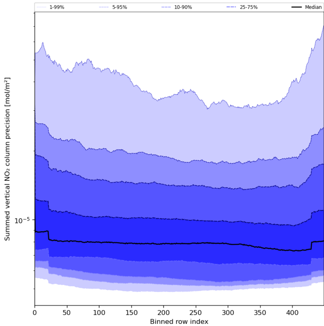
Figure 58: Along track statistics of “Summed vertical NO 2 column precision” for 2024-06-27 to 2024-06-29
