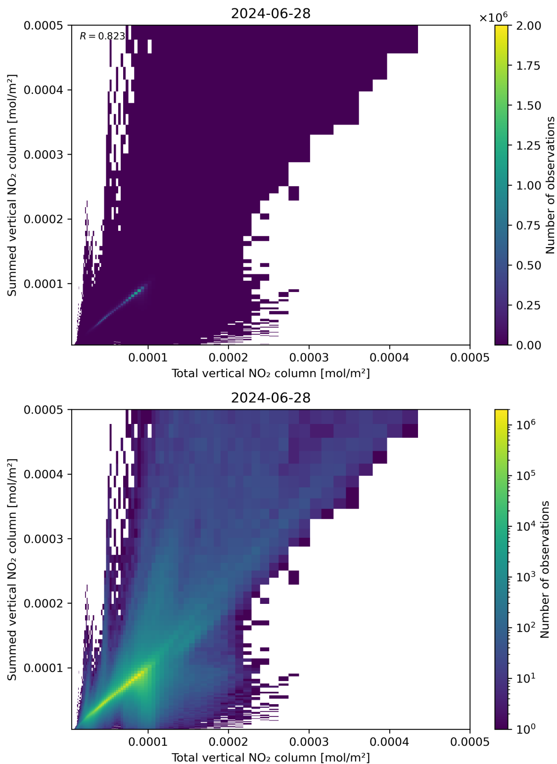
Figure 112: Scatter density plot of “Total vertical NO 2 column” against “Summed vertical NO 2 column” for 2024-06-27 to 2024-06-29.
