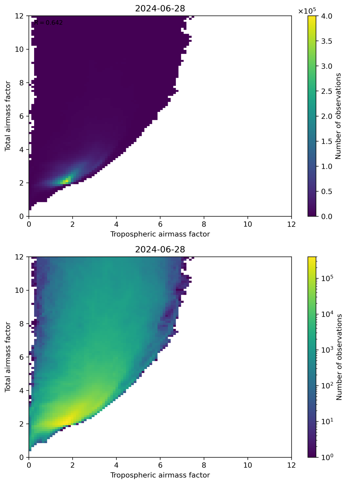
Figure 72: Scatter density plot of “Tropospheric airmass factor” against “Total airmass factor” for 2024-06-27 to 2024-06-29.
