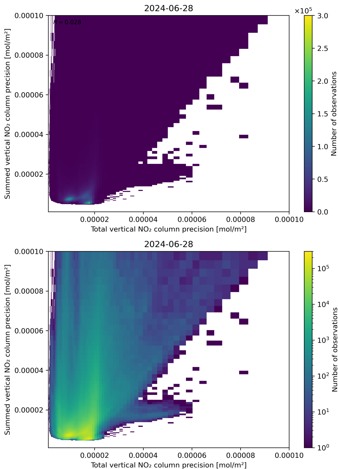
Figure 118: Scatter density plot of “Total vertical NO 2 column precision” against “Summed vertical NO 2 column precision” for 2024-06-27 to 2024-06-29.
