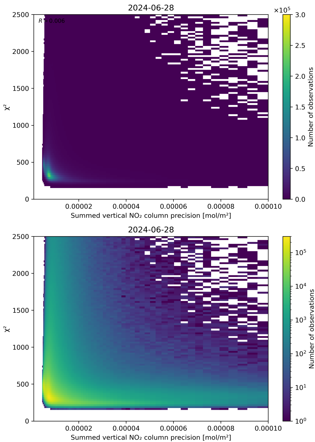
Figure 107: Scatter density plot of “Summed vertical NO 2 column precision” against “ \chi^2 ” for 2024-06-27 to 2024-06-29.
