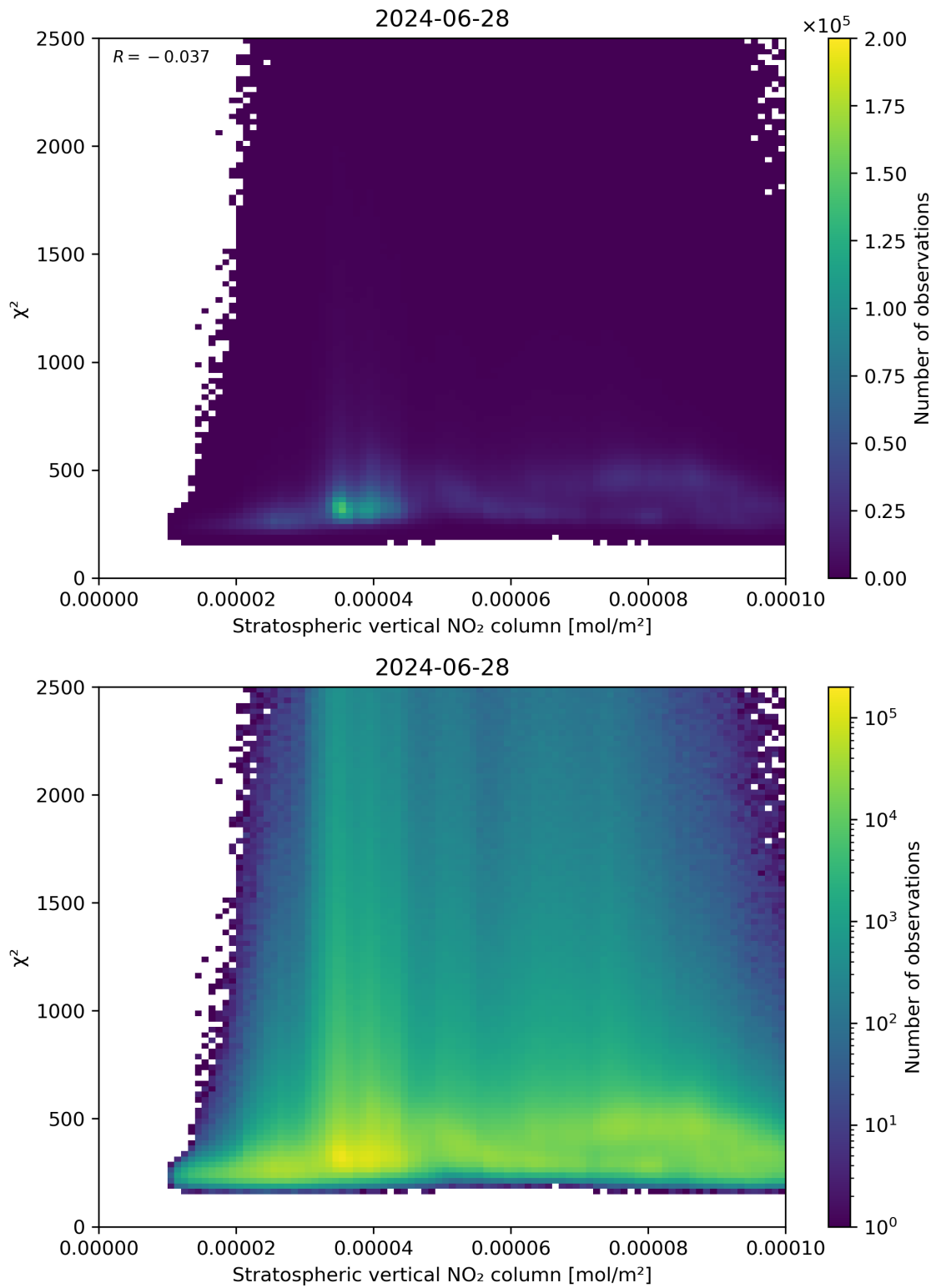
Figure 97: Scatter density plot of “Stratospheric vertical NO 2 column” against “ \chi^2 ” for 2024-06-27 to 2024-06-29.
