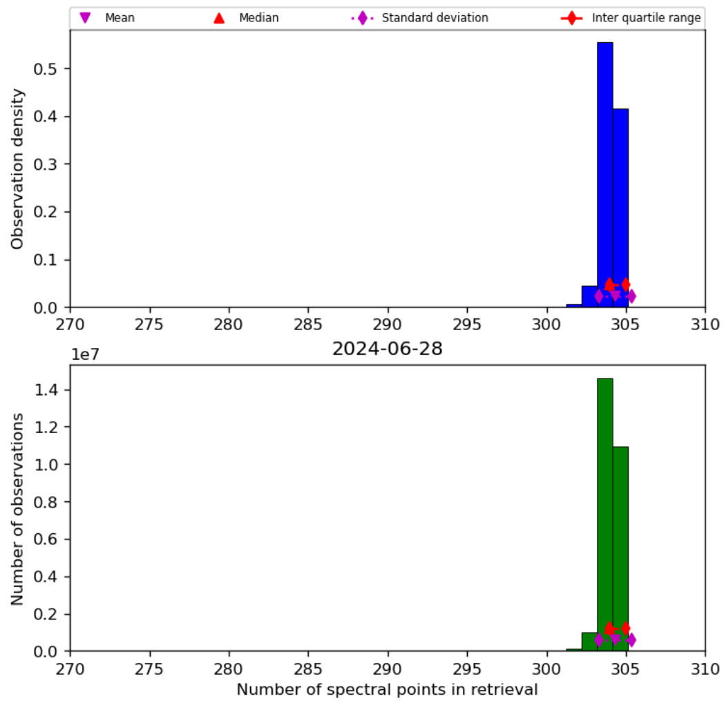
Figure 33: Histogram of “Number of spectral points in retrieval” for 2024-06-27 to 2024-06-29
