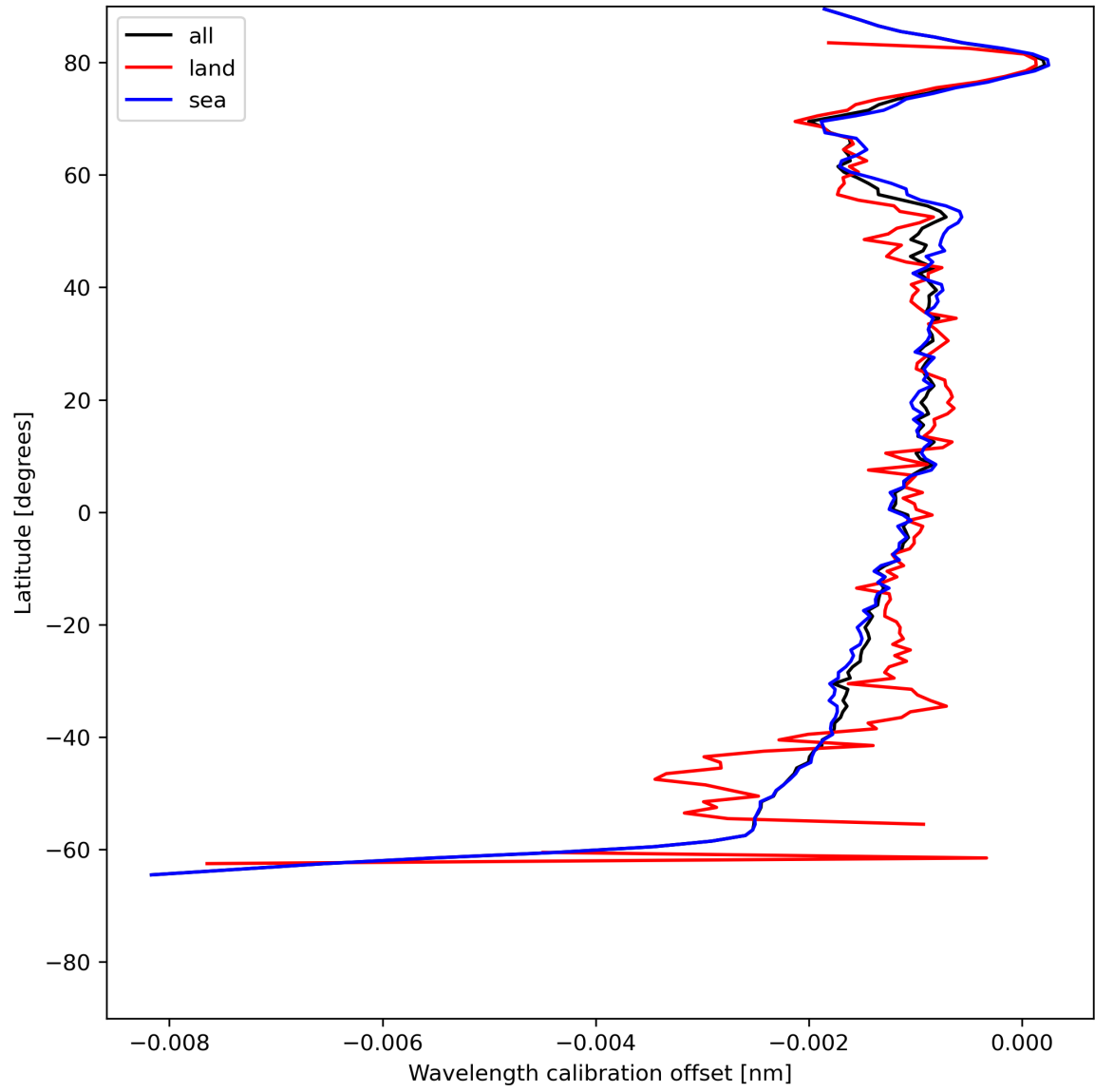
Figure 18: Zonal average of “Wavelength calibration offset” for 2024-06-27 to 2024-06-29.
