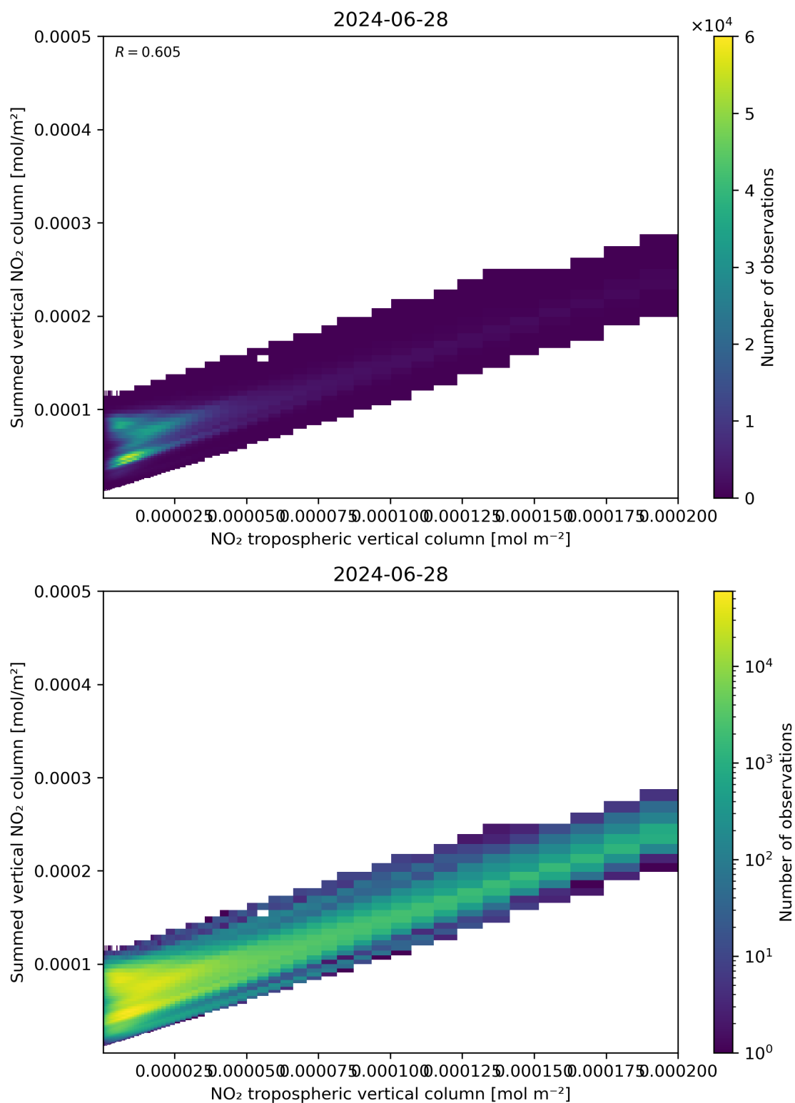
Figure 126: Scatter density plot of “NO 2 tropospheric vertical column” against “Summed vertical NO 2 column” for 2024-06-27 to 2024-06-29.
