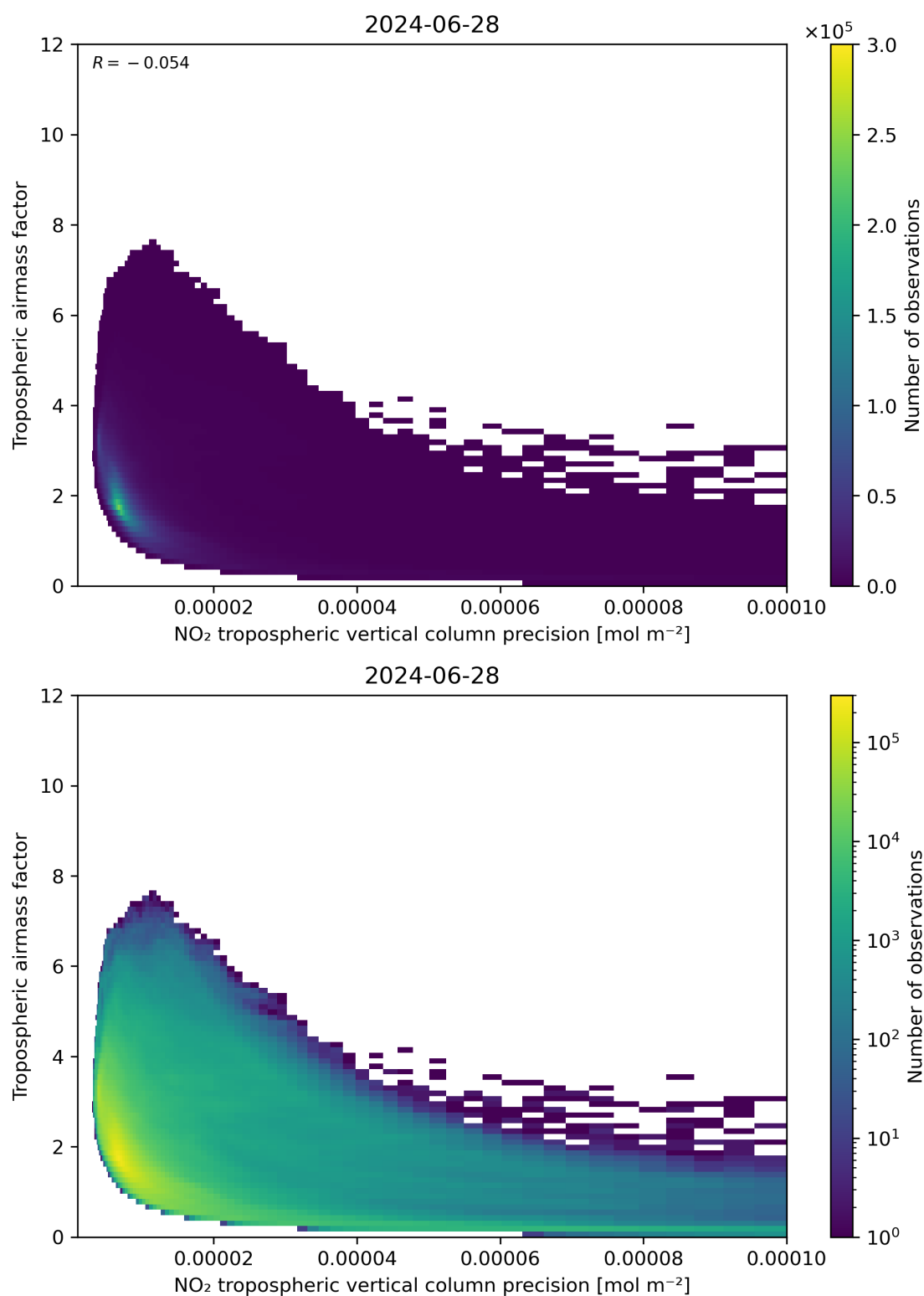
Figure 133: Scatter density plot of “NO 2 tropospheric vertical column precision” against “Tropospheric airmass factor” for 2024-06-27 to 2024-06-29.
