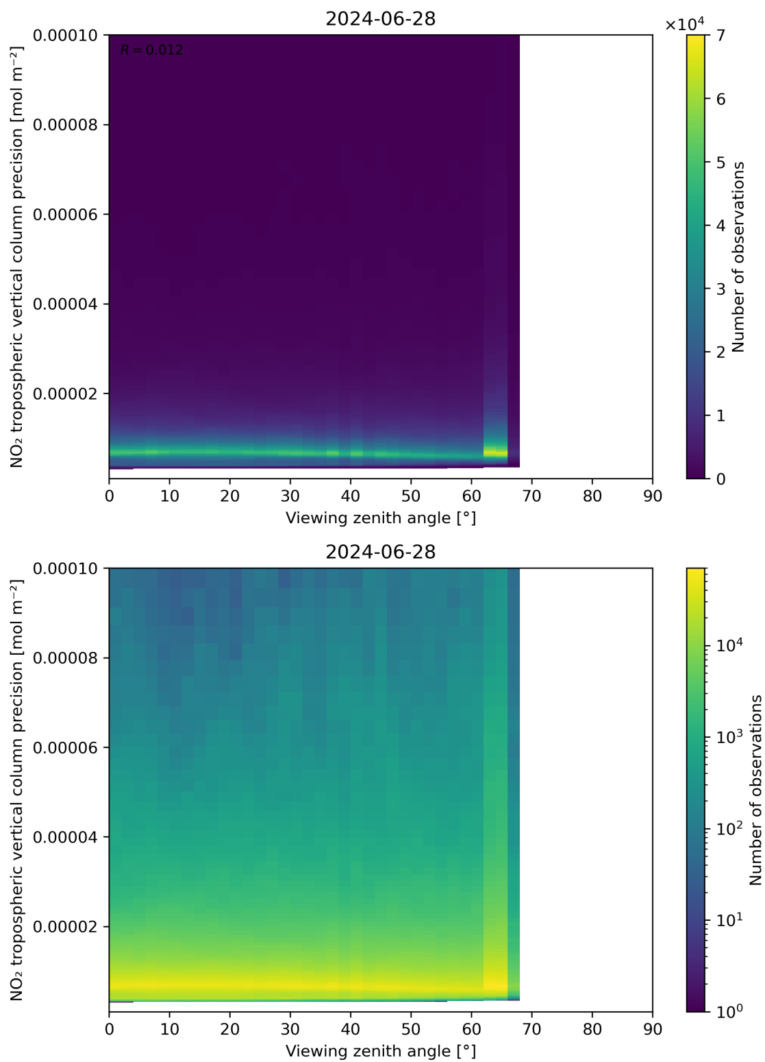
Figure 170: Scatter density plot of “Viewing zenith angle” against “NO 2 tropospheric vertical column precision” for 2024-06-27 to 2024-06-29.
