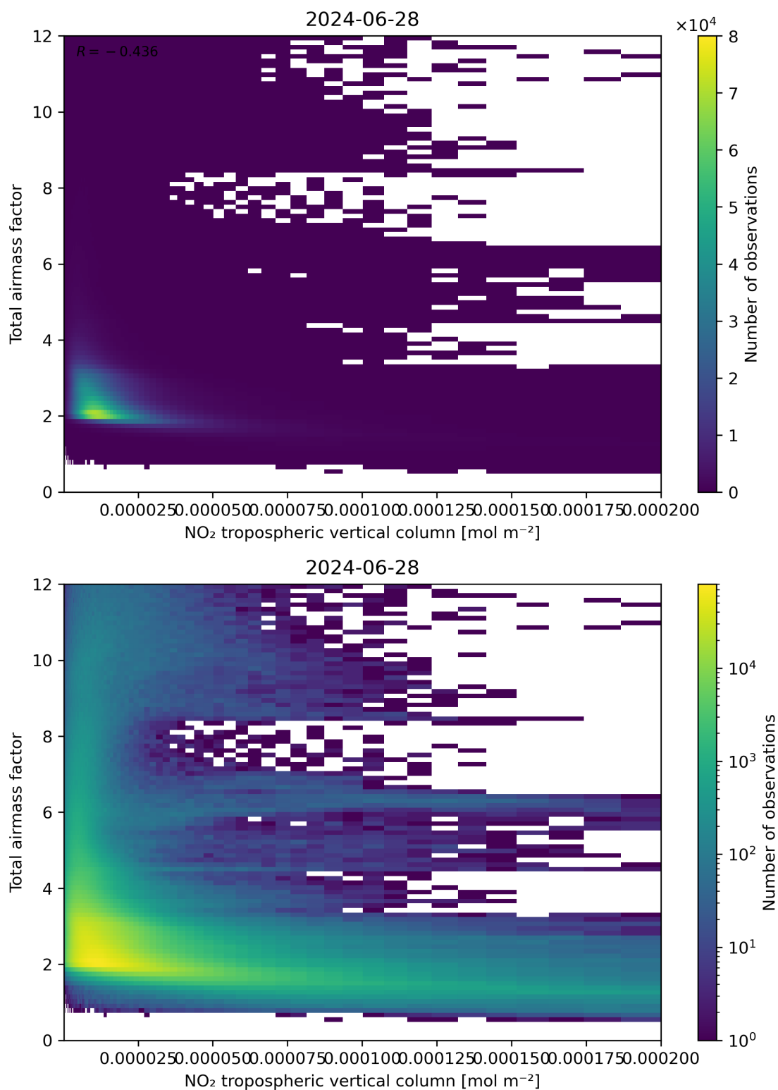
Figure 122: Scatter density plot of “NO 2 tropospheric vertical column” against “Total air mass factor” for 2024-06-27 to 2024-06-29.
