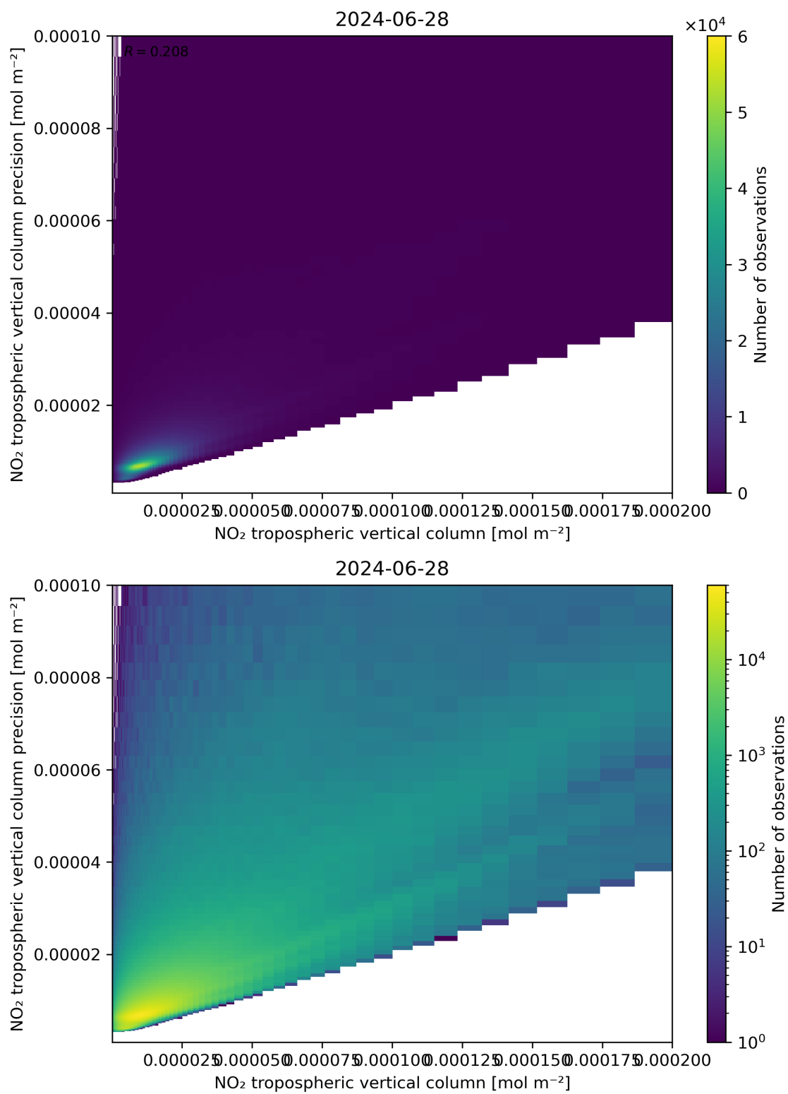
Figure 130: Scatter density plot of “NO 2 tropospheric vertical column” against “NO 2 tropospheric vertical column precision” for 2024-06-27 to 2024-06-29.
