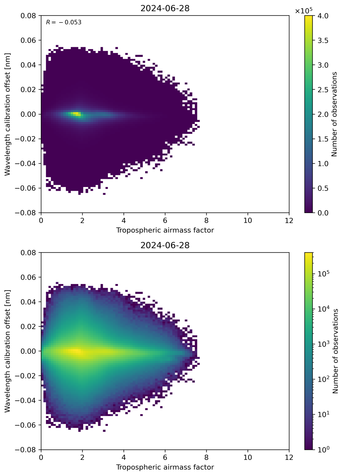
Figure 80: Scatter density plot of “Tropospheric air mass factor” against “Wavelength calibration offset” for 2024-06-27 to 2024-06-29.
