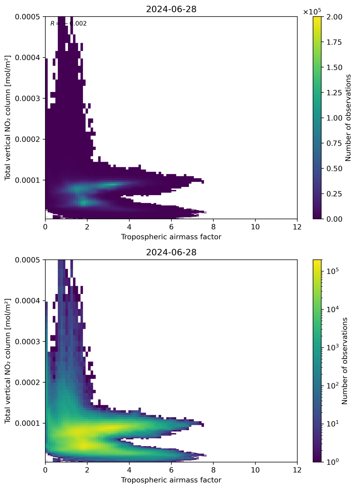
Figure 77: Scatter density plot of “Tropospheric airmass factor” against “Total vertical NO 2 column” for 2024-06-27 to 2024-06-29.
