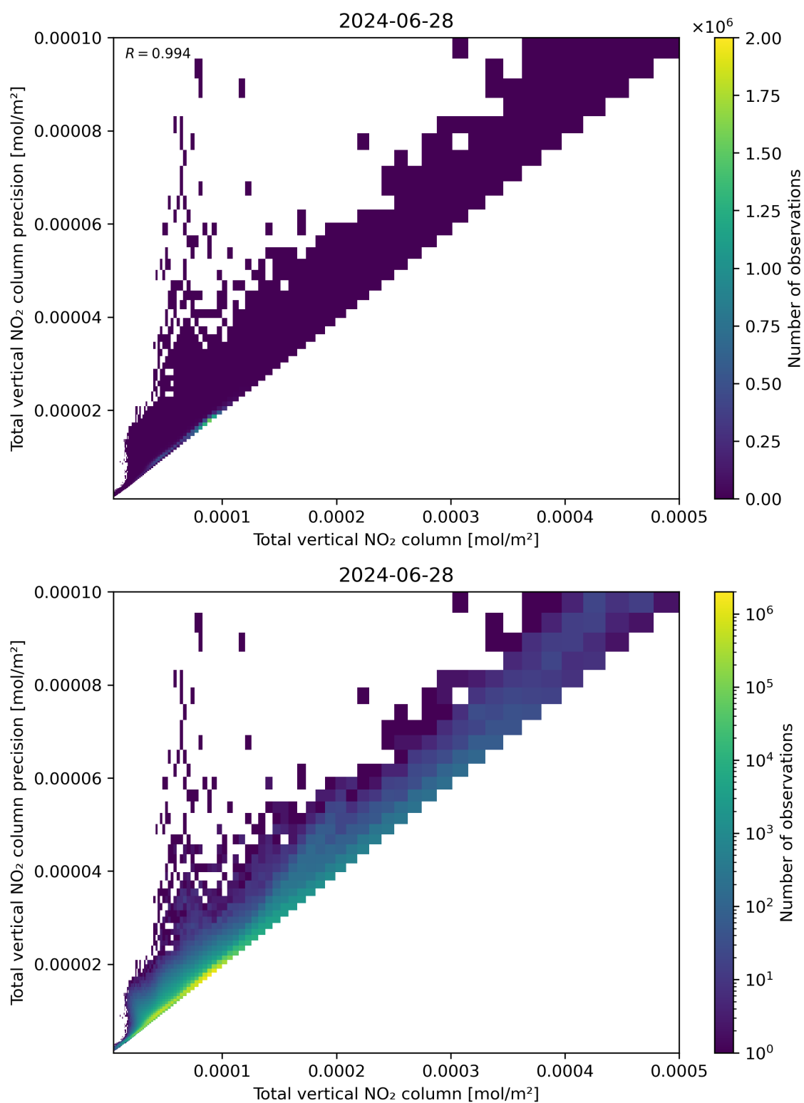
Figure 114: Scatter density plot of “Total vertical NO 2 column” against “Total vertical NO 2 column precision” for 2024-06-27 to 2024-06-29.
