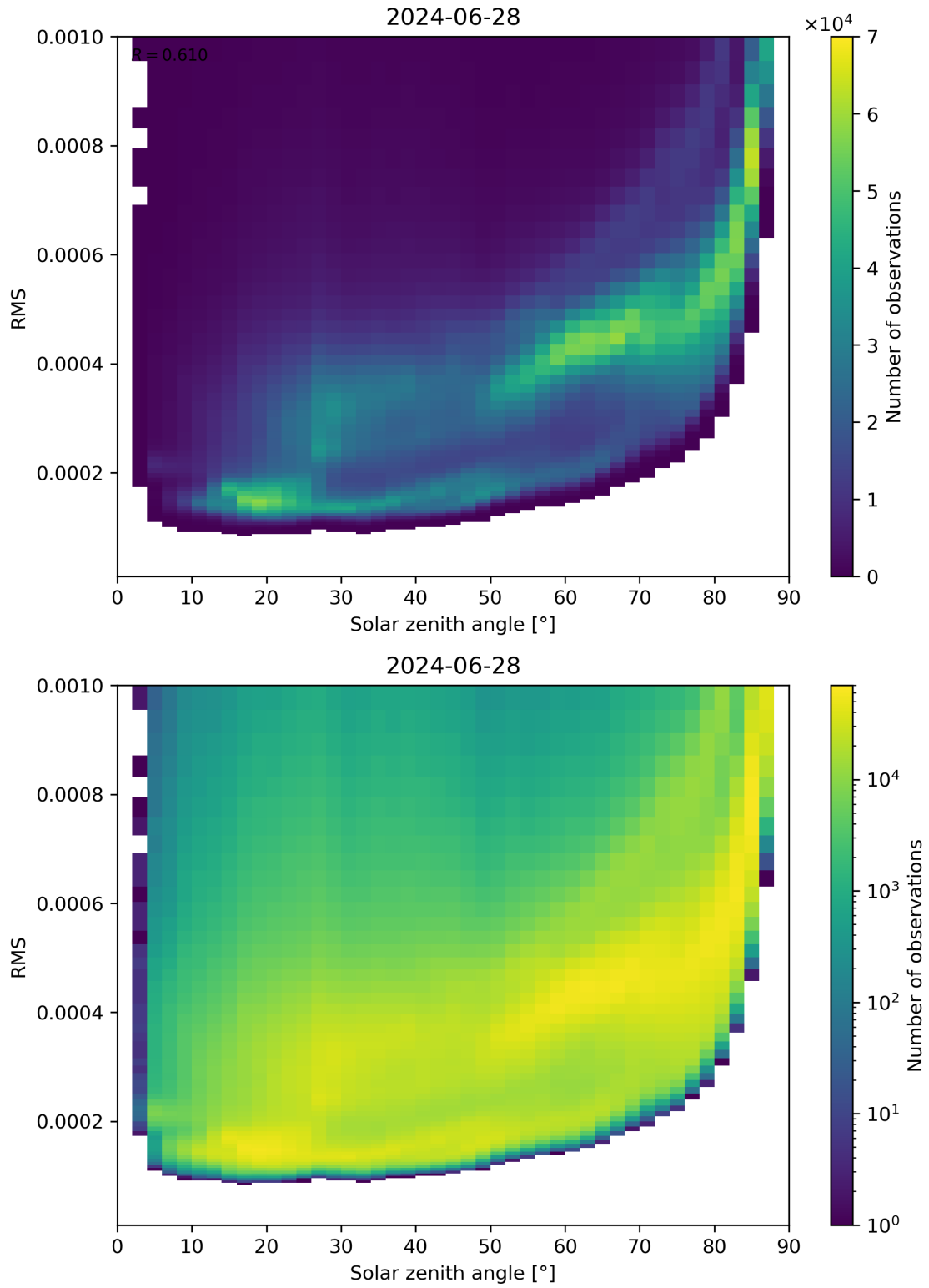
Figure 157: Scatter density plot of “Solar zenith angle” against “RMS” for 2024-06-27 to 2024-06-29.
