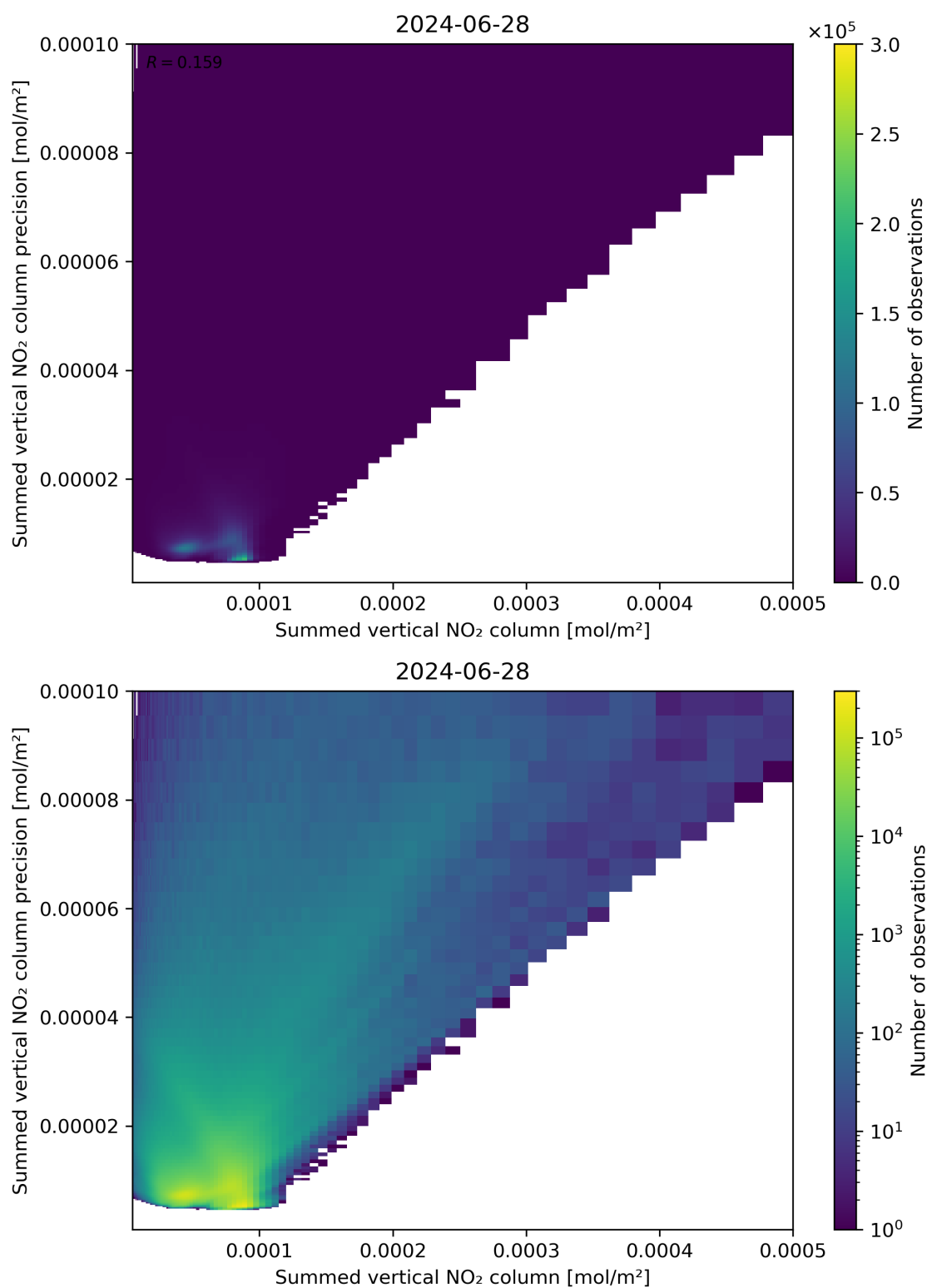
Figure 105: Scatter density plot of “Summed vertical NO 2 column” against “Summed vertical NO 2 column precision” for 2024-06-27 to 2024-06-29.
