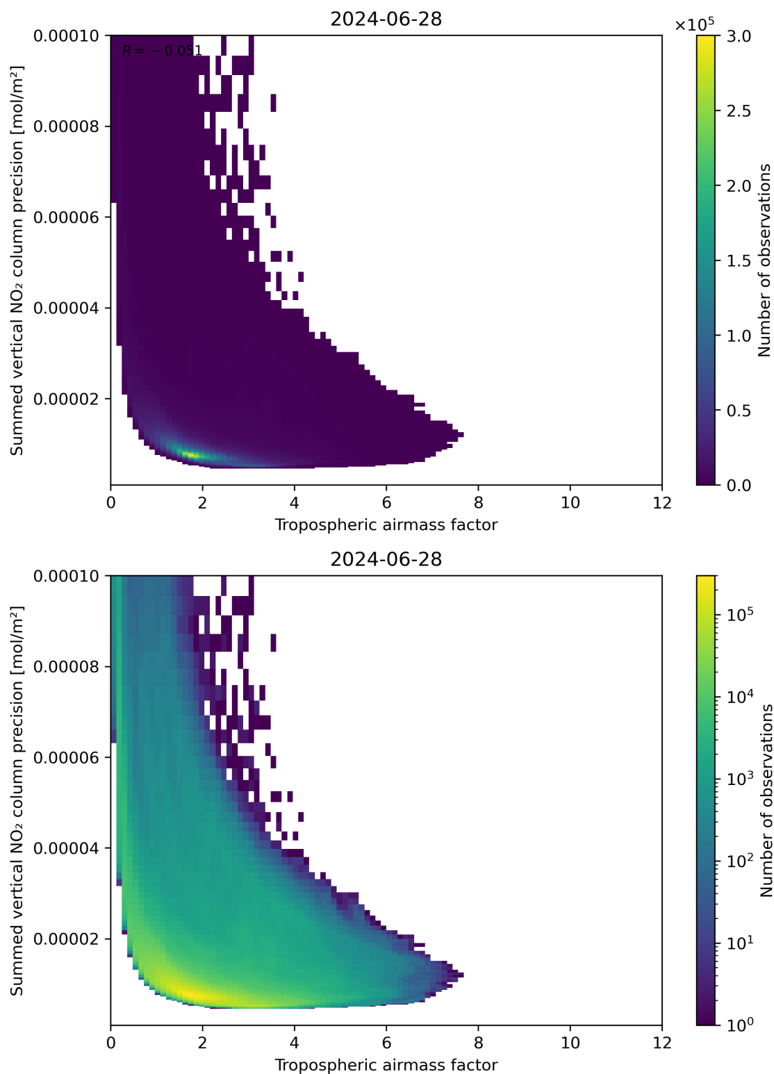
Figure 76: Scatter density plot of “Tropospheric air mass factor” against “Summed vertical NO 2 column precision” for 2024-06-27 to 2024-06-29.
