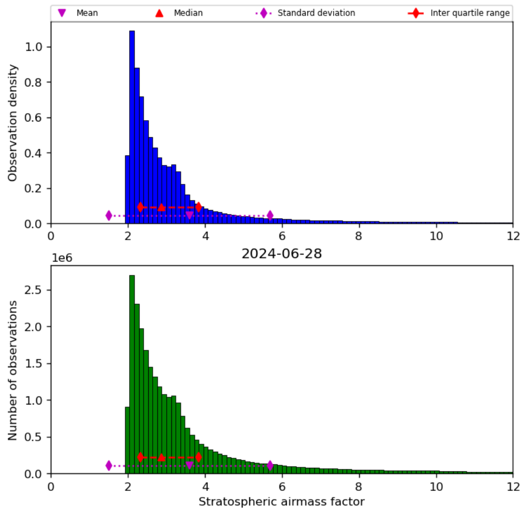
Figure 44: Histogram of “Stratospheric airmass factor” for 2024-06-27 to 2024-06-29
