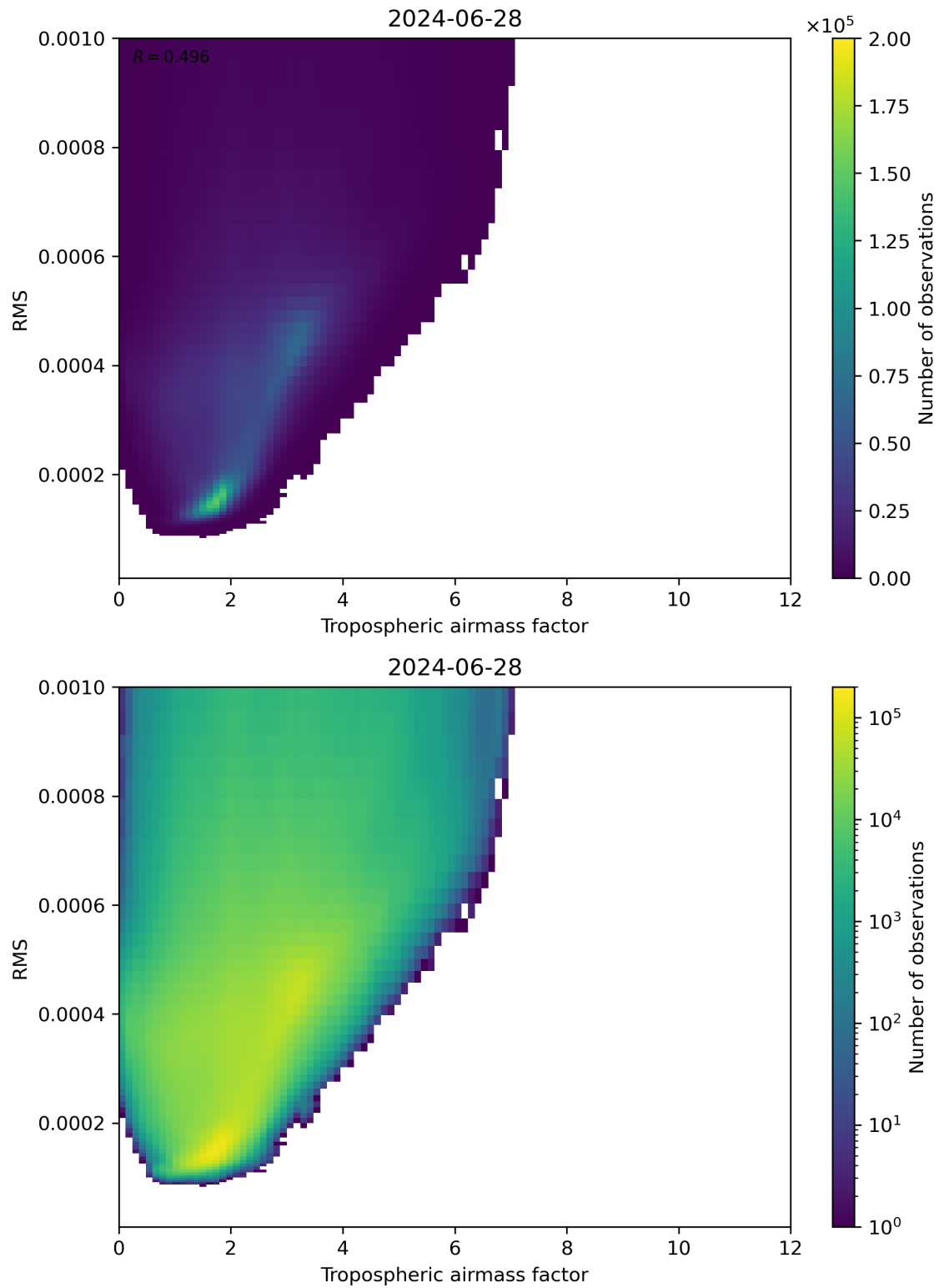
Figure 79: Scatter density plot of “Tropospheric airmass factor” against “RMS” for 2024-06-27 to 2024-06-29.
