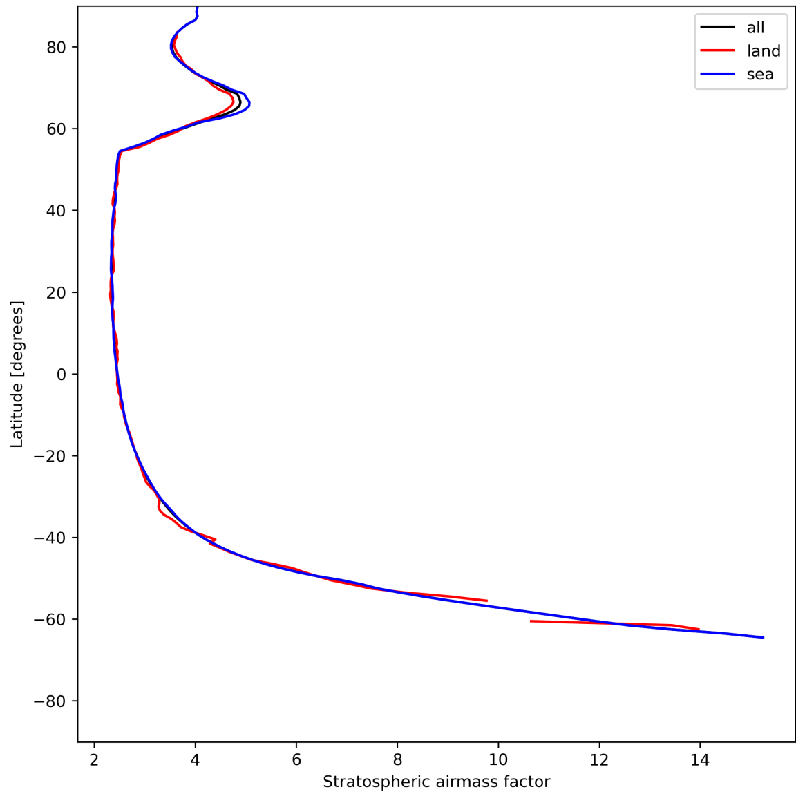
Figure 27: Zonal average of “Stratospheric airmass factor” for 2024-06-27 to 2024-06-29.
