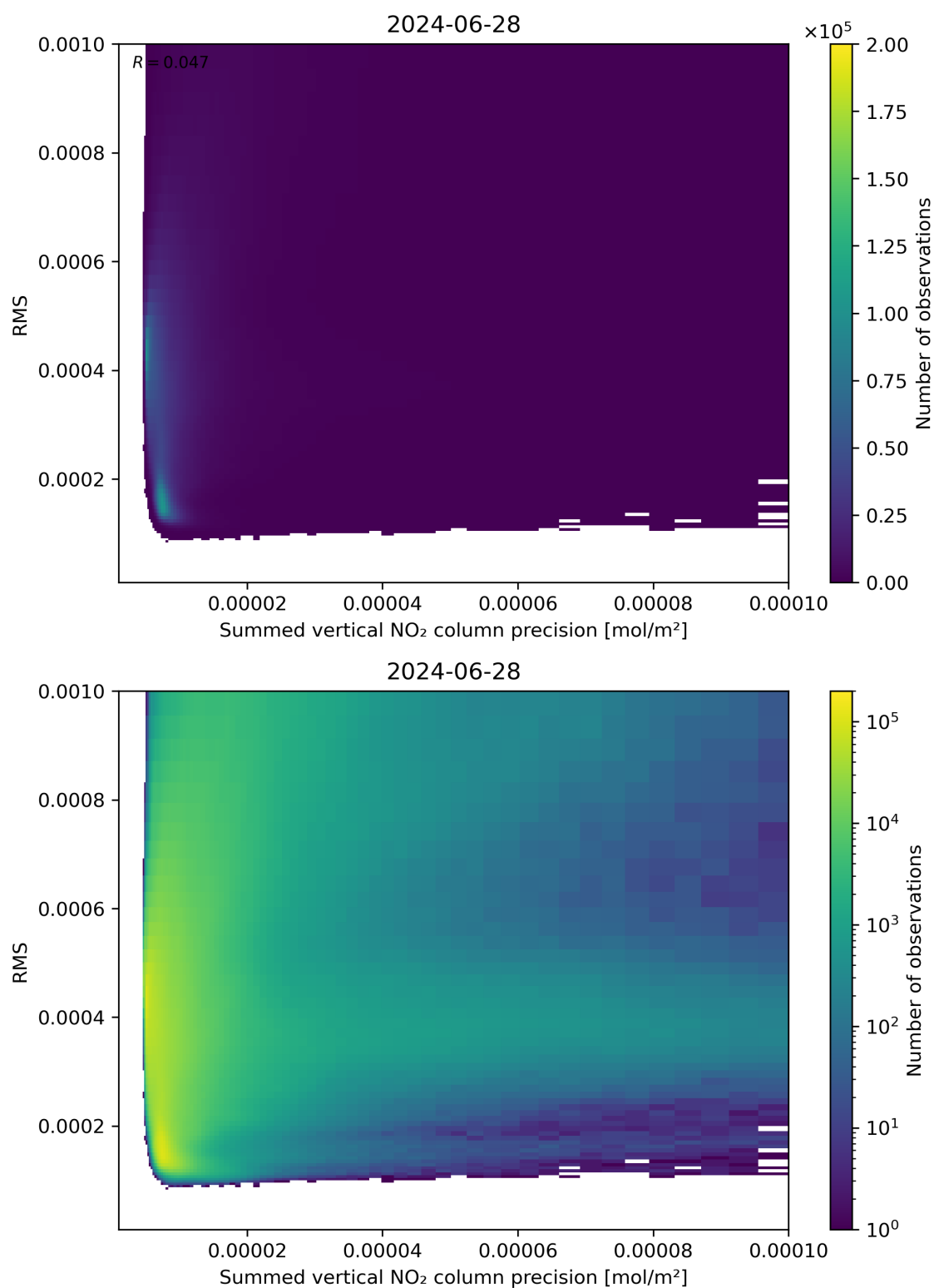
Figure 108: Scatter density plot of “Summed vertical NO 2 column precision” against “RMS” for 2024-06-27 to 2024-06-29.
