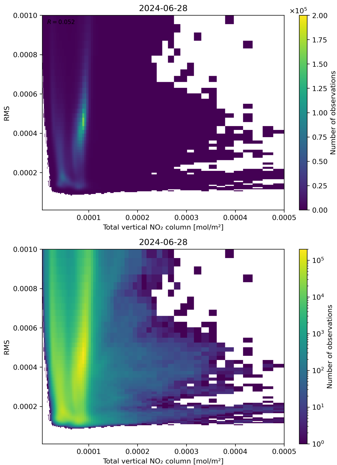
Figure 120: Scatter density plot of “Total vertical NO 2 column” against “RMS” for 2024-06-27 to 2024-06-29.
