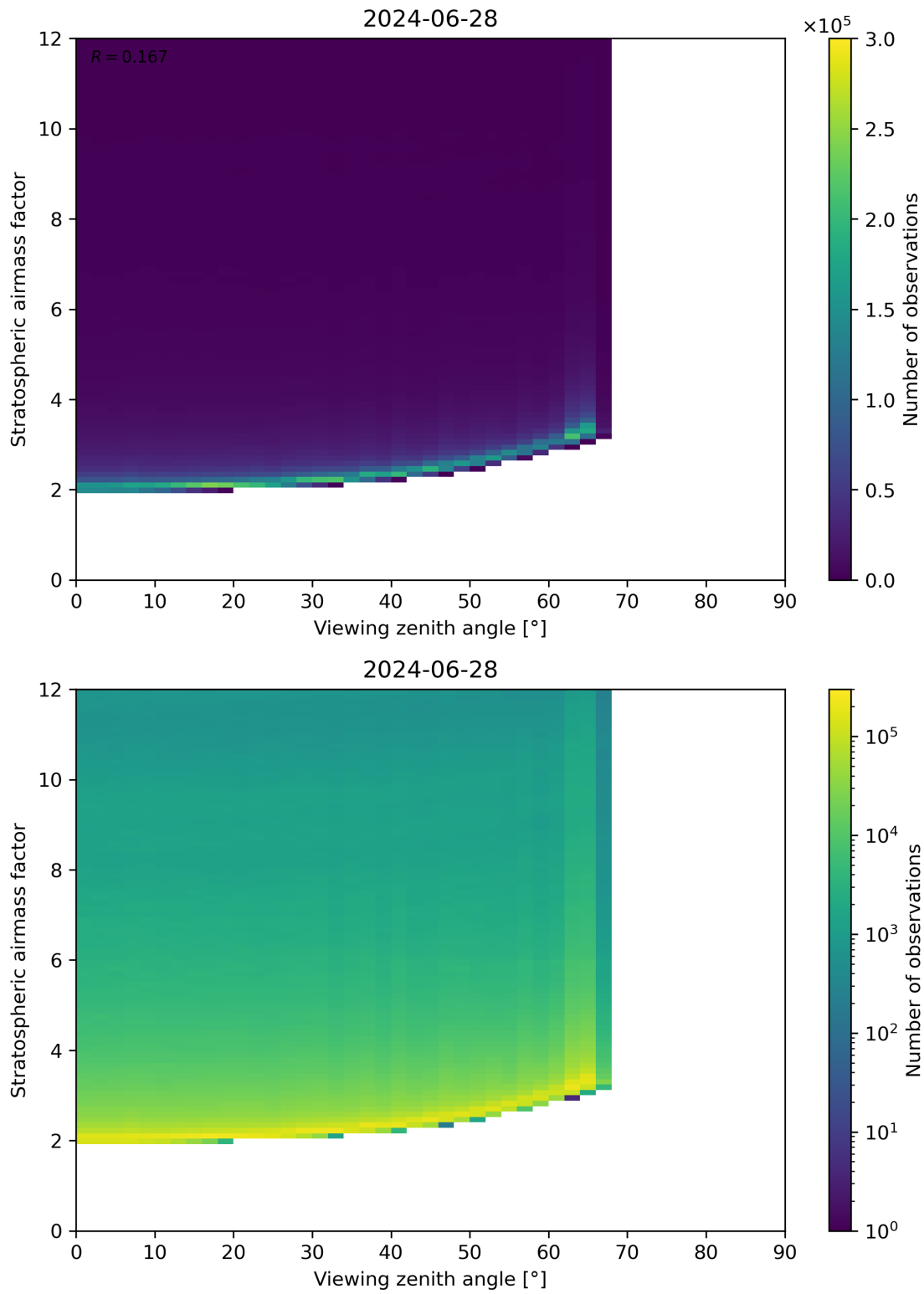
Figure 159: Scatter density plot of “Viewing zenith angle” against “Stratospheric airmass factor” for 2024-06-27 to 2024-06-29.
