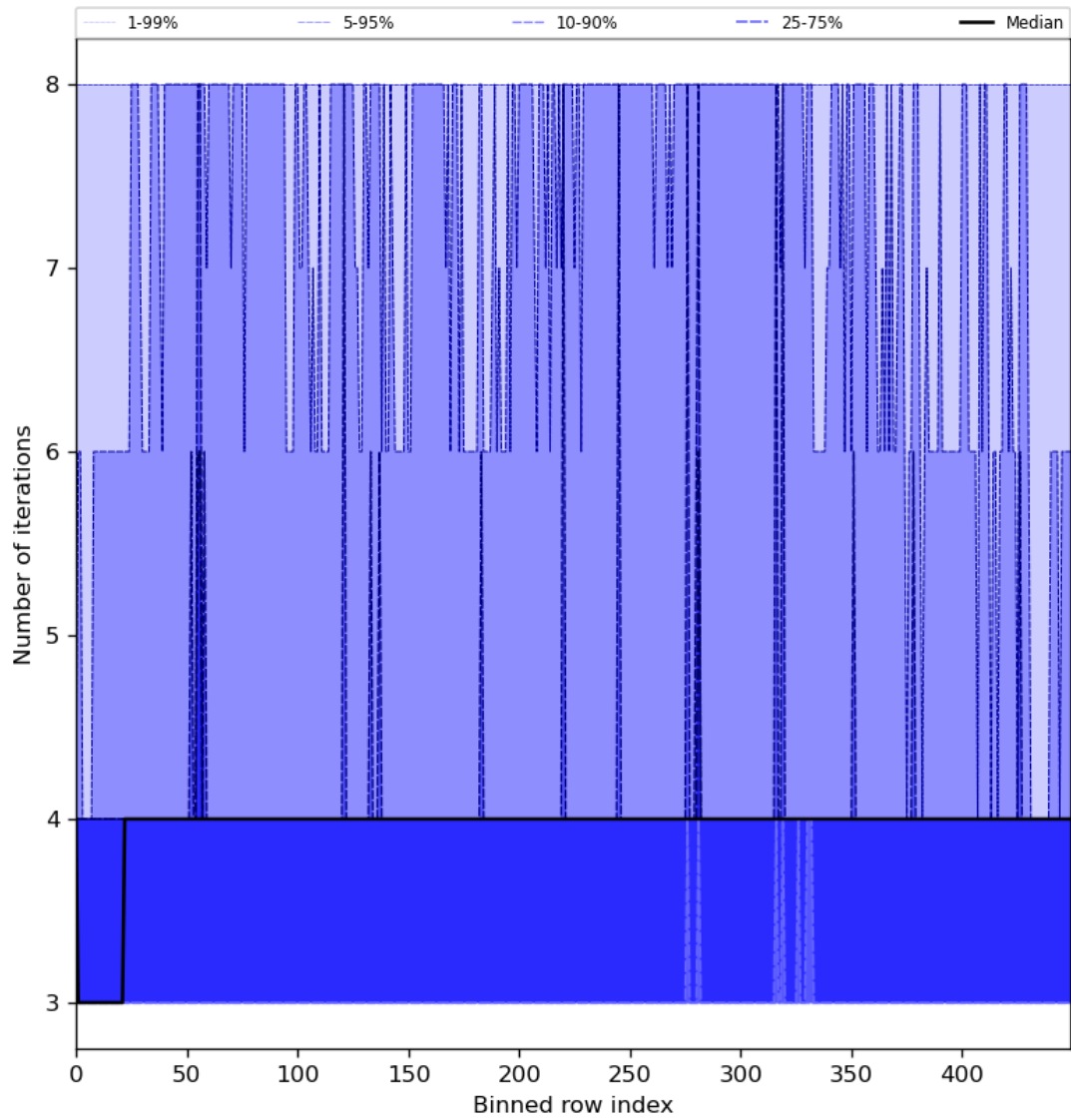
Figure 51: Along track statistics of “Number of iterations” for 2024-06-27 to 2024-06-29
