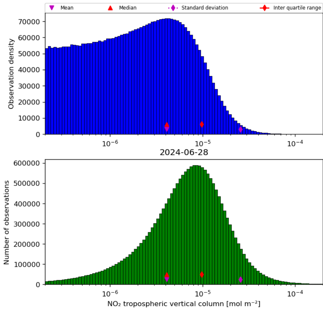
Figure 29: Histogram of “NO 2 tropospheric vertical column” for 2024-06-27 to 2024-06-29
