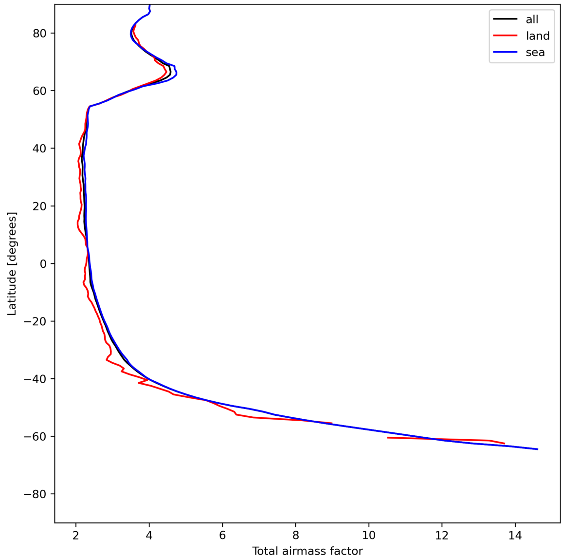
Figure 15: Zonal average of “Total airmass factor” for 2024-06-27 to 2024-06-29.
