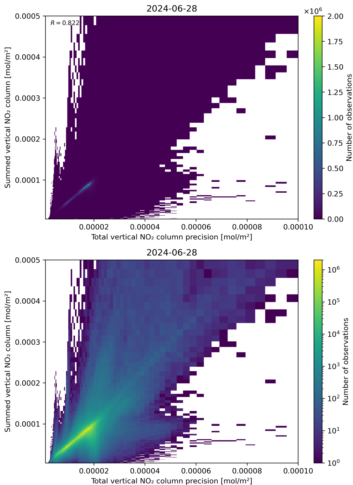
Figure 117: Scatter density plot of “Total vertical NO 2 column precision” against “Summed vertical NO 2 column” for 2024-06-27 to 2024-06-29.
