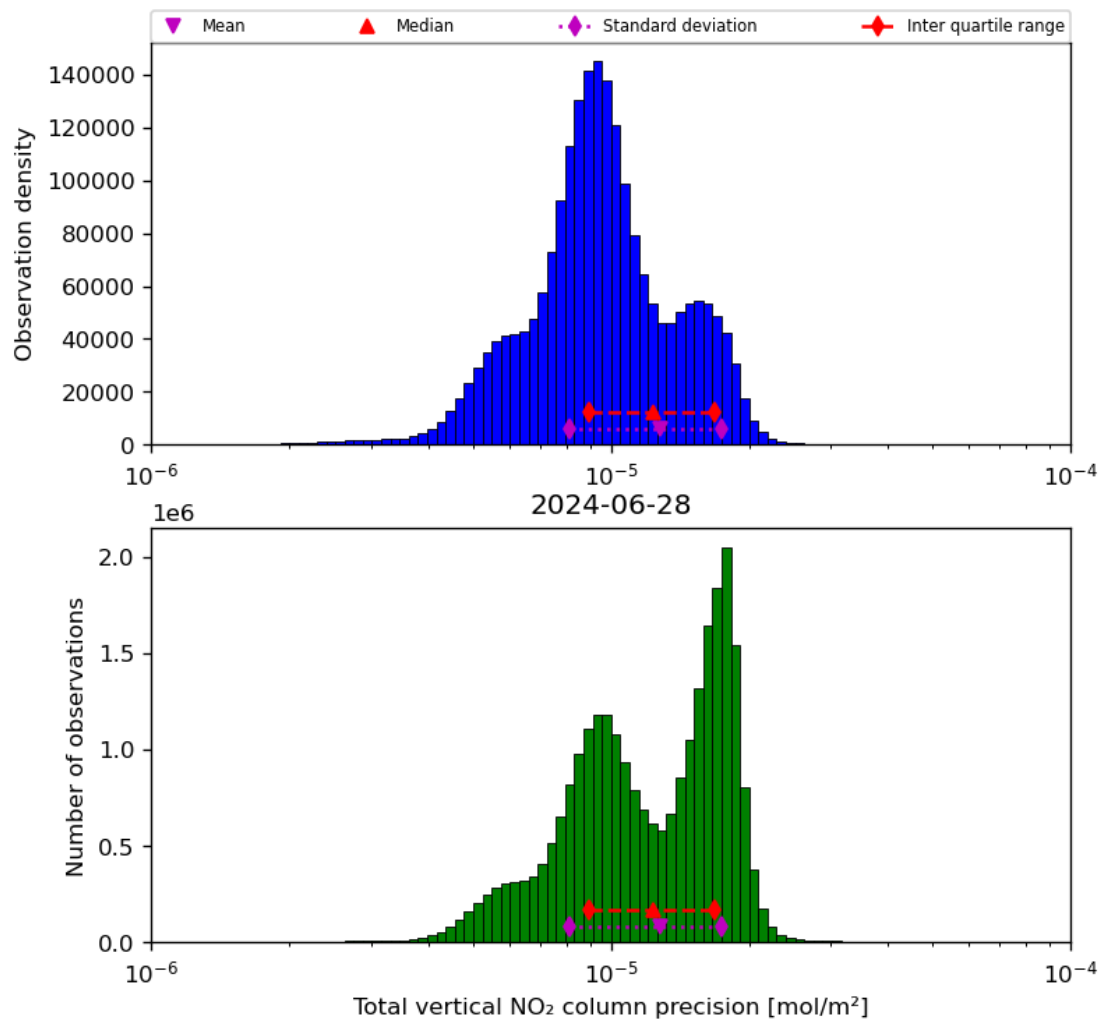
Figure 39: Histogram of “Total vertical NO 2 column precision” for 2024-06-27 to 2024-06-29
