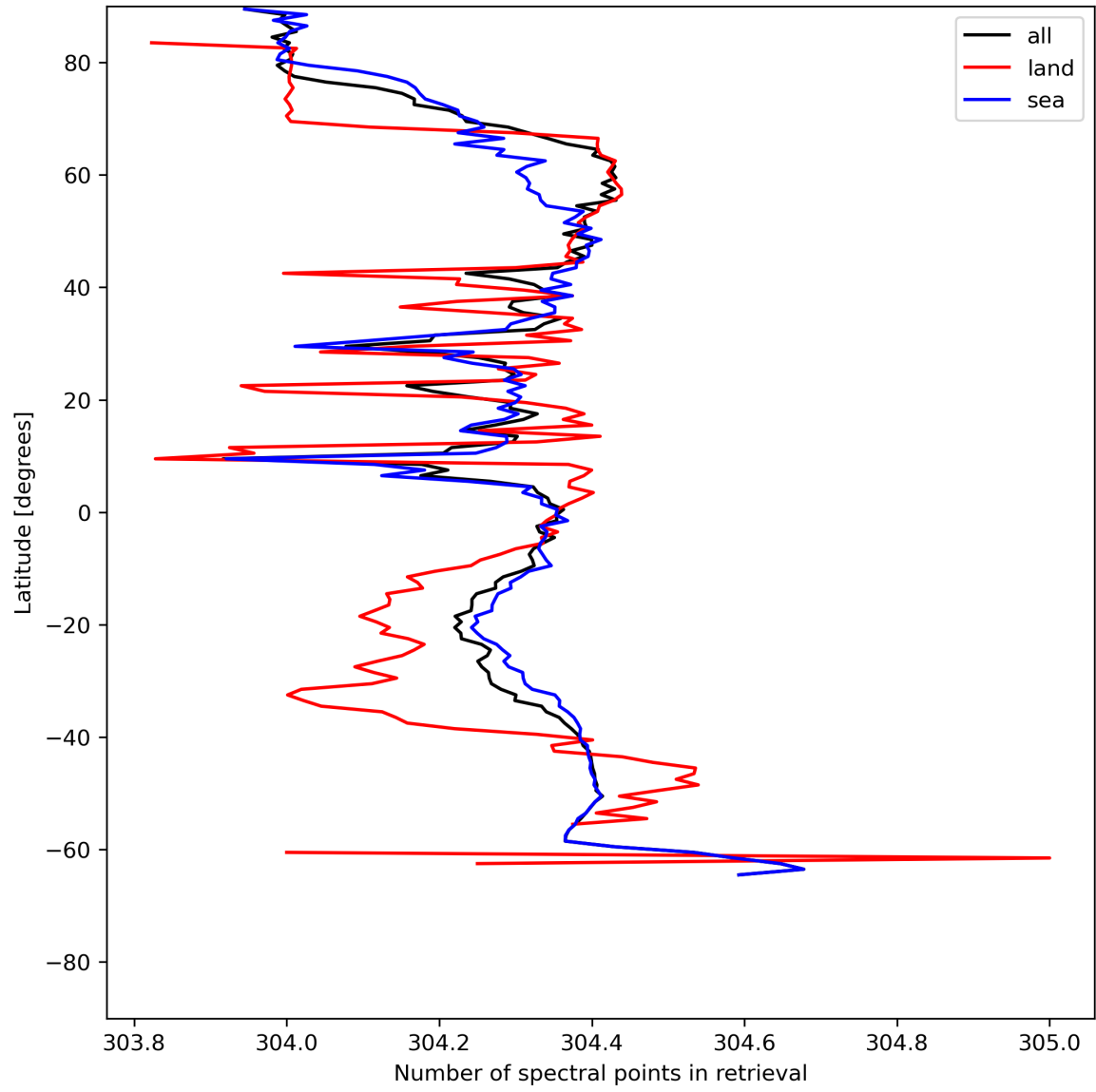
Figure 16: Zonal average of “Number of spectral points in retrieval” for 2024-06-27 to 2024-06-29.
