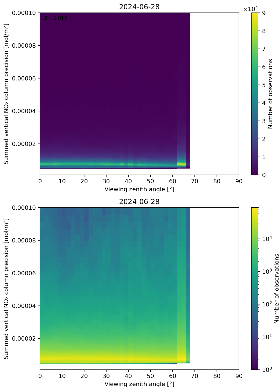
Figure 166: Scatter density plot of “Viewing zenith angle” against “Summed vertical NO 2 column precision” for 2024-06-27 to 2024-06-29.
