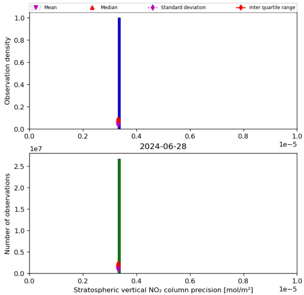
Figure 37: Histogram of “Stratospheric vertical NO 2 column precision” for 2024-06-27 to 2024-06-29
