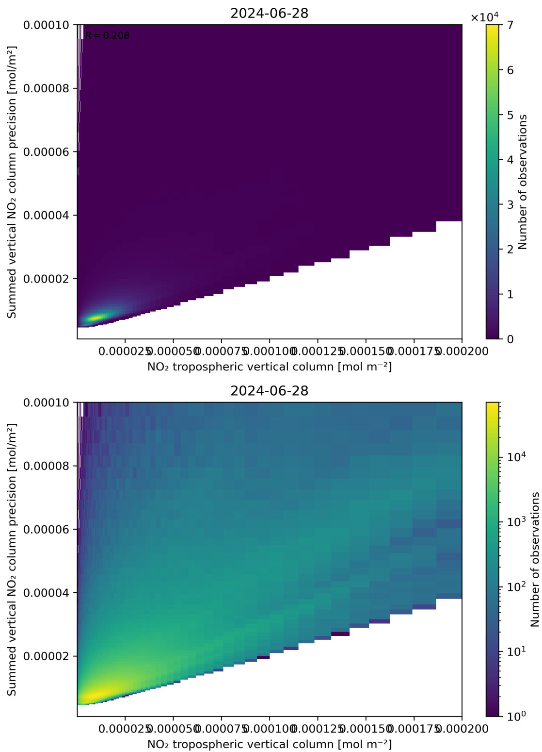
Figure 127: Scatter density plot of “NO 2 tropospheric vertical column” against “Summed vertical NO 2 column precision” for 2024-06-27 to 2024-06-29.
