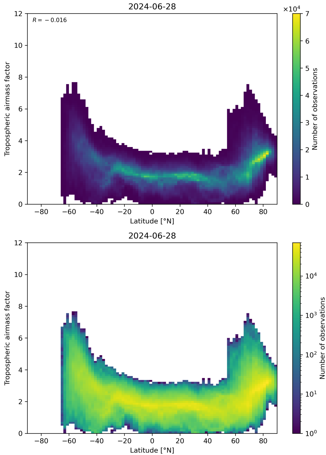
Figure 85: Scatter density plot of “Latitude” against “Tropospheric air mass factor” for 2024-06-27 to 2024-06-29.
