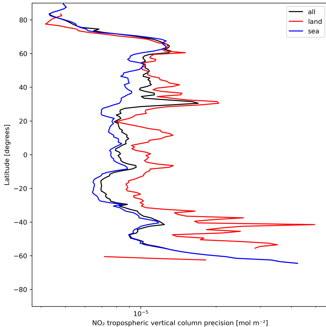
Figure 13: Zonal average of “NO 2 tropospheric vertical column precision” for 2024-06-27 to 2024-06-29.
