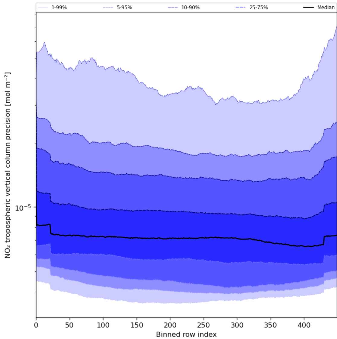
Figure 47: Along track statistics of “NO 2 tropospheric vertical column precision” for 2024-06-27 to 2024-06-29
