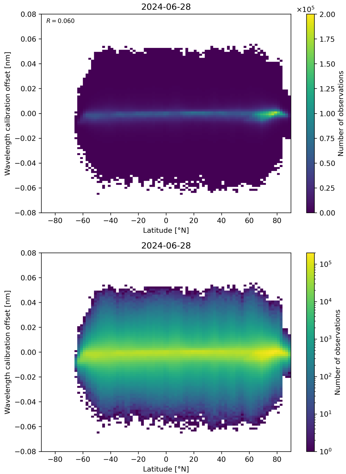
Figure 95: Scatter density plot of “Latitude” against “Wavelength calibration offset” for 2024-06-27 to 2024-06-29.
