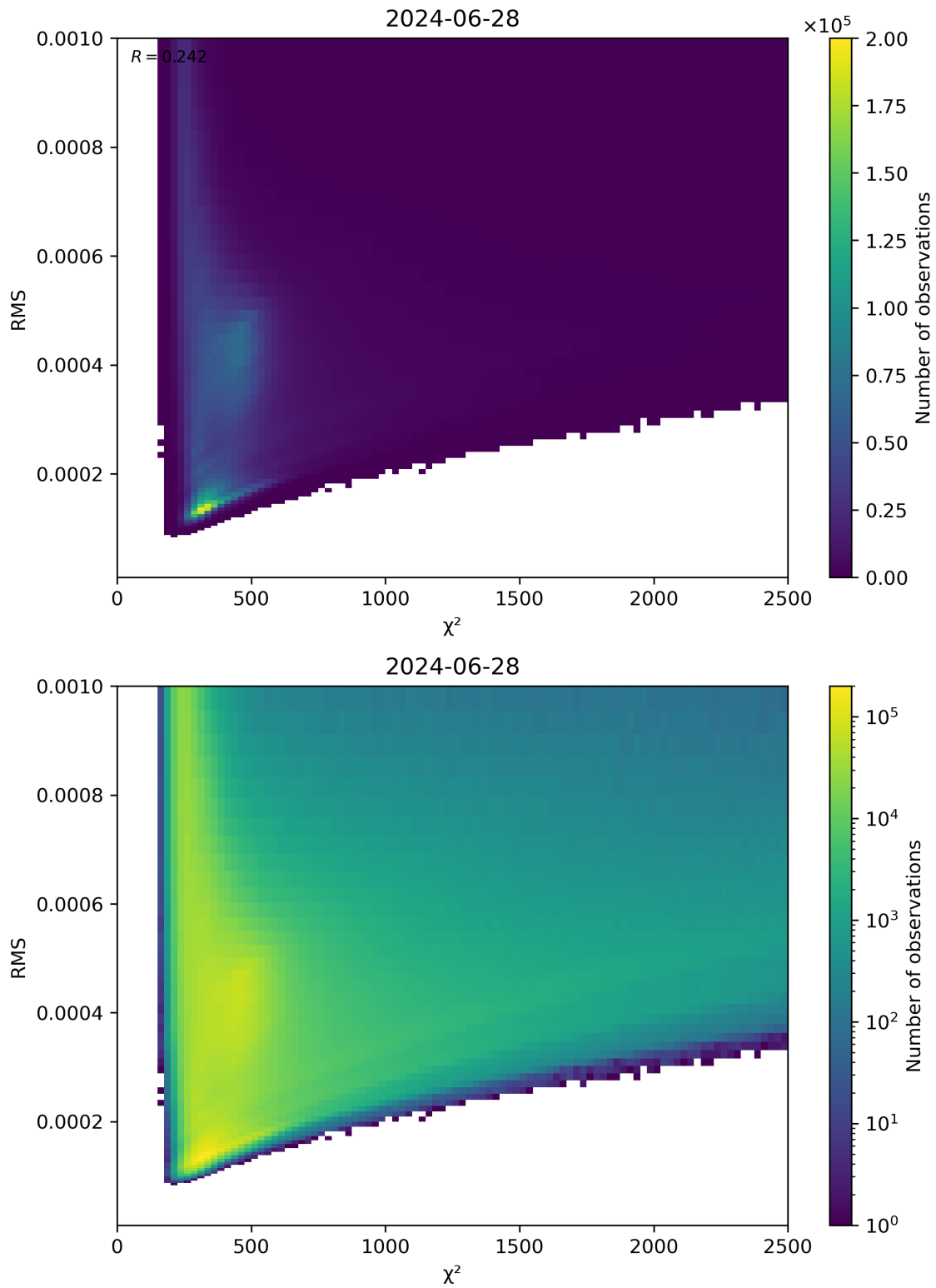
Figure 82: Scatter density plot of “ \chi^2 ” against “RMS” for 2024-06-27 to 2024-06-29.
