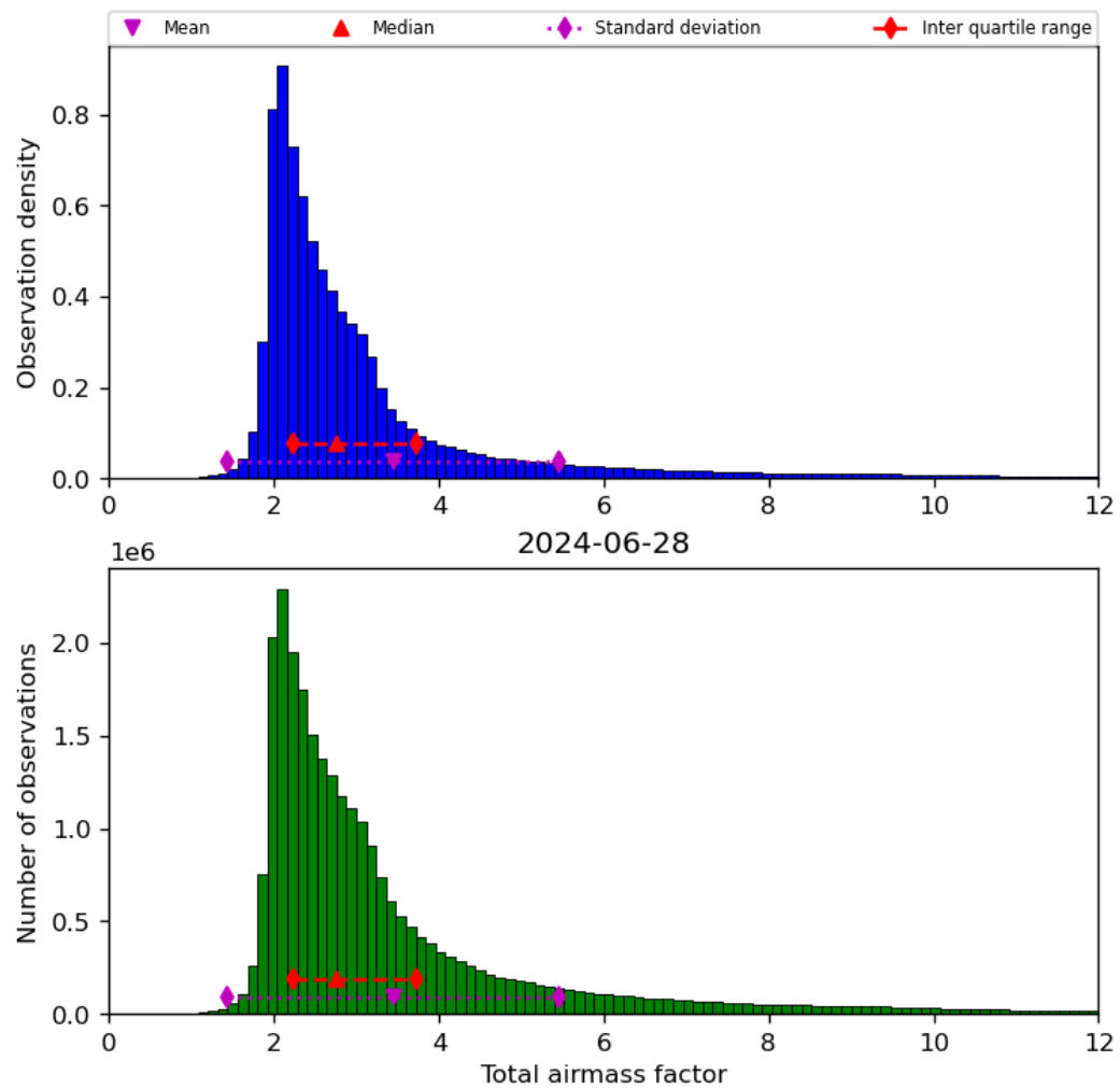
Figure 32: Histogram of “Total airmass factor” for 2024-06-27 to 2024-06-29
