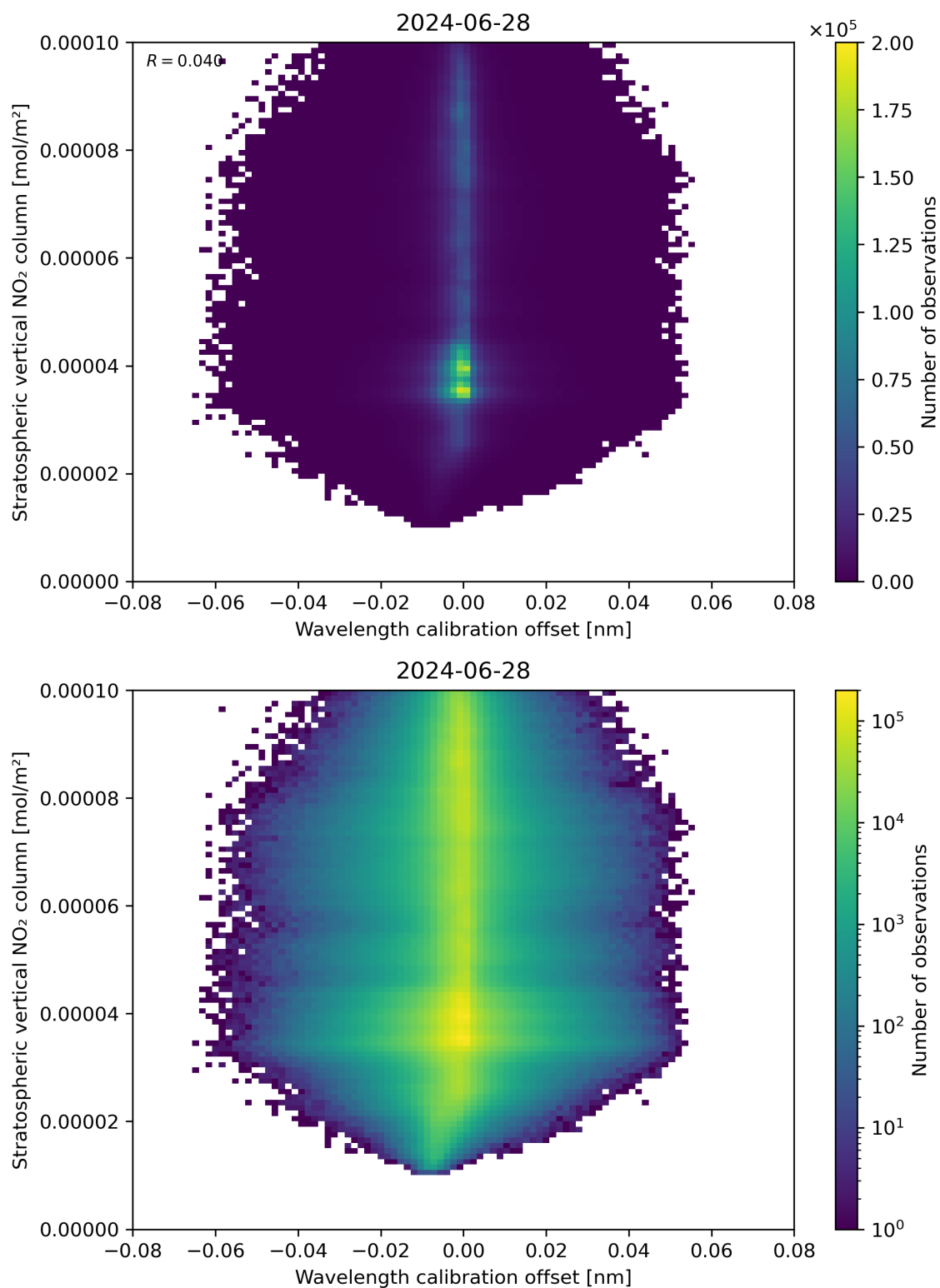
Figure 176: Scatter density plot of “Wavelength calibration offset” against “Stratospheric vertical NO 2 column” for 2024-06-27 to 2024-06-29.
