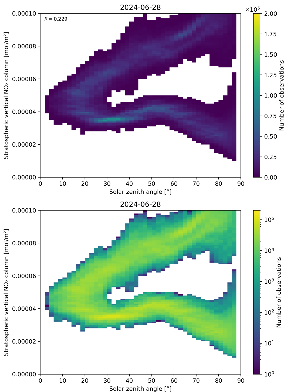
Figure 150: Scatter density plot of “Solar zenith angle” against “Stratospheric vertical NO 2 column” for 2024-06-27 to 2024-06-29.
