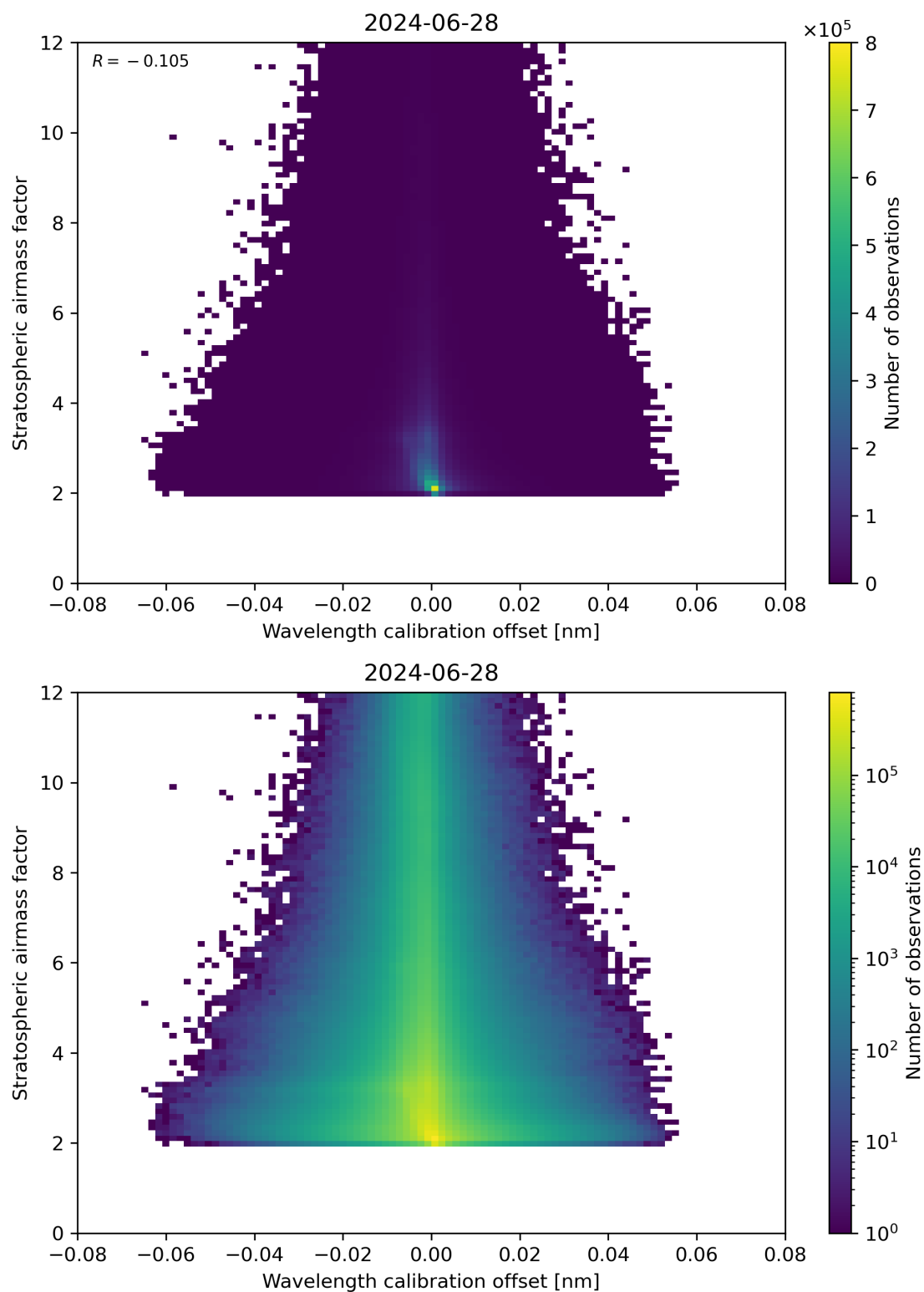
Figure 174: Scatter density plot of “Wavelength calibration offset” against “Stratospheric airmass factor” for 2024-06-27 to 2024-06-29.
