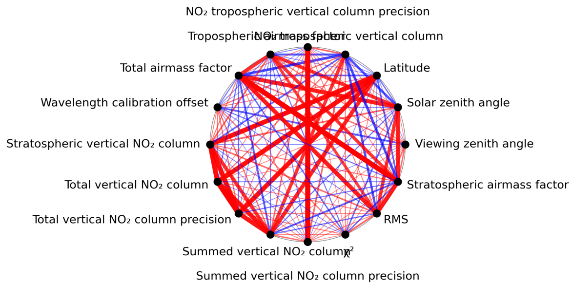
Figure 1: Map of correlation graph for 2024-06-27 to 2024-06-29.
