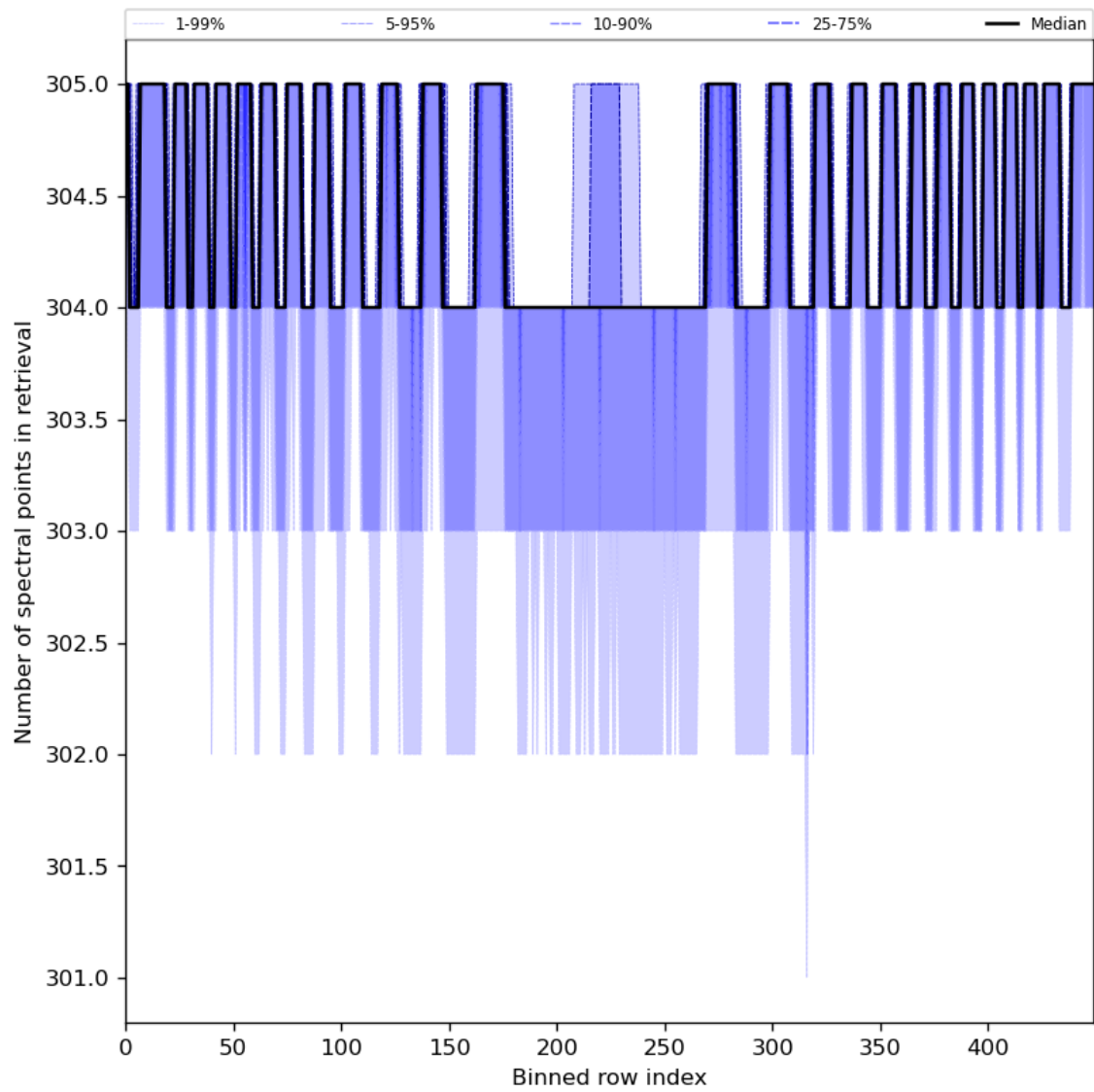
Figure 50: Along track statistics of “Number of spectral points in retrieval” for 2024-06-27 to 2024-06-29
