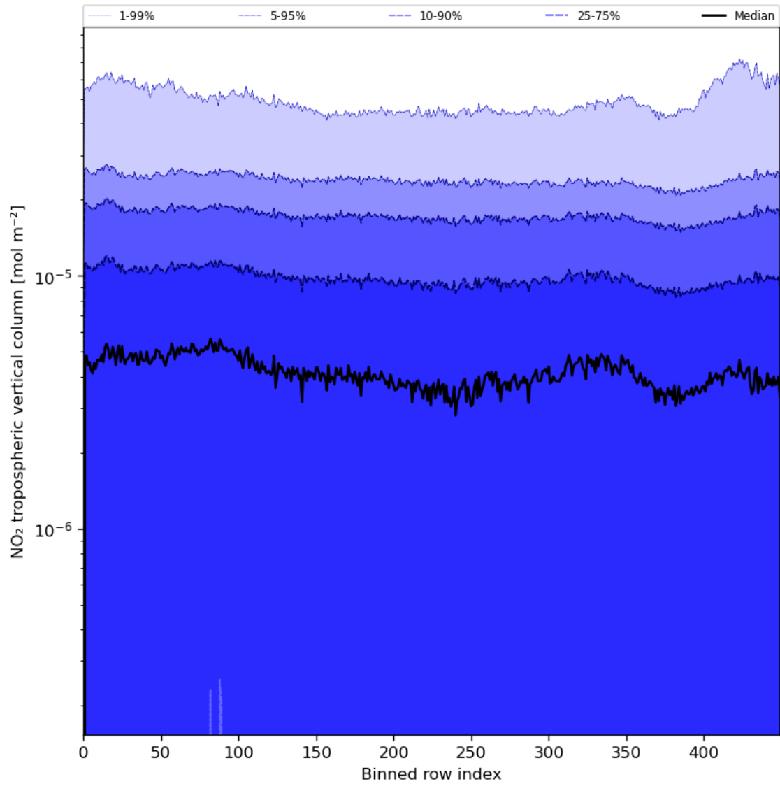
Figure 46: Along track statistics of “NO 2 tropospheric vertical column” for 2024-06-27 to 2024-06-29
