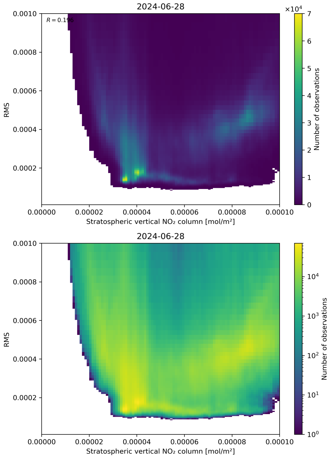
Figure 102: Scatter density plot of “Stratospheric vertical NO 2 column” against “RMS” for 2024-06-27 to 2024-06-29.
