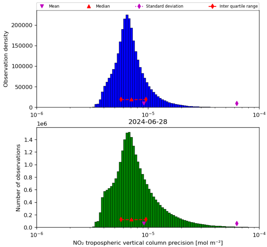
Figure 30: Histogram of “NO 2 tropospheric vertical column precision” for 2024-06-27 to 2024-06-29
