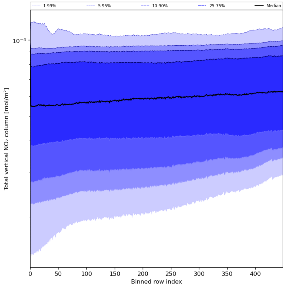
Figure 55: Along track statistics of "Total vertical NO 2 column" for 2024-06-27 to 2024-06-29
