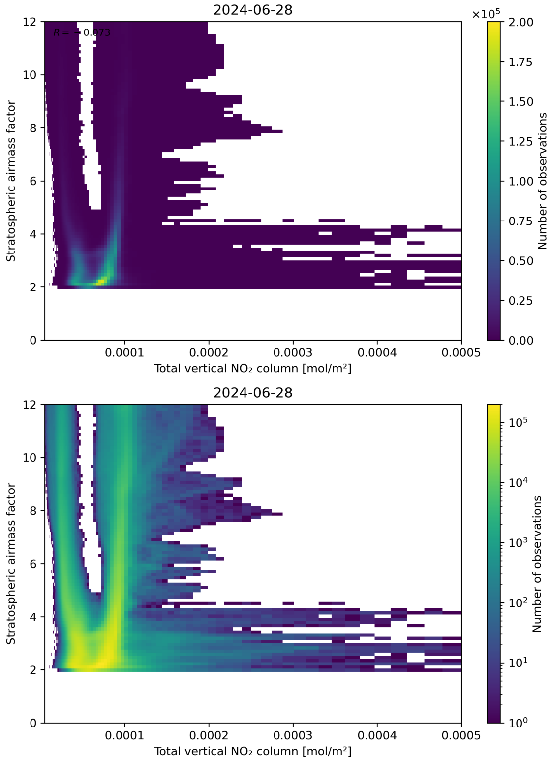
Figure 110: Scatter density plot of “Total vertical NO 2 column” against “Stratospheric airmass factor” for 2024-06-27 to 2024-06-29.
