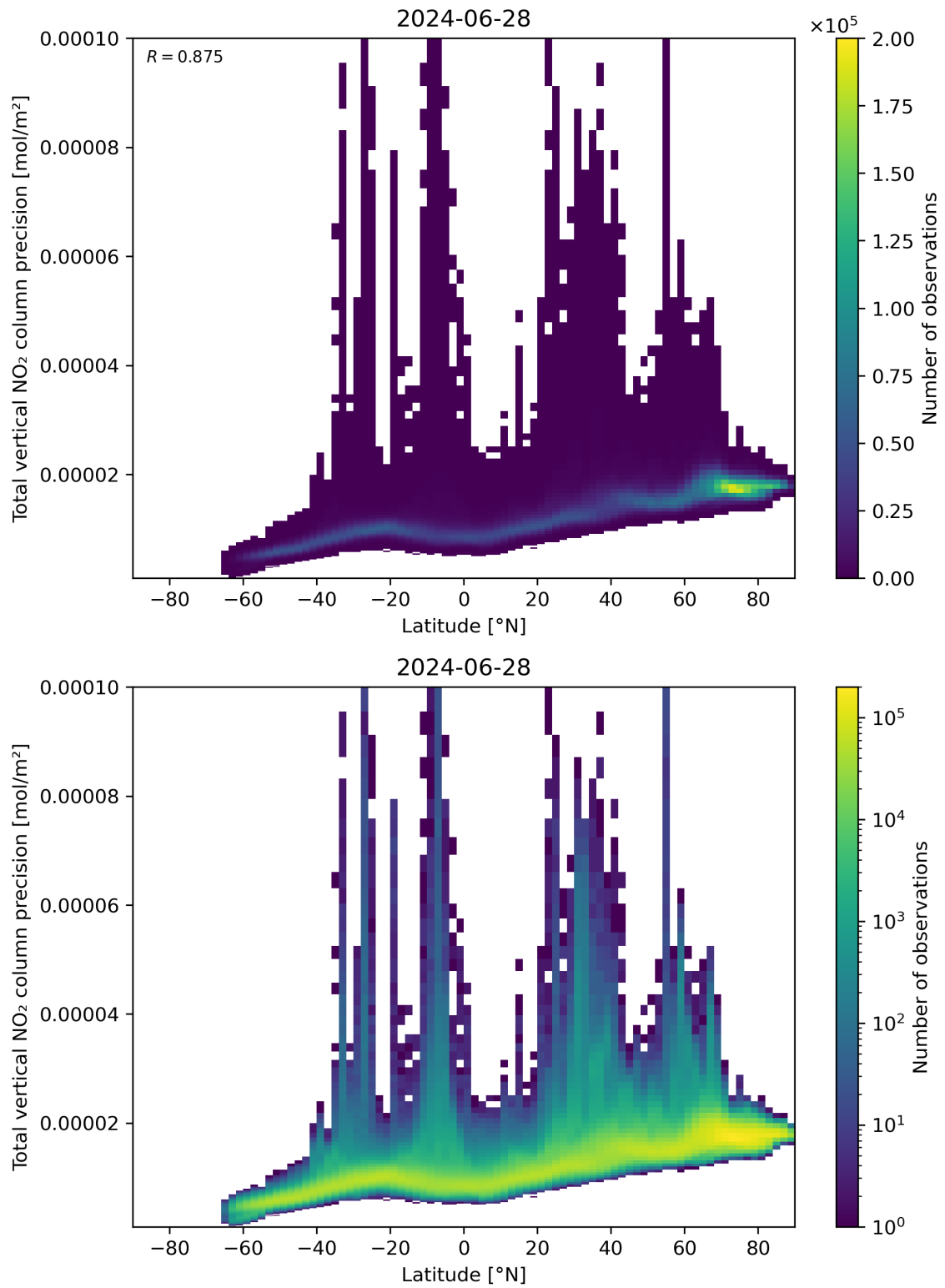
Figure 91: Scatter density plot of “Latitude” against “Total vertical NO 2 column precision” for 2024-06-27 to 2024-06-29.
