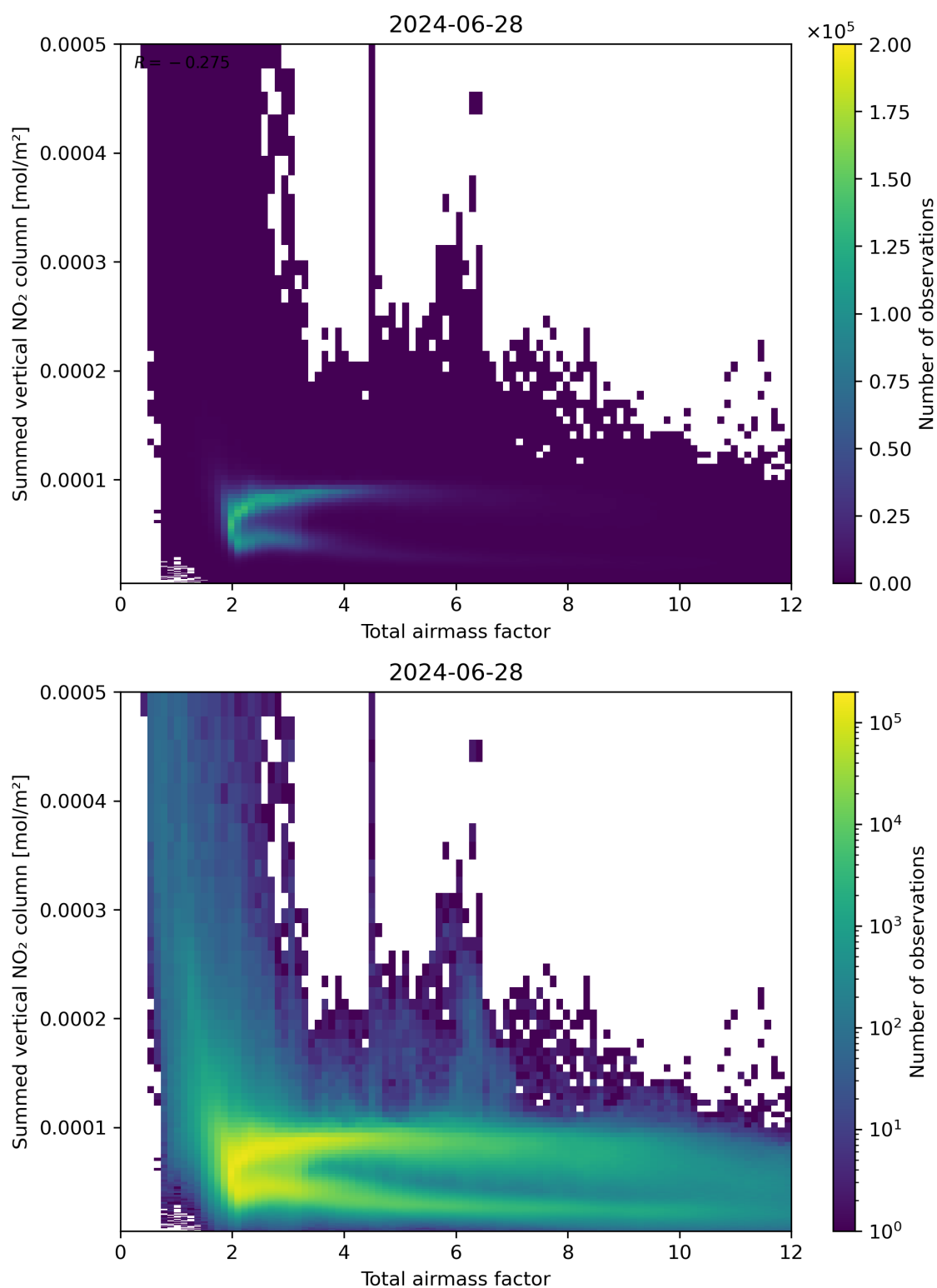
Figure 65: Scatter density plot of “Total airmass factor” against “Summed vertical NO 2 column” for 2024-06-27 to 2024-06-29.
