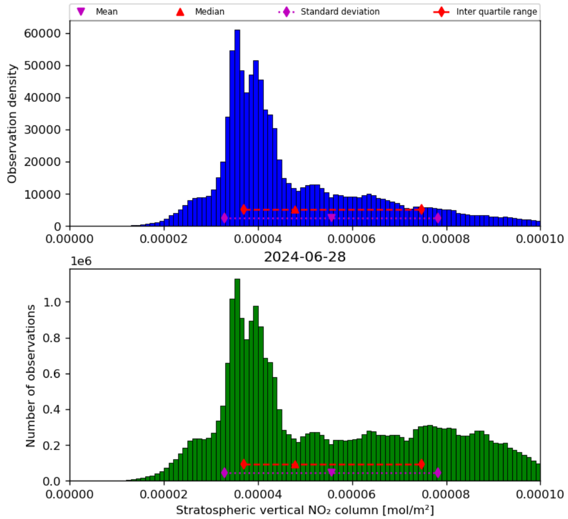
Figure 36: Histogram of “Stratospheric vertical NO 2 column” for 2024-06-27 to 2024-06-29
