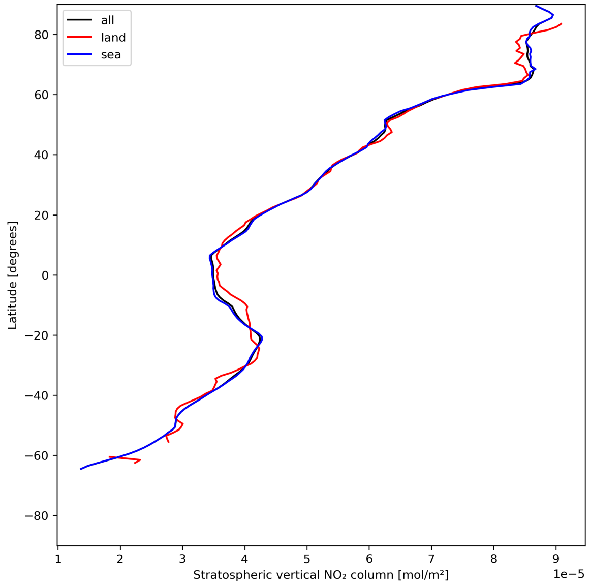
Figure 19: Zonal average of “Stratospheric vertical NO 2 column” for 2024-06-27 to 2024-06-29.
