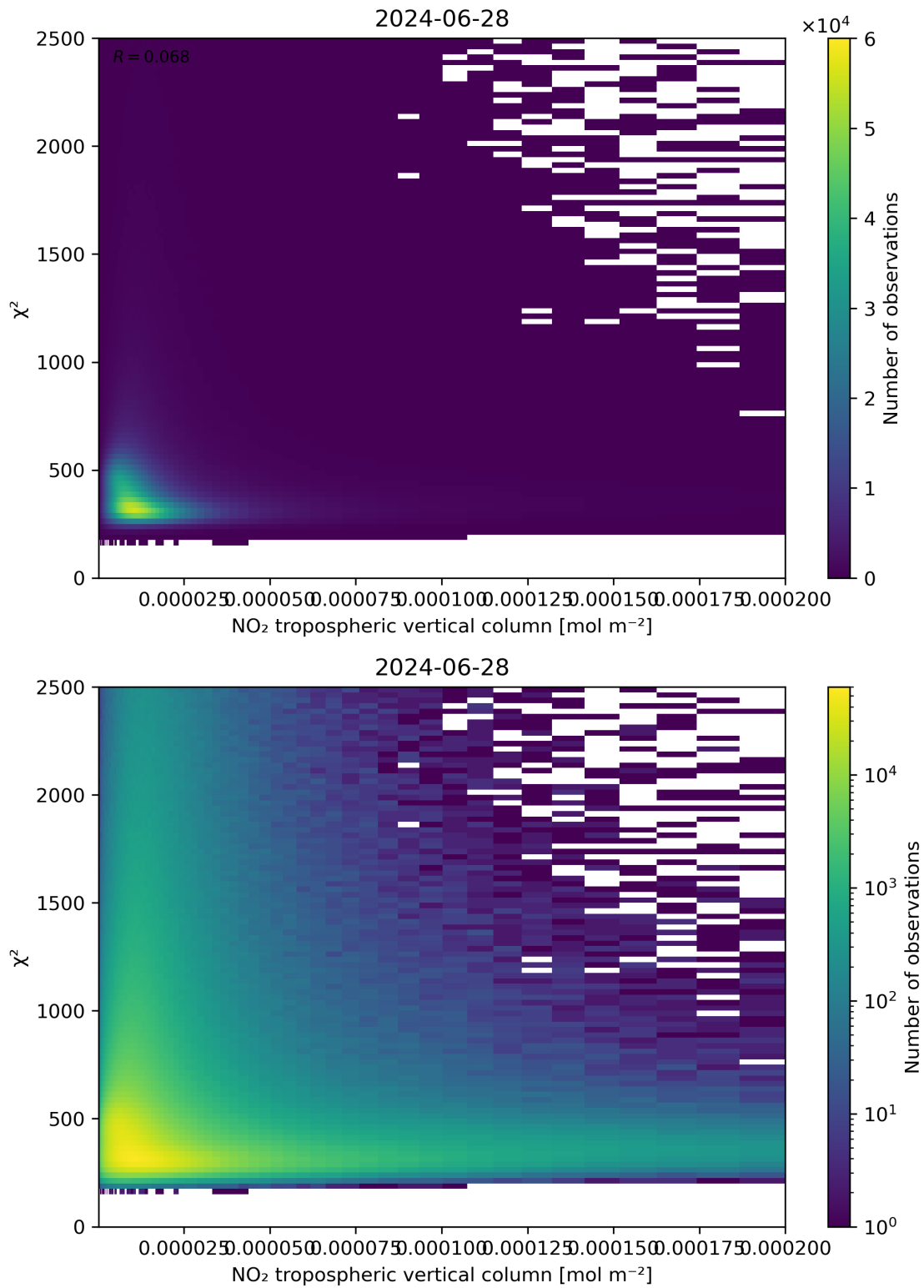
Figure 124: Scatter density plot of “NO 2 tropospheric vertical column” against “ \chi^2 ” for 2024-06-27 to 2024-06-29.
