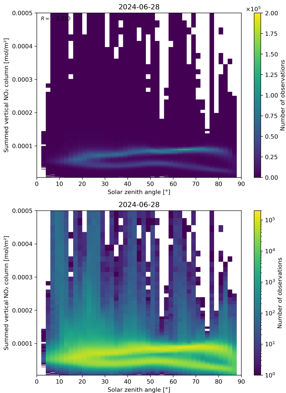
Figure 151: Scatter density plot of “Solar zenith angle” against “Summed vertical NO 2 column” for 2024-06-27 to 2024-06-29.
