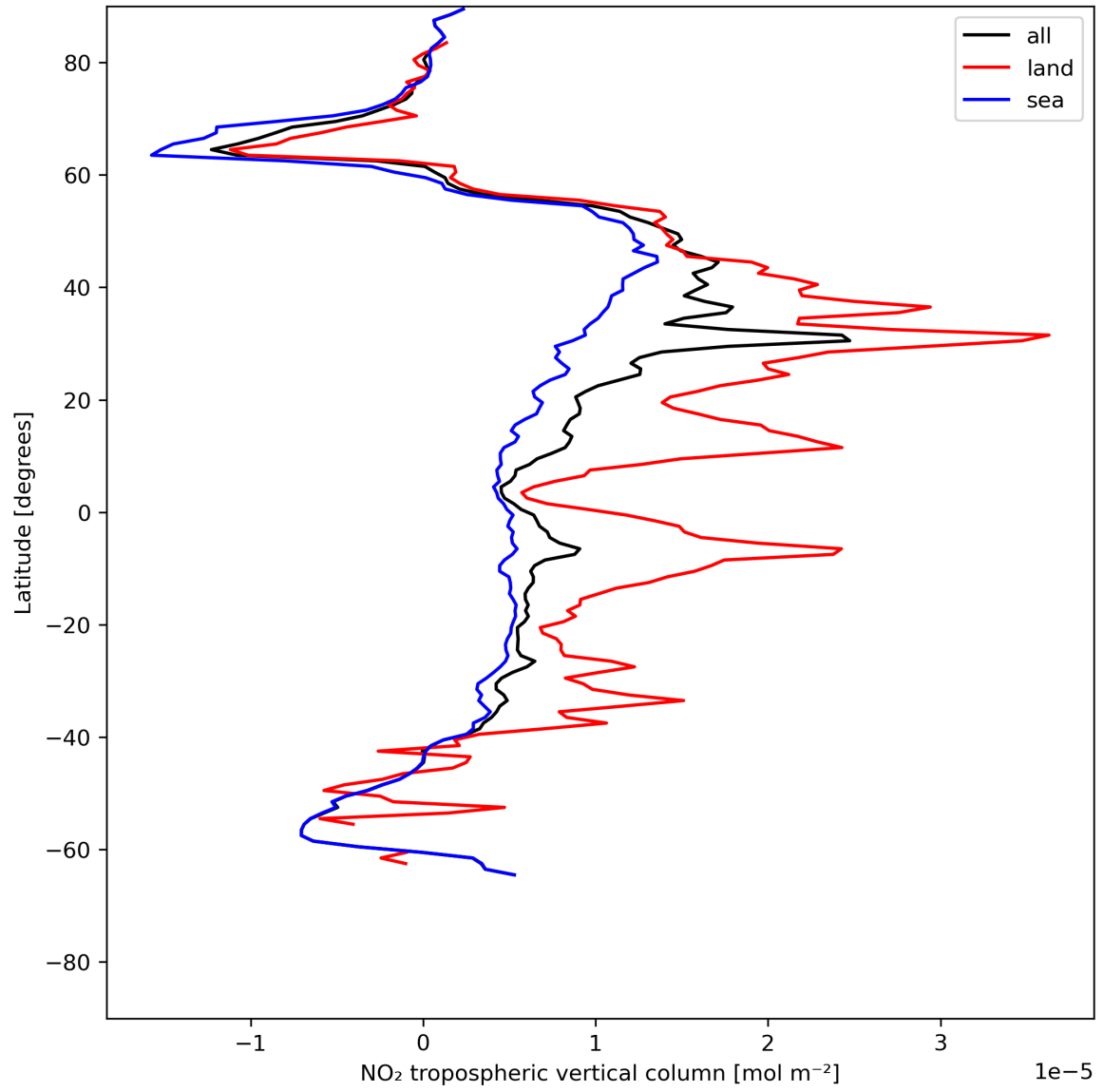
Figure 12: Zonal average of “NO 2 tropospheric vertical column” for 2024-06-27 to 2024-06-29.
