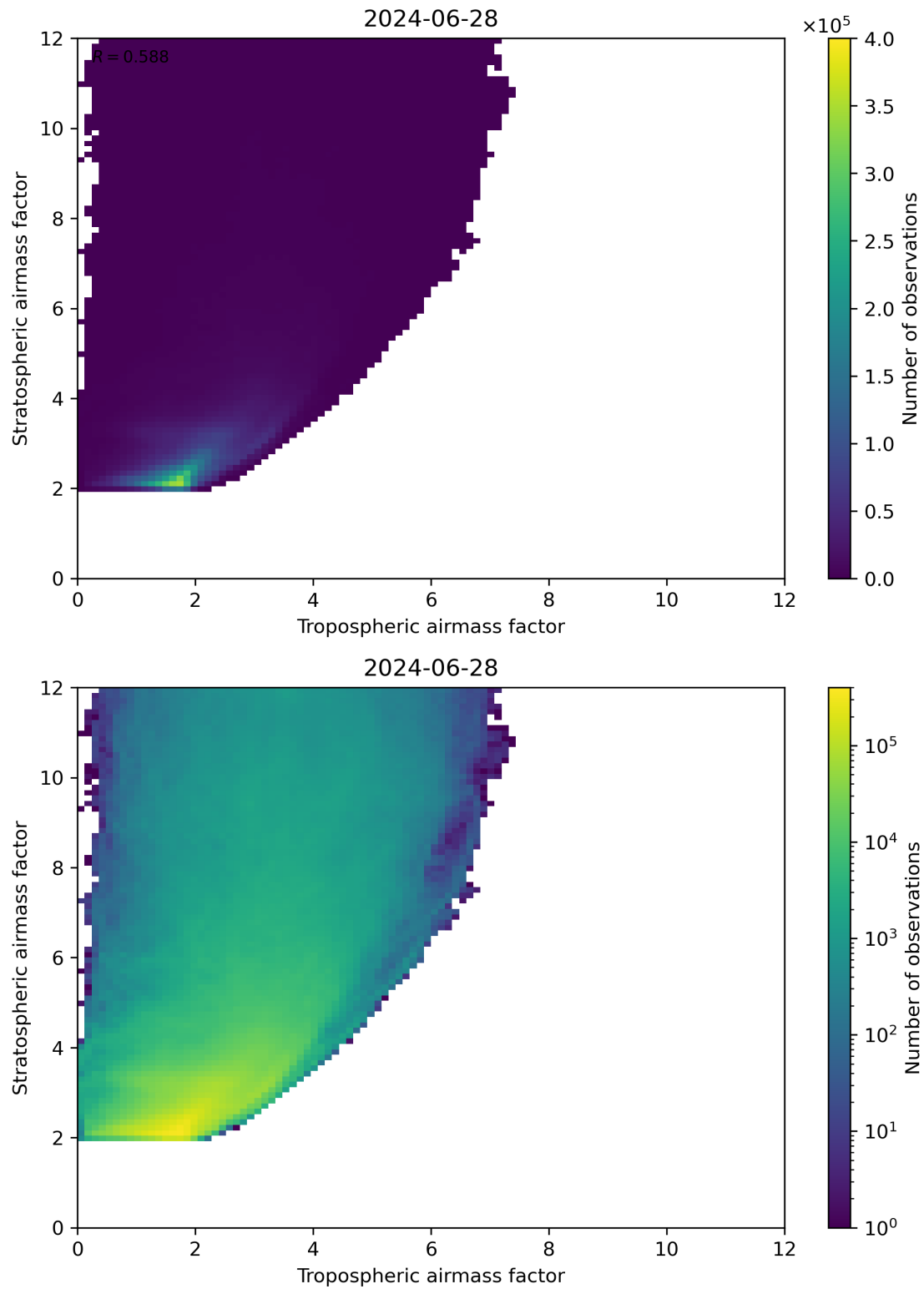
Figure 71: Scatter density plot of “Tropospheric airmass factor” against “Stratospheric airmass factor” for 2024-06-27 to 2024-06-29.
