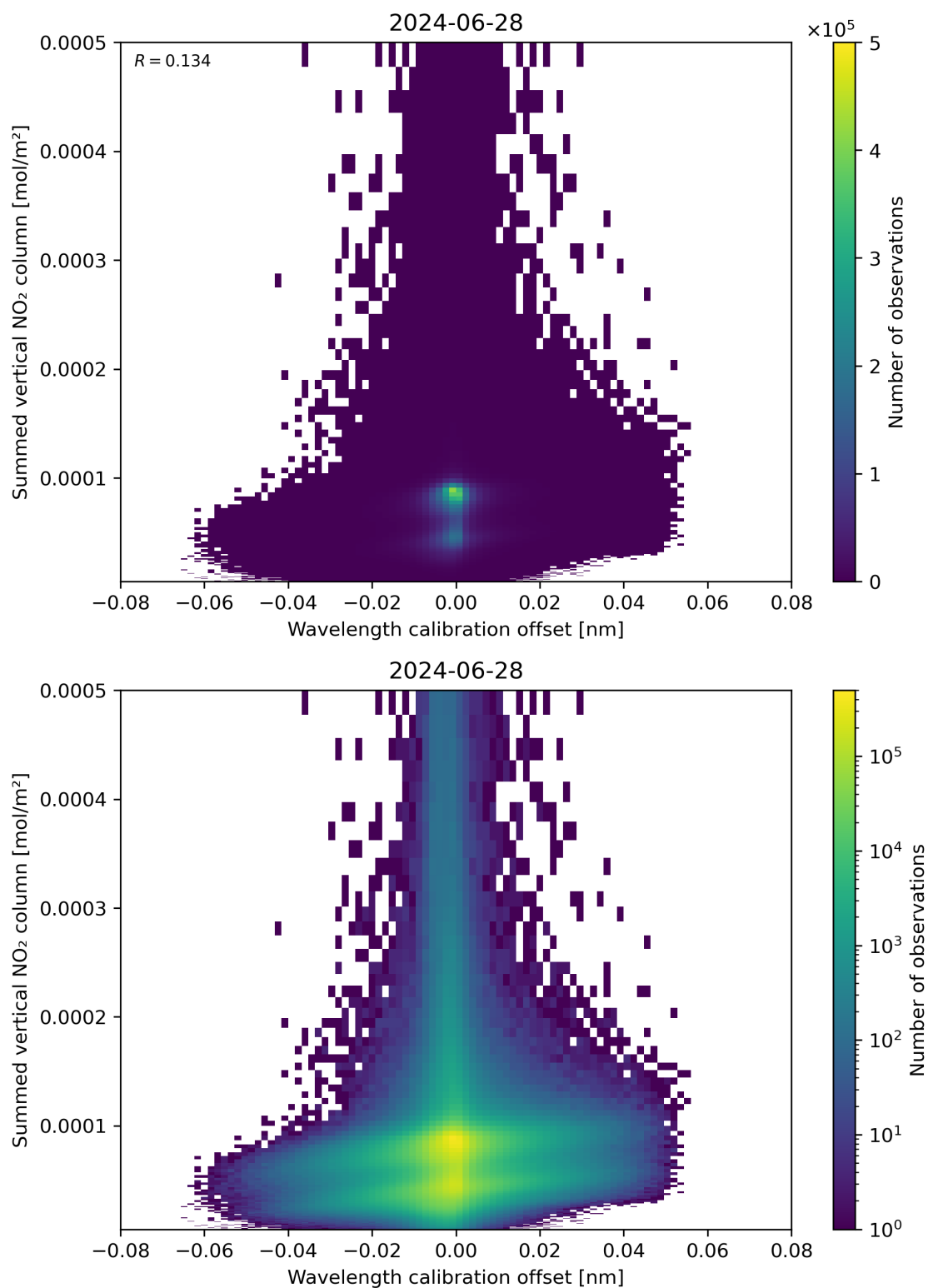
Figure 177: Scatter density plot of “Wavelength calibration offset” against “Summed vertical NO 2 column” for 2024-06-27 to 2024-06-29.
