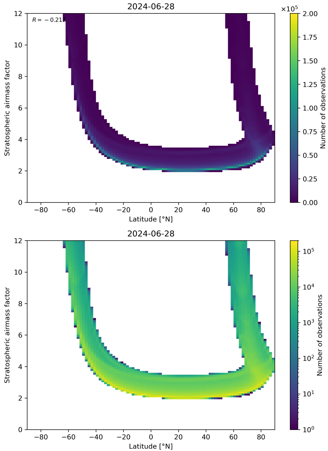
Figure 83: Scatter density plot of “Latitude” against “Stratospheric air mass factor” for 2024-06-27 to 2024-06-29.
