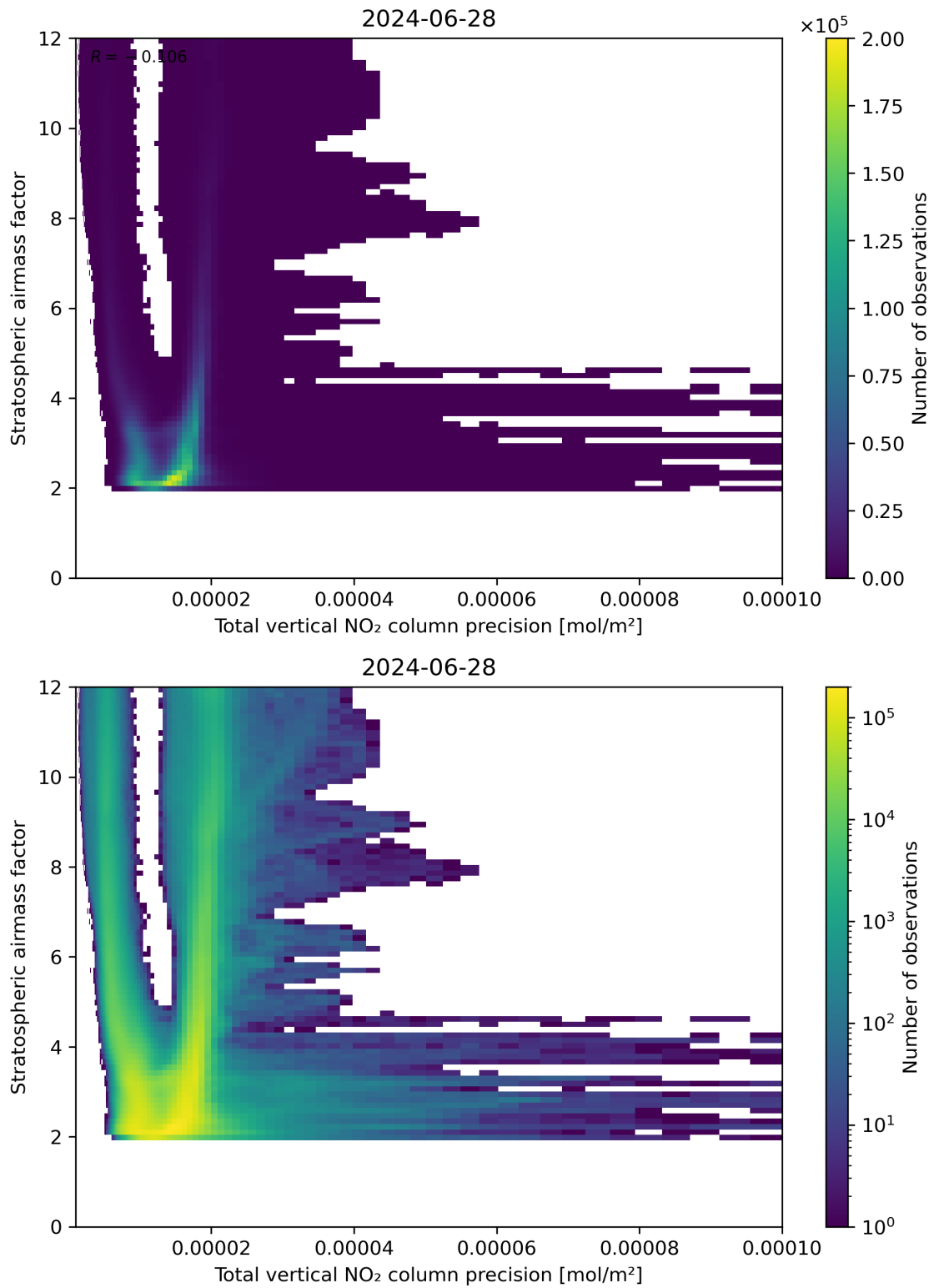
Figure 115: Scatter density plot of “Total vertical NO 2 column precision” against “Stratospheric air mass factor” for 2024-06-27 to 2024-06-29.
