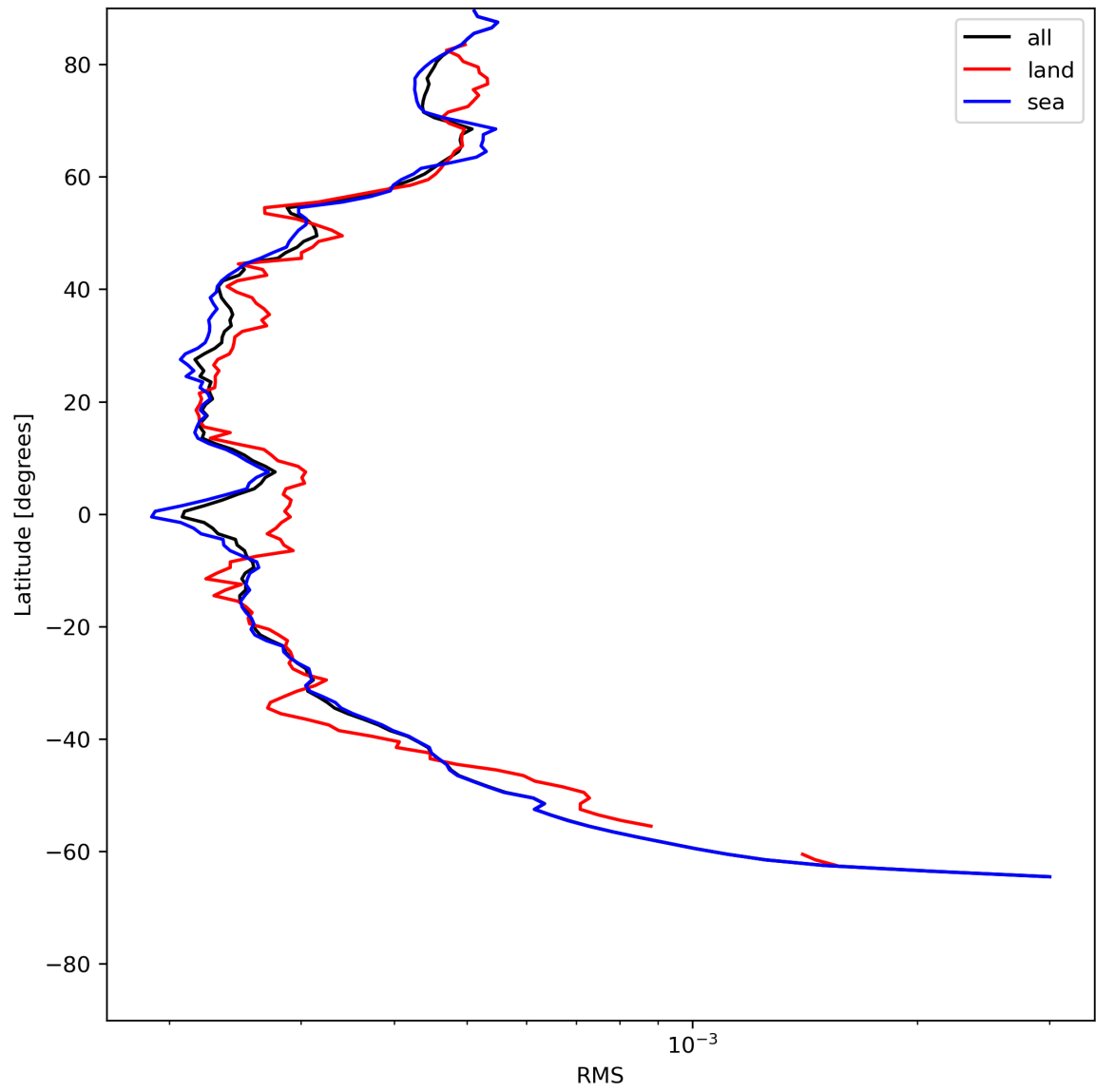
Figure 26: Zonal average of “RMS” for 2024-06-27 to 2024-06-29.
