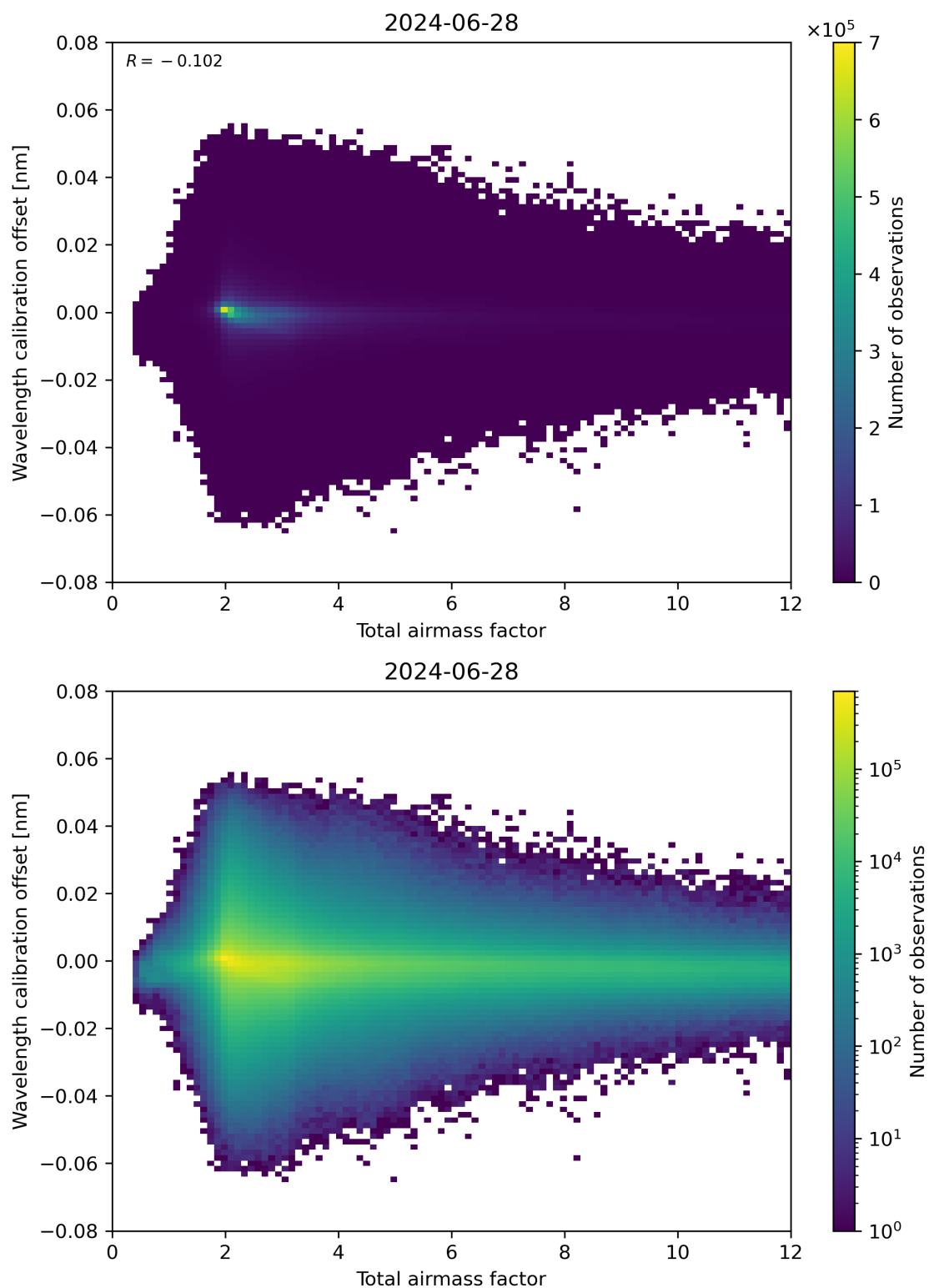
Figure 70: Scatter density plot of “Total airmass factor” against “Wavelength calibration offset” for 2024-06-27 to 2024-06-29.
