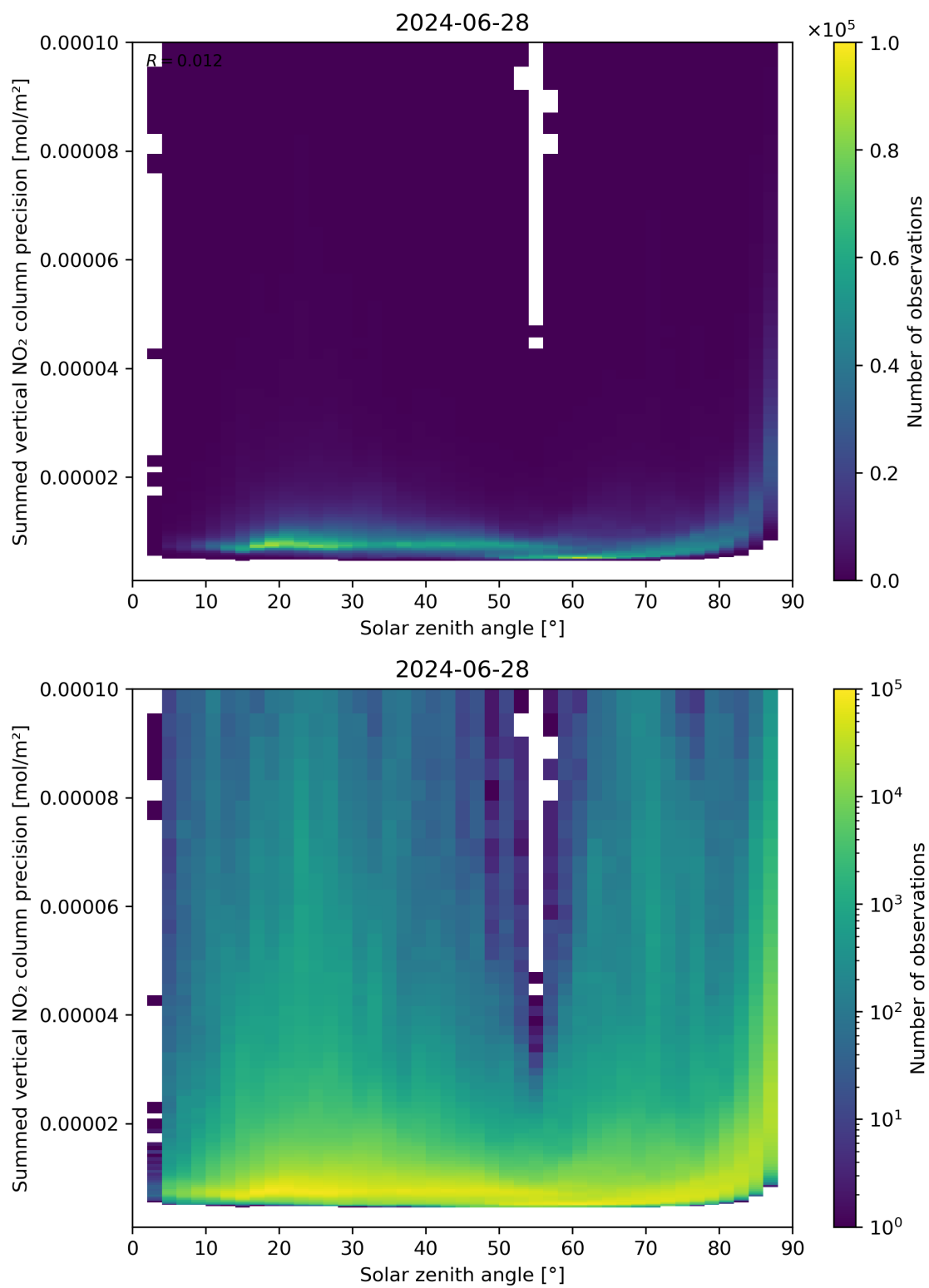
Figure 152: Scatter density plot of “Solar zenith angle” against “Summed vertical NO 2 column precision” for 2024-06-27 to 2024-06-29.
