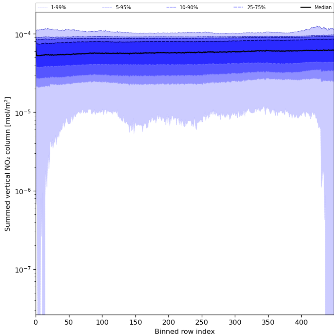
Figure 57: Along track statistics of “Summed vertical NO 2 column” for 2024-06-27 to 2024-06-29
