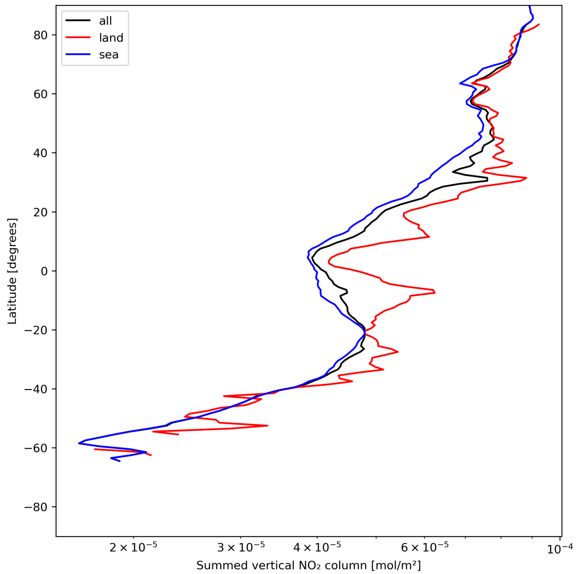
Figure 23: Zonal average of “Summed vertical NO 2 column” for 2024-06-27 to 2024-06-29.
