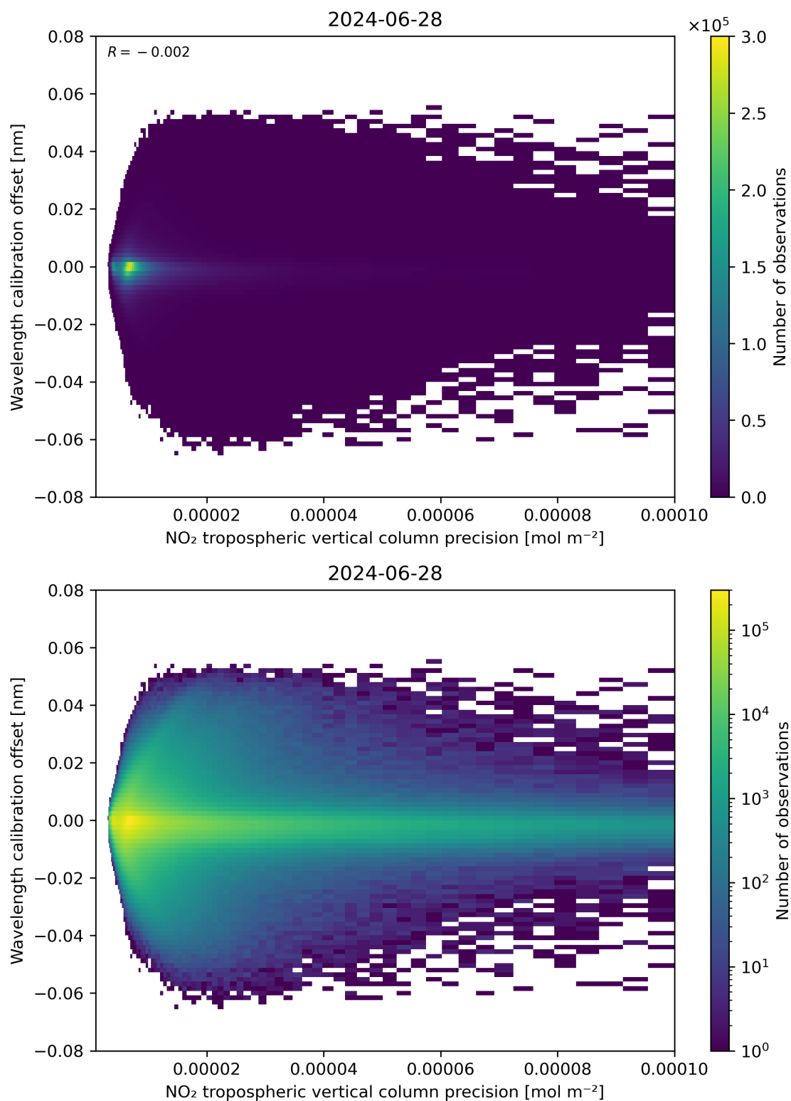
Figure 141: Scatter density plot of “NO 2 tropospheric vertical column precision” against “Wavelength calibration offset” for 2024-06-27 to 2024-06-29.
