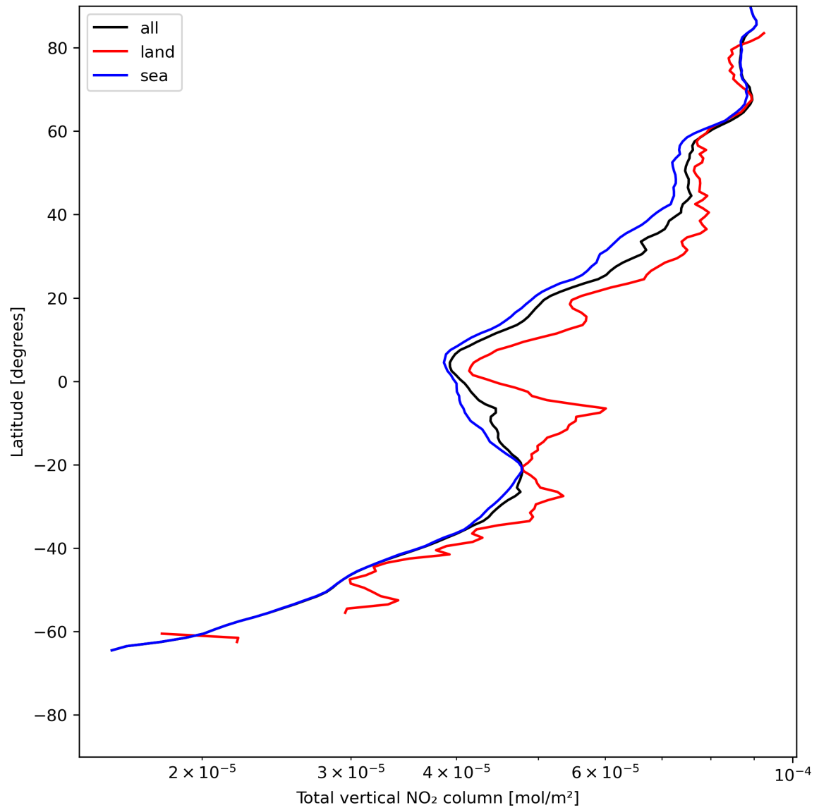
Figure 21: Zonal average of “Total vertical NO 2 column” for 2024-06-27 to 2024-06-29.
