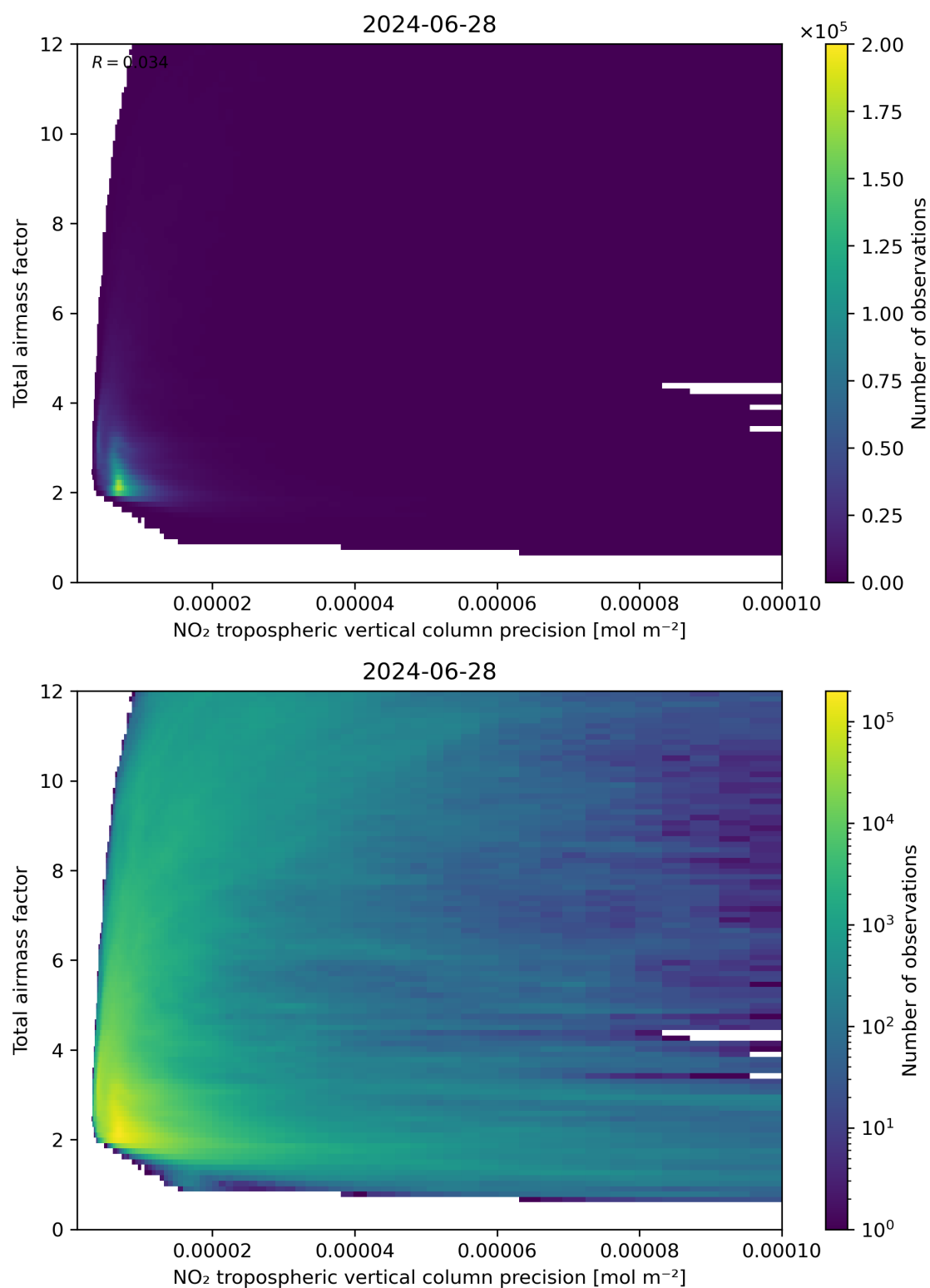
Figure 132: Scatter density plot of “NO 2 tropospheric vertical column precision” against “Total air mass factor” for 2024-06-27 to 2024-06-29.
