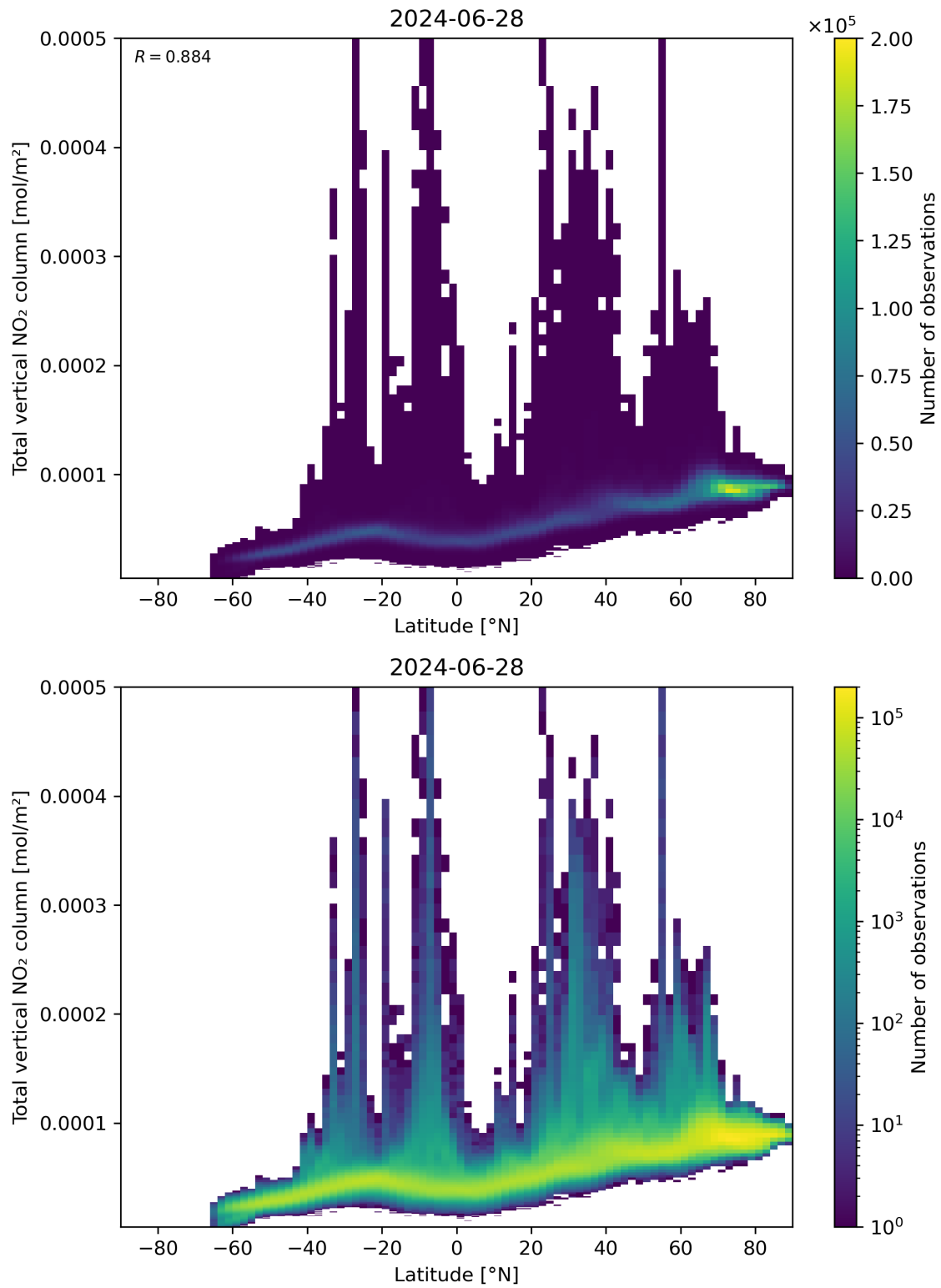
Figure 90: Scatter density plot of “Latitude” against “Total vertical NO 2 column” for 2024-06-27 to 2024-06-29.
