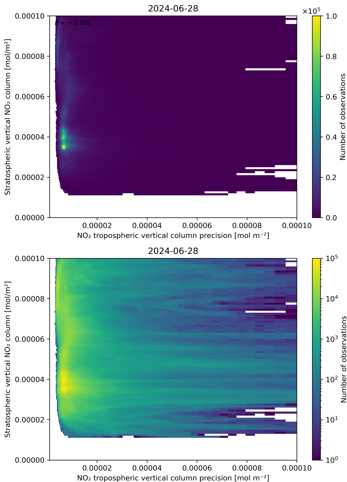
Figure 135: Scatter density plot of “NO 2 tropospheric vertical column precision” against “Stratospheric vertical NO 2 column” for 2024-06-27 to 2024-06-29.
