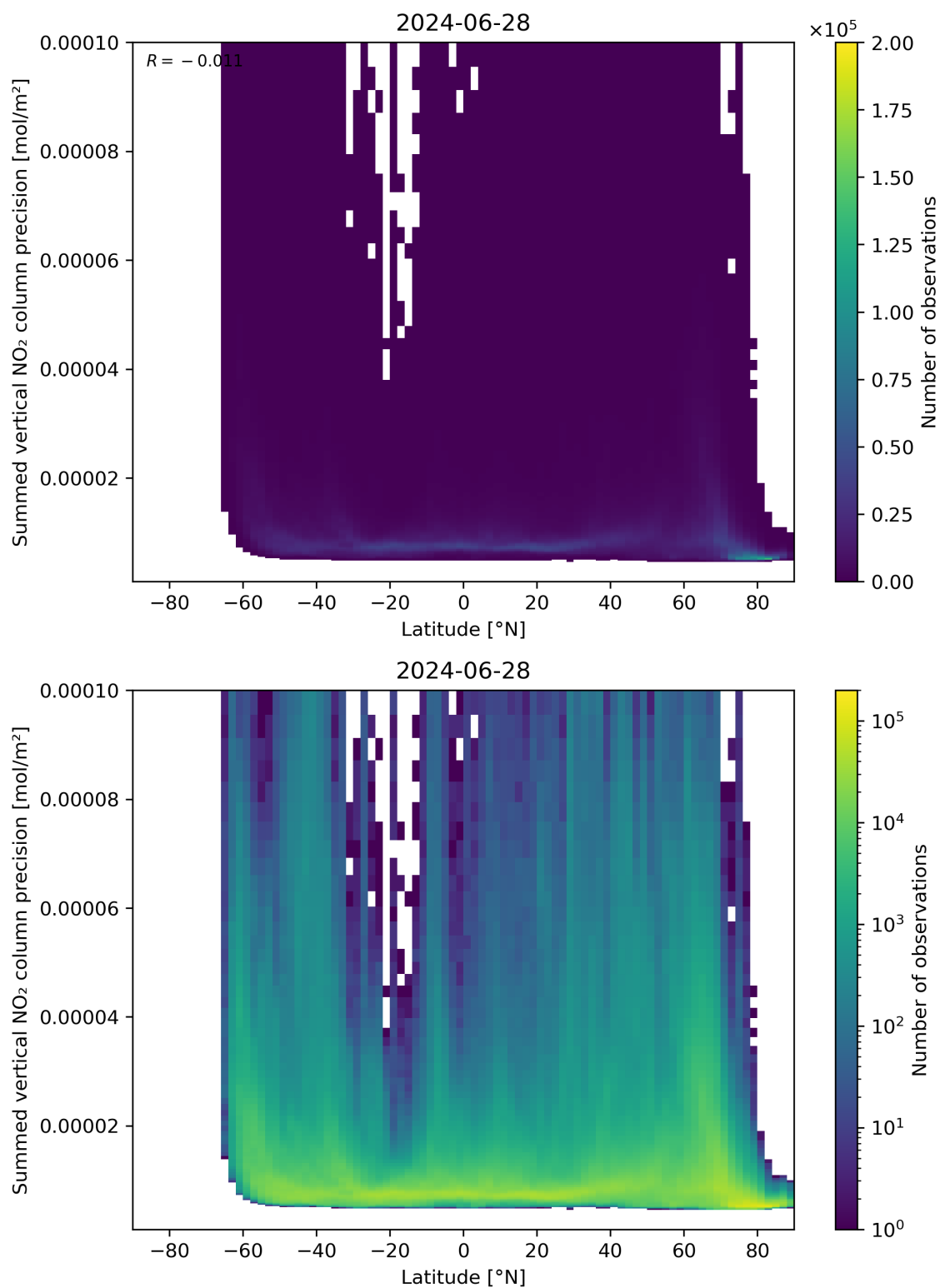
Figure 89: Scatter density plot of “Latitude” against “Summed vertical NO 2 column precision” for 2024-06-27 to 2024-06-29.
