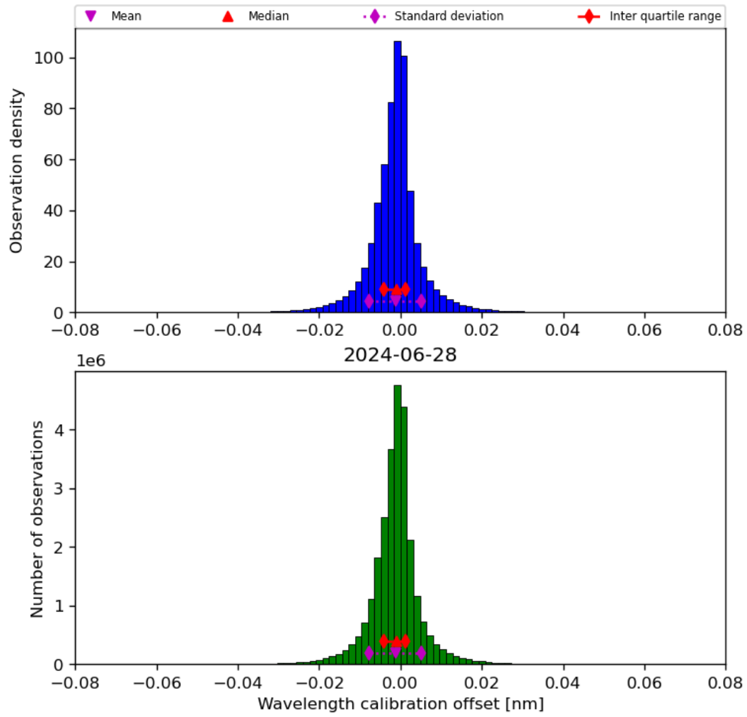
Figure 35: Histogram of “Wavelength calibration offset” for 2024-06-27 to 2024-06-29
