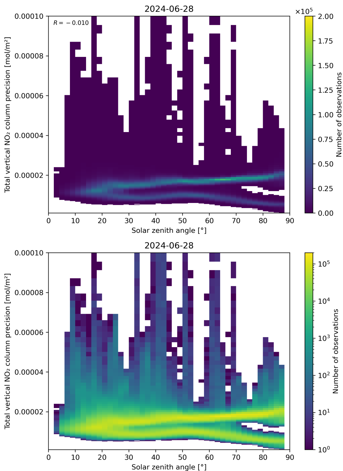
Figure 154: Scatter density plot of “Solar zenith angle” against “Total vertical NO 2 column precision” for 2024-06-27 to 2024-06-29.
