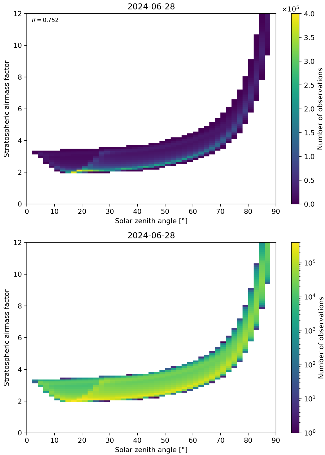
Figure 145: Scatter density plot of “Solar zenith angle” against “Stratospheric airmass factor” for 2024-06-27 to 2024-06-29.
