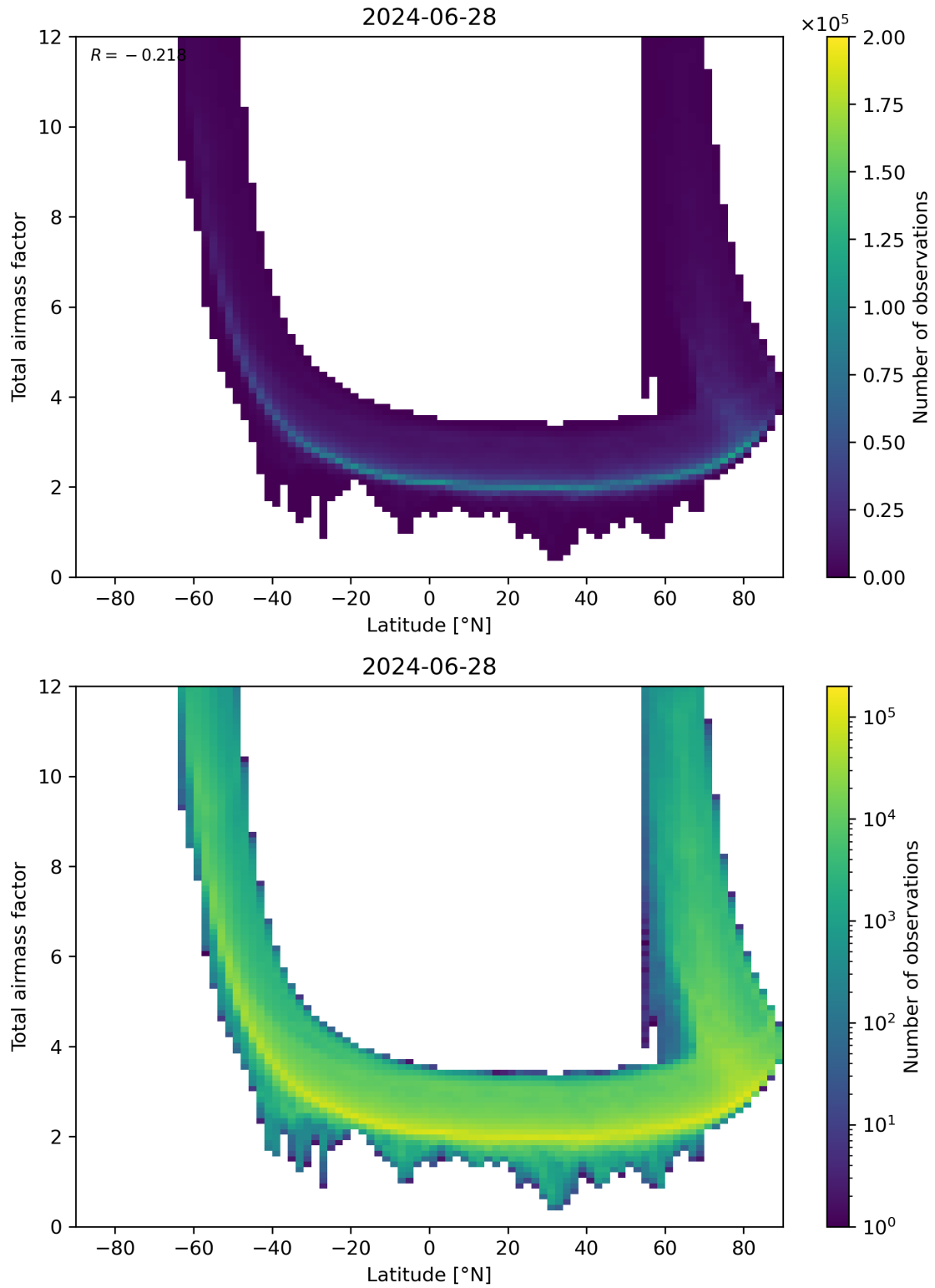
Figure 84: Scatter density plot of “Latitude” against “Total airmass factor” for 2024-06-27 to 2024-06-29.
