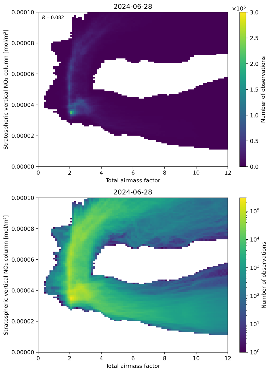
Figure 64: Scatter density plot of “Total airmass factor” against “Stratospheric vertical \text{NO}_2 column” for 2024-06-27 to 2024-06-29.
