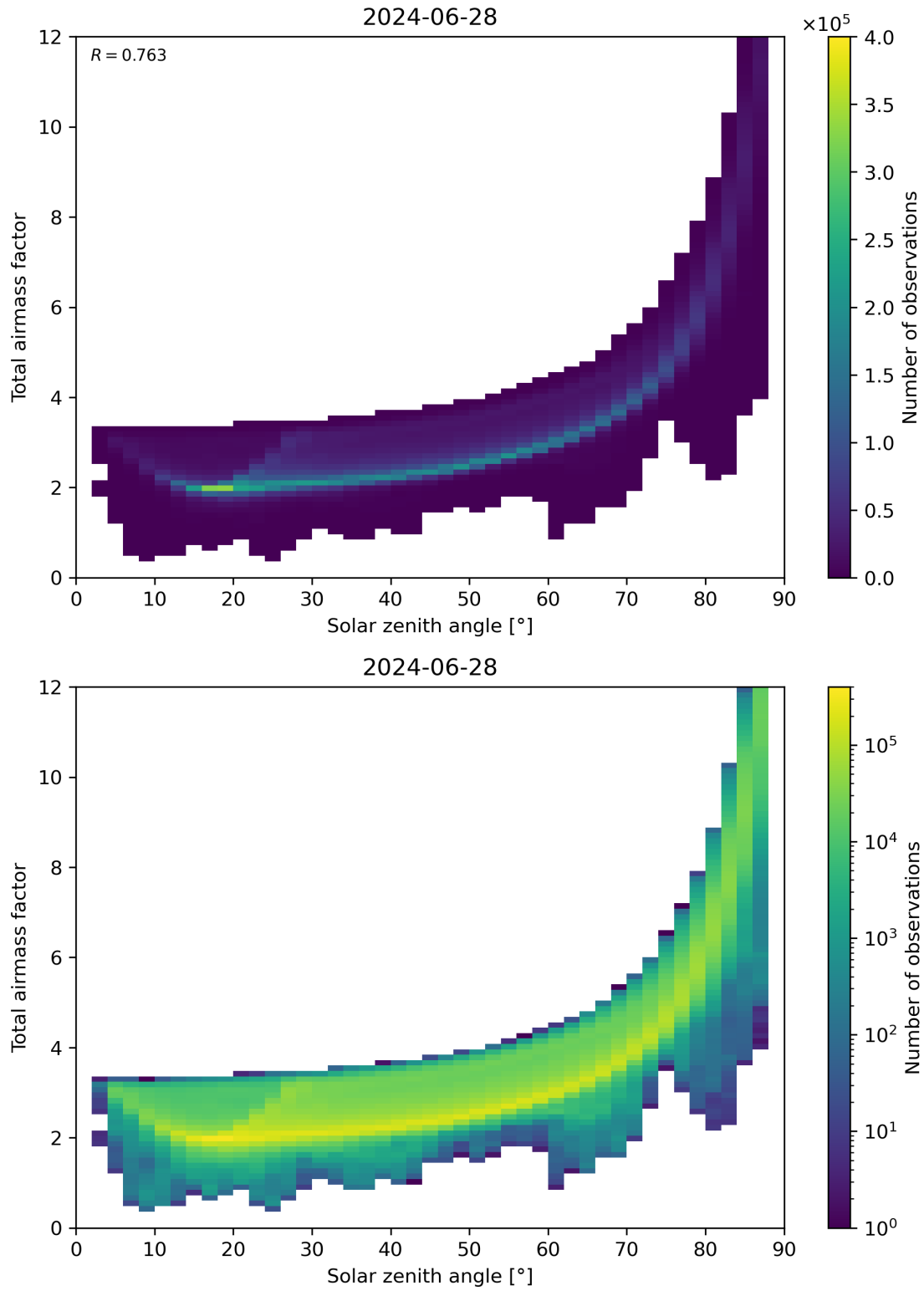
Figure 146: Scatter density plot of “Solar zenith angle” against “Total airmass factor” for 2024-06-27 to 2024-06-29.
