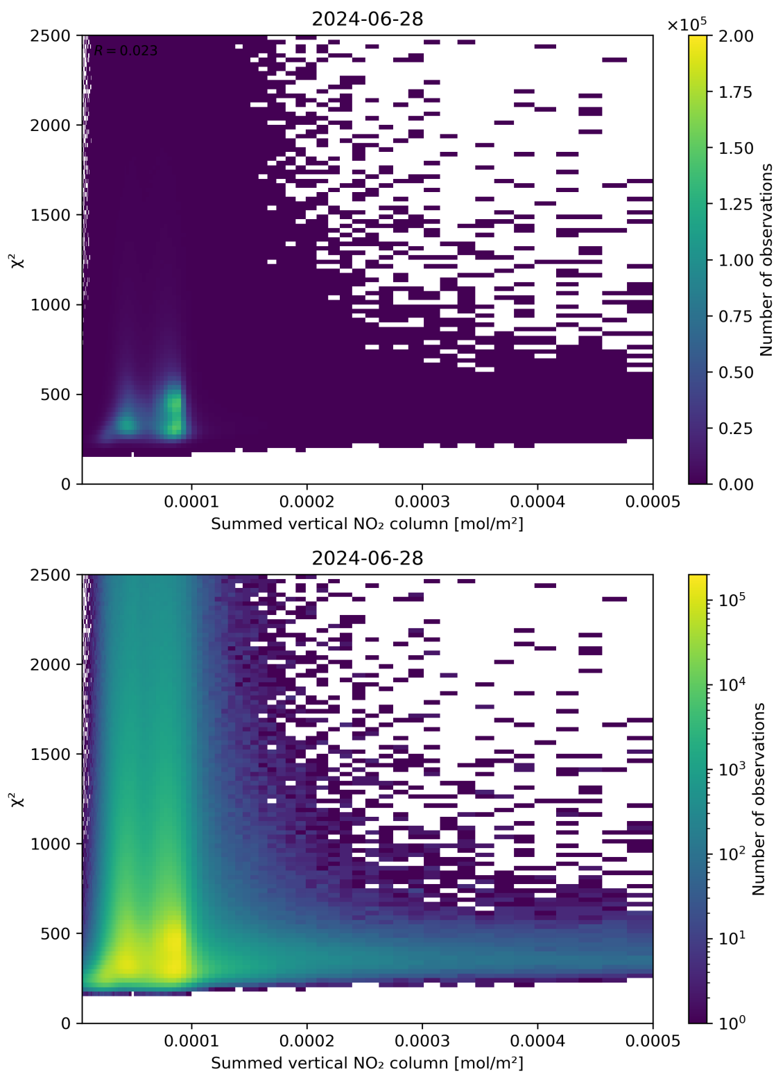
Figure 104: Scatter density plot of “Summed vertical NO 2 column” against “ \chi^2 ” for 2024-06-27 to 2024-06-29.
