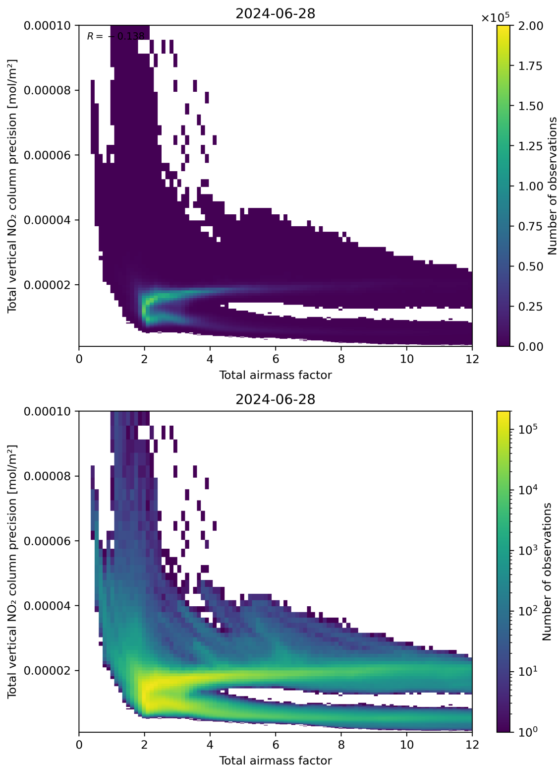
Figure 68: Scatter density plot of “Total airmass factor” against “Total vertical NO 2 column precision” for 2024-06-27 to 2024-06-29.
