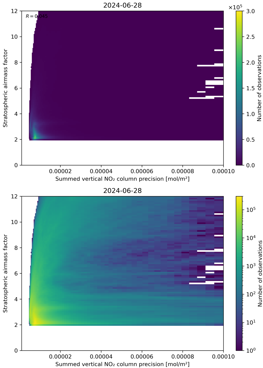
Figure 106: Scatter density plot of “Summed vertical NO 2 column precision” against “Stratospheric airmass factor” for 2024-06-27 to 2024-06-29.
