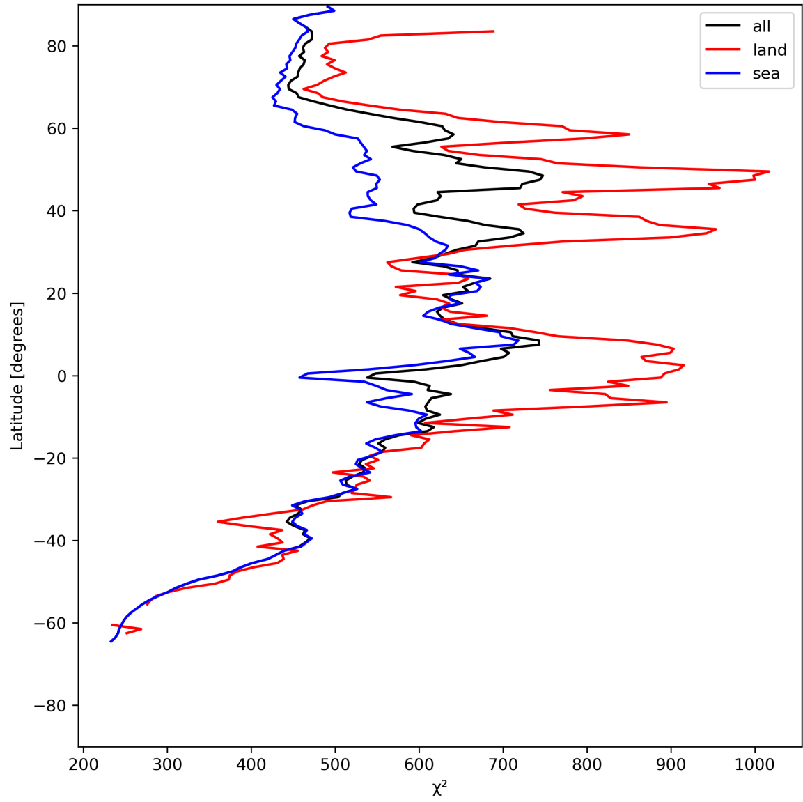
Figure 25: Zonal average of “ \chi^2 ” for 2024-06-27 to 2024-06-29.
