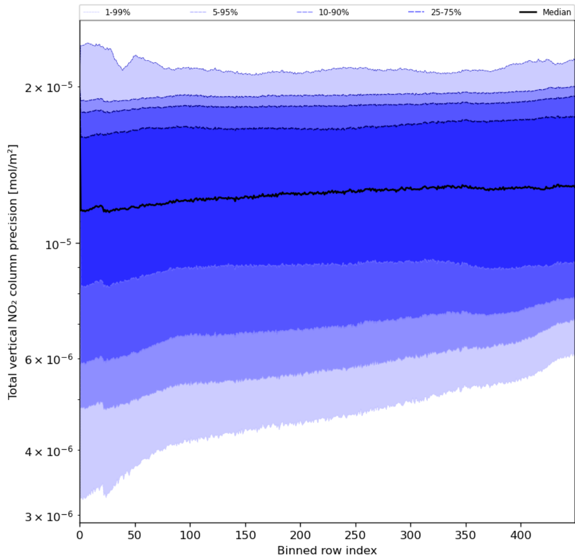
Figure 56: Along track statistics of “Total vertical NO 2 column precision” for 2024-06-27 to 2024-06-29
