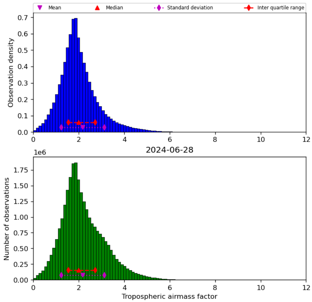
Figure 31: Histogram of “Tropospheric airmass factor” for 2024-06-27 to 2024-06-29
