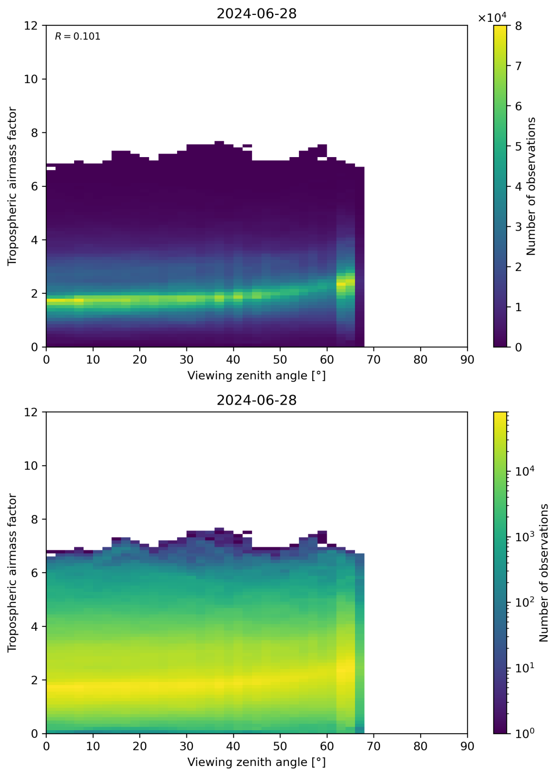
Figure 161: Scatter density plot of “Viewing zenith angle” against “Tropospheric airmass factor” for 2024-06-27 to 2024-06-29.
