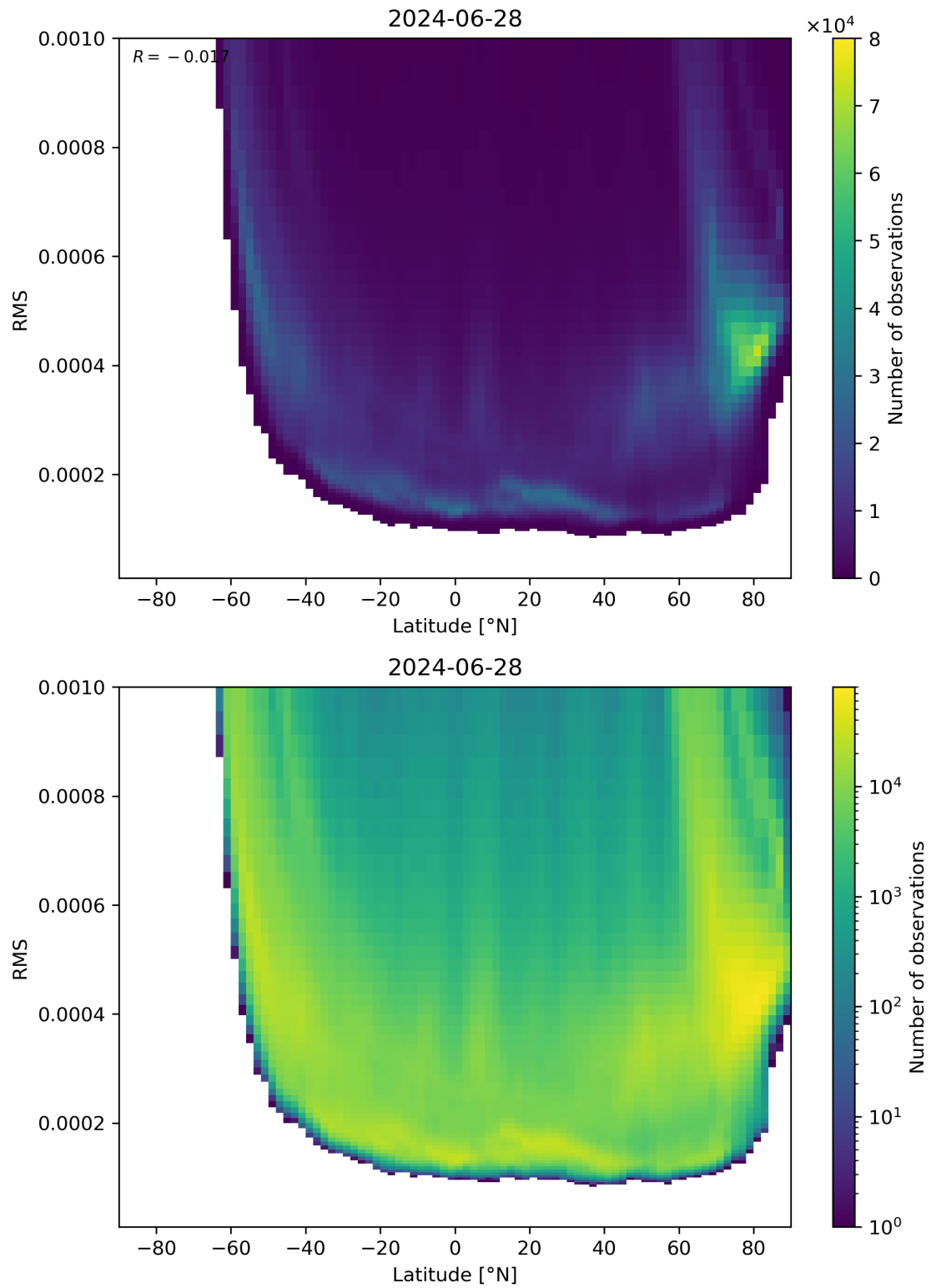
Figure 94: Scatter density plot of “Latitude” against “RMS” for 2024-06-27 to 2024-06-29.
