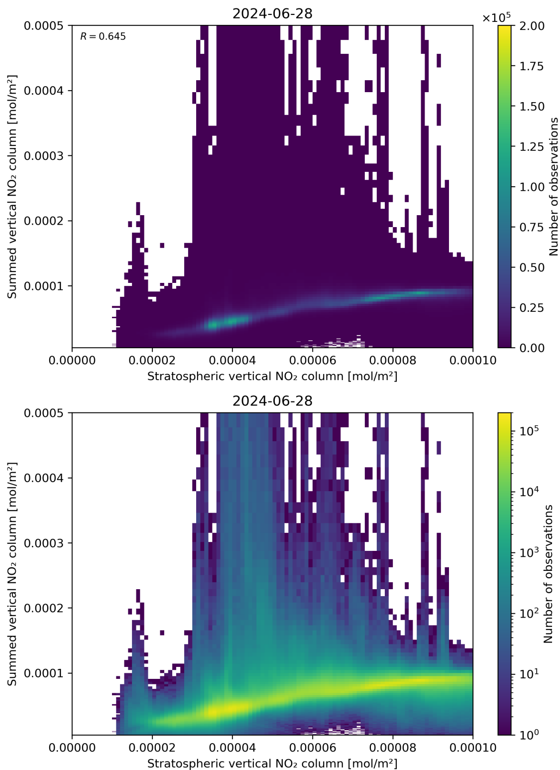
Figure 98: Scatter density plot of “Stratospheric vertical NO 2 column” against “Summed vertical NO 2 column” for 2024-06-27 to 2024-06-29.
