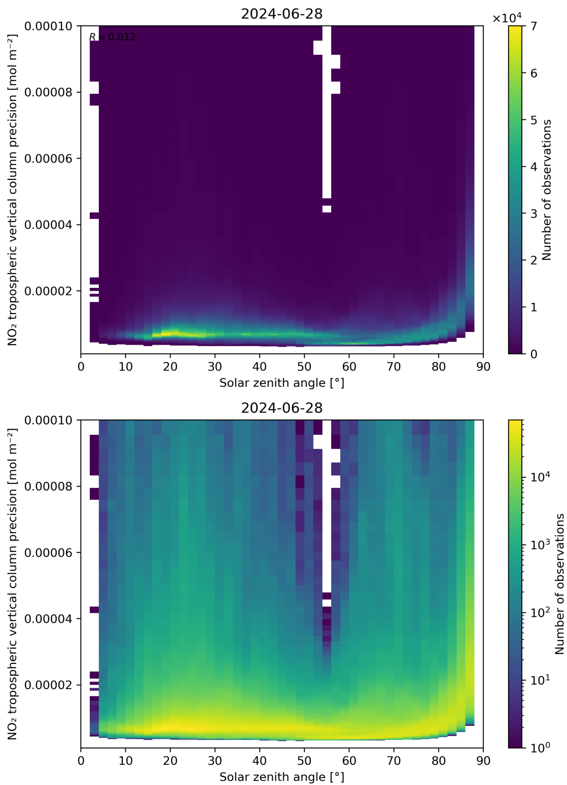
Figure 156: Scatter density plot of “Solar zenith angle” against “NO 2 tropospheric vertical column precision” for 2024-06-27 to 2024-06-29.
