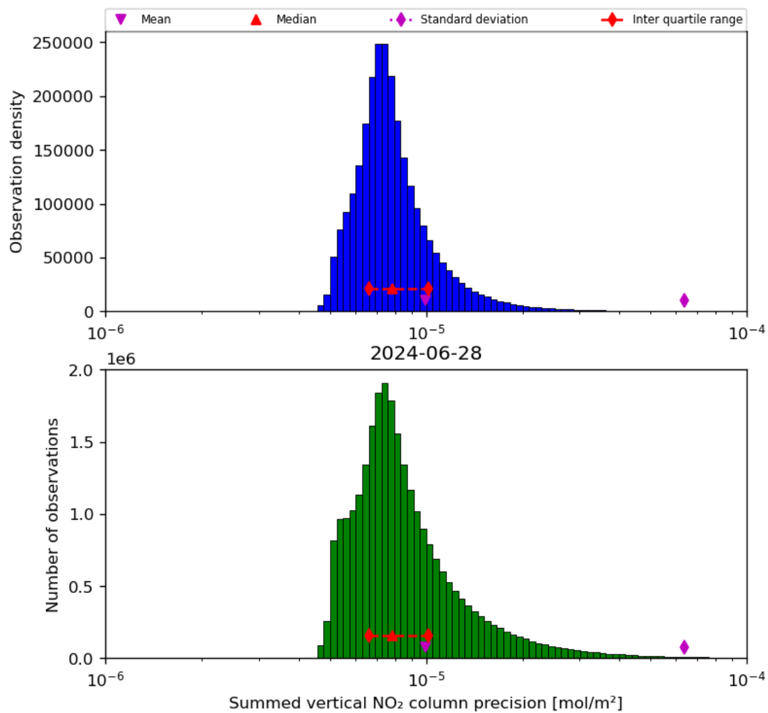
Figure 41: Histogram of "Summed vertical NO 2 column precision" for 2024-06-27 to 2024-06-29
