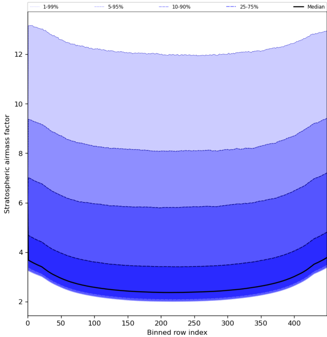
Figure 61: Along track statistics of “Stratospheric airmass factor” for 2024-06-27 to 2024-06-29
