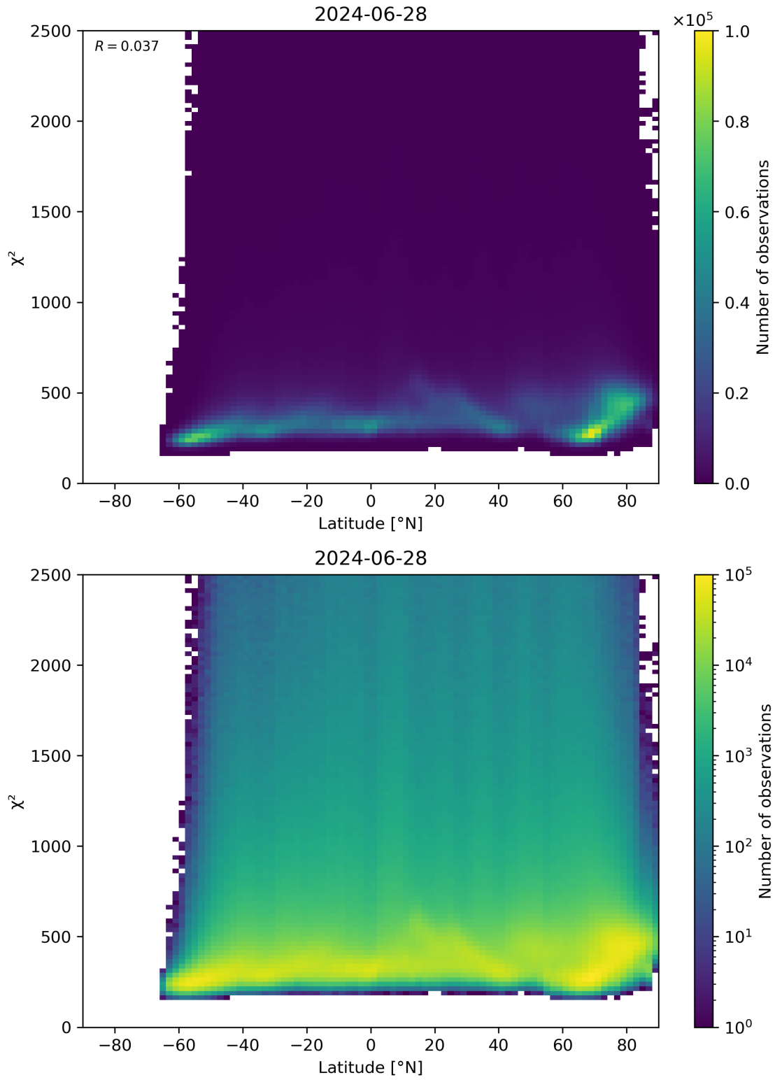
Figure 86: Scatter density plot of “Latitude” against “ \chi^2 ” for 2024-06-27 to 2024-06-29.
