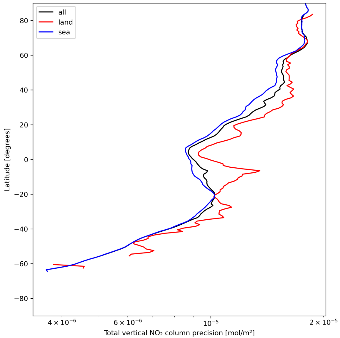
Figure 22: Zonal average of “Total vertical NO 2 column precision” for 2024-06-27 to 2024-06-29.
