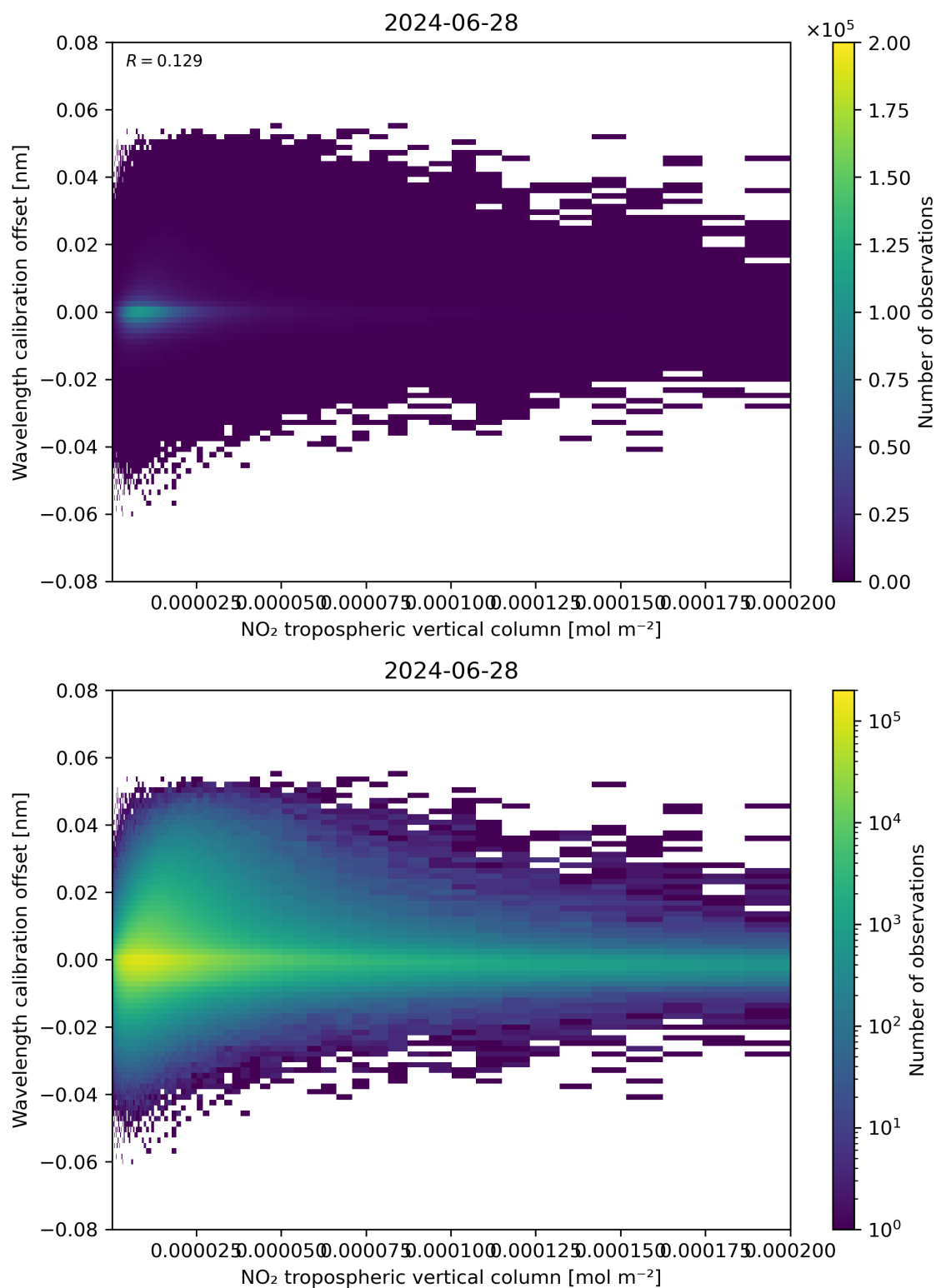
Figure 143: Scatter density plot of “NO 2 tropospheric vertical column” against “Wavelength calibration offset” for 2024-06-27 to 2024-06-29.
