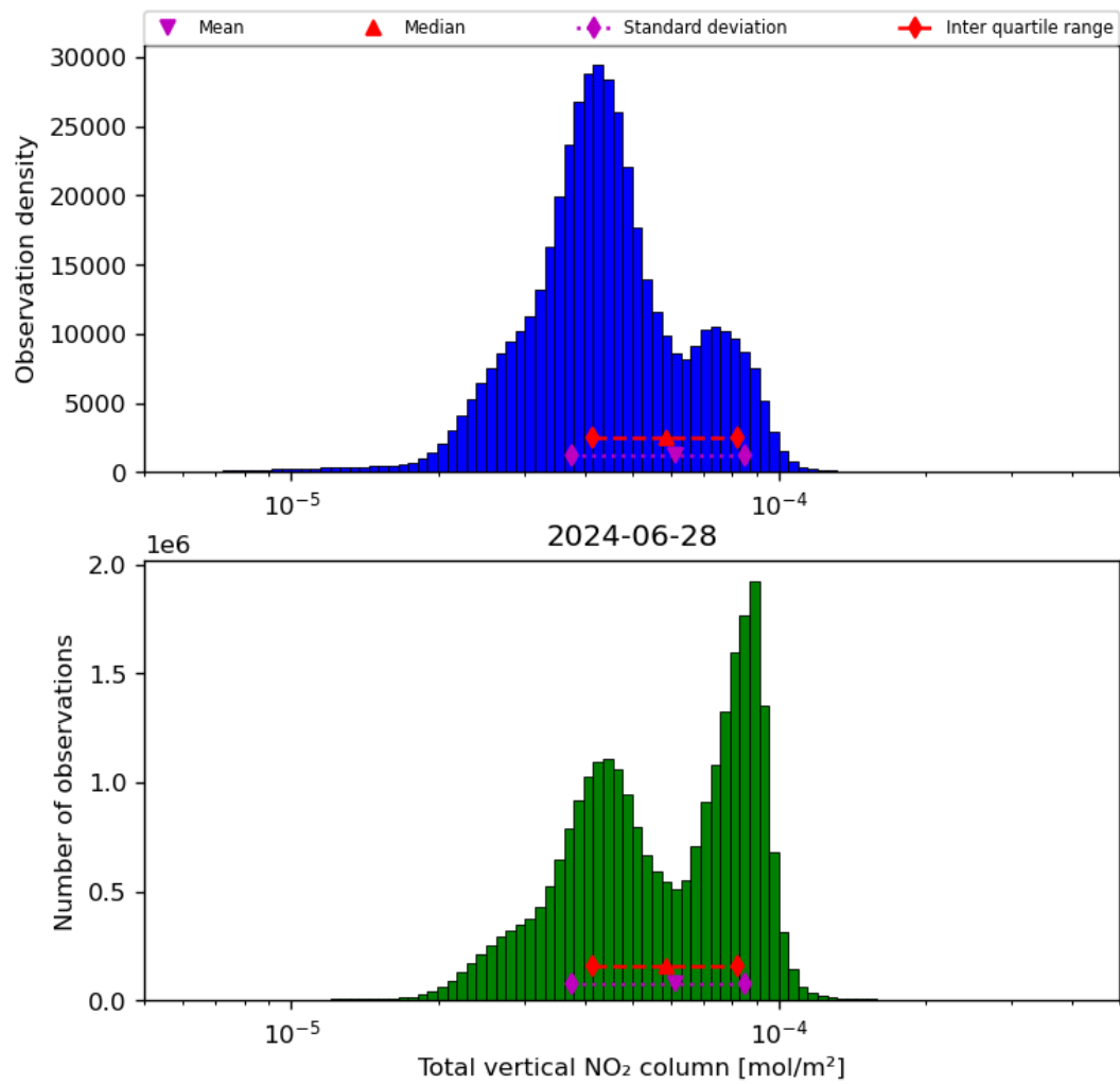
Figure 38: Histogram of “Total vertical NO 2 column” for 2024-06-27 to 2024-06-29
