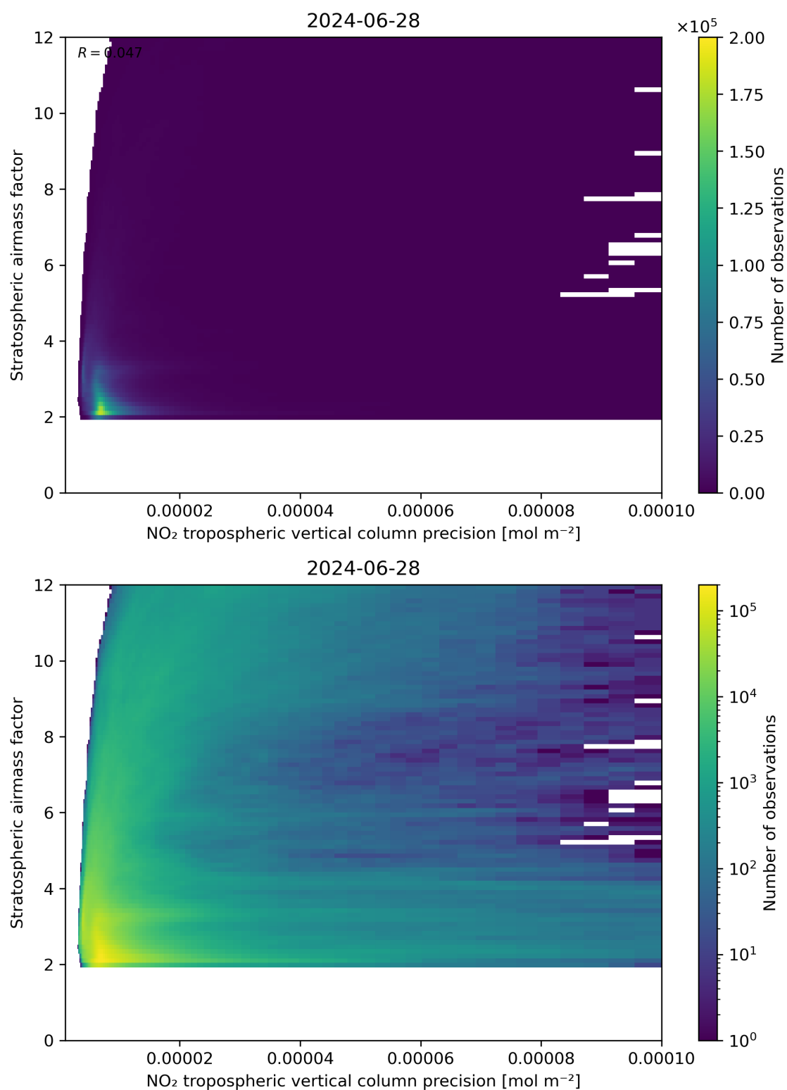
Figure 131: Scatter density plot of “NO 2 tropospheric vertical column precision” against “Stratospheric airmass factor” for 2024-06-27 to 2024-06-29.
