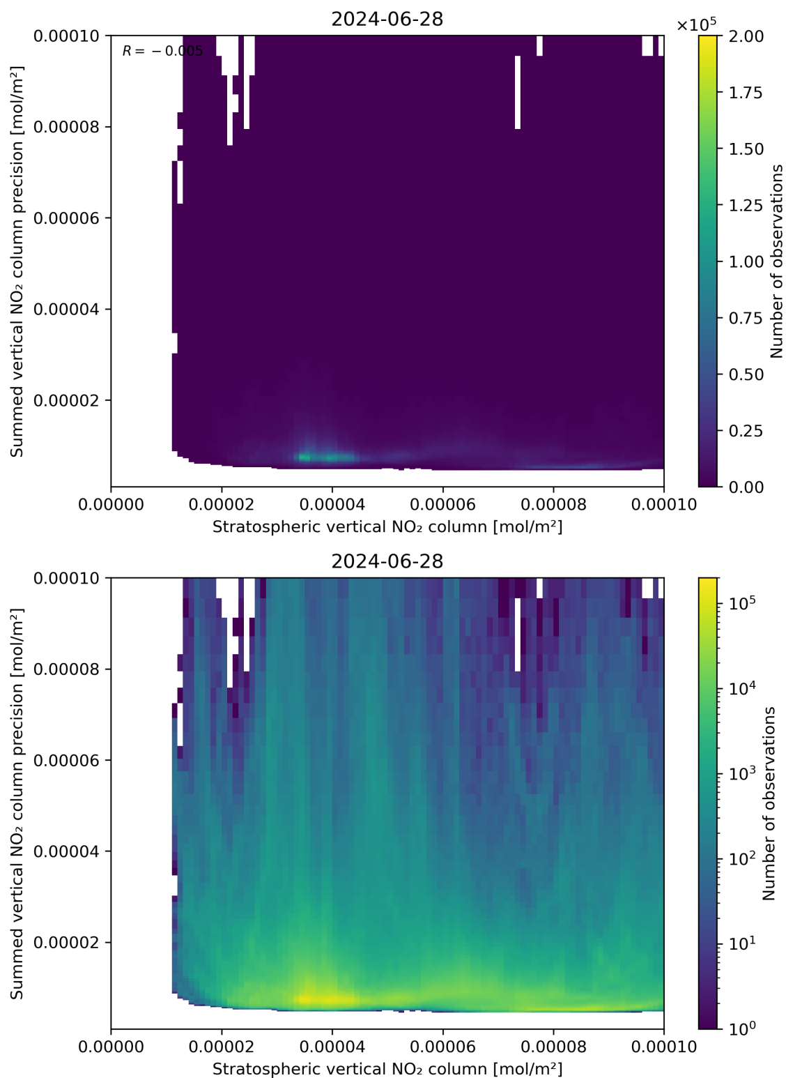
Figure 99: Scatter density plot of “Stratospheric vertical NO 2 column” against “Summed vertical NO 2 column precision” for 2024-06-27 to 2024-06-29.
