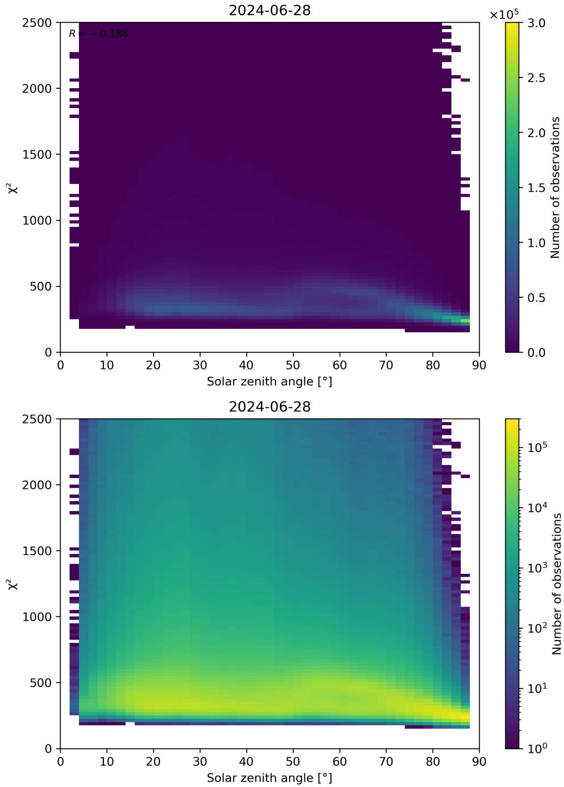
Figure 148: Scatter density plot of “Solar zenith angle” against “ \chi^2 ” for 2024-06-27 to 2024-06-29.
