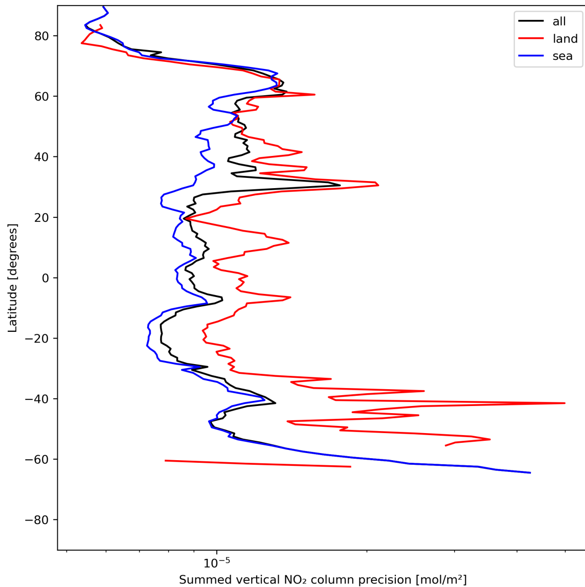
Figure 24: Zonal average of “Summed vertical NO 2 column precision” for 2024-06-27 to 2024-06-29.
