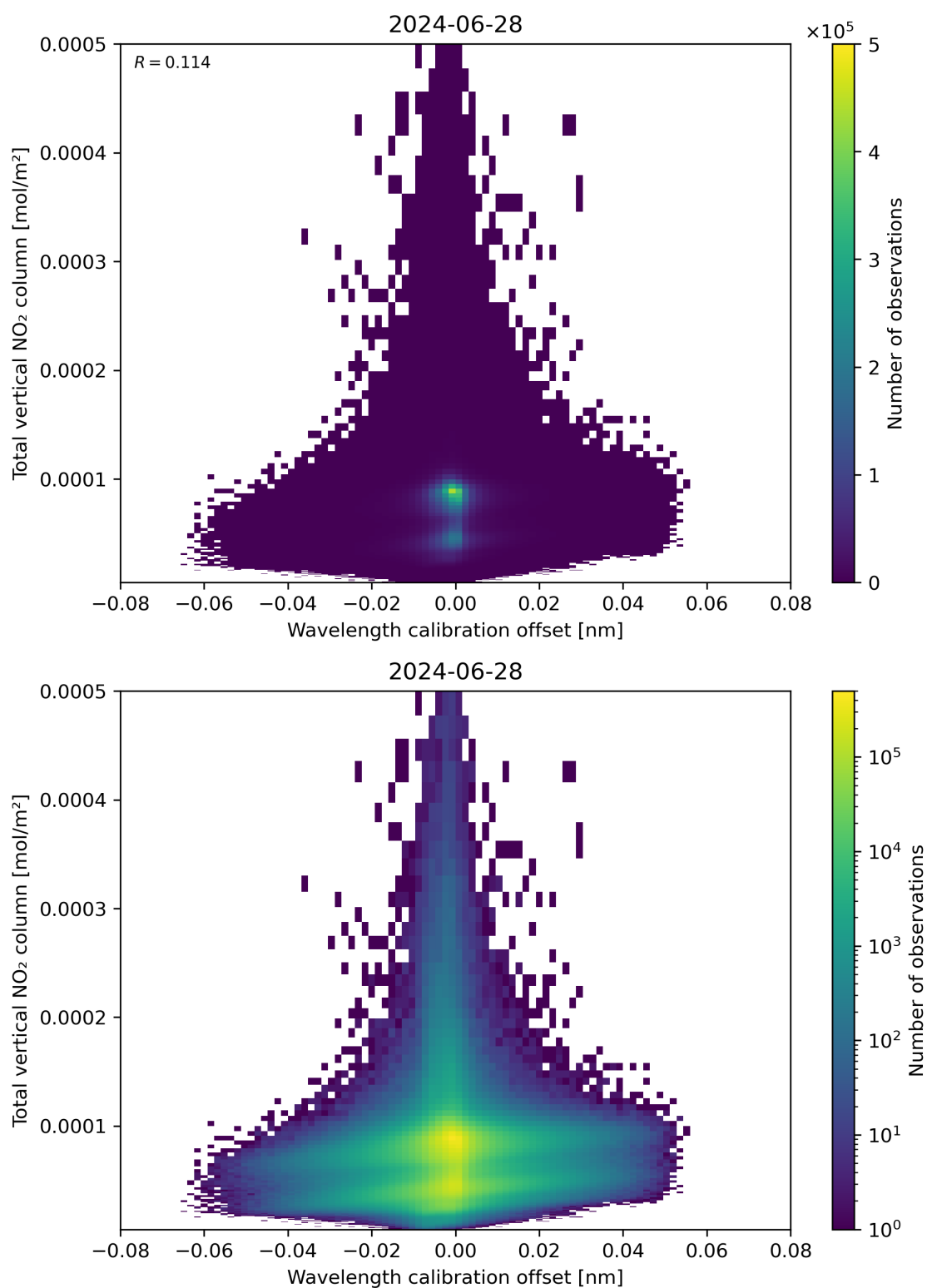
Figure 179: Scatter density plot of “Wavelength calibration offset” against “Total vertical NO 2 column” for 2024-06-27 to 2024-06-29.
