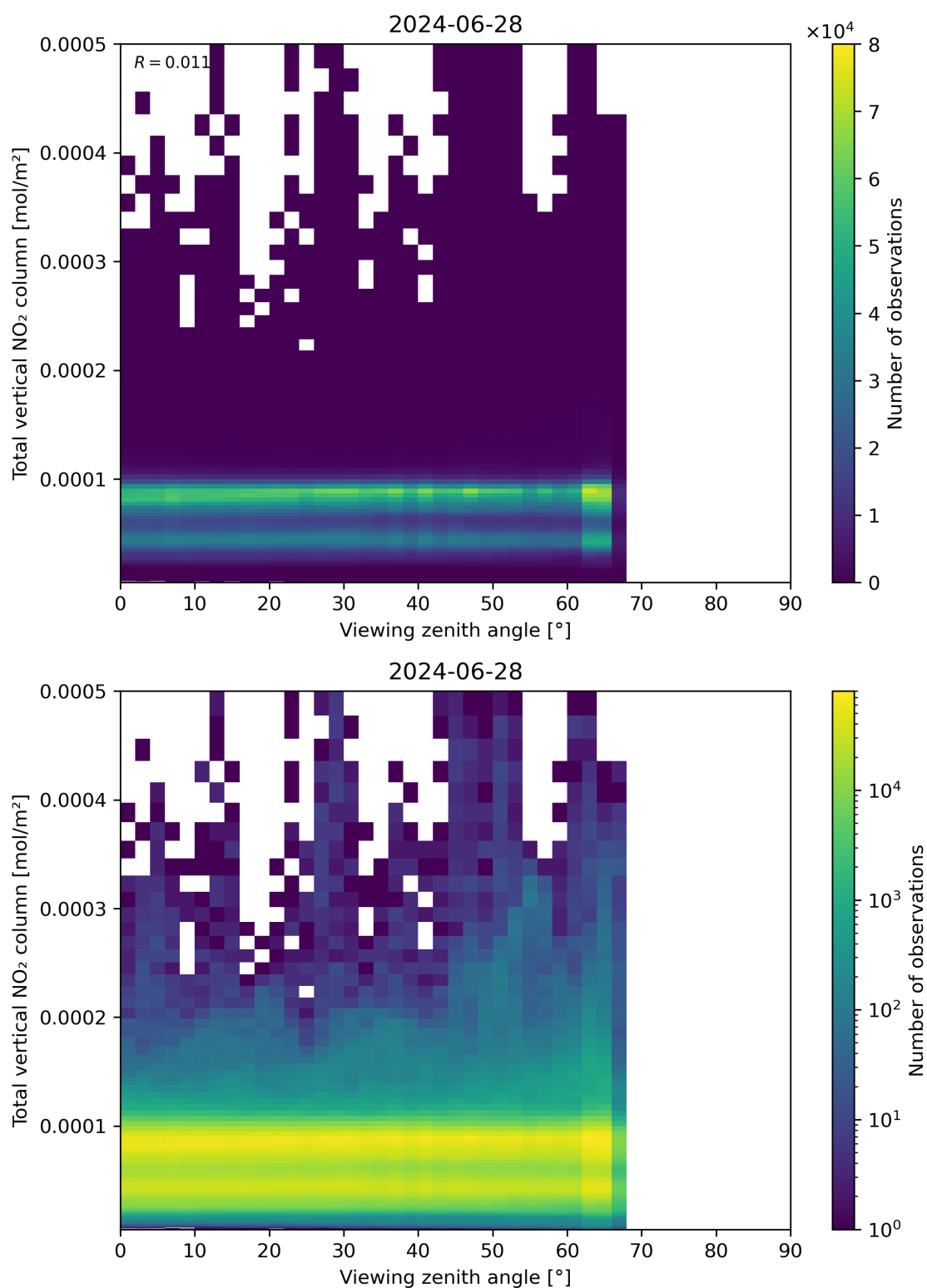
Figure 167: Scatter density plot of “Viewing zenith angle” against “Total vertical NO 2 column” for 2024-06-27 to 2024-06-29.
