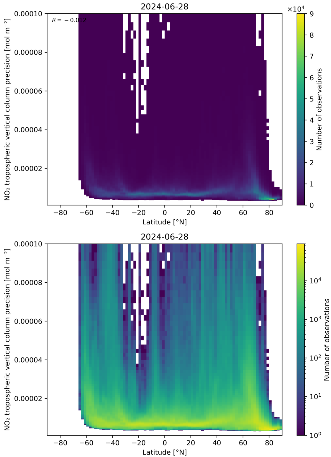
Figure 93: Scatter density plot of “Latitude” against “NO 2 tropospheric vertical column precision” for 2024-06-27 to 2024-06-29.
