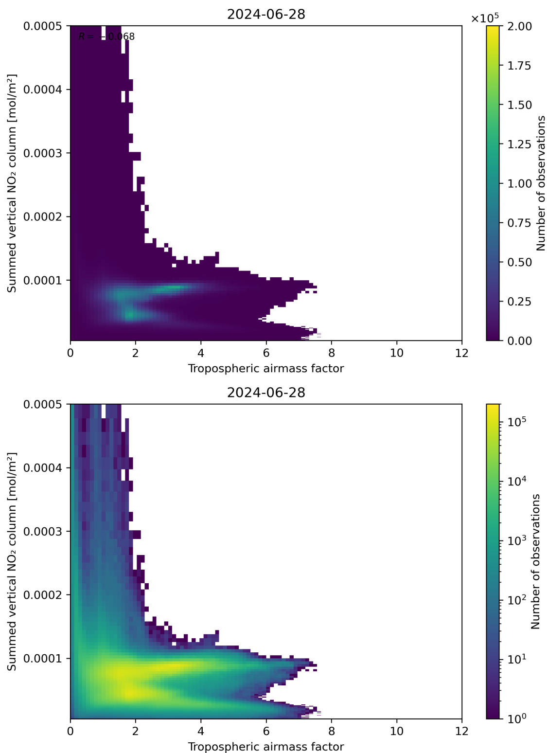
Figure 75: Scatter density plot of “Tropospheric airmass factor” against “Summed vertical NO 2 column” for 2024-06-27 to 2024-06-29.
