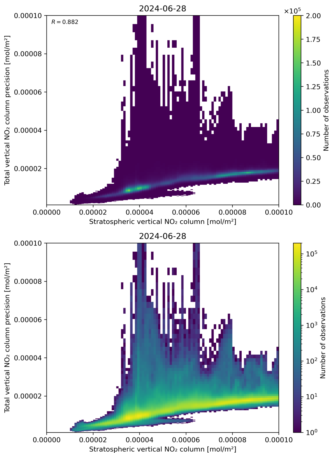
Figure 101: Scatter density plot of “Stratospheric vertical NO 2 column” against “Total vertical NO 2 column precision” for 2024-06-27 to 2024-06-29.
