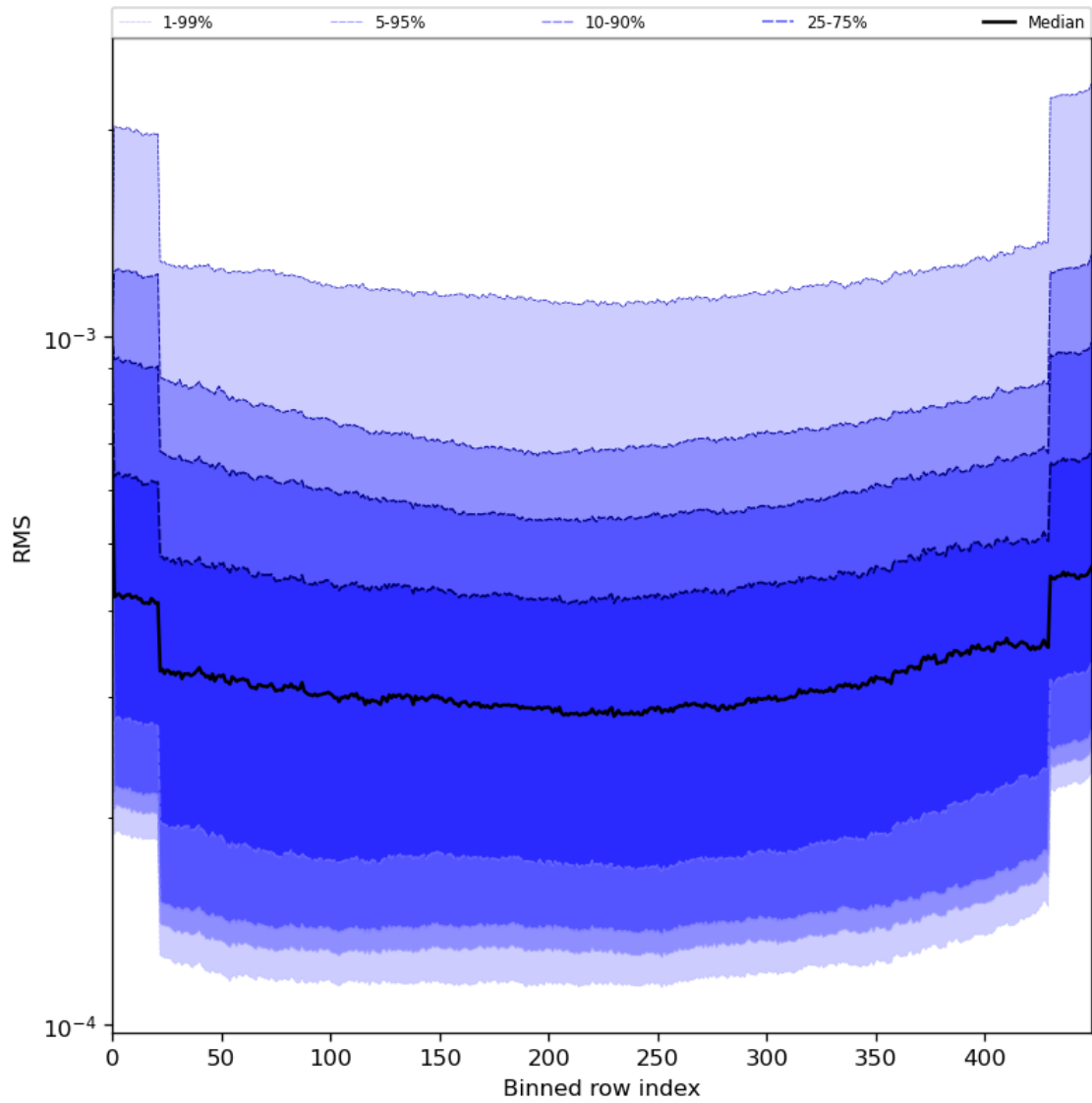
Figure 60: Along track statistics of “RMS” for 2024-06-27 to 2024-06-29
