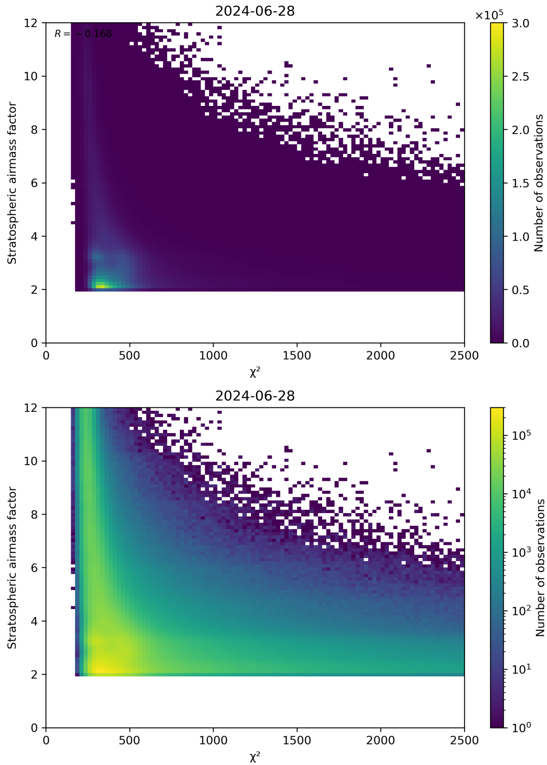
Figure 81: Scatter density plot of “ \chi^2 ” against “Stratospheric air mass factor” for 2024-06-27 to 2024-06-29.
