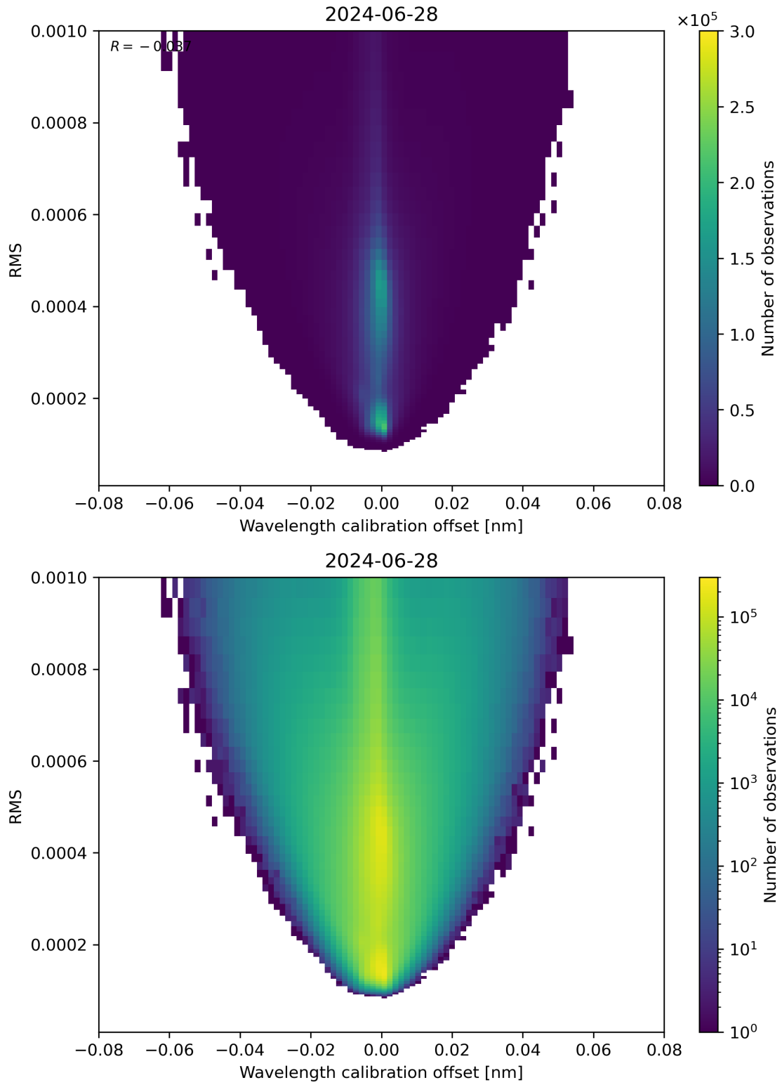
Figure 181: Scatter density plot of “Wavelength calibration offset” against “RMS” for 2024-06-27 to 2024-06-29.
