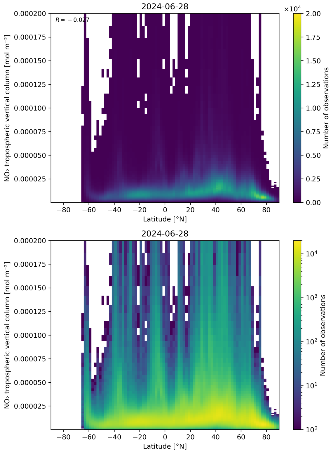
Figure 92: Scatter density plot of “Latitude” against “NO 2 tropospheric vertical column” for 2024-06-27 to 2024-06-29.
