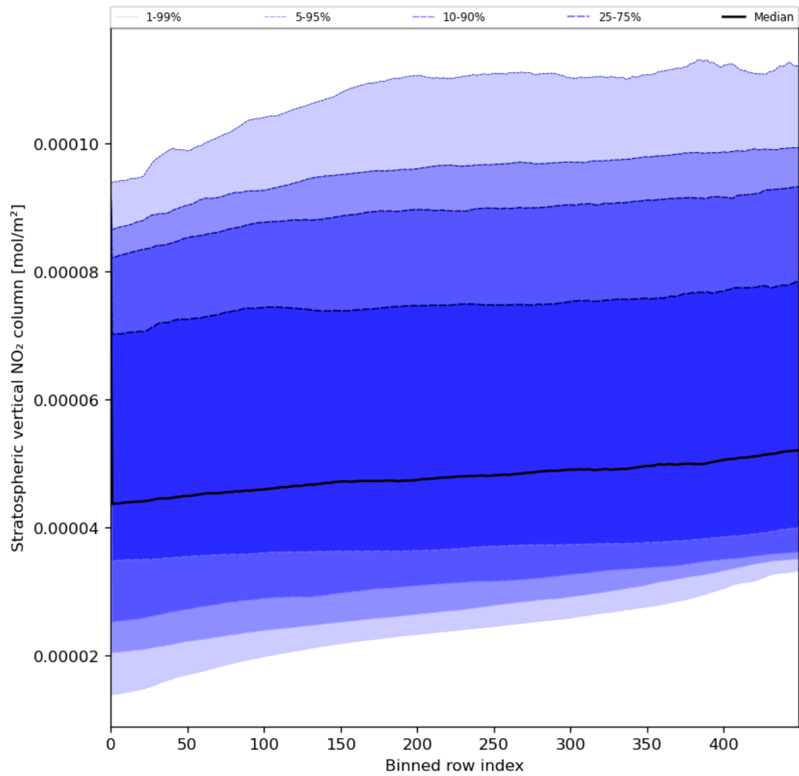
Figure 53: Along track statistics of “Stratospheric vertical NO 2 column” for 2024-06-27 to 2024-06-29
