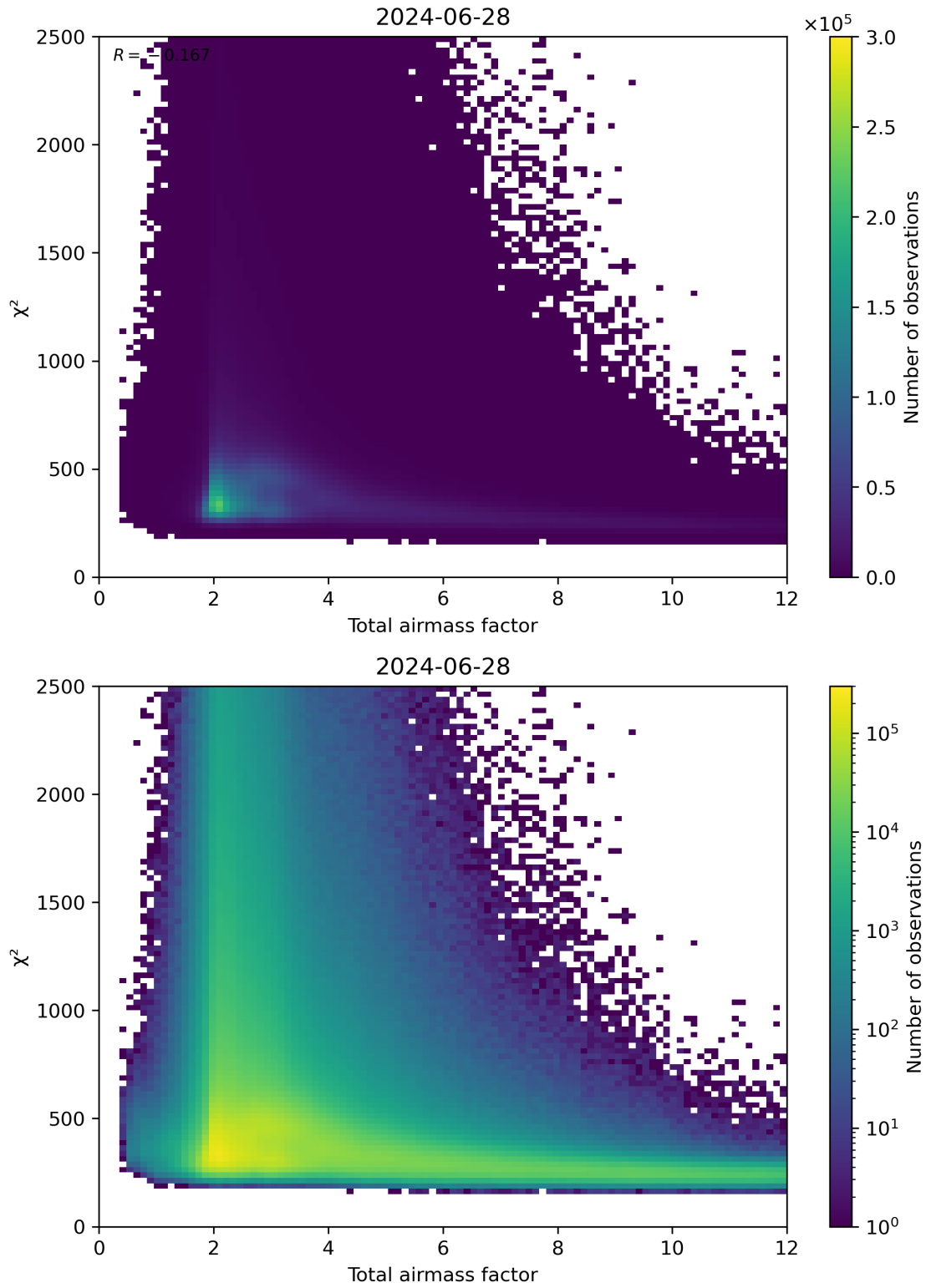
Figure 63: Scatter density plot of “Total airmass factor” against “ \chi^2 ” for 2024-06-27 to 2024-06-29.
