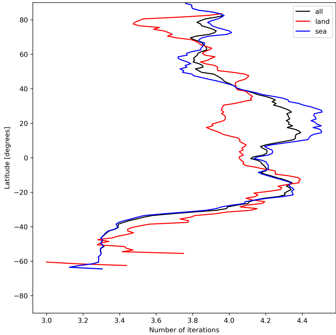
Figure 17: Zonal average of “Number of iterations” for 2024-06-27 to 2024-06-29.
