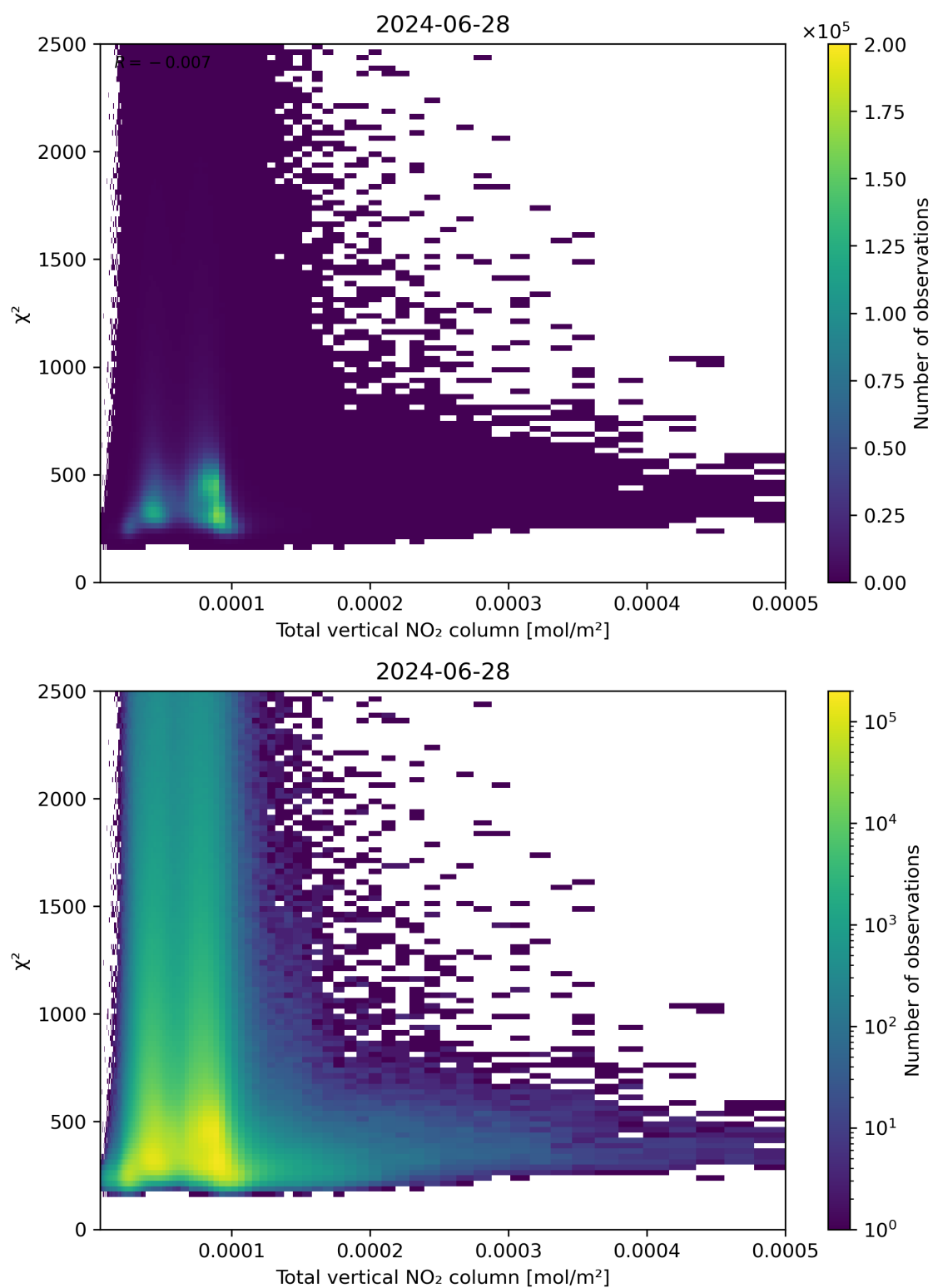
Figure 111: Scatter density plot of “Total vertical NO 2 column” against “ \chi^2 ” for 2024-06-27 to 2024-06-29.
