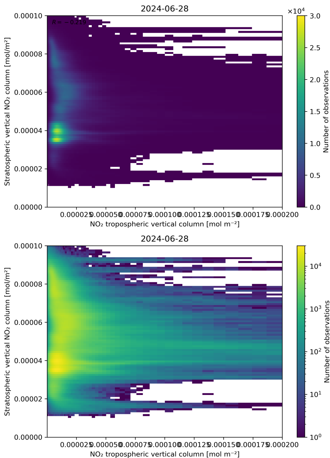
Figure 125: Scatter density plot of “NO 2 tropospheric vertical column” against “Stratospheric vertical NO 2 column” for 2024-06-27 to 2024-06-29.
