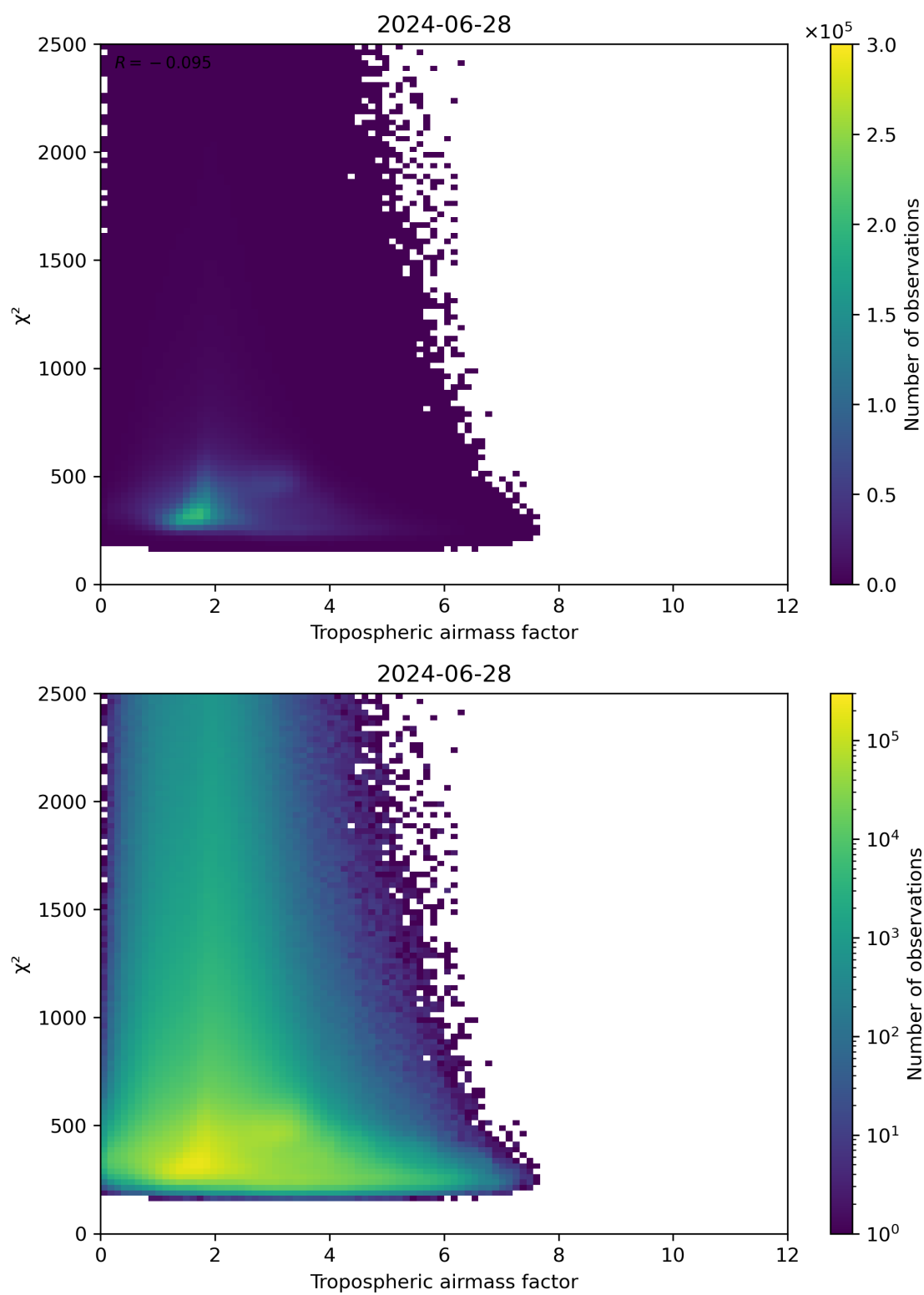
Figure 73: Scatter density plot of “Tropospheric airmass factor” against “ \chi^2 ” for 2024-06-27 to 2024-06-29.
