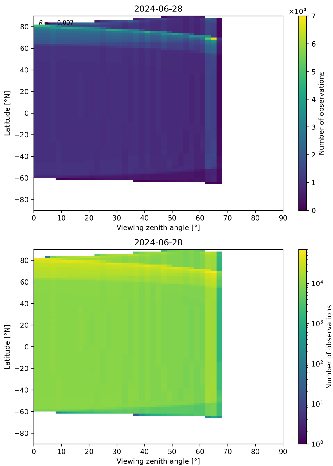
Figure 163: Scatter density plot of “Viewing zenith angle” against “Latitude” for 2024-06-27 to 2024-06-29.
