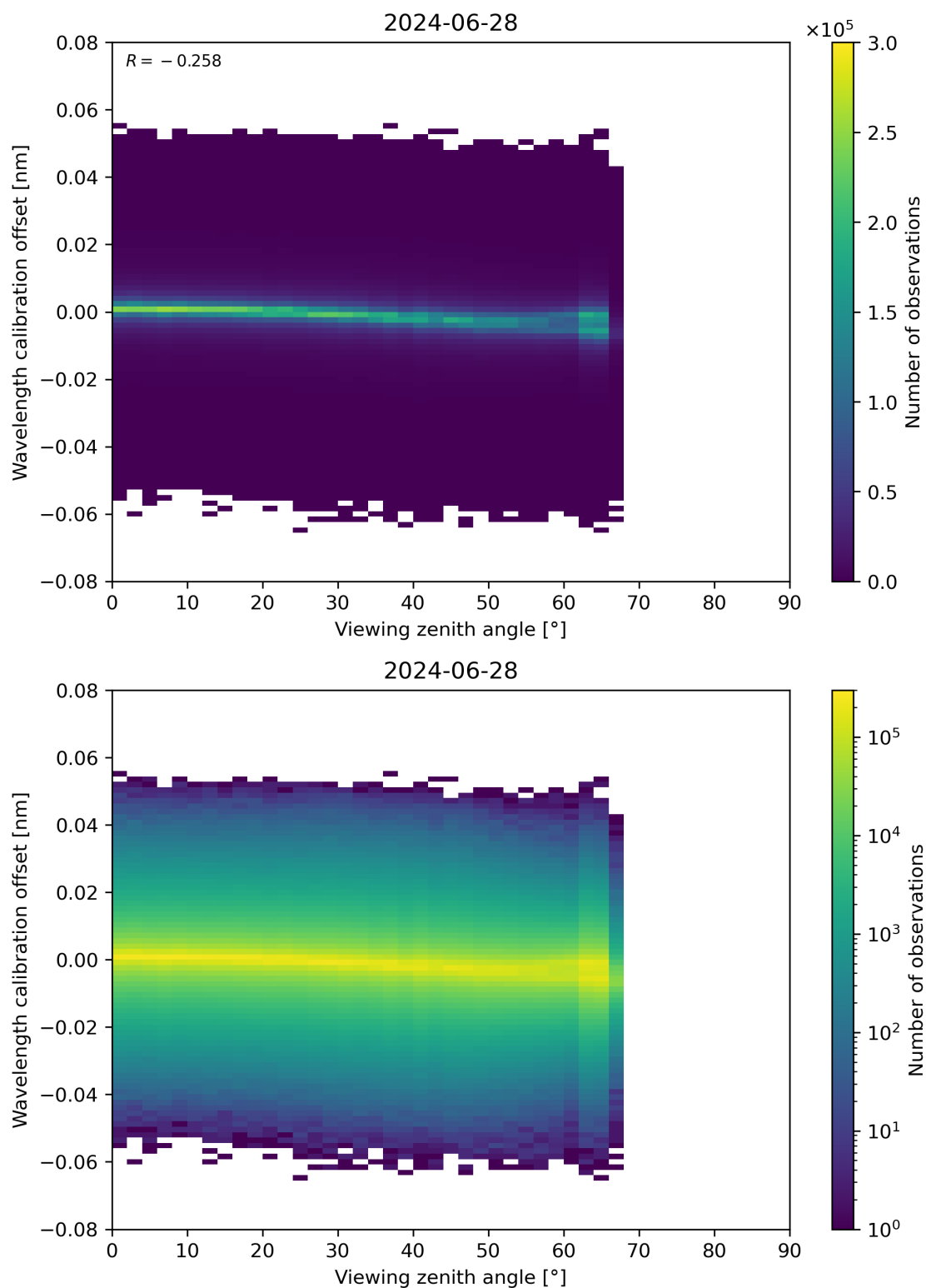
Figure 173: Scatter density plot of “Viewing zenith angle” against “Wavelength calibration offset” for 2024-06-27 to 2024-06-29.
