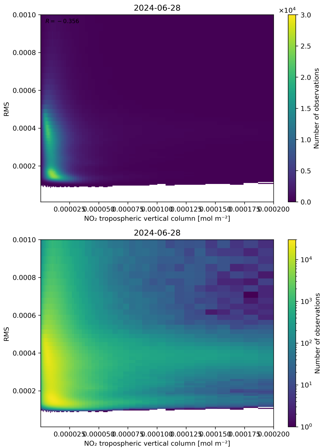
Figure 142: Scatter density plot of “NO 2 tropospheric vertical column” against “RMS” for 2024-06-27 to 2024-06-29.
