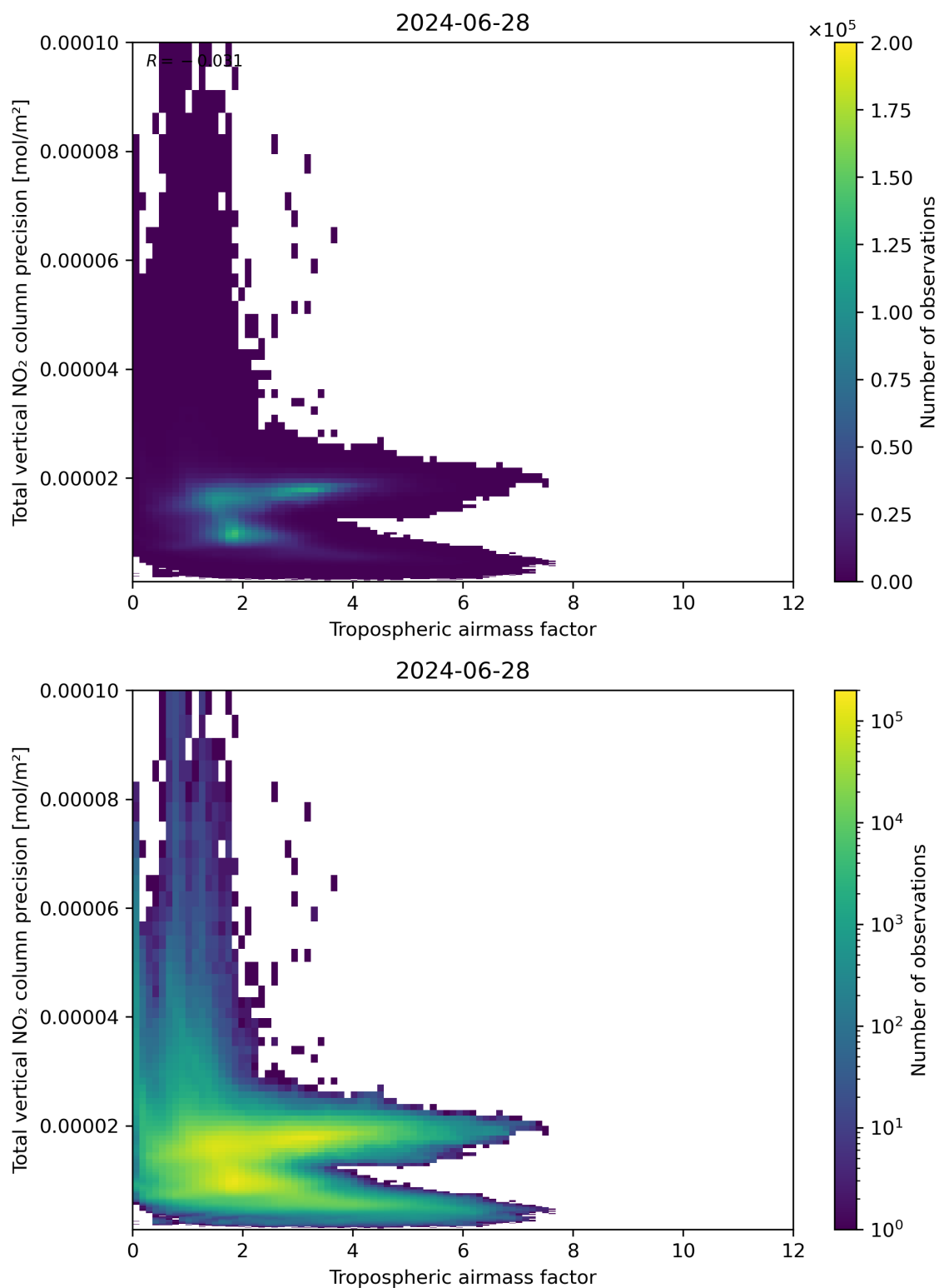
Figure 78: Scatter density plot of “Tropospheric air mass factor” against “Total vertical NO 2 column precision” for 2024-06-27 to 2024-06-29.
