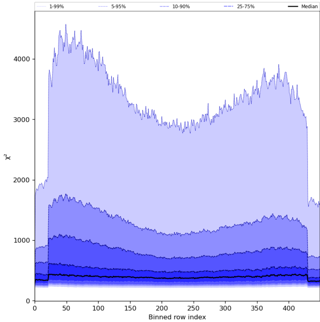
Figure 59: Along track statistics of “ \chi^2 ” for 2024-06-27 to 2024-06-29
