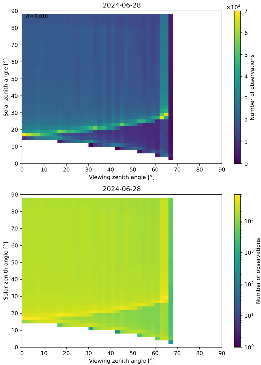
Figure 172: Scatter density plot of “Viewing zenith angle” against “Solar zenith angle” for 2024-06-27 to 2024-06-29.
