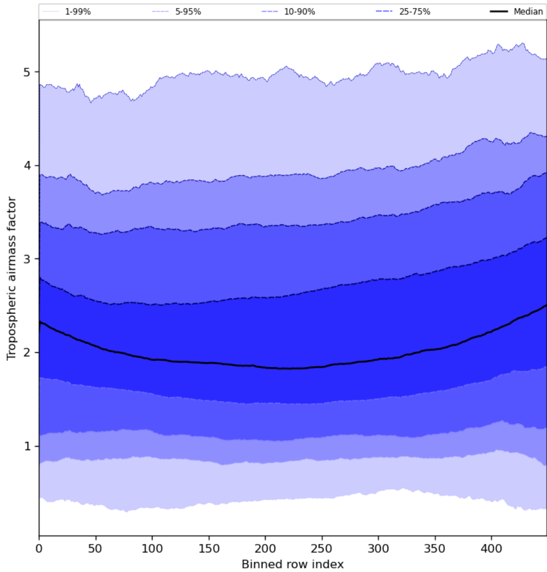
Figure 48: Along track statistics of “Tropospheric air mass factor” for 2024-06-27 to 2024-06-29
