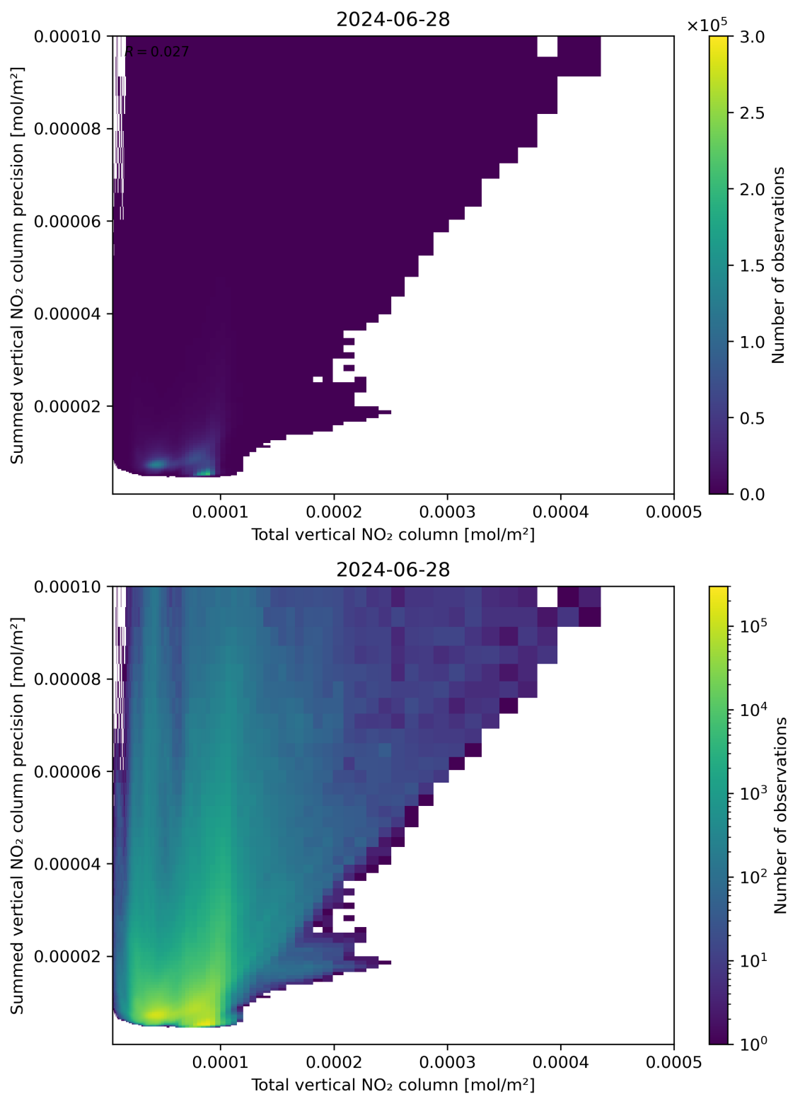
Figure 113: Scatter density plot of “Total vertical NO 2 column” against “Summed vertical NO 2 column precision” for 2024-06-27 to 2024-06-29.
