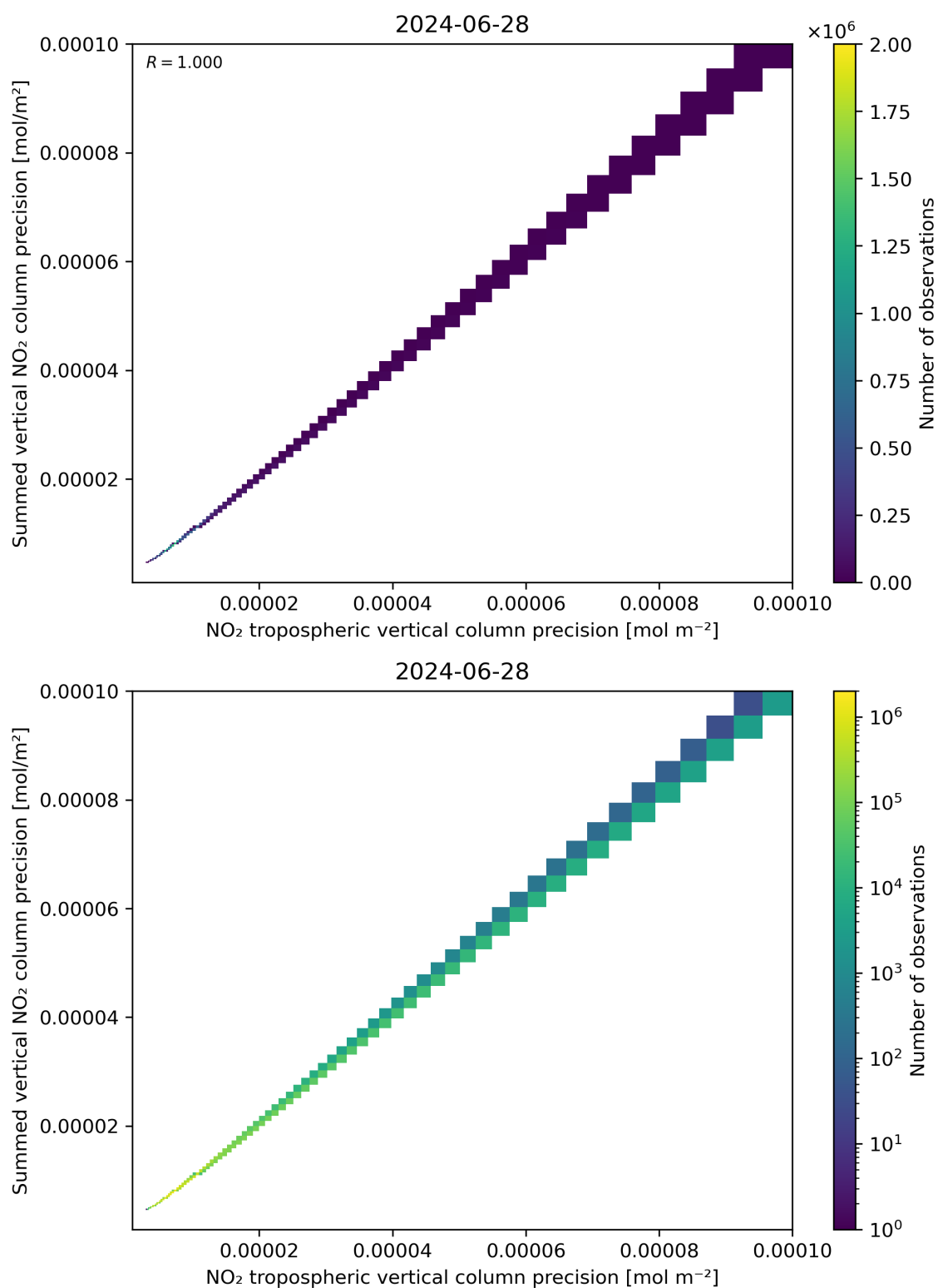
Figure 137: Scatter density plot of “NO 2 tropospheric vertical column precision” against “Summed vertical NO 2 column precision” for 2024-06-27 to 2024-06-29.
