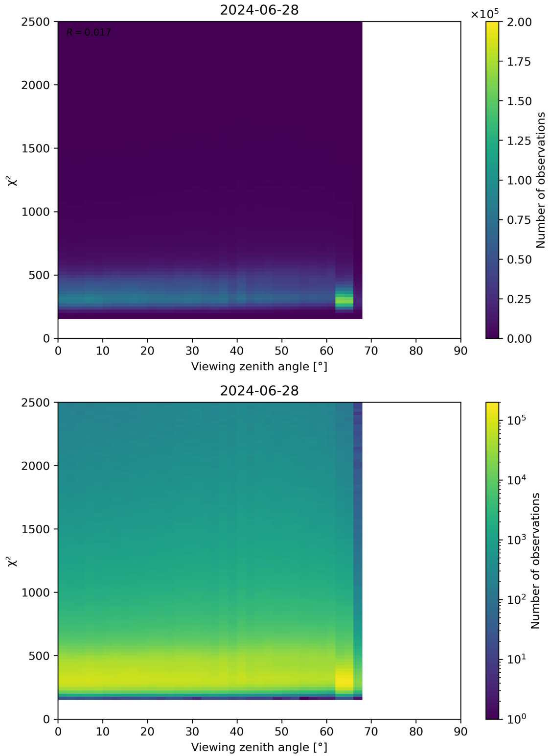
Figure 162: Scatter density plot of “Viewing zenith angle” against “ \chi^2 ” for 2024-06-27 to 2024-06-29.
