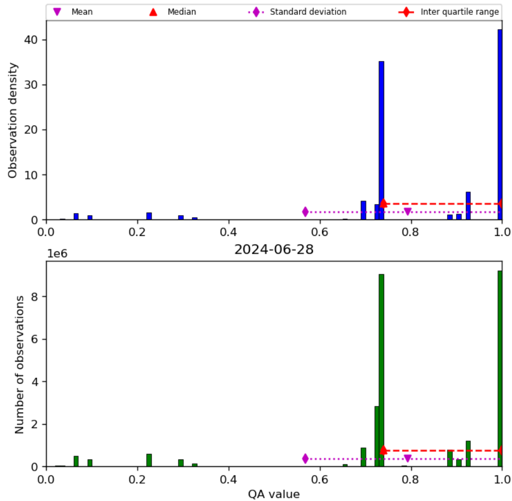
Figure 28: Histogram of “QA value” for 2024-06-27 to 2024-06-29
