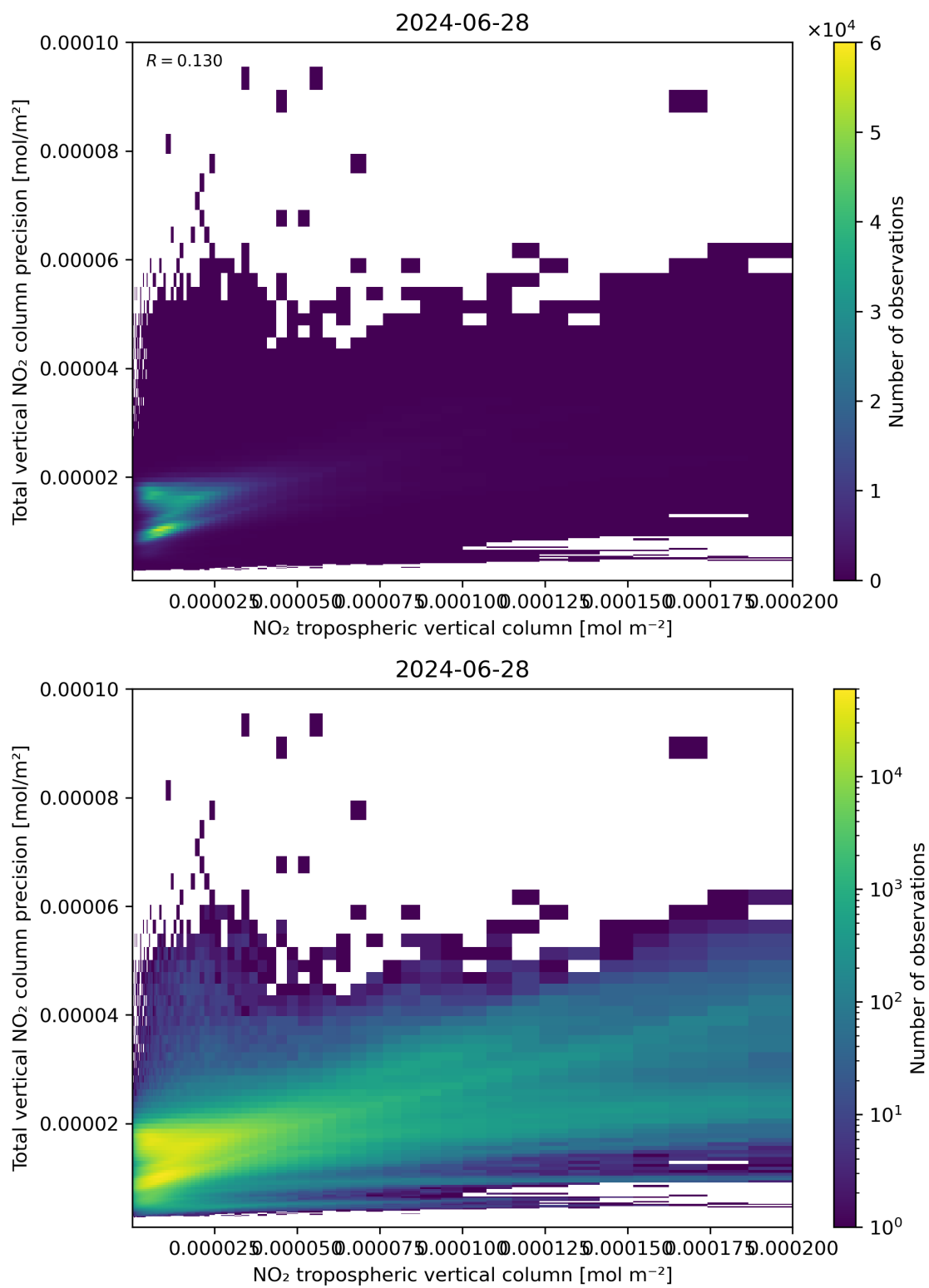
Figure 129: Scatter density plot of “NO 2 tropospheric vertical column” against “Total vertical NO 2 column precision” for 2024-06-27 to 2024-06-29.
