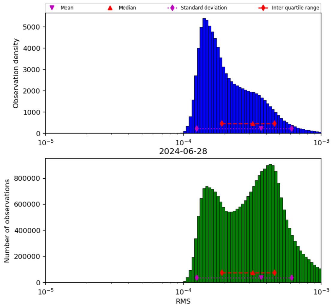
Figure 43: Histogram of “RMS” for 2024-06-27 to 2024-06-29
