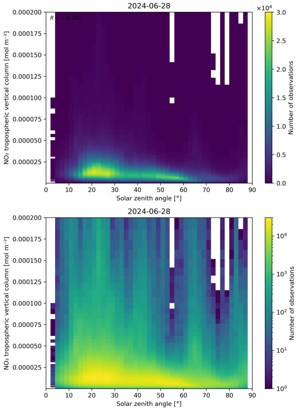
Figure 155: Scatter density plot of “Solar zenith angle” against “NO 2 tropospheric vertical column” for 2024-06-27 to 2024-06-29.
