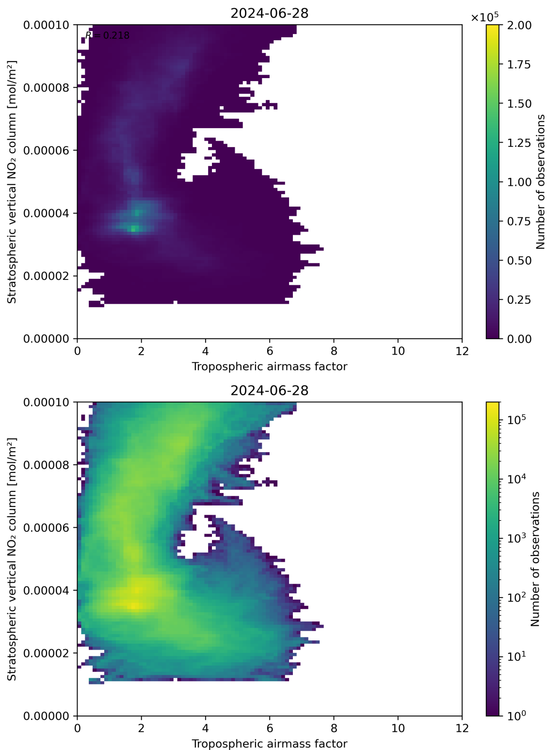
Figure 74: Scatter density plot of “Tropospheric air mass factor” against “Stratospheric vertical NO 2 column” for 2024-06-27 to 2024-06-29.
