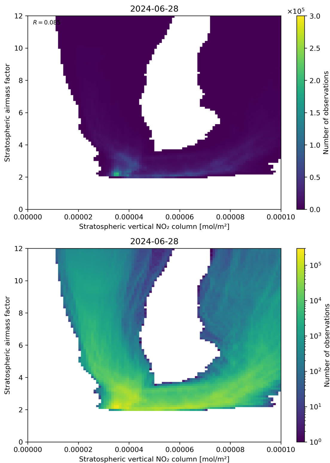
Figure 96: Scatter density plot of “Stratospheric vertical NO 2 column” against “Stratospheric airmass factor” for 2024-06-27 to 2024-06-29.
