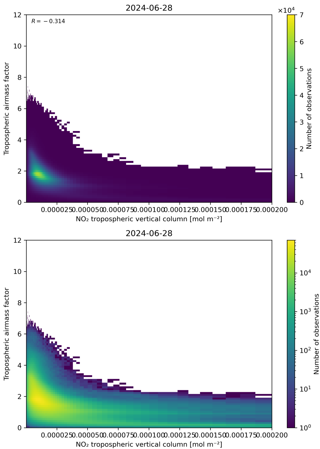
Figure 123: Scatter density plot of “NO 2 tropospheric vertical column” against “Tropospheric air mass factor” for 2024-06-27 to 2024-06-29.
