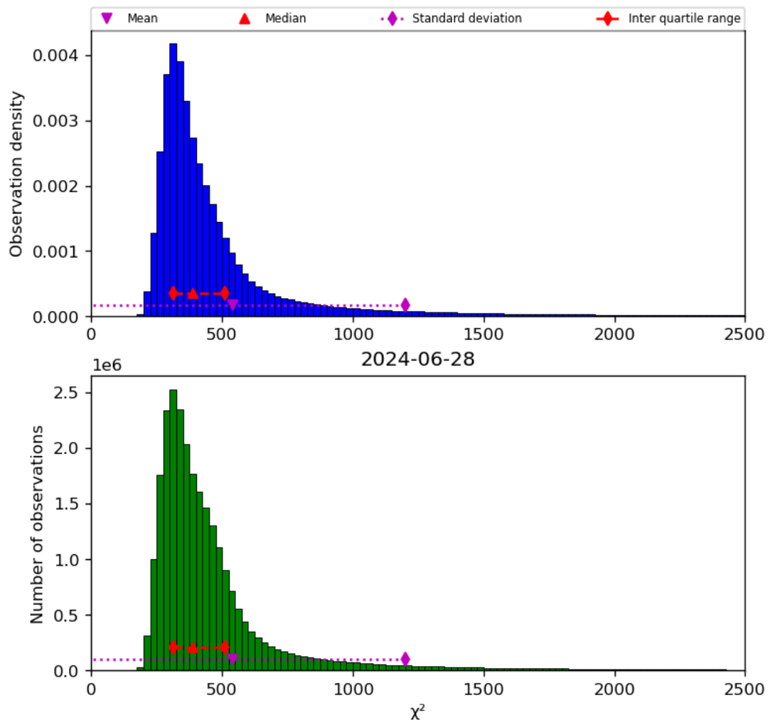
Figure 42: Histogram of “ \chi^2 ” for 2024-06-27 to 2024-06-29
