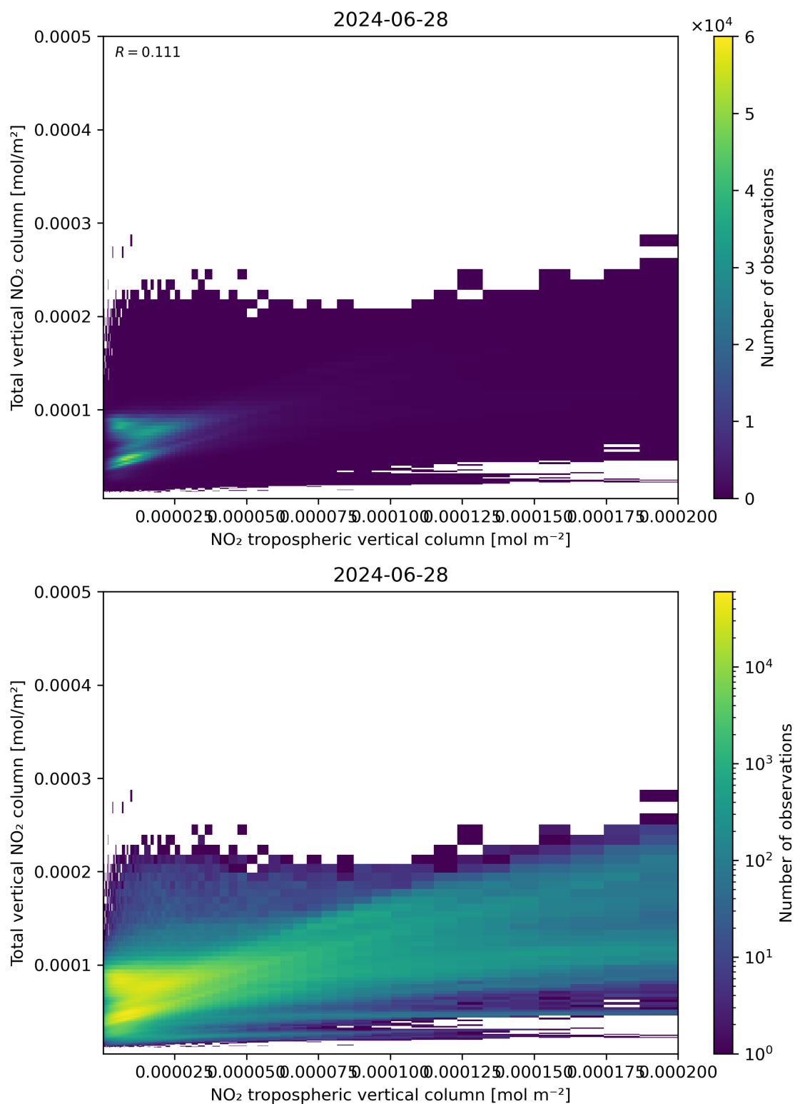
Figure 128: Scatter density plot of “NO 2 tropospheric vertical column” against “Total vertical NO 2 column” for 2024-06-27 to 2024-06-29.
