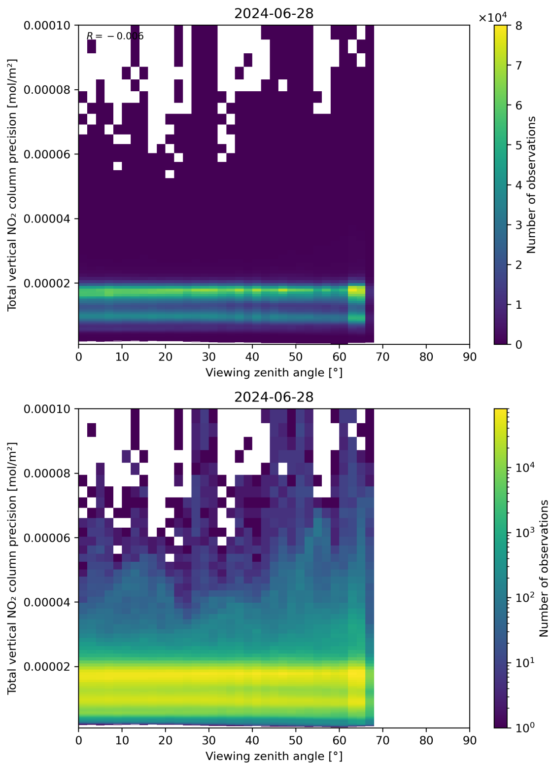
Figure 168: Scatter density plot of “Viewing zenith angle” against “Total vertical NO 2 column precision” for 2024-06-27 to 2024-06-29.
