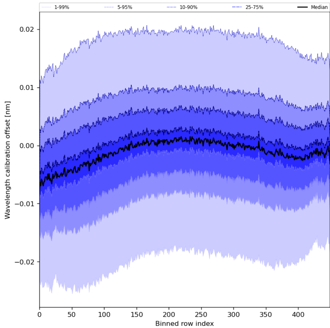
Figure 52: Along track statistics of “Wavelength calibration offset” for 2024-06-27 to 2024-06-29
