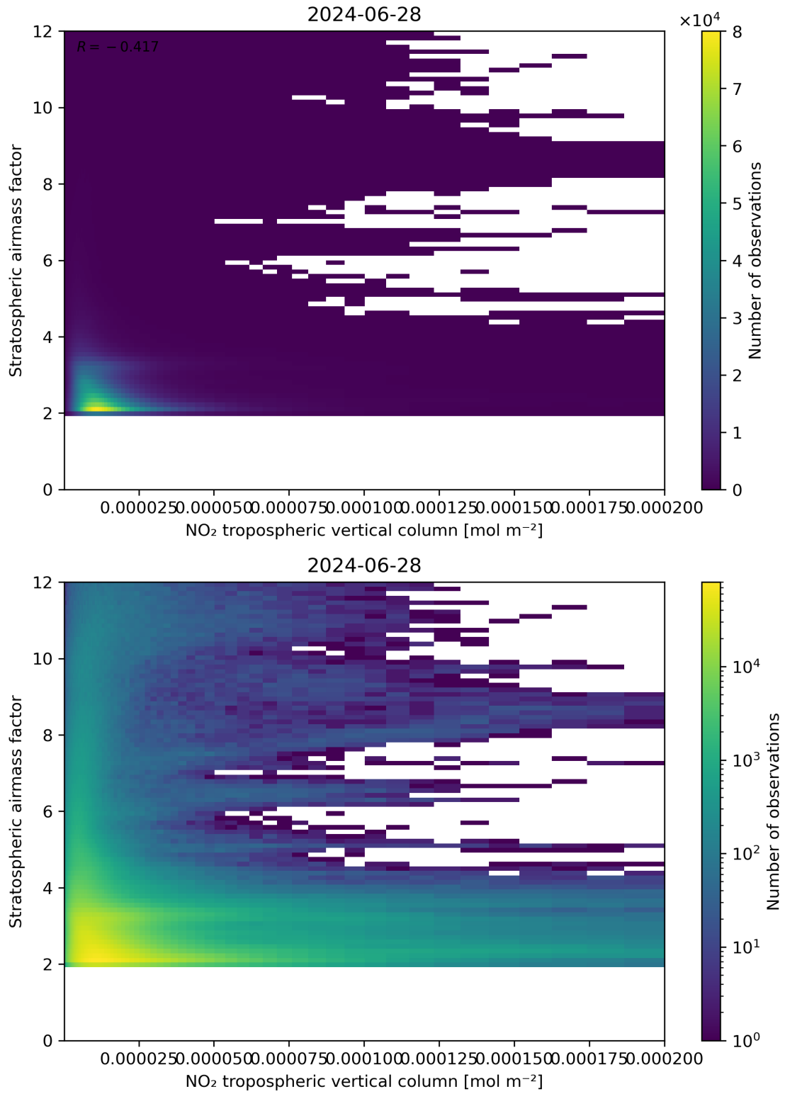
Figure 121: Scatter density plot of “NO 2 tropospheric vertical column” against “Stratospheric air mass factor” for 2024-06-27 to 2024-06-29.
