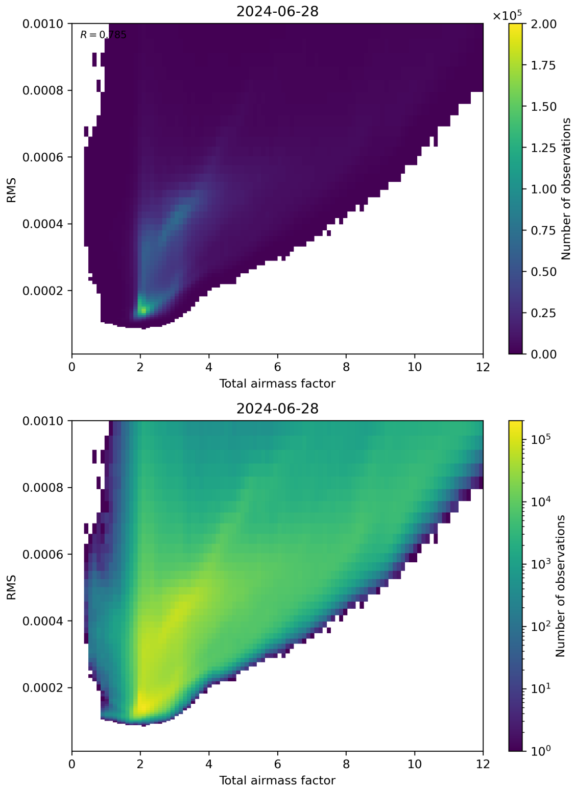
Figure 69: Scatter density plot of “Total airmass factor” against “RMS” for 2024-06-27 to 2024-06-29.
