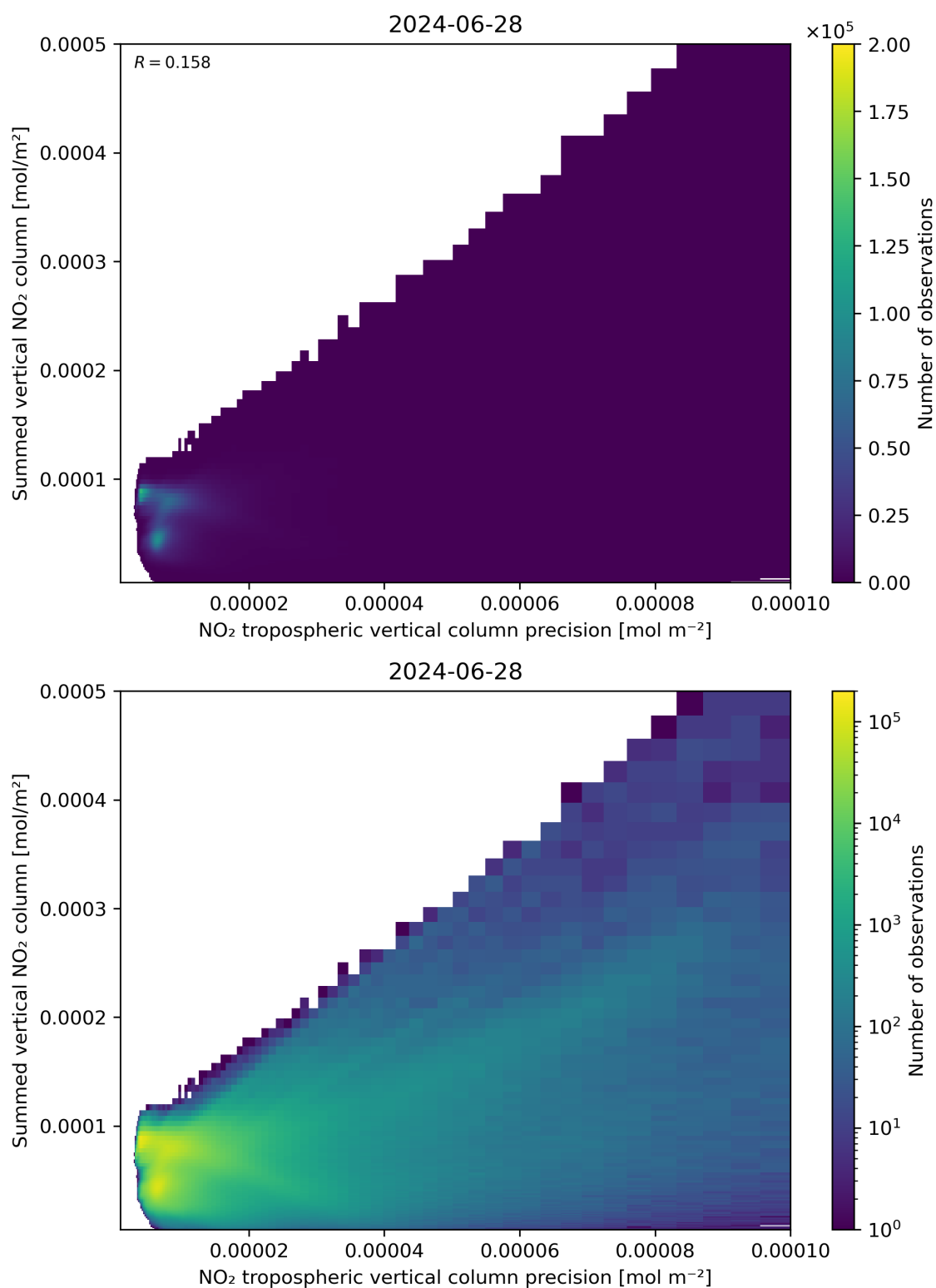
Figure 136: Scatter density plot of “NO 2 tropospheric vertical column precision” against “Summed vertical NO 2 column” for 2024-06-27 to 2024-06-29.
