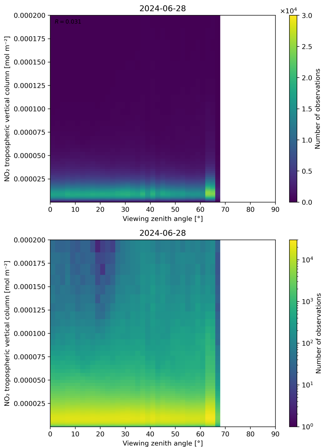
Figure 169: Scatter density plot of “Viewing zenith angle” against “NO 2 tropospheric vertical column” for 2024-06-27 to 2024-06-29.
