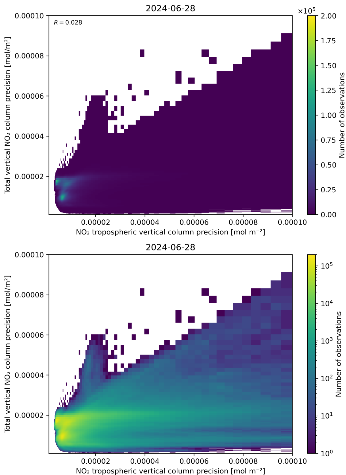
Figure 139: Scatter density plot of “NO 2 tropospheric vertical column precision” against “Total vertical NO 2 column precision” for 2024-06-27 to 2024-06-29.
