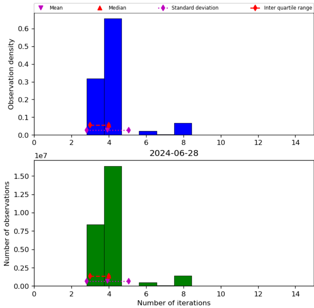
Figure 34: Histogram of “Number of iterations” for 2024-06-27 to 2024-06-29
