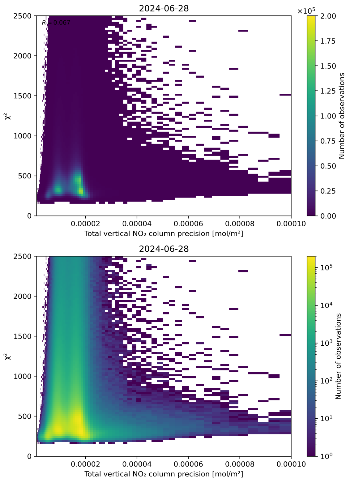
Figure 116: Scatter density plot of “Total vertical NO 2 column precision” against “ \chi^2 ” for 2024-06-27 to 2024-06-29.
