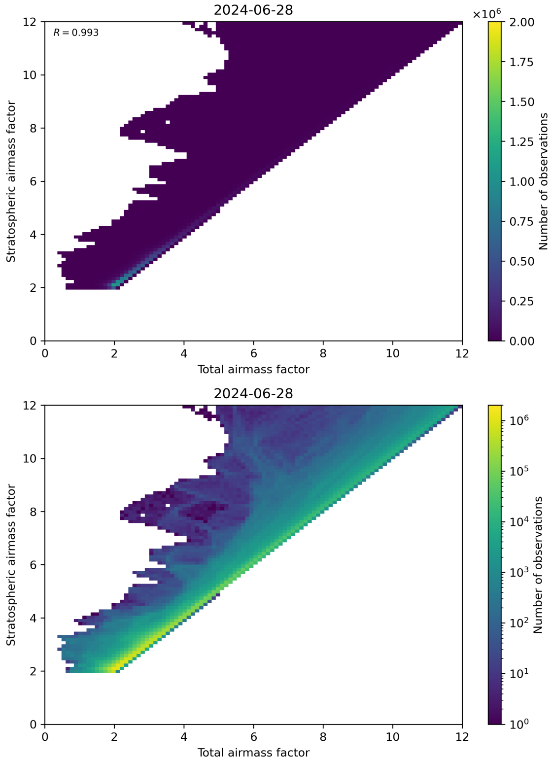
Figure 62: Scatter density plot of “Total airmass factor” against “Stratospheric airmass factor” for 2024-06-27 to 2024-06-29.
