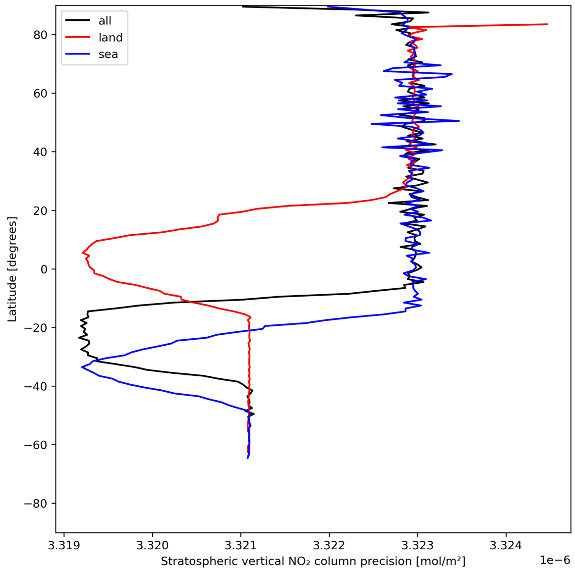
Figure 20: Zonal average of “Stratospheric vertical NO 2 column precision” for 2024-06-27 to 2024-06-29.
