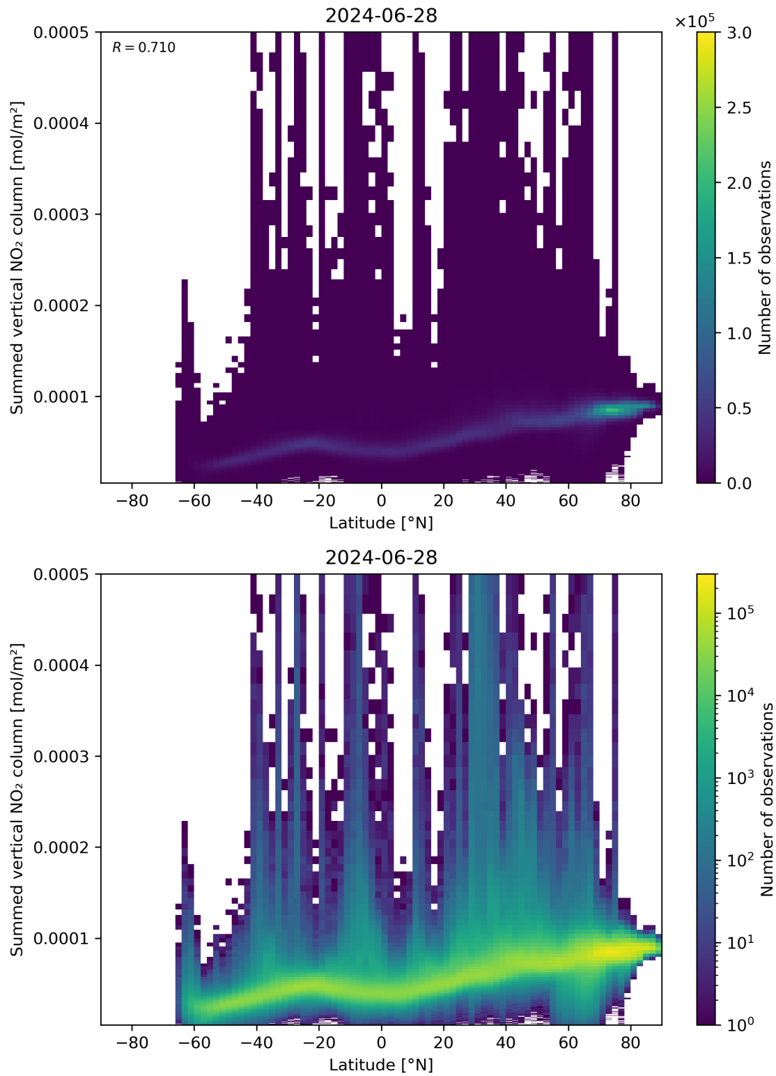
Figure 88: Scatter density plot of “Latitude” against “Summed vertical NO 2 column” for 2024-06-27 to 2024-06-29.
