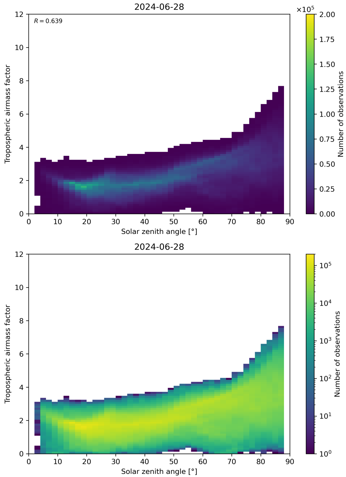
Figure 147: Scatter density plot of “Solar zenith angle” against “Tropospheric airmass factor” for 2024-06-27 to 2024-06-29.
