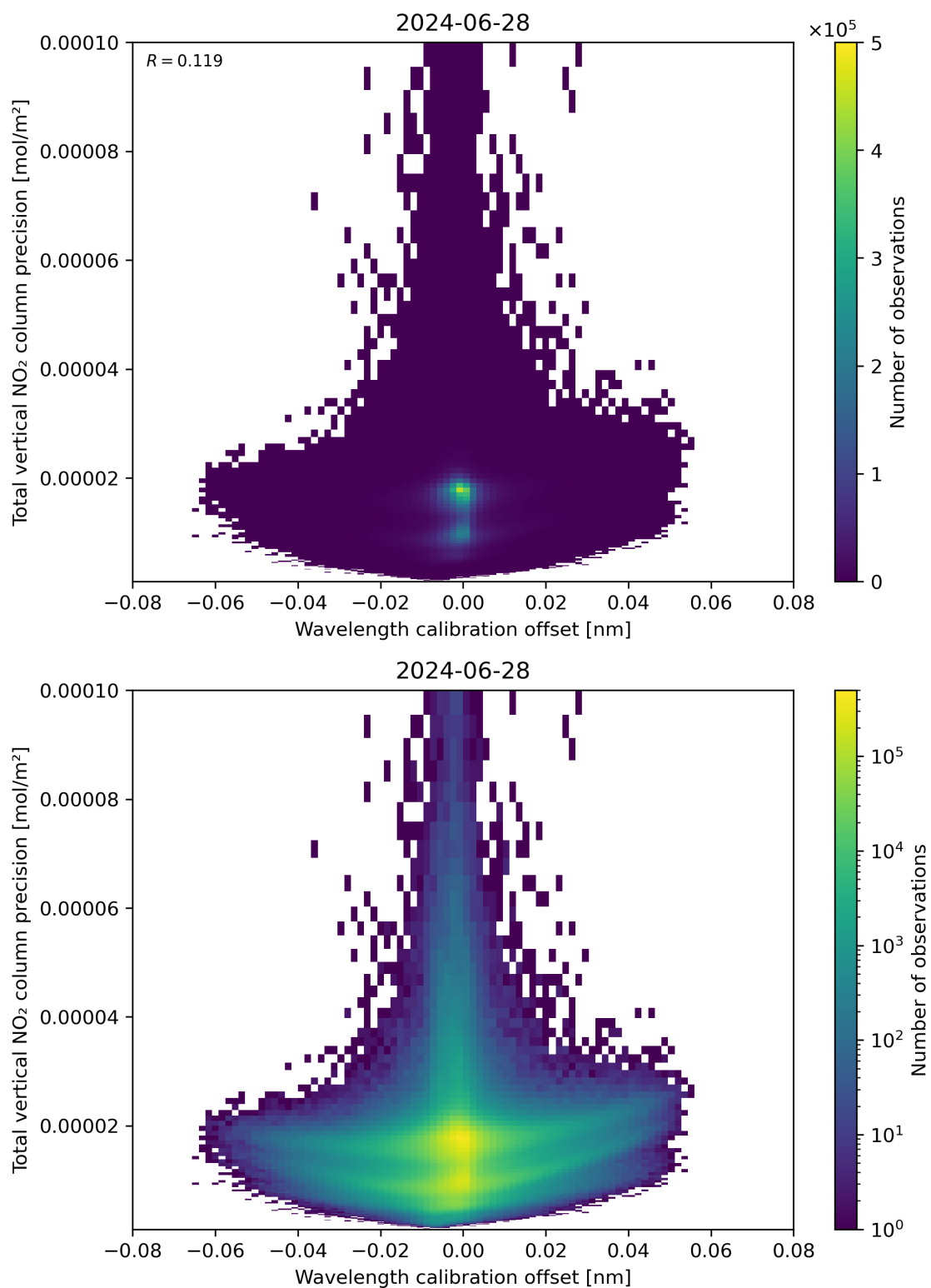
Figure 180: Scatter density plot of “Wavelength calibration offset” against “Total vertical NO 2 column precision” for 2024-06-27 to 2024-06-29.
