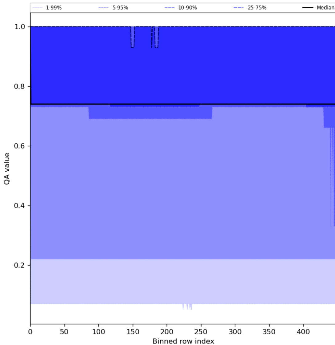
Figure 45: Along track statistics of “QA value” for 2024-06-27 to 2024-06-29
