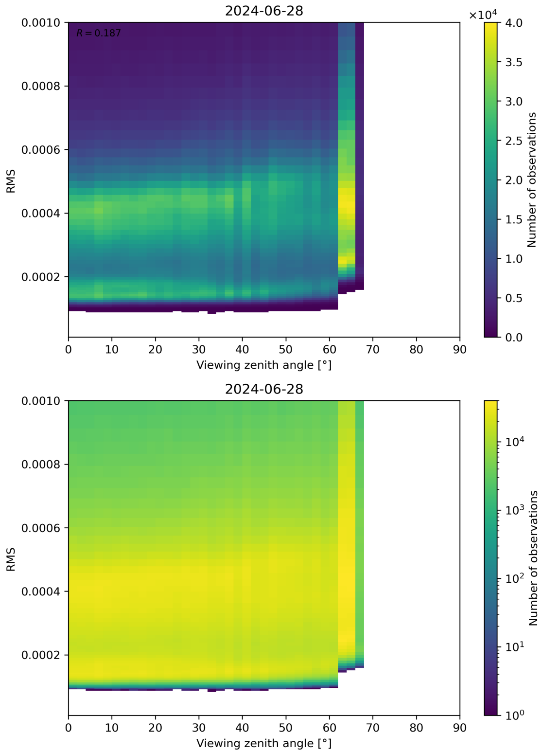
Figure 171: Scatter density plot of “Viewing zenith angle” against “RMS” for 2024-06-27 to 2024-06-29.
