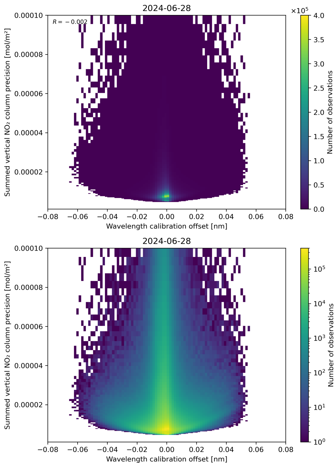
Figure 178: Scatter density plot of “Wavelength calibration offset” against “Summed vertical NO 2 column precision” for 2024-06-27 to 2024-06-29.
