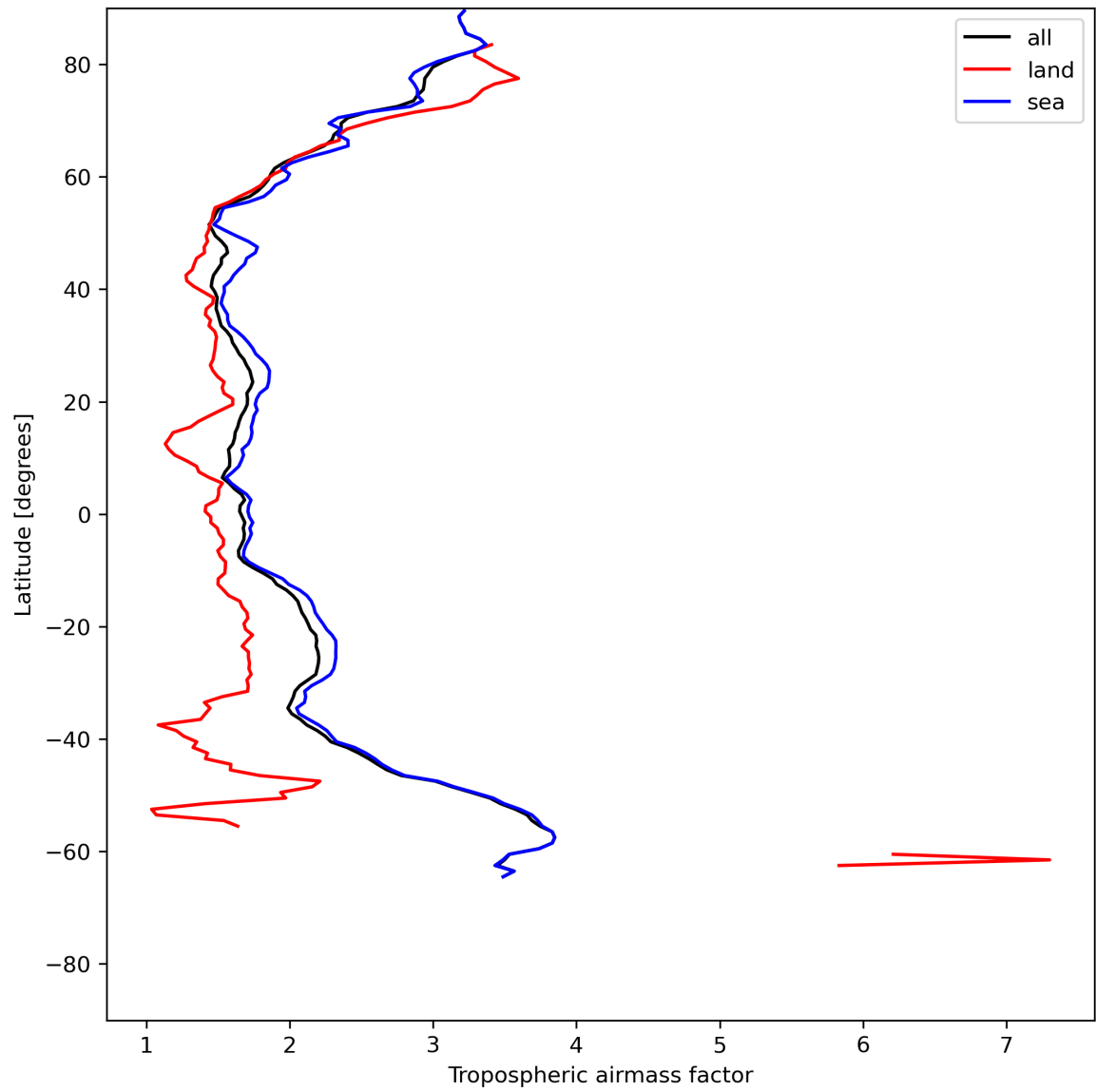
Figure 14: Zonal average of “Tropospheric airmass factor” for 2024-06-27 to 2024-06-29.
