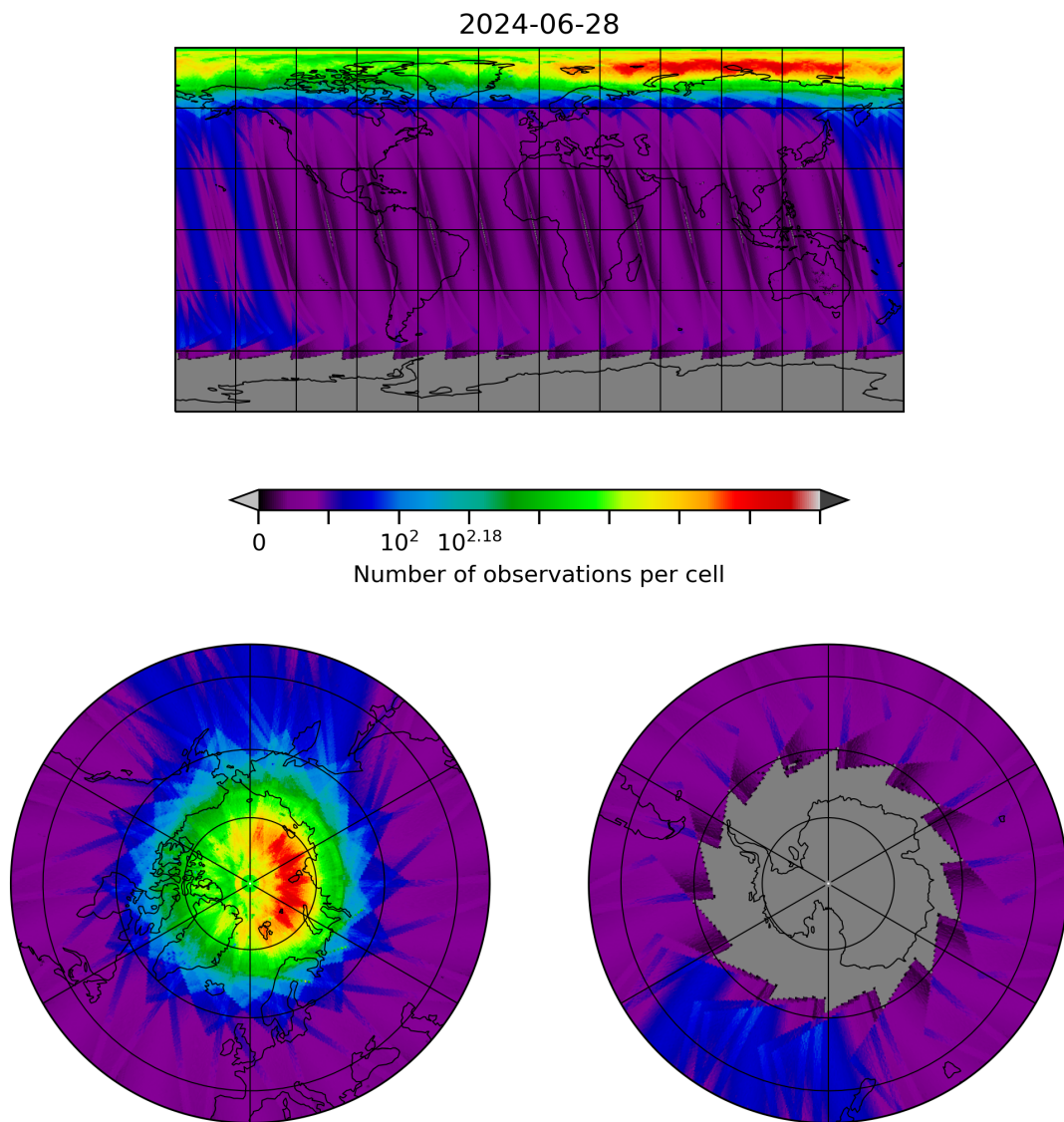
Figure 10: Map of the number of observations for 2024-06-27 to 2024-06-29
