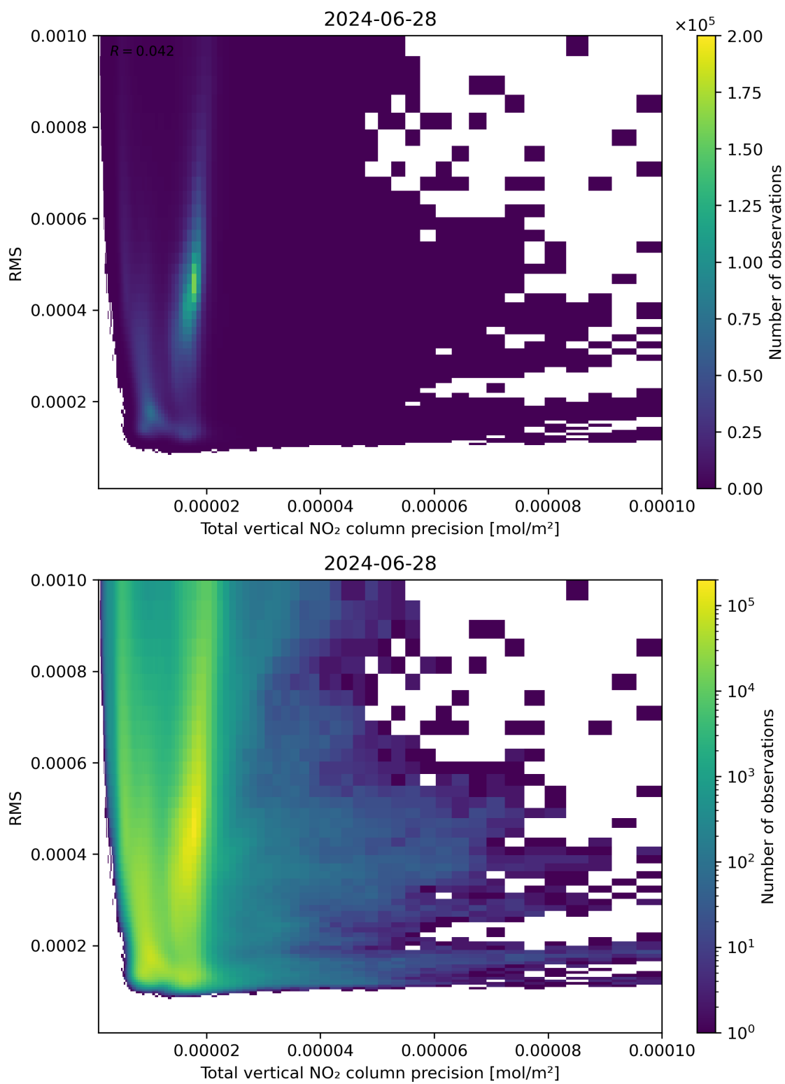
Figure 119: Scatter density plot of “Total vertical NO 2 column precision” against “RMS” for 2024-06-27 to 2024-06-29.
