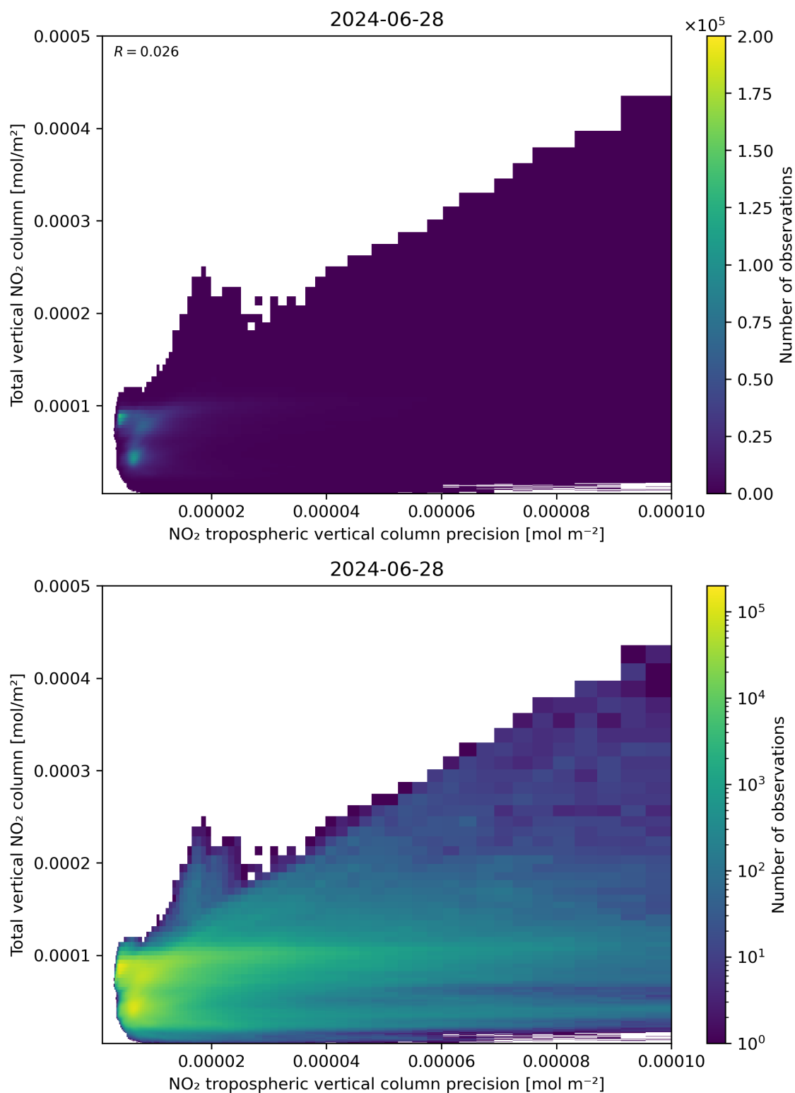
Figure 138: Scatter density plot of “NO 2 tropospheric vertical column precision” against “Total vertical NO 2 column” for 2024-06-27 to 2024-06-29.
