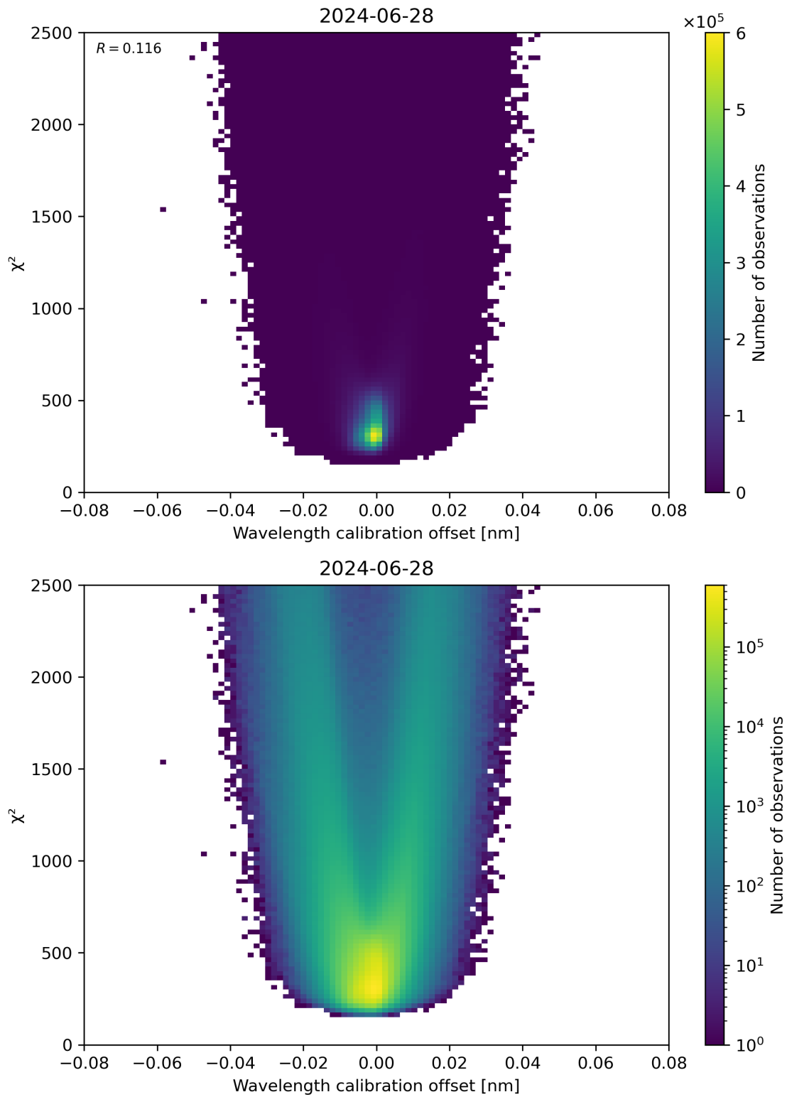
Figure 175: Scatter density plot of “Wavelength calibration offset” against “ \chi^2 ” for 2024-06-27 to 2024-06-29.
