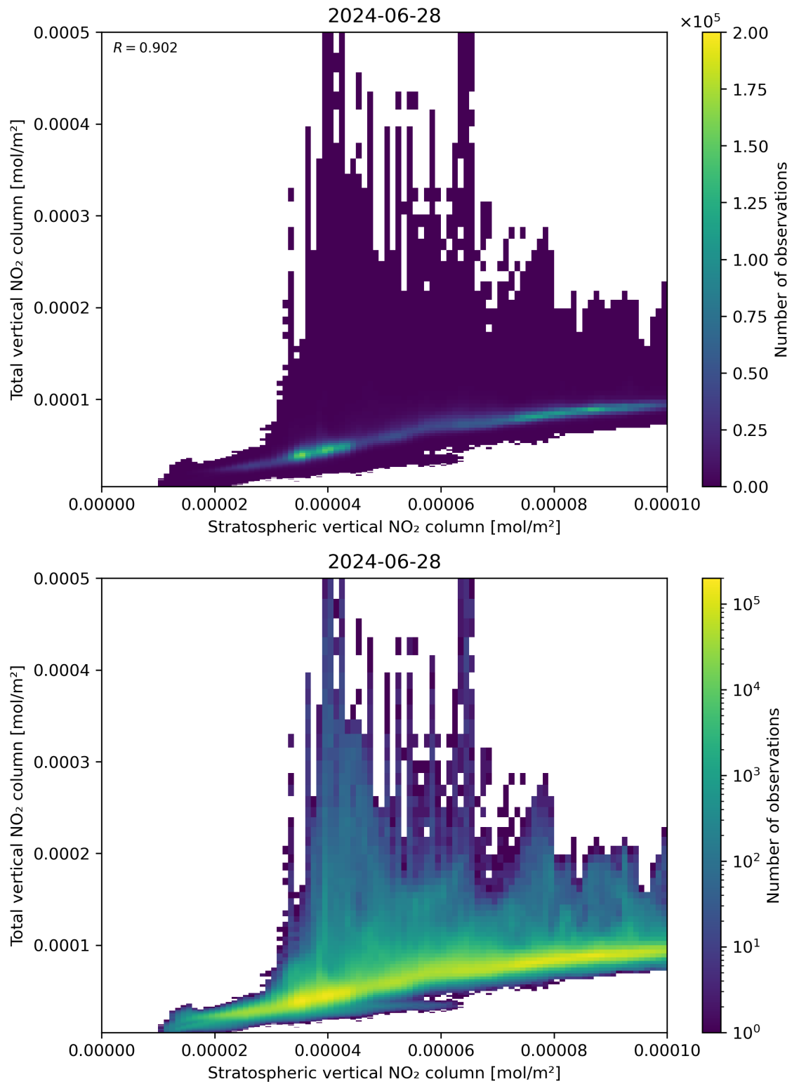
Figure 100: Scatter density plot of “Stratospheric vertical NO 2 column” against “Total vertical NO 2 column” for 2024-06-27 to 2024-06-29.
