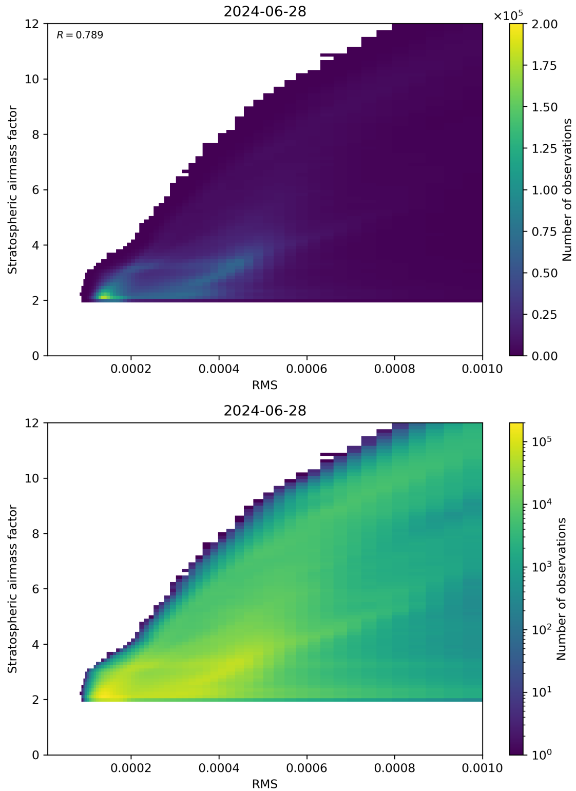
Figure 144: Scatter density plot of “RMS” against “Stratospheric airmass factor” for 2024-06-27 to 2024-06-29.
