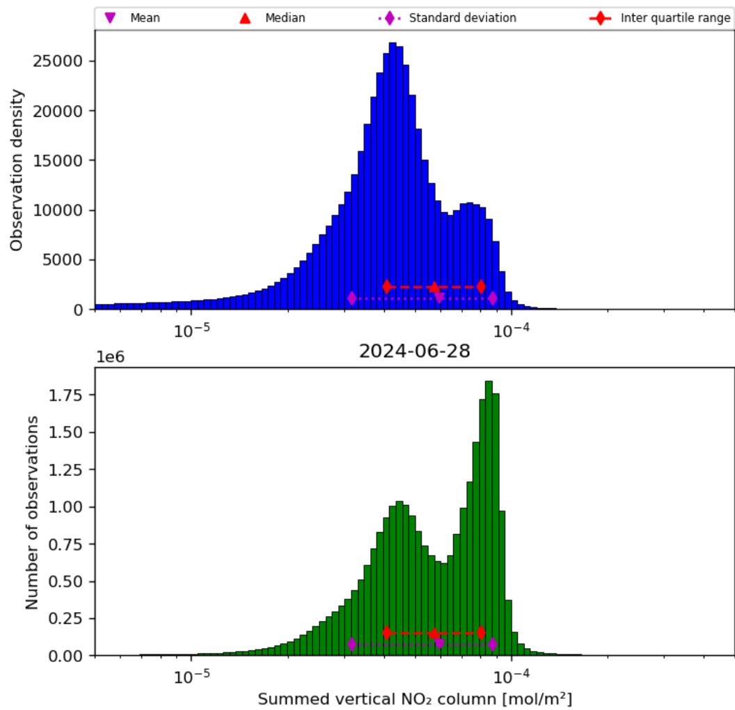
Figure 40: Histogram of “Summed vertical NO 2 column” for 2024-06-27 to 2024-06-29
