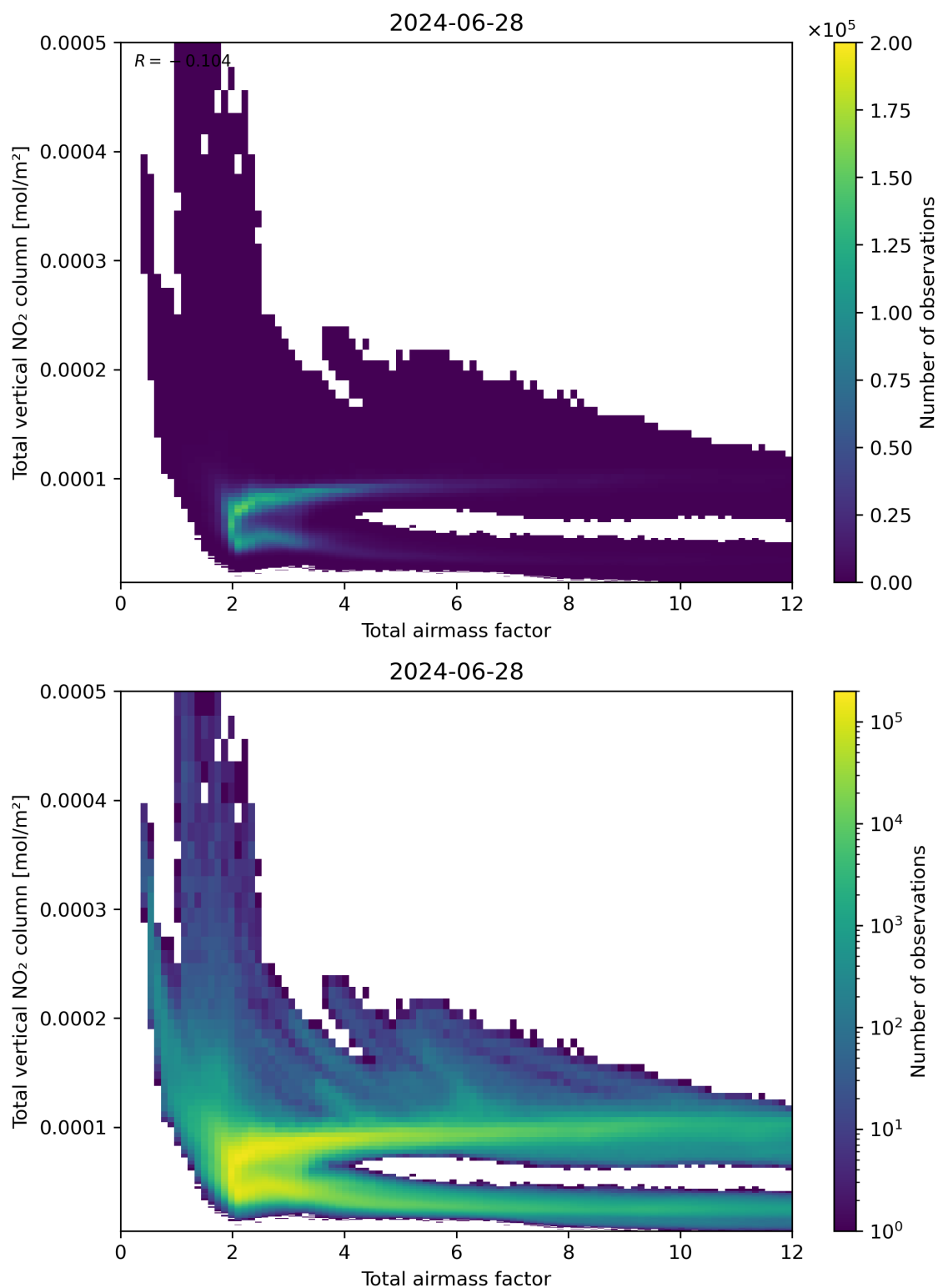
Figure 67: Scatter density plot of “Total airmass factor” against “Total vertical NO 2 column” for 2024-06-27 to 2024-06-29.
