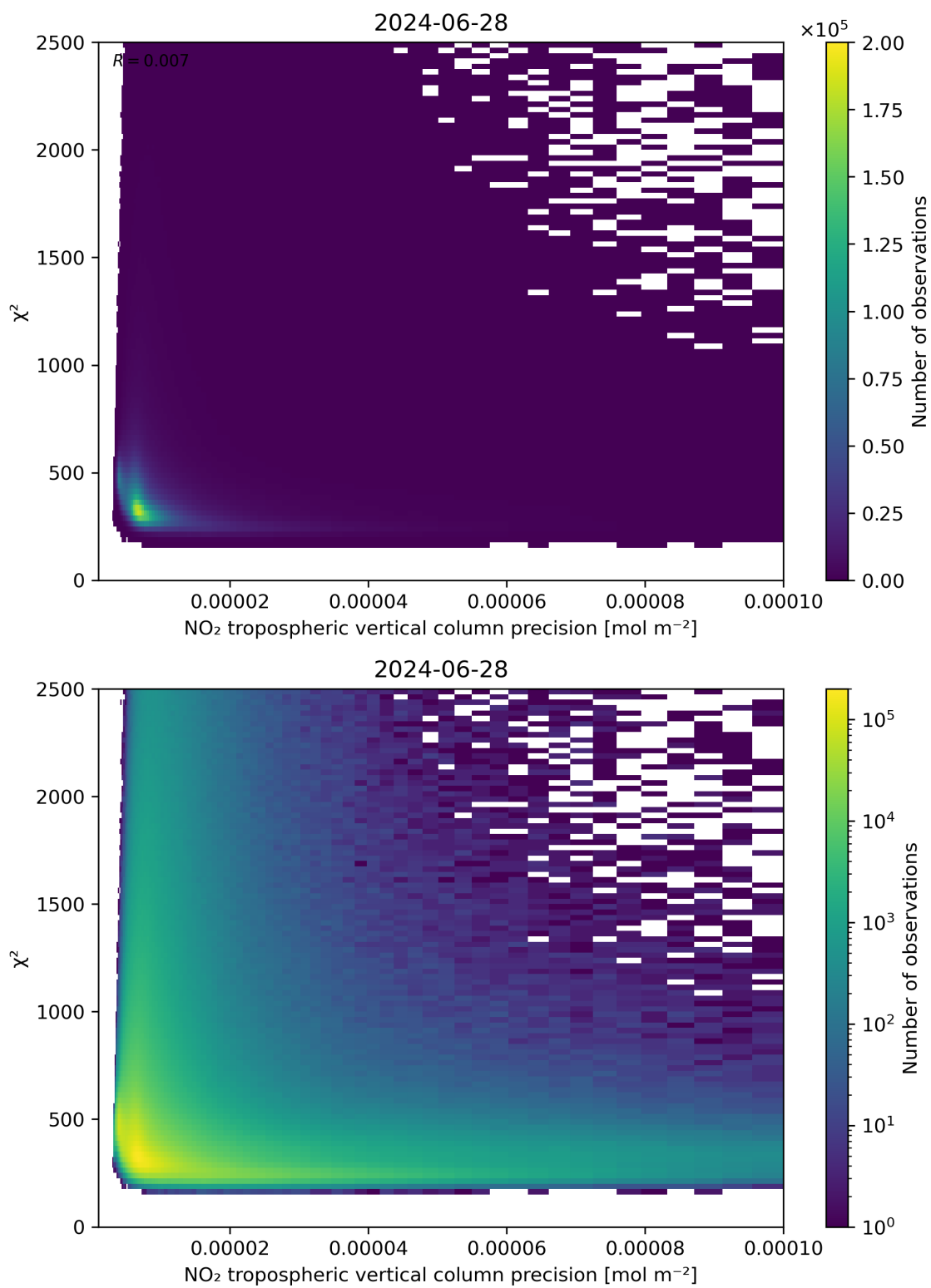
Figure 134: Scatter density plot of “NO 2 tropospheric vertical column precision” against “ \chi^2 ” for 2024-06-27 to 2024-06-29.
