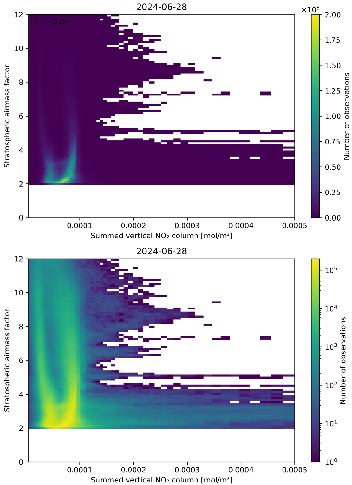
Figure 103: Scatter density plot of “Summed vertical NO 2 column” against “Stratospheric air mass factor” for 2024-06-27 to 2024-06-29.
