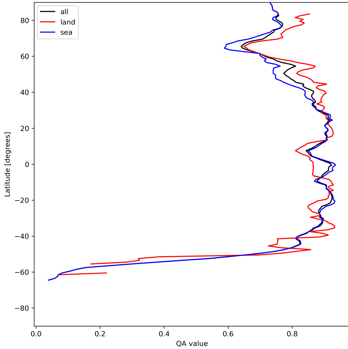
Figure 11: Zonal average of “QA value” for 2024-06-27 to 2024-06-29.
