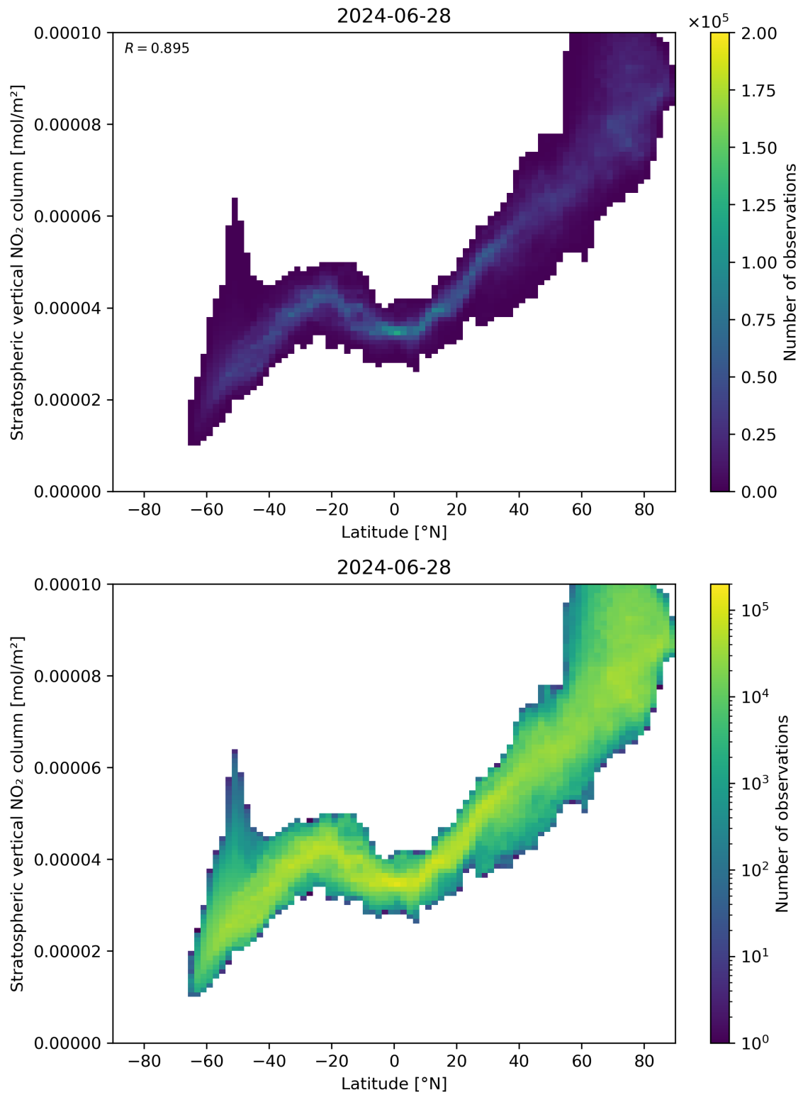
Figure 87: Scatter density plot of “Latitude” against “Stratospheric vertical \text{NO}_2 column” for 2024-06-27 to 2024-06-29.
