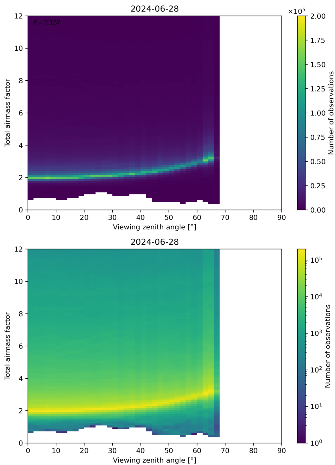
Figure 160: Scatter density plot of “Viewing zenith angle” against “Total airmass factor” for 2024-06-27 to 2024-06-29.
