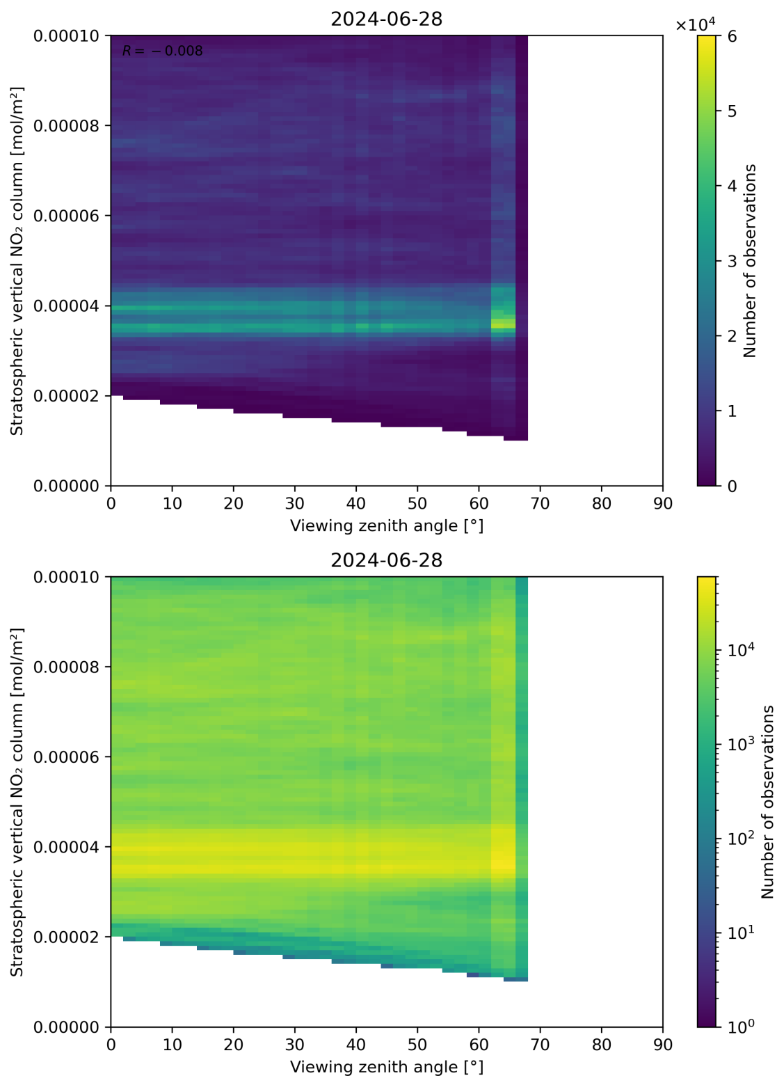
Figure 164: Scatter density plot of “Viewing zenith angle” against “Stratospheric vertical NO 2 column” for 2024-06-27 to 2024-06-29.
