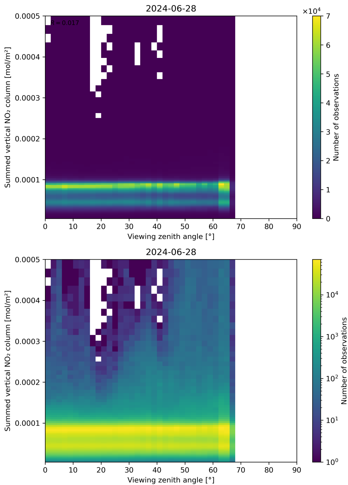
Figure 165: Scatter density plot of “Viewing zenith angle” against “Summed vertical NO 2 column” for 2024-06-27 to 2024-06-29.
