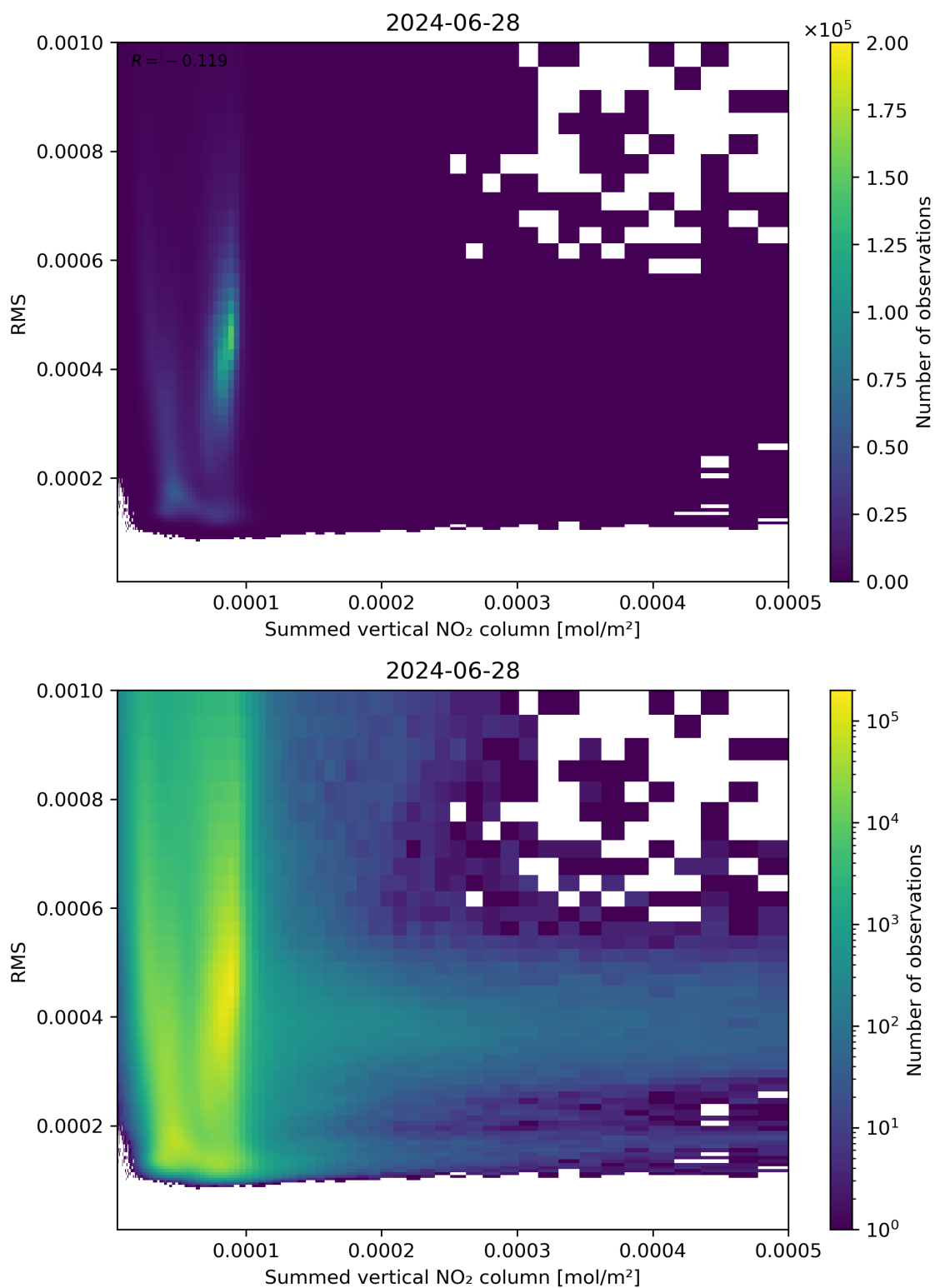
Figure 109: Scatter density plot of “Summed vertical NO 2 column” against “RMS” for 2024-06-27 to 2024-06-29.
