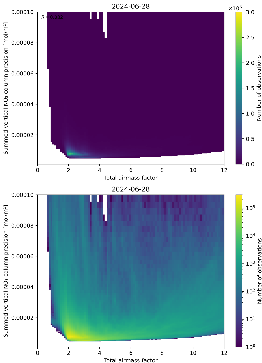
Figure 66: Scatter density plot of “Total airmass factor” against “Summed vertical NO 2 column precision” for 2024-06-27 to 2024-06-29.
