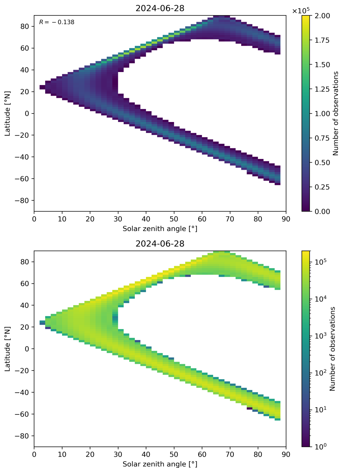
Figure 149: Scatter density plot of “Solar zenith angle” against “Latitude” for 2024-06-27 to 2024-06-29.
