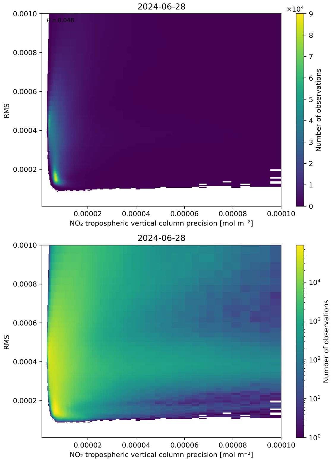
Figure 140: Scatter density plot of “NO 2 tropospheric vertical column precision” against “RMS” for 2024-06-27 to 2024-06-29.
