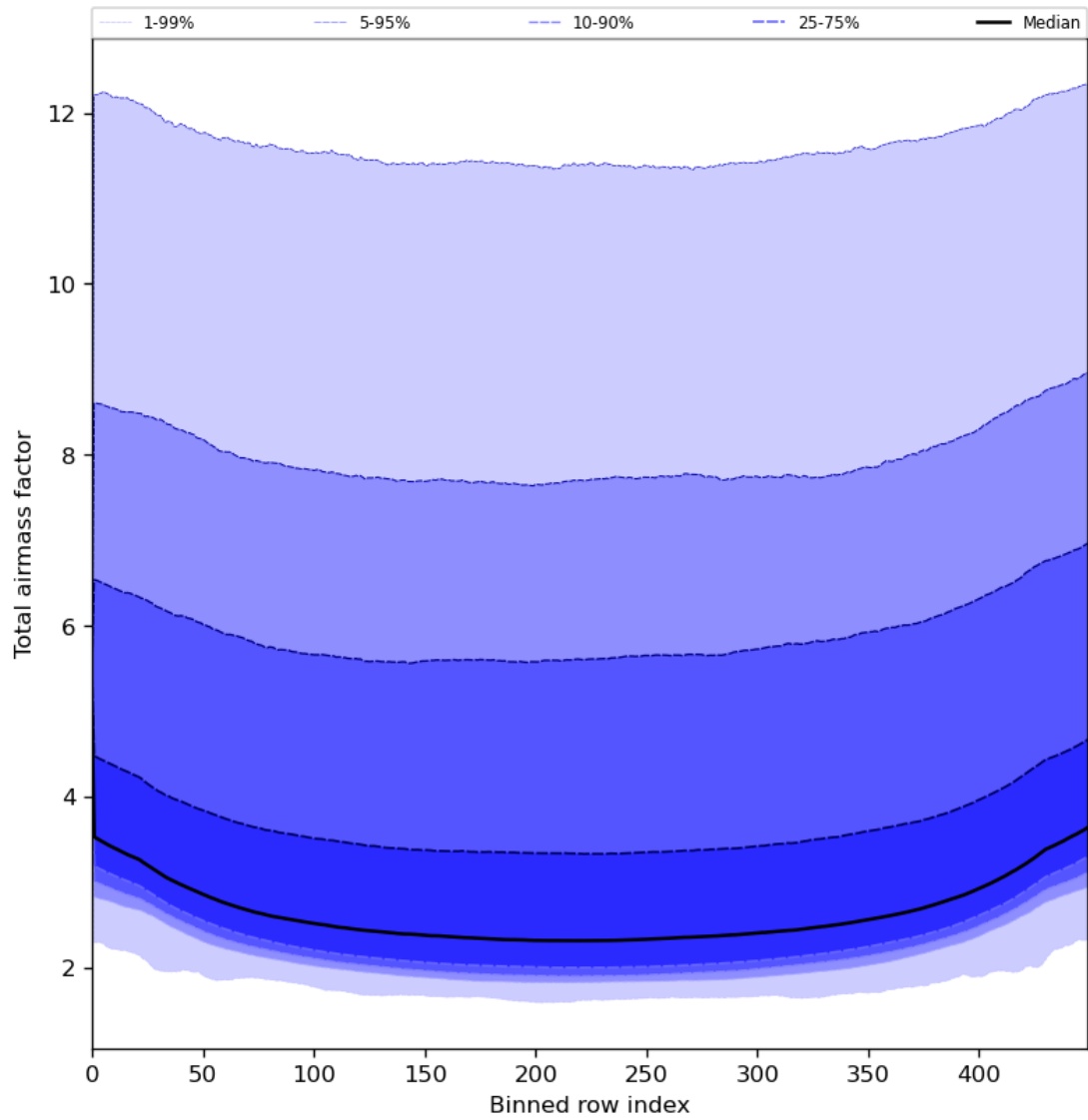
Figure 49: Along track statistics of “Total airmass factor” for 2024-06-27 to 2024-06-29
