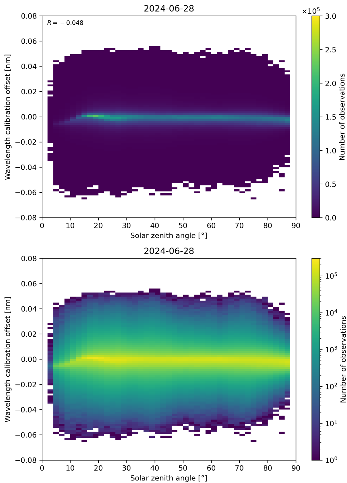
Figure 158: Scatter density plot of “Solar zenith angle” against “Wavelength calibration offset” for 2024-06-27 to 2024-06-29.
