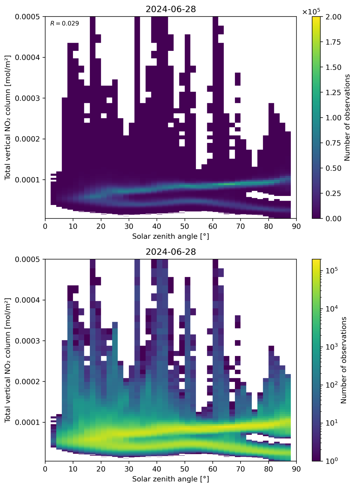
Figure 153: Scatter density plot of “Solar zenith angle” against “Total vertical NO 2 column” for 2024-06-27 to 2024-06-29.
