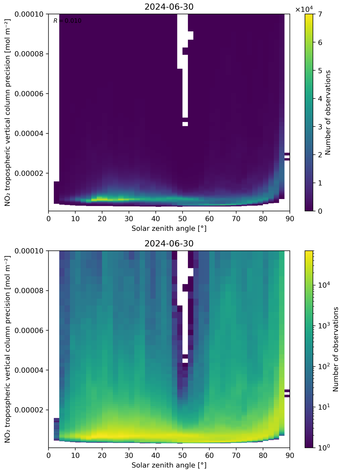
Figure 156: Scatter density plot of “Solar zenith angle” against “NO 2 tropospheric vertical column precision” for 2024-06-29 to 2024-07-01.
