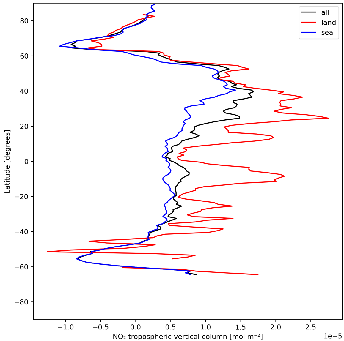
Figure 12: Zonal average of “NO 2 tropospheric vertical column” for 2024-06-29 to 2024-07-01.
