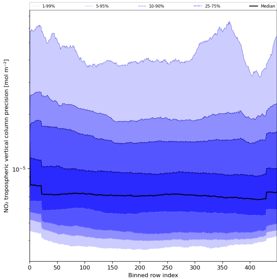
Figure 47: Along track statistics of “NO 2 tropospheric vertical column precision” for 2024-06-29 to 2024-07-01
