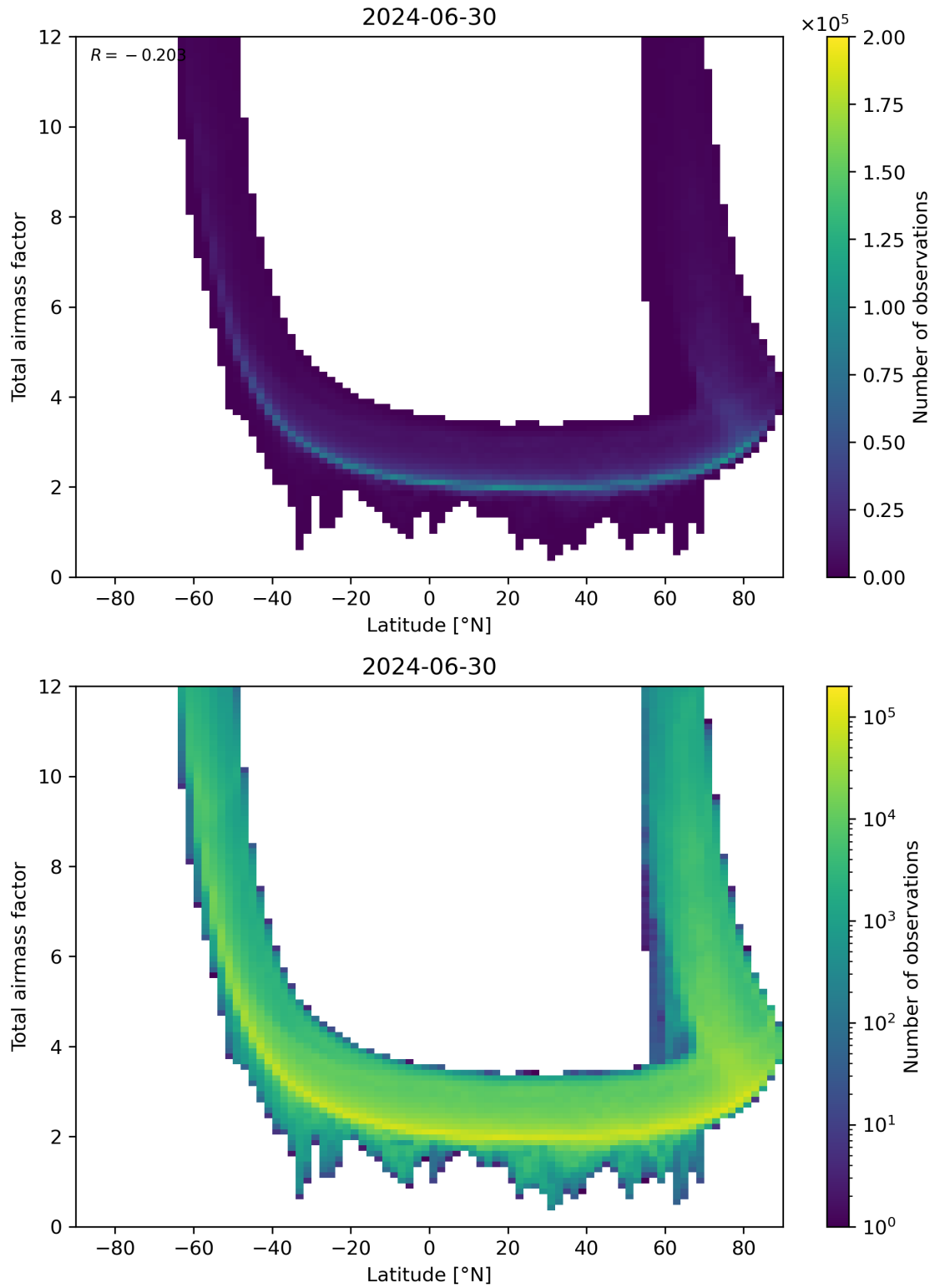
Figure 84: Scatter density plot of “Latitude” against “Total airmass factor” for 2024-06-29 to 2024-07-01.
