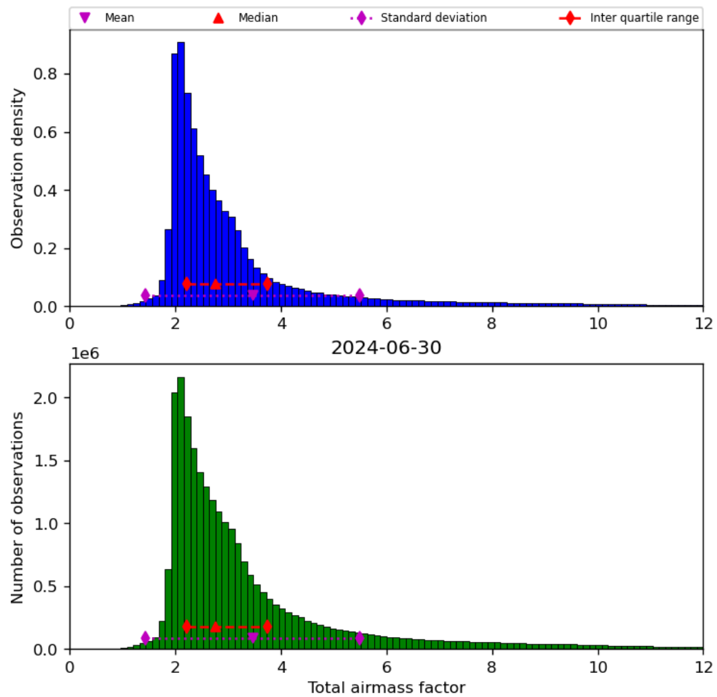
Figure 32: Histogram of “Total airmass factor” for 2024-06-29 to 2024-07-01
