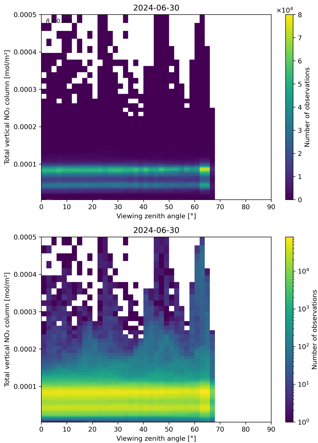
Figure 167: Scatter density plot of “Viewing zenith angle” against “Total vertical NO 2 column” for 2024-06-29 to 2024-07-01.
