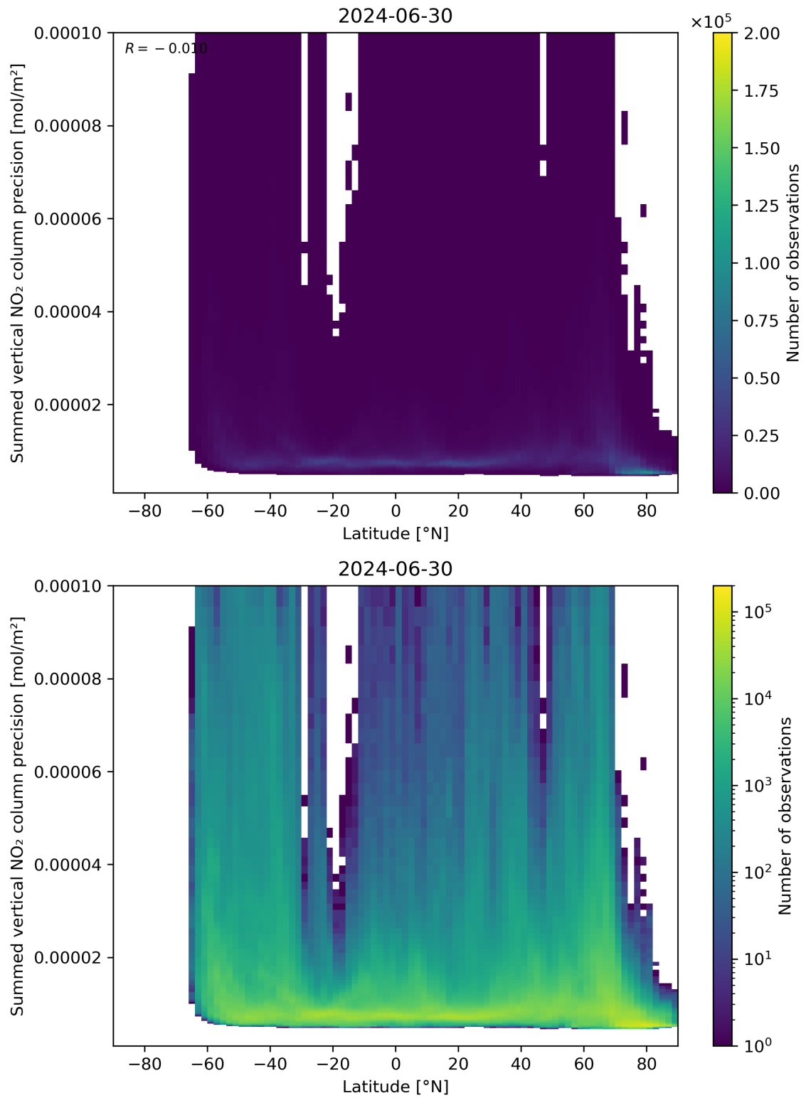
Figure 89: Scatter density plot of “Latitude” against “Summed vertical NO 2 column precision” for 2024-06-29 to 2024-07-01.
