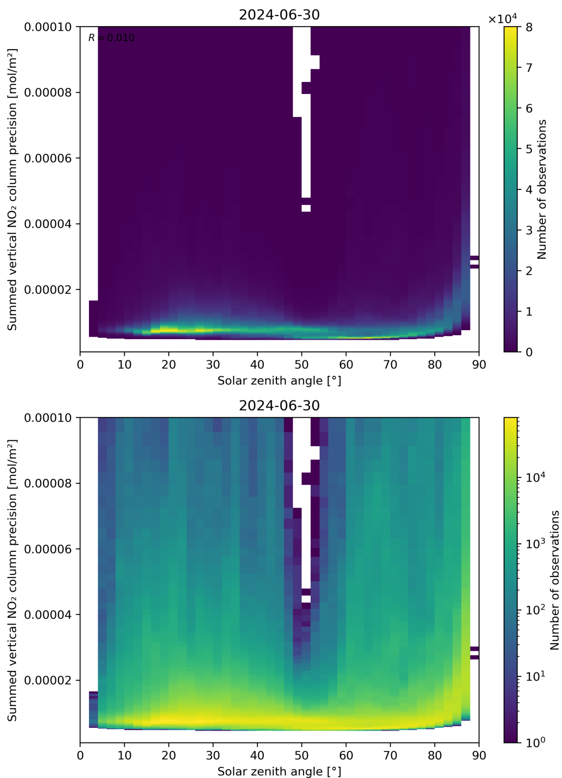
Figure 152: Scatter density plot of “Solar zenith angle” against “Summed vertical NO 2 column precision” for 2024-06-29 to 2024-07-01.
