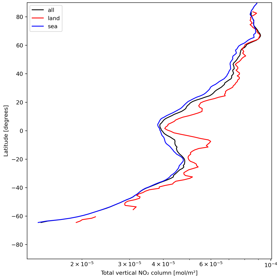
Figure 21: Zonal average of “Total vertical NO 2 column” for 2024-06-29 to 2024-07-01.
