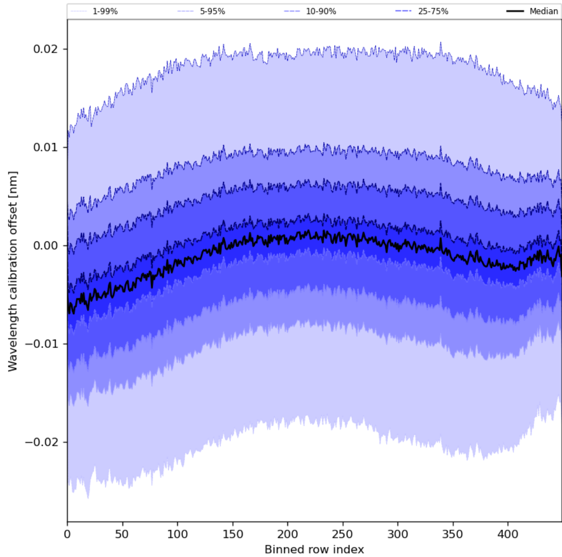
Figure 52: Along track statistics of “Wavelength calibration offset” for 2024-06-29 to 2024-07-01
