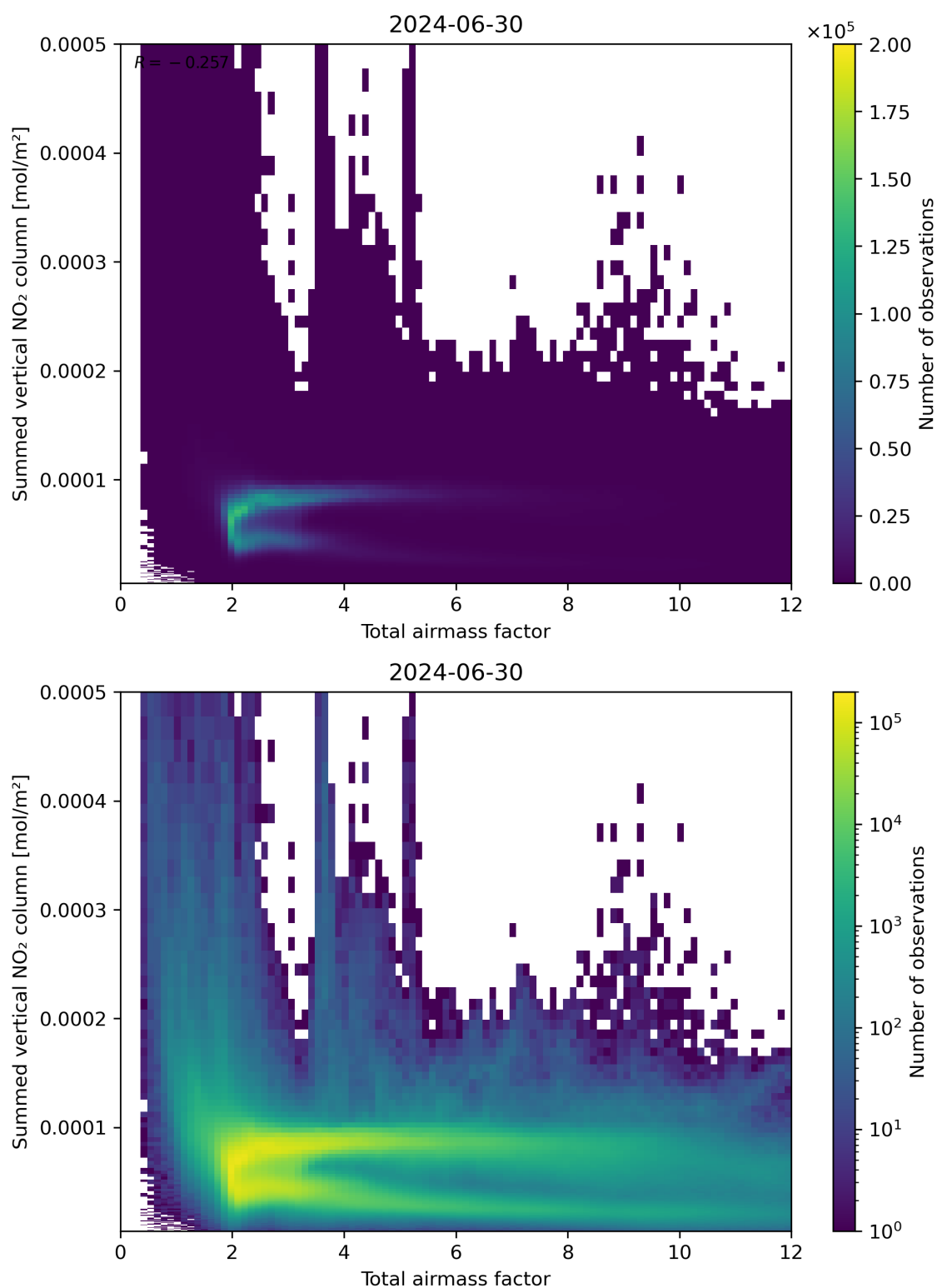
Figure 65: Scatter density plot of “Total airmass factor” against “Summed vertical NO 2 column” for 2024-06-29 to 2024-07-01.
