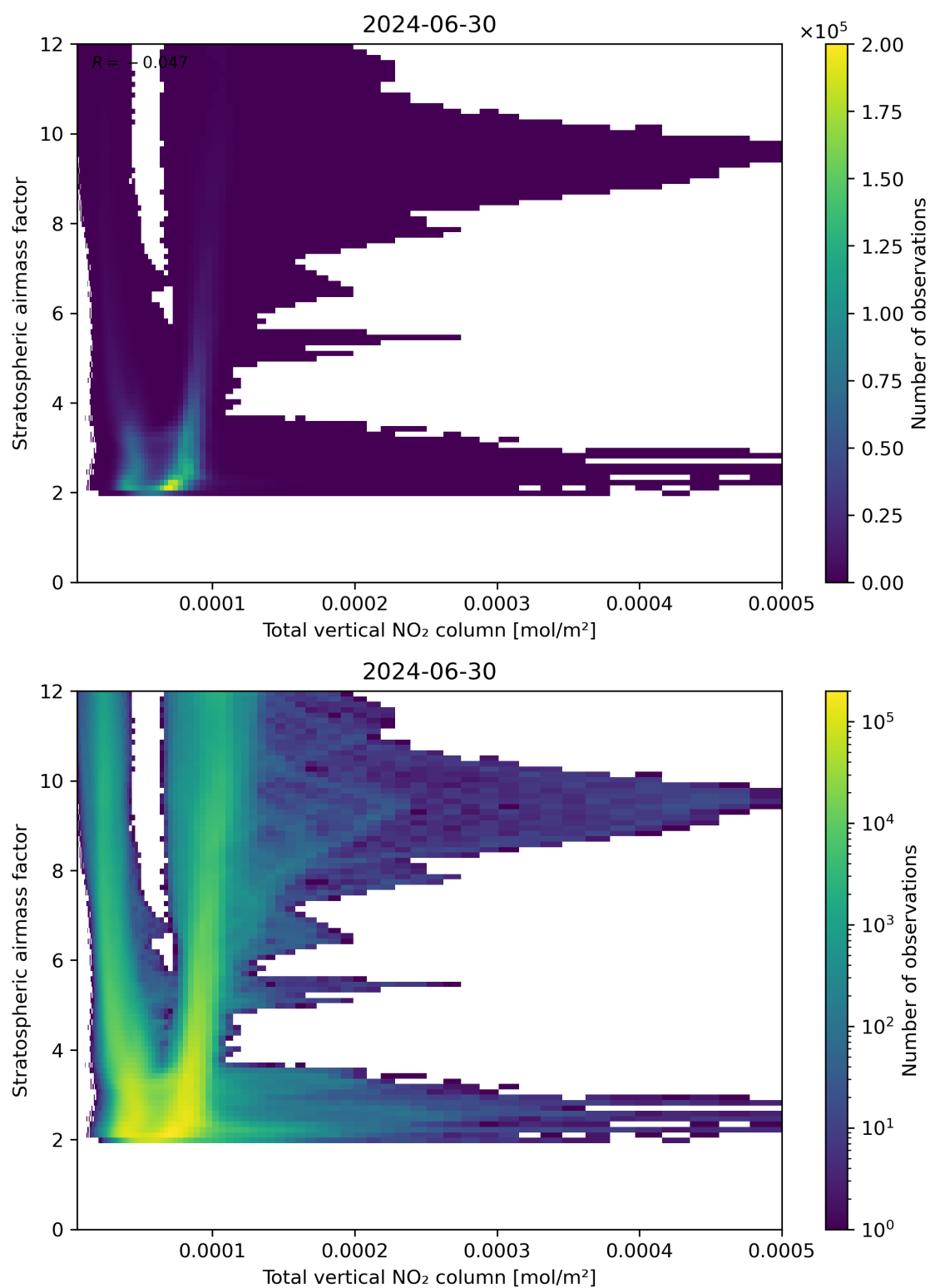
Figure 110: Scatter density plot of “Total vertical NO 2 column” against “Stratospheric air mass factor” for 2024-06-29 to 2024-07-01.
