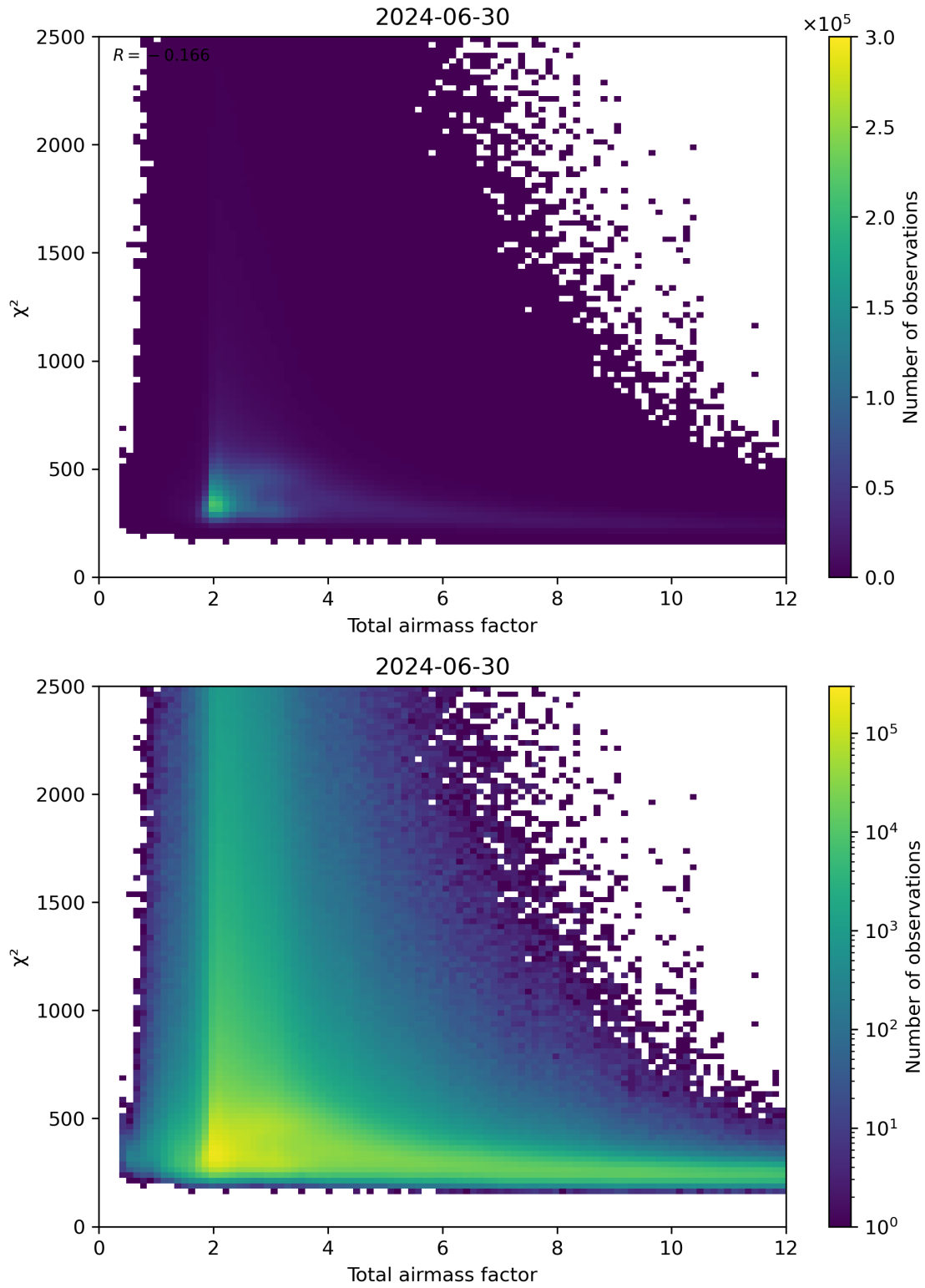
Figure 63: Scatter density plot of “Total airmass factor” against “ \chi^2 ” for 2024-06-29 to 2024-07-01.
