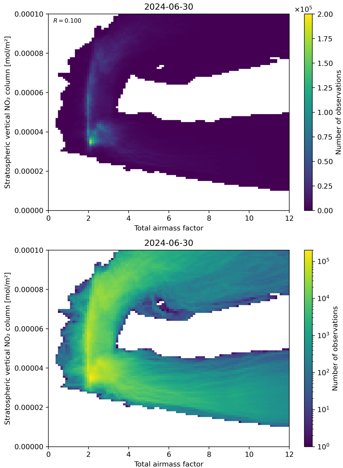
Figure 64: Scatter density plot of “Total airmass factor” against “Stratospheric vertical \text{NO}_2 column” for 2024-06-29 to 2024-07-01.
