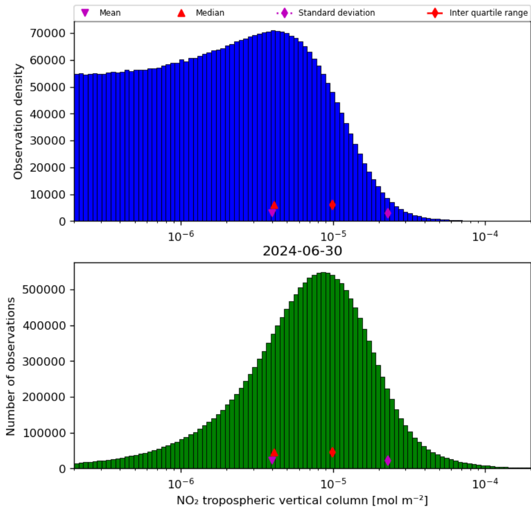
Figure 29: Histogram of “NO 2 tropospheric vertical column” for 2024-06-29 to 2024-07-01
