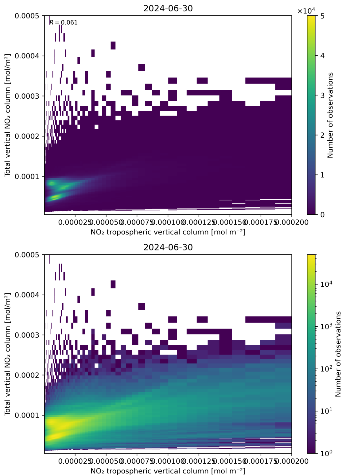
Figure 128: Scatter density plot of “NO 2 tropospheric vertical column” against “Total vertical NO 2 column” for 2024-06-29 to 2024-07-01.
