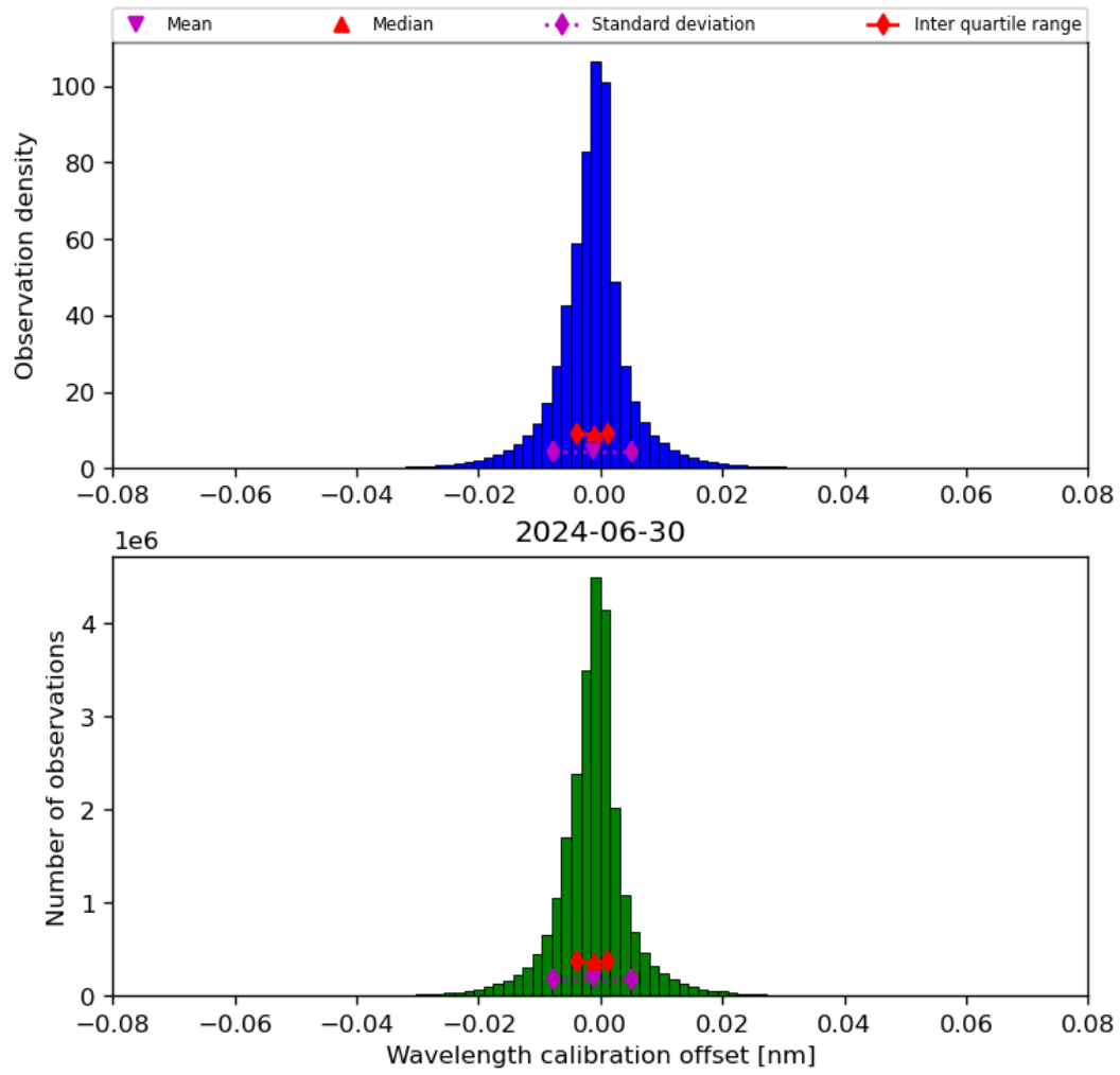
Figure 35: Histogram of “Wavelength calibration offset” for 2024-06-29 to 2024-07-01
