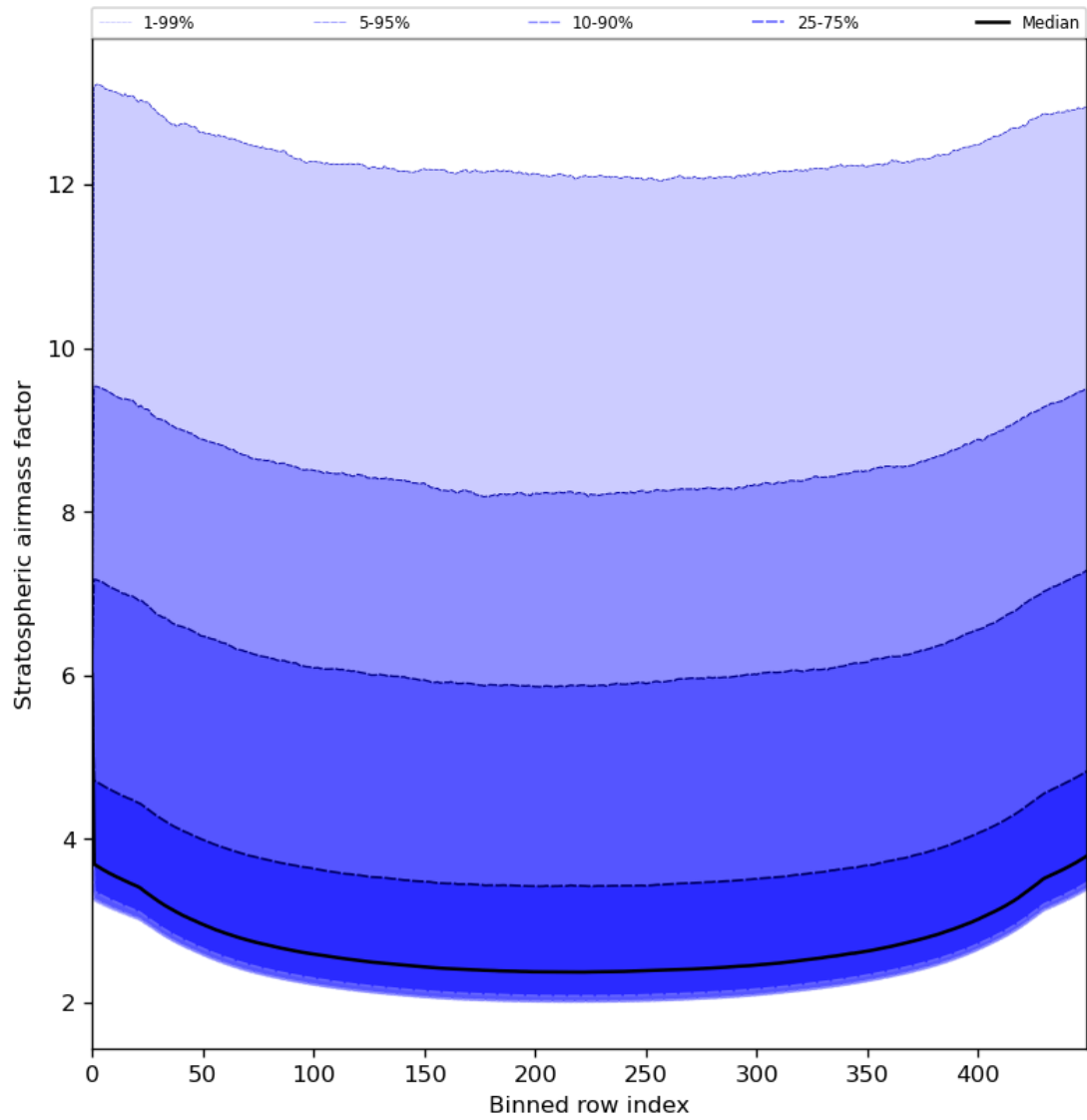
Figure 61: Along track statistics of “Stratospheric airmass factor” for 2024-06-29 to 2024-07-01
