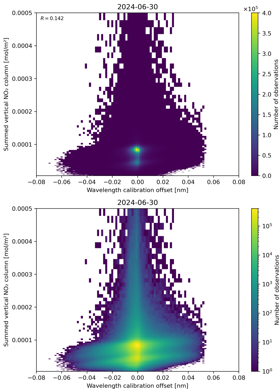
Figure 177: Scatter density plot of “Wavelength calibration offset” against “Summed vertical NO 2 column” for 2024-06-29 to 2024-07-01.
