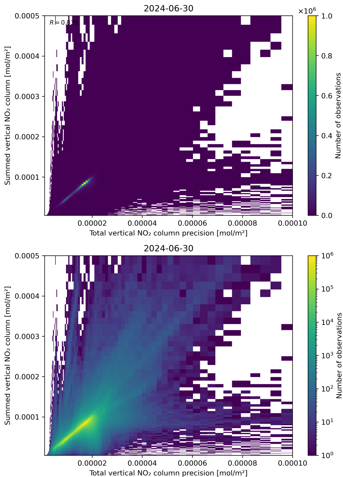
Figure 117: Scatter density plot of “Total vertical NO 2 column precision” against “Summed vertical NO 2 column” for 2024-06-29 to 2024-07-01.
