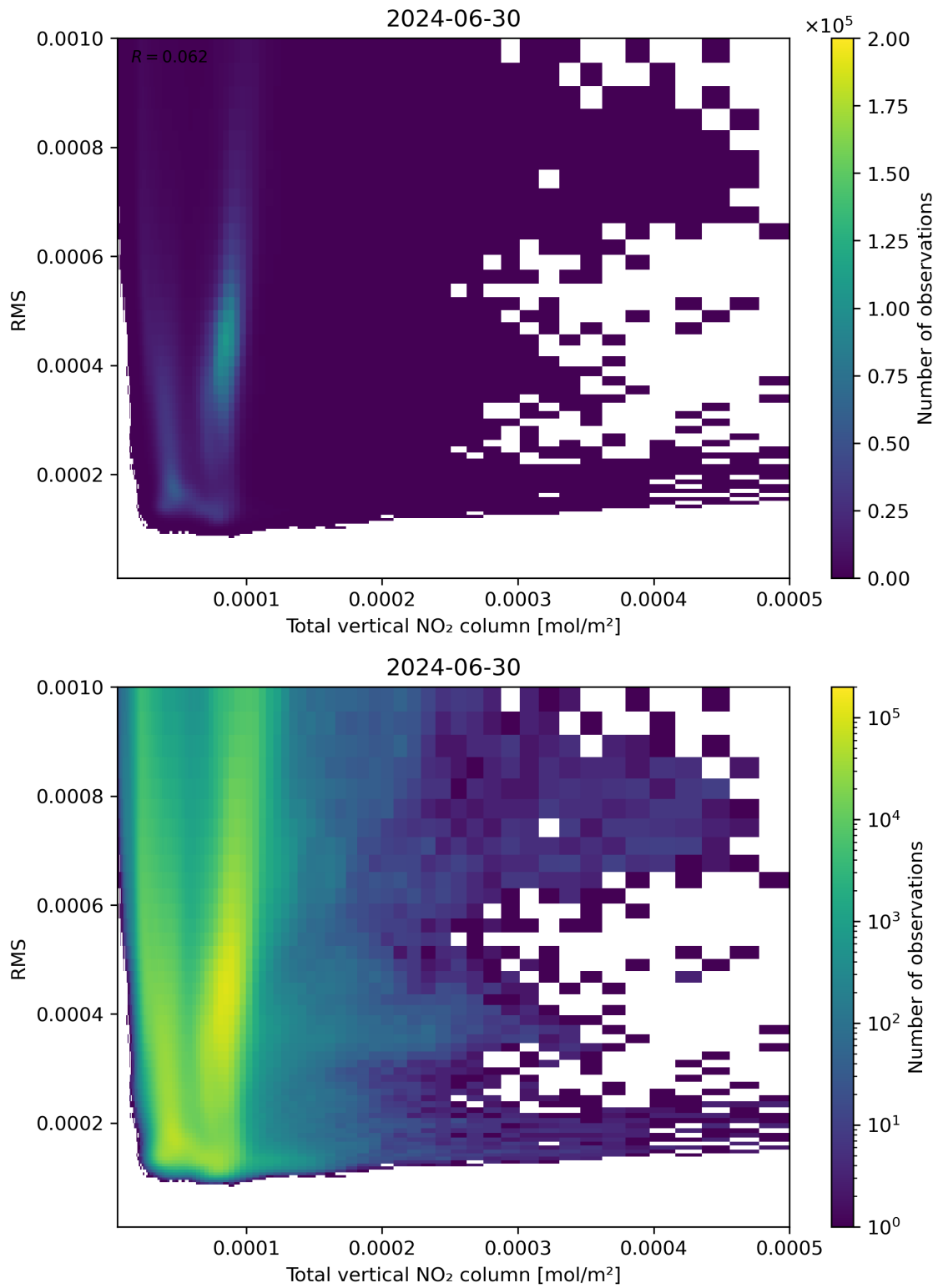
Figure 120: Scatter density plot of “Total vertical NO 2 column” against “RMS” for 2024-06-29 to 2024-07-01.
