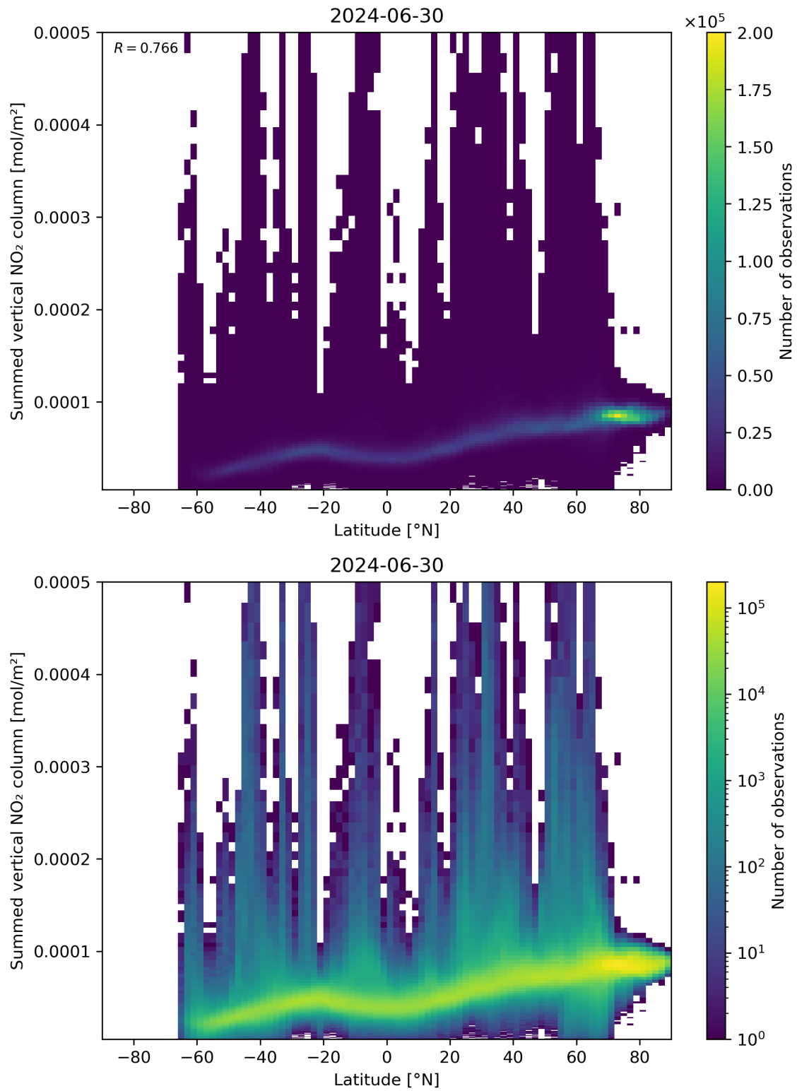
Figure 88: Scatter density plot of “Latitude” against “Summed vertical NO 2 column” for 2024-06-29 to 2024-07-01.
