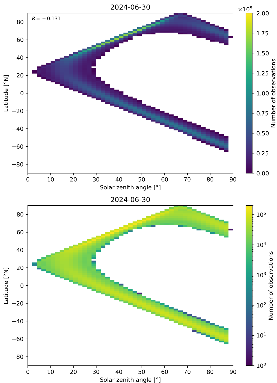
Figure 149: Scatter density plot of “Solar zenith angle” against “Latitude” for 2024-06-29 to 2024-07-01.
