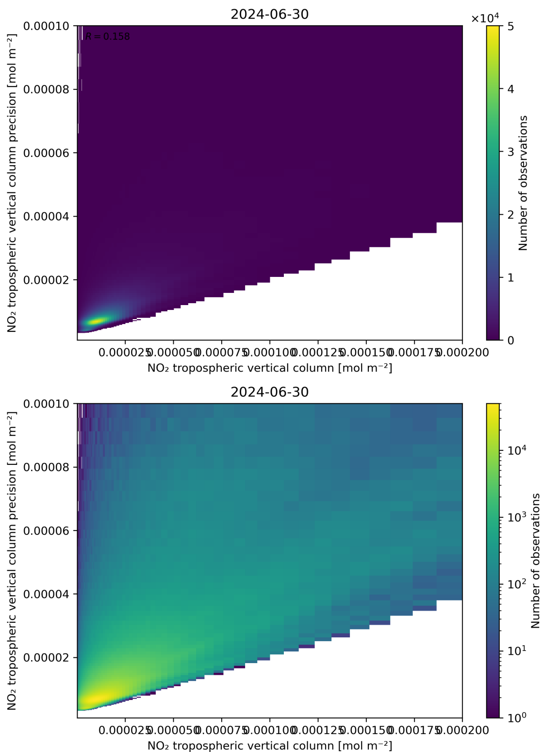
Figure 130: Scatter density plot of “NO 2 tropospheric vertical column” against “NO 2 tropospheric vertical column precision” for 2024-06-29 to 2024-07-01.
