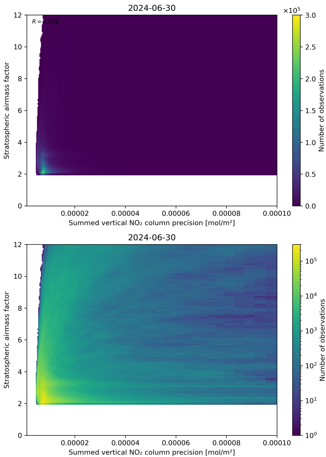
Figure 106: Scatter density plot of “Summed vertical NO 2 column precision” against “Stratospheric airmass factor” for 2024-06-29 to 2024-07-01.
