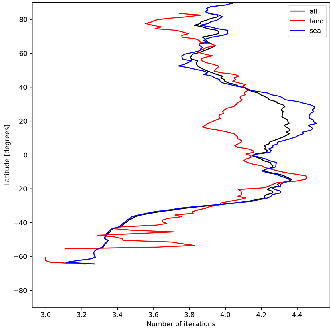
Figure 17: Zonal average of “Number of iterations” for 2024-06-29 to 2024-07-01.
