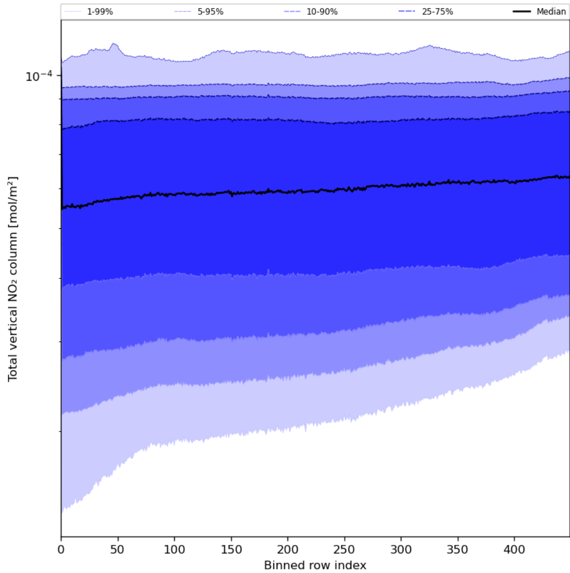
Figure 55: Along track statistics of “Total vertical NO 2 column” for 2024-06-29 to 2024-07-01
