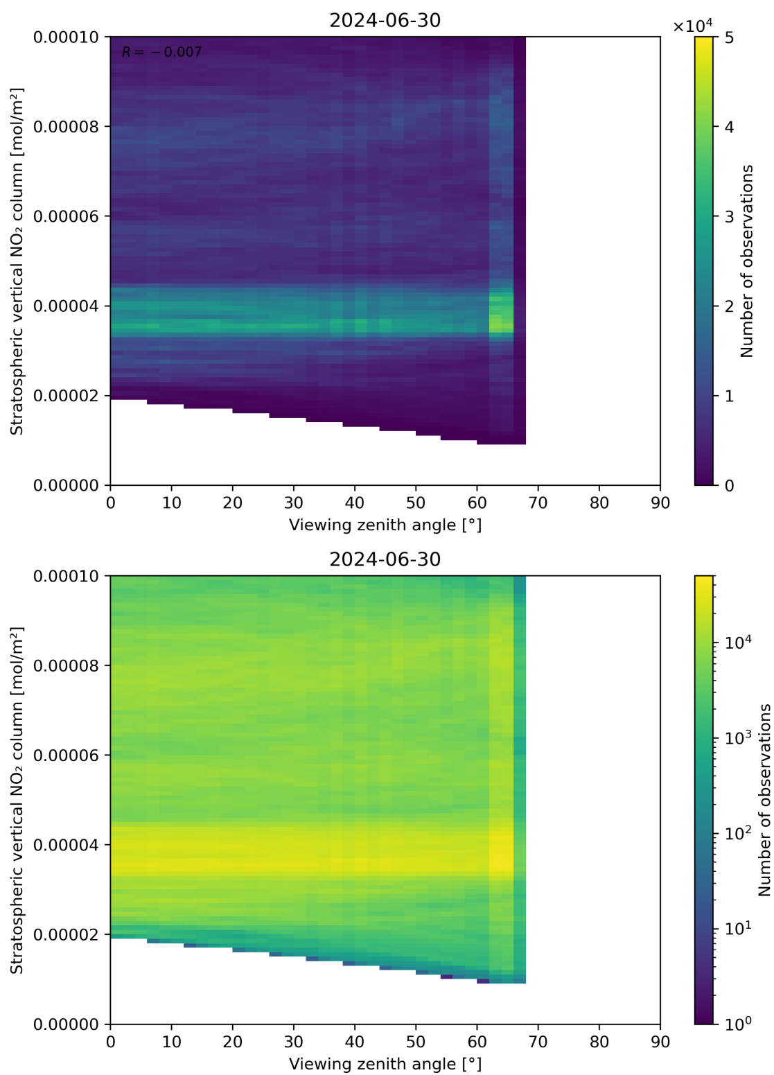
Figure 164: Scatter density plot of “Viewing zenith angle” against “Stratospheric vertical NO 2 column” for 2024-06-29 to 2024-07-01.
