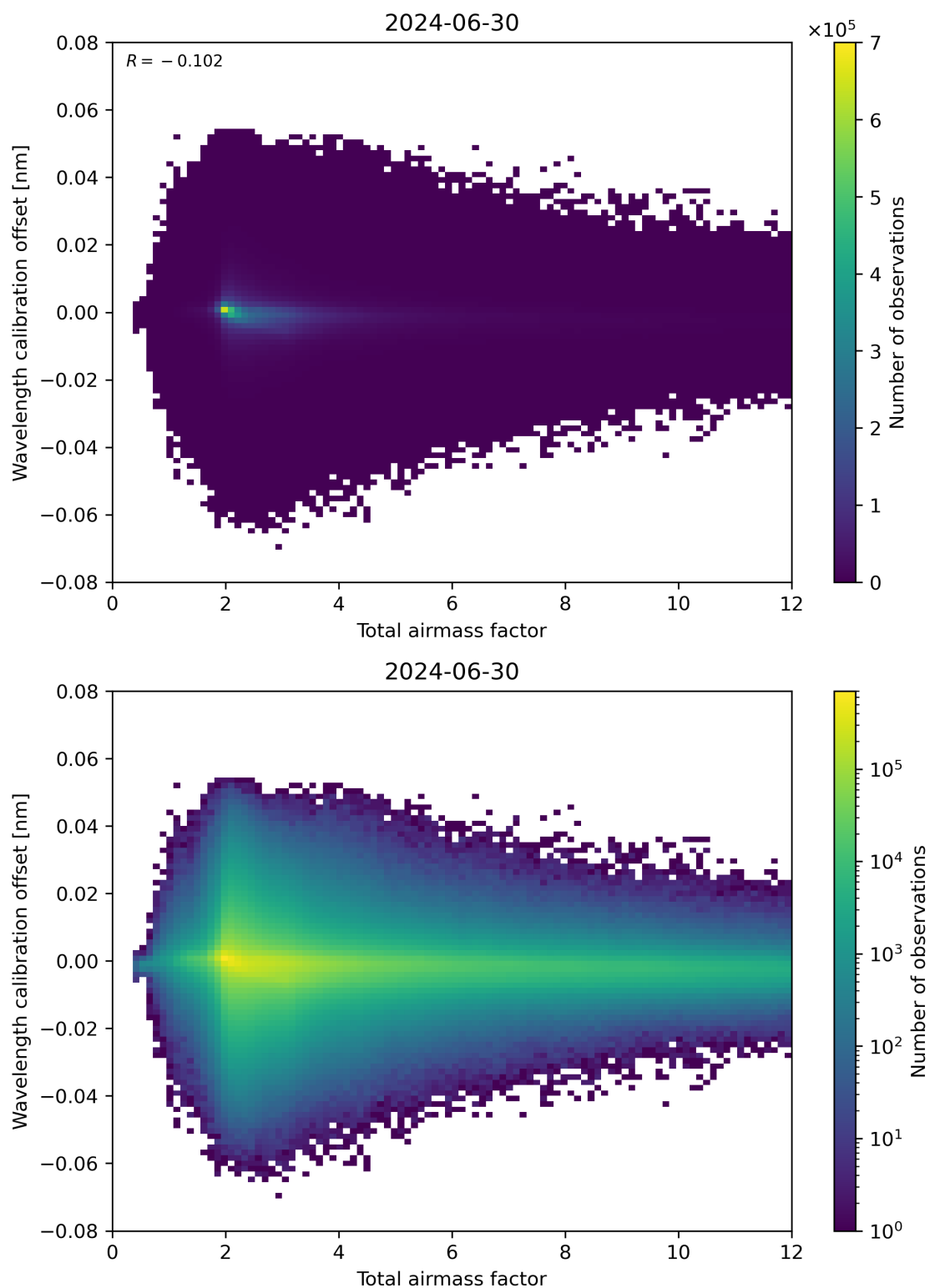
Figure 70: Scatter density plot of “Total airmass factor” against “Wavelength calibration offset” for 2024-06-29 to 2024-07-01.
