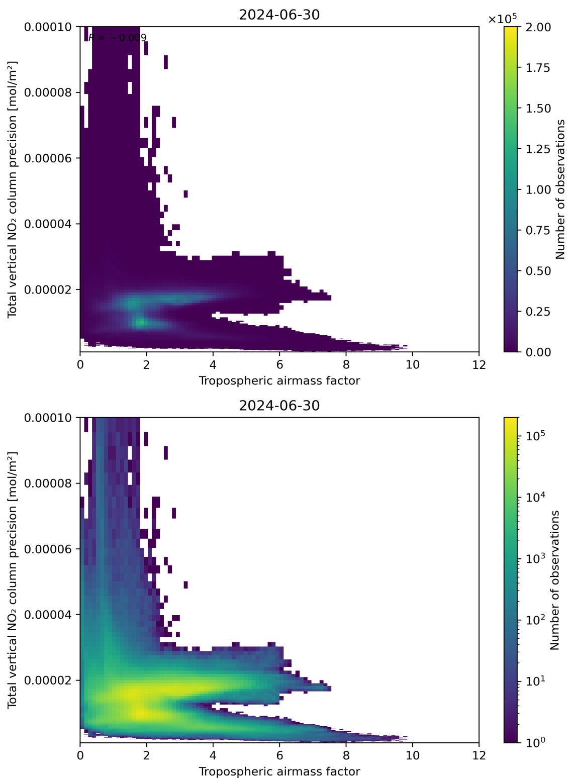
Figure 78: Scatter density plot of “Tropospheric air mass factor” against “Total vertical NO 2 column precision” for 2024-06-29 to 2024-07-01.
