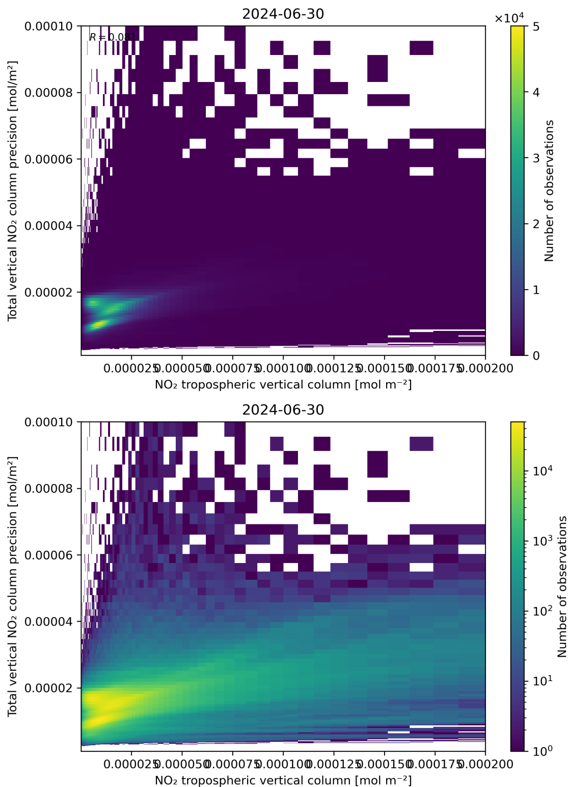
Figure 129: Scatter density plot of “NO 2 tropospheric vertical column” against “Total vertical NO 2 column precision” for 2024-06-29 to 2024-07-01.
