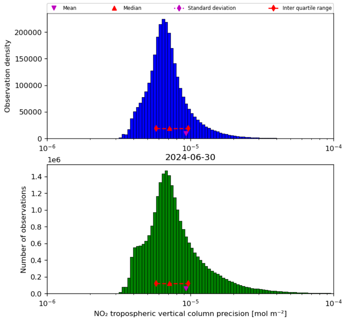
Figure 30: Histogram of “NO 2 tropospheric vertical column precision” for 2024-06-29 to 2024-07-01
