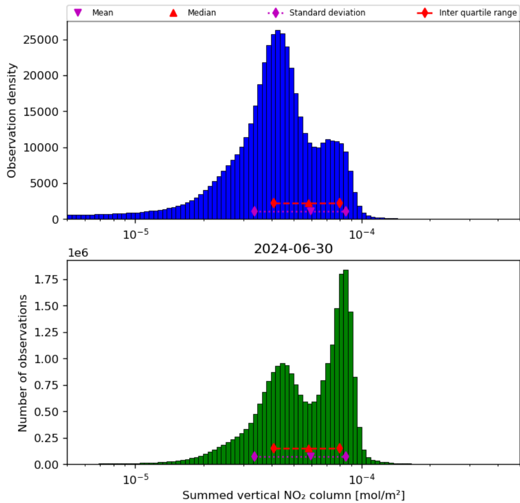
Figure 40: Histogram of “Summed vertical NO 2 column” for 2024-06-29 to 2024-07-01
