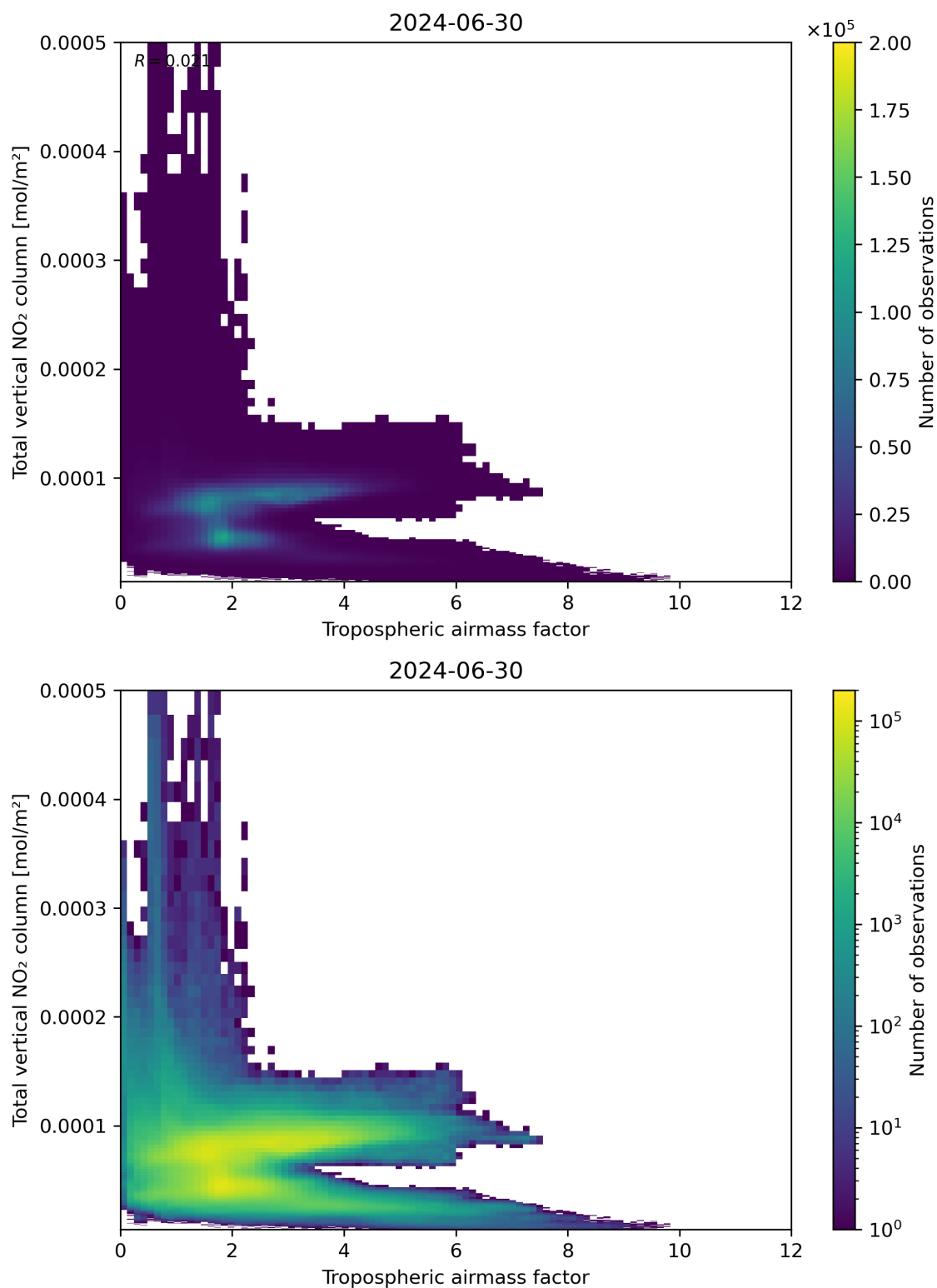
Figure 77: Scatter density plot of “Tropospheric airmass factor” against “Total vertical NO 2 column” for 2024-06-29 to 2024-07-01.
