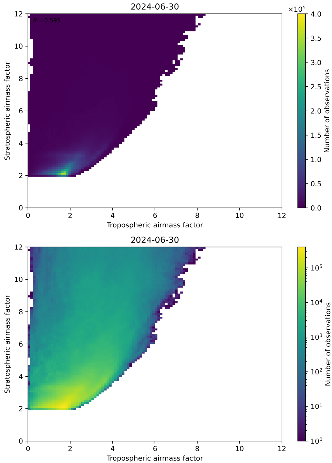
Figure 71: Scatter density plot of “Tropospheric airmass factor” against “Stratospheric airmass factor” for 2024-06-29 to 2024-07-01.
