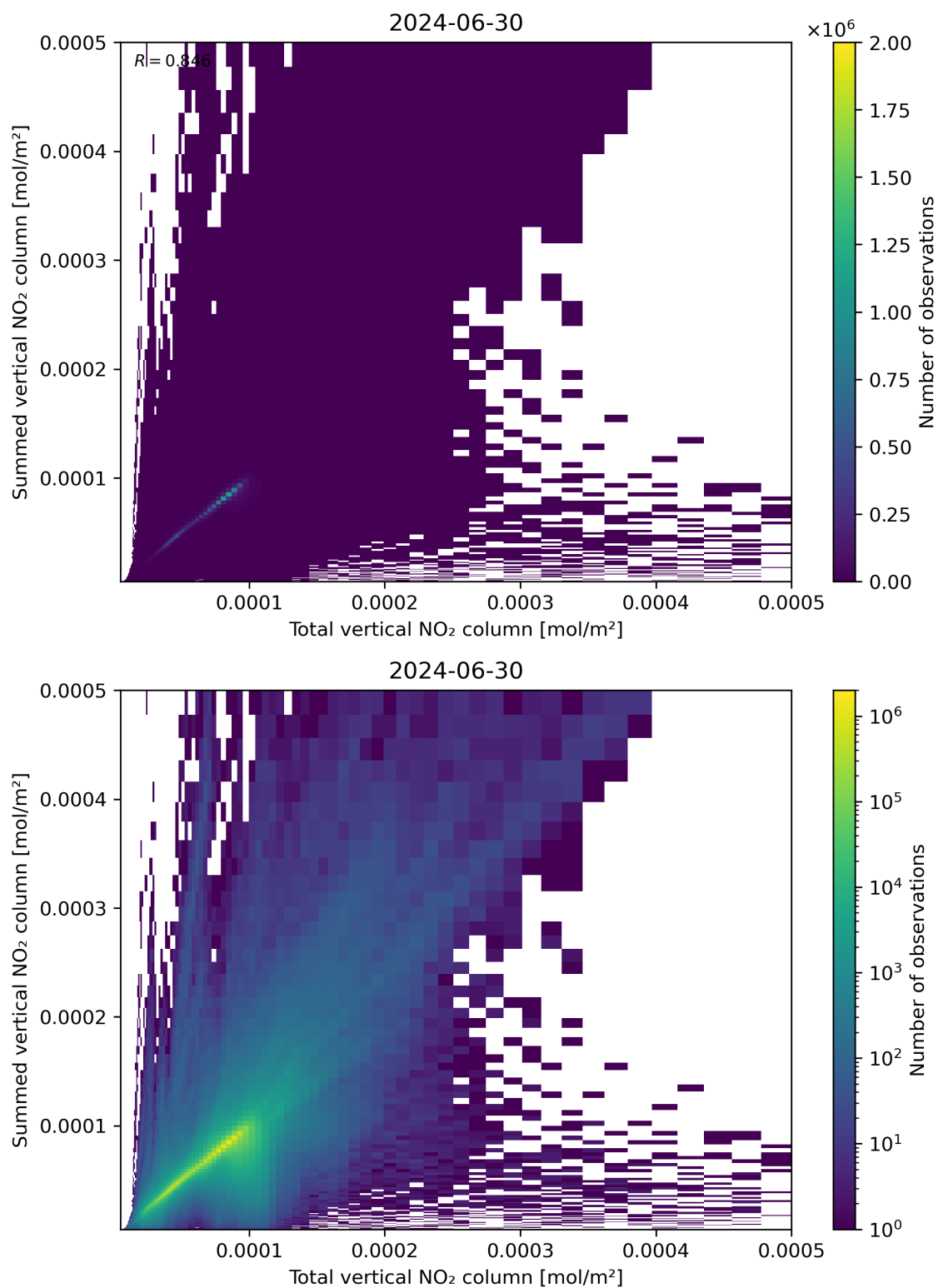
Figure 112: Scatter density plot of “Total vertical NO 2 column” against “Summed vertical NO 2 column” for 2024-06-29 to 2024-07-01.
