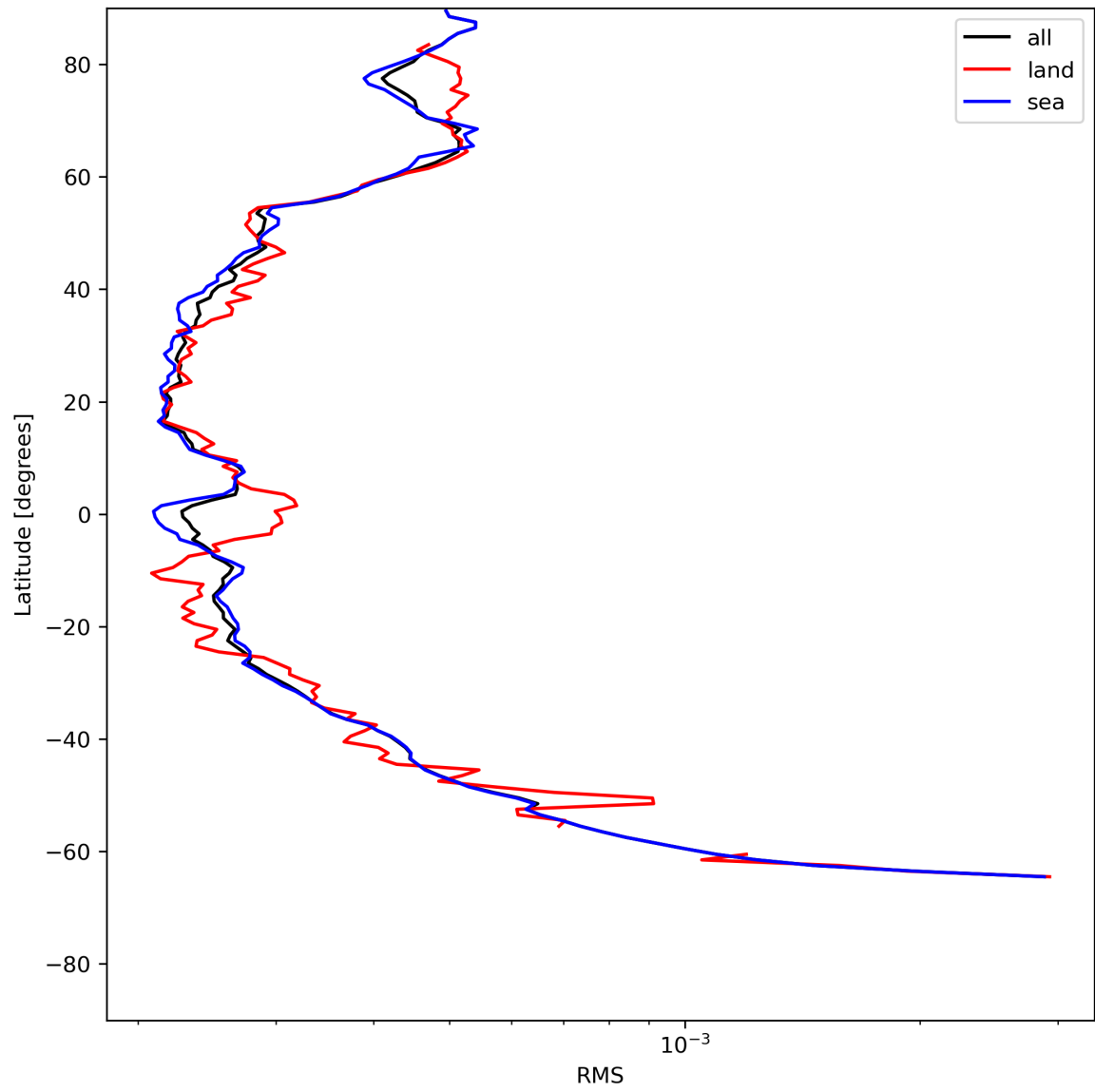
Figure 26: Zonal average of “RMS” for 2024-06-29 to 2024-07-01.
