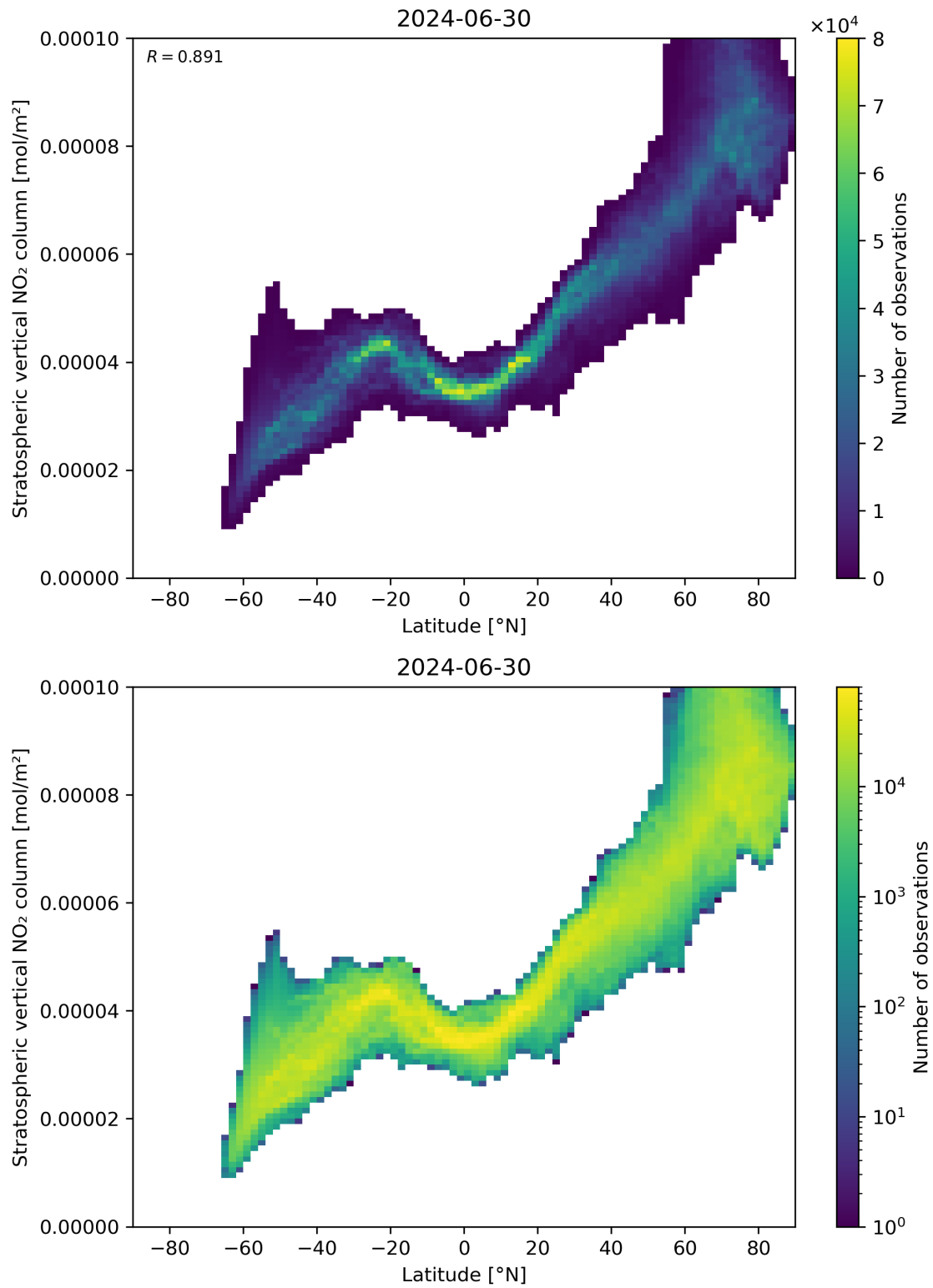
Figure 87: Scatter density plot of “Latitude” against “Stratospheric vertical NO 2 column” for 2024-06-29 to 2024-07-01.
