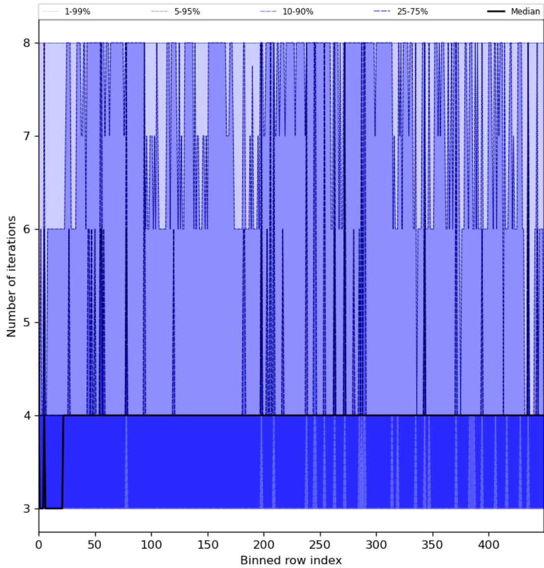
Figure 51: Along track statistics of “Number of iterations” for 2024-06-29 to 2024-07-01
