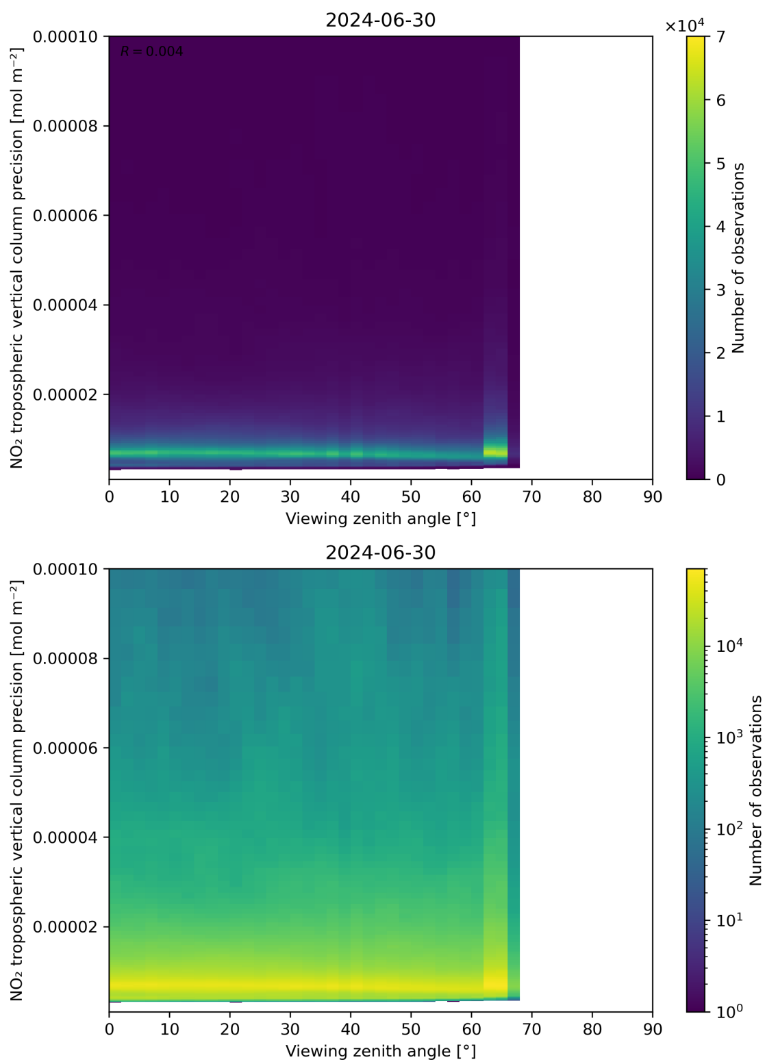
Figure 170: Scatter density plot of “Viewing zenith angle” against “NO 2 tropospheric vertical column precision” for 2024-06-29 to 2024-07-01.
