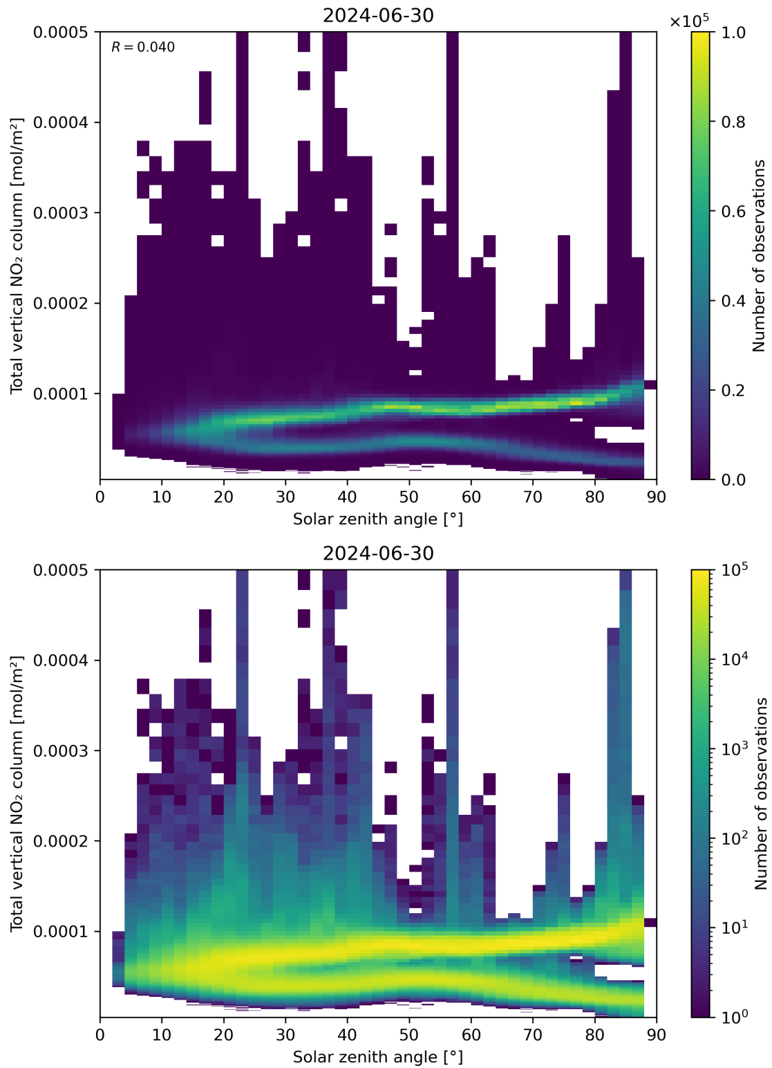
Figure 153: Scatter density plot of “Solar zenith angle” against “Total vertical NO 2 column” for 2024-06-29 to 2024-07-01.
