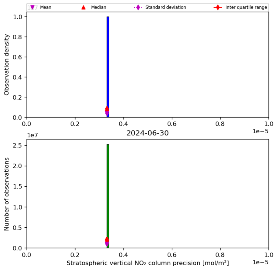
Figure 37: Histogram of “Stratospheric vertical NO 2 column precision” for 2024-06-29 to 2024-07-01
