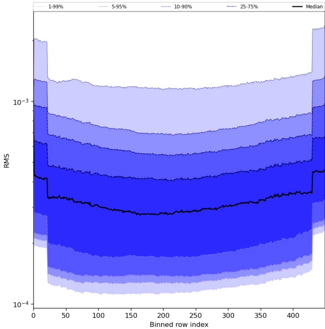
Figure 60: Along track statistics of “RMS” for 2024-06-29 to 2024-07-01
