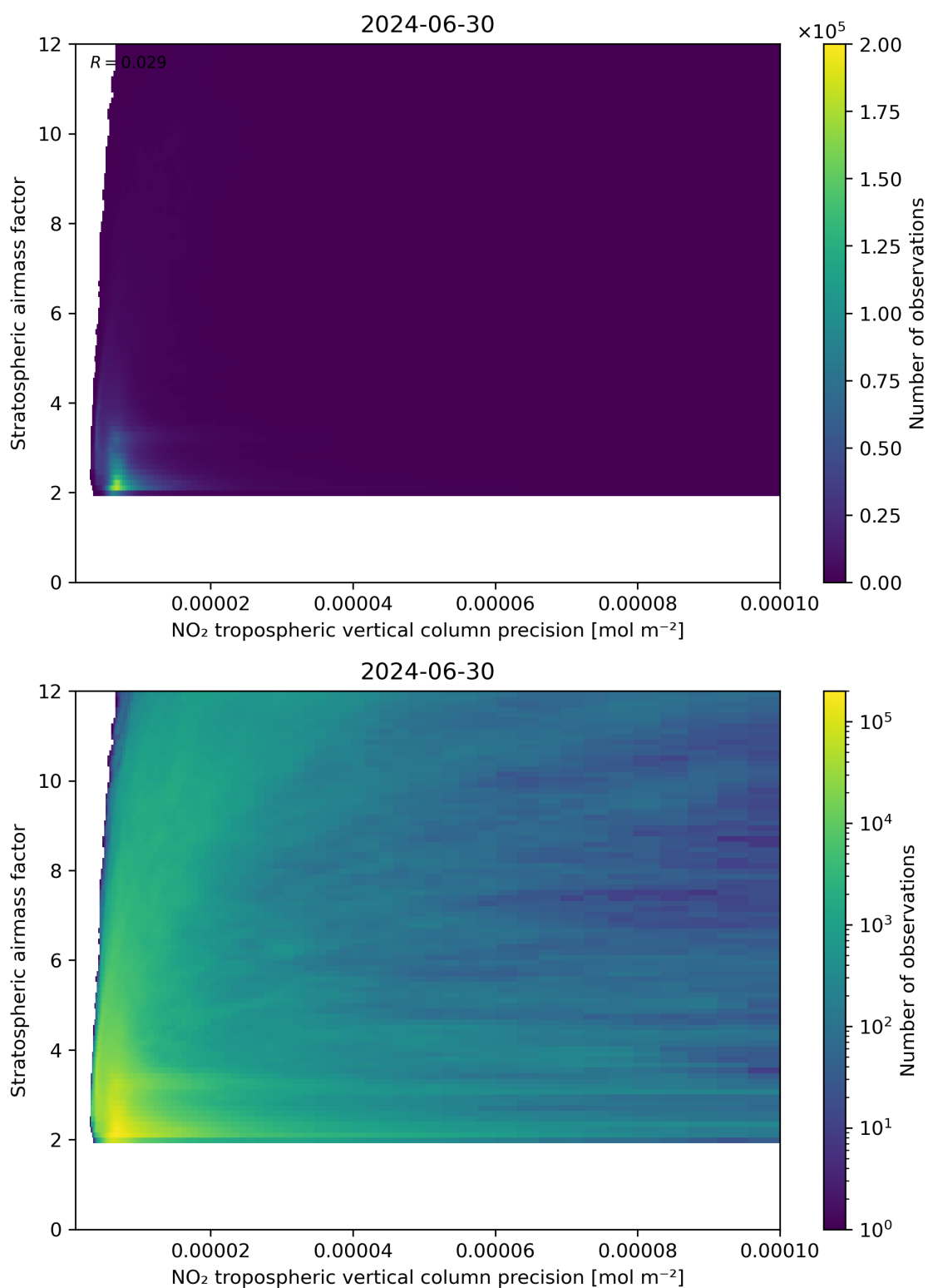
Figure 131: Scatter density plot of “NO 2 tropospheric vertical column precision” against “Stratospheric airmass factor” for 2024-06-29 to 2024-07-01.
