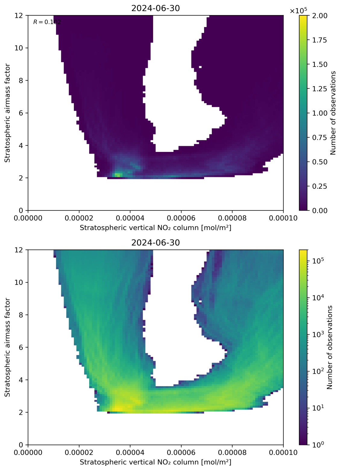
Figure 96: Scatter density plot of “Stratospheric vertical NO 2 column” against “Stratospheric airmass factor” for 2024-06-29 to 2024-07-01.
