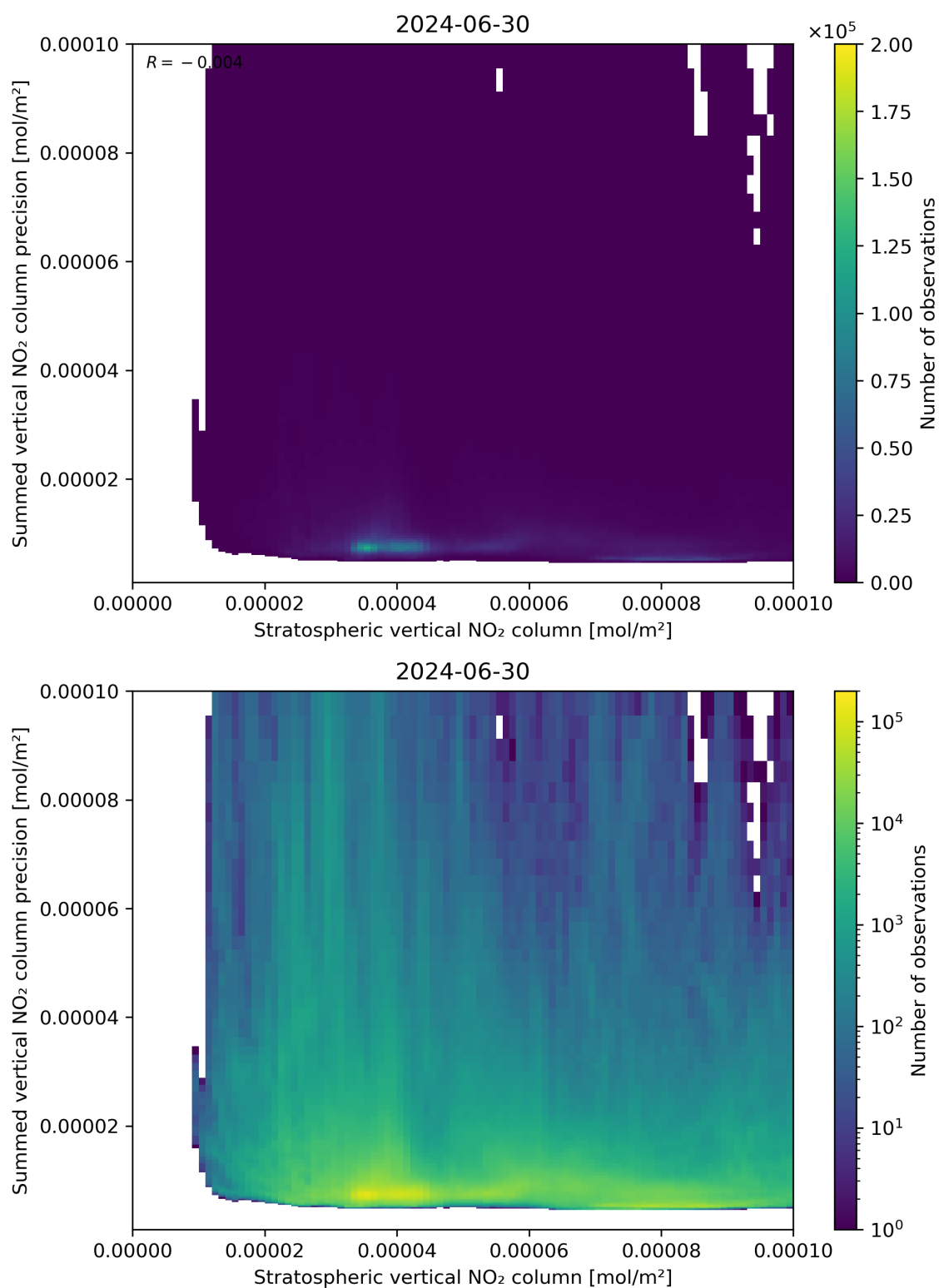
Figure 99: Scatter density plot of “Stratospheric vertical NO 2 column” against “Summed vertical NO 2 column precision” for 2024-06-29 to 2024-07-01.
