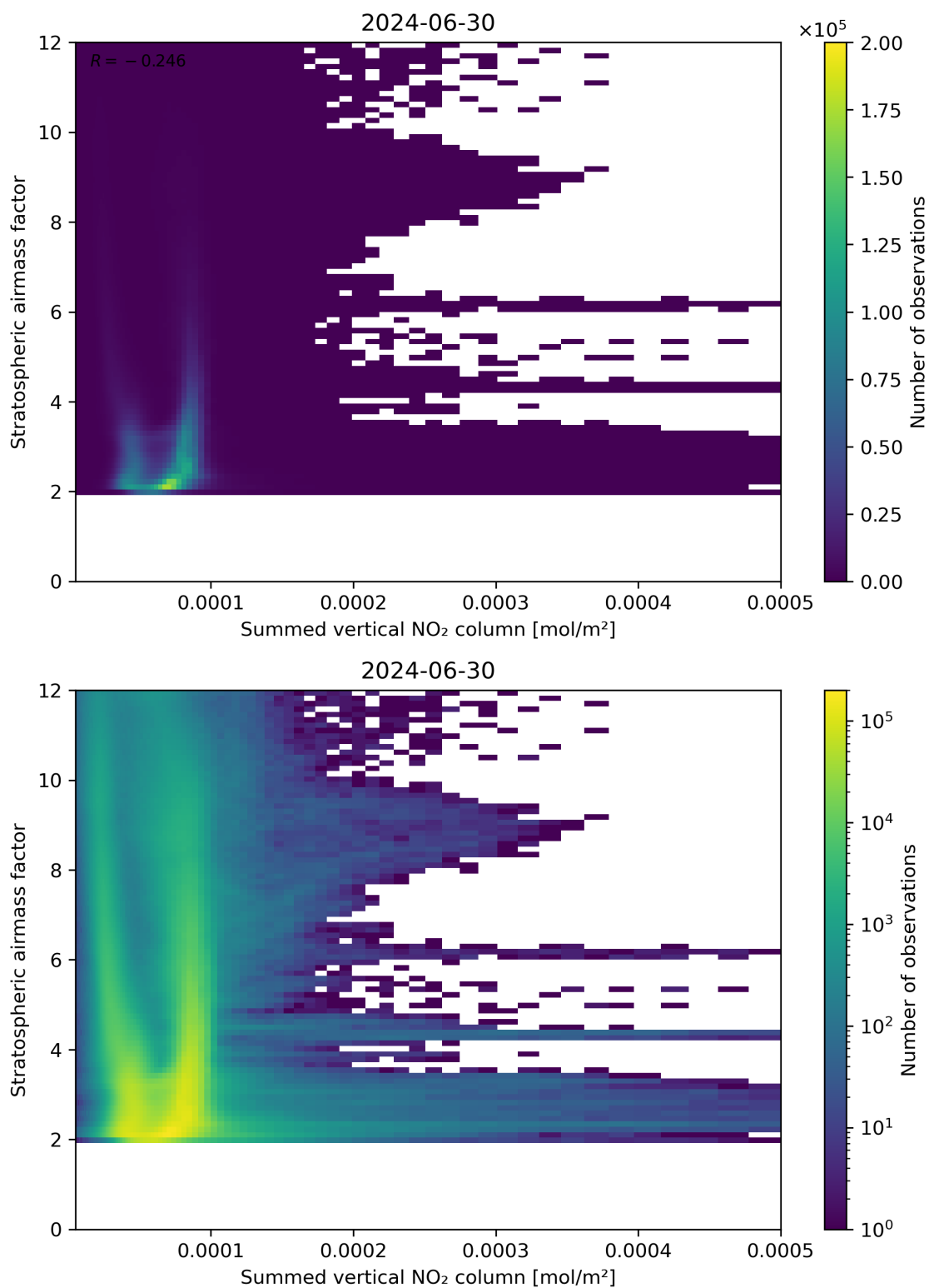
Figure 103: Scatter density plot of “Summed vertical NO 2 column” against “Stratospheric air mass factor” for 2024-06-29 to 2024-07-01.
