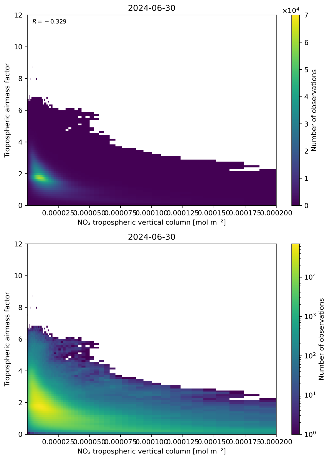
Figure 123: Scatter density plot of “NO 2 tropospheric vertical column” against “Tropospheric airmass factor” for 2024-06-29 to 2024-07-01.
