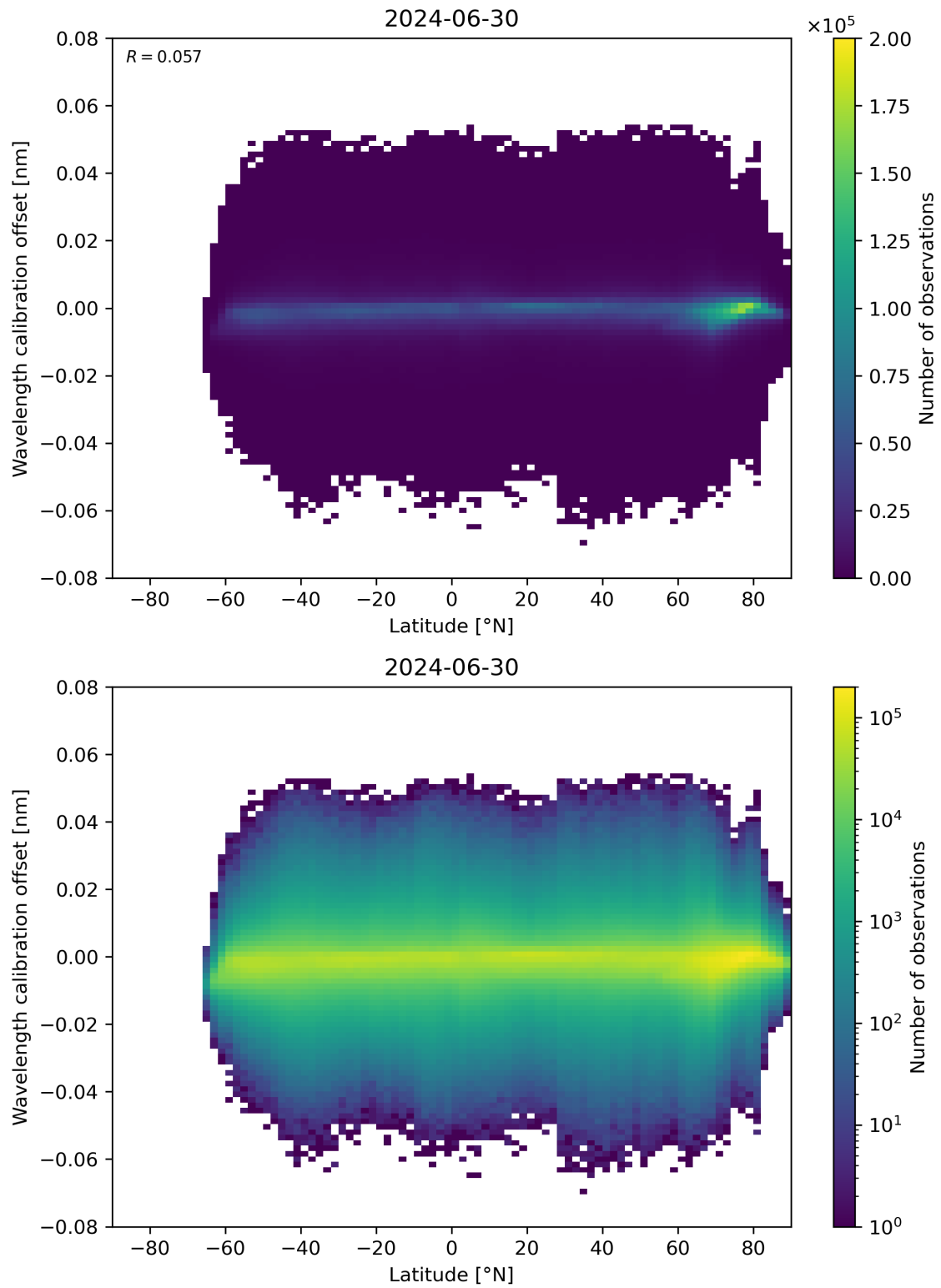
Figure 95: Scatter density plot of “Latitude” against “Wavelength calibration offset” for 2024-06-29 to 2024-07-01.
