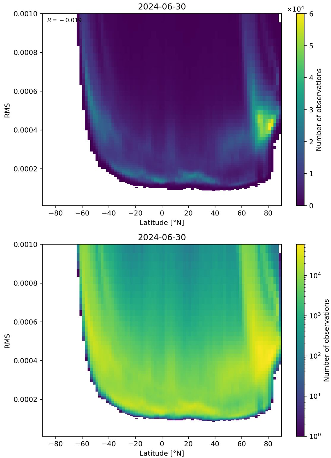
Figure 94: Scatter density plot of “Latitude” against “RMS” for 2024-06-29 to 2024-07-01.
