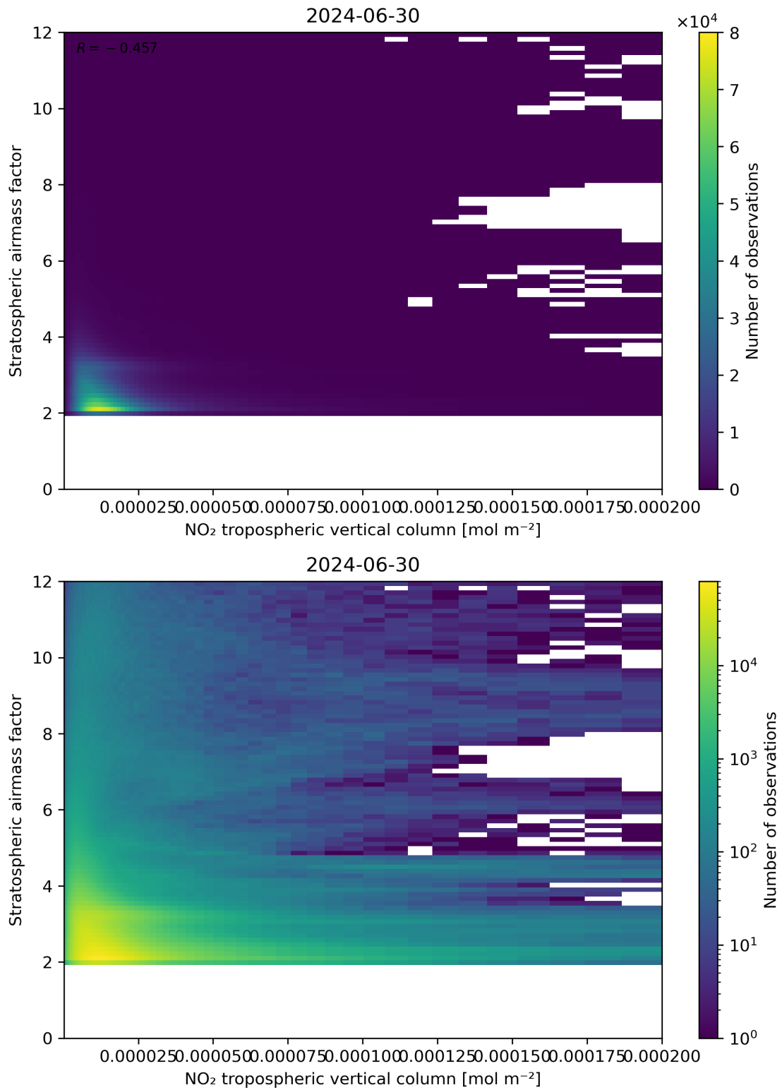
Figure 121: Scatter density plot of “NO 2 tropospheric vertical column” against “Stratospheric air mass factor” for 2024-06-29 to 2024-07-01.
