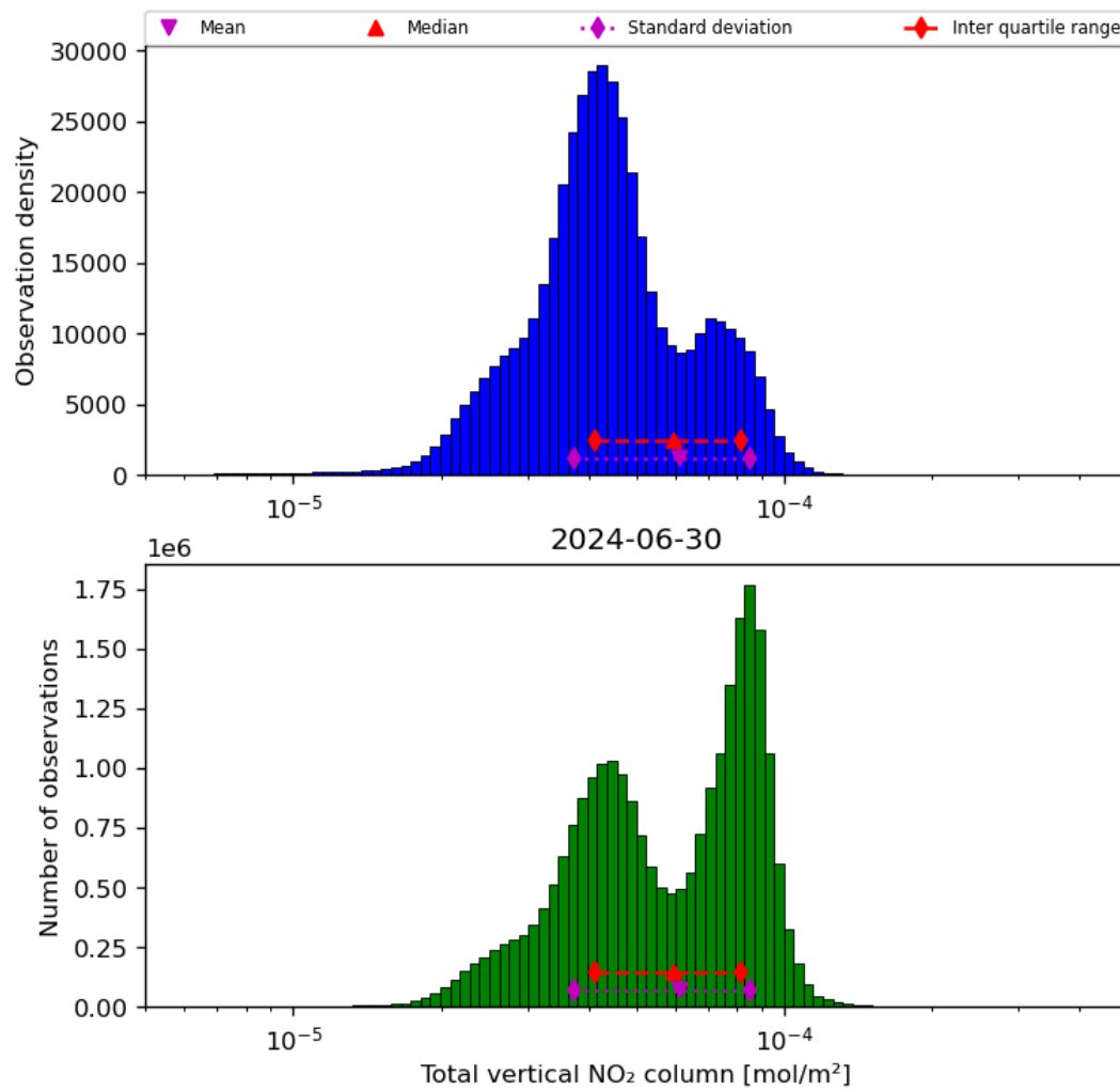
Figure 38: Histogram of “Total vertical NO 2 column” for 2024-06-29 to 2024-07-01
