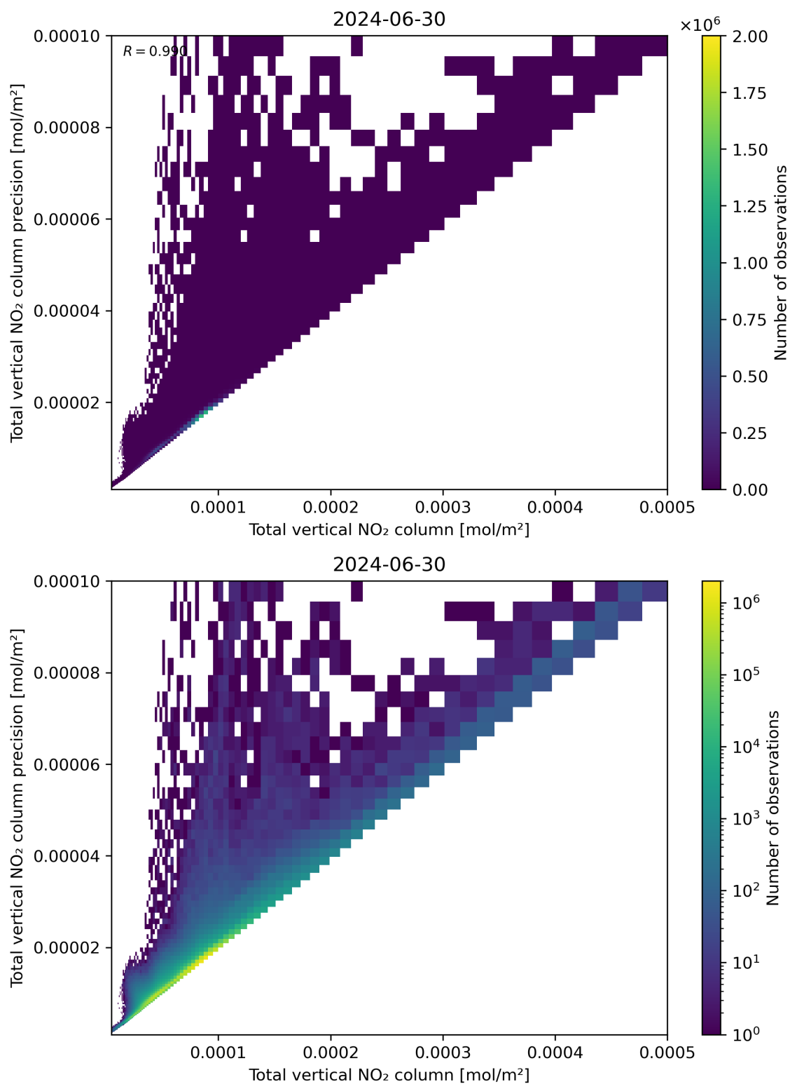
Figure 114: Scatter density plot of “Total vertical NO 2 column” against “Total vertical NO 2 column precision” for 2024-06-29 to 2024-07-01.
