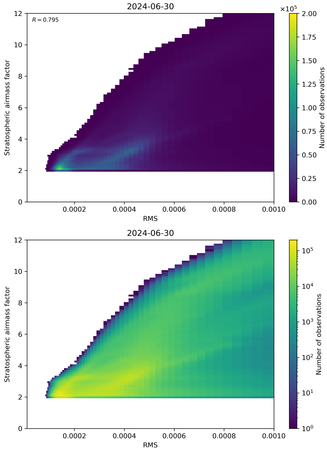
Figure 144: Scatter density plot of “RMS” against “Stratospheric airmass factor” for 2024-06-29 to 2024-07-01.
