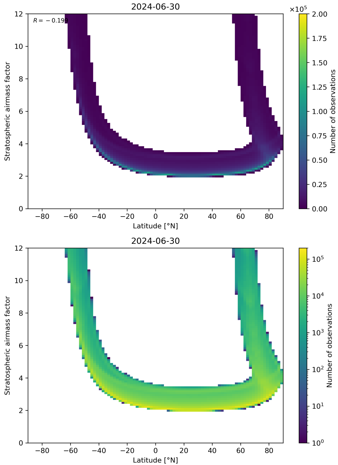
Figure 83: Scatter density plot of “Latitude” against “Stratospheric air mass factor” for 2024-06-29 to 2024-07-01.
