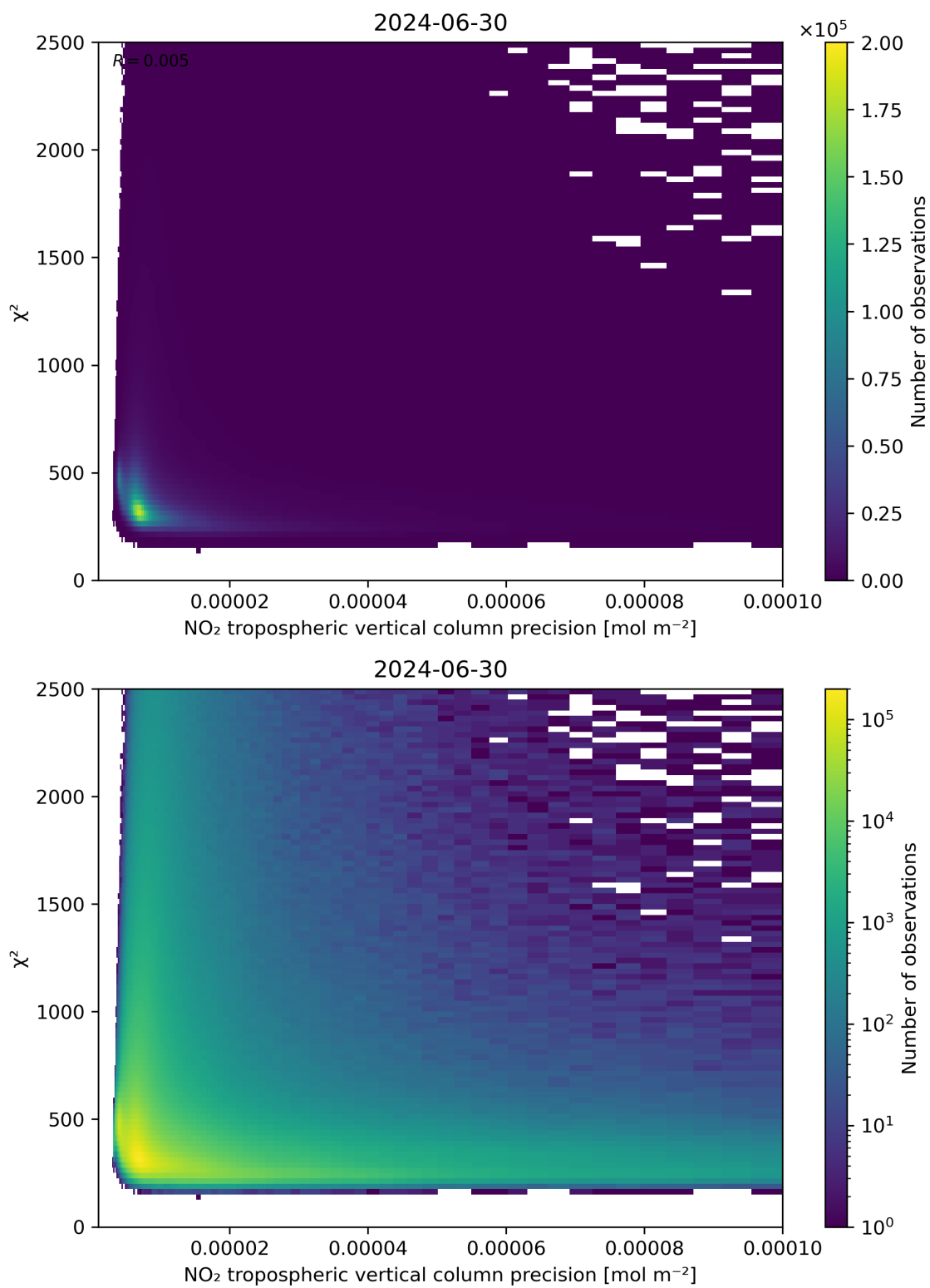
Figure 134: Scatter density plot of “NO 2 tropospheric vertical column precision” against “ \chi^2 ” for 2024-06-29 to 2024-07-01.
