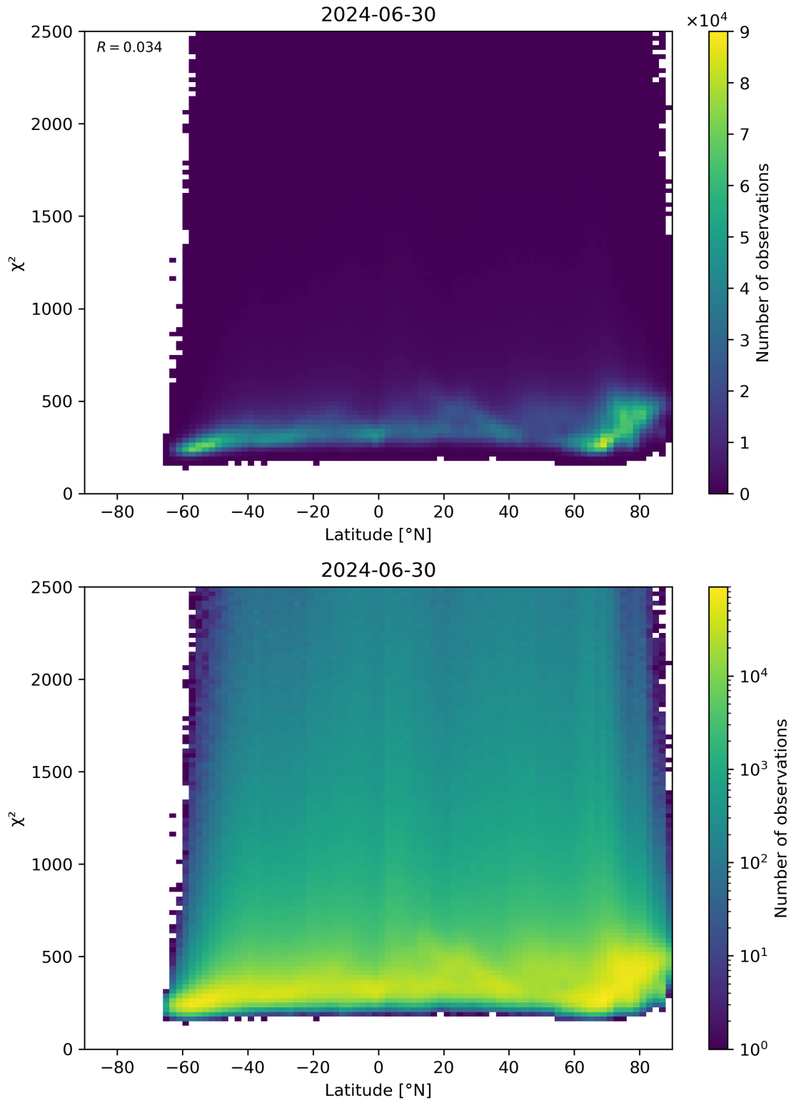
Figure 86: Scatter density plot of “Latitude” against “ \chi^2 ” for 2024-06-29 to 2024-07-01.
