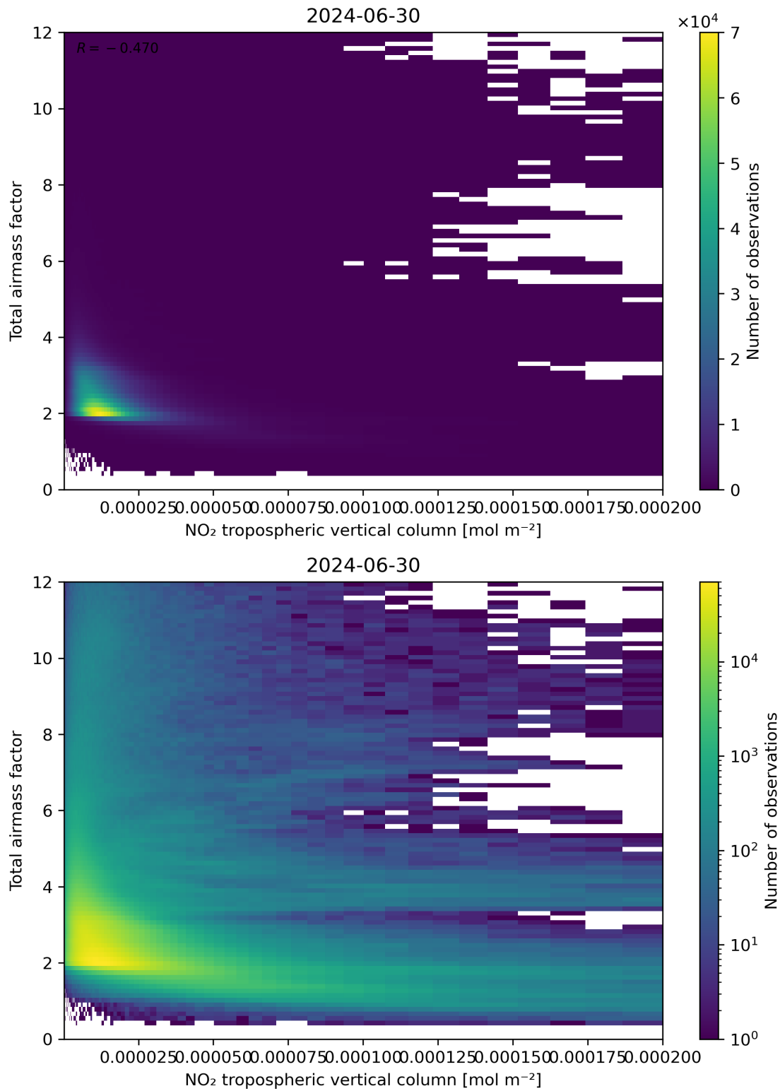
Figure 122: Scatter density plot of “NO 2 tropospheric vertical column” against “Total air mass factor” for 2024-06-29 to 2024-07-01.
