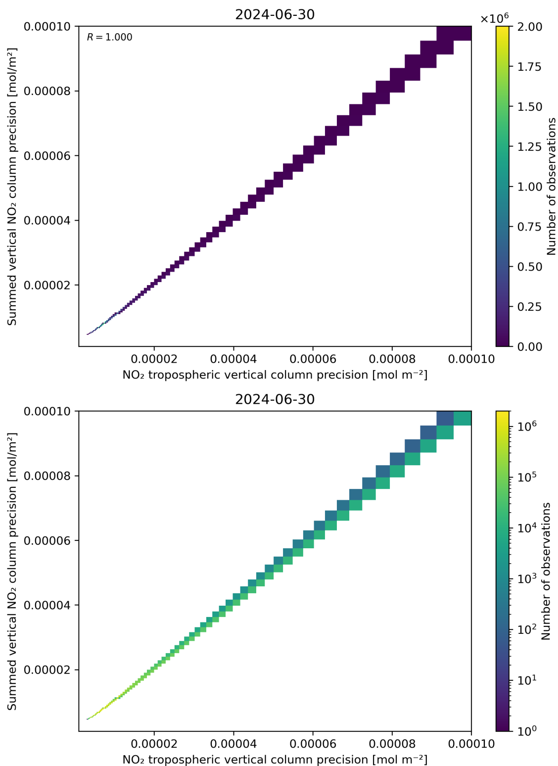
Figure 137: Scatter density plot of “NO 2 tropospheric vertical column precision” against “Summed vertical NO 2 column precision” for 2024-06-29 to 2024-07-01.
