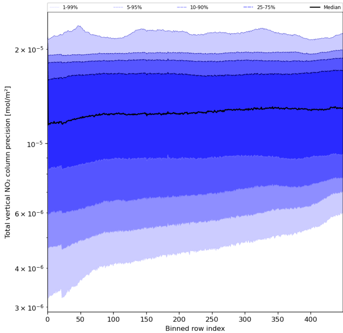
Figure 56: Along track statistics of “Total vertical NO 2 column precision” for 2024-06-29 to 2024-07-01
