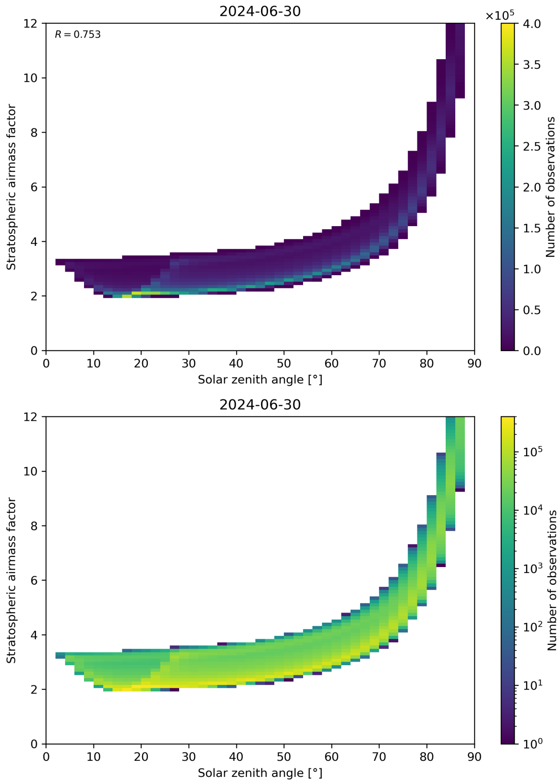
Figure 145: Scatter density plot of “Solar zenith angle” against “Stratospheric airmass factor” for 2024-06-29 to 2024-07-01.
