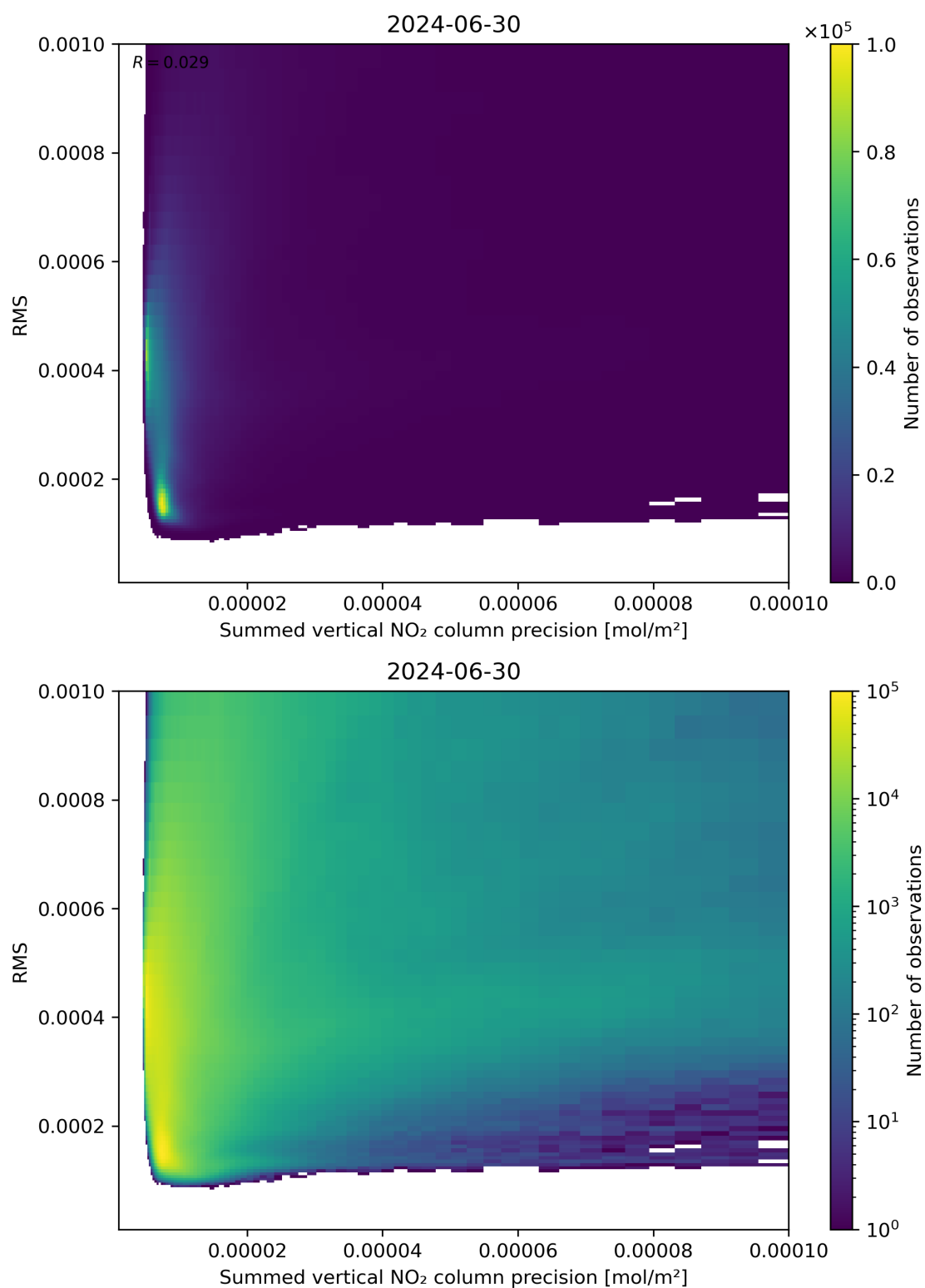
Figure 108: Scatter density plot of “Summed vertical NO 2 column precision” against “RMS” for 2024-06-29 to 2024-07-01.
