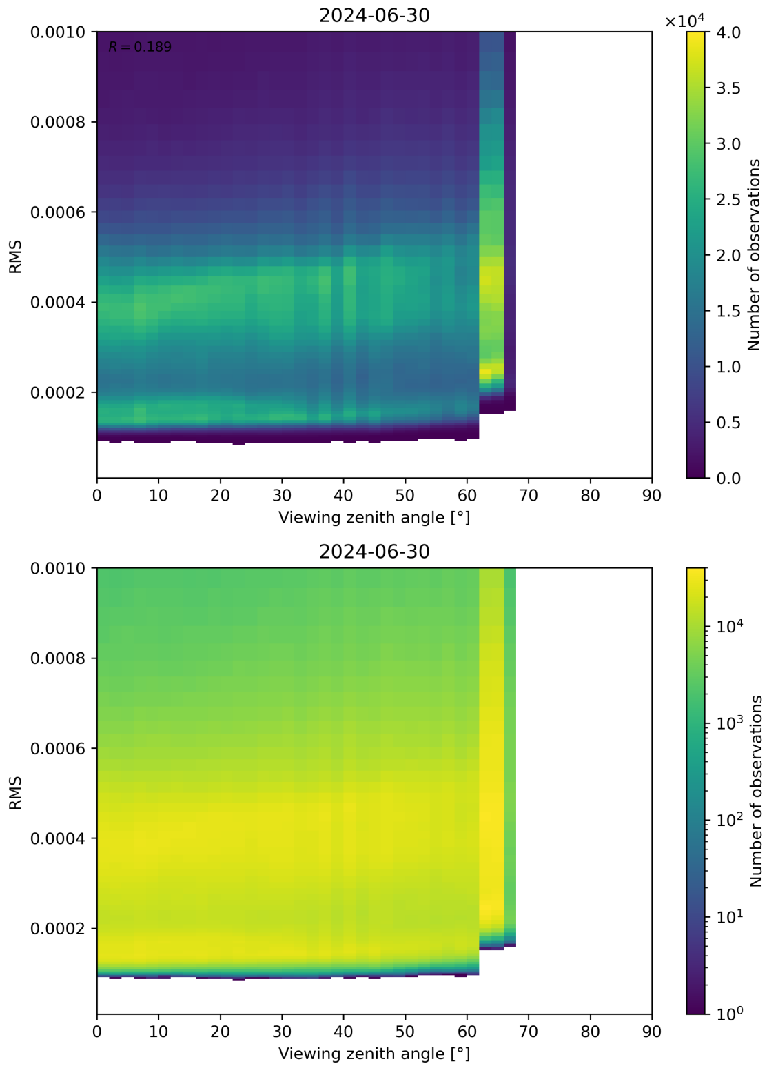
Figure 171: Scatter density plot of “Viewing zenith angle” against “RMS” for 2024-06-29 to 2024-07-01.
