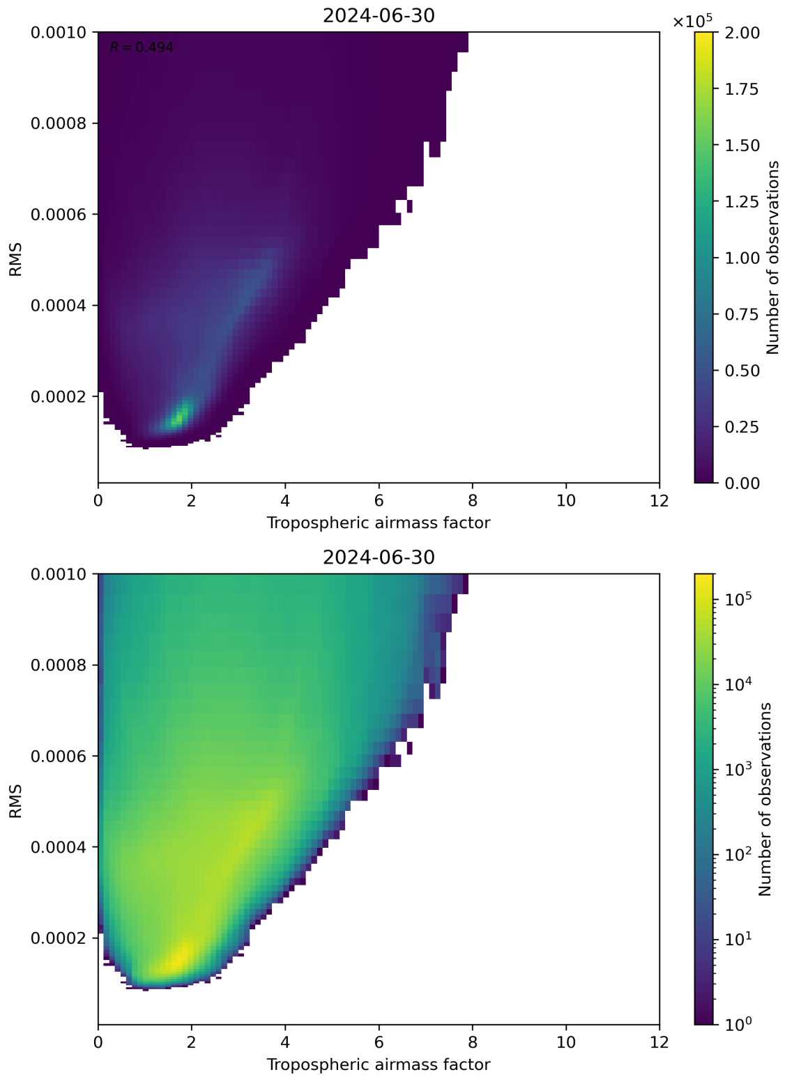
Figure 79: Scatter density plot of “Tropospheric airmass factor” against “RMS” for 2024-06-29 to 2024-07-01.
