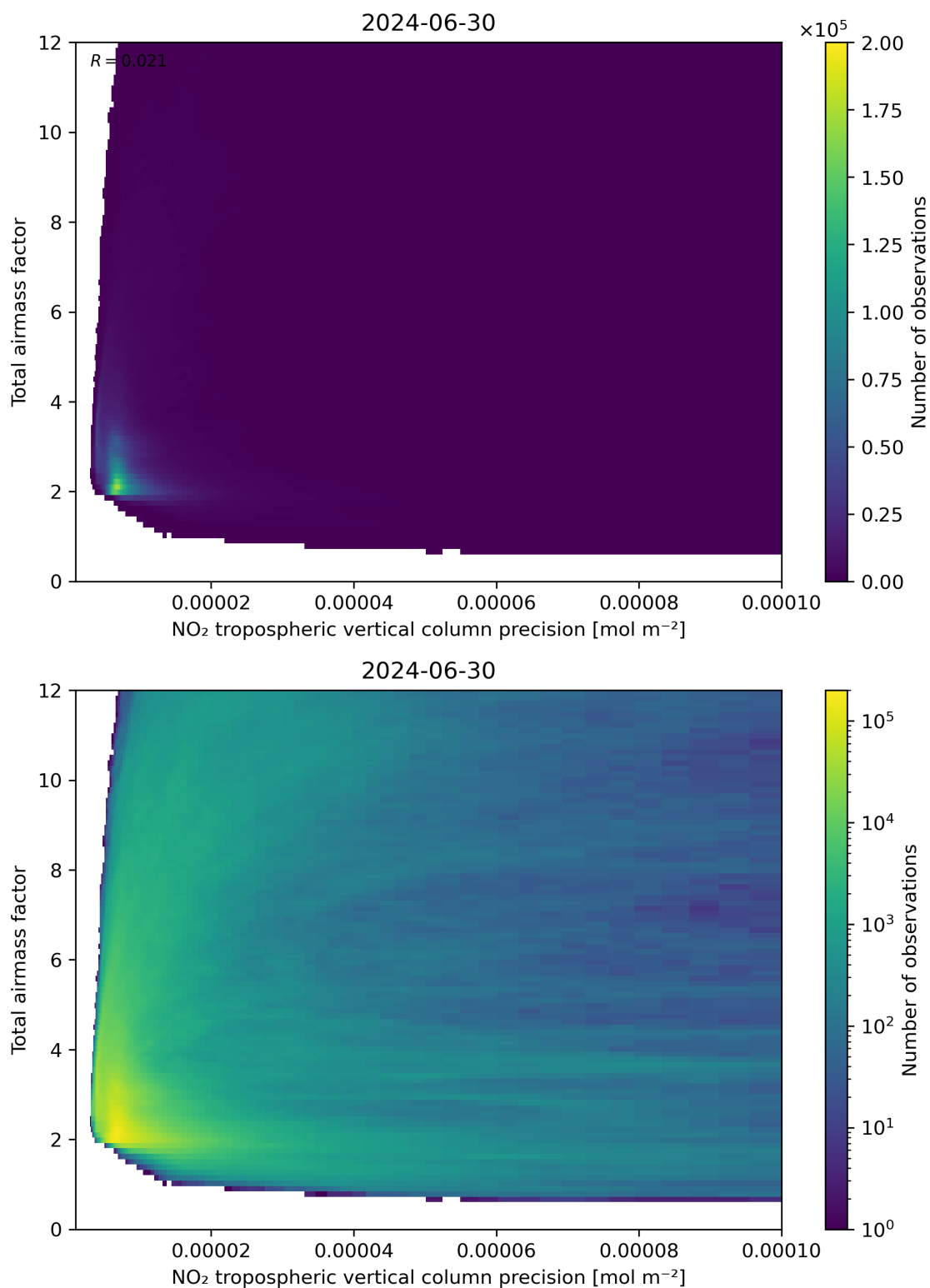
Figure 132: Scatter density plot of “NO 2 tropospheric vertical column precision” against “Total air mass factor” for 2024-06-29 to 2024-07-01.
