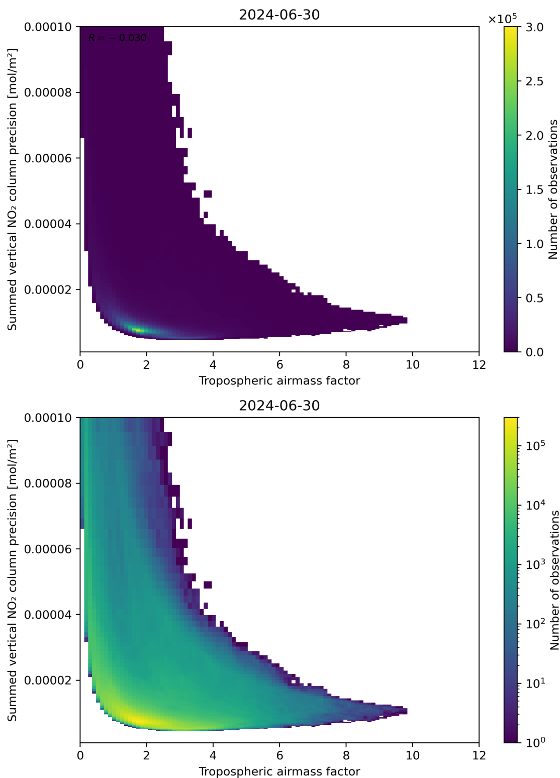
Figure 76: Scatter density plot of “Tropospheric air mass factor” against “Summed vertical NO 2 column precision” for 2024-06-29 to 2024-07-01.
