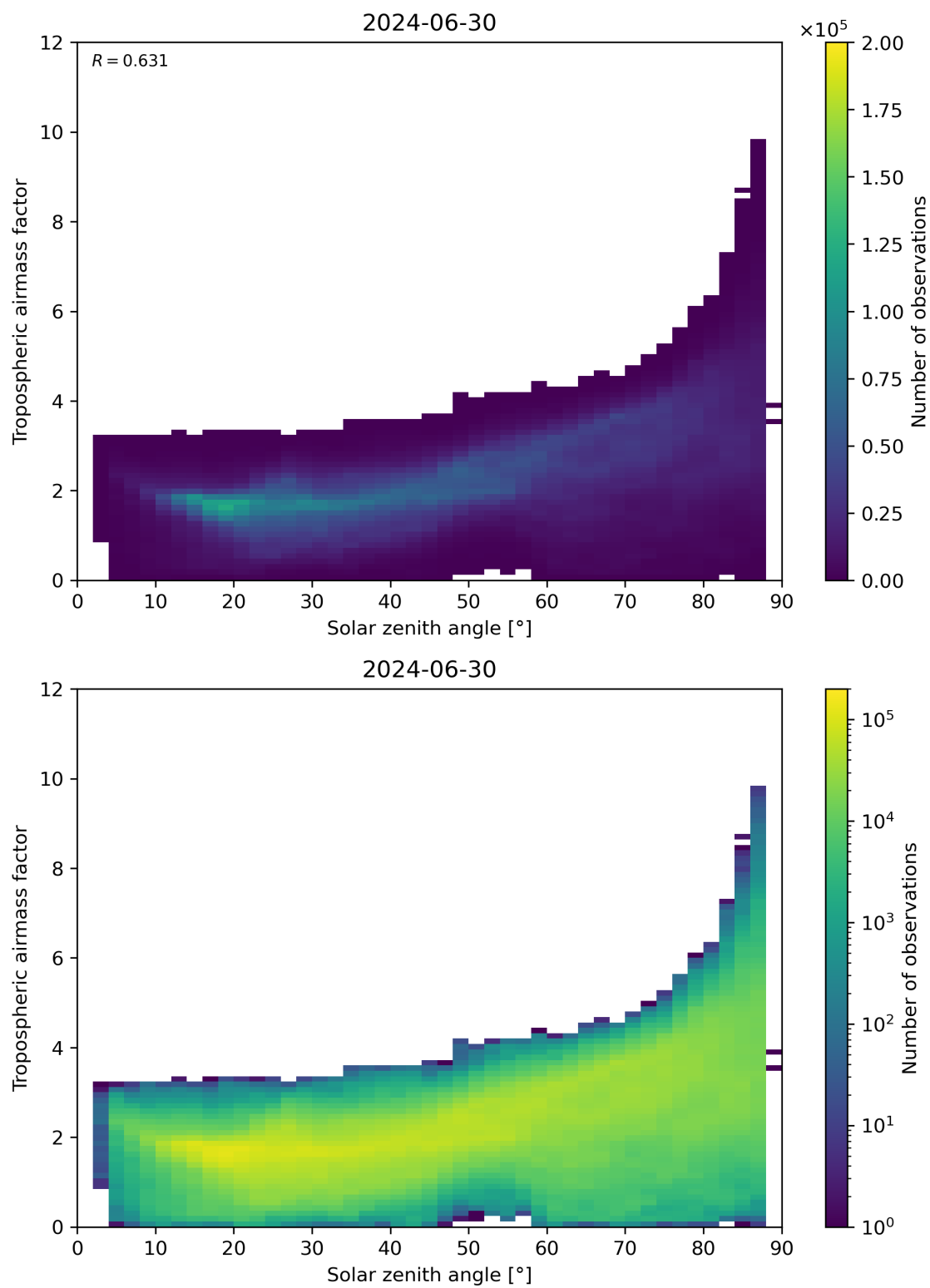
Figure 147: Scatter density plot of “Solar zenith angle” against “Tropospheric airmass factor” for 2024-06-29 to 2024-07-01.
