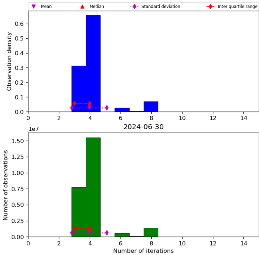
Figure 34: Histogram of “Number of iterations” for 2024-06-29 to 2024-07-01
