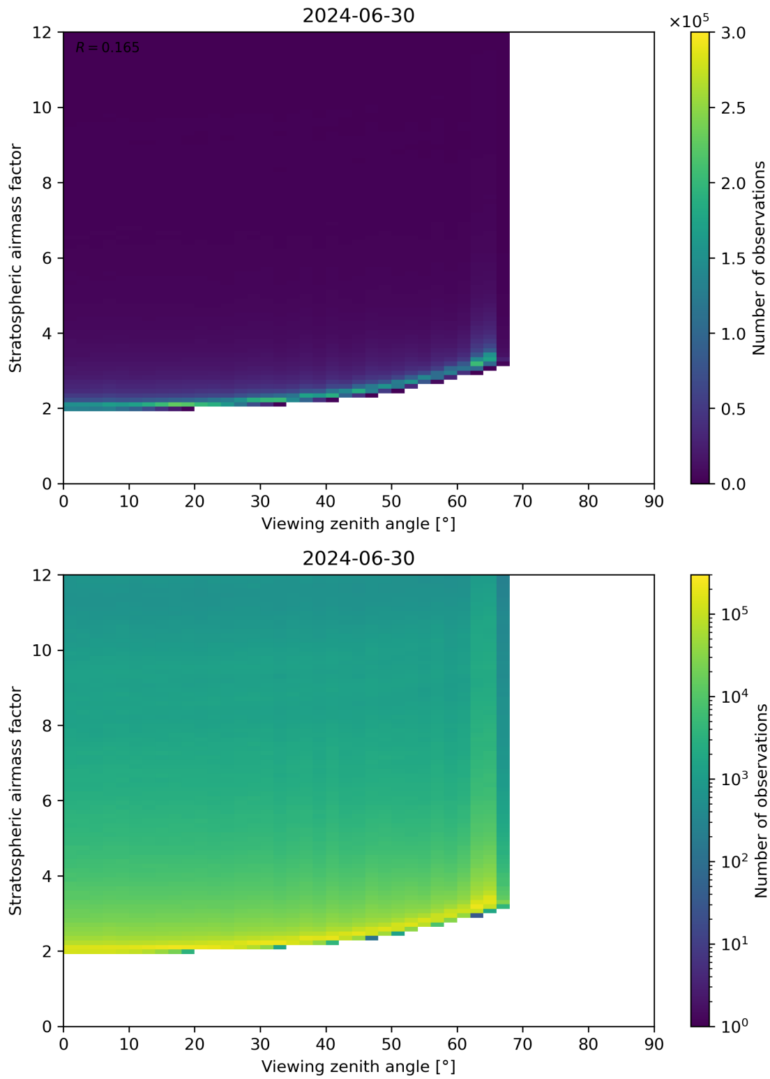
Figure 159: Scatter density plot of “Viewing zenith angle” against “Stratospheric airmass factor” for 2024-06-29 to 2024-07-01.
