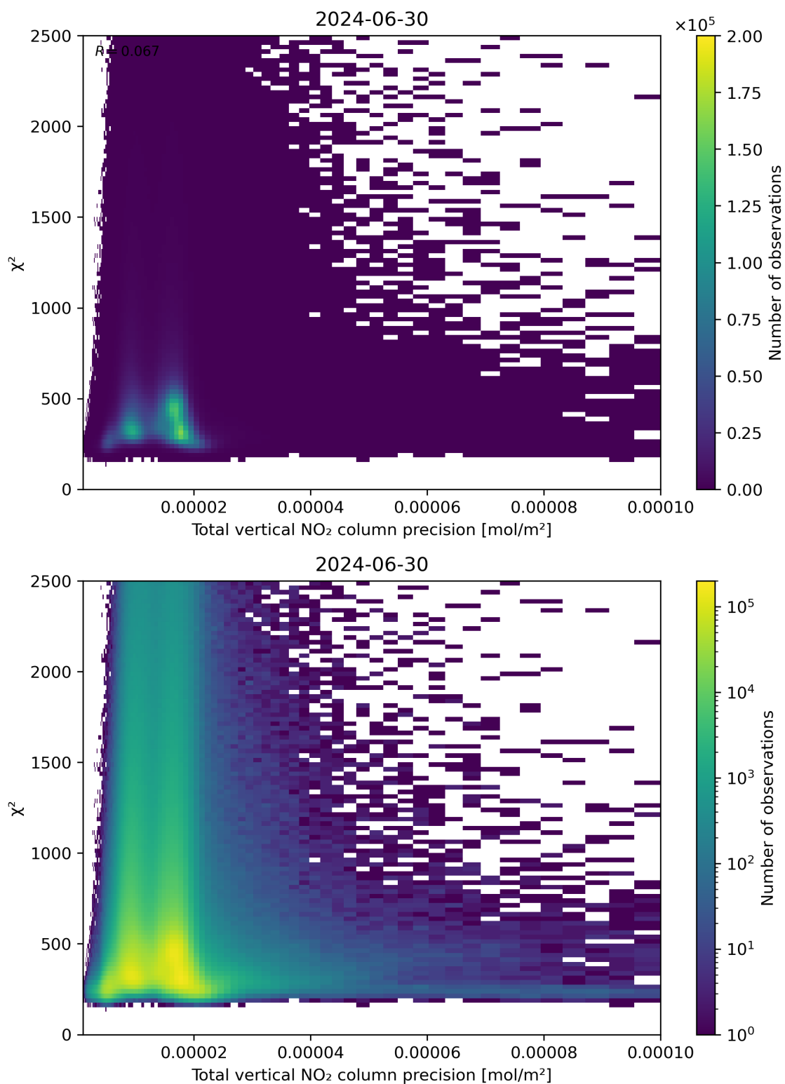
Figure 116: Scatter density plot of “Total vertical NO 2 column precision” against “ \chi^2 ” for 2024-06-29 to 2024-07-01.
