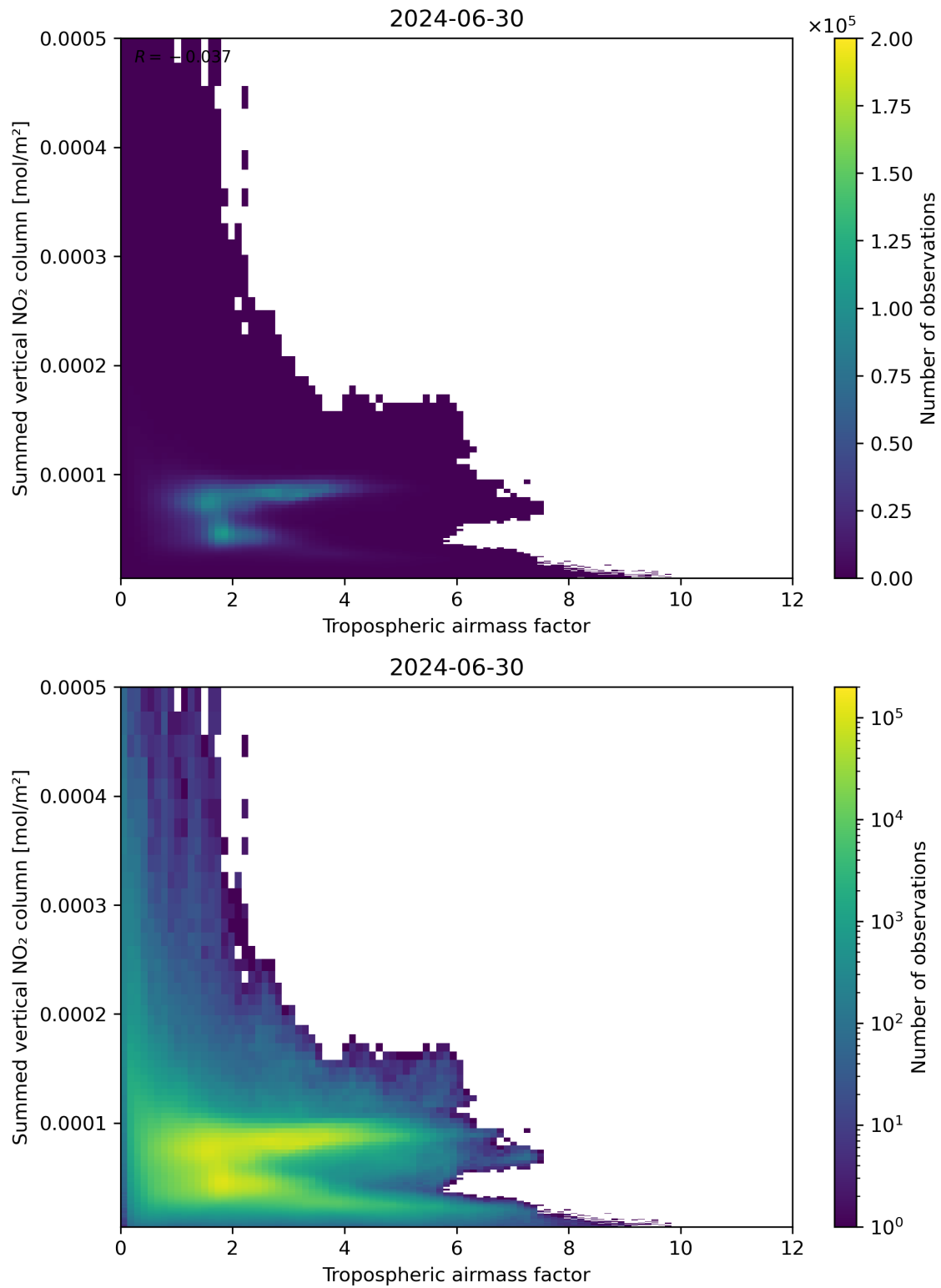
Figure 75: Scatter density plot of “Tropospheric air mass factor” against “Summed vertical NO 2 column” for 2024-06-29 to 2024-07-01.
