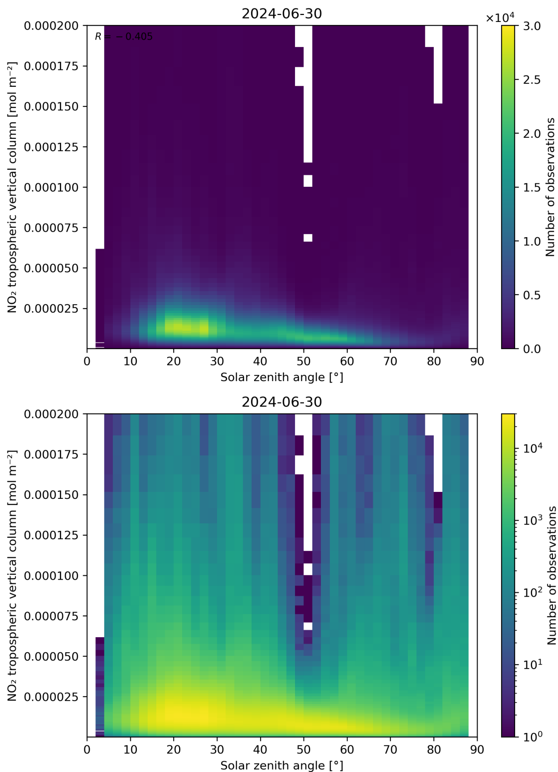
Figure 155: Scatter density plot of “Solar zenith angle” against “NO 2 tropospheric vertical column” for 2024-06-29 to 2024-07-01.
