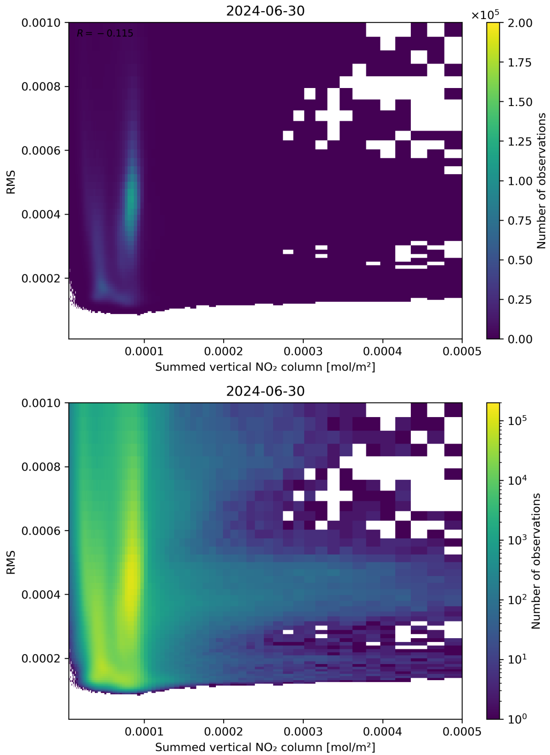
Figure 109: Scatter density plot of “Summed vertical NO 2 column” against “RMS” for 2024-06-29 to 2024-07-01.
