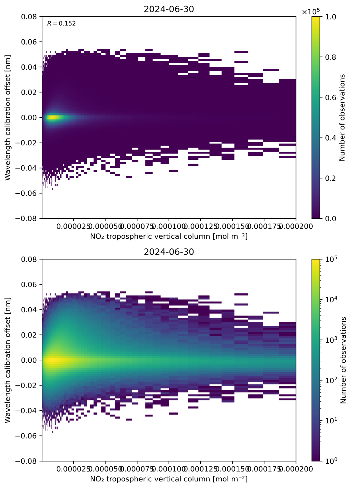
Figure 143: Scatter density plot of “NO 2 tropospheric vertical column” against “Wavelength calibration offset” for 2024-06-29 to 2024-07-01.
