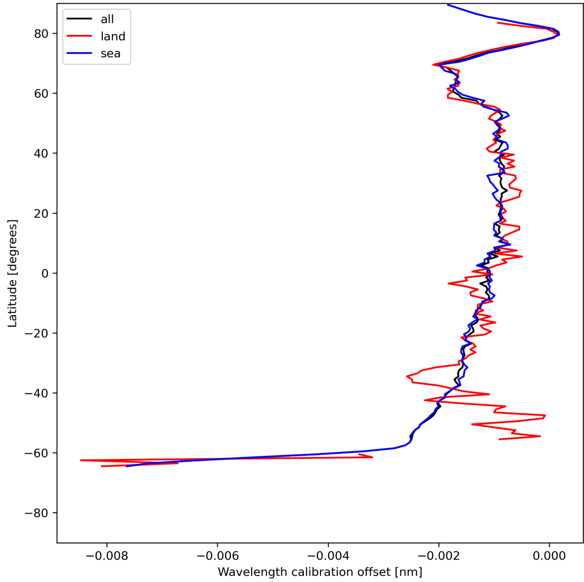
Figure 18: Zonal average of “Wavelength calibration offset” for 2024-06-29 to 2024-07-01.
