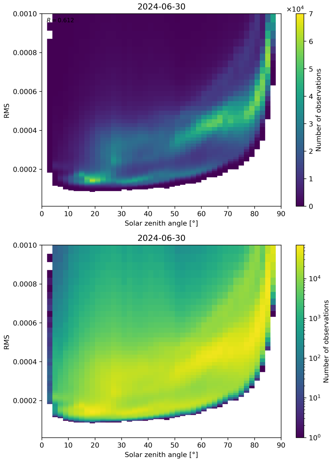
Figure 157: Scatter density plot of “Solar zenith angle” against “RMS” for 2024-06-29 to 2024-07-01.
