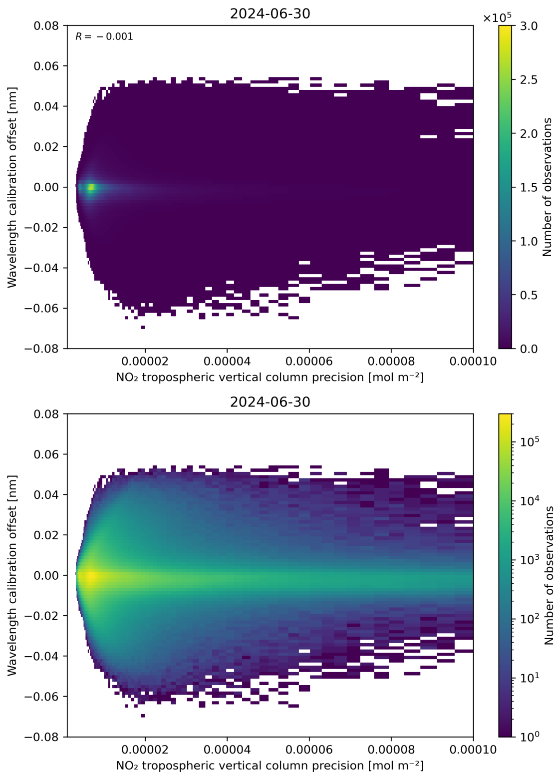
Figure 141: Scatter density plot of “NO 2 tropospheric vertical column precision” against “Wavelength calibration offset” for 2024-06-29 to 2024-07-01.
