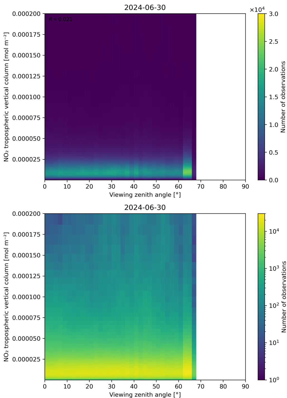
Figure 169: Scatter density plot of “Viewing zenith angle” against “NO 2 tropospheric vertical column” for 2024-06-29 to 2024-07-01.
