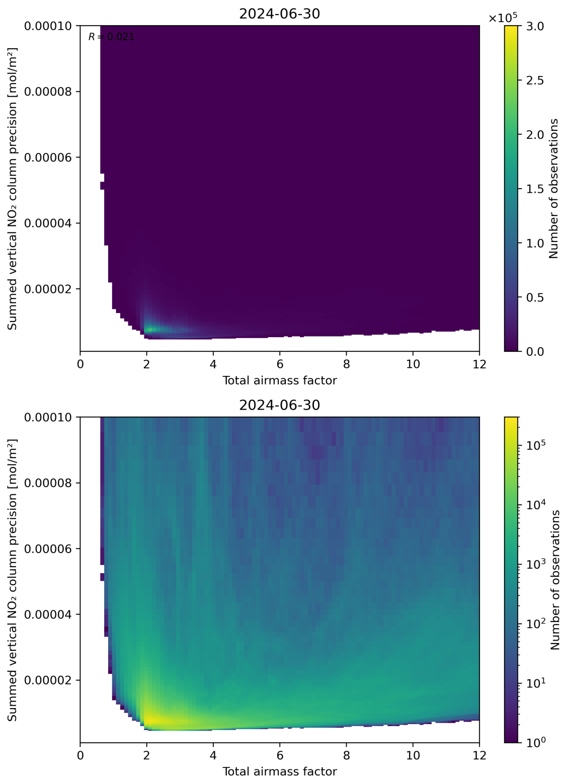
Figure 66: Scatter density plot of “Total airmass factor” against “Summed vertical NO 2 column precision” for 2024-06-29 to 2024-07-01.
