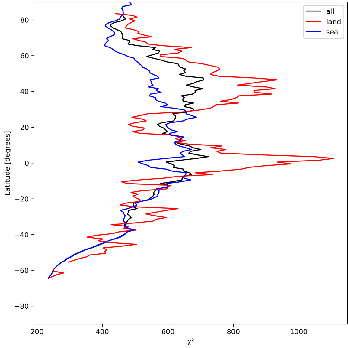
Figure 25: Zonal average of “ \chi^2 ” for 2024-06-29 to 2024-07-01.
