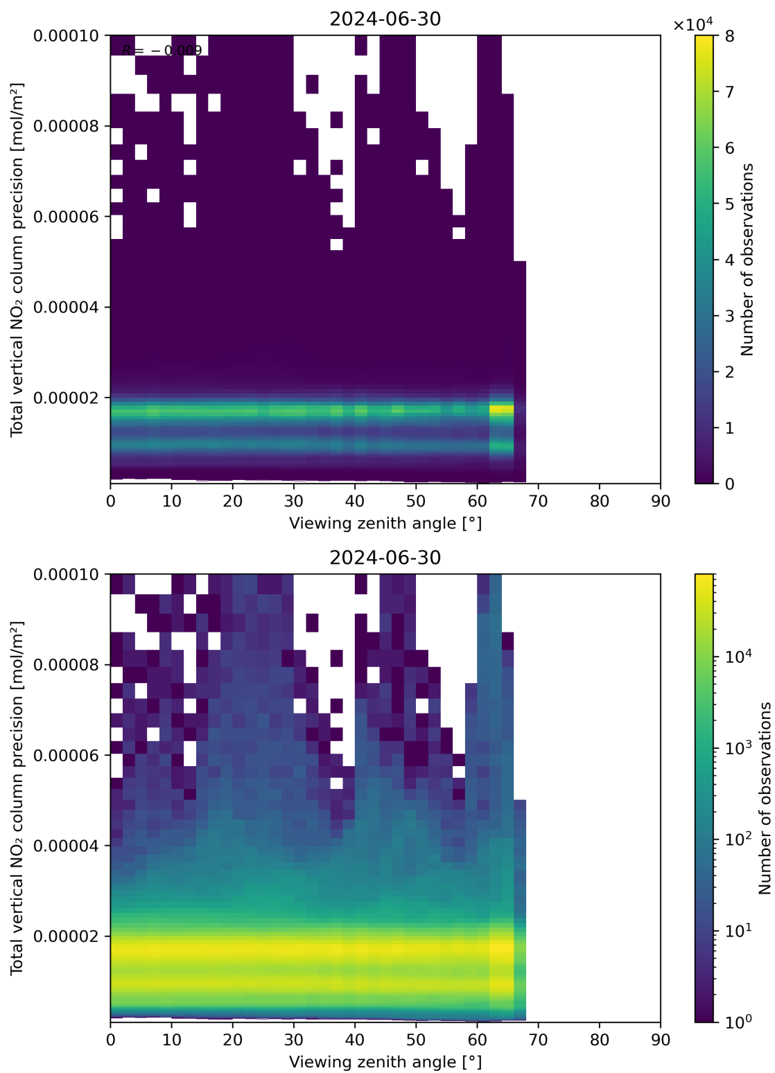
Figure 168: Scatter density plot of “Viewing zenith angle” against “Total vertical NO 2 column precision” for 2024-06-29 to 2024-07-01.
