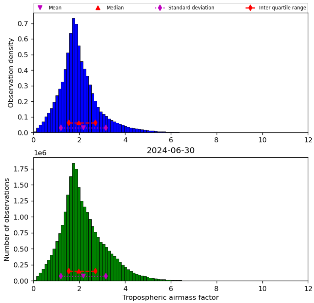
Figure 31: Histogram of “Tropospheric airmass factor” for 2024-06-29 to 2024-07-01
