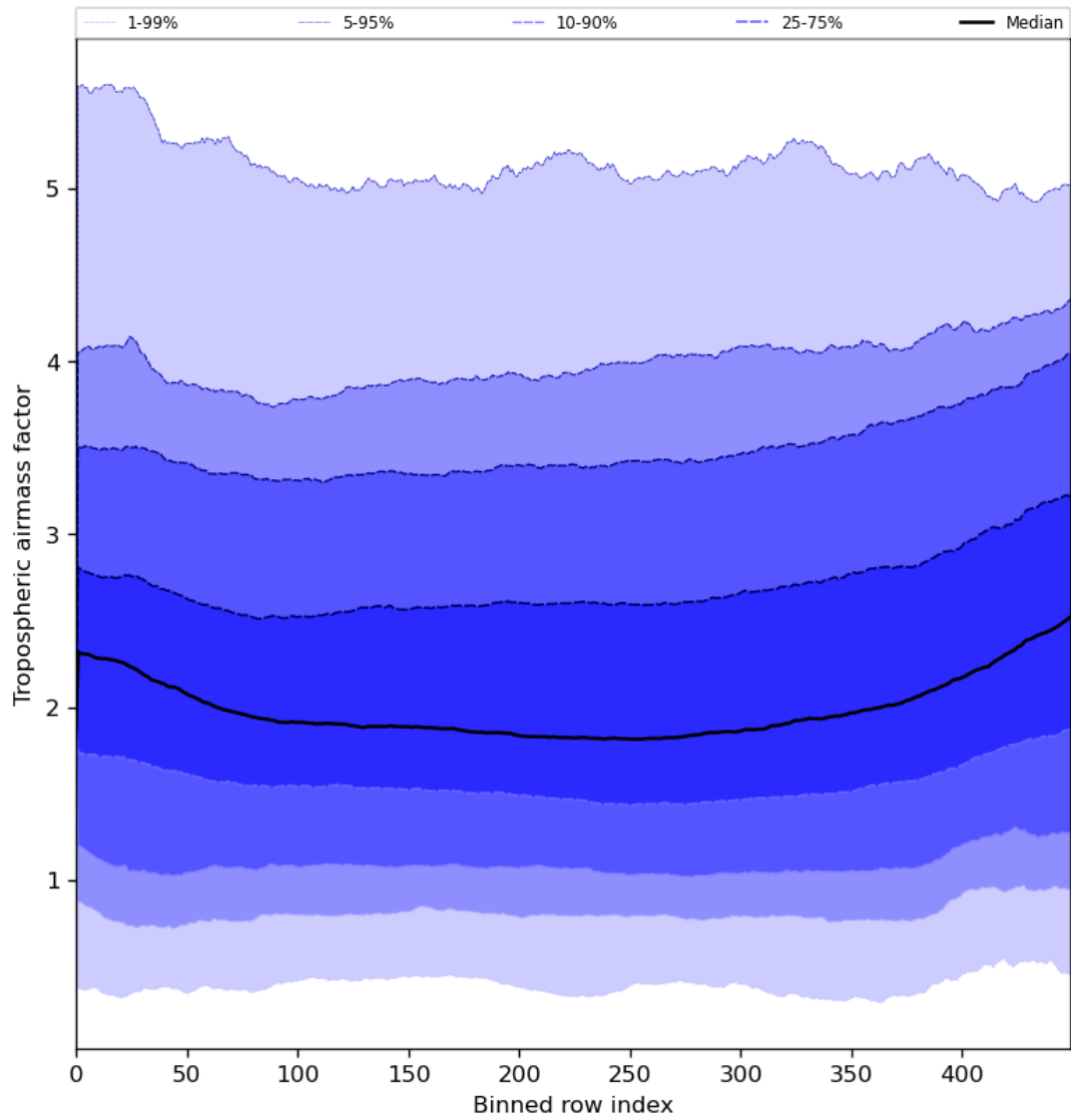
Figure 48: Along track statistics of “Tropospheric airmass factor” for 2024-06-29 to 2024-07-01
