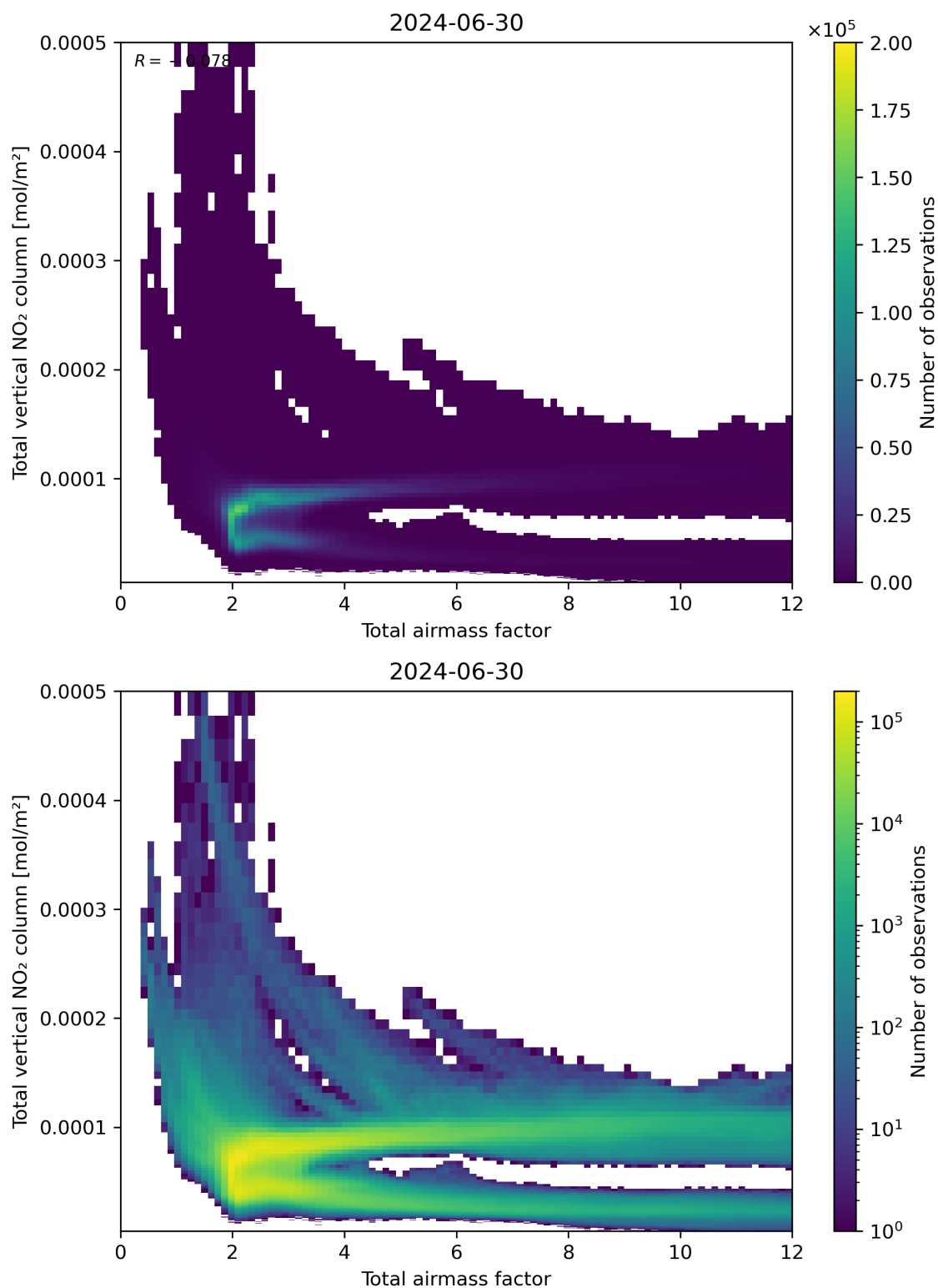
Figure 67: Scatter density plot of “Total airmass factor” against “Total vertical NO 2 column” for 2024-06-29 to 2024-07-01.
