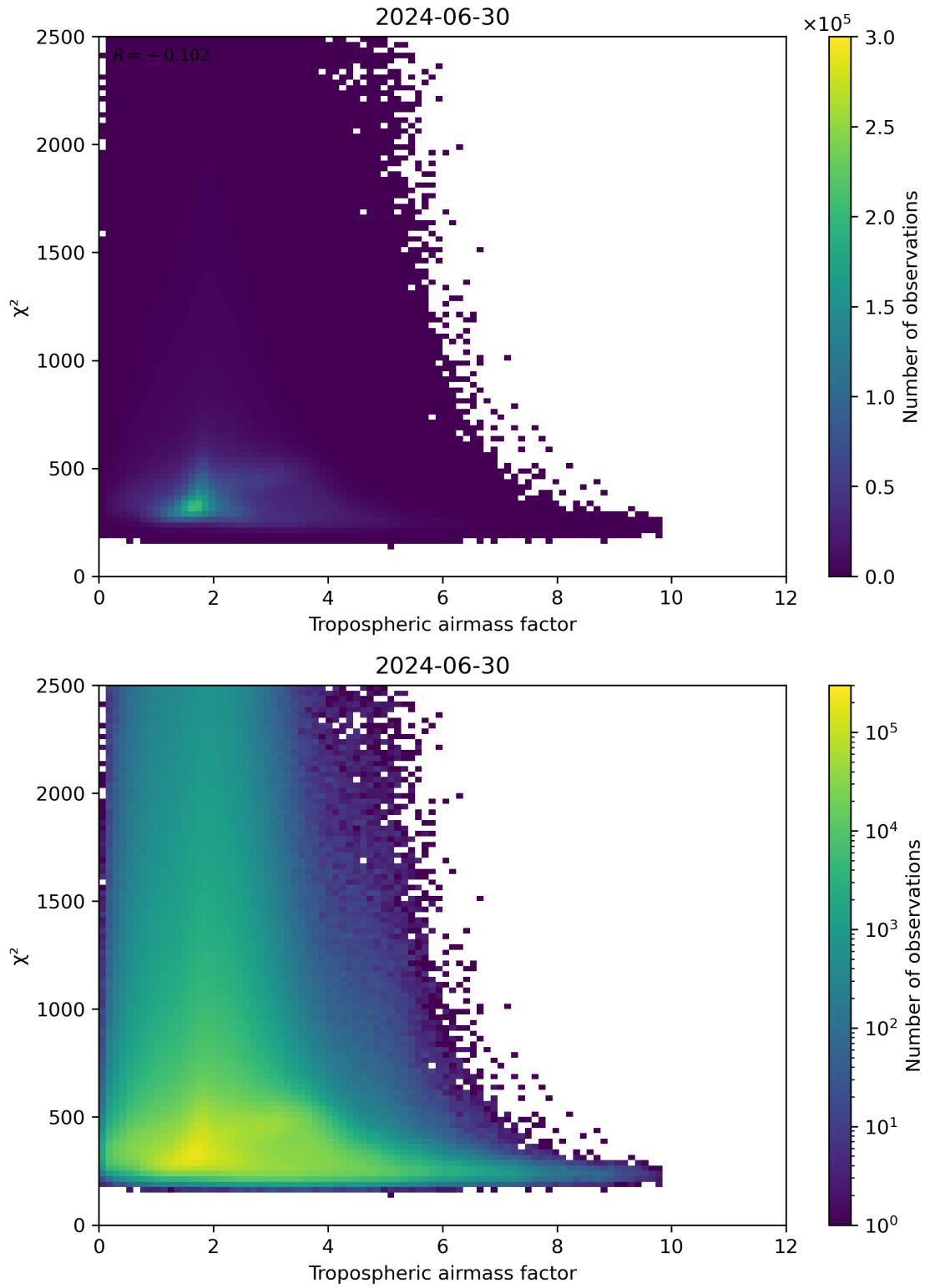
Figure 73: Scatter density plot of “Tropospheric airmass factor” against “ \chi^2 ” for 2024-06-29 to 2024-07-01.
