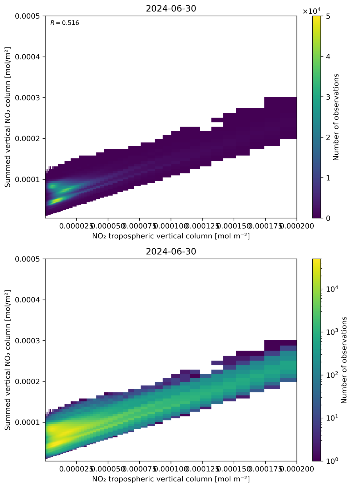
Figure 126: Scatter density plot of “NO 2 tropospheric vertical column” against “Summed vertical NO 2 column” for 2024-06-29 to 2024-07-01.
