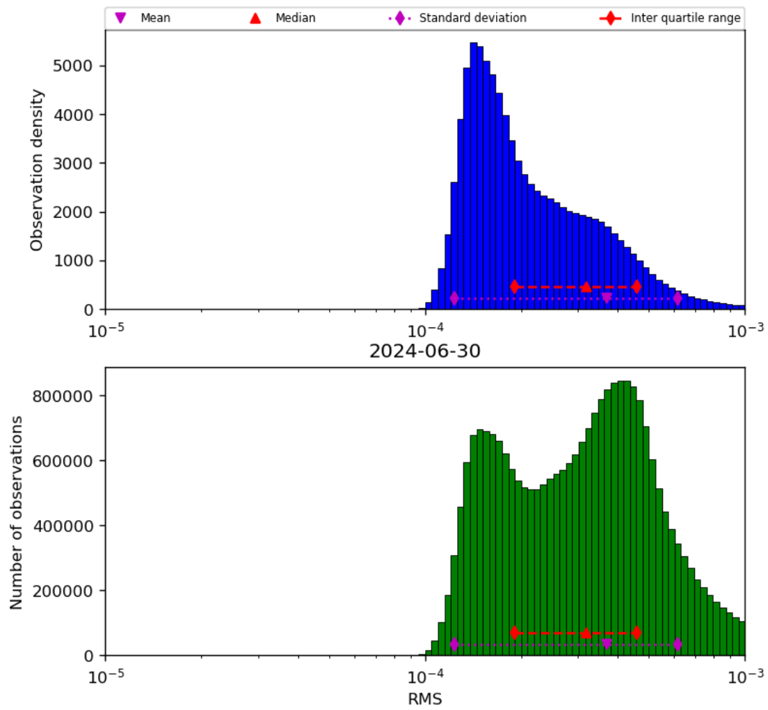
Figure 43: Histogram of “RMS” for 2024-06-29 to 2024-07-01
