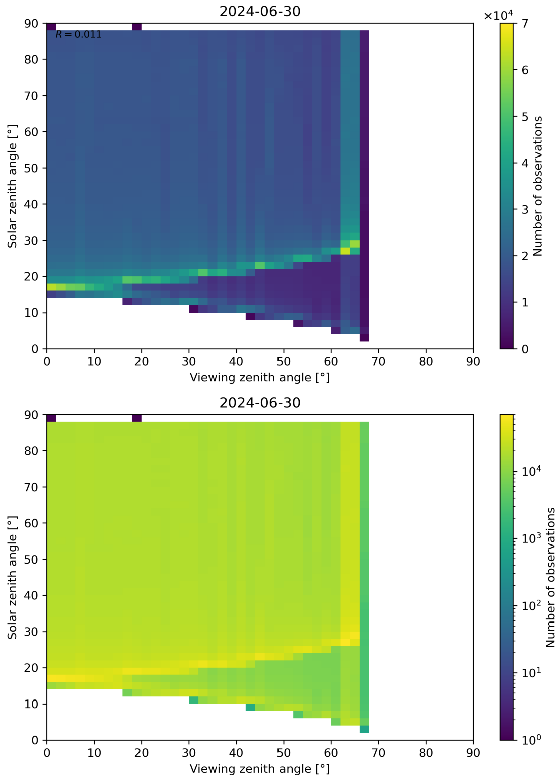
Figure 172: Scatter density plot of “Viewing zenith angle” against “Solar zenith angle” for 2024-06-29 to 2024-07-01.
