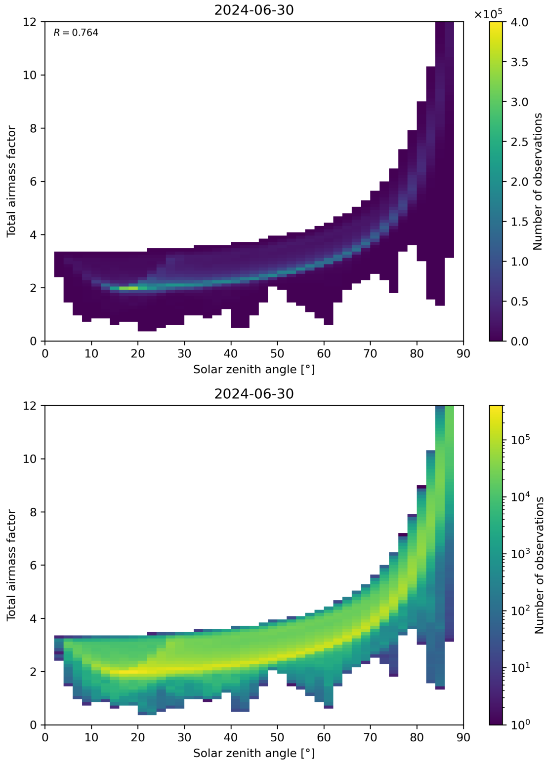
Figure 146: Scatter density plot of “Solar zenith angle” against “Total airmass factor” for 2024-06-29 to 2024-07-01.
