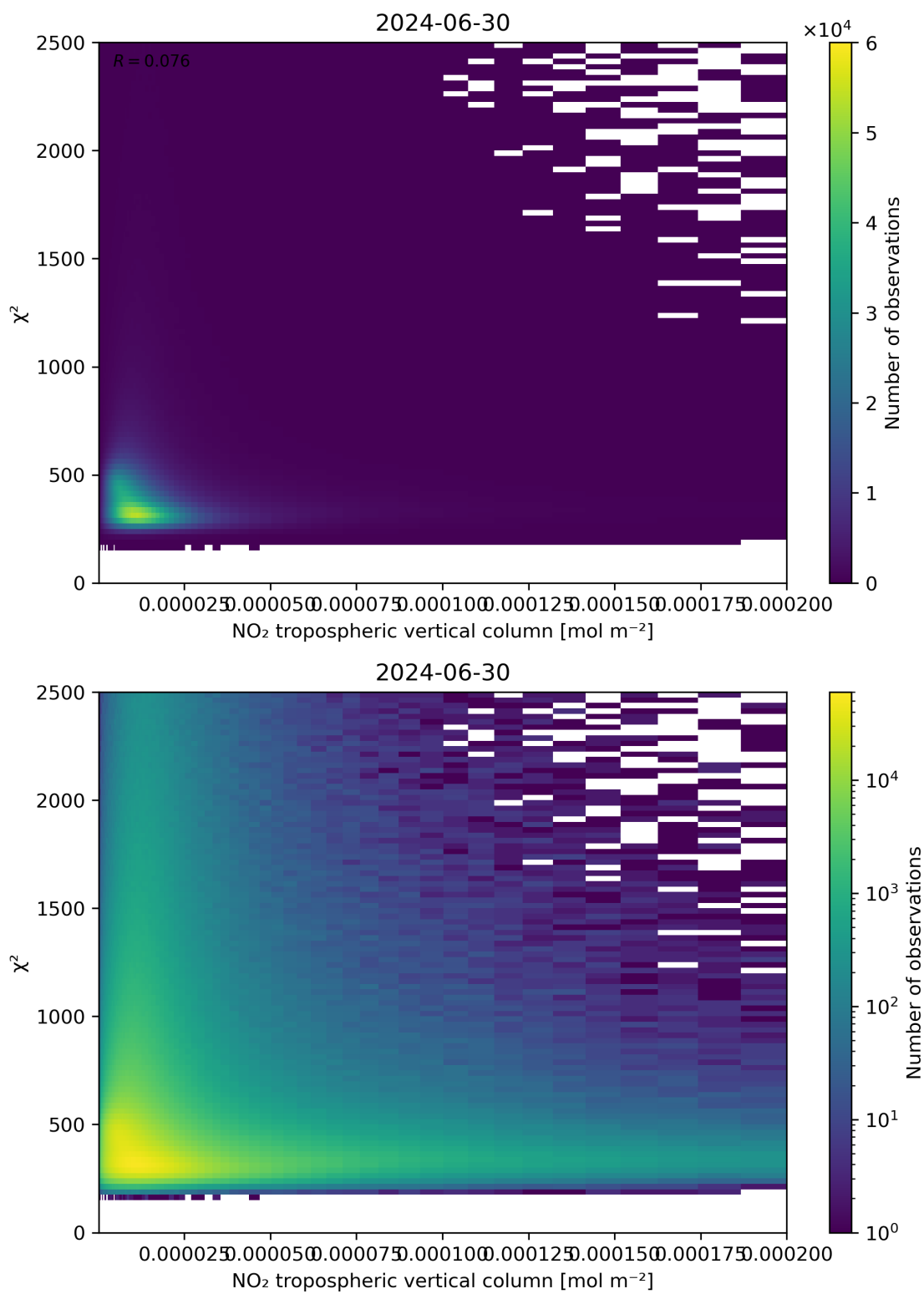
Figure 124: Scatter density plot of “NO 2 tropospheric vertical column” against “ \chi^2 ” for 2024-06-29 to 2024-07-01.
