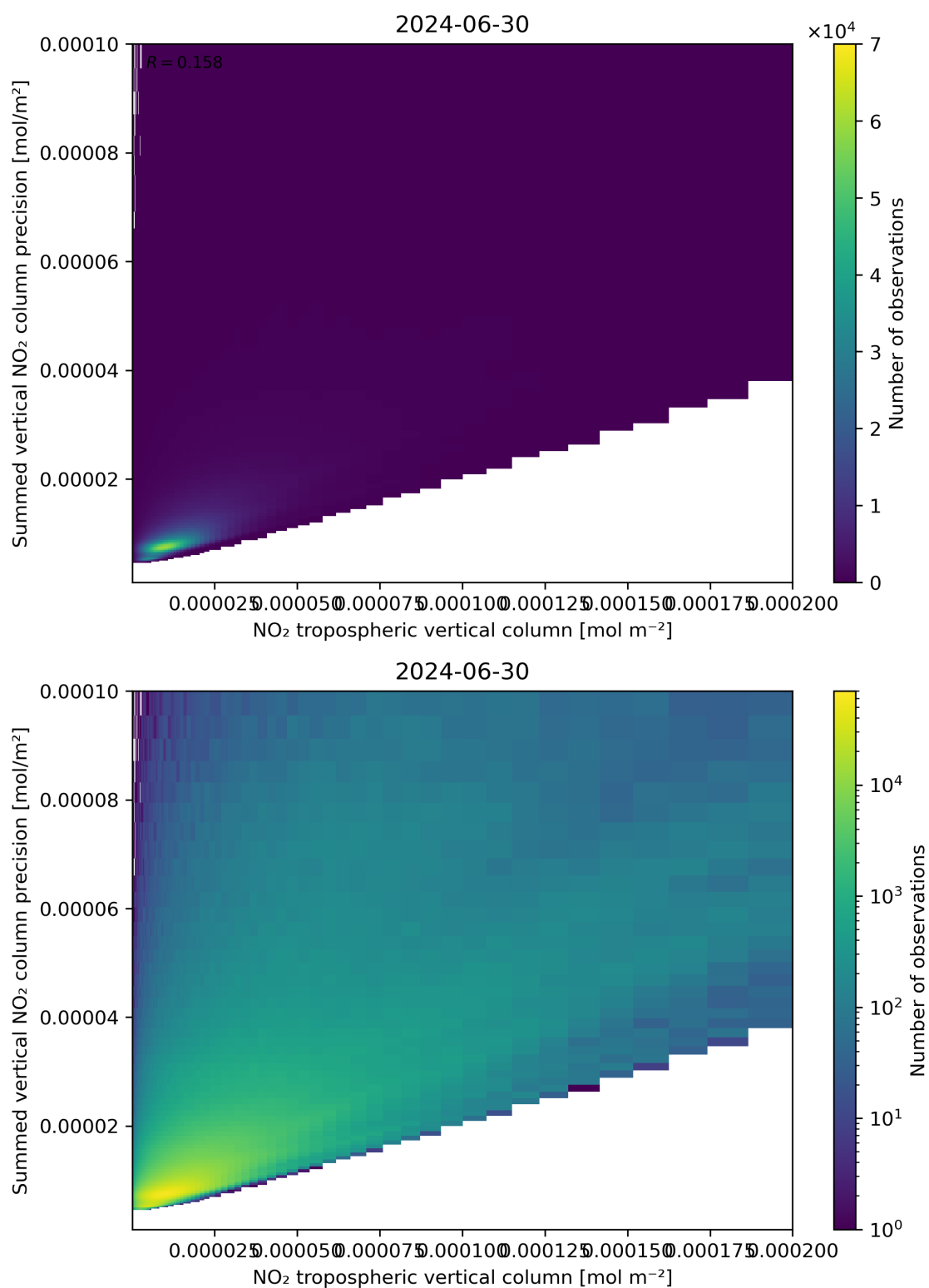
Figure 127: Scatter density plot of “NO 2 tropospheric vertical column” against “Summed vertical NO 2 column precision” for 2024-06-29 to 2024-07-01.
