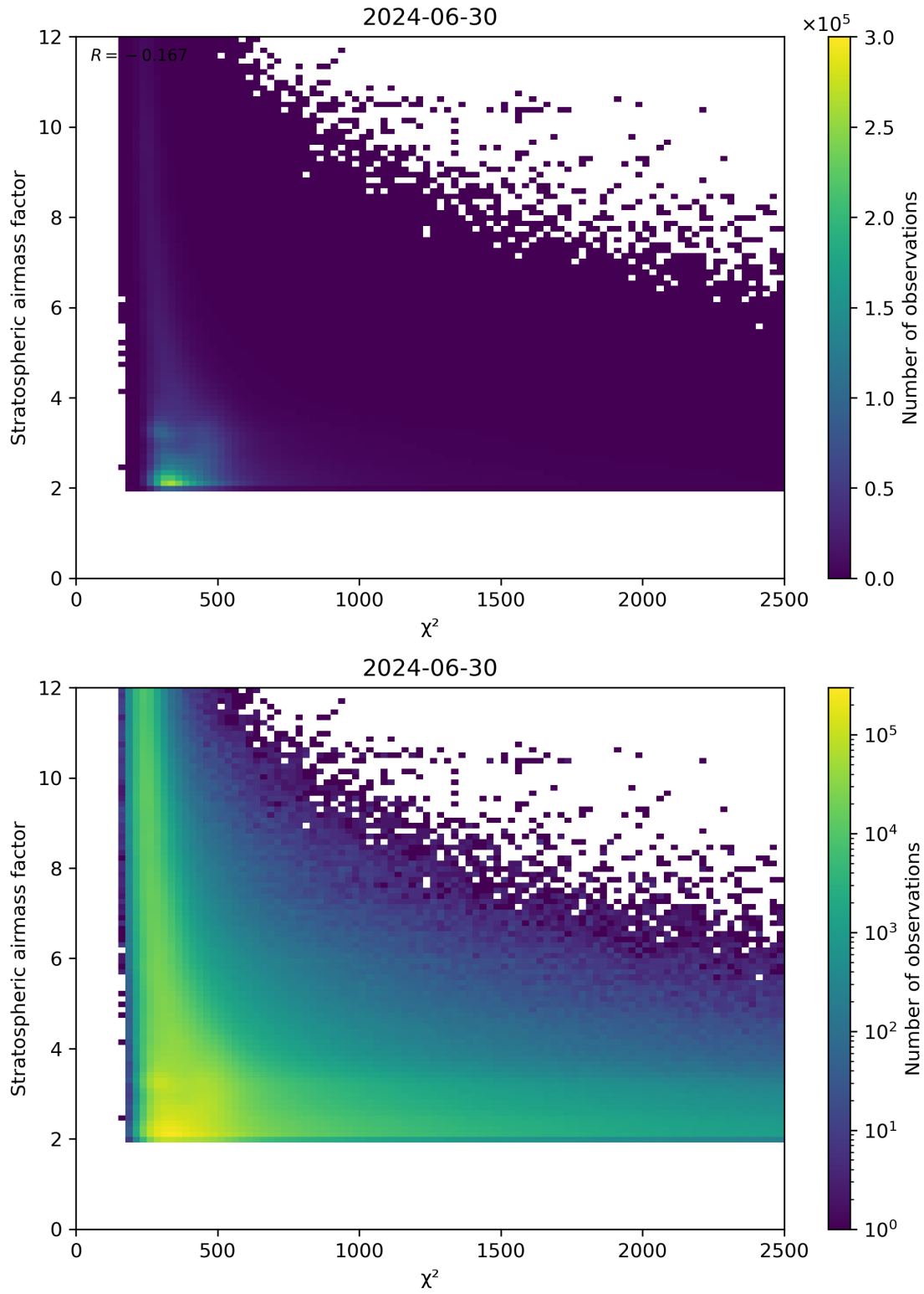
Figure 81: Scatter density plot of “ \chi^2 ” against “Stratospheric airmass factor” for 2024-06-29 to 2024-07-01.
