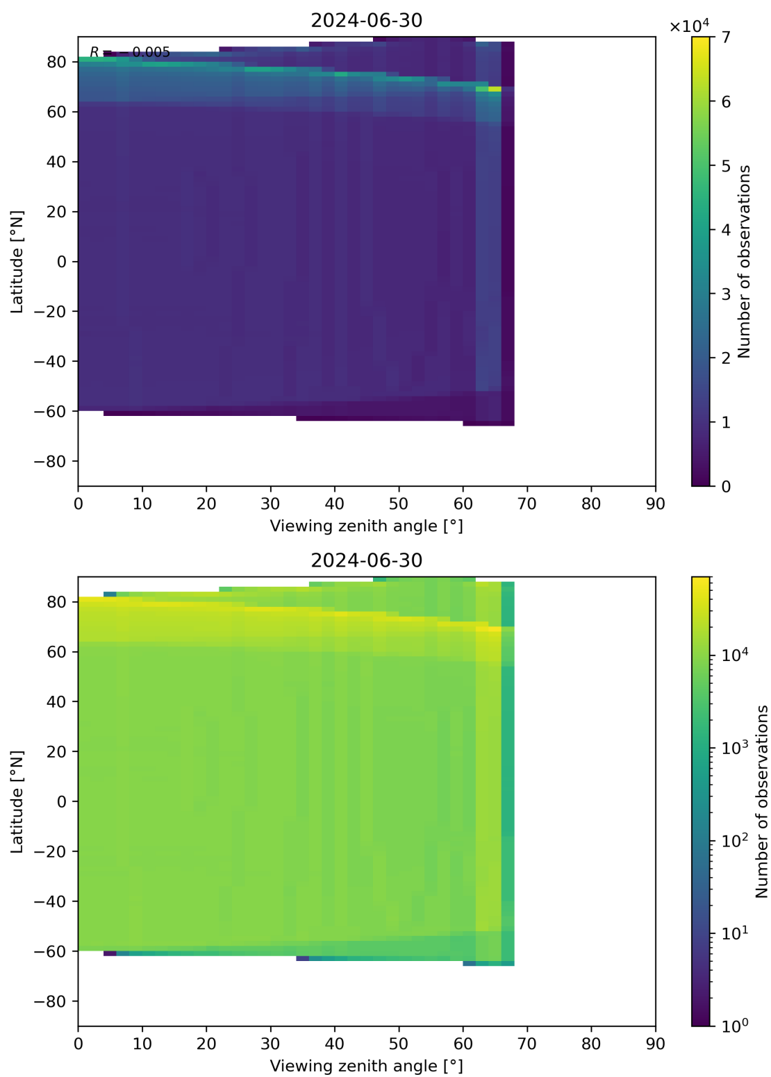
Figure 163: Scatter density plot of “Viewing zenith angle” against “Latitude” for 2024-06-29 to 2024-07-01.
