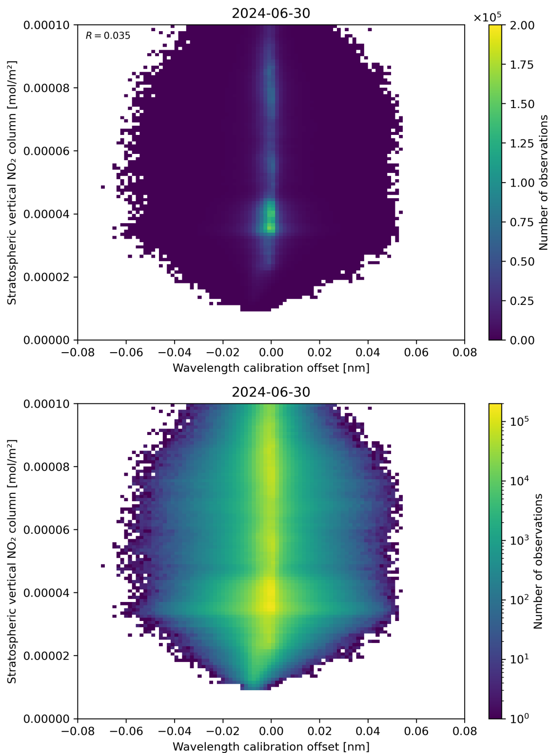
Figure 176: Scatter density plot of “Wavelength calibration offset” against “Stratospheric vertical NO 2 column” for 2024-06-29 to 2024-07-01.
