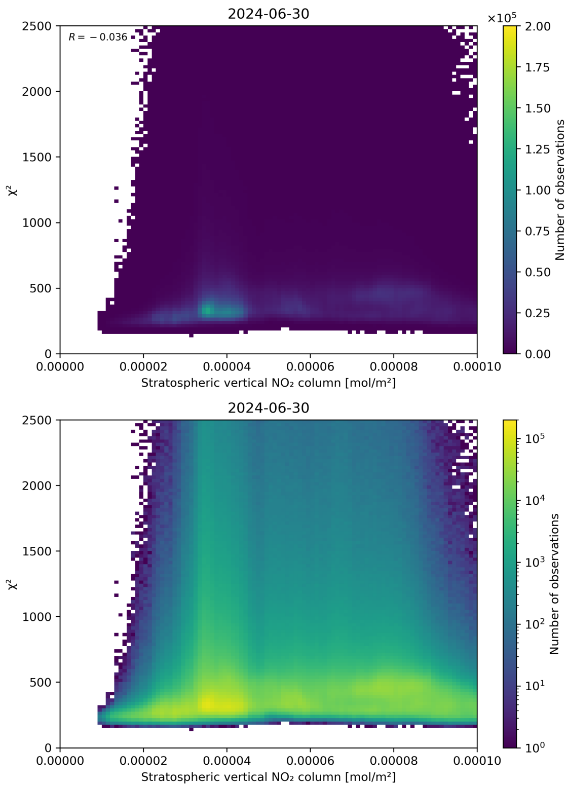
Figure 97: Scatter density plot of “Stratospheric vertical NO 2 column” against “ \chi^2 ” for 2024-06-29 to 2024-07-01.
