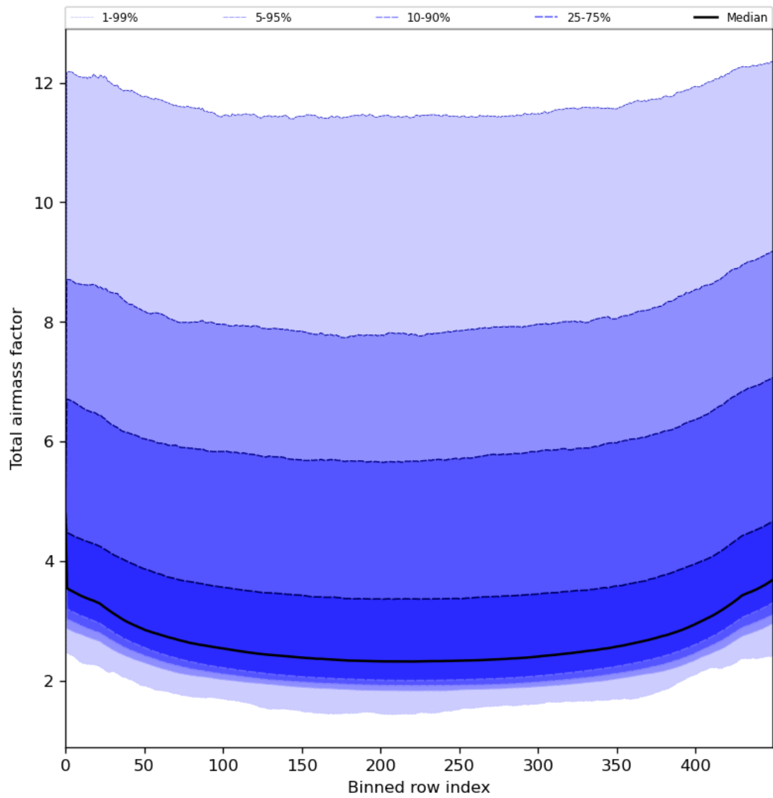
Figure 49: Along track statistics of “Total airmass factor” for 2024-06-29 to 2024-07-01
