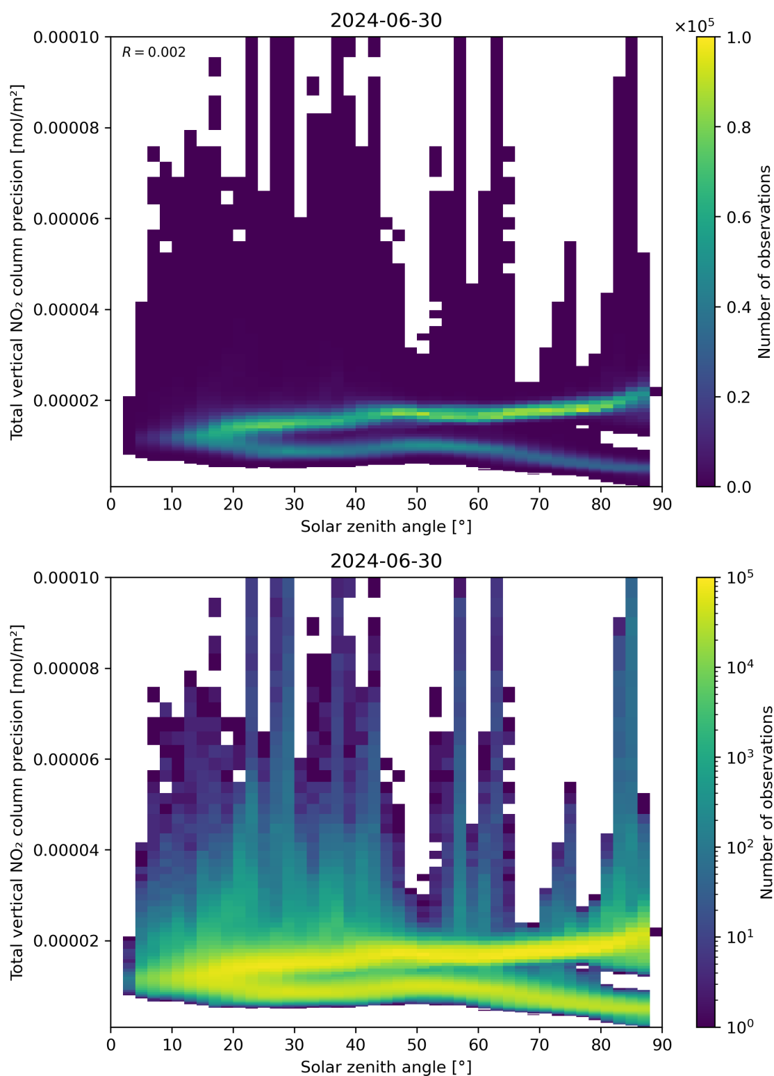
Figure 154: Scatter density plot of “Solar zenith angle” against “Total vertical NO 2 column precision” for 2024-06-29 to 2024-07-01.
