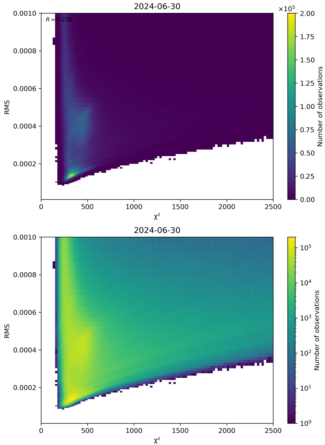
Figure 82: Scatter density plot of “ \chi^2 ” against “RMS” for 2024-06-29 to 2024-07-01.
