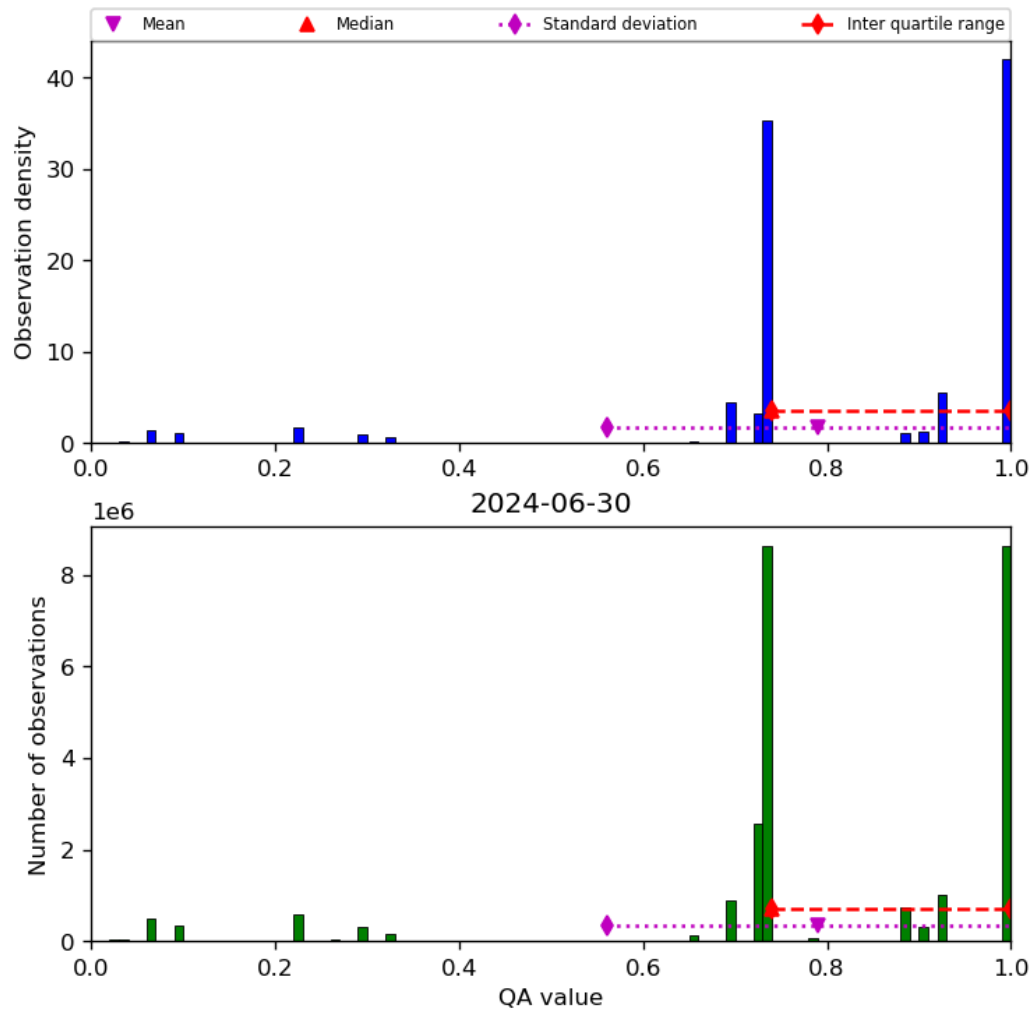
Figure 28: Histogram of “QA value” for 2024-06-29 to 2024-07-01
