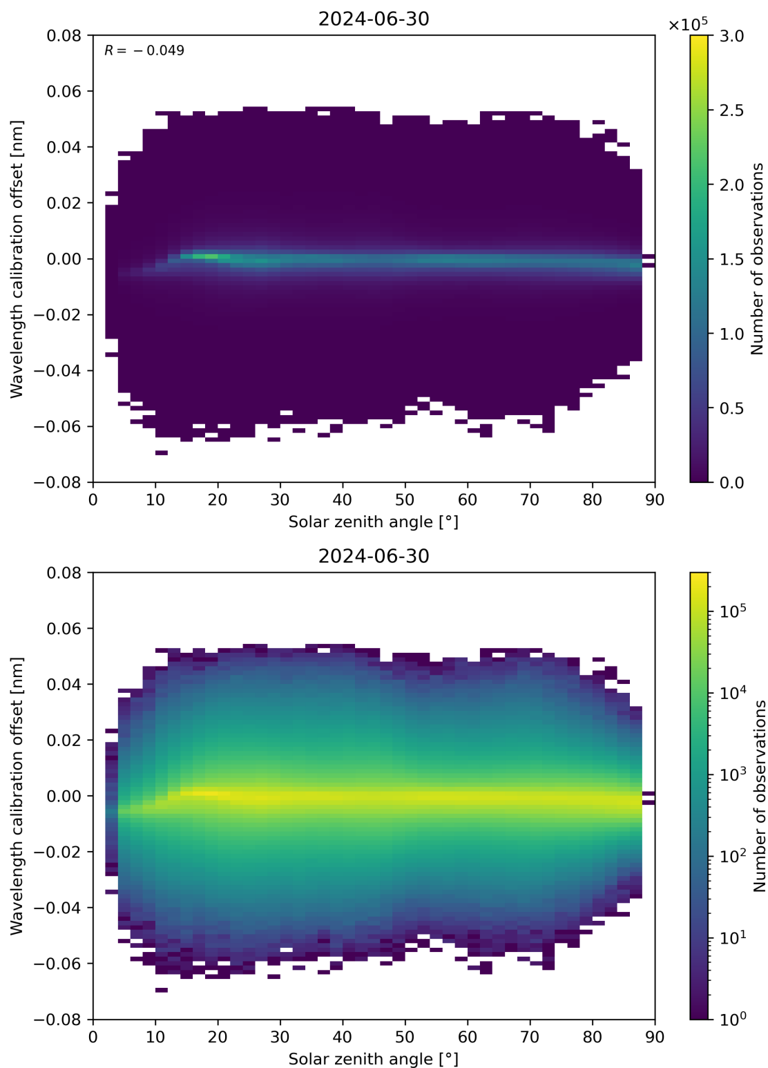
Figure 158: Scatter density plot of “Solar zenith angle” against “Wavelength calibration offset” for 2024-06-29 to 2024-07-01.
