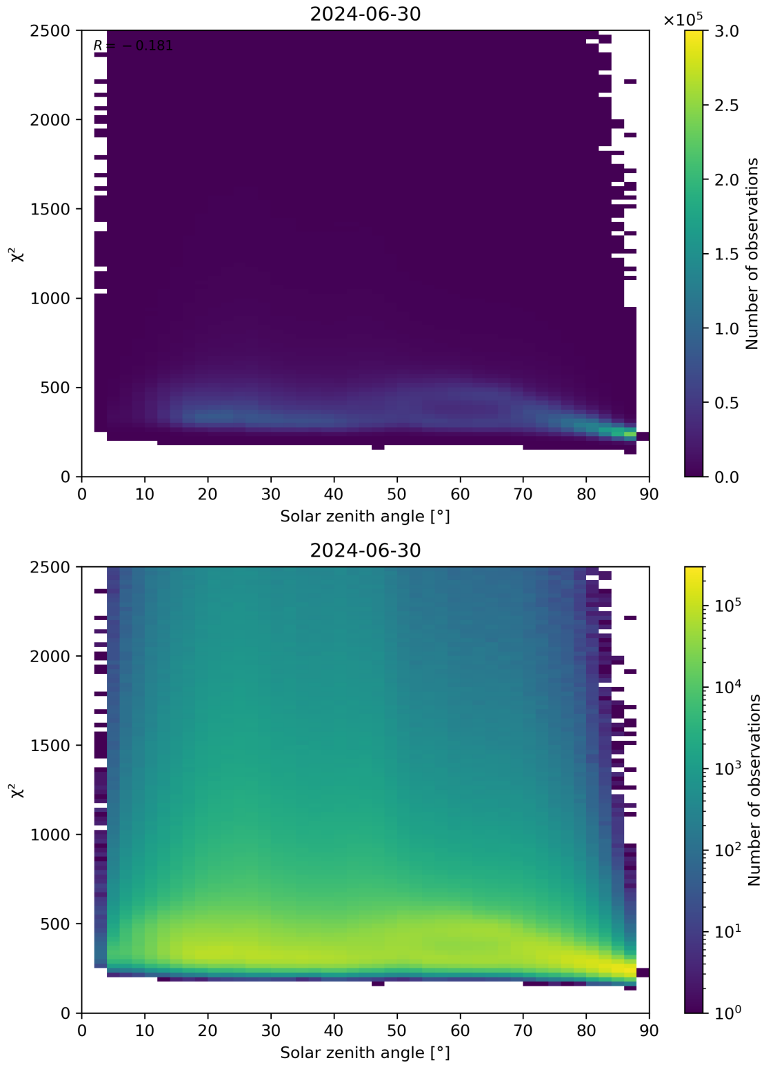
Figure 148: Scatter density plot of “Solar zenith angle” against “ \chi^2 ” for 2024-06-29 to 2024-07-01.
