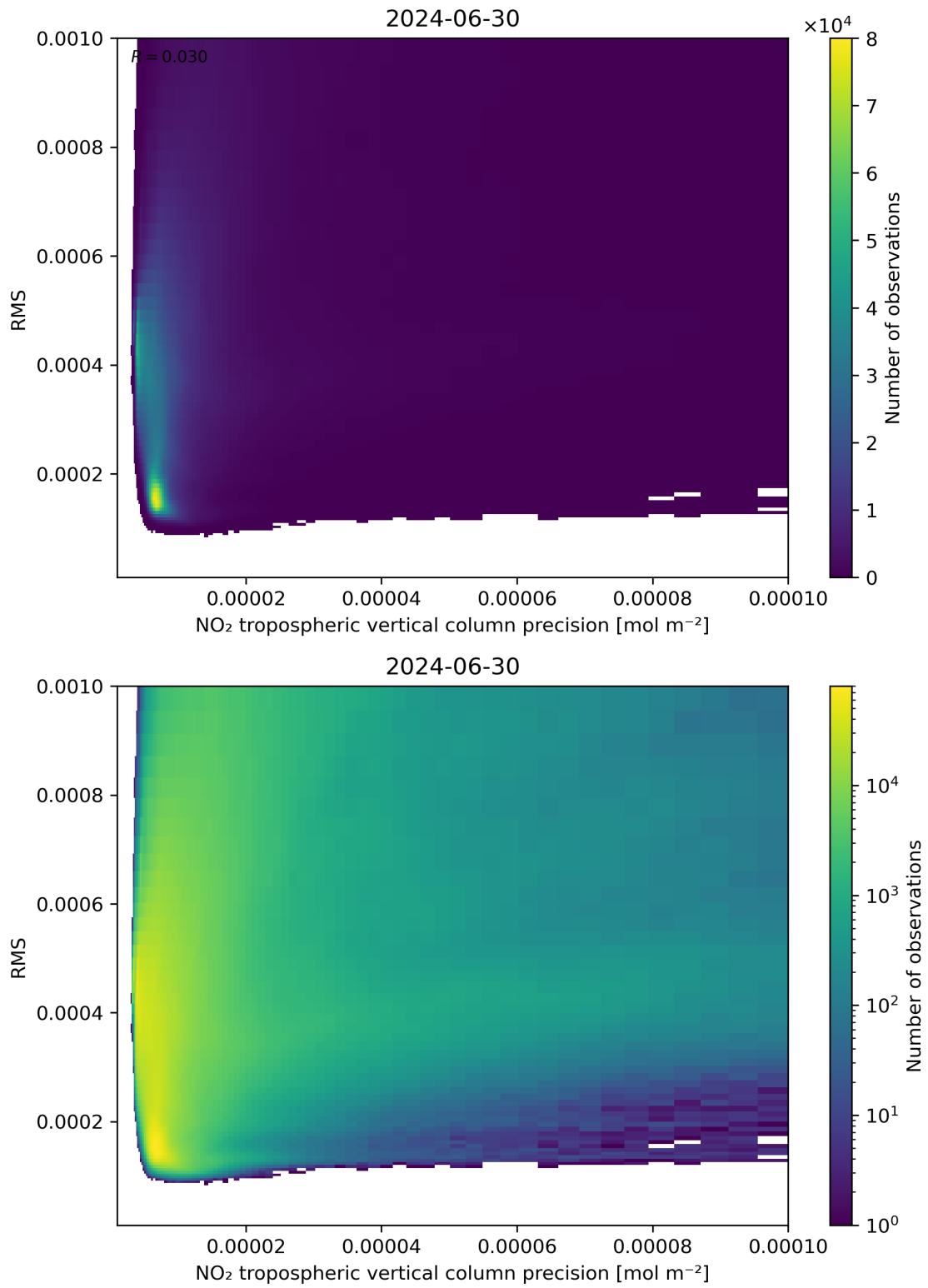
Figure 140: Scatter density plot of “NO 2 tropospheric vertical column precision” against “RMS” for 2024-06-29 to 2024-07-01.
