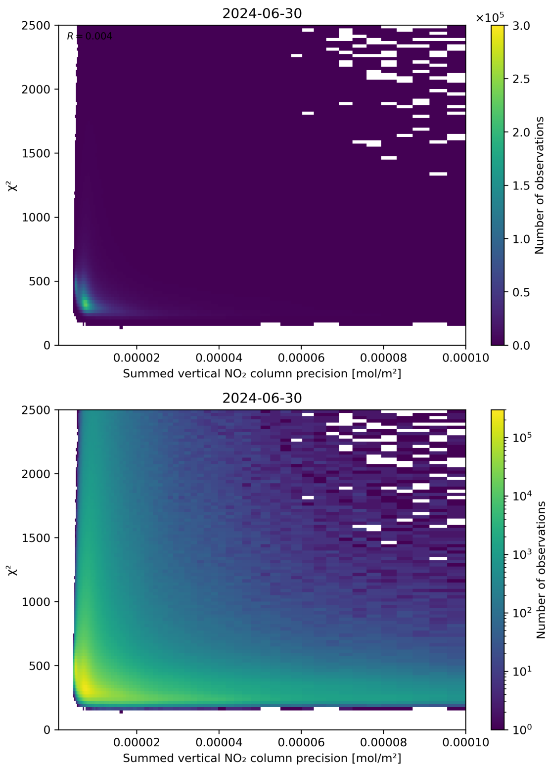
Figure 107: Scatter density plot of “Summed vertical NO 2 column precision” against “ \chi^2 ” for 2024-06-29 to 2024-07-01.
