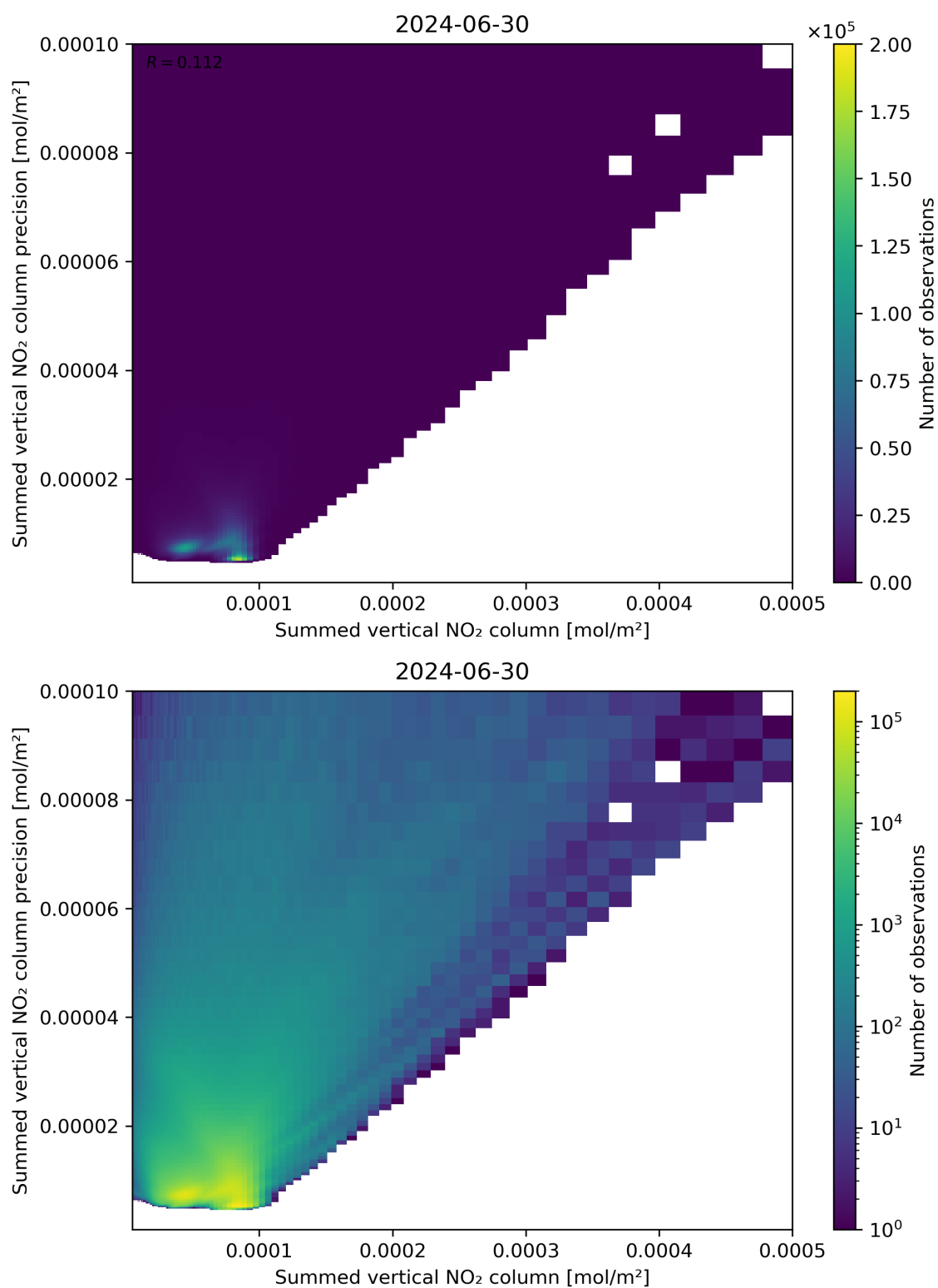
Figure 105: Scatter density plot of “Summed vertical NO 2 column” against “Summed vertical NO 2 column precision” for 2024-06-29 to 2024-07-01.
