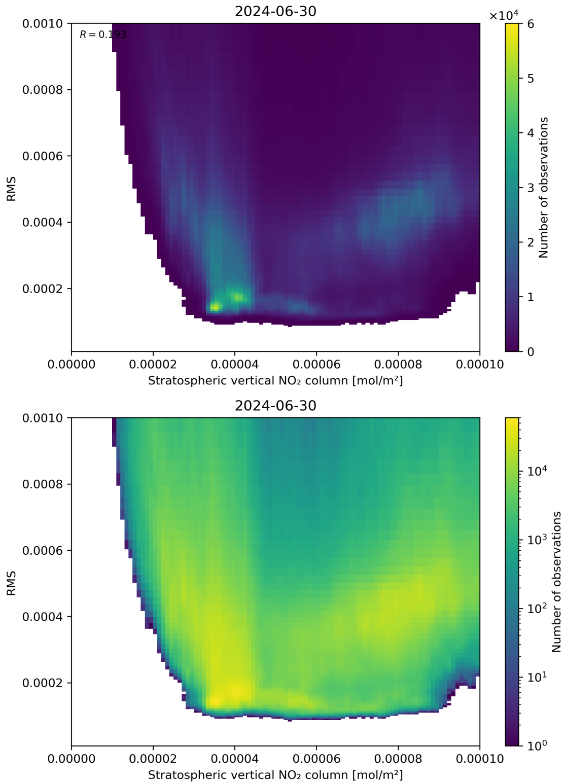
Figure 102: Scatter density plot of “Stratospheric vertical NO 2 column” against “RMS” for 2024-06-29 to 2024-07-01.
