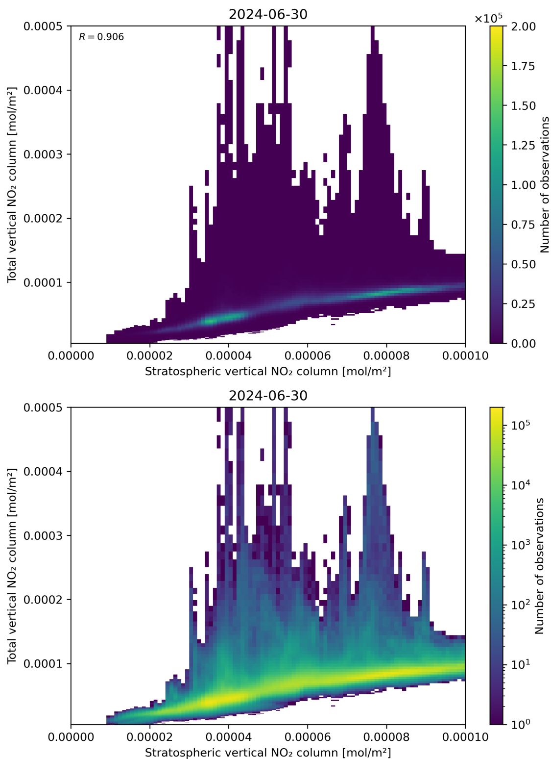
Figure 100: Scatter density plot of “Stratospheric vertical NO 2 column” against “Total vertical NO 2 column” for 2024-06-29 to 2024-07-01.
