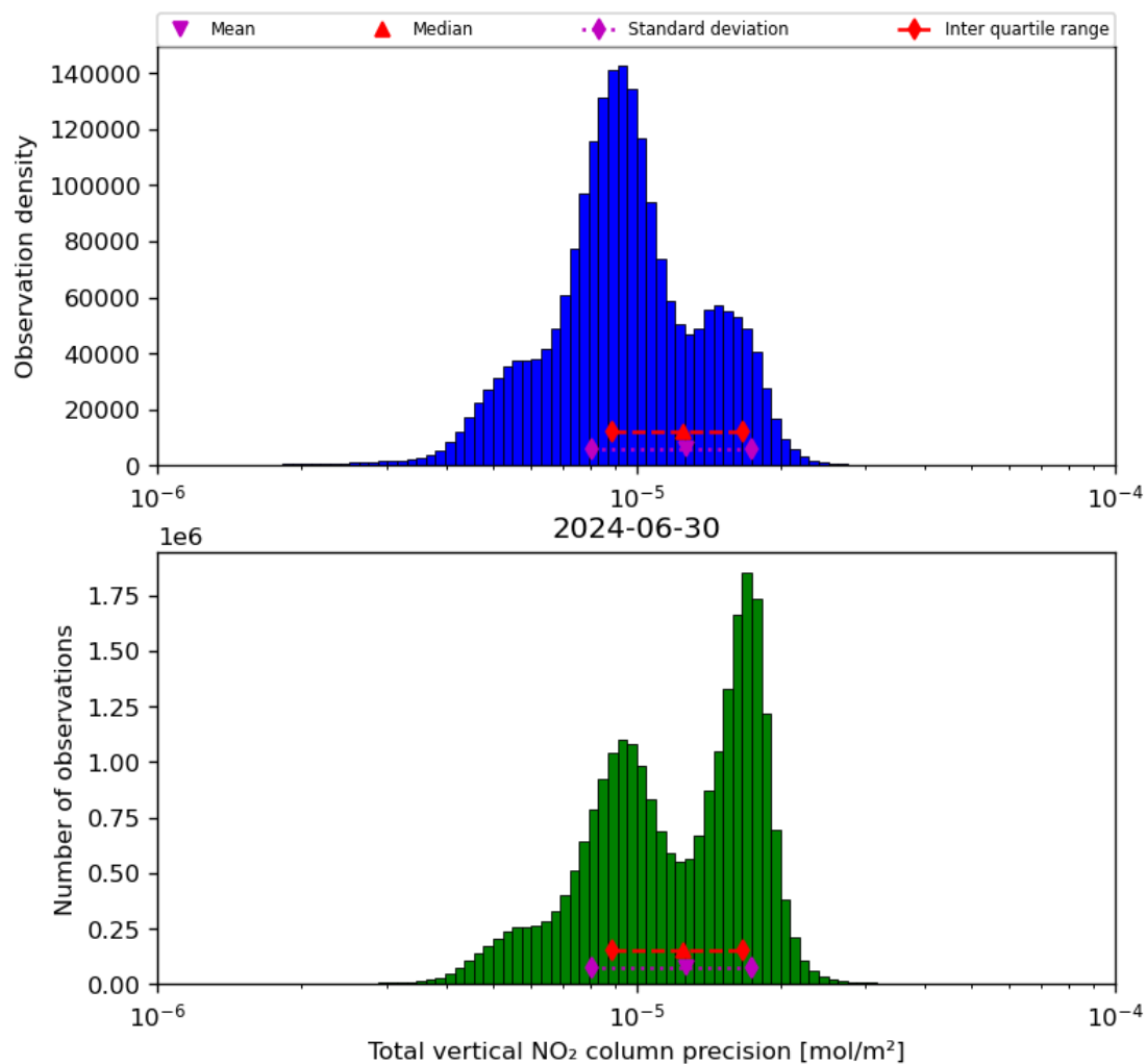
Figure 39: Histogram of "Total vertical NO 2 column precision" for 2024-06-29 to 2024-07-01
