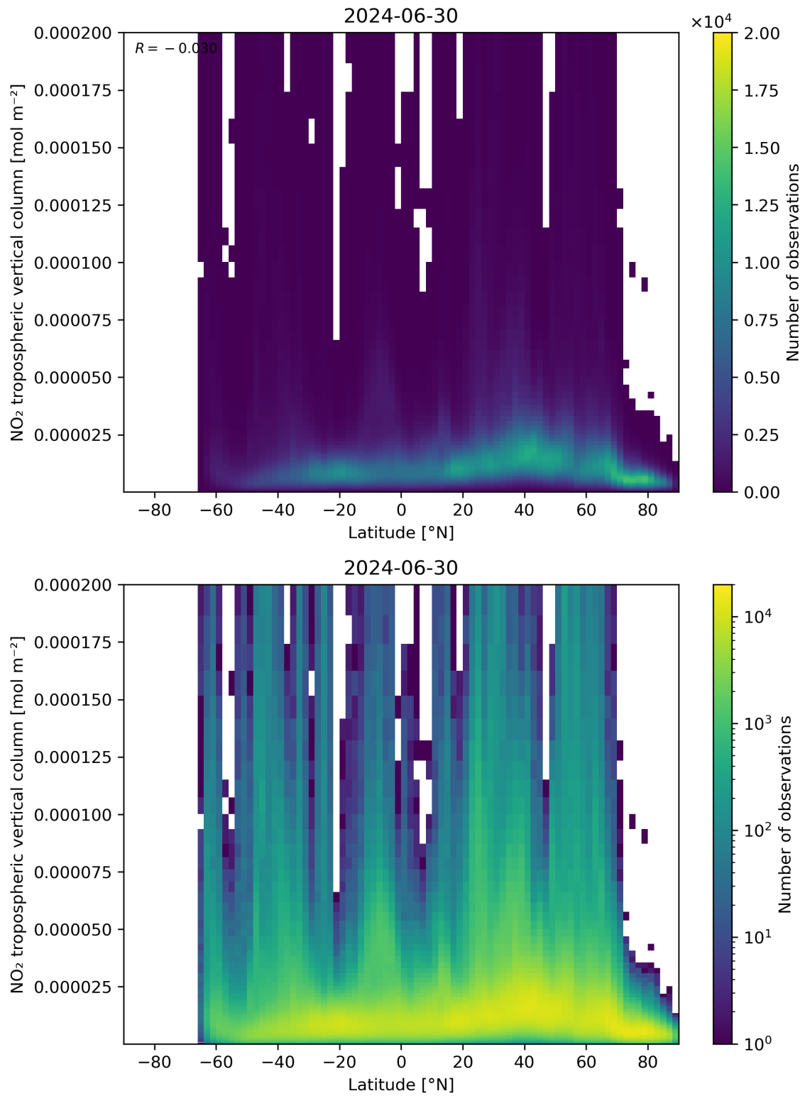
Figure 92: Scatter density plot of “Latitude” against “NO 2 tropospheric vertical column” for 2024-06-29 to 2024-07-01.
