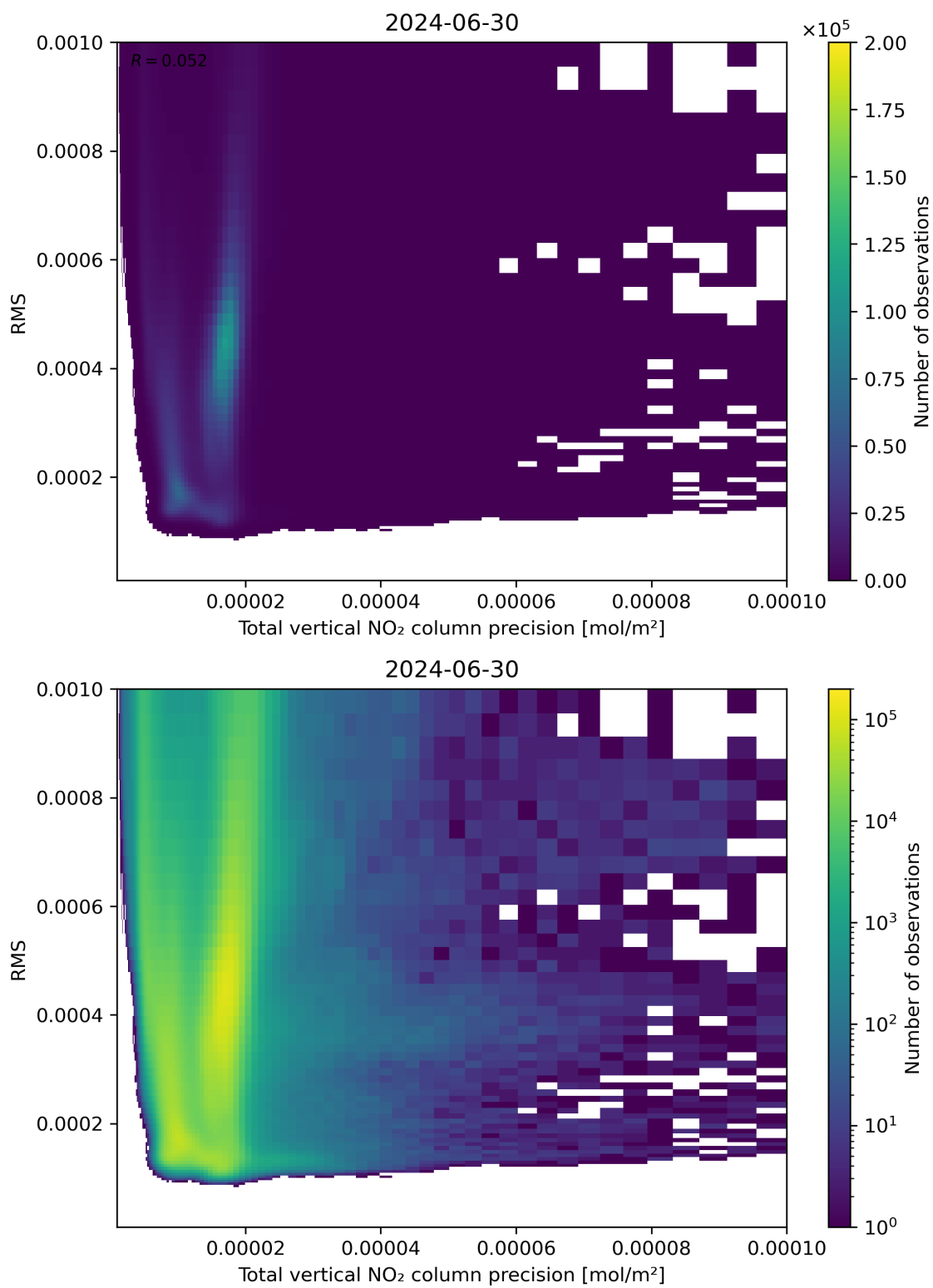
Figure 119: Scatter density plot of “Total vertical NO 2 column precision” against “RMS” for 2024-06-29 to 2024-07-01.
