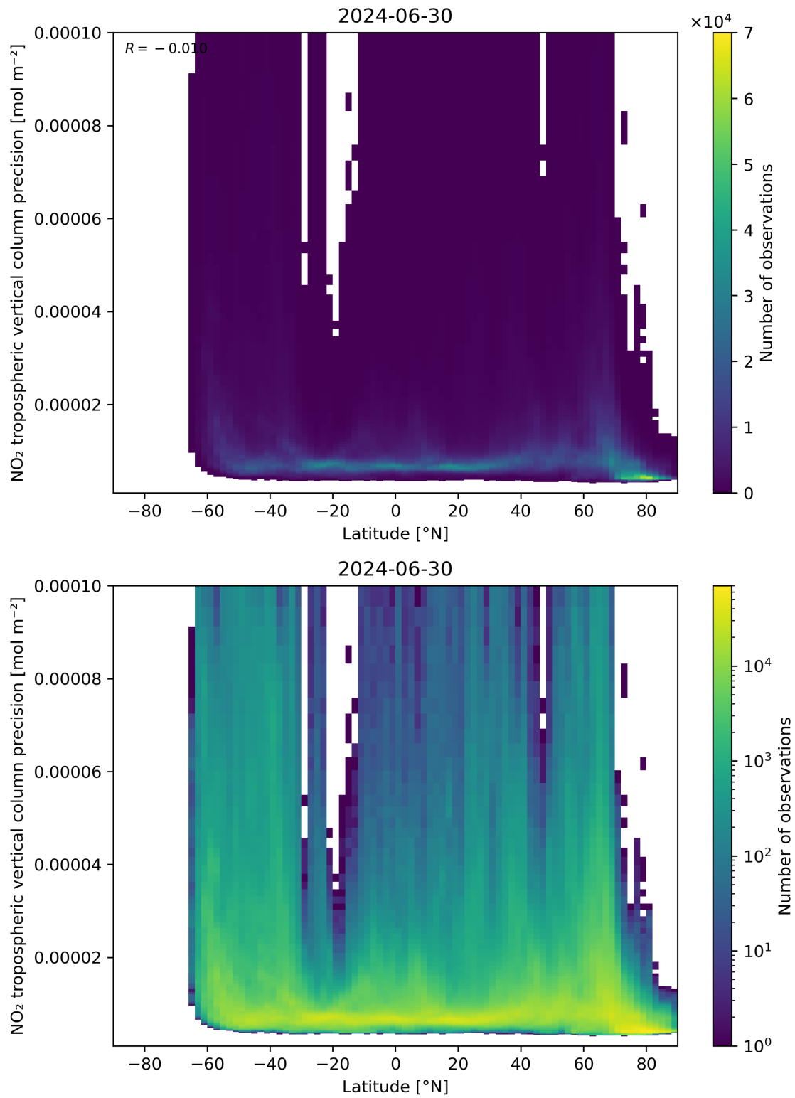
Figure 93: Scatter density plot of “Latitude” against “NO 2 tropospheric vertical column precision” for 2024-06-29 to 2024-07-01.
