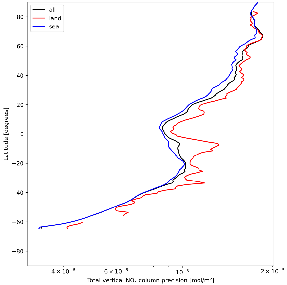
Figure 22: Zonal average of “Total vertical NO 2 column precision” for 2024-06-29 to 2024-07-01.
