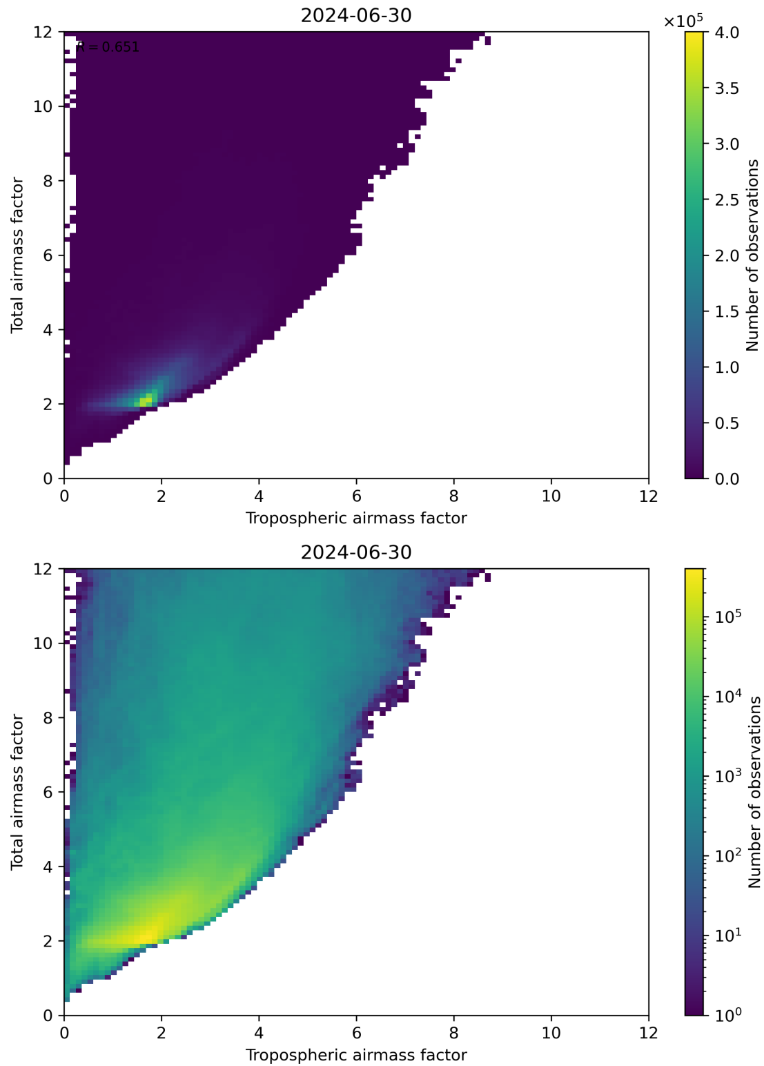
Figure 72: Scatter density plot of “Tropospheric airmass factor” against “Total airmass factor” for 2024-06-29 to 2024-07-01.
