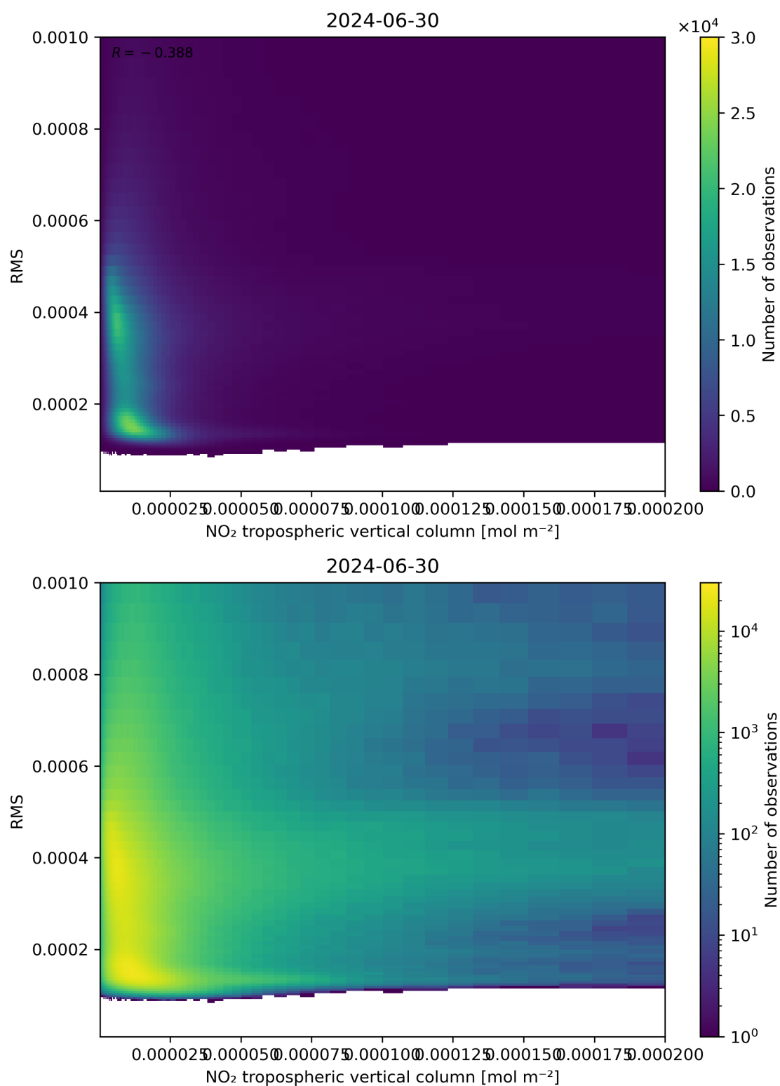
Figure 142: Scatter density plot of “NO 2 tropospheric vertical column” against “RMS” for 2024-06-29 to 2024-07-01.
