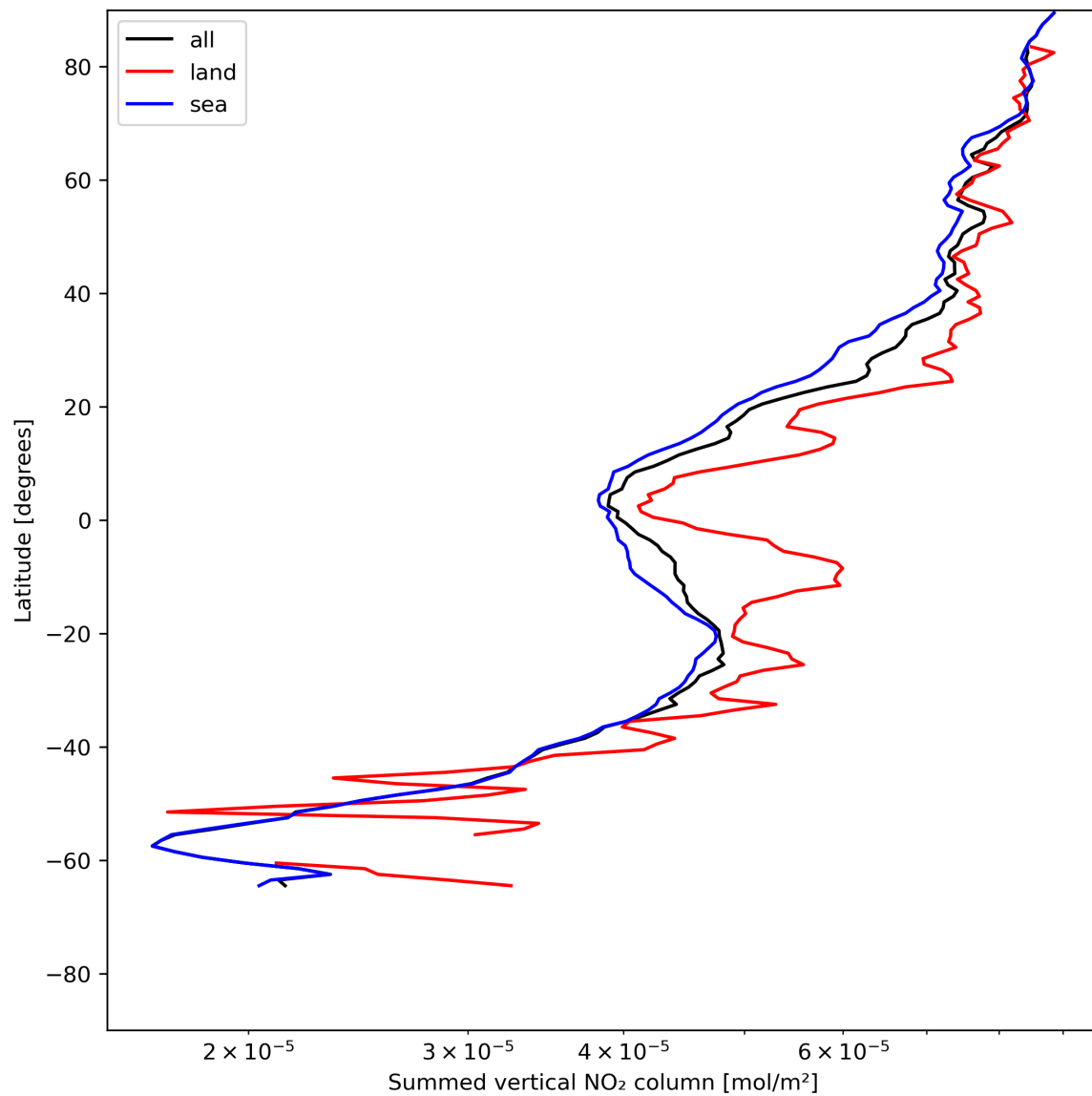
Figure 23: Zonal average of “Summed vertical NO 2 column” for 2024-06-29 to 2024-07-01.
