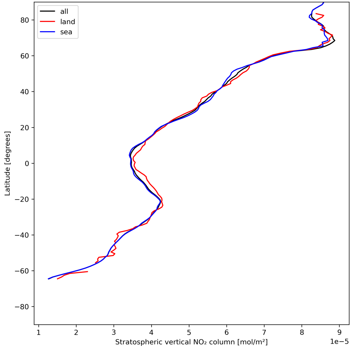
Figure 19: Zonal average of “Stratospheric vertical NO 2 column” for 2024-06-29 to 2024-07-01.
