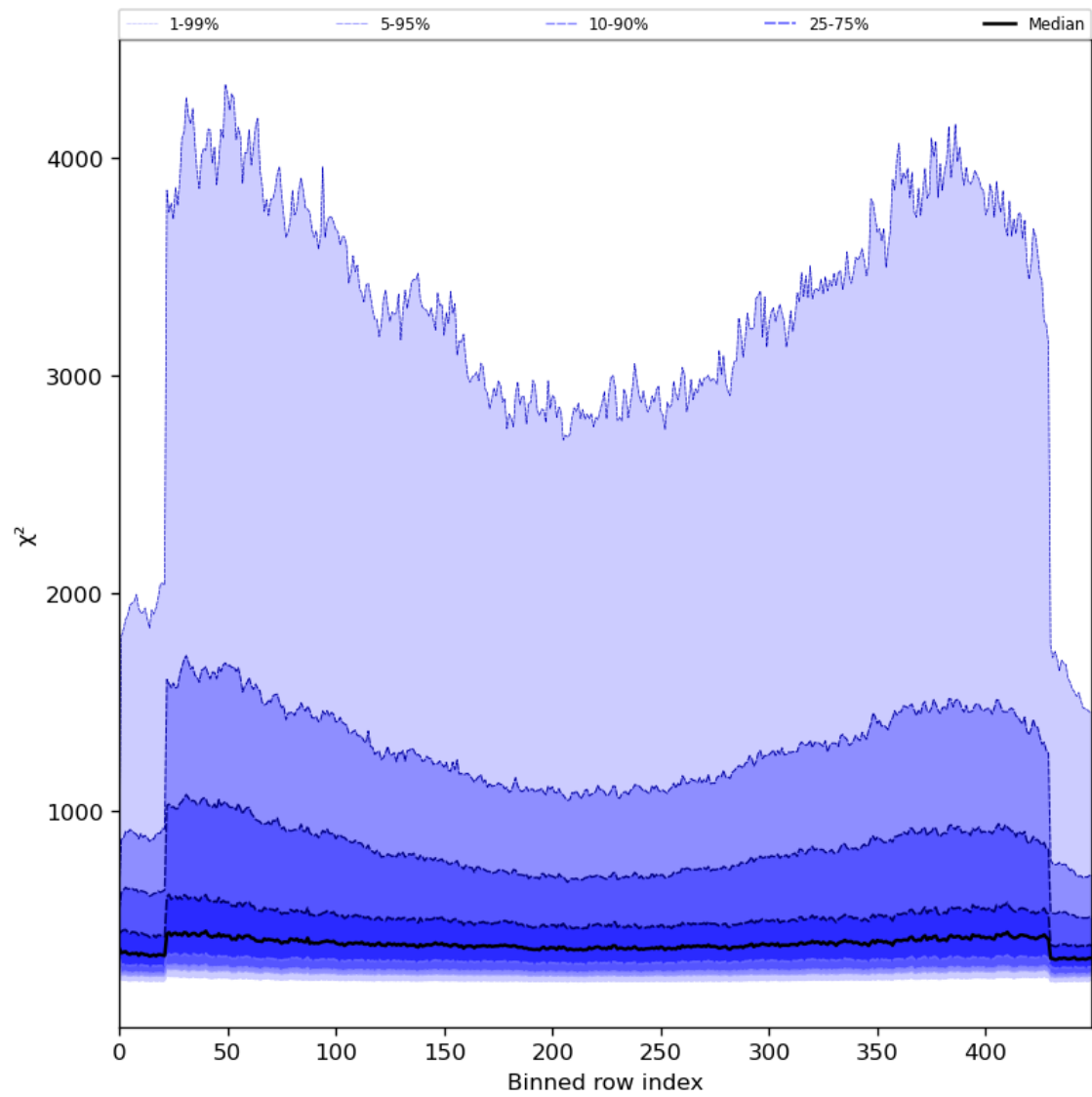
Figure 59: Along track statistics of “ \chi^2 ” for 2024-06-29 to 2024-07-01
