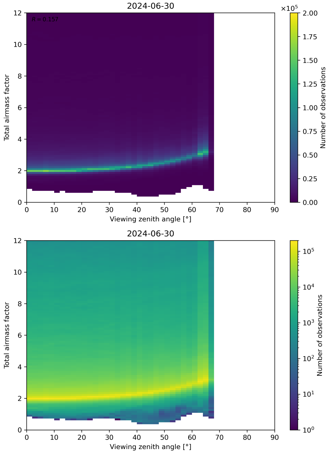
Figure 160: Scatter density plot of “Viewing zenith angle” against “Total airmass factor” for 2024-06-29 to 2024-07-01.
