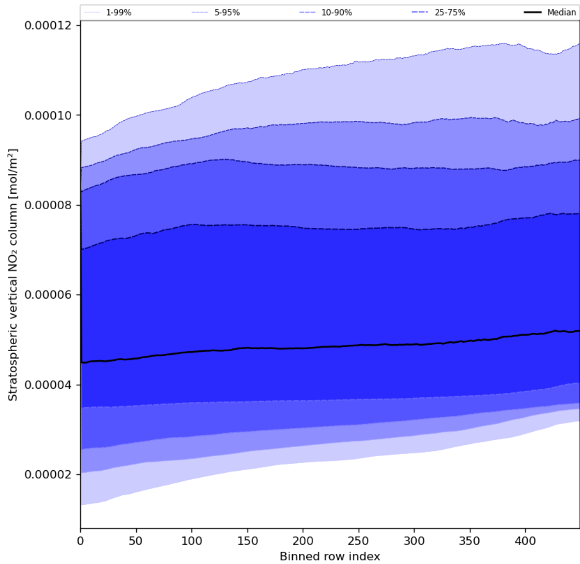
Figure 53: Along track statistics of “Stratospheric vertical NO 2 column” for 2024-06-29 to 2024-07-01
