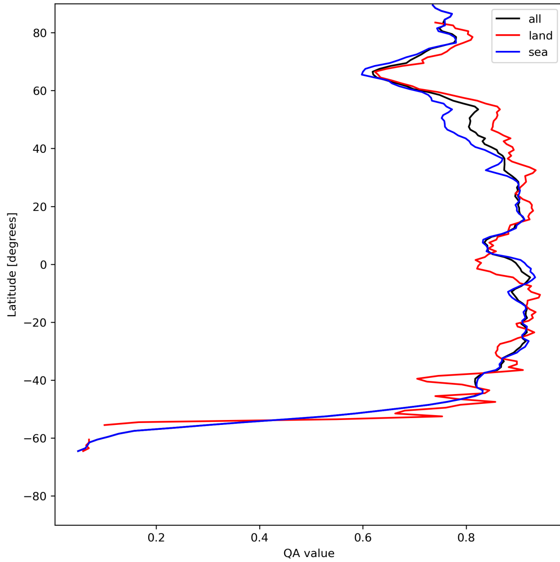
Figure 11: Zonal average of “QA value” for 2024-06-29 to 2024-07-01.
