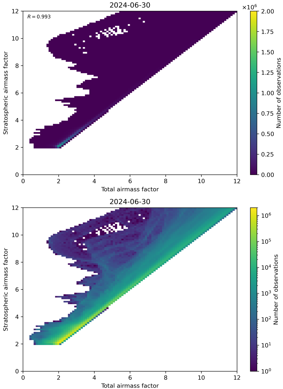
Figure 62: Scatter density plot of “Total airmass factor” against “Stratospheric airmass factor” for 2024-06-29 to 2024-07-01.
