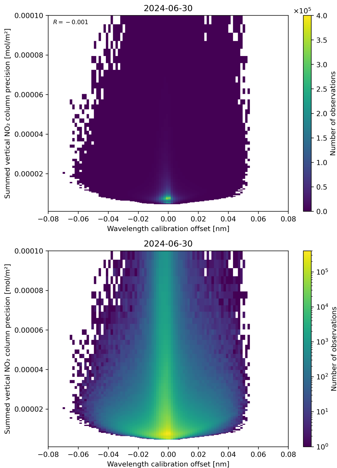
Figure 178: Scatter density plot of “Wavelength calibration offset” against “Summed vertical NO 2 column precision” for 2024-06-29 to 2024-07-01.
