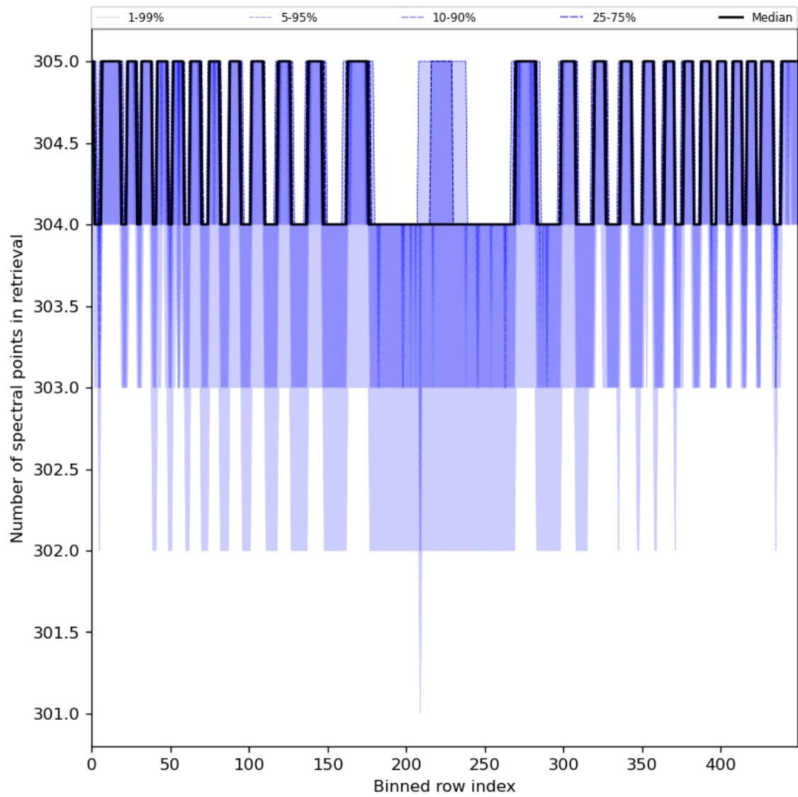
Figure 50: Along track statistics of “Number of spectral points in retrieval” for 2024-06-29 to 2024-07-01
