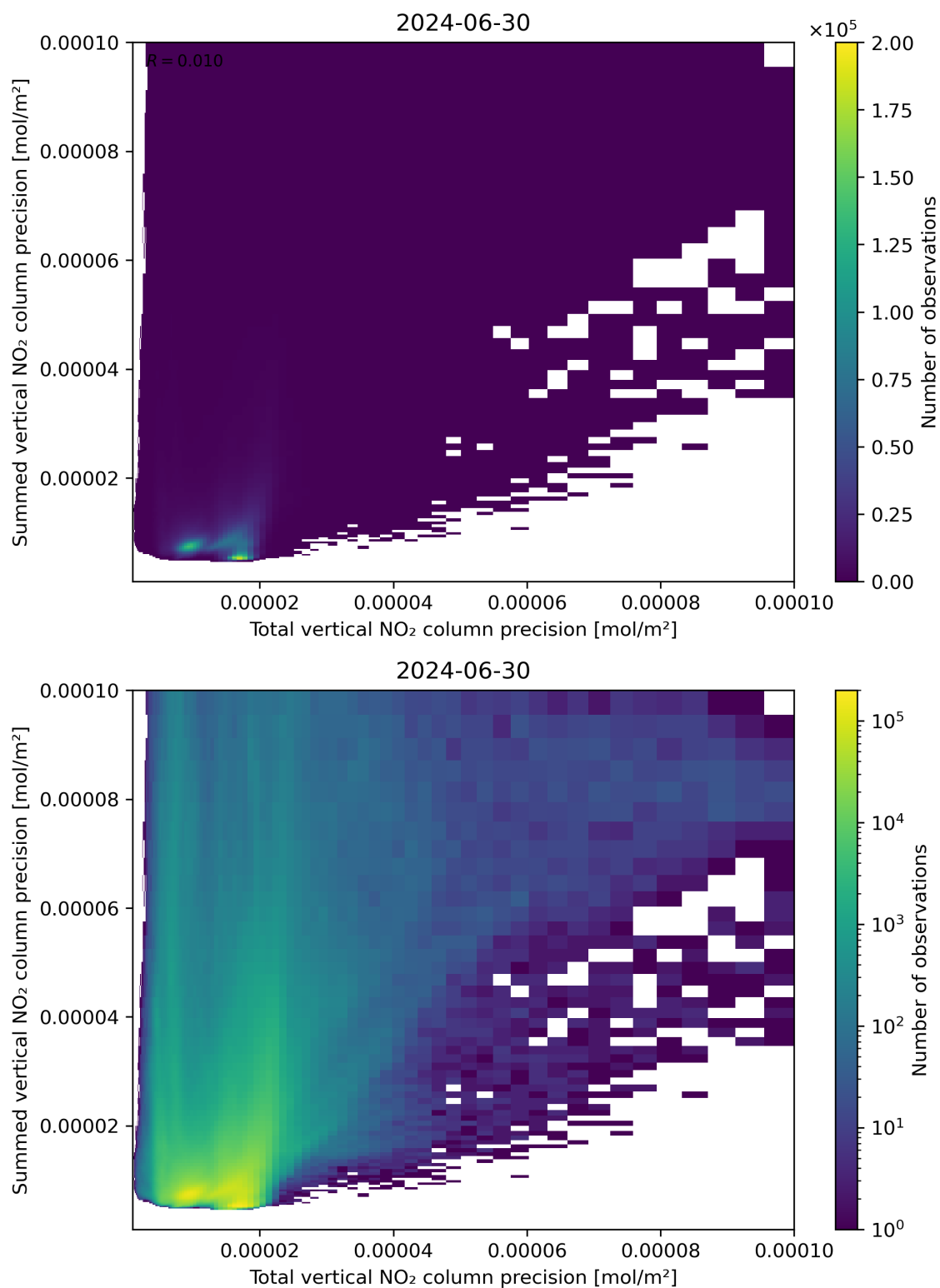
Figure 118: Scatter density plot of “Total vertical NO 2 column precision” against “Summed vertical NO 2 column precision” for 2024-06-29 to 2024-07-01.
