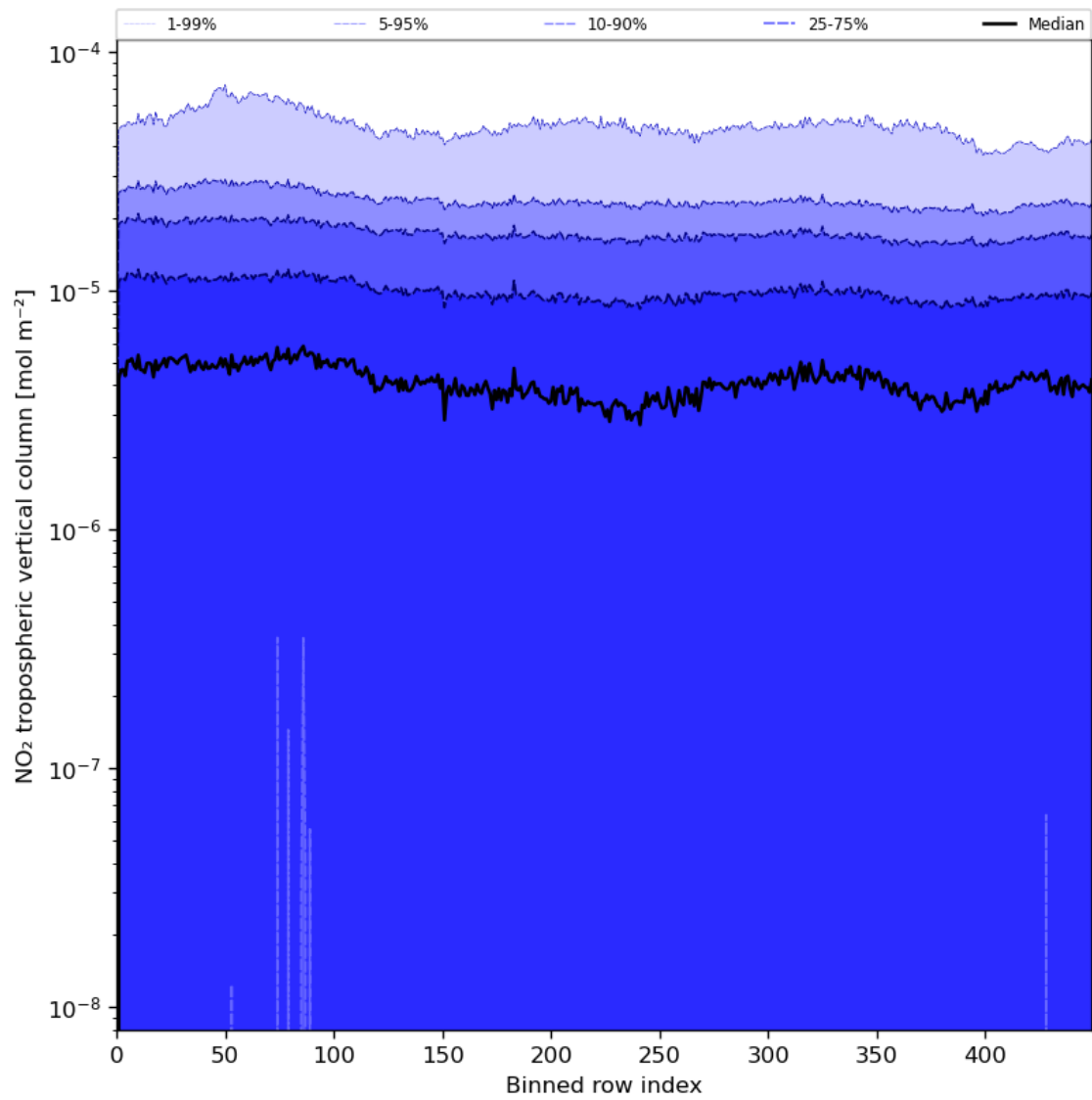
Figure 46: Along track statistics of “NO 2 tropospheric vertical column” for 2024-06-29 to 2024-07-01
