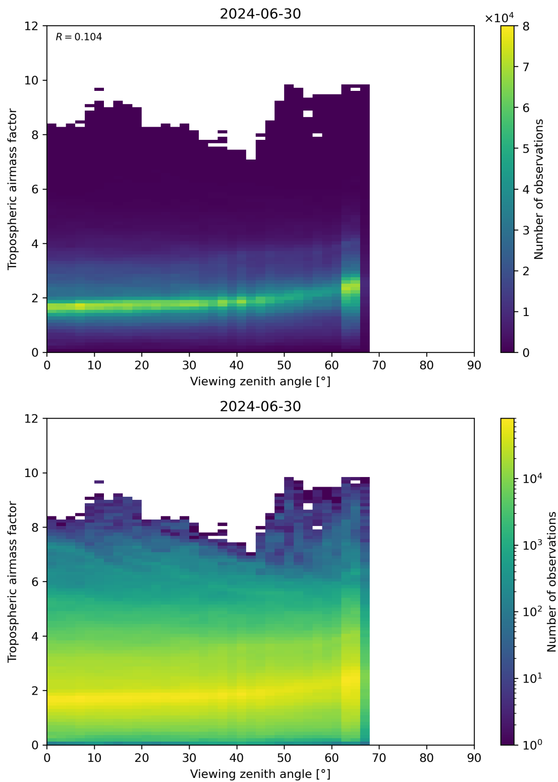
Figure 161: Scatter density plot of “Viewing zenith angle” against “Tropospheric airmass factor” for 2024-06-29 to 2024-07-01.
