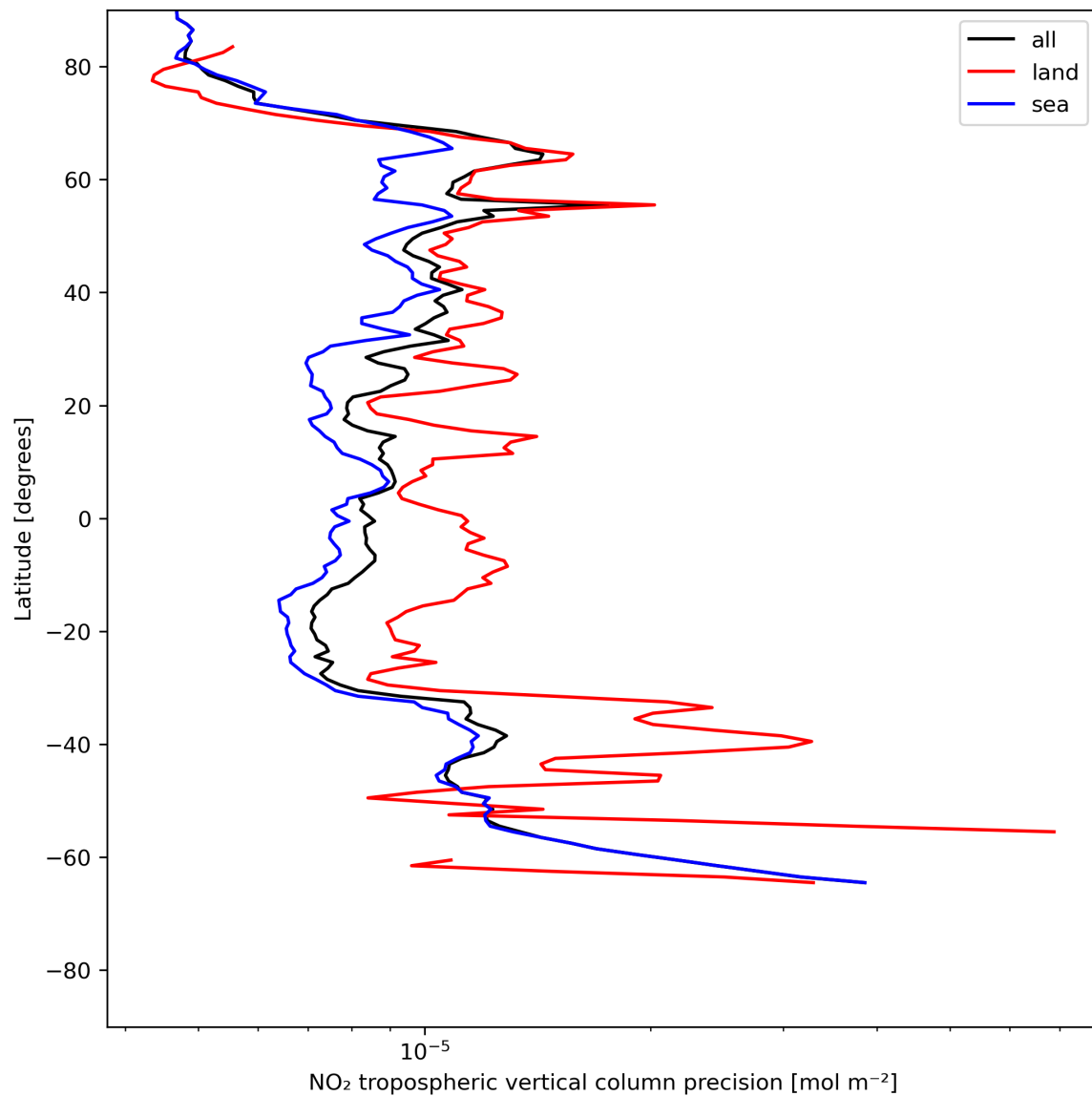
Figure 13: Zonal average of “NO 2 tropospheric vertical column precision” for 2024-06-29 to 2024-07-01.
