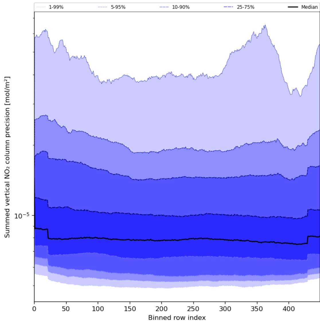
Figure 58: Along track statistics of “Summed vertical NO 2 column precision” for 2024-06-29 to 2024-07-01
