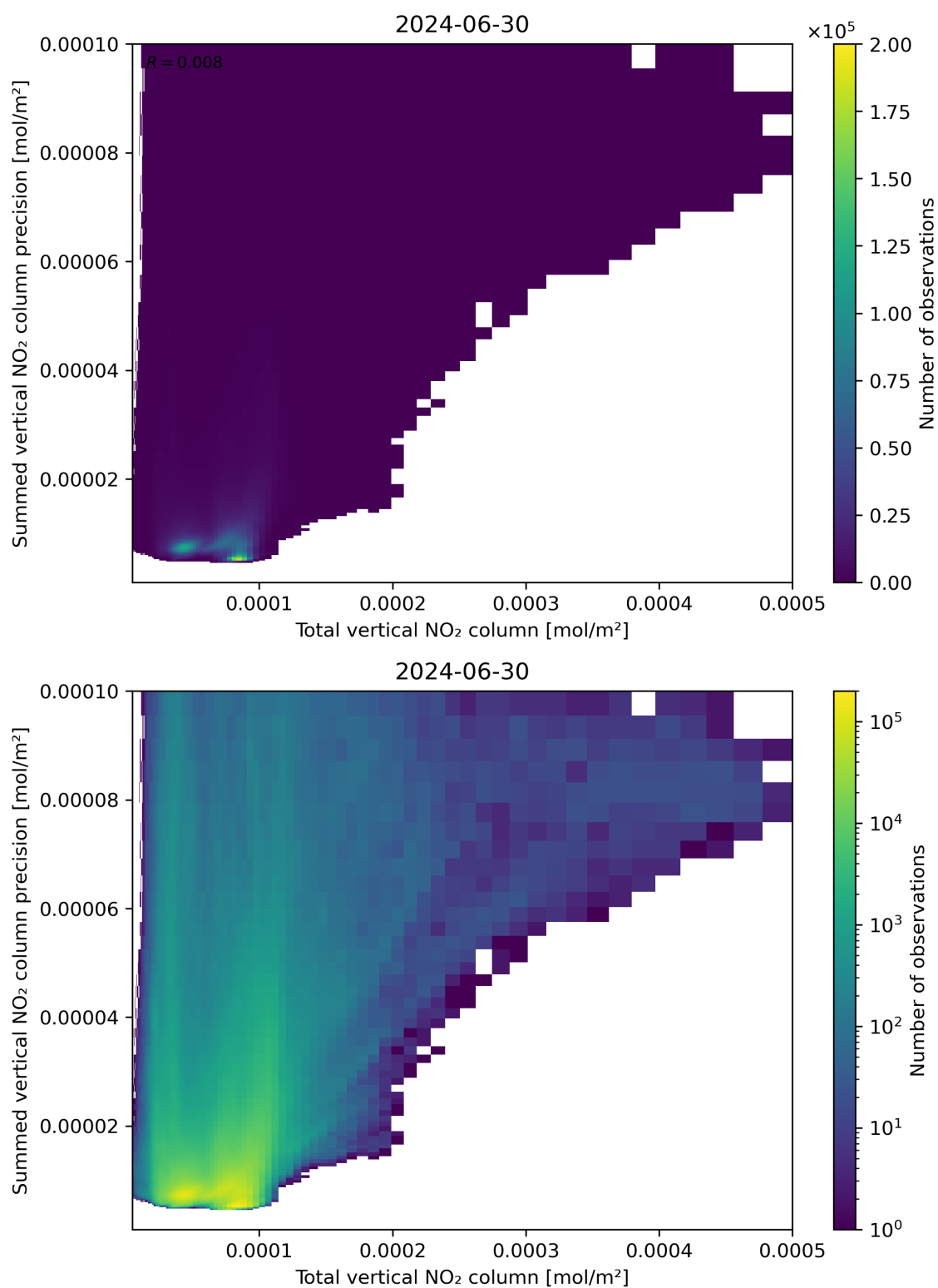
Figure 113: Scatter density plot of “Total vertical NO 2 column” against “Summed vertical NO 2 column precision” for 2024-06-29 to 2024-07-01.
