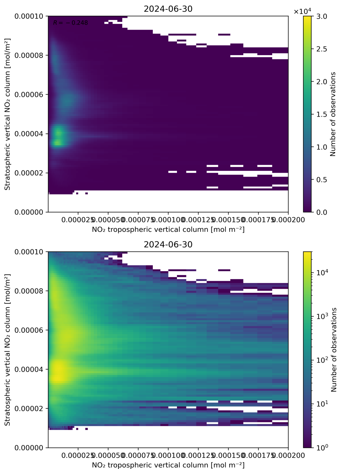
Figure 125: Scatter density plot of “NO 2 tropospheric vertical column” against “Stratospheric vertical NO 2 column” for 2024-06-29 to 2024-07-01.
