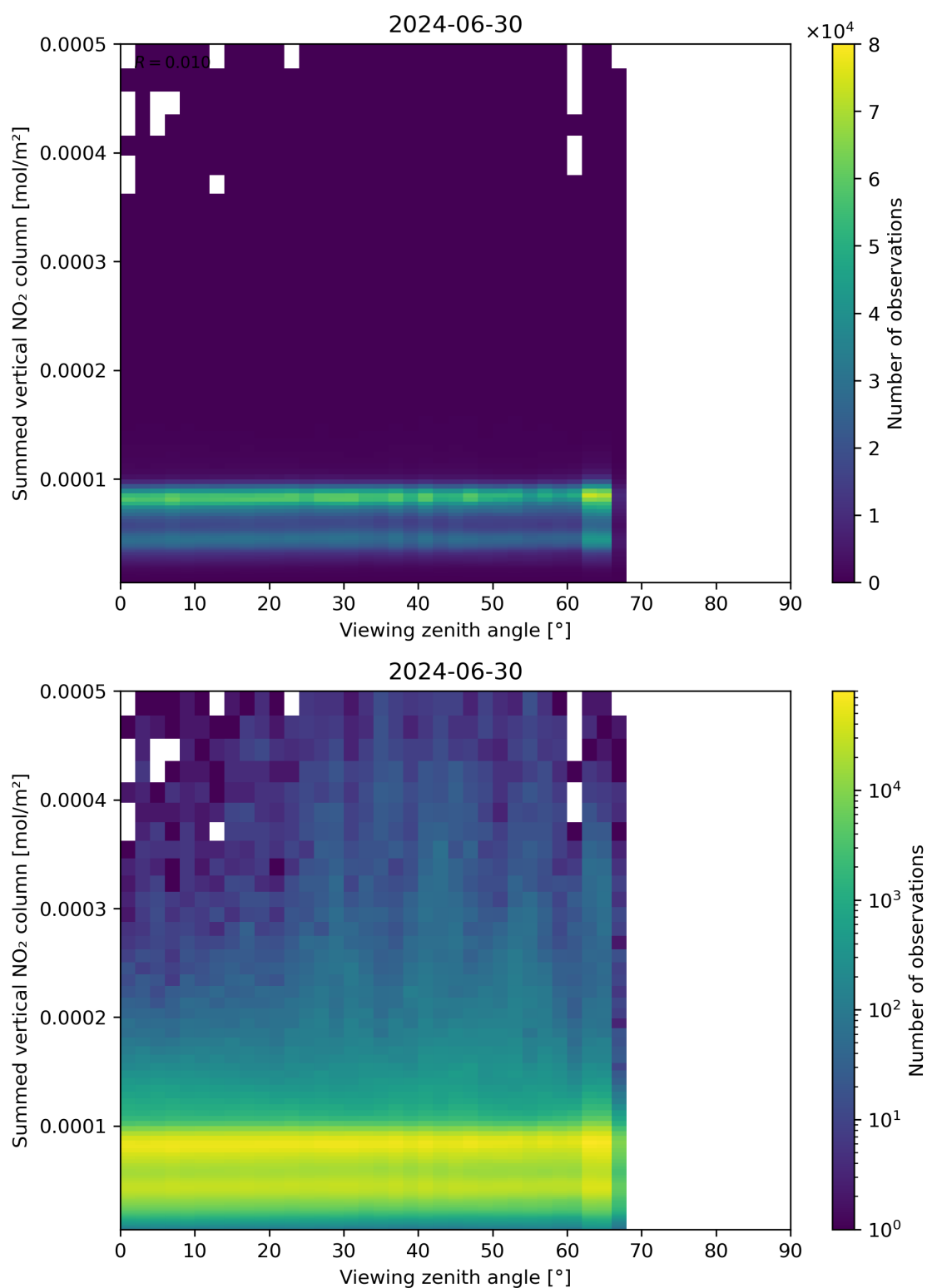
Figure 165: Scatter density plot of “Viewing zenith angle” against “Summed vertical NO 2 column” for 2024-06-29 to 2024-07-01.
