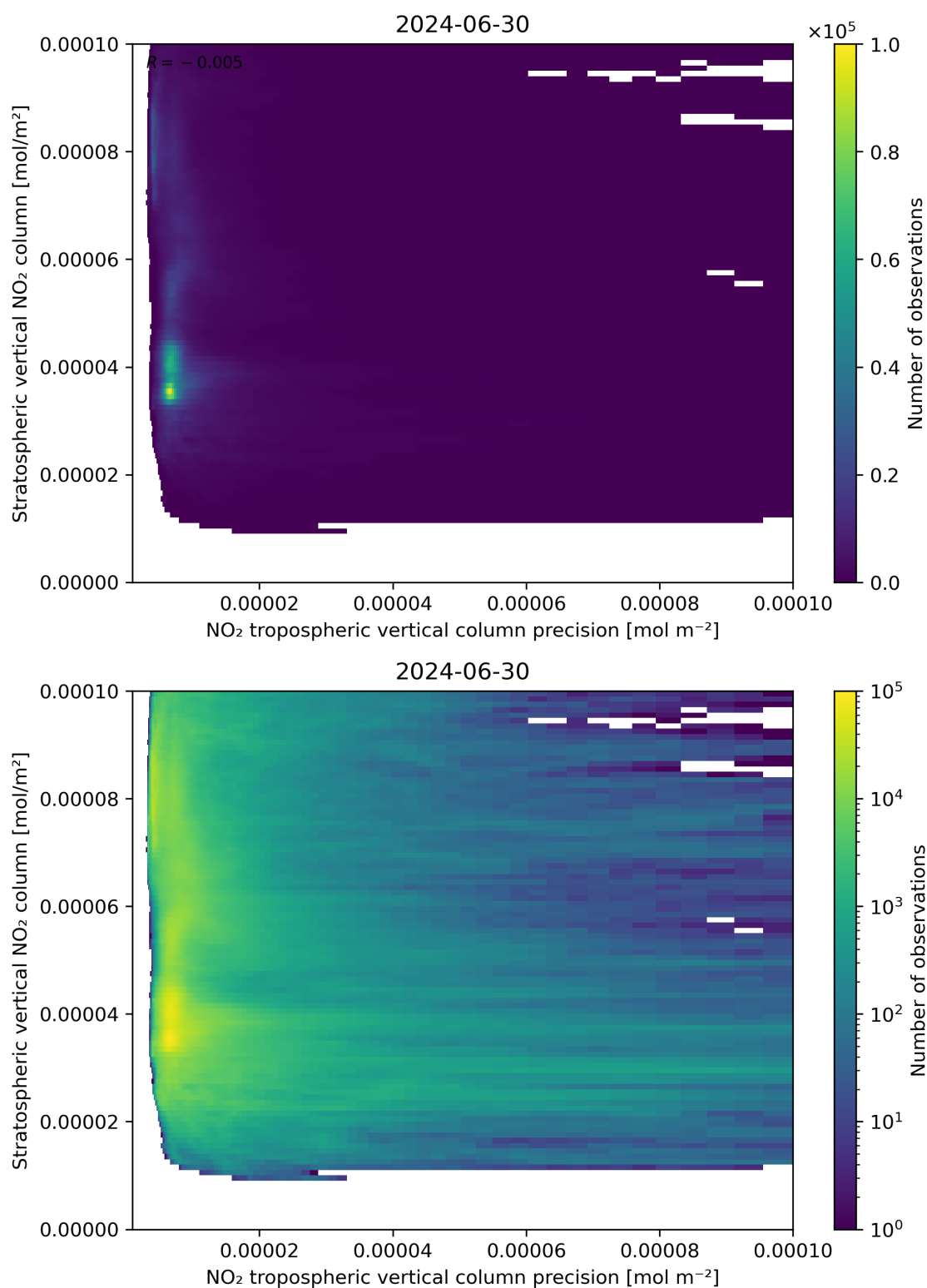
Figure 135: Scatter density plot of “NO 2 tropospheric vertical column precision” against “Stratospheric vertical NO 2 column” for 2024-06-29 to 2024-07-01.
