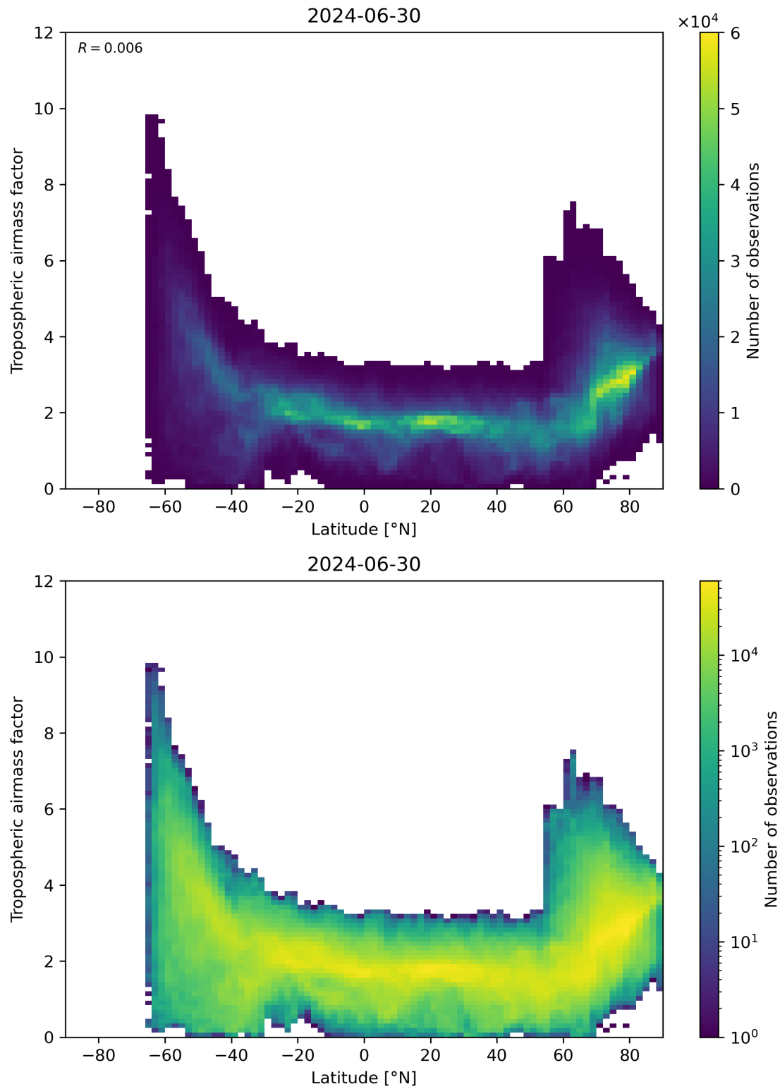
Figure 85: Scatter density plot of “Latitude” against “Tropospheric airmass factor” for 2024-06-29 to 2024-07-01.
