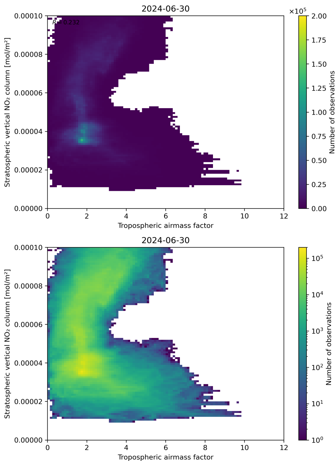
Figure 74: Scatter density plot of “Tropospheric air mass factor” against “Stratospheric vertical NO 2 column” for 2024-06-29 to 2024-07-01.
