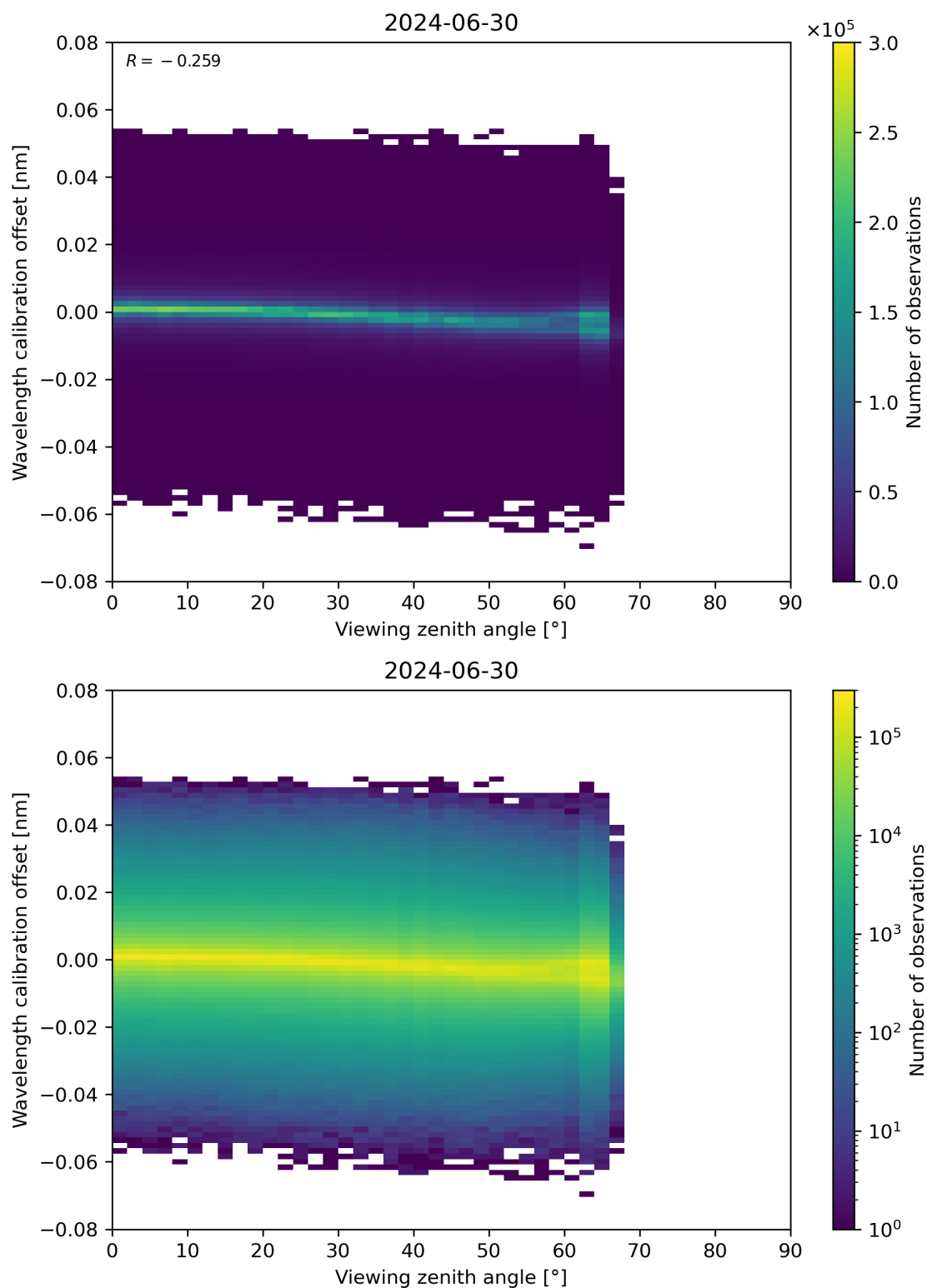
Figure 173: Scatter density plot of “Viewing zenith angle” against “Wavelength calibration offset” for 2024-06-29 to 2024-07-01.
