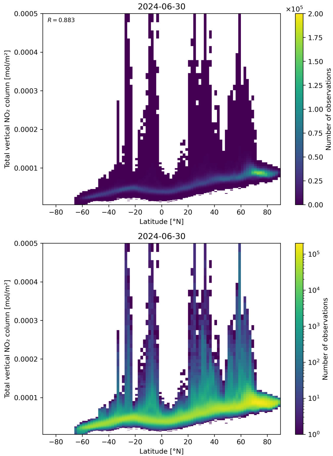
Figure 90: Scatter density plot of “Latitude” against “Total vertical NO 2 column” for 2024-06-29 to 2024-07-01.
