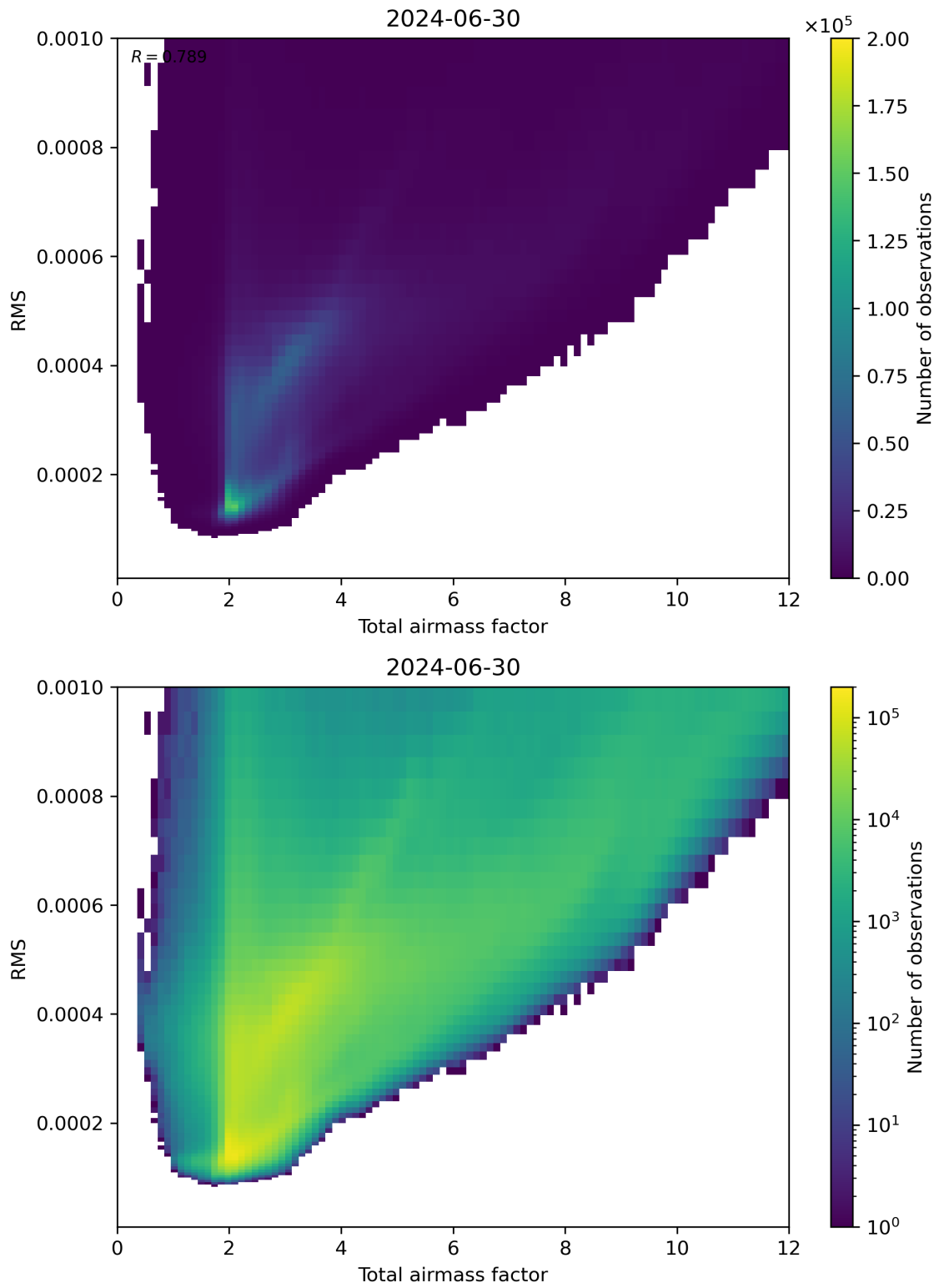
Figure 69: Scatter density plot of “Total airmass factor” against “RMS” for 2024-06-29 to 2024-07-01.
