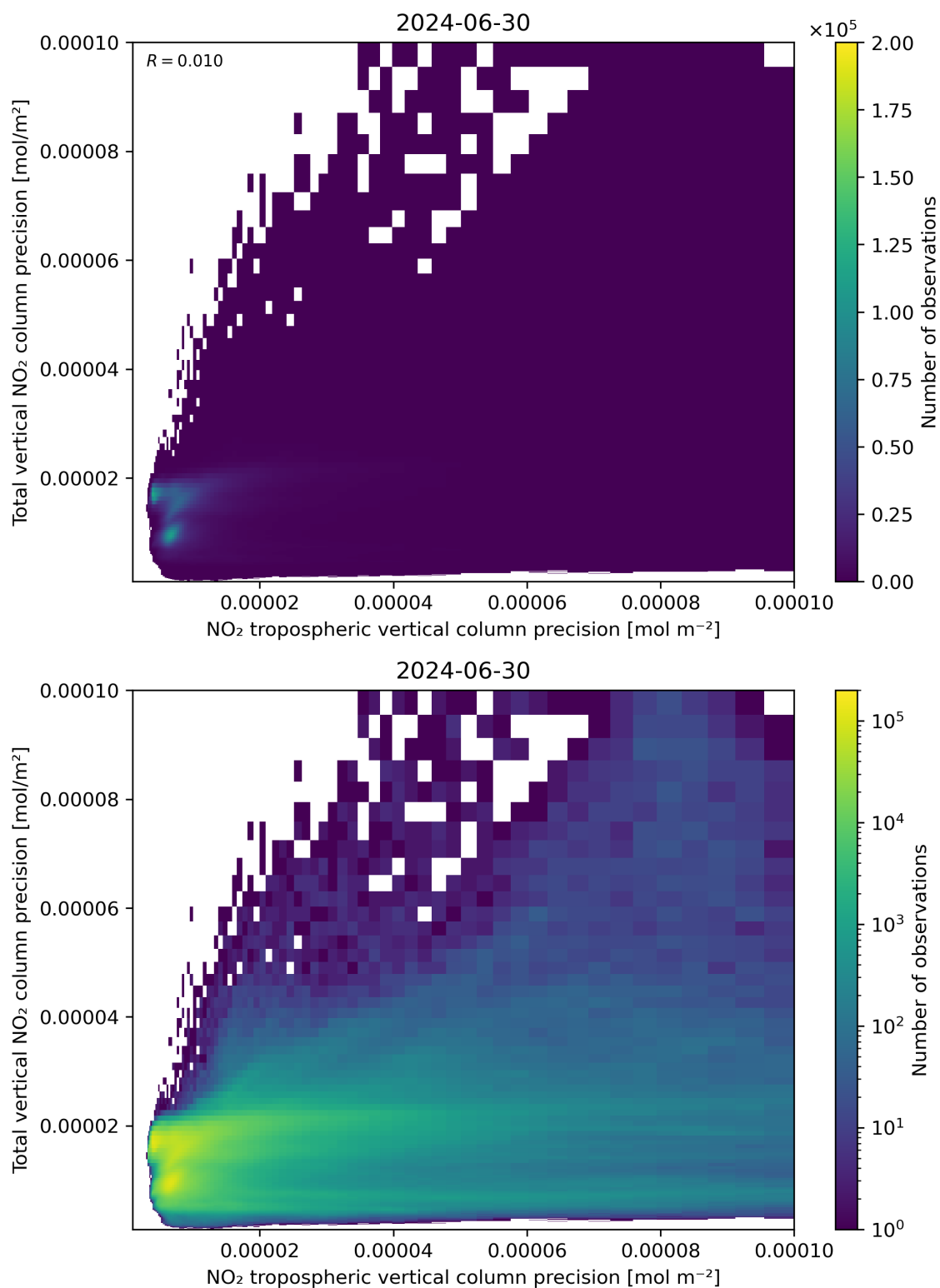
Figure 139: Scatter density plot of “NO 2 tropospheric vertical column precision” against “Total vertical NO 2 column precision” for 2024-06-29 to 2024-07-01.
