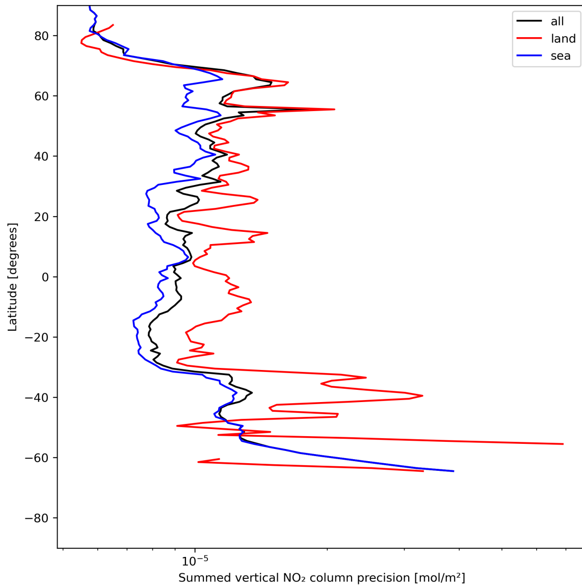
Figure 24: Zonal average of “Summed vertical NO 2 column precision” for 2024-06-29 to 2024-07-01.
