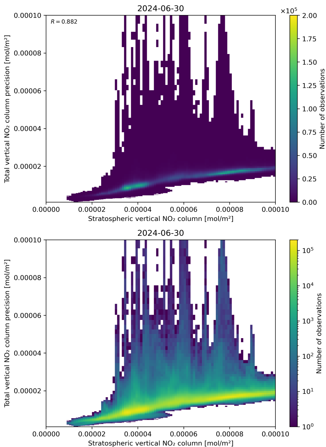
Figure 101: Scatter density plot of “Stratospheric vertical NO 2 column” against “Total vertical NO 2 column precision” for 2024-06-29 to 2024-07-01.
