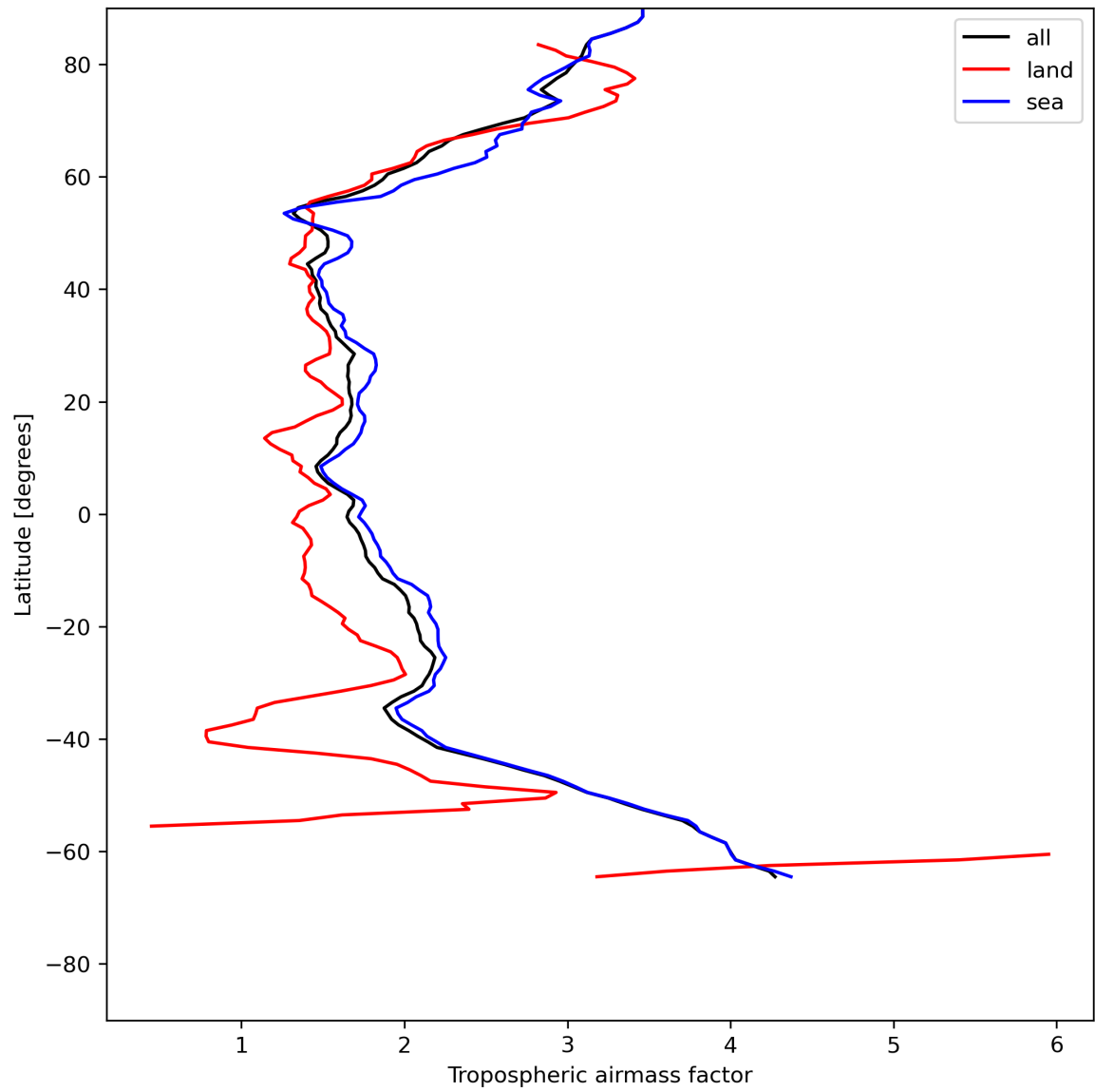
Figure 14: Zonal average of “Tropospheric airmass factor” for 2024-06-29 to 2024-07-01.
