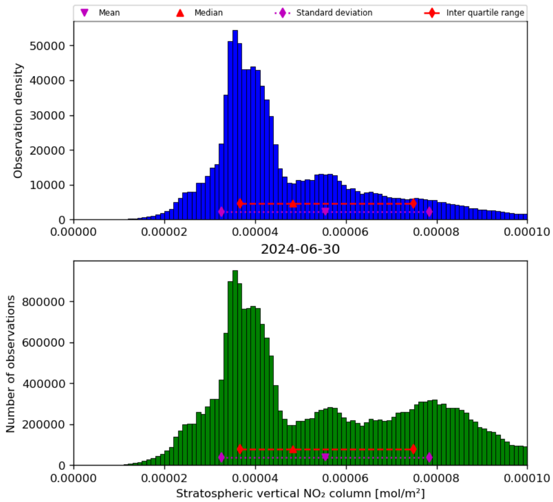
Figure 36: Histogram of “Stratospheric vertical NO 2 column” for 2024-06-29 to 2024-07-01
