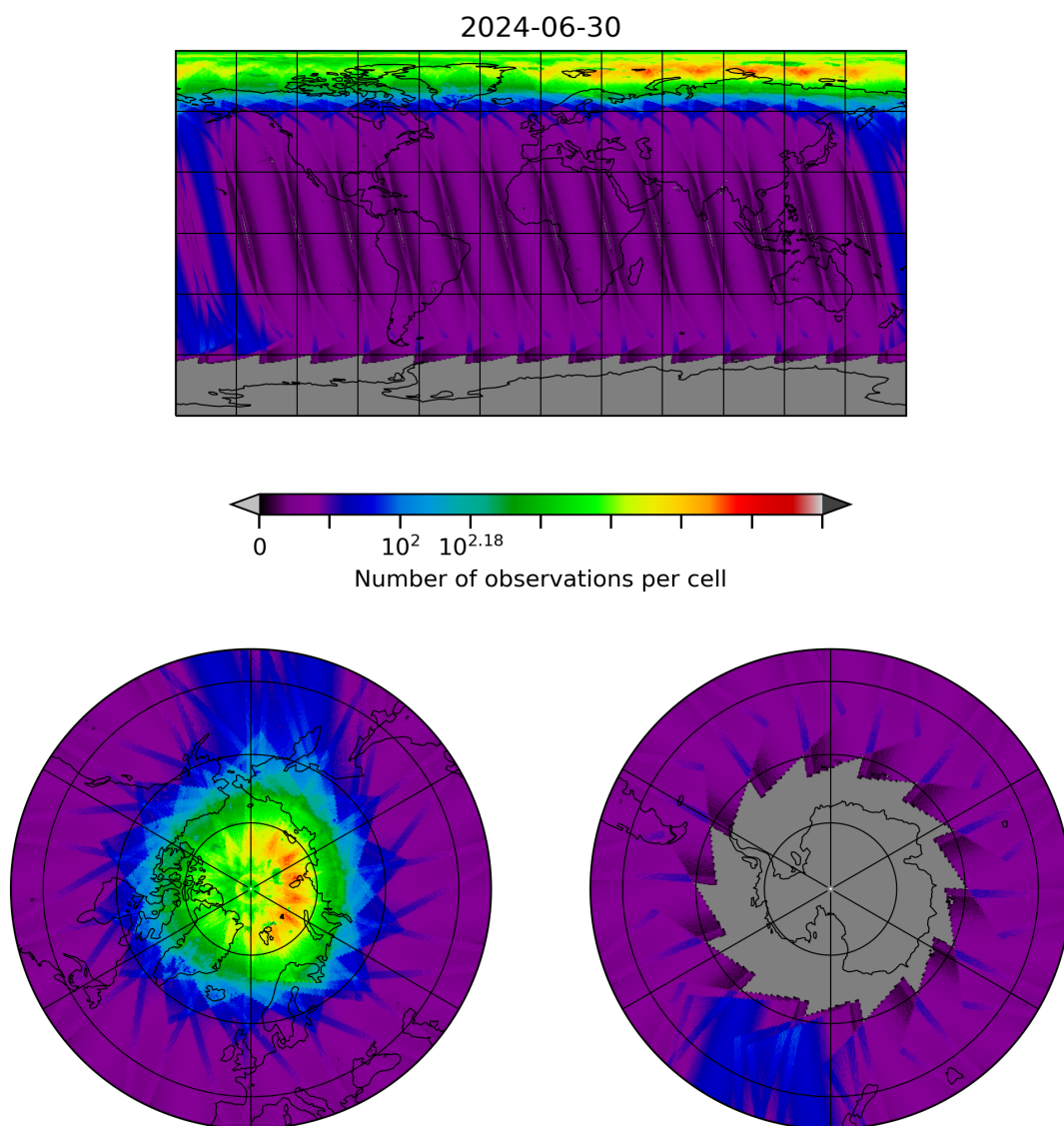
Figure 10: Map of the number of observations for 2024-06-29 to 2024-07-01
