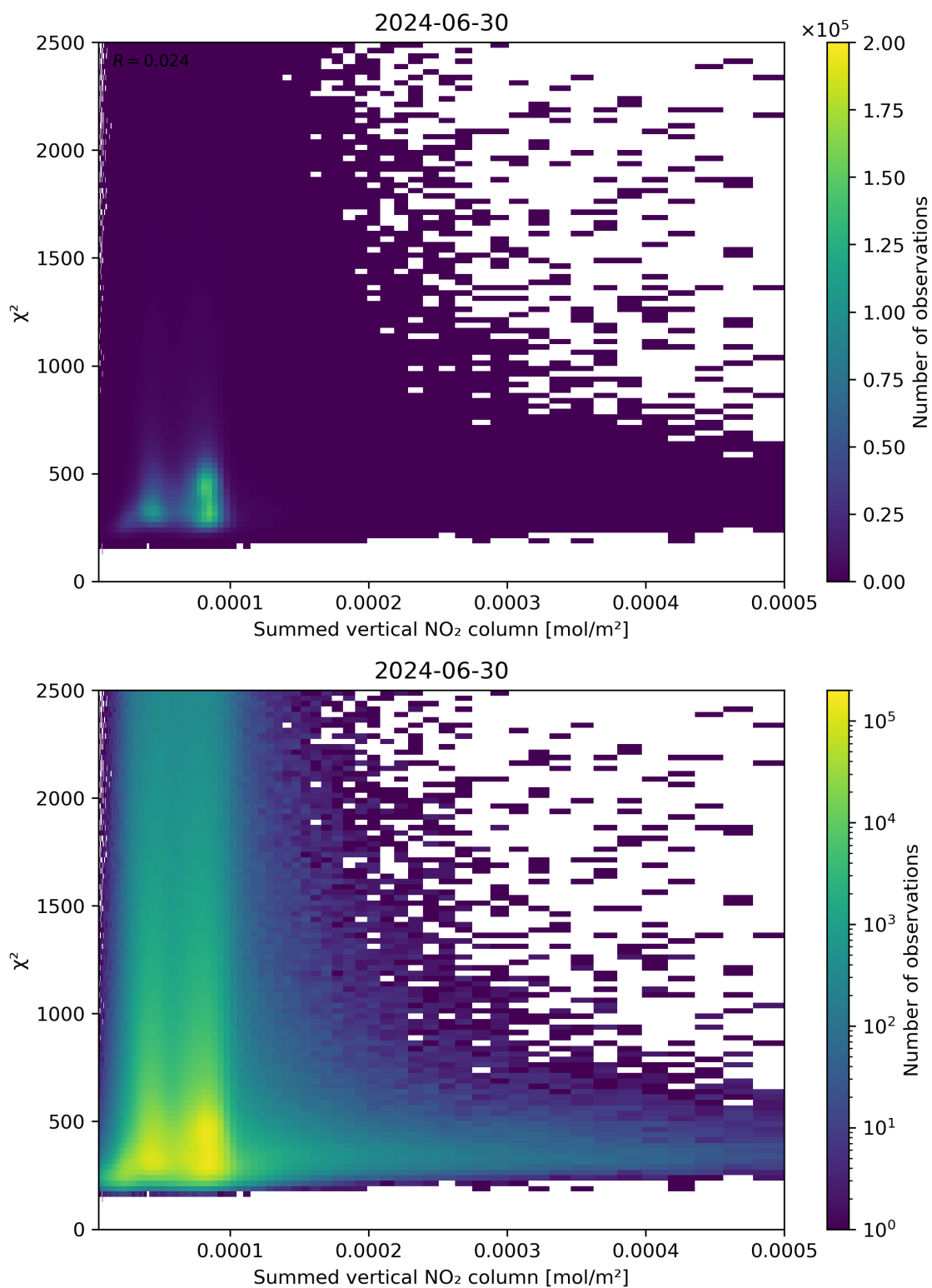
Figure 104: Scatter density plot of “Summed vertical NO 2 column” against “ \chi^2 ” for 2024-06-29 to 2024-07-01.
