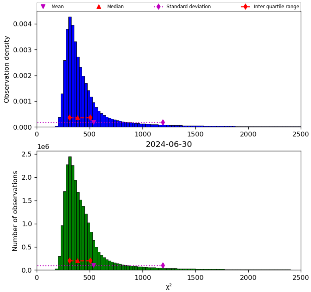
Figure 42: Histogram of “ \chi^2 ” for 2024-06-29 to 2024-07-01
