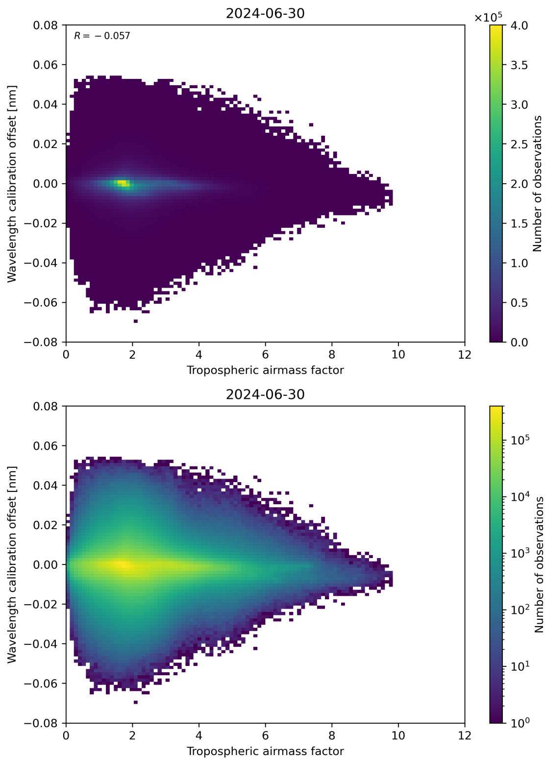
Figure 80: Scatter density plot of “Tropospheric airmass factor” against “Wavelength calibration offset” for 2024-06-29 to 2024-07-01.
