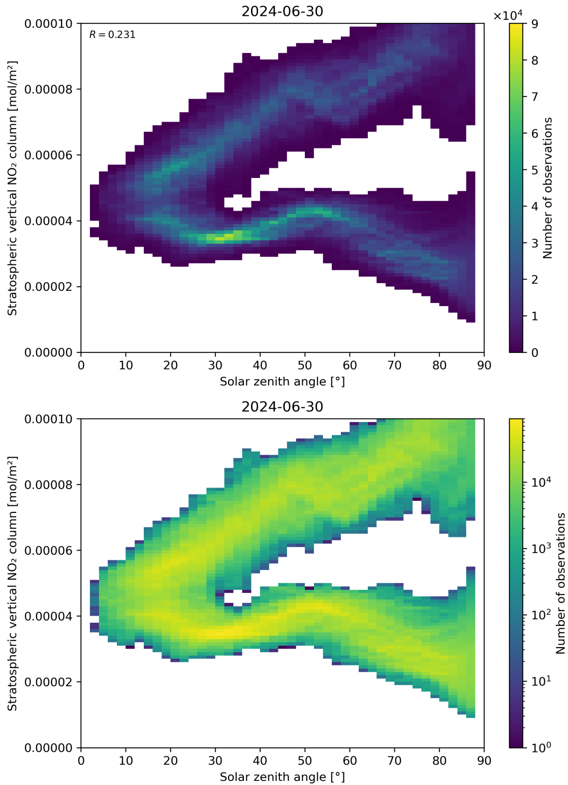
Figure 150: Scatter density plot of “Solar zenith angle” against “Stratospheric vertical NO 2 column” for 2024-06-29 to 2024-07-01.
