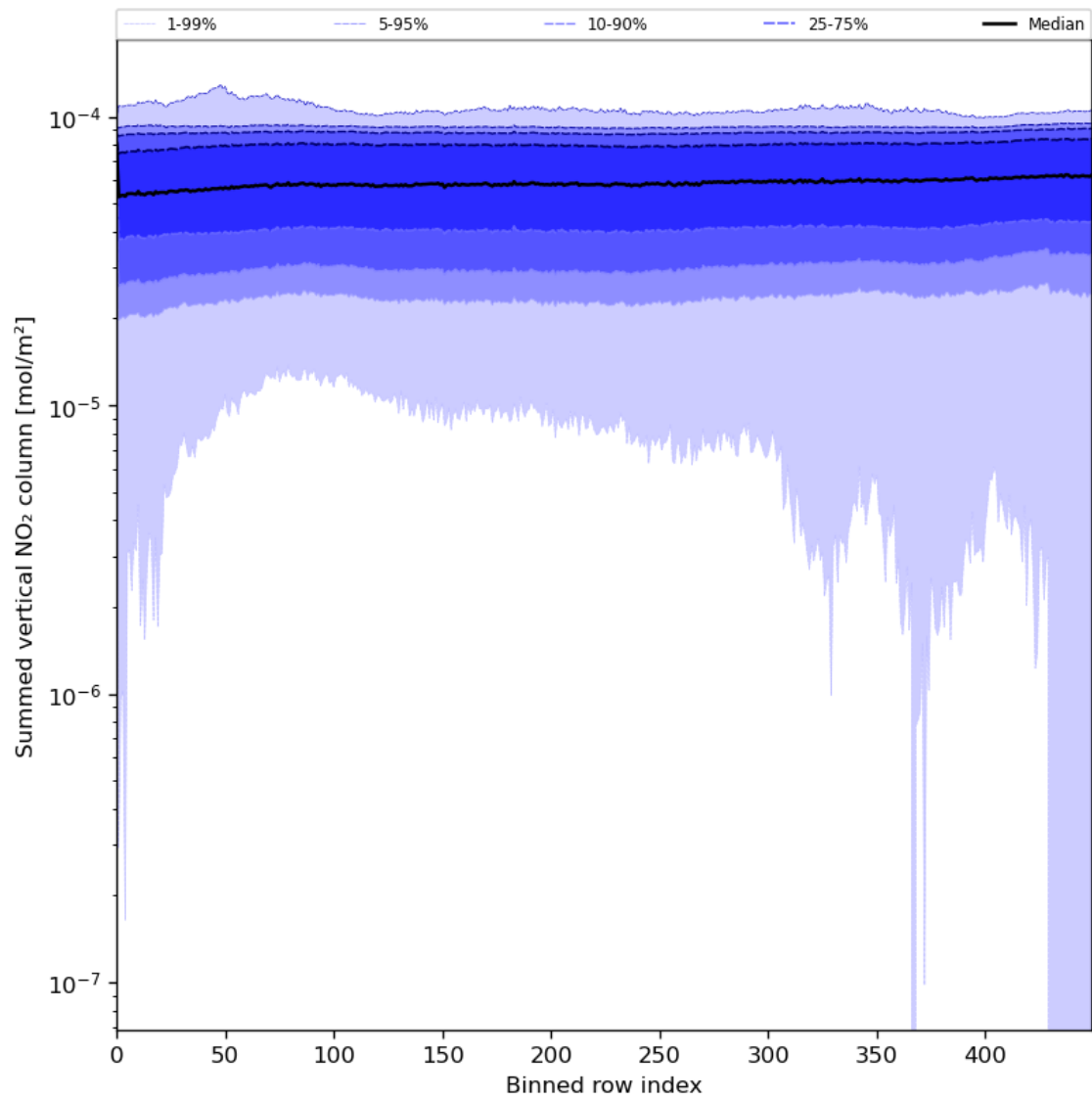
Figure 57: Along track statistics of “Summed vertical NO 2 column” for 2024-06-29 to 2024-07-01
