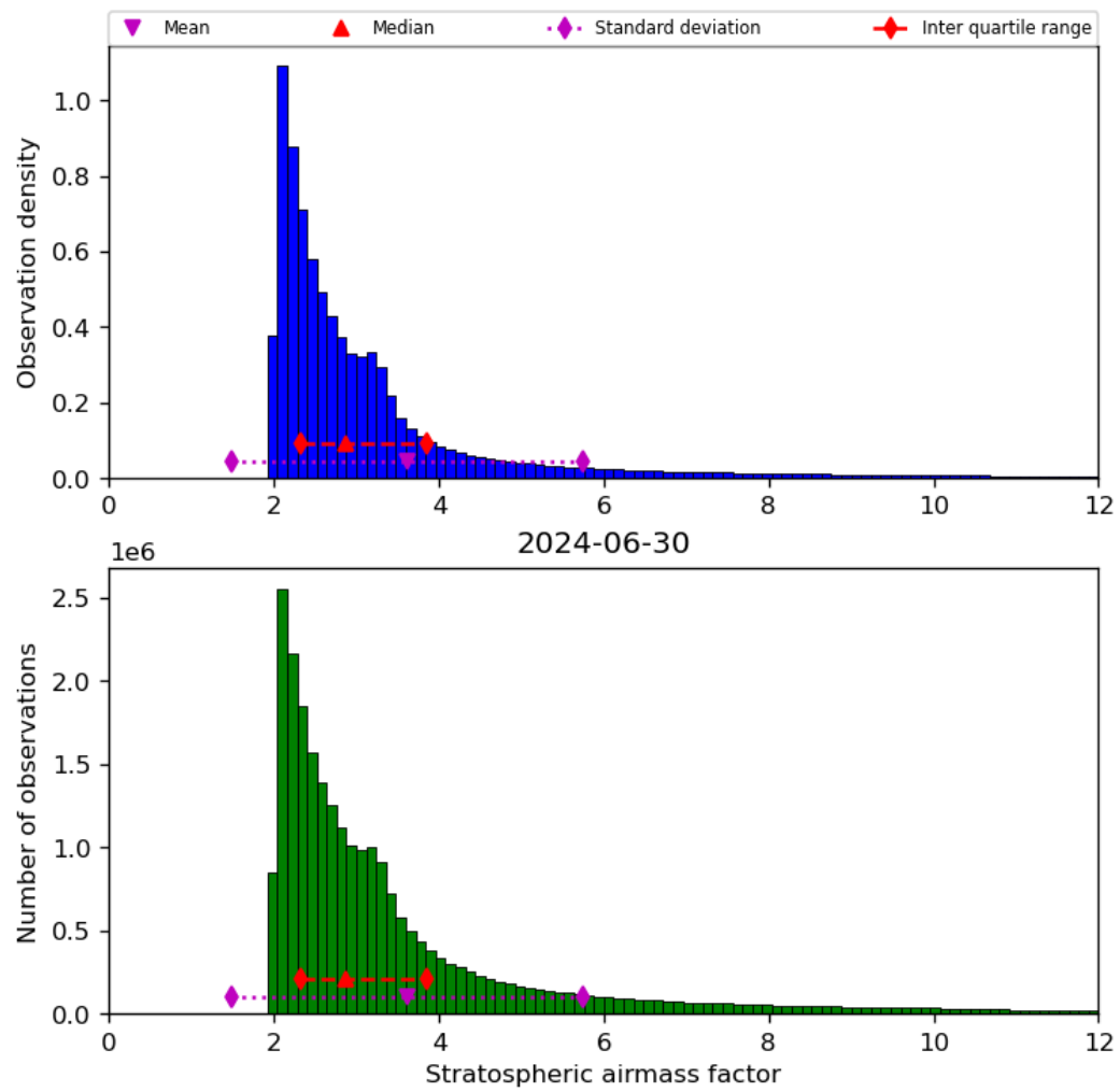
Figure 44: Histogram of “Stratospheric airmass factor” for 2024-06-29 to 2024-07-01
