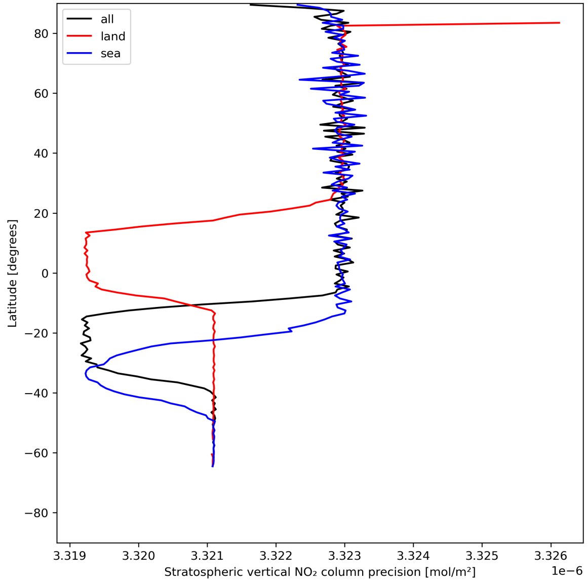
Figure 20: Zonal average of “Stratospheric vertical NO 2 column precision” for 2024-06-29 to 2024-07-01.
