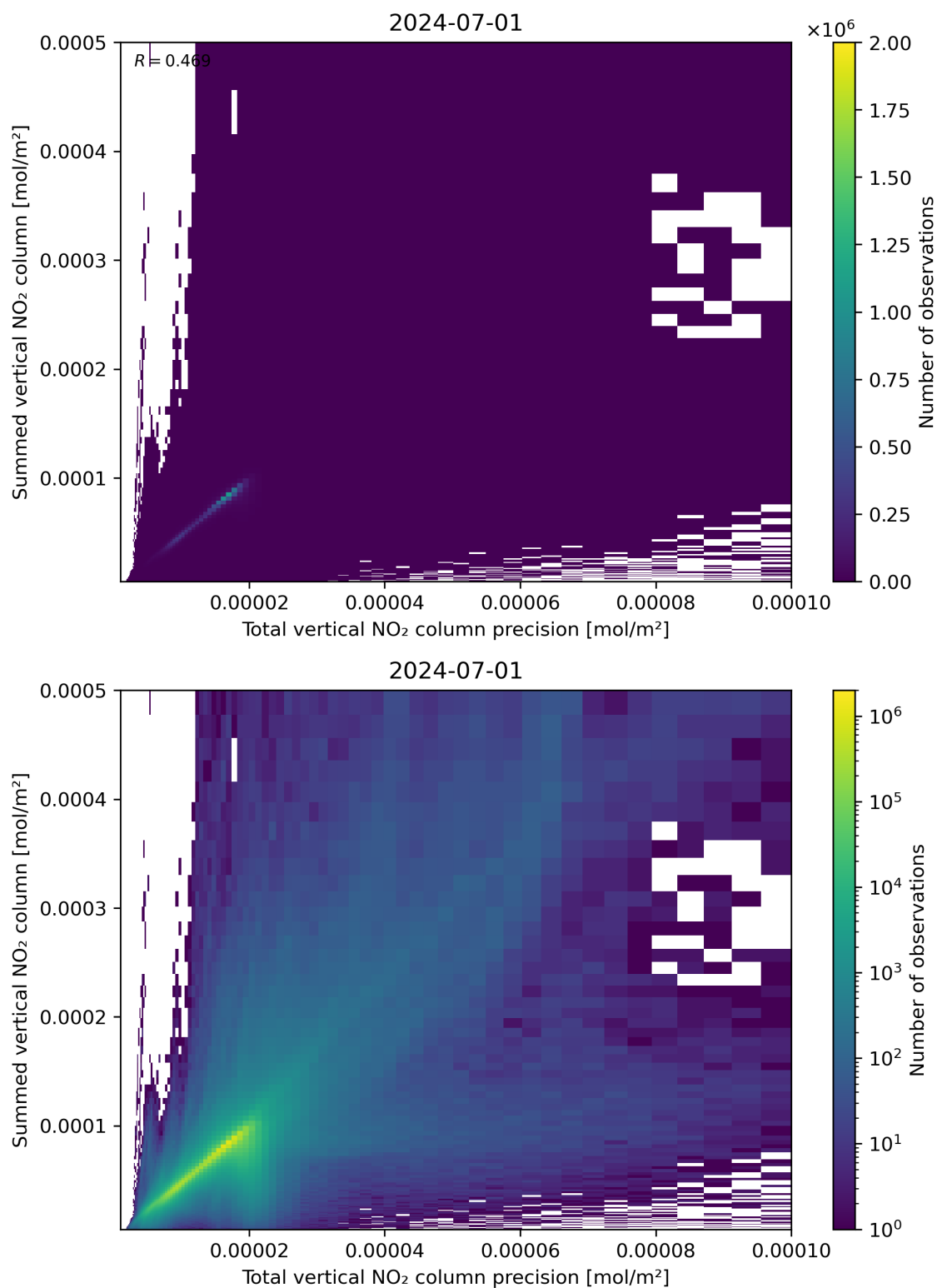
Figure 117: Scatter density plot of “Total vertical NO 2 column precision” against “Summed vertical NO 2 column” for 2024-06-30 to 2024-07-02.
