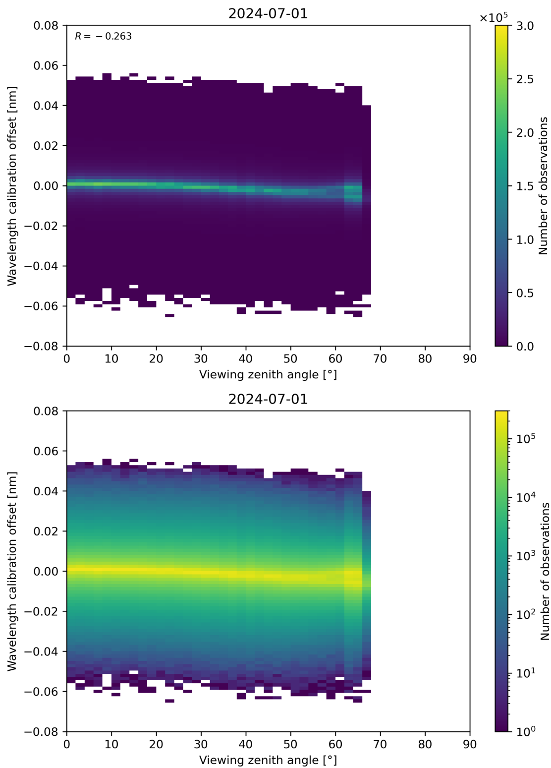
Figure 173: Scatter density plot of “Viewing zenith angle” against “Wavelength calibration offset” for 2024-06-30 to 2024-07-02.
