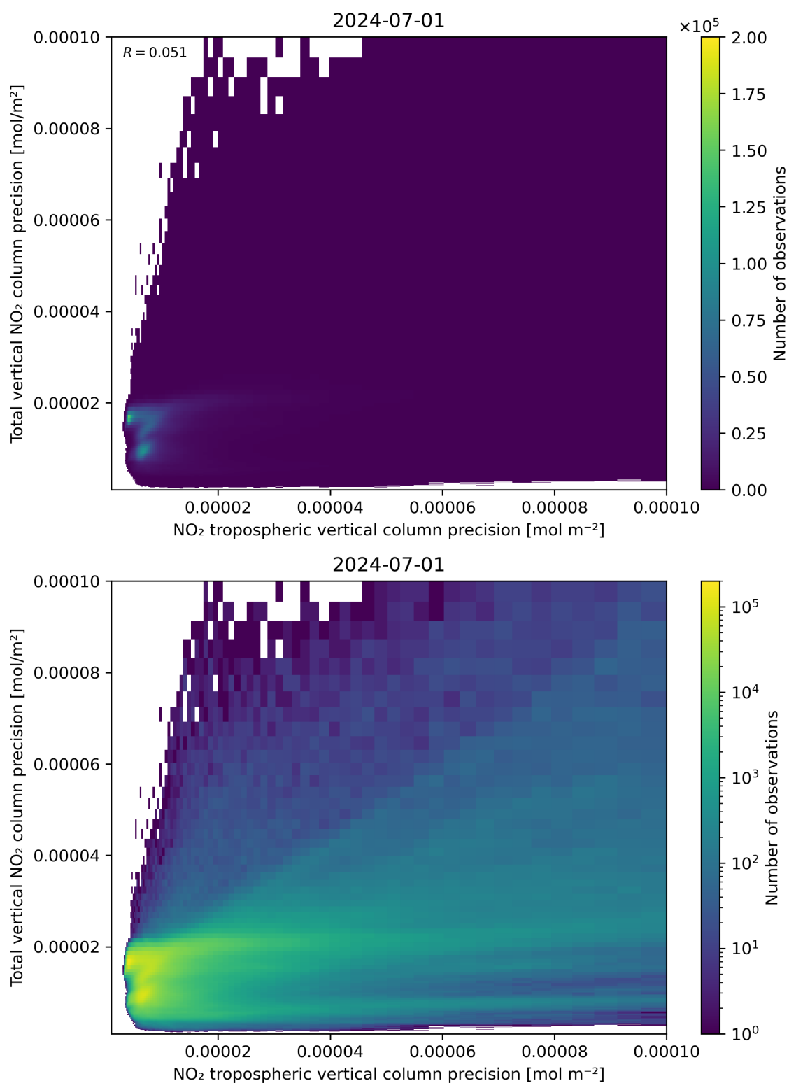
Figure 139: Scatter density plot of “NO 2 tropospheric vertical column precision” against “Total vertical NO 2 column precision” for 2024-06-30 to 2024-07-02.
