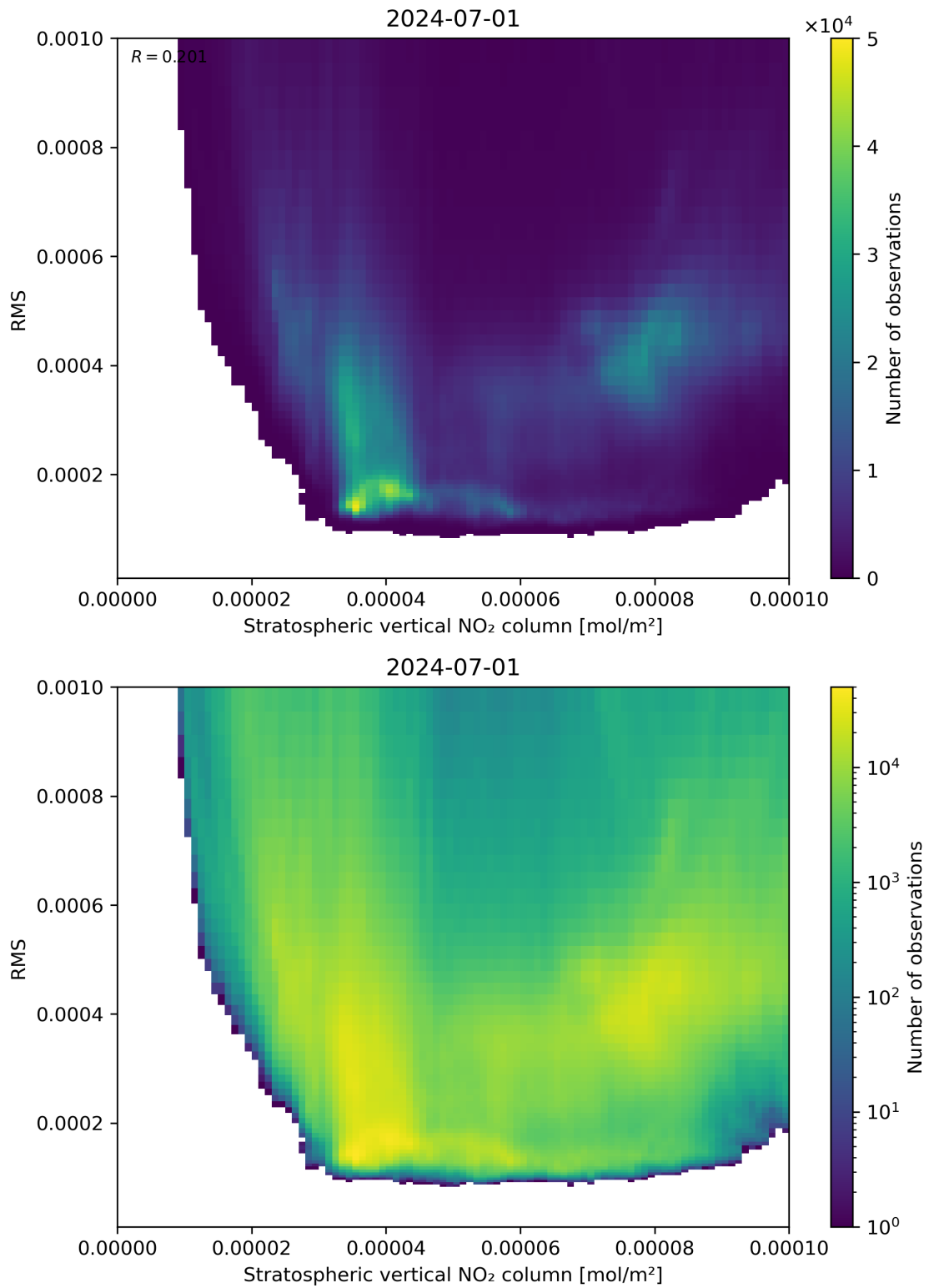
Figure 102: Scatter density plot of “Stratospheric vertical NO 2 column” against “RMS” for 2024-06-30 to 2024-07-02.
