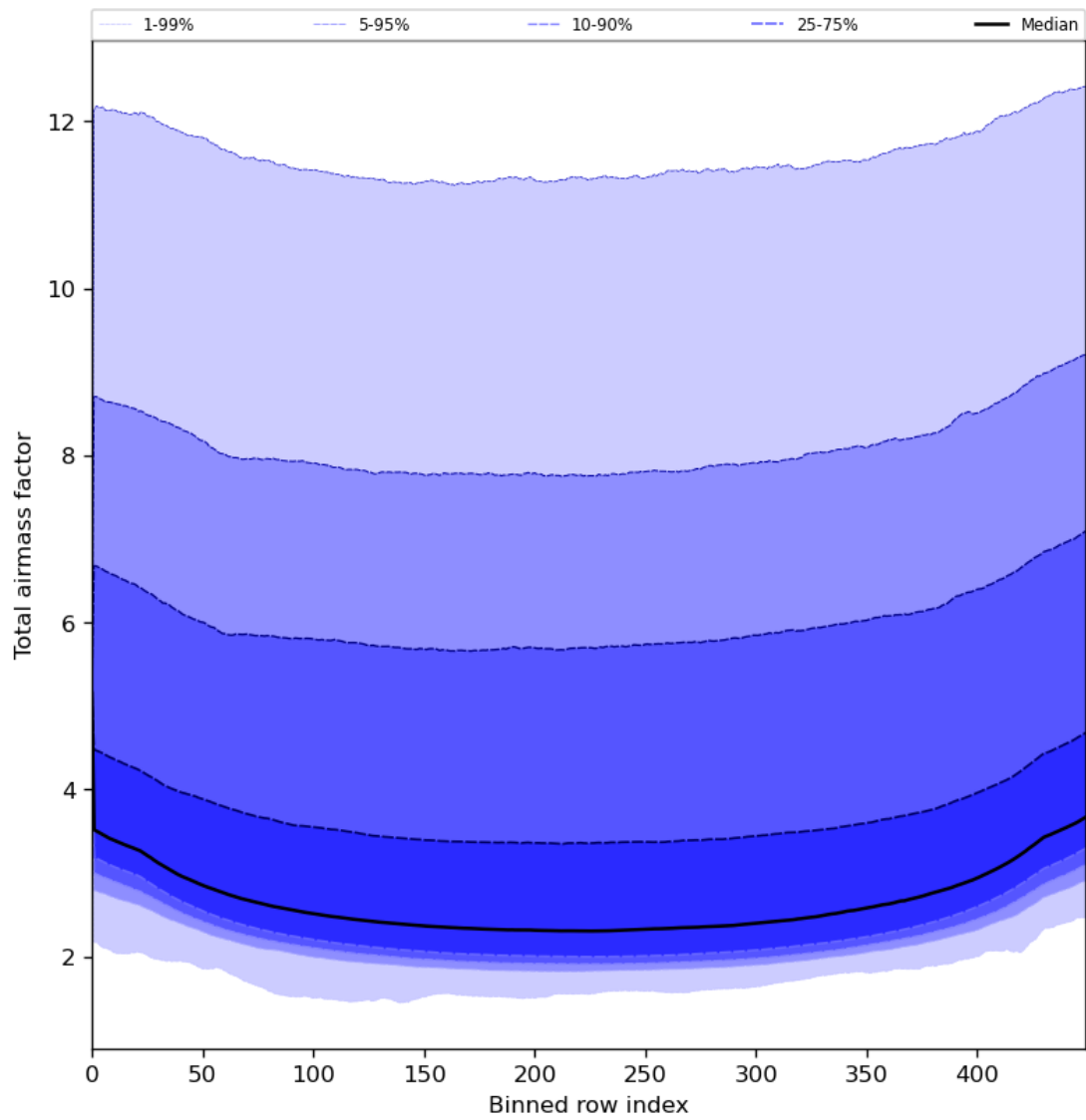
Figure 49: Along track statistics of “Total airmass factor” for 2024-06-30 to 2024-07-02
