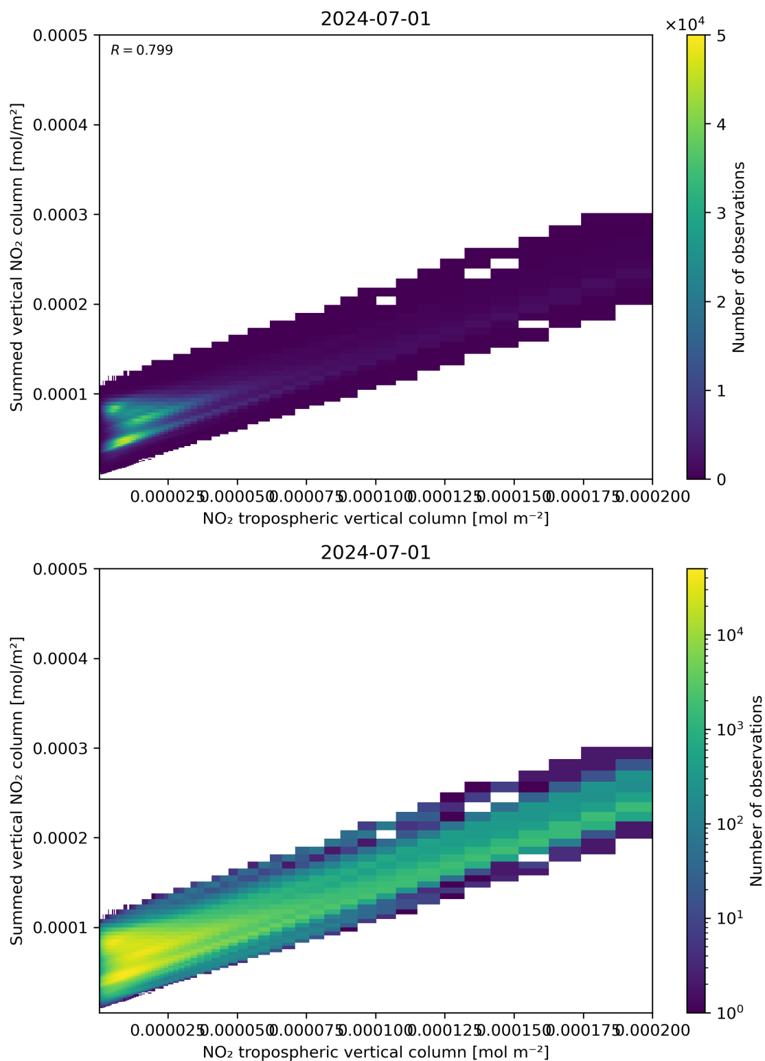
Figure 126: Scatter density plot of “NO 2 tropospheric vertical column” against “Summed vertical NO 2 column” for 2024-06-30 to 2024-07-02.
