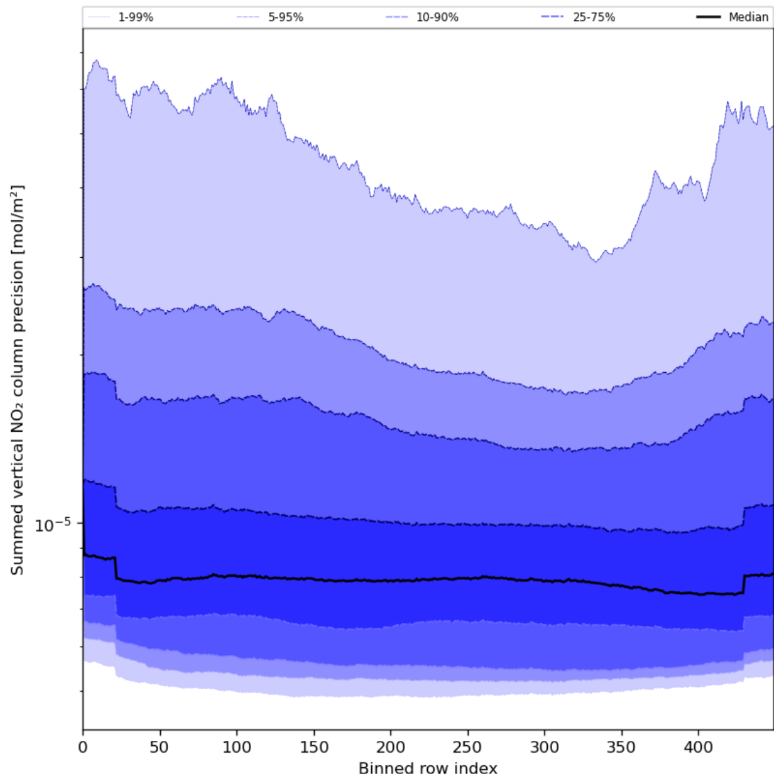
Figure 58: Along track statistics of “Summed vertical NO 2 column precision” for 2024-06-30 to 2024-07-02
