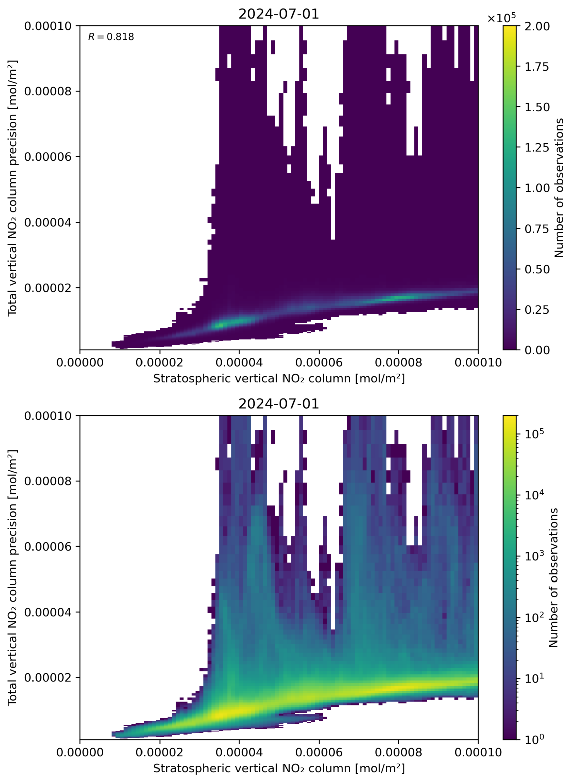
Figure 101: Scatter density plot of “Stratospheric vertical NO 2 column” against “Total vertical NO 2 column precision” for 2024-06-30 to 2024-07-02.
