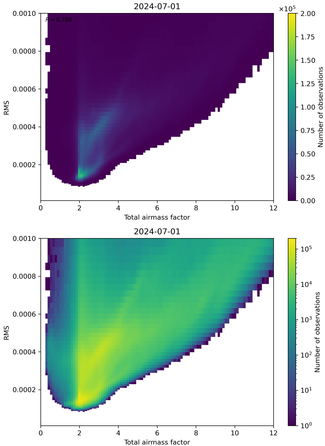
Figure 69: Scatter density plot of “Total airmass factor” against “RMS” for 2024-06-30 to 2024-07-02.
