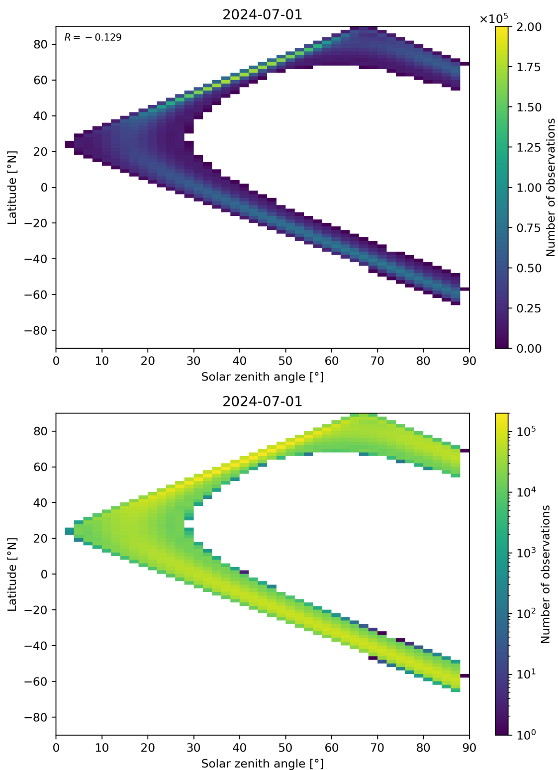
Figure 149: Scatter density plot of “Solar zenith angle” against “Latitude” for 2024-06-30 to 2024-07-02.
