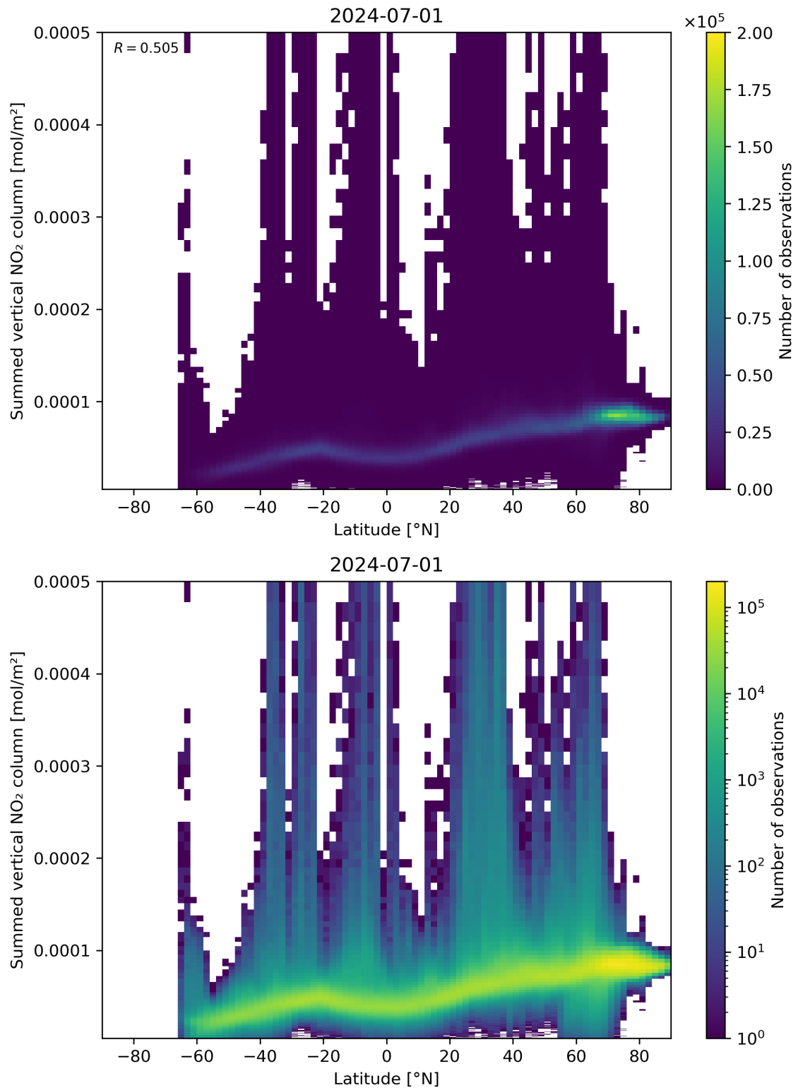
Figure 88: Scatter density plot of “Latitude” against “Summed vertical NO 2 column” for 2024-06-30 to 2024-07-02.
