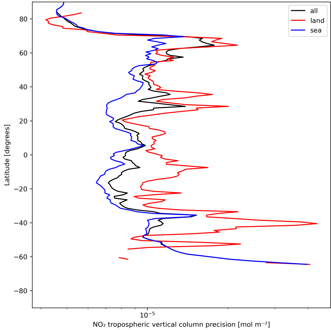
Figure 13: Zonal average of “NO 2 tropospheric vertical column precision” for 2024-06-30 to 2024-07-02.
