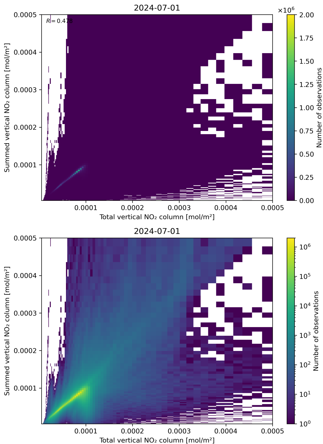
Figure 112: Scatter density plot of “Total vertical NO 2 column” against “Summed vertical NO 2 column” for 2024-06-30 to 2024-07-02.
