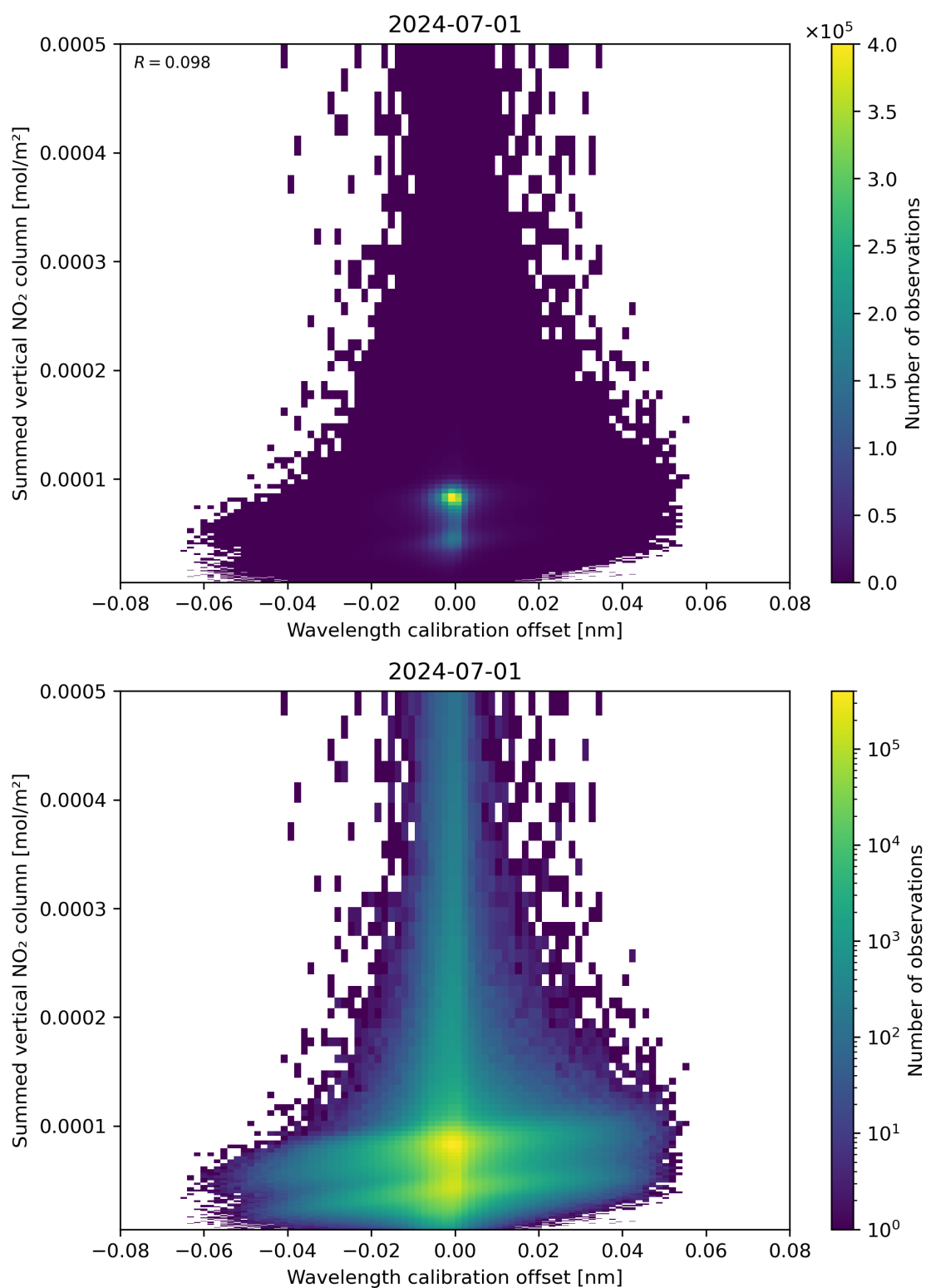
Figure 177: Scatter density plot of “Wavelength calibration offset” against “Summed vertical NO 2 column” for 2024-06-30 to 2024-07-02.
