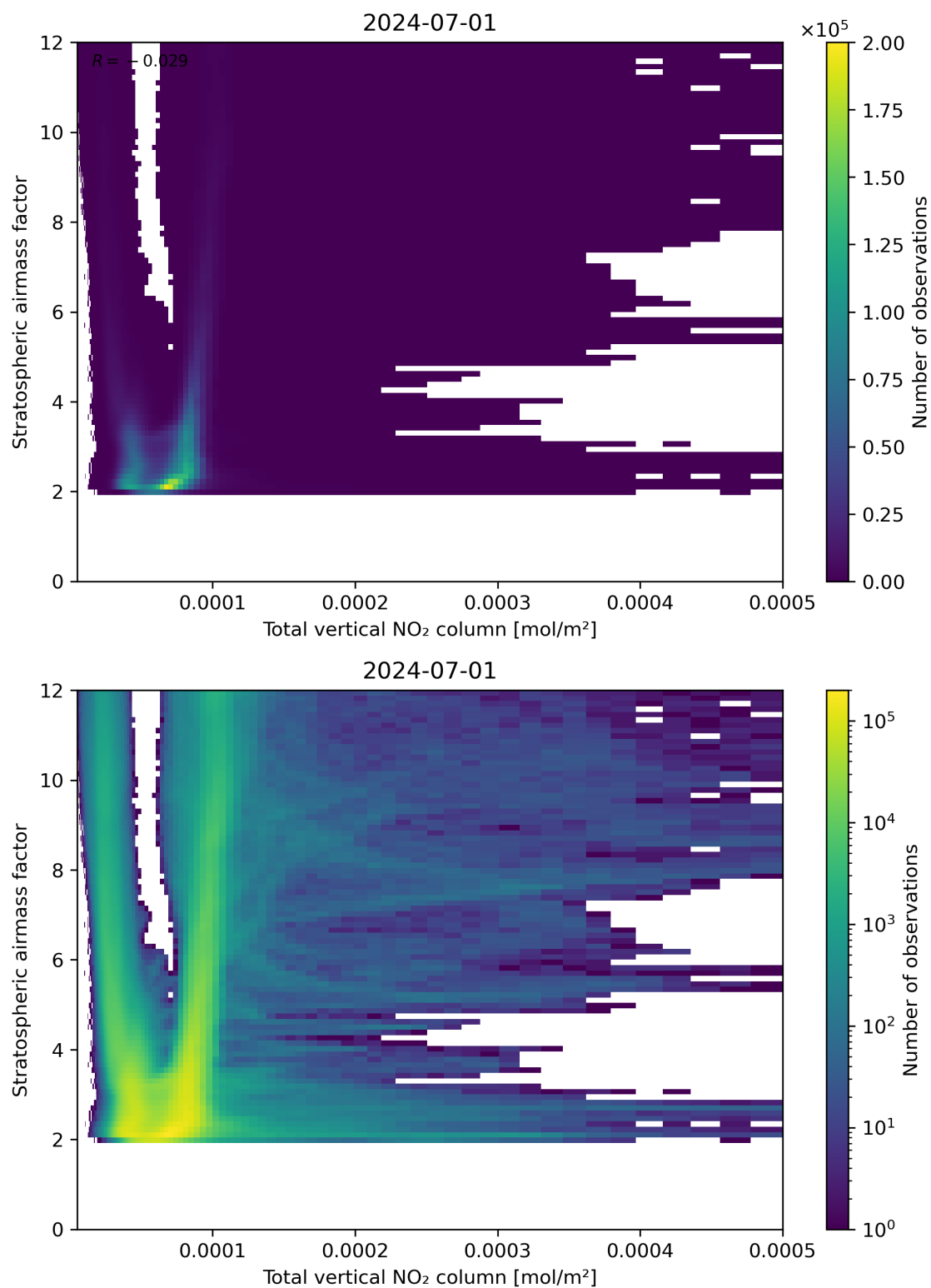
Figure 110: Scatter density plot of “Total vertical NO 2 column” against “Stratospheric airmass factor” for 2024-06-30 to 2024-07-02.
