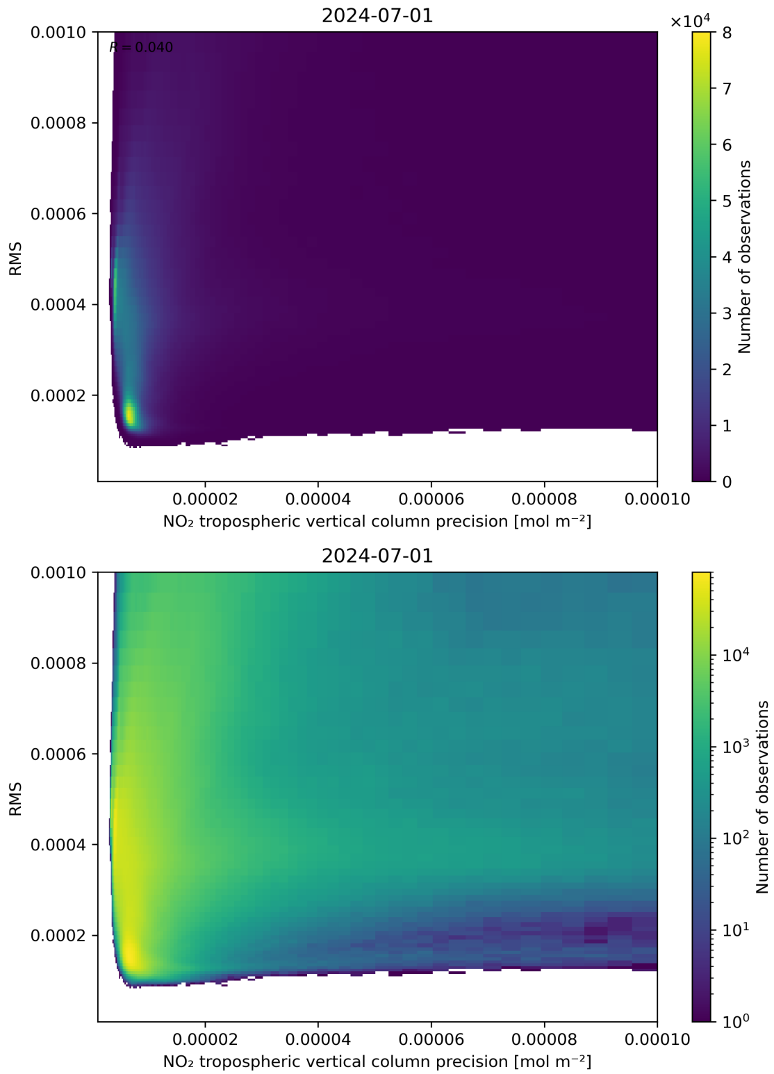
Figure 140: Scatter density plot of “NO 2 tropospheric vertical column precision” against “RMS” for 2024-06-30 to 2024-07-02.
