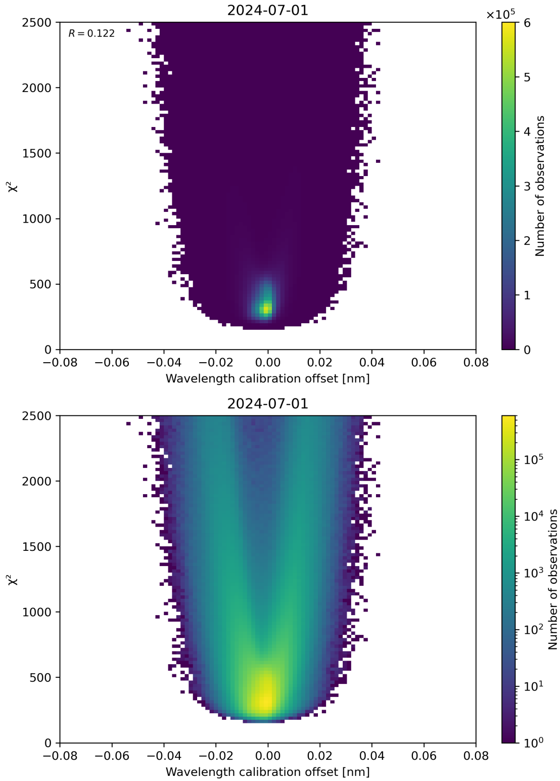
Figure 175: Scatter density plot of “Wavelength calibration offset” against “ \chi^2 ” for 2024-06-30 to 2024-07-02.
