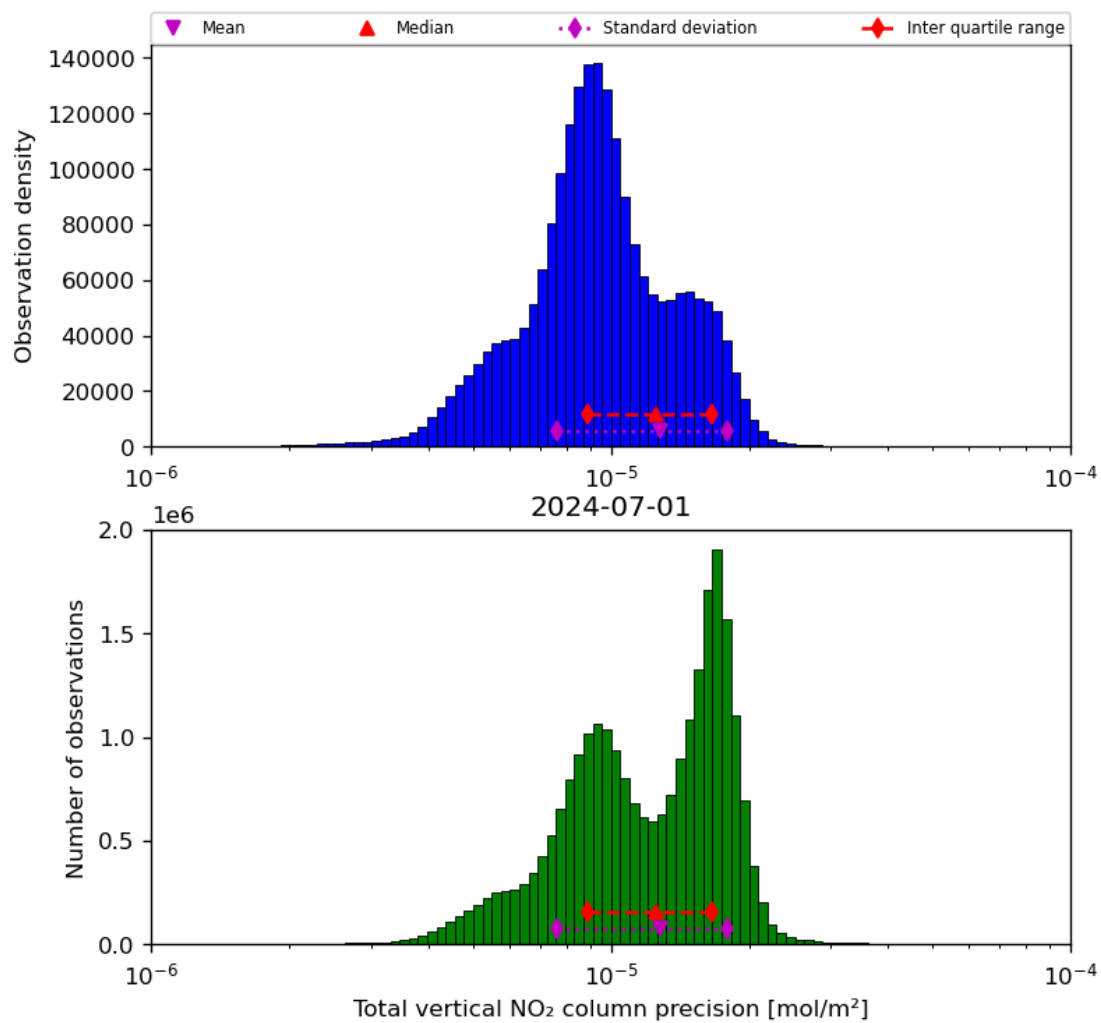
Figure 39: Histogram of “Total vertical NO 2 column precision” for 2024-06-30 to 2024-07-02
