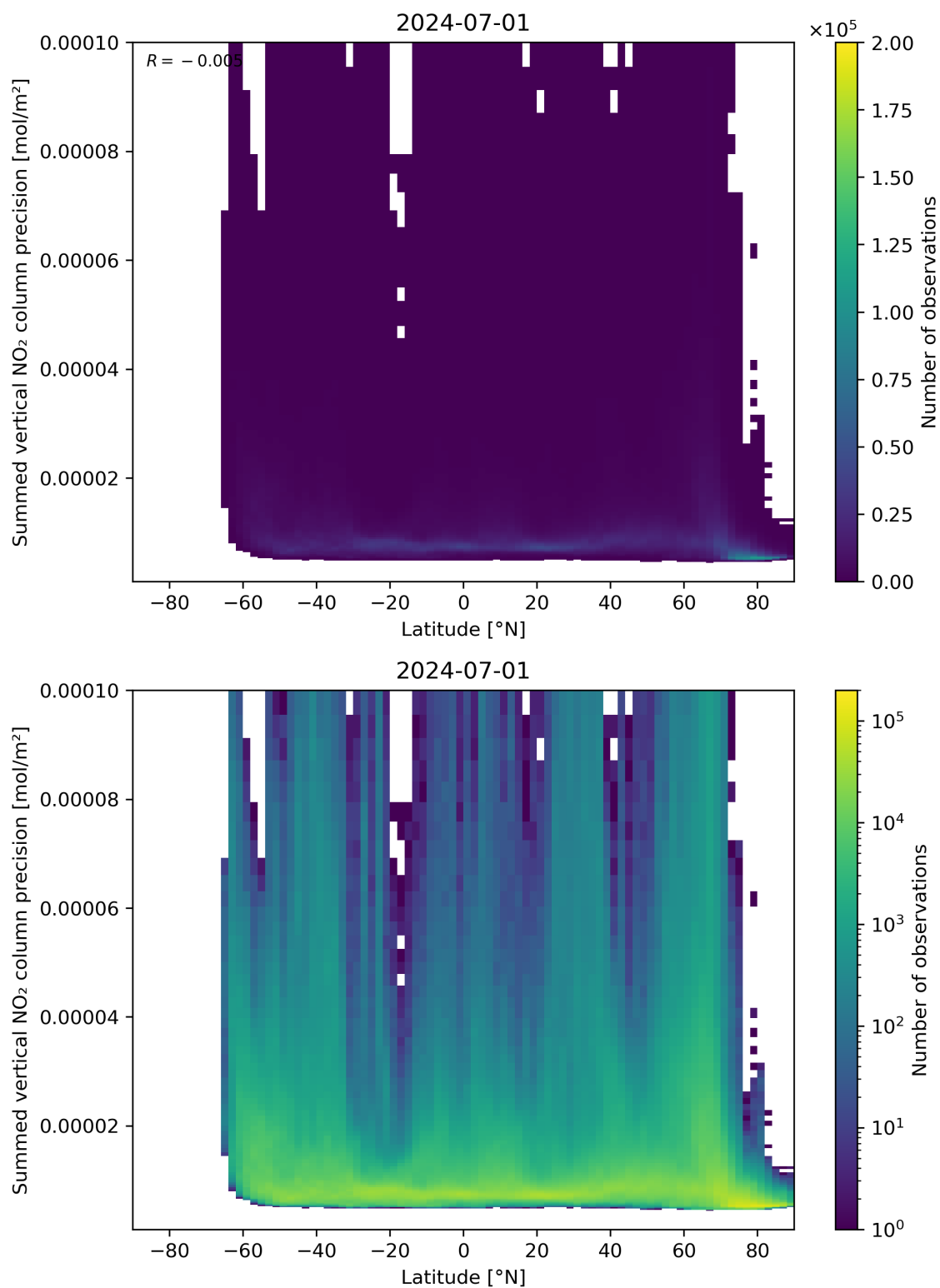
Figure 89: Scatter density plot of “Latitude” against “Summed vertical NO 2 column precision” for 2024-06-30 to 2024-07-02.
