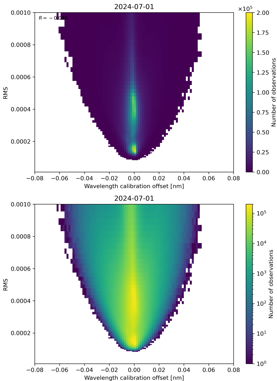
Figure 181: Scatter density plot of “Wavelength calibration offset” against “RMS” for 2024-06-30 to 2024-07-02.
