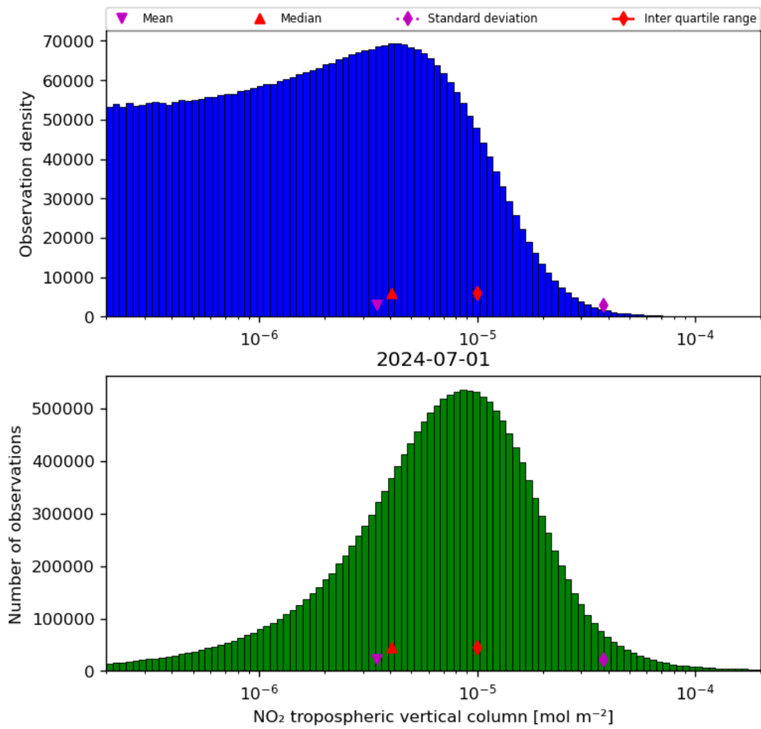
Figure 29: Histogram of “NO 2 tropospheric vertical column” for 2024-06-30 to 2024-07-02
