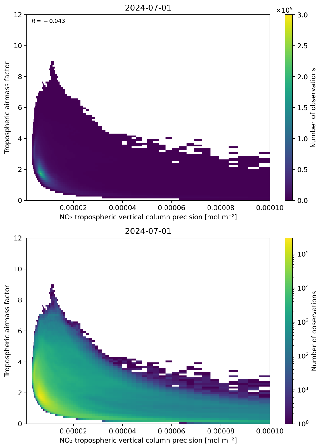
Figure 133: Scatter density plot of “NO 2 tropospheric vertical column precision” against “Tropospheric airmass factor” for 2024-06-30 to 2024-07-02.
