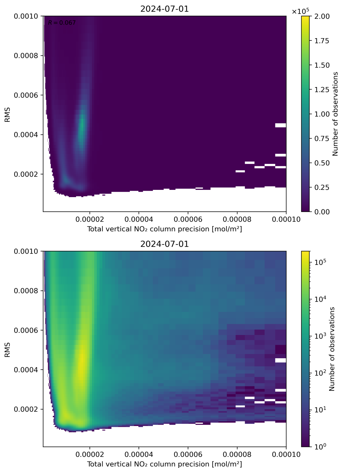
Figure 119: Scatter density plot of “Total vertical NO 2 column precision” against “RMS” for 2024-06-30 to 2024-07-02.
