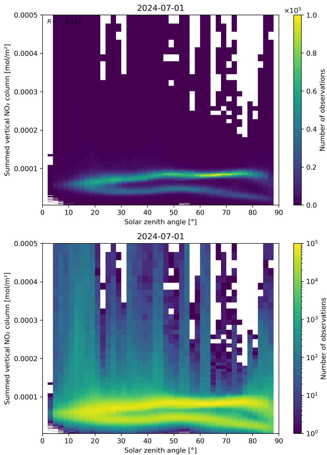
Figure 151: Scatter density plot of “Solar zenith angle” against “Summed vertical NO 2 column” for 2024-06-30 to 2024-07-02.
