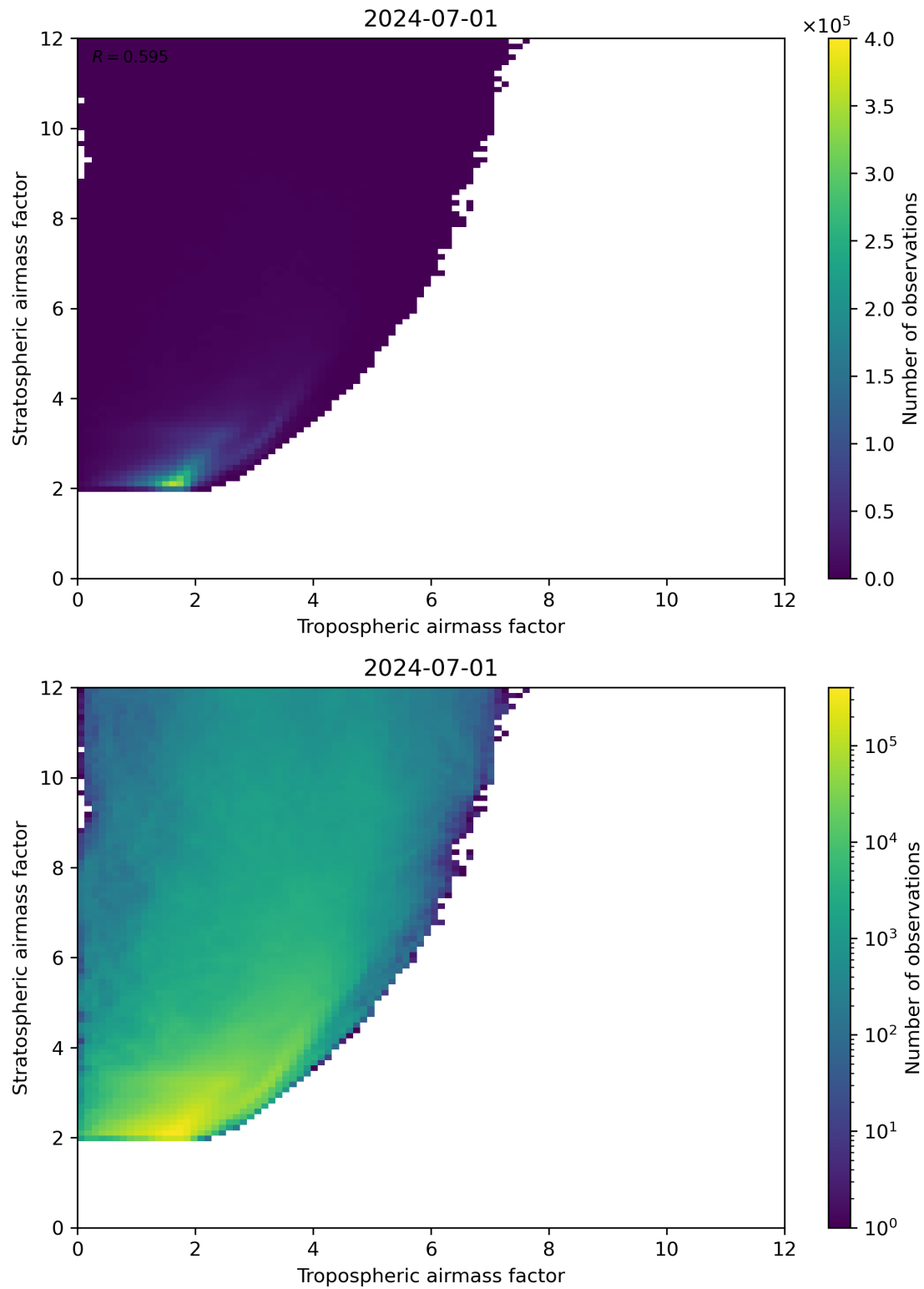
Figure 71: Scatter density plot of “Tropospheric airmass factor” against “Stratospheric airmass factor” for 2024-06-30 to 2024-07-02.
