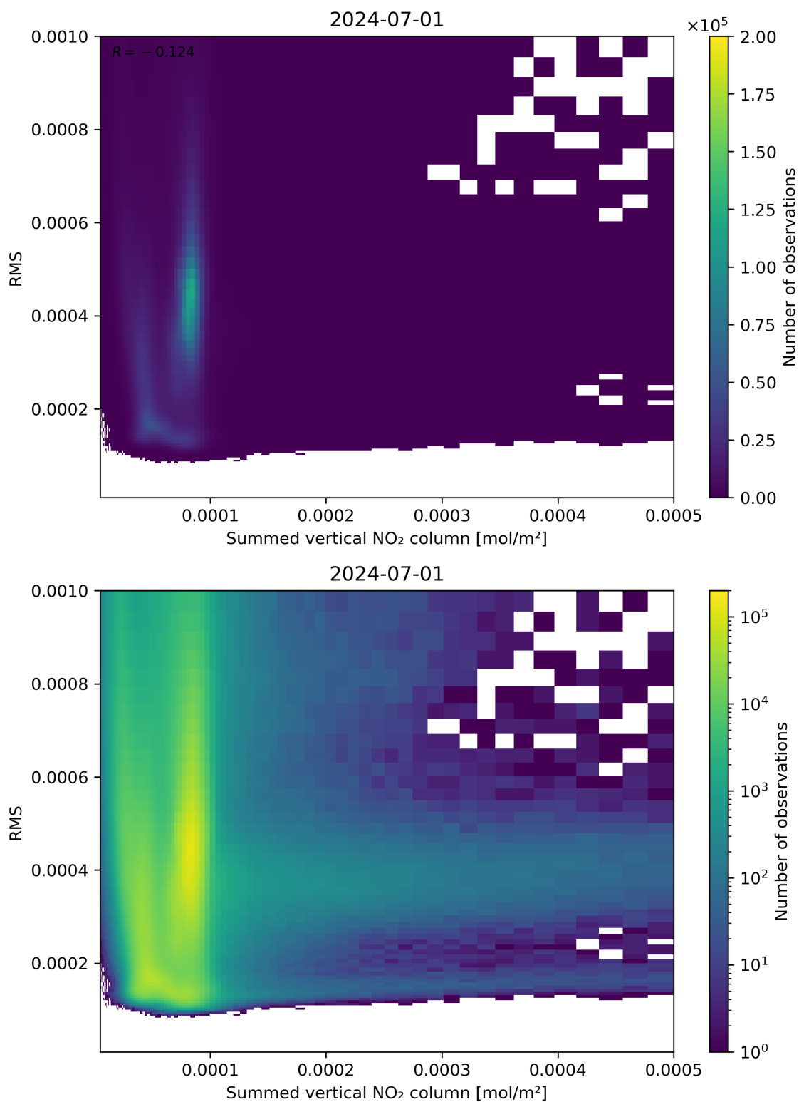
Figure 109: Scatter density plot of “Summed vertical NO 2 column” against “RMS” for 2024-06-30 to 2024-07-02.
