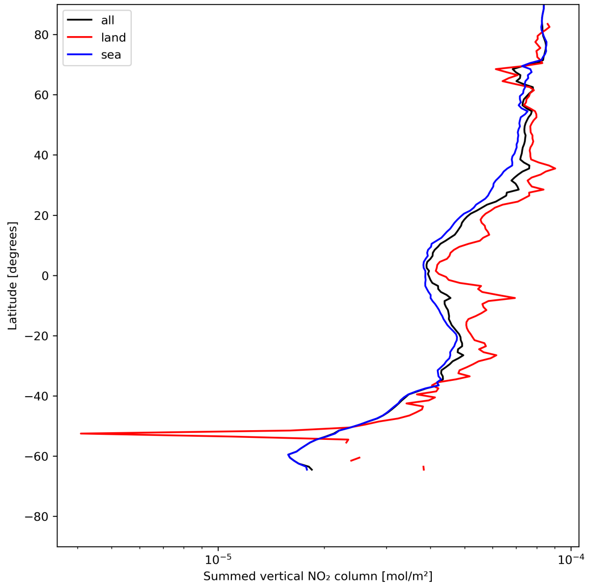
Figure 23: Zonal average of “Summed vertical NO 2 column” for 2024-06-30 to 2024-07-02.
