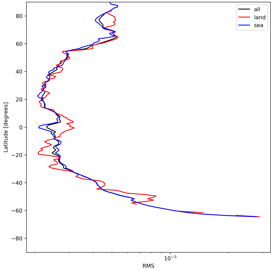
Figure 26: Zonal average of “RMS” for 2024-06-30 to 2024-07-02.
