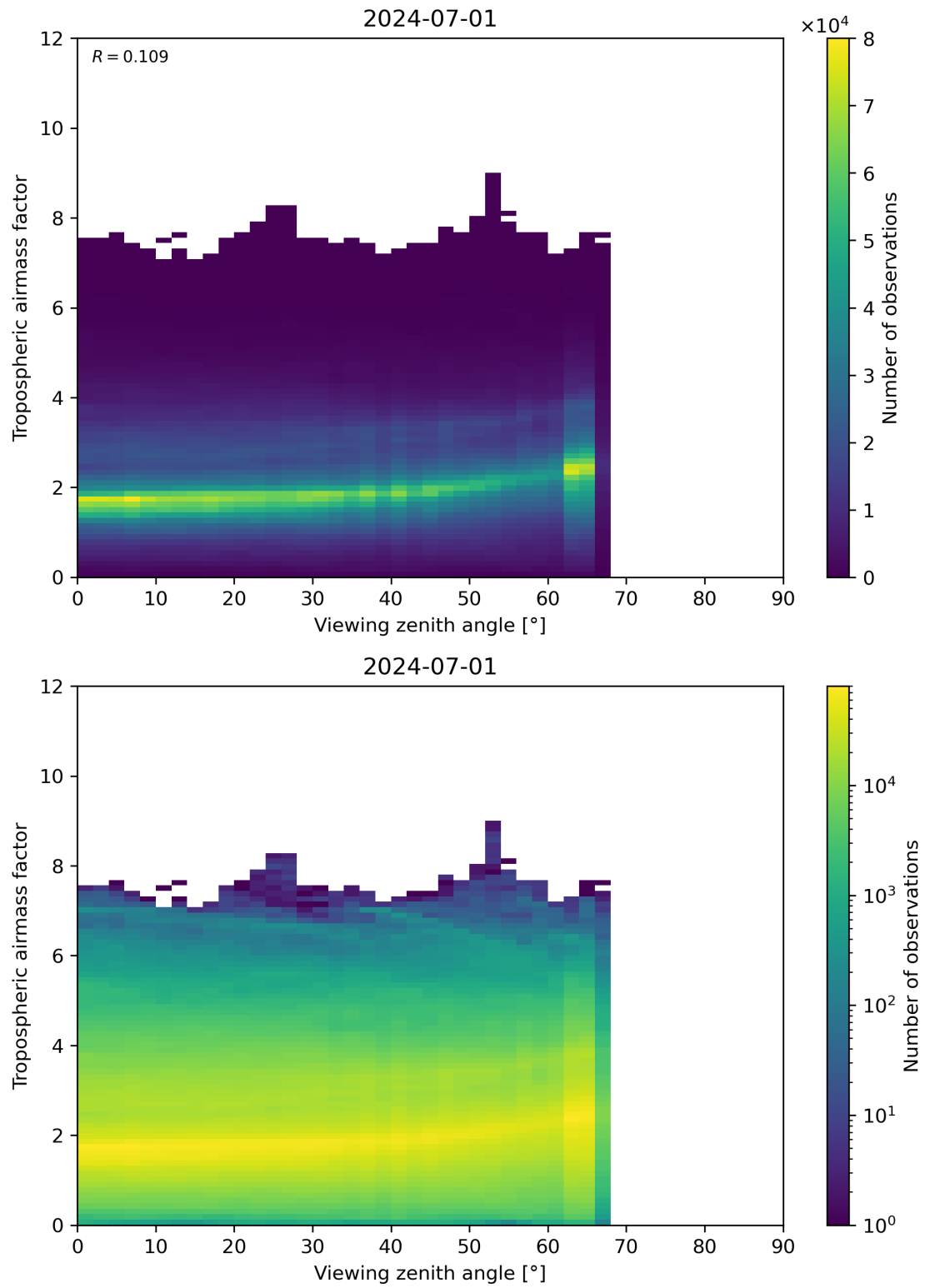
Figure 161: Scatter density plot of “Viewing zenith angle” against “Tropospheric airmass factor” for 2024-06-30 to 2024-07-02.
