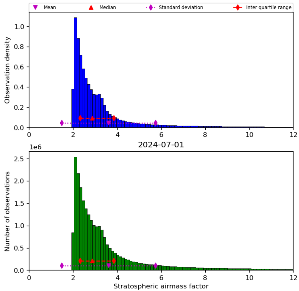
Figure 44: Histogram of “Stratospheric airmass factor” for 2024-06-30 to 2024-07-02
