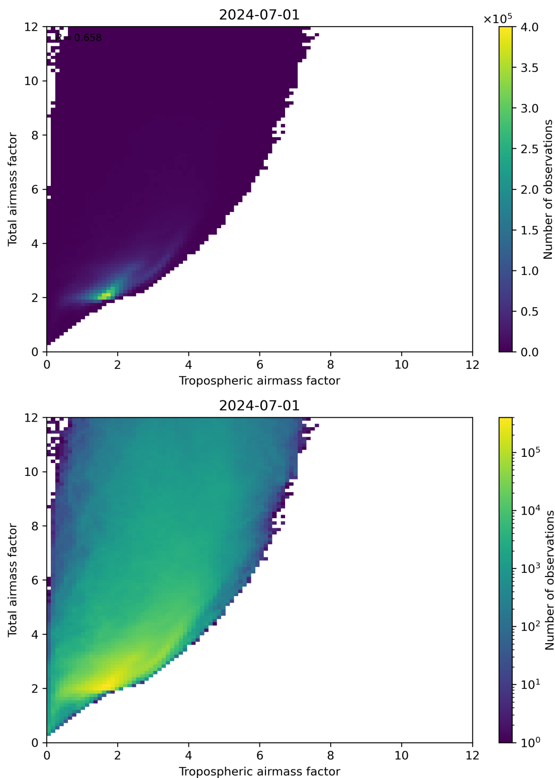
Figure 72: Scatter density plot of “Tropospheric airmass factor” against “Total airmass factor” for 2024-06-30 to 2024-07-02.
