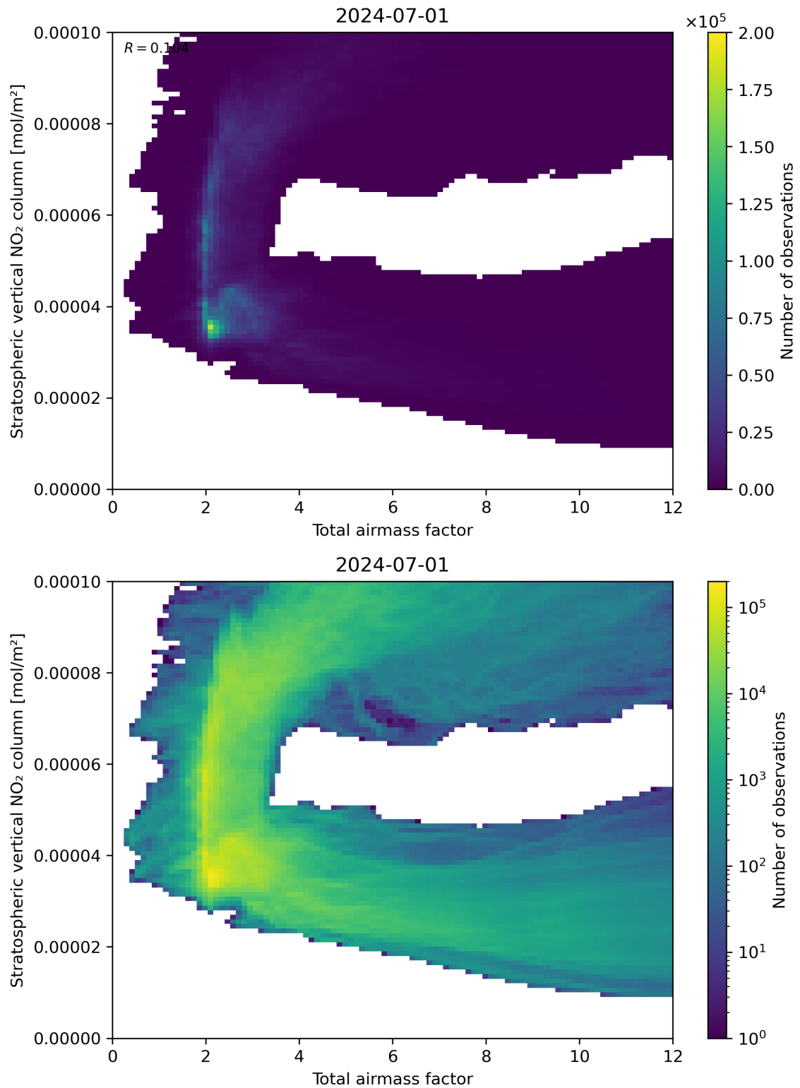
Figure 64: Scatter density plot of “Total airmass factor” against “Stratospheric vertical NO 2 column” for 2024-06-30 to 2024-07-02.
