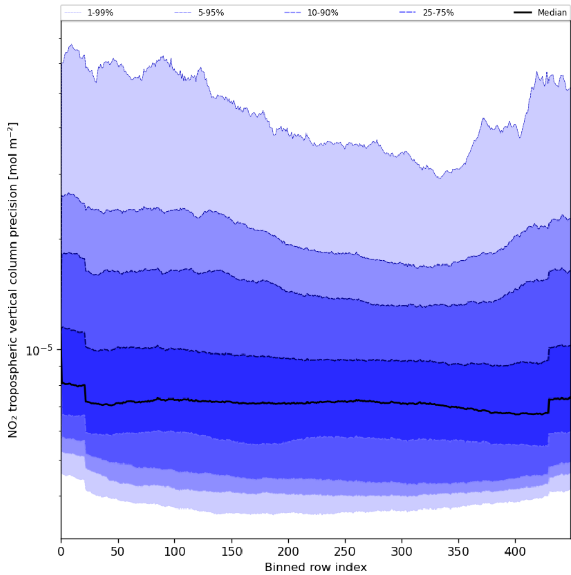
Figure 47: Along track statistics of “NO 2 tropospheric vertical column precision” for 2024-06-30 to 2024-07-02
