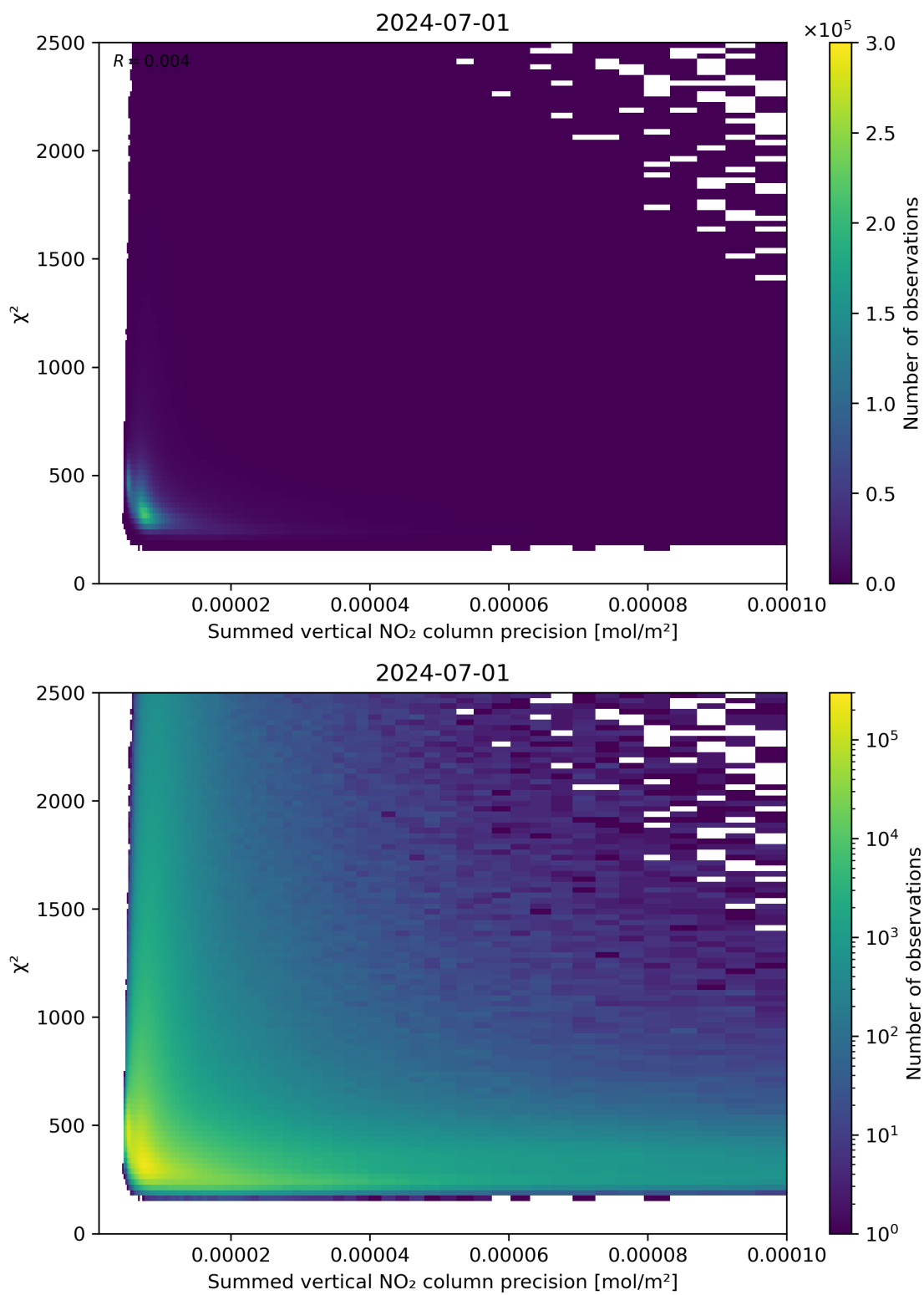
Figure 107: Scatter density plot of “Summed vertical NO 2 column precision” against “ \chi^2 ” for 2024-06-30 to 2024-07-02.
