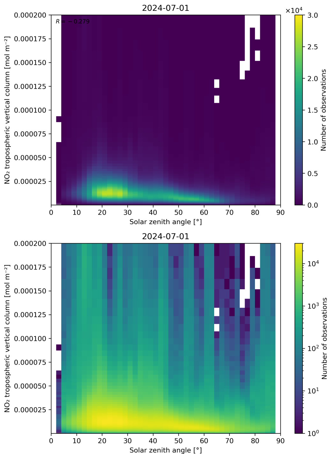
Figure 155: Scatter density plot of “Solar zenith angle” against “NO 2 tropospheric vertical column” for 2024-06-30 to 2024-07-02.
