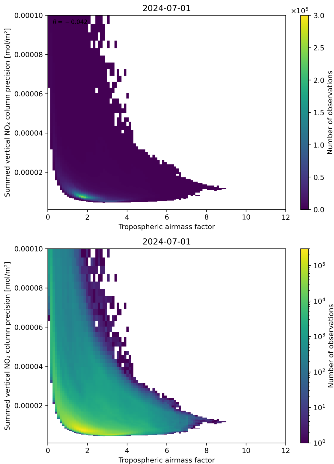
Figure 76: Scatter density plot of “Tropospheric air mass factor” against “Summed vertical NO 2 column precision” for 2024-06-30 to 2024-07-02.
