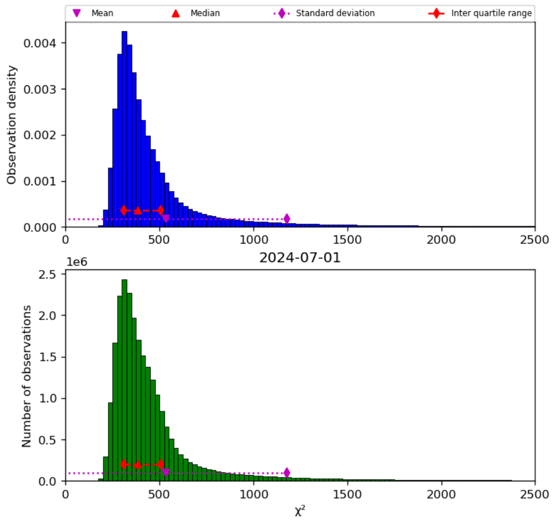
Figure 42: Histogram of “ \chi^2 ” for 2024-06-30 to 2024-07-02
