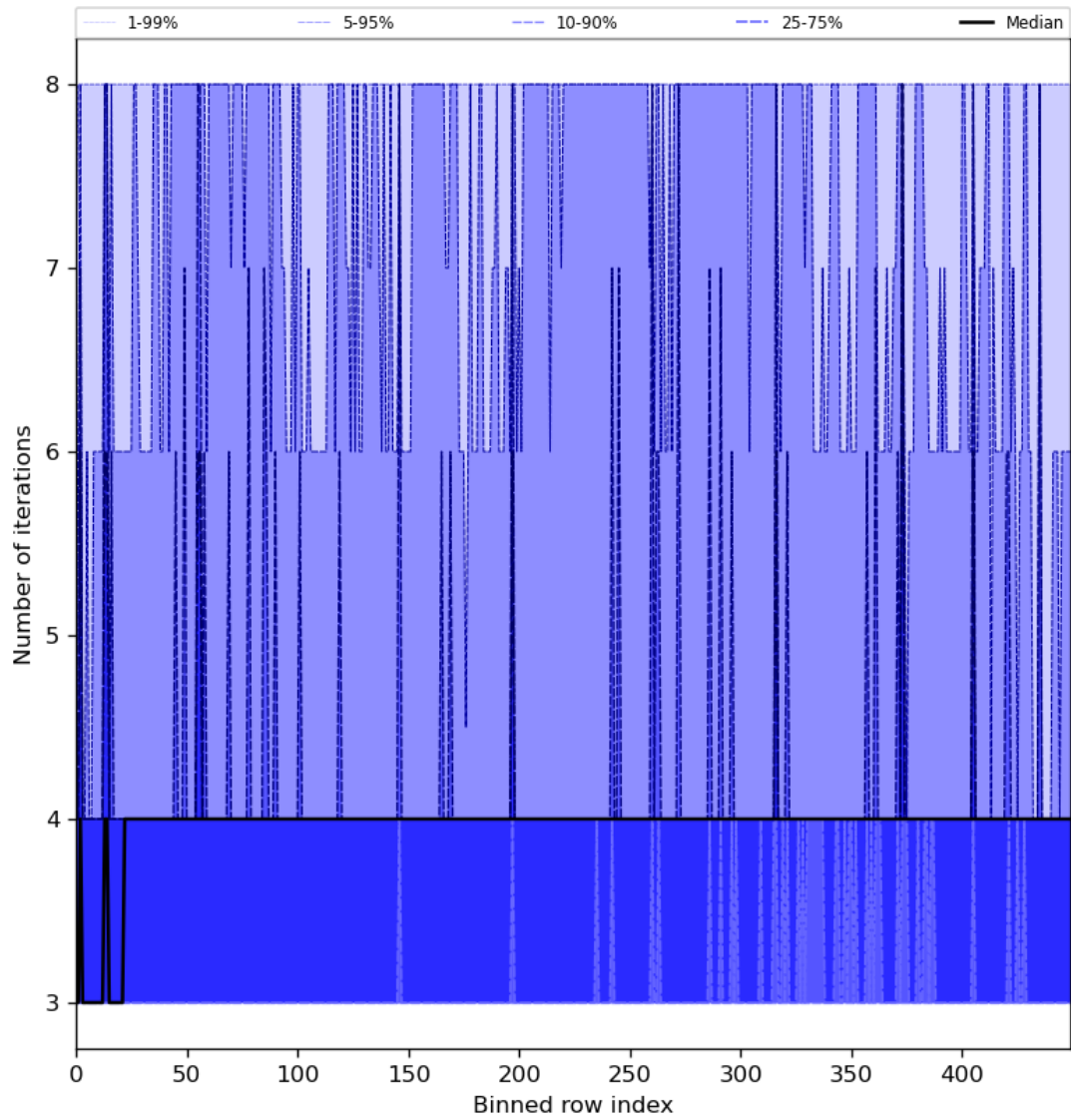
Figure 51: Along track statistics of “Number of iterations” for 2024-06-30 to 2024-07-02
