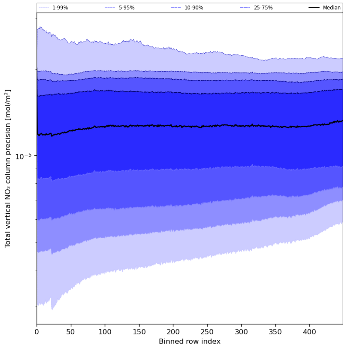
Figure 56: Along track statistics of “Total vertical NO 2 column precision” for 2024-06-30 to 2024-07-02
