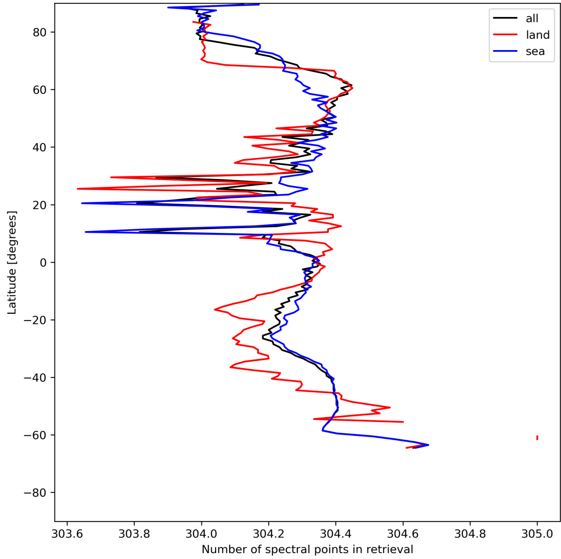
Figure 16: Zonal average of “Number of spectral points in retrieval” for 2024-06-30 to 2024-07-02.
