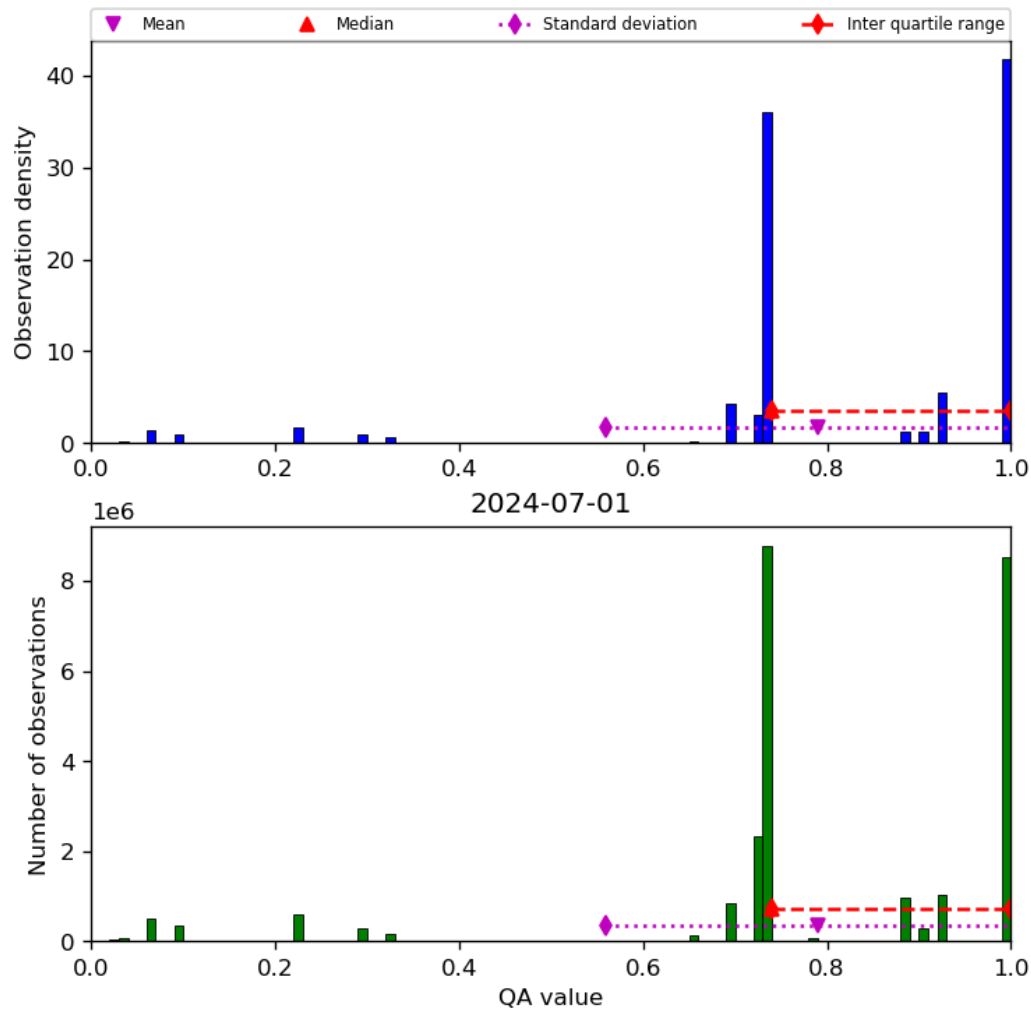
Figure 28: Histogram of “QA value” for 2024-06-30 to 2024-07-02
