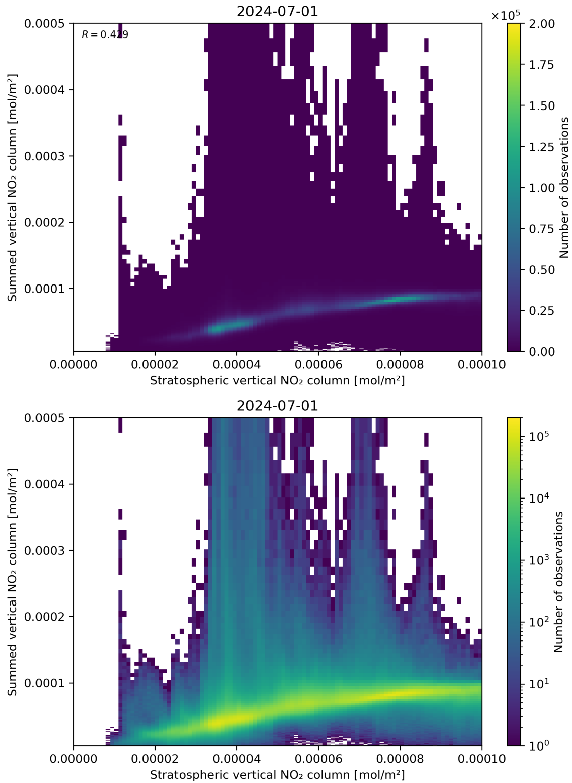
Figure 98: Scatter density plot of “Stratospheric vertical NO 2 column” against “Summed vertical NO 2 column” for 2024-06-30 to 2024-07-02.
