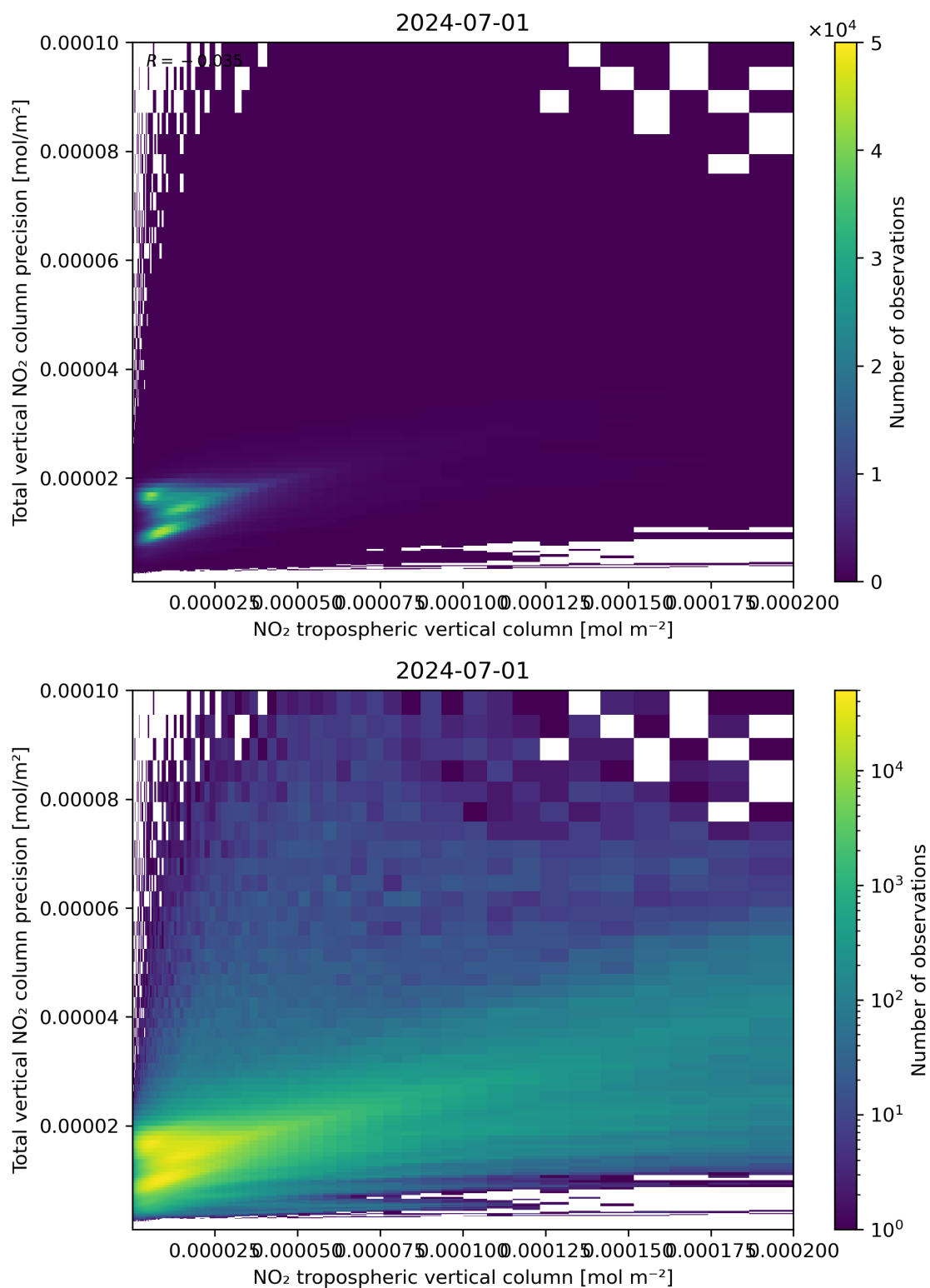
Figure 129: Scatter density plot of “NO 2 tropospheric vertical column” against “Total vertical NO 2 column precision” for 2024-06-30 to 2024-07-02.
