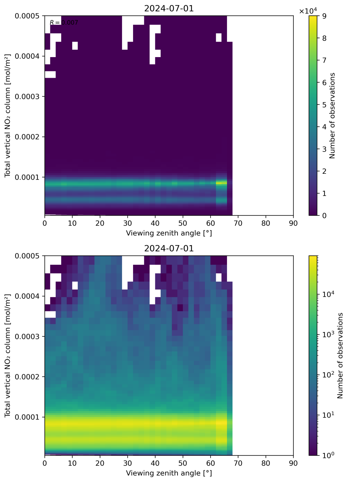
Figure 167: Scatter density plot of “Viewing zenith angle” against “Total vertical NO 2 column” for 2024-06-30 to 2024-07-02.
