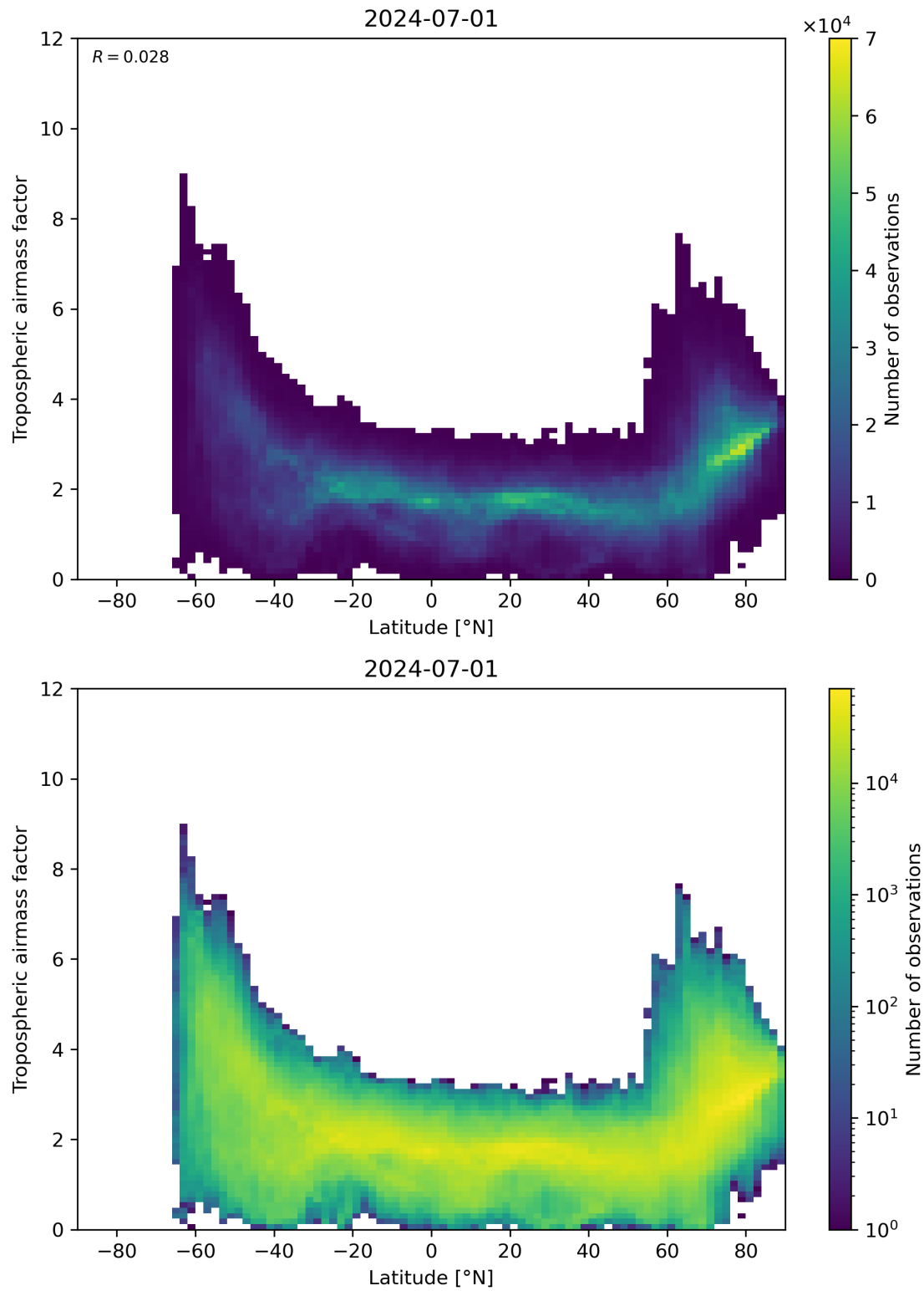
Figure 85: Scatter density plot of “Latitude” against “Tropospheric airmass factor” for 2024-06-30 to 2024-07-02.
