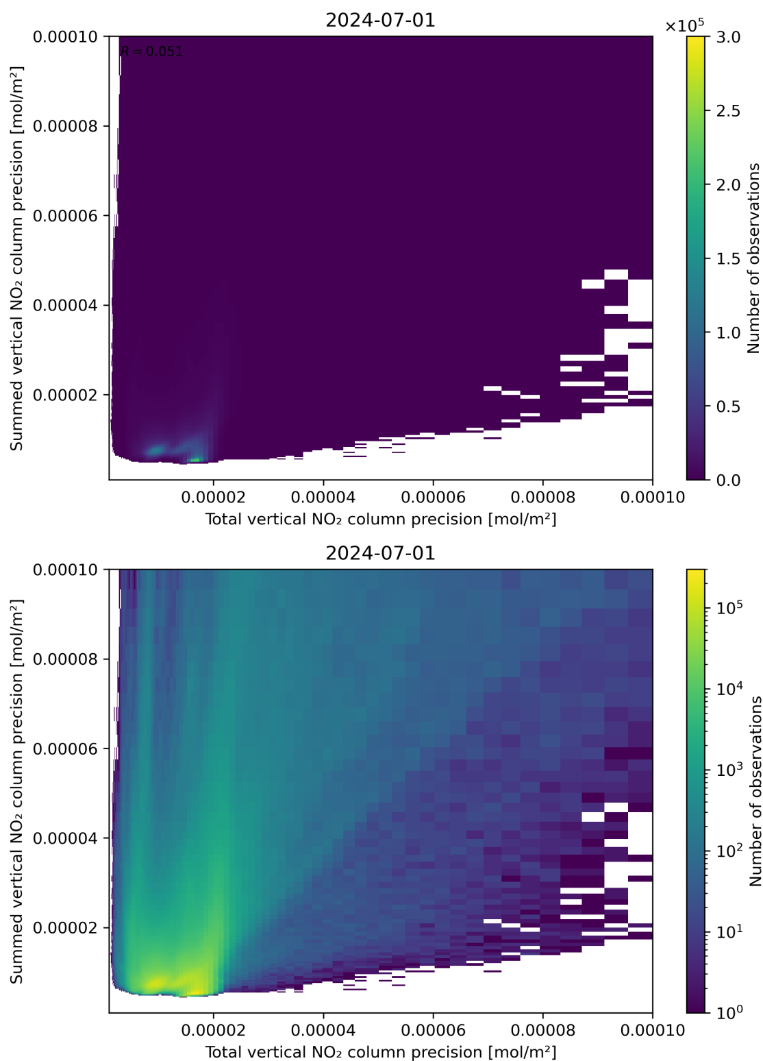
Figure 118: Scatter density plot of “Total vertical NO 2 column precision” against “Summed vertical NO 2 column precision” for 2024-06-30 to 2024-07-02.
