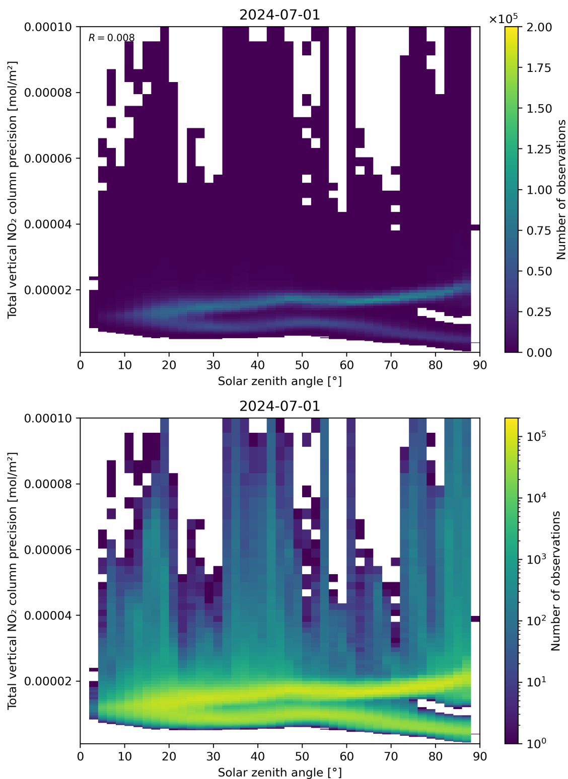
Figure 154: Scatter density plot of “Solar zenith angle” against “Total vertical NO 2 column precision” for 2024-06-30 to 2024-07-02.
