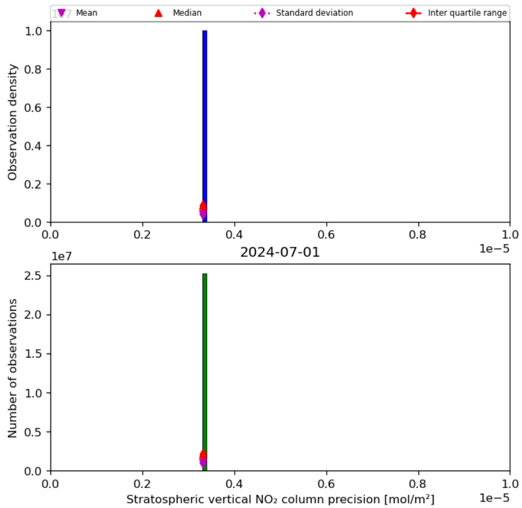
Figure 37: Histogram of “Stratospheric vertical NO 2 column precision” for 2024-06-30 to 2024-07-02
