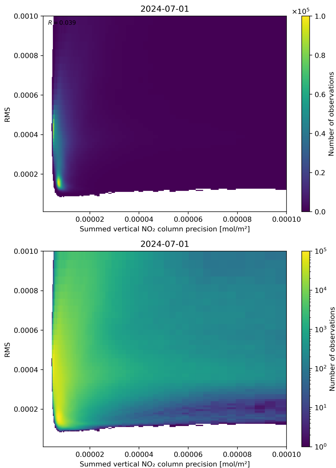
Figure 108: Scatter density plot of “Summed vertical NO 2 column precision” against “RMS” for 2024-06-30 to 2024-07-02.
