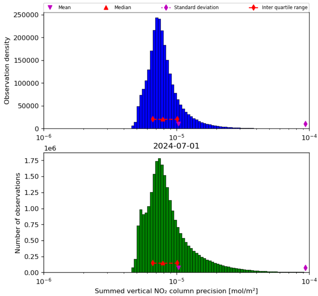
Figure 41: Histogram of "Summed vertical NO 2 column precision" for 2024-06-30 to 2024-07-02
