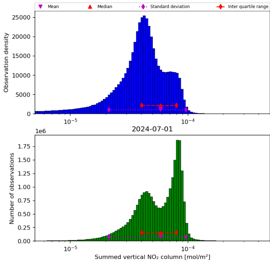
Figure 40: Histogram of "Summed vertical NO 2 column" for 2024-06-30 to 2024-07-02
