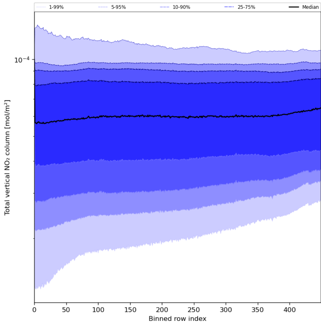
Figure 55: Along track statistics of “Total vertical NO 2 column” for 2024-06-30 to 2024-07-02
