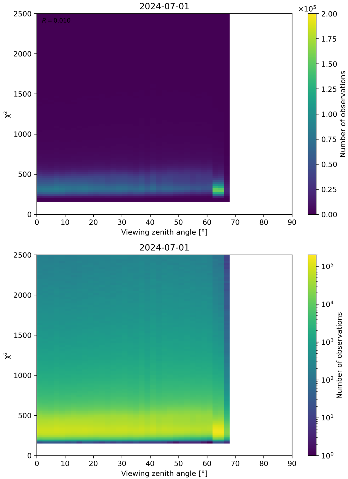
Figure 162: Scatter density plot of “Viewing zenith angle” against “ \chi^2 ” for 2024-06-30 to 2024-07-02.
