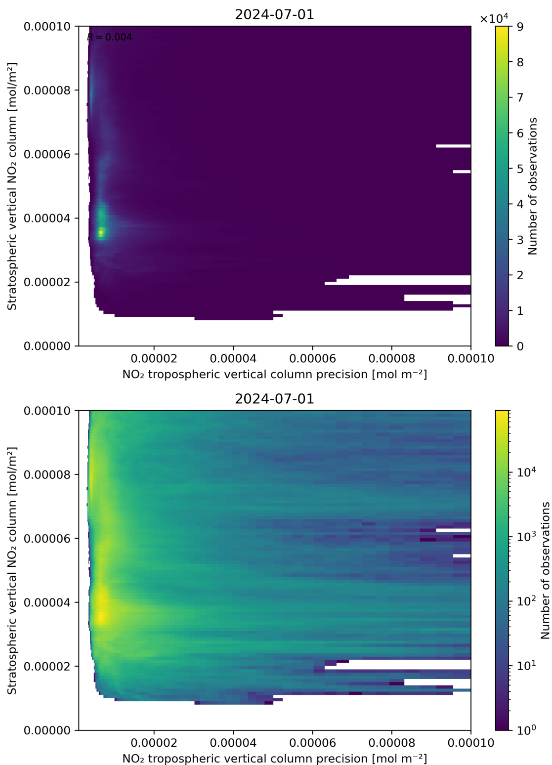
Figure 135: Scatter density plot of “NO 2 tropospheric vertical column precision” against “Stratospheric vertical NO 2 column” for 2024-06-30 to 2024-07-02.
