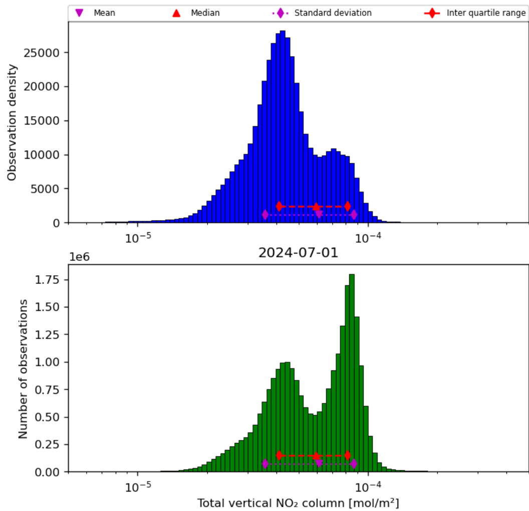
Figure 38: Histogram of “Total vertical NO 2 column” for 2024-06-30 to 2024-07-02
