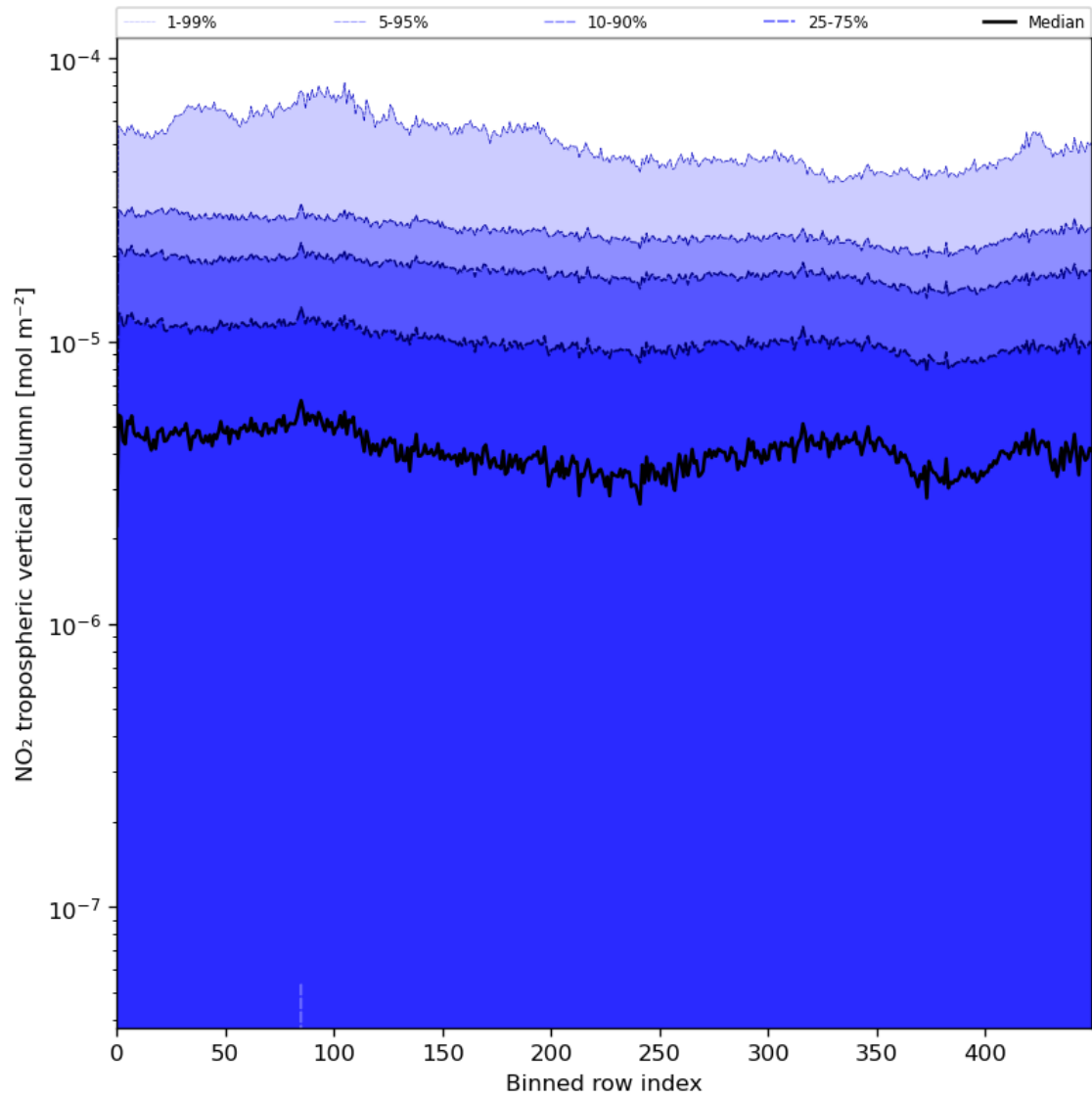
Figure 46: Along track statistics of “NO 2 tropospheric vertical column” for 2024-06-30 to 2024-07-02
