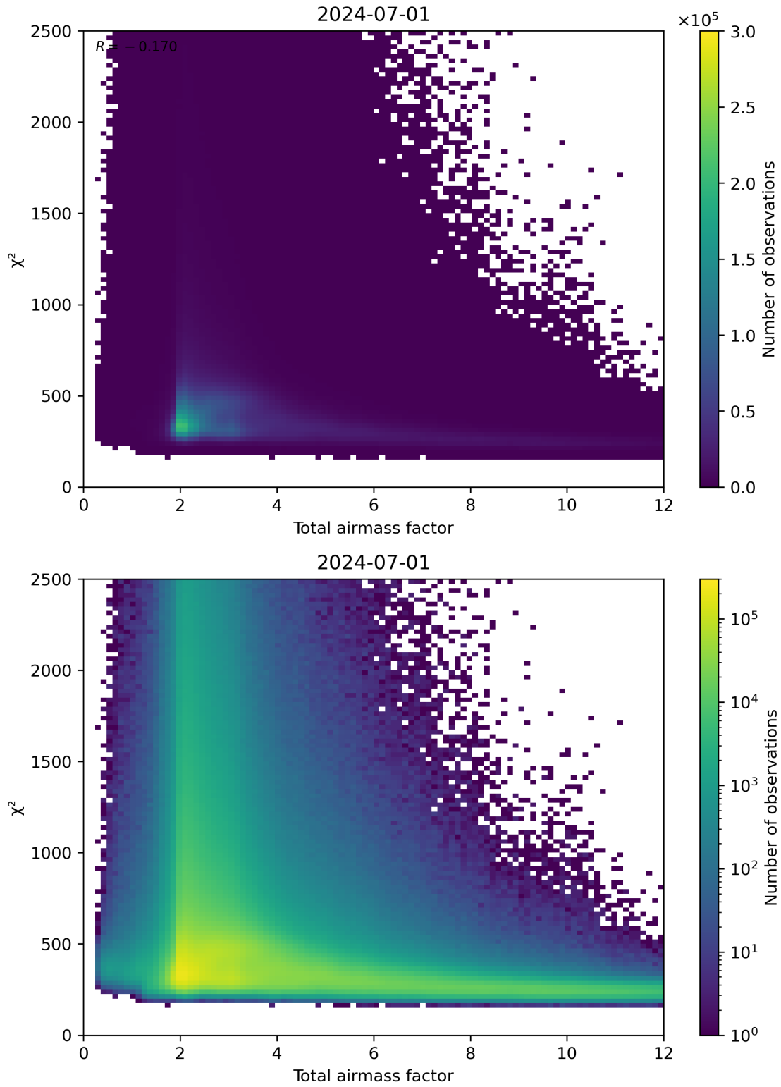
Figure 63: Scatter density plot of “Total airmass factor” against “ \chi^2 ” for 2024-06-30 to 2024-07-02.
