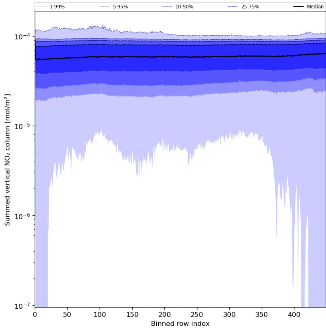
Figure 57: Along track statistics of “Summed vertical NO 2 column” for 2024-06-30 to 2024-07-02
