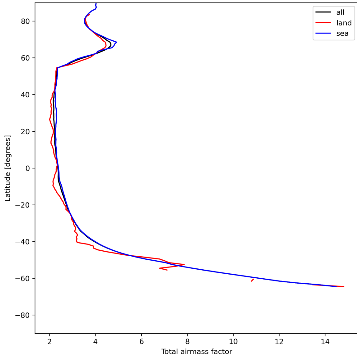
Figure 15: Zonal average of “Total airmass factor” for 2024-06-30 to 2024-07-02.
