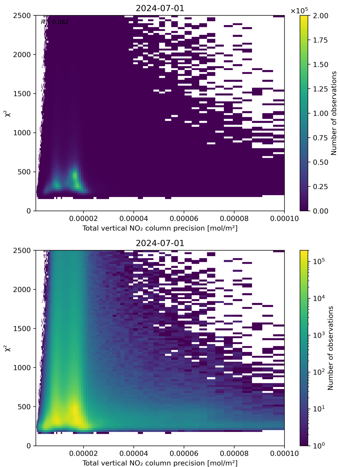
Figure 116: Scatter density plot of “Total vertical NO 2 column precision” against “ \chi^2 ” for 2024-06-30 to 2024-07-02.
