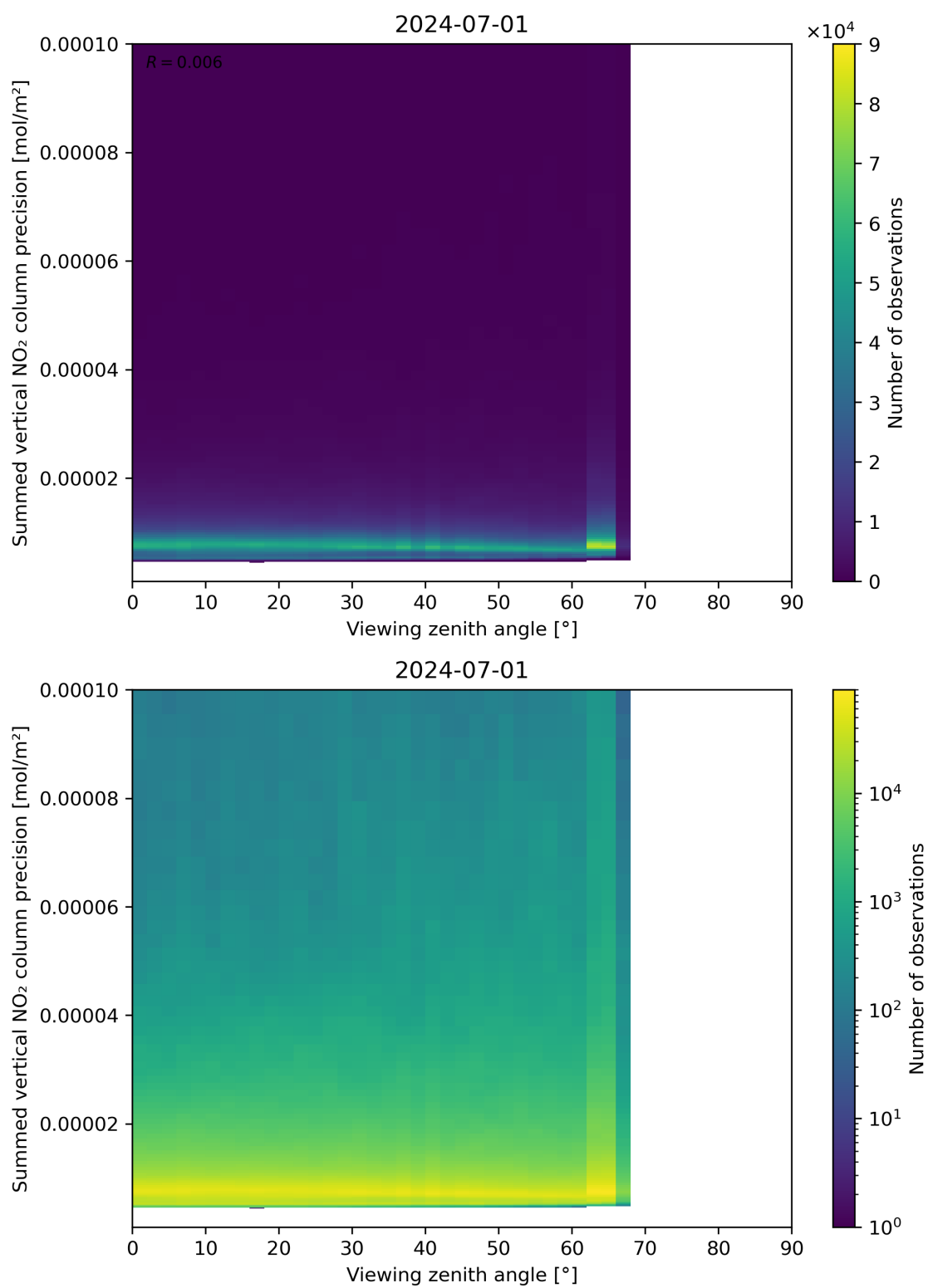
Figure 166: Scatter density plot of “Viewing zenith angle” against “Summed vertical NO 2 column precision” for 2024-06-30 to 2024-07-02.
