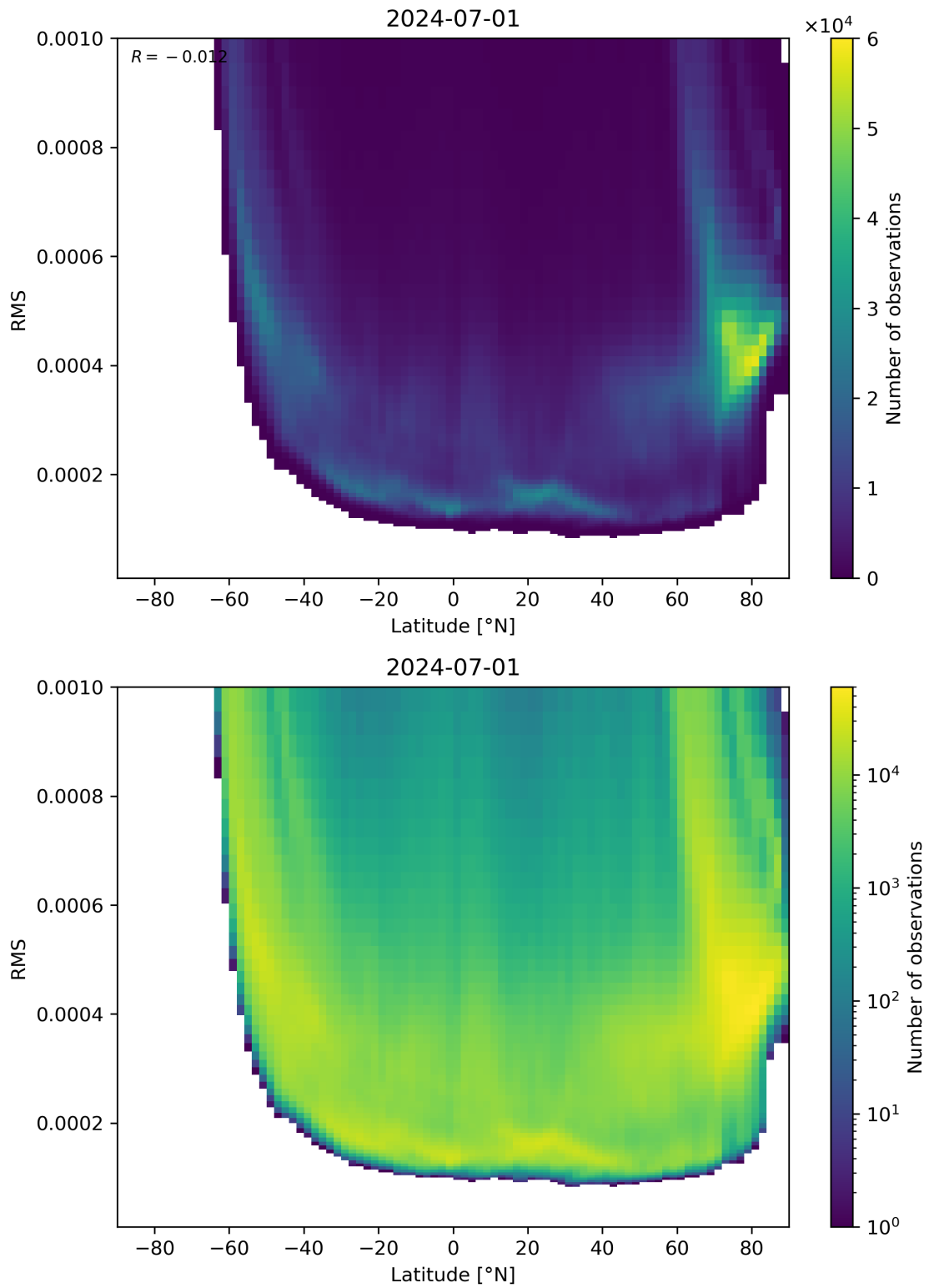
Figure 94: Scatter density plot of “Latitude” against “RMS” for 2024-06-30 to 2024-07-02.
