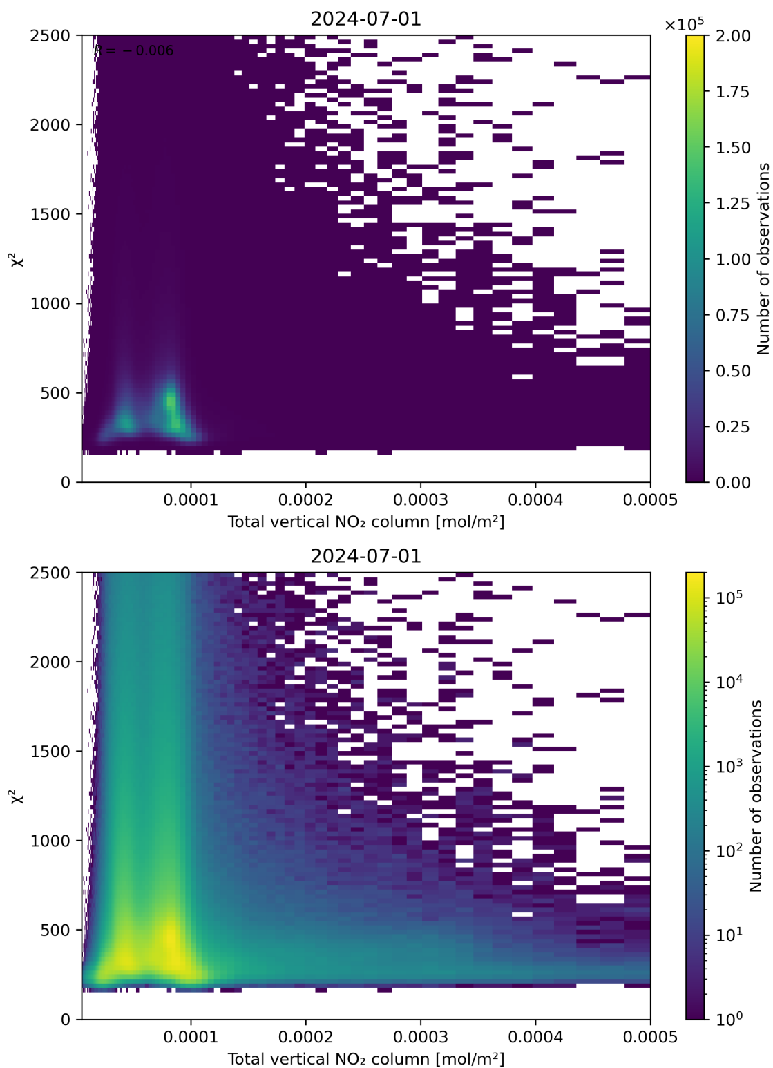
Figure 111: Scatter density plot of “Total vertical NO 2 column” against “ \chi^2 ” for 2024-06-30 to 2024-07-02.
