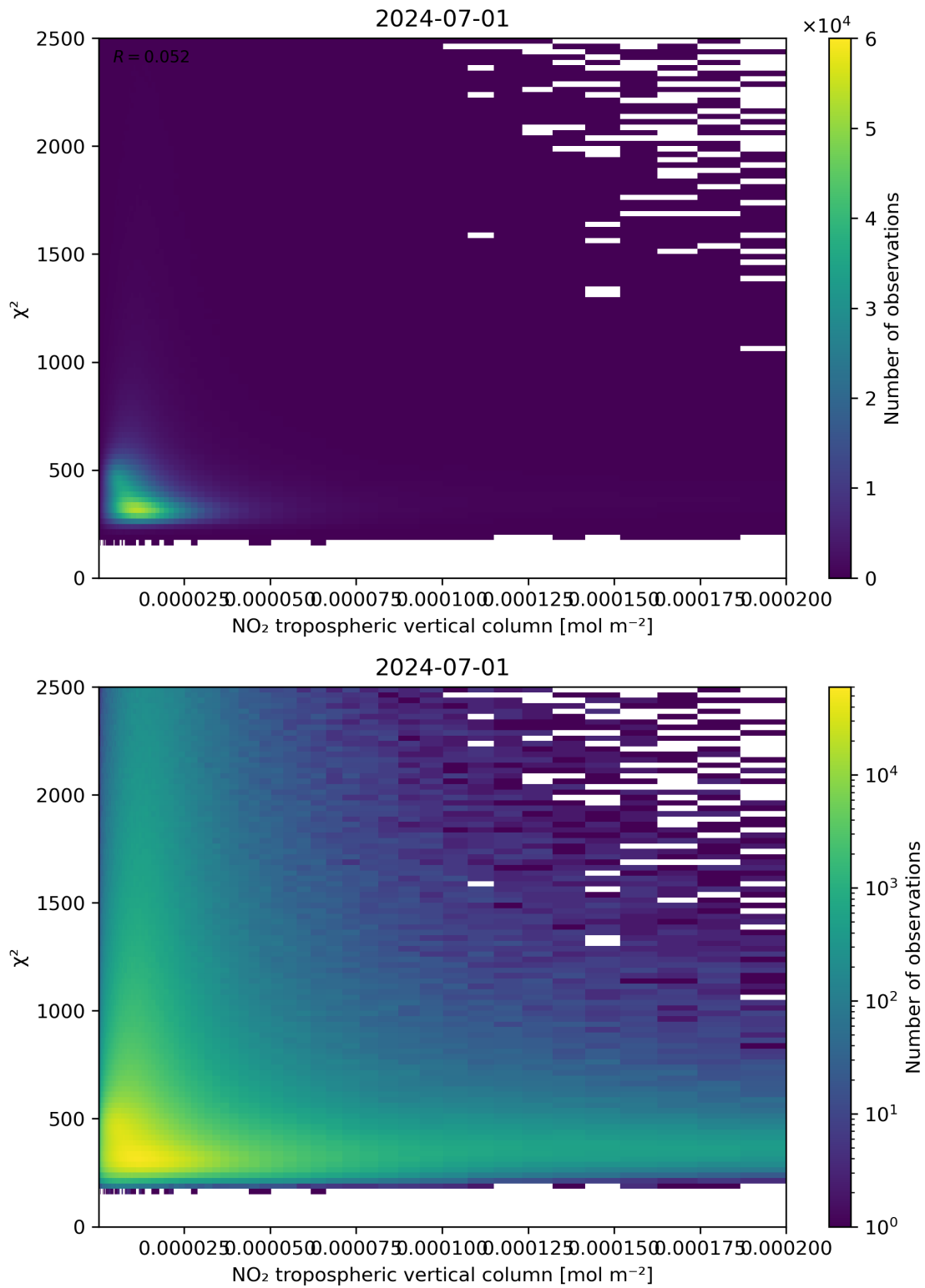
Figure 124: Scatter density plot of “NO 2 tropospheric vertical column” against “ \chi^2 ” for 2024-06-30 to 2024-07-02.
