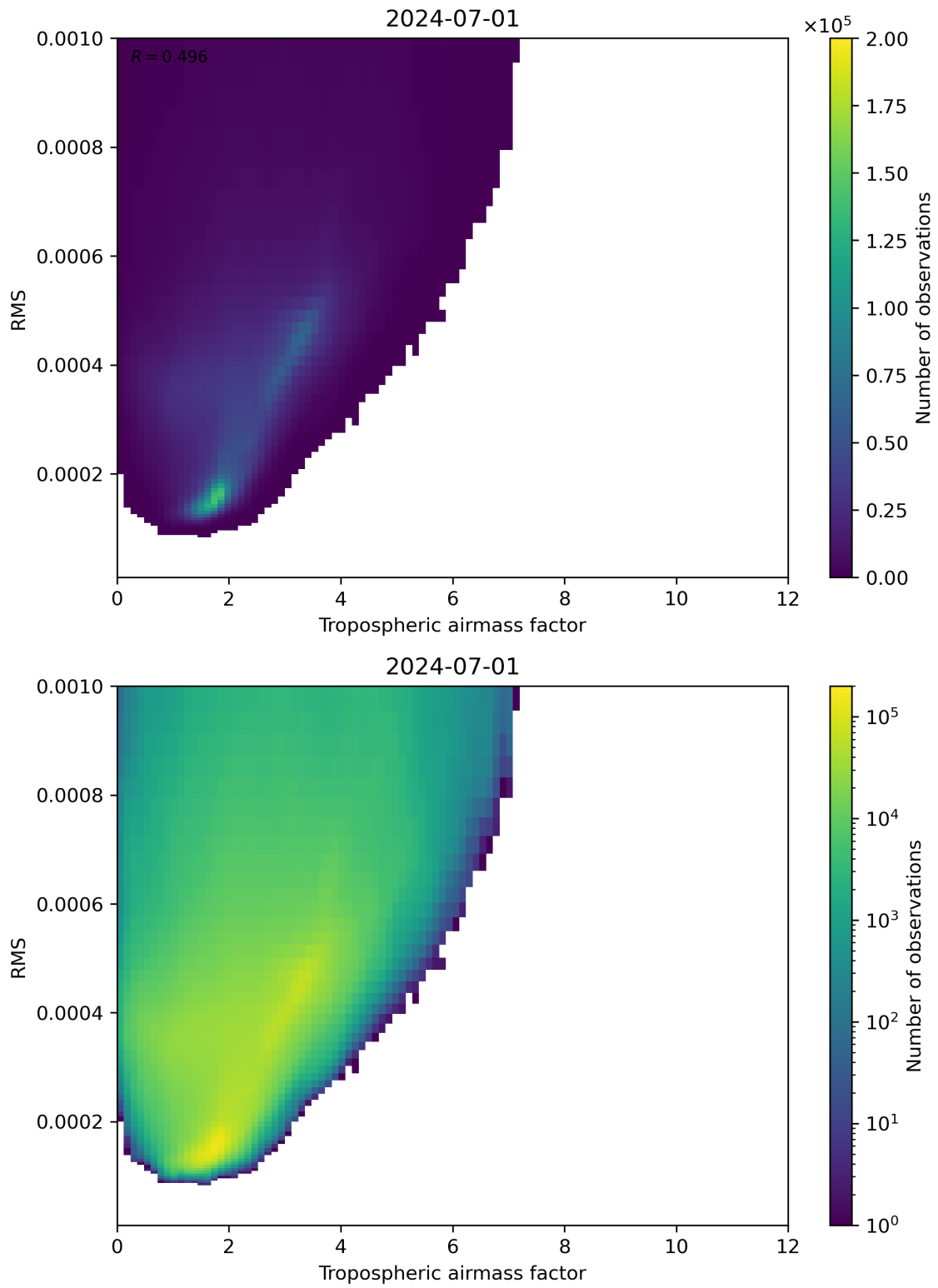
Figure 79: Scatter density plot of “Tropospheric airmass factor” against “RMS” for 2024-06-30 to 2024-07-02.
