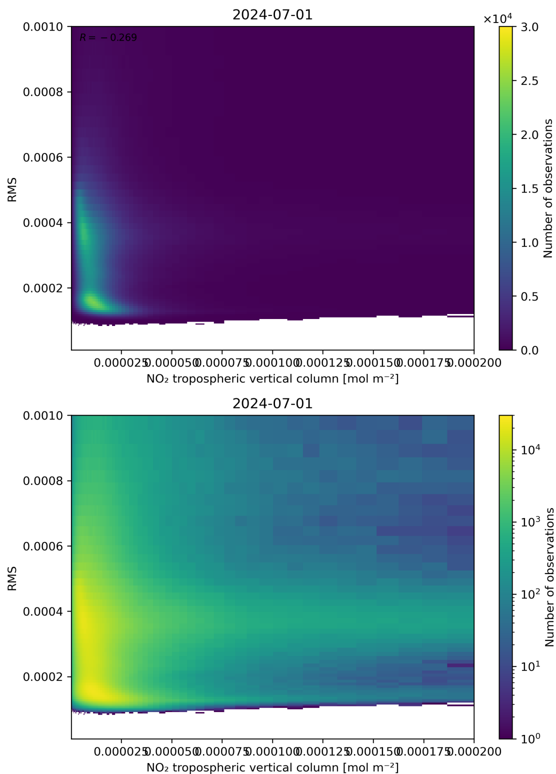
Figure 142: Scatter density plot of “NO 2 tropospheric vertical column” against “RMS” for 2024-06-30 to 2024-07-02.
