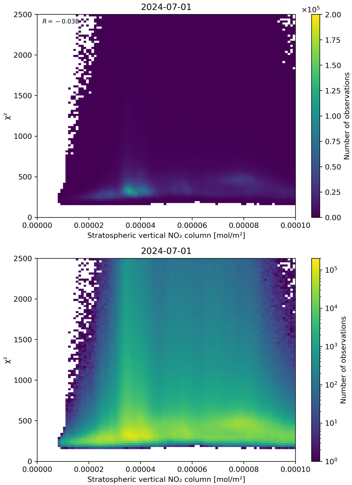
Figure 97: Scatter density plot of “Stratospheric vertical NO 2 column” against “ \chi^2 ” for 2024-06-30 to 2024-07-02.
