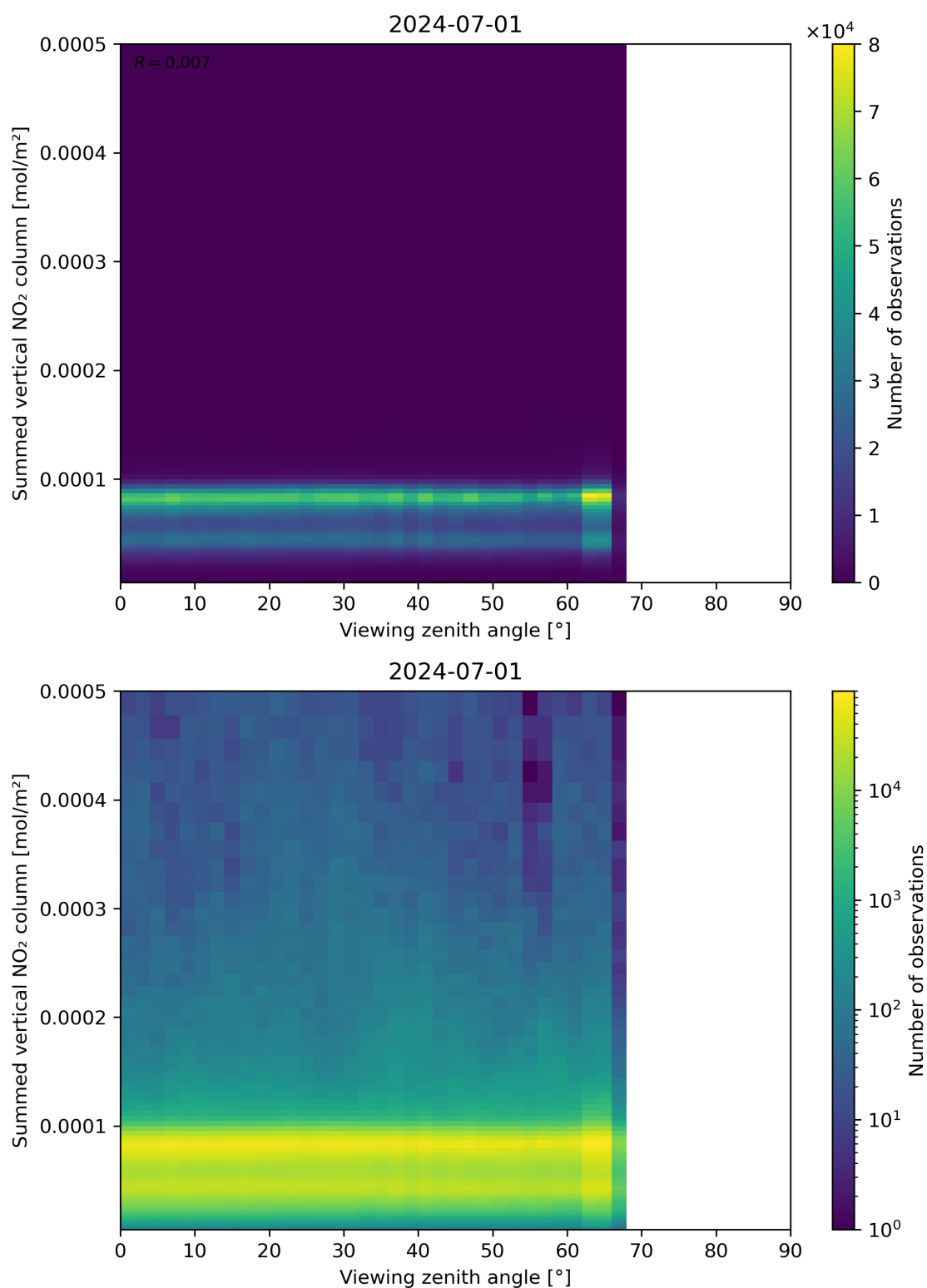
Figure 165: Scatter density plot of “Viewing zenith angle” against “Summed vertical NO 2 column” for 2024-06-30 to 2024-07-02.
