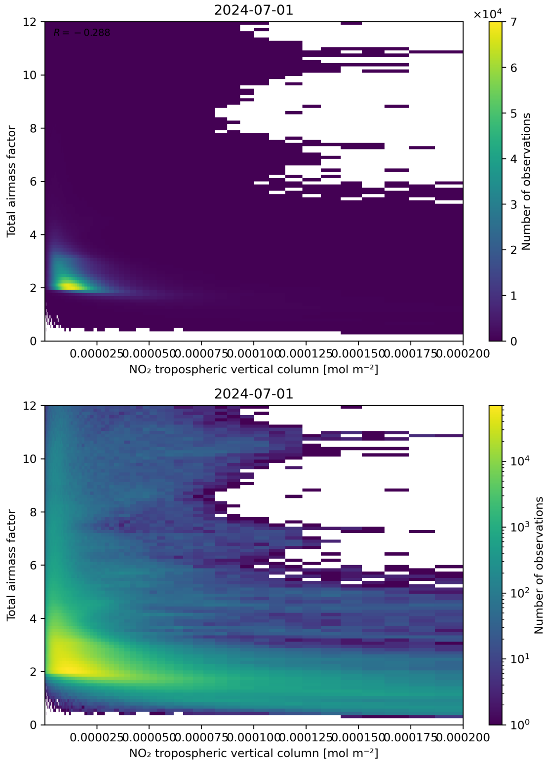
Figure 122: Scatter density plot of “NO 2 tropospheric vertical column” against “Total air mass factor” for 2024-06-30 to 2024-07-02.
