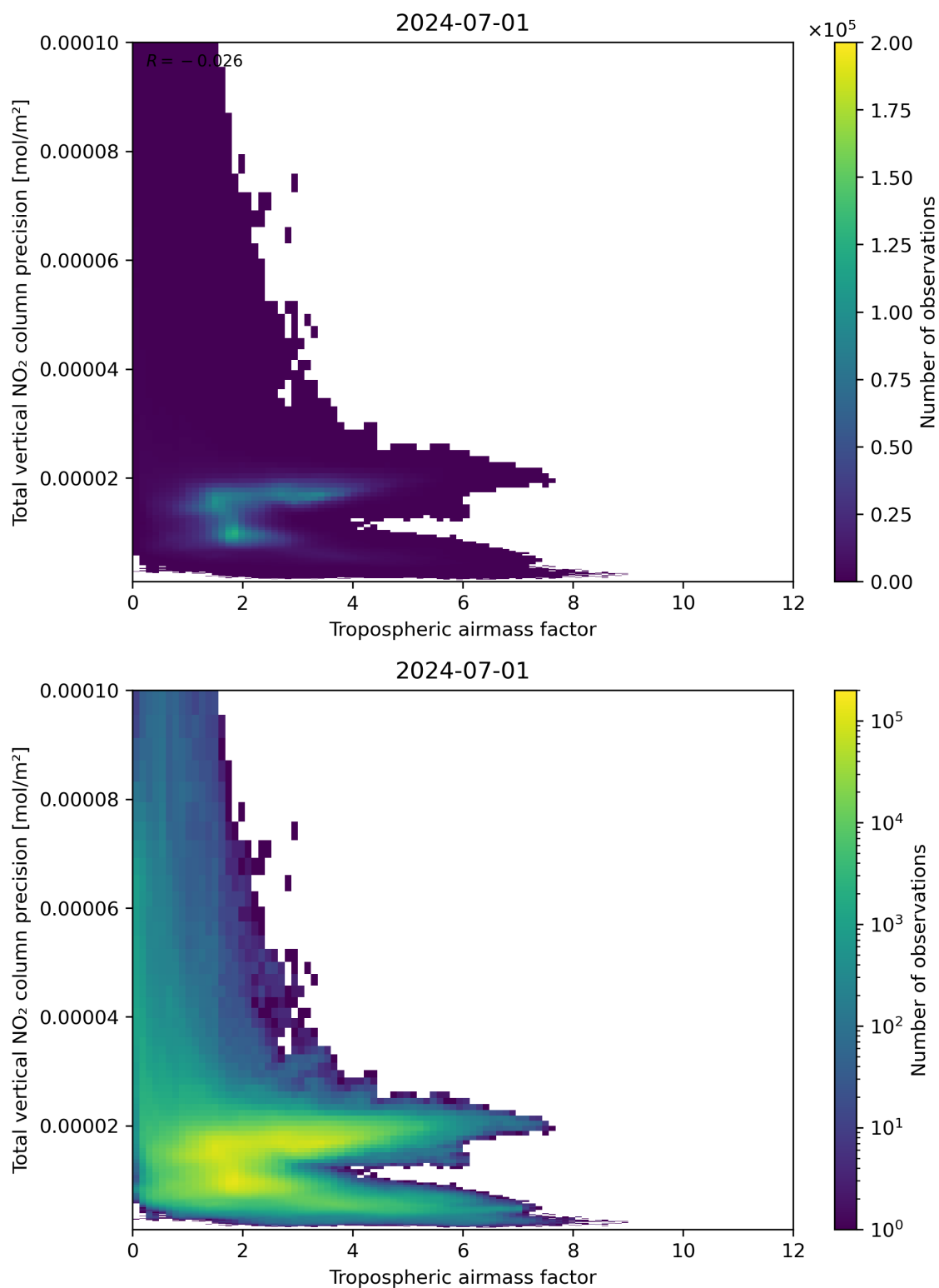
Figure 78: Scatter density plot of “Tropospheric air mass factor” against “Total vertical NO 2 column precision” for 2024-06-30 to 2024-07-02.
