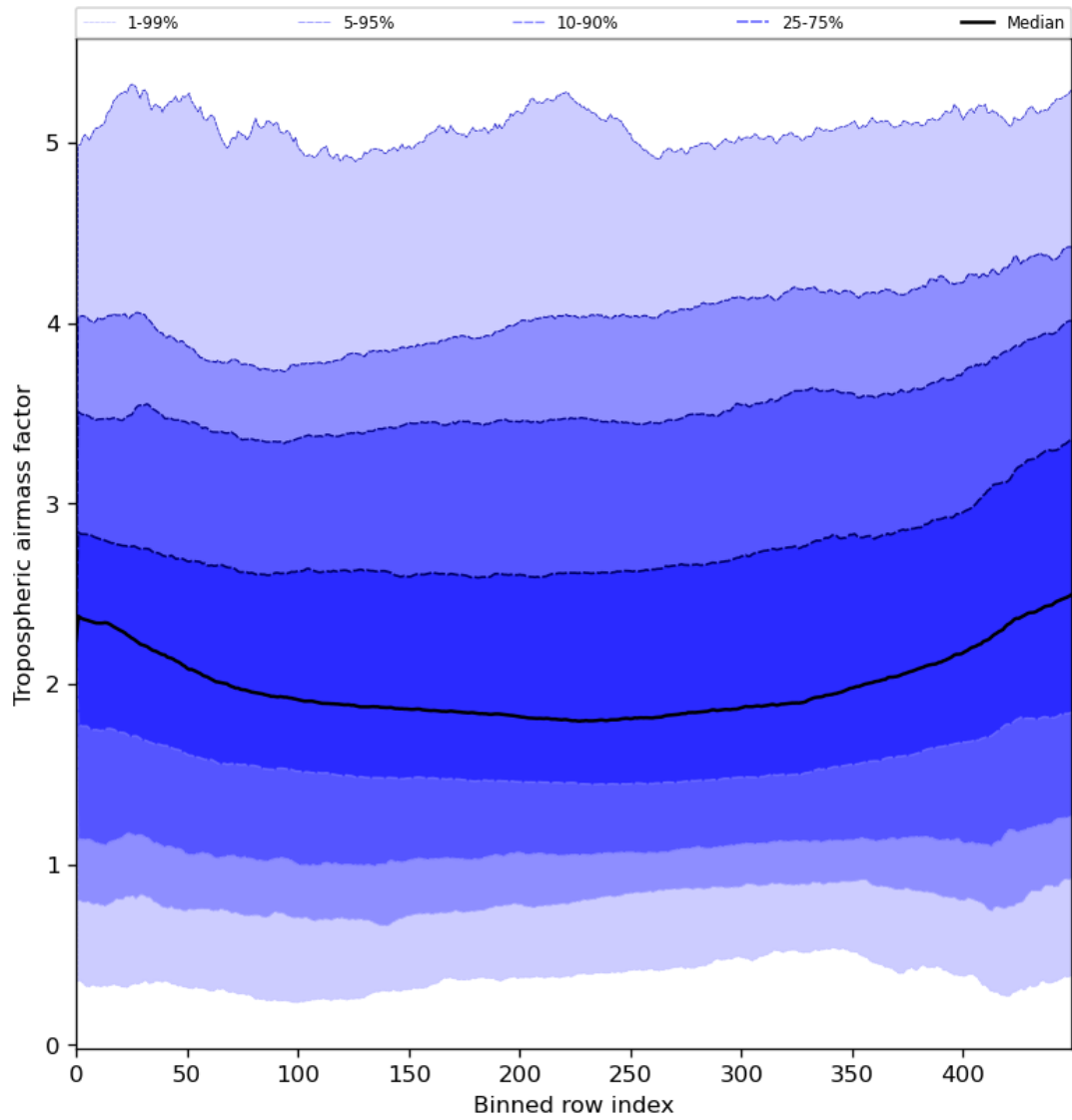
Figure 48: Along track statistics of “Tropospheric airmass factor” for 2024-06-30 to 2024-07-02
