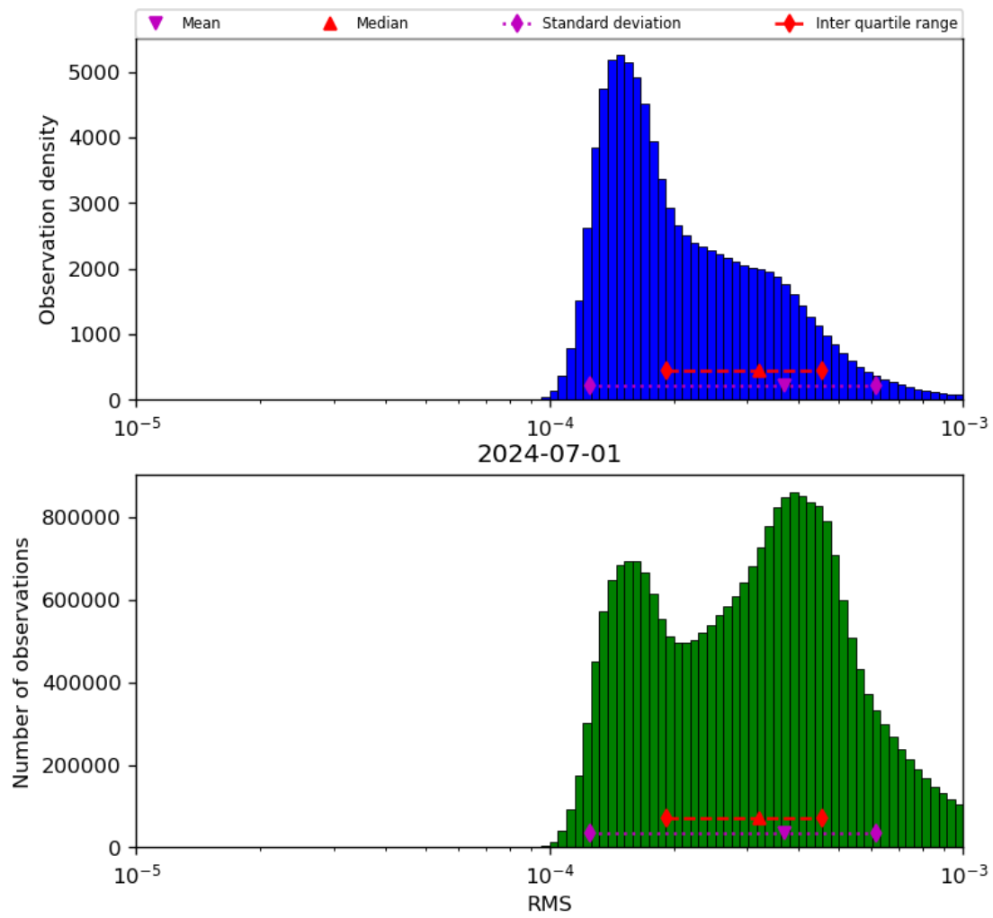
Figure 43: Histogram of “RMS” for 2024-06-30 to 2024-07-02
