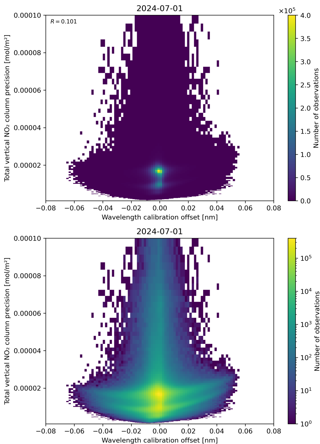
Figure 180: Scatter density plot of “Wavelength calibration offset” against “Total vertical NO 2 column precision” for 2024-06-30 to 2024-07-02.
