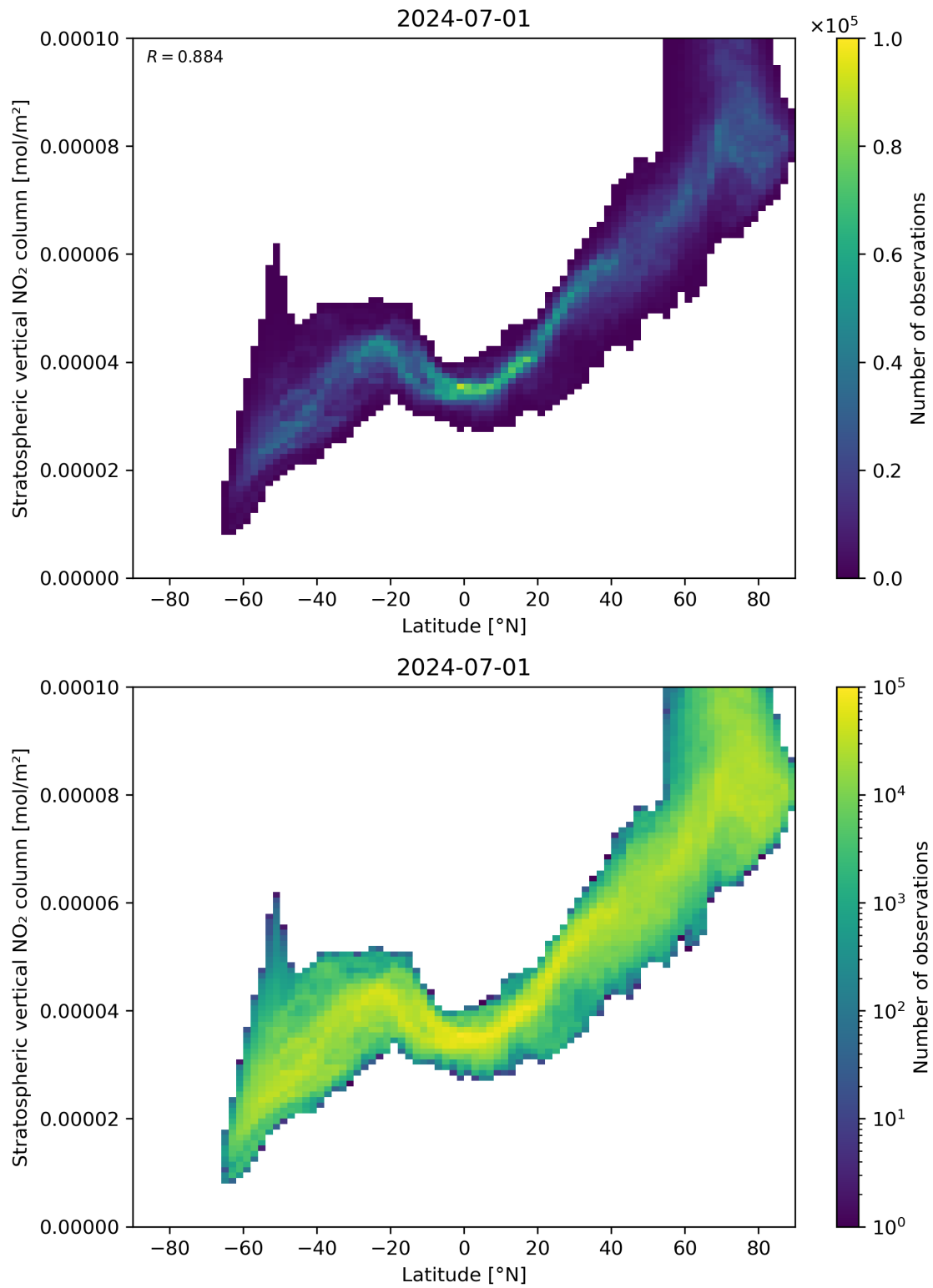
Figure 87: Scatter density plot of “Latitude” against “Stratospheric vertical NO 2 column” for 2024-06-30 to 2024-07-02.
