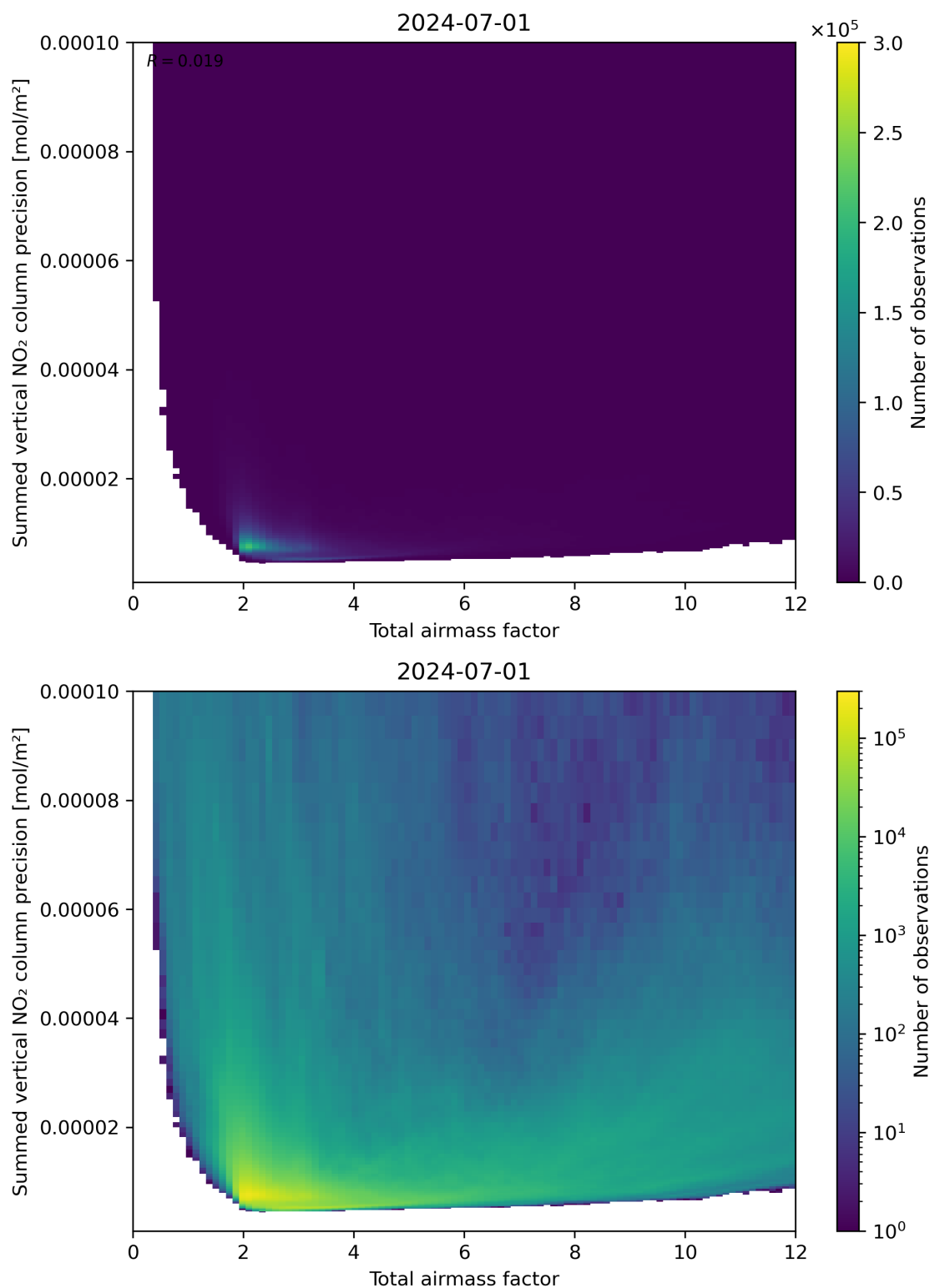
Figure 66: Scatter density plot of “Total airmass factor” against “Summed vertical NO 2 column precision” for 2024-06-30 to 2024-07-02.
