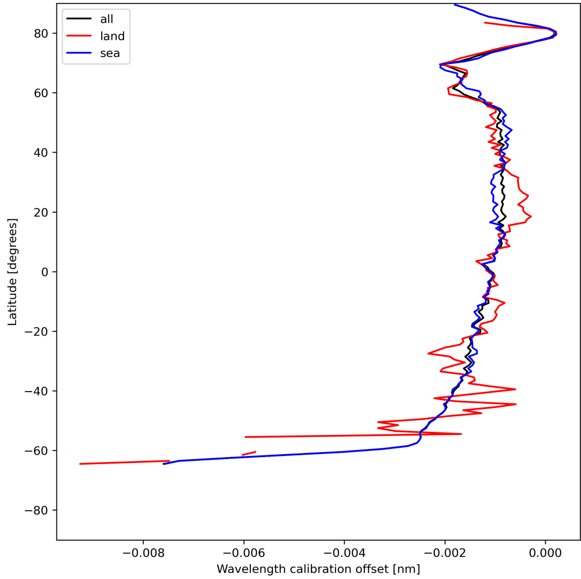
Figure 18: Zonal average of “Wavelength calibration offset” for 2024-06-30 to 2024-07-02.
