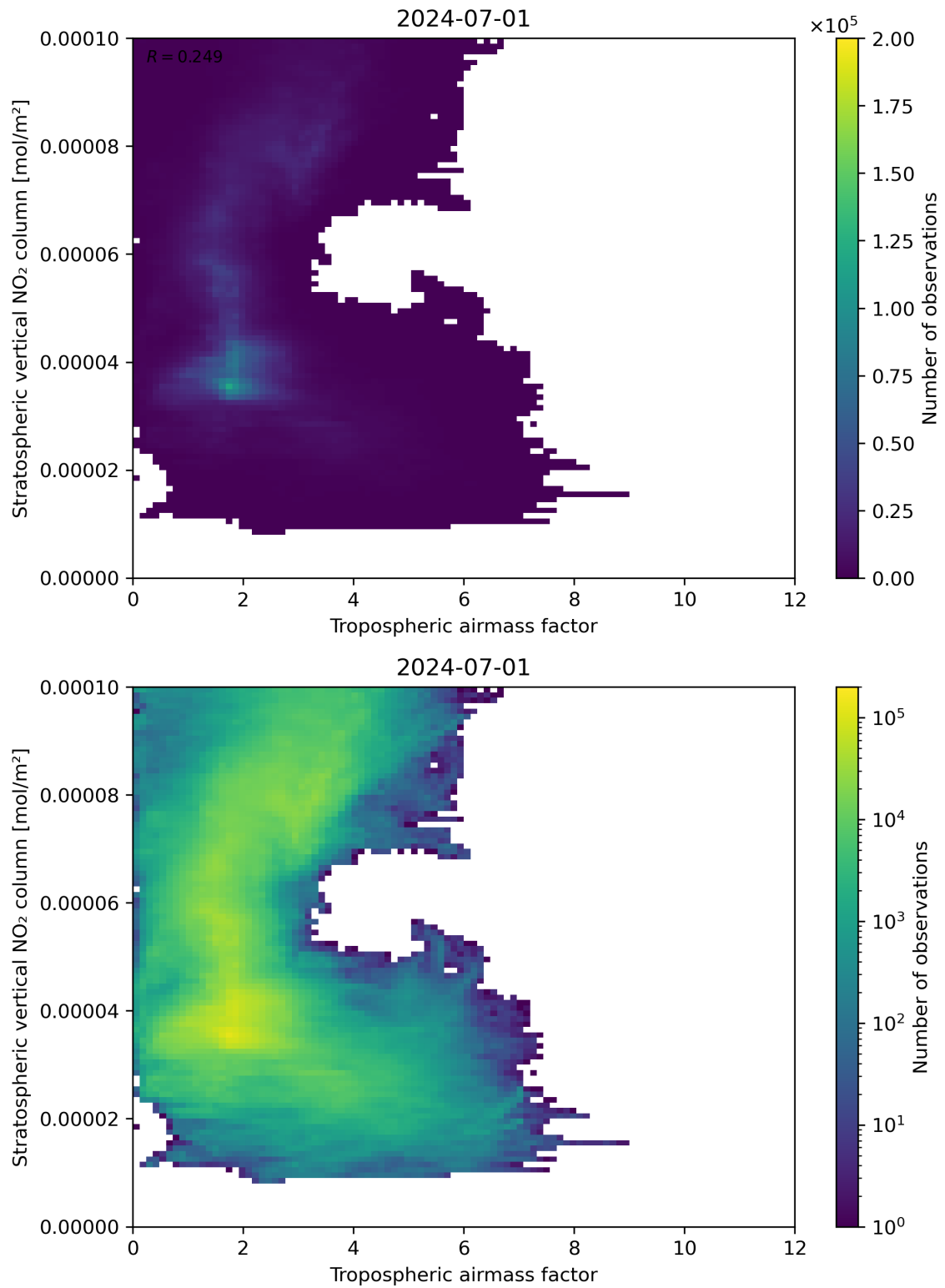
Figure 74: Scatter density plot of “Tropospheric air mass factor” against “Stratospheric vertical NO 2 column” for 2024-06-30 to 2024-07-02.
