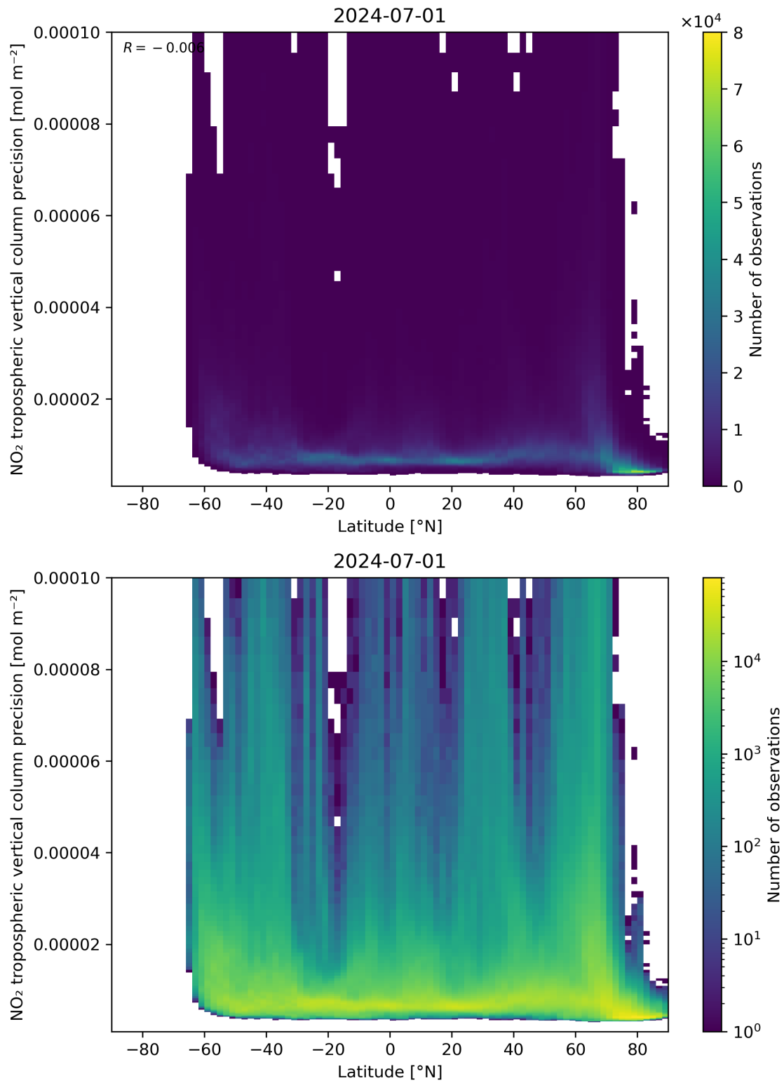
Figure 93: Scatter density plot of “Latitude” against “NO 2 tropospheric vertical column precision” for 2024-06-30 to 2024-07-02.
