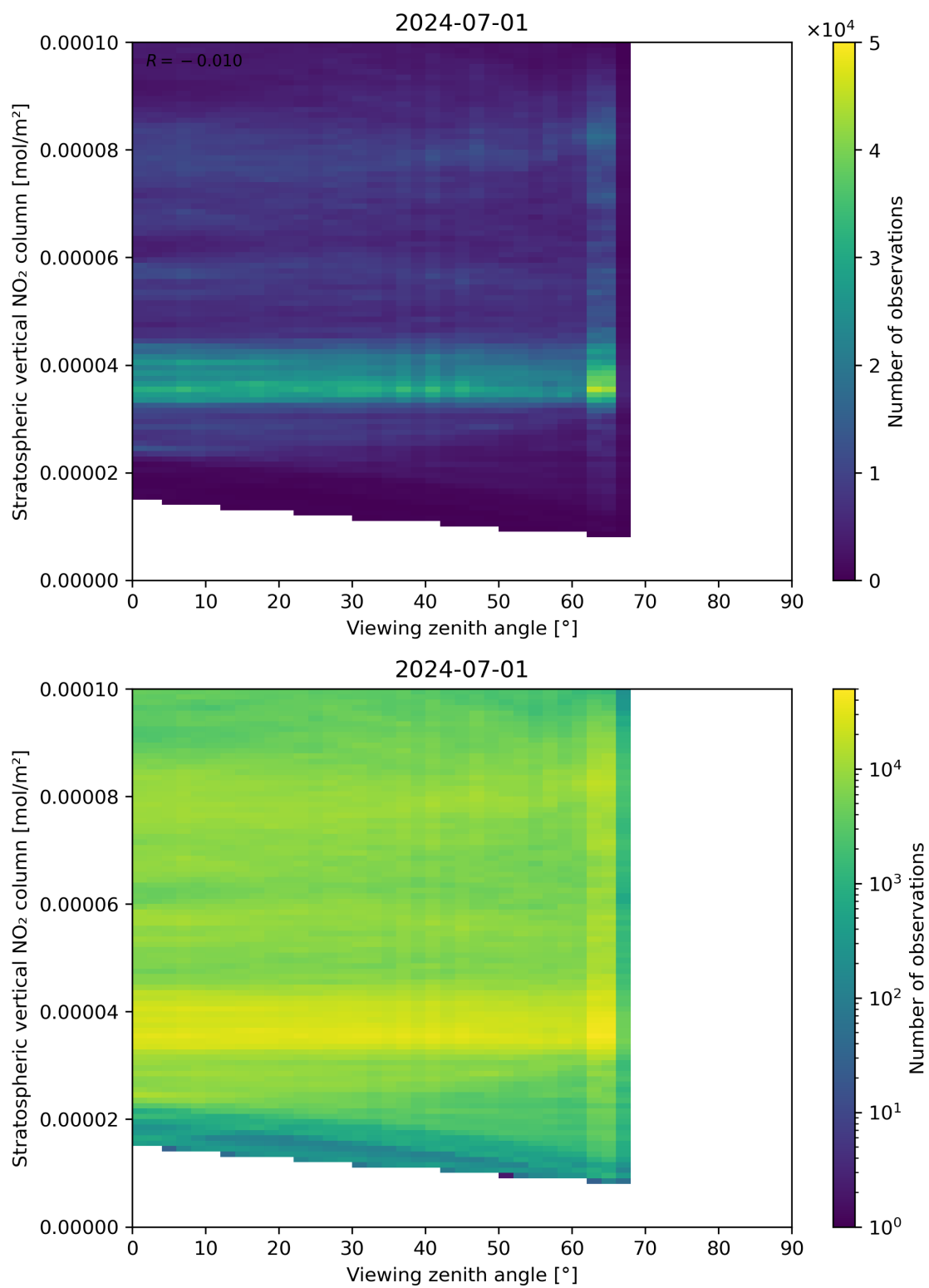
Figure 164: Scatter density plot of “Viewing zenith angle” against “Stratospheric vertical NO 2 column” for 2024-06-30 to 2024-07-02.
