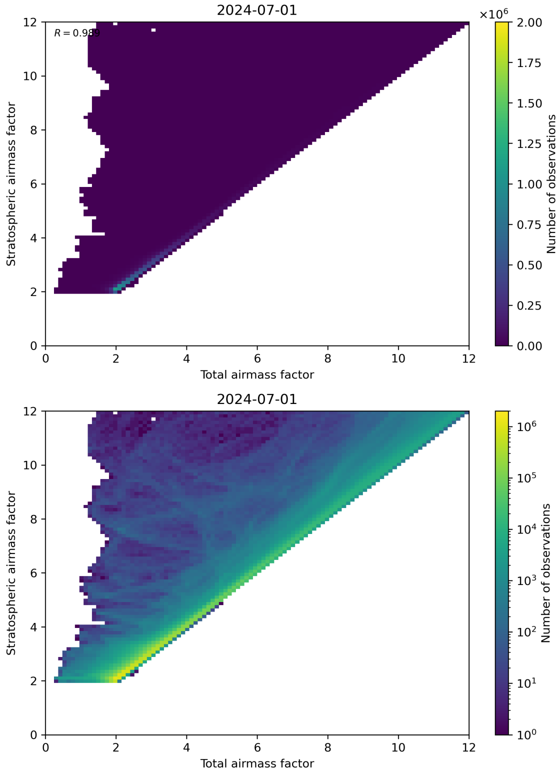
Figure 62: Scatter density plot of “Total air mass factor” against “Stratospheric air mass factor” for 2024-06-30 to 2024-07-02.
