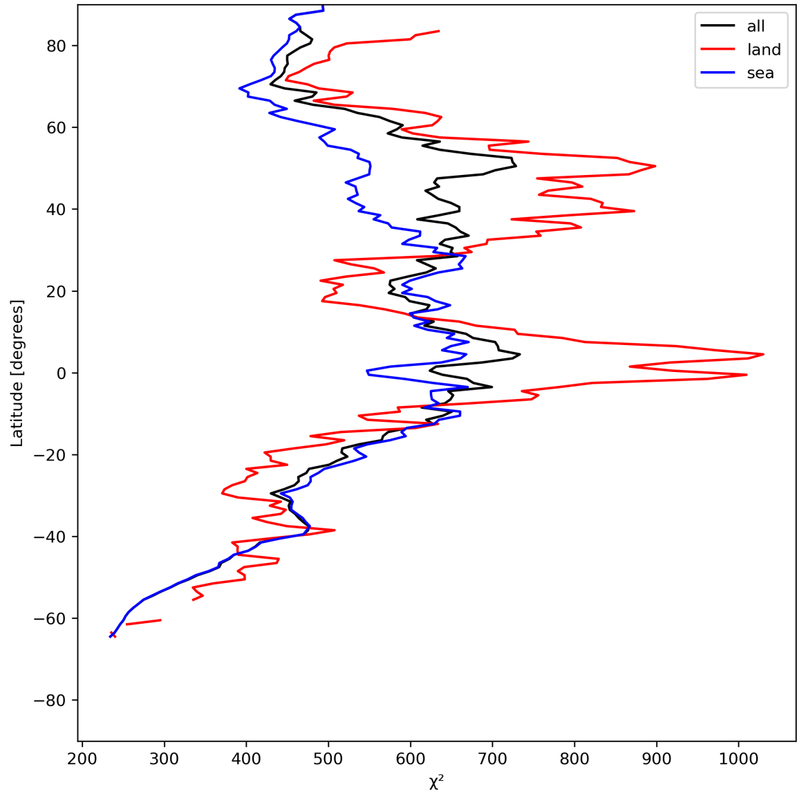
Figure 25: Zonal average of “ \chi^2 ” for 2024-06-30 to 2024-07-02.
