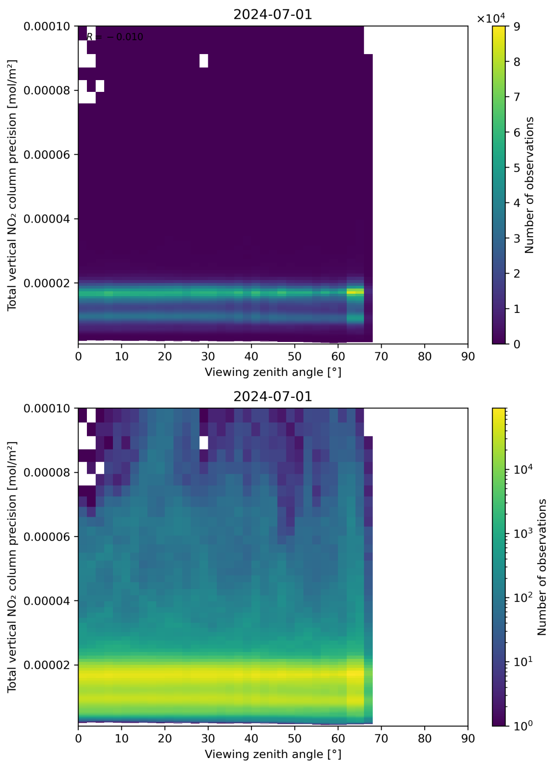
Figure 168: Scatter density plot of “Viewing zenith angle” against “Total vertical NO 2 column precision” for 2024-06-30 to 2024-07-02.
