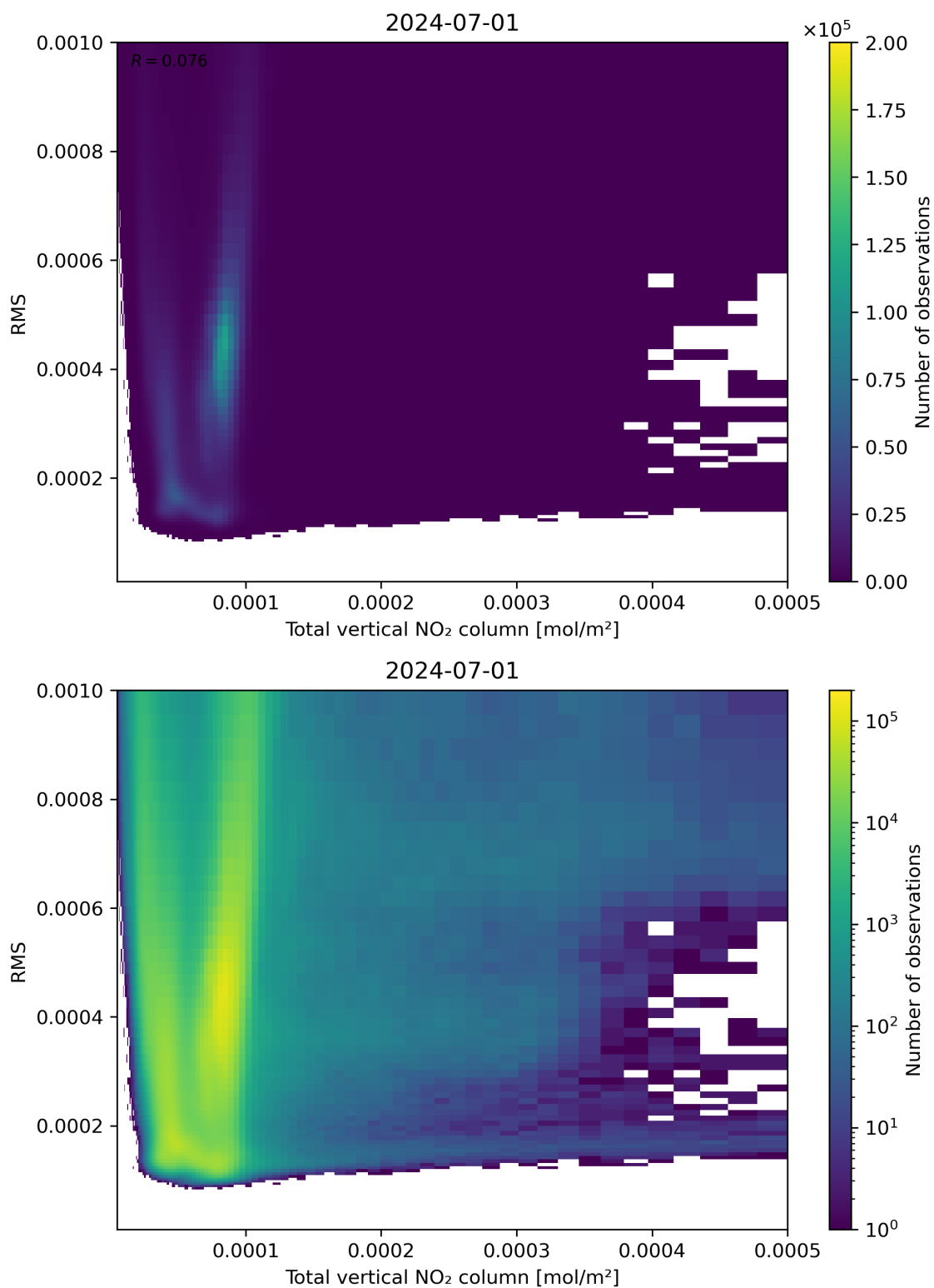
Figure 120: Scatter density plot of “Total vertical NO 2 column” against “RMS” for 2024-06-30 to 2024-07-02.
