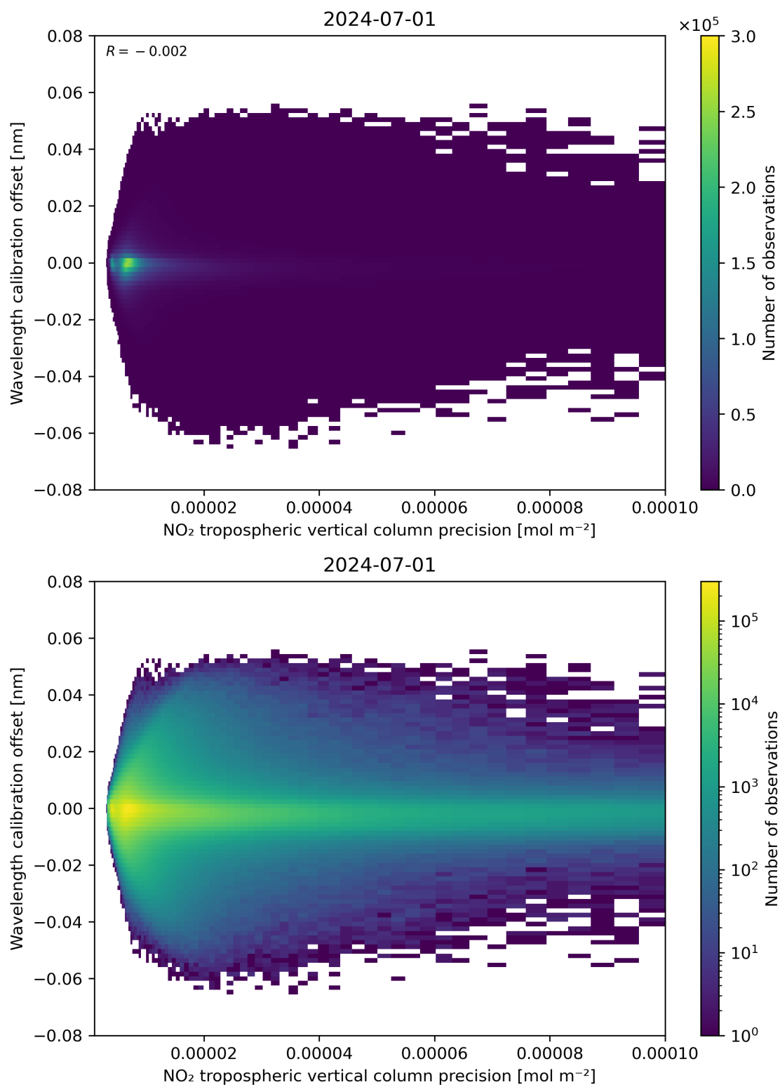
Figure 141: Scatter density plot of “NO 2 tropospheric vertical column precision” against “Wavelength calibration offset” for 2024-06-30 to 2024-07-02.
