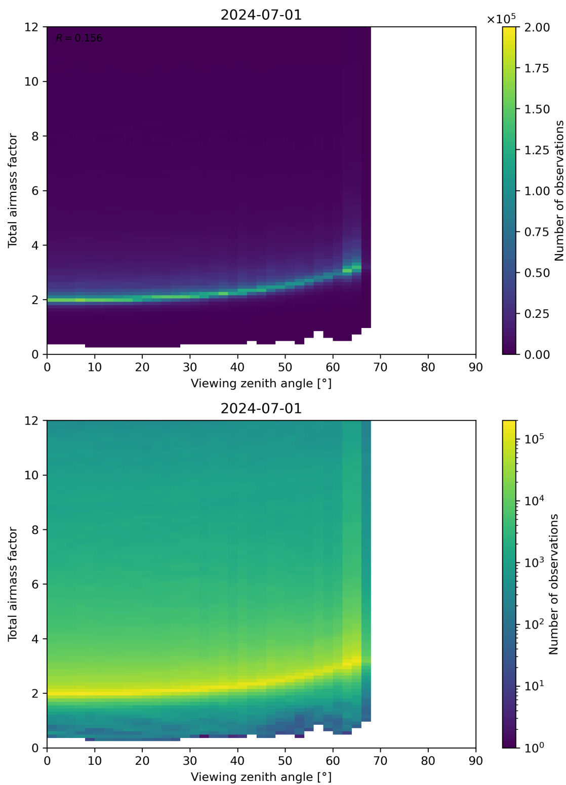
Figure 160: Scatter density plot of “Viewing zenith angle” against “Total airmass factor” for 2024-06-30 to 2024-07-02.
