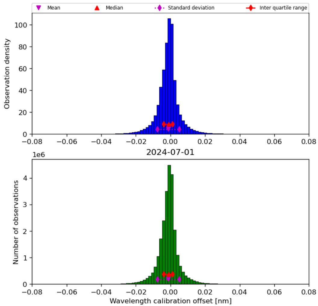
Figure 35: Histogram of “Wavelength calibration offset” for 2024-06-30 to 2024-07-02
