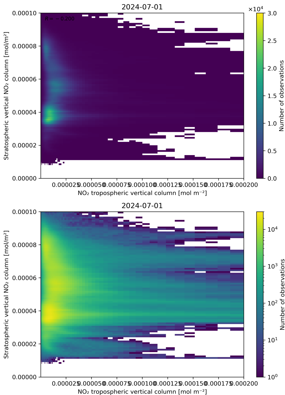
Figure 125: Scatter density plot of “NO 2 tropospheric vertical column” against “Stratospheric vertical NO 2 column” for 2024-06-30 to 2024-07-02.
