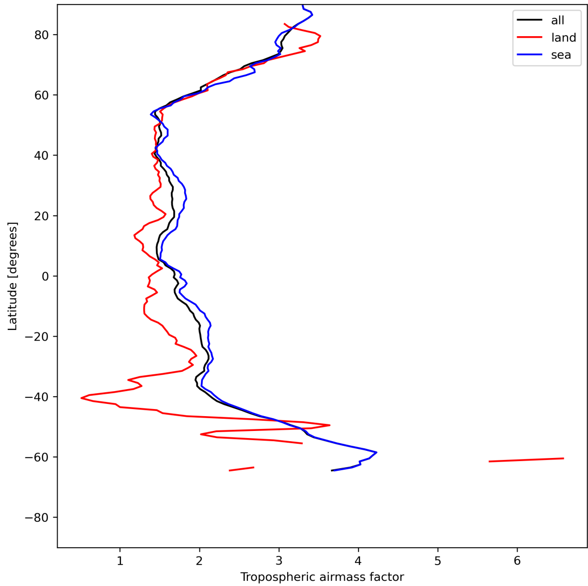
Figure 14: Zonal average of “Tropospheric airmass factor” for 2024-06-30 to 2024-07-02.
