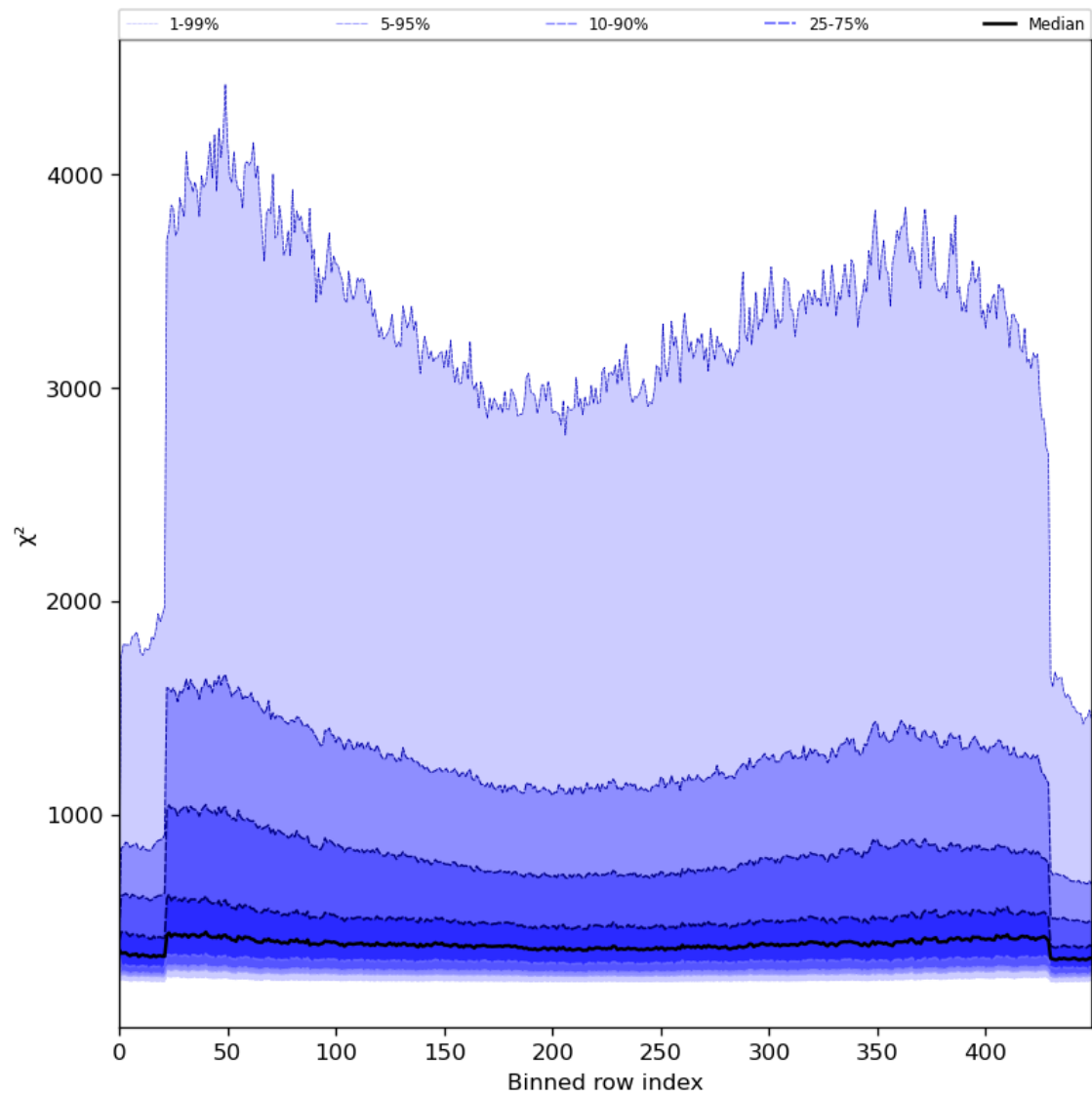
Figure 59: Along track statistics of “ \chi^2 ” for 2024-06-30 to 2024-07-02
