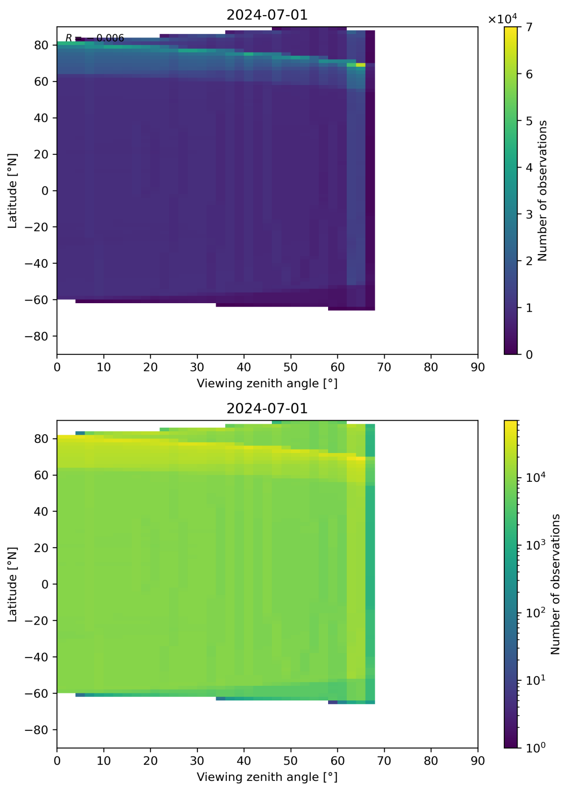
Figure 163: Scatter density plot of “Viewing zenith angle” against “Latitude” for 2024-06-30 to 2024-07-02.
