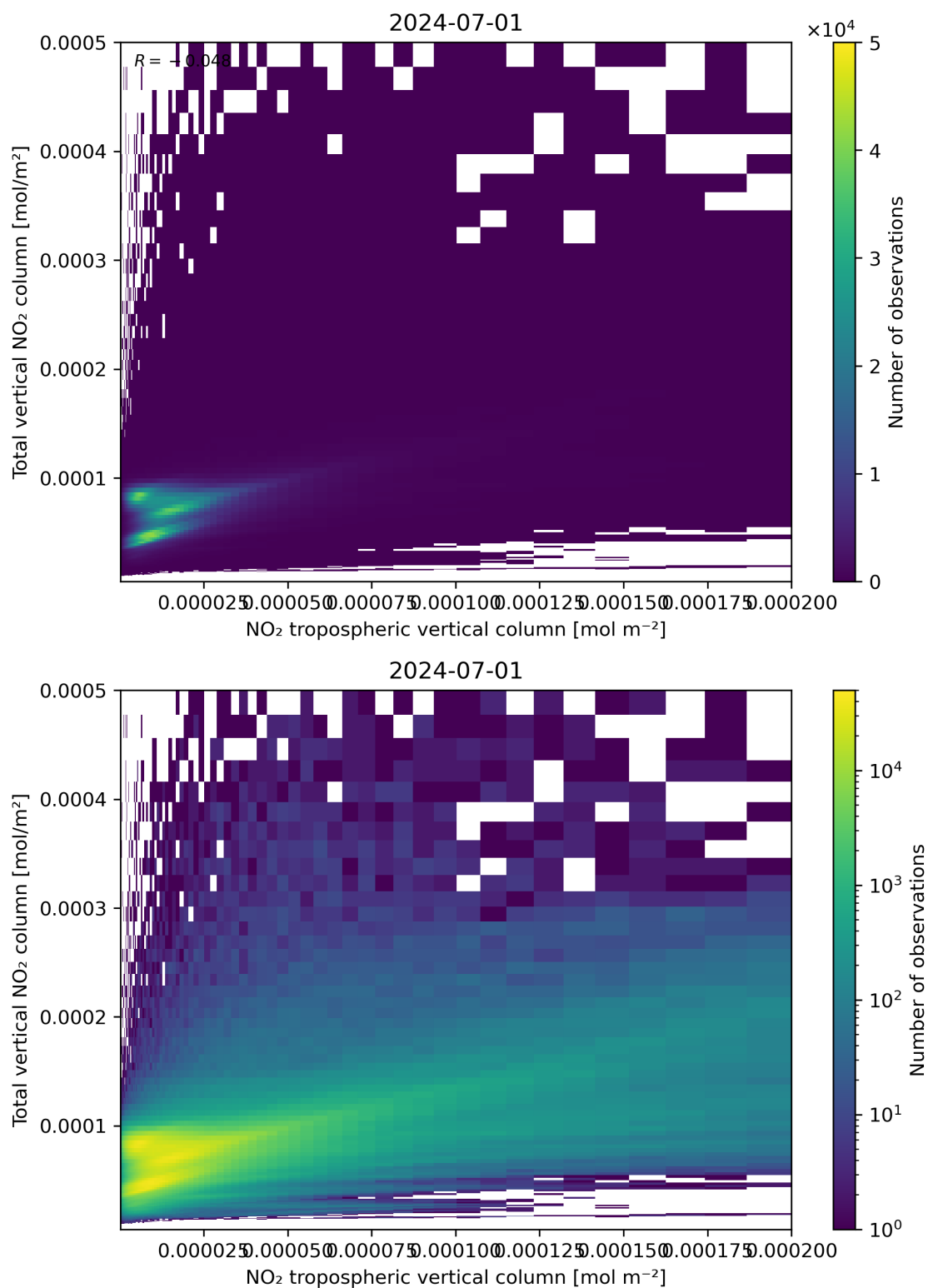
Figure 128: Scatter density plot of “NO 2 tropospheric vertical column” against “Total vertical NO 2 column” for 2024-06-30 to 2024-07-02.
