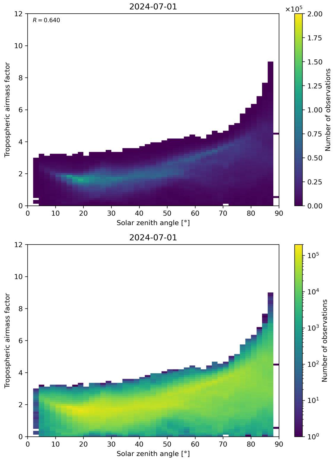
Figure 147: Scatter density plot of “Solar zenith angle” against “Tropospheric airmass factor” for 2024-06-30 to 2024-07-02.
