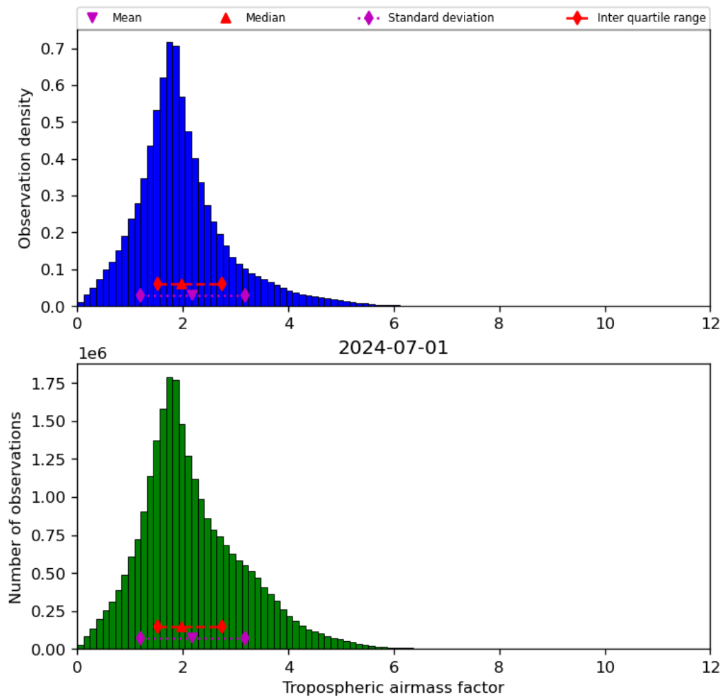
Figure 31: Histogram of “Tropospheric airmass factor” for 2024-06-30 to 2024-07-02
