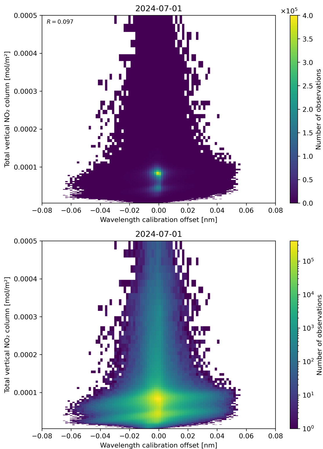
Figure 179: Scatter density plot of “Wavelength calibration offset” against “Total vertical NO 2 column” for 2024-06-30 to 2024-07-02.
