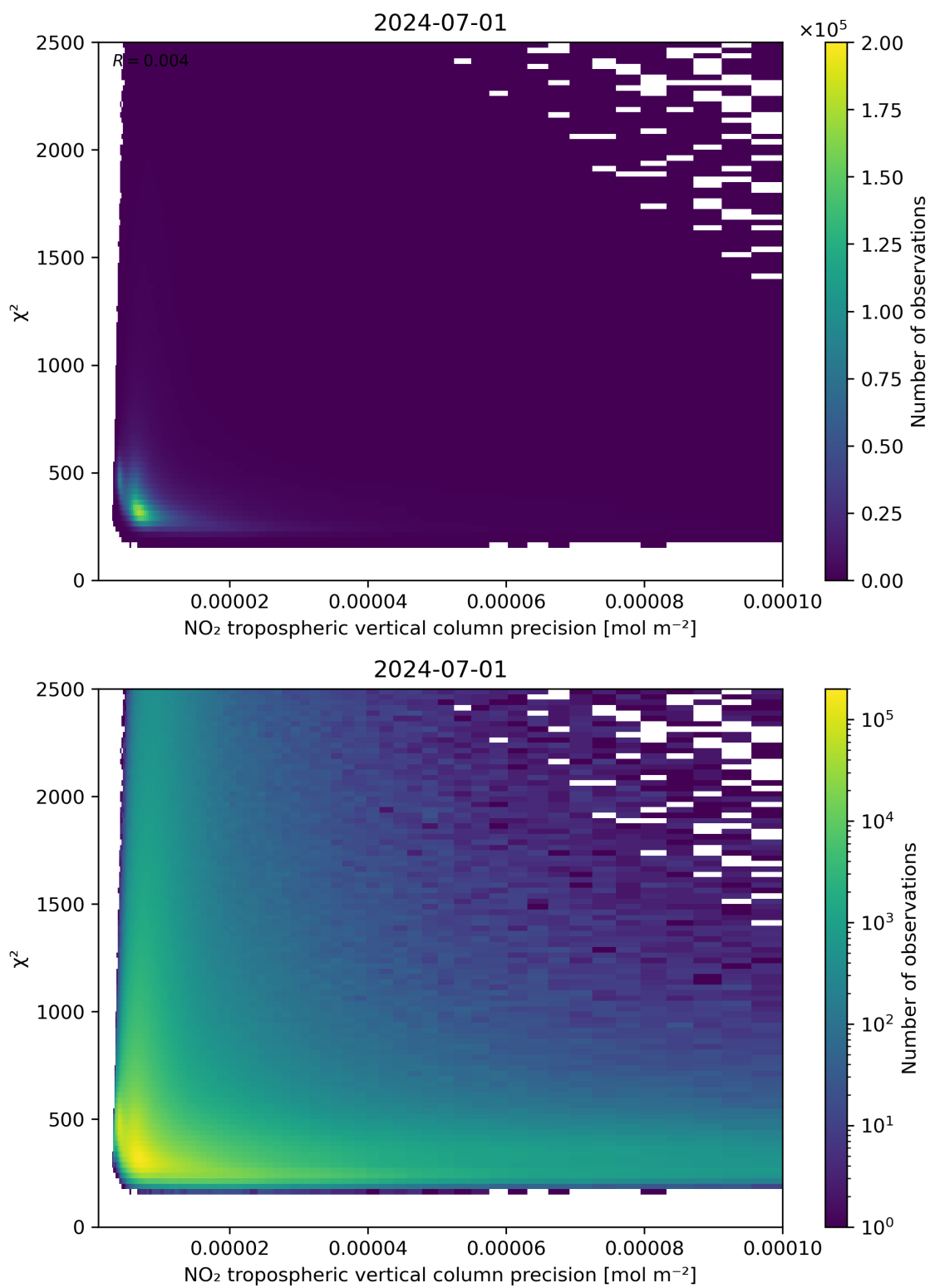
Figure 134: Scatter density plot of “NO 2 tropospheric vertical column precision” against “ \chi^2 ” for 2024-06-30 to 2024-07-02.
