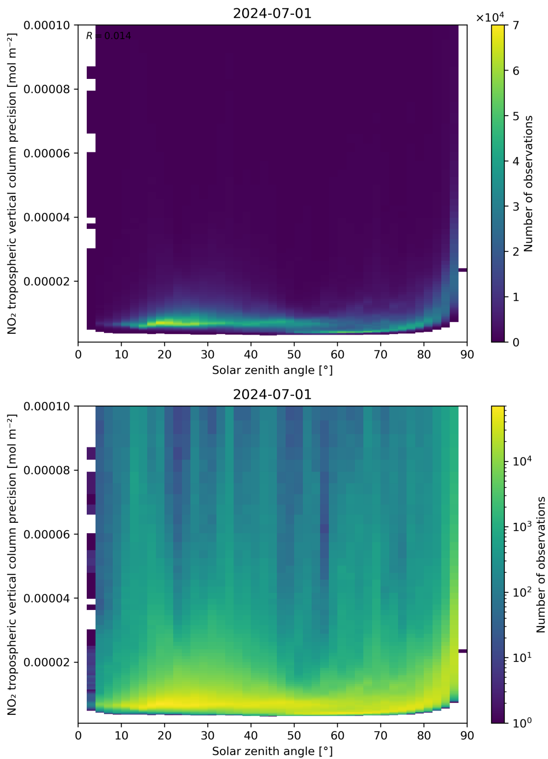
Figure 156: Scatter density plot of “Solar zenith angle” against “NO 2 tropospheric vertical column precision” for 2024-06-30 to 2024-07-02.
