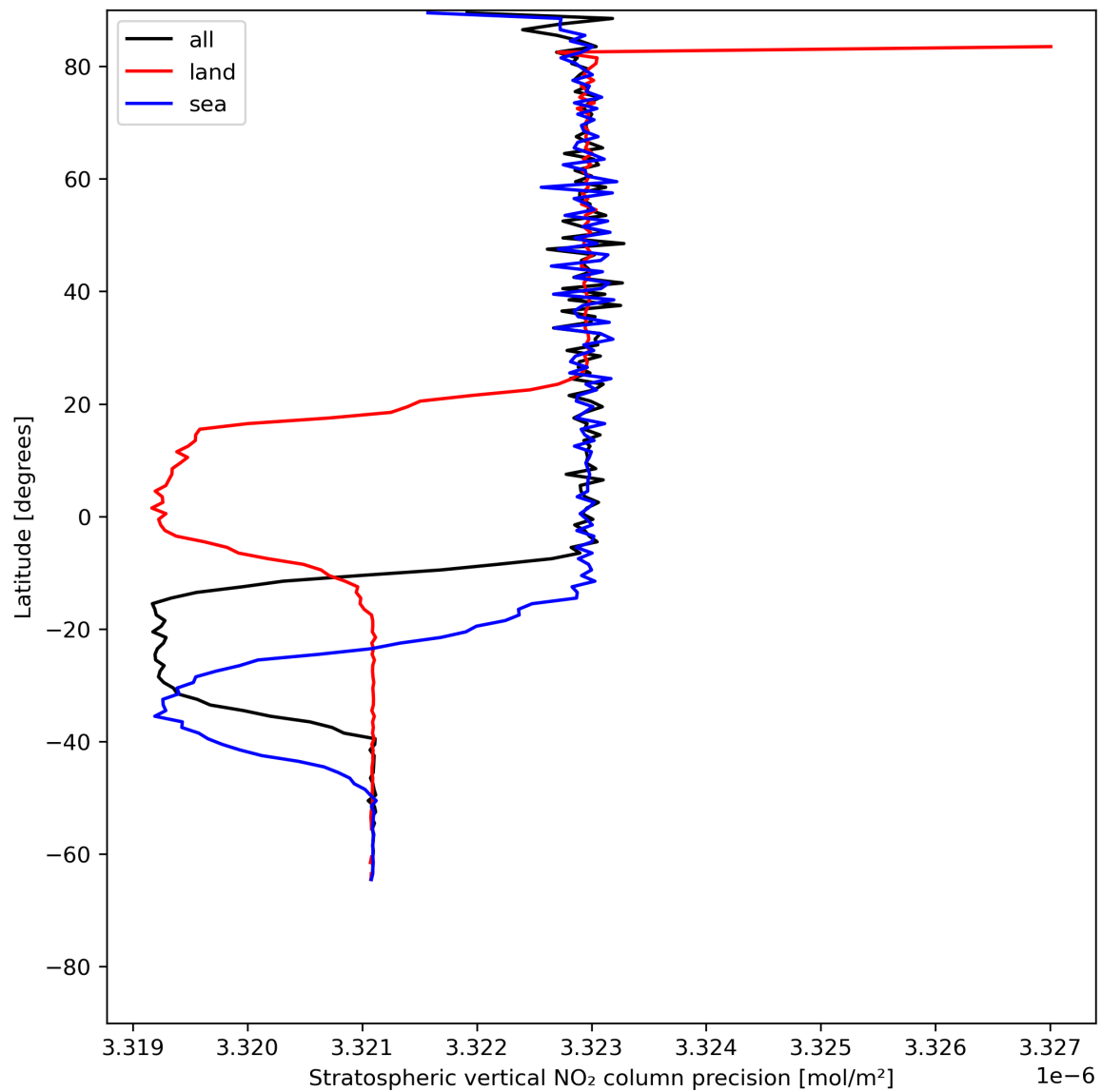
Figure 20: Zonal average of “Stratospheric vertical NO 2 column precision” for 2024-06-30 to 2024-07-02.
