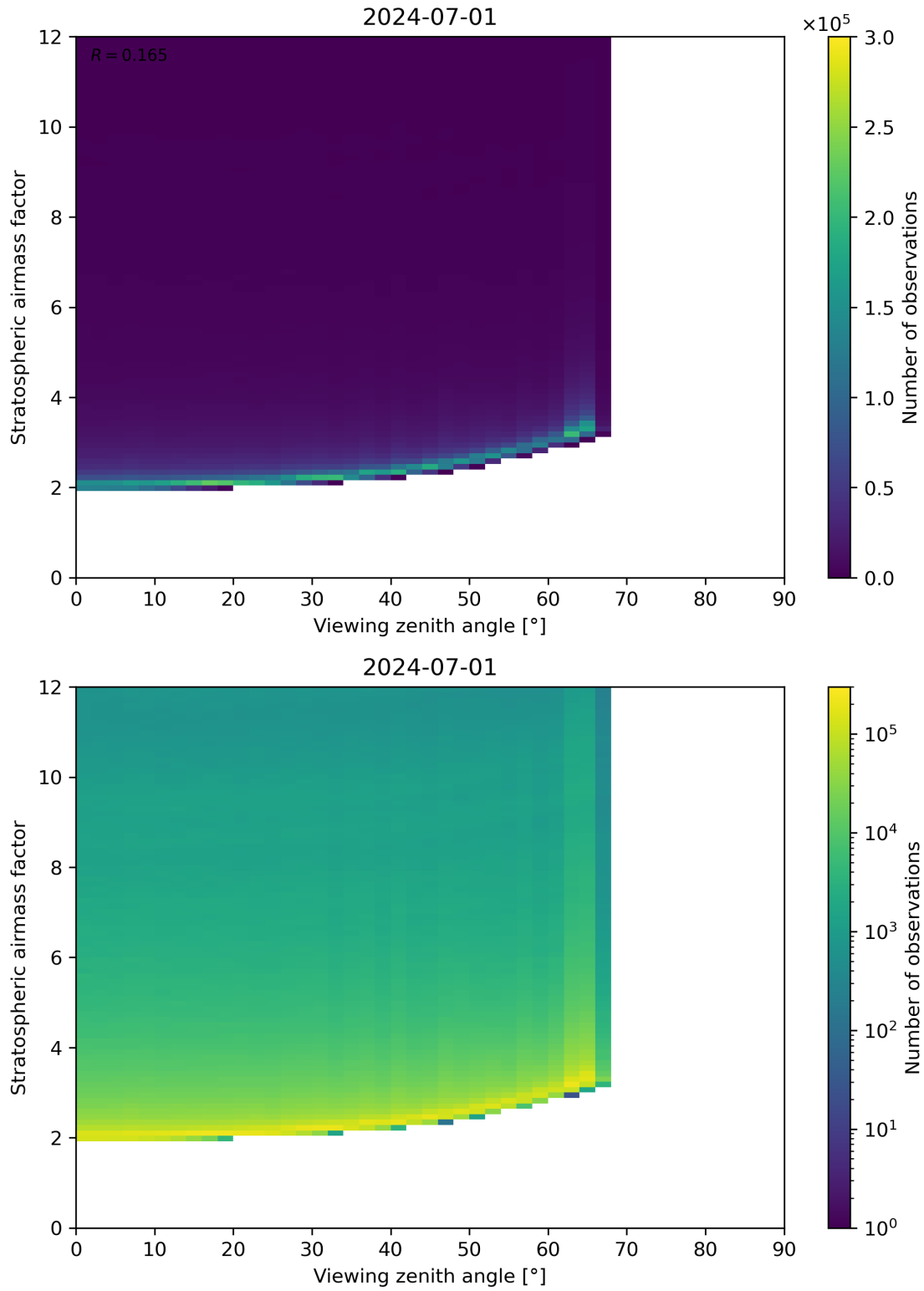
Figure 159: Scatter density plot of “Viewing zenith angle” against “Stratospheric airmass factor” for 2024-06-30 to 2024-07-02.
