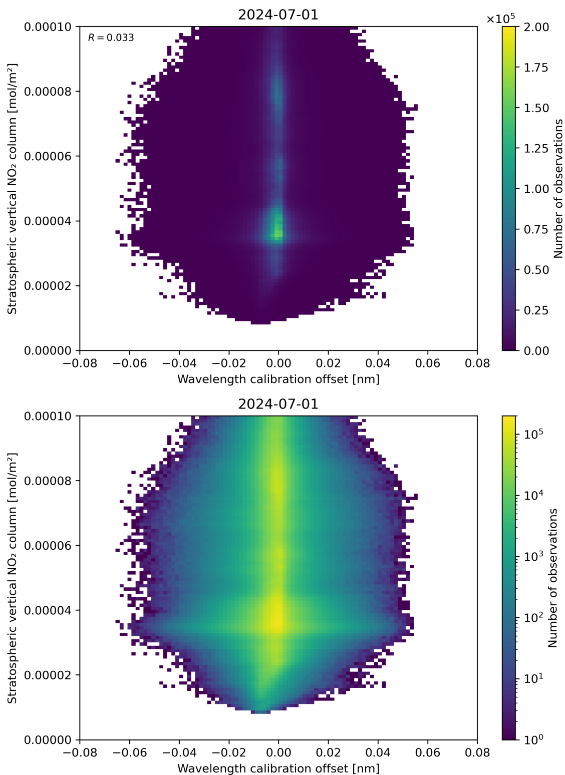
Figure 176: Scatter density plot of “Wavelength calibration offset” against “Stratospheric vertical NO 2 column” for 2024-06-30 to 2024-07-02.
