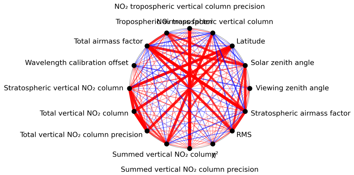
Figure 1: Map of correlation graph for 2024-06-30 to 2024-07-02.
