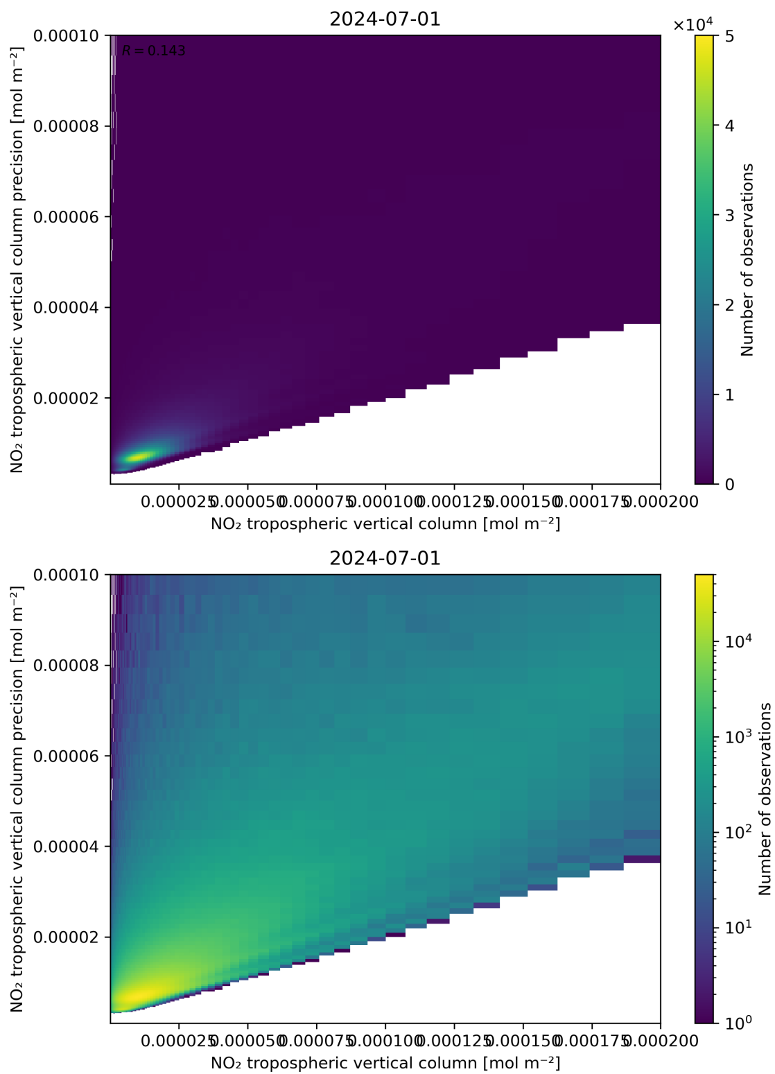
Figure 130: Scatter density plot of “NO 2 tropospheric vertical column” against “NO 2 tropospheric vertical column precision” for 2024-06-30 to 2024-07-02.
