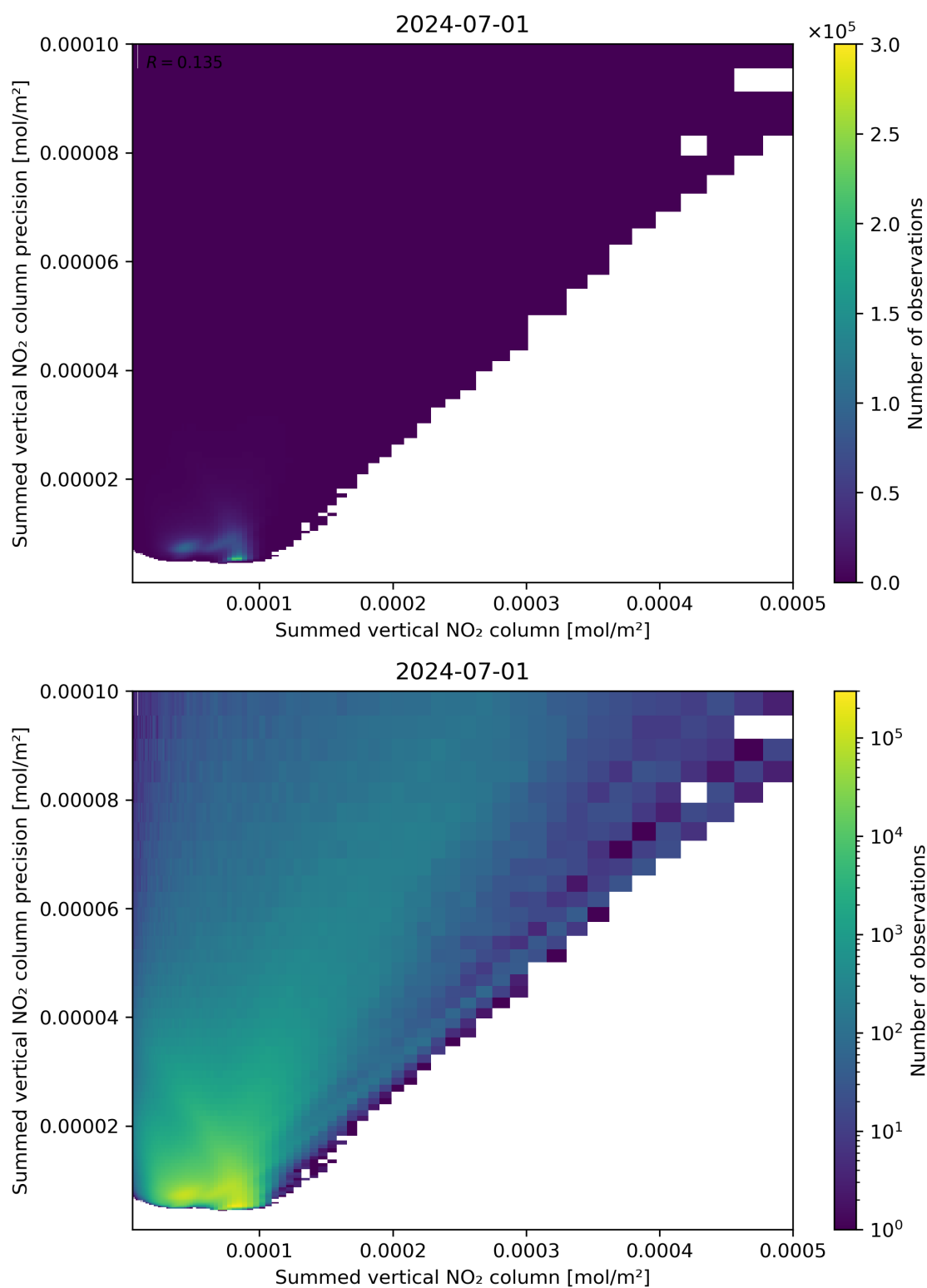
Figure 105: Scatter density plot of “Summed vertical NO 2 column” against “Summed vertical NO 2 column precision” for 2024-06-30 to 2024-07-02.
