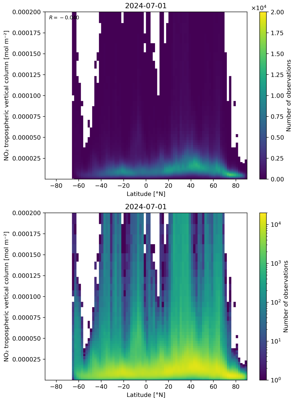
Figure 92: Scatter density plot of “Latitude” against “NO 2 tropospheric vertical column” for 2024-06-30 to 2024-07-02.
