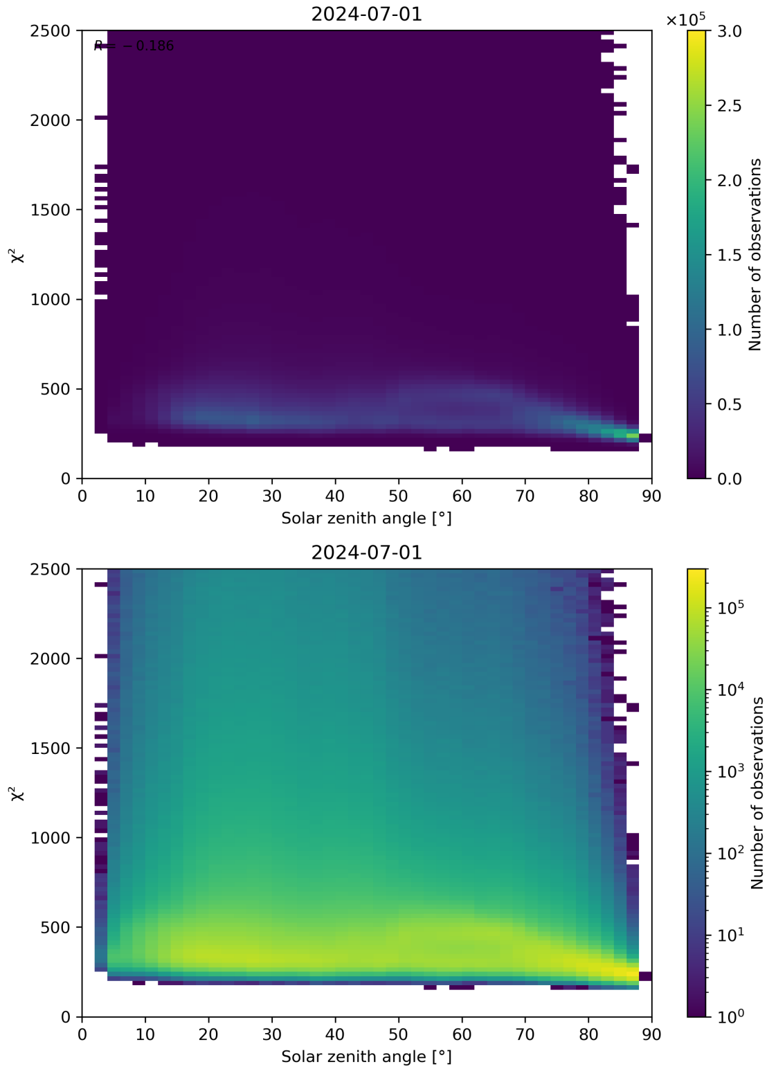
Figure 148: Scatter density plot of “Solar zenith angle” against “ \chi^2 ” for 2024-06-30 to 2024-07-02.
