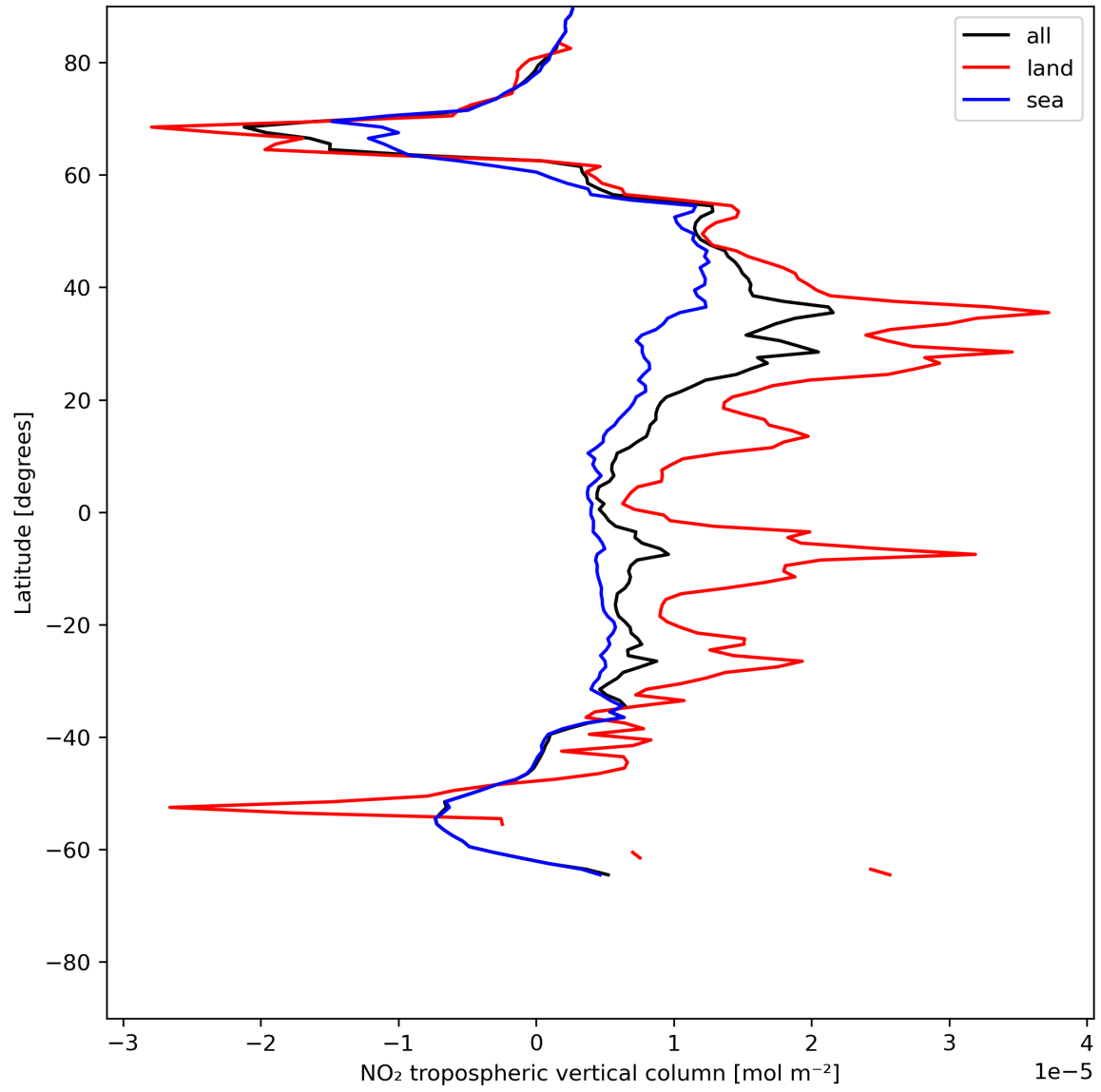
Figure 12: Zonal average of “NO 2 tropospheric vertical column” for 2024-06-30 to 2024-07-02.
