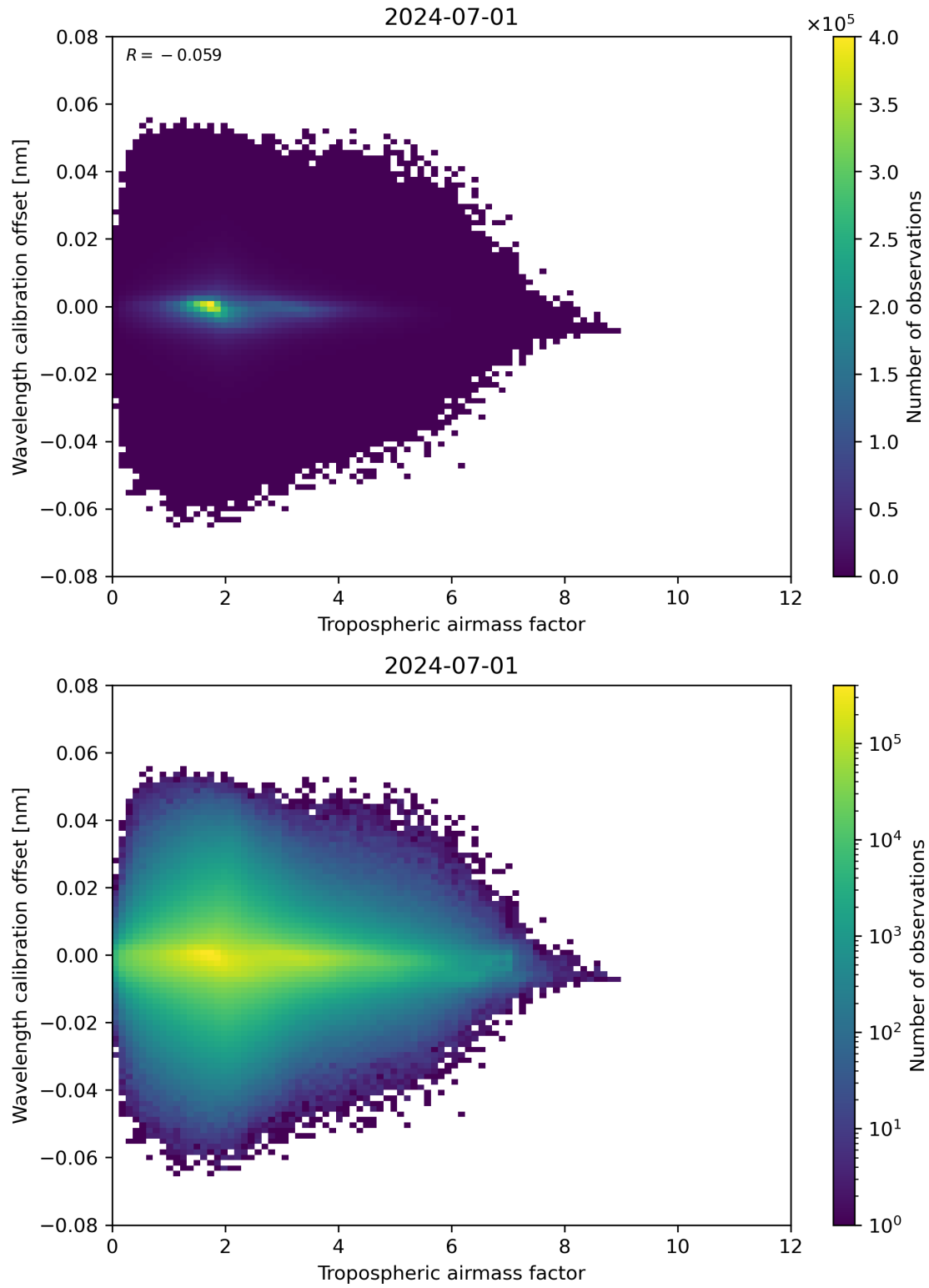
Figure 80: Scatter density plot of “Tropospheric airmass factor” against “Wavelength calibration offset” for 2024-06-30 to 2024-07-02.
