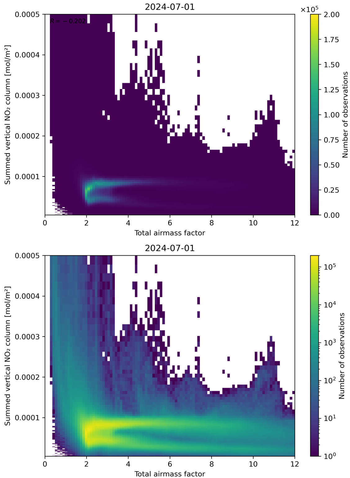
Figure 65: Scatter density plot of “Total airmass factor” against “Summed vertical NO 2 column” for 2024-06-30 to 2024-07-02.
