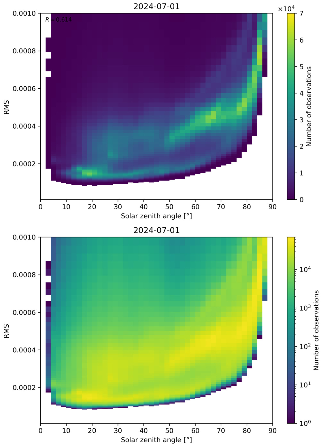
Figure 157: Scatter density plot of “Solar zenith angle” against “RMS” for 2024-06-30 to 2024-07-02.
