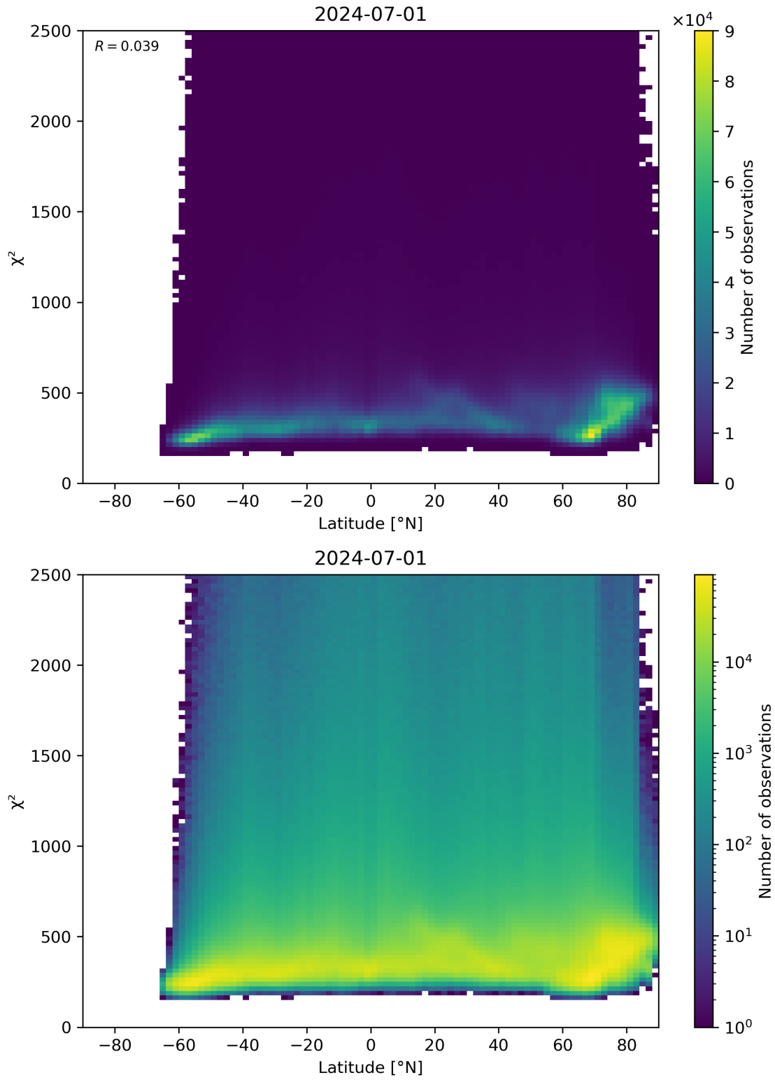
Figure 86: Scatter density plot of “Latitude” against “ \chi^2 ” for 2024-06-30 to 2024-07-02.
