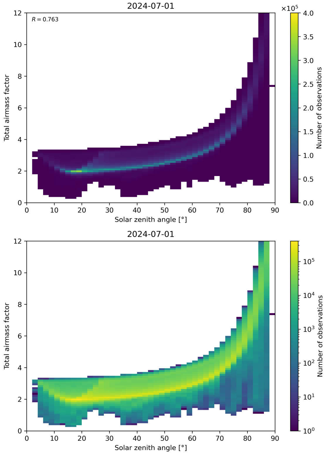
Figure 146: Scatter density plot of “Solar zenith angle” against “Total air mass factor” for 2024-06-30 to 2024-07-02.
