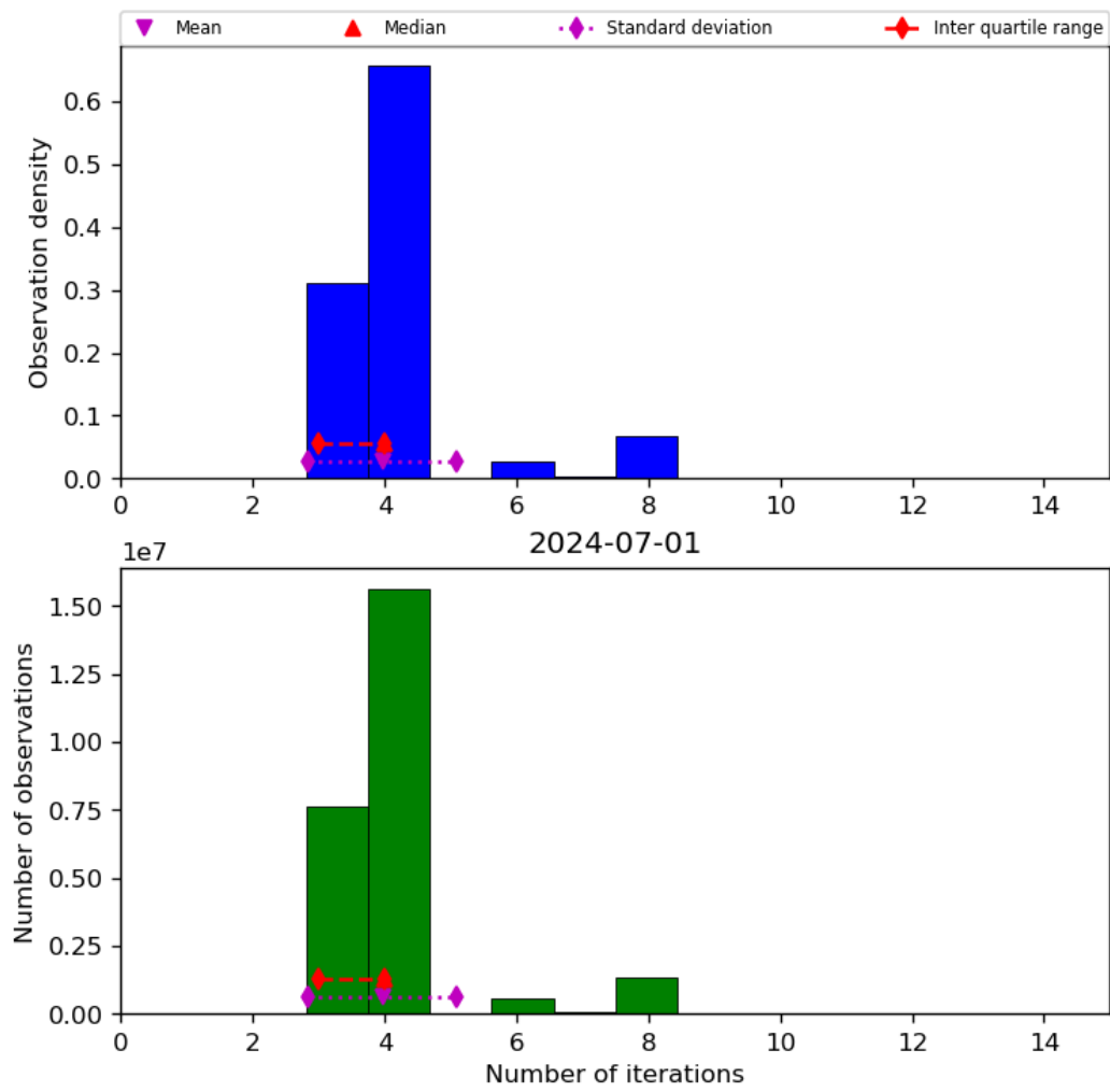
Figure 34: Histogram of "Number of iterations" for 2024-06-30 to 2024-07-02
