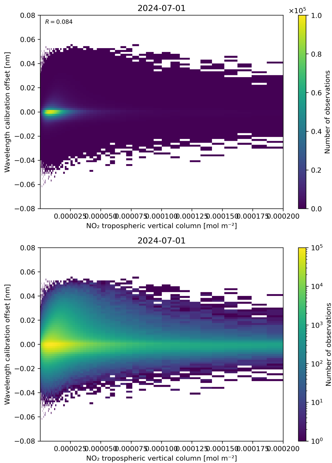
Figure 143: Scatter density plot of “NO 2 tropospheric vertical column” against “Wavelength calibration offset” for 2024-06-30 to 2024-07-02.
