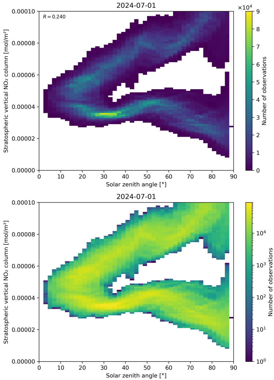
Figure 150: Scatter density plot of “Solar zenith angle” against “Stratospheric vertical NO 2 column” for 2024-06-30 to 2024-07-02.
