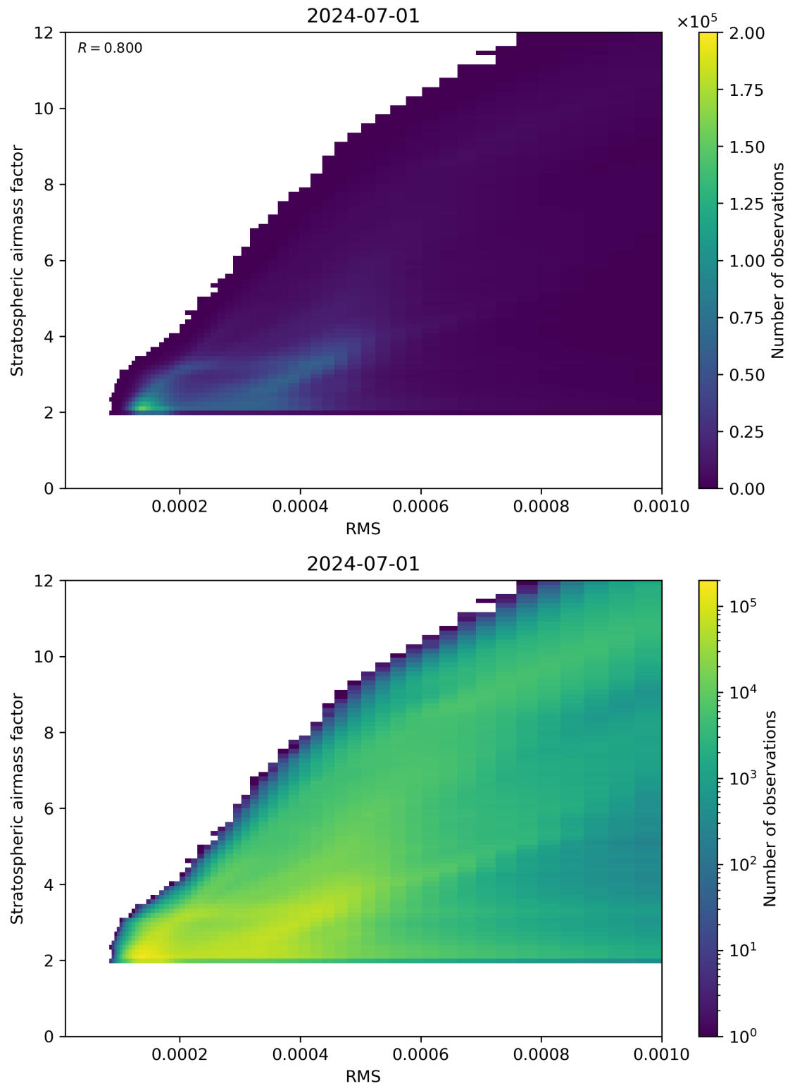
Figure 144: Scatter density plot of “RMS” against “Stratospheric airmass factor” for 2024-06-30 to 2024-07-02.
