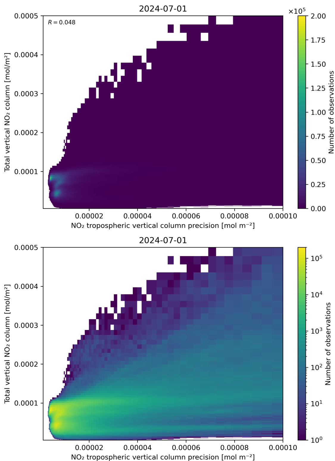
Figure 138: Scatter density plot of “NO 2 tropospheric vertical column precision” against “Total vertical NO 2 column” for 2024-06-30 to 2024-07-02.
