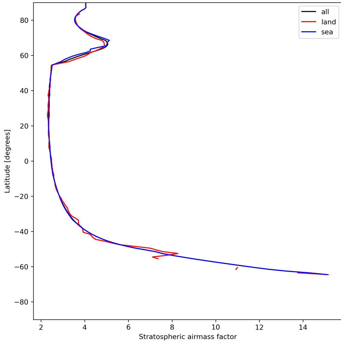
Figure 27: Zonal average of “Stratospheric airmass factor” for 2024-06-30 to 2024-07-02.
