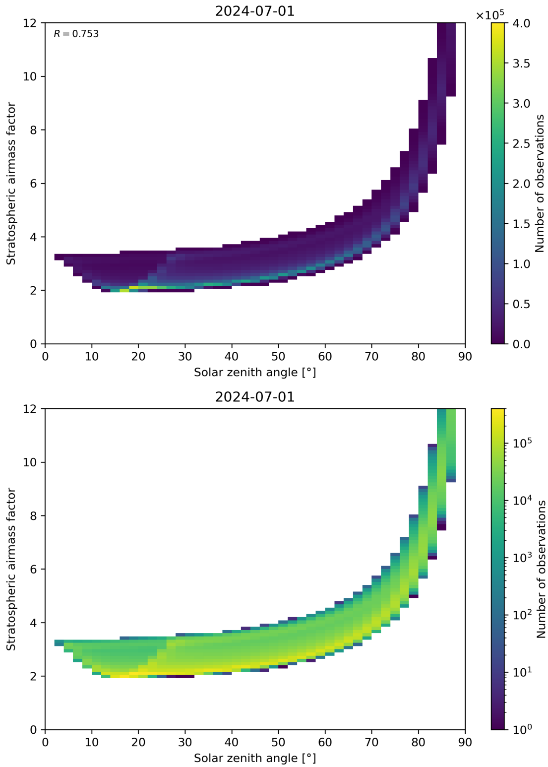
Figure 145: Scatter density plot of “Solar zenith angle” against “Stratospheric airmass factor” for 2024-06-30 to 2024-07-02.
