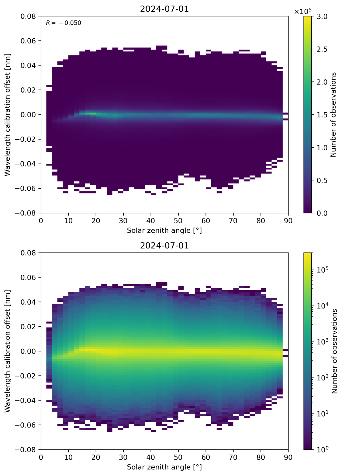
Figure 158: Scatter density plot of “Solar zenith angle” against “Wavelength calibration offset” for 2024-06-30 to 2024-07-02.
