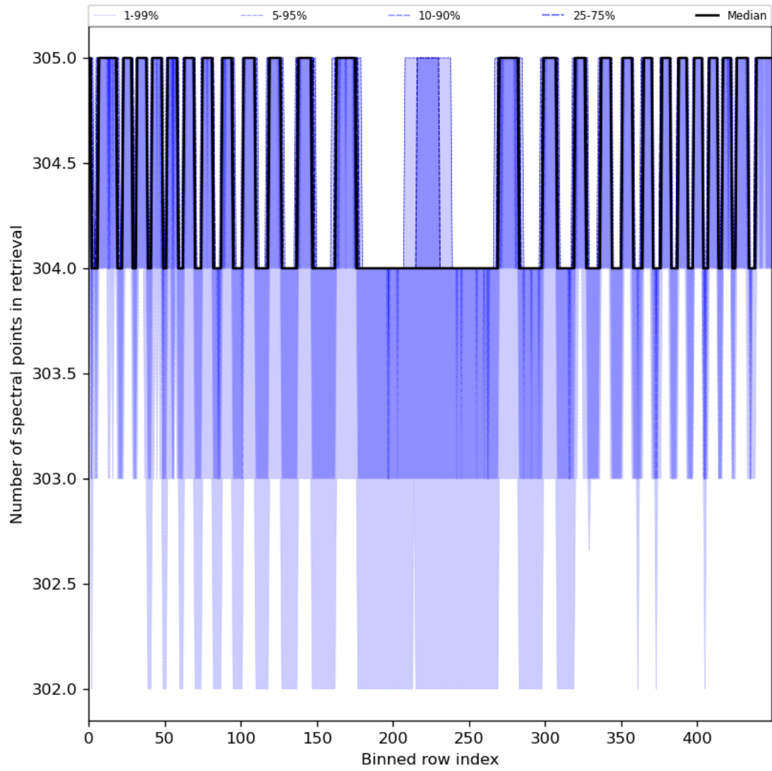
Figure 50: Along track statistics of “Number of spectral points in retrieval” for 2024-06-30 to 2024-07-02
