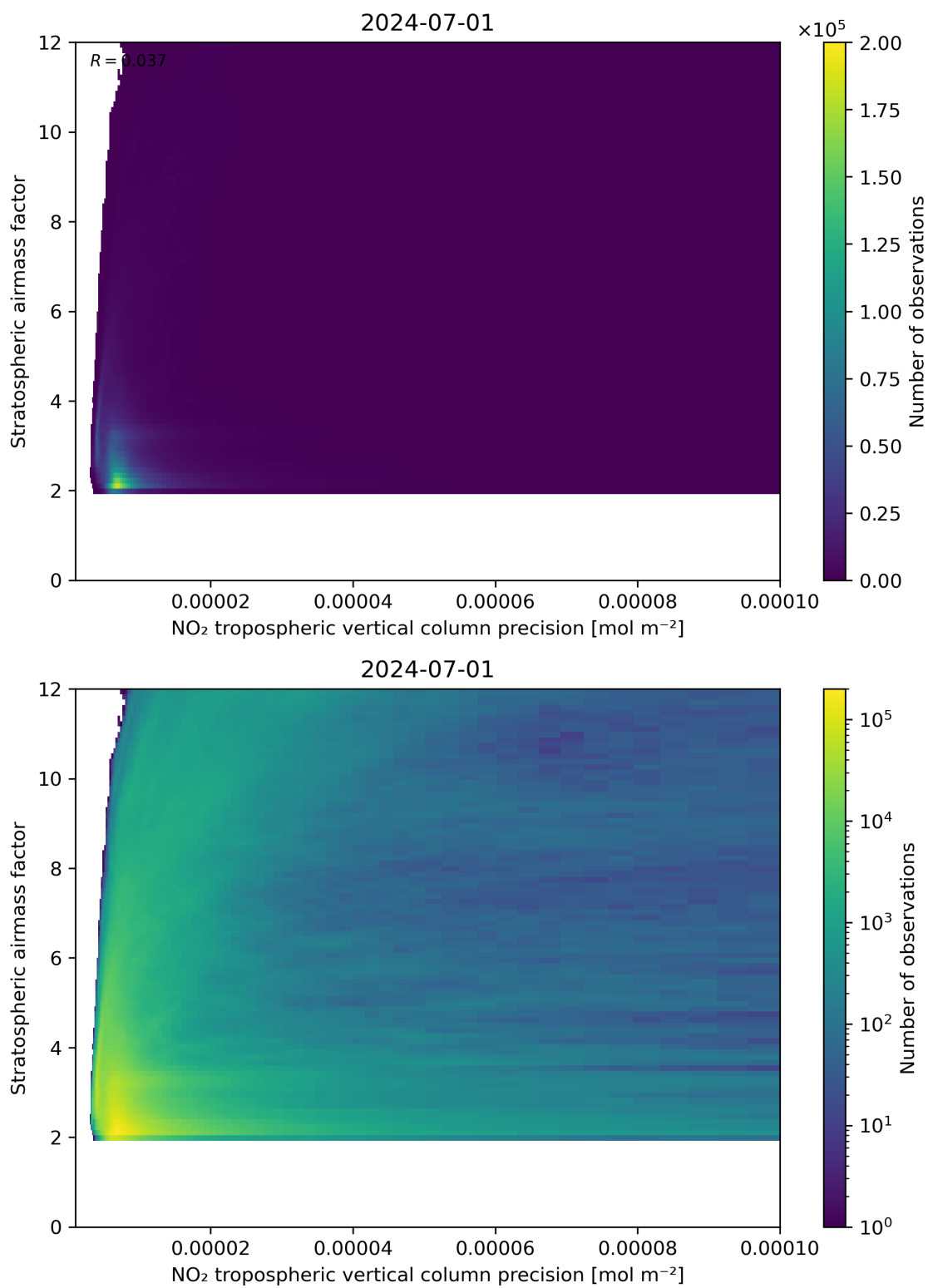
Figure 131: Scatter density plot of “NO 2 tropospheric vertical column precision” against “Stratospheric airmass factor” for 2024-06-30 to 2024-07-02.
