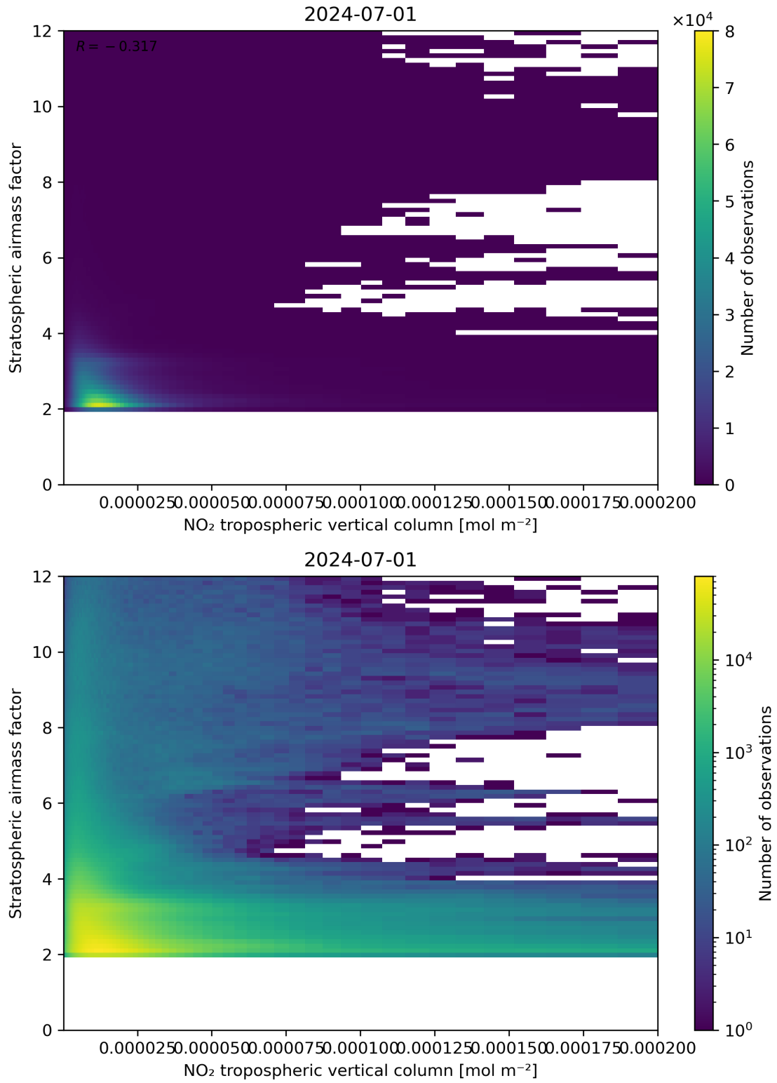
Figure 121: Scatter density plot of “NO 2 tropospheric vertical column” against “Stratospheric air mass factor” for 2024-06-30 to 2024-07-02.
