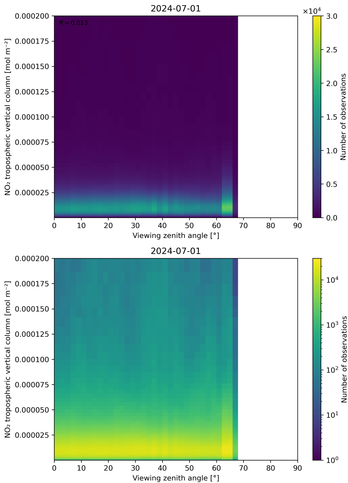
Figure 169: Scatter density plot of “Viewing zenith angle” against “NO 2 tropospheric vertical column” for 2024-06-30 to 2024-07-02.
