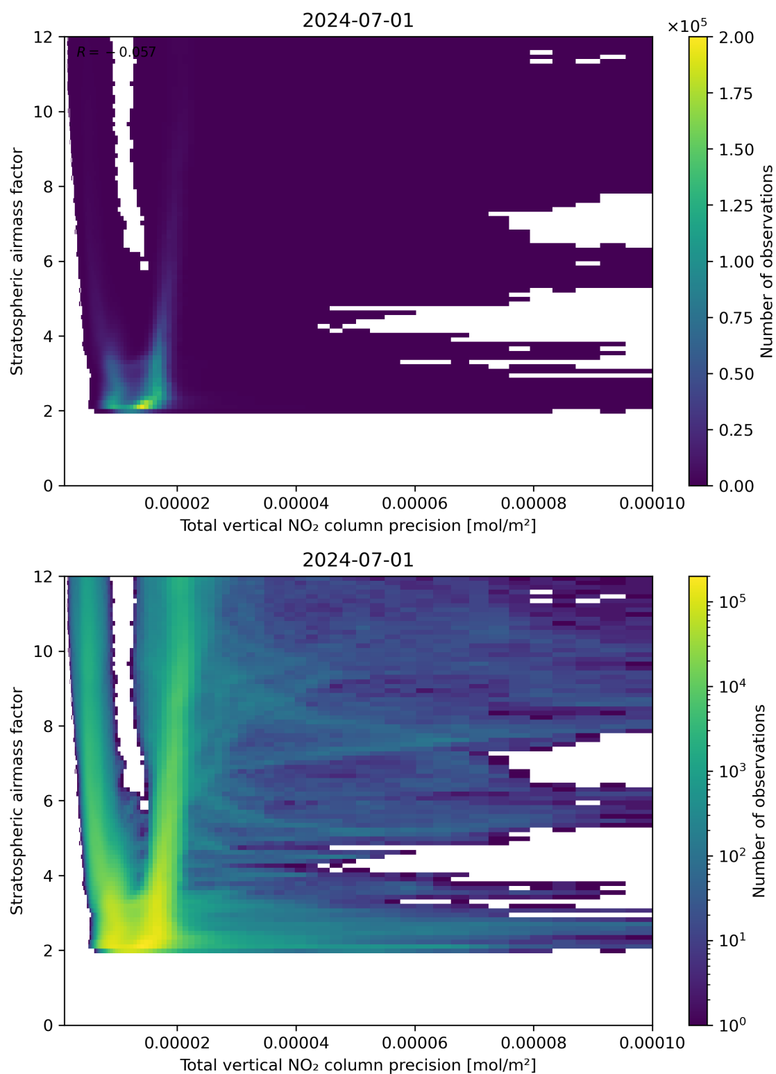
Figure 115: Scatter density plot of “Total vertical NO 2 column precision” against “Stratospheric air mass factor” for 2024-06-30 to 2024-07-02.
