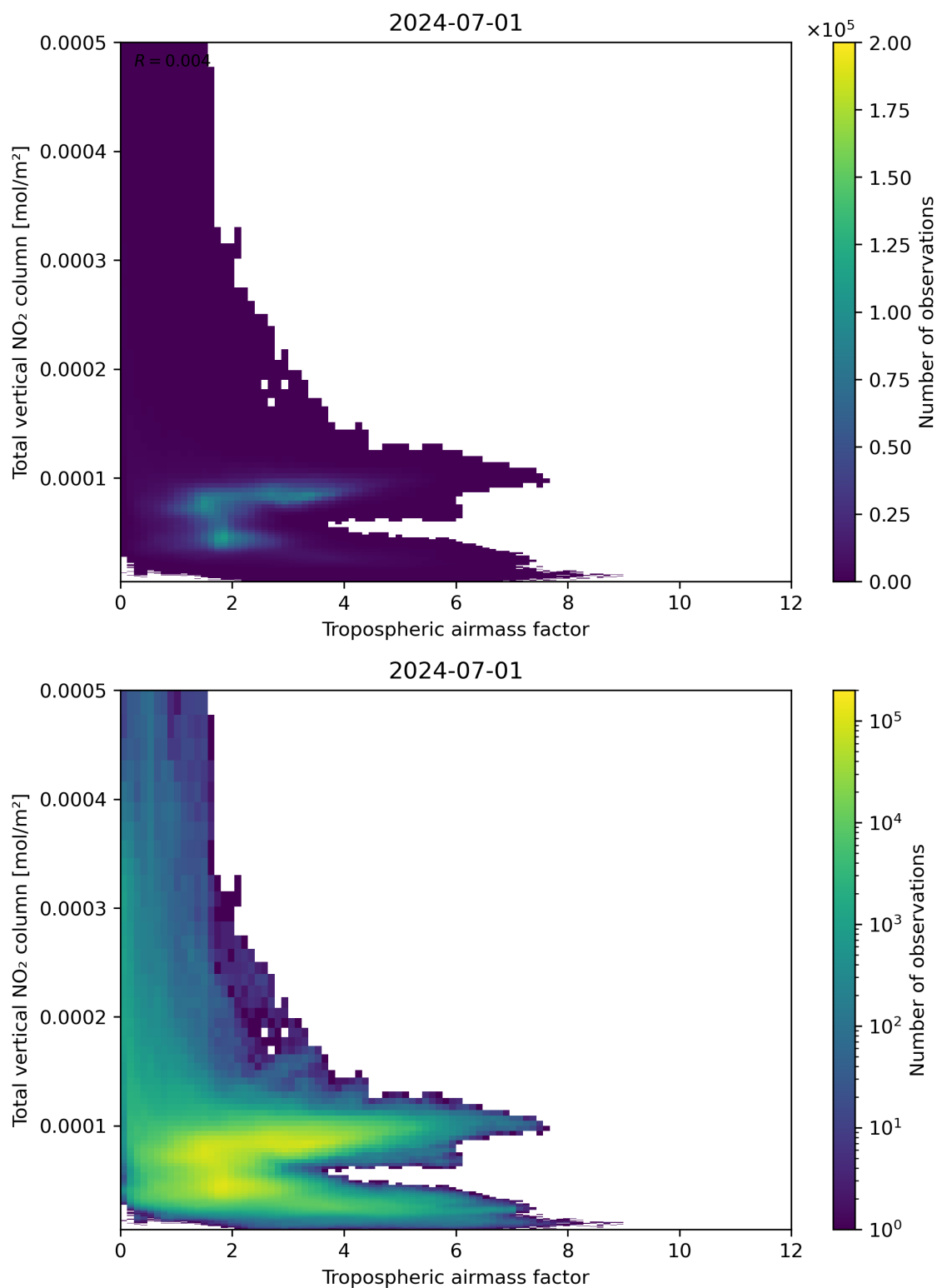
Figure 77: Scatter density plot of “Tropospheric airmass factor” against “Total vertical NO 2 column” for 2024-06-30 to 2024-07-02.
