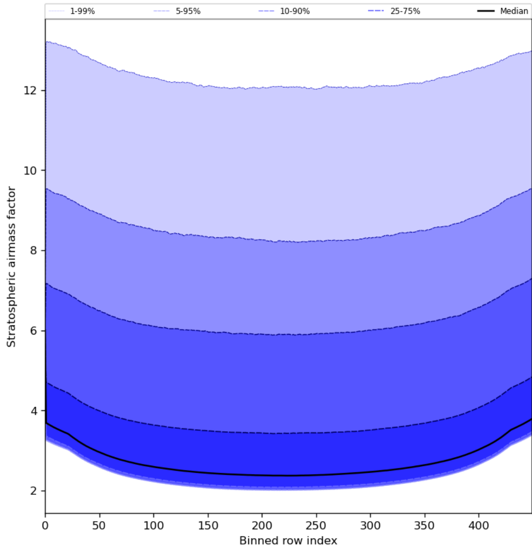
Figure 61: Along track statistics of “Stratospheric airmass factor” for 2024-06-30 to 2024-07-02
