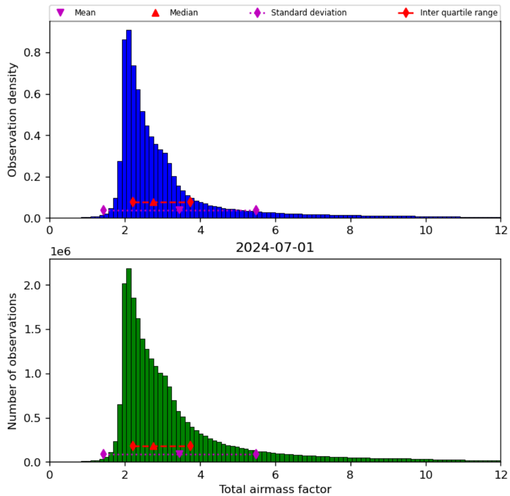
Figure 32: Histogram of “Total airmass factor” for 2024-06-30 to 2024-07-02
