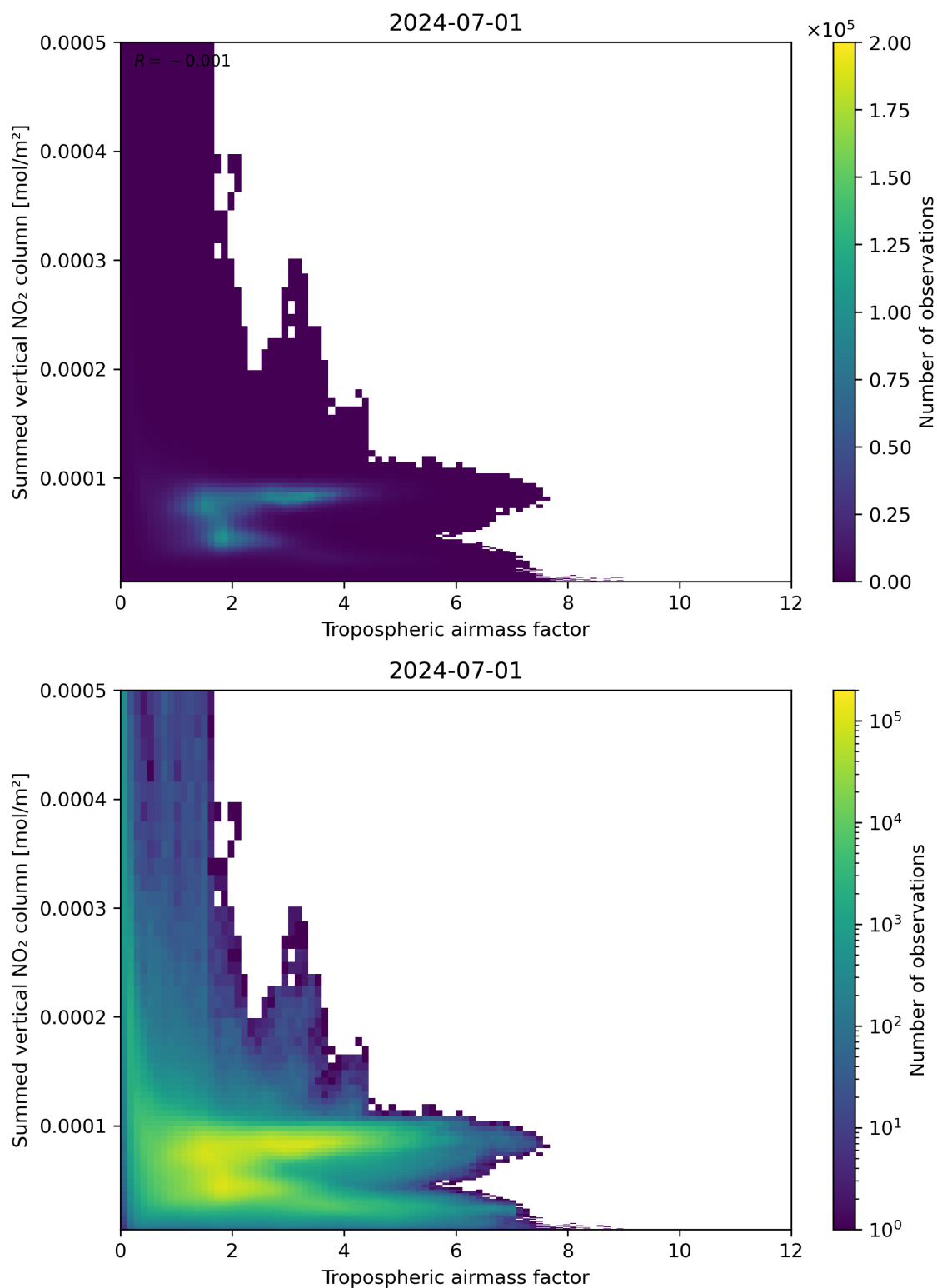
Figure 75: Scatter density plot of “Tropospheric airmass factor” against “Summed vertical NO 2 column” for 2024-06-30 to 2024-07-02.
