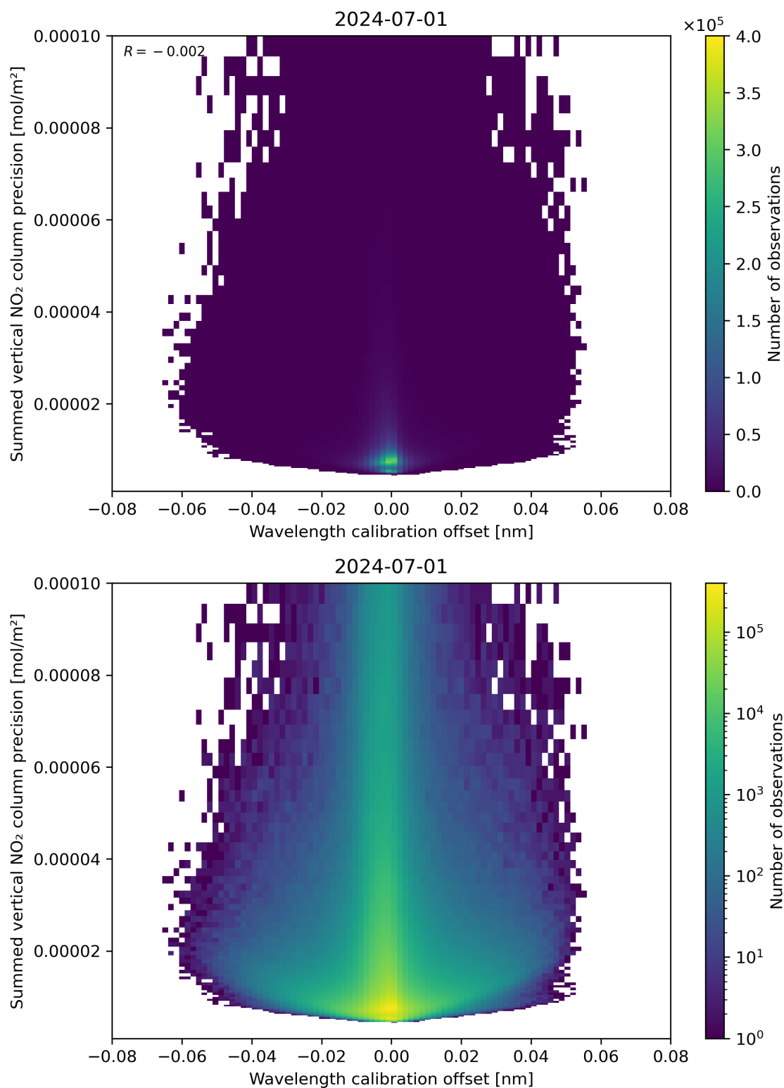
Figure 178: Scatter density plot of “Wavelength calibration offset” against “Summed vertical NO 2 column precision” for 2024-06-30 to 2024-07-02.
