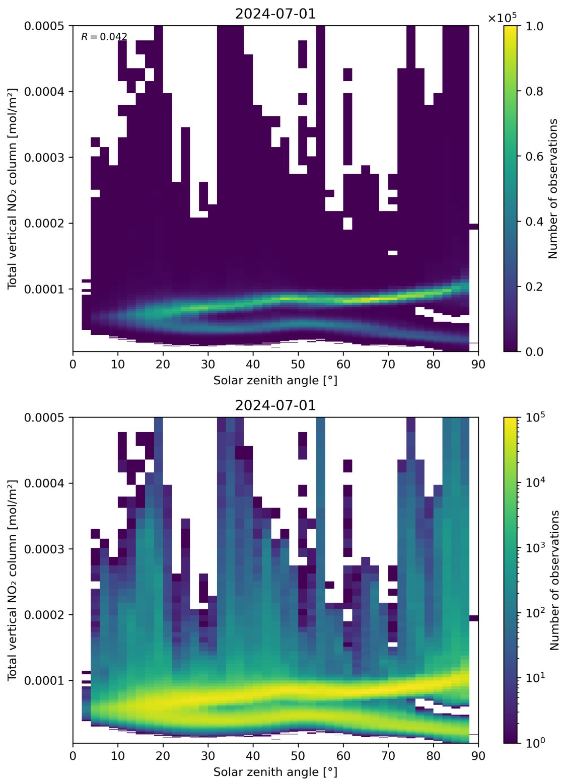
Figure 153: Scatter density plot of “Solar zenith angle” against “Total vertical NO 2 column” for 2024-06-30 to 2024-07-02.
