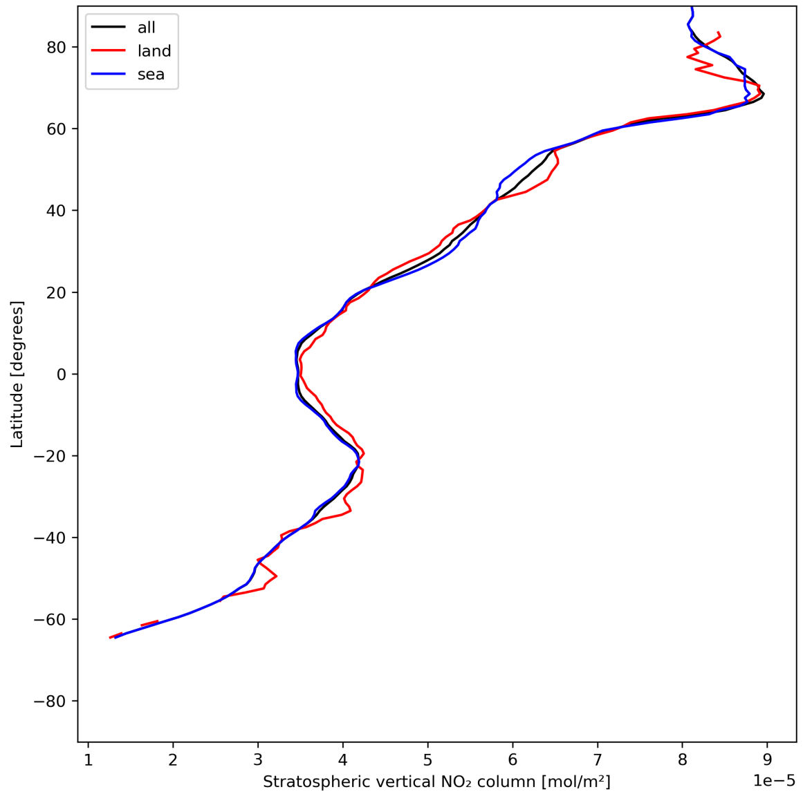
Figure 19: Zonal average of “Stratospheric vertical NO 2 column” for 2024-06-30 to 2024-07-02.
