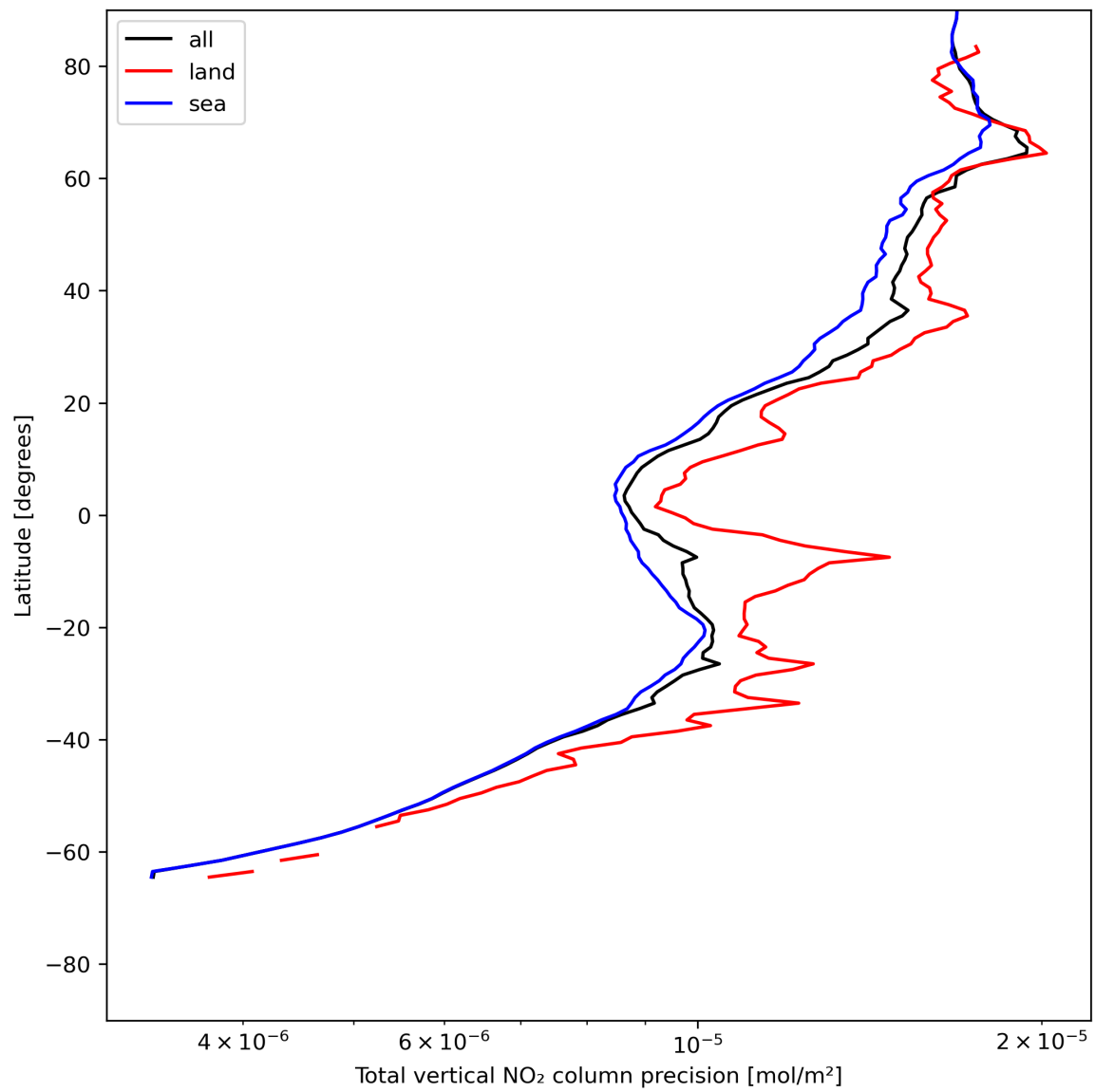
Figure 22: Zonal average of “Total vertical NO 2 column precision” for 2024-06-30 to 2024-07-02.
