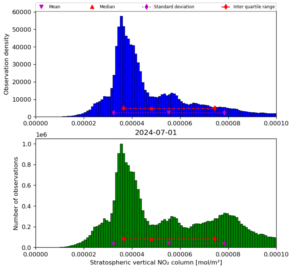
Figure 36: Histogram of “Stratospheric vertical NO 2 column” for 2024-06-30 to 2024-07-02
