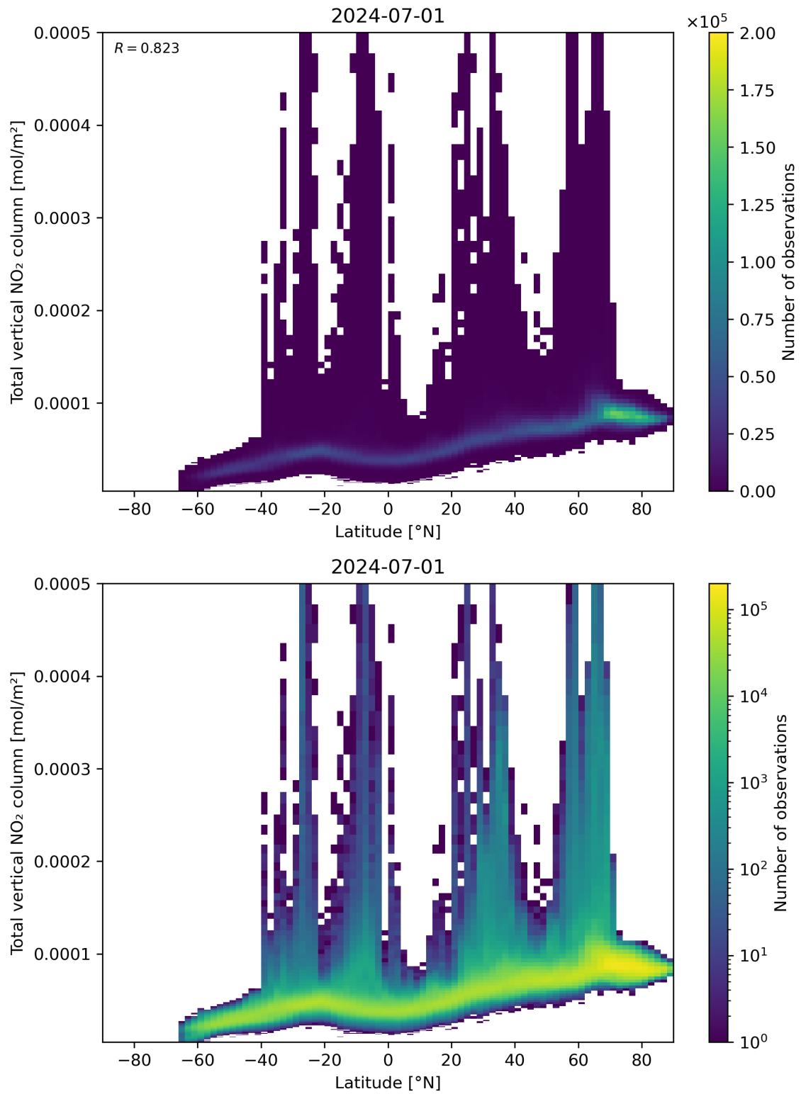
Figure 90: Scatter density plot of “Latitude” against “Total vertical NO 2 column” for 2024-06-30 to 2024-07-02.
