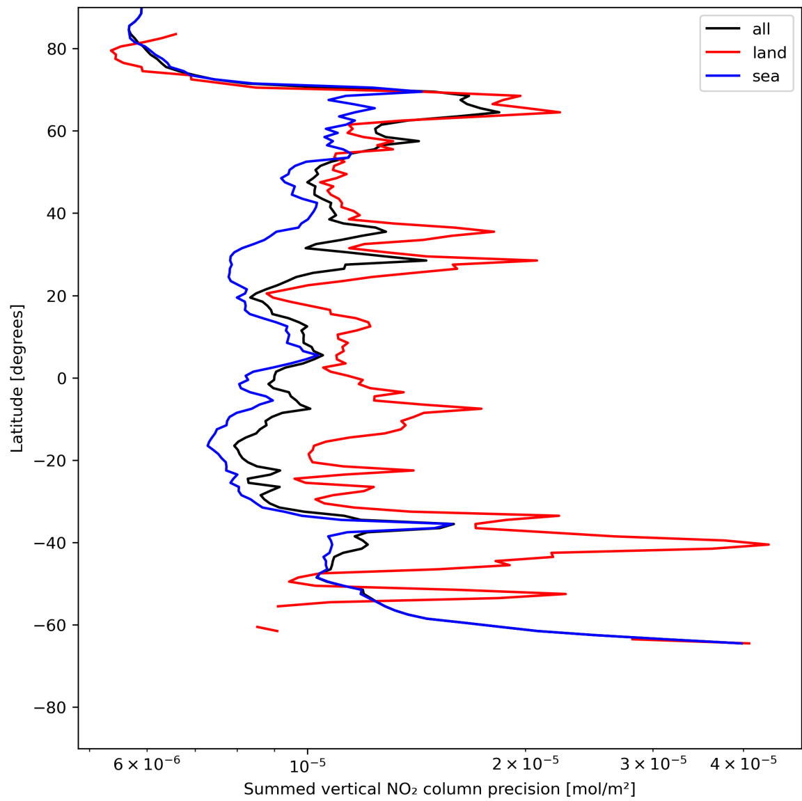
Figure 24: Zonal average of “Summed vertical NO 2 column precision” for 2024-06-30 to 2024-07-02.
