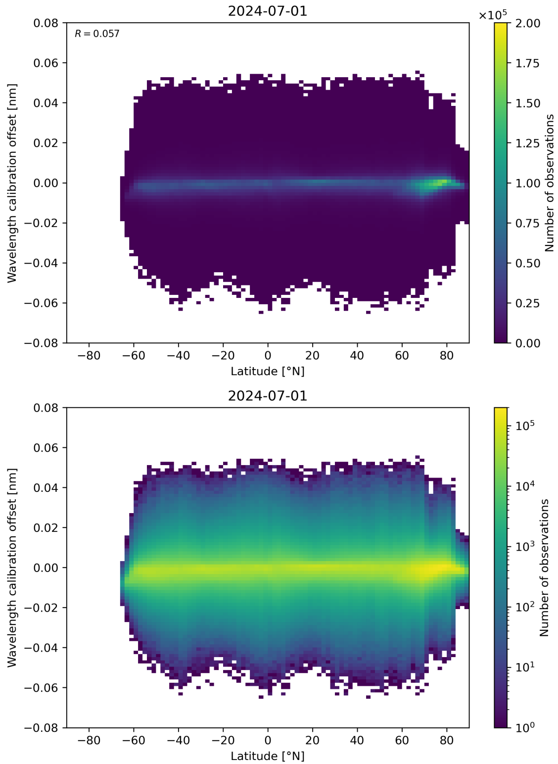
Figure 95: Scatter density plot of “Latitude” against “Wavelength calibration offset” for 2024-06-30 to 2024-07-02.
