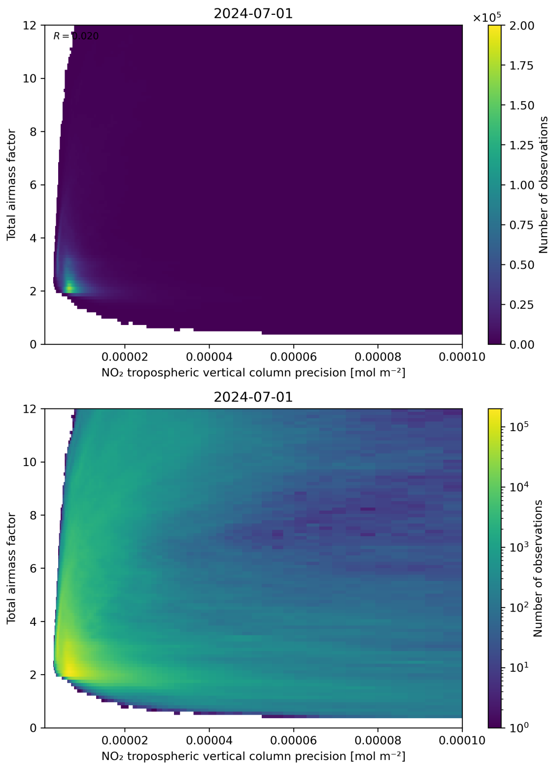
Figure 132: Scatter density plot of “NO 2 tropospheric vertical column precision” against “Total air mass factor” for 2024-06-30 to 2024-07-02.
