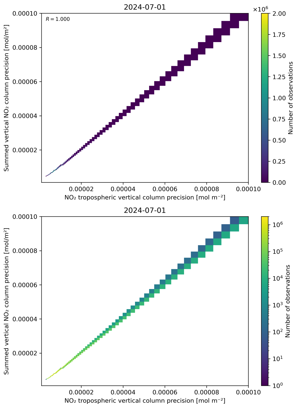
Figure 137: Scatter density plot of “NO 2 tropospheric vertical column precision” against “Summed vertical NO 2 column precision” for 2024-06-30 to 2024-07-02.
