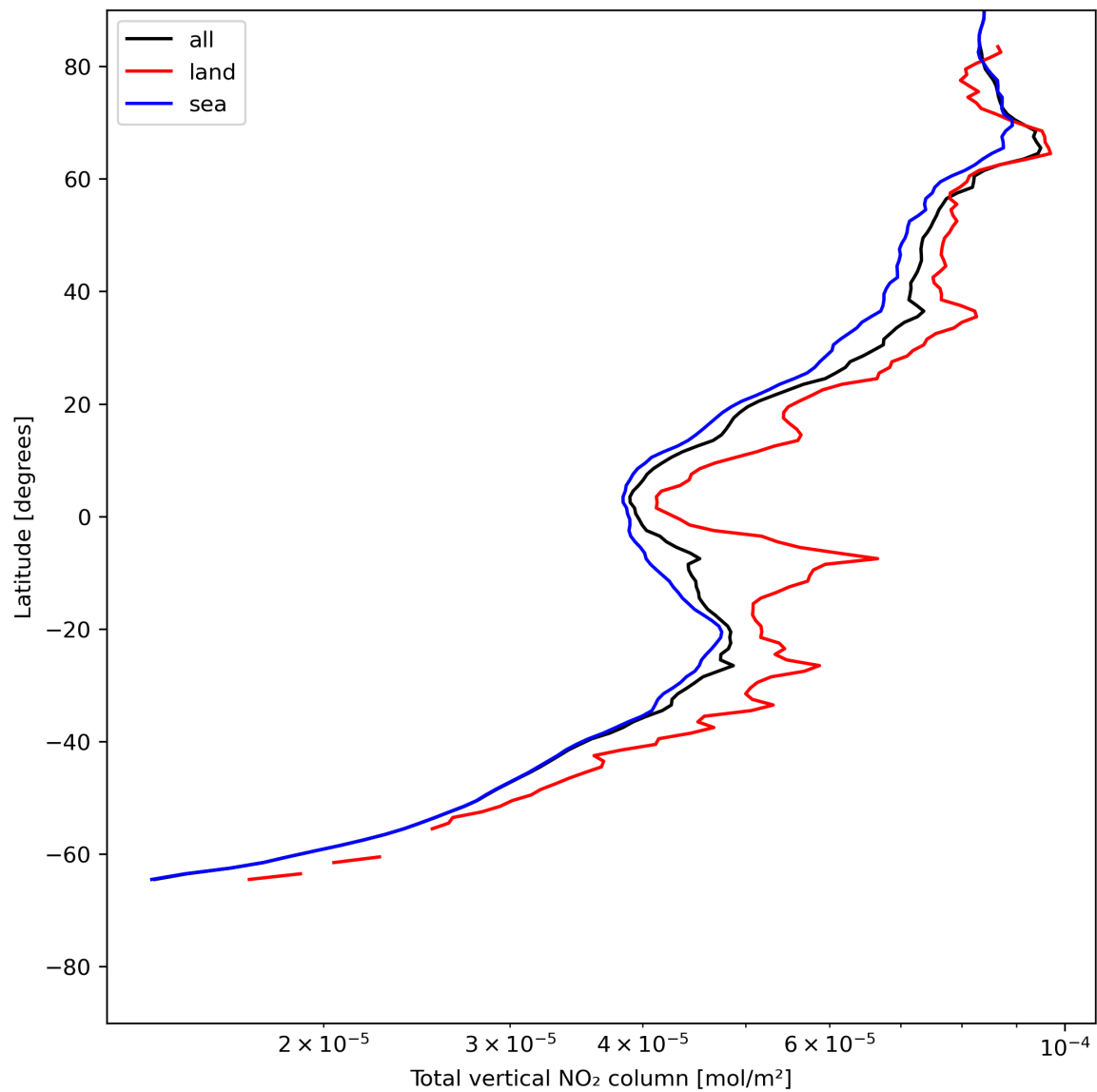
Figure 21: Zonal average of “Total vertical NO 2 column” for 2024-06-30 to 2024-07-02.
