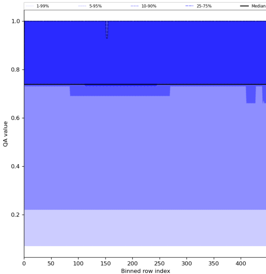
Figure 45: Along track statistics of “QA value” for 2024-06-30 to 2024-07-02
