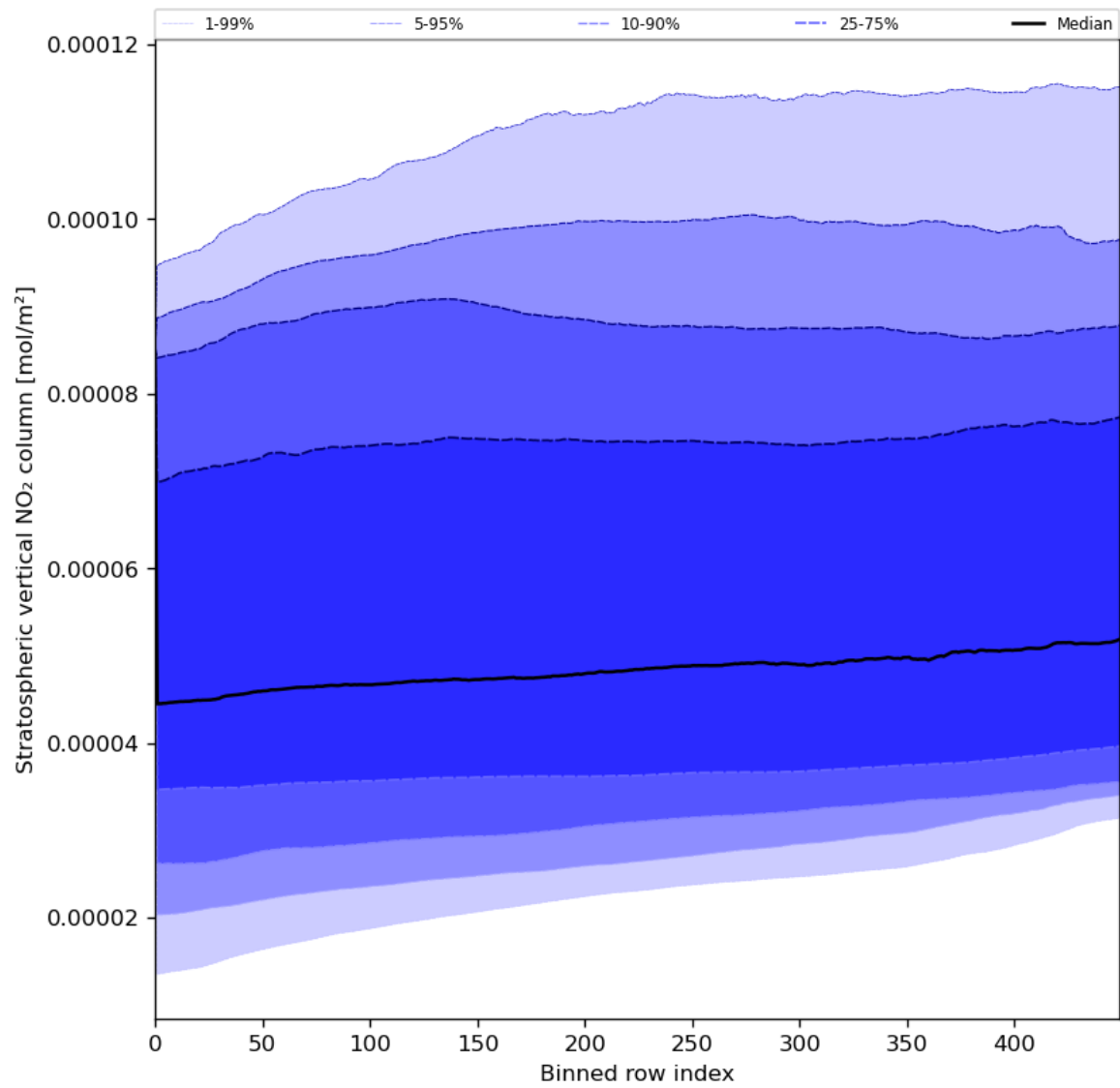
Figure 53: Along track statistics of “Stratospheric vertical NO 2 column” for 2024-06-30 to 2024-07-02
