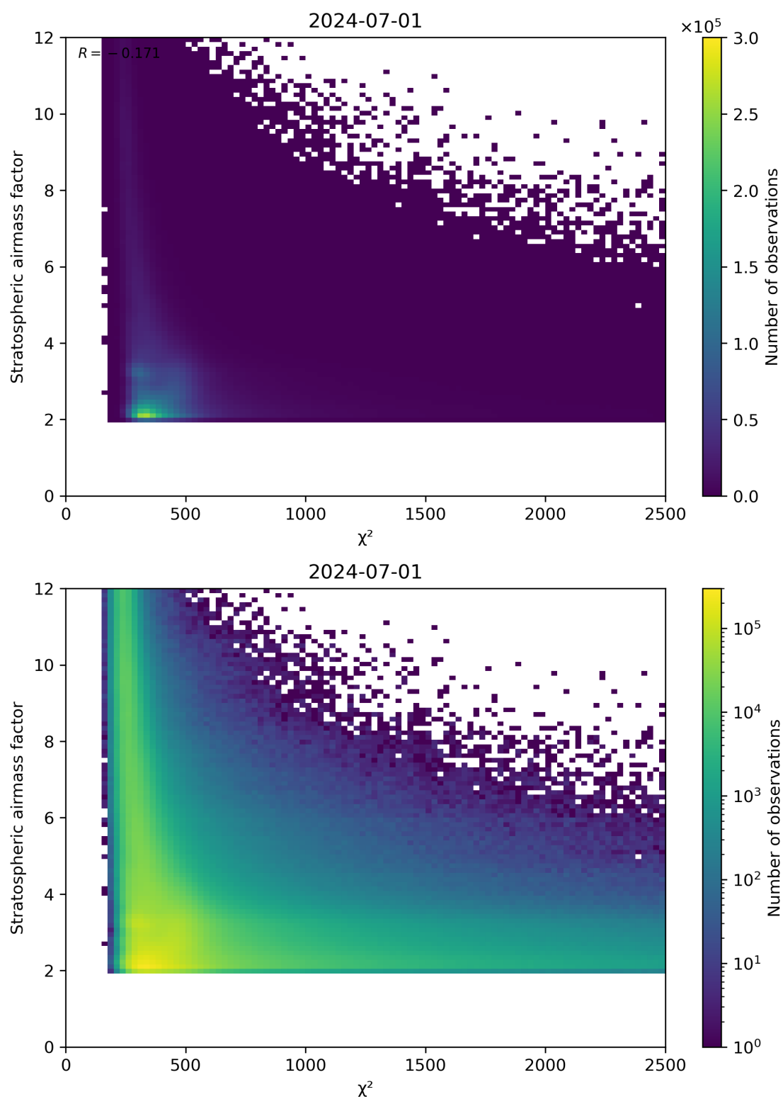
Figure 81: Scatter density plot of “ \chi^2 ” against “Stratospheric airmass factor” for 2024-06-30 to 2024-07-02.
