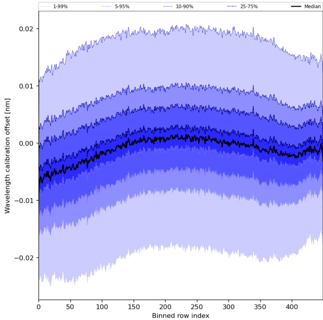
Figure 52: Along track statistics of “Wavelength calibration offset” for 2024-06-30 to 2024-07-02
