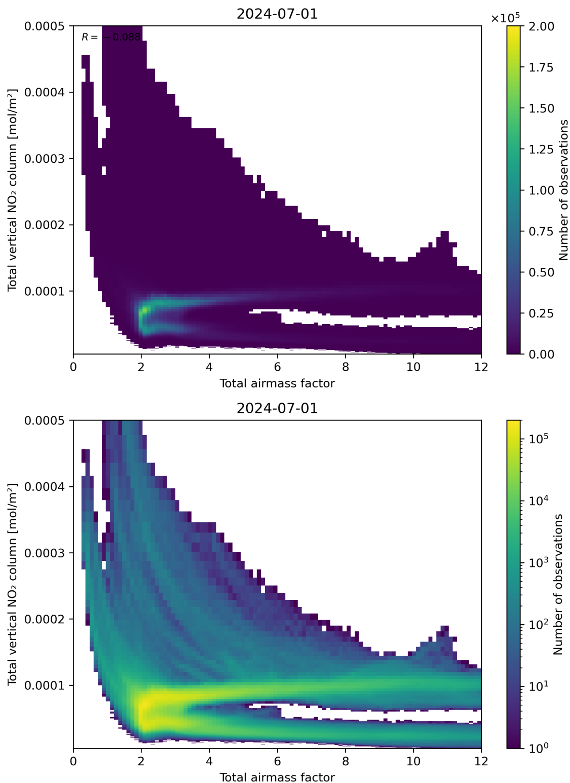
Figure 67: Scatter density plot of “Total airmass factor” against “Total vertical NO 2 column” for 2024-06-30 to 2024-07-02.
