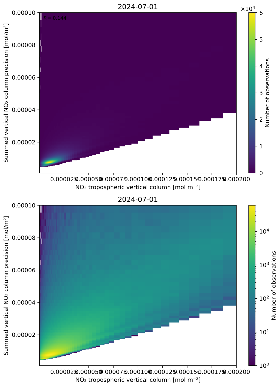
Figure 127: Scatter density plot of “NO 2 tropospheric vertical column” against “Summed vertical NO 2 column precision” for 2024-06-30 to 2024-07-02.
