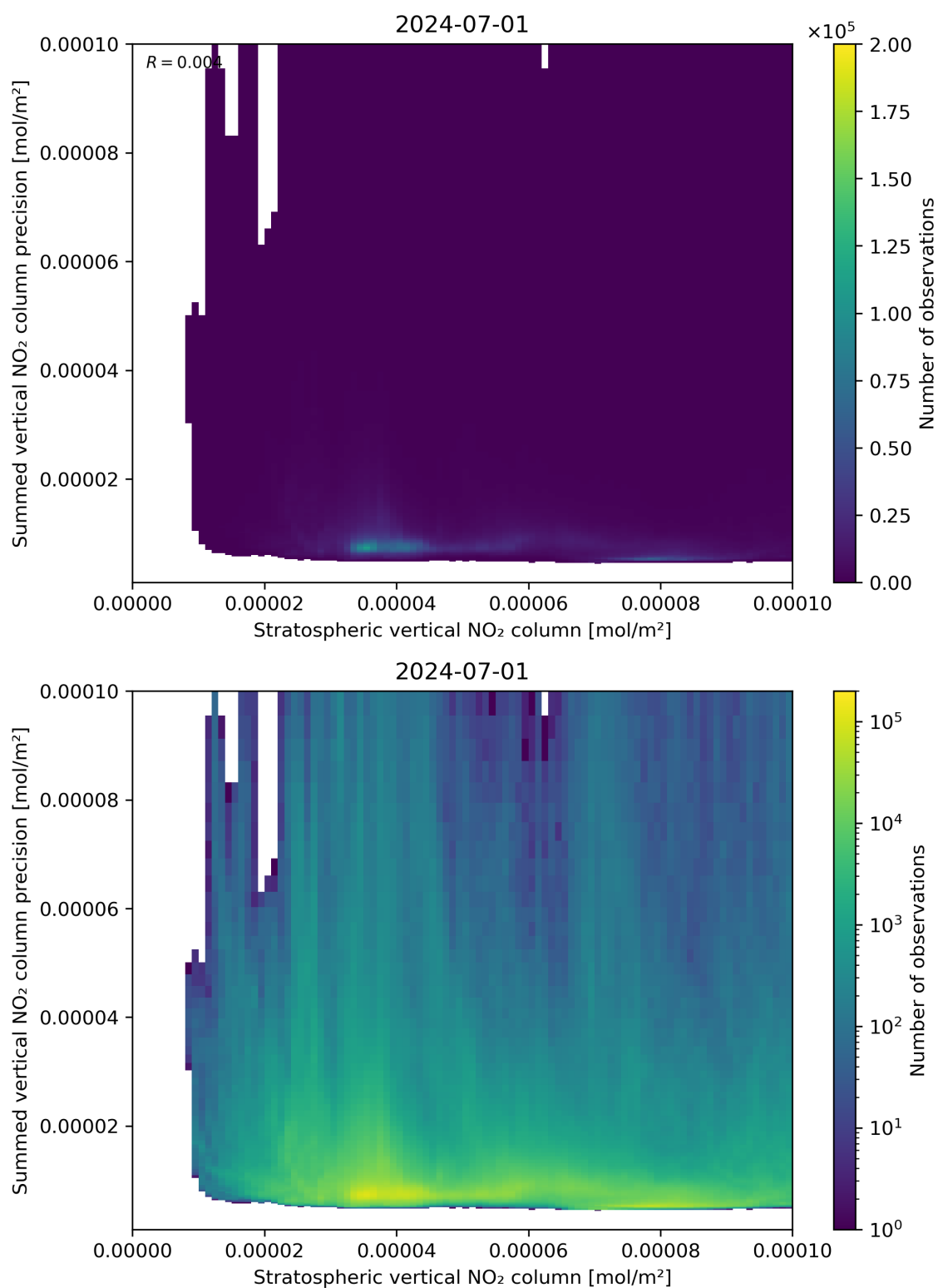
Figure 99: Scatter density plot of “Stratospheric vertical NO 2 column” against “Summed vertical NO 2 column precision” for 2024-06-30 to 2024-07-02.
