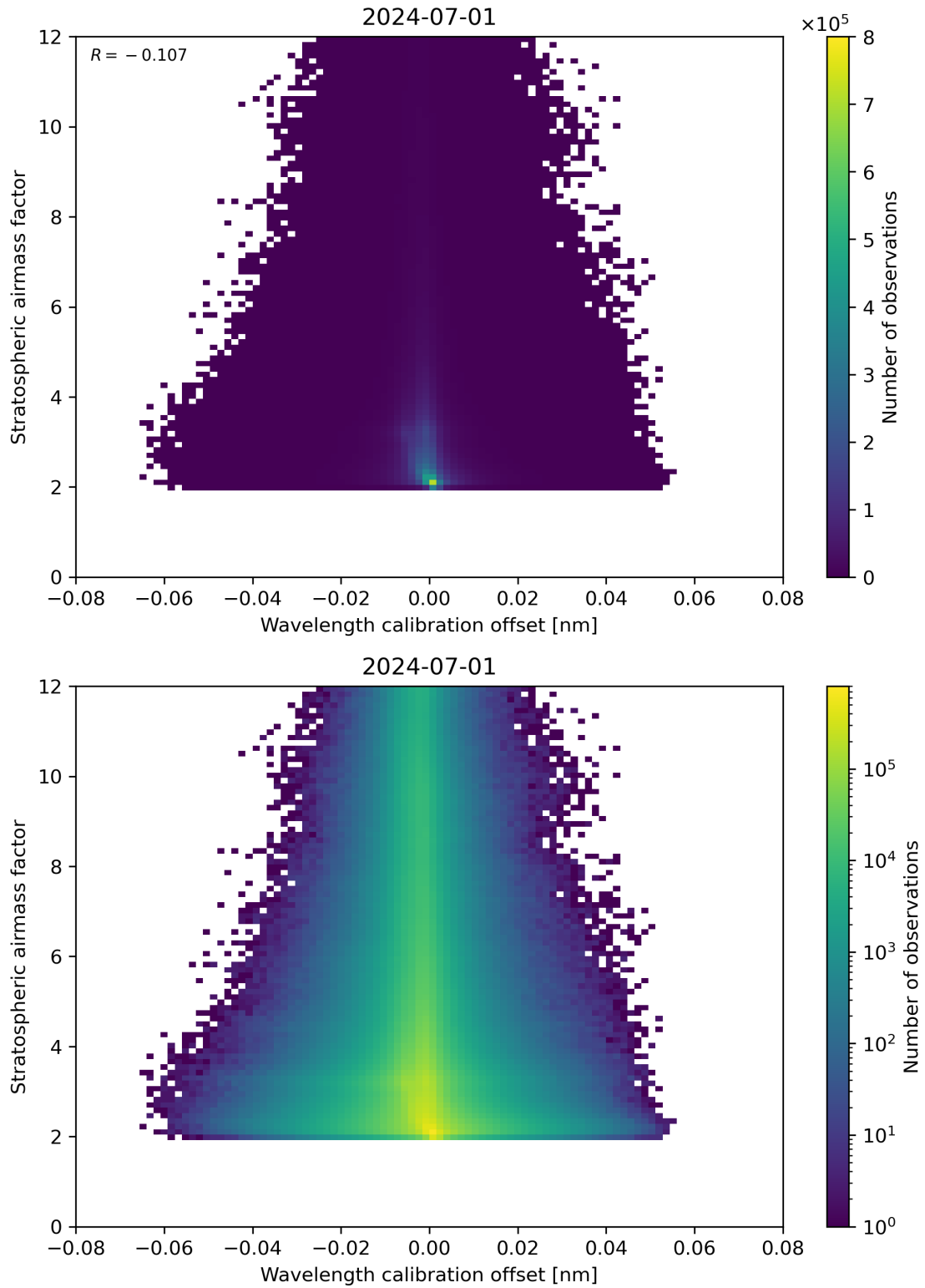
Figure 174: Scatter density plot of “Wavelength calibration offset” against “Stratospheric air mass factor” for 2024-06-30 to 2024-07-02.
