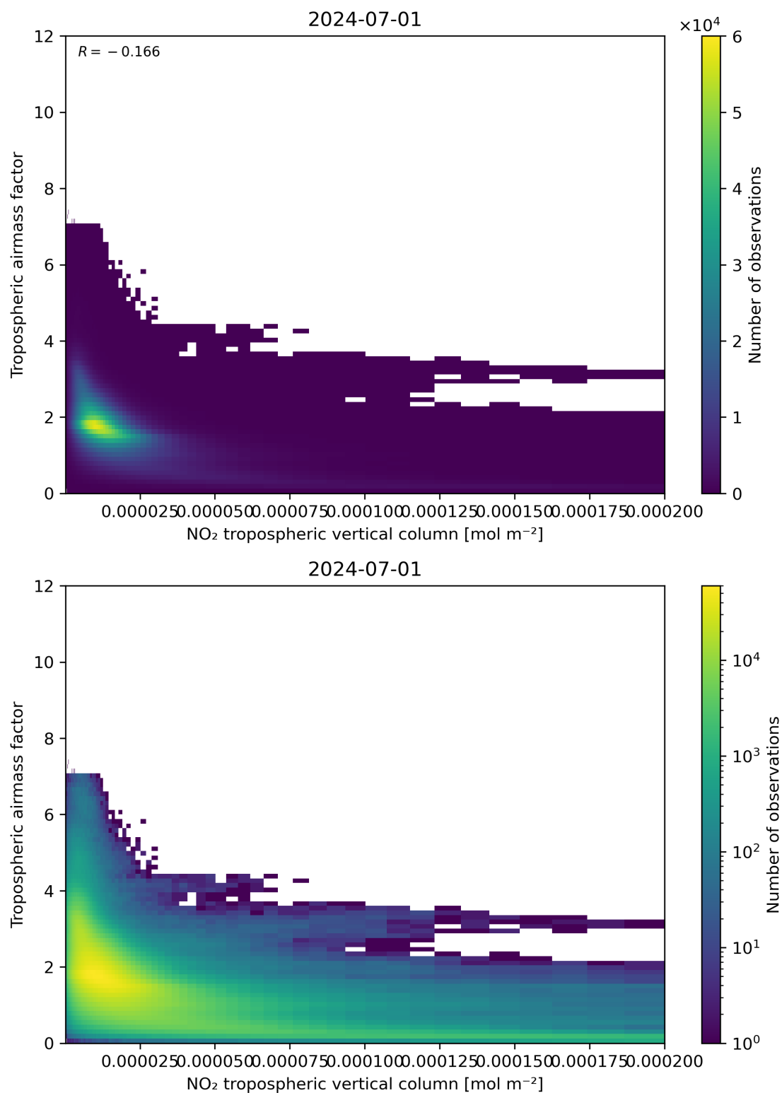
Figure 123: Scatter density plot of “NO 2 tropospheric vertical column” against “Tropospheric air mass factor” for 2024-06-30 to 2024-07-02.
