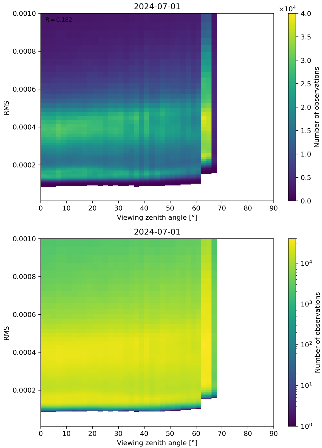
Figure 171: Scatter density plot of “Viewing zenith angle” against “RMS” for 2024-06-30 to 2024-07-02.
