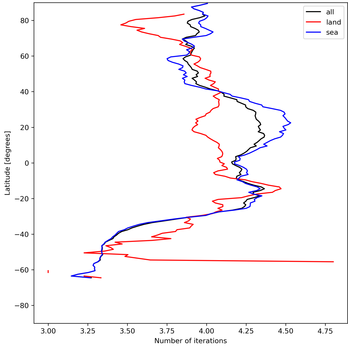
Figure 17: Zonal average of “Number of iterations” for 2024-06-30 to 2024-07-02.
