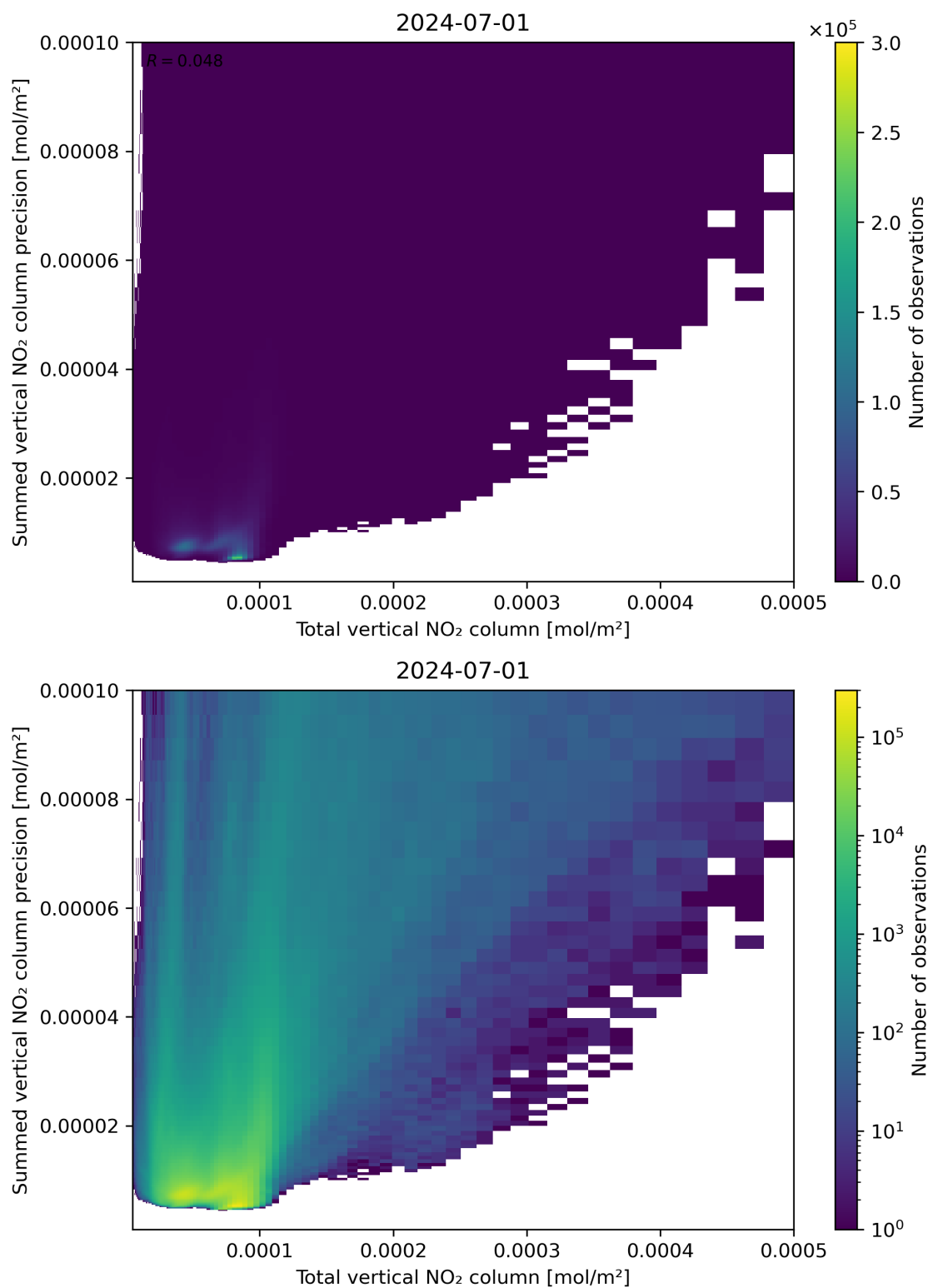
Figure 113: Scatter density plot of “Total vertical NO 2 column” against “Summed vertical NO 2 column precision” for 2024-06-30 to 2024-07-02.
