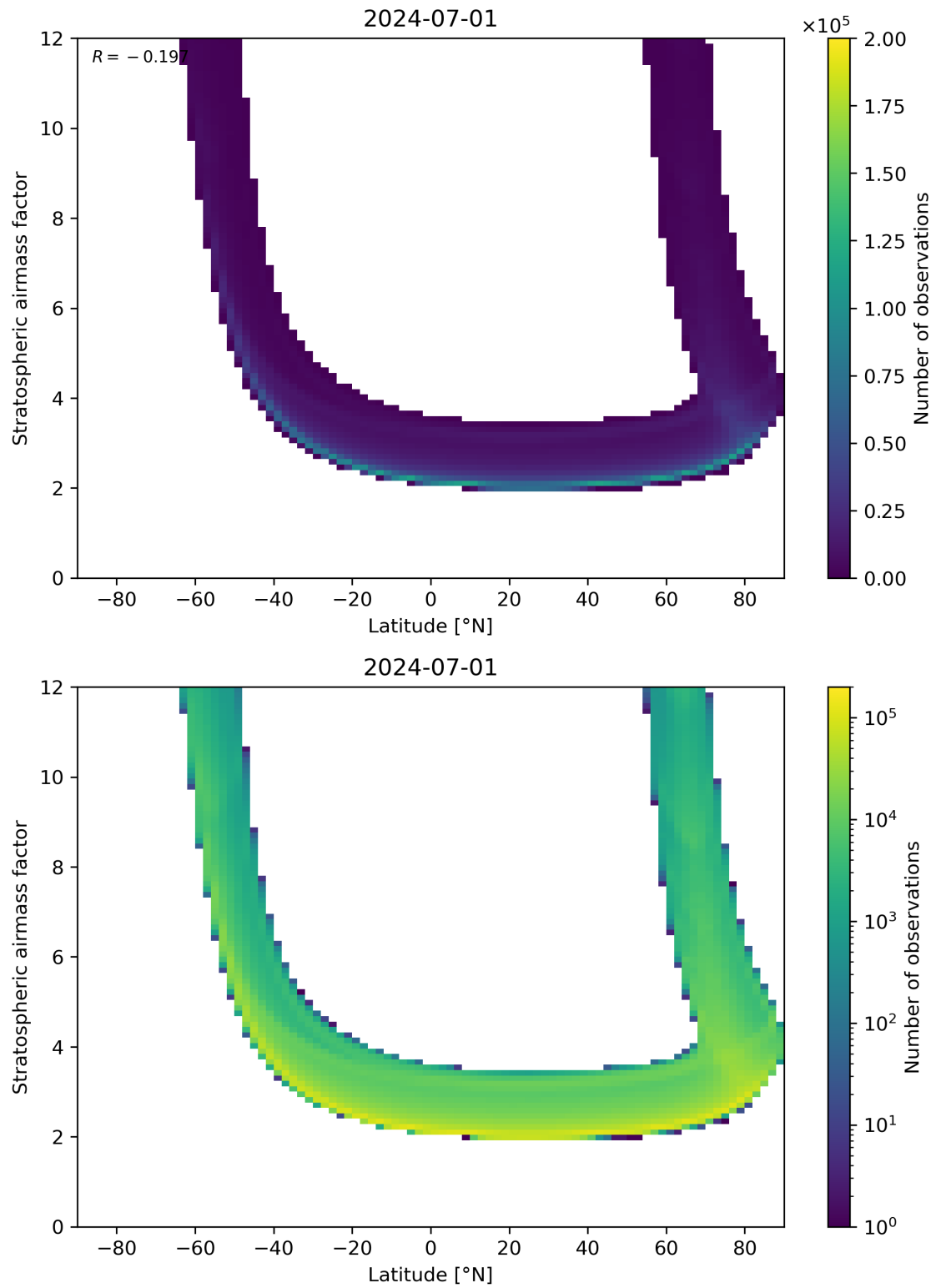
Figure 83: Scatter density plot of “Latitude” against “Stratospheric air mass factor” for 2024-06-30 to 2024-07-02.
