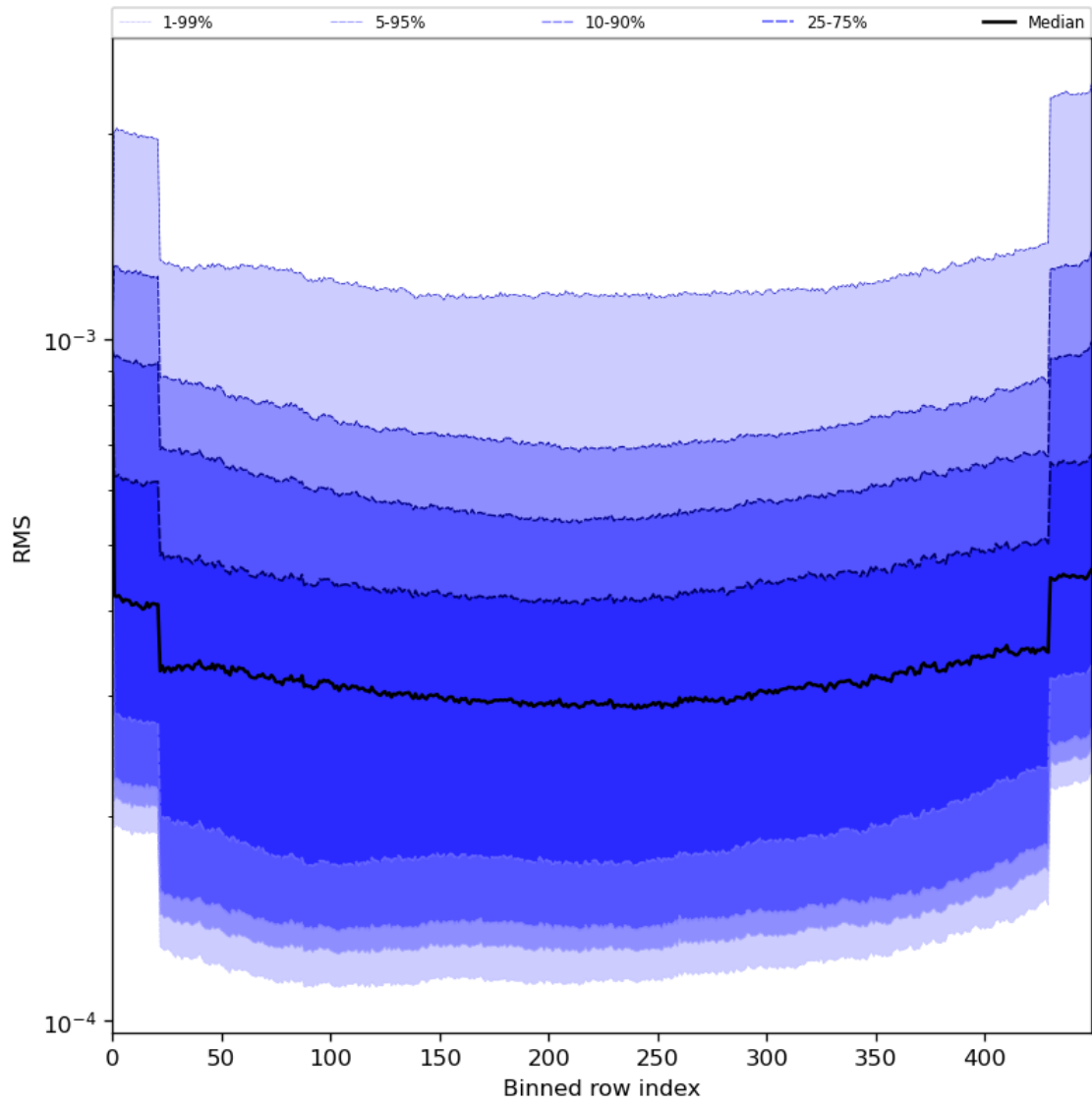
Figure 60: Along track statistics of “RMS” for 2024-06-30 to 2024-07-02
