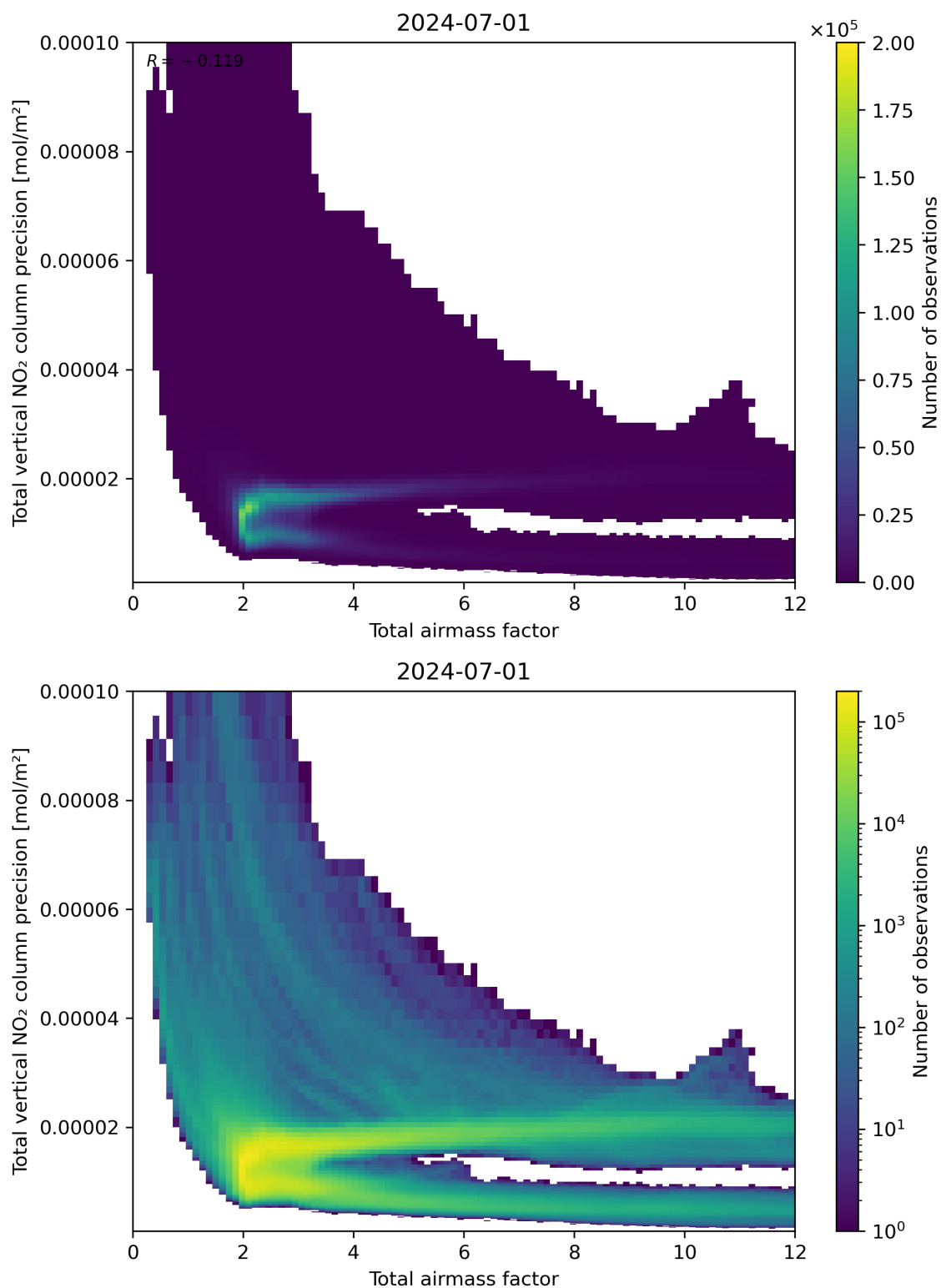
Figure 68: Scatter density plot of “Total airmass factor” against “Total vertical NO 2 column precision” for 2024-06-30 to 2024-07-02.
