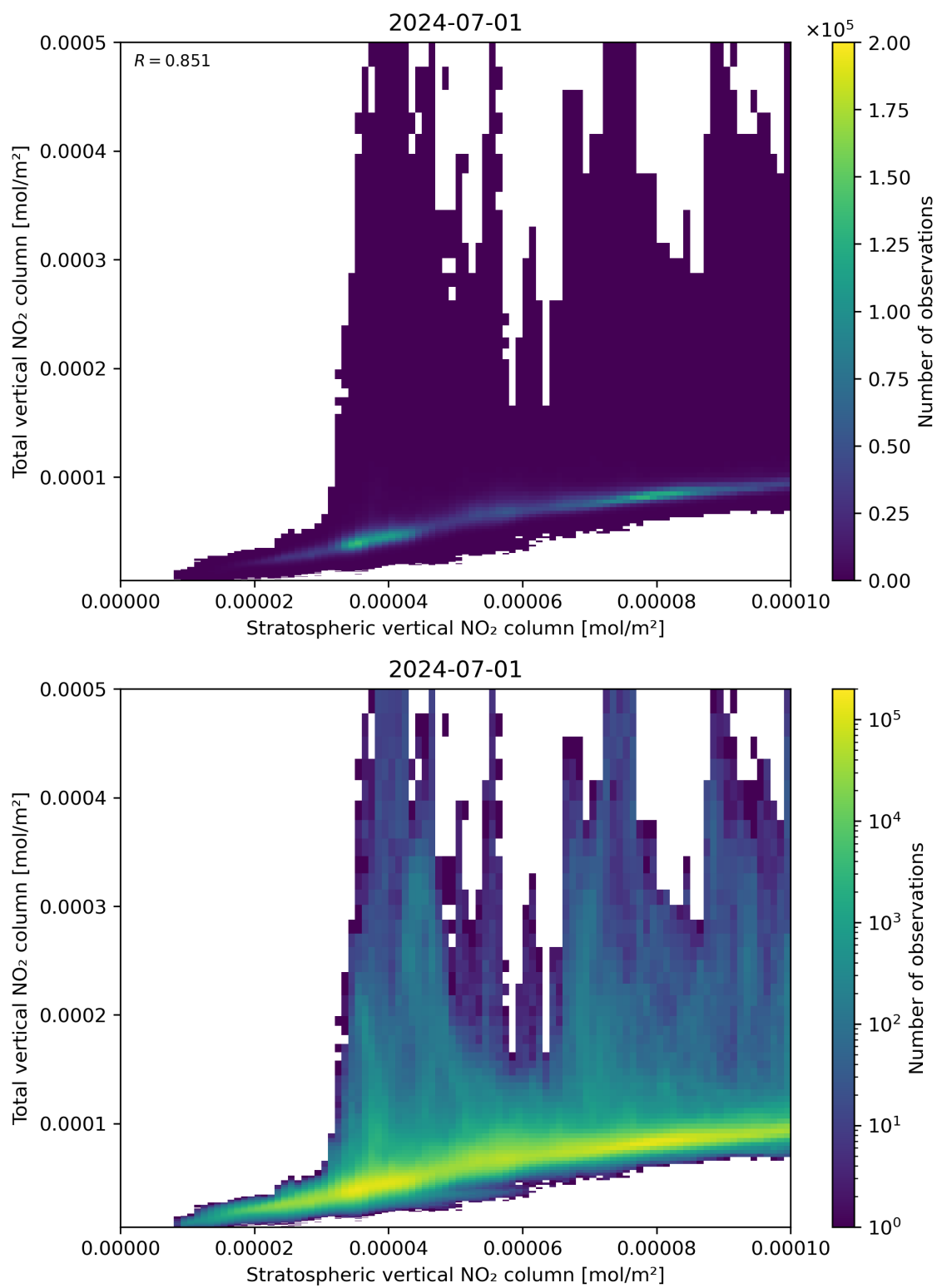
Figure 100: Scatter density plot of “Stratospheric vertical NO 2 column” against “Total vertical NO 2 column” for 2024-06-30 to 2024-07-02.
