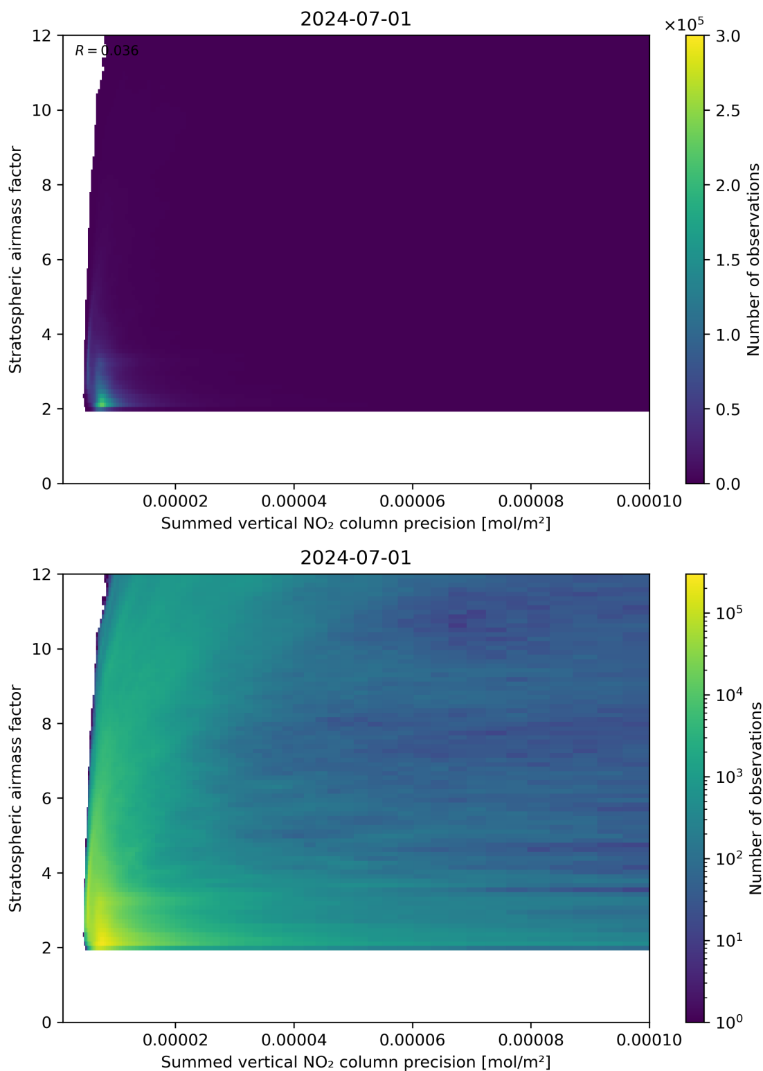
Figure 106: Scatter density plot of “Summed vertical NO 2 column precision” against “Stratospheric airmass factor” for 2024-06-30 to 2024-07-02.
