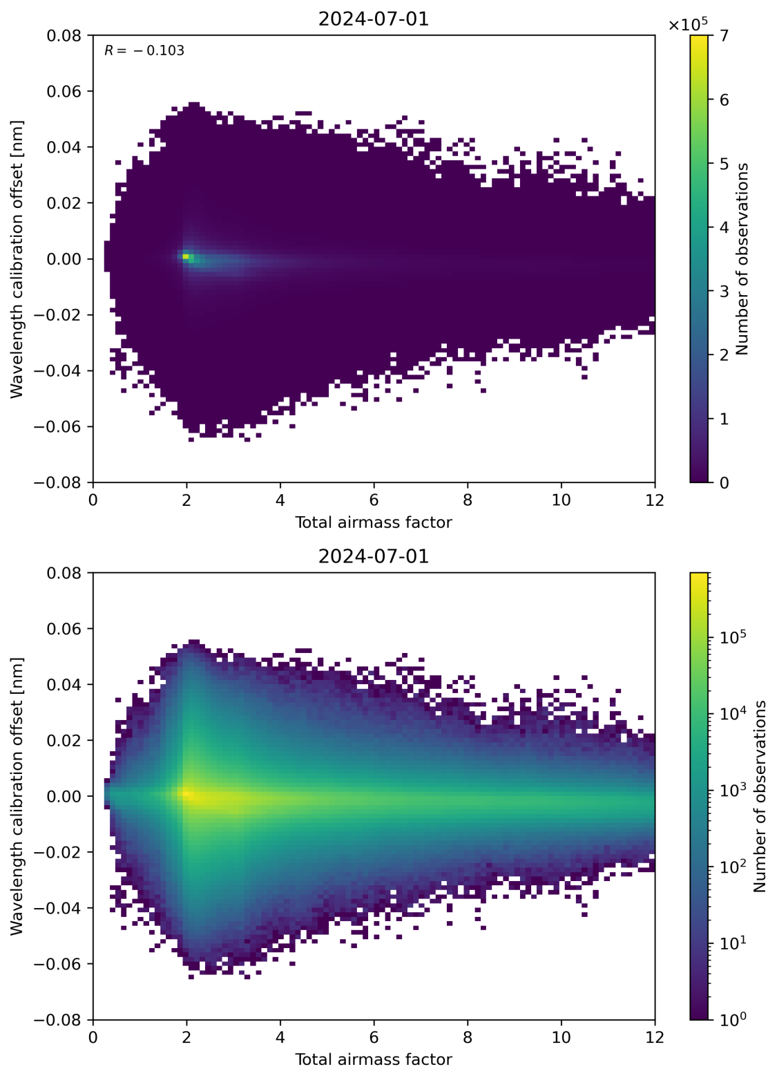
Figure 70: Scatter density plot of “Total airmass factor” against “Wavelength calibration offset” for 2024-06-30 to 2024-07-02.
