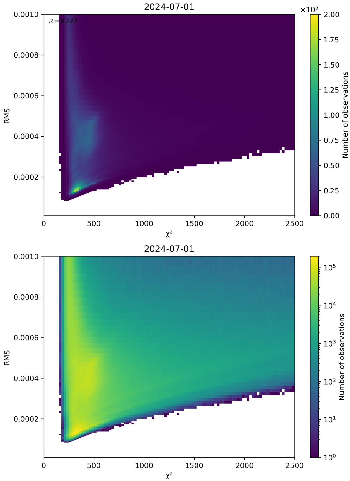
Figure 82: Scatter density plot of “ \chi^2 ” against “RMS” for 2024-06-30 to 2024-07-02.
