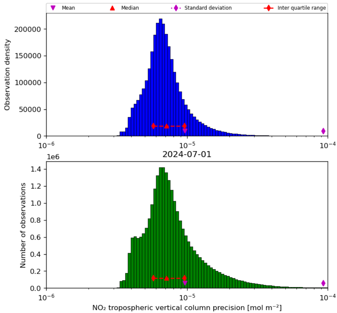
Figure 30: Histogram of “NO 2 tropospheric vertical column precision” for 2024-06-30 to 2024-07-02
