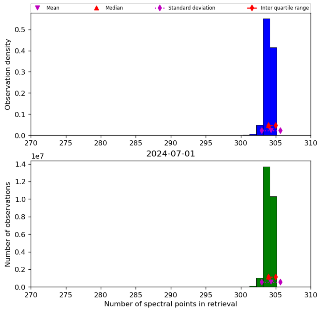
Figure 33: Histogram of “Number of spectral points in retrieval” for 2024-06-30 to 2024-07-02
