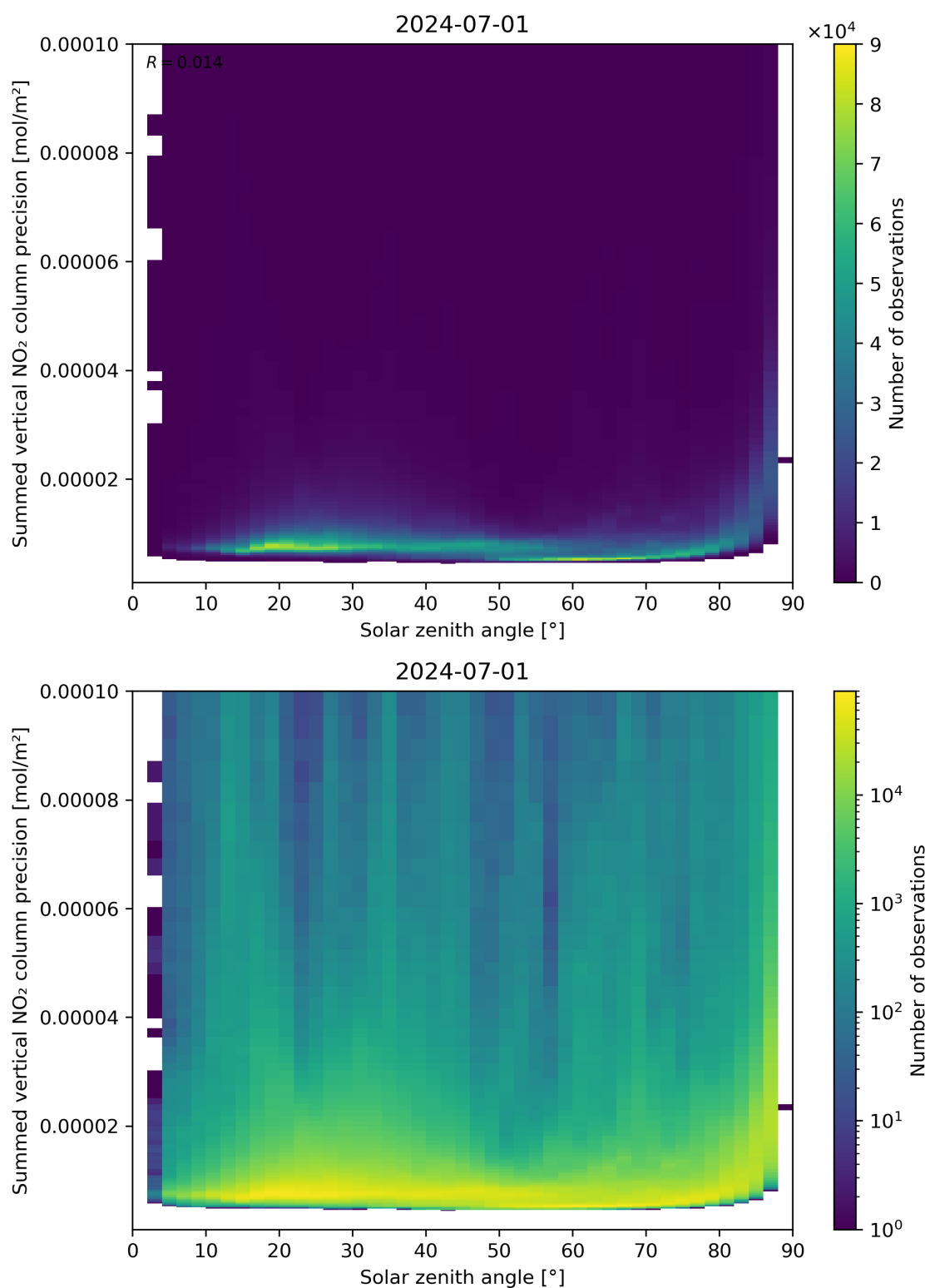
Figure 152: Scatter density plot of “Solar zenith angle” against “Summed vertical NO 2 column precision” for 2024-06-30 to 2024-07-02.
