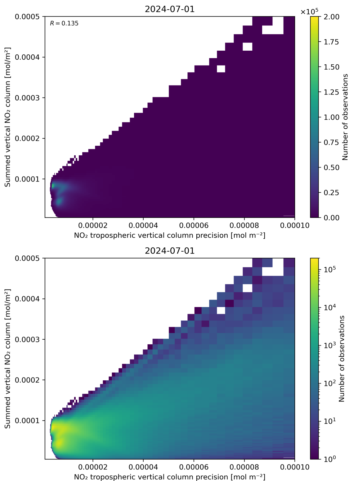
Figure 136: Scatter density plot of “NO 2 tropospheric vertical column precision” against “Summed vertical NO 2 column” for 2024-06-30 to 2024-07-02.
