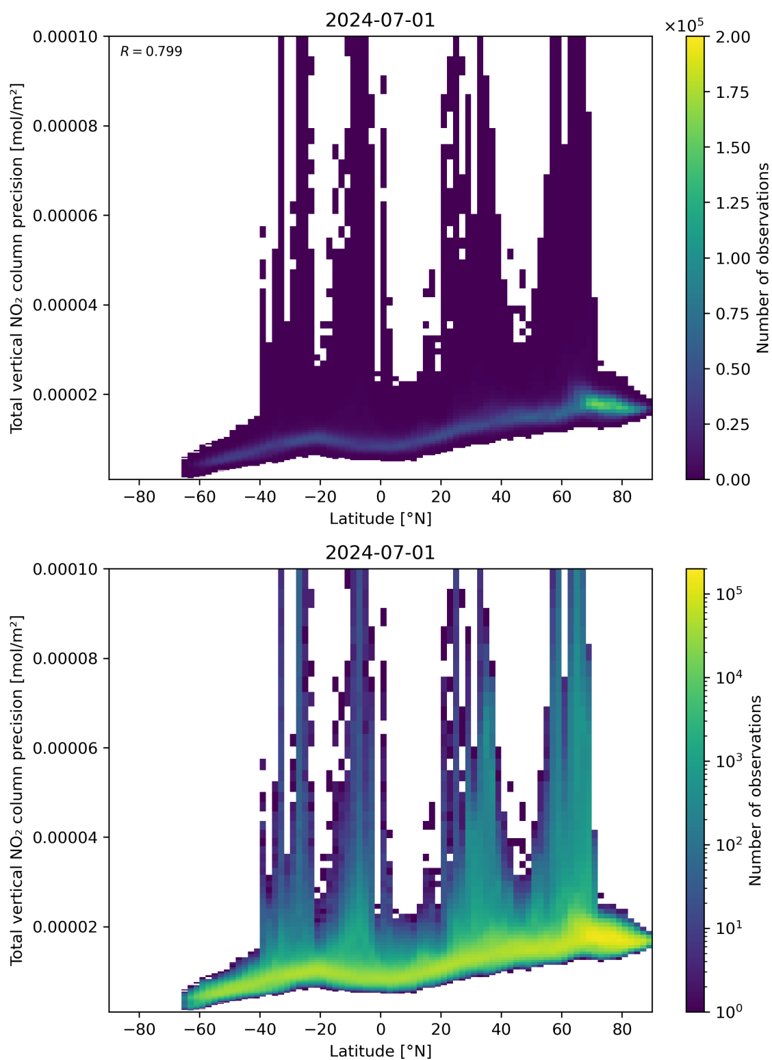
Figure 91: Scatter density plot of “Latitude” against “Total vertical NO 2 column precision” for 2024-06-30 to 2024-07-02.
