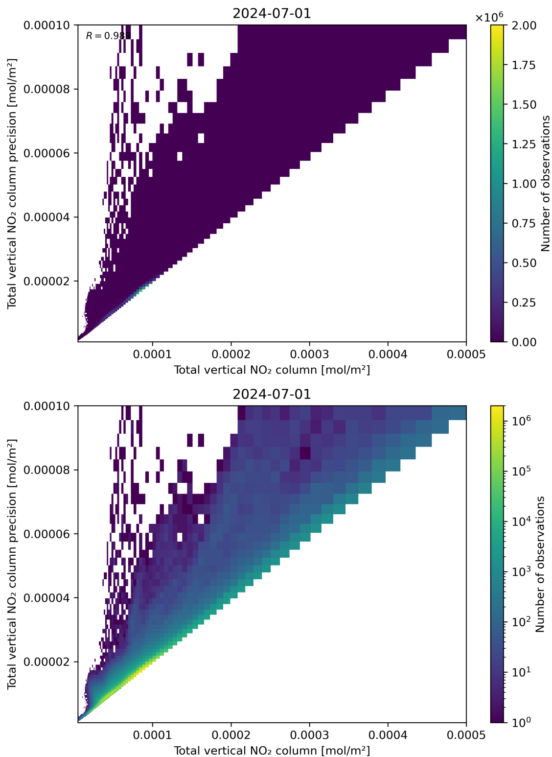
Figure 114: Scatter density plot of “Total vertical NO 2 column” against “Total vertical NO 2 column precision” for 2024-06-30 to 2024-07-02.
