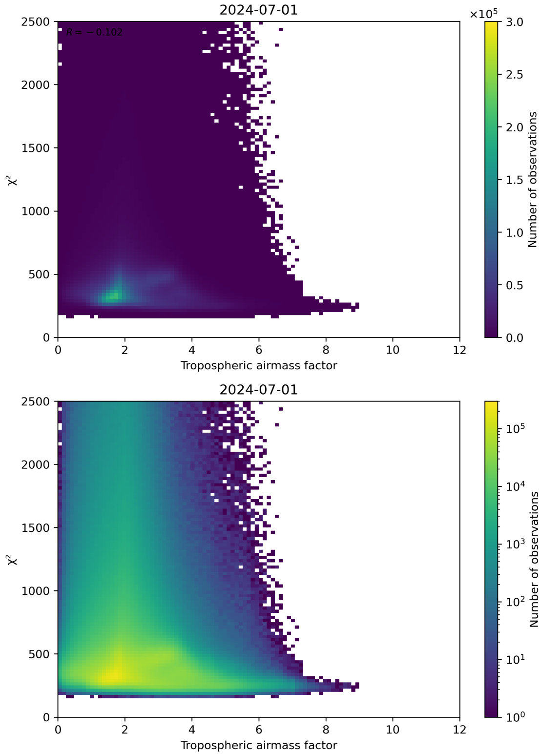
Figure 73: Scatter density plot of “Tropospheric airmass factor” against “ \chi^2 ” for 2024-06-30 to 2024-07-02.
