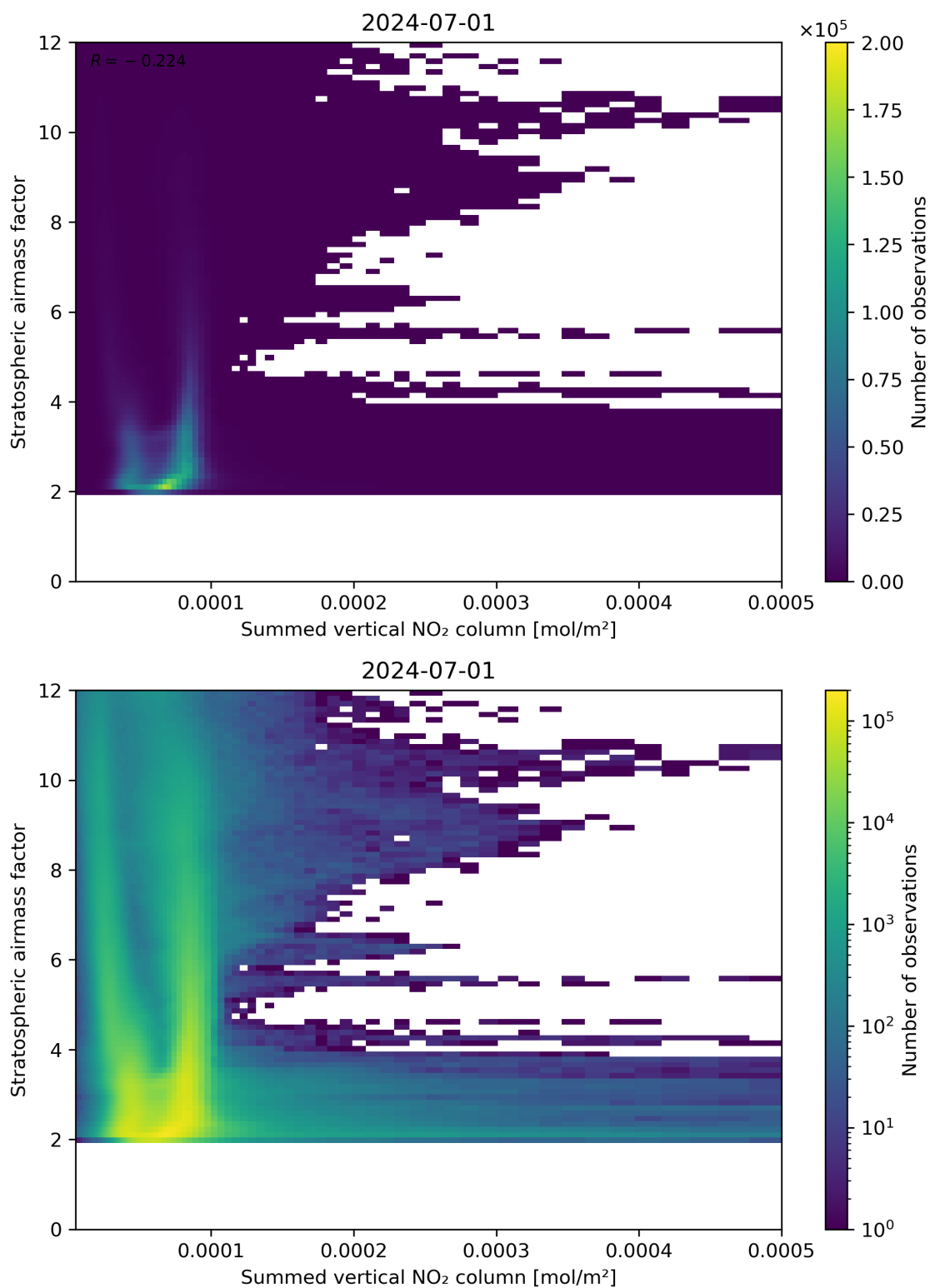
Figure 103: Scatter density plot of “Summed vertical NO 2 column” against “Stratospheric airmass factor” for 2024-06-30 to 2024-07-02.
