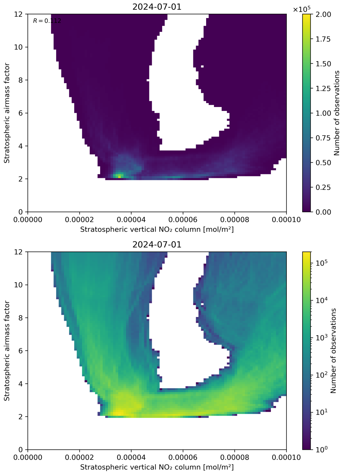
Figure 96: Scatter density plot of “Stratospheric vertical NO 2 column” against “Stratospheric airmass factor” for 2024-06-30 to 2024-07-02.
