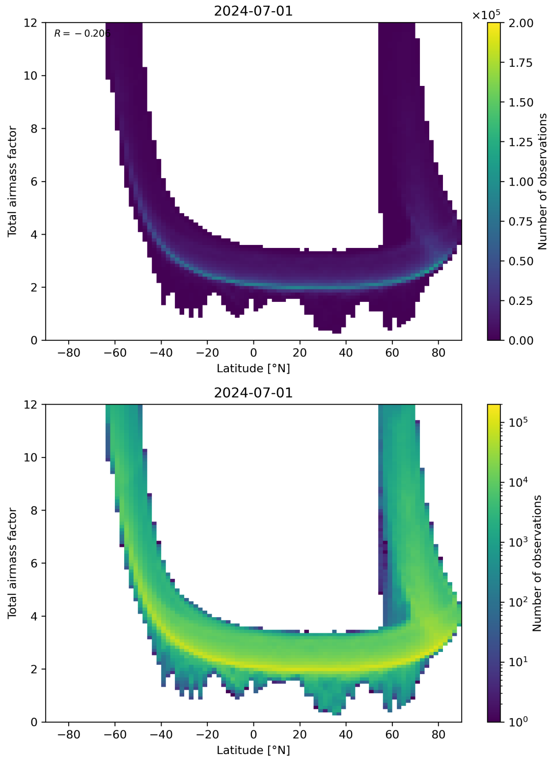
Figure 84: Scatter density plot of “Latitude” against “Total airmass factor” for 2024-06-30 to 2024-07-02.
