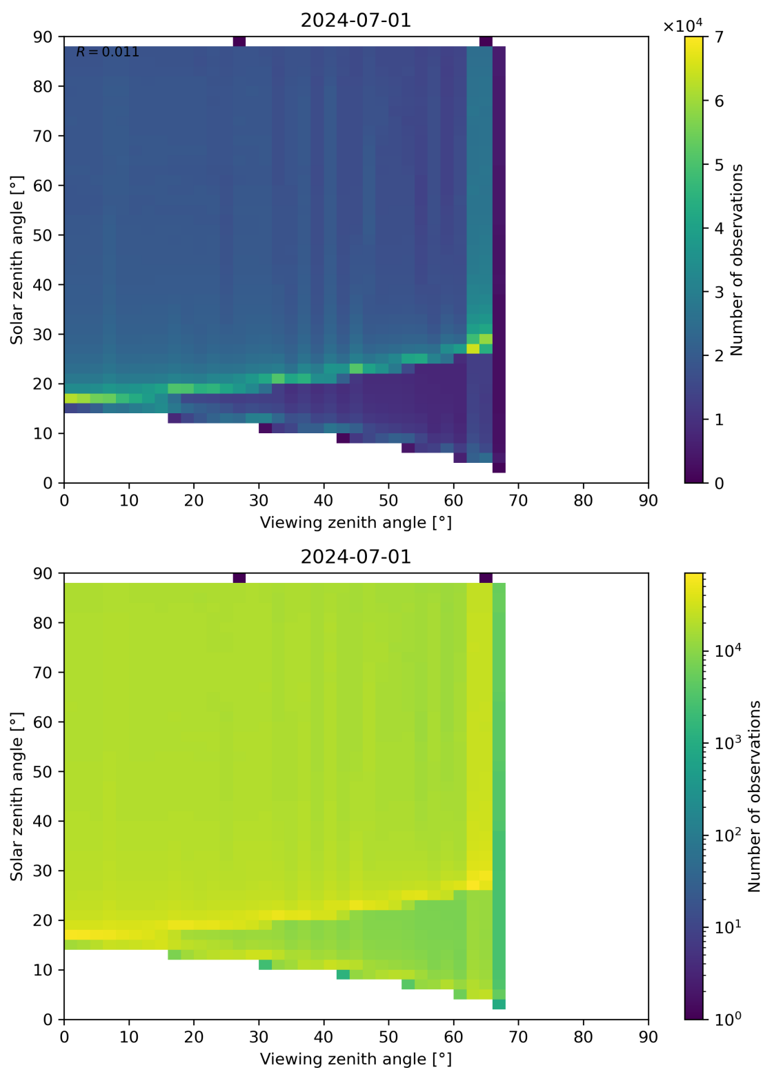
Figure 172: Scatter density plot of “Viewing zenith angle” against “Solar zenith angle” for 2024-06-30 to 2024-07-02.
