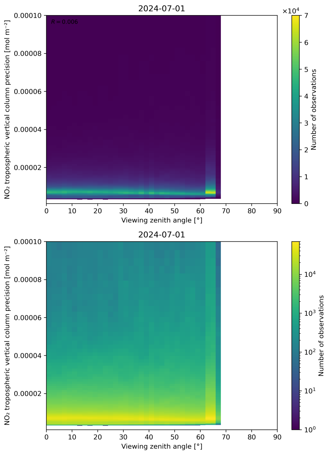
Figure 170: Scatter density plot of “Viewing zenith angle” against “NO 2 tropospheric vertical column precision” for 2024-06-30 to 2024-07-02.
