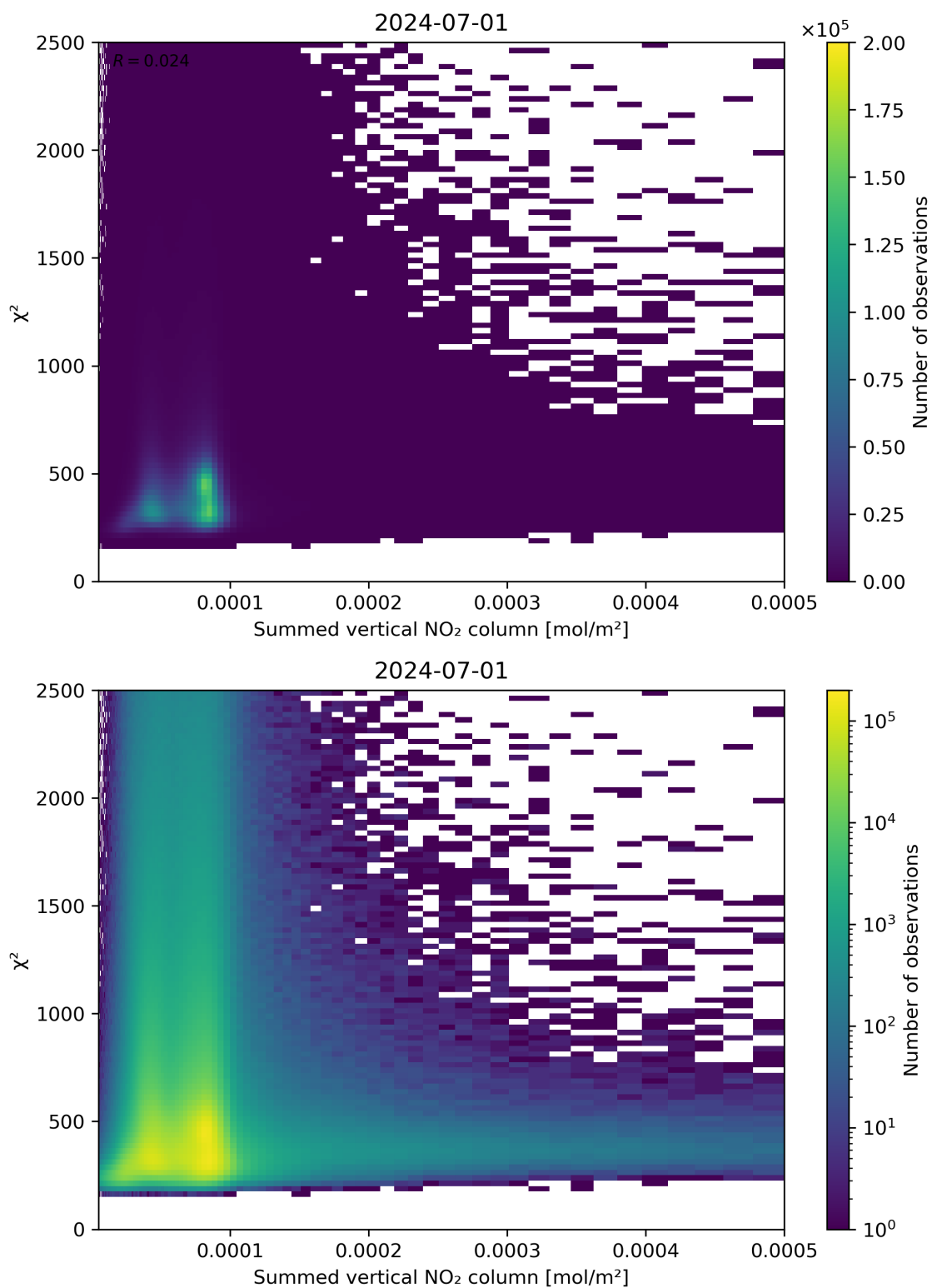
Figure 104: Scatter density plot of “Summed vertical NO 2 column” against “ \chi^2 ” for 2024-06-30 to 2024-07-02.
