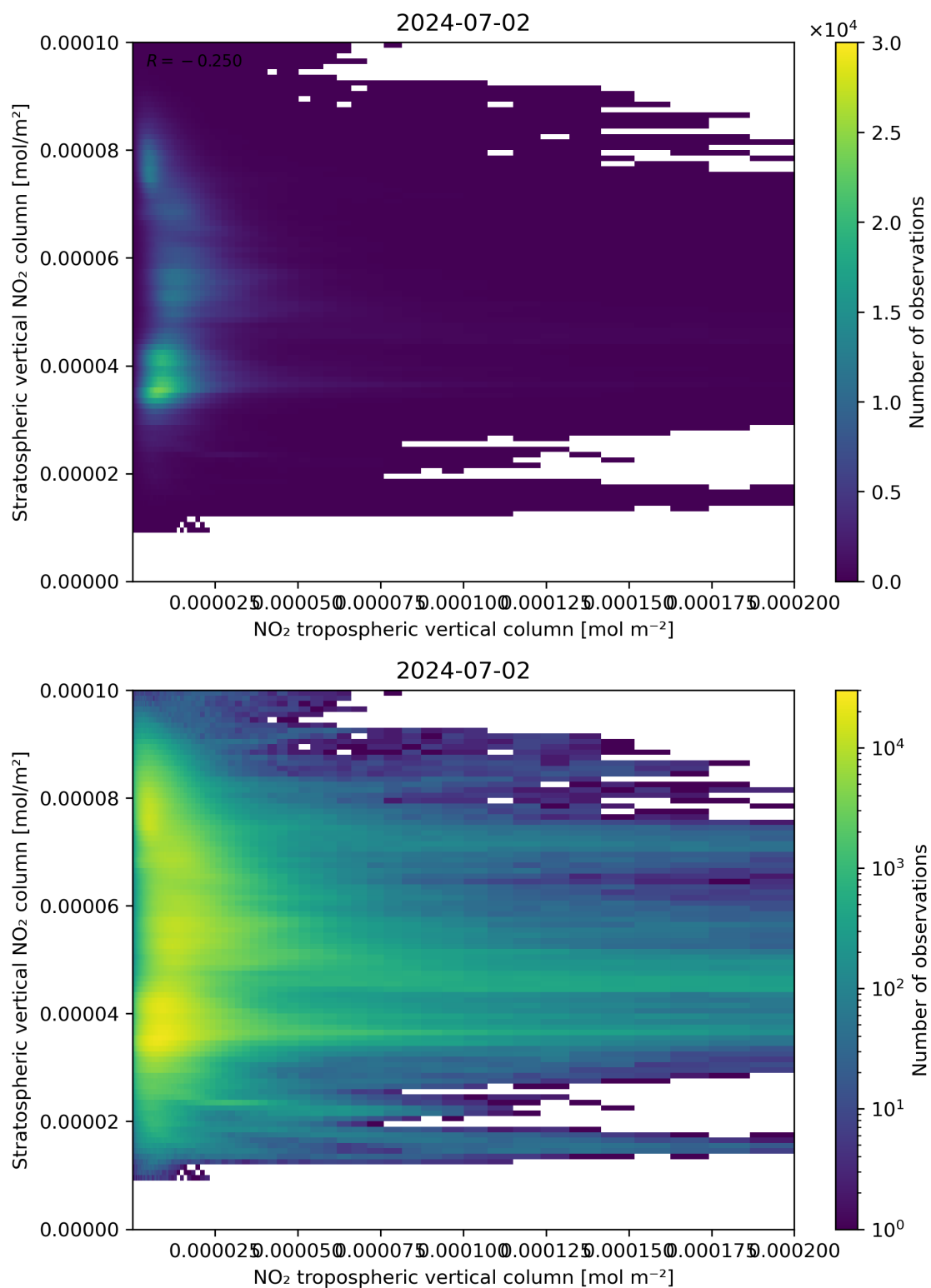
Figure 125: Scatter density plot of “NO 2 tropospheric vertical column” against “Stratospheric vertical NO 2 column” for 2024-07-01 to 2024-07-03.
