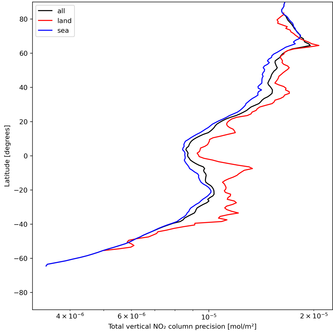
Figure 22: Zonal average of “Total vertical NO 2 column precision” for 2024-07-01 to 2024-07-03.
