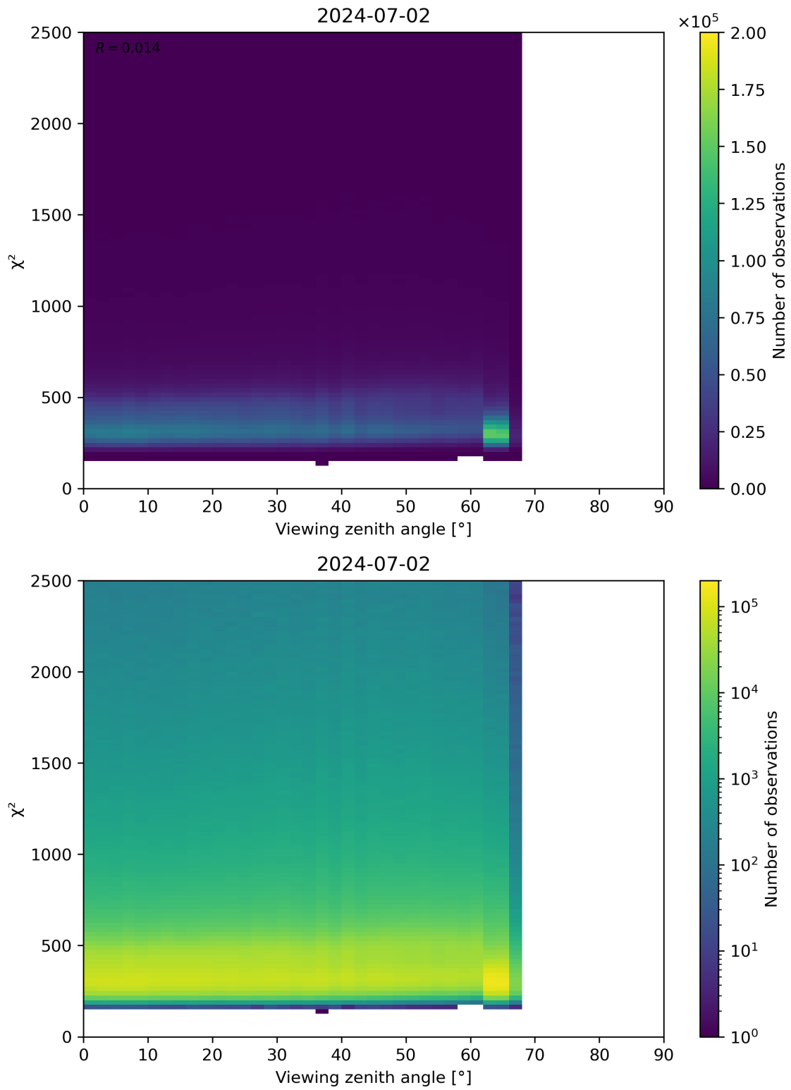
Figure 162: Scatter density plot of “Viewing zenith angle” against “ \chi^2 ” for 2024-07-01 to 2024-07-03.
