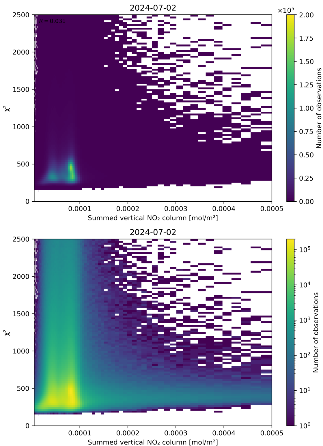
Figure 104: Scatter density plot of “Summed vertical NO 2 column” against “ \chi^2 ” for 2024-07-01 to 2024-07-03.
