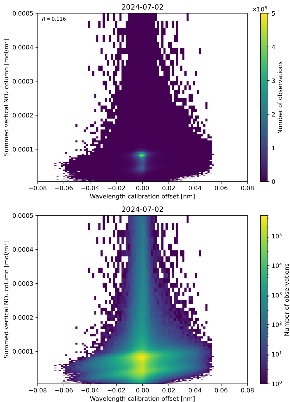
Figure 177: Scatter density plot of “Wavelength calibration offset” against “Summed vertical NO 2 column” for 2024-07-01 to 2024-07-03.
