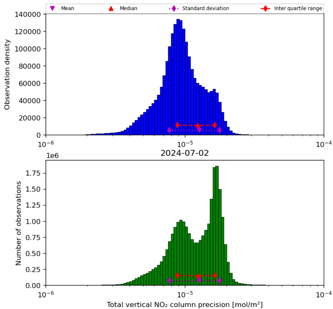
Figure 39: Histogram of “Total vertical NO 2 column precision” for 2024-07-01 to 2024-07-03
