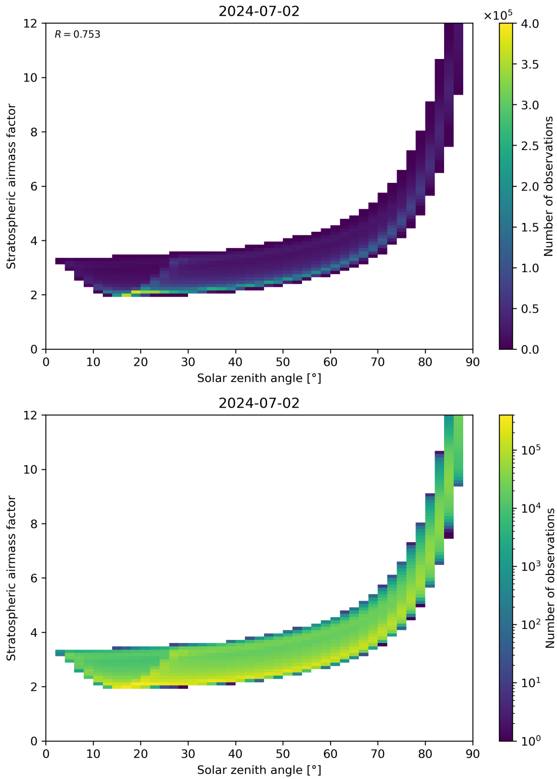
Figure 145: Scatter density plot of “Solar zenith angle” against “Stratospheric airmass factor” for 2024-07-01 to 2024-07-03.
