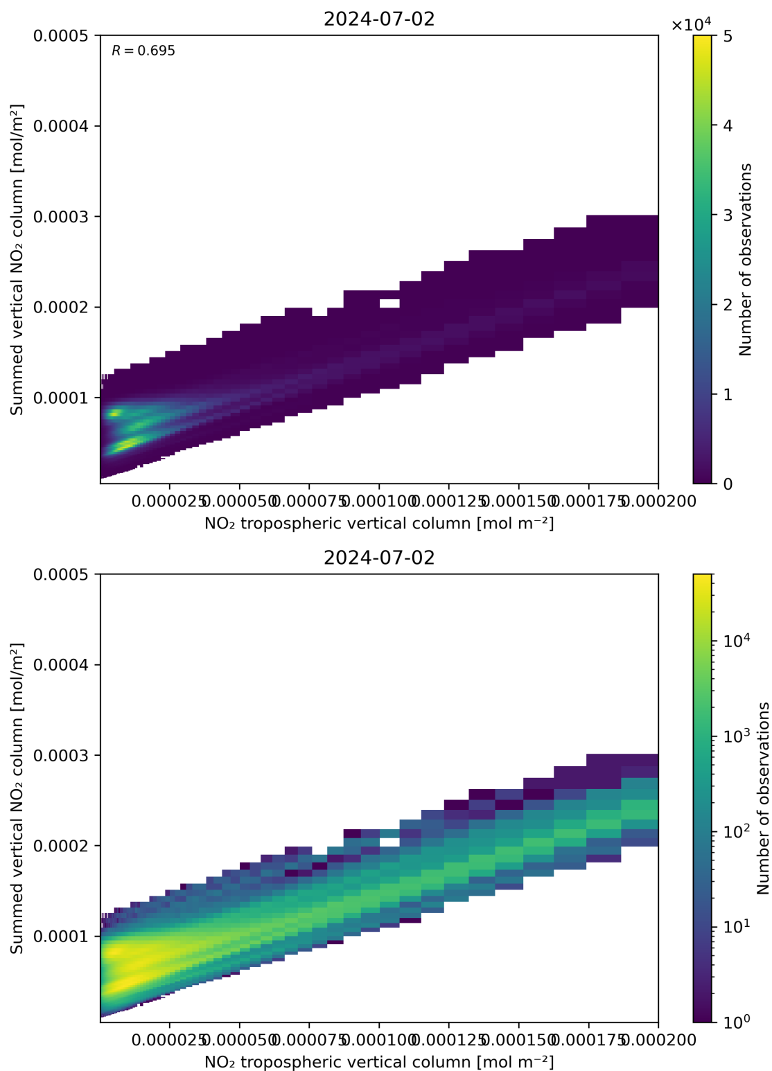
Figure 126: Scatter density plot of “NO 2 tropospheric vertical column” against “Summed vertical NO 2 column” for 2024-07-01 to 2024-07-03.
