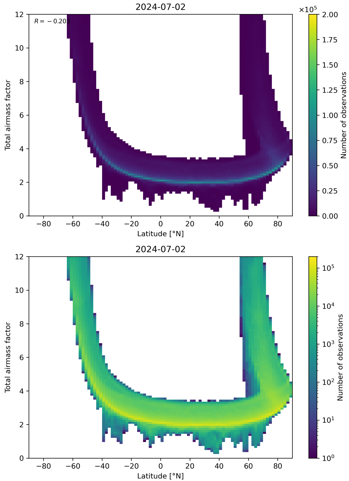
Figure 84: Scatter density plot of “Latitude” against “Total airmass factor” for 2024-07-01 to 2024-07-03.
