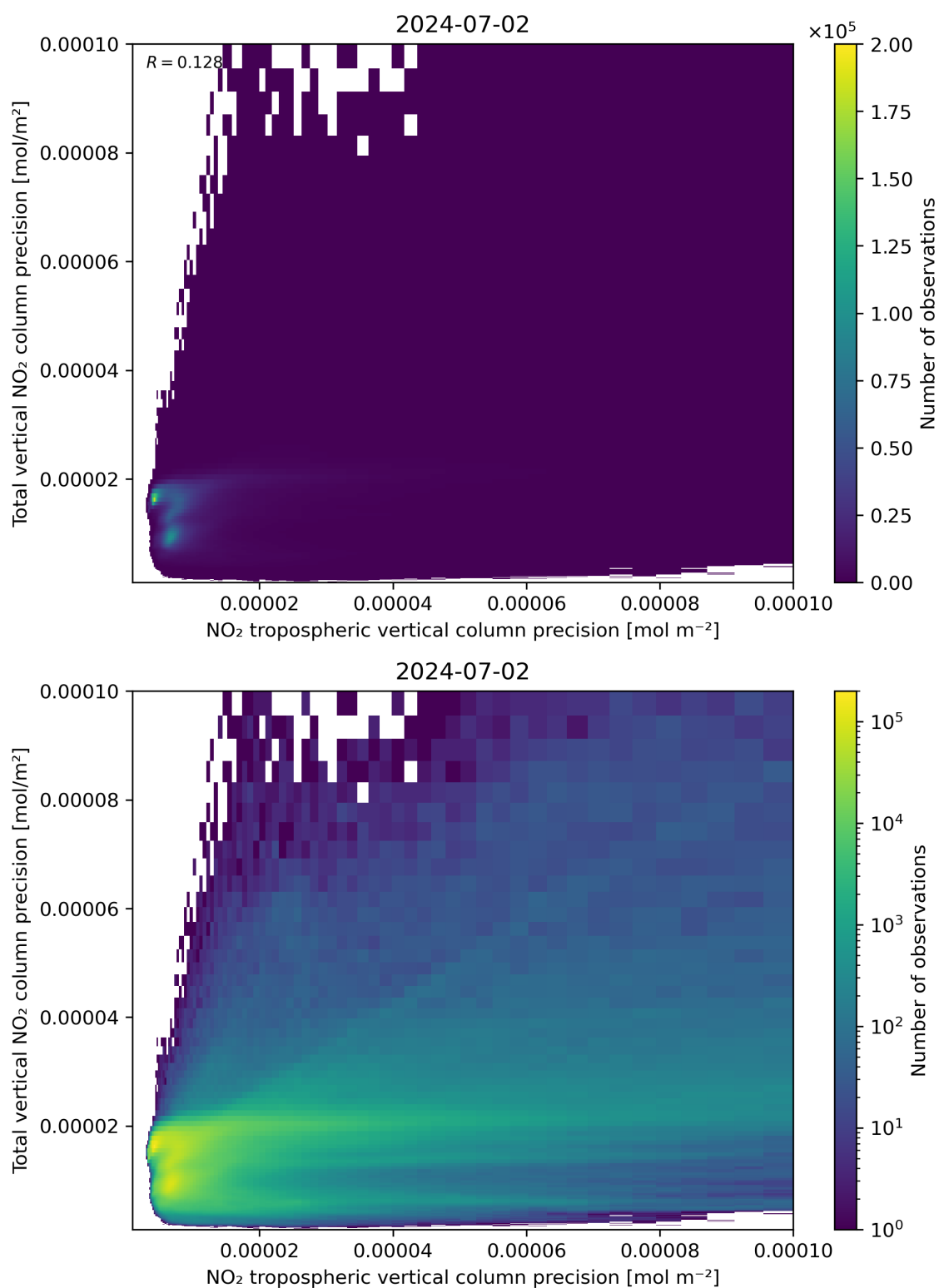
Figure 139: Scatter density plot of “NO 2 tropospheric vertical column precision” against “Total vertical NO 2 column precision” for 2024-07-01 to 2024-07-03.
