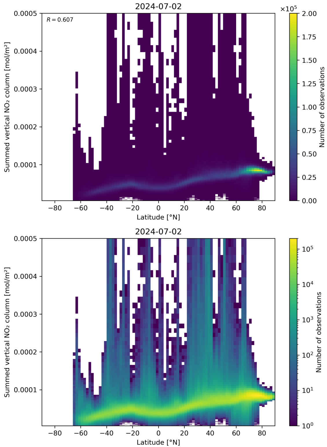
Figure 88: Scatter density plot of “Latitude” against “Summed vertical NO 2 column” for 2024-07-01 to 2024-07-03.
