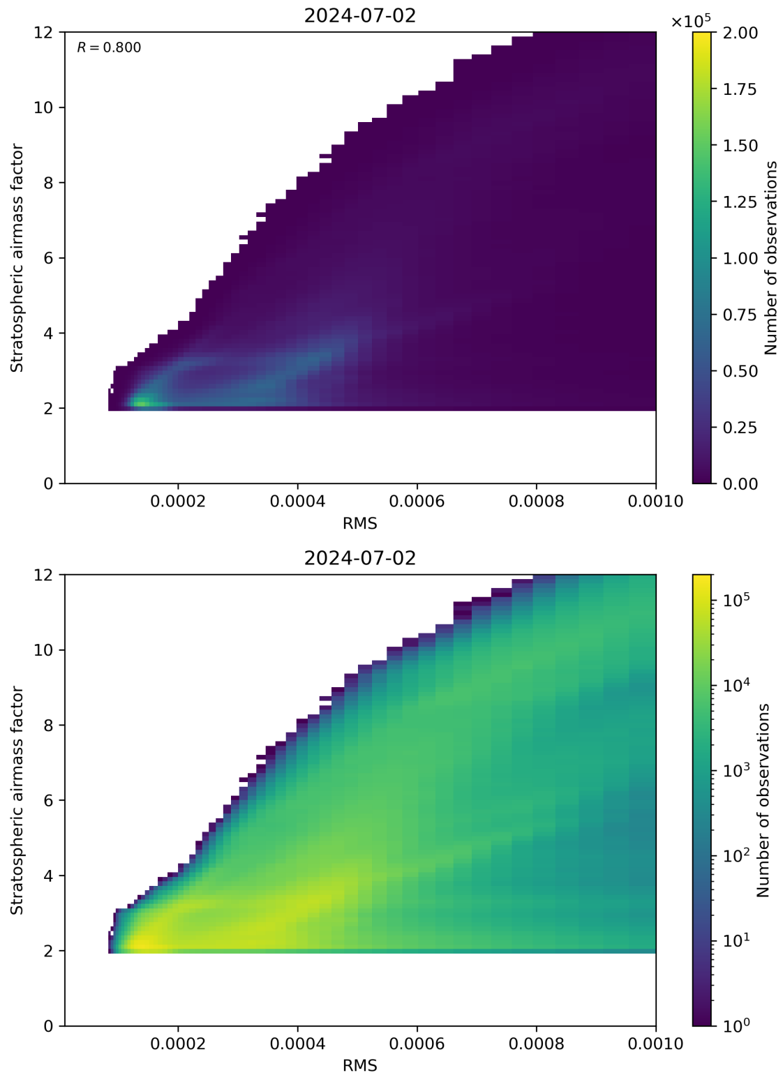
Figure 144: Scatter density plot of “RMS” against “Stratospheric airmass factor” for 2024-07-01 to 2024-07-03.
