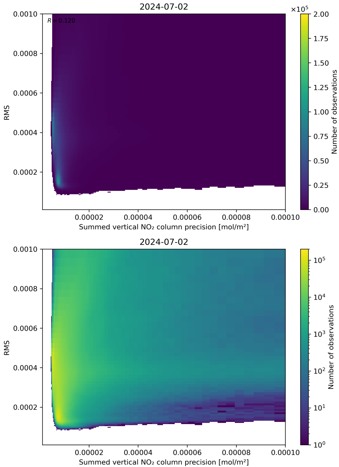
Figure 108: Scatter density plot of “Summed vertical NO 2 column precision” against “RMS” for 2024-07-01 to 2024-07-03.
