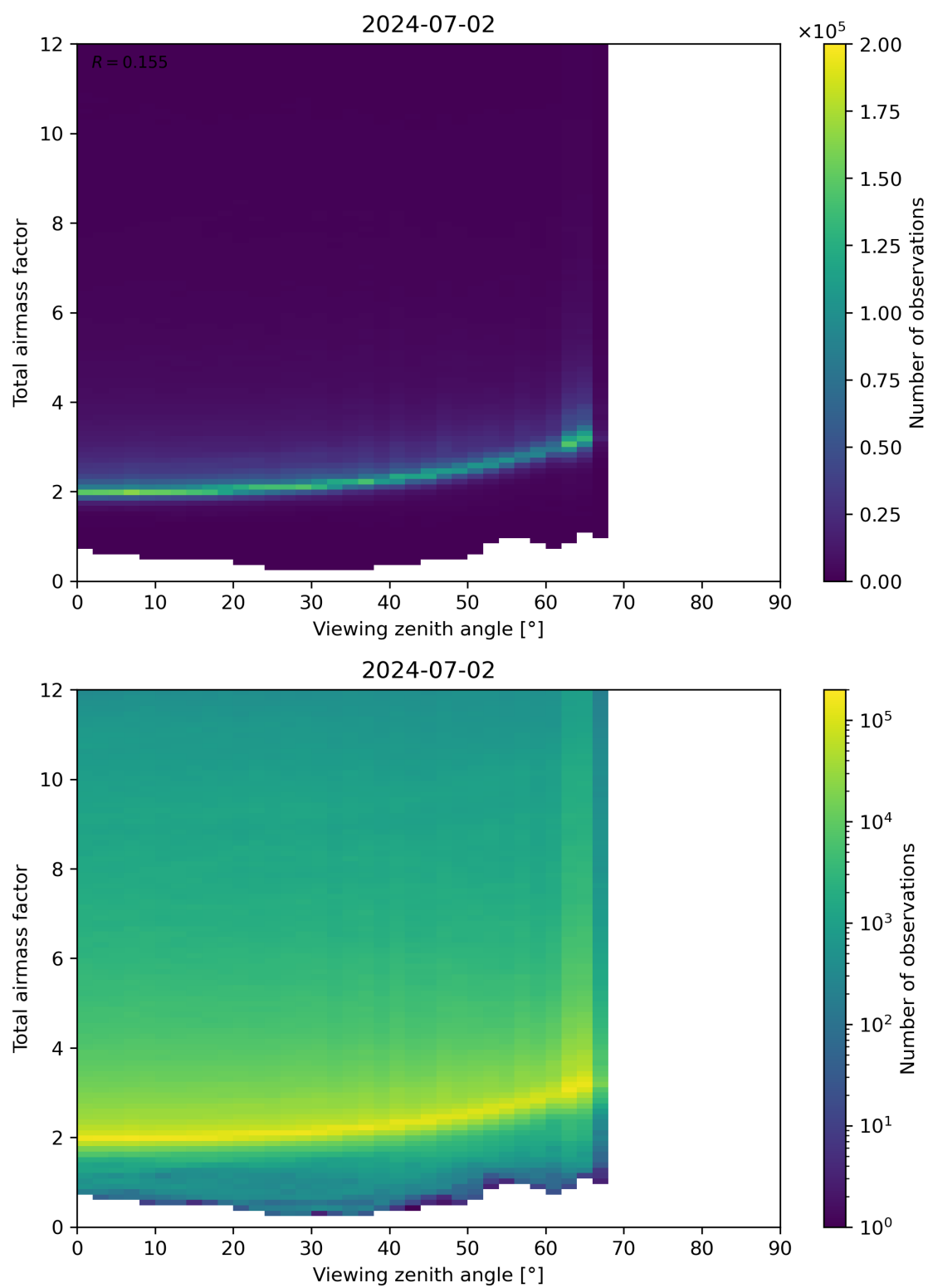
Figure 160: Scatter density plot of “Viewing zenith angle” against “Total airmass factor” for 2024-07-01 to 2024-07-03.
