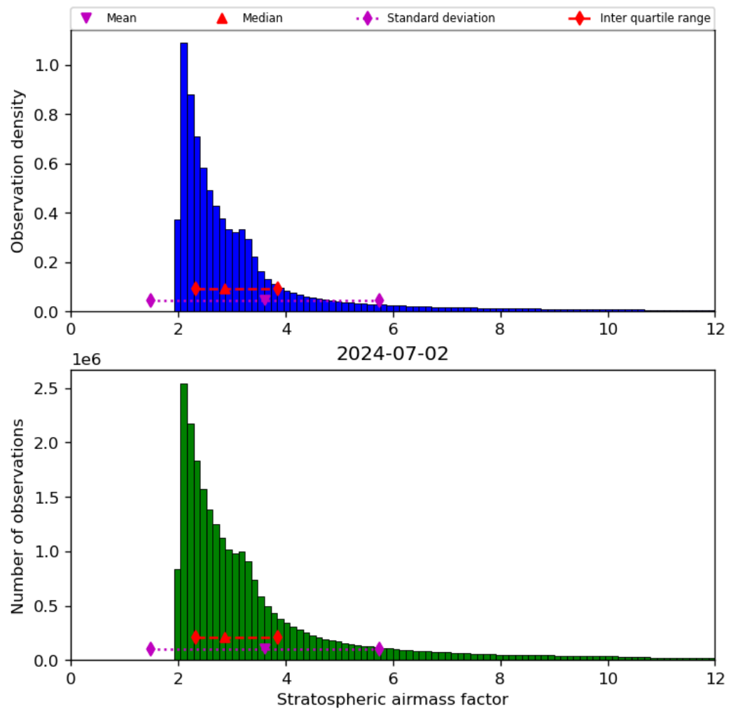
Figure 44: Histogram of “Stratospheric airmass factor” for 2024-07-01 to 2024-07-03
