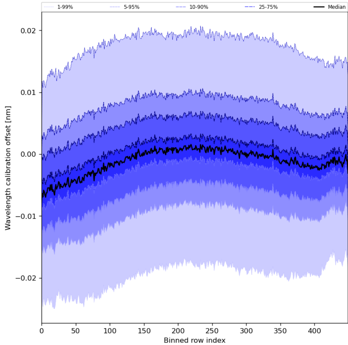
Figure 52: Along track statistics of “Wavelength calibration offset” for 2024-07-01 to 2024-07-03
