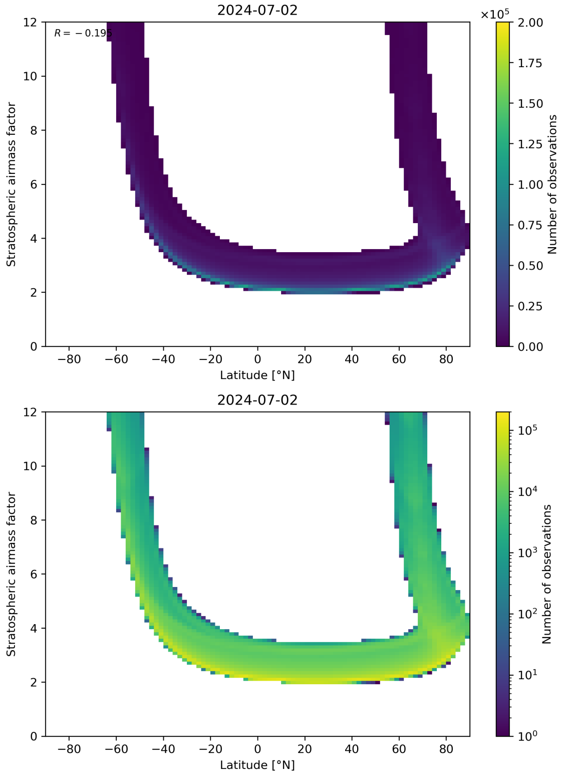
Figure 83: Scatter density plot of “Latitude” against “Stratospheric air mass factor” for 2024-07-01 to 2024-07-03.
