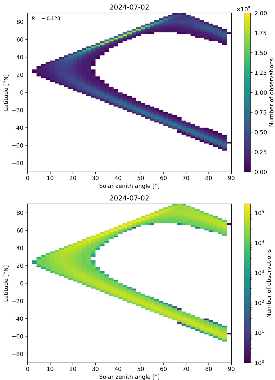
Figure 149: Scatter density plot of “Solar zenith angle” against “Latitude” for 2024-07-01 to 2024-07-03.
