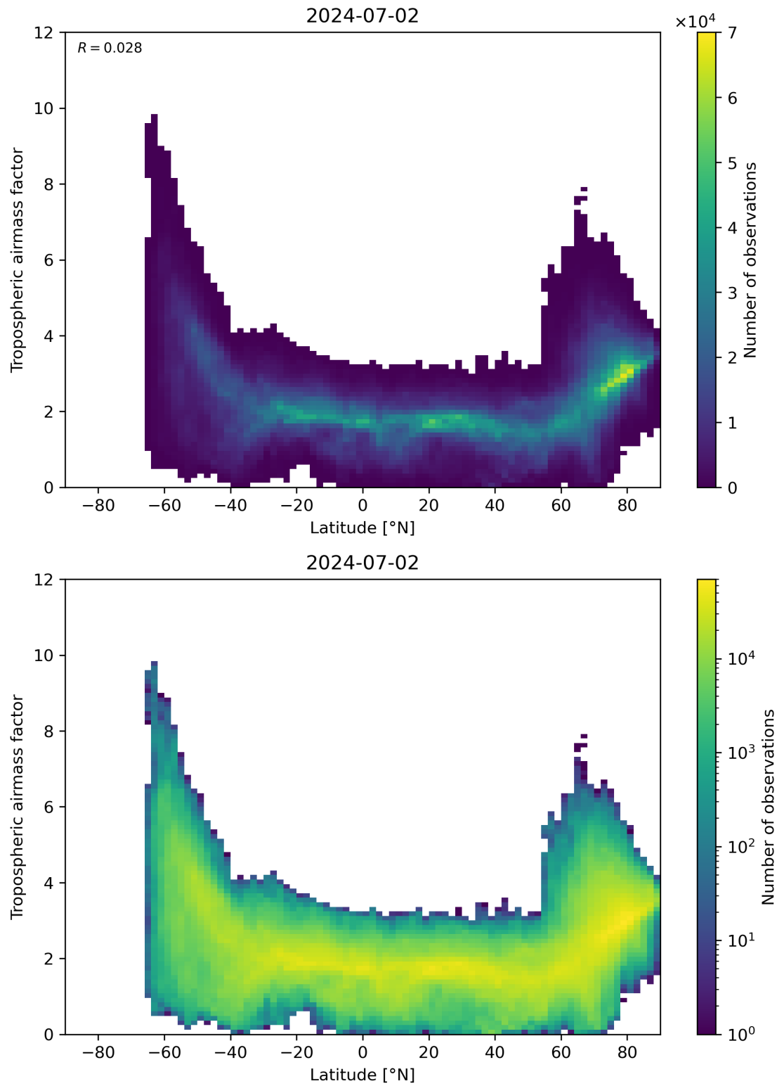
Figure 85: Scatter density plot of “Latitude” against “Tropospheric airmass factor” for 2024-07-01 to 2024-07-03.
