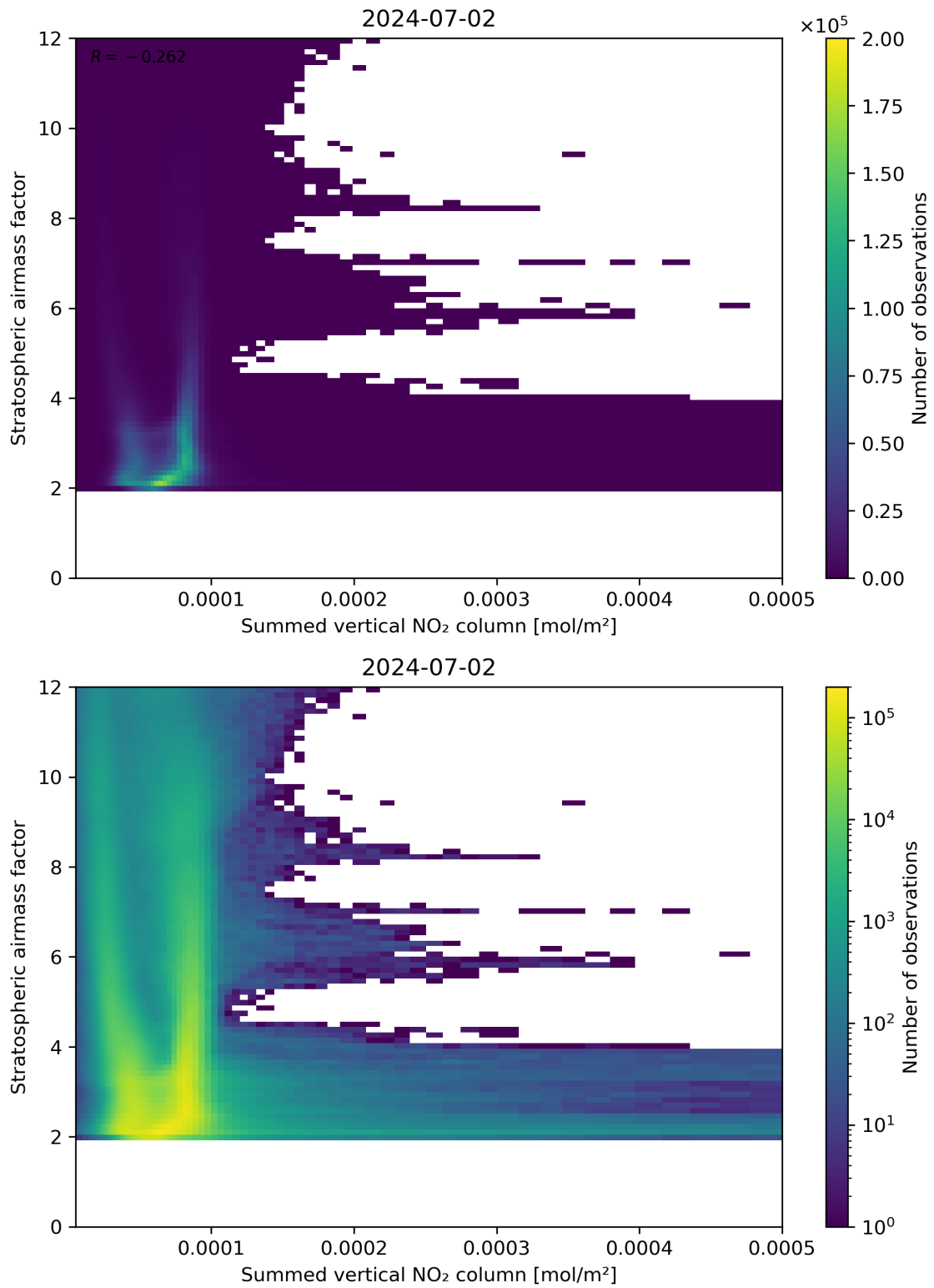
Figure 103: Scatter density plot of “Summed vertical NO 2 column” against “Stratospheric airmass factor” for 2024-07-01 to 2024-07-03.
