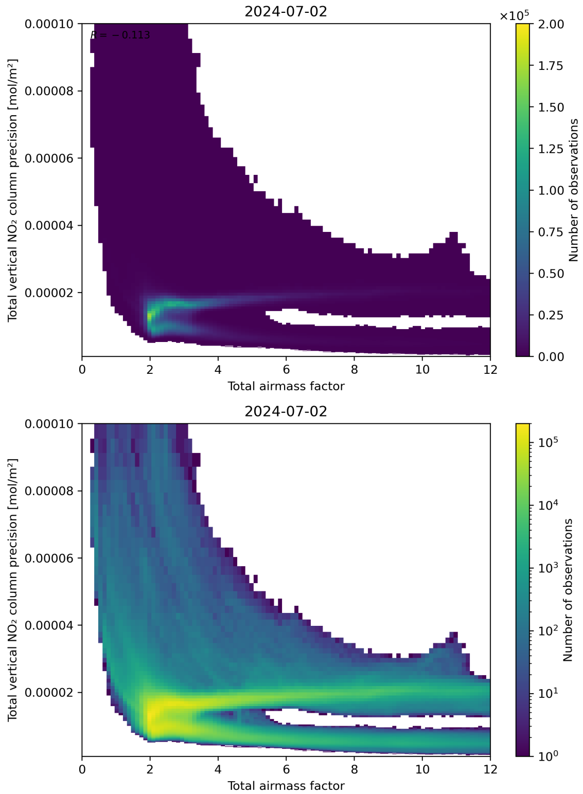
Figure 68: Scatter density plot of “Total airmass factor” against “Total vertical NO 2 column precision” for 2024-07-01 to 2024-07-03.
