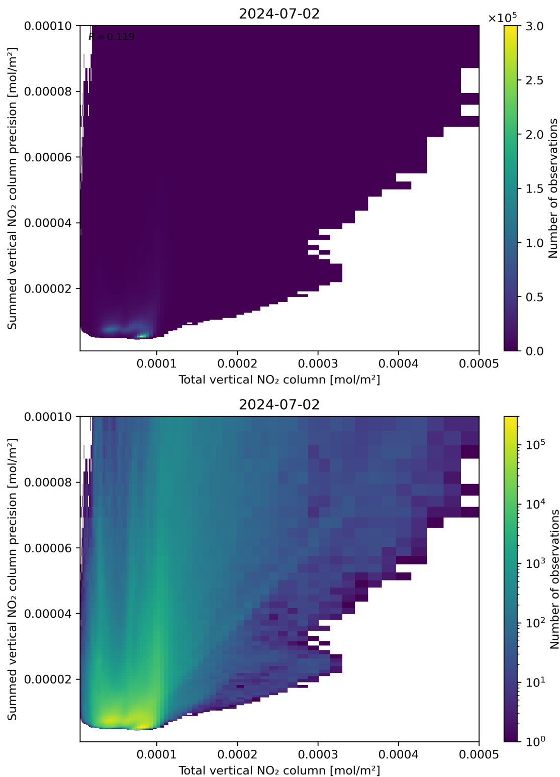
Figure 113: Scatter density plot of “Total vertical NO 2 column” against “Summed vertical NO 2 column precision” for 2024-07-01 to 2024-07-03.
