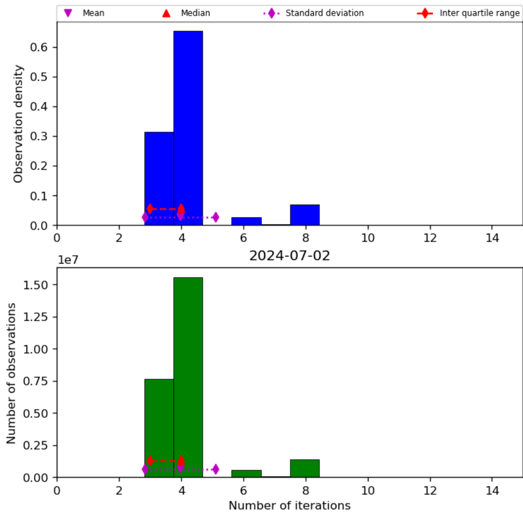
Figure 34: Histogram of “Number of iterations” for 2024-07-01 to 2024-07-03
