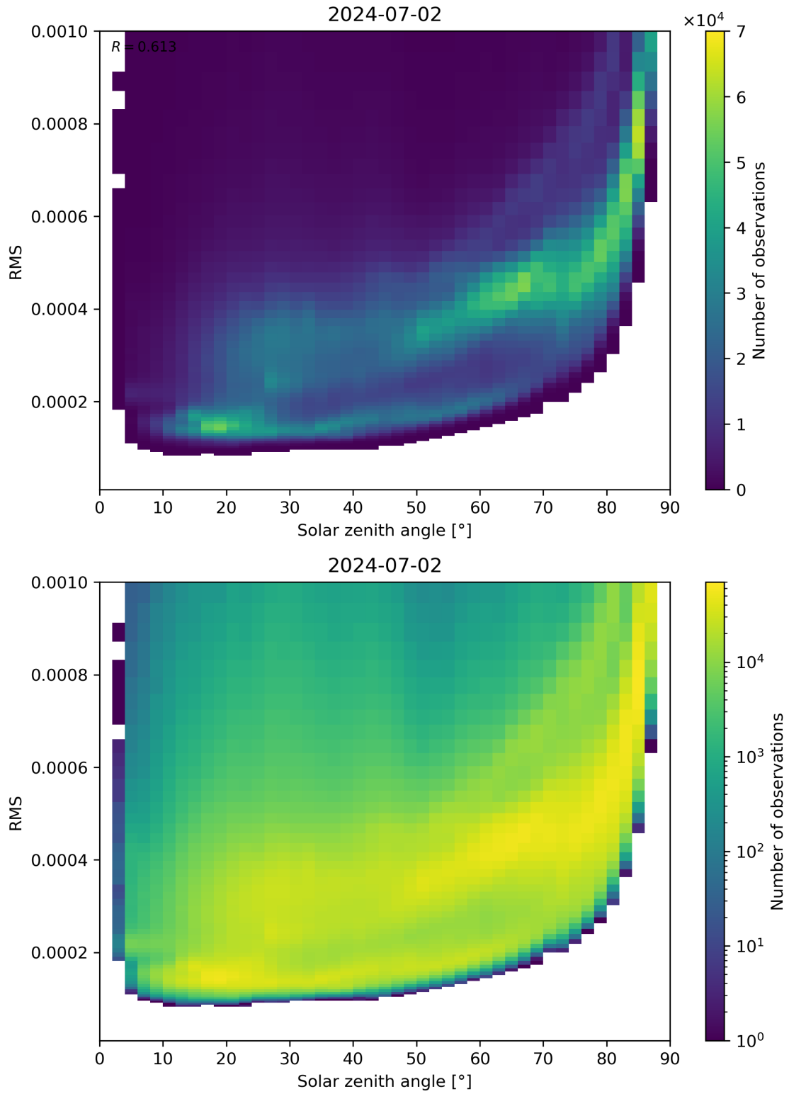
Figure 157: Scatter density plot of “Solar zenith angle” against “RMS” for 2024-07-01 to 2024-07-03.
