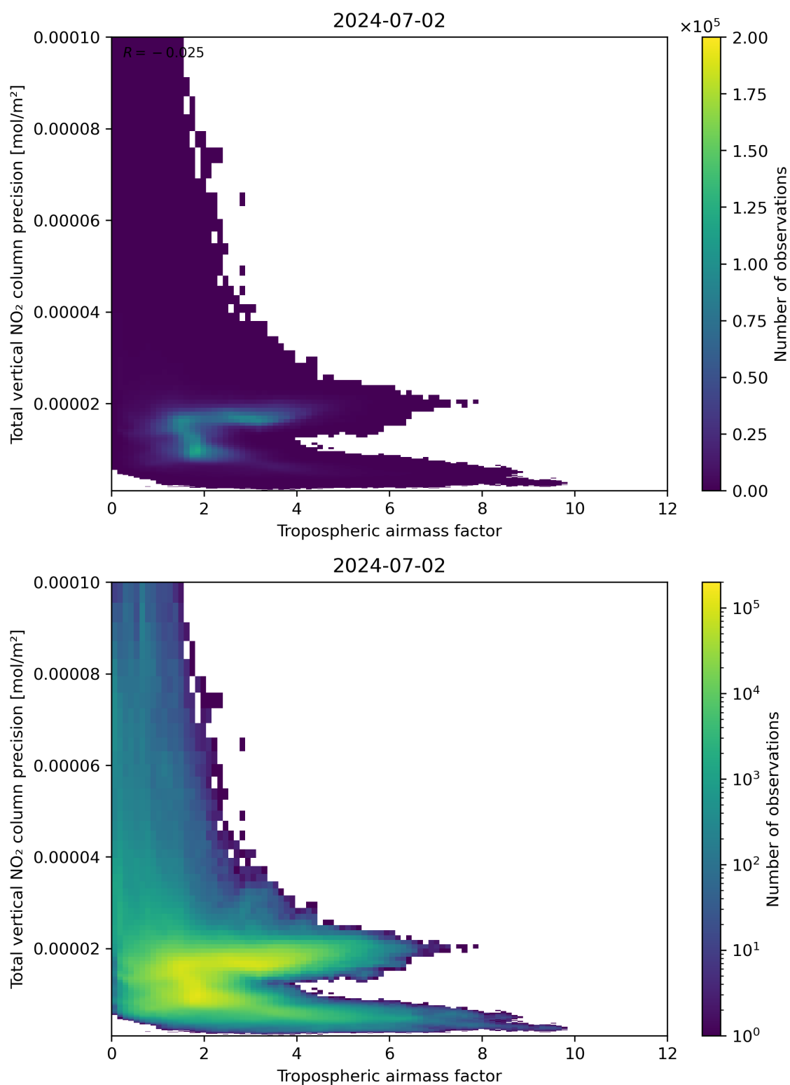
Figure 78: Scatter density plot of “Tropospheric air mass factor” against “Total vertical NO 2 column precision” for 2024-07-01 to 2024-07-03.
