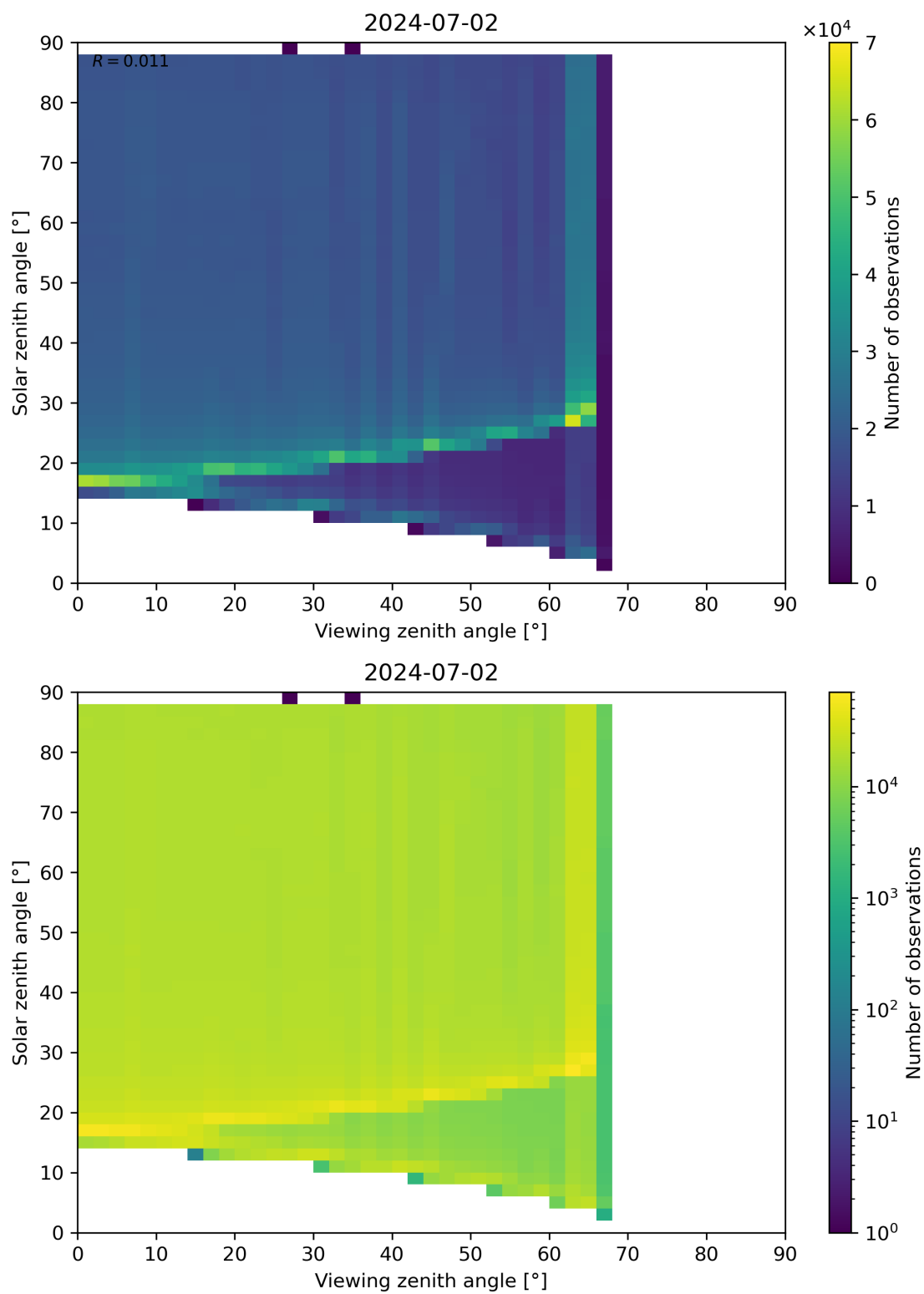
Figure 172: Scatter density plot of “Viewing zenith angle” against “Solar zenith angle” for 2024-07-01 to 2024-07-03.
