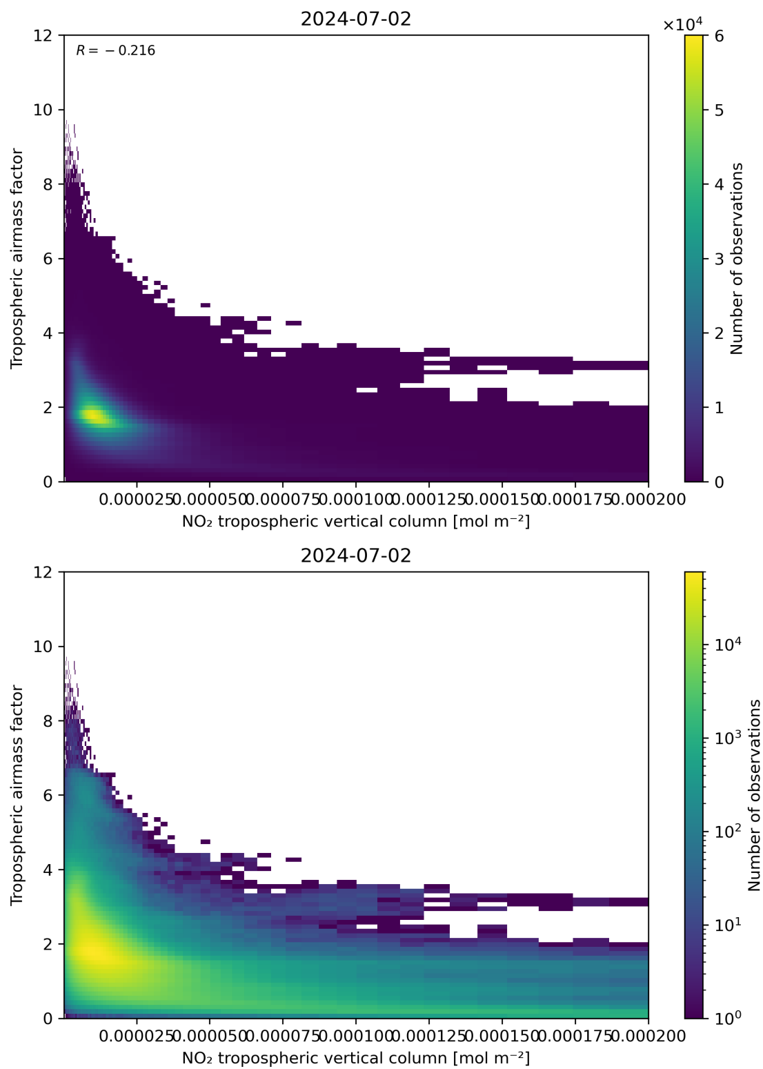
Figure 123: Scatter density plot of “NO 2 tropospheric vertical column” against “Tropospheric air mass factor” for 2024-07-01 to 2024-07-03.
