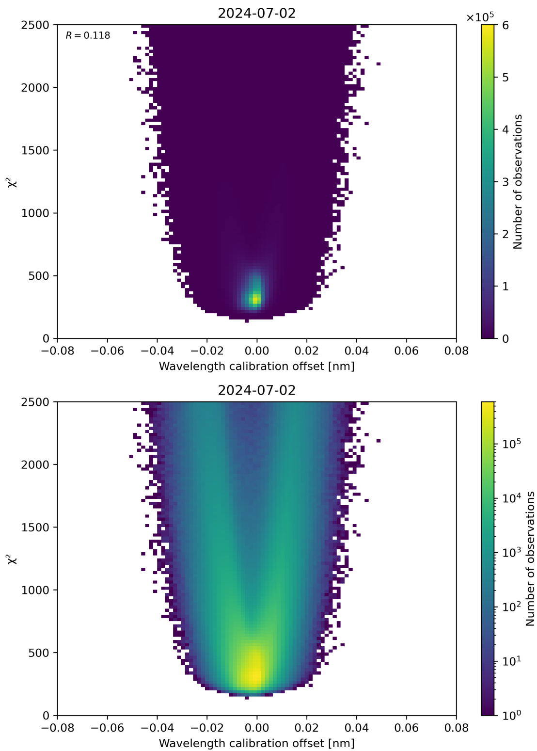
Figure 175: Scatter density plot of “Wavelength calibration offset” against “ \chi^2 ” for 2024-07-01 to 2024-07-03.
