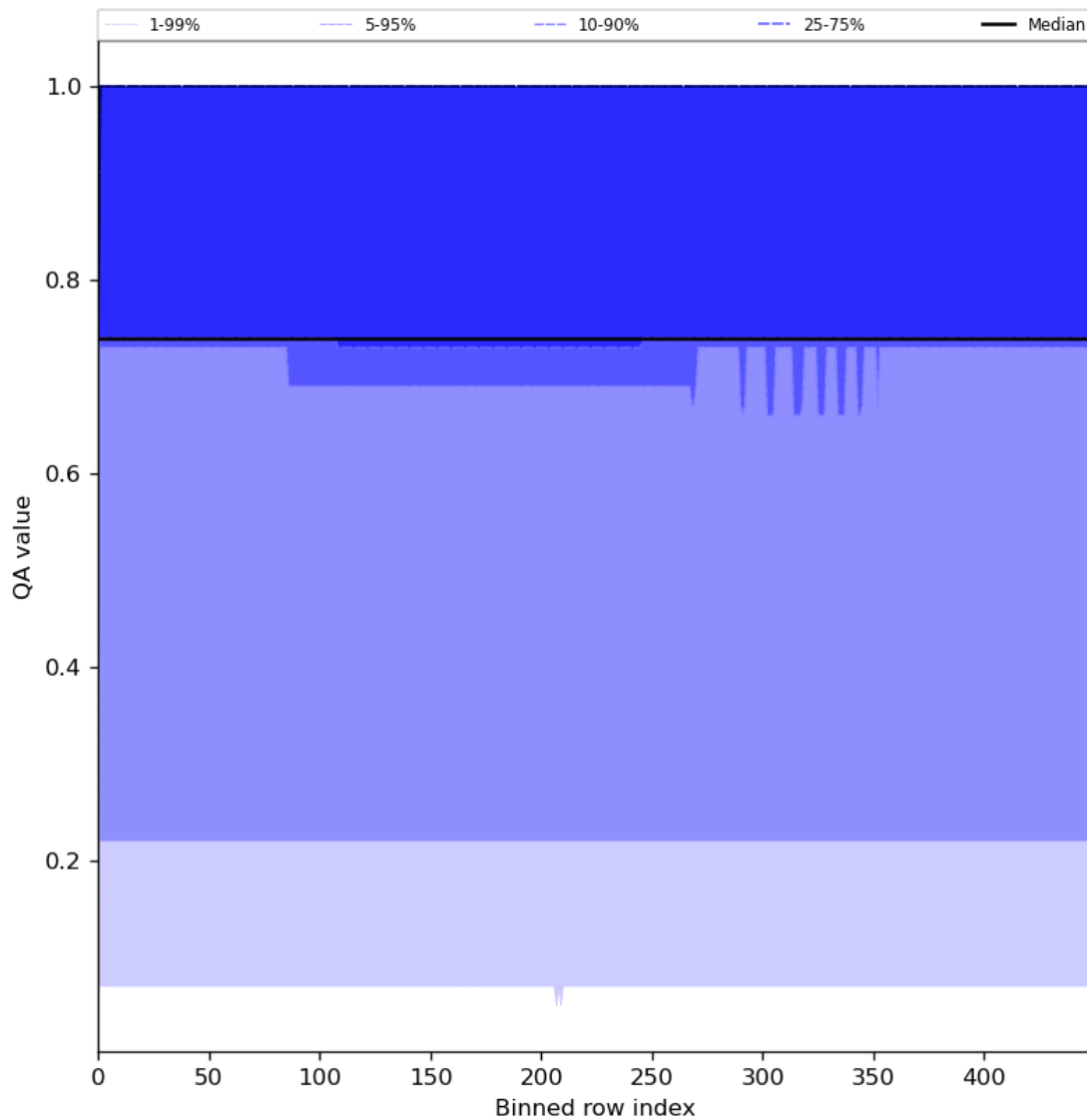
Figure 45: Along track statistics of “QA value” for 2024-07-01 to 2024-07-03
