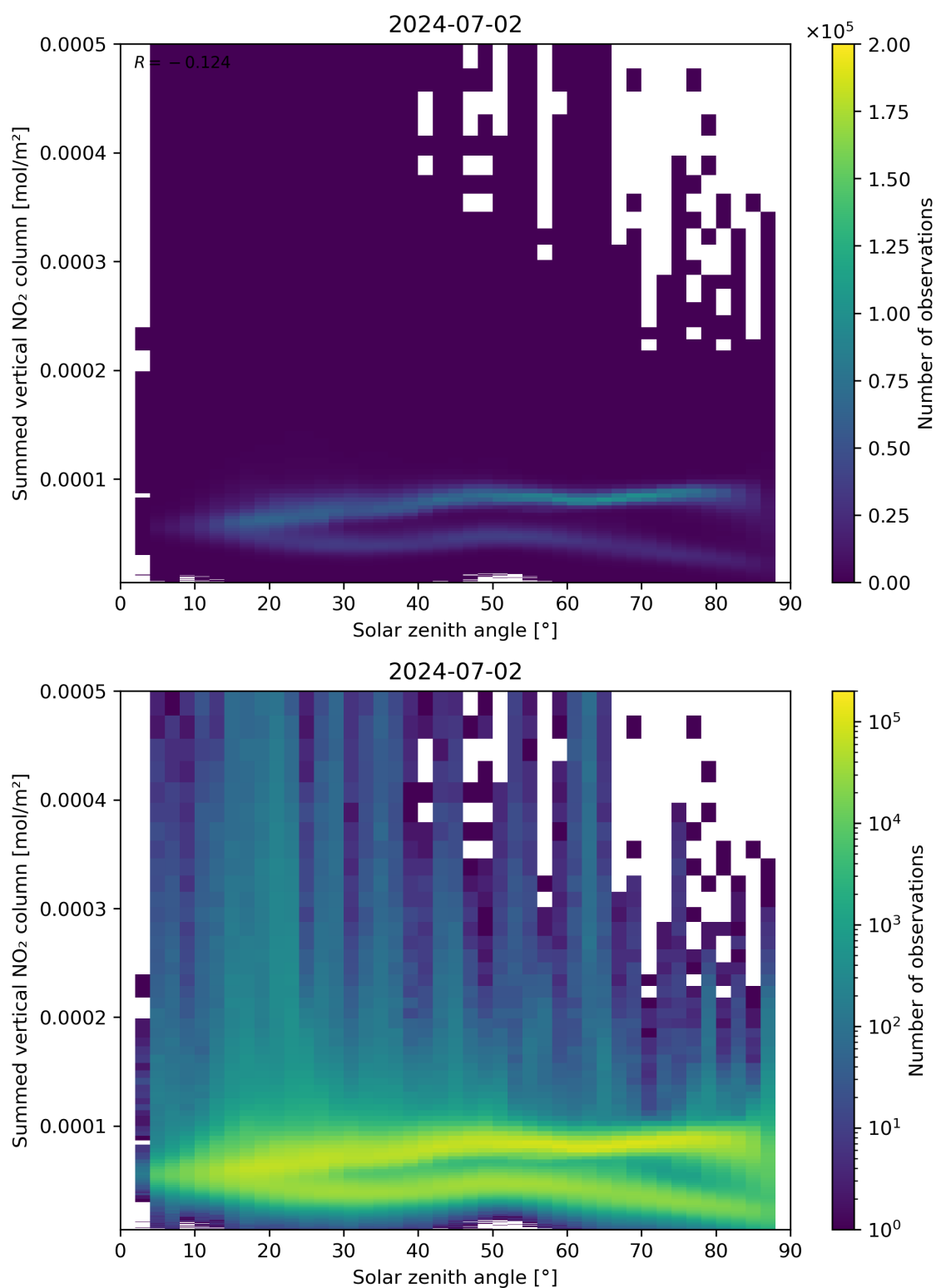
Figure 151: Scatter density plot of “Solar zenith angle” against “Summed vertical NO 2 column” for 2024-07-01 to 2024-07-03.
