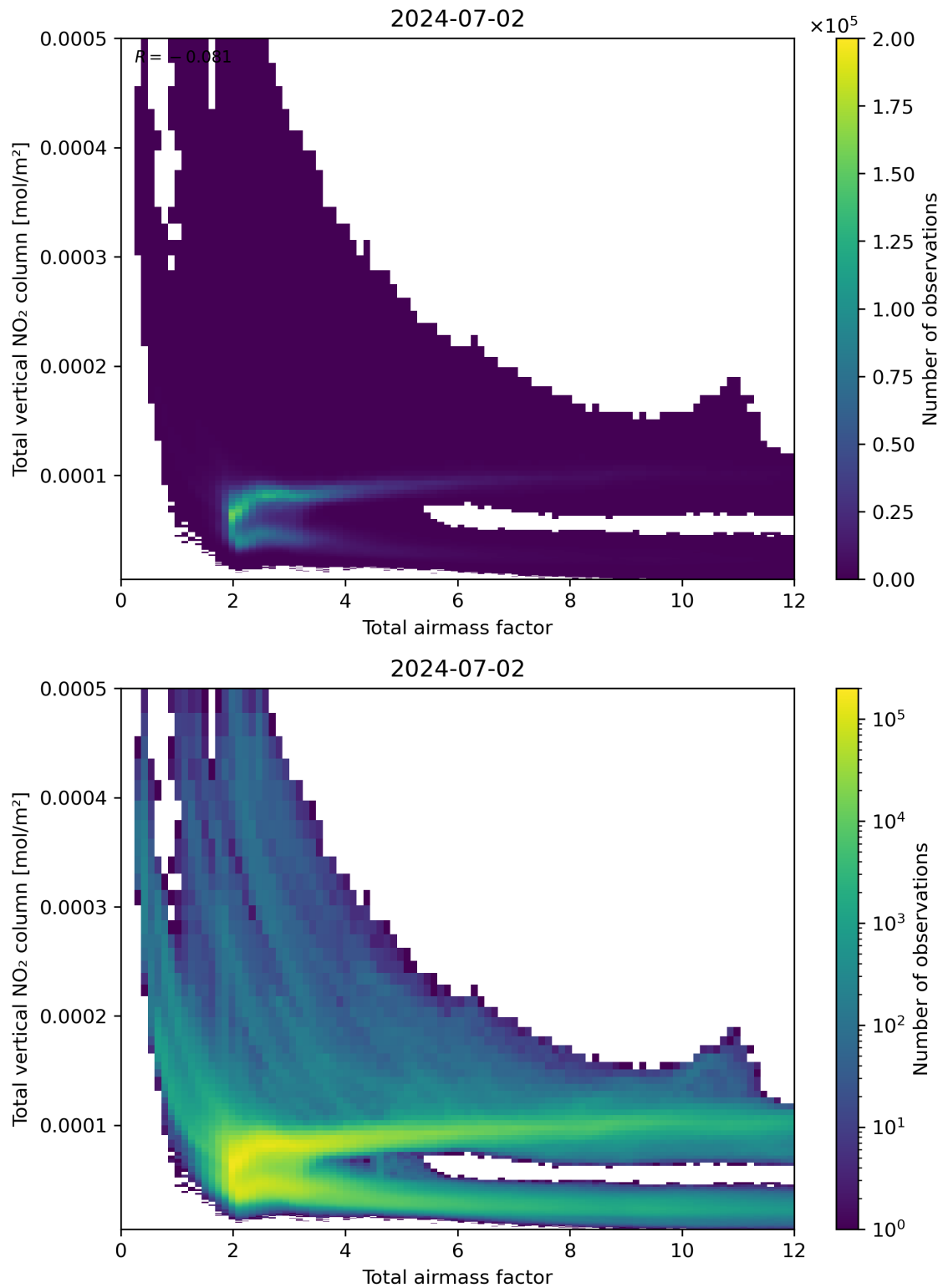
Figure 67: Scatter density plot of “Total airmass factor” against “Total vertical NO 2 column” for 2024-07-01 to 2024-07-03.
