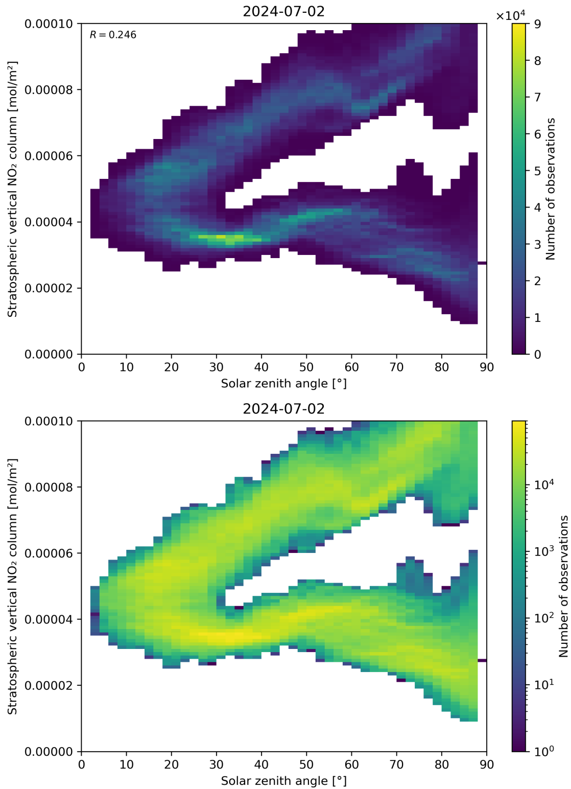
Figure 150: Scatter density plot of “Solar zenith angle” against “Stratospheric vertical NO 2 column” for 2024-07-01 to 2024-07-03.
