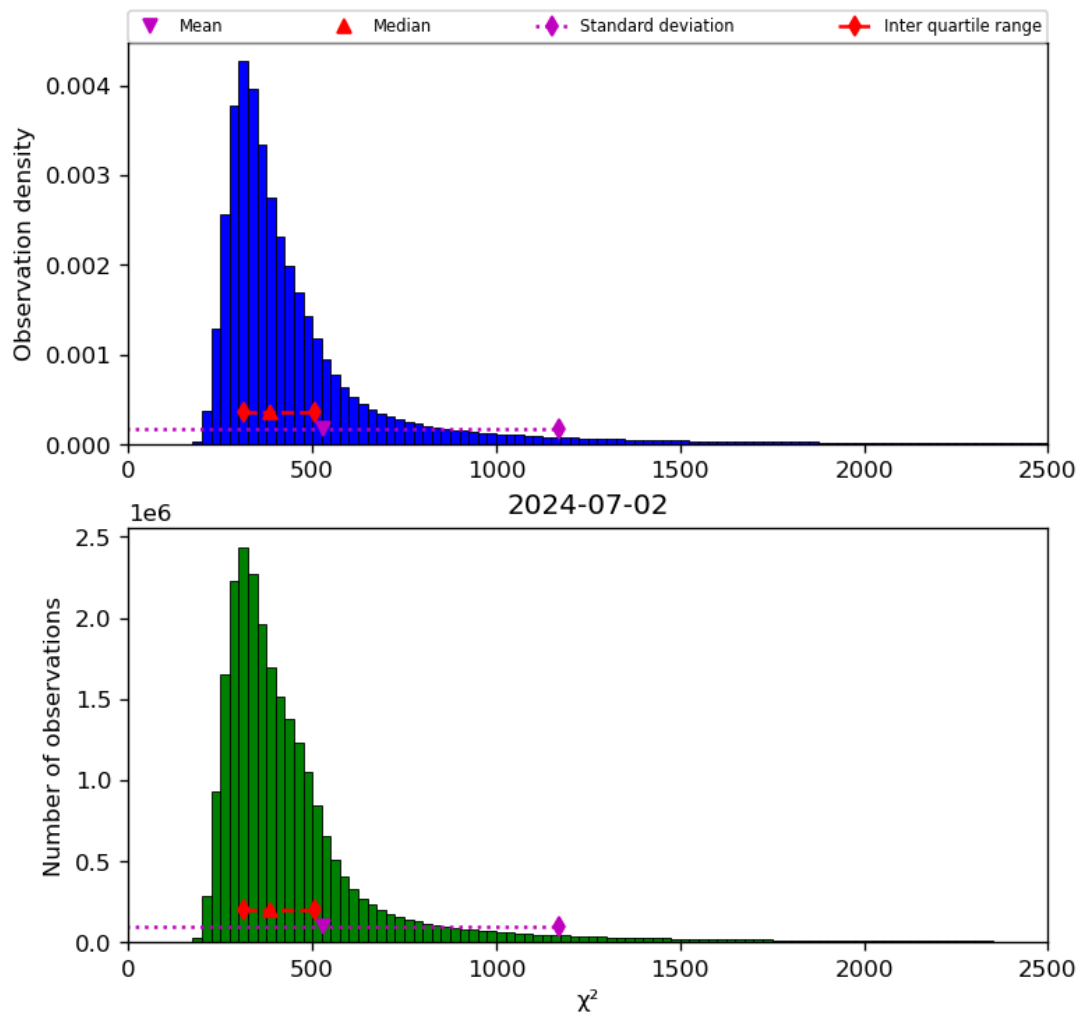
Figure 42: Histogram of “ \chi^2 ” for 2024-07-01 to 2024-07-03
