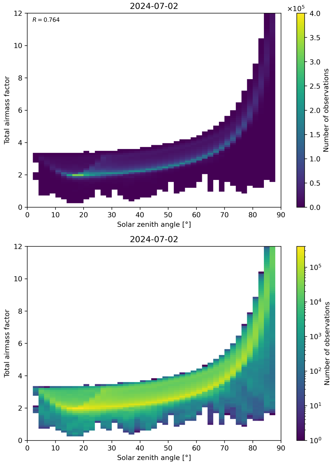
Figure 146: Scatter density plot of “Solar zenith angle” against “Total air mass factor” for 2024-07-01 to 2024-07-03.
