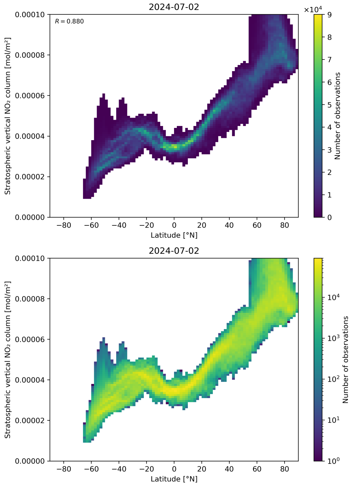
Figure 87: Scatter density plot of “Latitude” against “Stratospheric vertical NO 2 column” for 2024-07-01 to 2024-07-03.
