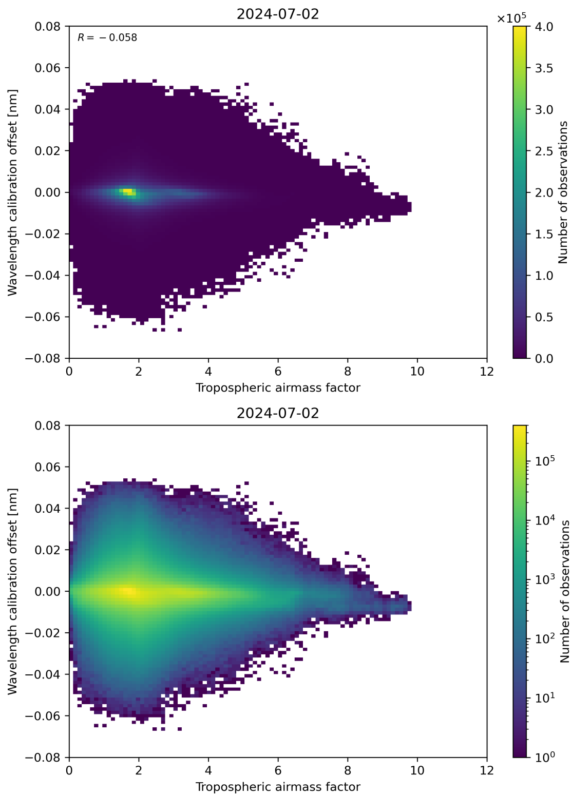
Figure 80: Scatter density plot of “Tropospheric airmass factor” against “Wavelength calibration offset” for 2024-07-01 to 2024-07-03.
