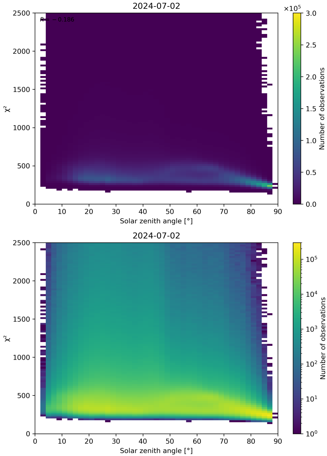
Figure 148: Scatter density plot of “Solar zenith angle” against “ \chi^2 ” for 2024-07-01 to 2024-07-03.
