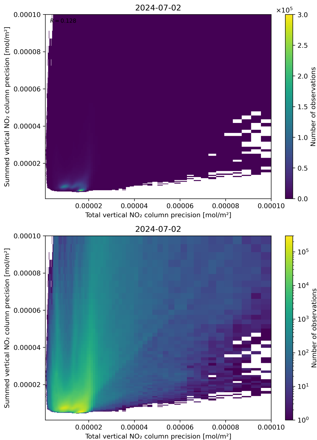
Figure 118: Scatter density plot of “Total vertical NO 2 column precision” against “Summed vertical NO 2 column precision” for 2024-07-01 to 2024-07-03.
