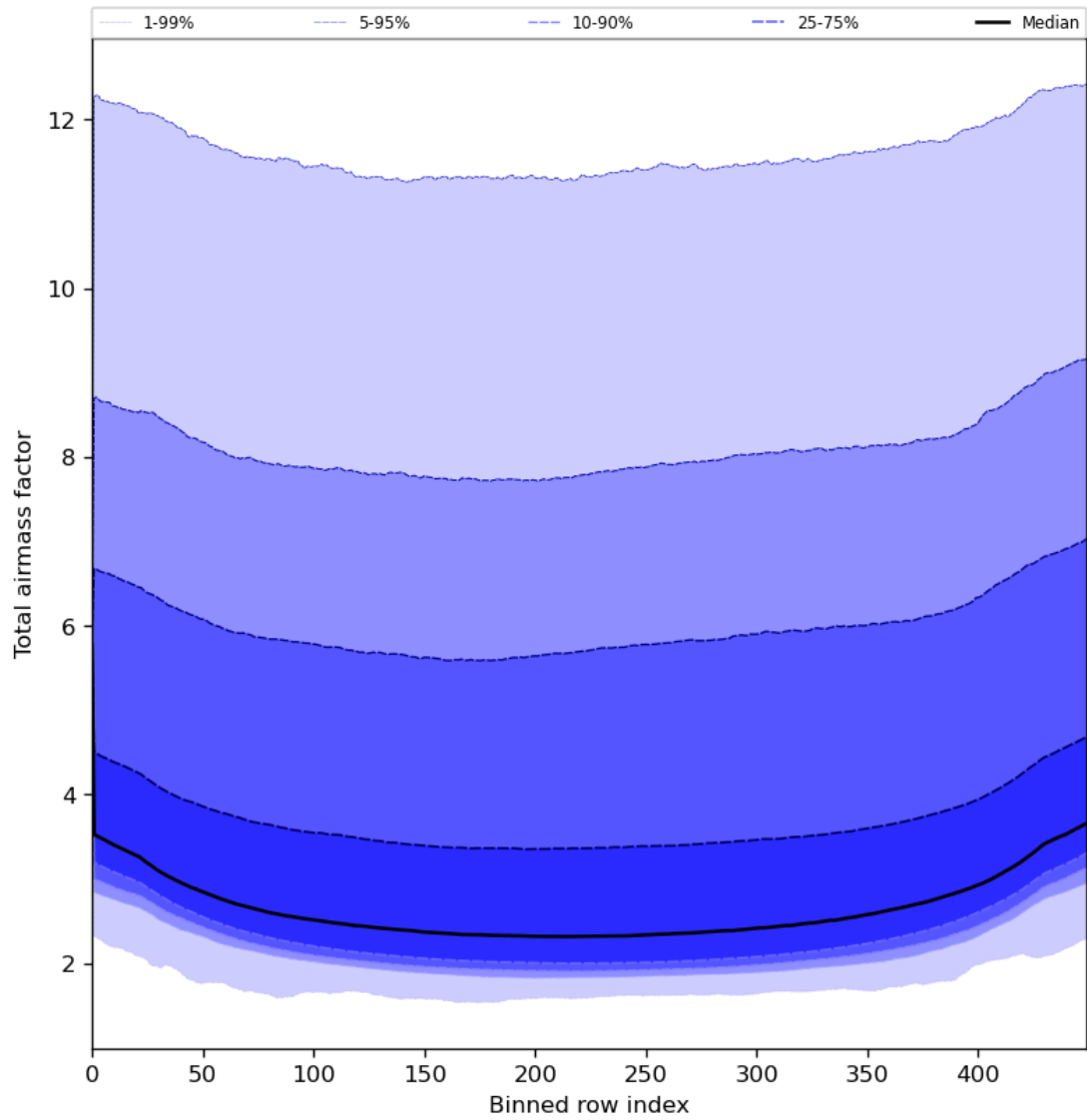
Figure 49: Along track statistics of “Total airmass factor” for 2024-07-01 to 2024-07-03
