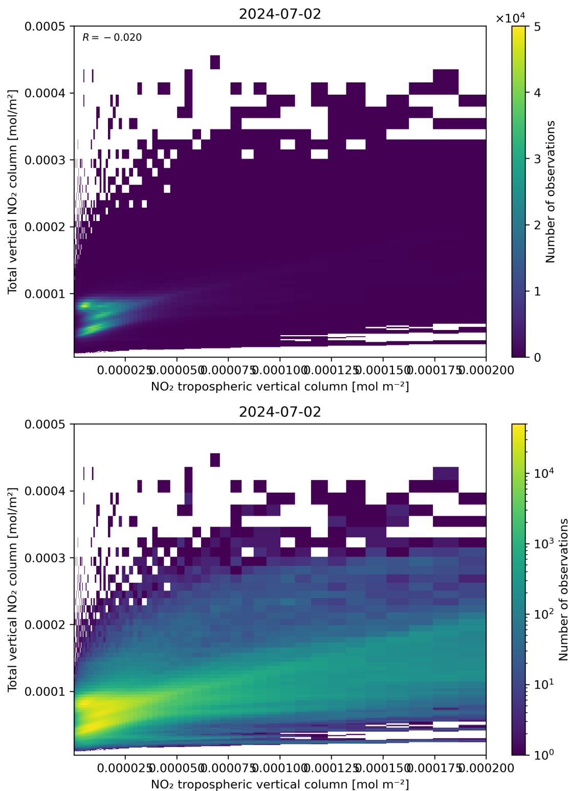
Figure 128: Scatter density plot of “NO 2 tropospheric vertical column” against “Total vertical NO 2 column” for 2024-07-01 to 2024-07-03.
