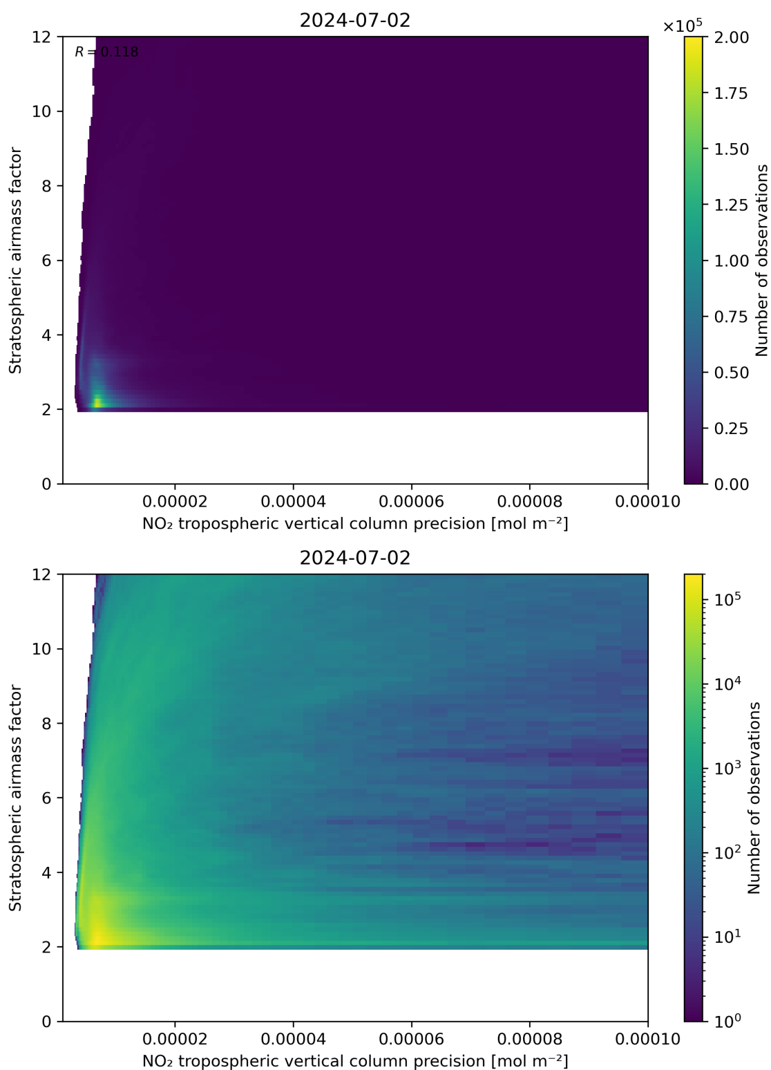
Figure 131: Scatter density plot of “NO 2 tropospheric vertical column precision” against “Stratospheric airmass factor” for 2024-07-01 to 2024-07-03.
