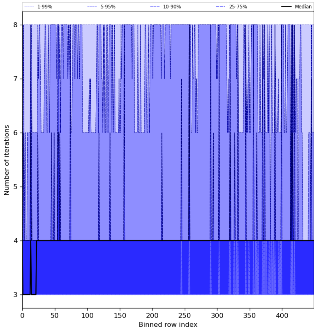
Figure 51: Along track statistics of “Number of iterations” for 2024-07-01 to 2024-07-03
