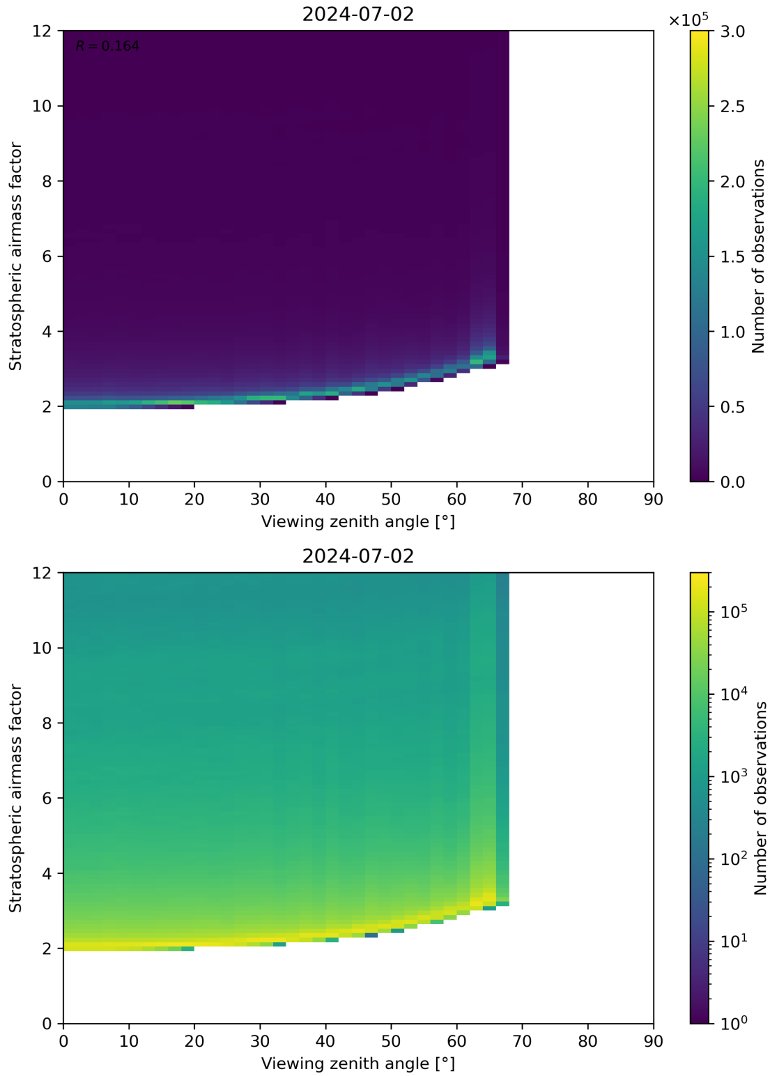
Figure 159: Scatter density plot of “Viewing zenith angle” against “Stratospheric airmass factor” for 2024-07-01 to 2024-07-03.
