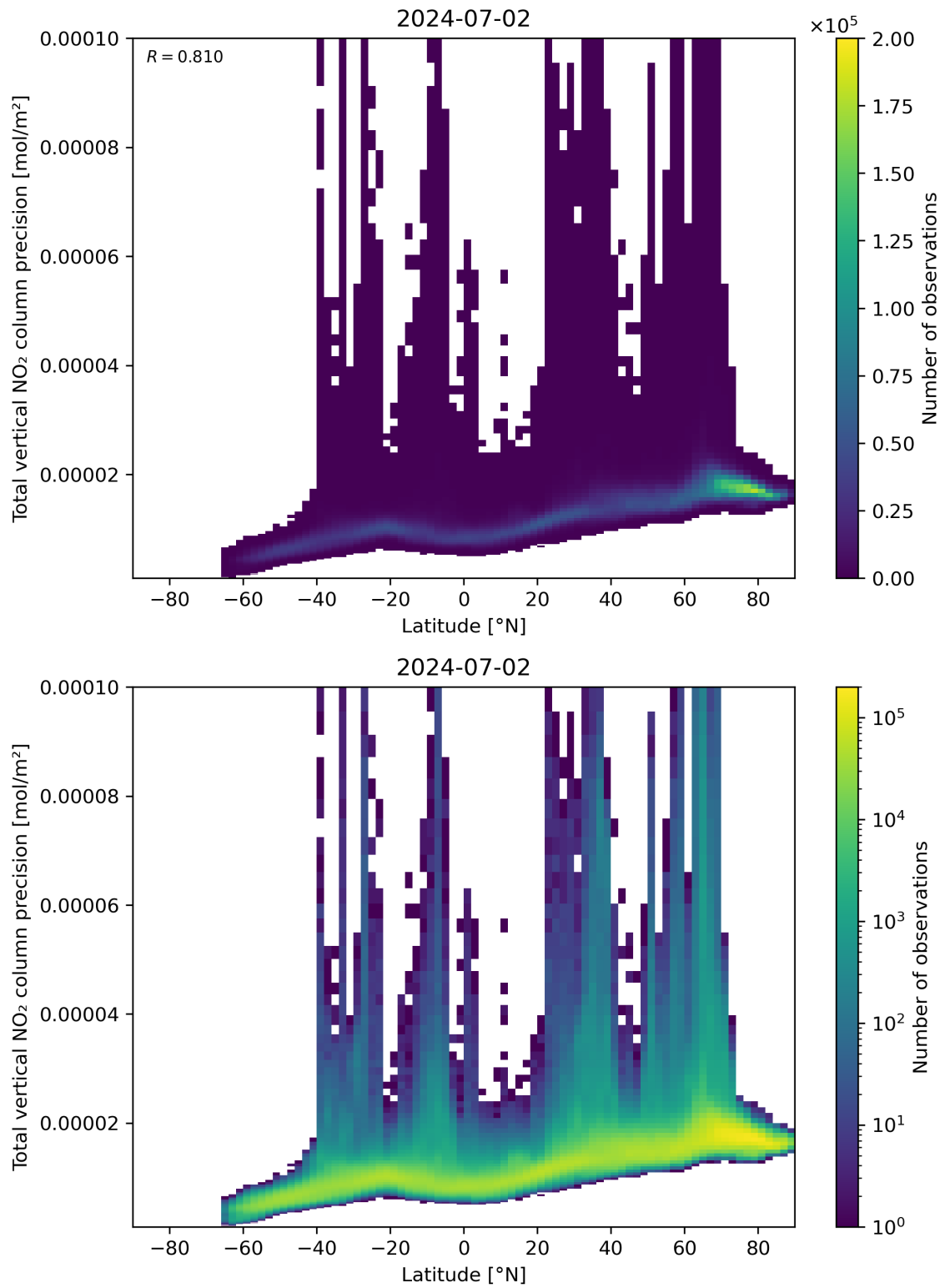
Figure 91: Scatter density plot of “Latitude” against “Total vertical NO 2 column precision” for 2024-07-01 to 2024-07-03.
