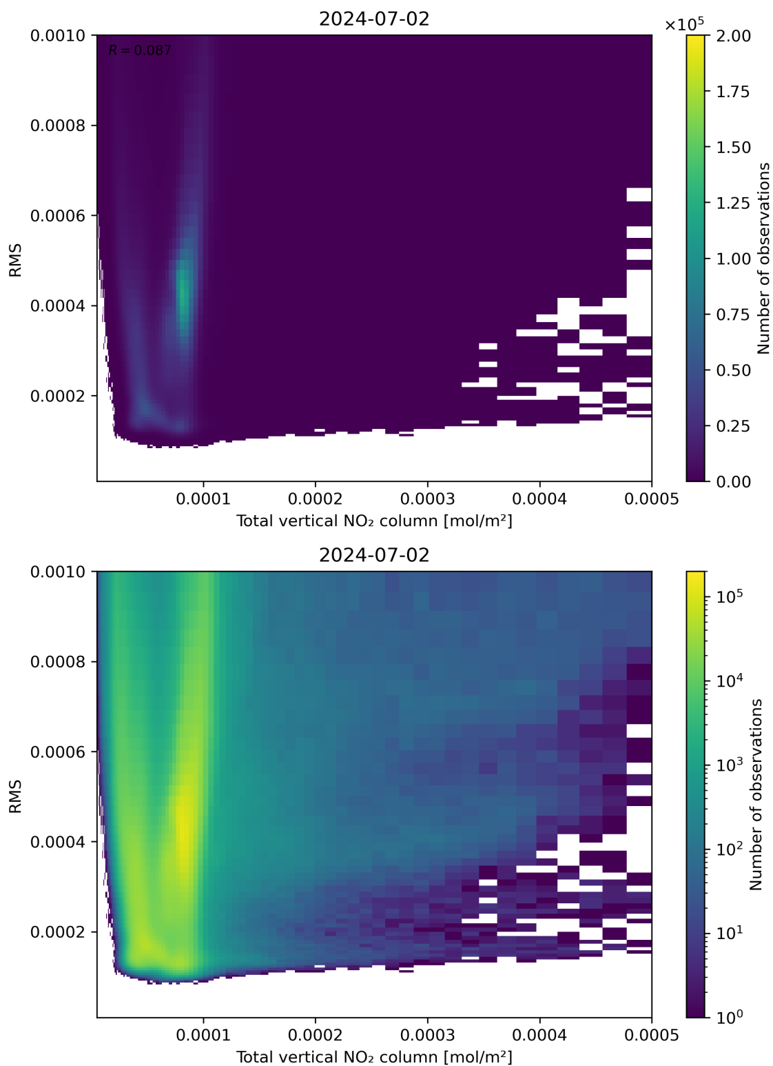
Figure 120: Scatter density plot of “Total vertical NO 2 column” against “RMS” for 2024-07-01 to 2024-07-03.
