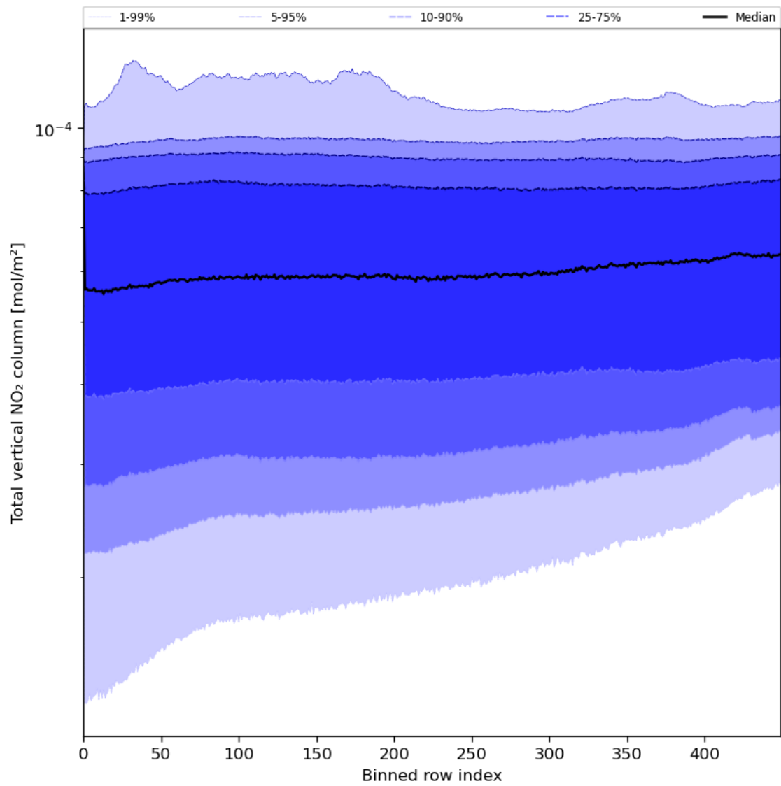
Figure 55: Along track statistics of “Total vertical NO 2 column” for 2024-07-01 to 2024-07-03
