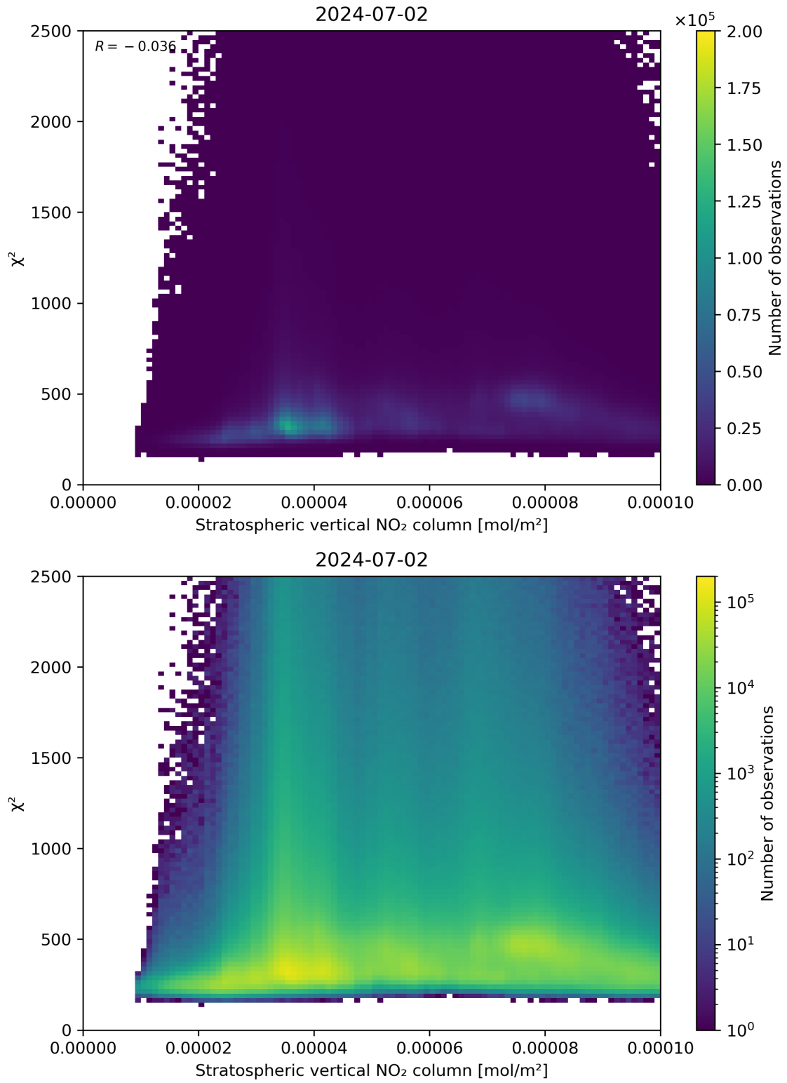
Figure 97: Scatter density plot of “Stratospheric vertical NO 2 column” against “ \chi^2 ” for 2024-07-01 to 2024-07-03.
