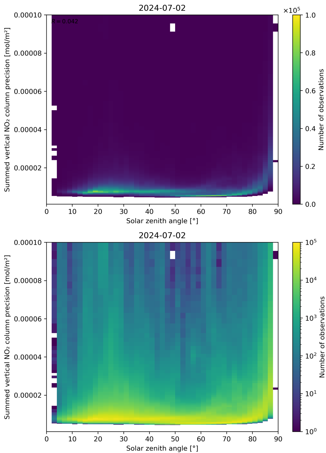
Figure 152: Scatter density plot of “Solar zenith angle” against “Summed vertical NO 2 column precision” for 2024-07-01 to 2024-07-03.
