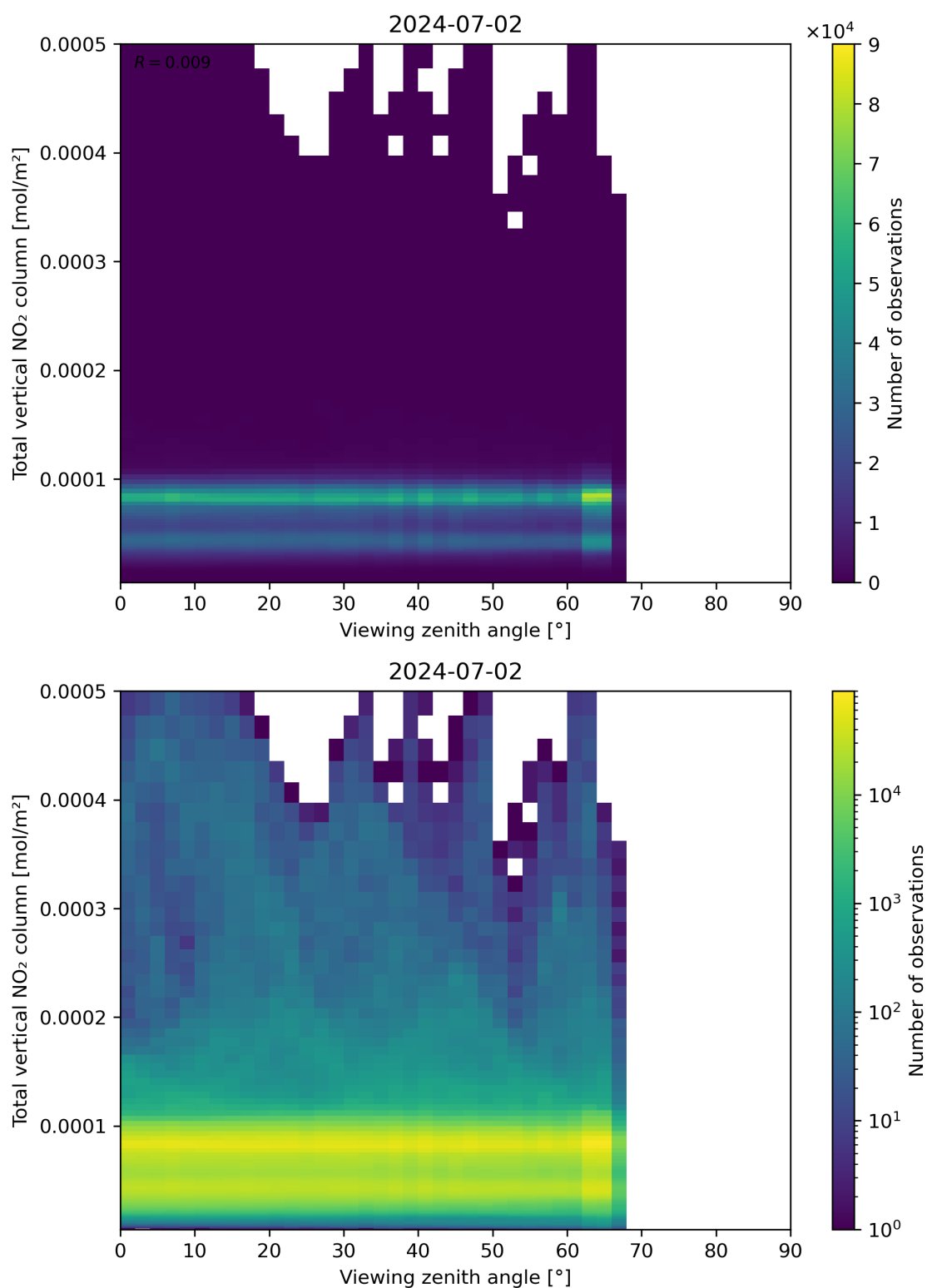
Figure 167: Scatter density plot of “Viewing zenith angle” against “Total vertical NO 2 column” for 2024-07-01 to 2024-07-03.
