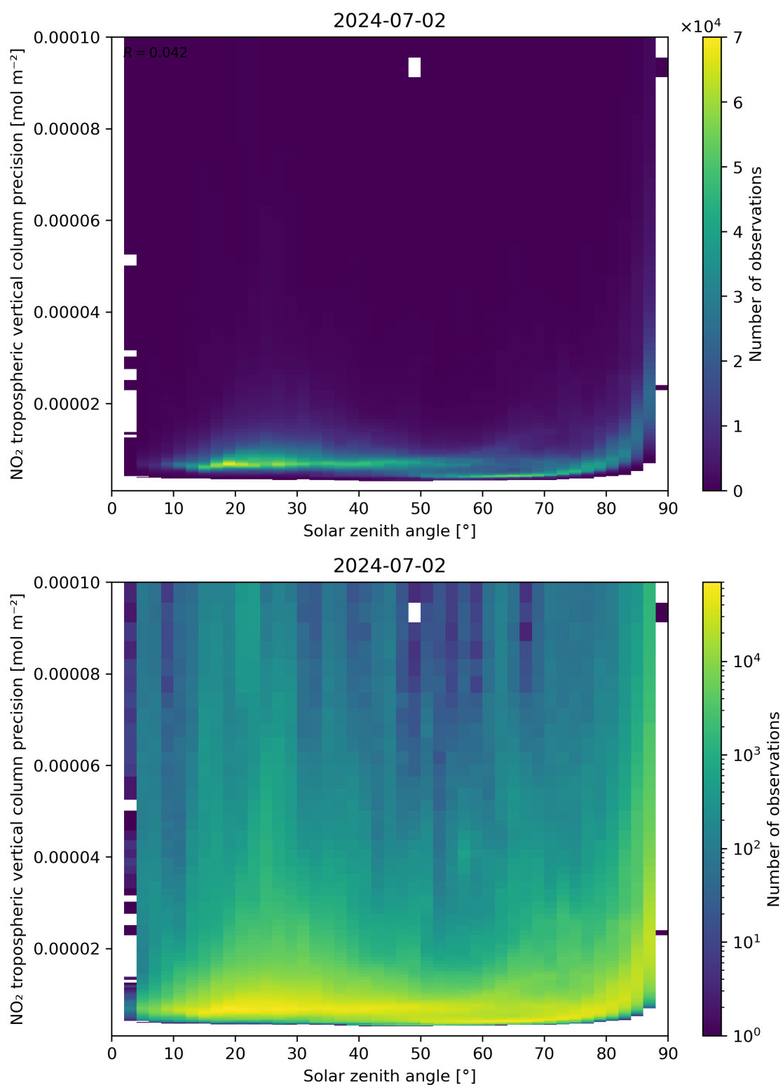
Figure 156: Scatter density plot of “Solar zenith angle” against “NO 2 tropospheric vertical column precision” for 2024-07-01 to 2024-07-03.
