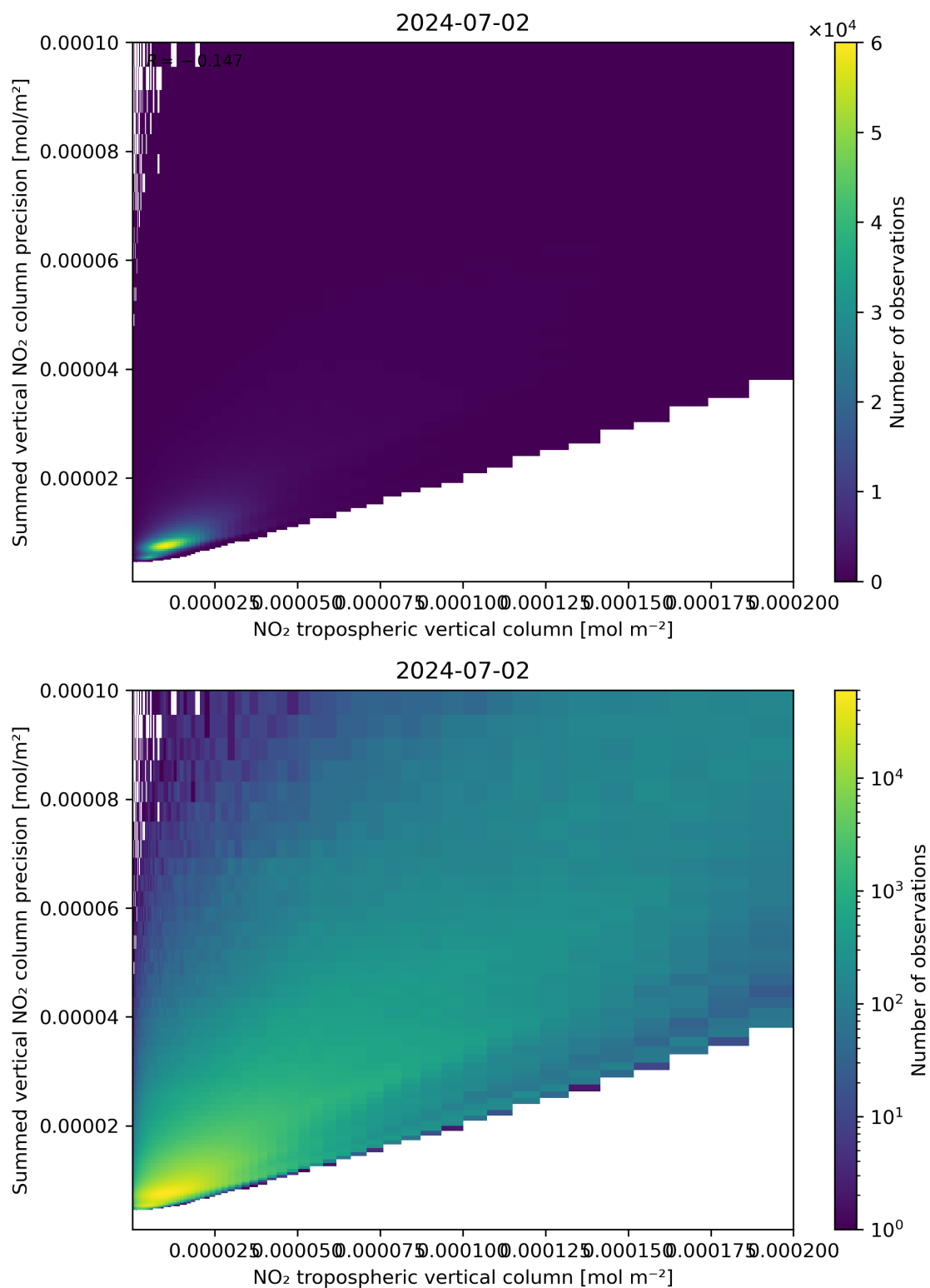
Figure 127: Scatter density plot of “NO 2 tropospheric vertical column” against “Summed vertical NO 2 column precision” for 2024-07-01 to 2024-07-03.
