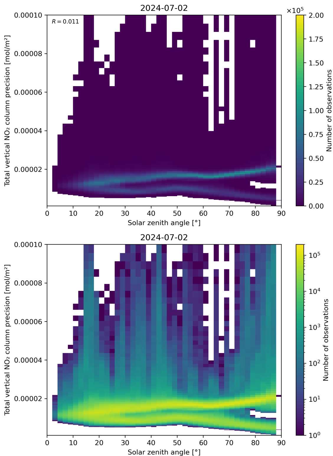
Figure 154: Scatter density plot of “Solar zenith angle” against “Total vertical NO 2 column precision” for 2024-07-01 to 2024-07-03.
