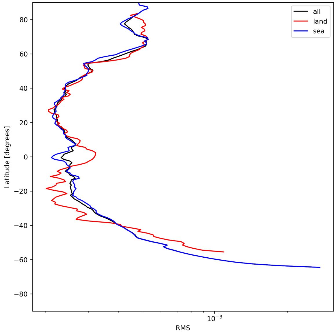
Figure 26: Zonal average of “RMS” for 2024-07-01 to 2024-07-03.
