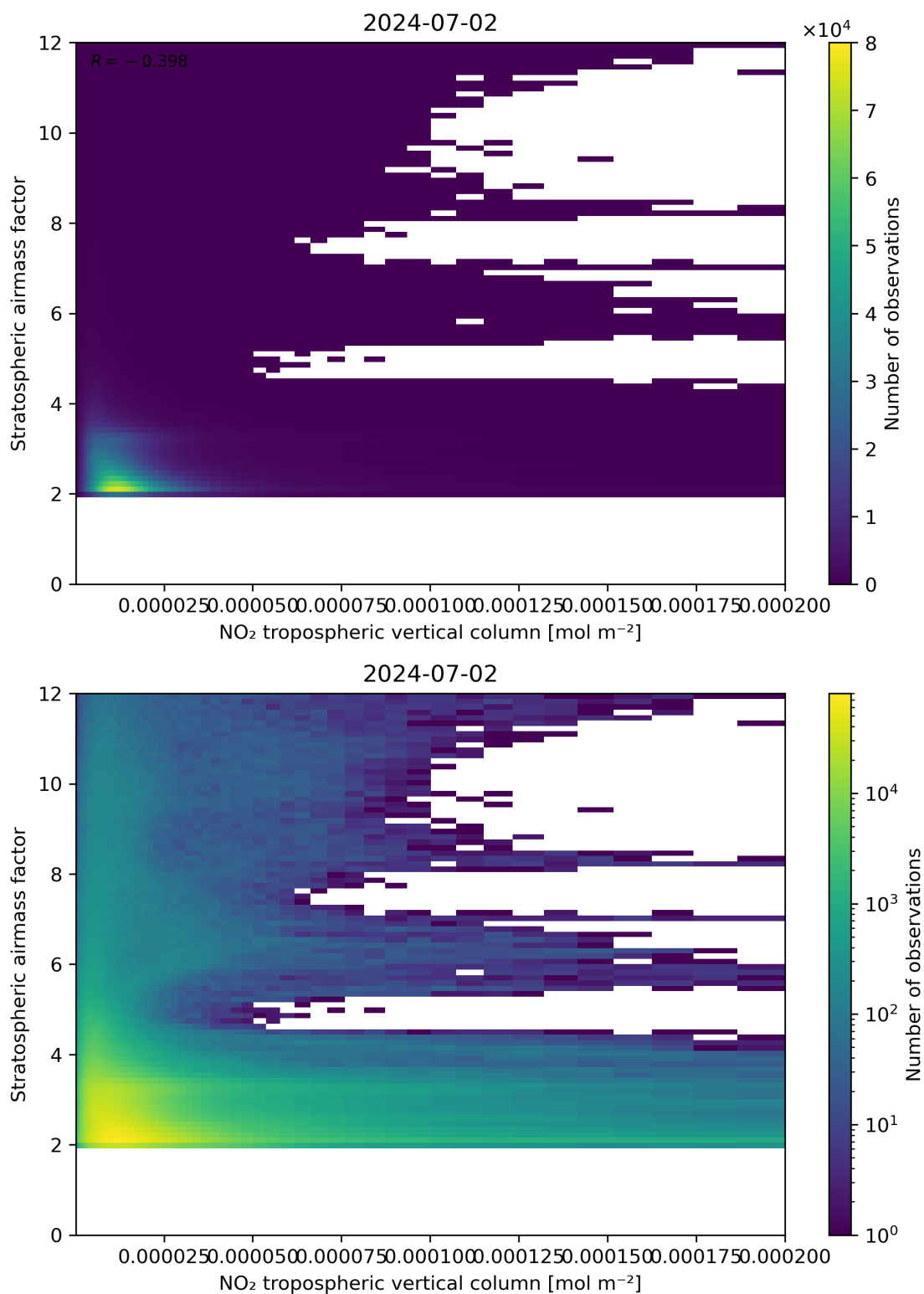
Figure 121: Scatter density plot of “NO 2 tropospheric vertical column” against “Stratospheric air mass factor” for 2024-07-01 to 2024-07-03.
