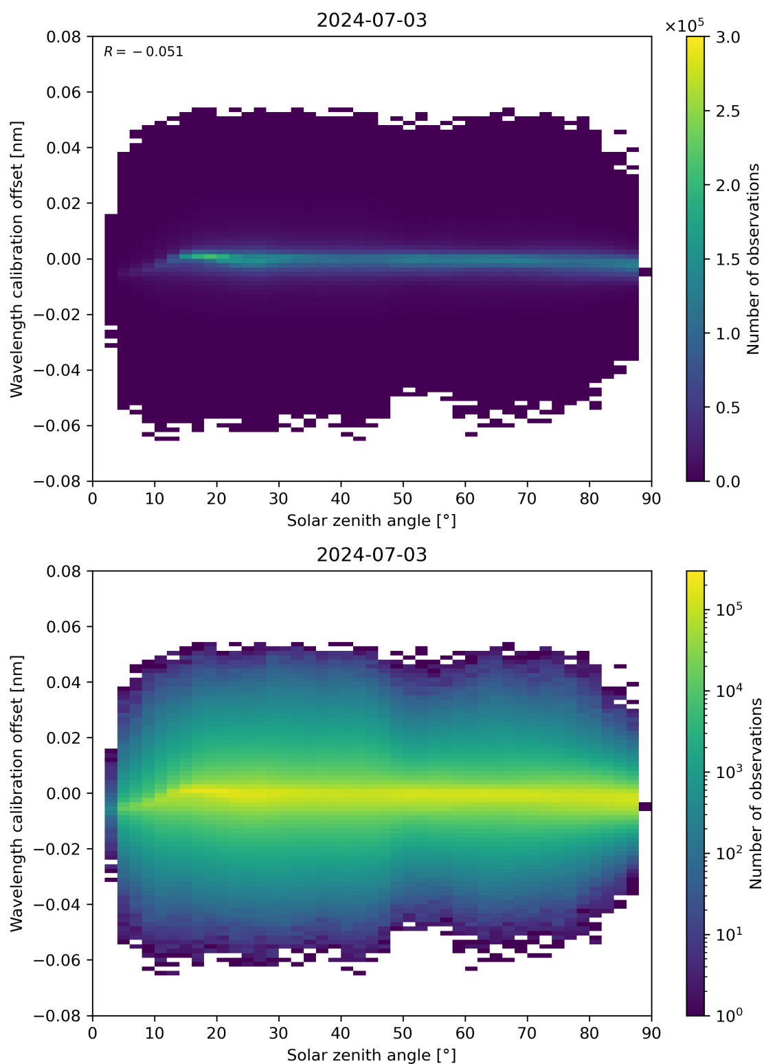
Figure 158: Scatter density plot of “Solar zenith angle” against “Wavelength calibration offset” for 2024-07-02 to 2024-07-04.
