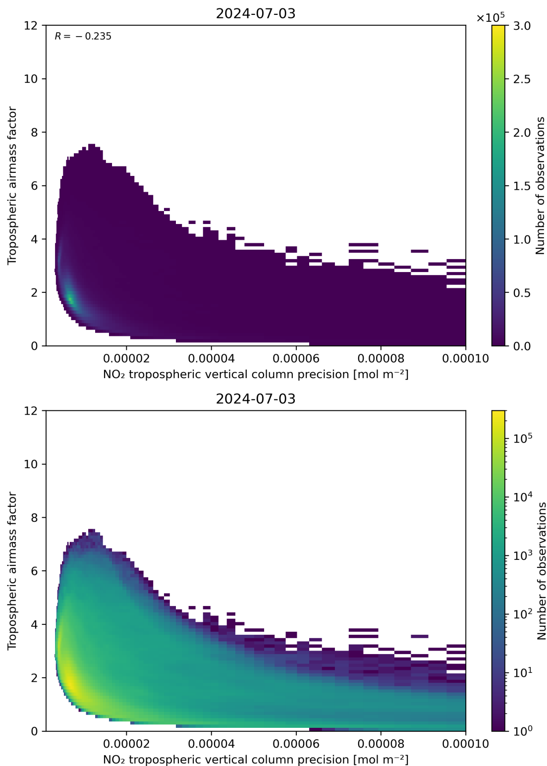
Figure 133: Scatter density plot of “NO 2 tropospheric vertical column precision” against “Tropospheric airmass factor” for 2024-07-02 to 2024-07-04.
