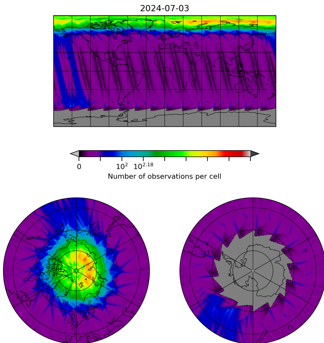
Figure 10: Map of the number of observations for 2024-07-02 to 2024-07-04
