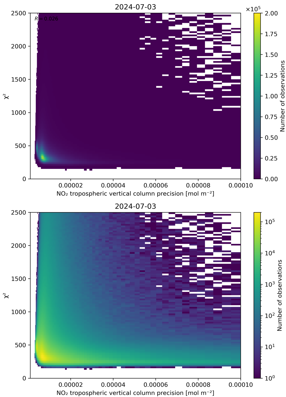
Figure 134: Scatter density plot of “NO 2 tropospheric vertical column precision” against “ \chi^2 ” for 2024-07-02 to 2024-07-04.
