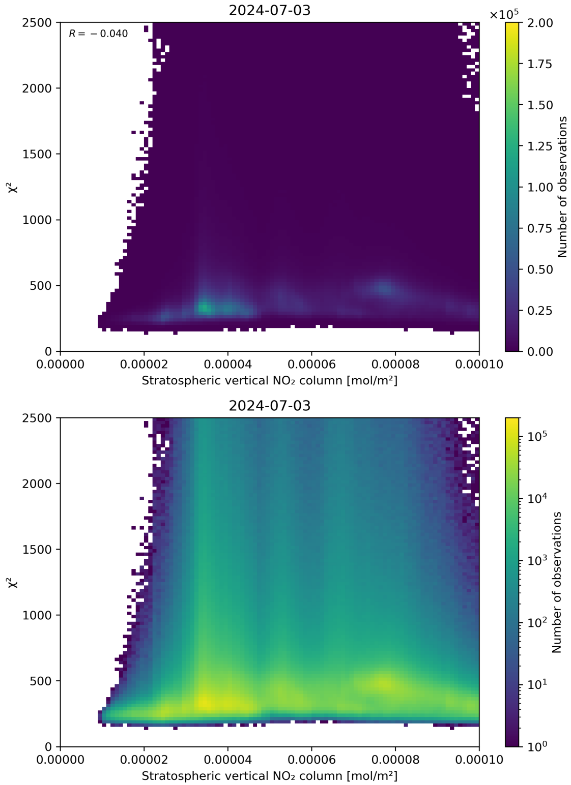
Figure 97: Scatter density plot of “Stratospheric vertical NO 2 column” against “ \chi^2 ” for 2024-07-02 to 2024-07-04.
