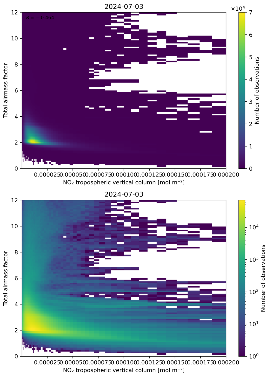
Figure 122: Scatter density plot of “NO 2 tropospheric vertical column” against “Total air mass factor” for 2024-07-02 to 2024-07-04.
