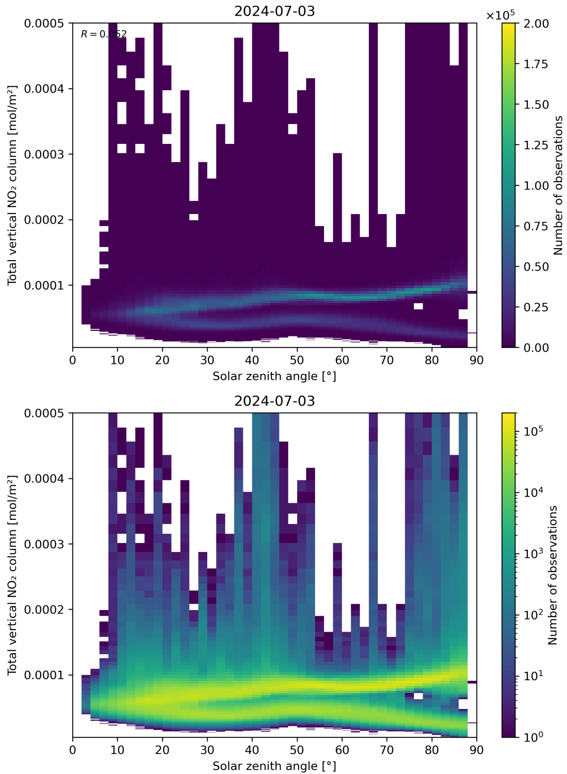
Figure 153: Scatter density plot of “Solar zenith angle” against “Total vertical NO 2 column” for 2024-07-02 to 2024-07-04.
