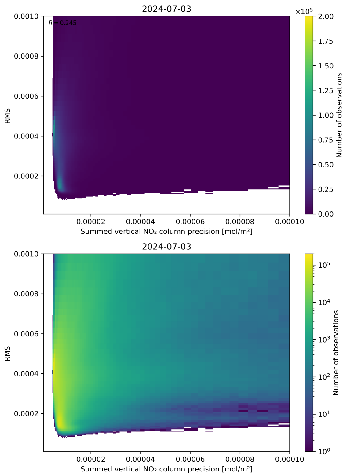
Figure 108: Scatter density plot of “Summed vertical NO 2 column precision” against “RMS” for 2024-07-02 to 2024-07-04.
