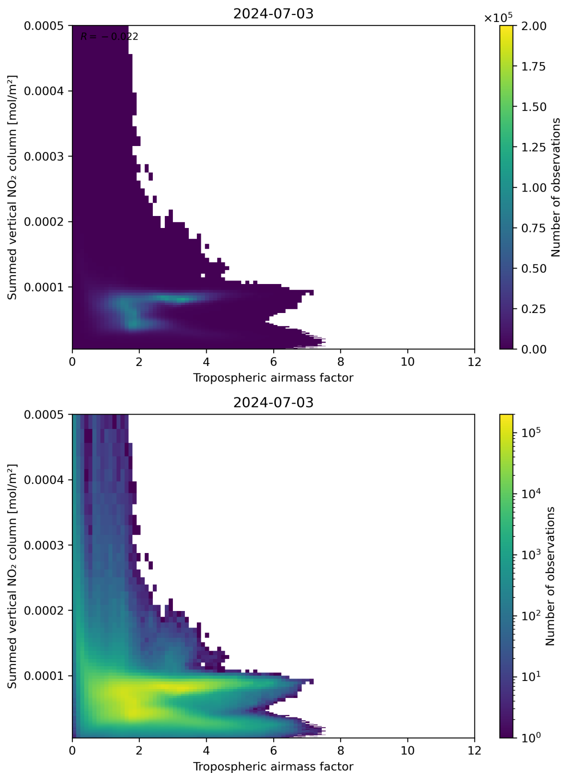
Figure 75: Scatter density plot of “Tropospheric airmass factor” against “Summed vertical NO 2 column” for 2024-07-02 to 2024-07-04.
