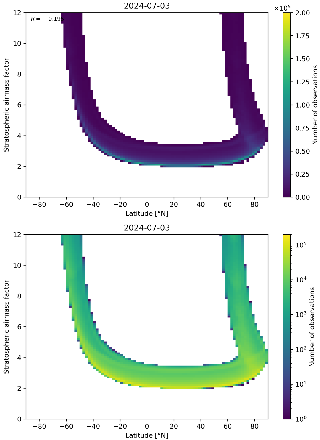
Figure 83: Scatter density plot of “Latitude” against “Stratospheric air mass factor” for 2024-07-02 to 2024-07-04.
