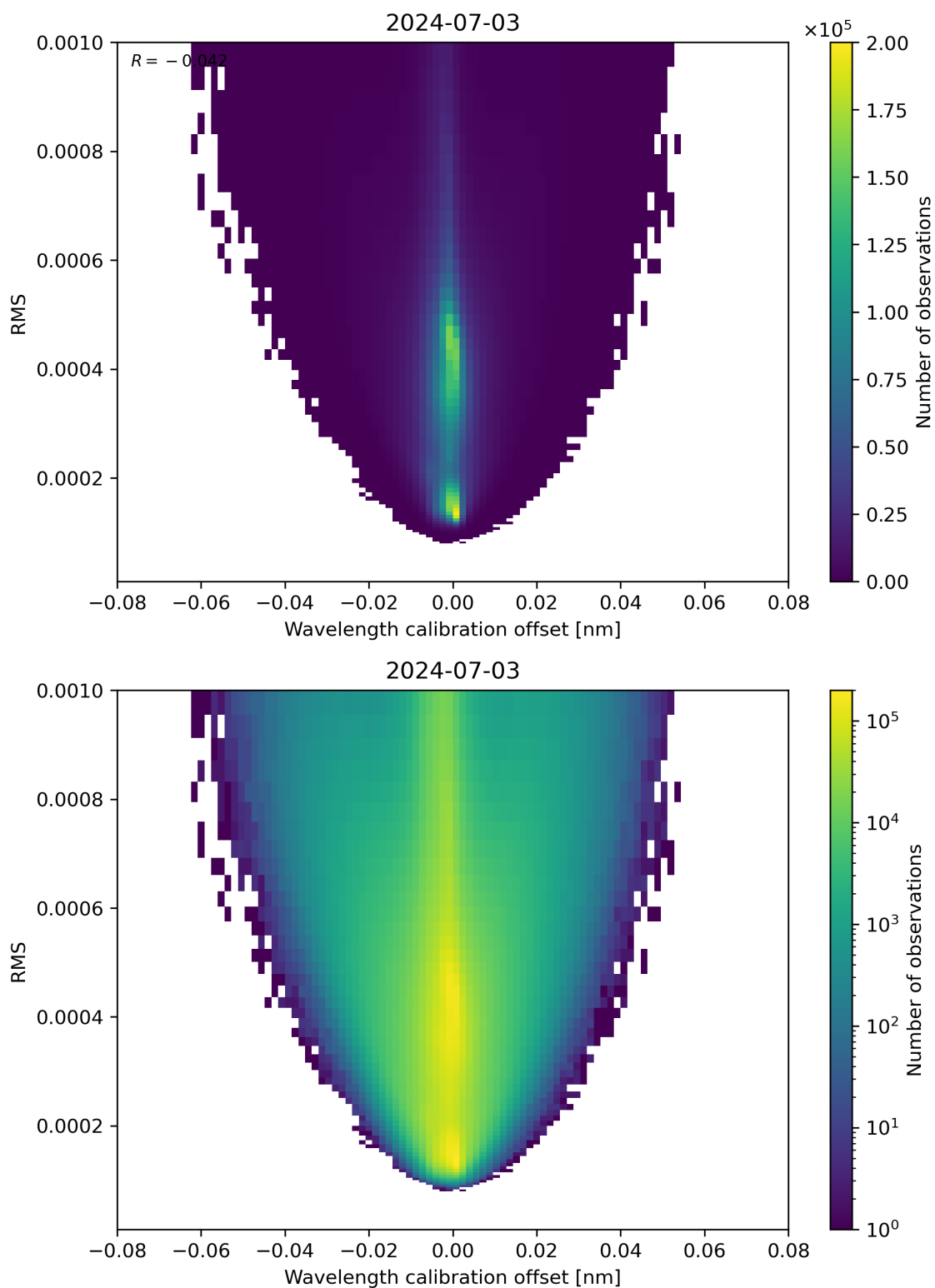
Figure 181: Scatter density plot of “Wavelength calibration offset” against “RMS” for 2024-07-02 to 2024-07-04.
