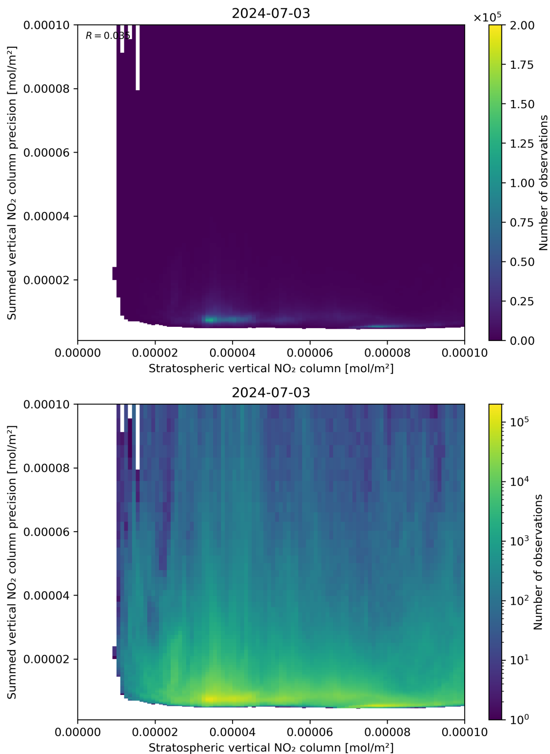
Figure 99: Scatter density plot of “Stratospheric vertical NO 2 column” against “Summed vertical NO 2 column precision” for 2024-07-02 to 2024-07-04.
