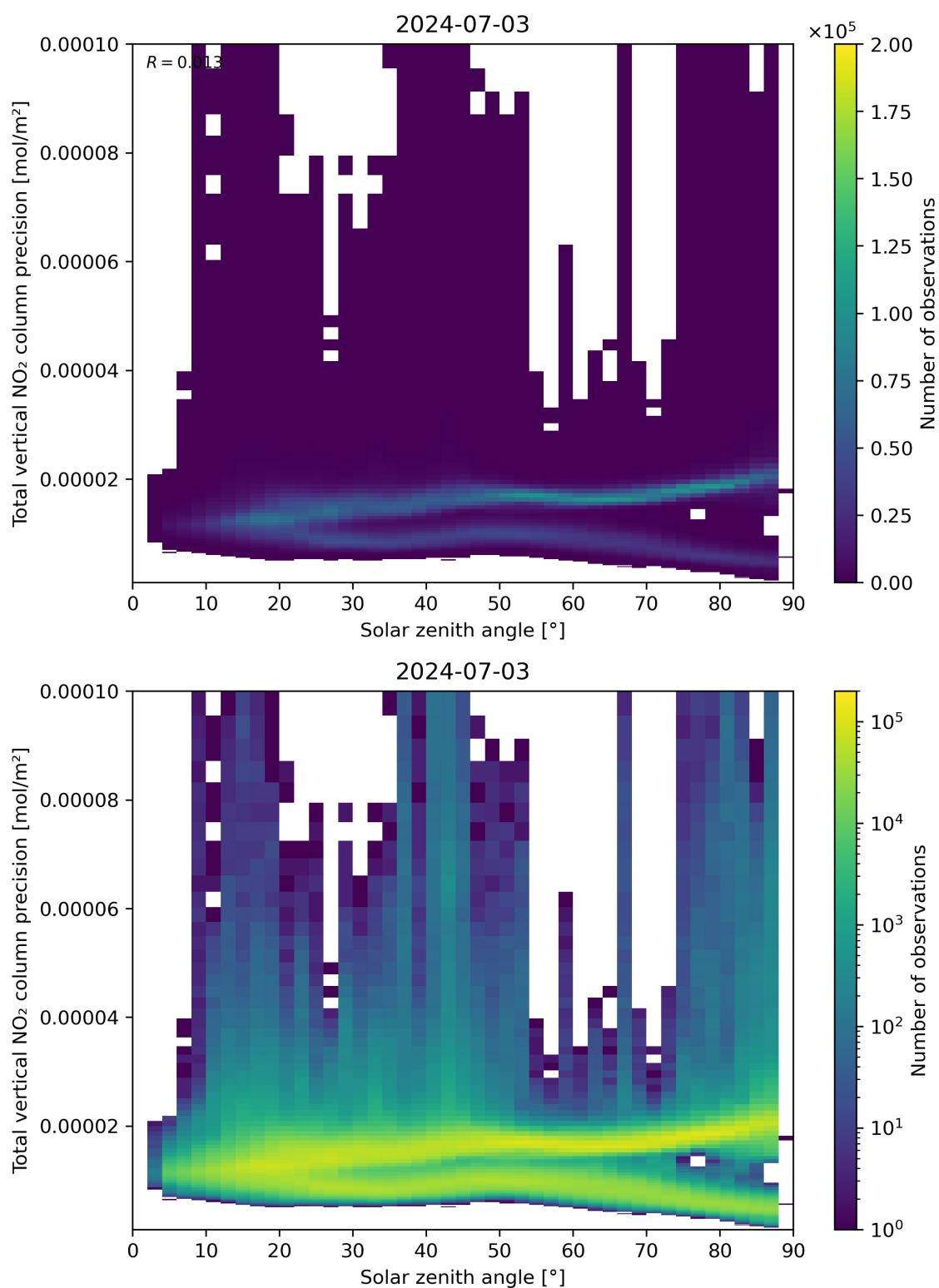
Figure 154: Scatter density plot of “Solar zenith angle” against “Total vertical NO 2 column precision” for 2024-07-02 to 2024-07-04.
