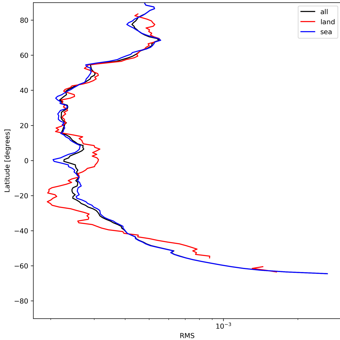
Figure 26: Zonal average of “RMS” for 2024-07-02 to 2024-07-04.
