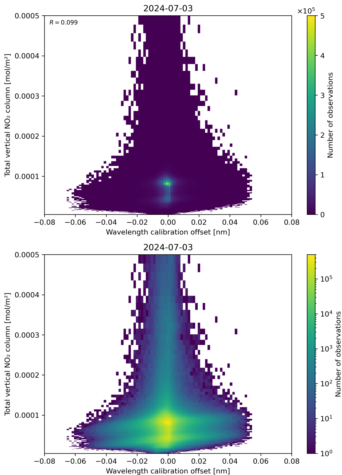
Figure 179: Scatter density plot of “Wavelength calibration offset” against “Total vertical NO 2 column” for 2024-07-02 to 2024-07-04.
