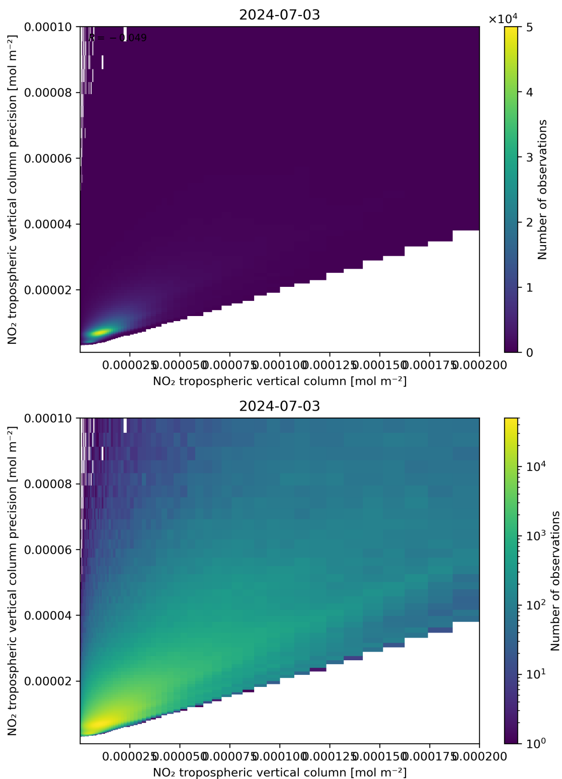
Figure 130: Scatter density plot of “NO 2 tropospheric vertical column” against “NO 2 tropospheric vertical column precision” for 2024-07-02 to 2024-07-04.
