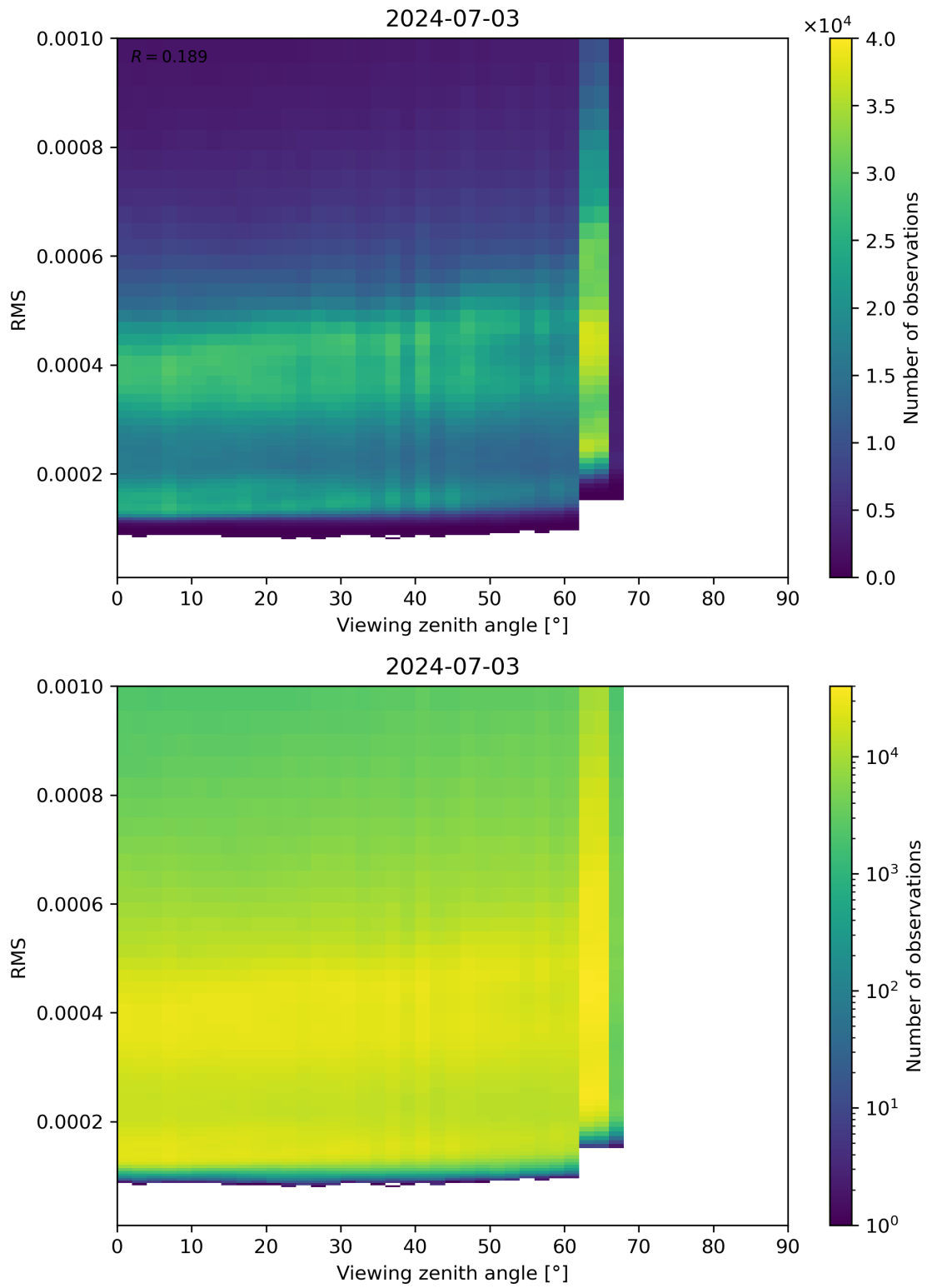
Figure 171: Scatter density plot of “Viewing zenith angle” against “RMS” for 2024-07-02 to 2024-07-04.
