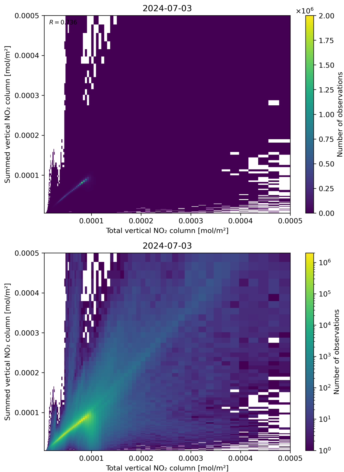
Figure 112: Scatter density plot of “Total vertical NO 2 column” against “Summed vertical NO 2 column” for 2024-07-02 to 2024-07-04.
