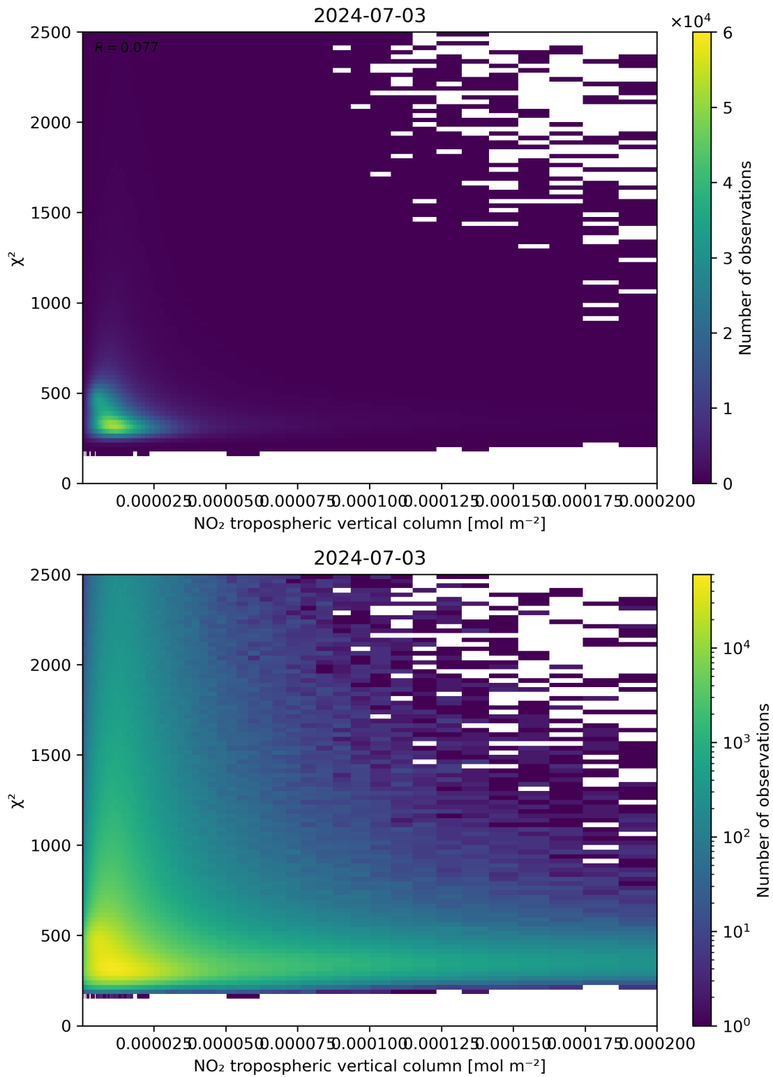
Figure 124: Scatter density plot of “NO 2 tropospheric vertical column” against “ \chi^2 ” for 2024-07-02 to 2024-07-04.
