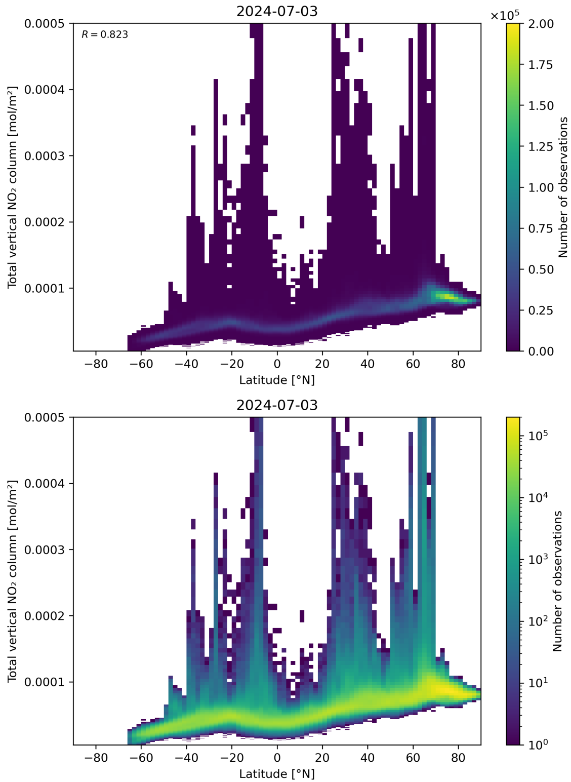
Figure 90: Scatter density plot of “Latitude” against “Total vertical NO 2 column” for 2024-07-02 to 2024-07-04.
