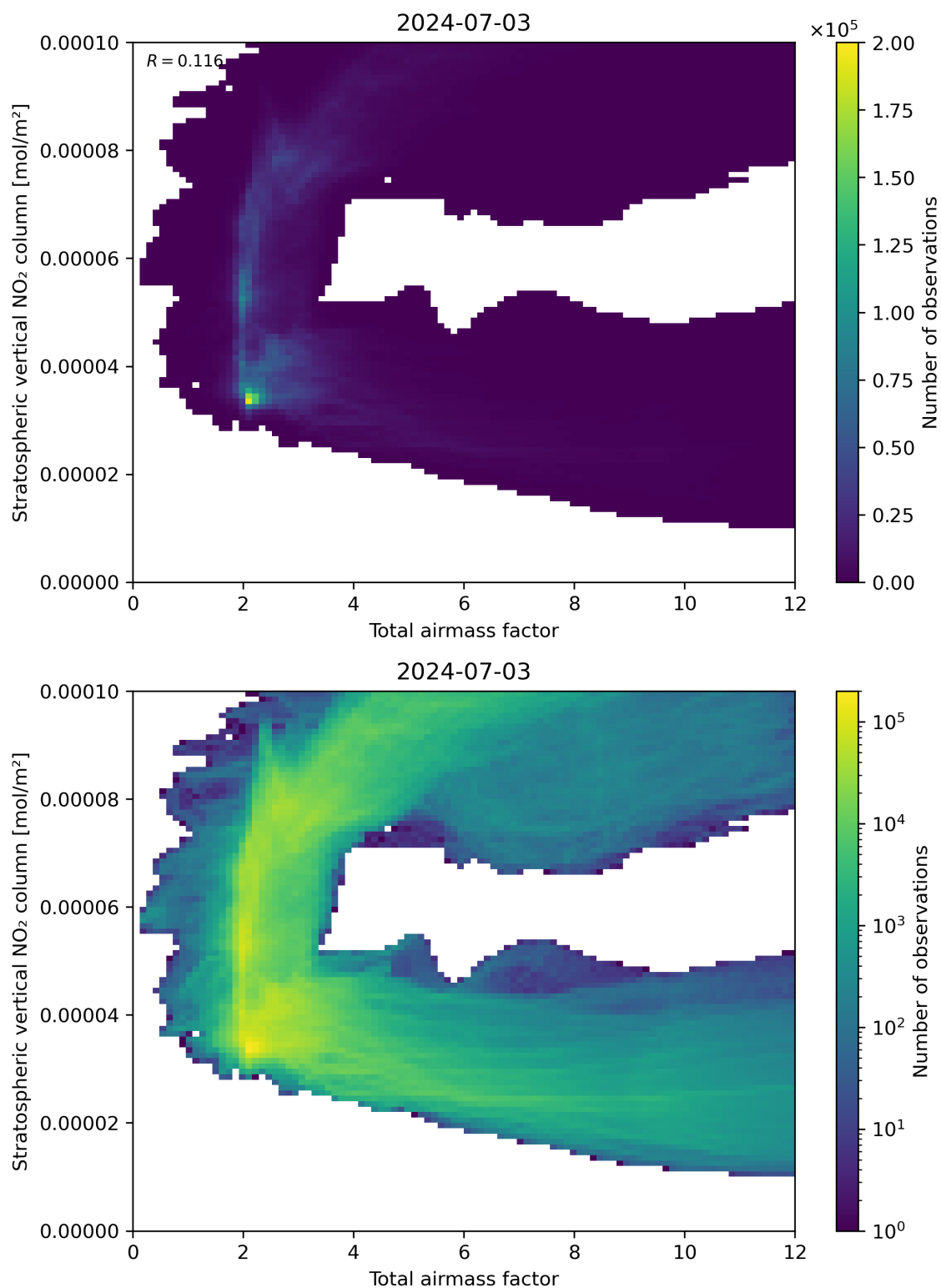
Figure 64: Scatter density plot of “Total airmass factor” against “Stratospheric vertical NO 2 column” for 2024-07-02 to 2024-07-04.
