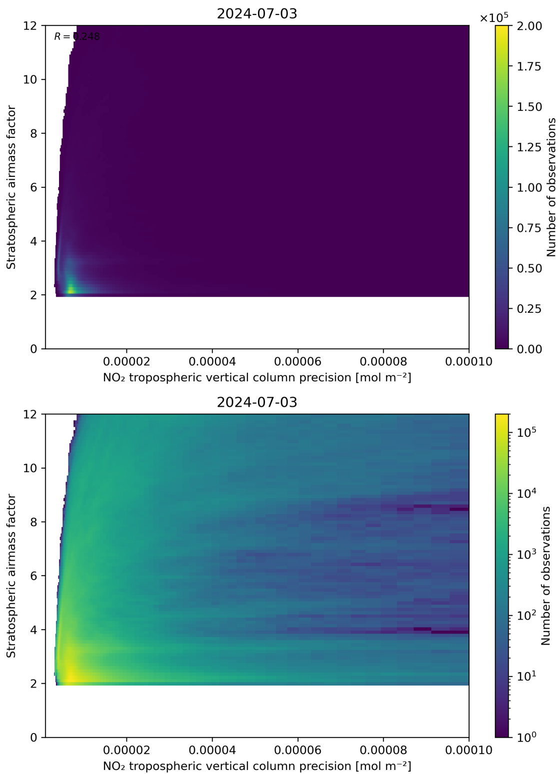
Figure 131: Scatter density plot of “NO 2 tropospheric vertical column precision” against “Stratospheric airmass factor” for 2024-07-02 to 2024-07-04.
