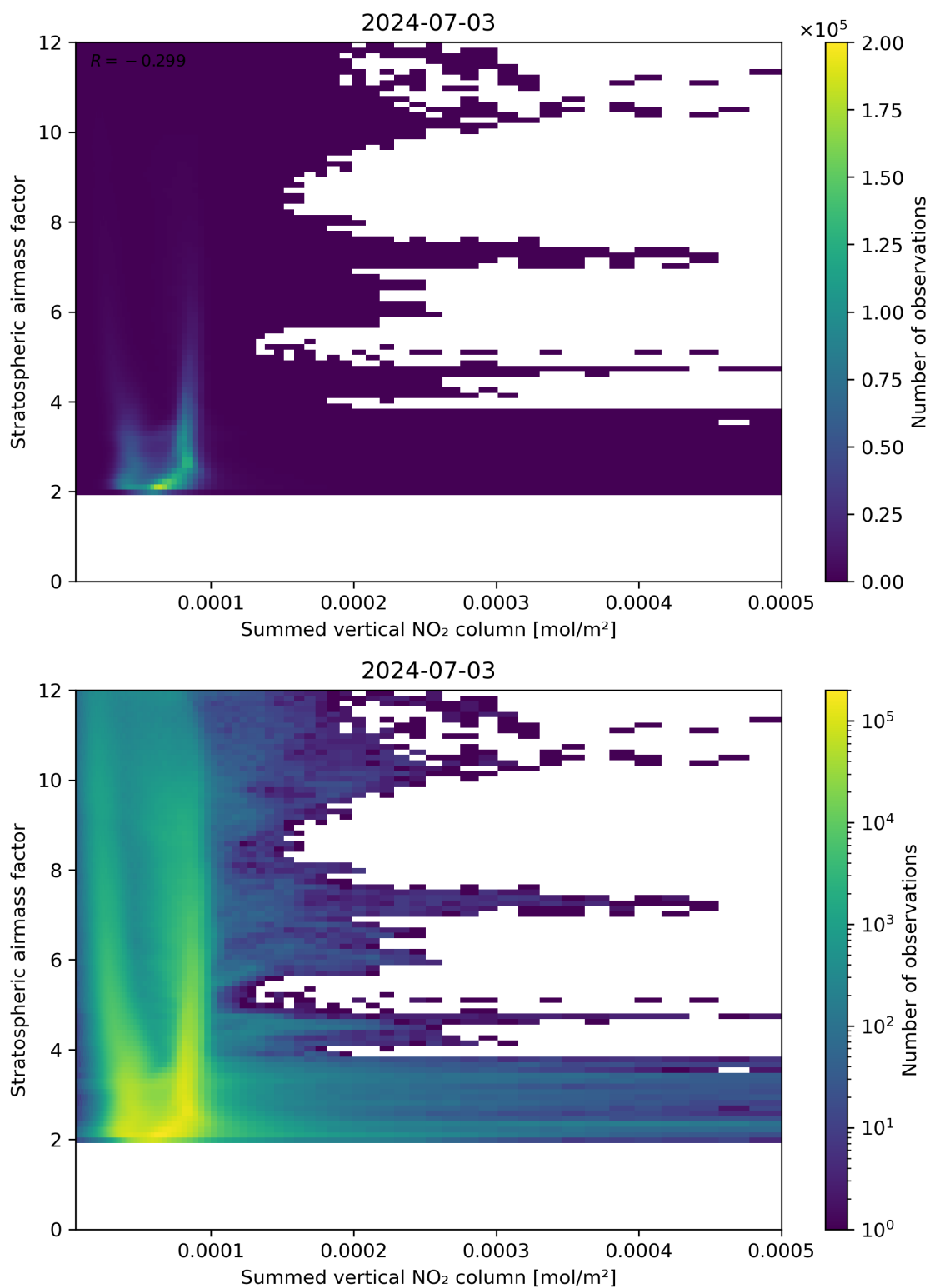
Figure 103: Scatter density plot of “Summed vertical NO 2 column” against “Stratospheric air mass factor” for 2024-07-02 to 2024-07-04.
