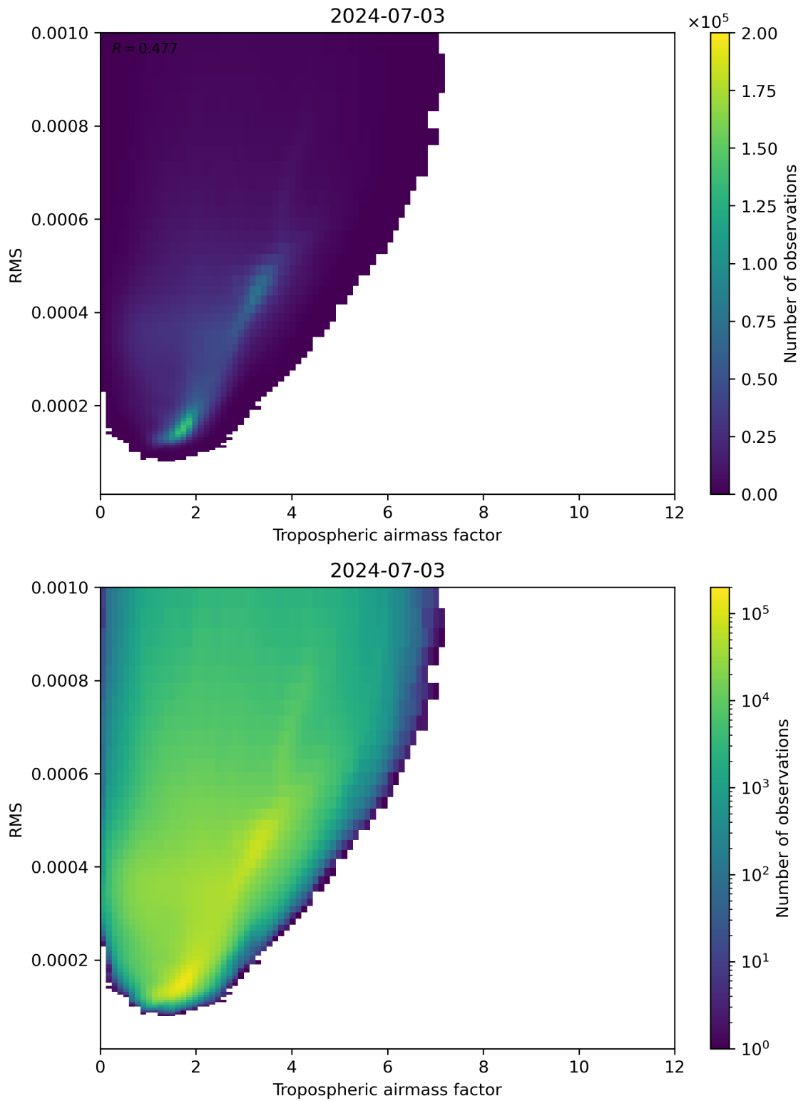
Figure 79: Scatter density plot of “Tropospheric airmass factor” against “RMS” for 2024-07-02 to 2024-07-04.
