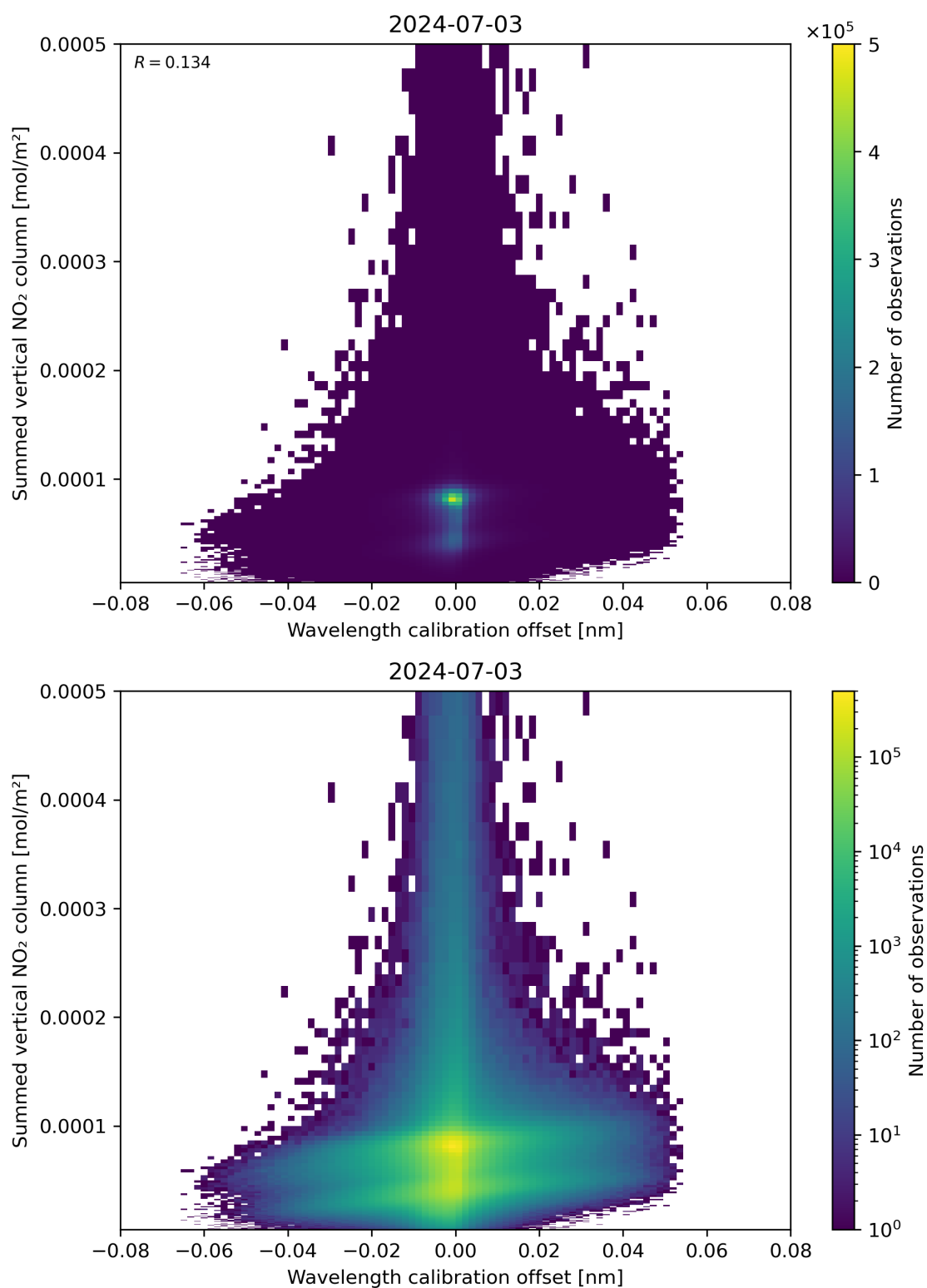
Figure 177: Scatter density plot of “Wavelength calibration offset” against “Summed vertical NO 2 column” for 2024-07-02 to 2024-07-04.
