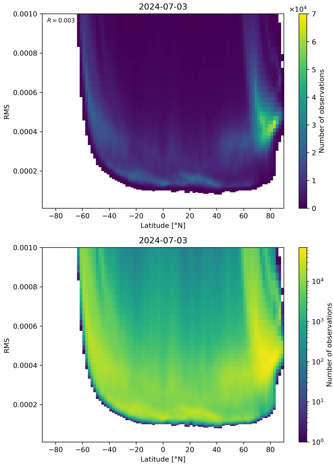
Figure 94: Scatter density plot of “Latitude” against “RMS” for 2024-07-02 to 2024-07-04.
