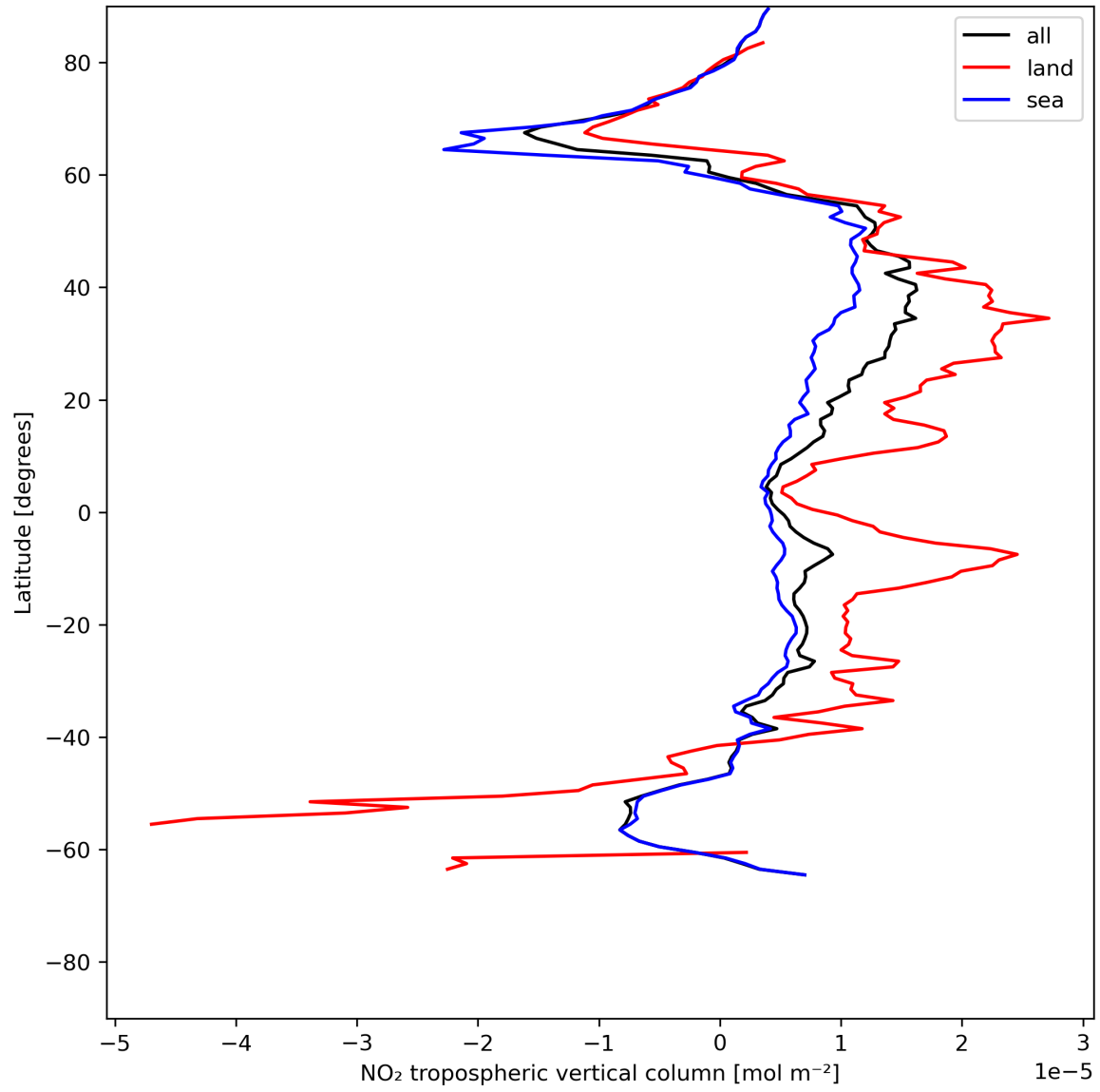
Figure 12: Zonal average of “NO 2 tropospheric vertical column” for 2024-07-02 to 2024-07-04.
