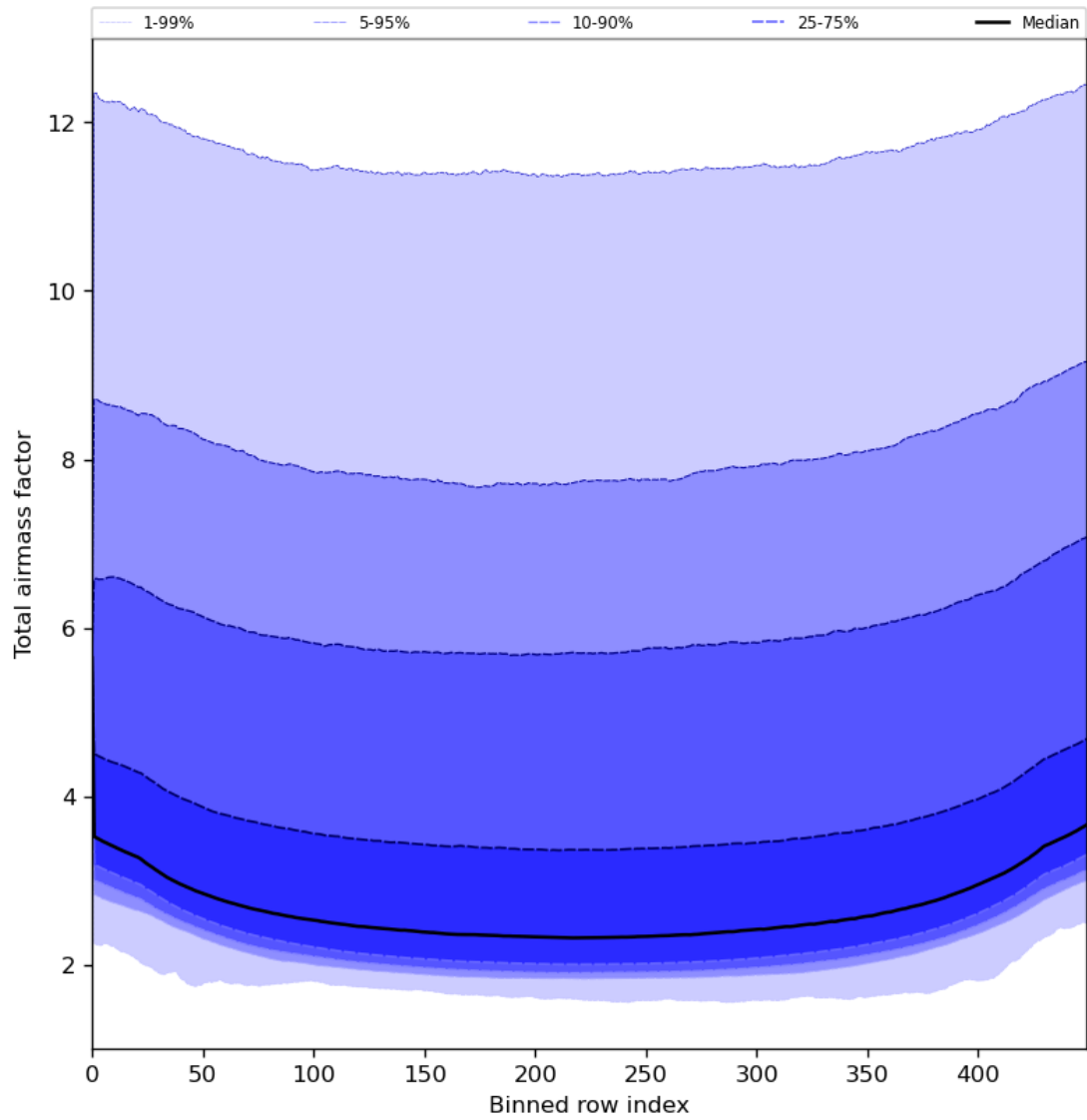
Figure 49: Along track statistics of “Total airmass factor” for 2024-07-02 to 2024-07-04
