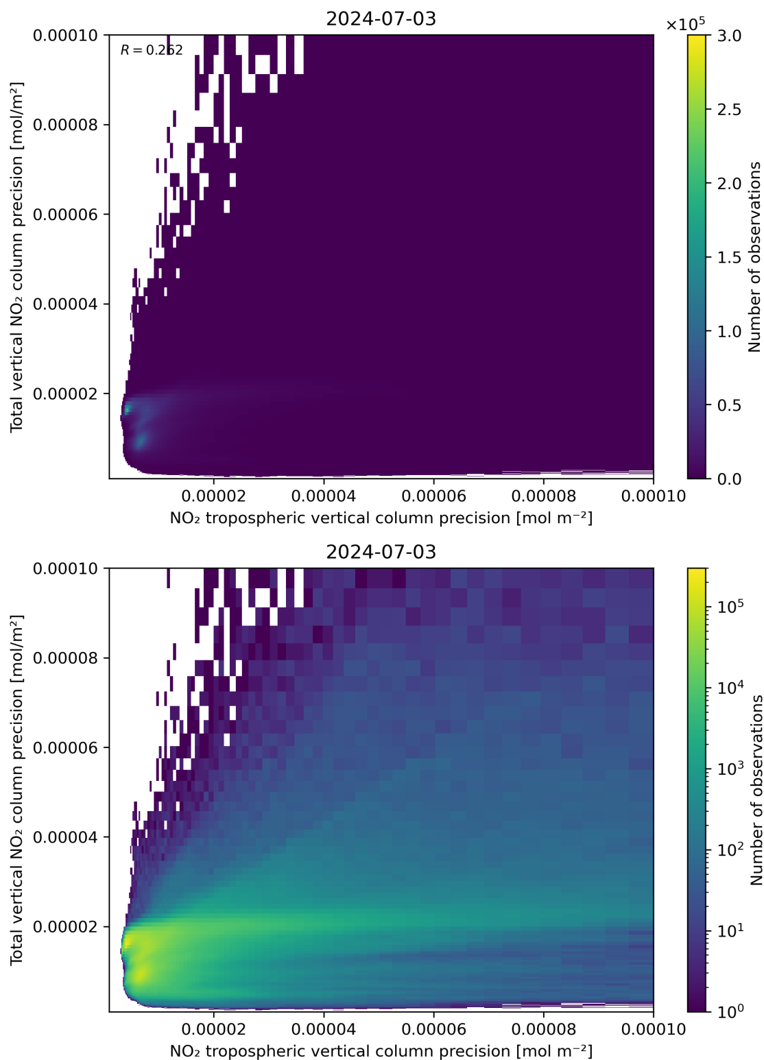
Figure 139: Scatter density plot of “NO 2 tropospheric vertical column precision” against “Total vertical NO 2 column precision” for 2024-07-02 to 2024-07-04.
