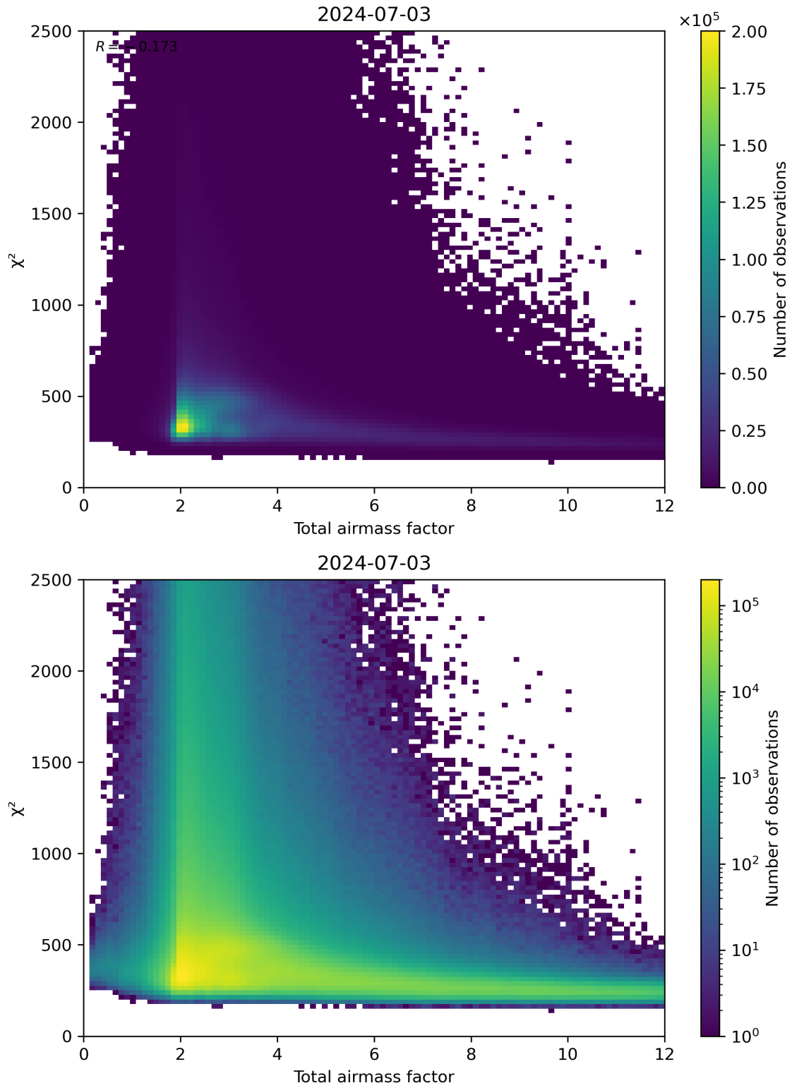
Figure 63: Scatter density plot of “Total airmass factor” against “ \chi^2 ” for 2024-07-02 to 2024-07-04.
