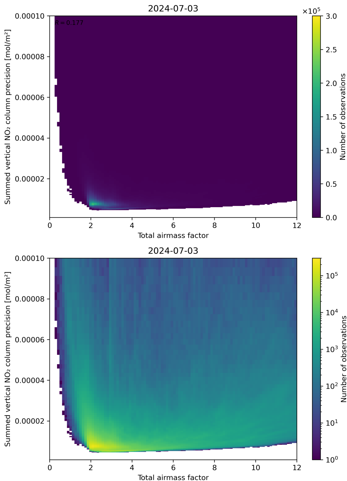
Figure 66: Scatter density plot of “Total airmass factor” against “Summed vertical NO 2 column precision” for 2024-07-02 to 2024-07-04.
