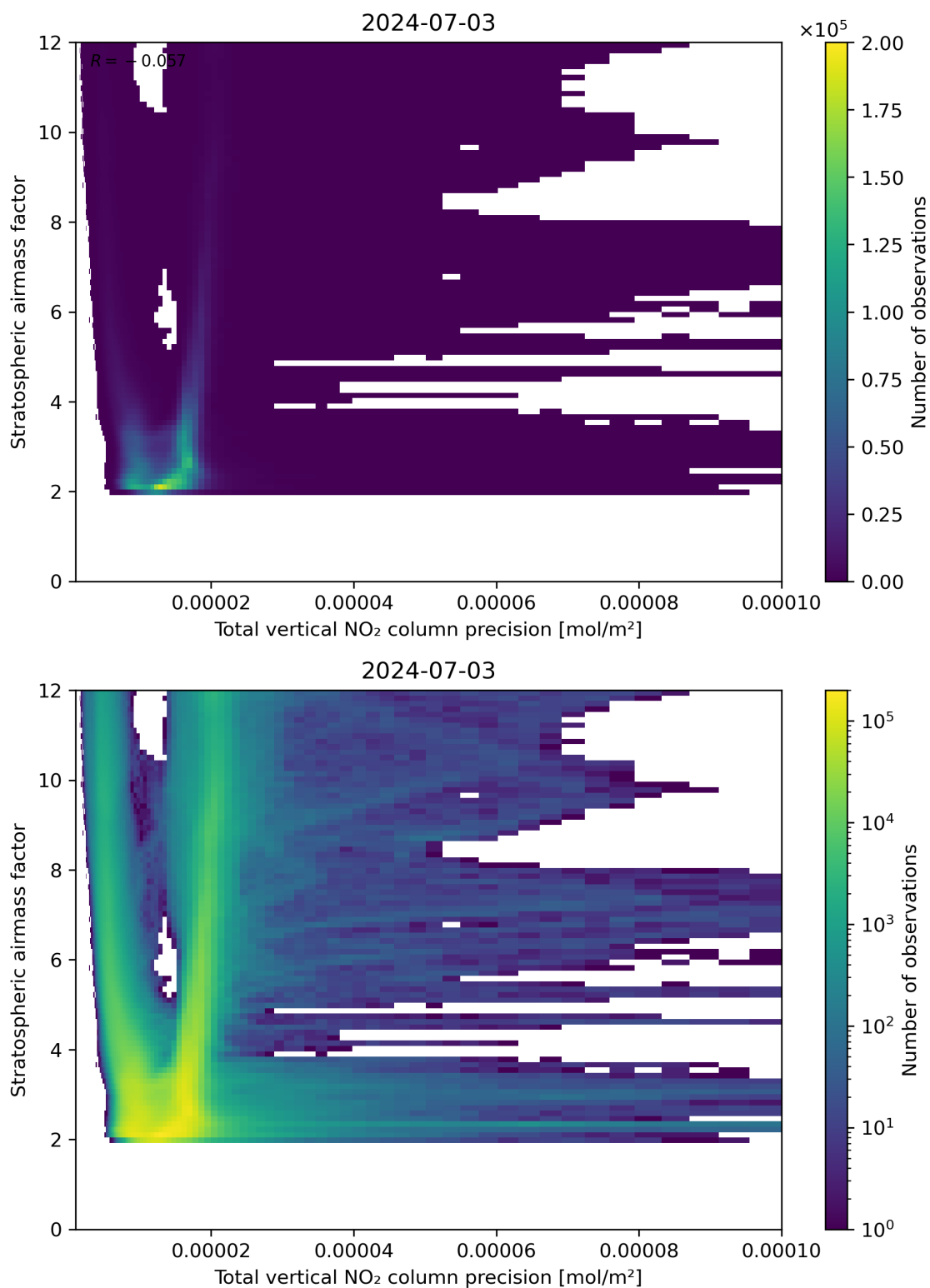
Figure 115: Scatter density plot of “Total vertical NO 2 column precision” against “Stratospheric air mass factor” for 2024-07-02 to 2024-07-04.
