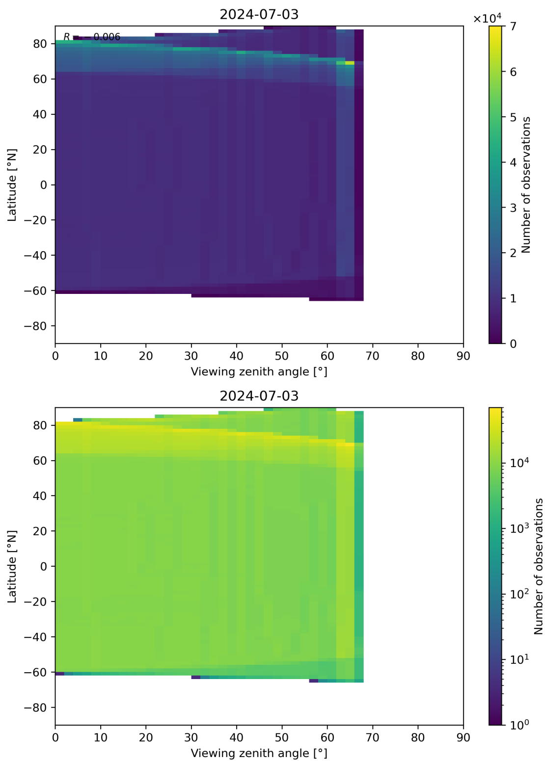
Figure 163: Scatter density plot of “Viewing zenith angle” against “Latitude” for 2024-07-02 to 2024-07-04.
