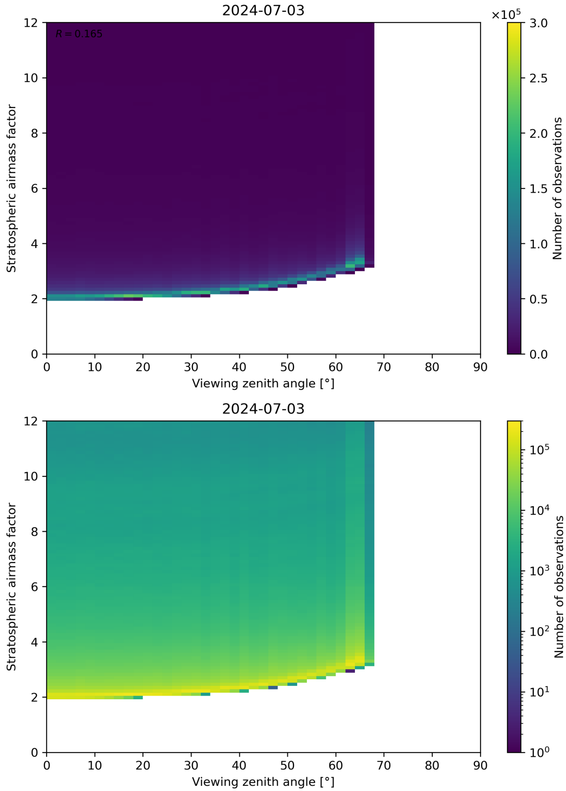
Figure 159: Scatter density plot of “Viewing zenith angle” against “Stratospheric airmass factor” for 2024-07-02 to 2024-07-04.
