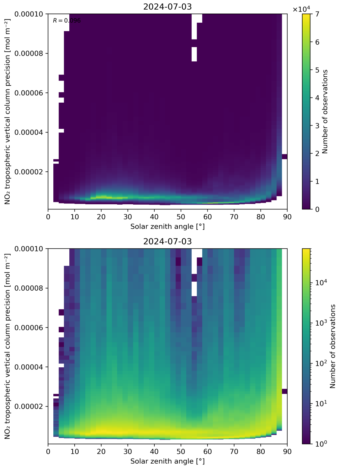
Figure 156: Scatter density plot of “Solar zenith angle” against “NO 2 tropospheric vertical column precision” for 2024-07-02 to 2024-07-04.
