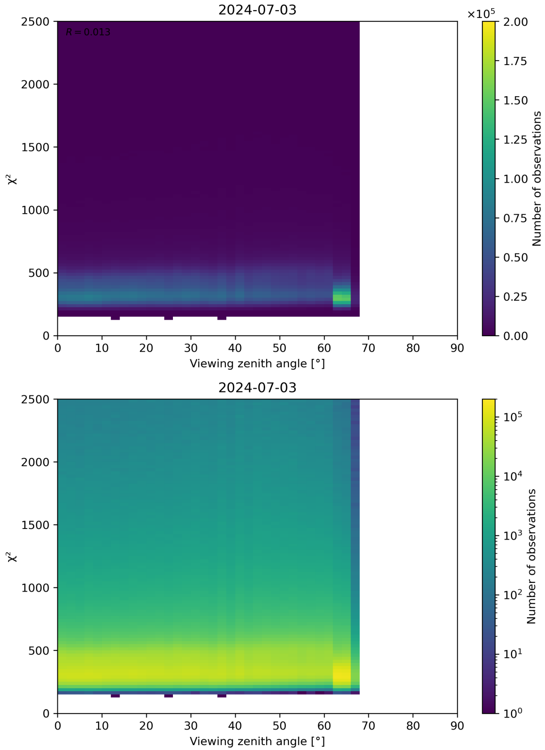
Figure 162: Scatter density plot of “Viewing zenith angle” against “ \chi^2 ” for 2024-07-02 to 2024-07-04.
