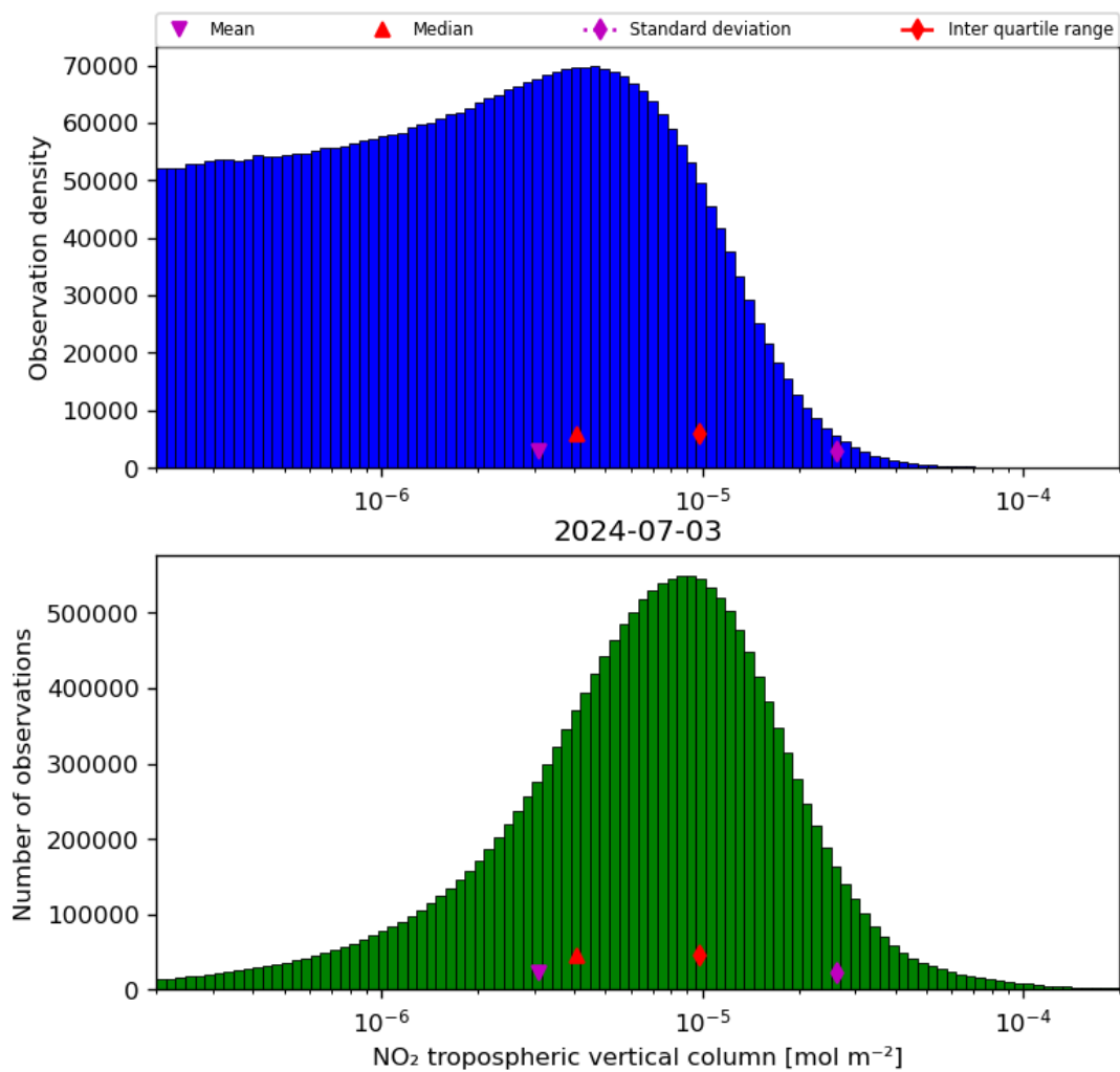
Figure 29: Histogram of “NO 2 tropospheric vertical column” for 2024-07-02 to 2024-07-04
