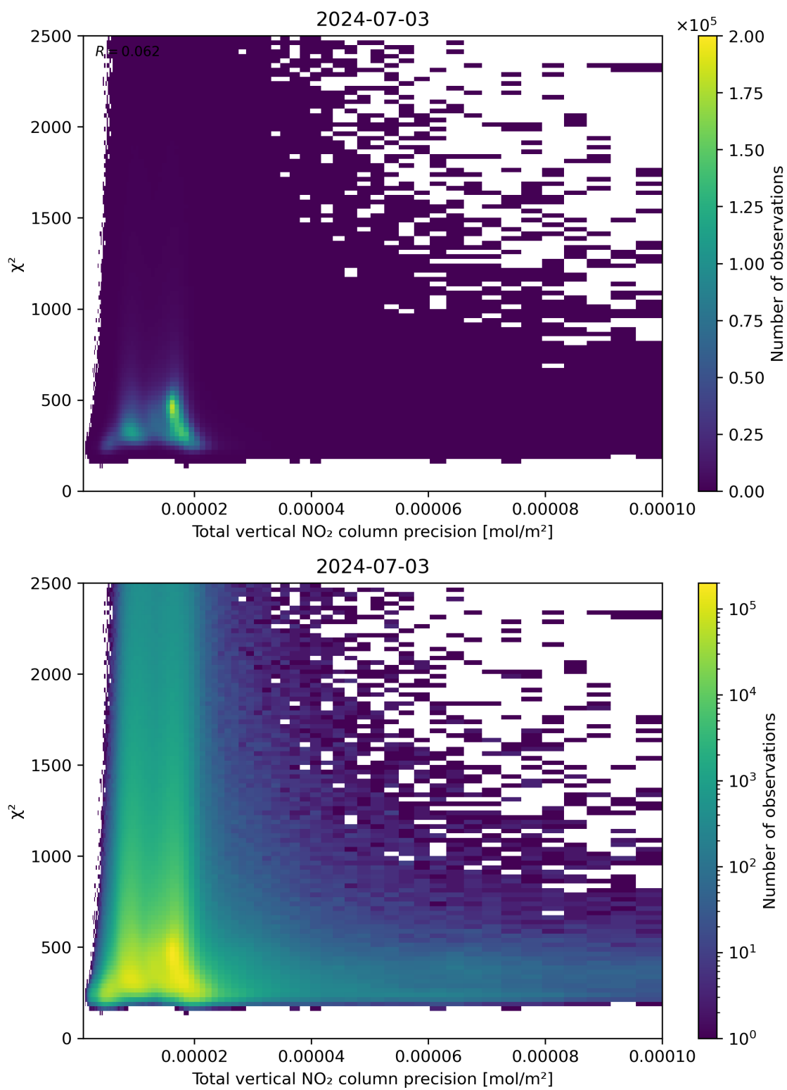
Figure 116: Scatter density plot of “Total vertical NO 2 column precision” against “ \chi^2 ” for 2024-07-02 to 2024-07-04.
