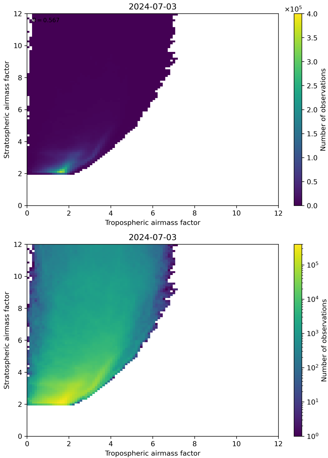
Figure 71: Scatter density plot of “Tropospheric airmass factor” against “Stratospheric airmass factor” for 2024-07-02 to 2024-07-04.
