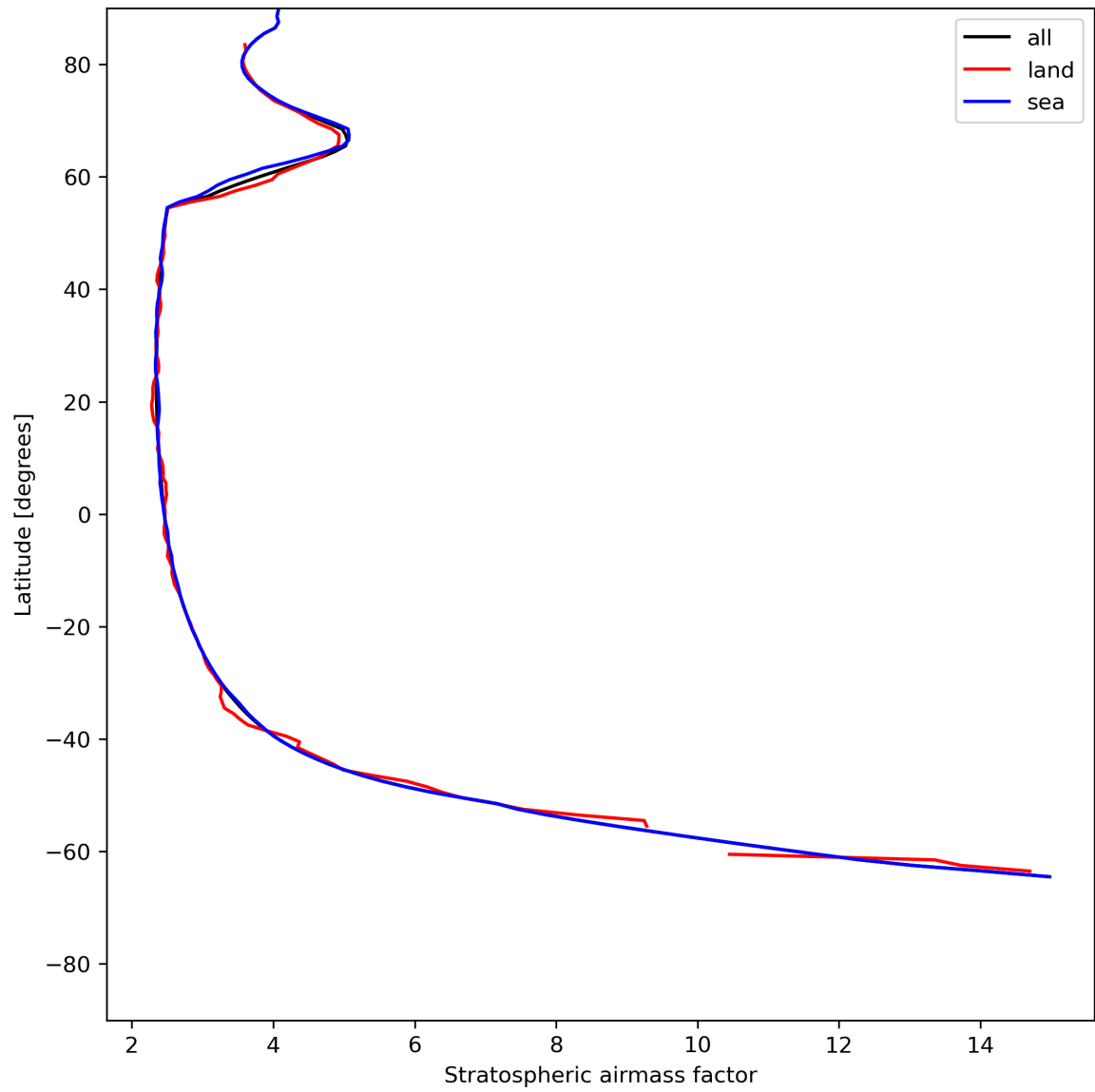
Figure 27: Zonal average of “Stratospheric airmass factor” for 2024-07-02 to 2024-07-04.
