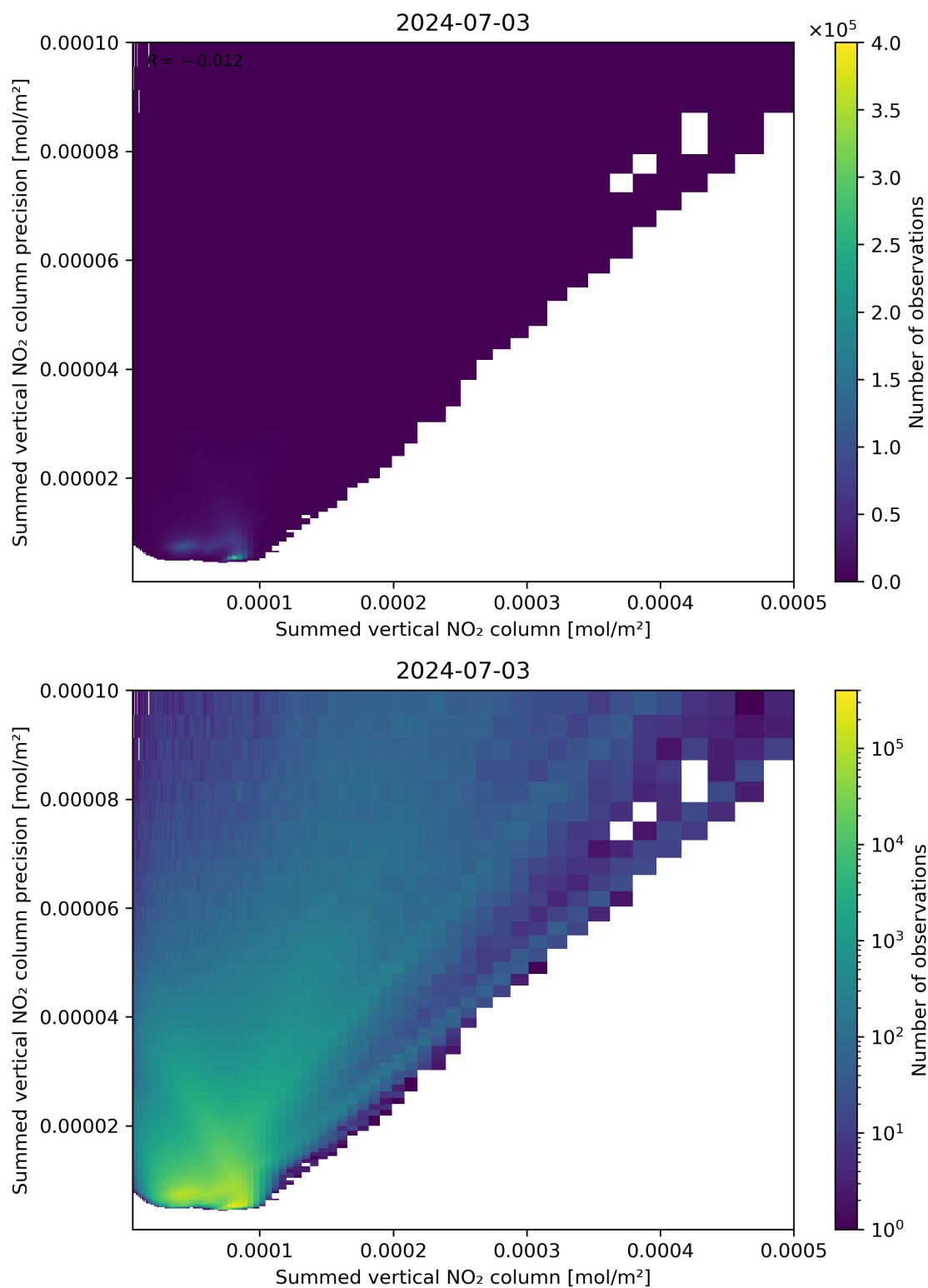
Figure 105: Scatter density plot of “Summed vertical NO 2 column” against “Summed vertical NO 2 column precision” for 2024-07-02 to 2024-07-04.
