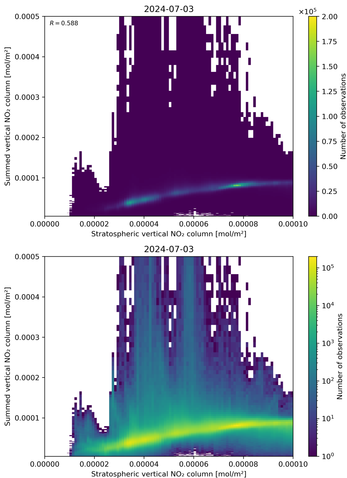
Figure 98: Scatter density plot of “Stratospheric vertical NO 2 column” against “Summed vertical NO 2 column” for 2024-07-02 to 2024-07-04.
