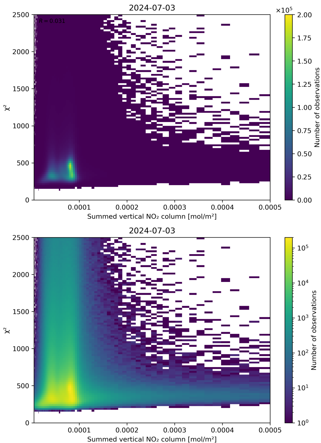
Figure 104: Scatter density plot of “Summed vertical NO 2 column” against “ \chi^2 ” for 2024-07-02 to 2024-07-04.
