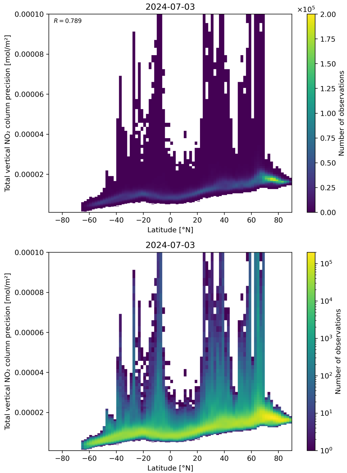
Figure 91: Scatter density plot of “Latitude” against “Total vertical NO 2 column precision” for 2024-07-02 to 2024-07-04.
