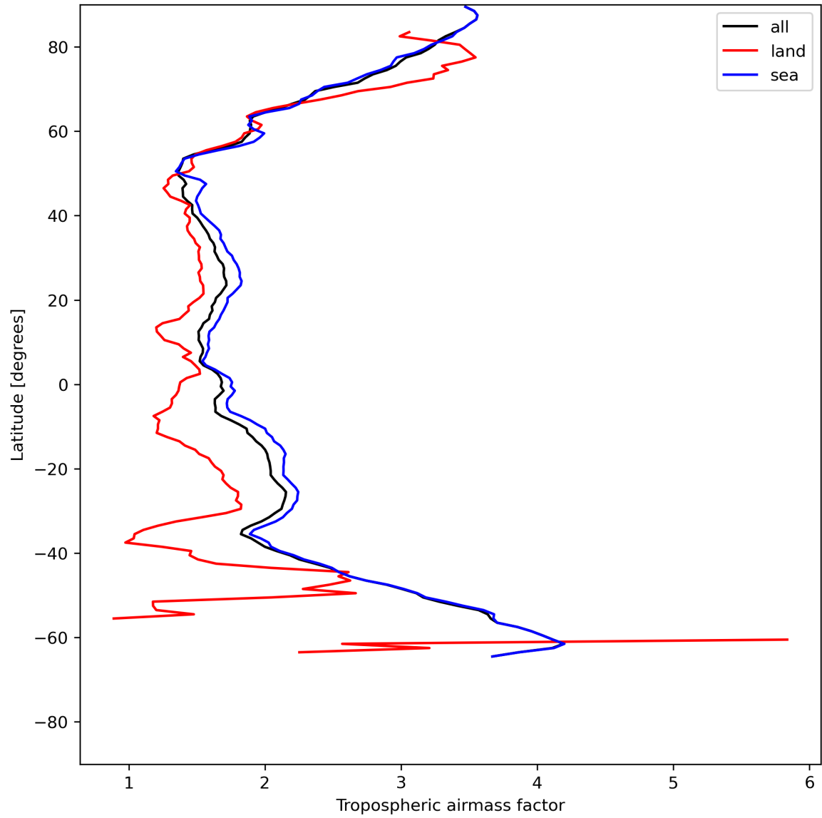
Figure 14: Zonal average of “Tropospheric airmass factor” for 2024-07-02 to 2024-07-04.
