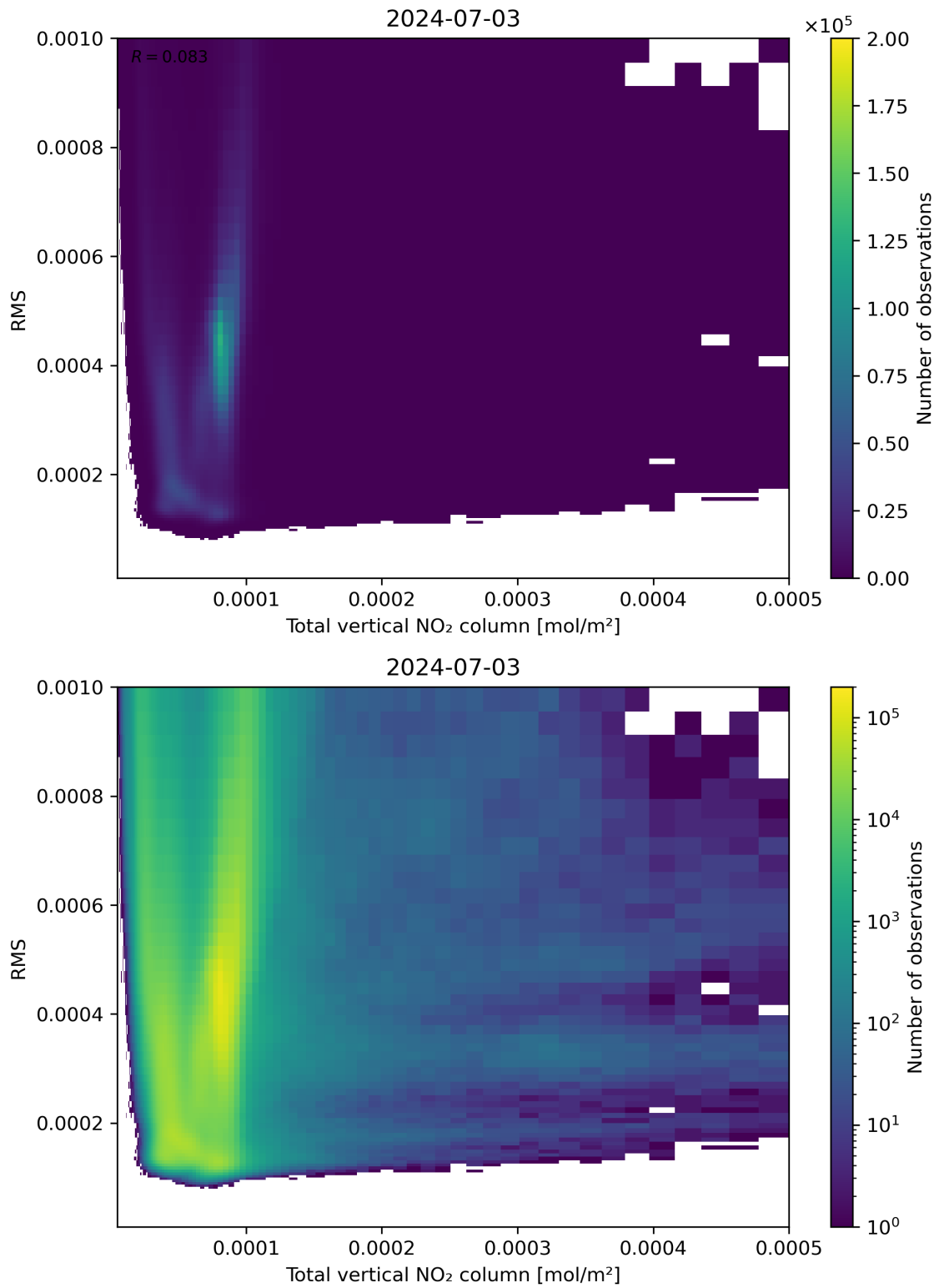
Figure 120: Scatter density plot of “Total vertical NO 2 column” against “RMS” for 2024-07-02 to 2024-07-04.
