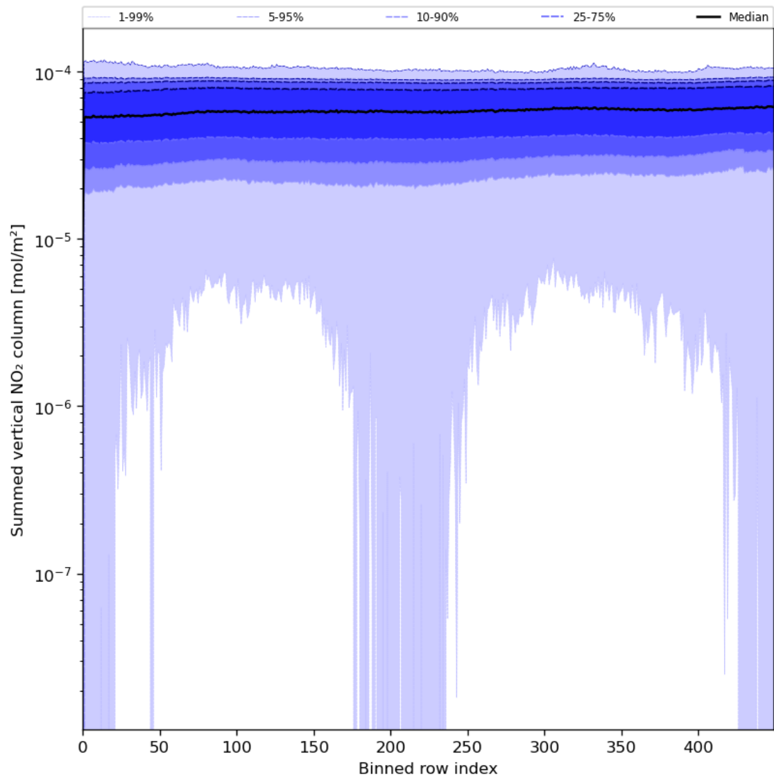
Figure 57: Along track statistics of “Summed vertical NO 2 column” for 2024-07-02 to 2024-07-04
