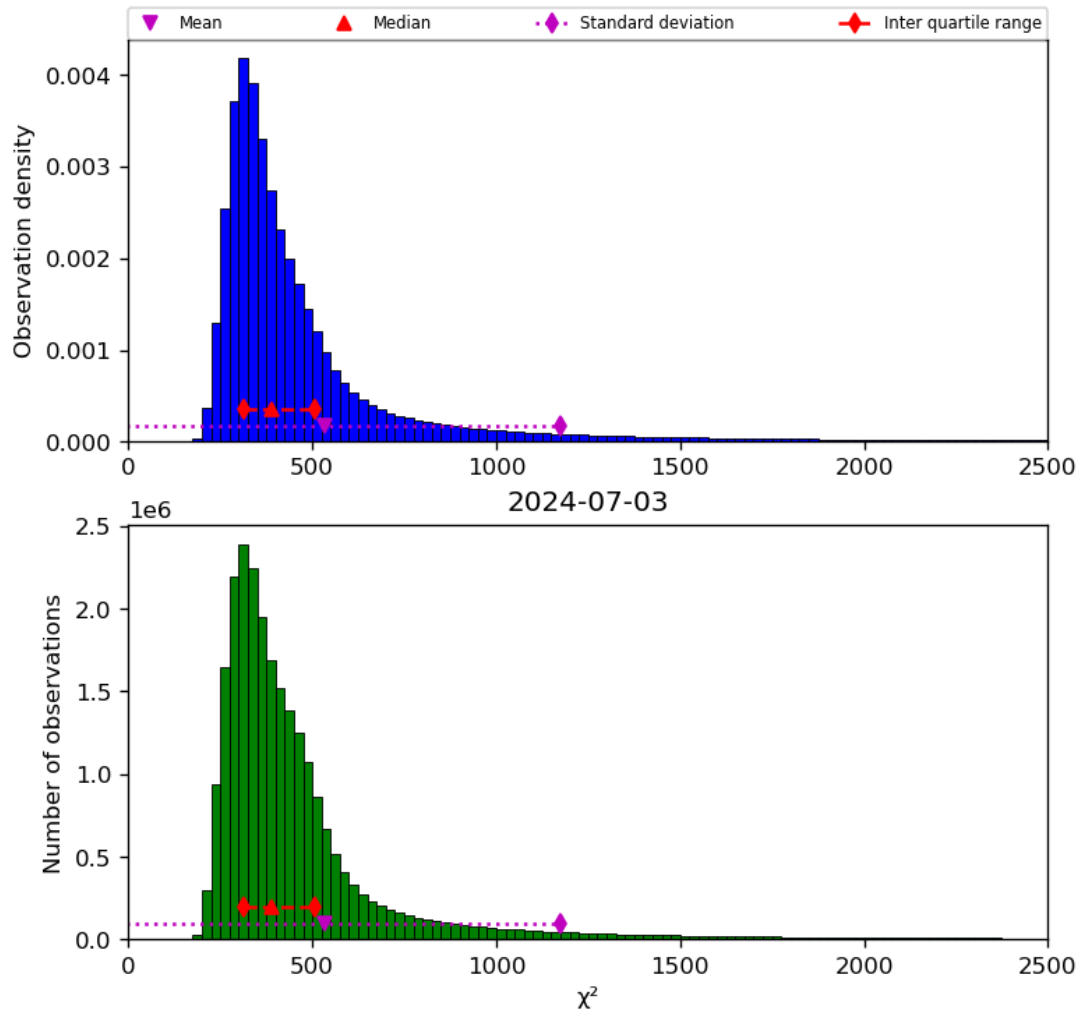
Figure 42: Histogram of “ \chi^2 ” for 2024-07-02 to 2024-07-04
