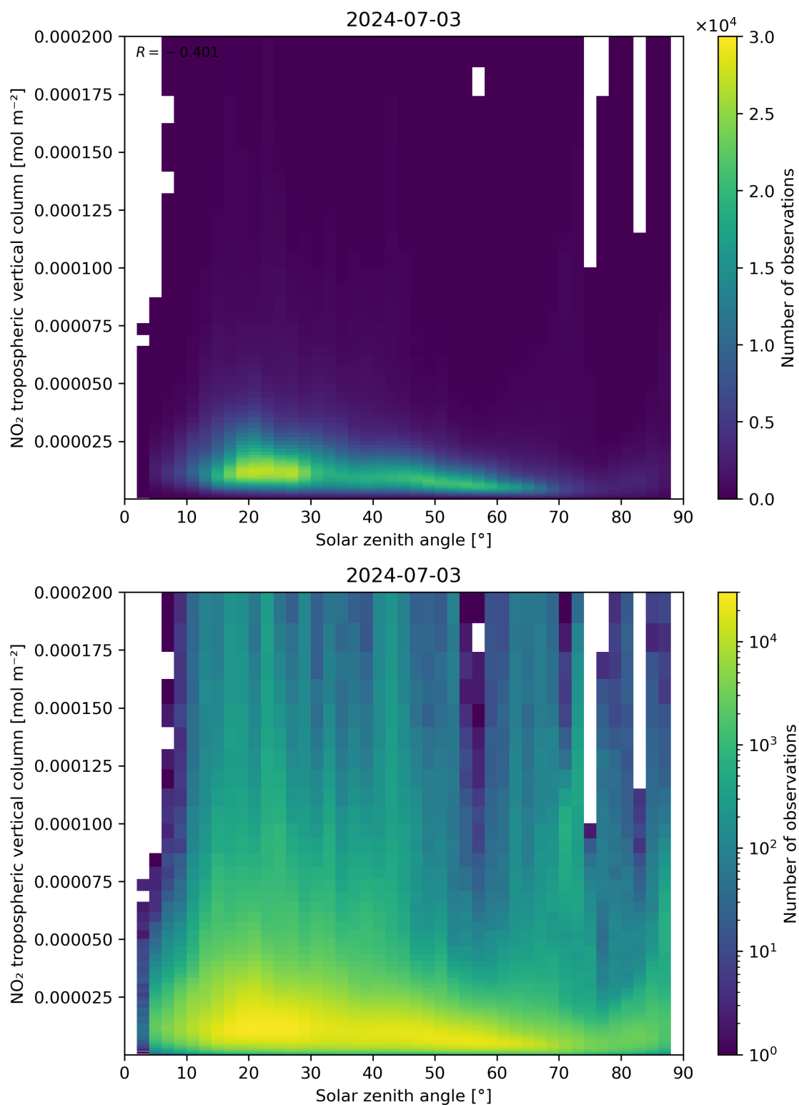
Figure 155: Scatter density plot of “Solar zenith angle” against “NO 2 tropospheric vertical column” for 2024-07-02 to 2024-07-04.
