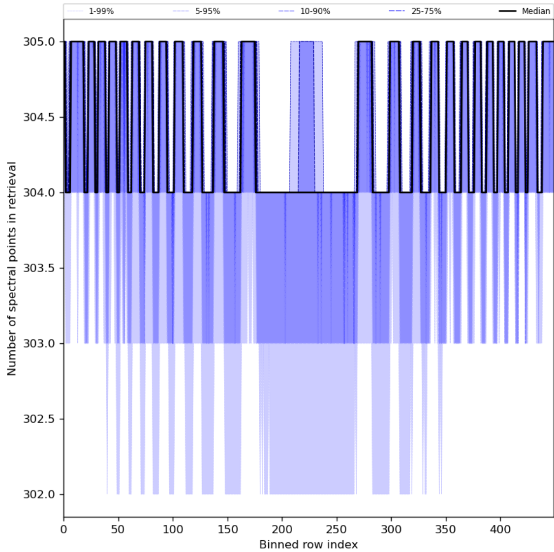
Figure 50: Along track statistics of “Number of spectral points in retrieval” for 2024-07-02 to 2024-07-04
