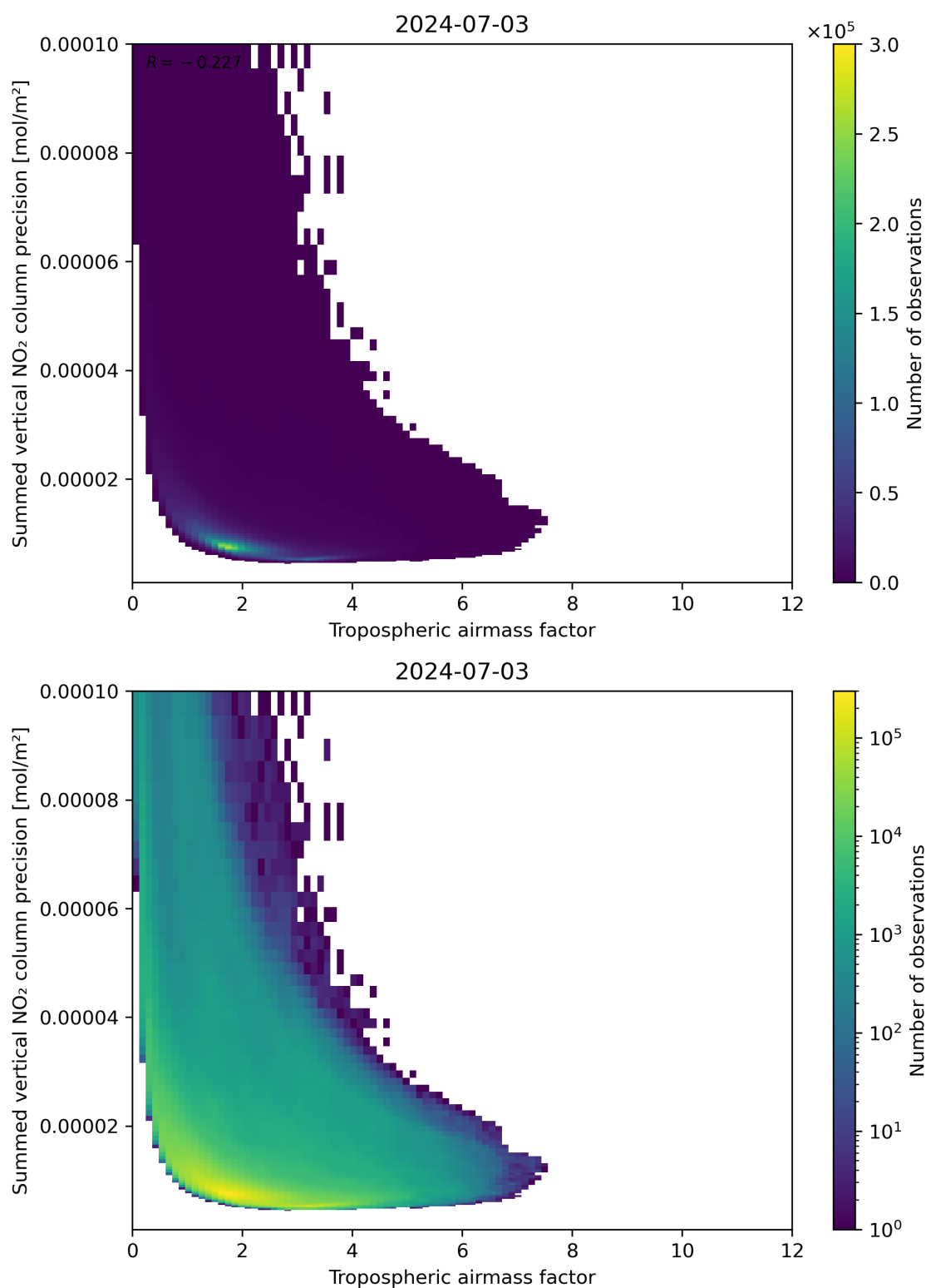
Figure 76: Scatter density plot of “Tropospheric air mass factor” against “Summed vertical NO 2 column precision” for 2024-07-02 to 2024-07-04.
