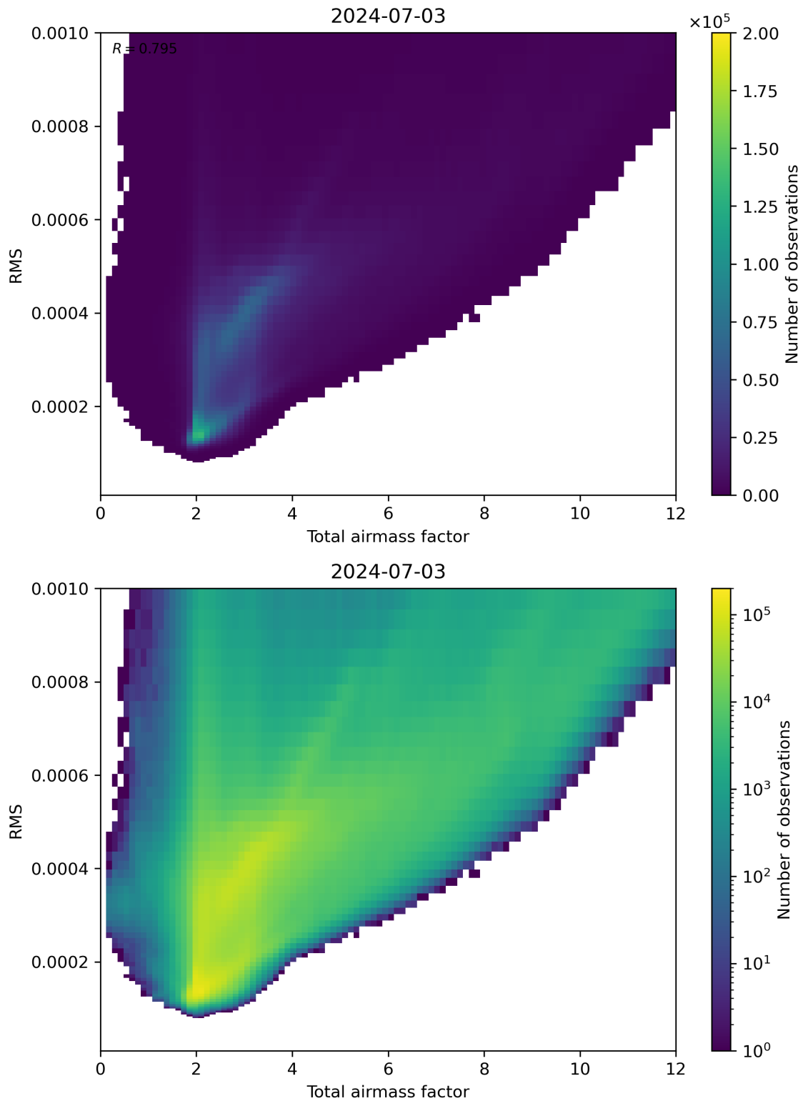
Figure 69: Scatter density plot of “Total airmass factor” against “RMS” for 2024-07-02 to 2024-07-04.
