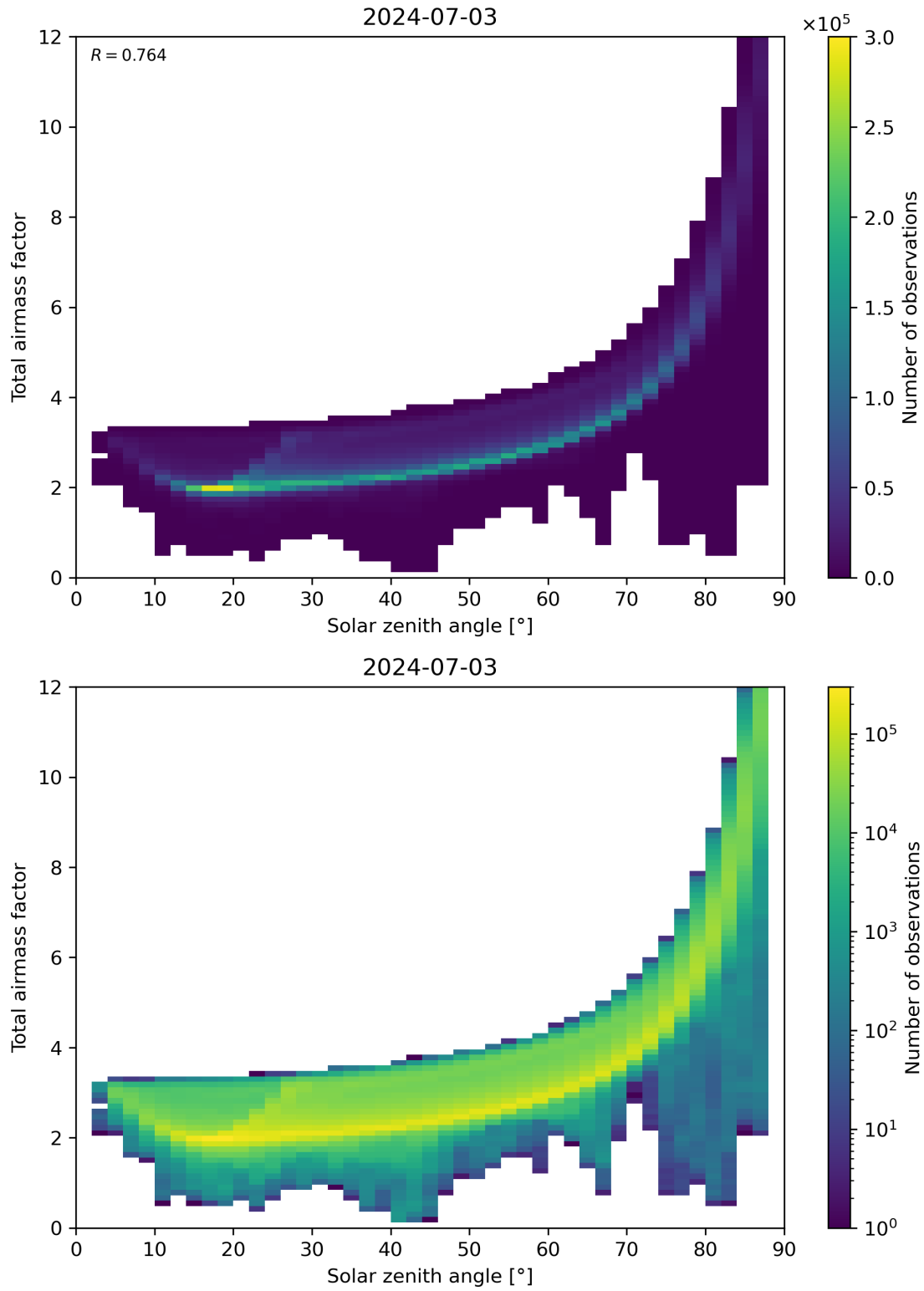
Figure 146: Scatter density plot of “Solar zenith angle” against “Total air mass factor” for 2024-07-02 to 2024-07-04.
