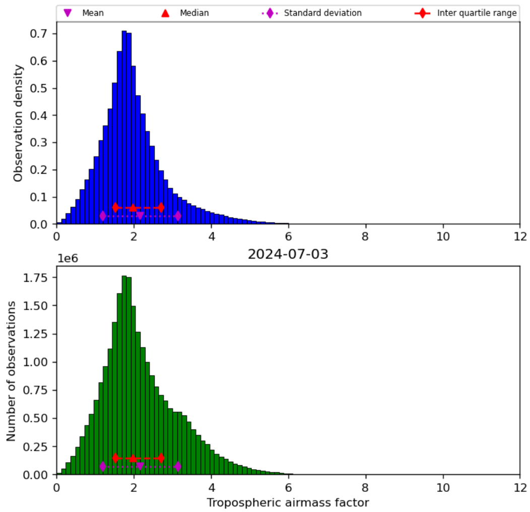
Figure 31: Histogram of “Tropospheric airmass factor” for 2024-07-02 to 2024-07-04
