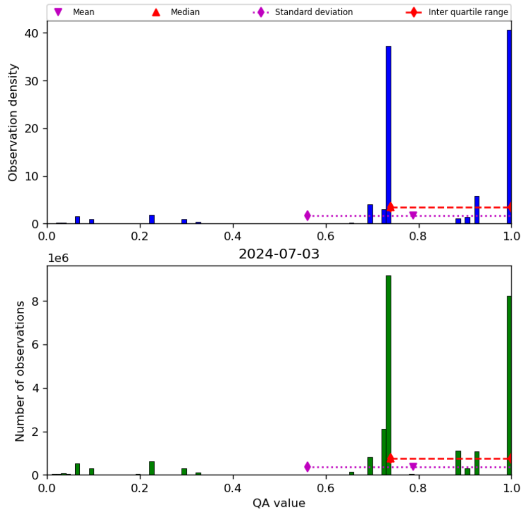
Figure 28: Histogram of “QA value” for 2024-07-02 to 2024-07-04
