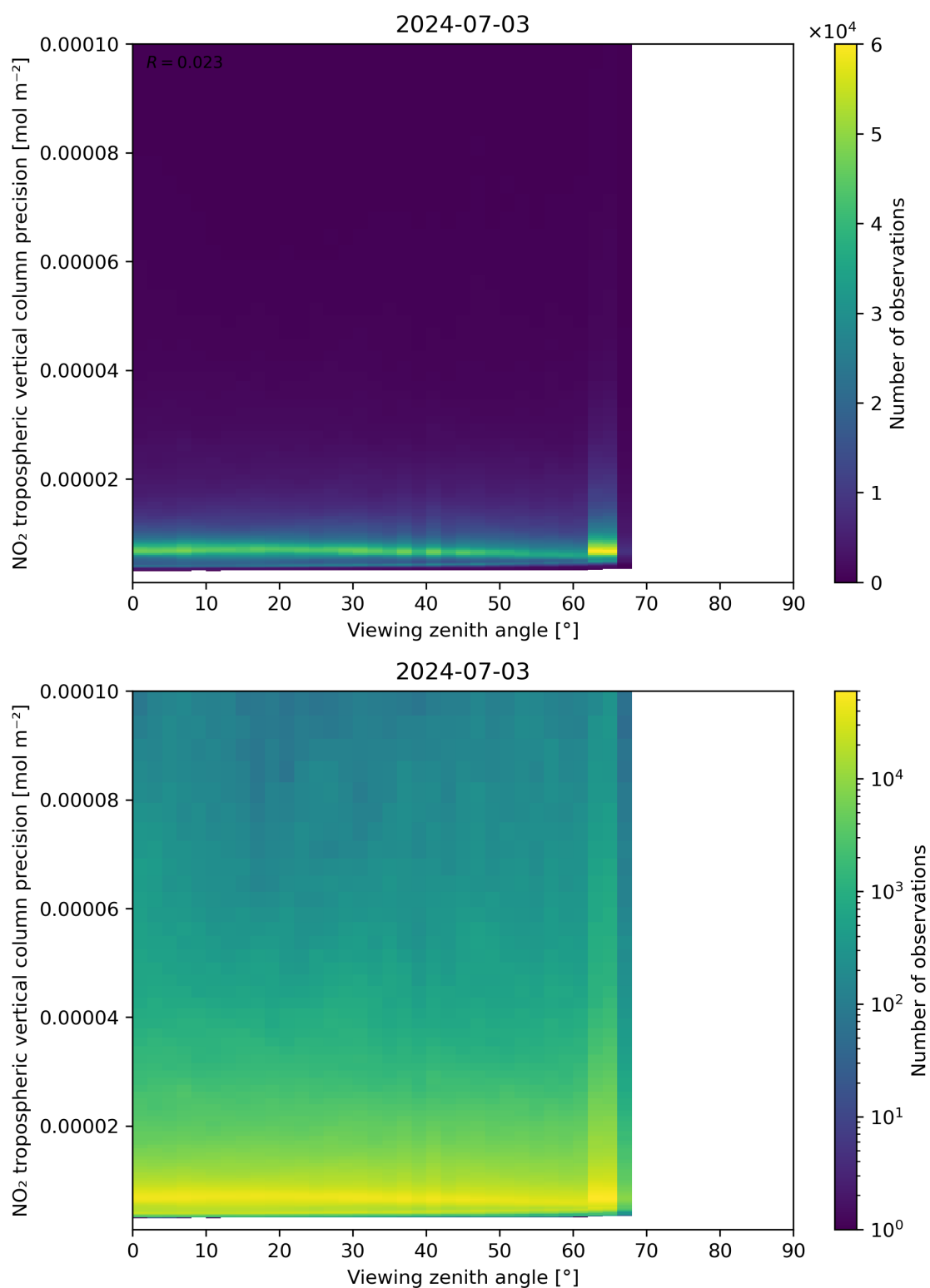
Figure 170: Scatter density plot of “Viewing zenith angle” against “NO 2 tropospheric vertical column precision” for 2024-07-02 to 2024-07-04.
