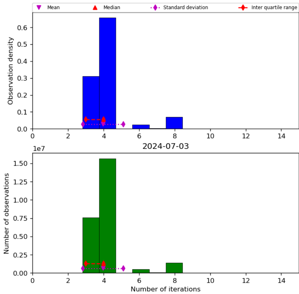
Figure 34: Histogram of “Number of iterations” for 2024-07-02 to 2024-07-04
