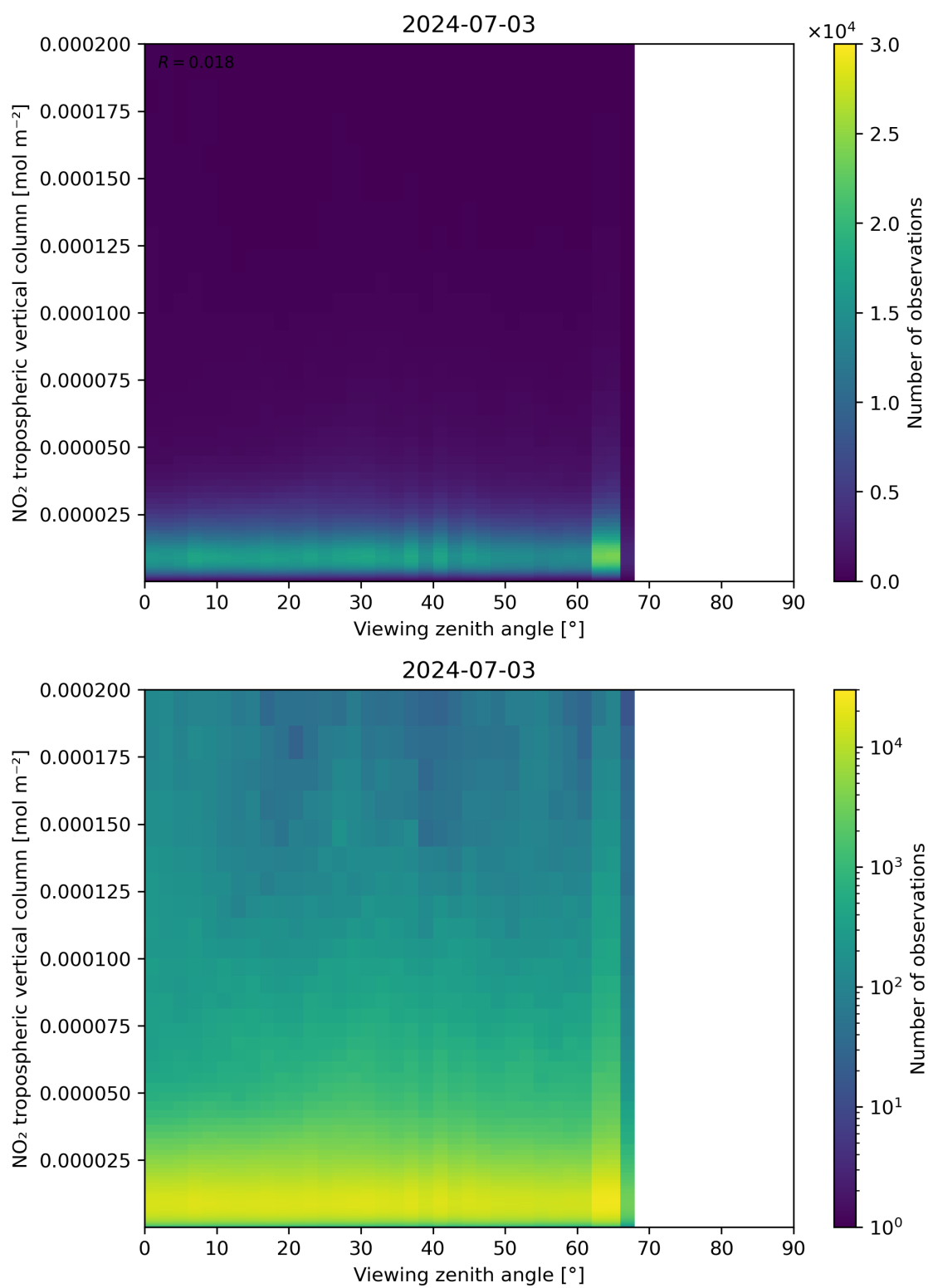
Figure 169: Scatter density plot of “Viewing zenith angle” against “NO 2 tropospheric vertical column” for 2024-07-02 to 2024-07-04.
