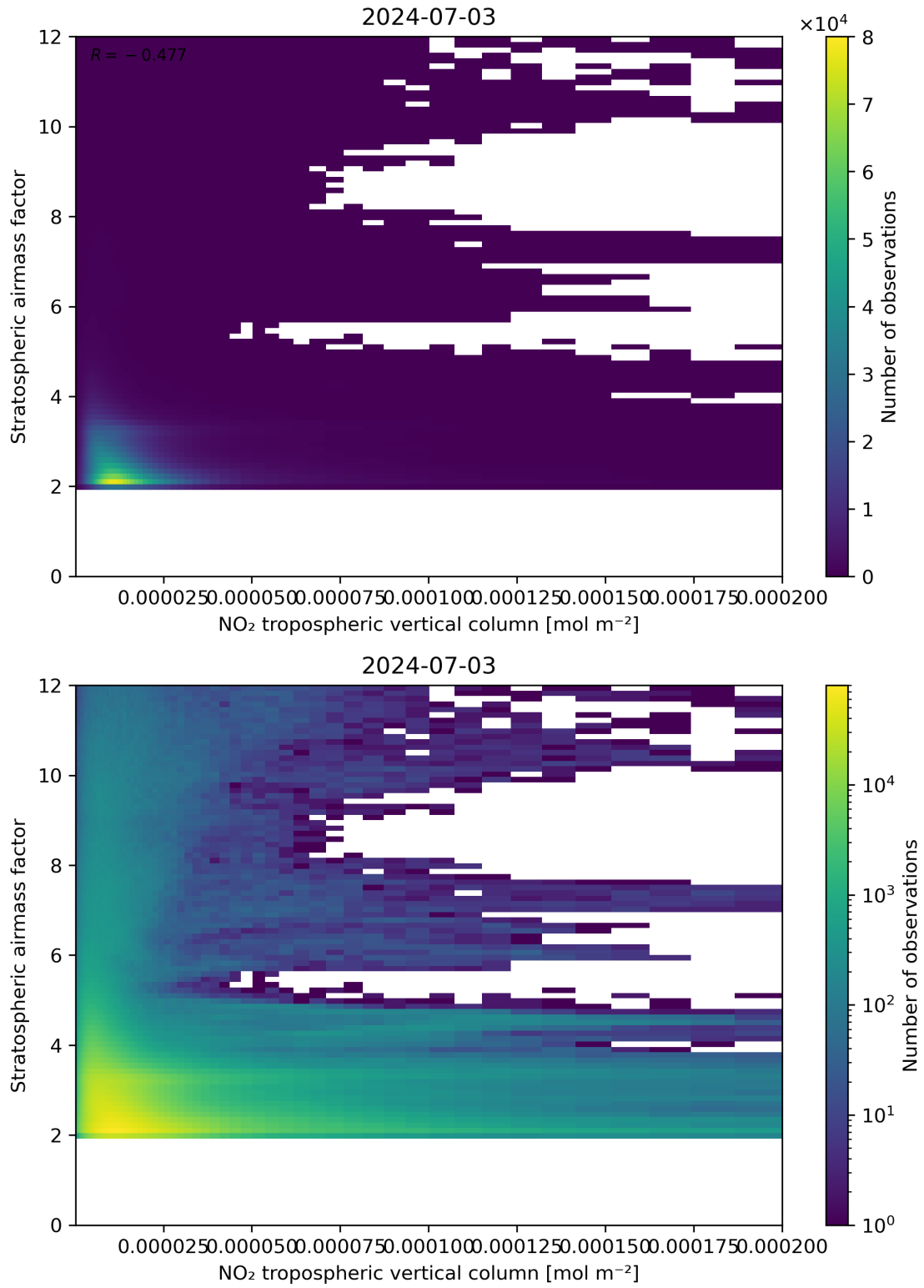
Figure 121: Scatter density plot of “NO 2 tropospheric vertical column” against “Stratospheric air mass factor” for 2024-07-02 to 2024-07-04.
