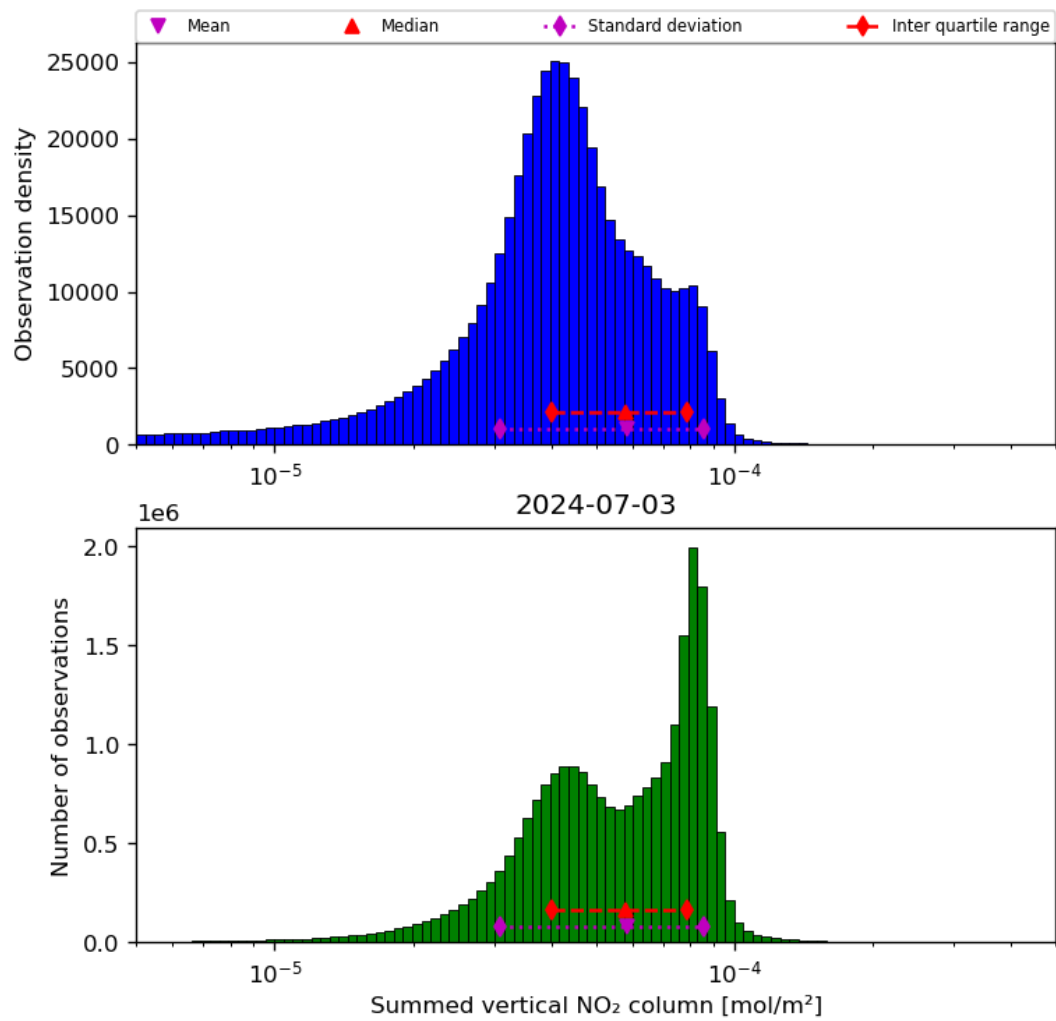
Figure 40: Histogram of “Summed vertical NO 2 column” for 2024-07-02 to 2024-07-04
