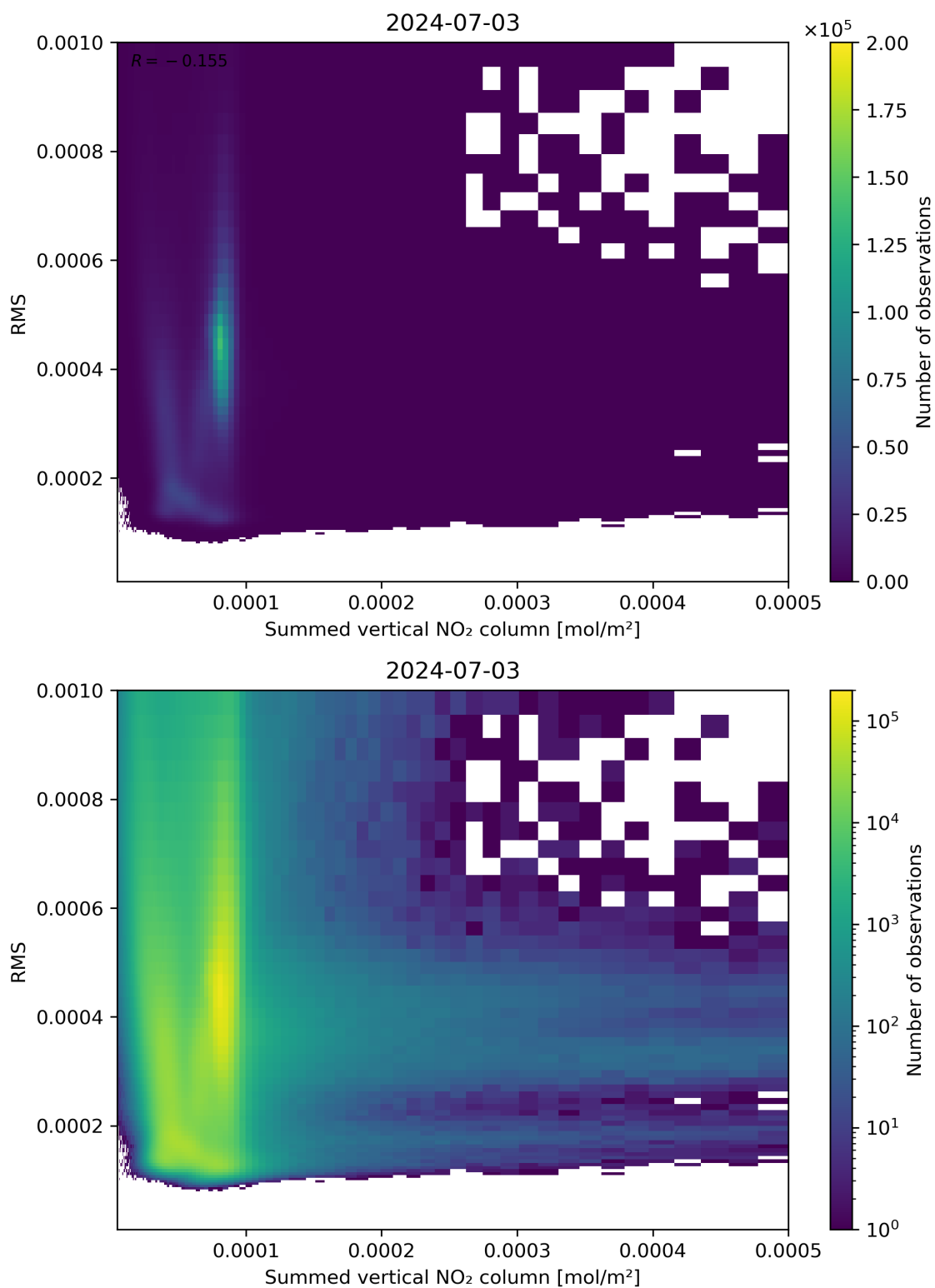
Figure 109: Scatter density plot of “Summed vertical NO 2 column” against “RMS” for 2024-07-02 to 2024-07-04.
