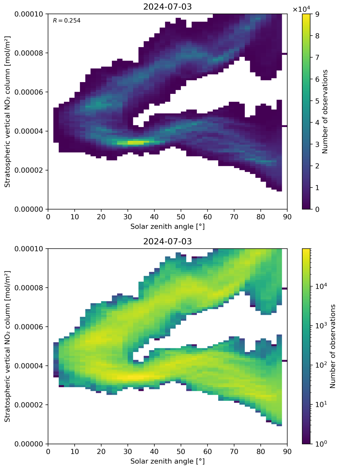
Figure 150: Scatter density plot of “Solar zenith angle” against “Stratospheric vertical NO 2 column” for 2024-07-02 to 2024-07-04.
