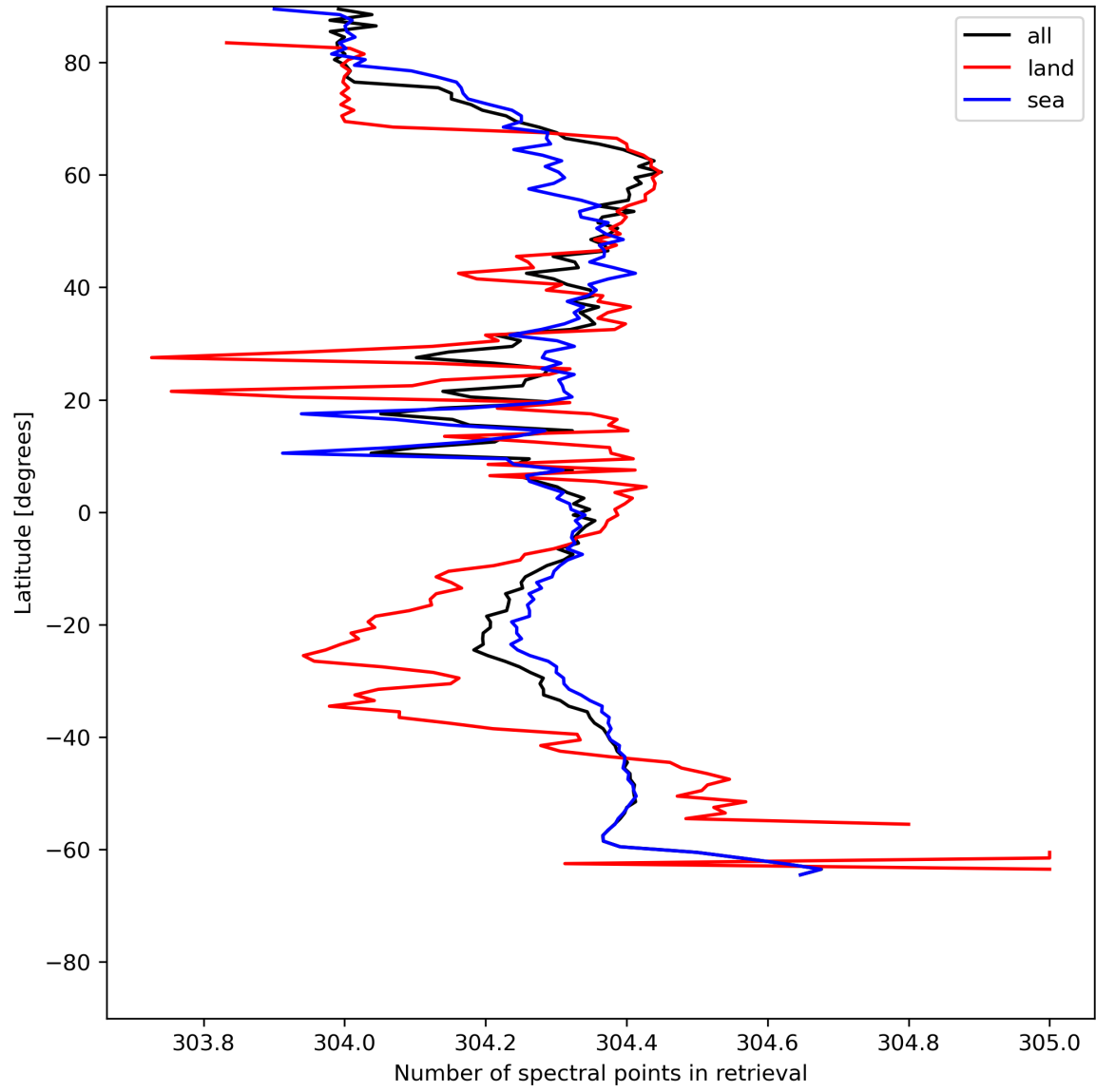
Figure 16: Zonal average of “Number of spectral points in retrieval” for 2024-07-02 to 2024-07-04.
