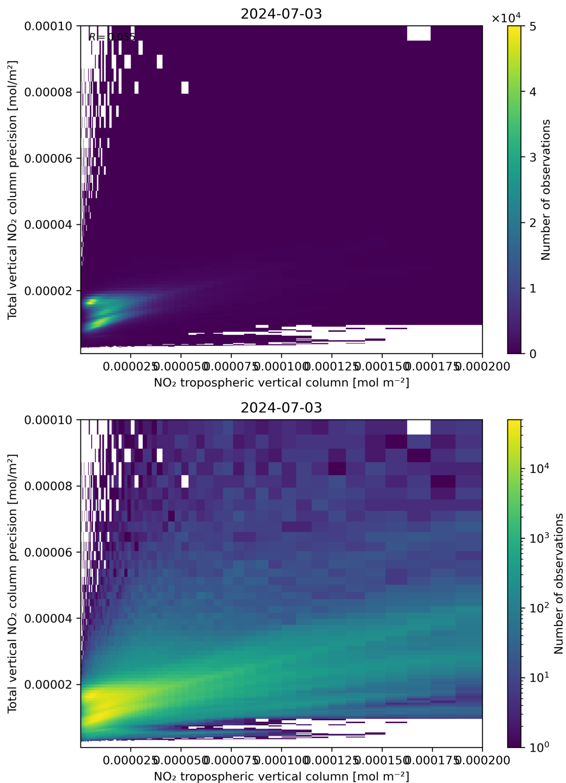
Figure 129: Scatter density plot of “NO 2 tropospheric vertical column” against “Total vertical NO 2 column precision” for 2024-07-02 to 2024-07-04.
