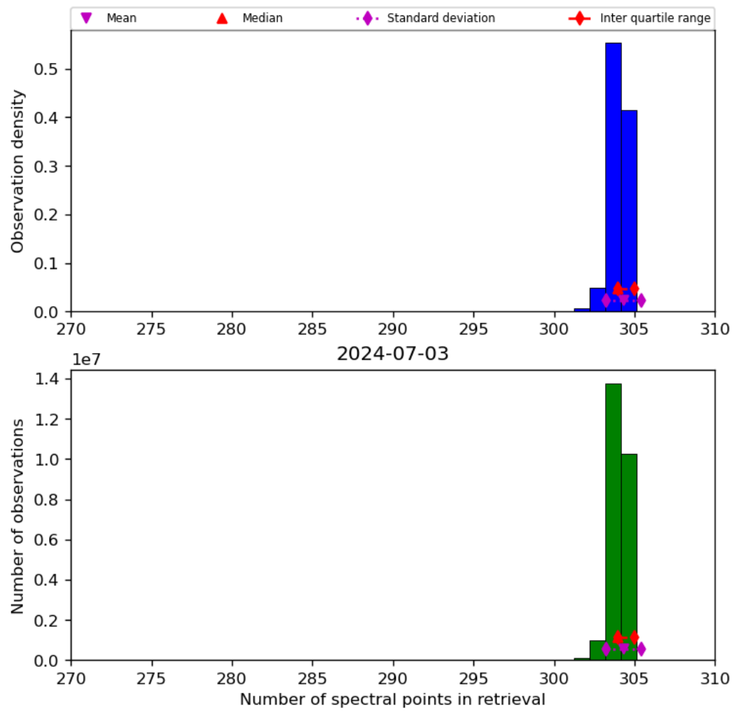
Figure 33: Histogram of “Number of spectral points in retrieval” for 2024-07-02 to 2024-07-04
