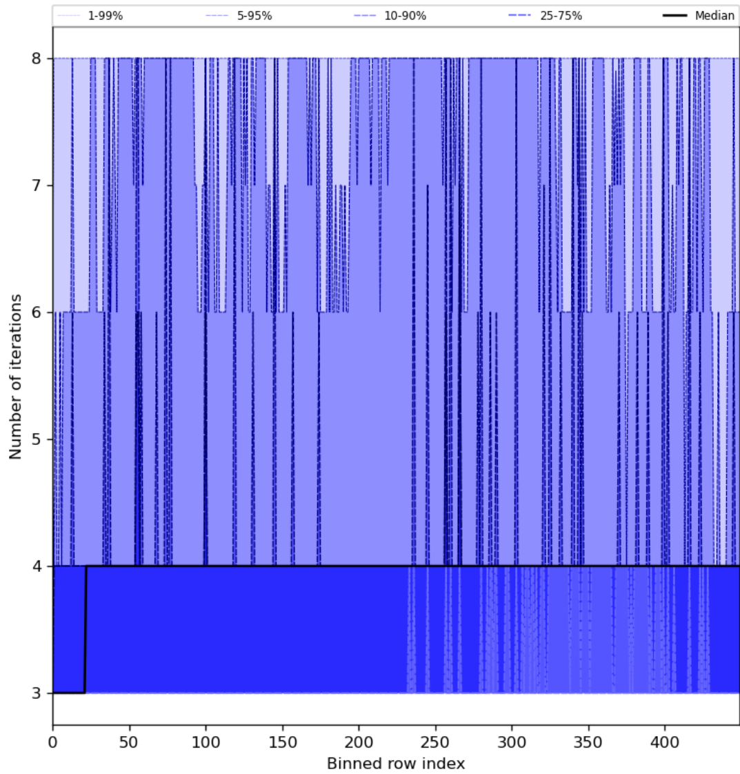
Figure 51: Along track statistics of “Number of iterations” for 2024-07-02 to 2024-07-04
