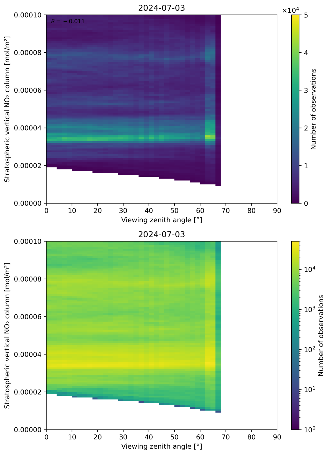
Figure 164: Scatter density plot of “Viewing zenith angle” against “Stratospheric vertical NO 2 column” for 2024-07-02 to 2024-07-04.
