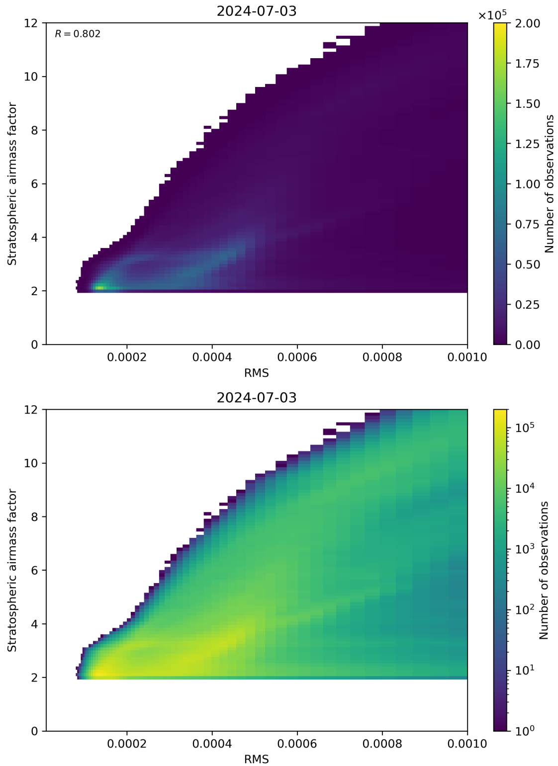
Figure 144: Scatter density plot of “RMS” against “Stratospheric airmass factor” for 2024-07-02 to 2024-07-04.
