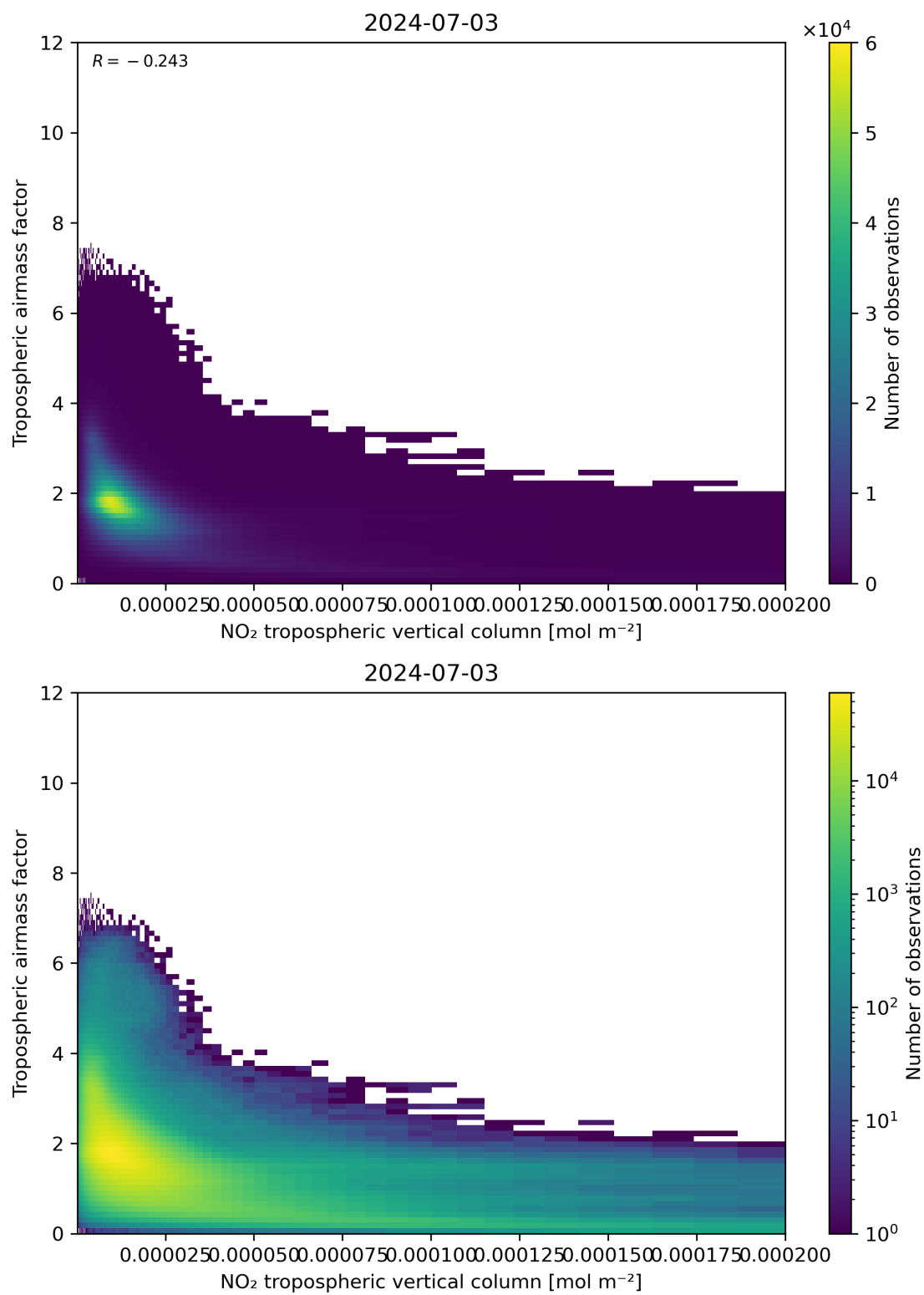
Figure 123: Scatter density plot of “NO 2 tropospheric vertical column” against “Tropospheric air mass factor” for 2024-07-02 to 2024-07-04.
