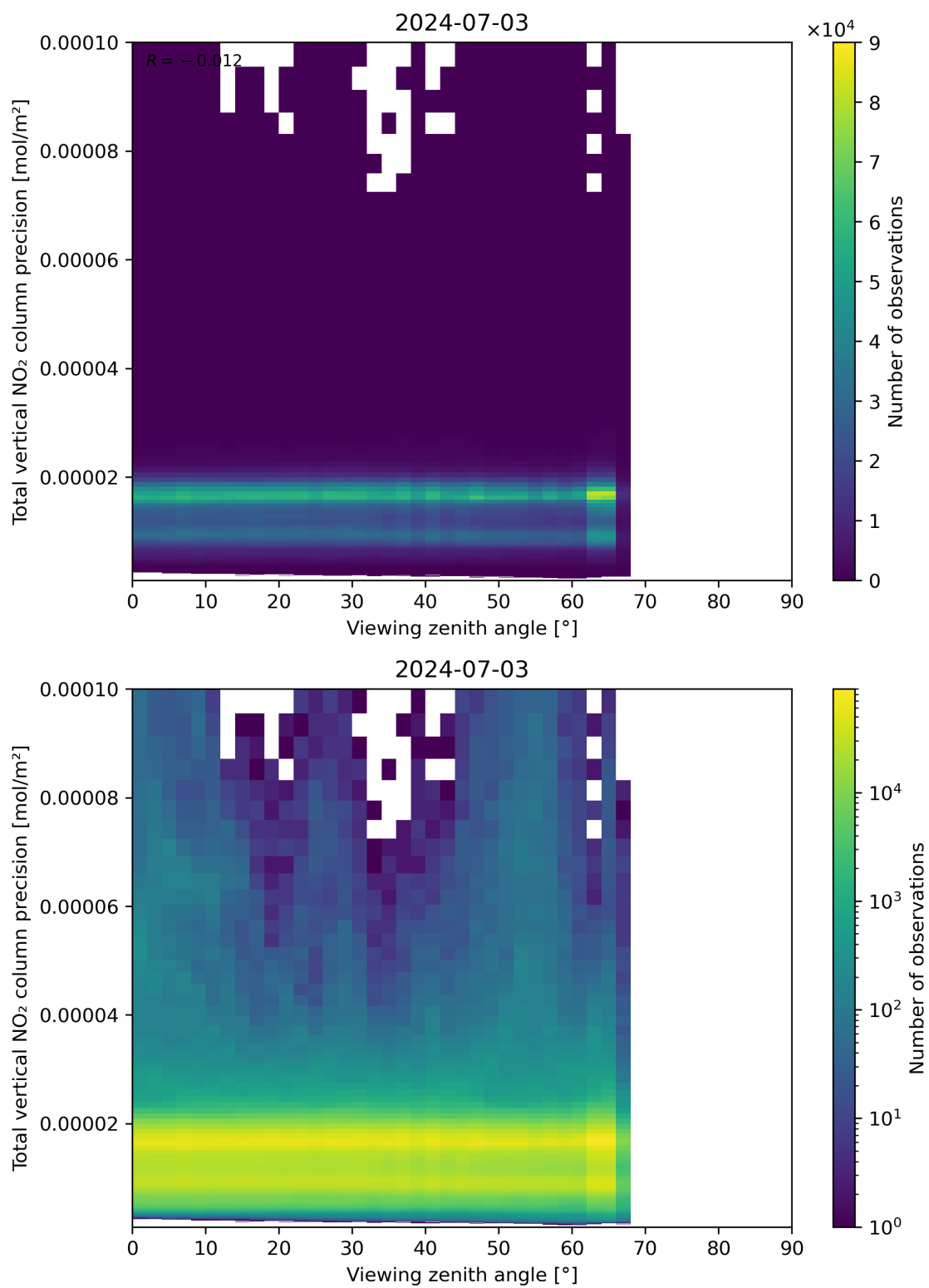
Figure 168: Scatter density plot of “Viewing zenith angle” against “Total vertical NO 2 column precision” for 2024-07-02 to 2024-07-04.
