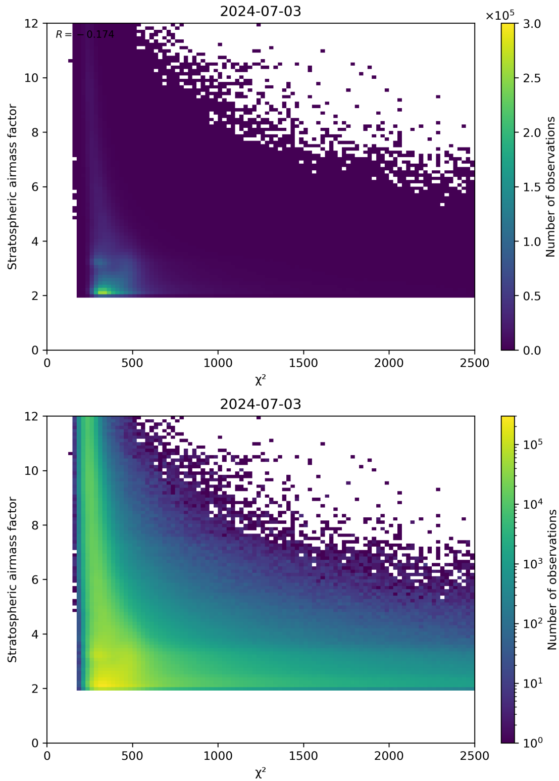
Figure 81: Scatter density plot of “ \chi^2 ” against “Stratospheric airmass factor” for 2024-07-02 to 2024-07-04.
