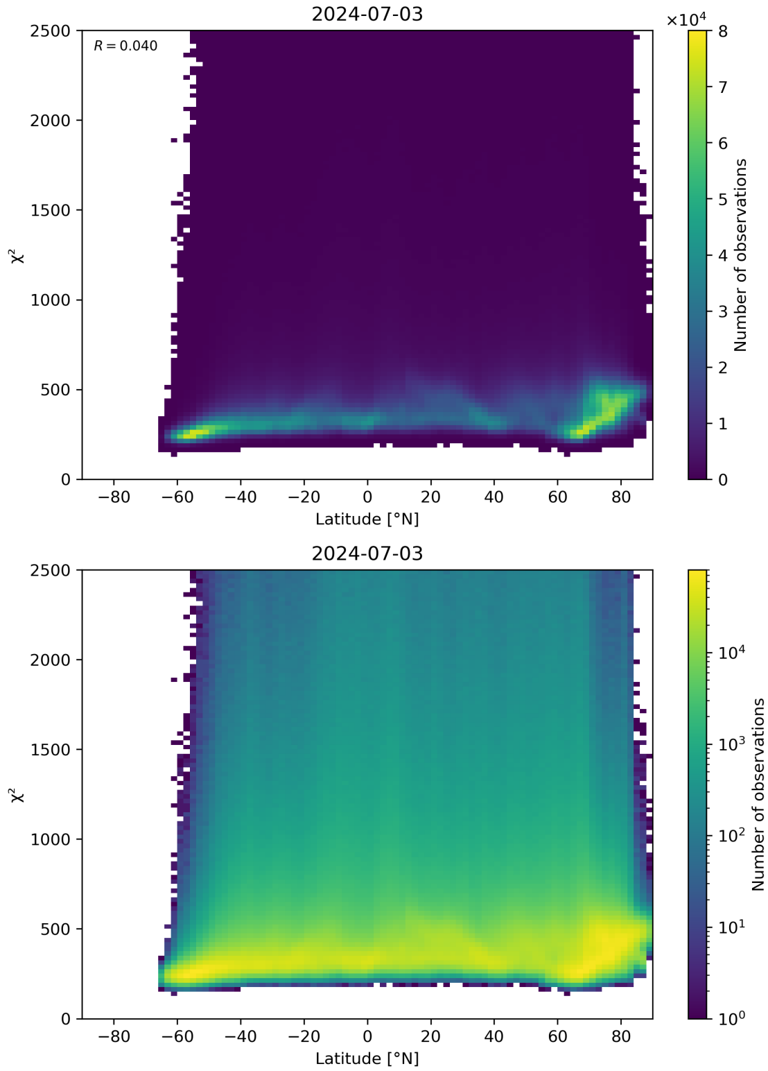
Figure 86: Scatter density plot of “Latitude” against “ \chi^2 ” for 2024-07-02 to 2024-07-04.
