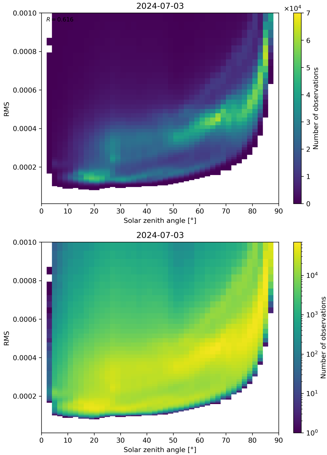
Figure 157: Scatter density plot of “Solar zenith angle” against “RMS” for 2024-07-02 to 2024-07-04.
