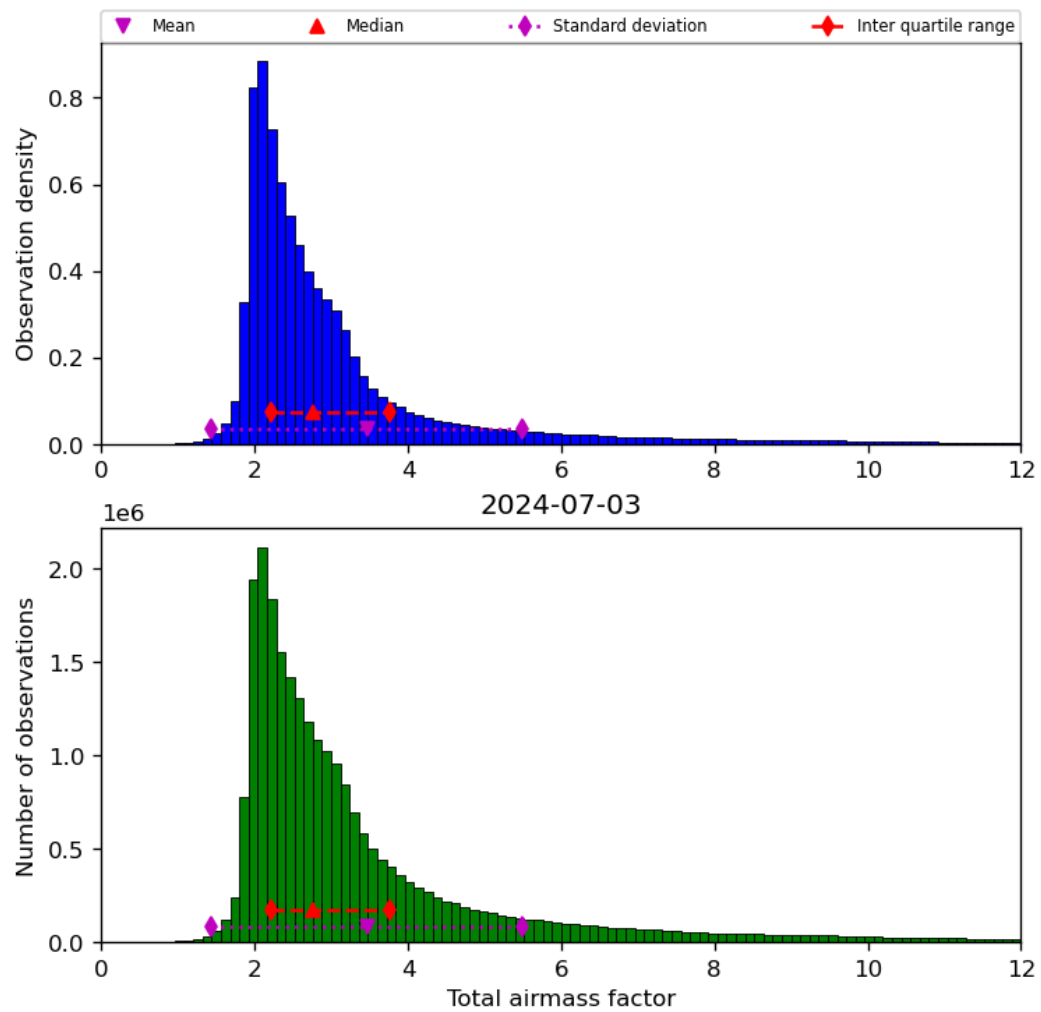
Figure 32: Histogram of “Total airmass factor” for 2024-07-02 to 2024-07-04
