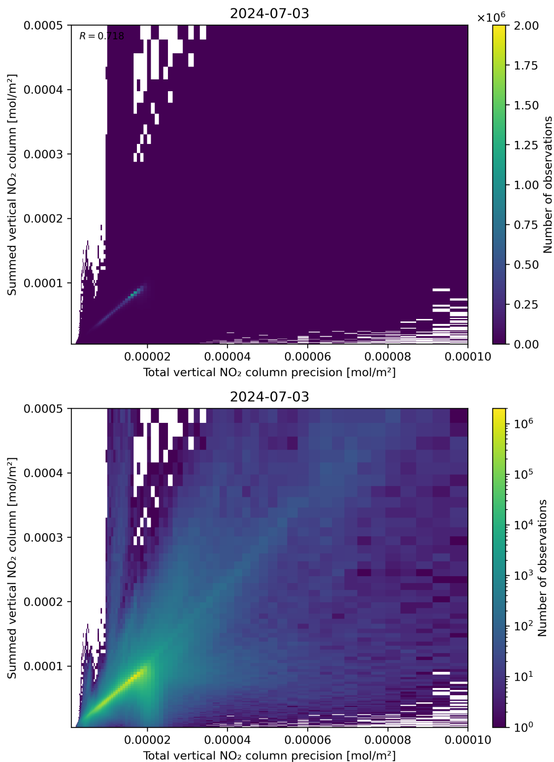
Figure 117: Scatter density plot of “Total vertical NO 2 column precision” against “Summed vertical NO 2 column” for 2024-07-02 to 2024-07-04.
