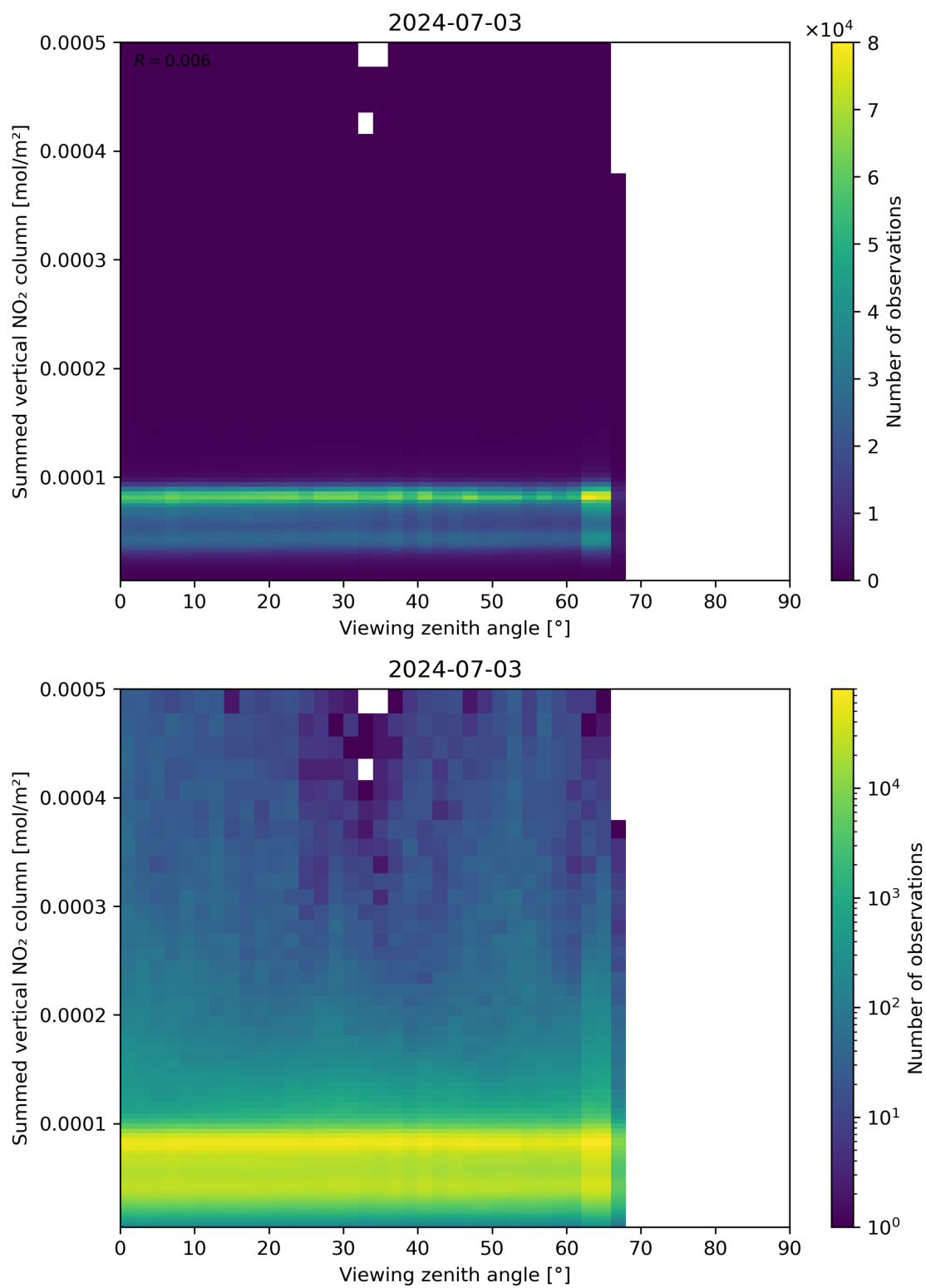
Figure 165: Scatter density plot of “Viewing zenith angle” against “Summed vertical NO 2 column” for 2024-07-02 to 2024-07-04.
