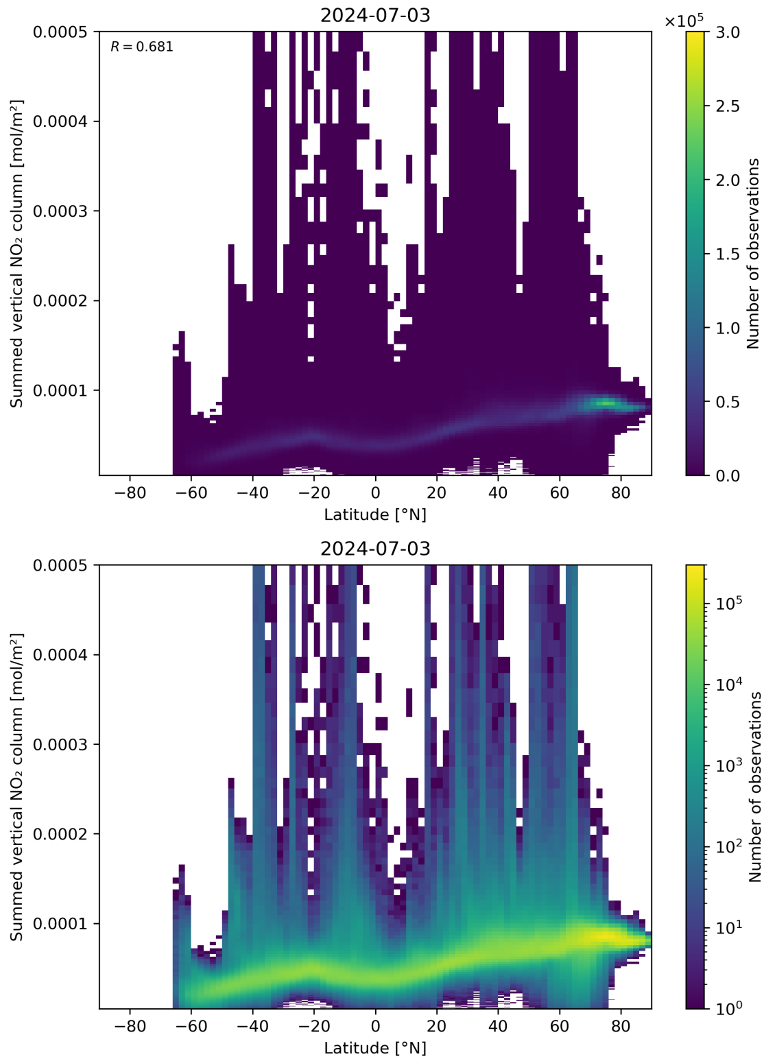
Figure 88: Scatter density plot of “Latitude” against “Summed vertical NO 2 column” for 2024-07-02 to 2024-07-04.
