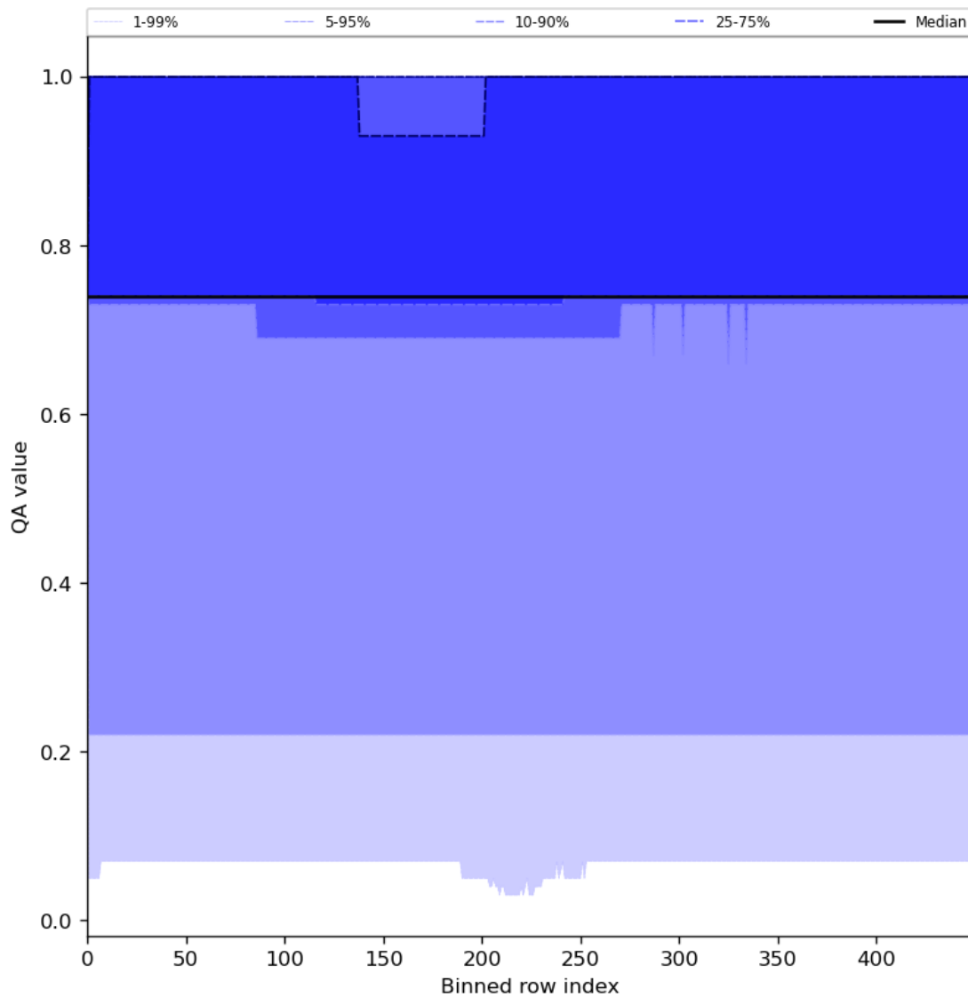
Figure 45: Along track statistics of “QA value” for 2024-07-02 to 2024-07-04
