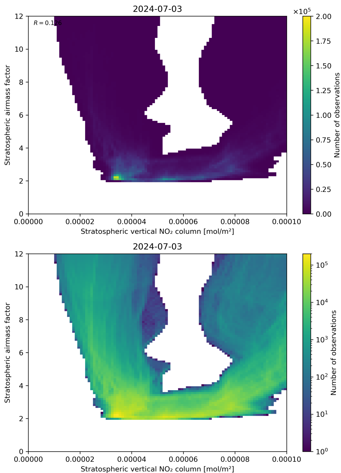
Figure 96: Scatter density plot of “Stratospheric vertical NO 2 column” against “Stratospheric airmass factor” for 2024-07-02 to 2024-07-04.
