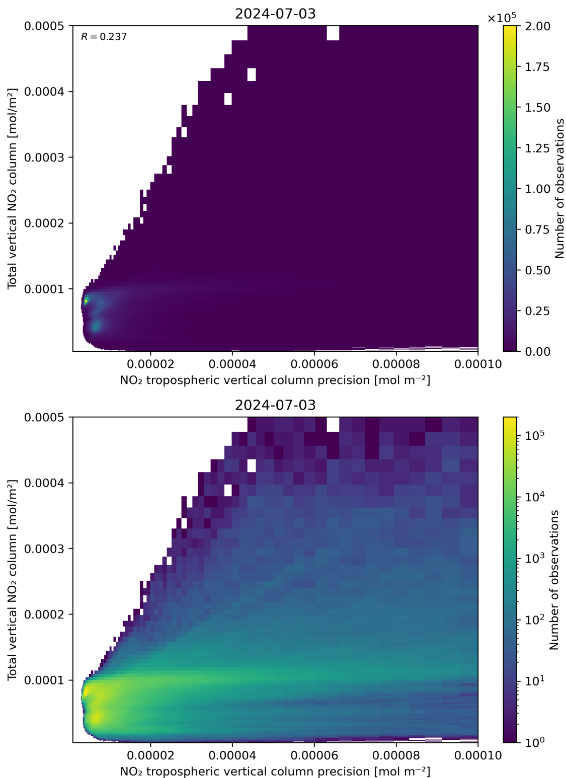
Figure 138: Scatter density plot of “NO 2 tropospheric vertical column precision” against “Total vertical NO 2 column” for 2024-07-02 to 2024-07-04.
