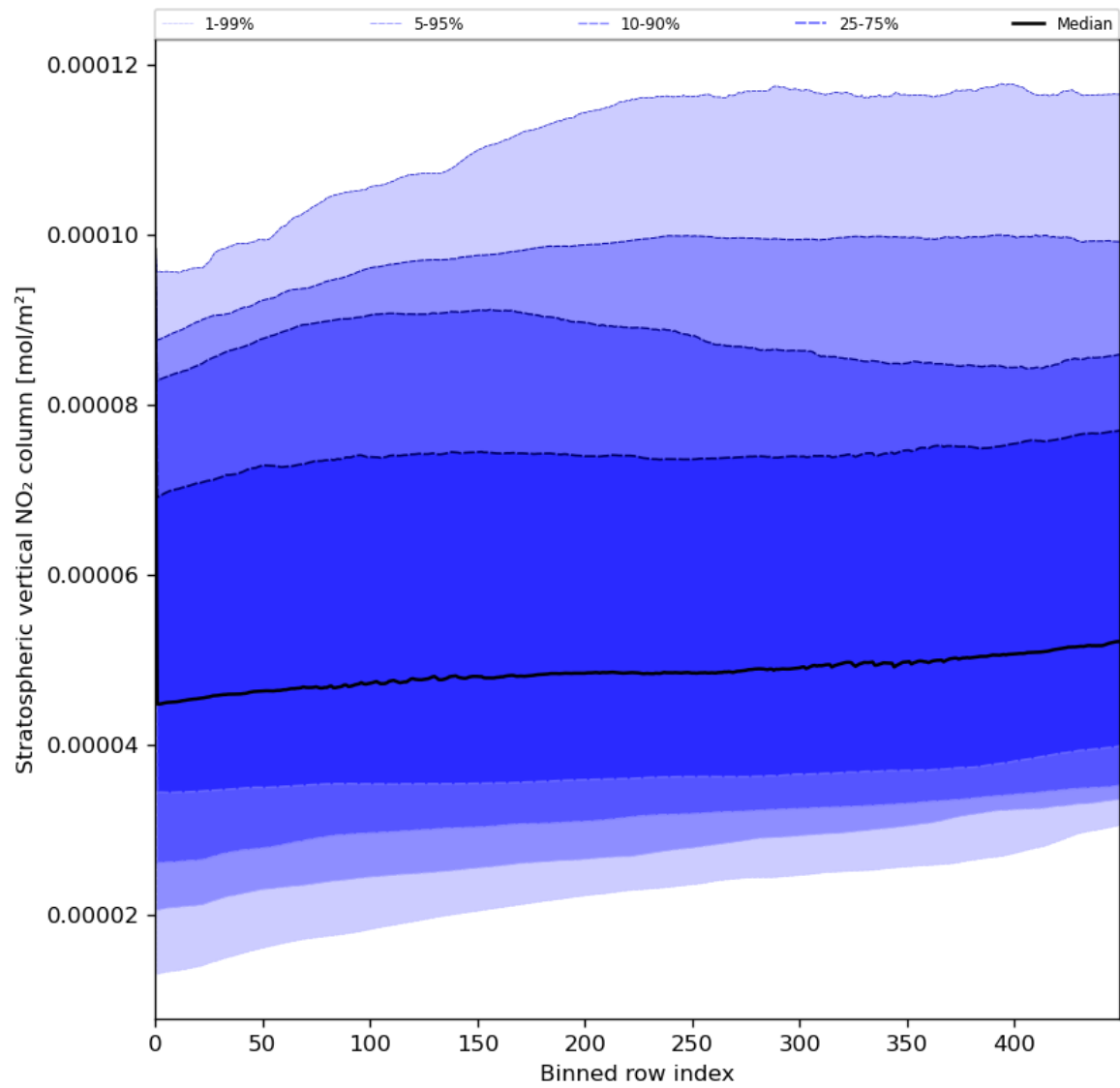
Figure 53: Along track statistics of “Stratospheric vertical NO 2 column” for 2024-07-02 to 2024-07-04
