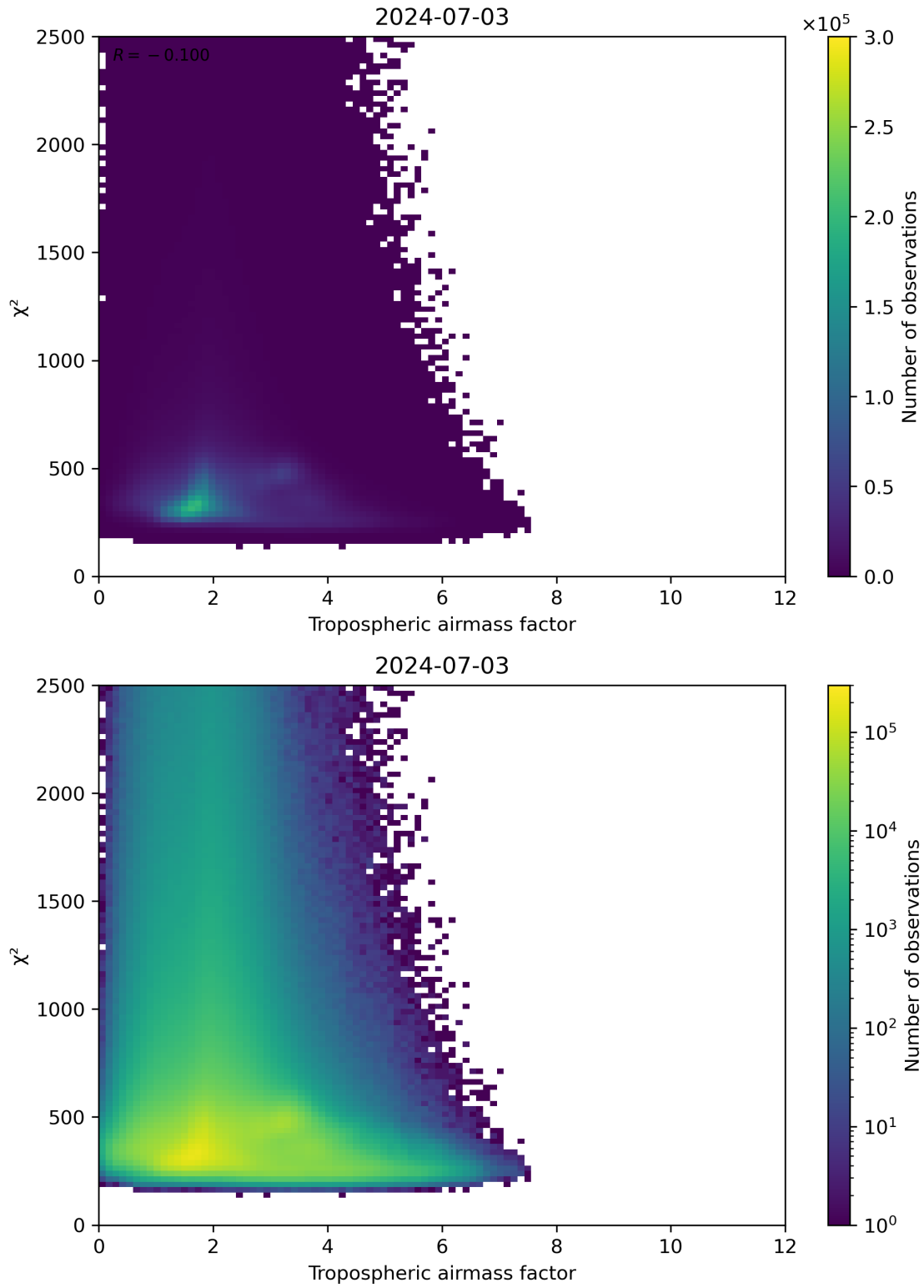
Figure 73: Scatter density plot of “Tropospheric airmass factor” against “ \chi^2 ” for 2024-07-02 to 2024-07-04.
