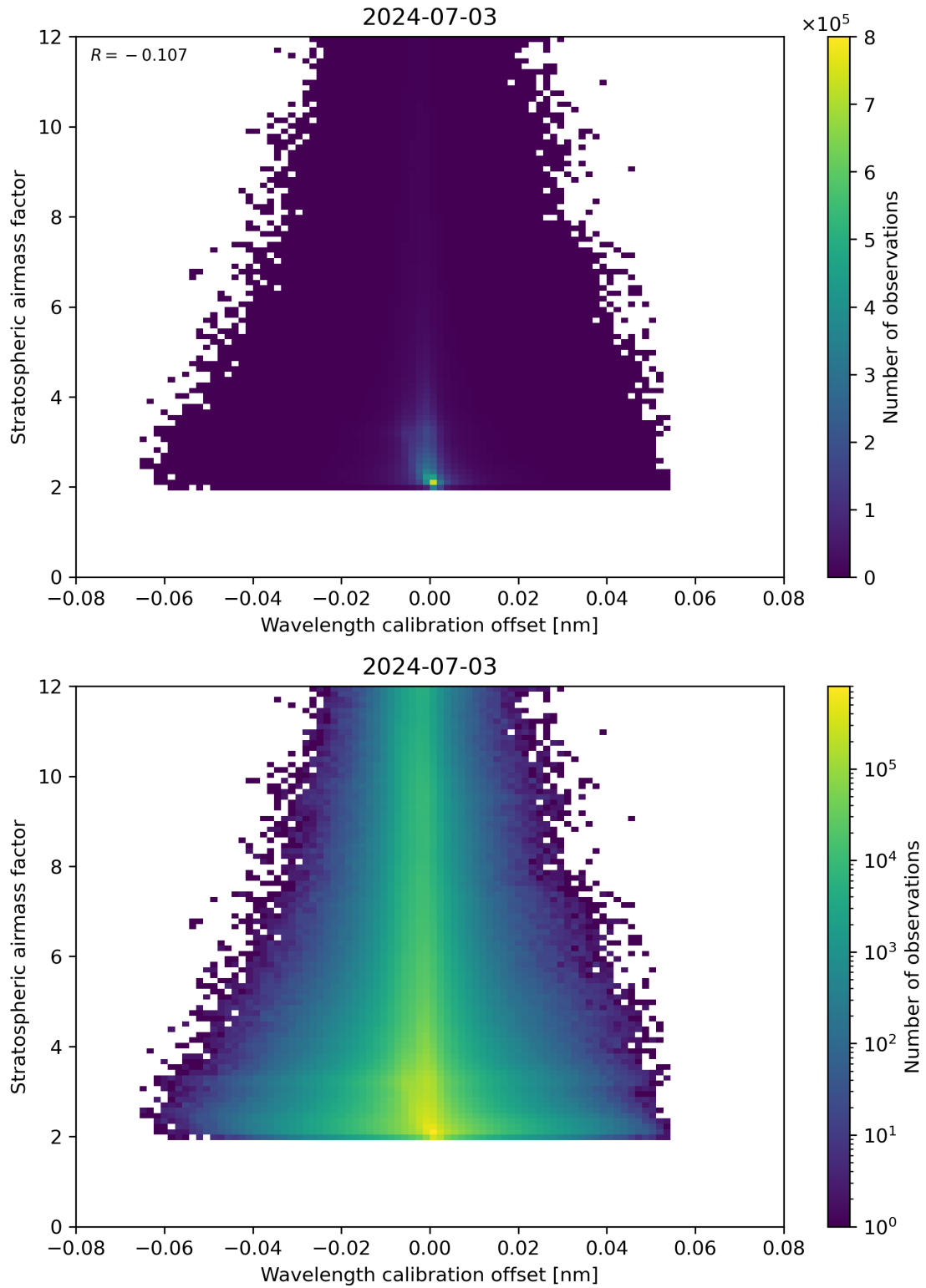
Figure 174: Scatter density plot of “Wavelength calibration offset” against “Stratospheric air mass factor” for 2024-07-02 to 2024-07-04.
