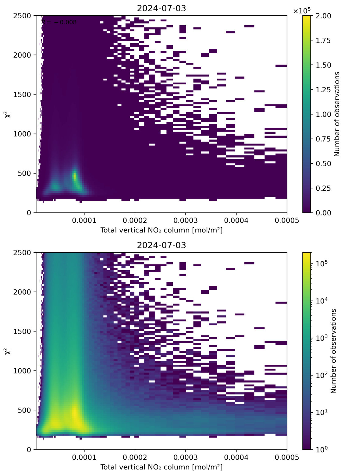
Figure 111: Scatter density plot of “Total vertical NO 2 column” against “ \chi^2 ” for 2024-07-02 to 2024-07-04.
