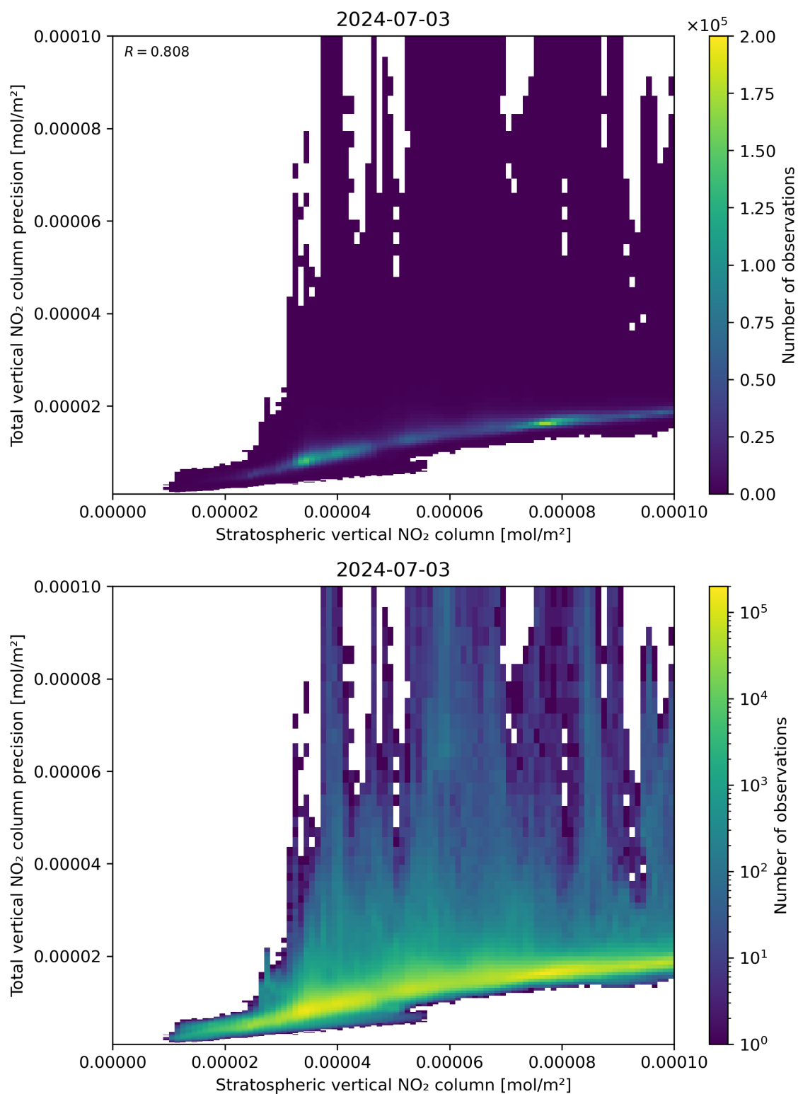
Figure 101: Scatter density plot of “Stratospheric vertical NO 2 column” against “Total vertical NO 2 column precision” for 2024-07-02 to 2024-07-04.
