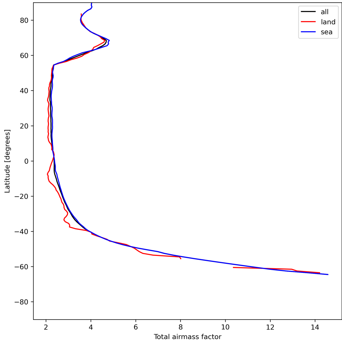
Figure 15: Zonal average of “Total airmass factor” for 2024-07-02 to 2024-07-04.
