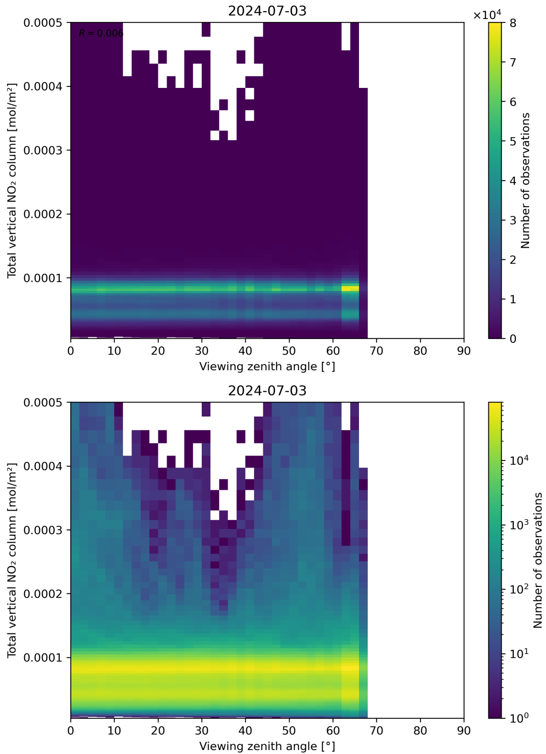
Figure 167: Scatter density plot of “Viewing zenith angle” against “Total vertical NO 2 column” for 2024-07-02 to 2024-07-04.
