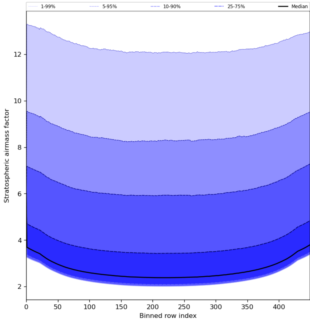
Figure 61: Along track statistics of “Stratospheric airmass factor” for 2024-07-02 to 2024-07-04
