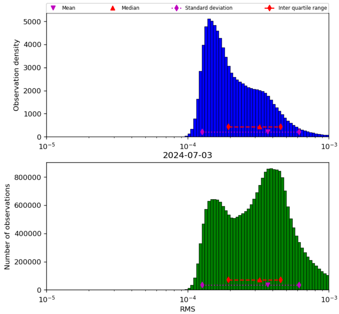
Figure 43: Histogram of “RMS” for 2024-07-02 to 2024-07-04
