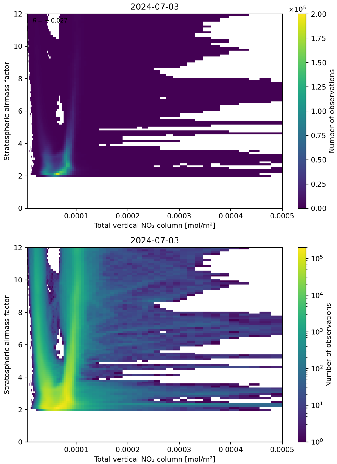
Figure 110: Scatter density plot of “Total vertical NO 2 column” against “Stratospheric air mass factor” for 2024-07-02 to 2024-07-04.
