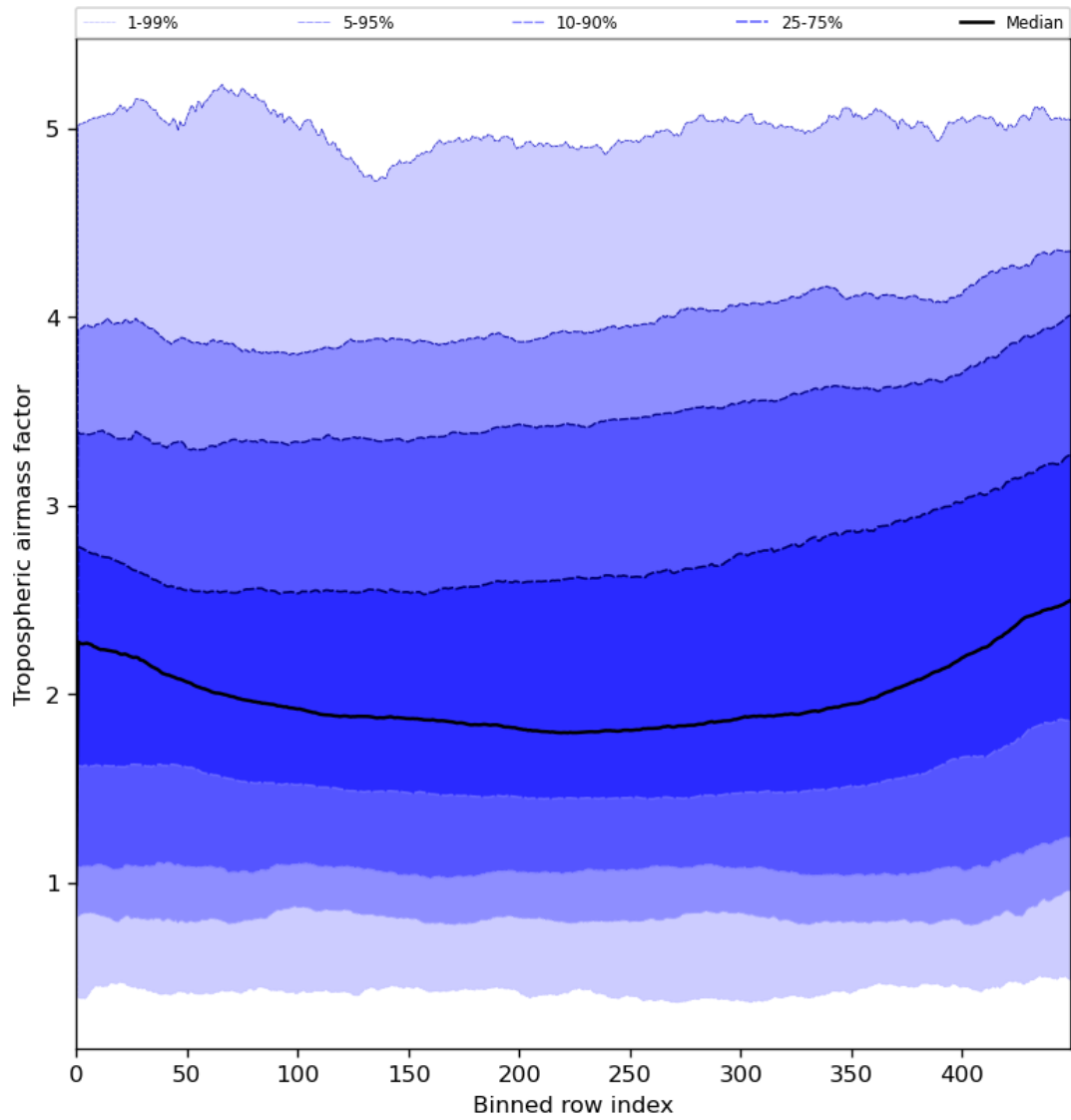
Figure 48: Along track statistics of “Tropospheric airmass factor” for 2024-07-02 to 2024-07-04
