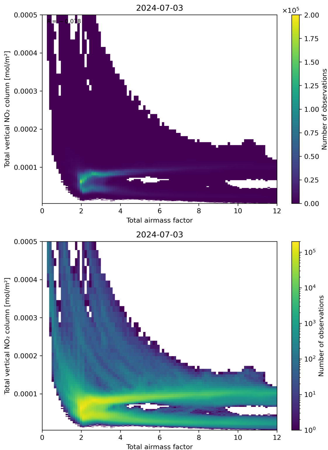
Figure 67: Scatter density plot of “Total airmass factor” against “Total vertical NO 2 column” for 2024-07-02 to 2024-07-04.
