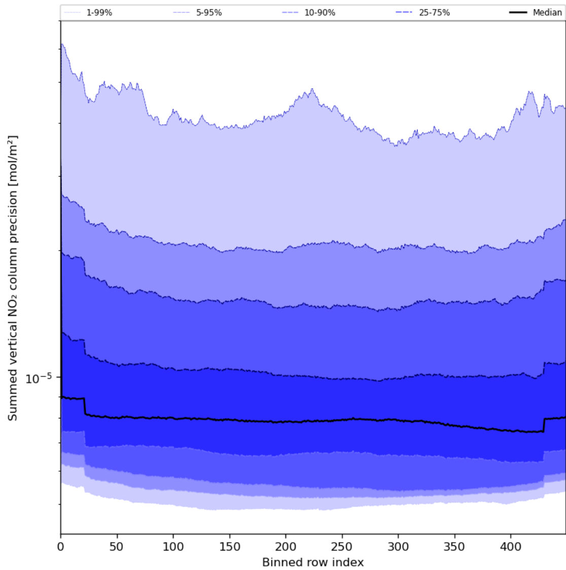
Figure 58: Along track statistics of “Summed vertical NO 2 column precision” for 2024-07-02 to 2024-07-04
