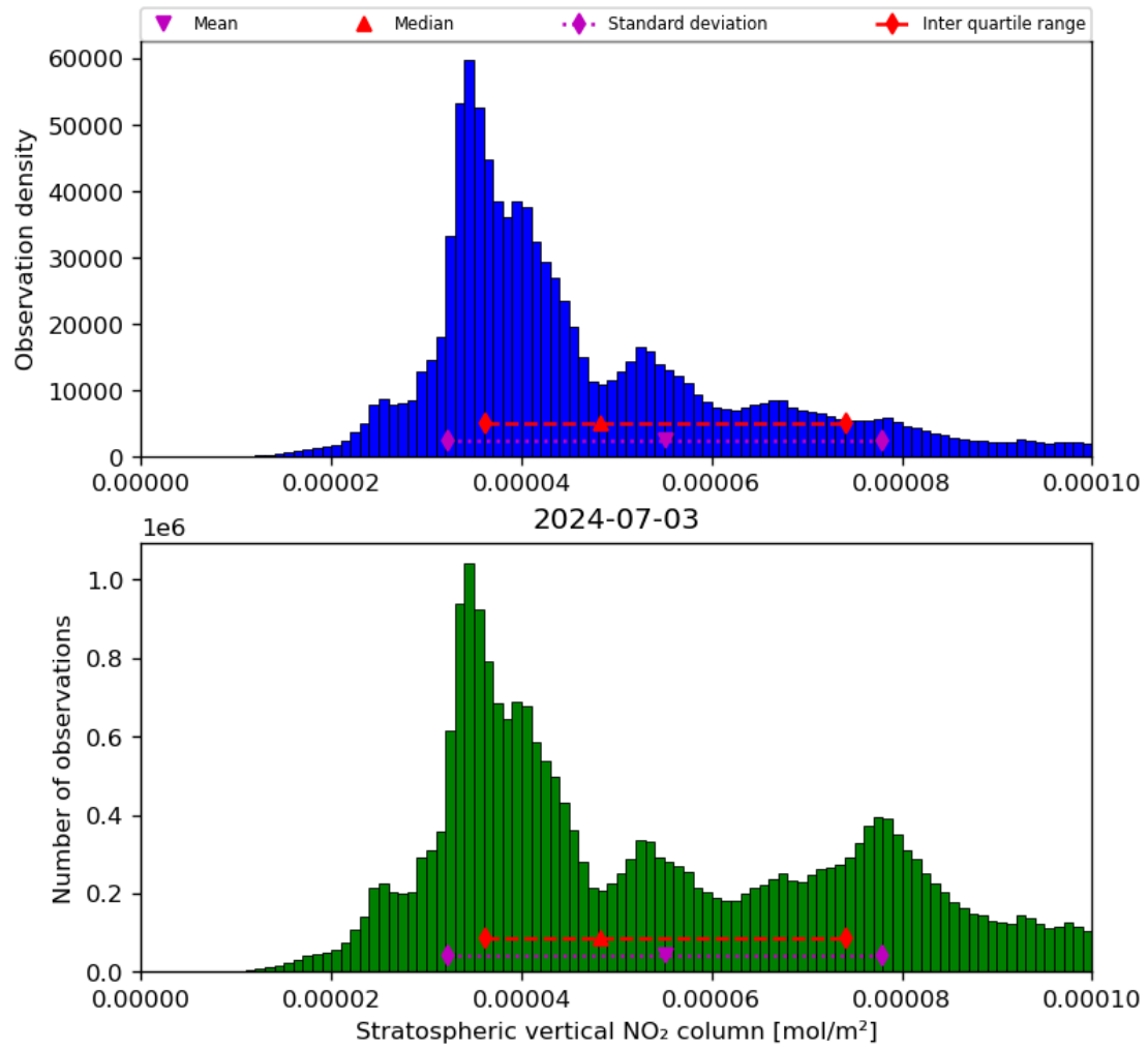
Figure 36: Histogram of “Stratospheric vertical NO 2 column” for 2024-07-02 to 2024-07-04
