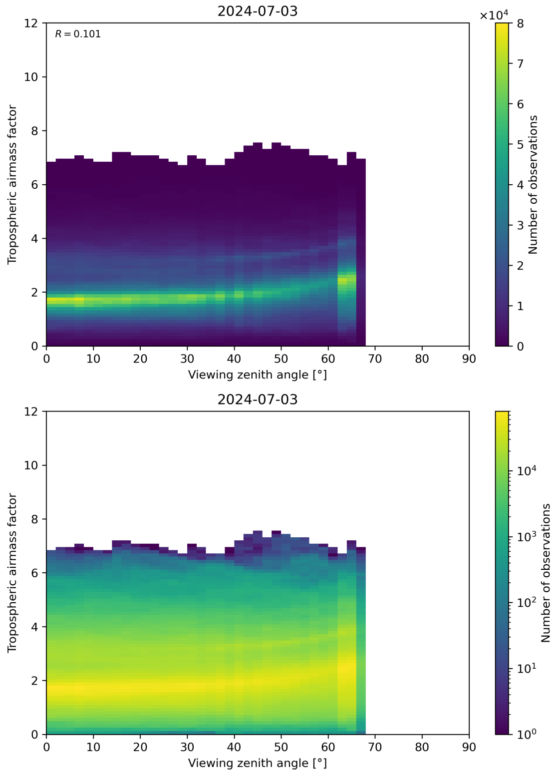
Figure 161: Scatter density plot of “Viewing zenith angle” against “Tropospheric airmass factor” for 2024-07-02 to 2024-07-04.
