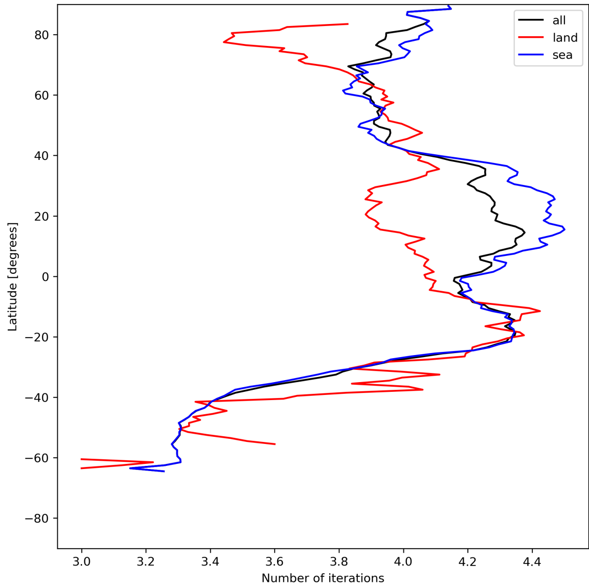
Figure 17: Zonal average of “Number of iterations” for 2024-07-02 to 2024-07-04.
