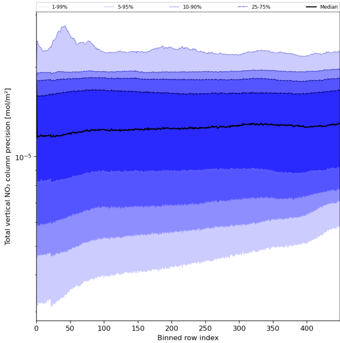
Figure 56: Along track statistics of “Total vertical NO 2 column precision” for 2024-07-02 to 2024-07-04
