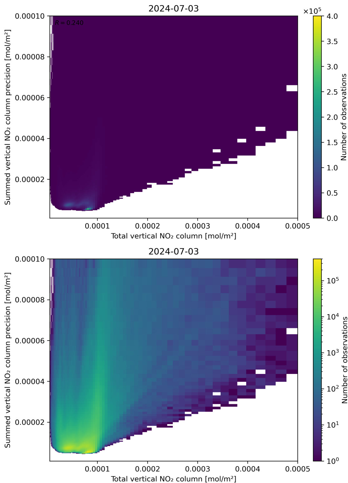
Figure 113: Scatter density plot of “Total vertical NO 2 column” against “Summed vertical NO 2 column precision” for 2024-07-02 to 2024-07-04.
