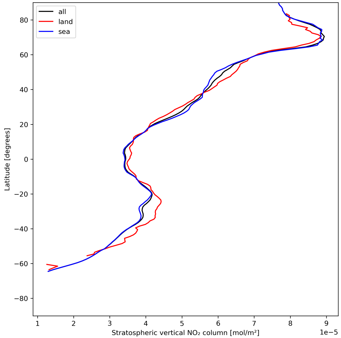
Figure 19: Zonal average of “Stratospheric vertical NO 2 column” for 2024-07-02 to 2024-07-04.
