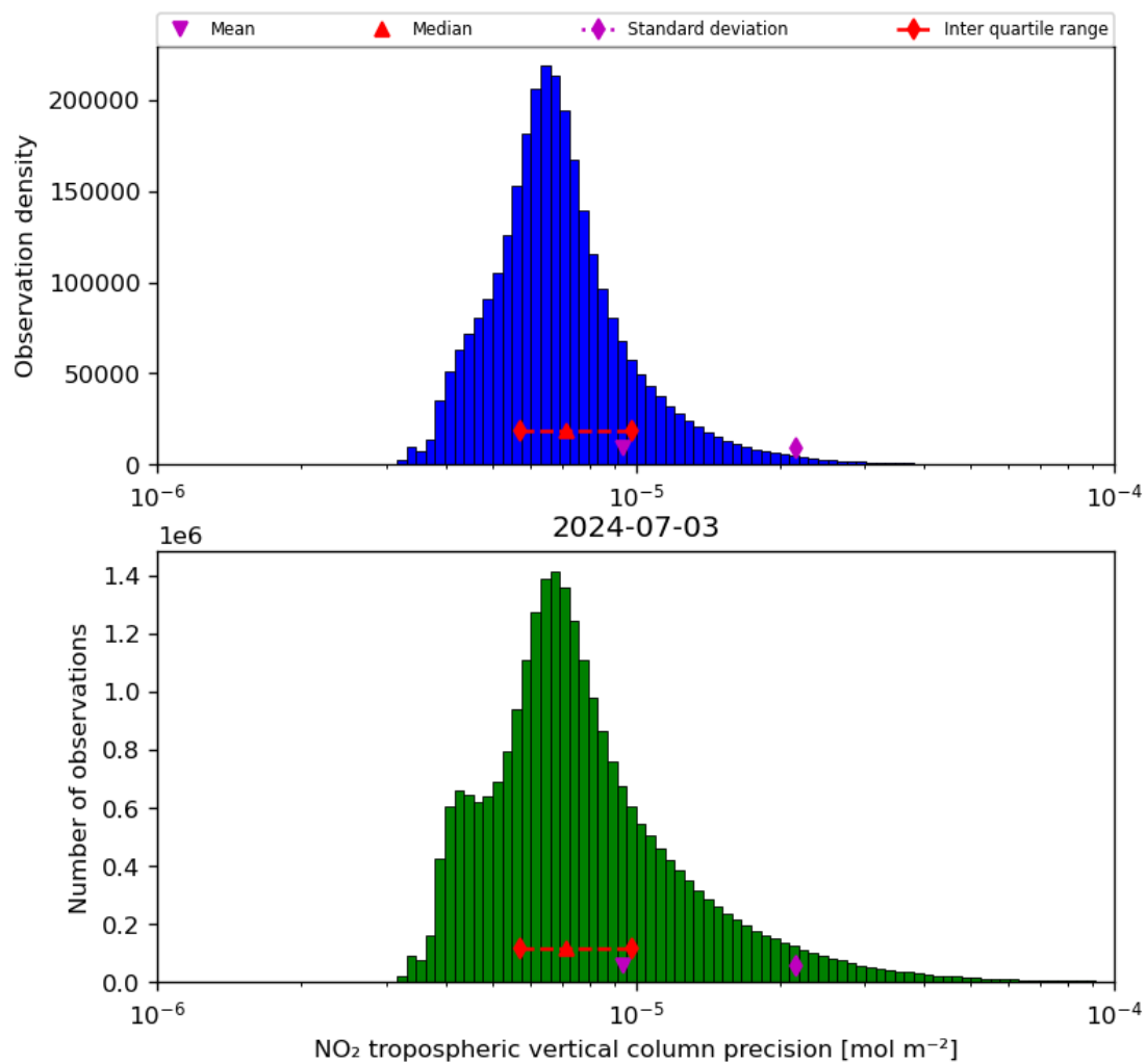
Figure 30: Histogram of “NO 2 tropospheric vertical column precision” for 2024-07-02 to 2024-07-04
