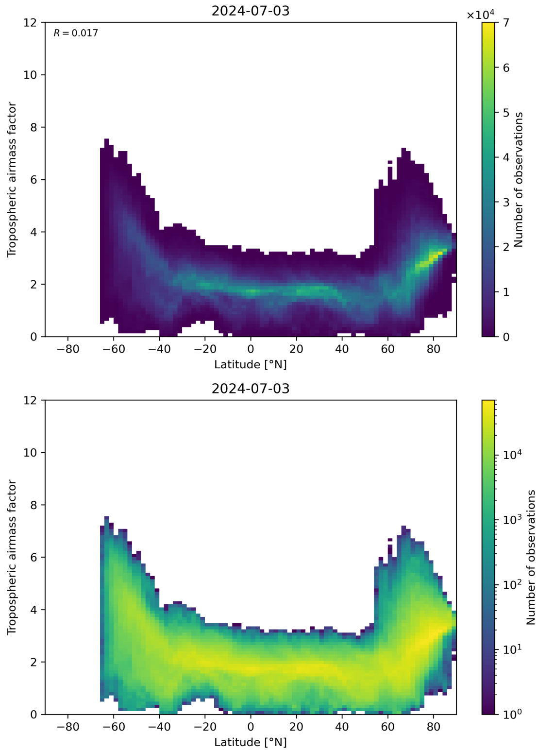
Figure 85: Scatter density plot of “Latitude” against “Tropospheric air mass factor” for 2024-07-02 to 2024-07-04.
