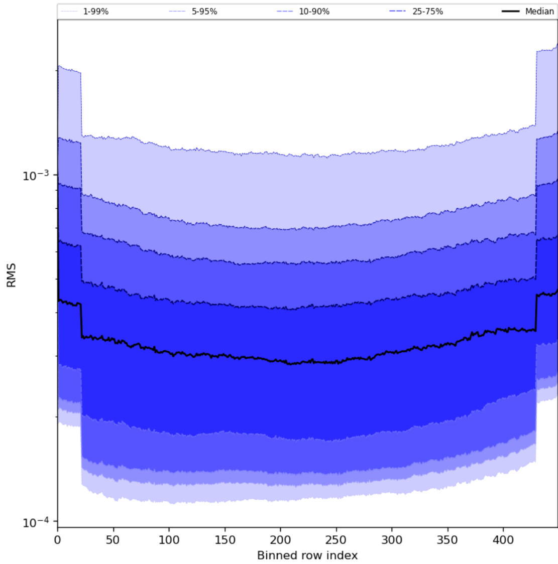
Figure 60: Along track statistics of “RMS” for 2024-07-02 to 2024-07-04
