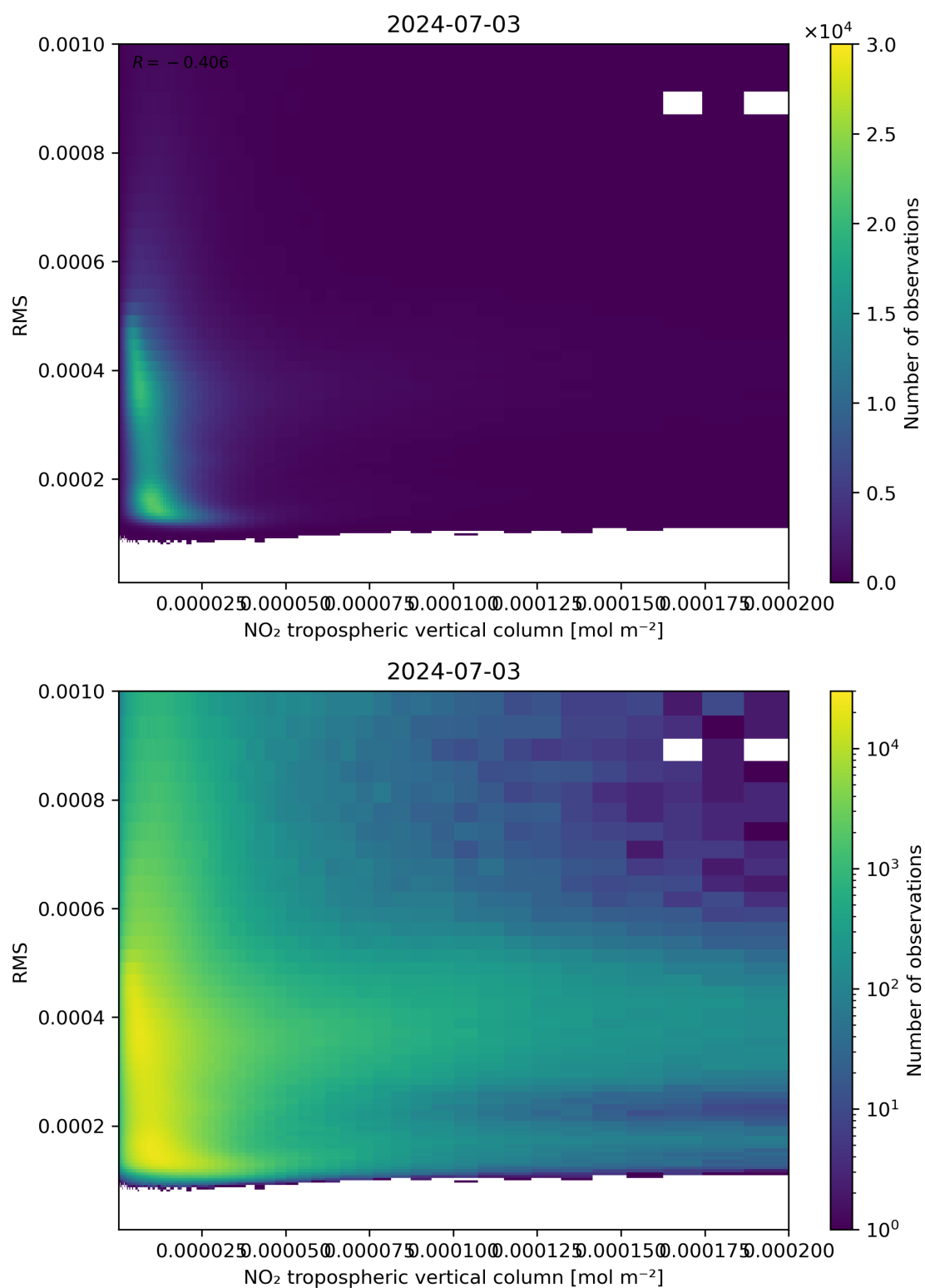
Figure 142: Scatter density plot of “NO 2 tropospheric vertical column” against “RMS” for 2024-07-02 to 2024-07-04.
