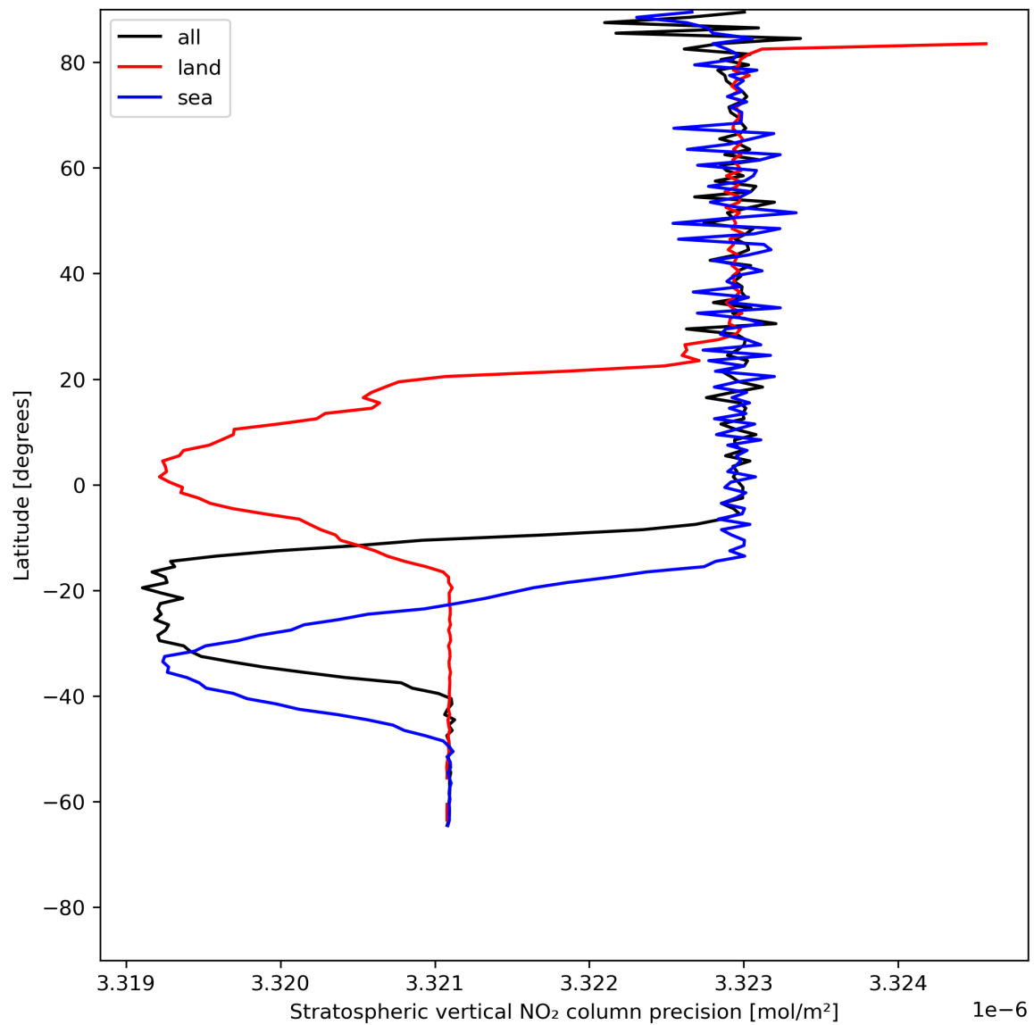
Figure 20: Zonal average of “Stratospheric vertical NO 2 column precision” for 2024-07-02 to 2024-07-04.
