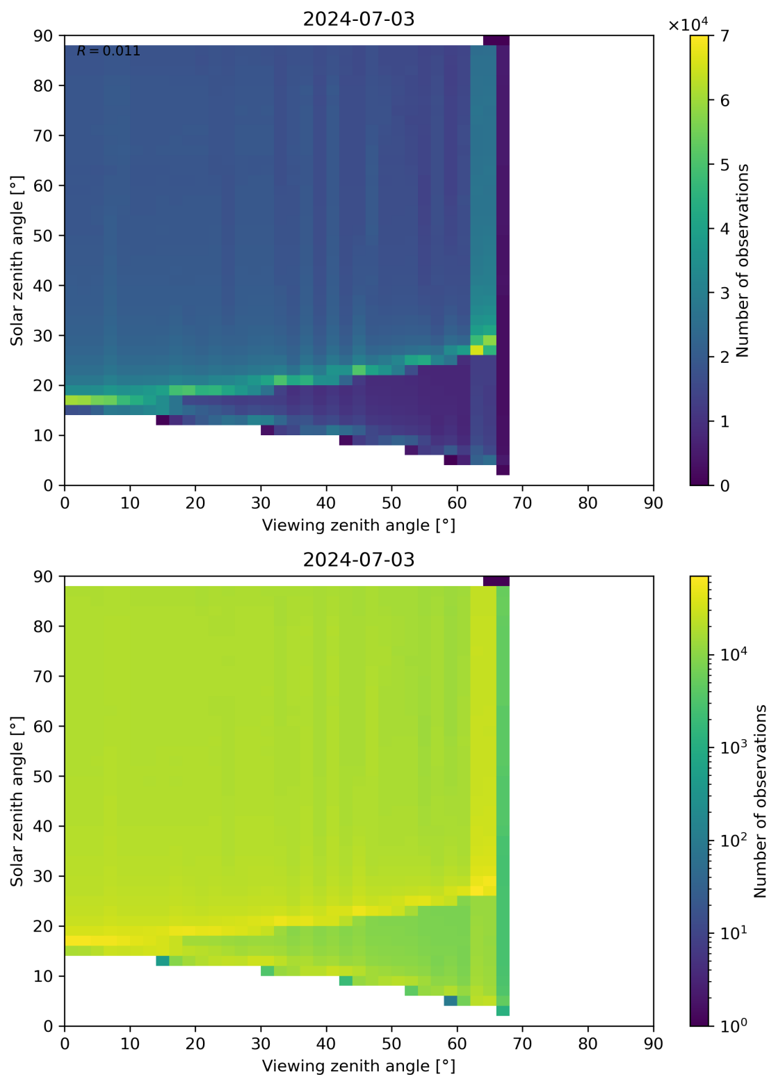
Figure 172: Scatter density plot of “Viewing zenith angle” against “Solar zenith angle” for 2024-07-02 to 2024-07-04.
