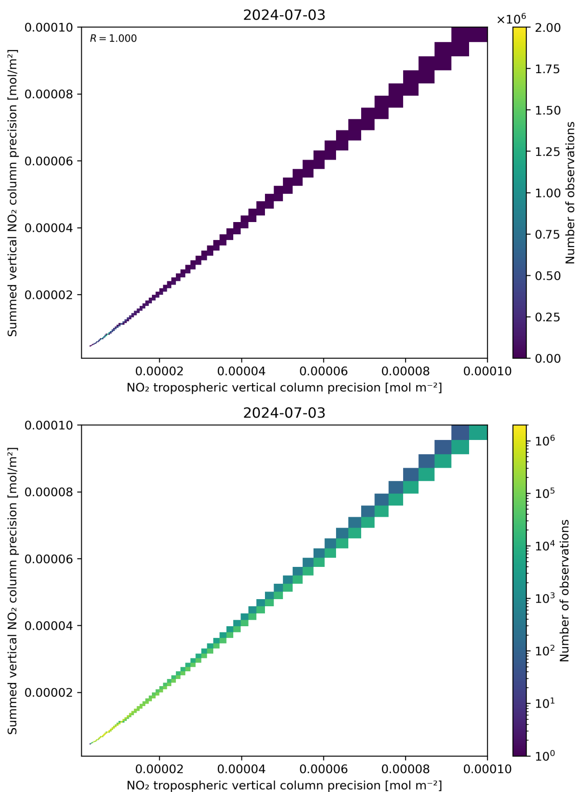
Figure 137: Scatter density plot of “NO 2 tropospheric vertical column precision” against “Summed vertical NO 2 column precision” for 2024-07-02 to 2024-07-04.
