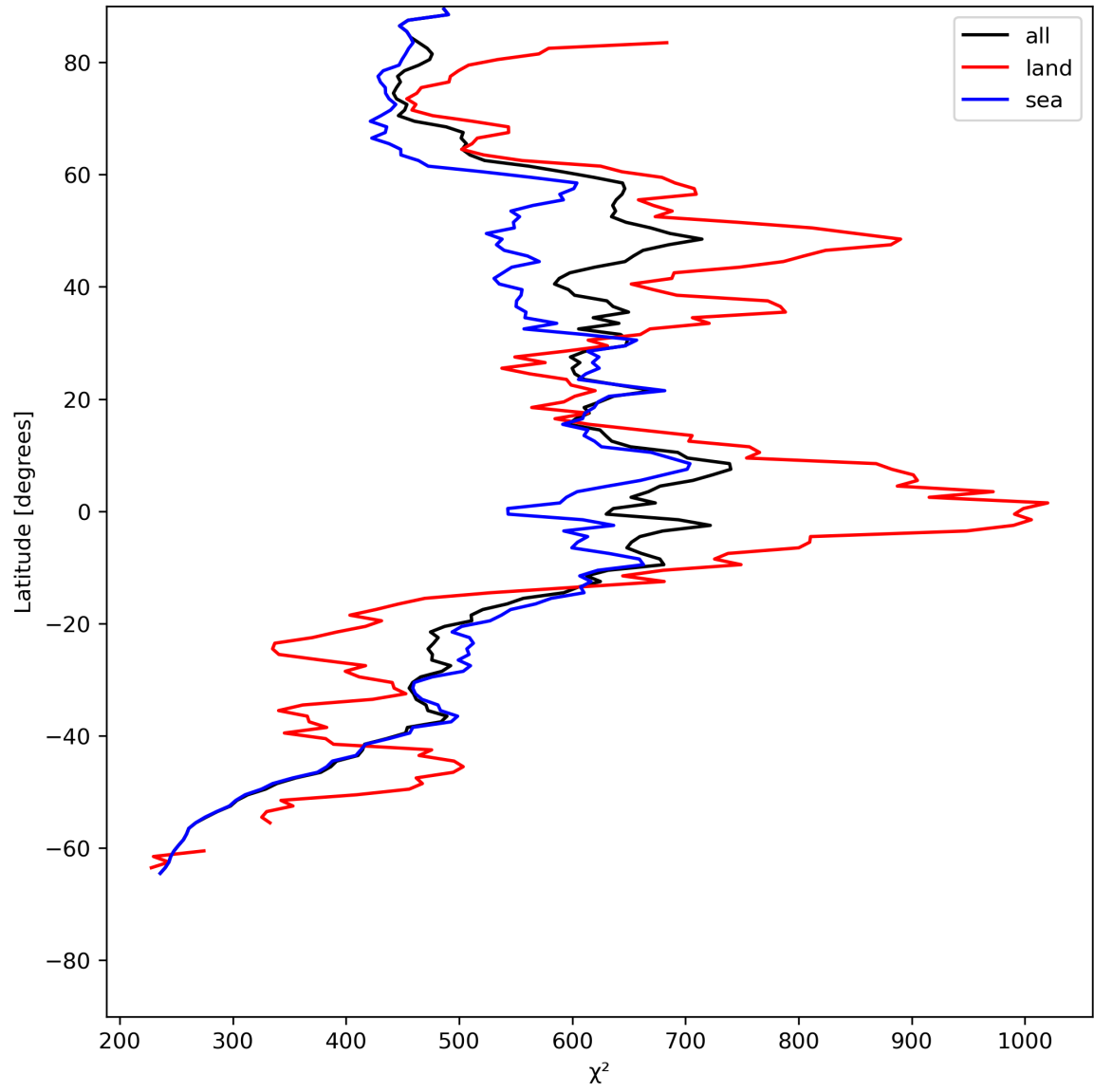
Figure 25: Zonal average of “ \chi^2 ” for 2024-07-02 to 2024-07-04.
