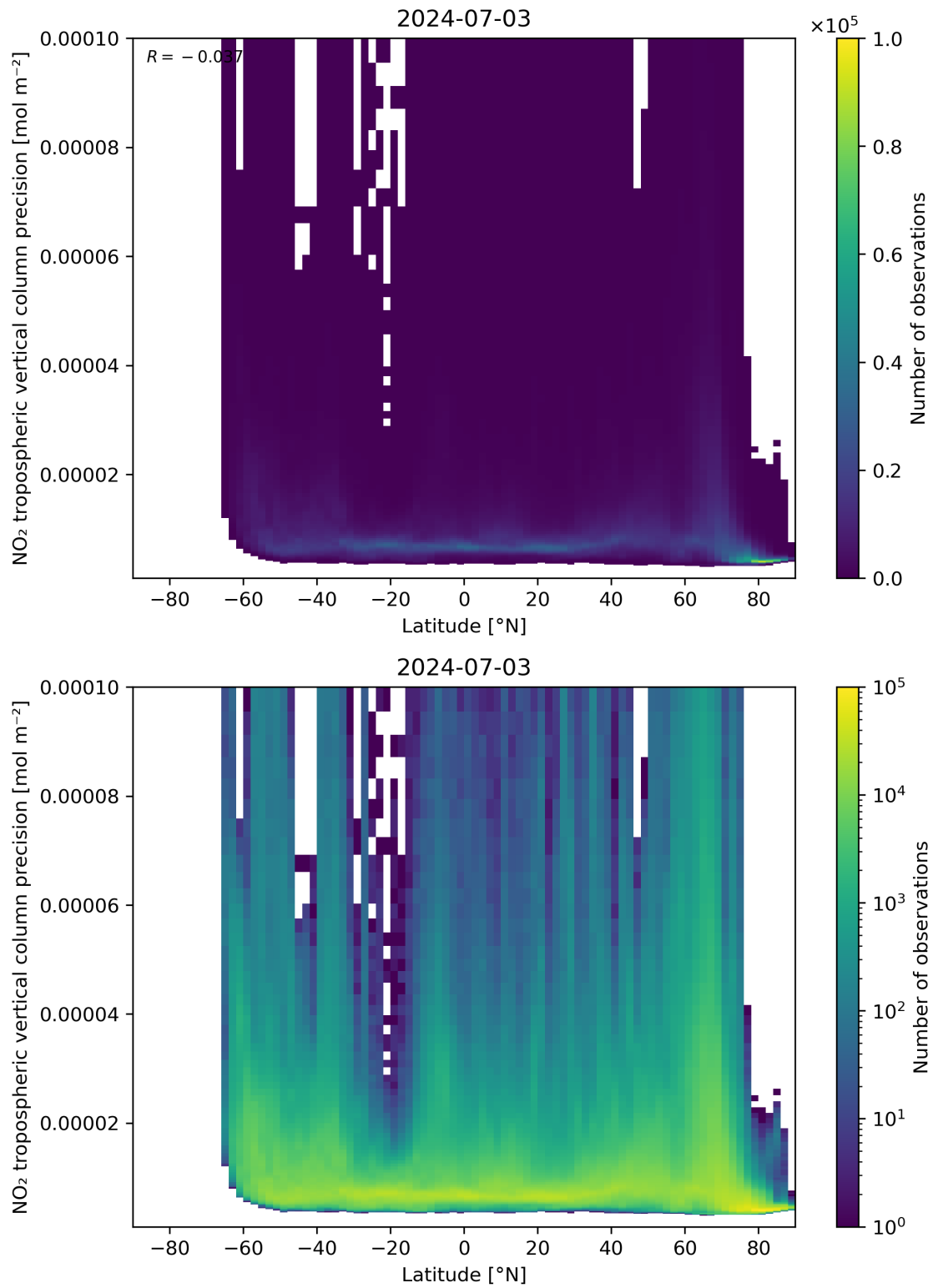
Figure 93: Scatter density plot of “Latitude” against “NO 2 tropospheric vertical column precision” for 2024-07-02 to 2024-07-04.
