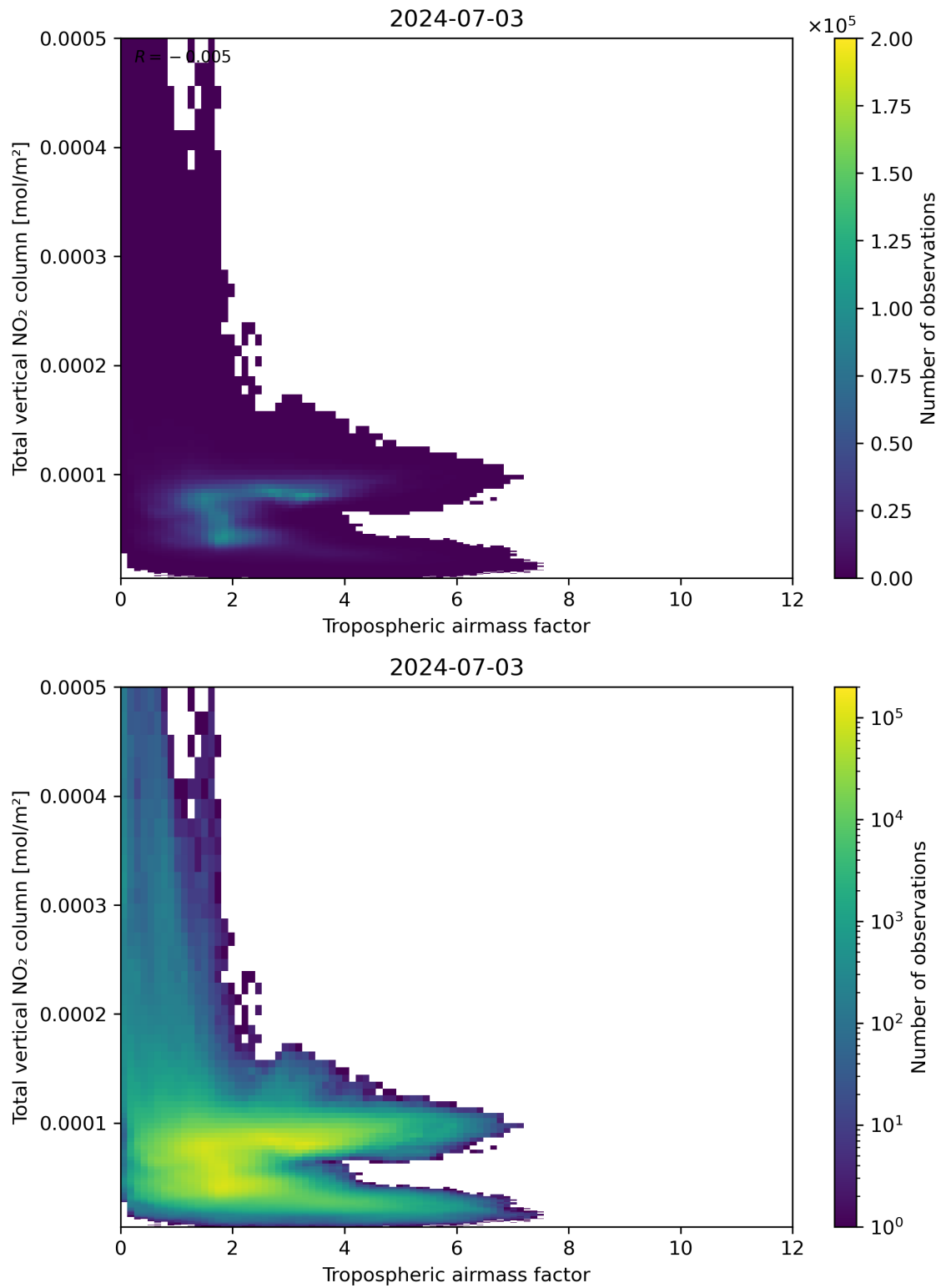
Figure 77: Scatter density plot of “Tropospheric airmass factor” against “Total vertical NO 2 column” for 2024-07-02 to 2024-07-04.
