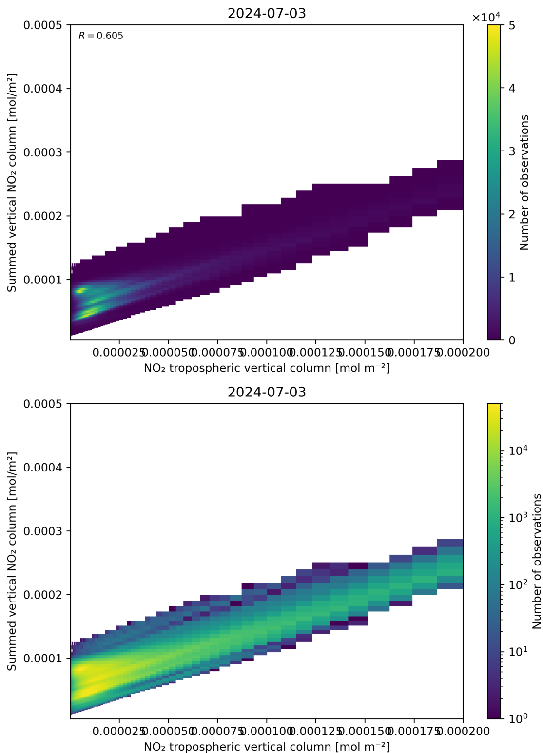
Figure 126: Scatter density plot of “NO 2 tropospheric vertical column” against “Summed vertical NO 2 column” for 2024-07-02 to 2024-07-04.
