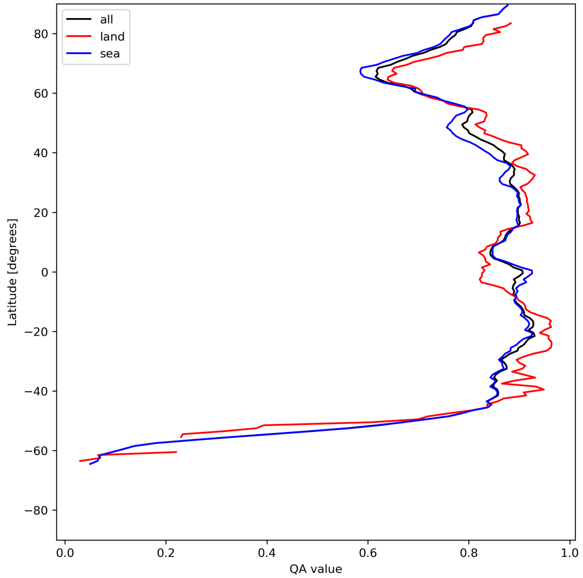
Figure 11: Zonal average of “QA value” for 2024-07-02 to 2024-07-04.
