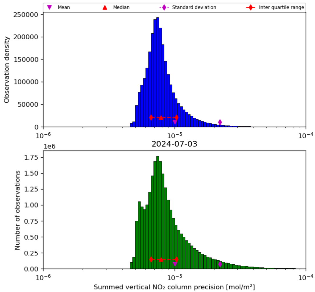
Figure 41: Histogram of "Summed vertical NO 2 column precision" for 2024-07-02 to 2024-07-04
