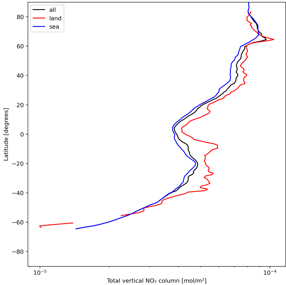
Figure 21: Zonal average of “Total vertical NO 2 column” for 2024-07-02 to 2024-07-04.
