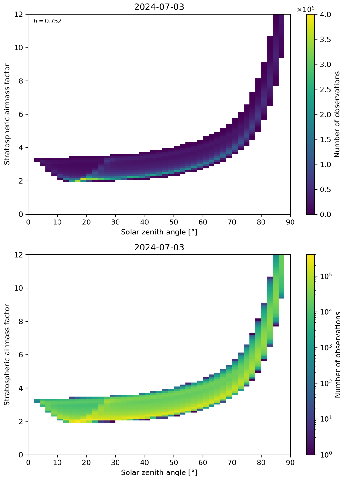
Figure 145: Scatter density plot of “Solar zenith angle” against “Stratospheric airmass factor” for 2024-07-02 to 2024-07-04.
