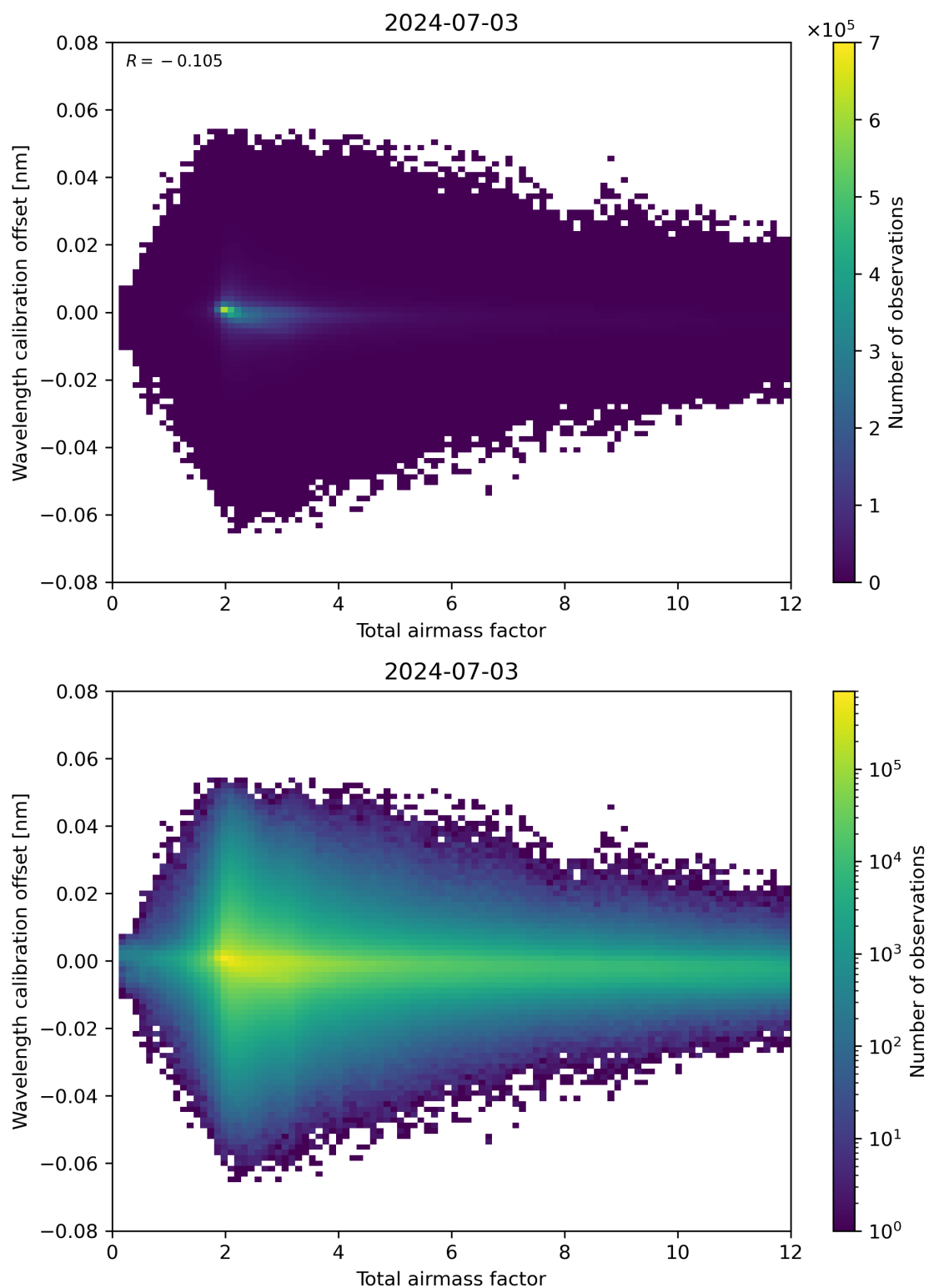
Figure 70: Scatter density plot of “Total airmass factor” against “Wavelength calibration offset” for 2024-07-02 to 2024-07-04.
