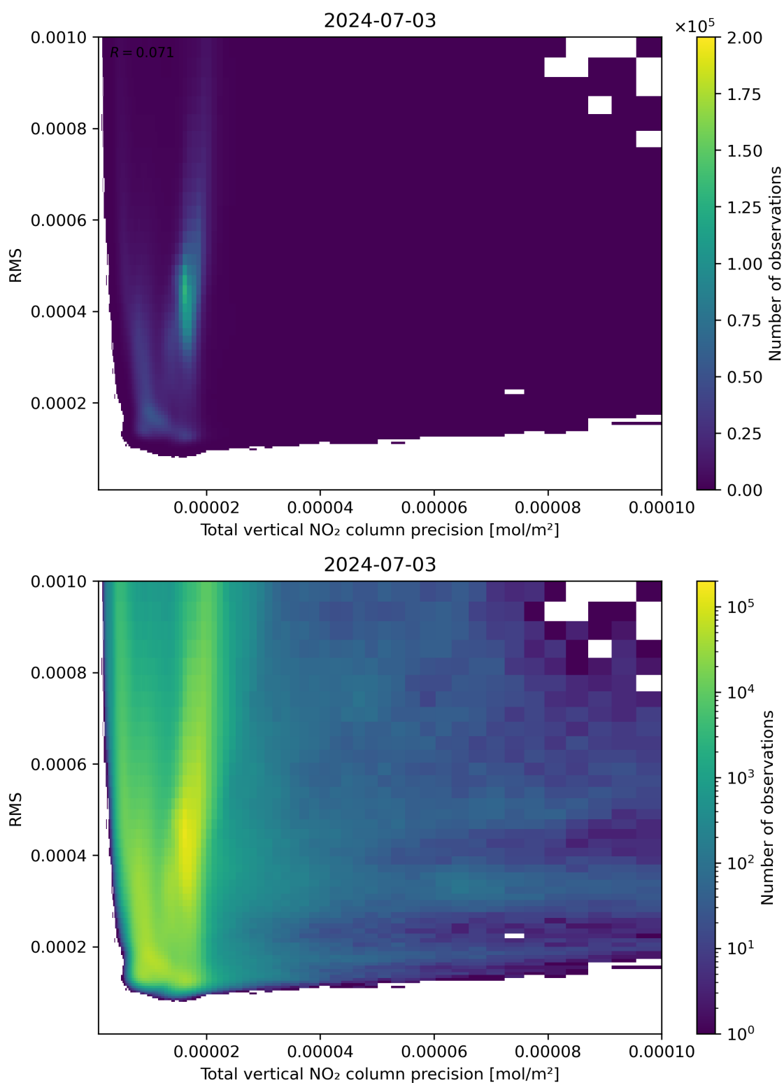
Figure 119: Scatter density plot of “Total vertical NO 2 column precision” against “RMS” for 2024-07-02 to 2024-07-04.
