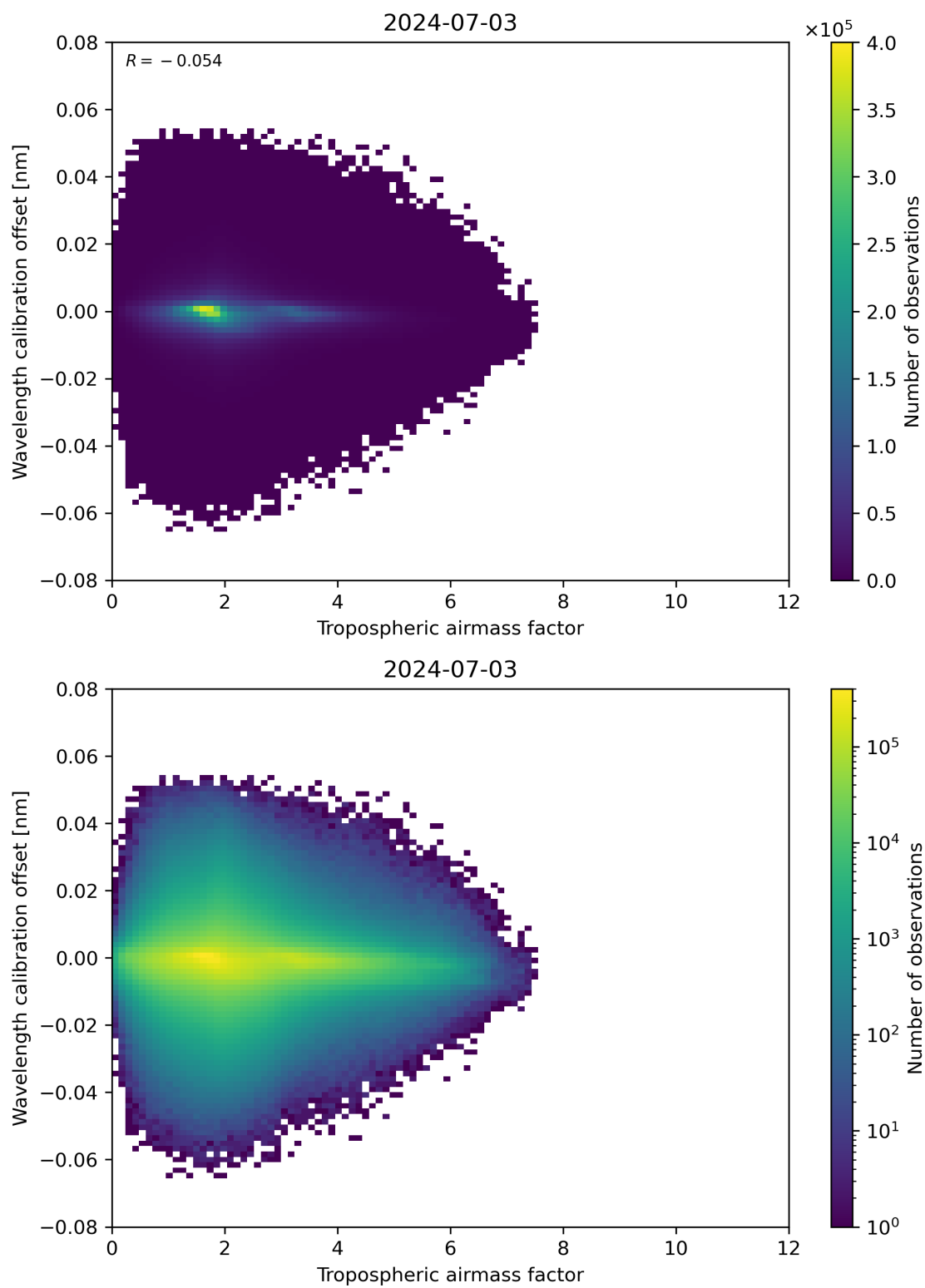
Figure 80: Scatter density plot of “Tropospheric airmass factor” against “Wavelength calibration offset” for 2024-07-02 to 2024-07-04.
