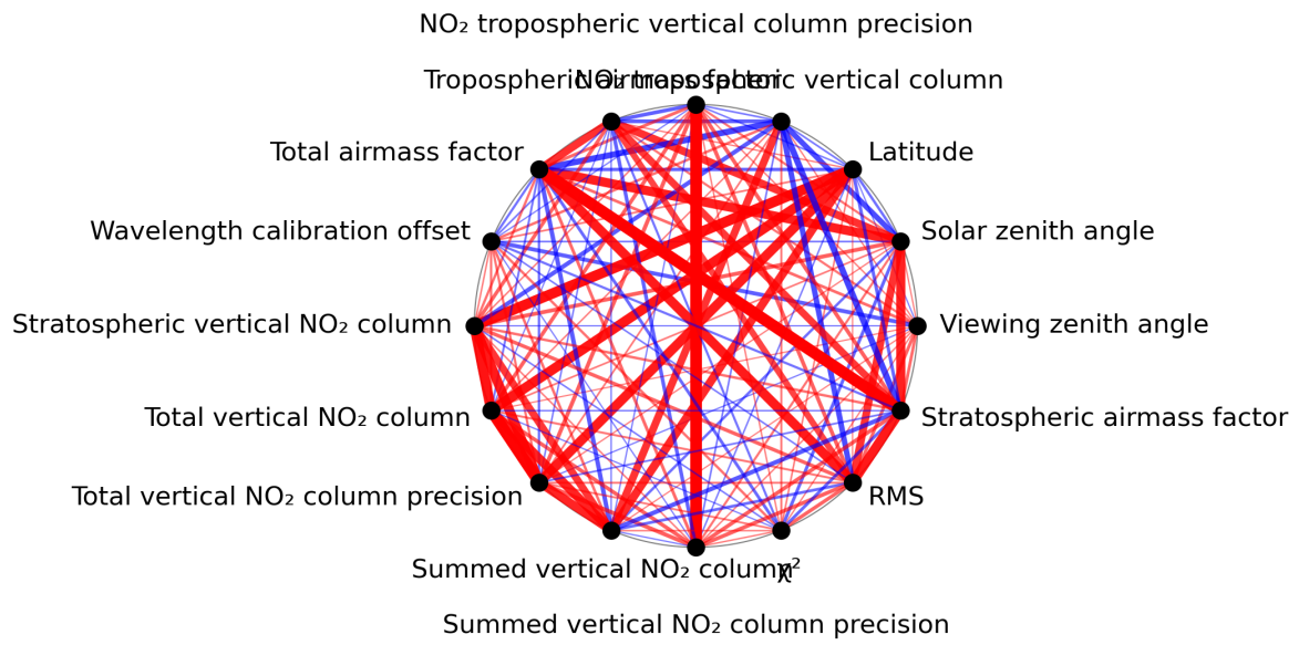
Figure 1: Map of correlation graph for 2024-07-02 to 2024-07-04.
