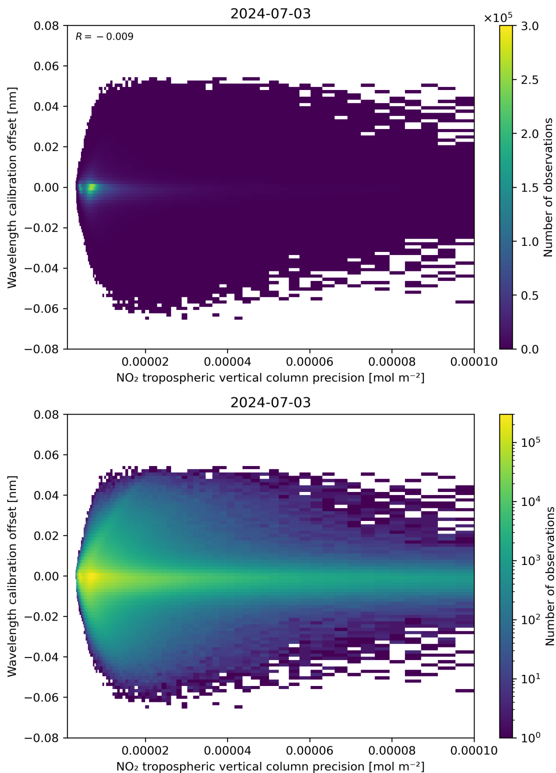
Figure 141: Scatter density plot of “NO 2 tropospheric vertical column precision” against “Wavelength calibration offset” for 2024-07-02 to 2024-07-04.
