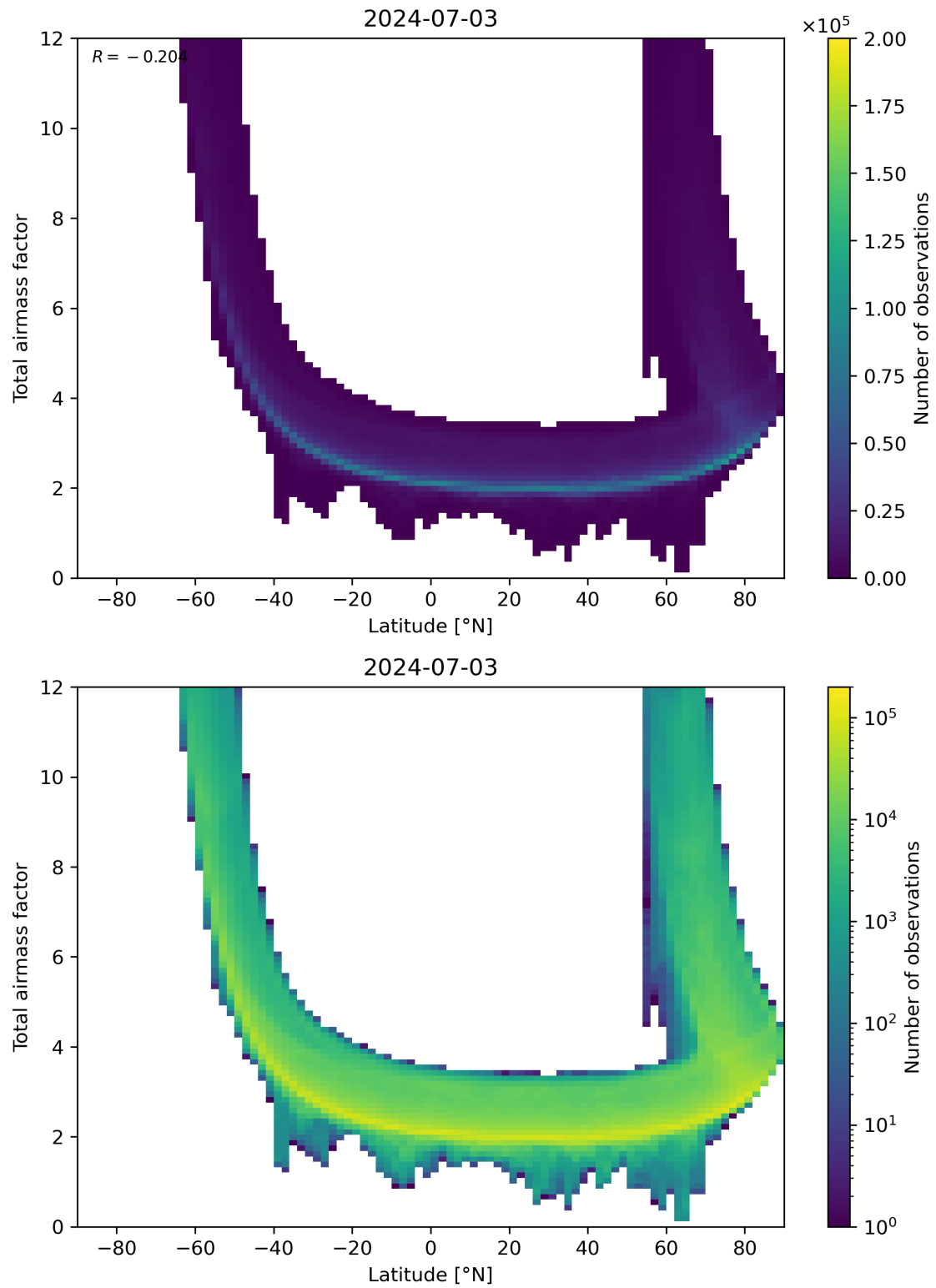
Figure 84: Scatter density plot of “Latitude” against “Total airmass factor” for 2024-07-02 to 2024-07-04.
