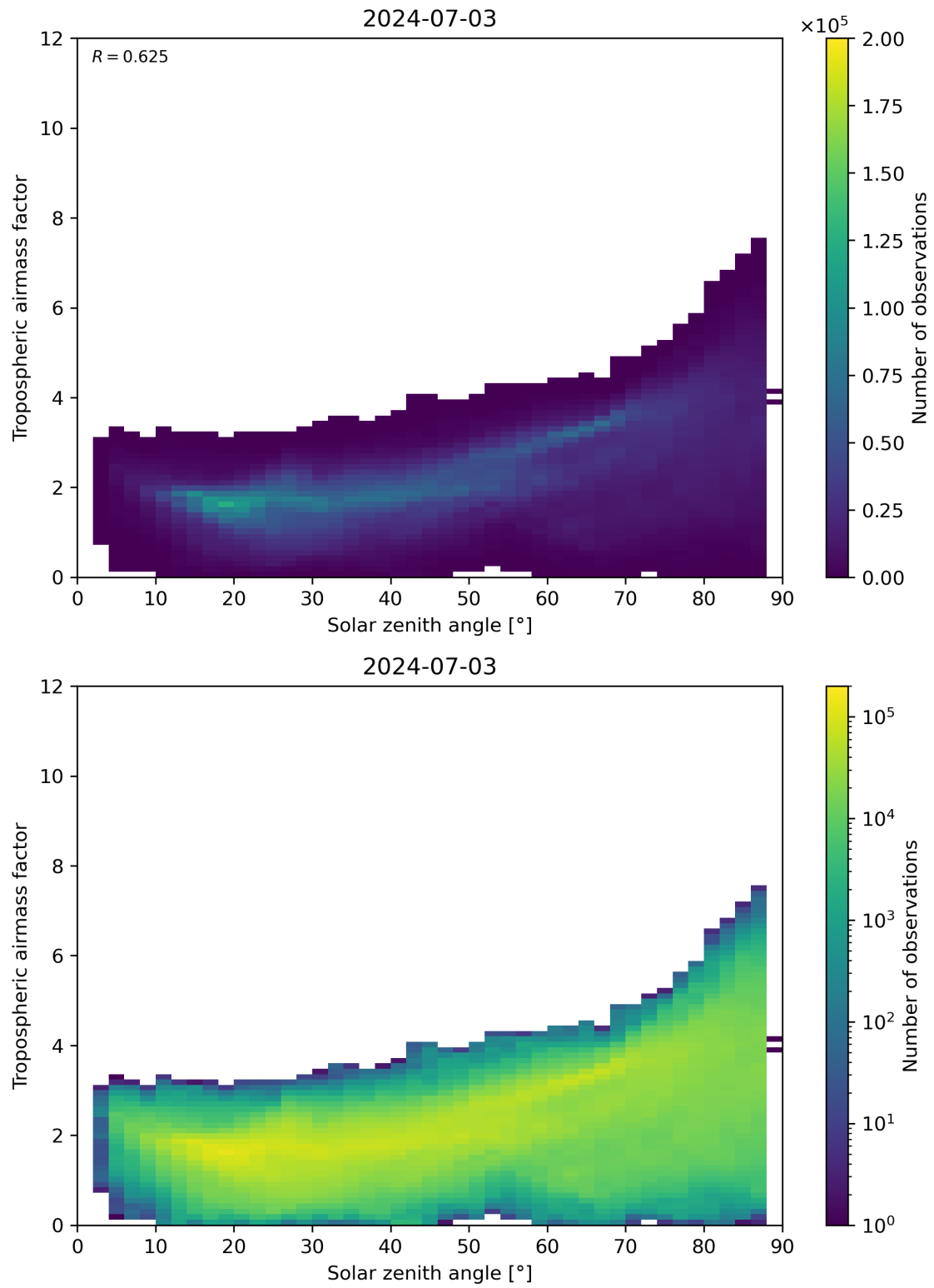
Figure 147: Scatter density plot of “Solar zenith angle” against “Tropospheric airmass factor” for 2024-07-02 to 2024-07-04.
