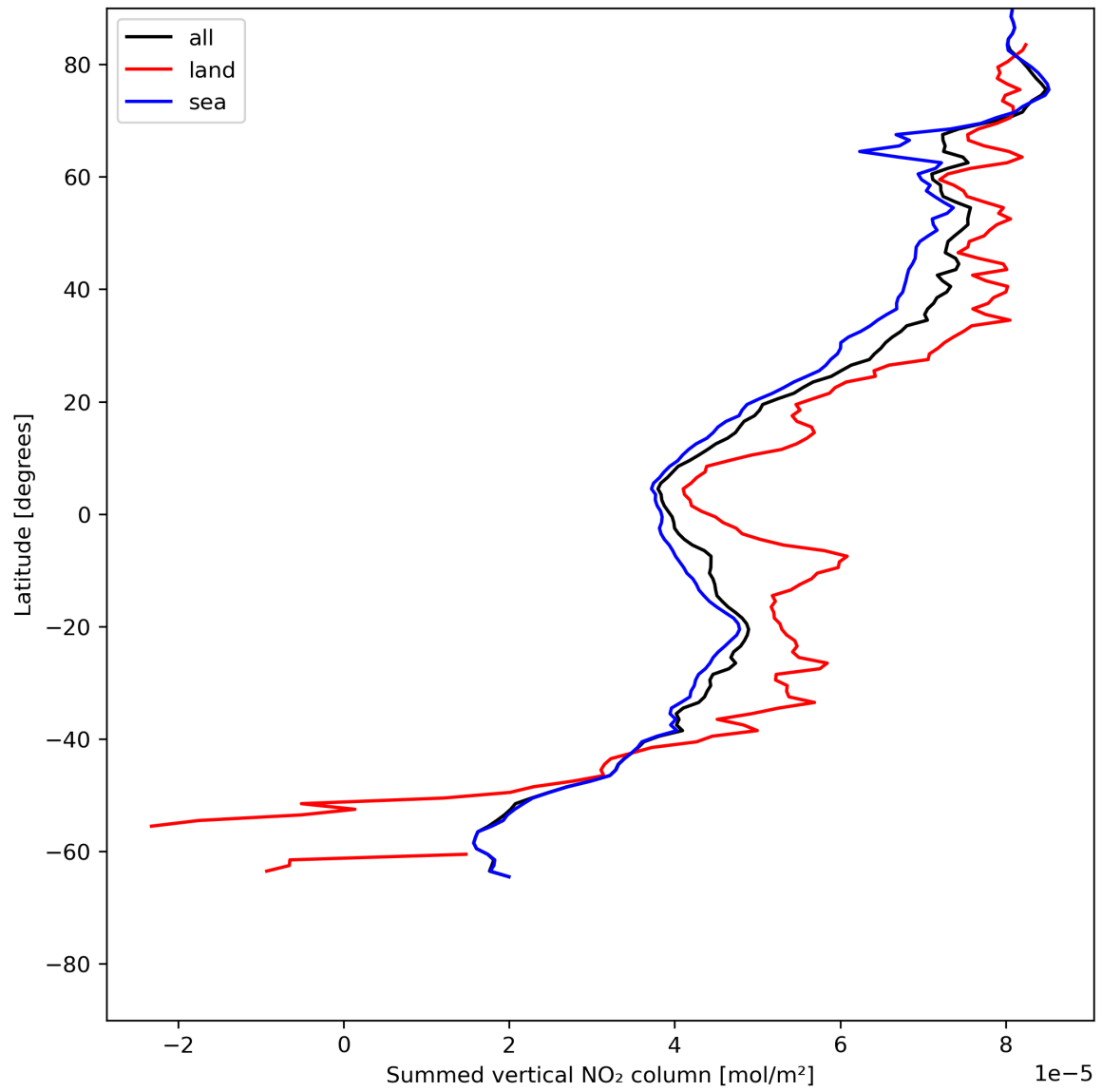
Figure 23: Zonal average of “Summed vertical NO 2 column” for 2024-07-02 to 2024-07-04.
