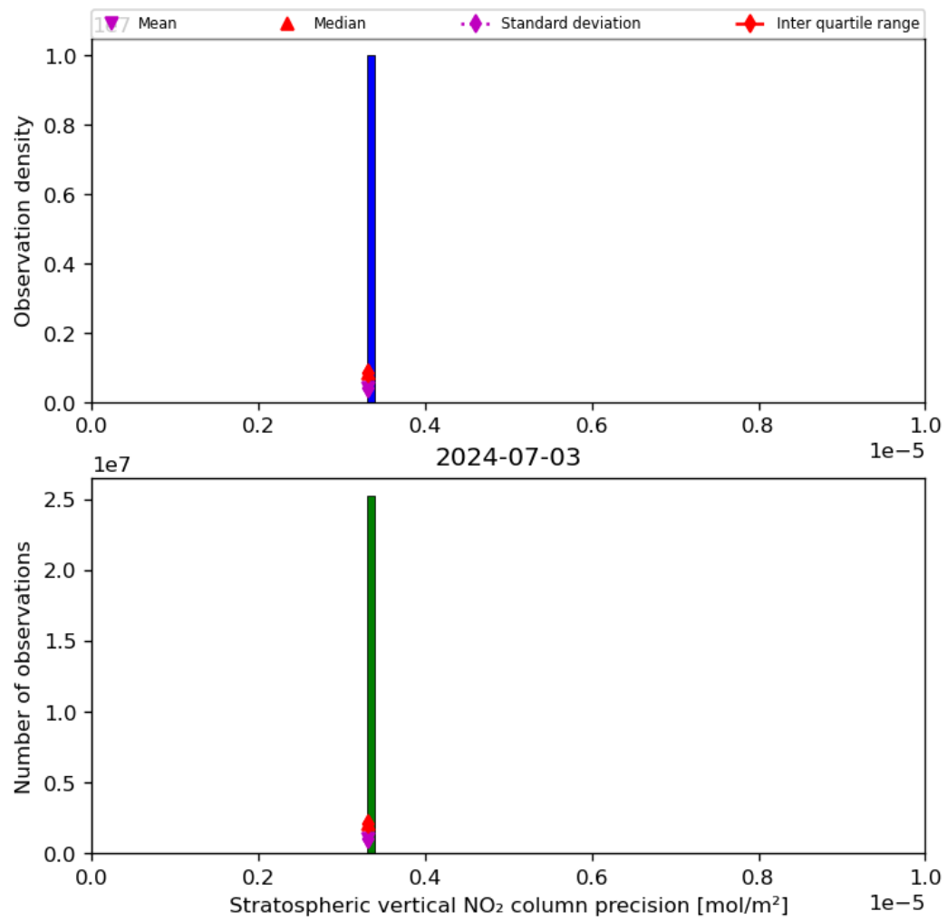
Figure 37: Histogram of “Stratospheric vertical NO 2 column precision” for 2024-07-02 to 2024-07-04
