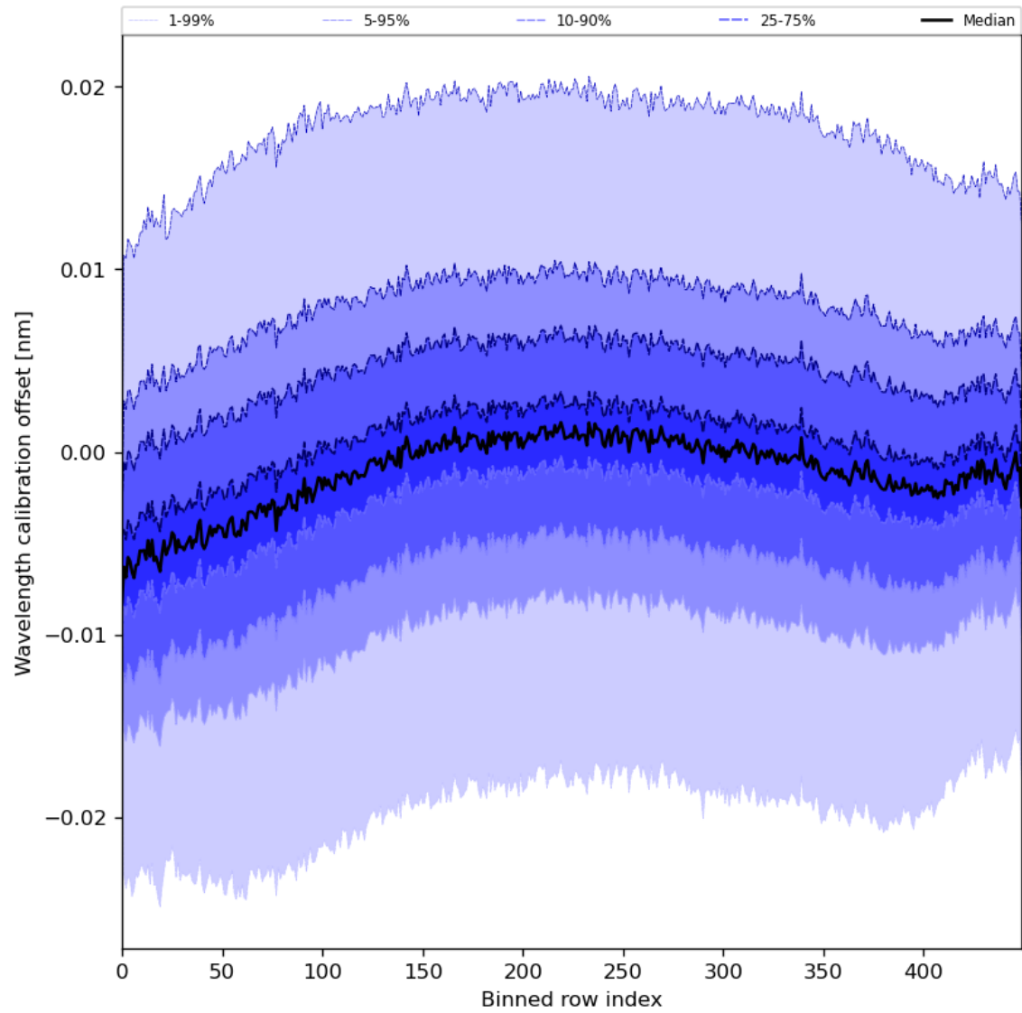
Figure 52: Along track statistics of “Wavelength calibration offset” for 2024-07-02 to 2024-07-04
