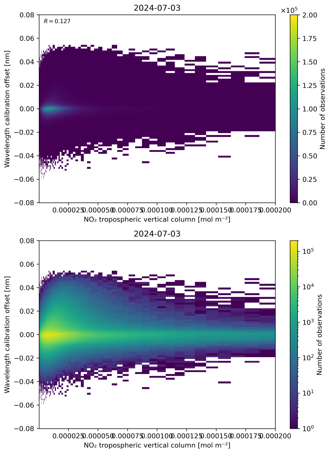
Figure 143: Scatter density plot of “NO 2 tropospheric vertical column” against “Wavelength calibration offset” for 2024-07-02 to 2024-07-04.
