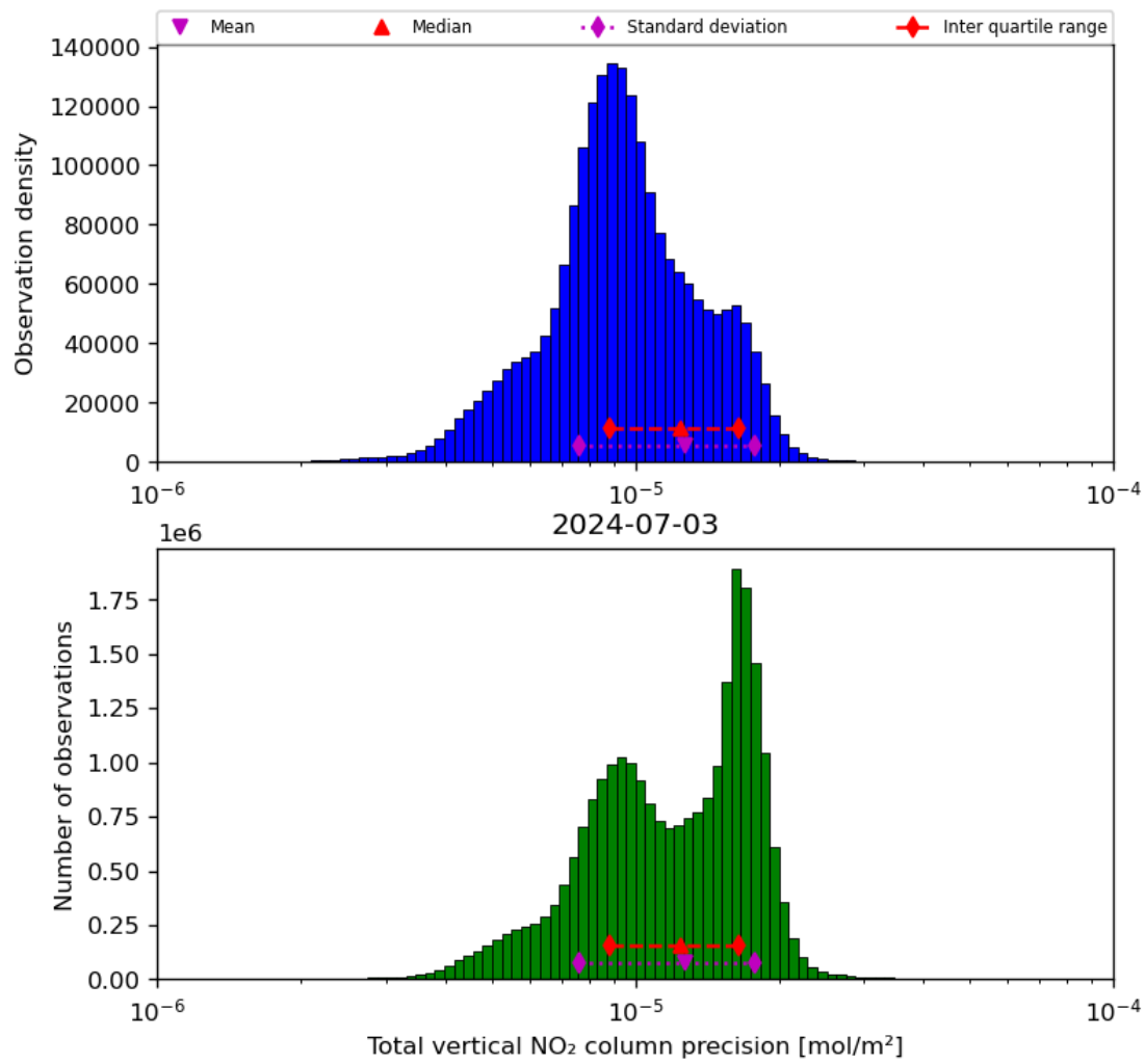
Figure 39: Histogram of “Total vertical NO 2 column precision” for 2024-07-02 to 2024-07-04
