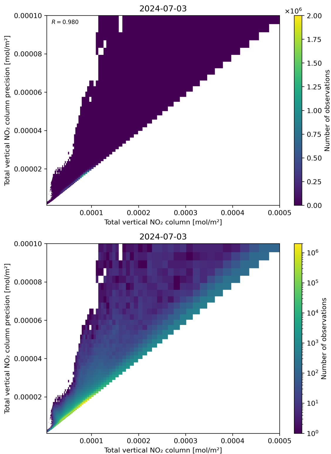
Figure 114: Scatter density plot of “Total vertical NO 2 column” against “Total vertical NO 2 column precision” for 2024-07-02 to 2024-07-04.
