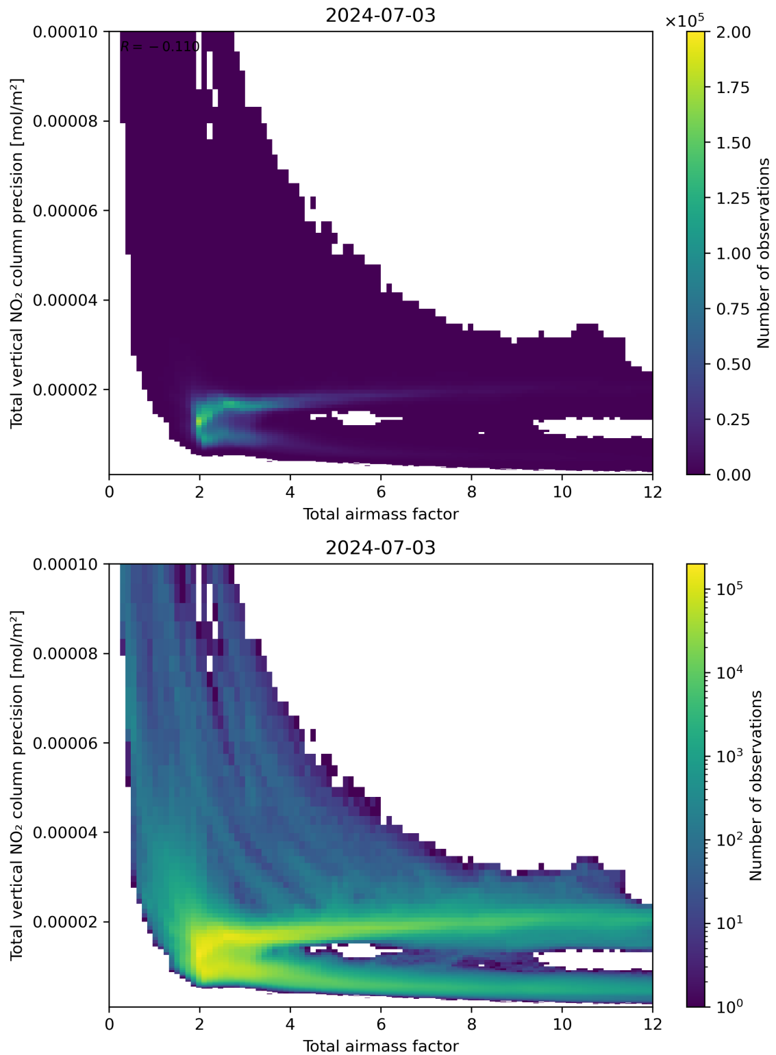
Figure 68: Scatter density plot of “Total airmass factor” against “Total vertical NO 2 column precision” for 2024-07-02 to 2024-07-04.
