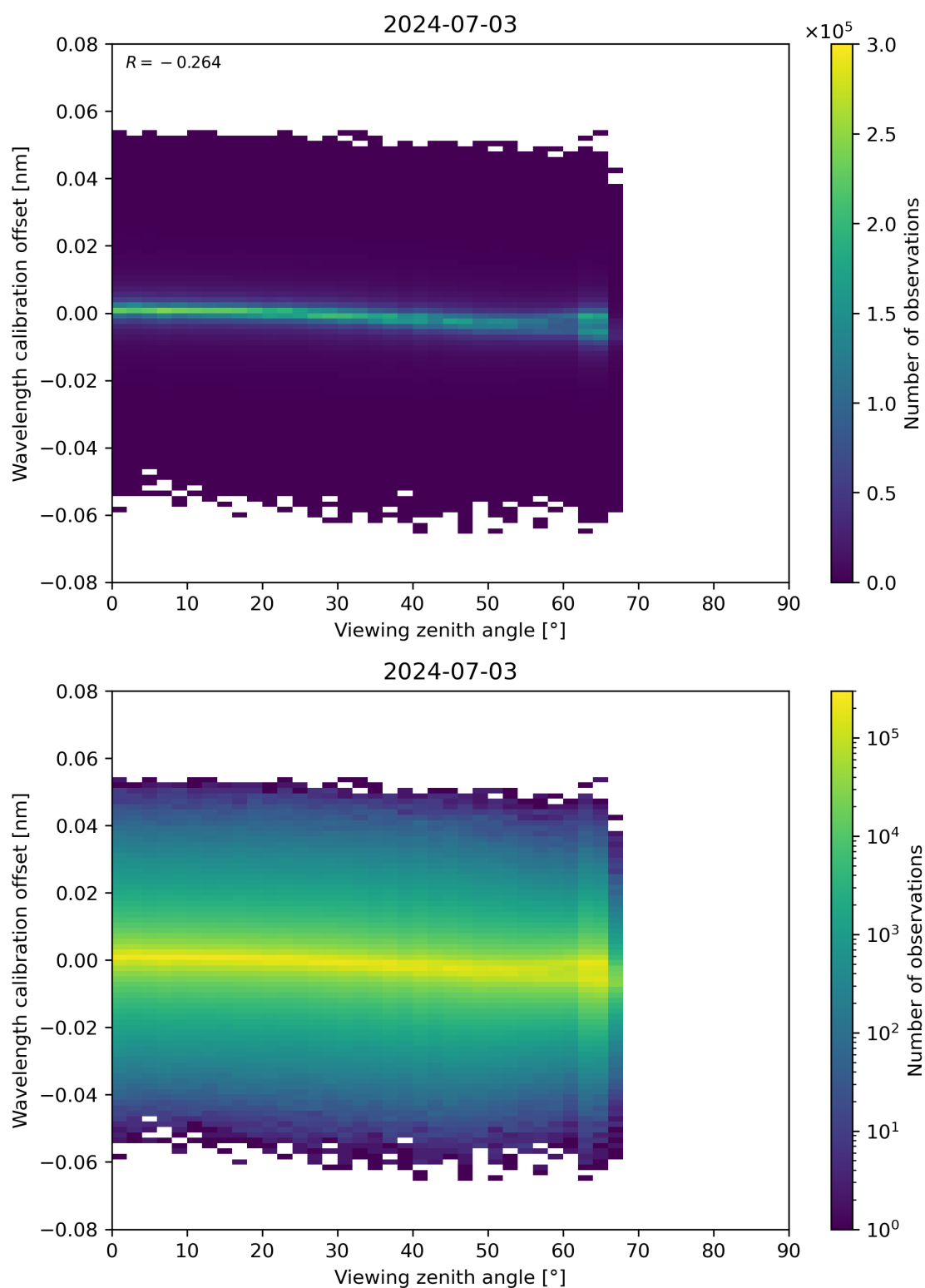
Figure 173: Scatter density plot of “Viewing zenith angle” against “Wavelength calibration offset” for 2024-07-02 to 2024-07-04.
