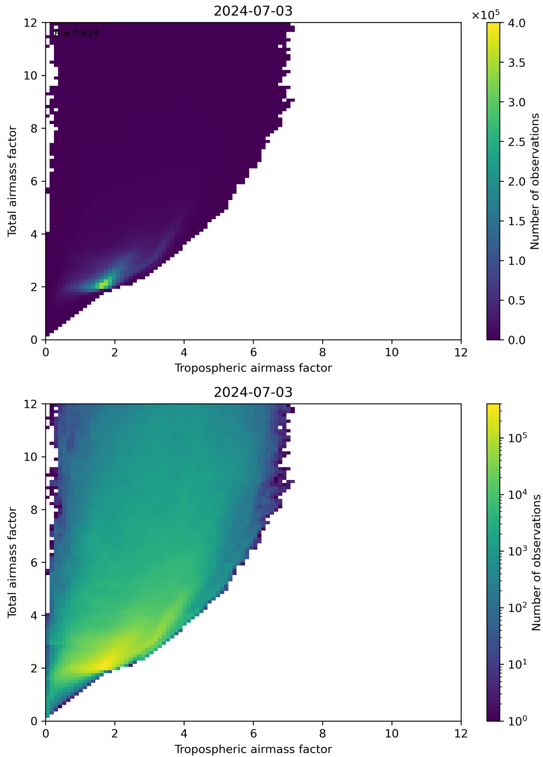
Figure 72: Scatter density plot of “Tropospheric airmass factor” against “Total airmass factor” for 2024-07-02 to 2024-07-04.
