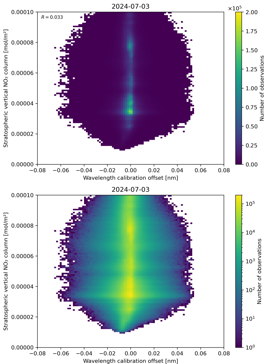
Figure 176: Scatter density plot of “Wavelength calibration offset” against “Stratospheric vertical NO 2 column” for 2024-07-02 to 2024-07-04.
