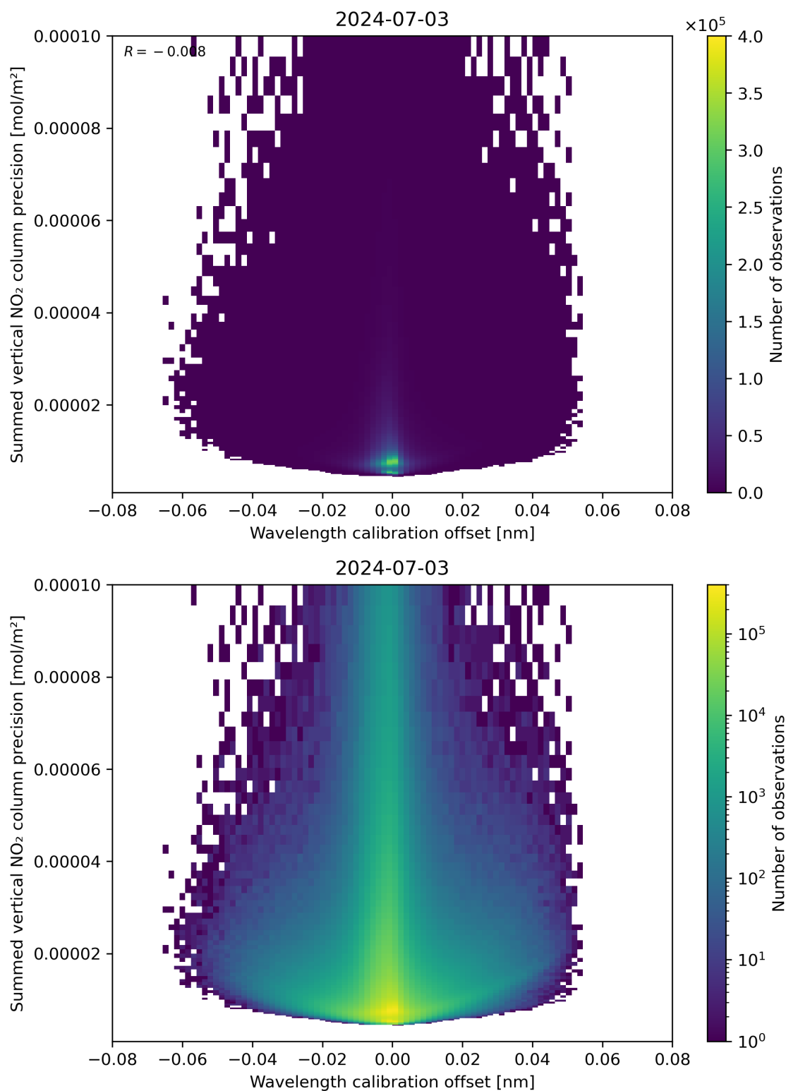
Figure 178: Scatter density plot of “Wavelength calibration offset” against “Summed vertical NO 2 column precision” for 2024-07-02 to 2024-07-04.
