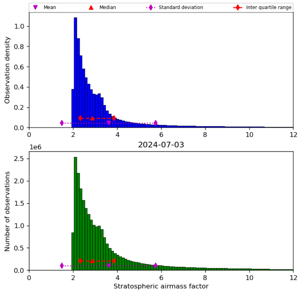
Figure 44: Histogram of “Stratospheric airmass factor” for 2024-07-02 to 2024-07-04
