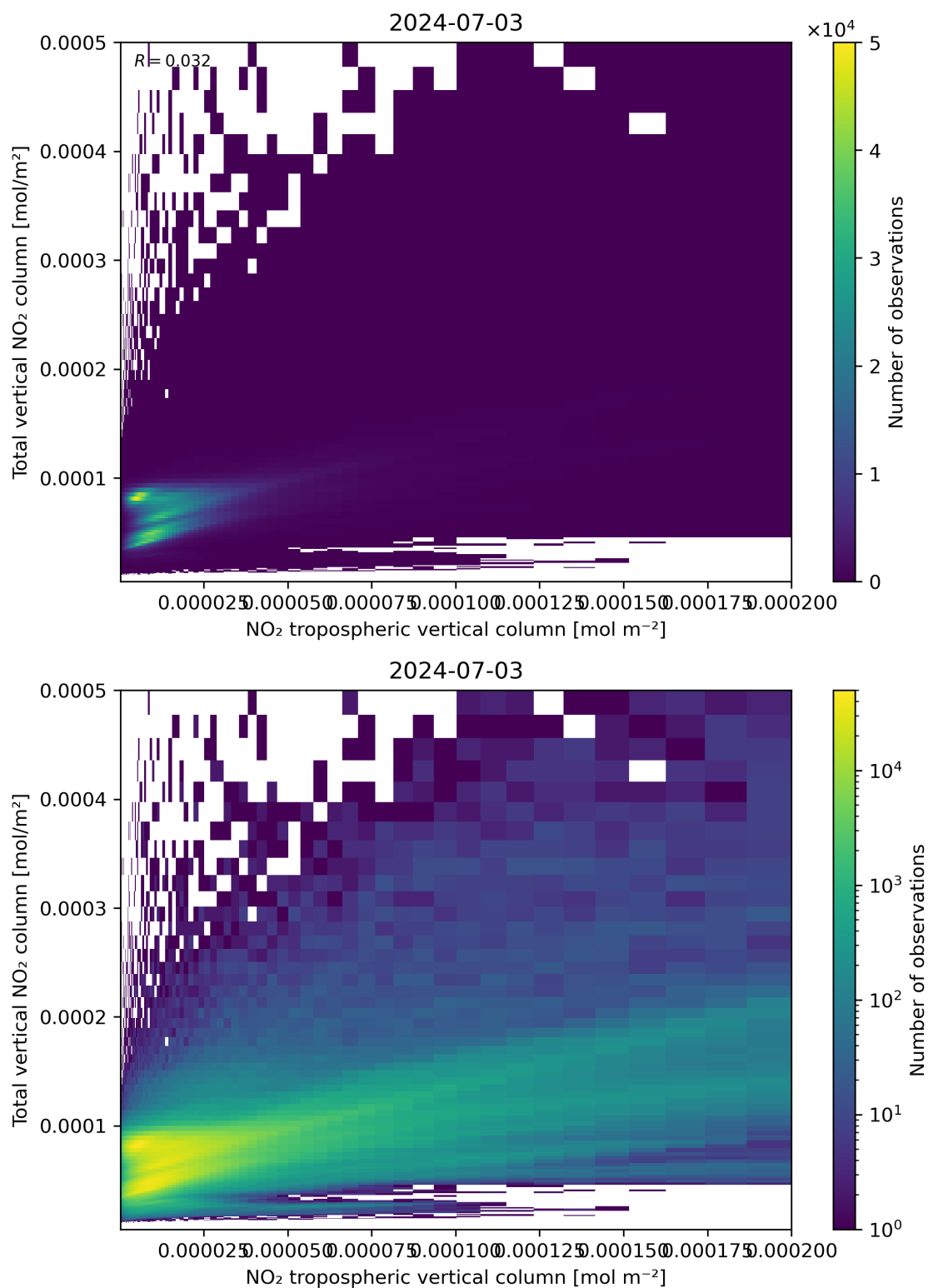
Figure 128: Scatter density plot of “NO 2 tropospheric vertical column” against “Total vertical NO 2 column” for 2024-07-02 to 2024-07-04.
