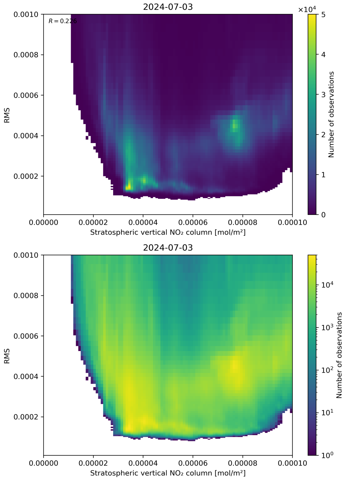
Figure 102: Scatter density plot of “Stratospheric vertical NO 2 column” against “RMS” for 2024-07-02 to 2024-07-04.
