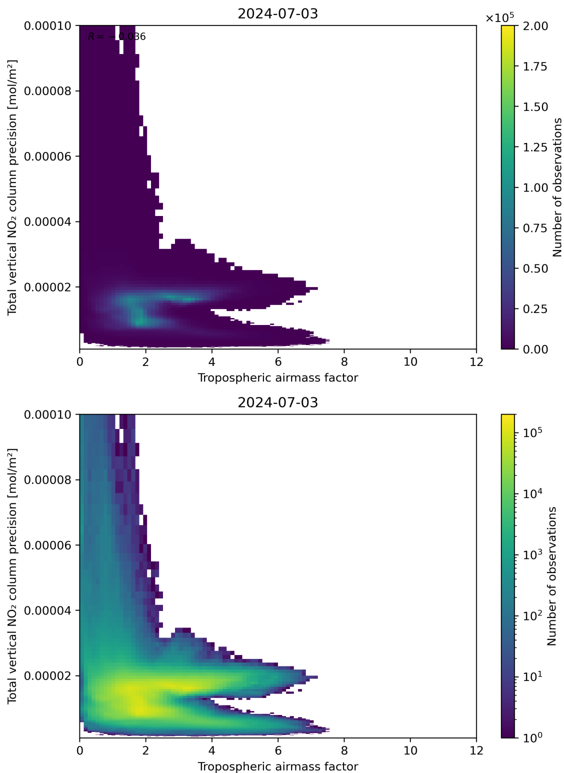
Figure 78: Scatter density plot of “Tropospheric airmass factor” against “Total vertical NO 2 column precision” for 2024-07-02 to 2024-07-04.
