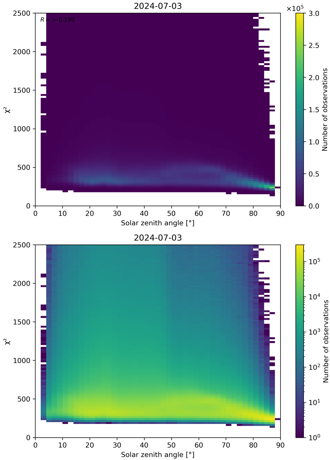
Figure 148: Scatter density plot of “Solar zenith angle” against “ \chi^2 ” for 2024-07-02 to 2024-07-04.
