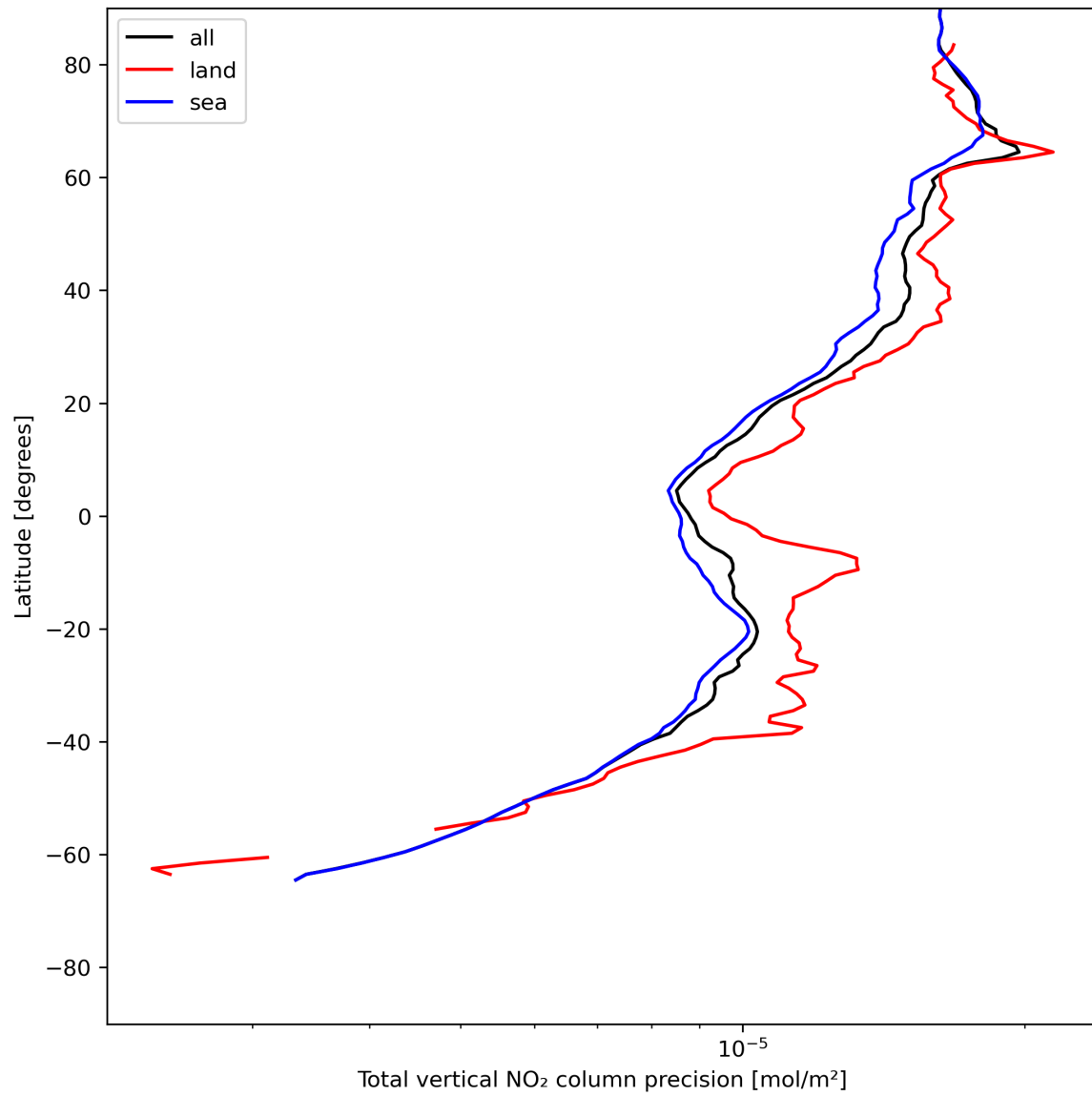
Figure 22: Zonal average of “Total vertical NO 2 column precision” for 2024-07-02 to 2024-07-04.
