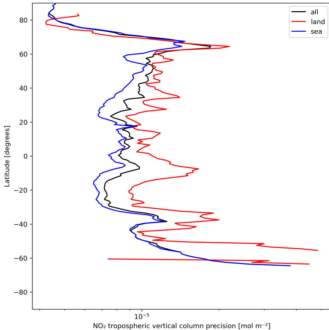
Figure 13: Zonal average of “NO 2 tropospheric vertical column precision” for 2024-07-02 to 2024-07-04.
