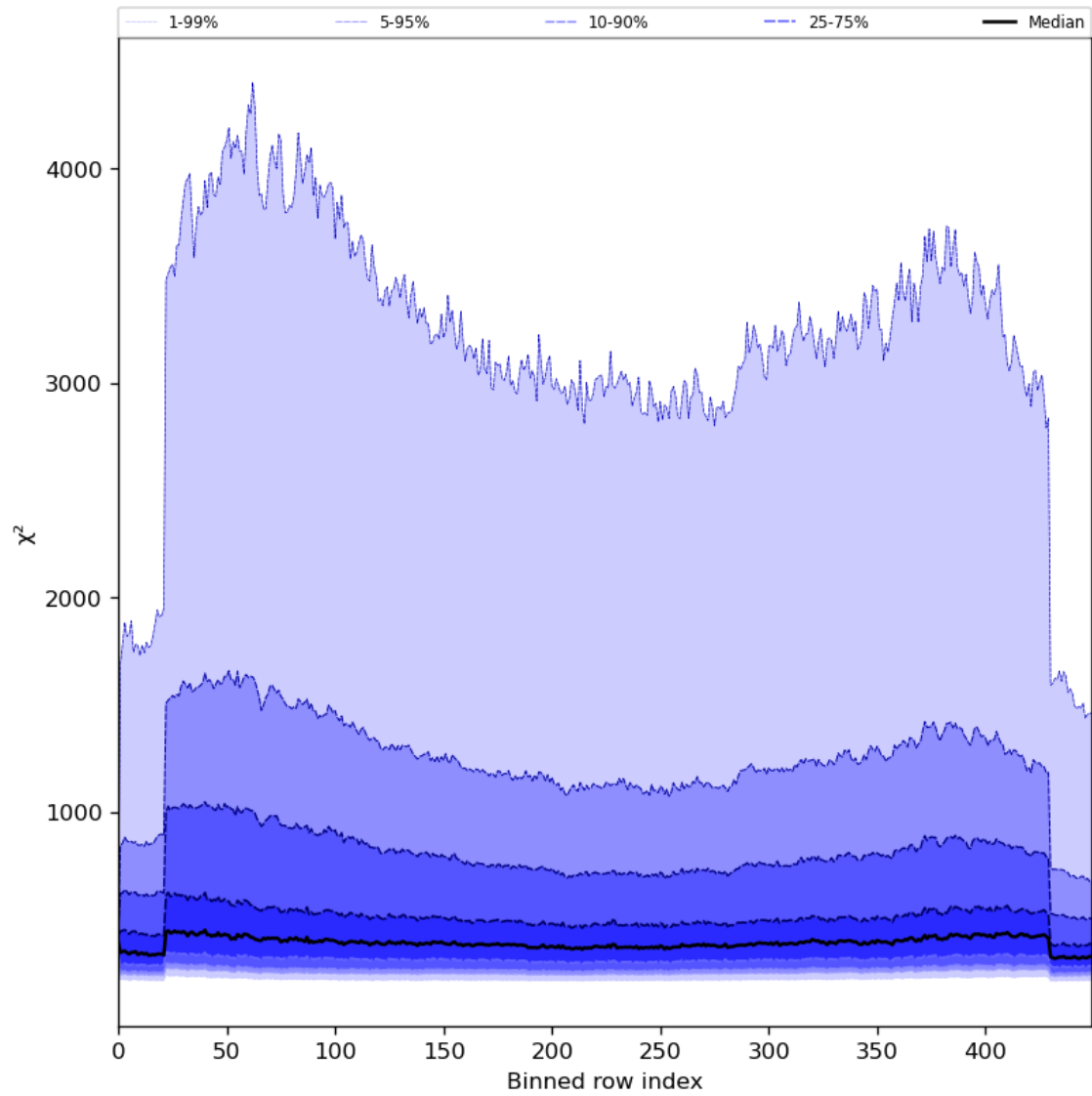
Figure 59: Along track statistics of “ \chi^2 ” for 2024-07-02 to 2024-07-04
