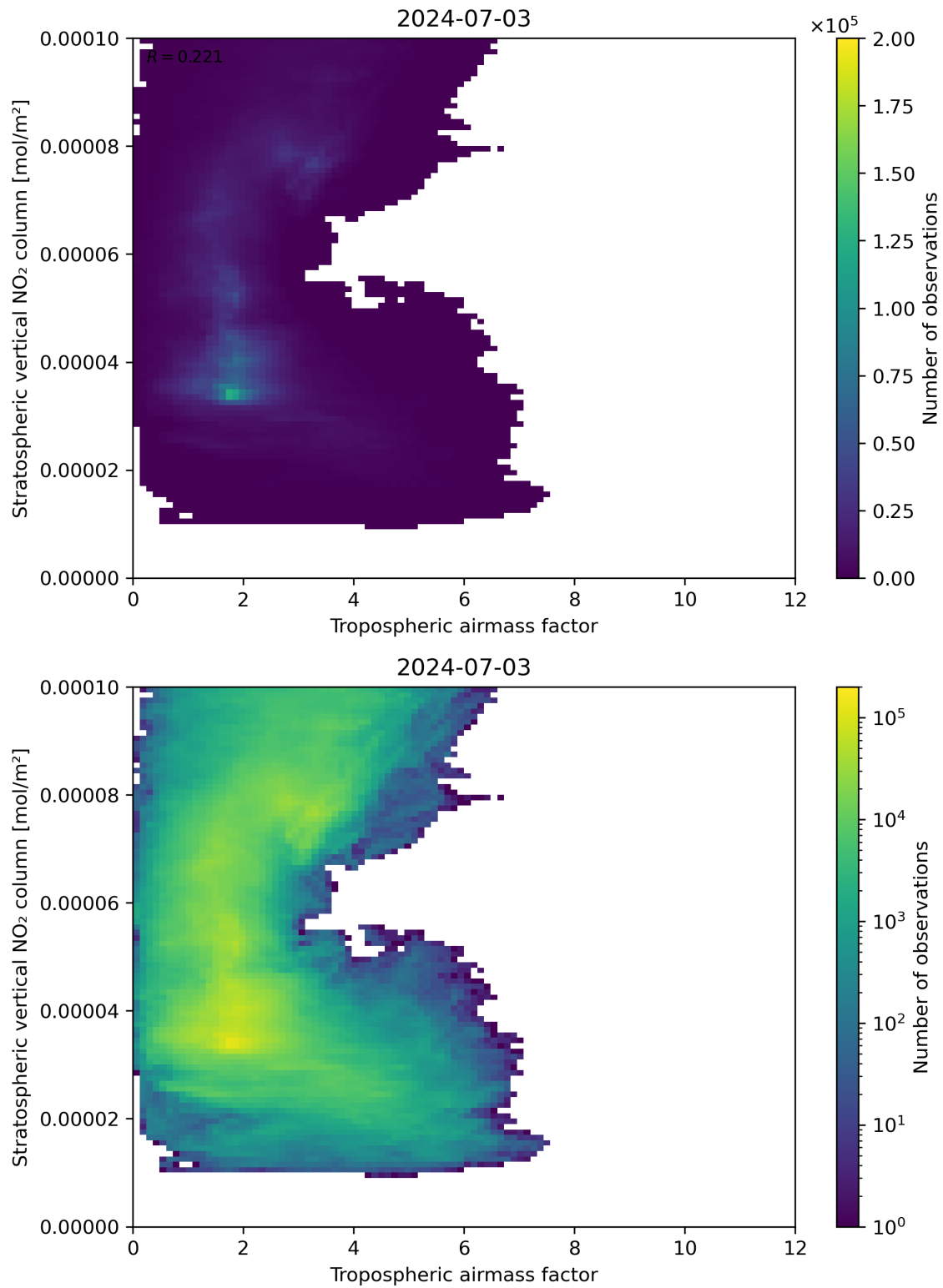
Figure 74: Scatter density plot of “Tropospheric air mass factor” against “Stratospheric vertical NO 2 column” for 2024-07-02 to 2024-07-04.
