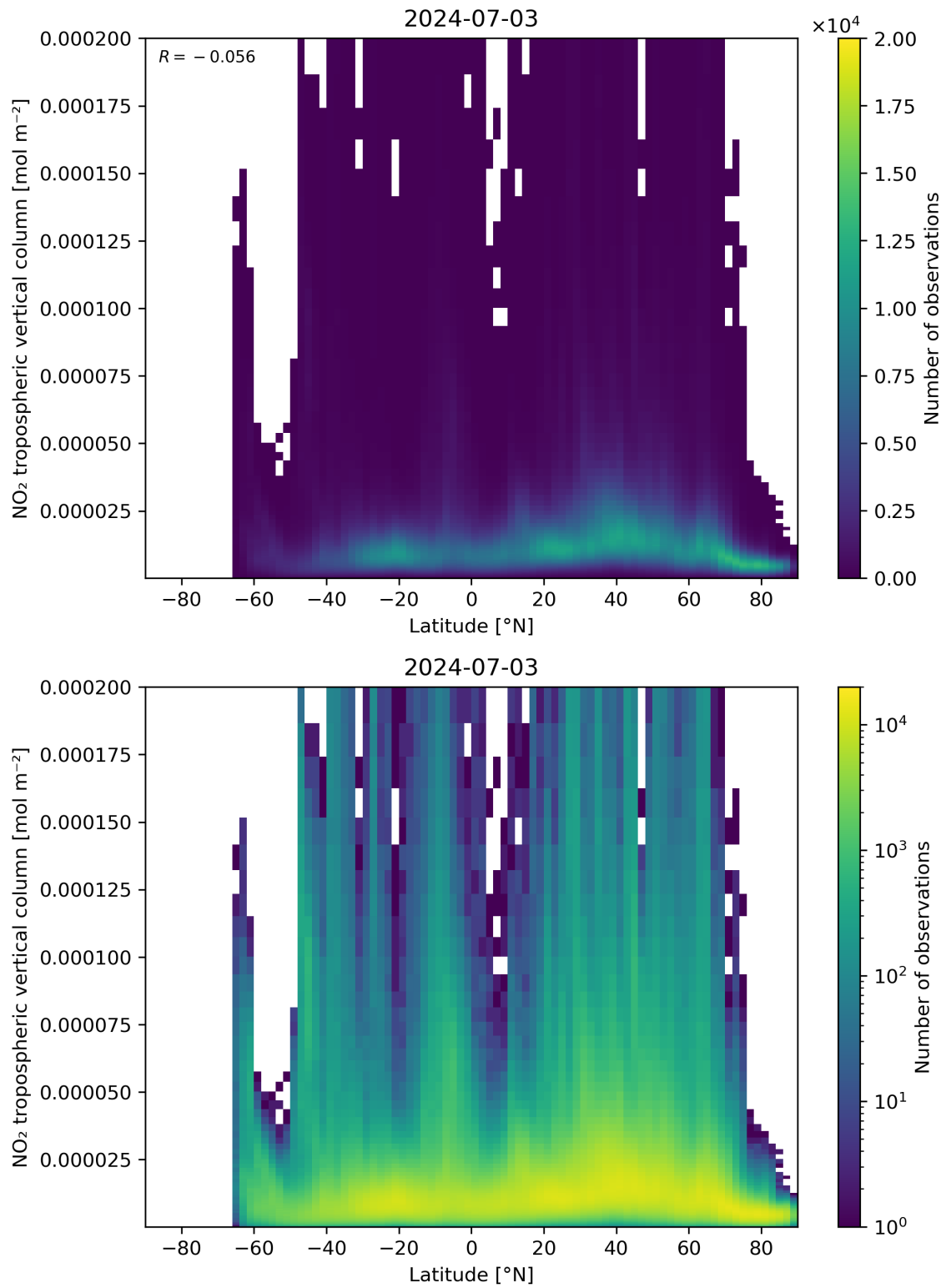
Figure 92: Scatter density plot of “Latitude” against “NO 2 tropospheric vertical column” for 2024-07-02 to 2024-07-04.
