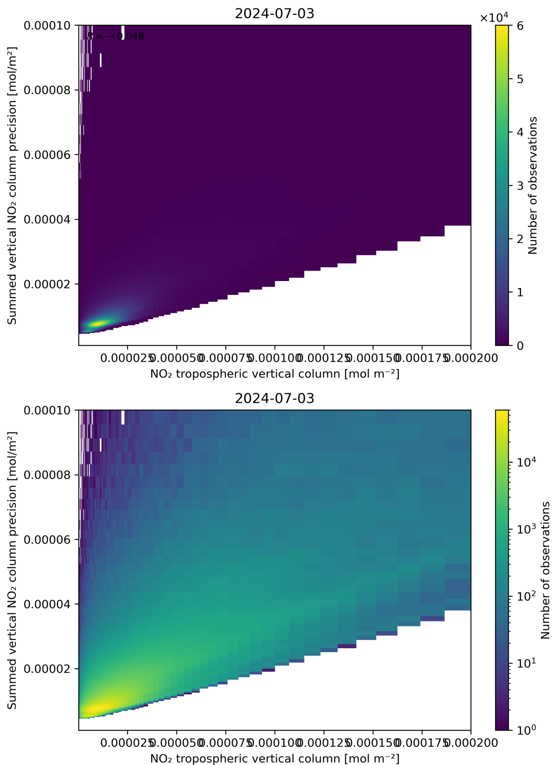
Figure 127: Scatter density plot of “NO 2 tropospheric vertical column” against “Summed vertical NO 2 column precision” for 2024-07-02 to 2024-07-04.
