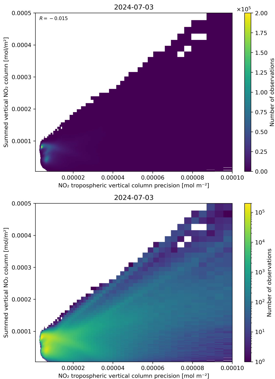
Figure 136: Scatter density plot of “NO 2 tropospheric vertical column precision” against “Summed vertical NO 2 column” for 2024-07-02 to 2024-07-04.
