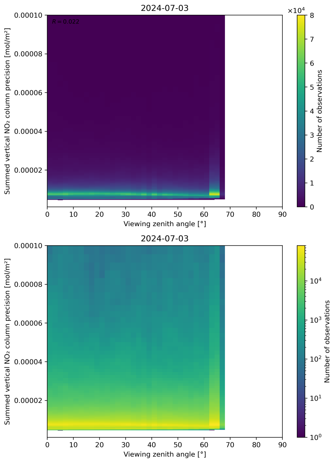
Figure 166: Scatter density plot of “Viewing zenith angle” against “Summed vertical NO 2 column precision” for 2024-07-02 to 2024-07-04.
