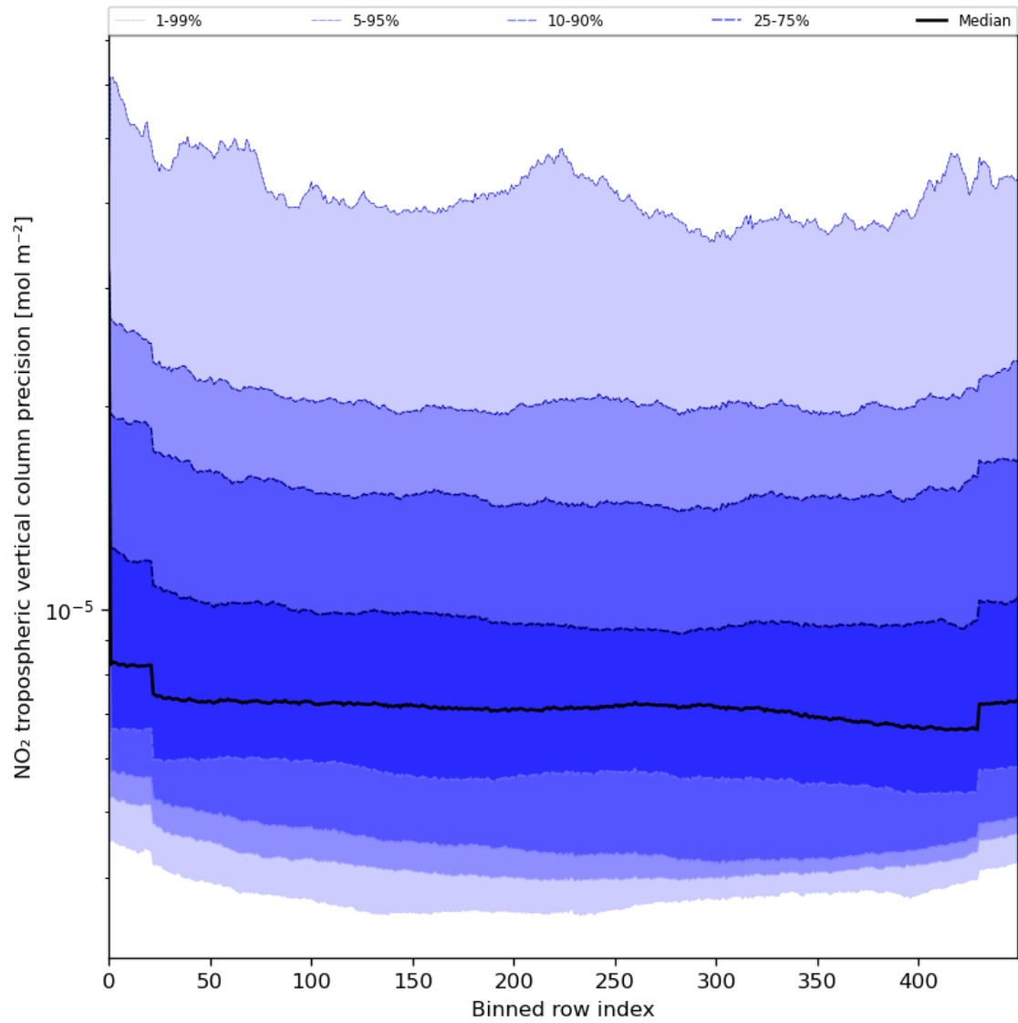
Figure 47: Along track statistics of “NO 2 tropospheric vertical column precision” for 2024-07-02 to 2024-07-04
