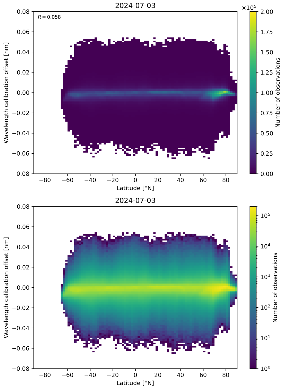
Figure 95: Scatter density plot of “Latitude” against “Wavelength calibration offset” for 2024-07-02 to 2024-07-04.
