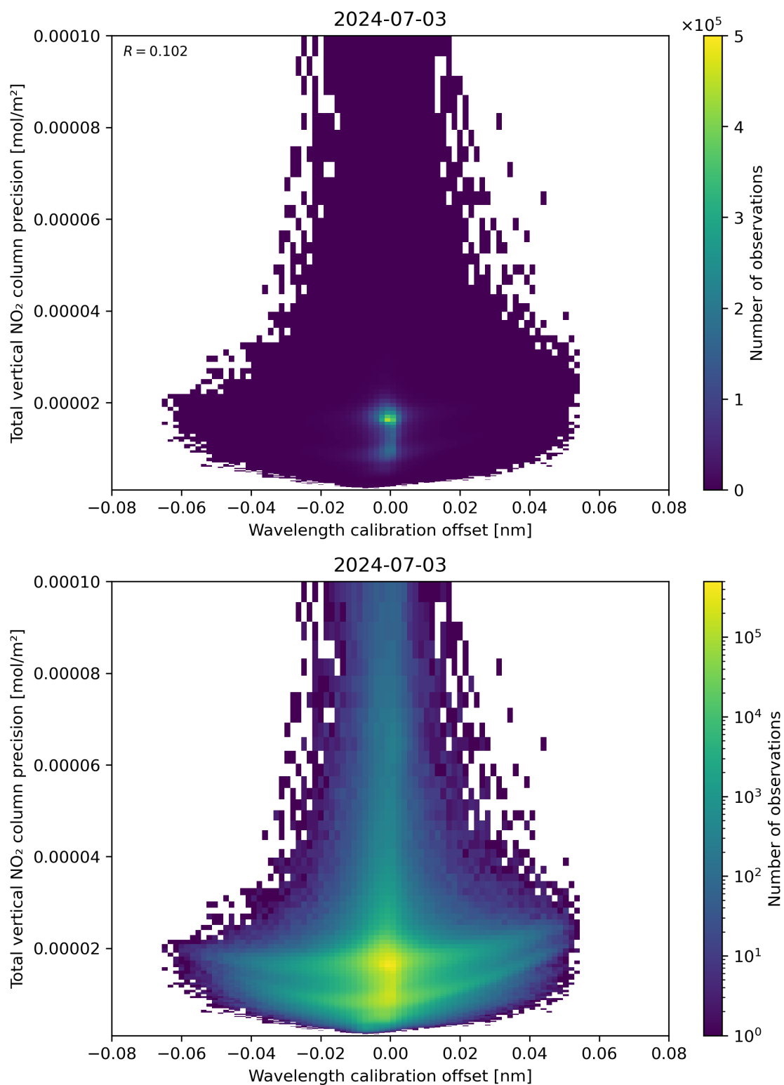
Figure 180: Scatter density plot of “Wavelength calibration offset” against “Total vertical NO 2 column precision” for 2024-07-02 to 2024-07-04.
