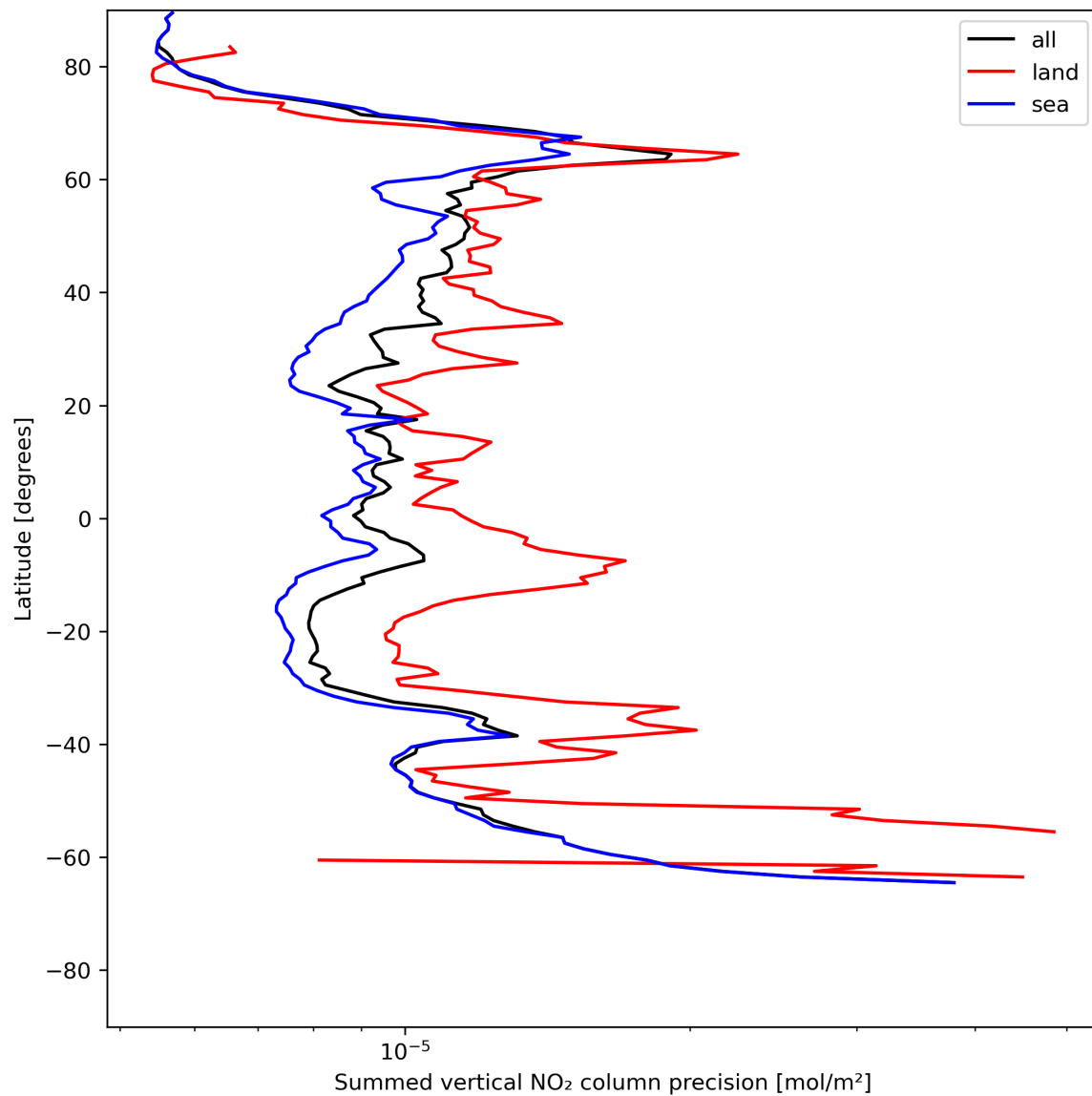
Figure 24: Zonal average of “Summed vertical NO 2 column precision” for 2024-07-02 to 2024-07-04.
