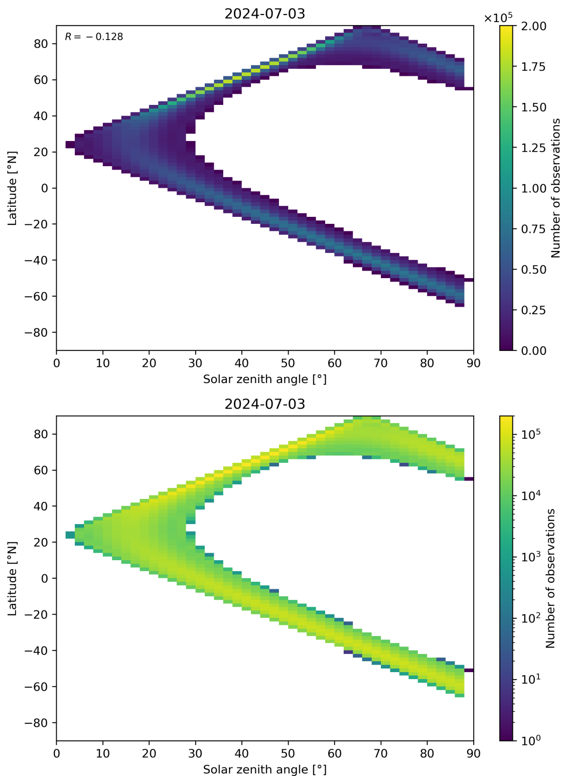
Figure 149: Scatter density plot of “Solar zenith angle” against “Latitude” for 2024-07-02 to 2024-07-04.
