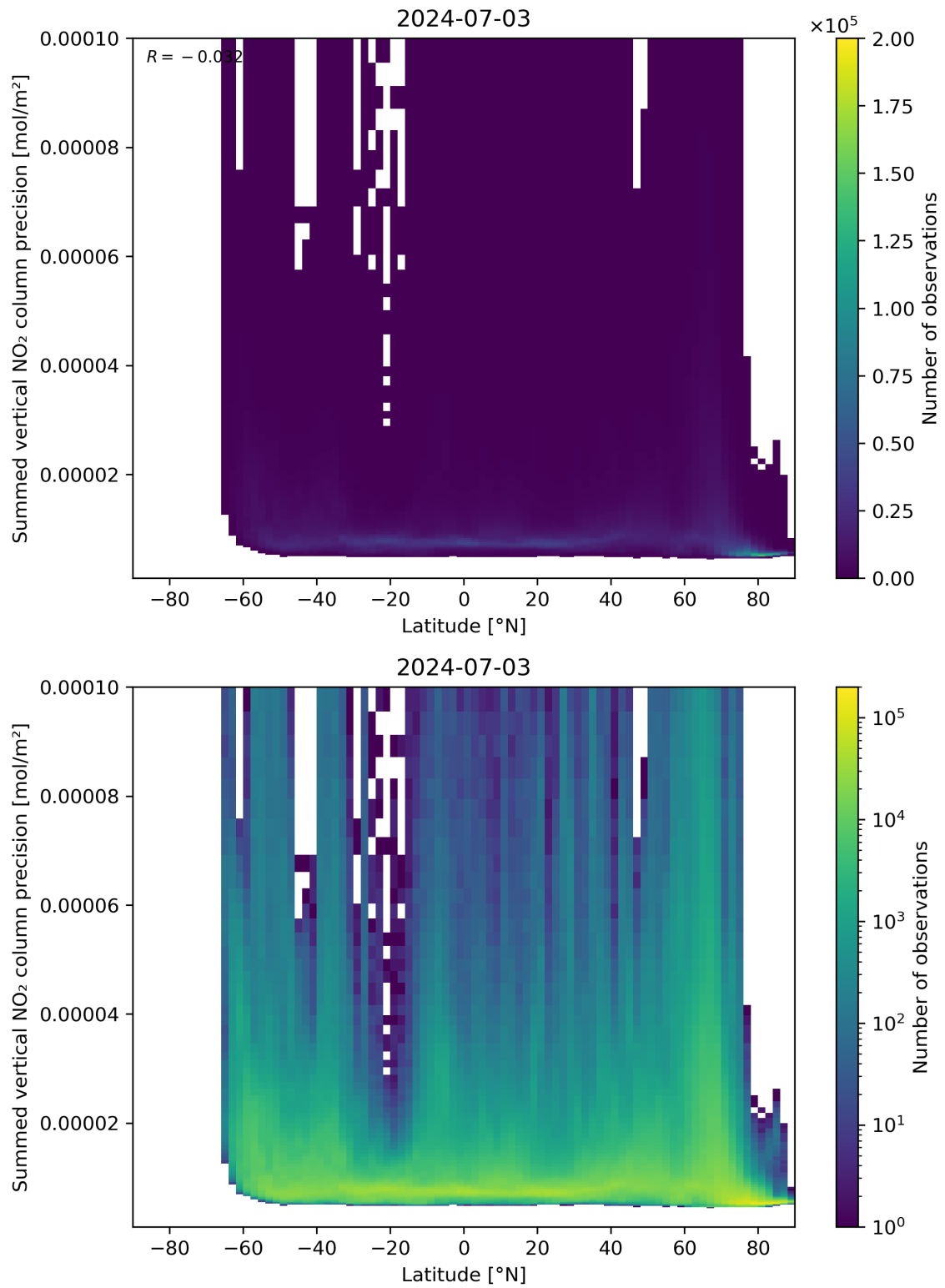
Figure 89: Scatter density plot of “Latitude” against “Summed vertical NO 2 column precision” for 2024-07-02 to 2024-07-04.
