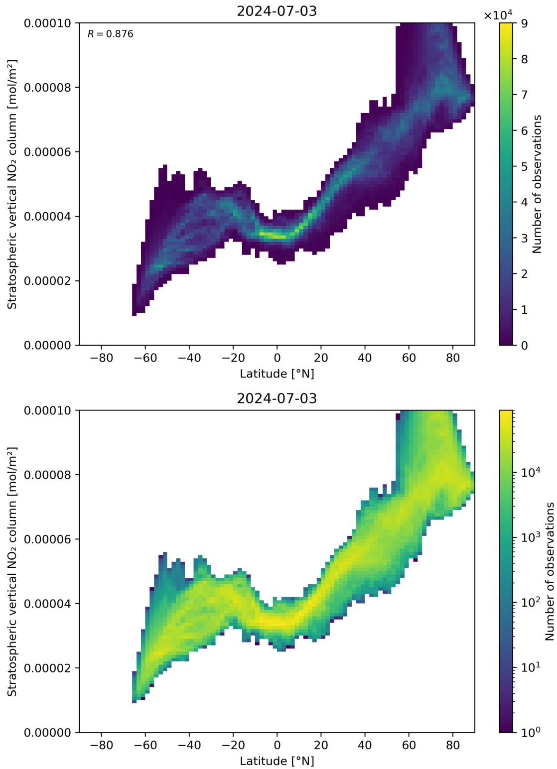
Figure 87: Scatter density plot of “Latitude” against “Stratospheric vertical NO 2 column” for 2024-07-02 to 2024-07-04.
