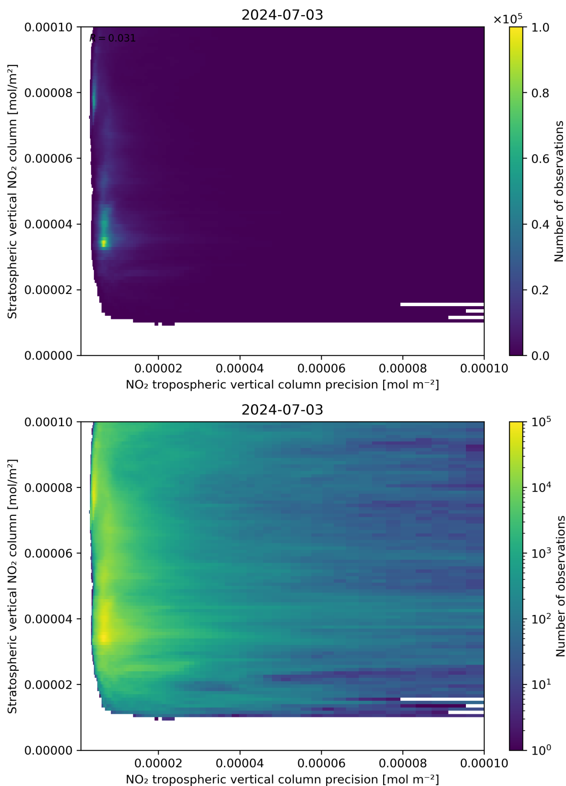
Figure 135: Scatter density plot of “NO 2 tropospheric vertical column precision” against “Stratospheric vertical NO 2 column” for 2024-07-02 to 2024-07-04.
