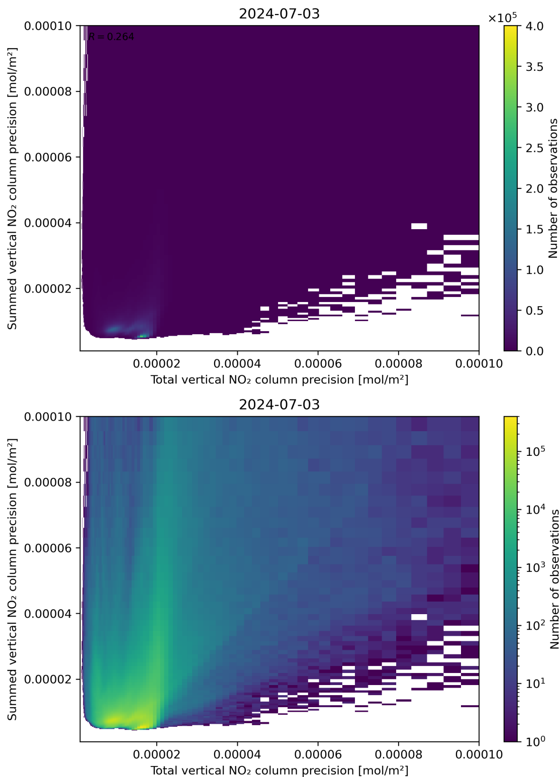
Figure 118: Scatter density plot of “Total vertical NO 2 column precision” against “Summed vertical NO 2 column precision” for 2024-07-02 to 2024-07-04.
