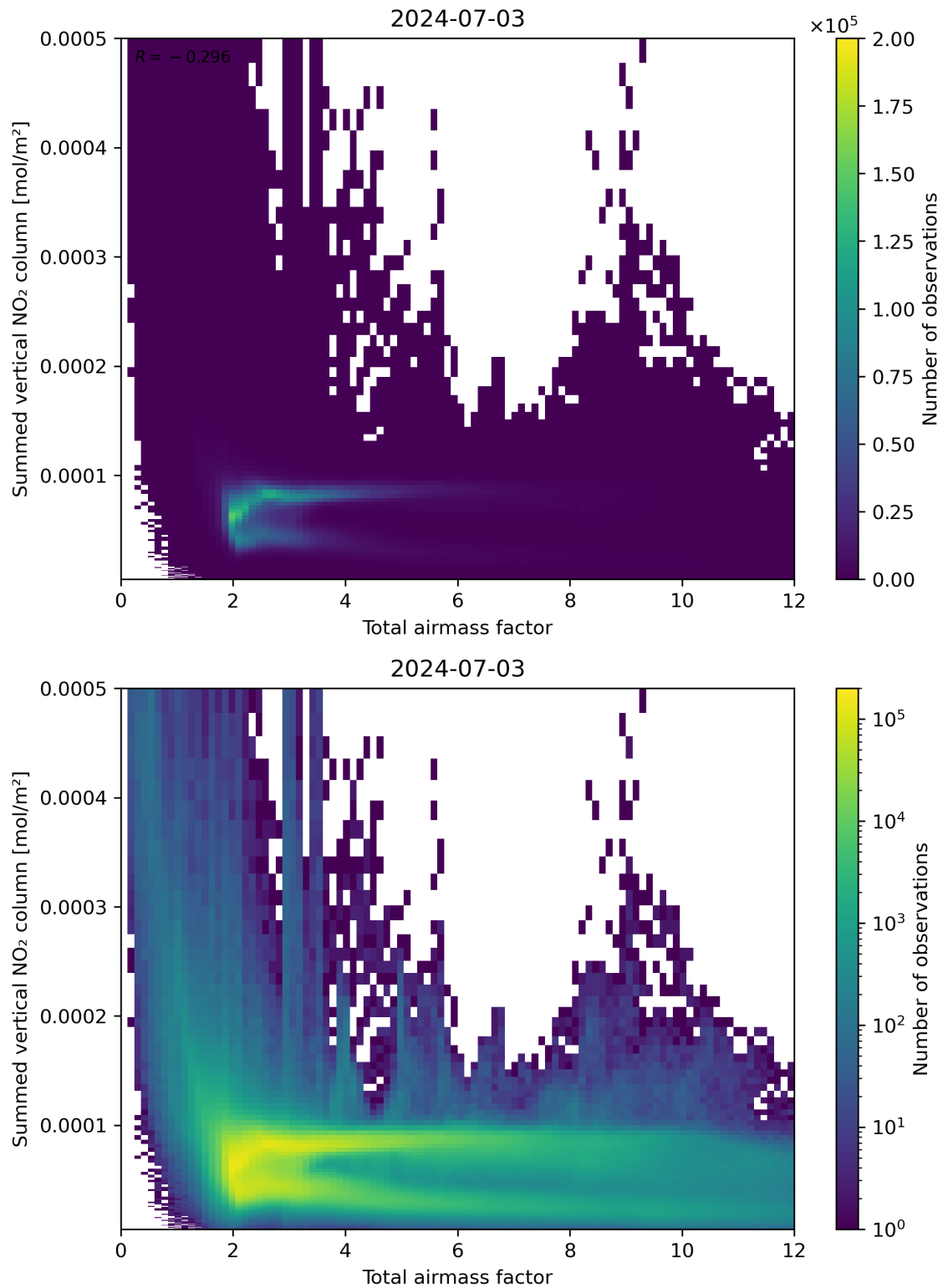
Figure 65: Scatter density plot of “Total airmass factor” against “Summed vertical NO 2 column” for 2024-07-02 to 2024-07-04.
