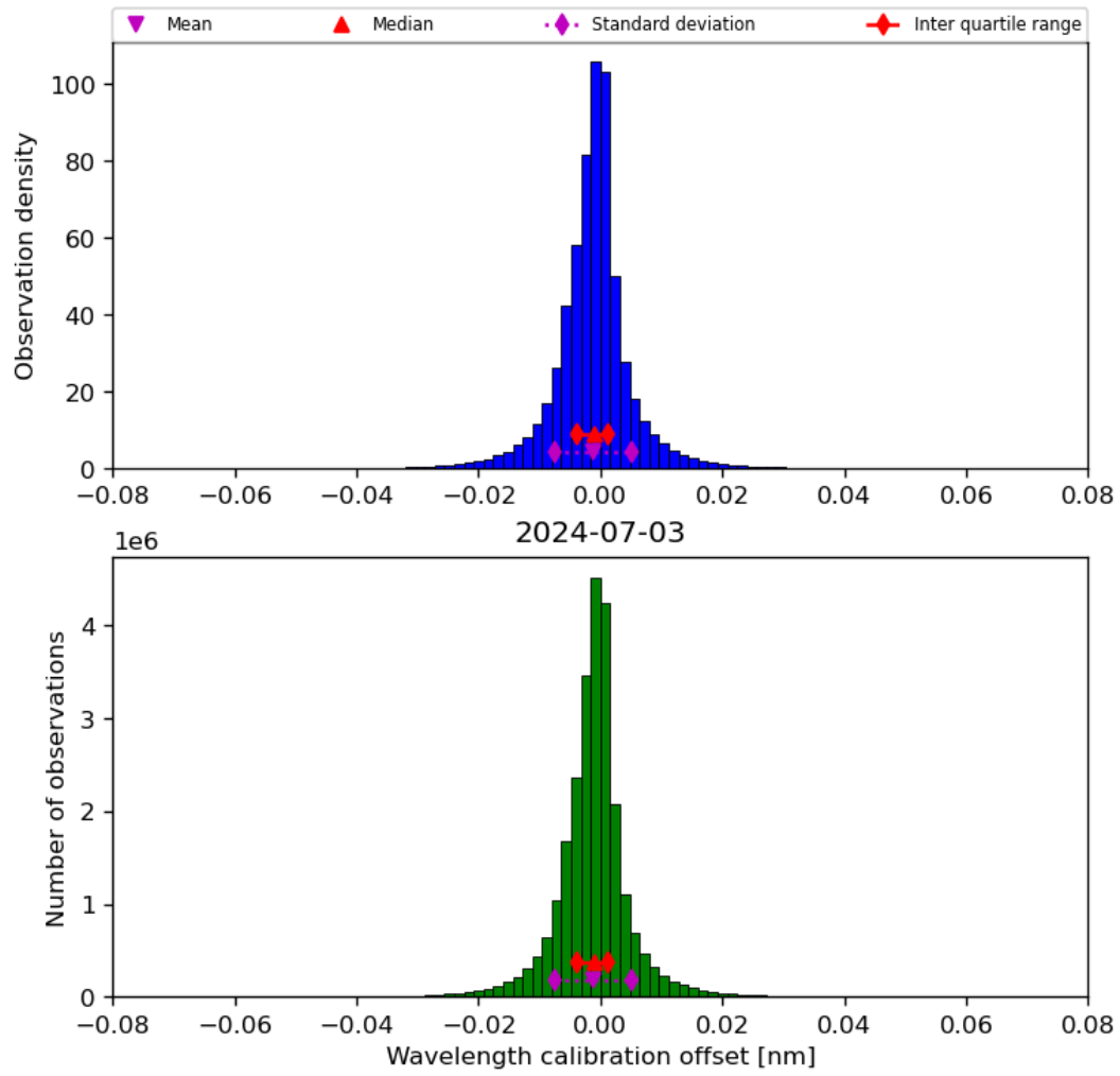
Figure 35: Histogram of “Wavelength calibration offset” for 2024-07-02 to 2024-07-04
