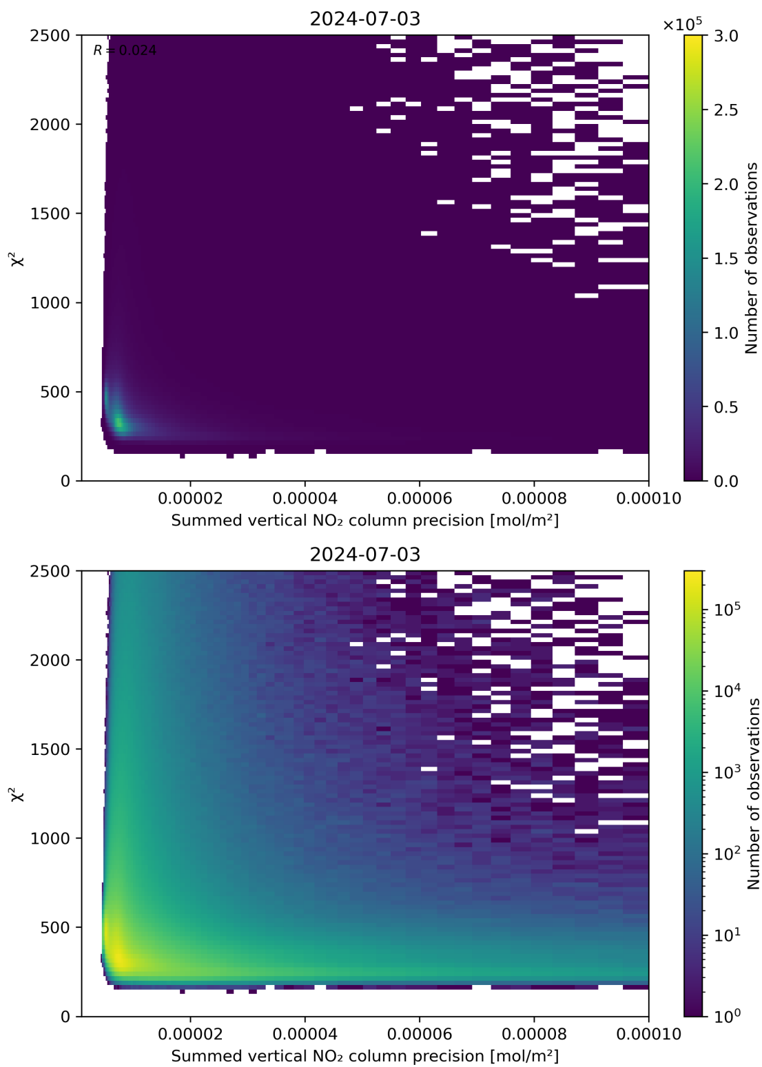
Figure 107: Scatter density plot of “Summed vertical NO 2 column precision” against “ \chi^2 ” for 2024-07-02 to 2024-07-04.
