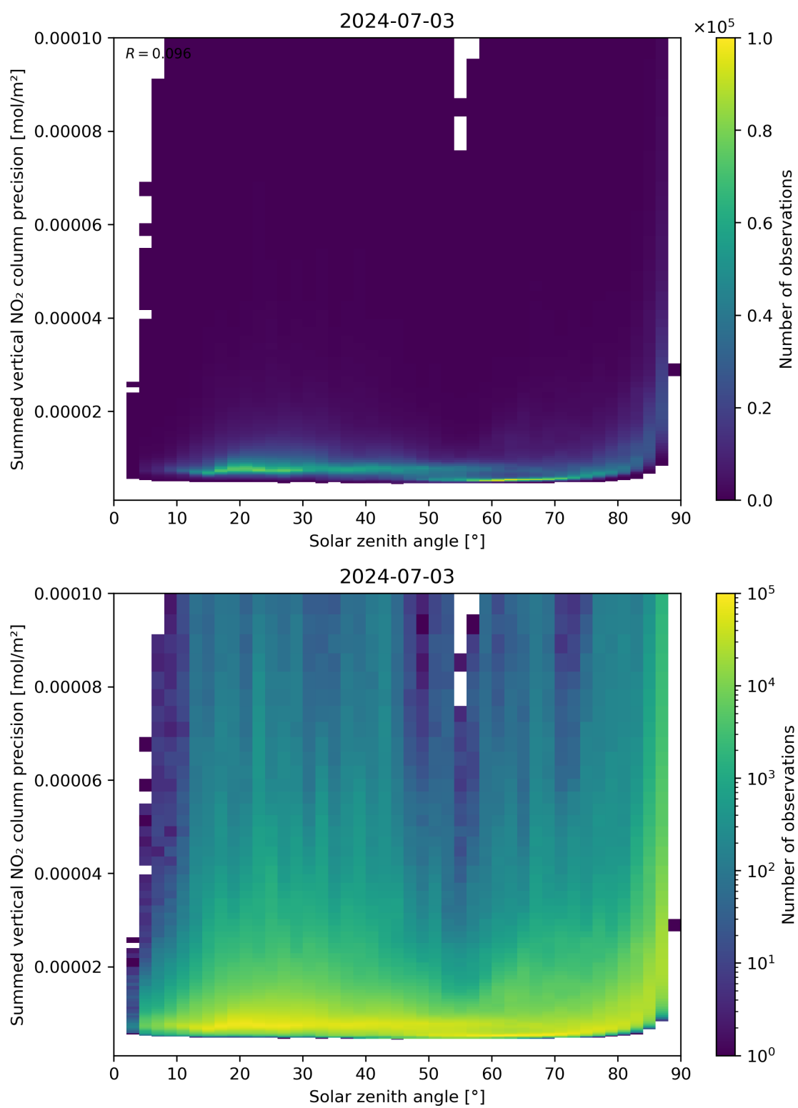
Figure 152: Scatter density plot of “Solar zenith angle” against “Summed vertical NO 2 column precision” for 2024-07-02 to 2024-07-04.
