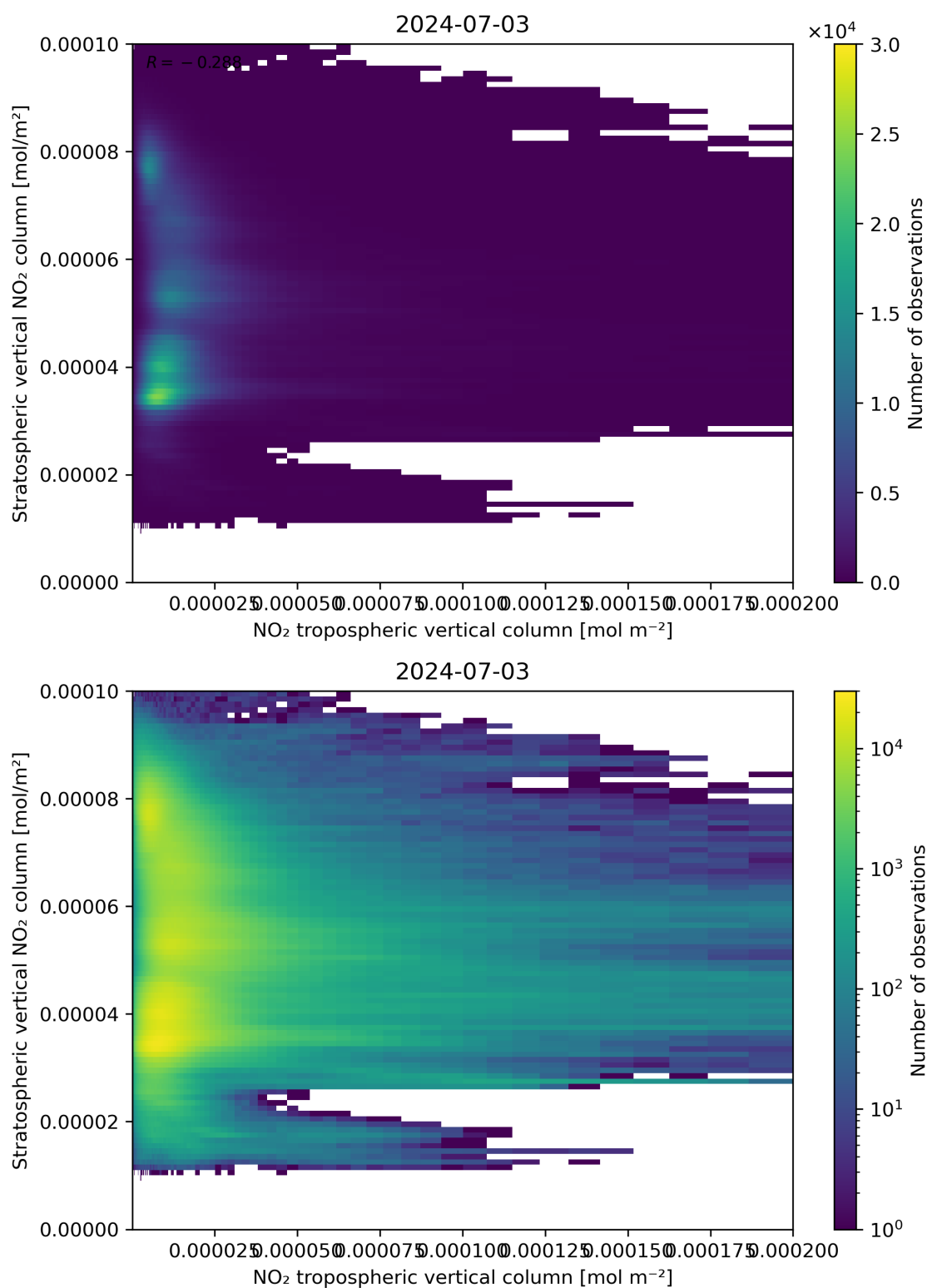
Figure 125: Scatter density plot of “NO 2 tropospheric vertical column” against “Stratospheric vertical NO 2 column” for 2024-07-02 to 2024-07-04.
