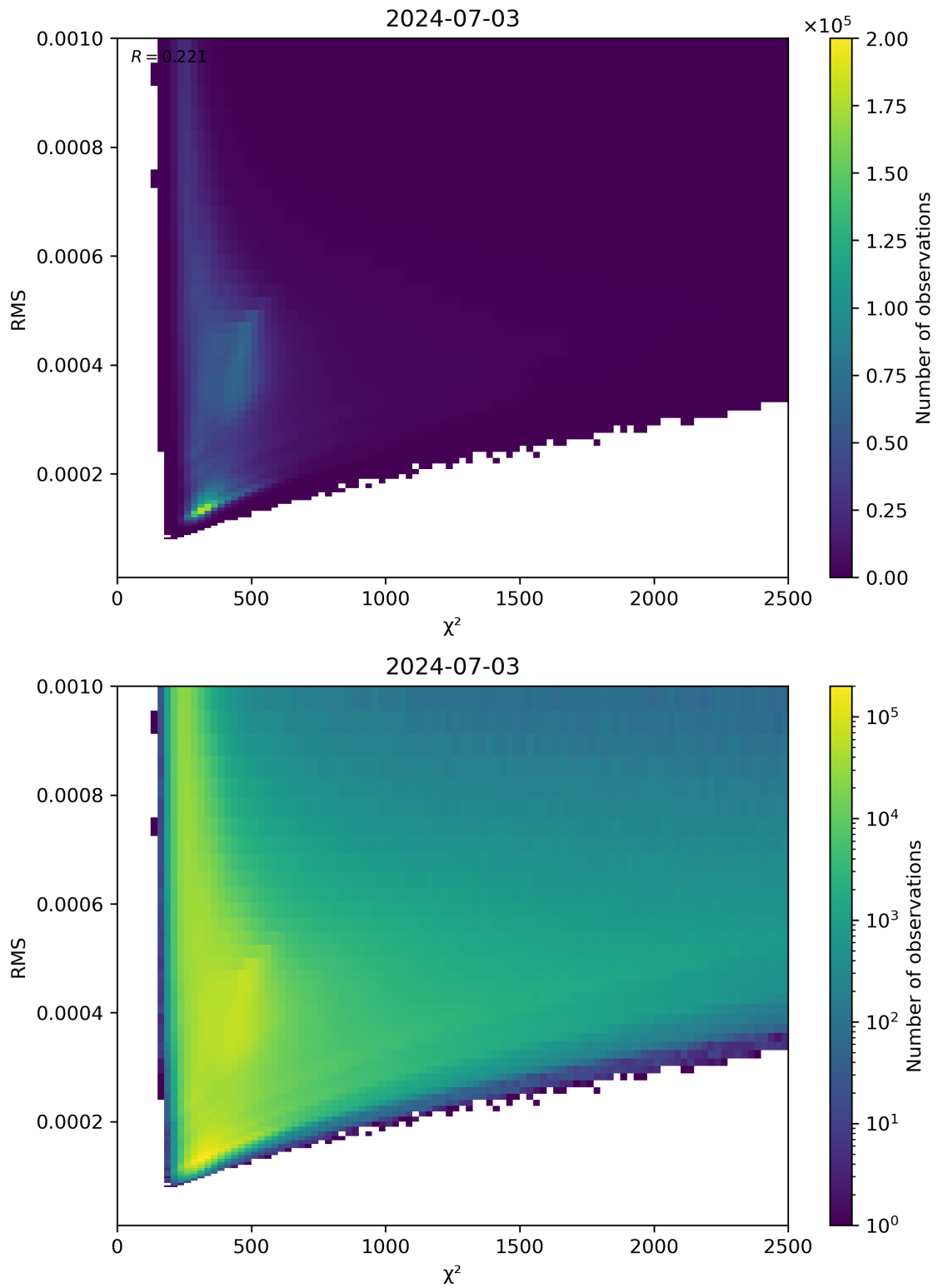
Figure 82: Scatter density plot of “ \chi^2 ” against “RMS” for 2024-07-02 to 2024-07-04.
