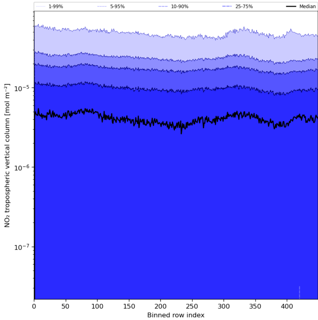
Figure 46: Along track statistics of “NO 2 tropospheric vertical column” for 2024-07-02 to 2024-07-04
