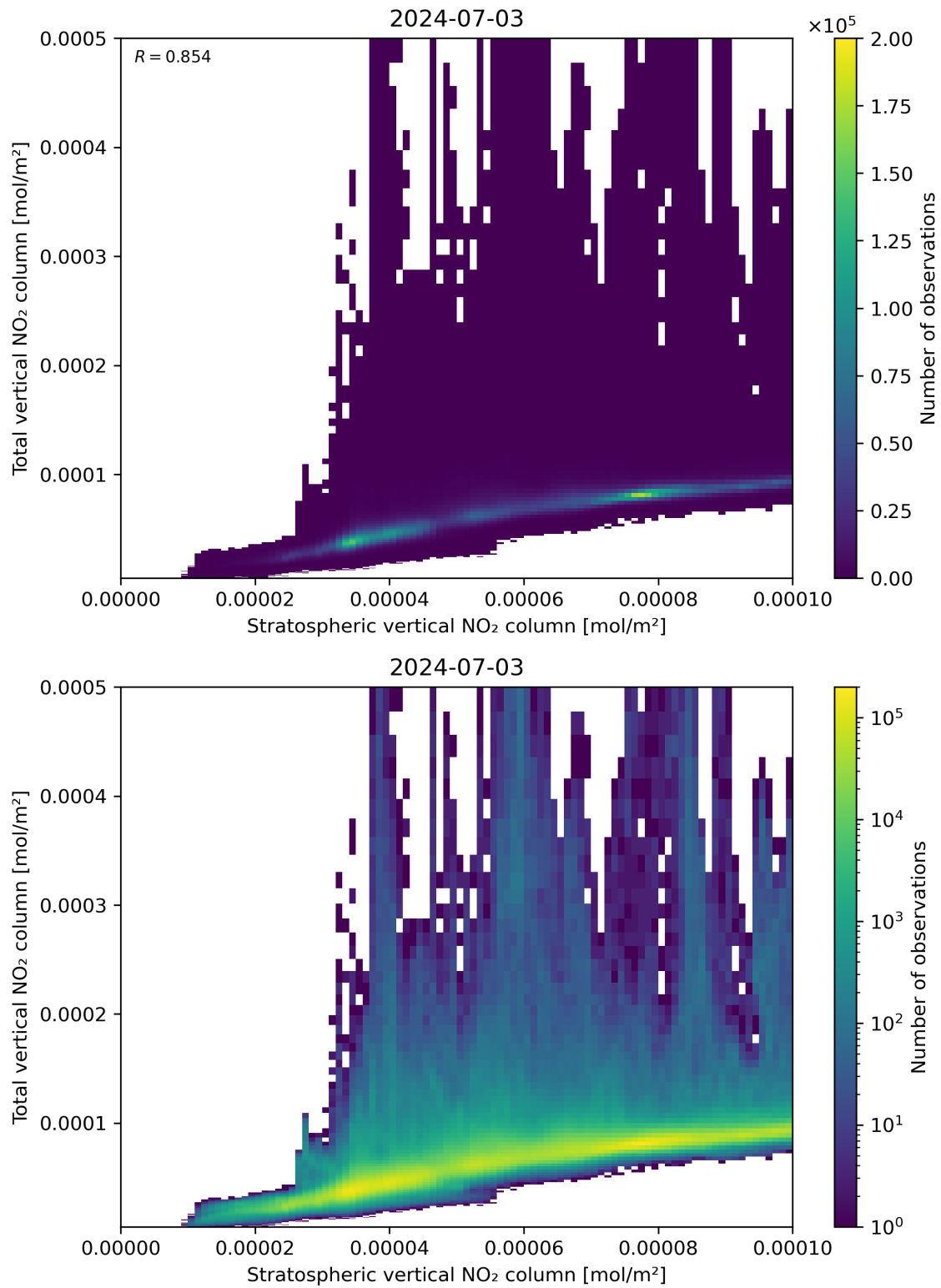
Figure 100: Scatter density plot of “Stratospheric vertical NO 2 column” against “Total vertical NO 2 column” for 2024-07-02 to 2024-07-04.
