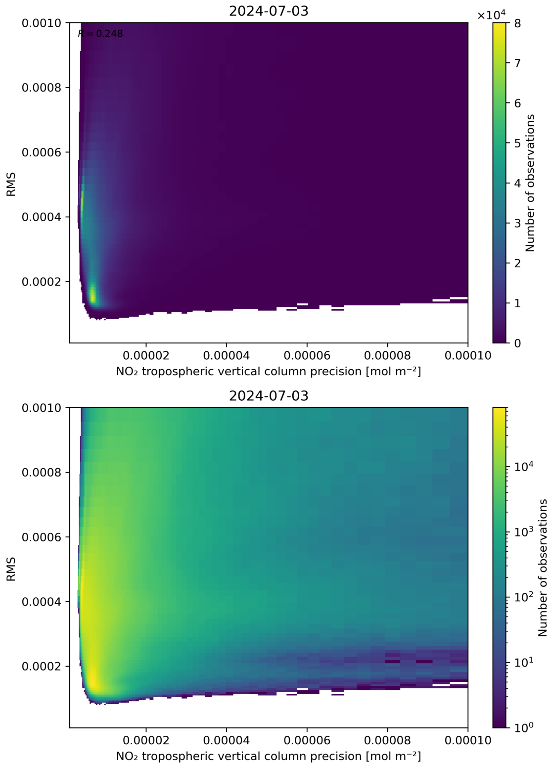
Figure 140: Scatter density plot of “NO 2 tropospheric vertical column precision” against “RMS” for 2024-07-02 to 2024-07-04.
