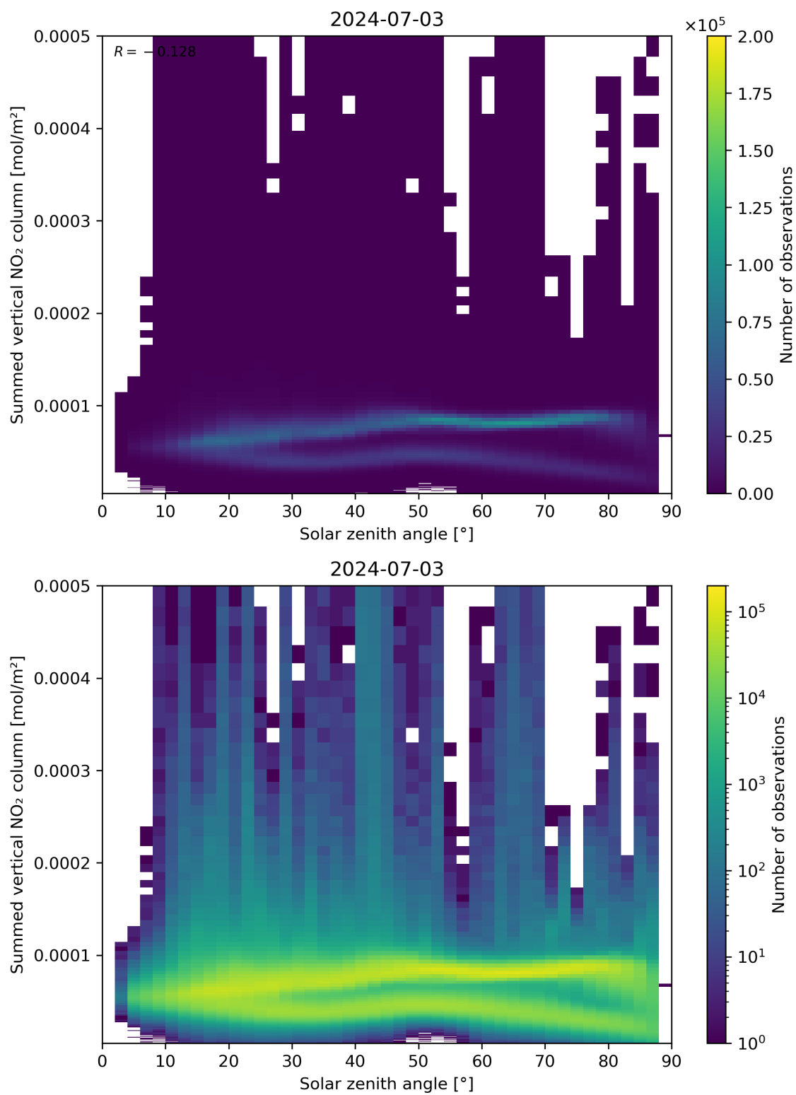
Figure 151: Scatter density plot of “Solar zenith angle” against “Summed vertical NO 2 column” for 2024-07-02 to 2024-07-04.
