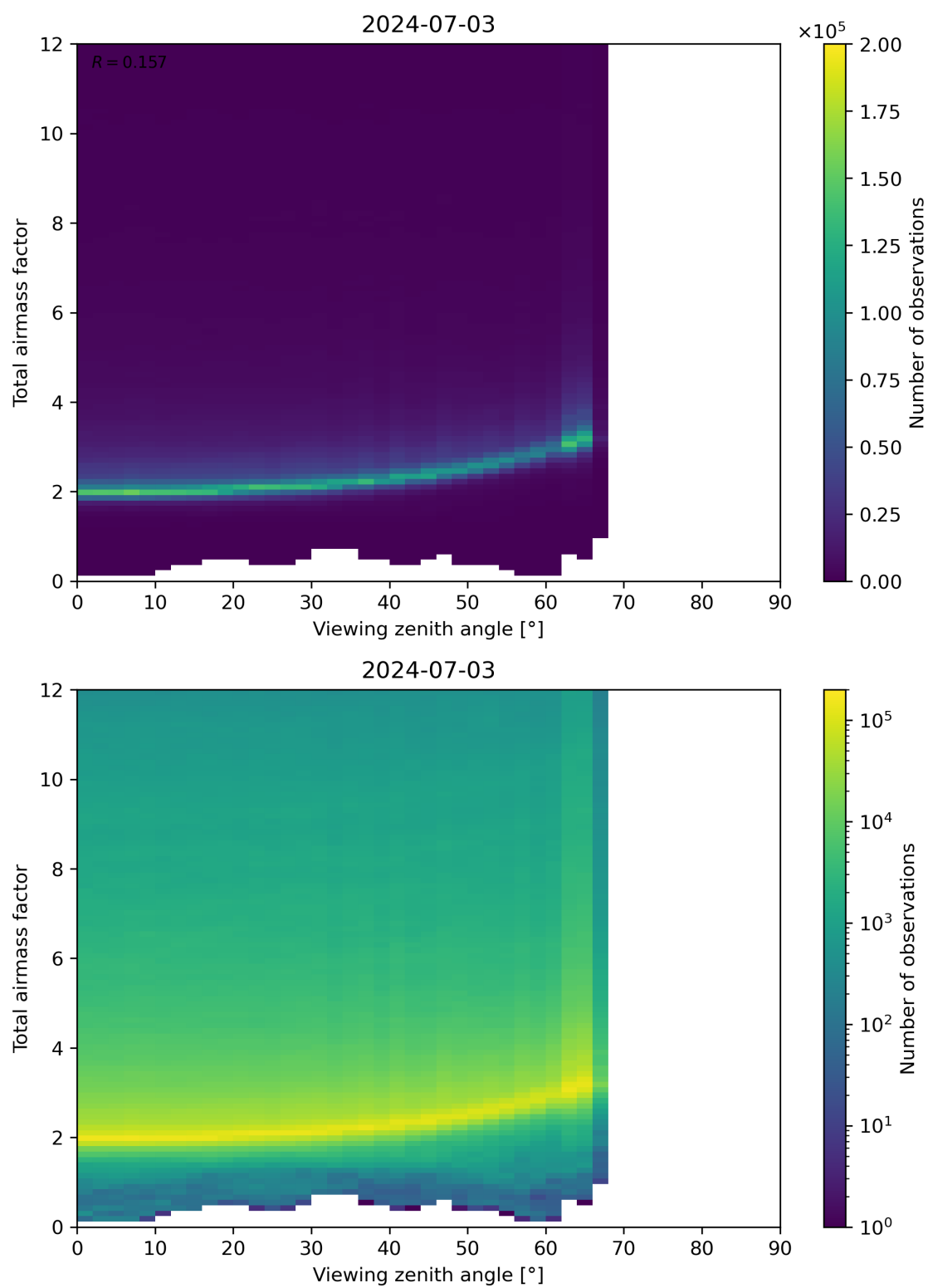
Figure 160: Scatter density plot of “Viewing zenith angle” against “Total airmass factor” for 2024-07-02 to 2024-07-04.
