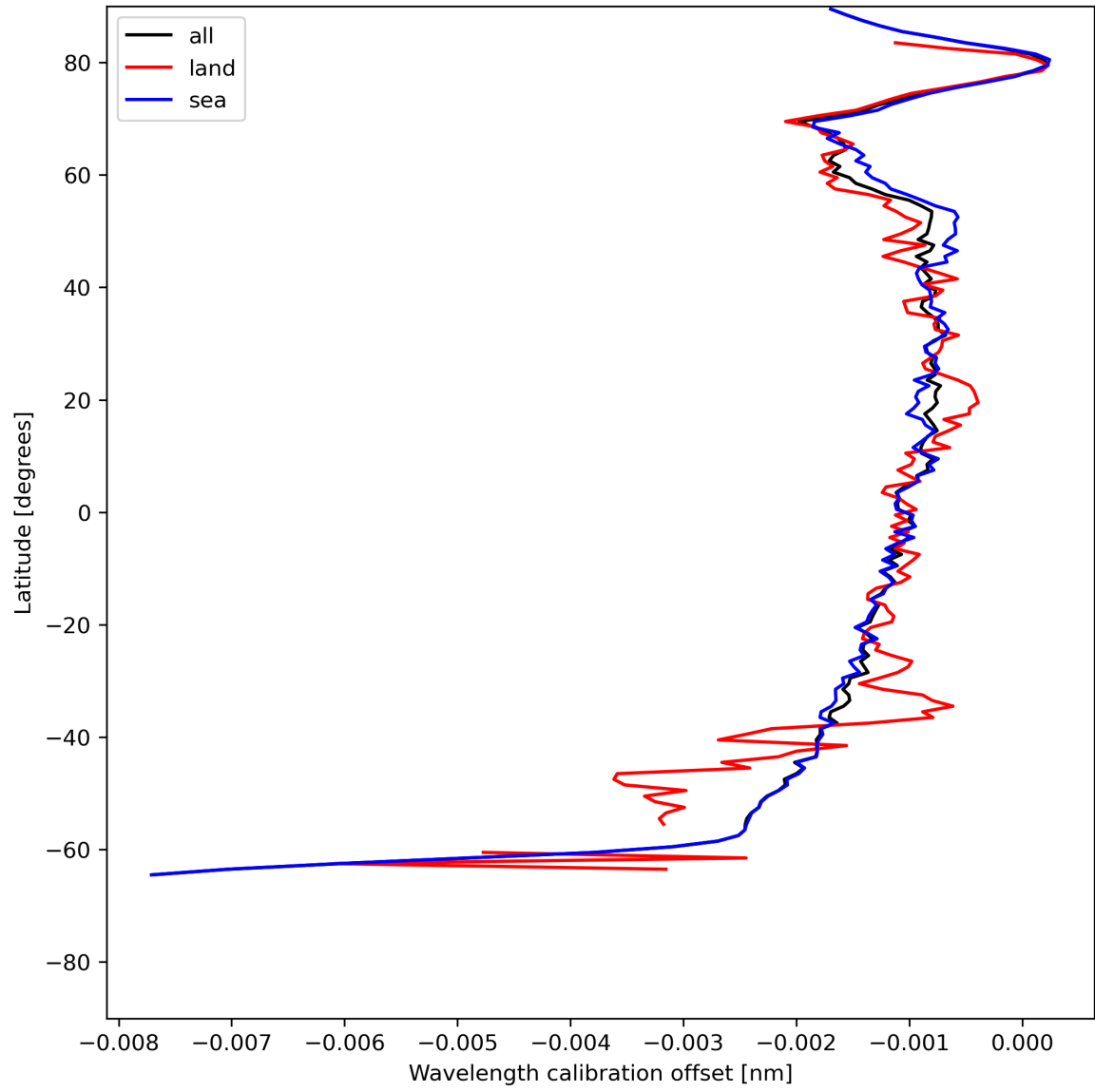
Figure 18: Zonal average of “Wavelength calibration offset” for 2024-07-02 to 2024-07-04.
