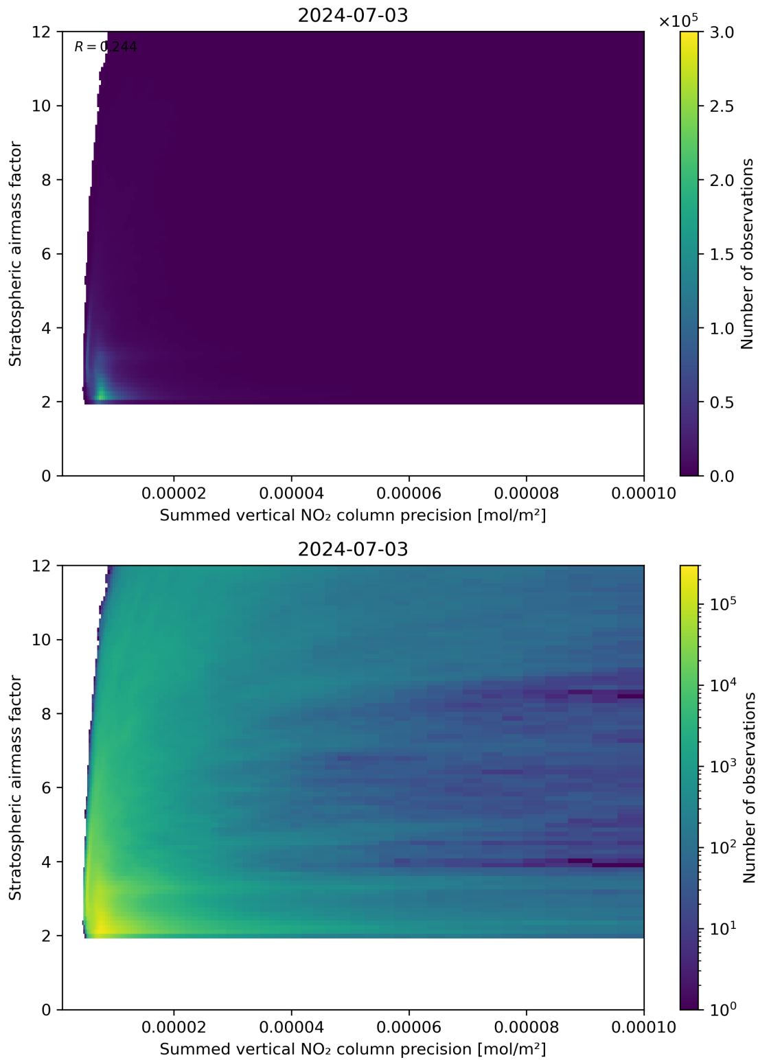
Figure 106: Scatter density plot of “Summed vertical NO 2 column precision” against “Stratospheric airmass factor” for 2024-07-02 to 2024-07-04.
