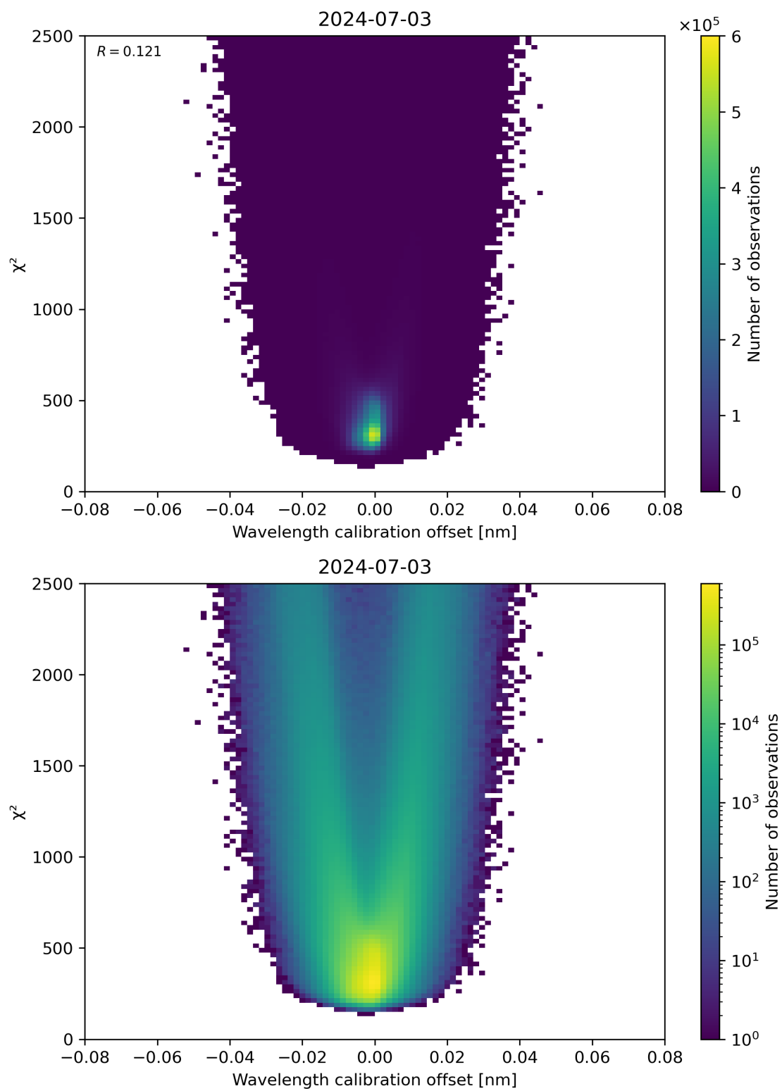
Figure 175: Scatter density plot of “Wavelength calibration offset” against “ \chi^2 ” for 2024-07-02 to 2024-07-04.
