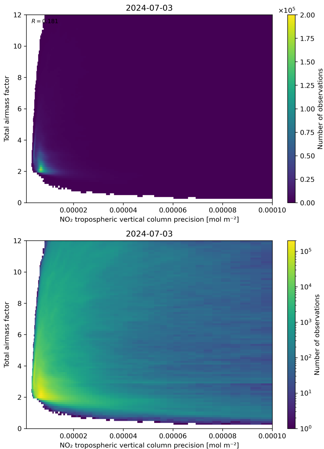
Figure 132: Scatter density plot of “NO 2 tropospheric vertical column precision” against “Total air mass factor” for 2024-07-02 to 2024-07-04.
