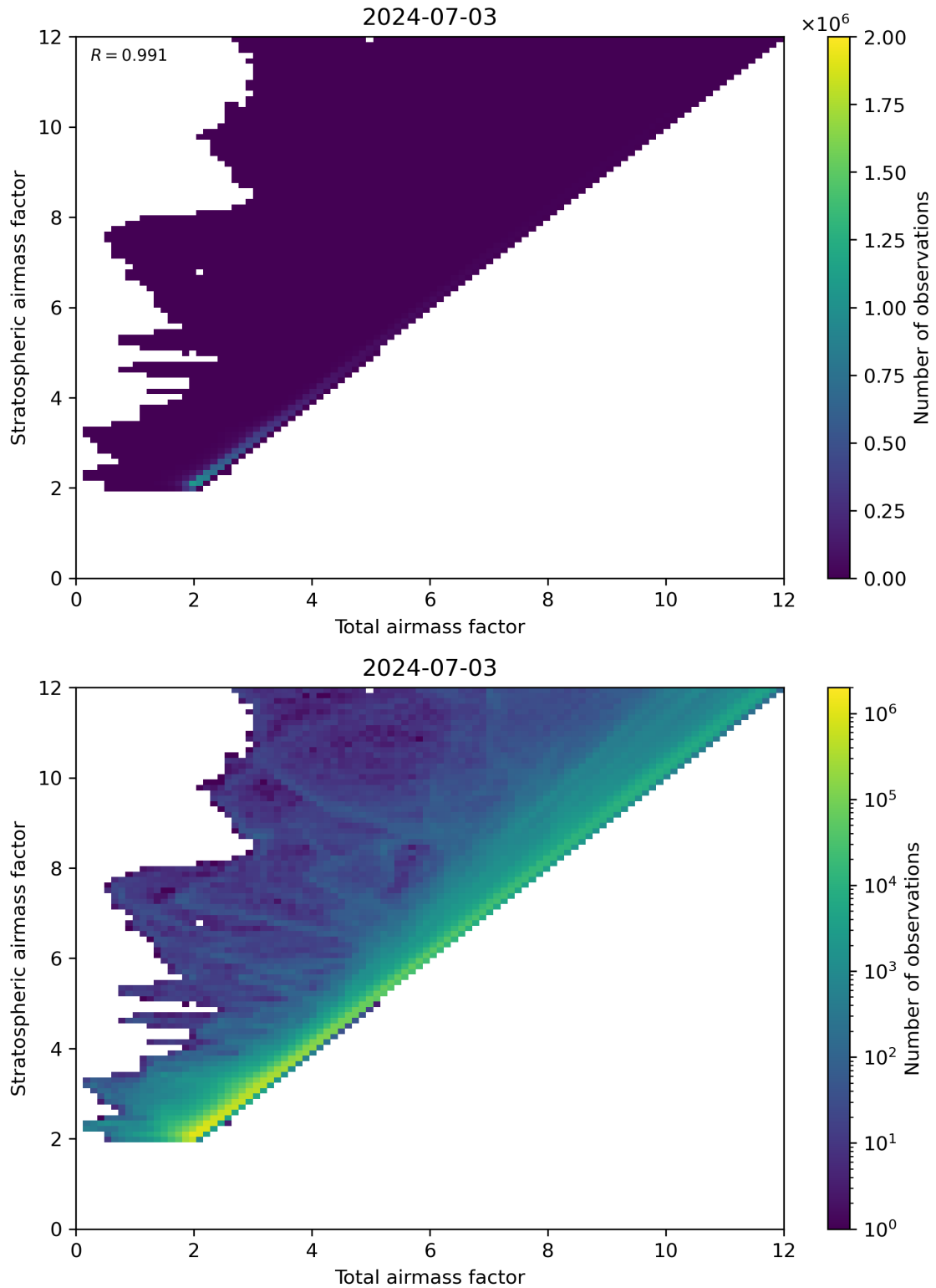
Figure 62: Scatter density plot of “Total airmass factor” against “Stratospheric airmass factor” for 2024-07-02 to 2024-07-04.
