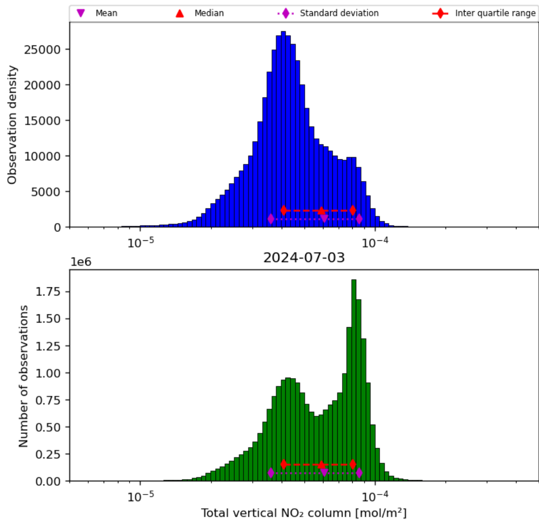
Figure 38: Histogram of “Total vertical NO 2 column” for 2024-07-02 to 2024-07-04
