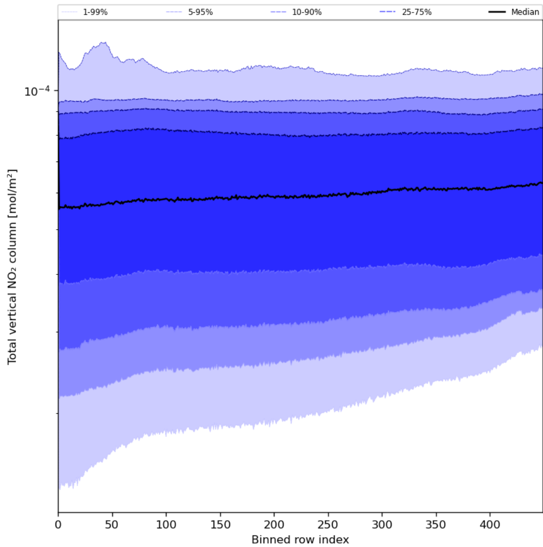
Figure 55: Along track statistics of “Total vertical NO 2 column” for 2024-07-02 to 2024-07-04
