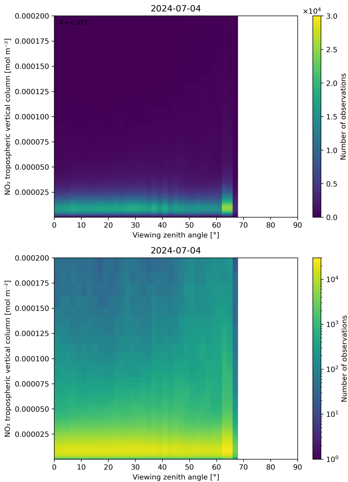
Figure 169: Scatter density plot of “Viewing zenith angle” against “NO 2 tropospheric vertical column” for 2024-07-03 to 2024-07-05.
