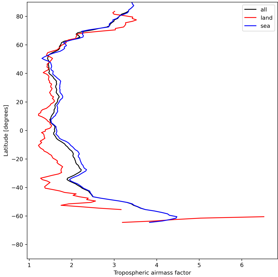
Figure 14: Zonal average of “Tropospheric air mass factor” for 2024-07-03 to 2024-07-05.
