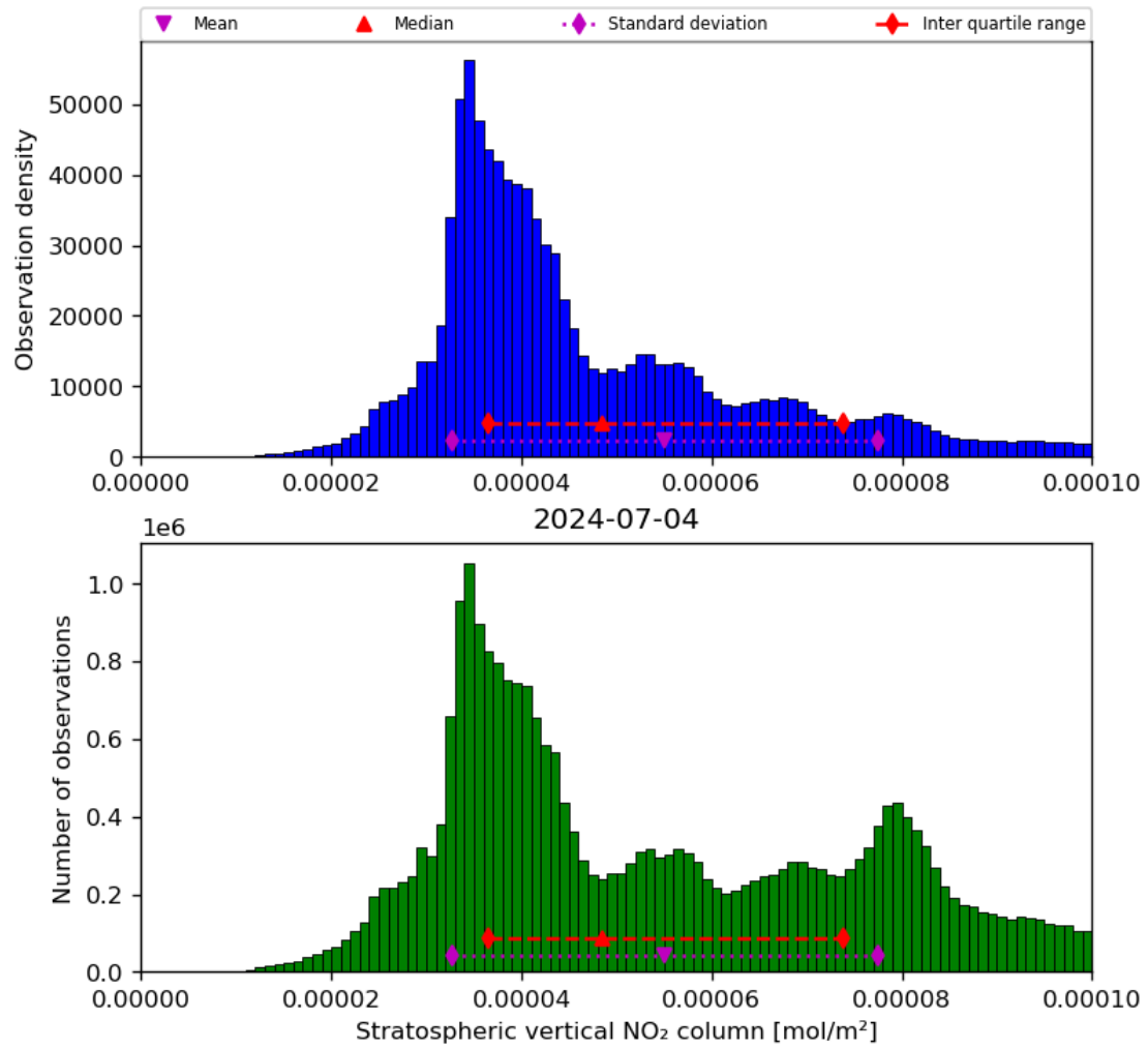
Figure 36: Histogram of “Stratospheric vertical NO 2 column” for 2024-07-03 to 2024-07-05
