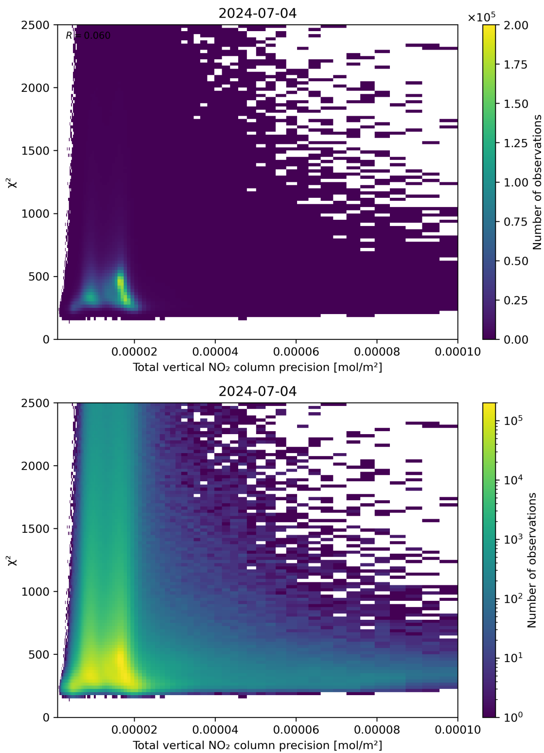
Figure 116: Scatter density plot of “Total vertical NO 2 column precision” against “ \chi^2 ” for 2024-07-03 to 2024-07-05.
