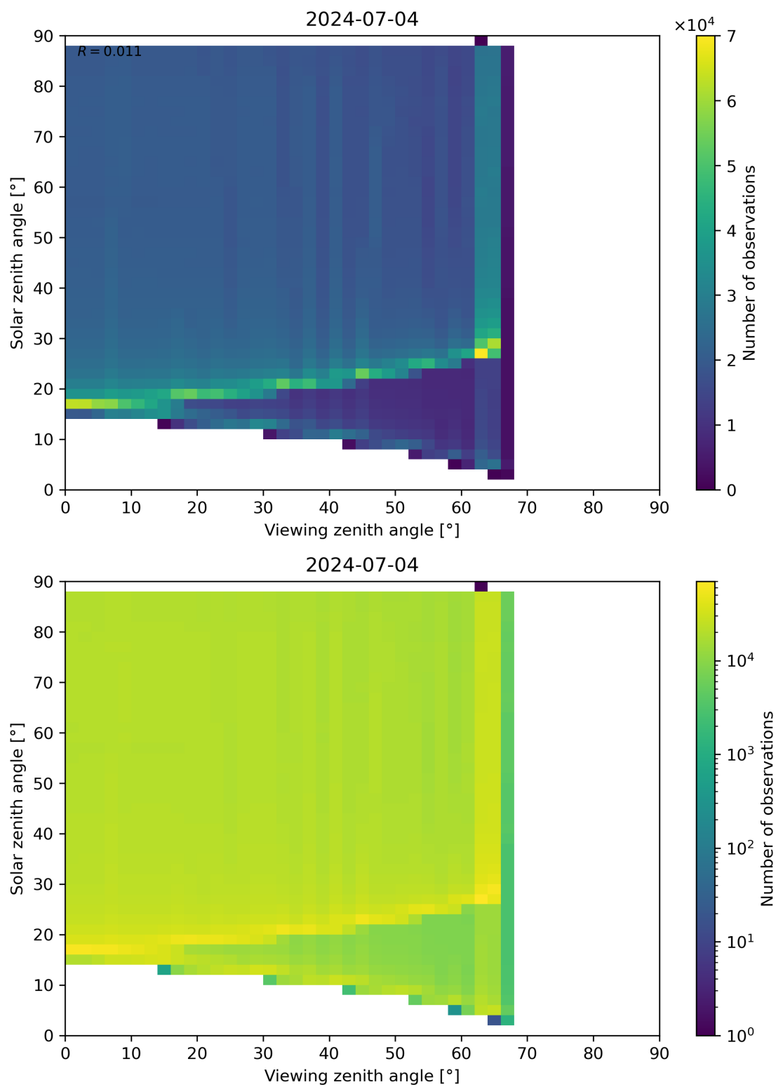
Figure 172: Scatter density plot of “Viewing zenith angle” against “Solar zenith angle” for 2024-07-03 to 2024-07-05.
