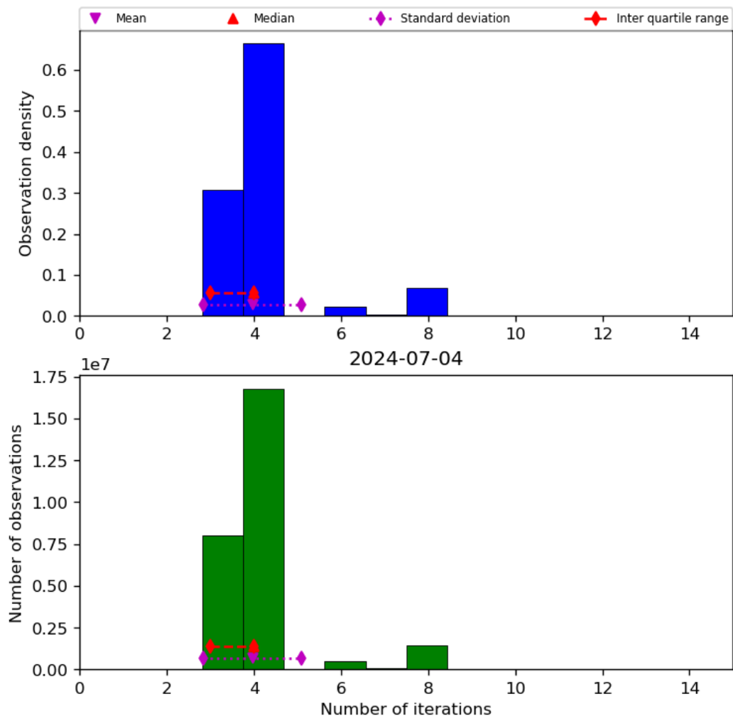
Figure 34: Histogram of “Number of iterations” for 2024-07-03 to 2024-07-05
