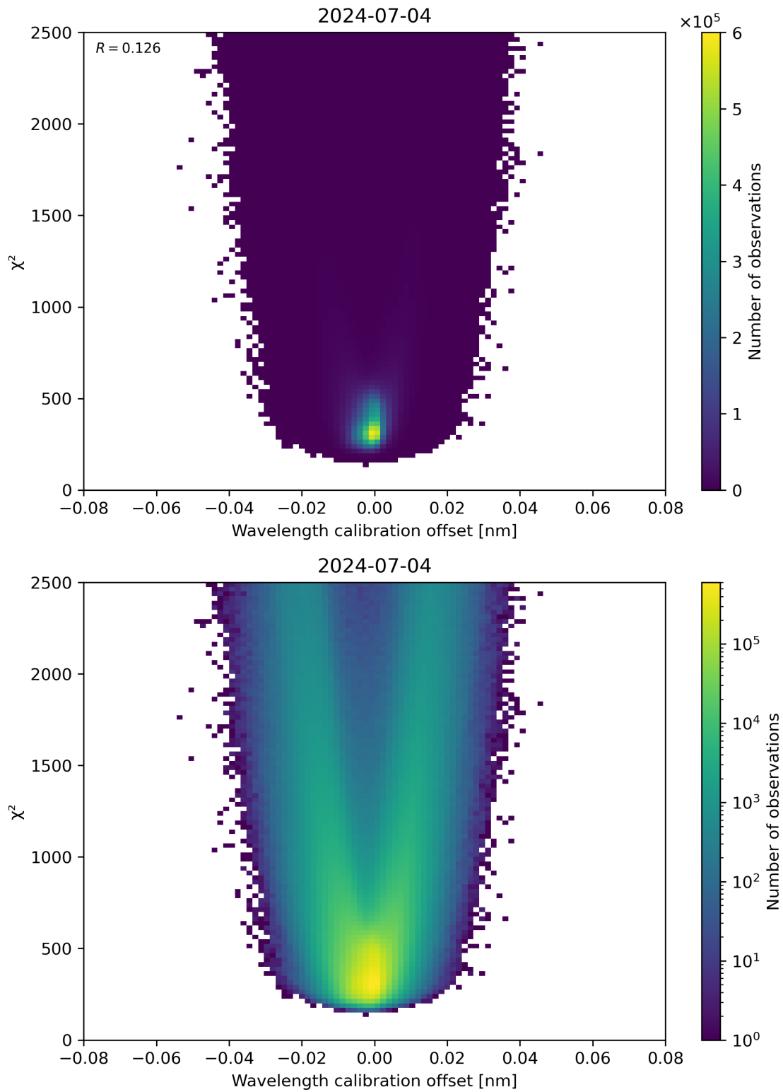
Figure 175: Scatter density plot of “Wavelength calibration offset” against “ \chi^2 ” for 2024-07-03 to 2024-07-05.
