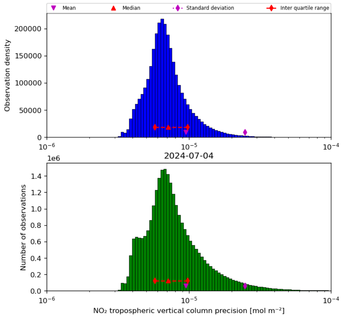
Figure 30: Histogram of “NO 2 tropospheric vertical column precision” for 2024-07-03 to 2024-07-05
