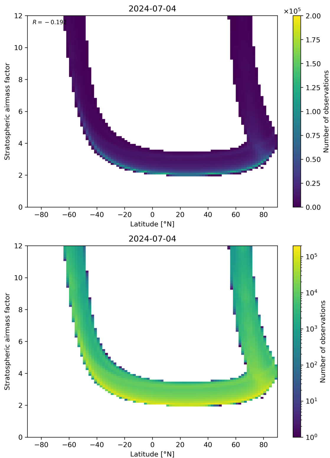
Figure 83: Scatter density plot of “Latitude” against “Stratospheric air mass factor” for 2024-07-03 to 2024-07-05.
