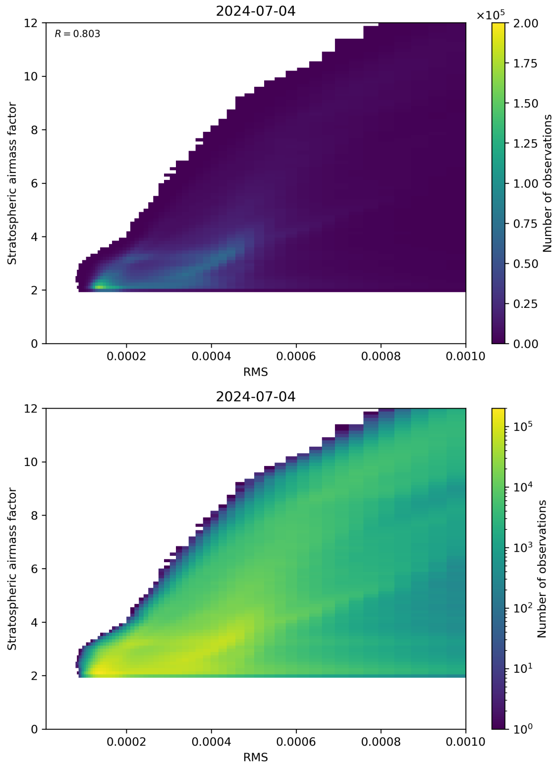
Figure 144: Scatter density plot of “RMS” against “Stratospheric airmass factor” for 2024-07-03 to 2024-07-05.
