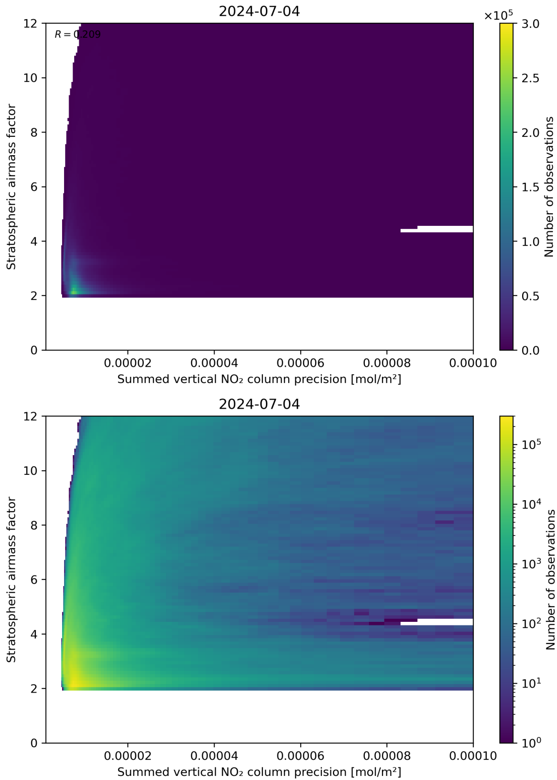
Figure 106: Scatter density plot of “Summed vertical NO 2 column precision” against “Stratospheric airmass factor” for 2024-07-03 to 2024-07-05.
