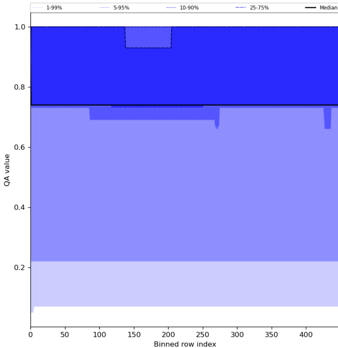
Figure 45: Along track statistics of “QA value” for 2024-07-03 to 2024-07-05
