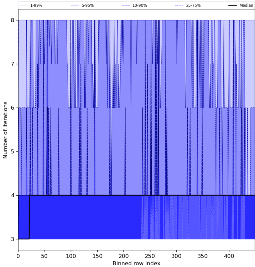
Figure 51: Along track statistics of “Number of iterations” for 2024-07-03 to 2024-07-05
