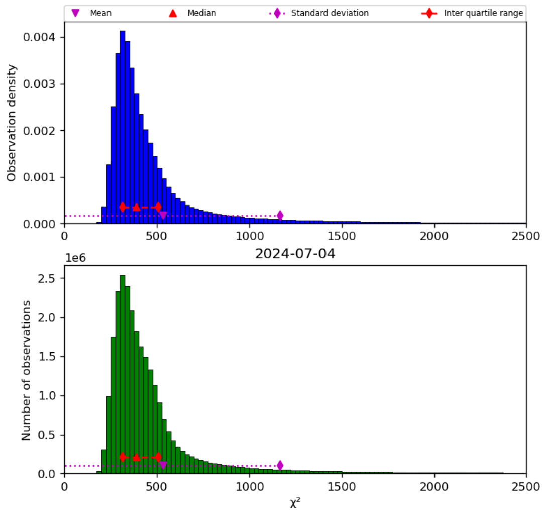
Figure 42: Histogram of “ \chi^2 ” for 2024-07-03 to 2024-07-05
