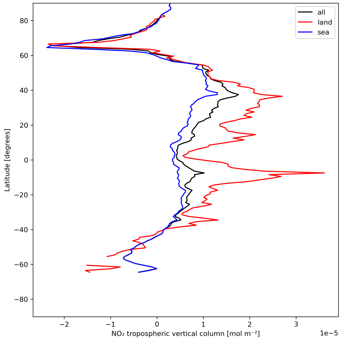
Figure 12: Zonal average of “NO 2 tropospheric vertical column” for 2024-07-03 to 2024-07-05.
