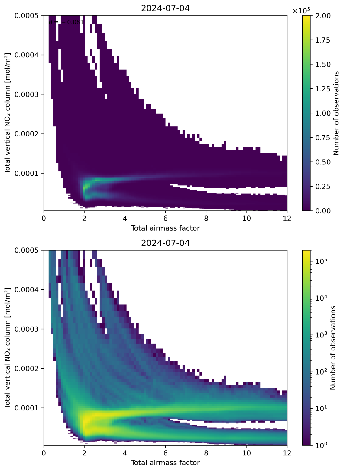
Figure 67: Scatter density plot of “Total airmass factor” against “Total vertical NO 2 column” for 2024-07-03 to 2024-07-05.
