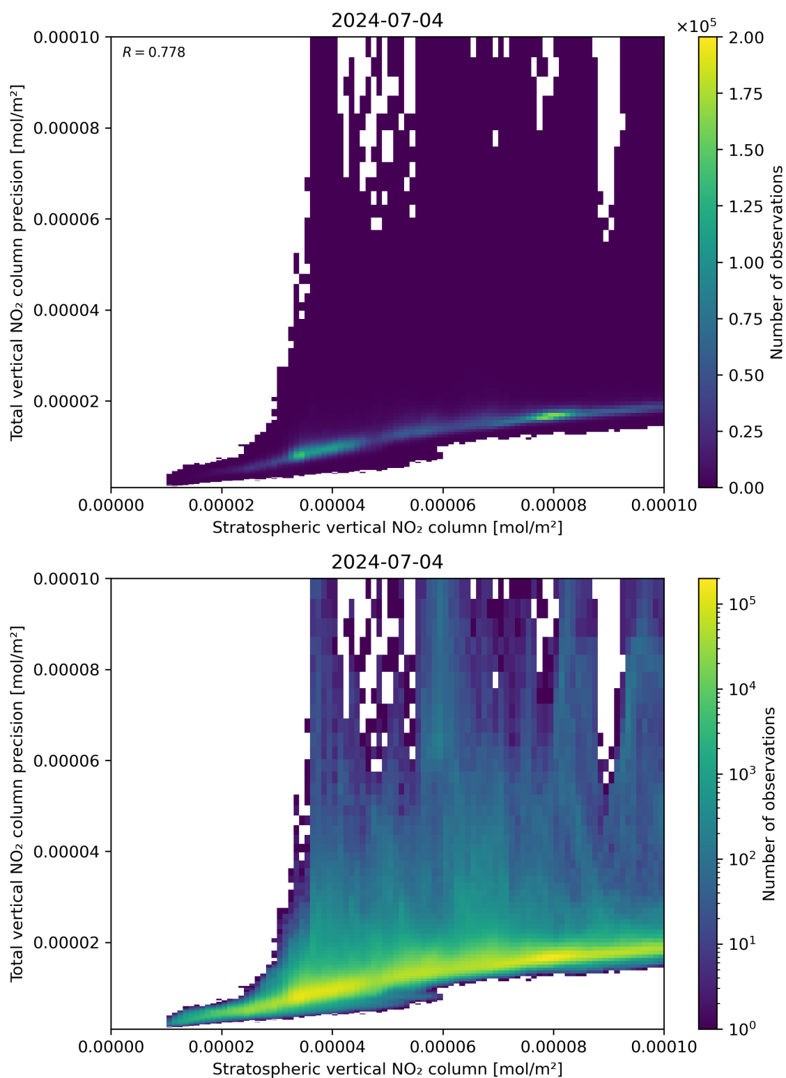
Figure 101: Scatter density plot of “Stratospheric vertical NO 2 column” against “Total vertical NO 2 column precision” for 2024-07-03 to 2024-07-05.
