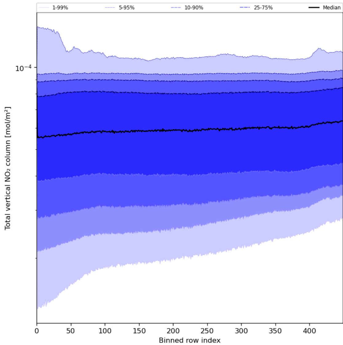
Figure 55: Along track statistics of “Total vertical NO 2 column” for 2024-07-03 to 2024-07-05
