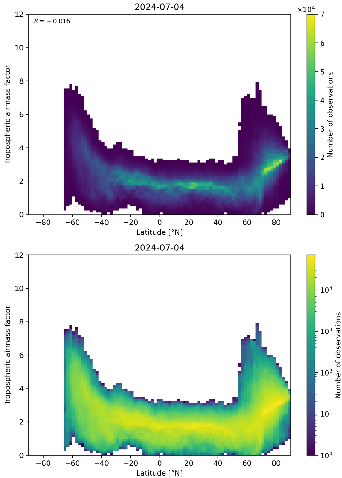
Figure 85: Scatter density plot of “Latitude” against “Tropospheric airmass factor” for 2024-07-03 to 2024-07-05.
