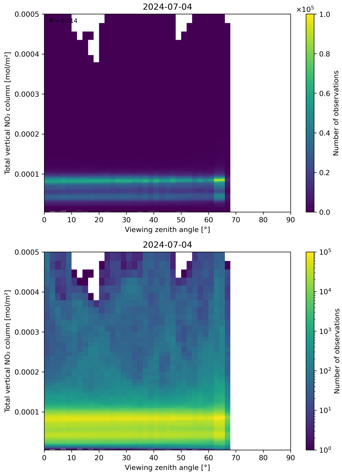
Figure 167: Scatter density plot of “Viewing zenith angle” against “Total vertical NO 2 column” for 2024-07-03 to 2024-07-05.
