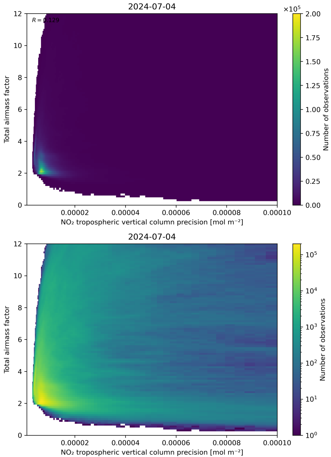
Figure 132: Scatter density plot of “NO 2 tropospheric vertical column precision” against “Total air mass factor” for 2024-07-03 to 2024-07-05.
