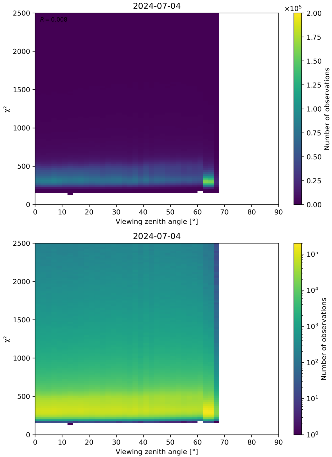
Figure 162: Scatter density plot of “Viewing zenith angle” against “ \chi^2 ” for 2024-07-03 to 2024-07-05.
