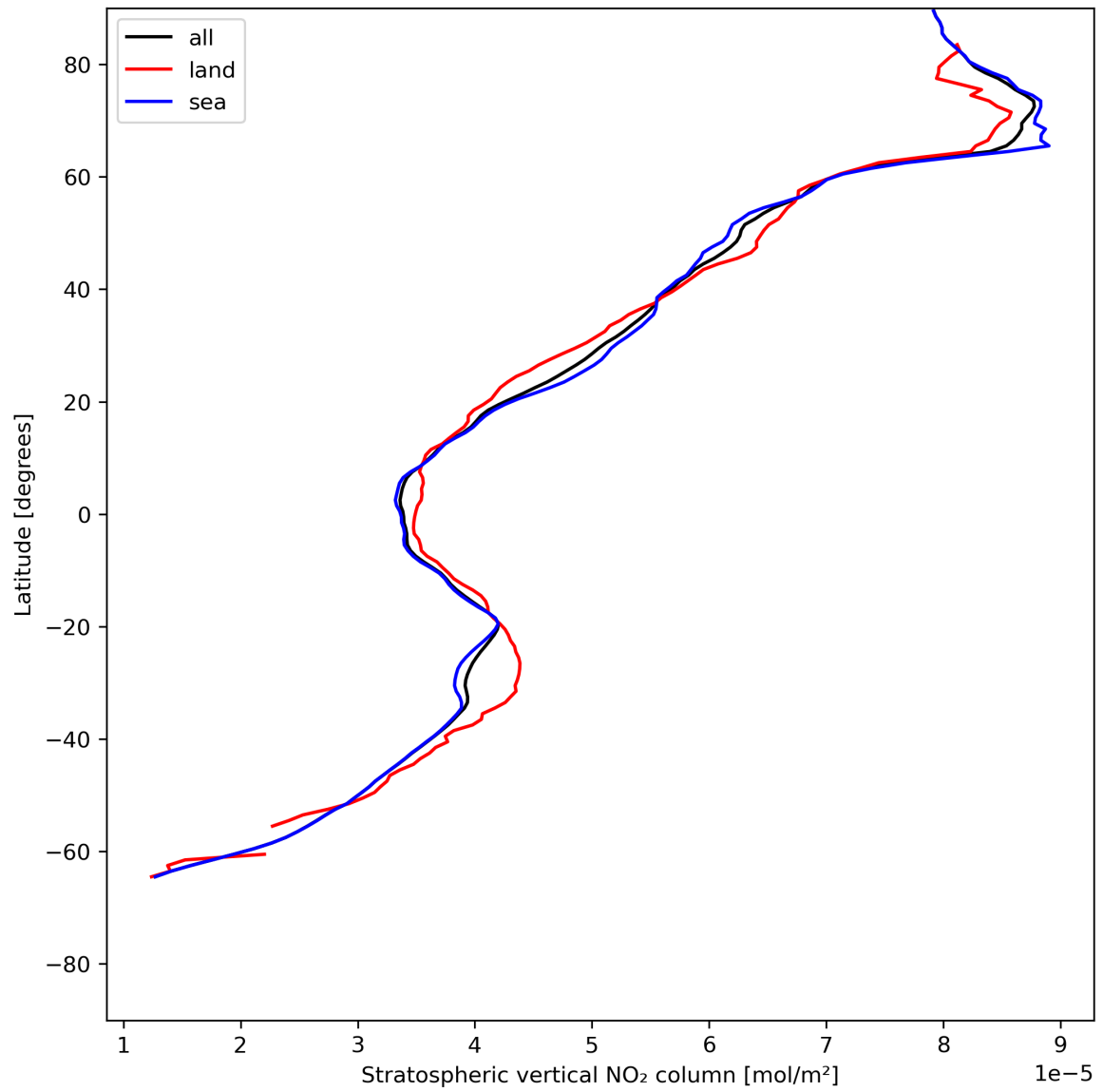
Figure 19: Zonal average of “Stratospheric vertical NO 2 column” for 2024-07-03 to 2024-07-05.
