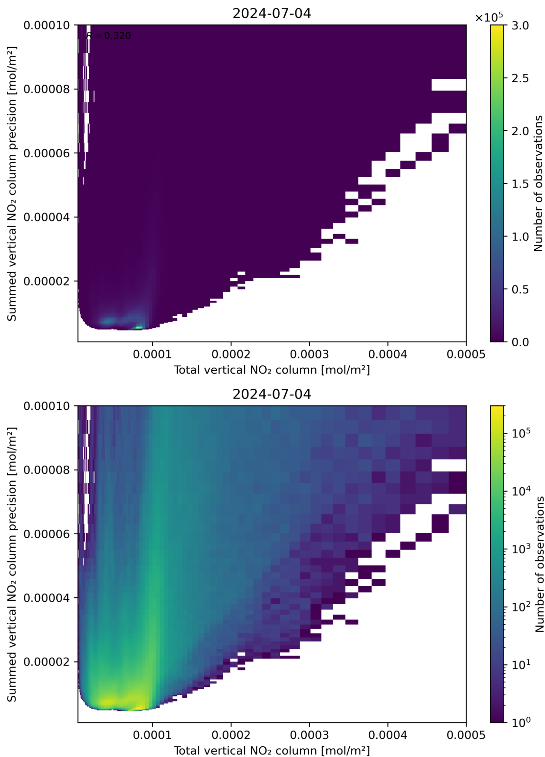
Figure 113: Scatter density plot of “Total vertical NO 2 column” against “Summed vertical NO 2 column precision” for 2024-07-03 to 2024-07-05.
