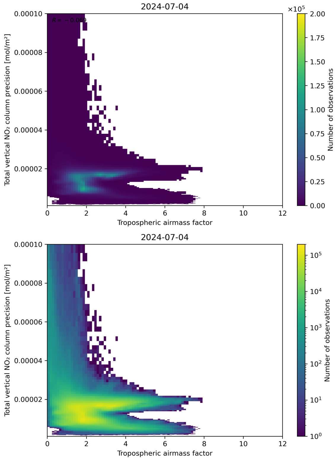
Figure 78: Scatter density plot of “Tropospheric airmass factor” against “Total vertical NO 2 column precision” for 2024-07-03 to 2024-07-05.
