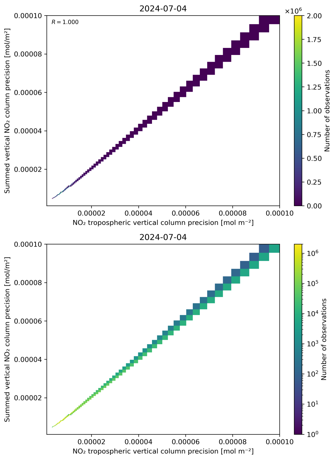
Figure 137: Scatter density plot of “NO 2 tropospheric vertical column precision” against “Summed vertical NO 2 column precision” for 2024-07-03 to 2024-07-05.
