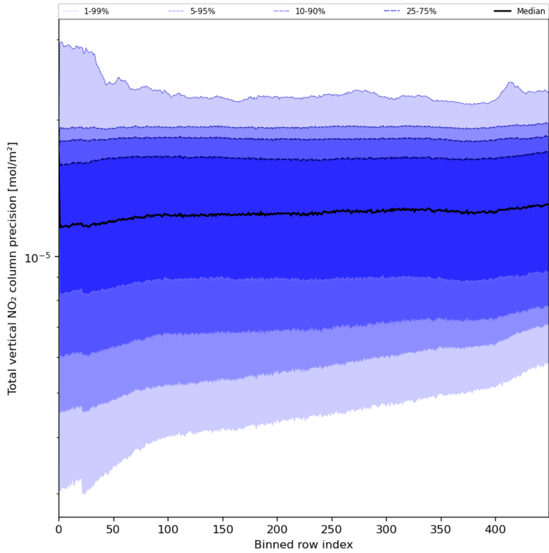
Figure 56: Along track statistics of “Total vertical NO 2 column precision” for 2024-07-03 to 2024-07-05
