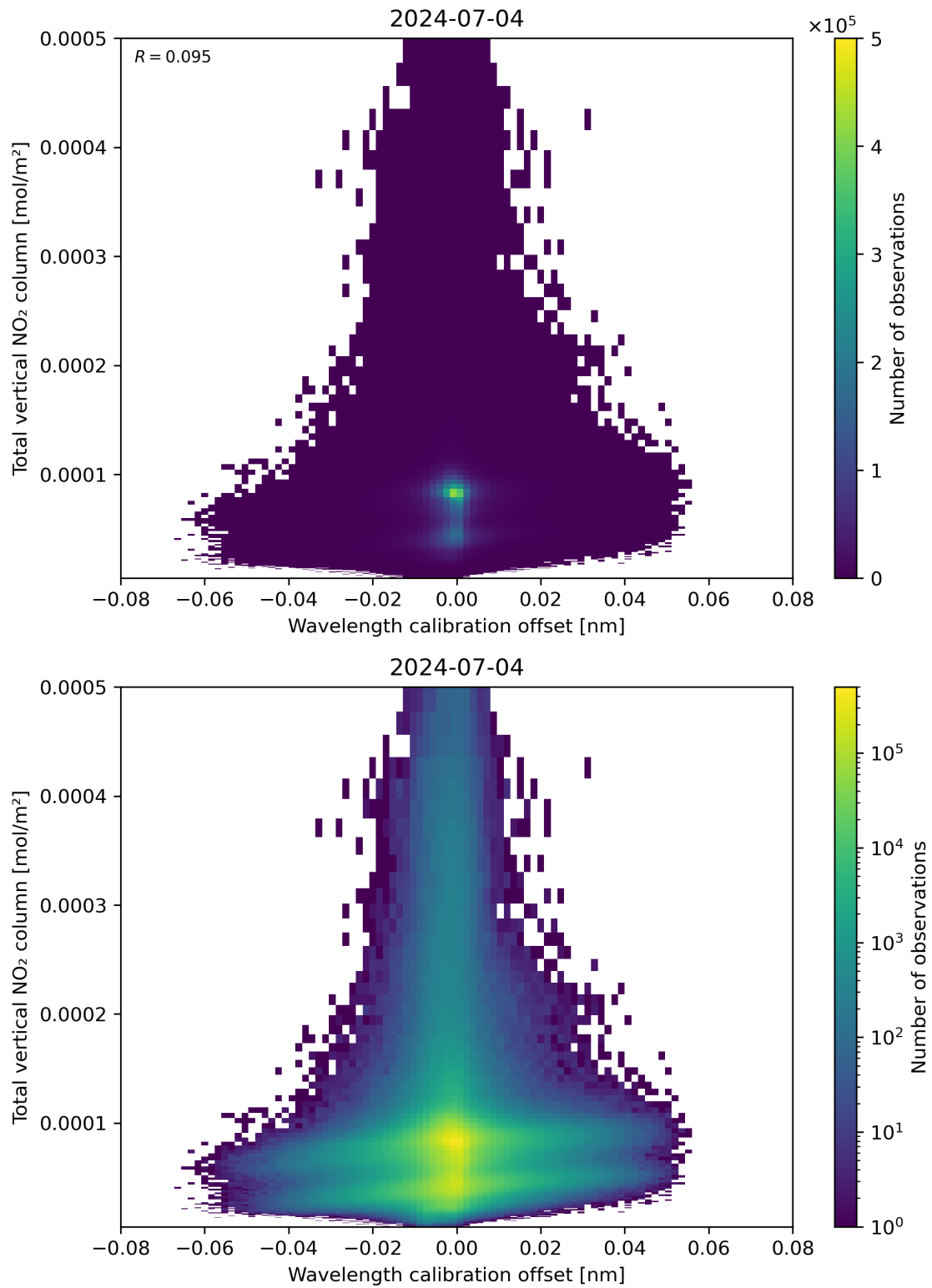
Figure 179: Scatter density plot of “Wavelength calibration offset” against “Total vertical NO 2 column” for 2024-07-03 to 2024-07-05.
