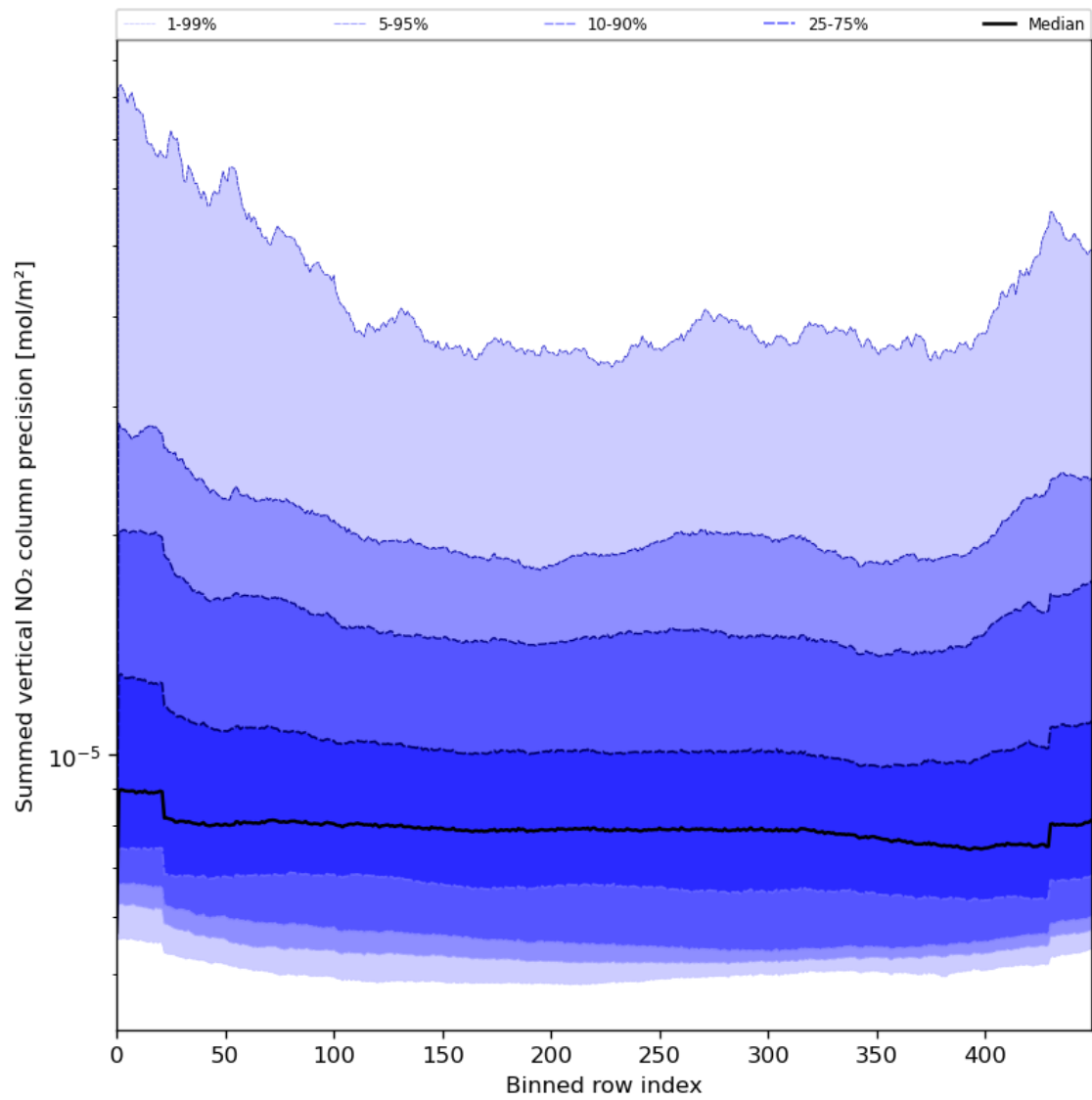
Figure 58: Along track statistics of “Summed vertical NO 2 column precision” for 2024-07-03 to 2024-07-05
