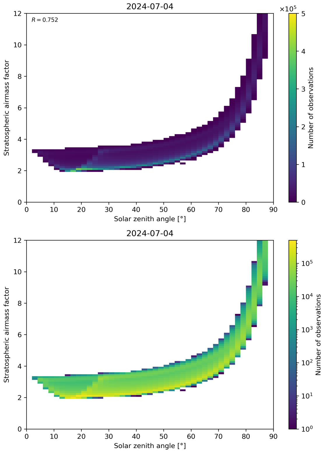
Figure 145: Scatter density plot of “Solar zenith angle” against “Stratospheric airmass factor” for 2024-07-03 to 2024-07-05.
