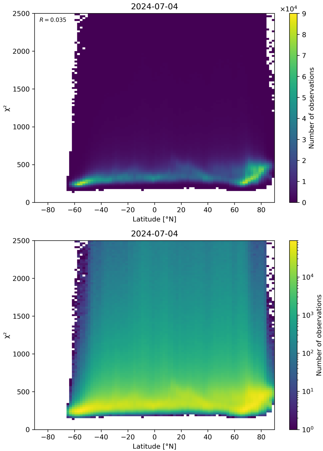
Figure 86: Scatter density plot of “Latitude” against “ \chi^2 ” for 2024-07-03 to 2024-07-05.
