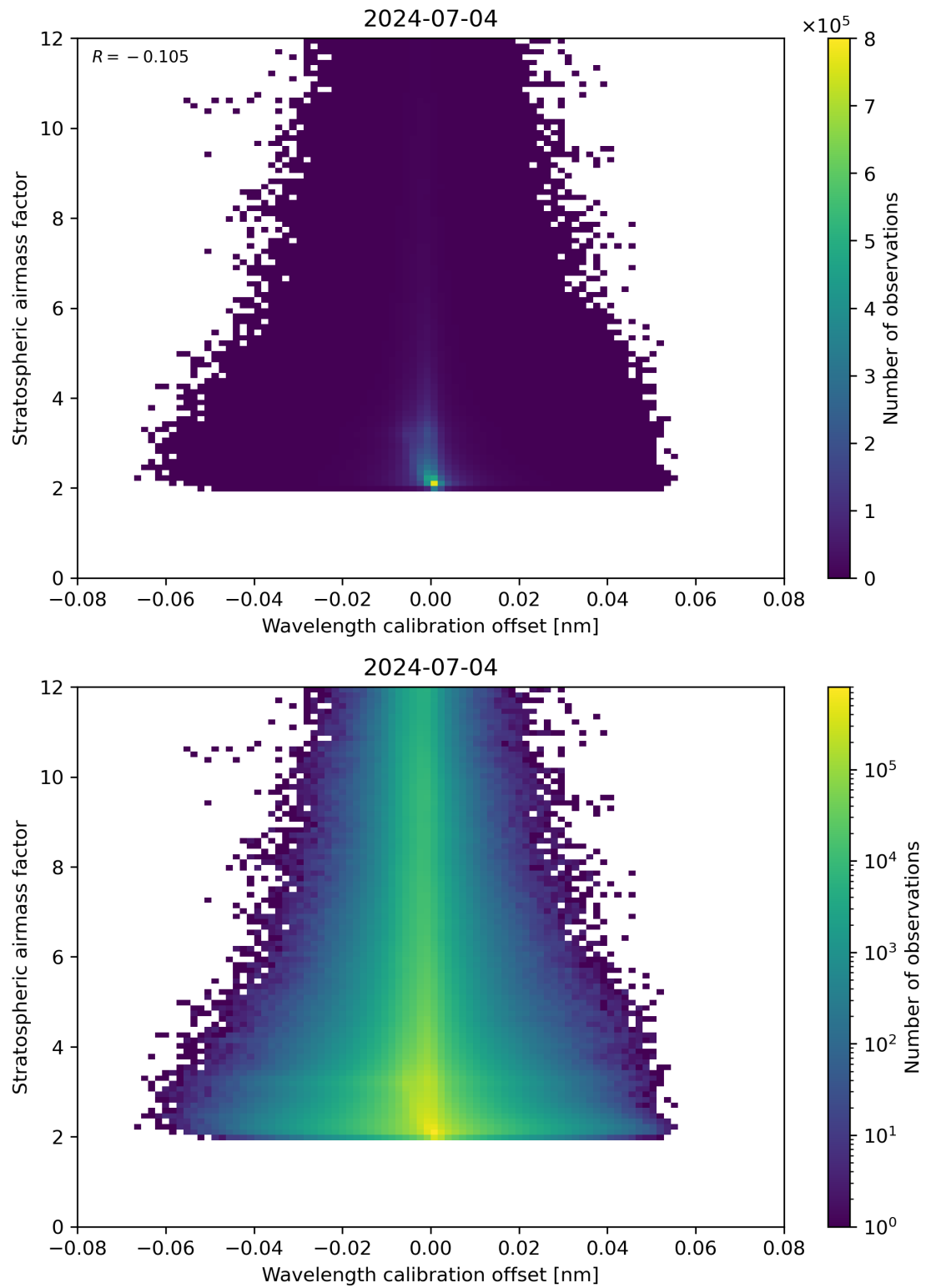
Figure 174: Scatter density plot of “Wavelength calibration offset” against “Stratospheric air mass factor” for 2024-07-03 to 2024-07-05.
