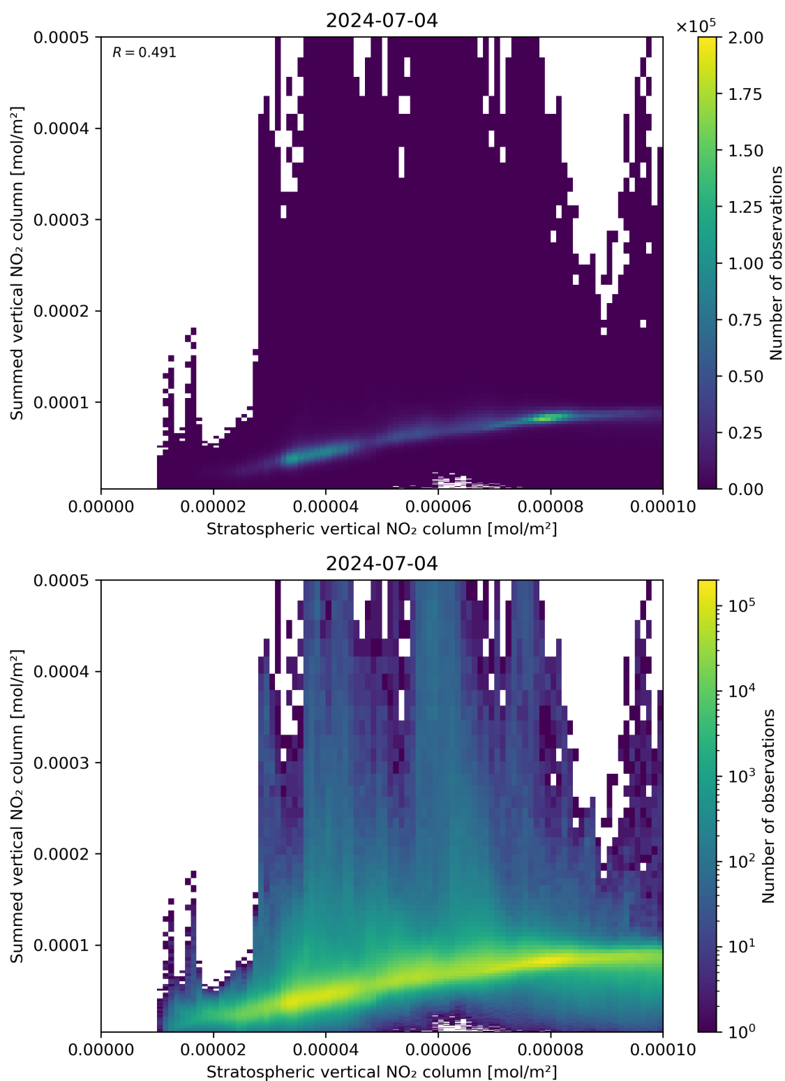
Figure 98: Scatter density plot of “Stratospheric vertical NO 2 column” against “Summed vertical NO 2 column” for 2024-07-03 to 2024-07-05.
