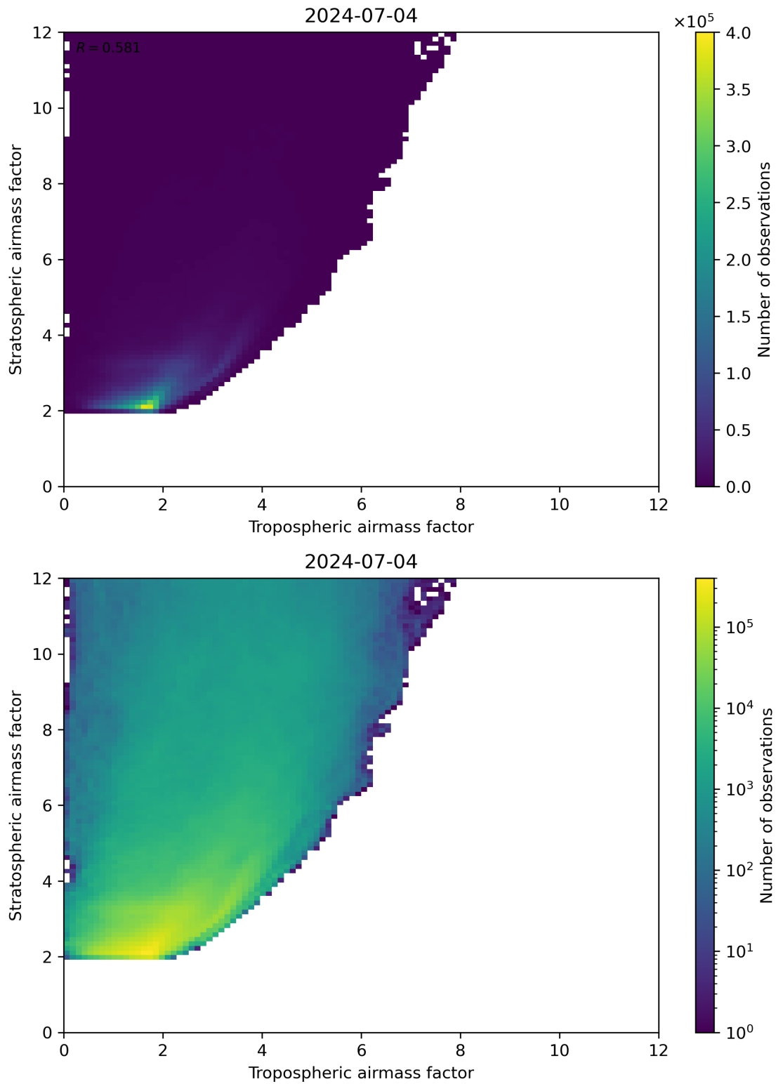
Figure 71: Scatter density plot of “Tropospheric airmass factor” against “Stratospheric airmass factor” for 2024-07-03 to 2024-07-05.
