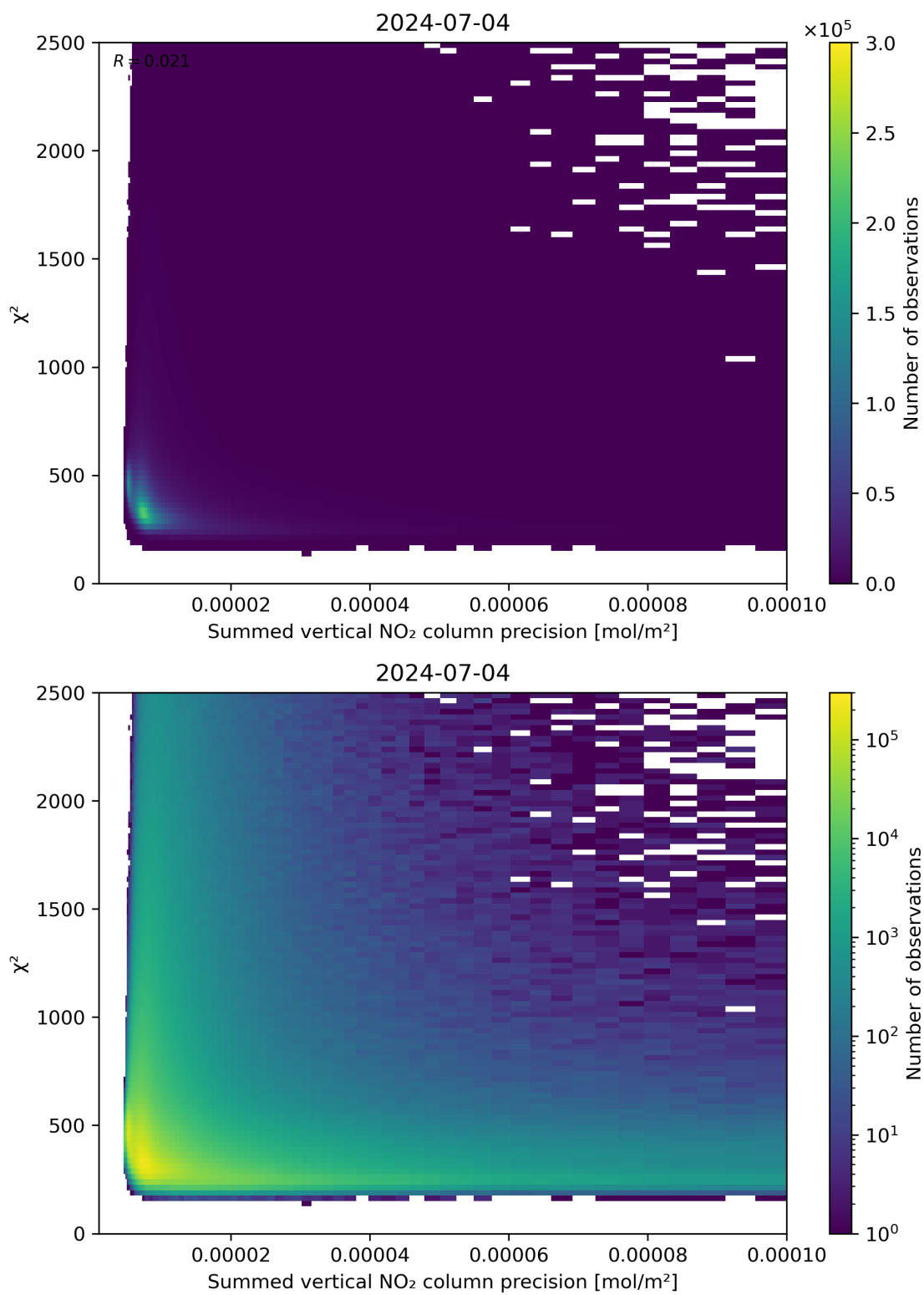
Figure 107: Scatter density plot of “Summed vertical NO 2 column precision” against “ \chi^2 ” for 2024-07-03 to 2024-07-05.
