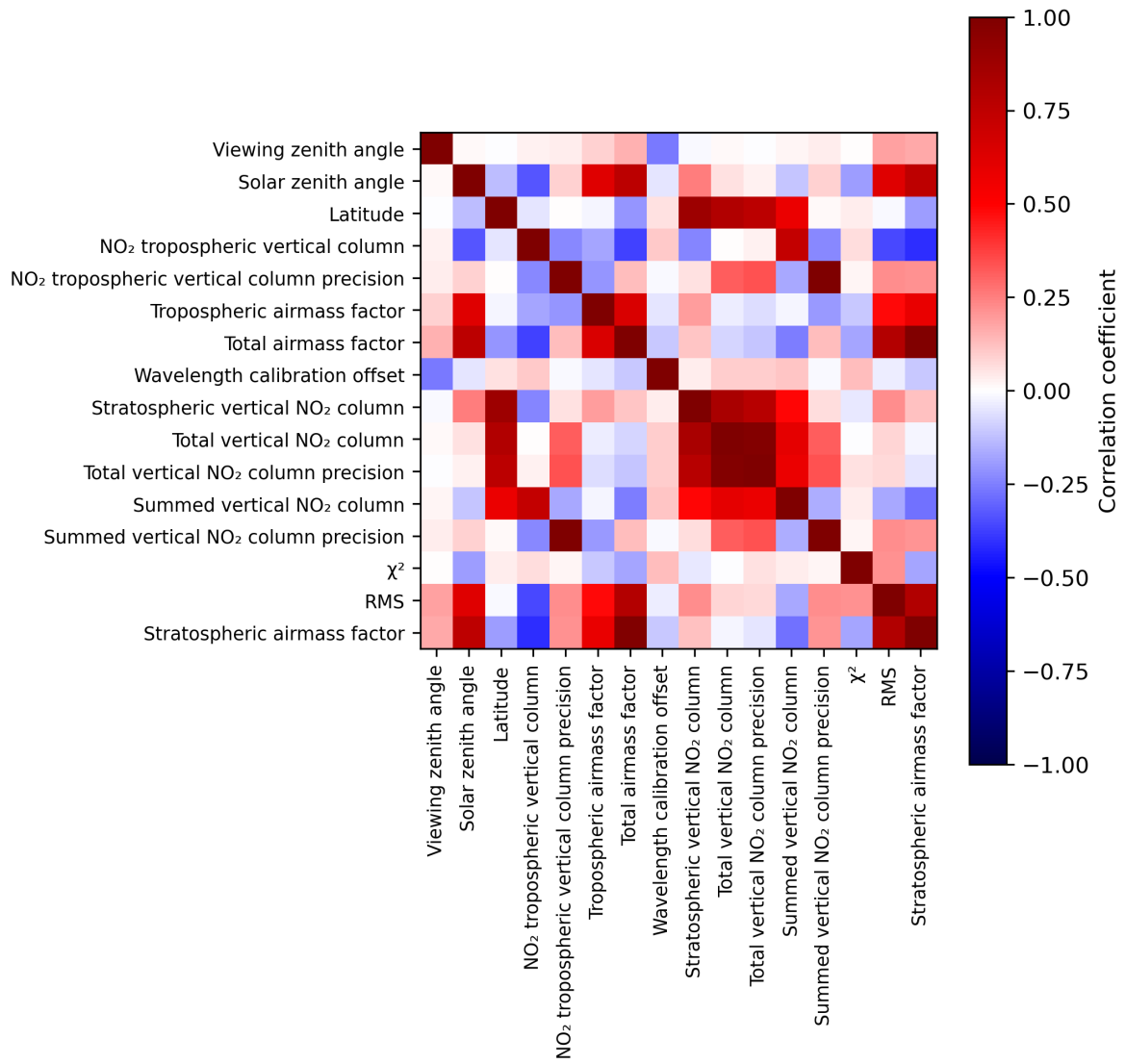
Figure 2: Map of correlation matrix for 2024-07-03 to 2024-07-05.
