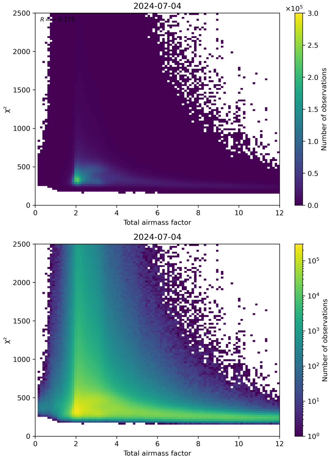
Figure 63: Scatter density plot of “Total airmass factor” against “ \chi^2 ” for 2024-07-03 to 2024-07-05.
