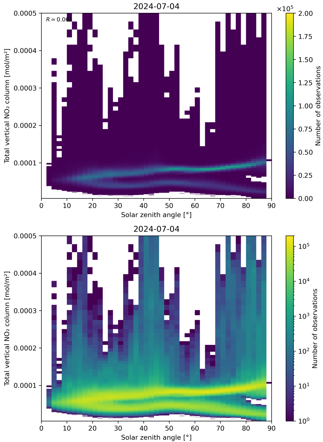
Figure 153: Scatter density plot of “Solar zenith angle” against “Total vertical NO 2 column” for 2024-07-03 to 2024-07-05.
