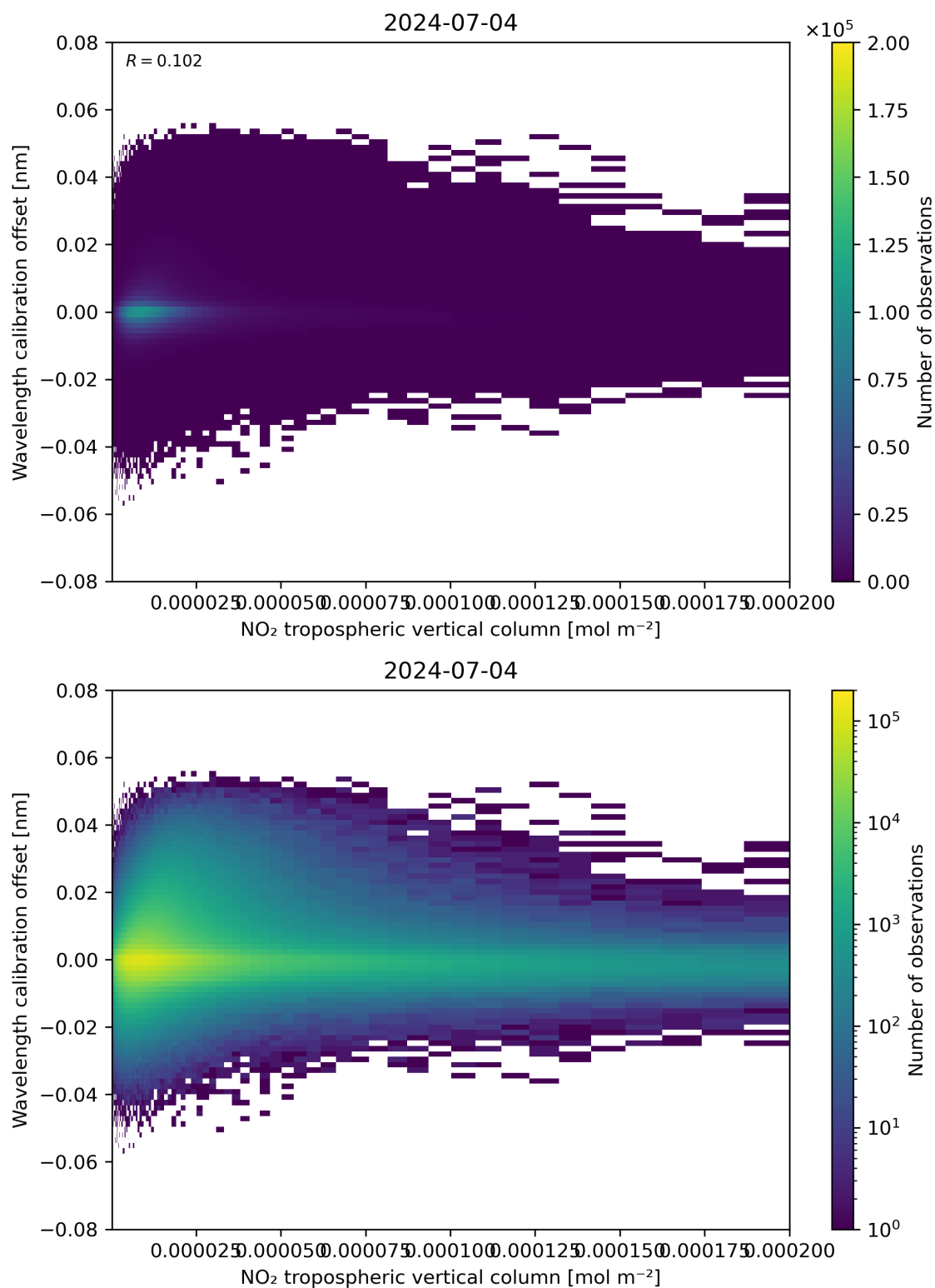
Figure 143: Scatter density plot of “NO 2 tropospheric vertical column” against “Wavelength calibration offset” for 2024-07-03 to 2024-07-05.
