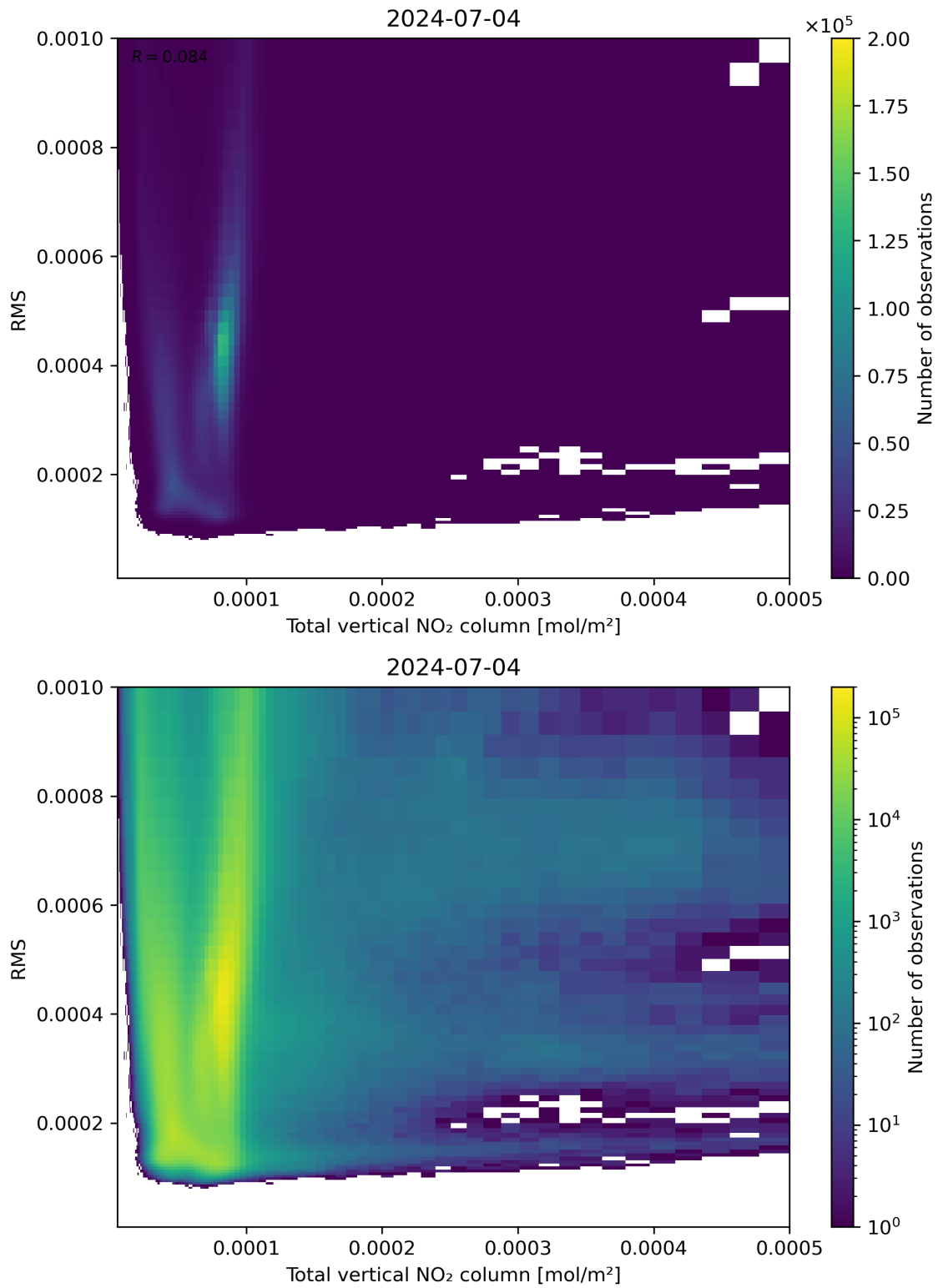
Figure 120: Scatter density plot of “Total vertical NO 2 column” against “RMS” for 2024-07-03 to 2024-07-05.
