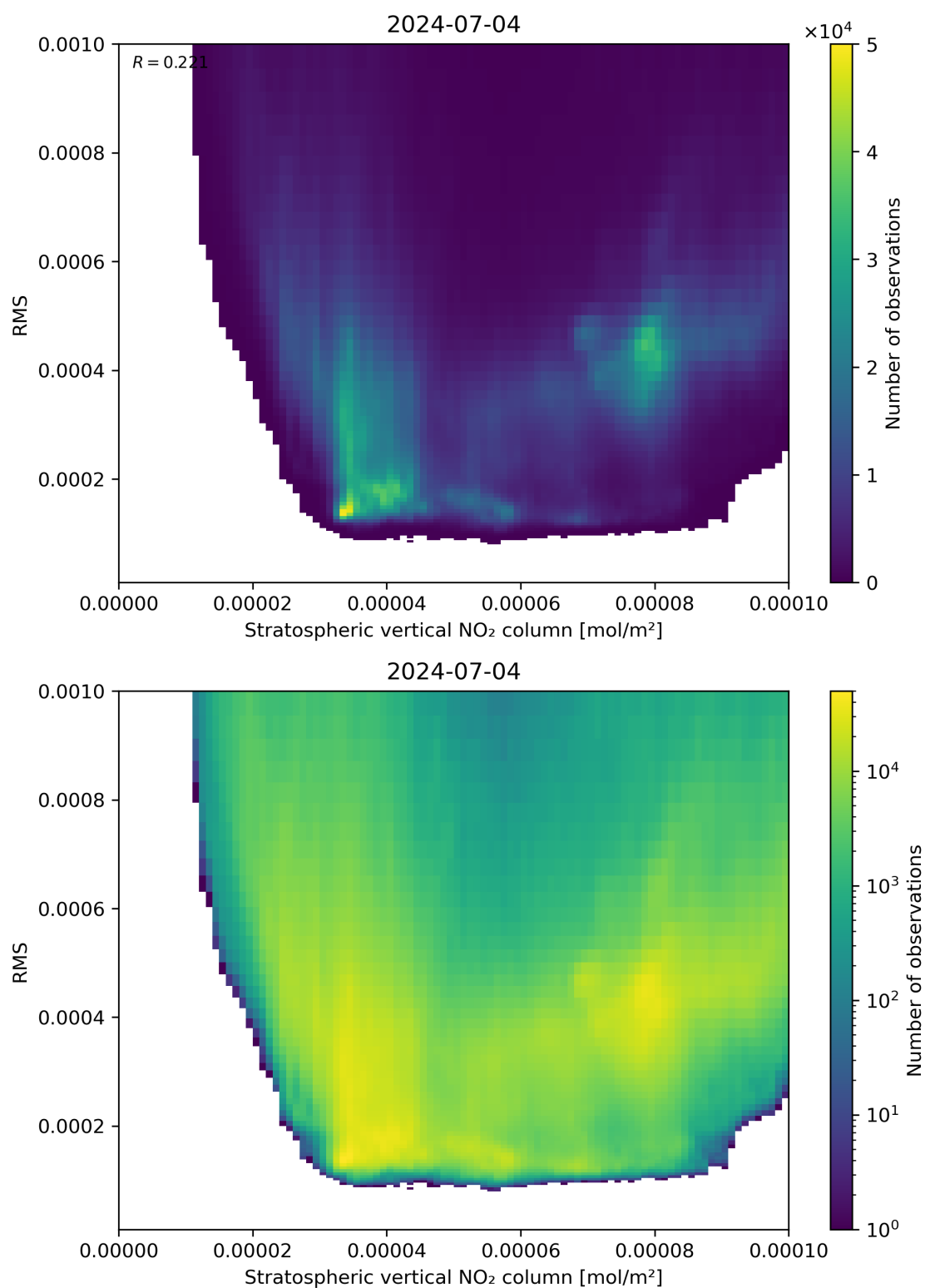
Figure 102: Scatter density plot of “Stratospheric vertical NO 2 column” against “RMS” for 2024-07-03 to 2024-07-05.
