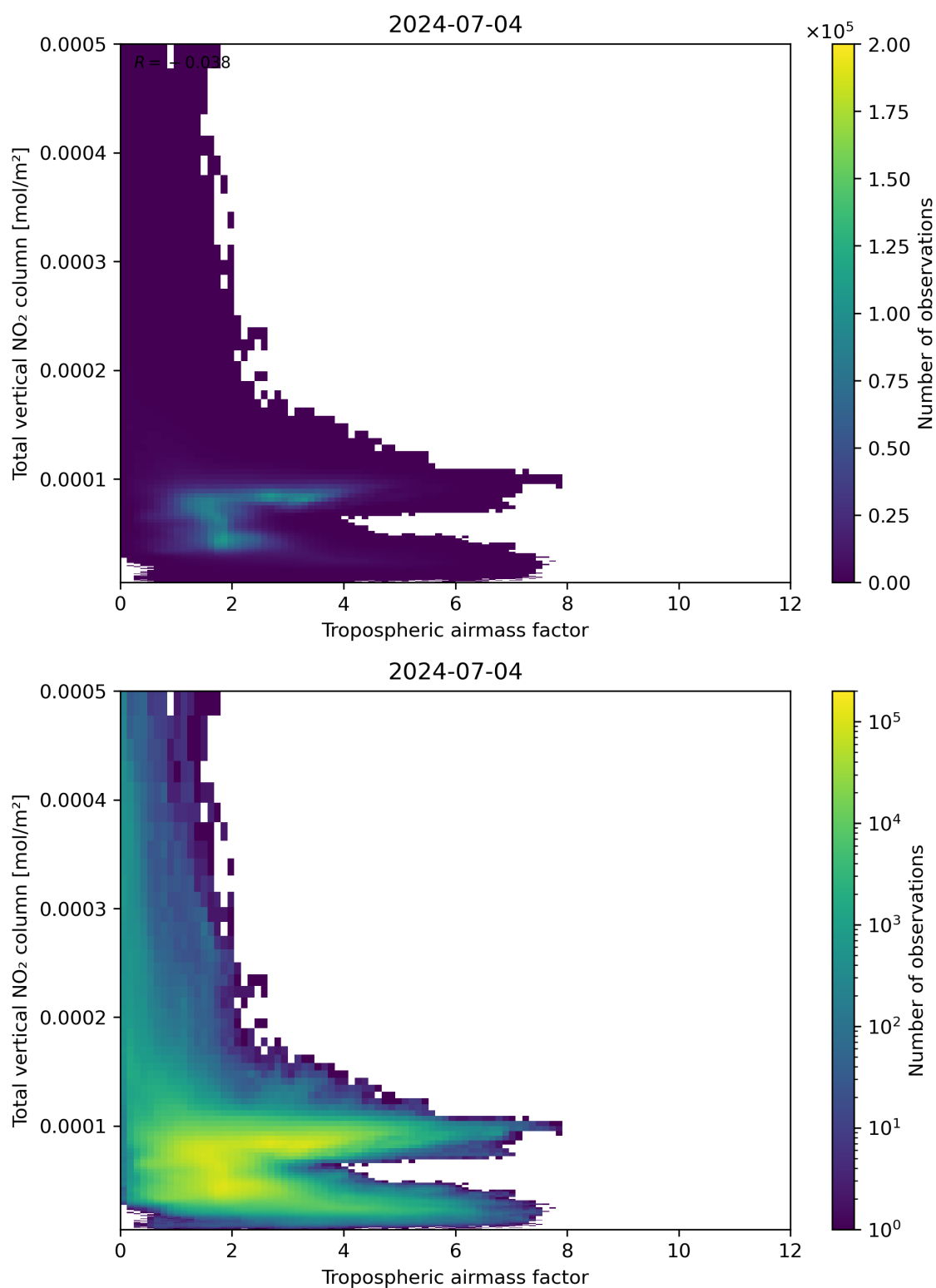
Figure 77: Scatter density plot of “Tropospheric airmass factor” against “Total vertical NO 2 column” for 2024-07-03 to 2024-07-05.
