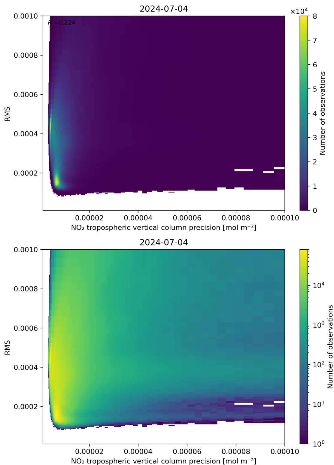
Figure 140: Scatter density plot of “NO 2 tropospheric vertical column precision” against “RMS” for 2024-07-03 to 2024-07-05.
