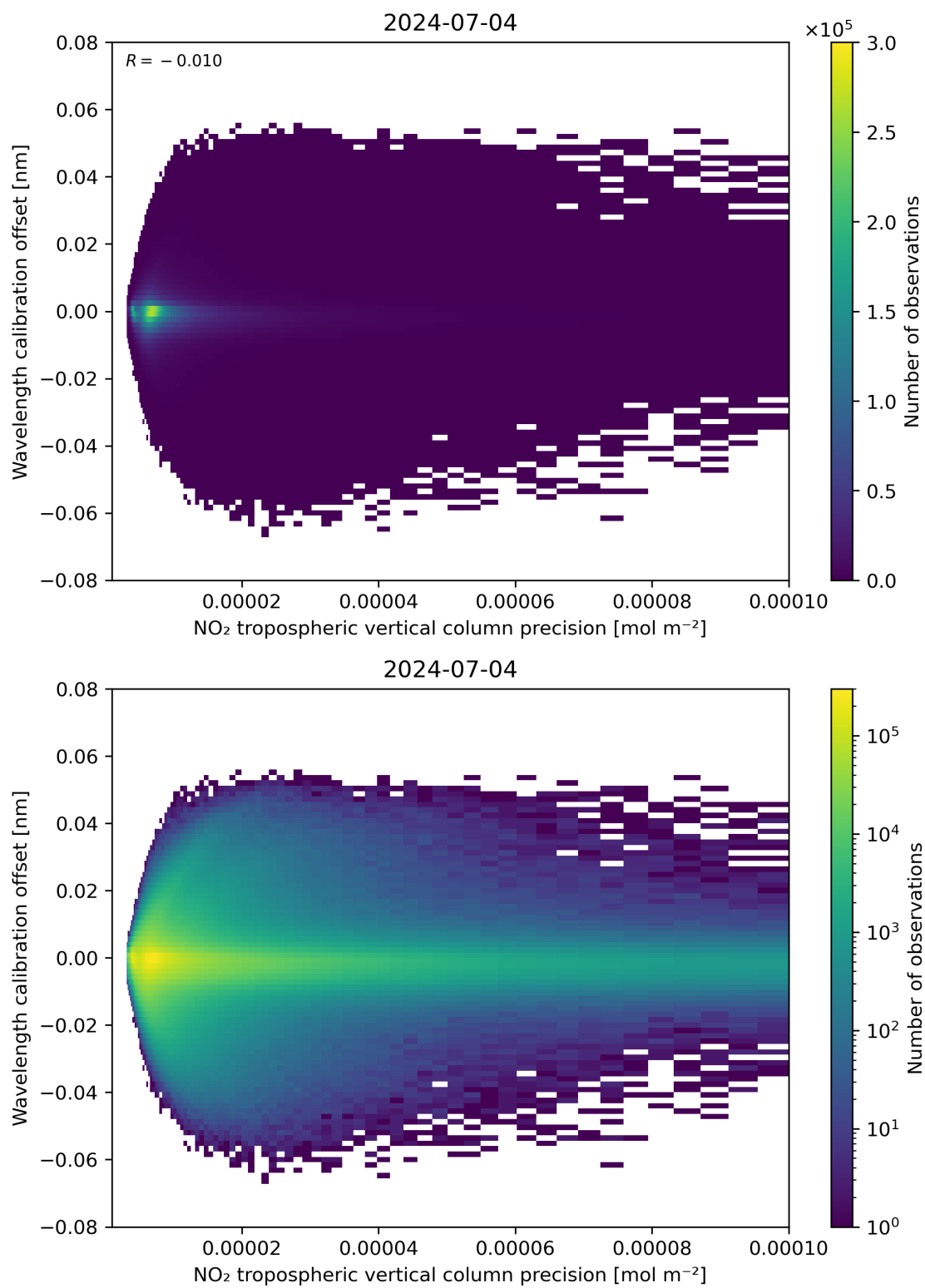
Figure 141: Scatter density plot of “NO 2 tropospheric vertical column precision” against “Wavelength calibration offset” for 2024-07-03 to 2024-07-05.
