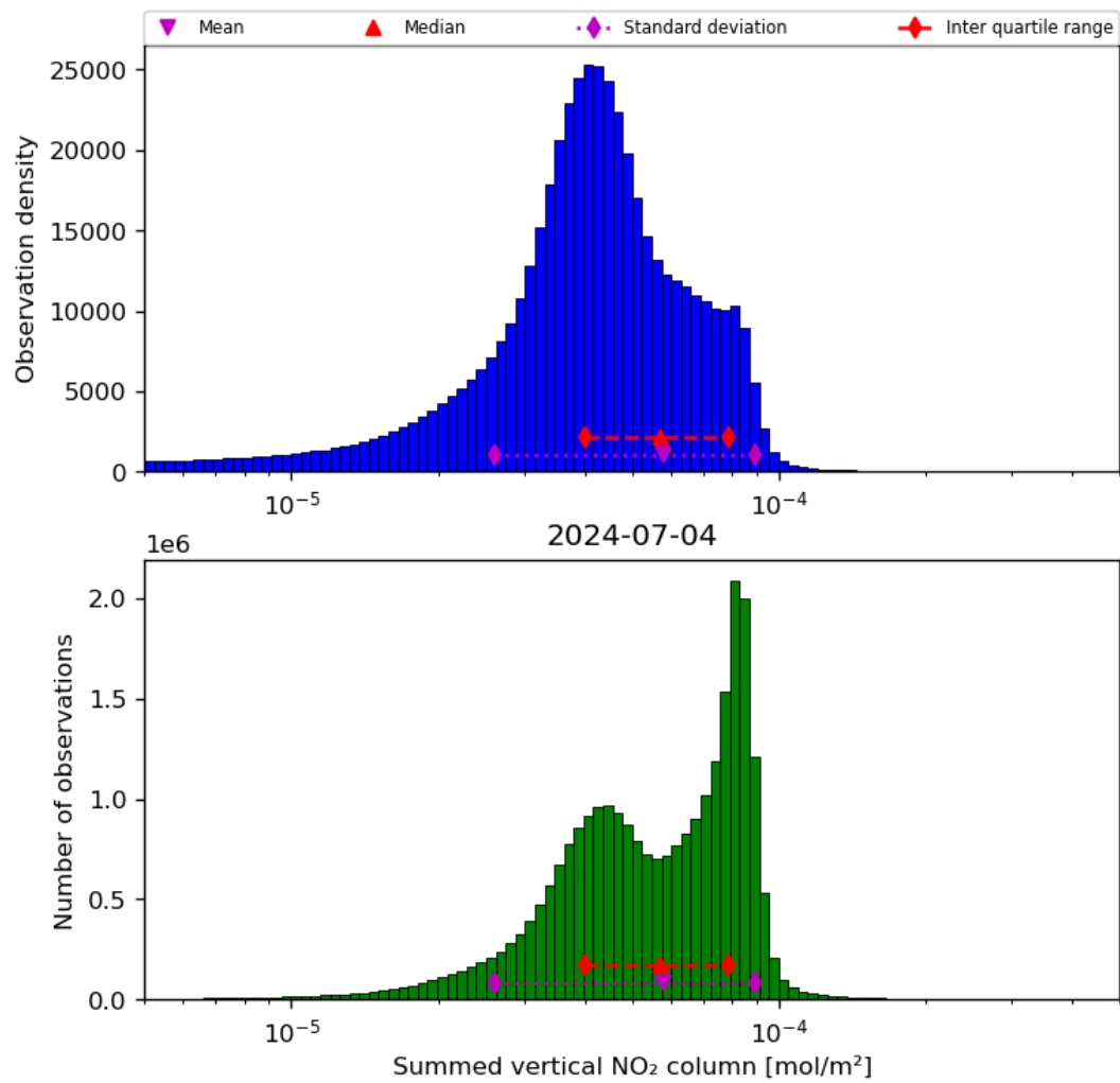
Figure 40: Histogram of “Summed vertical NO 2 column” for 2024-07-03 to 2024-07-05
