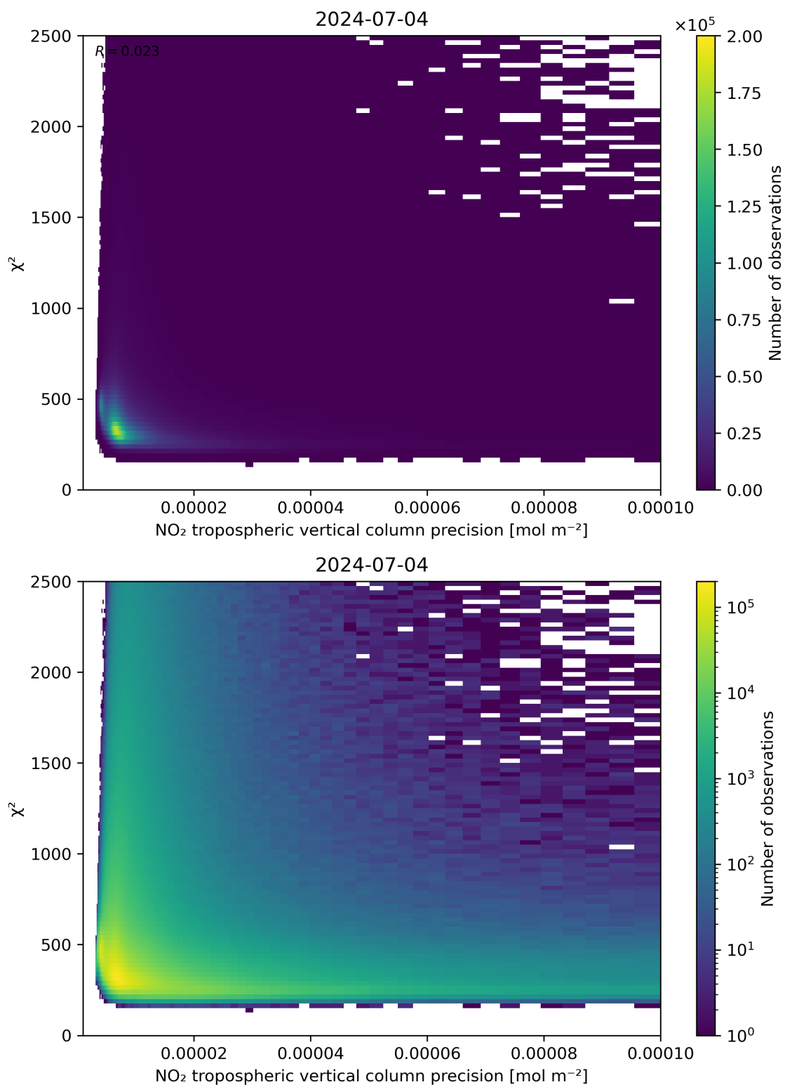
Figure 134: Scatter density plot of “NO 2 tropospheric vertical column precision” against “ \chi^2 ” for 2024-07-03 to 2024-07-05.
