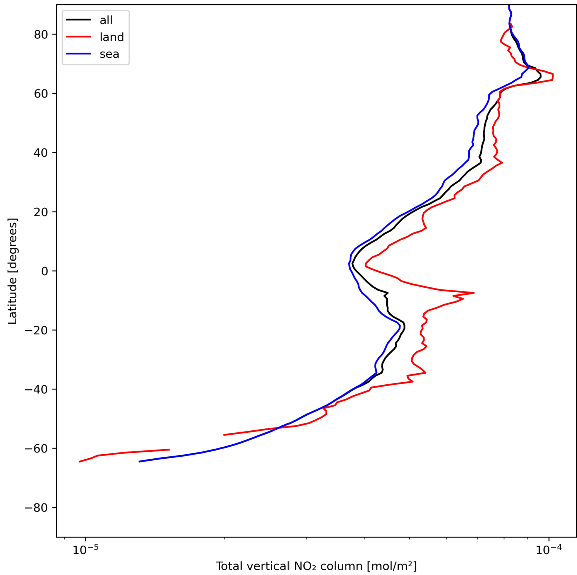
Figure 21: Zonal average of “Total vertical NO 2 column” for 2024-07-03 to 2024-07-05.
