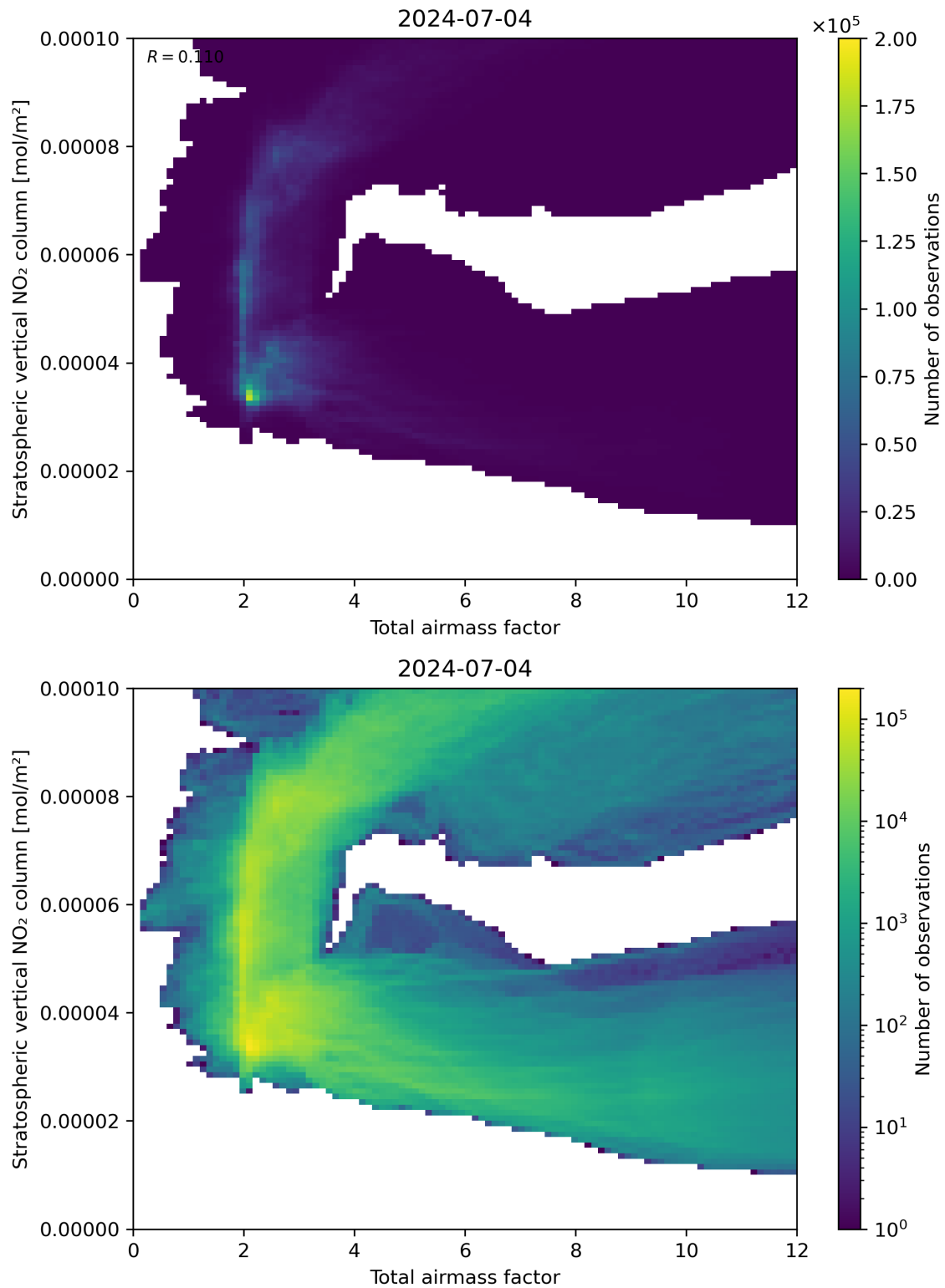
Figure 64: Scatter density plot of “Total airmass factor” against “Stratospheric vertical NO 2 column” for 2024-07-03 to 2024-07-05.
