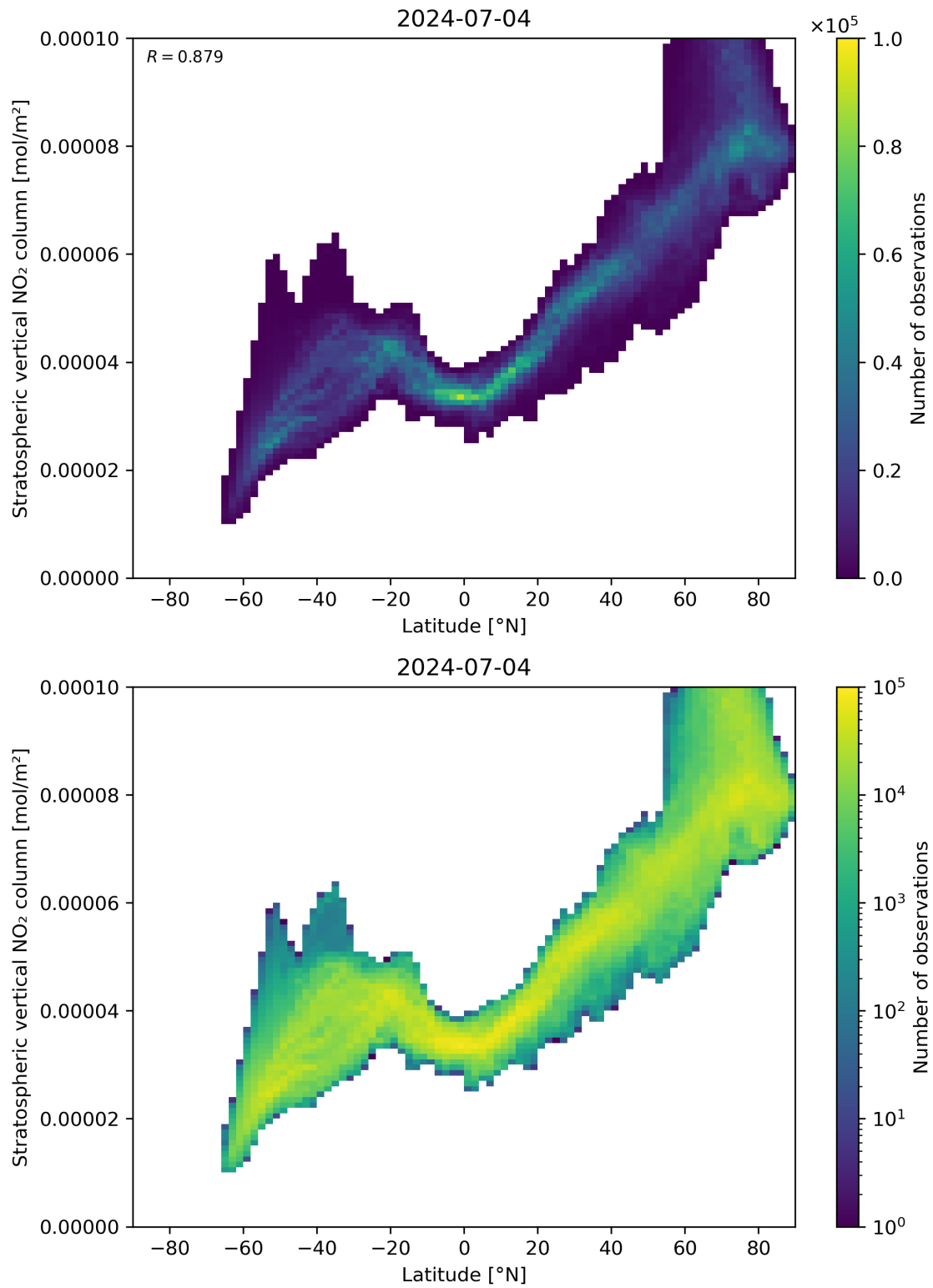
Figure 87: Scatter density plot of “Latitude” against “Stratospheric vertical NO 2 column” for 2024-07-03 to 2024-07-05.
