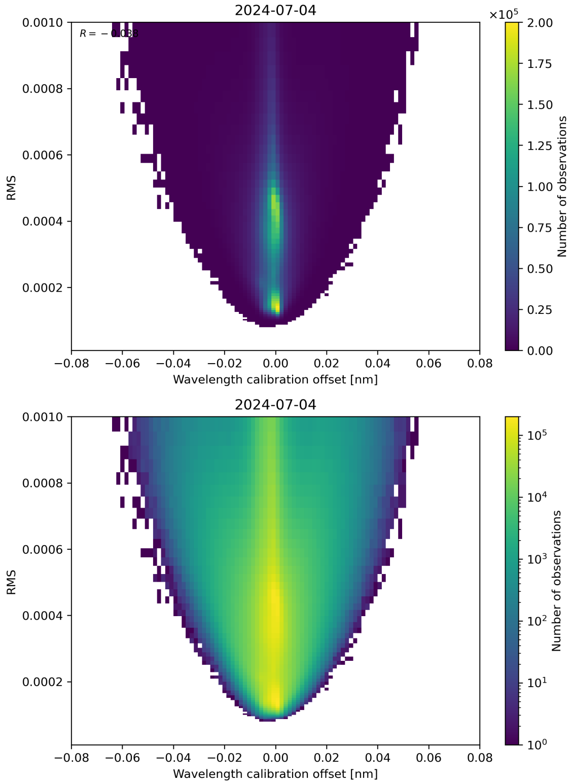
Figure 181: Scatter density plot of “Wavelength calibration offset” against “RMS” for 2024-07-03 to 2024-07-05.
