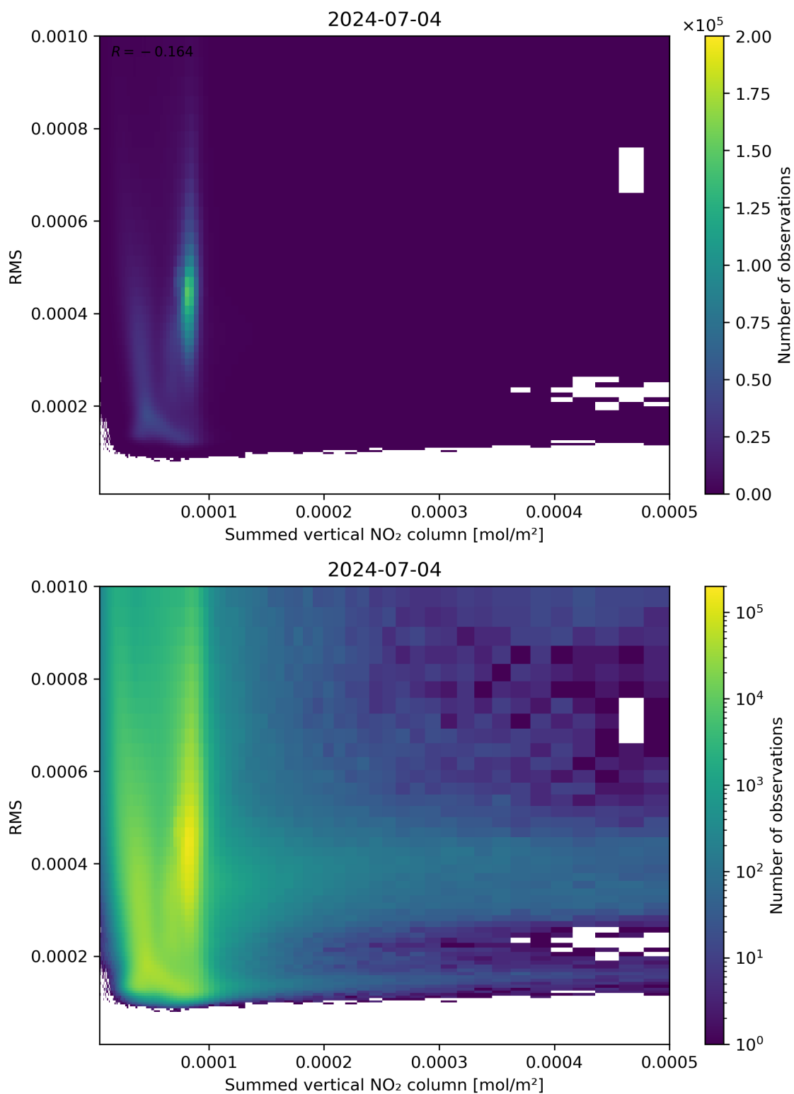
Figure 109: Scatter density plot of “Summed vertical NO 2 column” against “RMS” for 2024-07-03 to 2024-07-05.
