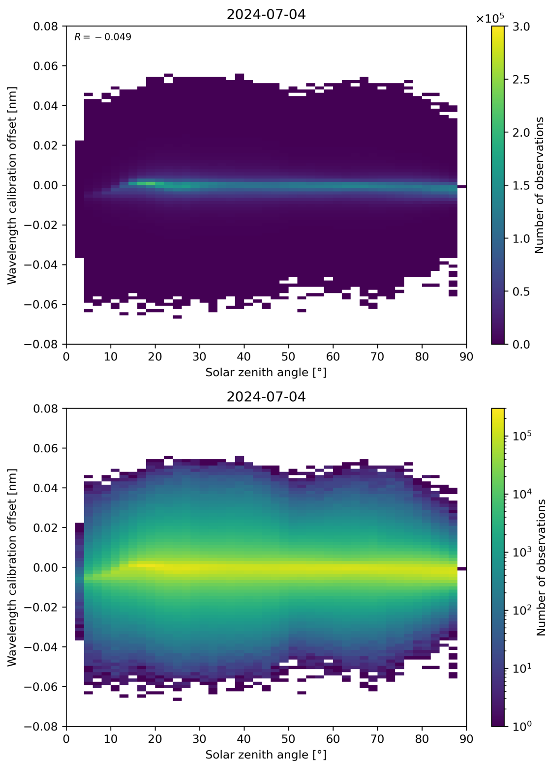
Figure 158: Scatter density plot of “Solar zenith angle” against “Wavelength calibration offset” for 2024-07-03 to 2024-07-05.
