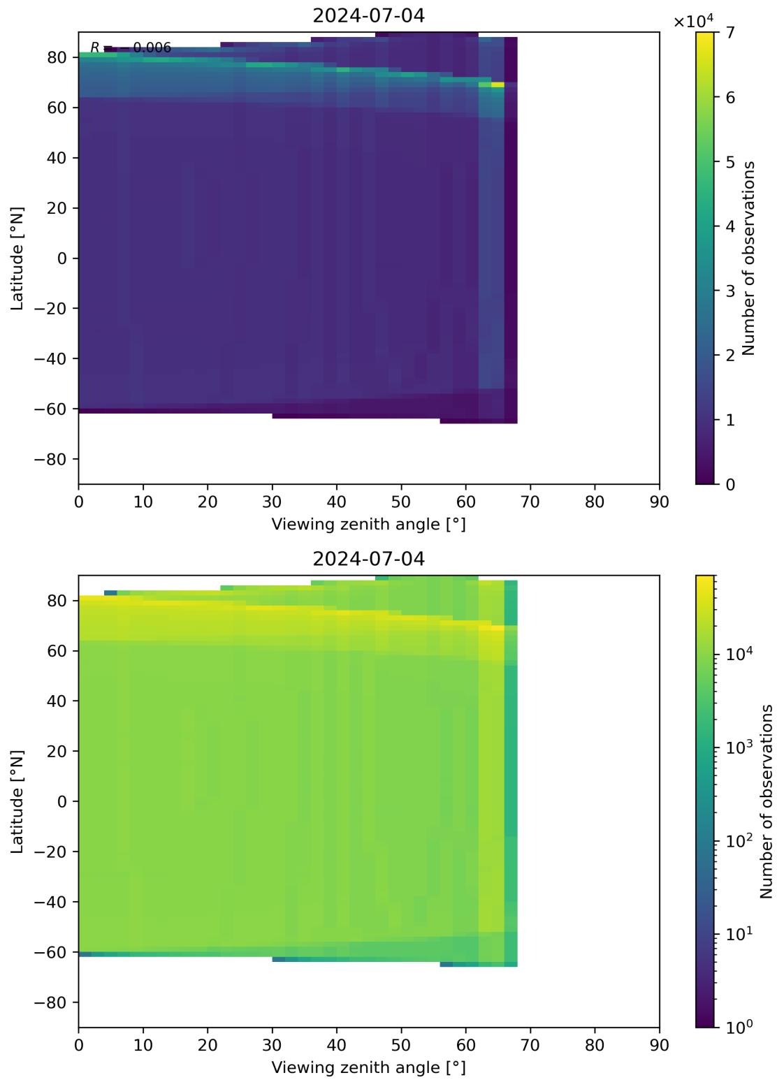
Figure 163: Scatter density plot of “Viewing zenith angle” against “Latitude” for 2024-07-03 to 2024-07-05.
