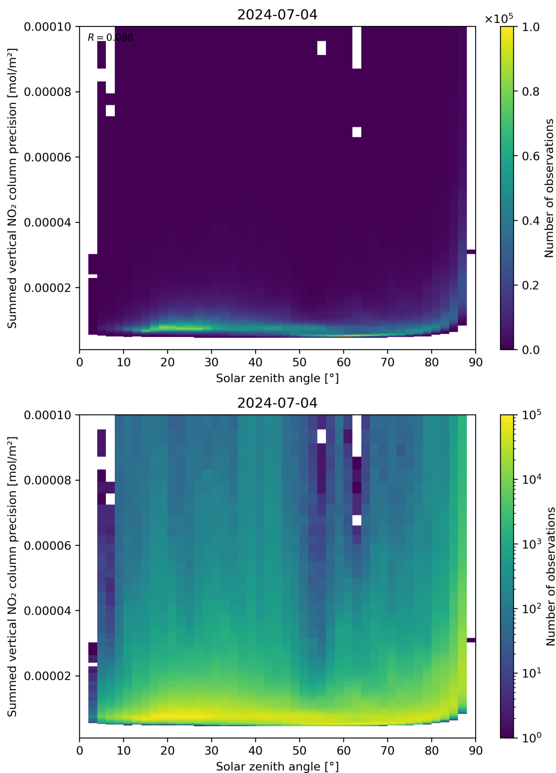
Figure 152: Scatter density plot of “Solar zenith angle” against “Summed vertical NO 2 column precision” for 2024-07-03 to 2024-07-05.
