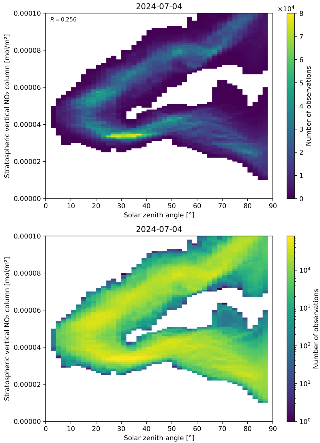
Figure 150: Scatter density plot of “Solar zenith angle” against “Stratospheric vertical NO 2 column” for 2024-07-03 to 2024-07-05.
