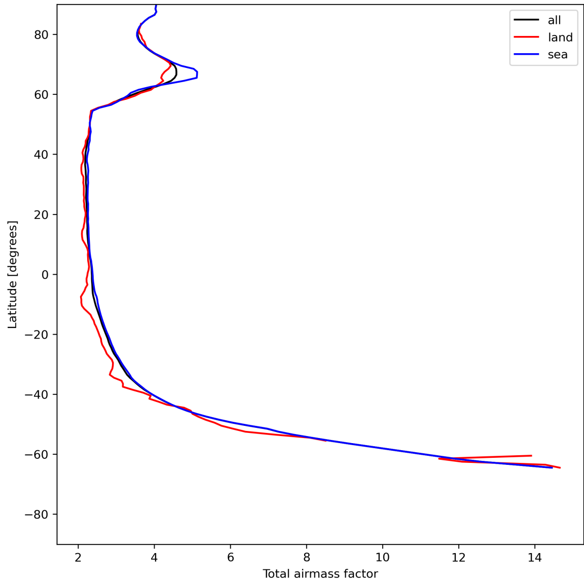
Figure 15: Zonal average of “Total airmass factor” for 2024-07-03 to 2024-07-05.
