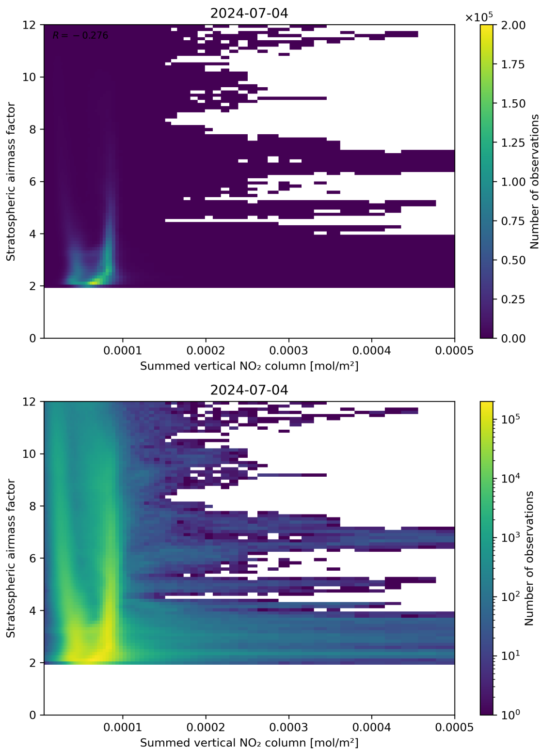
Figure 103: Scatter density plot of “Summed vertical NO 2 column” against “Stratospheric air mass factor” for 2024-07-03 to 2024-07-05.
