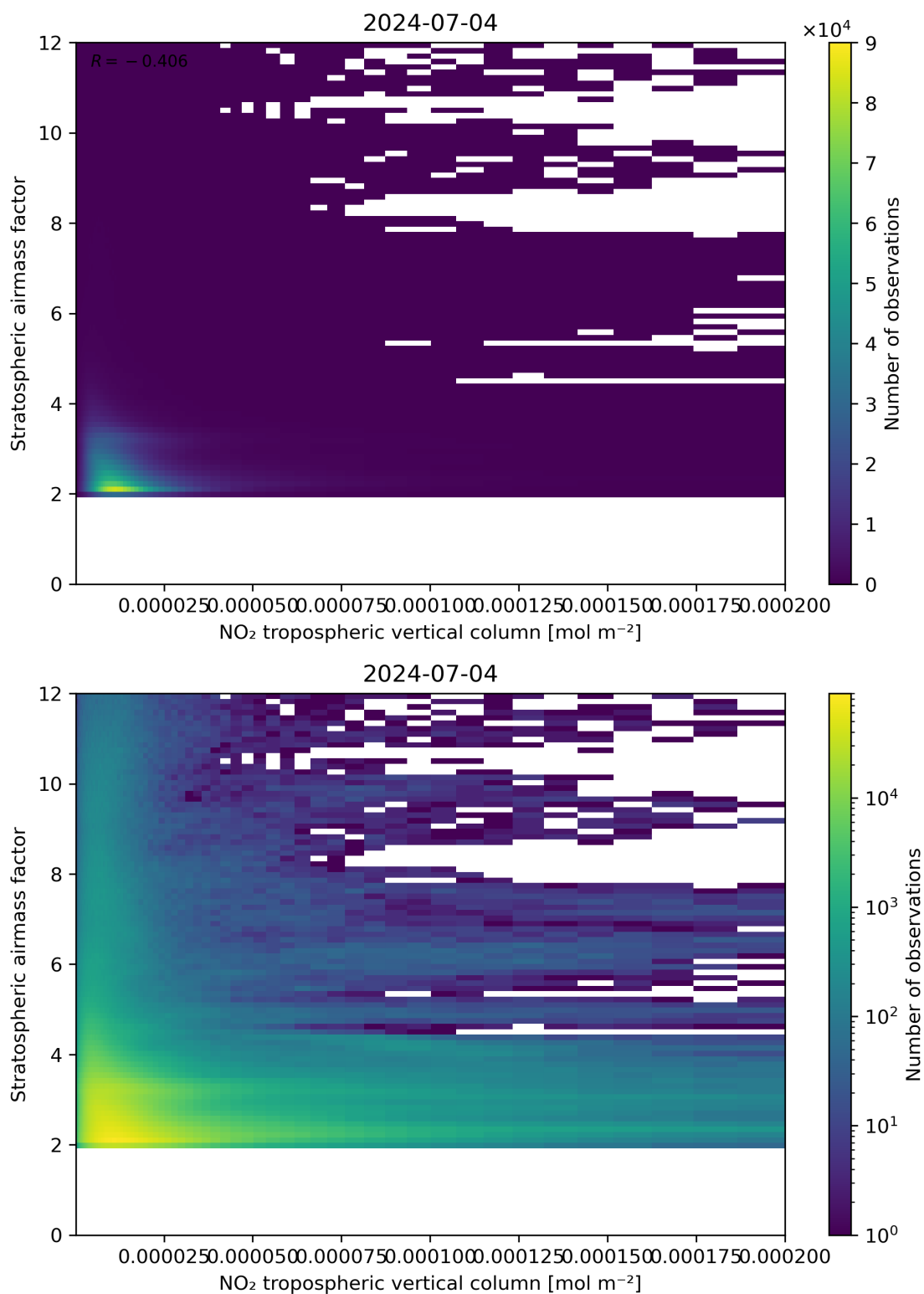
Figure 121: Scatter density plot of “NO 2 tropospheric vertical column” against “Stratospheric air mass factor” for 2024-07-03 to 2024-07-05.
