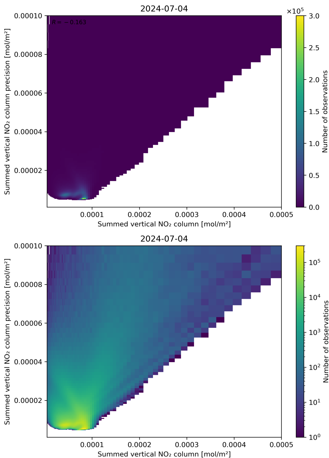
Figure 105: Scatter density plot of “Summed vertical NO 2 column” against “Summed vertical NO 2 column precision” for 2024-07-03 to 2024-07-05.
