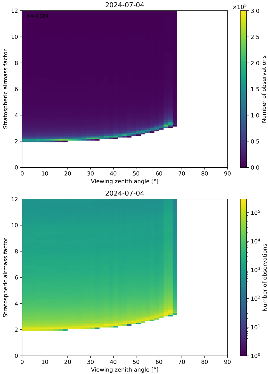
Figure 159: Scatter density plot of “Viewing zenith angle” against “Stratospheric airmass factor” for 2024-07-03 to 2024-07-05.
