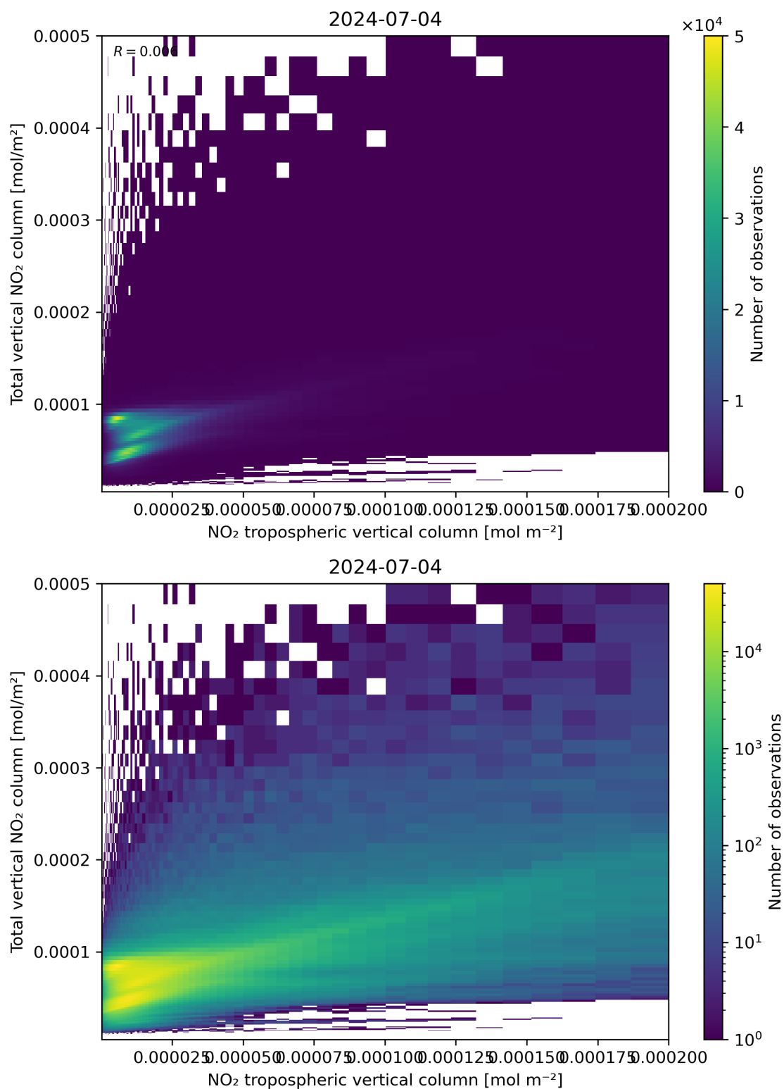
Figure 128: Scatter density plot of “NO 2 tropospheric vertical column” against “Total vertical NO 2 column” for 2024-07-03 to 2024-07-05.
