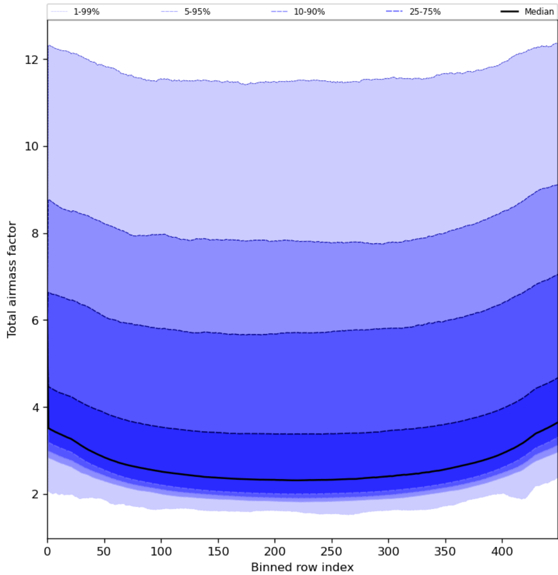
Figure 49: Along track statistics of “Total airmass factor” for 2024-07-03 to 2024-07-05
