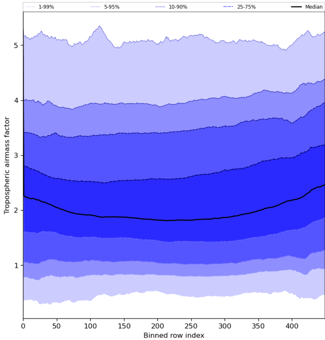
Figure 48: Along track statistics of “Tropospheric air mass factor” for 2024-07-03 to 2024-07-05
