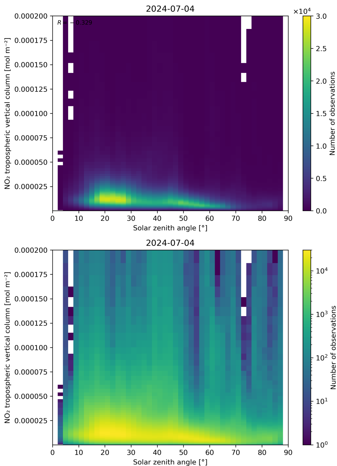
Figure 155: Scatter density plot of “Solar zenith angle” against “NO 2 tropospheric vertical column” for 2024-07-03 to 2024-07-05.
