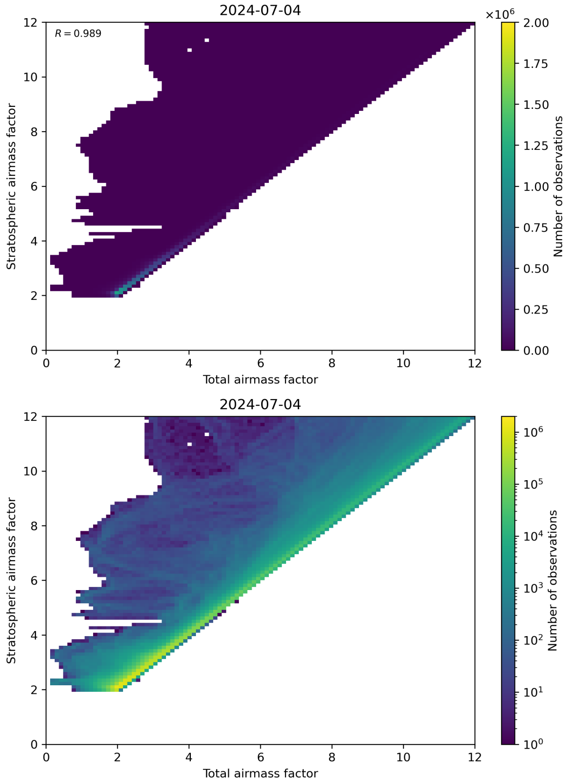
Figure 62: Scatter density plot of “Total airmass factor” against “Stratospheric airmass factor” for 2024-07-03 to 2024-07-05.
