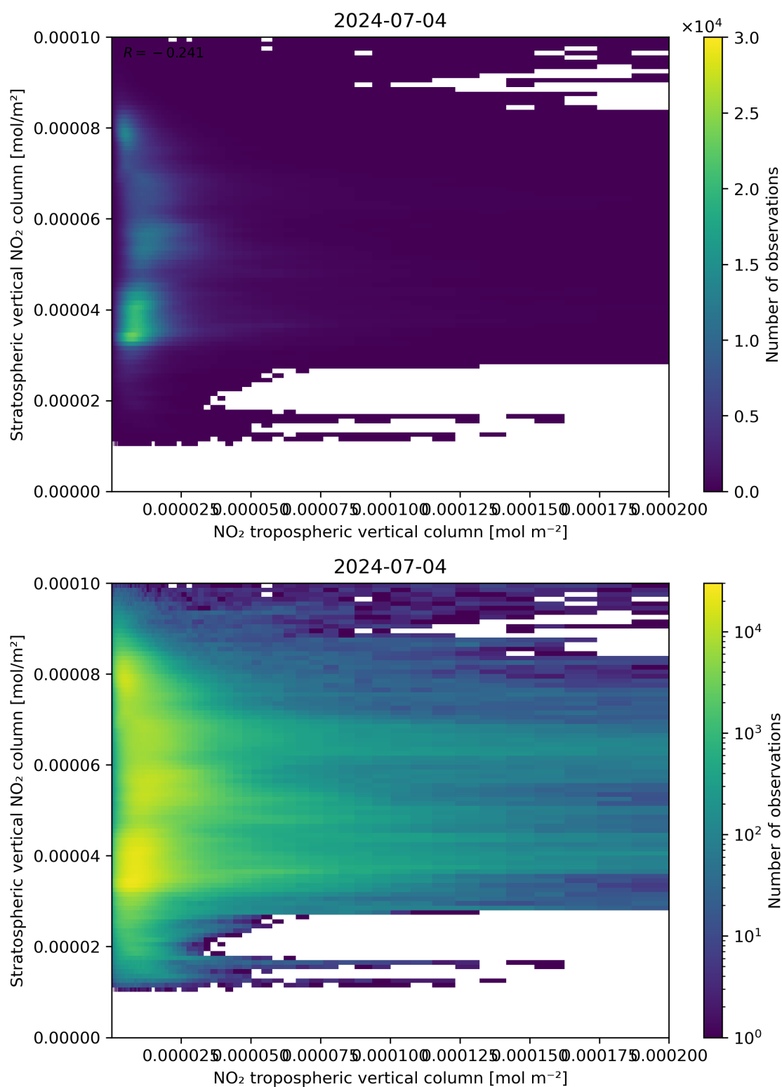
Figure 125: Scatter density plot of “NO 2 tropospheric vertical column” against “Stratospheric vertical NO 2 column” for 2024-07-03 to 2024-07-05.
