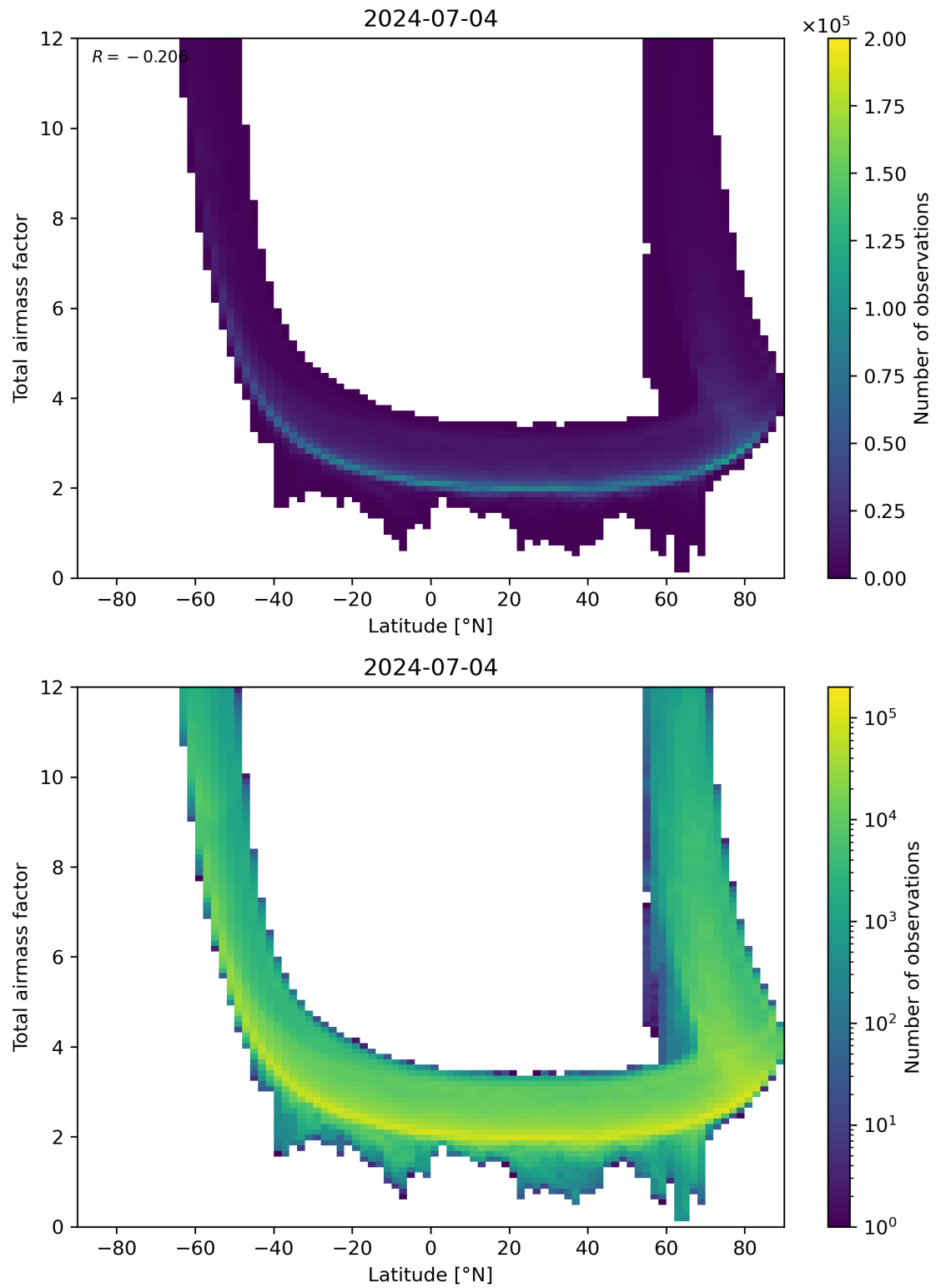
Figure 84: Scatter density plot of “Latitude” against “Total airmass factor” for 2024-07-03 to 2024-07-05.
