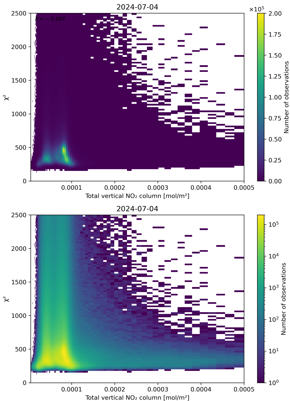
Figure 111: Scatter density plot of “Total vertical NO 2 column” against “ \chi^2 ” for 2024-07-03 to 2024-07-05.
