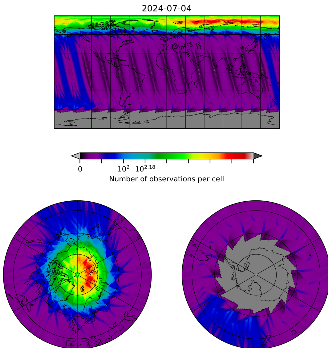
Figure 10: Map of the number of observations for 2024-07-03 to 2024-07-05
