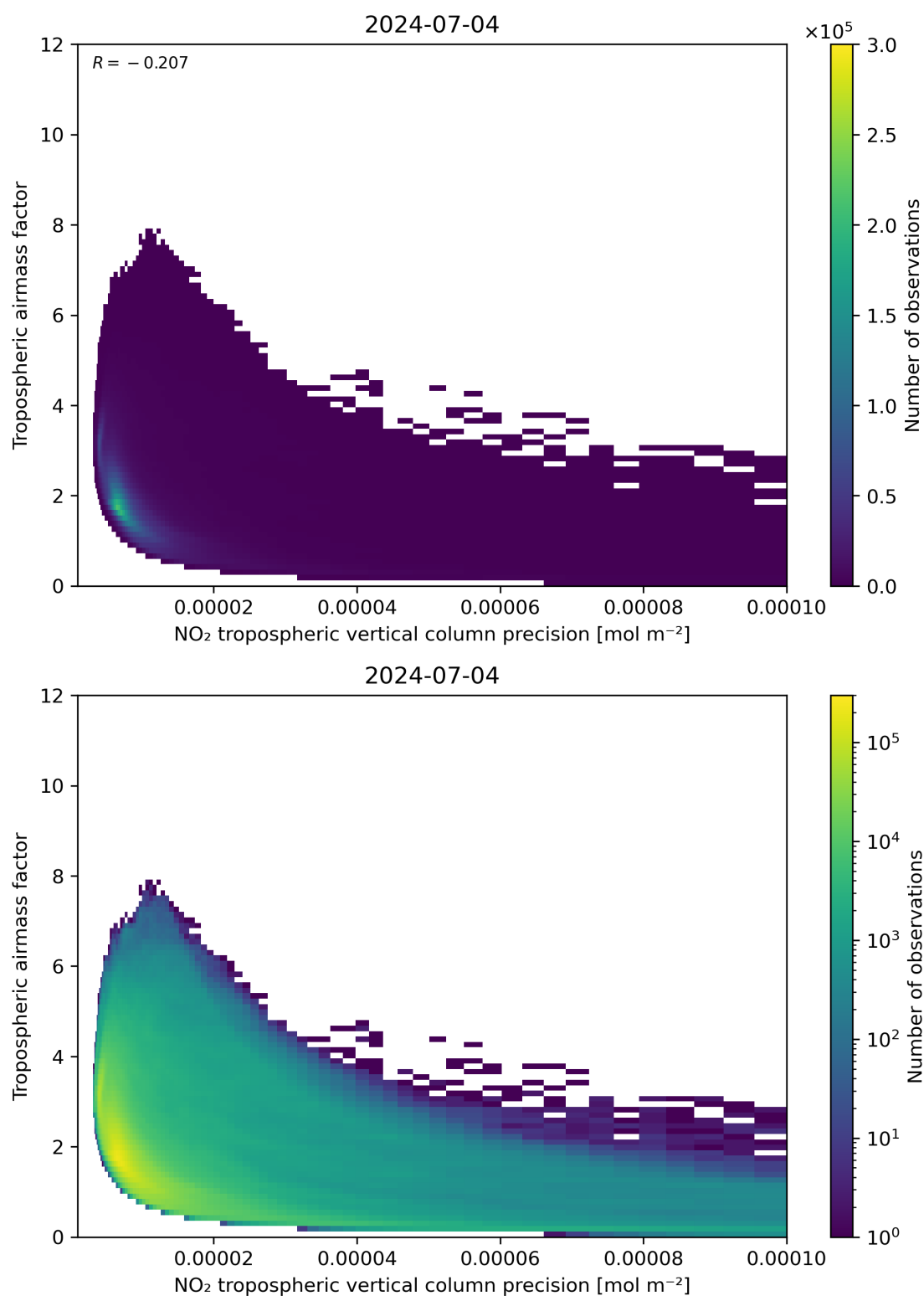
Figure 133: Scatter density plot of “NO 2 tropospheric vertical column precision” against “Tropospheric air mass factor” for 2024-07-03 to 2024-07-05.
