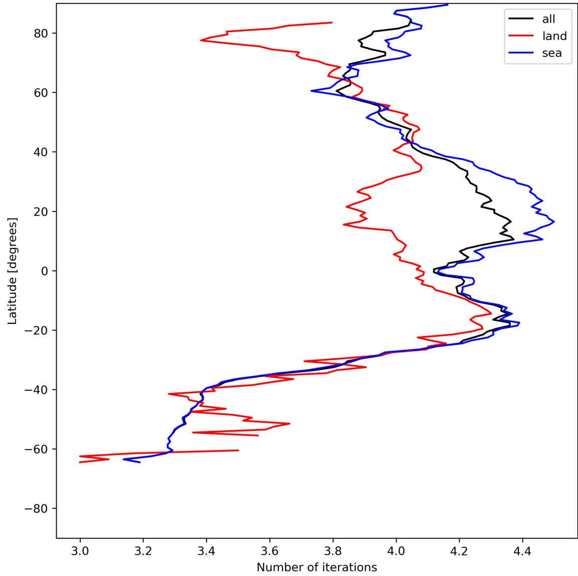
Figure 17: Zonal average of “Number of iterations” for 2024-07-03 to 2024-07-05.
