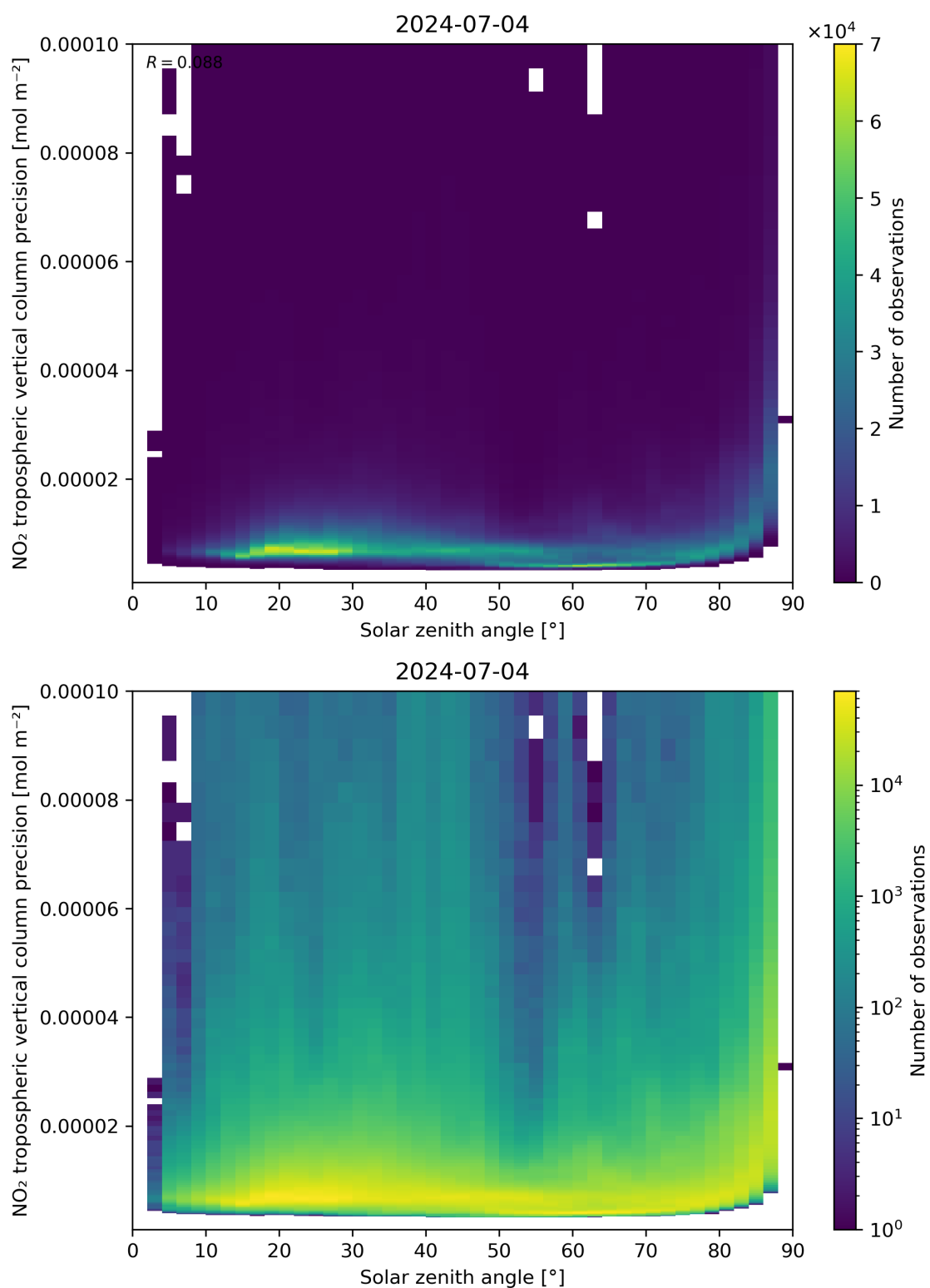
Figure 156: Scatter density plot of “Solar zenith angle” against “NO 2 tropospheric vertical column precision” for 2024-07-03 to 2024-07-05.
