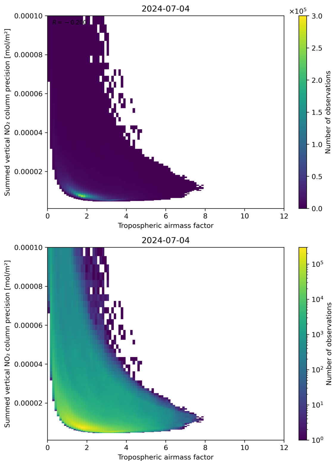
Figure 76: Scatter density plot of “Tropospheric air mass factor” against “Summed vertical NO 2 column precision” for 2024-07-03 to 2024-07-05.
