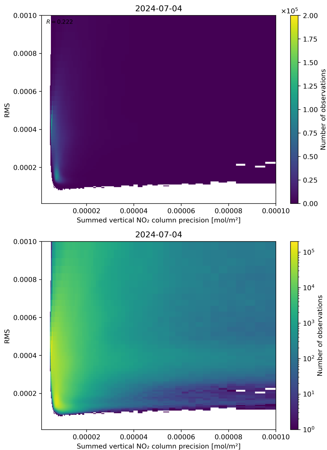
Figure 108: Scatter density plot of “Summed vertical NO 2 column precision” against “RMS” for 2024-07-03 to 2024-07-05.
