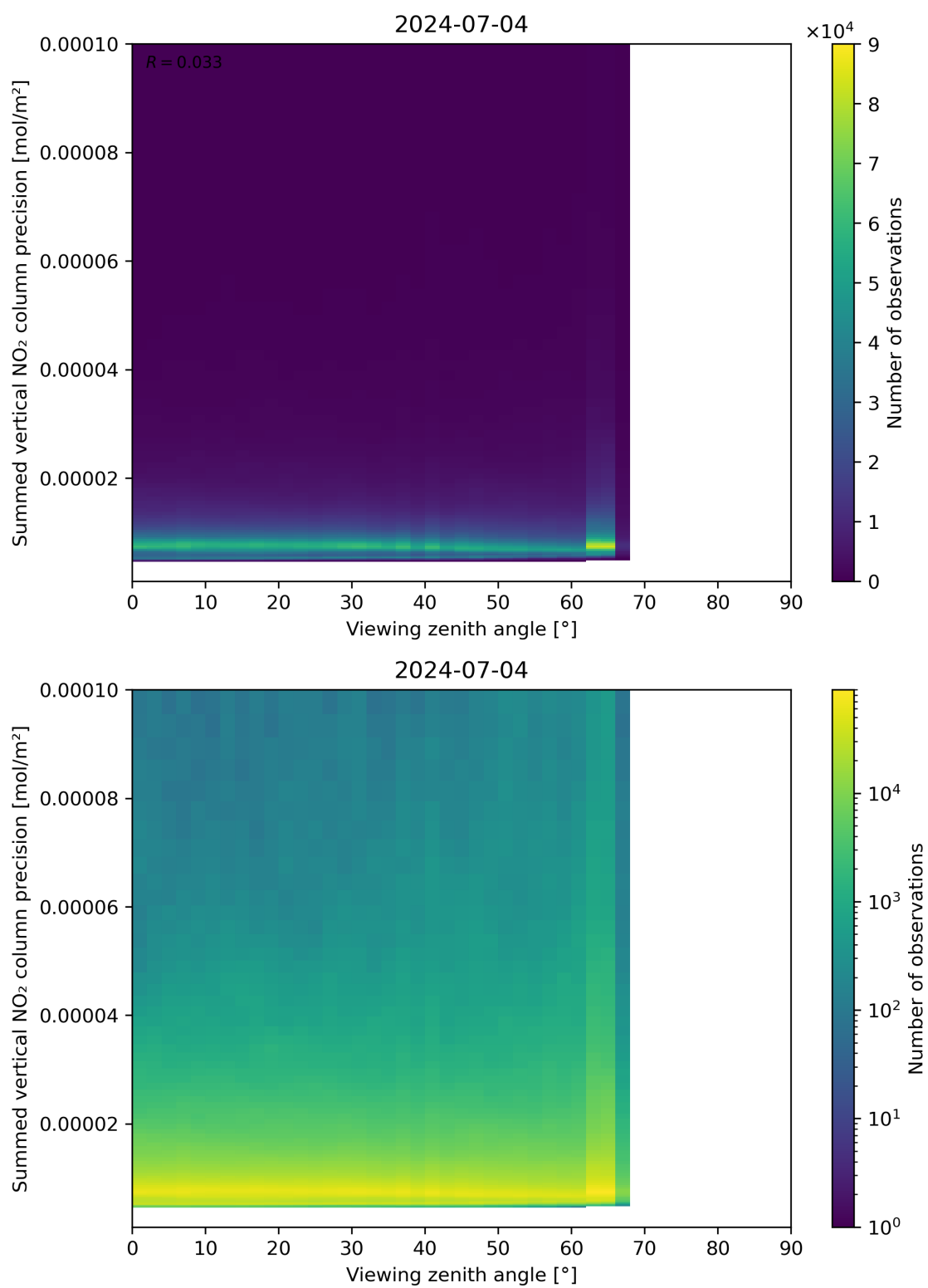
Figure 166: Scatter density plot of “Viewing zenith angle” against “Summed vertical NO 2 column precision” for 2024-07-03 to 2024-07-05.
