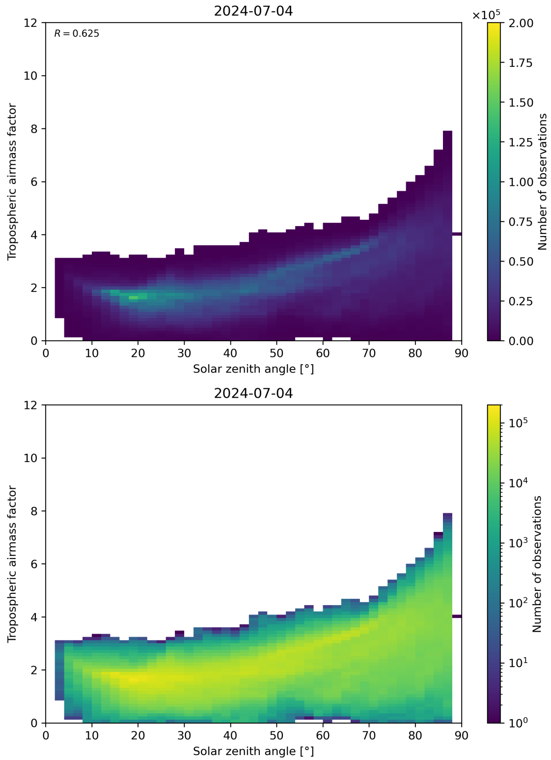
Figure 147: Scatter density plot of “Solar zenith angle” against “Tropospheric airmass factor” for 2024-07-03 to 2024-07-05.
