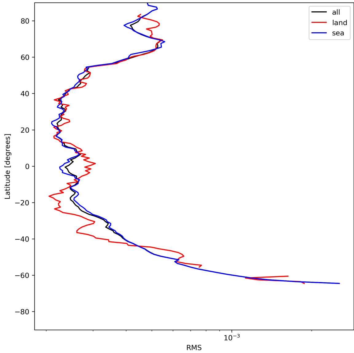
Figure 26: Zonal average of “RMS” for 2024-07-03 to 2024-07-05.
