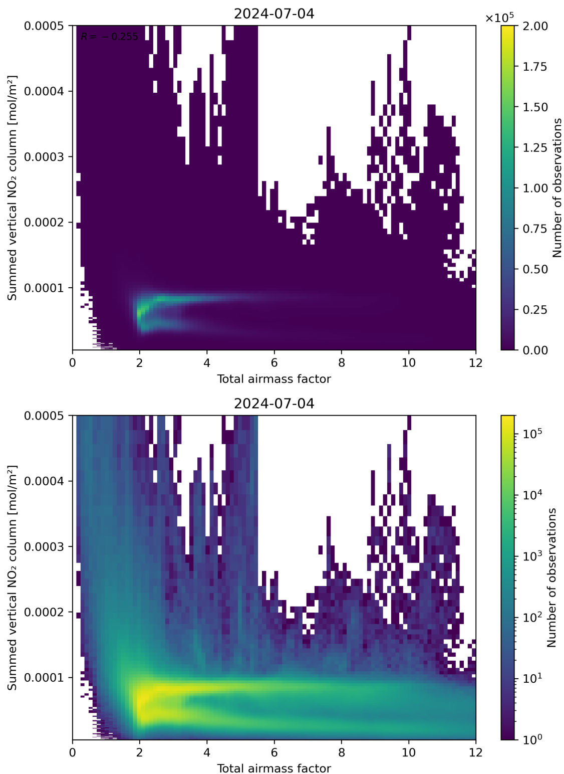
Figure 65: Scatter density plot of “Total airmass factor” against “Summed vertical NO 2 column” for 2024-07-03 to 2024-07-05.
