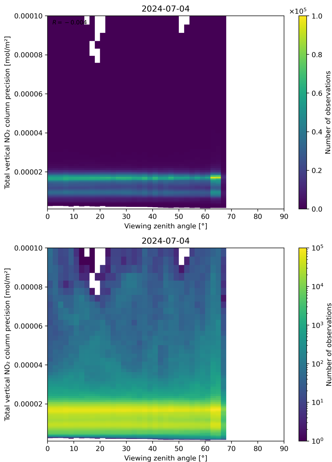
Figure 168: Scatter density plot of “Viewing zenith angle” against “Total vertical NO 2 column precision” for 2024-07-03 to 2024-07-05.
