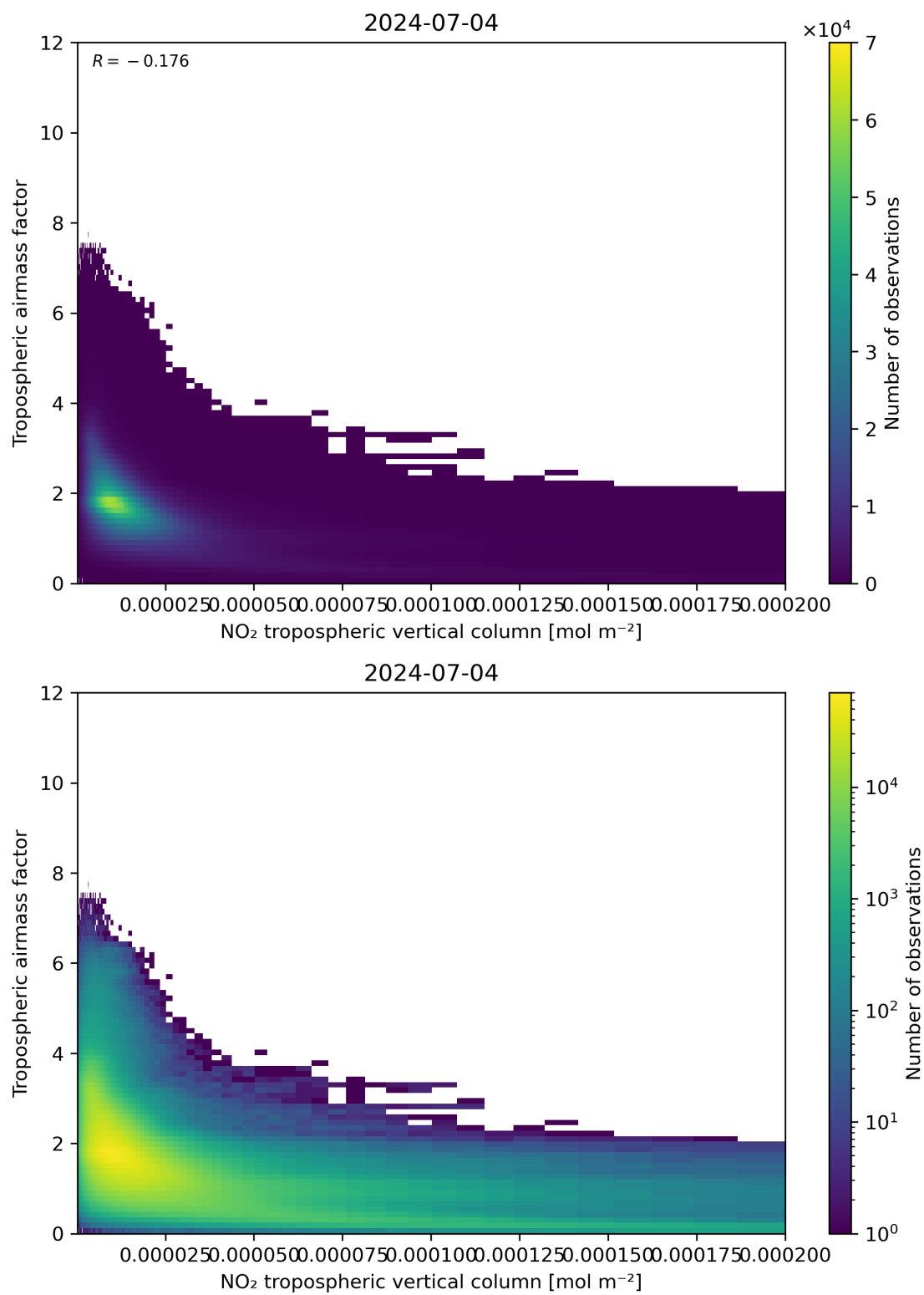
Figure 123: Scatter density plot of “NO 2 tropospheric vertical column” against “Tropospheric air mass factor” for 2024-07-03 to 2024-07-05.
