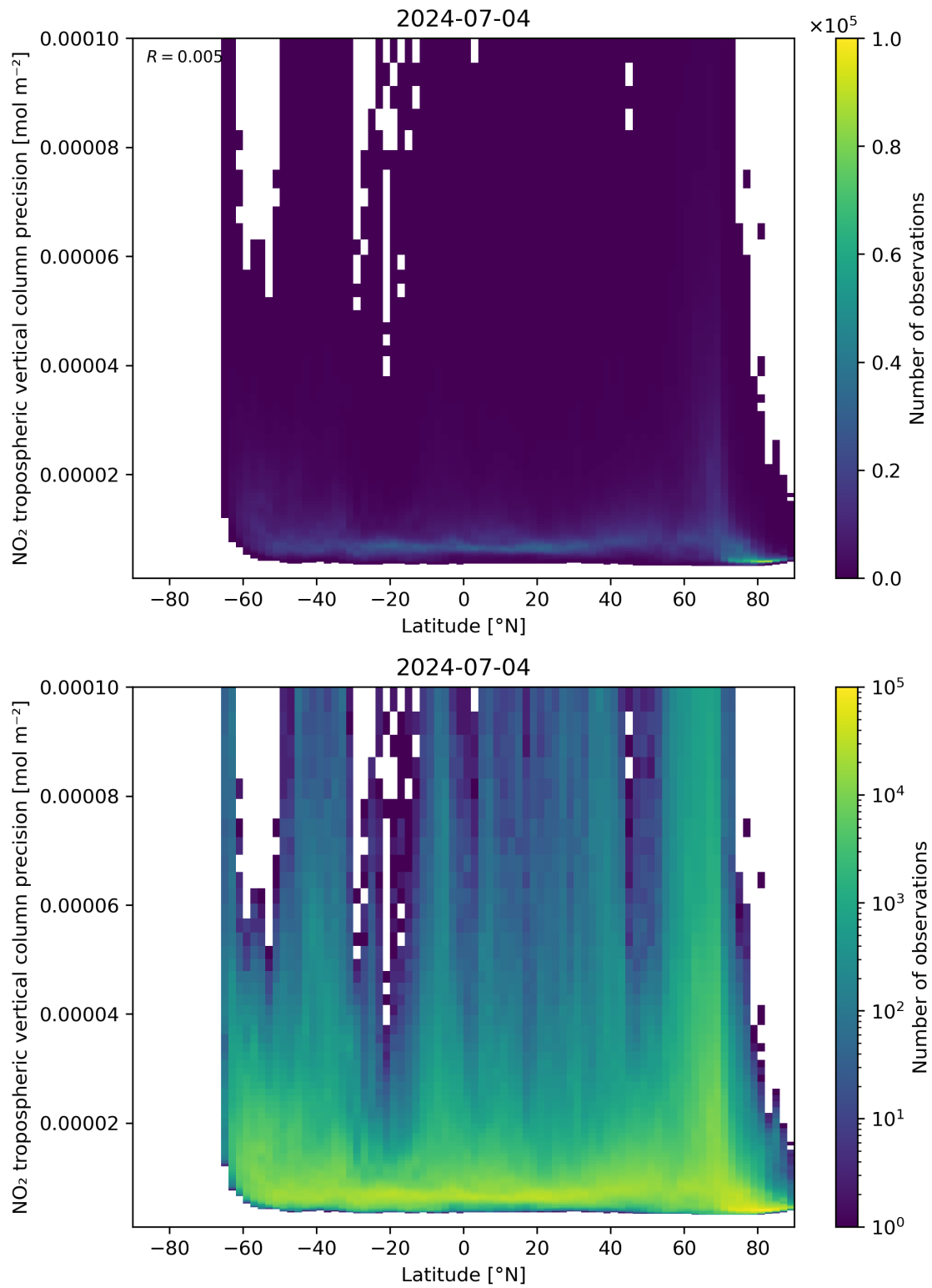
Figure 93: Scatter density plot of “Latitude” against “NO 2 tropospheric vertical column precision” for 2024-07-03 to 2024-07-05.
