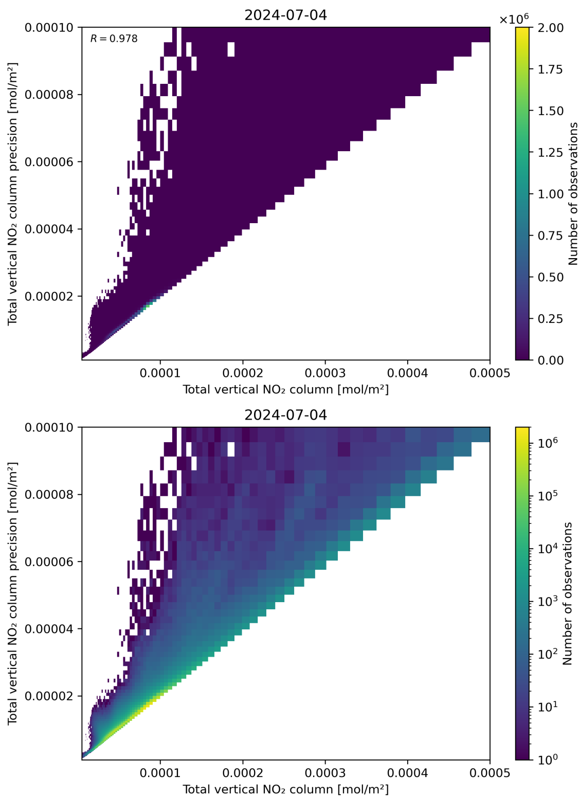
Figure 114: Scatter density plot of “Total vertical NO 2 column” against “Total vertical NO 2 column precision” for 2024-07-03 to 2024-07-05.
