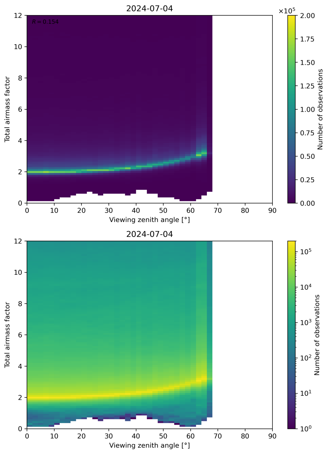
Figure 160: Scatter density plot of “Viewing zenith angle” against “Total airmass factor” for 2024-07-03 to 2024-07-05.
