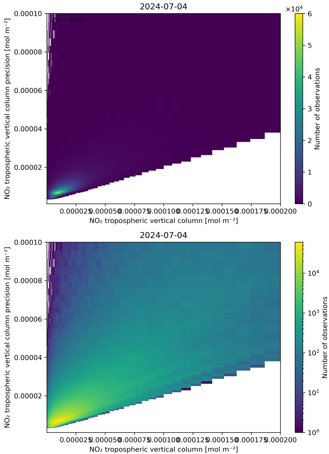
Figure 130: Scatter density plot of “NO 2 tropospheric vertical column” against “NO 2 tropospheric vertical column precision” for 2024-07-03 to 2024-07-05.
