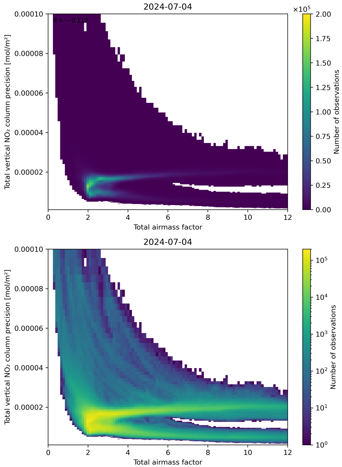
Figure 68: Scatter density plot of “Total airmass factor” against “Total vertical NO 2 column precision” for 2024-07-03 to 2024-07-05.
