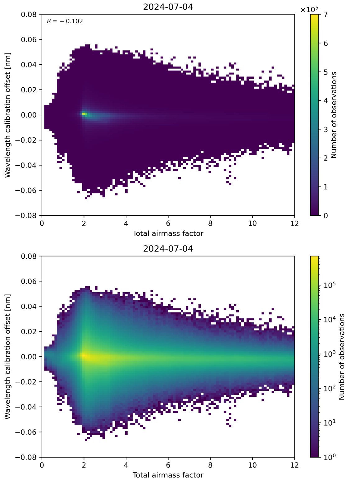
Figure 70: Scatter density plot of “Total airmass factor” against “Wavelength calibration offset” for 2024-07-03 to 2024-07-05.
