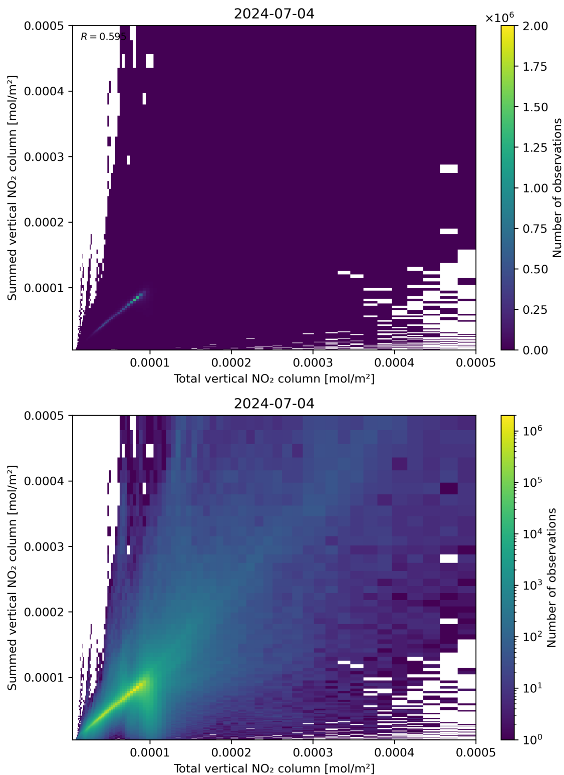
Figure 112: Scatter density plot of “Total vertical NO 2 column” against “Summed vertical NO 2 column” for 2024-07-03 to 2024-07-05.
