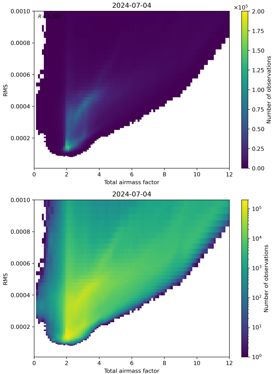
Figure 69: Scatter density plot of “Total airmass factor” against “RMS” for 2024-07-03 to 2024-07-05.
