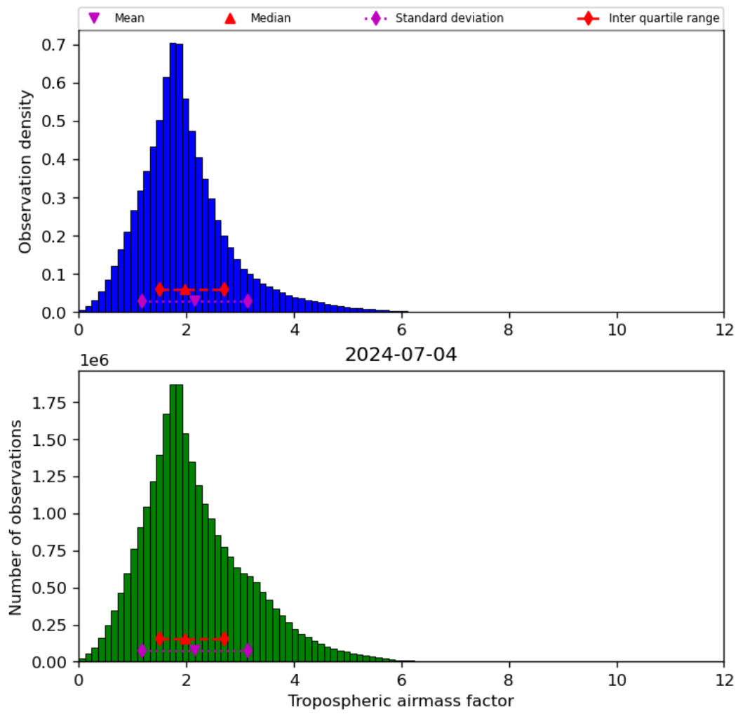
Figure 31: Histogram of “Tropospheric airmass factor” for 2024-07-03 to 2024-07-05
