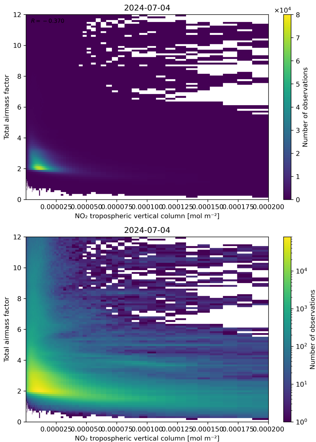
Figure 122: Scatter density plot of “NO 2 tropospheric vertical column” against “Total air mass factor” for 2024-07-03 to 2024-07-05.
