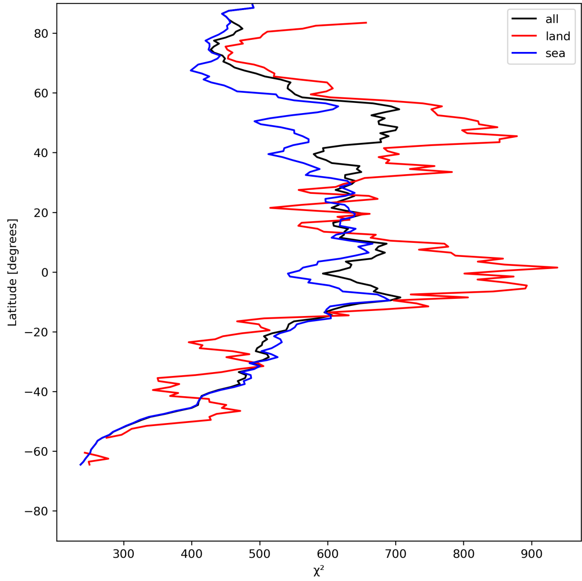
Figure 25: Zonal average of “ \chi^2 ” for 2024-07-03 to 2024-07-05.
