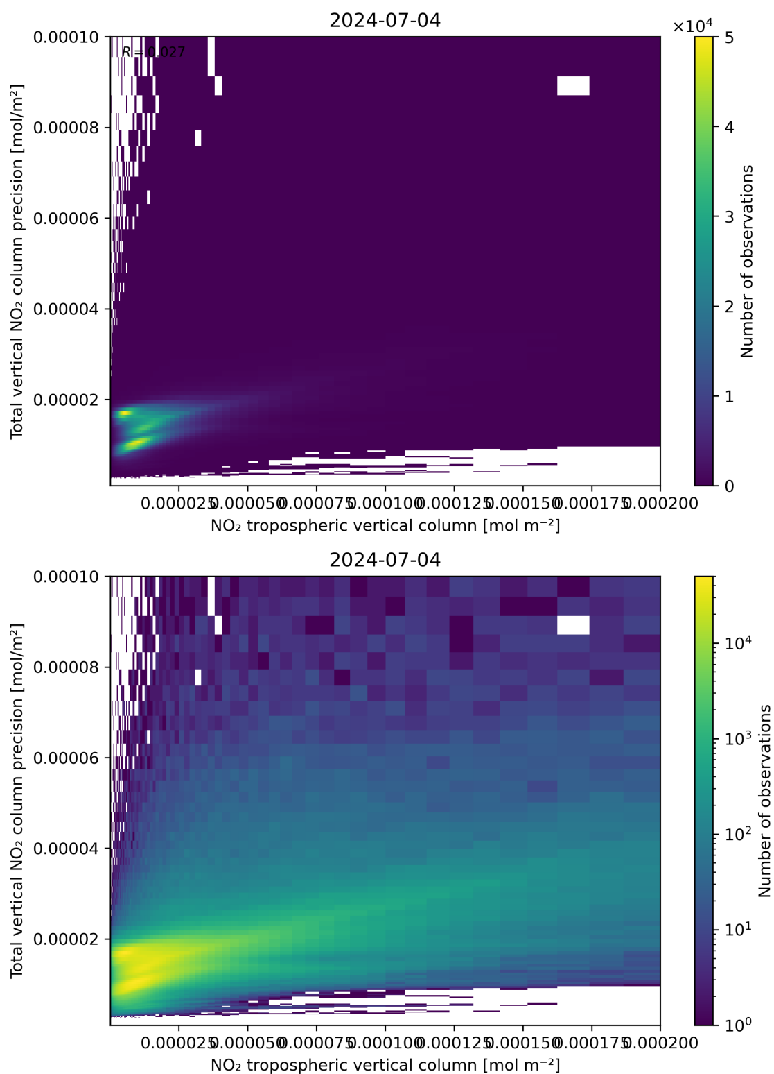
Figure 129: Scatter density plot of “NO 2 tropospheric vertical column” against “Total vertical NO 2 column precision” for 2024-07-03 to 2024-07-05.
