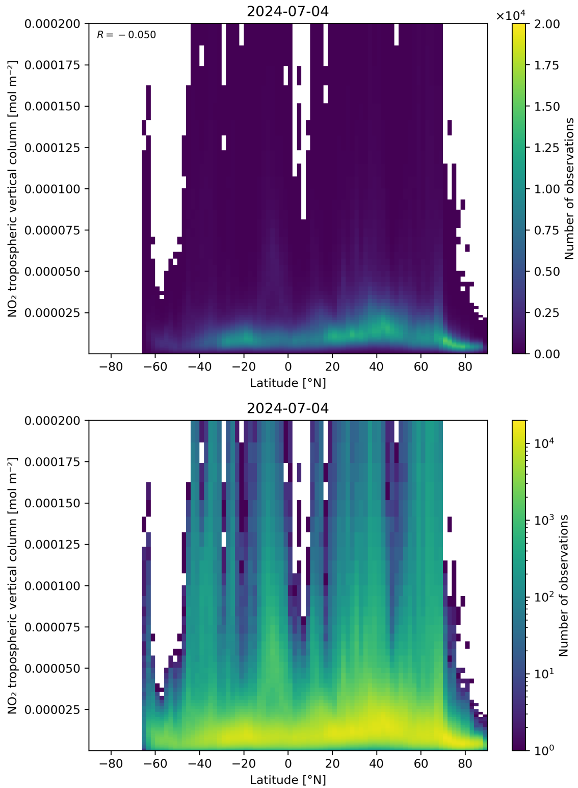
Figure 92: Scatter density plot of “Latitude” against “NO 2 tropospheric vertical column” for 2024-07-03 to 2024-07-05.
