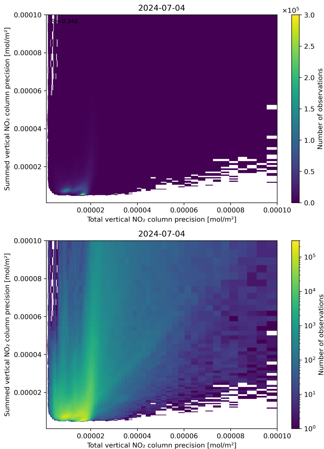
Figure 118: Scatter density plot of “Total vertical NO 2 column precision” against “Summed vertical NO 2 column precision” for 2024-07-03 to 2024-07-05.
