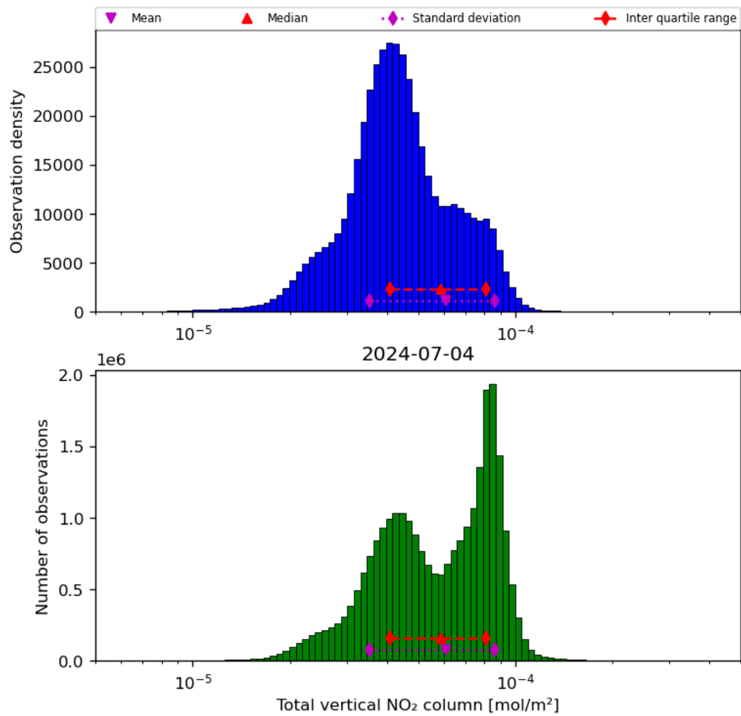
Figure 38: Histogram of “Total vertical NO 2 column” for 2024-07-03 to 2024-07-05
