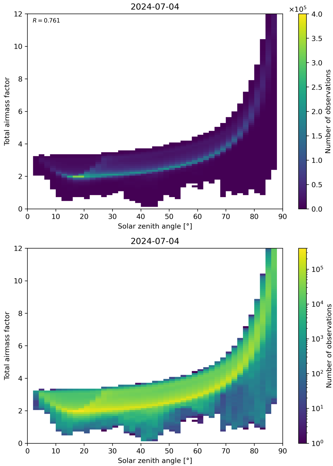
Figure 146: Scatter density plot of “Solar zenith angle” against “Total air mass factor” for 2024-07-03 to 2024-07-05.
