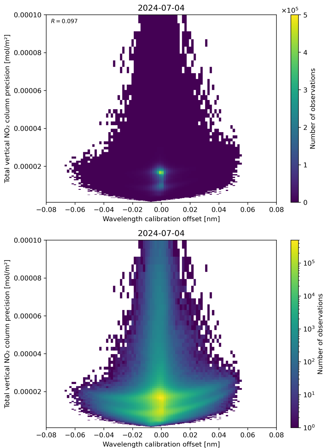
Figure 180: Scatter density plot of “Wavelength calibration offset” against “Total vertical NO 2 column precision” for 2024-07-03 to 2024-07-05.
