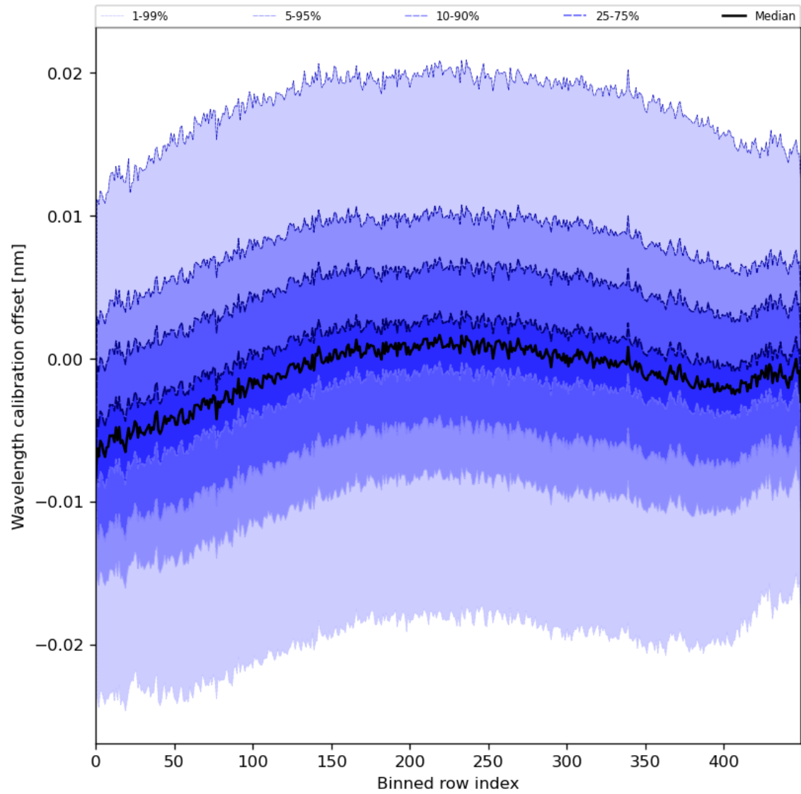
Figure 52: Along track statistics of “Wavelength calibration offset” for 2024-07-03 to 2024-07-05
