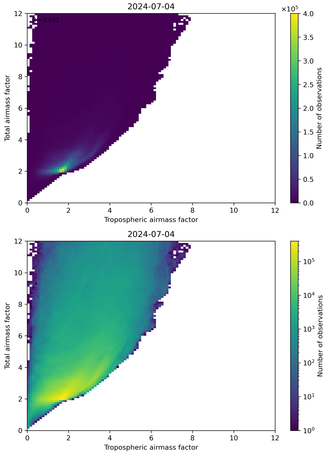
Figure 72: Scatter density plot of “Tropospheric airmass factor” against “Total airmass factor” for 2024-07-03 to 2024-07-05.
