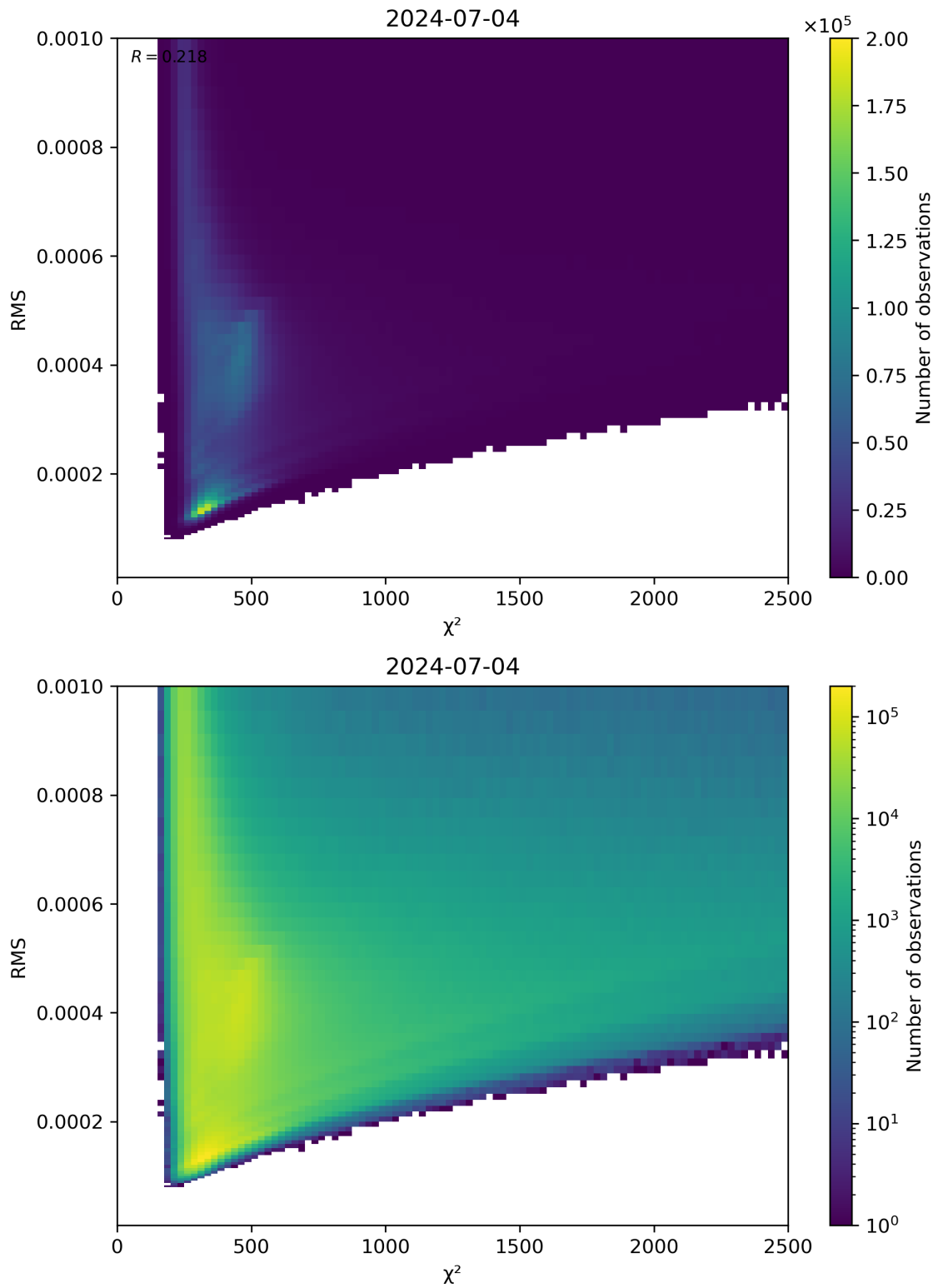
Figure 82: Scatter density plot of “ \chi^2 ” against “RMS” for 2024-07-03 to 2024-07-05.
