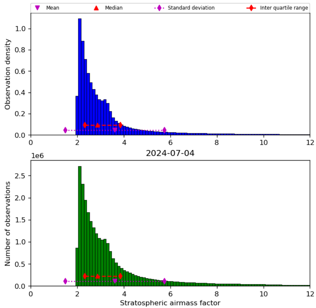
Figure 44: Histogram of “Stratospheric airmass factor” for 2024-07-03 to 2024-07-05
