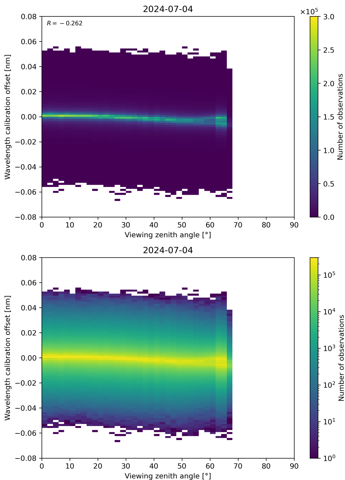
Figure 173: Scatter density plot of “Viewing zenith angle” against “Wavelength calibration offset” for 2024-07-03 to 2024-07-05.
