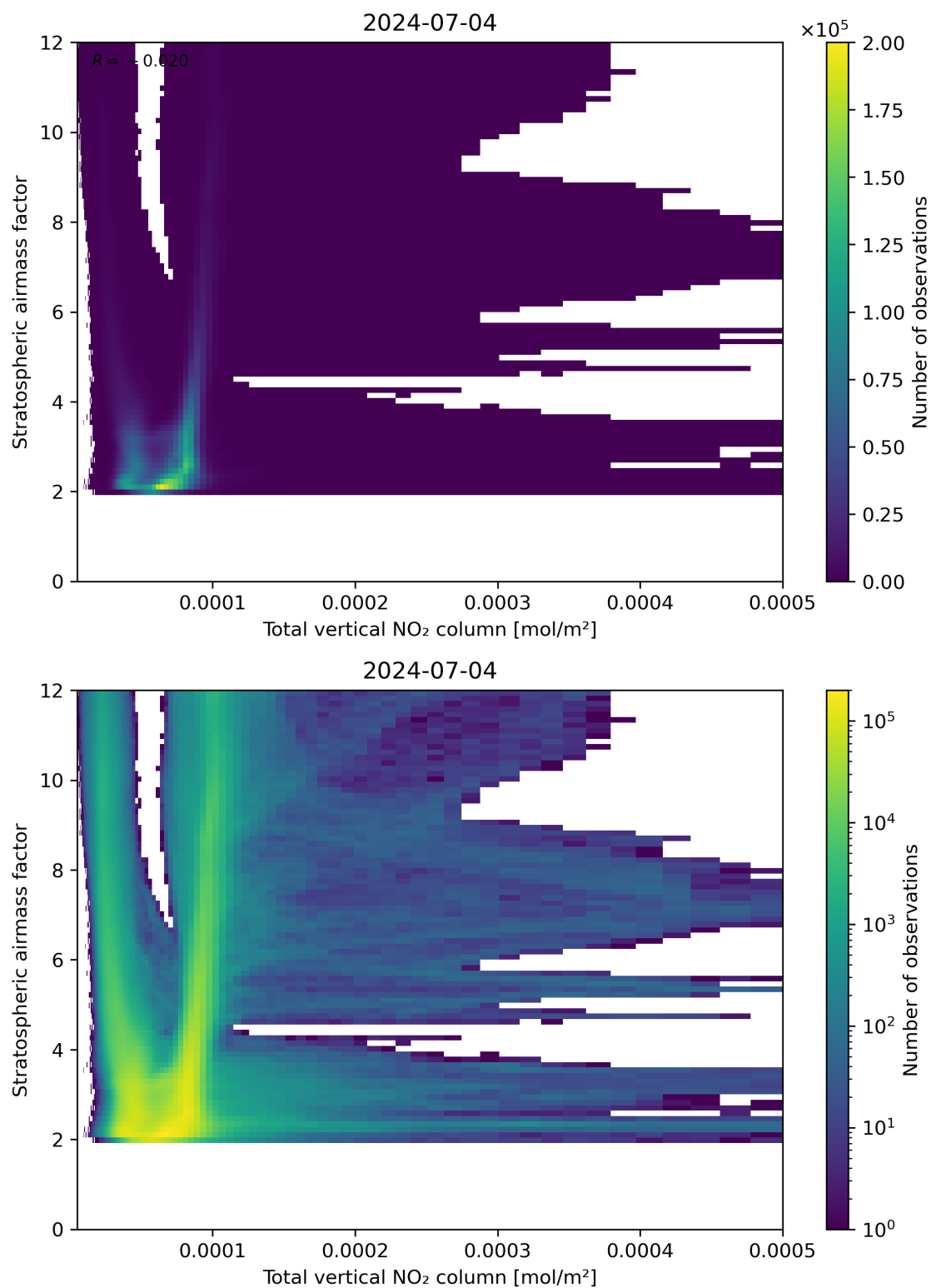
Figure 110: Scatter density plot of “Total vertical NO 2 column” against “Stratospheric airmass factor” for 2024-07-03 to 2024-07-05.
