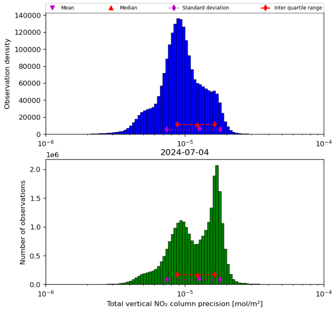
Figure 39: Histogram of “Total vertical NO 2 column precision” for 2024-07-03 to 2024-07-05
