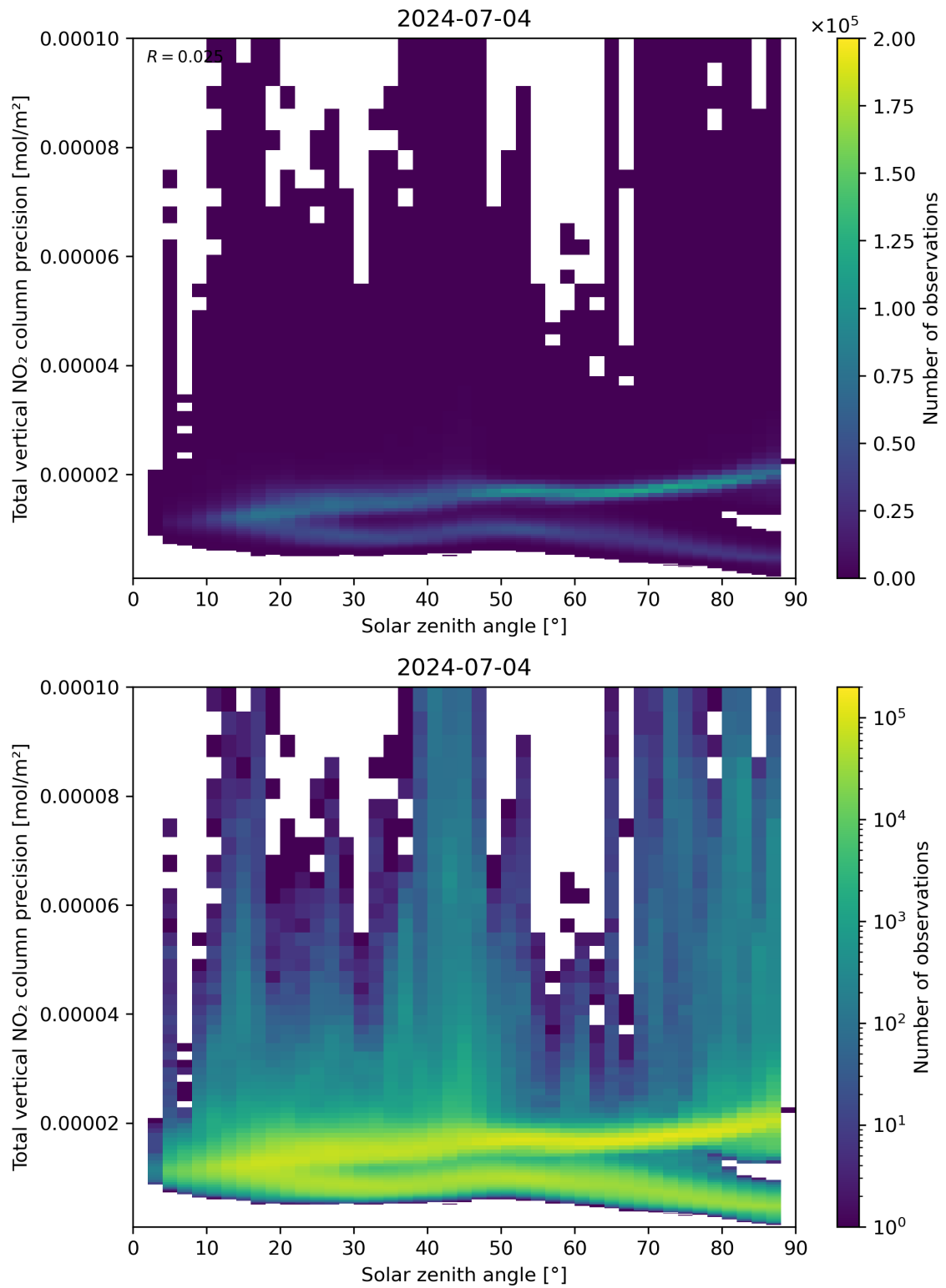
Figure 154: Scatter density plot of “Solar zenith angle” against “Total vertical NO 2 column precision” for 2024-07-03 to 2024-07-05.
