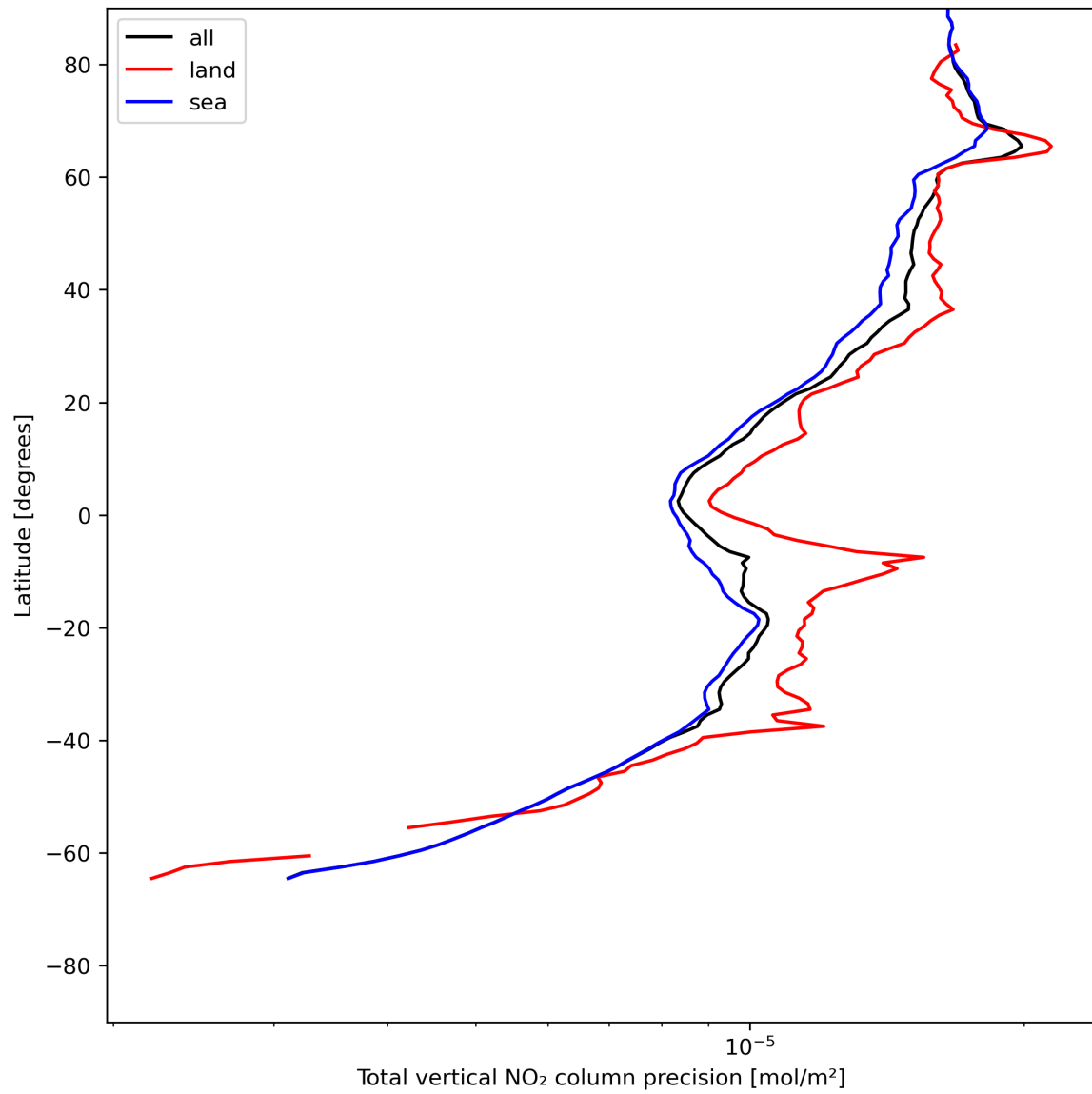
Figure 22: Zonal average of “Total vertical NO 2 column precision” for 2024-07-03 to 2024-07-05.
