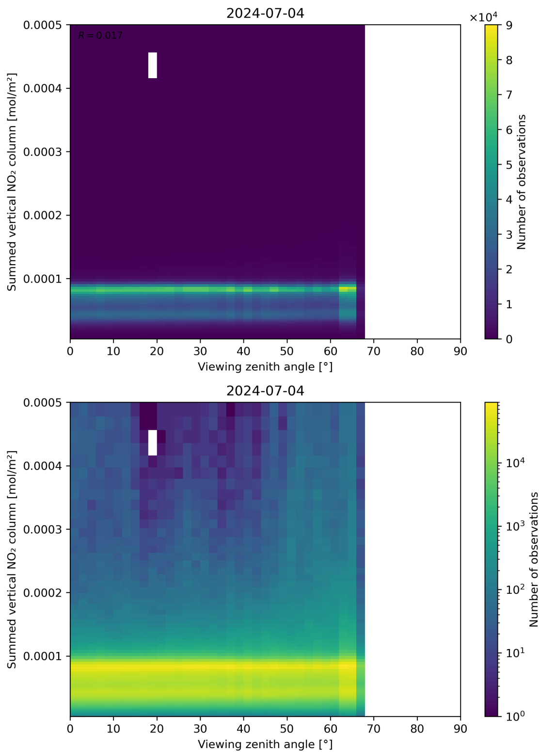
Figure 165: Scatter density plot of “Viewing zenith angle” against “Summed vertical NO 2 column” for 2024-07-03 to 2024-07-05.
