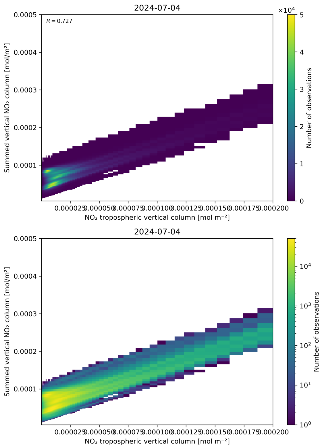
Figure 126: Scatter density plot of “NO 2 tropospheric vertical column” against “Summed vertical NO 2 column” for 2024-07-03 to 2024-07-05.
