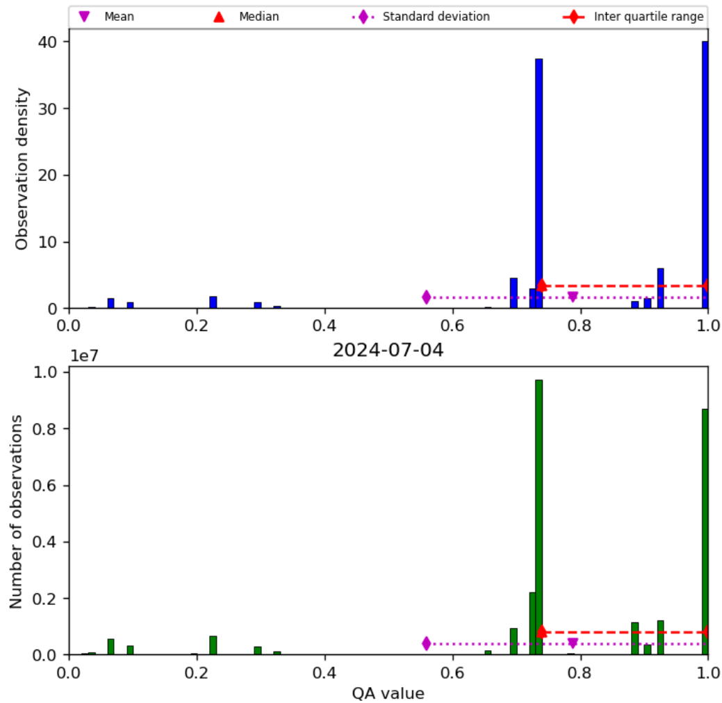
Figure 28: Histogram of “QA value” for 2024-07-03 to 2024-07-05
