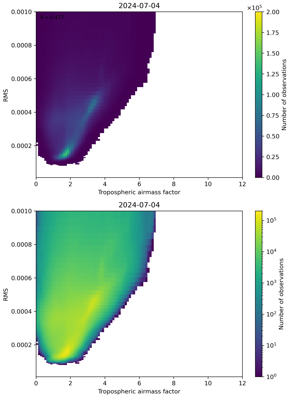
Figure 79: Scatter density plot of “Tropospheric airmass factor” against “RMS” for 2024-07-03 to 2024-07-05.
