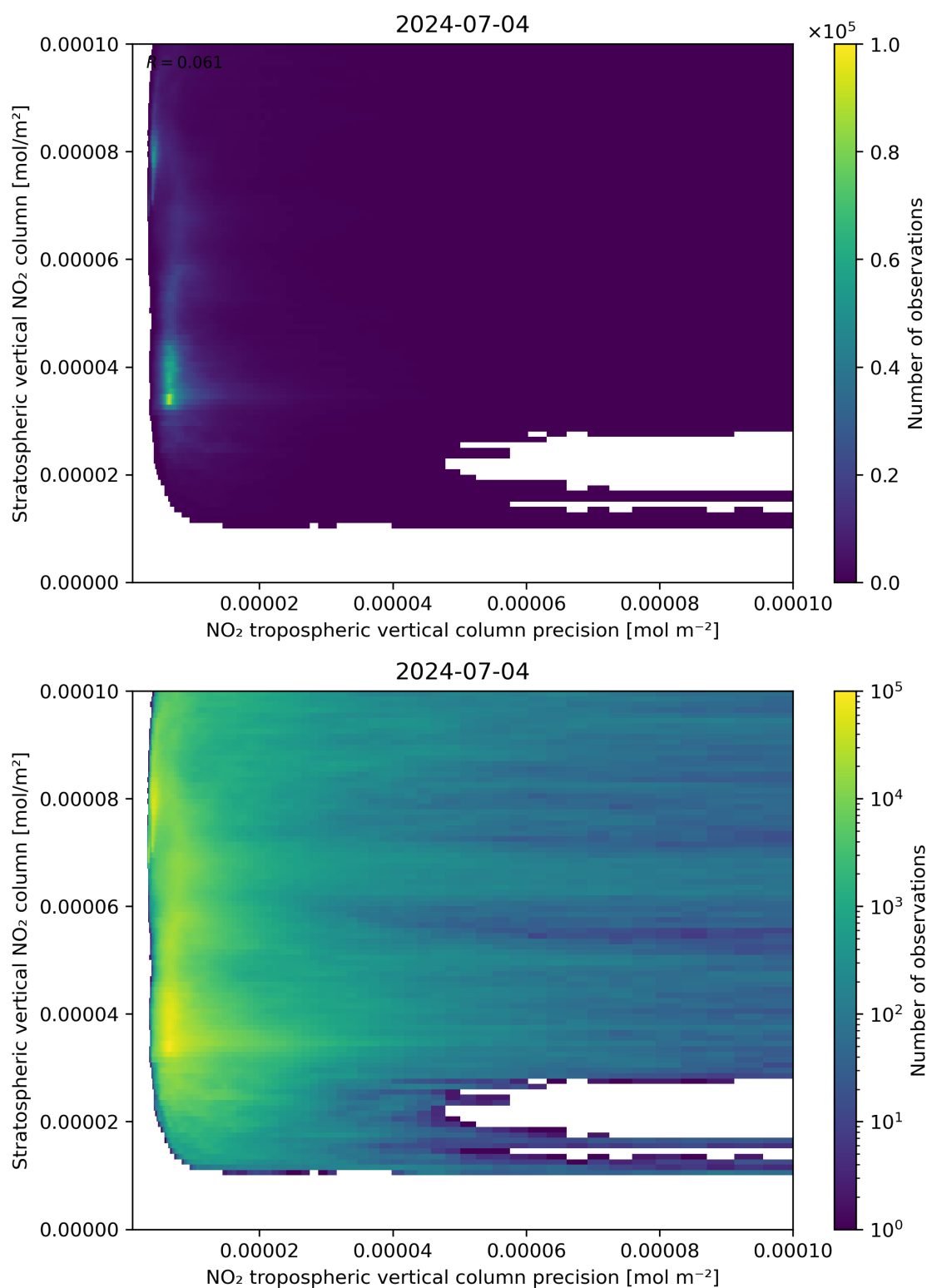
Figure 135: Scatter density plot of “NO 2 tropospheric vertical column precision” against “Stratospheric vertical NO 2 column” for 2024-07-03 to 2024-07-05.
