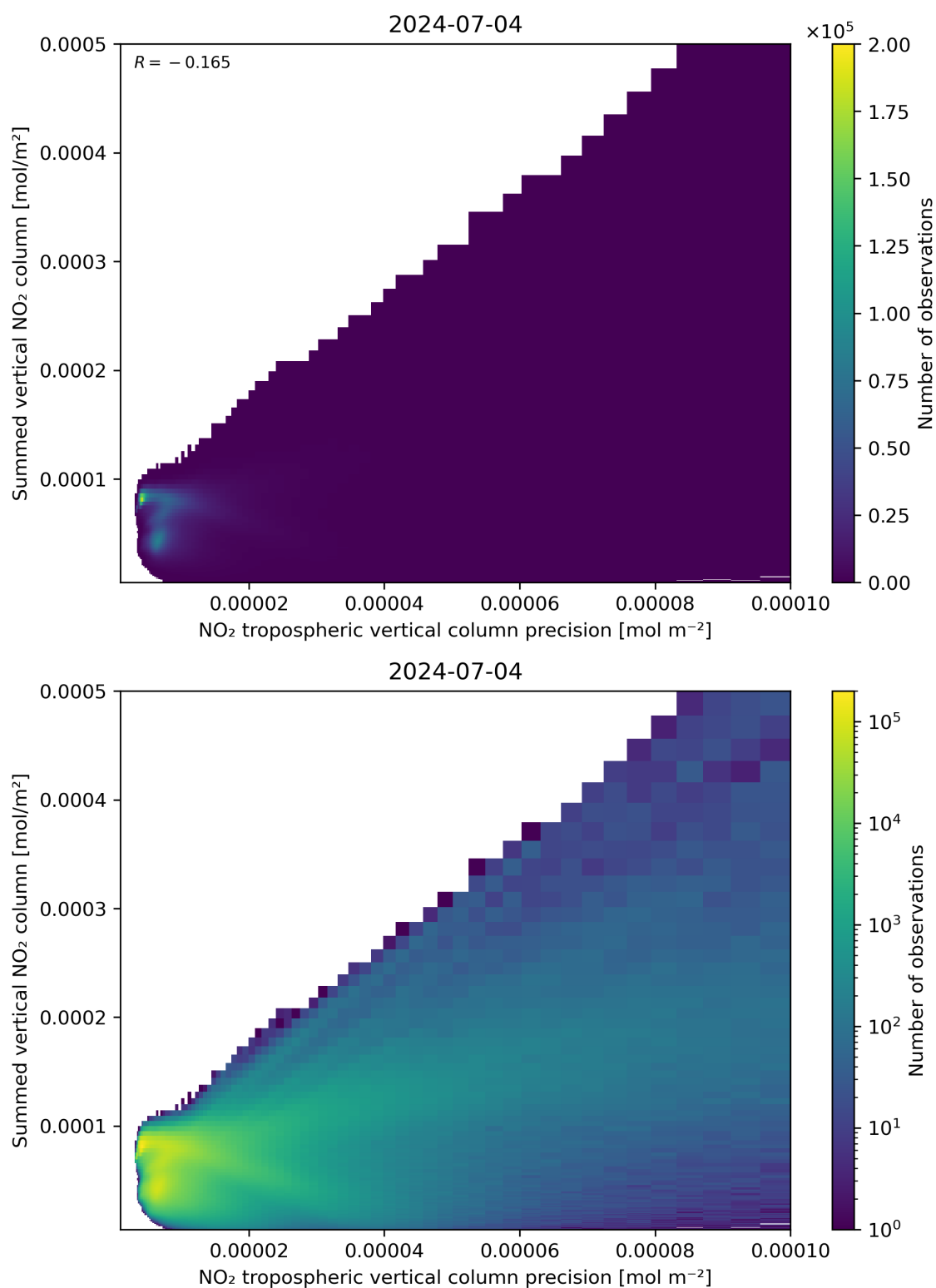
Figure 136: Scatter density plot of “NO 2 tropospheric vertical column precision” against “Summed vertical NO 2 column” for 2024-07-03 to 2024-07-05.
