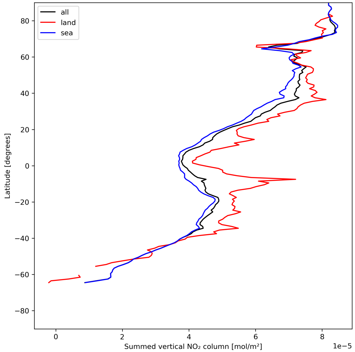
Figure 23: Zonal average of “Summed vertical NO 2 column” for 2024-07-03 to 2024-07-05.
