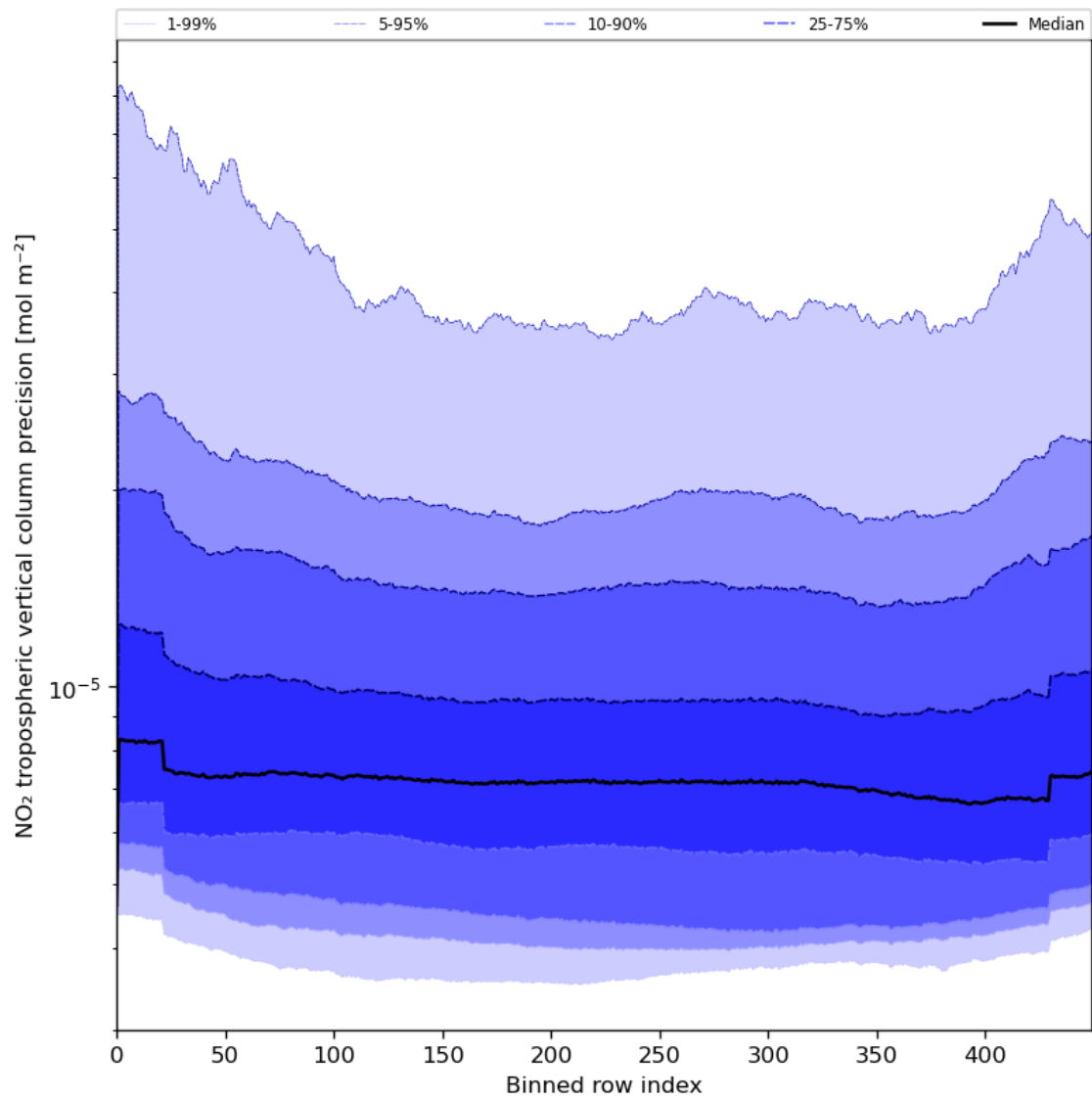
Figure 47: Along track statistics of “NO 2 tropospheric vertical column precision” for 2024-07-03 to 2024-07-05
