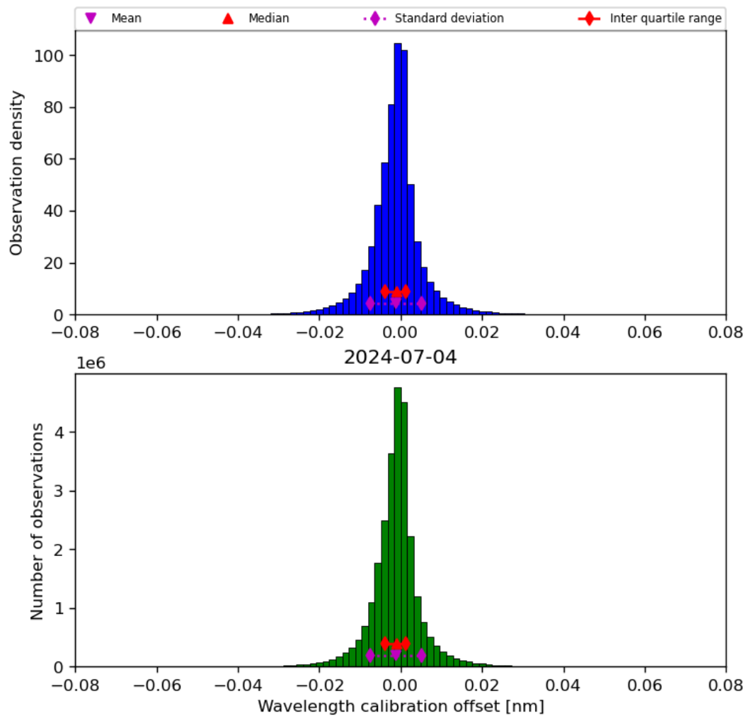
Figure 35: Histogram of “Wavelength calibration offset” for 2024-07-03 to 2024-07-05
