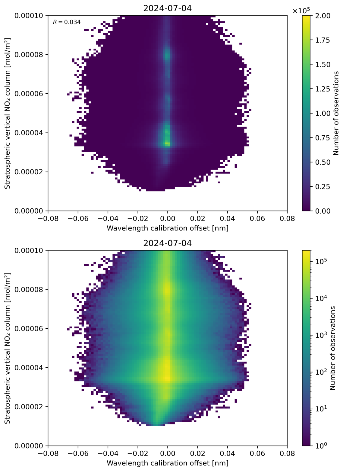
Figure 176: Scatter density plot of “Wavelength calibration offset” against “Stratospheric vertical NO 2 column” for 2024-07-03 to 2024-07-05.
