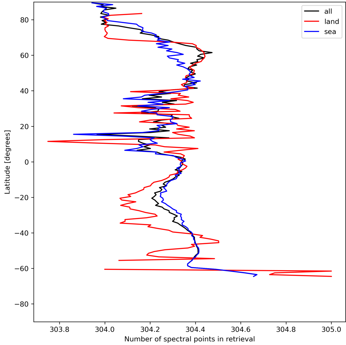
Figure 16: Zonal average of “Number of spectral points in retrieval” for 2024-07-03 to 2024-07-05.
