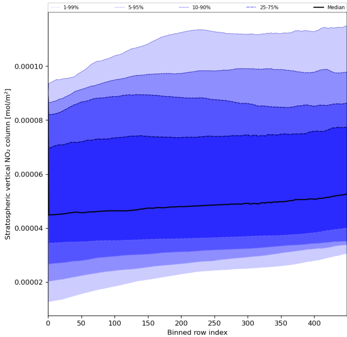
Figure 53: Along track statistics of “Stratospheric vertical NO 2 column” for 2024-07-03 to 2024-07-05
