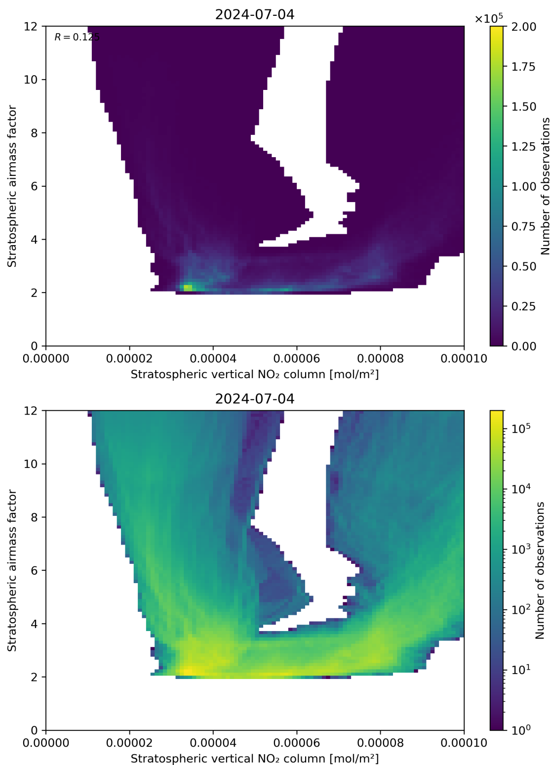
Figure 96: Scatter density plot of “Stratospheric vertical NO 2 column” against “Stratospheric airmass factor” for 2024-07-03 to 2024-07-05.
