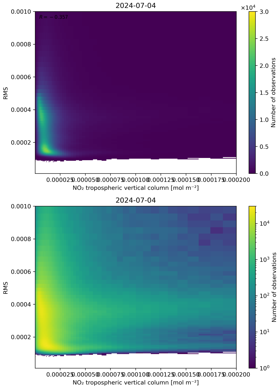
Figure 142: Scatter density plot of “NO 2 tropospheric vertical column” against “RMS” for 2024-07-03 to 2024-07-05.
