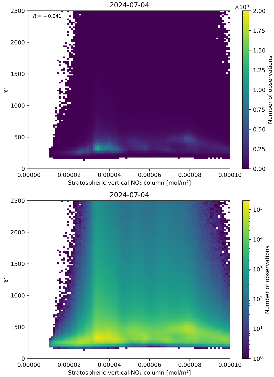
Figure 97: Scatter density plot of “Stratospheric vertical NO 2 column” against “ \chi^2 ” for 2024-07-03 to 2024-07-05.
