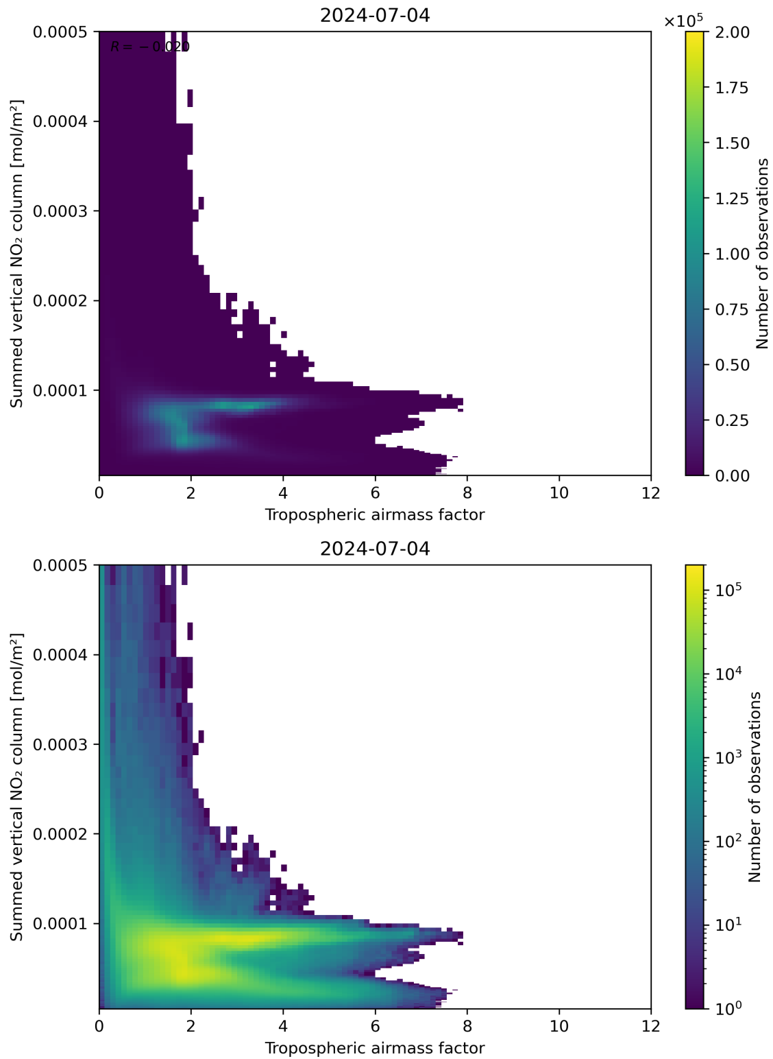
Figure 75: Scatter density plot of “Tropospheric airmass factor” against “Summed vertical NO 2 column” for 2024-07-03 to 2024-07-05.
