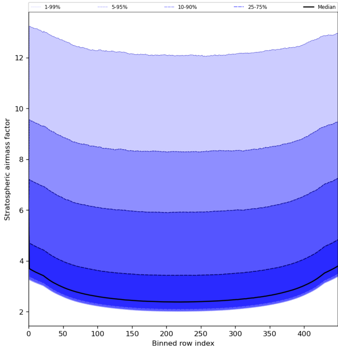
Figure 61: Along track statistics of “Stratospheric airmass factor” for 2024-07-03 to 2024-07-05
