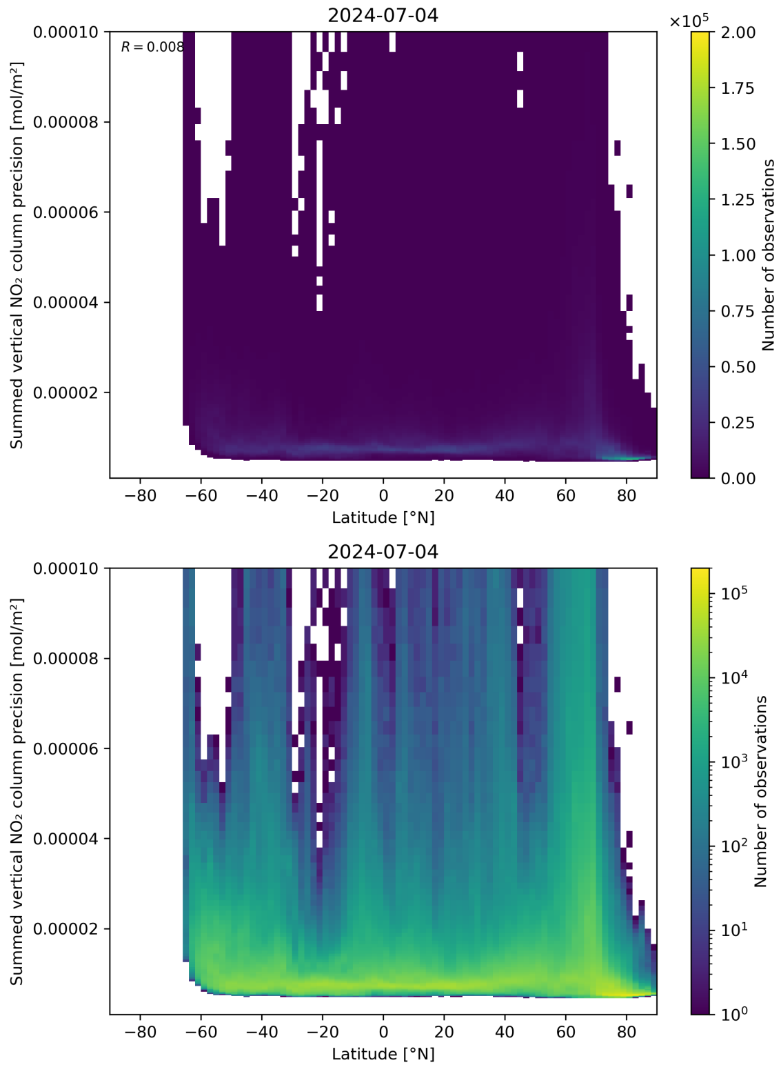
Figure 89: Scatter density plot of “Latitude” against “Summed vertical NO 2 column precision” for 2024-07-03 to 2024-07-05.
