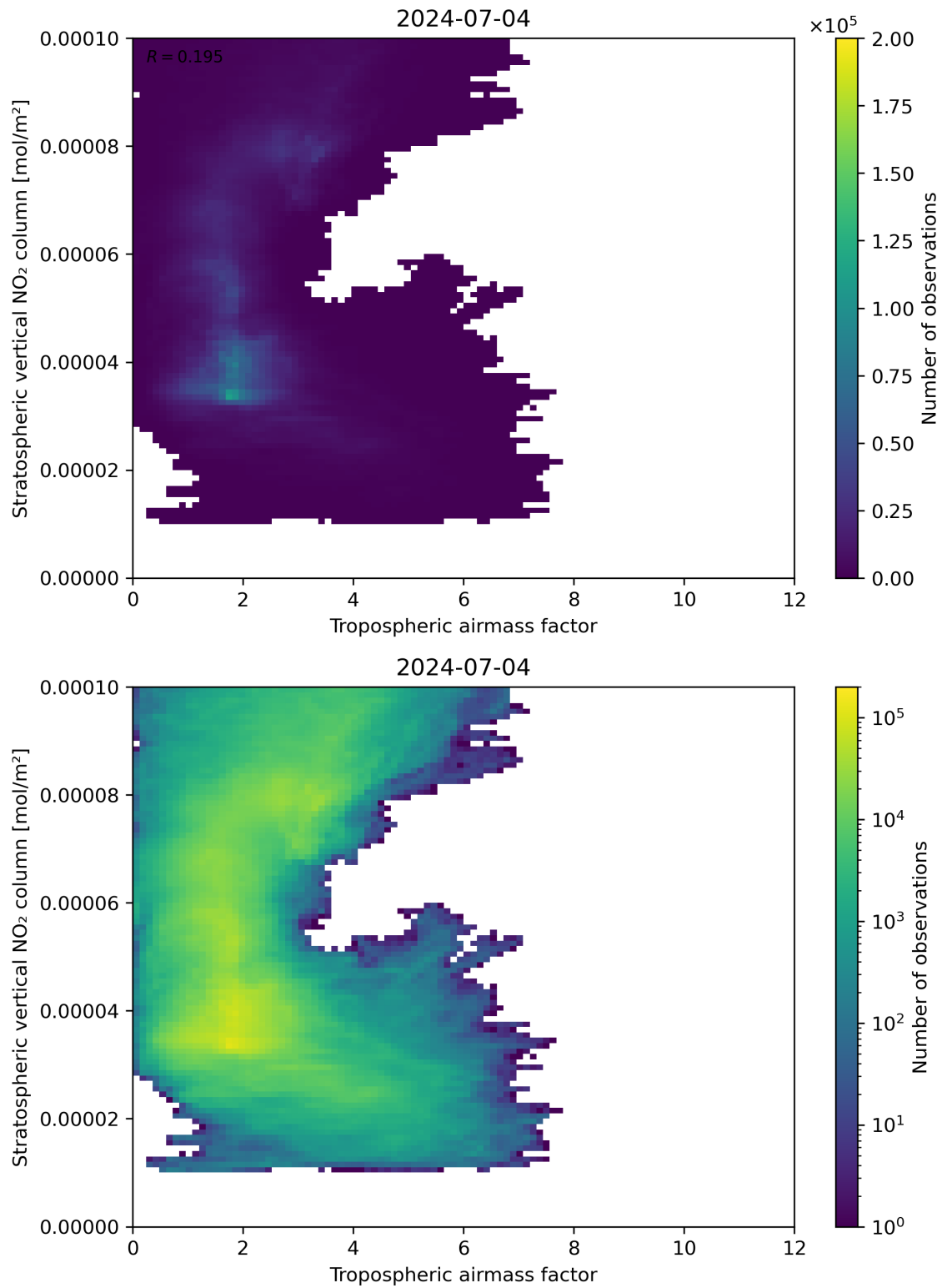
Figure 74: Scatter density plot of “Tropospheric air mass factor” against “Stratospheric vertical NO 2 column” for 2024-07-03 to 2024-07-05.
