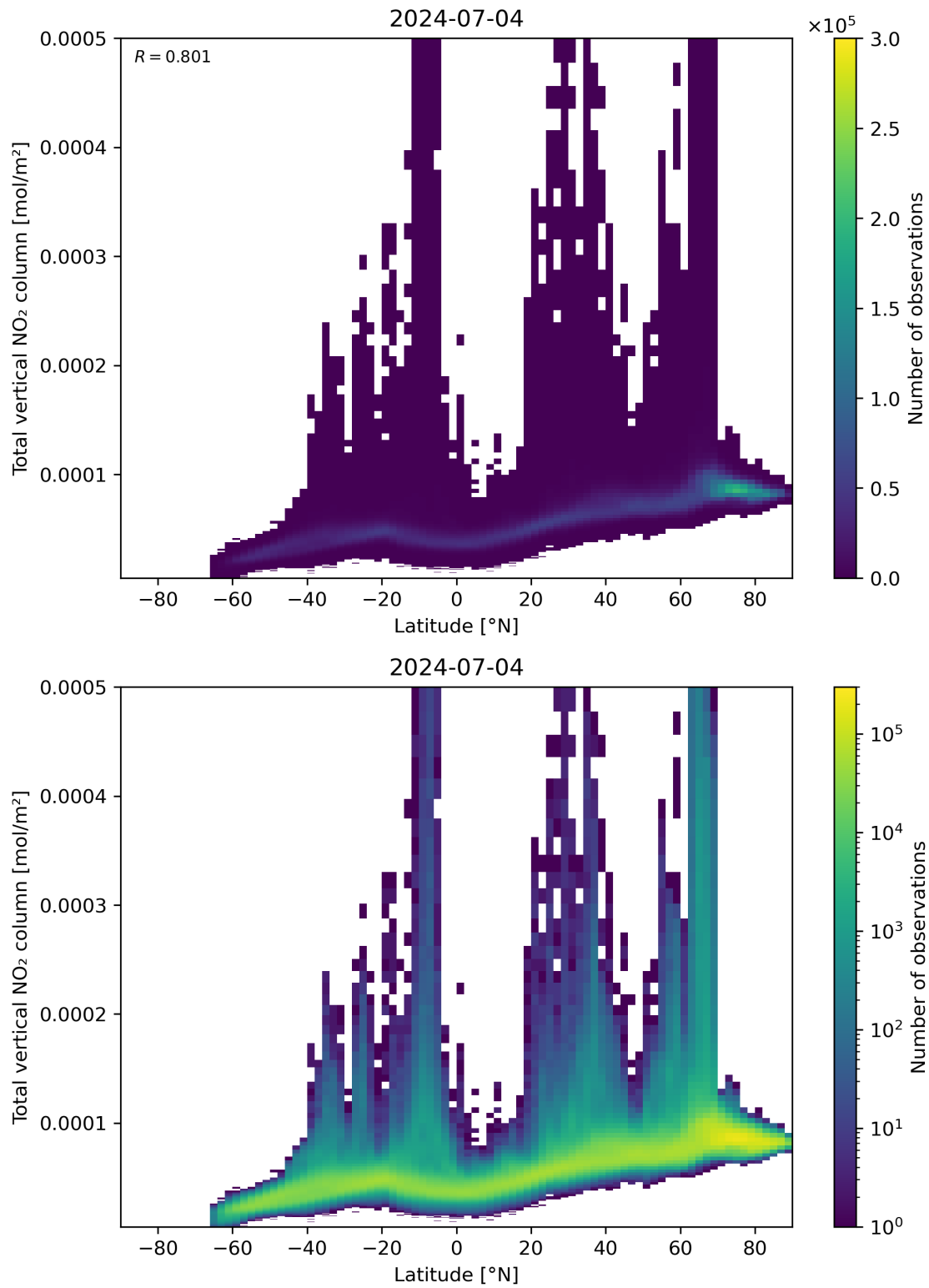
Figure 90: Scatter density plot of “Latitude” against “Total vertical NO 2 column” for 2024-07-03 to 2024-07-05.
