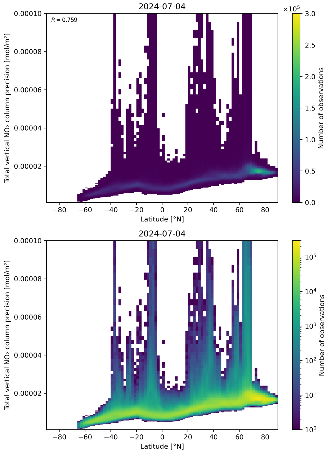
Figure 91: Scatter density plot of “Latitude” against “Total vertical NO 2 column precision” for 2024-07-03 to 2024-07-05.
