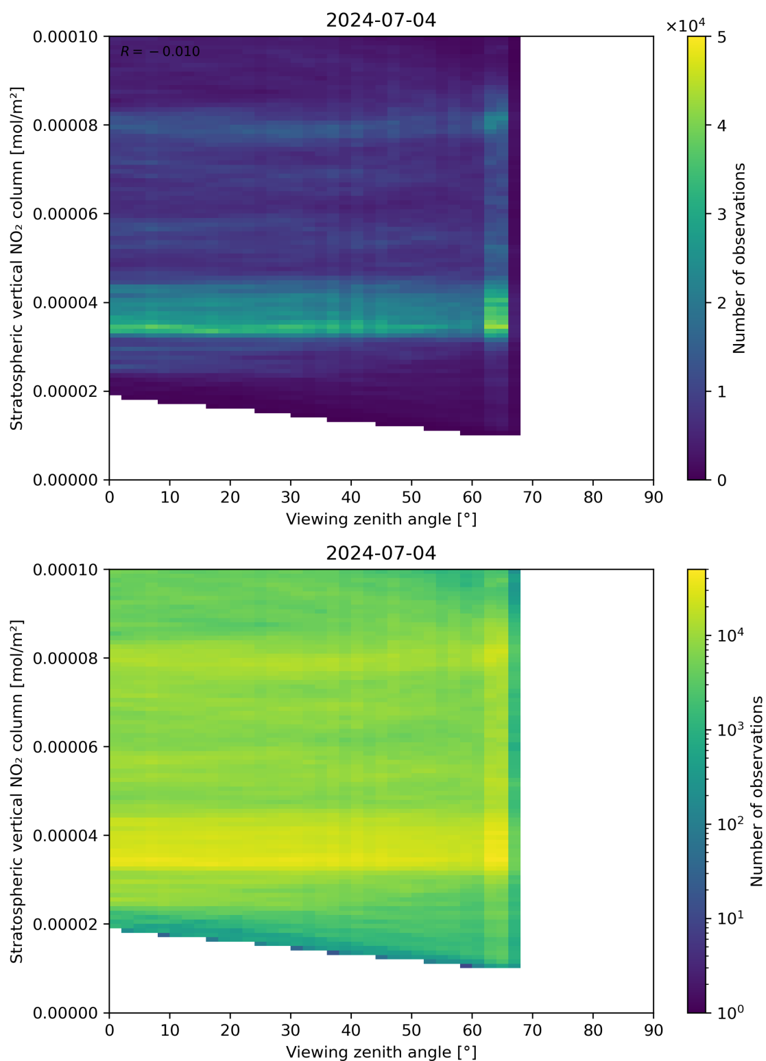
Figure 164: Scatter density plot of “Viewing zenith angle” against “Stratospheric vertical NO 2 column” for 2024-07-03 to 2024-07-05.
