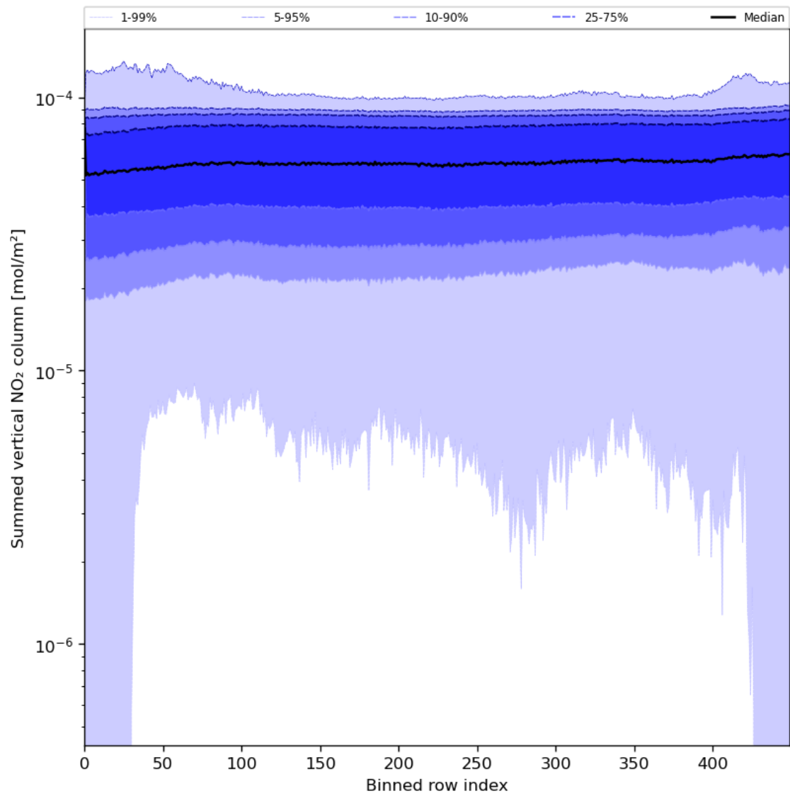
Figure 57: Along track statistics of “Summed vertical NO 2 column” for 2024-07-03 to 2024-07-05
