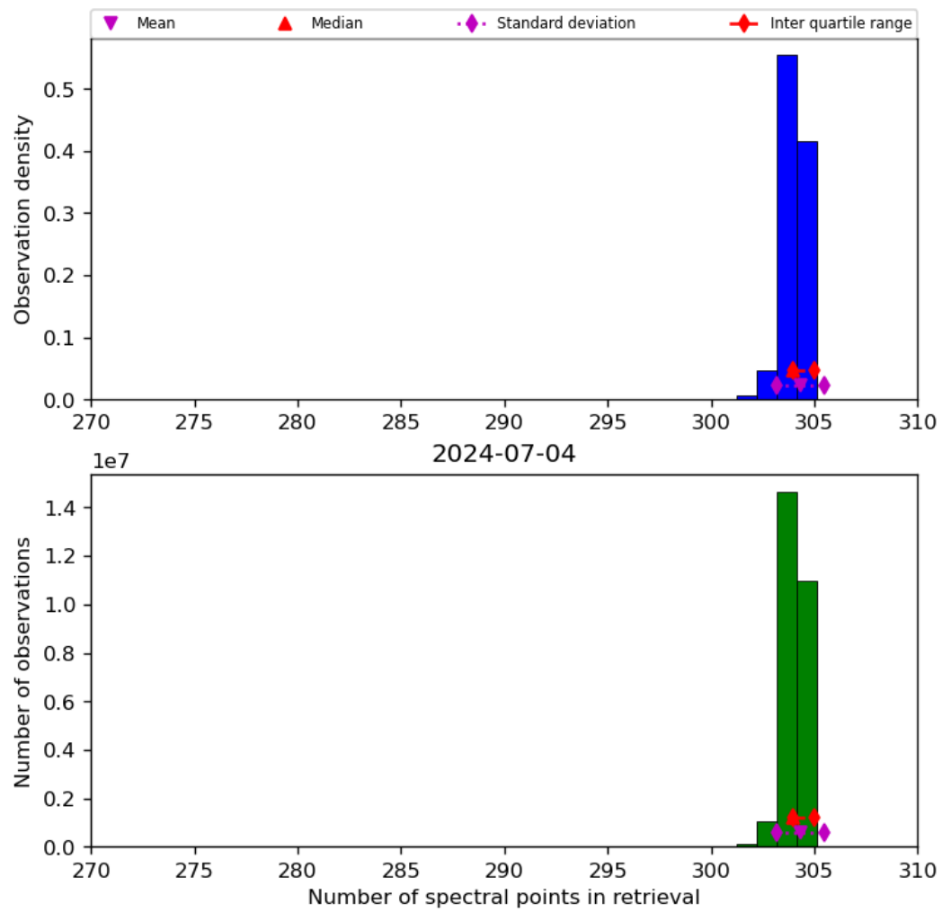
Figure 33: Histogram of “Number of spectral points in retrieval” for 2024-07-03 to 2024-07-05
