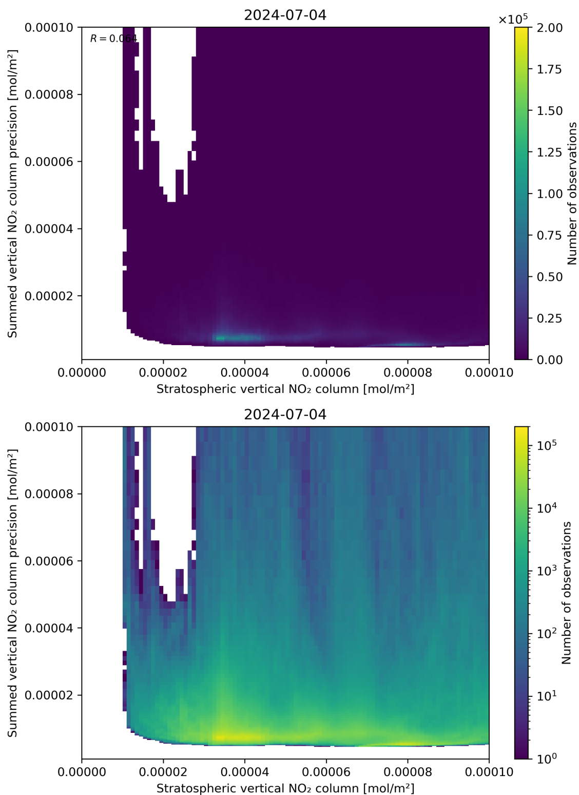
Figure 99: Scatter density plot of “Stratospheric vertical NO 2 column” against “Summed vertical NO 2 column precision” for 2024-07-03 to 2024-07-05.
