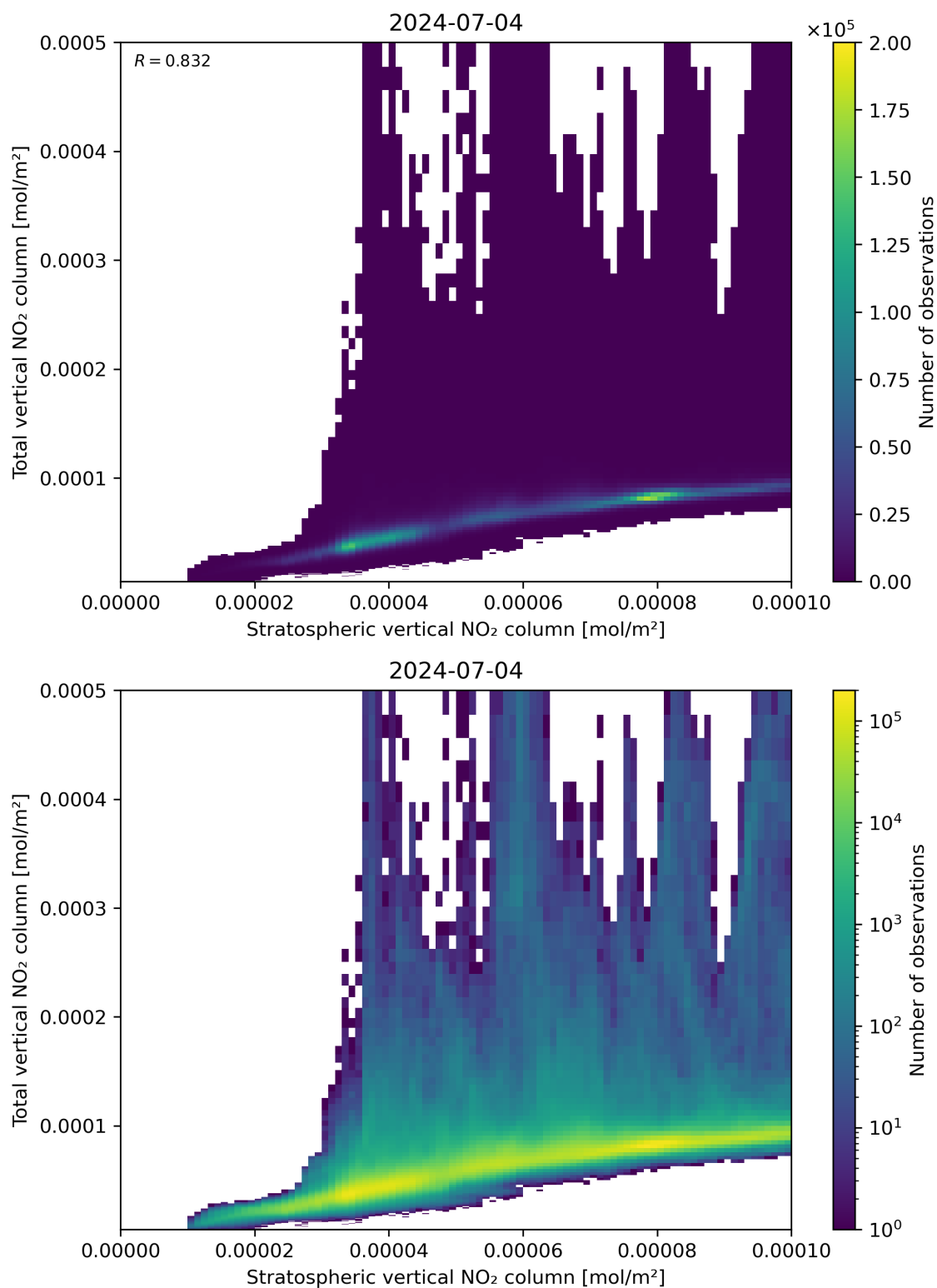
Figure 100: Scatter density plot of “Stratospheric vertical NO 2 column” against “Total vertical NO 2 column” for 2024-07-03 to 2024-07-05.
