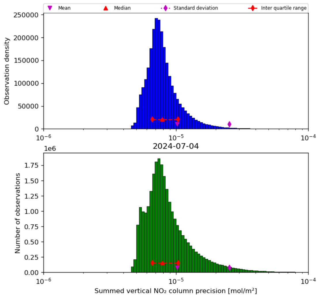
Figure 41: Histogram of “Summed vertical NO 2 column precision” for 2024-07-03 to 2024-07-05
