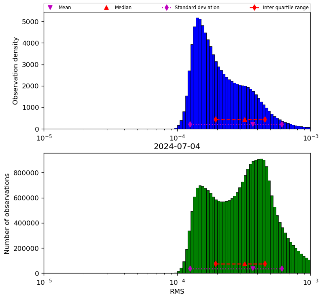
Figure 43: Histogram of “RMS” for 2024-07-03 to 2024-07-05
