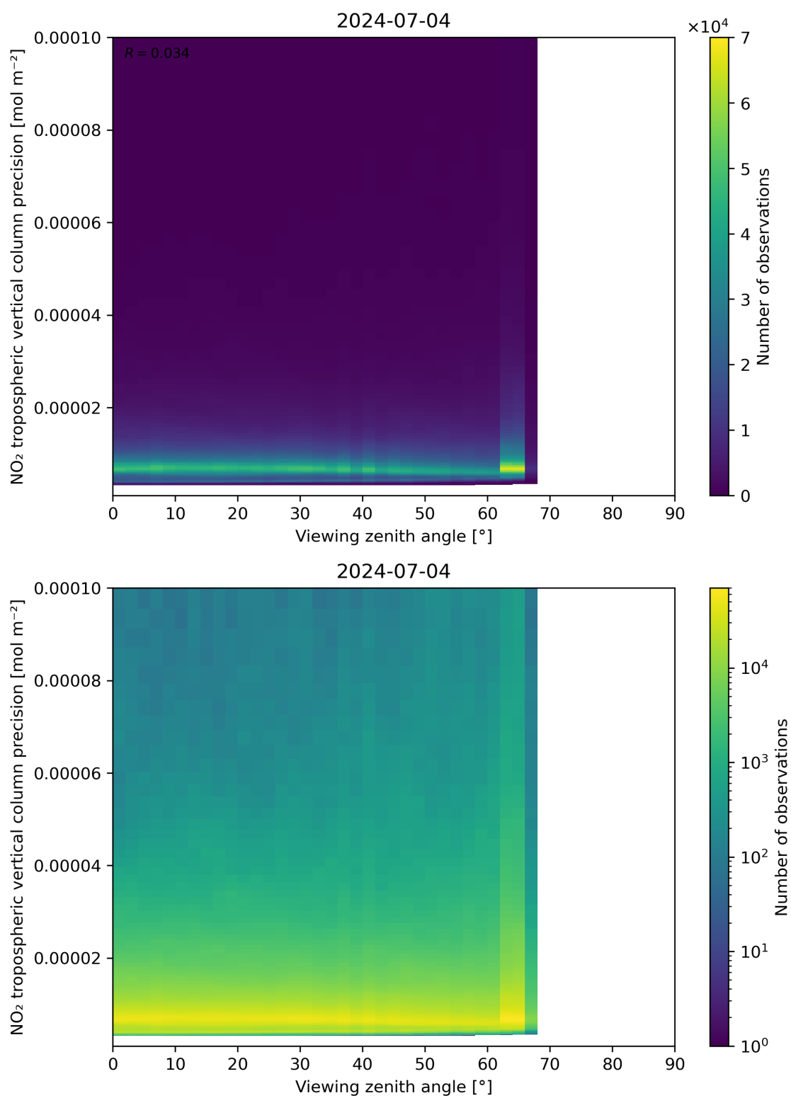
Figure 170: Scatter density plot of “Viewing zenith angle” against “NO 2 tropospheric vertical column precision” for 2024-07-03 to 2024-07-05.
