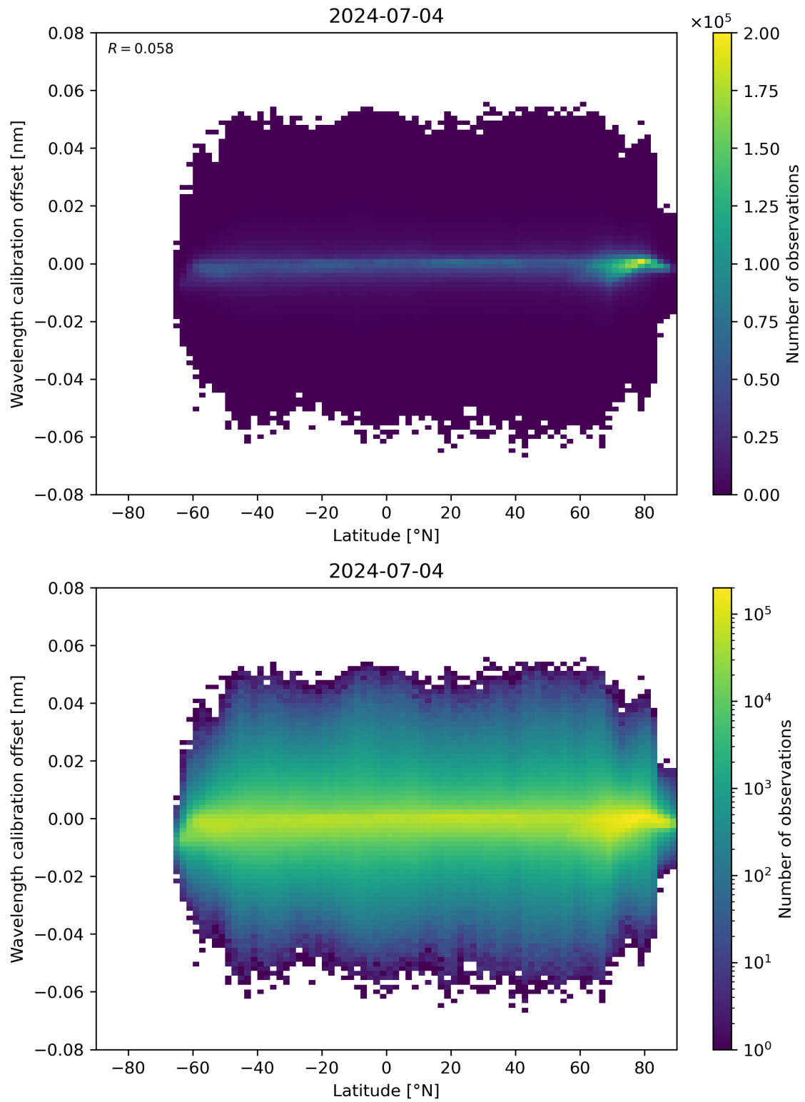
Figure 95: Scatter density plot of “Latitude” against “Wavelength calibration offset” for 2024-07-03 to 2024-07-05.
