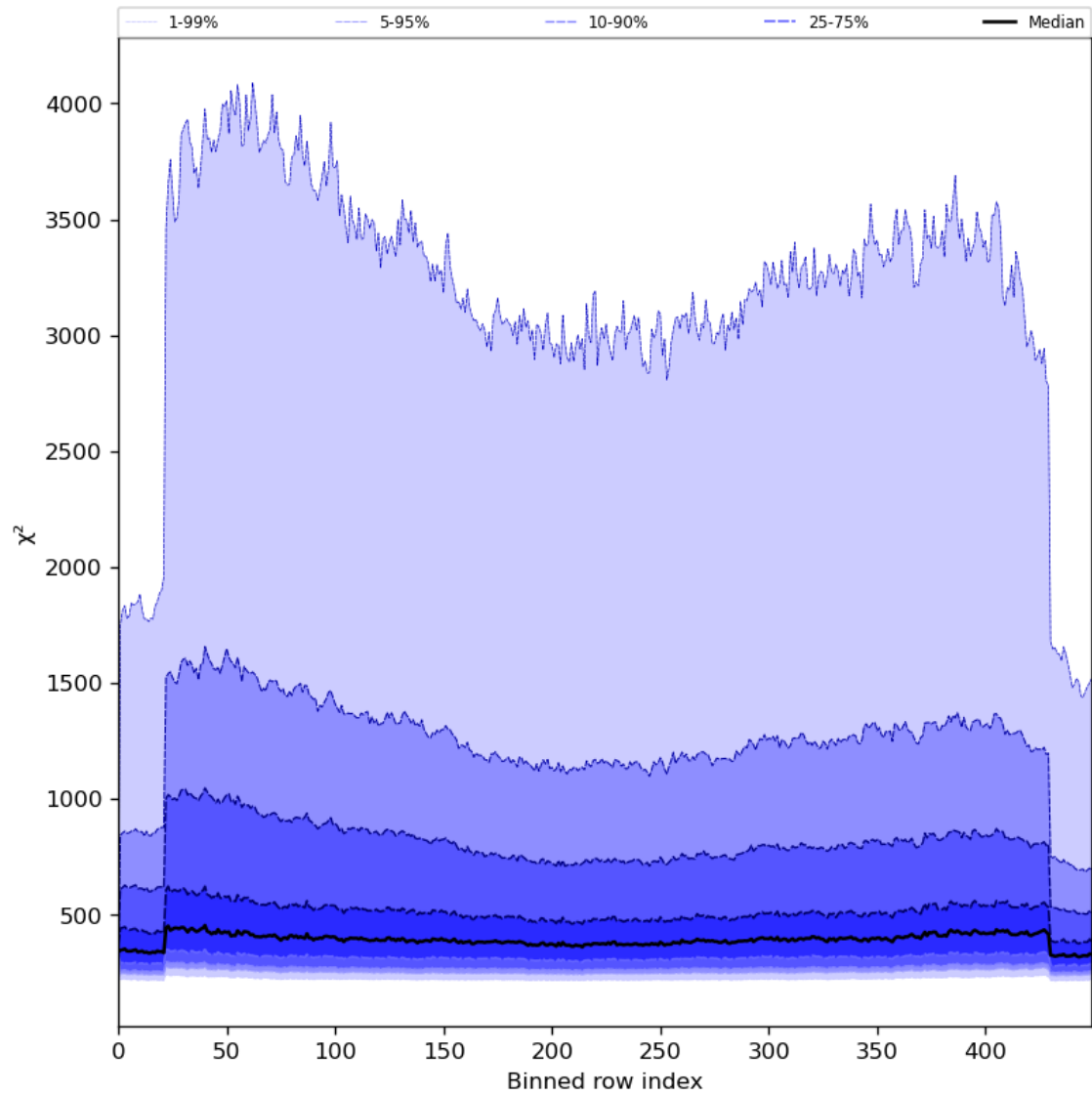
Figure 59: Along track statistics of “ \chi^2 ” for 2024-07-03 to 2024-07-05
