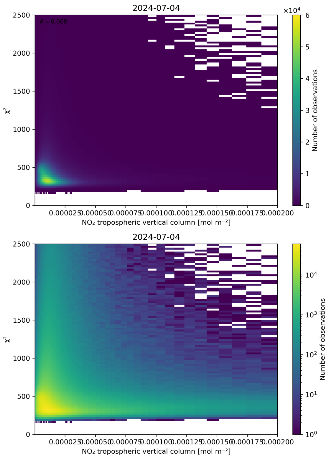
Figure 124: Scatter density plot of “NO 2 tropospheric vertical column” against “ \chi^2 ” for 2024-07-03 to 2024-07-05.
