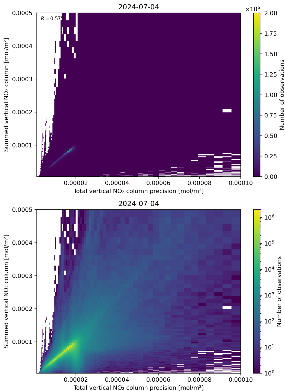
Figure 117: Scatter density plot of “Total vertical NO 2 column precision” against “Summed vertical NO 2 column” for 2024-07-03 to 2024-07-05.
