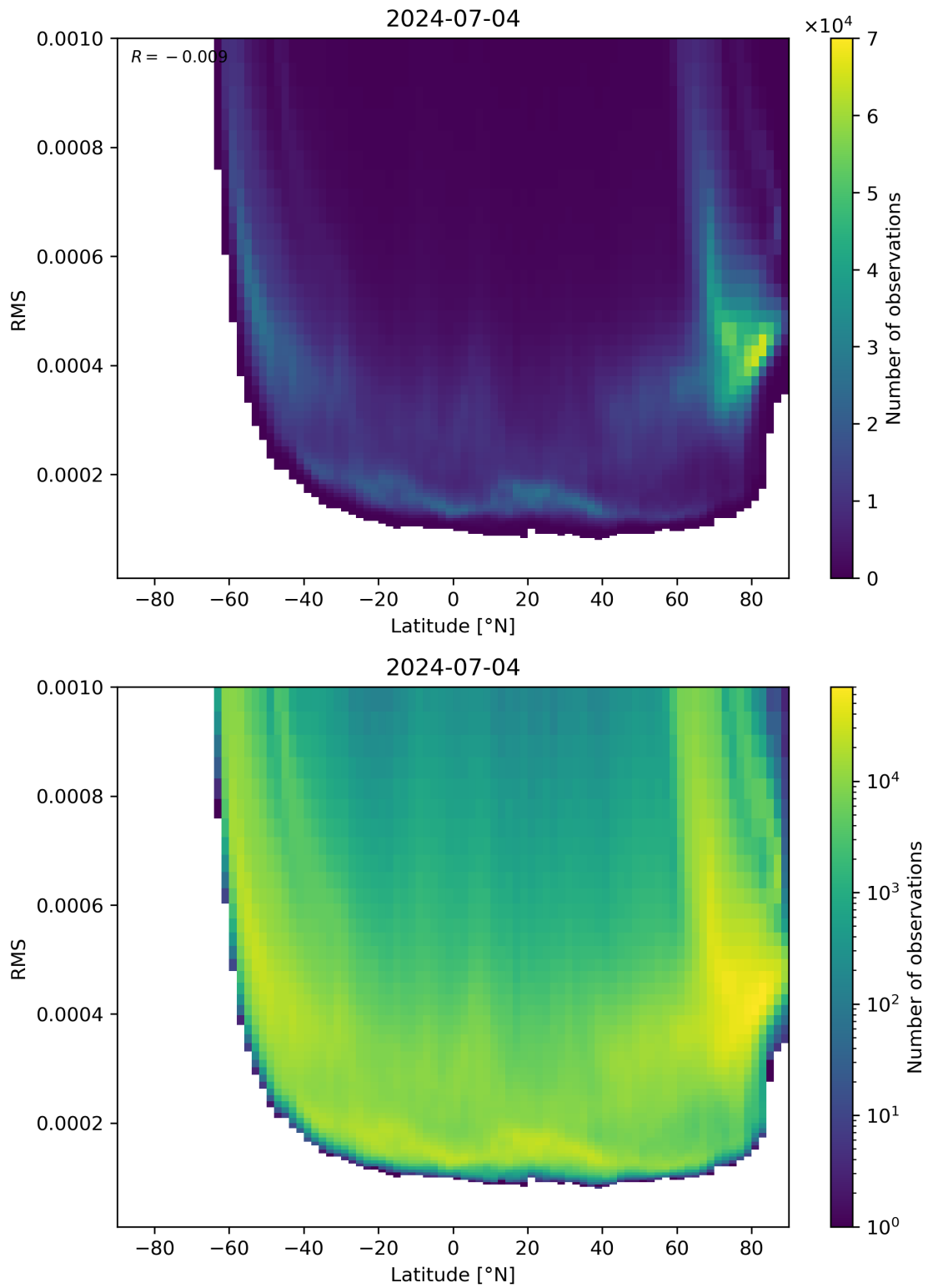
Figure 94: Scatter density plot of “Latitude” against “RMS” for 2024-07-03 to 2024-07-05.
