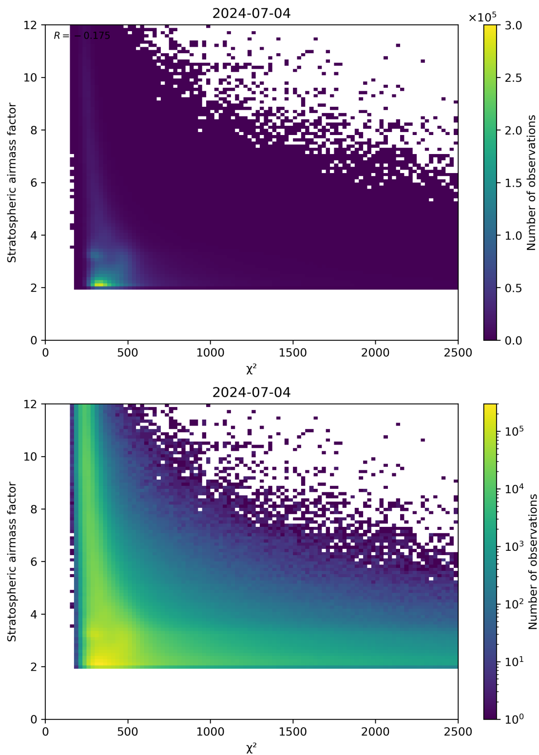
Figure 81: Scatter density plot of “ \chi^2 ” against “Stratospheric airmass factor” for 2024-07-03 to 2024-07-05.
