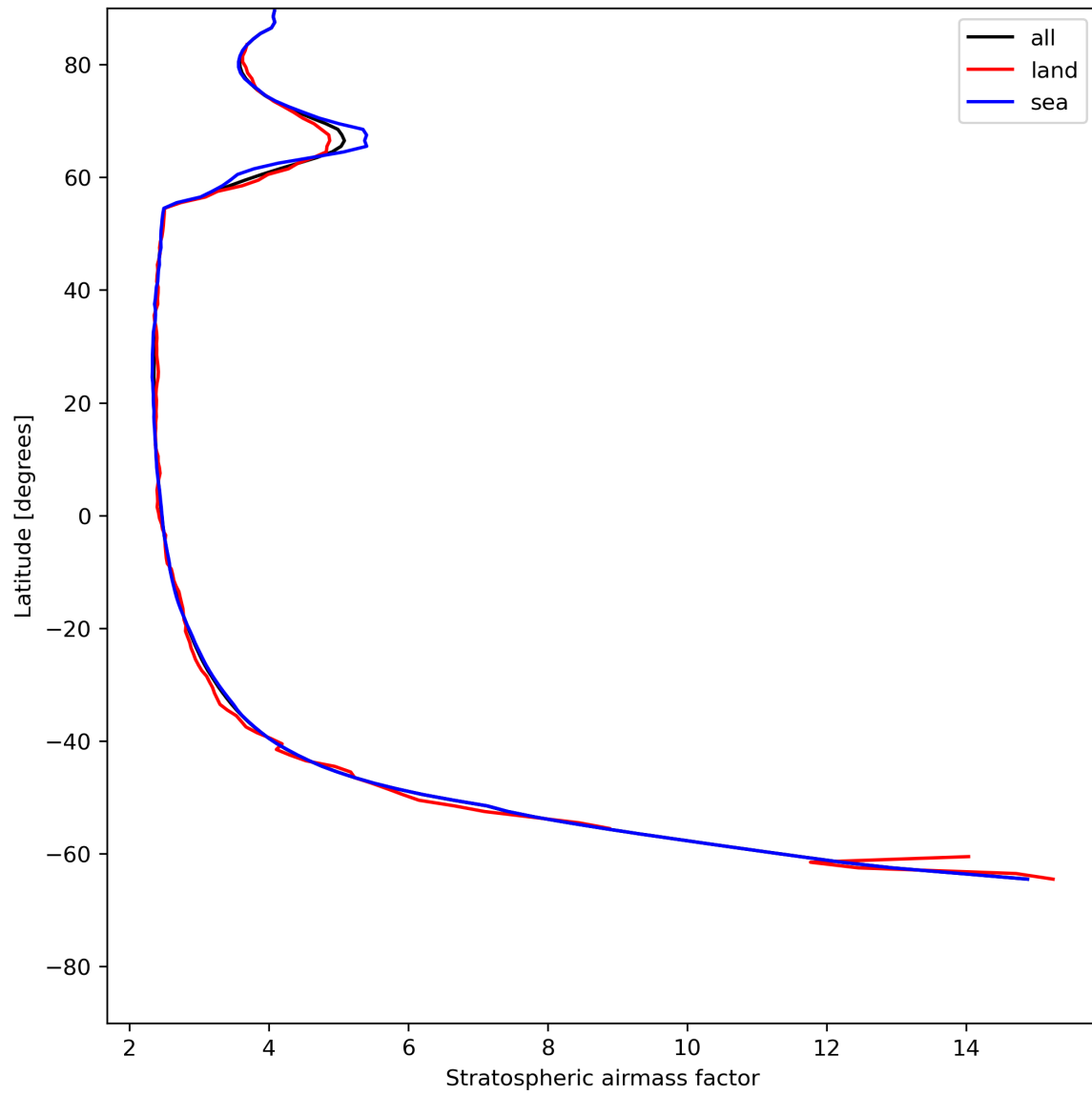
Figure 27: Zonal average of “Stratospheric air mass factor” for 2024-07-03 to 2024-07-05.
