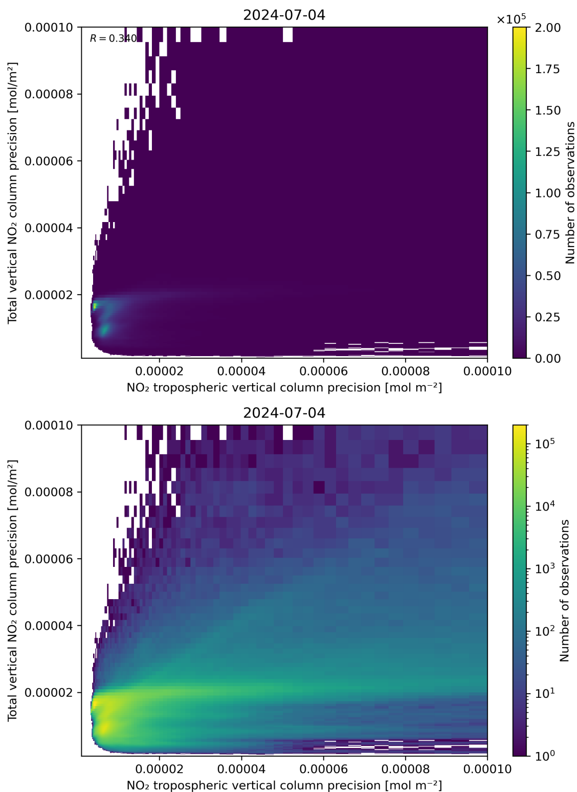
Figure 139: Scatter density plot of “NO 2 tropospheric vertical column precision” against “Total vertical NO 2 column precision” for 2024-07-03 to 2024-07-05.
