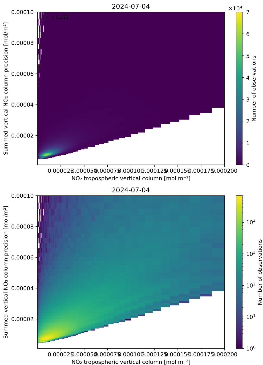
Figure 127: Scatter density plot of “NO 2 tropospheric vertical column” against “Summed vertical NO 2 column precision” for 2024-07-03 to 2024-07-05.
