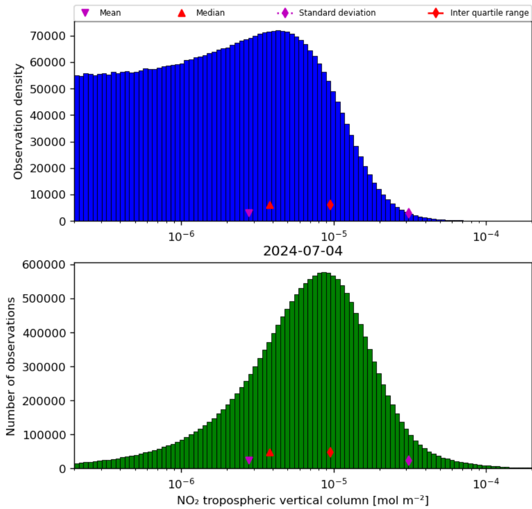
Figure 29: Histogram of “NO 2 tropospheric vertical column” for 2024-07-03 to 2024-07-05
