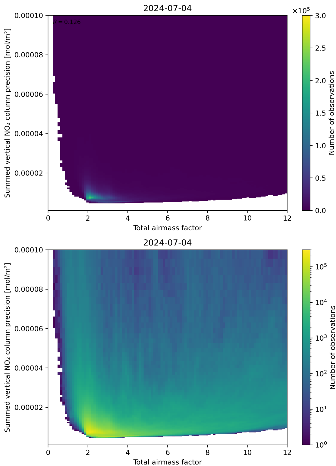
Figure 66: Scatter density plot of “Total airmass factor” against “Summed vertical NO 2 column precision” for 2024-07-03 to 2024-07-05.
