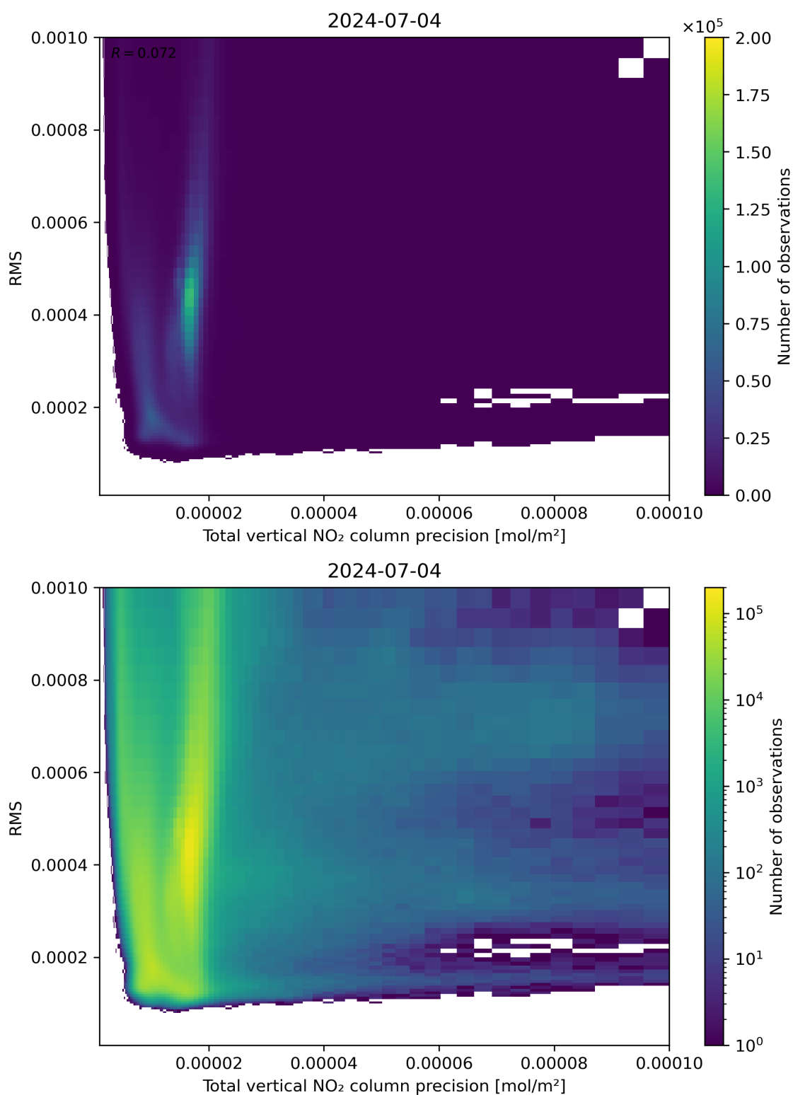
Figure 119: Scatter density plot of “Total vertical NO 2 column precision” against “RMS” for 2024-07-03 to 2024-07-05.
