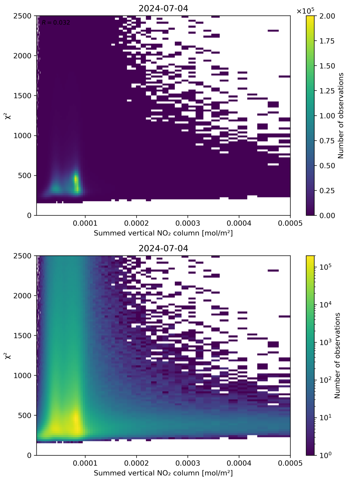
Figure 104: Scatter density plot of “Summed vertical NO 2 column” against “ \chi^2 ” for 2024-07-03 to 2024-07-05.
