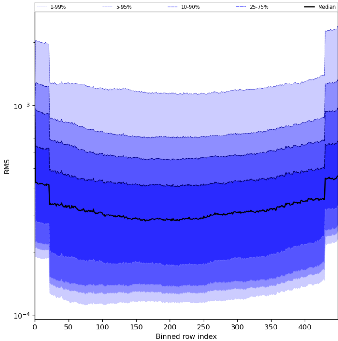
Figure 60: Along track statistics of “RMS” for 2024-07-03 to 2024-07-05
