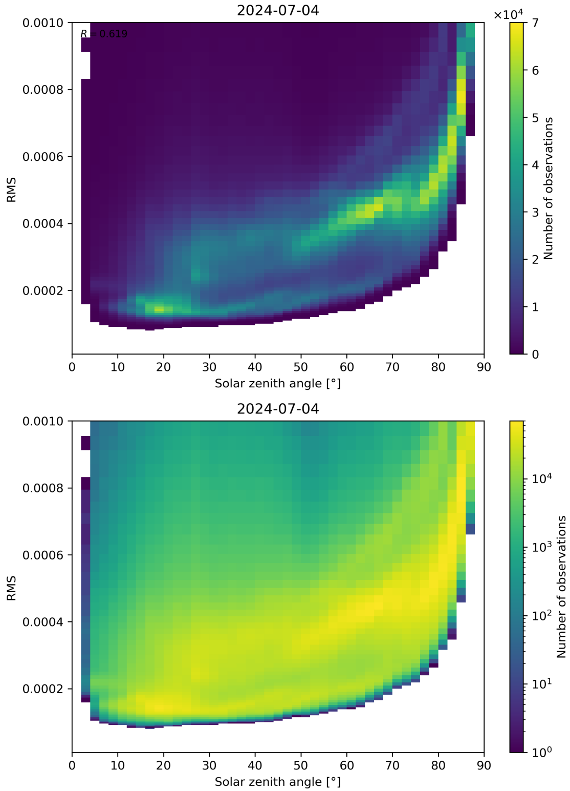
Figure 157: Scatter density plot of “Solar zenith angle” against “RMS” for 2024-07-03 to 2024-07-05.
