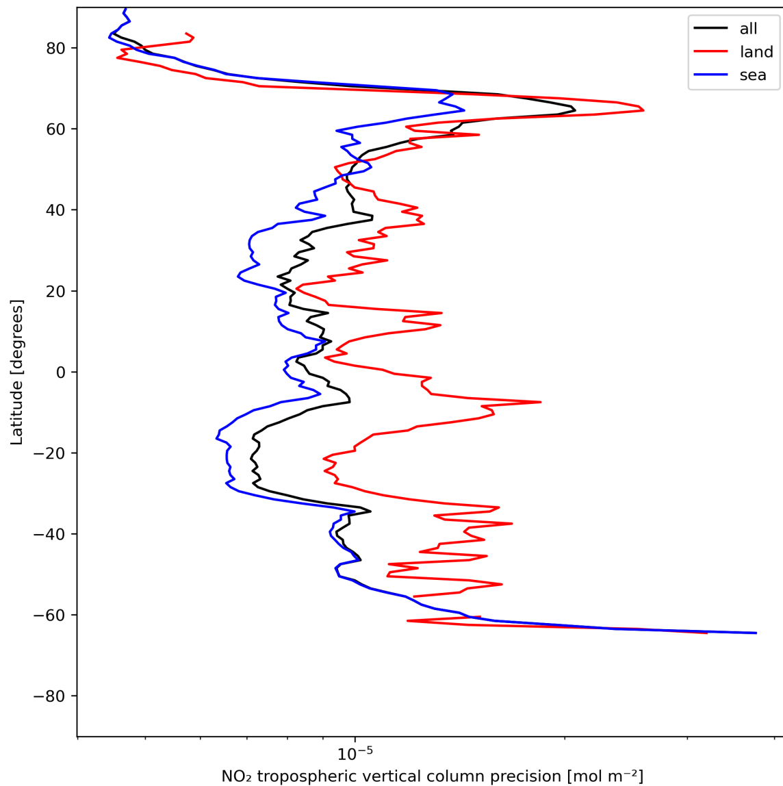
Figure 13: Zonal average of “NO 2 tropospheric vertical column precision” for 2024-07-03 to 2024-07-05.
