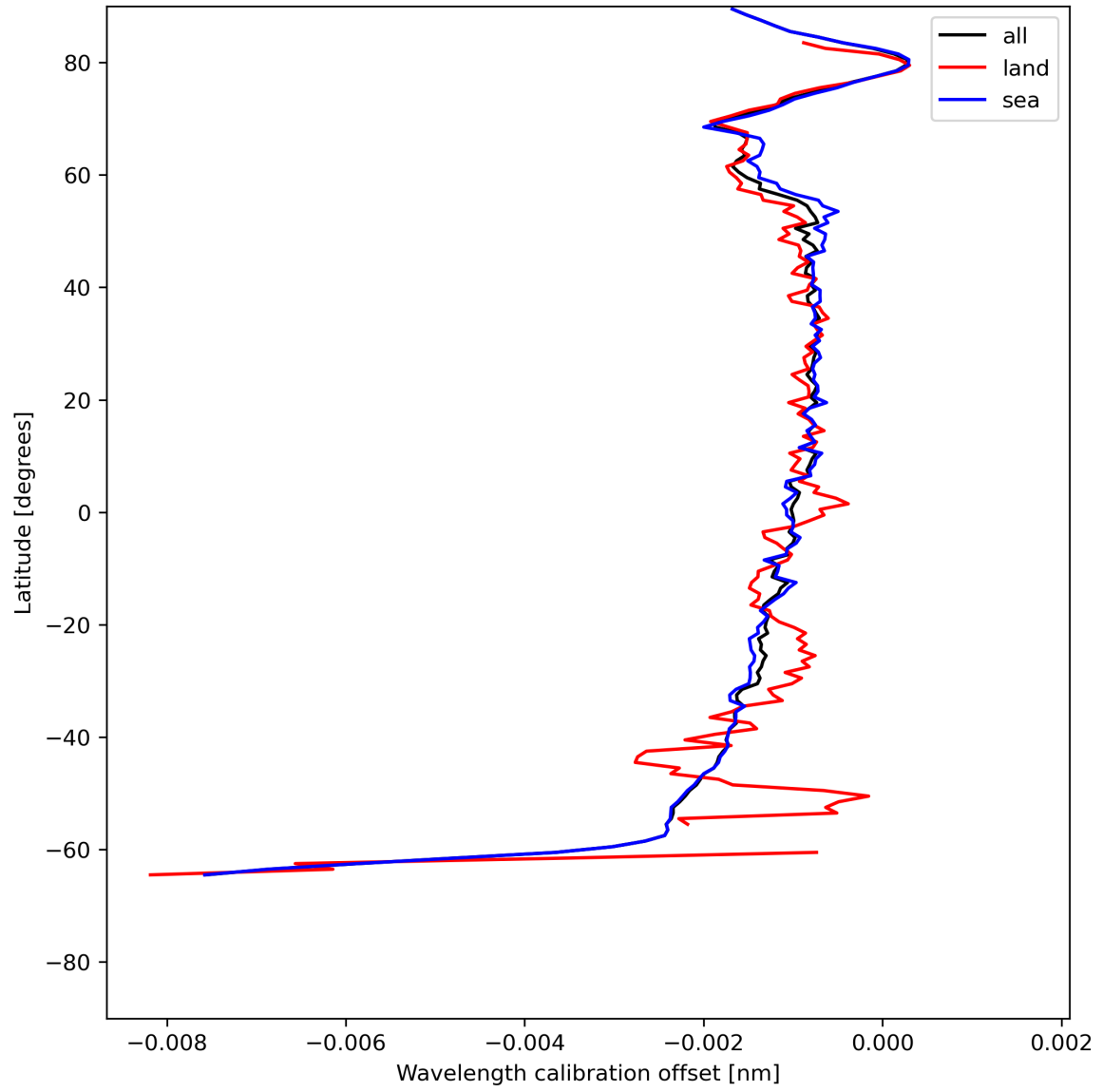
Figure 18: Zonal average of “Wavelength calibration offset” for 2024-07-03 to 2024-07-05.
