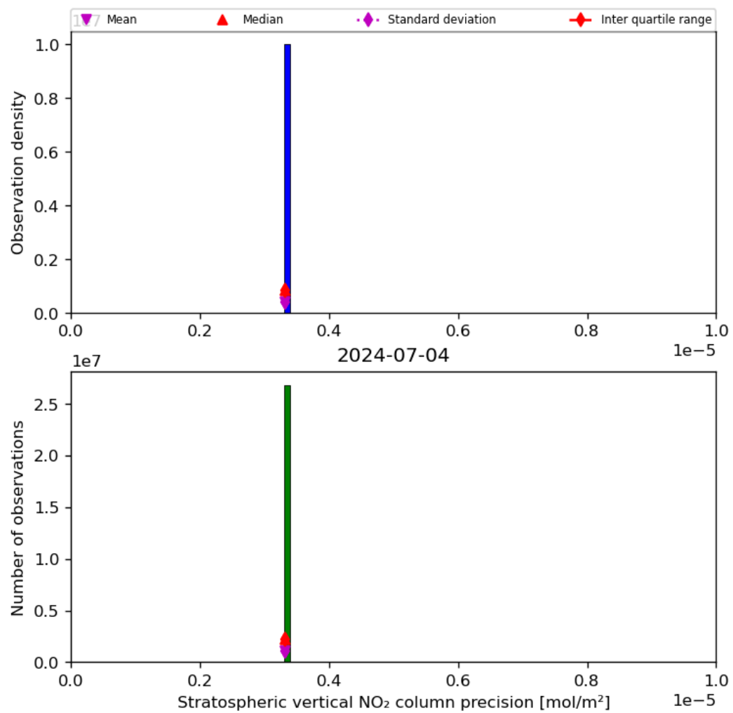
Figure 37: Histogram of “Stratospheric vertical NO 2 column precision” for 2024-07-03 to 2024-07-05
