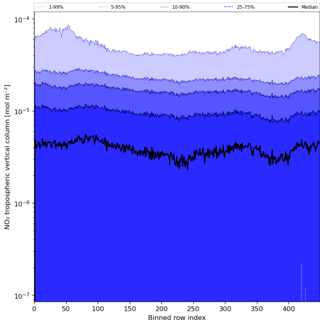
Figure 46: Along track statistics of “NO 2 tropospheric vertical column” for 2024-07-03 to 2024-07-05
