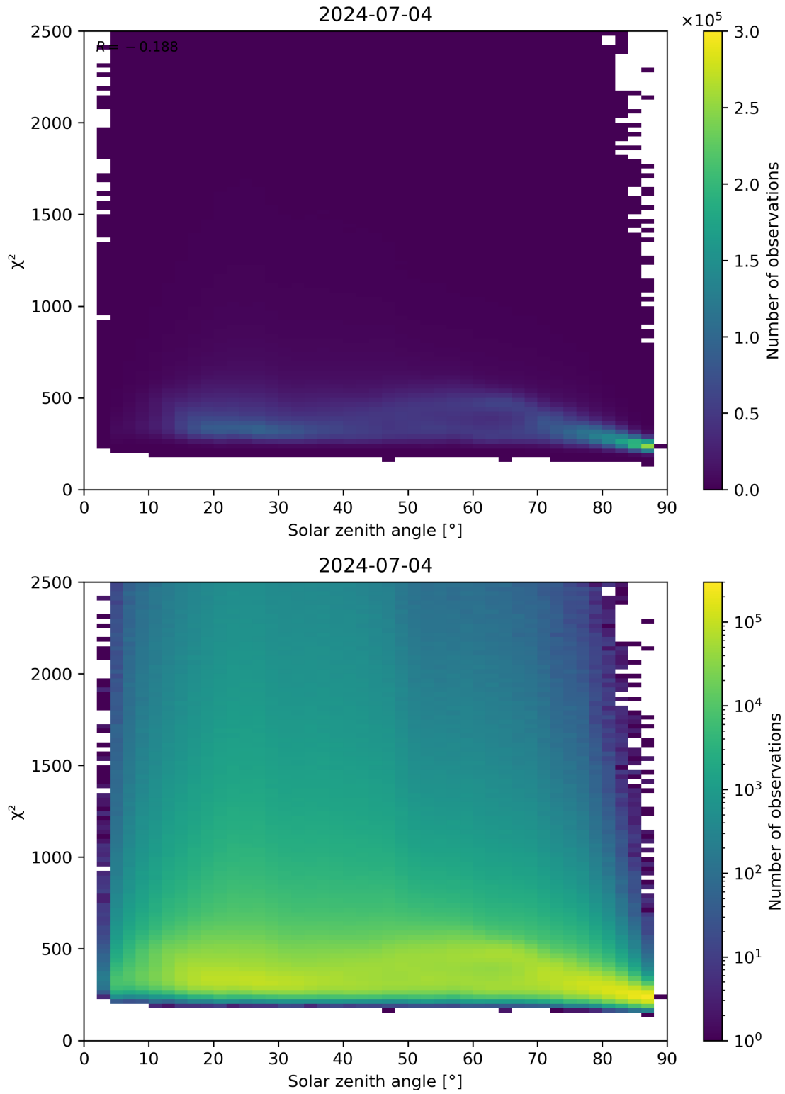
Figure 148: Scatter density plot of “Solar zenith angle” against “ \chi^2 ” for 2024-07-03 to 2024-07-05.
