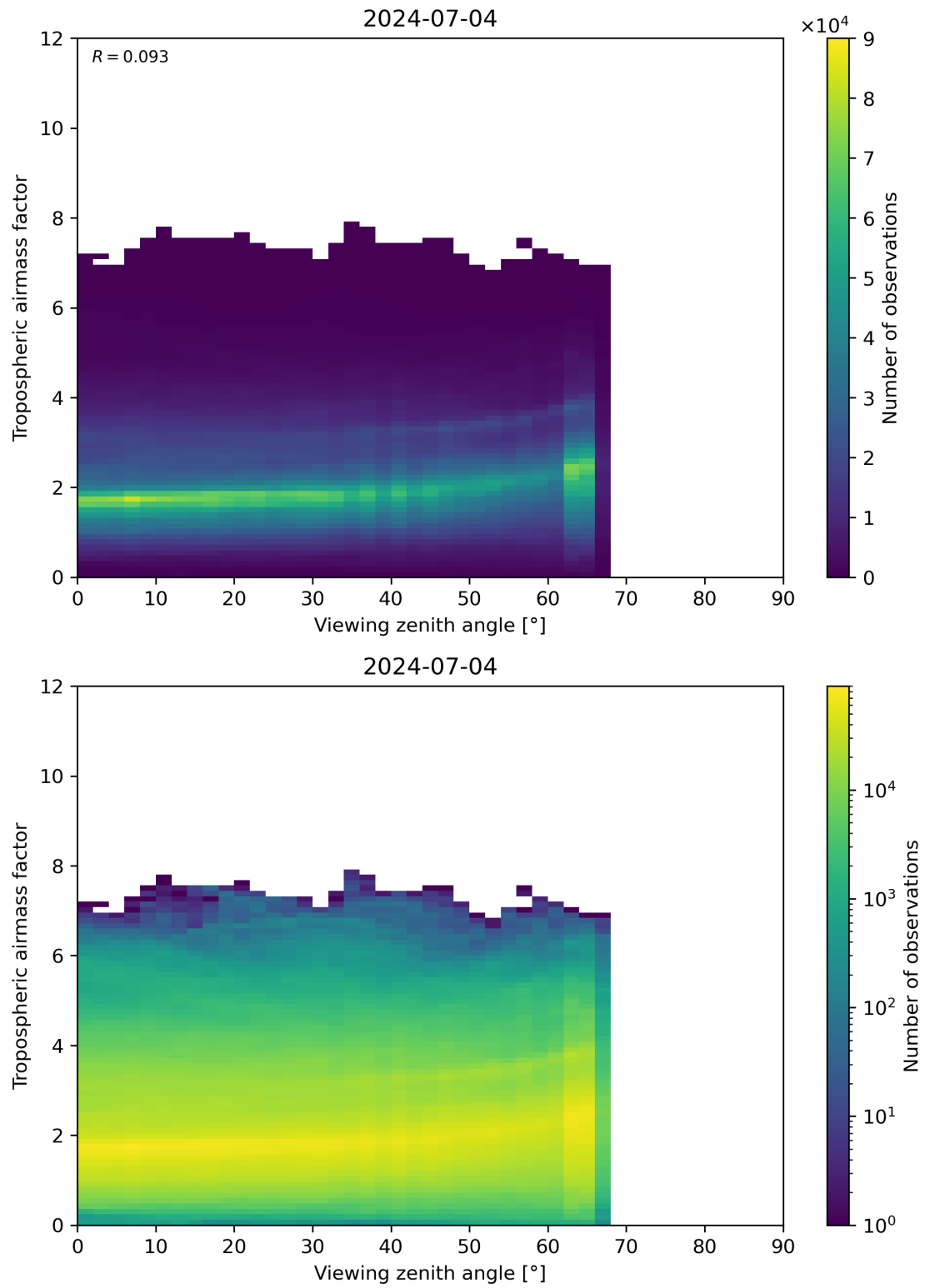
Figure 161: Scatter density plot of “Viewing zenith angle” against “Tropospheric airmass factor” for 2024-07-03 to 2024-07-05.
