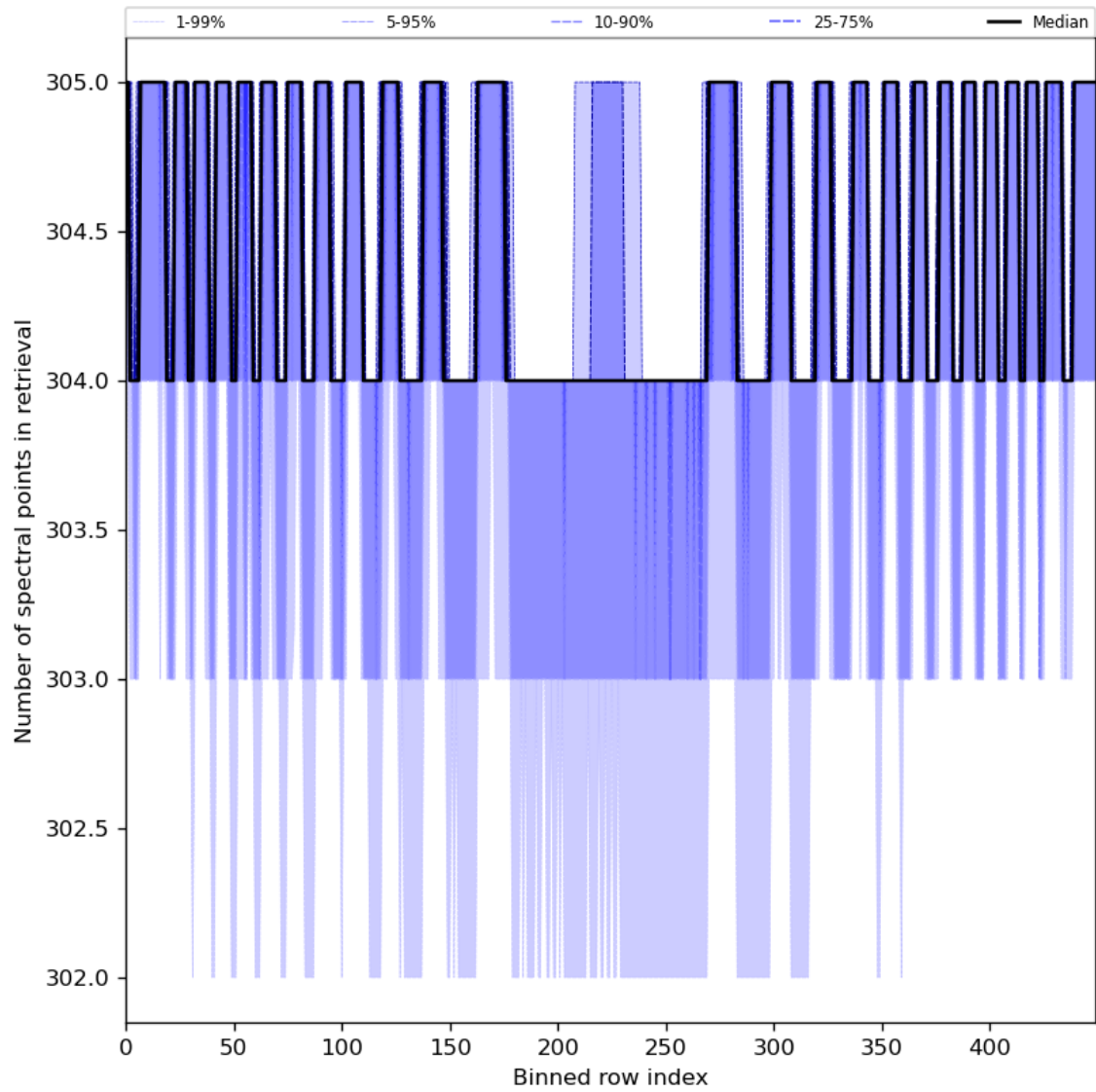
Figure 50: Along track statistics of “Number of spectral points in retrieval” for 2024-07-03 to 2024-07-05
