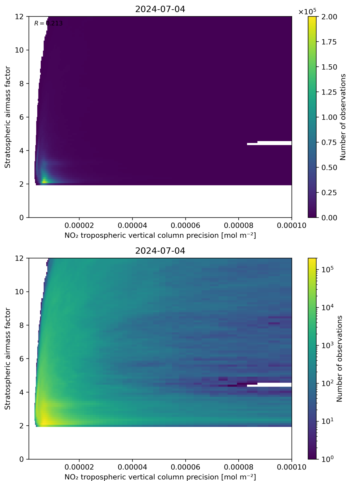
Figure 131: Scatter density plot of “NO 2 tropospheric vertical column precision” against “Stratospheric airmass factor” for 2024-07-03 to 2024-07-05.
