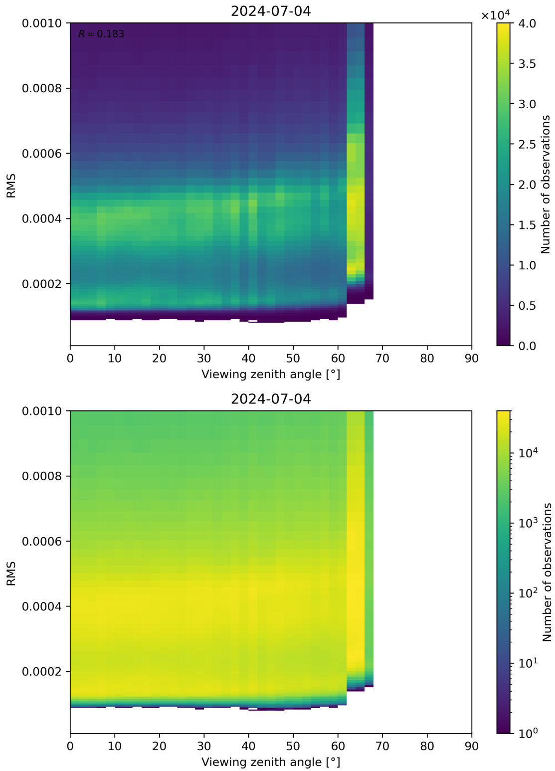
Figure 171: Scatter density plot of “Viewing zenith angle” against “RMS” for 2024-07-03 to 2024-07-05.
