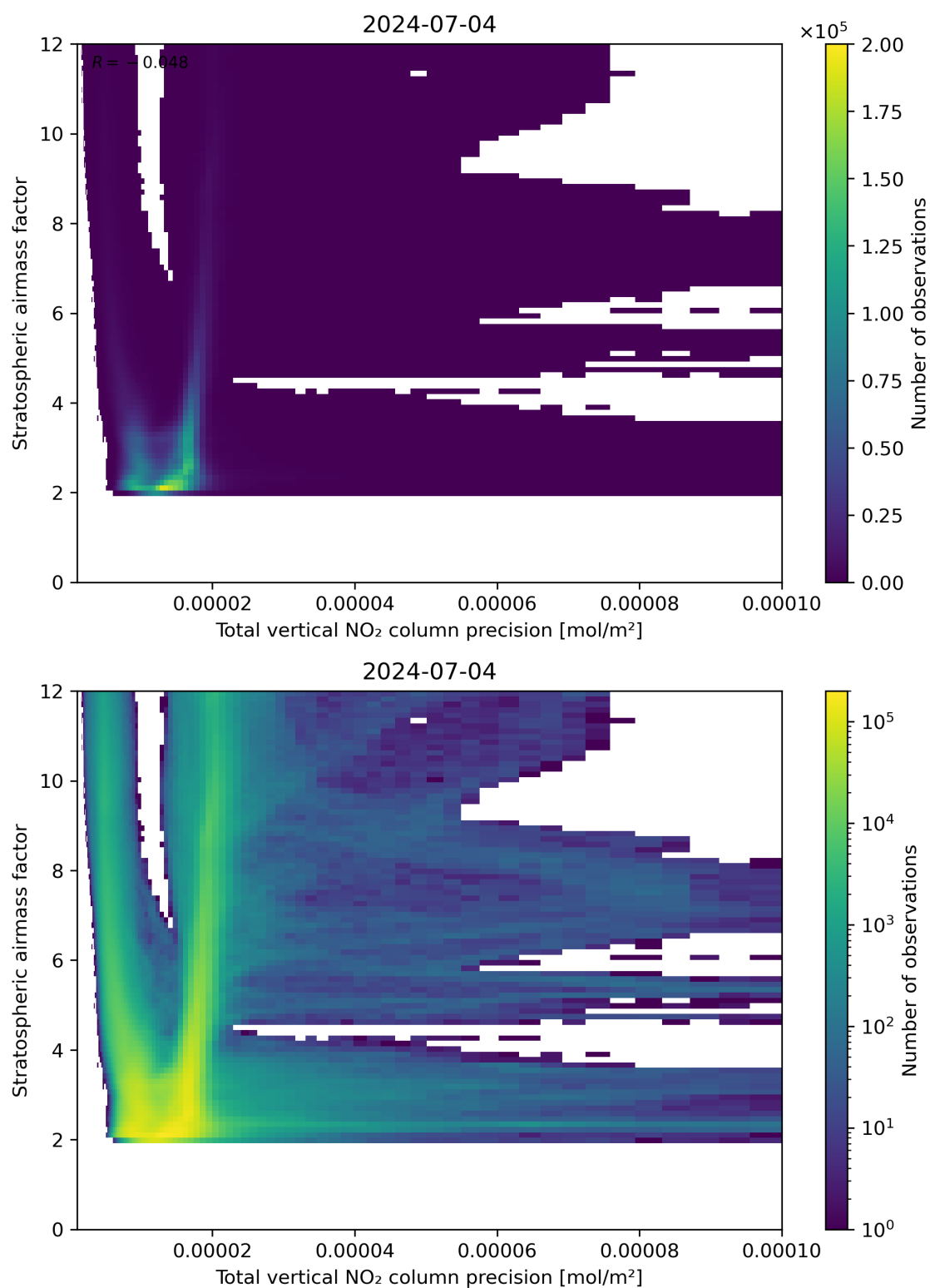
Figure 115: Scatter density plot of “Total vertical NO 2 column precision” against “Stratospheric air mass factor” for 2024-07-03 to 2024-07-05.
