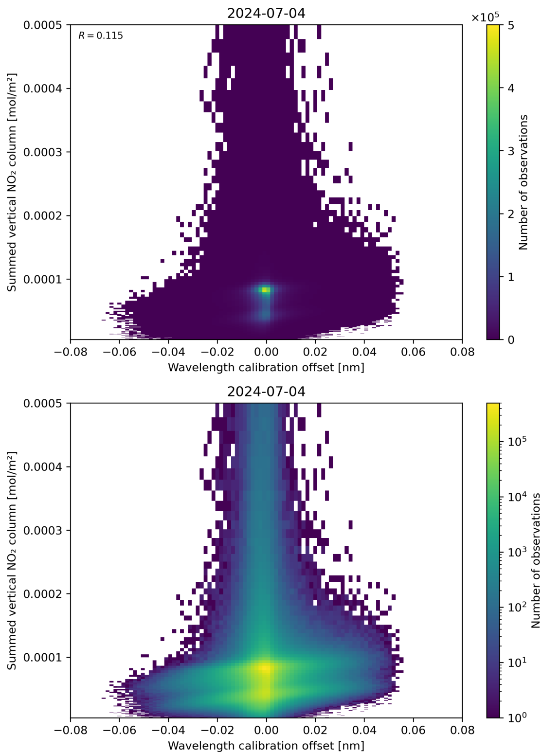
Figure 177: Scatter density plot of “Wavelength calibration offset” against “Summed vertical NO 2 column” for 2024-07-03 to 2024-07-05.
