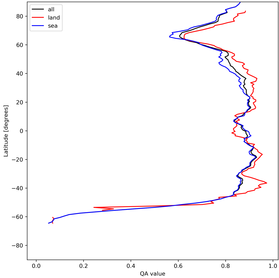
Figure 11: Zonal average of “QA value” for 2024-07-03 to 2024-07-05.
