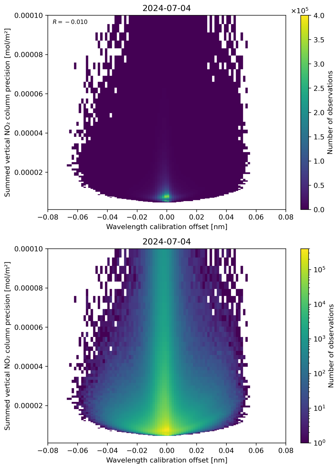
Figure 178: Scatter density plot of “Wavelength calibration offset” against “Summed vertical NO 2 column precision” for 2024-07-03 to 2024-07-05.
