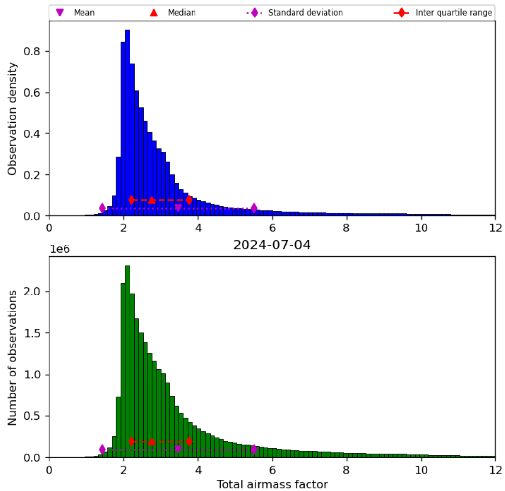
Figure 32: Histogram of “Total airmass factor” for 2024-07-03 to 2024-07-05
