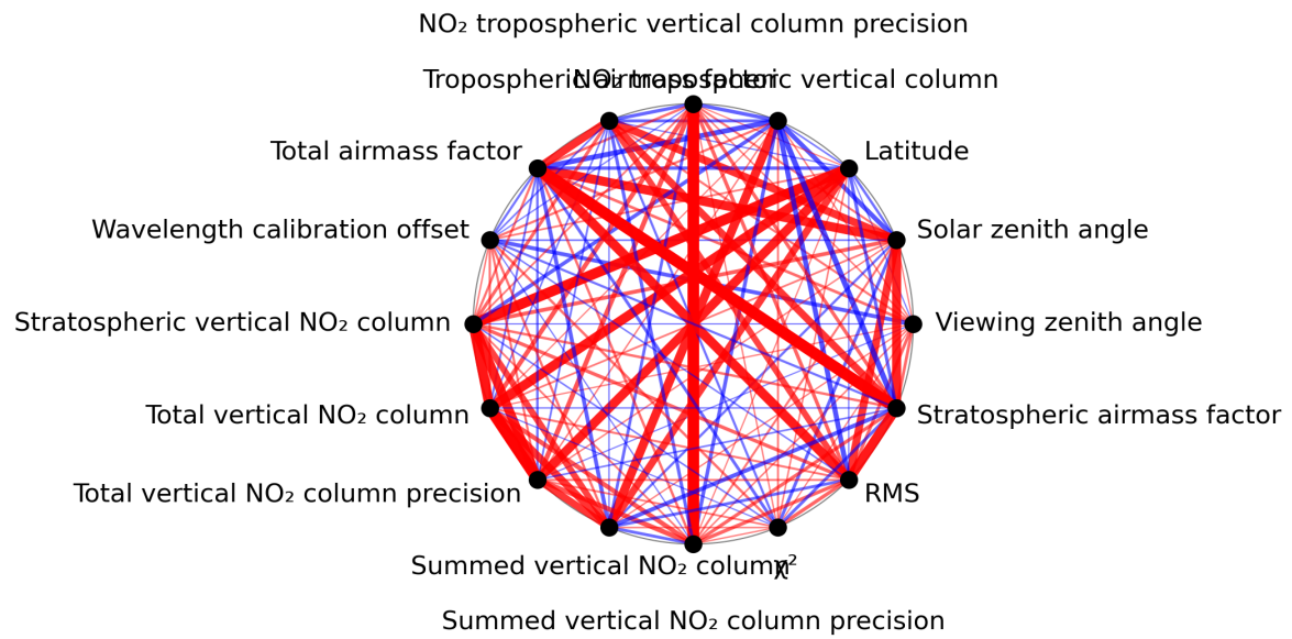
Figure 1: Map of correlation graph for 2024-07-03 to 2024-07-05.
