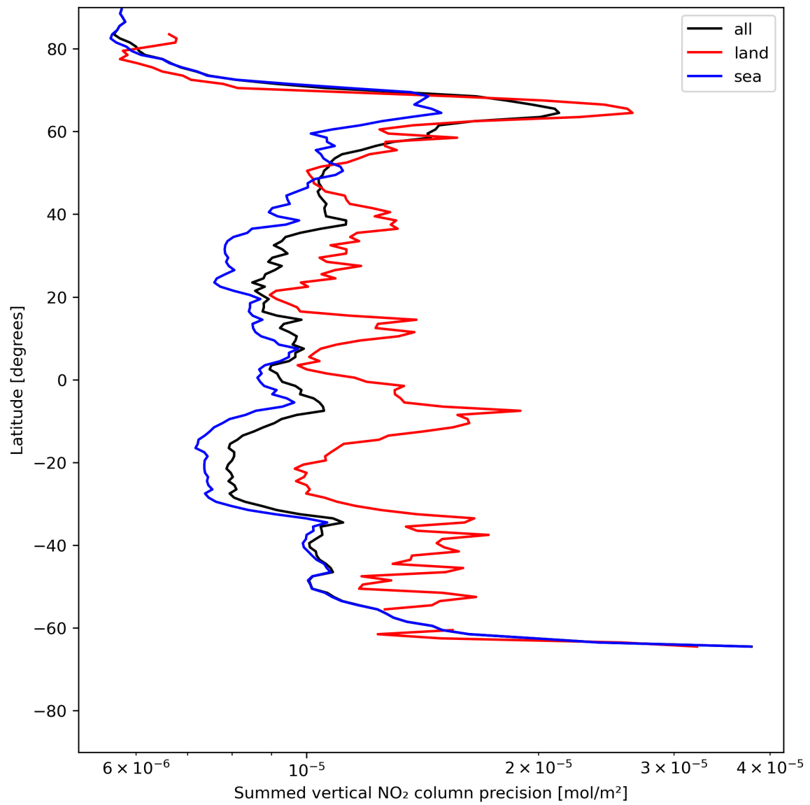
Figure 24: Zonal average of “Summed vertical NO 2 column precision” for 2024-07-03 to 2024-07-05.
