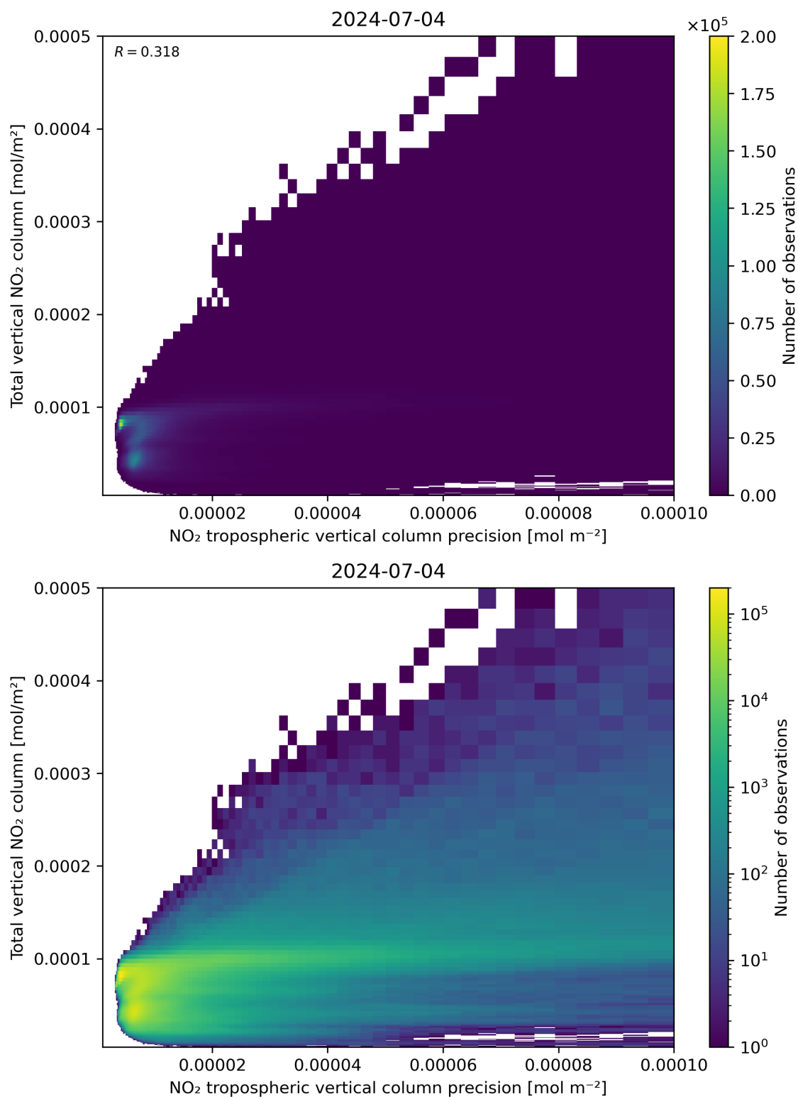
Figure 138: Scatter density plot of “NO 2 tropospheric vertical column precision” against “Total vertical NO 2 column” for 2024-07-03 to 2024-07-05.
