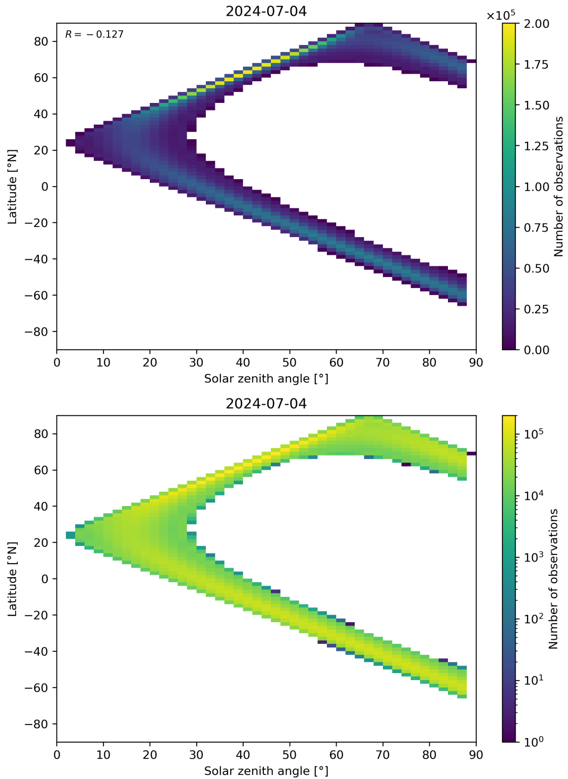
Figure 149: Scatter density plot of “Solar zenith angle” against “Latitude” for 2024-07-03 to 2024-07-05.
