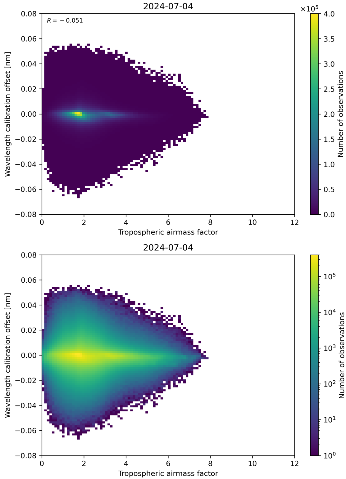
Figure 80: Scatter density plot of “Tropospheric air mass factor” against “Wavelength calibration offset” for 2024-07-03 to 2024-07-05.
