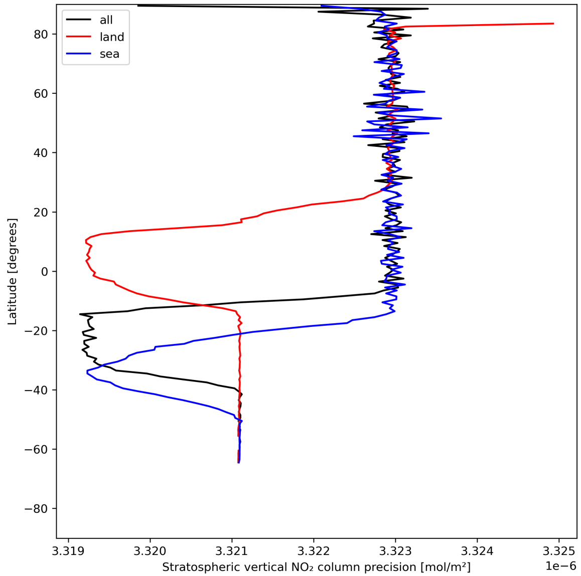
Figure 20: Zonal average of “Stratospheric vertical NO 2 column precision” for 2024-07-03 to 2024-07-05.
