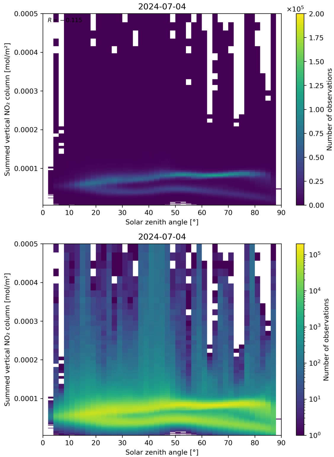
Figure 151: Scatter density plot of “Solar zenith angle” against “Summed vertical NO 2 column” for 2024-07-03 to 2024-07-05.
