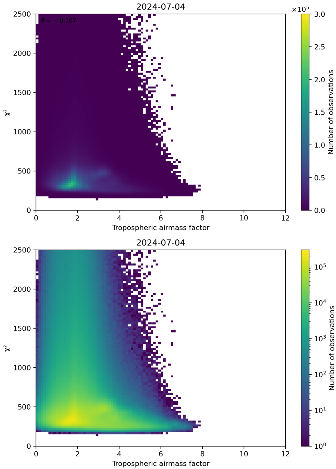
Figure 73: Scatter density plot of “Tropospheric airmass factor” against “ \chi^2 ” for 2024-07-03 to 2024-07-05.
