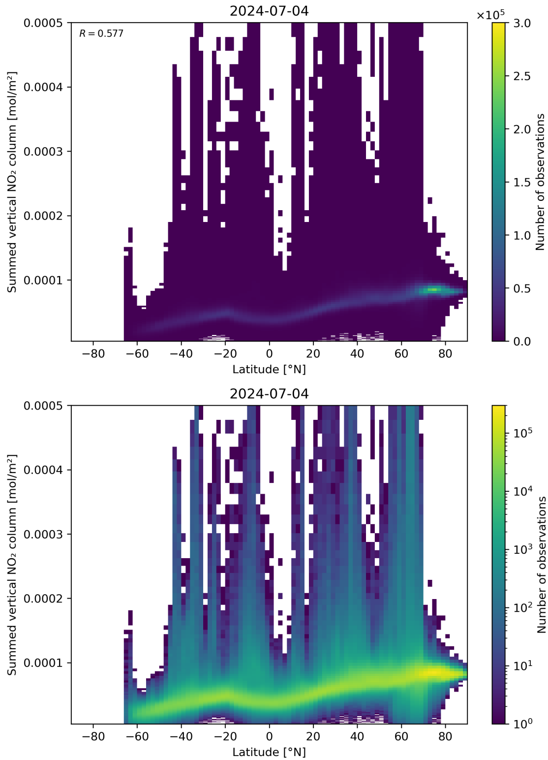
Figure 88: Scatter density plot of “Latitude” against “Summed vertical NO 2 column” for 2024-07-03 to 2024-07-05.
