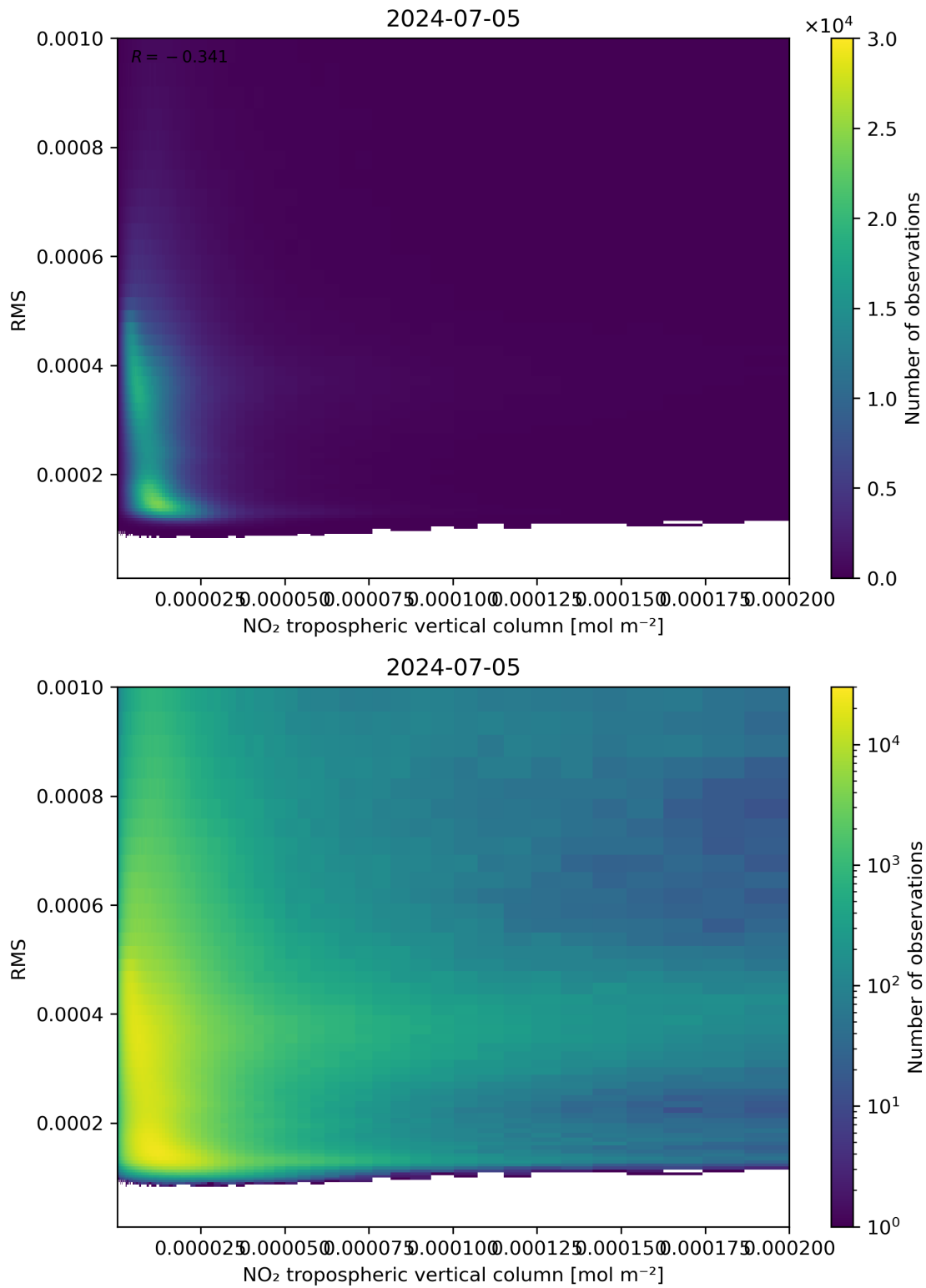
Figure 142: Scatter density plot of “NO 2 tropospheric vertical column” against “RMS” for 2024-07-05 to 2024-07-06.
