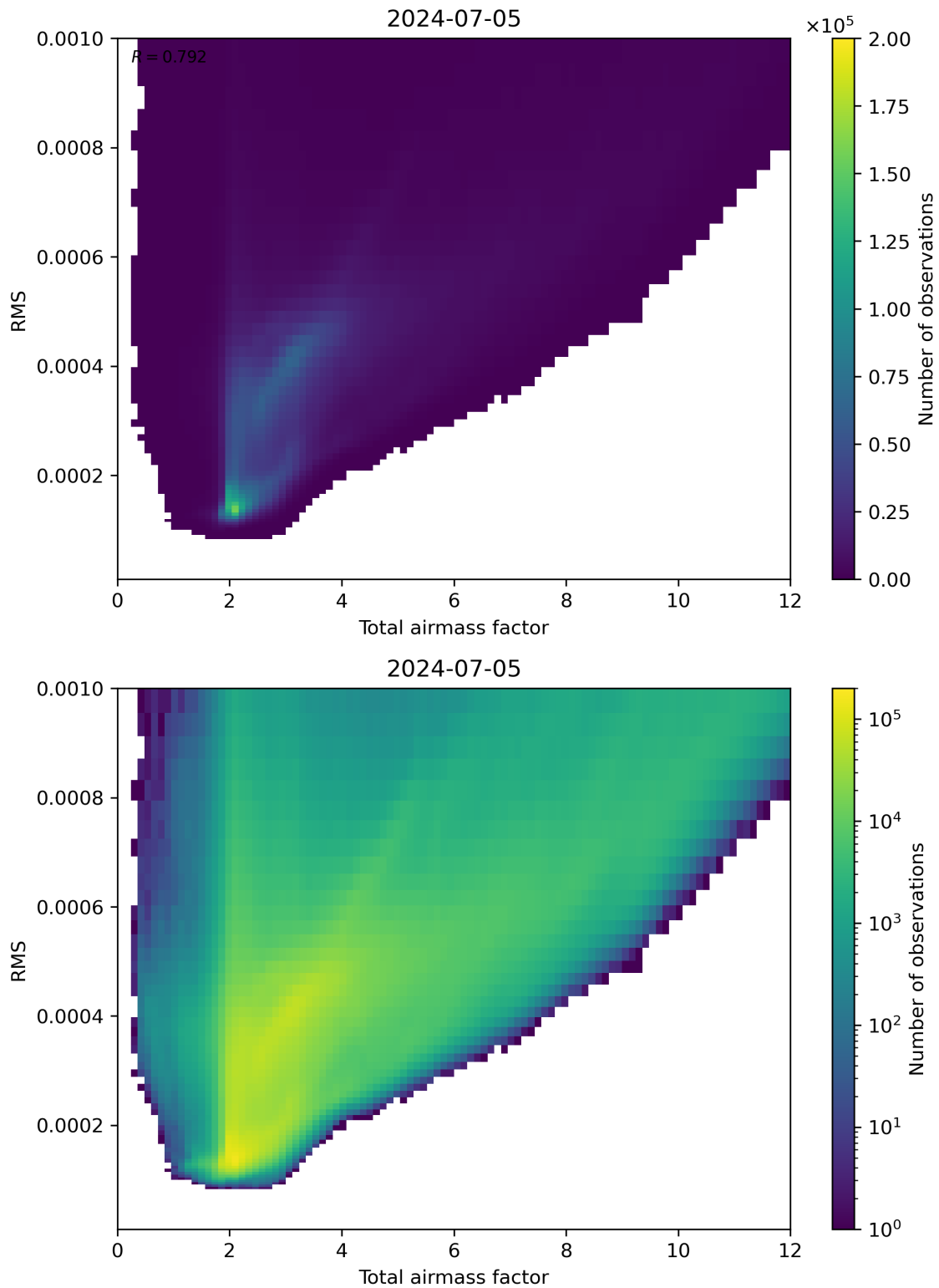
Figure 69: Scatter density plot of “Total airmass factor” against “RMS” for 2024-07-05 to 2024-07-06.
