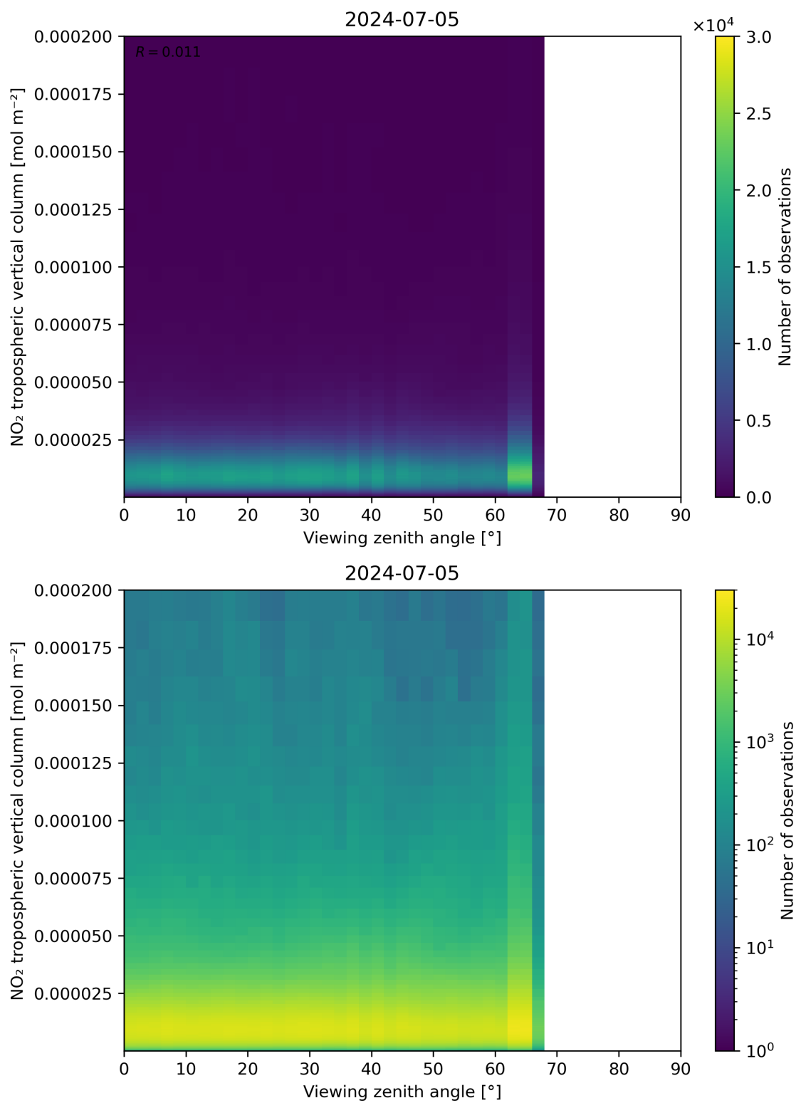
Figure 169: Scatter density plot of “Viewing zenith angle” against “NO 2 tropospheric vertical column” for 2024-07-05 to 2024-07-06.
