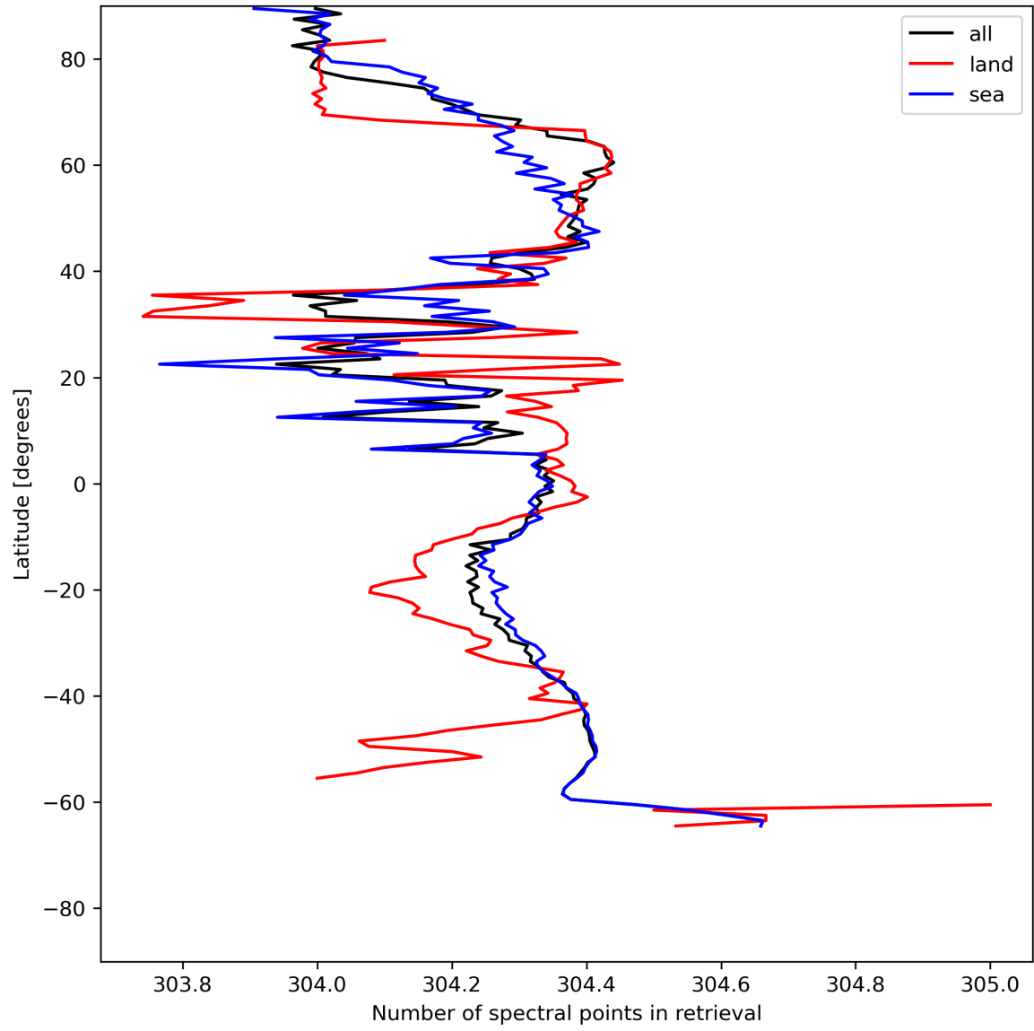
Figure 16: Zonal average of “Number of spectral points in retrieval” for 2024-07-05 to 2024-07-06.
