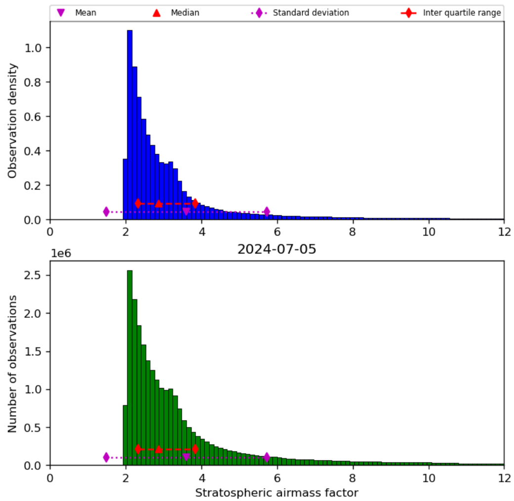
Figure 44: Histogram of “Stratospheric airmass factor” for 2024-07-05 to 2024-07-06
