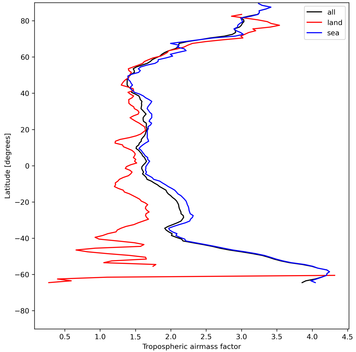
Figure 14: Zonal average of “Tropospheric airmass factor” for 2024-07-05 to 2024-07-06.
