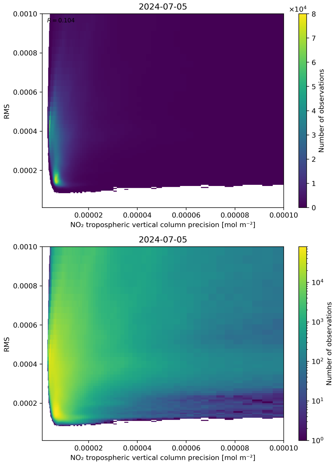
Figure 140: Scatter density plot of “NO 2 tropospheric vertical column precision” against “RMS” for 2024-07-05 to 2024-07-06.
