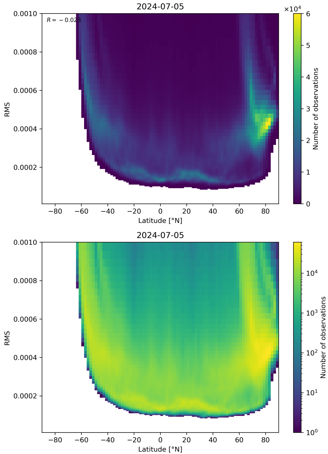
Figure 94: Scatter density plot of “Latitude” against “RMS” for 2024-07-05 to 2024-07-06.
