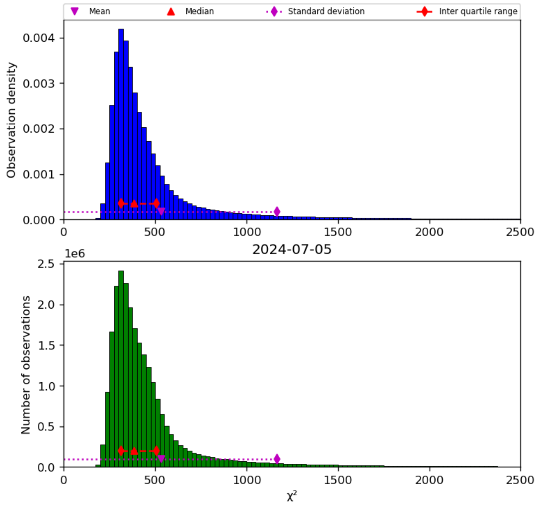
Figure 42: Histogram of “ \chi^2 ” for 2024-07-05 to 2024-07-06
