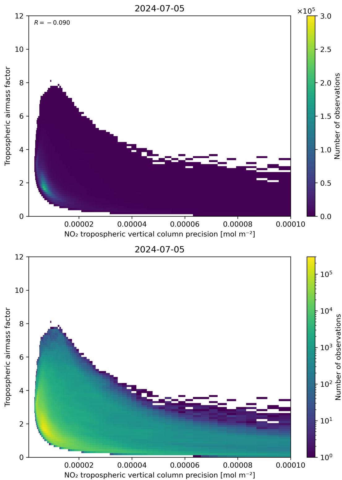
Figure 133: Scatter density plot of “NO 2 tropospheric vertical column precision” against “Tropospheric air mass factor” for 2024-07-05 to 2024-07-06.
