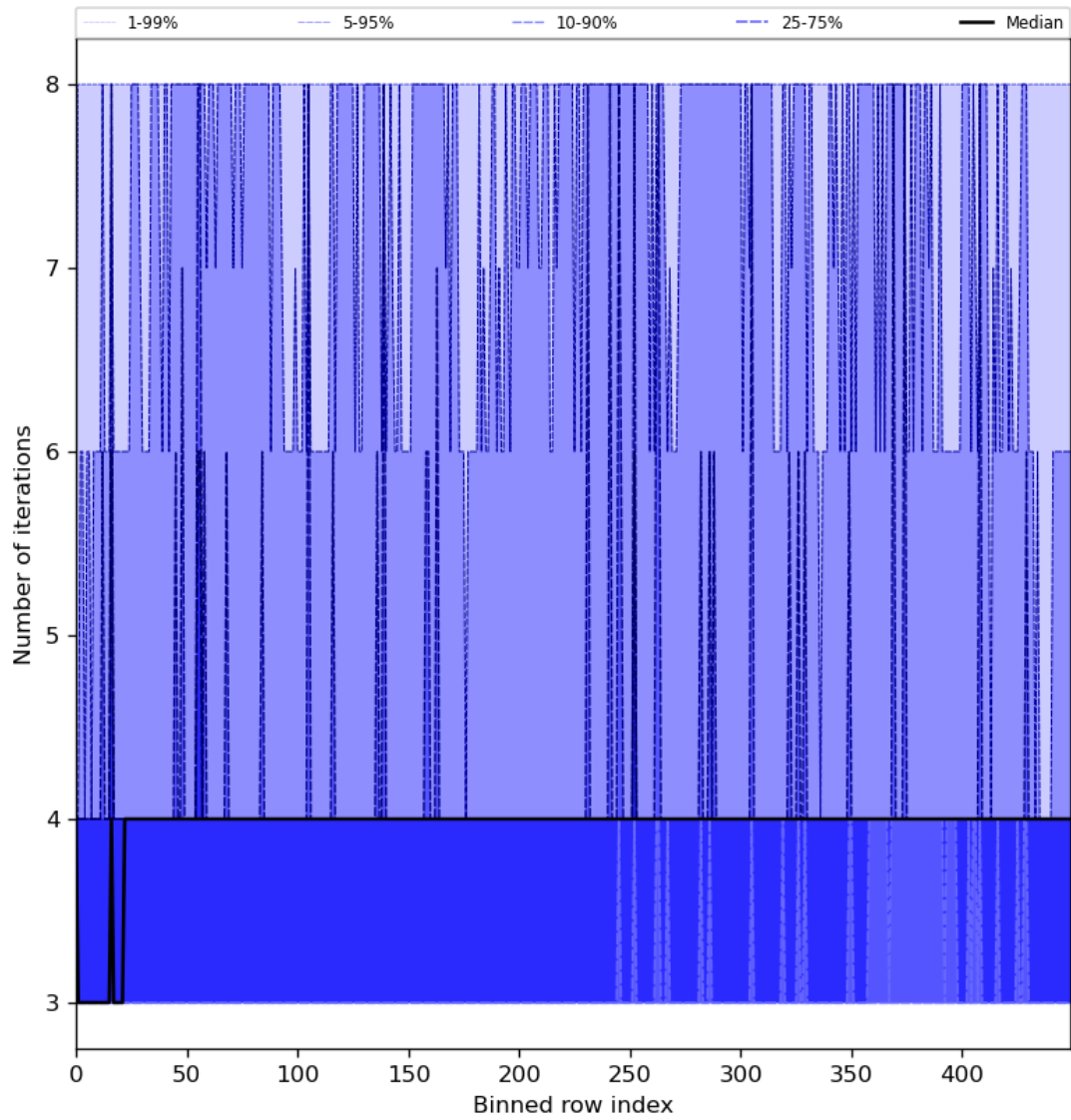
Figure 51: Along track statistics of “Number of iterations” for 2024-07-05 to 2024-07-06
