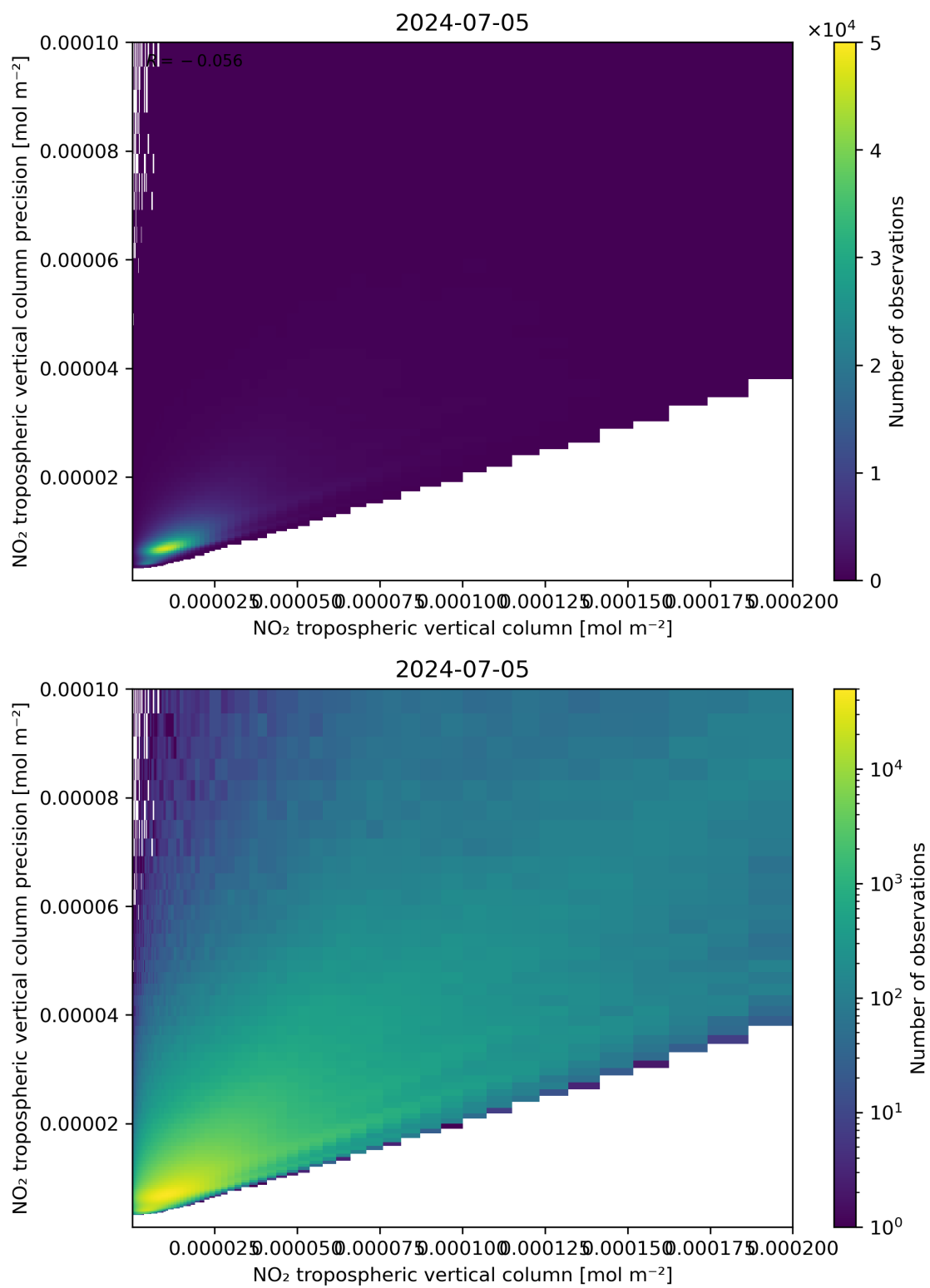
Figure 130: Scatter density plot of “NO 2 tropospheric vertical column” against “NO 2 tropospheric vertical column precision” for 2024-07-05 to 2024-07-06.
