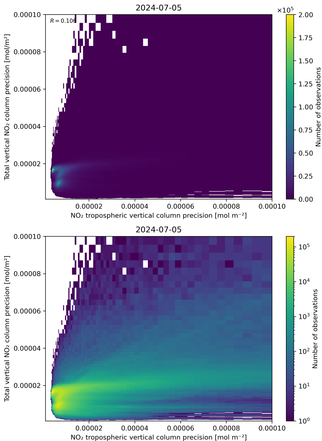
Figure 139: Scatter density plot of “NO 2 tropospheric vertical column precision” against “Total vertical NO 2 column precision” for 2024-07-05 to 2024-07-06.
