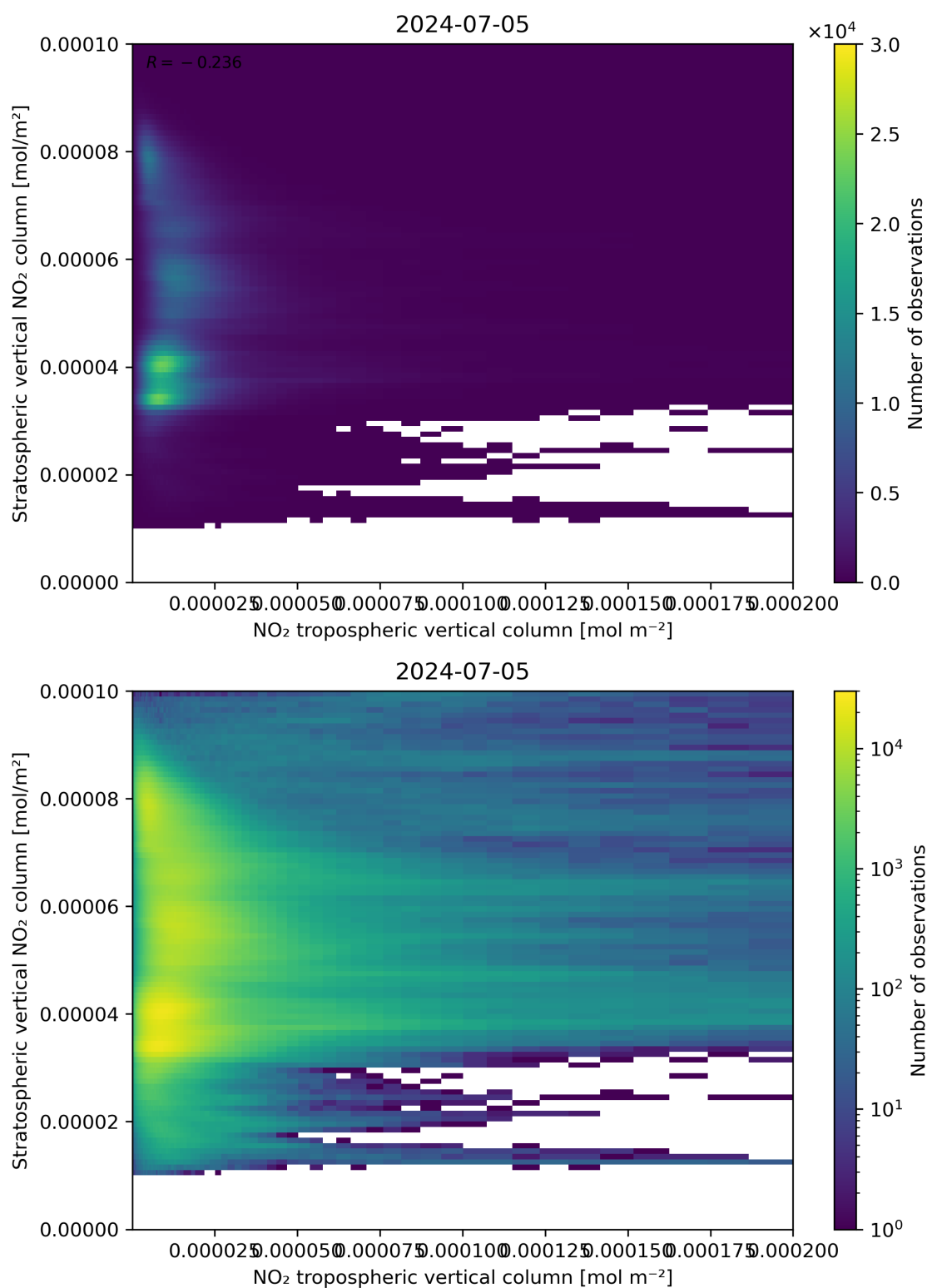
Figure 125: Scatter density plot of “NO 2 tropospheric vertical column” against “Stratospheric vertical NO 2 column” for 2024-07-05 to 2024-07-06.
