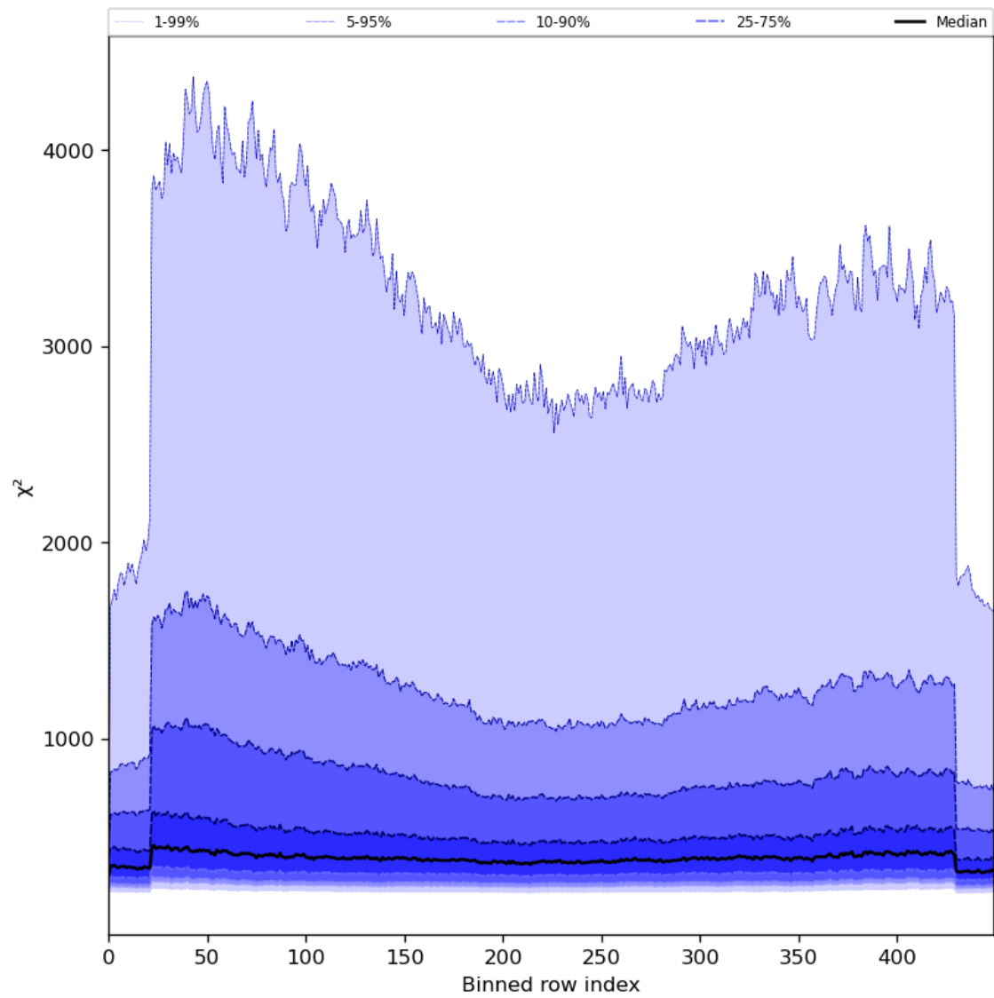
Figure 59: Along track statistics of “ \chi^2 ” for 2024-07-05 to 2024-07-06
