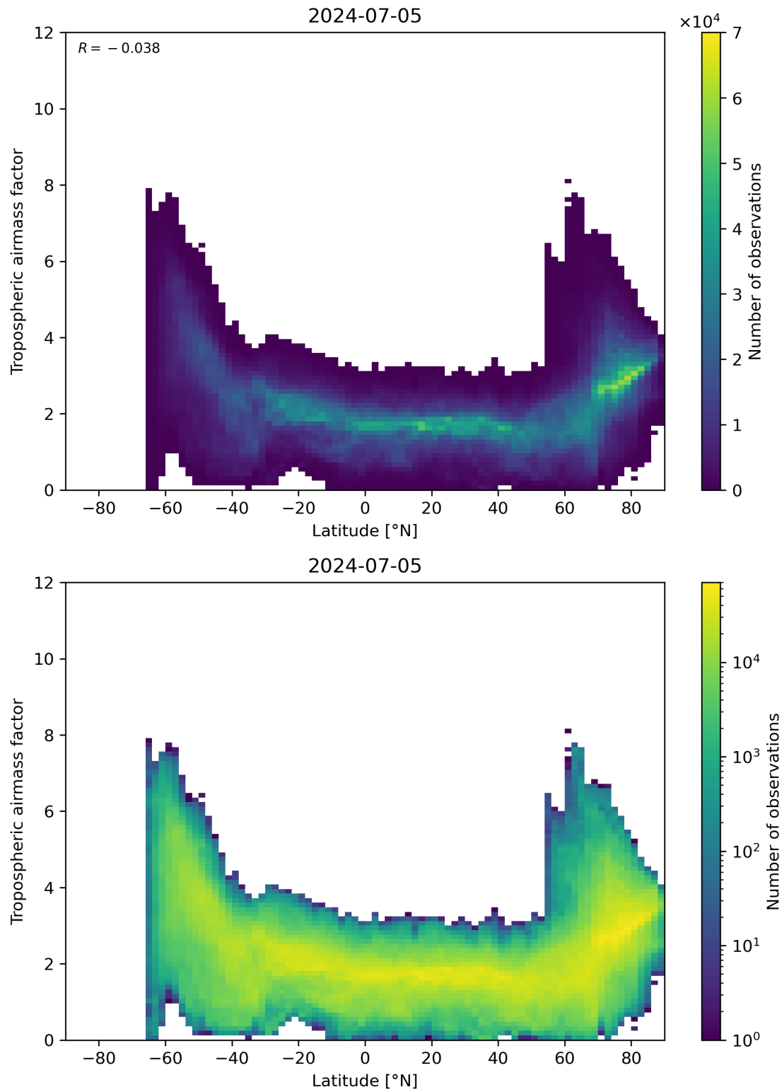
Figure 85: Scatter density plot of “Latitude” against “Tropospheric airmass factor” for 2024-07-05 to 2024-07-06.
