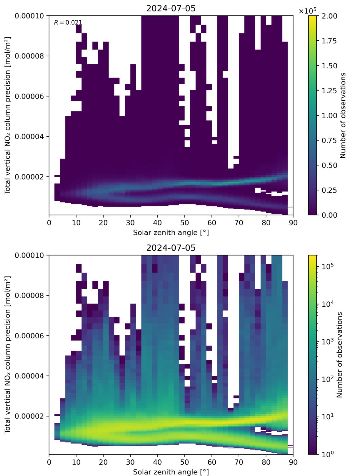
Figure 154: Scatter density plot of “Solar zenith angle” against “Total vertical NO 2 column precision” for 2024-07-05 to 2024-07-06.
