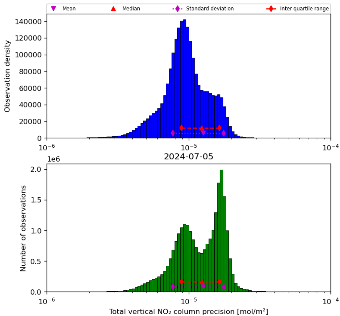
Figure 39: Histogram of “Total vertical NO 2 column precision” for 2024-07-05 to 2024-07-06
