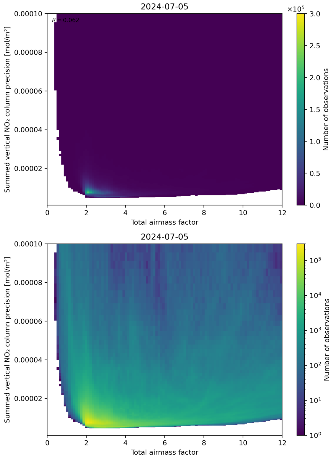
Figure 66: Scatter density plot of “Total airmass factor” against “Summed vertical NO 2 column precision” for 2024-07-05 to 2024-07-06.
