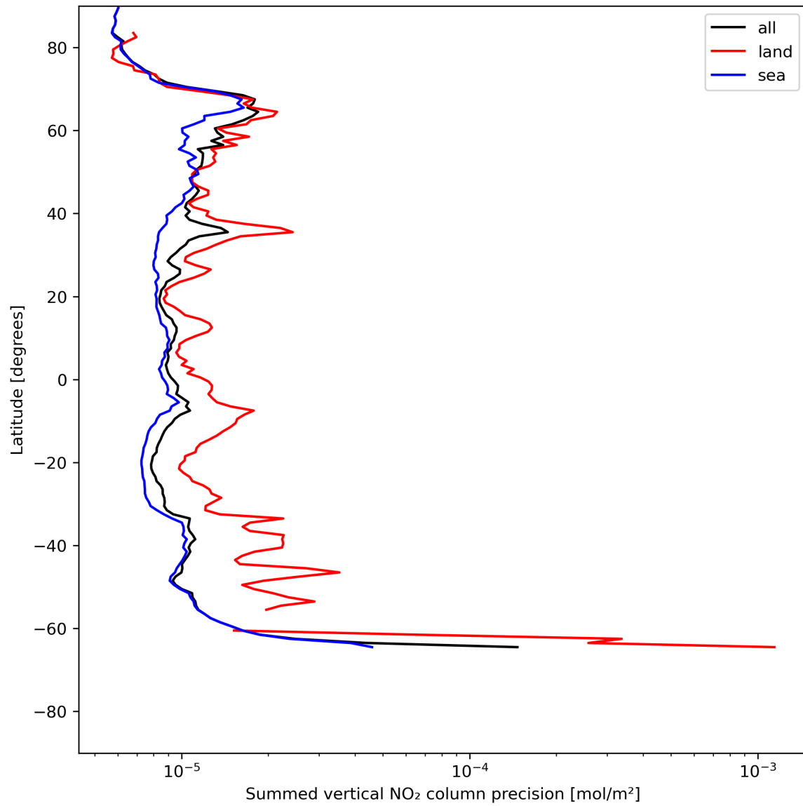
Figure 24: Zonal average of “Summed vertical NO 2 column precision” for 2024-07-05 to 2024-07-06.
