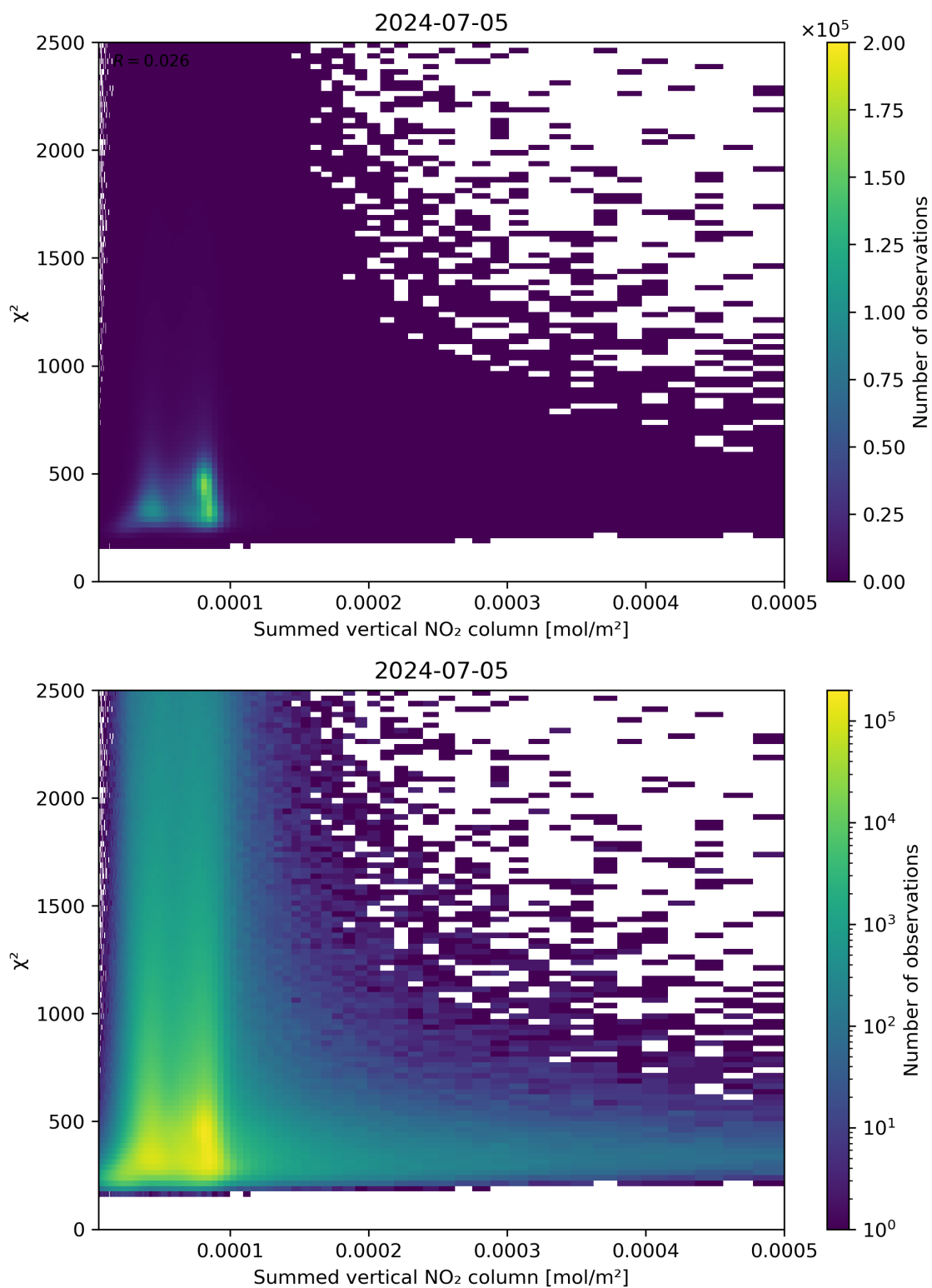
Figure 104: Scatter density plot of “Summed vertical NO 2 column” against “ \chi^2 ” for 2024-07-05 to 2024-07-06.
