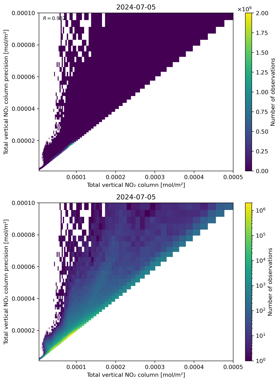
Figure 114: Scatter density plot of “Total vertical NO 2 column” against “Total vertical NO 2 column precision” for 2024-07-05 to 2024-07-06.
