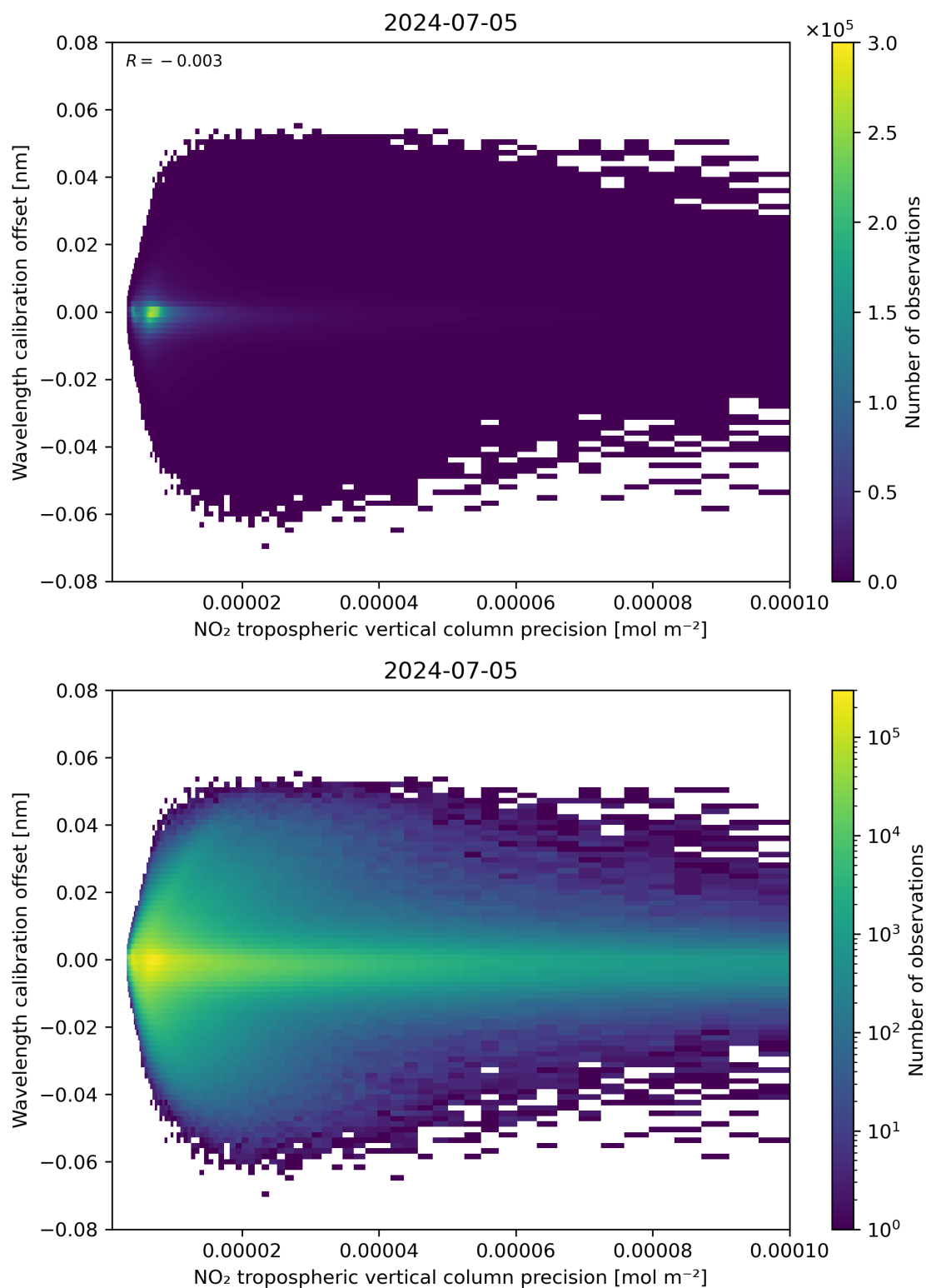
Figure 141: Scatter density plot of “NO 2 tropospheric vertical column precision” against “Wavelength calibration offset” for 2024-07-05 to 2024-07-06.
