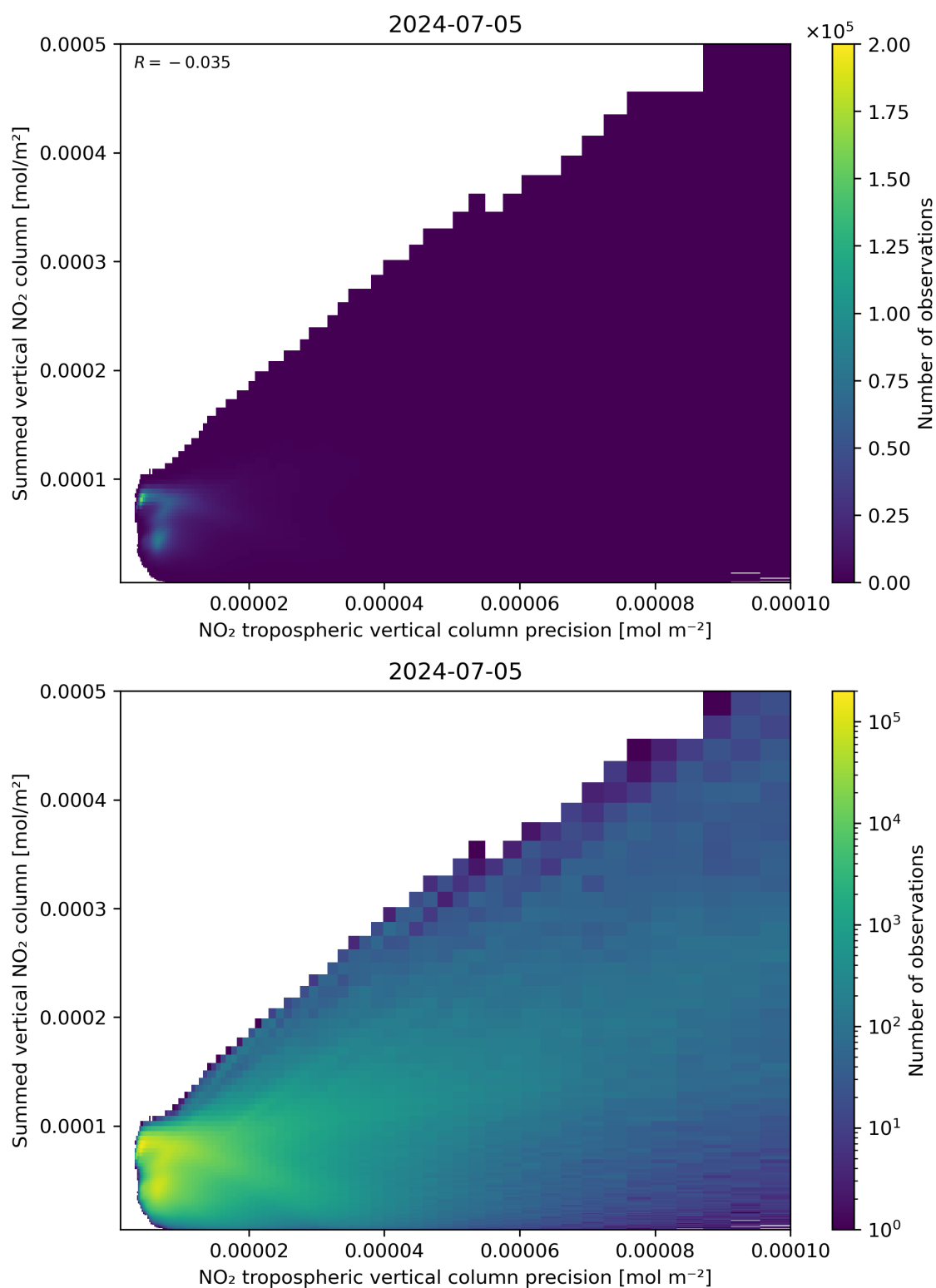
Figure 136: Scatter density plot of “NO 2 tropospheric vertical column precision” against “Summed vertical NO 2 column” for 2024-07-05 to 2024-07-06.
