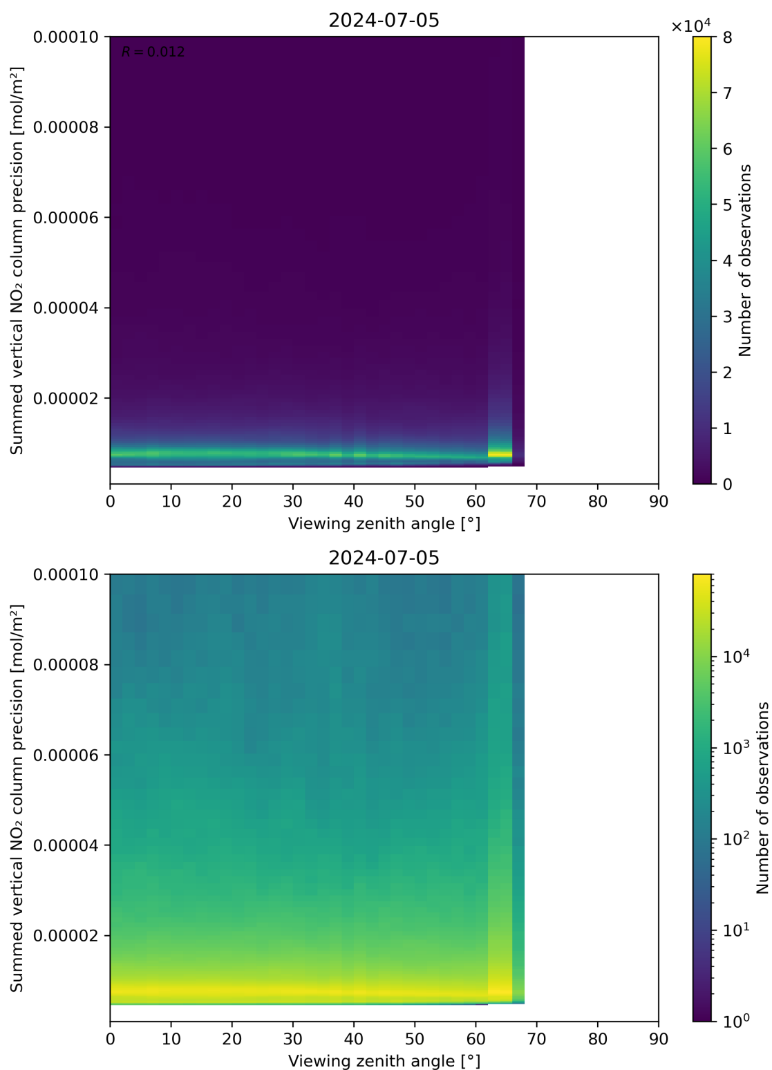
Figure 166: Scatter density plot of “Viewing zenith angle” against “Summed vertical NO 2 column precision” for 2024-07-05 to 2024-07-06.
