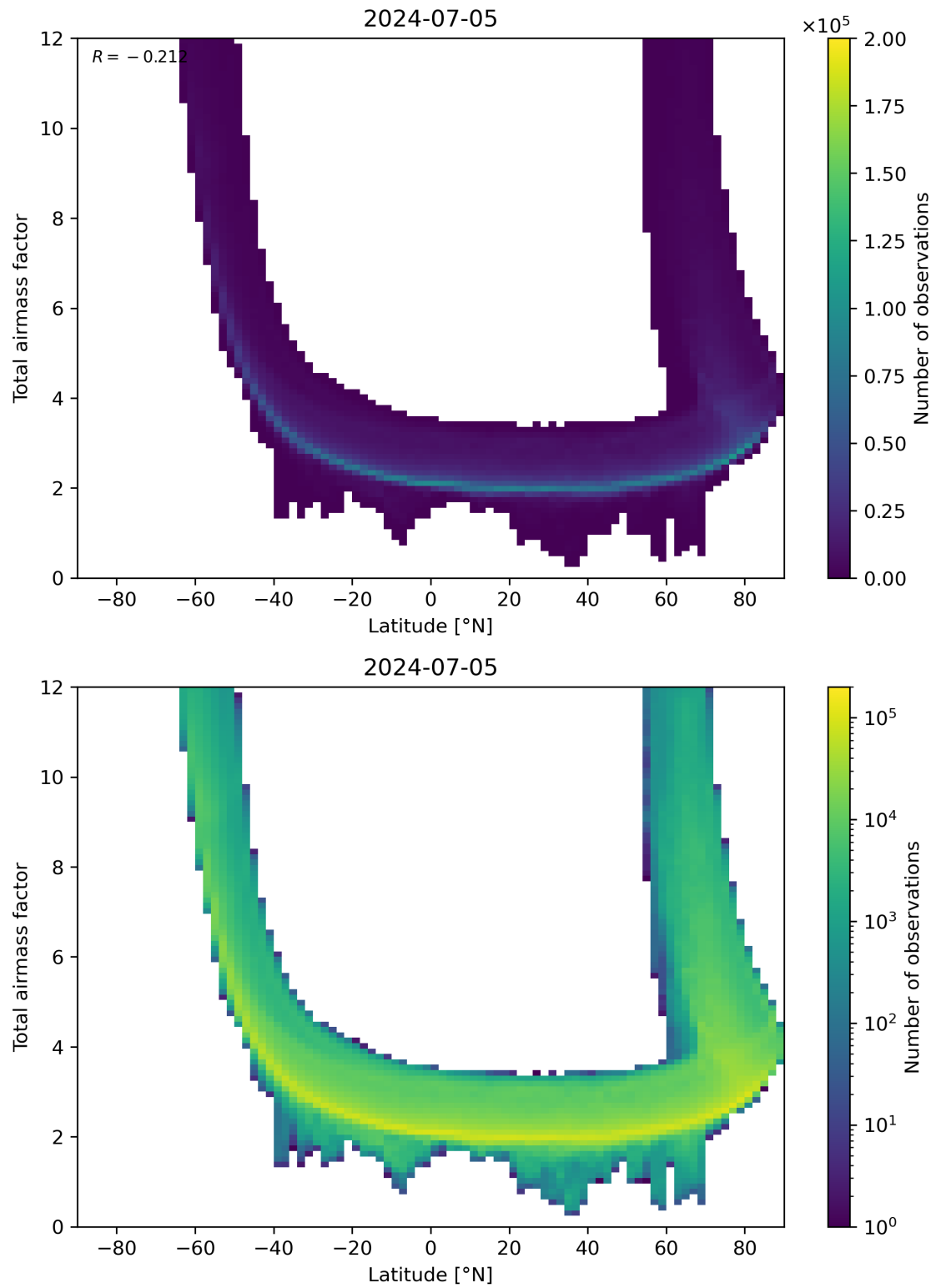
Figure 84: Scatter density plot of “Latitude” against “Total airmass factor” for 2024-07-05 to 2024-07-06.
