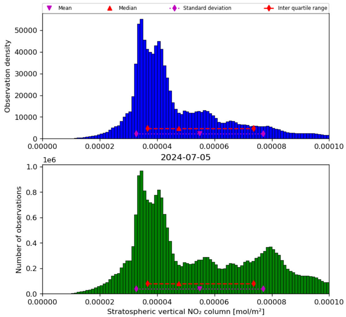
Figure 36: Histogram of “Stratospheric vertical NO 2 column” for 2024-07-05 to 2024-07-06
