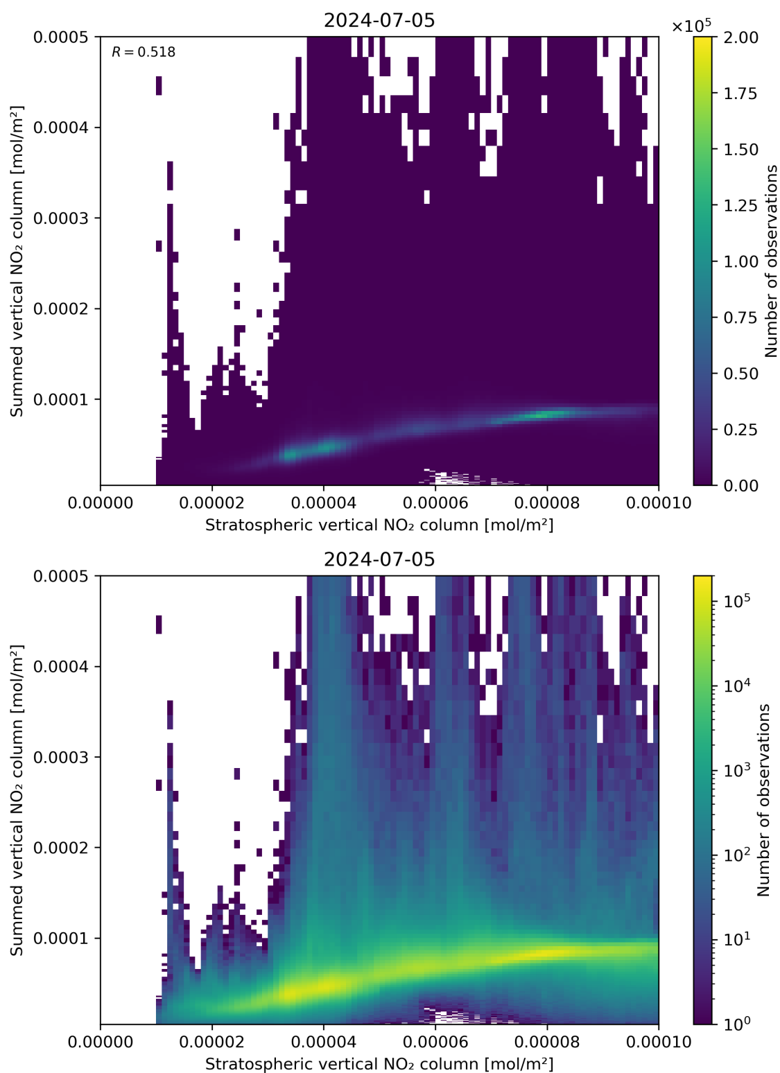
Figure 98: Scatter density plot of “Stratospheric vertical NO 2 column” against “Summed vertical NO 2 column” for 2024-07-05 to 2024-07-06.
