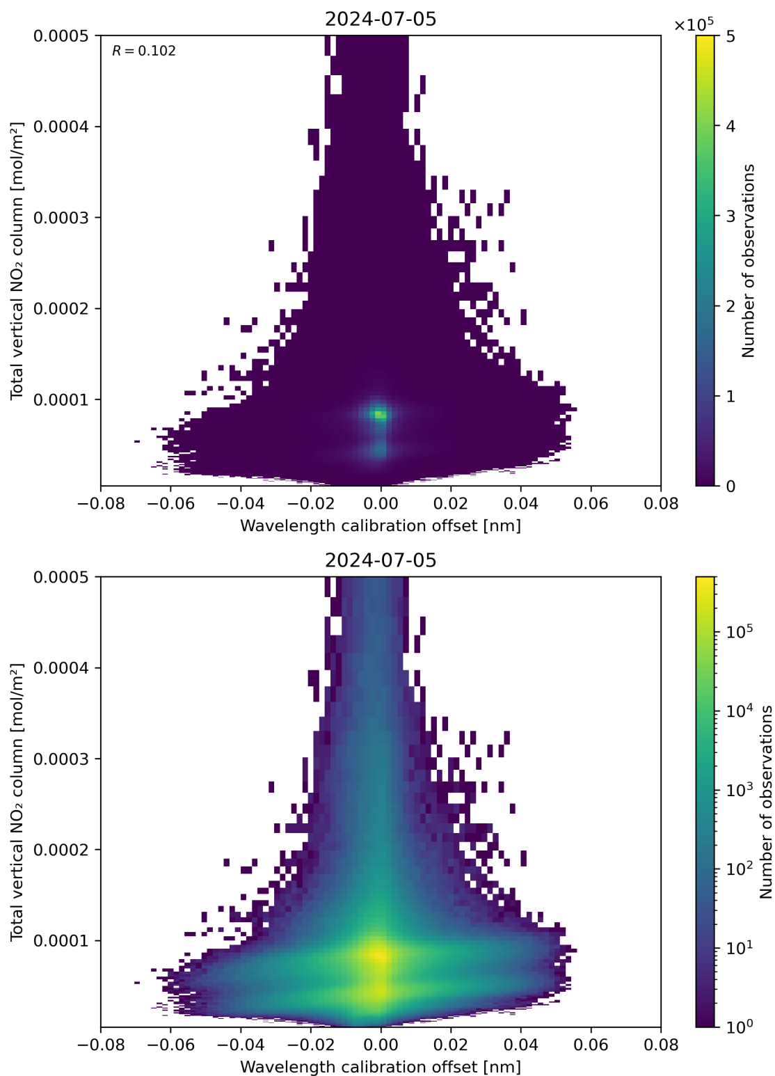
Figure 179: Scatter density plot of “Wavelength calibration offset” against “Total vertical NO 2 column” for 2024-07-05 to 2024-07-06.
