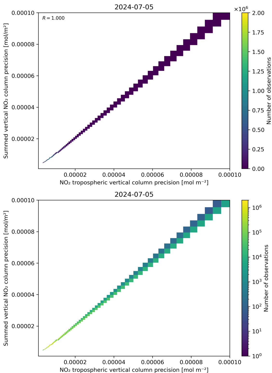
Figure 137: Scatter density plot of “NO 2 tropospheric vertical column precision” against “Summed vertical NO 2 column precision” for 2024-07-05 to 2024-07-06.
