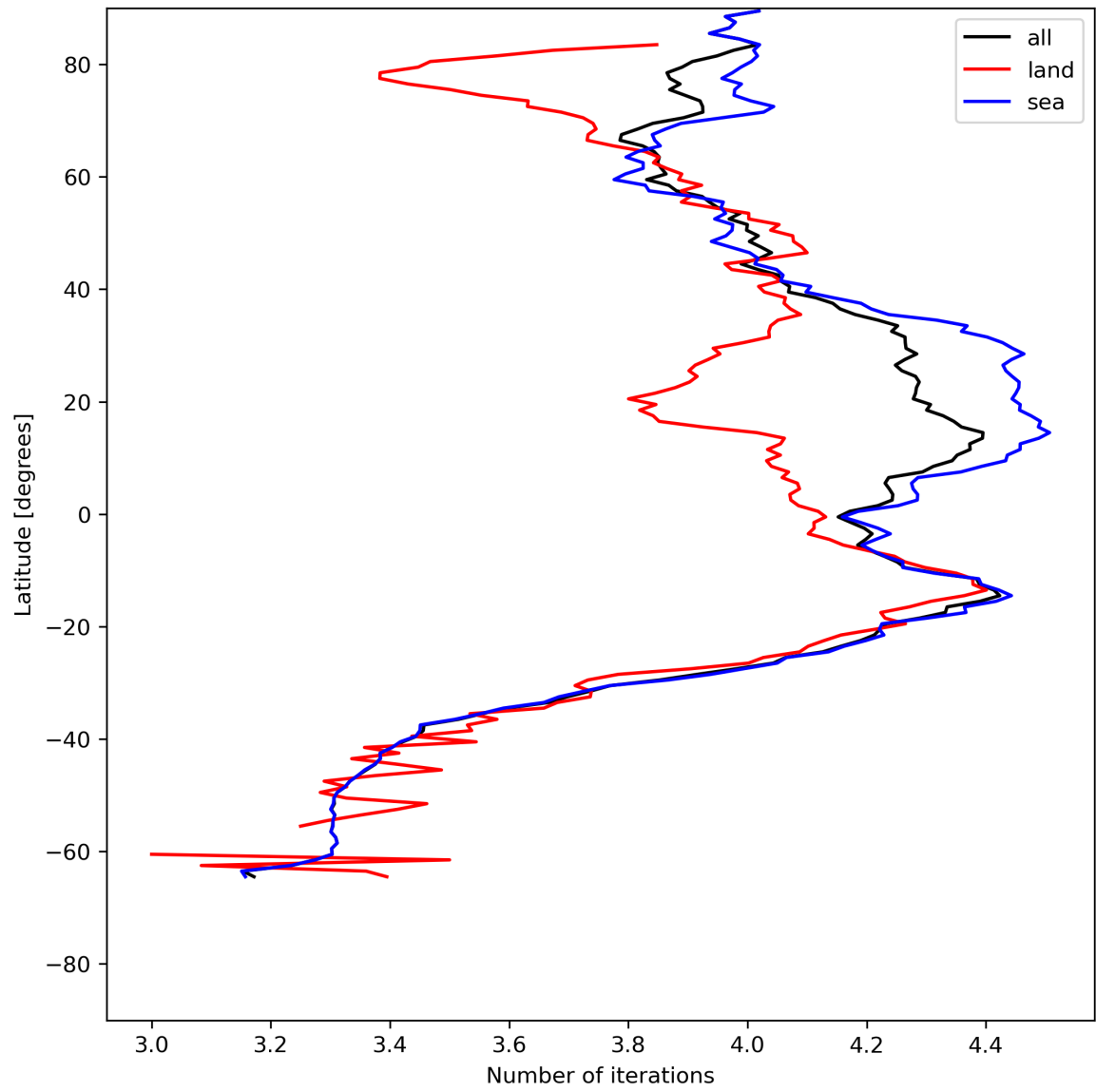
Figure 17: Zonal average of “Number of iterations” for 2024-07-05 to 2024-07-06.
