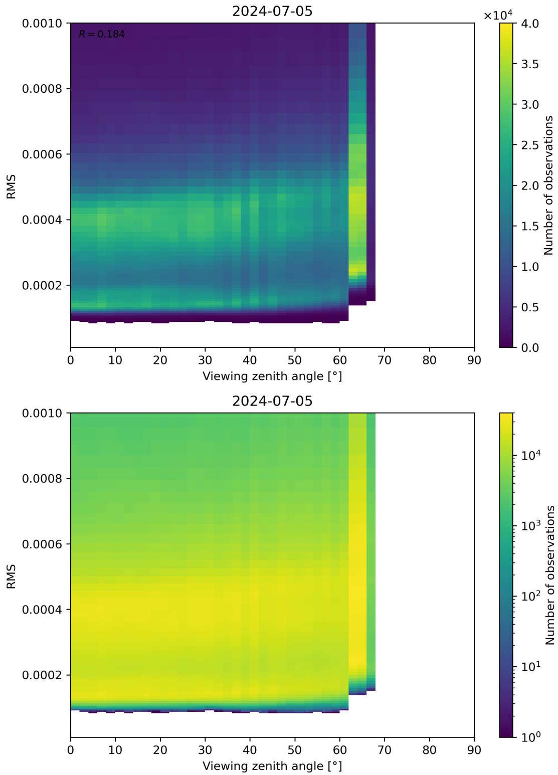
Figure 171: Scatter density plot of “Viewing zenith angle” against “RMS” for 2024-07-05 to 2024-07-06.
