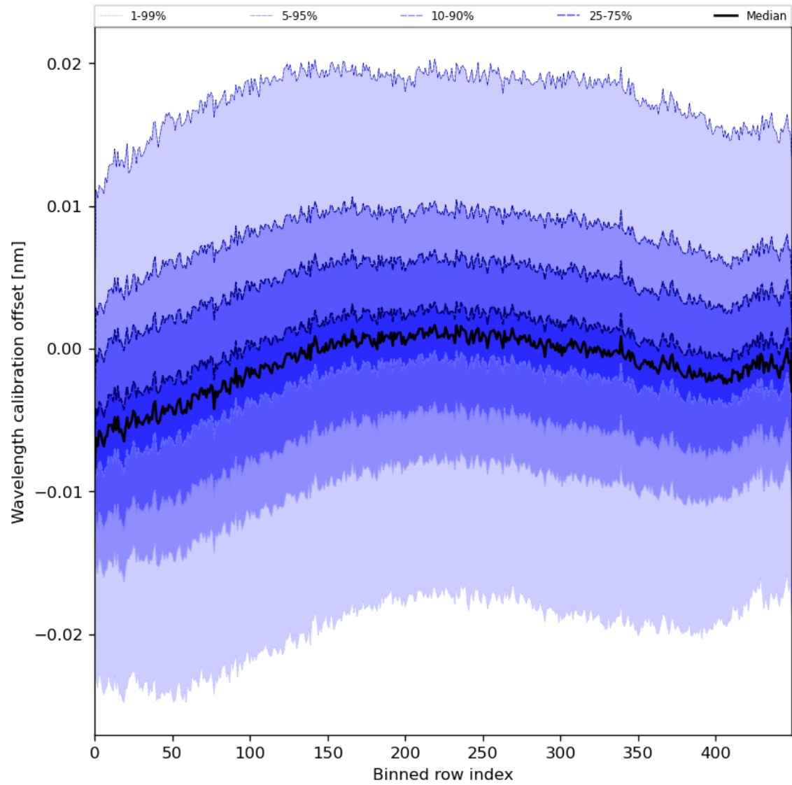
Figure 52: Along track statistics of “Wavelength calibration offset” for 2024-07-05 to 2024-07-06
