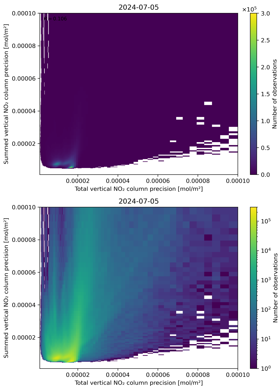
Figure 118: Scatter density plot of “Total vertical NO 2 column precision” against “Summed vertical NO 2 column precision” for 2024-07-05 to 2024-07-06.
