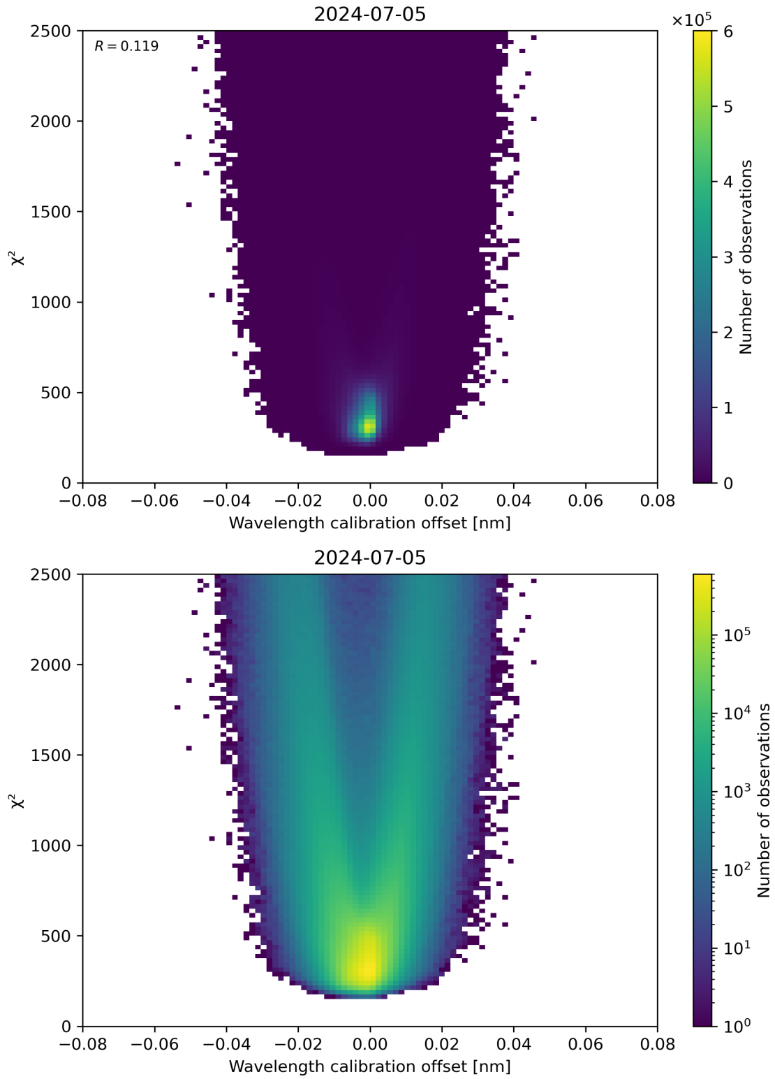
Figure 175: Scatter density plot of “Wavelength calibration offset” against “ \chi^2 ” for 2024-07-05 to 2024-07-06.
