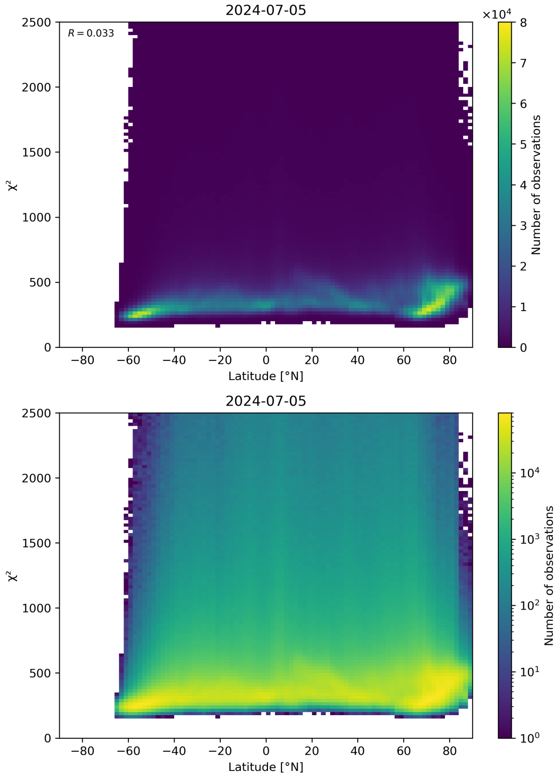
Figure 86: Scatter density plot of “Latitude” against “ \chi^2 ” for 2024-07-05 to 2024-07-06.
