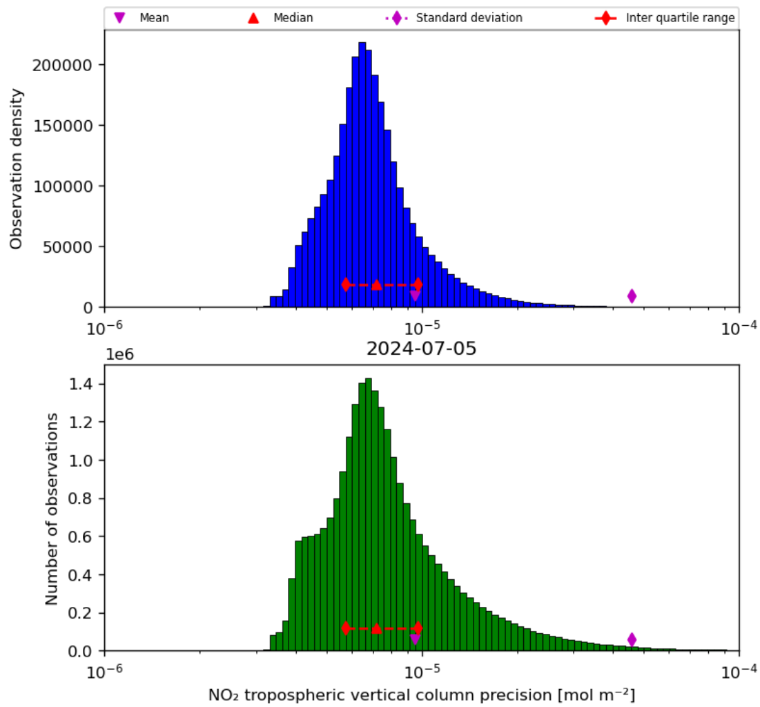
Figure 30: Histogram of “NO 2 tropospheric vertical column precision” for 2024-07-05 to 2024-07-06
