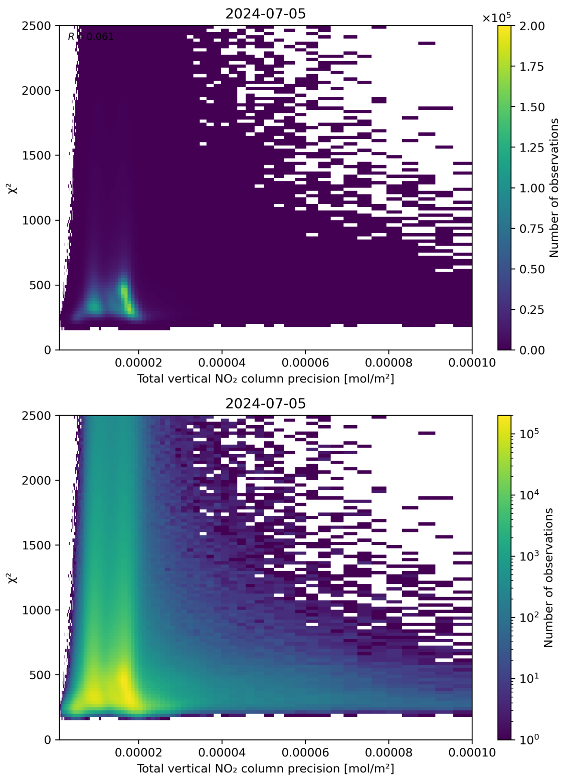
Figure 116: Scatter density plot of “Total vertical NO 2 column precision” against “ \chi^2 ” for 2024-07-05 to 2024-07-06.
