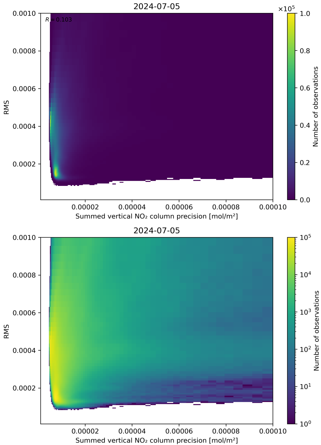
Figure 108: Scatter density plot of “Summed vertical NO 2 column precision” against “RMS” for 2024-07-05 to 2024-07-06.
