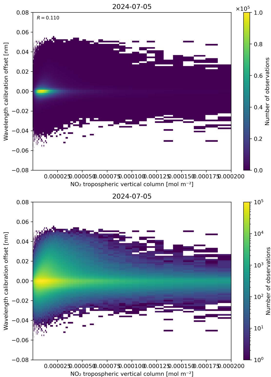
Figure 143: Scatter density plot of “NO 2 tropospheric vertical column” against “Wavelength calibration offset” for 2024-07-05 to 2024-07-06.
