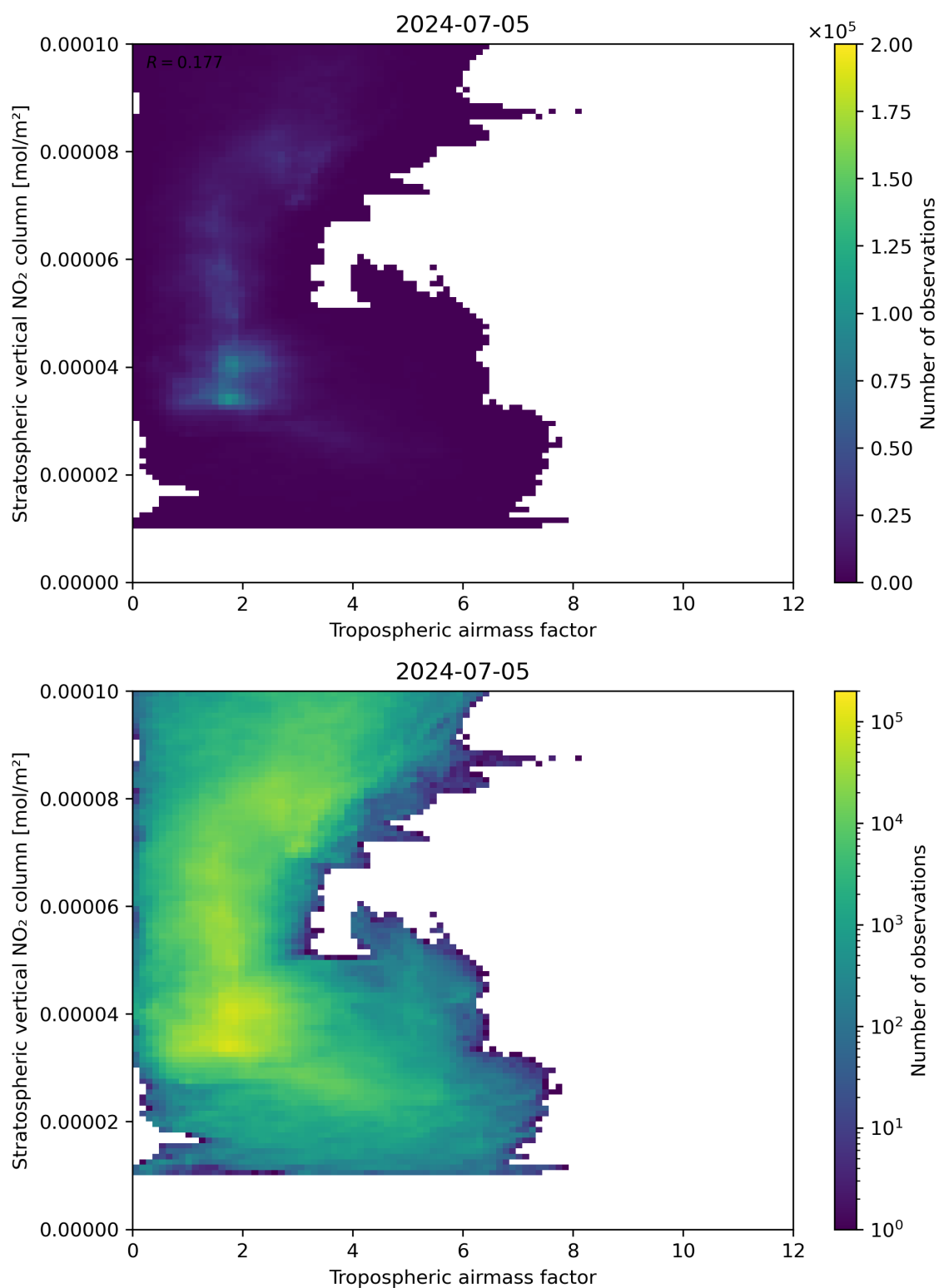
Figure 74: Scatter density plot of “Tropospheric air mass factor” against “Stratospheric vertical NO 2 column” for 2024-07-05 to 2024-07-06.
