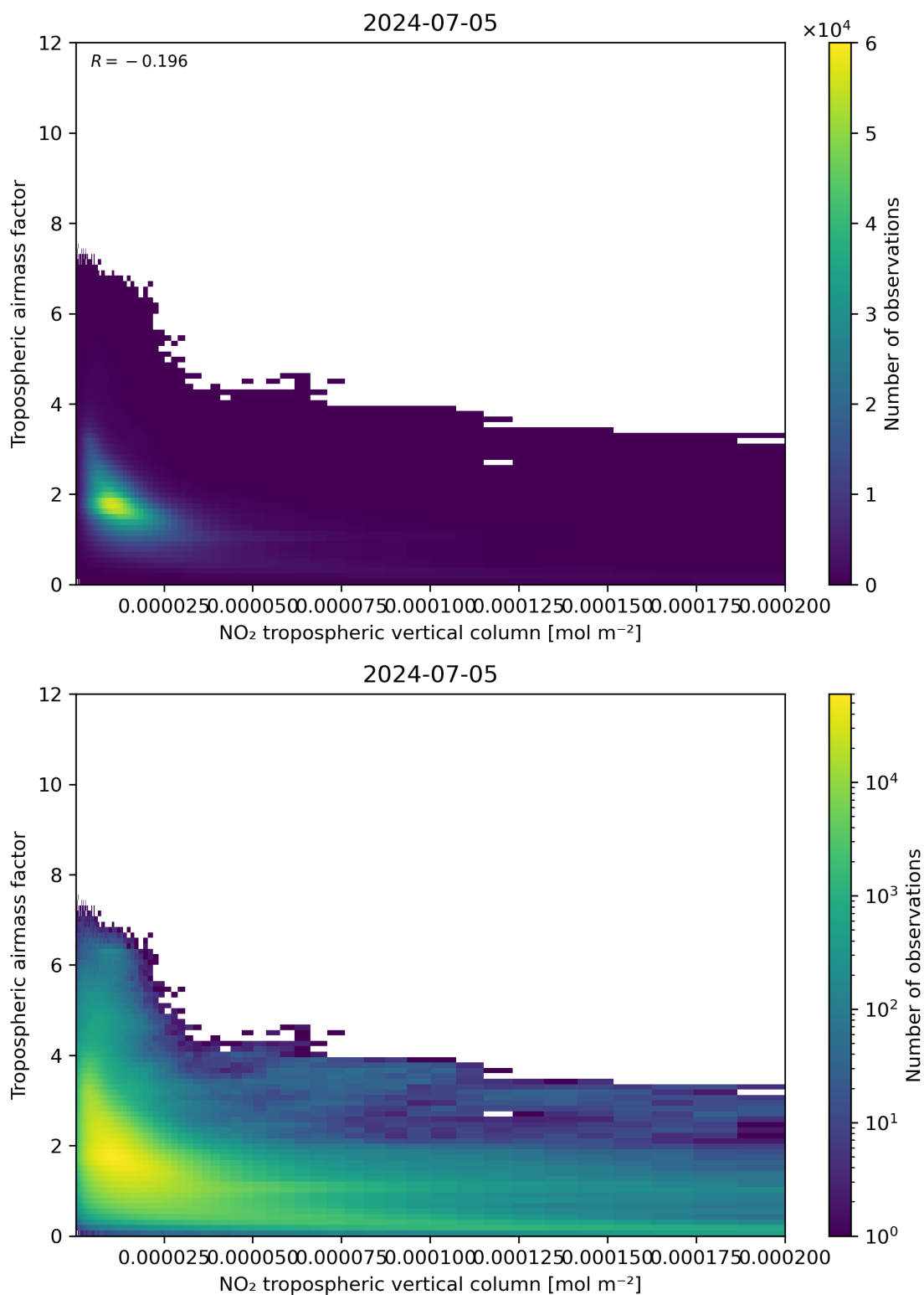
Figure 123: Scatter density plot of “NO 2 tropospheric vertical column” against “Tropospheric airmass factor” for 2024-07-05 to 2024-07-06.
