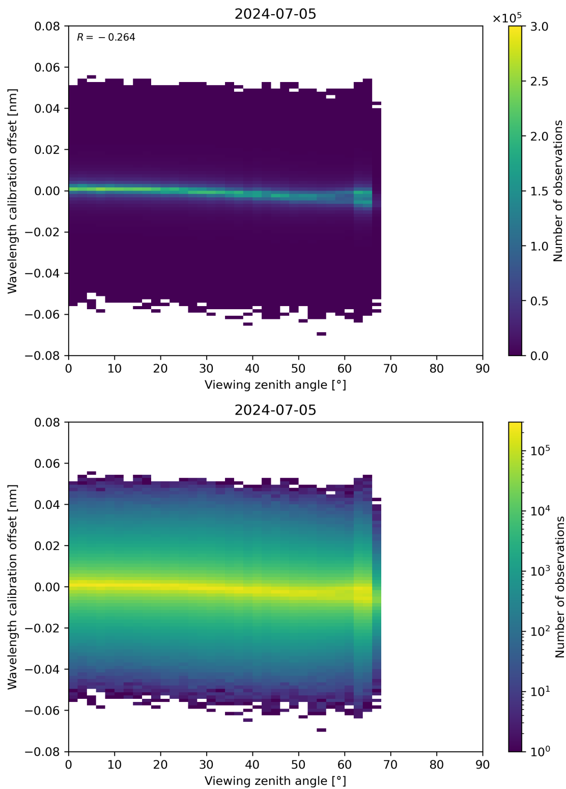
Figure 173: Scatter density plot of “Viewing zenith angle” against “Wavelength calibration offset” for 2024-07-05 to 2024-07-06.
