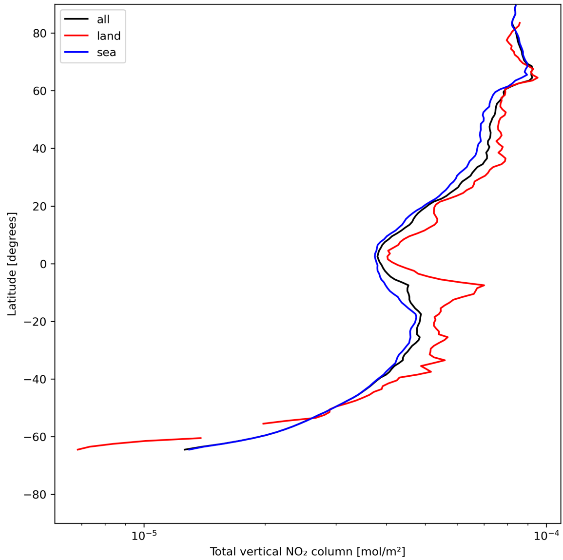
Figure 21: Zonal average of “Total vertical NO 2 column” for 2024-07-05 to 2024-07-06.
