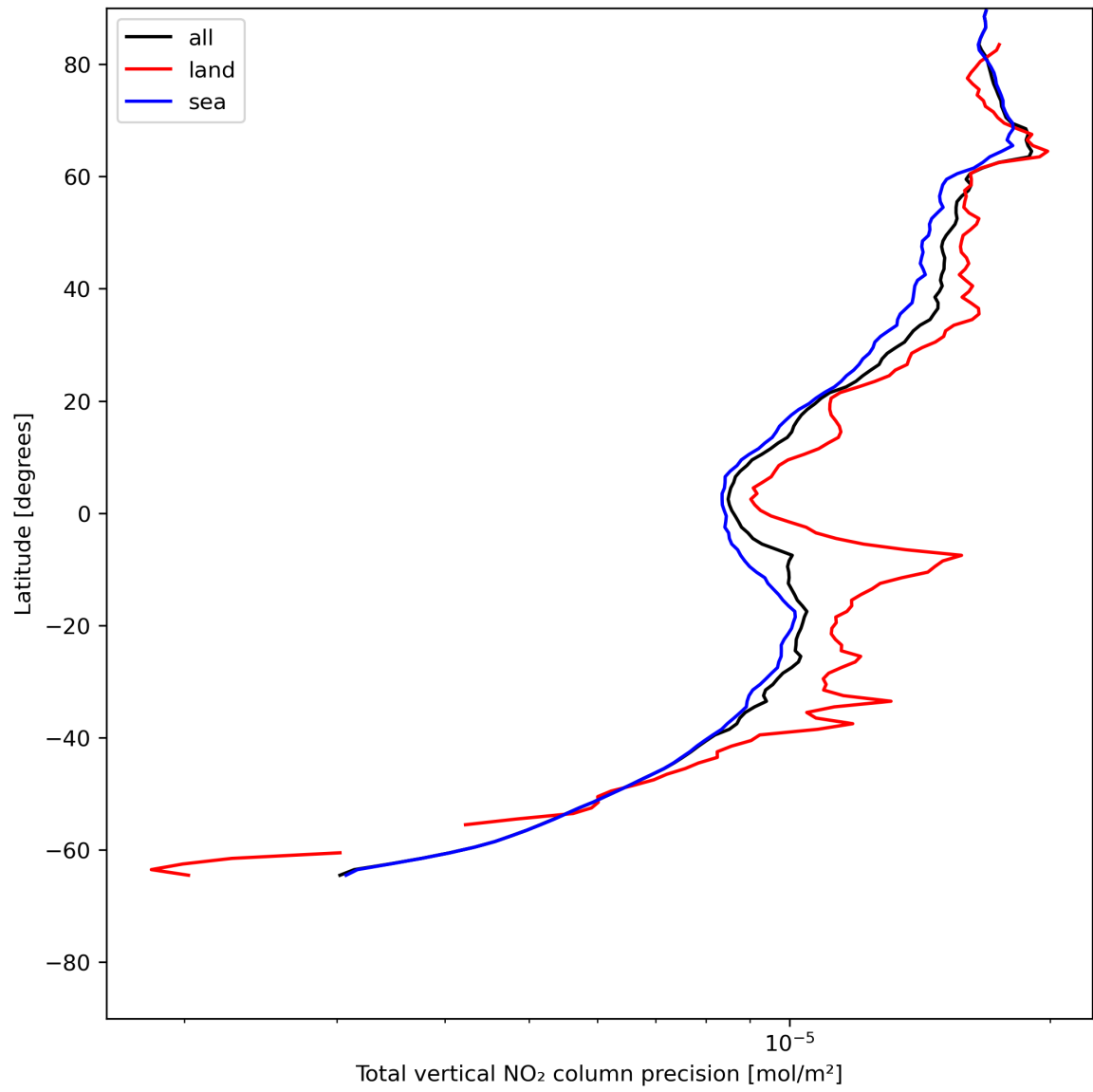
Figure 22: Zonal average of “Total vertical NO 2 column precision” for 2024-07-05 to 2024-07-06.
