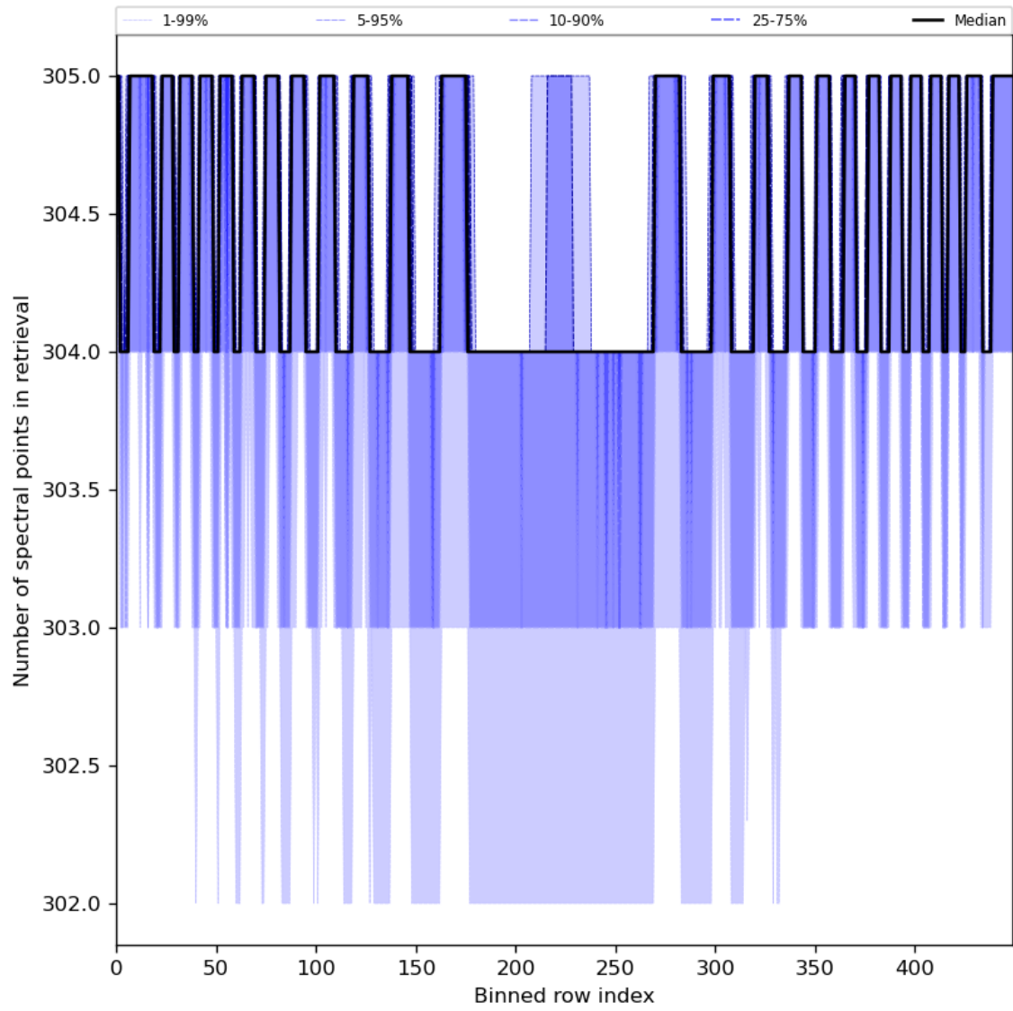
Figure 50: Along track statistics of “Number of spectral points in retrieval” for 2024-07-05 to 2024-07-06
