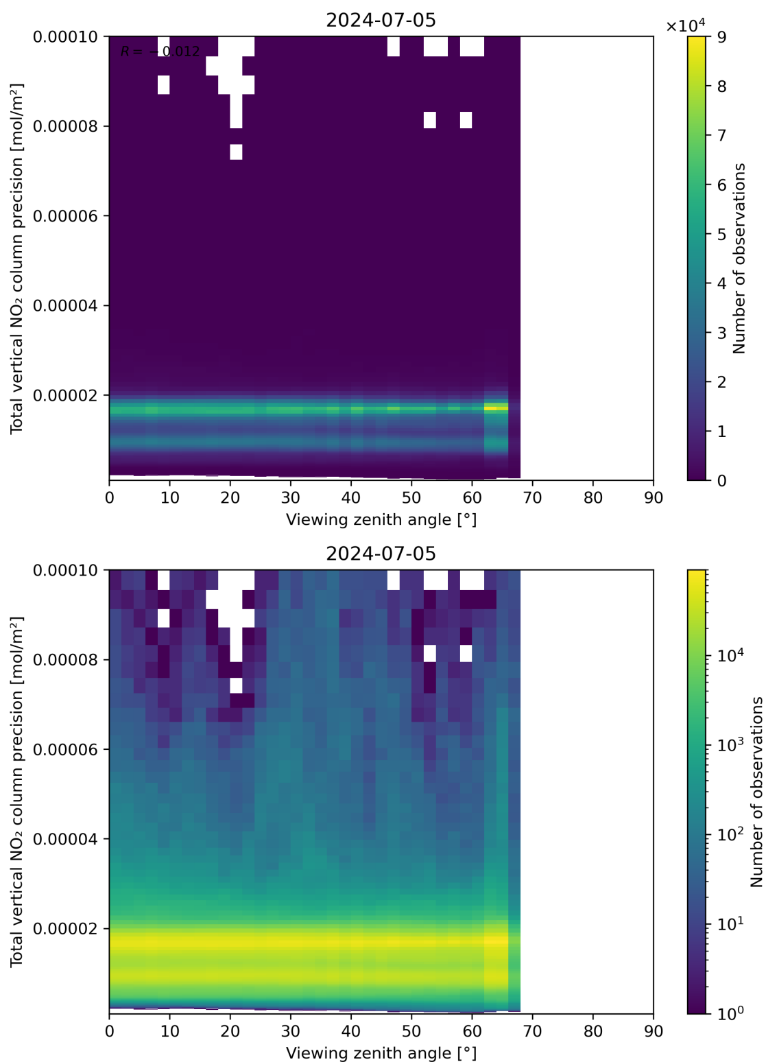
Figure 168: Scatter density plot of “Viewing zenith angle” against “Total vertical NO 2 column precision” for 2024-07-05 to 2024-07-06.
