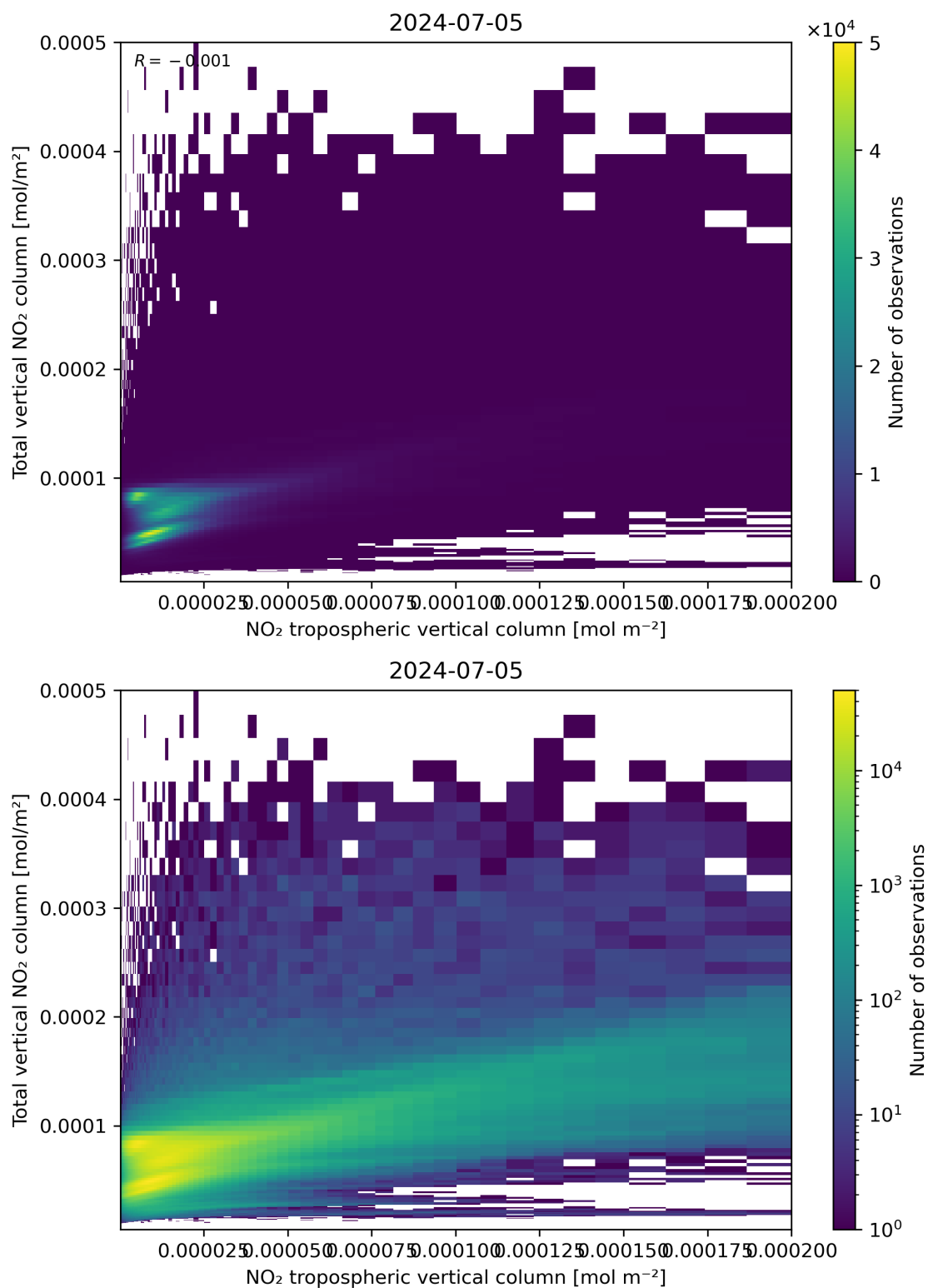
Figure 128: Scatter density plot of “NO 2 tropospheric vertical column” against “Total vertical NO 2 column” for 2024-07-05 to 2024-07-06.
