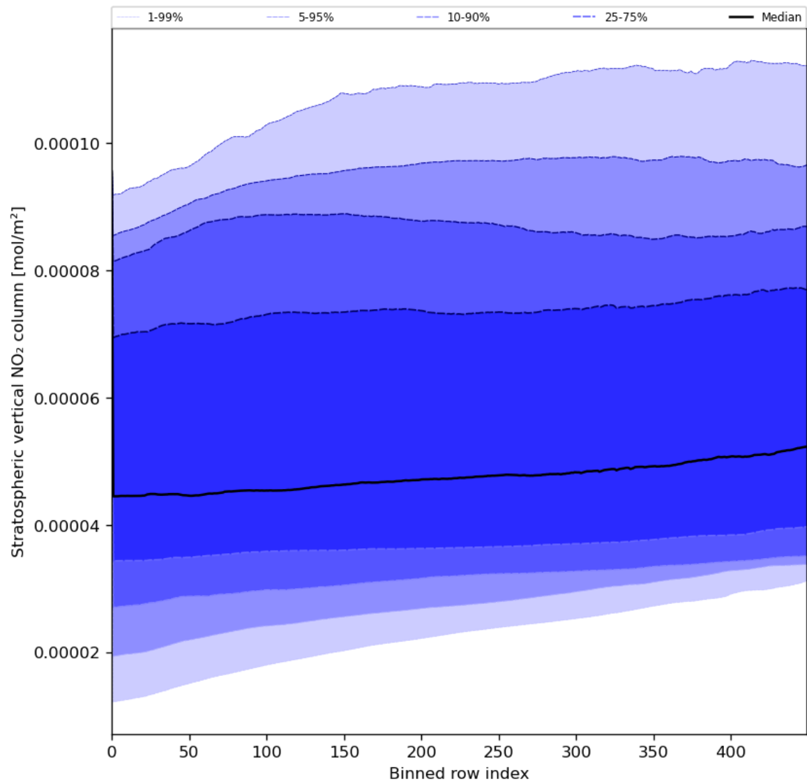
Figure 53: Along track statistics of “Stratospheric vertical NO 2 column” for 2024-07-05 to 2024-07-06
