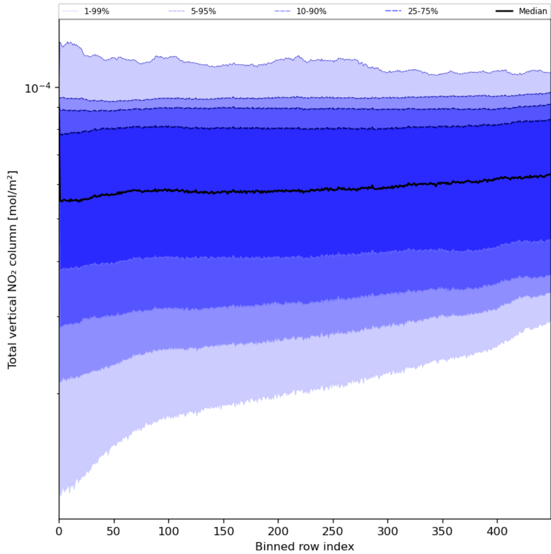
Figure 55: Along track statistics of “Total vertical NO 2 column” for 2024-07-05 to 2024-07-06
