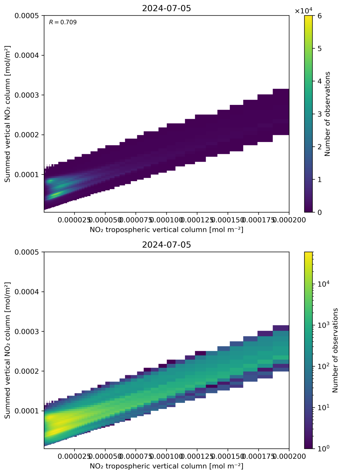
Figure 126: Scatter density plot of “NO 2 tropospheric vertical column” against “Summed vertical NO 2 column” for 2024-07-05 to 2024-07-06.
