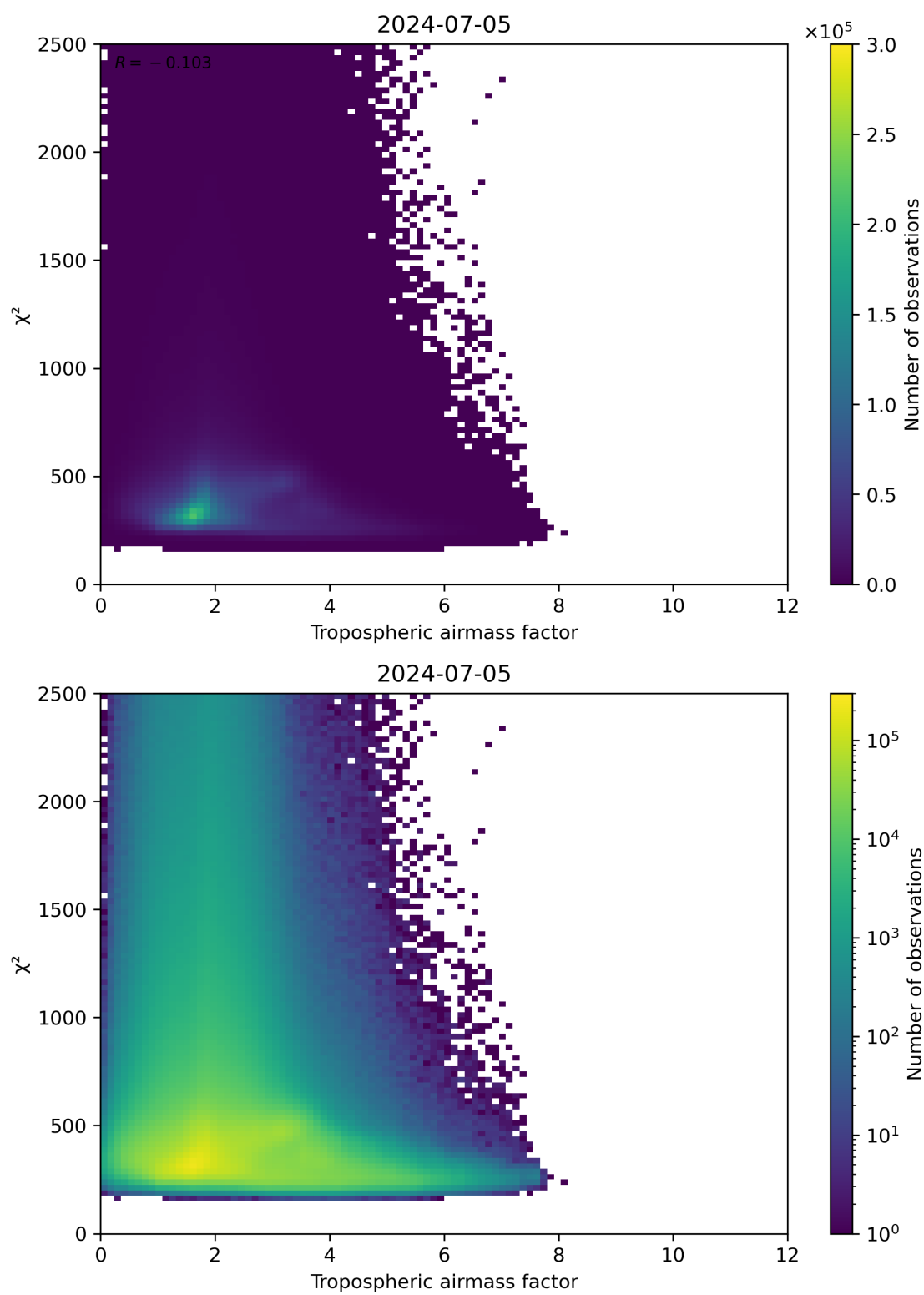
Figure 73: Scatter density plot of “Tropospheric airmass factor” against “ \chi^2 ” for 2024-07-05 to 2024-07-06.
