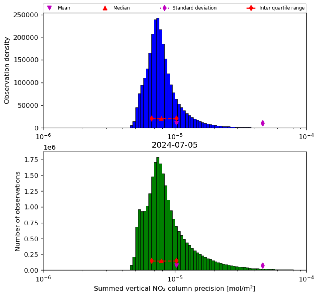
Figure 41: Histogram of “Summed vertical NO 2 column precision” for 2024-07-05 to 2024-07-06
