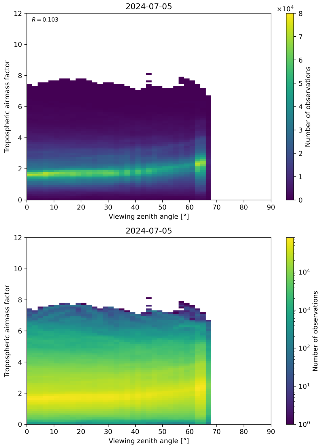
Figure 161: Scatter density plot of “Viewing zenith angle” against “Tropospheric airmass factor” for 2024-07-05 to 2024-07-06.
