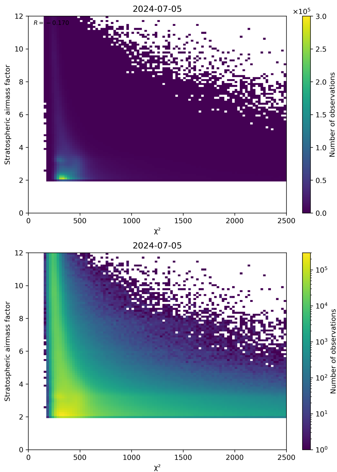
Figure 81: Scatter density plot of “ \chi^2 ” against “Stratospheric airmass factor” for 2024-07-05 to 2024-07-06.
