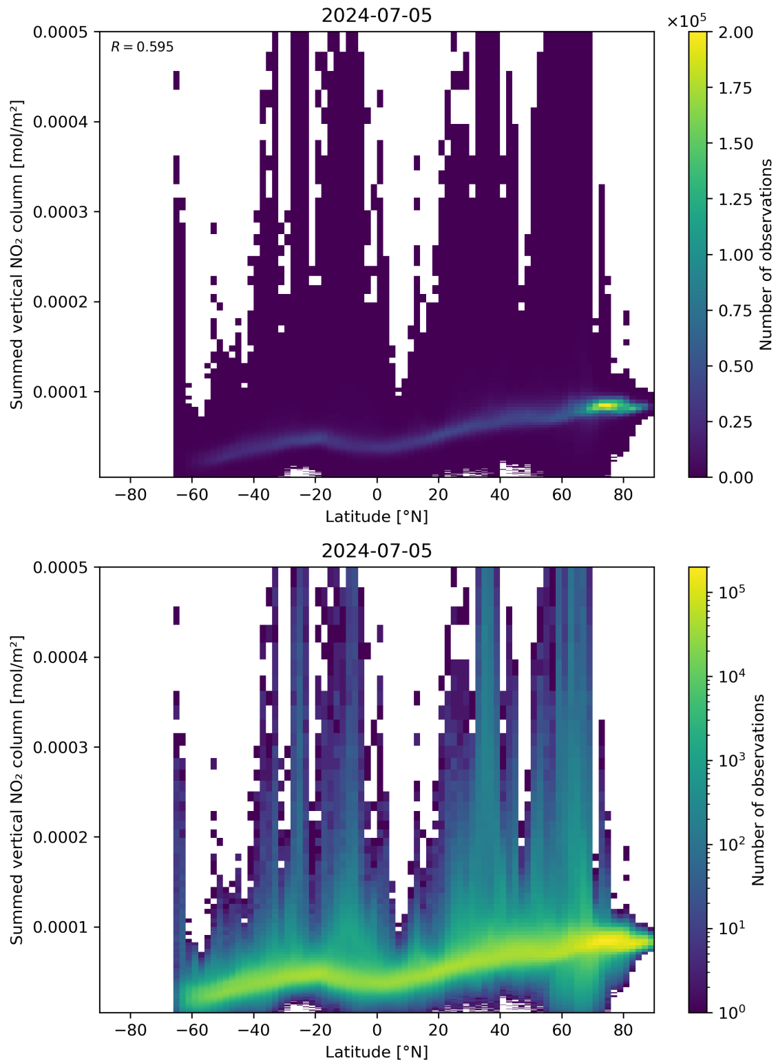
Figure 88: Scatter density plot of “Latitude” against “Summed vertical NO 2 column” for 2024-07-05 to 2024-07-06.
