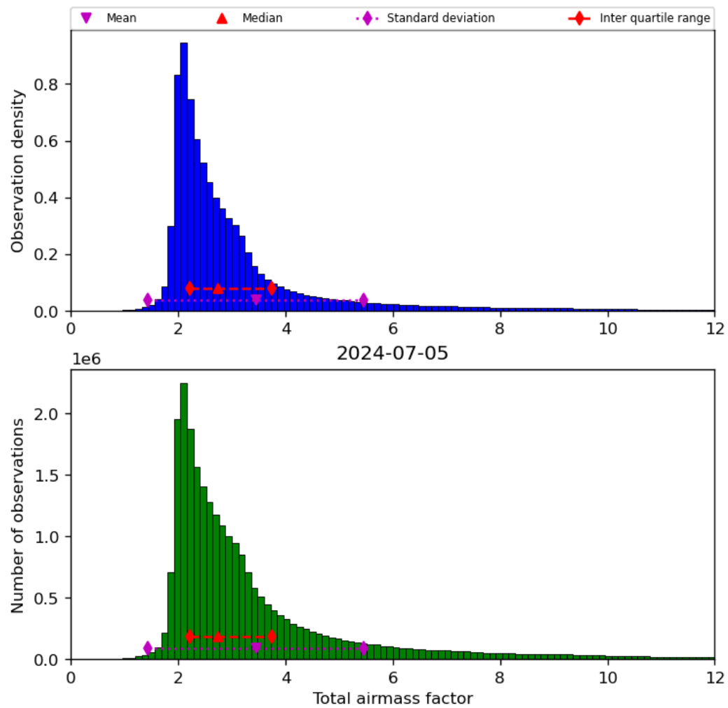
Figure 32: Histogram of “Total airmass factor” for 2024-07-05 to 2024-07-06
