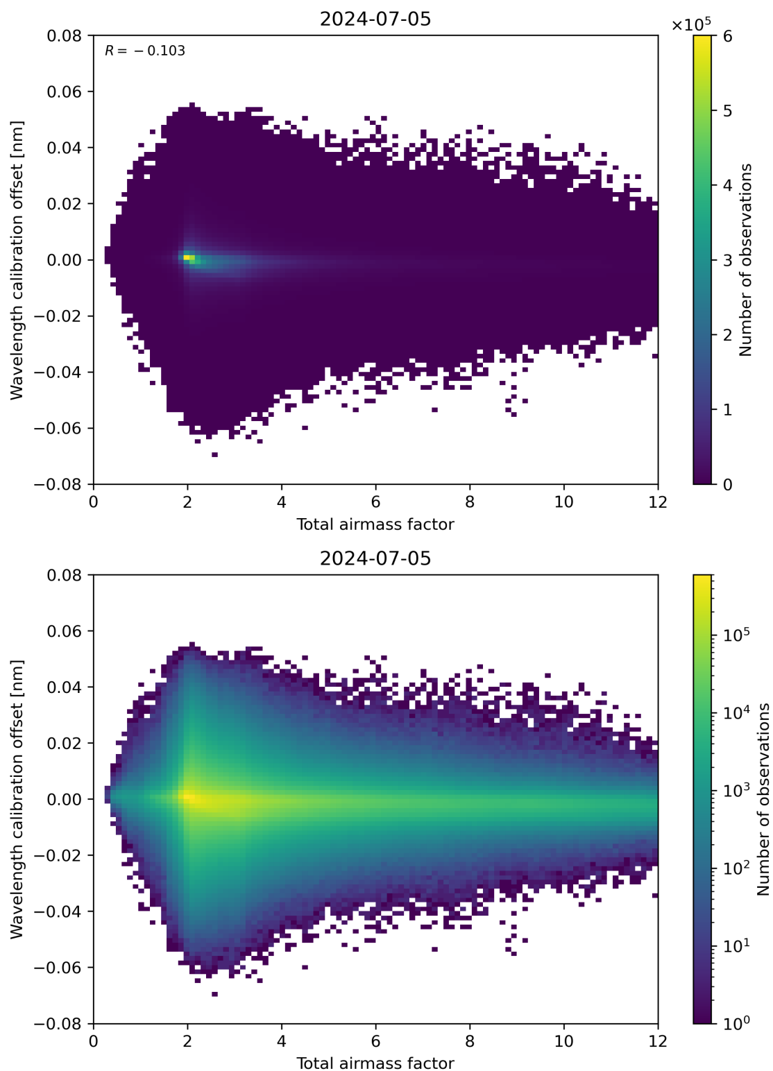
Figure 70: Scatter density plot of “Total airmass factor” against “Wavelength calibration offset” for 2024-07-05 to 2024-07-06.
