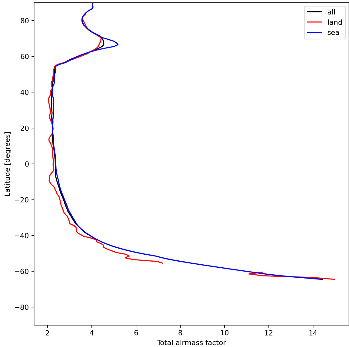
Figure 15: Zonal average of “Total airmass factor” for 2024-07-05 to 2024-07-06.
