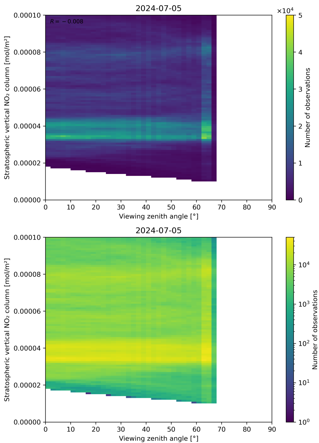
Figure 164: Scatter density plot of “Viewing zenith angle” against “Stratospheric vertical NO 2 column” for 2024-07-05 to 2024-07-06.
