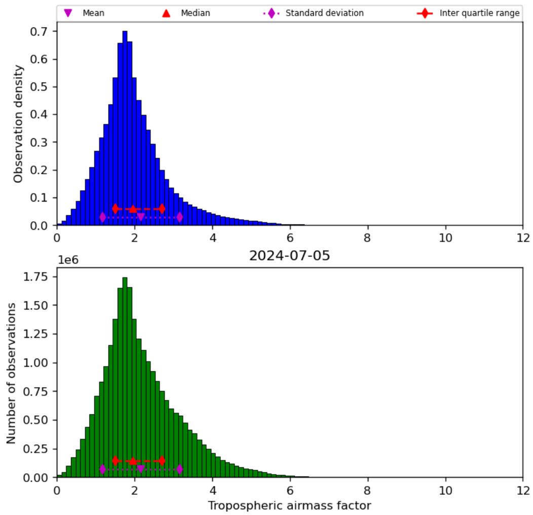
Figure 31: Histogram of “Tropospheric airmass factor” for 2024-07-05 to 2024-07-06
