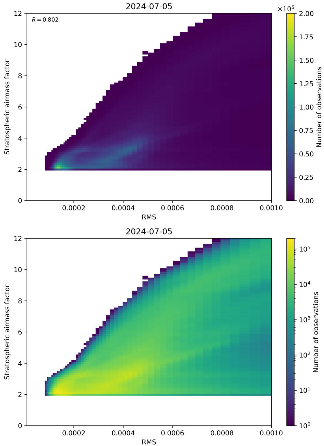
Figure 144: Scatter density plot of “RMS” against “Stratospheric airmass factor” for 2024-07-05 to 2024-07-06.
