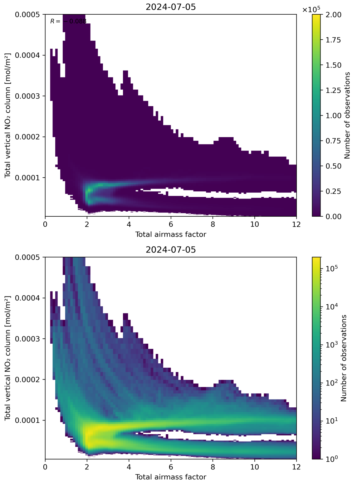
Figure 67: Scatter density plot of “Total airmass factor” against “Total vertical NO 2 column” for 2024-07-05 to 2024-07-06.
