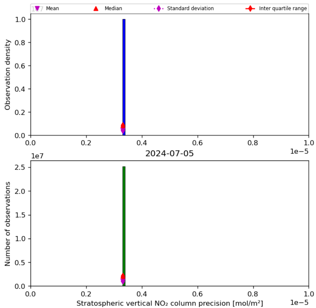
Figure 37: Histogram of “Stratospheric vertical NO 2 column precision” for 2024-07-05 to 2024-07-06
