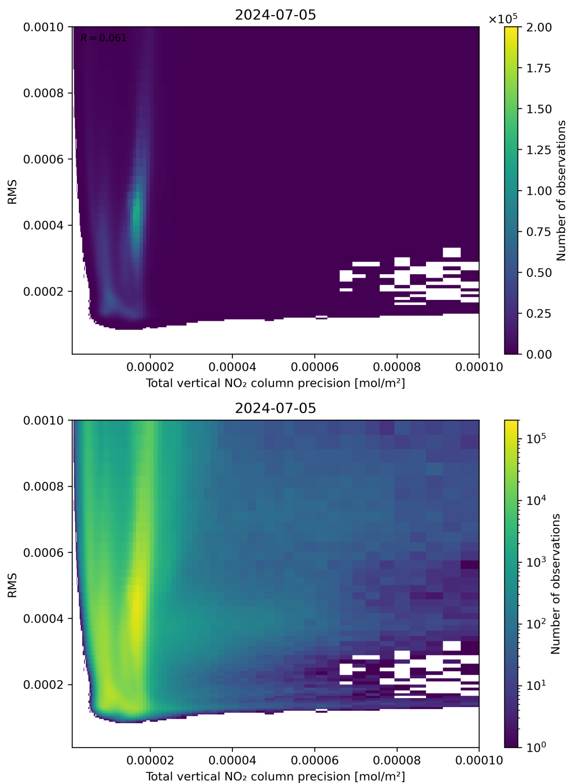
Figure 119: Scatter density plot of “Total vertical NO 2 column precision” against “RMS” for 2024-07-05 to 2024-07-06.
