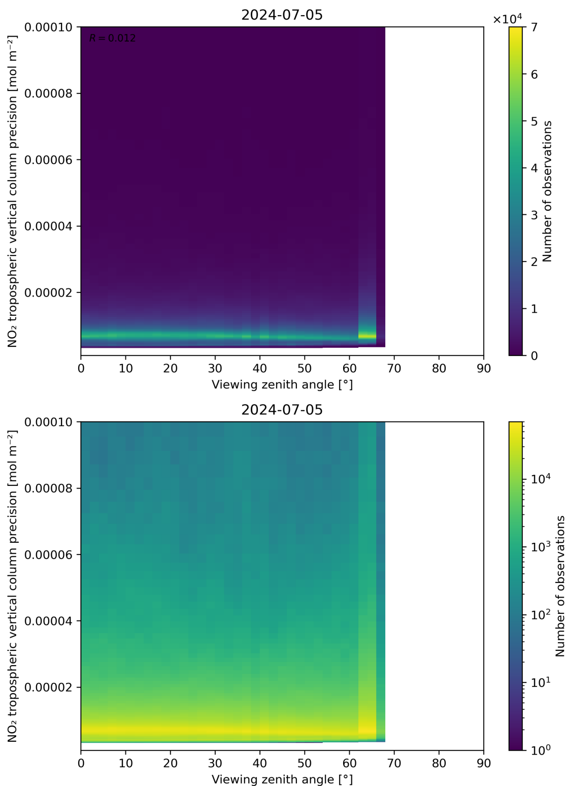
Figure 170: Scatter density plot of “Viewing zenith angle” against “NO 2 tropospheric vertical column precision” for 2024-07-05 to 2024-07-06.
