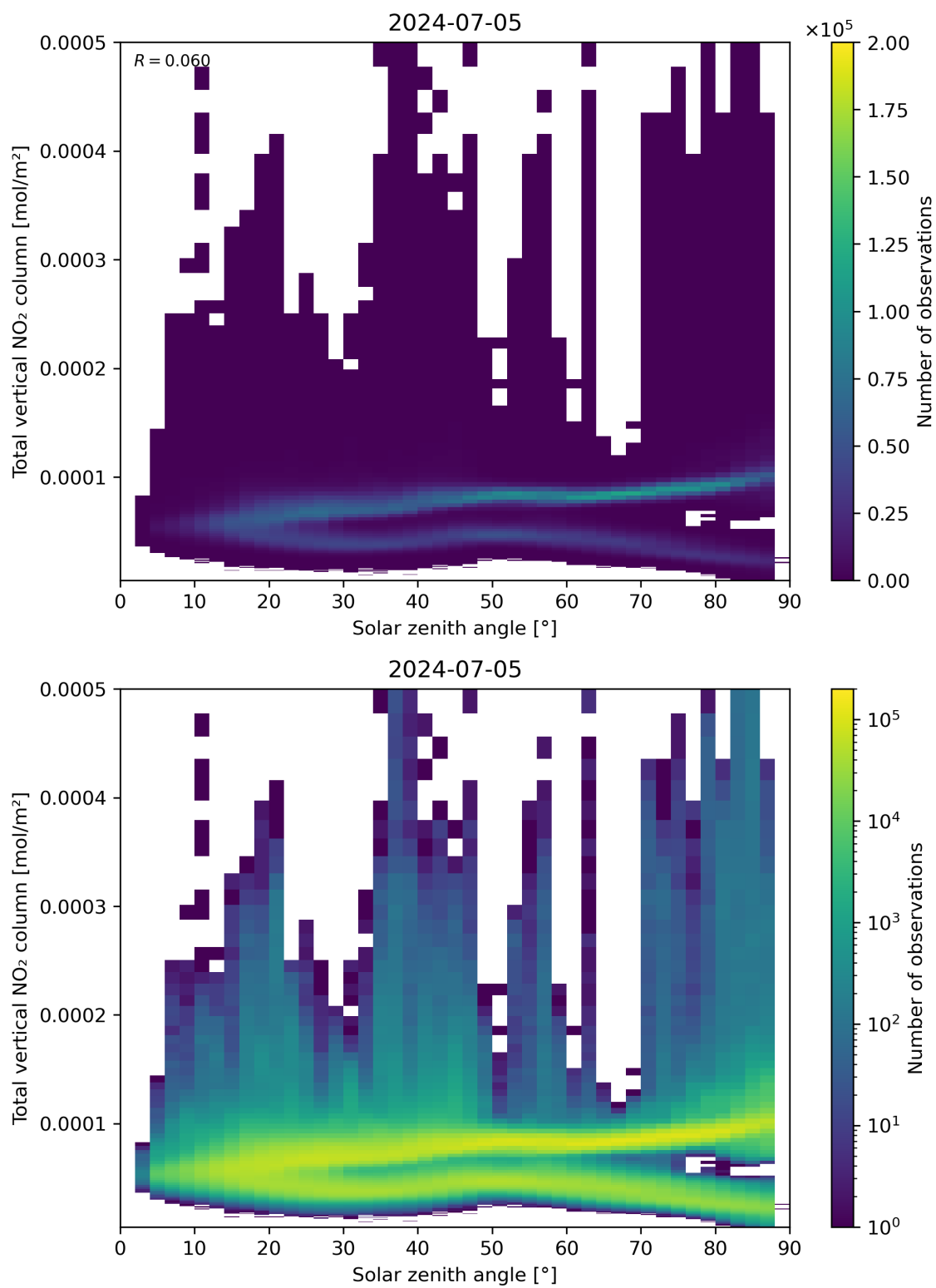
Figure 153: Scatter density plot of “Solar zenith angle” against “Total vertical NO 2 column” for 2024-07-05 to 2024-07-06.
