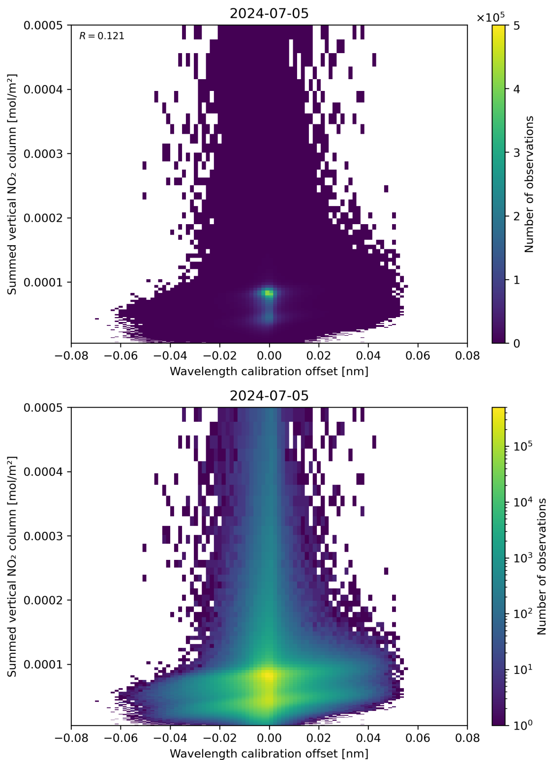
Figure 177: Scatter density plot of “Wavelength calibration offset” against “Summed vertical NO 2 column” for 2024-07-05 to 2024-07-06.
