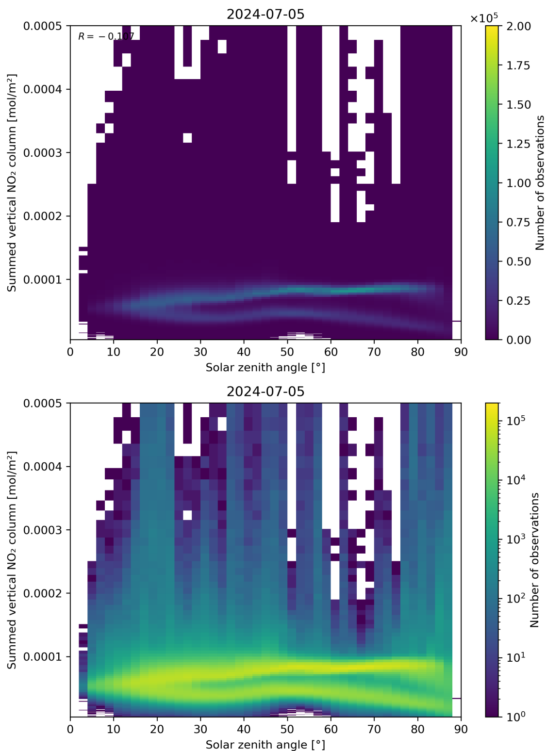
Figure 151: Scatter density plot of “Solar zenith angle” against “Summed vertical NO 2 column” for 2024-07-05 to 2024-07-06.
