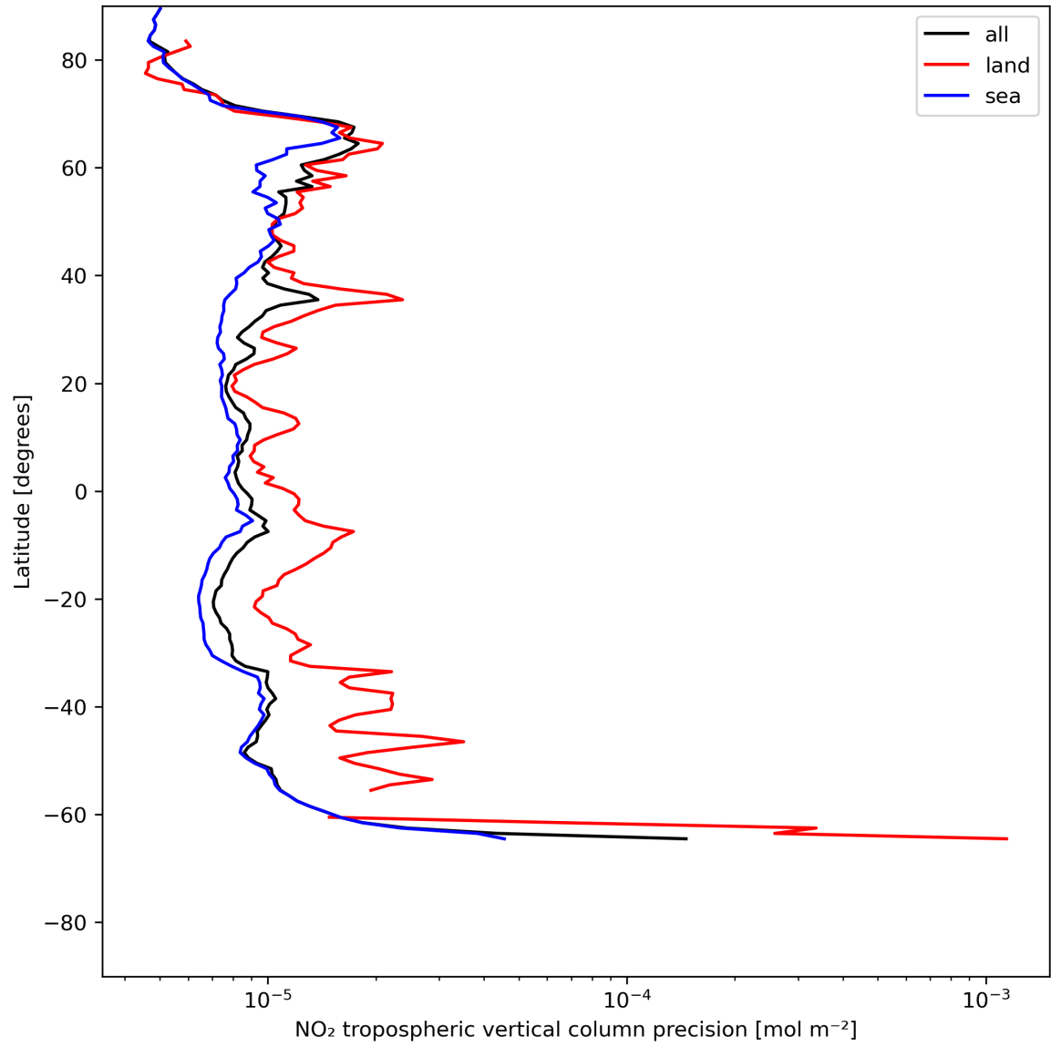
Figure 13: Zonal average of “NO 2 tropospheric vertical column precision” for 2024-07-05 to 2024-07-06.
