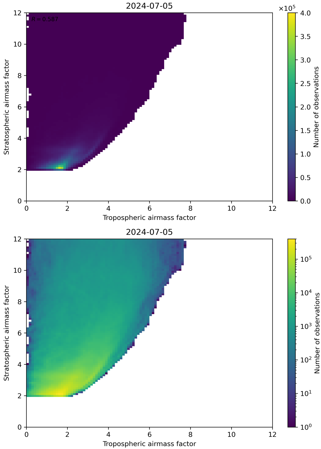
Figure 71: Scatter density plot of “Tropospheric airmass factor” against “Stratospheric airmass factor” for 2024-07-05 to 2024-07-06.
