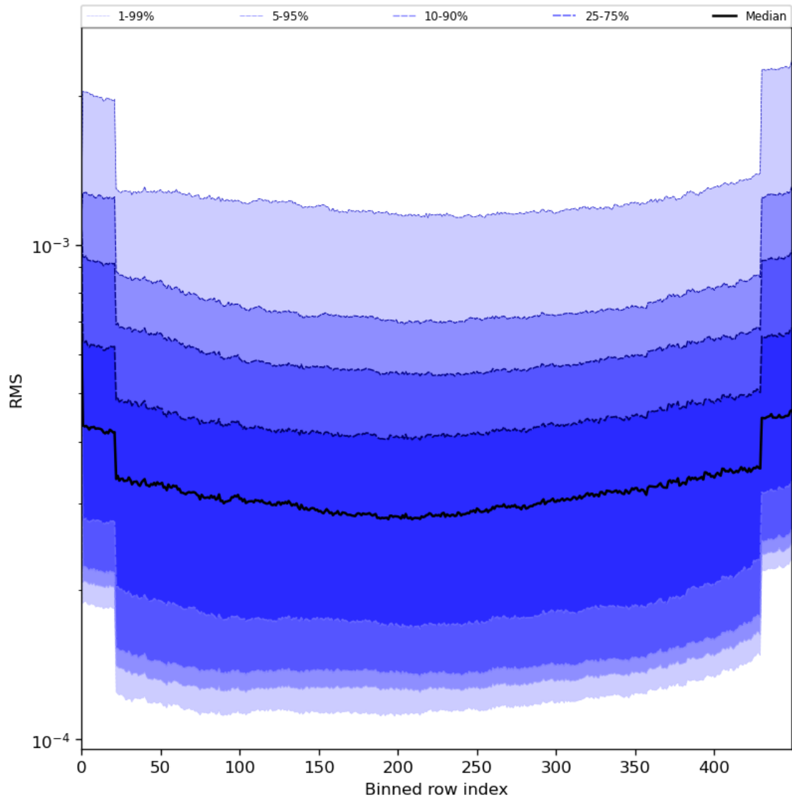
Figure 60: Along track statistics of “RMS” for 2024-07-05 to 2024-07-06
