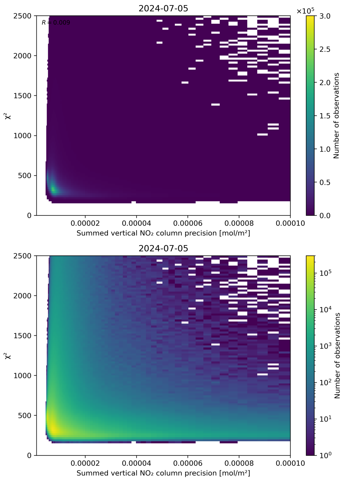
Figure 107: Scatter density plot of “Summed vertical NO 2 column precision” against “ \chi^2 ” for 2024-07-05 to 2024-07-06.
