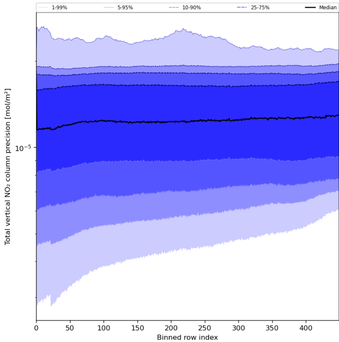
Figure 56: Along track statistics of “Total vertical NO 2 column precision” for 2024-07-05 to 2024-07-06
