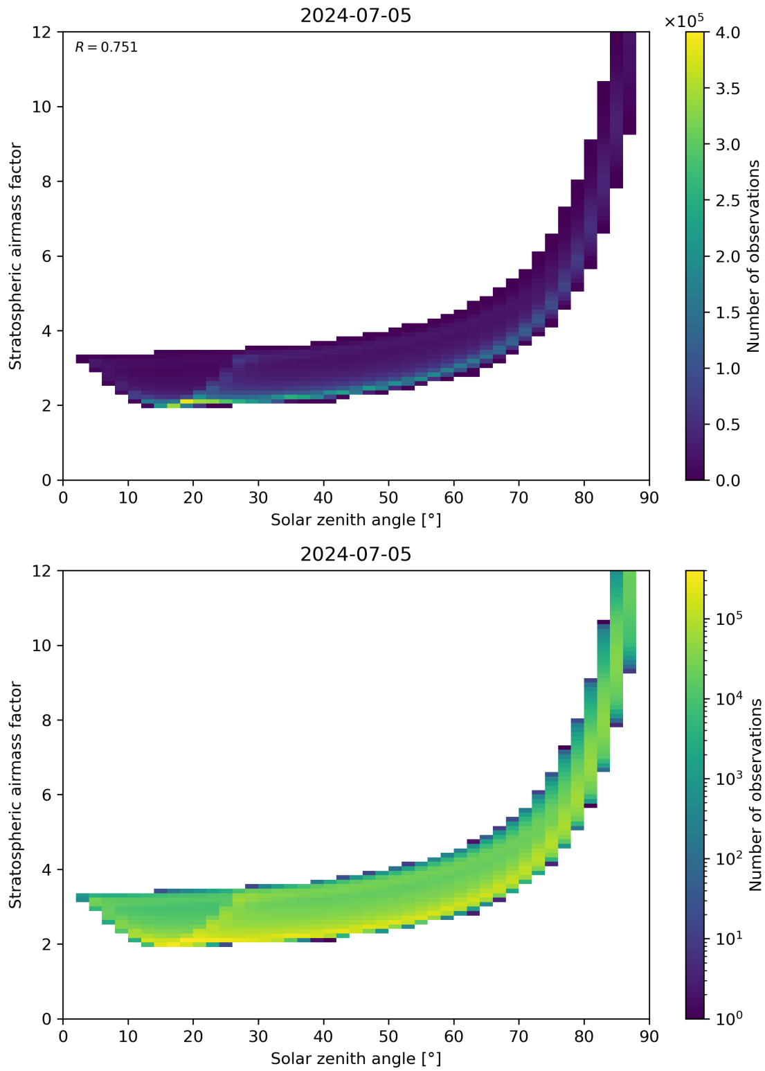
Figure 145: Scatter density plot of “Solar zenith angle” against “Stratospheric airmass factor” for 2024-07-05 to 2024-07-06.
