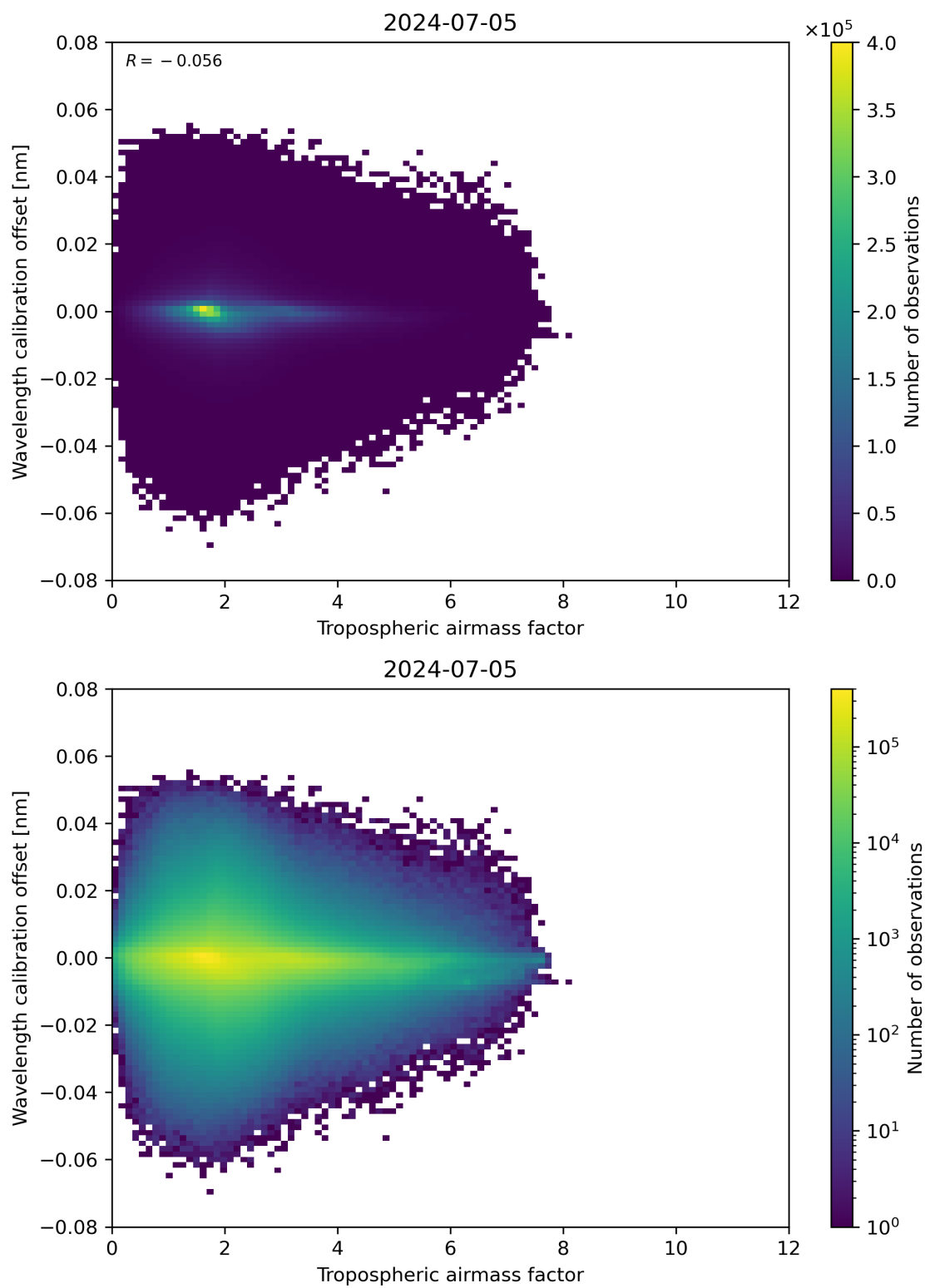
Figure 80: Scatter density plot of “Tropospheric airmass factor” against “Wavelength calibration offset” for 2024-07-05 to 2024-07-06.
