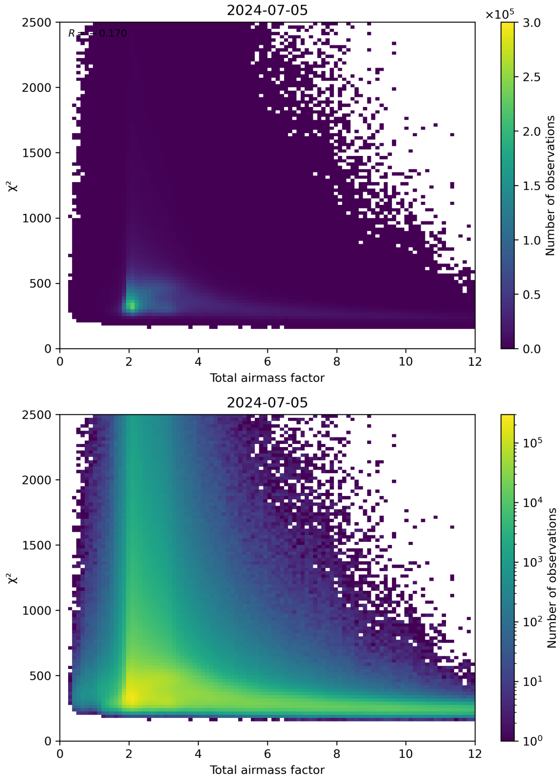
Figure 63: Scatter density plot of “Total airmass factor” against “ \chi^2 ” for 2024-07-05 to 2024-07-06.
