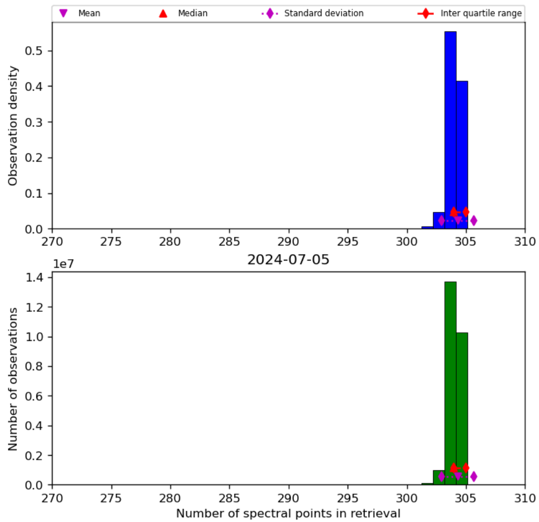
Figure 33: Histogram of “Number of spectral points in retrieval” for 2024-07-05 to 2024-07-06
