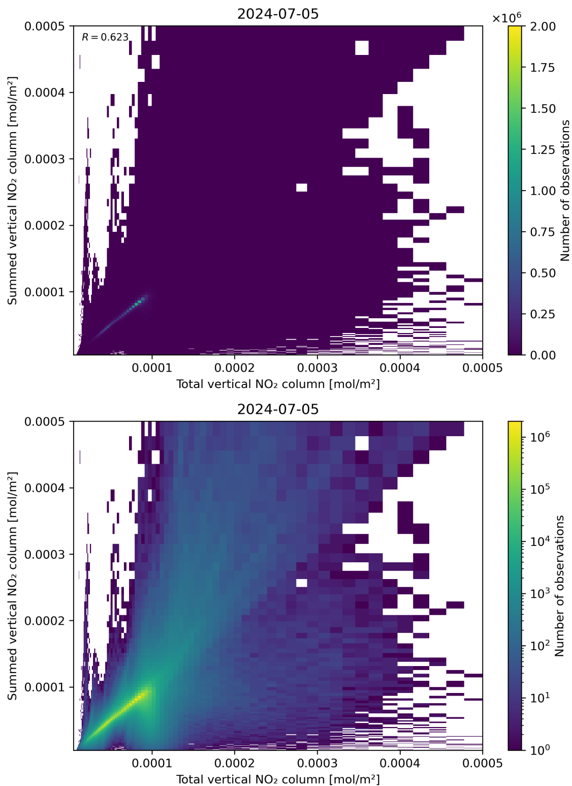
Figure 112: Scatter density plot of “Total vertical NO 2 column” against “Summed vertical NO 2 column” for 2024-07-05 to 2024-07-06.
