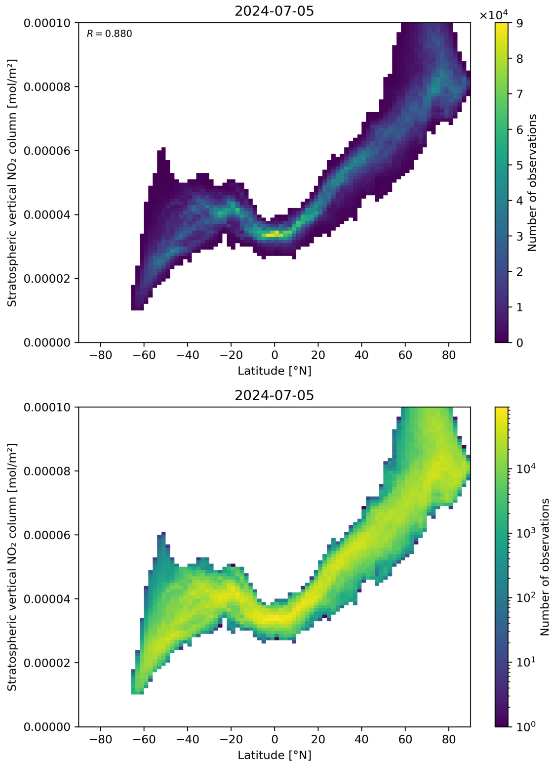
Figure 87: Scatter density plot of “Latitude” against “Stratospheric vertical NO 2 column” for 2024-07-05 to 2024-07-06.
