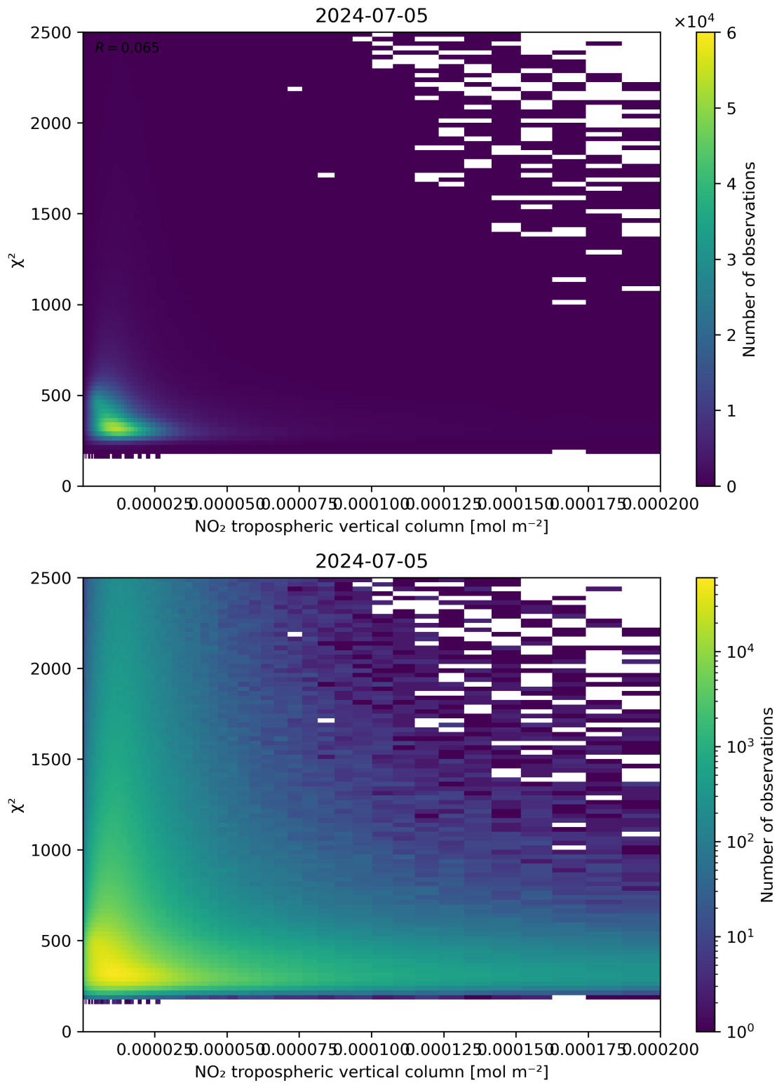
Figure 124: Scatter density plot of “NO 2 tropospheric vertical column” against “ \chi^2 ” for 2024-07-05 to 2024-07-06.
