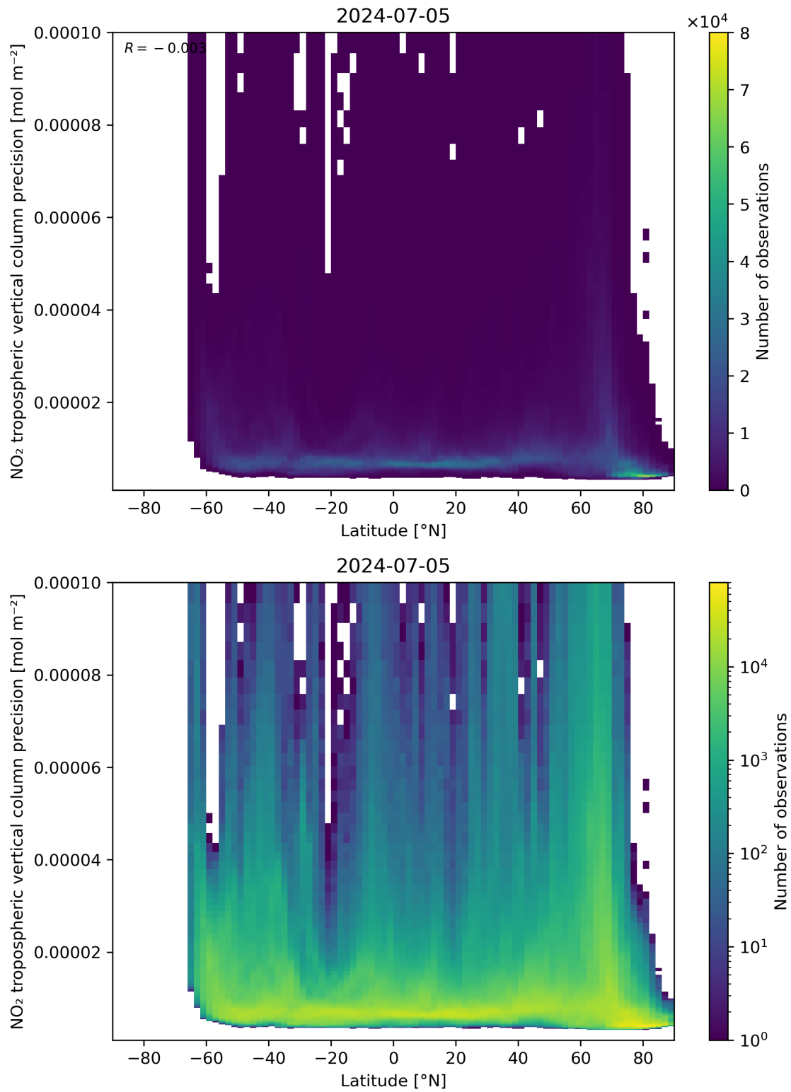
Figure 93: Scatter density plot of “Latitude” against “NO 2 tropospheric vertical column precision” for 2024-07-05 to 2024-07-06.
