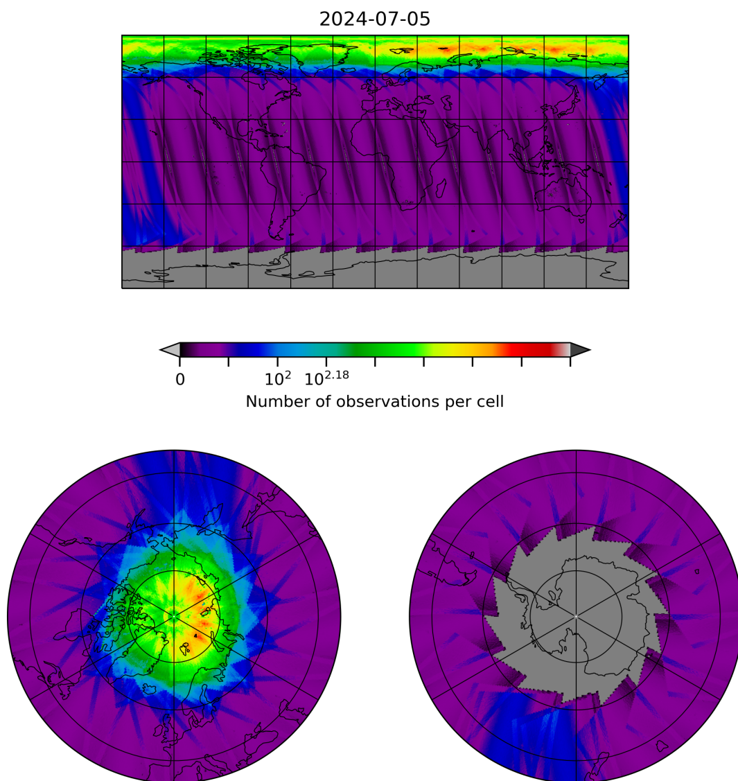
Figure 10: Map of the number of observations for 2024-07-05 to 2024-07-06
