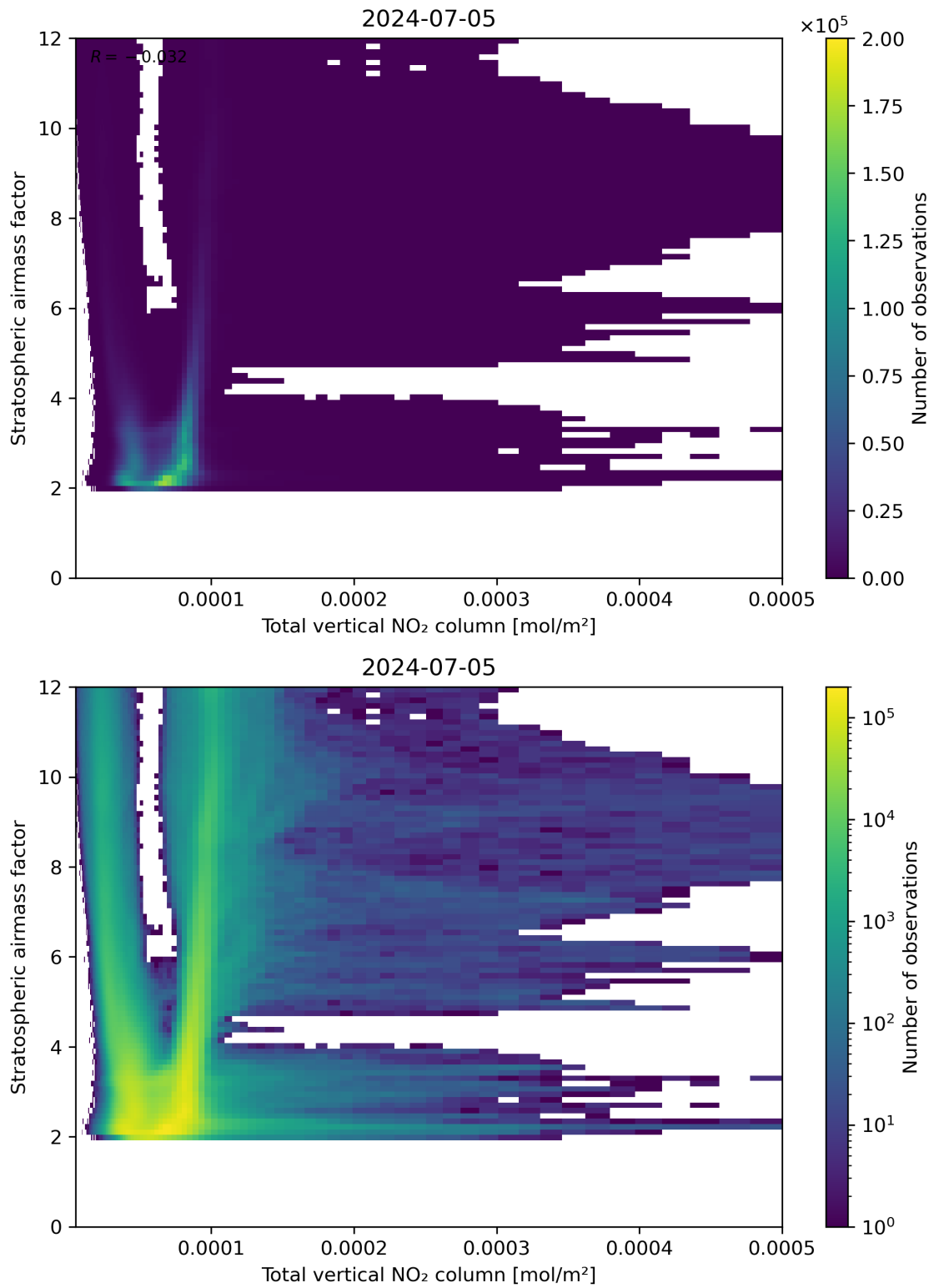
Figure 110: Scatter density plot of “Total vertical NO 2 column” against “Stratospheric airmass factor” for 2024-07-05 to 2024-07-06.
