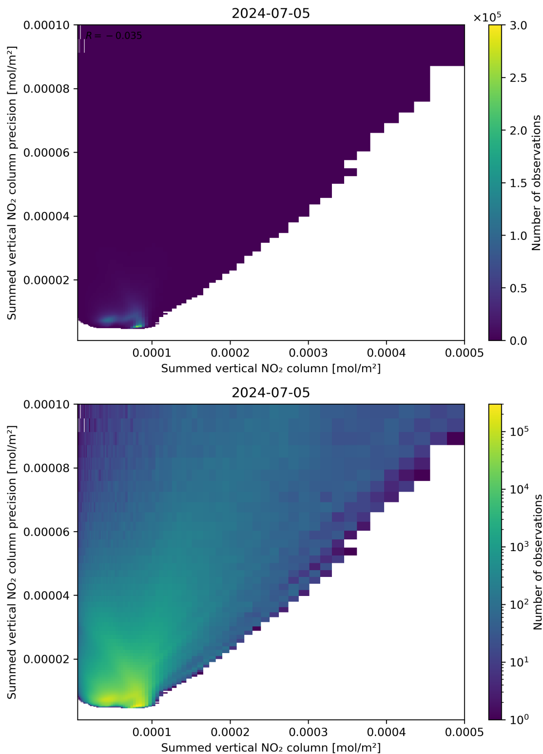
Figure 105: Scatter density plot of “Summed vertical NO 2 column” against “Summed vertical NO 2 column precision” for 2024-07-05 to 2024-07-06.
