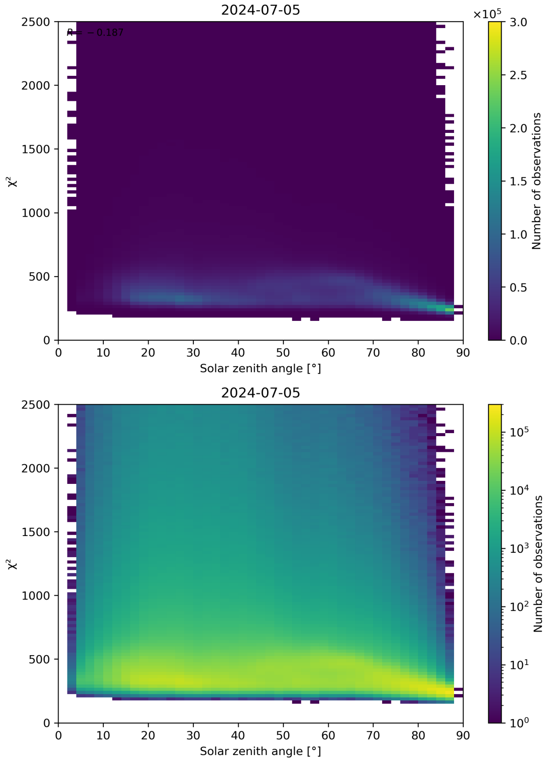
Figure 148: Scatter density plot of “Solar zenith angle” against “ \chi^2 ” for 2024-07-05 to 2024-07-06.
