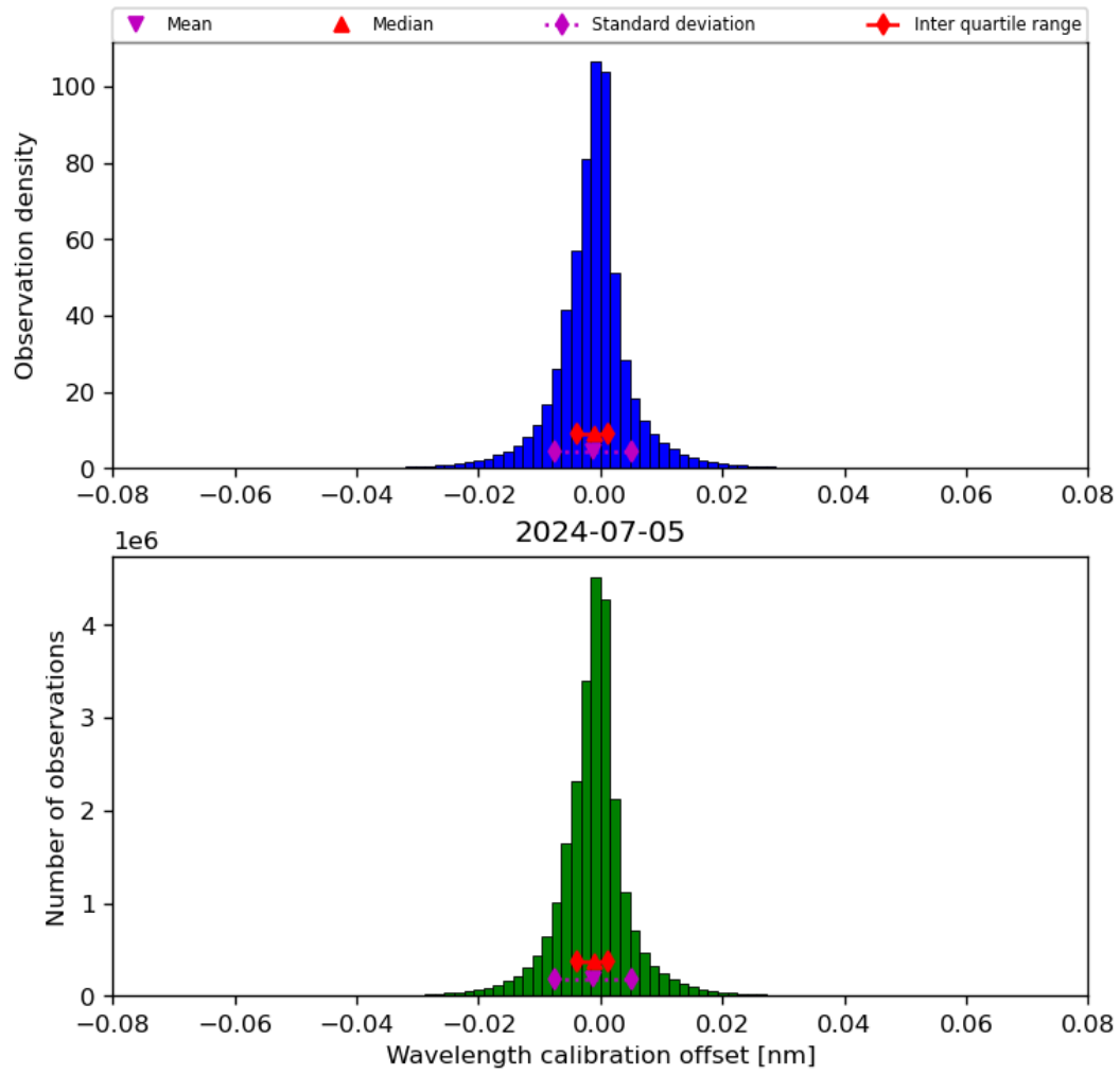
Figure 35: Histogram of “Wavelength calibration offset” for 2024-07-05 to 2024-07-06
