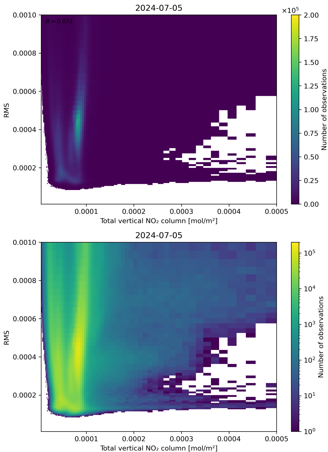
Figure 120: Scatter density plot of “Total vertical NO 2 column” against “RMS” for 2024-07-05 to 2024-07-06.
