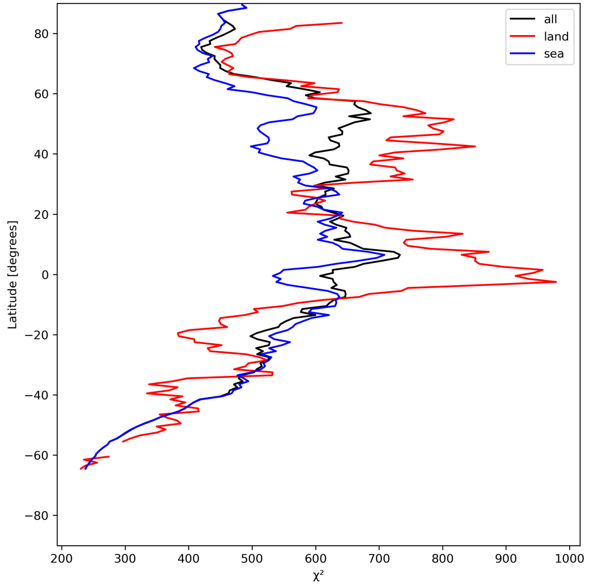
Figure 25: Zonal average of “ \chi^2 ” for 2024-07-05 to 2024-07-06.
