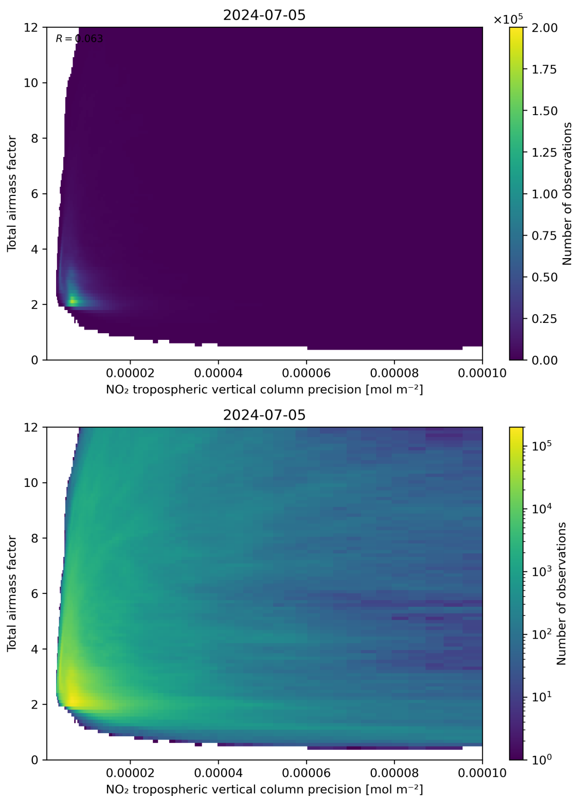
Figure 132: Scatter density plot of “NO 2 tropospheric vertical column precision” against “Total airmass factor” for 2024-07-05 to 2024-07-06.
