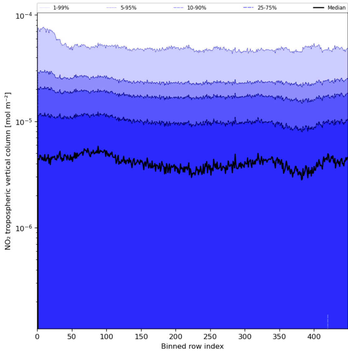
Figure 46: Along track statistics of “NO 2 tropospheric vertical column” for 2024-07-05 to 2024-07-06
