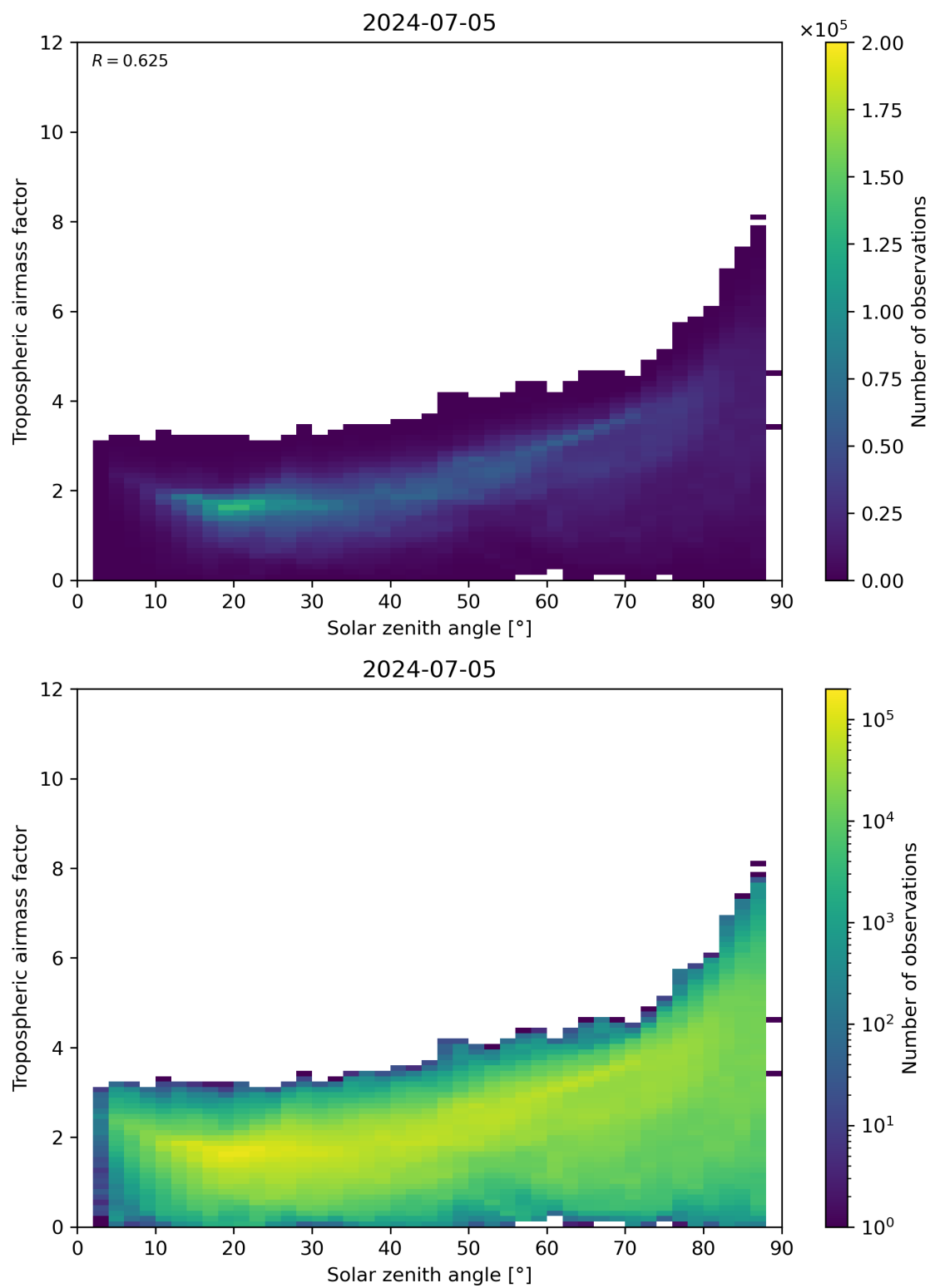
Figure 147: Scatter density plot of “Solar zenith angle” against “Tropospheric airmass factor” for 2024-07-05 to 2024-07-06.
