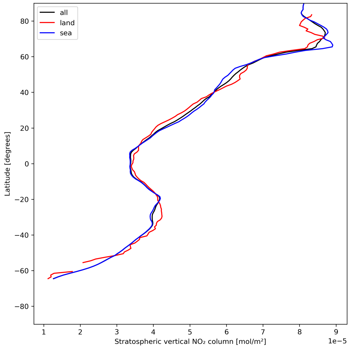
Figure 19: Zonal average of “Stratospheric vertical NO 2 column” for 2024-07-05 to 2024-07-06.
