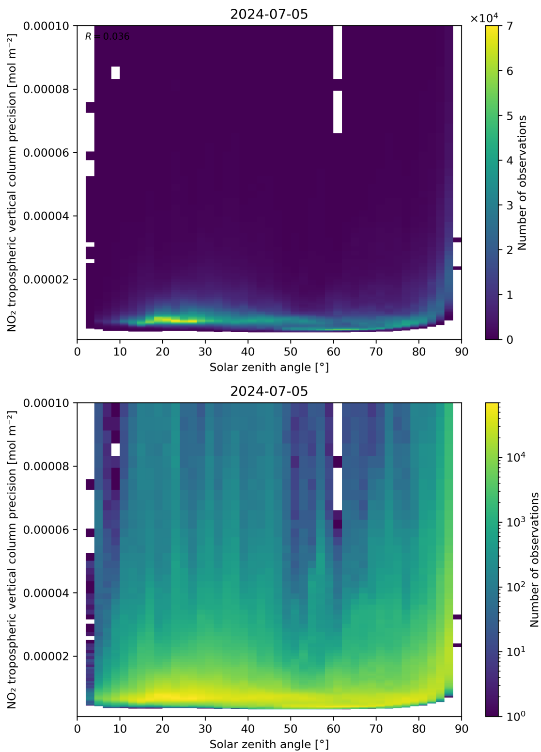
Figure 156: Scatter density plot of “Solar zenith angle” against “NO 2 tropospheric vertical column precision” for 2024-07-05 to 2024-07-06.
