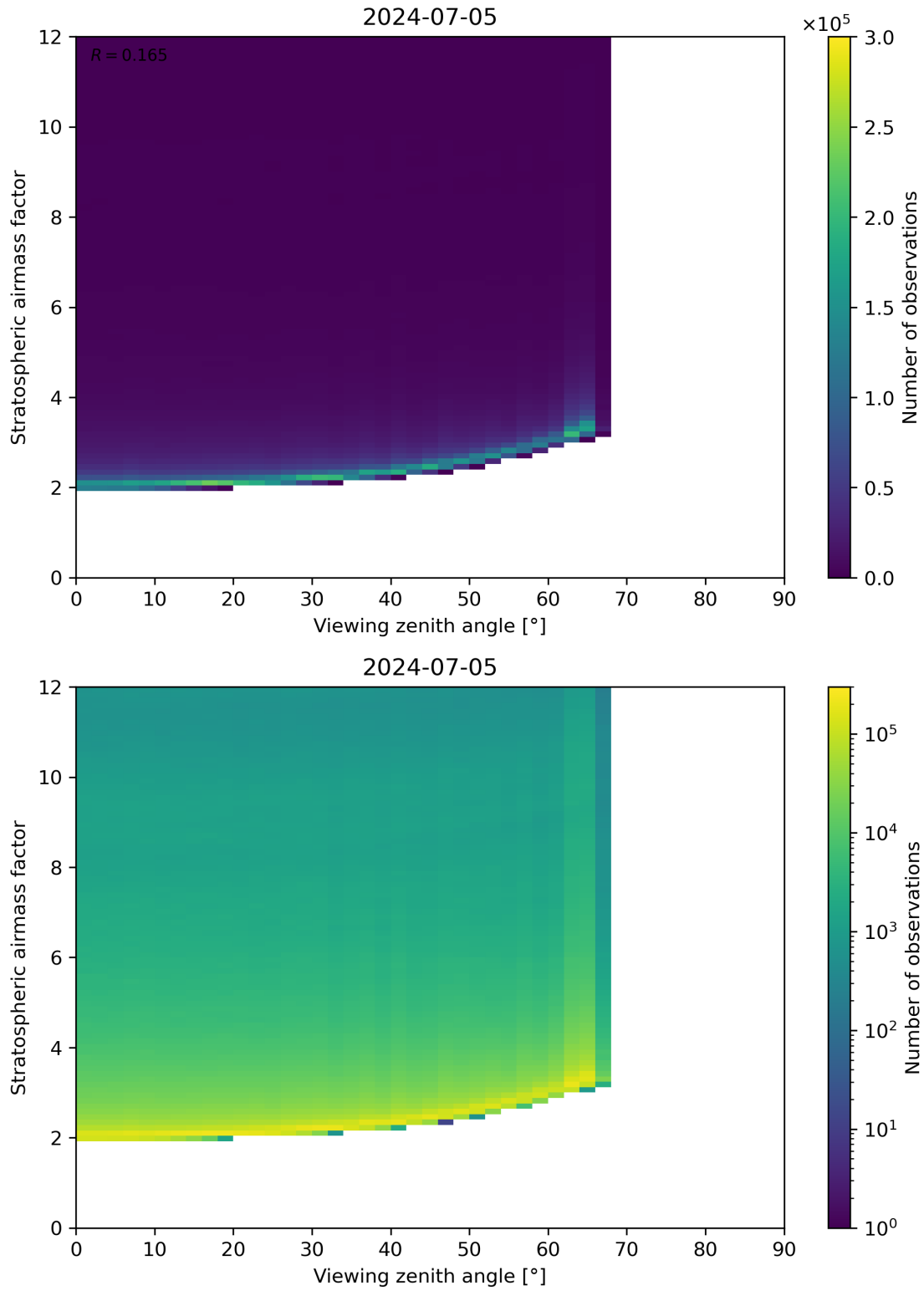
Figure 159: Scatter density plot of “Viewing zenith angle” against “Stratospheric airmass factor” for 2024-07-05 to 2024-07-06.
