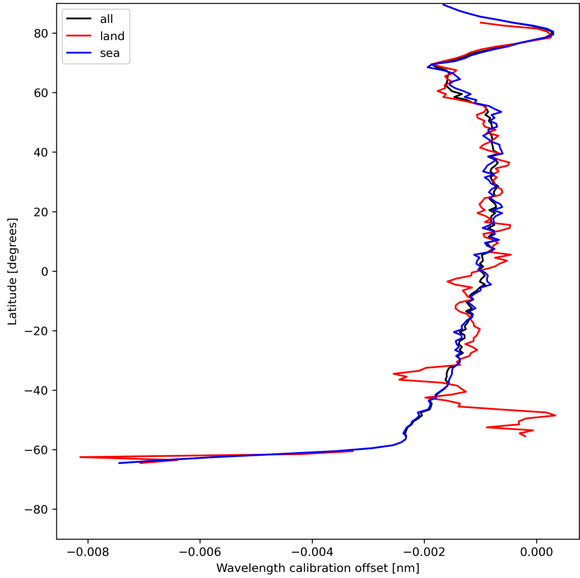
Figure 18: Zonal average of “Wavelength calibration offset” for 2024-07-05 to 2024-07-06.
