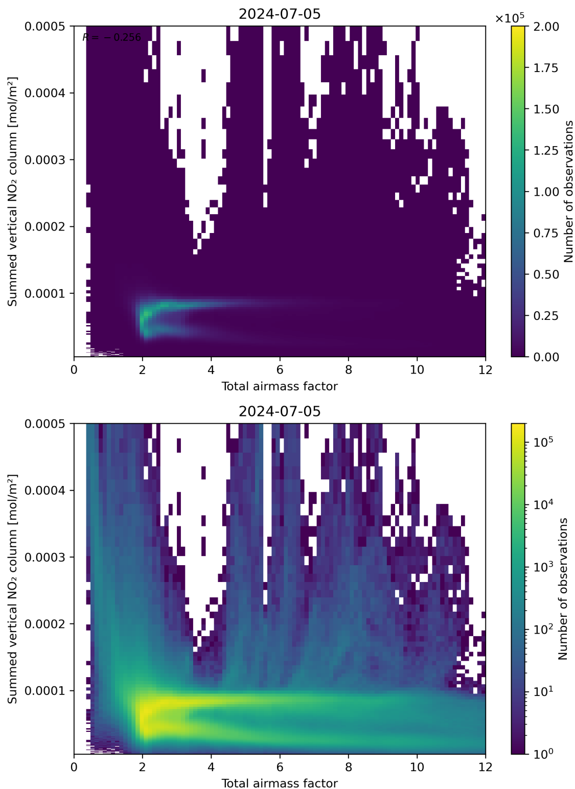
Figure 65: Scatter density plot of “Total airmass factor” against “Summed vertical NO 2 column” for 2024-07-05 to 2024-07-06.
