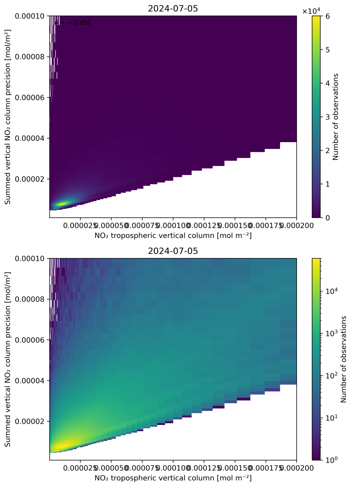
Figure 127: Scatter density plot of “NO 2 tropospheric vertical column” against “Summed vertical NO 2 column precision” for 2024-07-05 to 2024-07-06.
