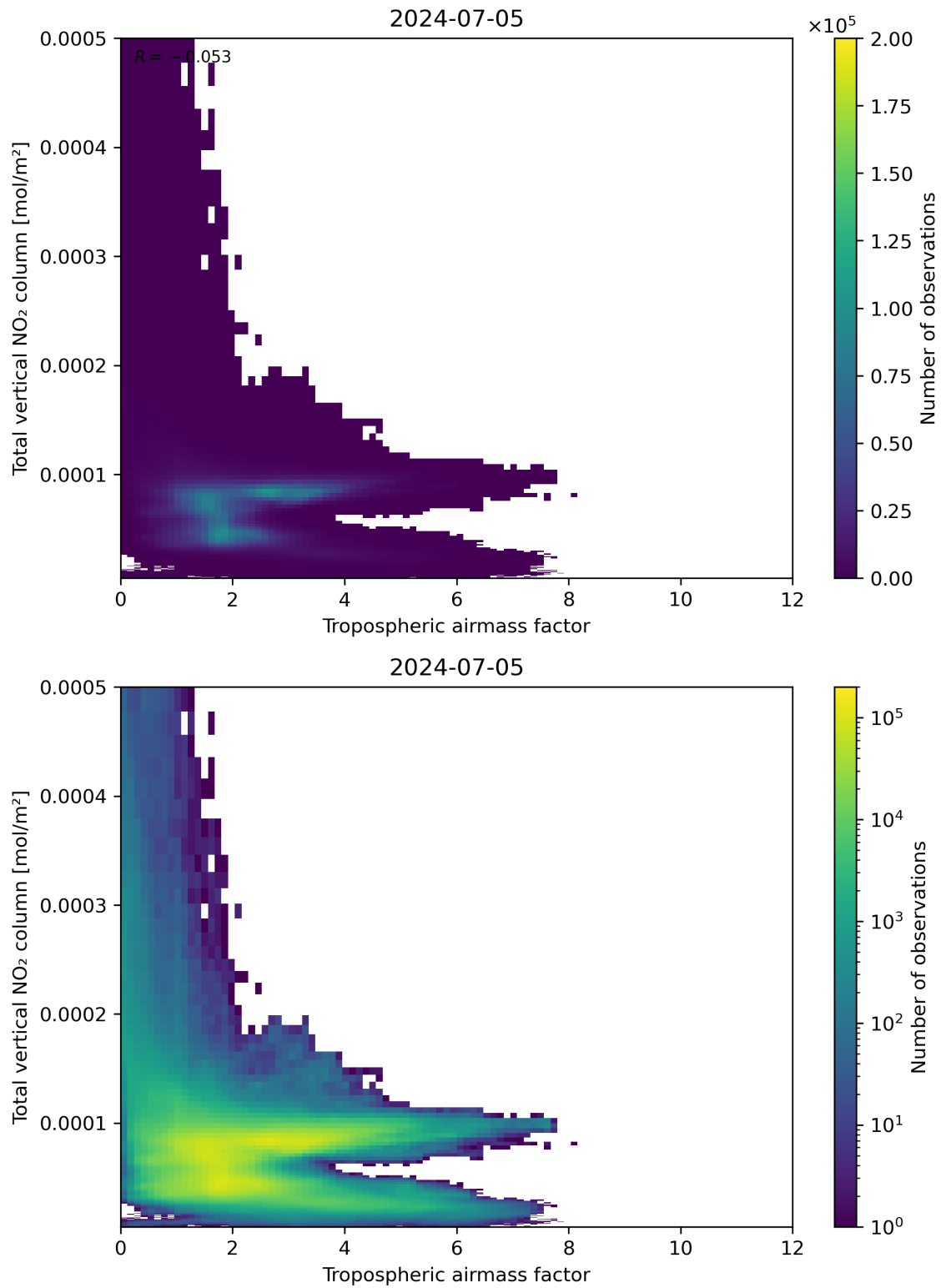
Figure 77: Scatter density plot of “Tropospheric airmass factor” against “Total vertical NO 2 column” for 2024-07-05 to 2024-07-06.
