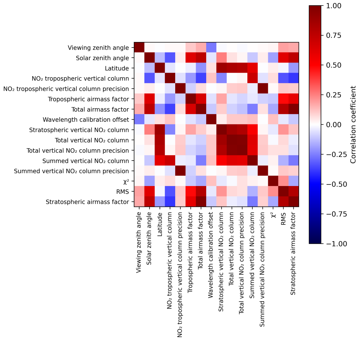
Figure 2: Map of correlation matrix for 2024-07-05 to 2024-07-06.
