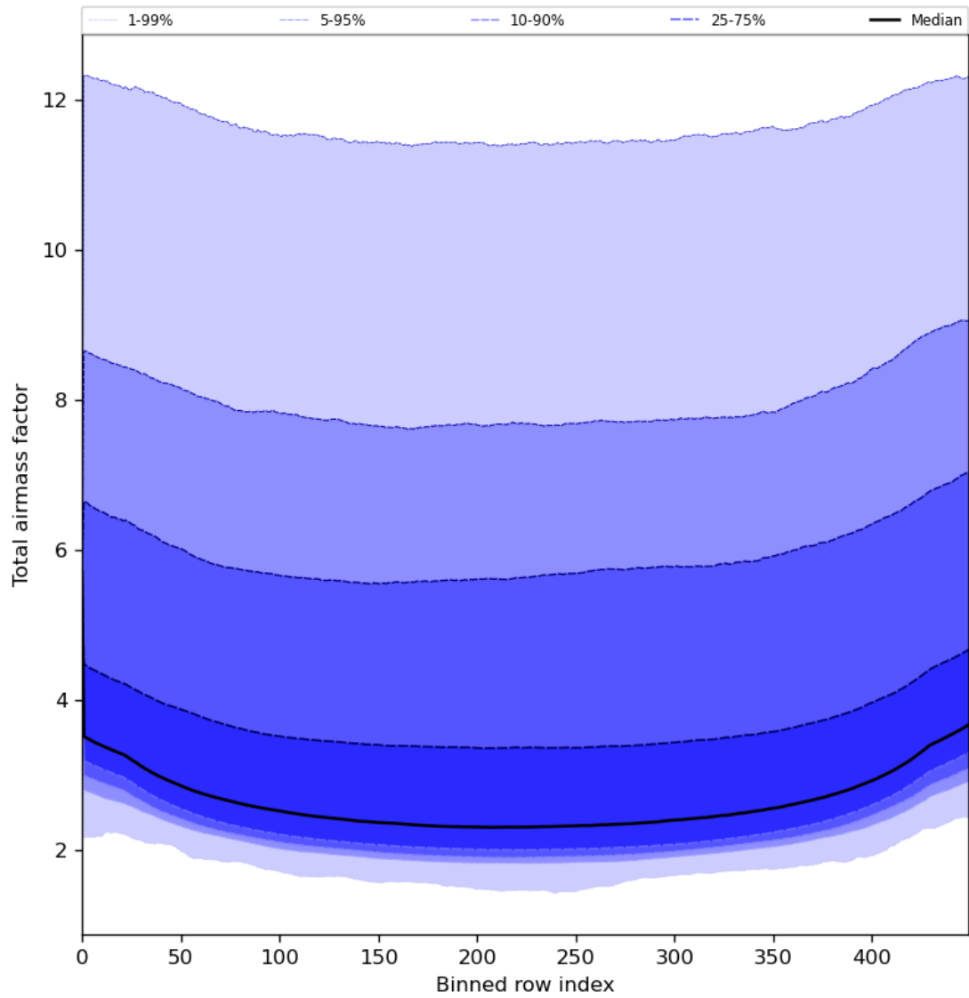
Figure 49: Along track statistics of “Total airmass factor” for 2024-07-05 to 2024-07-06
