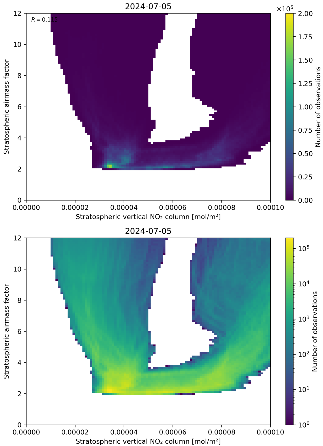
Figure 96: Scatter density plot of “Stratospheric vertical NO 2 column” against “Stratospheric airmass factor” for 2024-07-05 to 2024-07-06.
