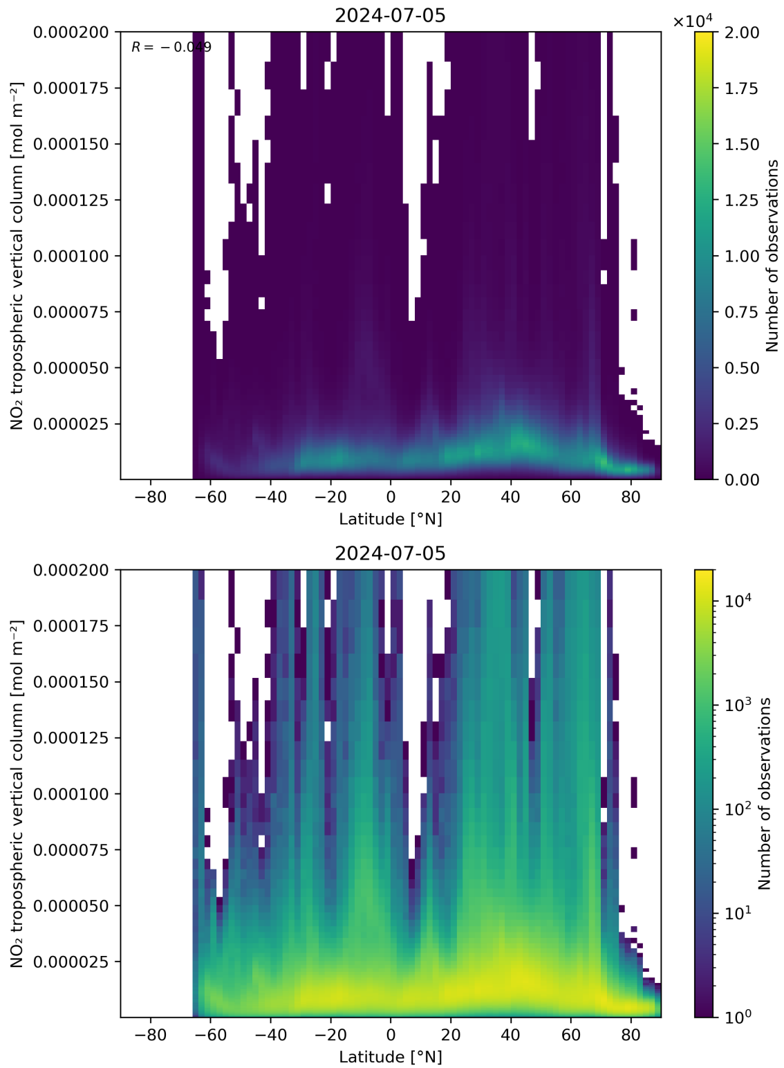
Figure 92: Scatter density plot of “Latitude” against “NO 2 tropospheric vertical column” for 2024-07-05 to 2024-07-06.
