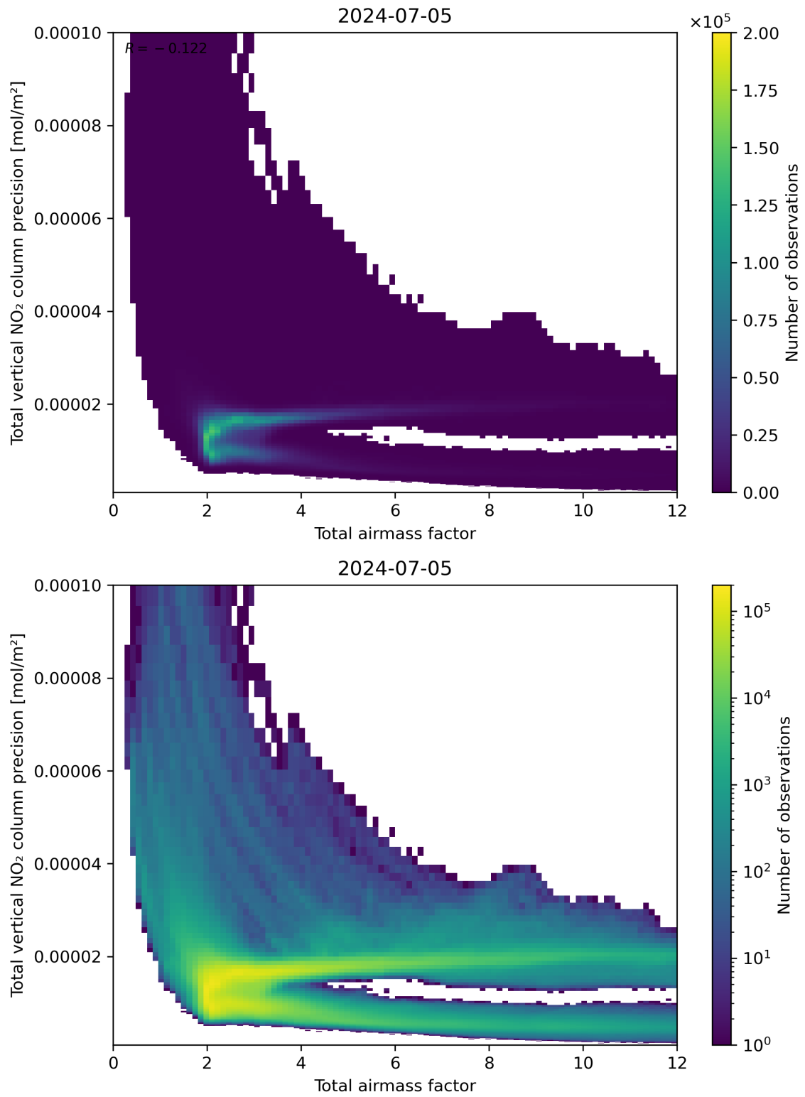
Figure 68: Scatter density plot of “Total airmass factor” against “Total vertical NO 2 column precision” for 2024-07-05 to 2024-07-06.
