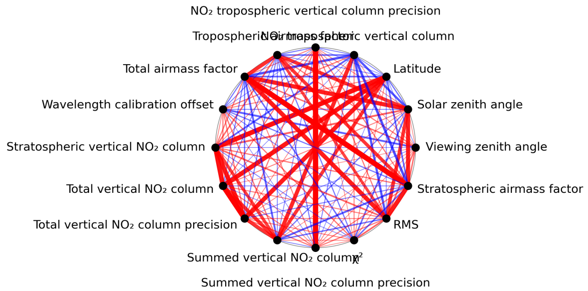
Figure 1: Map of correlation graph for 2024-07-05 to 2024-07-06.
