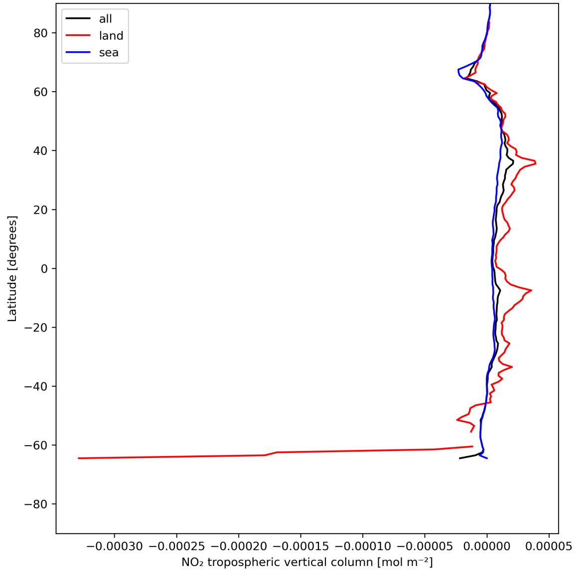
Figure 12: Zonal average of “NO 2 tropospheric vertical column” for 2024-07-05 to 2024-07-06.
