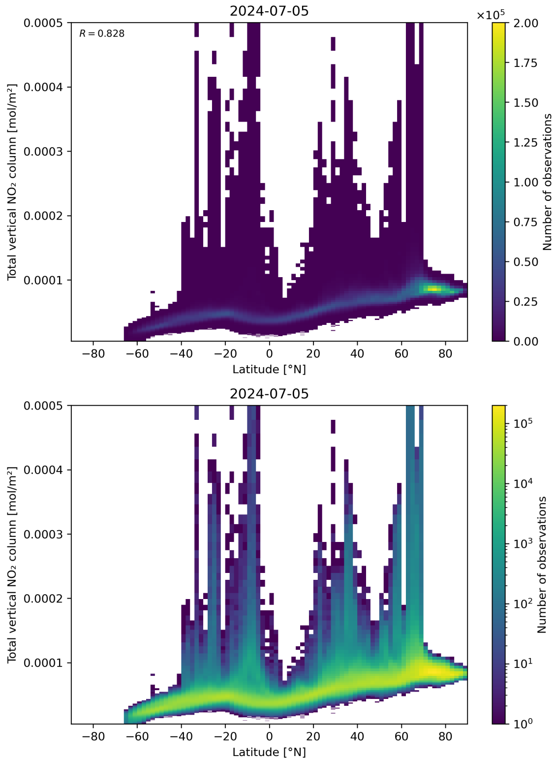
Figure 90: Scatter density plot of “Latitude” against “Total vertical NO 2 column” for 2024-07-05 to 2024-07-06.
