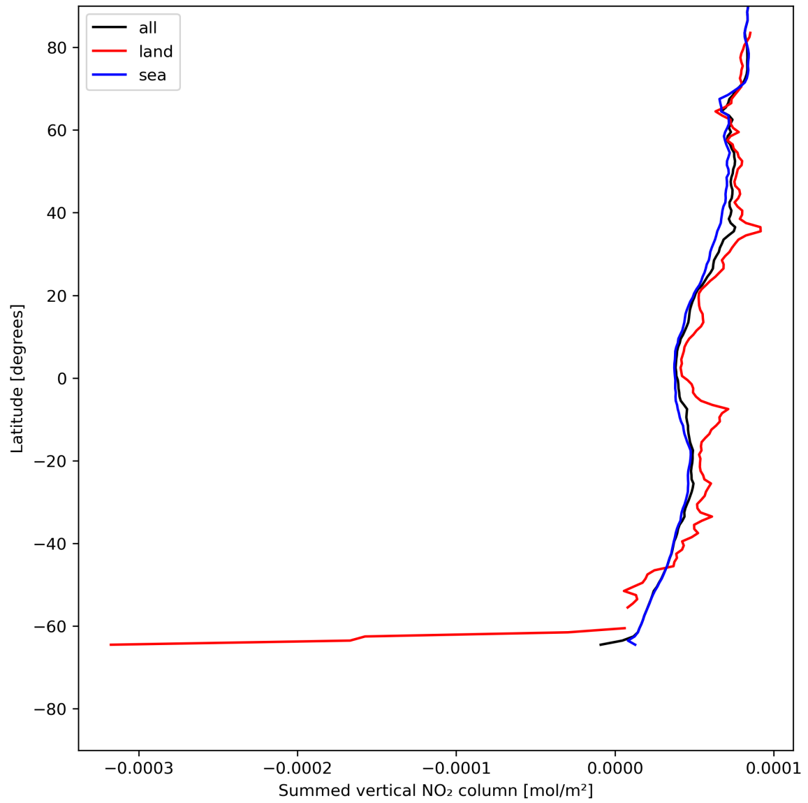
Figure 23: Zonal average of “Summed vertical NO 2 column” for 2024-07-05 to 2024-07-06.
