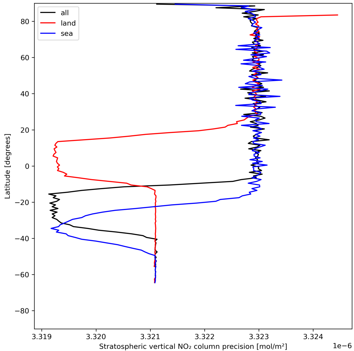
Figure 20: Zonal average of “Stratospheric vertical NO 2 column precision” for 2024-07-05 to 2024-07-06.
