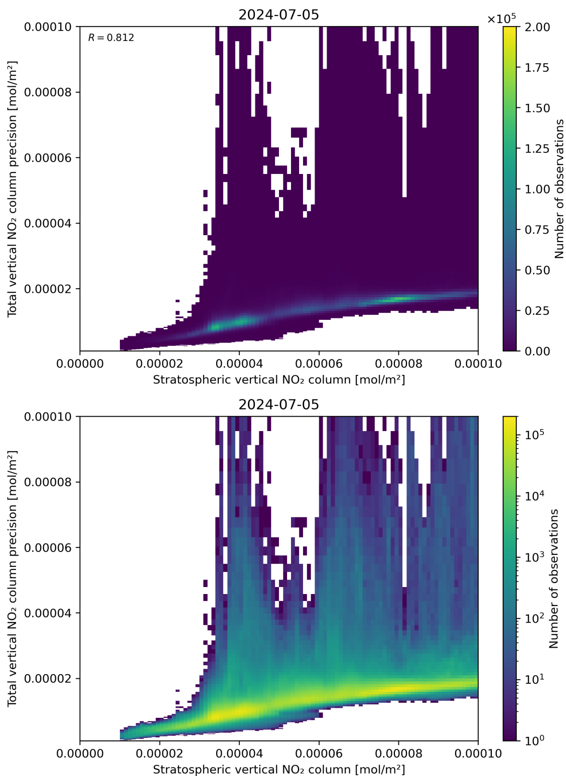
Figure 101: Scatter density plot of “Stratospheric vertical NO 2 column” against “Total vertical NO 2 column precision” for 2024-07-05 to 2024-07-06.
