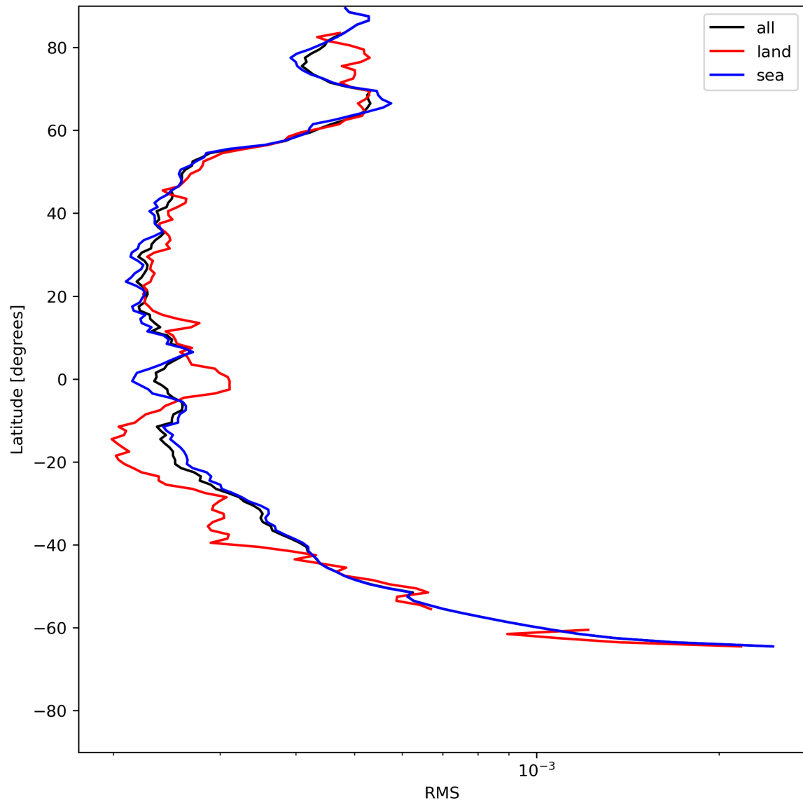
Figure 26: Zonal average of “RMS” for 2024-07-05 to 2024-07-06.
