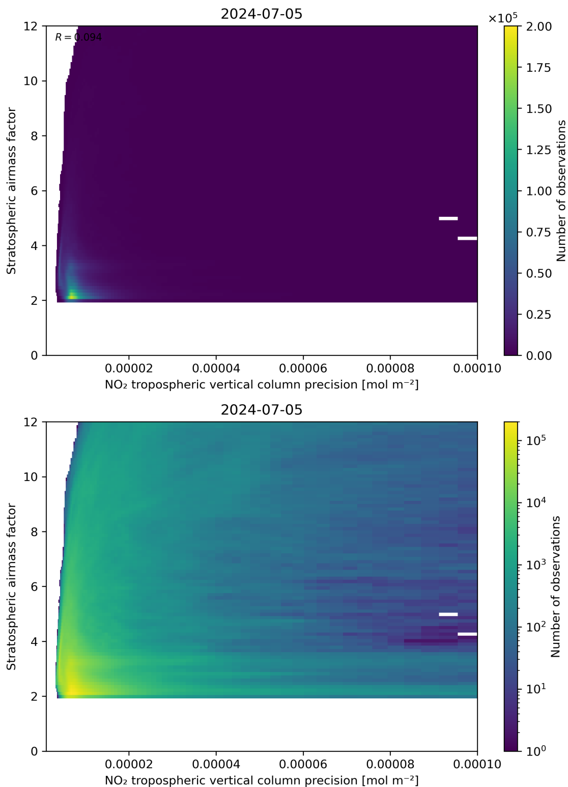
Figure 131: Scatter density plot of “NO 2 tropospheric vertical column precision” against “Stratospheric airmass factor” for 2024-07-05 to 2024-07-06.
