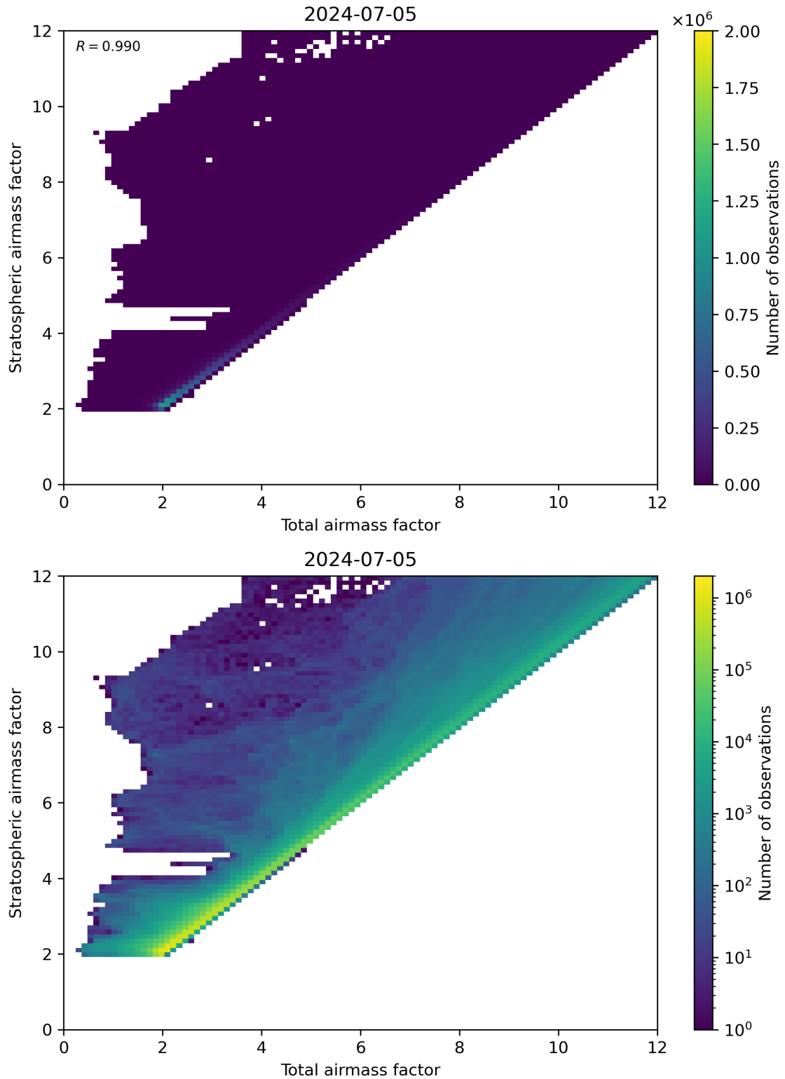
Figure 62: Scatter density plot of “Total airmass factor” against “Stratospheric airmass factor” for 2024-07-05 to 2024-07-06.
