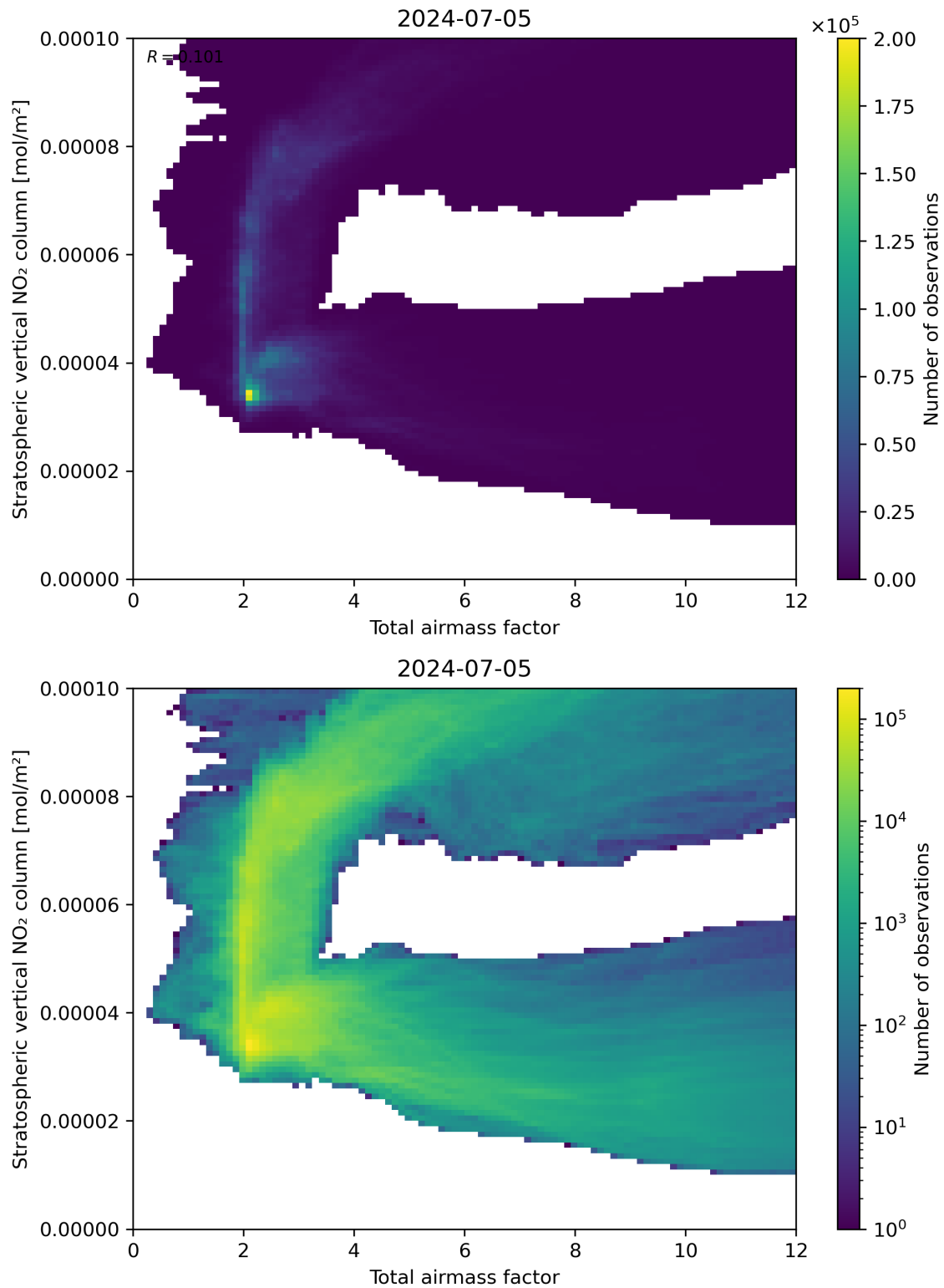
Figure 64: Scatter density plot of “Total airmass factor” against “Stratospheric vertical NO 2 column” for 2024-07-05 to 2024-07-06.
