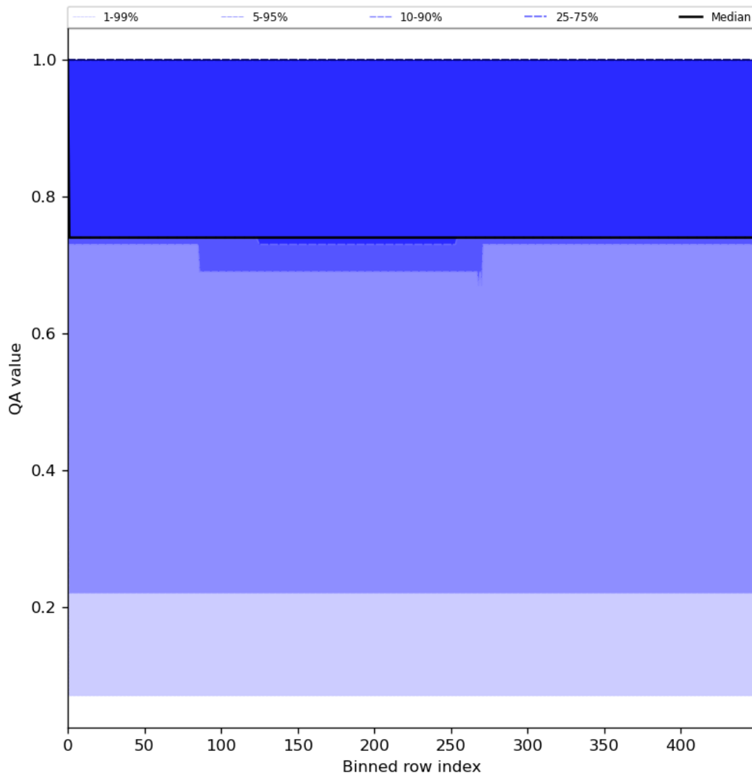
Figure 45: Along track statistics of “QA value” for 2024-07-05 to 2024-07-06
