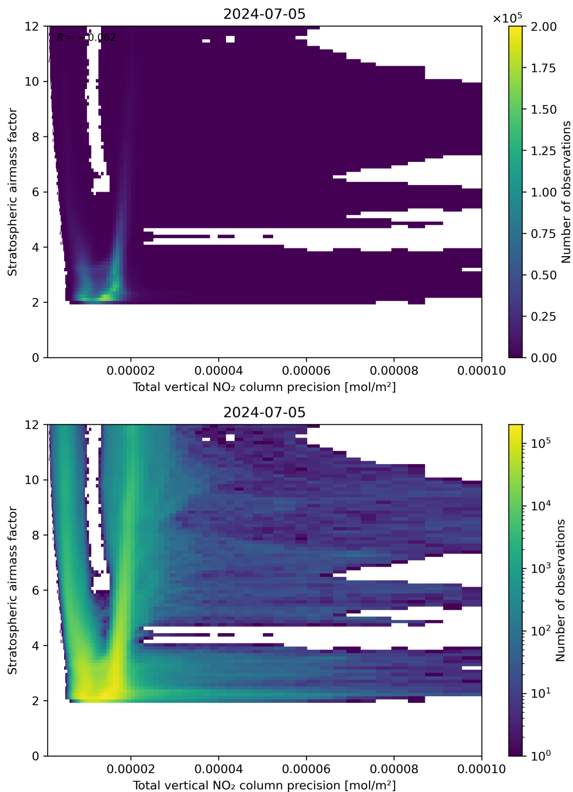
Figure 115: Scatter density plot of “Total vertical NO 2 column precision” against “Stratospheric airmass factor” for 2024-07-05 to 2024-07-06.
