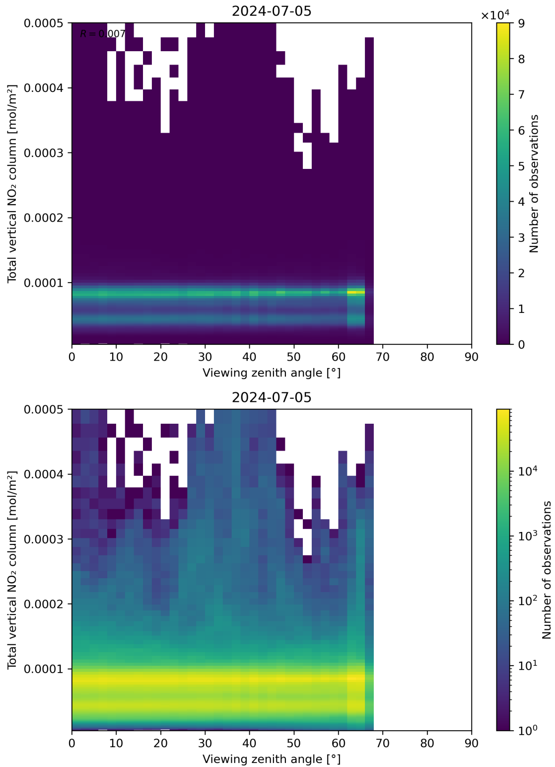
Figure 167: Scatter density plot of “Viewing zenith angle” against “Total vertical NO 2 column” for 2024-07-05 to 2024-07-06.
