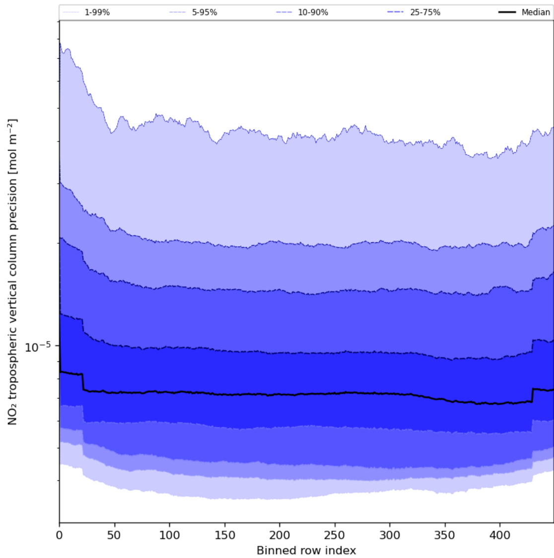
Figure 47: Along track statistics of “NO 2 tropospheric vertical column precision” for 2024-07-05 to 2024-07-06
