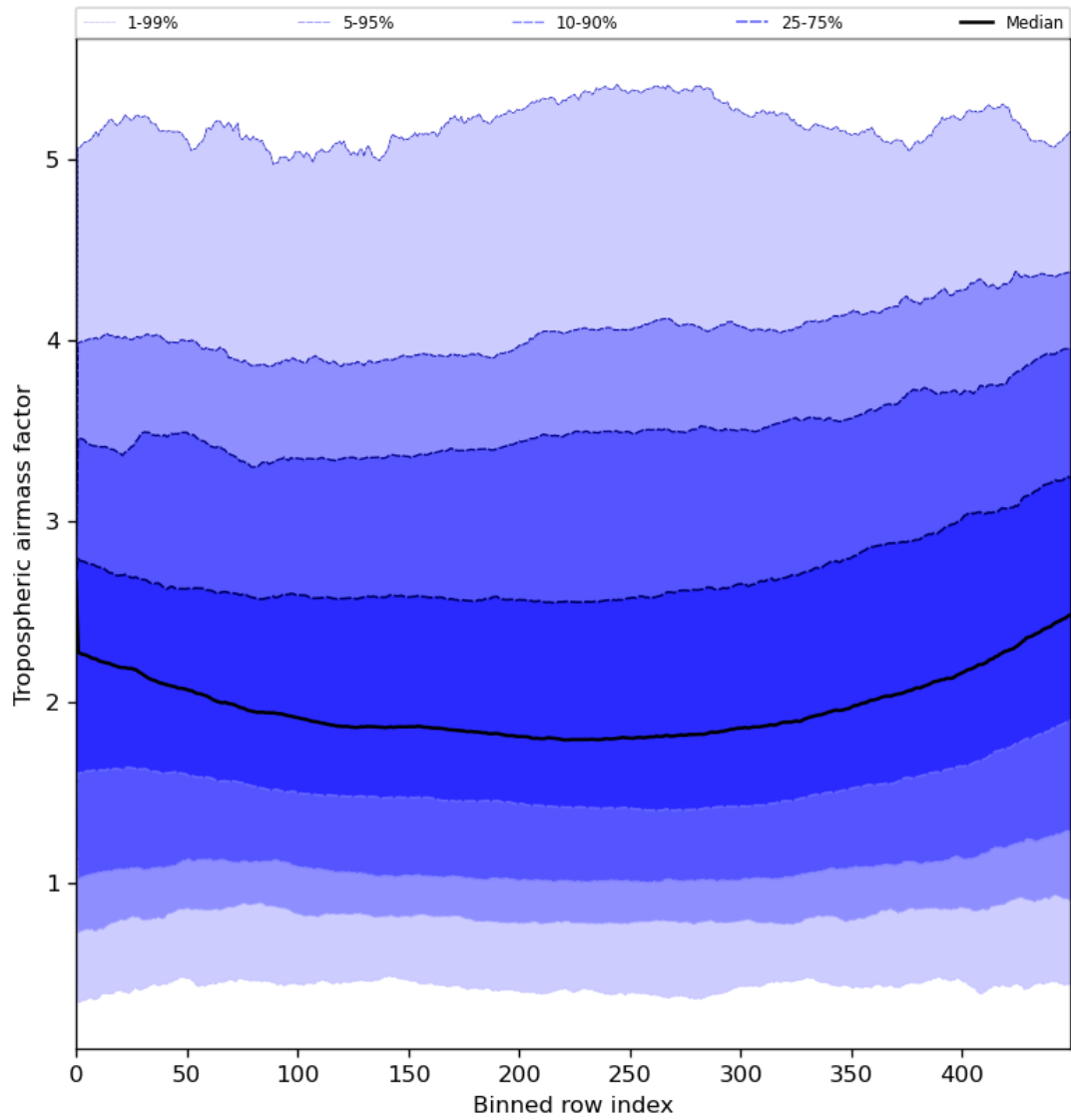
Figure 48: Along track statistics of “Tropospheric airmass factor” for 2024-07-05 to 2024-07-06
