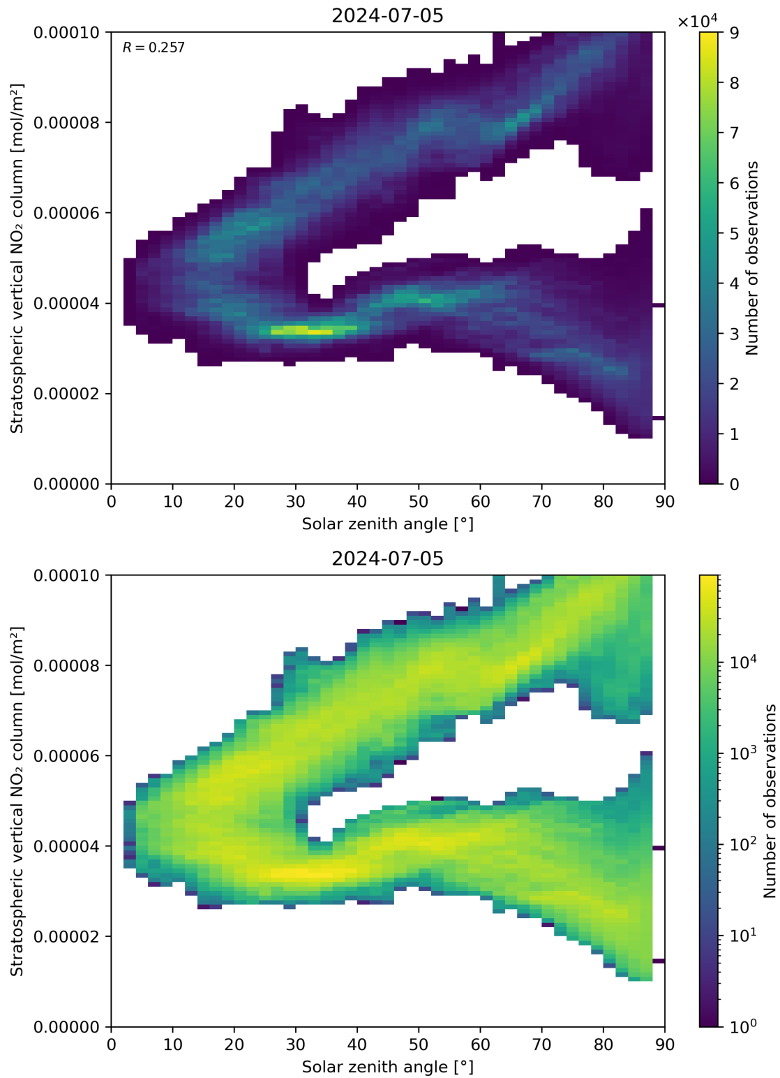
Figure 150: Scatter density plot of “Solar zenith angle” against “Stratospheric vertical NO 2 column” for 2024-07-05 to 2024-07-06.
