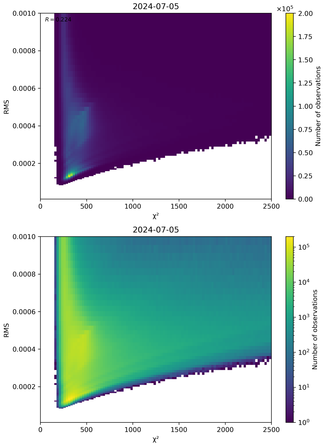
Figure 82: Scatter density plot of “ \chi^2 ” against “RMS” for 2024-07-05 to 2024-07-06.
