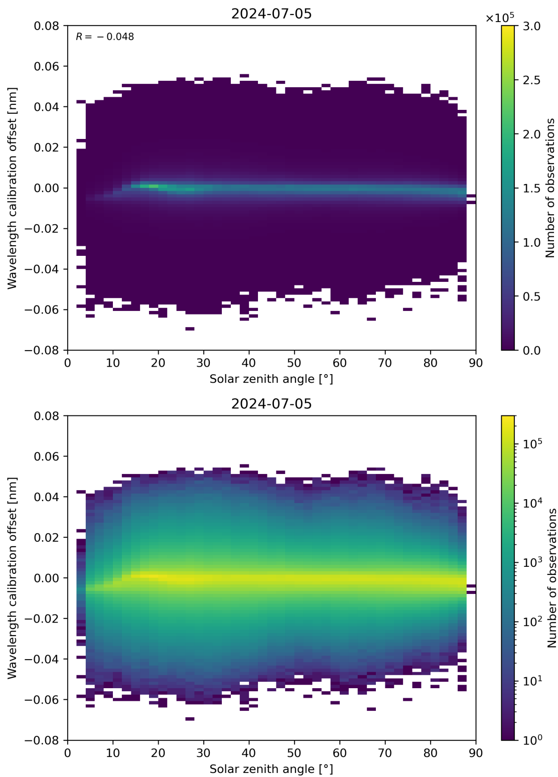
Figure 158: Scatter density plot of “Solar zenith angle” against “Wavelength calibration offset” for 2024-07-05 to 2024-07-06.
