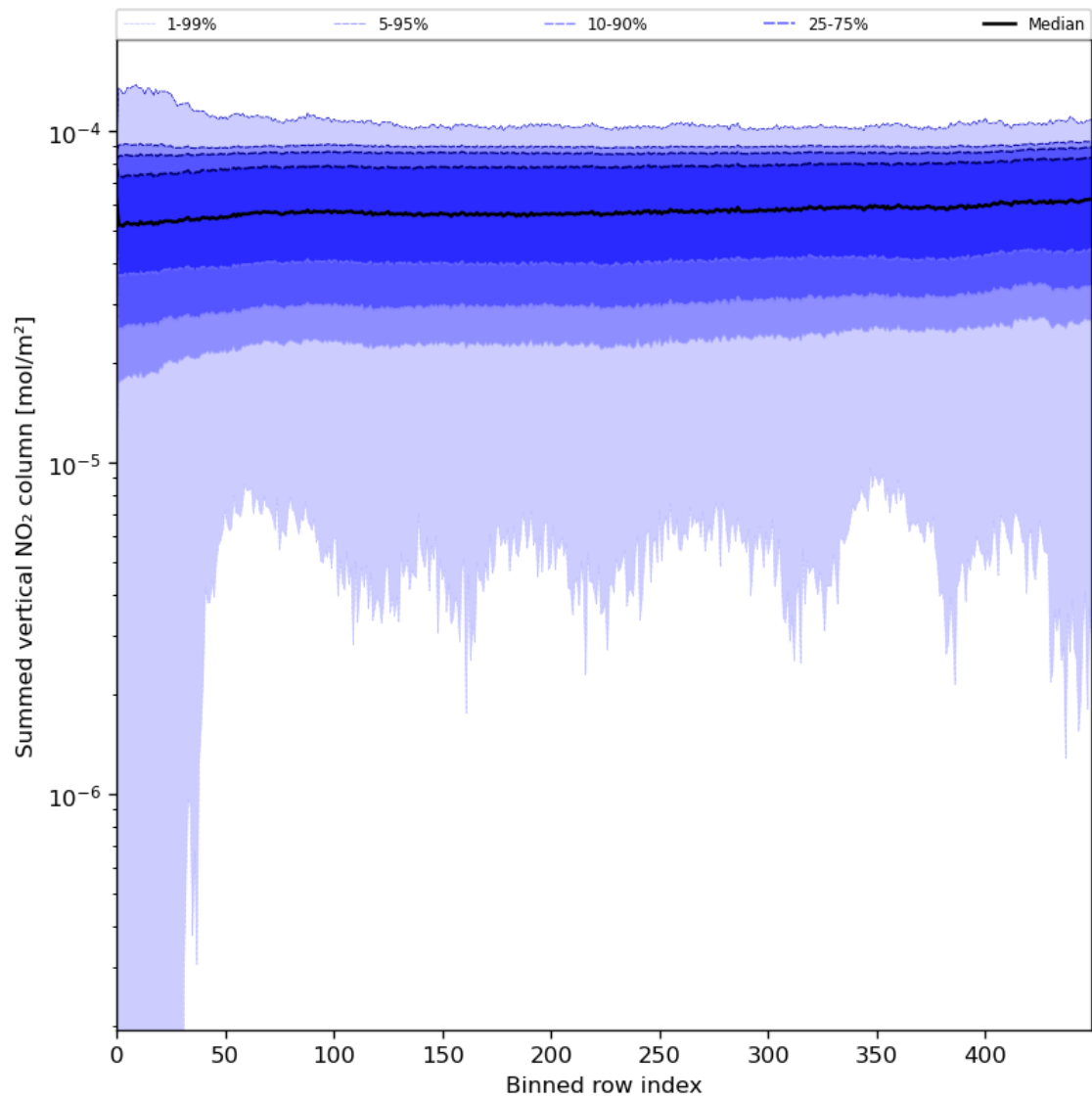
Figure 57: Along track statistics of “Summed vertical NO 2 column” for 2024-07-05 to 2024-07-06
