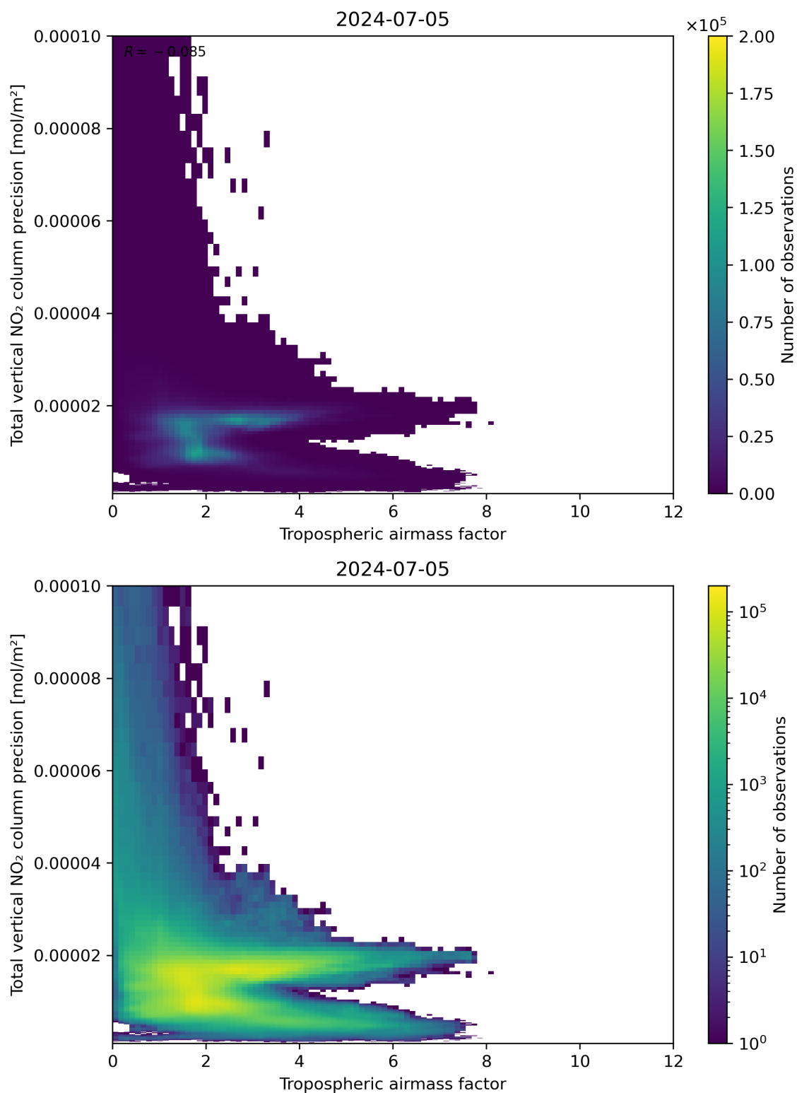
Figure 78: Scatter density plot of “Tropospheric air mass factor” against “Total vertical NO 2 column precision” for 2024-07-05 to 2024-07-06.
