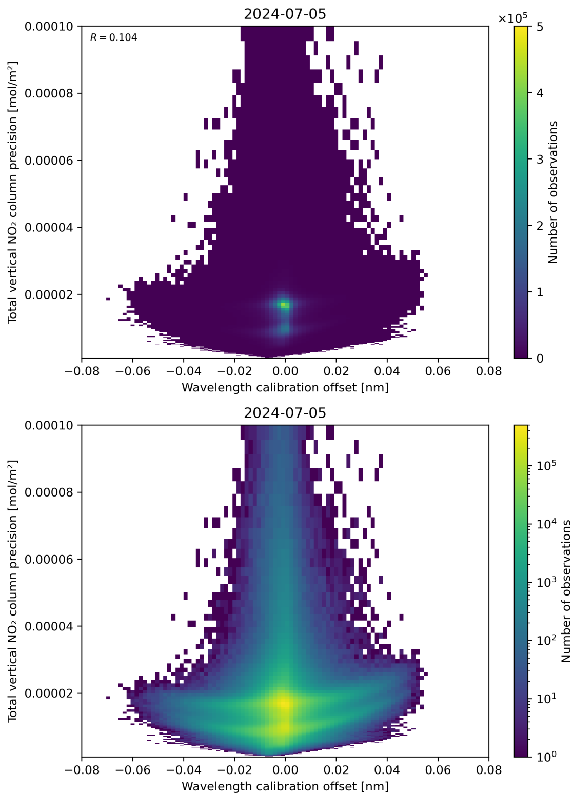
Figure 180: Scatter density plot of “Wavelength calibration offset” against “Total vertical NO 2 column precision” for 2024-07-05 to 2024-07-06.
