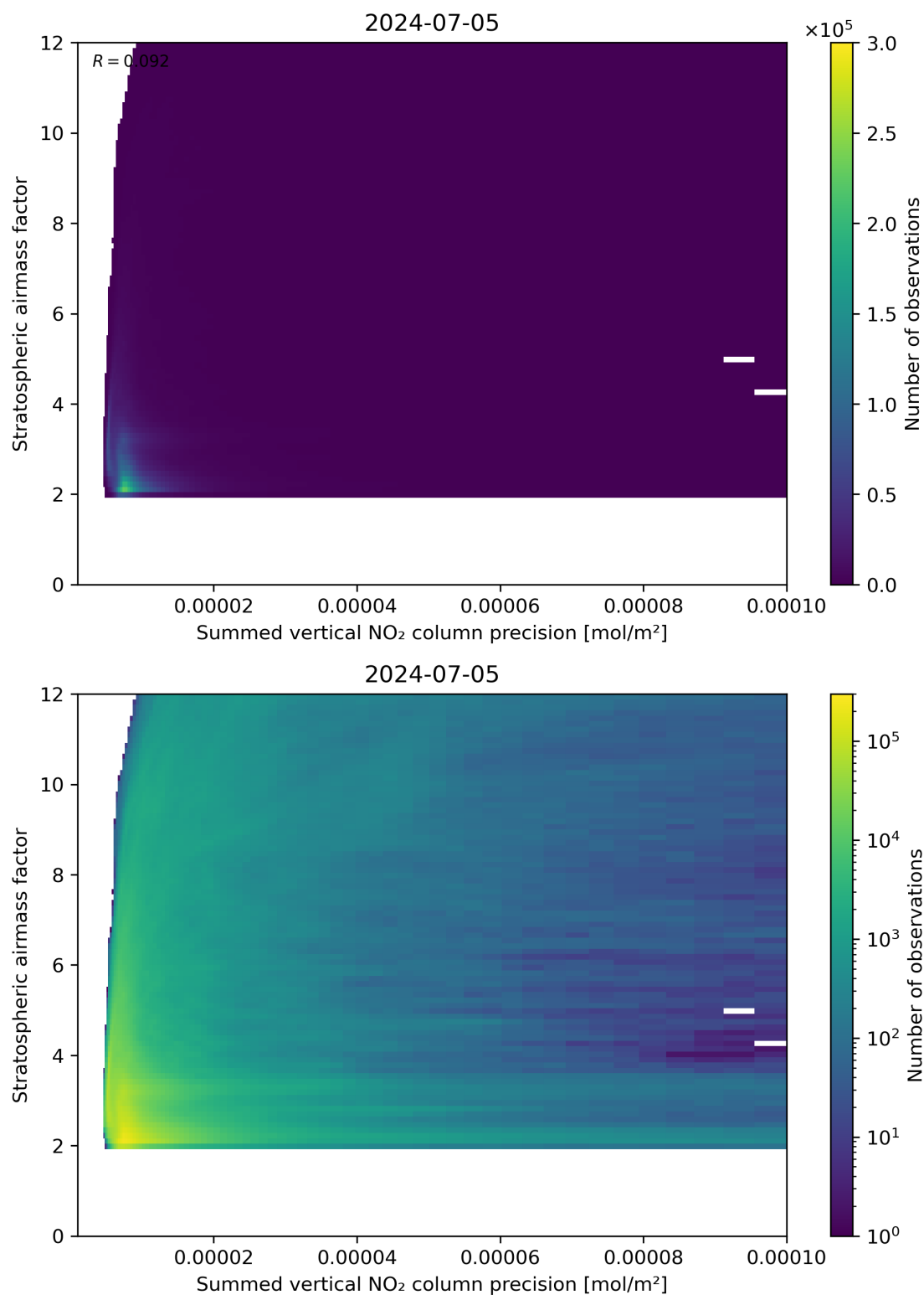
Figure 106: Scatter density plot of “Summed vertical NO 2 column precision” against “Stratospheric airmass factor” for 2024-07-05 to 2024-07-06.
