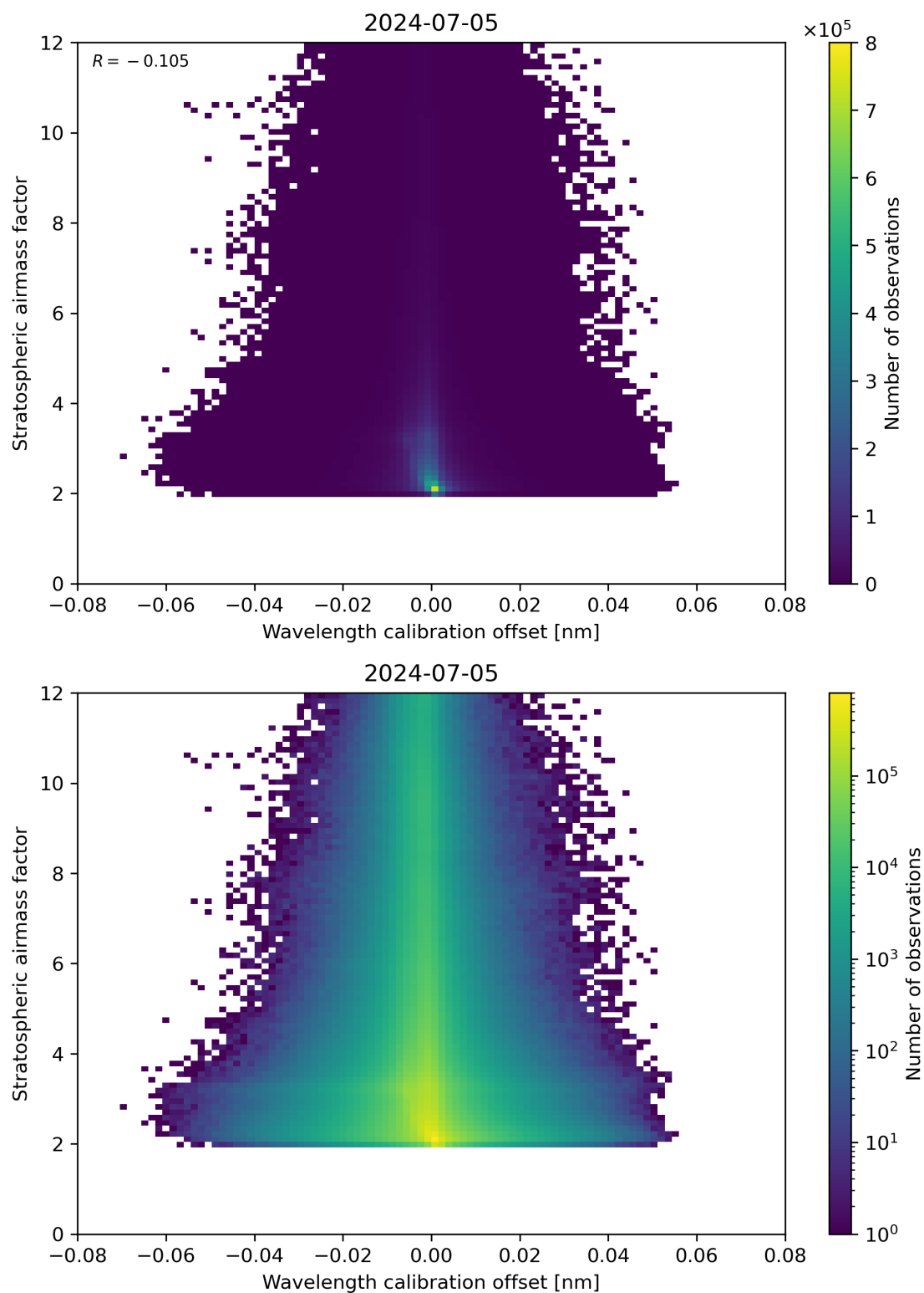
Figure 174: Scatter density plot of “Wavelength calibration offset” against “Stratospheric air mass factor” for 2024-07-05 to 2024-07-06.
