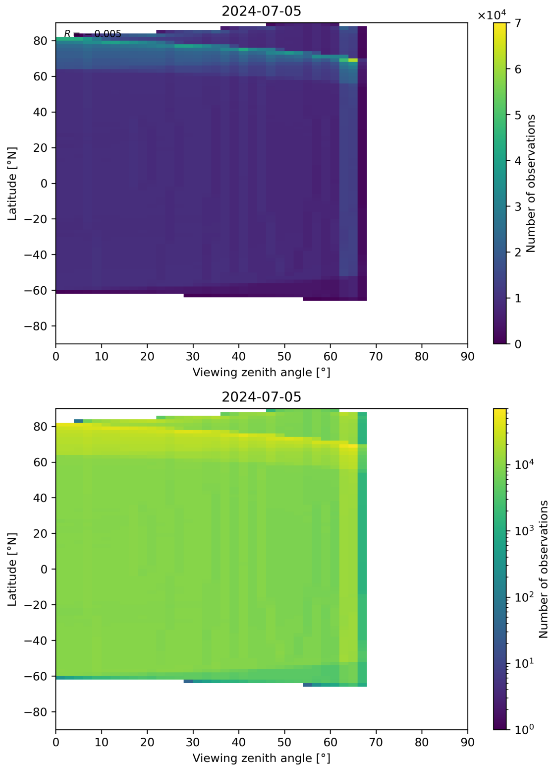
Figure 163: Scatter density plot of “Viewing zenith angle” against “Latitude” for 2024-07-05 to 2024-07-06.
