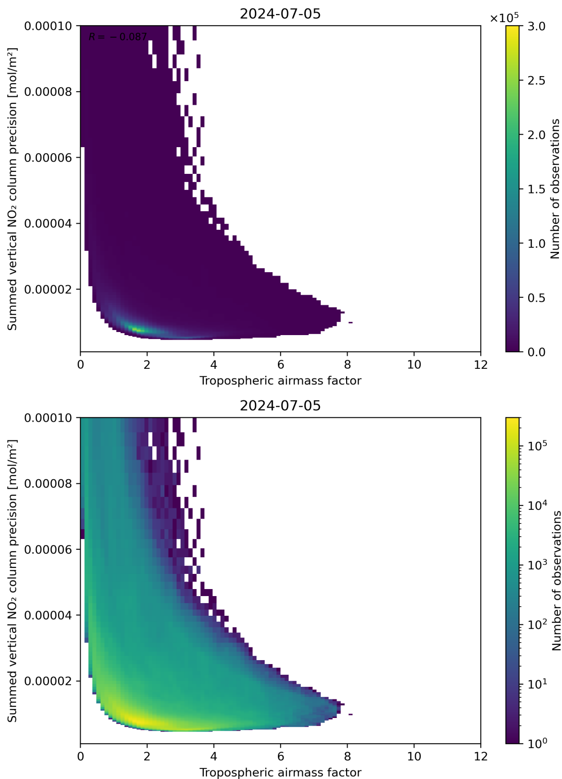
Figure 76: Scatter density plot of “Tropospheric air mass factor” against “Summed vertical NO 2 column precision” for 2024-07-05 to 2024-07-06.
