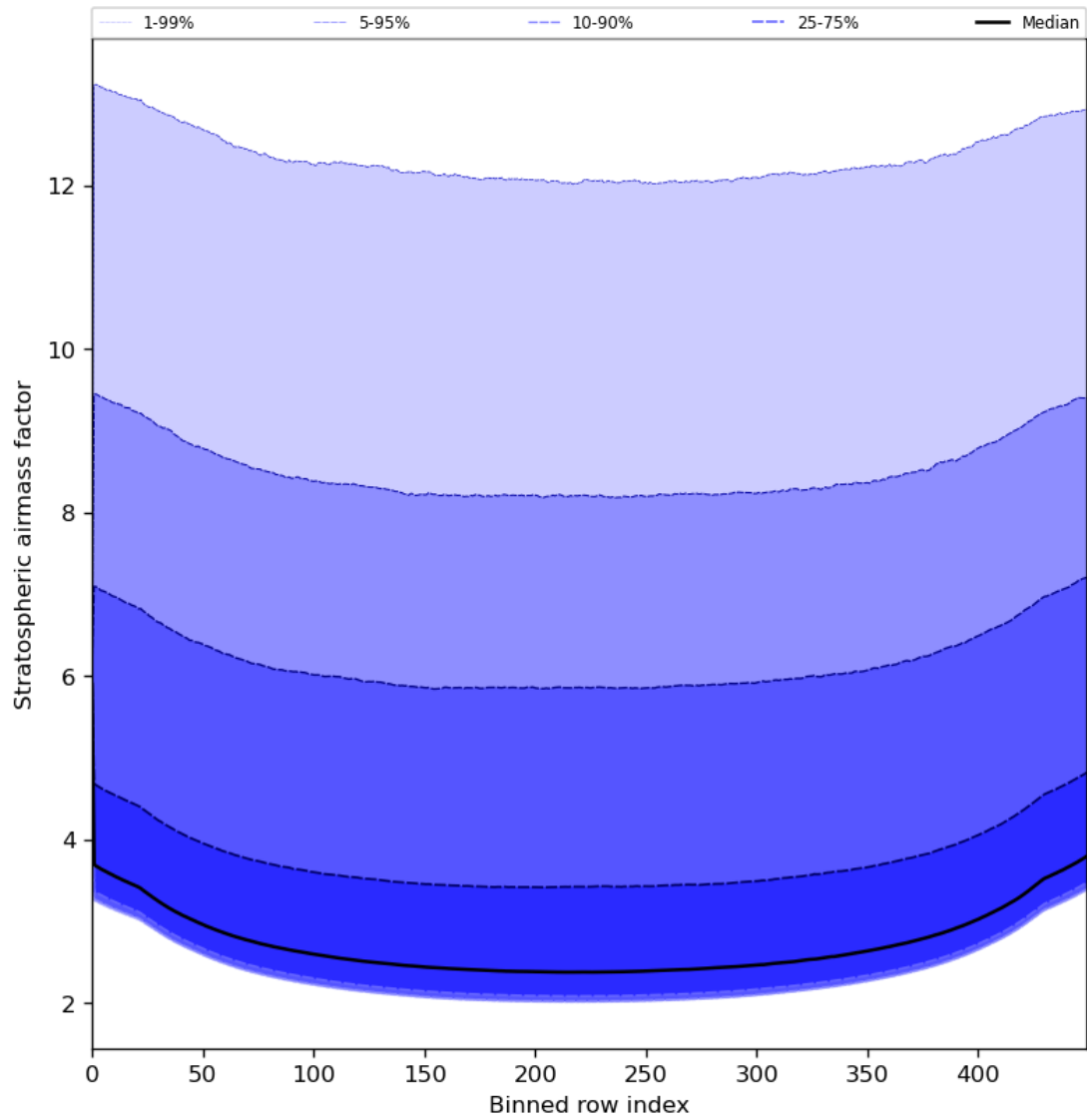
Figure 61: Along track statistics of “Stratospheric airmass factor” for 2024-07-05 to 2024-07-06
