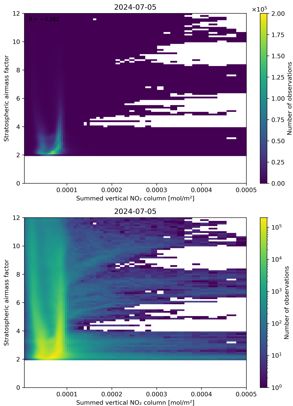
Figure 103: Scatter density plot of “Summed vertical NO 2 column” against “Stratospheric airmass factor” for 2024-07-05 to 2024-07-06.
