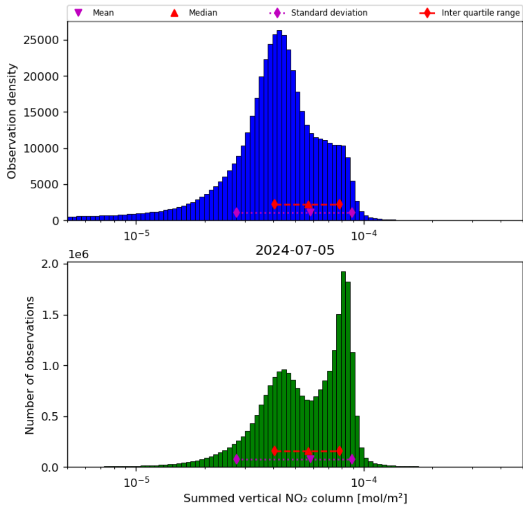
Figure 40: Histogram of “Summed vertical NO 2 column” for 2024-07-05 to 2024-07-06
