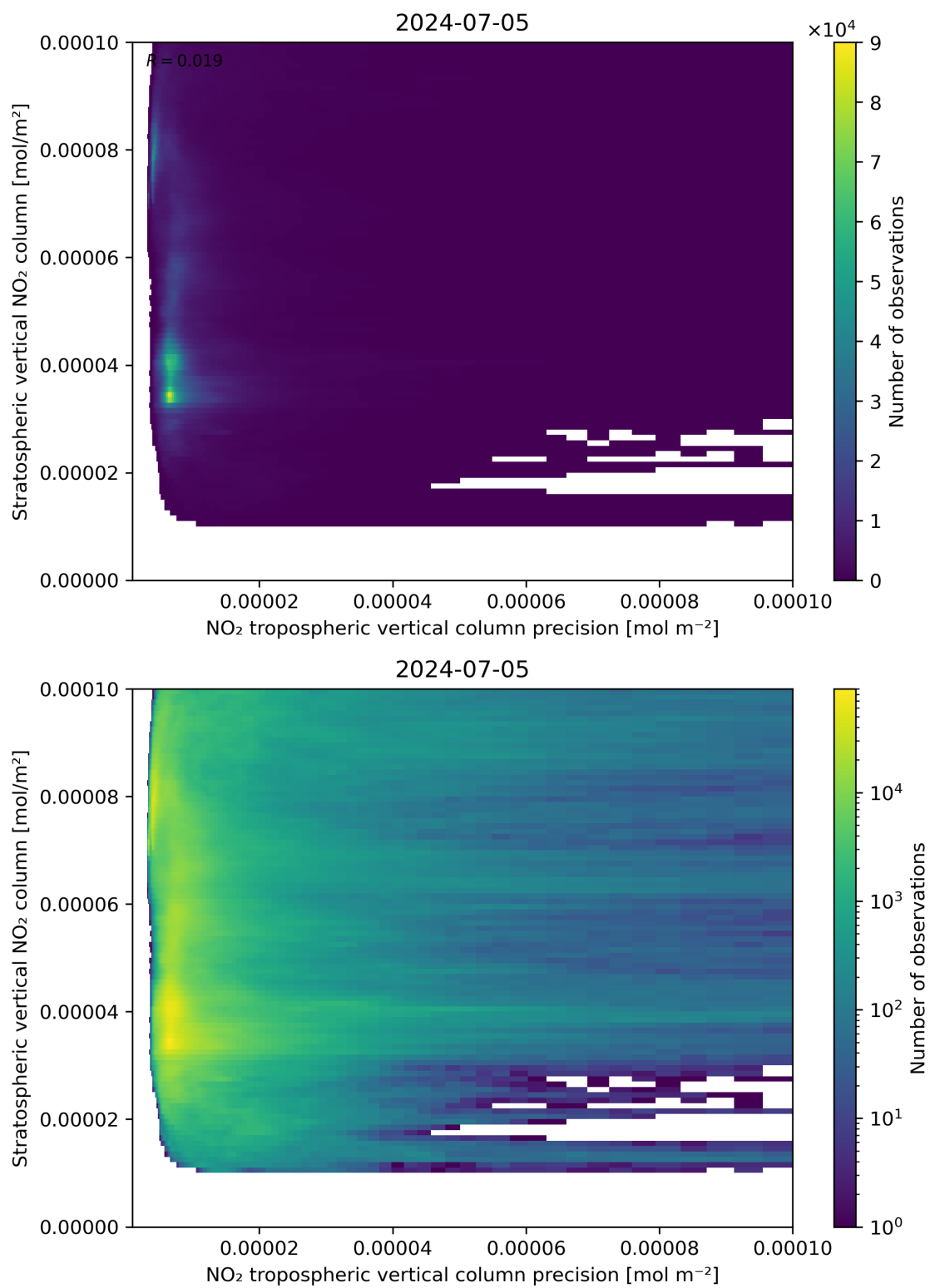
Figure 135: Scatter density plot of “NO 2 tropospheric vertical column precision” against “Stratospheric vertical NO 2 column” for 2024-07-05 to 2024-07-06.
