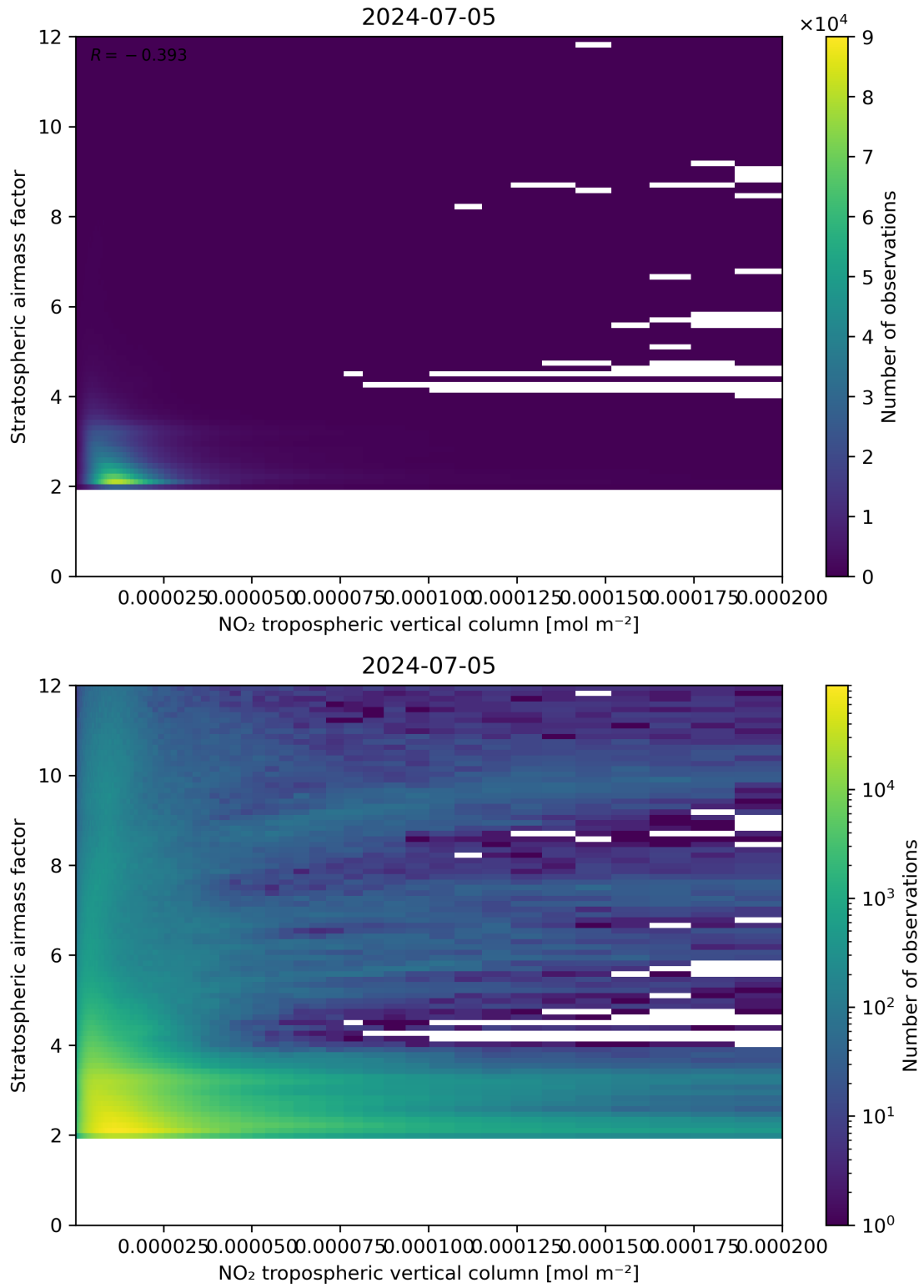
Figure 121: Scatter density plot of “NO 2 tropospheric vertical column” against “Stratospheric air mass factor” for 2024-07-05 to 2024-07-06.
