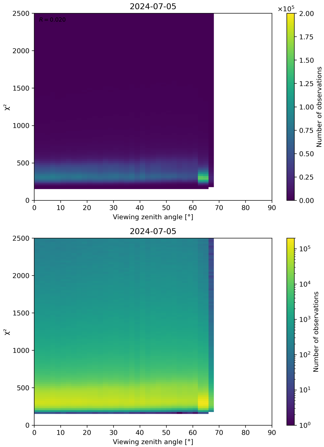
Figure 162: Scatter density plot of “Viewing zenith angle” against “ \chi^2 ” for 2024-07-05 to 2024-07-06.
