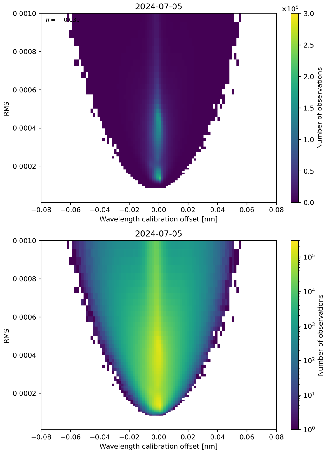
Figure 181: Scatter density plot of “Wavelength calibration offset” against “RMS” for 2024-07-05 to 2024-07-06.
