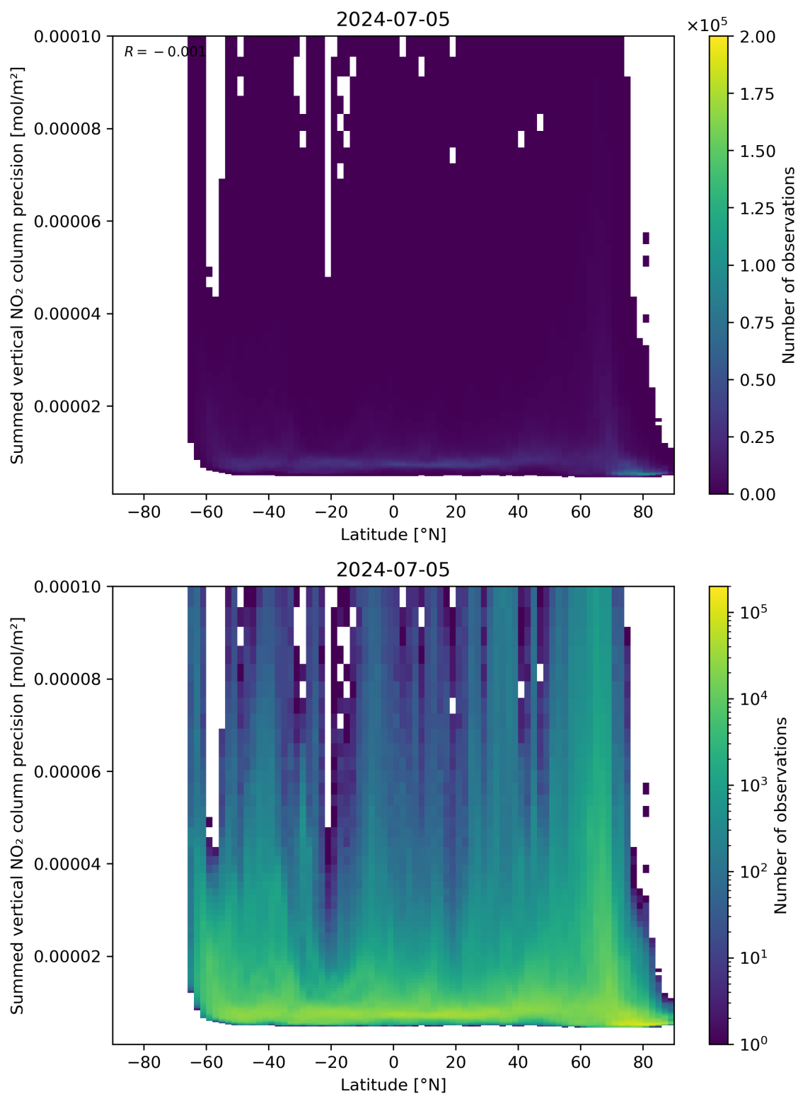
Figure 89: Scatter density plot of “Latitude” against “Summed vertical NO 2 column precision” for 2024-07-05 to 2024-07-06.
