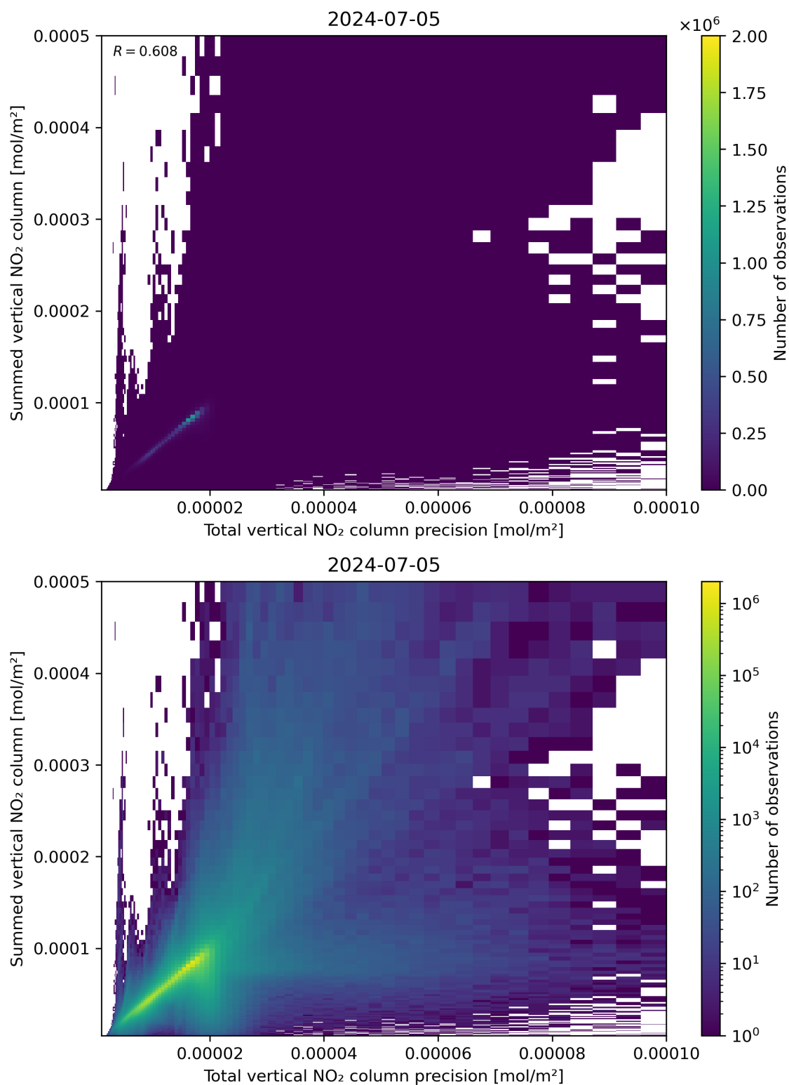
Figure 117: Scatter density plot of “Total vertical NO 2 column precision” against “Summed vertical NO 2 column” for 2024-07-05 to 2024-07-06.
