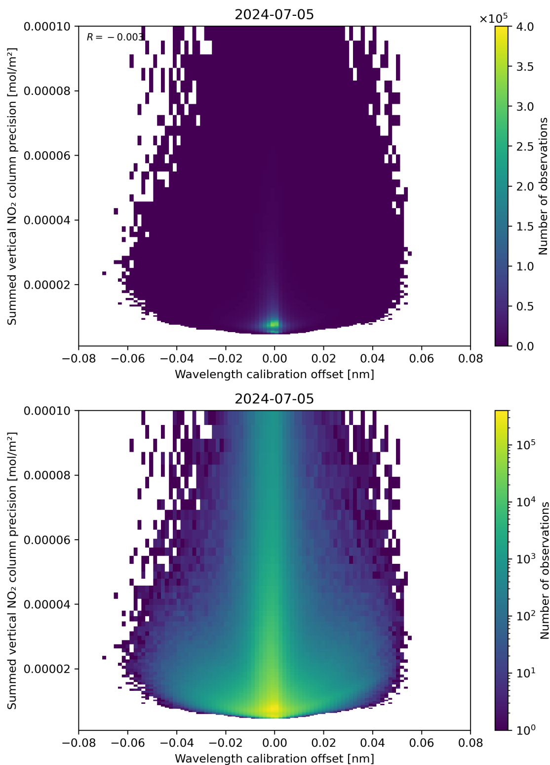
Figure 178: Scatter density plot of “Wavelength calibration offset” against “Summed vertical NO 2 column precision” for 2024-07-05 to 2024-07-06.
