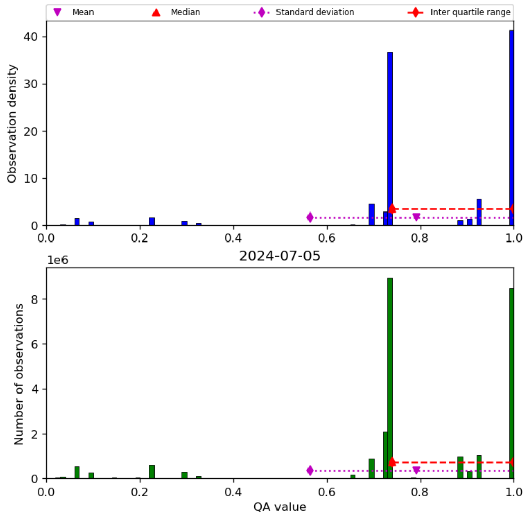
Figure 28: Histogram of “QA value” for 2024-07-05 to 2024-07-06
