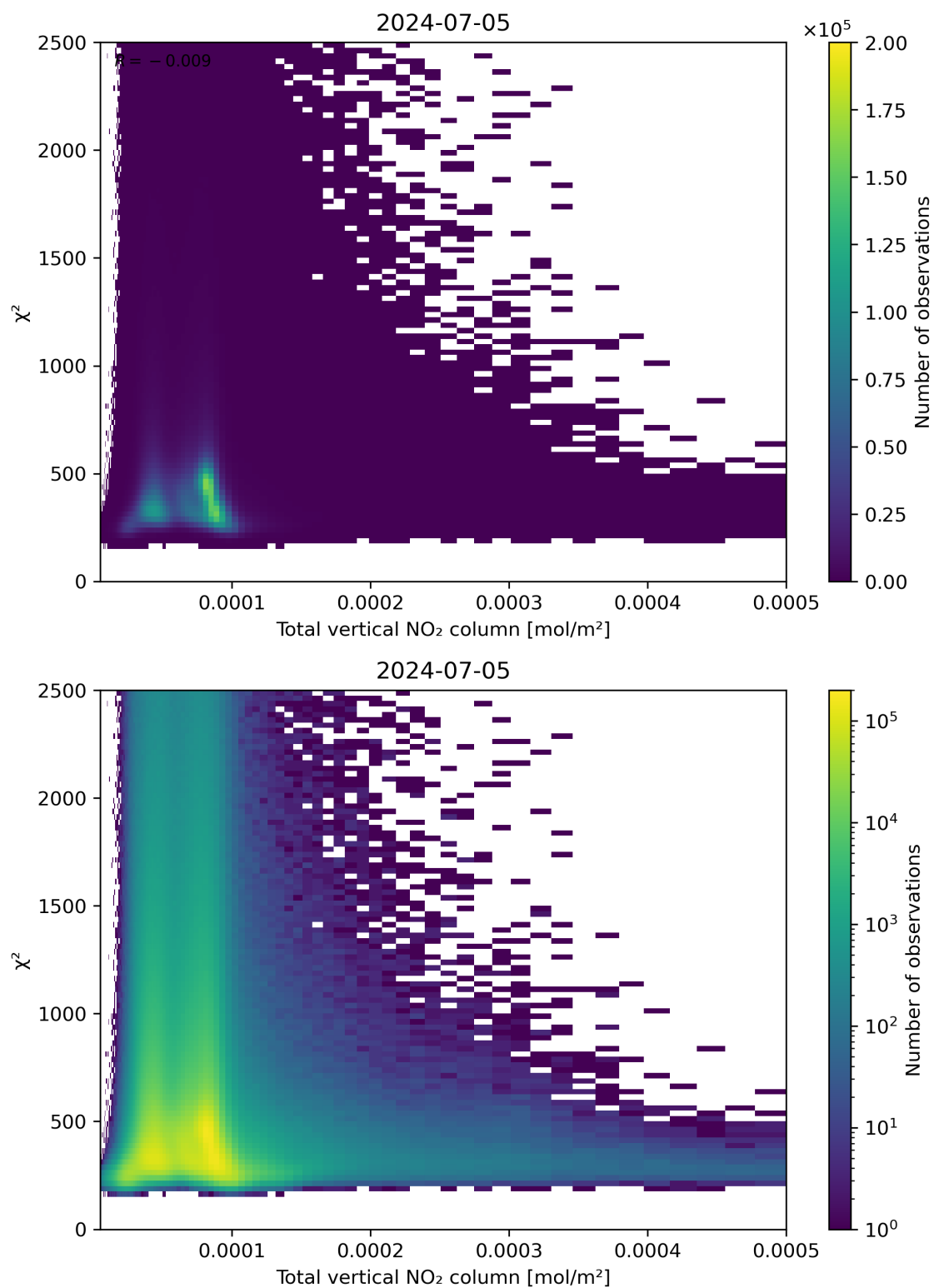
Figure 111: Scatter density plot of “Total vertical NO 2 column” against “ \chi^2 ” for 2024-07-05 to 2024-07-06.
