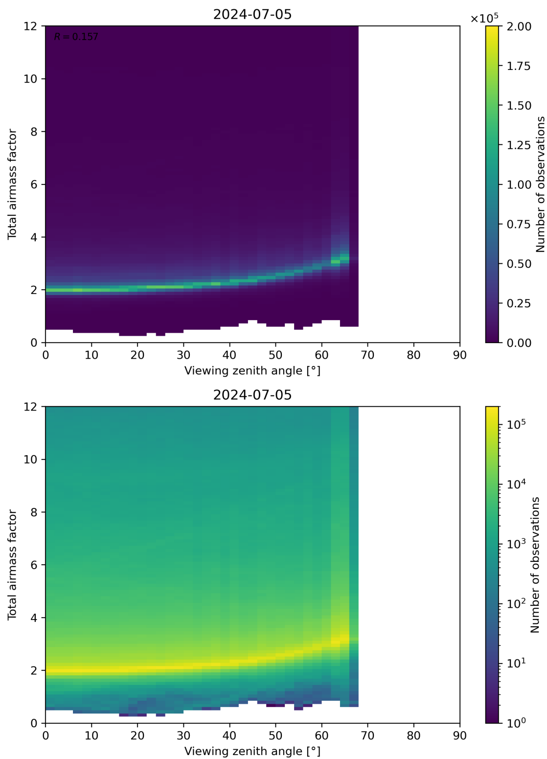
Figure 160: Scatter density plot of “Viewing zenith angle” against “Total airmass factor” for 2024-07-05 to 2024-07-06.
