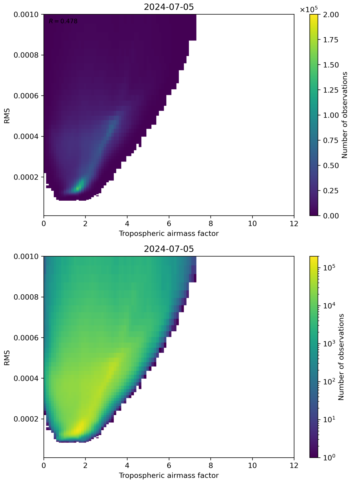
Figure 79: Scatter density plot of “Tropospheric airmass factor” against “RMS” for 2024-07-05 to 2024-07-06.
