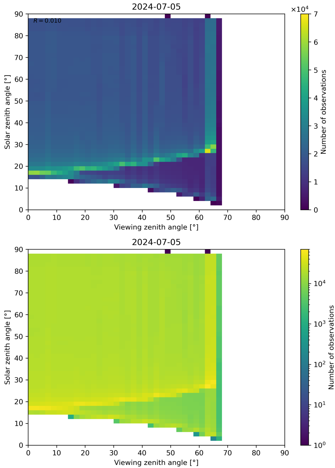
Figure 172: Scatter density plot of “Viewing zenith angle” against “Solar zenith angle” for 2024-07-05 to 2024-07-06.
