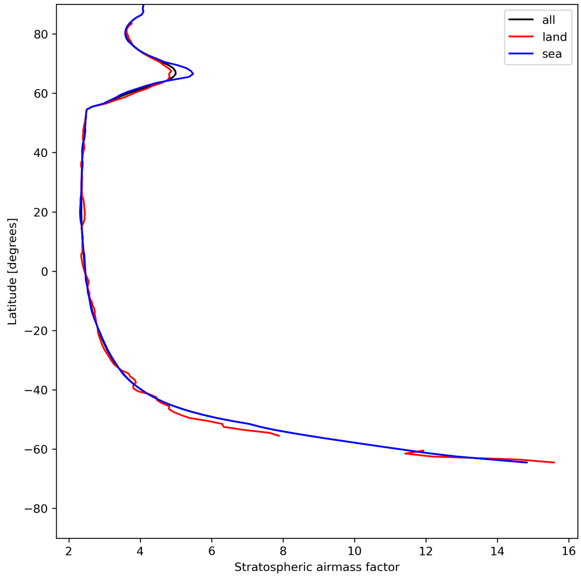
Figure 27: Zonal average of “Stratospheric airmass factor” for 2024-07-05 to 2024-07-06.
