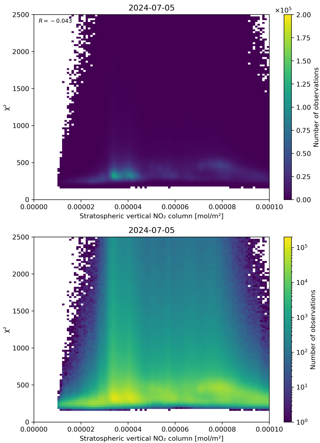
Figure 97: Scatter density plot of “Stratospheric vertical NO 2 column” against “ \chi^2 ” for 2024-07-05 to 2024-07-06.
