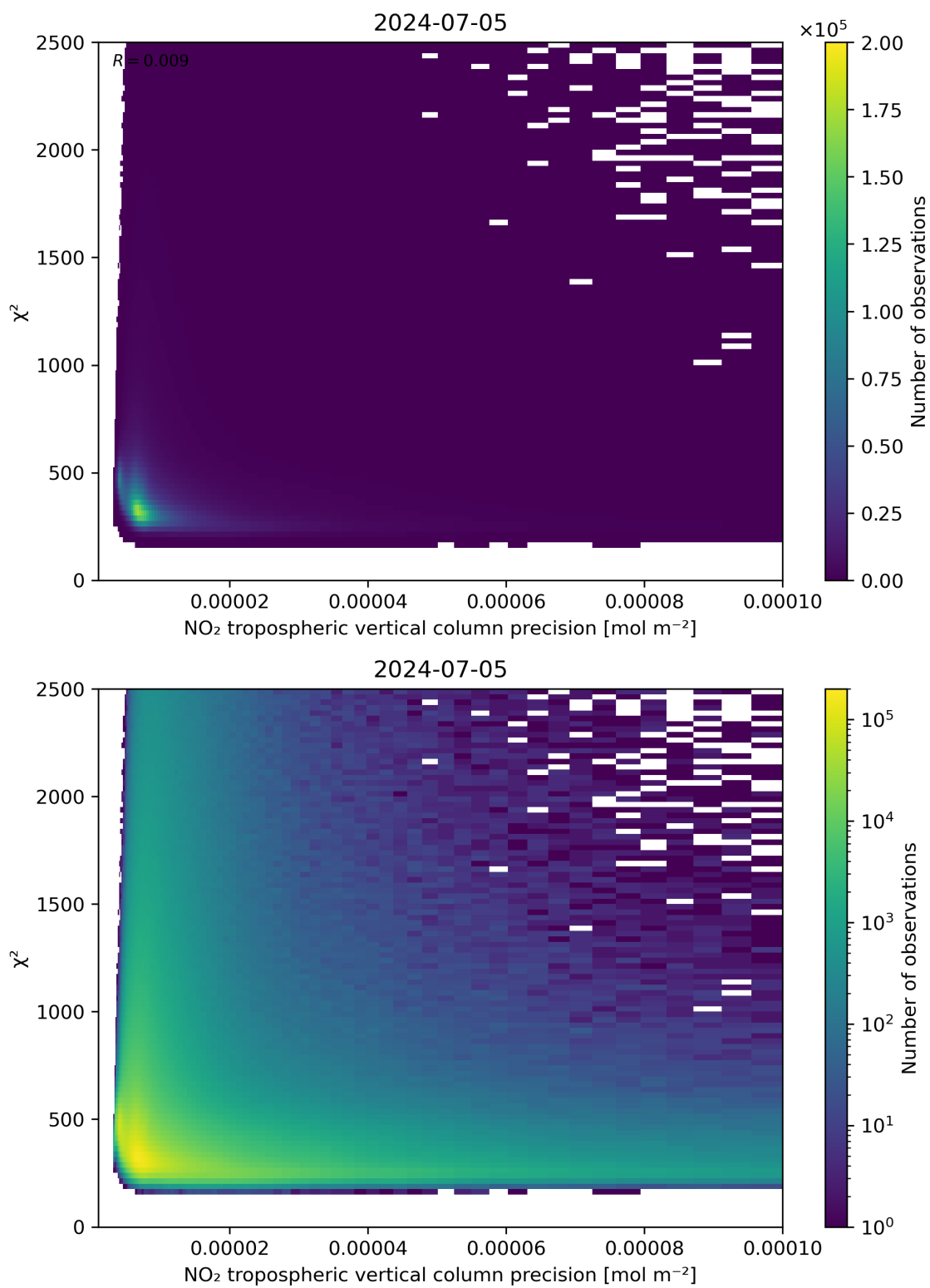
Figure 134: Scatter density plot of “NO 2 tropospheric vertical column precision” against “ \chi^2 ” for 2024-07-05 to 2024-07-06.
