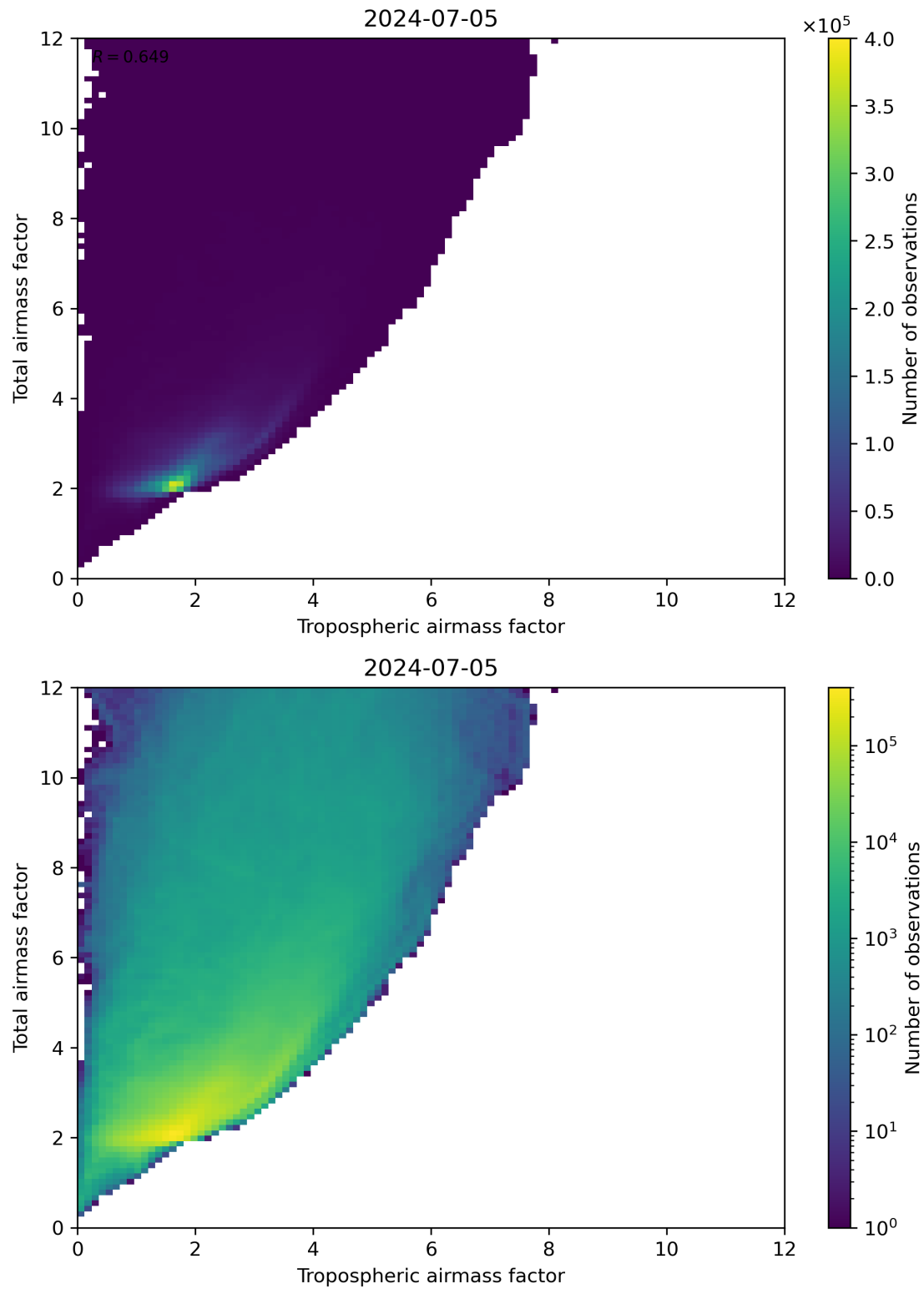
Figure 72: Scatter density plot of “Tropospheric airmass factor” against “Total airmass factor” for 2024-07-05 to 2024-07-06.
