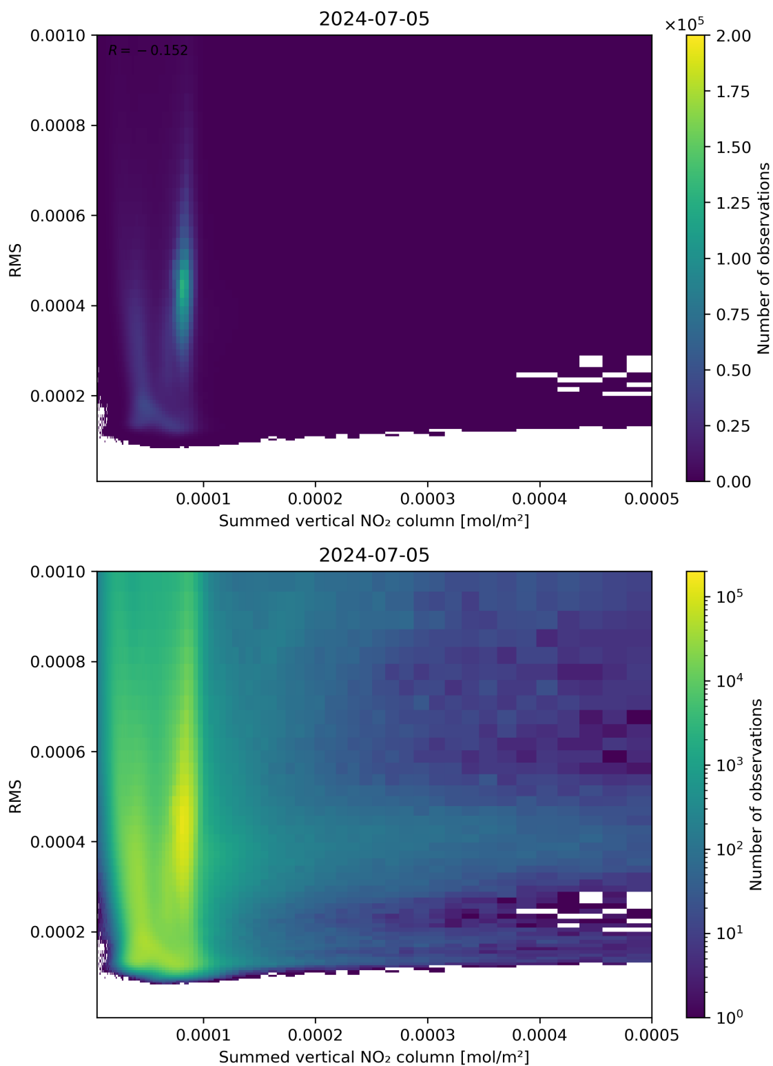
Figure 109: Scatter density plot of “Summed vertical NO 2 column” against “RMS” for 2024-07-05 to 2024-07-06.
