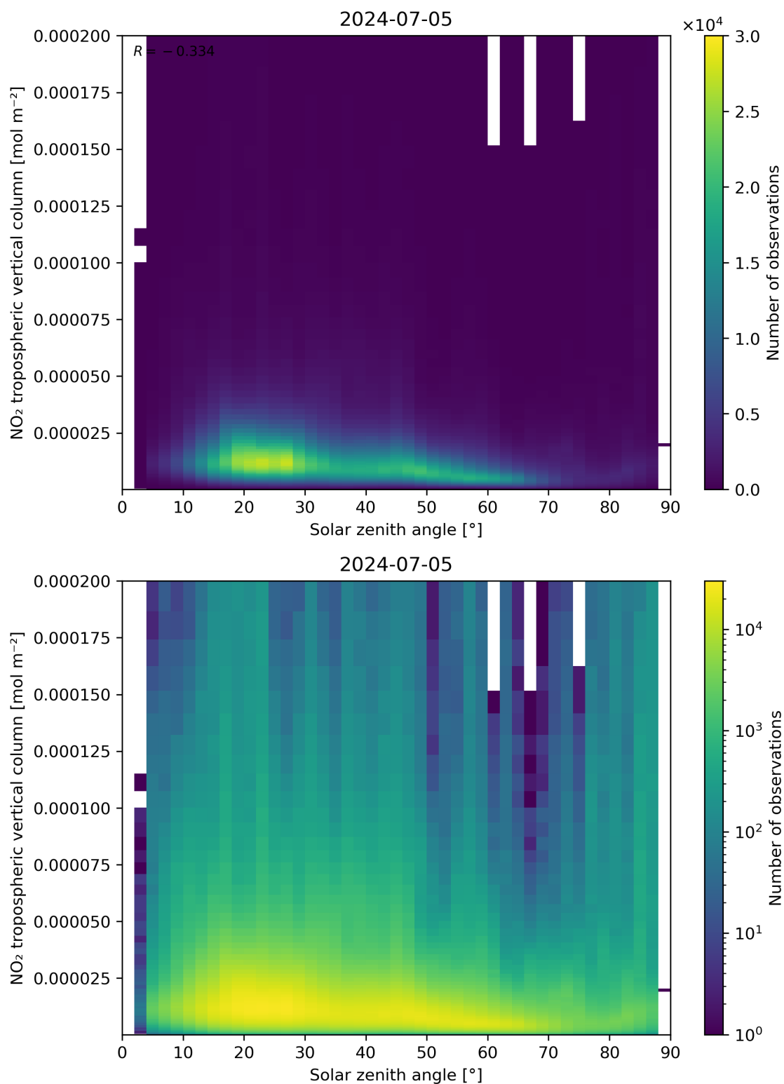
Figure 155: Scatter density plot of “Solar zenith angle” against “NO 2 tropospheric vertical column” for 2024-07-05 to 2024-07-06.
