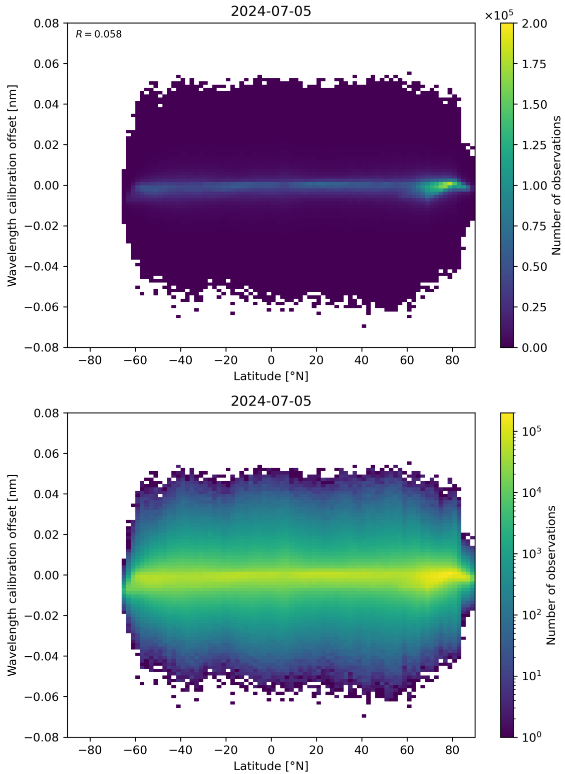
Figure 95: Scatter density plot of “Latitude” against “Wavelength calibration offset” for 2024-07-05 to 2024-07-06.
