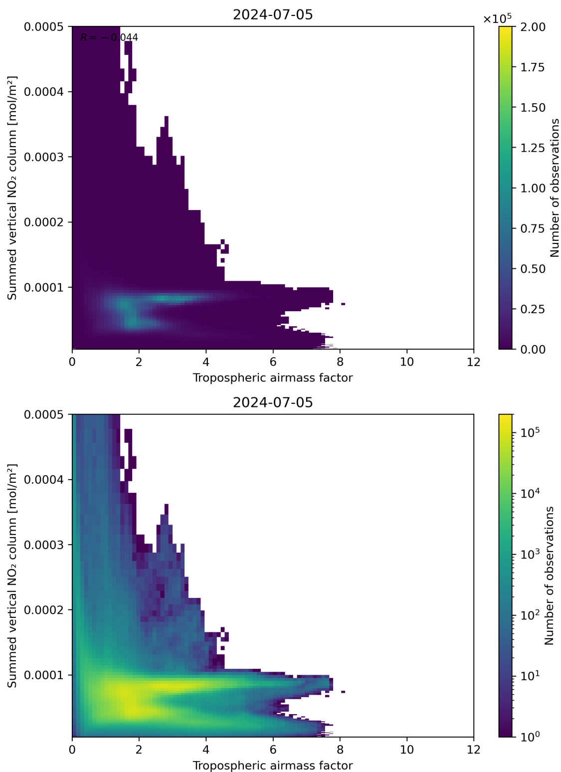
Figure 75: Scatter density plot of “Tropospheric airmass factor” against “Summed vertical NO 2 column” for 2024-07-05 to 2024-07-06.
