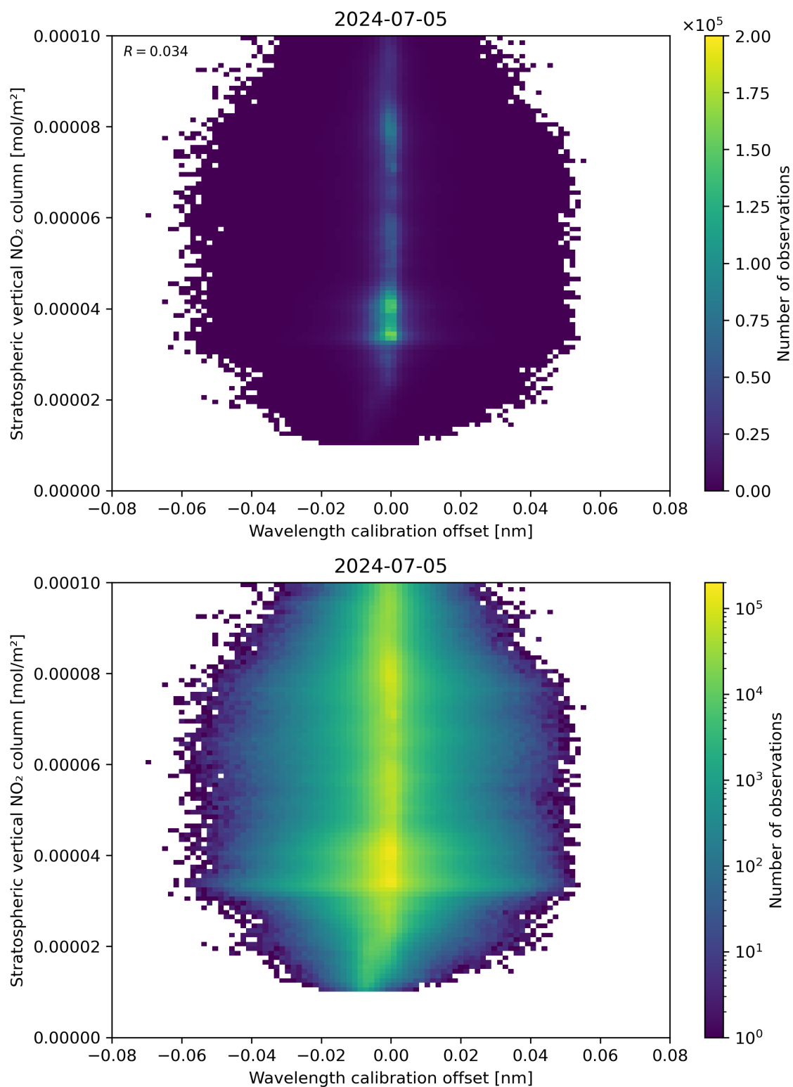
Figure 176: Scatter density plot of “Wavelength calibration offset” against “Stratospheric vertical NO 2 column” for 2024-07-05 to 2024-07-06.
