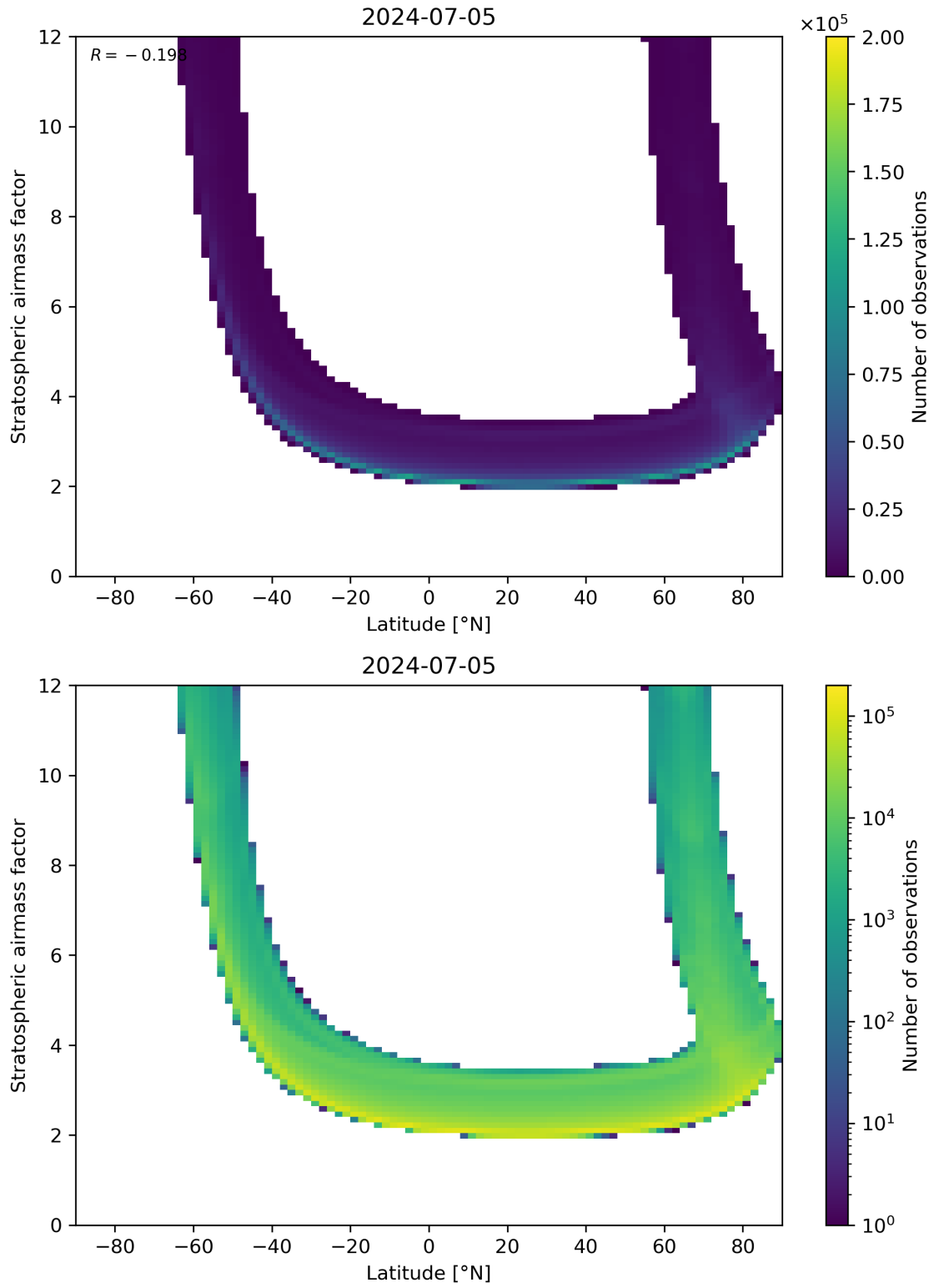
Figure 83: Scatter density plot of “Latitude” against “Stratospheric air mass factor” for 2024-07-05 to 2024-07-06.
