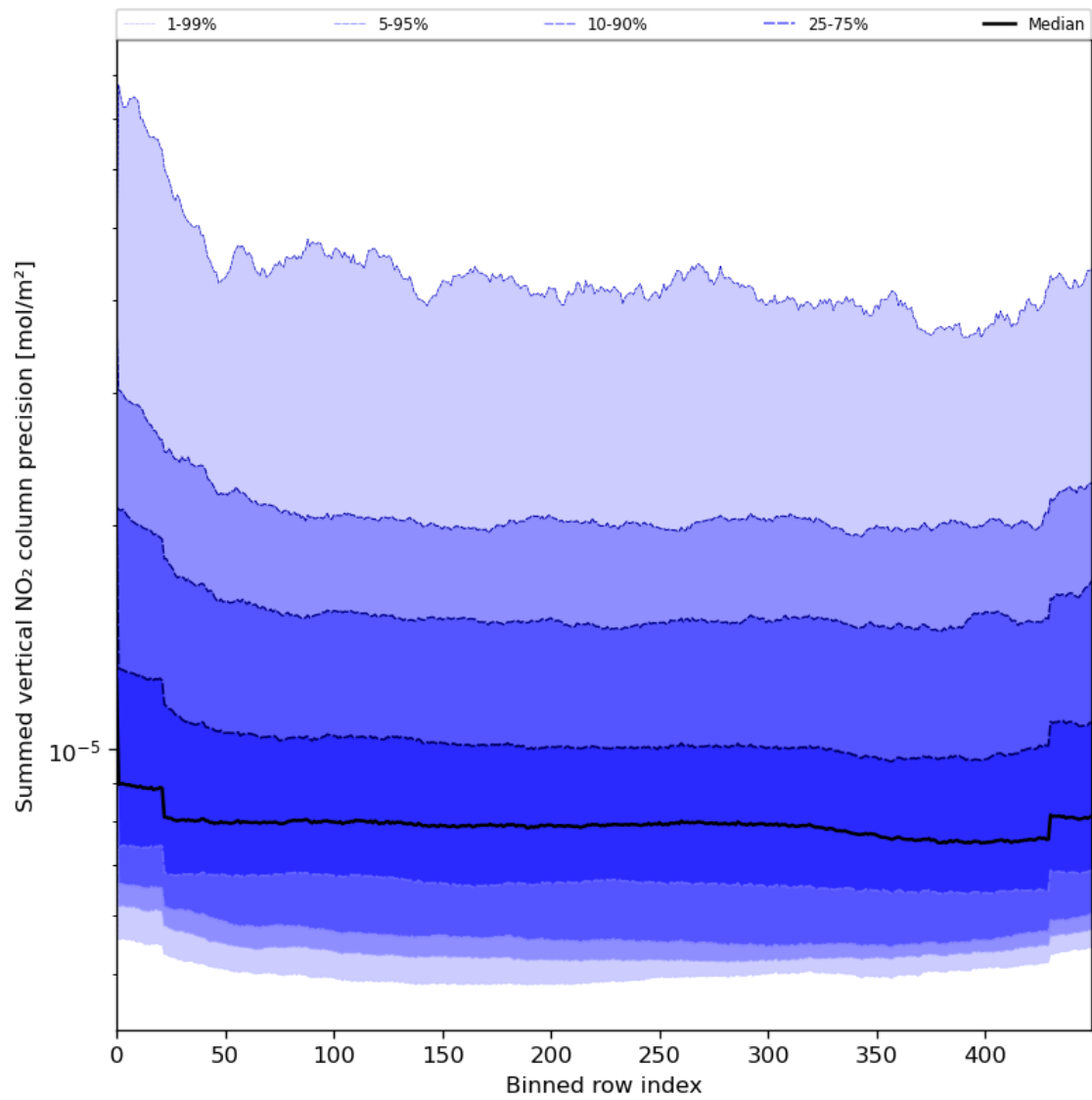
Figure 58: Along track statistics of “Summed vertical NO 2 column precision” for 2024-07-05 to 2024-07-06
