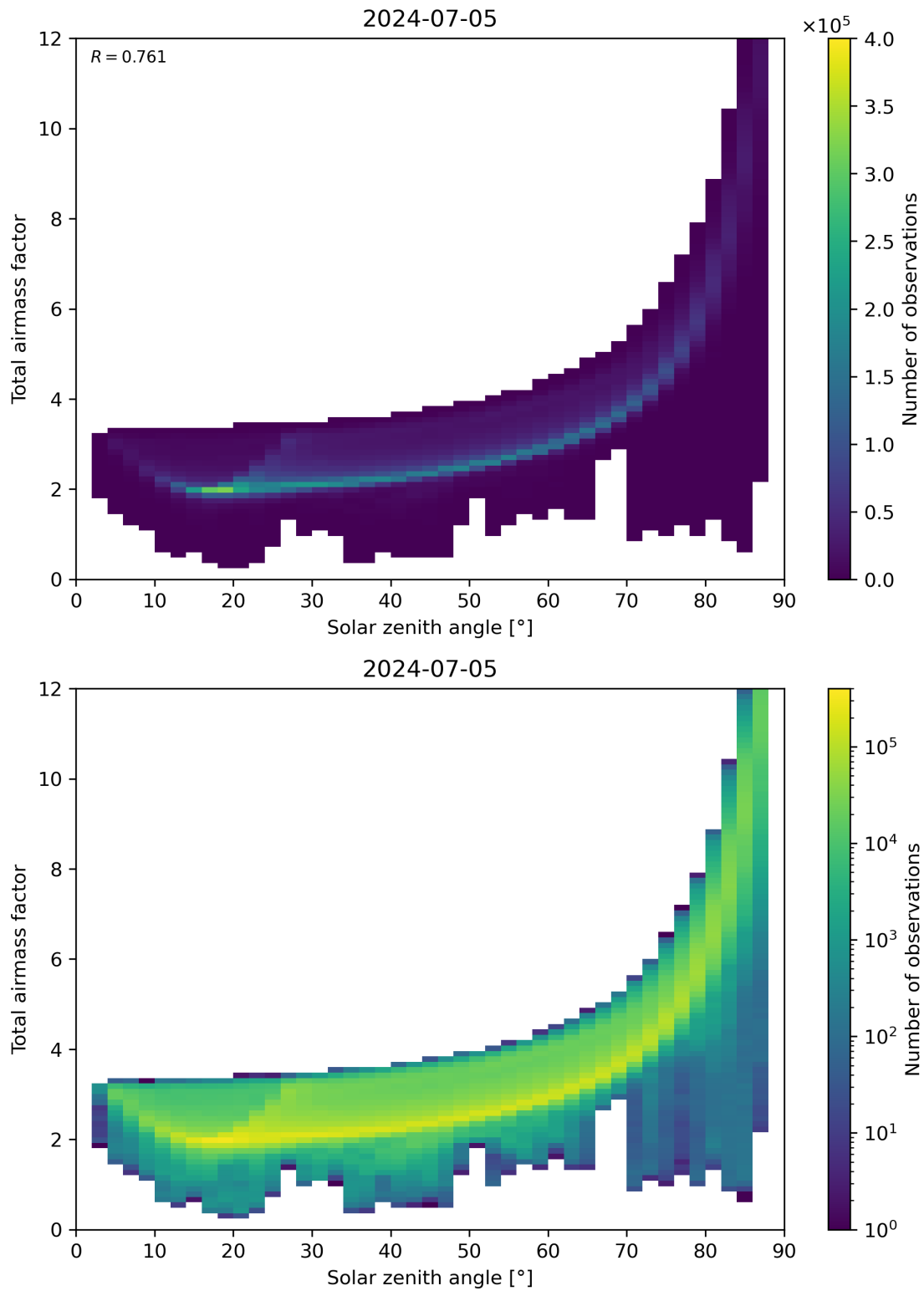
Figure 146: Scatter density plot of “Solar zenith angle” against “Total air mass factor” for 2024-07-05 to 2024-07-06.
