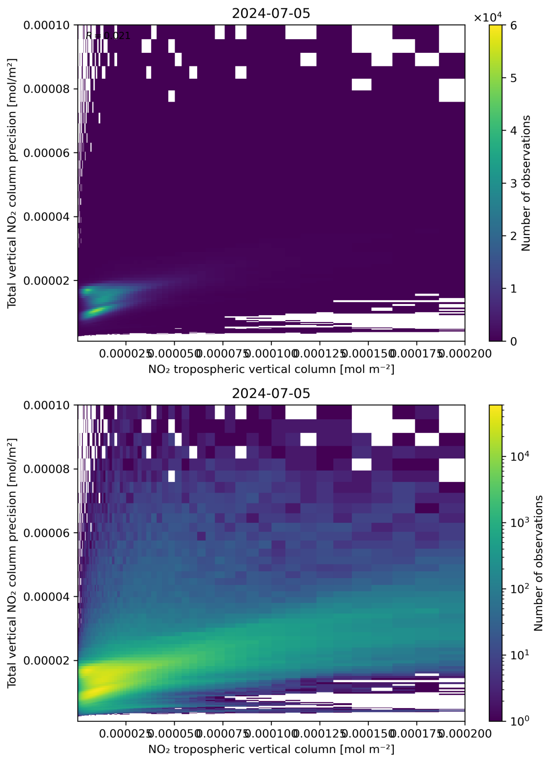
Figure 129: Scatter density plot of “NO 2 tropospheric vertical column” against “Total vertical NO 2 column precision” for 2024-07-05 to 2024-07-06.
