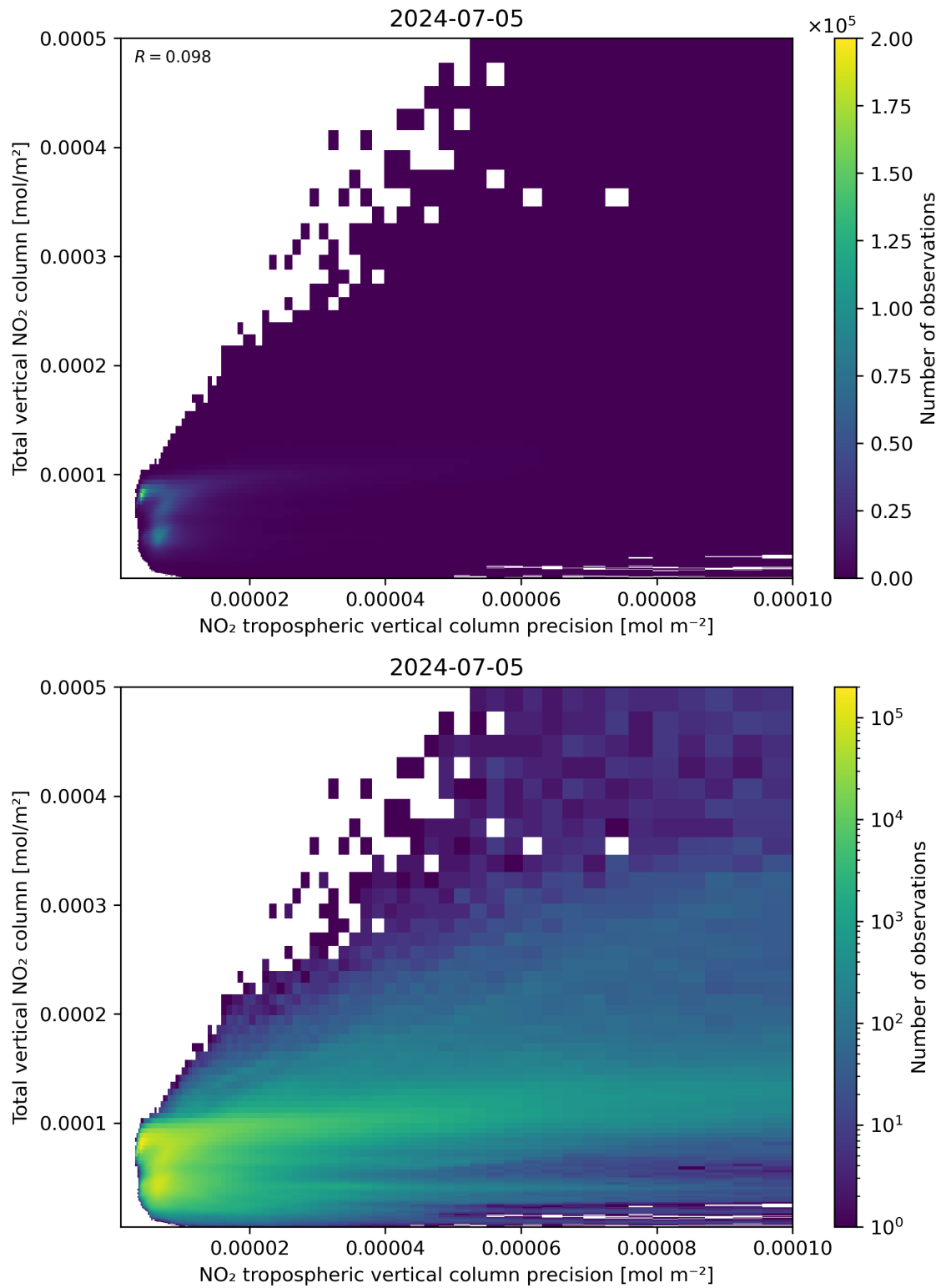
Figure 138: Scatter density plot of “NO 2 tropospheric vertical column precision” against “Total vertical NO 2 column” for 2024-07-05 to 2024-07-06.
