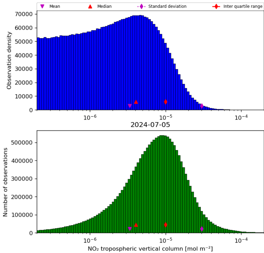
Figure 29: Histogram of “NO 2 tropospheric vertical column” for 2024-07-05 to 2024-07-06
