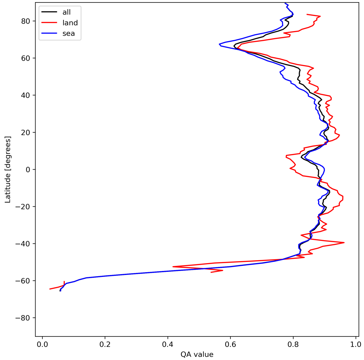
Figure 11: Zonal average of “QA value” for 2024-07-05 to 2024-07-07.
