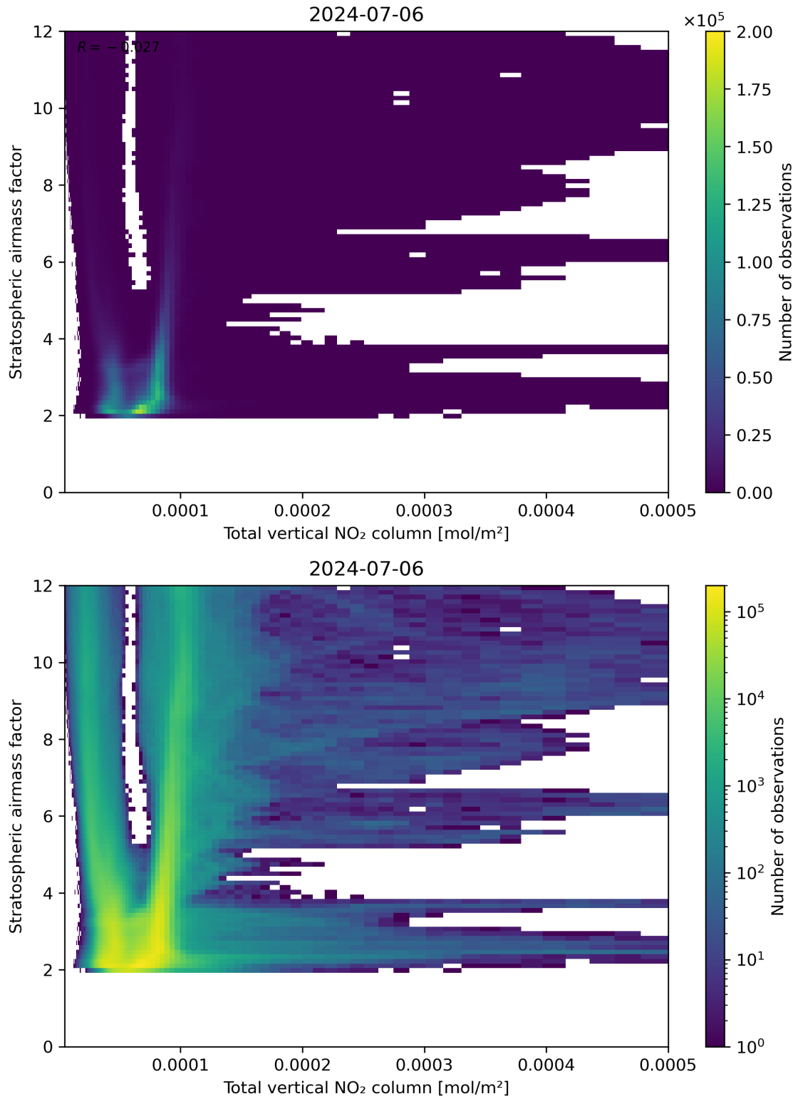
Figure 110: Scatter density plot of “Total vertical NO 2 column” against “Stratospheric airmass factor” for 2024-07-05 to 2024-07-07.
