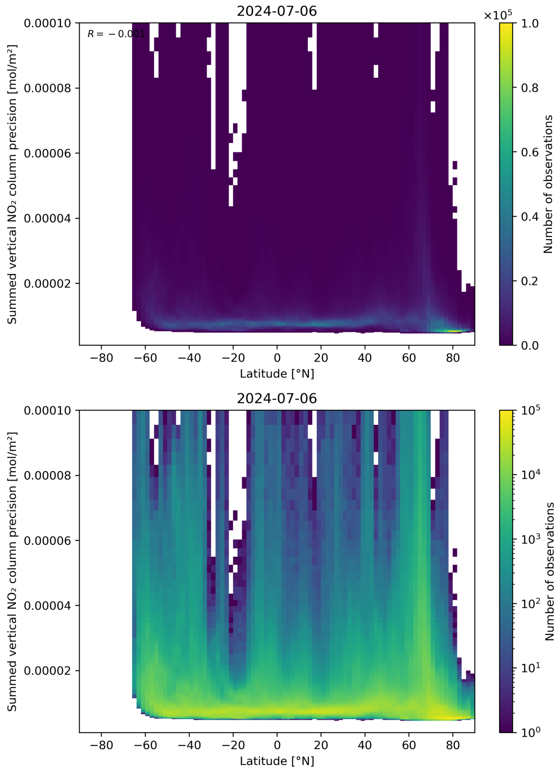
Figure 89: Scatter density plot of “Latitude” against “Summed vertical NO 2 column precision” for 2024-07-05 to 2024-07-07.
