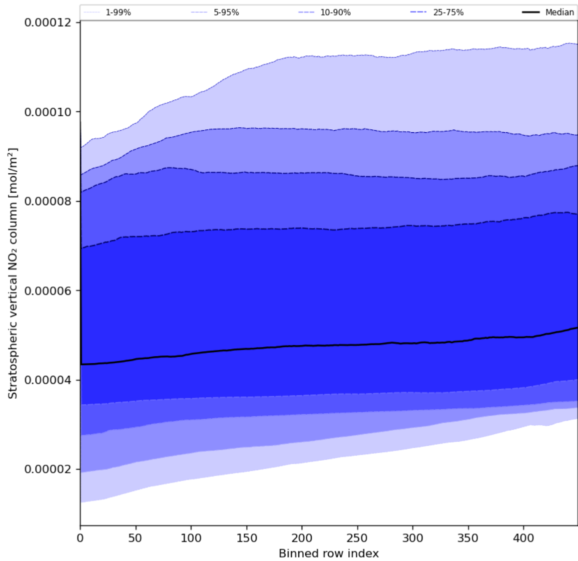
Figure 53: Along track statistics of “Stratospheric vertical NO 2 column” for 2024-07-05 to 2024-07-07
