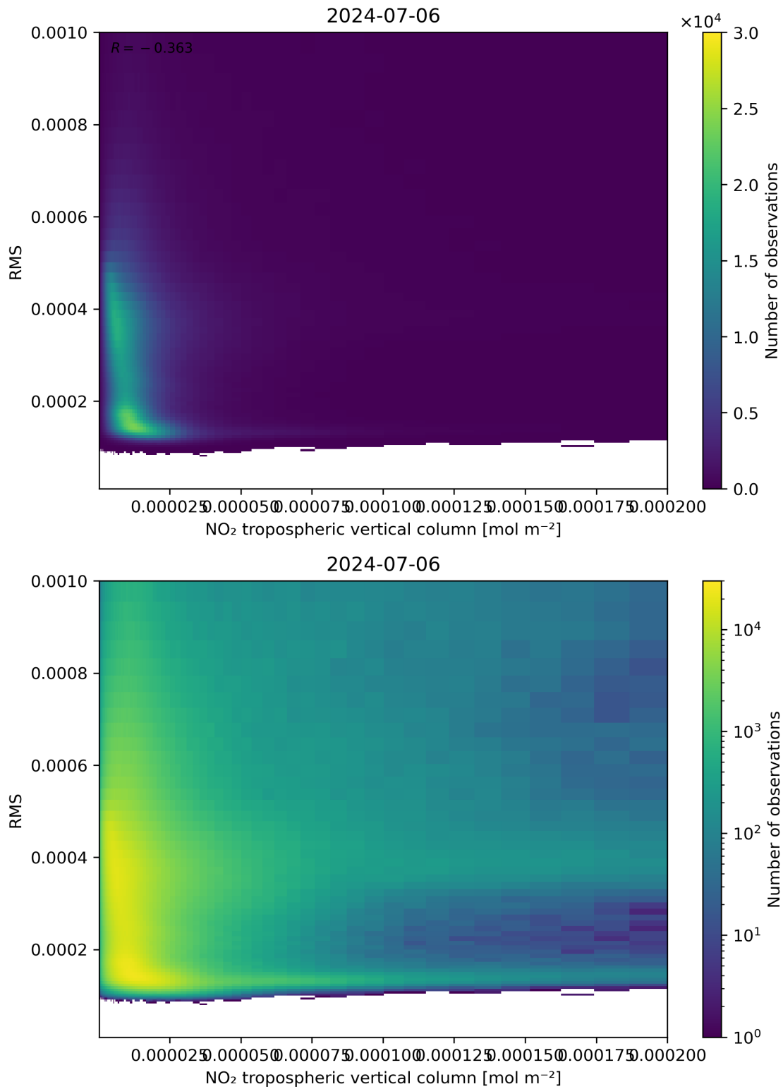
Figure 142: Scatter density plot of “NO 2 tropospheric vertical column” against “RMS” for 2024-07-05 to 2024-07-07.
