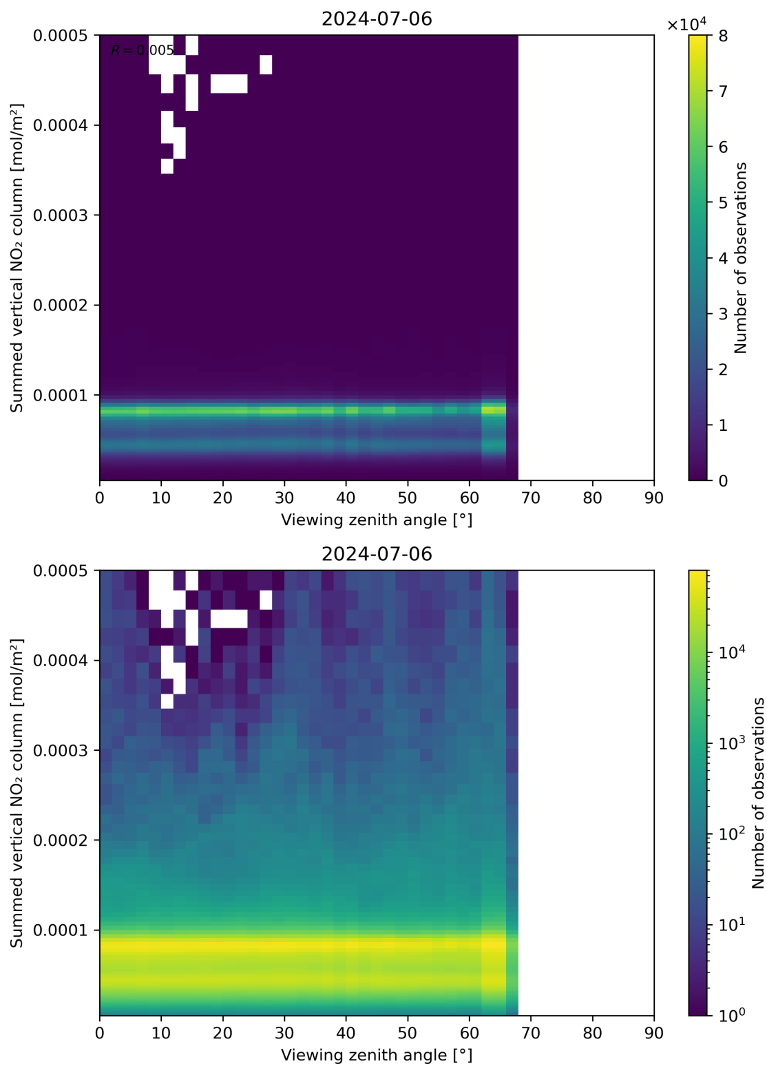
Figure 165: Scatter density plot of “Viewing zenith angle” against “Summed vertical NO 2 column” for 2024-07-05 to 2024-07-07.
