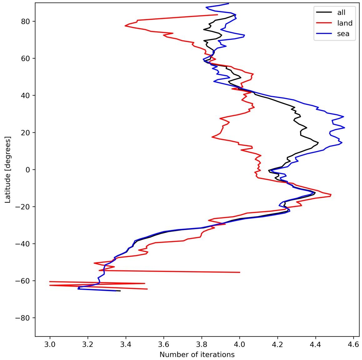
Figure 17: Zonal average of “Number of iterations” for 2024-07-05 to 2024-07-07.
