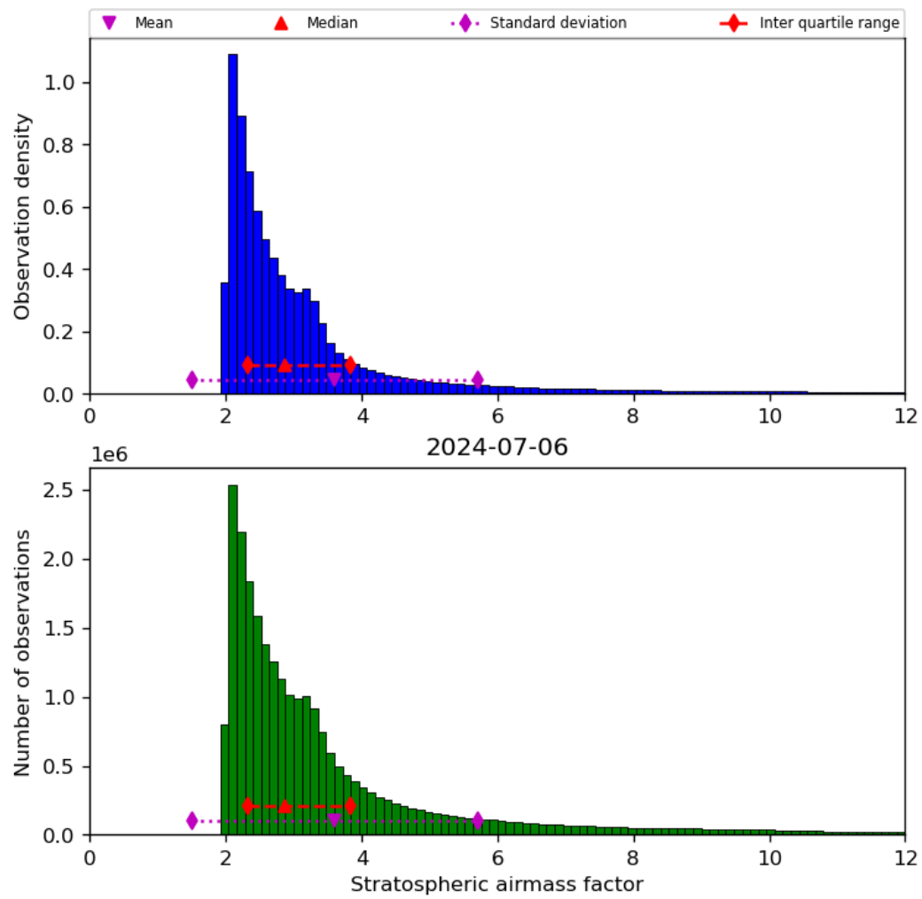
Figure 44: Histogram of “Stratospheric airmass factor” for 2024-07-05 to 2024-07-07
