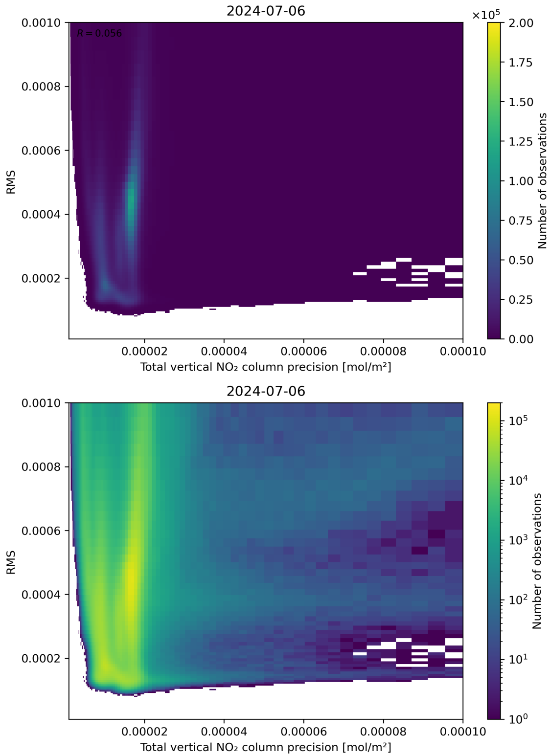
Figure 119: Scatter density plot of “Total vertical NO 2 column precision” against “RMS” for 2024-07-05 to 2024-07-07.
