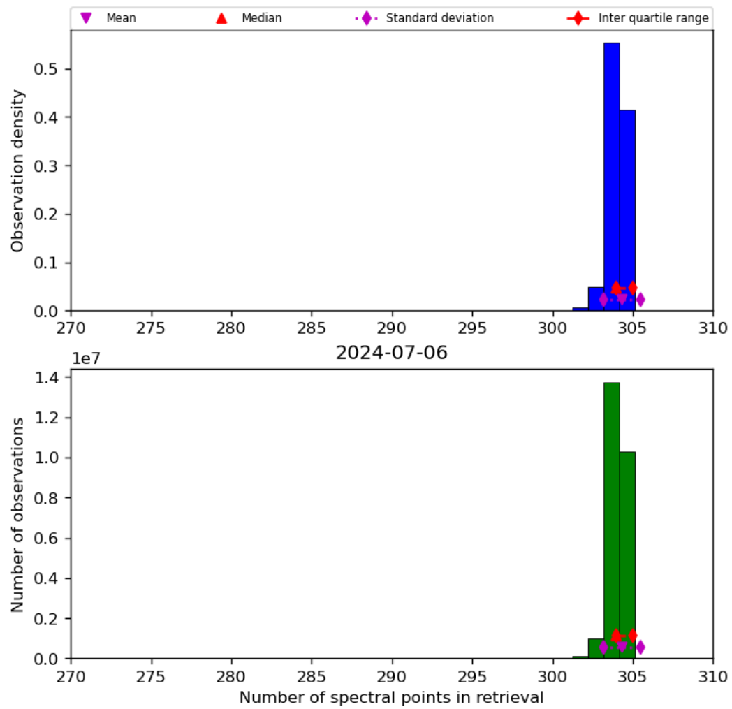
Figure 33: Histogram of “Number of spectral points in retrieval” for 2024-07-05 to 2024-07-07
