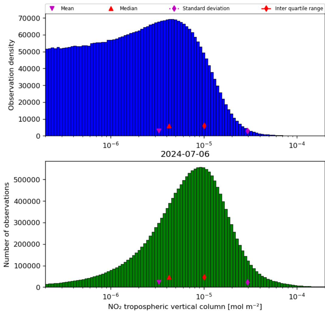
Figure 29: Histogram of “ \text{NO}_2 tropospheric vertical column” for 2024-07-05 to 2024-07-07
