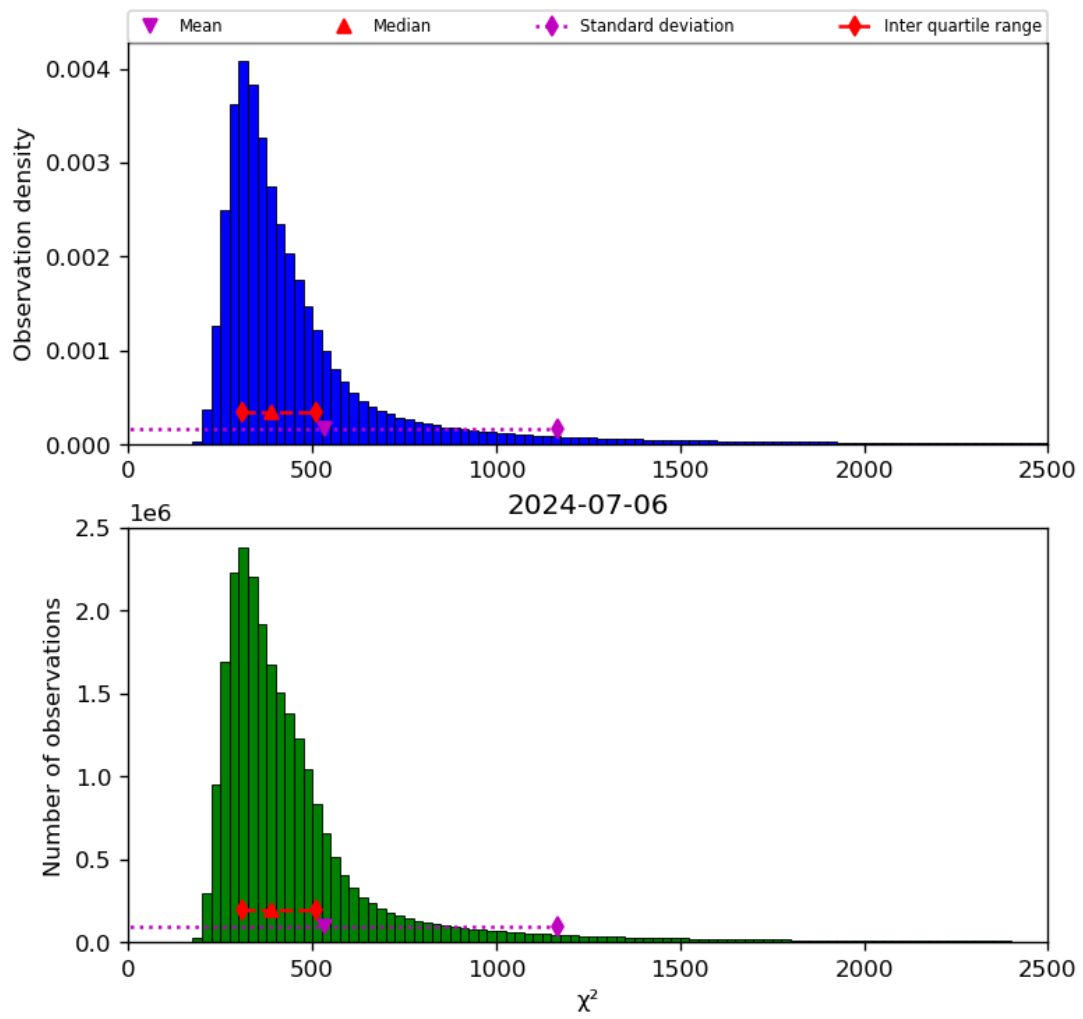
Figure 42: Histogram of “ \chi^2 ” for 2024-07-05 to 2024-07-07
