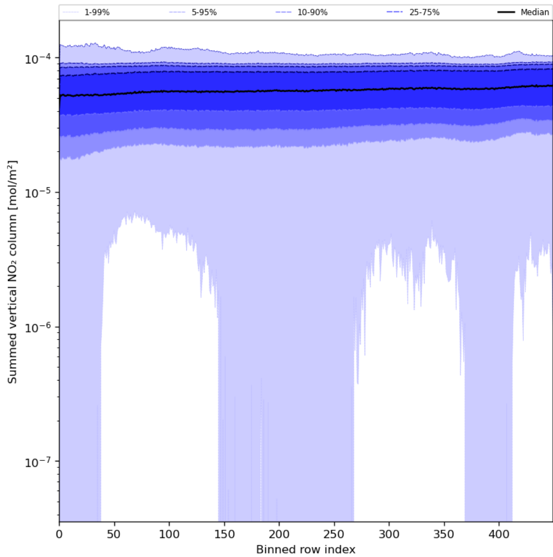
Figure 57: Along track statistics of “Summed vertical NO 2 column” for 2024-07-05 to 2024-07-07
