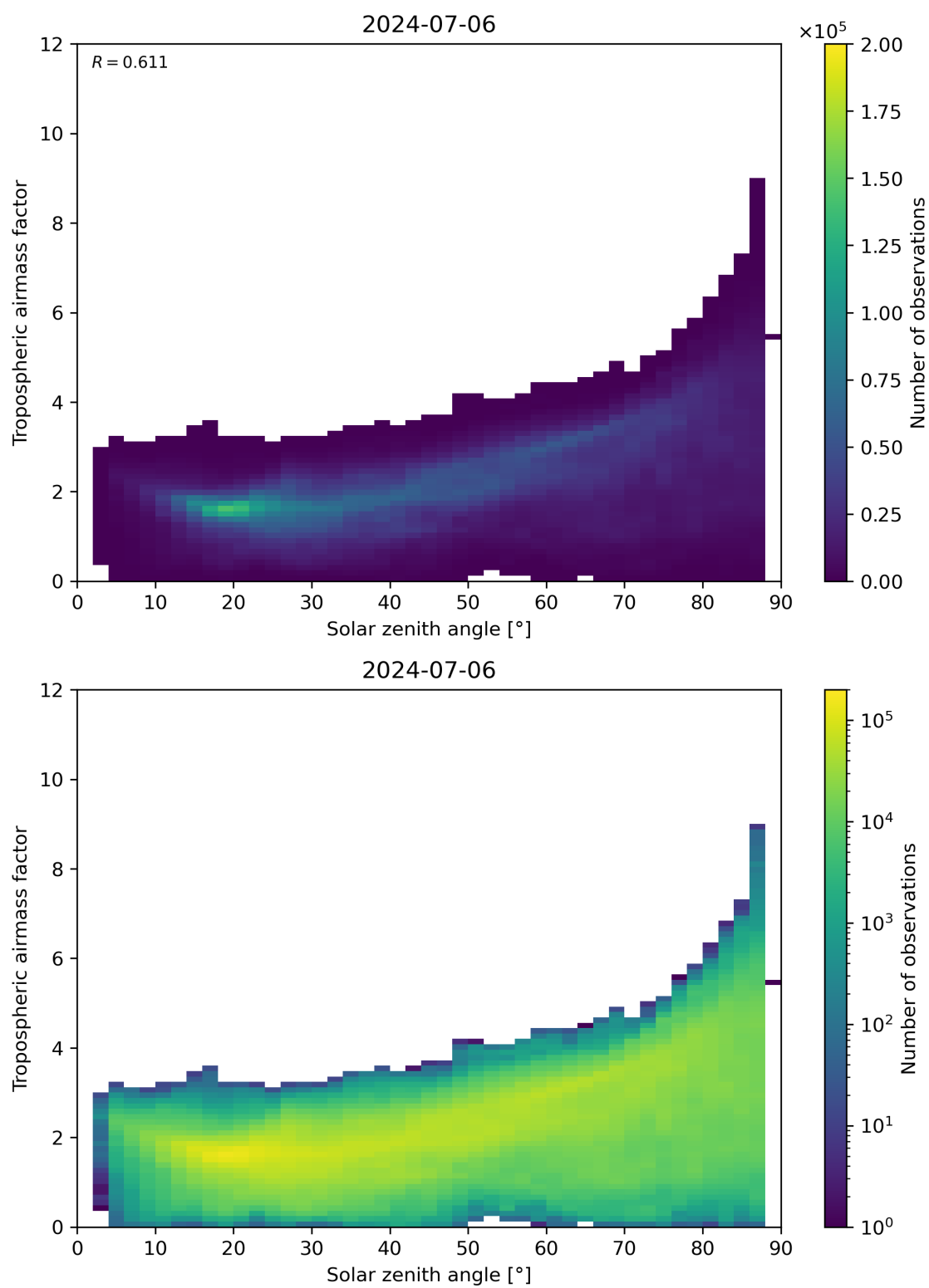
Figure 147: Scatter density plot of “Solar zenith angle” against “Tropospheric airmass factor” for 2024-07-05 to 2024-07-07.
