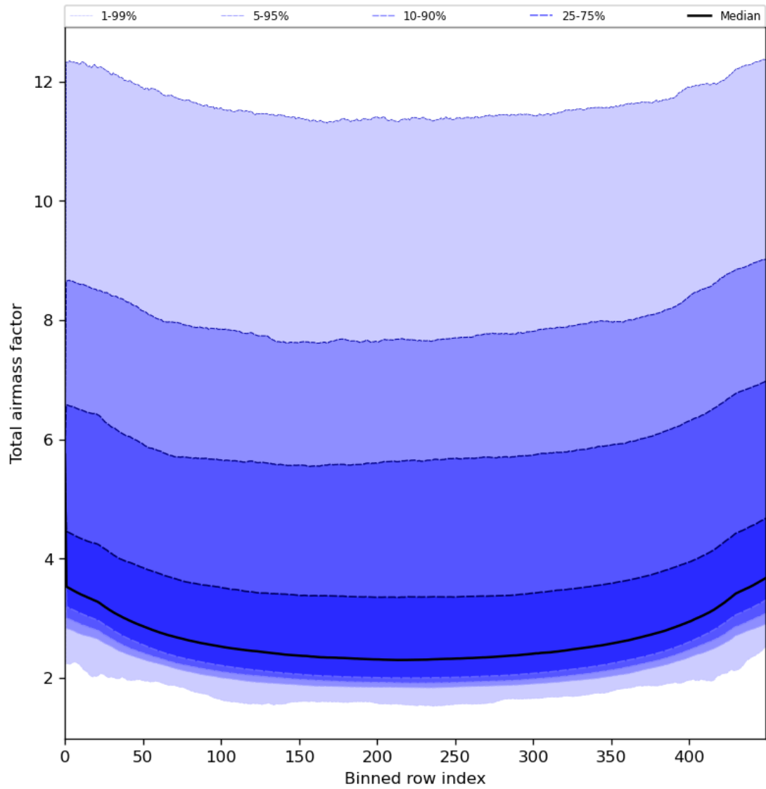
Figure 49: Along track statistics of “Total airmass factor” for 2024-07-05 to 2024-07-07
