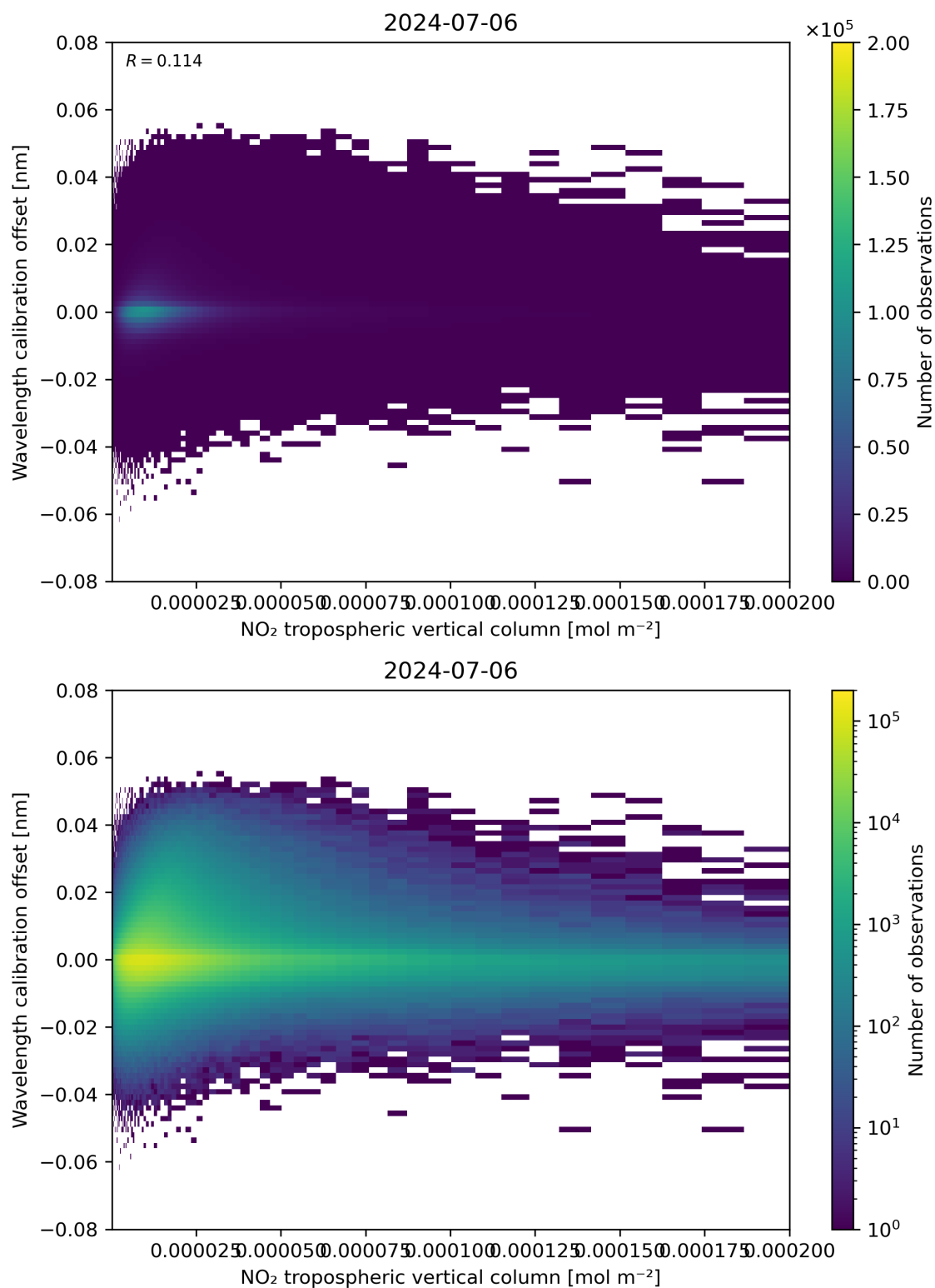
Figure 143: Scatter density plot of “NO 2 tropospheric vertical column” against “Wavelength calibration offset” for 2024-07-05 to 2024-07-07.
