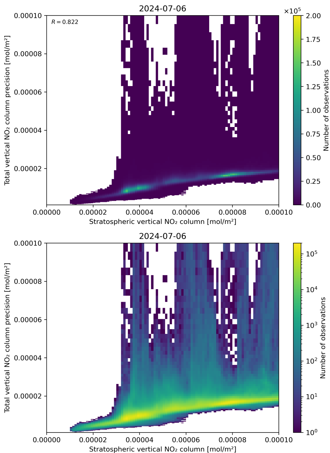
Figure 101: Scatter density plot of “Stratospheric vertical NO 2 column” against “Total vertical NO 2 column precision” for 2024-07-05 to 2024-07-07.
