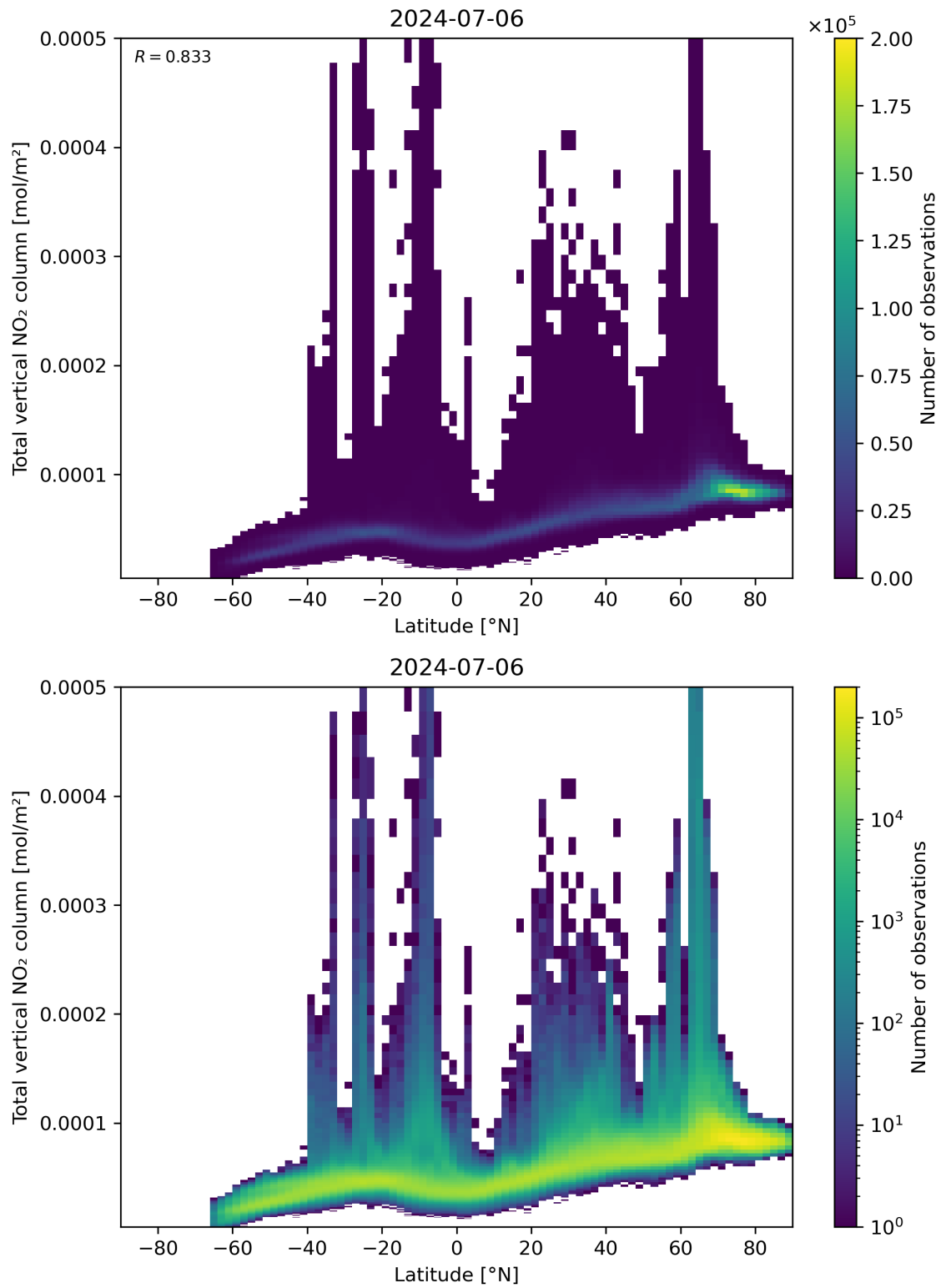
Figure 90: Scatter density plot of “Latitude” against “Total vertical NO 2 column” for 2024-07-05 to 2024-07-07.
