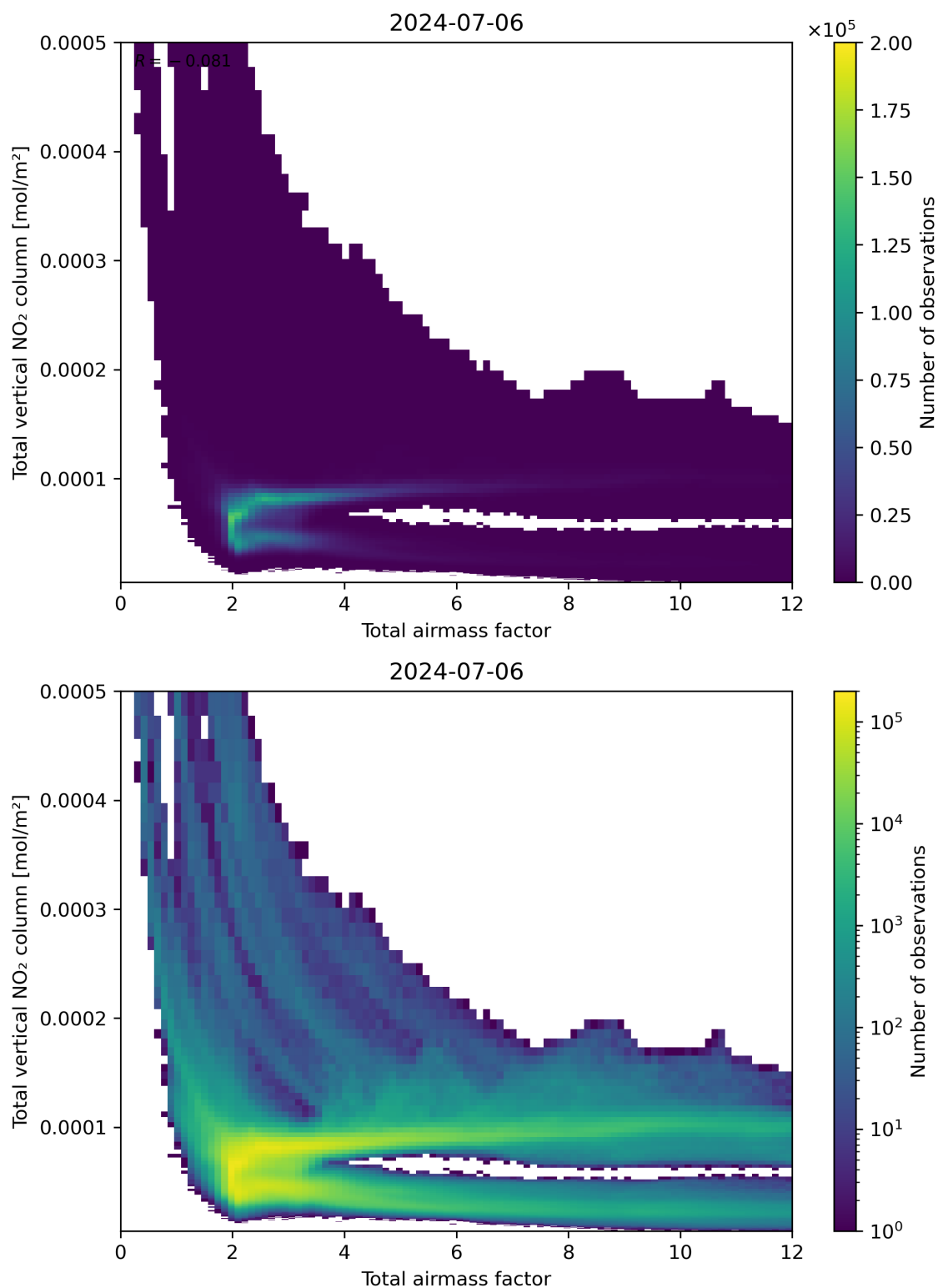
Figure 67: Scatter density plot of “Total airmass factor” against “Total vertical NO 2 column” for 2024-07-05 to 2024-07-07.
