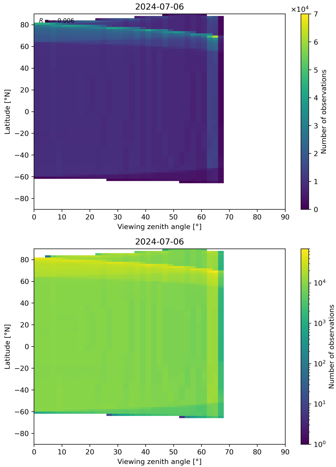
Figure 163: Scatter density plot of “Viewing zenith angle” against “Latitude” for 2024-07-05 to 2024-07-07.
