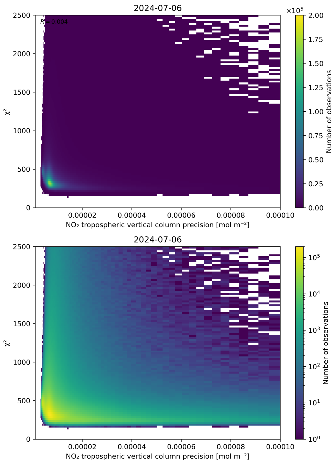
Figure 134: Scatter density plot of “NO 2 tropospheric vertical column precision” against “ \chi^2 ” for 2024-07-05 to 2024-07-07.
