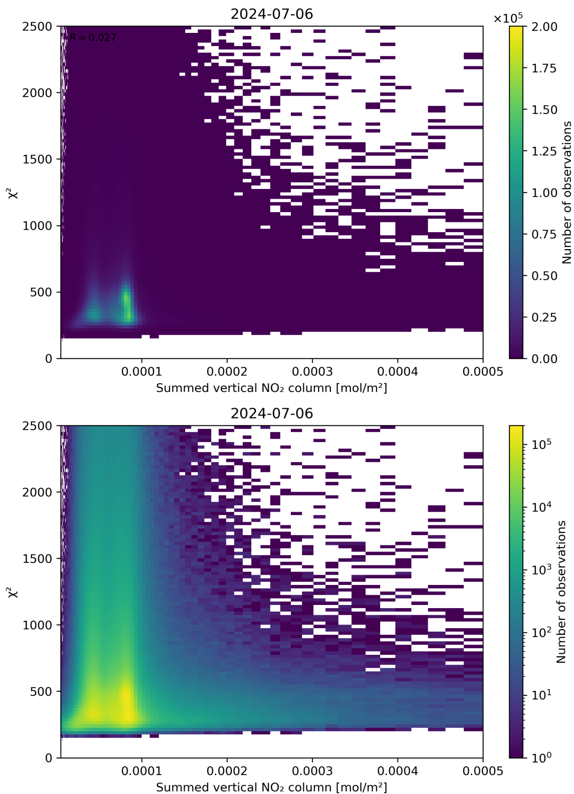
Figure 104: Scatter density plot of “Summed vertical NO 2 column” against “ \chi^2 ” for 2024-07-05 to 2024-07-07.
