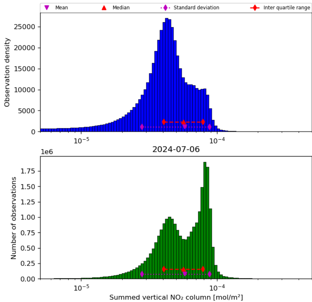
Figure 40: Histogram of “Summed vertical NO 2 column” for 2024-07-05 to 2024-07-07
