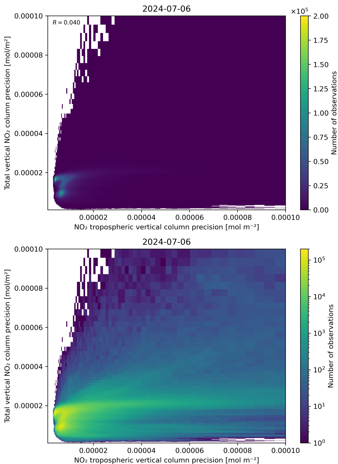
Figure 139: Scatter density plot of “NO 2 tropospheric vertical column precision” against “Total vertical NO 2 column precision” for 2024-07-05 to 2024-07-07.
