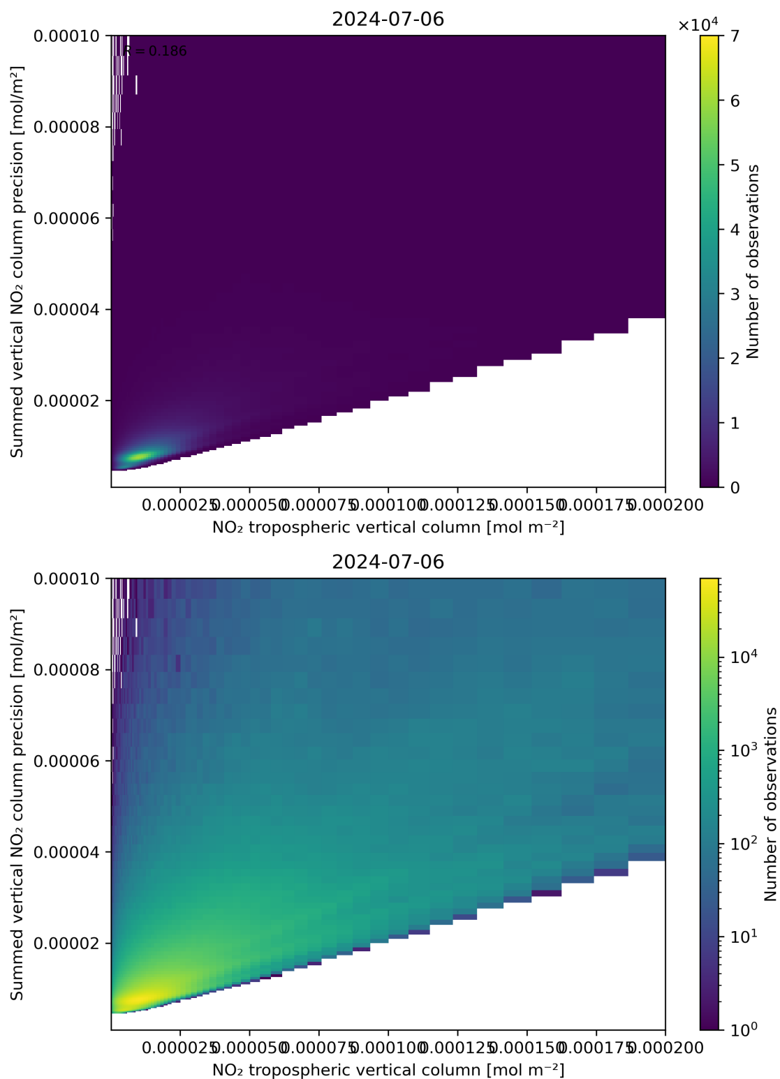
Figure 127: Scatter density plot of “NO 2 tropospheric vertical column” against “Summed vertical NO 2 column precision” for 2024-07-05 to 2024-07-07.
