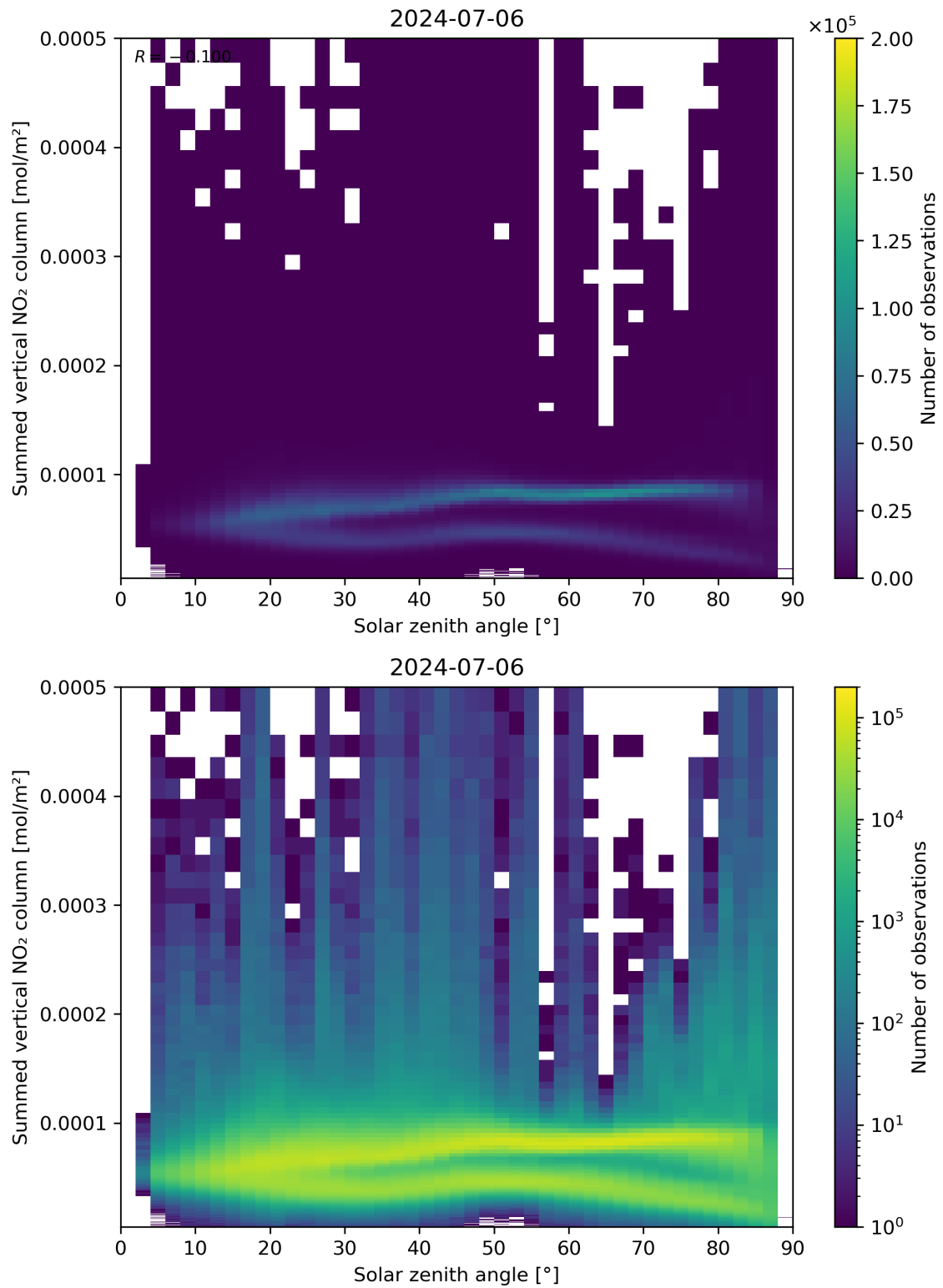
Figure 151: Scatter density plot of “Solar zenith angle” against “Summed vertical NO 2 column” for 2024-07-05 to 2024-07-07.
