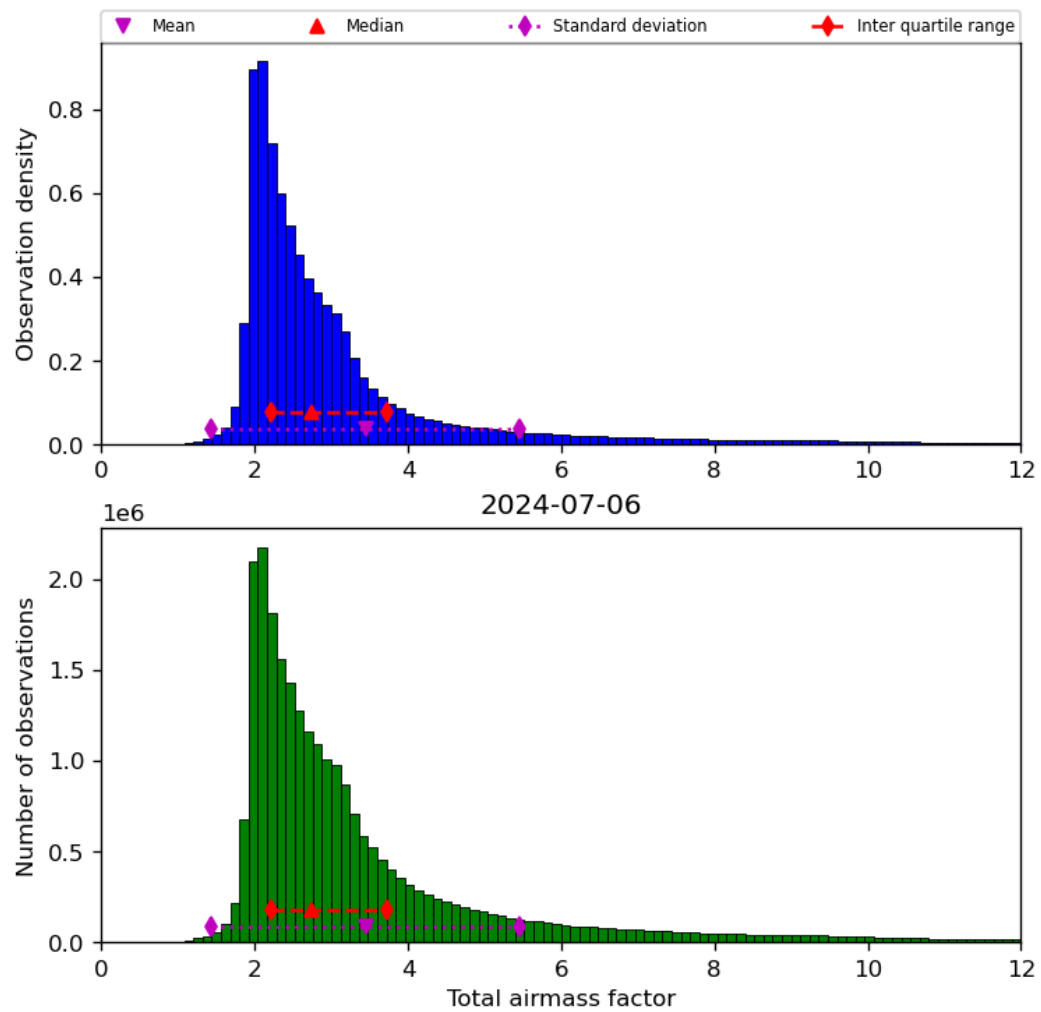
Figure 32: Histogram of “Total airmass factor” for 2024-07-05 to 2024-07-07
