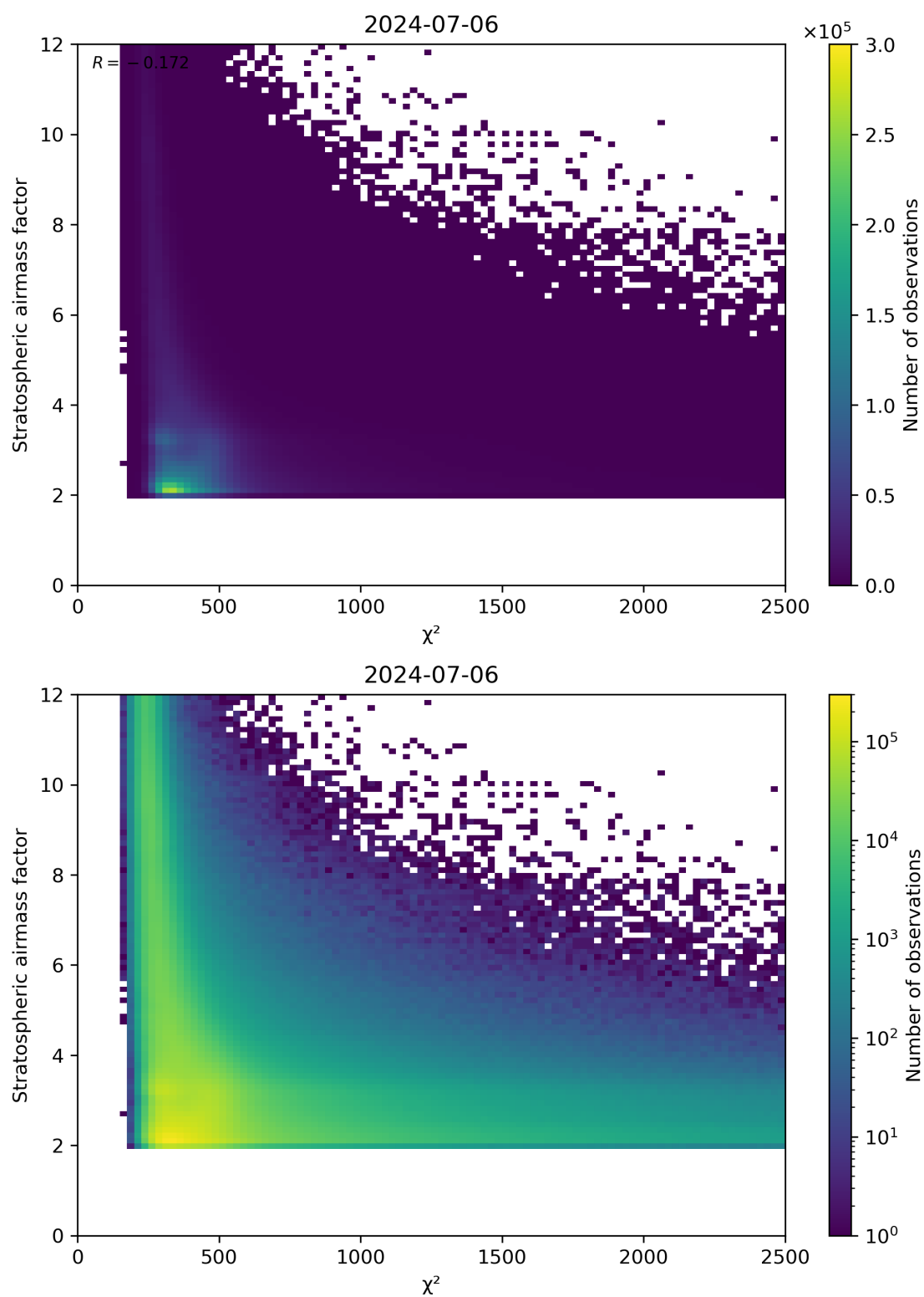
Figure 81: Scatter density plot of “ \chi^2 ” against “Stratospheric airmass factor” for 2024-07-05 to 2024-07-07.
