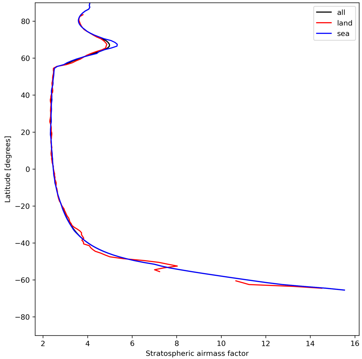
Figure 27: Zonal average of “Stratospheric airmass factor” for 2024-07-05 to 2024-07-07.
