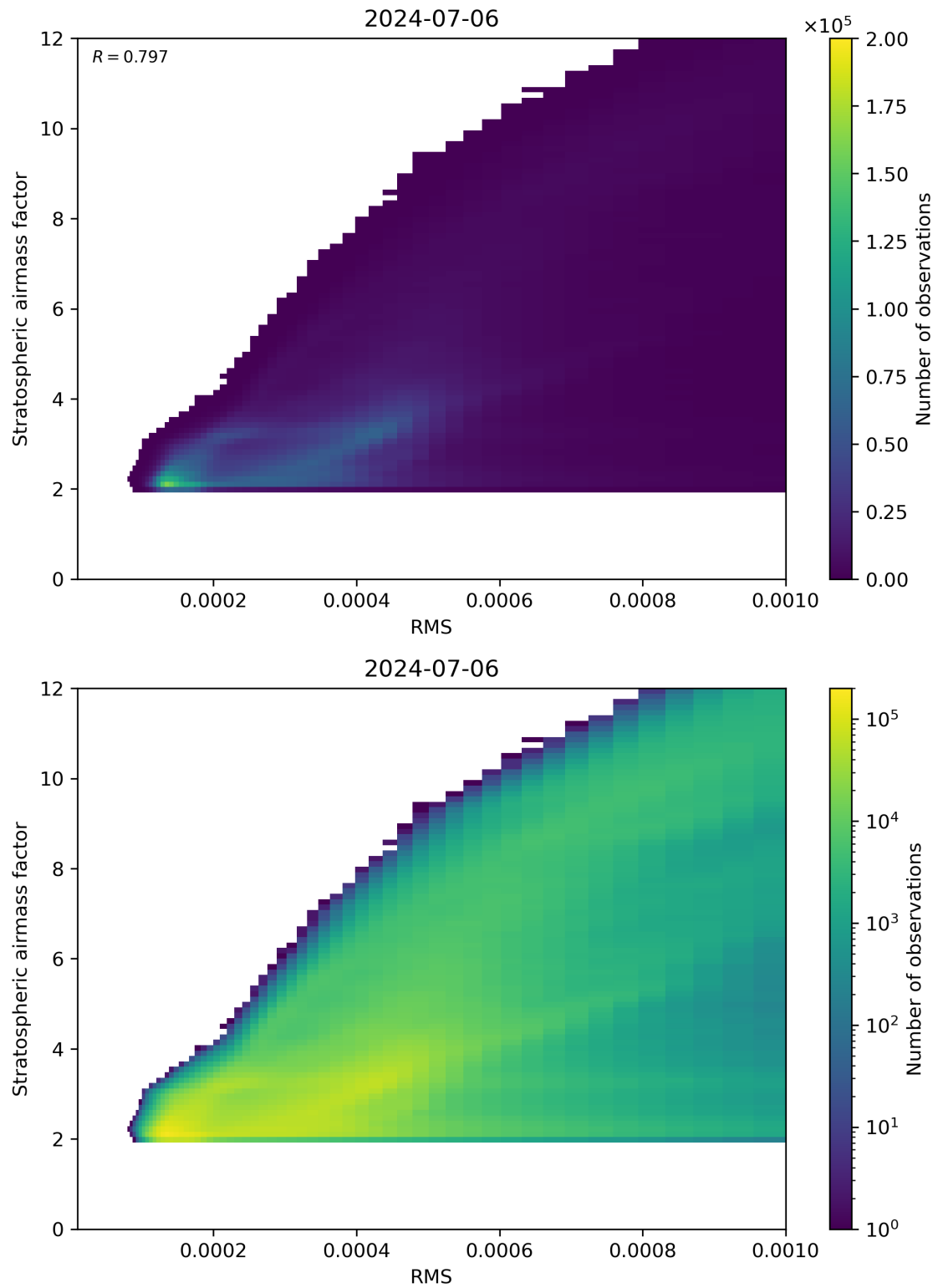
Figure 144: Scatter density plot of “RMS” against “Stratospheric airmass factor” for 2024-07-05 to 2024-07-07.
