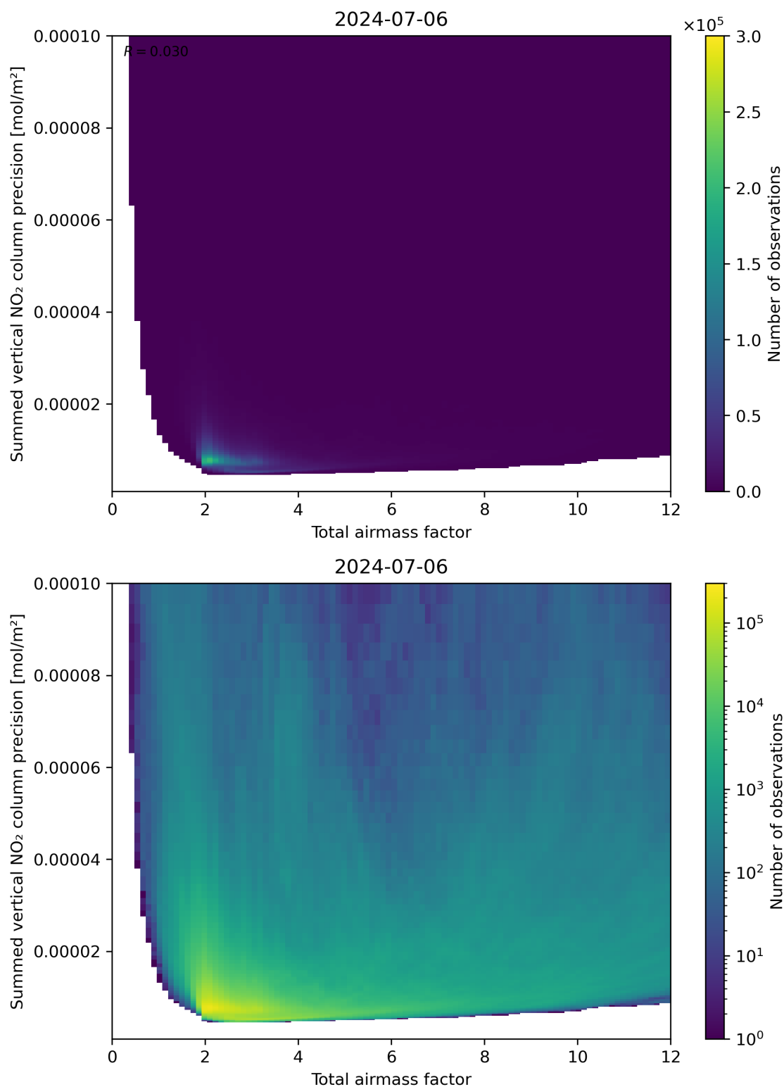
Figure 66: Scatter density plot of “Total airmass factor” against “Summed vertical NO 2 column precision” for 2024-07-05 to 2024-07-07.
