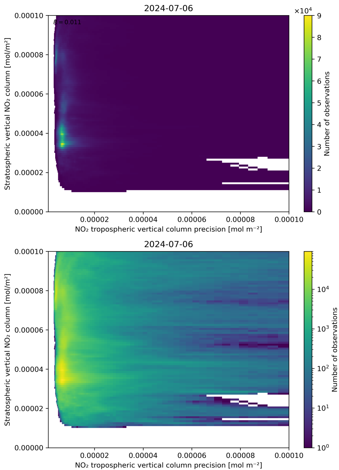
Figure 135: Scatter density plot of “NO 2 tropospheric vertical column precision” against “Stratospheric vertical NO 2 column” for 2024-07-05 to 2024-07-07.
