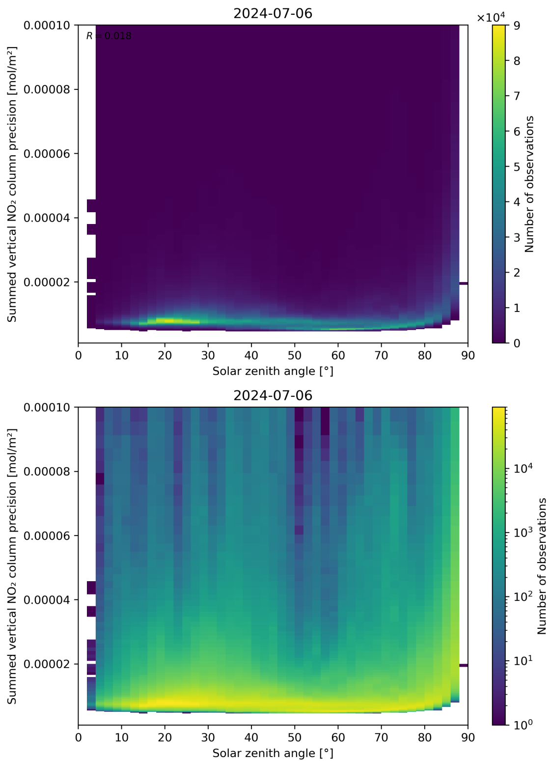
Figure 152: Scatter density plot of “Solar zenith angle” against “Summed vertical NO 2 column precision” for 2024-07-05 to 2024-07-07.
