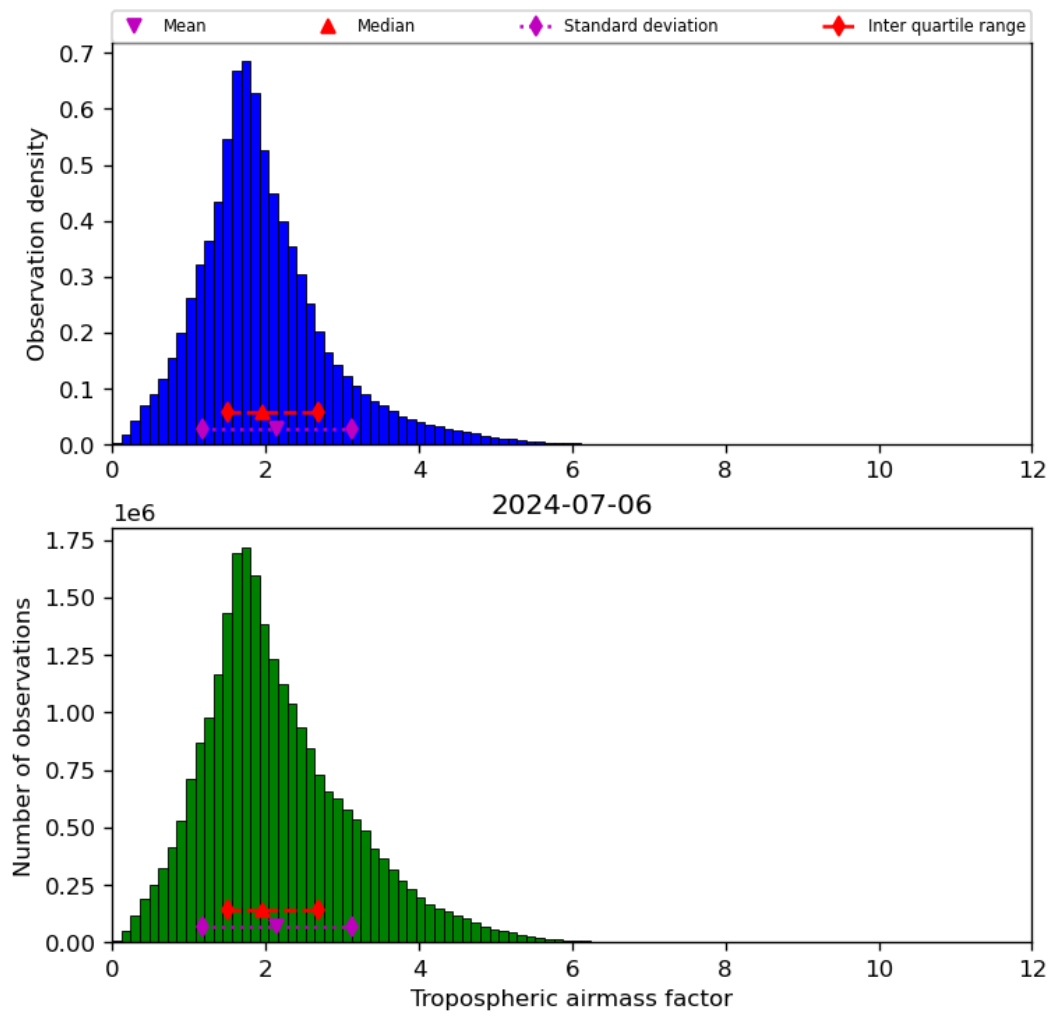
Figure 31: Histogram of “Tropospheric airmass factor” for 2024-07-05 to 2024-07-07
