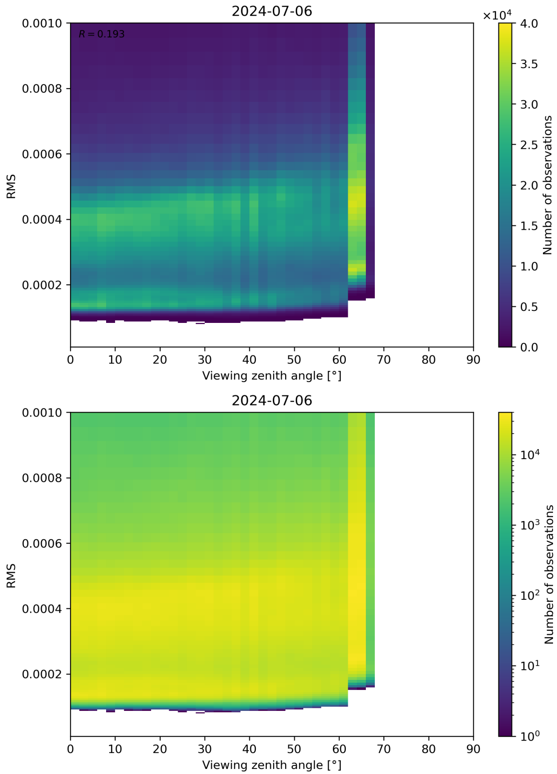
Figure 171: Scatter density plot of “Viewing zenith angle” against “RMS” for 2024-07-05 to 2024-07-07.
