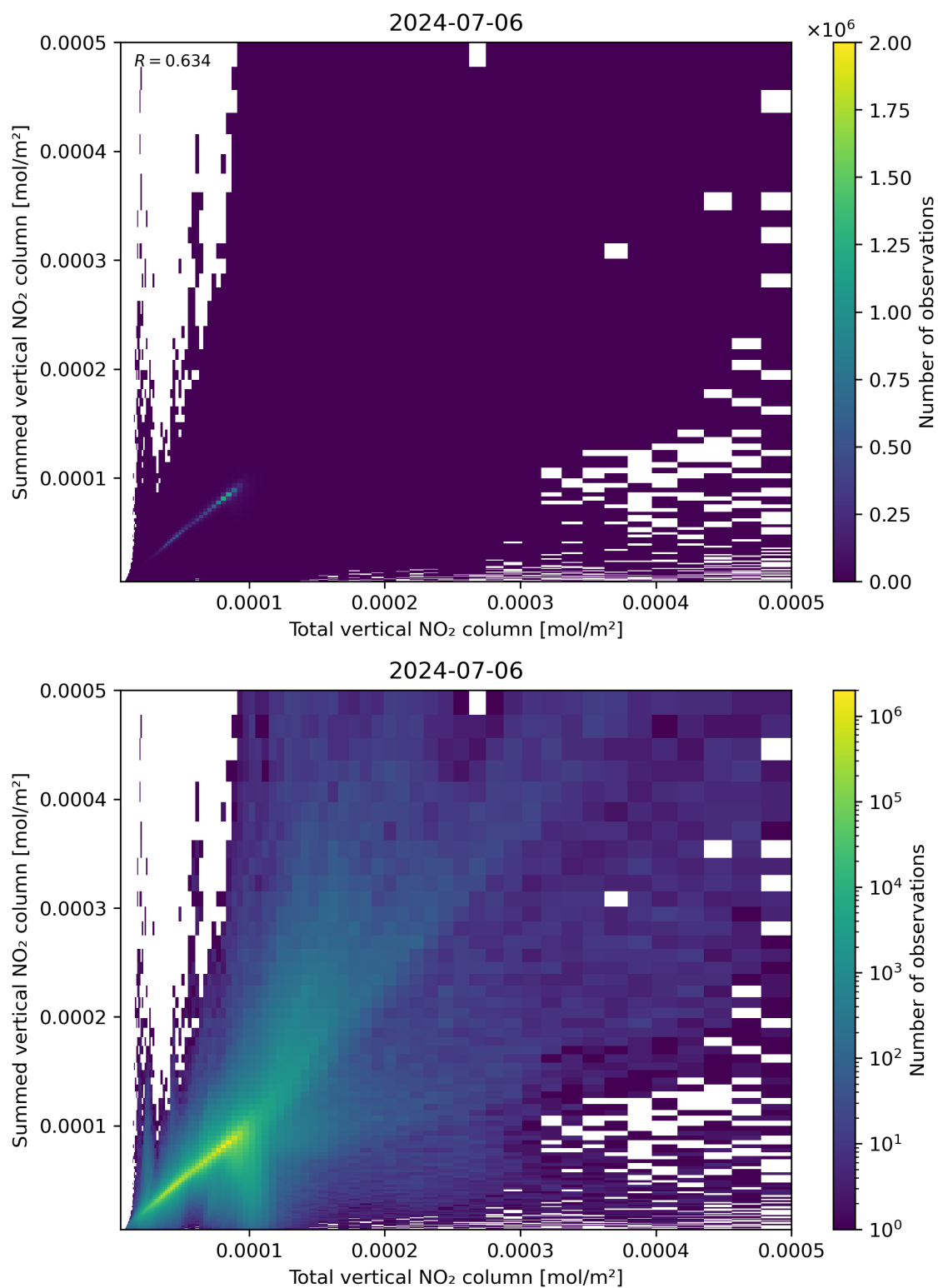
Figure 112: Scatter density plot of “Total vertical NO 2 column” against “Summed vertical NO 2 column” for 2024-07-05 to 2024-07-07.
