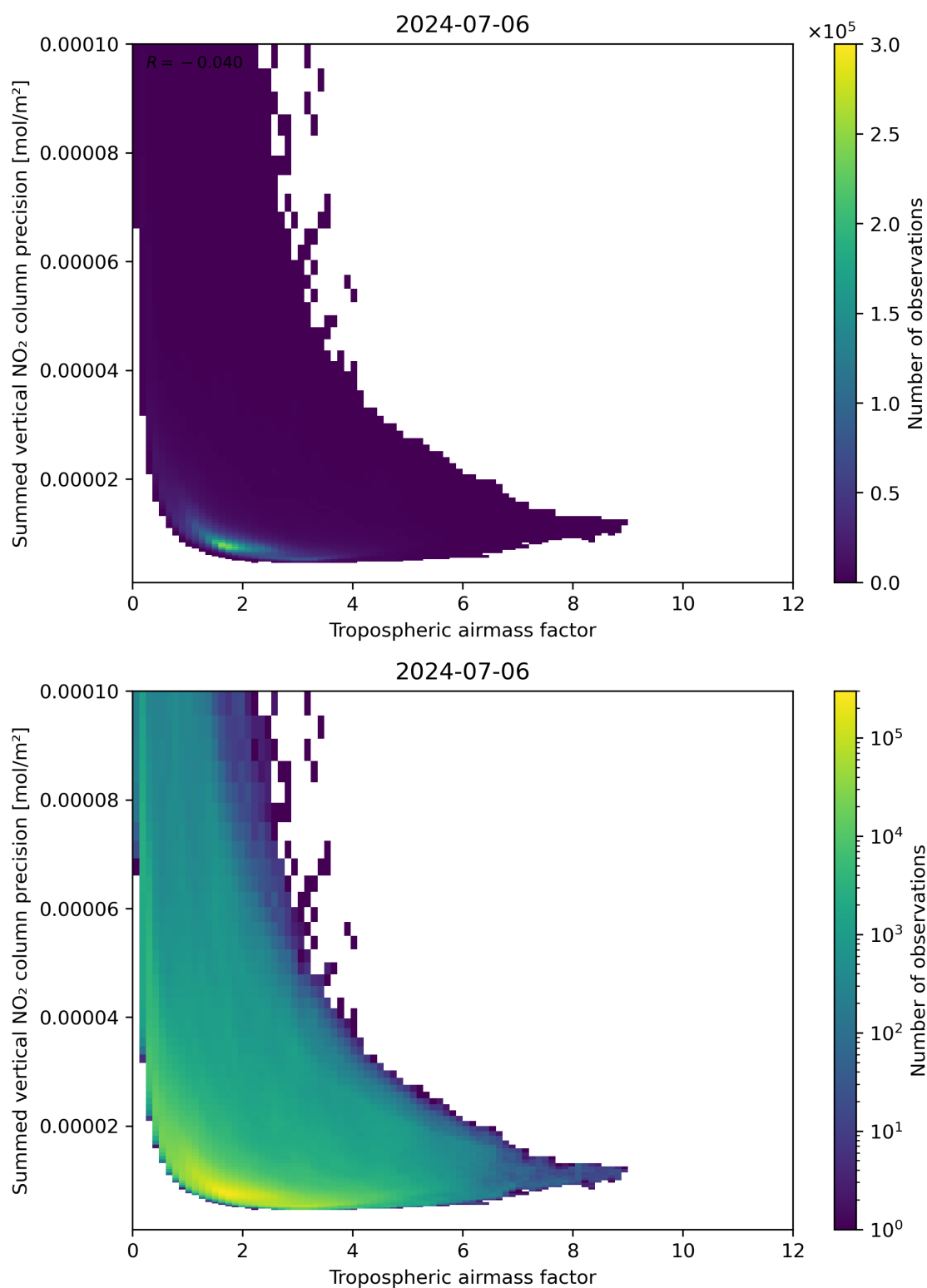
Figure 76: Scatter density plot of “Tropospheric airmass factor” against “Summed vertical NO 2 column precision” for 2024-07-05 to 2024-07-07.
