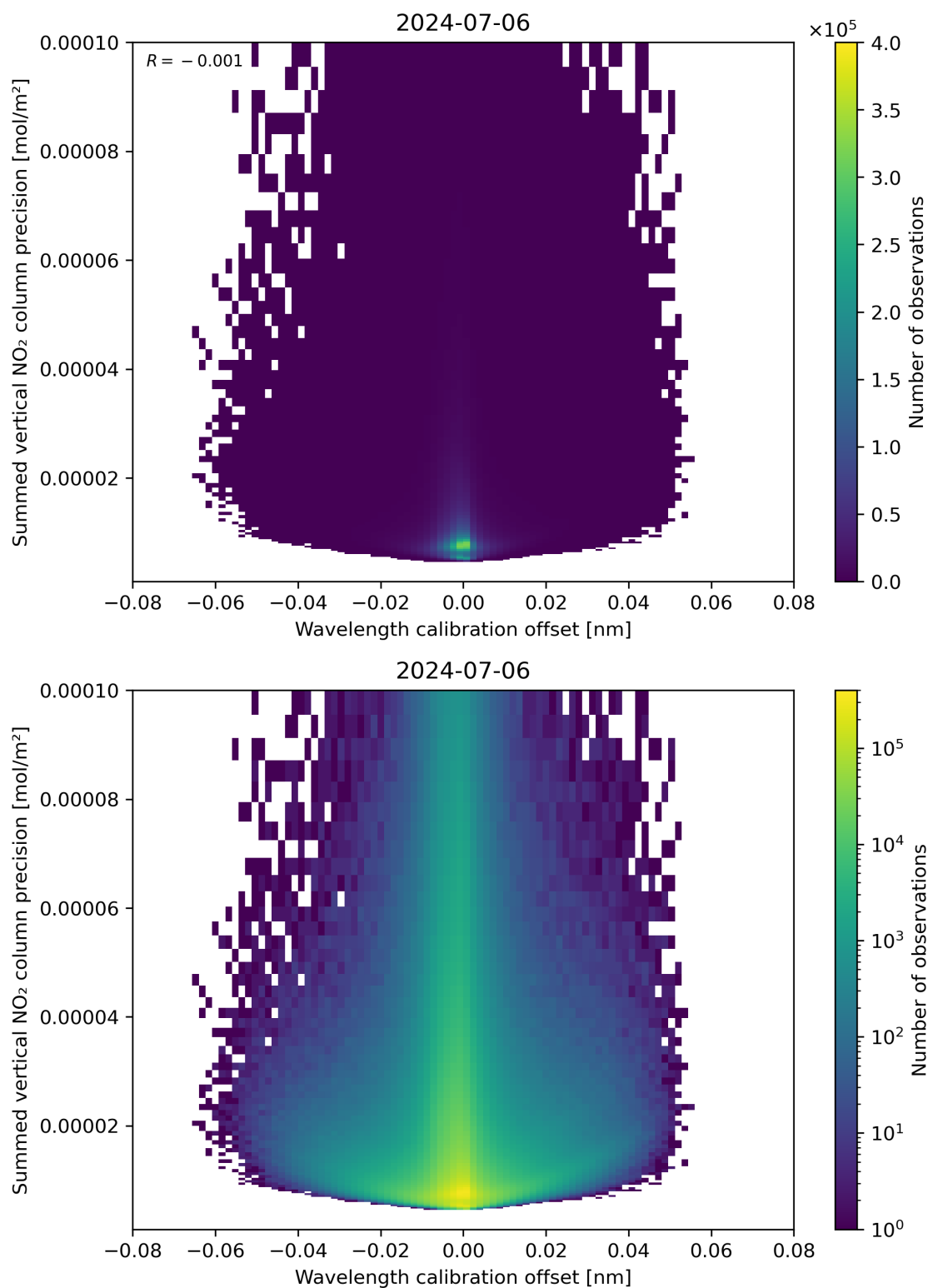
Figure 178: Scatter density plot of “Wavelength calibration offset” against “Summed vertical NO 2 column precision” for 2024-07-05 to 2024-07-07.
