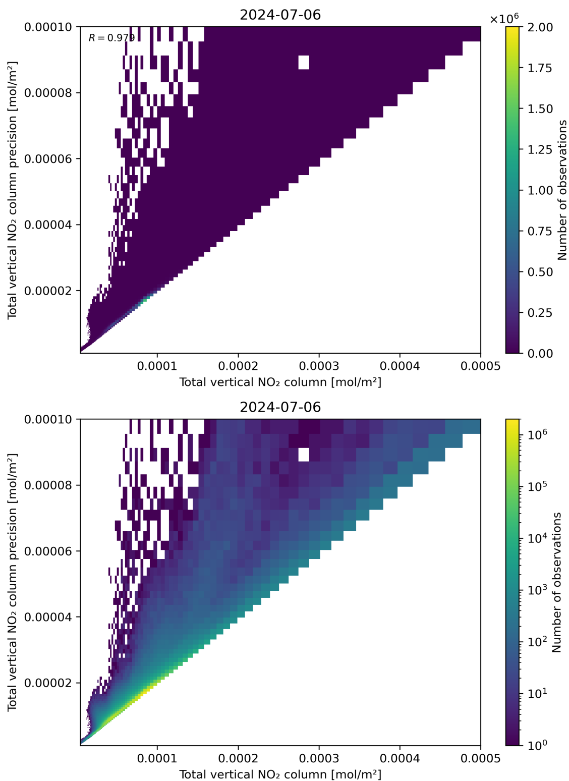
Figure 114: Scatter density plot of “Total vertical NO 2 column” against “Total vertical NO 2 column precision” for 2024-07-05 to 2024-07-07.
