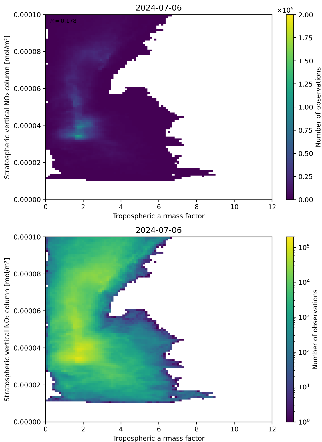
Figure 74: Scatter density plot of “Tropospheric airmass factor” against “Stratospheric vertical NO 2 column” for 2024-07-05 to 2024-07-07.
