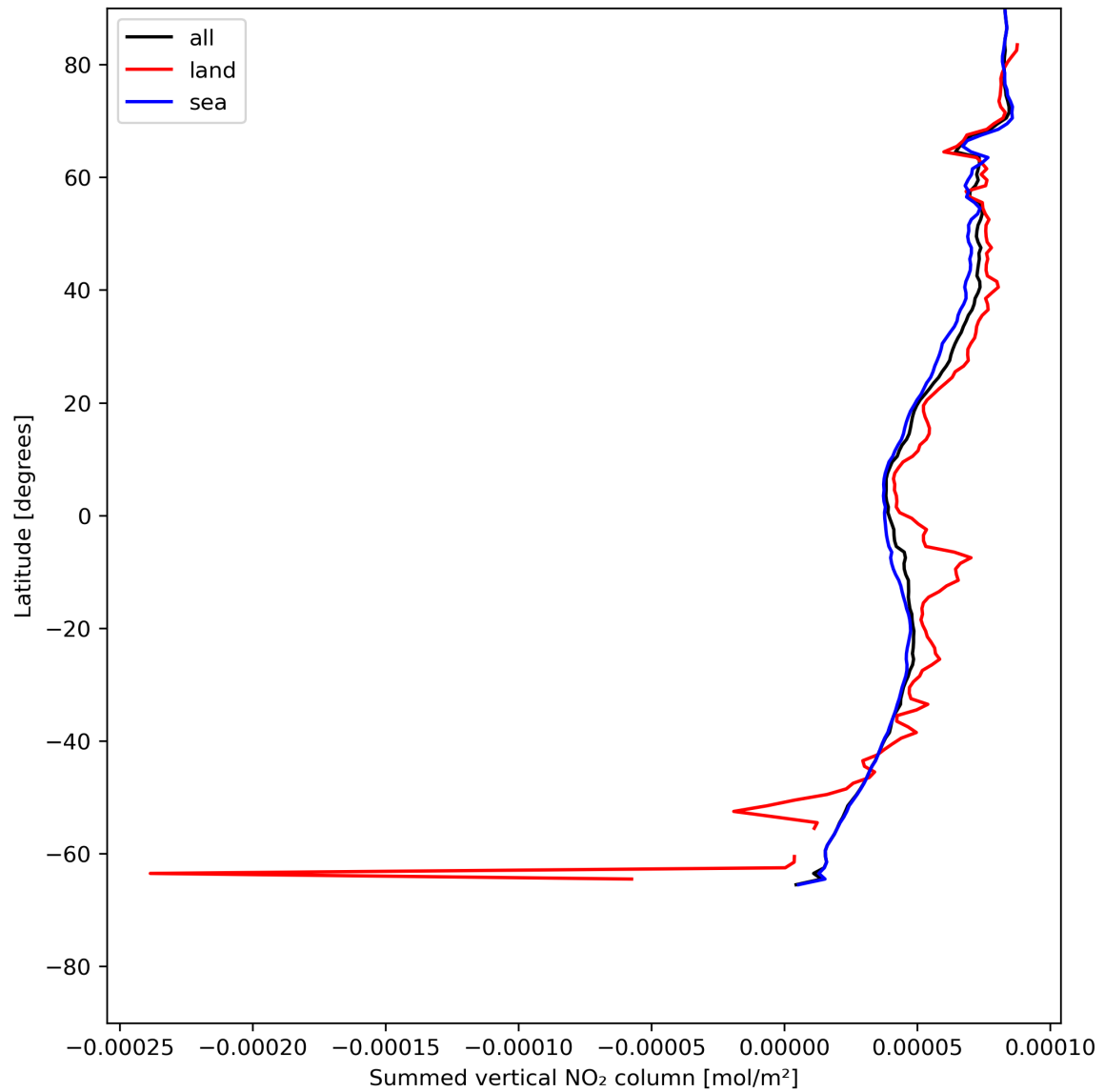
Figure 23: Zonal average of “Summed vertical NO 2 column” for 2024-07-05 to 2024-07-07.
