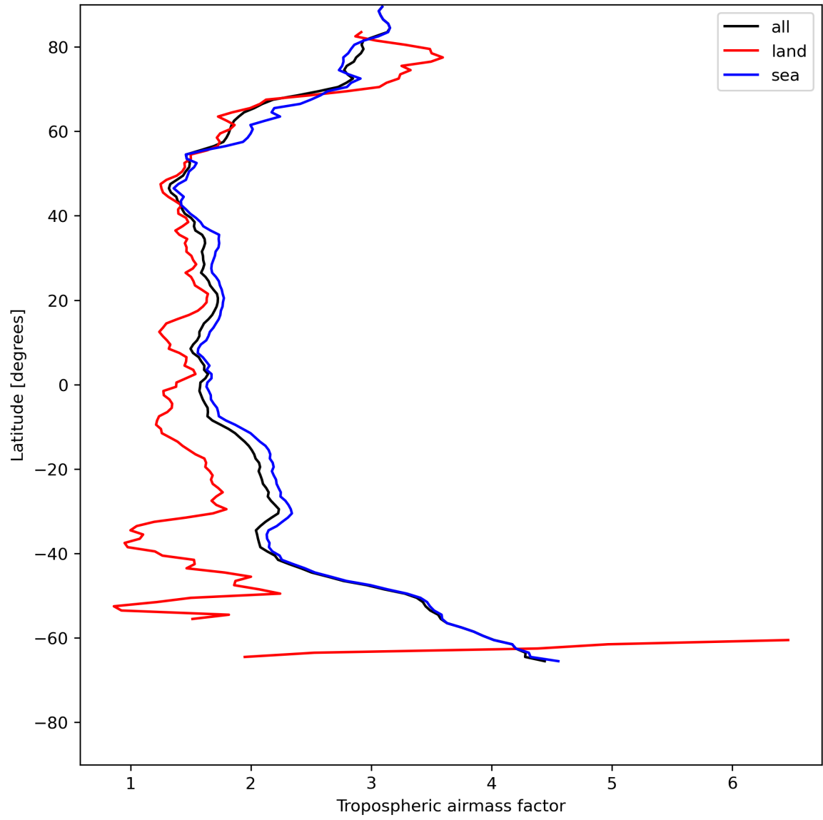
Figure 14: Zonal average of “Tropospheric airmass factor” for 2024-07-05 to 2024-07-07.
