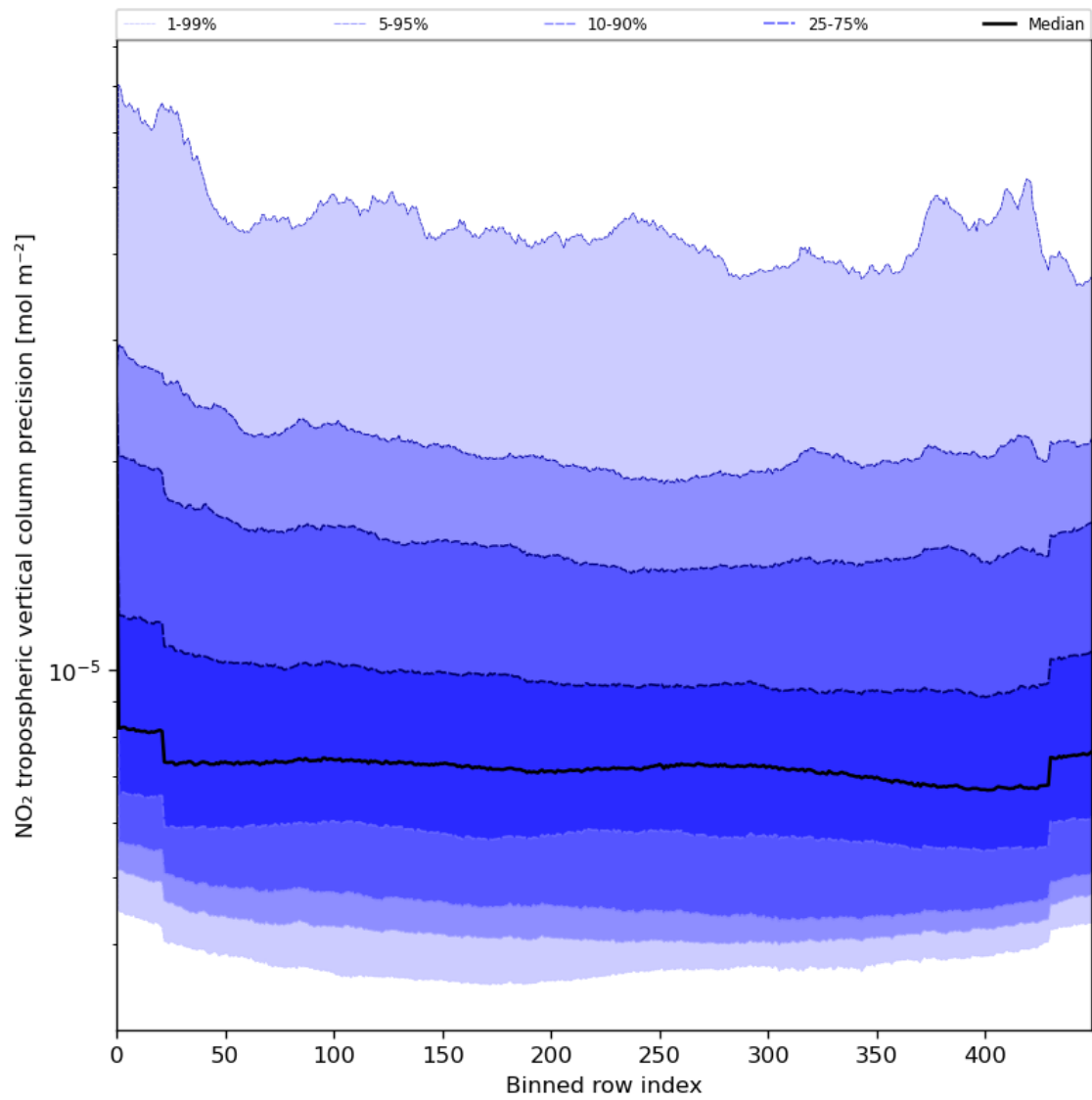
Figure 47: Along track statistics of “NO 2 tropospheric vertical column precision” for 2024-07-05 to 2024-07-07
