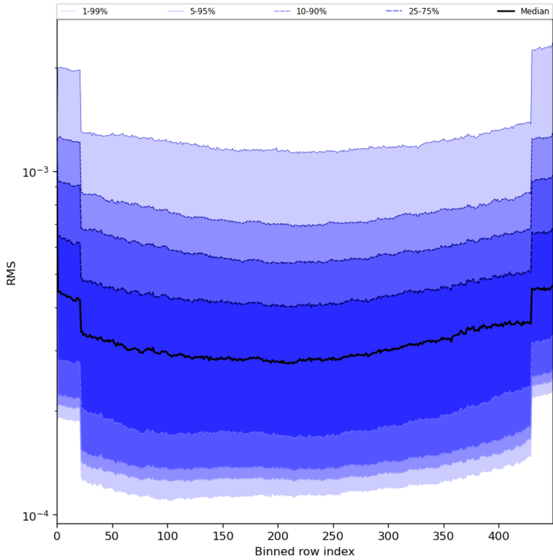
Figure 60: Along track statistics of “RMS” for 2024-07-05 to 2024-07-07
