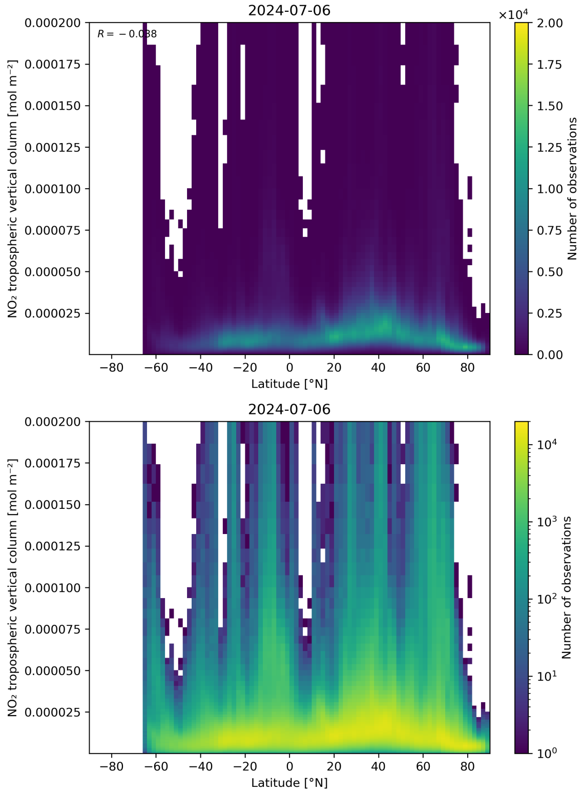
Figure 92: Scatter density plot of “Latitude” against “NO 2 tropospheric vertical column” for 2024-07-05 to 2024-07-07.
