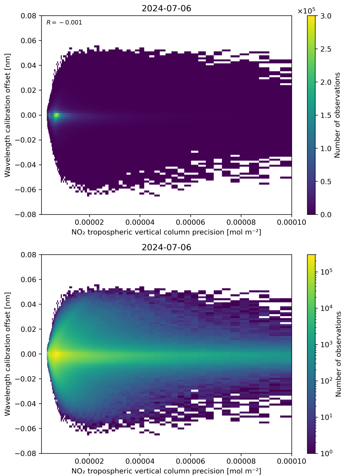
Figure 141: Scatter density plot of “NO 2 tropospheric vertical column precision” against “Wavelength calibration offset” for 2024-07-05 to 2024-07-07.
