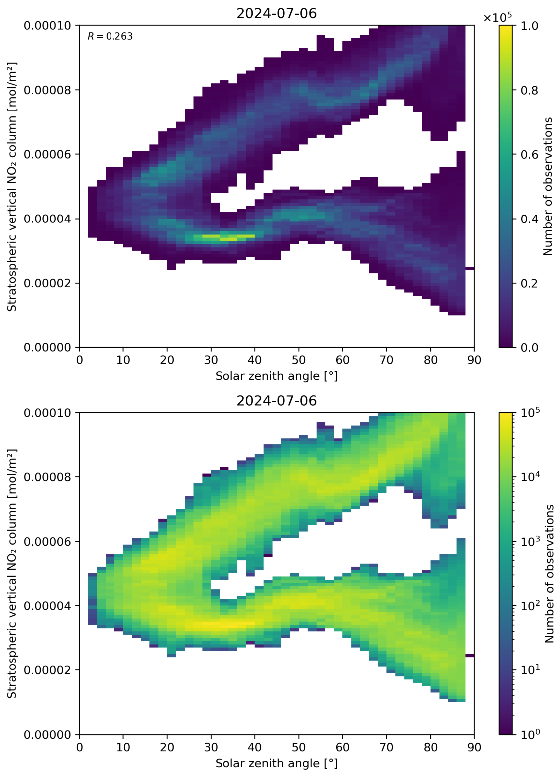
Figure 150: Scatter density plot of “Solar zenith angle” against “Stratospheric vertical NO 2 column” for 2024-07-05 to 2024-07-07.
