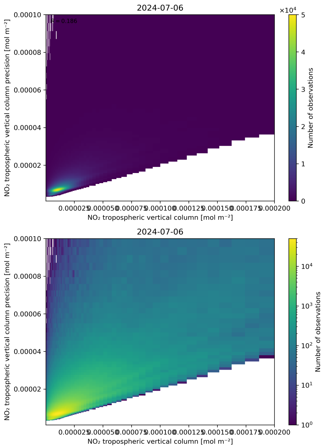
Figure 130: Scatter density plot of “NO 2 tropospheric vertical column” against “NO 2 tropospheric vertical column precision” for 2024-07-05 to 2024-07-07.
