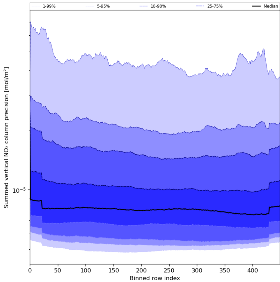
Figure 58: Along track statistics of “Summed vertical NO 2 column precision” for 2024-07-05 to 2024-07-07
