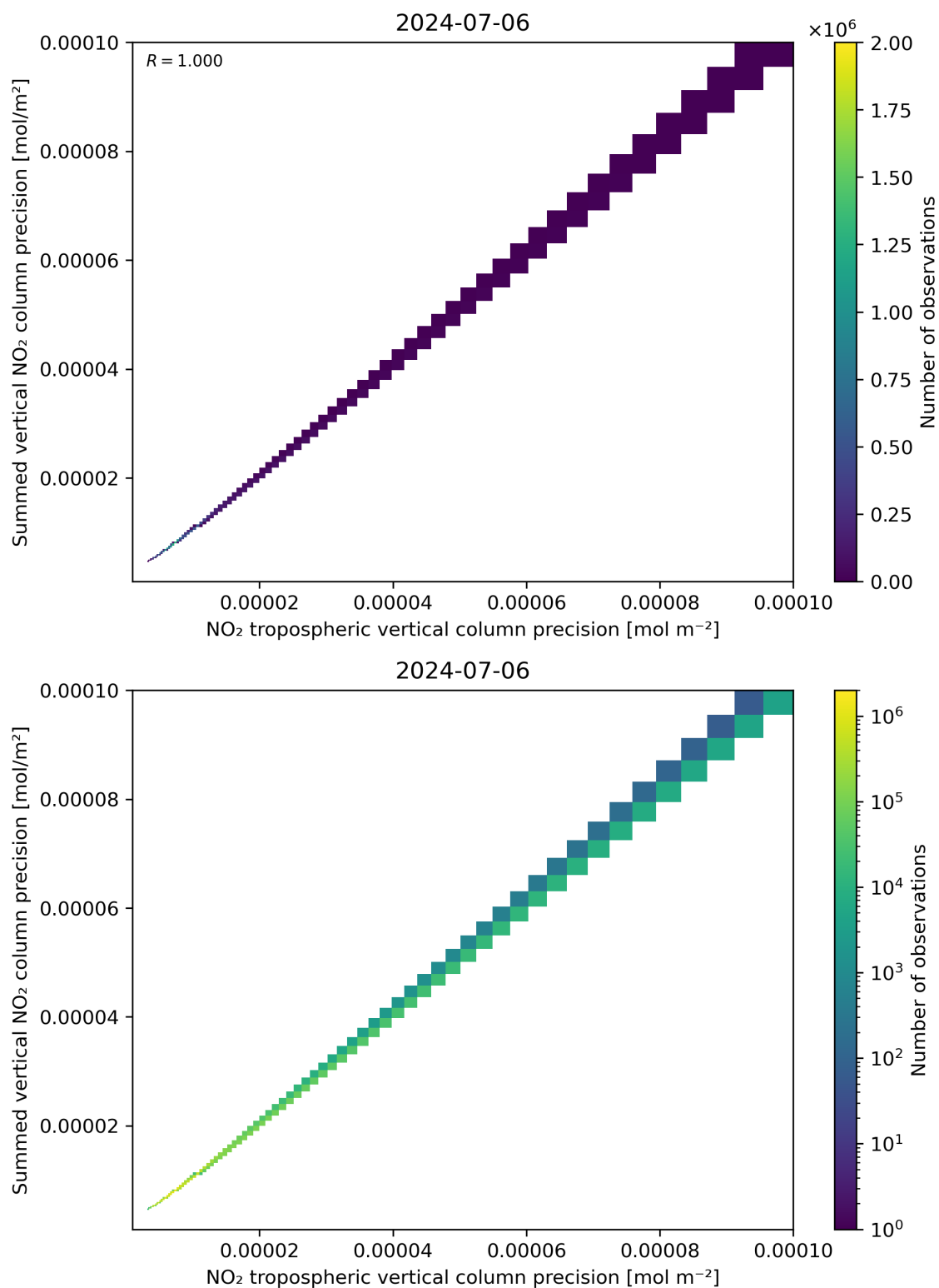
Figure 137: Scatter density plot of “NO 2 tropospheric vertical column precision” against “Summed vertical NO 2 column precision” for 2024-07-05 to 2024-07-07.
