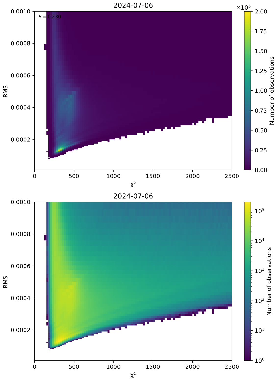
Figure 82: Scatter density plot of “ \chi^2 ” against “RMS” for 2024-07-05 to 2024-07-07.
