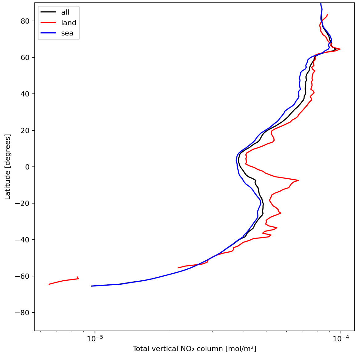
Figure 21: Zonal average of “Total vertical NO 2 column” for 2024-07-05 to 2024-07-07.
