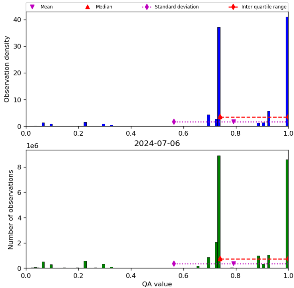
Figure 28: Histogram of “QA value” for 2024-07-05 to 2024-07-07
