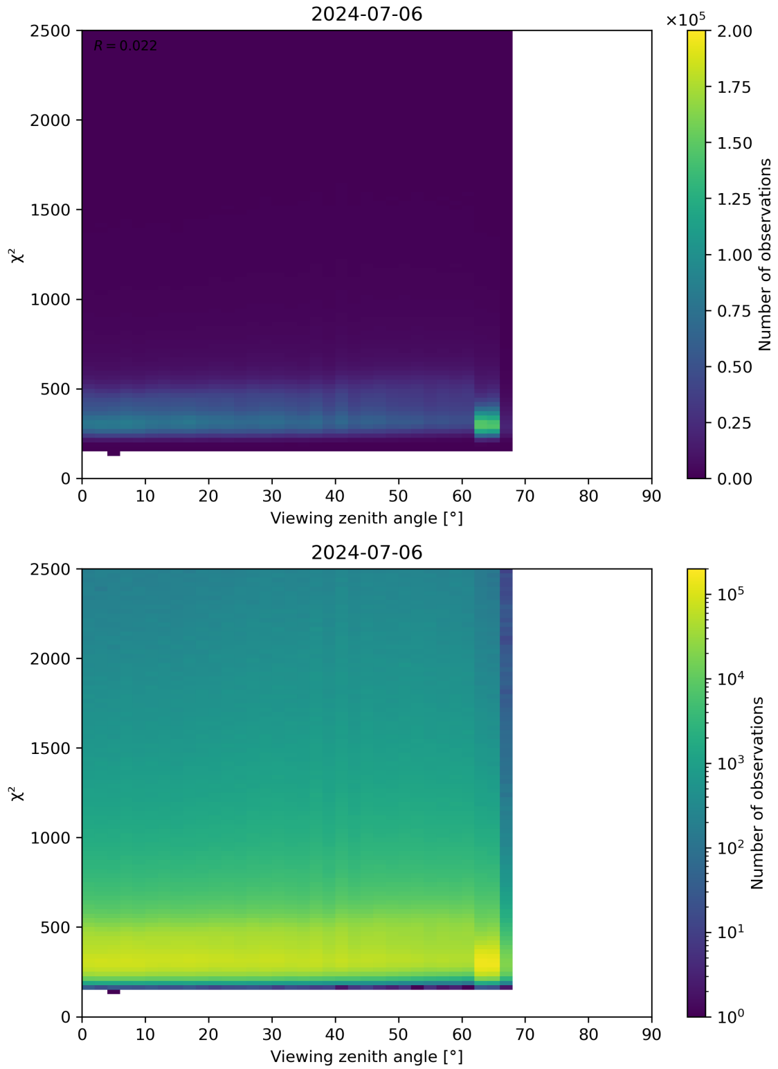
Figure 162: Scatter density plot of “Viewing zenith angle” against “ \chi^2 ” for 2024-07-05 to 2024-07-07.
