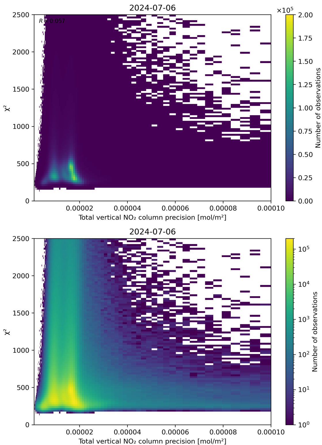
Figure 116: Scatter density plot of “Total vertical NO 2 column precision” against “ \chi^2 ” for 2024-07-05 to 2024-07-07.
