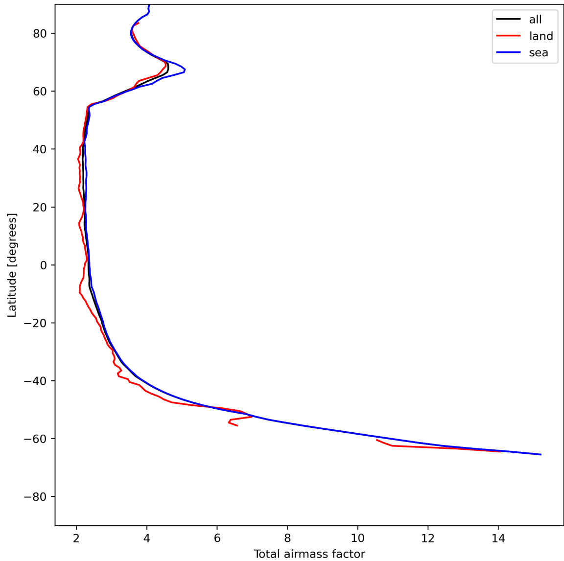
Figure 15: Zonal average of “Total airmass factor” for 2024-07-05 to 2024-07-07.
