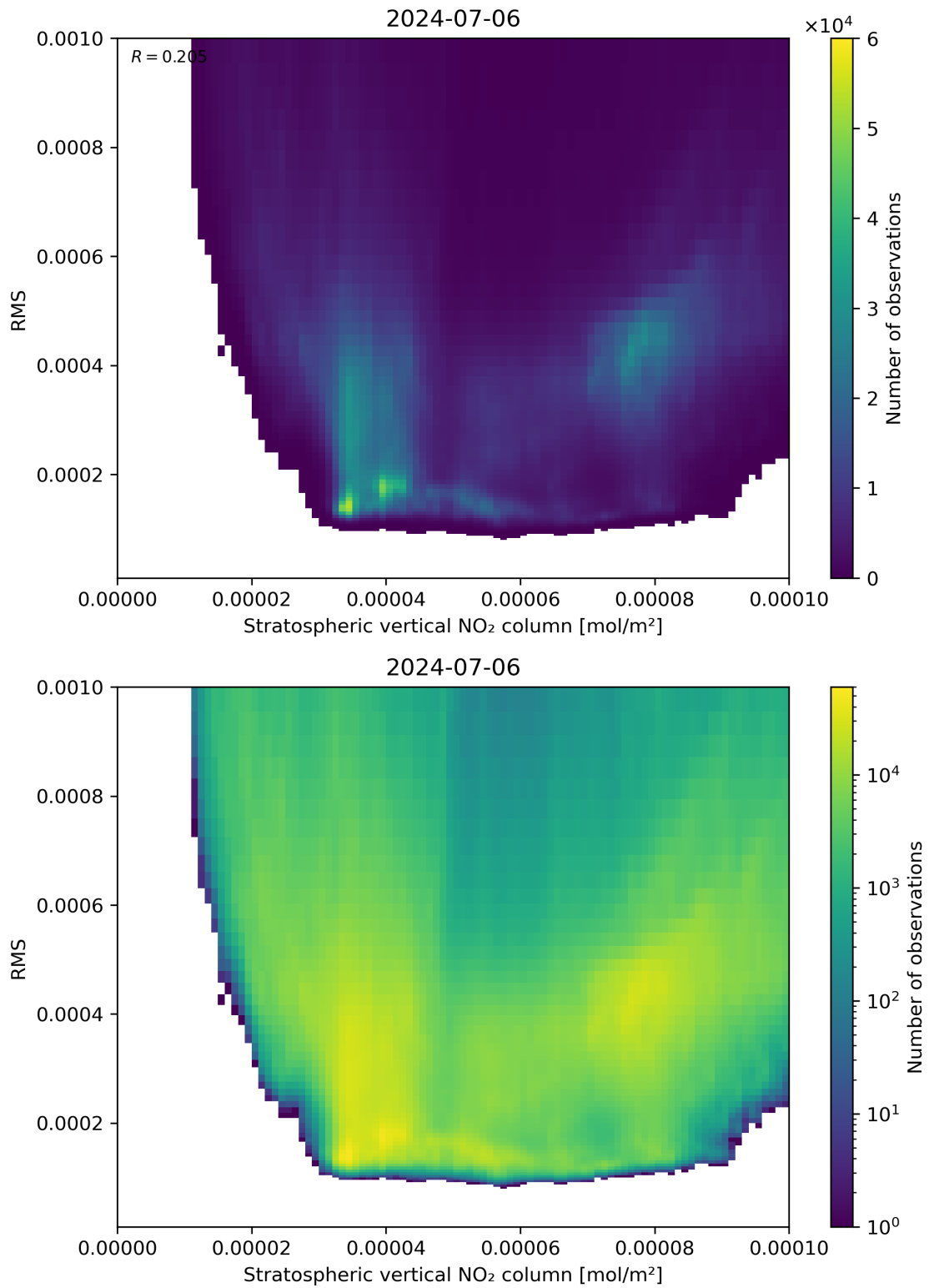
Figure 102: Scatter density plot of “Stratospheric vertical NO 2 column” against “RMS” for 2024-07-05 to 2024-07-07.
