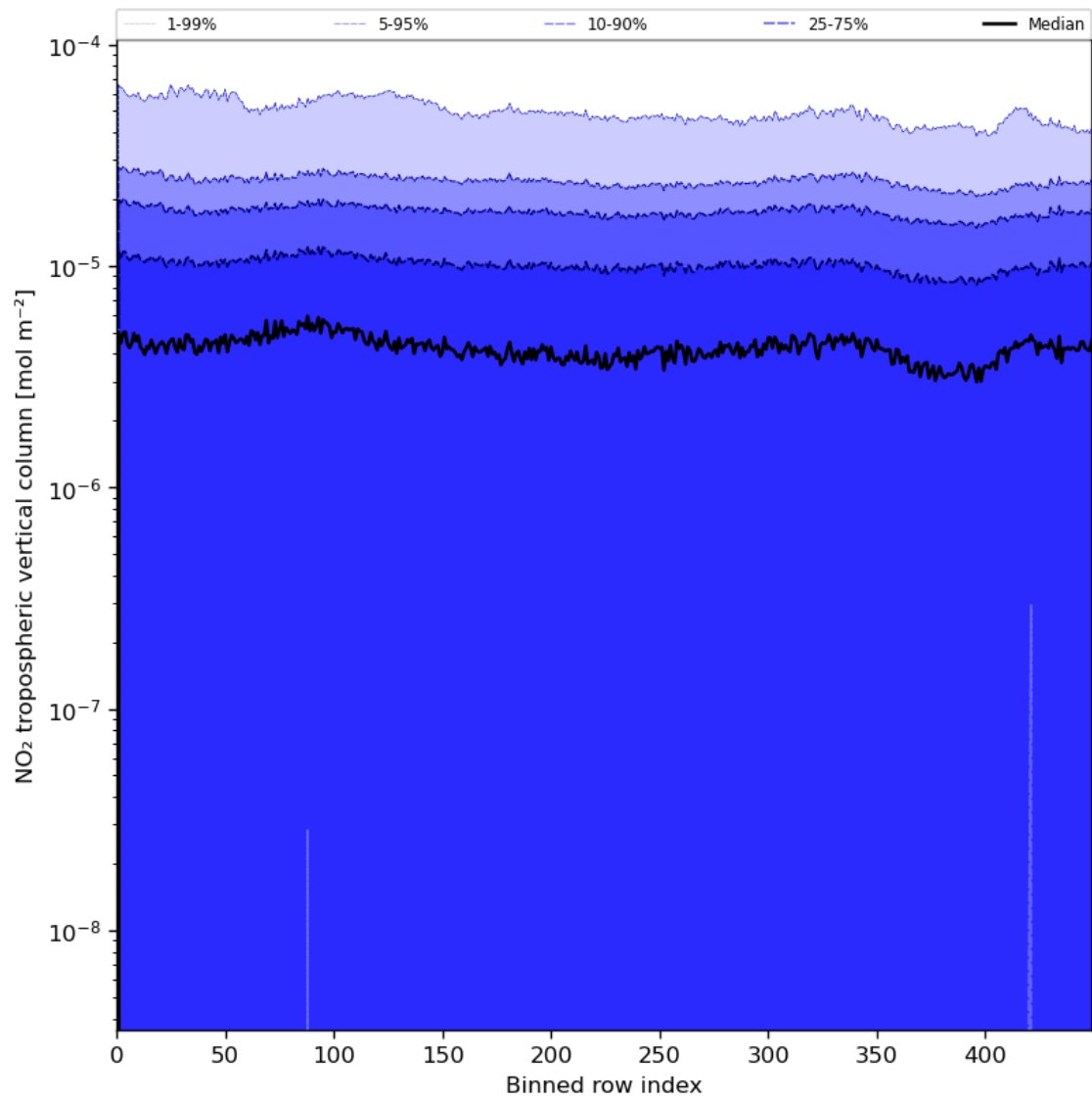
Figure 46: Along track statistics of “NO 2 tropospheric vertical column” for 2024-07-05 to 2024-07-07
