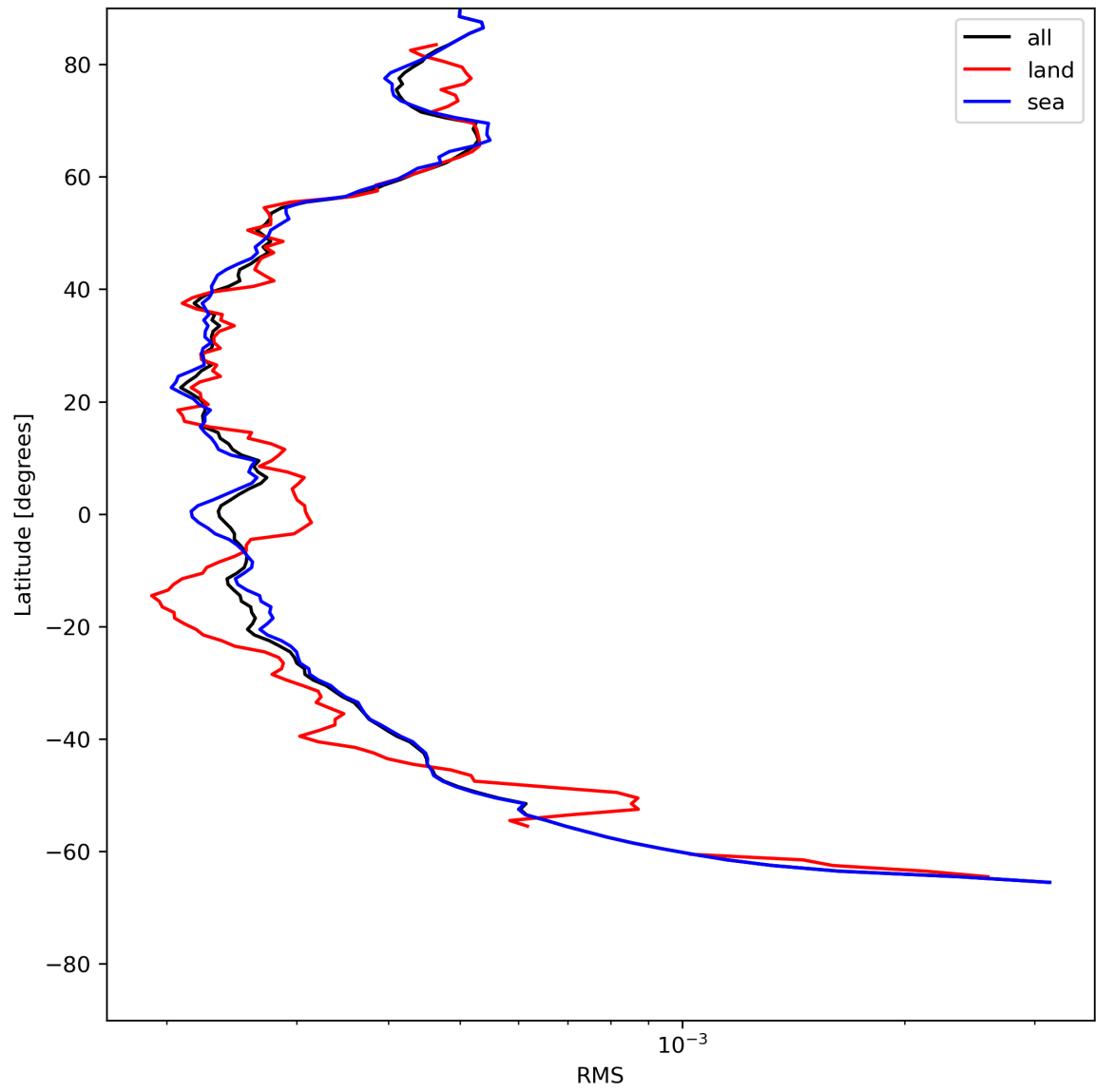
Figure 26: Zonal average of “RMS” for 2024-07-05 to 2024-07-07.
