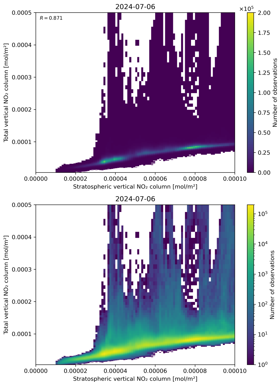
Figure 100: Scatter density plot of “Stratospheric vertical NO 2 column” against “Total vertical NO 2 column” for 2024-07-05 to 2024-07-07.
