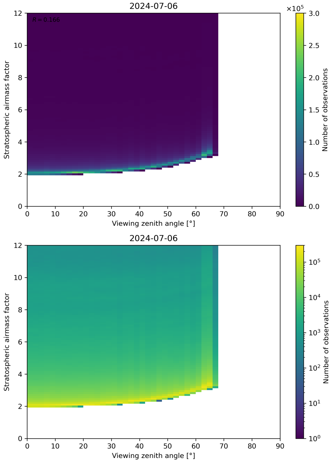
Figure 159: Scatter density plot of “Viewing zenith angle” against “Stratospheric airmass factor” for 2024-07-05 to 2024-07-07.
