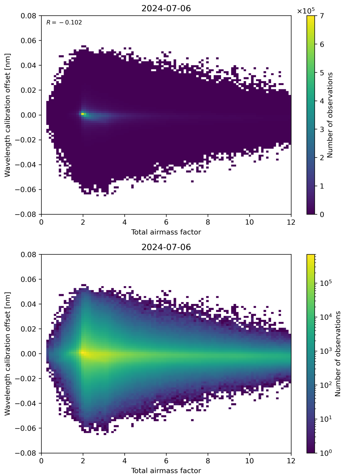
Figure 70: Scatter density plot of “Total airmass factor” against “Wavelength calibration offset” for 2024-07-05 to 2024-07-07.
