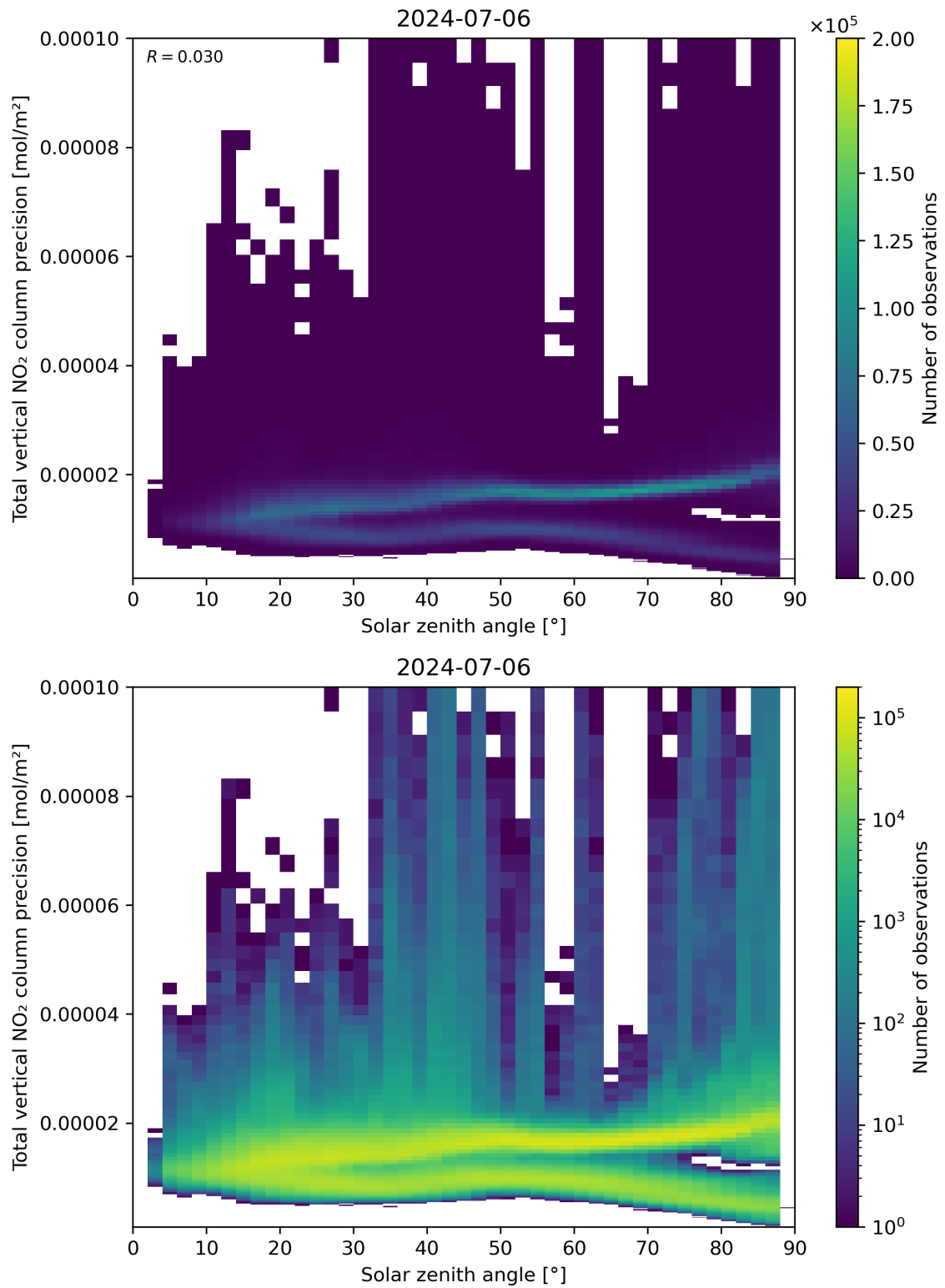
Figure 154: Scatter density plot of “Solar zenith angle” against “Total vertical NO 2 column precision” for 2024-07-05 to 2024-07-07.
