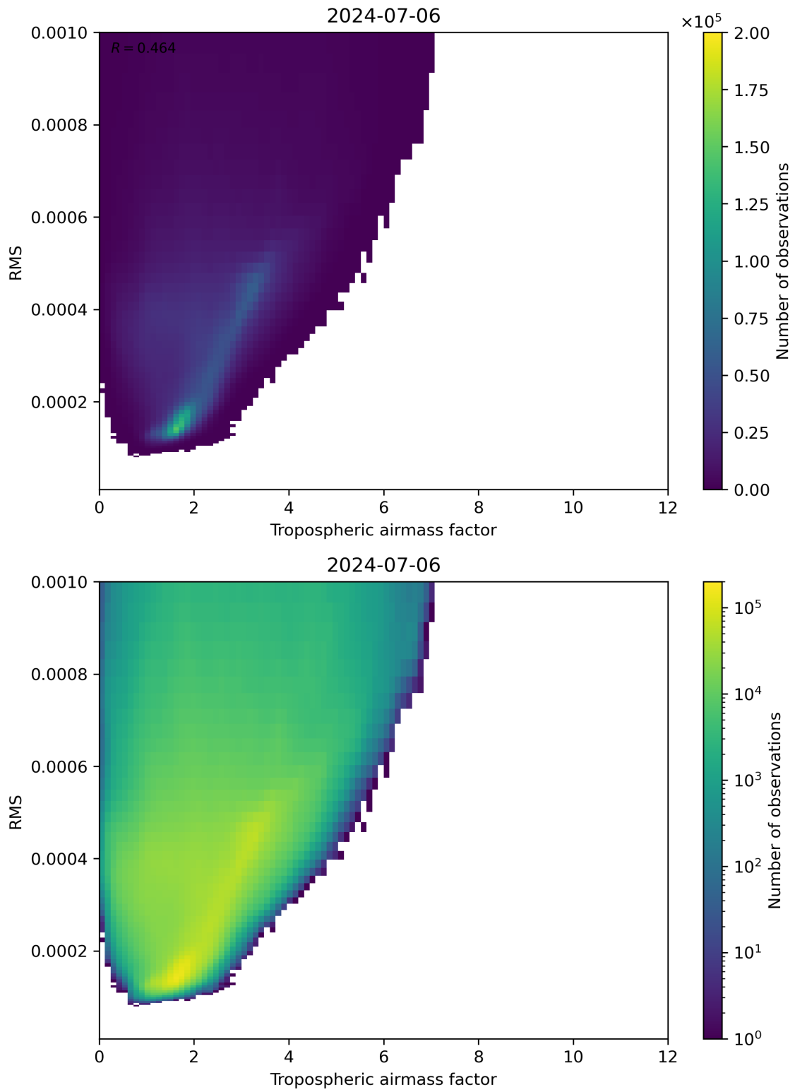
Figure 79: Scatter density plot of “Tropospheric airmass factor” against “RMS” for 2024-07-05 to 2024-07-07.
