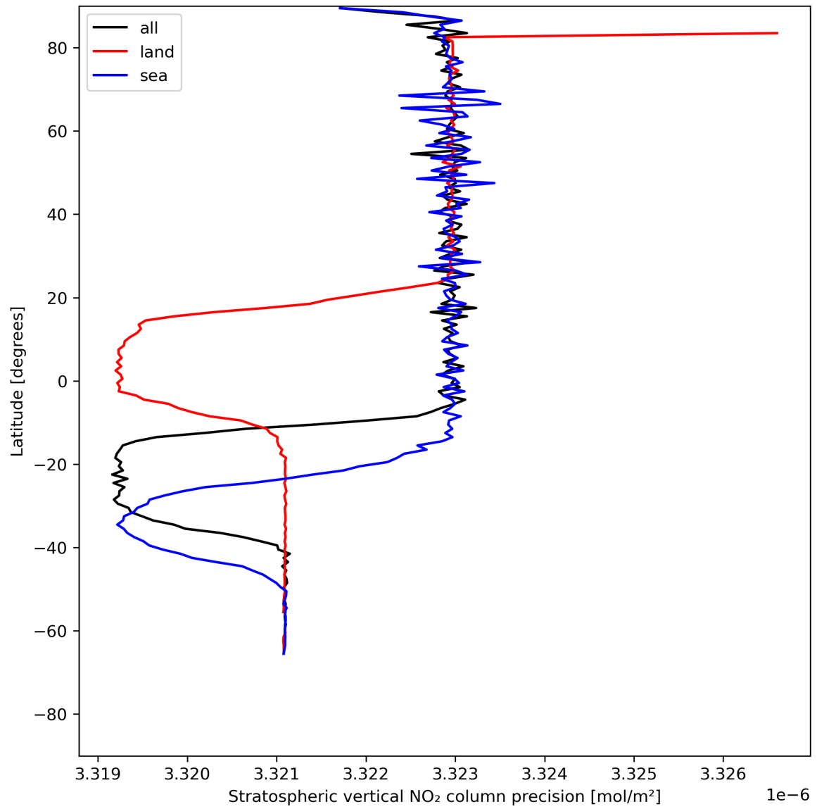
Figure 20: Zonal average of “Stratospheric vertical NO 2 column precision” for 2024-07-05 to 2024-07-07.
