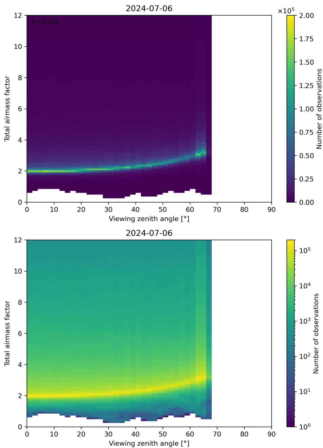
Figure 160: Scatter density plot of “Viewing zenith angle” against “Total airmass factor” for 2024-07-05 to 2024-07-07.
