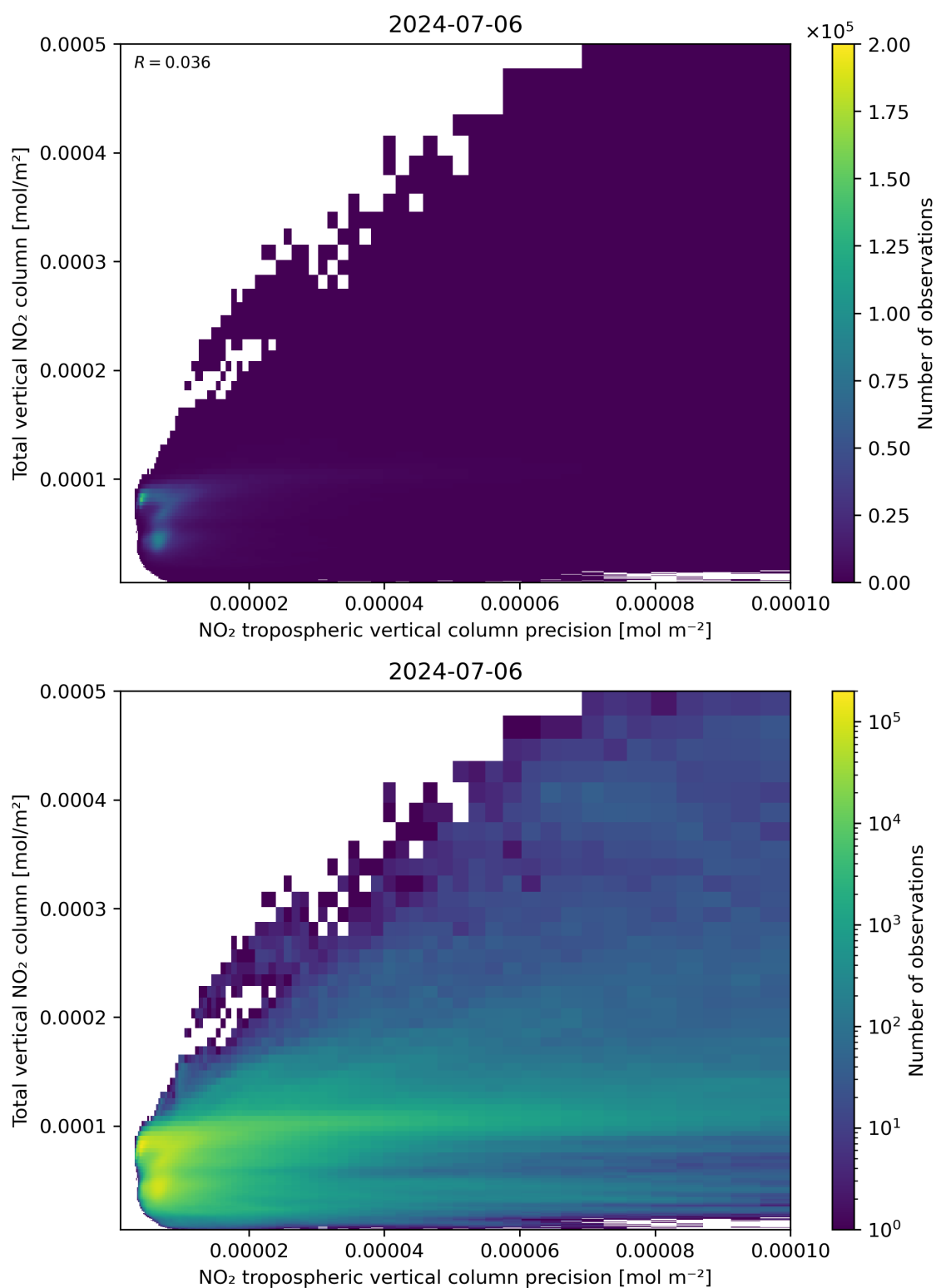
Figure 138: Scatter density plot of “NO 2 tropospheric vertical column precision” against “Total vertical NO 2 column” for 2024-07-05 to 2024-07-07.
