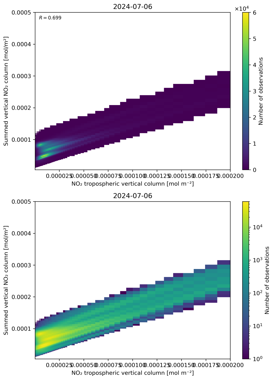
Figure 126: Scatter density plot of “NO 2 tropospheric vertical column” against “Summed vertical NO 2 column” for 2024-07-05 to 2024-07-07.
