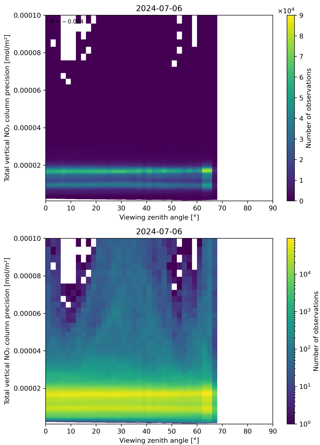
Figure 168: Scatter density plot of “Viewing zenith angle” against “Total vertical NO 2 column precision” for 2024-07-05 to 2024-07-07.
