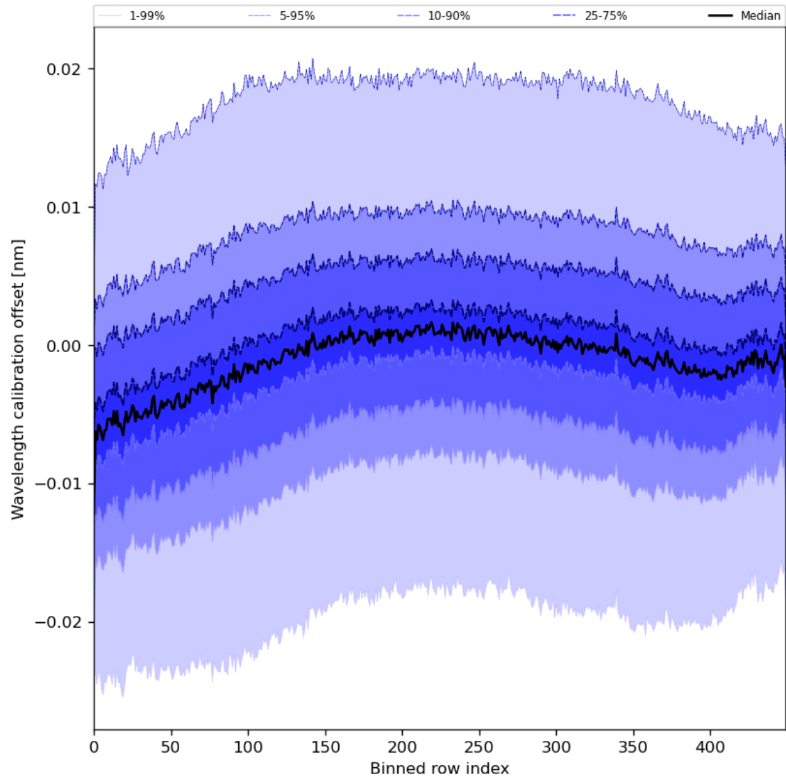
Figure 52: Along track statistics of “Wavelength calibration offset” for 2024-07-05 to 2024-07-07
