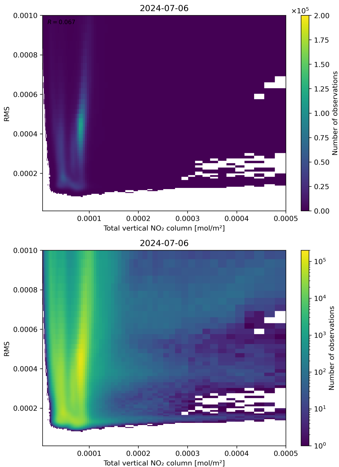
Figure 120: Scatter density plot of “Total vertical NO 2 column” against “RMS” for 2024-07-05 to 2024-07-07.
