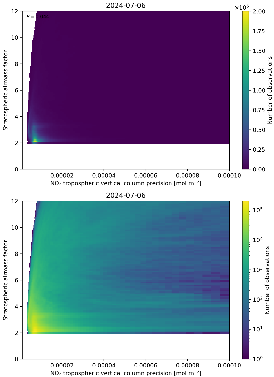
Figure 131: Scatter density plot of “NO 2 tropospheric vertical column precision” against “Stratospheric airmass factor” for 2024-07-05 to 2024-07-07.
