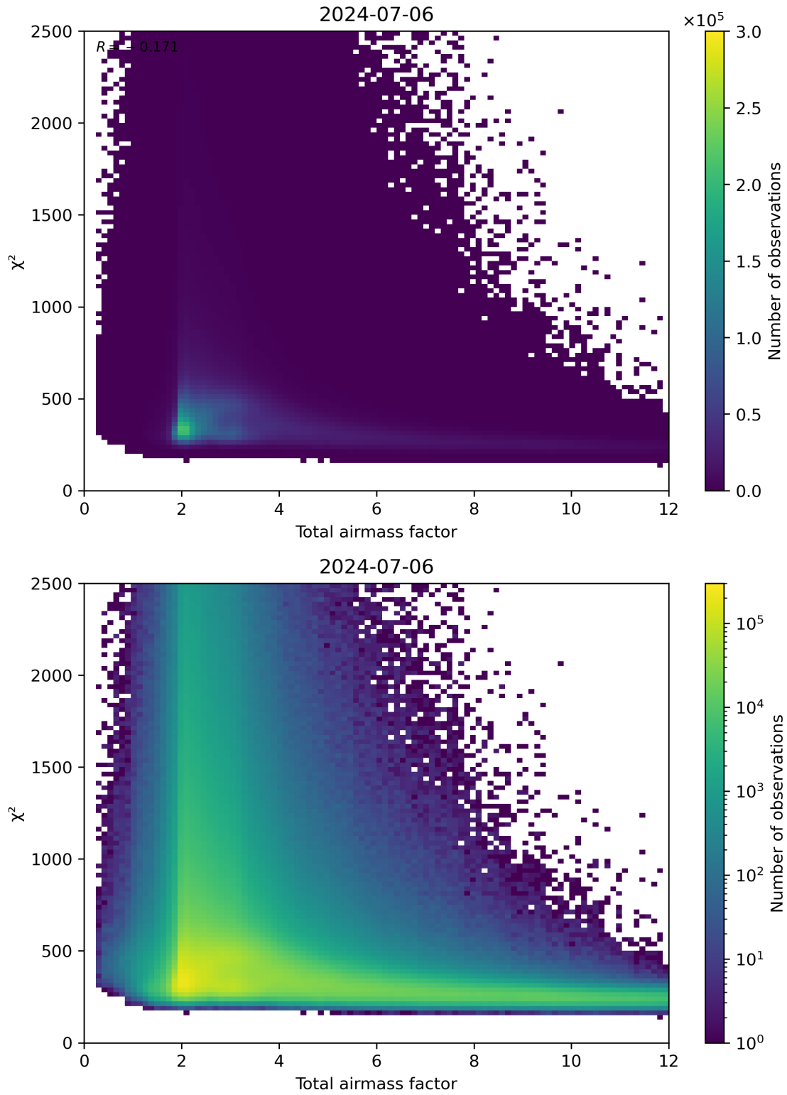
Figure 63: Scatter density plot of “Total airmass factor” against “ \chi^2 ” for 2024-07-05 to 2024-07-07.
