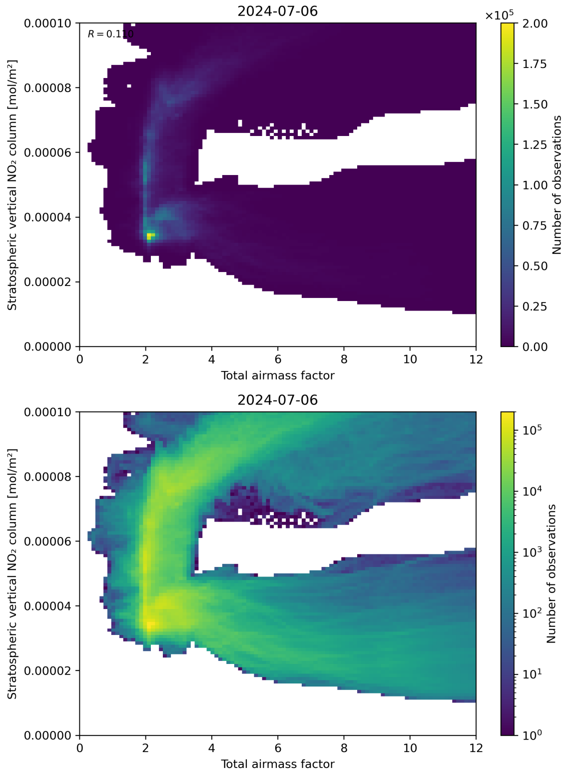
Figure 64: Scatter density plot of “Total airmass factor” against “Stratospheric vertical NO 2 column” for 2024-07-05 to 2024-07-07.
