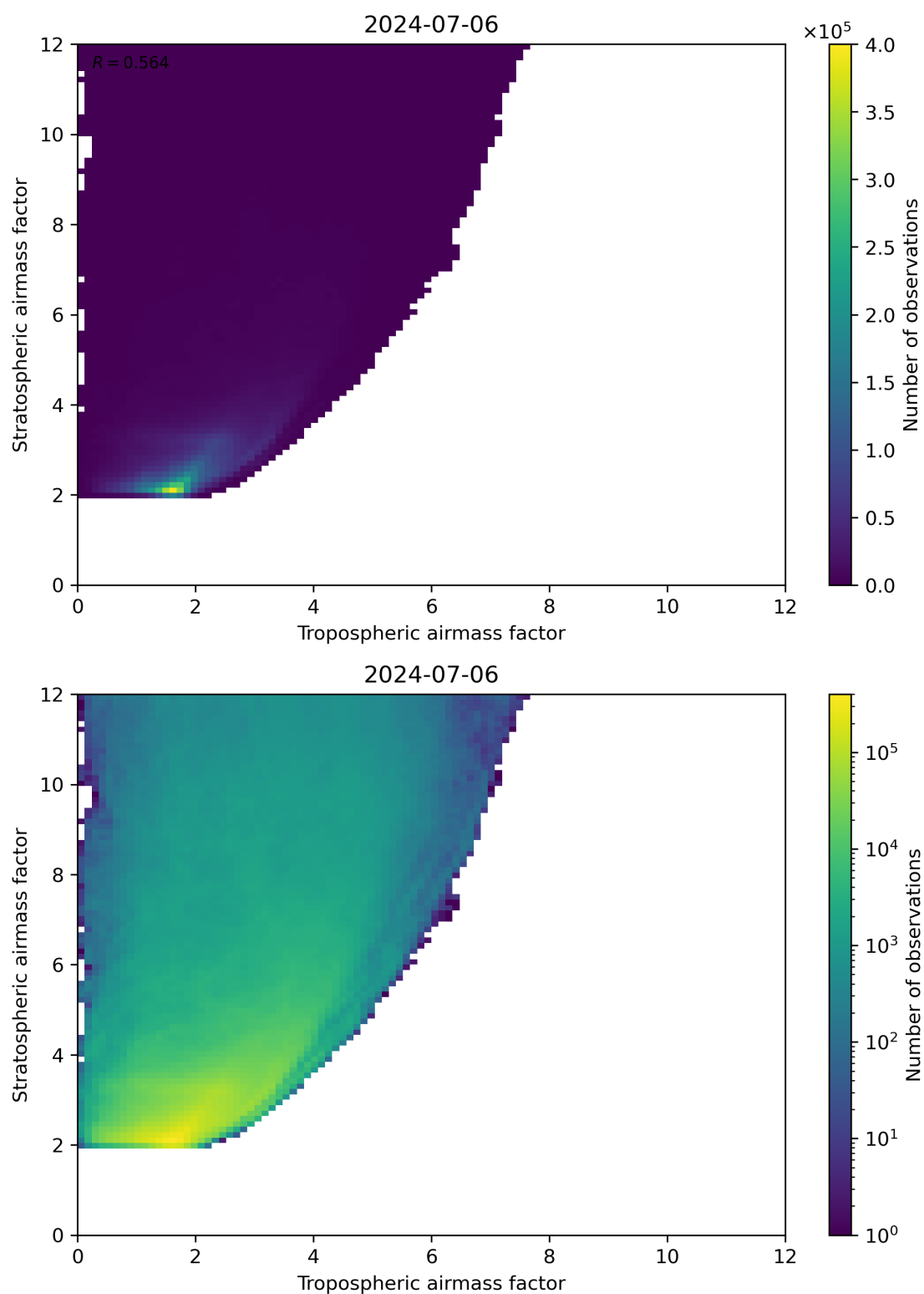
Figure 71: Scatter density plot of “Tropospheric airmass factor” against “Stratospheric airmass factor” for 2024-07-05 to 2024-07-07.
