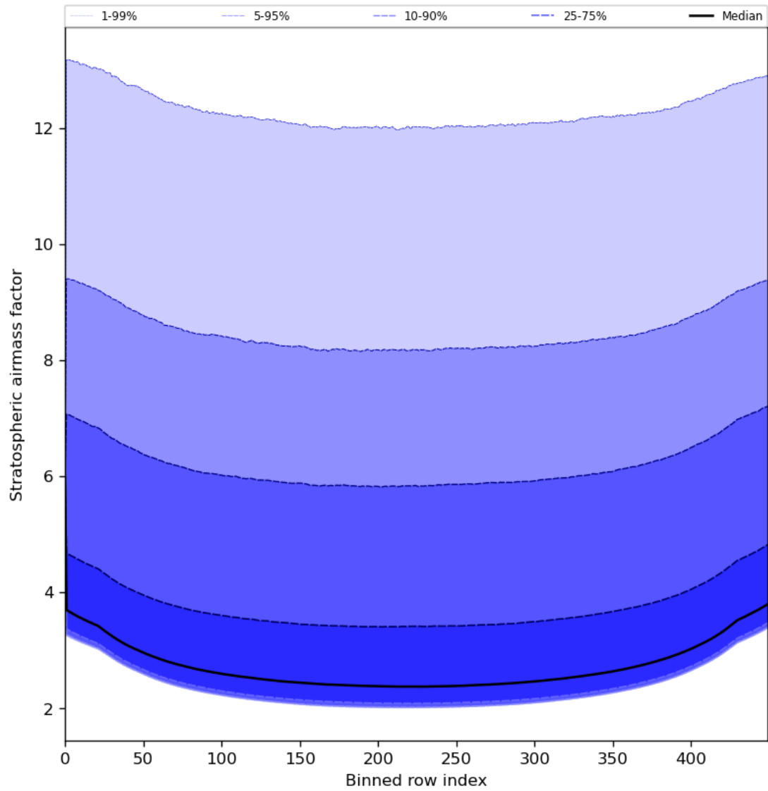
Figure 61: Along track statistics of “Stratospheric airmass factor” for 2024-07-05 to 2024-07-07
