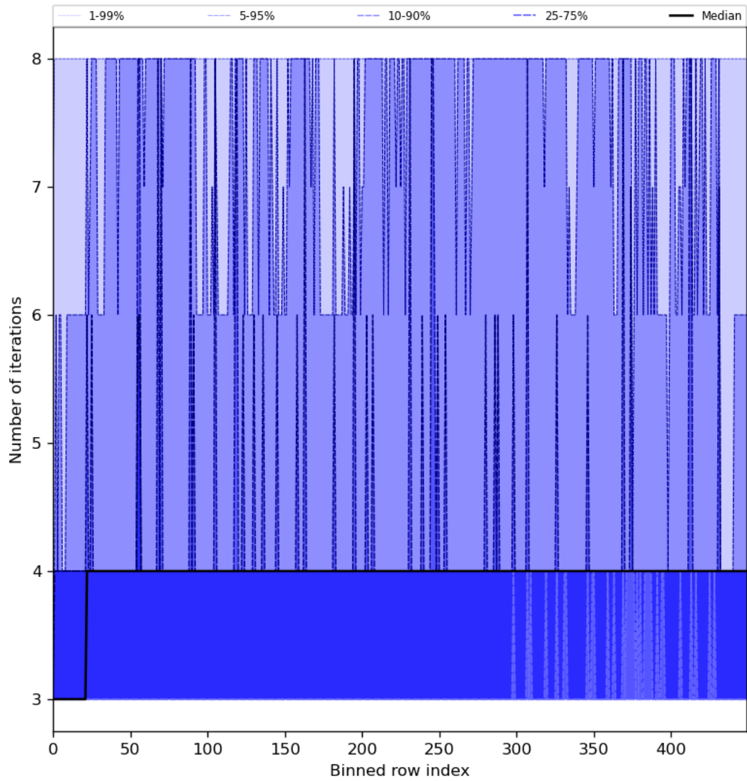
Figure 51: Along track statistics of “Number of iterations” for 2024-07-05 to 2024-07-07
