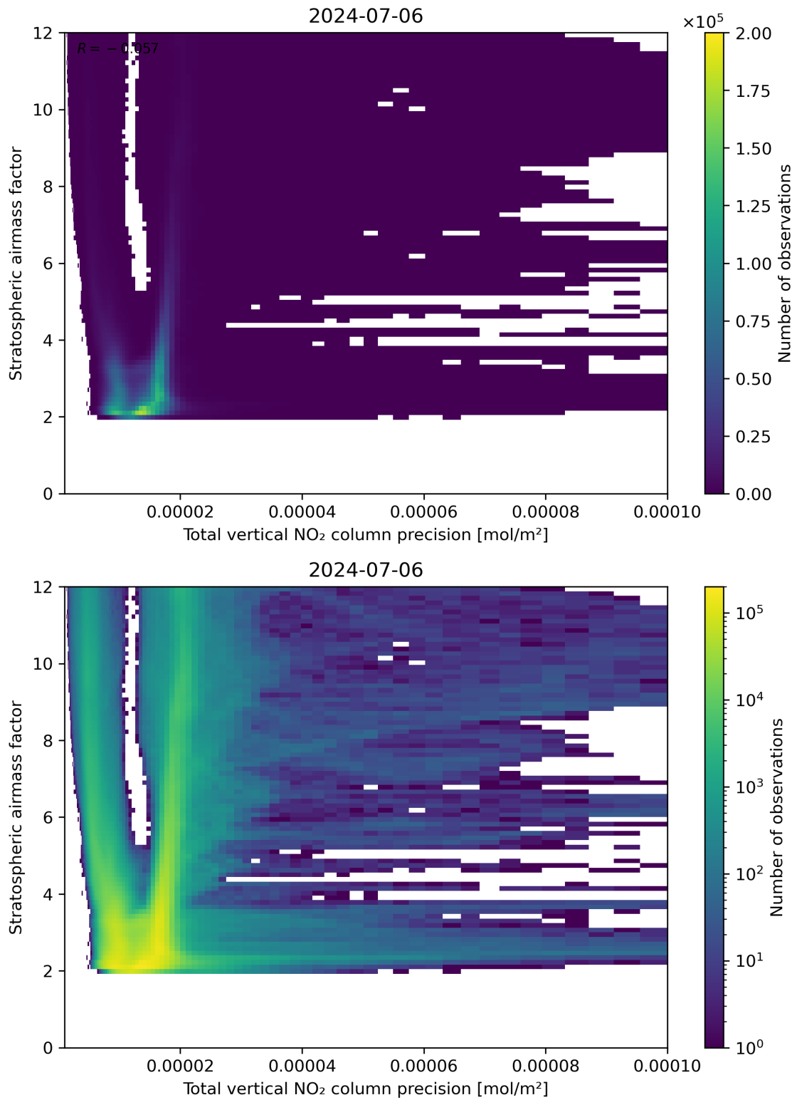
Figure 115: Scatter density plot of “Total vertical NO 2 column precision” against “Stratospheric air mass factor” for 2024-07-05 to 2024-07-07.
