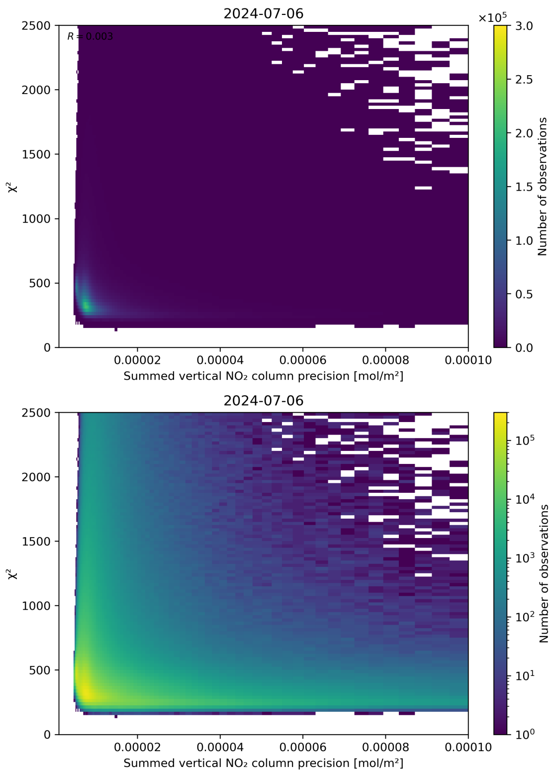
Figure 107: Scatter density plot of “Summed vertical NO 2 column precision” against “ \chi^2 ” for 2024-07-05 to 2024-07-07.
