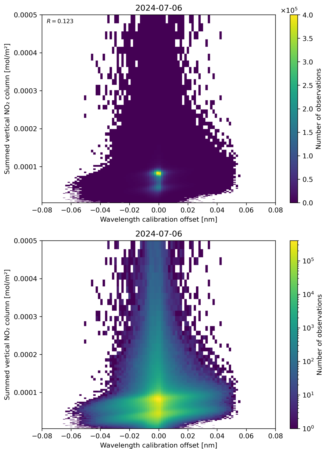
Figure 177: Scatter density plot of “Wavelength calibration offset” against “Summed vertical NO 2 column” for 2024-07-05 to 2024-07-07.
