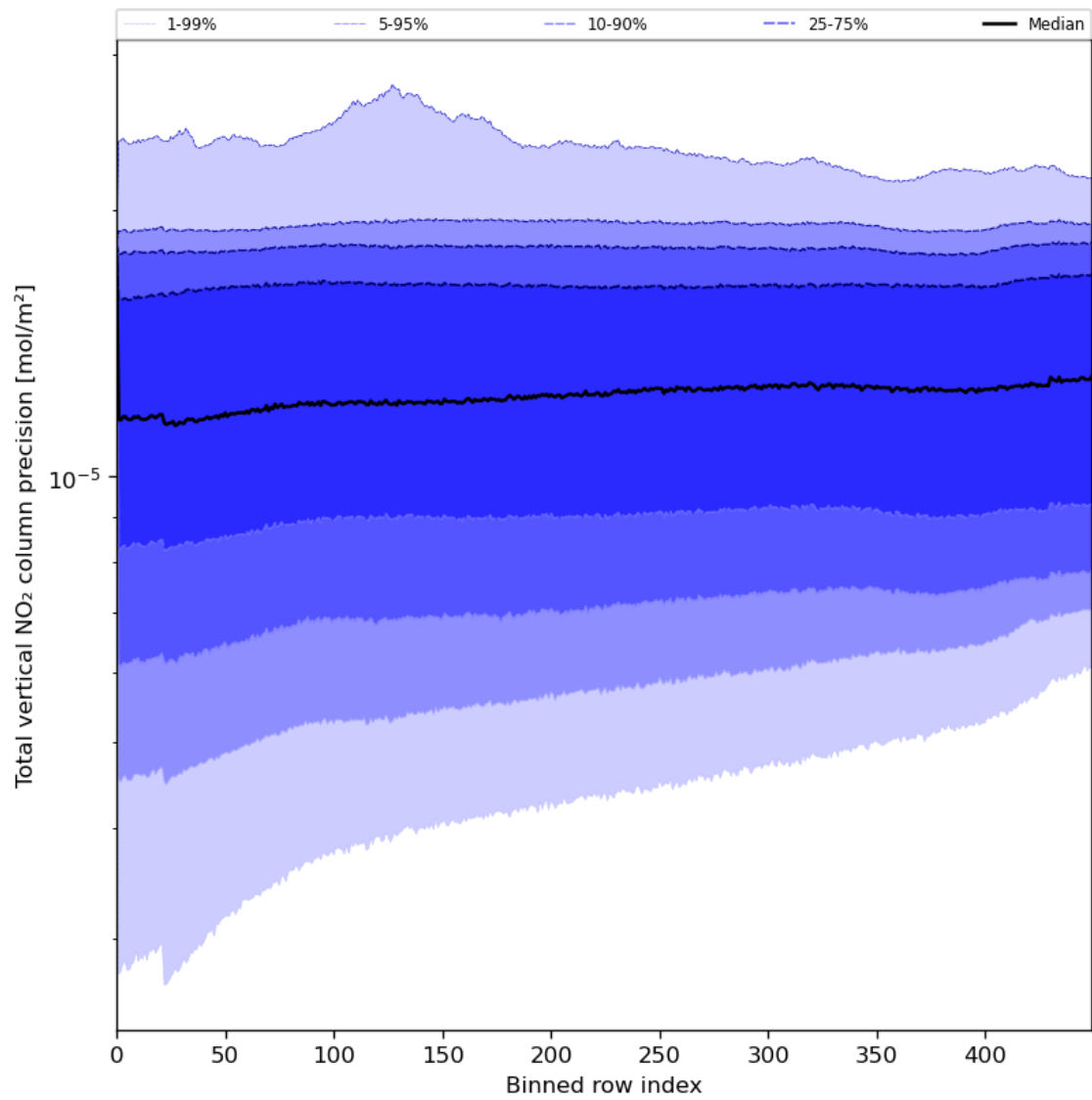
Figure 56: Along track statistics of “Total vertical NO 2 column precision” for 2024-07-05 to 2024-07-07
