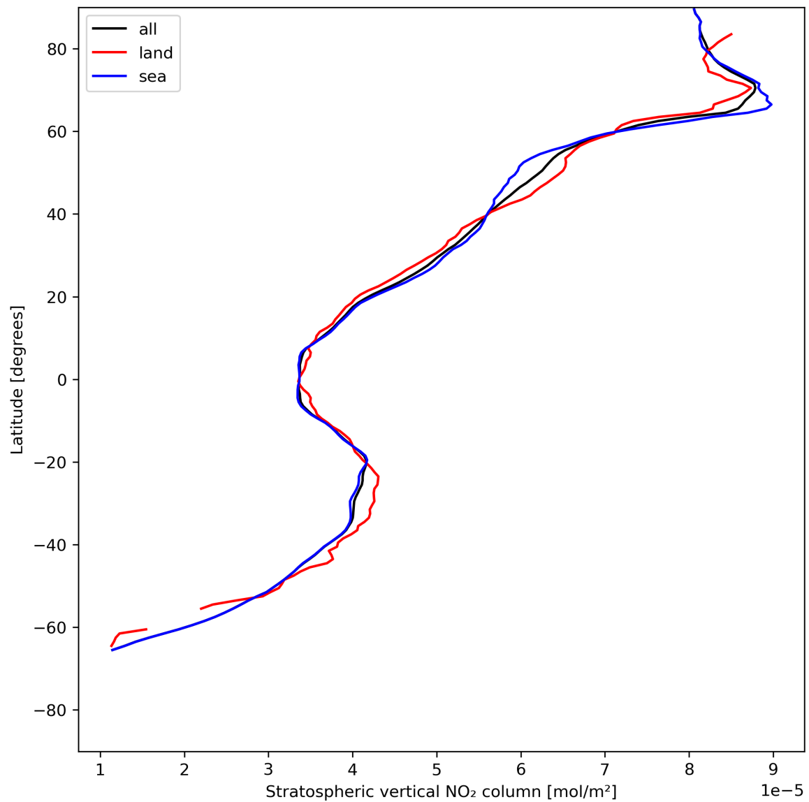
Figure 19: Zonal average of “Stratospheric vertical NO 2 column” for 2024-07-05 to 2024-07-07.
