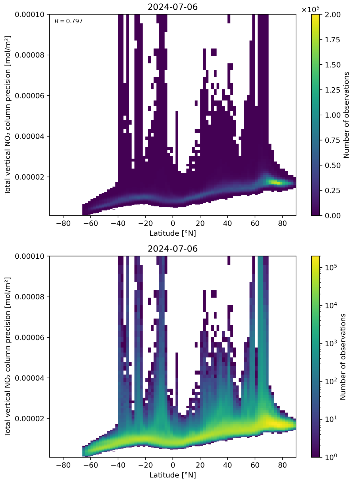
Figure 91: Scatter density plot of “Latitude” against “Total vertical NO 2 column precision” for 2024-07-05 to 2024-07-07.
