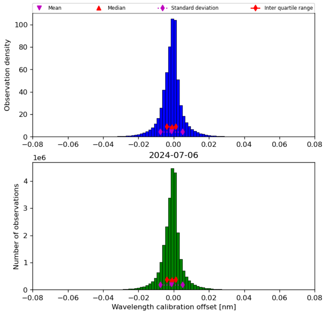
Figure 35: Histogram of “Wavelength calibration offset” for 2024-07-05 to 2024-07-07
