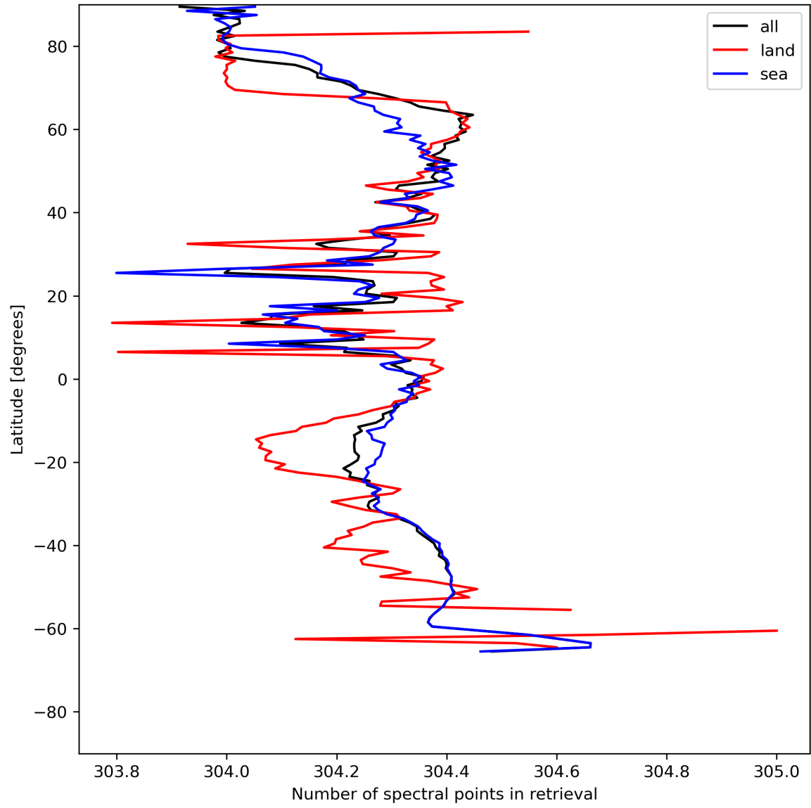
Figure 16: Zonal average of “Number of spectral points in retrieval” for 2024-07-05 to 2024-07-07.
