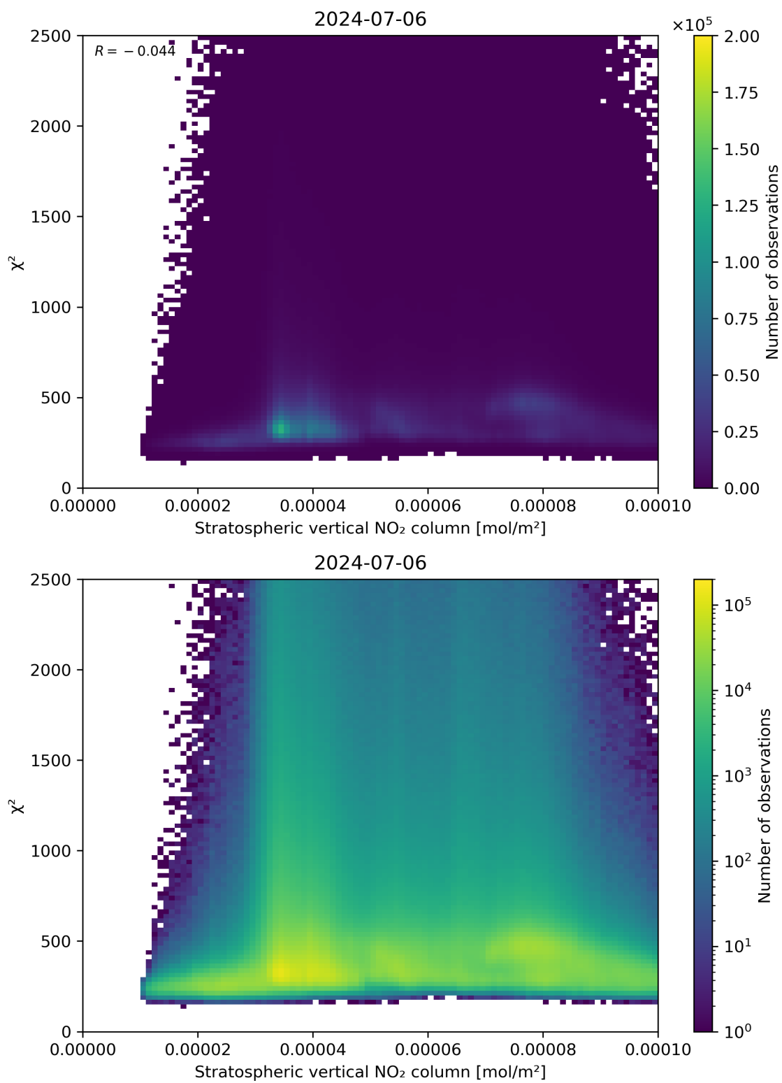
Figure 97: Scatter density plot of “Stratospheric vertical NO 2 column” against “ \chi^2 ” for 2024-07-05 to 2024-07-07.
