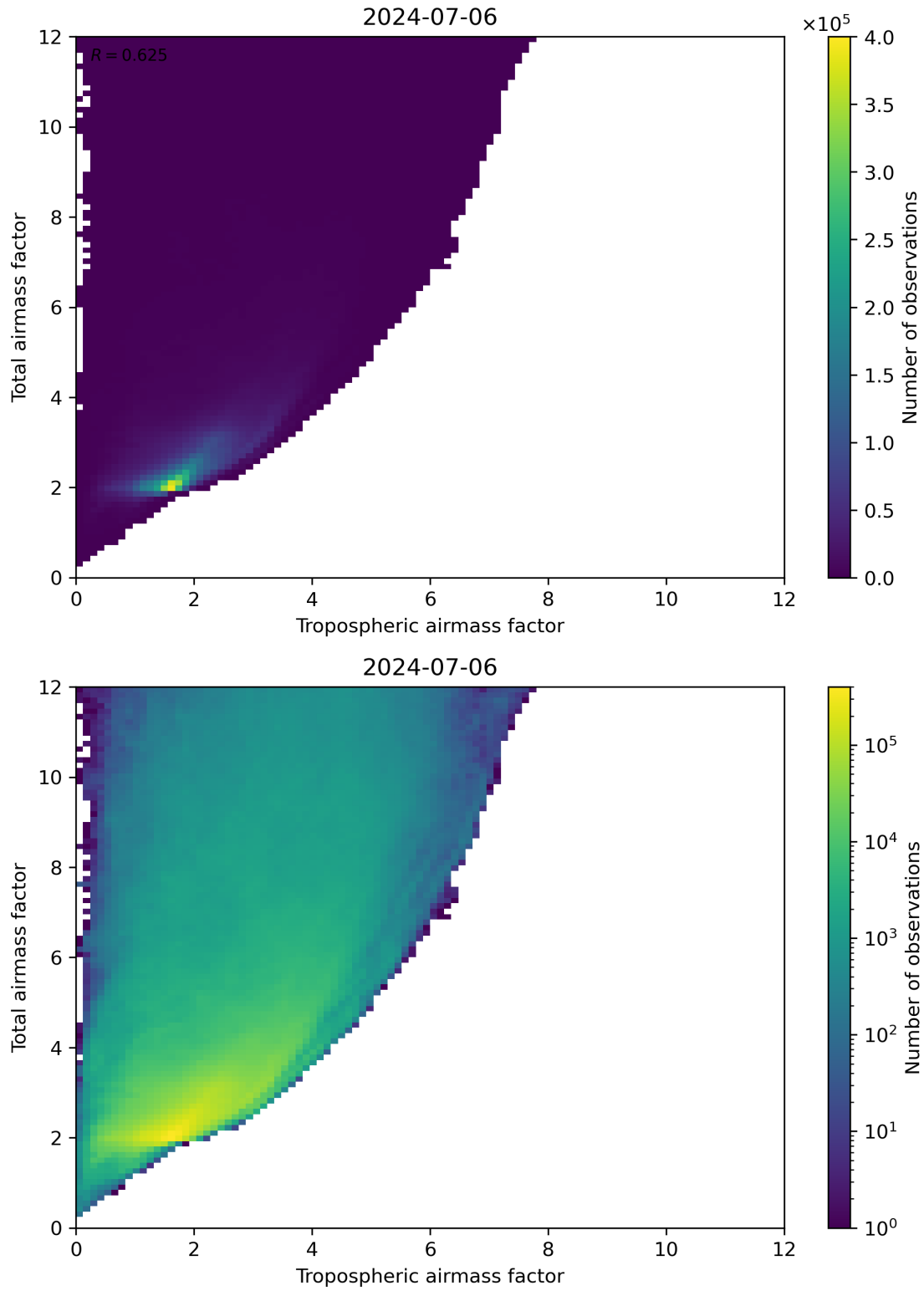
Figure 72: Scatter density plot of “Tropospheric airmass factor” against “Total airmass factor” for 2024-07-05 to 2024-07-07.
