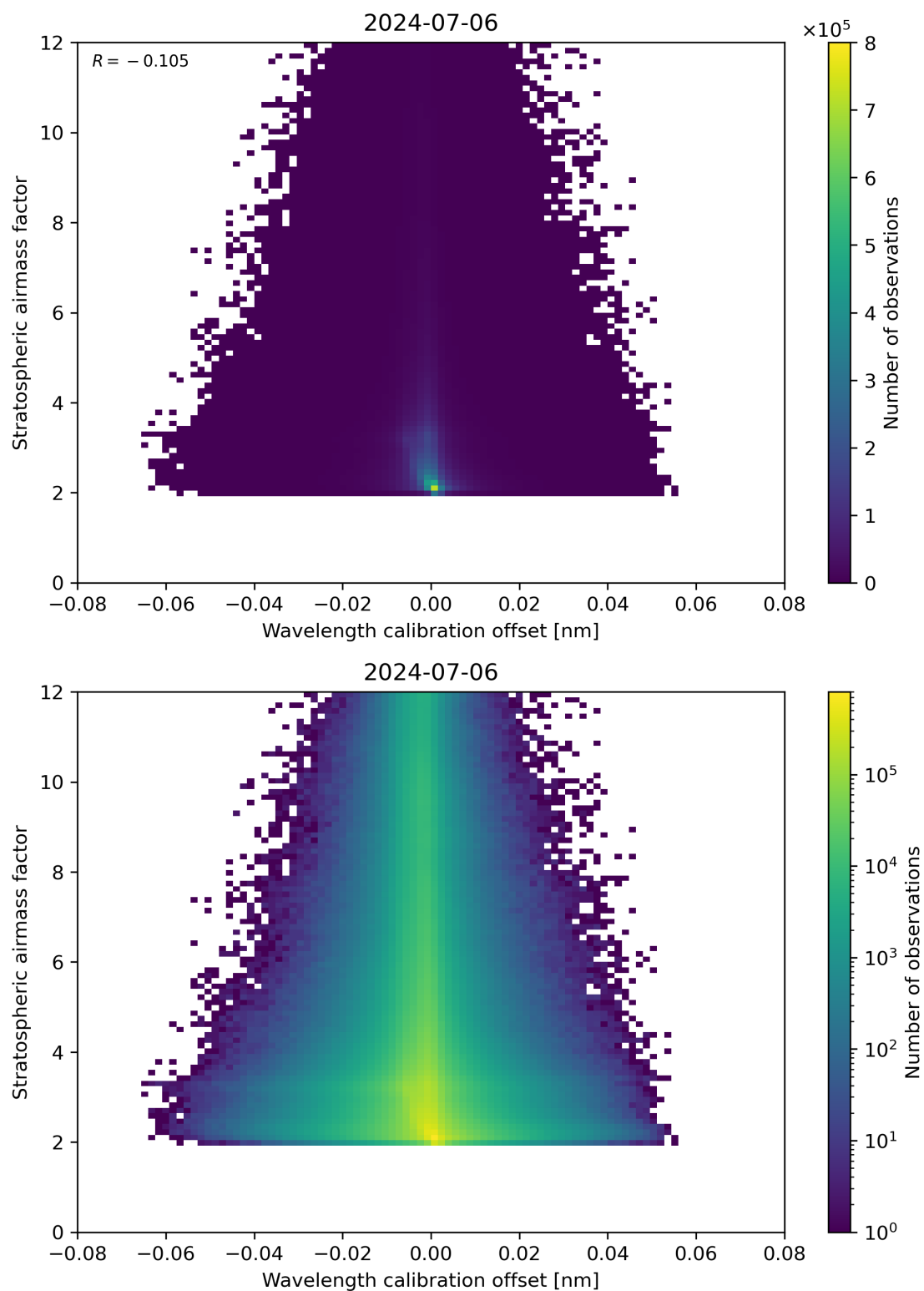
Figure 174: Scatter density plot of “Wavelength calibration offset” against “Stratospheric airmass factor” for 2024-07-05 to 2024-07-07.
