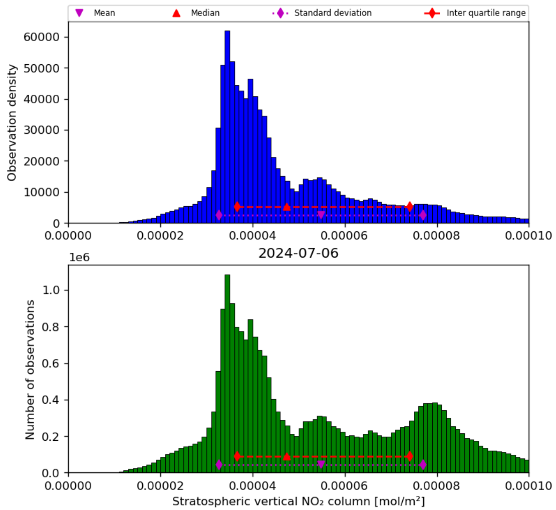
Figure 36: Histogram of “Stratospheric vertical NO 2 column” for 2024-07-05 to 2024-07-07
