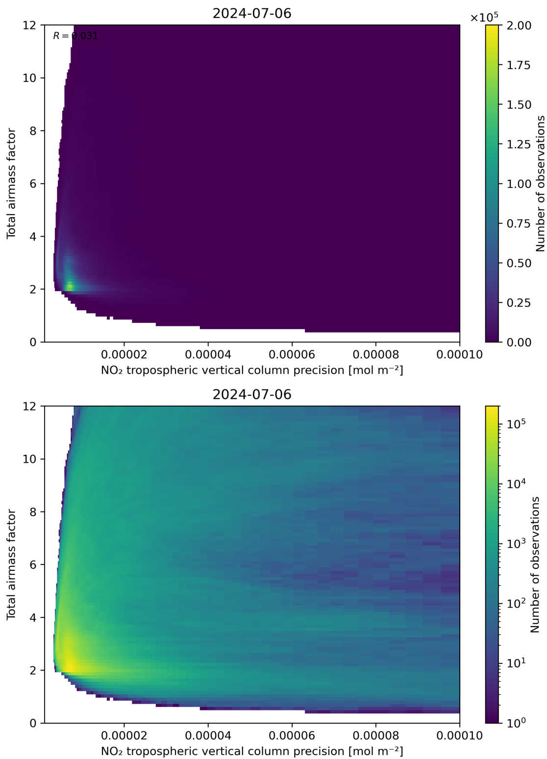
Figure 132: Scatter density plot of “NO 2 tropospheric vertical column precision” against “Total airmass factor” for 2024-07-05 to 2024-07-07.
