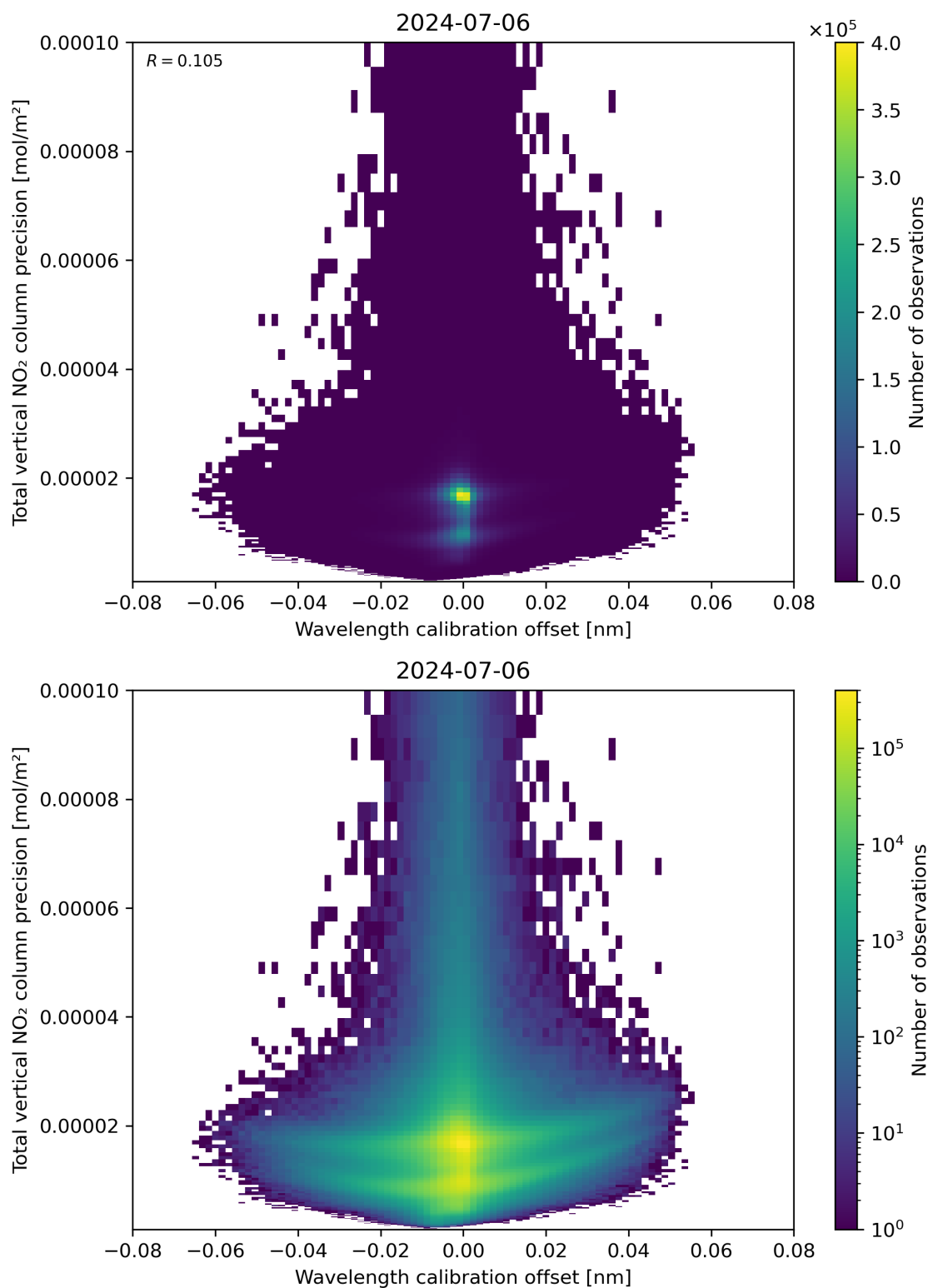
Figure 180: Scatter density plot of “Wavelength calibration offset” against “Total vertical NO 2 column precision” for 2024-07-05 to 2024-07-07.
