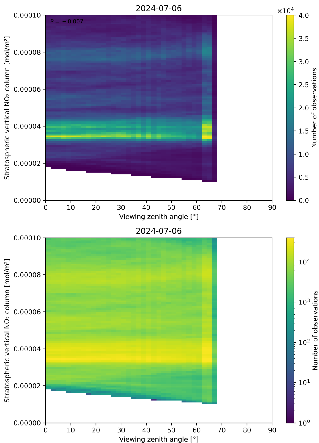
Figure 164: Scatter density plot of “Viewing zenith angle” against “Stratospheric vertical NO 2 column” for 2024-07-05 to 2024-07-07.
