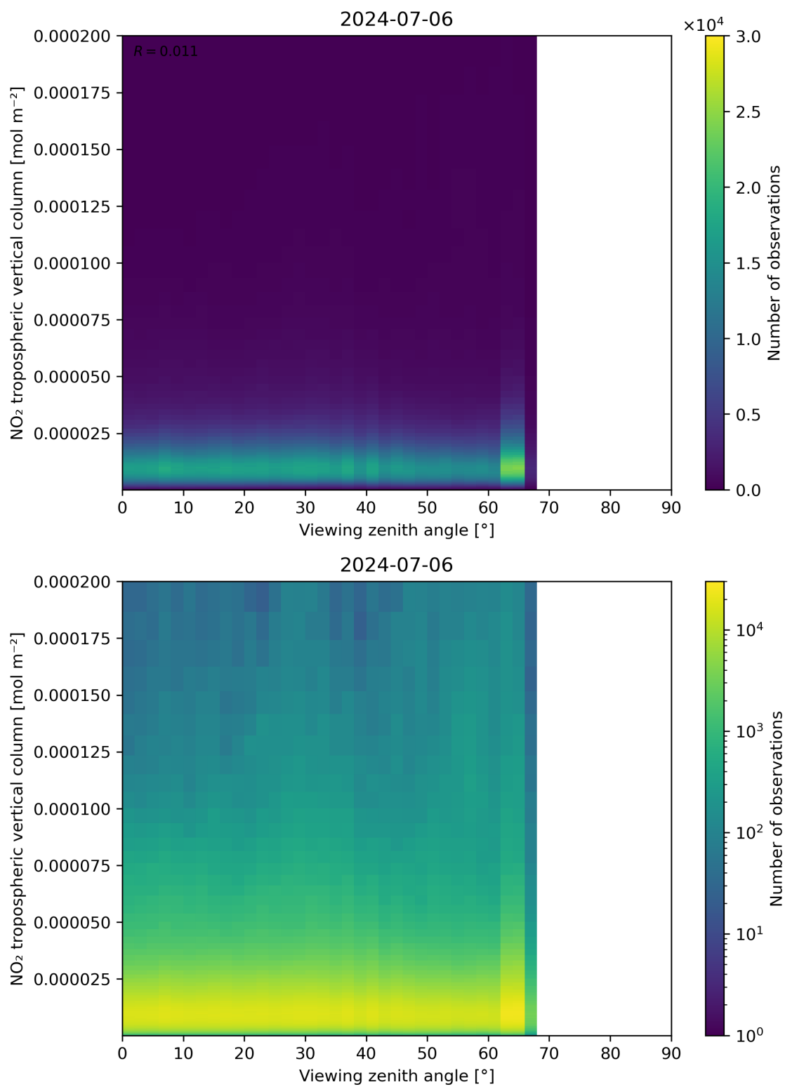
Figure 169: Scatter density plot of “Viewing zenith angle” against “NO 2 tropospheric vertical column” for 2024-07-05 to 2024-07-07.
