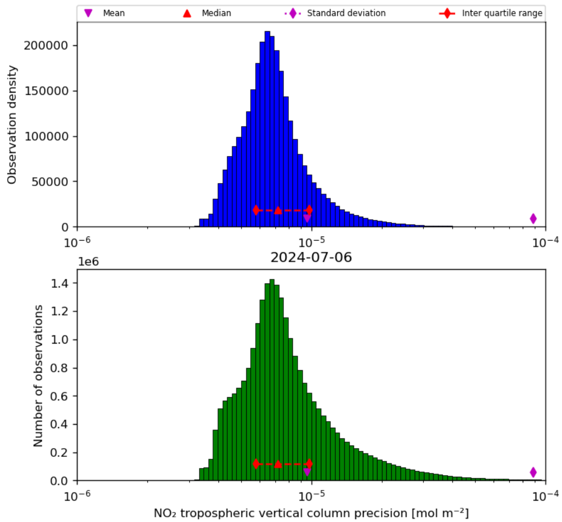
Figure 30: Histogram of “NO 2 tropospheric vertical column precision” for 2024-07-05 to 2024-07-07
