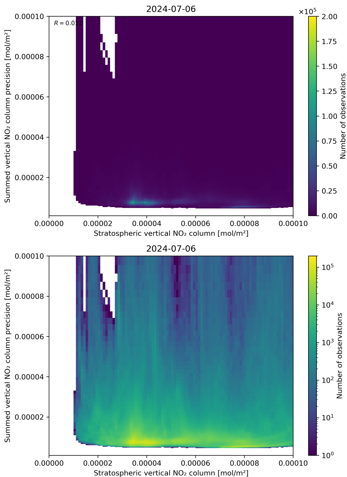
Figure 99: Scatter density plot of “Stratospheric vertical NO 2 column” against “Summed vertical NO 2 column precision” for 2024-07-05 to 2024-07-07.
