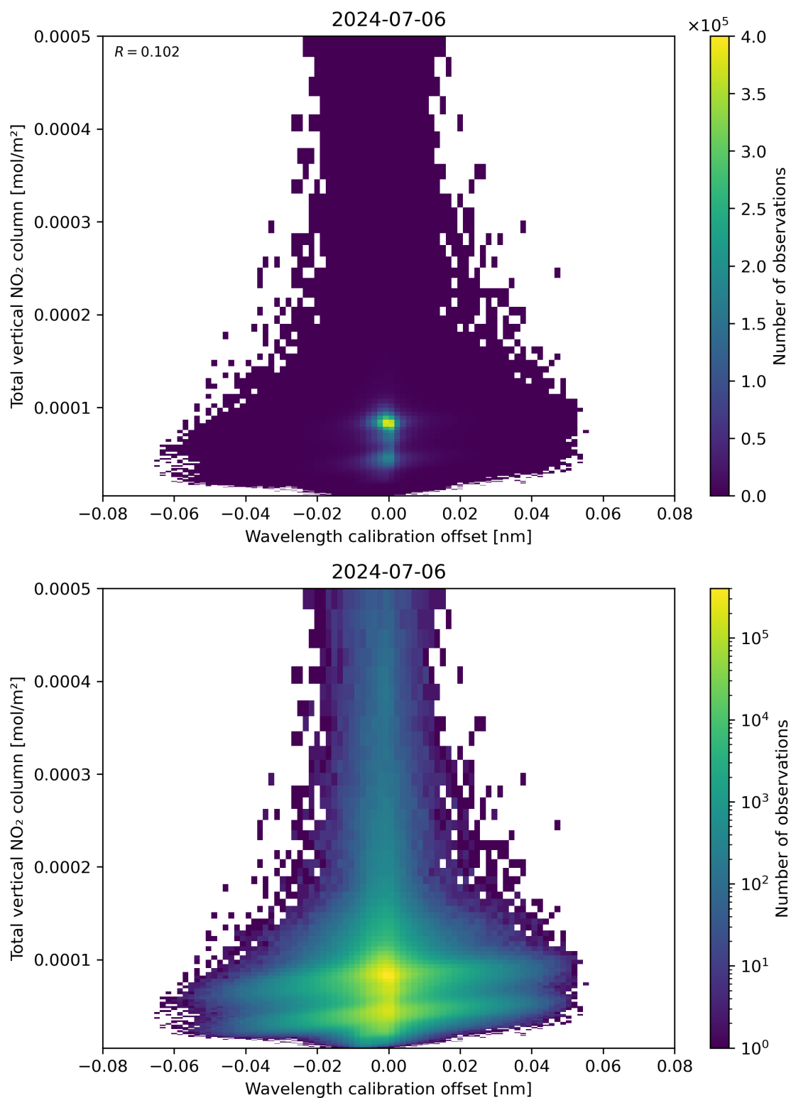
Figure 179: Scatter density plot of “Wavelength calibration offset” against “Total vertical NO 2 column” for 2024-07-05 to 2024-07-07.
