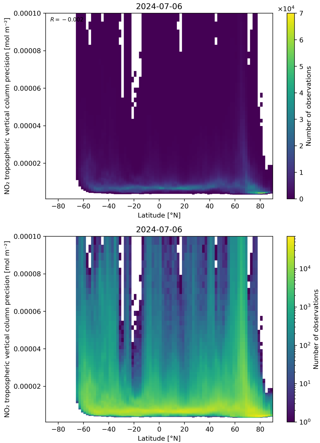
Figure 93: Scatter density plot of “Latitude” against “NO 2 tropospheric vertical column precision” for 2024-07-05 to 2024-07-07.
