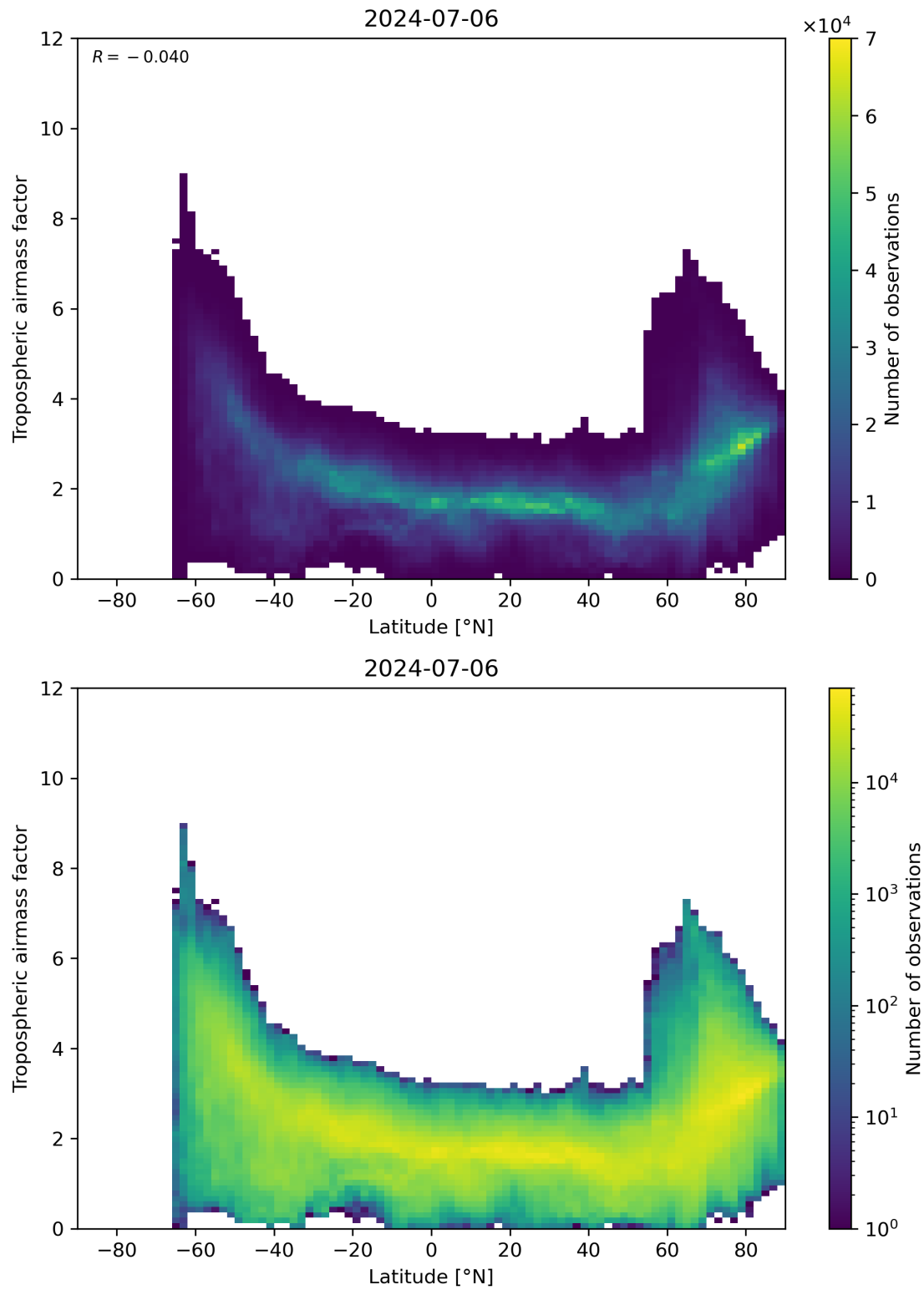
Figure 85: Scatter density plot of “Latitude” against “Tropospheric airmass factor” for 2024-07-05 to 2024-07-07.
