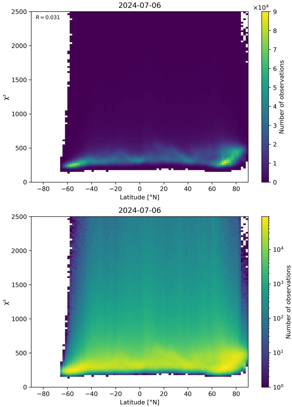
Figure 86: Scatter density plot of “Latitude” against “ \chi^2 ” for 2024-07-05 to 2024-07-07.
