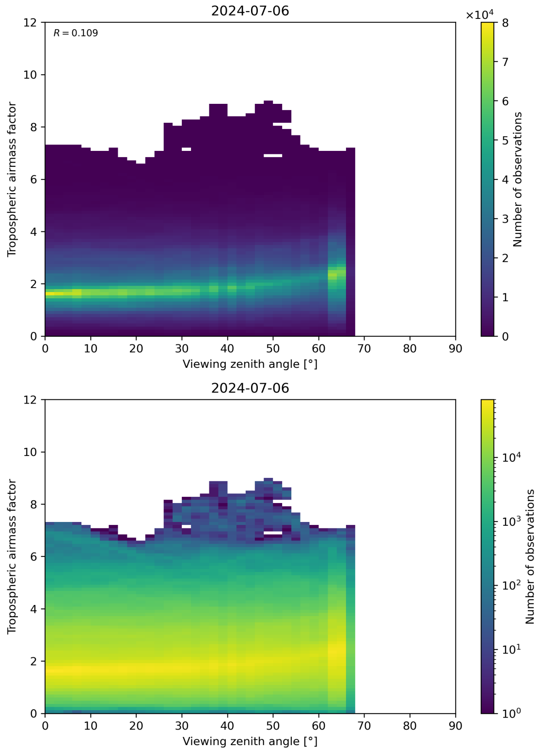
Figure 161: Scatter density plot of “Viewing zenith angle” against “Tropospheric airmass factor” for 2024-07-05 to 2024-07-07.
