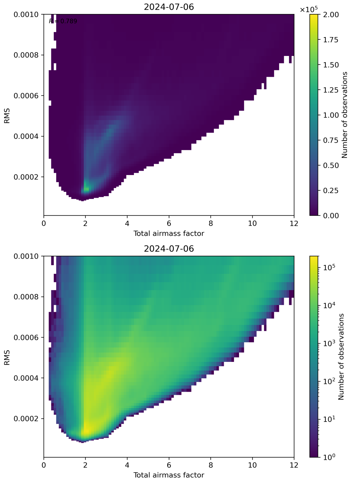
Figure 69: Scatter density plot of “Total airmass factor” against “RMS” for 2024-07-05 to 2024-07-07.
