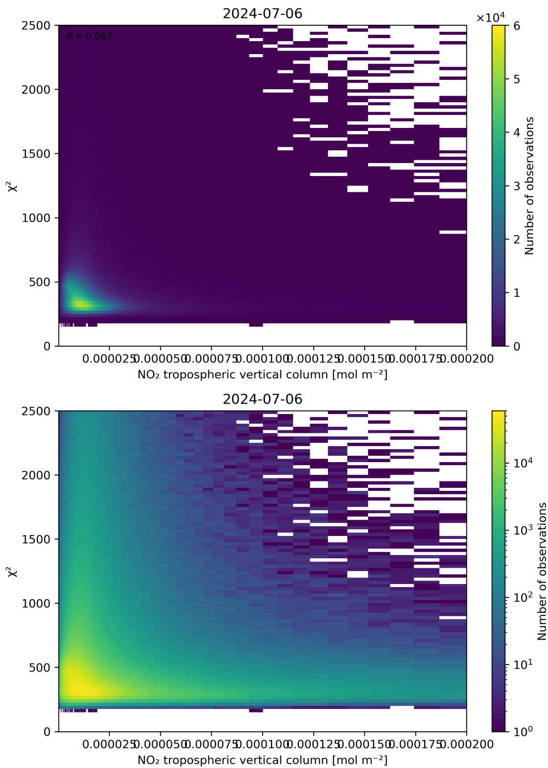
Figure 124: Scatter density plot of “NO 2 tropospheric vertical column” against “ \chi^2 ” for 2024-07-05 to 2024-07-07.
