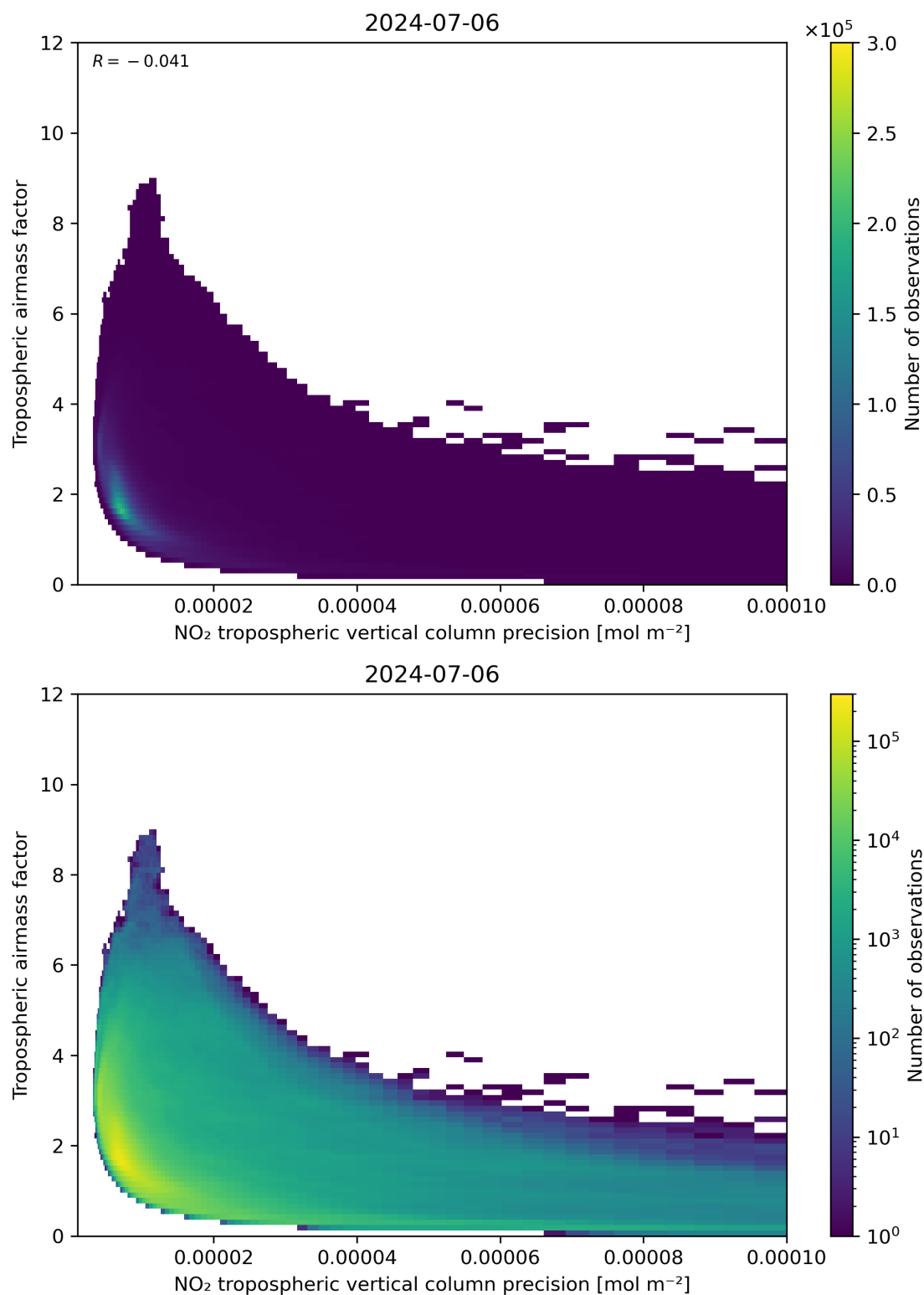
Figure 133: Scatter density plot of “NO 2 tropospheric vertical column precision” against “Tropospheric airmass factor” for 2024-07-05 to 2024-07-07.
