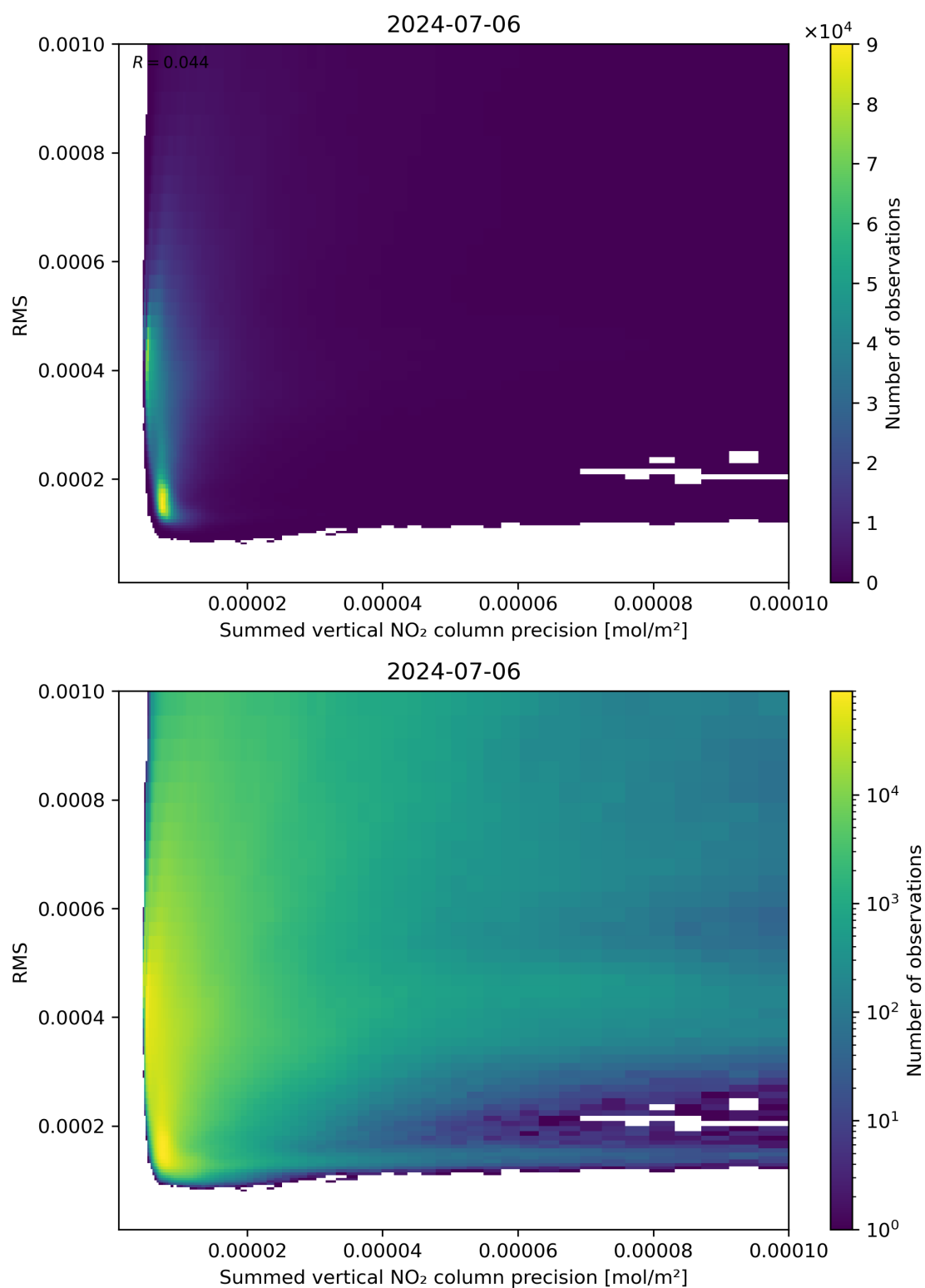
Figure 108: Scatter density plot of “Summed vertical NO 2 column precision” against “RMS” for 2024-07-05 to 2024-07-07.
