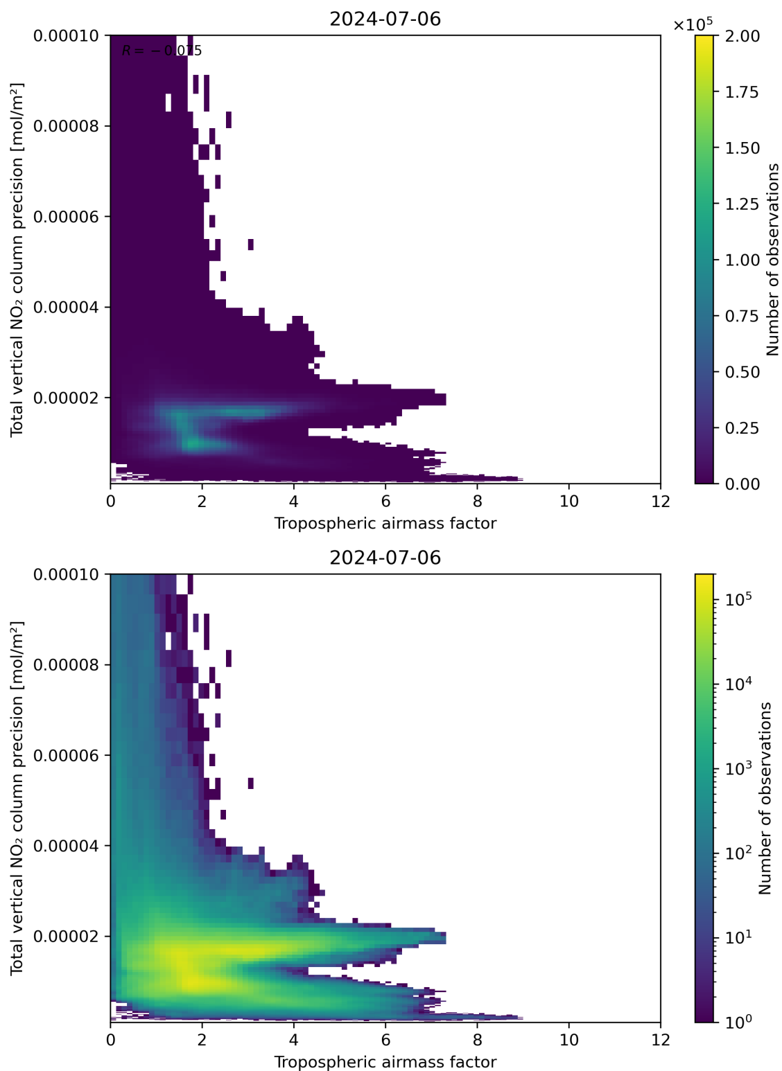
Figure 78: Scatter density plot of “Tropospheric air mass factor” against “Total vertical NO 2 column precision” for 2024-07-05 to 2024-07-07.
