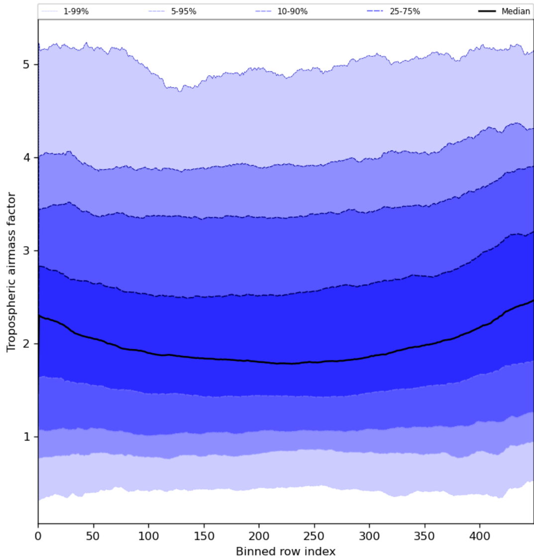
Figure 48: Along track statistics of “Tropospheric airmass factor” for 2024-07-05 to 2024-07-07
