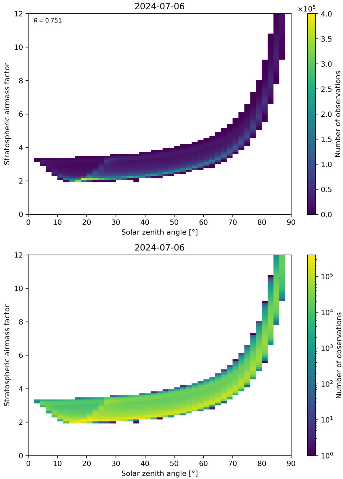
Figure 145: Scatter density plot of “Solar zenith angle” against “Stratospheric airmass factor” for 2024-07-05 to 2024-07-07.
