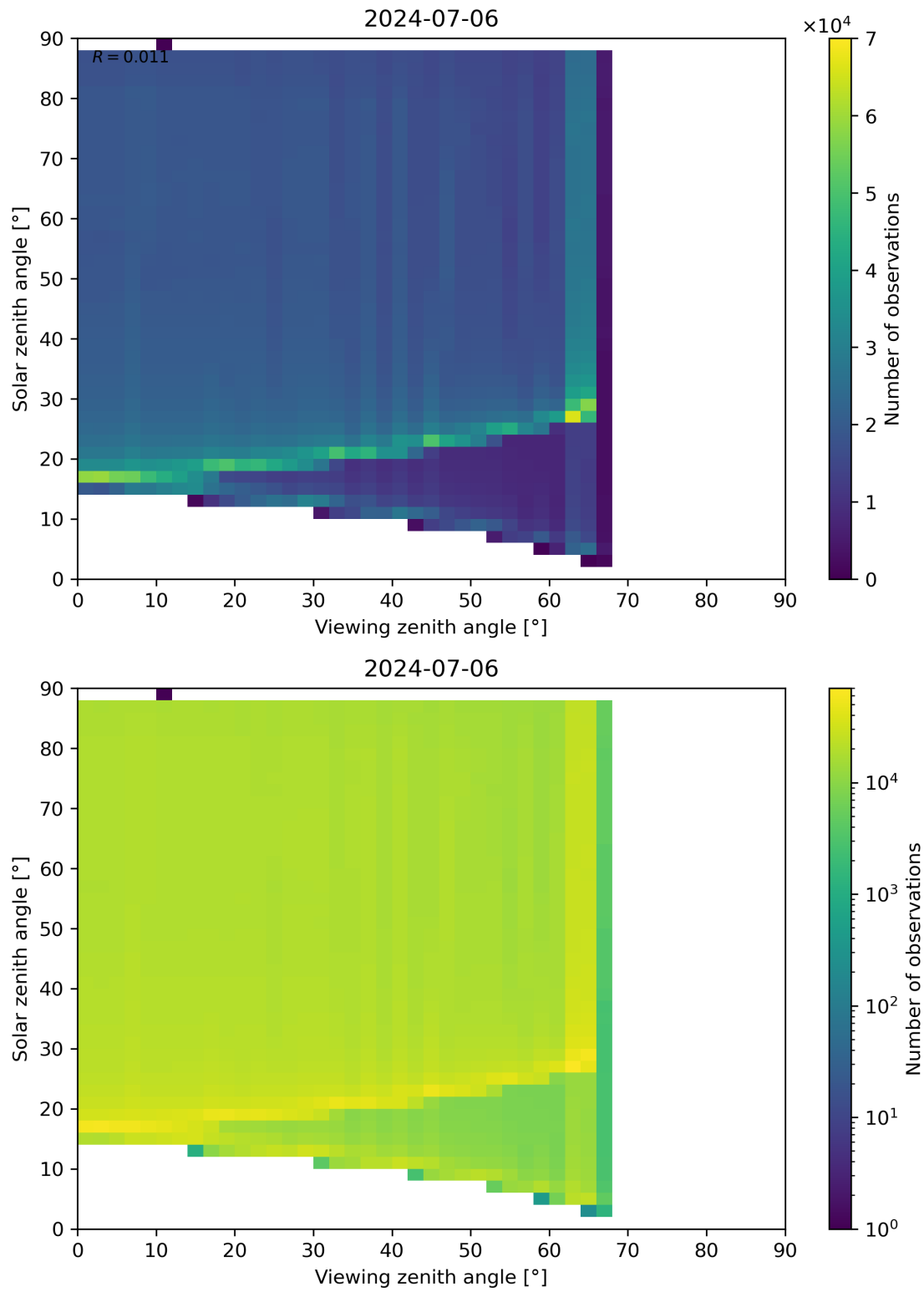
Figure 172: Scatter density plot of “Viewing zenith angle” against “Solar zenith angle” for 2024-07-05 to 2024-07-07.
