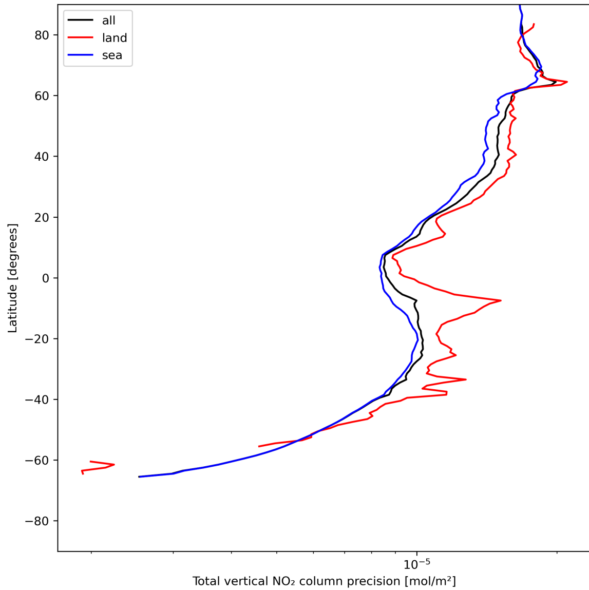
Figure 22: Zonal average of “Total vertical NO 2 column precision” for 2024-07-05 to 2024-07-07.
