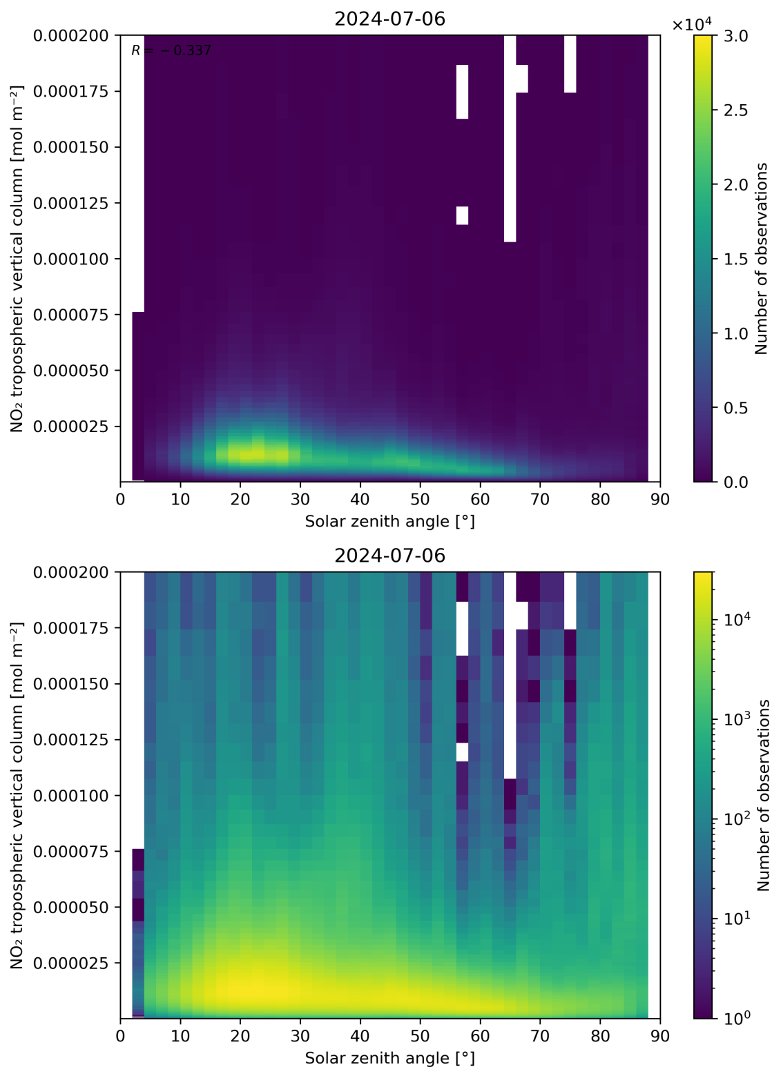
Figure 155: Scatter density plot of “Solar zenith angle” against “NO 2 tropospheric vertical column” for 2024-07-05 to 2024-07-07.
