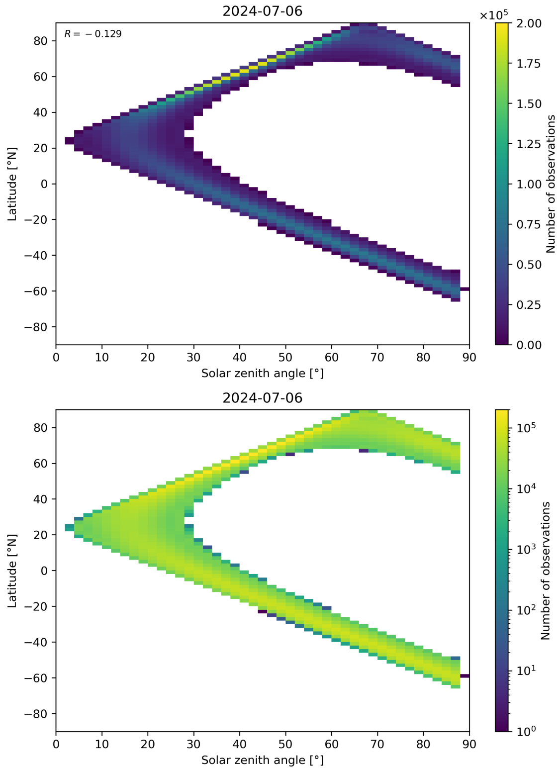
Figure 149: Scatter density plot of “Solar zenith angle” against “Latitude” for 2024-07-05 to 2024-07-07.
