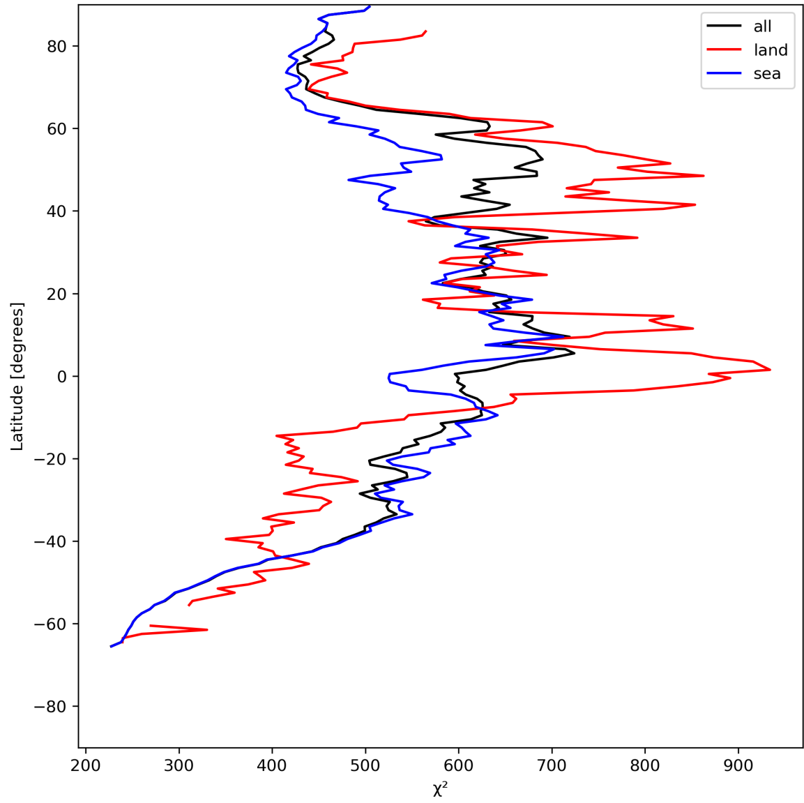
Figure 25: Zonal average of “ \chi^2 ” for 2024-07-05 to 2024-07-07.
