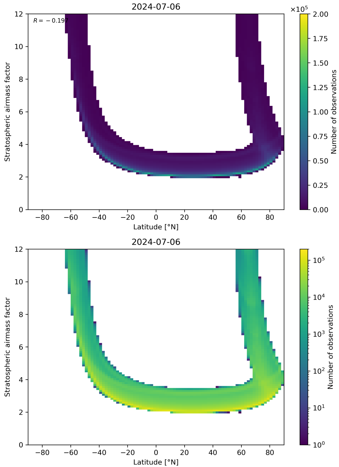
Figure 83: Scatter density plot of “Latitude” against “Stratospheric air mass factor” for 2024-07-05 to 2024-07-07.
