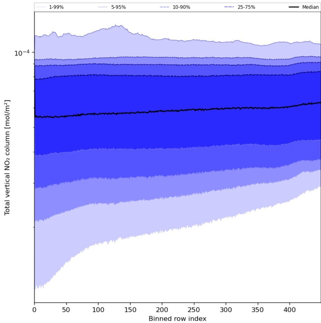
Figure 55: Along track statistics of “Total vertical NO 2 column” for 2024-07-05 to 2024-07-07
