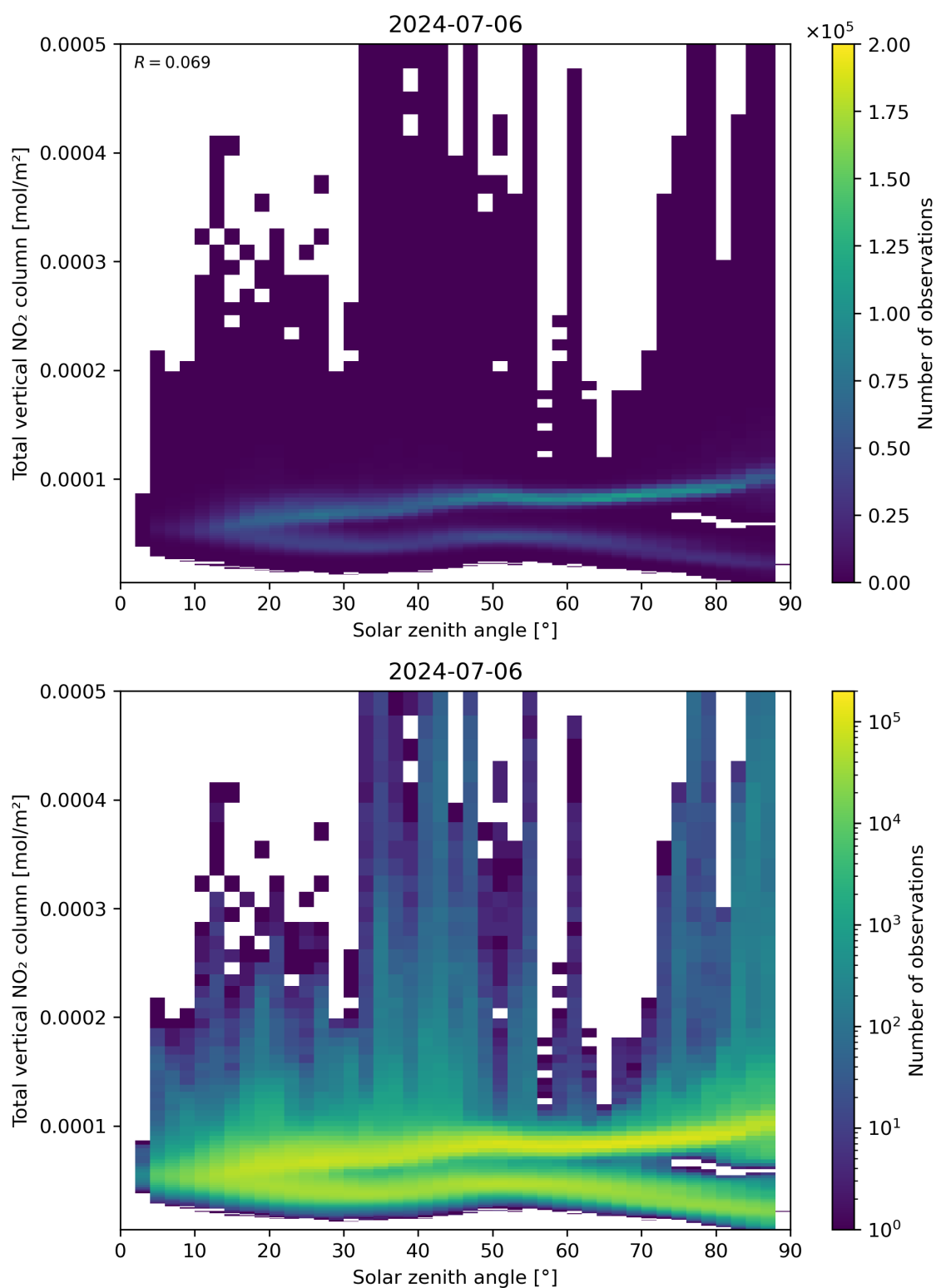
Figure 153: Scatter density plot of “Solar zenith angle” against “Total vertical NO 2 column” for 2024-07-05 to 2024-07-07.
