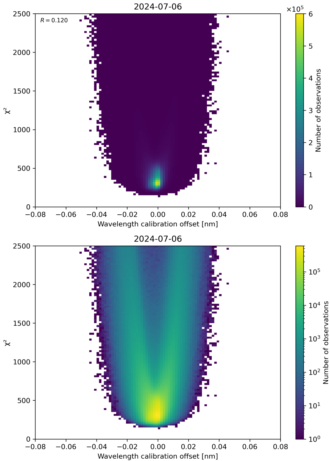
Figure 175: Scatter density plot of “Wavelength calibration offset” against “ \chi^2 ” for 2024-07-05 to 2024-07-07.
