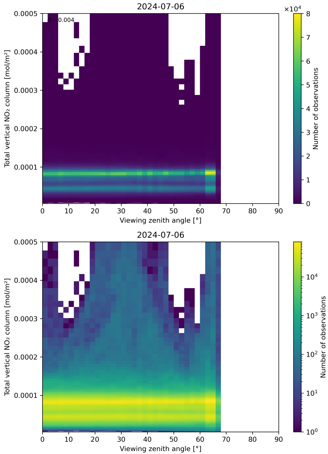
Figure 167: Scatter density plot of “Viewing zenith angle” against “Total vertical NO 2 column” for 2024-07-05 to 2024-07-07.
