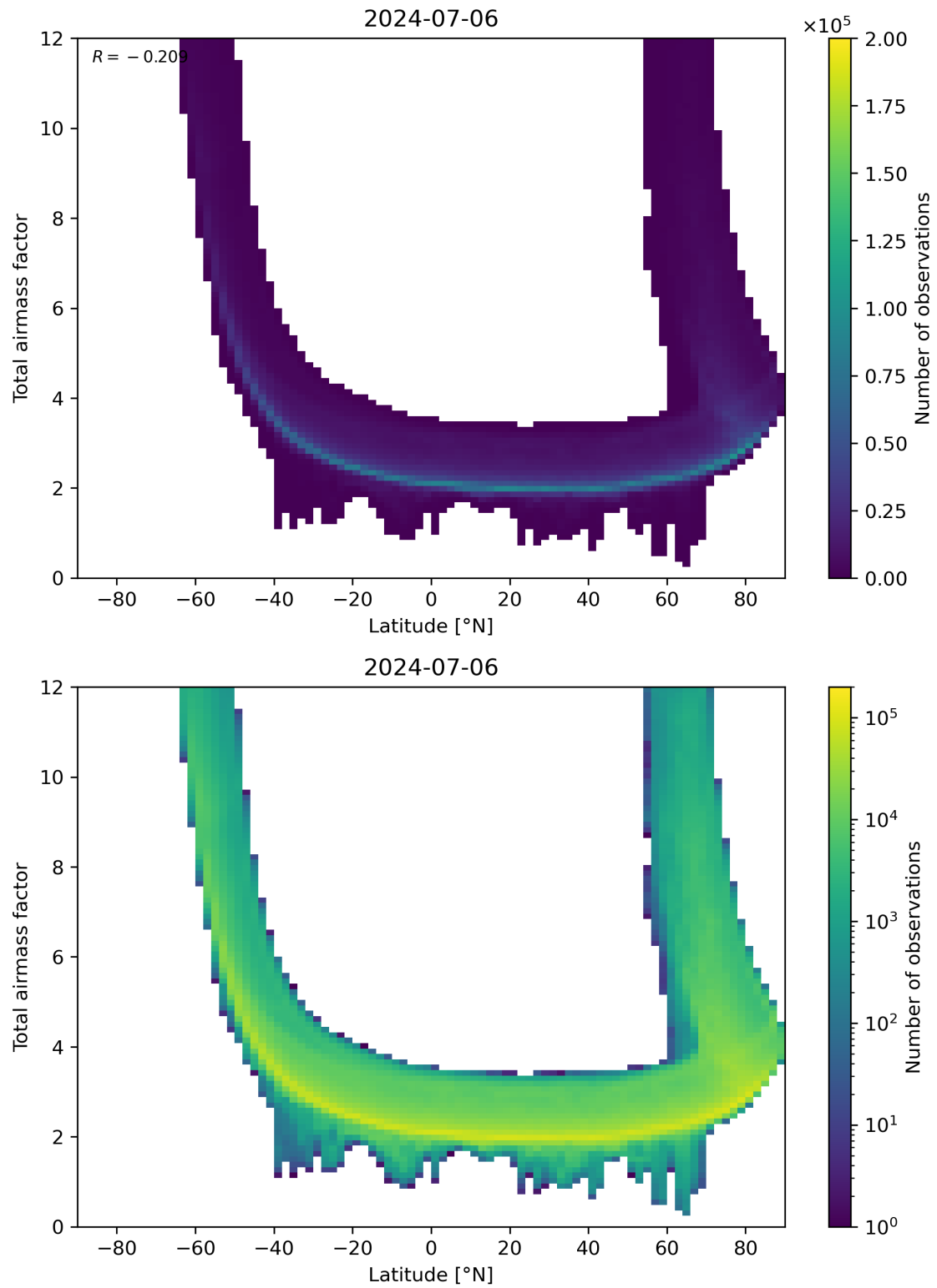
Figure 84: Scatter density plot of “Latitude” against “Total airmass factor” for 2024-07-05 to 2024-07-07.
