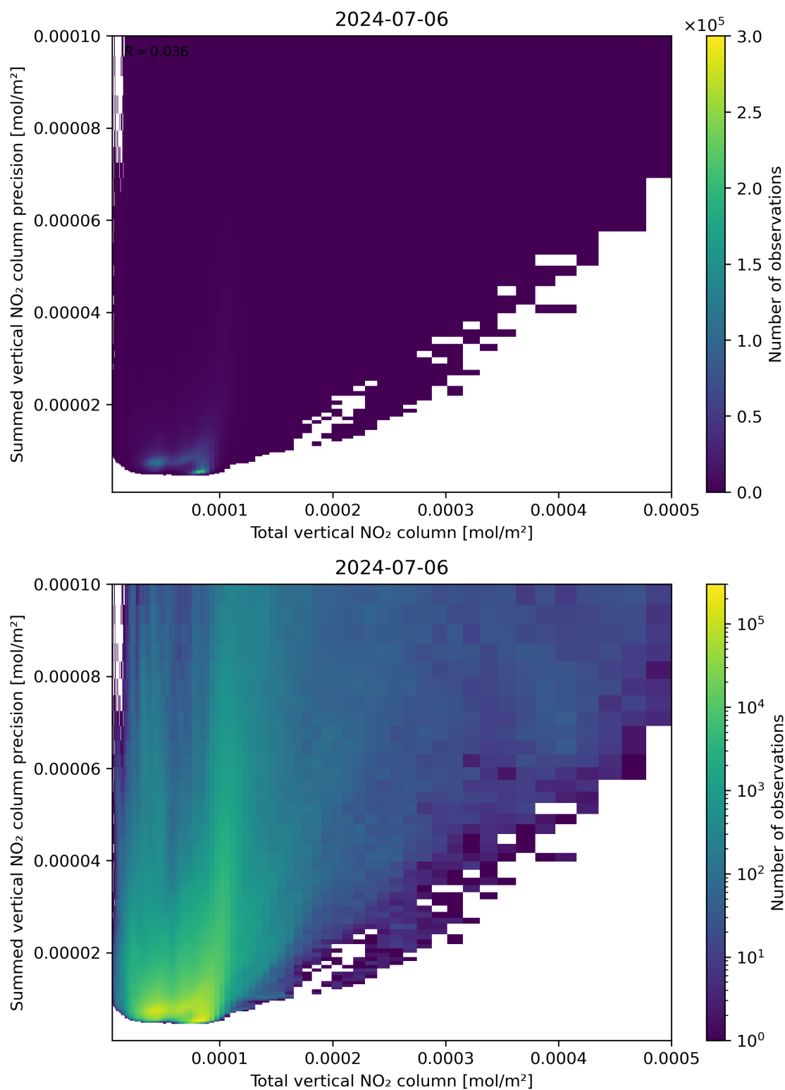
Figure 113: Scatter density plot of “Total vertical NO 2 column” against “Summed vertical NO 2 column precision” for 2024-07-05 to 2024-07-07.
