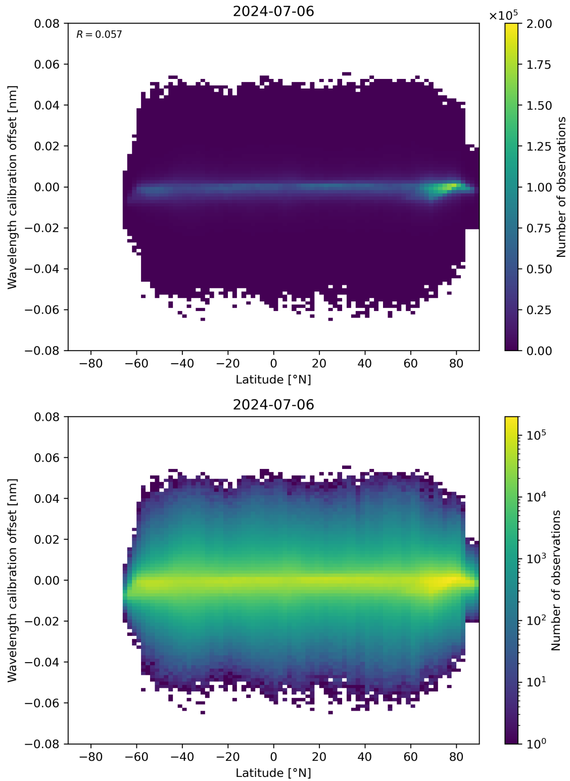
Figure 95: Scatter density plot of “Latitude” against “Wavelength calibration offset” for 2024-07-05 to 2024-07-07.
