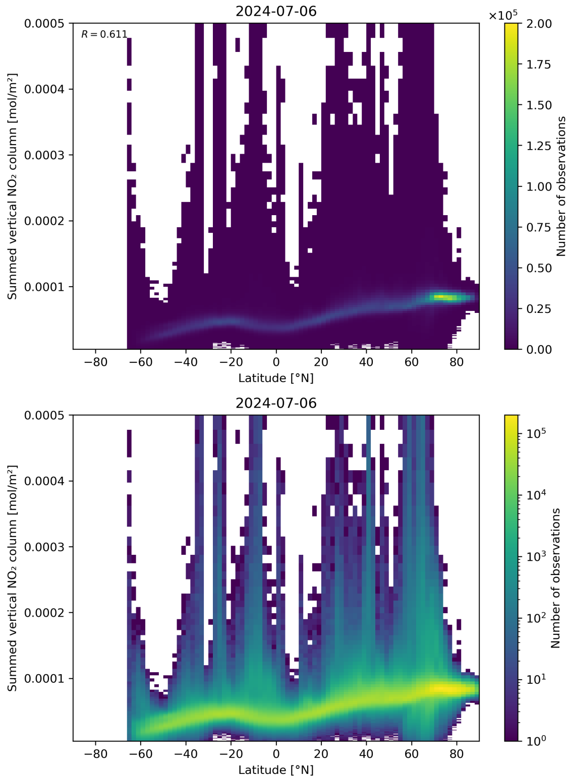
Figure 88: Scatter density plot of “Latitude” against “Summed vertical NO 2 column” for 2024-07-05 to 2024-07-07.
