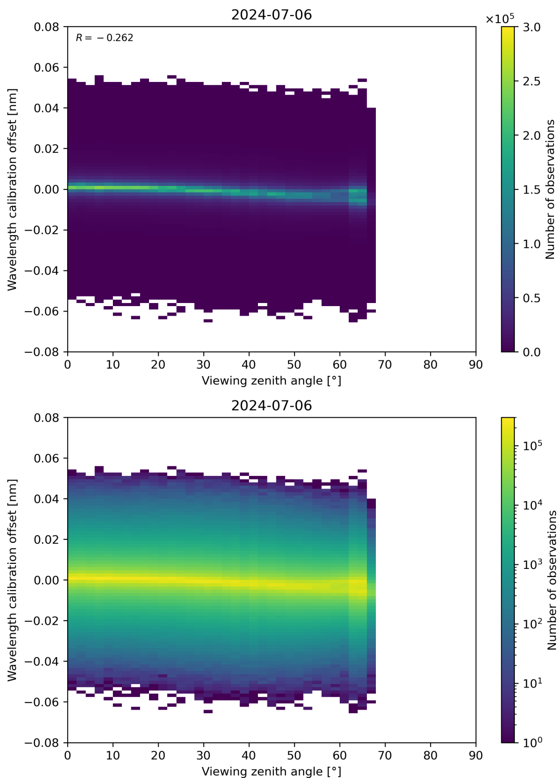
Figure 173: Scatter density plot of “Viewing zenith angle” against “Wavelength calibration offset” for 2024-07-05 to 2024-07-07.
