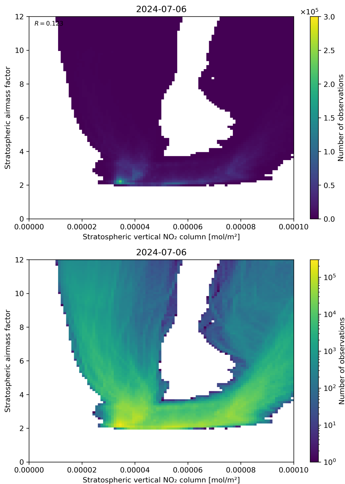
Figure 96: Scatter density plot of “Stratospheric vertical NO 2 column” against “Stratospheric airmass factor” for 2024-07-05 to 2024-07-07.
