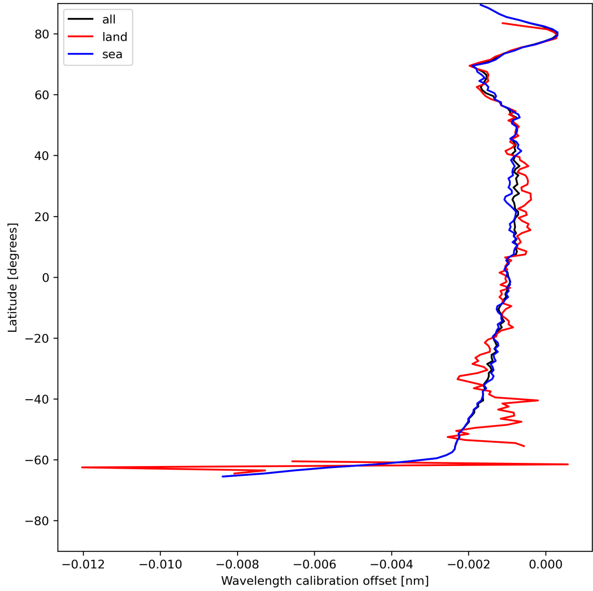
Figure 18: Zonal average of “Wavelength calibration offset” for 2024-07-05 to 2024-07-07.
