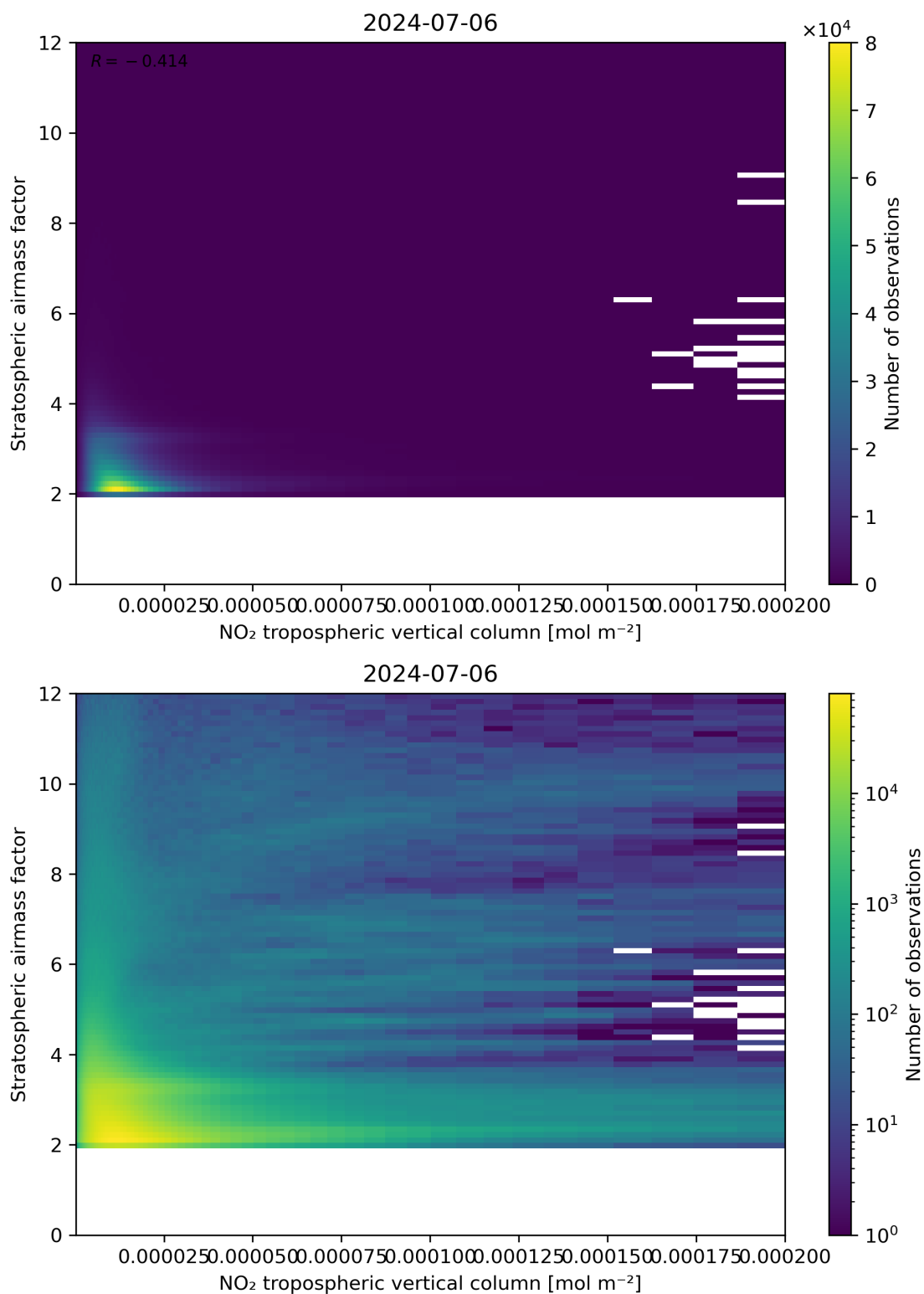
Figure 121: Scatter density plot of “NO 2 tropospheric vertical column” against “Stratospheric air mass factor” for 2024-07-05 to 2024-07-07.
