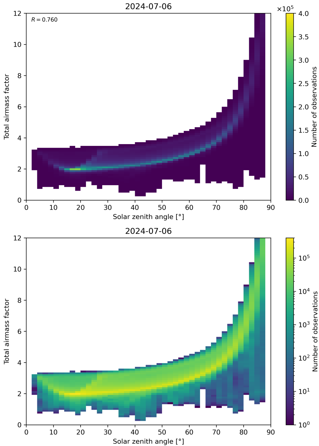
Figure 146: Scatter density plot of “Solar zenith angle” against “Total air mass factor” for 2024-07-05 to 2024-07-07.
