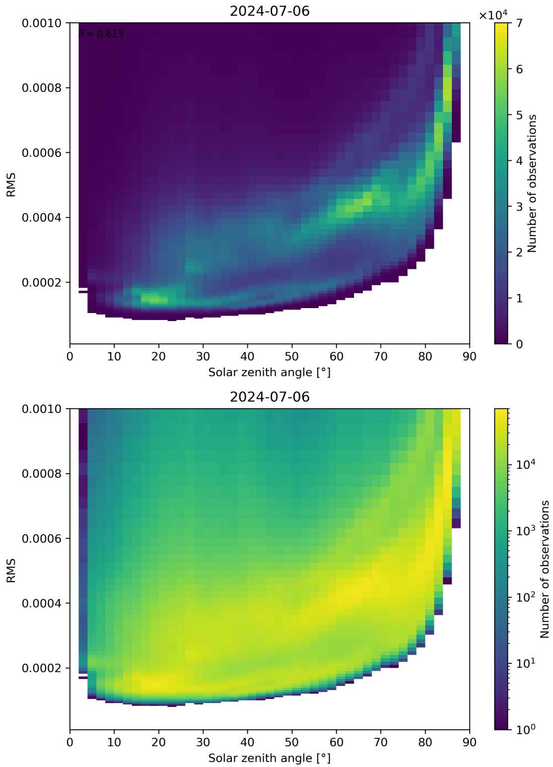
Figure 157: Scatter density plot of “Solar zenith angle” against “RMS” for 2024-07-05 to 2024-07-07.
