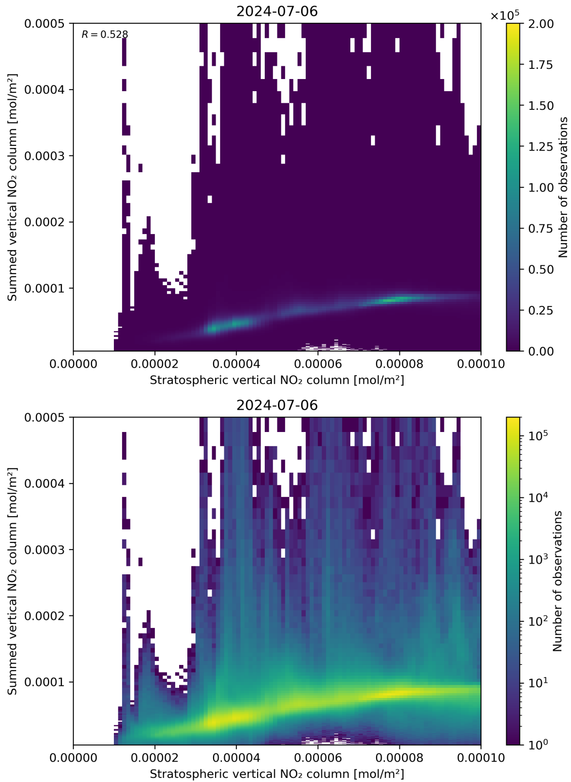
Figure 98: Scatter density plot of “Stratospheric vertical NO 2 column” against “Summed vertical NO 2 column” for 2024-07-05 to 2024-07-07.
