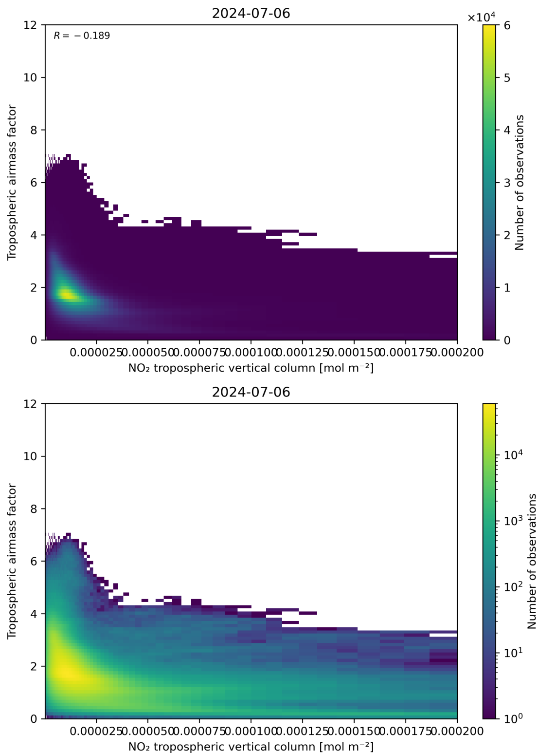
Figure 123: Scatter density plot of “NO 2 tropospheric vertical column” against “Tropospheric airmass factor” for 2024-07-05 to 2024-07-07.
