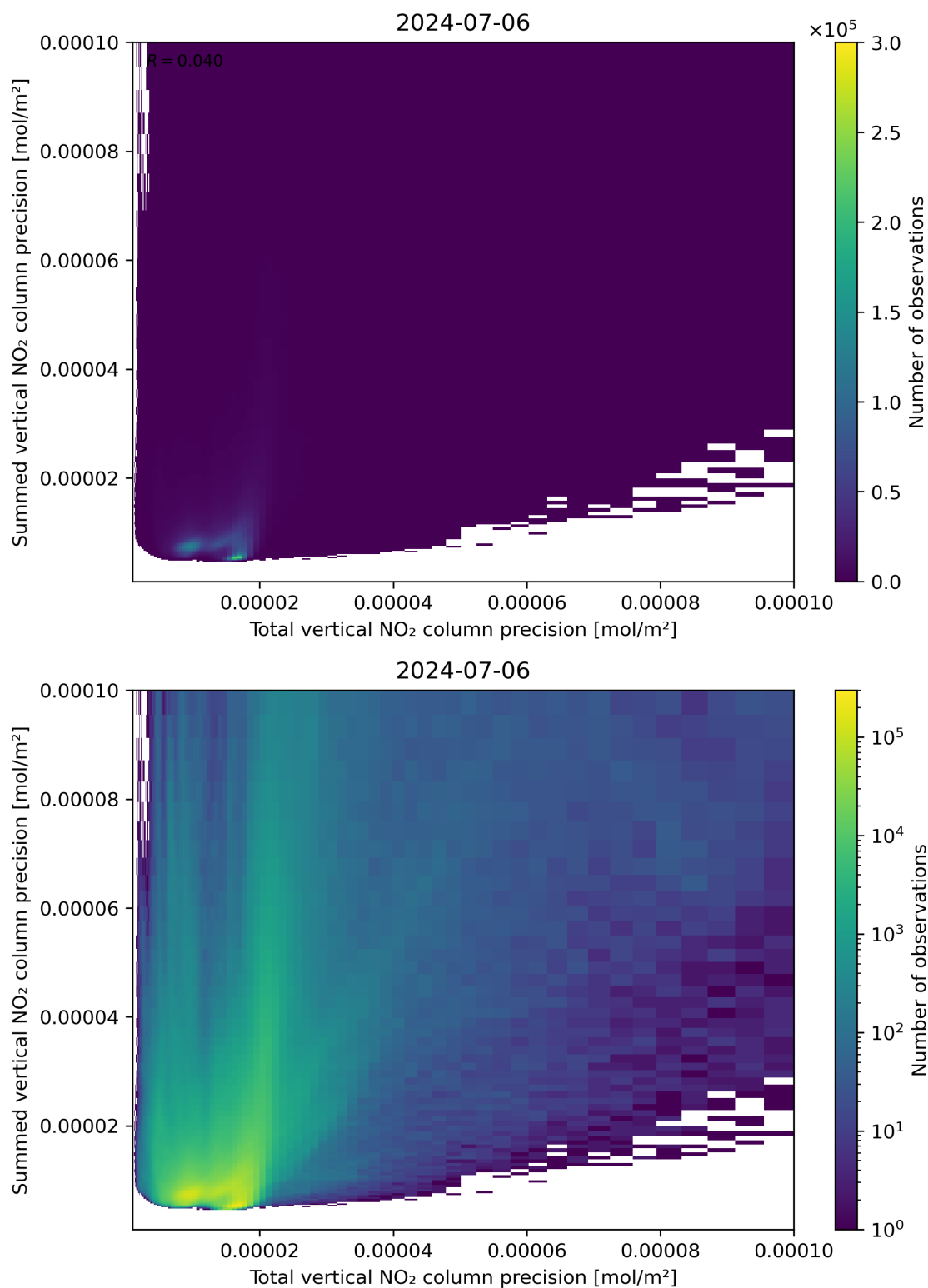
Figure 118: Scatter density plot of “Total vertical NO 2 column precision” against “Summed vertical NO 2 column precision” for 2024-07-05 to 2024-07-07.
