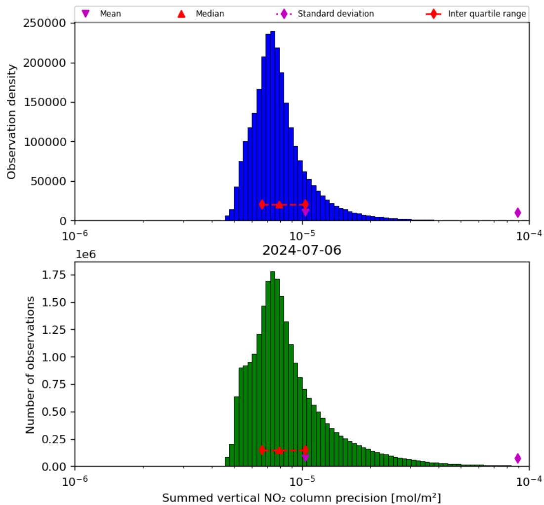
Figure 41: Histogram of "Summed vertical NO 2 column precision" for 2024-07-05 to 2024-07-07
