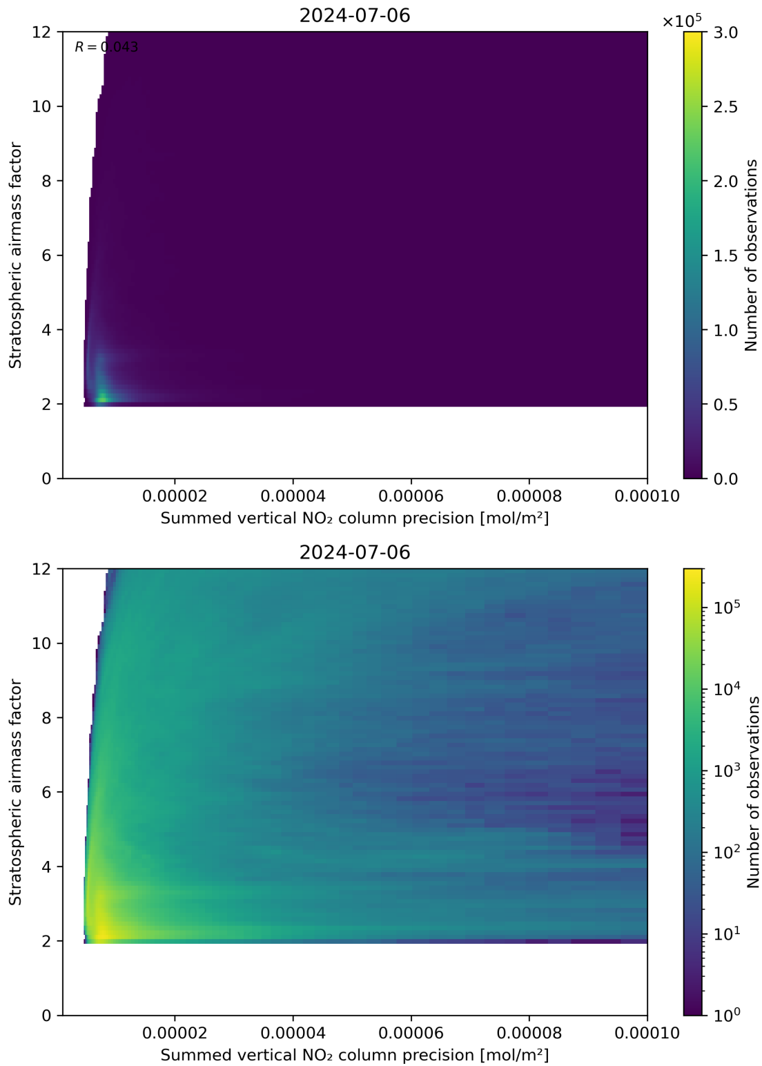
Figure 106: Scatter density plot of “Summed vertical NO 2 column precision” against “Stratospheric airmass factor” for 2024-07-05 to 2024-07-07.
