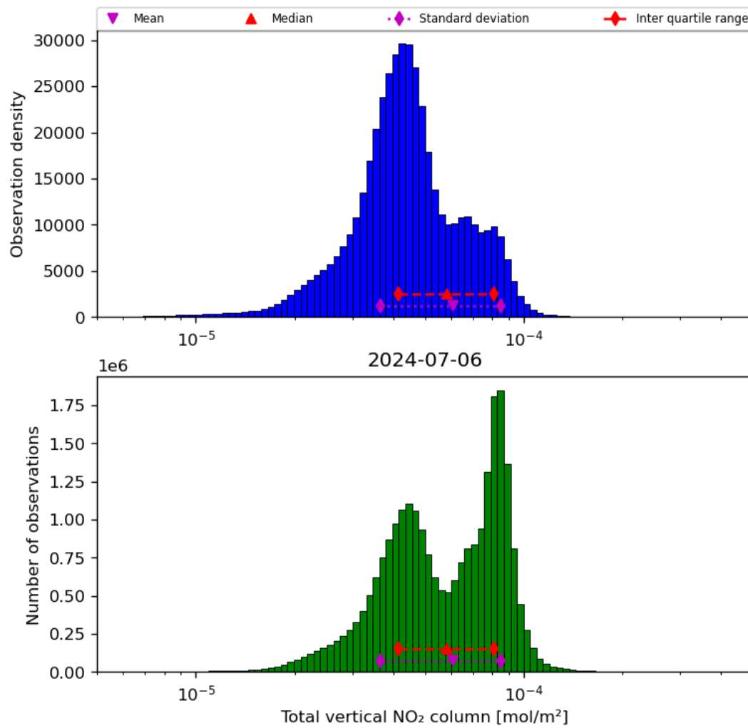
Figure 38: Histogram of “Total vertical NO 2 column” for 2024-07-05 to 2024-07-07
