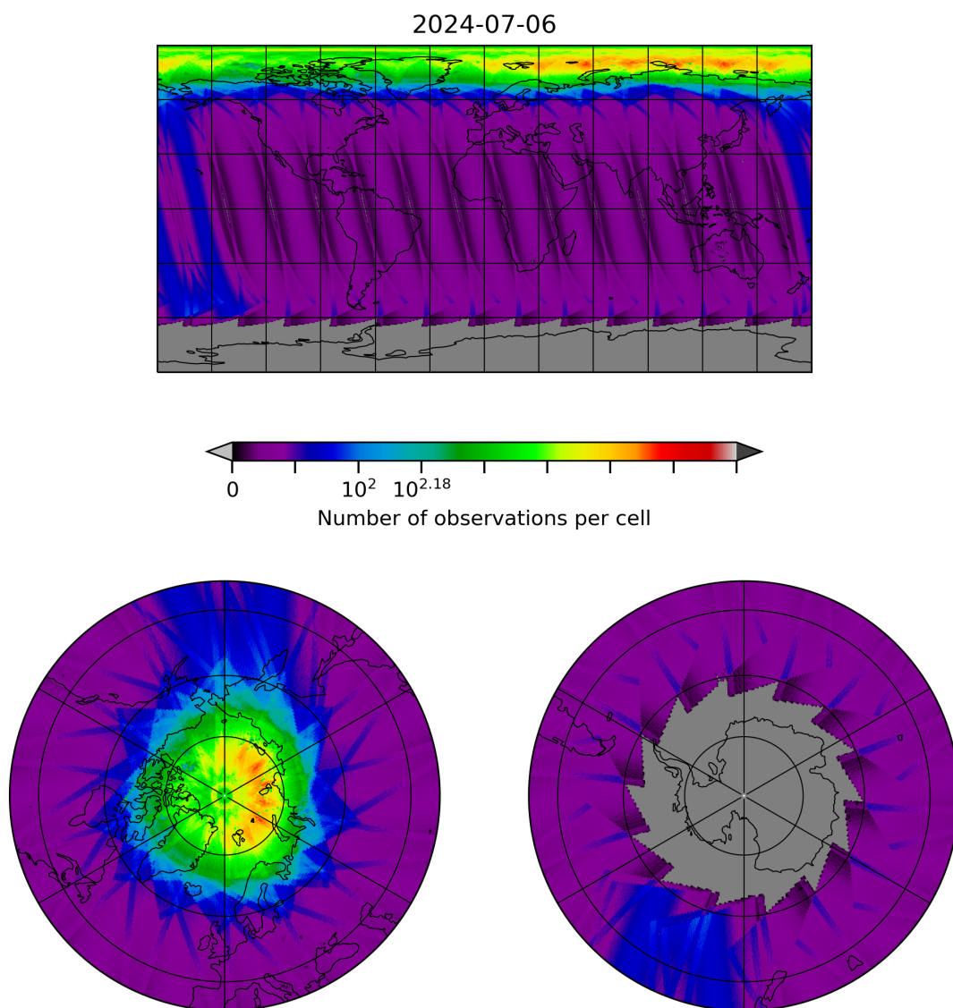
Figure 10: Map of the number of observations for 2024-07-05 to 2024-07-07
