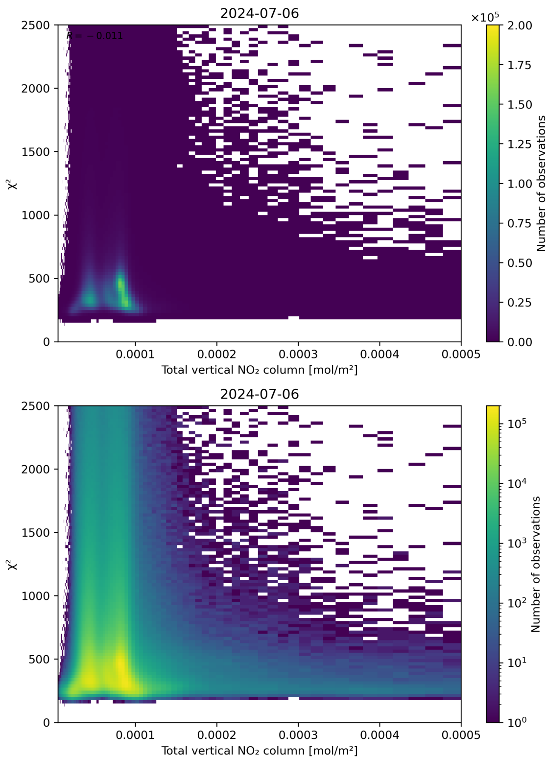
Figure 111: Scatter density plot of “Total vertical NO 2 column” against “ \chi^2 ” for 2024-07-05 to 2024-07-07.
