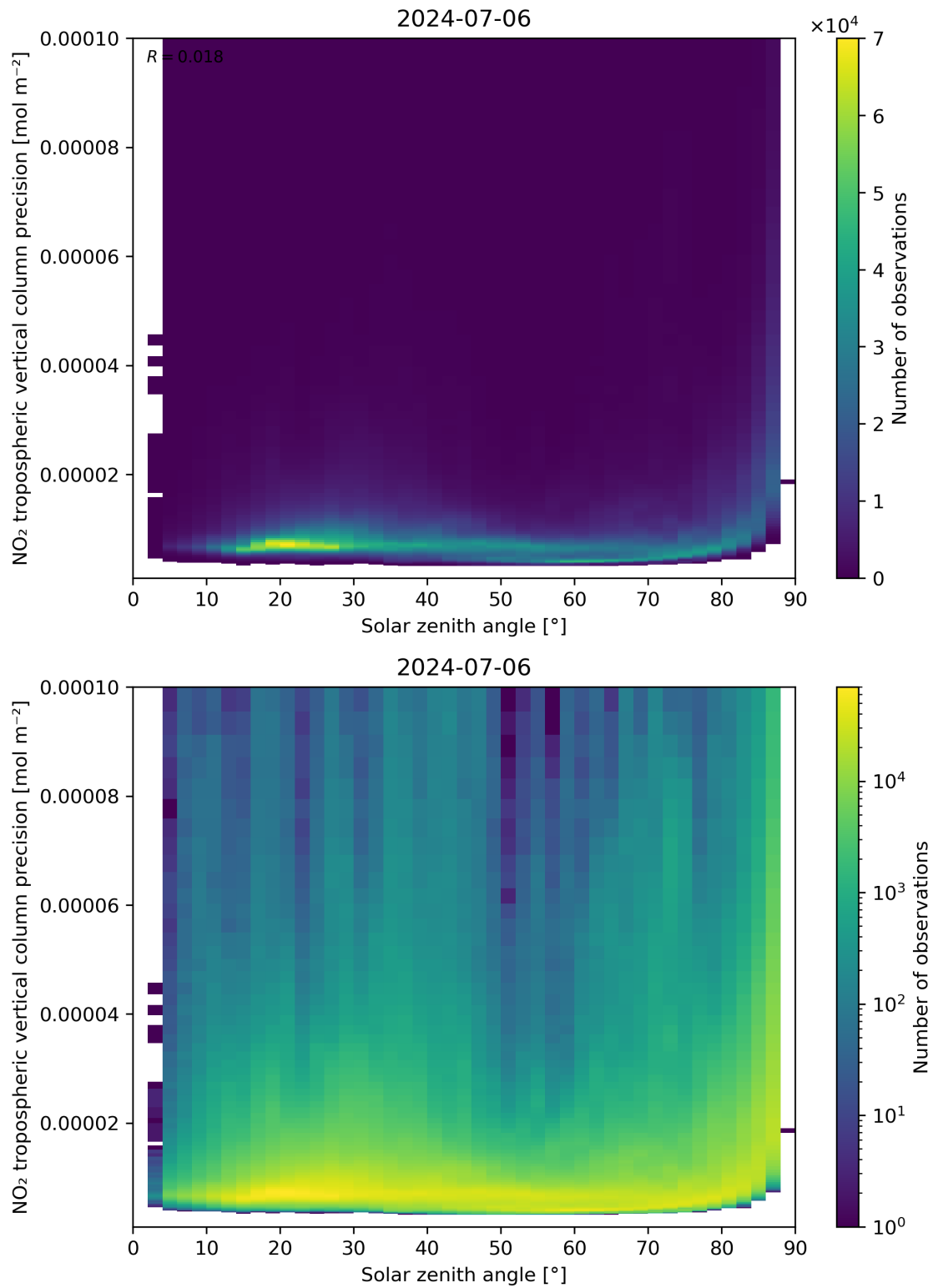
Figure 156: Scatter density plot of “Solar zenith angle” against “NO 2 tropospheric vertical column precision” for 2024-07-05 to 2024-07-07.
