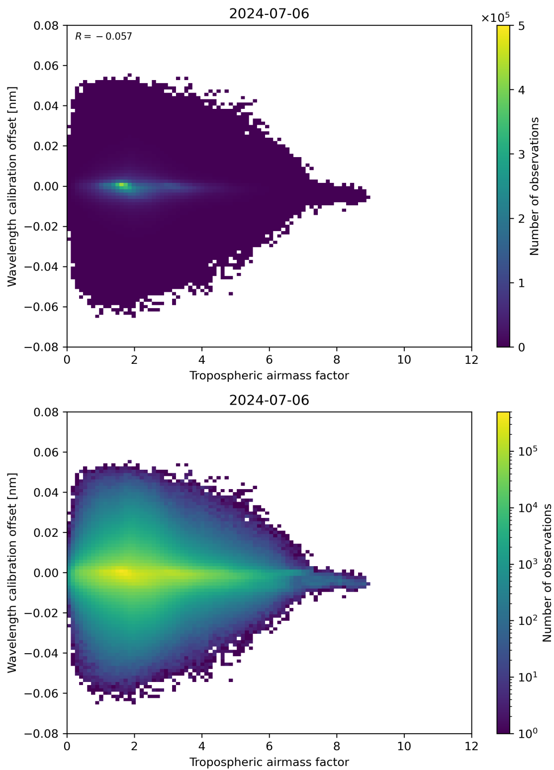
Figure 80: Scatter density plot of “Tropospheric airmass factor” against “Wavelength calibration offset” for 2024-07-05 to 2024-07-07.
