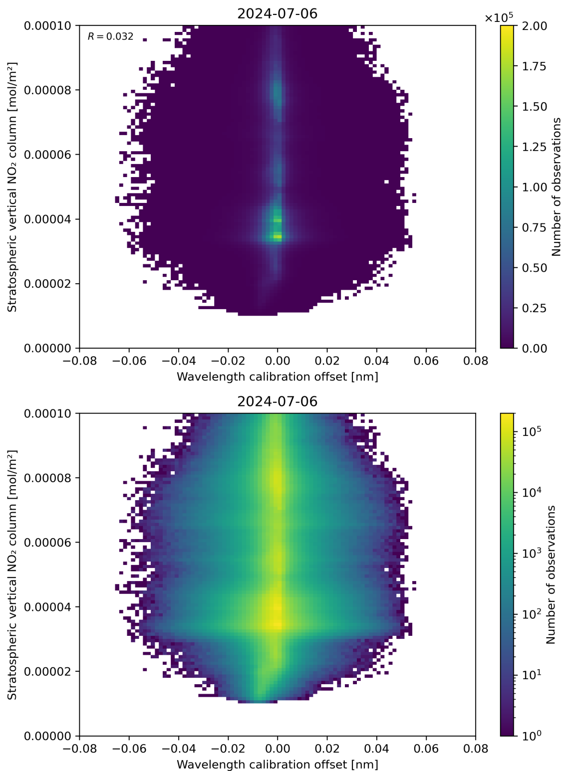
Figure 176: Scatter density plot of “Wavelength calibration offset” against “Stratospheric vertical NO 2 column” for 2024-07-05 to 2024-07-07.
