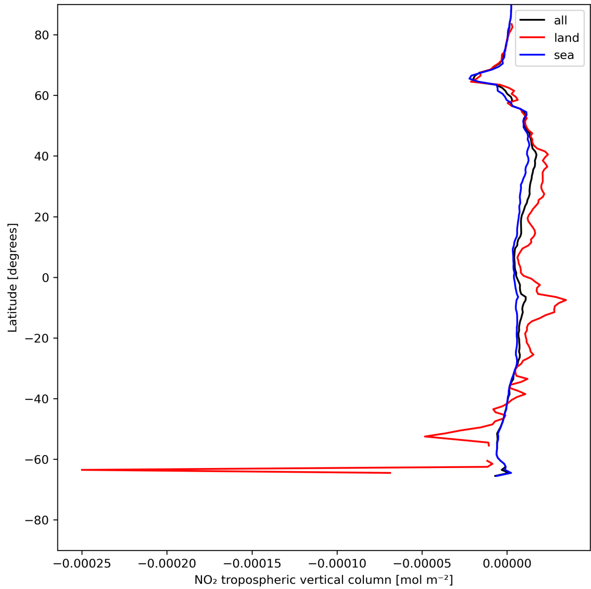
Figure 12: Zonal average of “NO 2 tropospheric vertical column” for 2024-07-05 to 2024-07-07.
