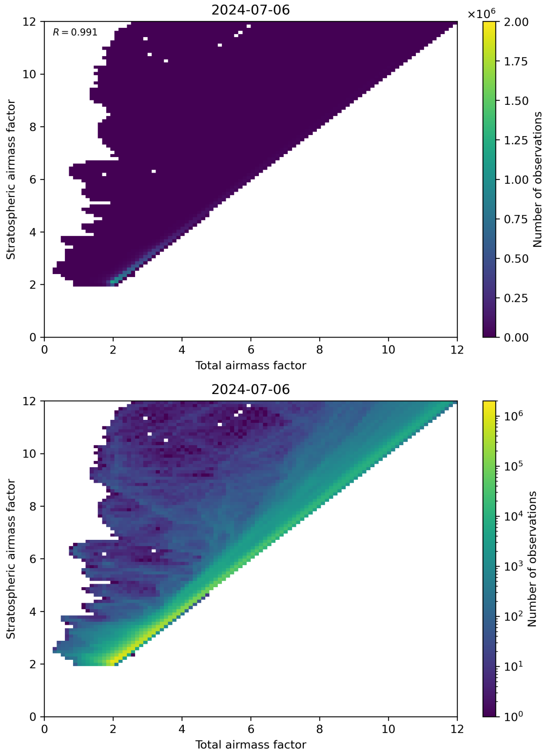
Figure 62: Scatter density plot of “Total airmass factor” against “Stratospheric airmass factor” for 2024-07-05 to 2024-07-07.
