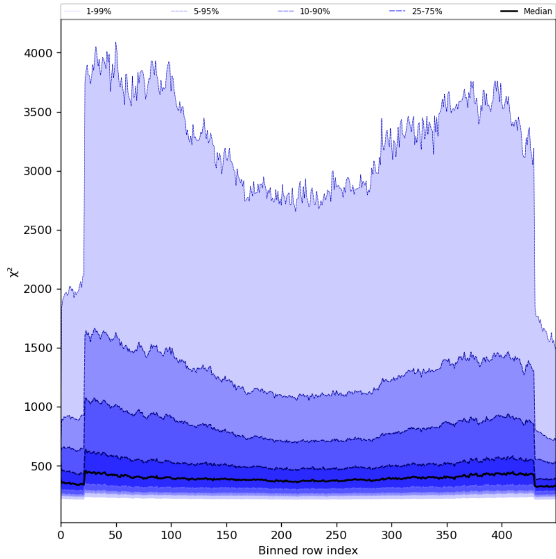
Figure 59: Along track statistics of “ \chi^2 ” for 2024-07-05 to 2024-07-07
