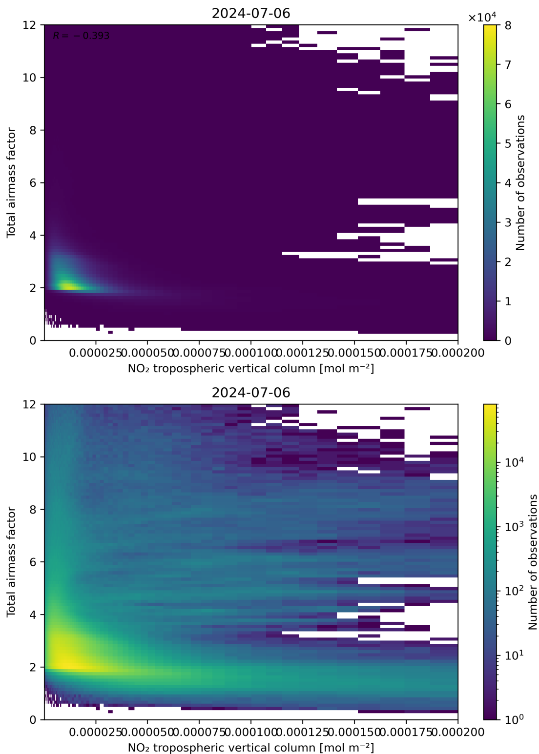
Figure 122: Scatter density plot of “NO 2 tropospheric vertical column” against “Total air mass factor” for 2024-07-05 to 2024-07-07.
