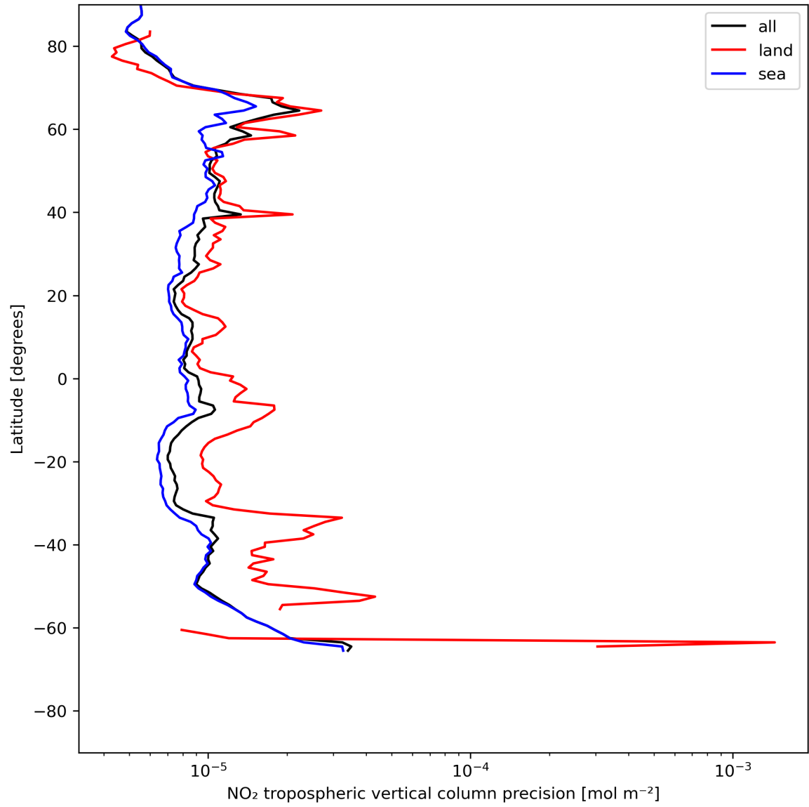
Figure 13: Zonal average of “NO 2 tropospheric vertical column precision” for 2024-07-05 to 2024-07-07.
