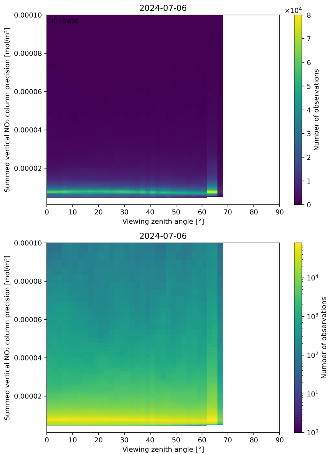
Figure 166: Scatter density plot of “Viewing zenith angle” against “Summed vertical NO 2 column precision” for 2024-07-05 to 2024-07-07.
