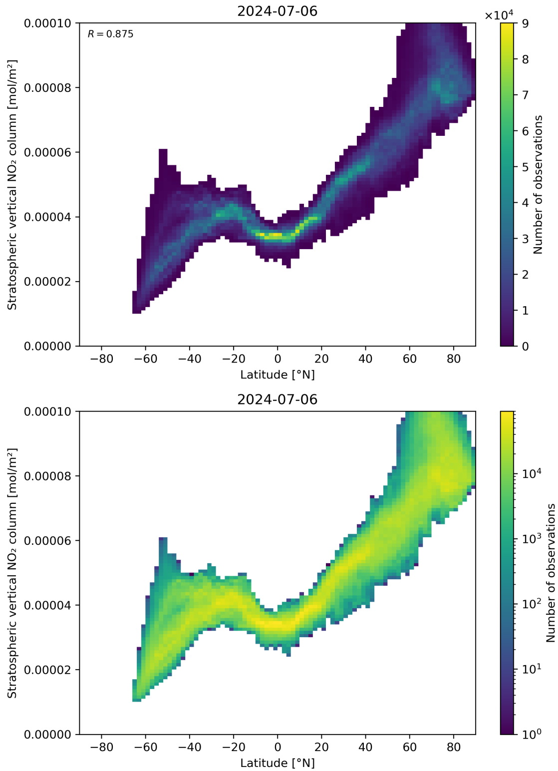
Figure 87: Scatter density plot of “Latitude” against “Stratospheric vertical NO 2 column” for 2024-07-05 to 2024-07-07.
