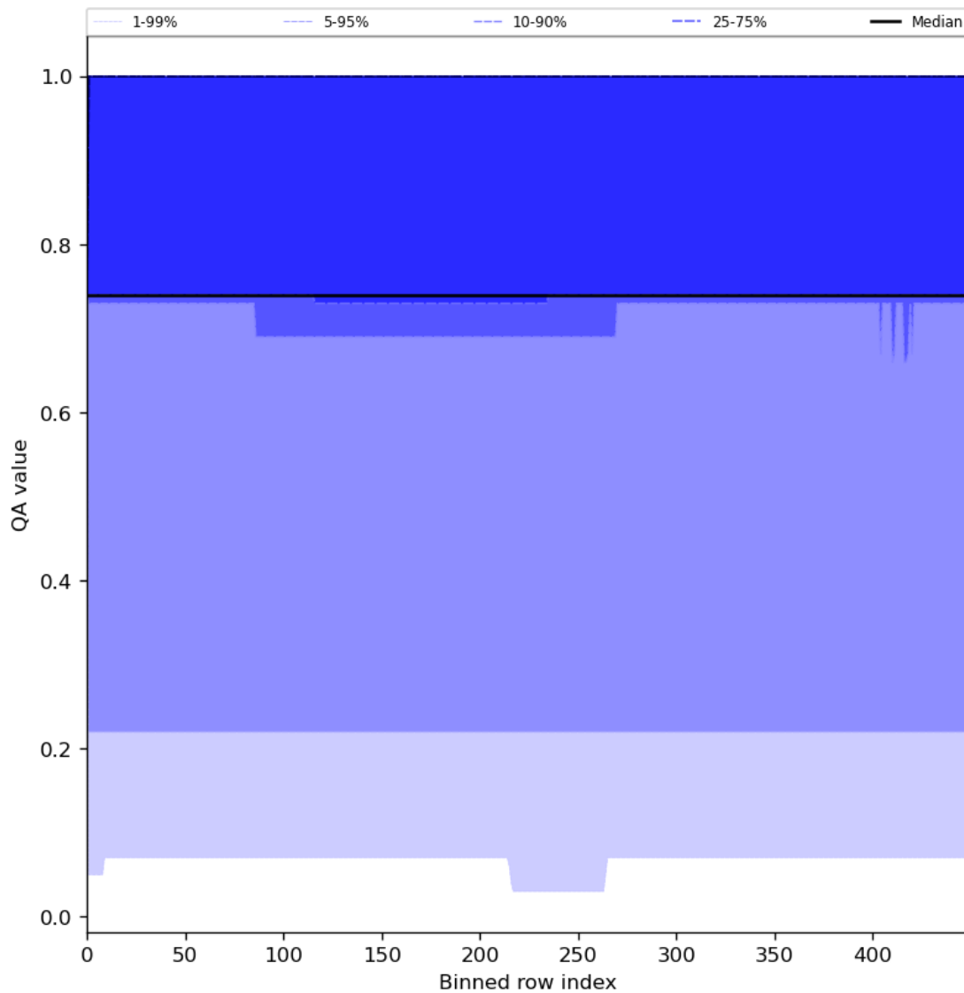
Figure 45: Along track statistics of “QA value” for 2024-07-05 to 2024-07-07
