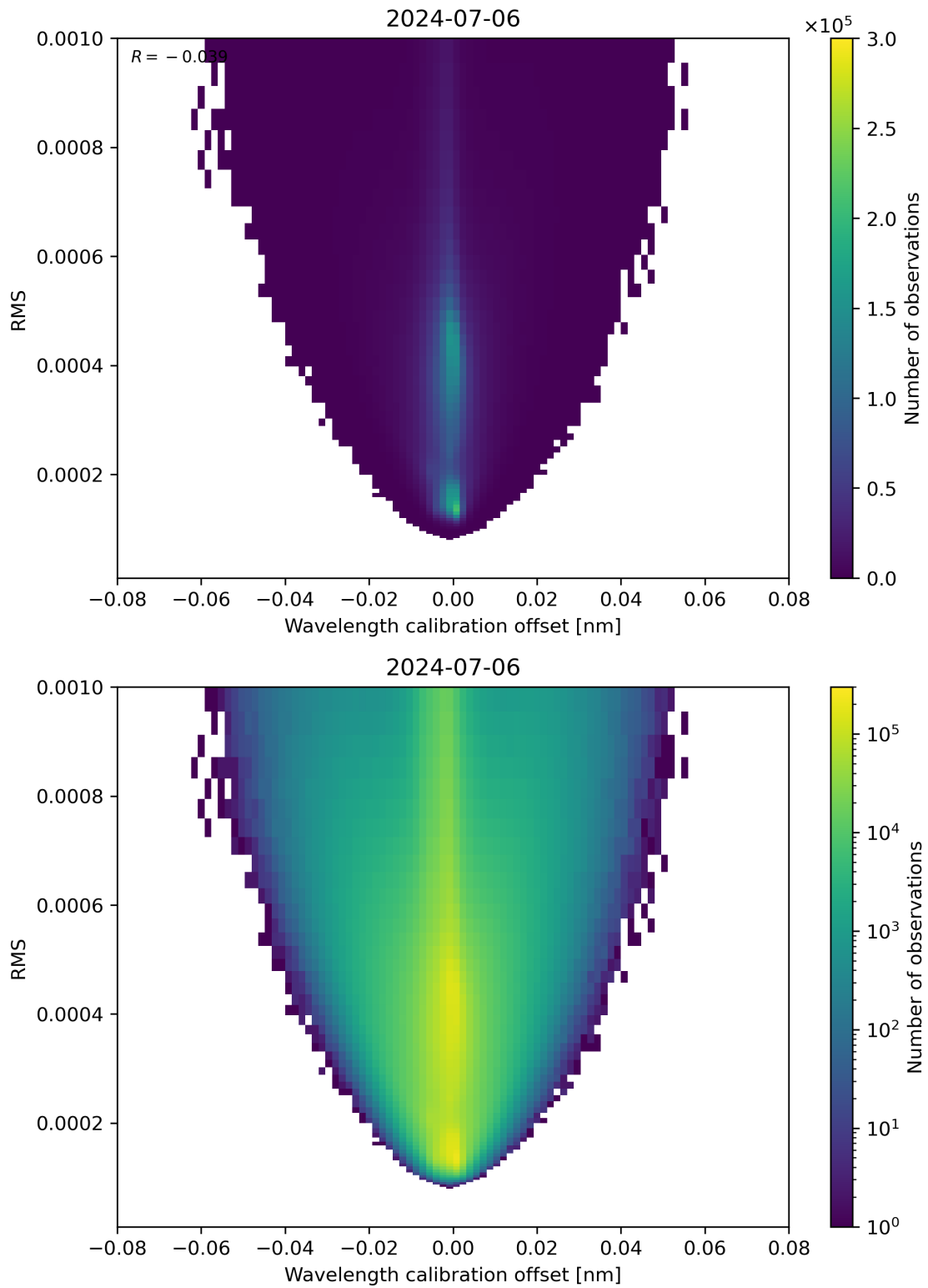
Figure 181: Scatter density plot of “Wavelength calibration offset” against “RMS” for 2024-07-05 to 2024-07-07.
