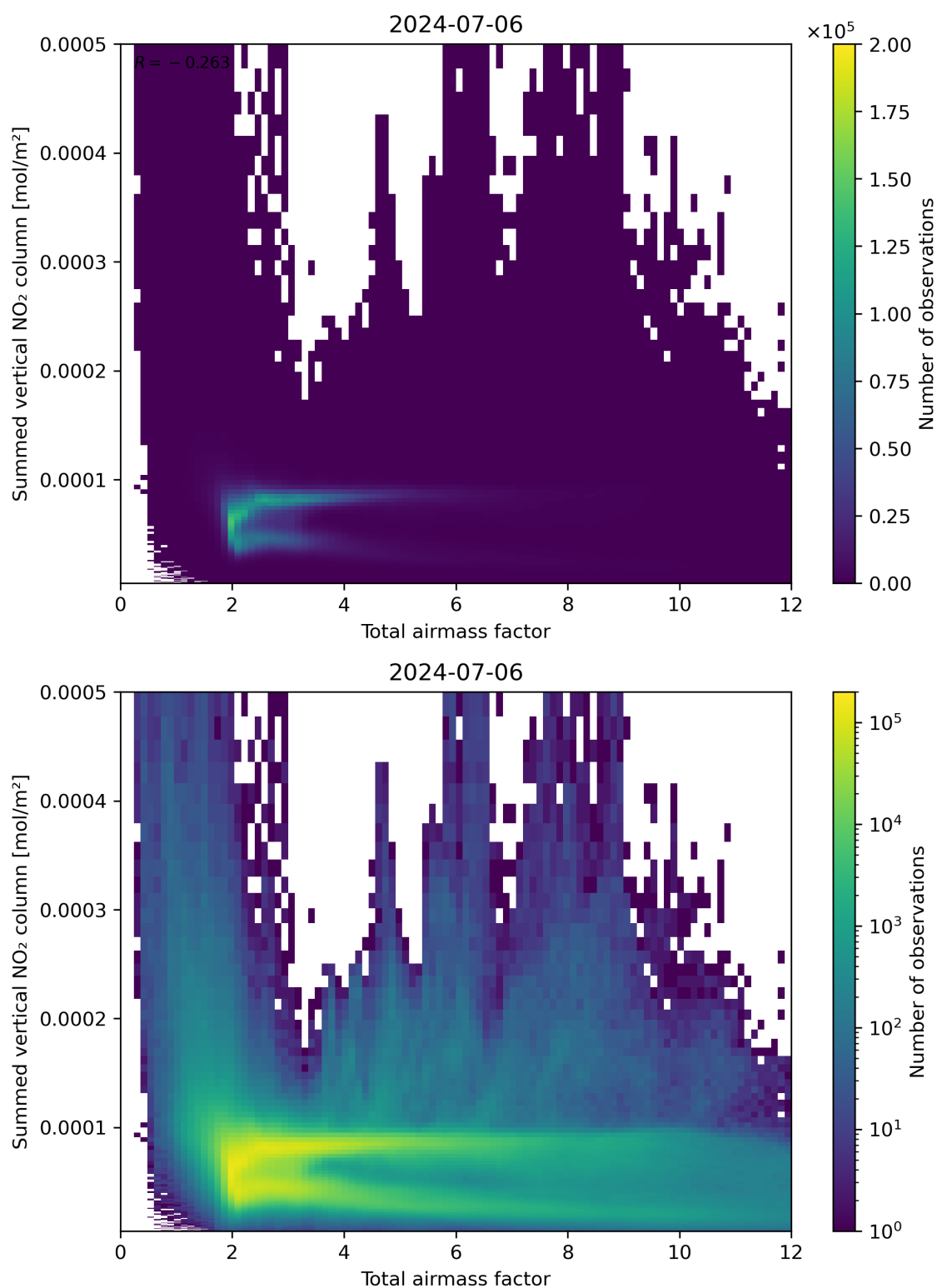
Figure 65: Scatter density plot of “Total airmass factor” against “Summed vertical NO 2 column” for 2024-07-05 to 2024-07-07.
