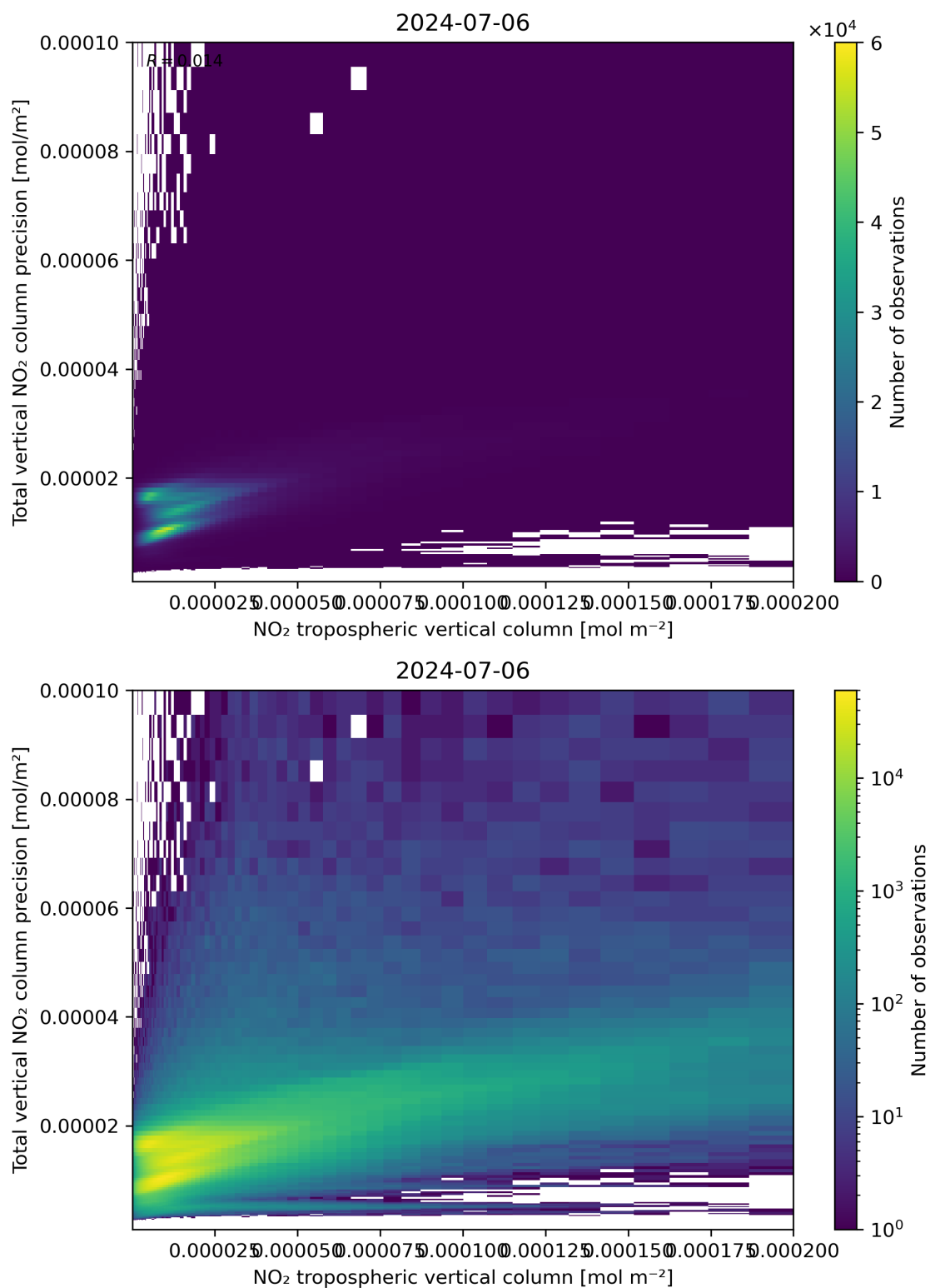
Figure 129: Scatter density plot of “NO 2 tropospheric vertical column” against “Total vertical NO 2 column precision” for 2024-07-05 to 2024-07-07.
