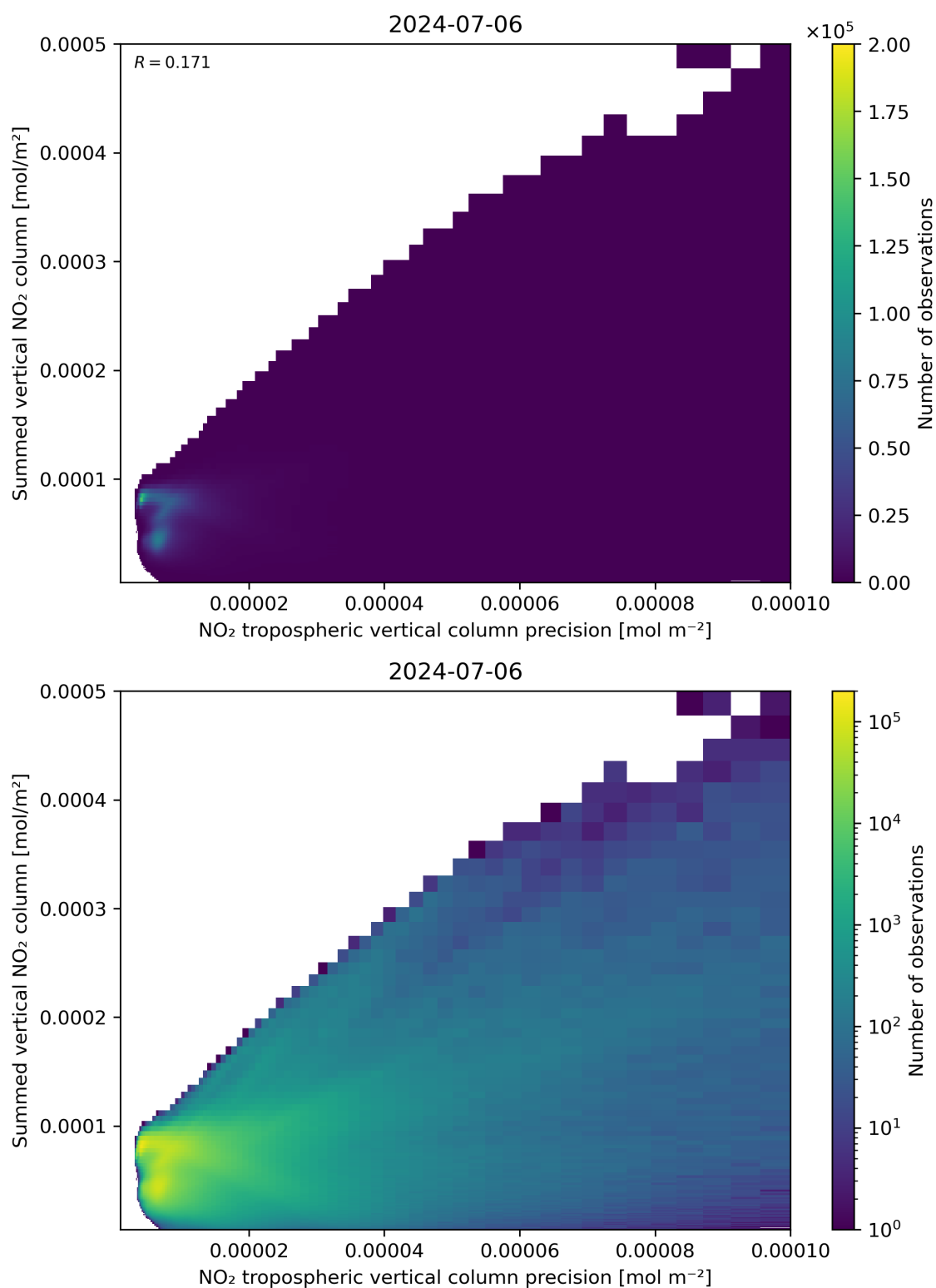
Figure 136: Scatter density plot of “NO 2 tropospheric vertical column precision” against “Summed vertical NO 2 column” for 2024-07-05 to 2024-07-07.
