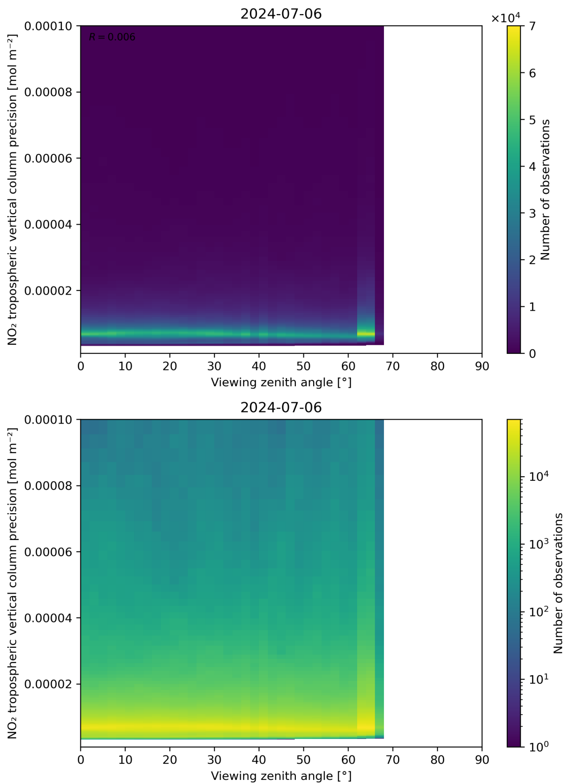
Figure 170: Scatter density plot of “Viewing zenith angle” against “NO 2 tropospheric vertical column precision” for 2024-07-05 to 2024-07-07.
