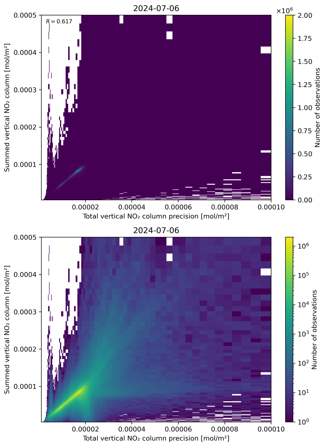
Figure 117: Scatter density plot of “Total vertical NO 2 column precision” against “Summed vertical NO 2 column” for 2024-07-05 to 2024-07-07.
