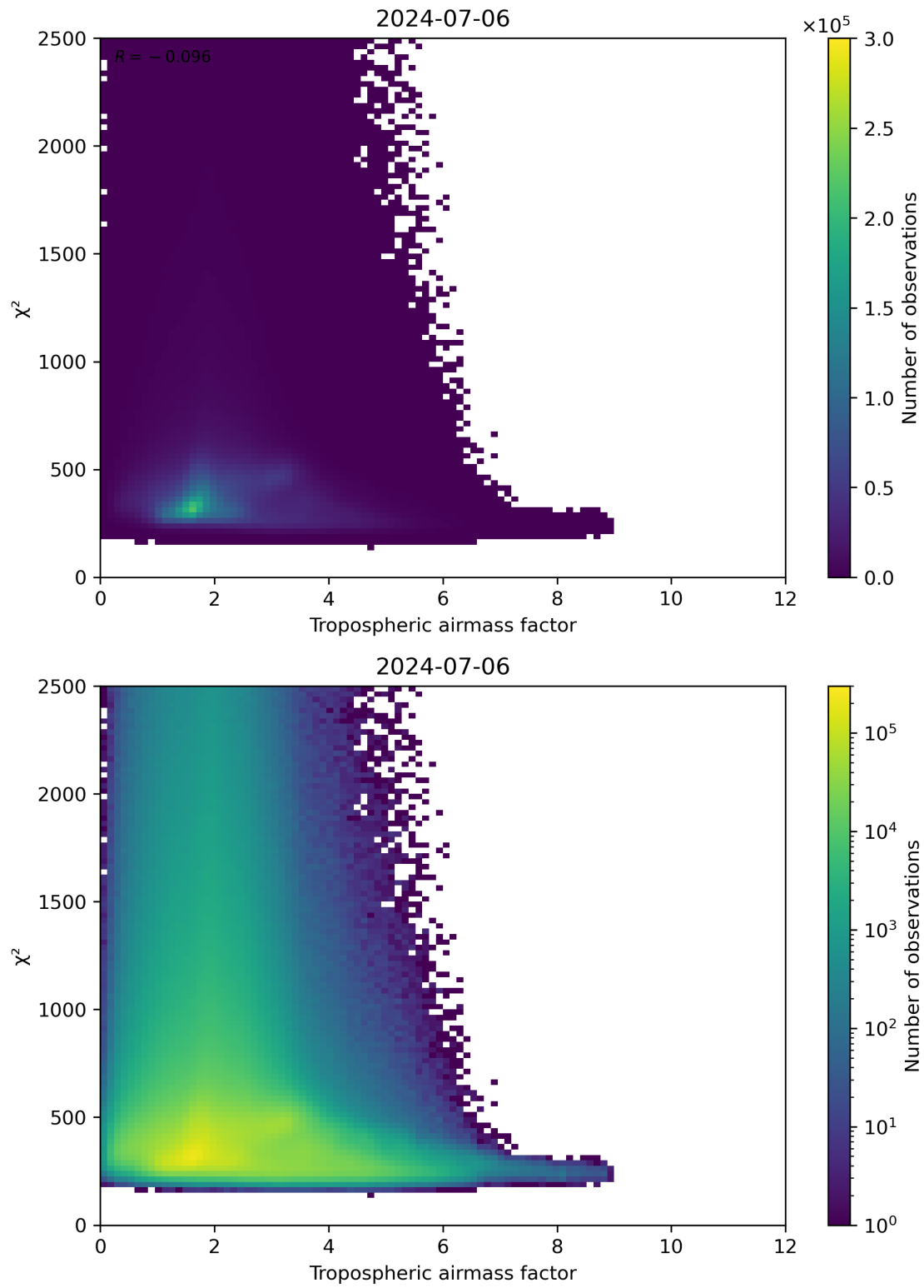
Figure 73: Scatter density plot of “Tropospheric airmass factor” against “ \chi^2 ” for 2024-07-05 to 2024-07-07.
