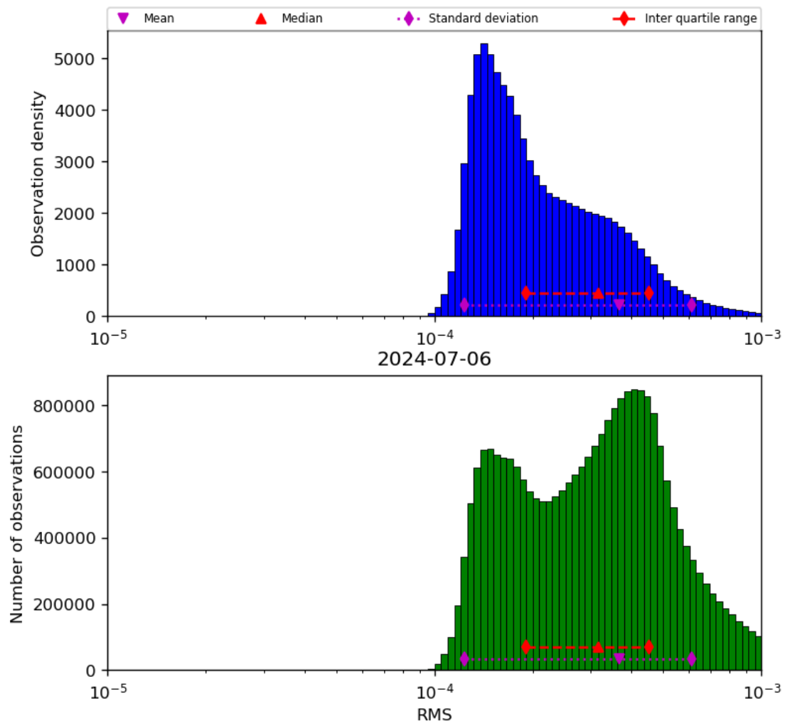
Figure 43: Histogram of “RMS” for 2024-07-05 to 2024-07-07
