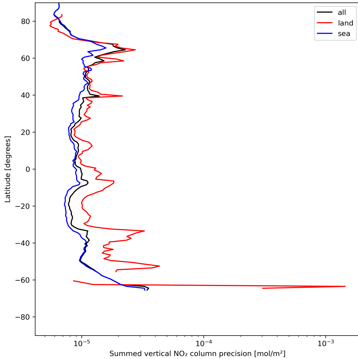
Figure 24: Zonal average of “Summed vertical NO 2 column precision” for 2024-07-05 to 2024-07-07.
