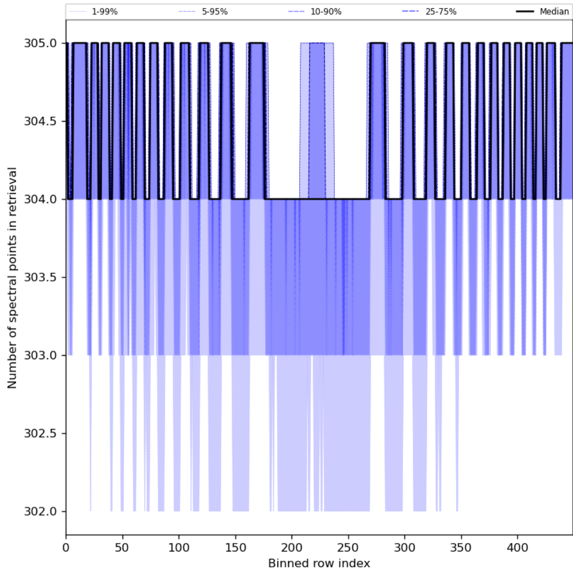
Figure 50: Along track statistics of “Number of spectral points in retrieval” for 2024-07-05 to 2024-07-07
