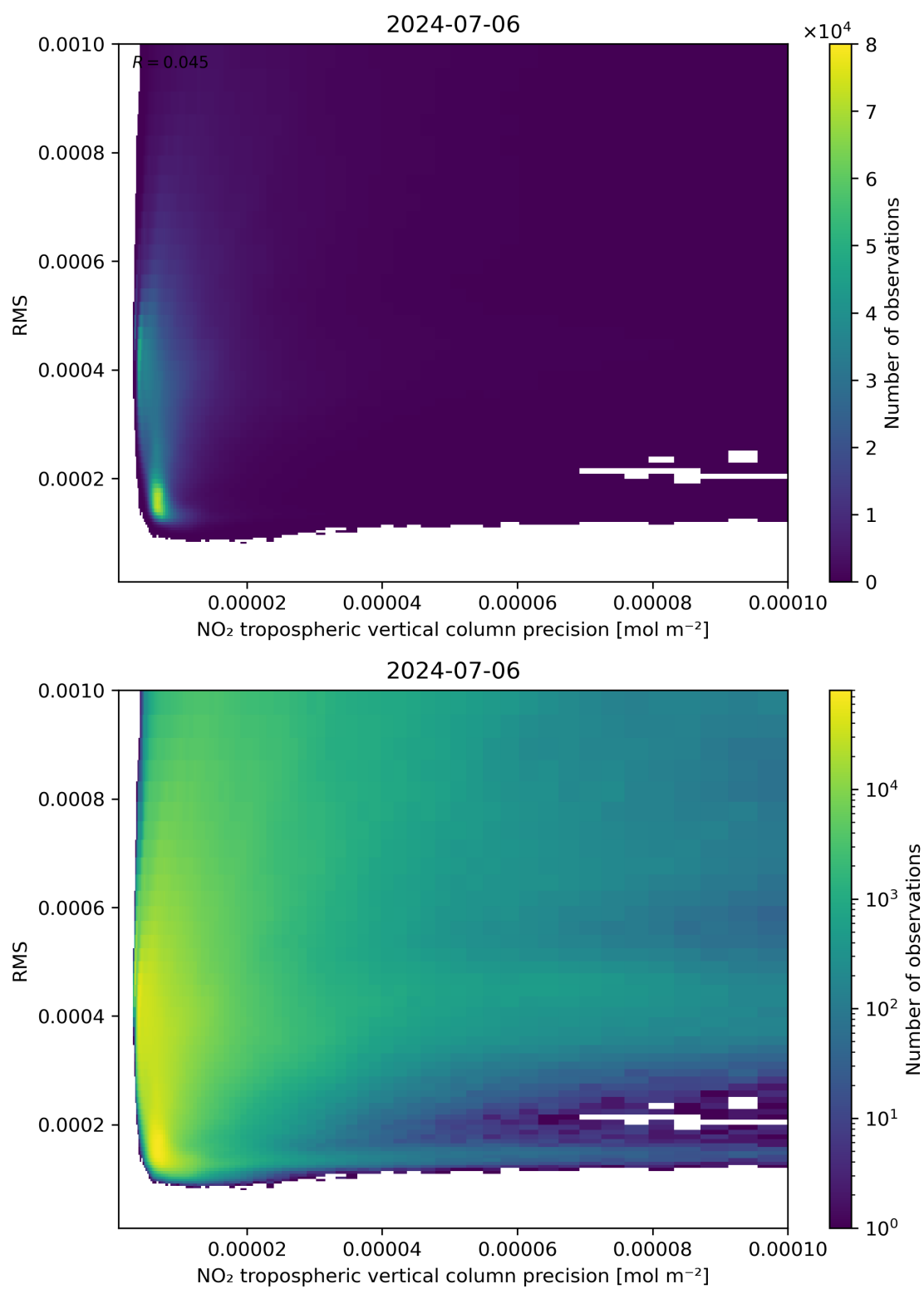
Figure 140: Scatter density plot of “NO 2 tropospheric vertical column precision” against “RMS” for 2024-07-05 to 2024-07-07.
