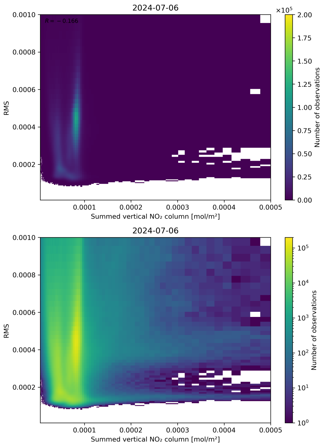
Figure 109: Scatter density plot of “Summed vertical NO 2 column” against “RMS” for 2024-07-05 to 2024-07-07.
