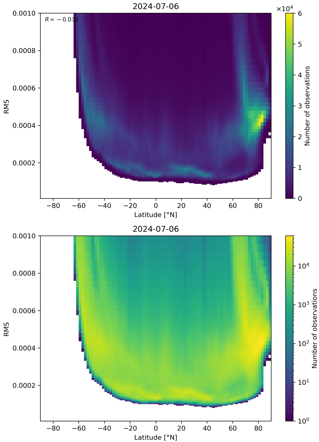
Figure 94: Scatter density plot of “Latitude” against “RMS” for 2024-07-05 to 2024-07-07.
