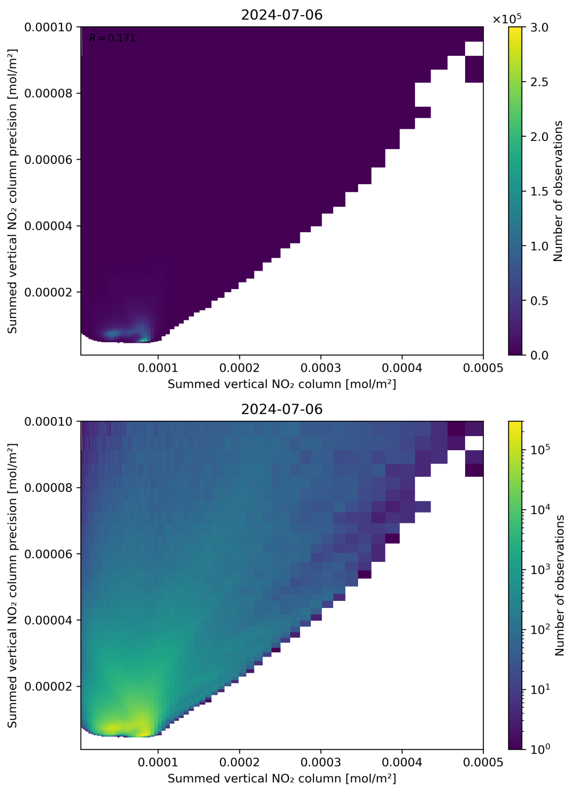
Figure 105: Scatter density plot of “Summed vertical NO 2 column” against “Summed vertical NO 2 column precision” for 2024-07-05 to 2024-07-07.
