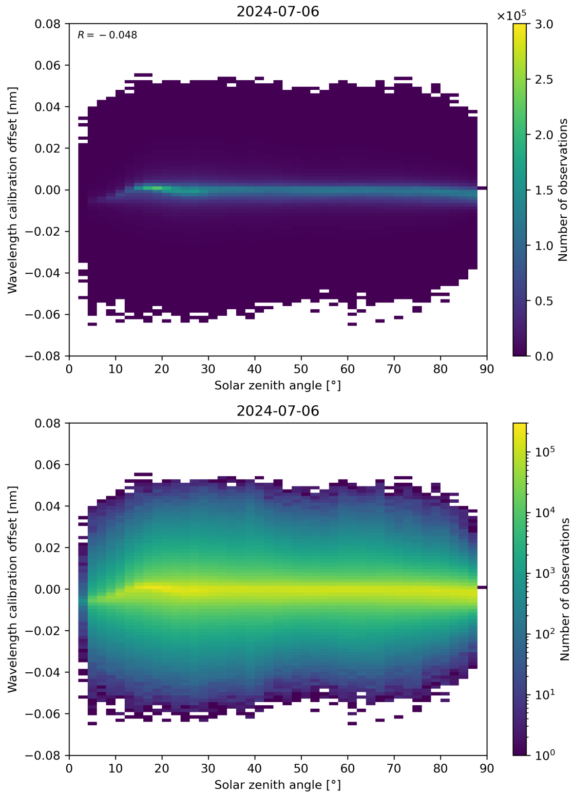
Figure 158: Scatter density plot of “Solar zenith angle” against “Wavelength calibration offset” for 2024-07-05 to 2024-07-07.
