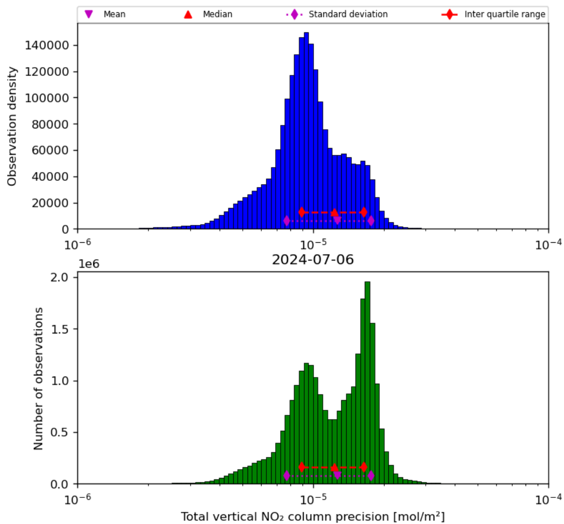
Figure 39: Histogram of "Total vertical NO 2 column precision" for 2024-07-05 to 2024-07-07
