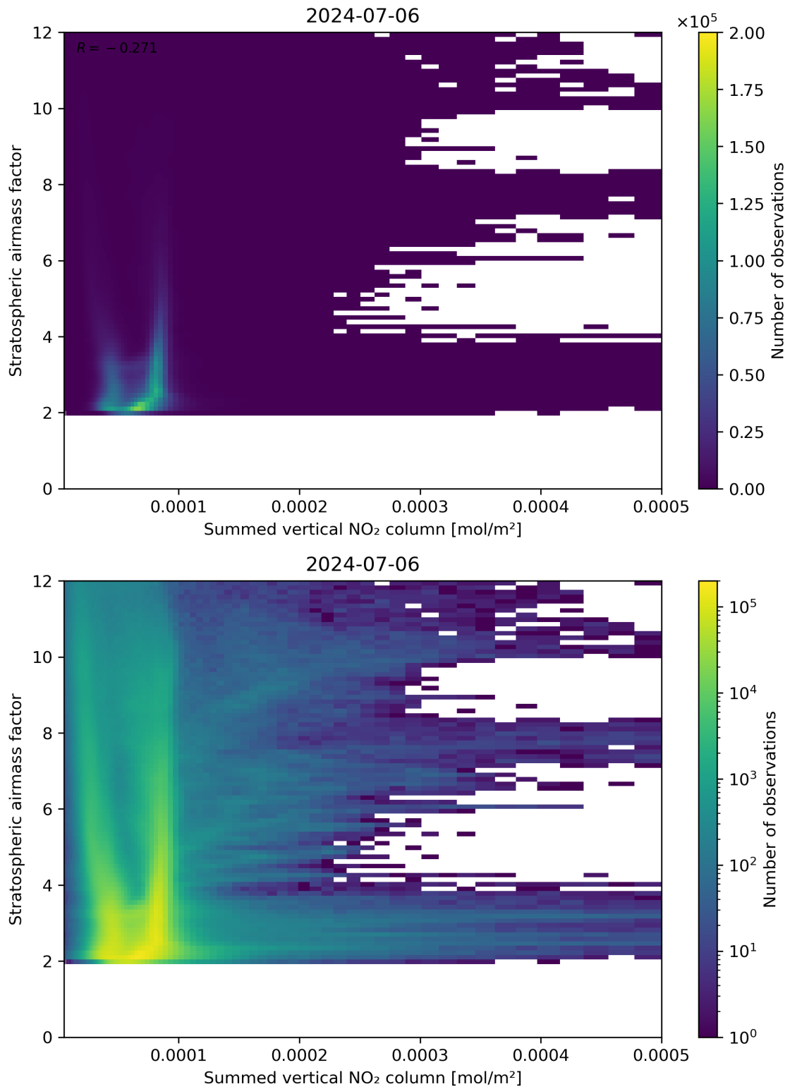
Figure 103: Scatter density plot of “Summed vertical NO 2 column” against “Stratospheric airmass factor” for 2024-07-05 to 2024-07-07.
