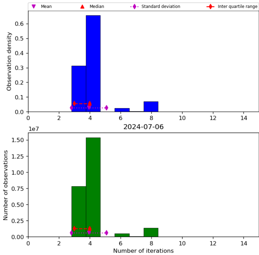
Figure 34: Histogram of “Number of iterations” for 2024-07-05 to 2024-07-07
