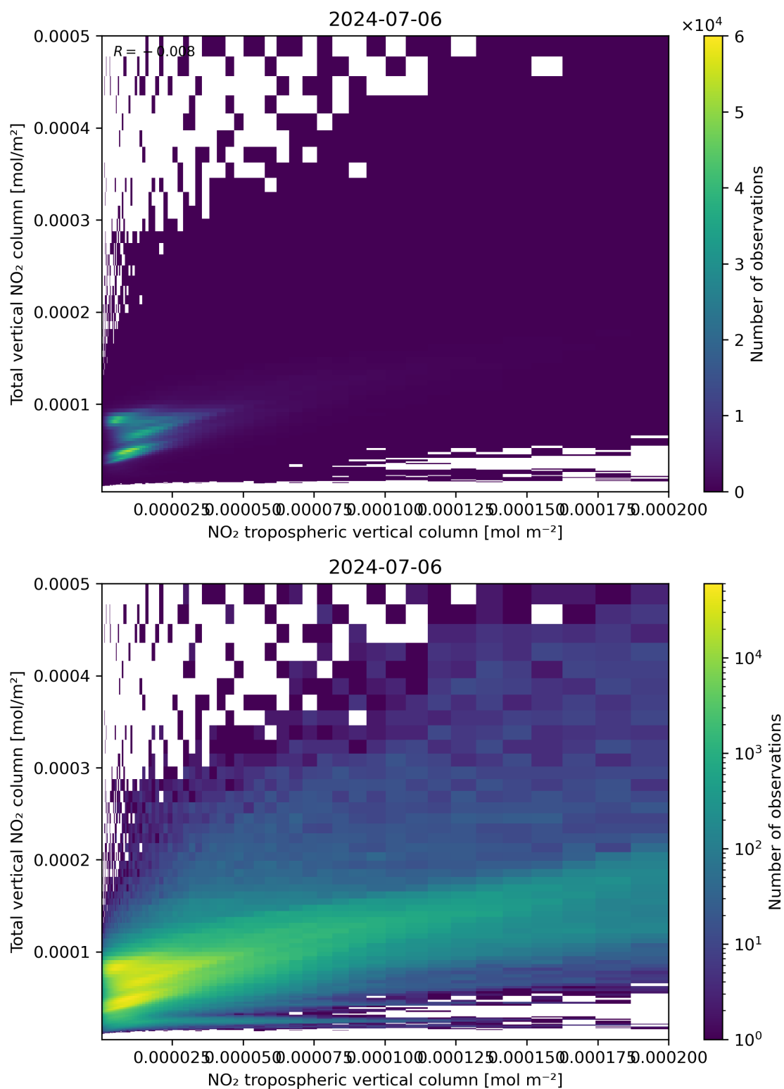
Figure 128: Scatter density plot of “NO 2 tropospheric vertical column” against “Total vertical NO 2 column” for 2024-07-05 to 2024-07-07.
