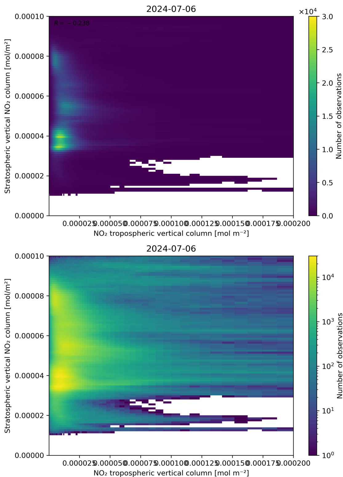
Figure 125: Scatter density plot of “NO 2 tropospheric vertical column” against “Stratospheric vertical NO 2 column” for 2024-07-05 to 2024-07-07.
