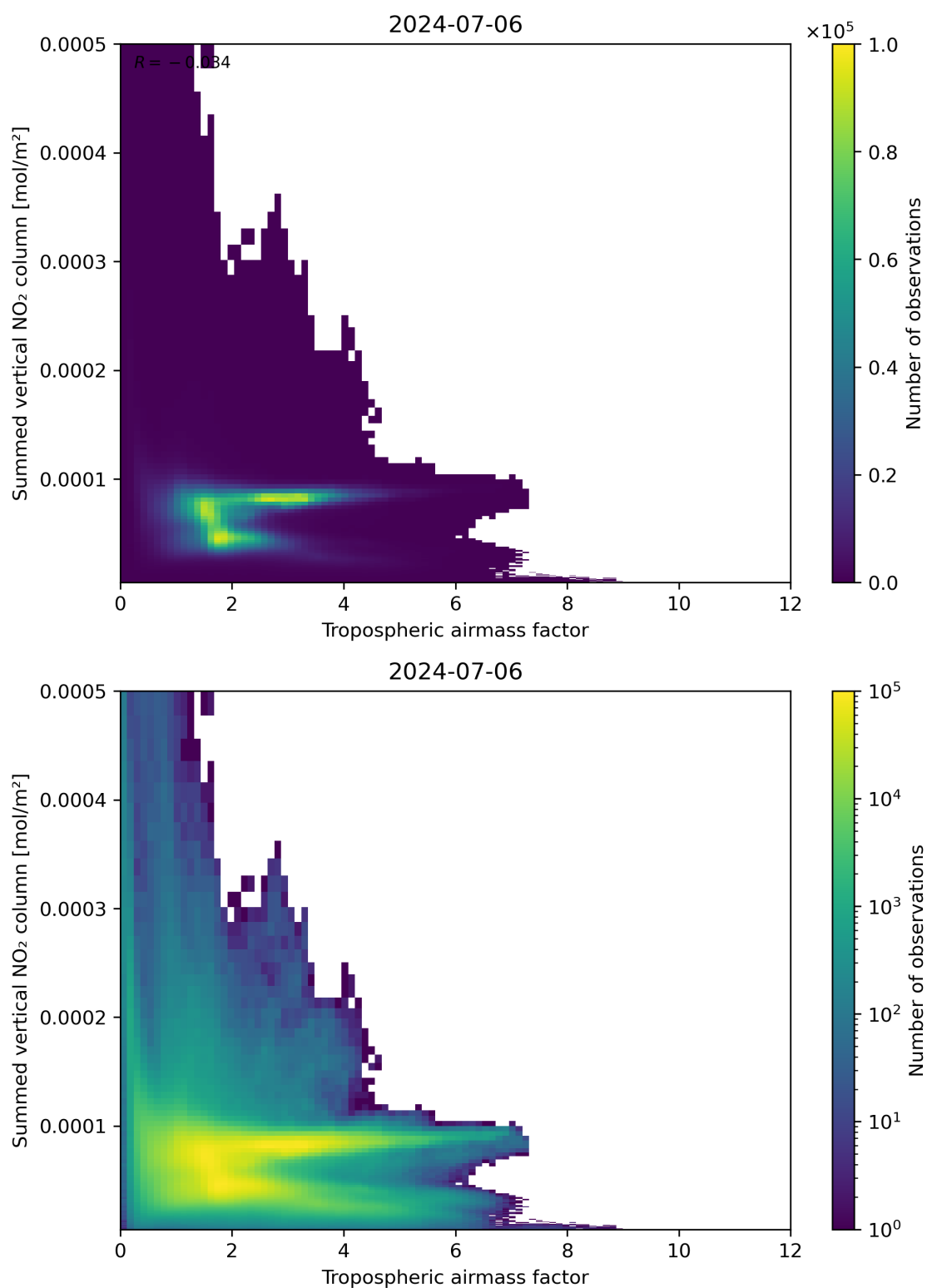
Figure 75: Scatter density plot of “Tropospheric airmass factor” against “Summed vertical NO 2 column” for 2024-07-05 to 2024-07-07.
