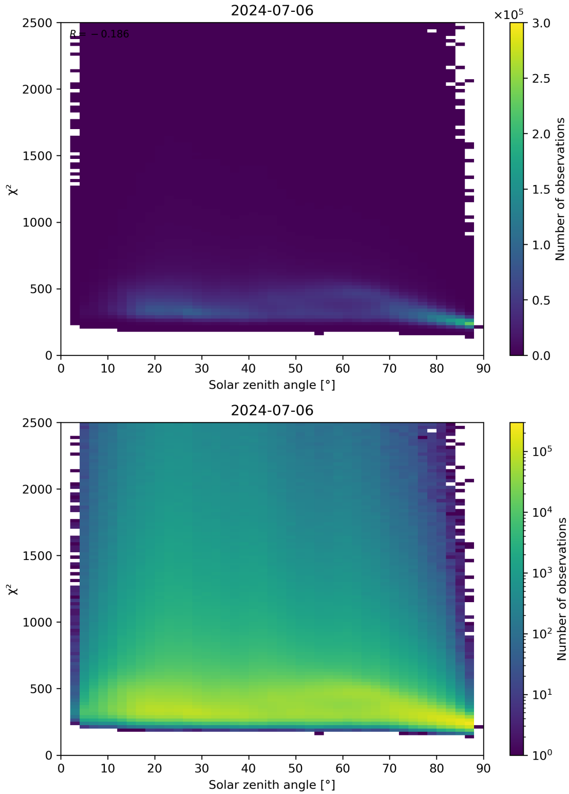
Figure 148: Scatter density plot of “Solar zenith angle” against “ \chi^2 ” for 2024-07-05 to 2024-07-07.
