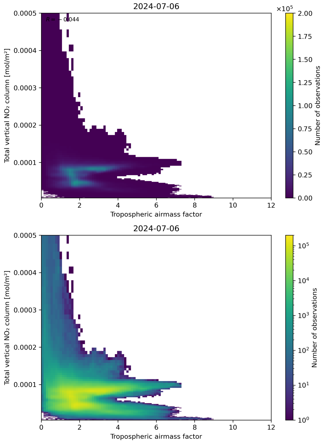
Figure 77: Scatter density plot of “Tropospheric airmass factor” against “Total vertical NO 2 column” for 2024-07-05 to 2024-07-07.
