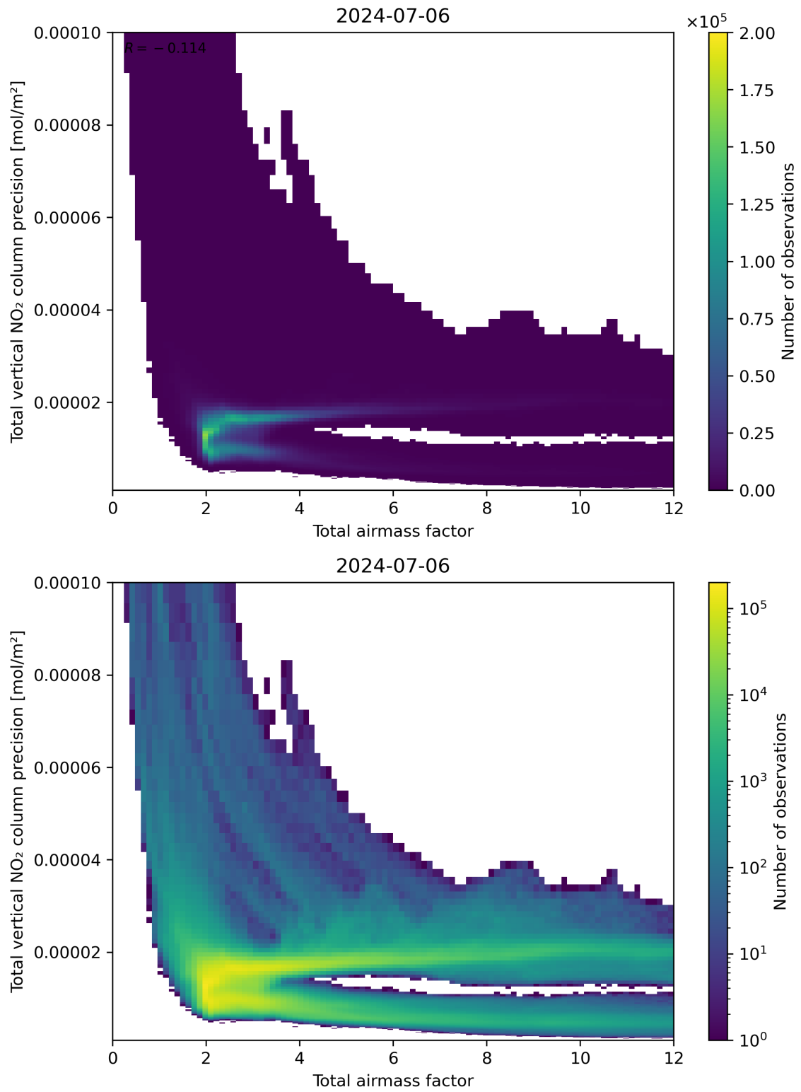
Figure 68: Scatter density plot of “Total airmass factor” against “Total vertical NO 2 column precision” for 2024-07-05 to 2024-07-07.
