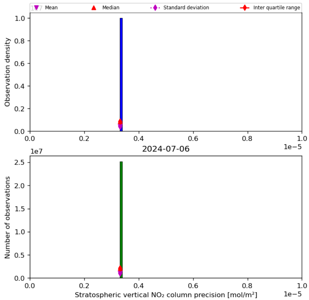
Figure 37: Histogram of “Stratospheric vertical NO 2 column precision” for 2024-07-05 to 2024-07-07
