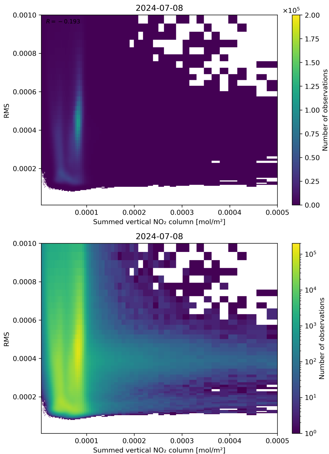
Figure 109: Scatter density plot of “Summed vertical NO 2 column” against “RMS” for 2024-07-07 to 2024-07-09.
