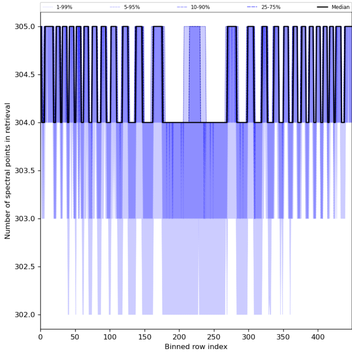
Figure 50: Along track statistics of “Number of spectral points in retrieval” for 2024-07-07 to 2024-07-09
