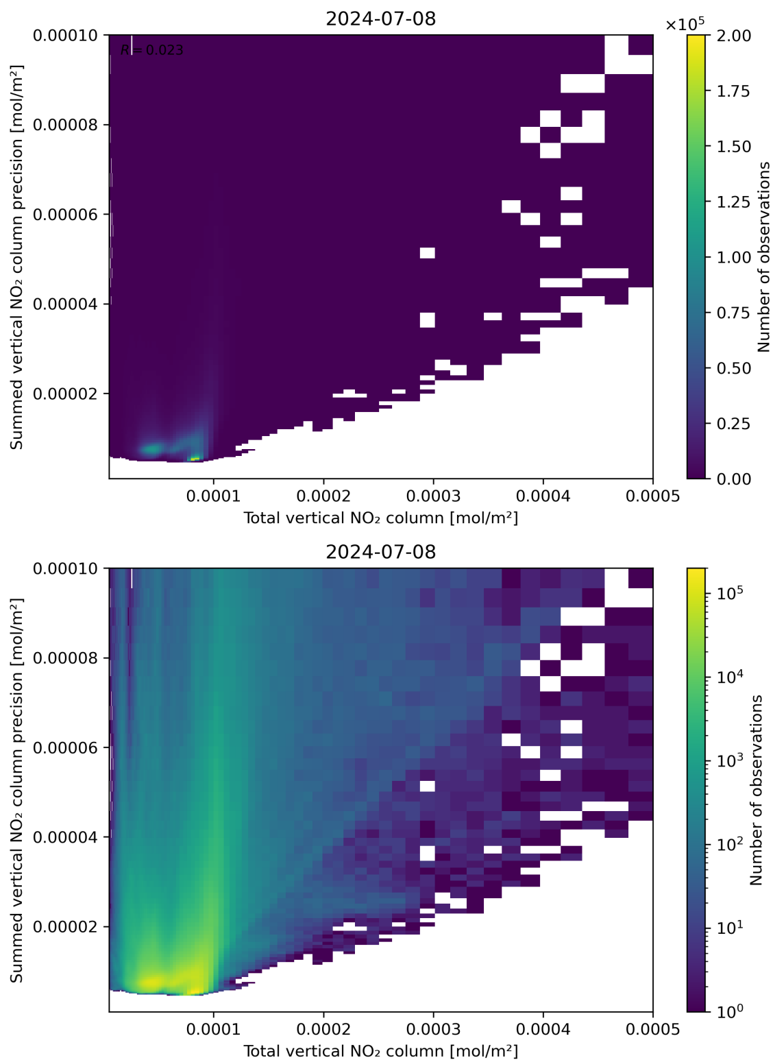
Figure 113: Scatter density plot of “Total vertical NO 2 column” against “Summed vertical NO 2 column precision” for 2024-07-07 to 2024-07-09.
