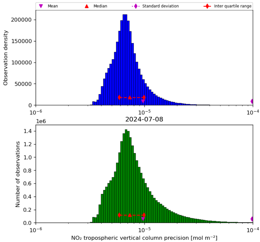
Figure 30: Histogram of “NO 2 tropospheric vertical column precision” for 2024-07-07 to 2024-07-09
