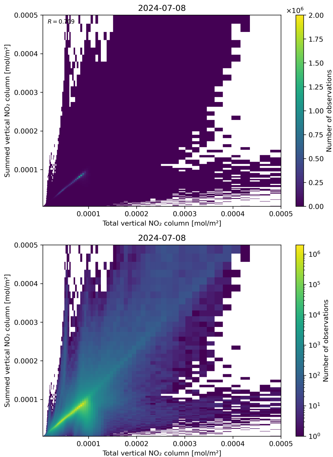
Figure 112: Scatter density plot of “Total vertical NO 2 column” against “Summed vertical NO 2 column” for 2024-07-07 to 2024-07-09.
