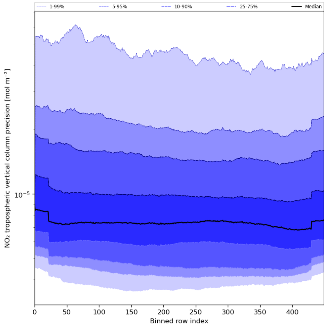
Figure 47: Along track statistics of “NO 2 tropospheric vertical column precision” for 2024-07-07 to 2024-07-09
