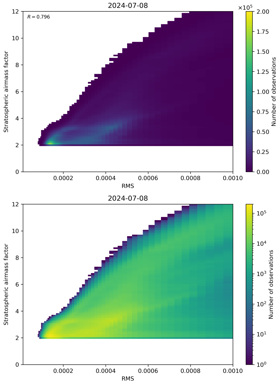
Figure 144: Scatter density plot of “RMS” against “Stratospheric airmass factor” for 2024-07-07 to 2024-07-09.
