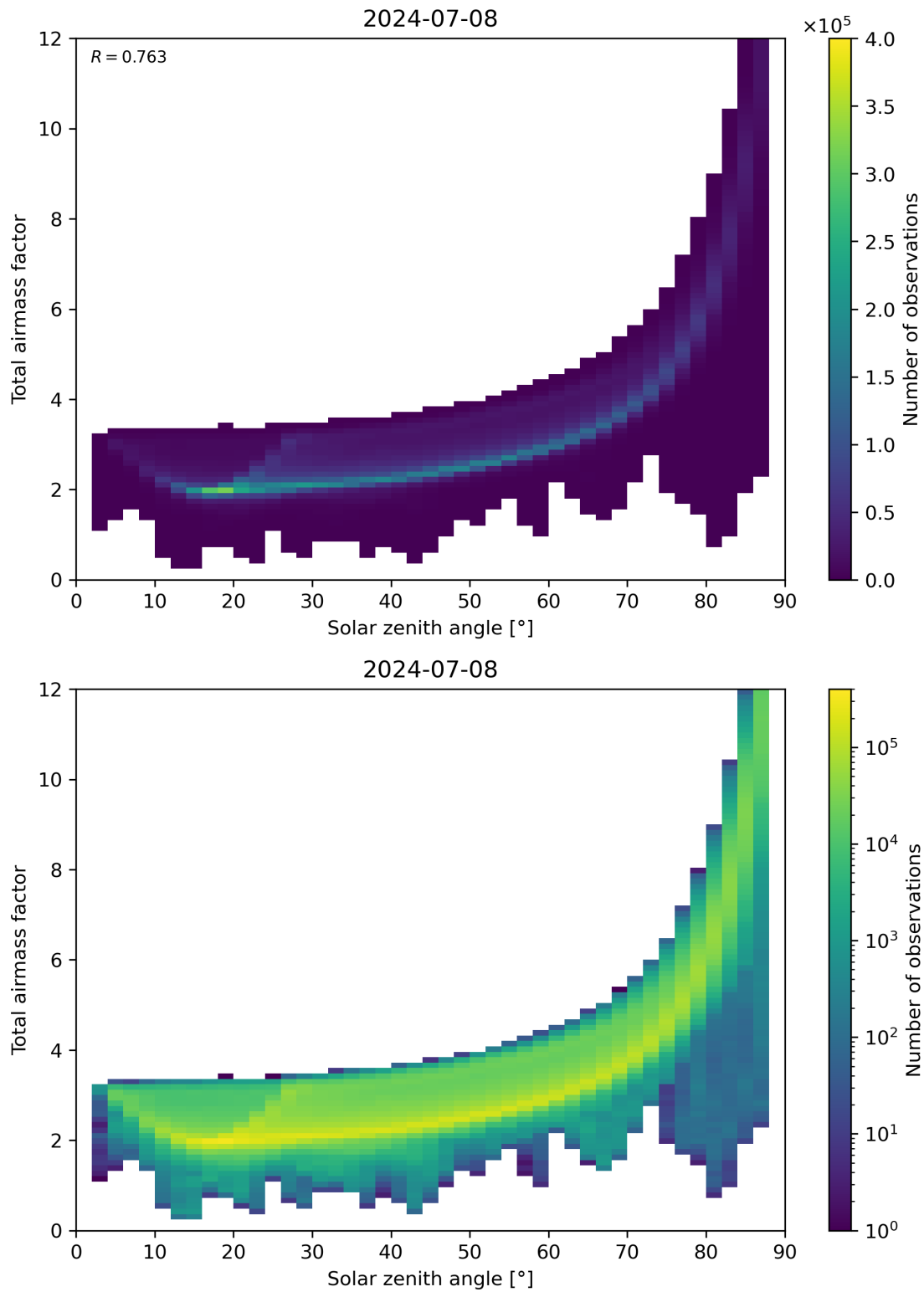
Figure 146: Scatter density plot of “Solar zenith angle” against “Total air mass factor” for 2024-07-07 to 2024-07-09.
