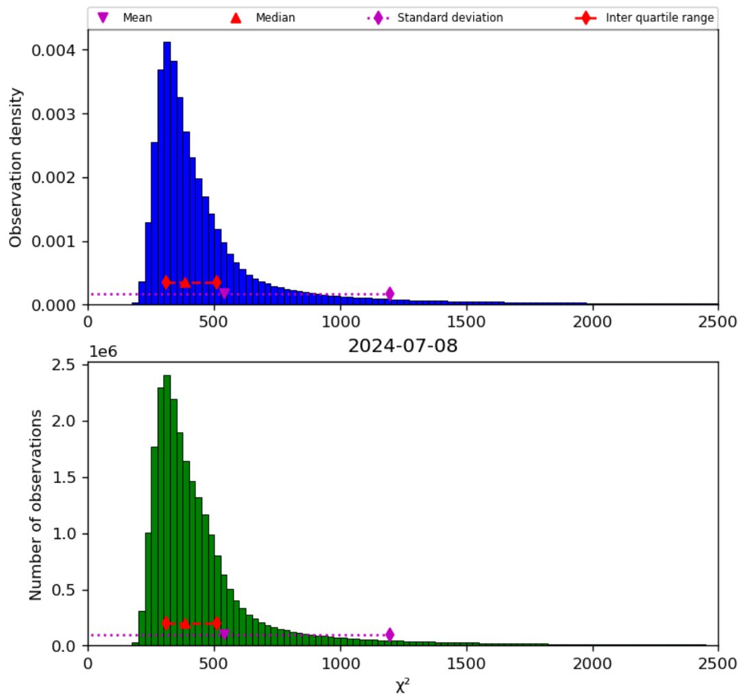
Figure 42: Histogram of “ \chi^2 ” for 2024-07-07 to 2024-07-09
