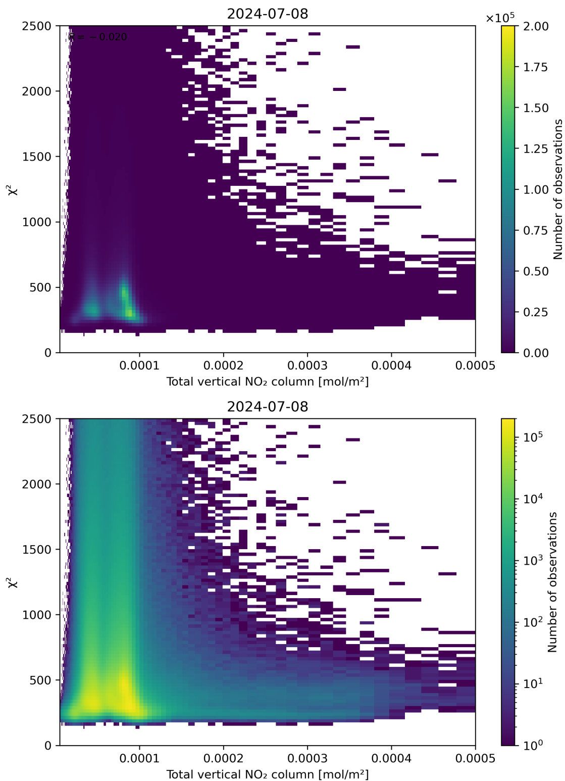
Figure 111: Scatter density plot of “Total vertical NO 2 column” against “ \chi^2 ” for 2024-07-07 to 2024-07-09.
