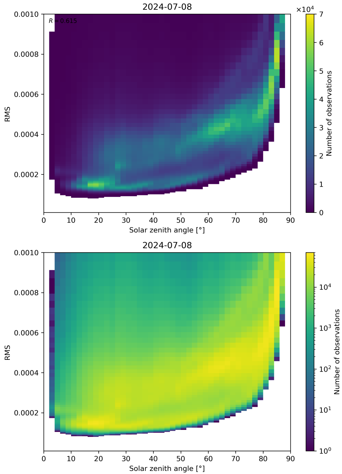
Figure 157: Scatter density plot of “Solar zenith angle” against “RMS” for 2024-07-07 to 2024-07-09.
