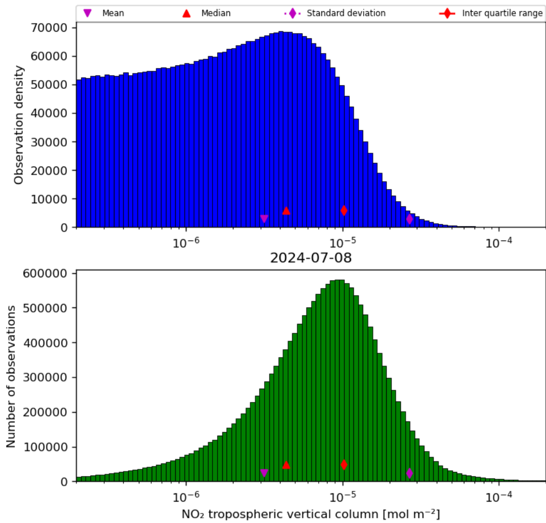
Figure 29: Histogram of “NO 2 tropospheric vertical column” for 2024-07-07 to 2024-07-09
