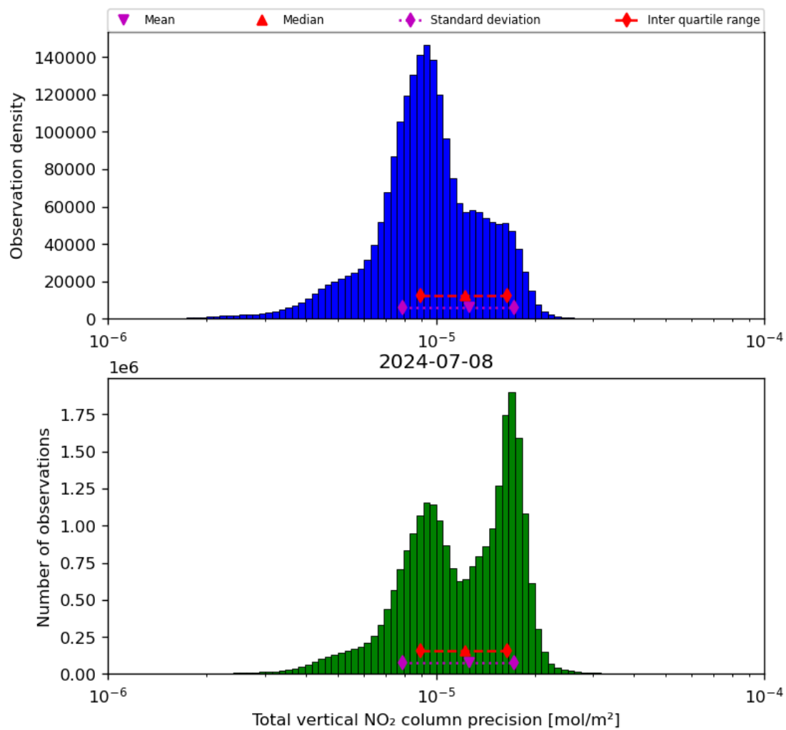
Figure 39: Histogram of “Total vertical NO 2 column precision” for 2024-07-07 to 2024-07-09
