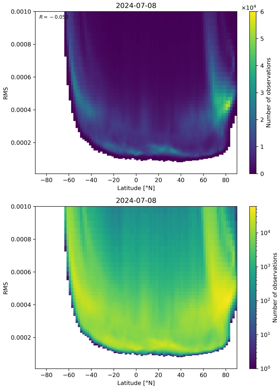
Figure 94: Scatter density plot of “Latitude” against “RMS” for 2024-07-07 to 2024-07-09.
