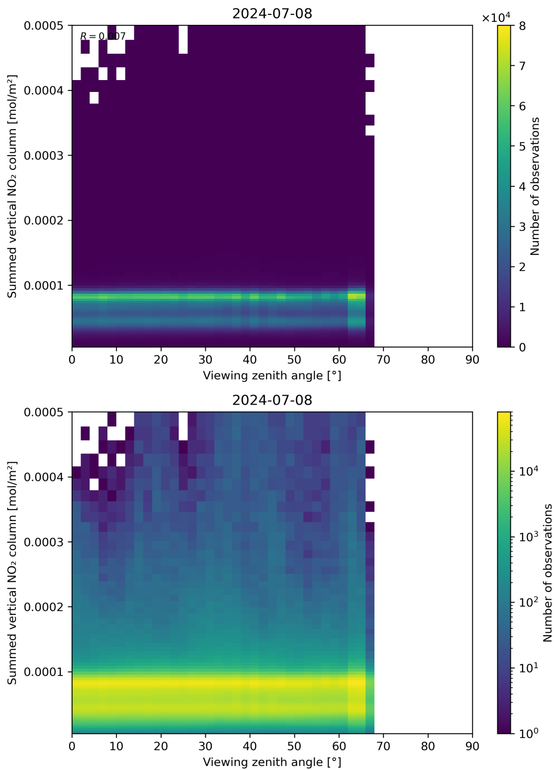
Figure 165: Scatter density plot of “Viewing zenith angle” against “Summed vertical NO 2 column” for 2024-07-07 to 2024-07-09.
