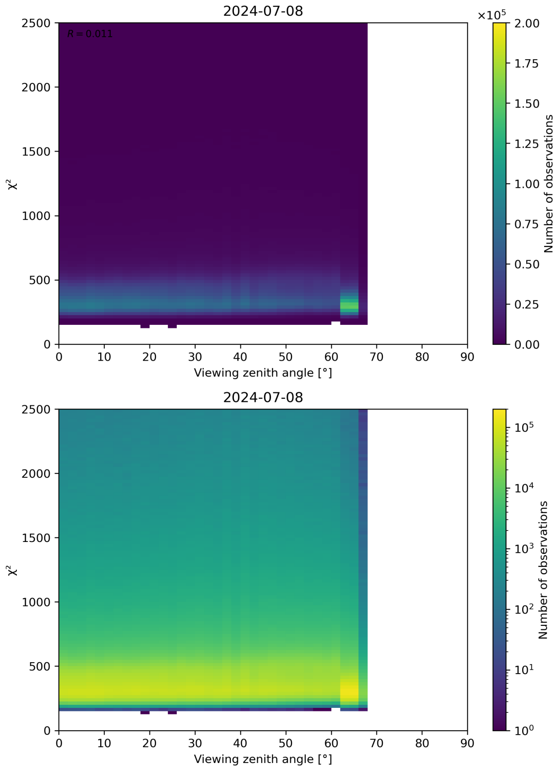
Figure 162: Scatter density plot of “Viewing zenith angle” against “ \chi^2 ” for 2024-07-07 to 2024-07-09.
