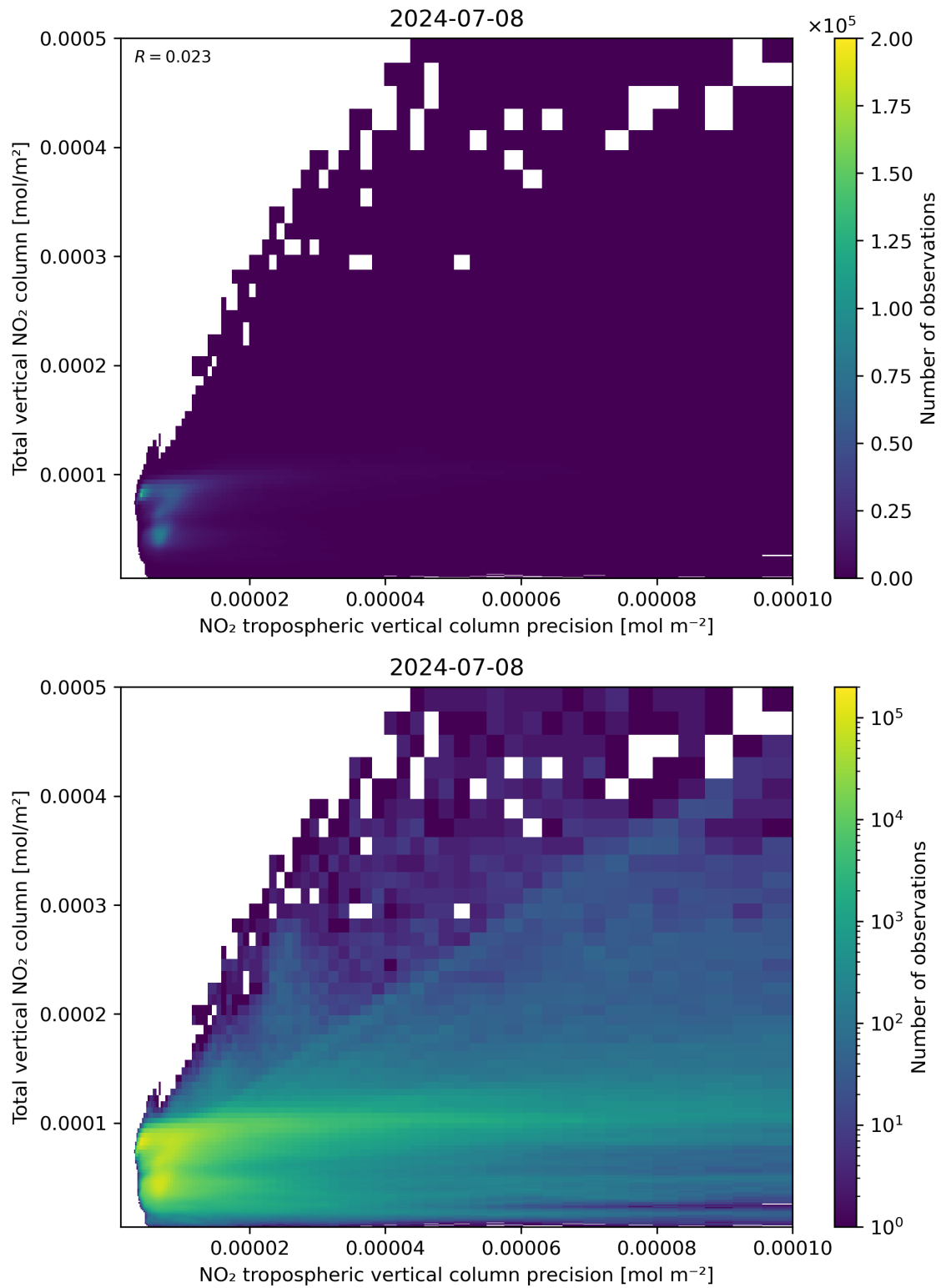
Figure 138: Scatter density plot of “NO 2 tropospheric vertical column precision” against “Total vertical NO 2 column” for 2024-07-07 to 2024-07-09.
