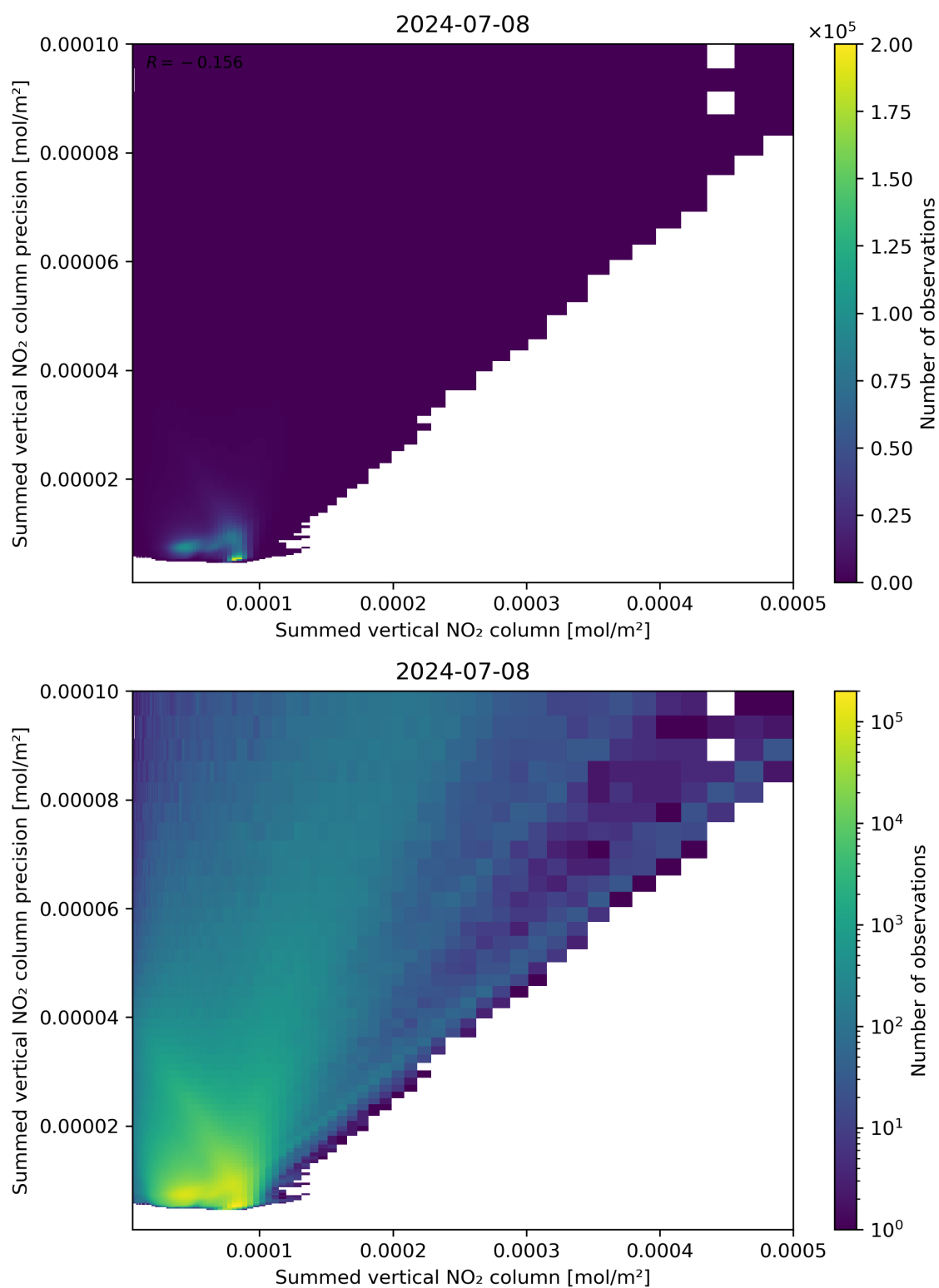
Figure 105: Scatter density plot of “Summed vertical NO 2 column” against “Summed vertical NO 2 column precision” for 2024-07-07 to 2024-07-09.
