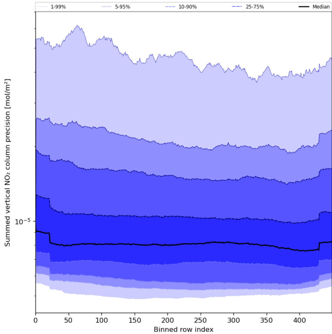
Figure 58: Along track statistics of “Summed vertical NO 2 column precision” for 2024-07-07 to 2024-07-09
