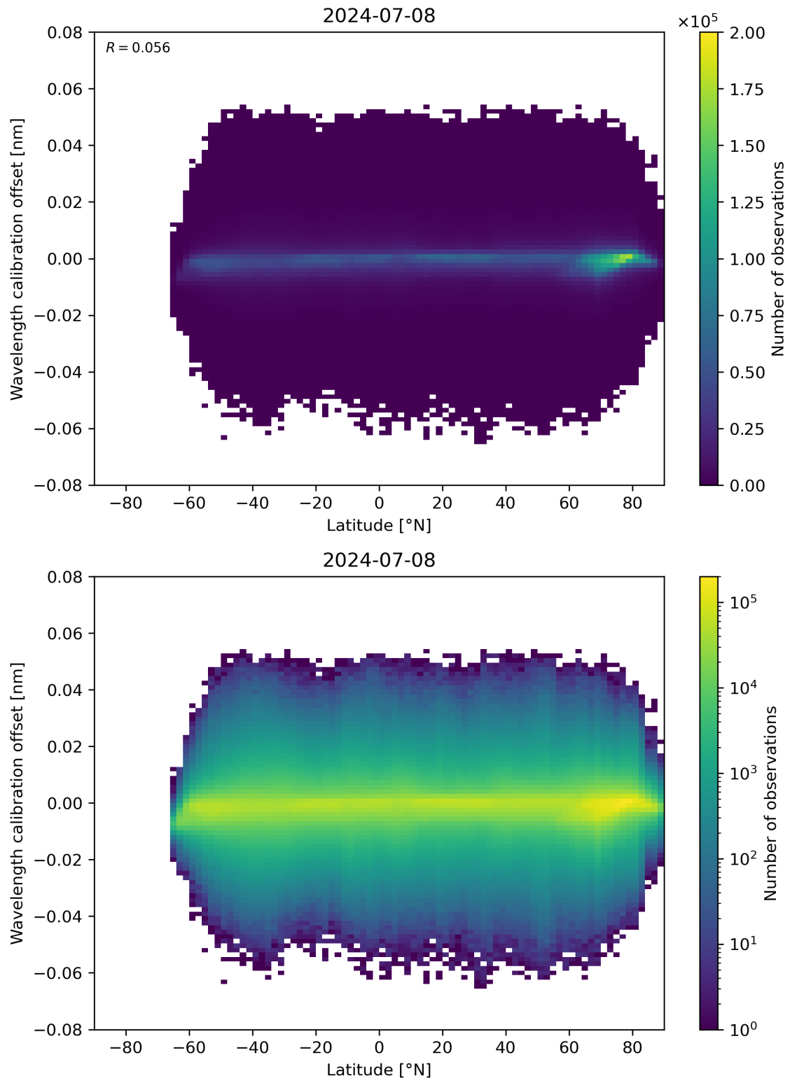
Figure 95: Scatter density plot of “Latitude” against “Wavelength calibration offset” for 2024-07-07 to 2024-07-09.
