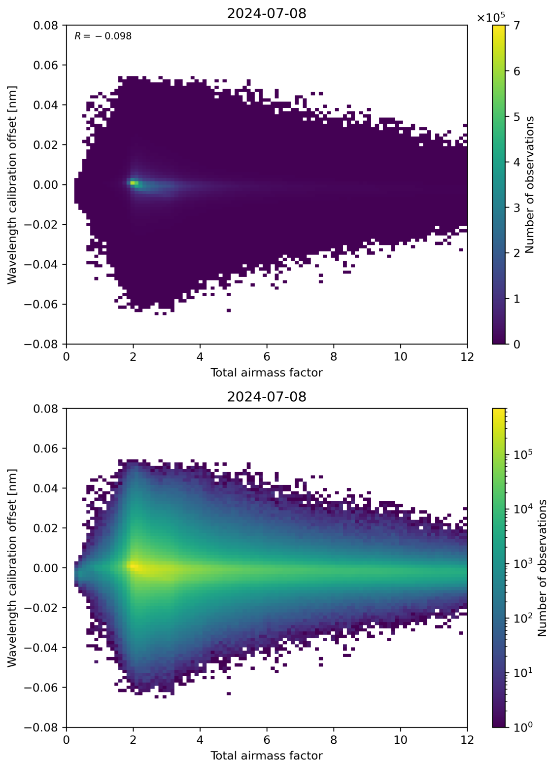
Figure 70: Scatter density plot of “Total airmass factor” against “Wavelength calibration offset” for 2024-07-07 to 2024-07-09.
