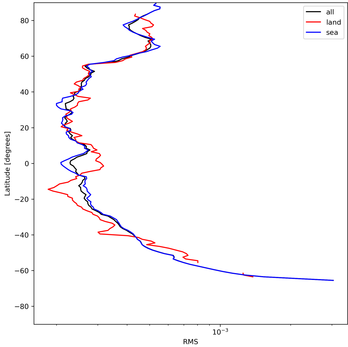
Figure 26: Zonal average of “RMS” for 2024-07-07 to 2024-07-09.
