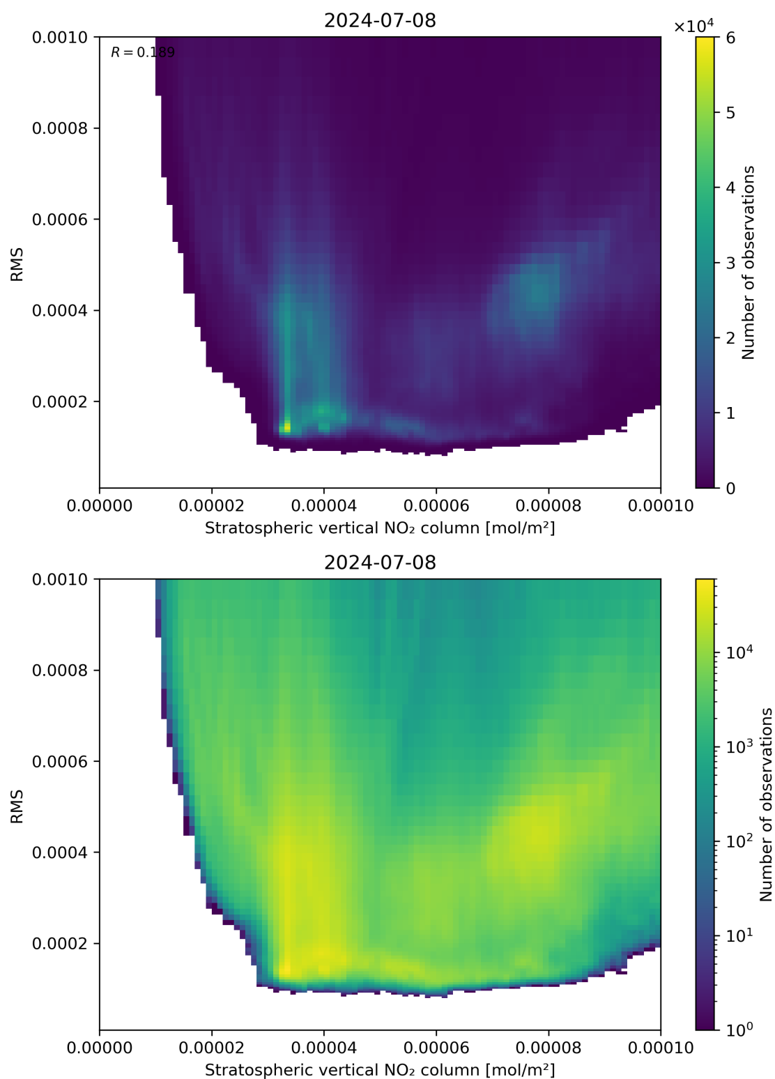
Figure 102: Scatter density plot of “Stratospheric vertical NO 2 column” against “RMS” for 2024-07-07 to 2024-07-09.
