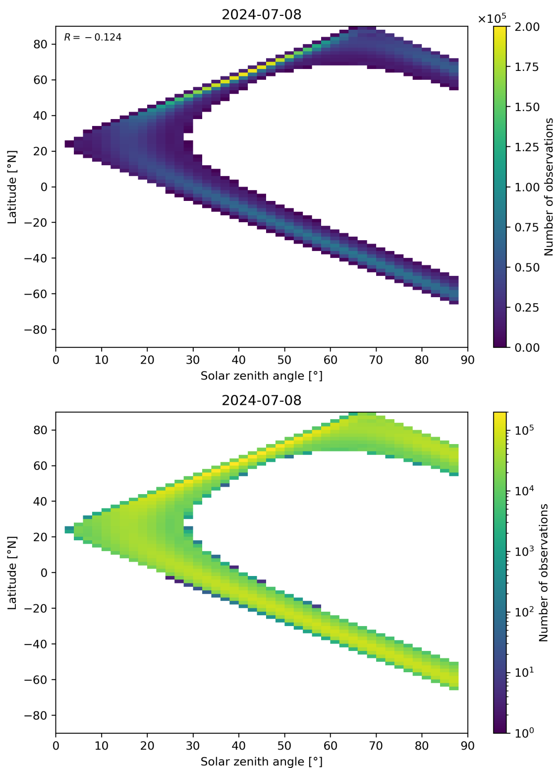
Figure 149: Scatter density plot of “Solar zenith angle” against “Latitude” for 2024-07-07 to 2024-07-09.
