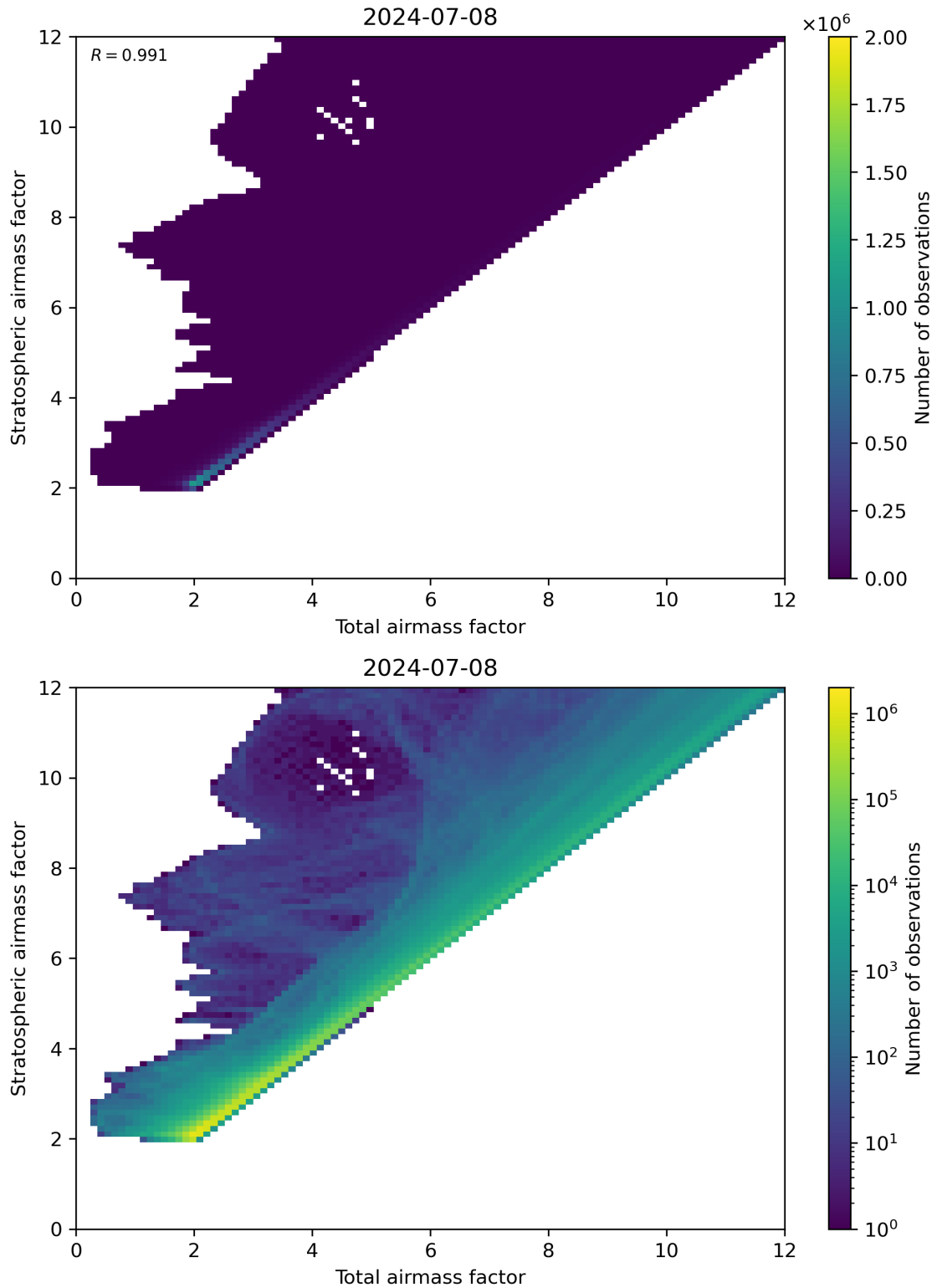
Figure 62: Scatter density plot of “Total airmass factor” against “Stratospheric airmass factor” for 2024-07-07 to 2024-07-09.
