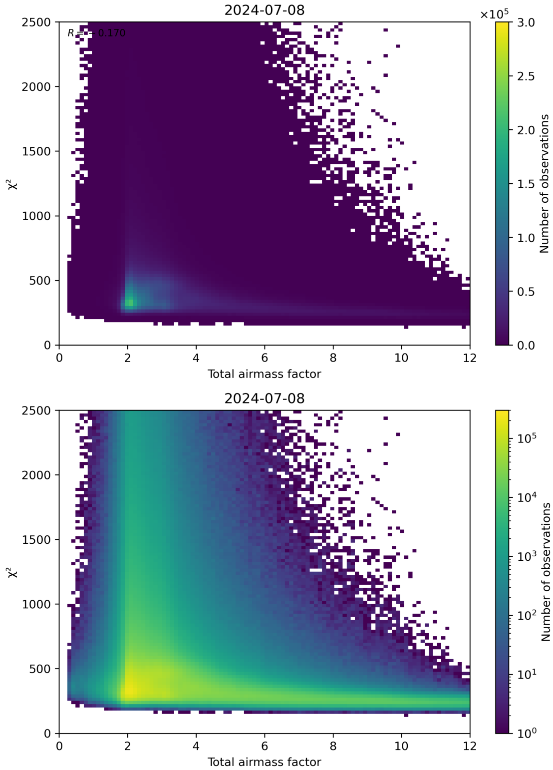
Figure 63: Scatter density plot of “Total airmass factor” against “ \chi^2 ” for 2024-07-07 to 2024-07-09.
