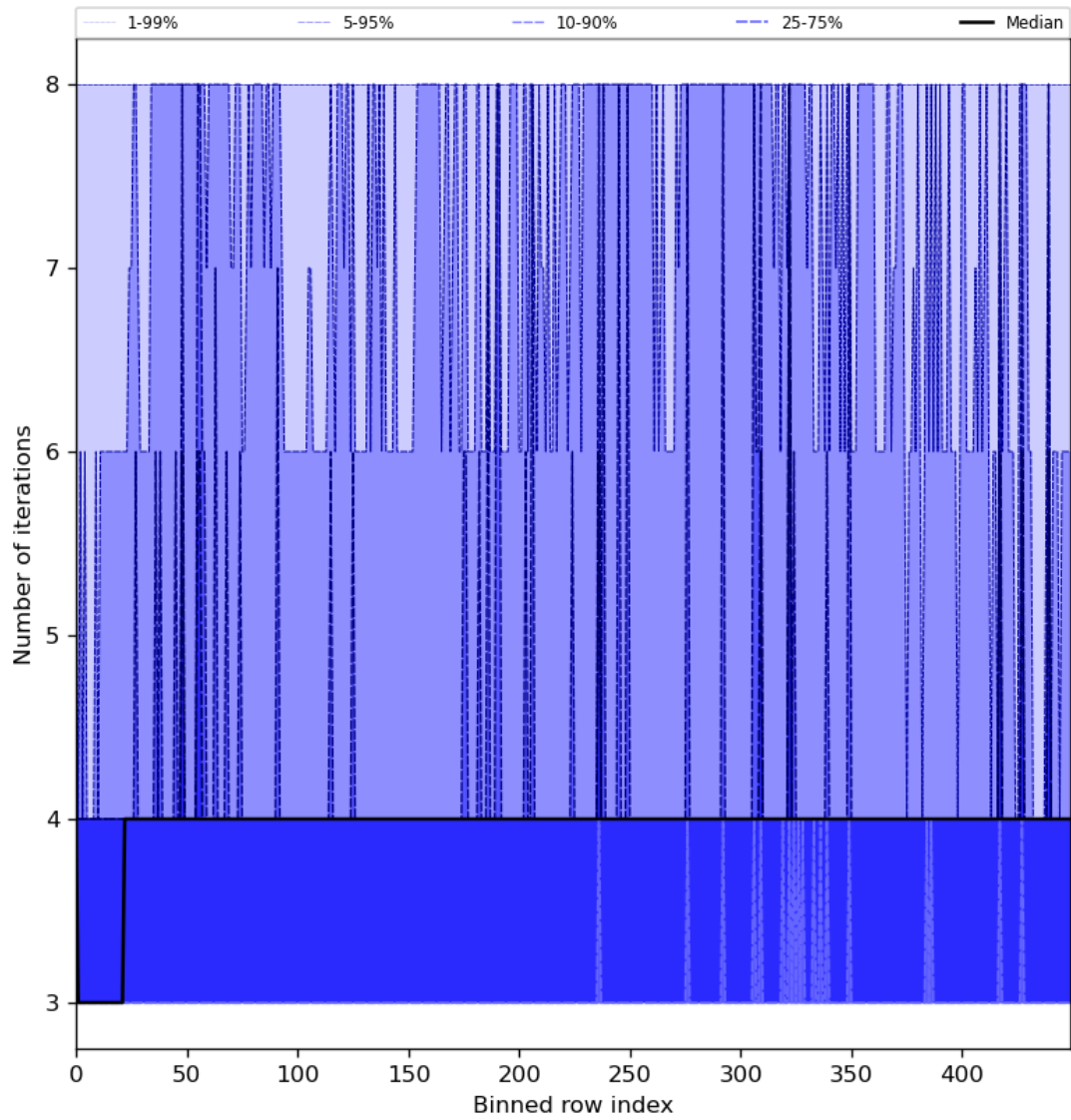
Figure 51: Along track statistics of “Number of iterations” for 2024-07-07 to 2024-07-09
