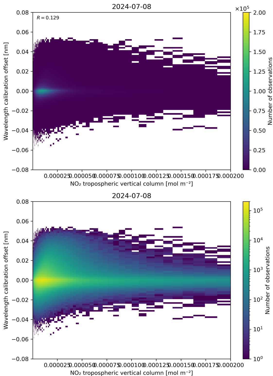
Figure 143: Scatter density plot of “NO 2 tropospheric vertical column” against “Wavelength calibration offset” for 2024-07-07 to 2024-07-09.
