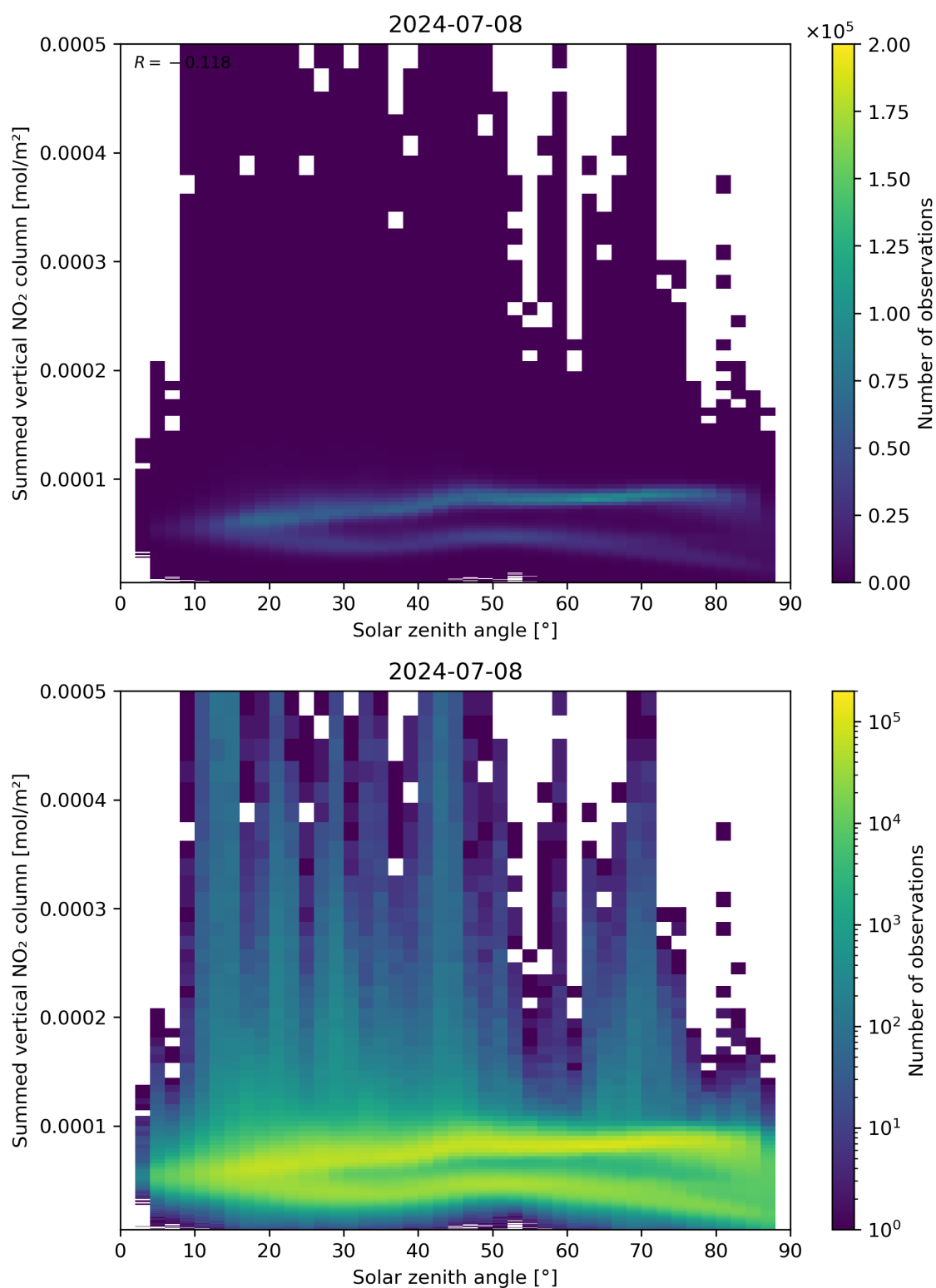
Figure 151: Scatter density plot of “Solar zenith angle” against “Summed vertical NO 2 column” for 2024-07-07 to 2024-07-09.
