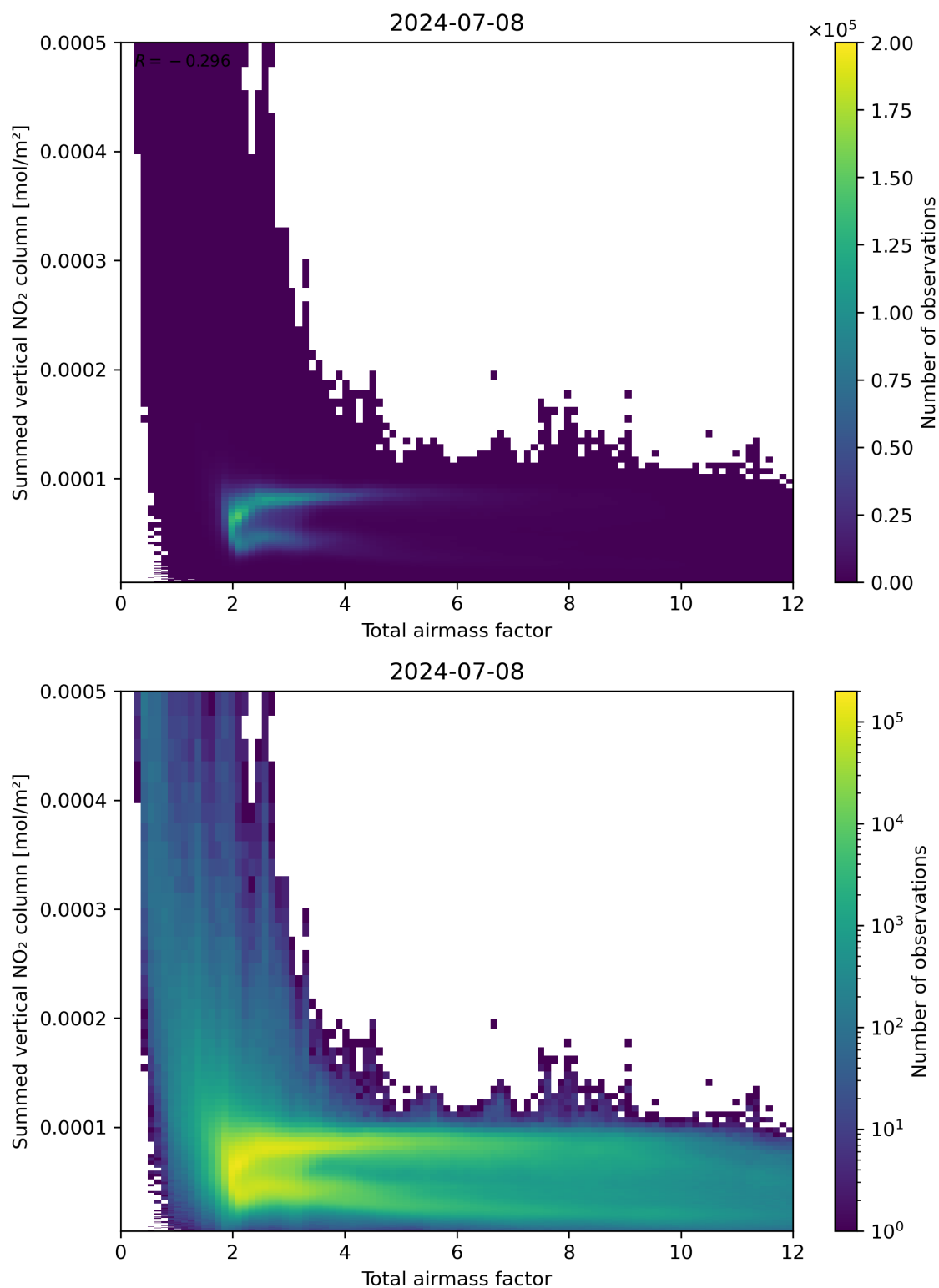
Figure 65: Scatter density plot of “Total airmass factor” against “Summed vertical NO 2 column” for 2024-07-07 to 2024-07-09.
