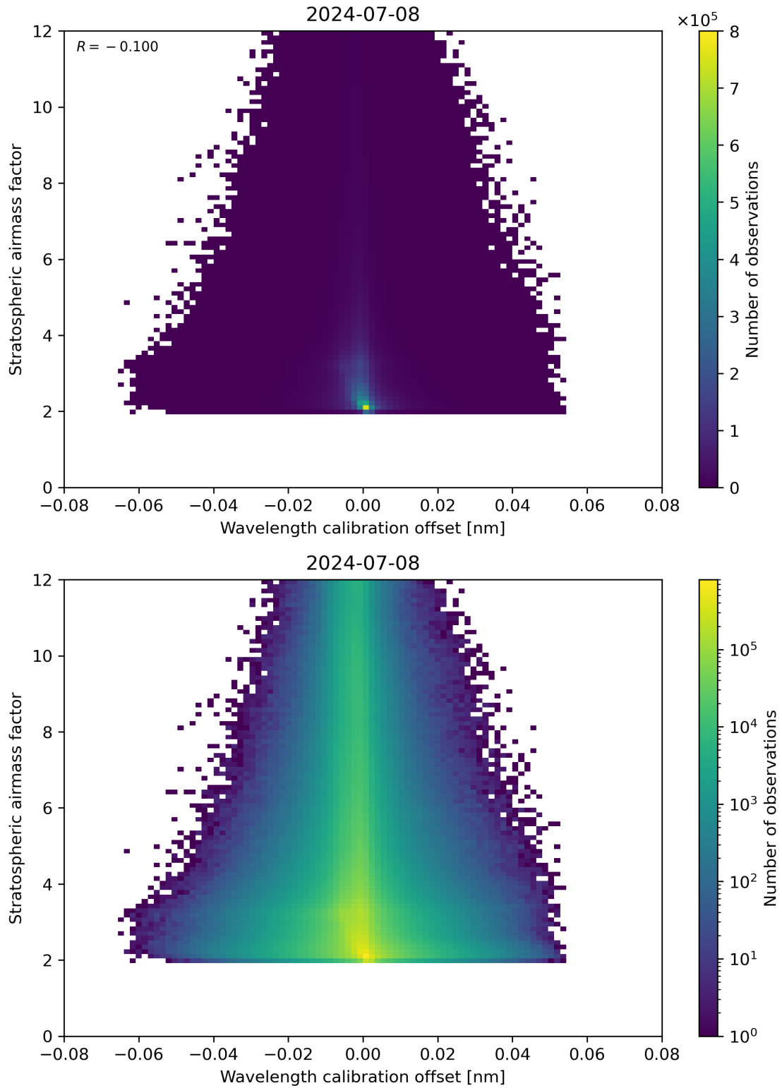
Figure 174: Scatter density plot of “Wavelength calibration offset” against “Stratospheric air mass factor” for 2024-07-07 to 2024-07-09.
