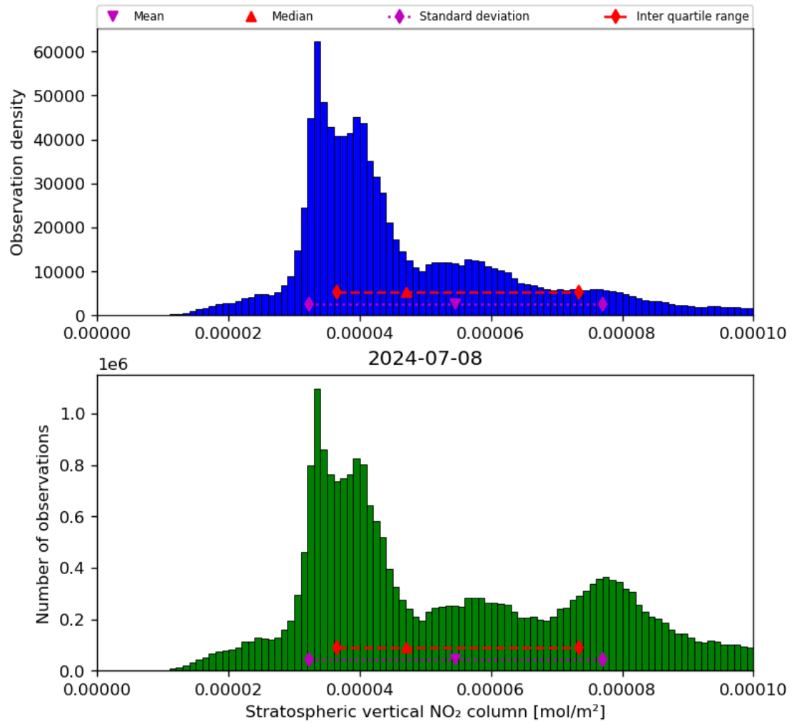
Figure 36: Histogram of “Stratospheric vertical NO 2 column” for 2024-07-07 to 2024-07-09
