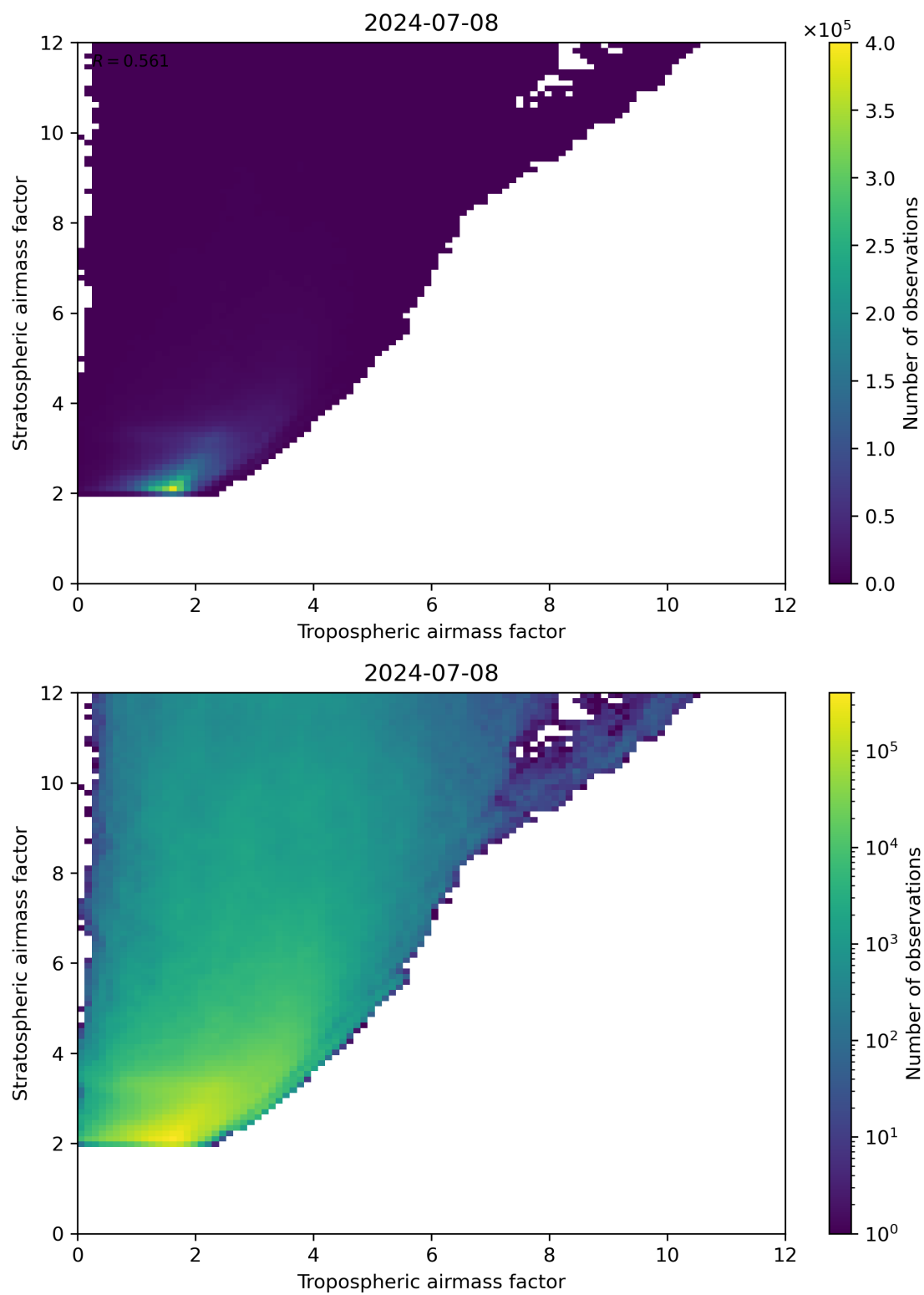
Figure 71: Scatter density plot of “Tropospheric airmass factor” against “Stratospheric airmass factor” for 2024-07-07 to 2024-07-09.
