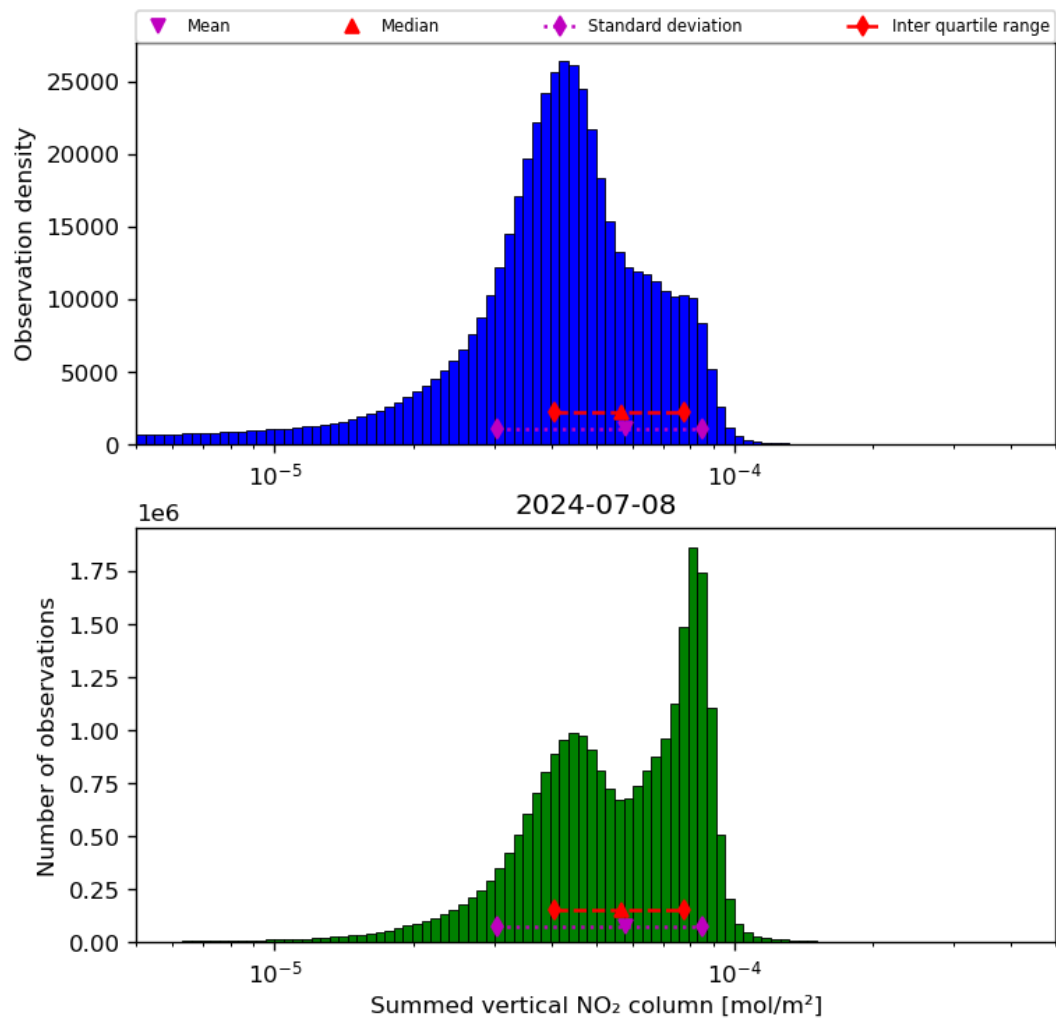
Figure 40: Histogram of “Summed vertical NO 2 column” for 2024-07-07 to 2024-07-09
