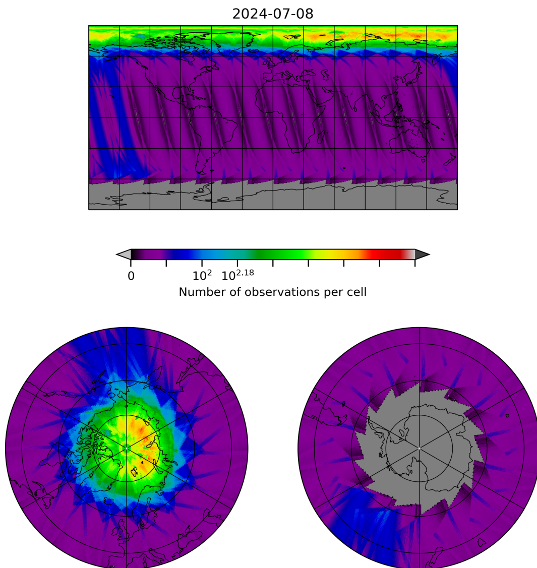
Figure 10: Map of the number of observations for 2024-07-07 to 2024-07-09
