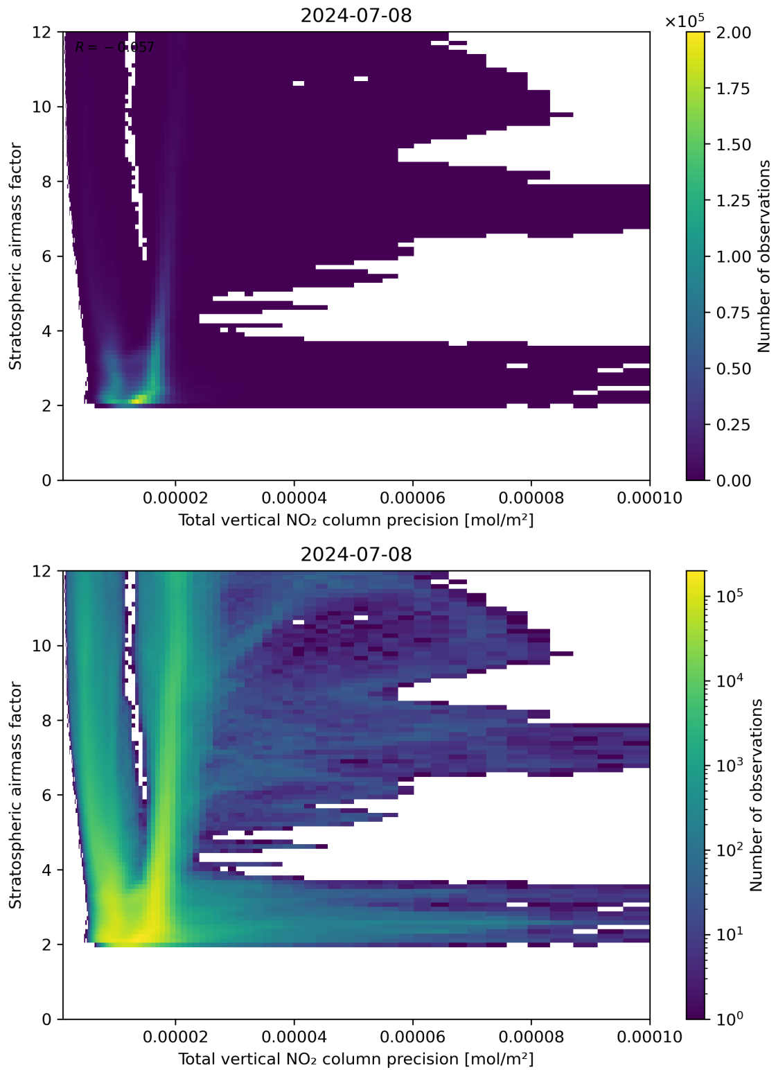
Figure 115: Scatter density plot of “Total vertical NO 2 column precision” against “Stratospheric air mass factor” for 2024-07-07 to 2024-07-09.
