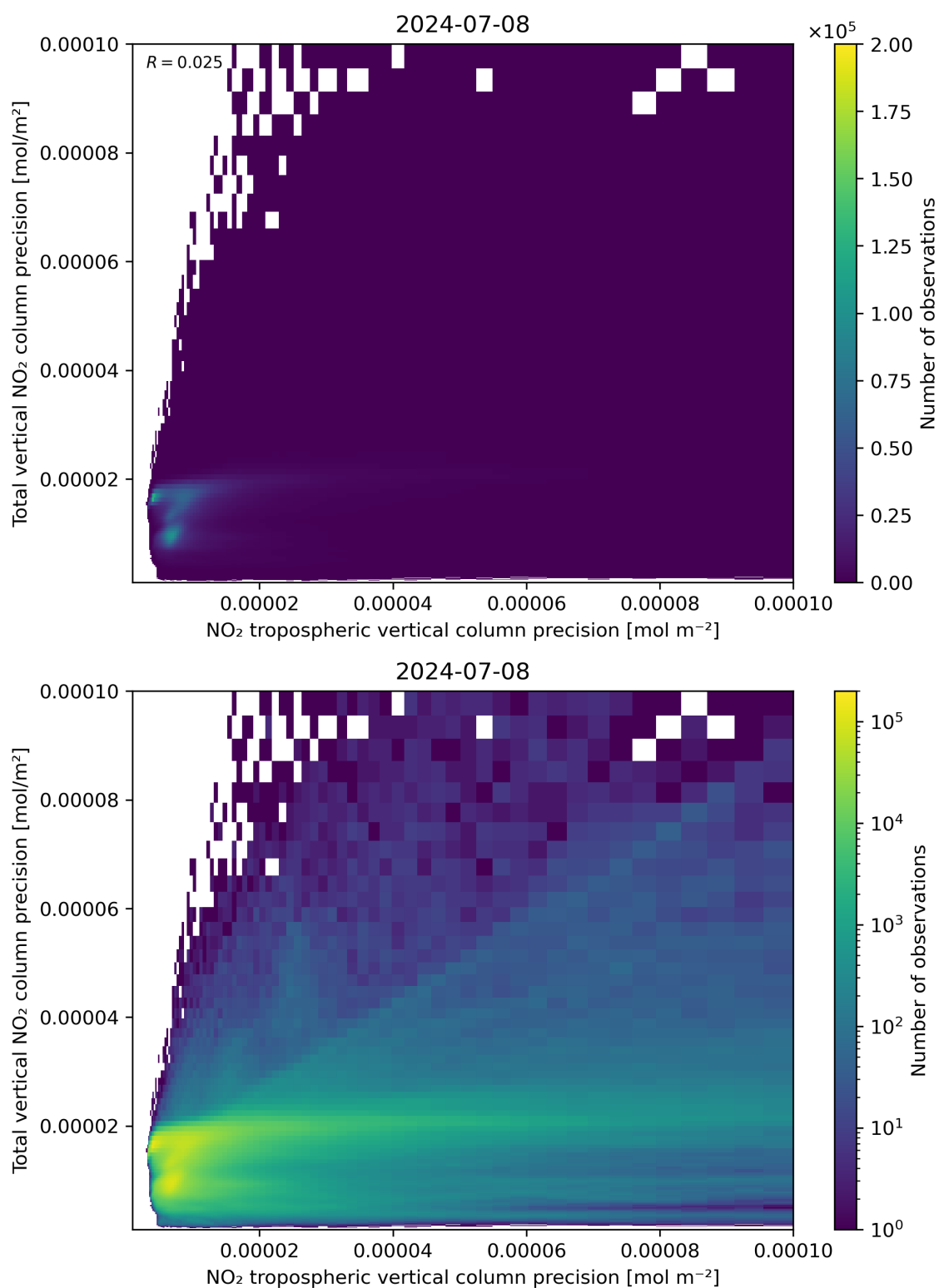
Figure 139: Scatter density plot of “NO 2 tropospheric vertical column precision” against “Total vertical NO 2 column precision” for 2024-07-07 to 2024-07-09.
