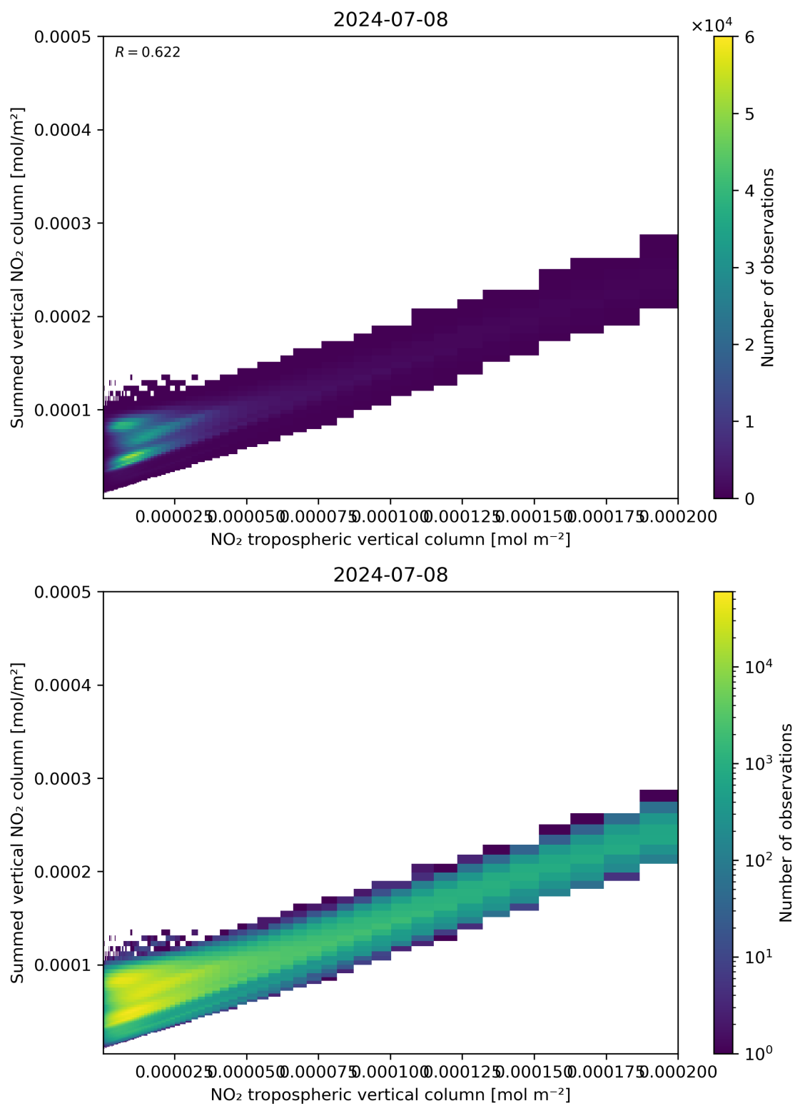
Figure 126: Scatter density plot of “NO 2 tropospheric vertical column” against “Summed vertical NO 2 column” for 2024-07-07 to 2024-07-09.
