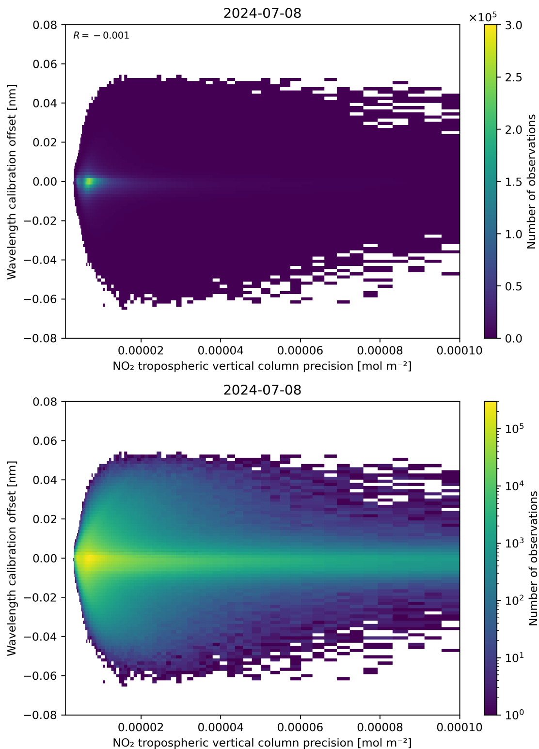
Figure 141: Scatter density plot of “NO 2 tropospheric vertical column precision” against “Wavelength calibration offset” for 2024-07-07 to 2024-07-09.
