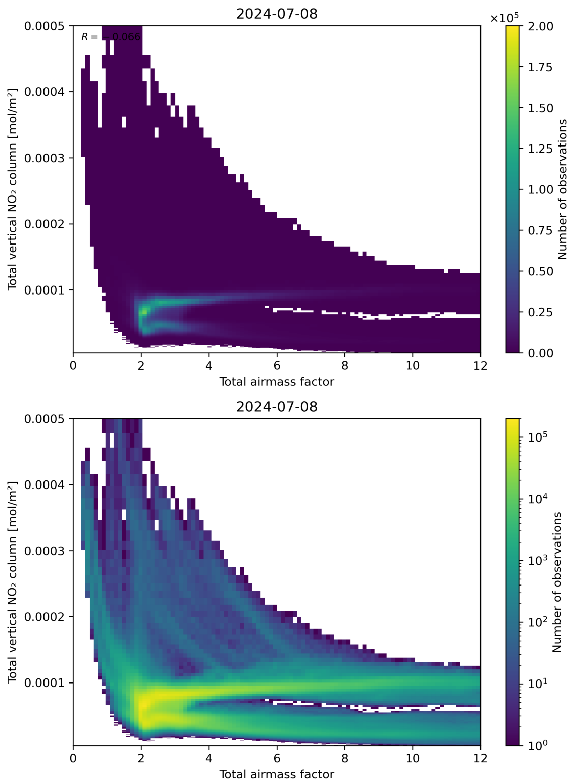
Figure 67: Scatter density plot of “Total airmass factor” against “Total vertical NO 2 column” for 2024-07-07 to 2024-07-09.
