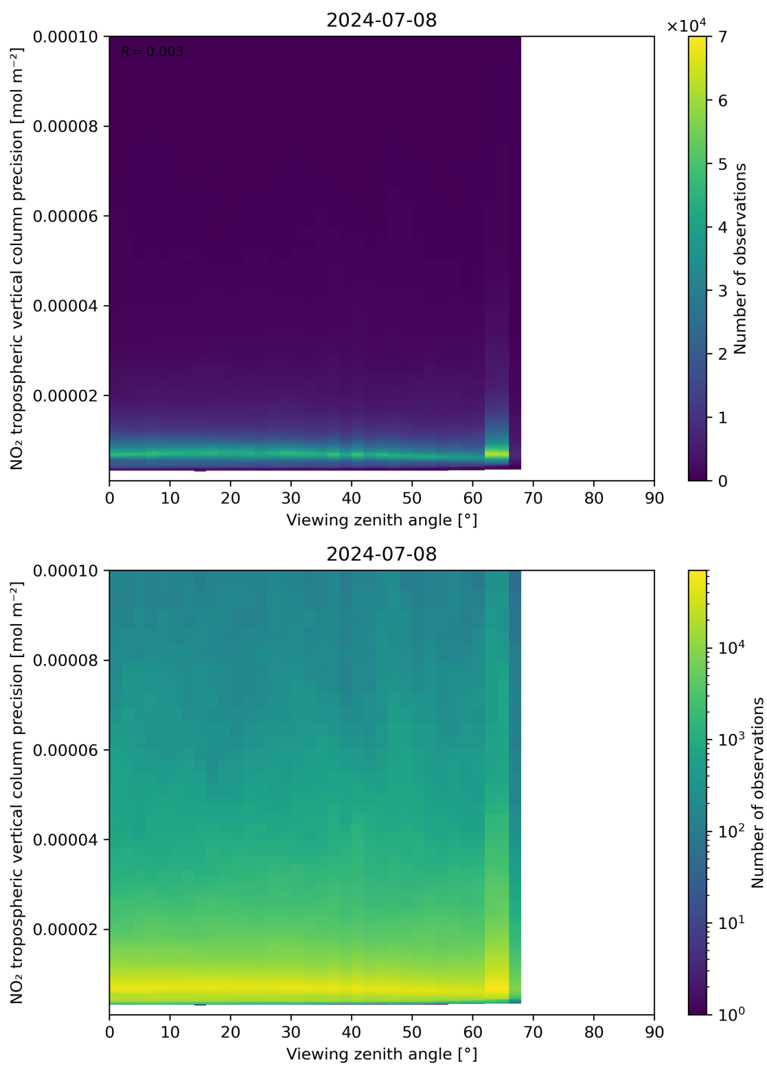
Figure 170: Scatter density plot of “Viewing zenith angle” against “NO 2 tropospheric vertical column precision” for 2024-07-07 to 2024-07-09.
