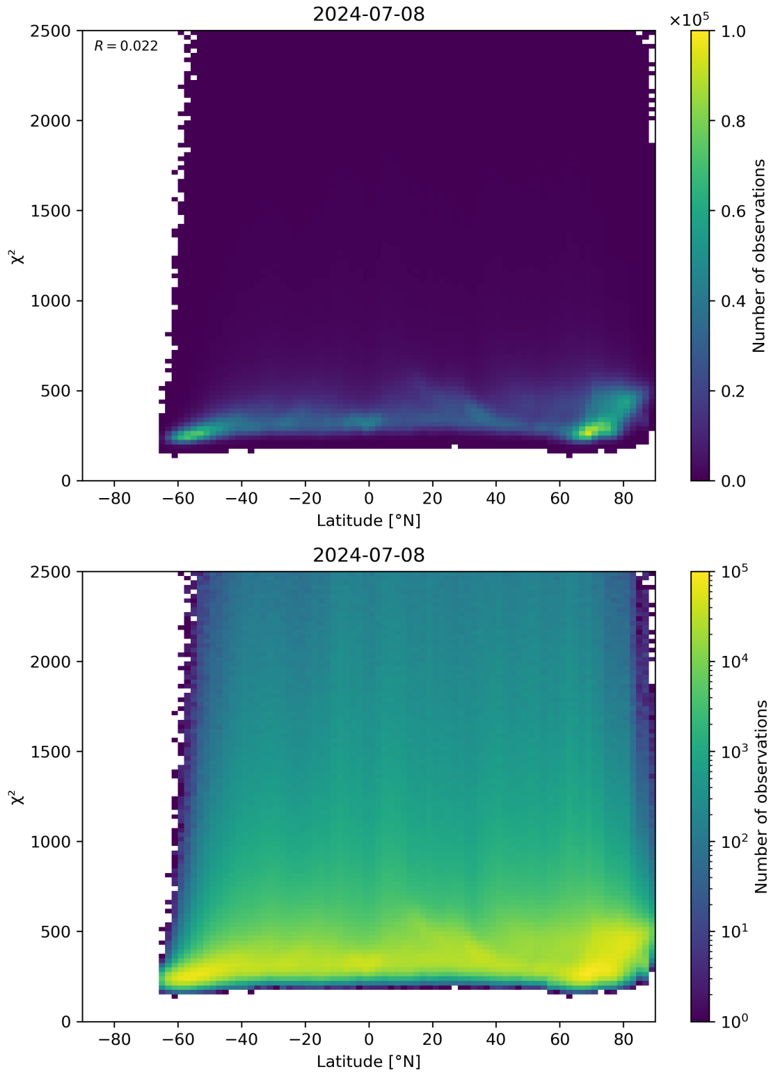
Figure 86: Scatter density plot of “Latitude” against “ \chi^2 ” for 2024-07-07 to 2024-07-09.
