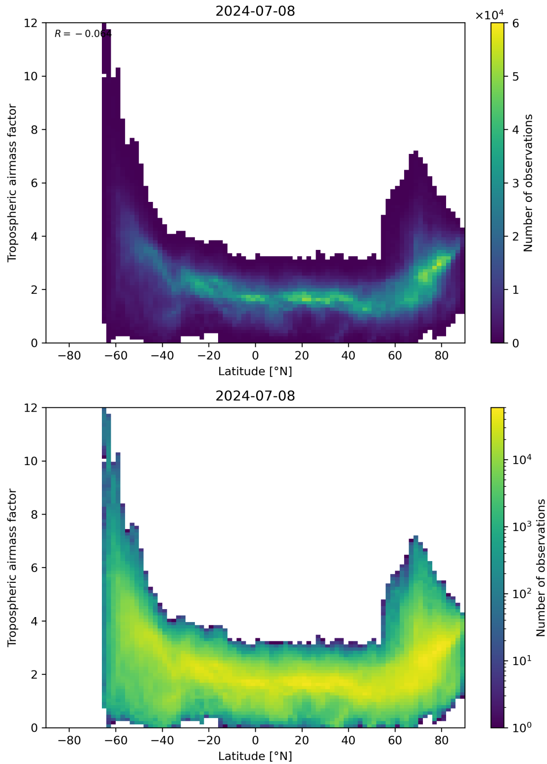
Figure 85: Scatter density plot of “Latitude” against “Tropospheric airmass factor” for 2024-07-07 to 2024-07-09.
