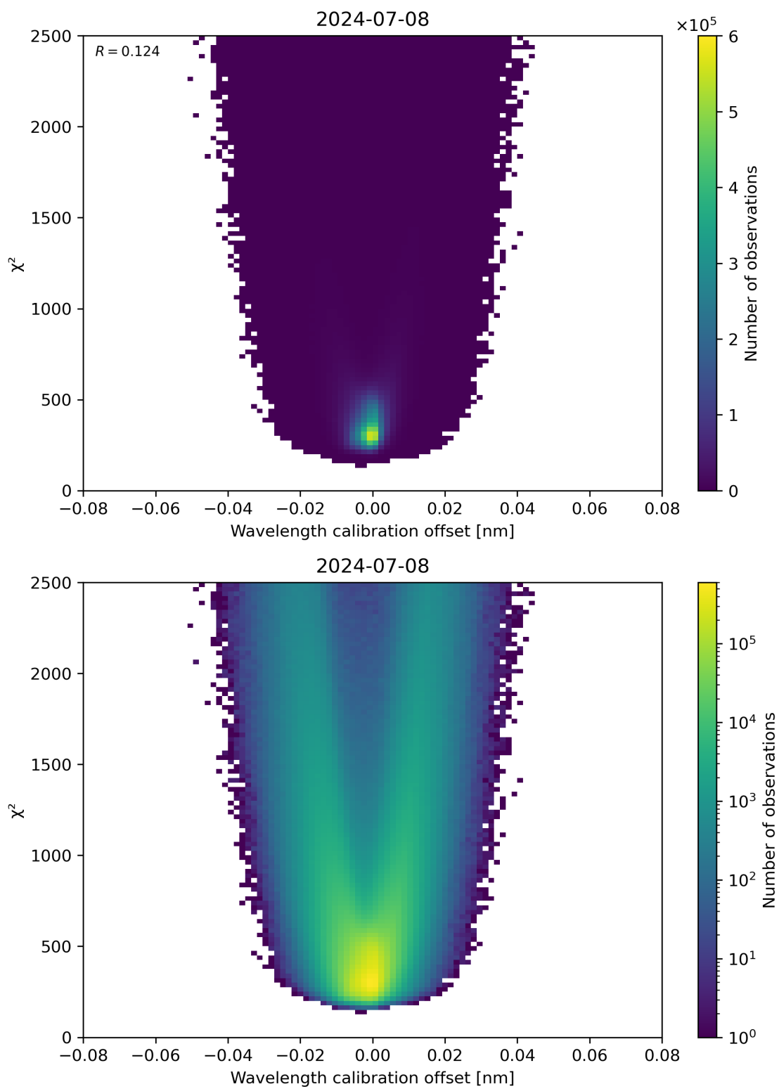
Figure 175: Scatter density plot of “Wavelength calibration offset” against “ \chi^2 ” for 2024-07-07 to 2024-07-09.
