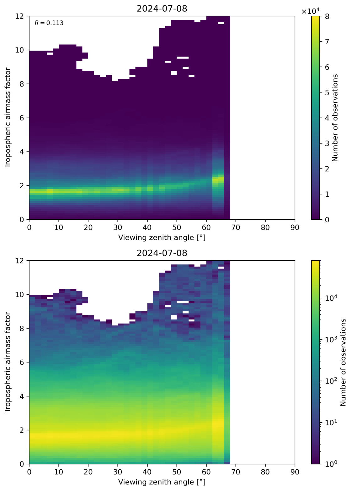
Figure 161: Scatter density plot of “Viewing zenith angle” against “Tropospheric airmass factor” for 2024-07-07 to 2024-07-09.
