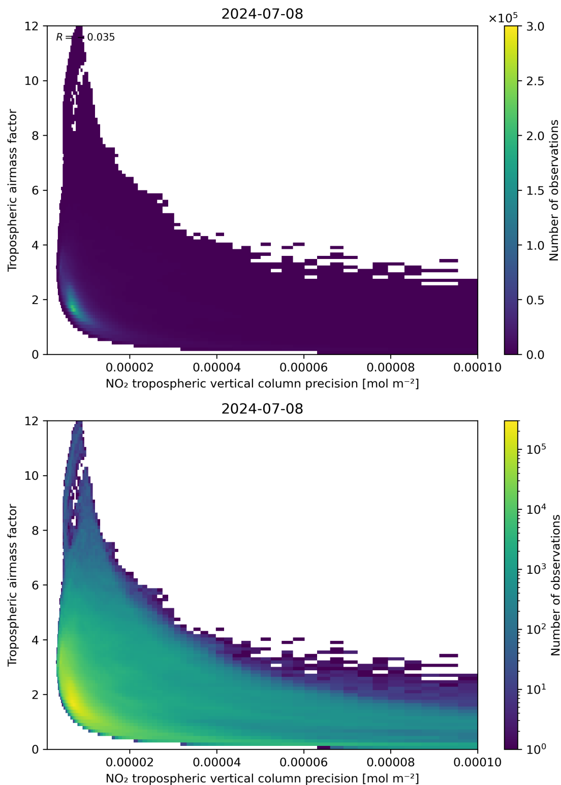
Figure 133: Scatter density plot of “NO 2 tropospheric vertical column precision” against “Tropospheric airmass factor” for 2024-07-07 to 2024-07-09.
