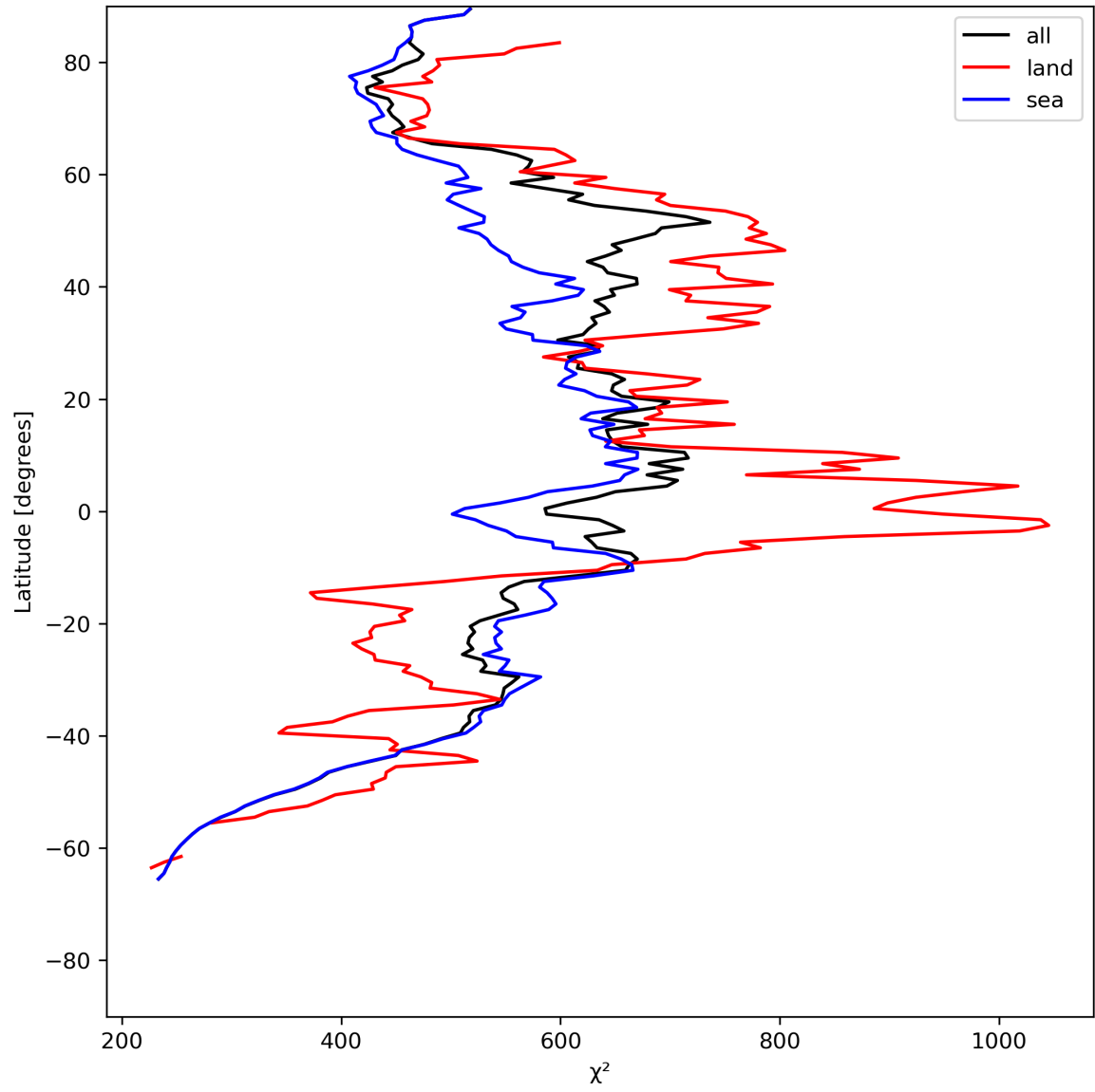
Figure 25: Zonal average of “ \chi^2 ” for 2024-07-07 to 2024-07-09.
