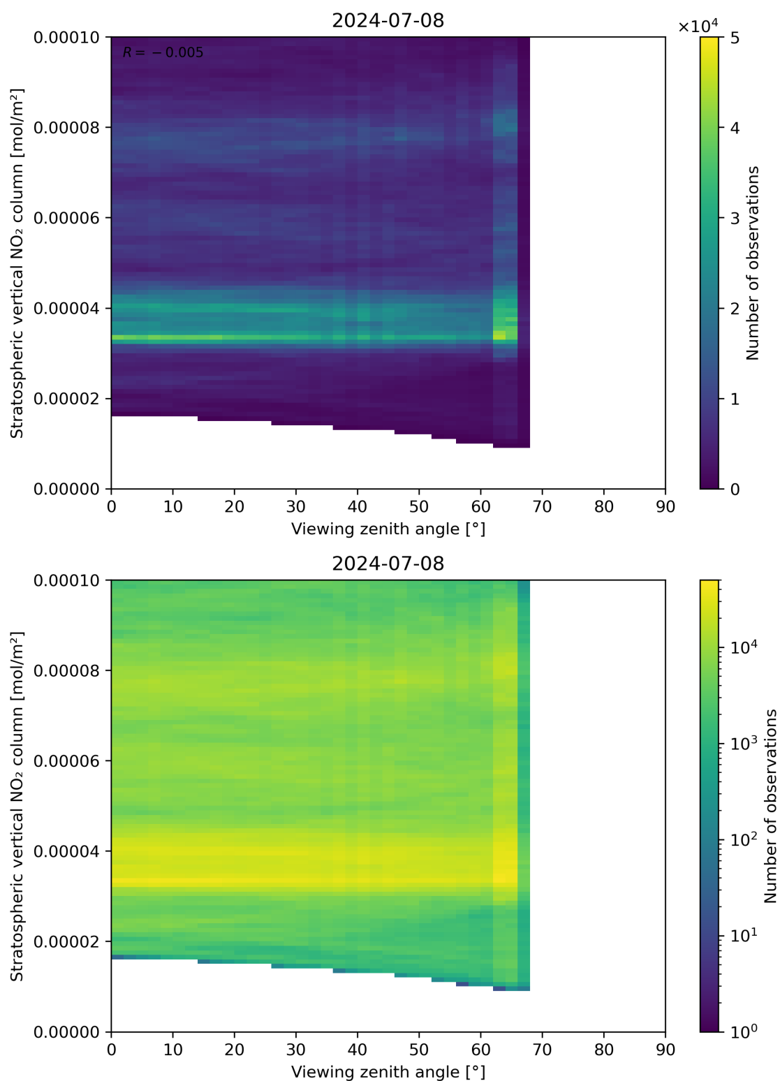
Figure 164: Scatter density plot of “Viewing zenith angle” against “Stratospheric vertical NO 2 column” for 2024-07-07 to 2024-07-09.
