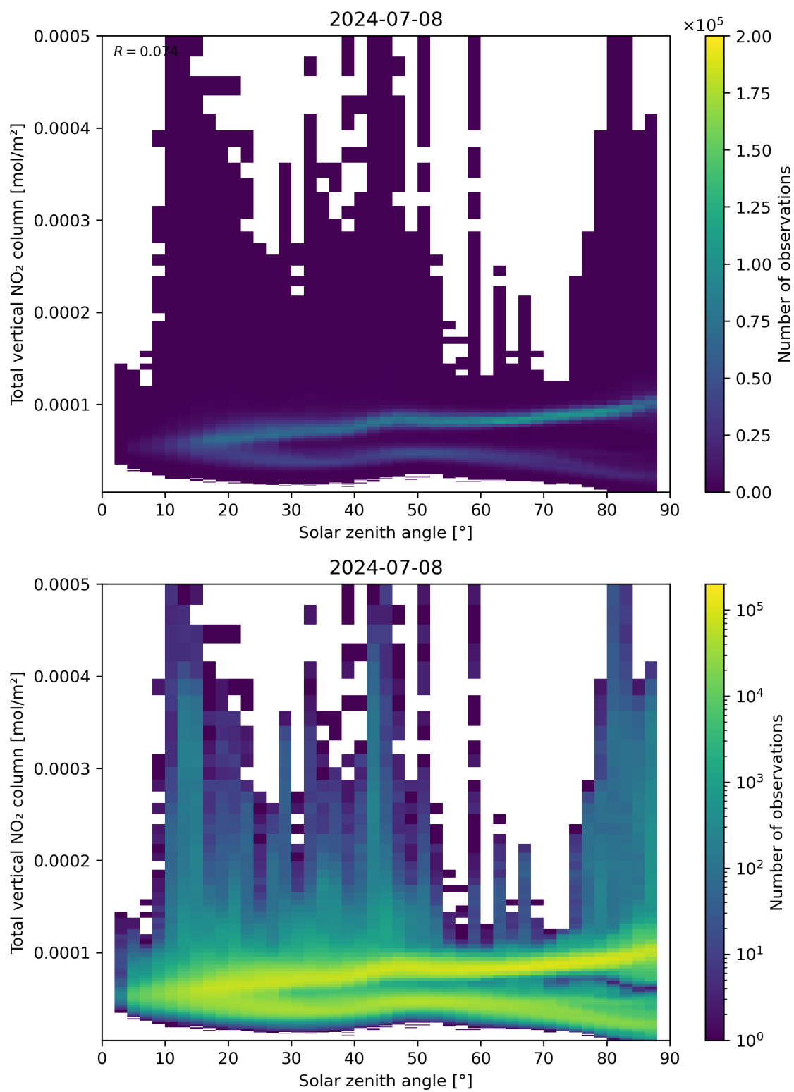
Figure 153: Scatter density plot of “Solar zenith angle” against “Total vertical NO 2 column” for 2024-07-07 to 2024-07-09.
