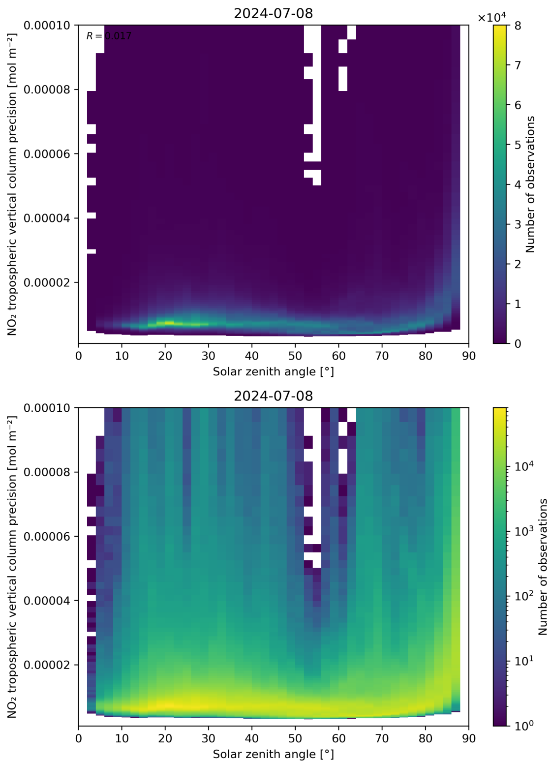
Figure 156: Scatter density plot of “Solar zenith angle” against “NO 2 tropospheric vertical column precision” for 2024-07-07 to 2024-07-09.
