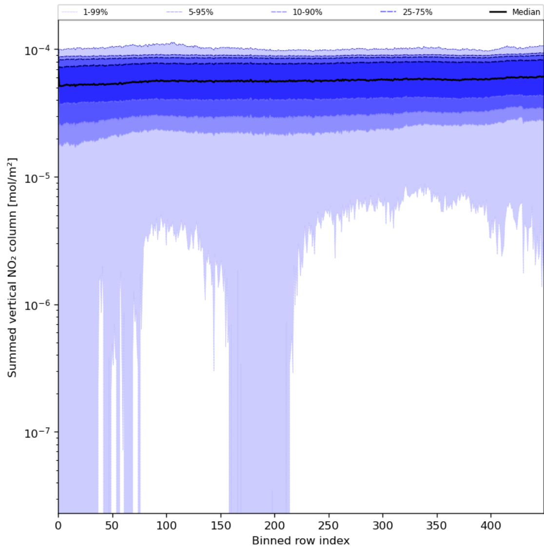
Figure 57: Along track statistics of “Summed vertical NO 2 column” for 2024-07-07 to 2024-07-09
