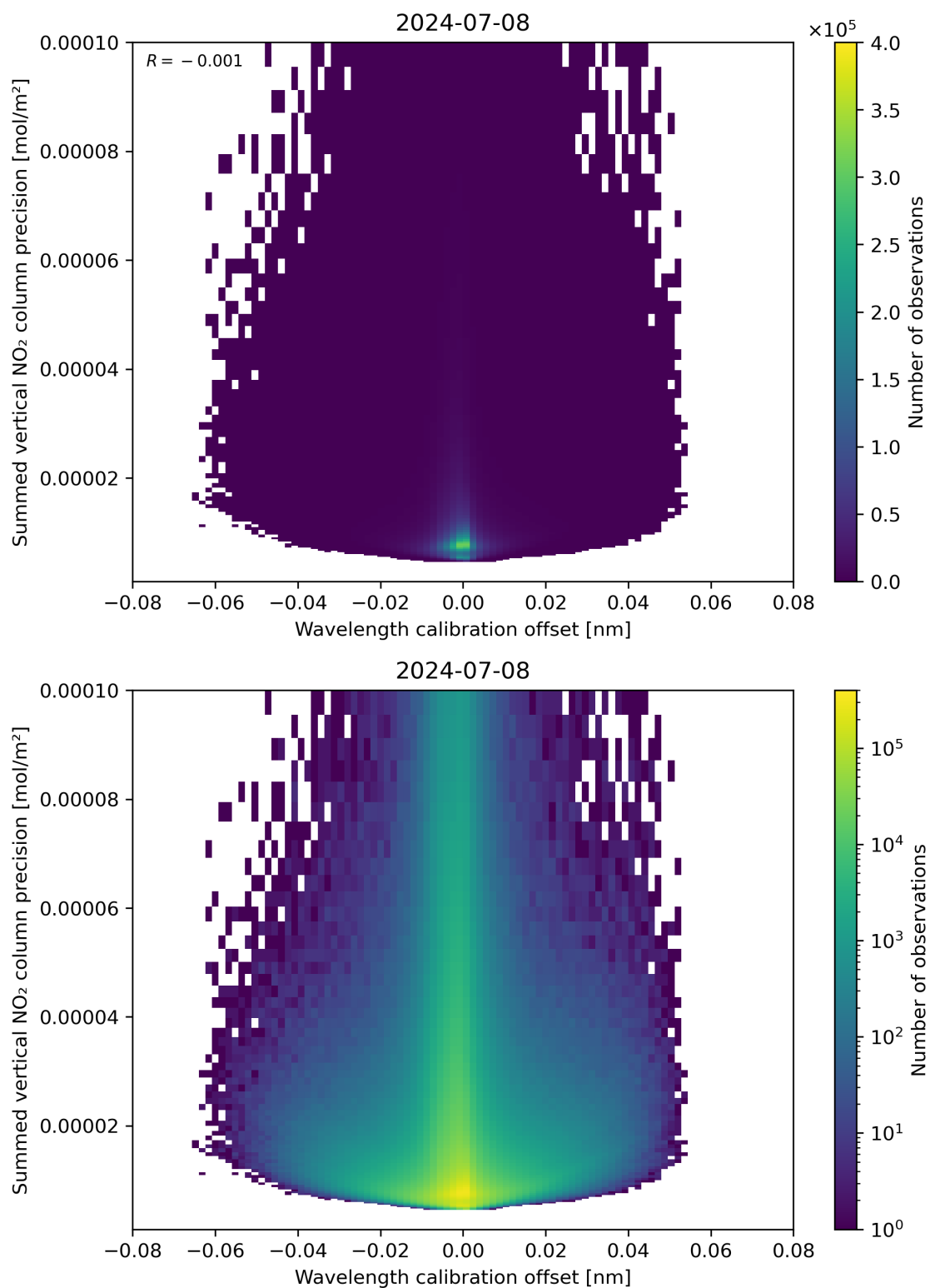
Figure 178: Scatter density plot of “Wavelength calibration offset” against “Summed vertical NO 2 column precision” for 2024-07-07 to 2024-07-09.
