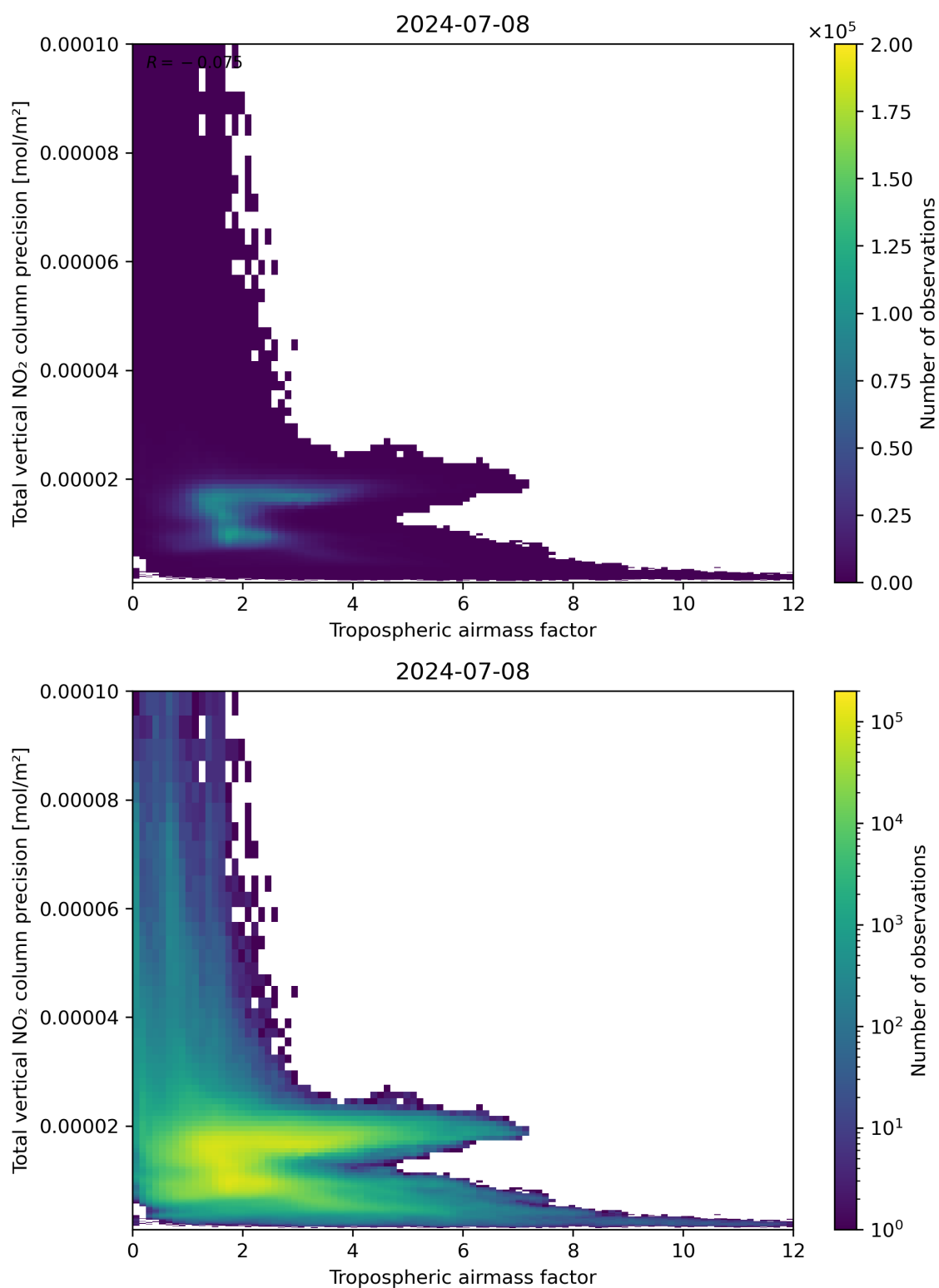
Figure 78: Scatter density plot of “Tropospheric air mass factor” against “Total vertical NO 2 column precision” for 2024-07-07 to 2024-07-09.
