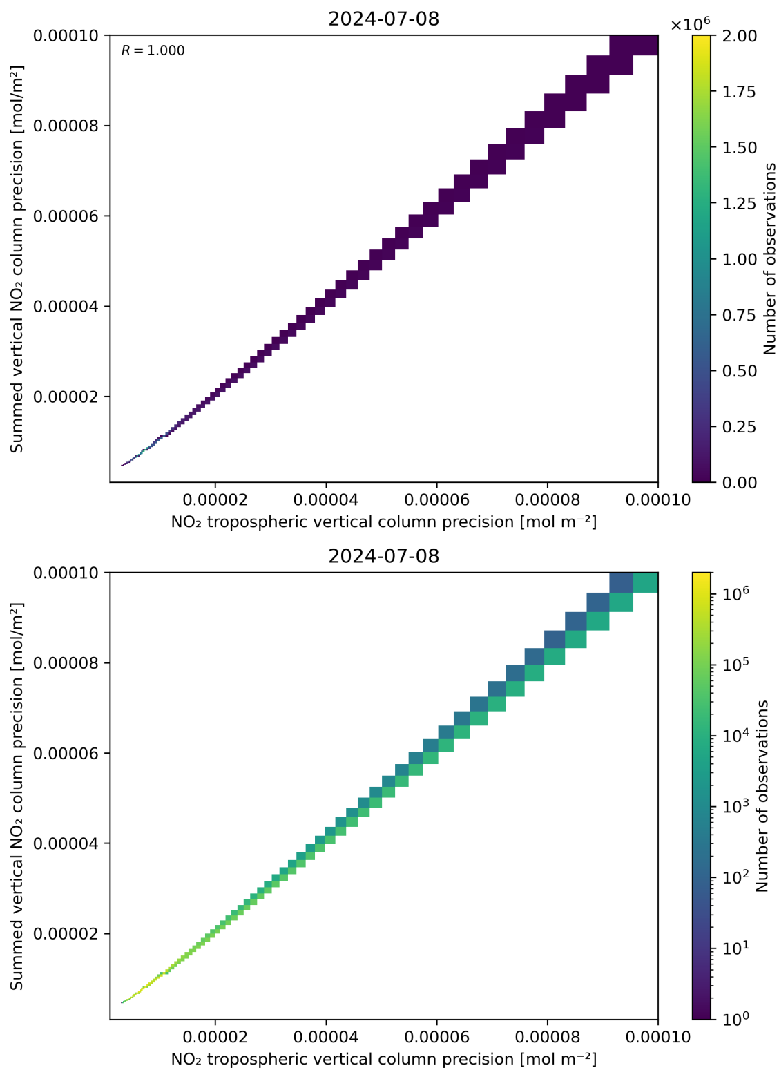
Figure 137: Scatter density plot of “NO 2 tropospheric vertical column precision” against “Summed vertical NO 2 column precision” for 2024-07-07 to 2024-07-09.
