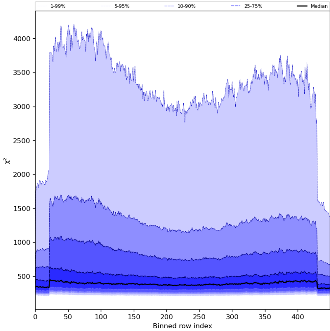
Figure 59: Along track statistics of “ \chi^2 ” for 2024-07-07 to 2024-07-09
