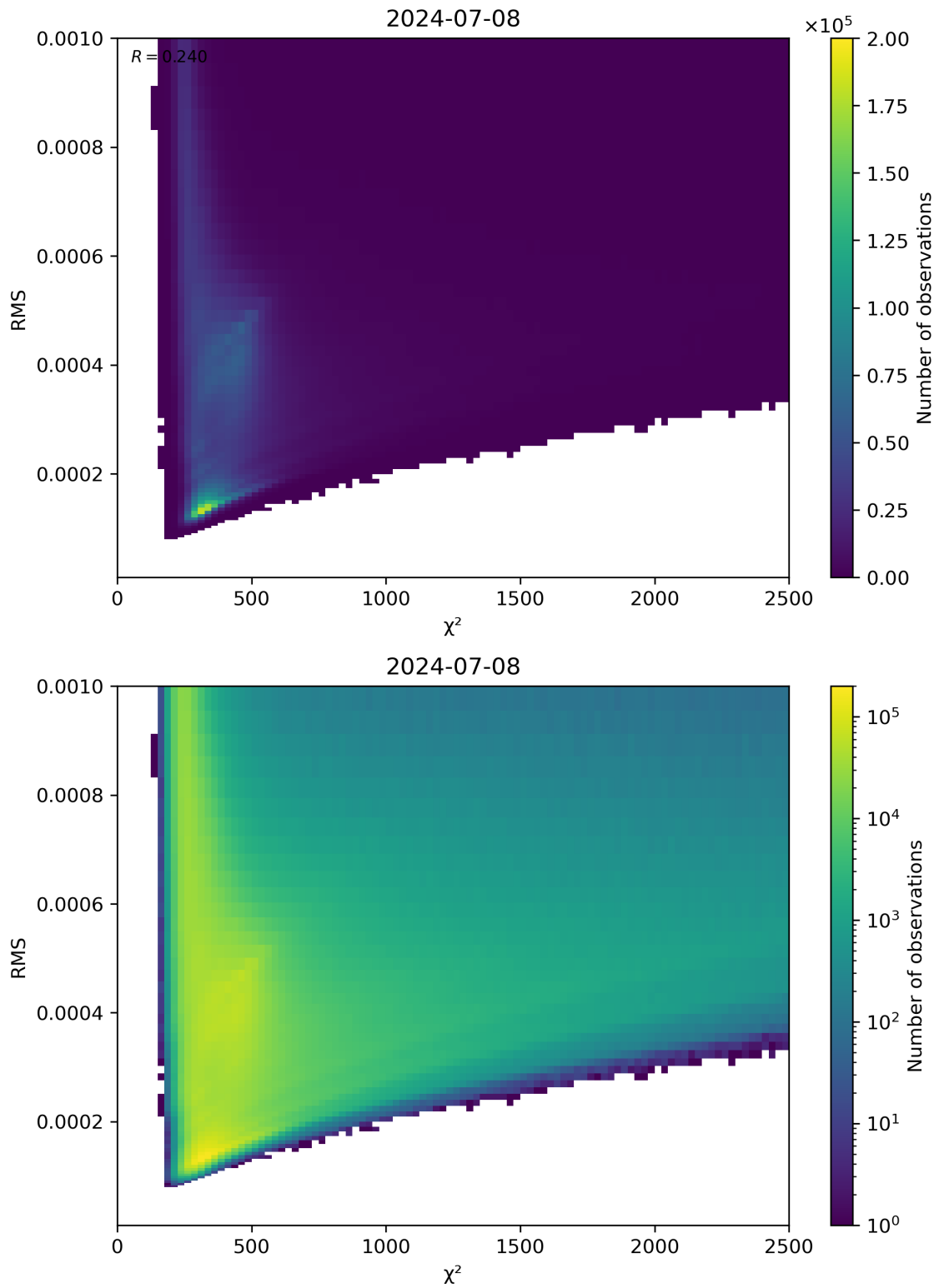
Figure 82: Scatter density plot of “ \chi^2 ” against “RMS” for 2024-07-07 to 2024-07-09.
