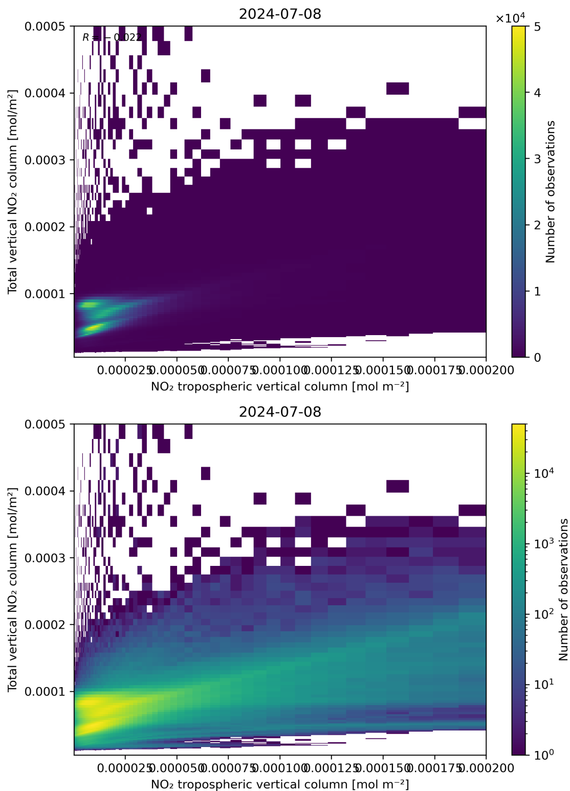
Figure 128: Scatter density plot of “NO 2 tropospheric vertical column” against “Total vertical NO 2 column” for 2024-07-07 to 2024-07-09.
