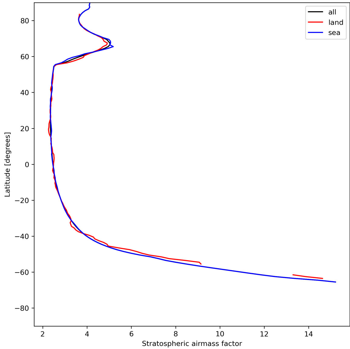
Figure 27: Zonal average of “Stratospheric air mass factor” for 2024-07-07 to 2024-07-09.
