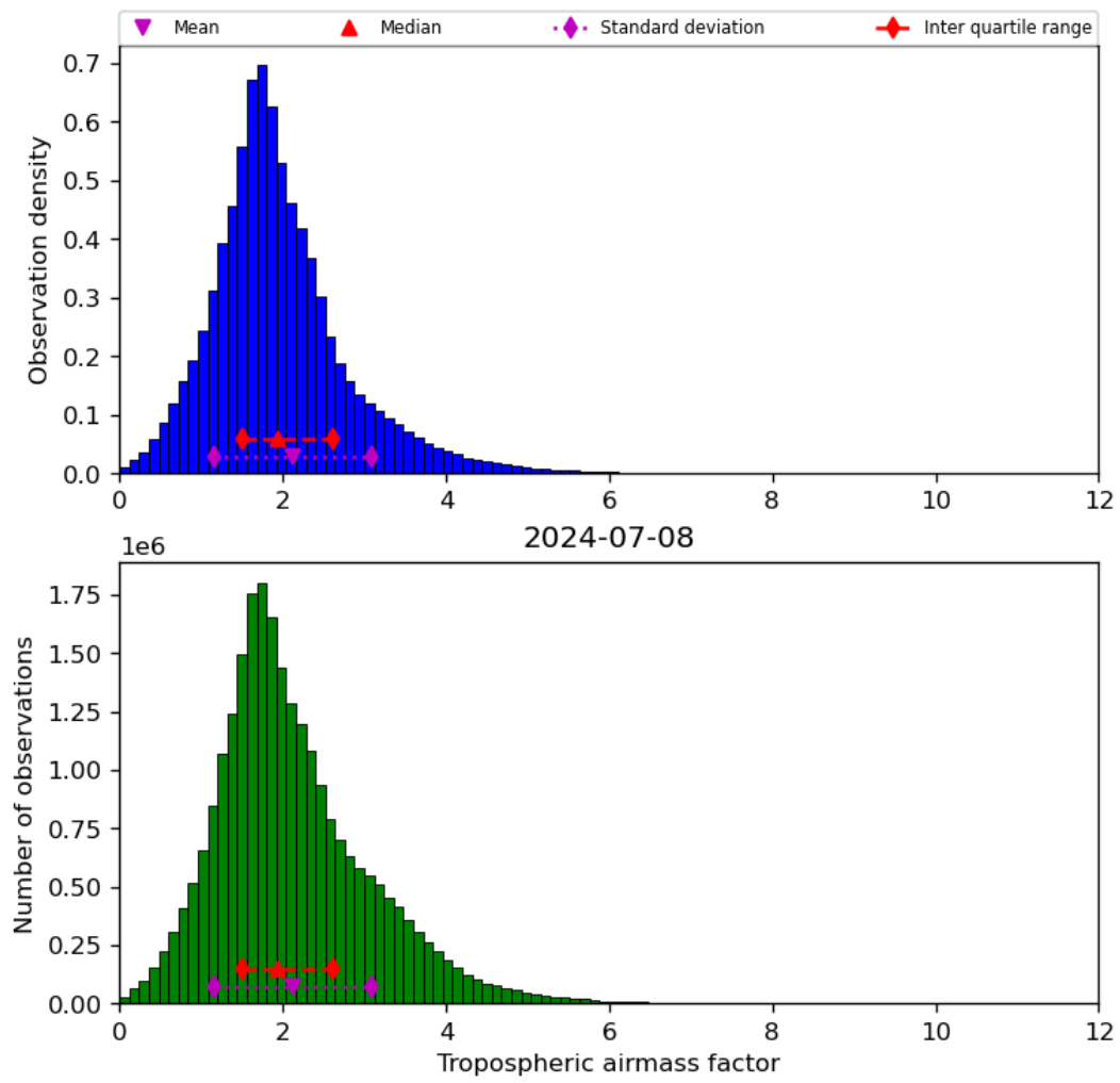
Figure 31: Histogram of “Tropospheric airmass factor” for 2024-07-07 to 2024-07-09
