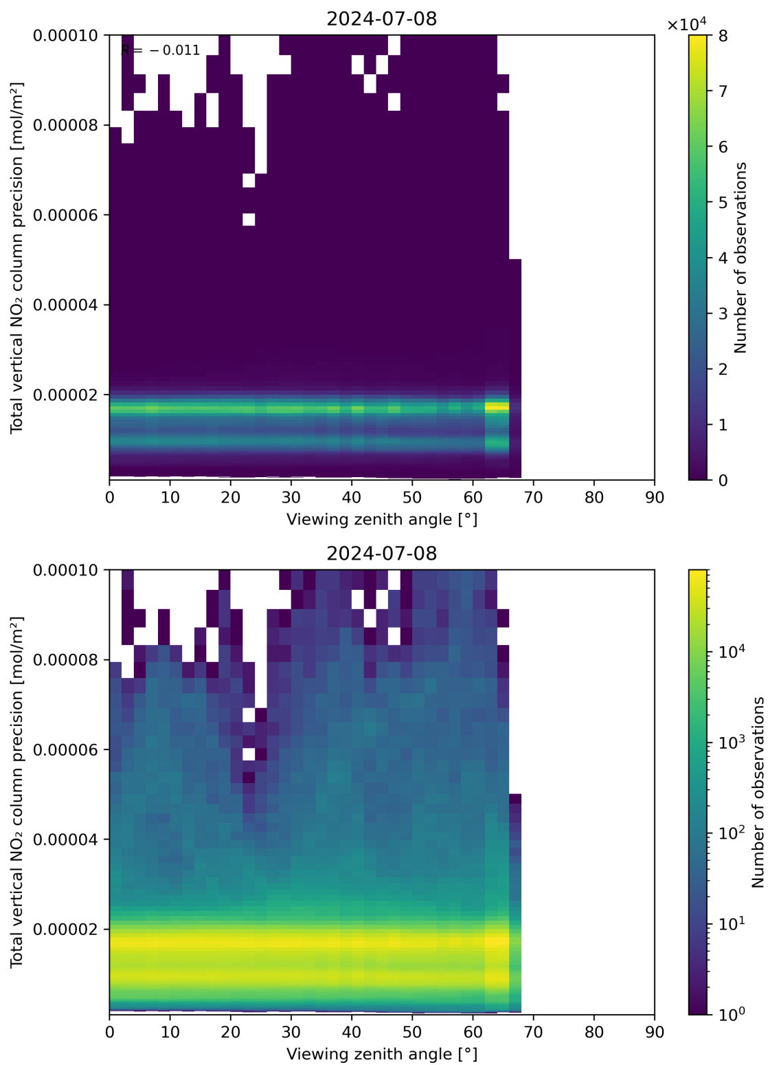
Figure 168: Scatter density plot of “Viewing zenith angle” against “Total vertical NO 2 column precision” for 2024-07-07 to 2024-07-09.
