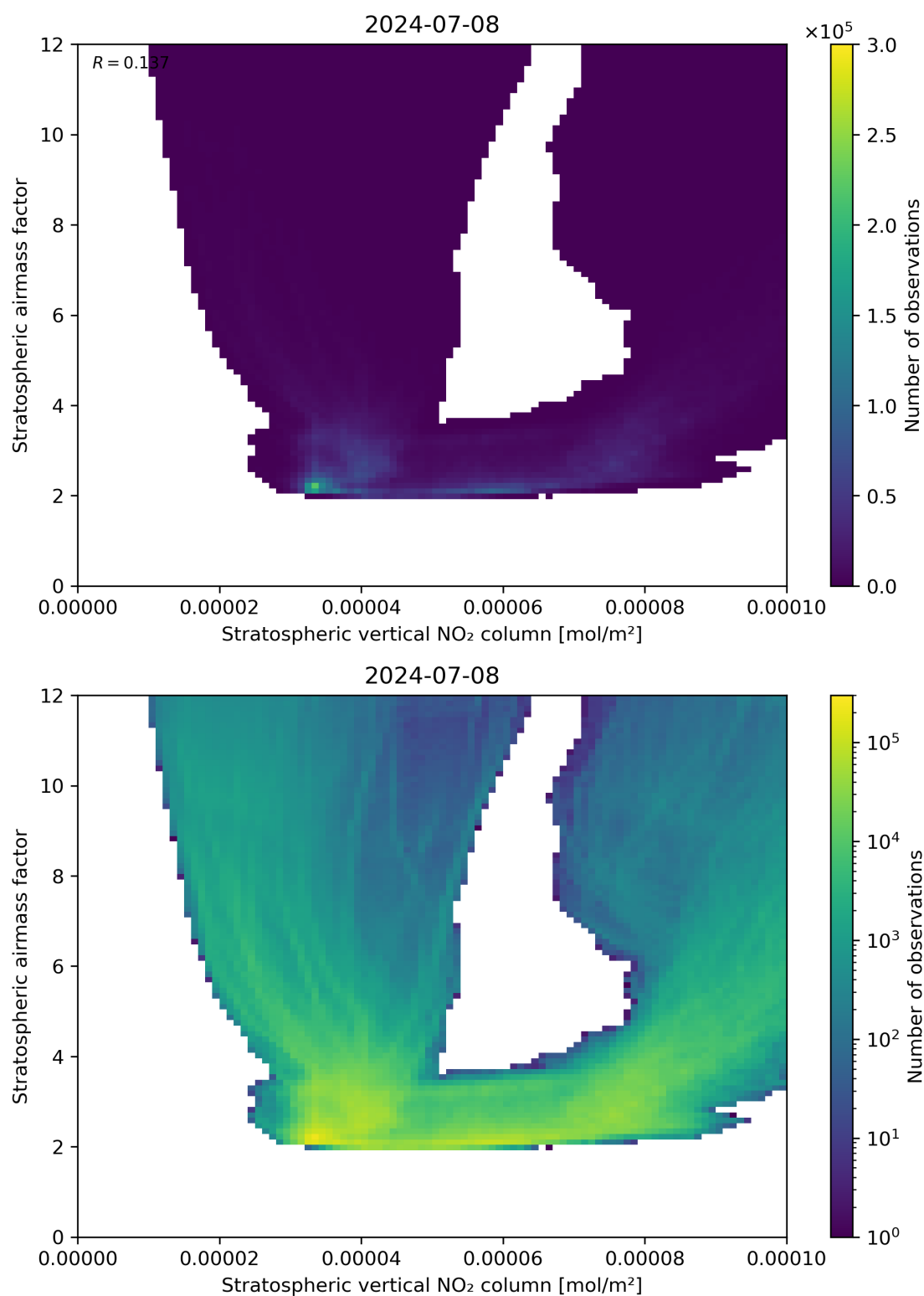
Figure 96: Scatter density plot of “Stratospheric vertical NO 2 column” against “Stratospheric airmass factor” for 2024-07-07 to 2024-07-09.
