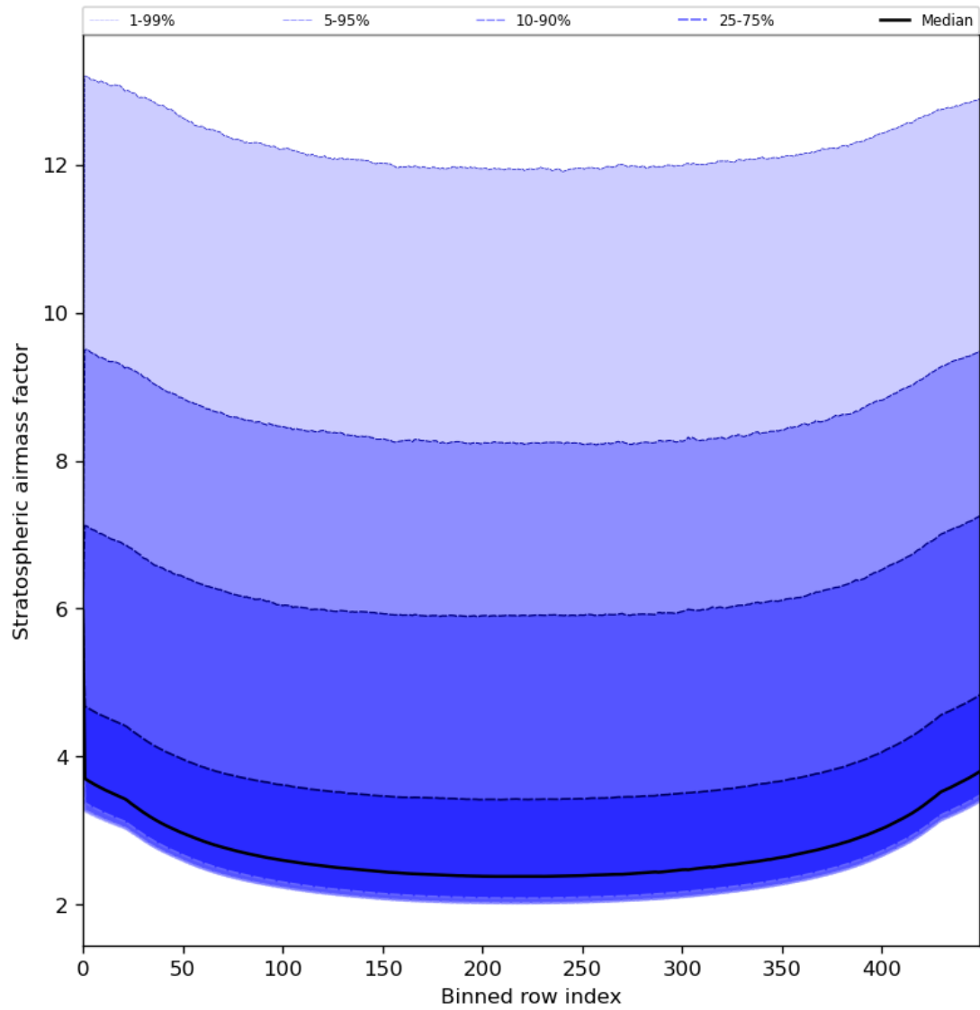
Figure 61: Along track statistics of “Stratospheric airmass factor” for 2024-07-07 to 2024-07-09
