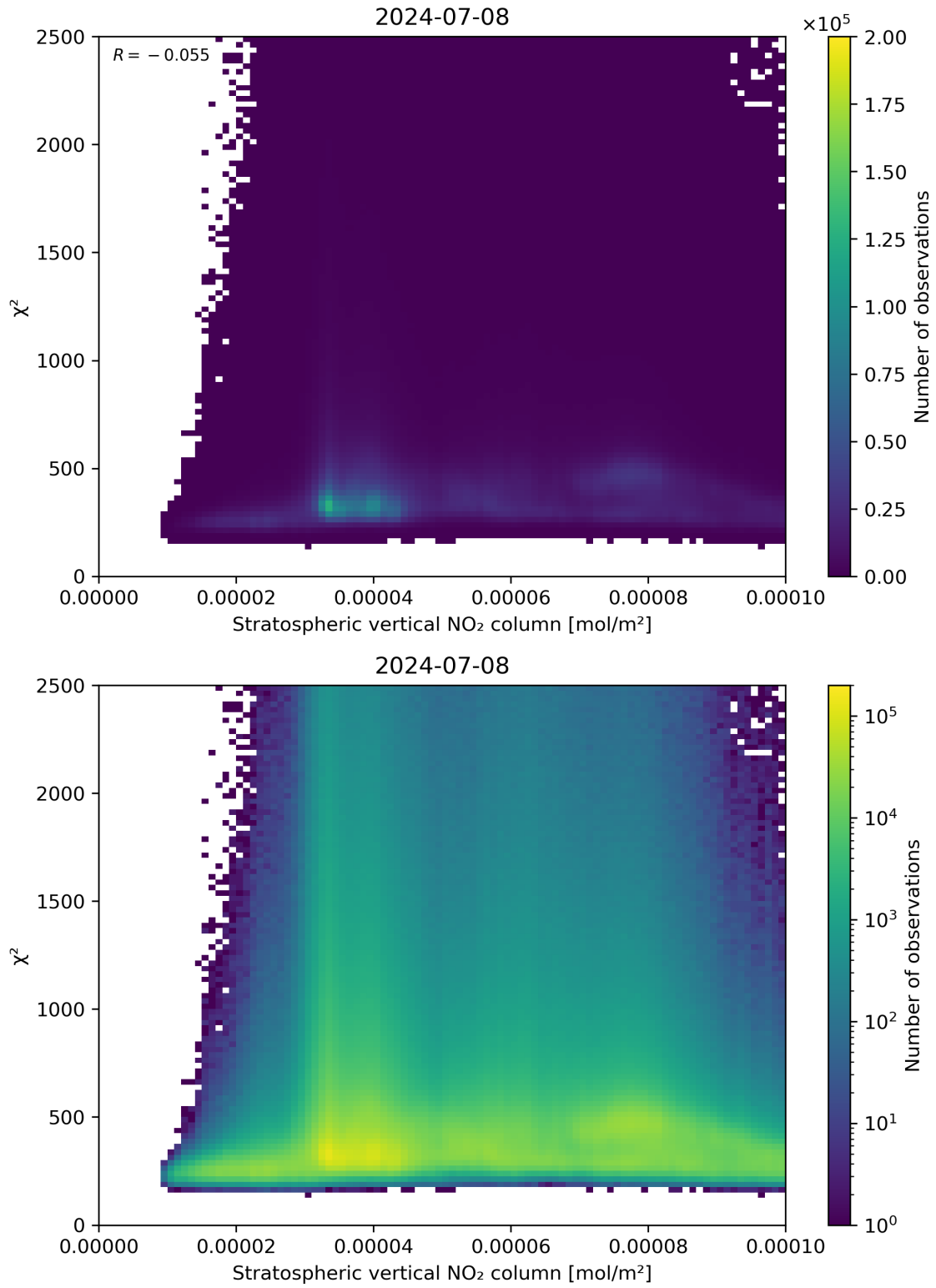
Figure 97: Scatter density plot of “Stratospheric vertical NO 2 column” against “ \chi^2 ” for 2024-07-07 to 2024-07-09.
