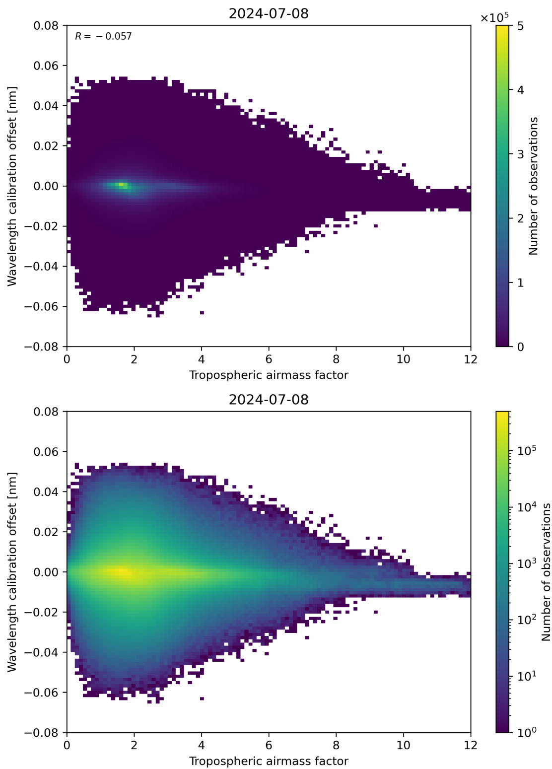
Figure 80: Scatter density plot of “Tropospheric air mass factor” against “Wavelength calibration offset” for 2024-07-07 to 2024-07-09.
