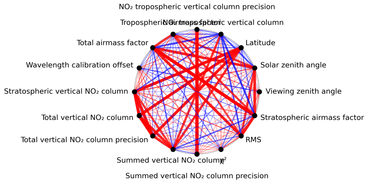
Figure 1: Map of correlation graph for 2024-07-07 to 2024-07-09.
