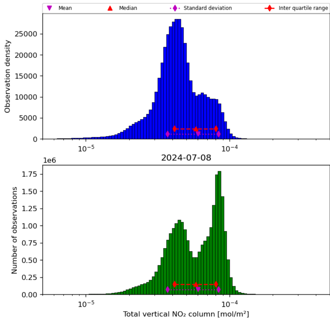
Figure 38: Histogram of “Total vertical NO 2 column” for 2024-07-07 to 2024-07-09
