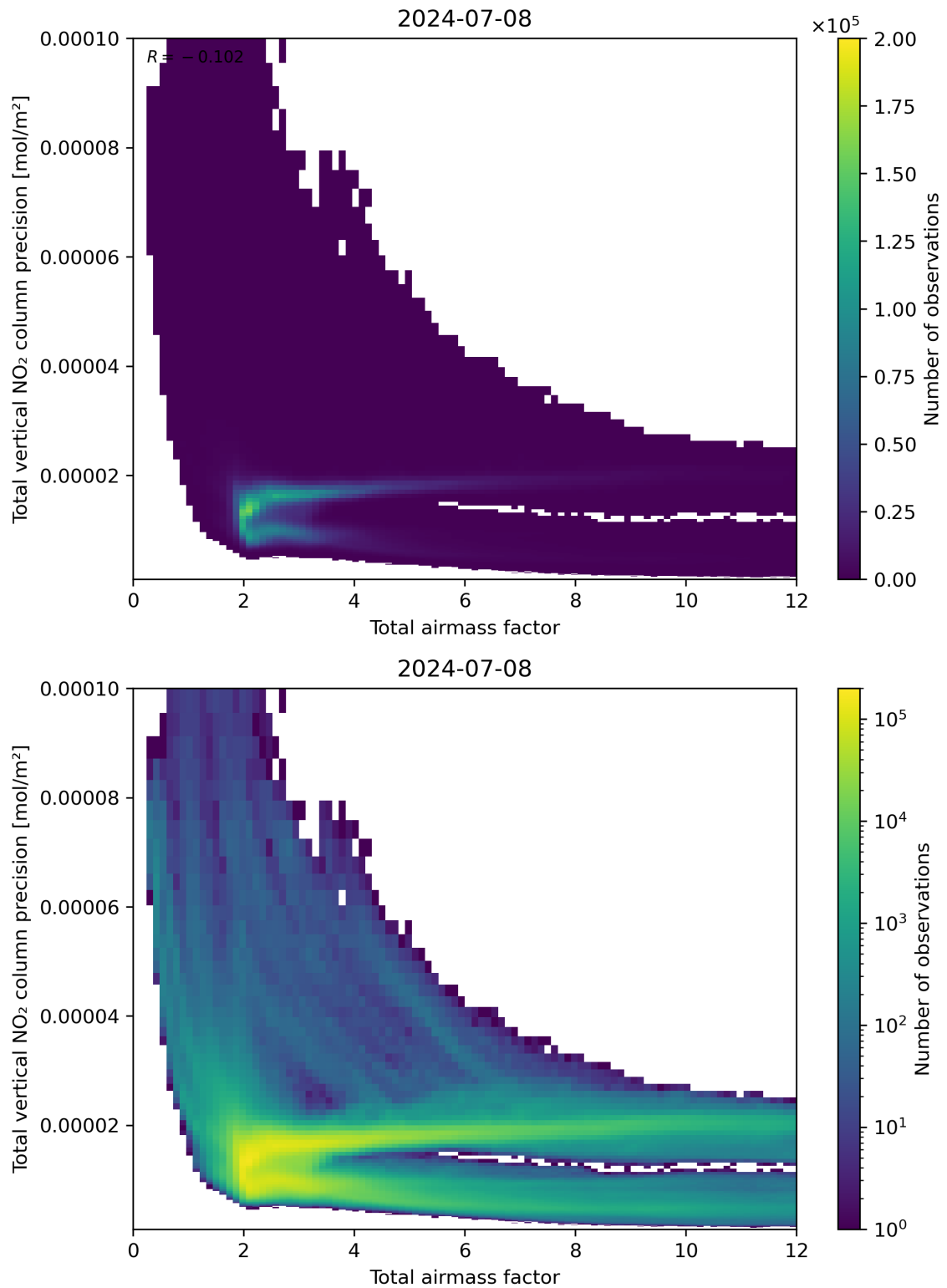
Figure 68: Scatter density plot of “Total airmass factor” against “Total vertical NO 2 column precision” for 2024-07-07 to 2024-07-09.
