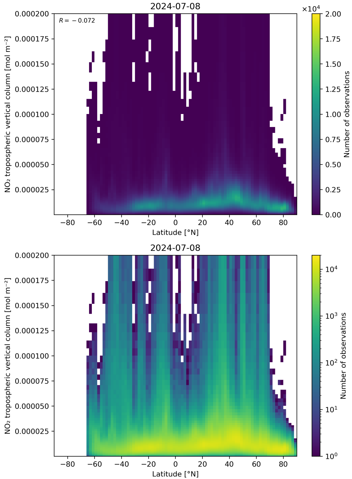
Figure 92: Scatter density plot of “Latitude” against “NO 2 tropospheric vertical column” for 2024-07-07 to 2024-07-09.
