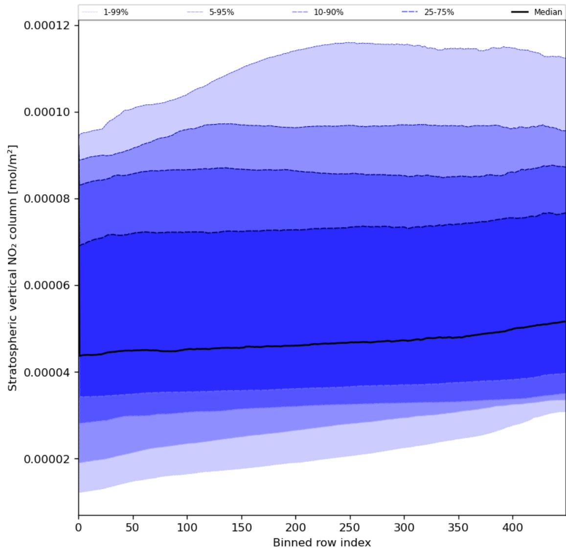
Figure 53: Along track statistics of “Stratospheric vertical NO 2 column” for 2024-07-07 to 2024-07-09
