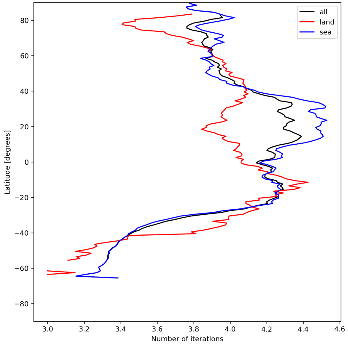
Figure 17: Zonal average of “Number of iterations” for 2024-07-07 to 2024-07-09.
