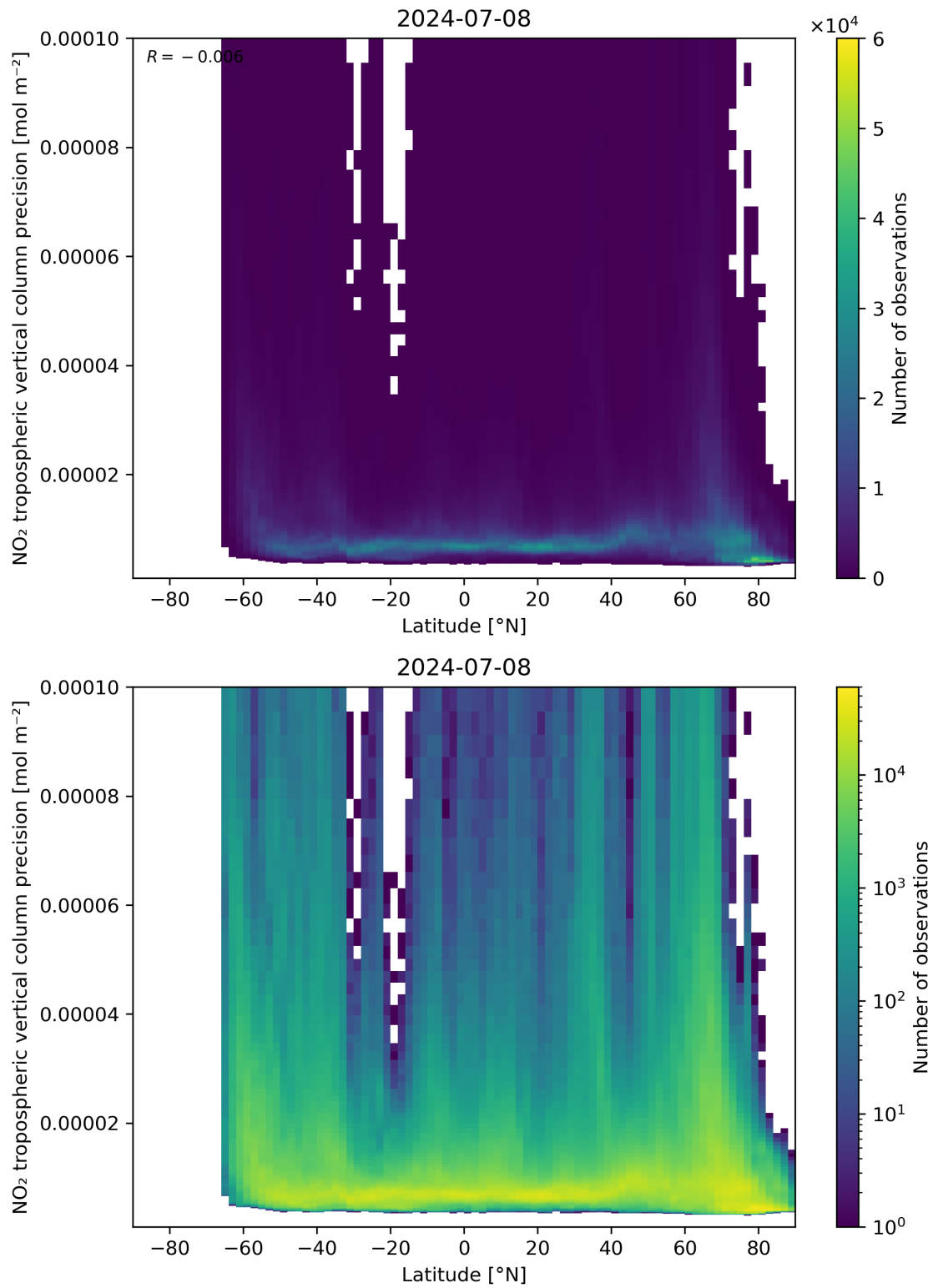
Figure 93: Scatter density plot of “Latitude” against “NO 2 tropospheric vertical column precision” for 2024-07-07 to 2024-07-09.
