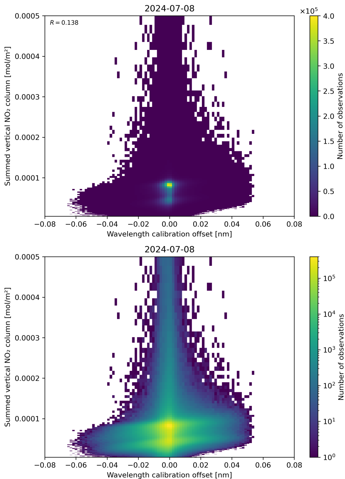
Figure 177: Scatter density plot of “Wavelength calibration offset” against “Summed vertical NO 2 column” for 2024-07-07 to 2024-07-09.
