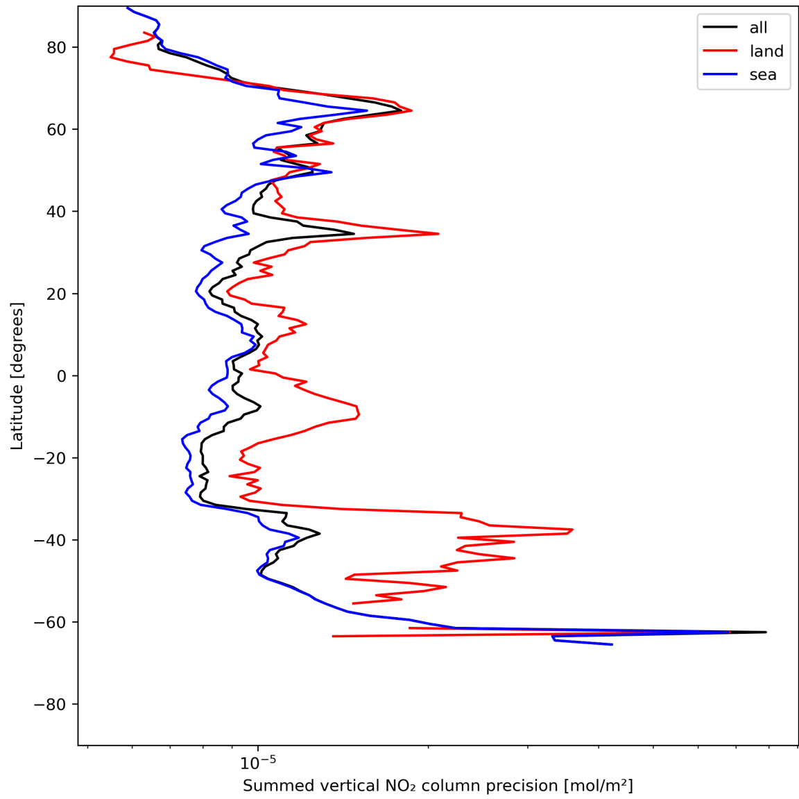
Figure 24: Zonal average of “Summed vertical NO 2 column precision” for 2024-07-07 to 2024-07-09.
