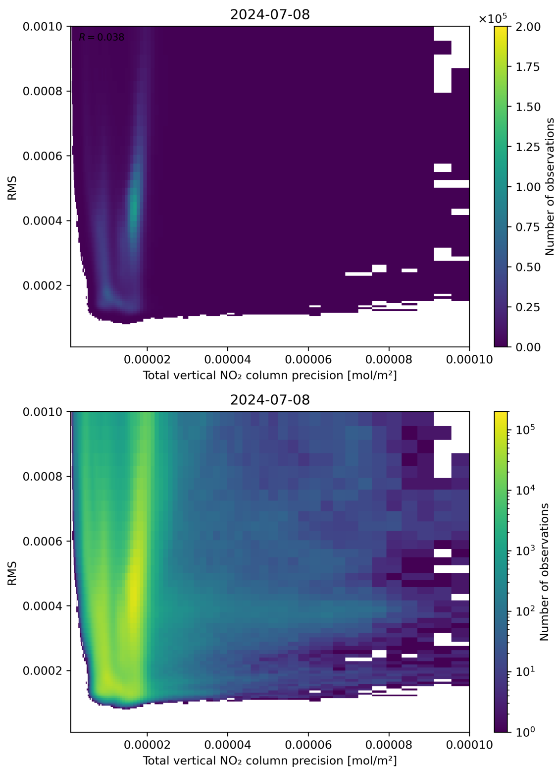
Figure 119: Scatter density plot of “Total vertical NO 2 column precision” against “RMS” for 2024-07-07 to 2024-07-09.
