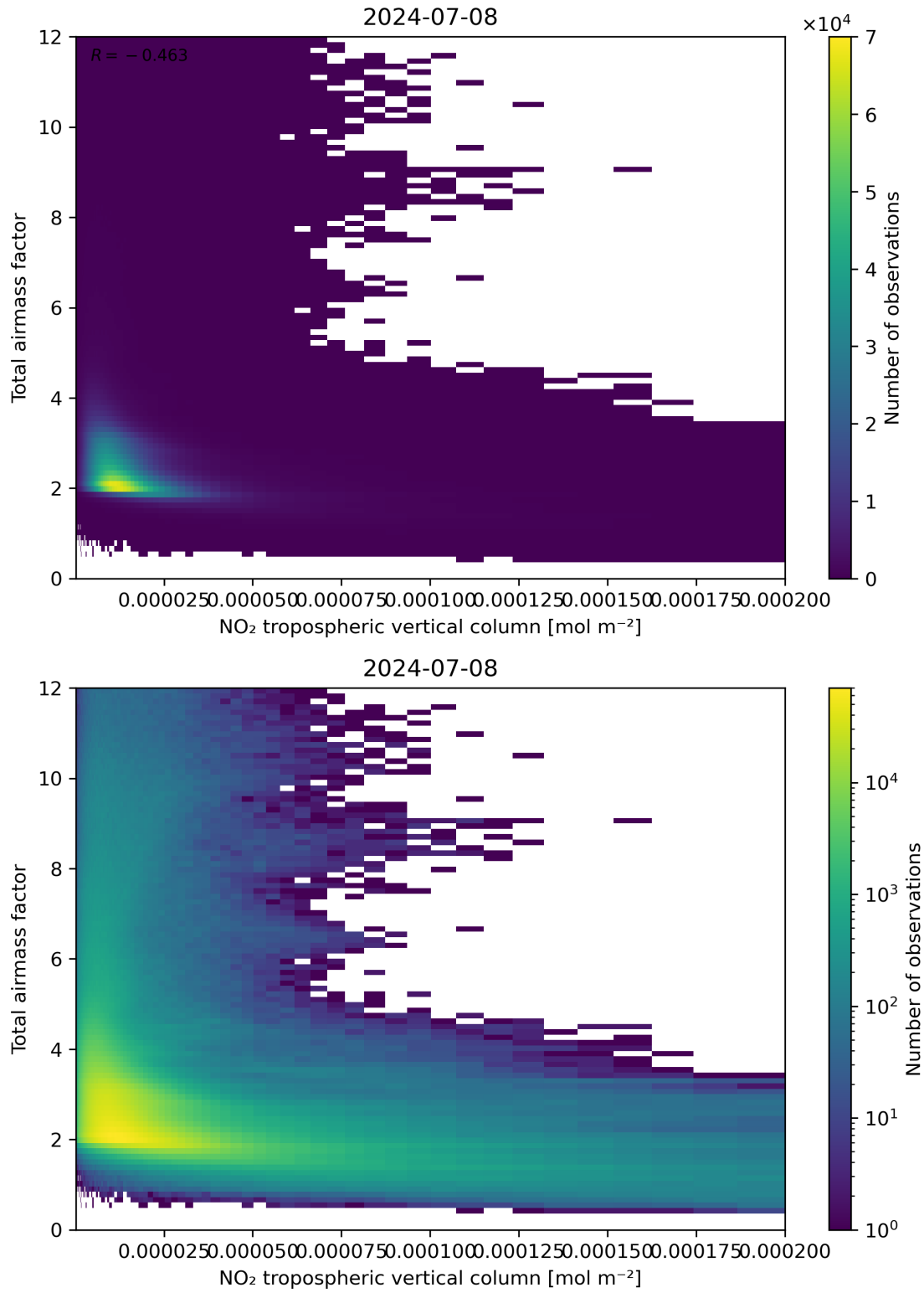
Figure 122: Scatter density plot of “NO 2 tropospheric vertical column” against “Total air mass factor” for 2024-07-07 to 2024-07-09.
