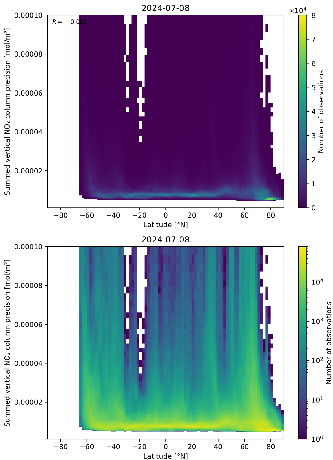
Figure 89: Scatter density plot of “Latitude” against “Summed vertical NO 2 column precision” for 2024-07-07 to 2024-07-09.
