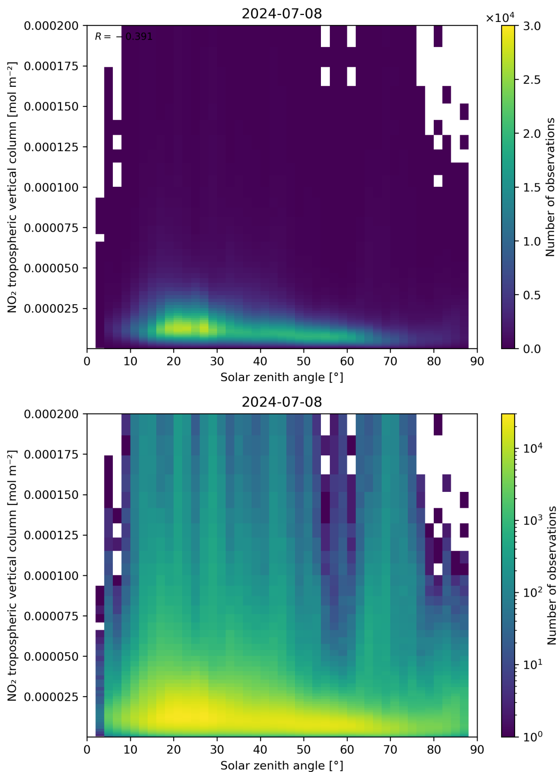
Figure 155: Scatter density plot of “Solar zenith angle” against “NO 2 tropospheric vertical column” for 2024-07-07 to 2024-07-09.
