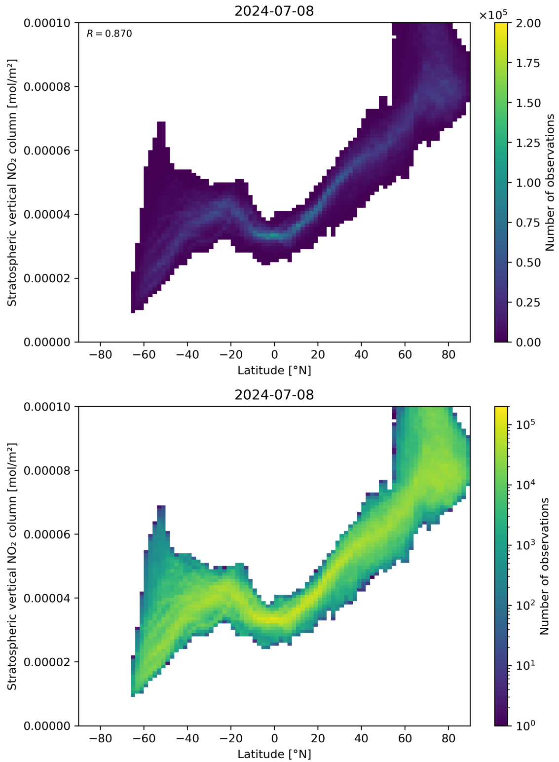
Figure 87: Scatter density plot of “Latitude” against “Stratospheric vertical NO 2 column” for 2024-07-07 to 2024-07-09.
