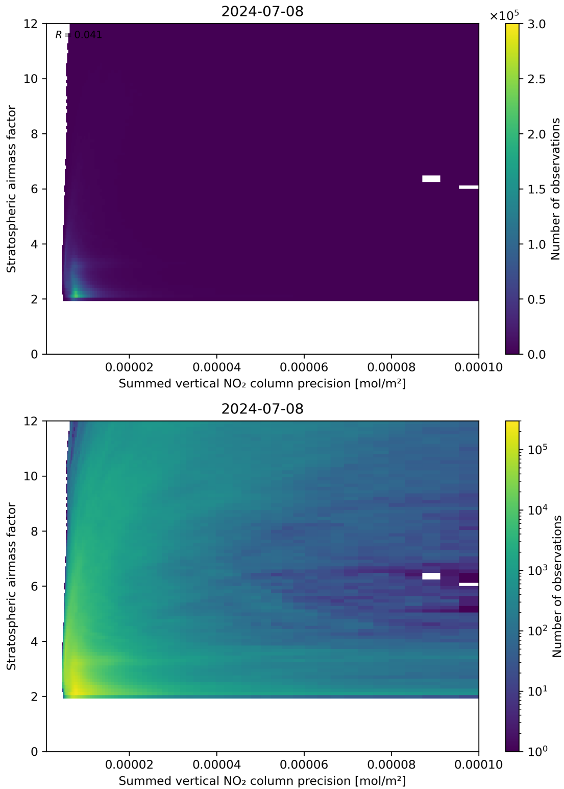
Figure 106: Scatter density plot of “Summed vertical NO 2 column precision” against “Stratospheric airmass factor” for 2024-07-07 to 2024-07-09.
