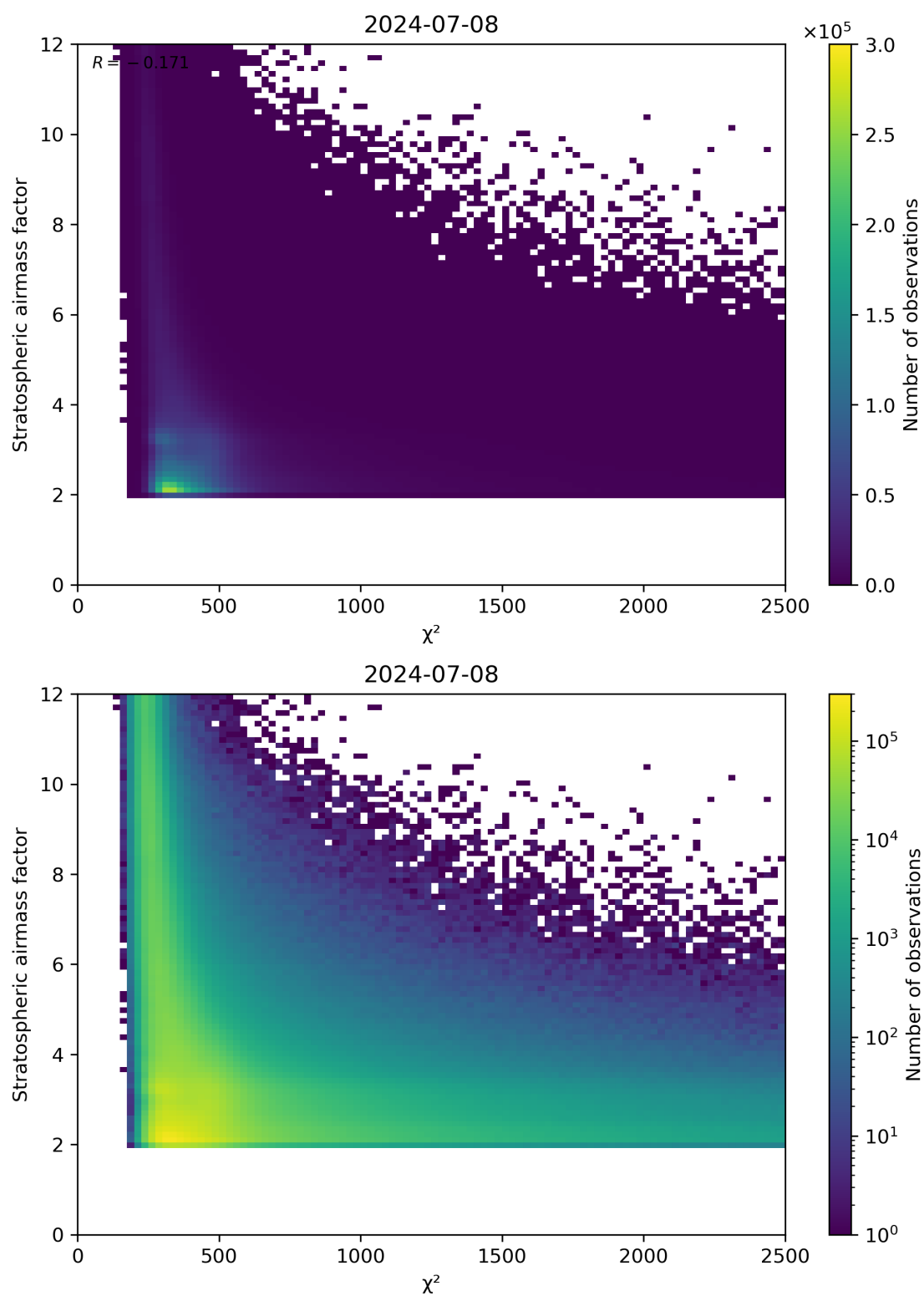
Figure 81: Scatter density plot of “ \chi^2 ” against “Stratospheric airmass factor” for 2024-07-07 to 2024-07-09.
