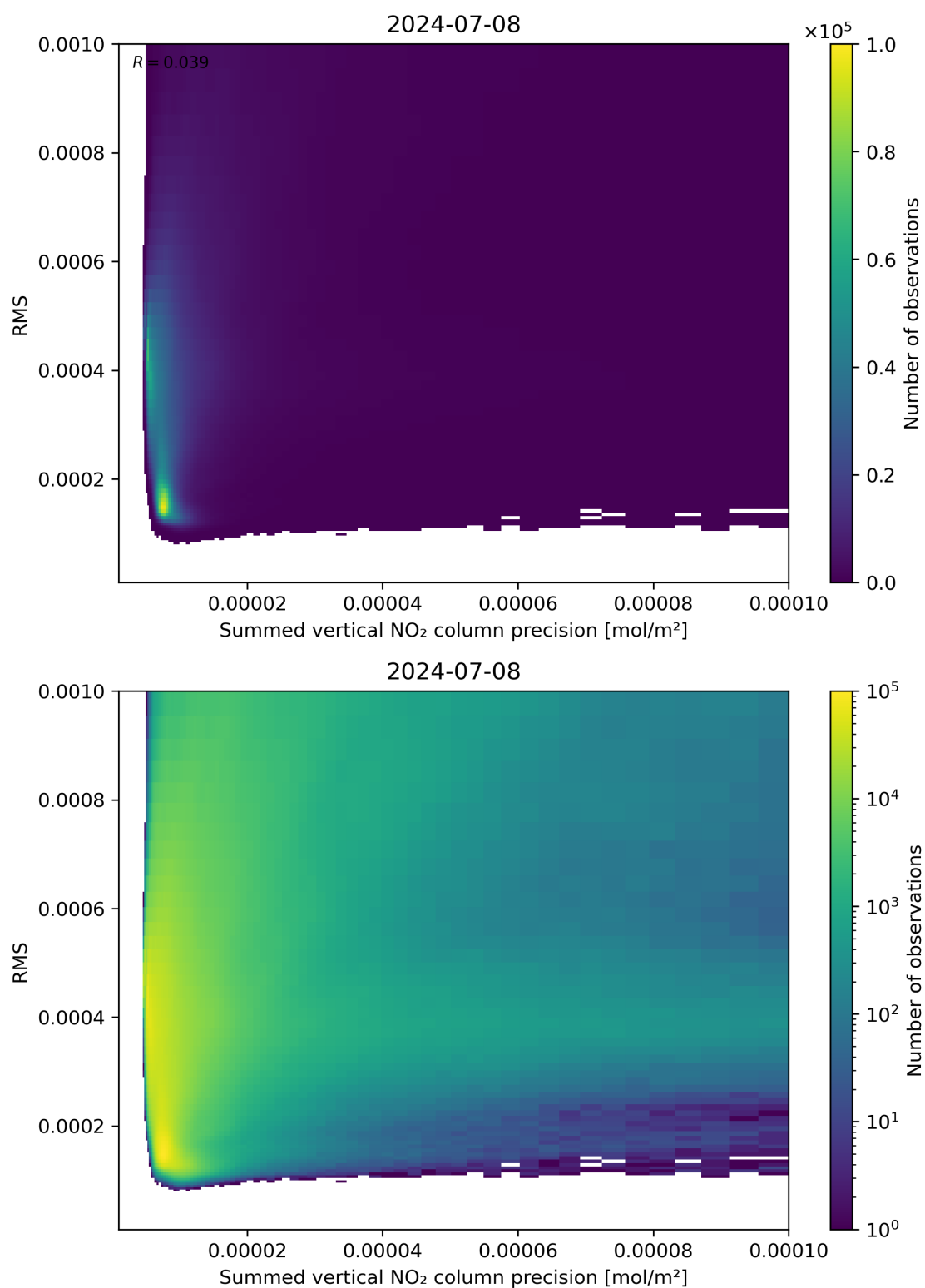
Figure 108: Scatter density plot of “Summed vertical NO 2 column precision” against “RMS” for 2024-07-07 to 2024-07-09.
