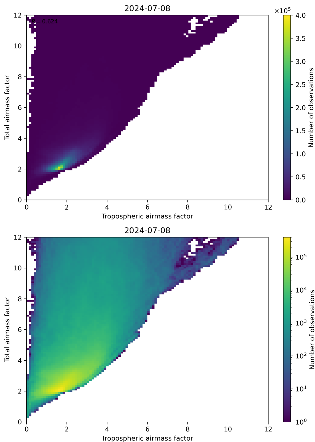
Figure 72: Scatter density plot of “Tropospheric airmass factor” against “Total airmass factor” for 2024-07-07 to 2024-07-09.
