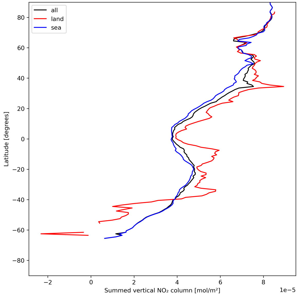
Figure 23: Zonal average of “Summed vertical NO 2 column” for 2024-07-07 to 2024-07-09.
