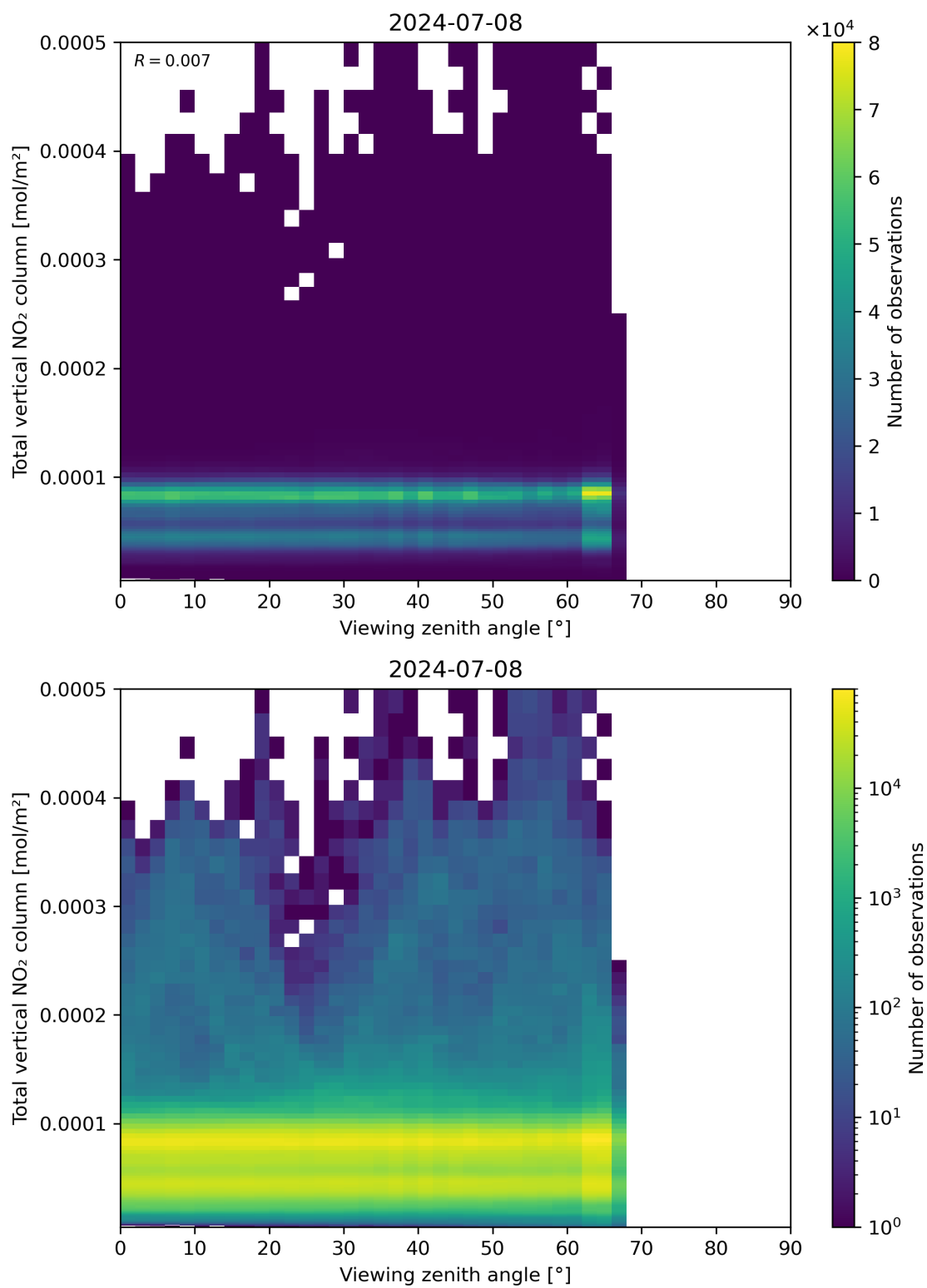
Figure 167: Scatter density plot of “Viewing zenith angle” against “Total vertical NO 2 column” for 2024-07-07 to 2024-07-09.
