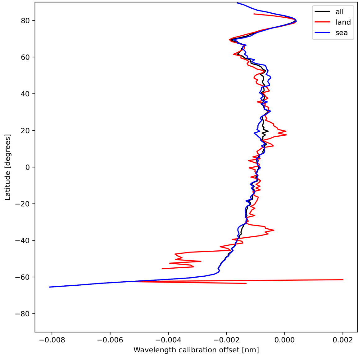
Figure 18: Zonal average of “Wavelength calibration offset” for 2024-07-07 to 2024-07-09.
