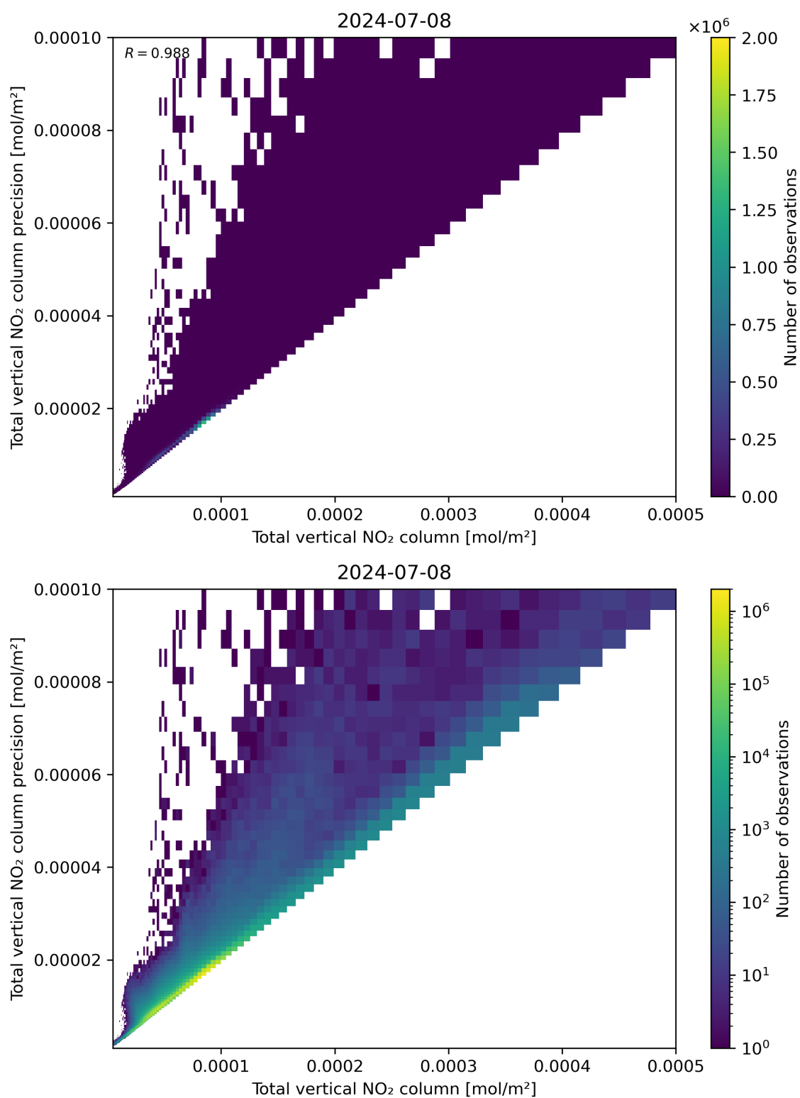
Figure 114: Scatter density plot of “Total vertical NO 2 column” against “Total vertical NO 2 column precision” for 2024-07-07 to 2024-07-09.
