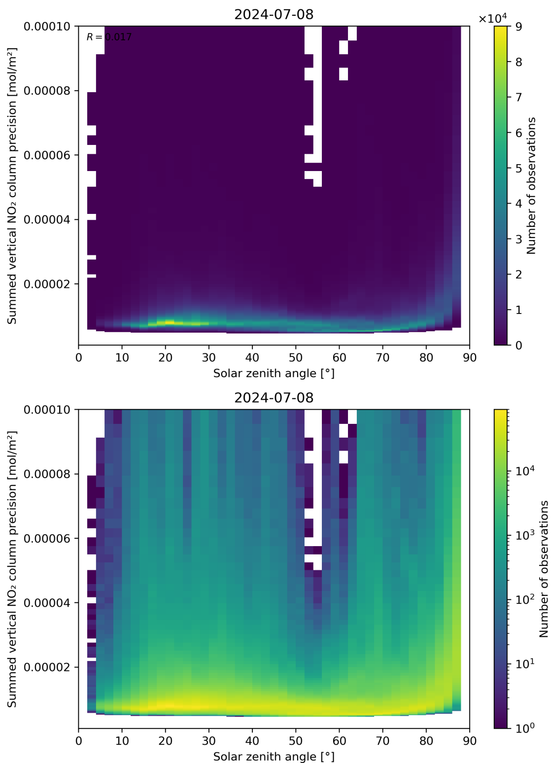
Figure 152: Scatter density plot of “Solar zenith angle” against “Summed vertical NO 2 column precision” for 2024-07-07 to 2024-07-09.
