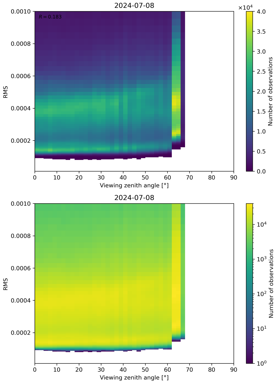
Figure 171: Scatter density plot of “Viewing zenith angle” against “RMS” for 2024-07-07 to 2024-07-09.
