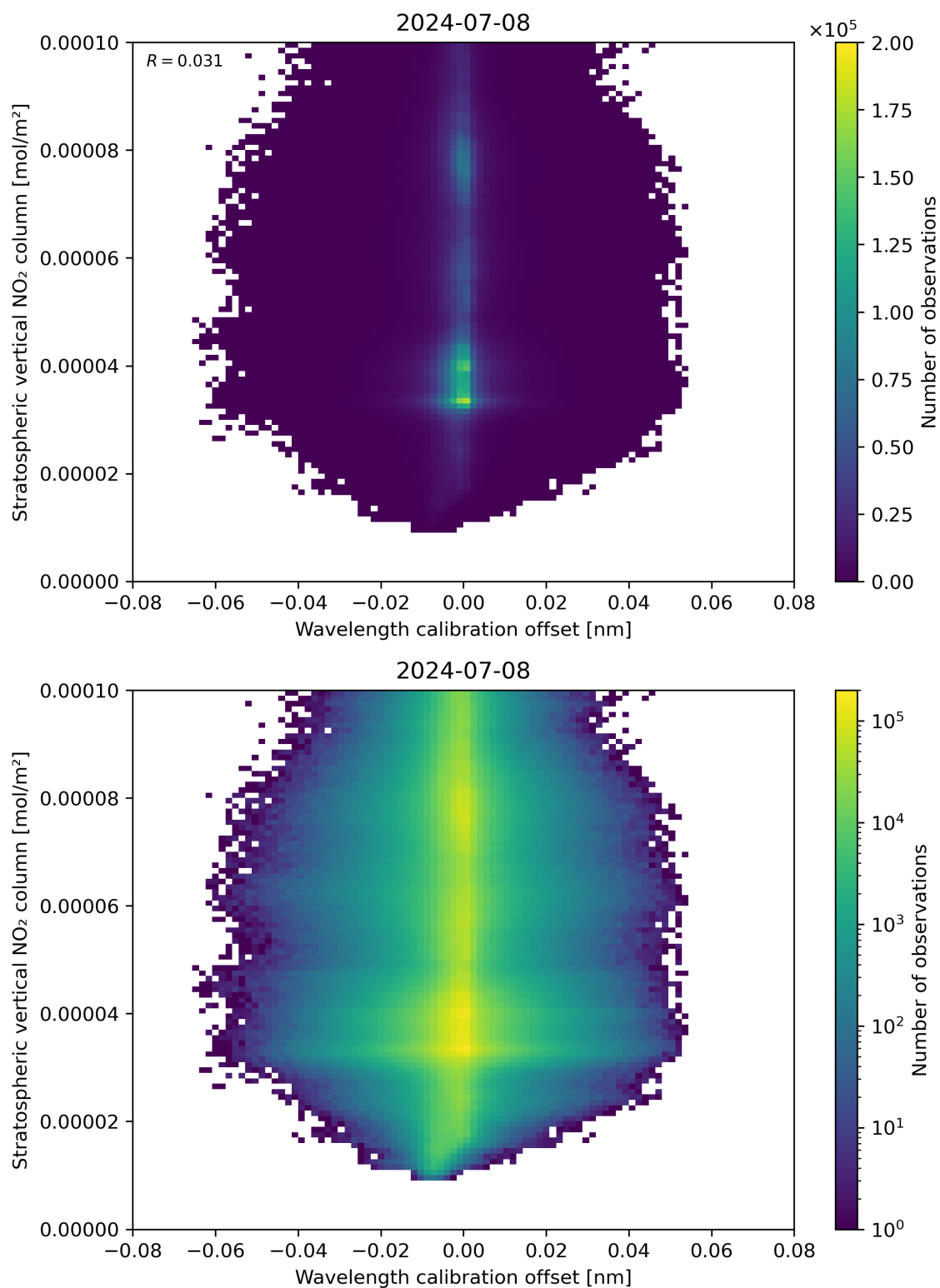
Figure 176: Scatter density plot of “Wavelength calibration offset” against “Stratospheric vertical NO 2 column” for 2024-07-07 to 2024-07-09.
