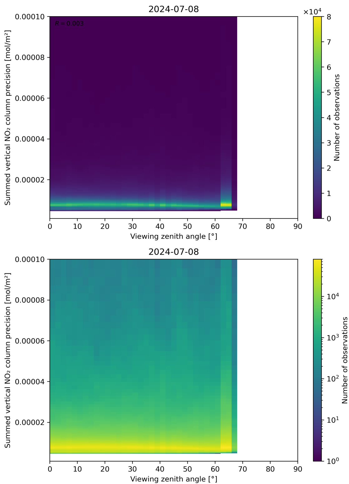
Figure 166: Scatter density plot of “Viewing zenith angle” against “Summed vertical NO 2 column precision” for 2024-07-07 to 2024-07-09.
