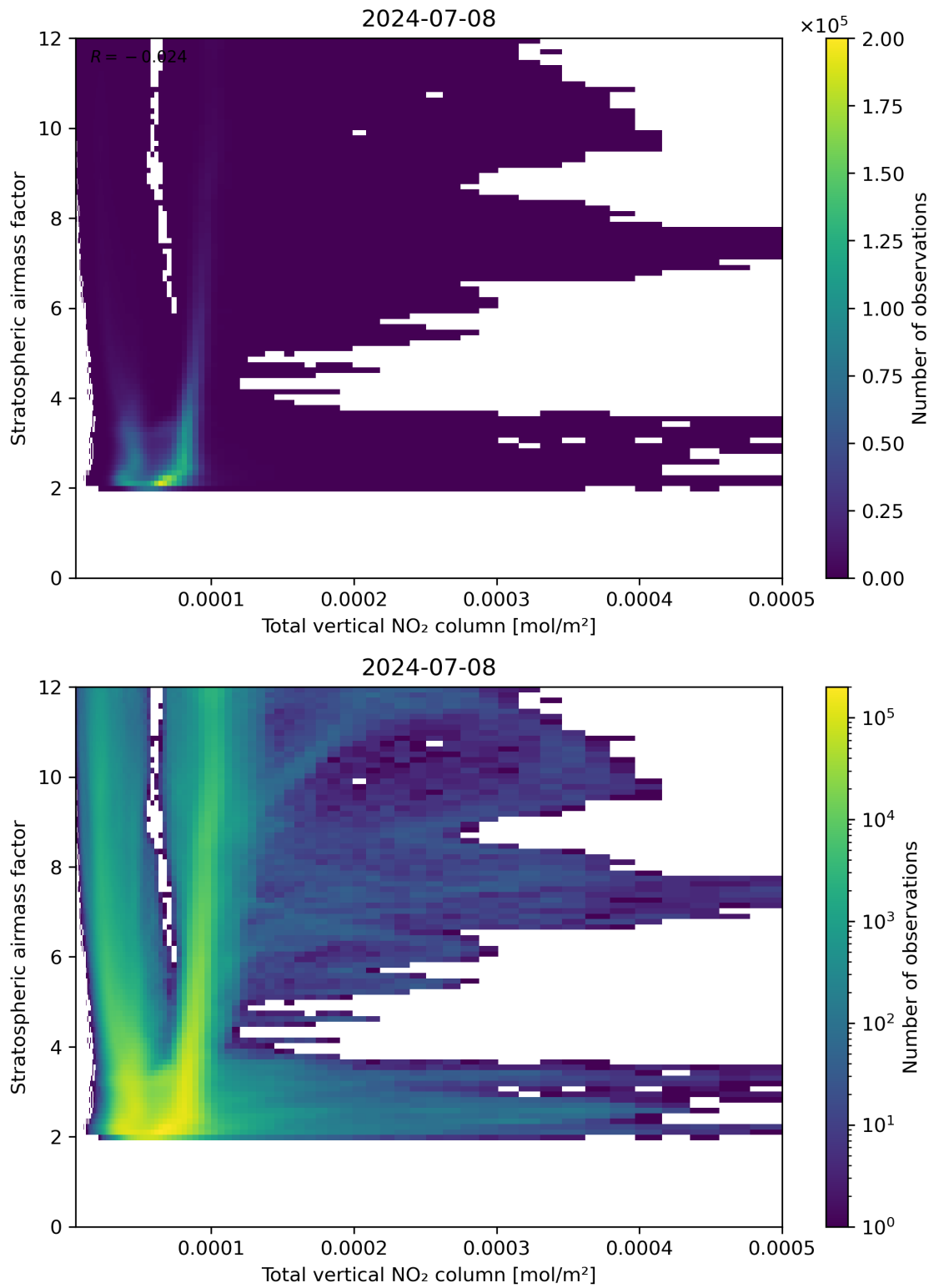
Figure 110: Scatter density plot of “Total vertical NO 2 column” against “Stratospheric airmass factor” for 2024-07-07 to 2024-07-09.
