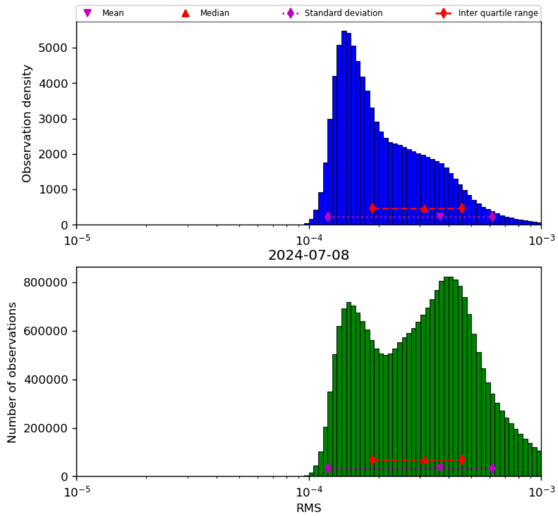
Figure 43: Histogram of “RMS” for 2024-07-07 to 2024-07-09
