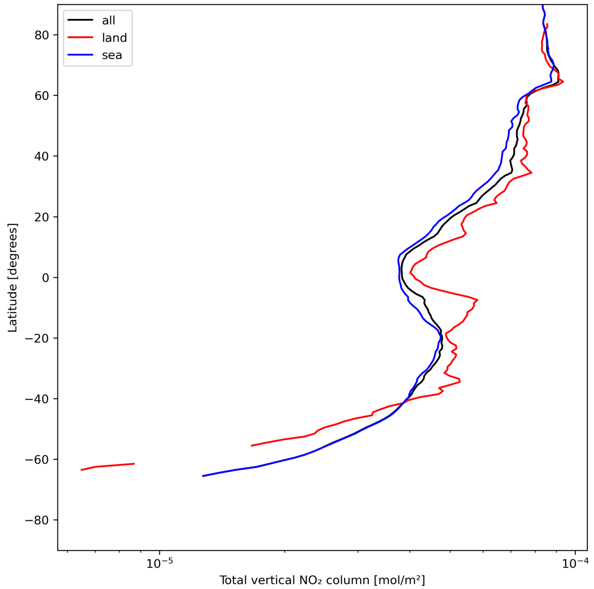
Figure 21: Zonal average of “Total vertical NO 2 column” for 2024-07-07 to 2024-07-09.
