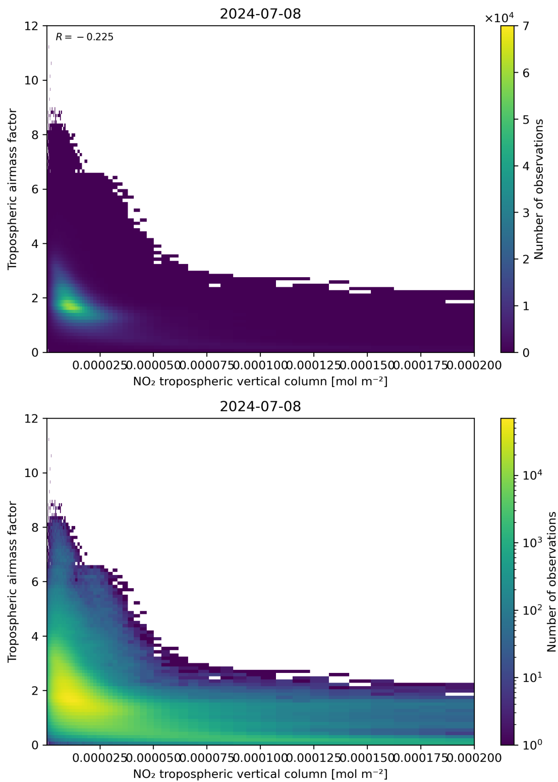
Figure 123: Scatter density plot of “NO 2 tropospheric vertical column” against “Tropospheric air mass factor” for 2024-07-07 to 2024-07-09.
