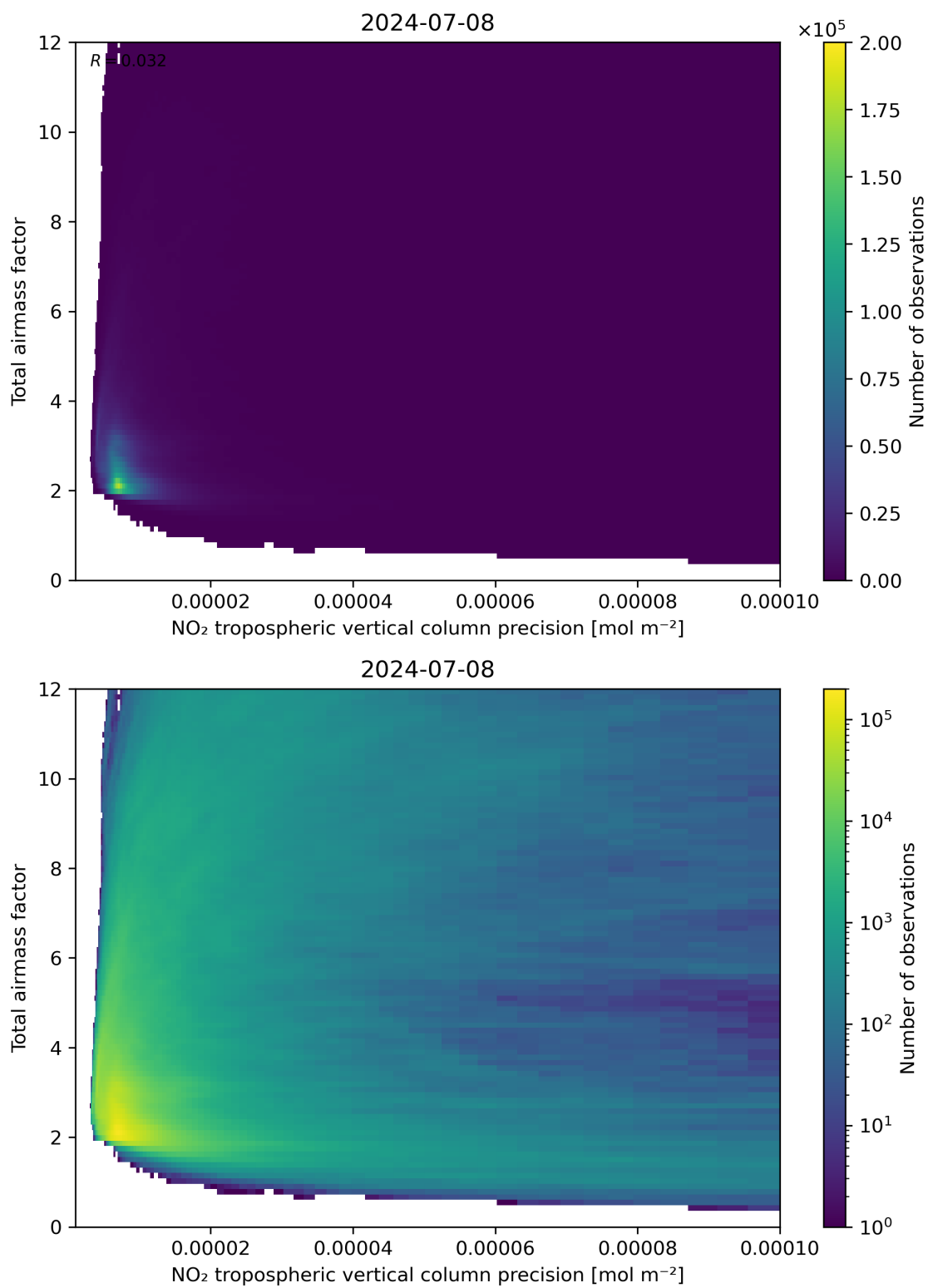
Figure 132: Scatter density plot of “NO 2 tropospheric vertical column precision” against “Total air mass factor” for 2024-07-07 to 2024-07-09.
