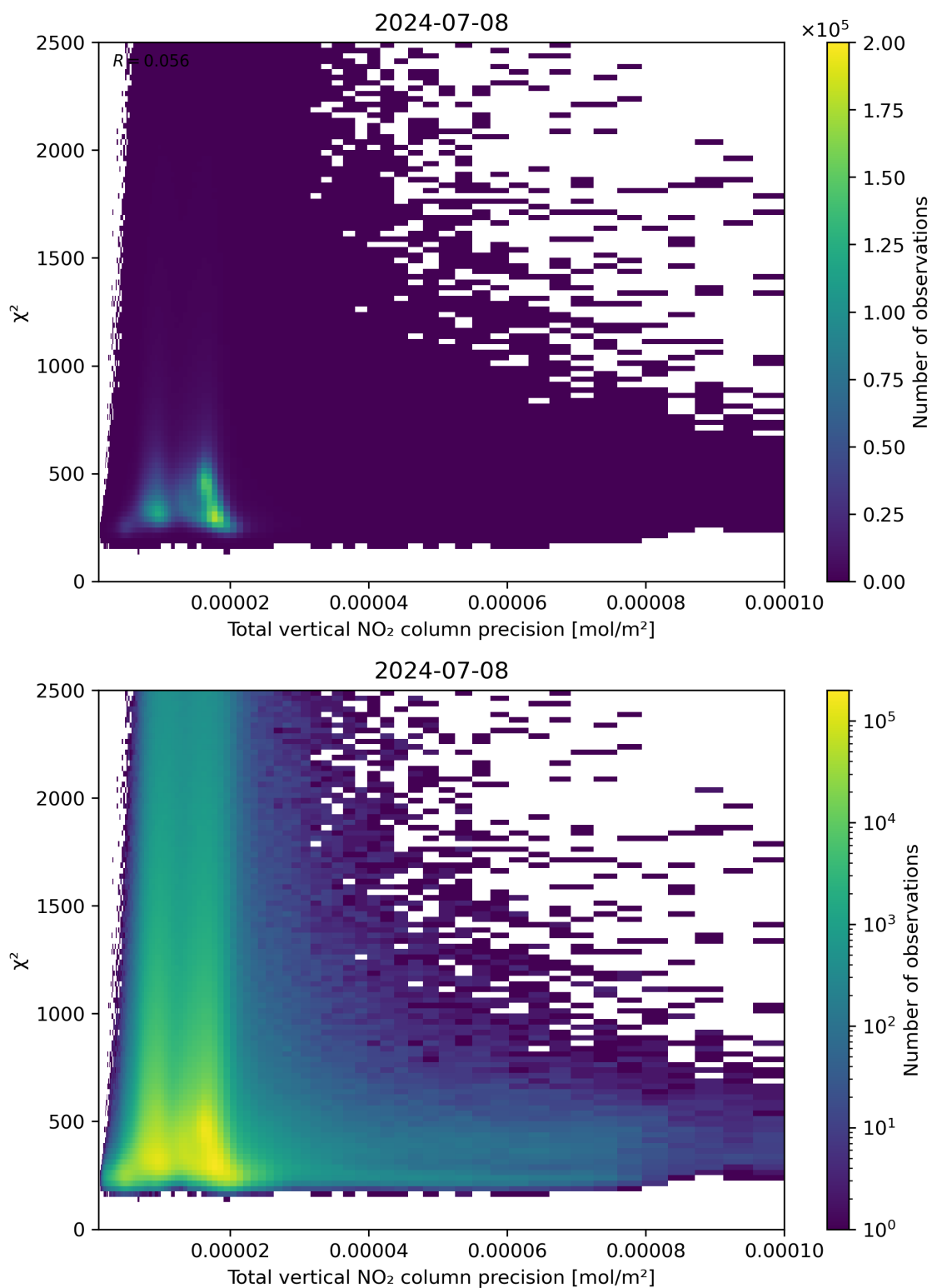
Figure 116: Scatter density plot of “Total vertical NO 2 column precision” against “ \chi^2 ” for 2024-07-07 to 2024-07-09.
