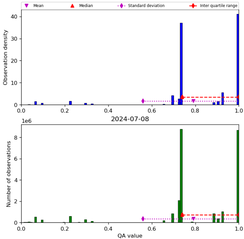
Figure 28: Histogram of “QA value” for 2024-07-07 to 2024-07-09
