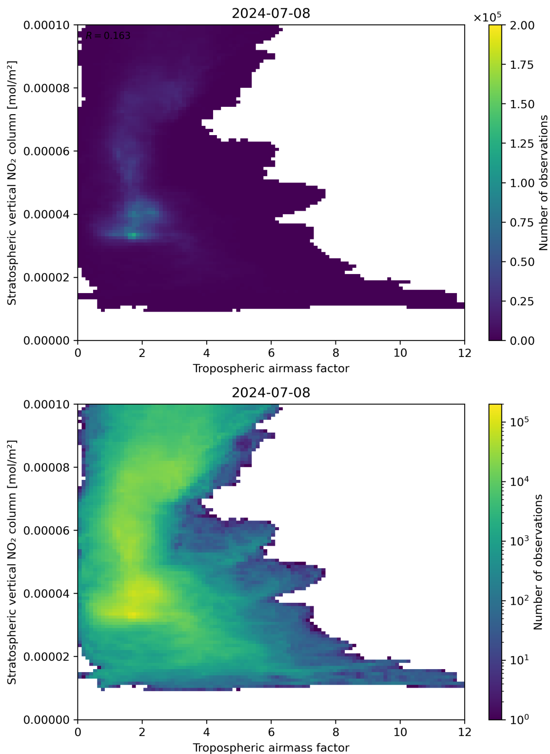
Figure 74: Scatter density plot of “Tropospheric air mass factor” against “Stratospheric vertical NO 2 column” for 2024-07-07 to 2024-07-09.
