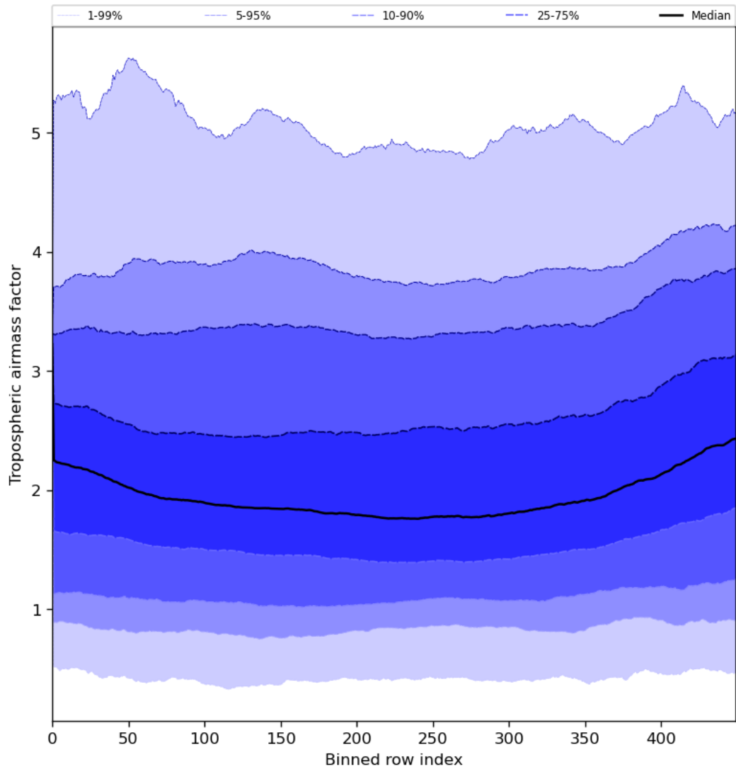
Figure 48: Along track statistics of “Tropospheric airmass factor” for 2024-07-07 to 2024-07-09
