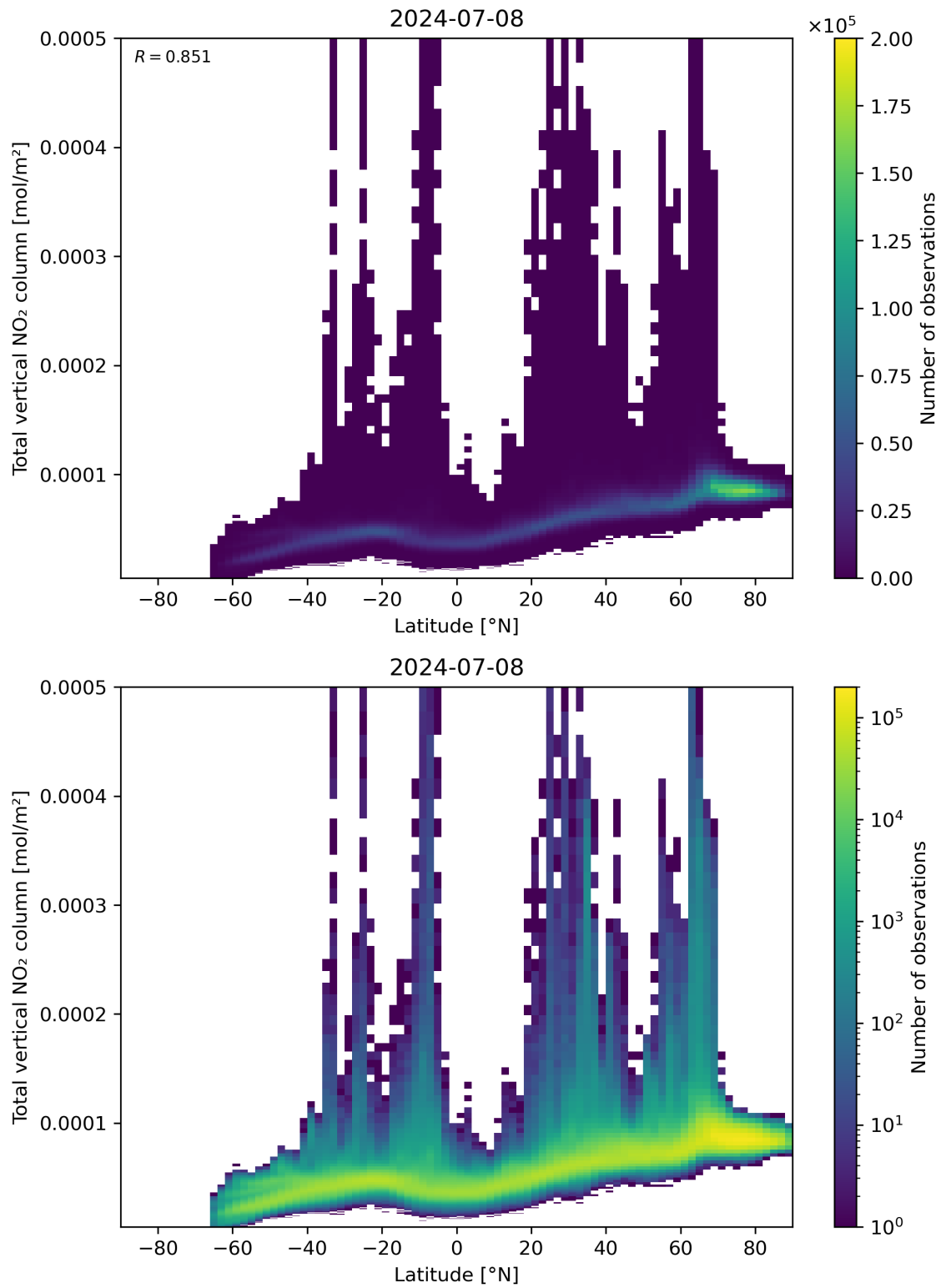
Figure 90: Scatter density plot of “Latitude” against “Total vertical NO 2 column” for 2024-07-07 to 2024-07-09.
