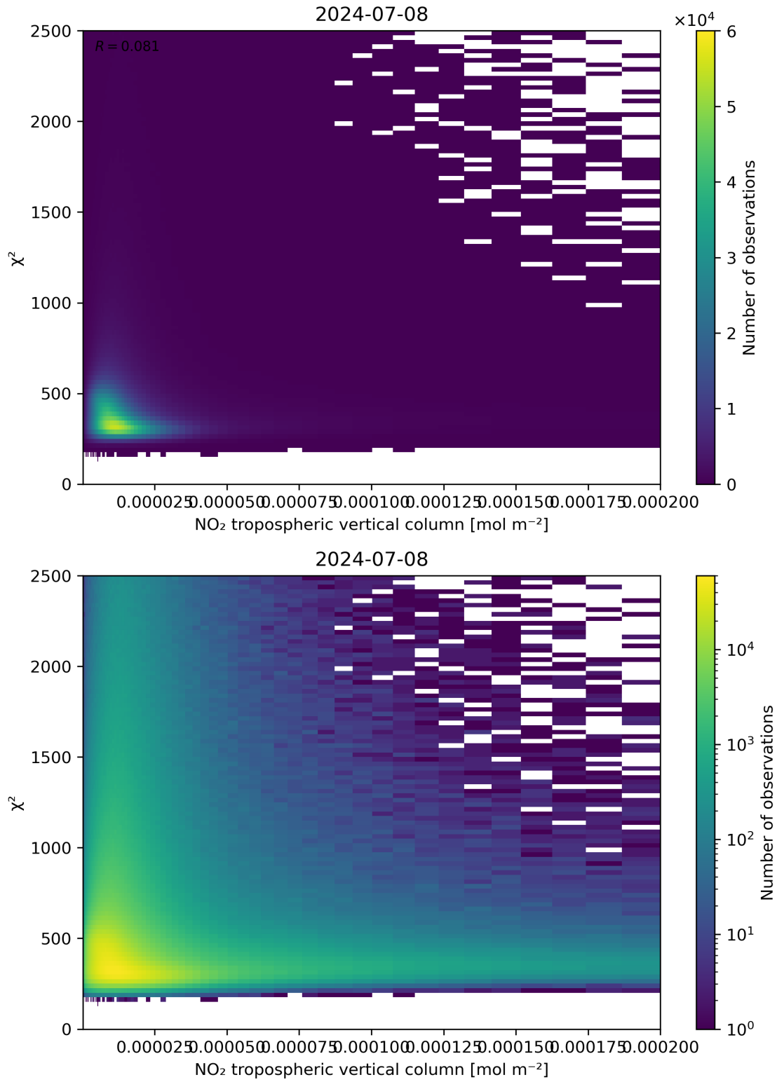
Figure 124: Scatter density plot of “NO 2 tropospheric vertical column” against “ \chi^2 ” for 2024-07-07 to 2024-07-09.
