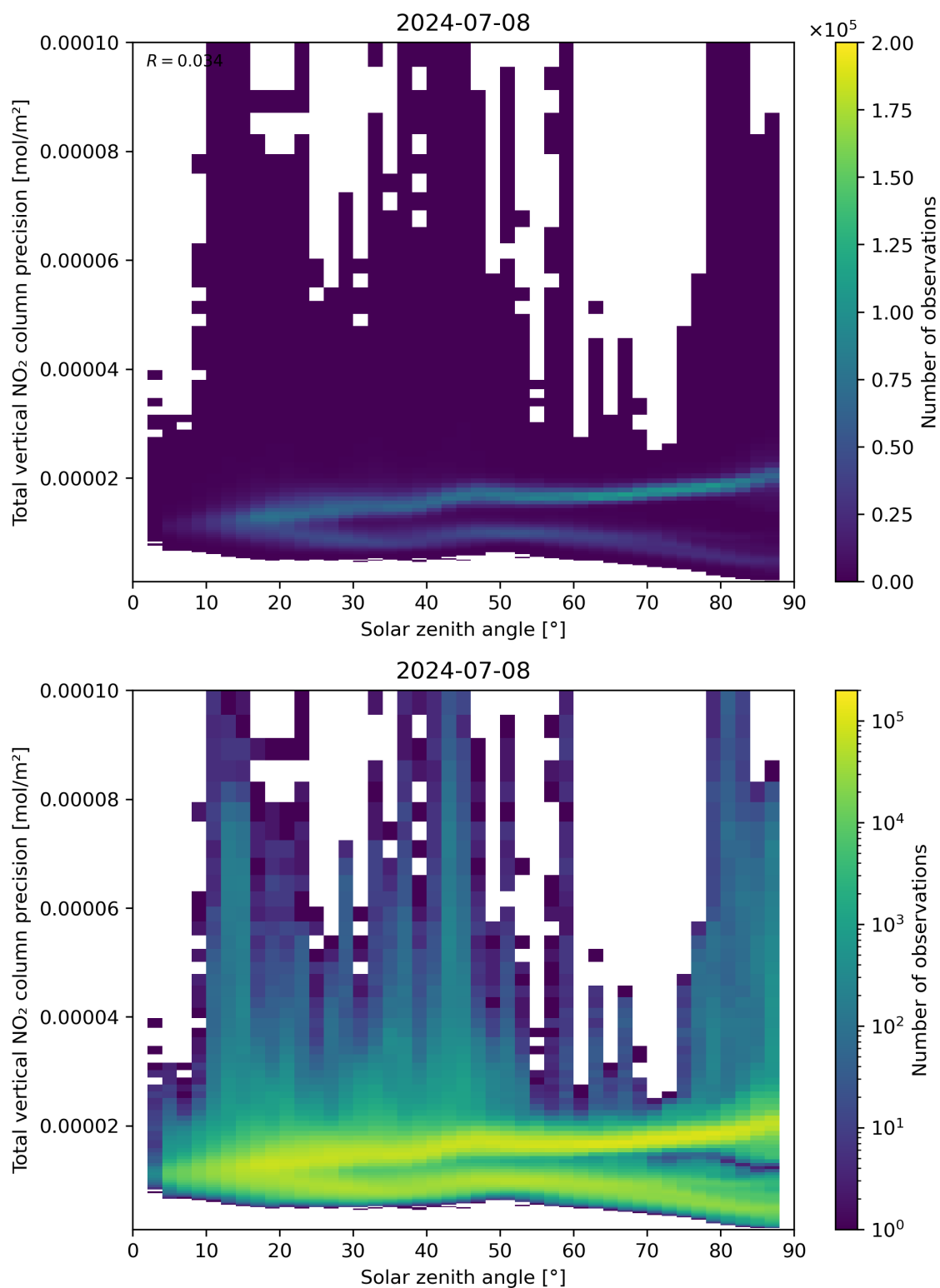
Figure 154: Scatter density plot of “Solar zenith angle” against “Total vertical NO 2 column precision” for 2024-07-07 to 2024-07-09.
