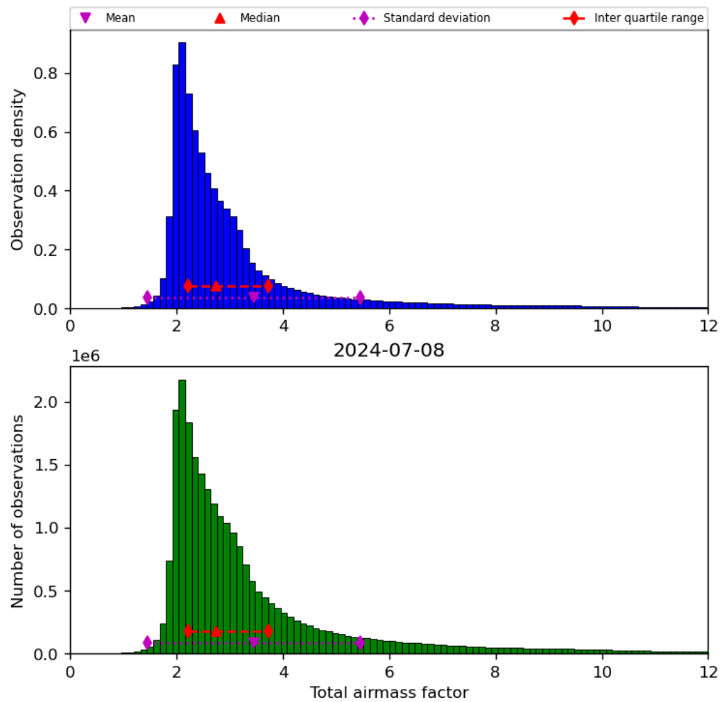
Figure 32: Histogram of “Total airmass factor” for 2024-07-07 to 2024-07-09
