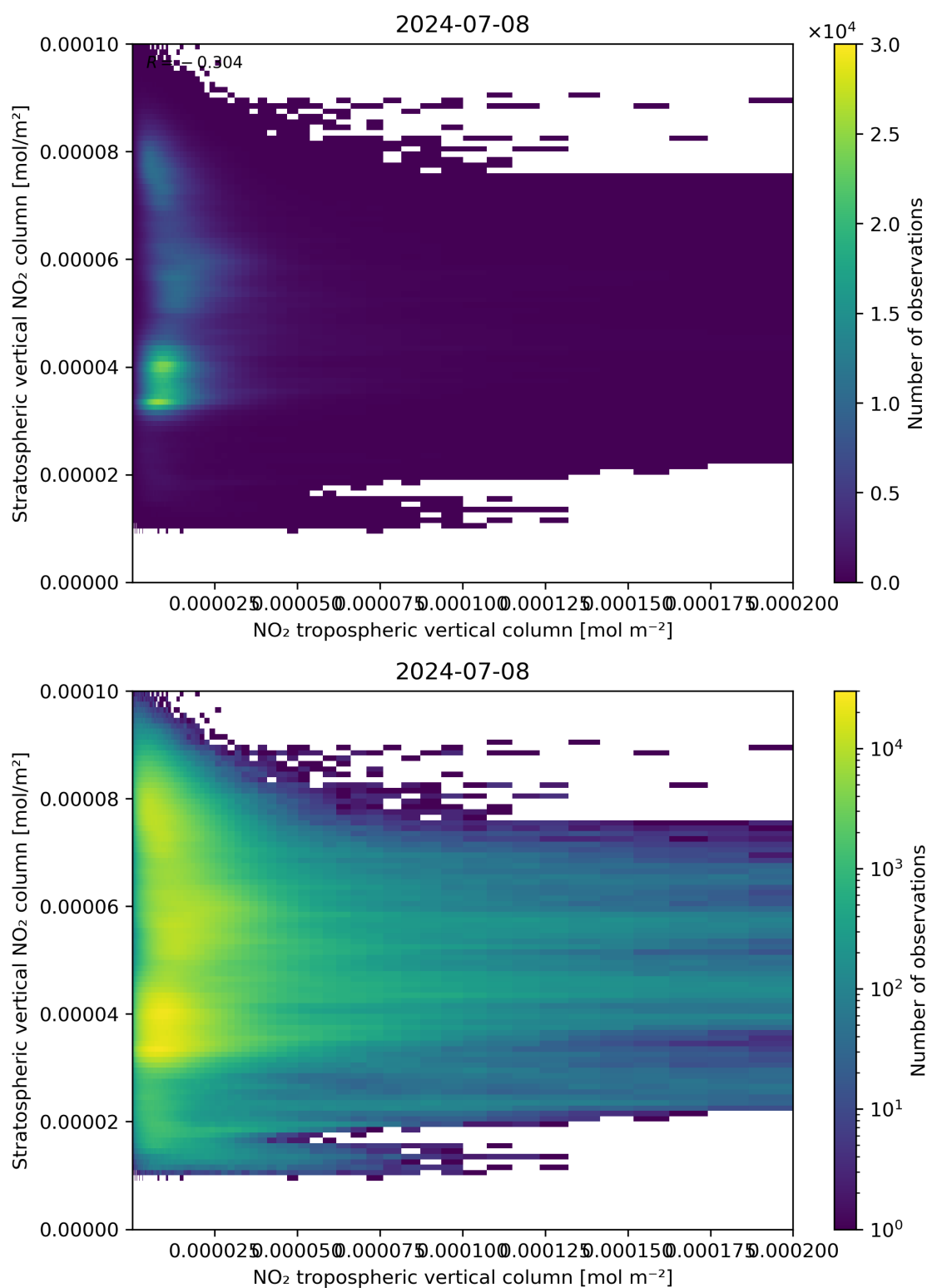
Figure 125: Scatter density plot of “NO 2 tropospheric vertical column” against “Stratospheric vertical NO 2 column” for 2024-07-07 to 2024-07-09.
