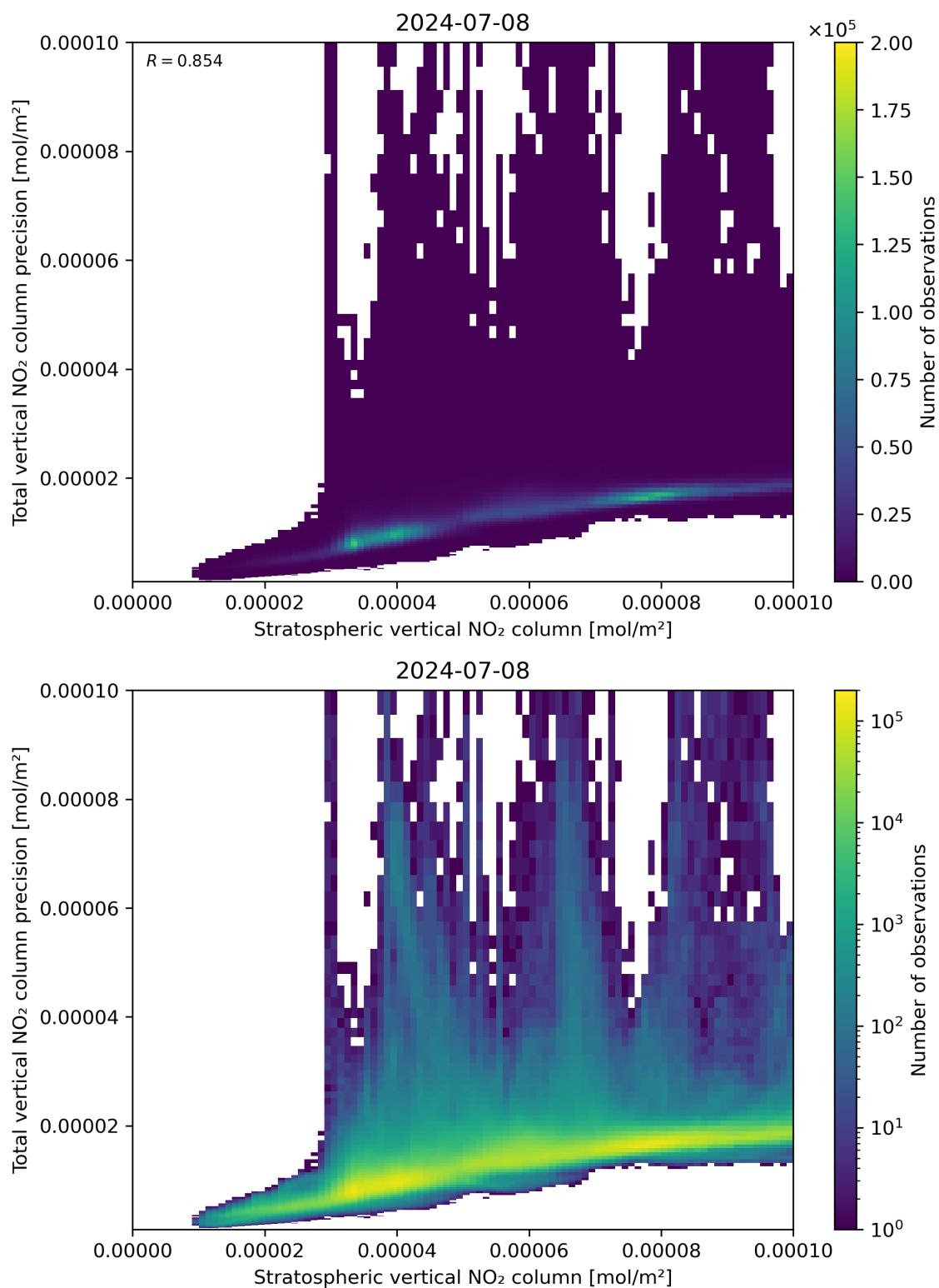
Figure 101: Scatter density plot of “Stratospheric vertical NO 2 column” against “Total vertical NO 2 column precision” for 2024-07-07 to 2024-07-09.
