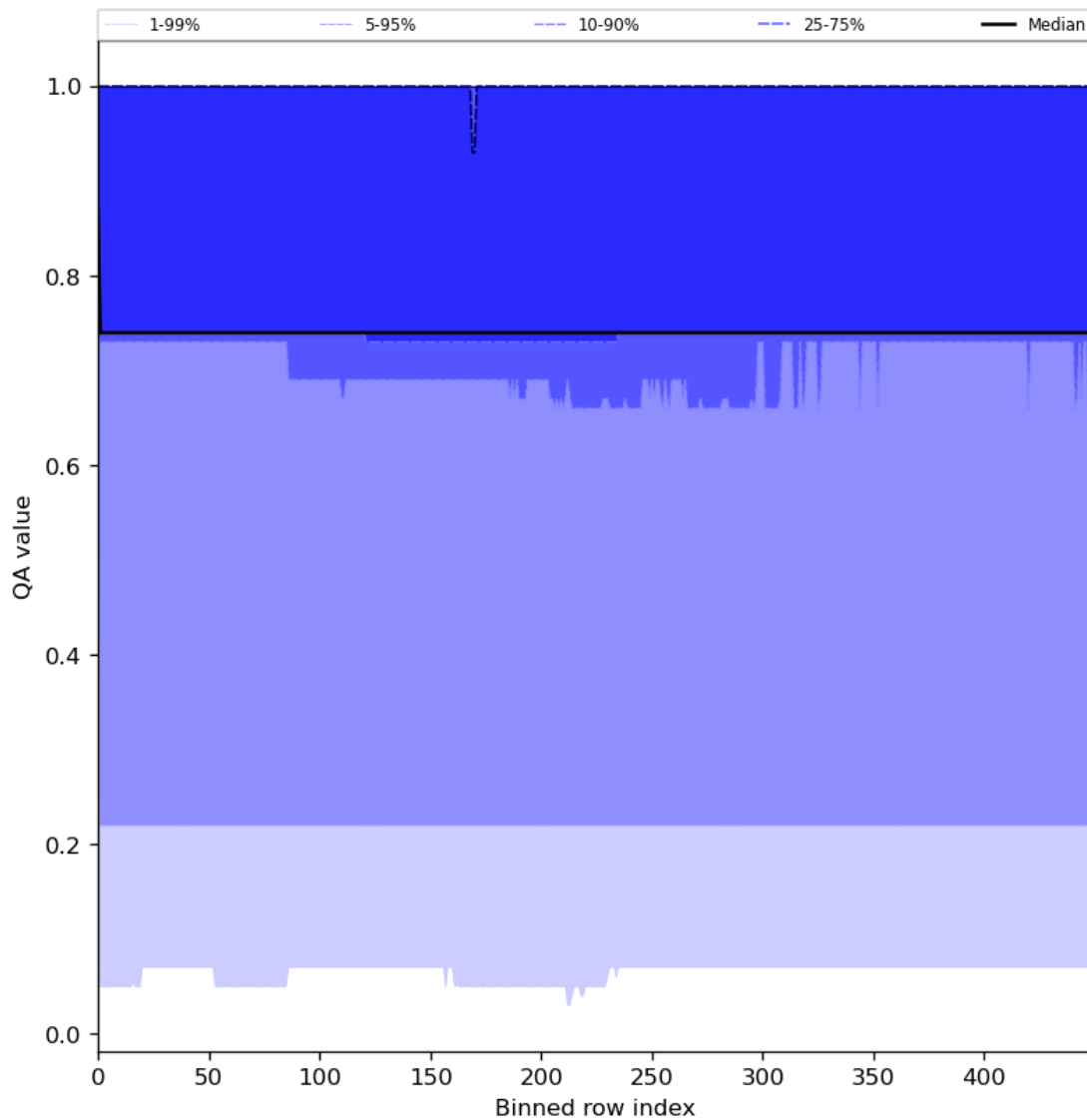
Figure 45: Along track statistics of “QA value” for 2024-07-07 to 2024-07-09
