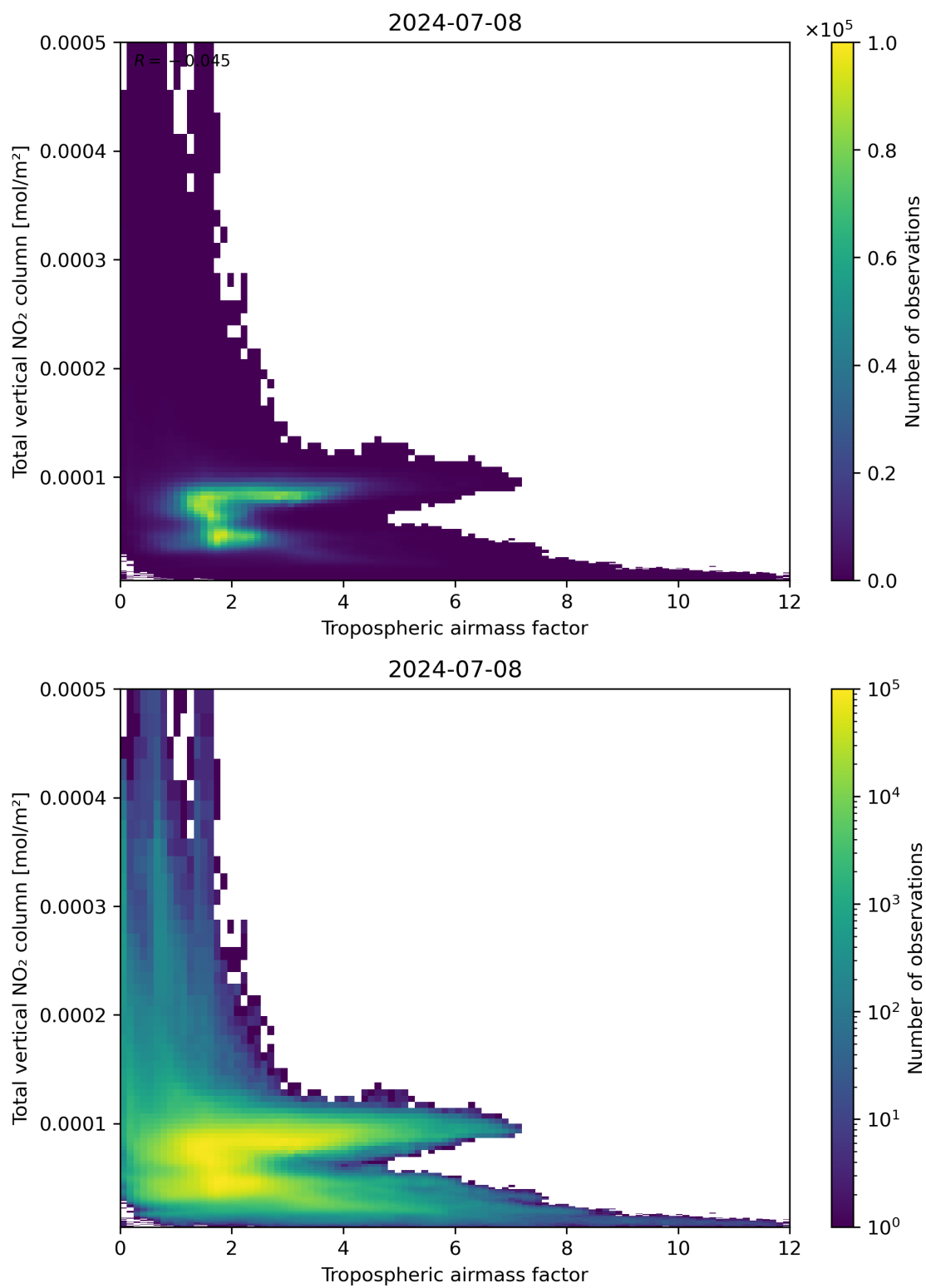
Figure 77: Scatter density plot of “Tropospheric airmass factor” against “Total vertical NO 2 column” for 2024-07-07 to 2024-07-09.
