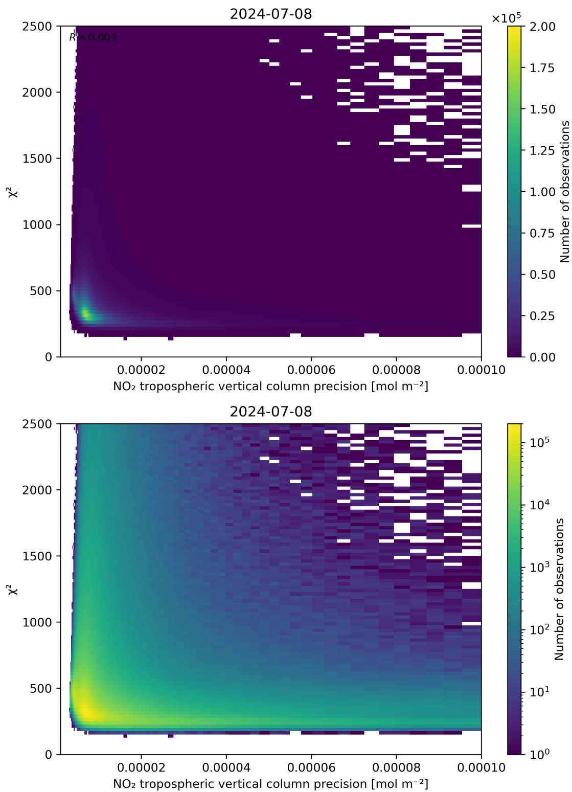
Figure 134: Scatter density plot of “NO 2 tropospheric vertical column precision” against “ \chi^2 ” for 2024-07-07 to 2024-07-09.
