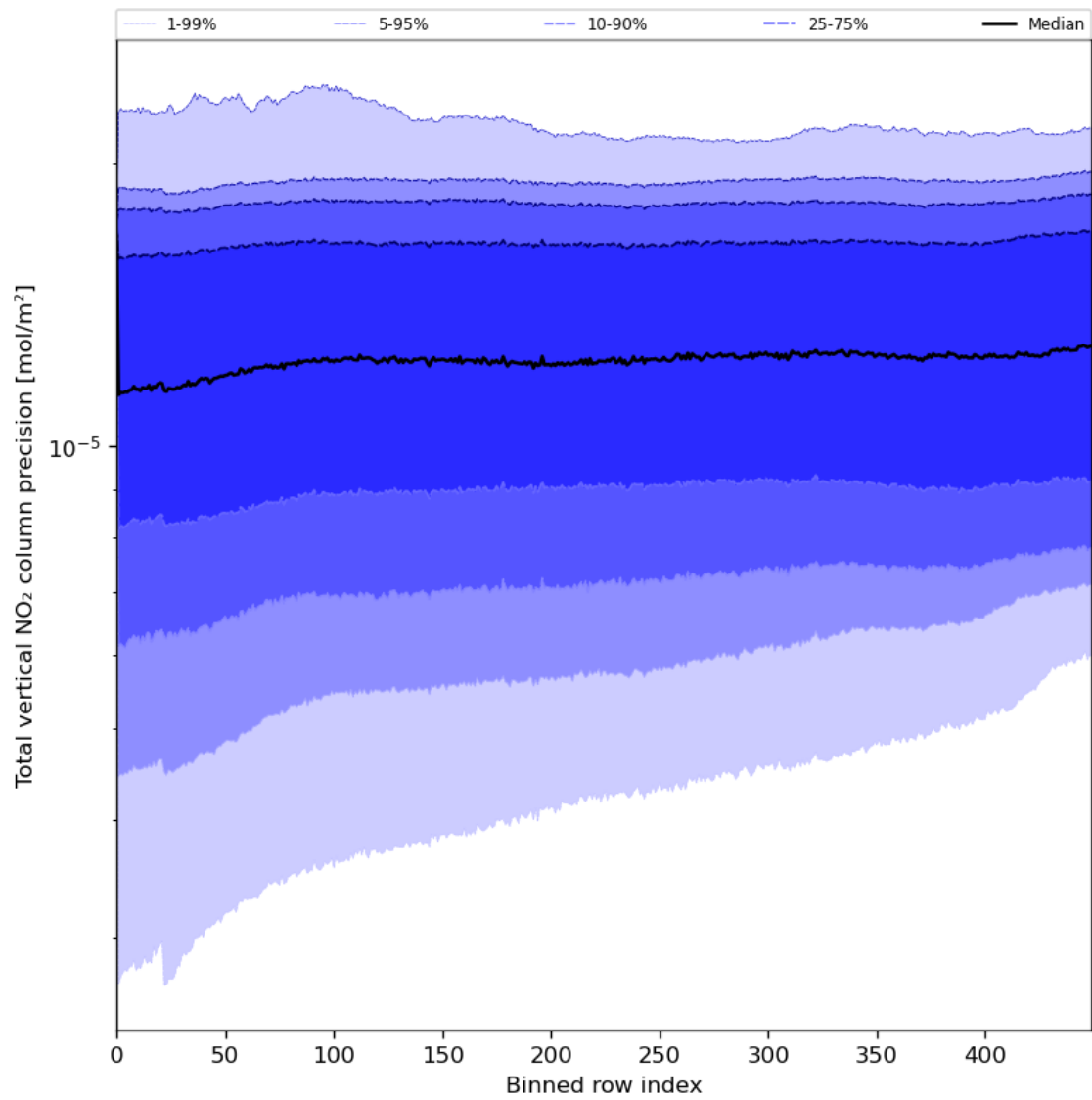
Figure 56: Along track statistics of “Total vertical NO 2 column precision” for 2024-07-07 to 2024-07-09
