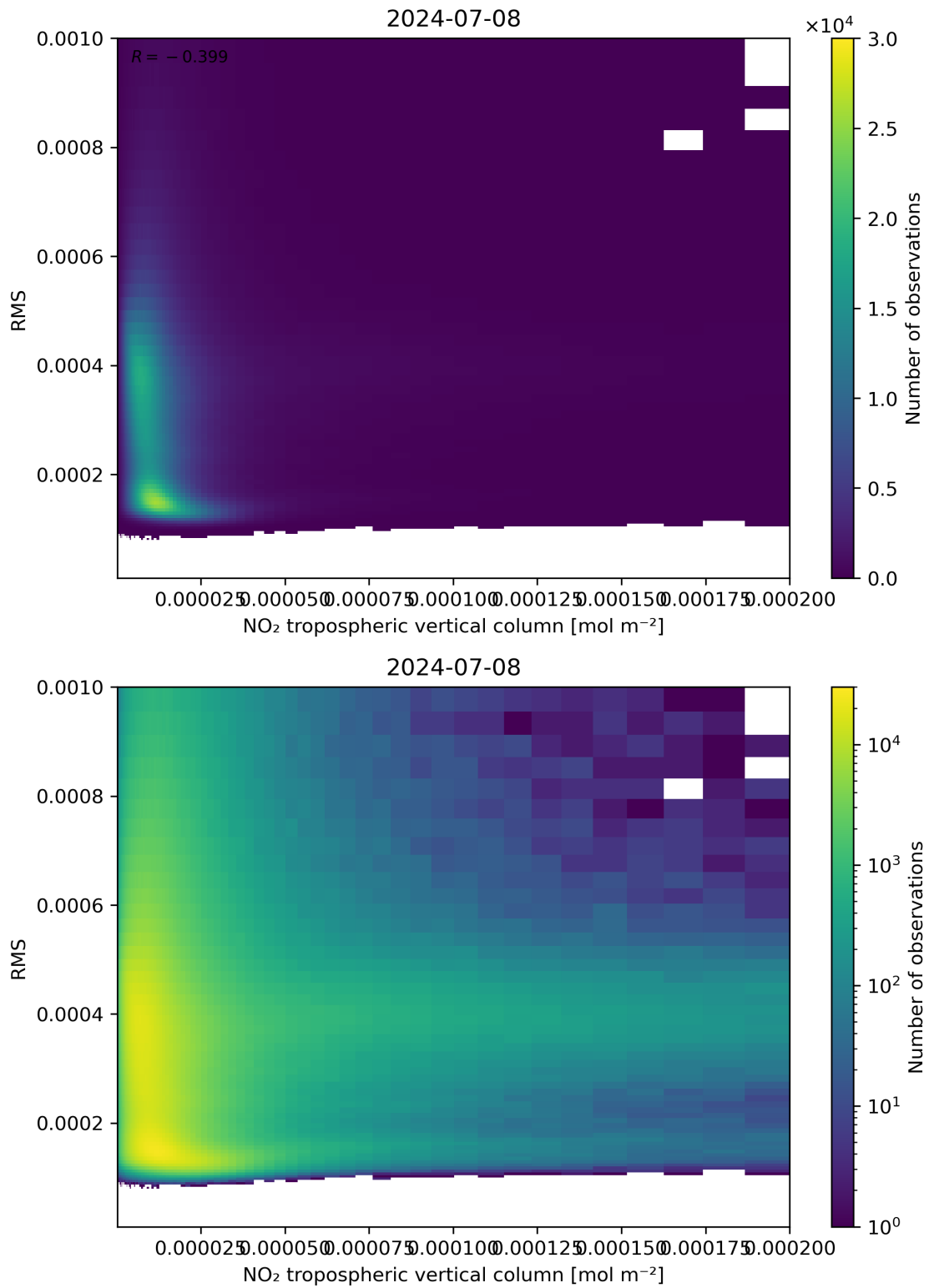
Figure 142: Scatter density plot of “NO 2 tropospheric vertical column” against “RMS” for 2024-07-07 to 2024-07-09.
