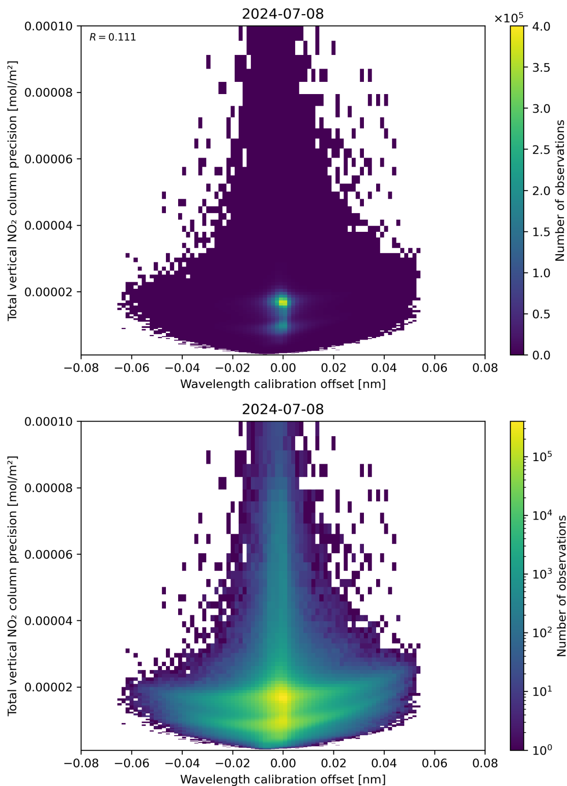
Figure 180: Scatter density plot of “Wavelength calibration offset” against “Total vertical NO 2 column precision” for 2024-07-07 to 2024-07-09.
