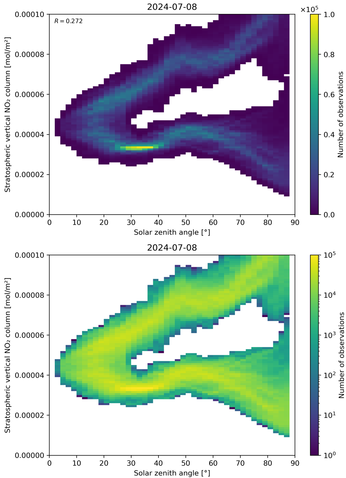
Figure 150: Scatter density plot of “Solar zenith angle” against “Stratospheric vertical NO 2 column” for 2024-07-07 to 2024-07-09.
