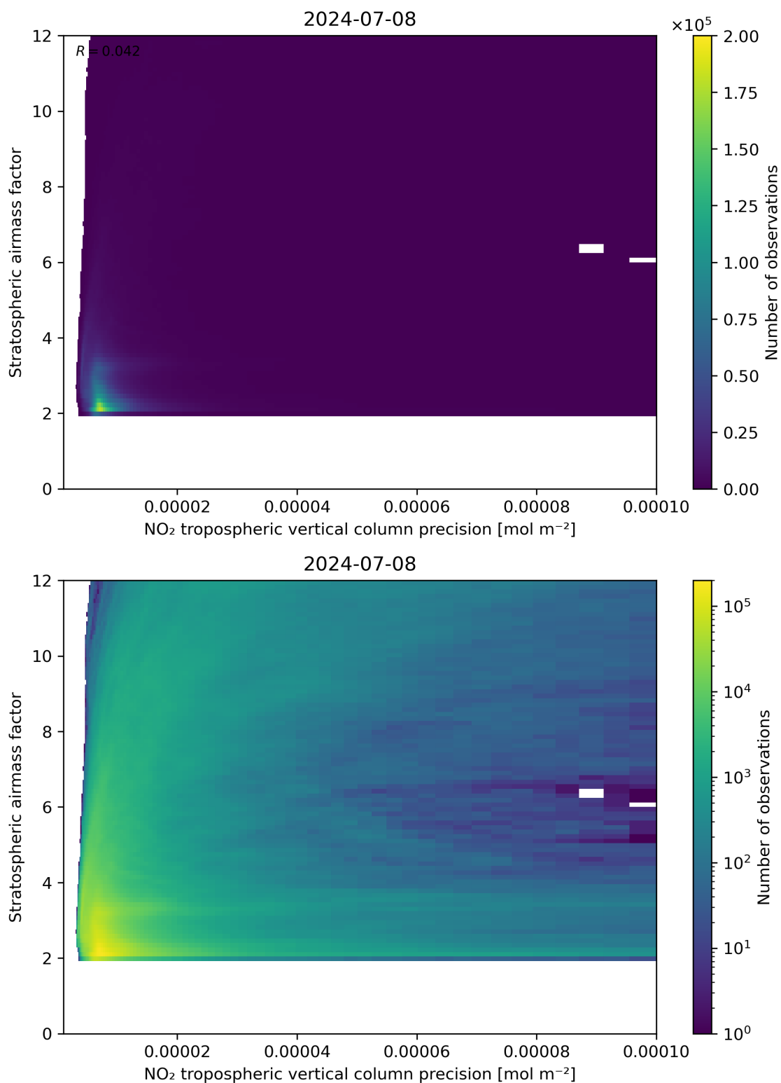
Figure 131: Scatter density plot of “NO 2 tropospheric vertical column precision” against “Stratospheric airmass factor” for 2024-07-07 to 2024-07-09.
