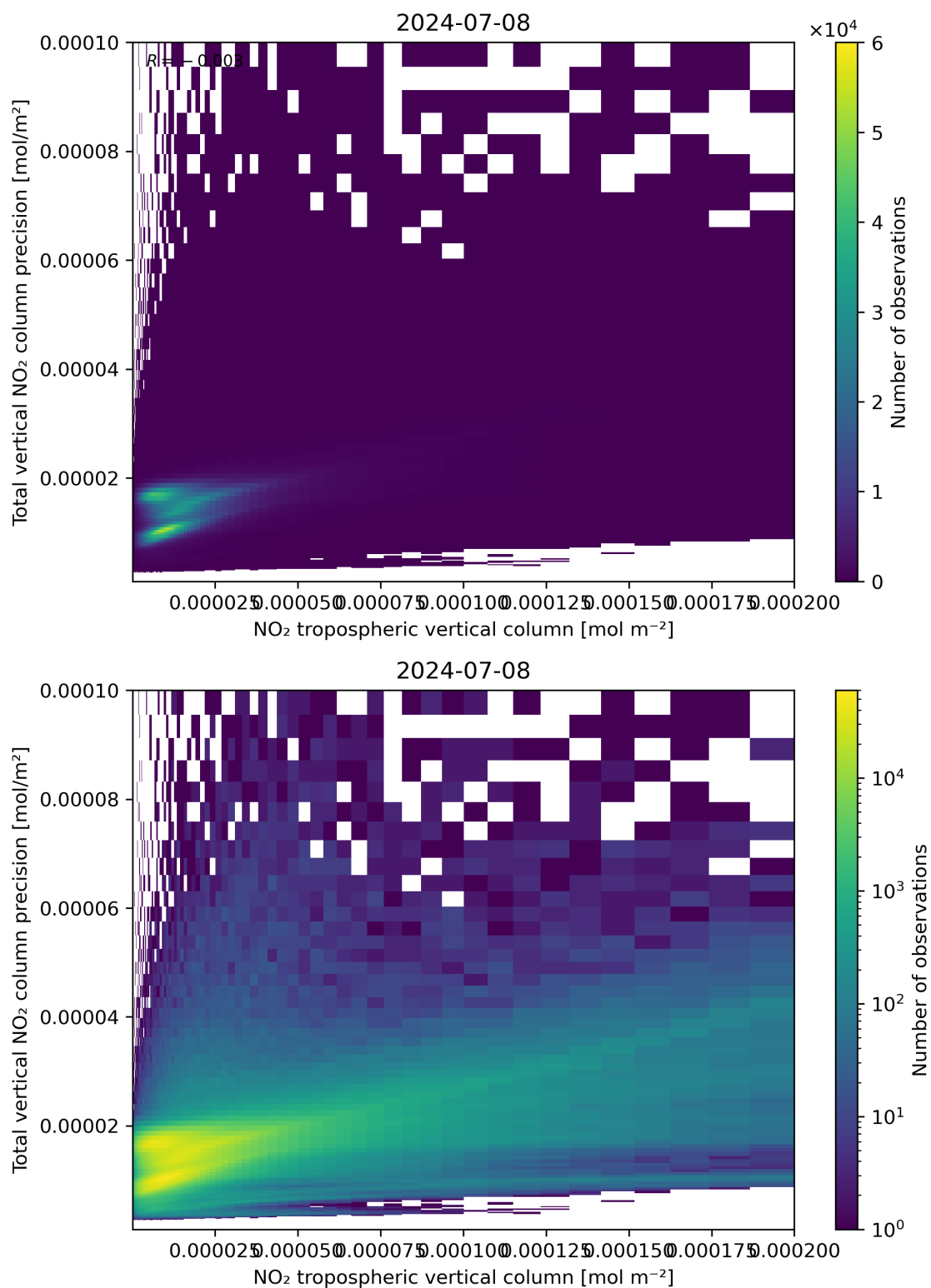
Figure 129: Scatter density plot of “NO 2 tropospheric vertical column” against “Total vertical NO 2 column precision” for 2024-07-07 to 2024-07-09.
