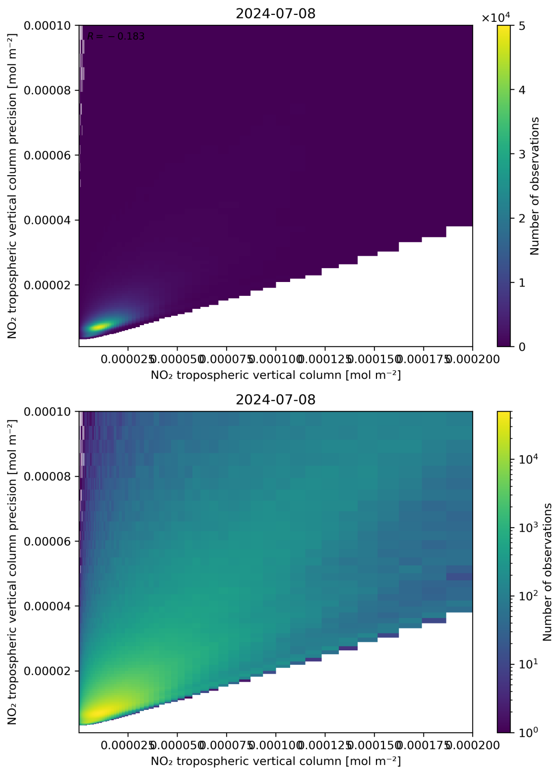
Figure 130: Scatter density plot of “NO 2 tropospheric vertical column” against “NO 2 tropospheric vertical column precision” for 2024-07-07 to 2024-07-09.
