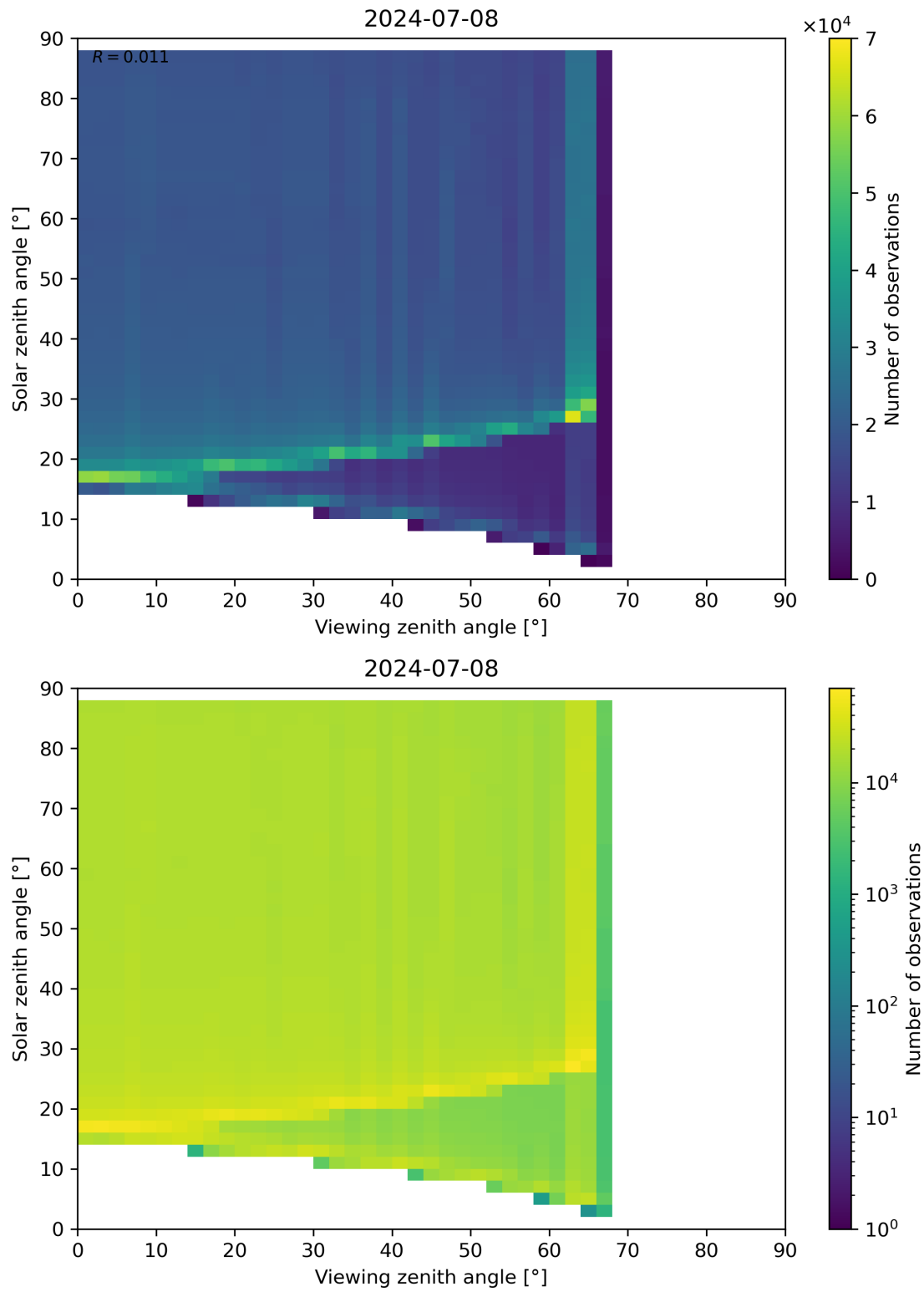
Figure 172: Scatter density plot of “Viewing zenith angle” against “Solar zenith angle” for 2024-07-07 to 2024-07-09.
