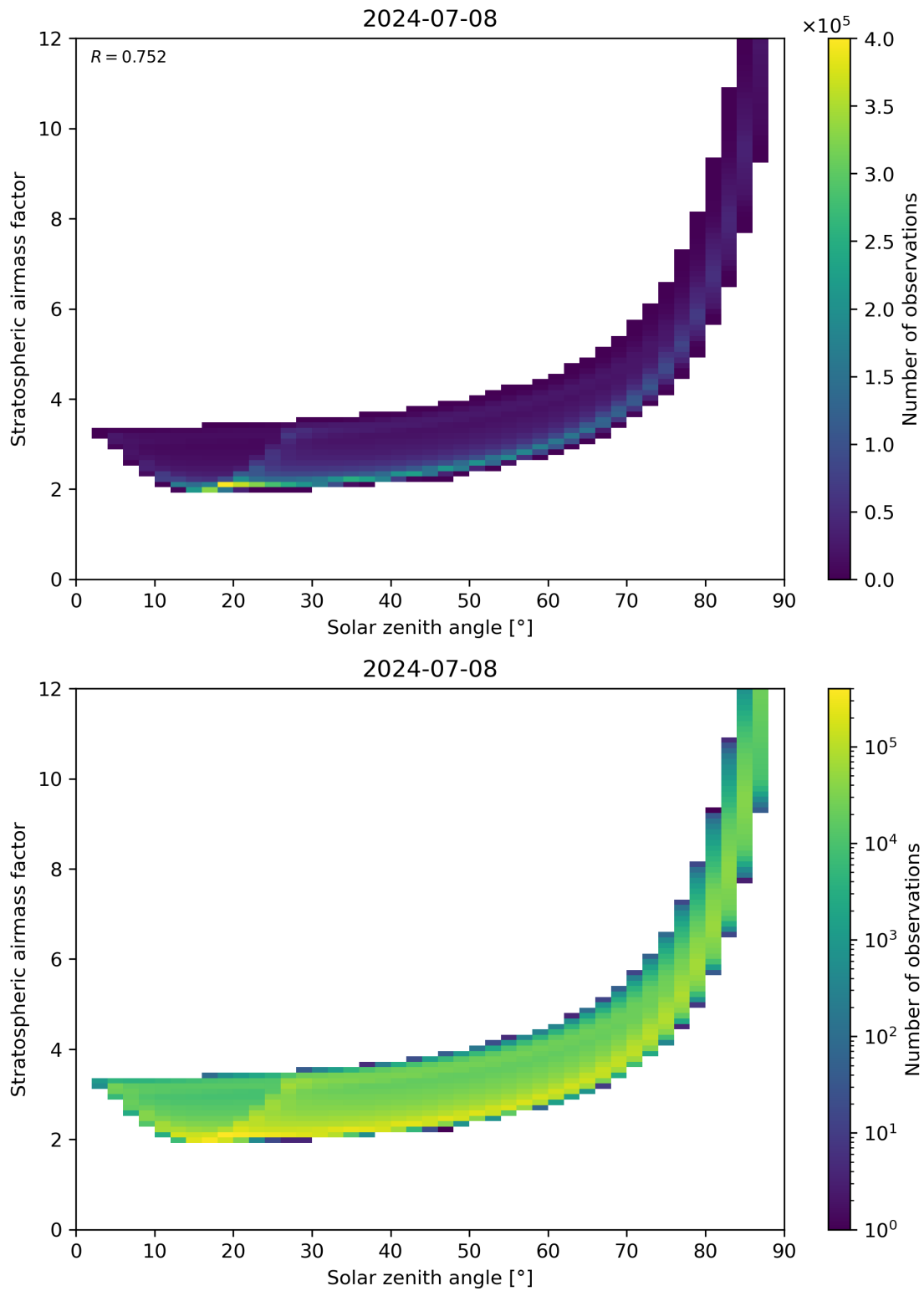
Figure 145: Scatter density plot of “Solar zenith angle” against “Stratospheric airmass factor” for 2024-07-07 to 2024-07-09.
