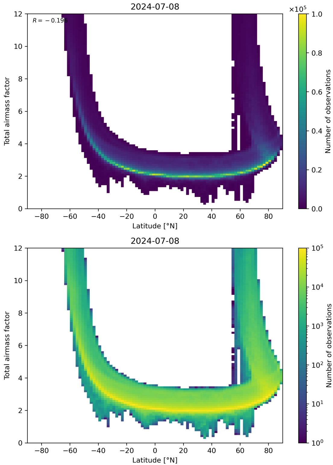
Figure 84: Scatter density plot of “Latitude” against “Total airmass factor” for 2024-07-07 to 2024-07-09.
