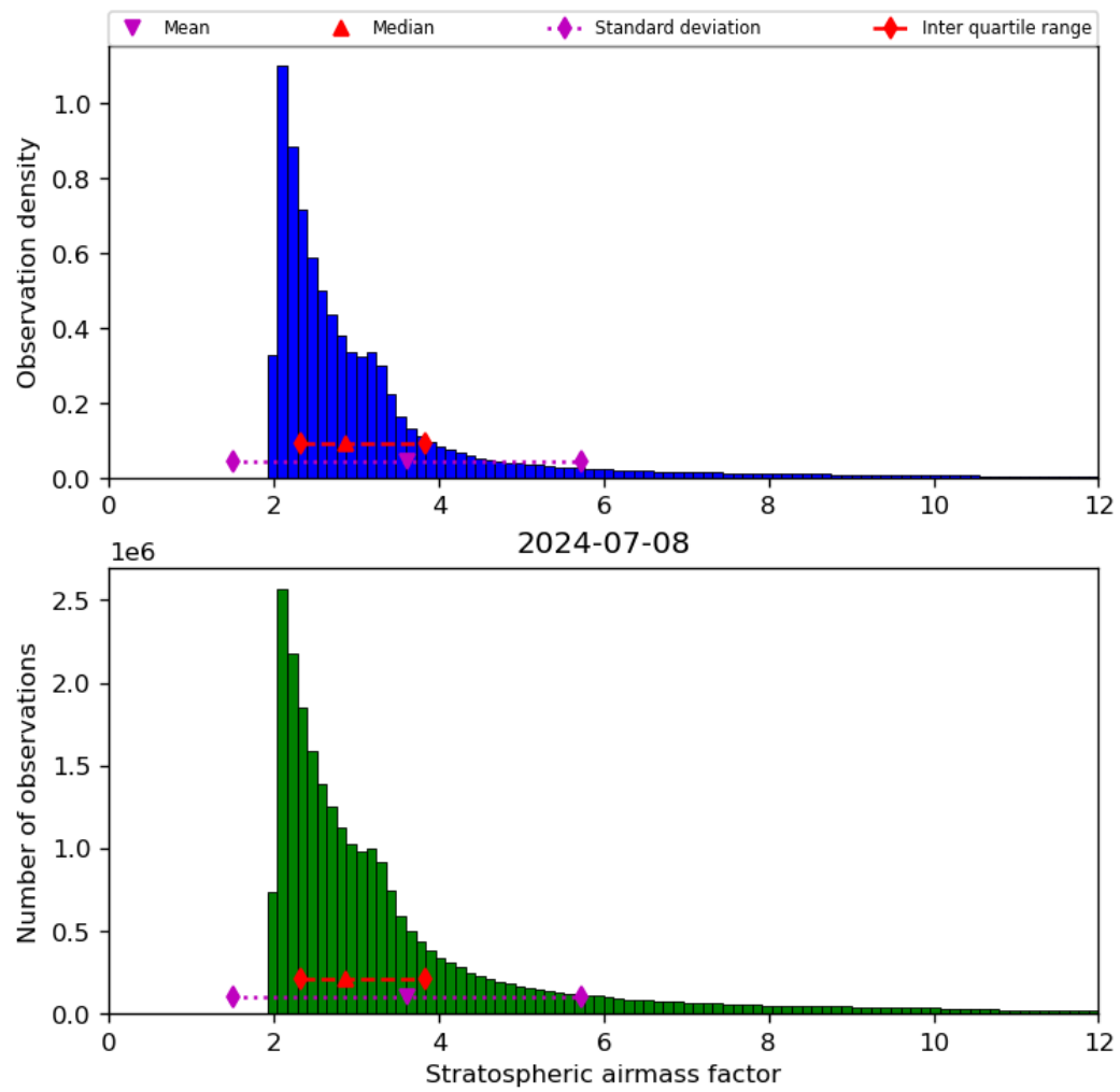
Figure 44: Histogram of “Stratospheric airmass factor” for 2024-07-07 to 2024-07-09
