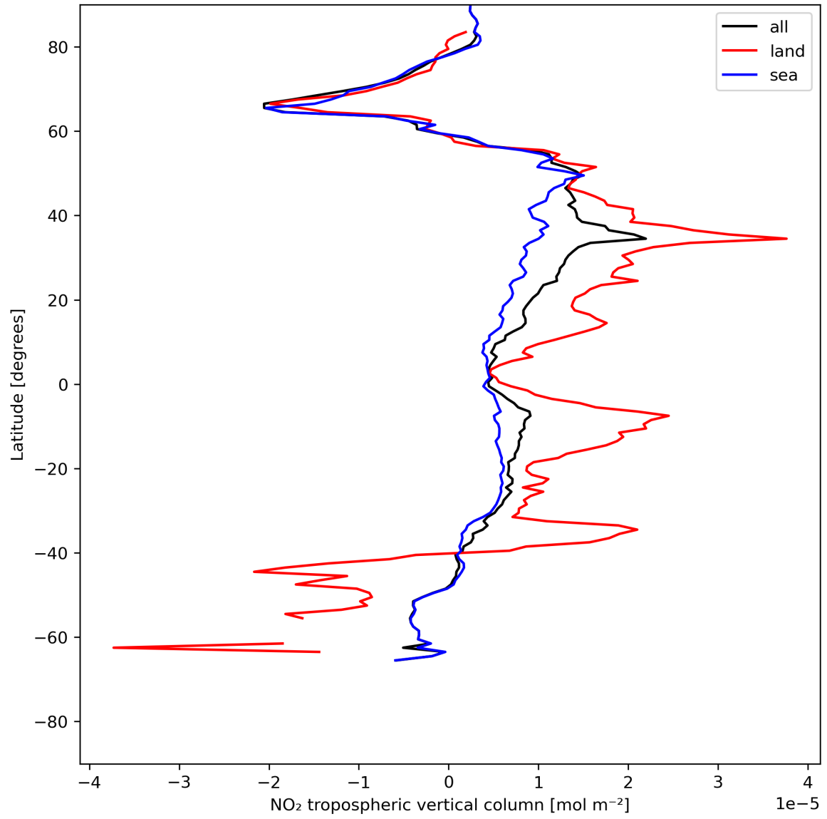
Figure 12: Zonal average of “NO 2 tropospheric vertical column” for 2024-07-07 to 2024-07-09.
