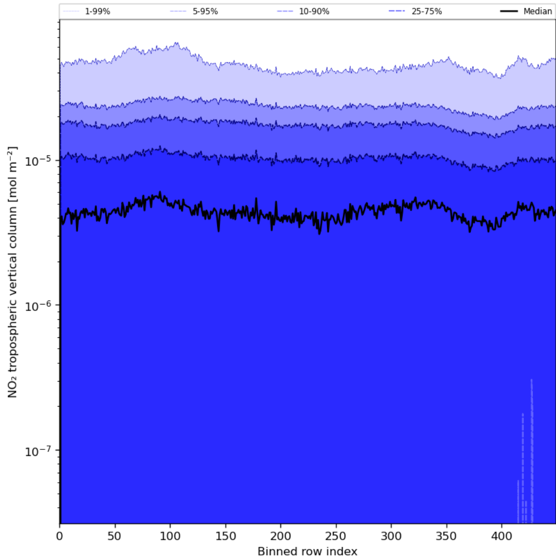
Figure 46: Along track statistics of “NO 2 tropospheric vertical column” for 2024-07-07 to 2024-07-09
