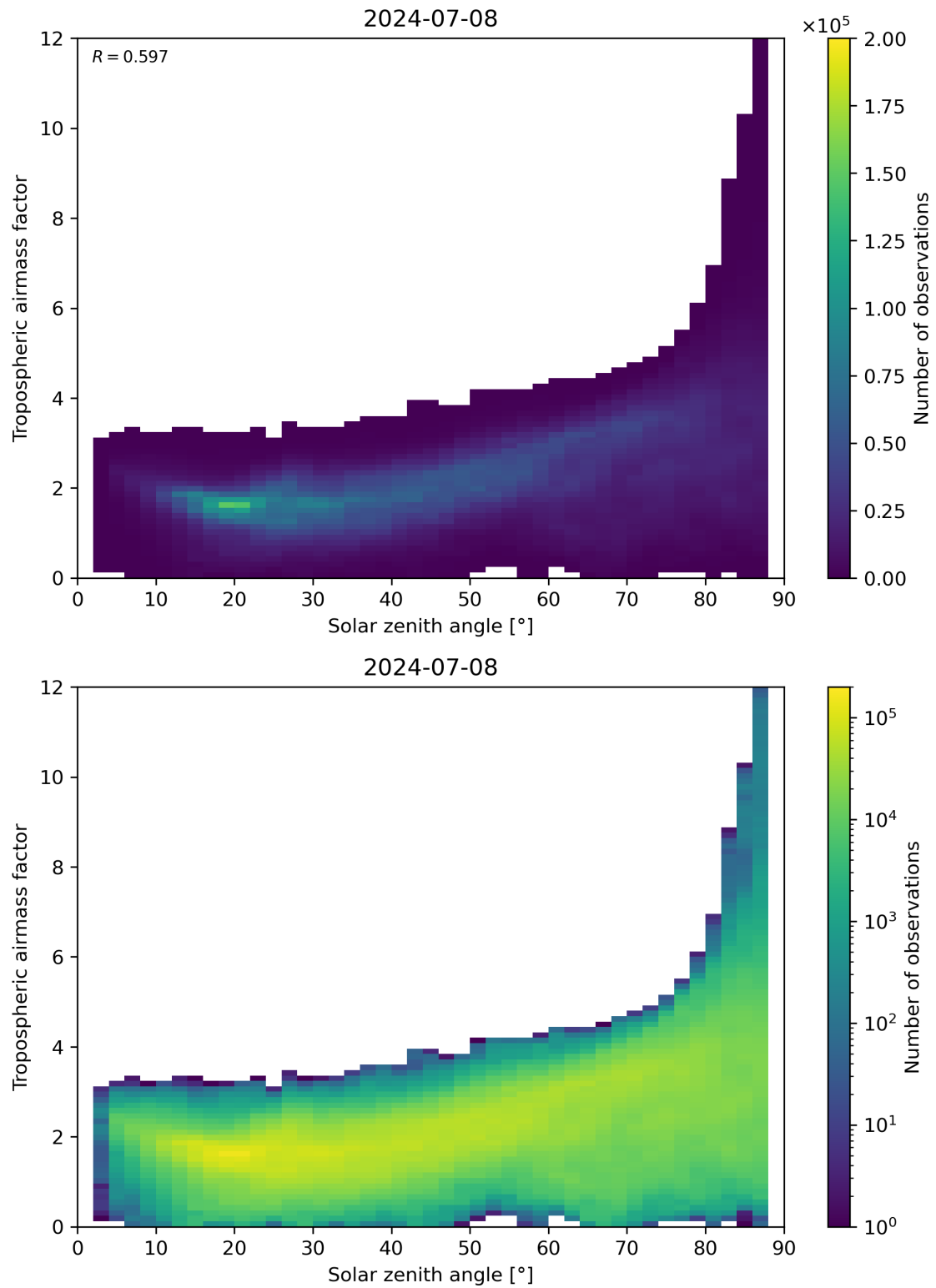
Figure 147: Scatter density plot of “Solar zenith angle” against “Tropospheric airmass factor” for 2024-07-07 to 2024-07-09.
