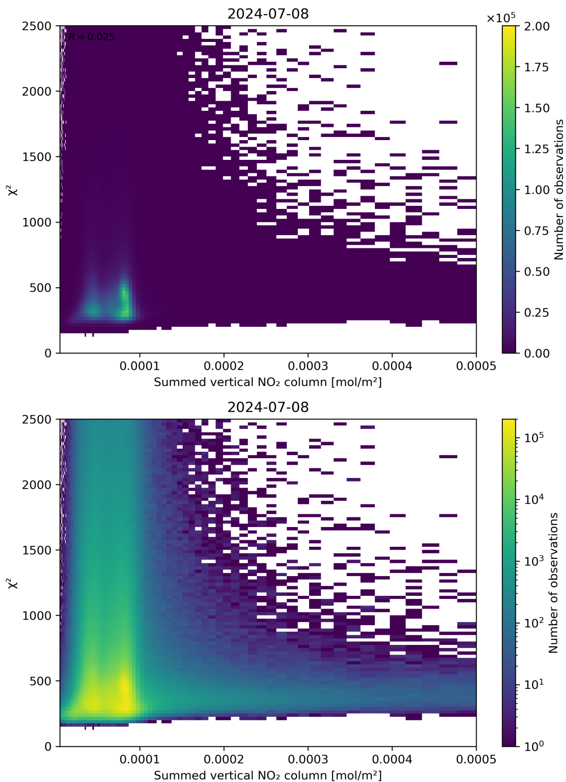
Figure 104: Scatter density plot of “Summed vertical NO 2 column” against “ \chi^2 ” for 2024-07-07 to 2024-07-09.
