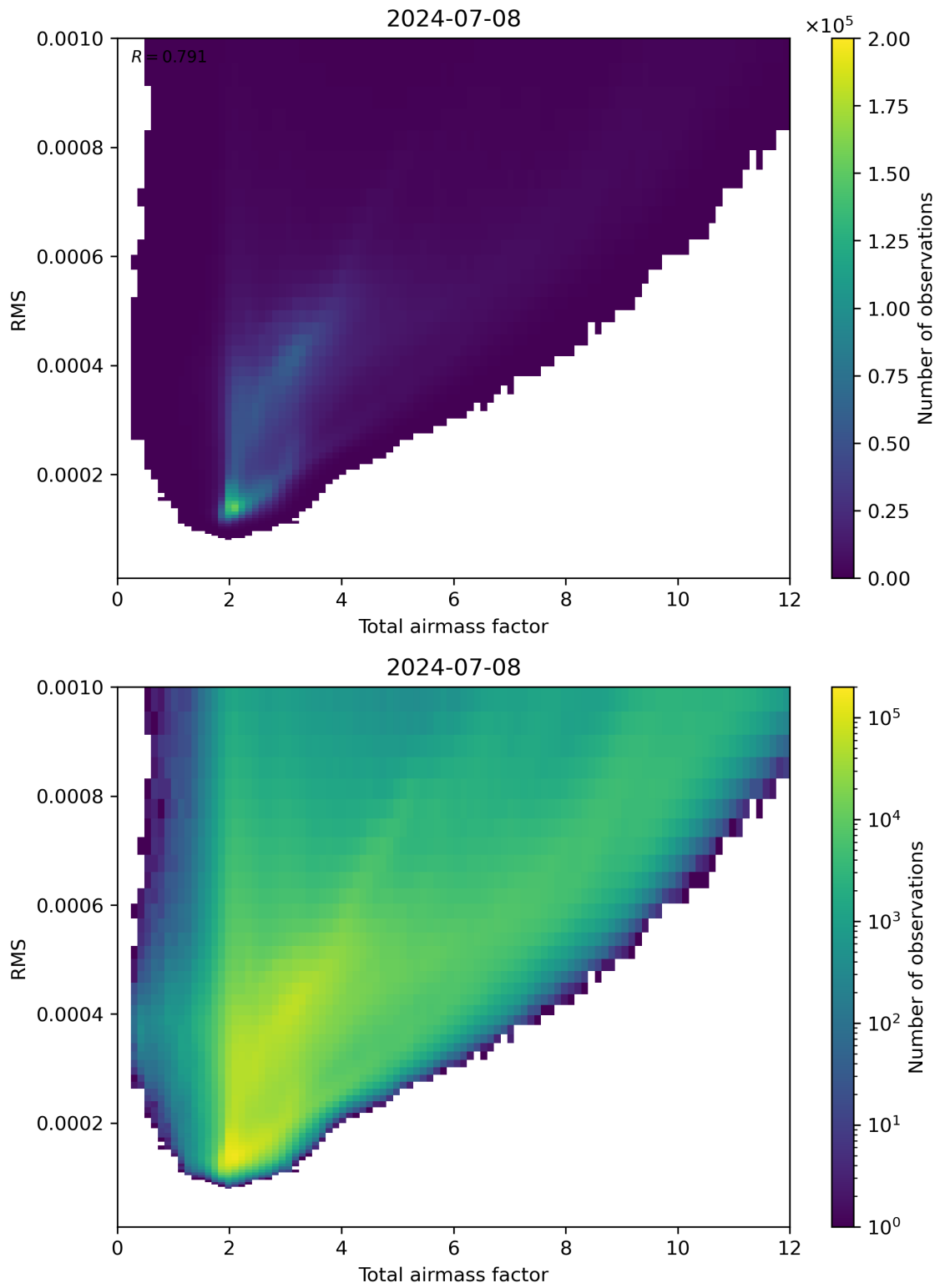
Figure 69: Scatter density plot of “Total airmass factor” against “RMS” for 2024-07-07 to 2024-07-09.
