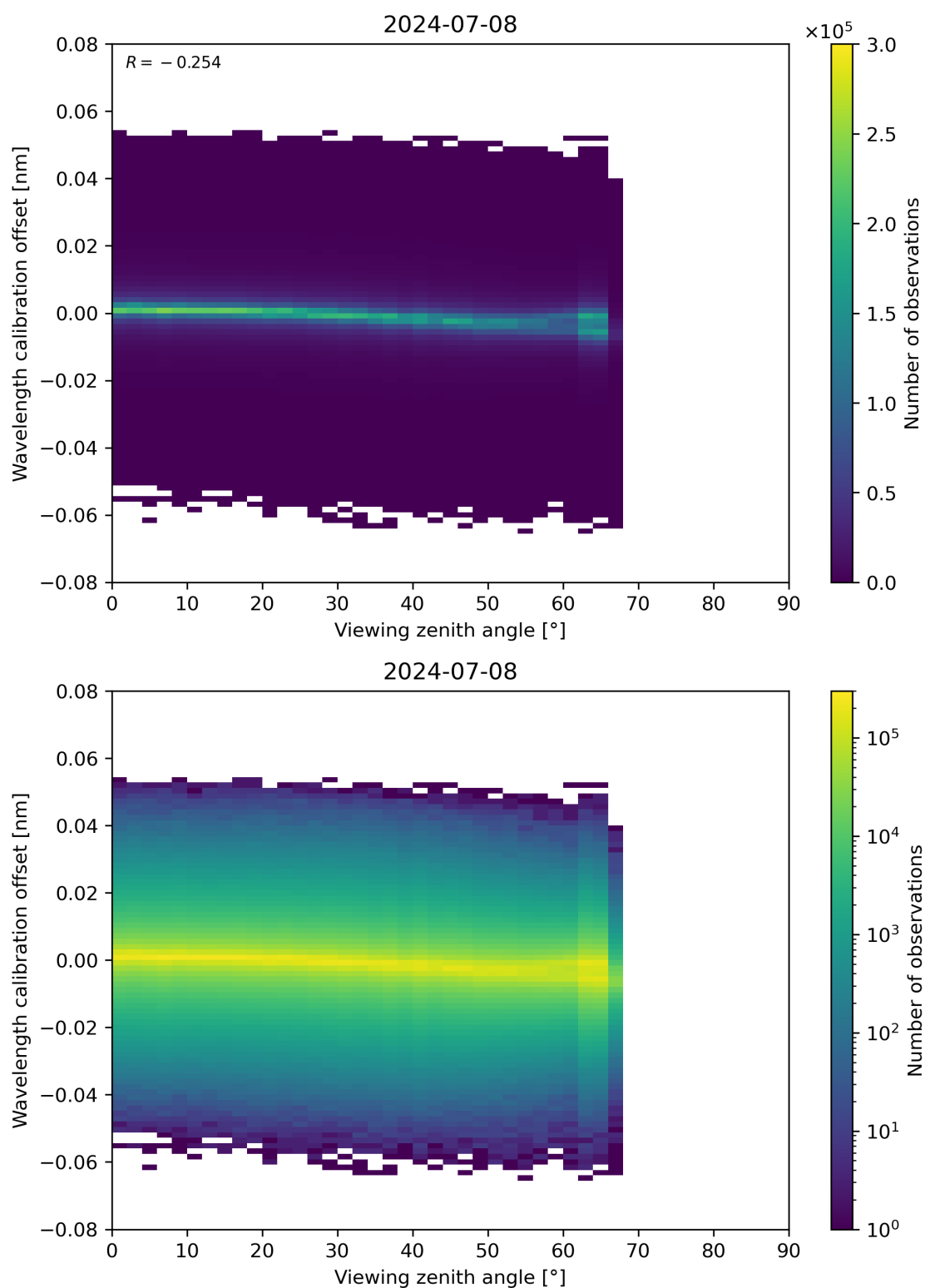
Figure 173: Scatter density plot of “Viewing zenith angle” against “Wavelength calibration offset” for 2024-07-07 to 2024-07-09.
