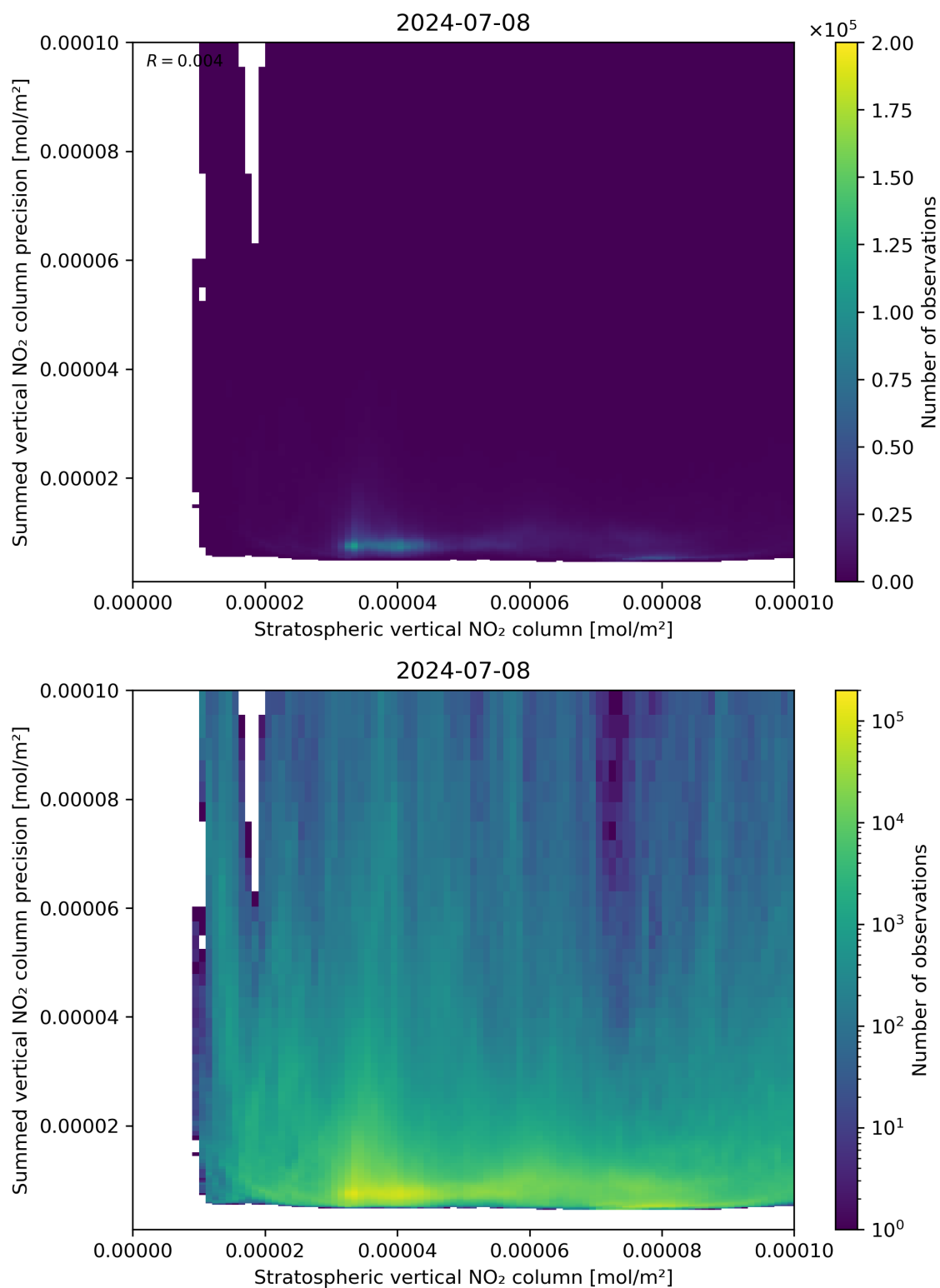
Figure 99: Scatter density plot of “Stratospheric vertical NO 2 column” against “Summed vertical NO 2 column precision” for 2024-07-07 to 2024-07-09.
