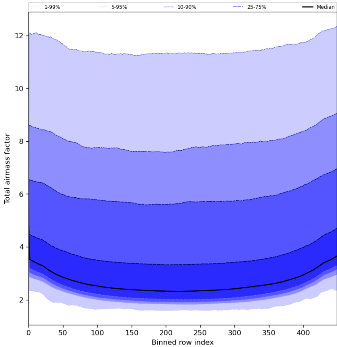
Figure 49: Along track statistics of “Total airmass factor” for 2024-07-07 to 2024-07-09
