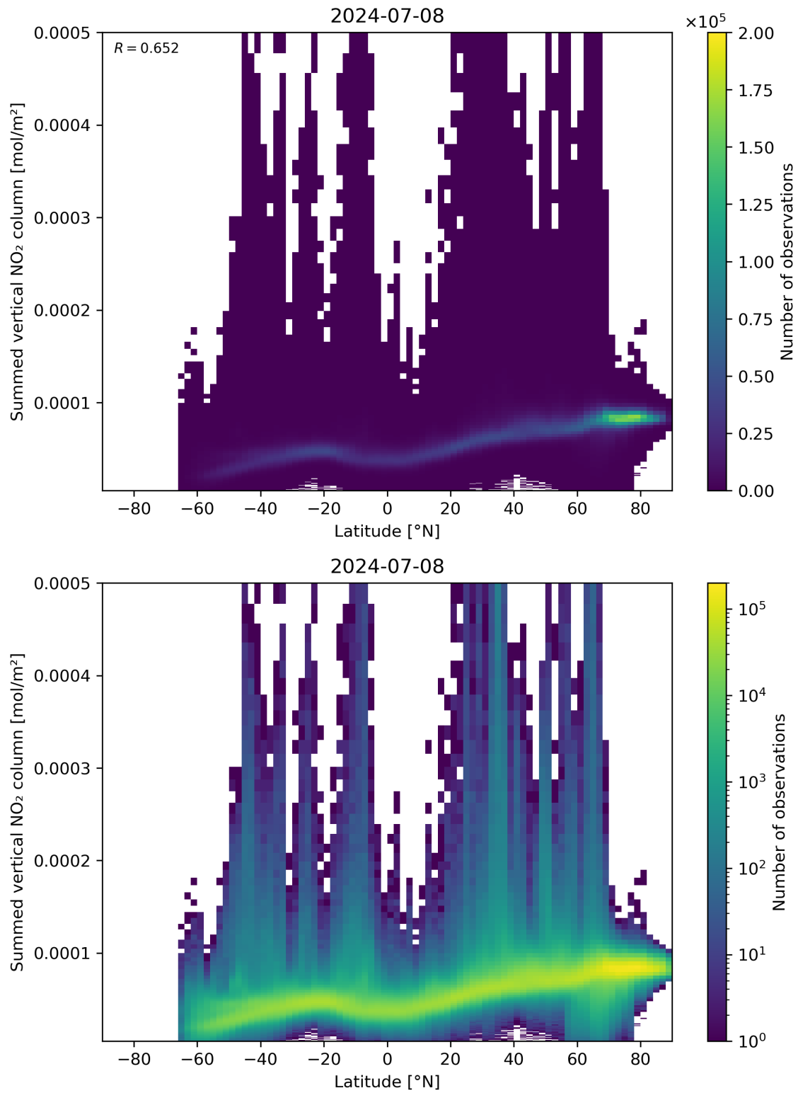
Figure 88: Scatter density plot of “Latitude” against “Summed vertical NO 2 column” for 2024-07-07 to 2024-07-09.
