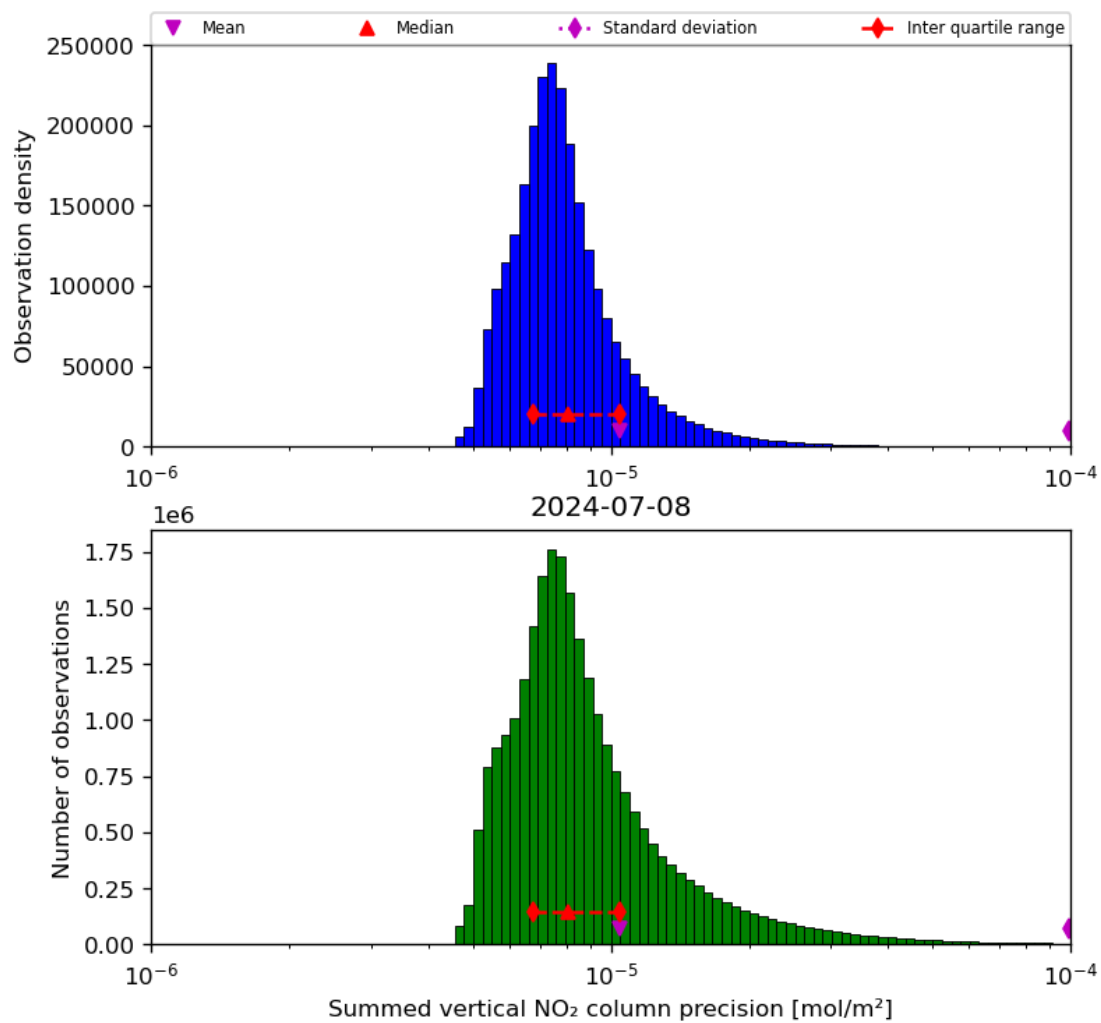
Figure 41: Histogram of “Summed vertical NO 2 column precision” for 2024-07-07 to 2024-07-09
