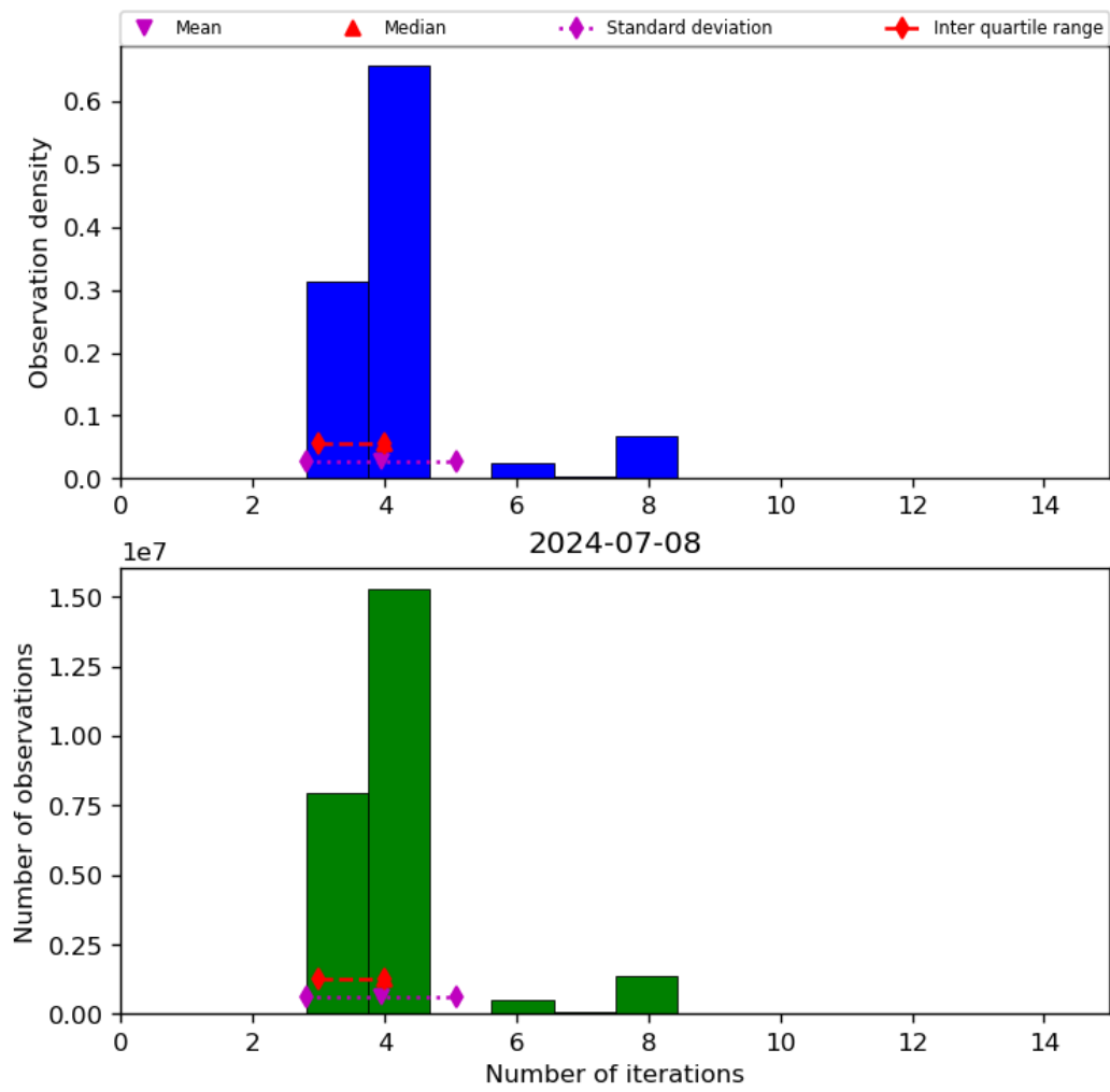
Figure 34: Histogram of “Number of iterations” for 2024-07-07 to 2024-07-09
