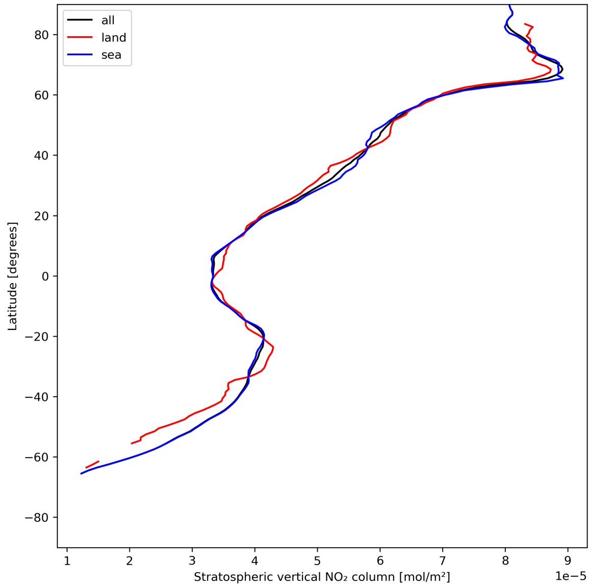
Figure 19: Zonal average of “Stratospheric vertical NO 2 column” for 2024-07-07 to 2024-07-09.
