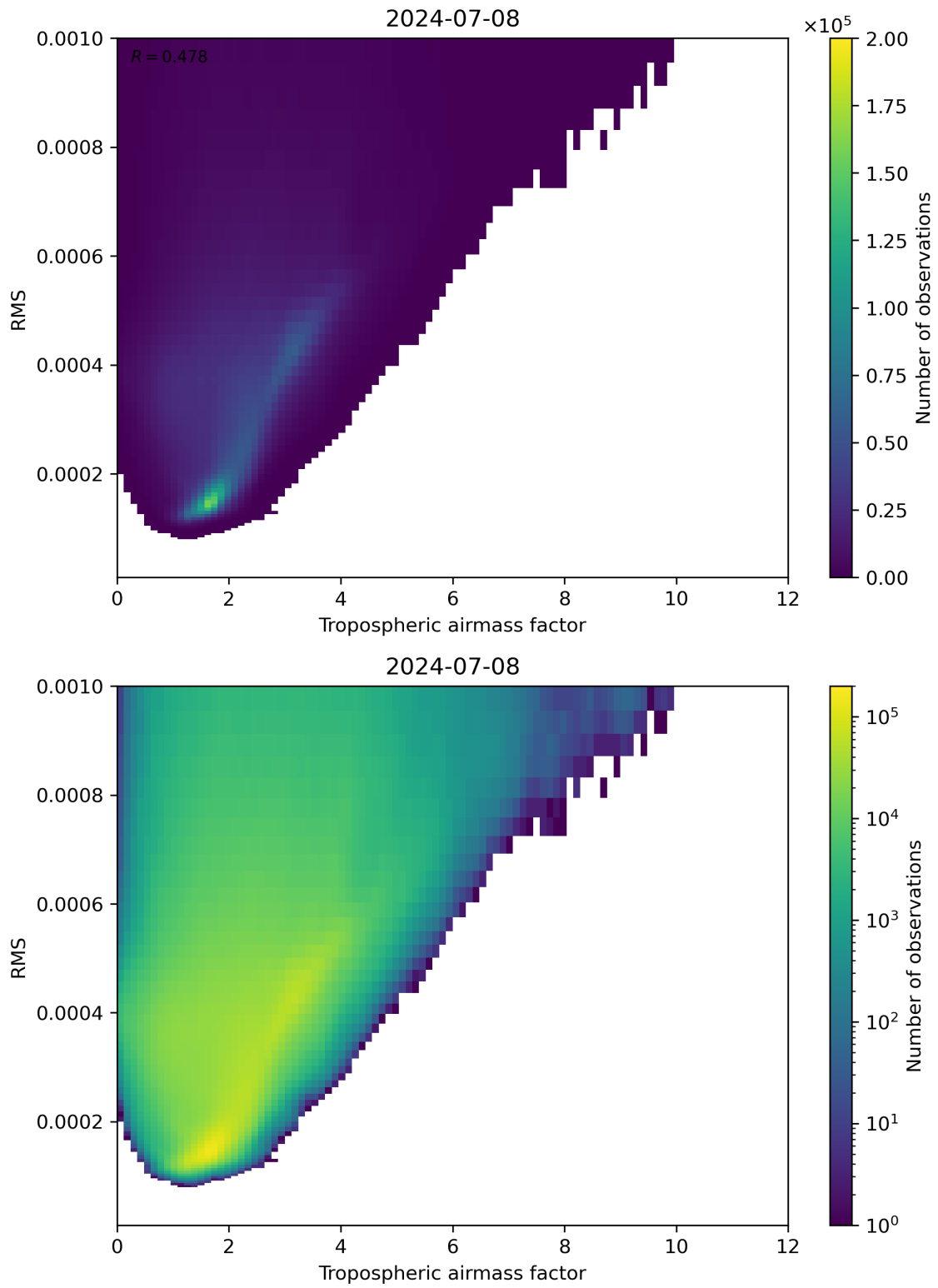
Figure 79: Scatter density plot of “Tropospheric airmass factor” against “RMS” for 2024-07-07 to 2024-07-09.
