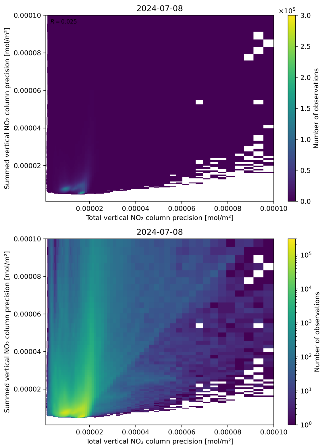
Figure 118: Scatter density plot of “Total vertical NO 2 column precision” against “Summed vertical NO 2 column precision” for 2024-07-07 to 2024-07-09.
