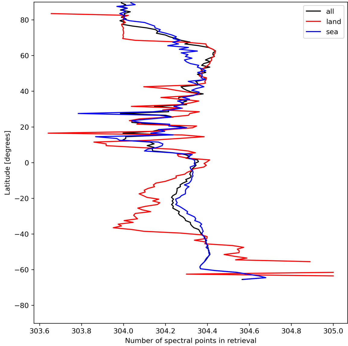
Figure 16: Zonal average of “Number of spectral points in retrieval” for 2024-07-07 to 2024-07-09.
