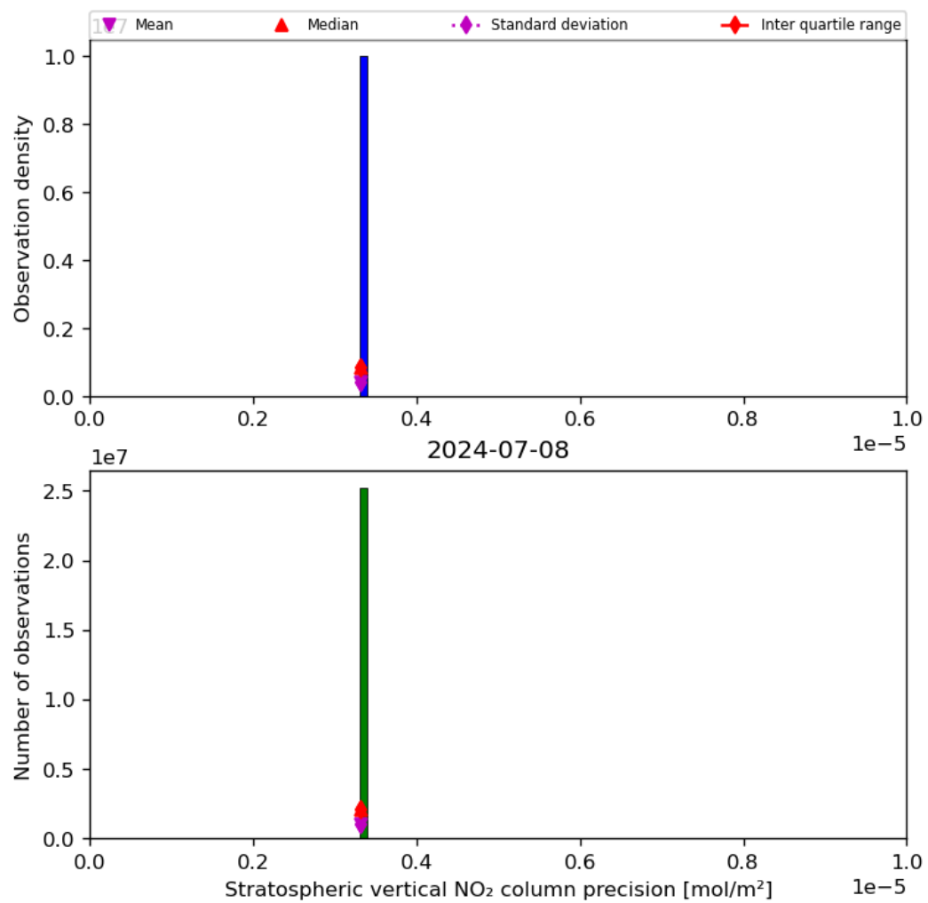
Figure 37: Histogram of “Stratospheric vertical NO 2 column precision” for 2024-07-07 to 2024-07-09
