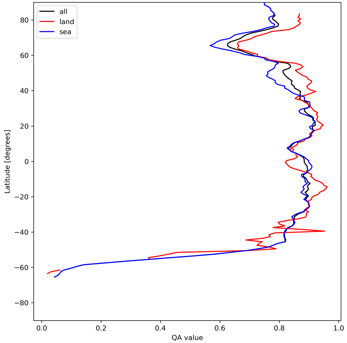
Figure 11: Zonal average of “QA value” for 2024-07-07 to 2024-07-09.
