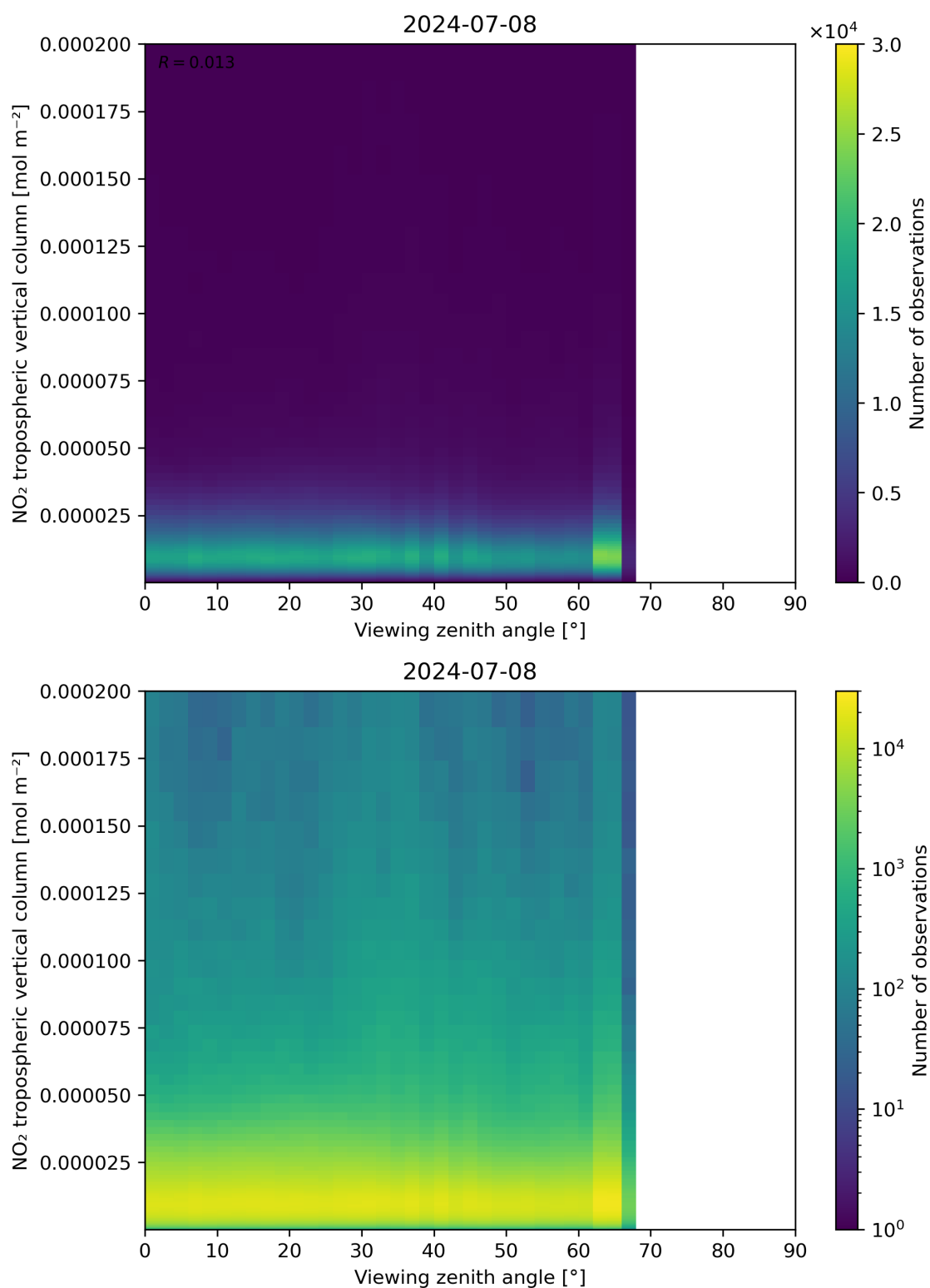
Figure 169: Scatter density plot of “Viewing zenith angle” against “NO 2 tropospheric vertical column” for 2024-07-07 to 2024-07-09.
