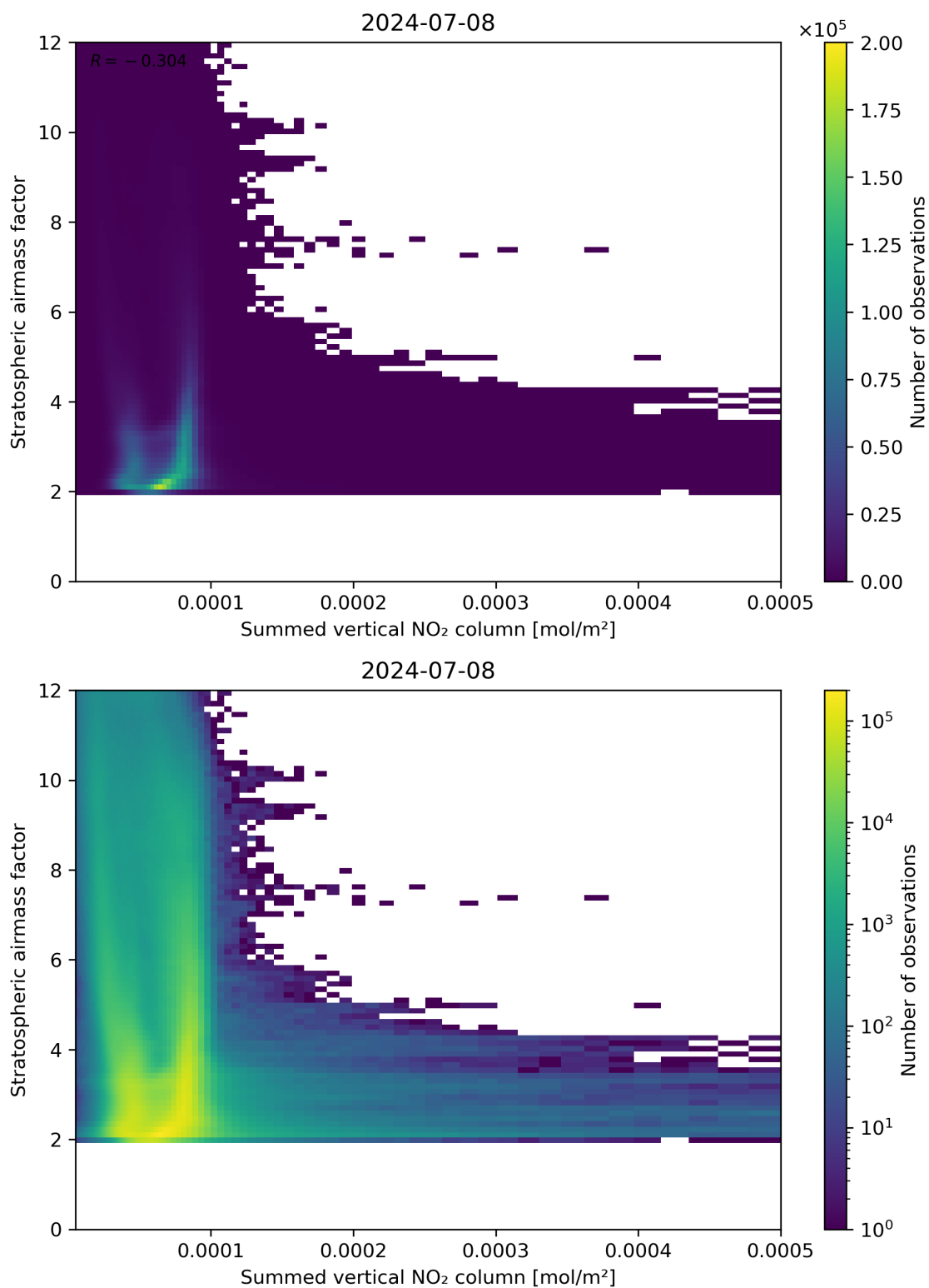
Figure 103: Scatter density plot of “Summed vertical NO 2 column” against “Stratospheric air mass factor” for 2024-07-07 to 2024-07-09.
