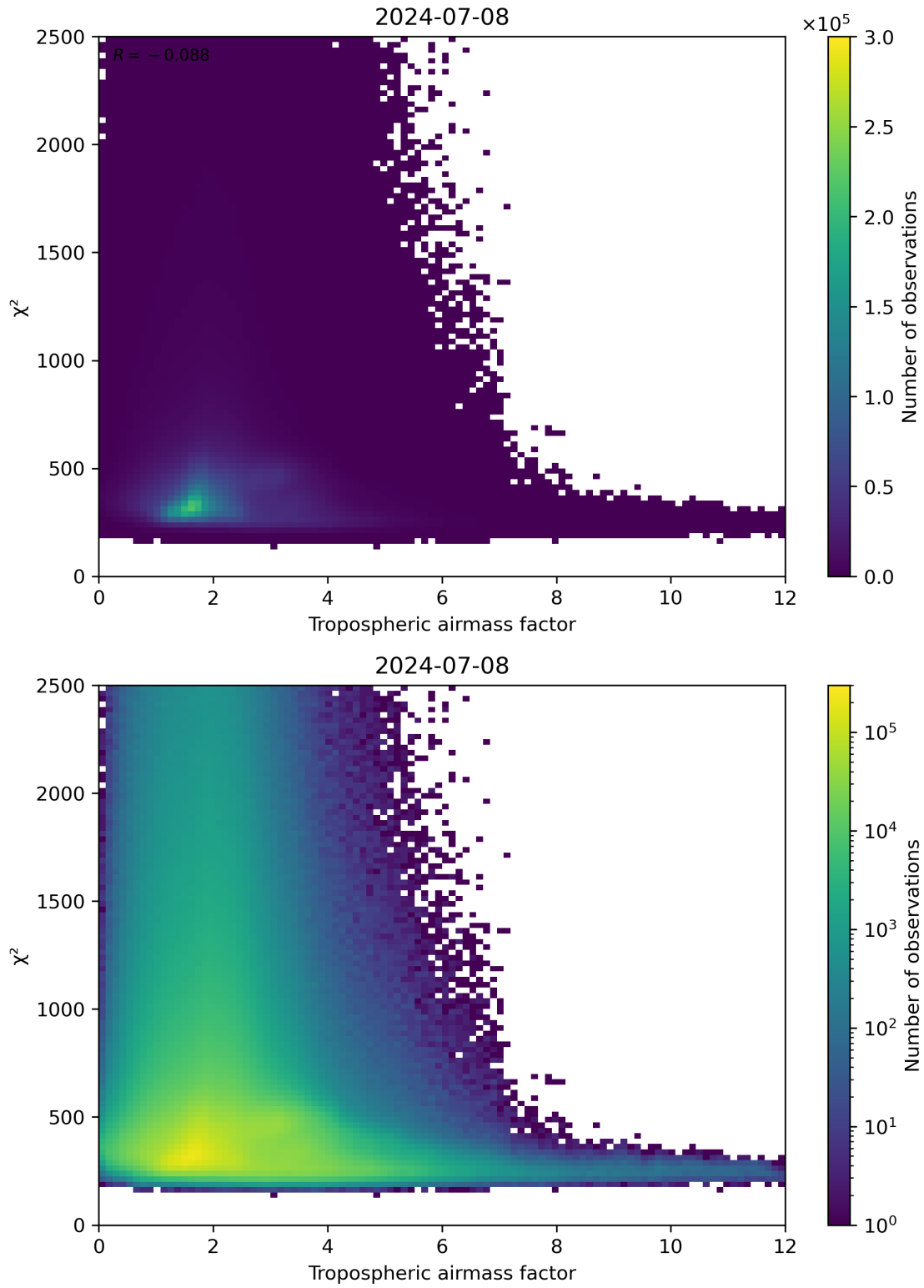
Figure 73: Scatter density plot of “Tropospheric airmass factor” against “ \chi^2 ” for 2024-07-07 to 2024-07-09.
