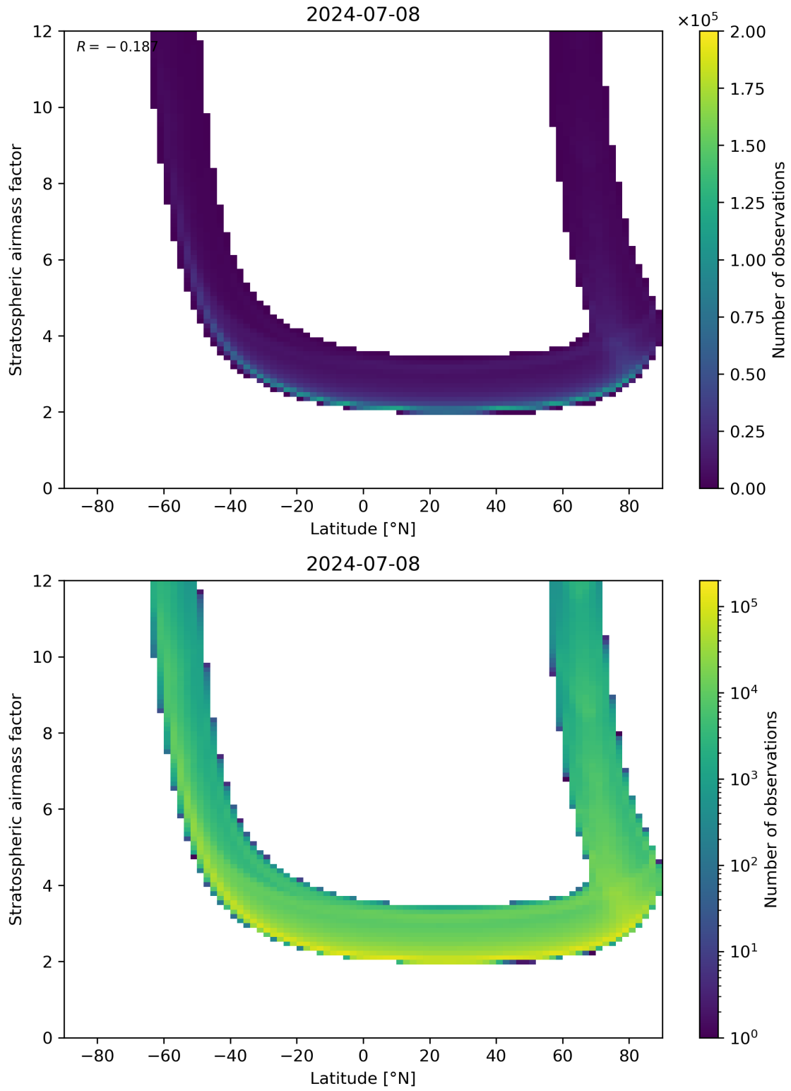
Figure 83: Scatter density plot of “Latitude” against “Stratospheric air mass factor” for 2024-07-07 to 2024-07-09.
