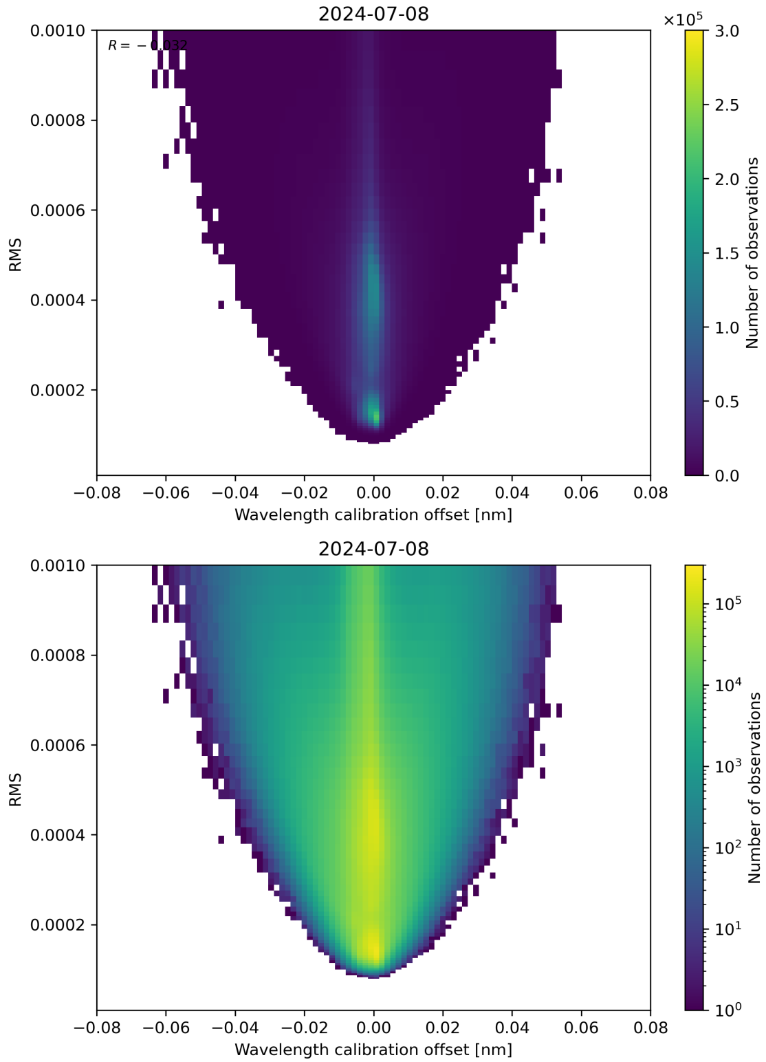
Figure 181: Scatter density plot of “Wavelength calibration offset” against “RMS” for 2024-07-07 to 2024-07-09.
