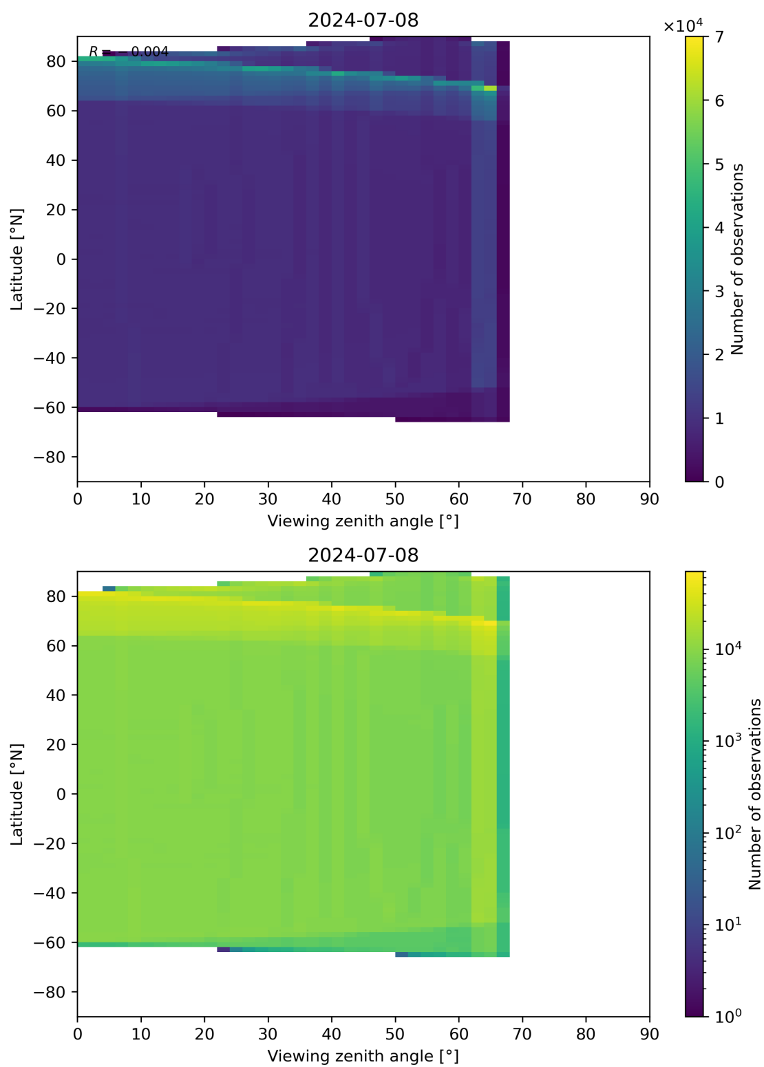
Figure 163: Scatter density plot of “Viewing zenith angle” against “Latitude” for 2024-07-07 to 2024-07-09.
