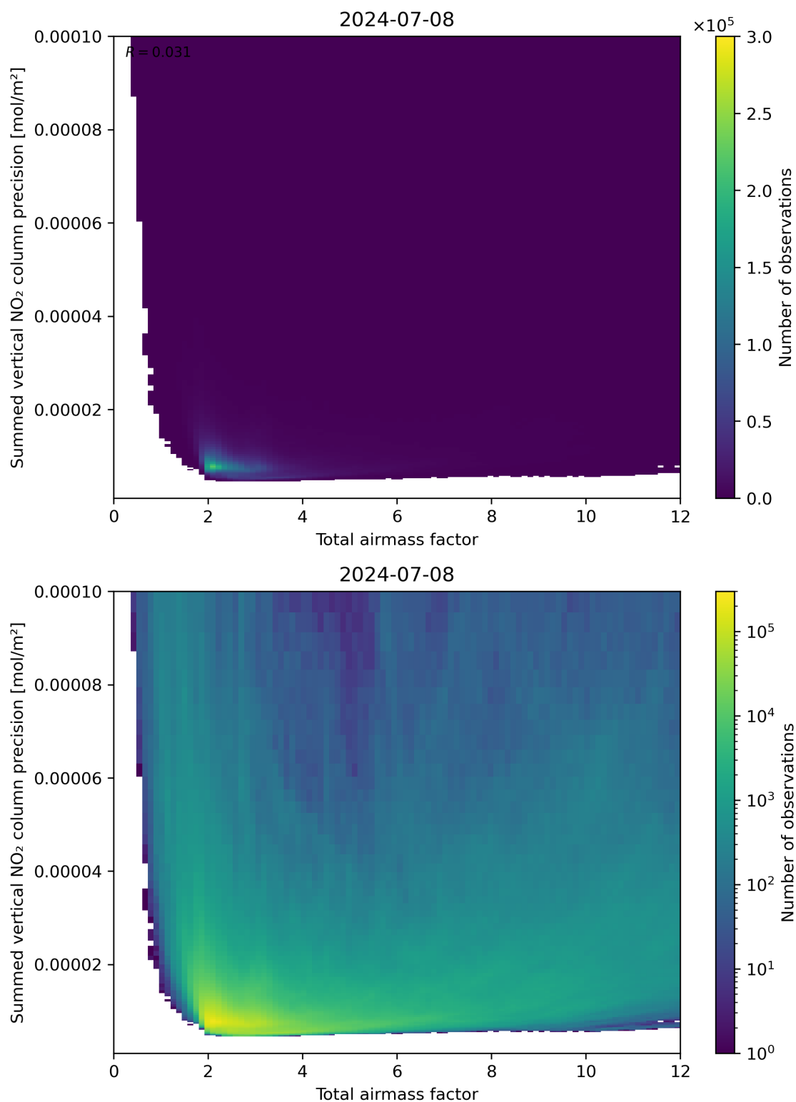
Figure 66: Scatter density plot of “Total airmass factor” against “Summed vertical NO 2 column precision” for 2024-07-07 to 2024-07-09.
