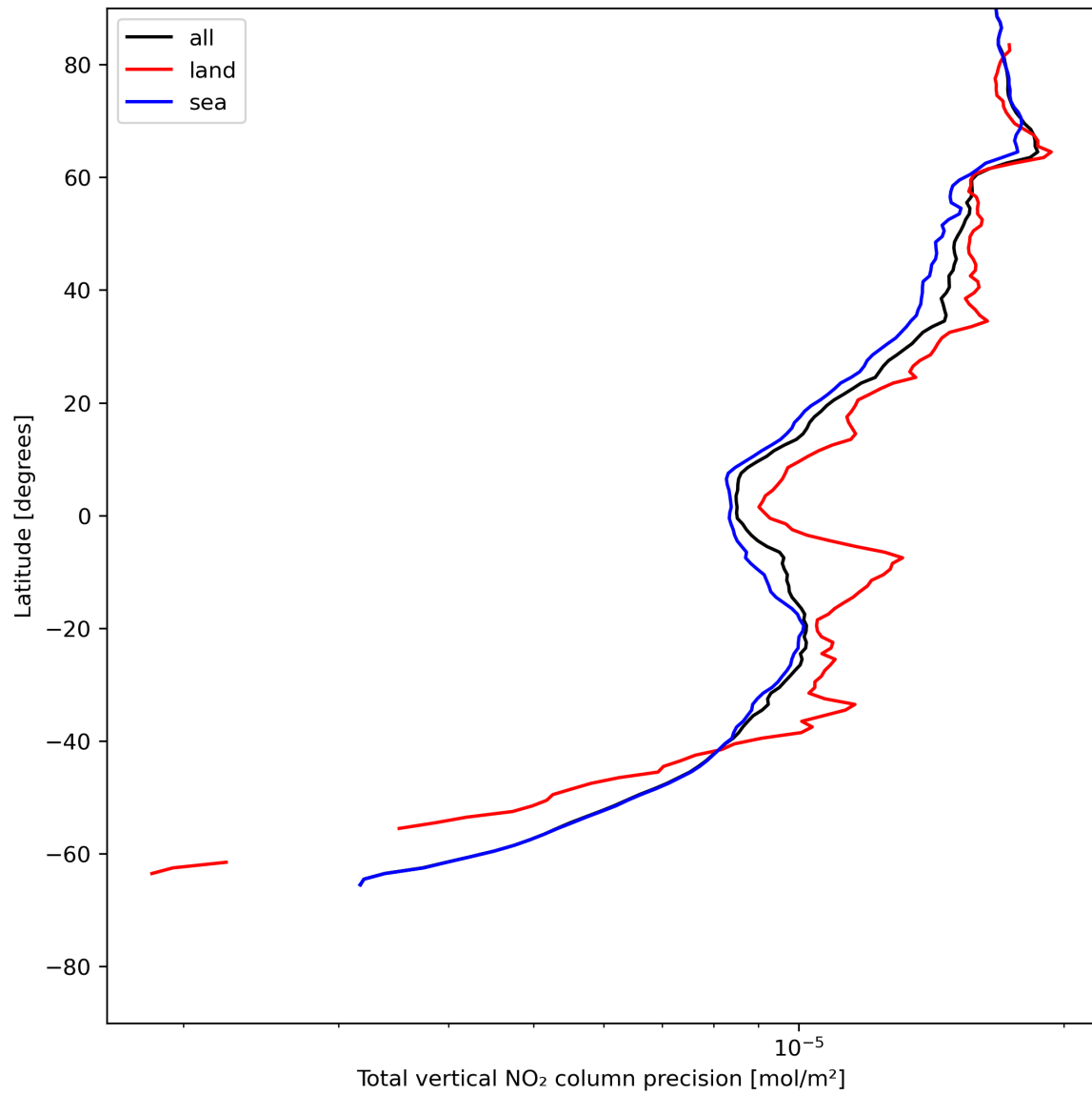
Figure 22: Zonal average of “Total vertical NO 2 column precision” for 2024-07-07 to 2024-07-09.
