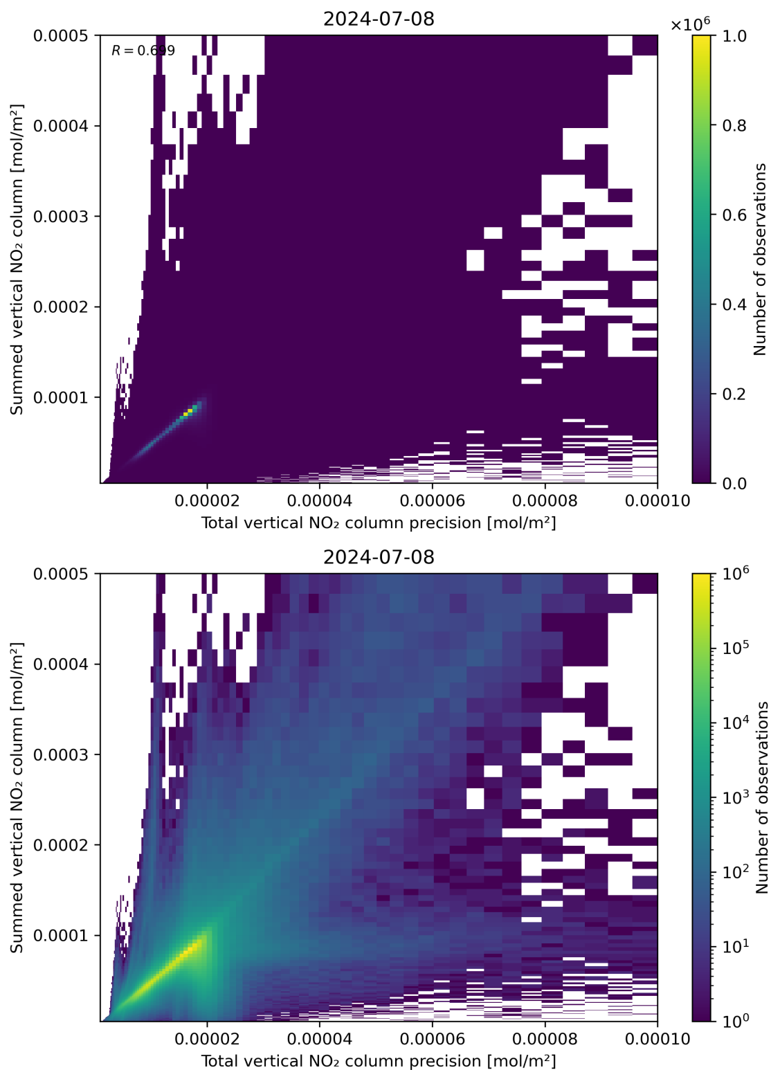
Figure 117: Scatter density plot of “Total vertical NO 2 column precision” against “Summed vertical NO 2 column” for 2024-07-07 to 2024-07-09.
