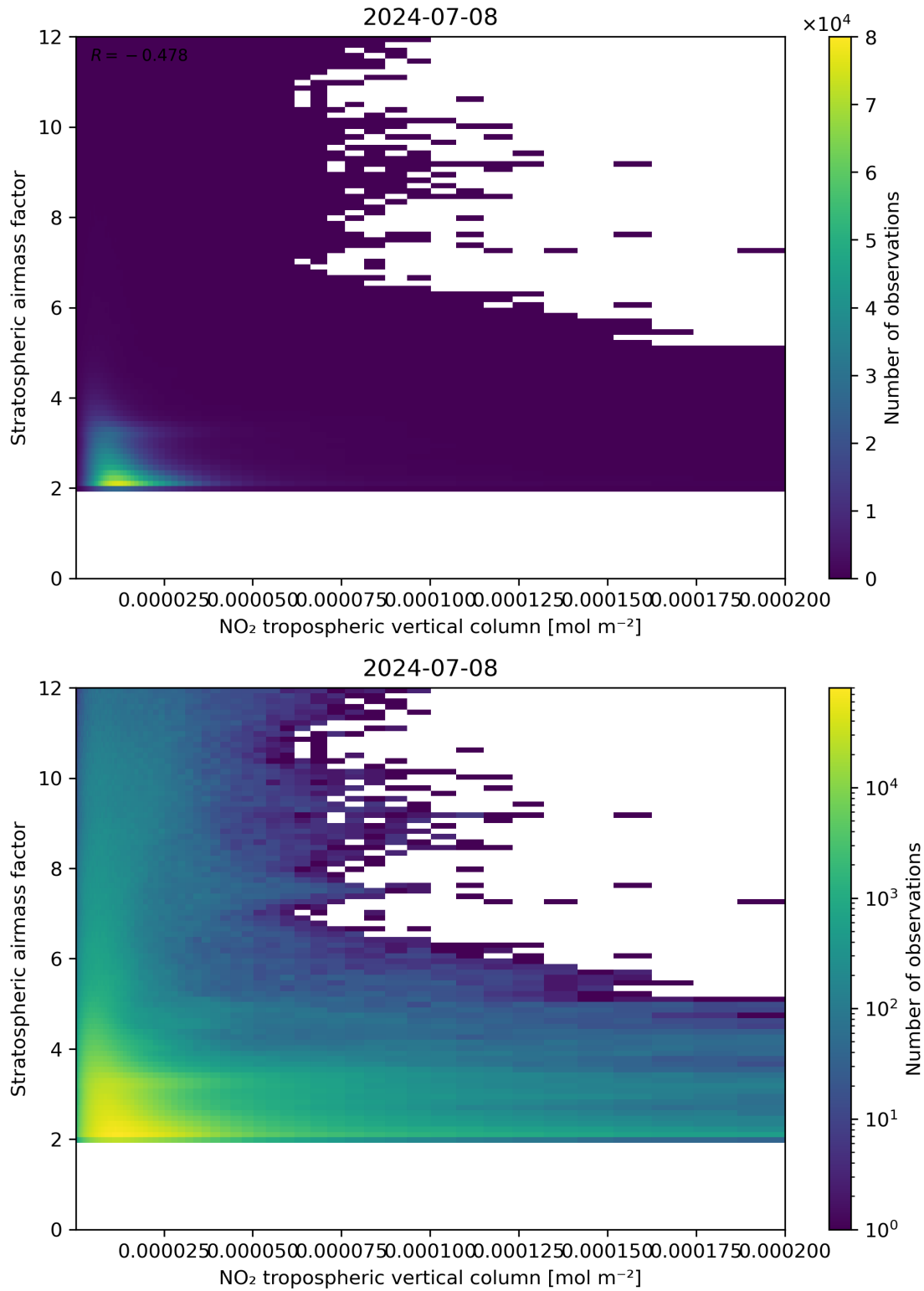
Figure 121: Scatter density plot of “NO 2 tropospheric vertical column” against “Stratospheric air mass factor” for 2024-07-07 to 2024-07-09.
