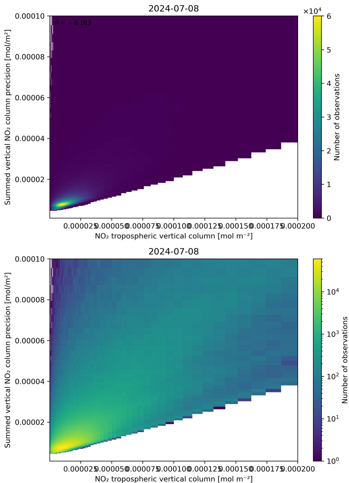
Figure 127: Scatter density plot of “NO 2 tropospheric vertical column” against “Summed vertical NO 2 column precision” for 2024-07-07 to 2024-07-09.
