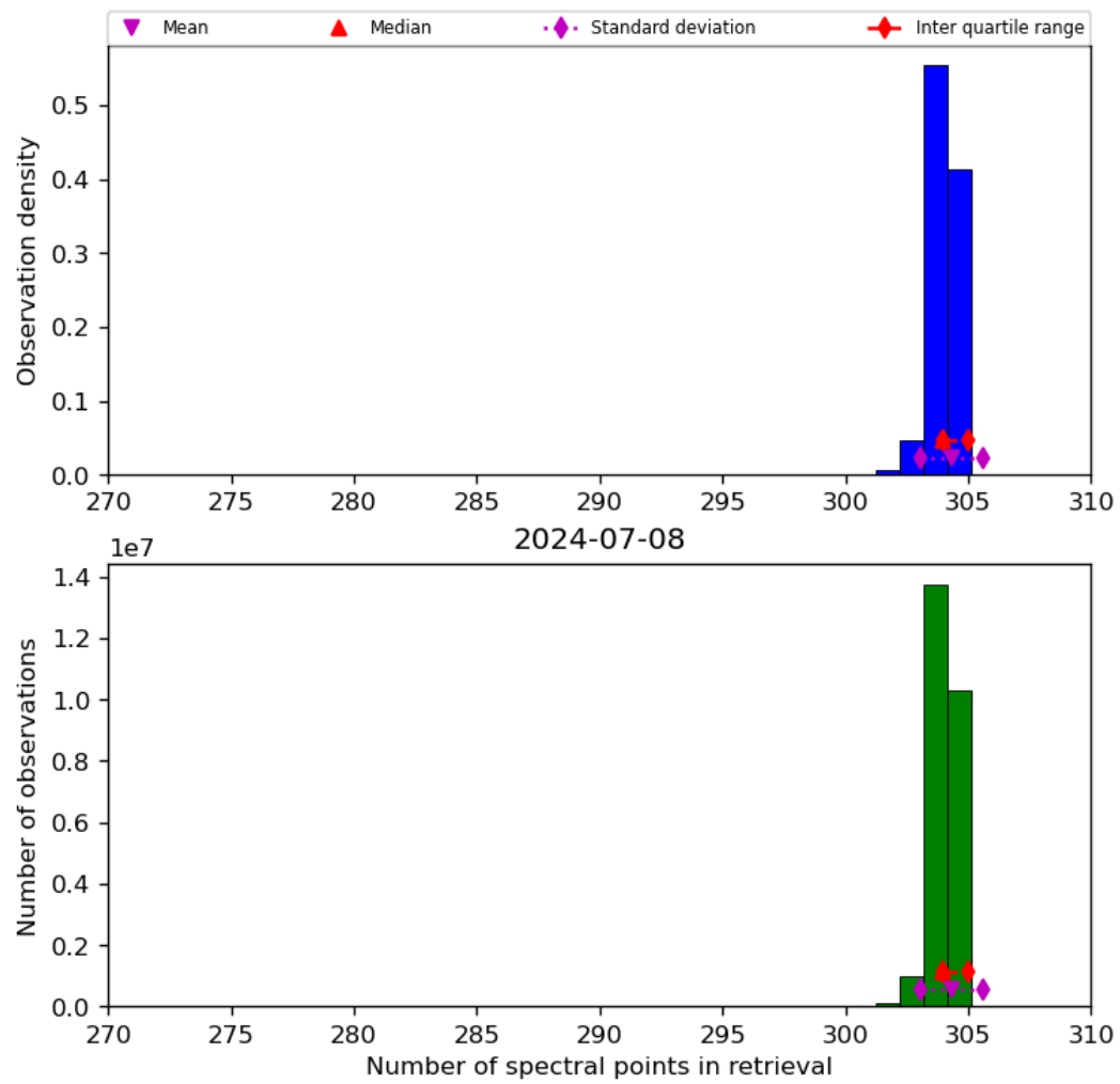
Figure 33: Histogram of “Number of spectral points in retrieval” for 2024-07-07 to 2024-07-09
