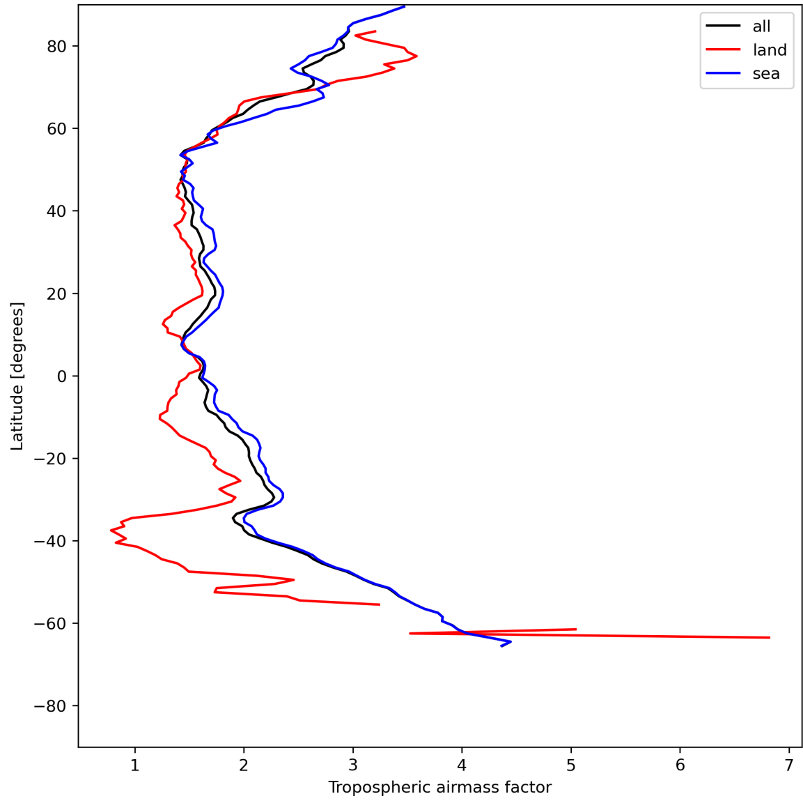
Figure 14: Zonal average of “Tropospheric airmass factor” for 2024-07-07 to 2024-07-09.
