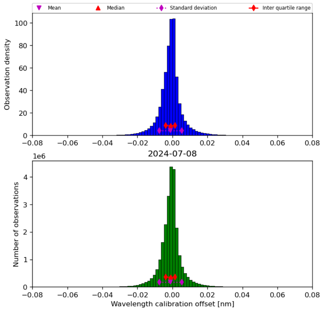
Figure 35: Histogram of “Wavelength calibration offset” for 2024-07-07 to 2024-07-09
