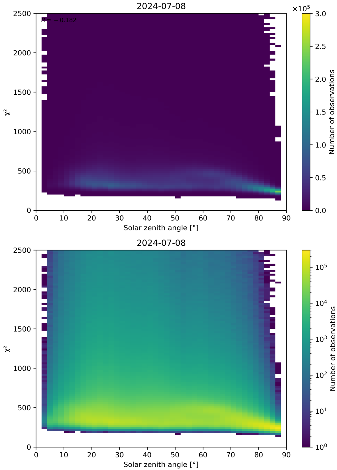
Figure 148: Scatter density plot of “Solar zenith angle” against “ \chi^2 ” for 2024-07-07 to 2024-07-09.
