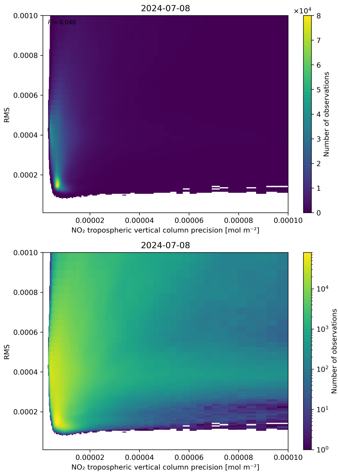
Figure 140: Scatter density plot of “NO 2 tropospheric vertical column precision” against “RMS” for 2024-07-07 to 2024-07-09.
