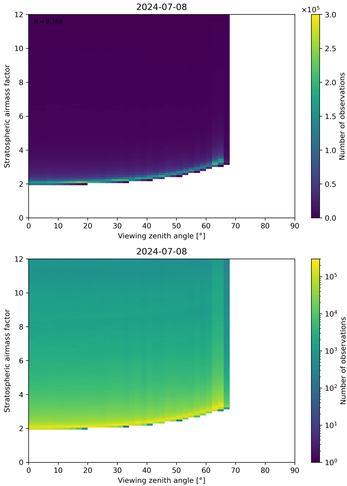
Figure 159: Scatter density plot of “Viewing zenith angle” against “Stratospheric airmass factor” for 2024-07-07 to 2024-07-09.
