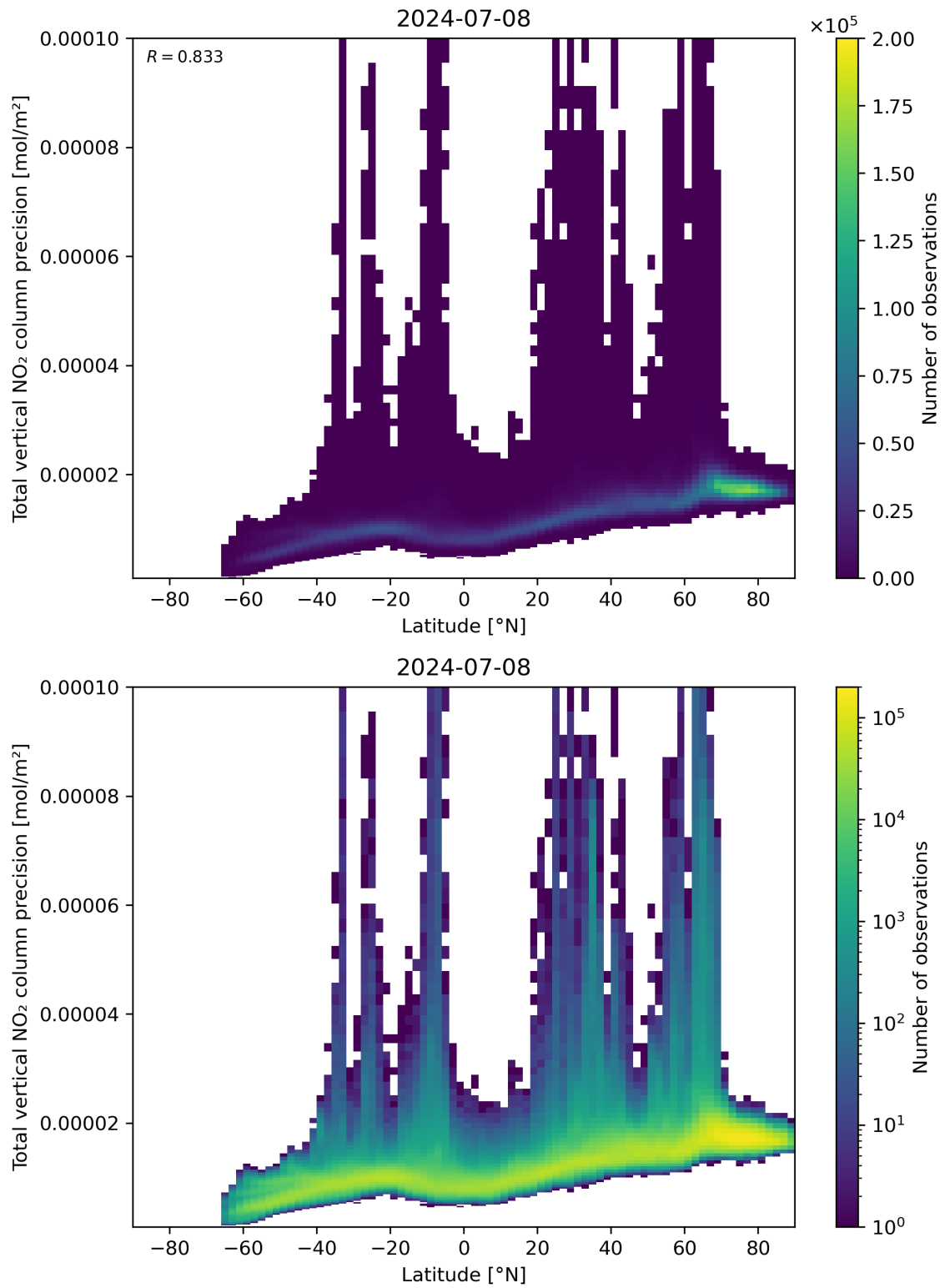
Figure 91: Scatter density plot of “Latitude” against “Total vertical NO 2 column precision” for 2024-07-07 to 2024-07-09.
