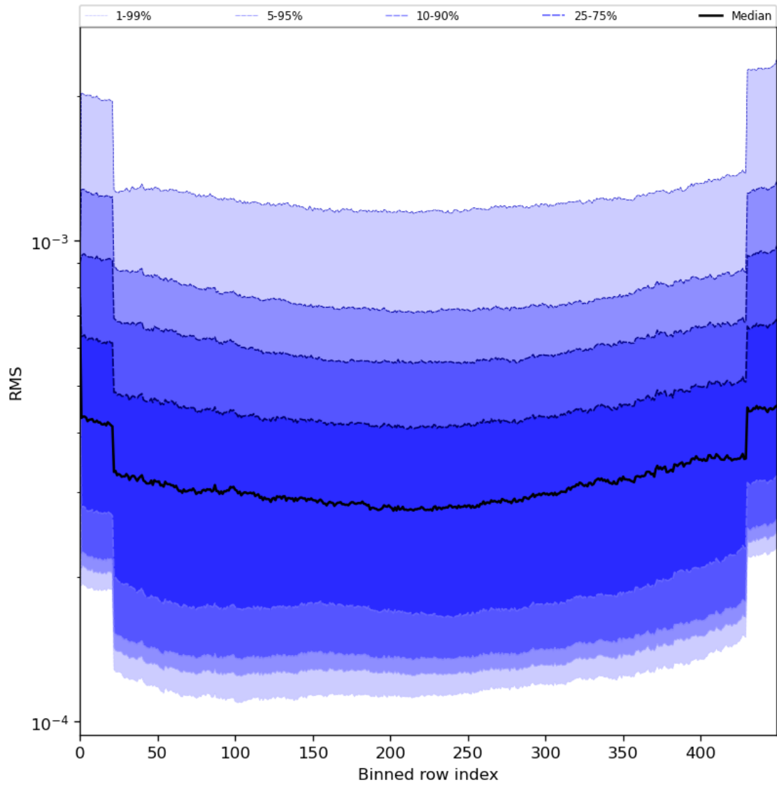
Figure 60: Along track statistics of “RMS” for 2024-07-07 to 2024-07-09
