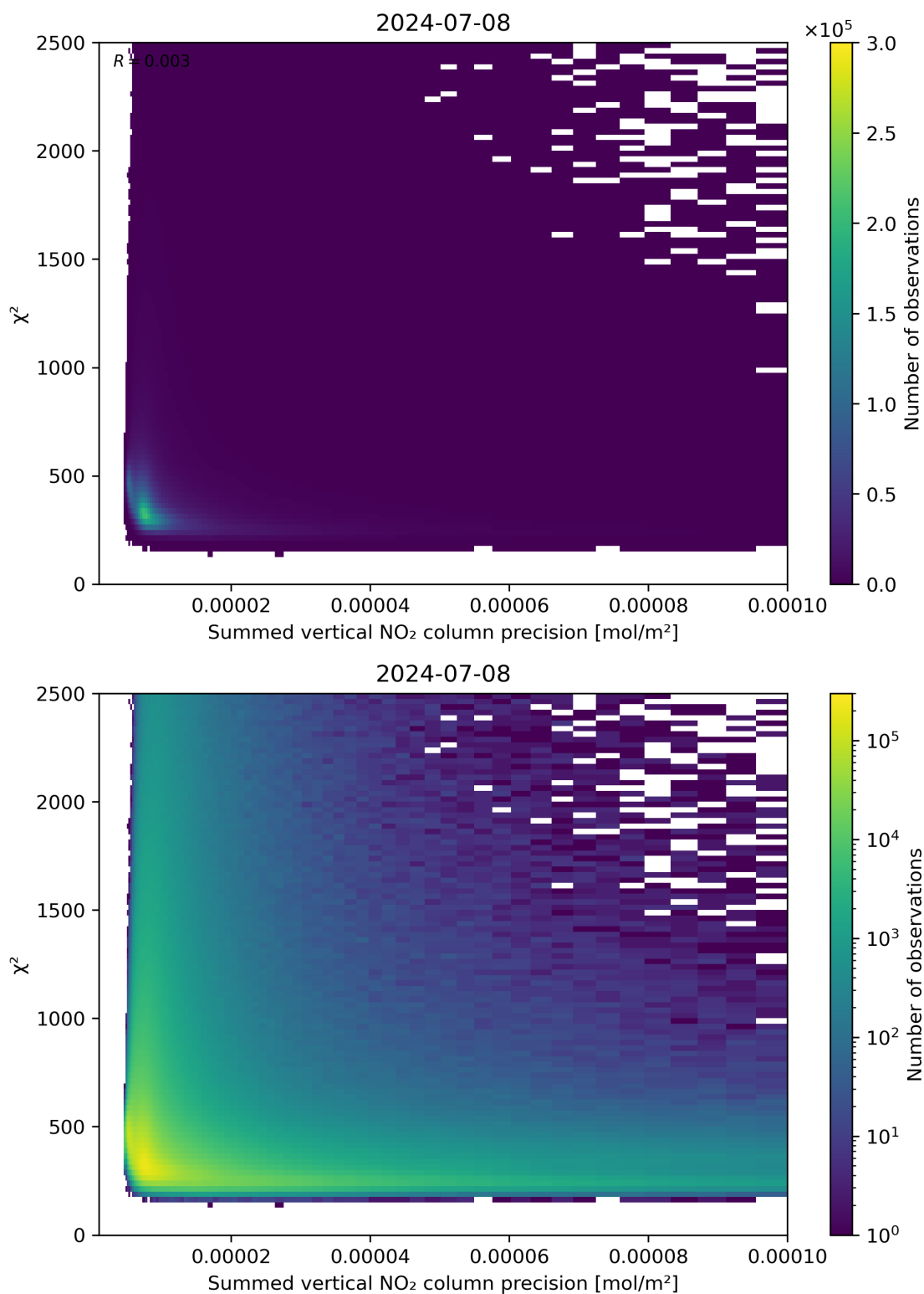
Figure 107: Scatter density plot of “Summed vertical NO 2 column precision” against “ \chi^2 ” for 2024-07-07 to 2024-07-09.
