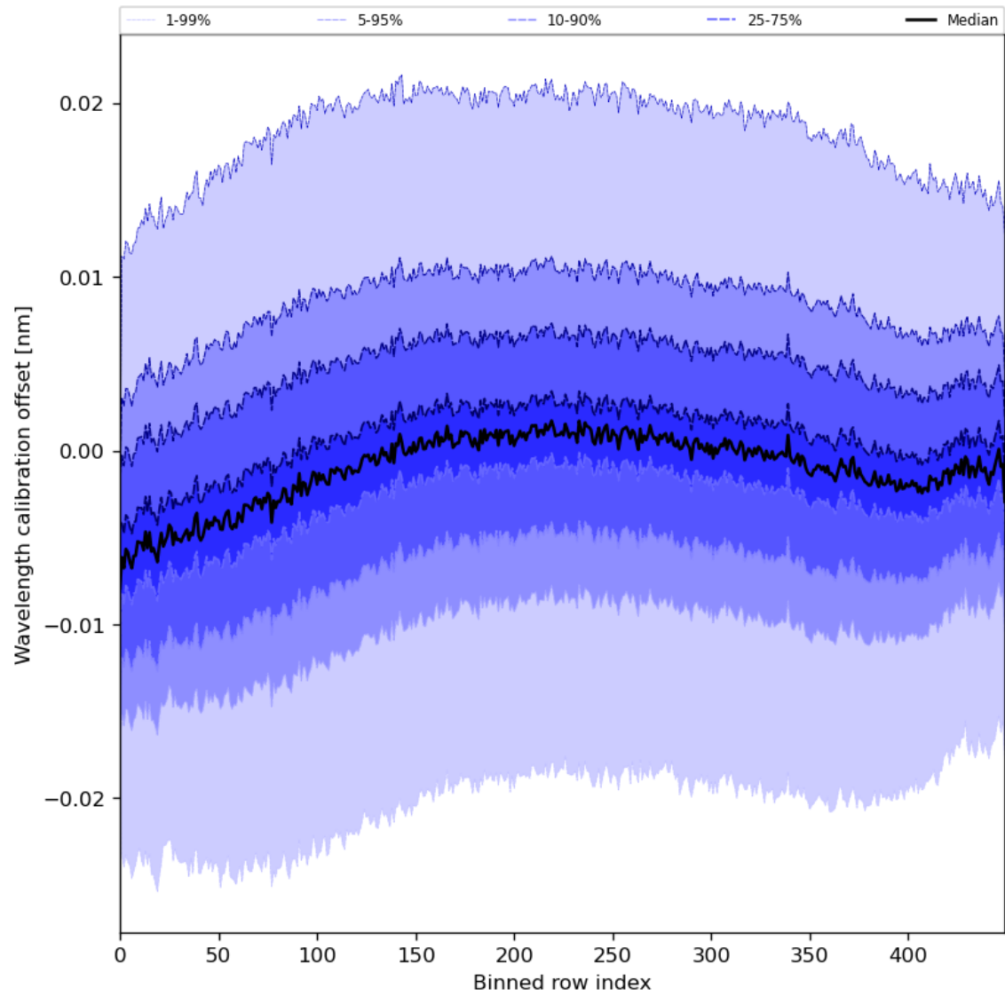
Figure 52: Along track statistics of “Wavelength calibration offset” for 2024-07-07 to 2024-07-09
