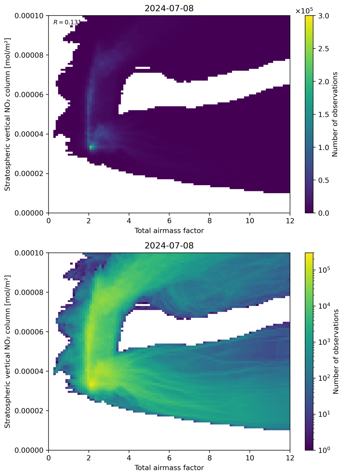
Figure 64: Scatter density plot of “Total airmass factor” against “Stratospheric vertical NO 2 column” for 2024-07-07 to 2024-07-09.
