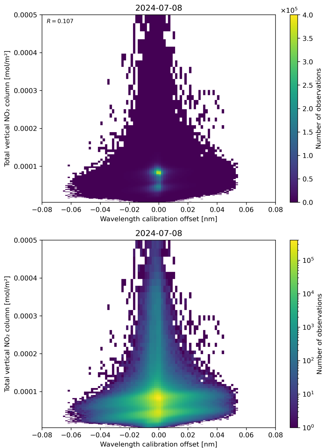
Figure 179: Scatter density plot of “Wavelength calibration offset” against “Total vertical NO 2 column” for 2024-07-07 to 2024-07-09.
