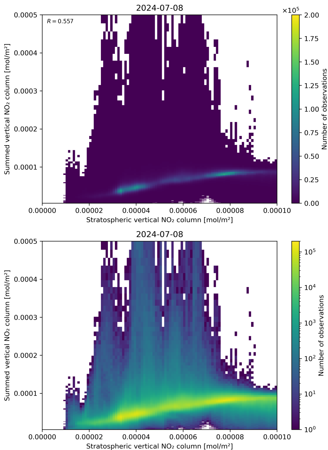
Figure 98: Scatter density plot of “Stratospheric vertical NO 2 column” against “Summed vertical NO 2 column” for 2024-07-07 to 2024-07-09.
