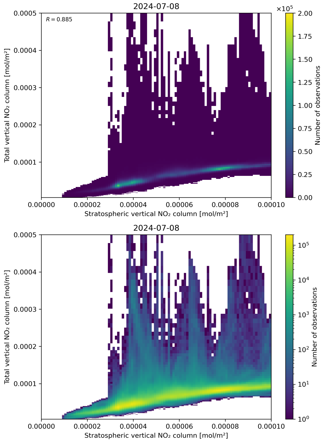
Figure 100: Scatter density plot of “Stratospheric vertical NO 2 column” against “Total vertical NO 2 column” for 2024-07-07 to 2024-07-09.
