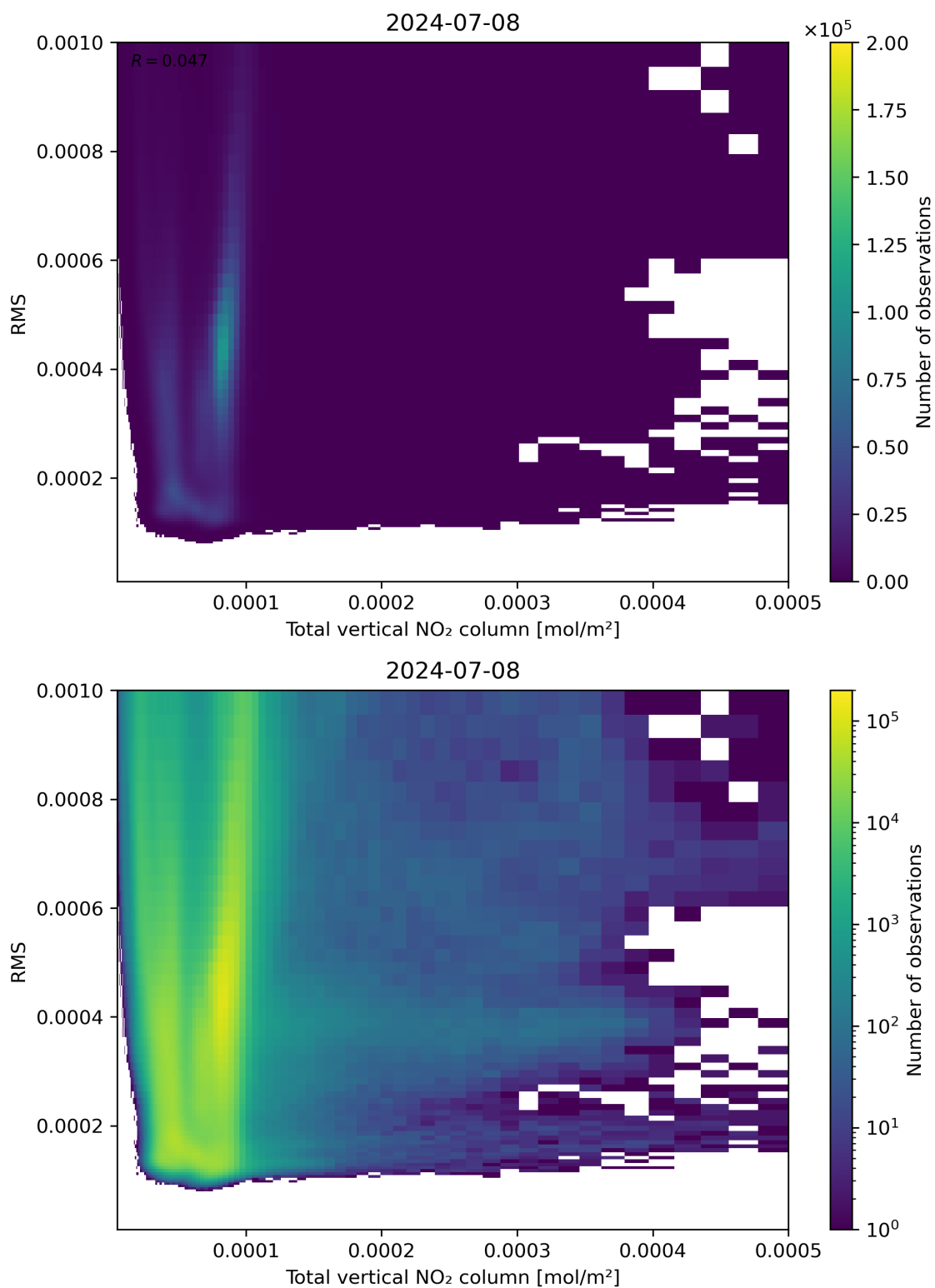
Figure 120: Scatter density plot of “Total vertical NO 2 column” against “RMS” for 2024-07-07 to 2024-07-09.
