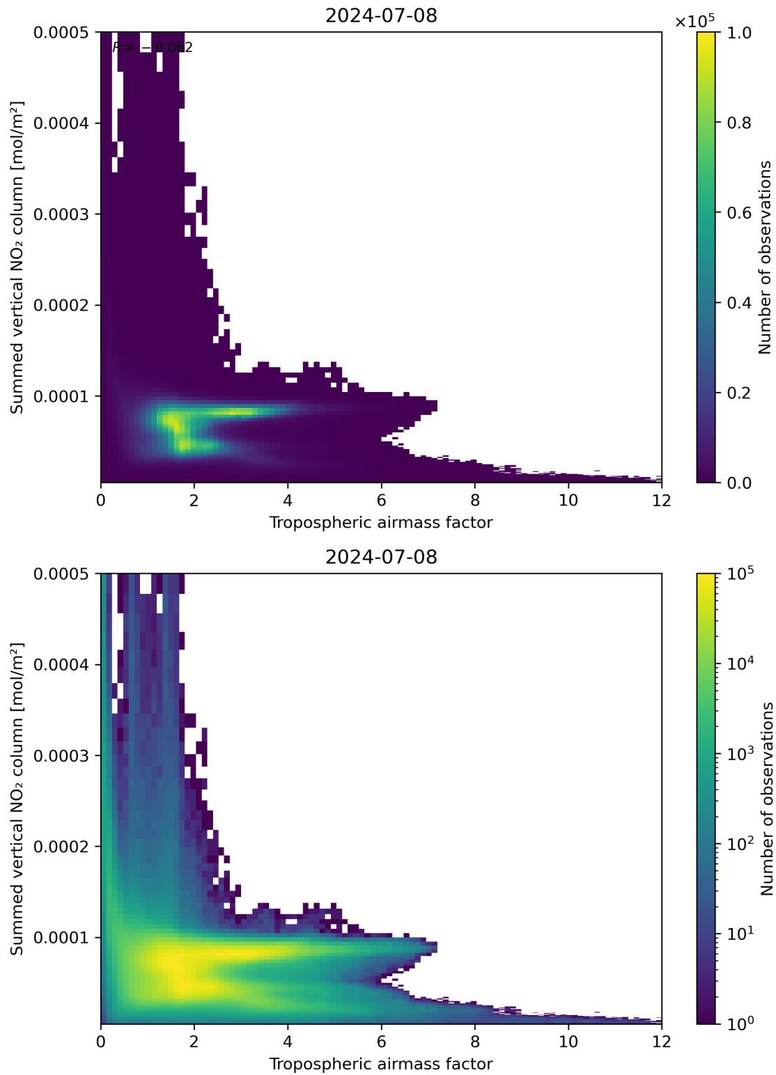
Figure 75: Scatter density plot of “Tropospheric airmass factor” against “Summed vertical NO 2 column” for 2024-07-07 to 2024-07-09.
