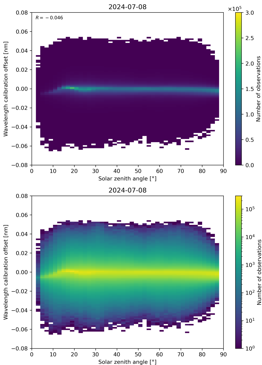
Figure 158: Scatter density plot of “Solar zenith angle” against “Wavelength calibration offset” for 2024-07-07 to 2024-07-09.
