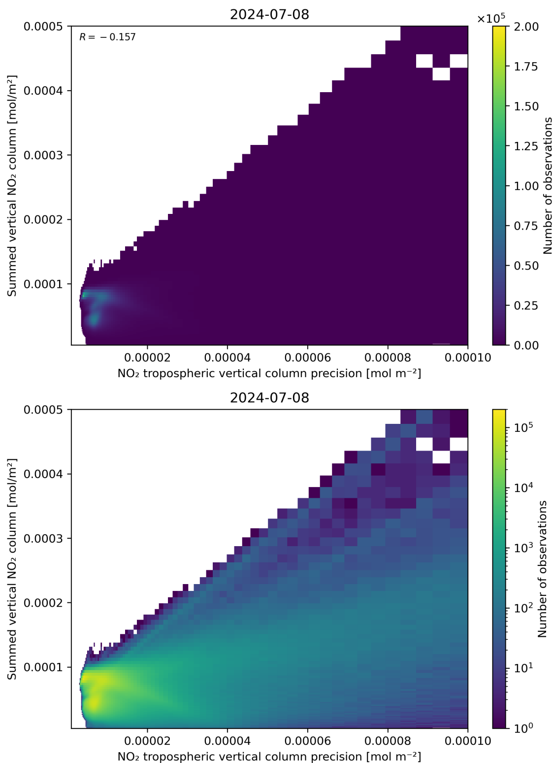
Figure 136: Scatter density plot of “NO 2 tropospheric vertical column precision” against “Summed vertical NO 2 column” for 2024-07-07 to 2024-07-09.
