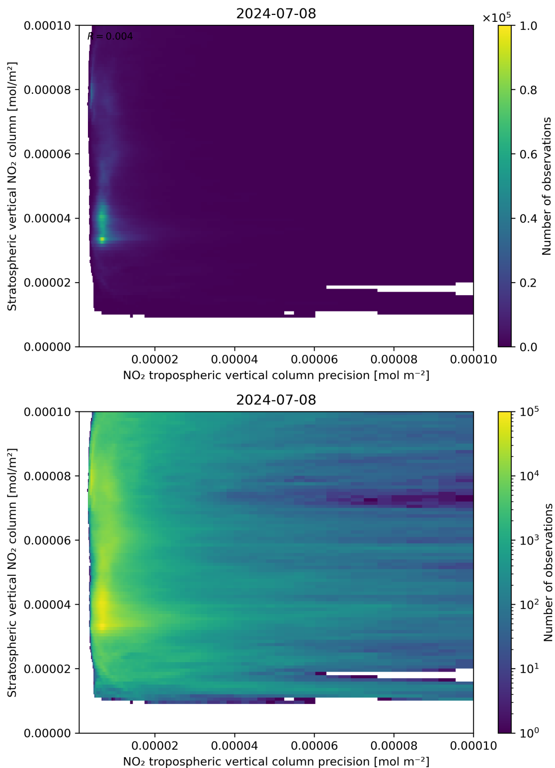
Figure 135: Scatter density plot of “NO 2 tropospheric vertical column precision” against “Stratospheric vertical NO 2 column” for 2024-07-07 to 2024-07-09.
