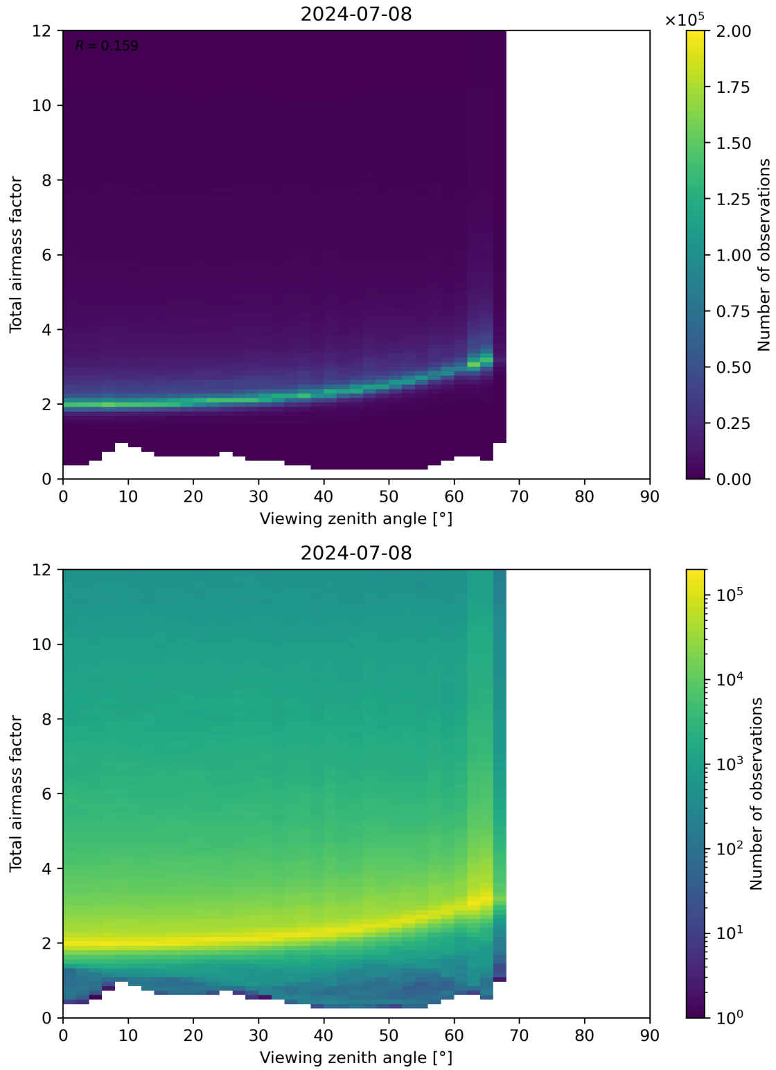
Figure 160: Scatter density plot of “Viewing zenith angle” against “Total airmass factor” for 2024-07-07 to 2024-07-09.
