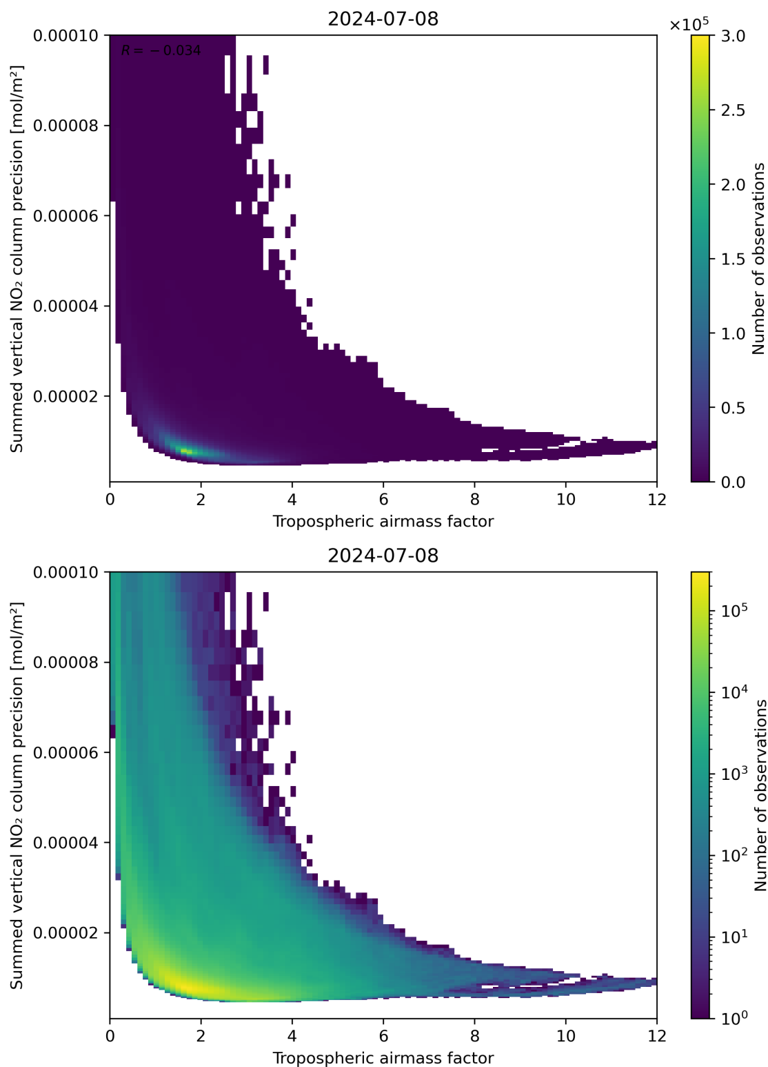
Figure 76: Scatter density plot of “Tropospheric air mass factor” against “Summed vertical NO 2 column precision” for 2024-07-07 to 2024-07-09.
