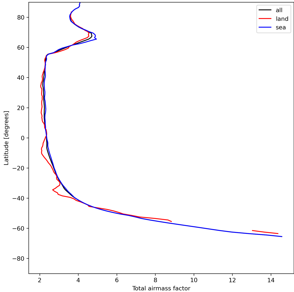
Figure 15: Zonal average of “Total airmass factor” for 2024-07-07 to 2024-07-09.
