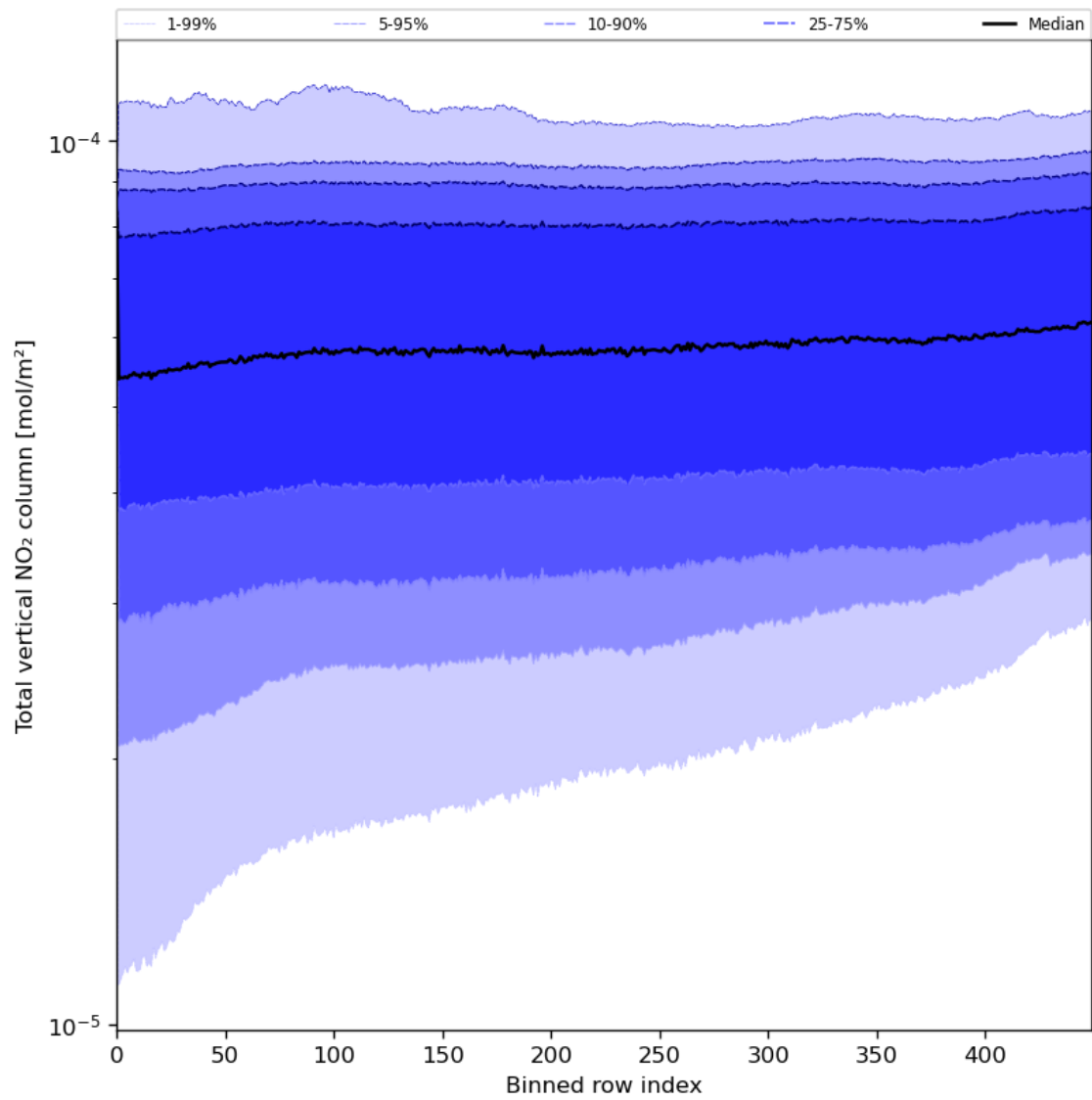
Figure 55: Along track statistics of "Total vertical NO 2 column" for 2024-07-07 to 2024-07-09
