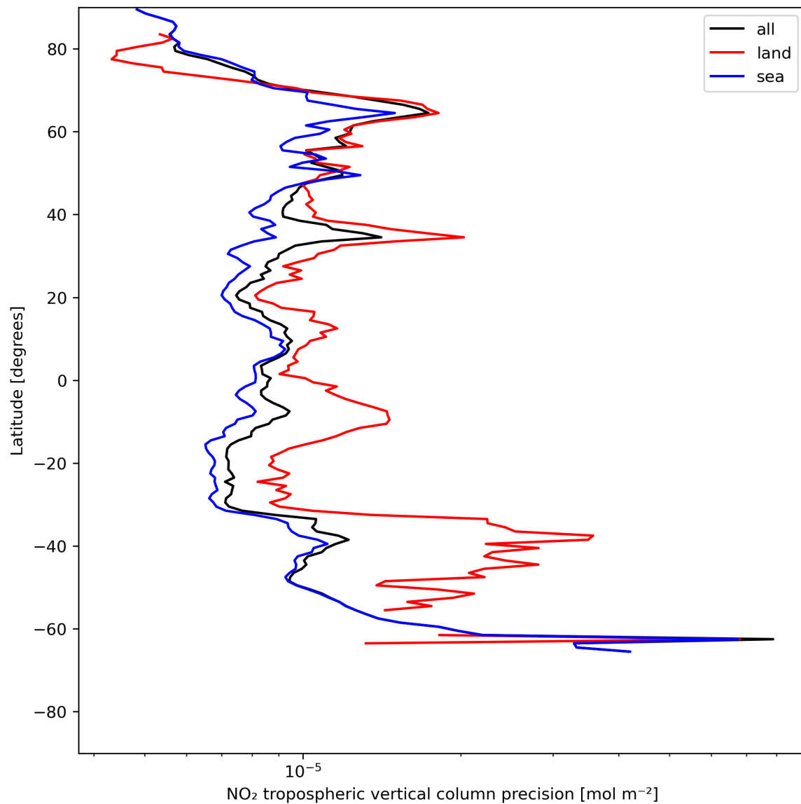
Figure 13: Zonal average of “NO 2 tropospheric vertical column precision” for 2024-07-07 to 2024-07-09.
