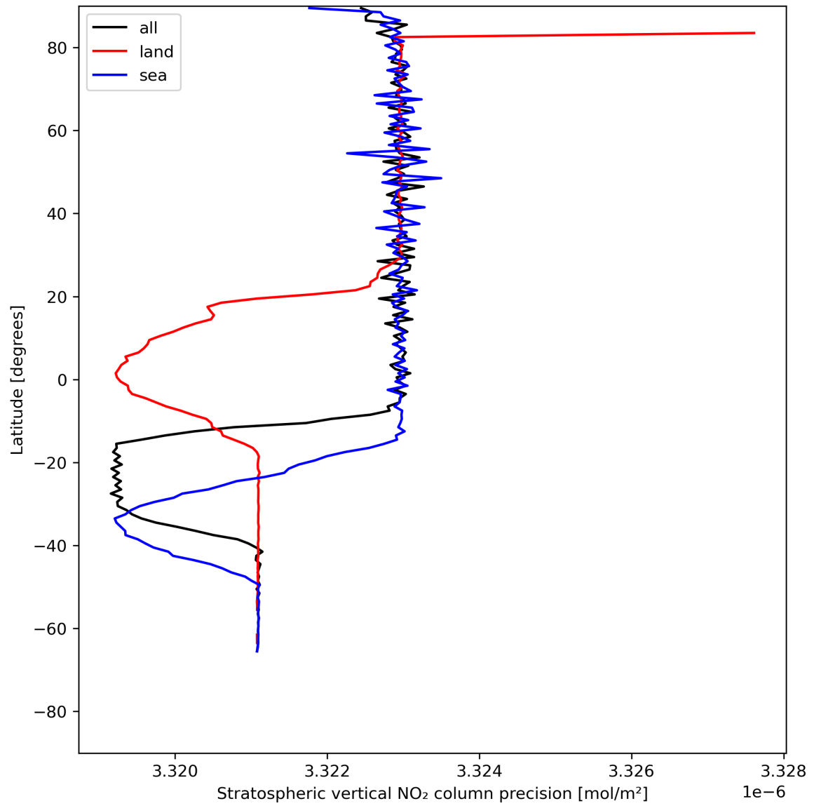
Figure 20: Zonal average of “Stratospheric vertical NO 2 column precision” for 2024-07-07 to 2024-07-09.
