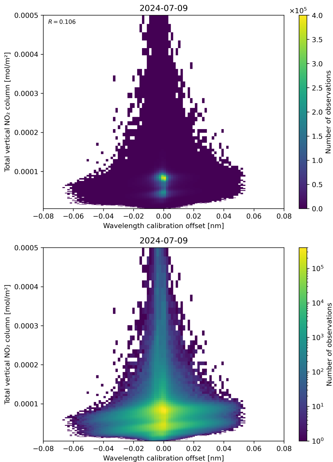
Figure 179: Scatter density plot of “Wavelength calibration offset” against “Total vertical NO 2 column” for 2024-07-08 to 2024-07-10.
