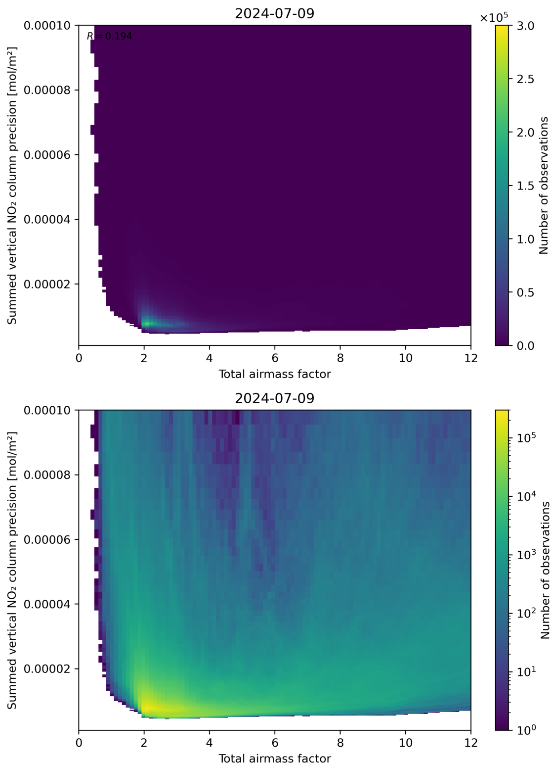
Figure 66: Scatter density plot of “Total airmass factor” against “Summed vertical NO 2 column precision” for 2024-07-08 to 2024-07-10.
