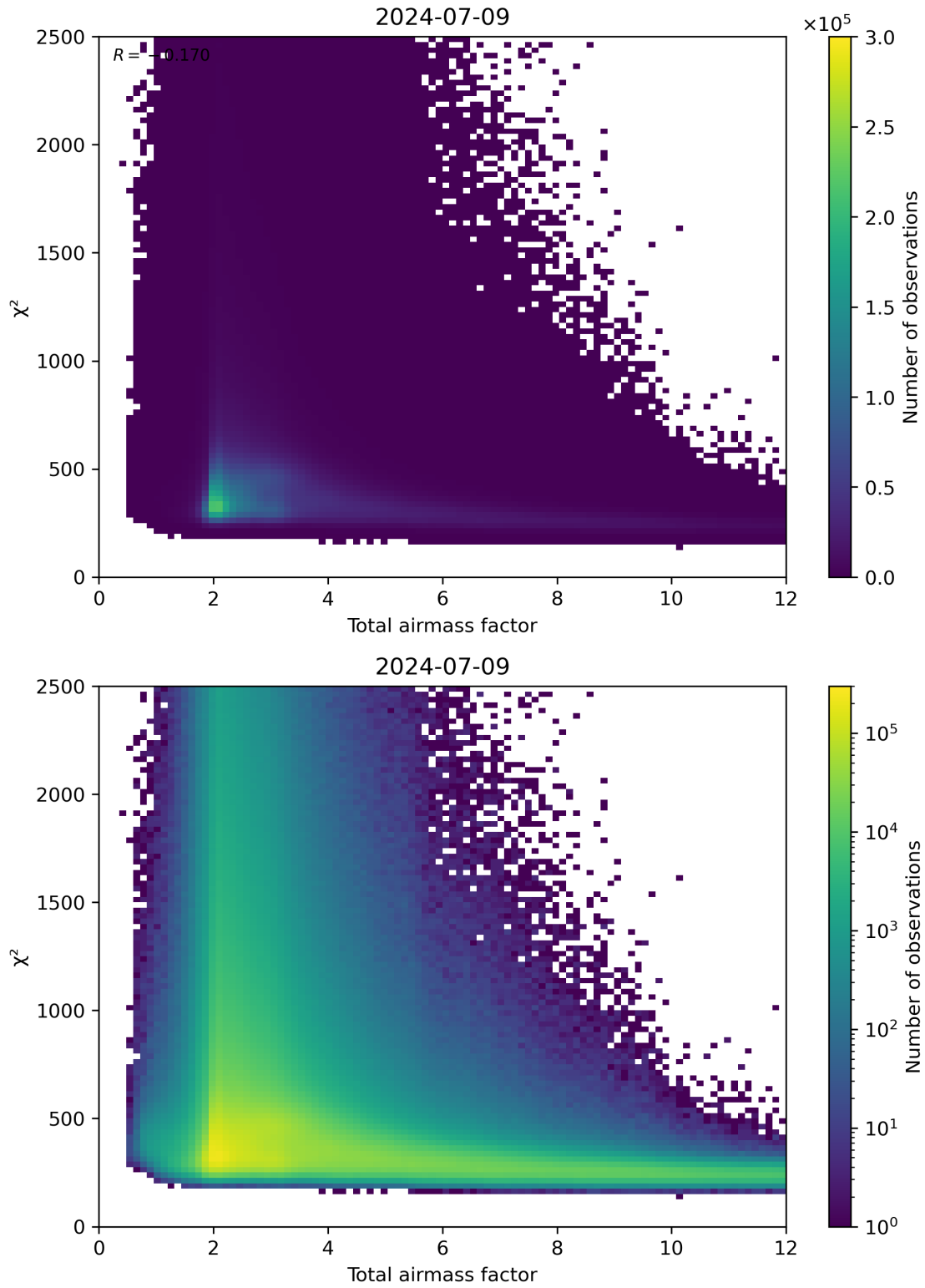
Figure 63: Scatter density plot of “Total airmass factor” against “ \chi^2 ” for 2024-07-08 to 2024-07-10.
