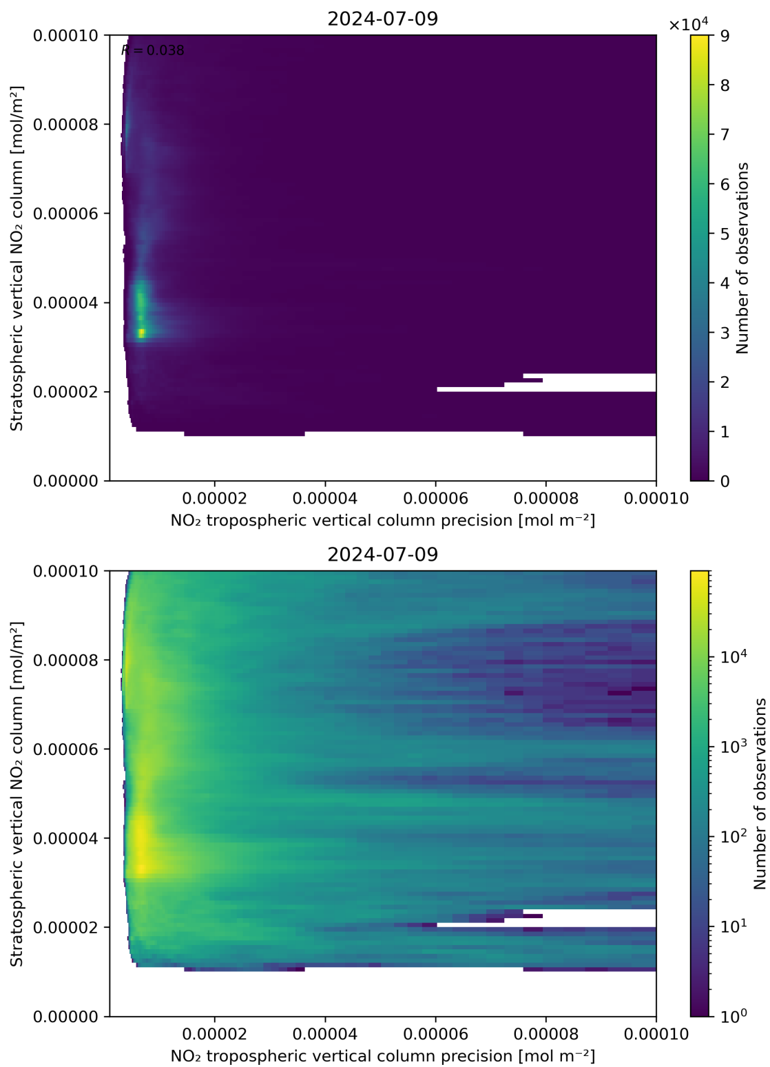
Figure 135: Scatter density plot of “NO 2 tropospheric vertical column precision” against “Stratospheric vertical NO 2 column” for 2024-07-08 to 2024-07-10.
