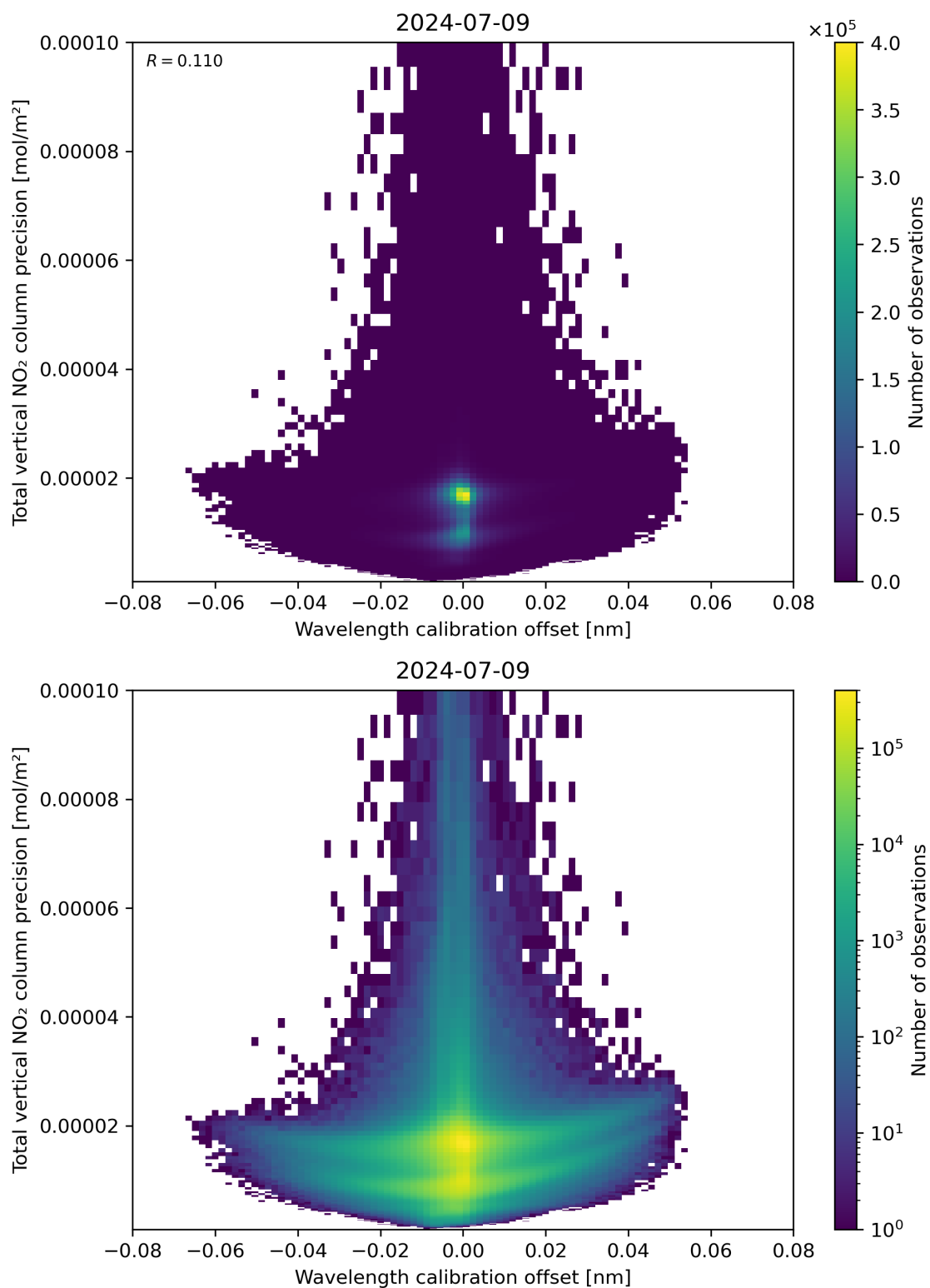
Figure 180: Scatter density plot of “Wavelength calibration offset” against “Total vertical NO 2 column precision” for 2024-07-08 to 2024-07-10.
