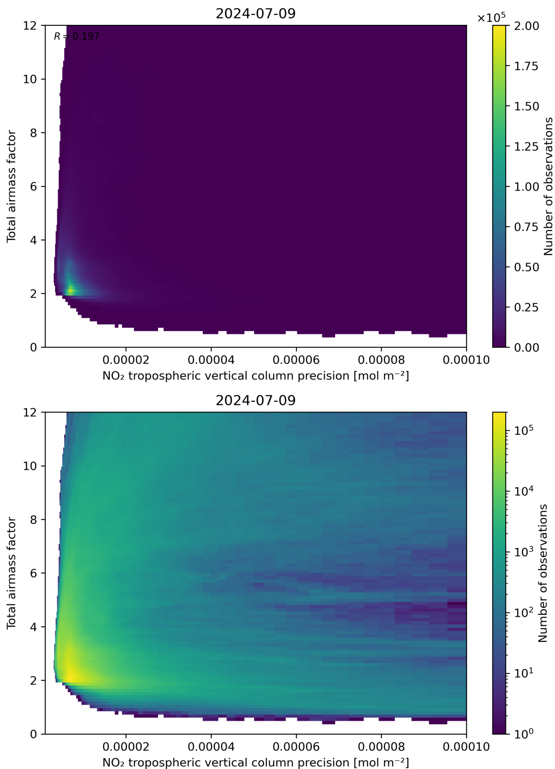
Figure 132: Scatter density plot of “NO 2 tropospheric vertical column precision” against “Total air mass factor” for 2024-07-08 to 2024-07-10.
