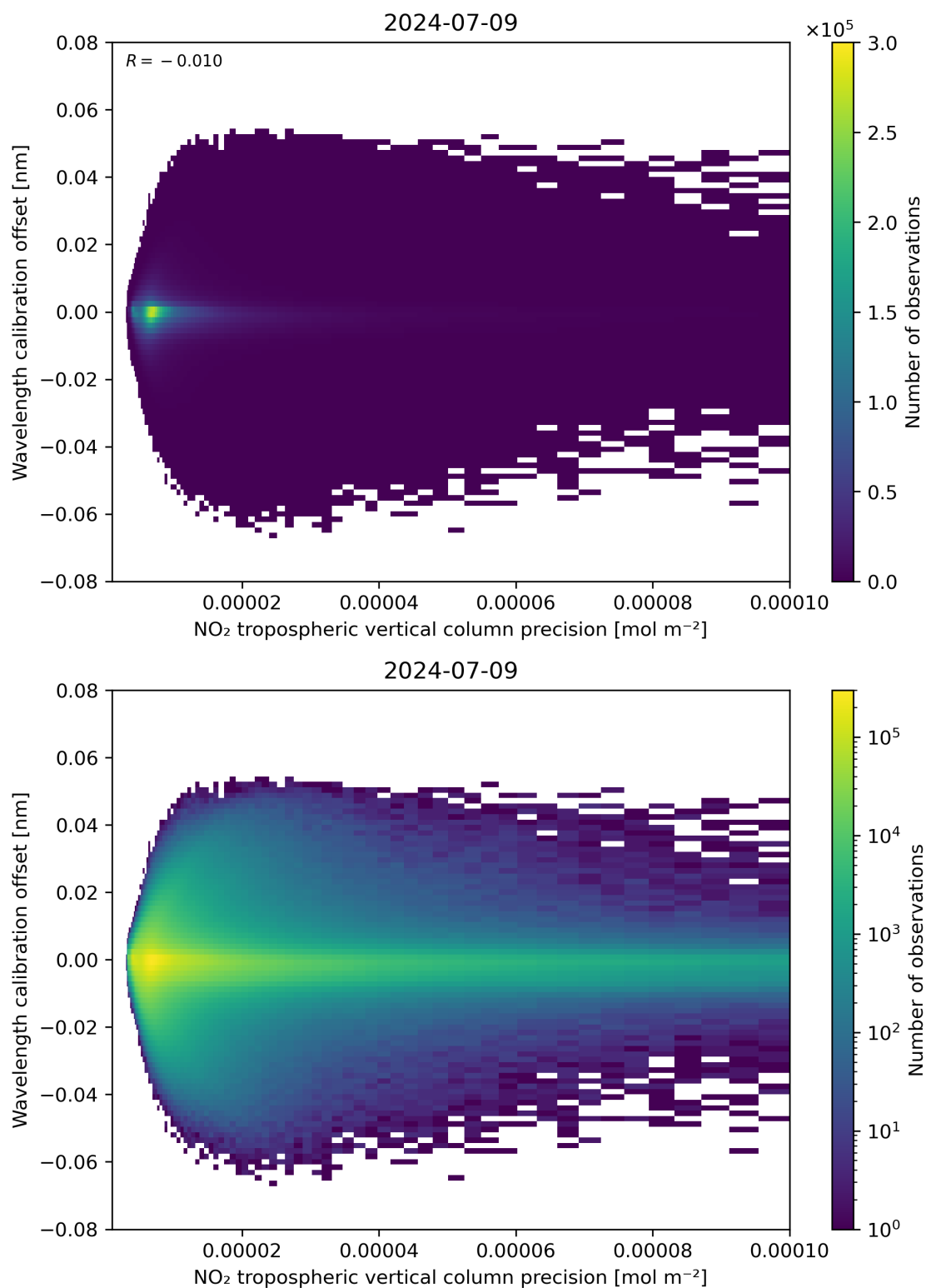
Figure 141: Scatter density plot of “NO 2 tropospheric vertical column precision” against “Wavelength calibration offset” for 2024-07-08 to 2024-07-10.
