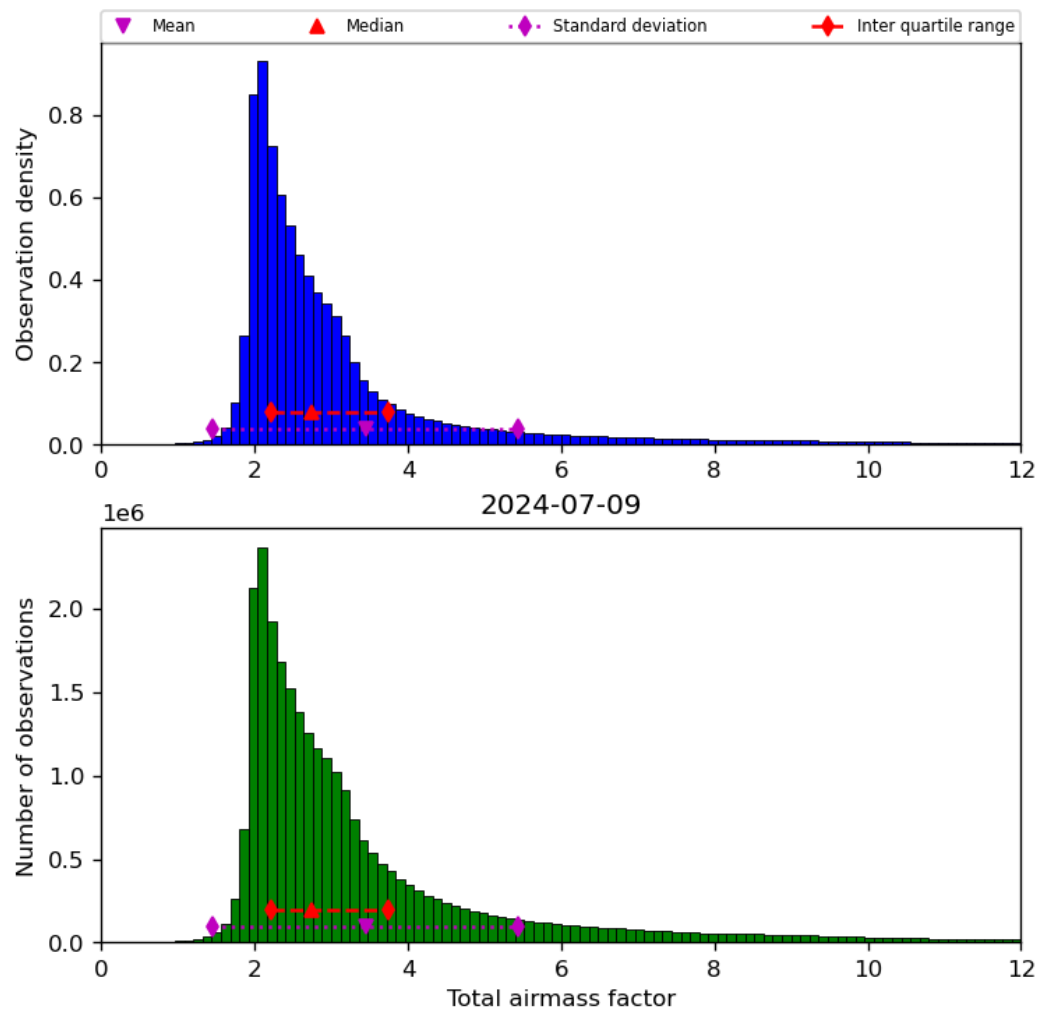
Figure 32: Histogram of “Total airmass factor” for 2024-07-08 to 2024-07-10
