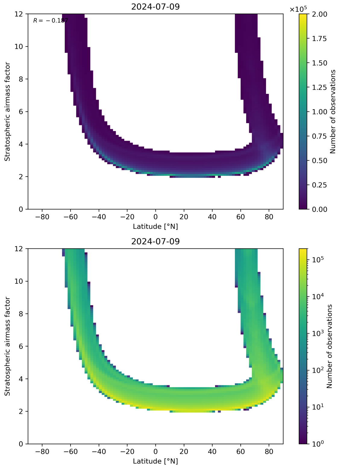
Figure 83: Scatter density plot of “Latitude” against “Stratospheric air mass factor” for 2024-07-08 to 2024-07-10.
