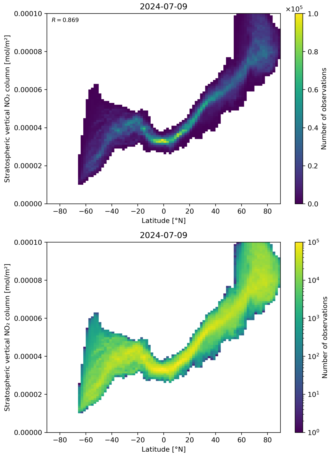
Figure 87: Scatter density plot of “Latitude” against “Stratospheric vertical NO 2 column” for 2024-07-08 to 2024-07-10.
