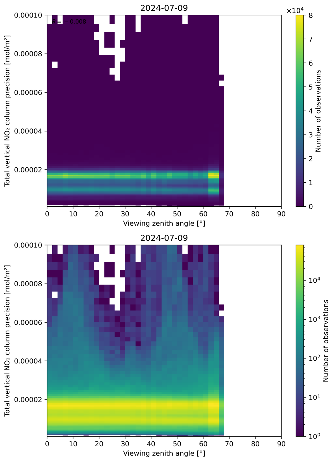
Figure 168: Scatter density plot of “Viewing zenith angle” against “Total vertical NO 2 column precision” for 2024-07-08 to 2024-07-10.
