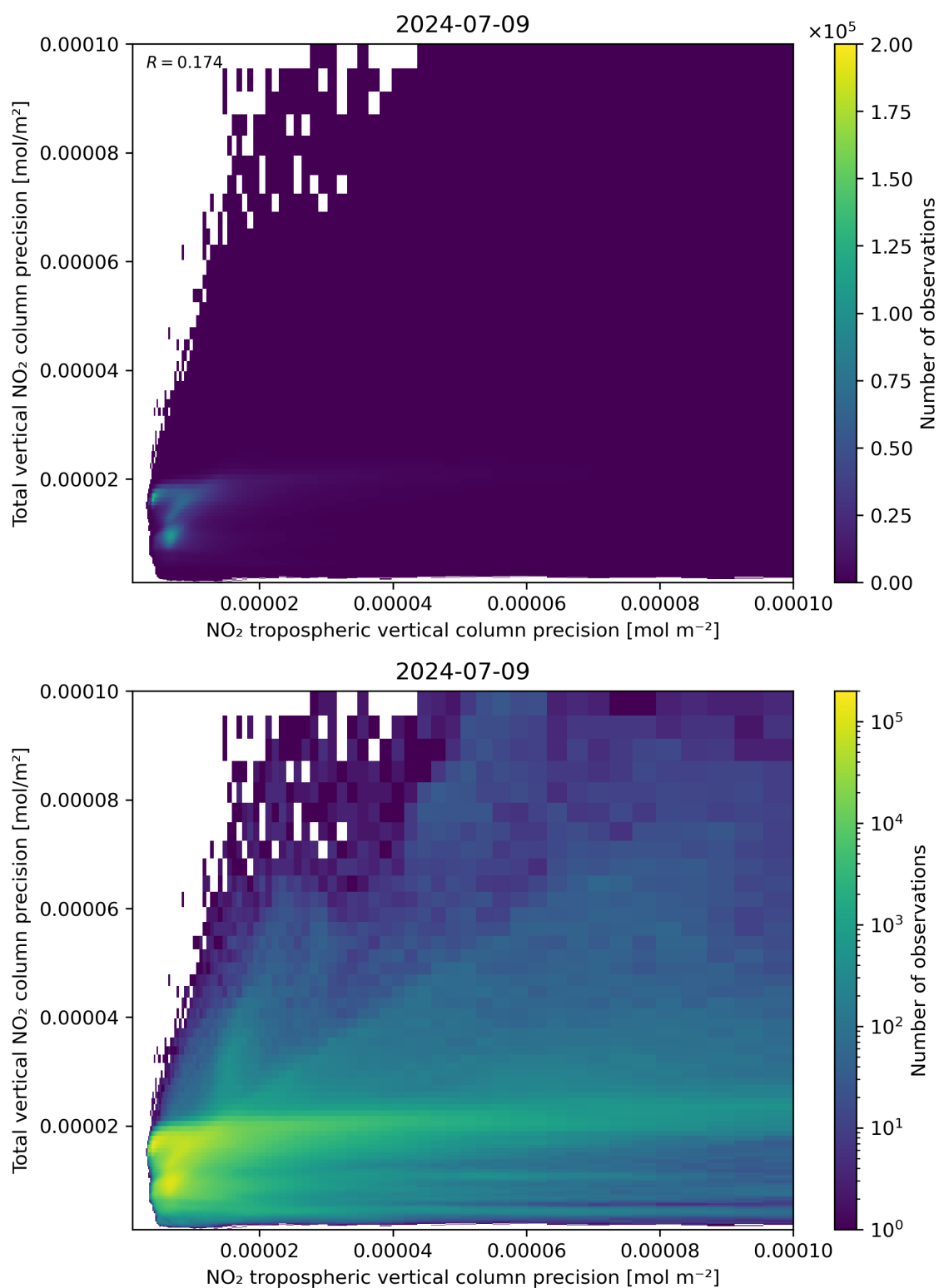
Figure 139: Scatter density plot of “NO 2 tropospheric vertical column precision” against “Total vertical NO 2 column precision” for 2024-07-08 to 2024-07-10.
