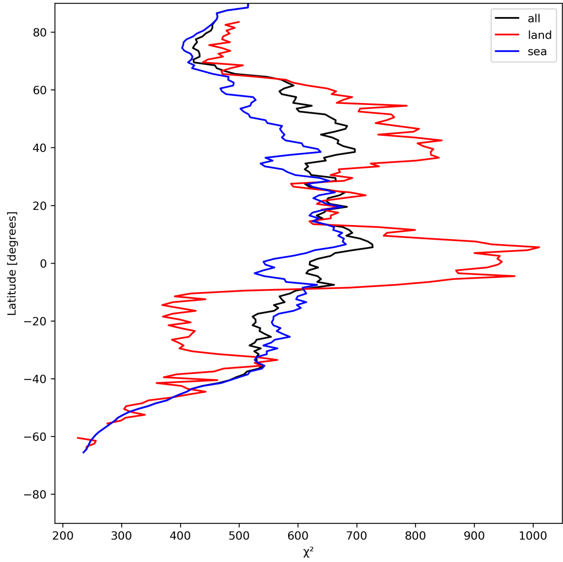
Figure 25: Zonal average of “ \chi^2 ” for 2024-07-08 to 2024-07-10.
