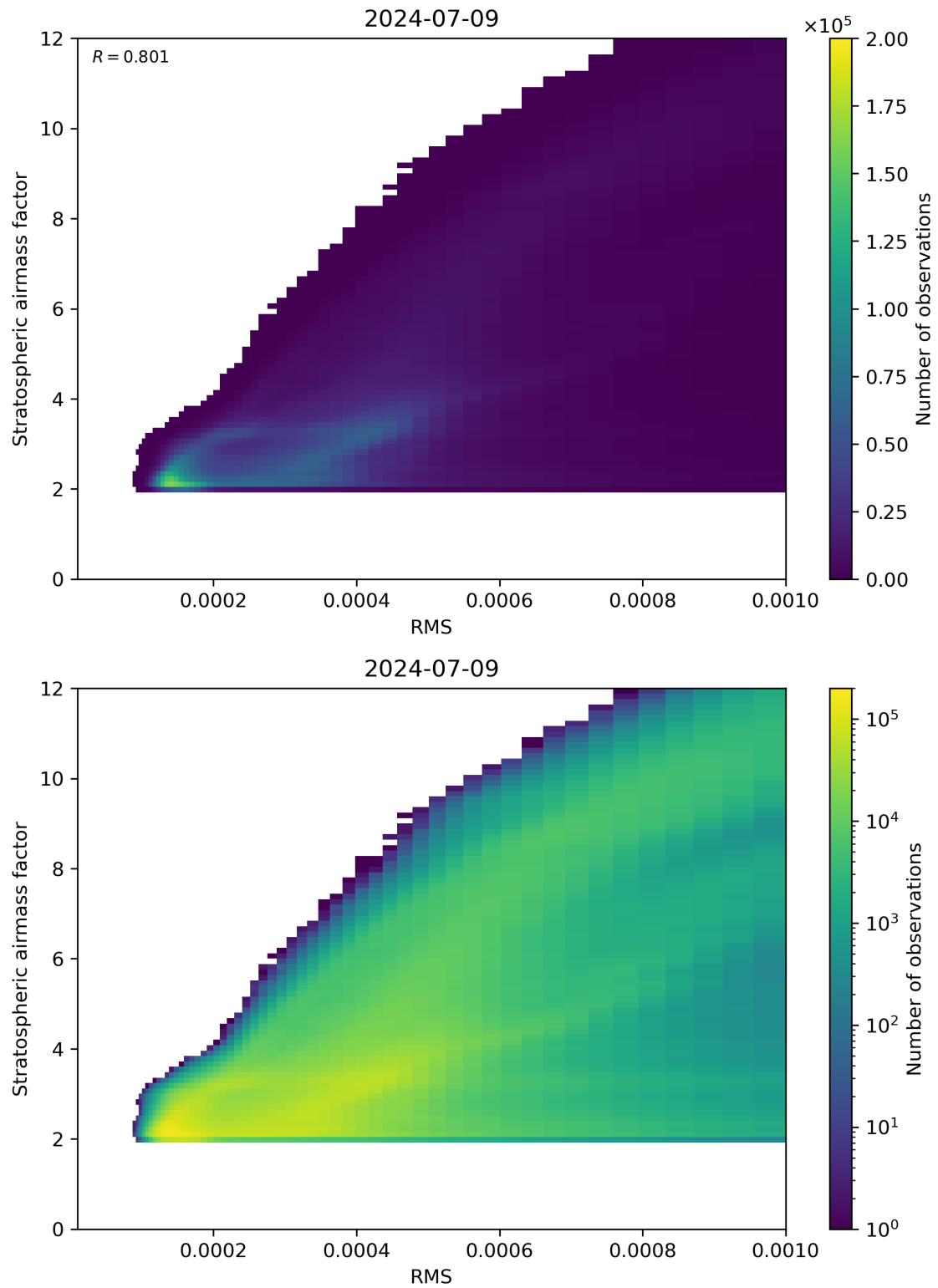
Figure 144: Scatter density plot of “RMS” against “Stratospheric airmass factor” for 2024-07-08 to 2024-07-10.
