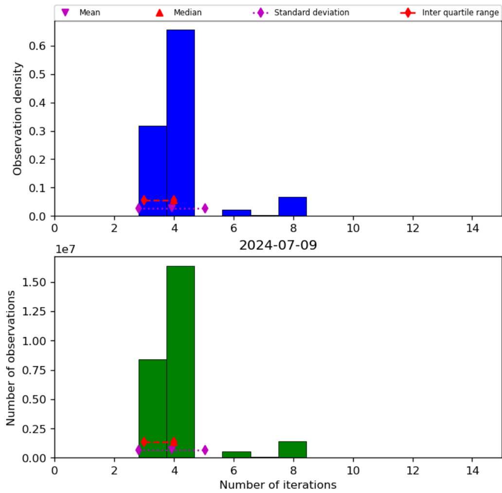
Figure 34: Histogram of “Number of iterations” for 2024-07-08 to 2024-07-10
