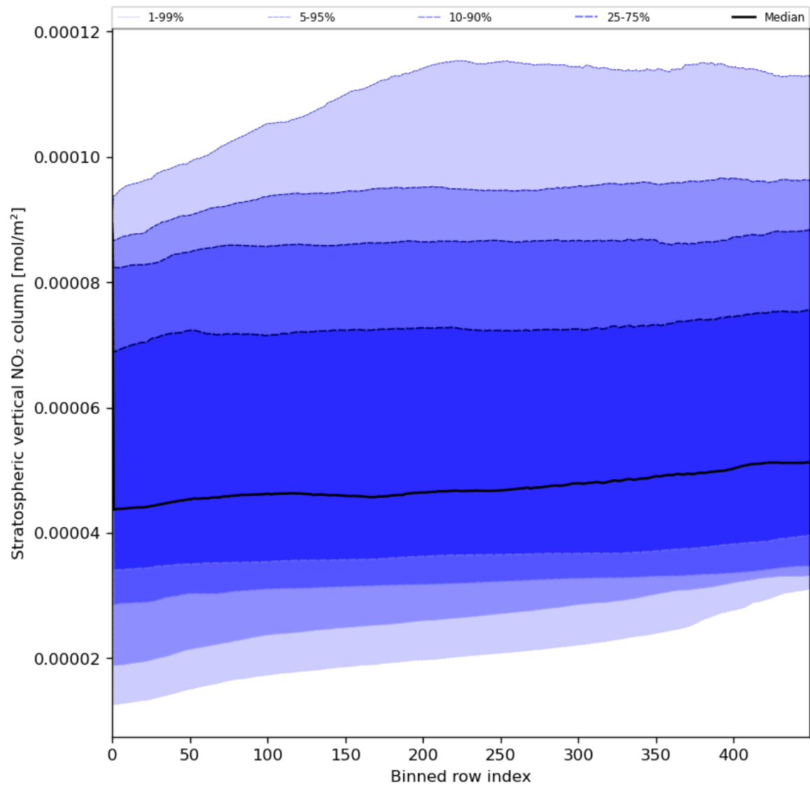
Figure 53: Along track statistics of “Stratospheric vertical NO 2 column” for 2024-07-08 to 2024-07-10
