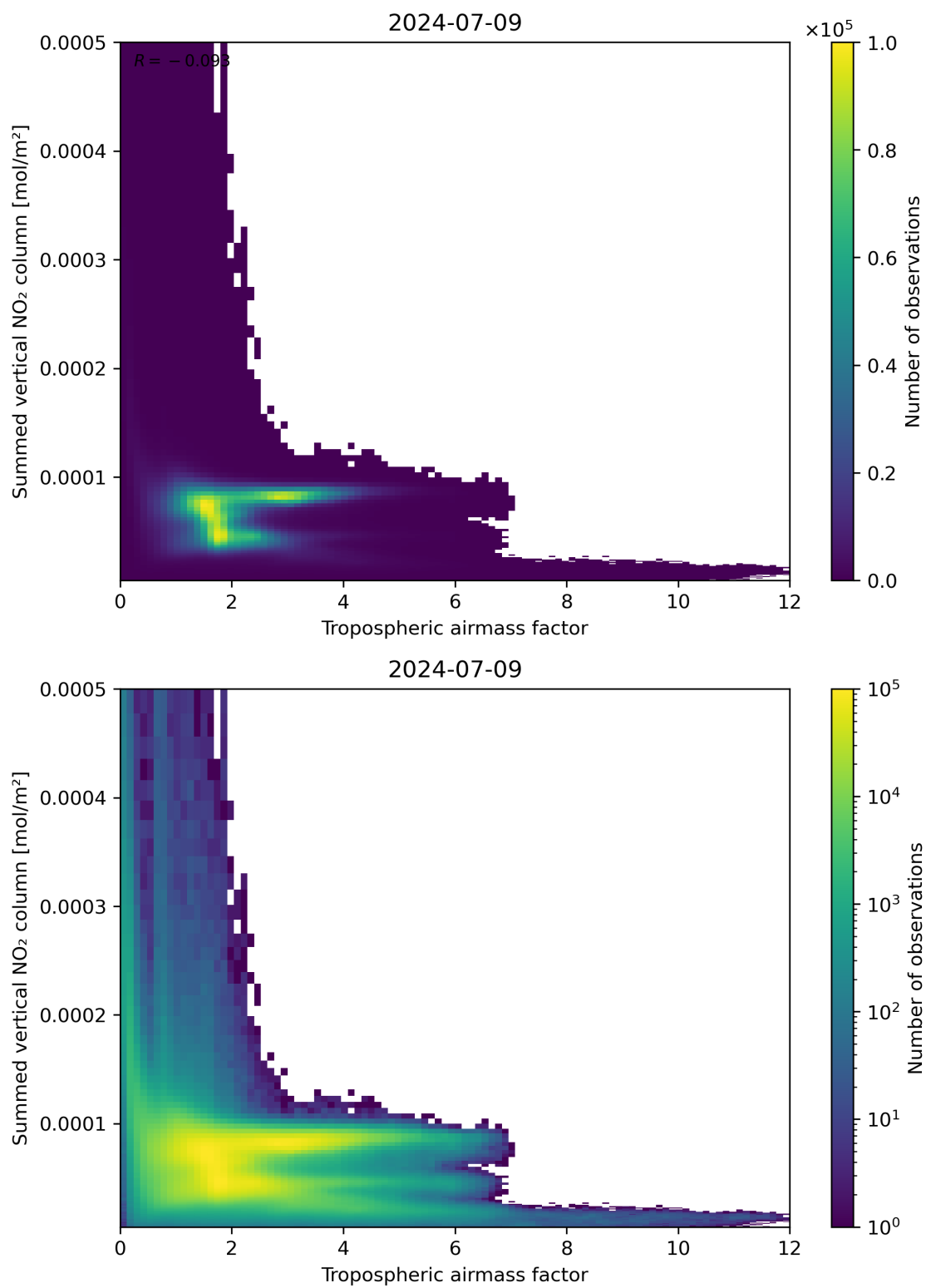
Figure 75: Scatter density plot of “Tropospheric airmass factor” against “Summed vertical NO 2 column” for 2024-07-08 to 2024-07-10.
