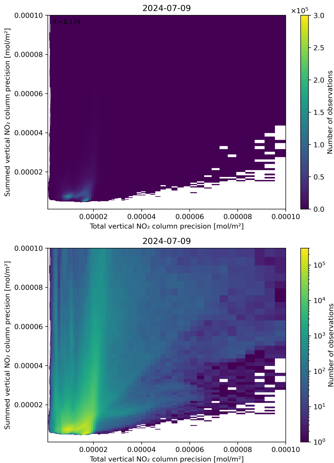
Figure 118: Scatter density plot of “Total vertical NO 2 column precision” against “Summed vertical NO 2 column precision” for 2024-07-08 to 2024-07-10.
