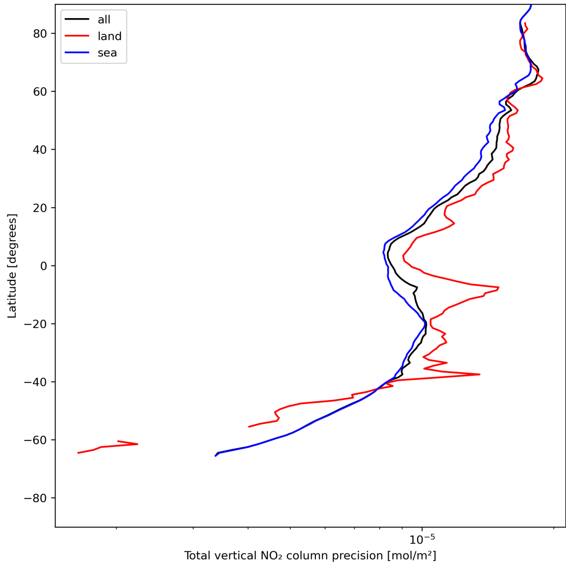
Figure 22: Zonal average of “Total vertical NO 2 column precision” for 2024-07-08 to 2024-07-10.
