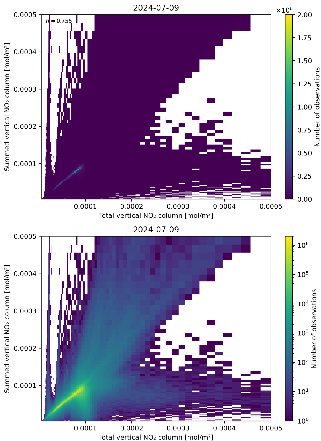
Figure 112: Scatter density plot of “Total vertical NO 2 column” against “Summed vertical NO 2 column” for 2024-07-08 to 2024-07-10.
