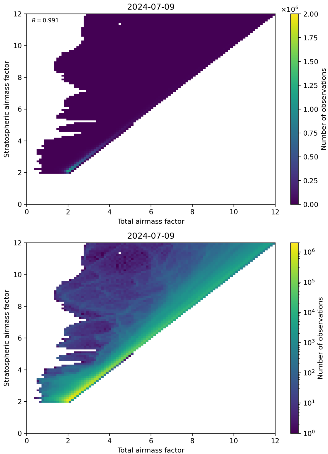
Figure 62: Scatter density plot of “Total airmass factor” against “Stratospheric airmass factor” for 2024-07-08 to 2024-07-10.
