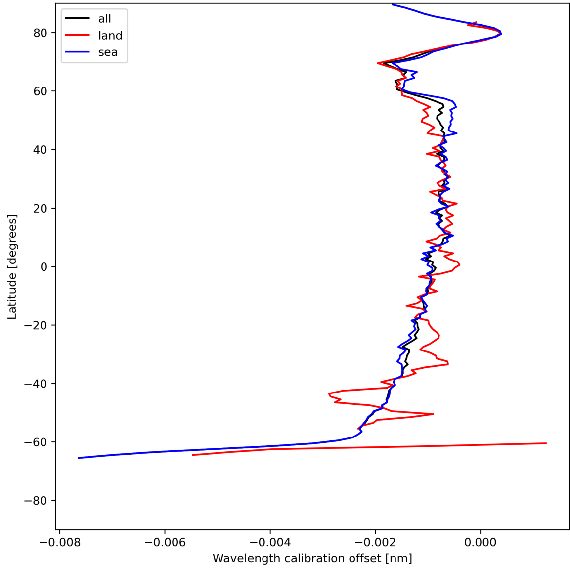
Figure 18: Zonal average of “Wavelength calibration offset” for 2024-07-08 to 2024-07-10.
