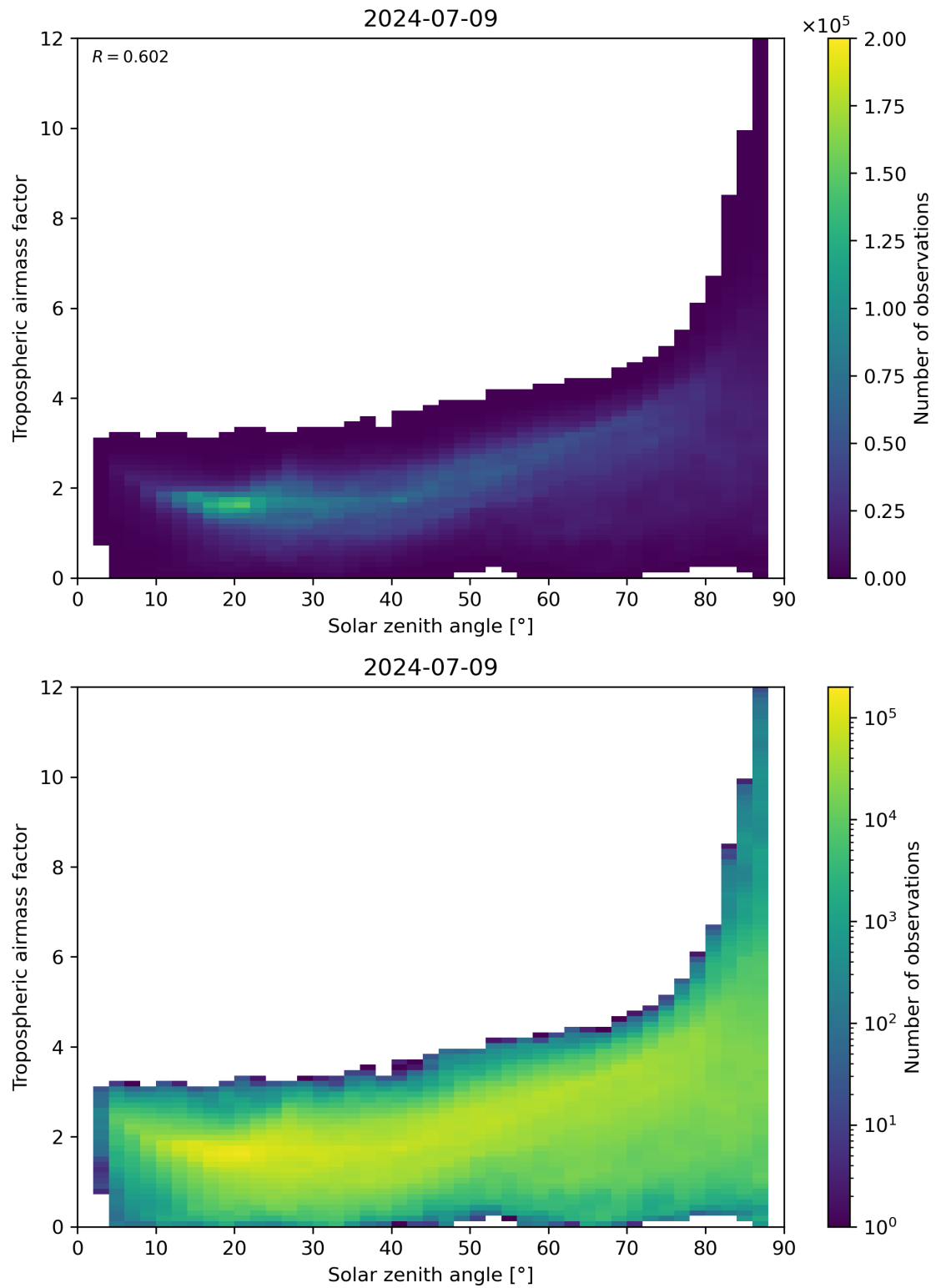
Figure 147: Scatter density plot of “Solar zenith angle” against “Tropospheric airmass factor” for 2024-07-08 to 2024-07-10.
