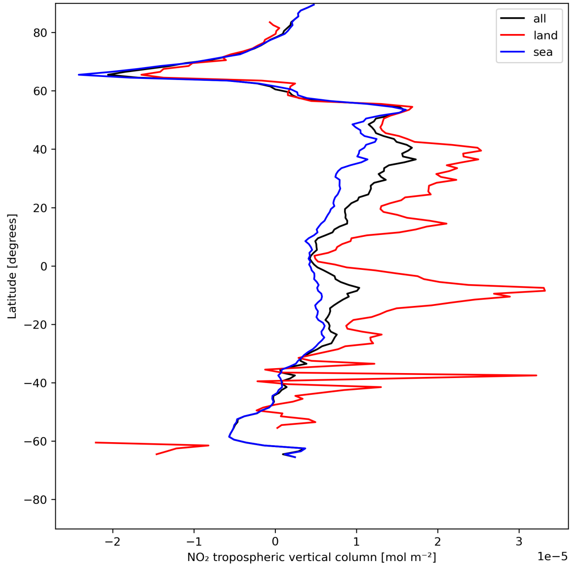
Figure 12: Zonal average of “NO 2 tropospheric vertical column” for 2024-07-08 to 2024-07-10.
