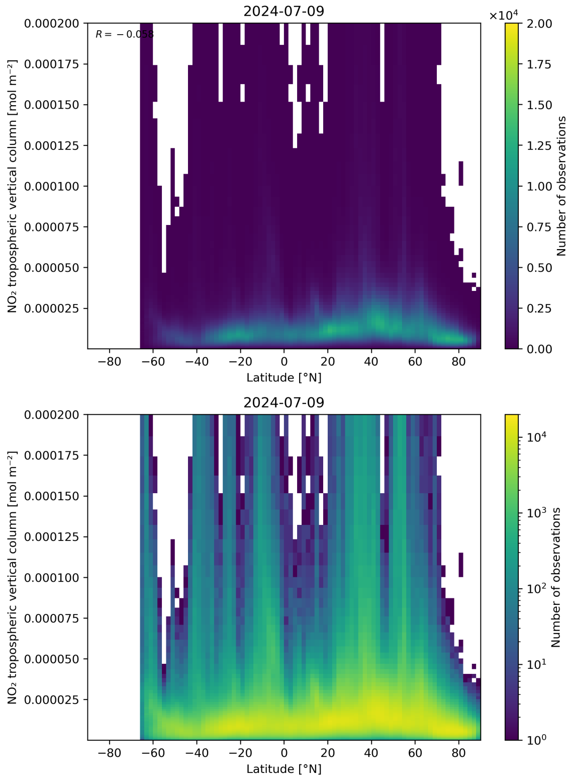
Figure 92: Scatter density plot of “Latitude” against “NO 2 tropospheric vertical column” for 2024-07-08 to 2024-07-10.
