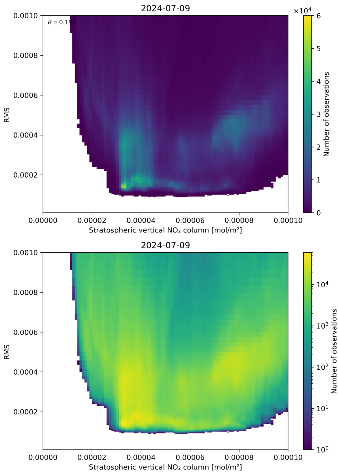
Figure 102: Scatter density plot of “Stratospheric vertical NO 2 column” against “RMS” for 2024-07-08 to 2024-07-10.
