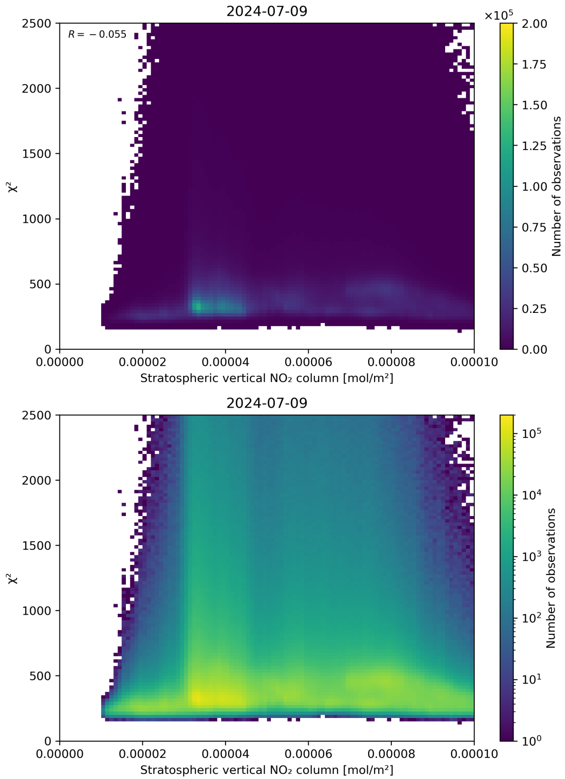
Figure 97: Scatter density plot of “Stratospheric vertical NO 2 column” against “ \chi^2 ” for 2024-07-08 to 2024-07-10.
