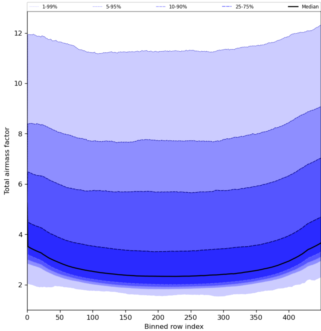
Figure 49: Along track statistics of “Total airmass factor” for 2024-07-08 to 2024-07-10
