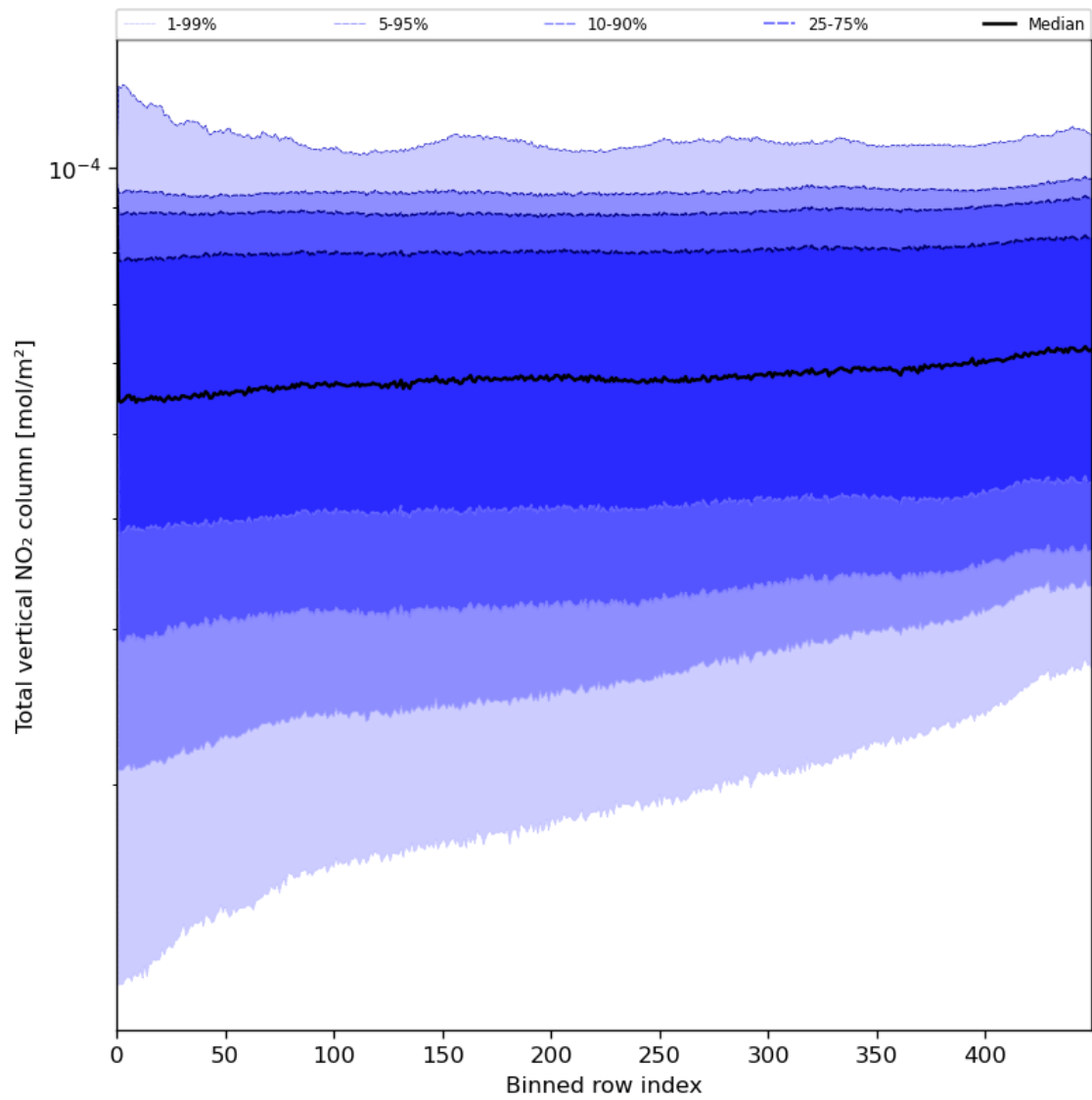
Figure 55: Along track statistics of “Total vertical NO 2 column” for 2024-07-08 to 2024-07-10
