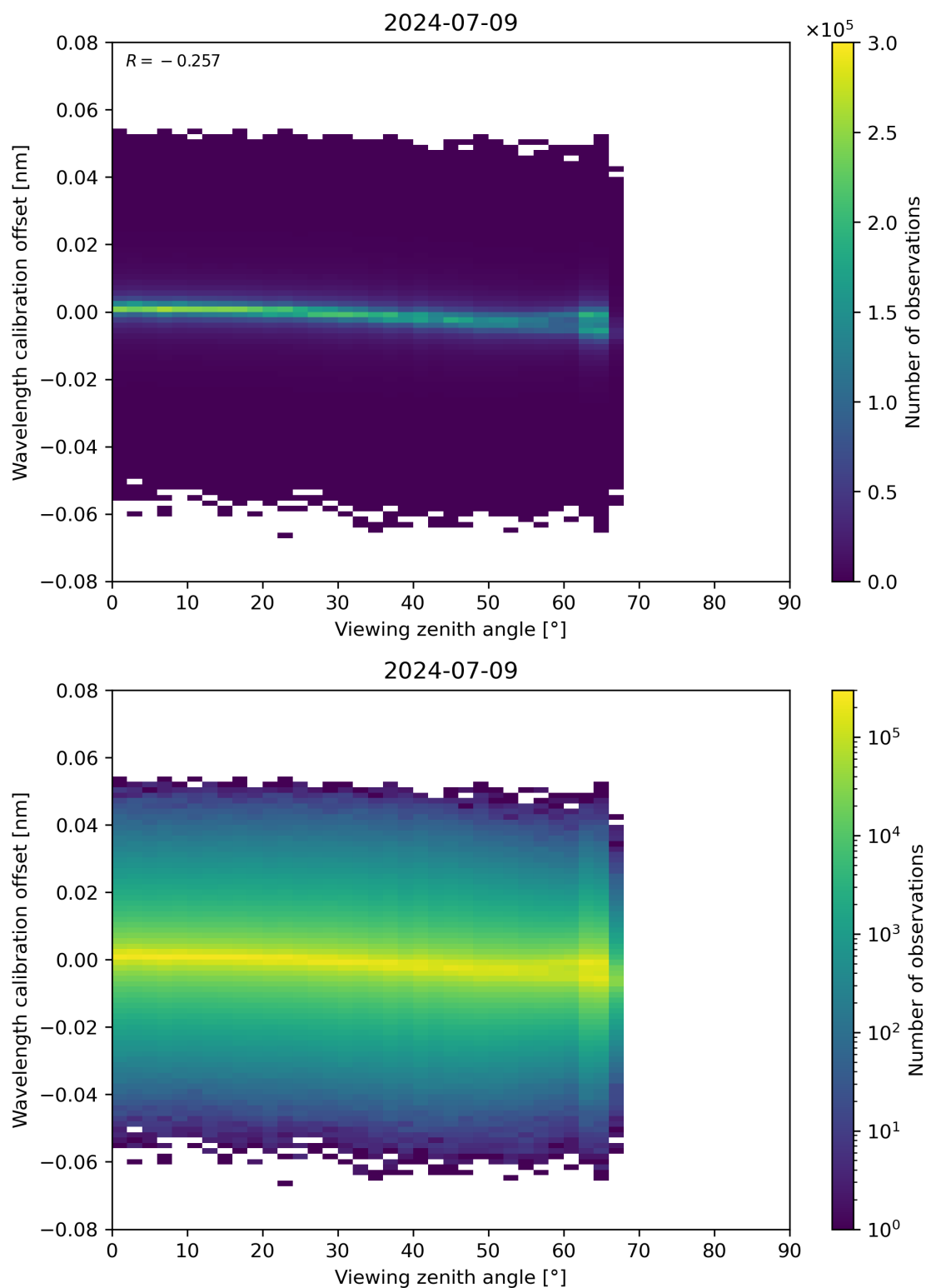
Figure 173: Scatter density plot of “Viewing zenith angle” against “Wavelength calibration offset” for 2024-07-08 to 2024-07-10.
