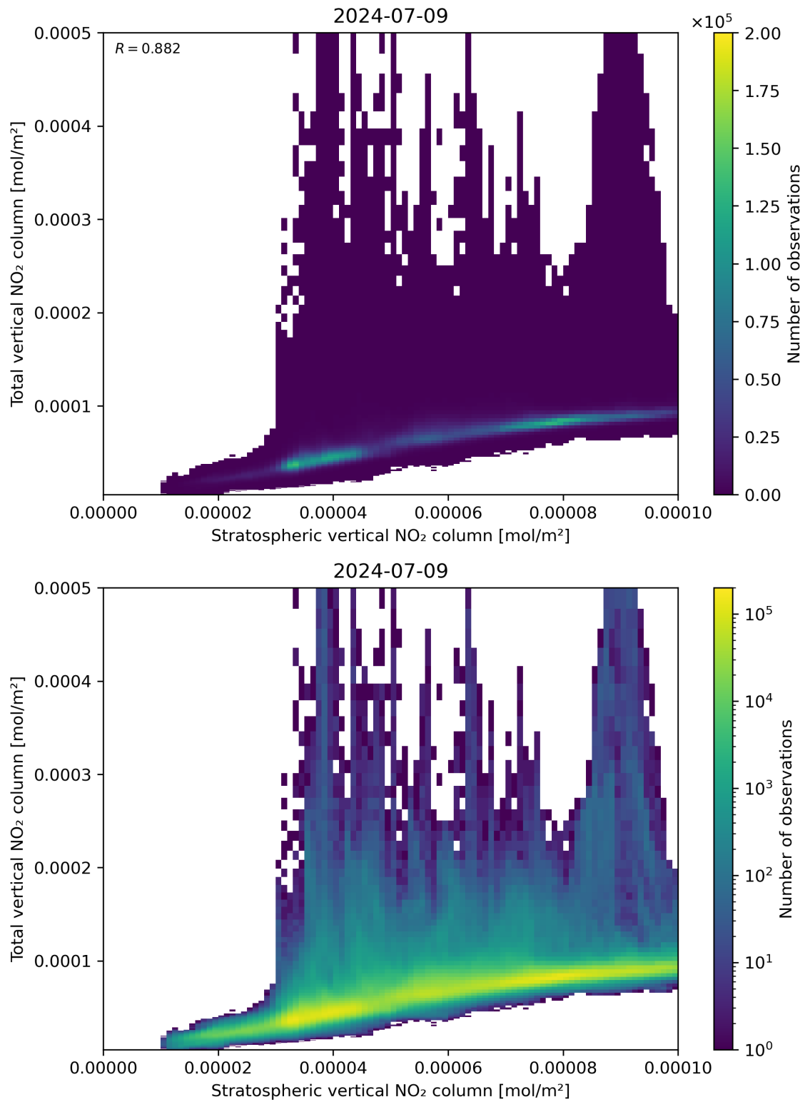
Figure 100: Scatter density plot of “Stratospheric vertical NO 2 column” against “Total vertical NO 2 column” for 2024-07-08 to 2024-07-10.
