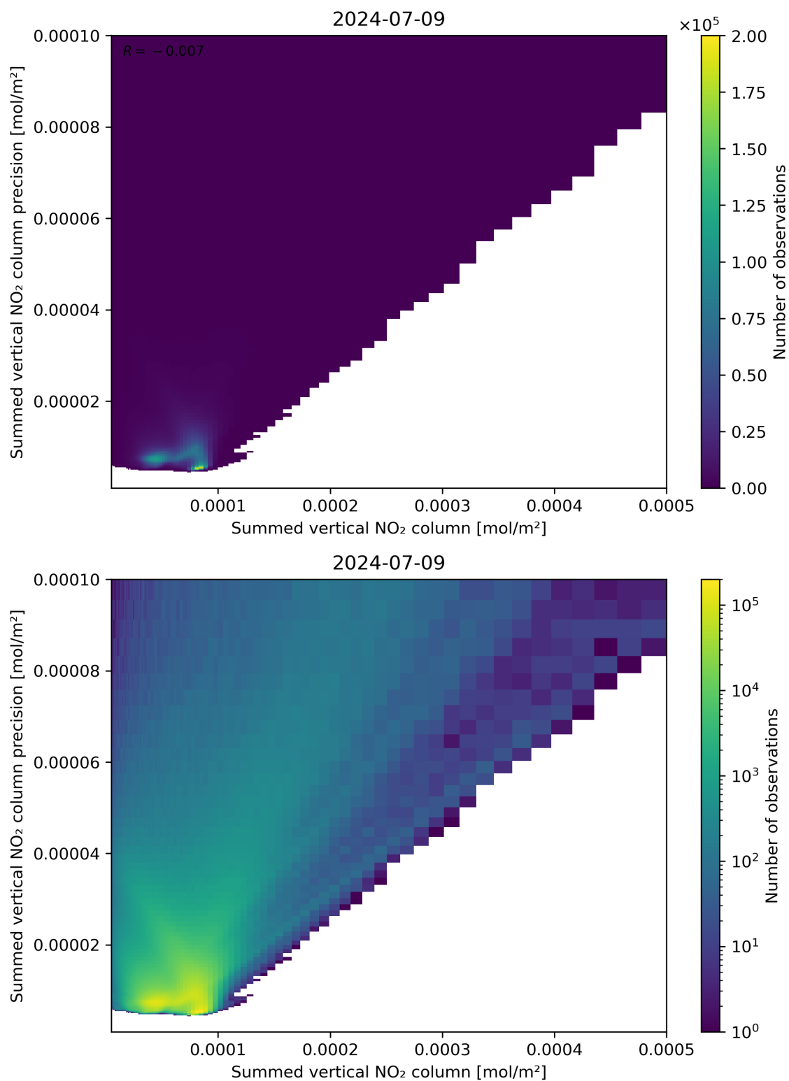
Figure 105: Scatter density plot of “Summed vertical NO 2 column” against “Summed vertical NO 2 column precision” for 2024-07-08 to 2024-07-10.
