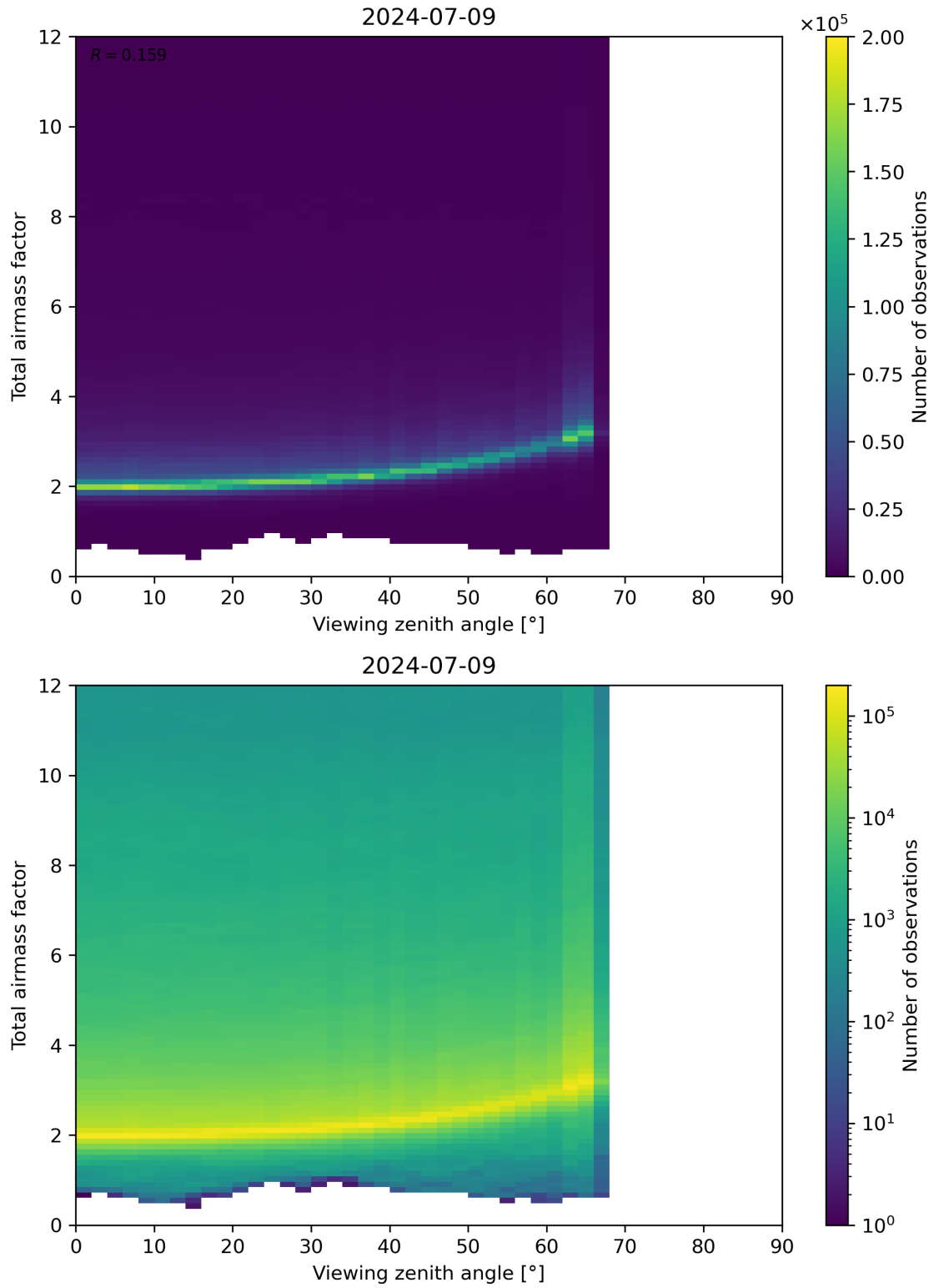
Figure 160: Scatter density plot of “Viewing zenith angle” against “Total airmass factor” for 2024-07-08 to 2024-07-10.
