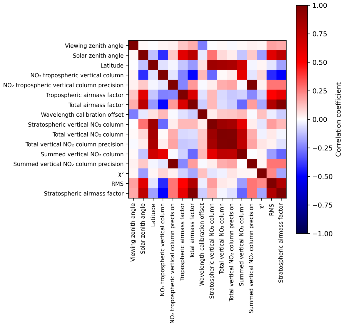
Figure 2: Map of correlation matrix for 2024-07-08 to 2024-07-10.
