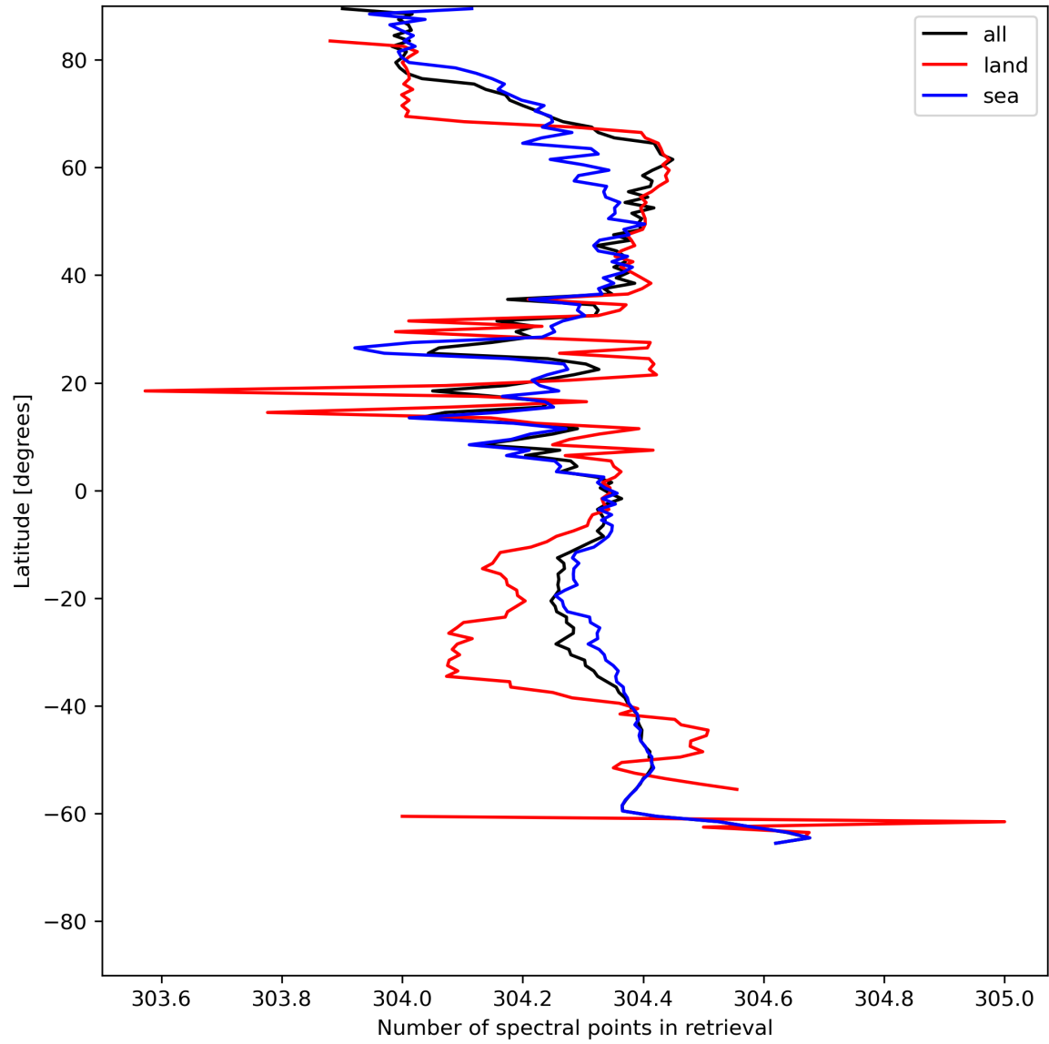
Figure 16: Zonal average of “Number of spectral points in retrieval” for 2024-07-08 to 2024-07-10.
