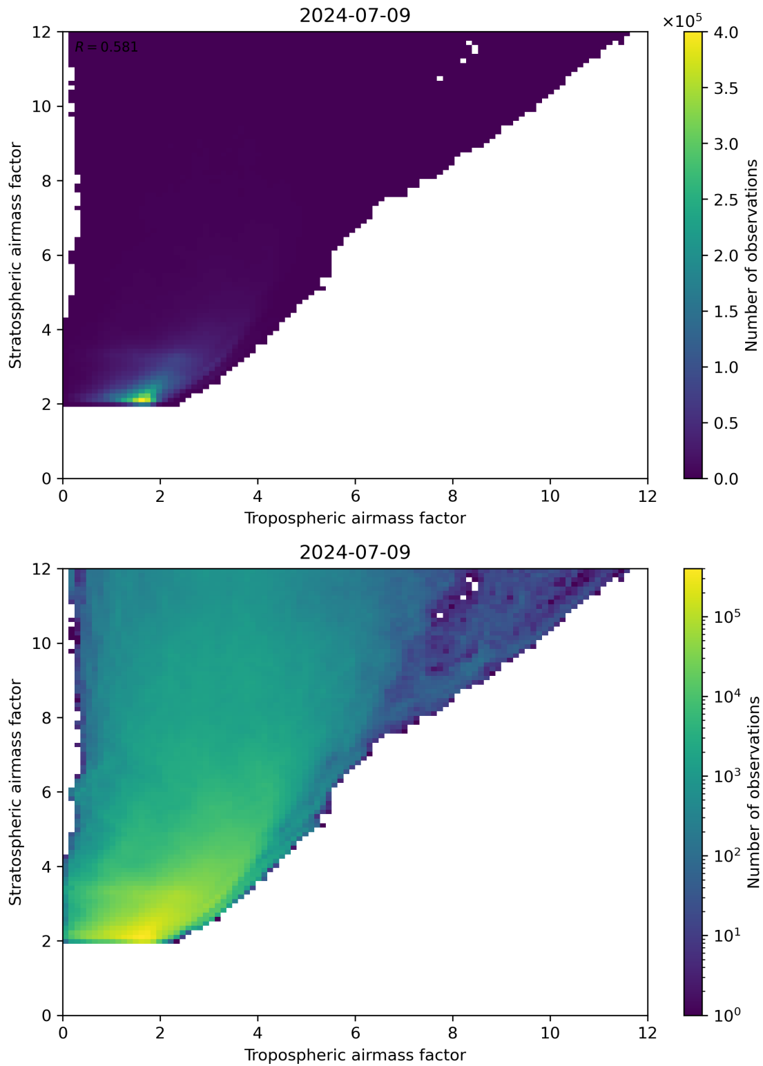
Figure 71: Scatter density plot of “Tropospheric airmass factor” against “Stratospheric airmass factor” for 2024-07-08 to 2024-07-10.
