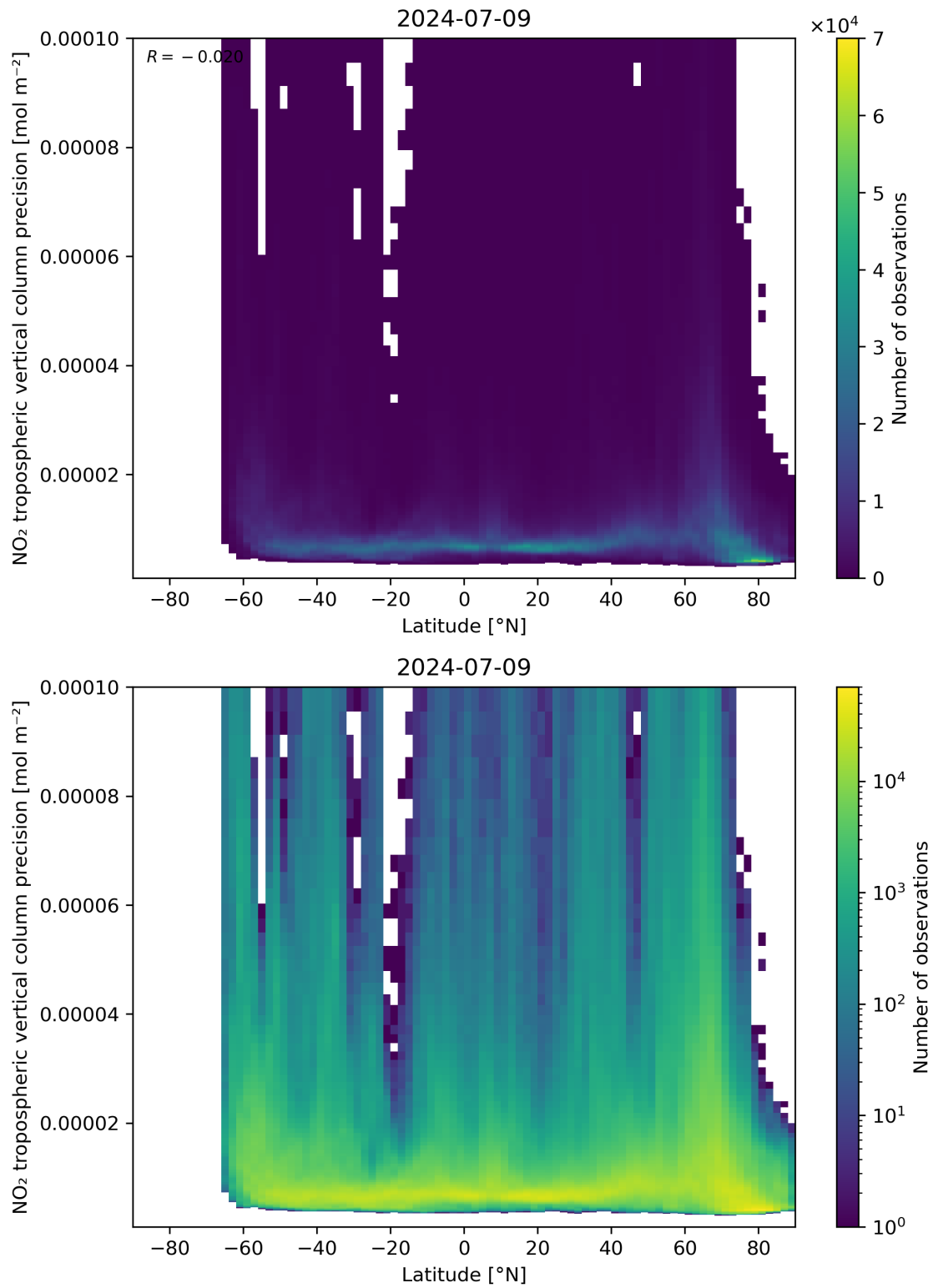
Figure 93: Scatter density plot of “Latitude” against “NO 2 tropospheric vertical column precision” for 2024-07-08 to 2024-07-10.
