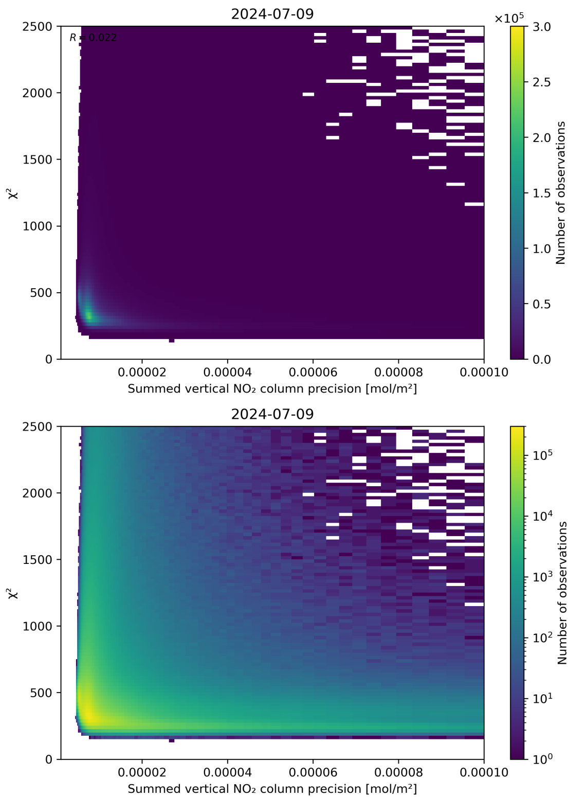
Figure 107: Scatter density plot of “Summed vertical NO 2 column precision” against “ \chi^2 ” for 2024-07-08 to 2024-07-10.
