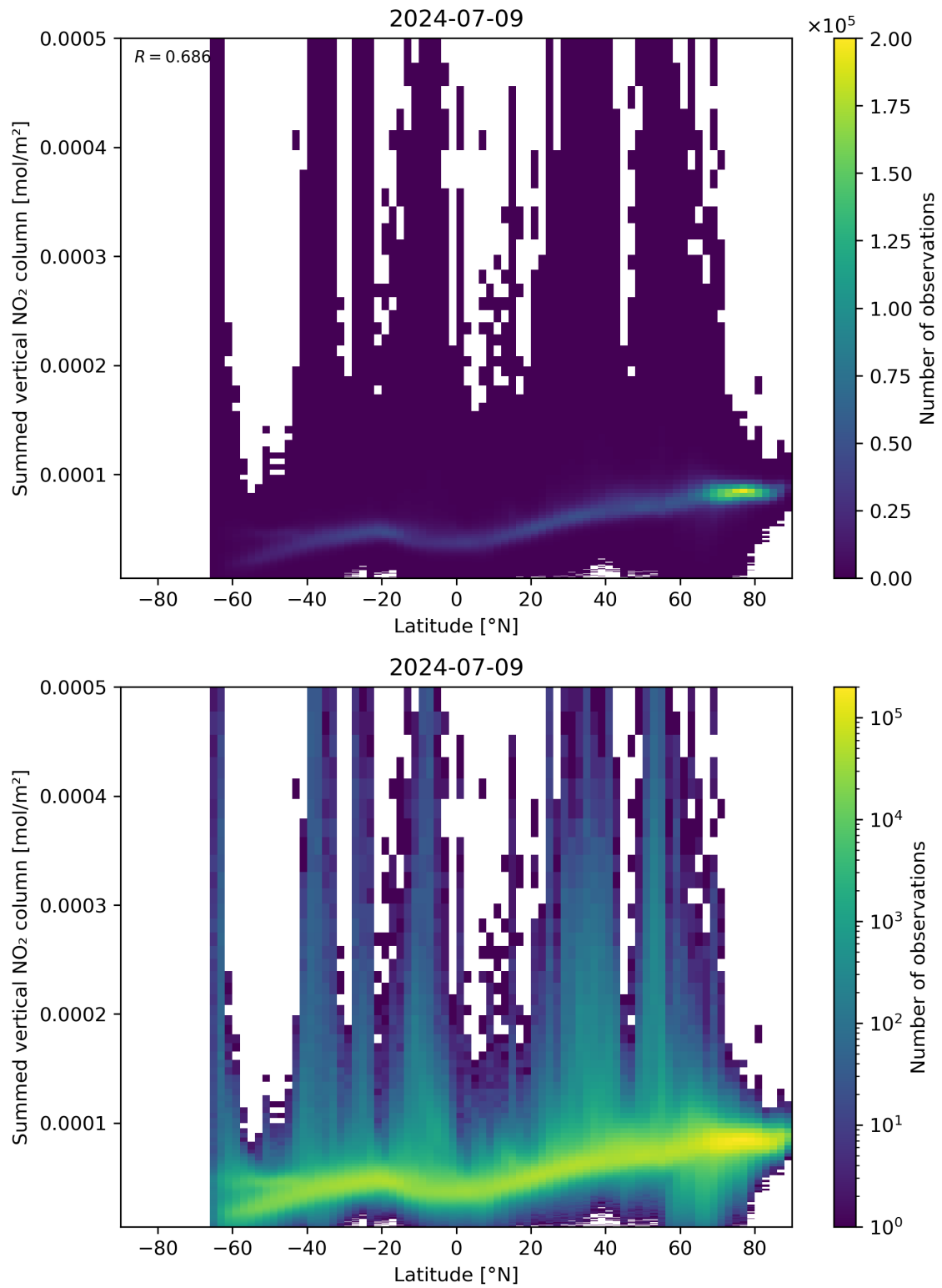
Figure 88: Scatter density plot of “Latitude” against “Summed vertical NO 2 column” for 2024-07-08 to 2024-07-10.
