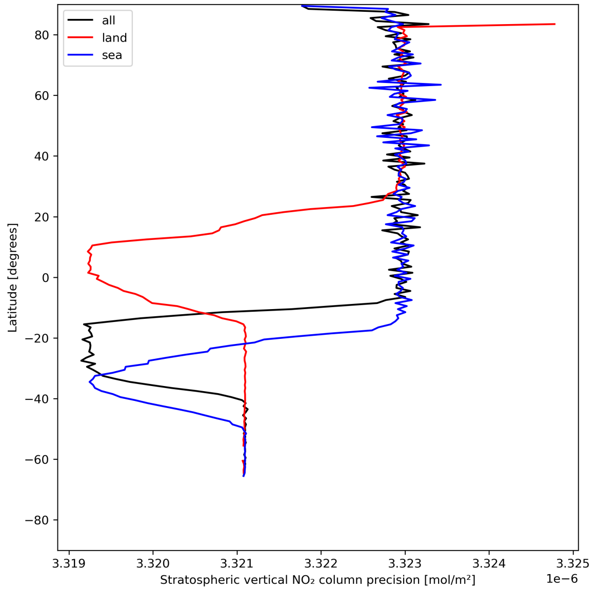
Figure 20: Zonal average of “Stratospheric vertical NO 2 column precision” for 2024-07-08 to 2024-07-10.
