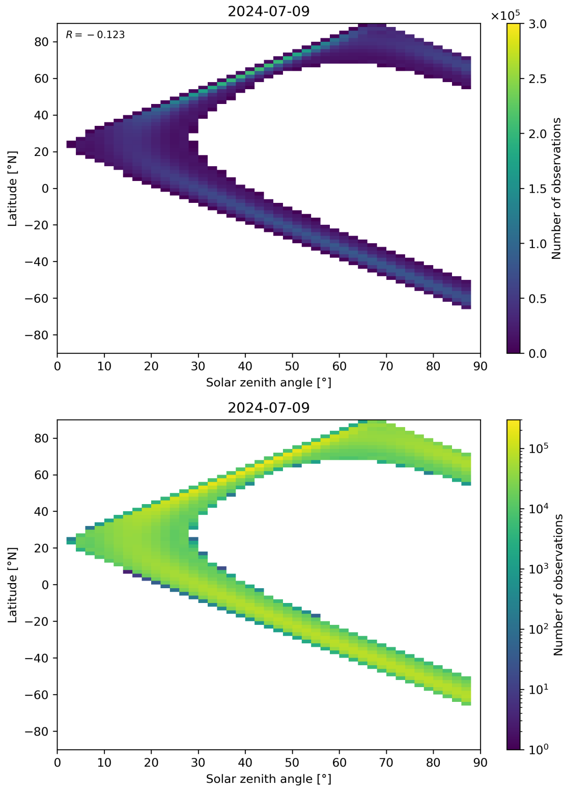
Figure 149: Scatter density plot of “Solar zenith angle” against “Latitude” for 2024-07-08 to 2024-07-10.
