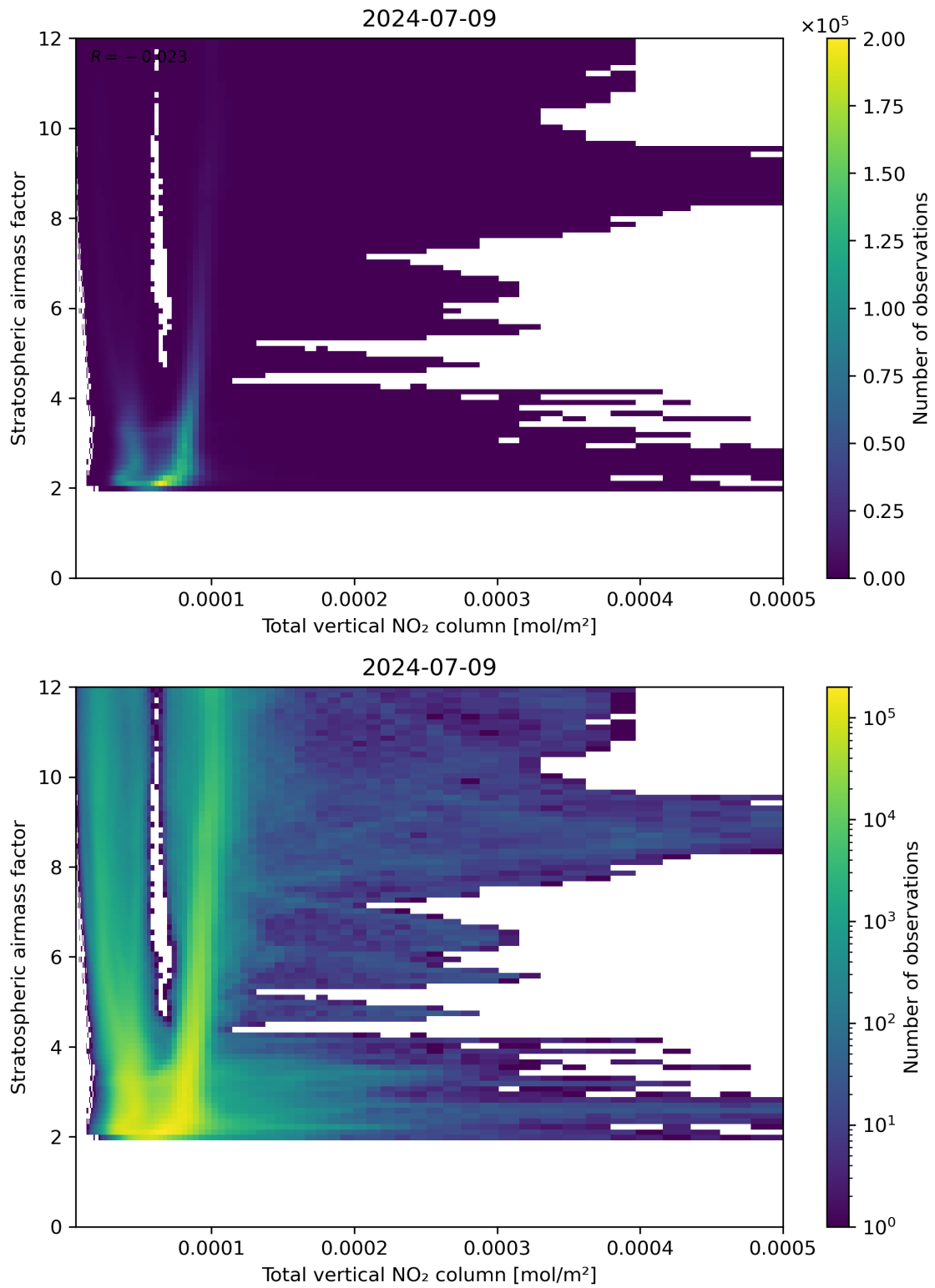
Figure 110: Scatter density plot of “Total vertical NO 2 column” against “Stratospheric airmass factor” for 2024-07-08 to 2024-07-10.
