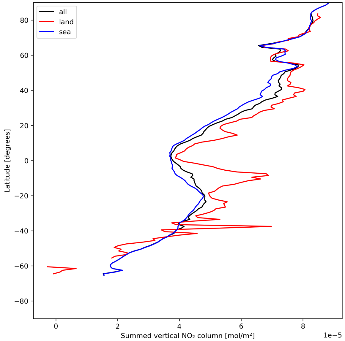
Figure 23: Zonal average of “Summed vertical NO 2 column” for 2024-07-08 to 2024-07-10.
