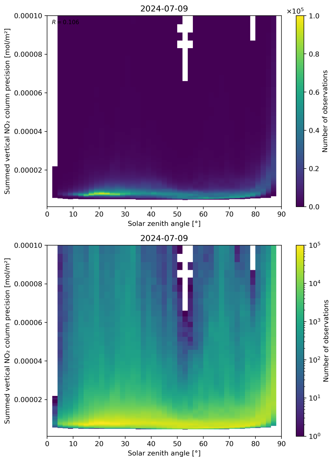
Figure 152: Scatter density plot of “Solar zenith angle” against “Summed vertical NO 2 column precision” for 2024-07-08 to 2024-07-10.
