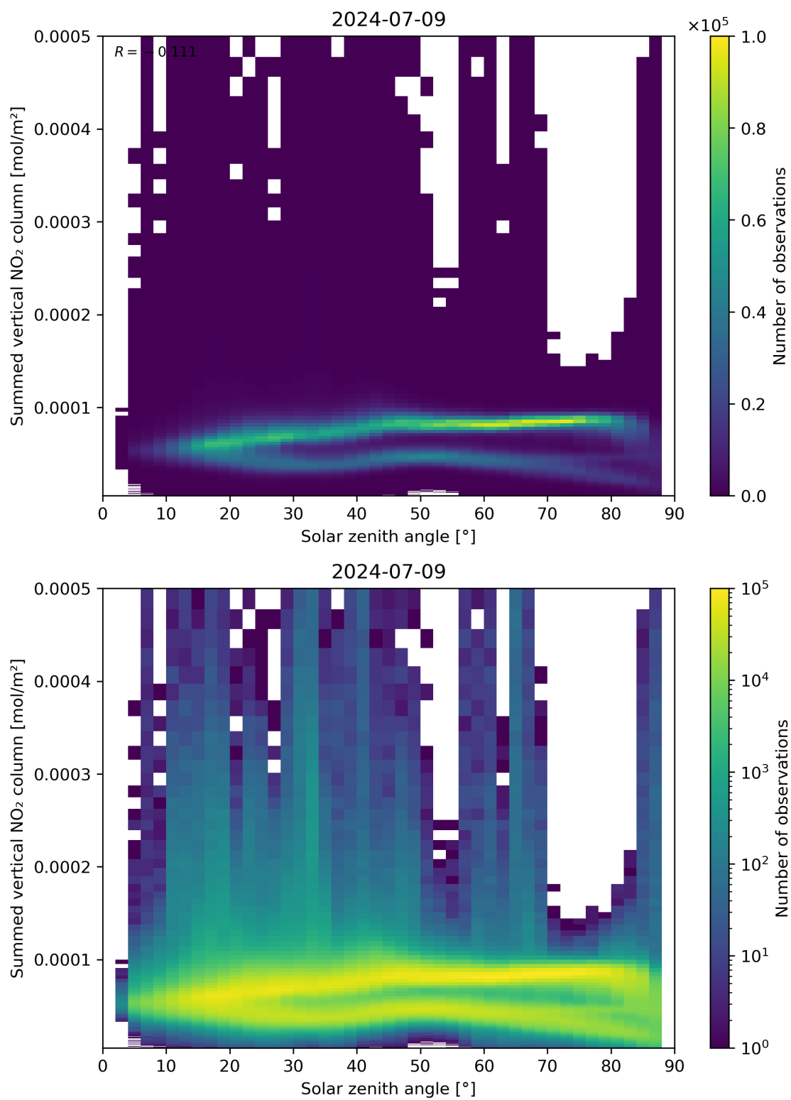
Figure 151: Scatter density plot of “Solar zenith angle” against “Summed vertical NO 2 column” for 2024-07-08 to 2024-07-10.
