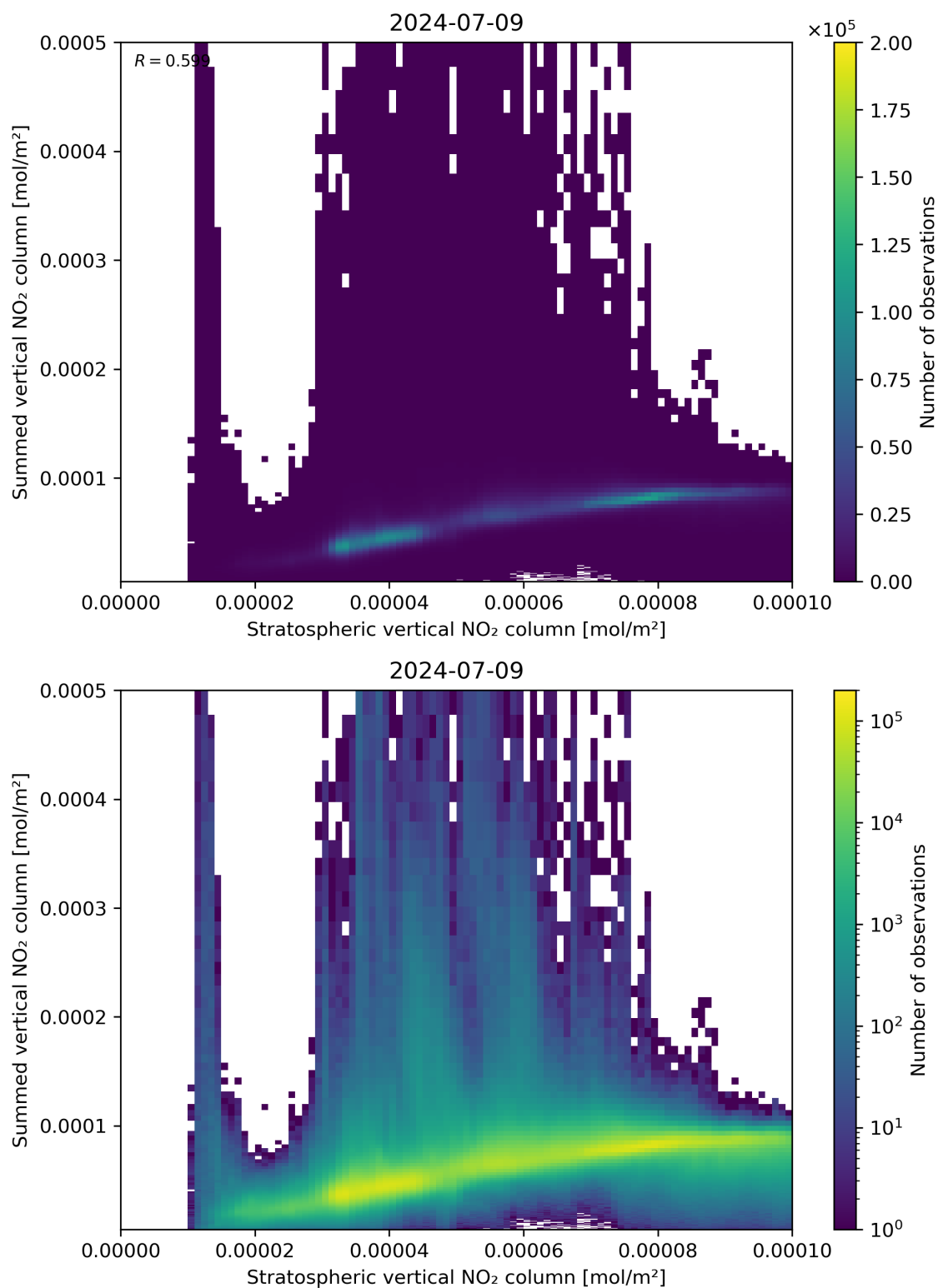
Figure 98: Scatter density plot of “Stratospheric vertical NO 2 column” against “Summed vertical NO 2 column” for 2024-07-08 to 2024-07-10.
