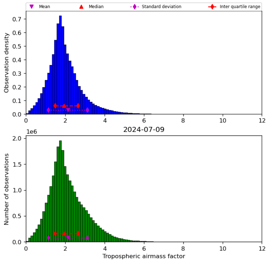
Figure 31: Histogram of “Tropospheric airmass factor” for 2024-07-08 to 2024-07-10
