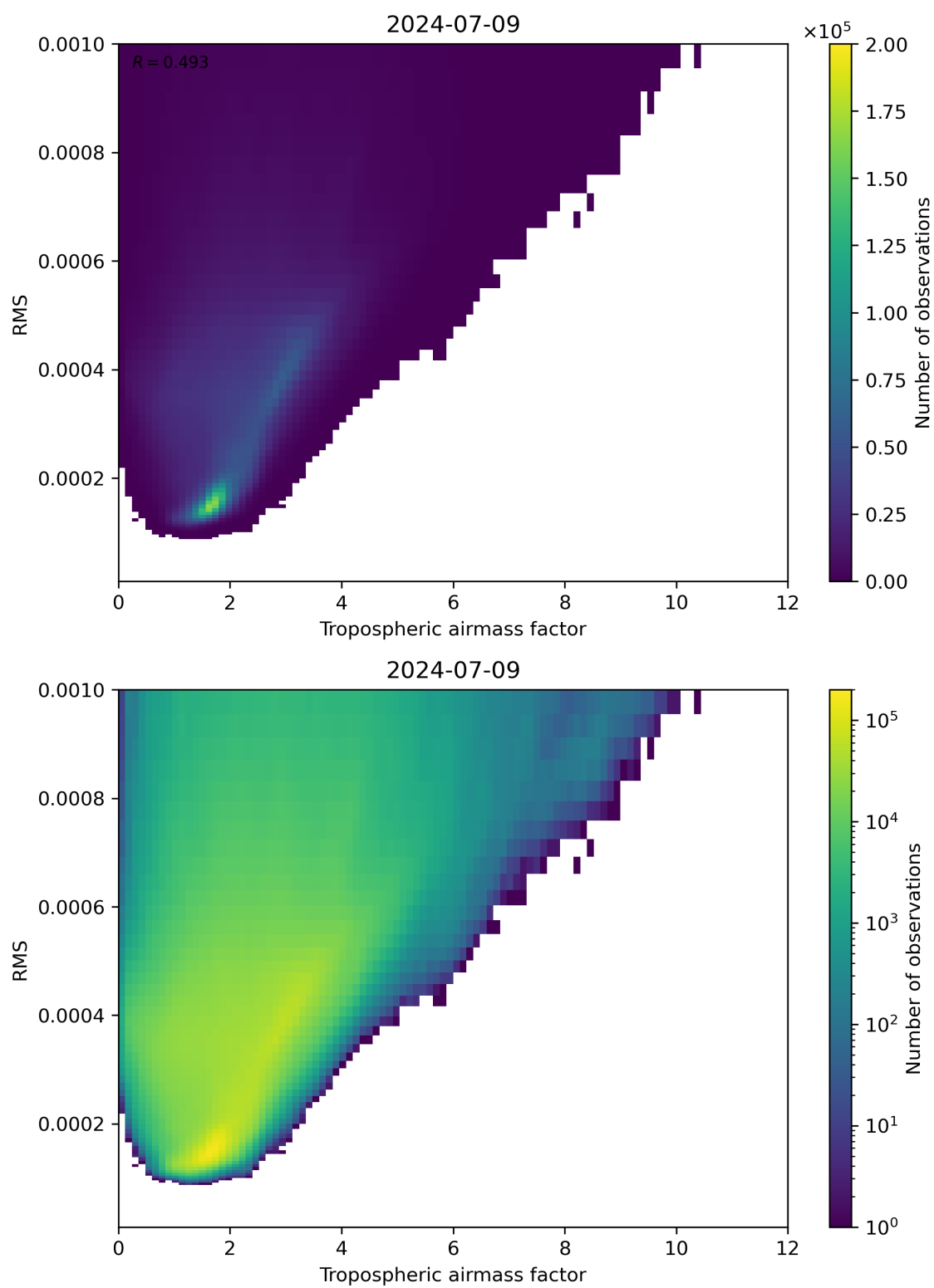
Figure 79: Scatter density plot of “Tropospheric airmass factor” against “RMS” for 2024-07-08 to 2024-07-10.
