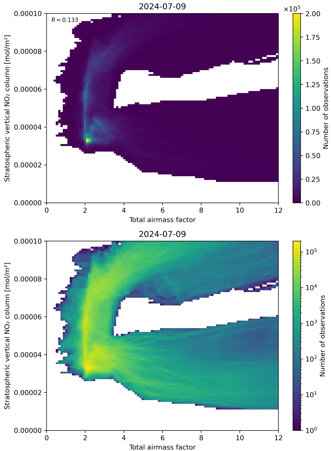
Figure 64: Scatter density plot of “Total airmass factor” against “Stratospheric vertical NO 2 column” for 2024-07-08 to 2024-07-10.
