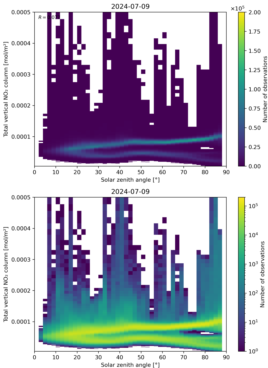
Figure 153: Scatter density plot of “Solar zenith angle” against “Total vertical NO 2 column” for 2024-07-08 to 2024-07-10.
