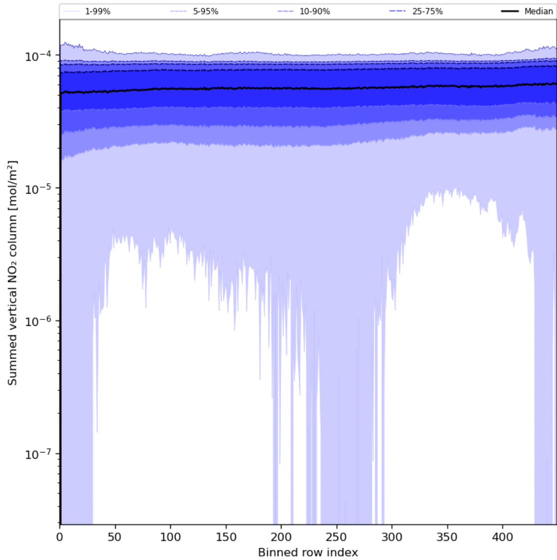
Figure 57: Along track statistics of “Summed vertical NO 2 column” for 2024-07-08 to 2024-07-10
