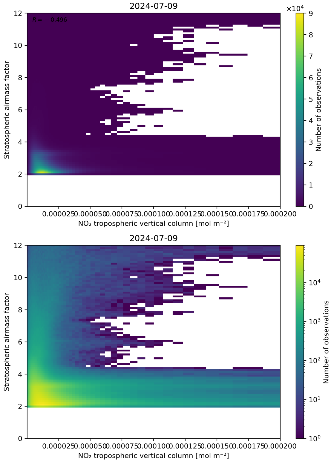
Figure 121: Scatter density plot of “NO 2 tropospheric vertical column” against “Stratospheric air mass factor” for 2024-07-08 to 2024-07-10.
