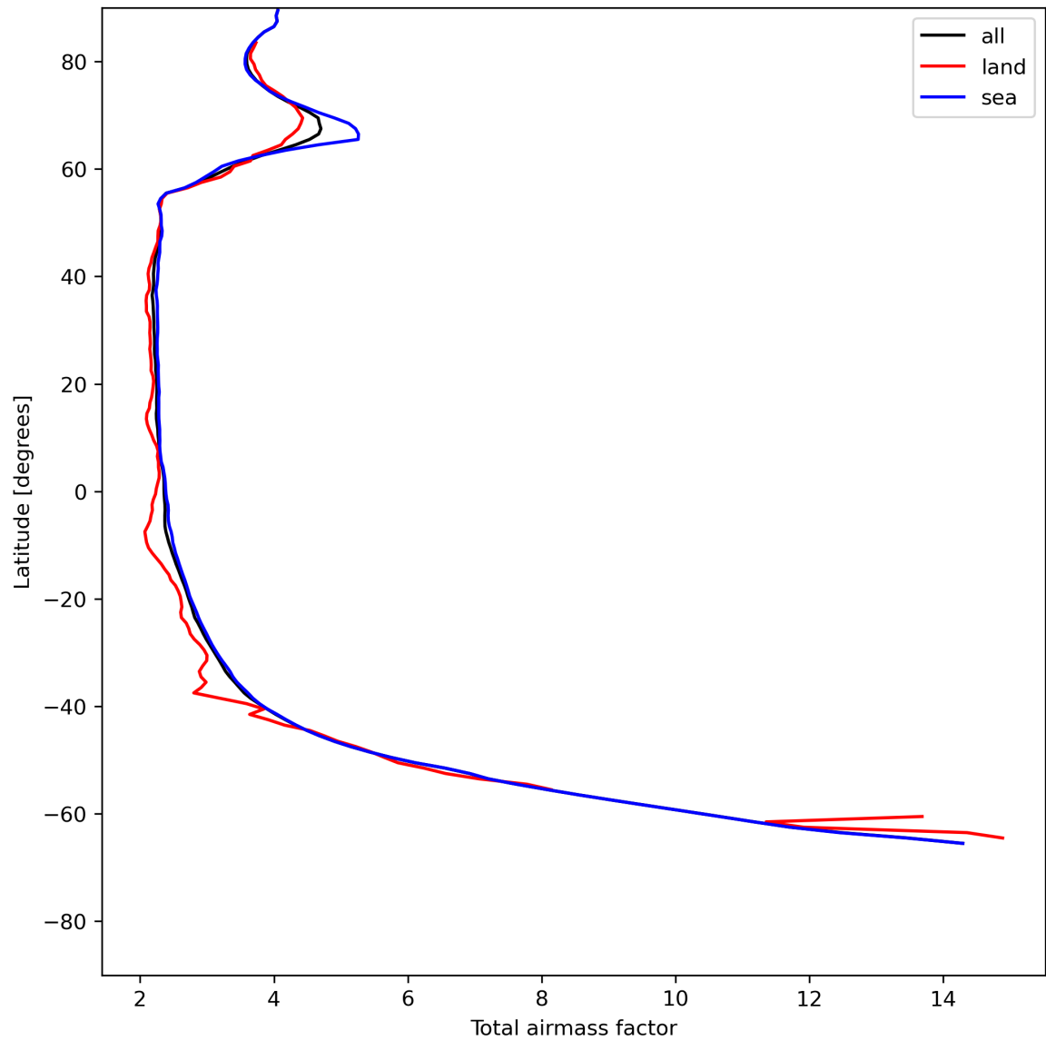
Figure 15: Zonal average of “Total airmass factor” for 2024-07-08 to 2024-07-10.
