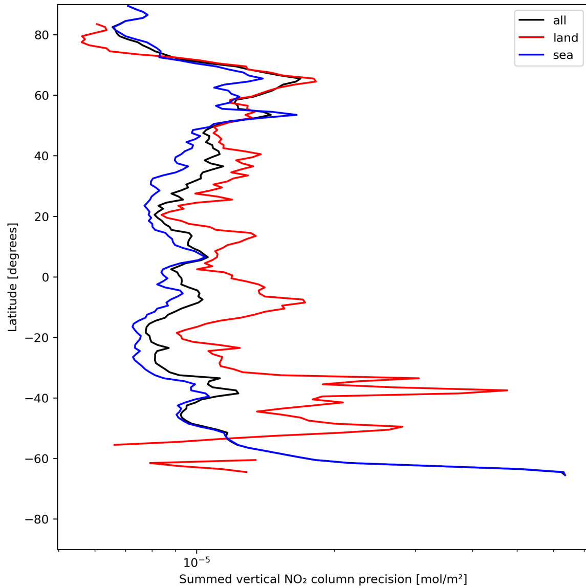
Figure 24: Zonal average of “Summed vertical NO 2 column precision” for 2024-07-08 to 2024-07-10.
