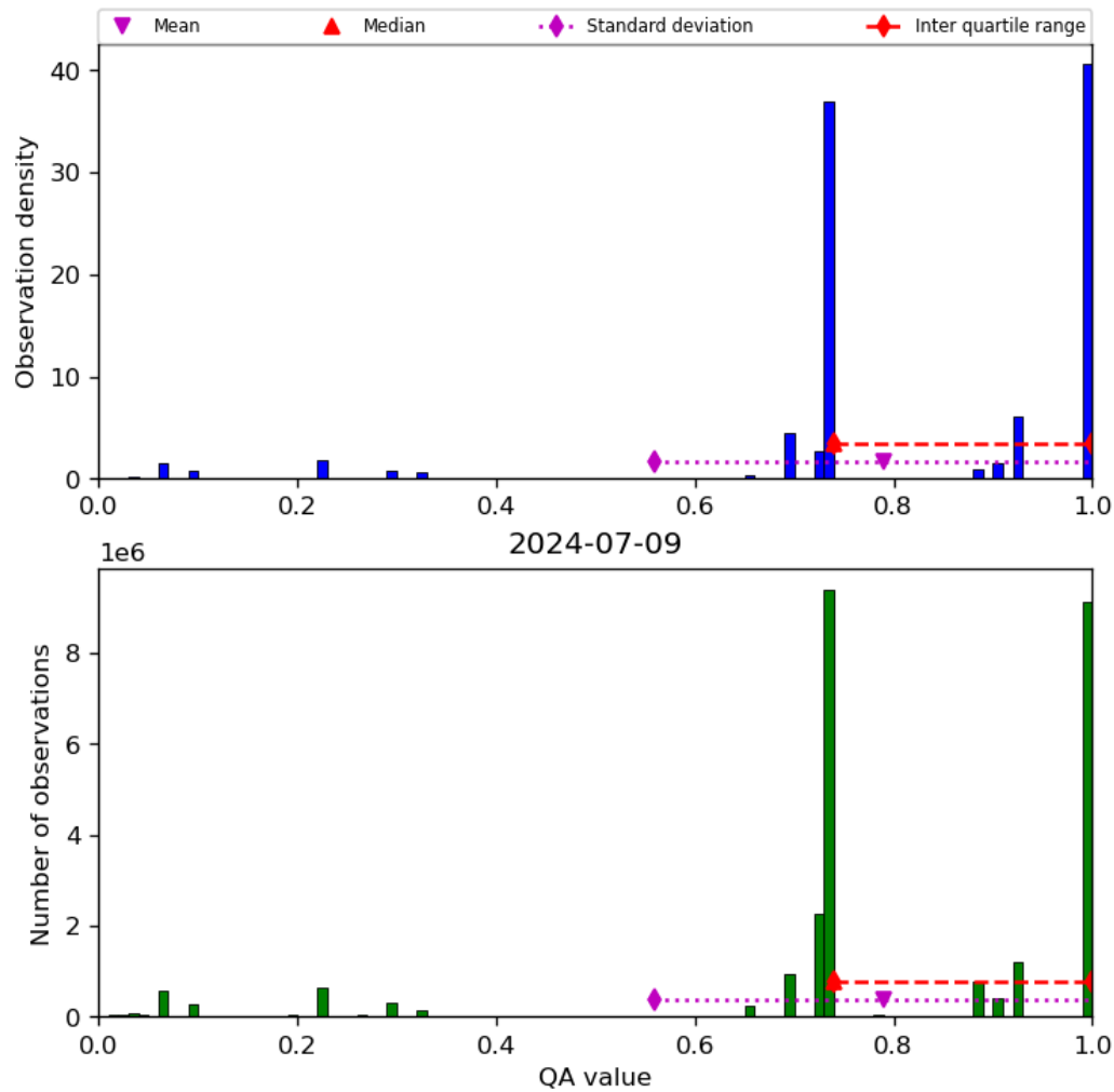
Figure 28: Histogram of “QA value” for 2024-07-08 to 2024-07-10
