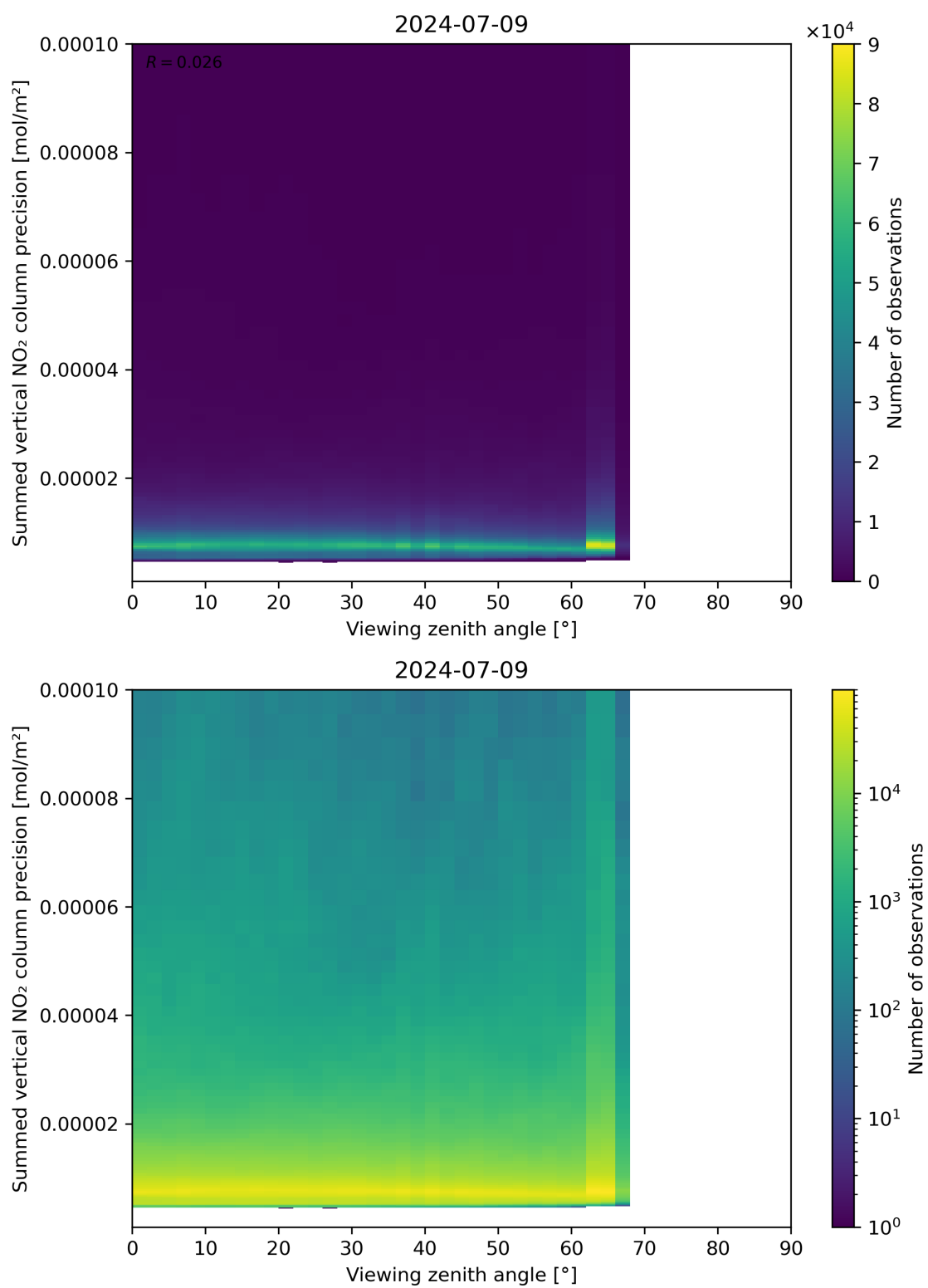
Figure 166: Scatter density plot of “Viewing zenith angle” against “Summed vertical NO 2 column precision” for 2024-07-08 to 2024-07-10.
