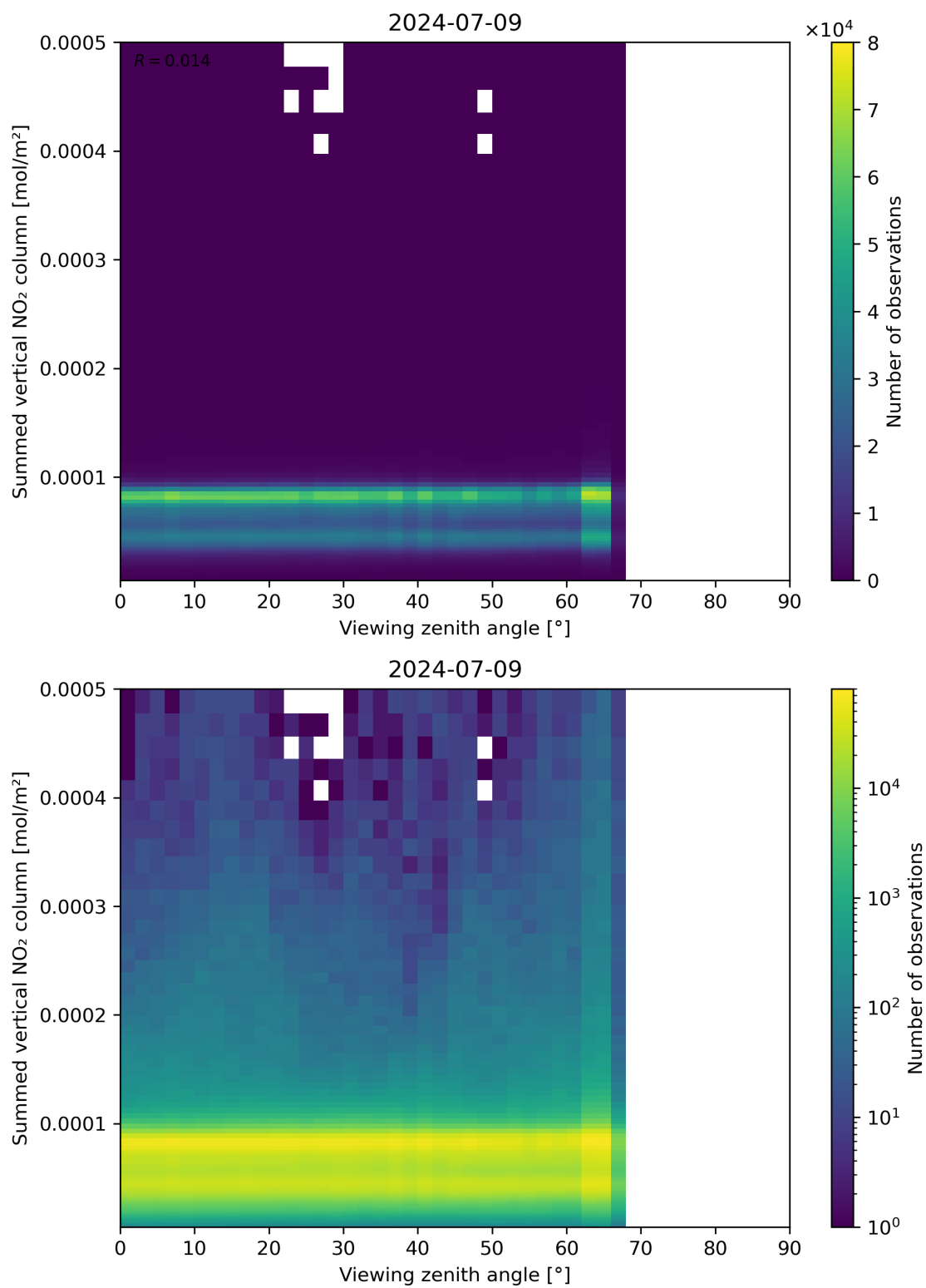
Figure 165: Scatter density plot of “Viewing zenith angle” against “Summed vertical NO 2 column” for 2024-07-08 to 2024-07-10.
