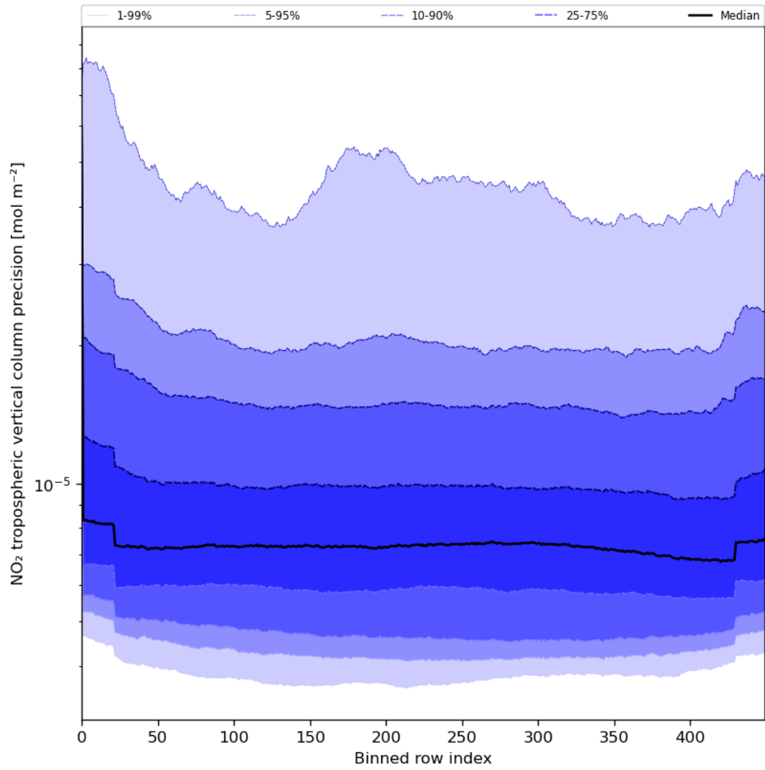
Figure 47: Along track statistics of “NO 2 tropospheric vertical column precision” for 2024-07-08 to 2024-07-10
