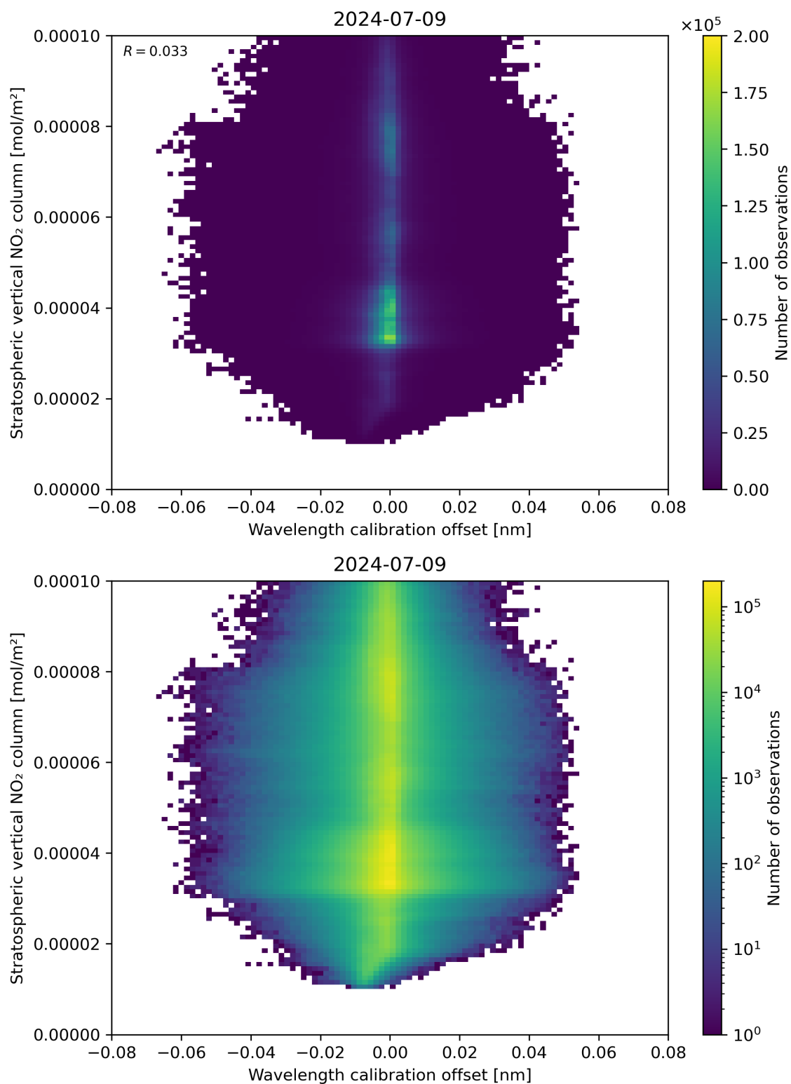
Figure 176: Scatter density plot of “Wavelength calibration offset” against “Stratospheric vertical NO 2 column” for 2024-07-08 to 2024-07-10.
