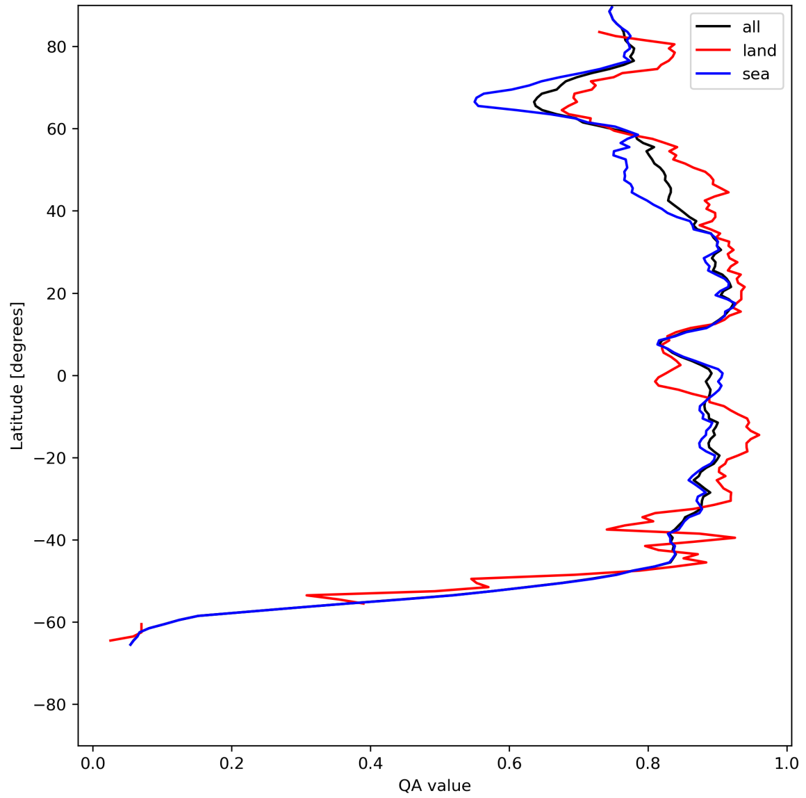
Figure 11: Zonal average of “QA value” for 2024-07-08 to 2024-07-10.
