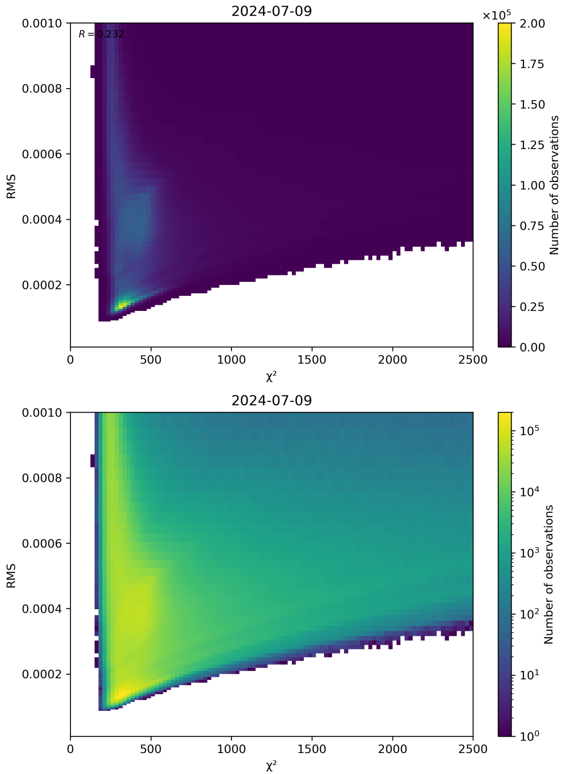
Figure 82: Scatter density plot of “ \chi^2 ” against “RMS” for 2024-07-08 to 2024-07-10.
