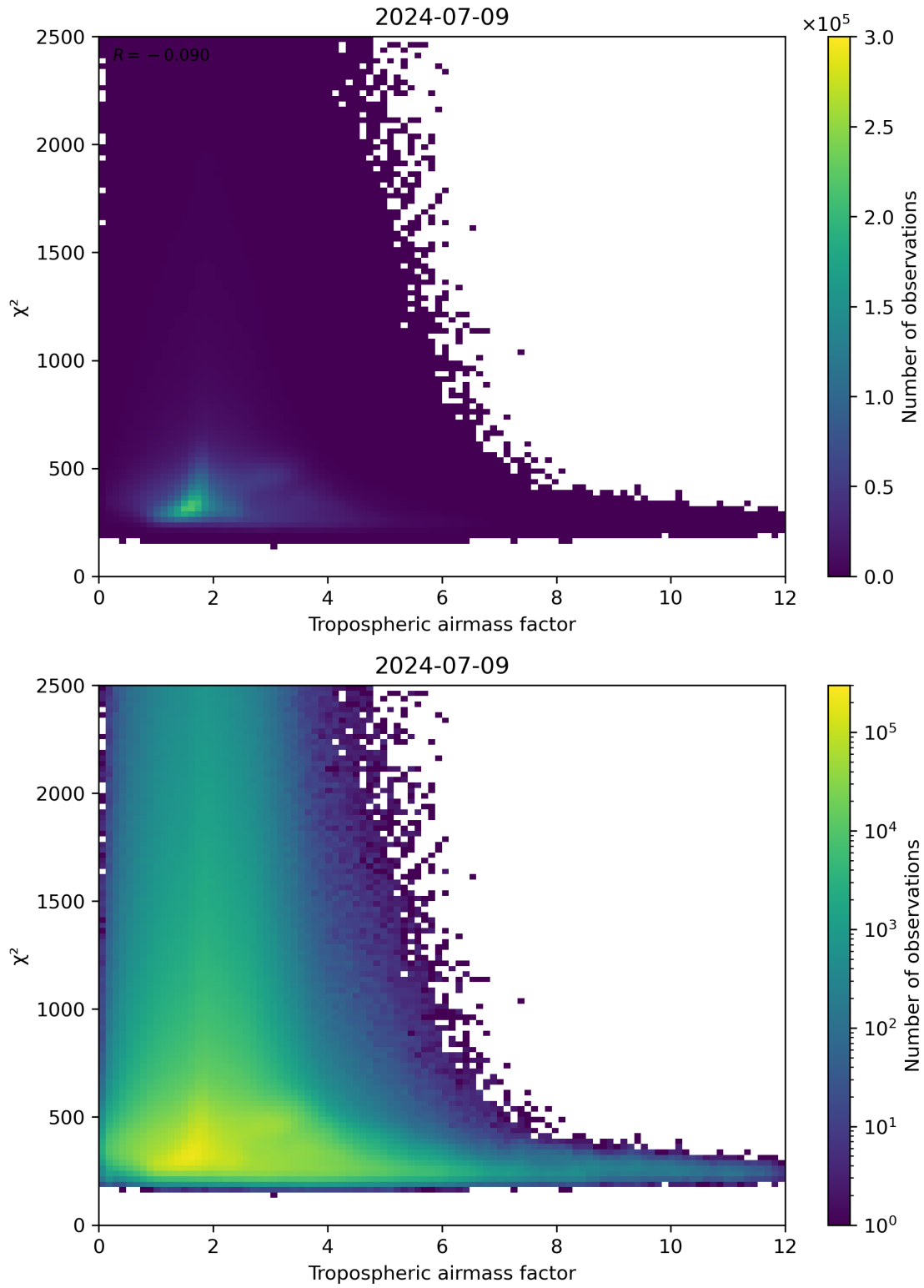
Figure 73: Scatter density plot of “Tropospheric airmass factor” against “ \chi^2 ” for 2024-07-08 to 2024-07-10.
