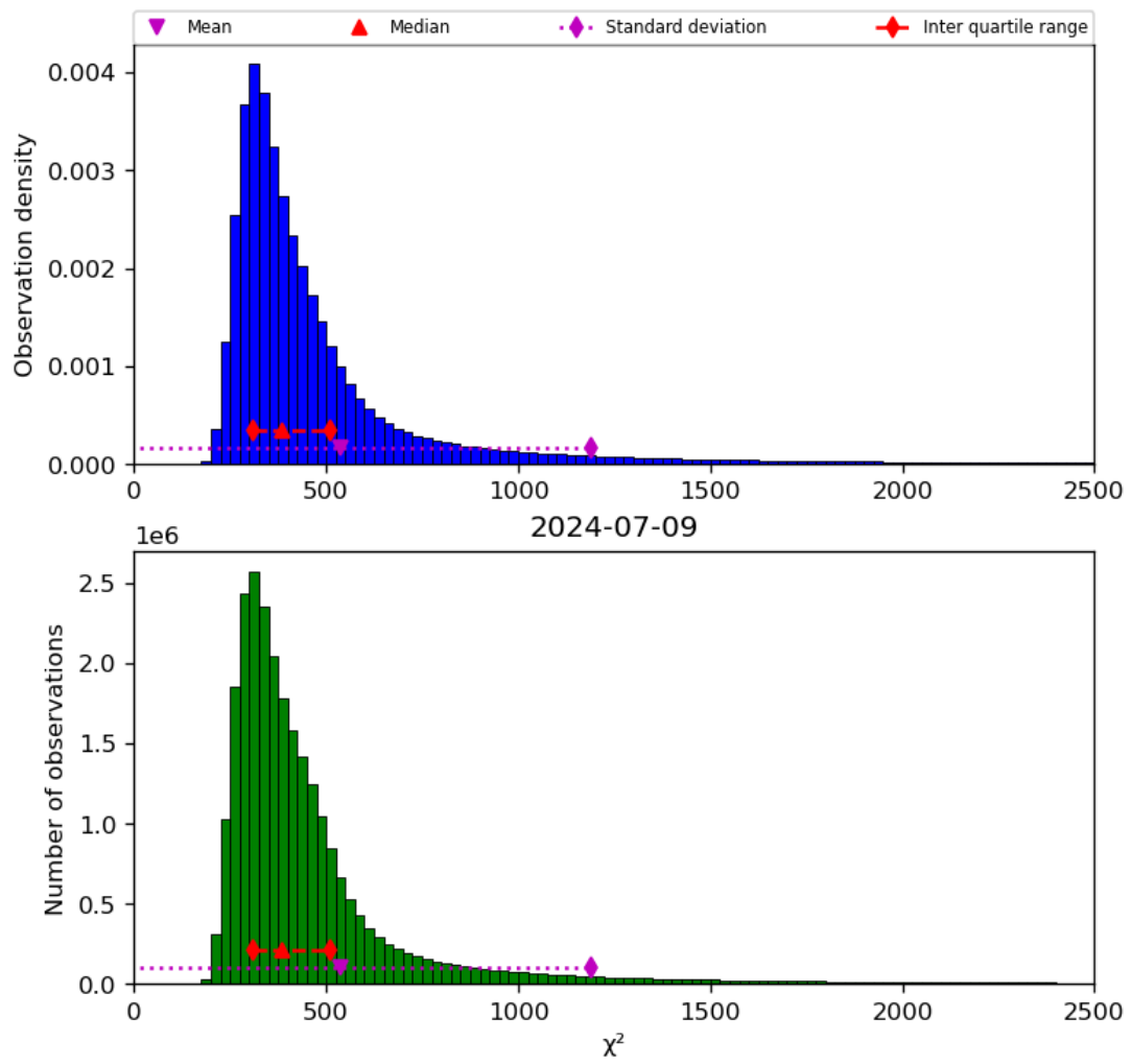
Figure 42: Histogram of “ \chi^2 ” for 2024-07-08 to 2024-07-10
