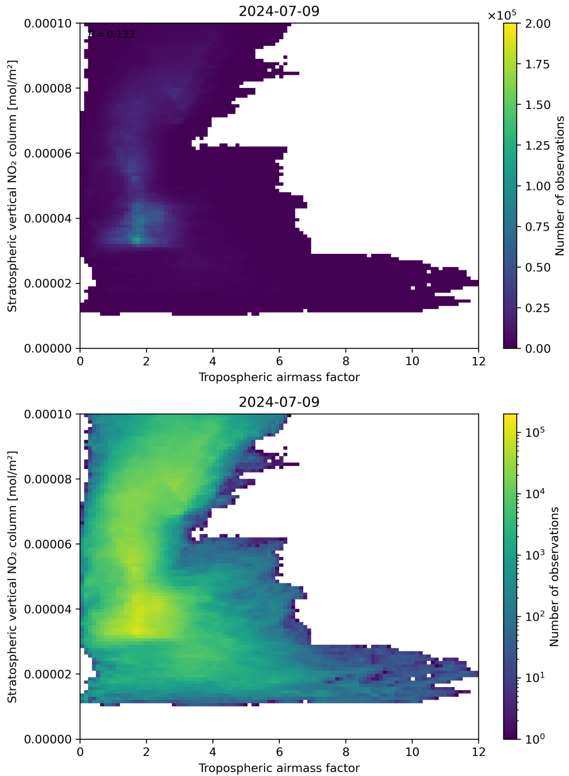
Figure 74: Scatter density plot of “Tropospheric air mass factor” against “Stratospheric vertical NO 2 column” for 2024-07-08 to 2024-07-10.
