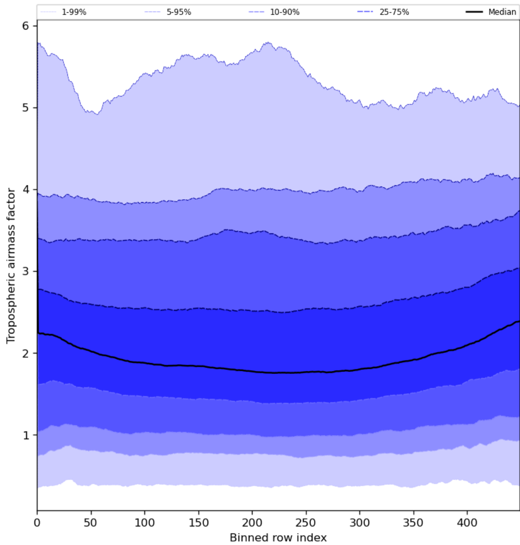
Figure 48: Along track statistics of “Tropospheric airmass factor” for 2024-07-10 to 2024-07-11
