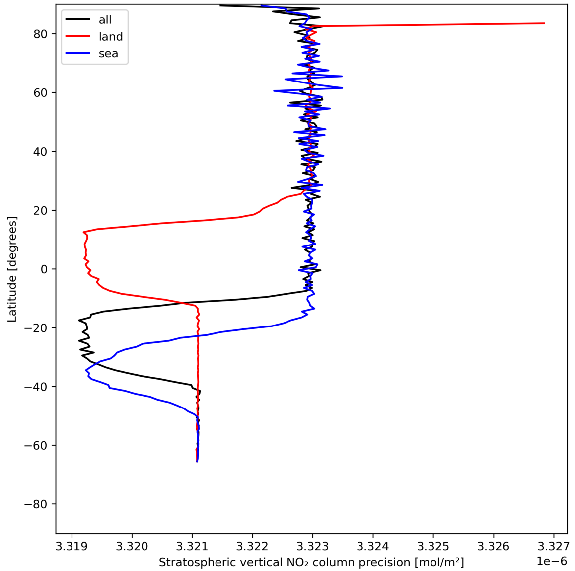
Figure 20: Zonal average of “Stratospheric vertical NO 2 column precision” for 2024-07-10 to 2024-07-11.
