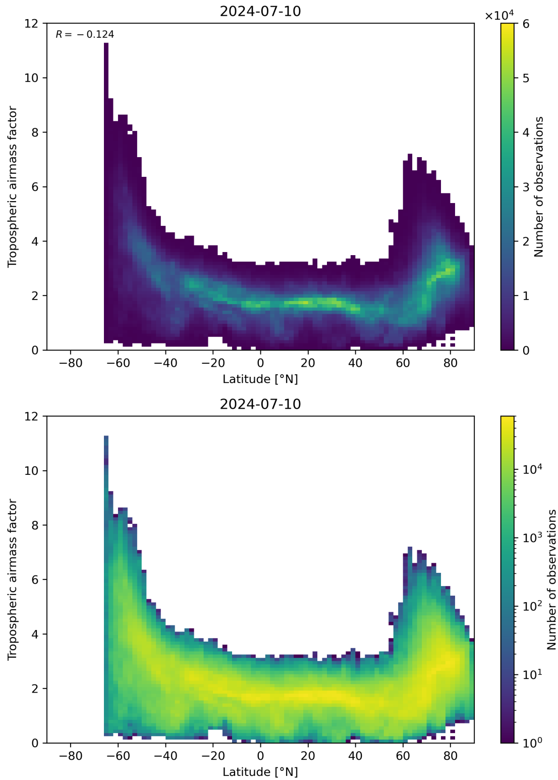
Figure 85: Scatter density plot of “Latitude” against “Tropospheric air mass factor” for 2024-07-10 to 2024-07-11.
