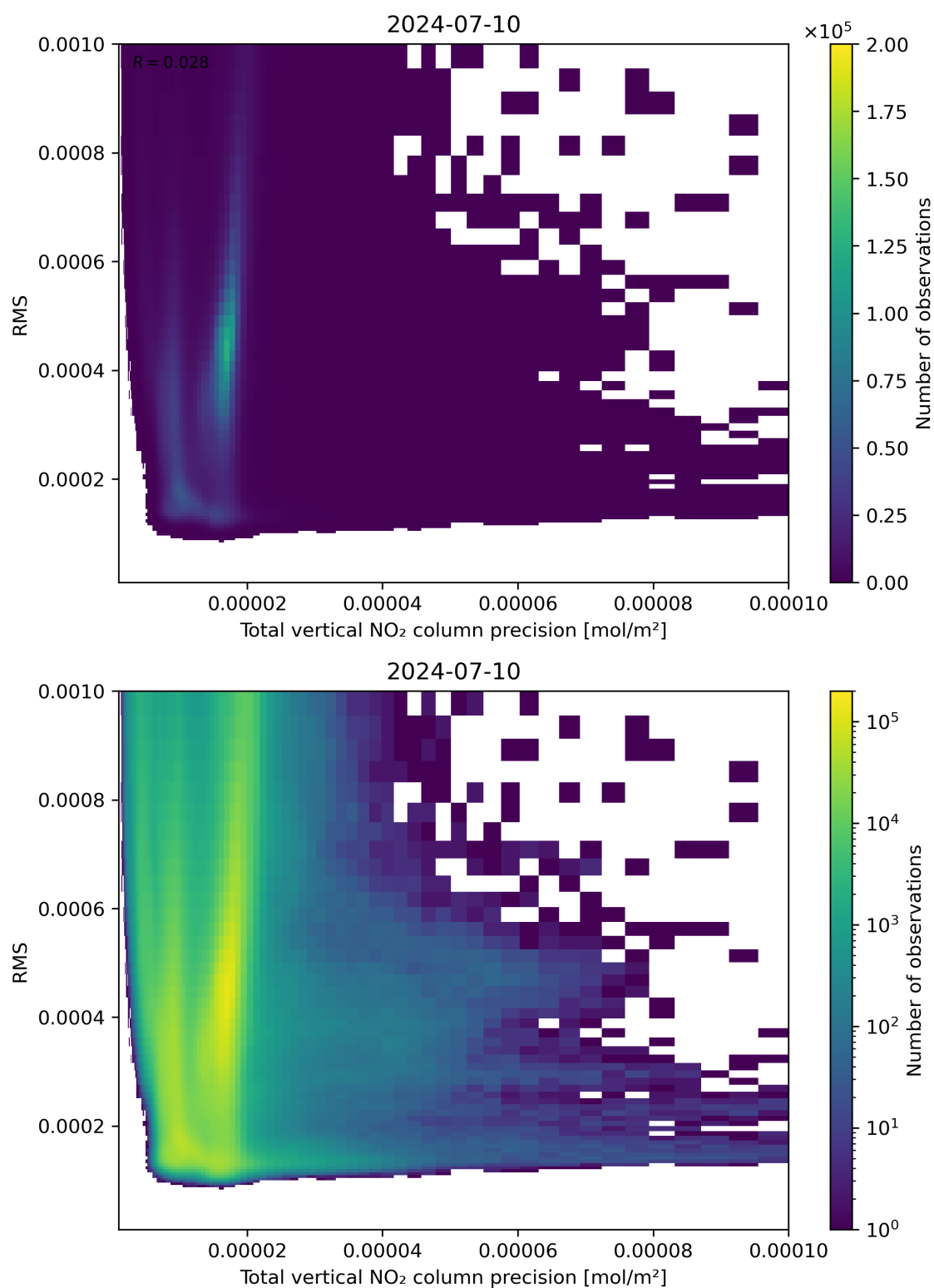
Figure 119: Scatter density plot of “Total vertical NO 2 column precision” against “RMS” for 2024-07-10 to 2024-07-11.
