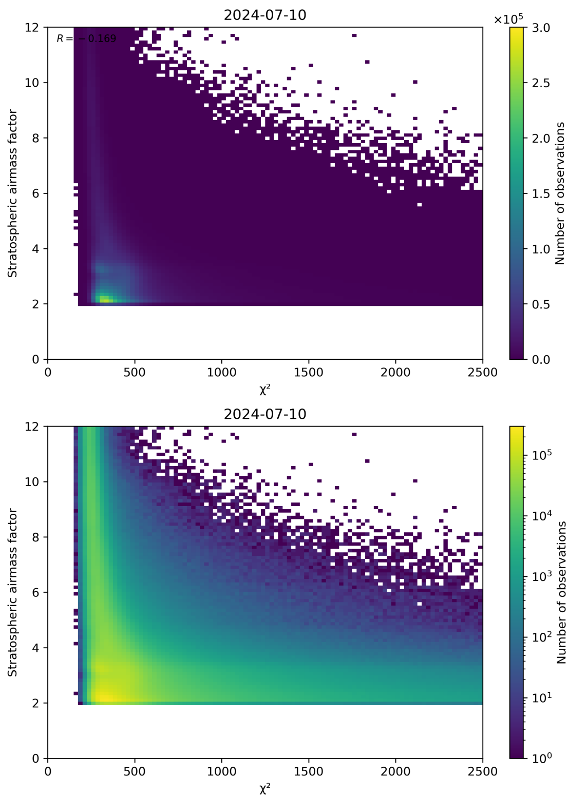
Figure 81: Scatter density plot of “ \chi^2 ” against “Stratospheric airmass factor” for 2024-07-10 to 2024-07-11.
