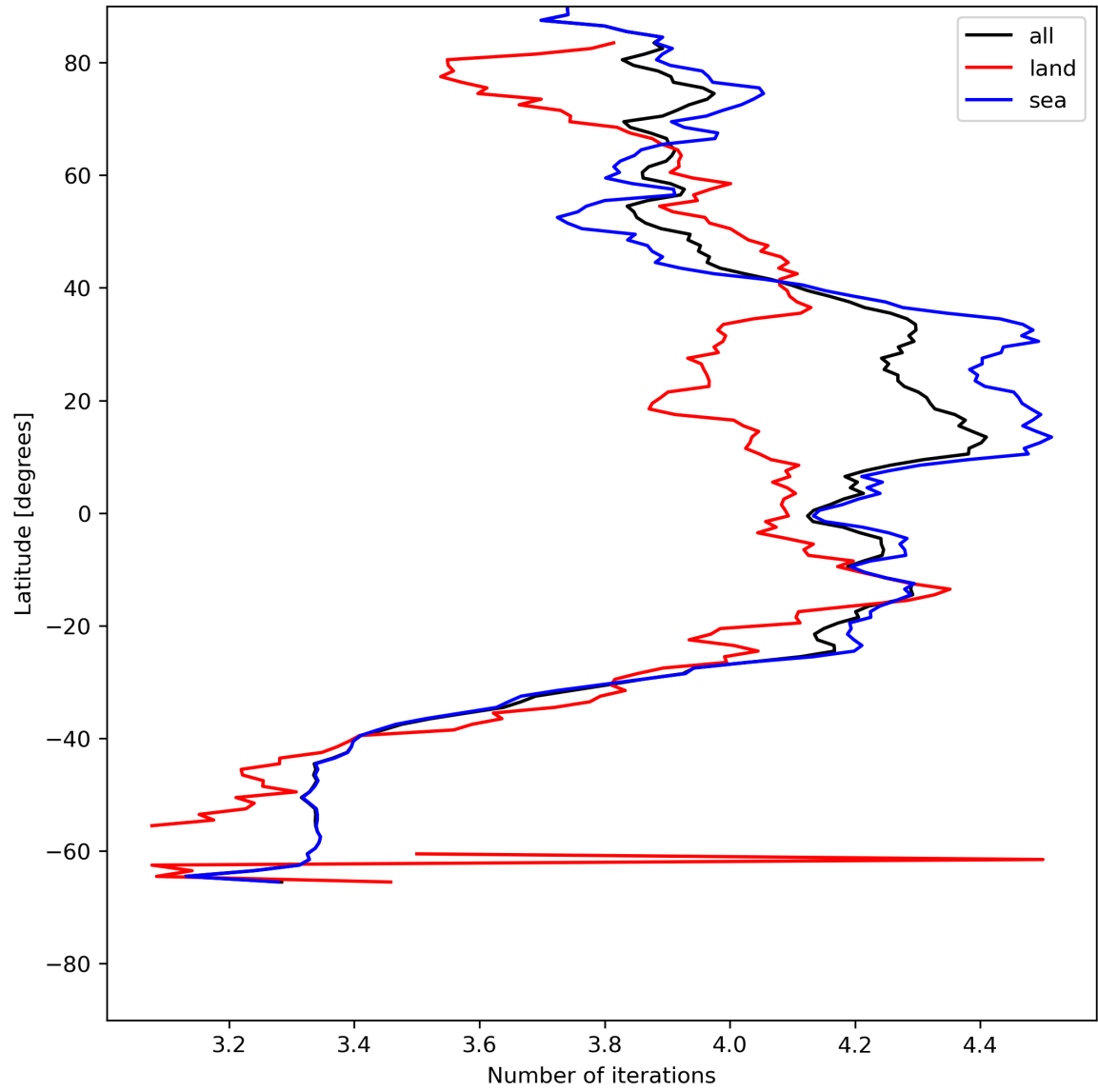
Figure 17: Zonal average of “Number of iterations” for 2024-07-10 to 2024-07-11.
