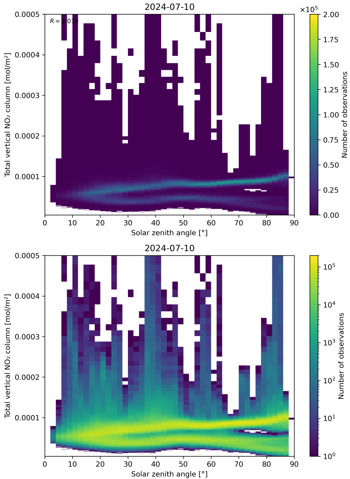
Figure 153: Scatter density plot of “Solar zenith angle” against “Total vertical NO 2 column” for 2024-07-10 to 2024-07-11.
