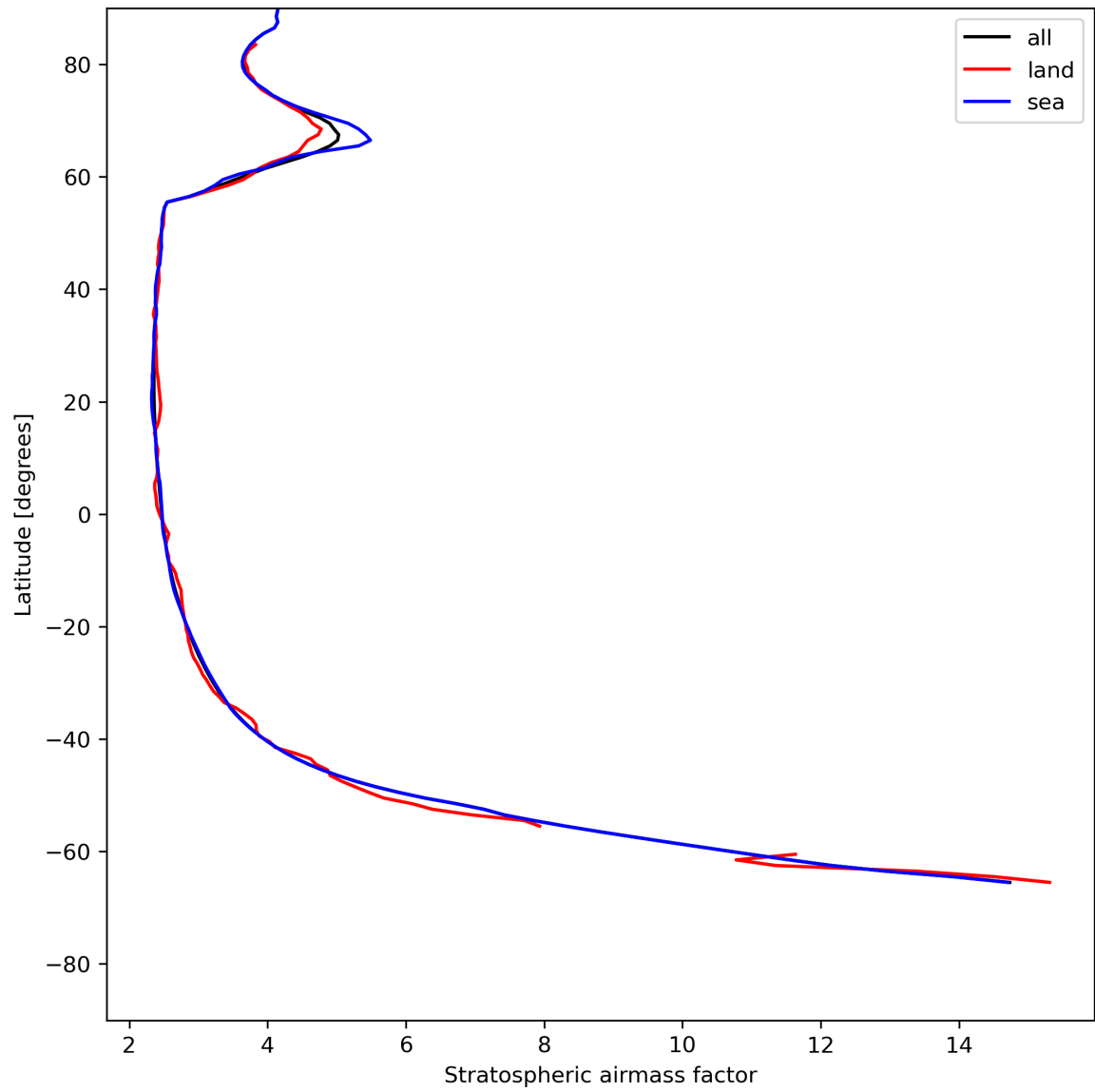
Figure 27: Zonal average of “Stratospheric airmass factor” for 2024-07-10 to 2024-07-11.
