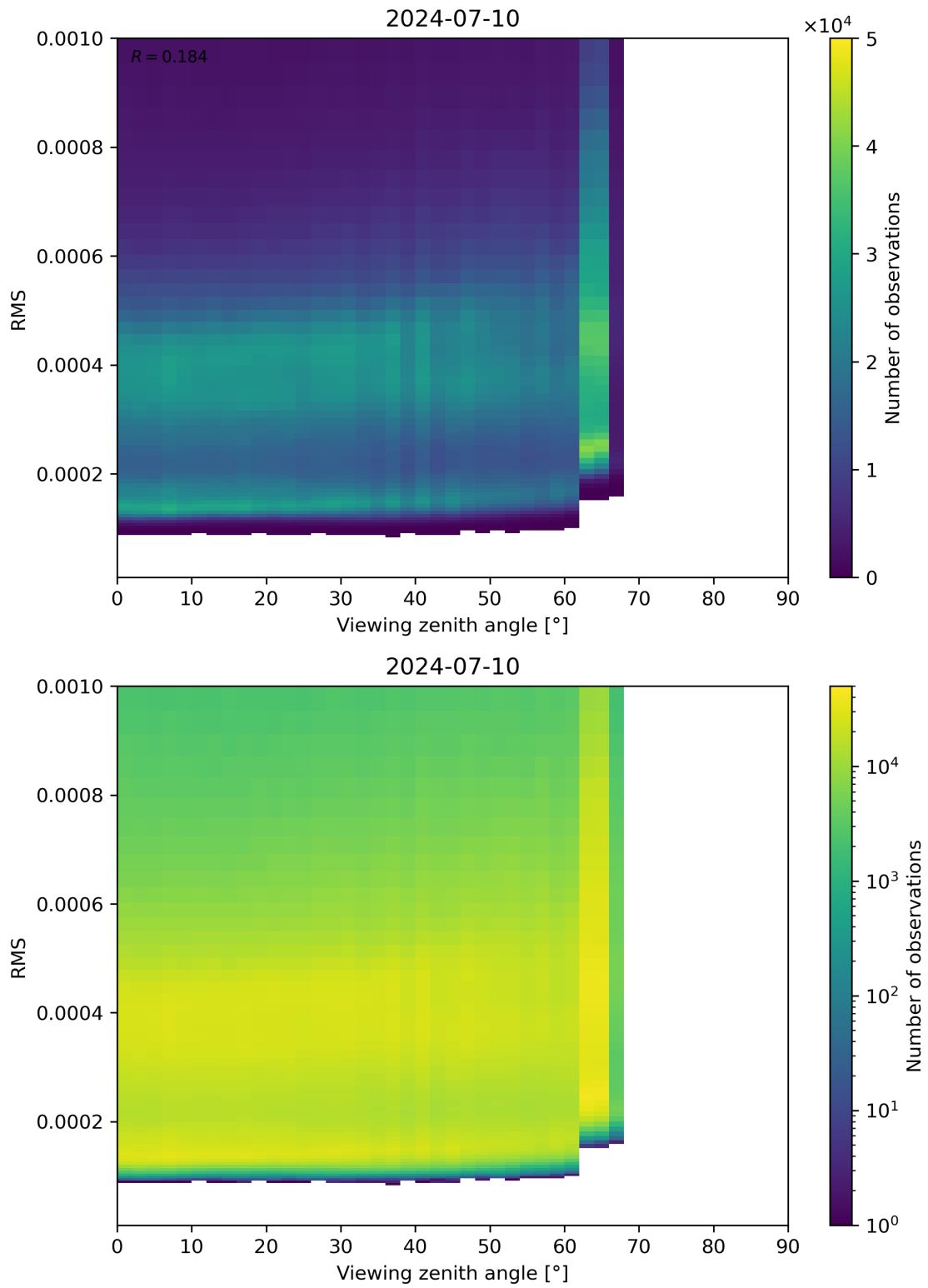
Figure 171: Scatter density plot of “Viewing zenith angle” against “RMS” for 2024-07-10 to 2024-07-11.
