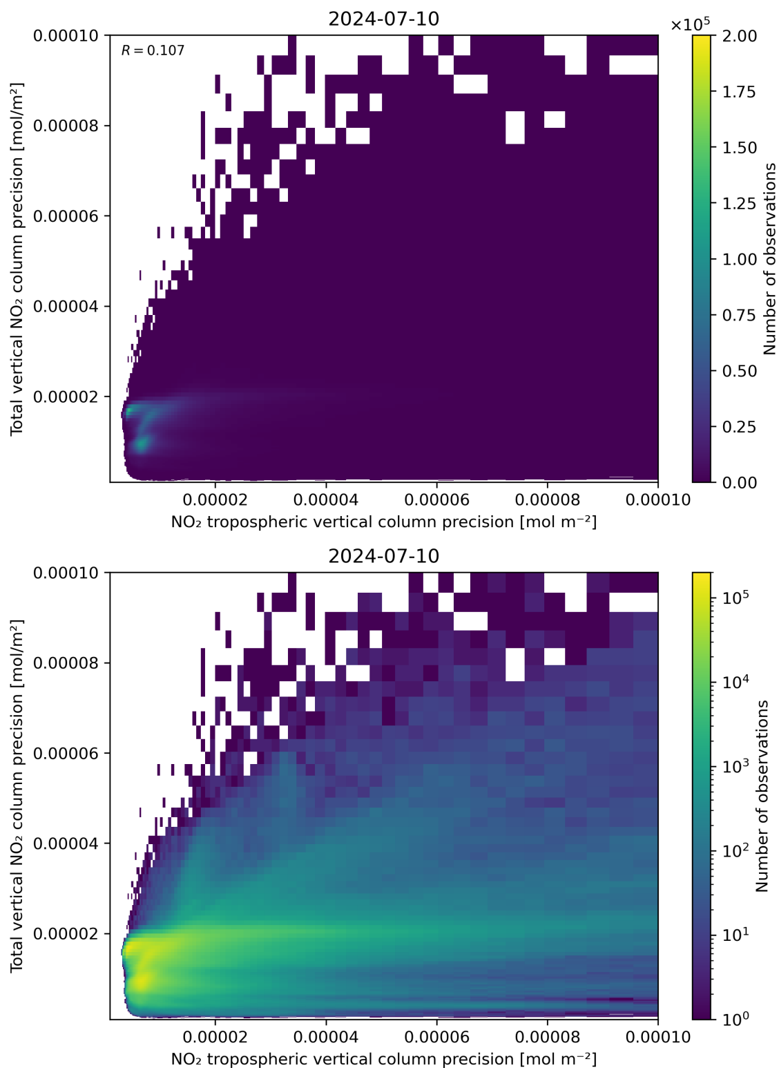
Figure 139: Scatter density plot of “NO 2 tropospheric vertical column precision” against “Total vertical NO 2 column precision” for 2024-07-10 to 2024-07-11.
