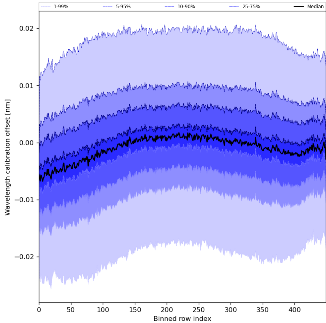
Figure 52: Along track statistics of “Wavelength calibration offset” for 2024-07-10 to 2024-07-11
