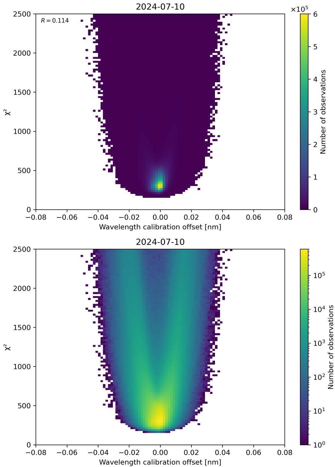
Figure 175: Scatter density plot of “Wavelength calibration offset” against “ \chi^2 ” for 2024-07-10 to 2024-07-11.
