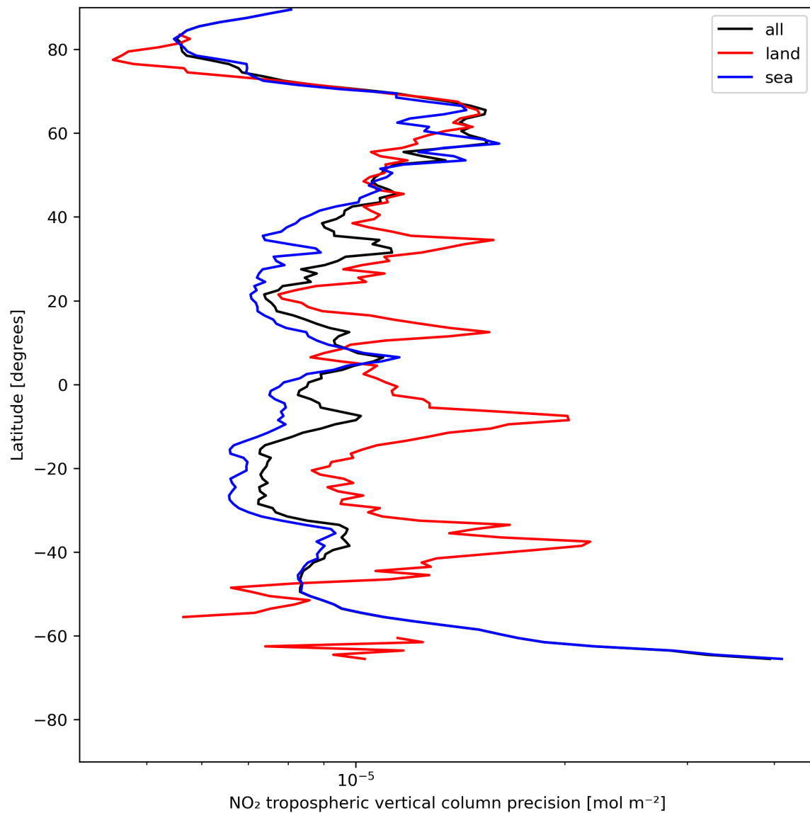
Figure 13: Zonal average of “NO 2 tropospheric vertical column precision” for 2024-07-10 to 2024-07-11.
