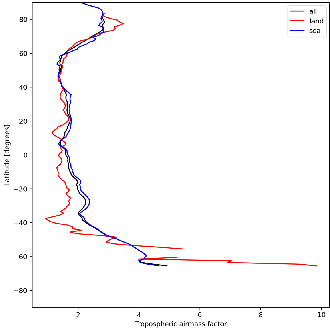
Figure 14: Zonal average of “Tropospheric airmass factor” for 2024-07-10 to 2024-07-11.
