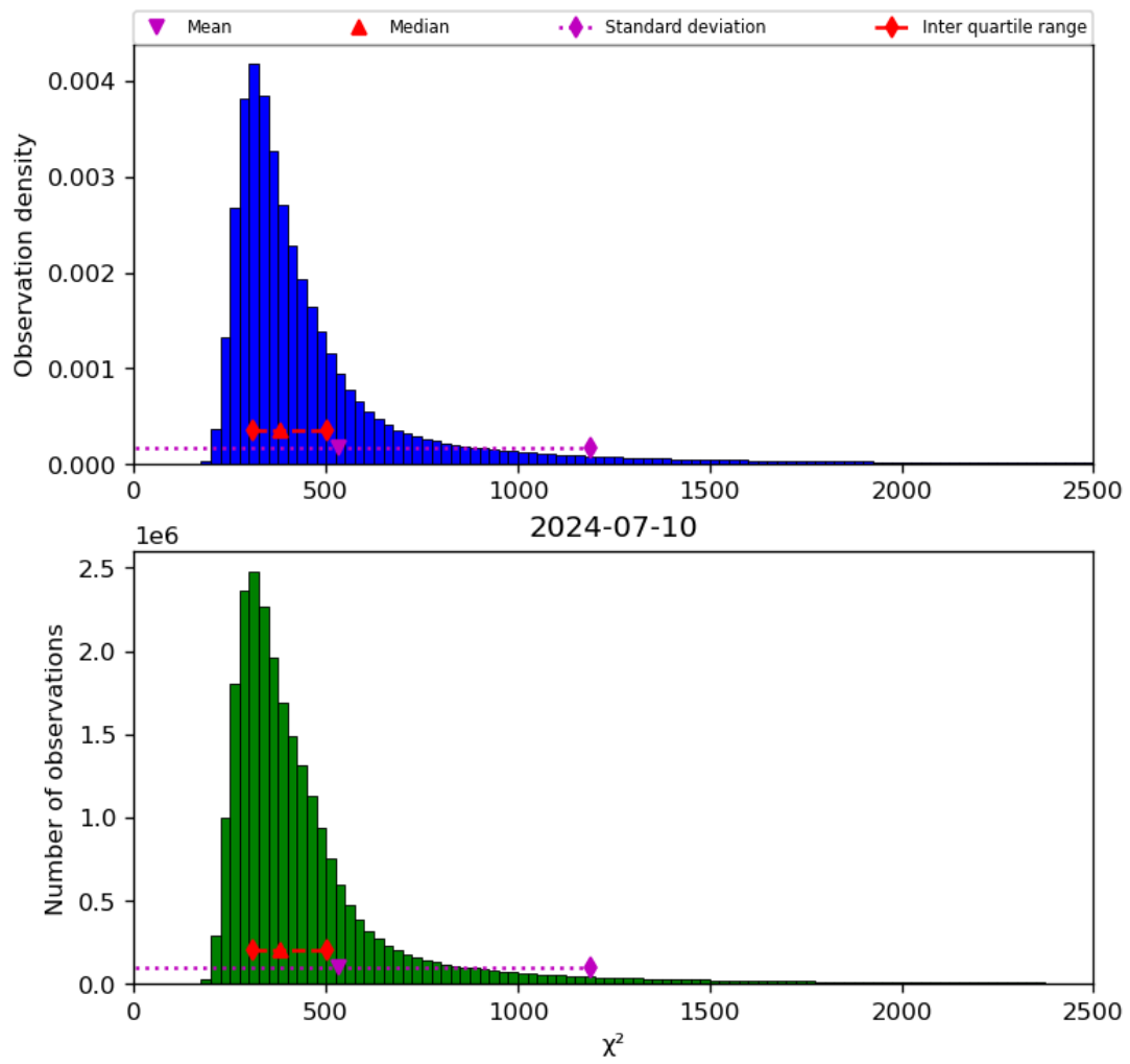
Figure 42: Histogram of “ \chi^2 ” for 2024-07-10 to 2024-07-11
