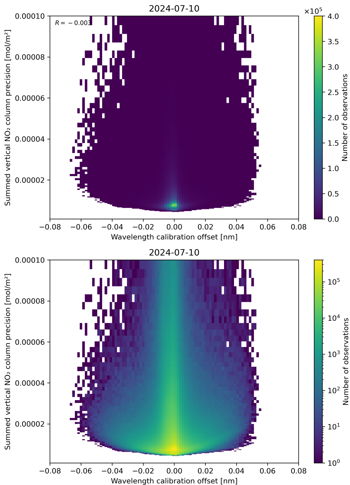
Figure 178: Scatter density plot of “Wavelength calibration offset” against “Summed vertical NO 2 column precision” for 2024-07-10 to 2024-07-11.
