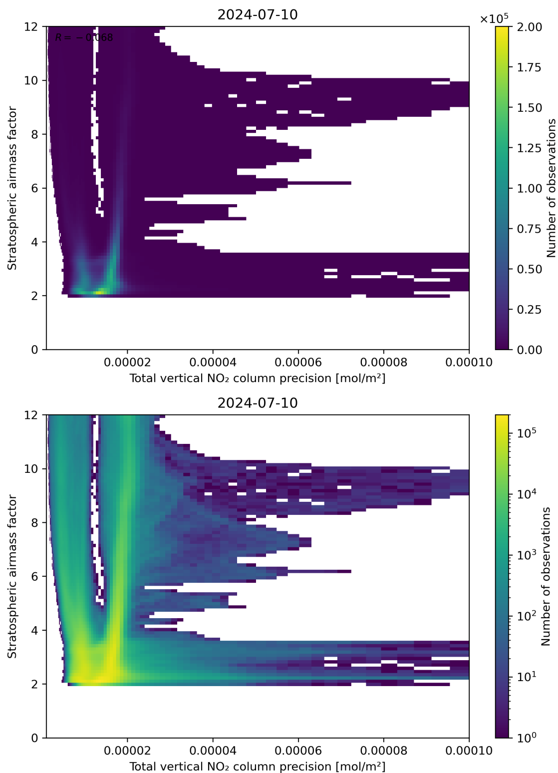
Figure 115: Scatter density plot of “Total vertical NO 2 column precision” against “Stratospheric air mass factor” for 2024-07-10 to 2024-07-11.
