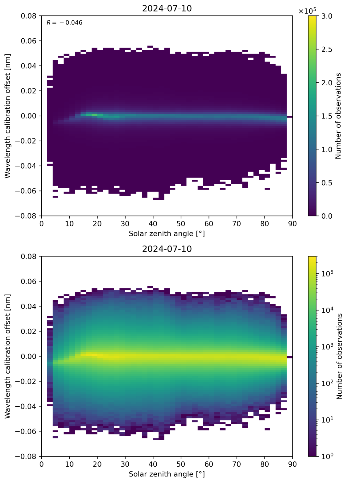
Figure 158: Scatter density plot of “Solar zenith angle” against “Wavelength calibration offset” for 2024-07-10 to 2024-07-11.
