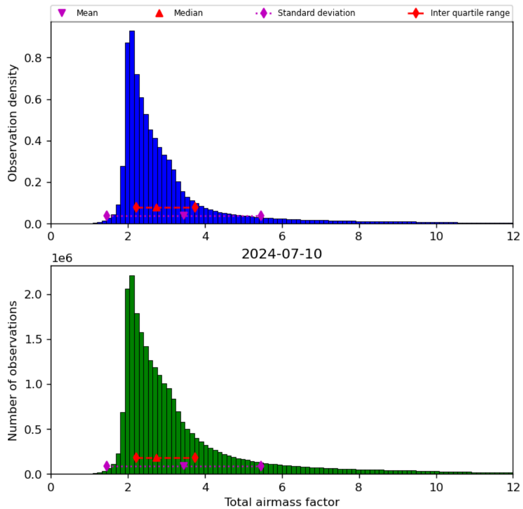
Figure 32: Histogram of “Total airmass factor” for 2024-07-10 to 2024-07-11
