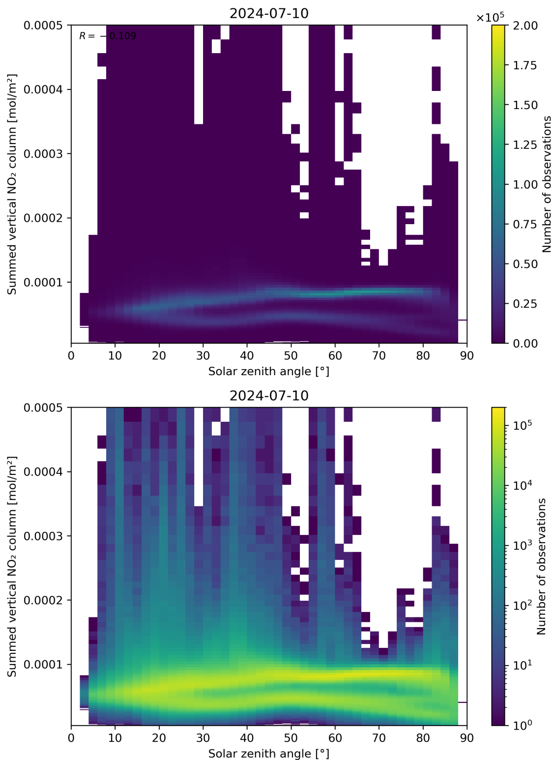
Figure 151: Scatter density plot of “Solar zenith angle” against “Summed vertical NO 2 column” for 2024-07-10 to 2024-07-11.
