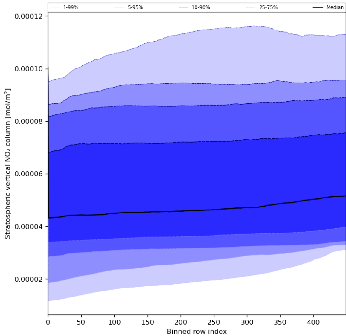
Figure 53: Along track statistics of “Stratospheric vertical NO 2 column” for 2024-07-10 to 2024-07-11
