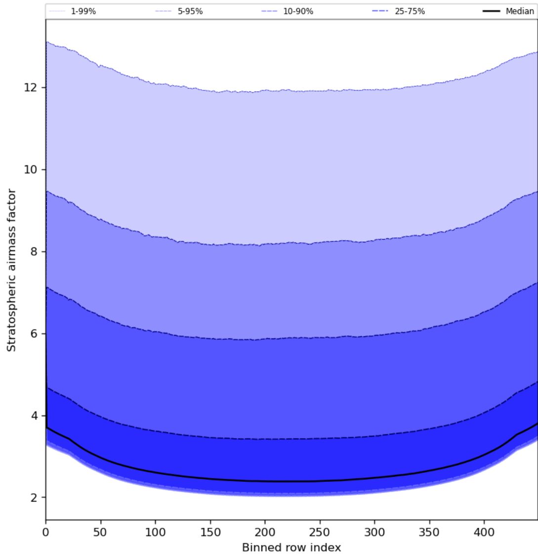
Figure 61: Along track statistics of “Stratospheric airmass factor” for 2024-07-10 to 2024-07-11
