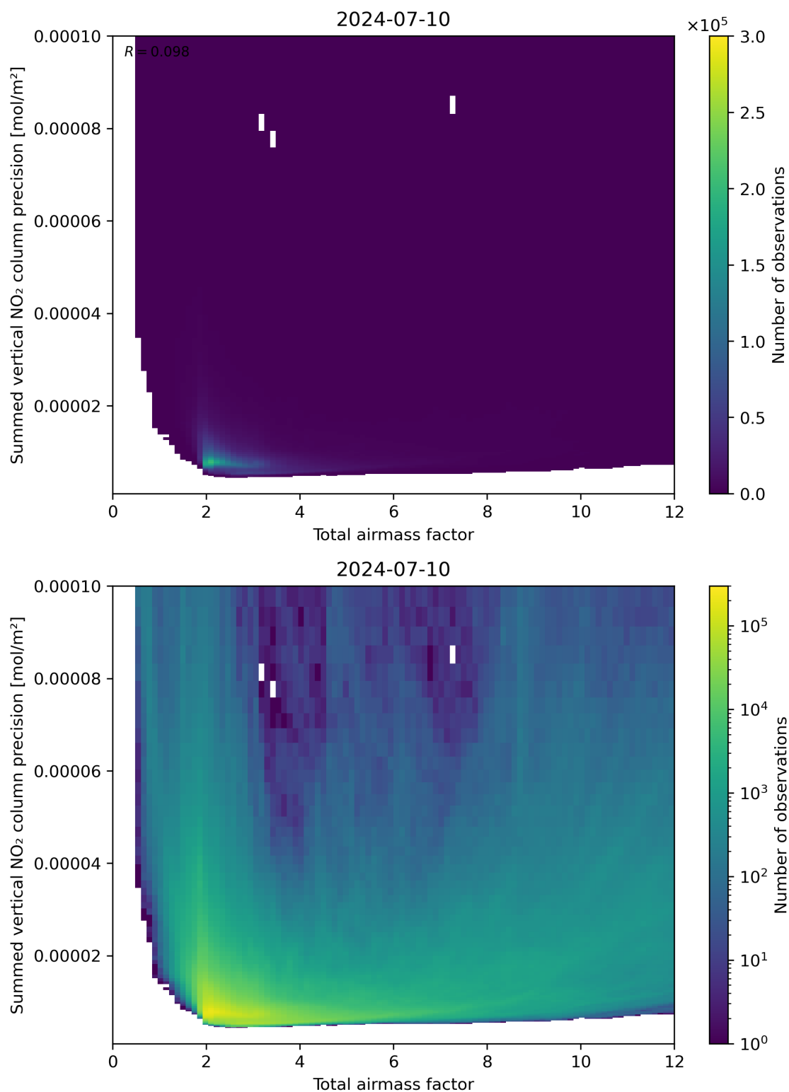
Figure 66: Scatter density plot of “Total airmass factor” against “Summed vertical NO 2 column precision” for 2024-07-10 to 2024-07-11.
