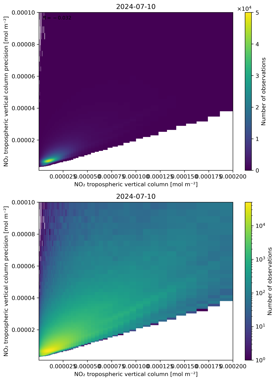
Figure 130: Scatter density plot of “NO 2 tropospheric vertical column” against “NO 2 tropospheric vertical column precision” for 2024-07-10 to 2024-07-11.
