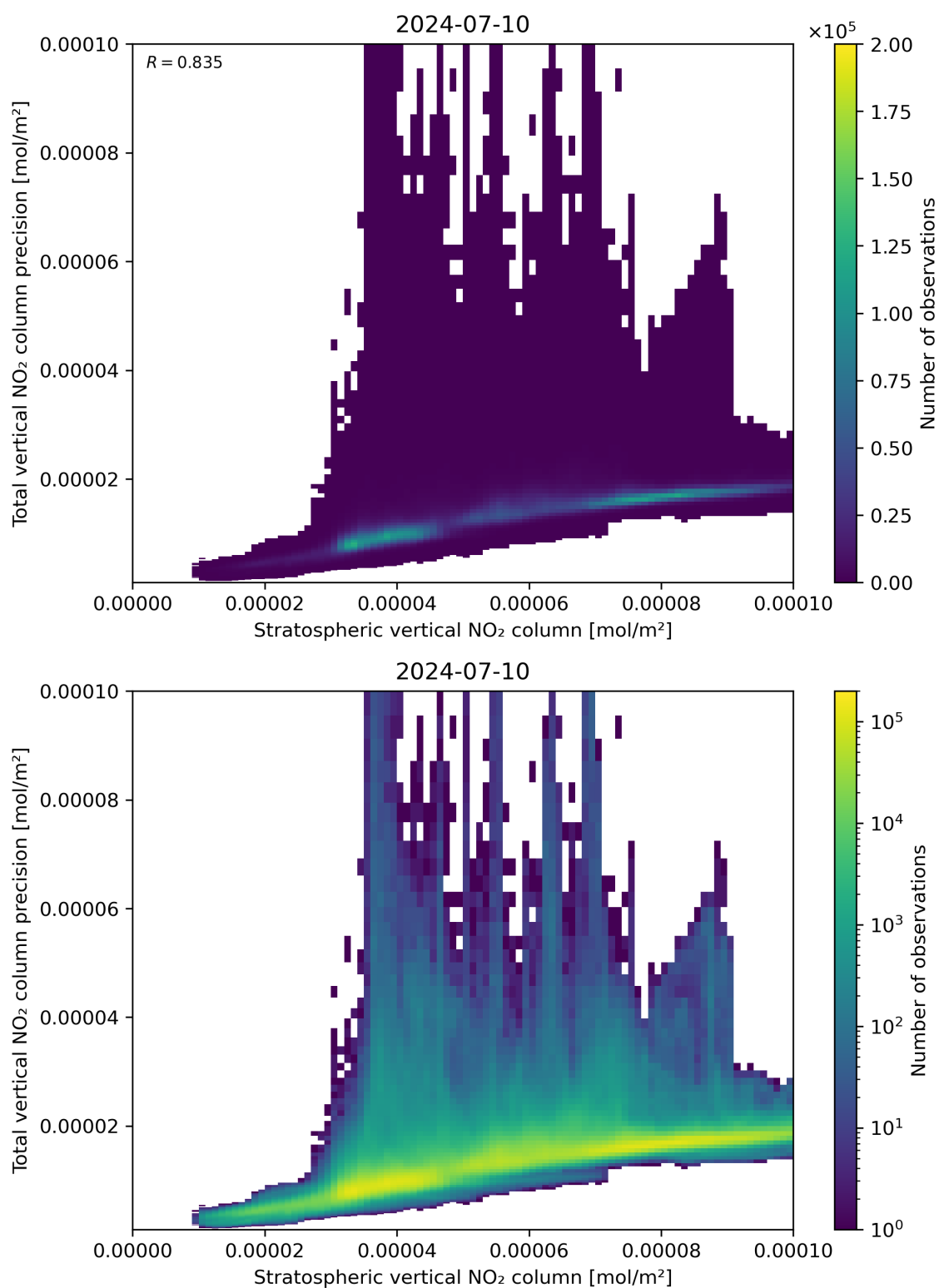
Figure 101: Scatter density plot of “Stratospheric vertical NO 2 column” against “Total vertical NO 2 column precision” for 2024-07-10 to 2024-07-11.
