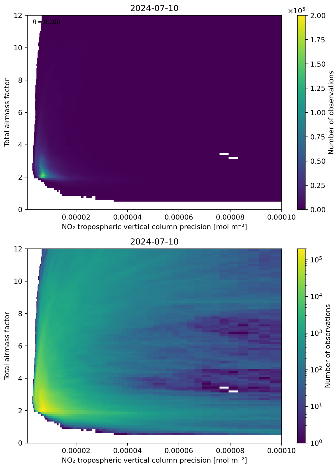
Figure 132: Scatter density plot of “NO 2 tropospheric vertical column precision” against “Total air mass factor” for 2024-07-10 to 2024-07-11.
