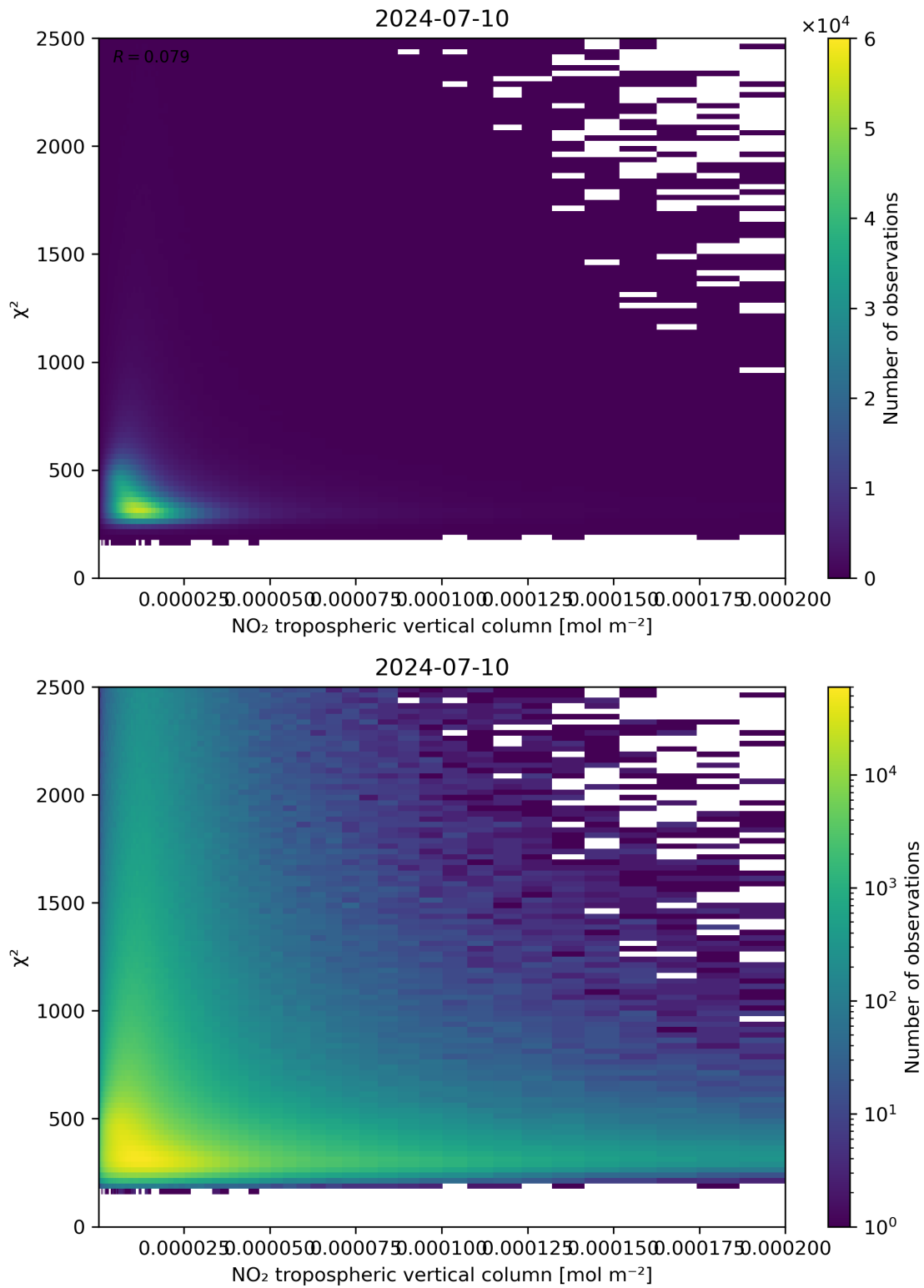
Figure 124: Scatter density plot of “NO 2 tropospheric vertical column” against “ \chi^2 ” for 2024-07-10 to 2024-07-11.
