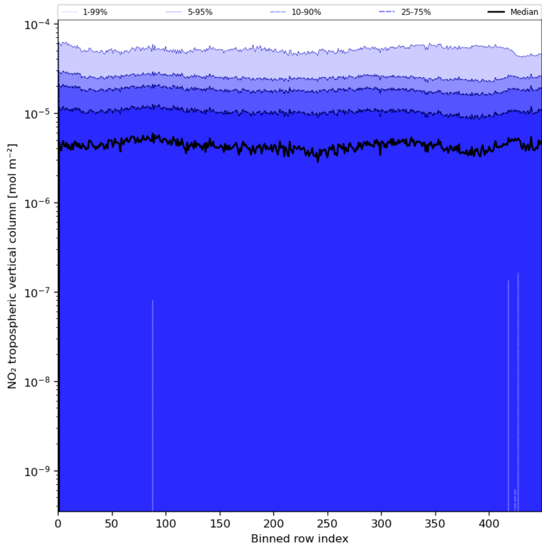
Figure 46: Along track statistics of “NO 2 tropospheric vertical column” for 2024-07-10 to 2024-07-11
