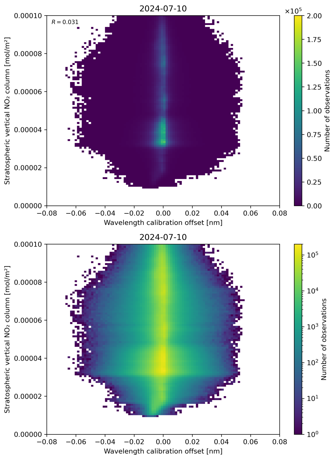
Figure 176: Scatter density plot of “Wavelength calibration offset” against “Stratospheric vertical NO 2 column” for 2024-07-10 to 2024-07-11.
