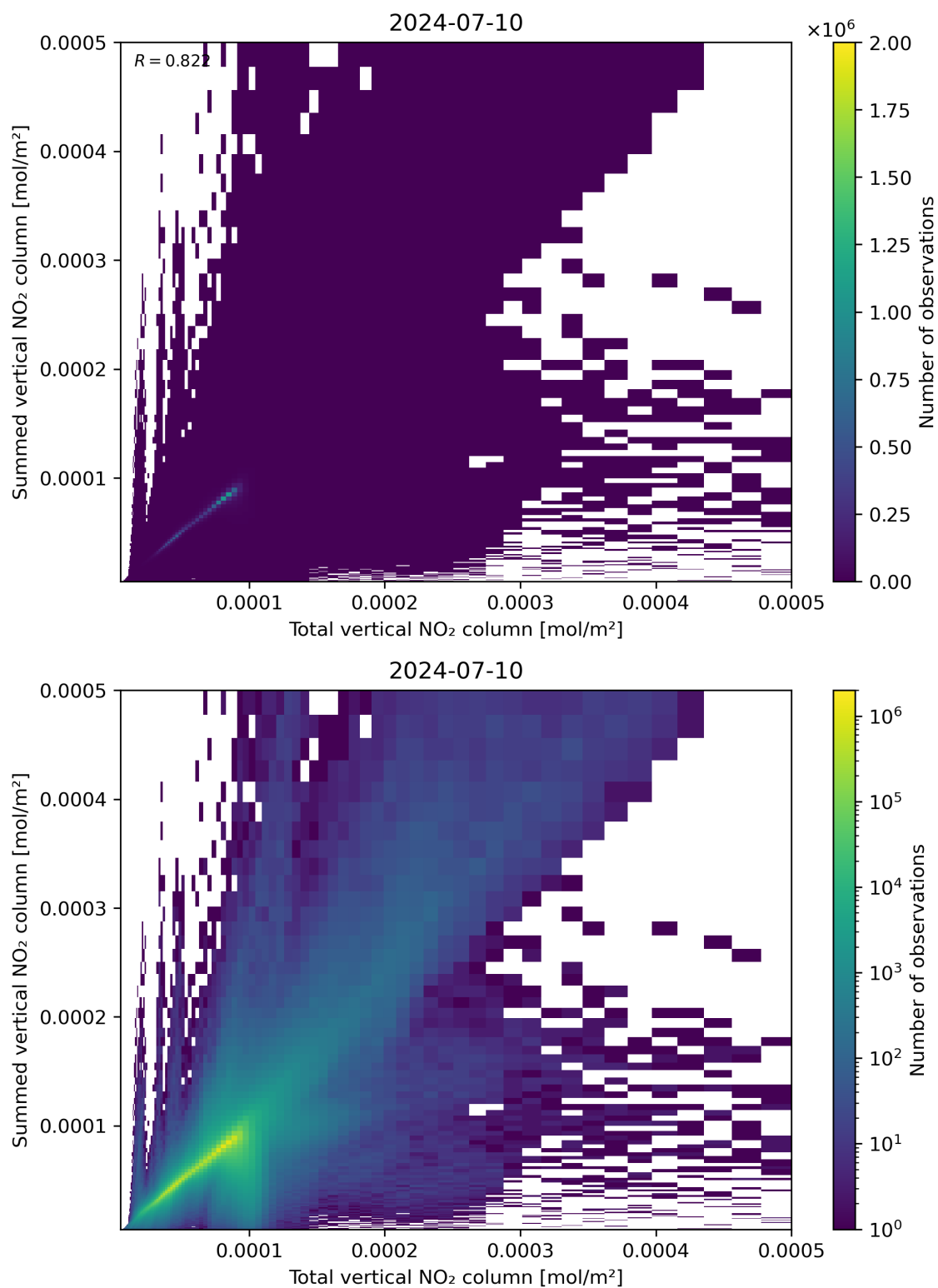
Figure 112: Scatter density plot of “Total vertical NO 2 column” against “Summed vertical NO 2 column” for 2024-07-10 to 2024-07-11.
