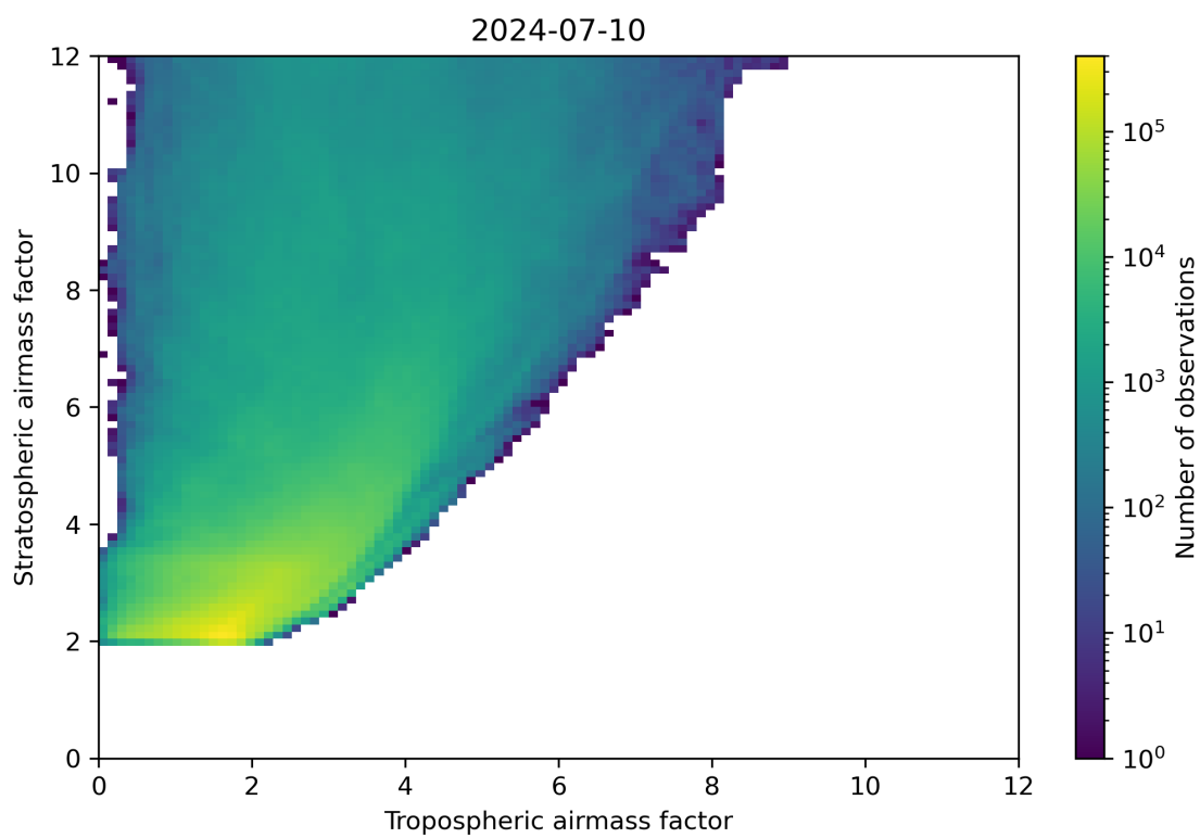
Figure 71: Scatter density plot of “Tropospheric airmass factor” against “Stratospheric airmass factor” for 2024-07-10 to 2024-07-11.
