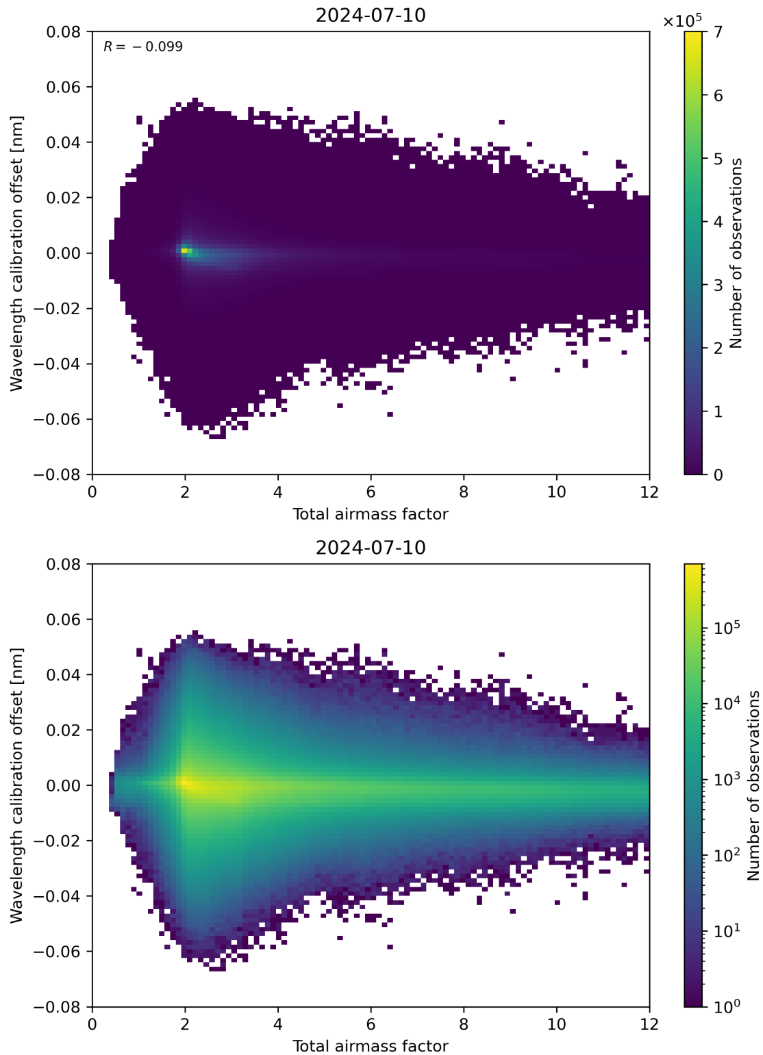
Figure 70: Scatter density plot of “Total airmass factor” against “Wavelength calibration offset” for 2024-07-10 to 2024-07-11.
