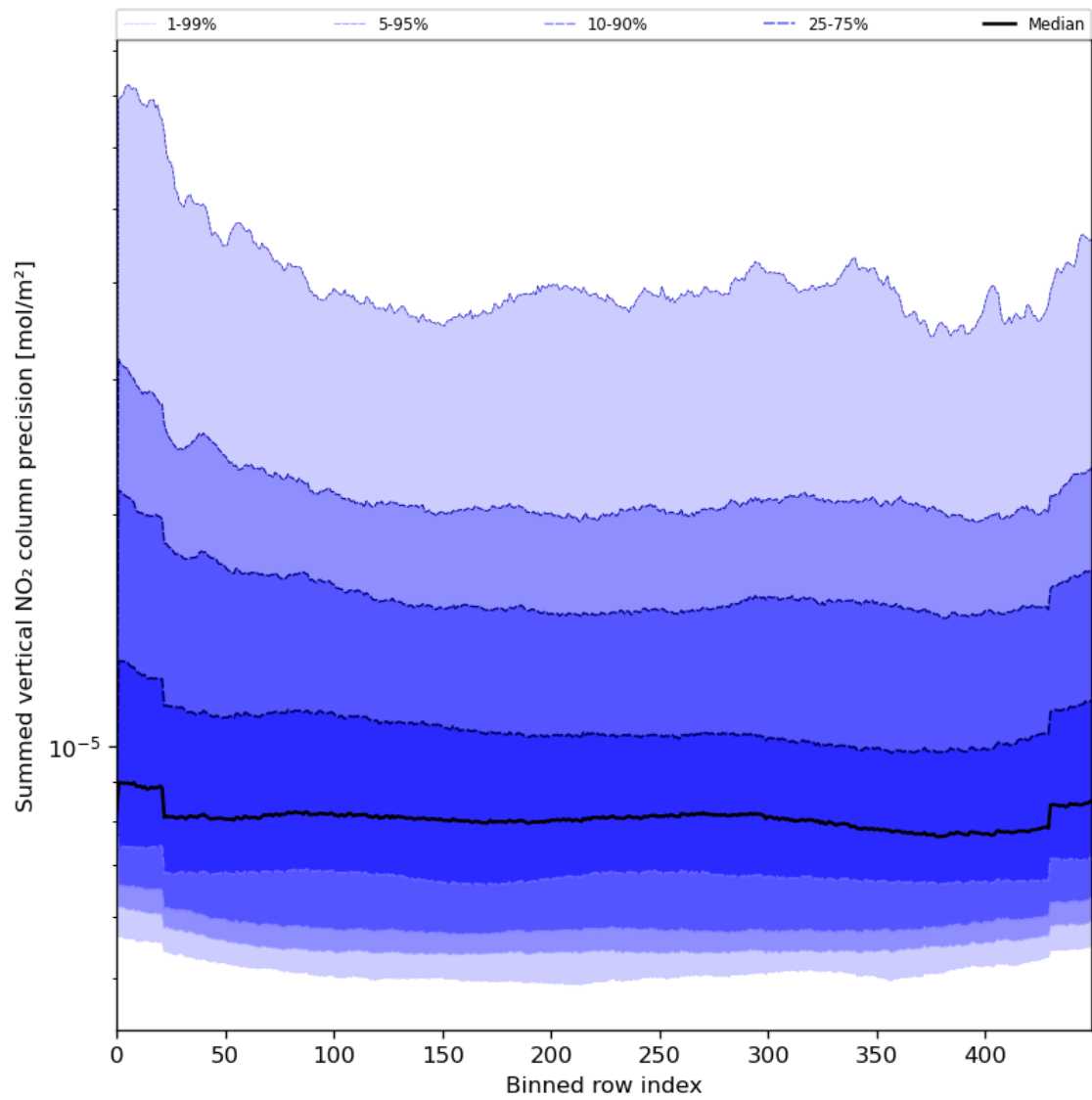
Figure 58: Along track statistics of “Summed vertical NO 2 column precision” for 2024-07-10 to 2024-07-11
