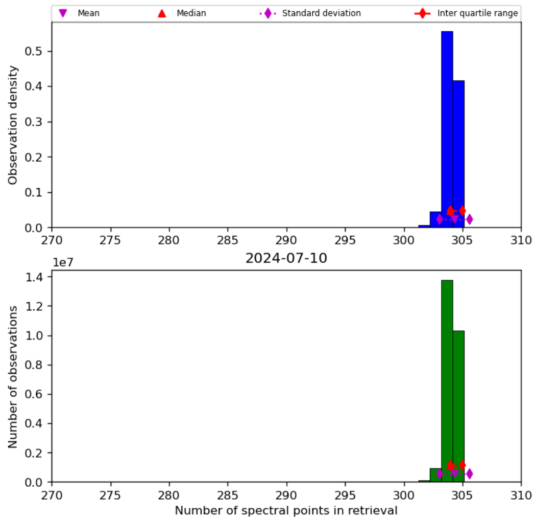
Figure 33: Histogram of “Number of spectral points in retrieval” for 2024-07-10 to 2024-07-11
