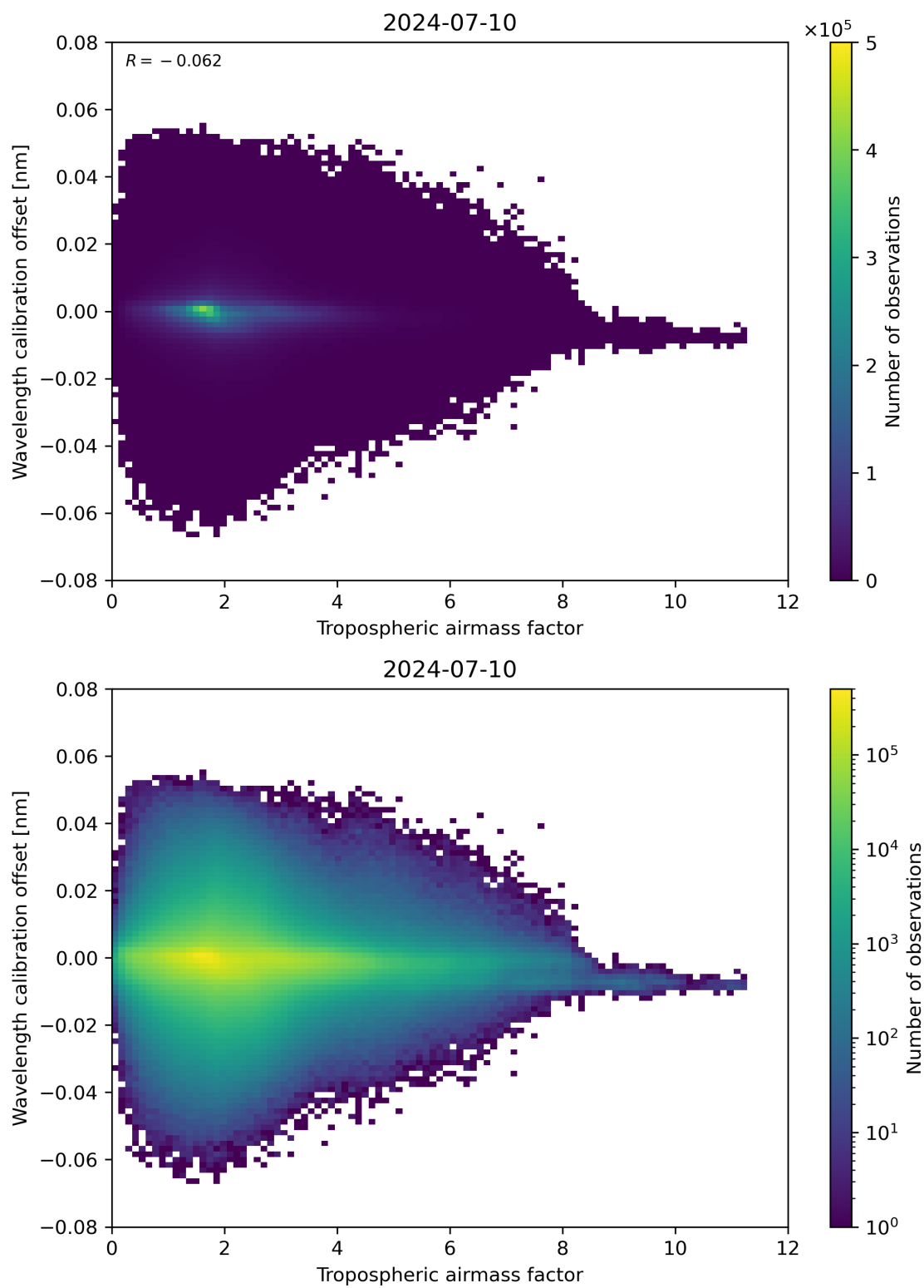
Figure 80: Scatter density plot of “Tropospheric airmass factor” against “Wavelength calibration offset” for 2024-07-10 to 2024-07-11.
