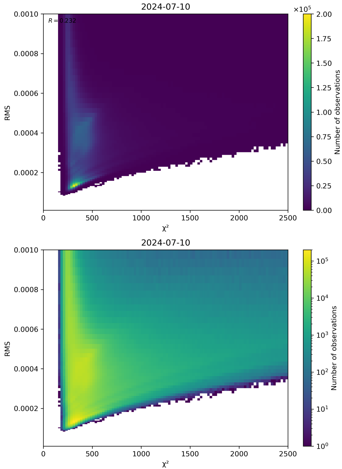
Figure 82: Scatter density plot of “ \chi^2 ” against “RMS” for 2024-07-10 to 2024-07-11.
