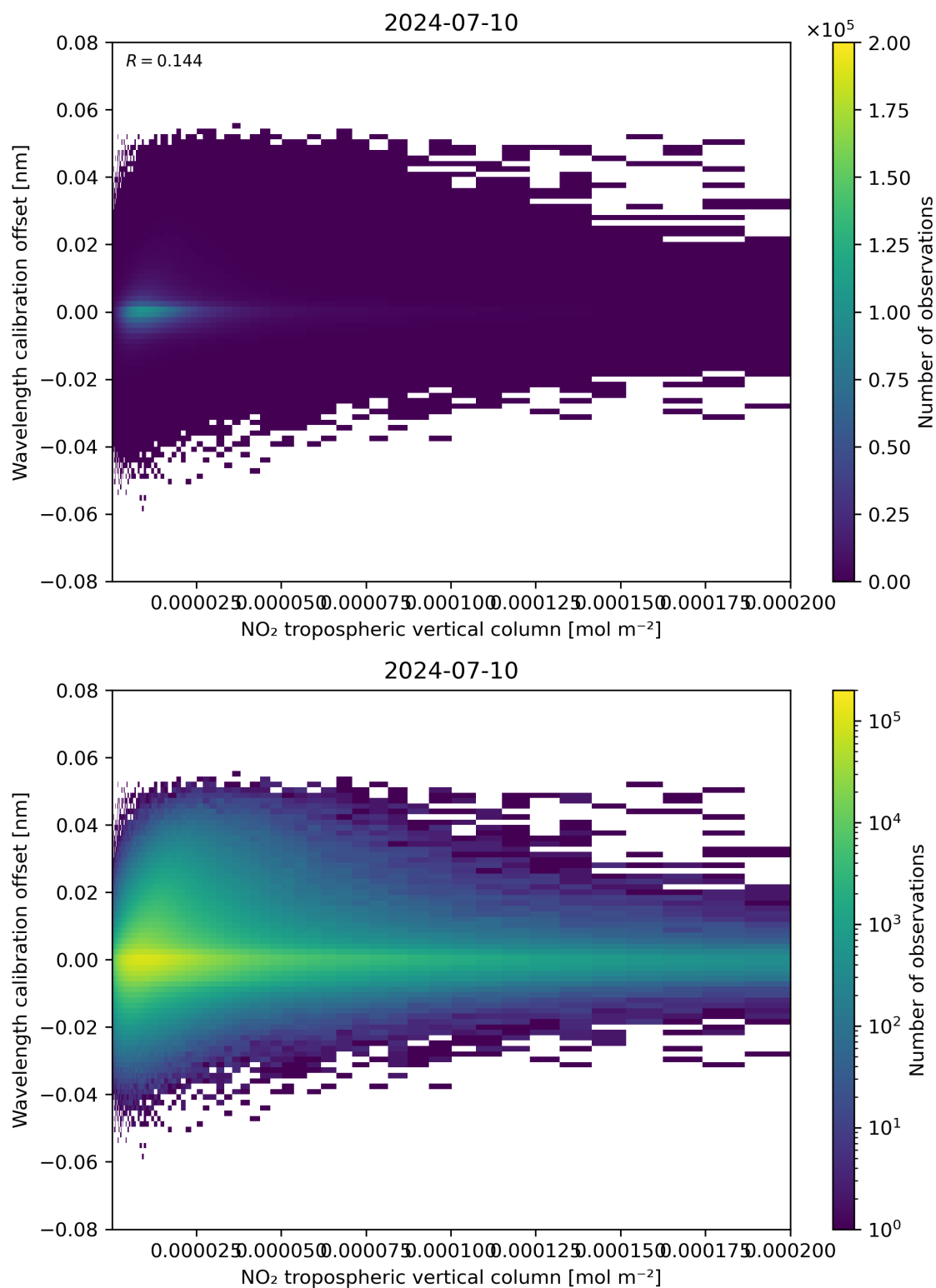
Figure 143: Scatter density plot of “NO 2 tropospheric vertical column” against “Wavelength calibration offset” for 2024-07-10 to 2024-07-11.
