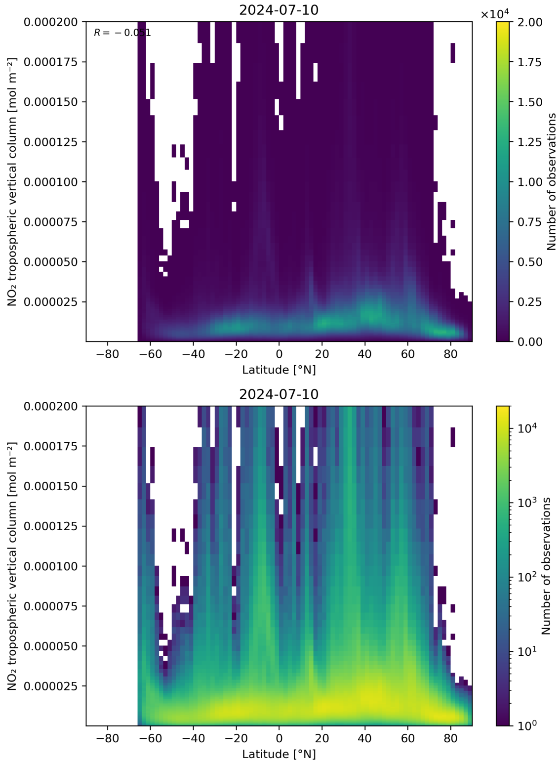
Figure 92: Scatter density plot of “Latitude” against “NO 2 tropospheric vertical column” for 2024-07-10 to 2024-07-11.
