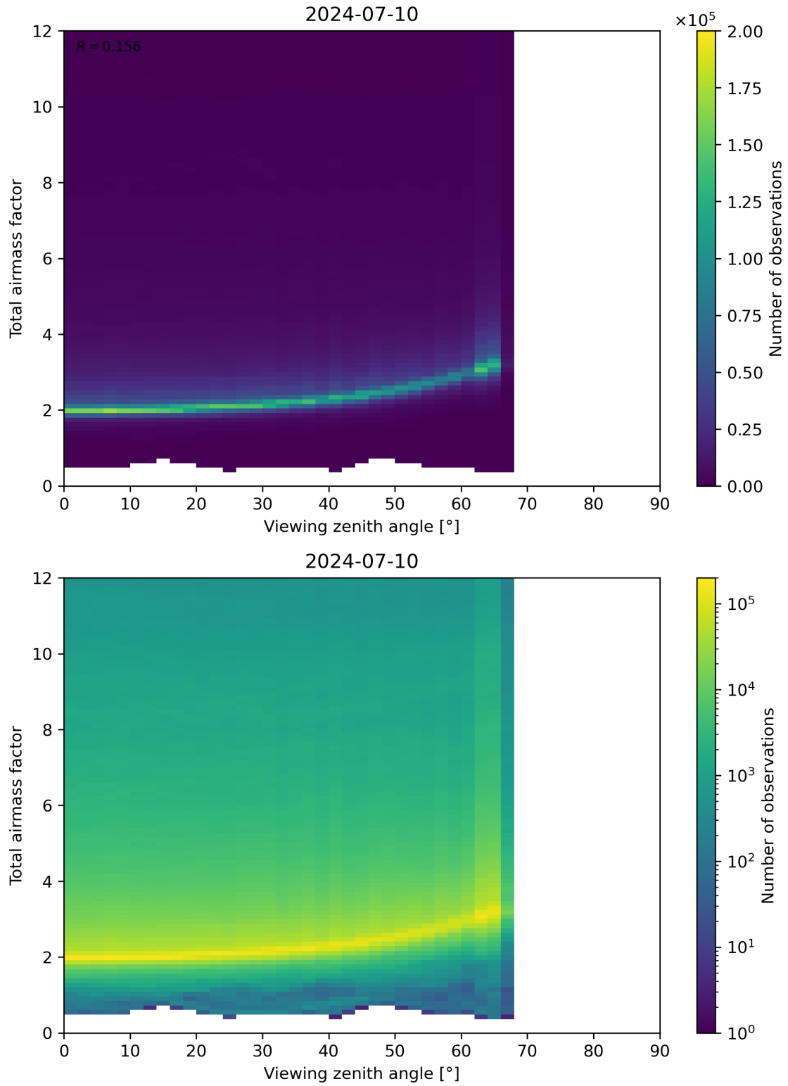
Figure 160: Scatter density plot of “Viewing zenith angle” against “Total airmass factor” for 2024-07-10 to 2024-07-11.
