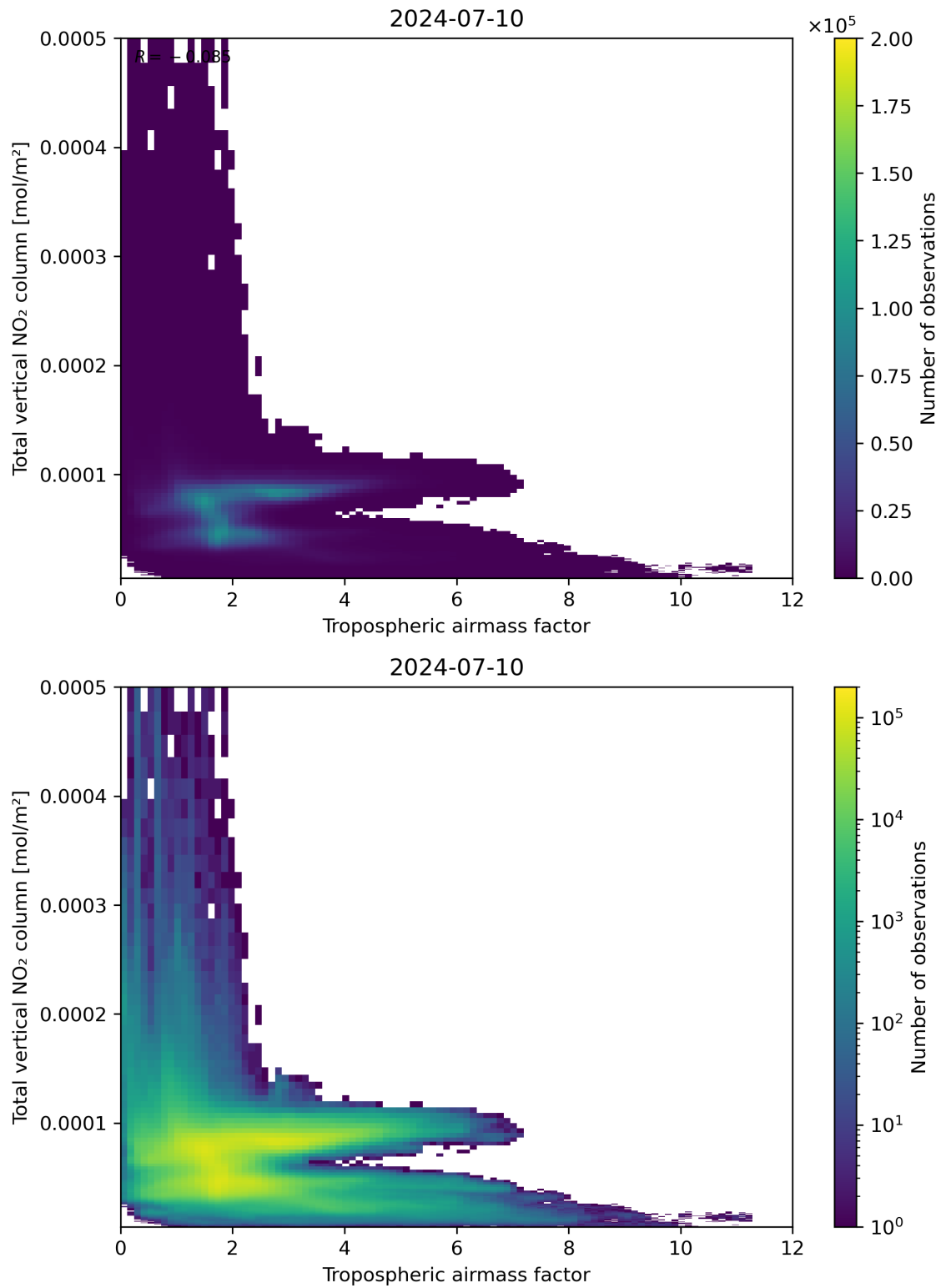
Figure 77: Scatter density plot of “Tropospheric airmass factor” against “Total vertical NO 2 column” for 2024-07-10 to 2024-07-11.
