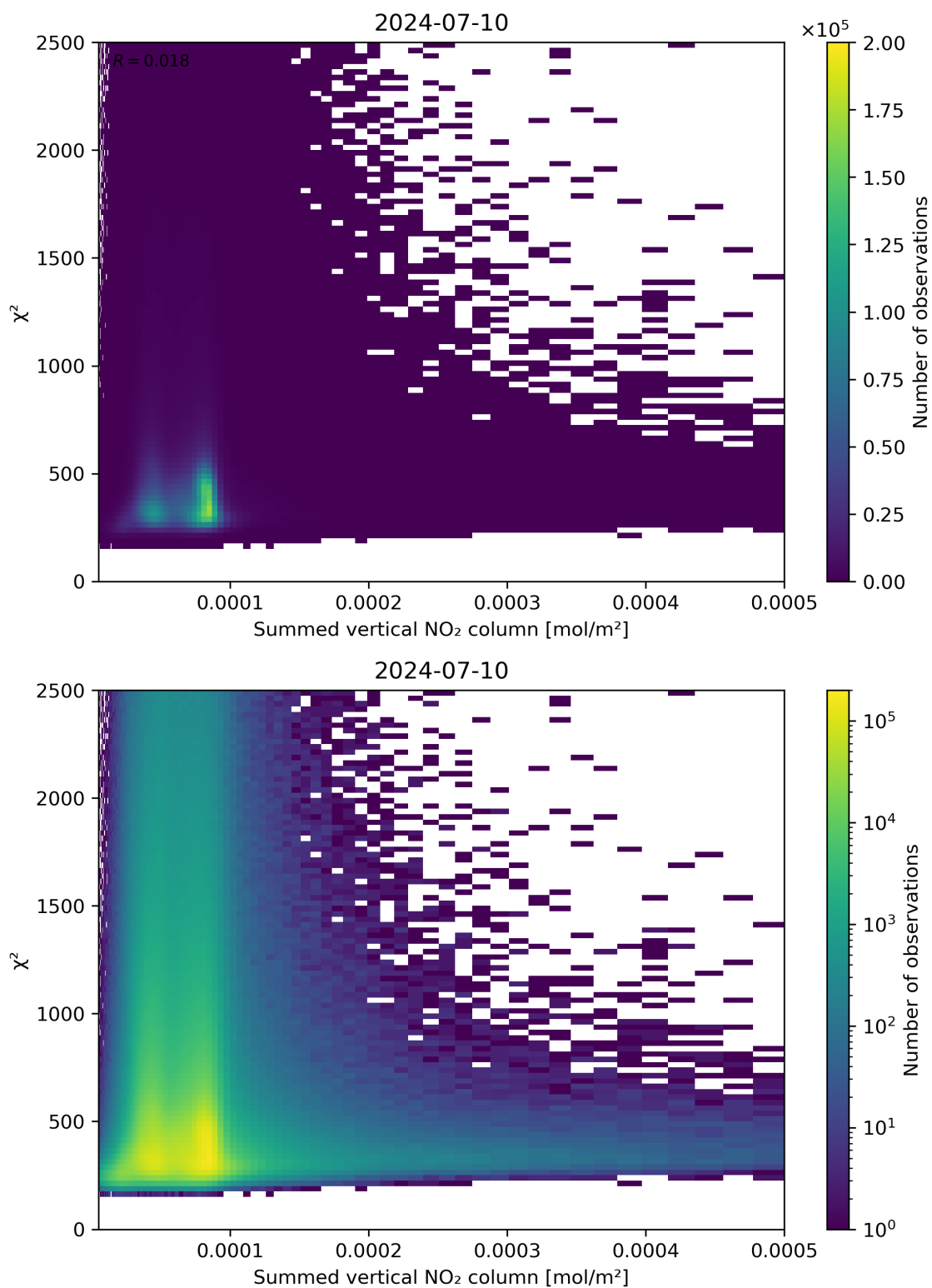
Figure 104: Scatter density plot of “Summed vertical NO 2 column” against “ \chi^2 ” for 2024-07-10 to 2024-07-11.
