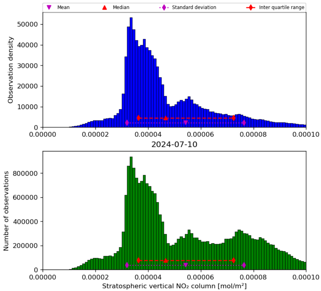
Figure 36: Histogram of “Stratospheric vertical NO 2 column” for 2024-07-10 to 2024-07-11
