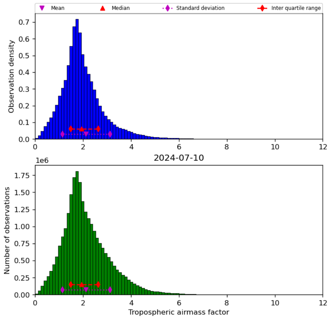
Figure 31: Histogram of “Tropospheric airmass factor” for 2024-07-10 to 2024-07-11
