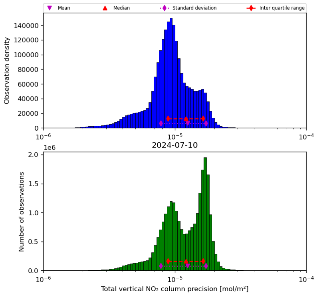
Figure 39: Histogram of “Total vertical NO 2 column precision” for 2024-07-10 to 2024-07-11
