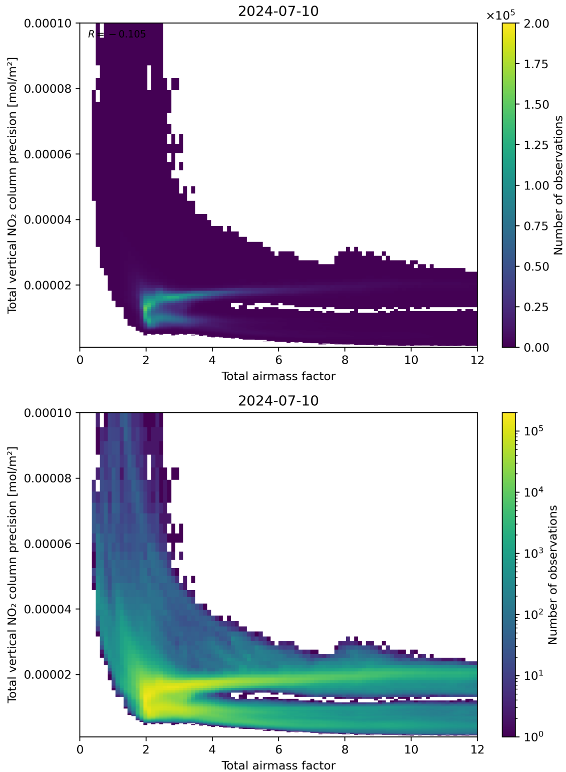
Figure 68: Scatter density plot of “Total airmass factor” against “Total vertical NO 2 column precision” for 2024-07-10 to 2024-07-11.
