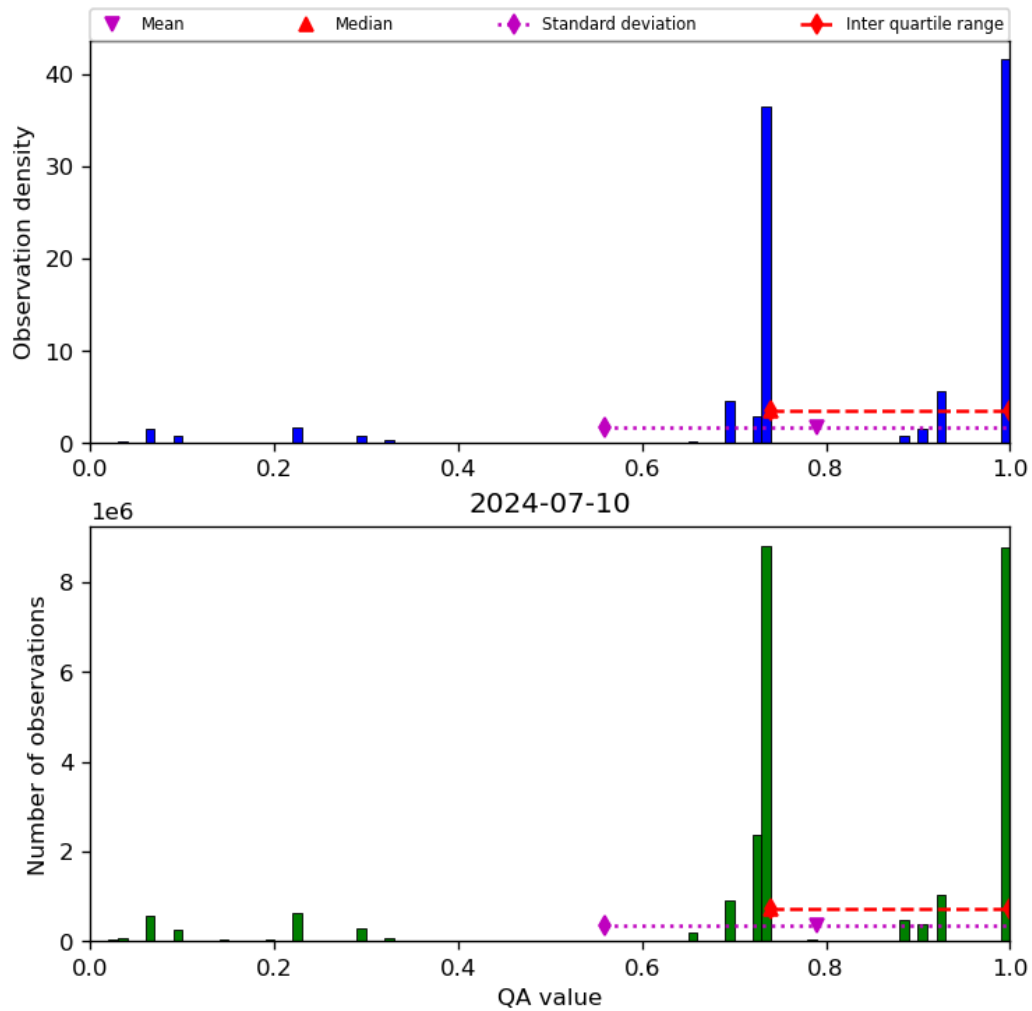
Figure 28: Histogram of “QA value” for 2024-07-10 to 2024-07-11
