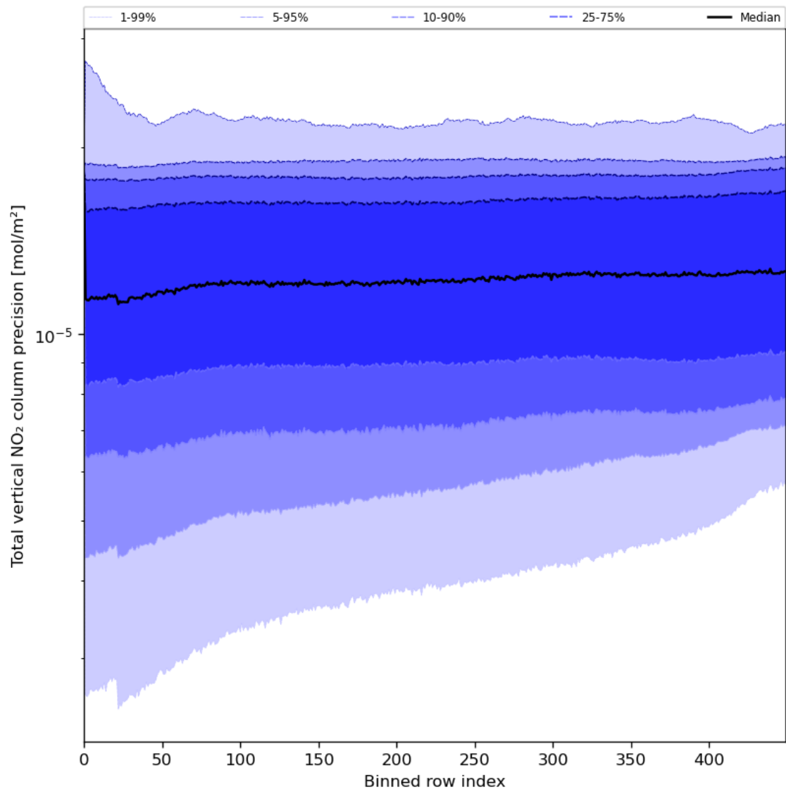
Figure 56: Along track statistics of “Total vertical NO 2 column precision” for 2024-07-10 to 2024-07-11
