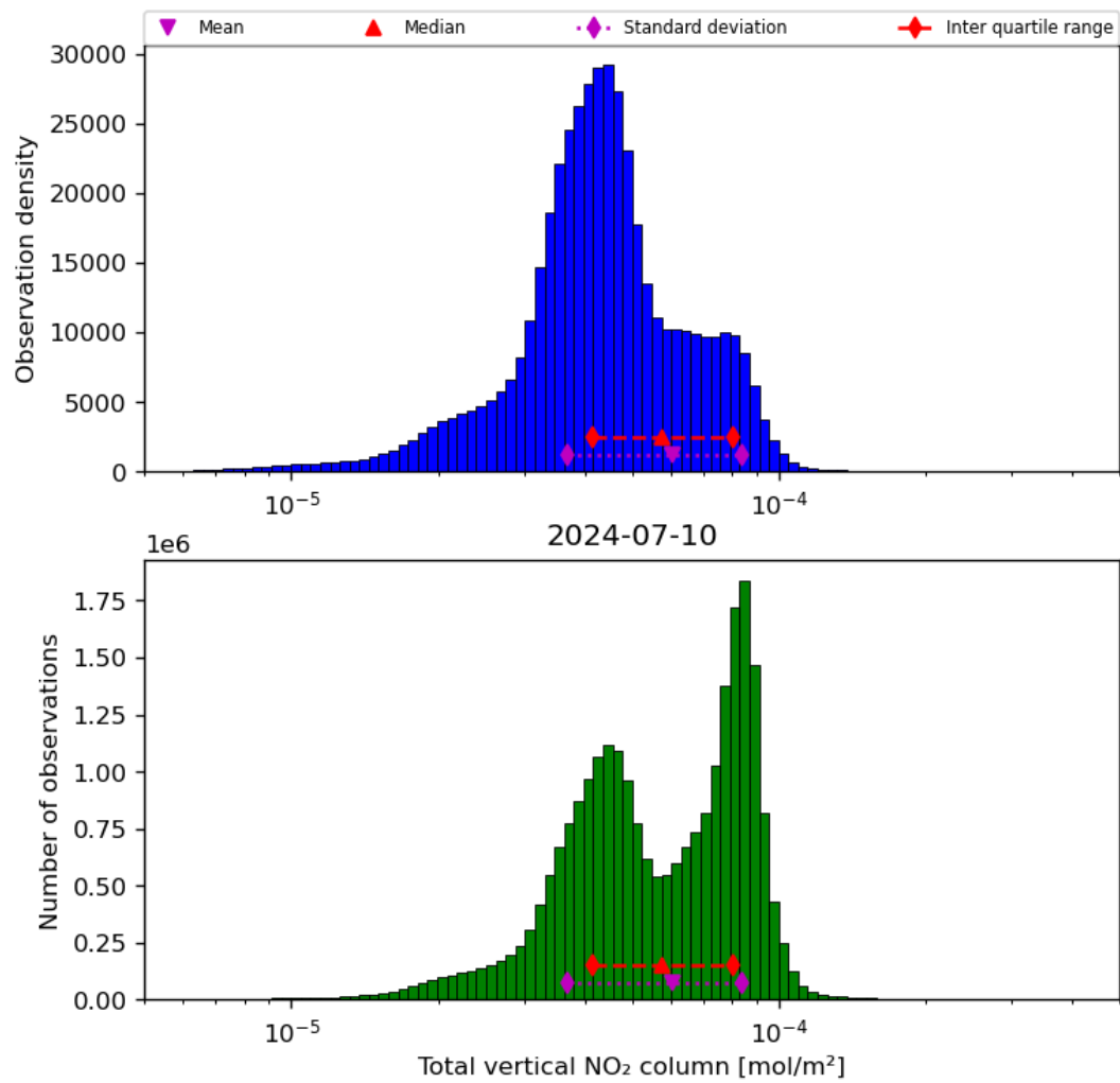
Figure 38: Histogram of “Total vertical NO 2 column” for 2024-07-10 to 2024-07-11
