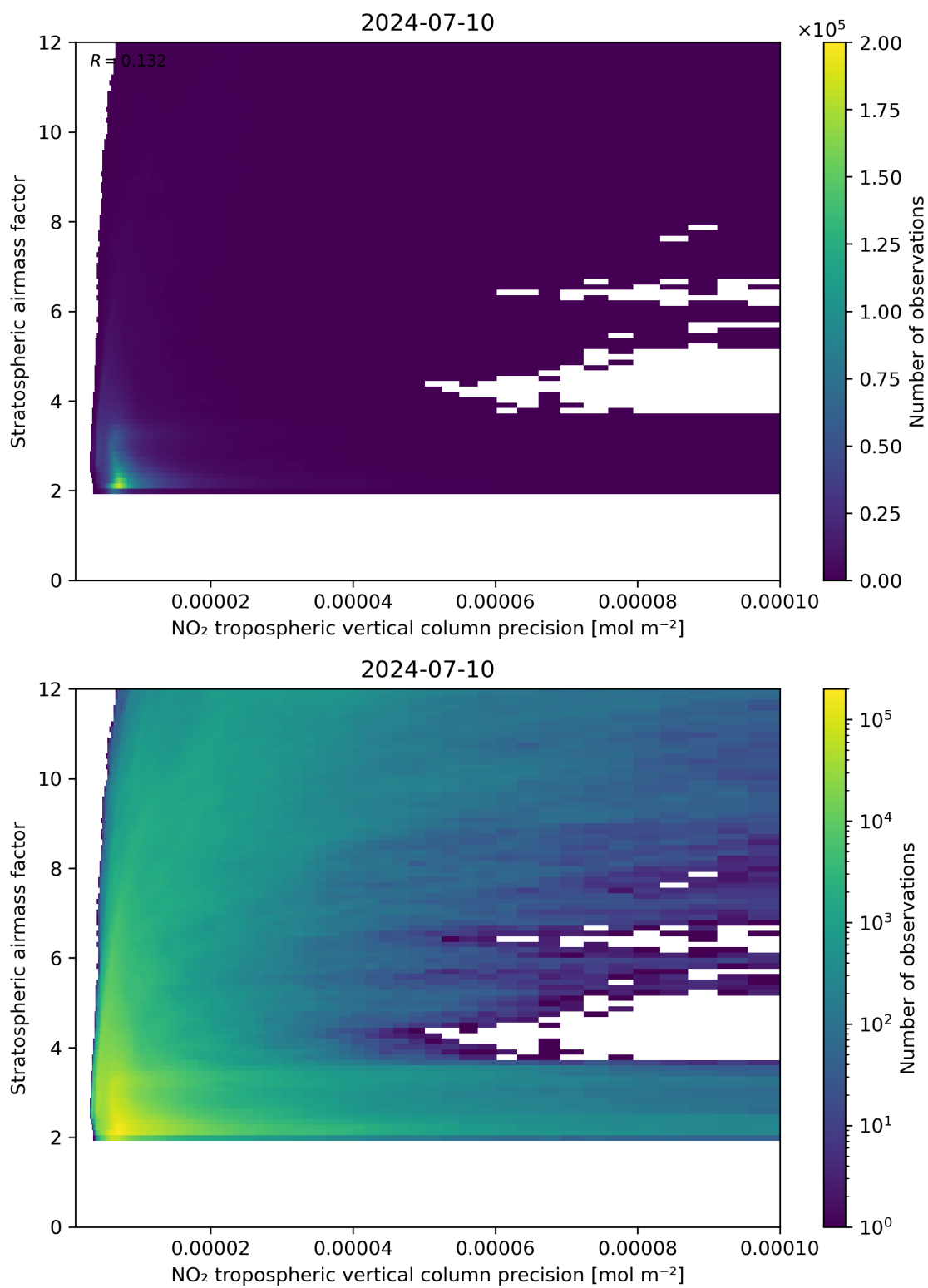
Figure 131: Scatter density plot of “NO 2 tropospheric vertical column precision” against “Stratospheric airmass factor” for 2024-07-10 to 2024-07-11.
