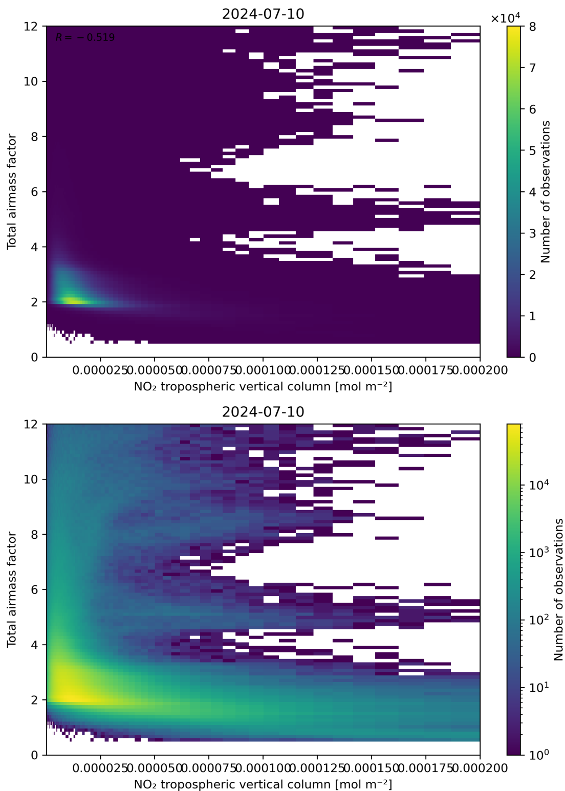
Figure 122: Scatter density plot of “NO 2 tropospheric vertical column” against “Total air mass factor” for 2024-07-10 to 2024-07-11.
