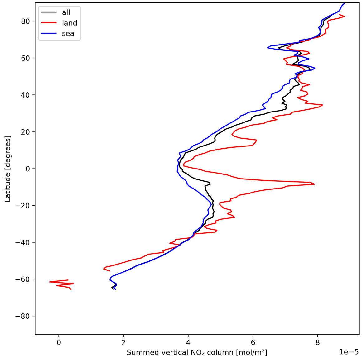
Figure 23: Zonal average of “Summed vertical NO 2 column” for 2024-07-10 to 2024-07-11.
