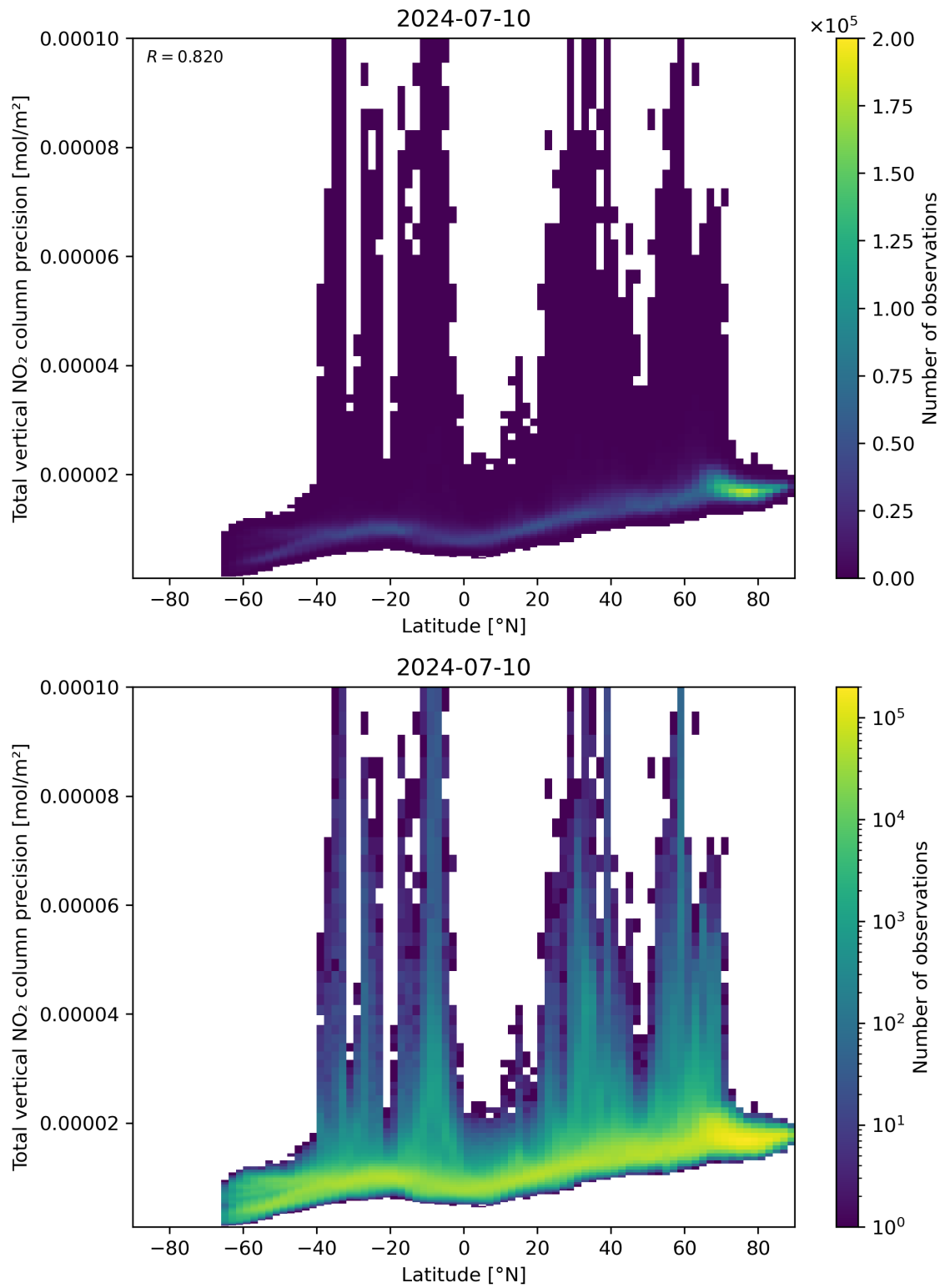
Figure 91: Scatter density plot of “Latitude” against “Total vertical NO 2 column precision” for 2024-07-10 to 2024-07-11.
