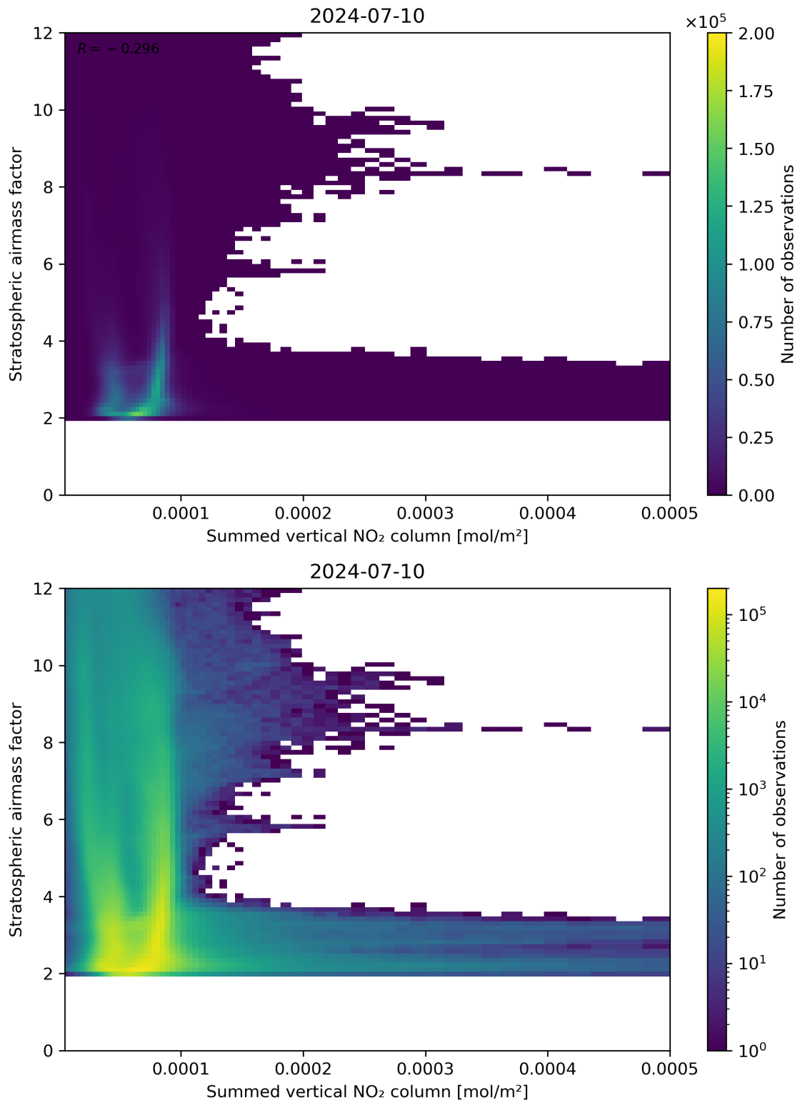
Figure 103: Scatter density plot of “Summed vertical NO 2 column” against “Stratospheric air mass factor” for 2024-07-10 to 2024-07-11.
