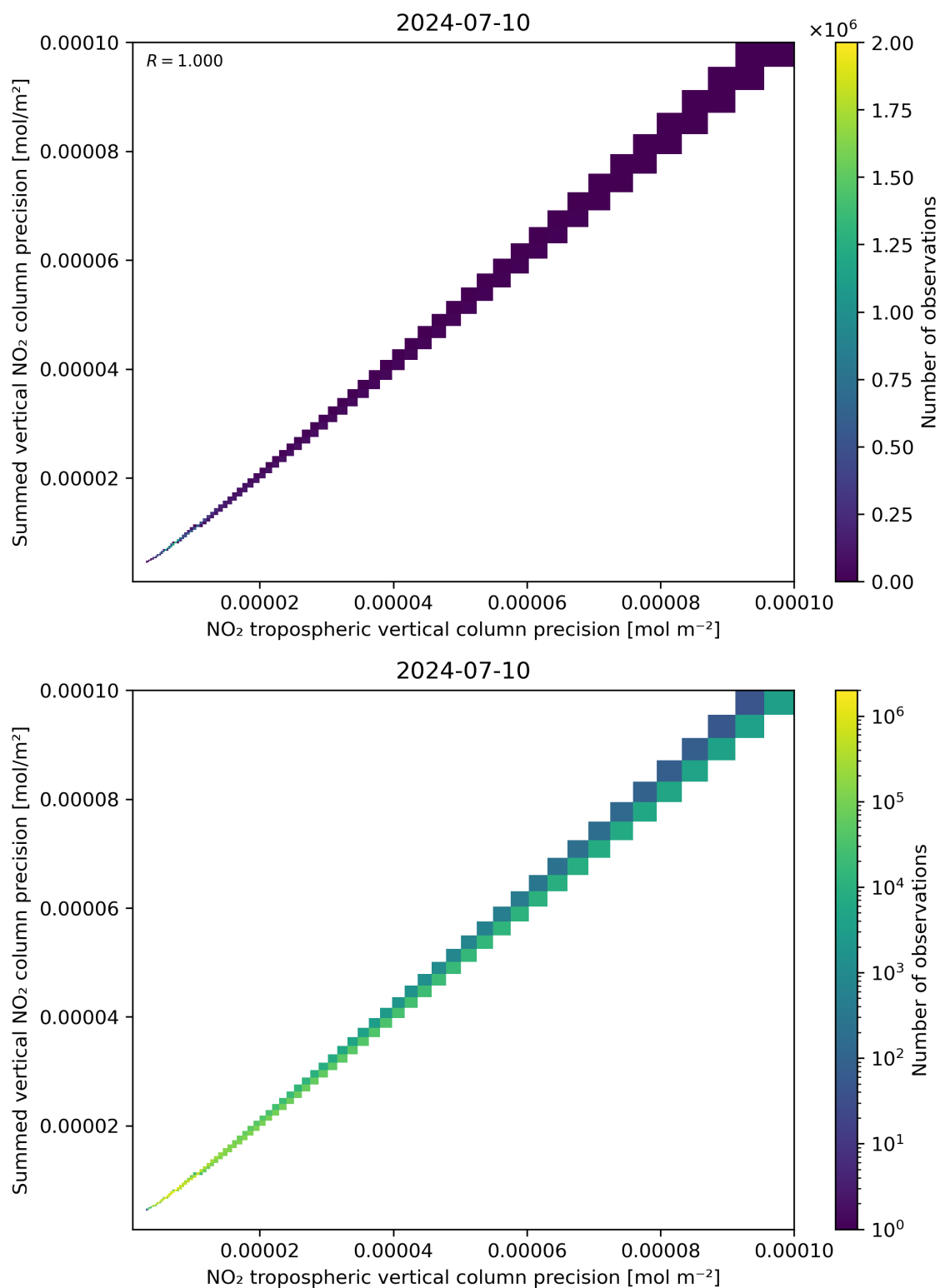
Figure 137: Scatter density plot of “NO 2 tropospheric vertical column precision” against “Summed vertical NO 2 column precision” for 2024-07-10 to 2024-07-11.
