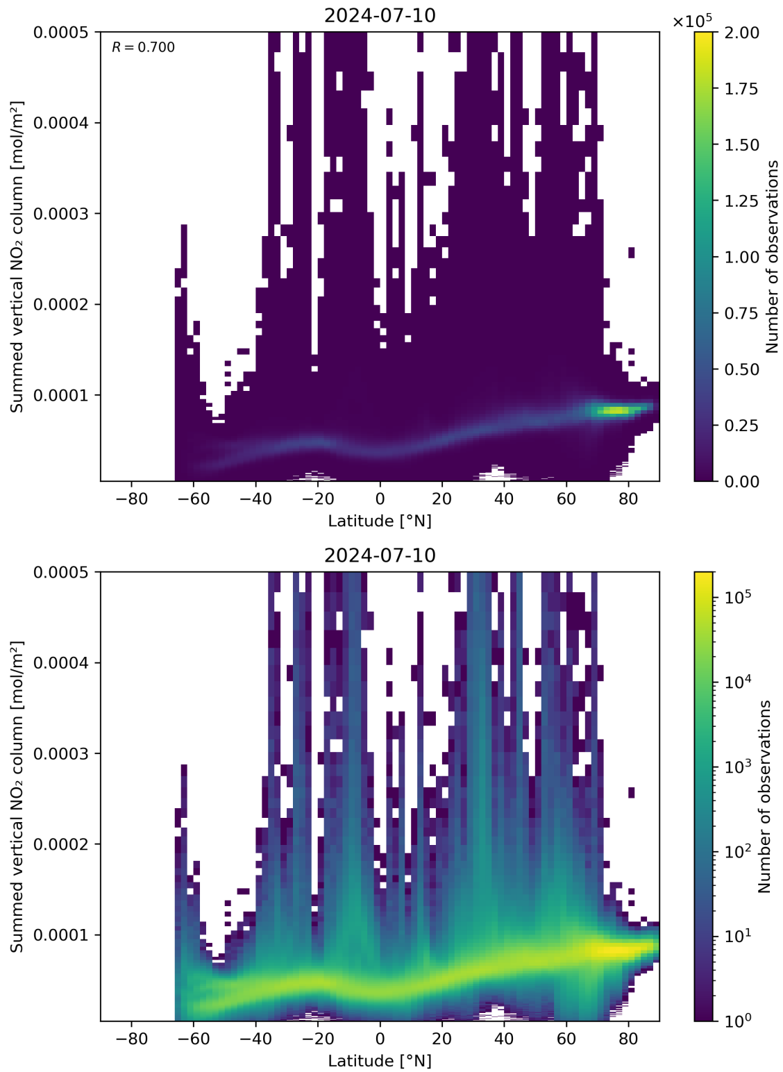
Figure 88: Scatter density plot of “Latitude” against “Summed vertical NO 2 column” for 2024-07-10 to 2024-07-11.
