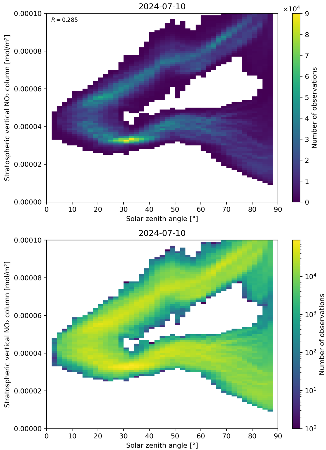
Figure 150: Scatter density plot of “Solar zenith angle” against “Stratospheric vertical NO 2 column” for 2024-07-10 to 2024-07-11.
