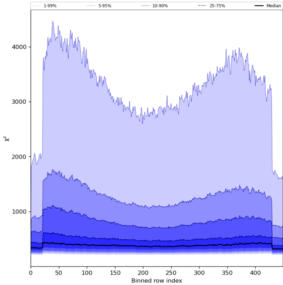
Figure 59: Along track statistics of “ \chi^2 ” for 2024-07-10 to 2024-07-11
