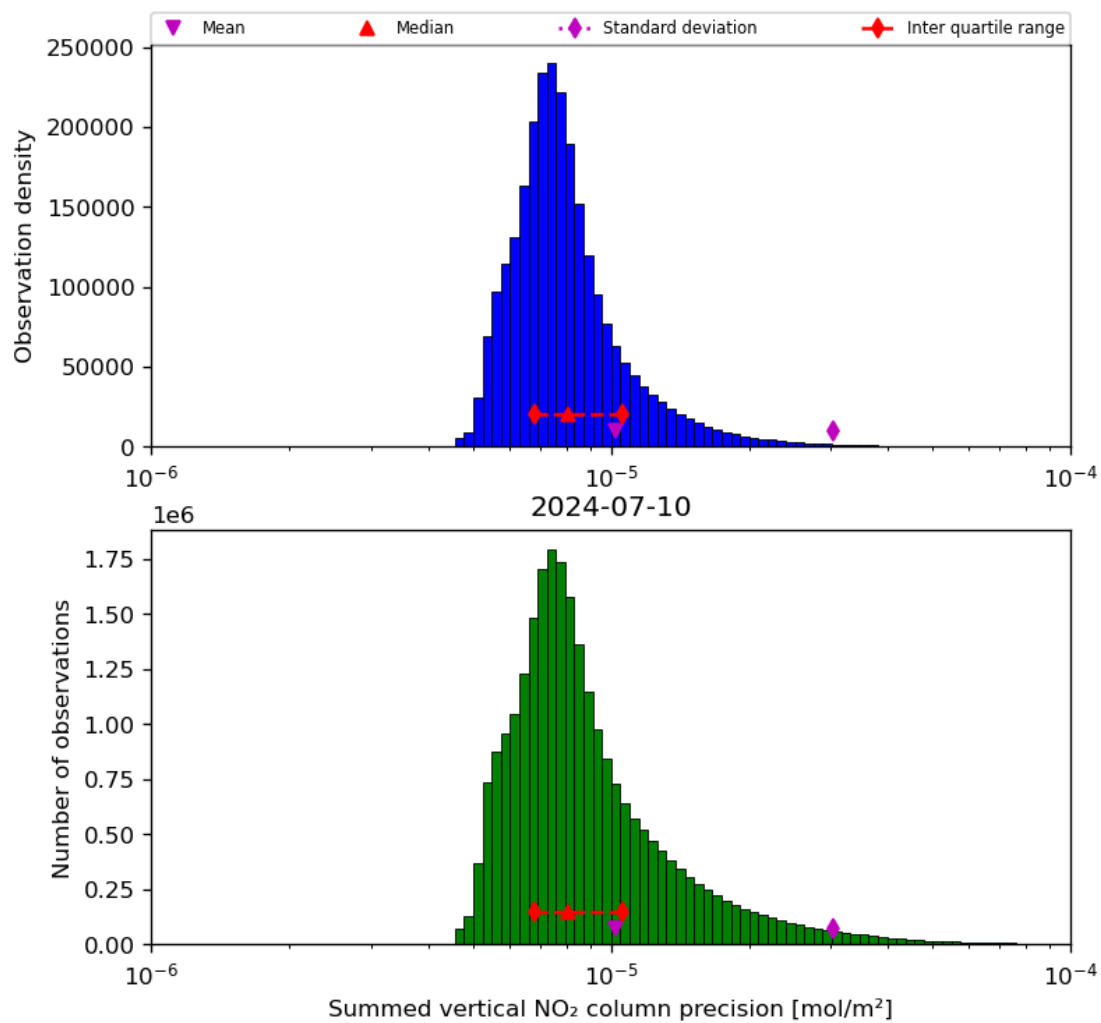
Figure 41: Histogram of "Summed vertical NO 2 column precision" for 2024-07-10 to 2024-07-11
