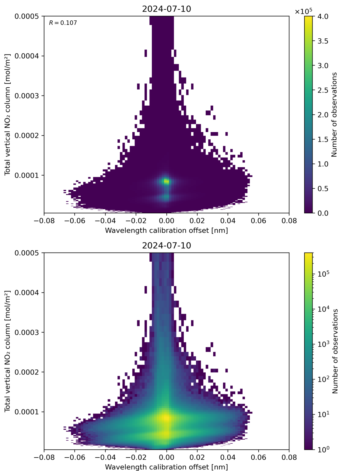
Figure 179: Scatter density plot of “Wavelength calibration offset” against “Total vertical NO 2 column” for 2024-07-10 to 2024-07-11.
