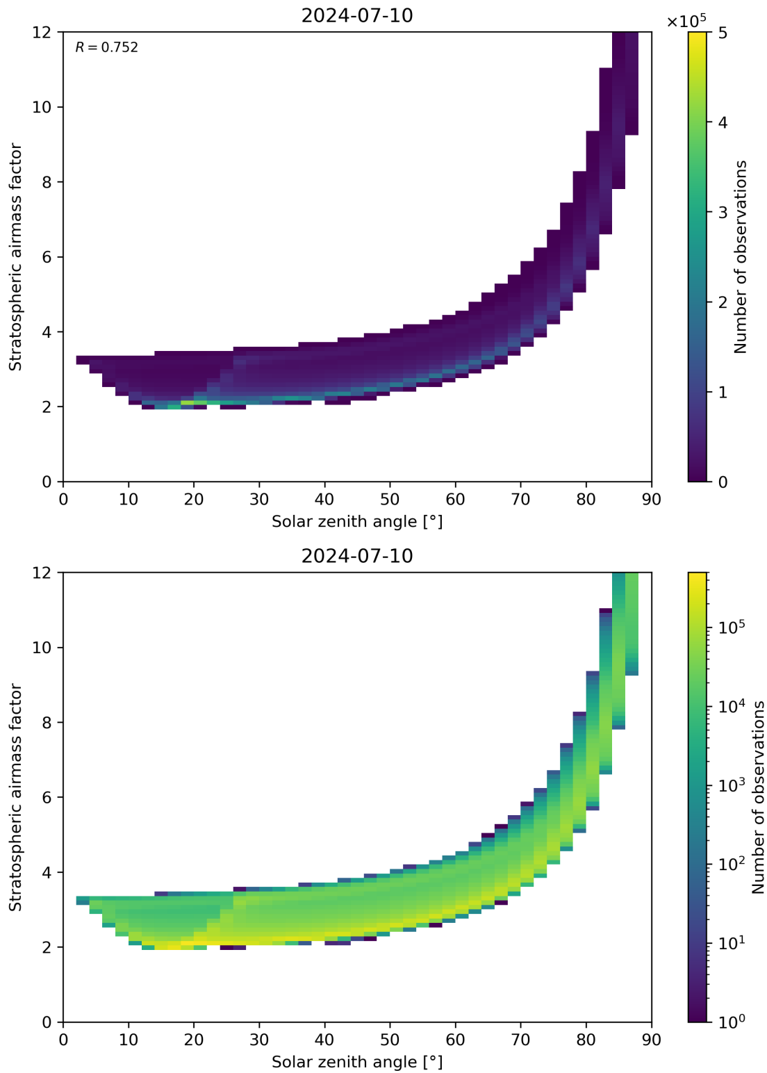
Figure 145: Scatter density plot of “Solar zenith angle” against “Stratospheric airmass factor” for 2024-07-10 to 2024-07-11.
