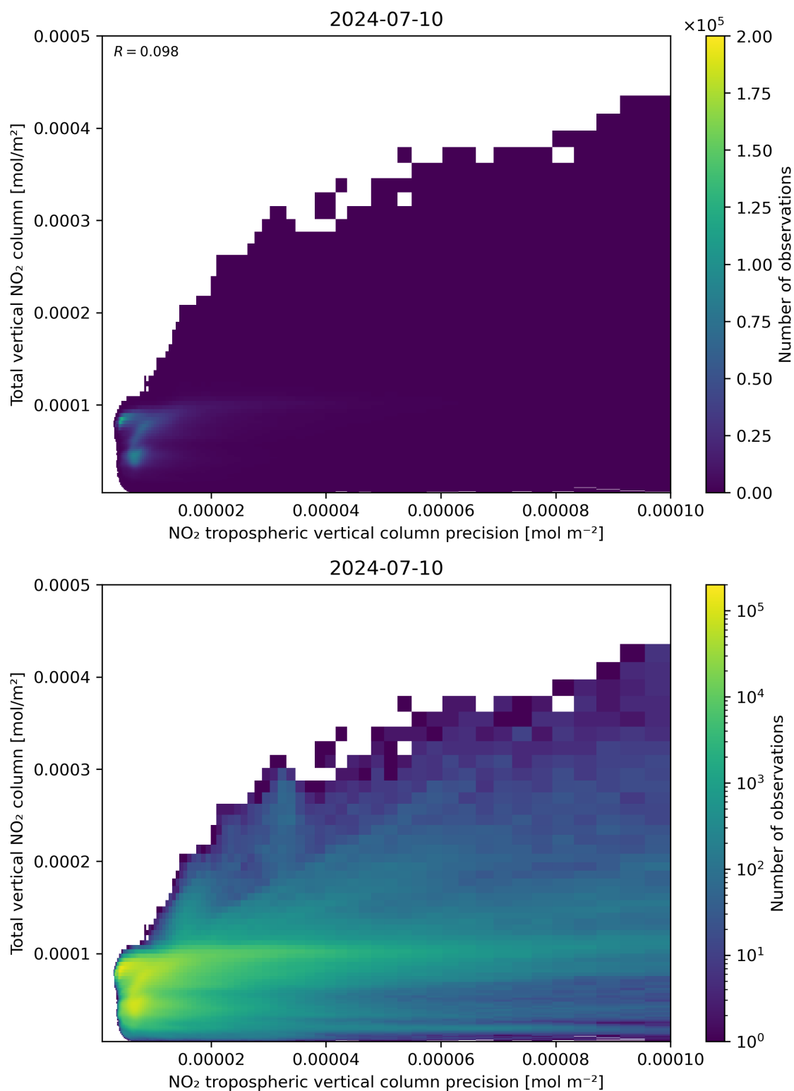
Figure 138: Scatter density plot of “NO 2 tropospheric vertical column precision” against “Total vertical NO 2 column” for 2024-07-10 to 2024-07-11.
