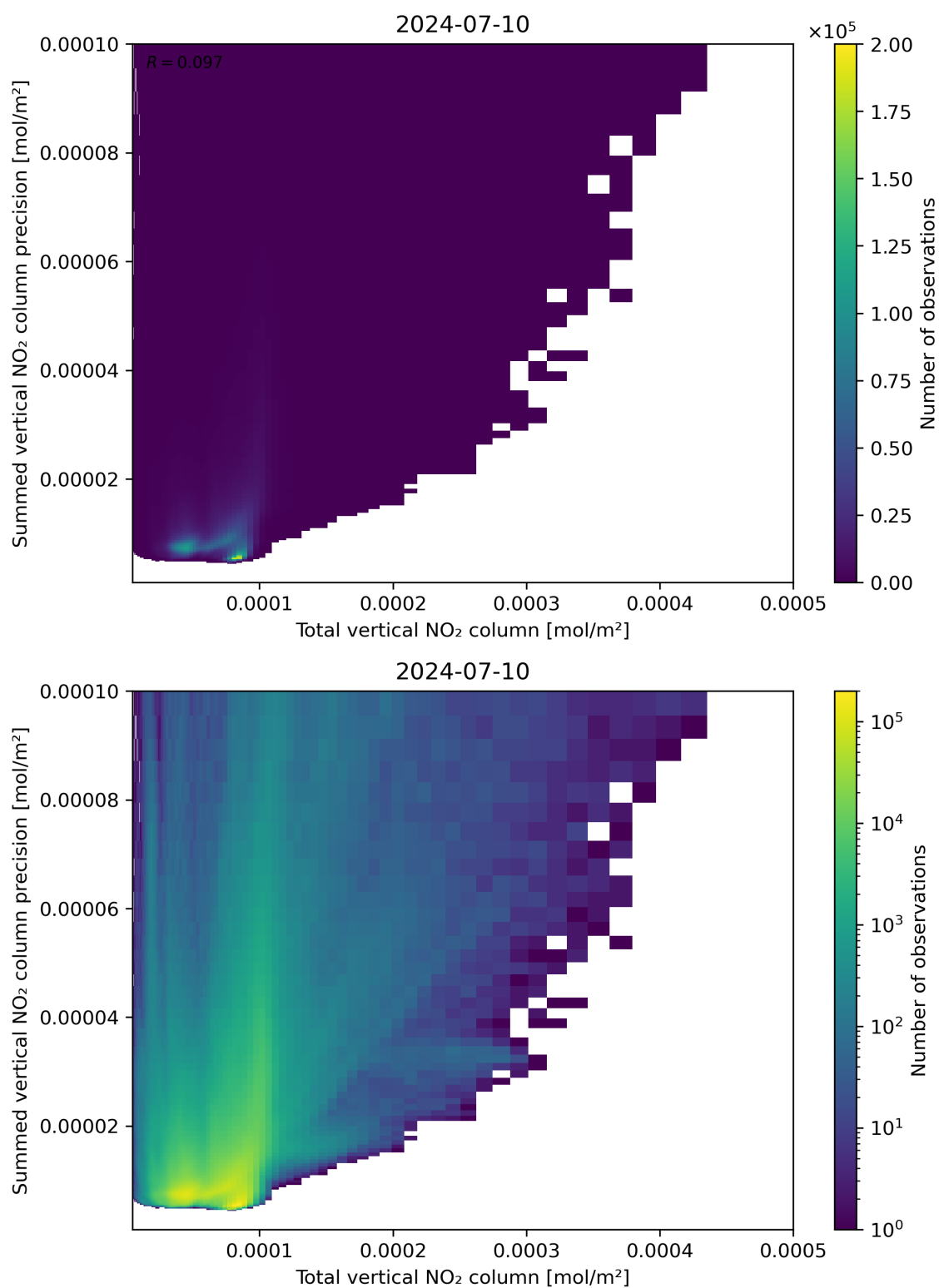
Figure 113: Scatter density plot of “Total vertical NO 2 column” against “Summed vertical NO 2 column precision” for 2024-07-10 to 2024-07-11.
