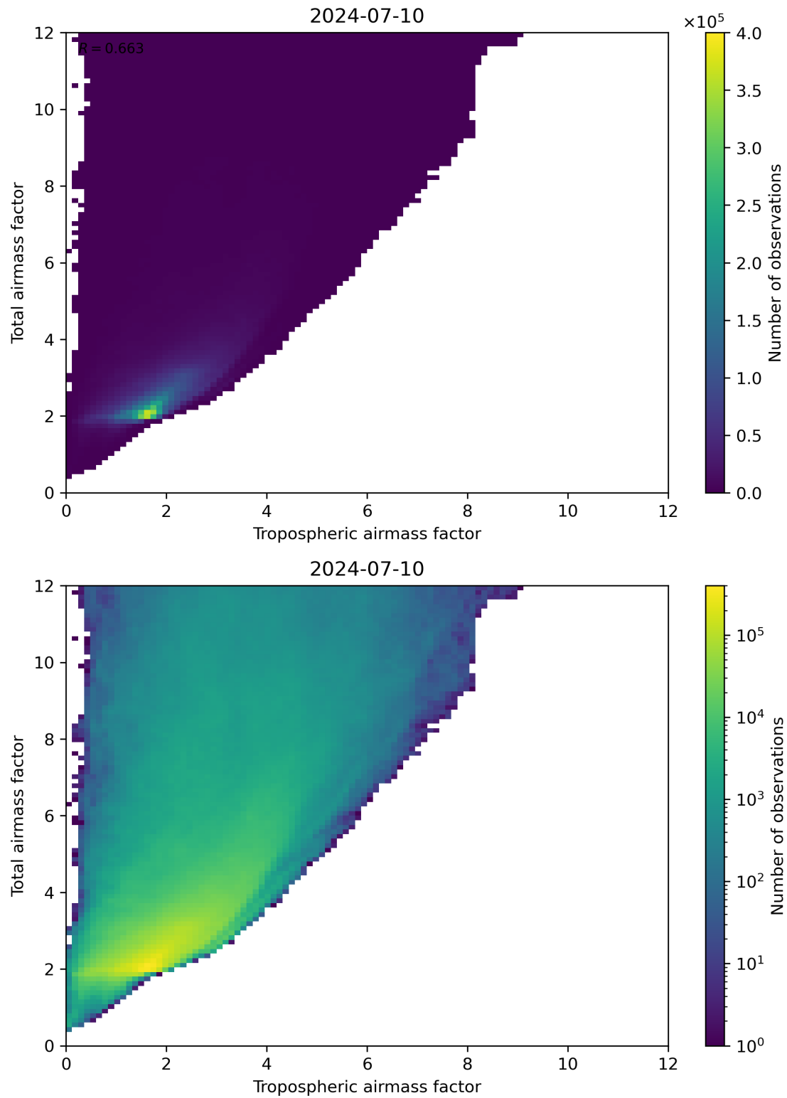
Figure 72: Scatter density plot of “Tropospheric airmass factor” against “Total airmass factor” for 2024-07-10 to 2024-07-11.
