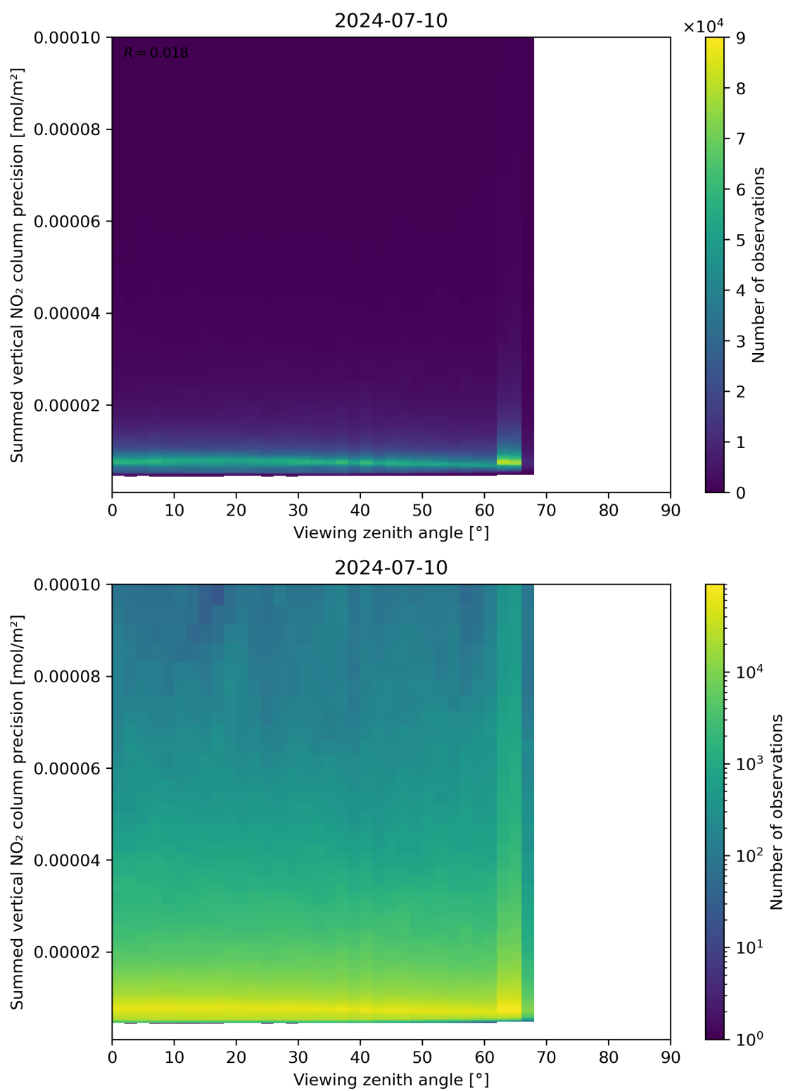
Figure 166: Scatter density plot of “Viewing zenith angle” against “Summed vertical NO 2 column precision” for 2024-07-10 to 2024-07-11.
