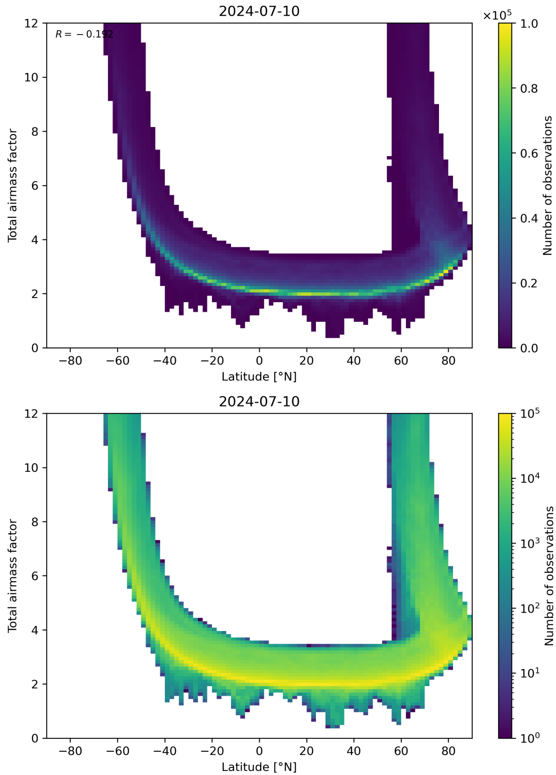
Figure 84: Scatter density plot of “Latitude” against “Total airmass factor” for 2024-07-10 to 2024-07-11.
