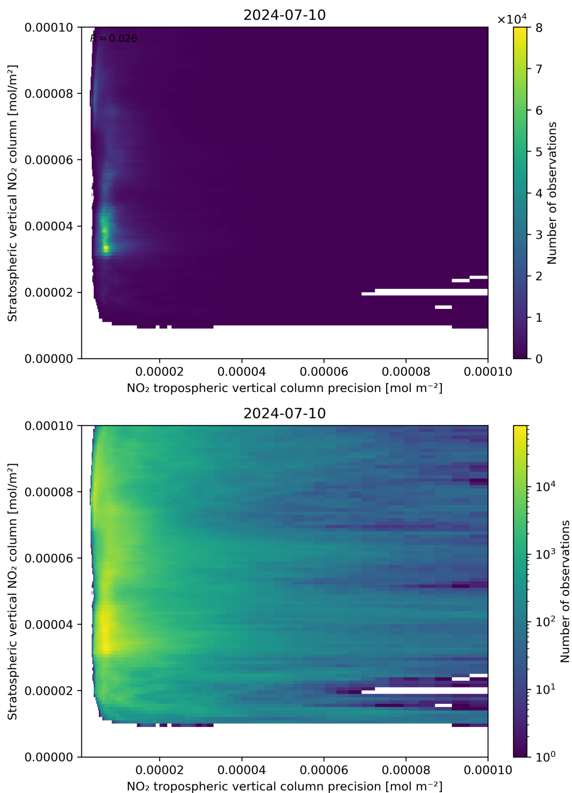
Figure 135: Scatter density plot of “NO 2 tropospheric vertical column precision” against “Stratospheric vertical NO 2 column” for 2024-07-10 to 2024-07-11.
