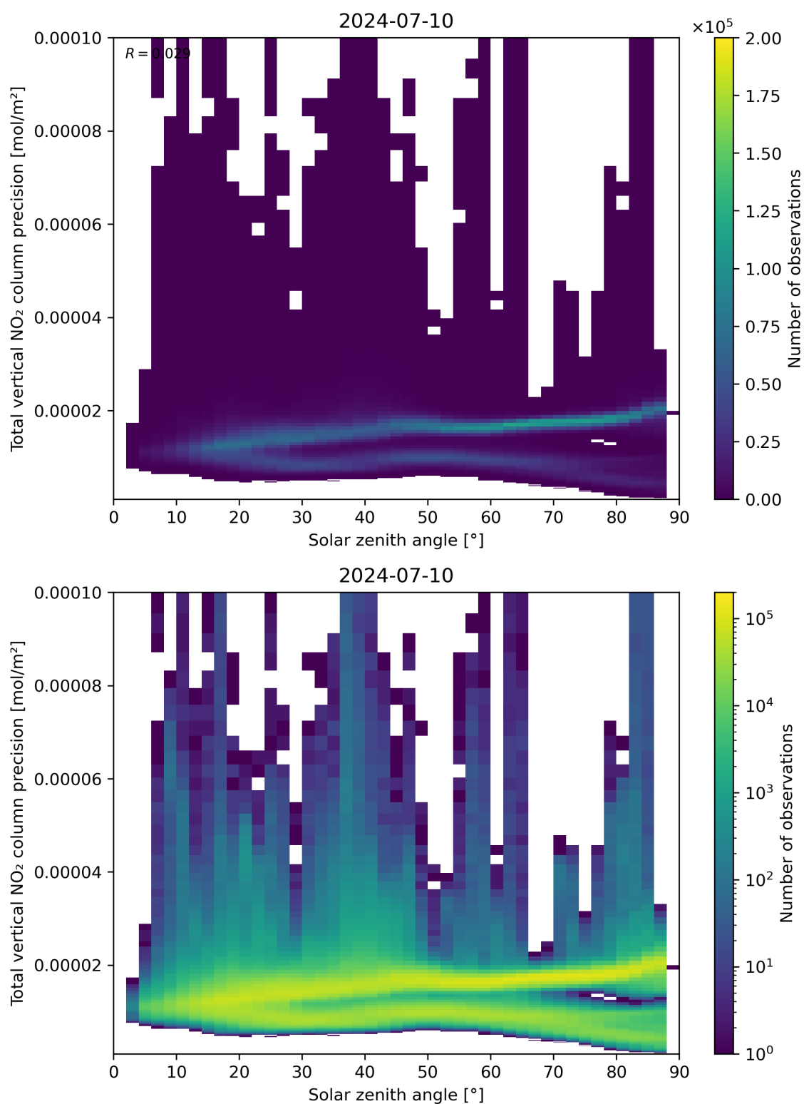
Figure 154: Scatter density plot of “Solar zenith angle” against “Total vertical NO 2 column precision” for 2024-07-10 to 2024-07-11.
