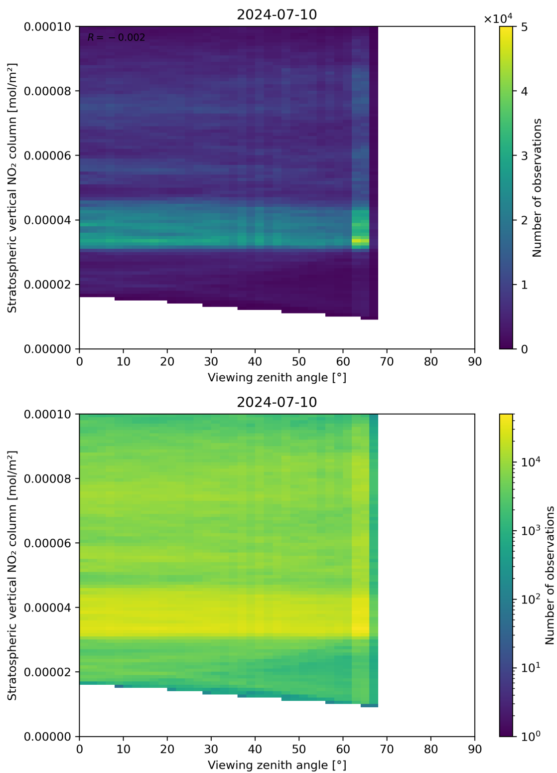
Figure 164: Scatter density plot of “Viewing zenith angle” against “Stratospheric vertical NO 2 column” for 2024-07-10 to 2024-07-11.
