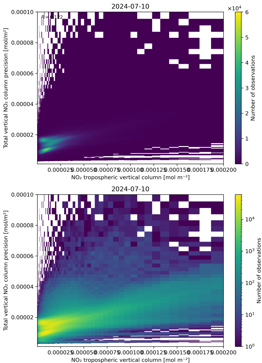
Figure 129: Scatter density plot of “NO 2 tropospheric vertical column” against “Total vertical NO 2 column precision” for 2024-07-10 to 2024-07-11.
