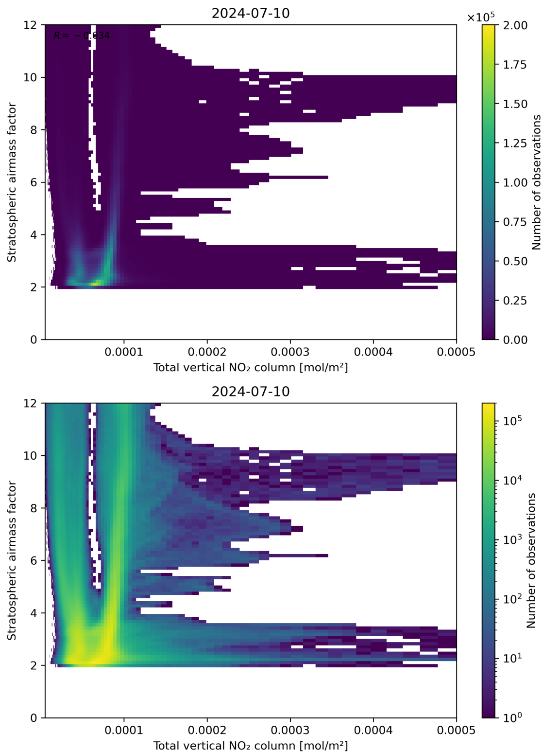
Figure 110: Scatter density plot of “Total vertical NO 2 column” against “Stratospheric air mass factor” for 2024-07-10 to 2024-07-11.
