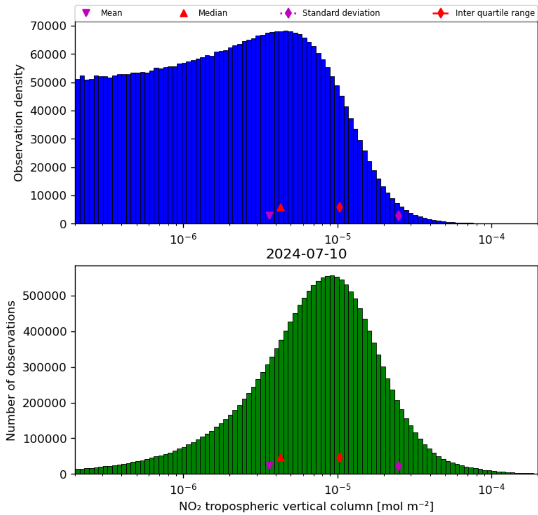
Figure 29: Histogram of “NO 2 tropospheric vertical column” for 2024-07-10 to 2024-07-11
