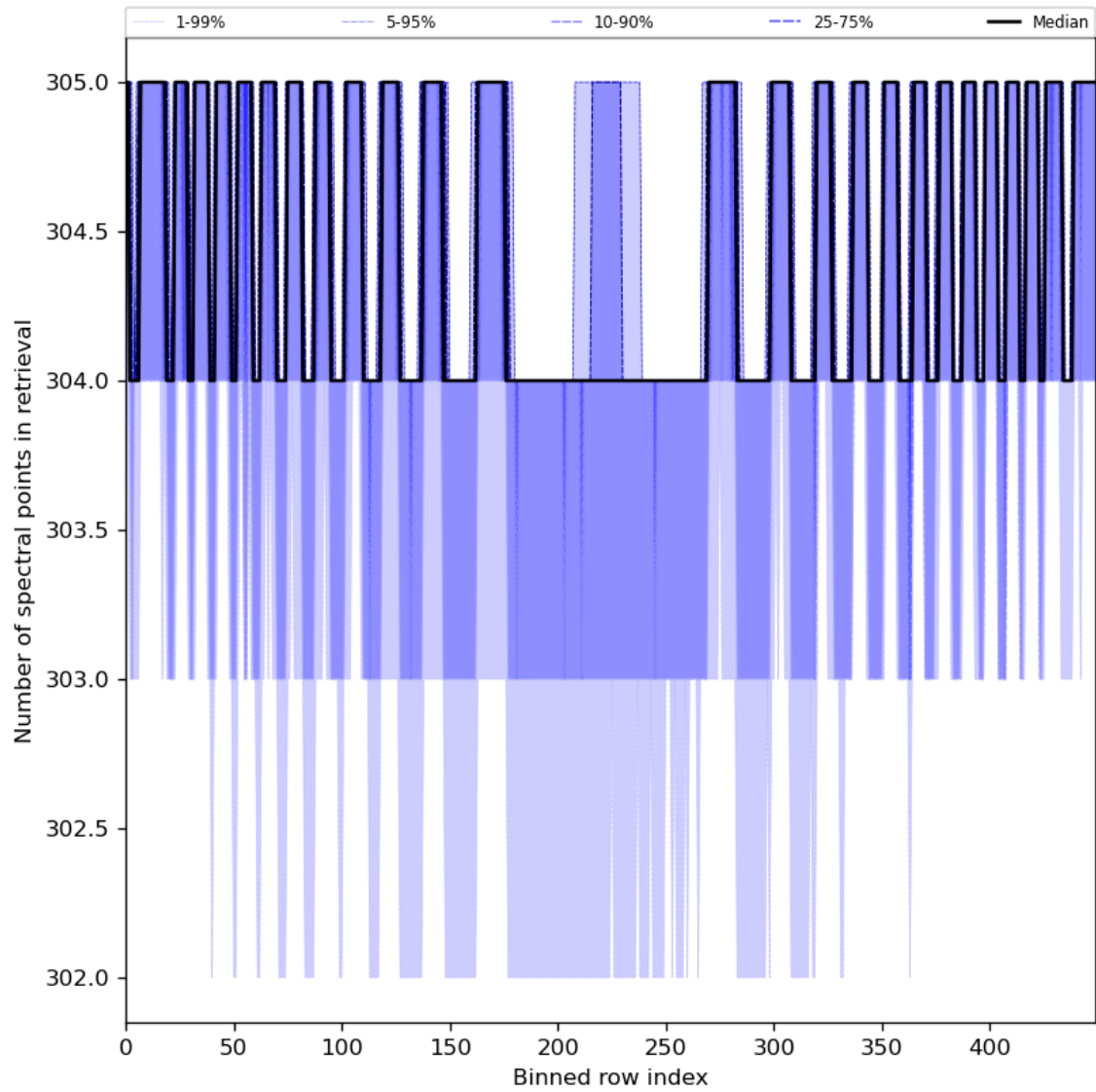
Figure 50: Along track statistics of “Number of spectral points in retrieval” for 2024-07-10 to 2024-07-11
