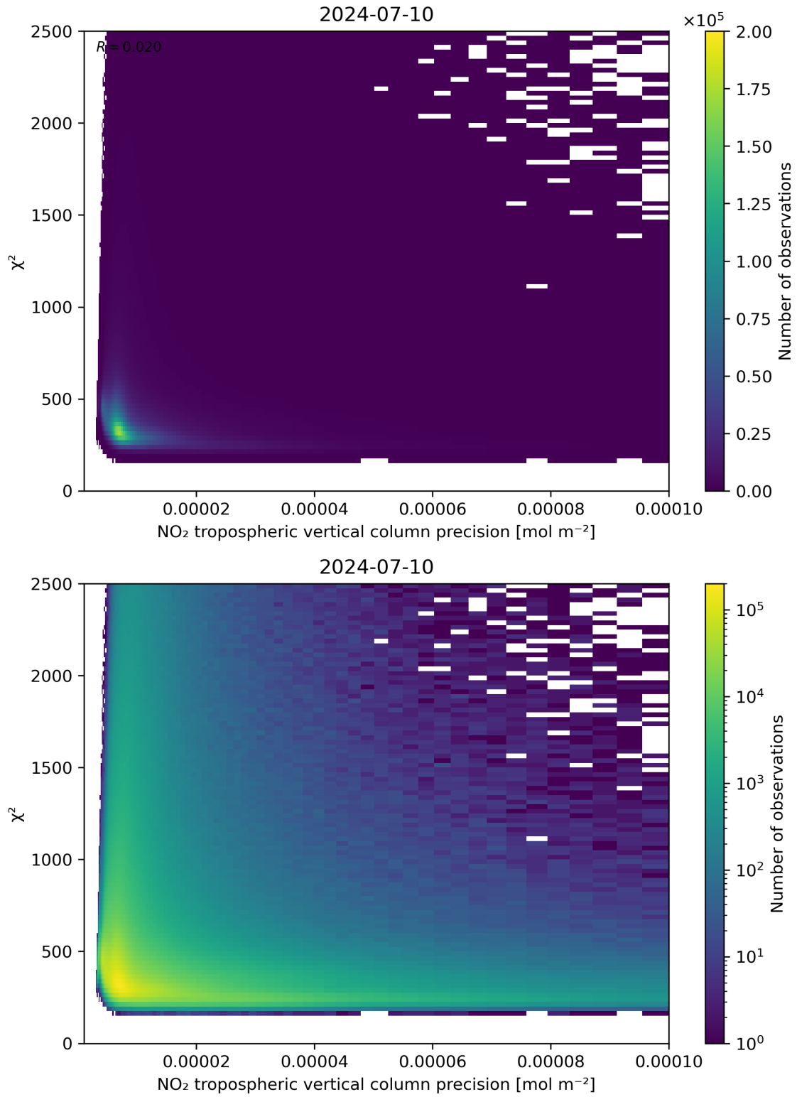
Figure 134: Scatter density plot of “NO 2 tropospheric vertical column precision” against “ \chi^2 ” for 2024-07-10 to 2024-07-11.
