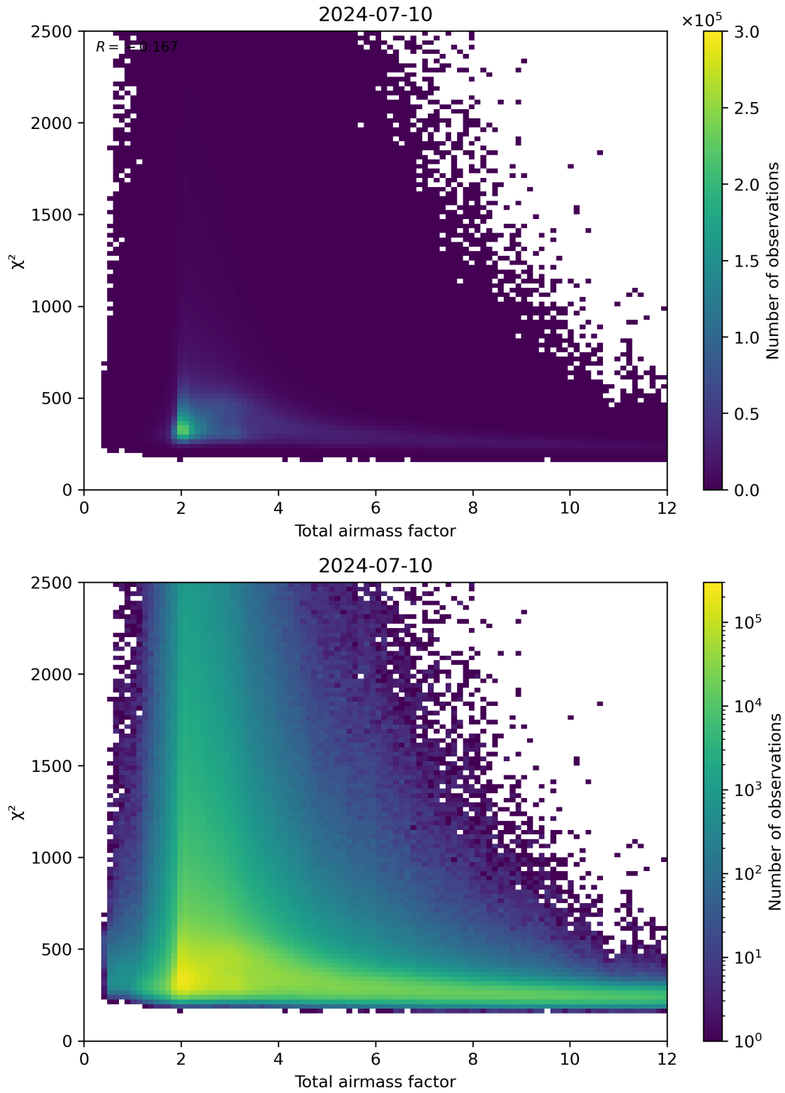
Figure 63: Scatter density plot of “Total airmass factor” against “ \chi^2 ” for 2024-07-10 to 2024-07-11.
