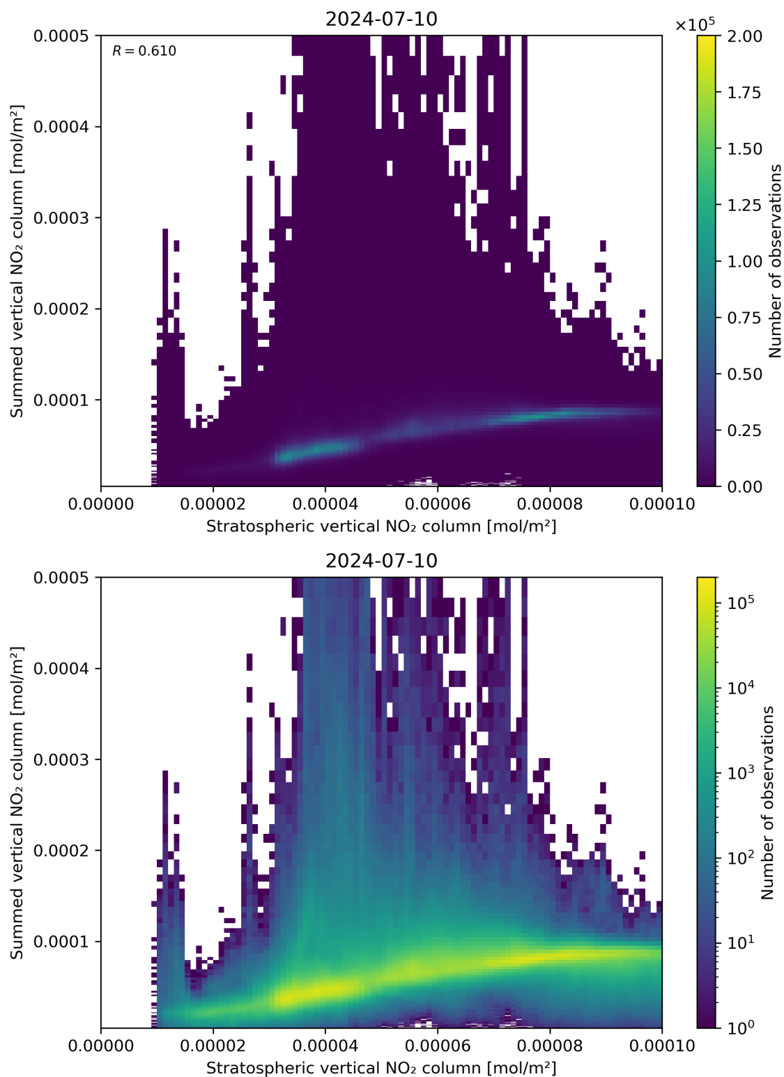
Figure 98: Scatter density plot of “Stratospheric vertical NO 2 column” against “Summed vertical NO 2 column” for 2024-07-10 to 2024-07-11.
