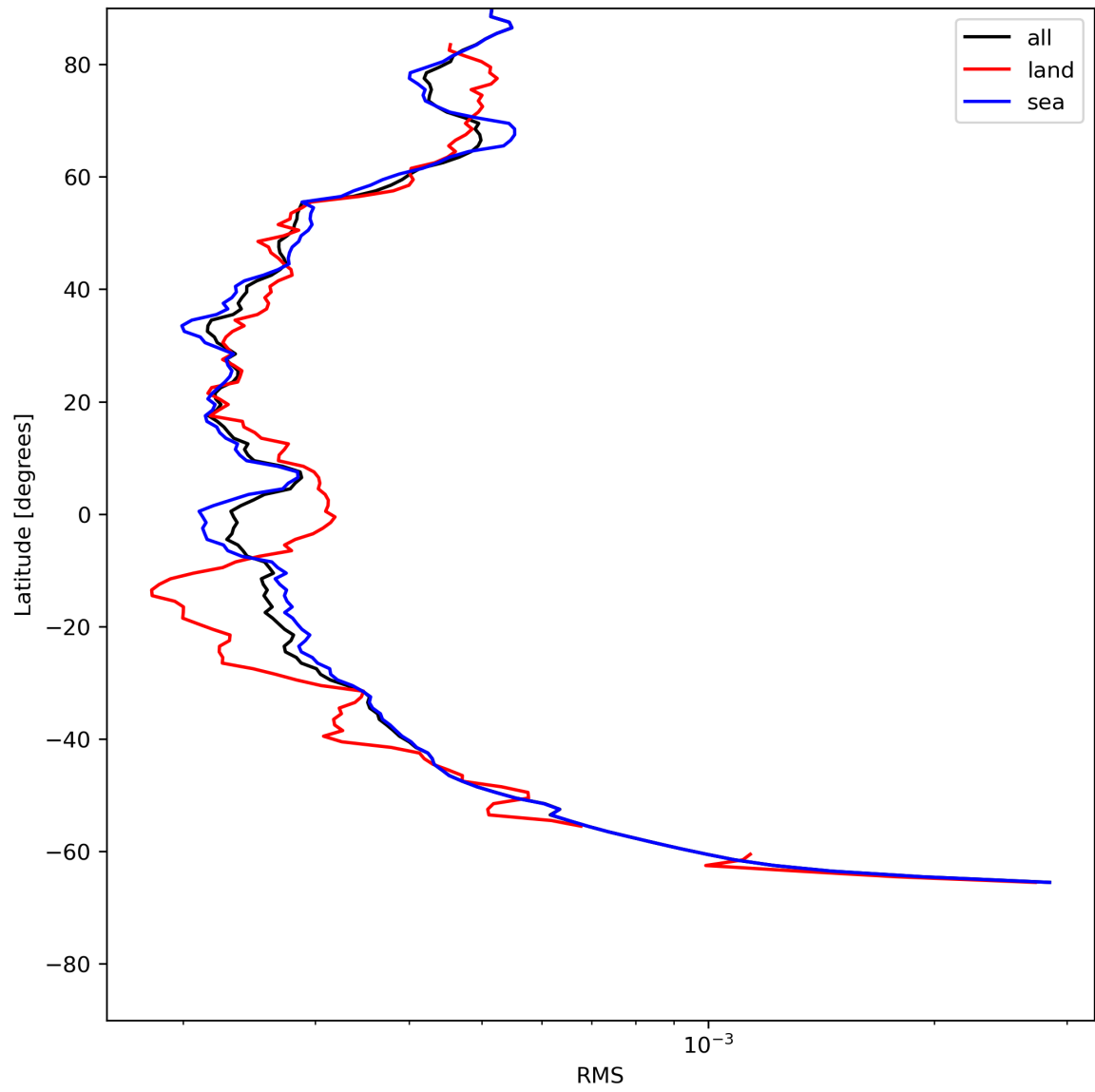
Figure 26: Zonal average of “RMS” for 2024-07-10 to 2024-07-11.
