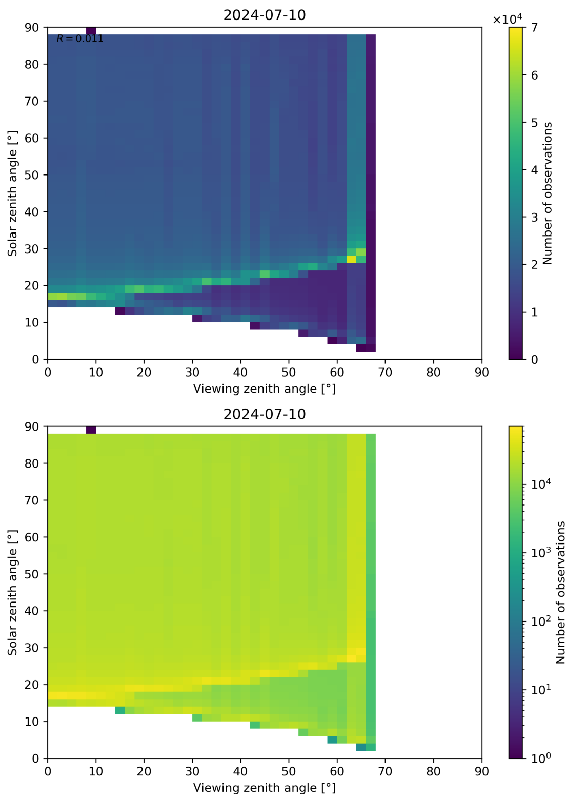
Figure 172: Scatter density plot of “Viewing zenith angle” against “Solar zenith angle” for 2024-07-10 to 2024-07-11.
