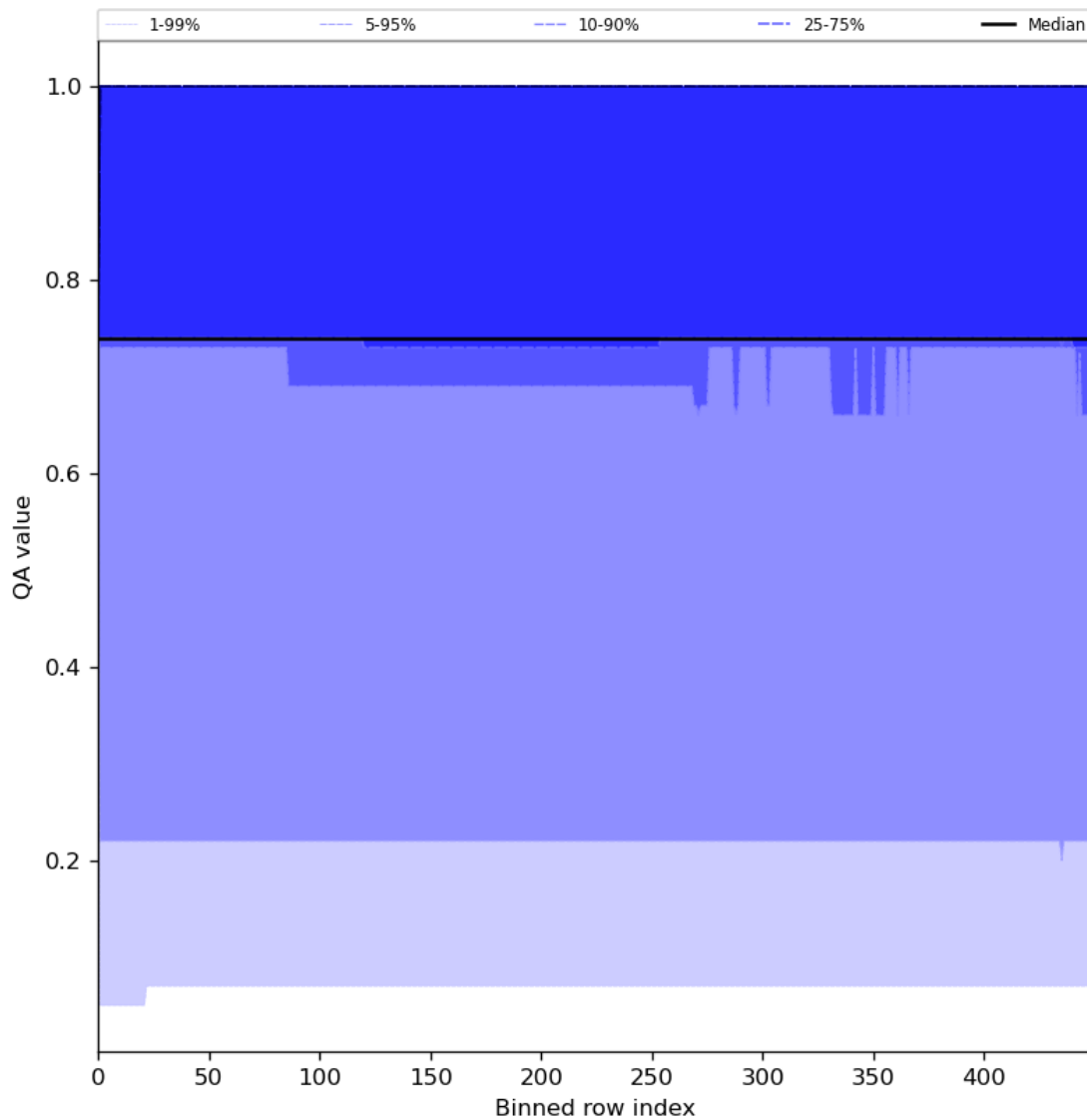
Figure 45: Along track statistics of “QA value” for 2024-07-10 to 2024-07-11
