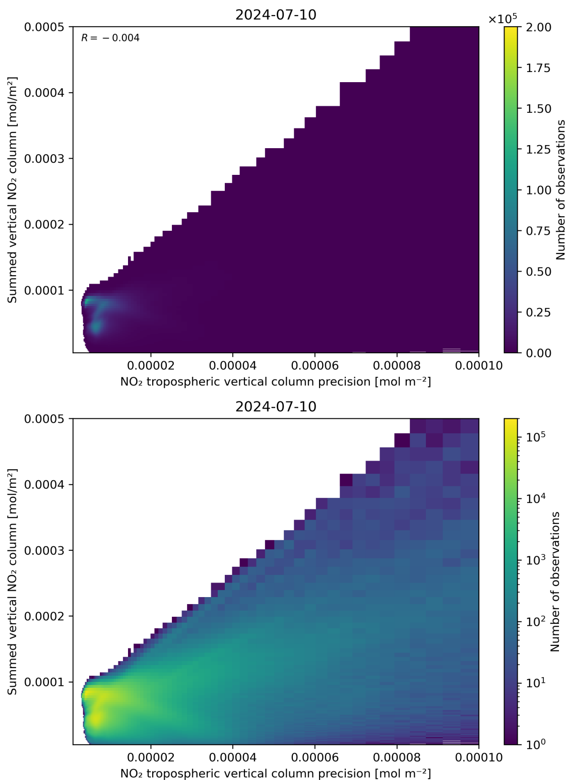
Figure 136: Scatter density plot of “NO 2 tropospheric vertical column precision” against “Summed vertical NO 2 column” for 2024-07-10 to 2024-07-11.
