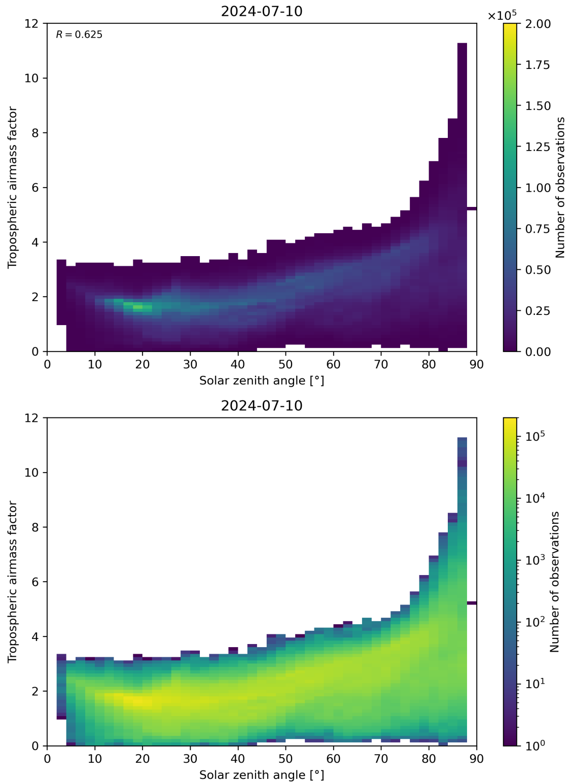
Figure 147: Scatter density plot of “Solar zenith angle” against “Tropospheric airmass factor” for 2024-07-10 to 2024-07-11.
