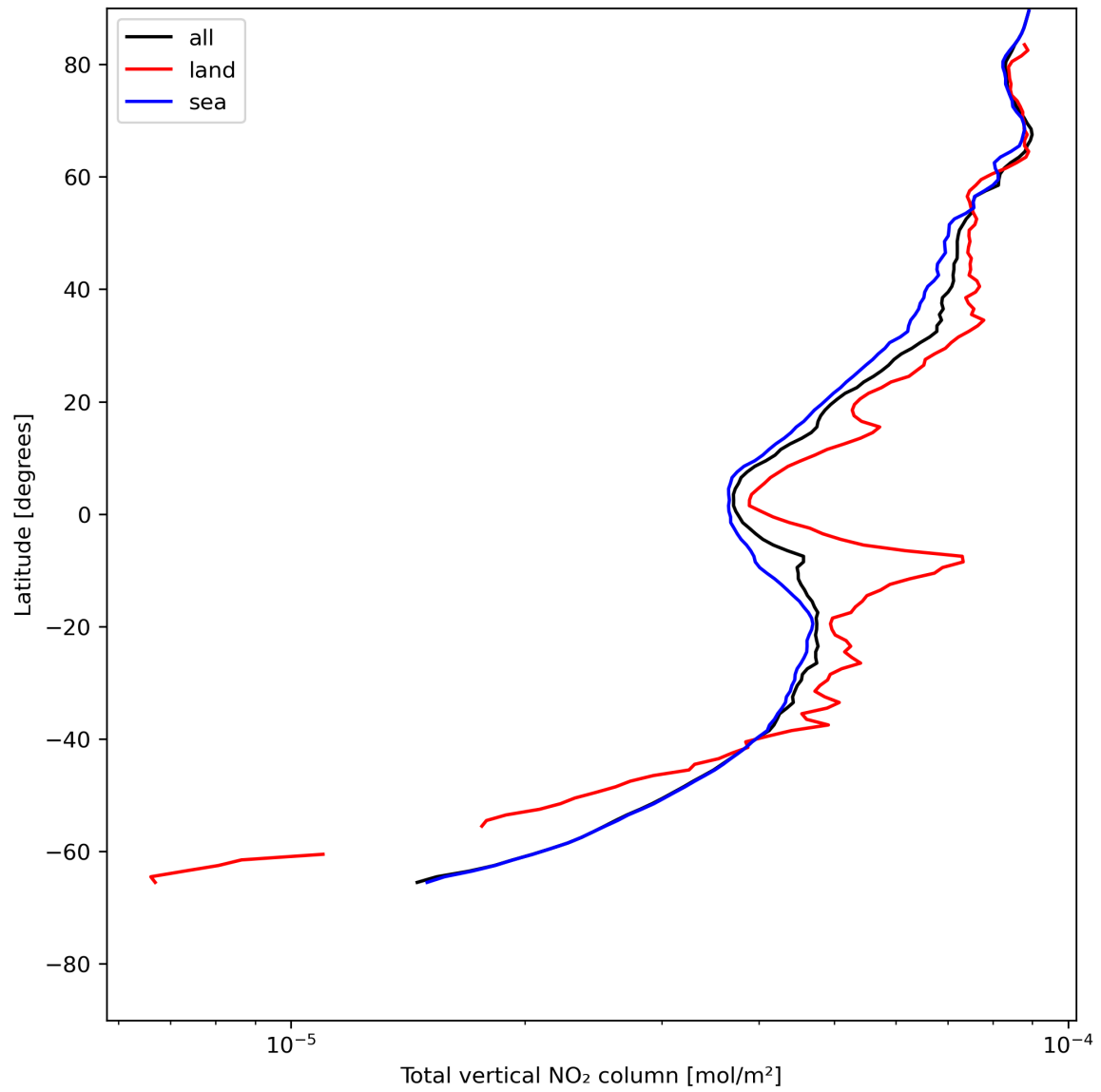
Figure 21: Zonal average of “Total vertical NO 2 column” for 2024-07-10 to 2024-07-11.
