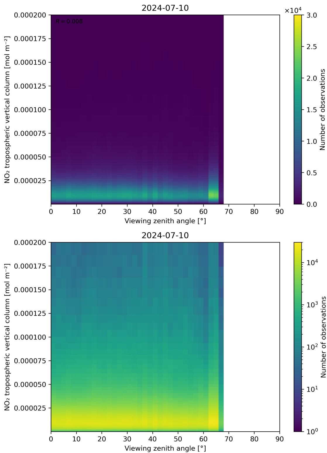
Figure 169: Scatter density plot of “Viewing zenith angle” against “NO 2 tropospheric vertical column” for 2024-07-10 to 2024-07-11.
