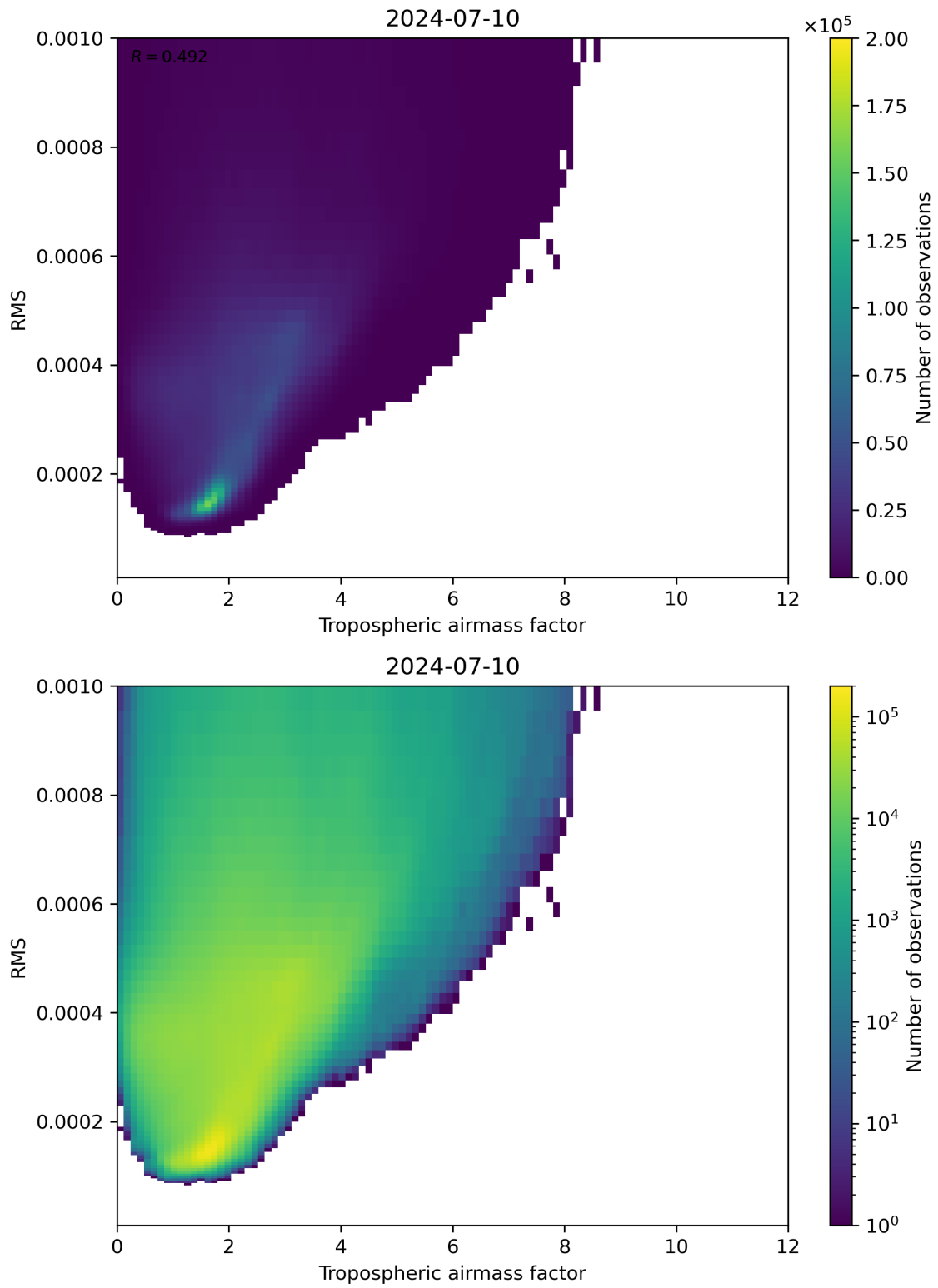
Figure 79: Scatter density plot of “Tropospheric airmass factor” against “RMS” for 2024-07-10 to 2024-07-11.
