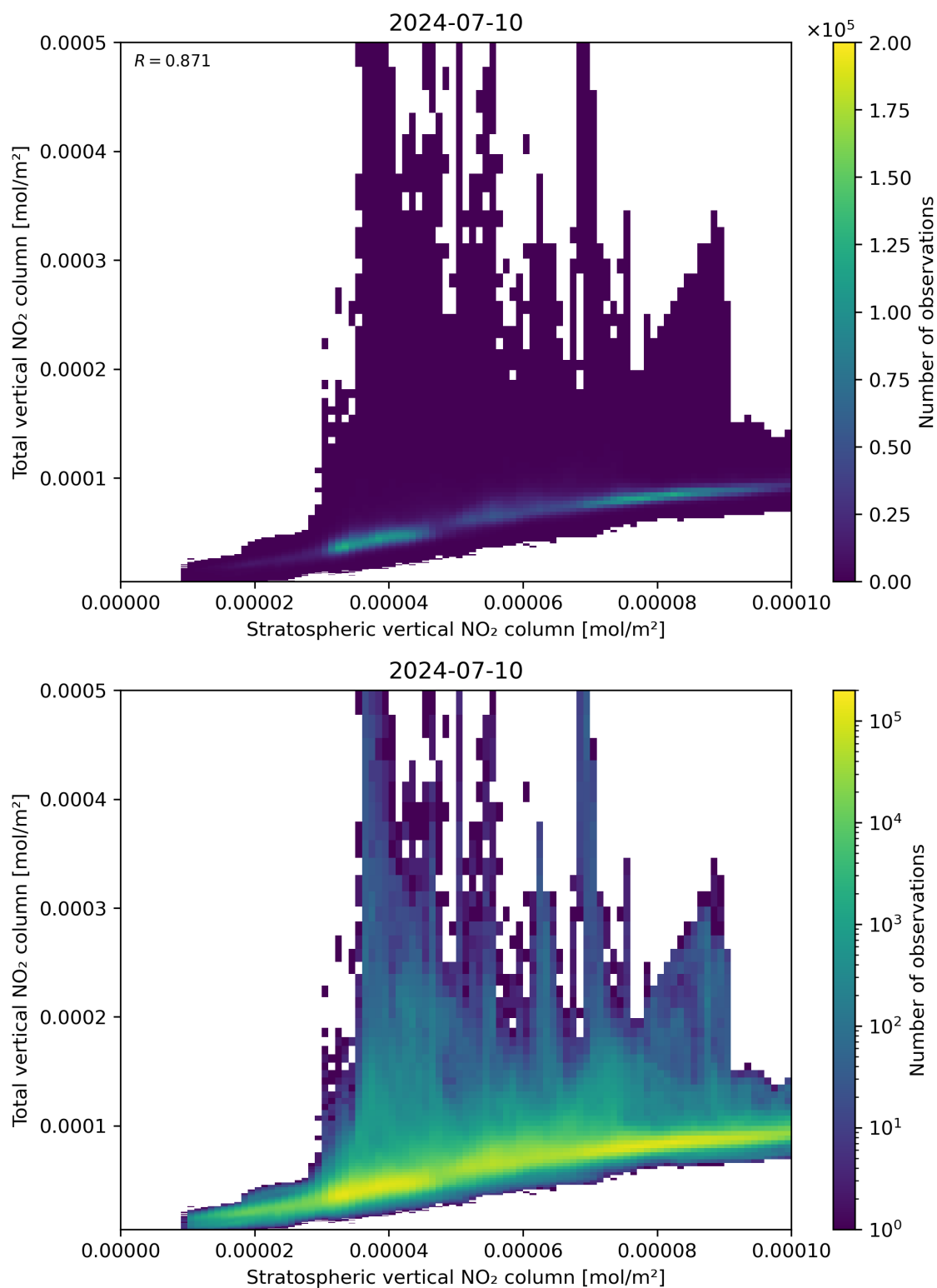
Figure 100: Scatter density plot of “Stratospheric vertical NO 2 column” against “Total vertical NO 2 column” for 2024-07-10 to 2024-07-11.
