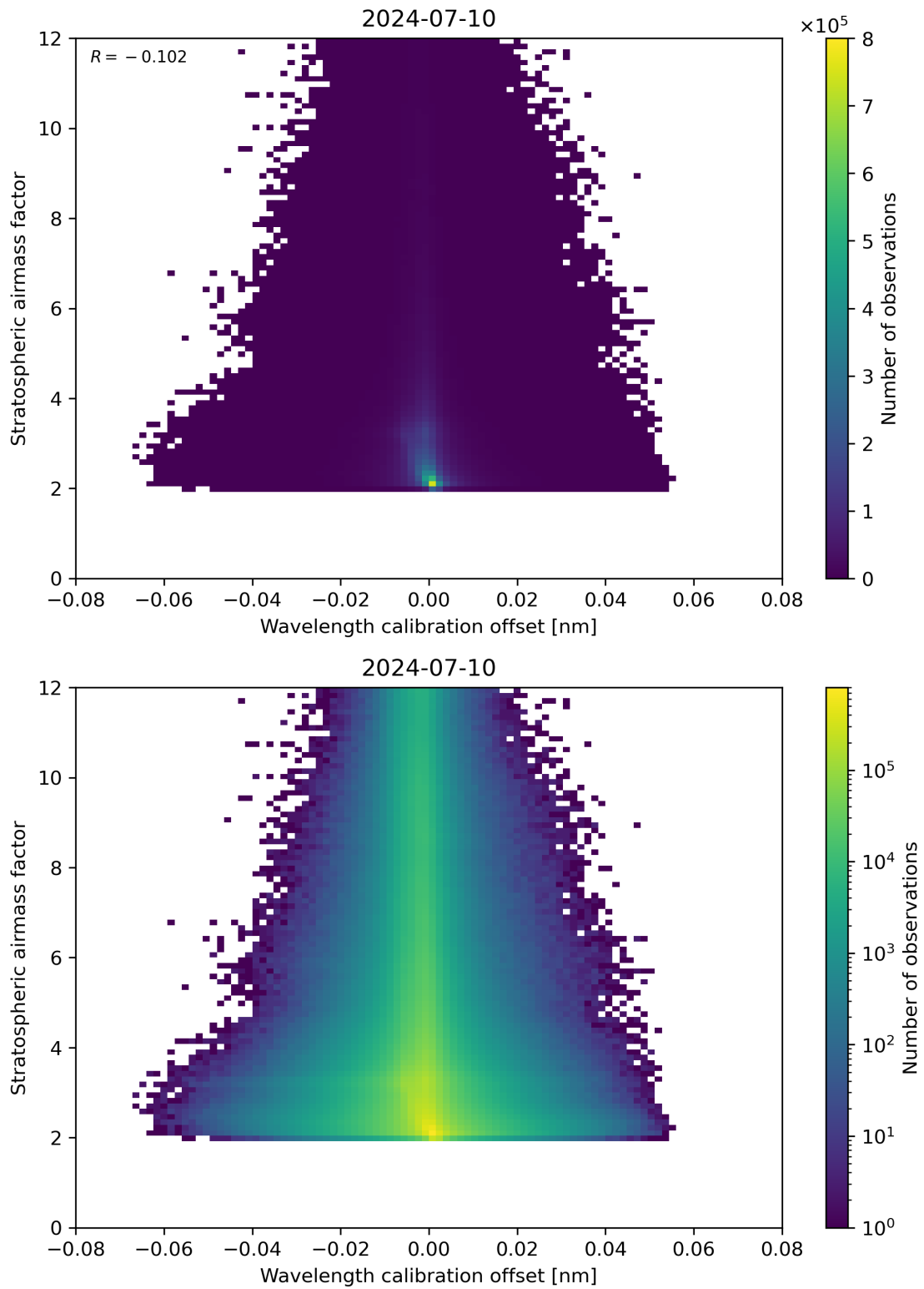
Figure 174: Scatter density plot of “Wavelength calibration offset” against “Stratospheric airmass factor” for 2024-07-10 to 2024-07-11.
