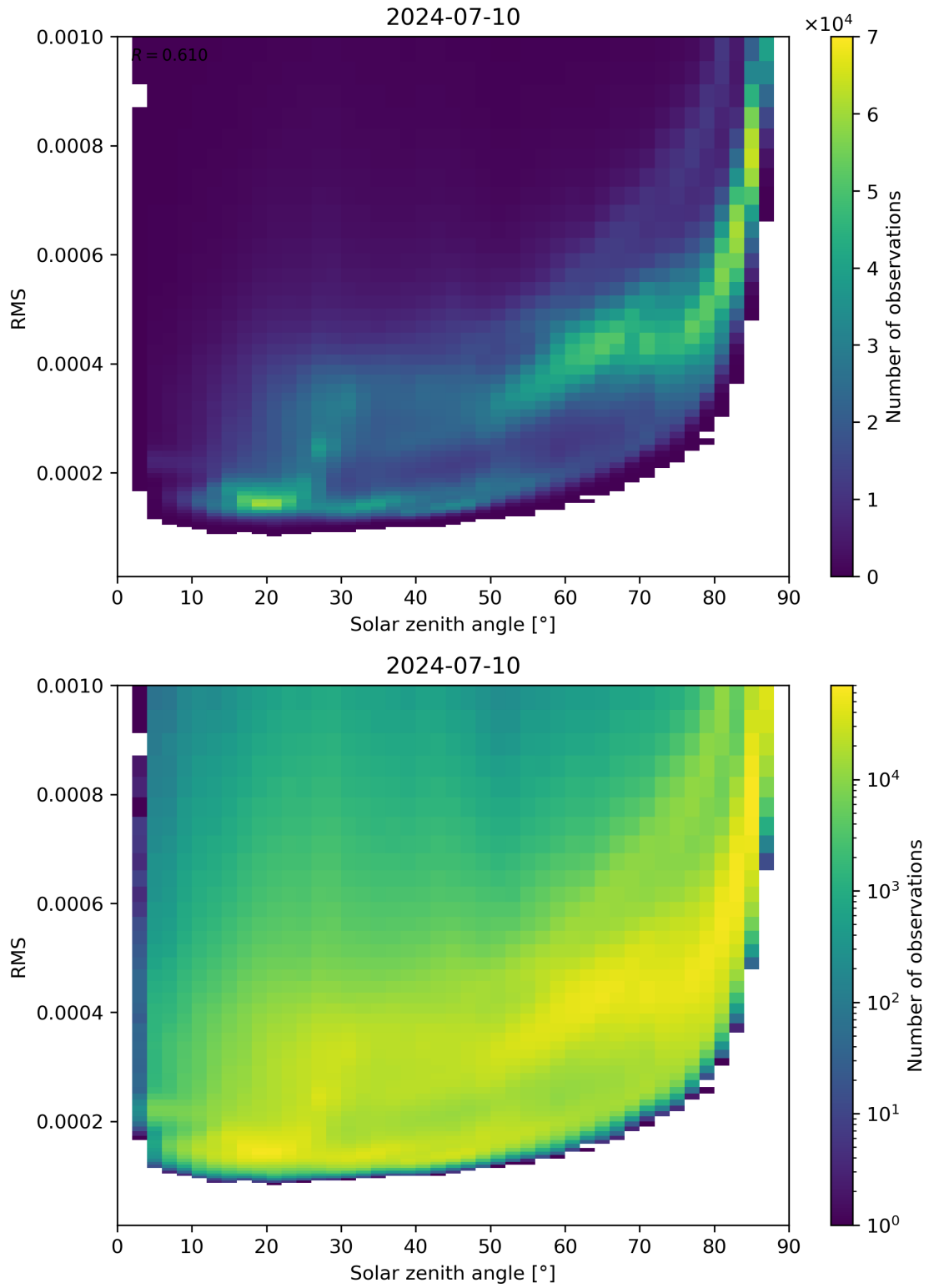
Figure 157: Scatter density plot of “Solar zenith angle” against “RMS” for 2024-07-10 to 2024-07-11.
