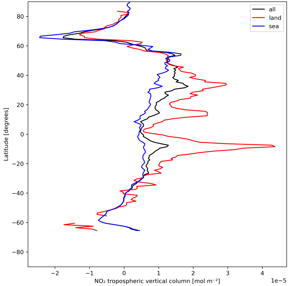
Figure 12: Zonal average of “NO 2 tropospheric vertical column” for 2024-07-10 to 2024-07-11.
