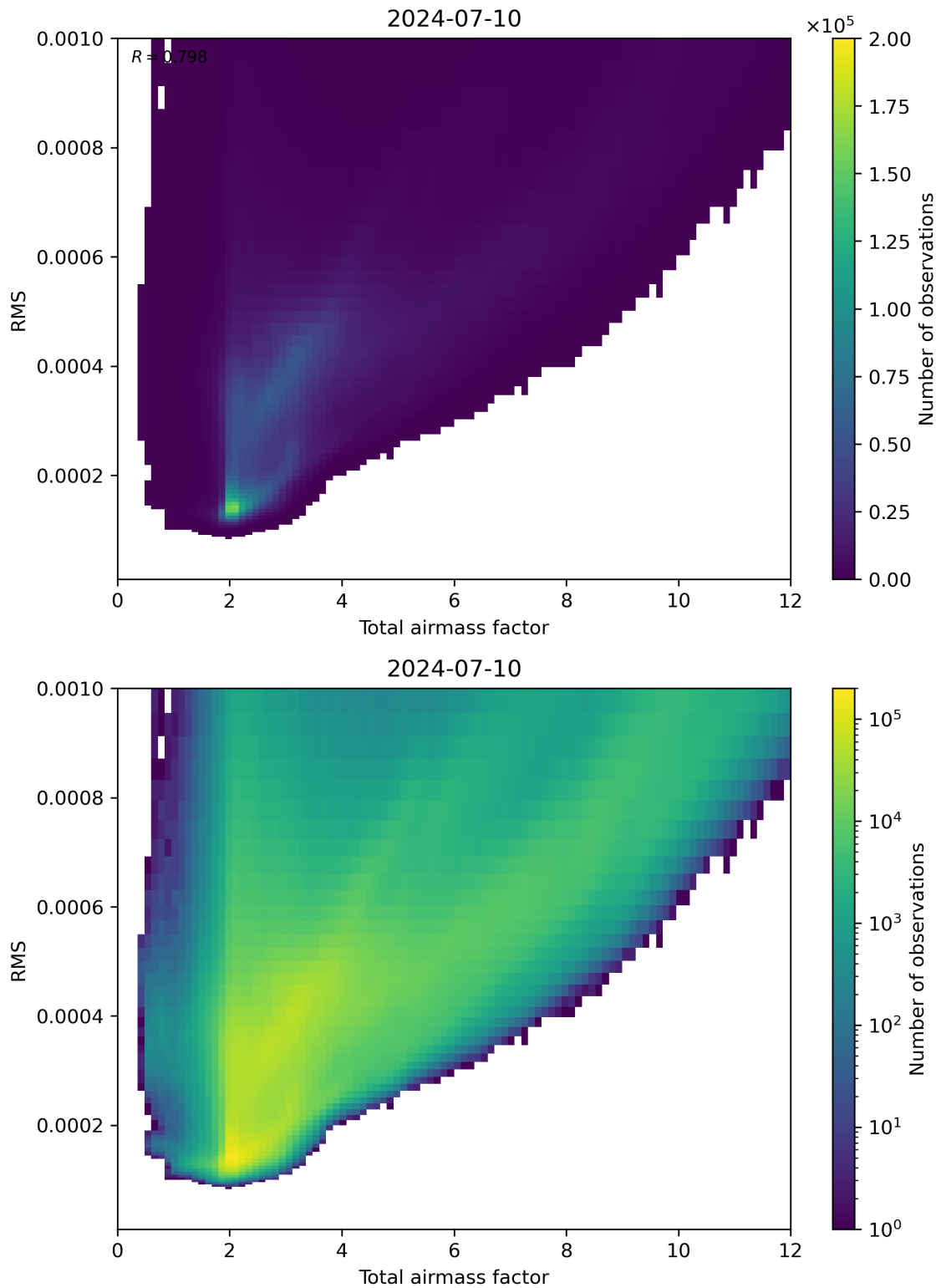
Figure 69: Scatter density plot of “Total airmass factor” against “RMS” for 2024-07-10 to 2024-07-11.
