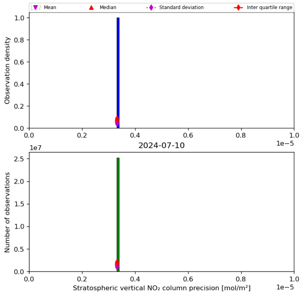
Figure 37: Histogram of “Stratospheric vertical NO 2 column precision” for 2024-07-10 to 2024-07-11
