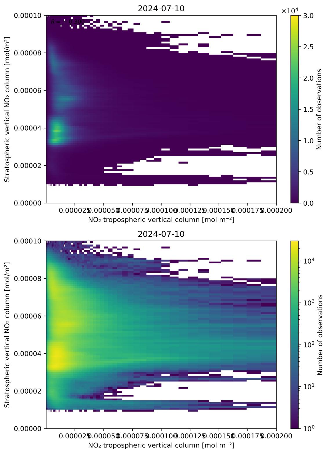
Figure 125: Scatter density plot of “NO 2 tropospheric vertical column” against “Stratospheric vertical NO 2 column” for 2024-07-10 to 2024-07-11.
