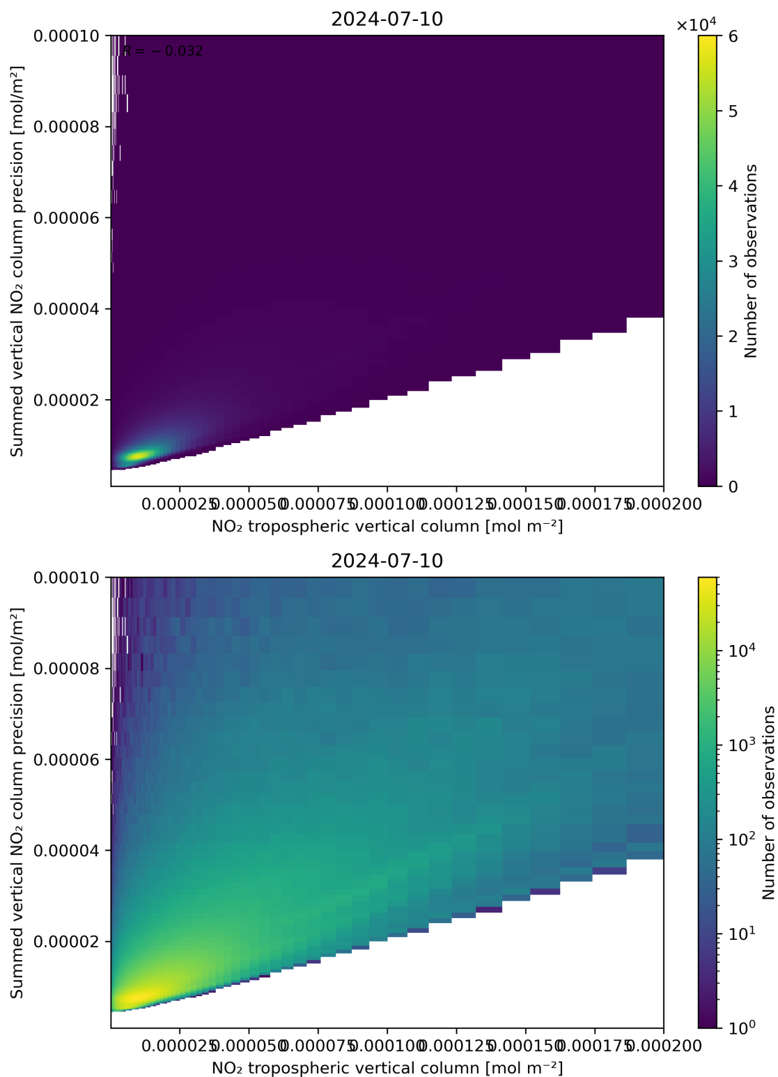
Figure 127: Scatter density plot of “NO 2 tropospheric vertical column” against “Summed vertical NO 2 column precision” for 2024-07-10 to 2024-07-11.
