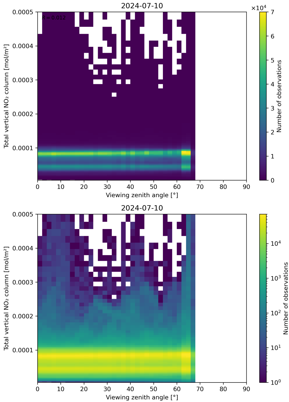
Figure 167: Scatter density plot of “Viewing zenith angle” against “Total vertical NO 2 column” for 2024-07-10 to 2024-07-11.
