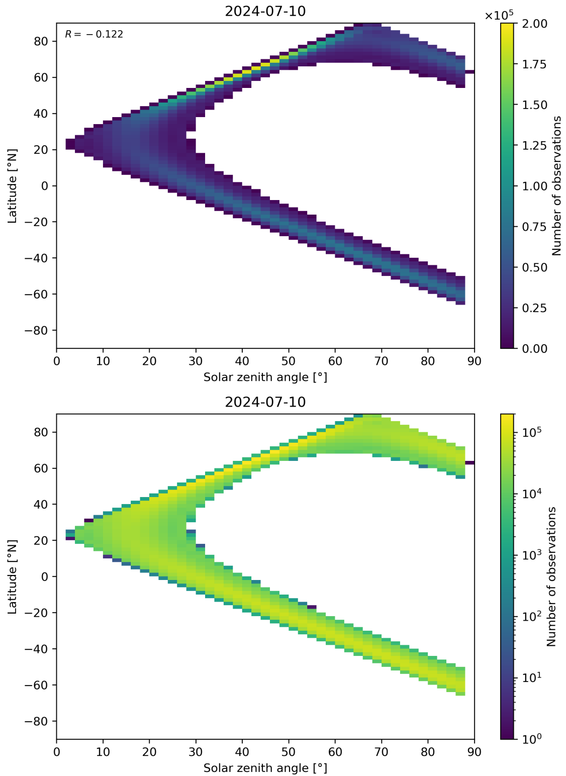
Figure 149: Scatter density plot of “Solar zenith angle” against “Latitude” for 2024-07-10 to 2024-07-11.
