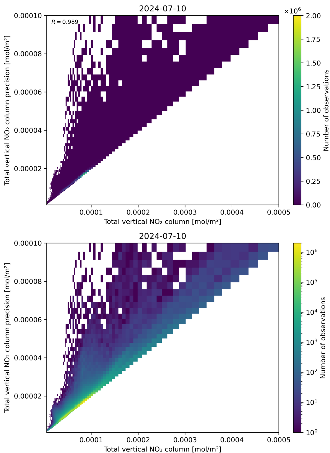
Figure 114: Scatter density plot of “Total vertical NO 2 column” against “Total vertical NO 2 column precision” for 2024-07-10 to 2024-07-11.
