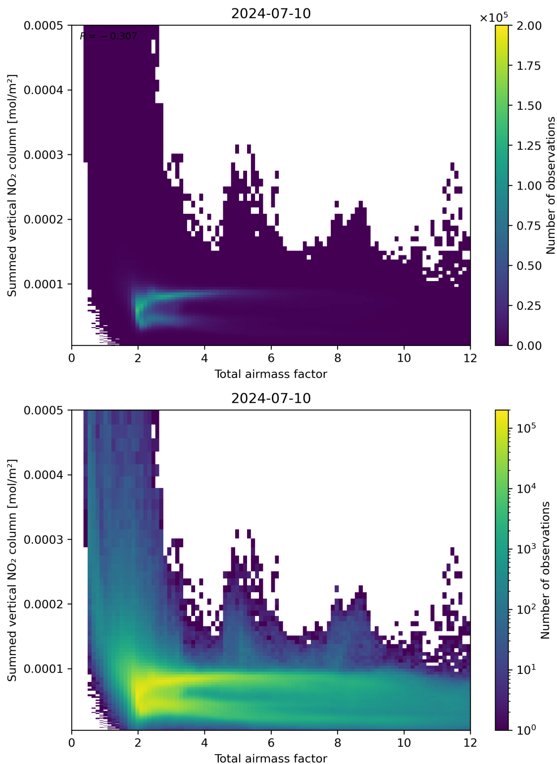
Figure 65: Scatter density plot of “Total airmass factor” against “Summed vertical NO 2 column” for 2024-07-10 to 2024-07-11.
