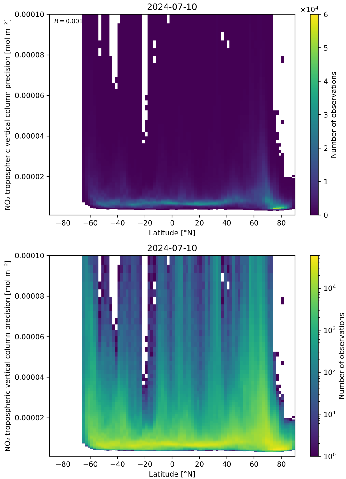
Figure 93: Scatter density plot of “Latitude” against “NO 2 tropospheric vertical column precision” for 2024-07-10 to 2024-07-11.
