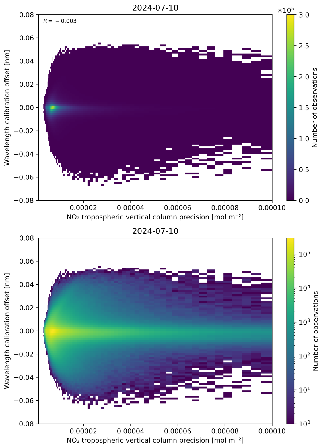
Figure 141: Scatter density plot of “NO 2 tropospheric vertical column precision” against “Wavelength calibration offset” for 2024-07-10 to 2024-07-11.
