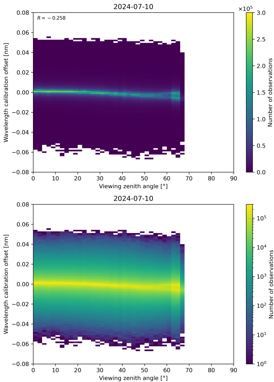
Figure 173: Scatter density plot of “Viewing zenith angle” against “Wavelength calibration offset” for 2024-07-10 to 2024-07-11.
