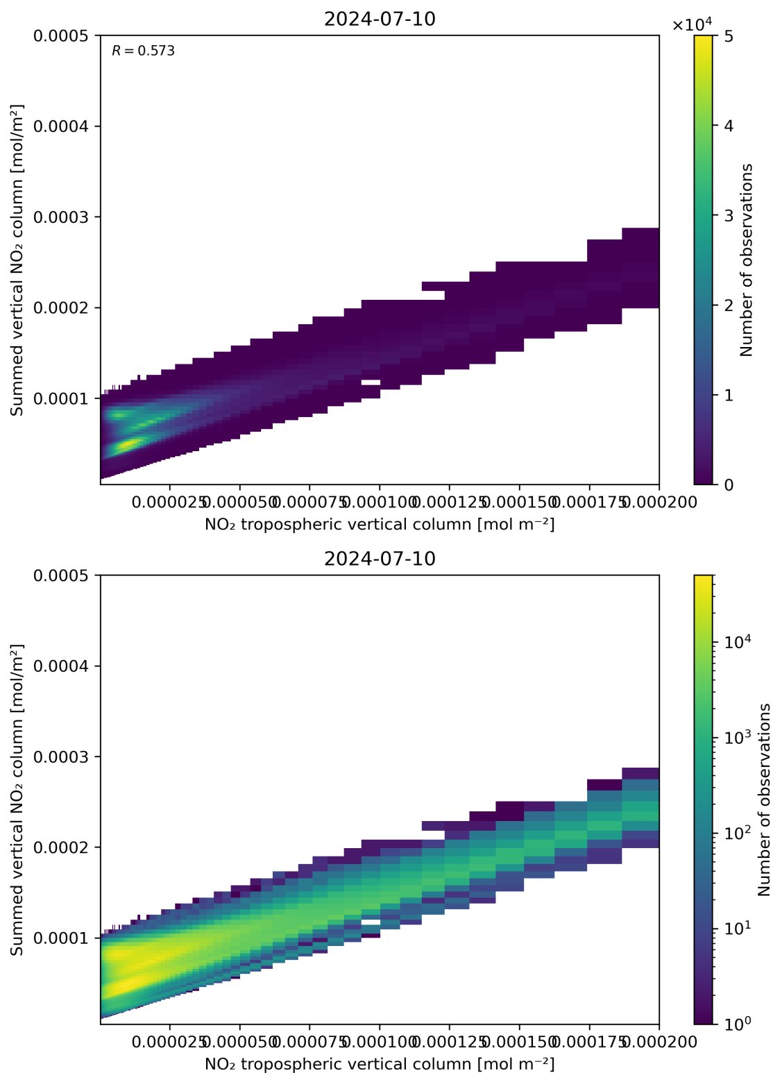
Figure 126: Scatter density plot of “NO 2 tropospheric vertical column” against “Summed vertical NO 2 column” for 2024-07-10 to 2024-07-11.
