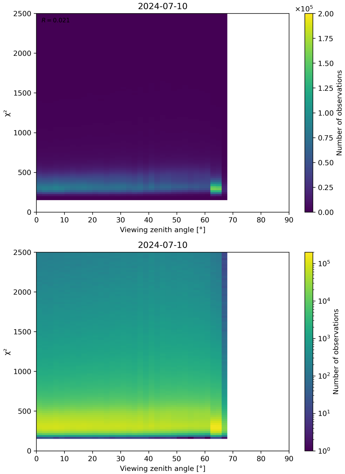
Figure 162: Scatter density plot of “Viewing zenith angle” against “ \chi^2 ” for 2024-07-10 to 2024-07-11.
