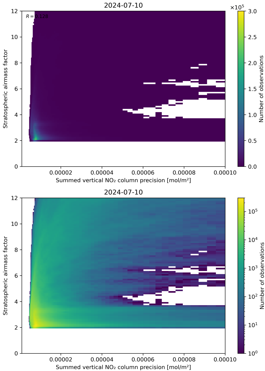
Figure 106: Scatter density plot of “Summed vertical NO 2 column precision” against “Stratospheric airmass factor” for 2024-07-10 to 2024-07-11.
