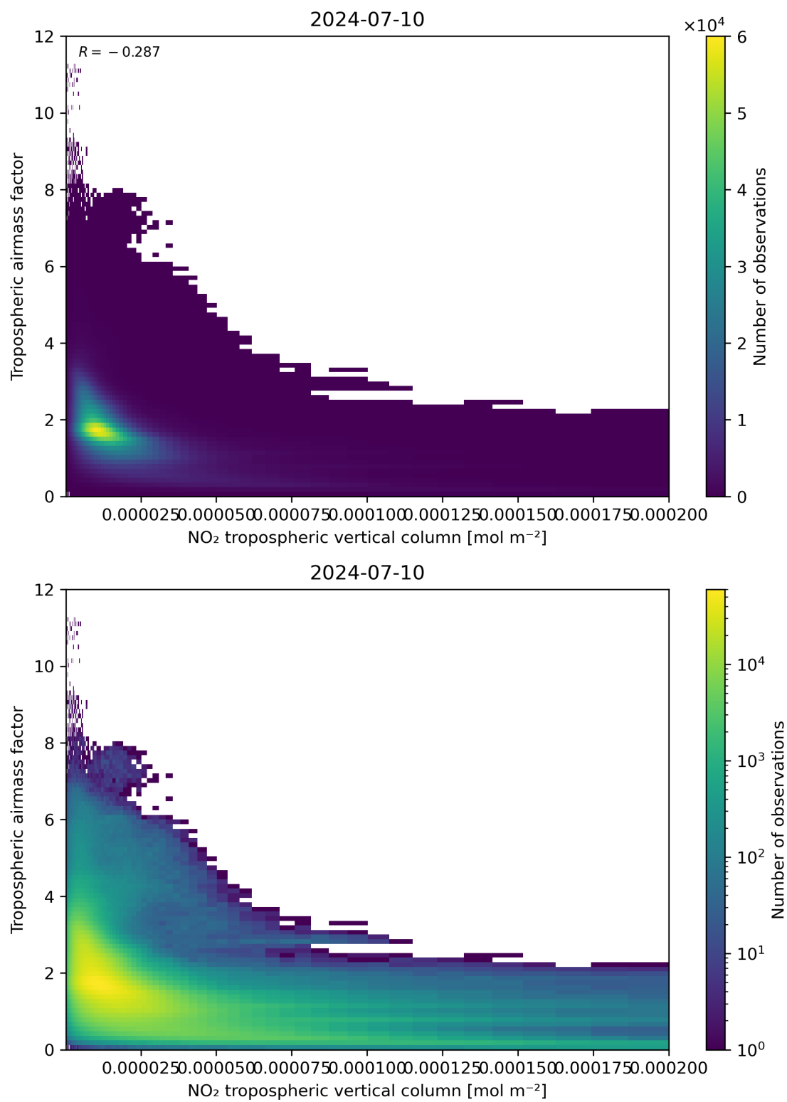
Figure 123: Scatter density plot of “NO 2 tropospheric vertical column” against “Tropospheric air mass factor” for 2024-07-10 to 2024-07-11.
