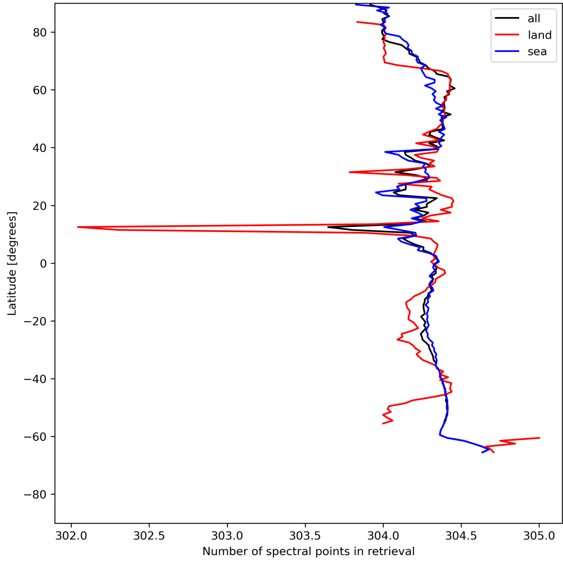
Figure 16: Zonal average of “Number of spectral points in retrieval” for 2024-07-10 to 2024-07-11.
