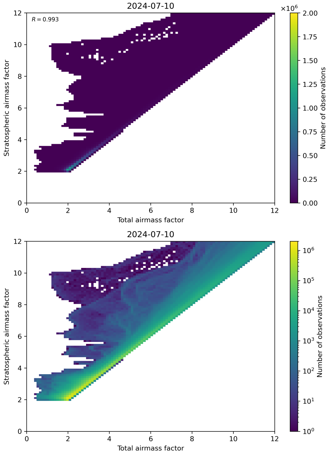
Figure 62: Scatter density plot of “Total airmass factor” against “Stratospheric airmass factor” for 2024-07-10 to 2024-07-11.
