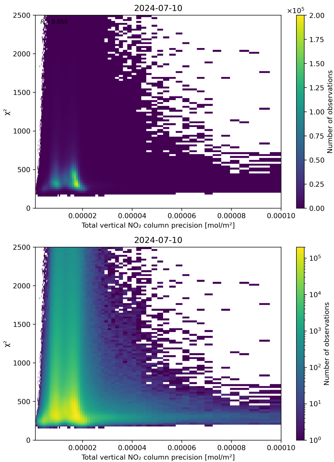
Figure 116: Scatter density plot of “Total vertical NO 2 column precision” against “ \chi^2 ” for 2024-07-10 to 2024-07-11.
