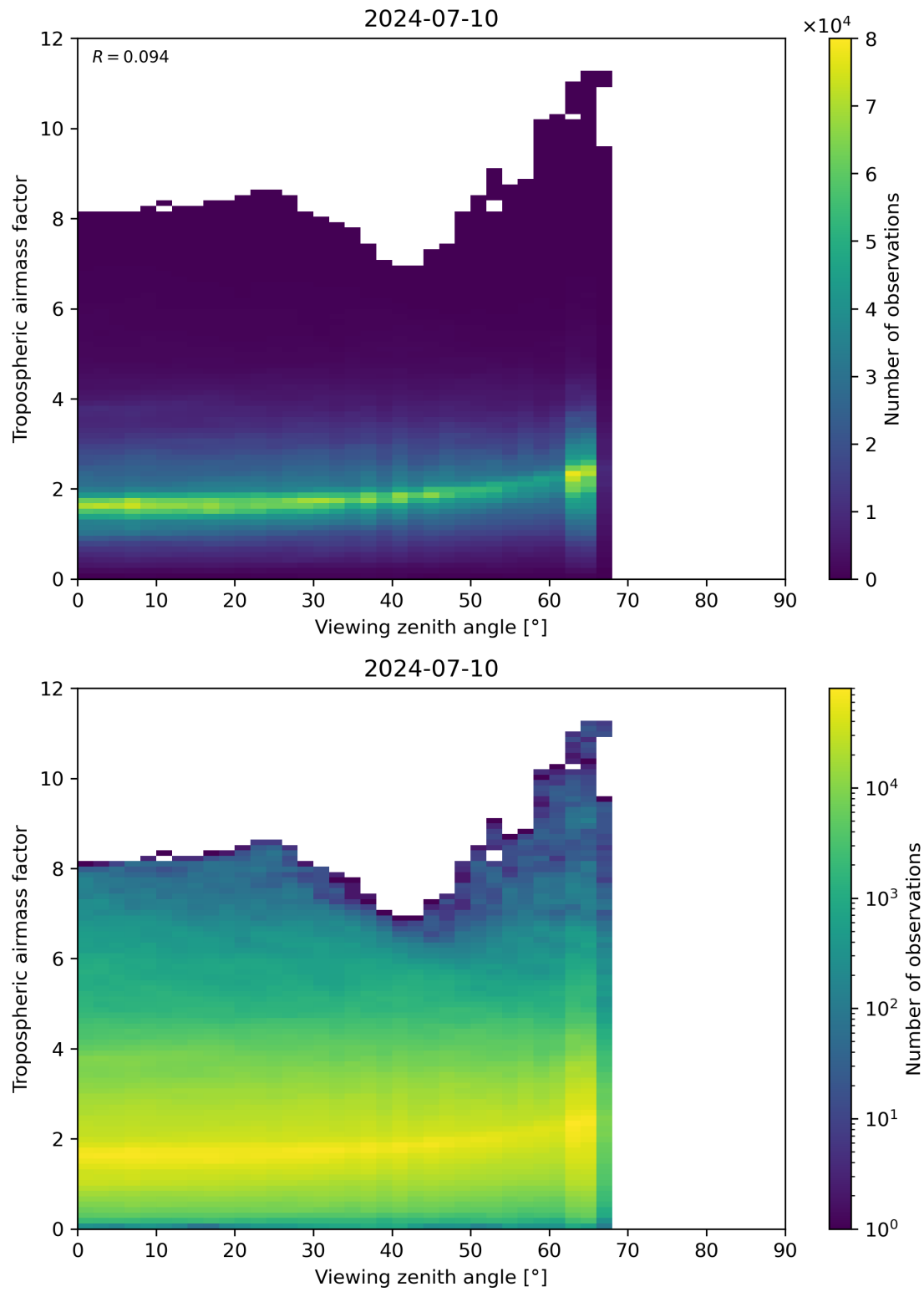
Figure 161: Scatter density plot of “Viewing zenith angle” against “Tropospheric airmass factor” for 2024-07-10 to 2024-07-11.
