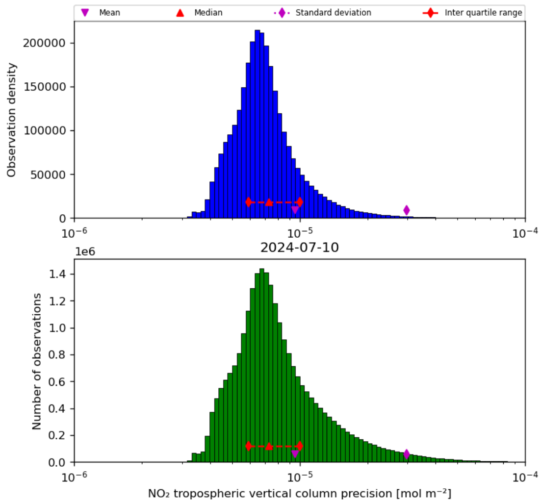
Figure 30: Histogram of “NO 2 tropospheric vertical column precision” for 2024-07-10 to 2024-07-11
