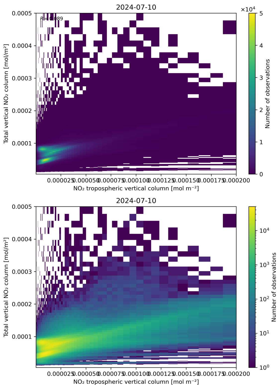
Figure 128: Scatter density plot of “NO 2 tropospheric vertical column” against “Total vertical NO 2 column” for 2024-07-10 to 2024-07-11.
