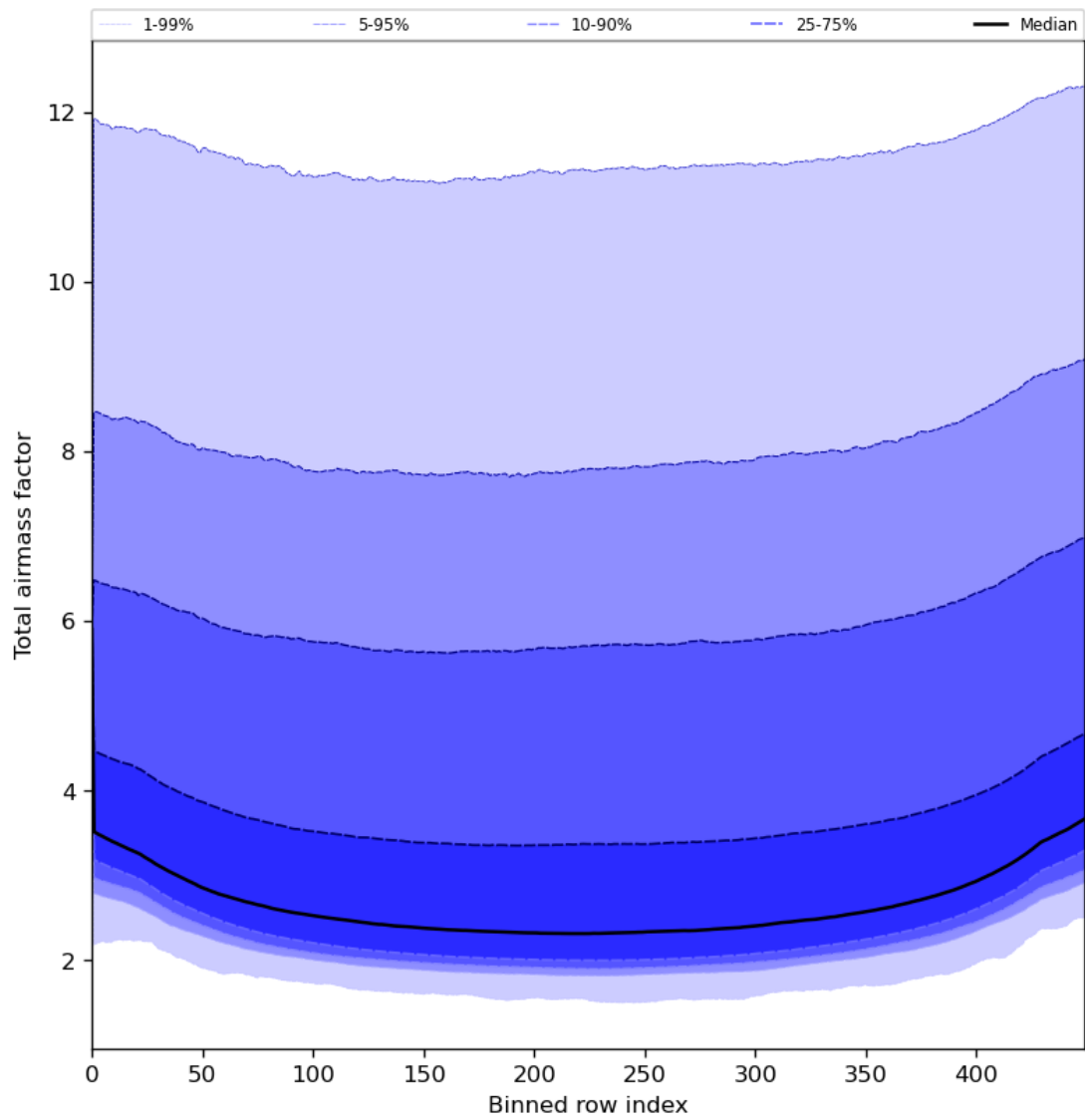
Figure 49: Along track statistics of “Total airmass factor” for 2024-07-10 to 2024-07-11
