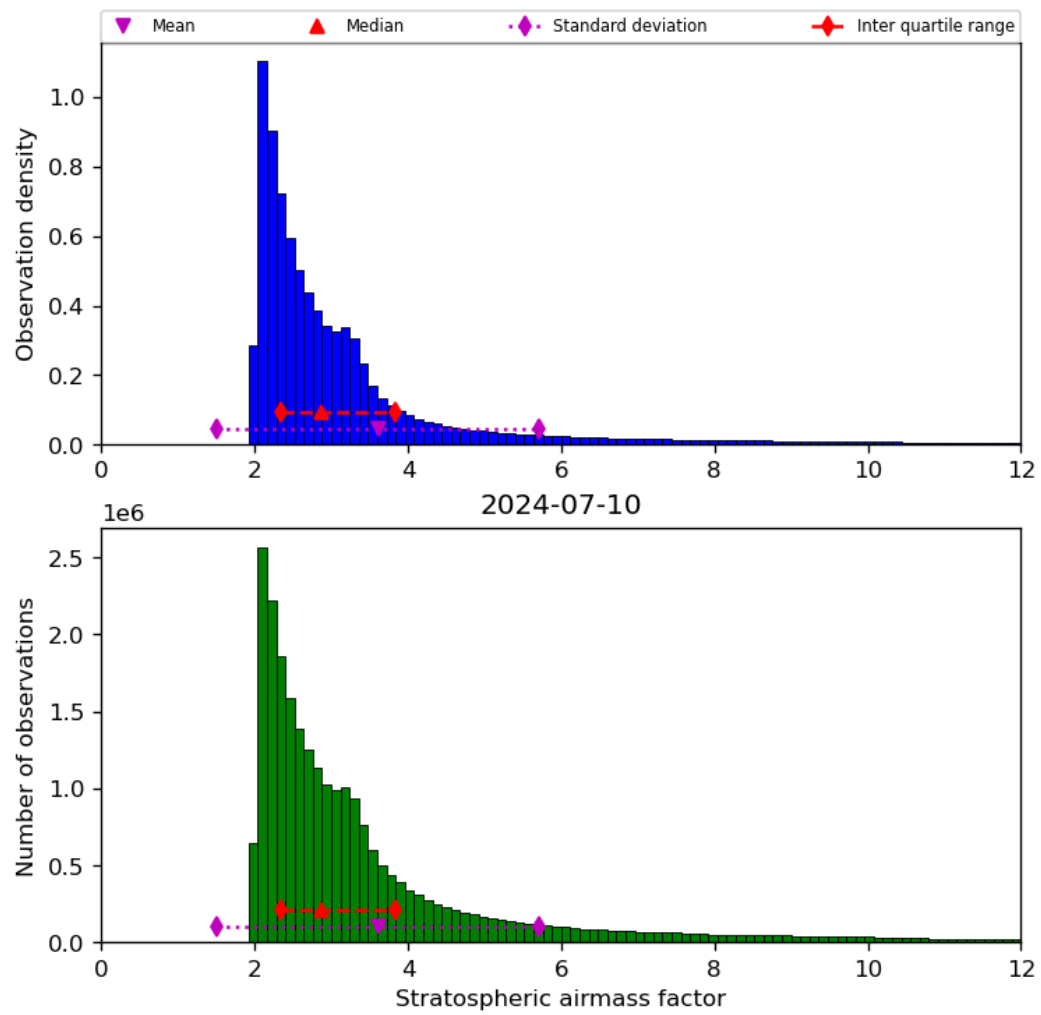
Figure 44: Histogram of “Stratospheric airmass factor” for 2024-07-10 to 2024-07-11
