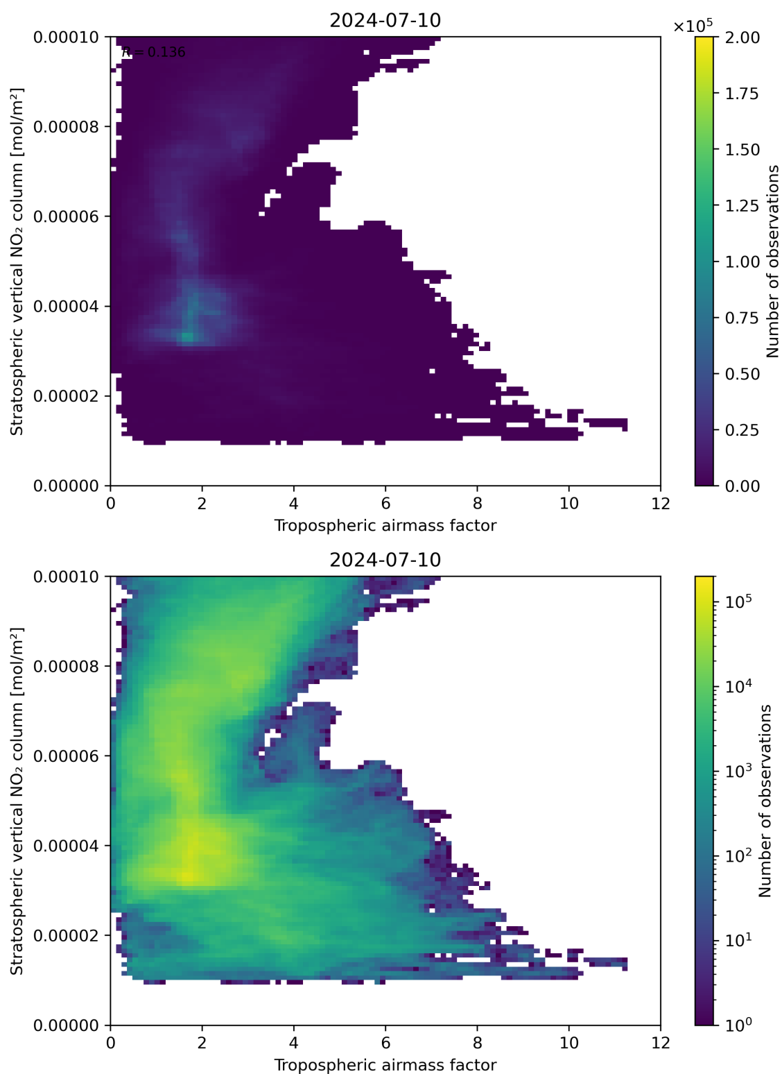
Figure 74: Scatter density plot of “Tropospheric air mass factor” against “Stratospheric vertical NO 2 column” for 2024-07-10 to 2024-07-11.
