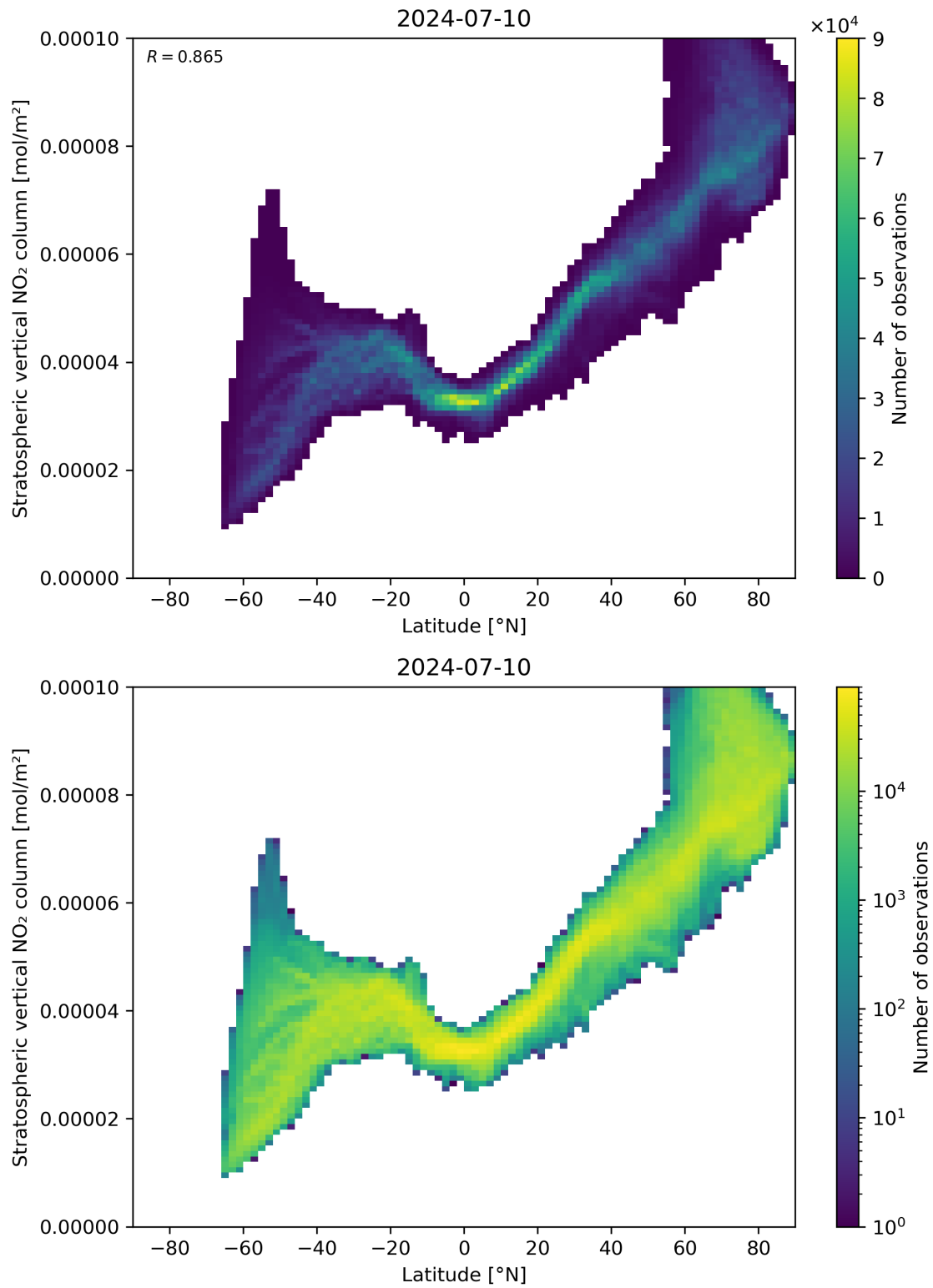
Figure 87: Scatter density plot of “Latitude” against “Stratospheric vertical NO 2 column” for 2024-07-10 to 2024-07-11.
