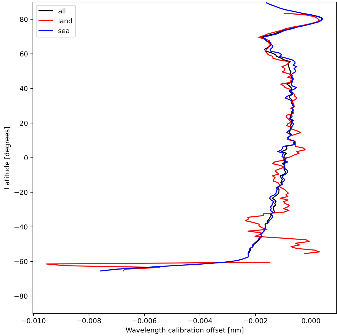
Figure 18: Zonal average of “Wavelength calibration offset” for 2024-07-10 to 2024-07-11.
