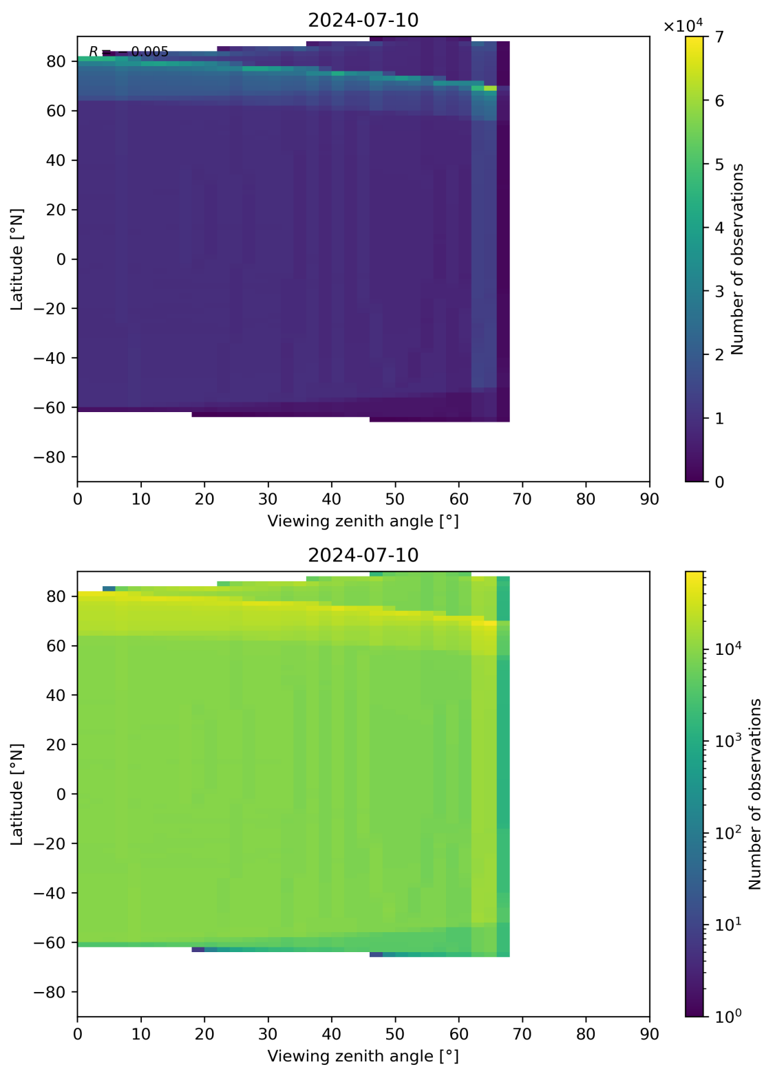
Figure 163: Scatter density plot of “Viewing zenith angle” against “Latitude” for 2024-07-10 to 2024-07-11.
