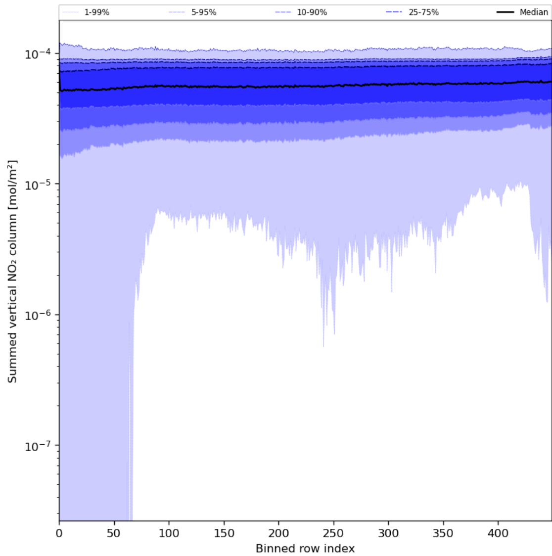
Figure 57: Along track statistics of “Summed vertical NO 2 column” for 2024-07-10 to 2024-07-11
