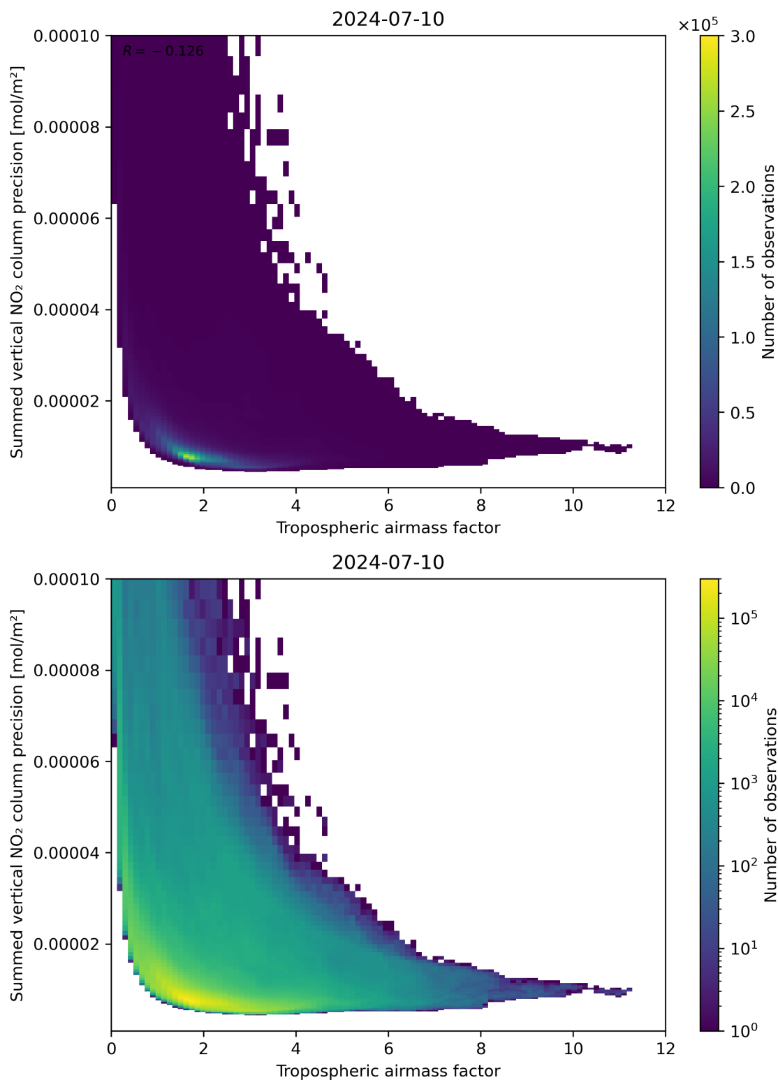
Figure 76: Scatter density plot of “Tropospheric air mass factor” against “Summed vertical NO 2 column precision” for 2024-07-10 to 2024-07-11.
