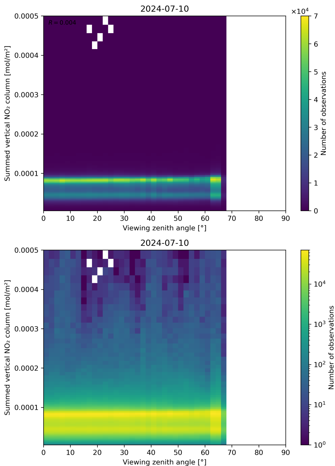
Figure 165: Scatter density plot of “Viewing zenith angle” against “Summed vertical NO 2 column” for 2024-07-10 to 2024-07-11.
