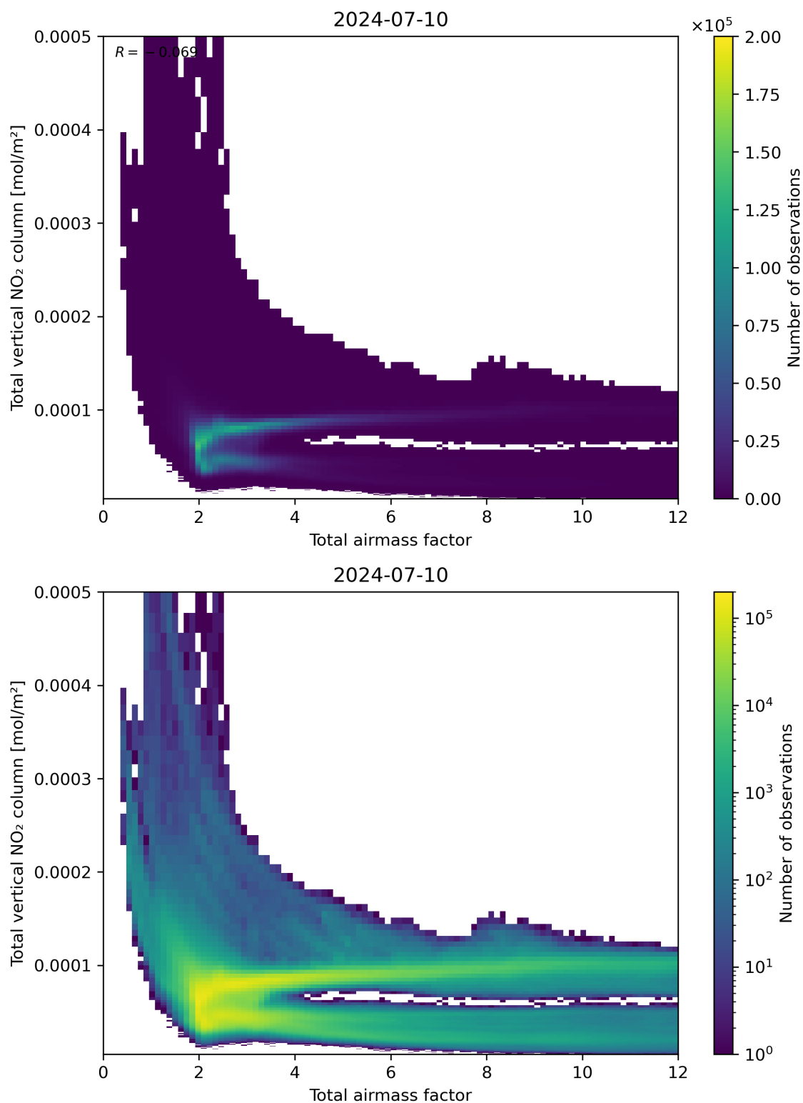
Figure 67: Scatter density plot of “Total airmass factor” against “Total vertical NO 2 column” for 2024-07-10 to 2024-07-11.
