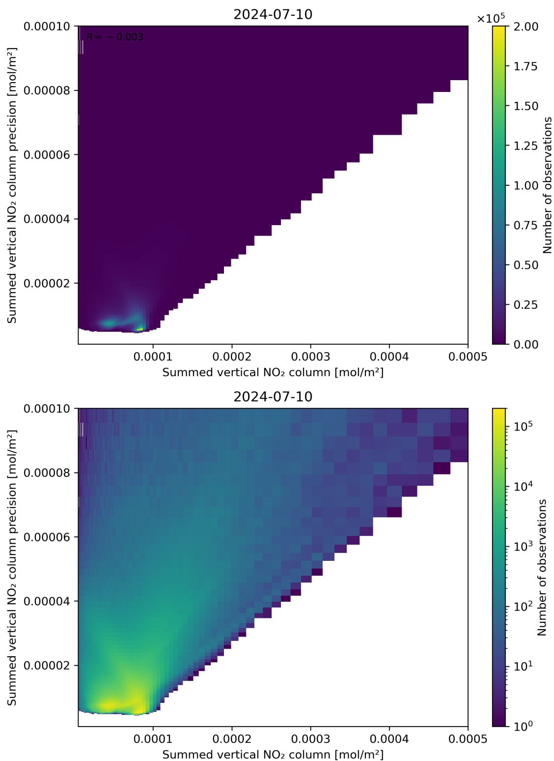
Figure 105: Scatter density plot of “Summed vertical NO 2 column” against “Summed vertical NO 2 column precision” for 2024-07-10 to 2024-07-11.
