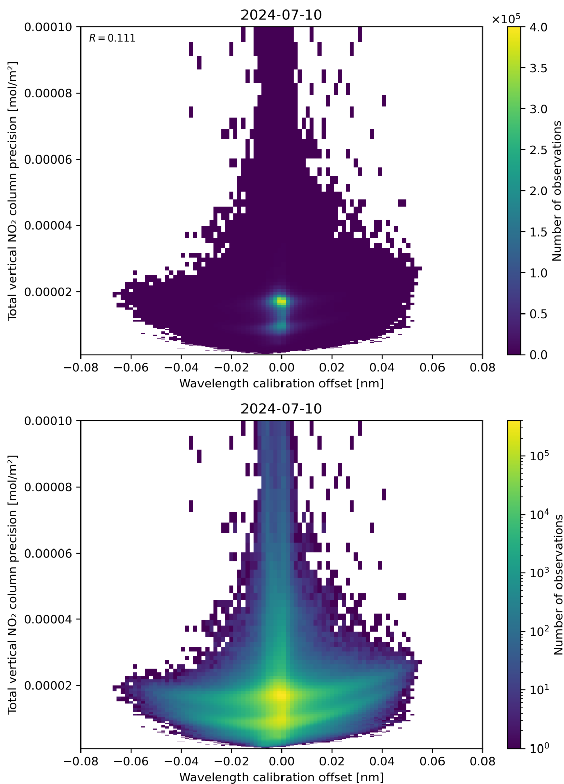
Figure 180: Scatter density plot of “Wavelength calibration offset” against “Total vertical NO 2 column precision” for 2024-07-10 to 2024-07-11.
