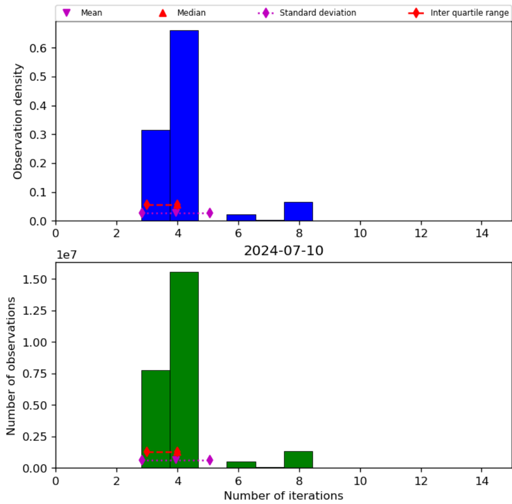
Figure 34: Histogram of “Number of iterations” for 2024-07-10 to 2024-07-11
