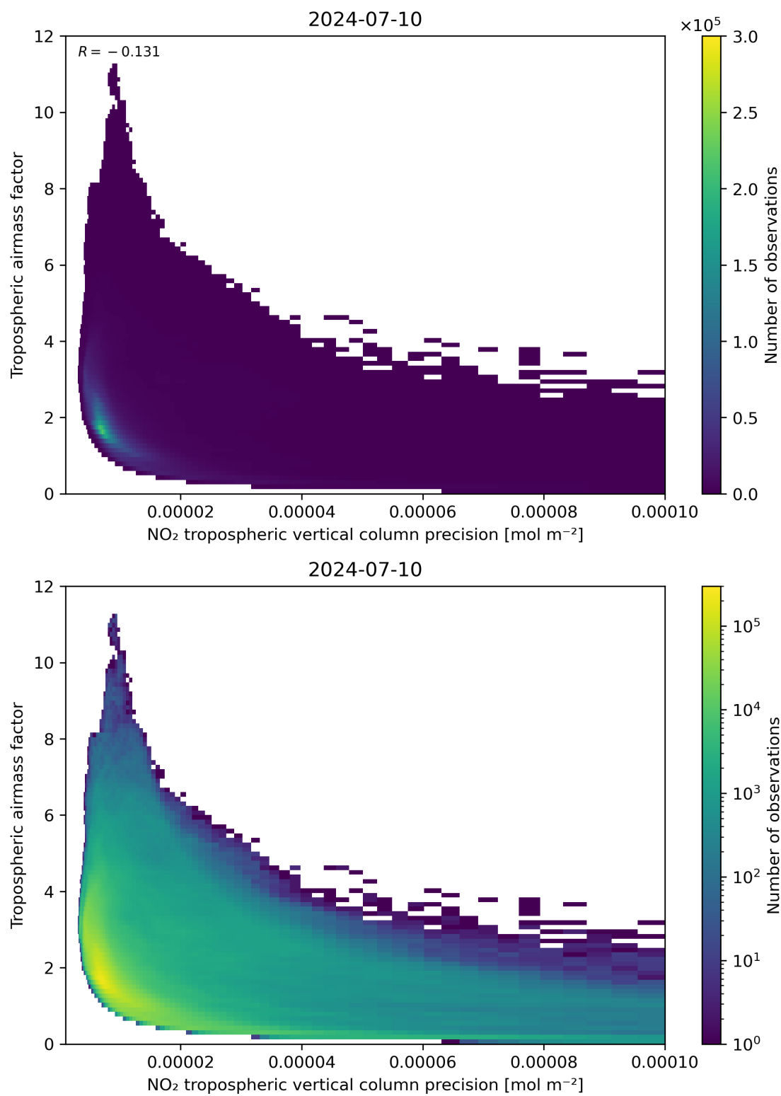
Figure 133: Scatter density plot of “NO 2 tropospheric vertical column precision” against “Tropospheric air mass factor” for 2024-07-10 to 2024-07-11.
