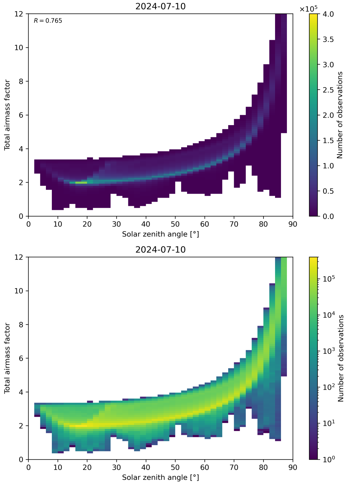
Figure 146: Scatter density plot of “Solar zenith angle” against “Total air mass factor” for 2024-07-10 to 2024-07-11.
