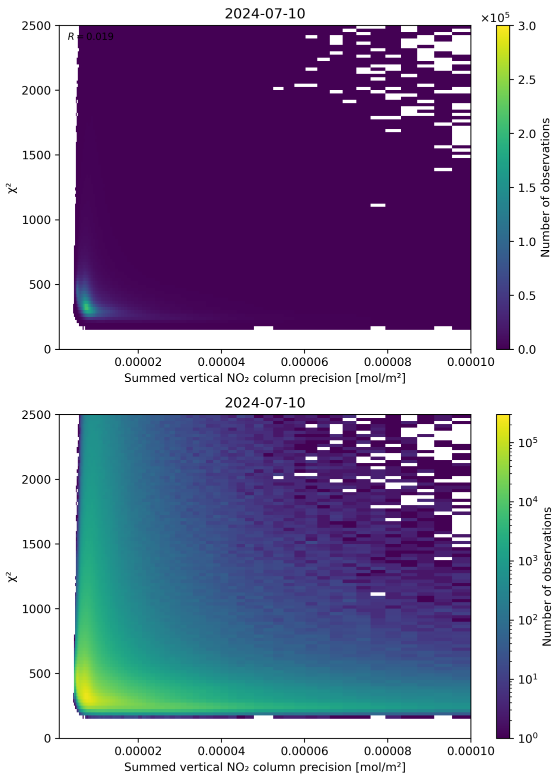
Figure 107: Scatter density plot of “Summed vertical NO 2 column precision” against “ \chi^2 ” for 2024-07-10 to 2024-07-11.
