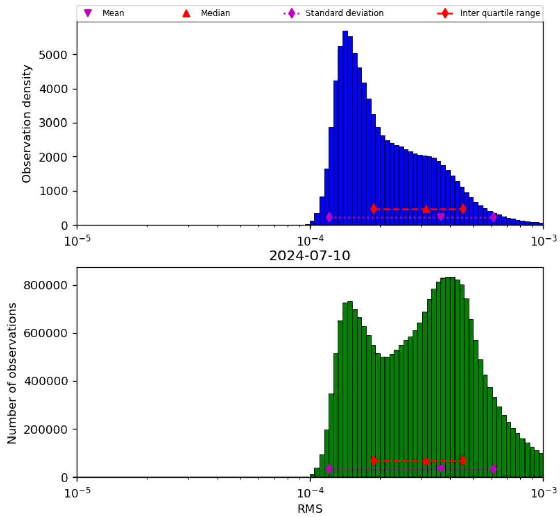
Figure 43: Histogram of “RMS” for 2024-07-10 to 2024-07-11
