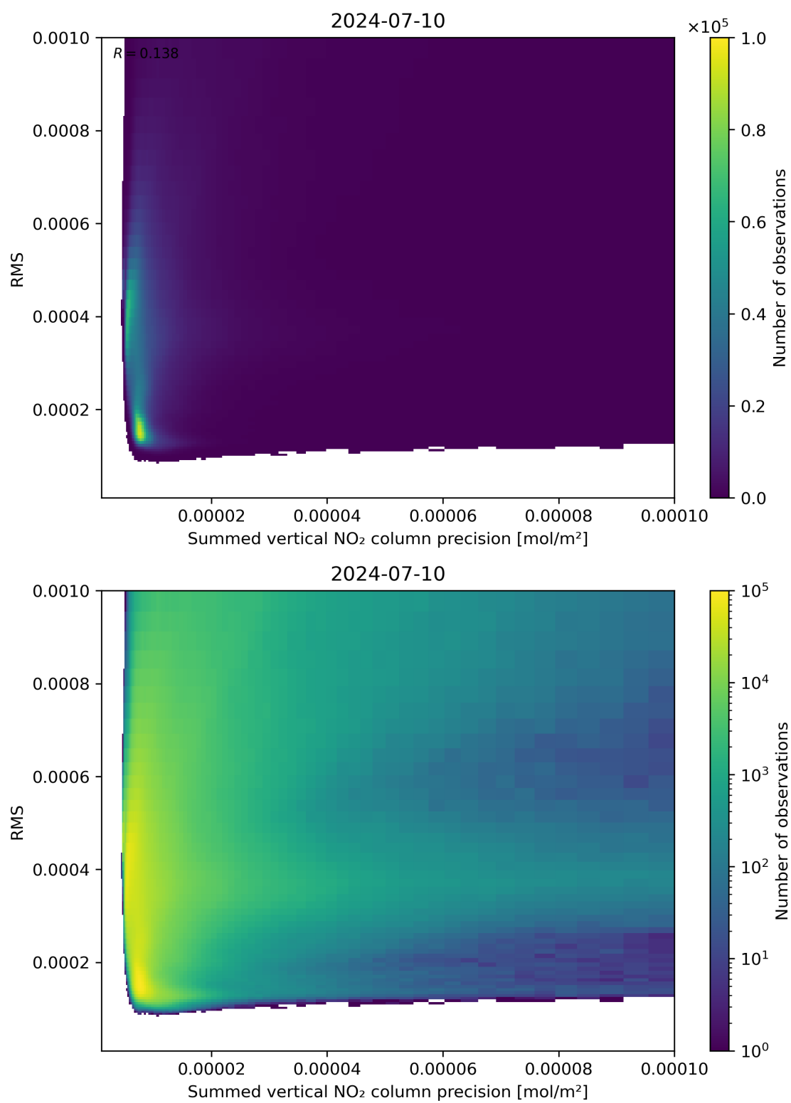
Figure 108: Scatter density plot of “Summed vertical NO 2 column precision” against “RMS” for 2024-07-10 to 2024-07-11.
