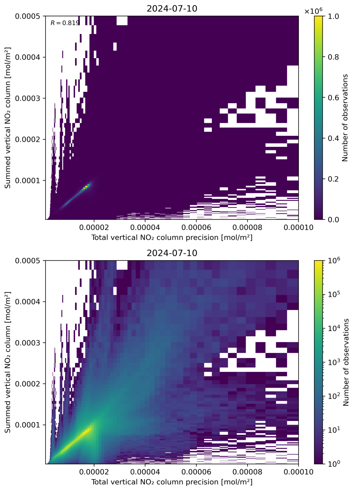
Figure 117: Scatter density plot of “Total vertical NO 2 column precision” against “Summed vertical NO 2 column” for 2024-07-10 to 2024-07-11.
