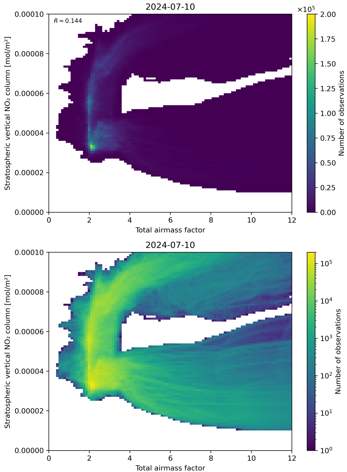
Figure 64: Scatter density plot of “Total airmass factor” against “Stratospheric vertical NO 2 column” for 2024-07-10 to 2024-07-11.
