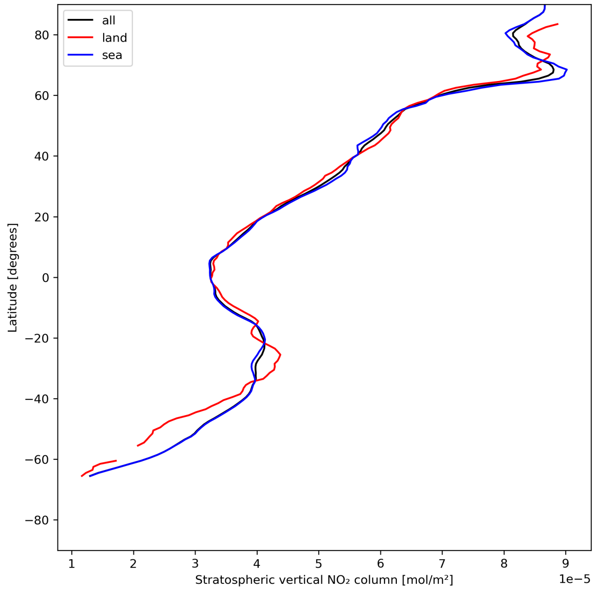
Figure 19: Zonal average of “Stratospheric vertical NO 2 column” for 2024-07-10 to 2024-07-11.
