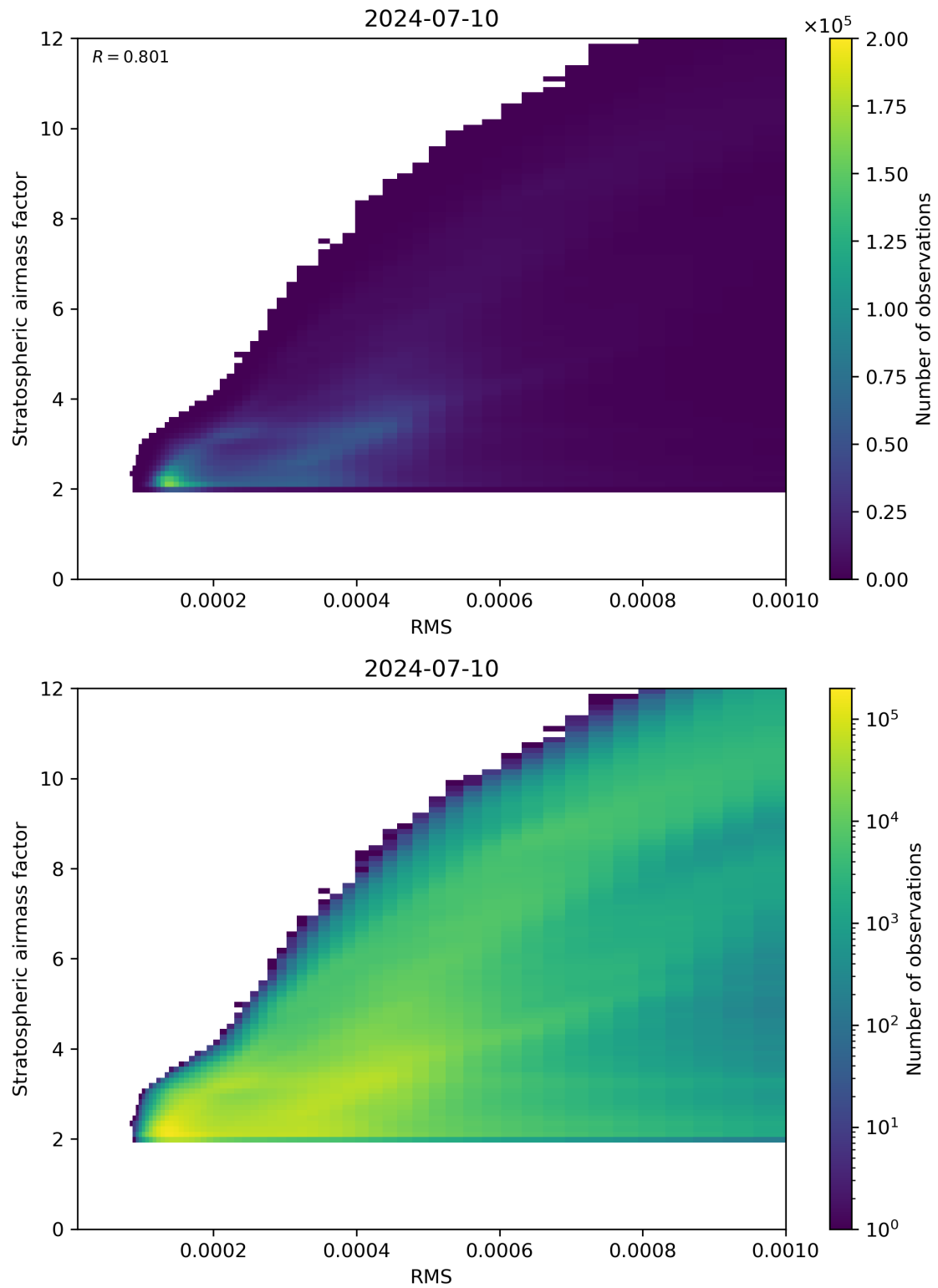
Figure 144: Scatter density plot of “RMS” against “Stratospheric airmass factor” for 2024-07-10 to 2024-07-11.
