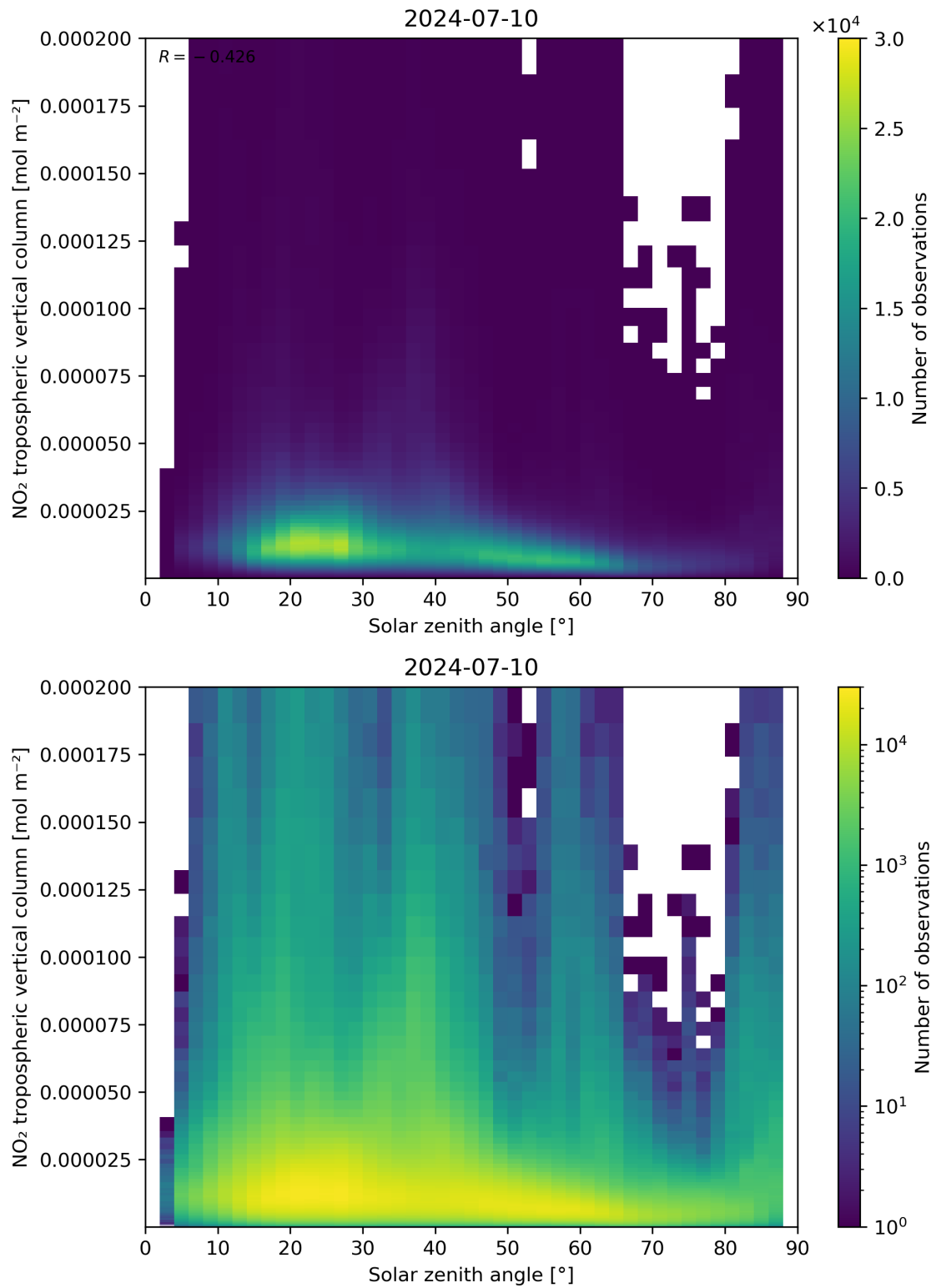
Figure 155: Scatter density plot of “Solar zenith angle” against “NO 2 tropospheric vertical column” for 2024-07-10 to 2024-07-11.
