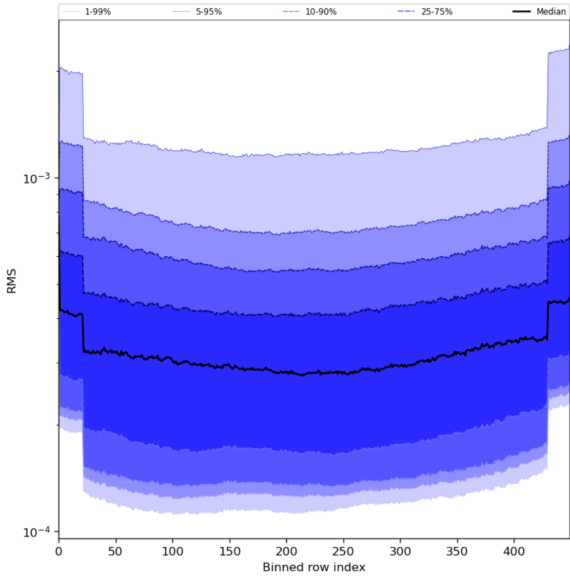
Figure 60: Along track statistics of “RMS” for 2024-07-10 to 2024-07-11
