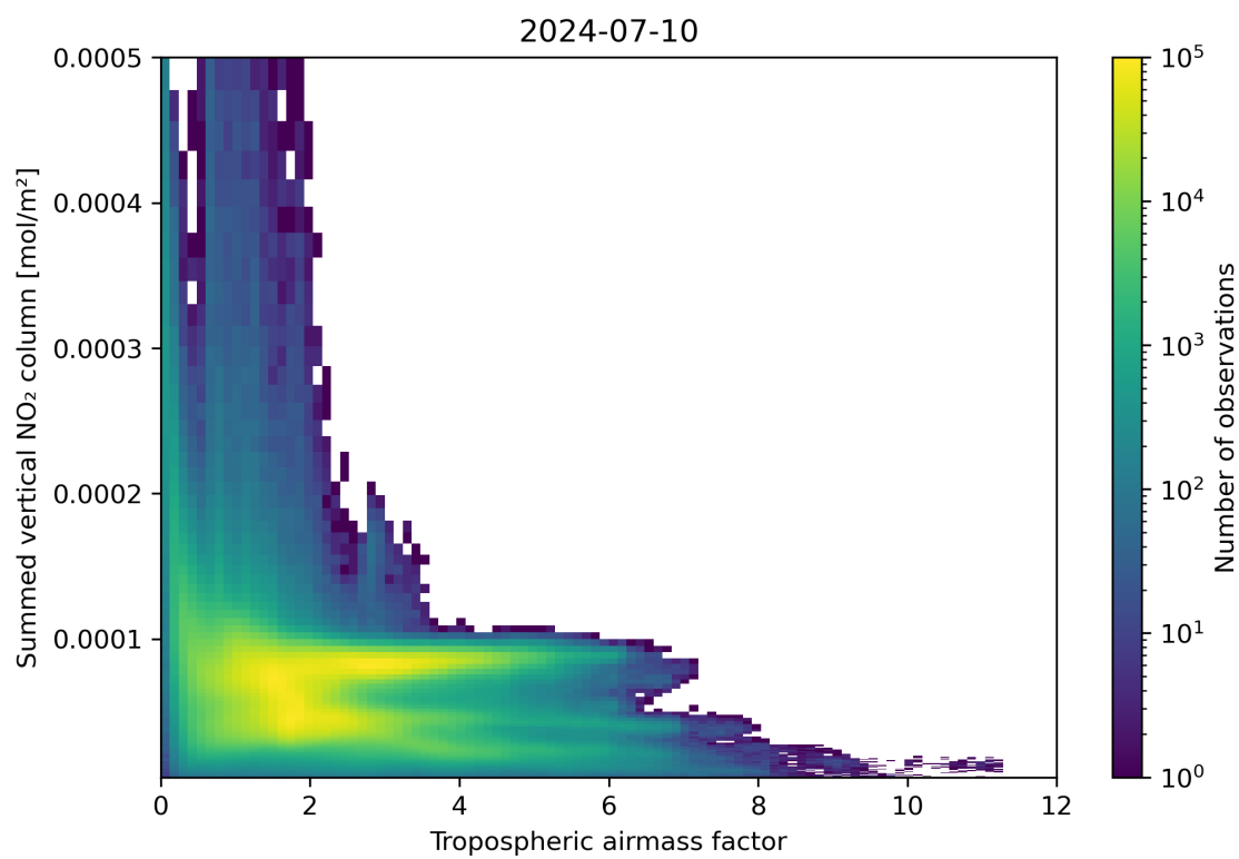
Figure 75: Scatter density plot of “Tropospheric airmass factor” against “Summed vertical NO 2 column” for 2024-07-10 to 2024-07-11.
