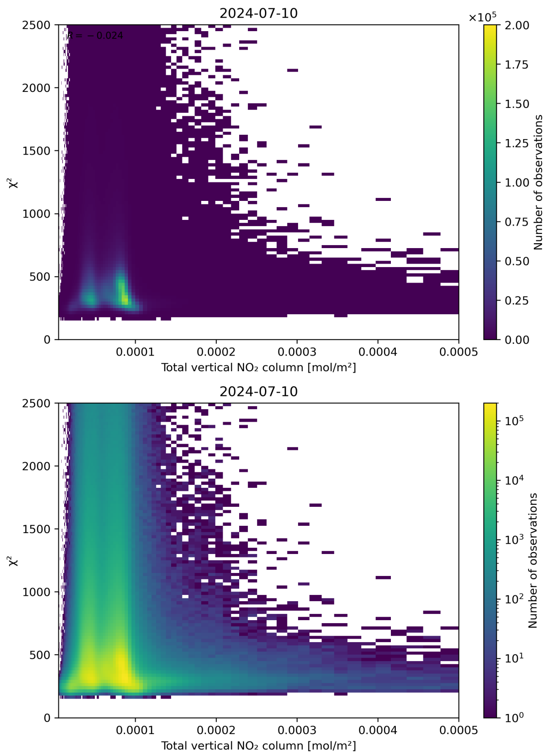
Figure 111: Scatter density plot of “Total vertical NO 2 column” against “ \chi^2 ” for 2024-07-10 to 2024-07-11.
