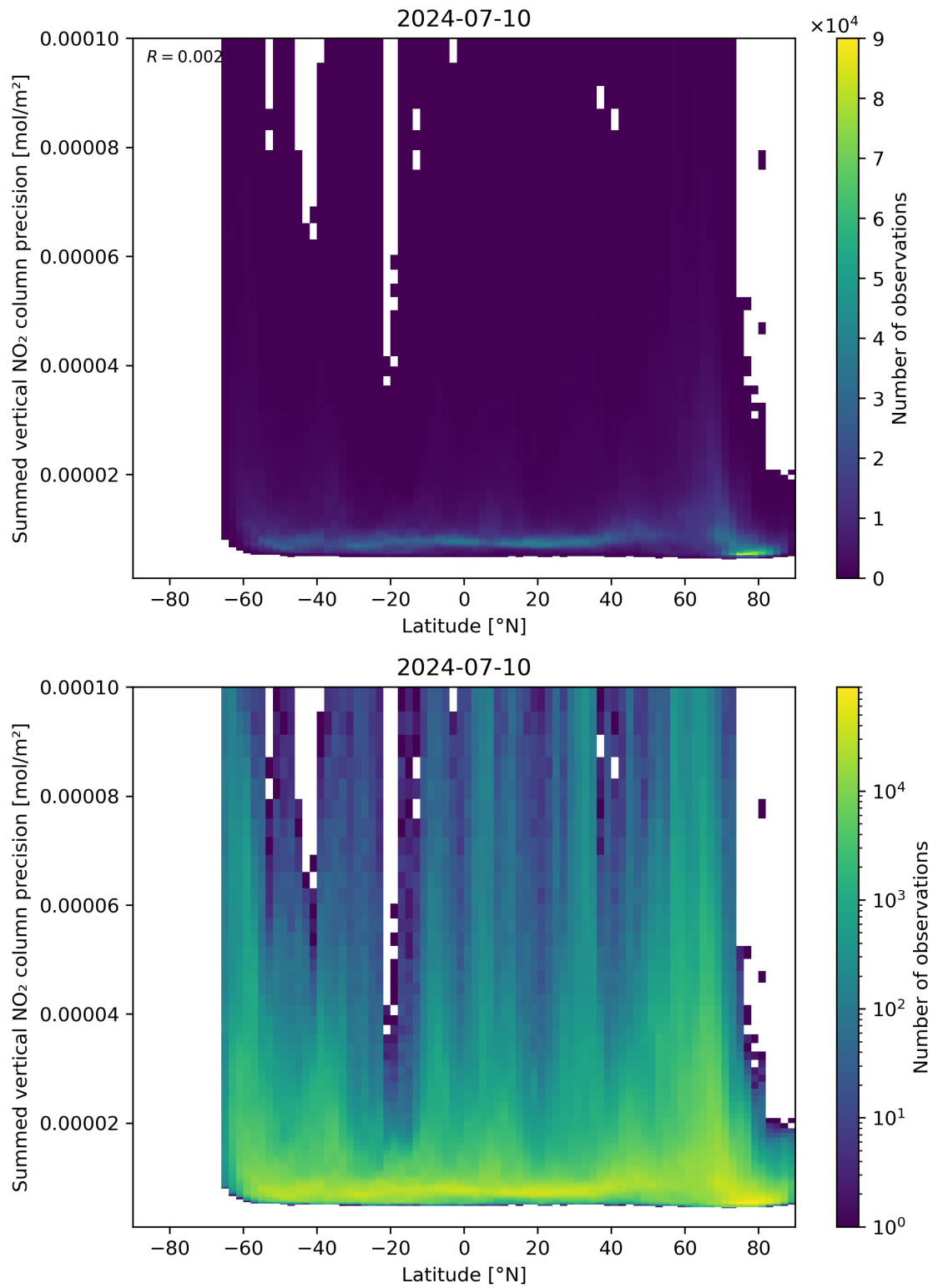
Figure 89: Scatter density plot of “Latitude” against “Summed vertical NO 2 column precision” for 2024-07-10 to 2024-07-11.
