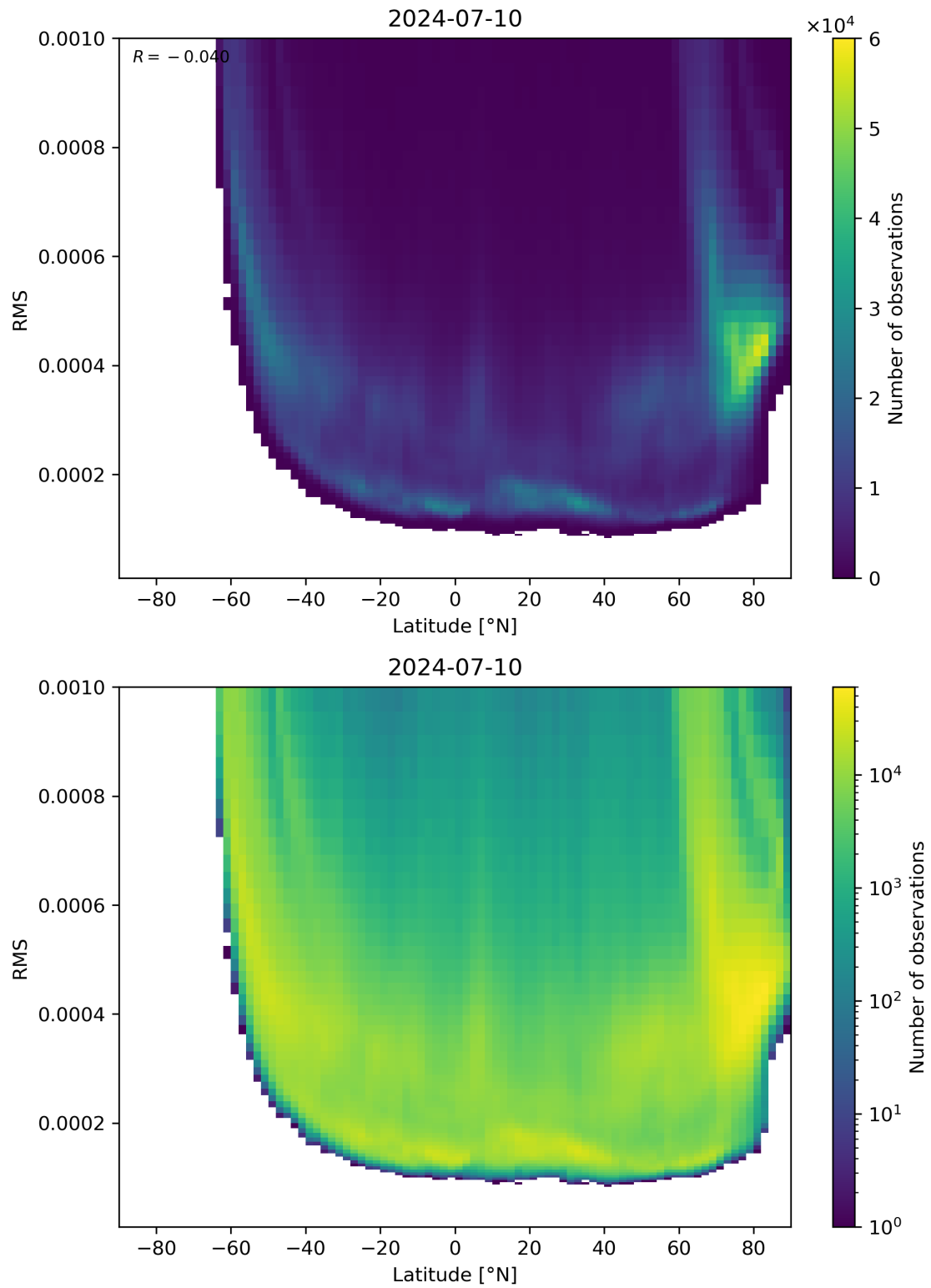
Figure 94: Scatter density plot of “Latitude” against “RMS” for 2024-07-10 to 2024-07-11.
