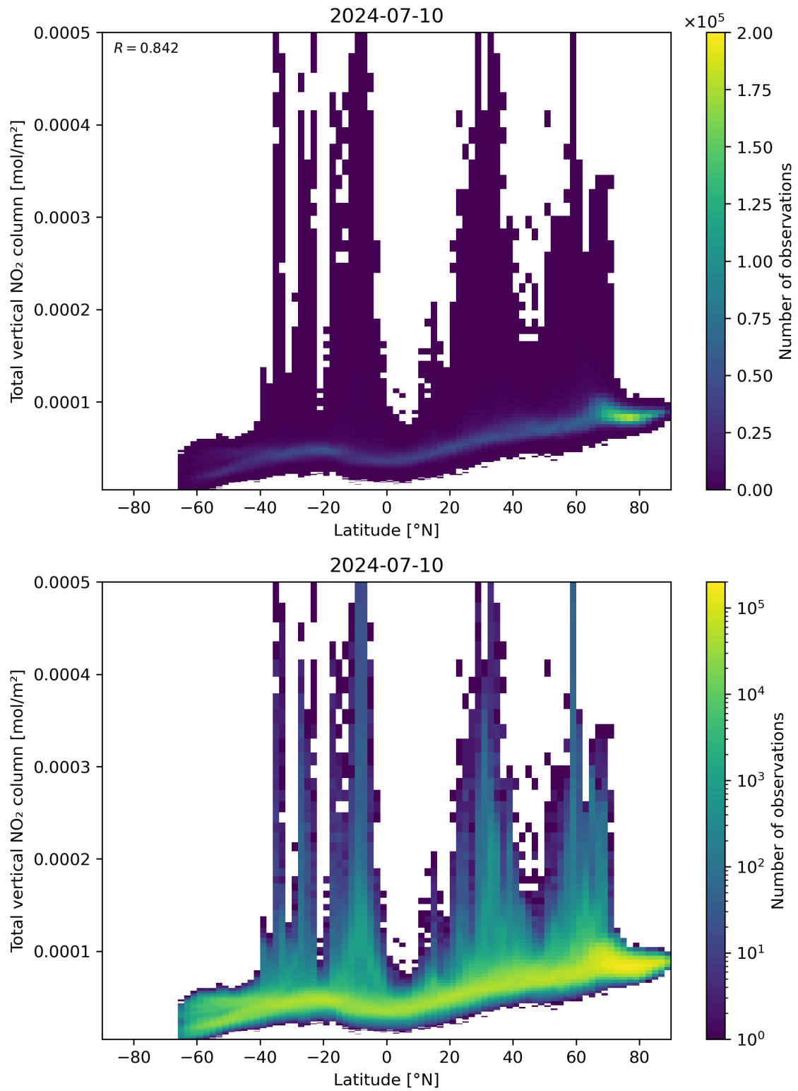
Figure 90: Scatter density plot of “Latitude” against “Total vertical NO 2 column” for 2024-07-10 to 2024-07-11.
