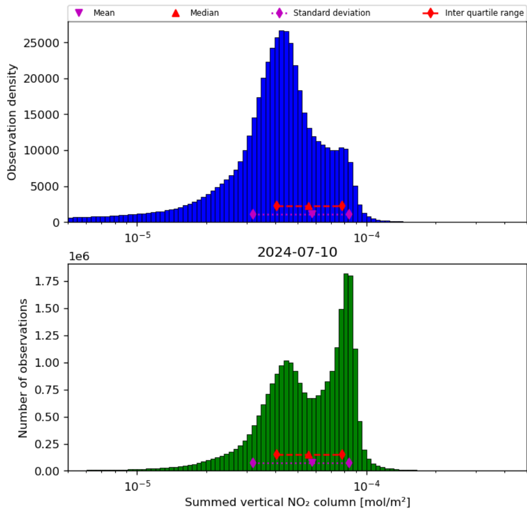
Figure 40: Histogram of “Summed vertical NO 2 column” for 2024-07-10 to 2024-07-11
