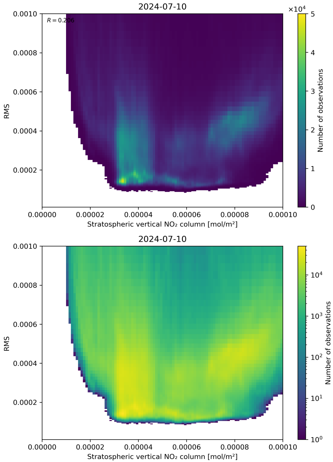
Figure 102: Scatter density plot of “Stratospheric vertical NO 2 column” against “RMS” for 2024-07-10 to 2024-07-11.
