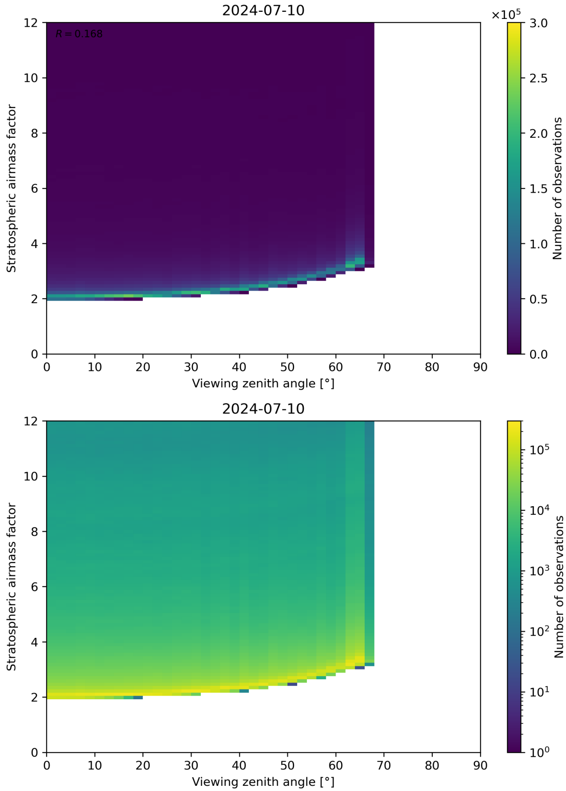
Figure 159: Scatter density plot of “Viewing zenith angle” against “Stratospheric airmass factor” for 2024-07-10 to 2024-07-11.
