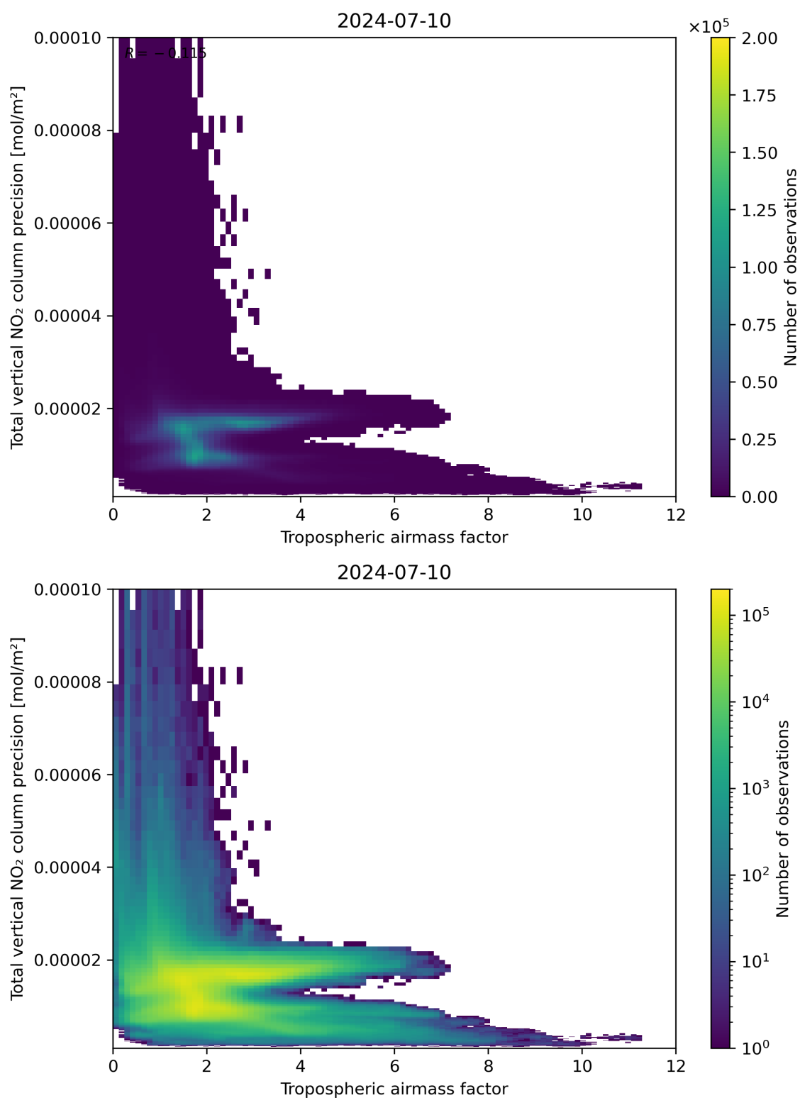
Figure 78: Scatter density plot of “Tropospheric air mass factor” against “Total vertical NO 2 column precision” for 2024-07-10 to 2024-07-11.
