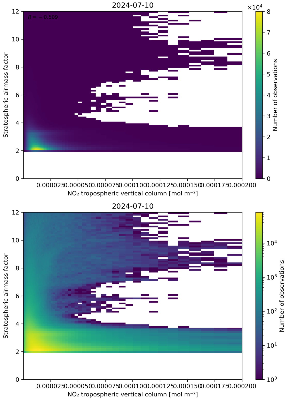
Figure 121: Scatter density plot of “NO 2 tropospheric vertical column” against “Stratospheric air mass factor” for 2024-07-10 to 2024-07-11.
