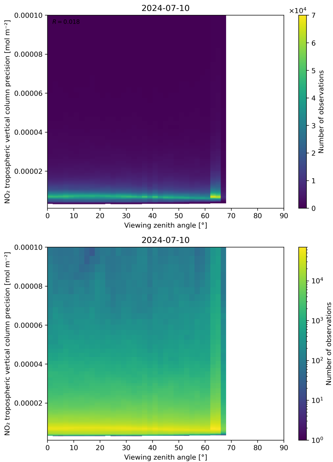
Figure 170: Scatter density plot of “Viewing zenith angle” against “NO 2 tropospheric vertical column precision” for 2024-07-10 to 2024-07-11.
