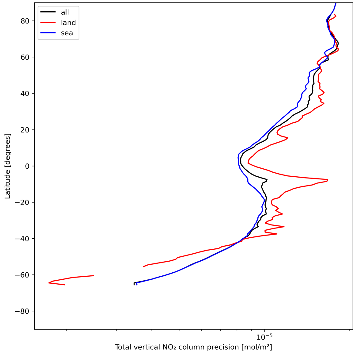
Figure 22: Zonal average of “Total vertical NO 2 column precision” for 2024-07-10 to 2024-07-11.
