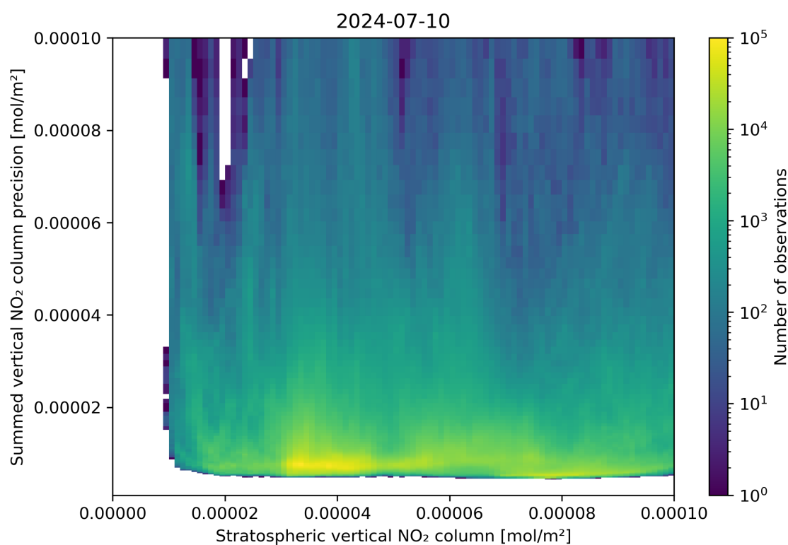
Figure 99: Scatter density plot of “Stratospheric vertical NO 2 column” against “Summed vertical NO 2 column precision” for 2024-07-10 to 2024-07-11.
