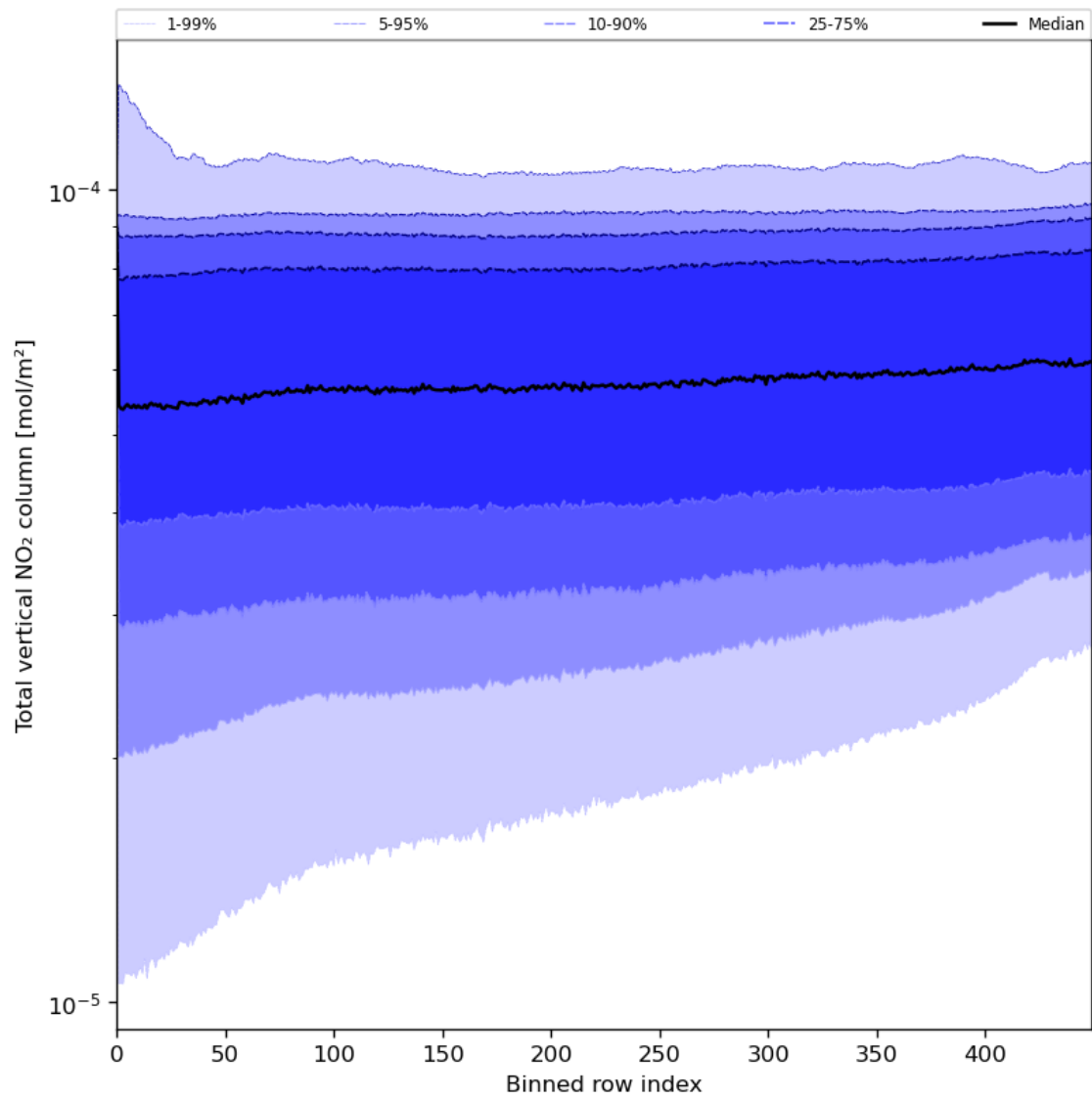
Figure 55: Along track statistics of “Total vertical NO 2 column” for 2024-07-10 to 2024-07-11
