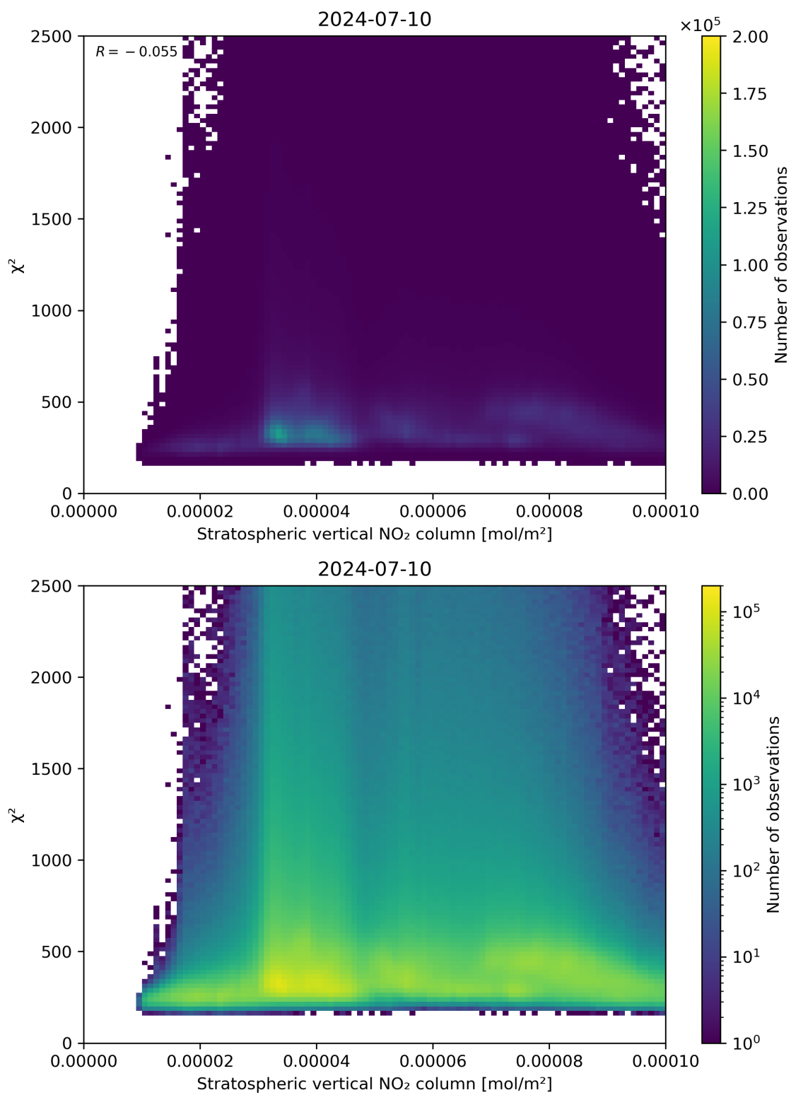
Figure 97: Scatter density plot of “Stratospheric vertical NO 2 column” against “ \chi^2 ” for 2024-07-10 to 2024-07-11.
