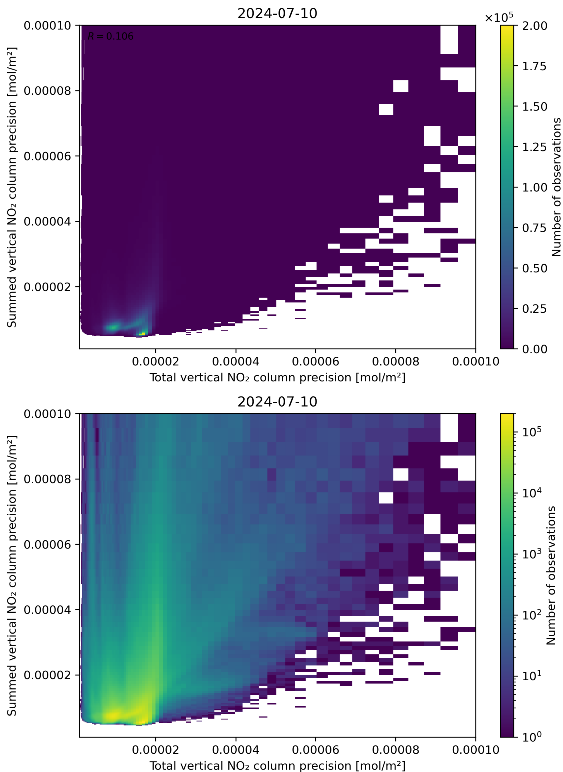
Figure 118: Scatter density plot of “Total vertical NO 2 column precision” against “Summed vertical NO 2 column precision” for 2024-07-10 to 2024-07-11.
