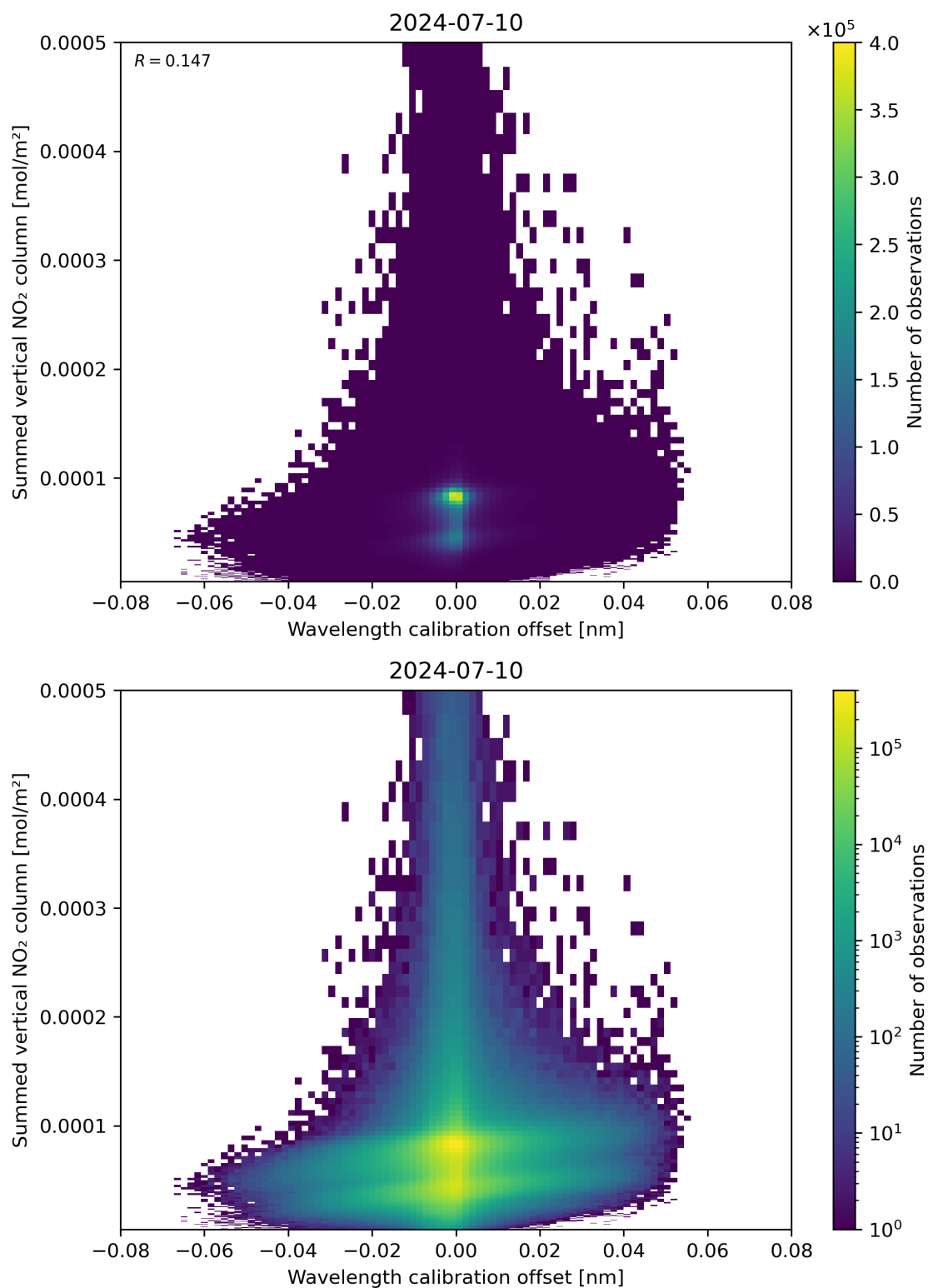
Figure 177: Scatter density plot of “Wavelength calibration offset” against “Summed vertical NO 2 column” for 2024-07-10 to 2024-07-11.
