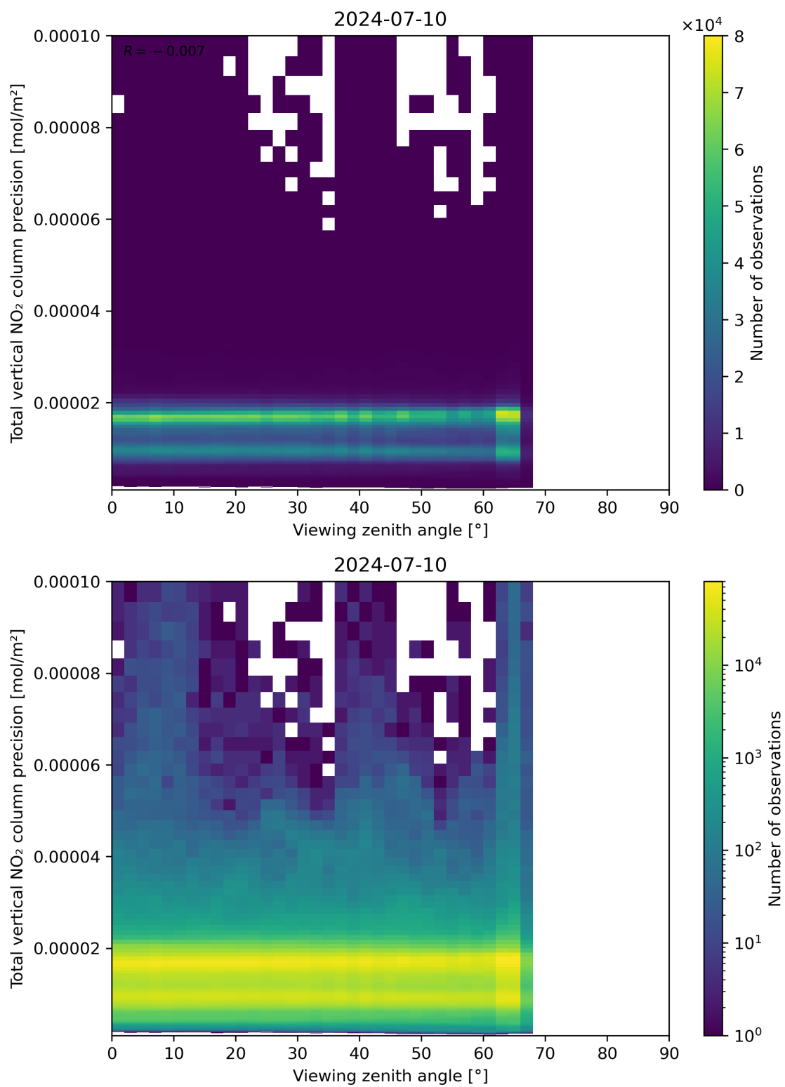
Figure 168: Scatter density plot of “Viewing zenith angle” against “Total vertical NO 2 column precision” for 2024-07-10 to 2024-07-11.
