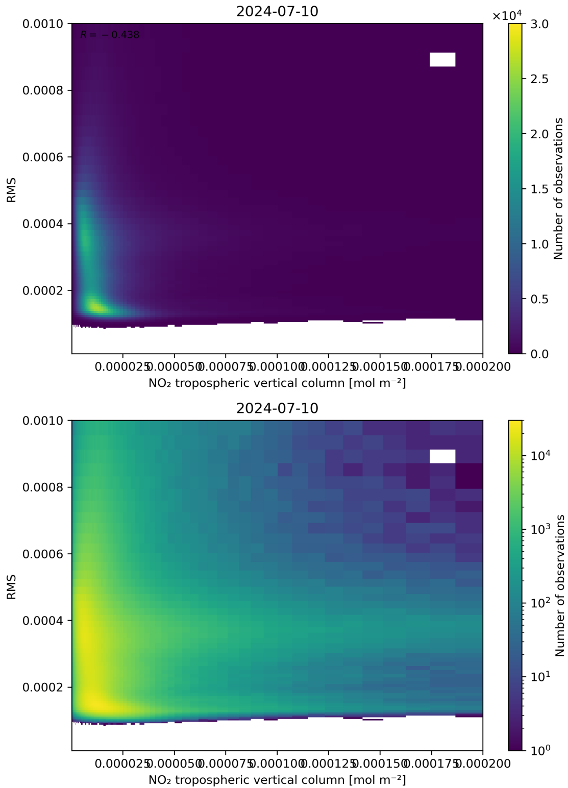
Figure 142: Scatter density plot of “NO 2 tropospheric vertical column” against “RMS” for 2024-07-10 to 2024-07-11.
