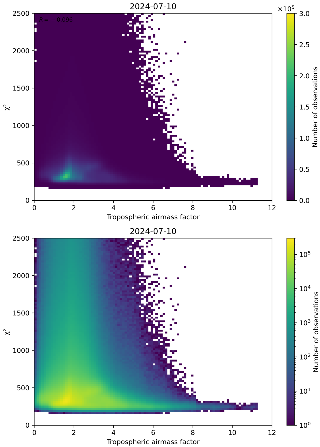
Figure 73: Scatter density plot of “Tropospheric airmass factor” against “ \chi^2 ” for 2024-07-10 to 2024-07-11.
