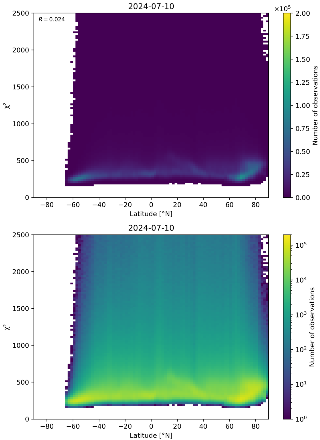
Figure 86: Scatter density plot of “Latitude” against “ \chi^2 ” for 2024-07-10 to 2024-07-11.
