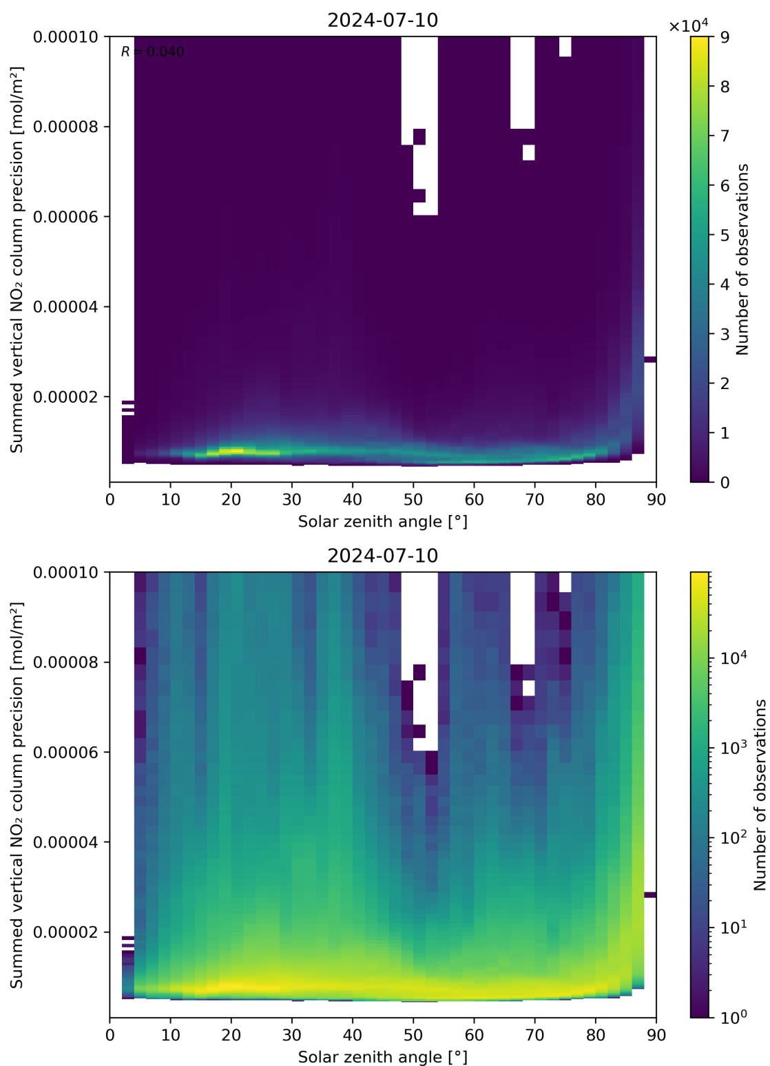
Figure 152: Scatter density plot of “Solar zenith angle” against “Summed vertical NO 2 column precision” for 2024-07-10 to 2024-07-11.
