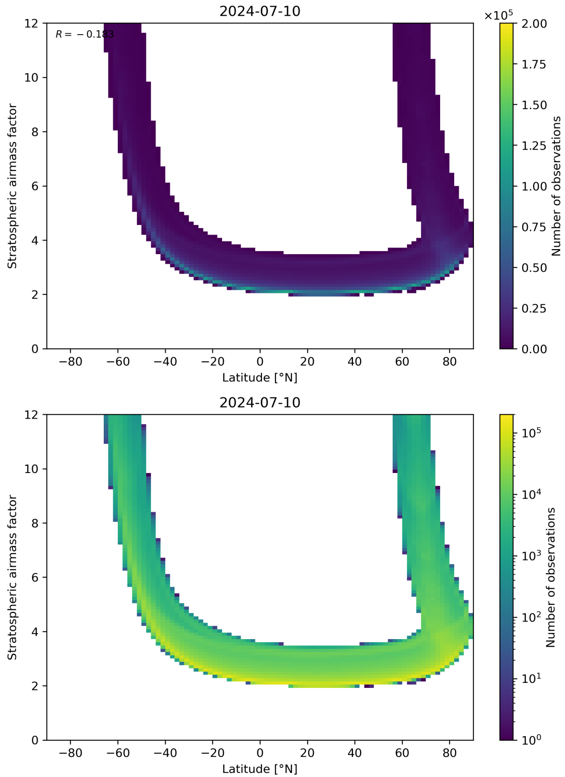
Figure 83: Scatter density plot of “Latitude” against “Stratospheric air mass factor” for 2024-07-10 to 2024-07-11.
