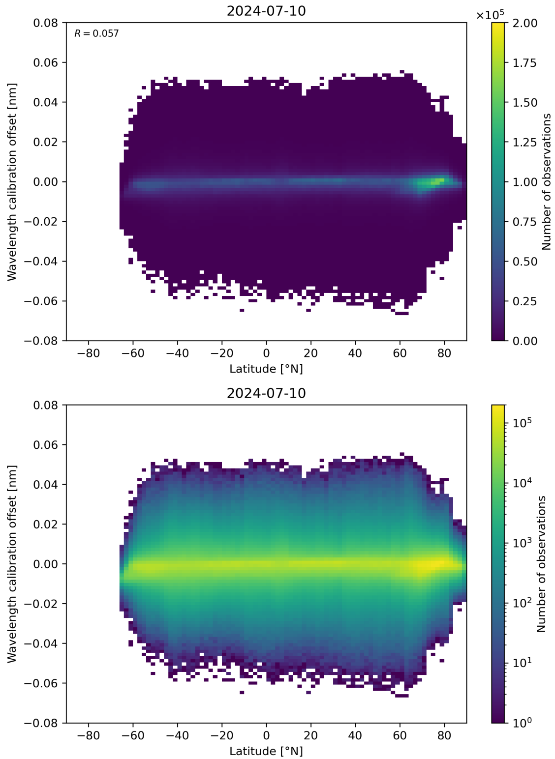
Figure 95: Scatter density plot of “Latitude” against “Wavelength calibration offset” for 2024-07-10 to 2024-07-11.
