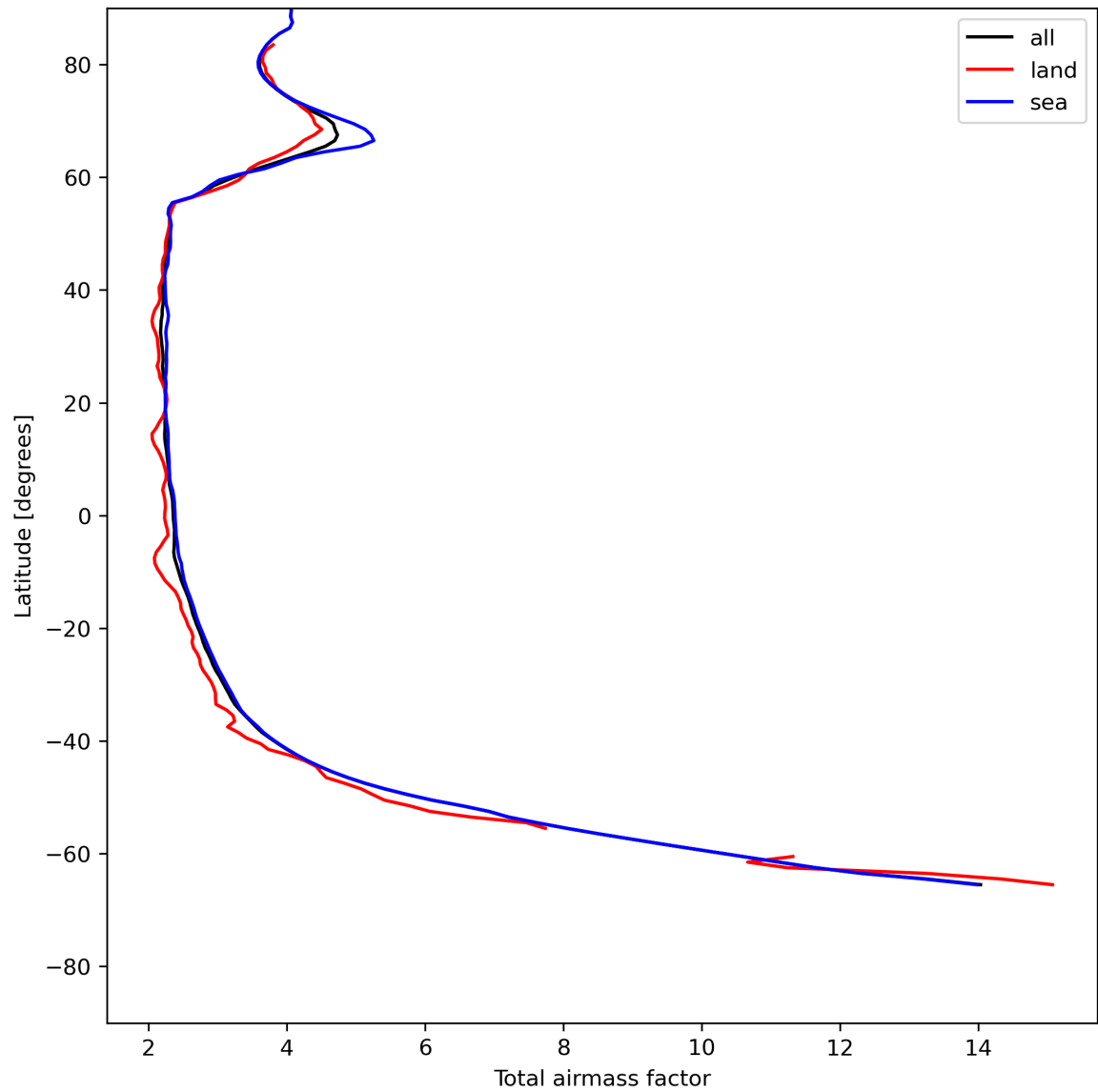
Figure 15: Zonal average of “Total airmass factor” for 2024-07-10 to 2024-07-11.
