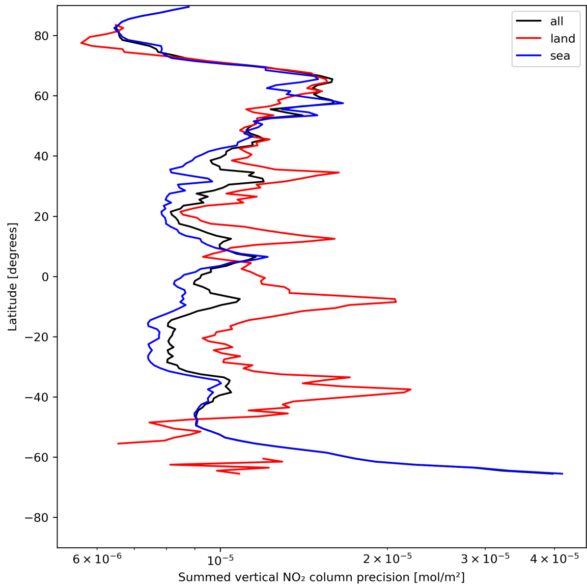
Figure 24: Zonal average of “Summed vertical NO 2 column precision” for 2024-07-10 to 2024-07-11.
