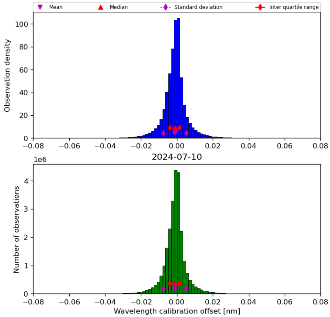
Figure 35: Histogram of “Wavelength calibration offset” for 2024-07-10 to 2024-07-11
