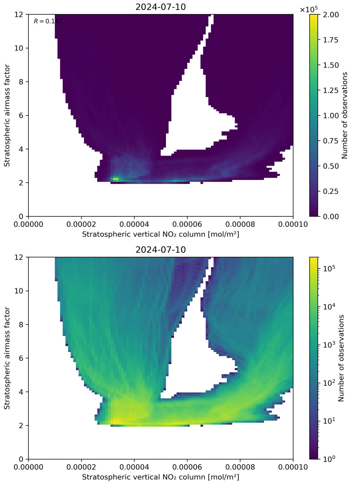
Figure 96: Scatter density plot of “Stratospheric vertical NO 2 column” against “Stratospheric airmass factor” for 2024-07-10 to 2024-07-11.
