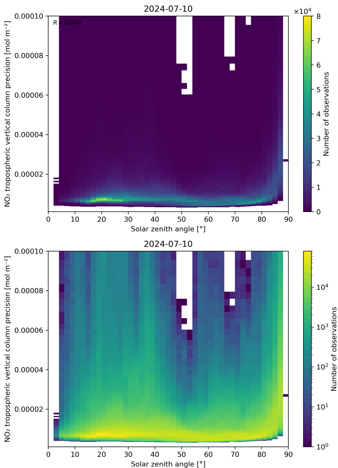
Figure 156: Scatter density plot of “Solar zenith angle” against “NO 2 tropospheric vertical column precision” for 2024-07-10 to 2024-07-11.
