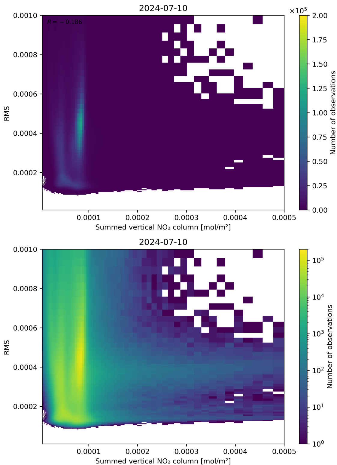
Figure 109: Scatter density plot of “Summed vertical NO 2 column” against “RMS” for 2024-07-10 to 2024-07-11.
