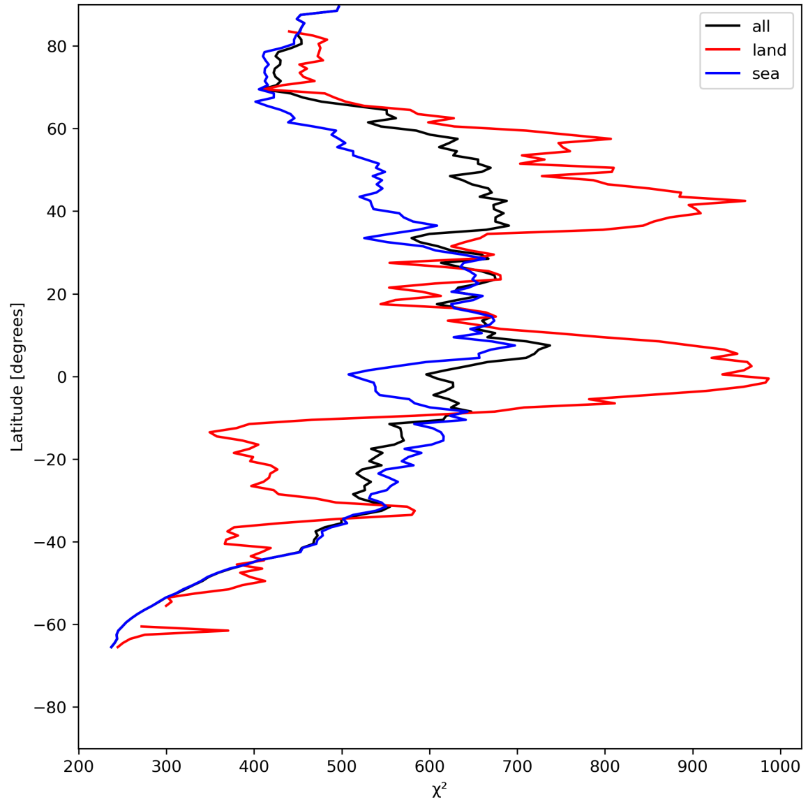
Figure 25: Zonal average of “ \chi^2 ” for 2024-07-10 to 2024-07-11.
