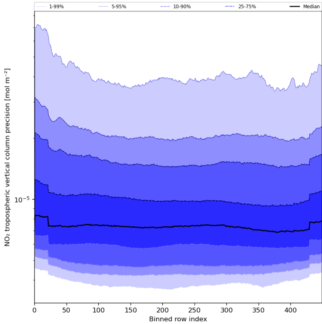
Figure 47: Along track statistics of “NO 2 tropospheric vertical column precision” for 2024-07-10 to 2024-07-11
