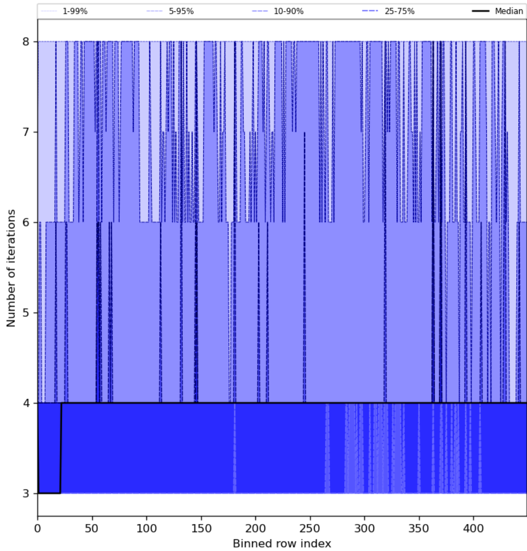
Figure 51: Along track statistics of “Number of iterations” for 2024-07-10 to 2024-07-11
