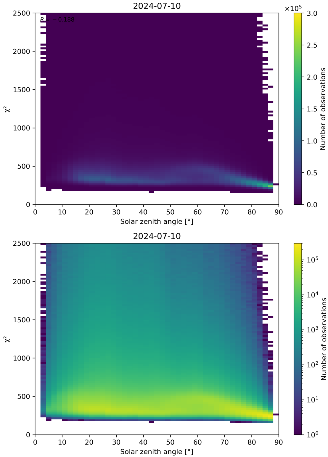
Figure 148: Scatter density plot of “Solar zenith angle” against “ \chi^2 ” for 2024-07-10 to 2024-07-11.
