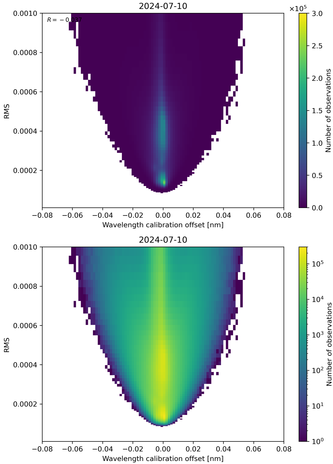
Figure 181: Scatter density plot of “Wavelength calibration offset” against “RMS” for 2024-07-10 to 2024-07-11.
