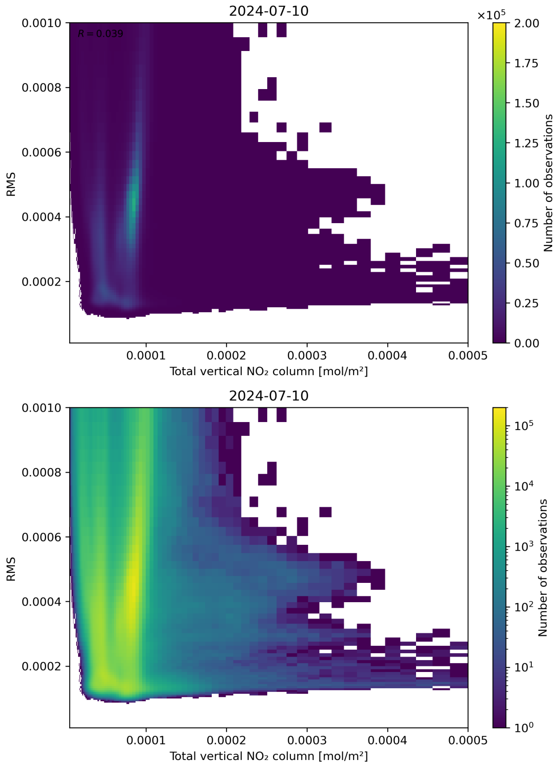
Figure 120: Scatter density plot of “Total vertical NO 2 column” against “RMS” for 2024-07-10 to 2024-07-11.
