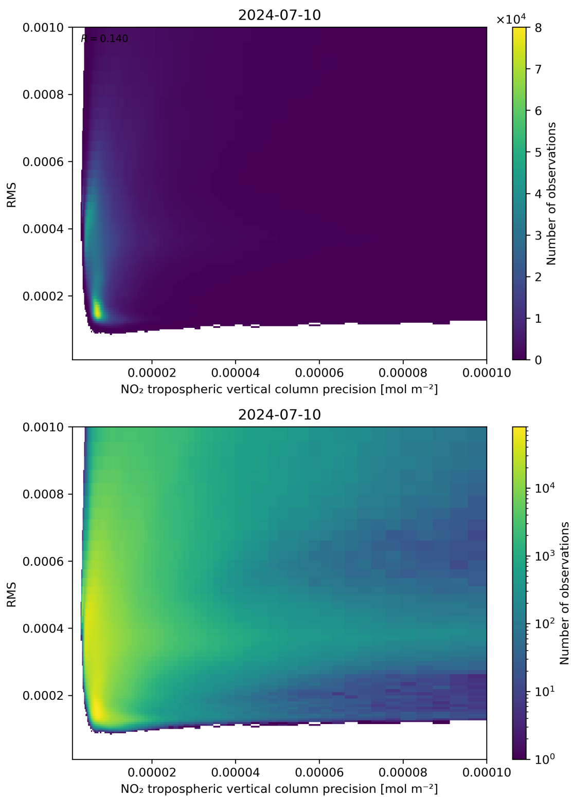
Figure 140: Scatter density plot of “NO 2 tropospheric vertical column precision” against “RMS” for 2024-07-10 to 2024-07-11.
