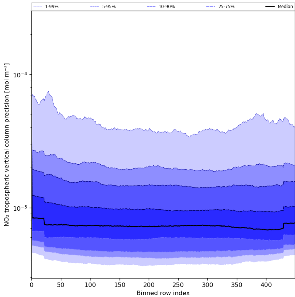
Figure 47: Along track statistics of “NO 2 tropospheric vertical column precision” for 2024-07-10 to 2024-07-12
