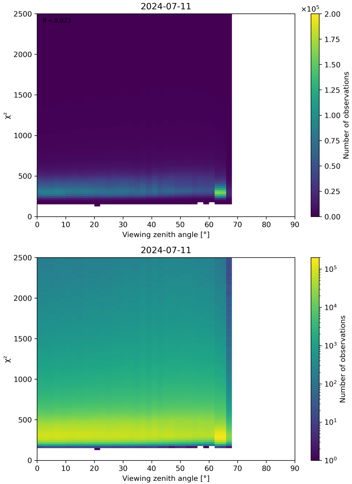
Figure 162: Scatter density plot of “Viewing zenith angle” against “ \chi^2 ” for 2024-07-10 to 2024-07-12.
