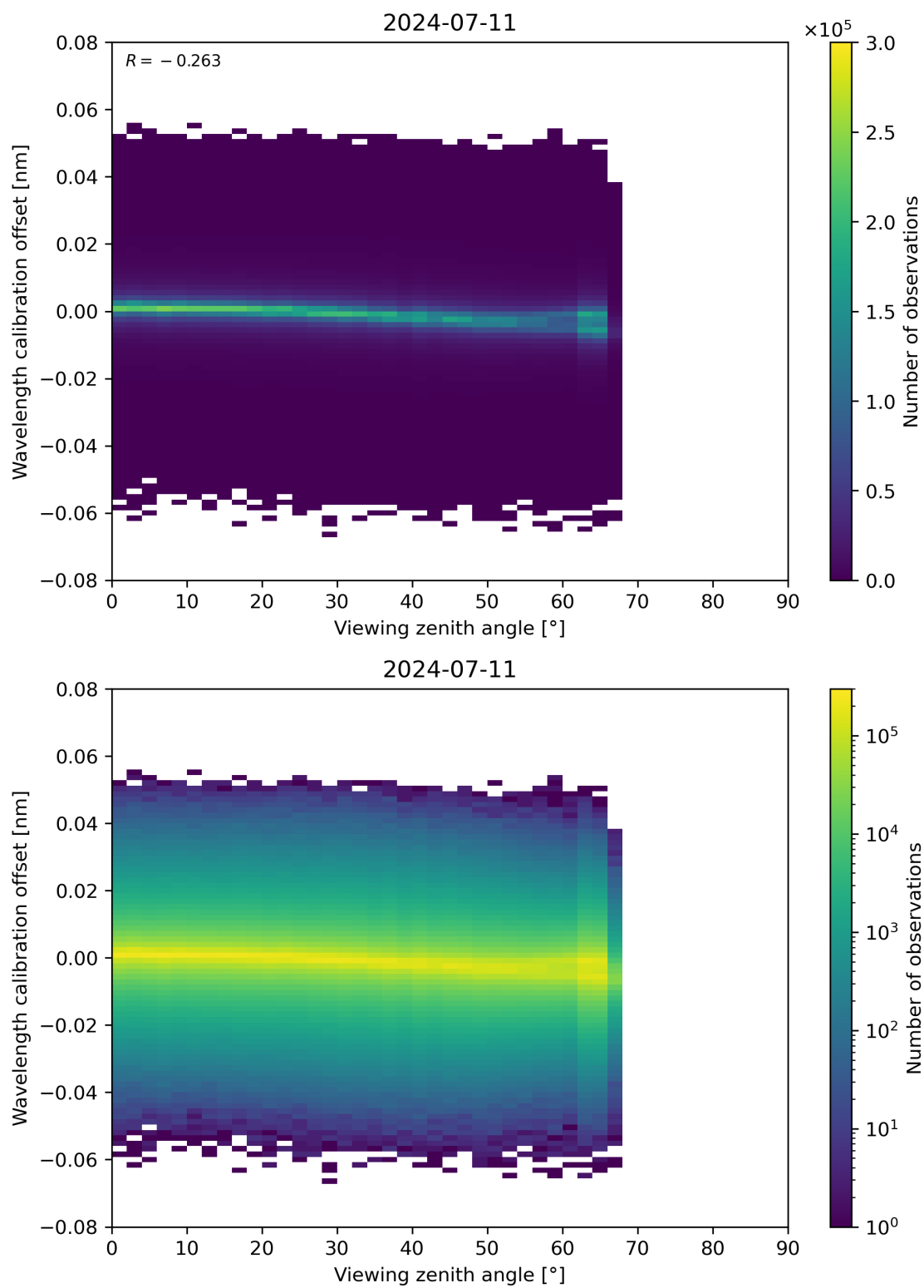
Figure 173: Scatter density plot of “Viewing zenith angle” against “Wavelength calibration offset” for 2024-07-10 to 2024-07-12.
