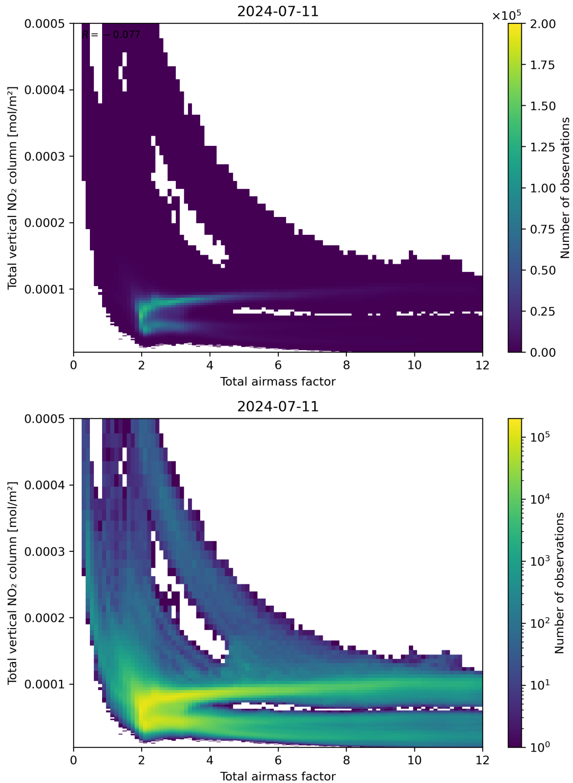
Figure 67: Scatter density plot of “Total airmass factor” against “Total vertical NO 2 column” for 2024-07-10 to 2024-07-12.
