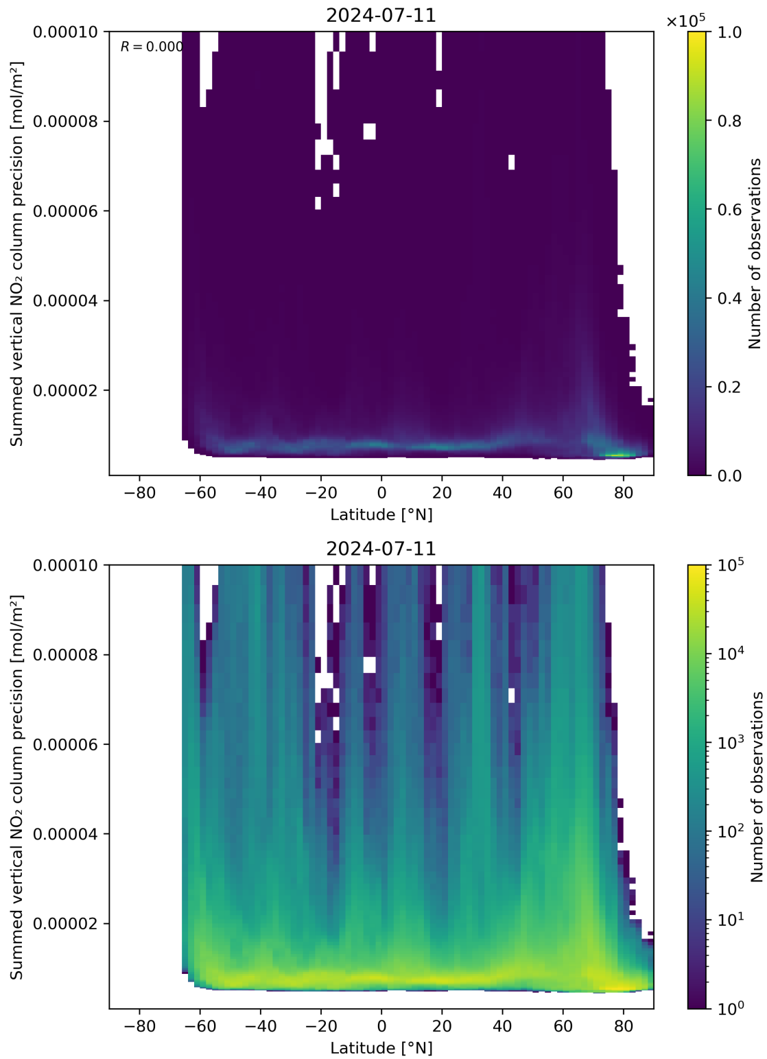
Figure 89: Scatter density plot of “Latitude” against “Summed vertical NO 2 column precision” for 2024-07-10 to 2024-07-12.
