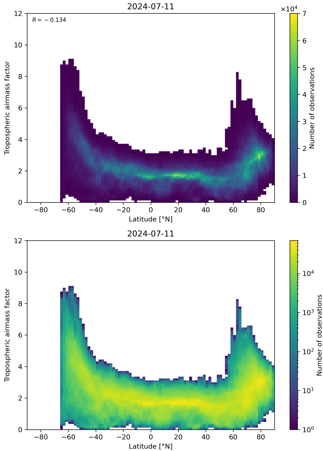
Figure 85: Scatter density plot of “Latitude” against “Tropospheric airmass factor” for 2024-07-10 to 2024-07-12.
