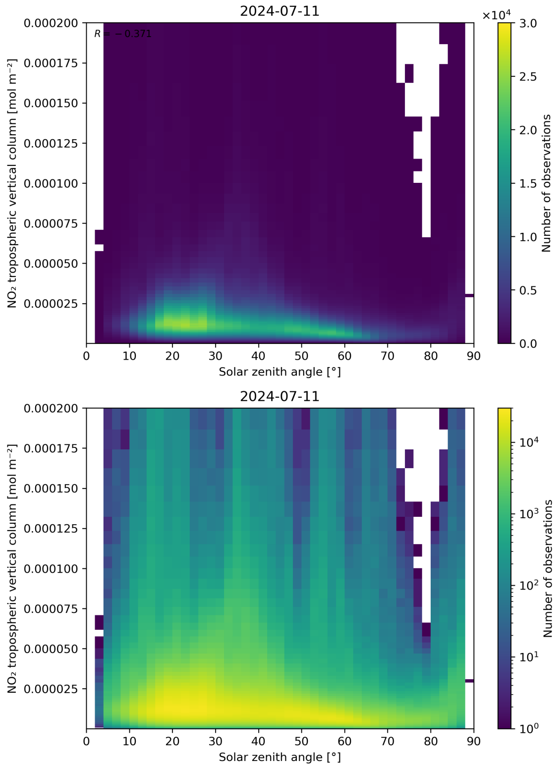
Figure 155: Scatter density plot of “Solar zenith angle” against “NO 2 tropospheric vertical column” for 2024-07-10 to 2024-07-12.
