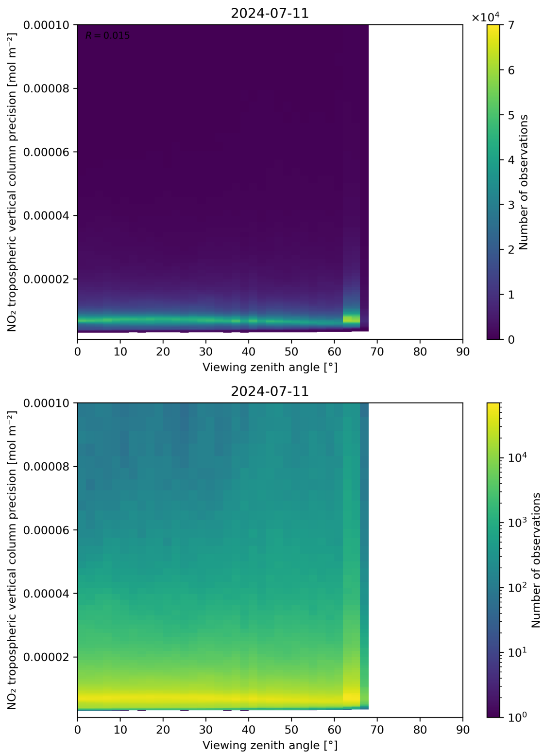
Figure 170: Scatter density plot of “Viewing zenith angle” against “NO 2 tropospheric vertical column precision” for 2024-07-10 to 2024-07-12.
