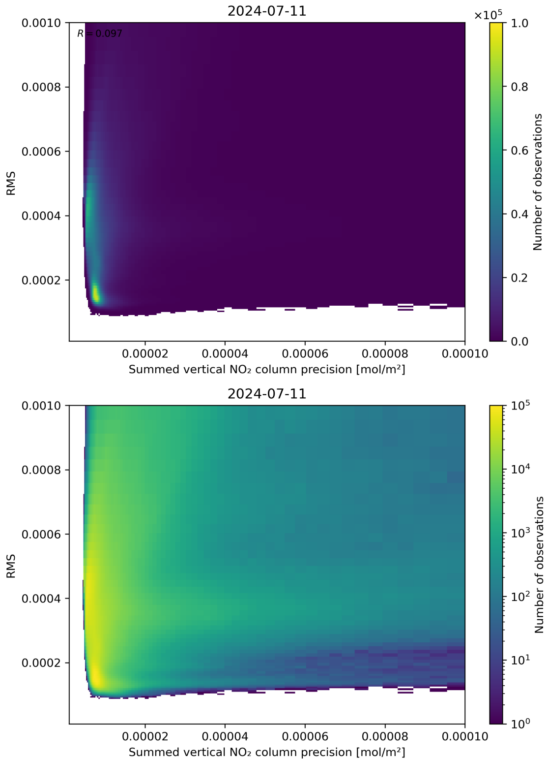
Figure 108: Scatter density plot of “Summed vertical NO 2 column precision” against “RMS” for 2024-07-10 to 2024-07-12.
