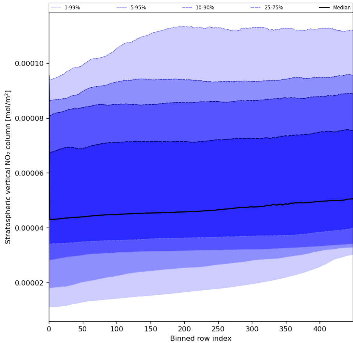
Figure 53: Along track statistics of “Stratospheric vertical NO 2 column” for 2024-07-10 to 2024-07-12
