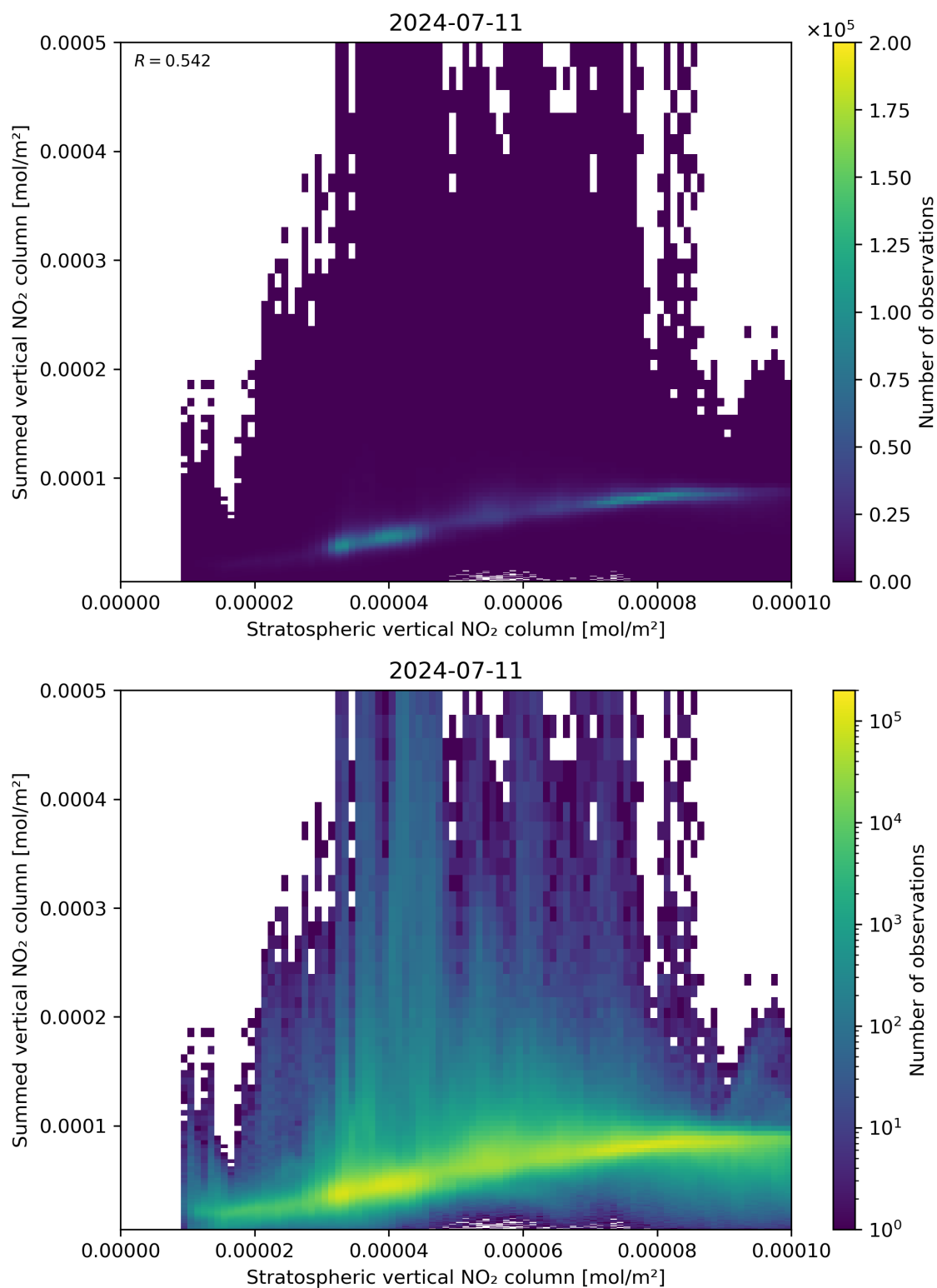
Figure 98: Scatter density plot of “Stratospheric vertical NO 2 column” against “Summed vertical NO 2 column” for 2024-07-10 to 2024-07-12.
