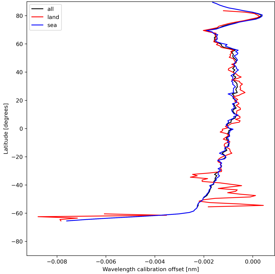
Figure 18: Zonal average of “Wavelength calibration offset” for 2024-07-10 to 2024-07-12.
