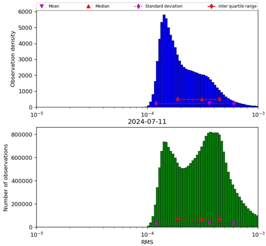
Figure 43: Histogram of “RMS” for 2024-07-10 to 2024-07-12
