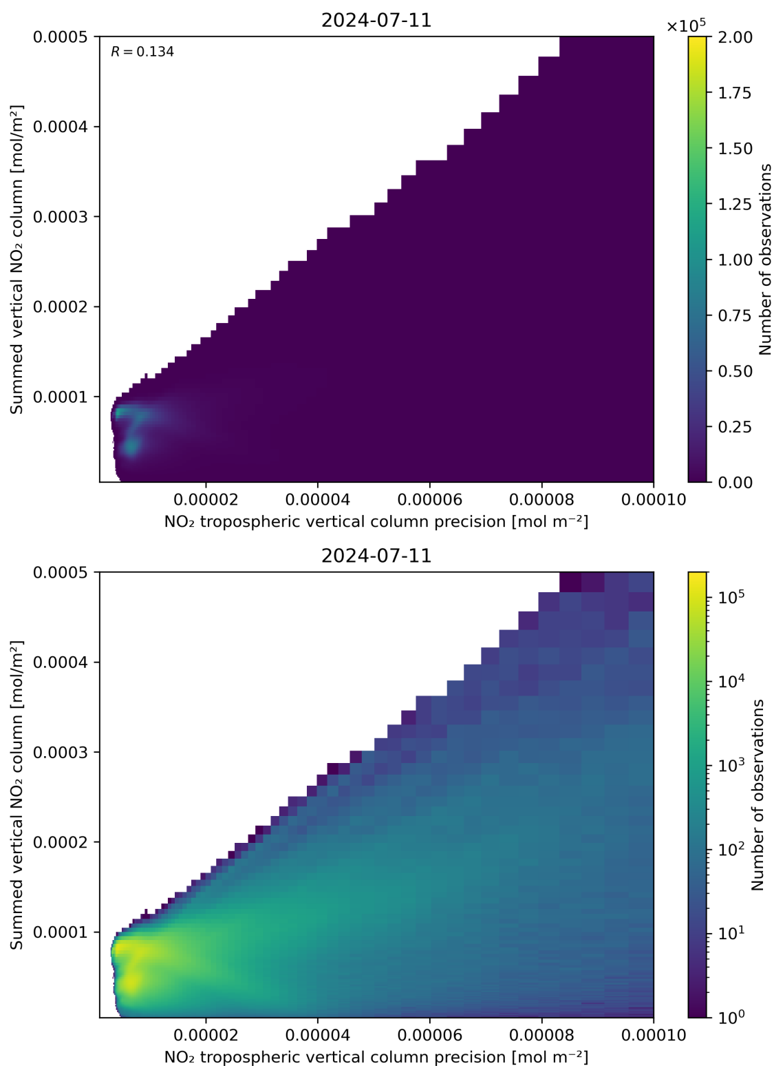
Figure 136: Scatter density plot of “NO 2 tropospheric vertical column precision” against “Summed vertical NO 2 column” for 2024-07-10 to 2024-07-12.
