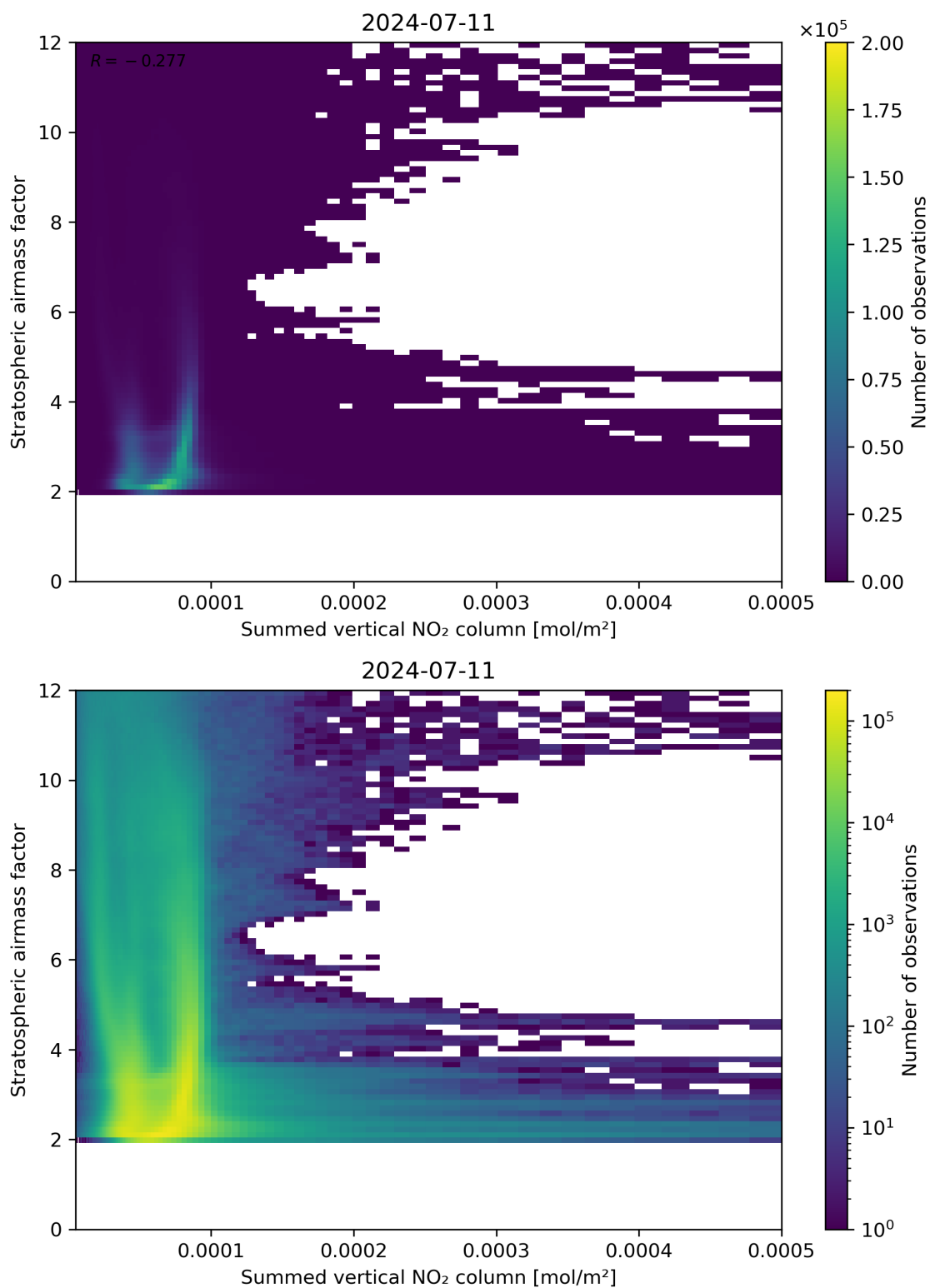
Figure 103: Scatter density plot of “Summed vertical NO 2 column” against “Stratospheric air mass factor” for 2024-07-10 to 2024-07-12.
