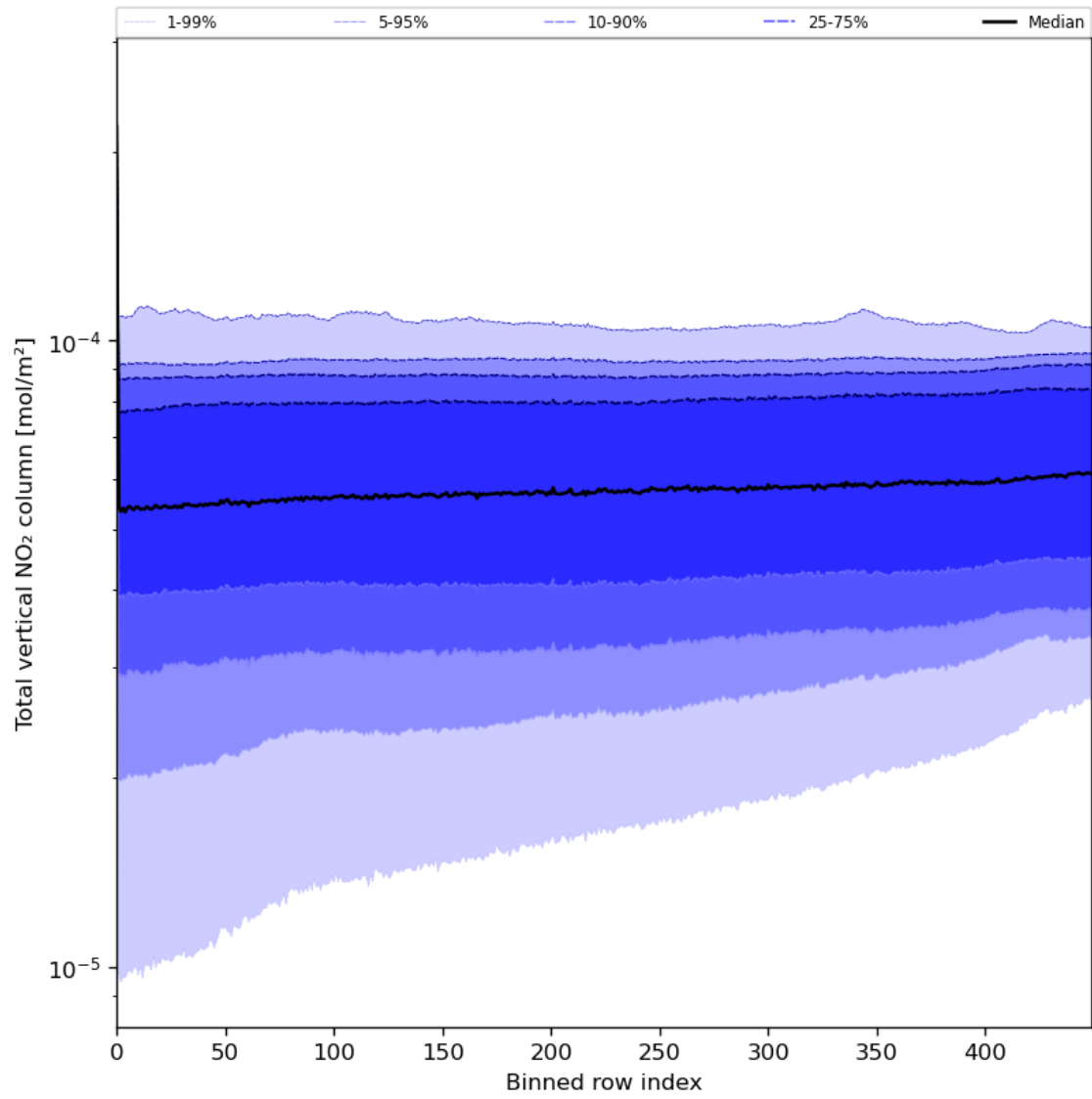
Figure 55: Along track statistics of “Total vertical NO 2 column” for 2024-07-10 to 2024-07-12
