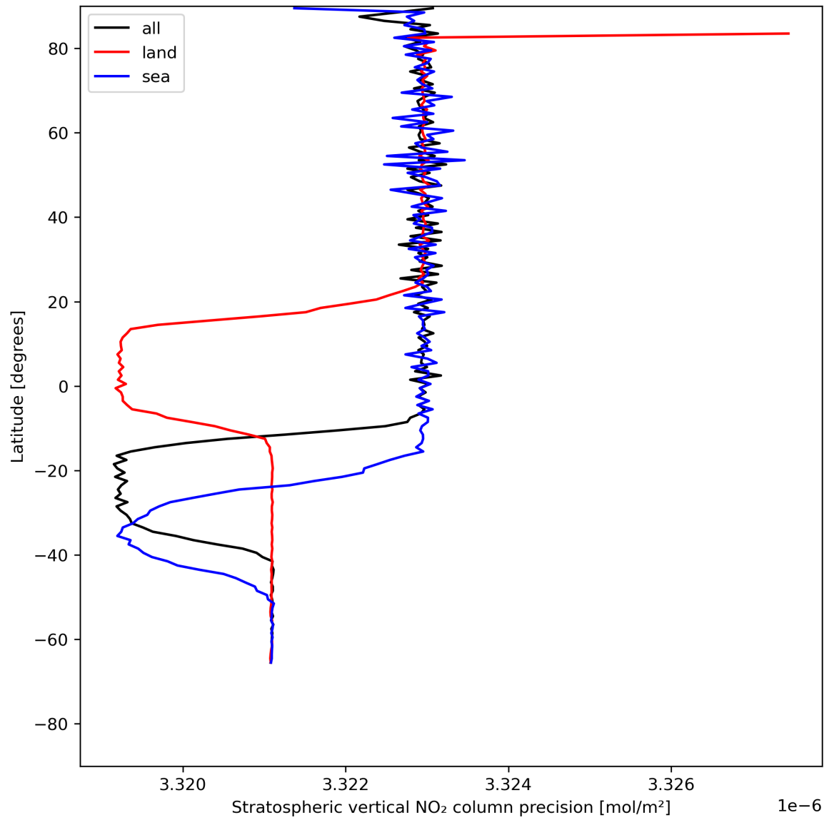
Figure 20: Zonal average of “Stratospheric vertical NO 2 column precision” for 2024-07-10 to 2024-07-12.
