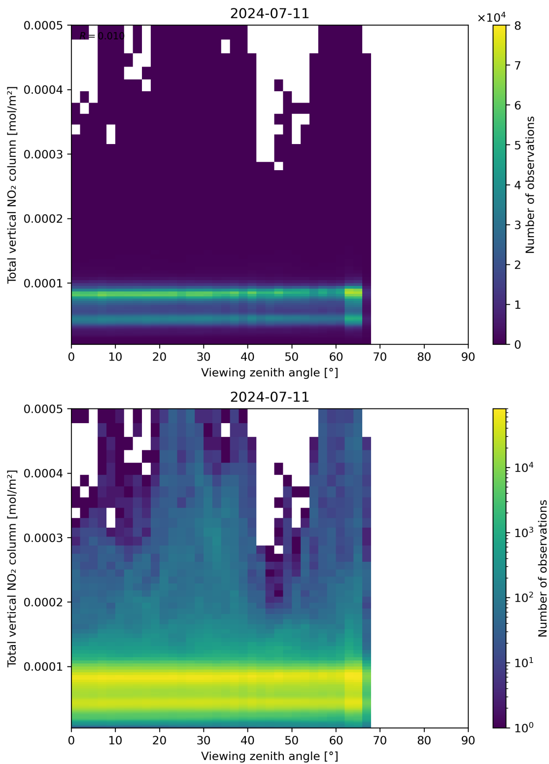
Figure 167: Scatter density plot of “Viewing zenith angle” against “Total vertical NO 2 column” for 2024-07-10 to 2024-07-12.
