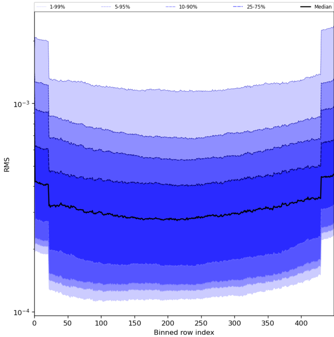
Figure 60: Along track statistics of “RMS” for 2024-07-10 to 2024-07-12
