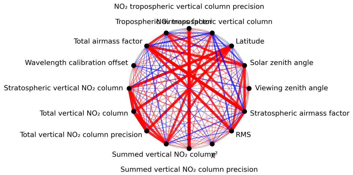
Figure 1: Map of correlation graph for 2024-07-10 to 2024-07-12.
