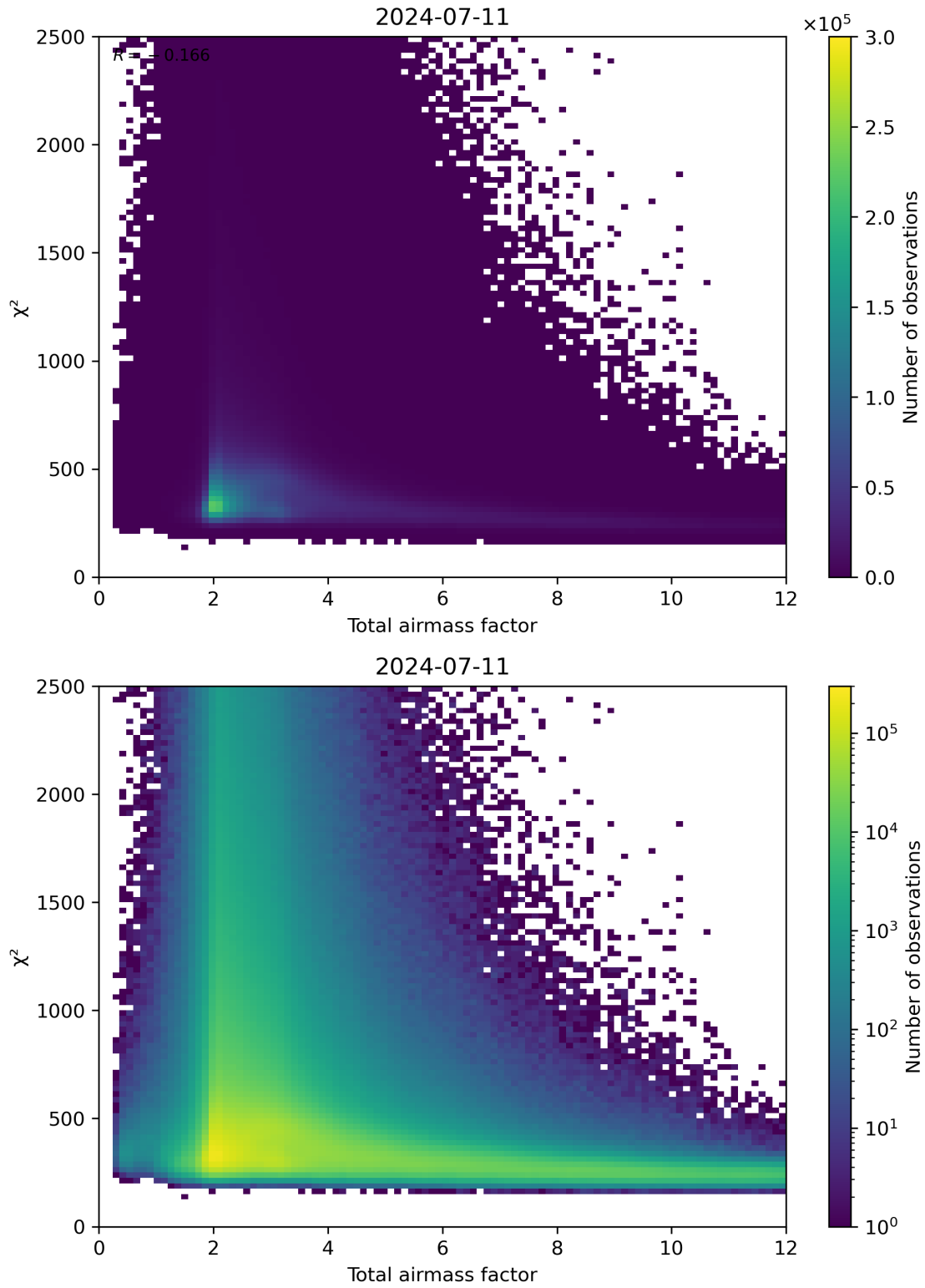
Figure 63: Scatter density plot of “Total airmass factor” against “ \chi^2 ” for 2024-07-10 to 2024-07-12.
