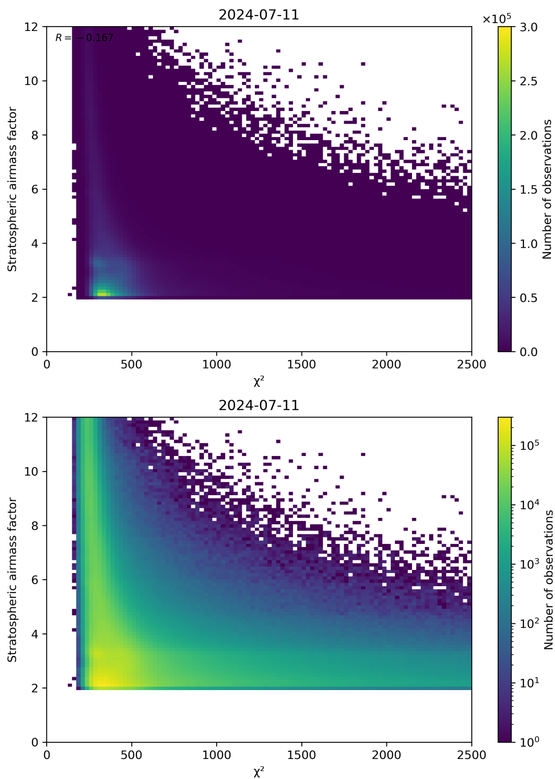
Figure 81: Scatter density plot of “ \chi^2 ” against “Stratospheric airmass factor” for 2024-07-10 to 2024-07-12.
