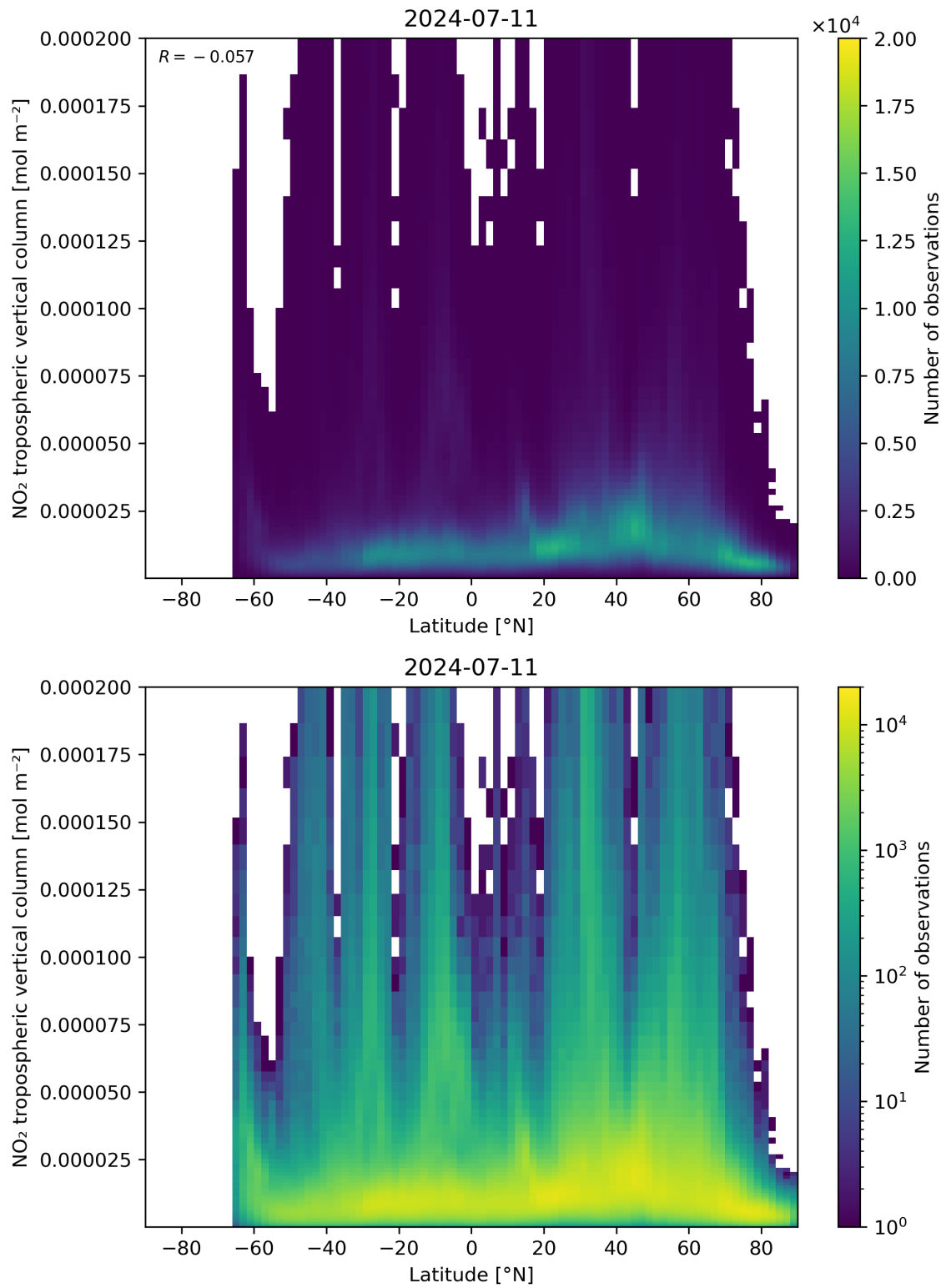
Figure 92: Scatter density plot of “Latitude” against “NO 2 tropospheric vertical column” for 2024-07-10 to 2024-07-12.
