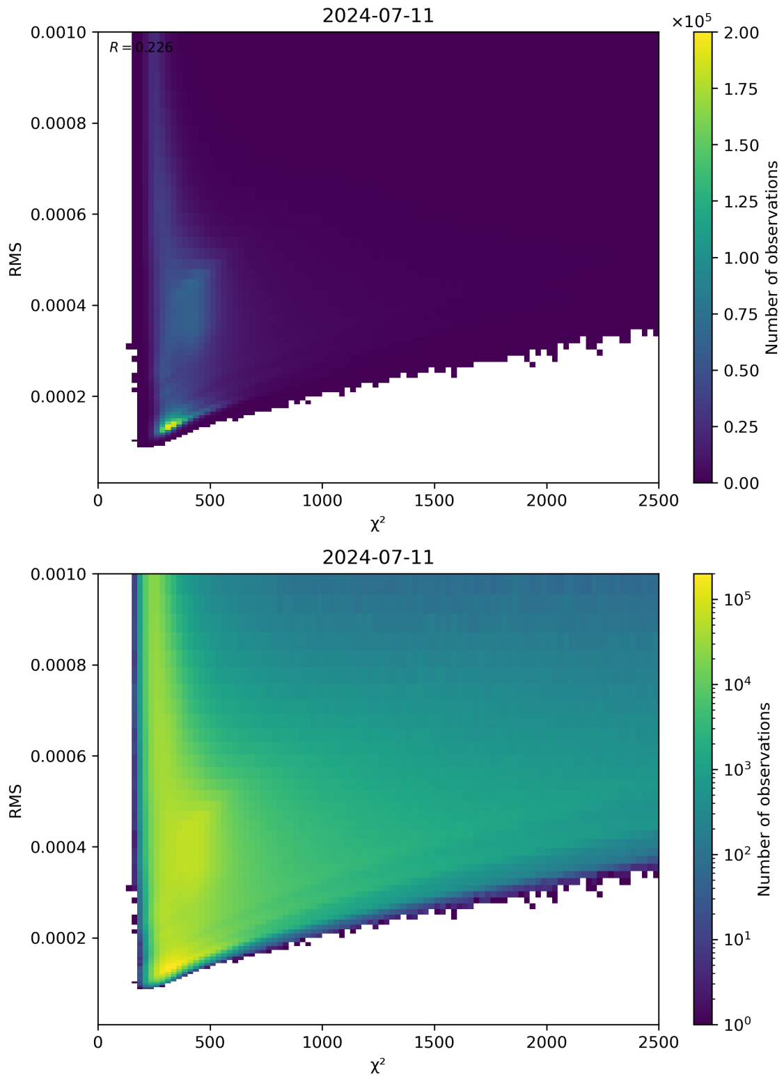
Figure 82: Scatter density plot of “ \chi^2 ” against “RMS” for 2024-07-10 to 2024-07-12.
