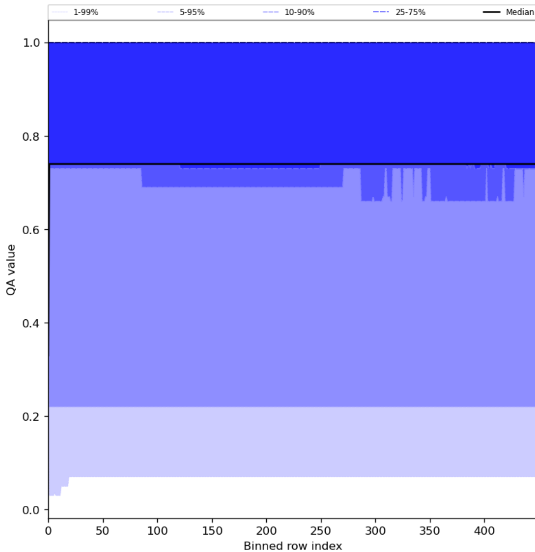
Figure 45: Along track statistics of “QA value” for 2024-07-10 to 2024-07-12
