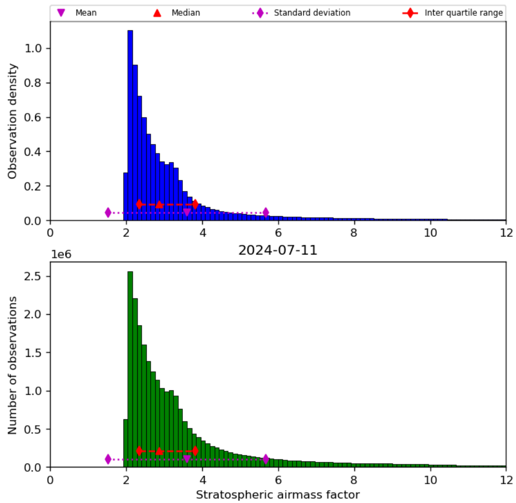
Figure 44: Histogram of “Stratospheric airmass factor” for 2024-07-10 to 2024-07-12
