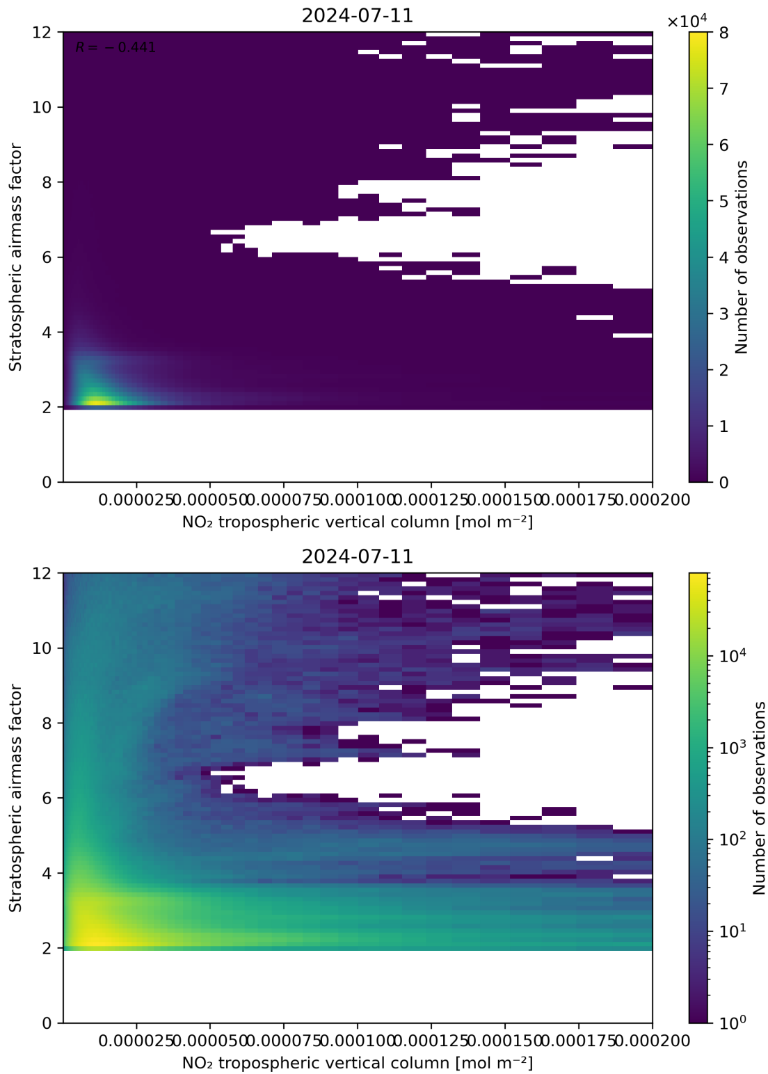
Figure 121: Scatter density plot of “NO 2 tropospheric vertical column” against “Stratospheric air mass factor” for 2024-07-10 to 2024-07-12.
