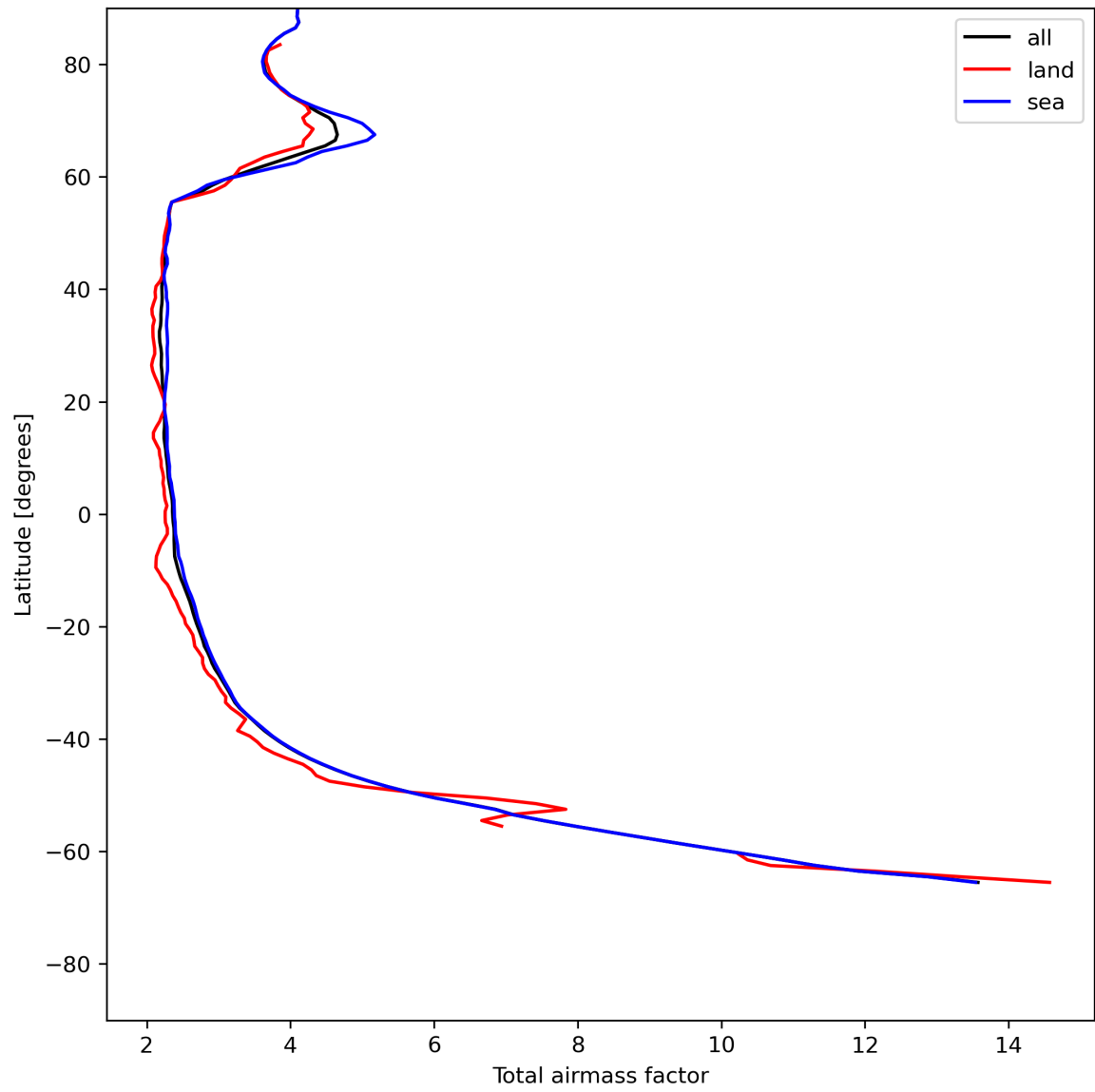
Figure 15: Zonal average of “Total airmass factor” for 2024-07-10 to 2024-07-12.
