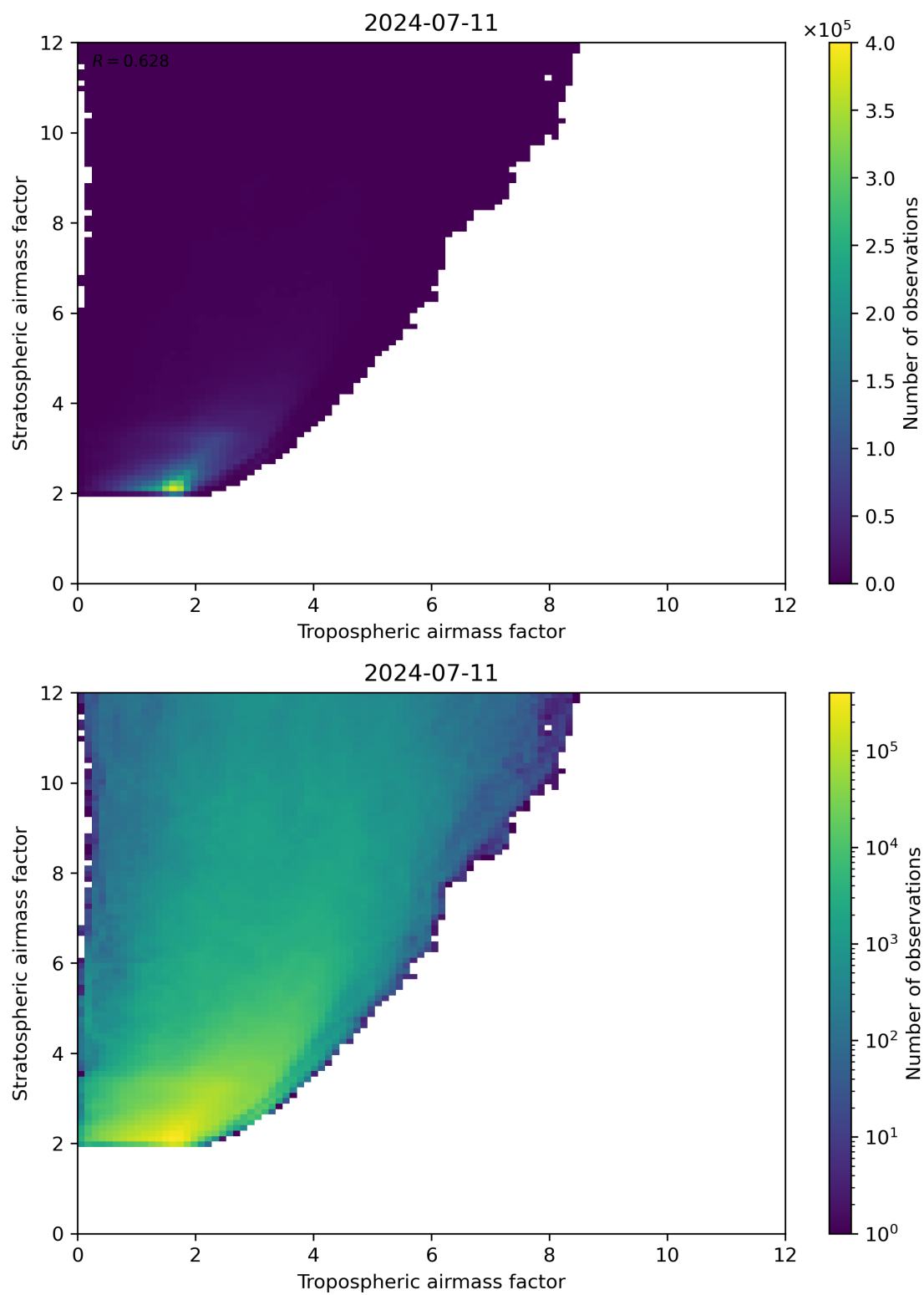
Figure 71: Scatter density plot of “Tropospheric airmass factor” against “Stratospheric airmass factor” for 2024-07-10 to 2024-07-12.
