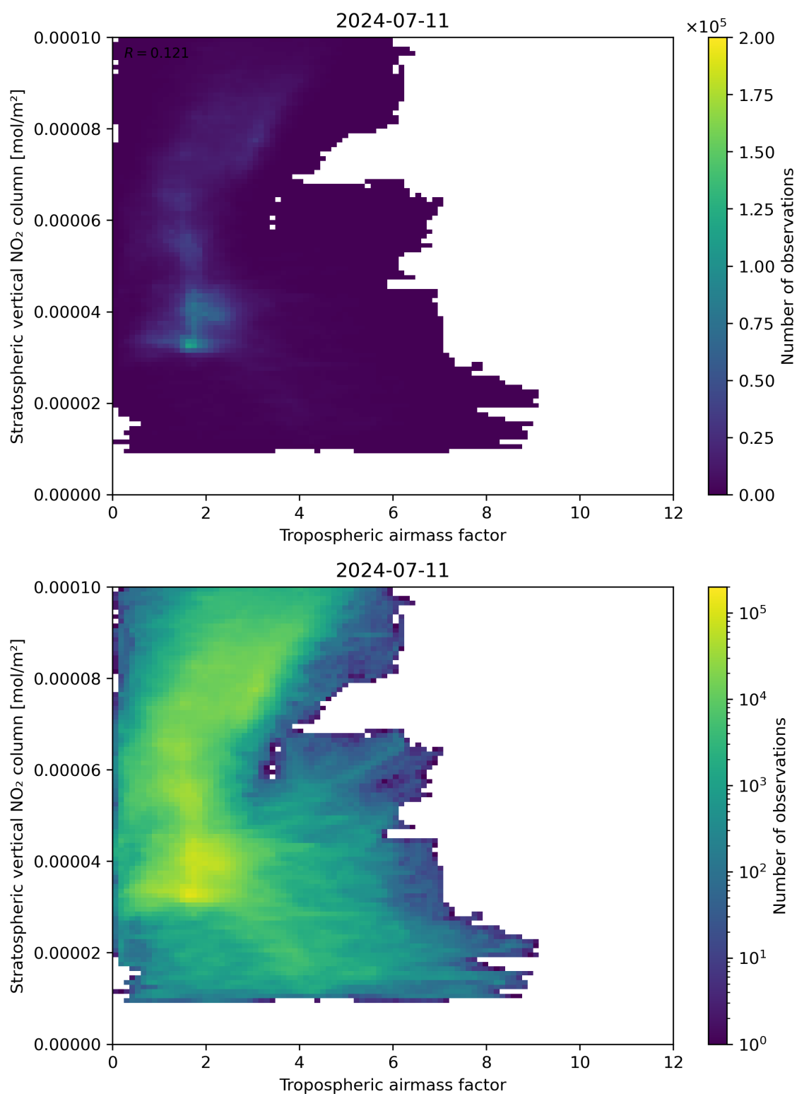
Figure 74: Scatter density plot of “Tropospheric airmass factor” against “Stratospheric vertical NO 2 column” for 2024-07-10 to 2024-07-12.
