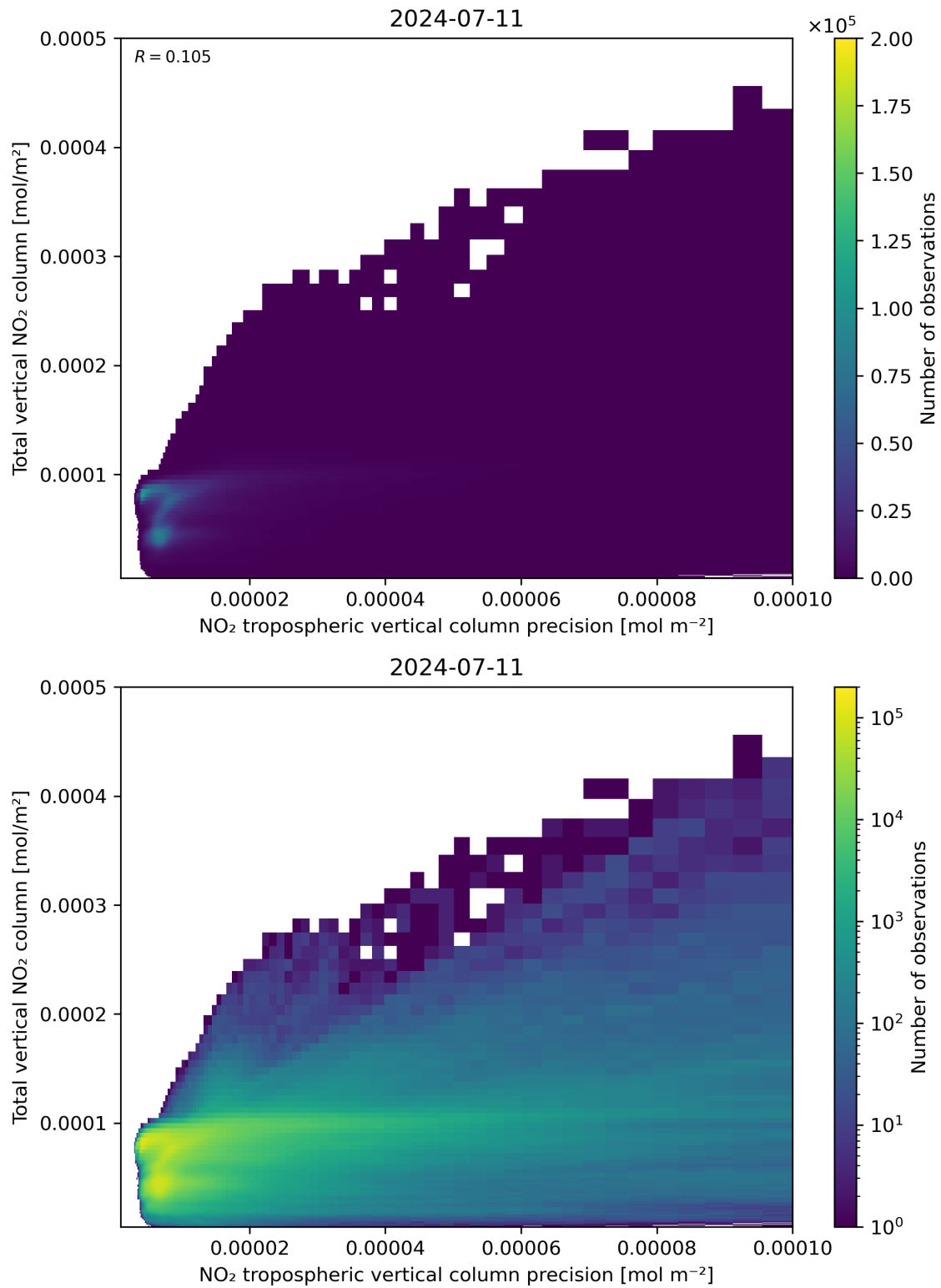
Figure 138: Scatter density plot of “NO 2 tropospheric vertical column precision” against “Total vertical NO 2 column” for 2024-07-10 to 2024-07-12.
