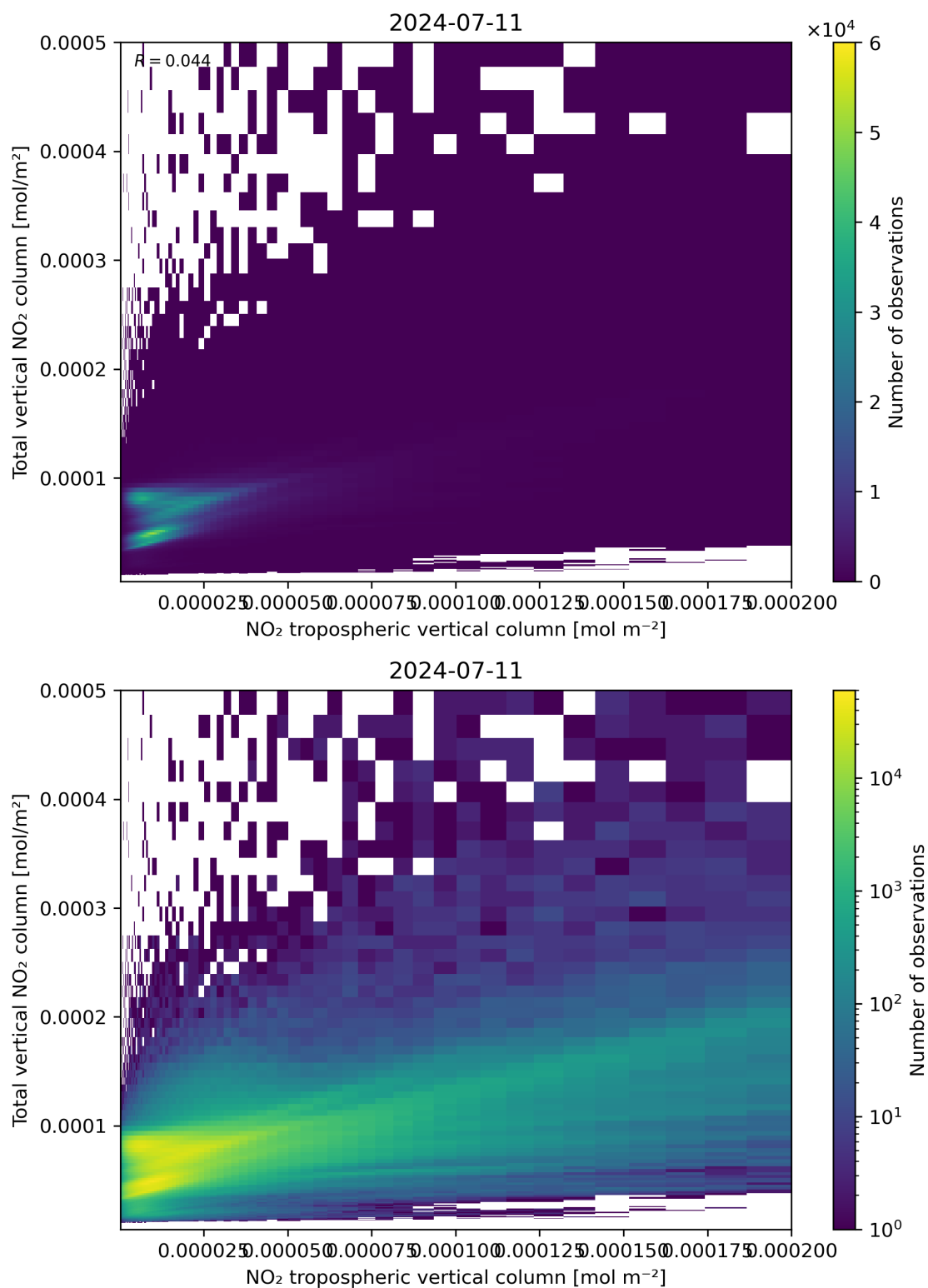
Figure 128: Scatter density plot of “NO 2 tropospheric vertical column” against “Total vertical NO 2 column” for 2024-07-10 to 2024-07-12.
