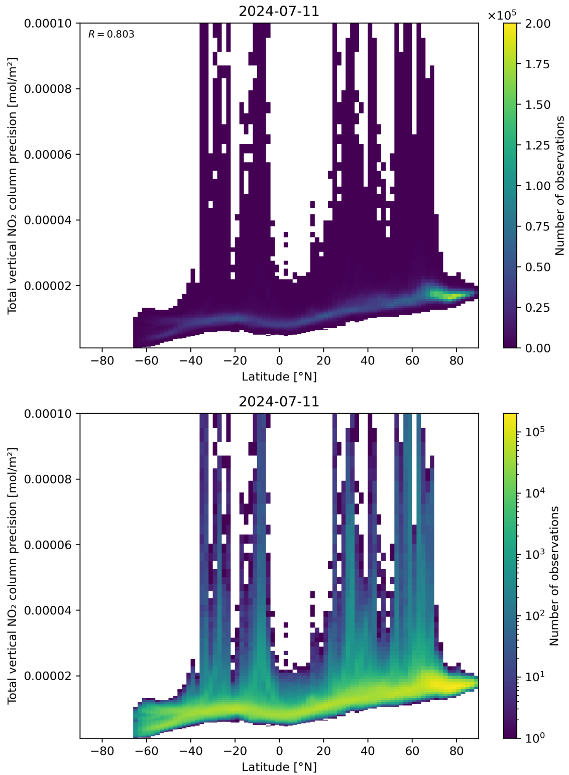
Figure 91: Scatter density plot of “Latitude” against “Total vertical NO 2 column precision” for 2024-07-10 to 2024-07-12.
