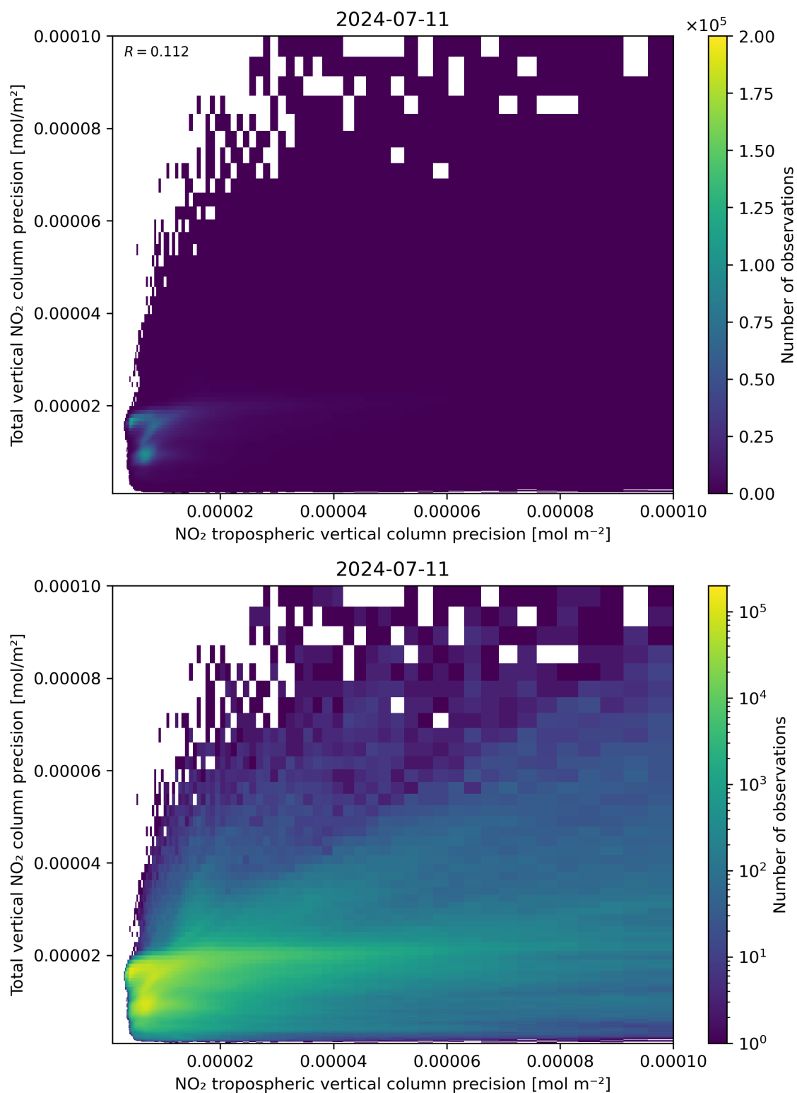
Figure 139: Scatter density plot of “NO 2 tropospheric vertical column precision” against “Total vertical NO 2 column precision” for 2024-07-10 to 2024-07-12.
