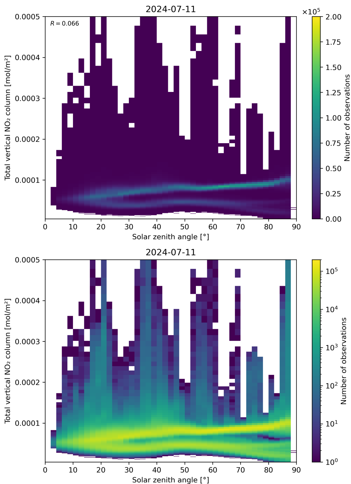
Figure 153: Scatter density plot of “Solar zenith angle” against “Total vertical \text{NO}_2 column” for 2024-07-10 to 2024-07-12.
