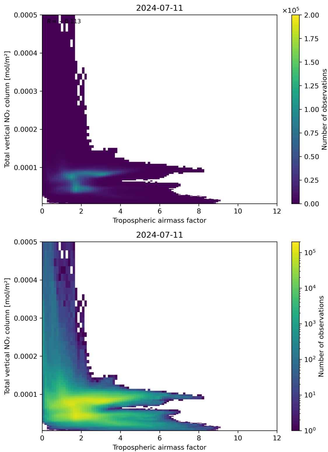
Figure 77: Scatter density plot of “Tropospheric airmass factor” against “Total vertical NO 2 column” for 2024-07-10 to 2024-07-12.
