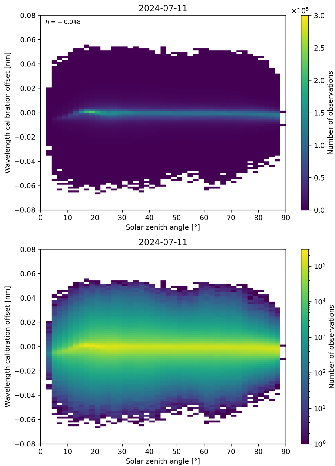
Figure 158: Scatter density plot of “Solar zenith angle” against “Wavelength calibration offset” for 2024-07-10 to 2024-07-12.
