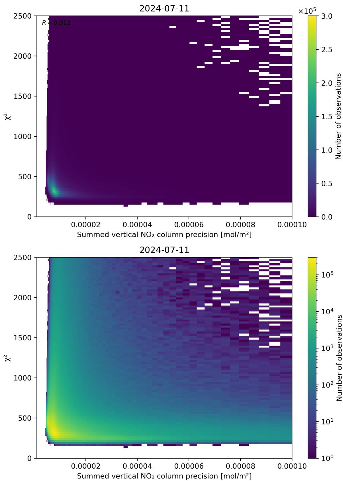
Figure 107: Scatter density plot of “Summed vertical NO 2 column precision” against “ \chi^2 ” for 2024-07-10 to 2024-07-12.
