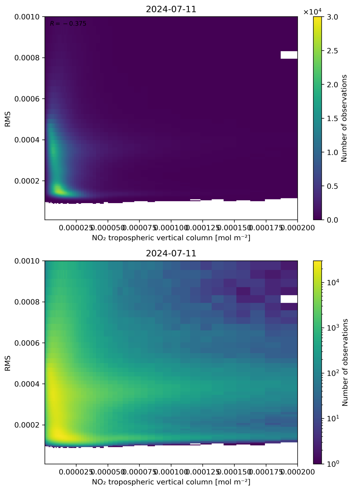
Figure 142: Scatter density plot of “NO 2 tropospheric vertical column” against “RMS” for 2024-07-10 to 2024-07-12.
