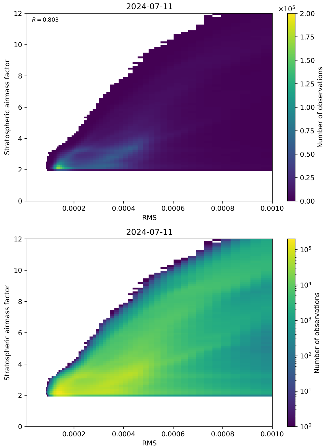
Figure 144: Scatter density plot of “RMS” against “Stratospheric airmass factor” for 2024-07-10 to 2024-07-12.
