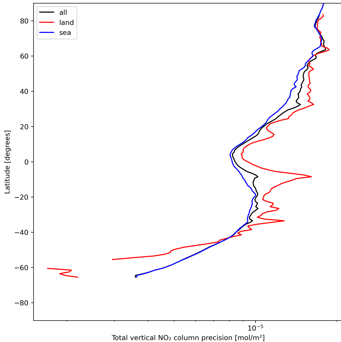
Figure 22: Zonal average of “Total vertical NO 2 column precision” for 2024-07-10 to 2024-07-12.
