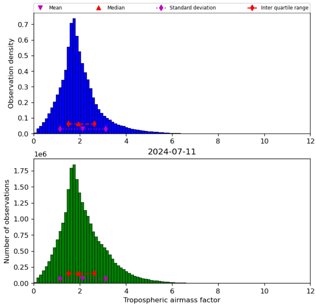
Figure 31: Histogram of “Tropospheric airmass factor” for 2024-07-10 to 2024-07-12
