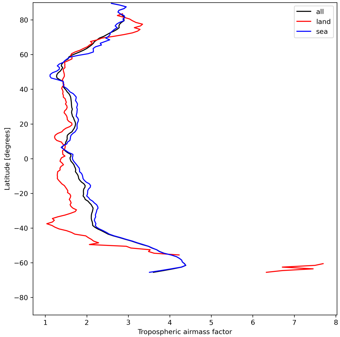
Figure 14: Zonal average of “Tropospheric airmass factor” for 2024-07-10 to 2024-07-12.
