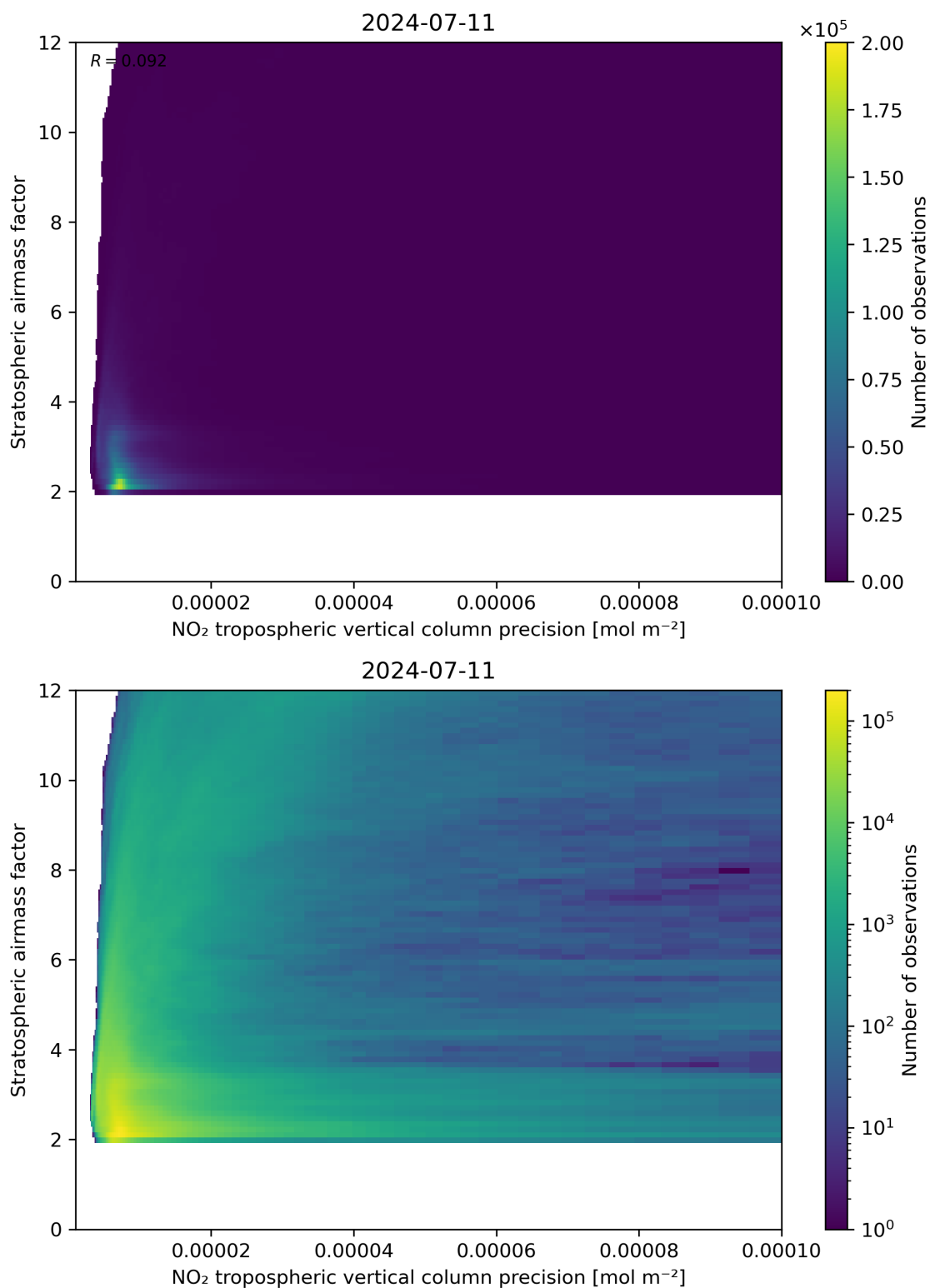
Figure 131: Scatter density plot of “NO 2 tropospheric vertical column precision” against “Stratospheric airmass factor” for 2024-07-10 to 2024-07-12.
