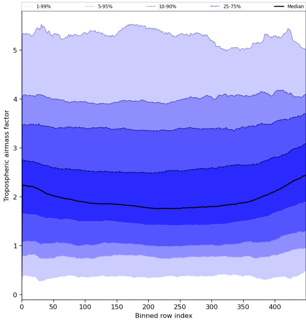
Figure 48: Along track statistics of “Tropospheric airmass factor” for 2024-07-10 to 2024-07-12
