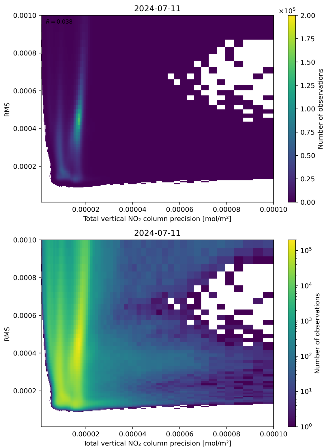
Figure 119: Scatter density plot of “Total vertical NO 2 column precision” against “RMS” for 2024-07-10 to 2024-07-12.
