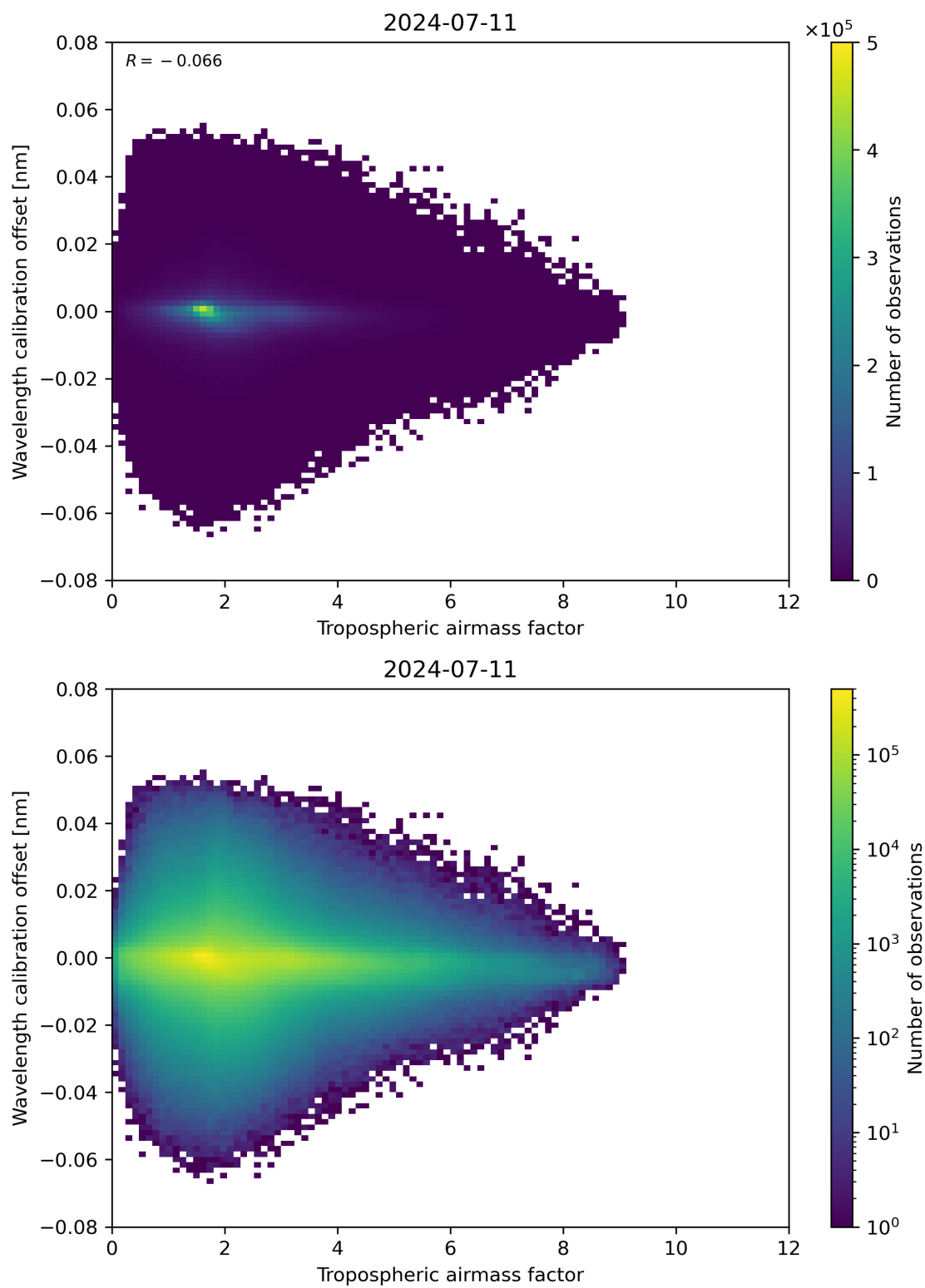
Figure 80: Scatter density plot of “Tropospheric air mass factor” against “Wavelength calibration offset” for 2024-07-10 to 2024-07-12.
