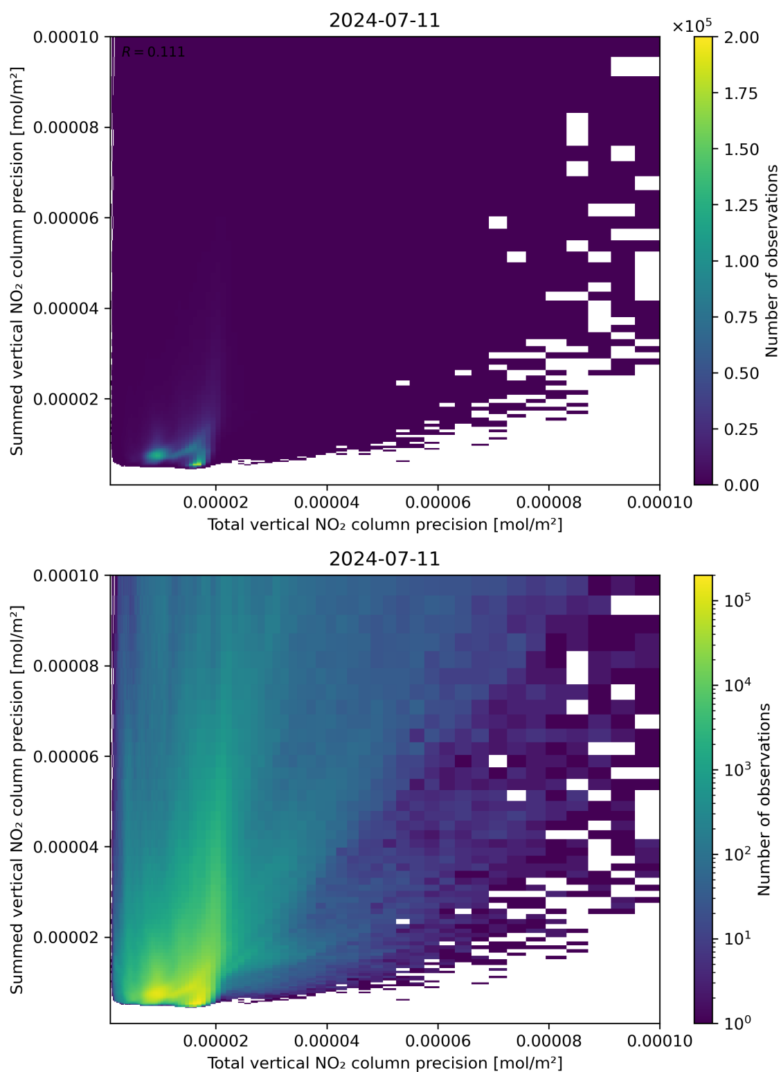
Figure 118: Scatter density plot of “Total vertical NO 2 column precision” against “Summed vertical NO 2 column precision” for 2024-07-10 to 2024-07-12.
