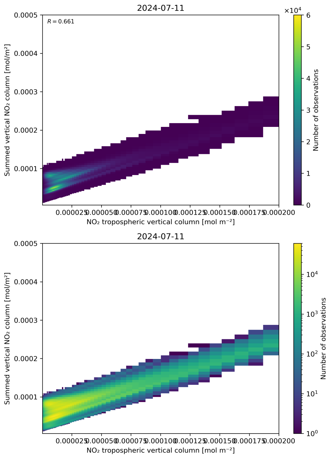
Figure 126: Scatter density plot of “NO 2 tropospheric vertical column” against “Summed vertical NO 2 column” for 2024-07-10 to 2024-07-12.
