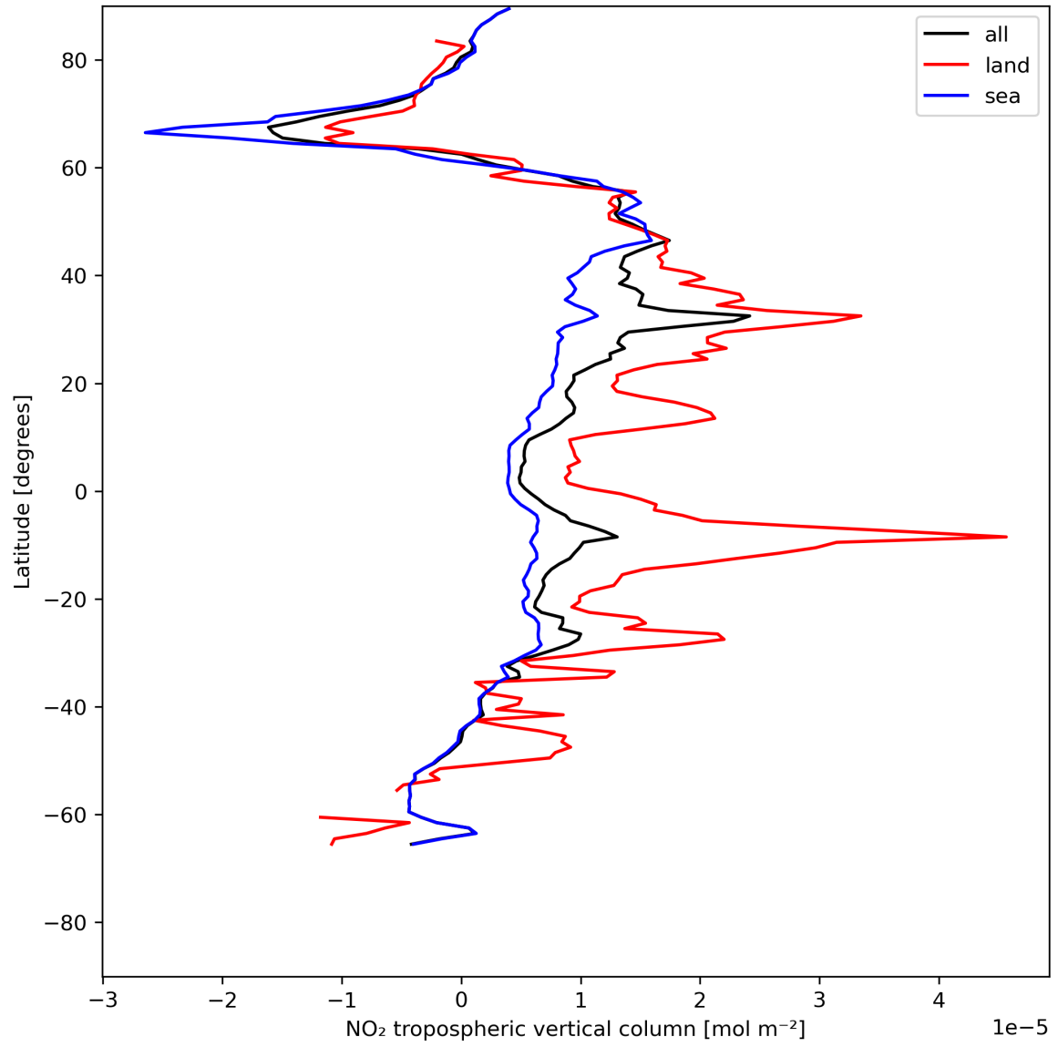
Figure 12: Zonal average of “NO 2 tropospheric vertical column” for 2024-07-10 to 2024-07-12.
