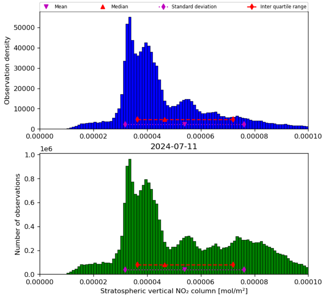
Figure 36: Histogram of “Stratospheric vertical NO 2 column” for 2024-07-10 to 2024-07-12
