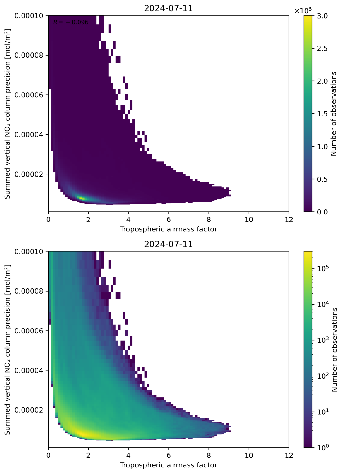
Figure 76: Scatter density plot of “Tropospheric air mass factor” against “Summed vertical NO 2 column precision” for 2024-07-10 to 2024-07-12.
