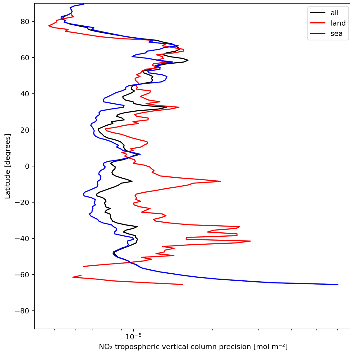
Figure 13: Zonal average of “NO 2 tropospheric vertical column precision” for 2024-07-10 to 2024-07-12.
