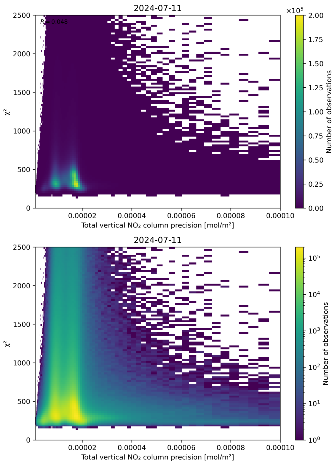
Figure 116: Scatter density plot of “Total vertical NO 2 column precision” against “ \chi^2 ” for 2024-07-10 to 2024-07-12.
