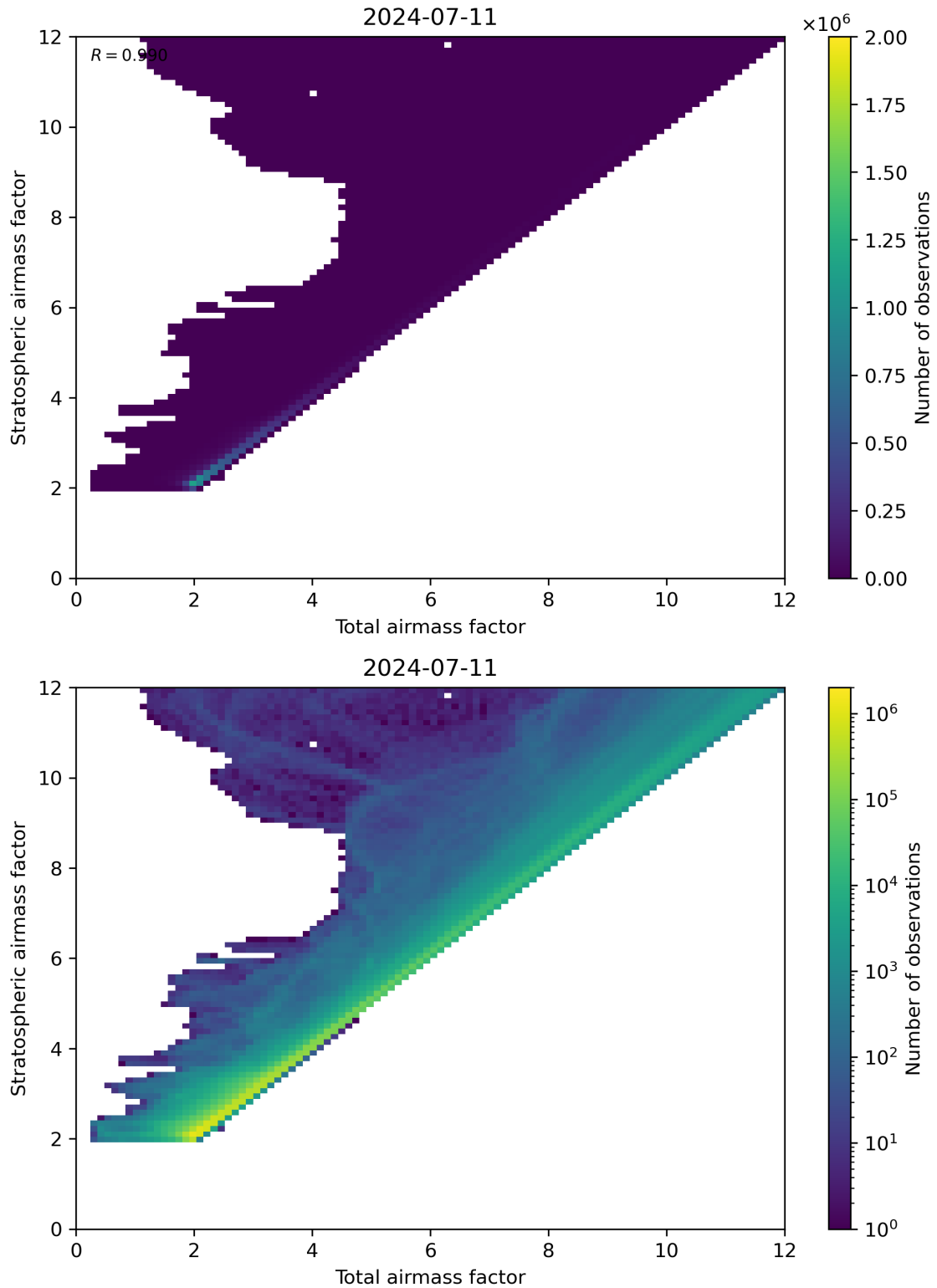
Figure 62: Scatter density plot of “Total airmass factor” against “Stratospheric airmass factor” for 2024-07-10 to 2024-07-12.
