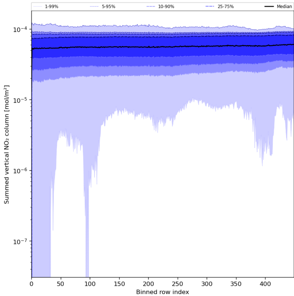
Figure 57: Along track statistics of “Summed vertical NO 2 column” for 2024-07-10 to 2024-07-12
