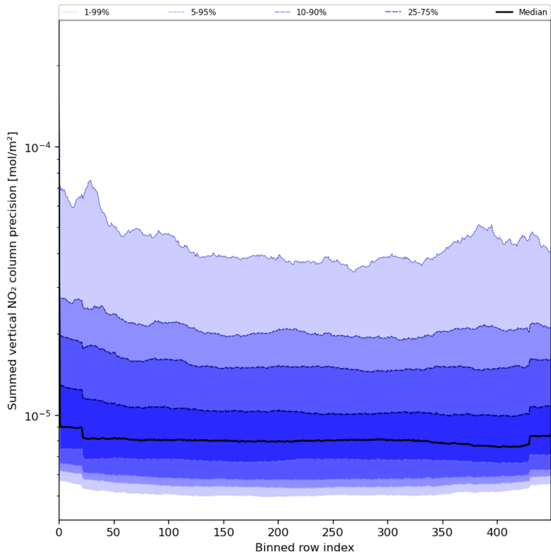
Figure 58: Along track statistics of “Summed vertical NO 2 column precision” for 2024-07-10 to 2024-07-12
