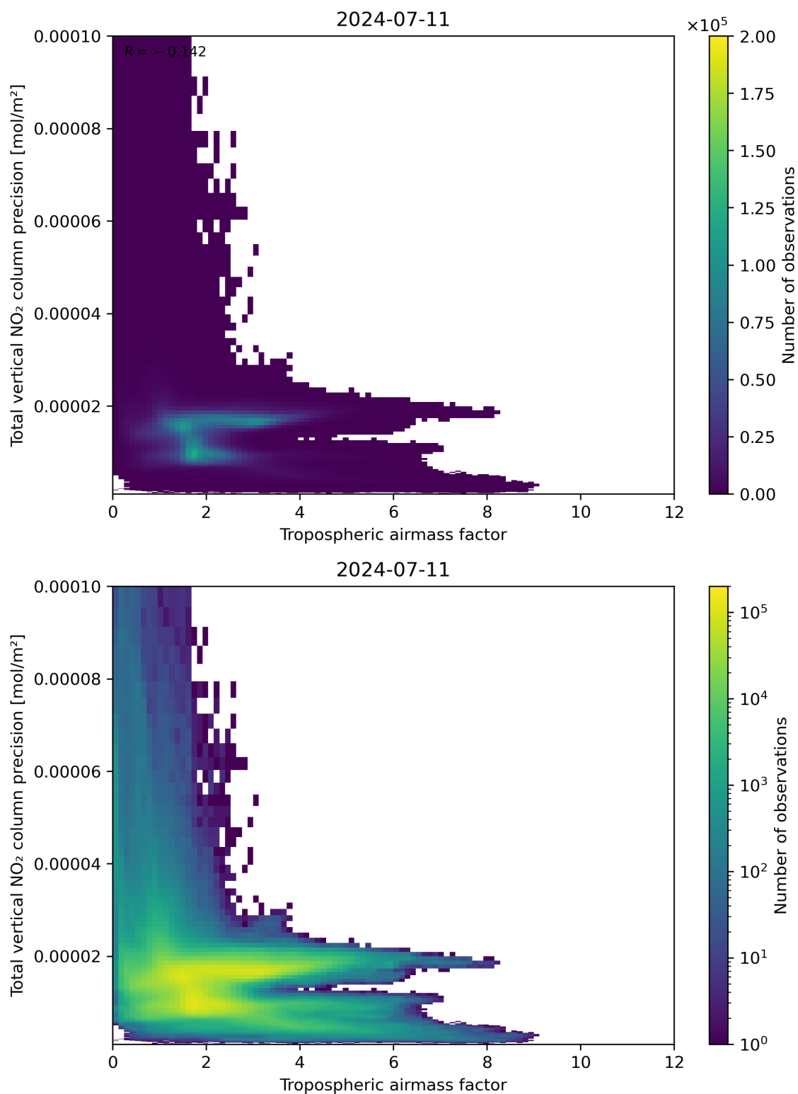
Figure 78: Scatter density plot of “Tropospheric air mass factor” against “Total vertical NO 2 column precision” for 2024-07-10 to 2024-07-12.
