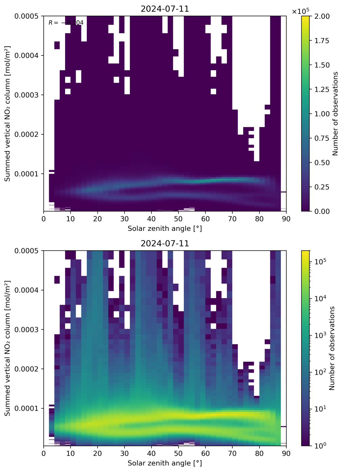
Figure 151: Scatter density plot of “Solar zenith angle” against “Summed vertical NO 2 column” for 2024-07-10 to 2024-07-12.
