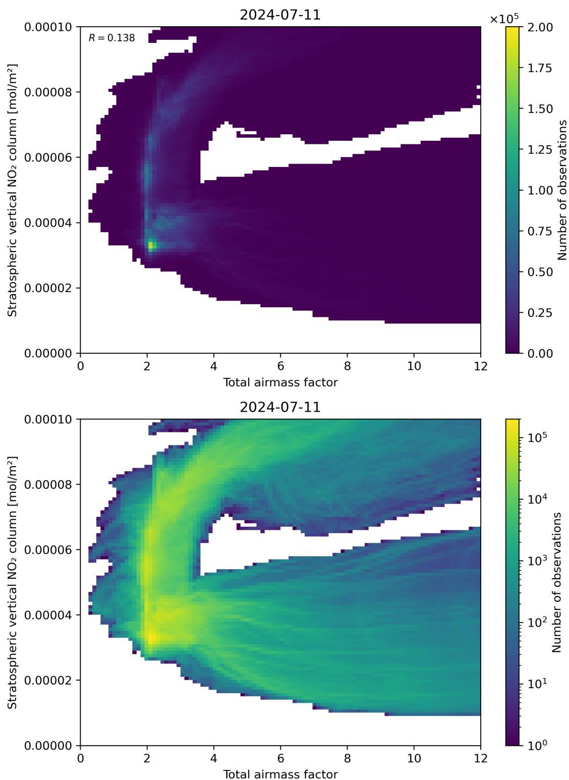
Figure 64: Scatter density plot of “Total airmass factor” against “Stratospheric vertical \text{NO}_2 column” for 2024-07-10 to 2024-07-12.
