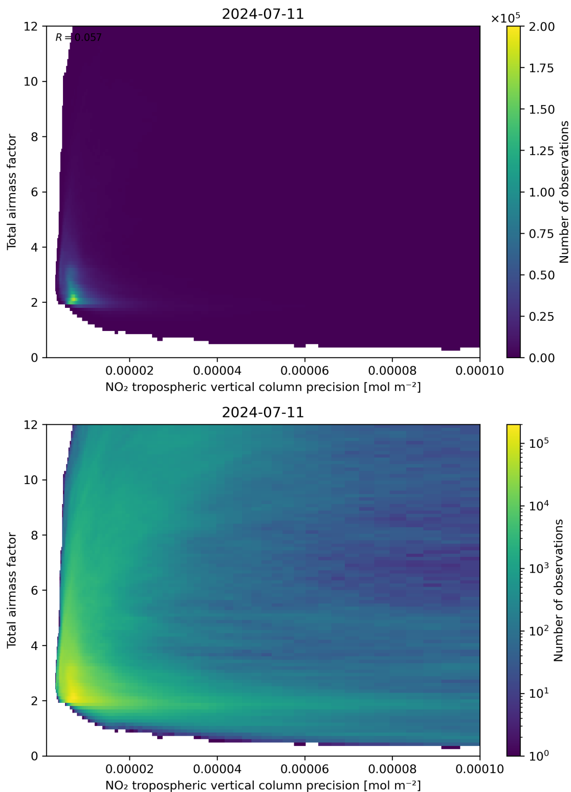
Figure 132: Scatter density plot of “NO 2 tropospheric vertical column precision” against “Total air mass factor” for 2024-07-10 to 2024-07-12.
