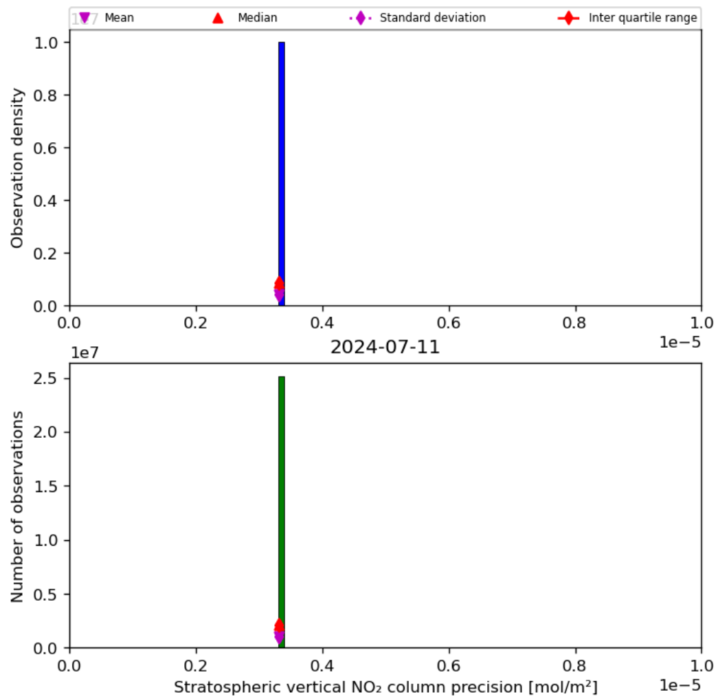
Figure 37: Histogram of “Stratospheric vertical NO 2 column precision” for 2024-07-10 to 2024-07-12
