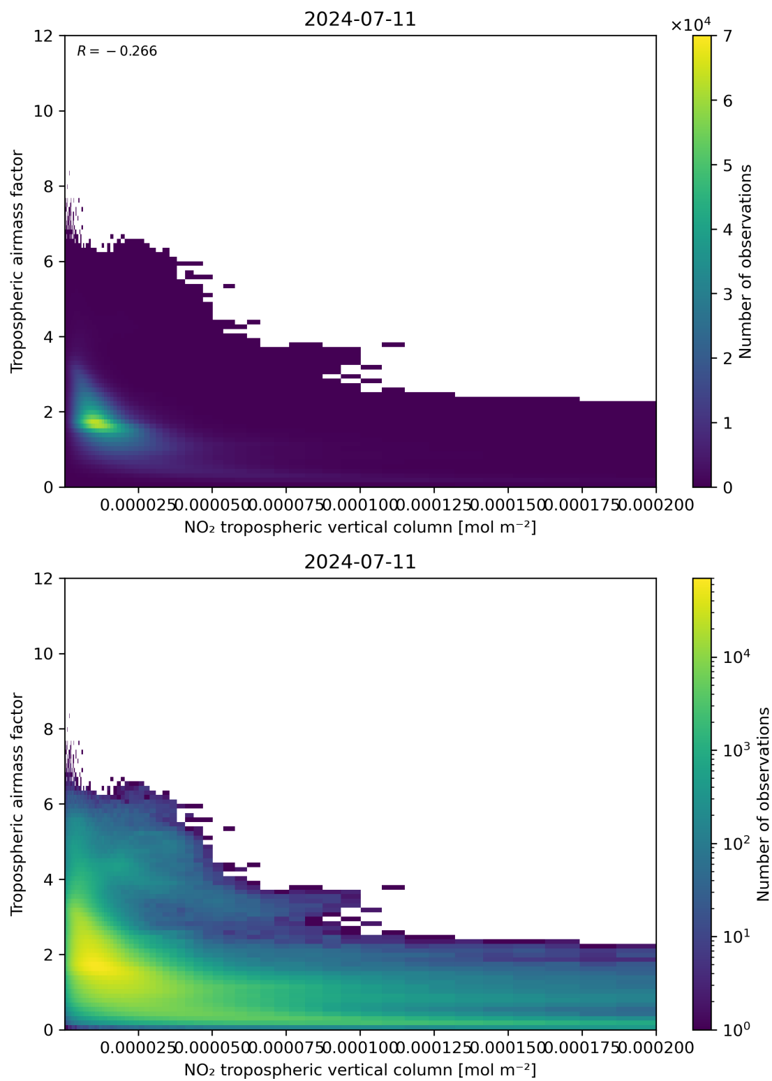
Figure 123: Scatter density plot of “NO 2 tropospheric vertical column” against “Tropospheric air mass factor” for 2024-07-10 to 2024-07-12.
