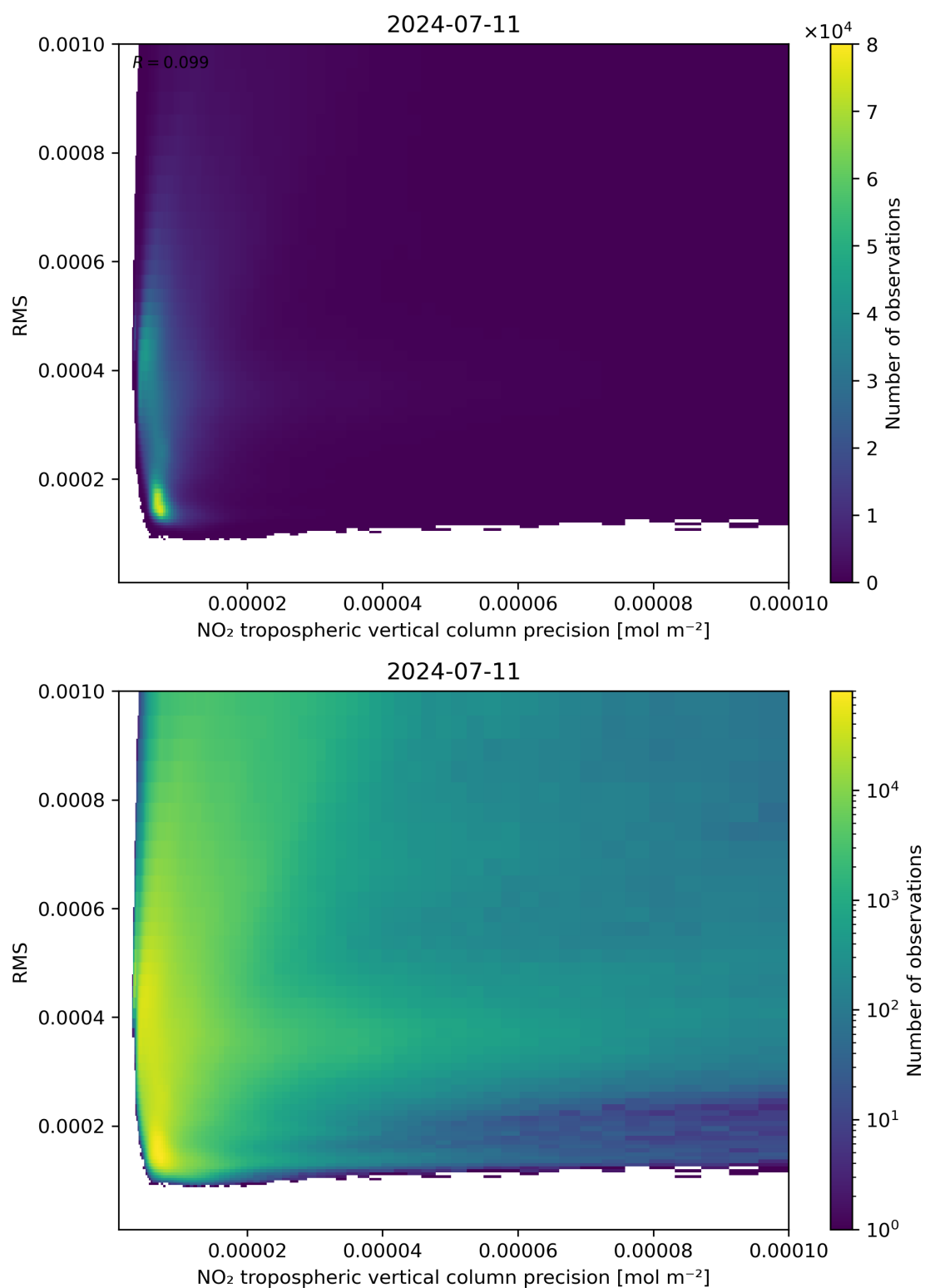
Figure 140: Scatter density plot of “NO 2 tropospheric vertical column precision” against “RMS” for 2024-07-10 to 2024-07-12.
