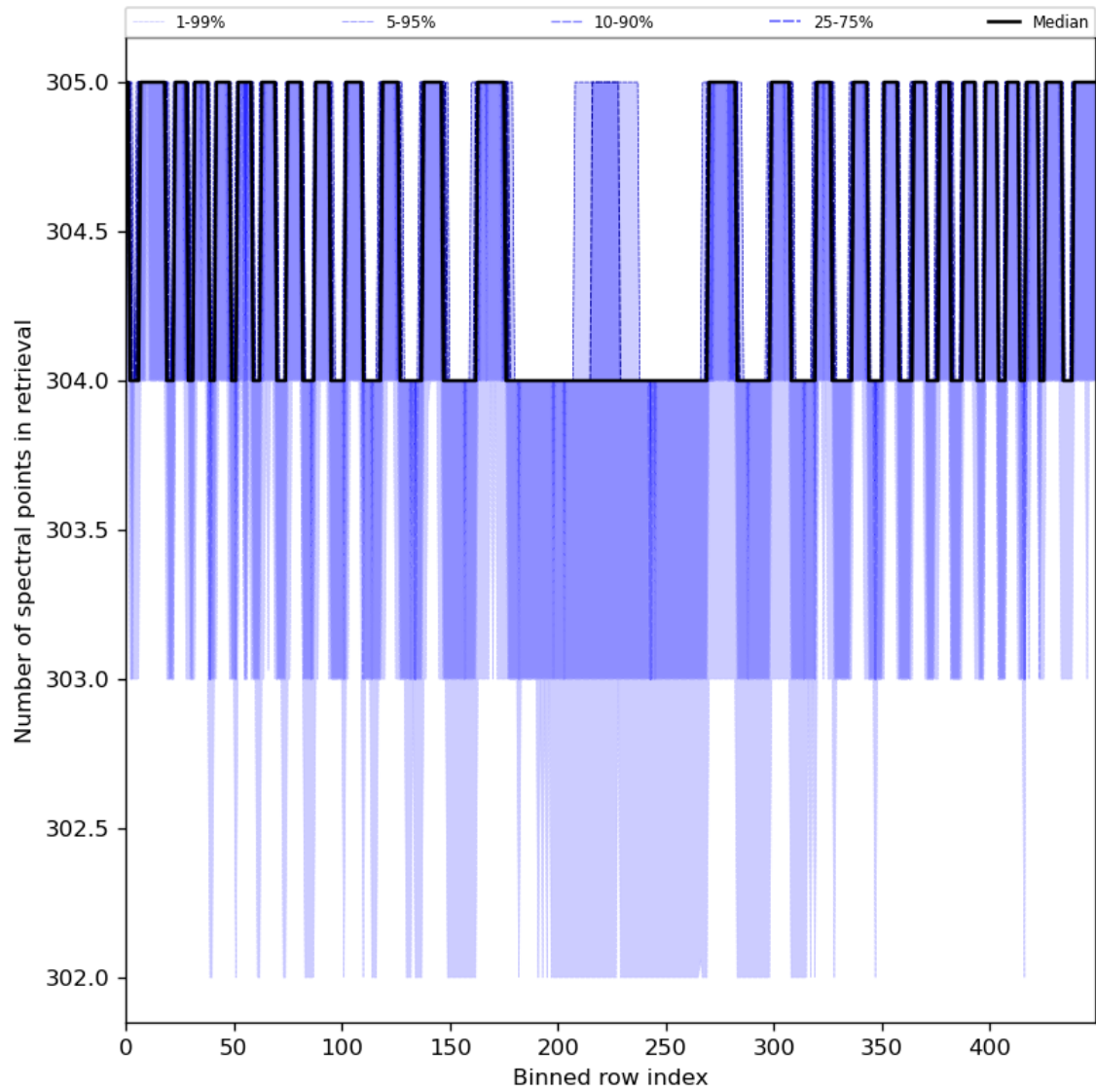
Figure 50: Along track statistics of “Number of spectral points in retrieval” for 2024-07-10 to 2024-07-12
