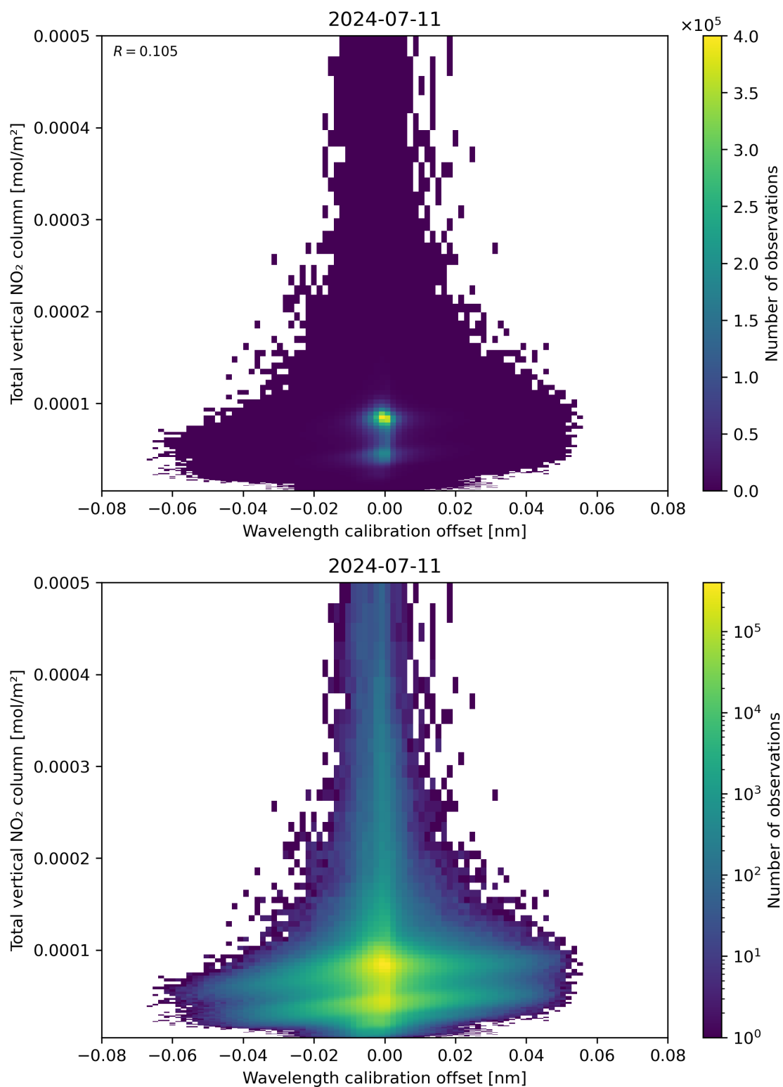
Figure 179: Scatter density plot of “Wavelength calibration offset” against “Total vertical NO 2 column” for 2024-07-10 to 2024-07-12.
