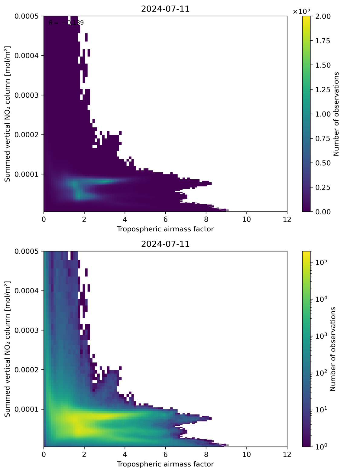
Figure 75: Scatter density plot of “Tropospheric airmass factor” against “Summed vertical NO 2 column” for 2024-07-10 to 2024-07-12.
