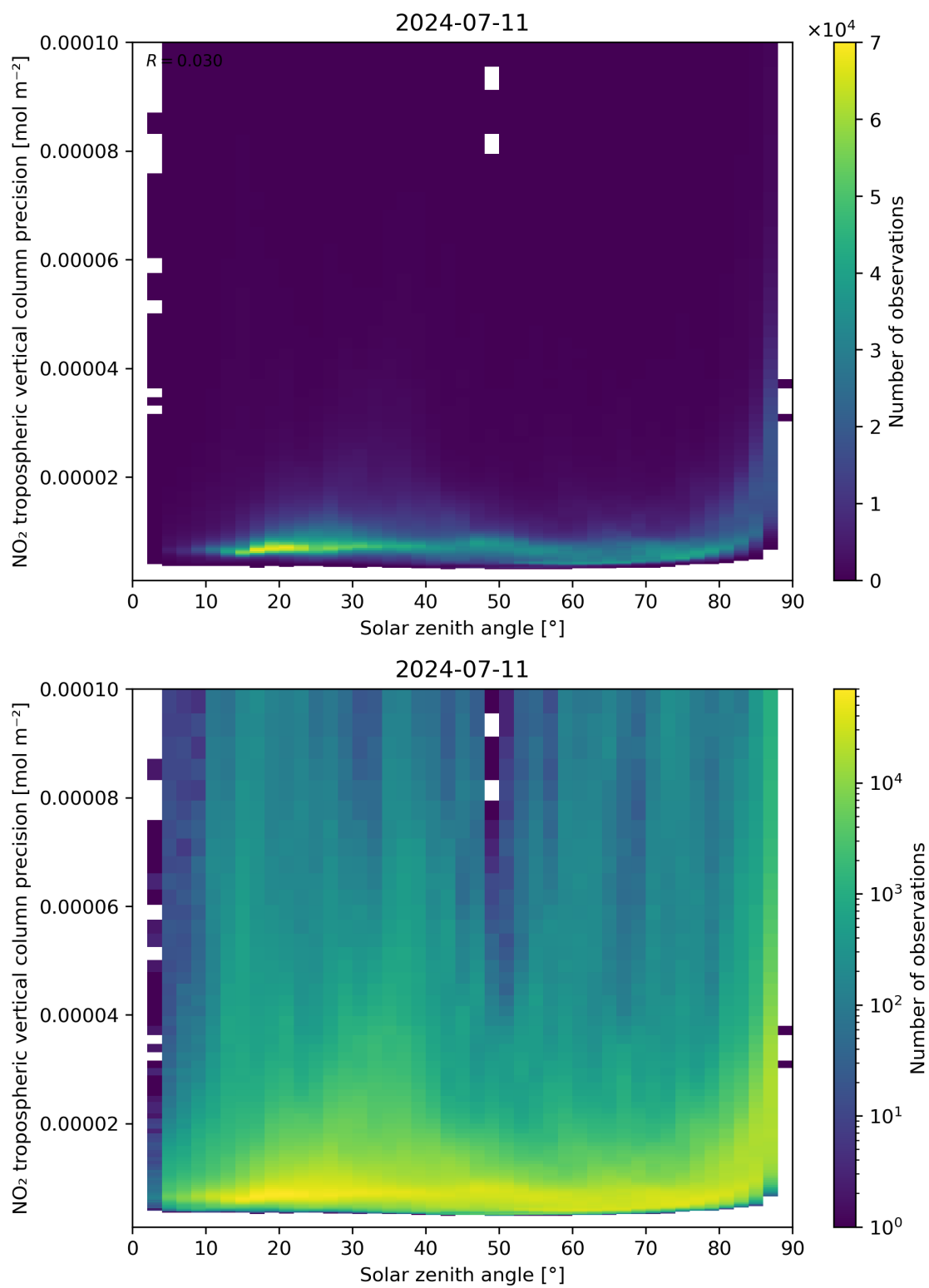
Figure 156: Scatter density plot of “Solar zenith angle” against “NO 2 tropospheric vertical column precision” for 2024-07-10 to 2024-07-12.
