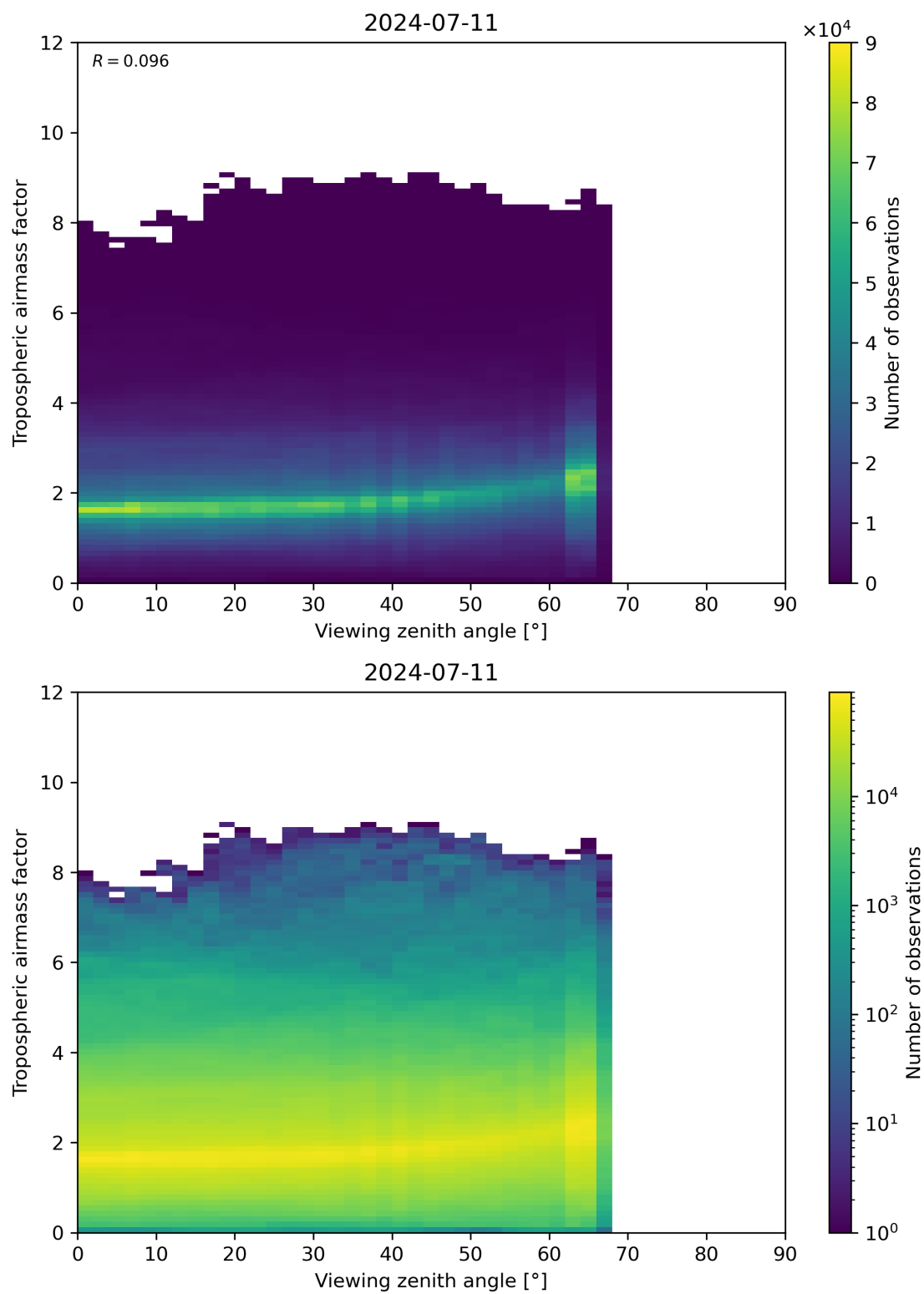
Figure 161: Scatter density plot of “Viewing zenith angle” against “Tropospheric airmass factor” for 2024-07-10 to 2024-07-12.
