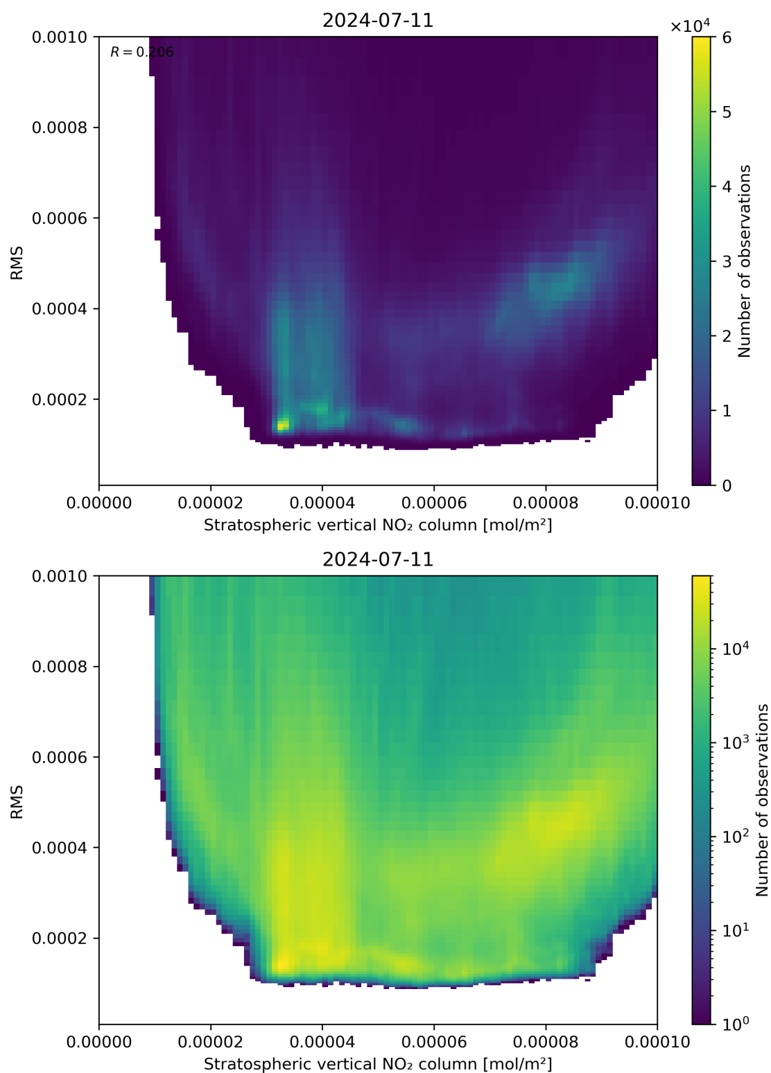
Figure 102: Scatter density plot of “Stratospheric vertical NO 2 column” against “RMS” for 2024-07-10 to 2024-07-12.
