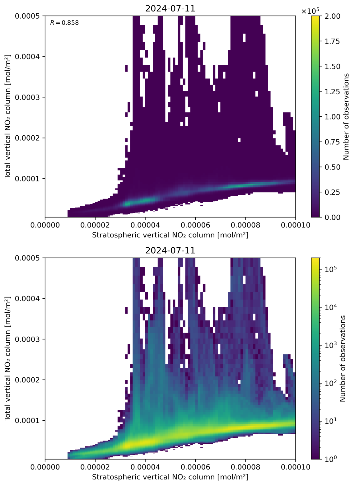
Figure 100: Scatter density plot of “Stratospheric vertical NO 2 column” against “Total vertical NO 2 column” for 2024-07-10 to 2024-07-12.
