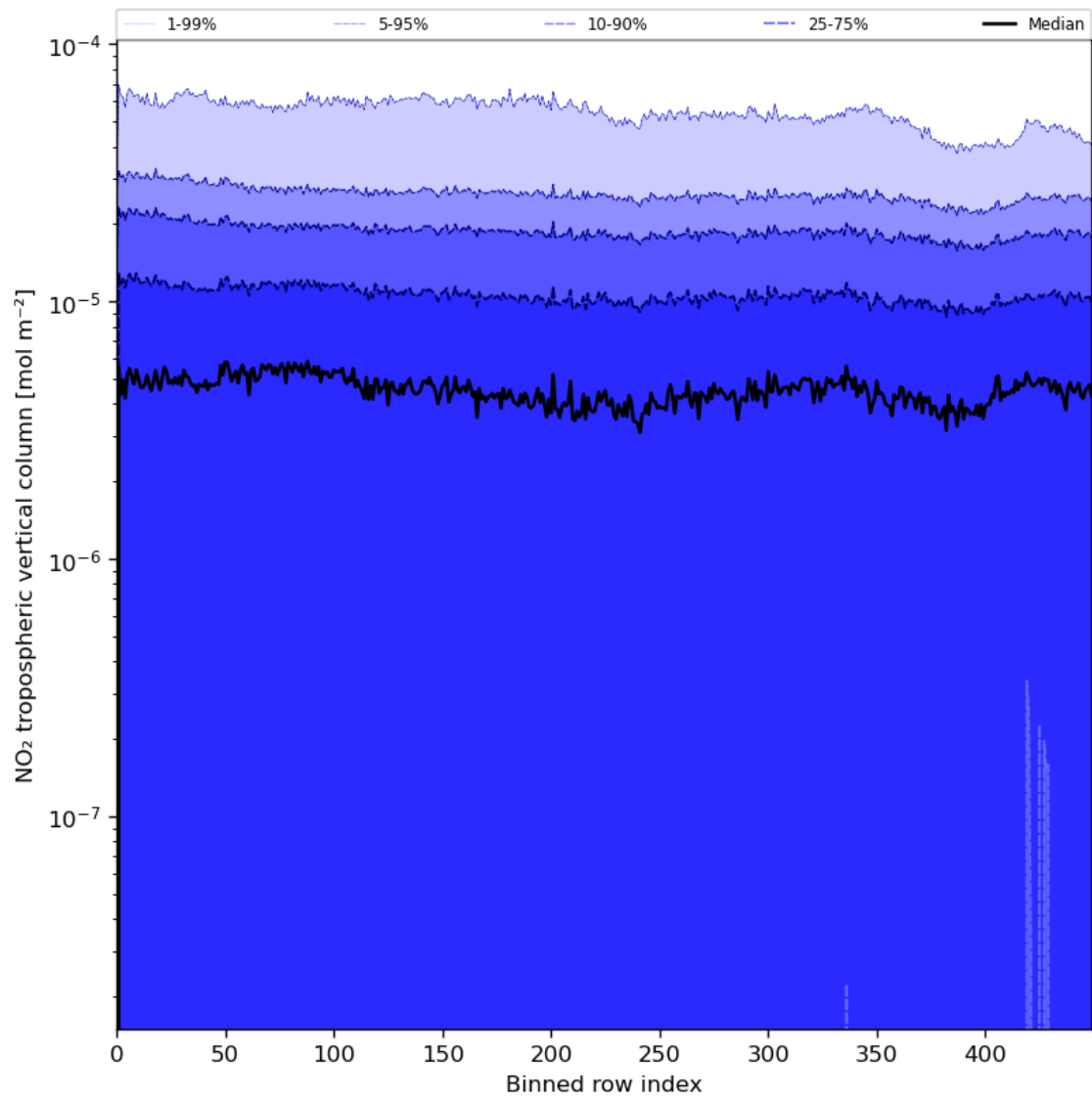
Figure 46: Along track statistics of “NO 2 tropospheric vertical column” for 2024-07-10 to 2024-07-12
