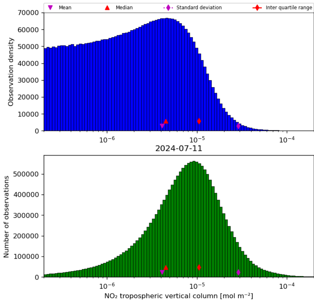
Figure 29: Histogram of “NO 2 tropospheric vertical column” for 2024-07-10 to 2024-07-12
