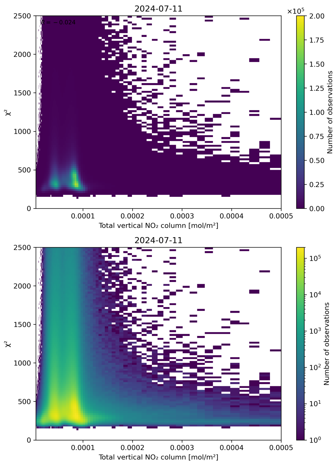
Figure 111: Scatter density plot of “Total vertical NO 2 column” against “ \chi^2 ” for 2024-07-10 to 2024-07-12.
