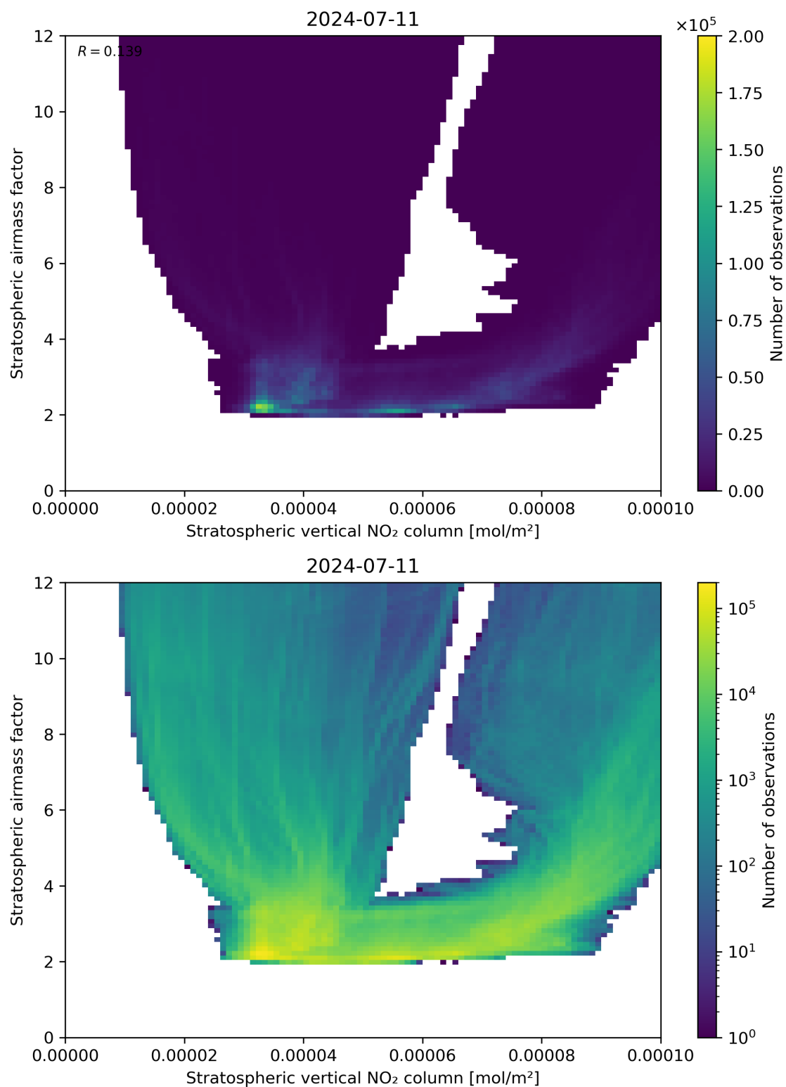
Figure 96: Scatter density plot of “Stratospheric vertical NO 2 column” against “Stratospheric airmass factor” for 2024-07-10 to 2024-07-12.
