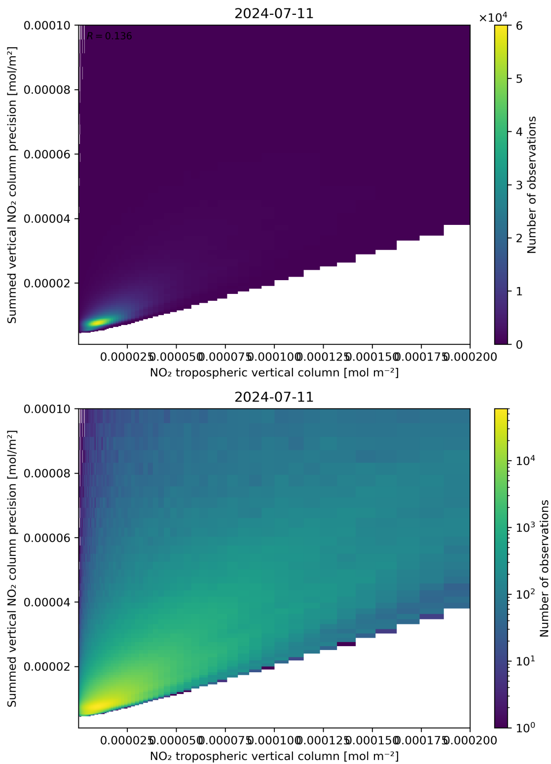
Figure 127: Scatter density plot of “NO 2 tropospheric vertical column” against “Summed vertical NO 2 column precision” for 2024-07-10 to 2024-07-12.
