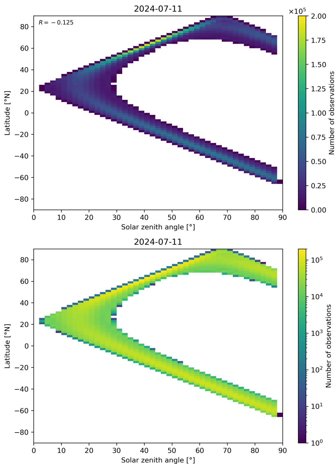
Figure 149: Scatter density plot of “Solar zenith angle” against “Latitude” for 2024-07-10 to 2024-07-12.
