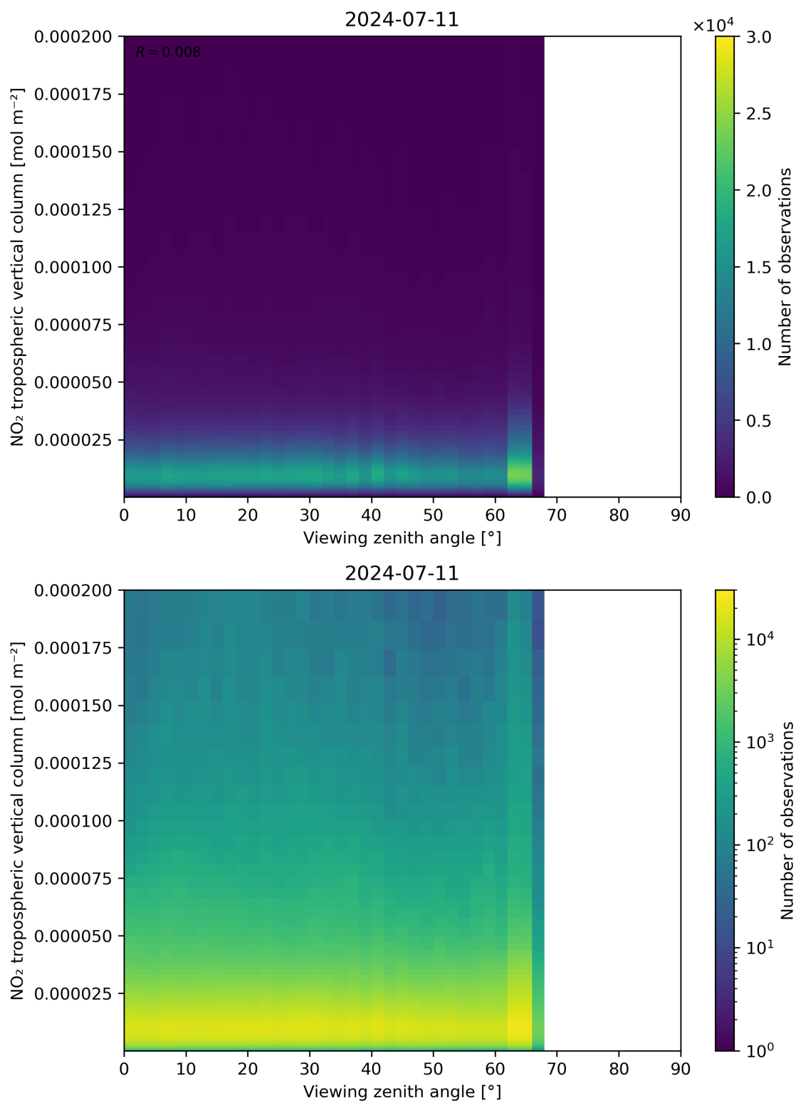
Figure 169: Scatter density plot of “Viewing zenith angle” against “NO 2 tropospheric vertical column” for 2024-07-10 to 2024-07-12.
