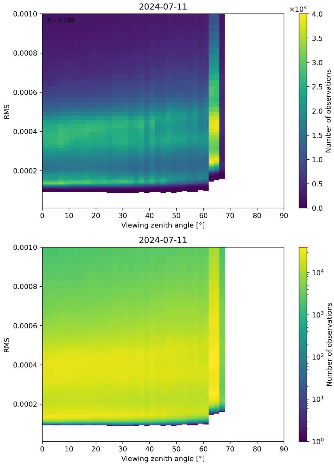
Figure 171: Scatter density plot of “Viewing zenith angle” against “RMS” for 2024-07-10 to 2024-07-12.
