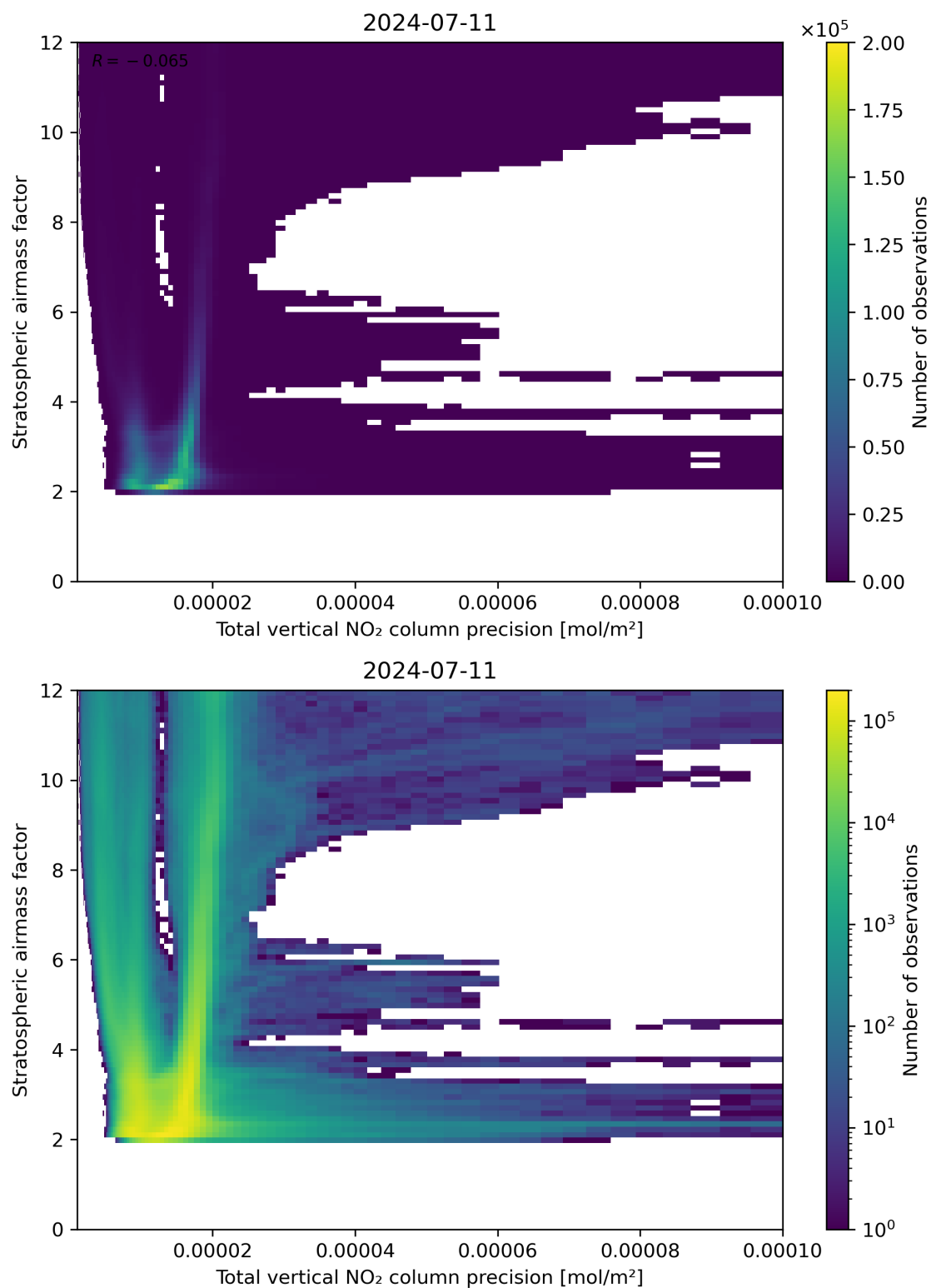
Figure 115: Scatter density plot of “Total vertical NO 2 column precision” against “Stratospheric air mass factor” for 2024-07-10 to 2024-07-12.
