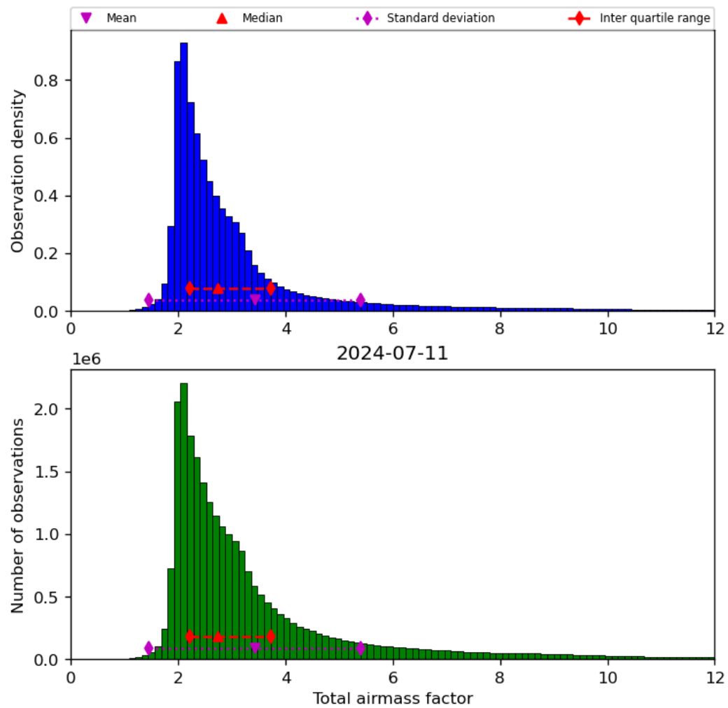
Figure 32: Histogram of “Total airmass factor” for 2024-07-10 to 2024-07-12
