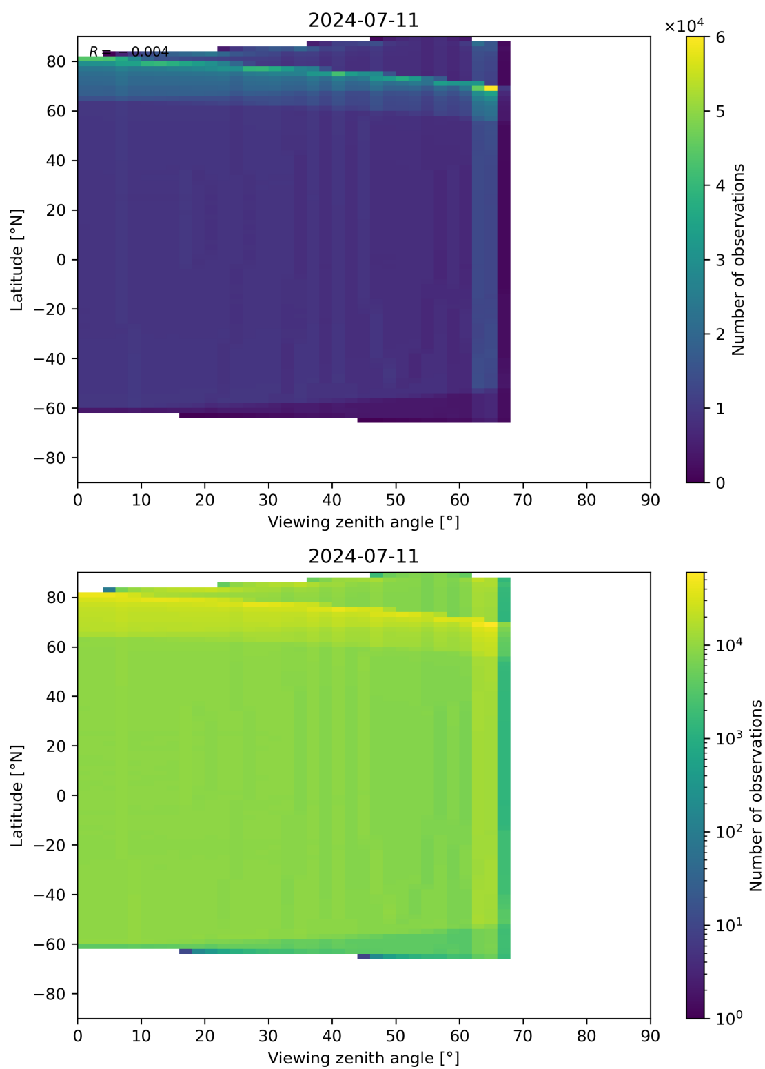
Figure 163: Scatter density plot of “Viewing zenith angle” against “Latitude” for 2024-07-10 to 2024-07-12.
