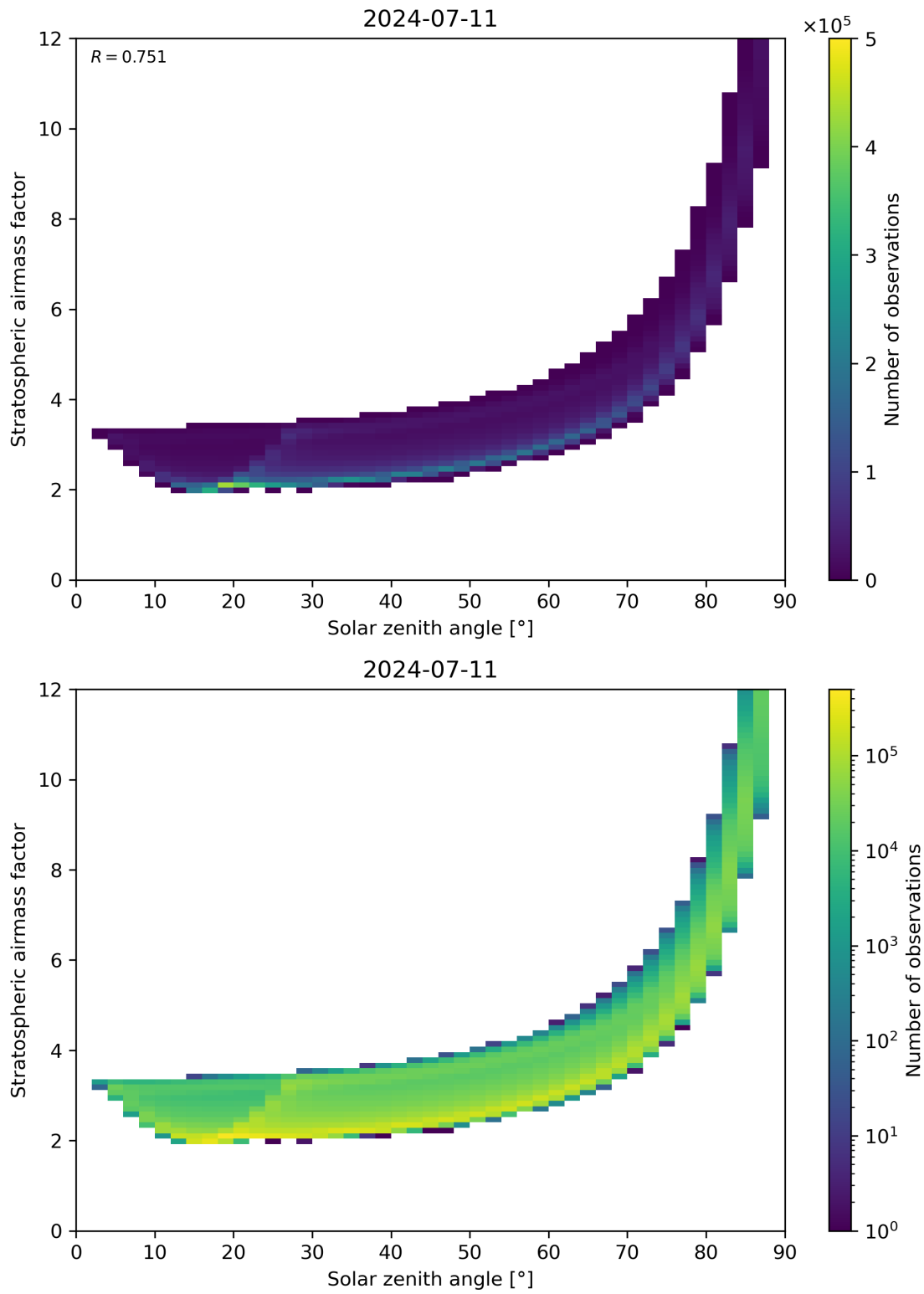
Figure 145: Scatter density plot of “Solar zenith angle” against “Stratospheric airmass factor” for 2024-07-10 to 2024-07-12.
