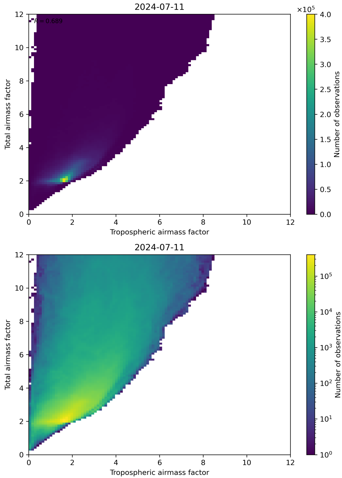
Figure 72: Scatter density plot of “Tropospheric airmass factor” against “Total airmass factor” for 2024-07-10 to 2024-07-12.
