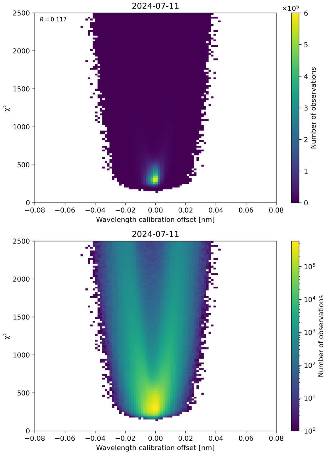
Figure 175: Scatter density plot of “Wavelength calibration offset” against “ \chi^2 ” for 2024-07-10 to 2024-07-12.
