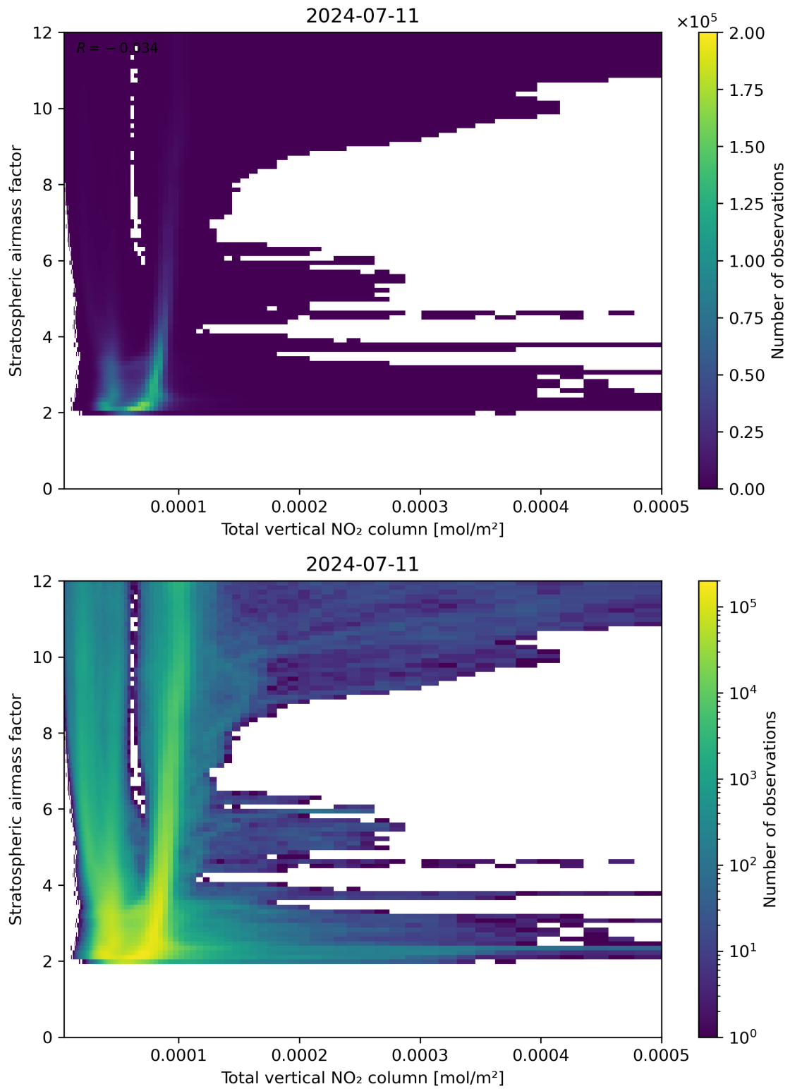
Figure 110: Scatter density plot of “Total vertical NO 2 column” against “Stratospheric airmass factor” for 2024-07-10 to 2024-07-12.
