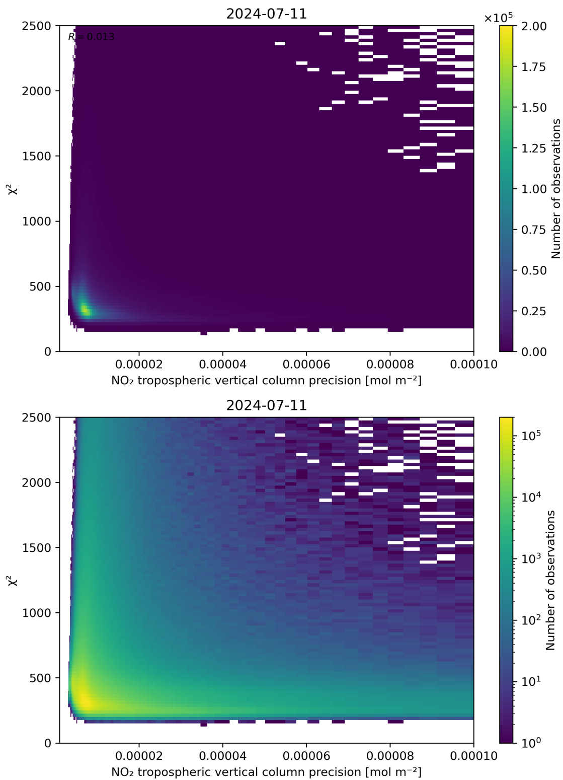
Figure 134: Scatter density plot of “NO 2 tropospheric vertical column precision” against “ \chi^2 ” for 2024-07-10 to 2024-07-12.
