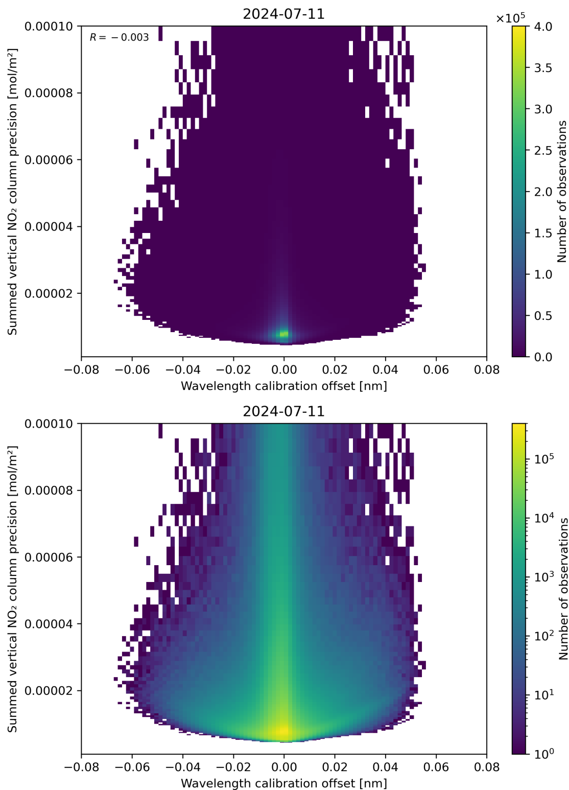
Figure 178: Scatter density plot of “Wavelength calibration offset” against “Summed vertical NO 2 column precision” for 2024-07-10 to 2024-07-12.
