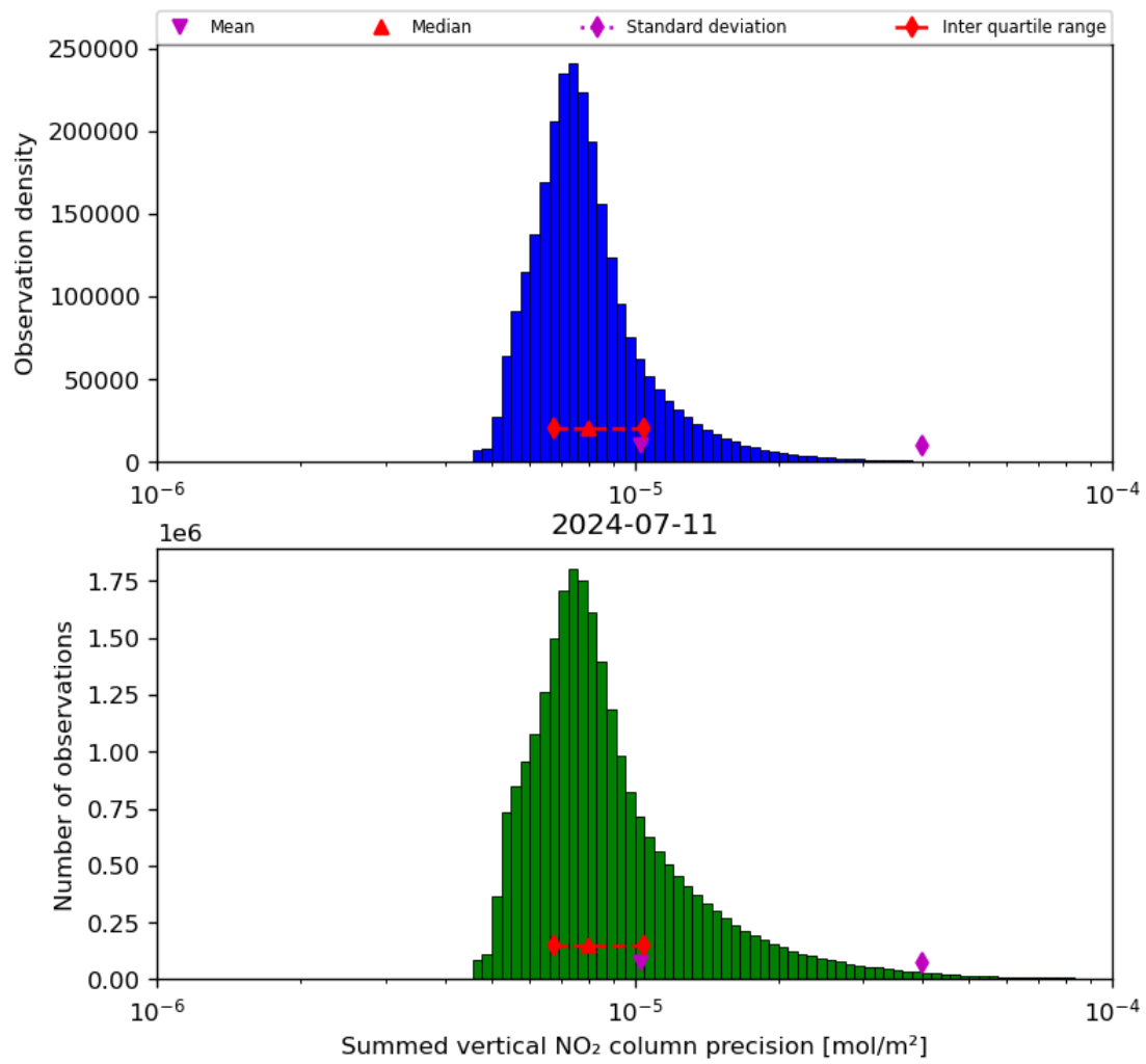
Figure 41: Histogram of "Summed vertical NO 2 column precision" for 2024-07-10 to 2024-07-12
