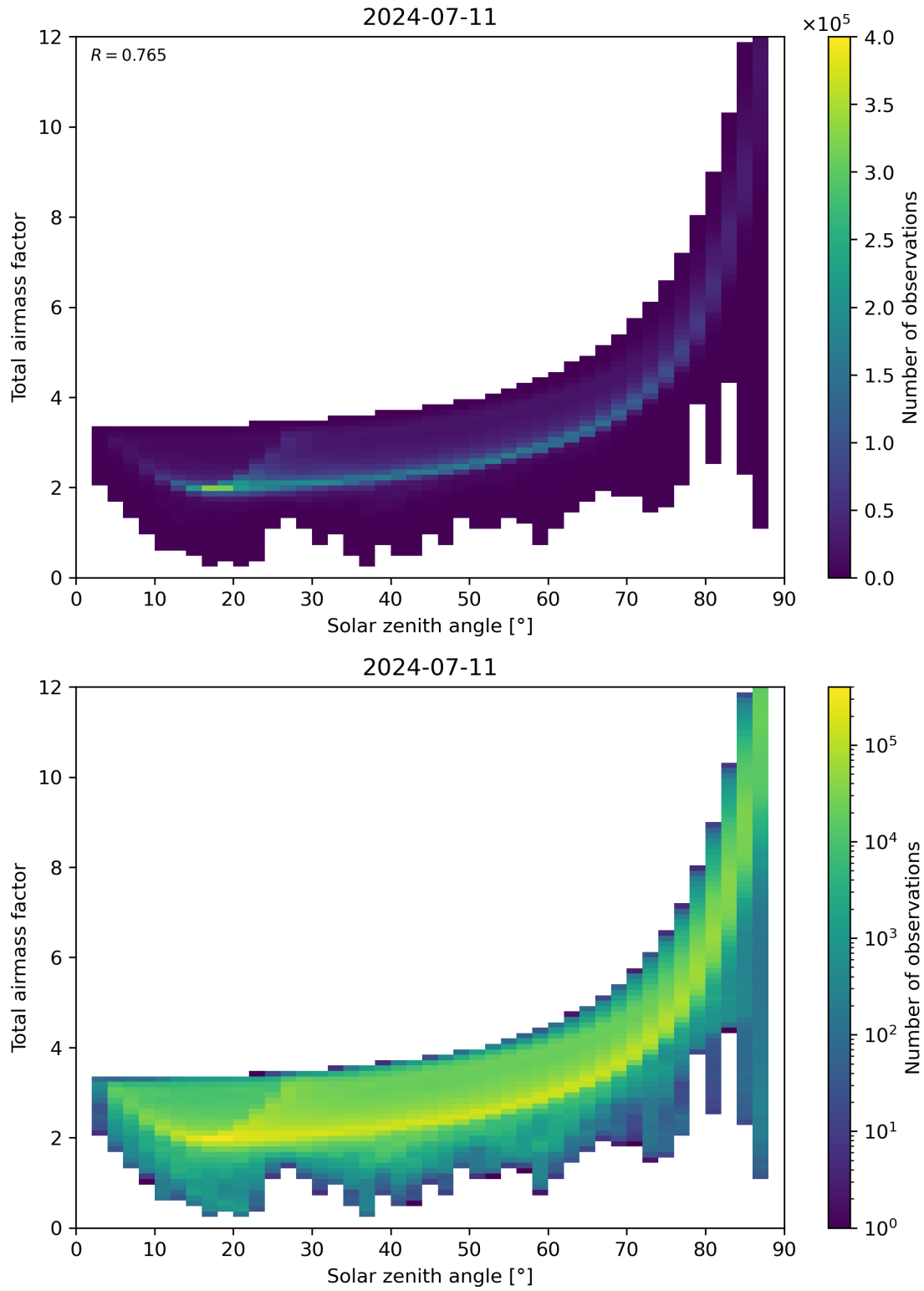
Figure 146: Scatter density plot of “Solar zenith angle” against “Total air mass factor” for 2024-07-10 to 2024-07-12.
