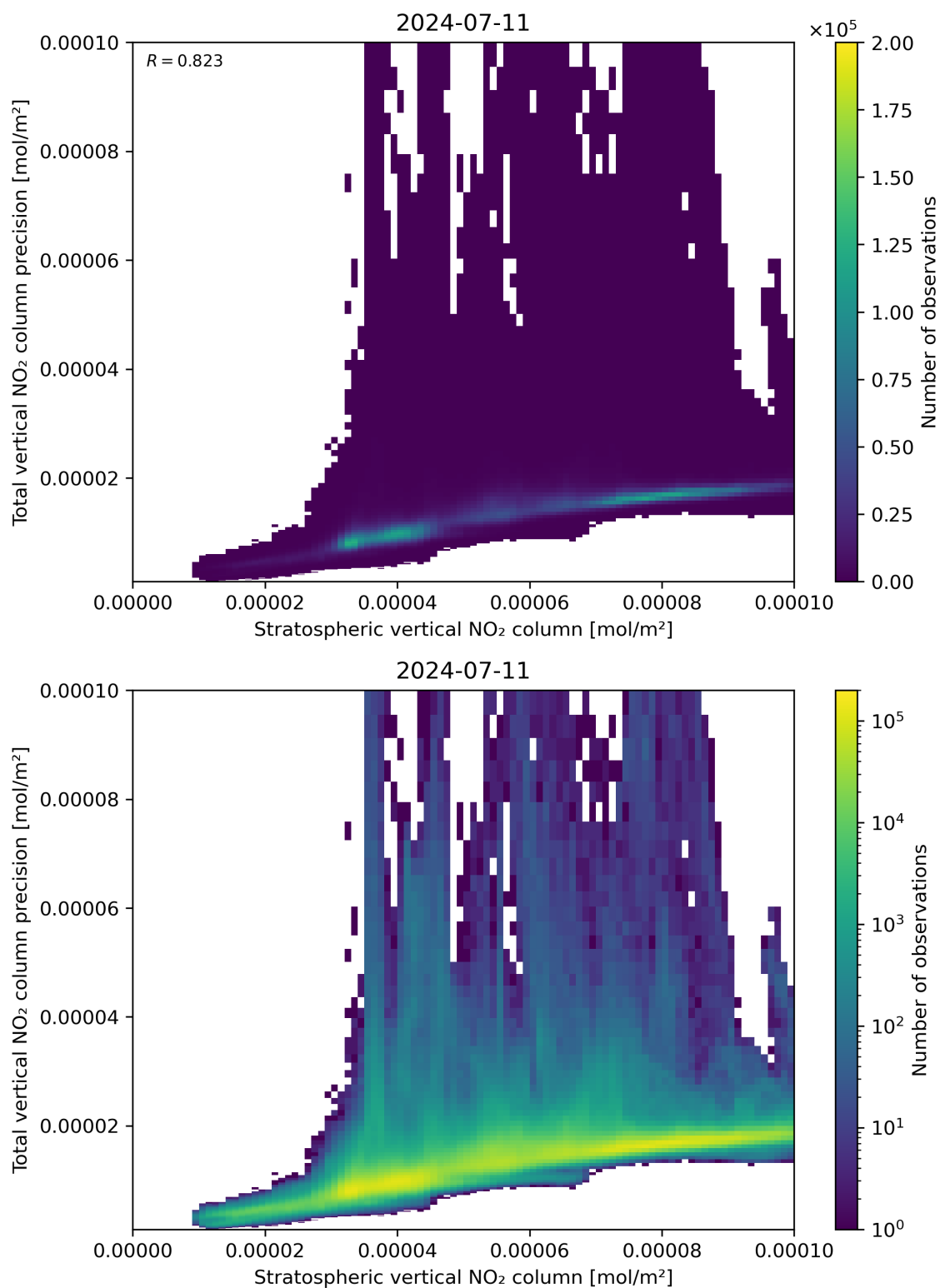
Figure 101: Scatter density plot of “Stratospheric vertical NO 2 column” against “Total vertical NO 2 column precision” for 2024-07-10 to 2024-07-12.
