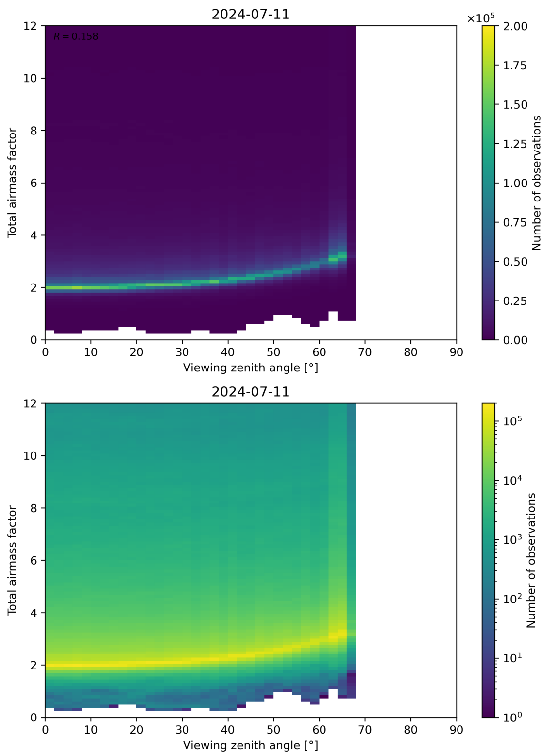
Figure 160: Scatter density plot of “Viewing zenith angle” against “Total airmass factor” for 2024-07-10 to 2024-07-12.
