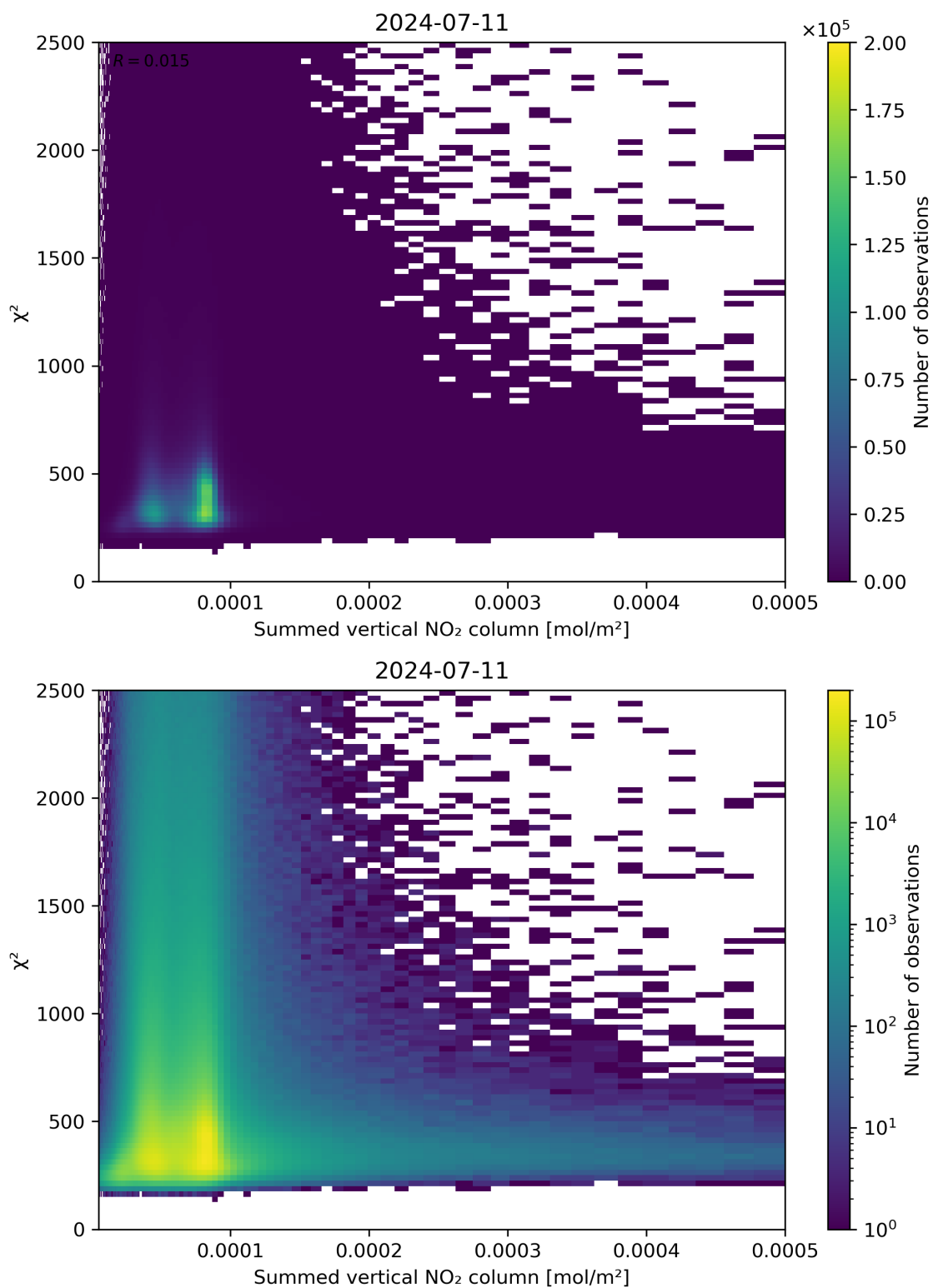
Figure 104: Scatter density plot of “Summed vertical NO 2 column” against “ \chi^2 ” for 2024-07-10 to 2024-07-12.
