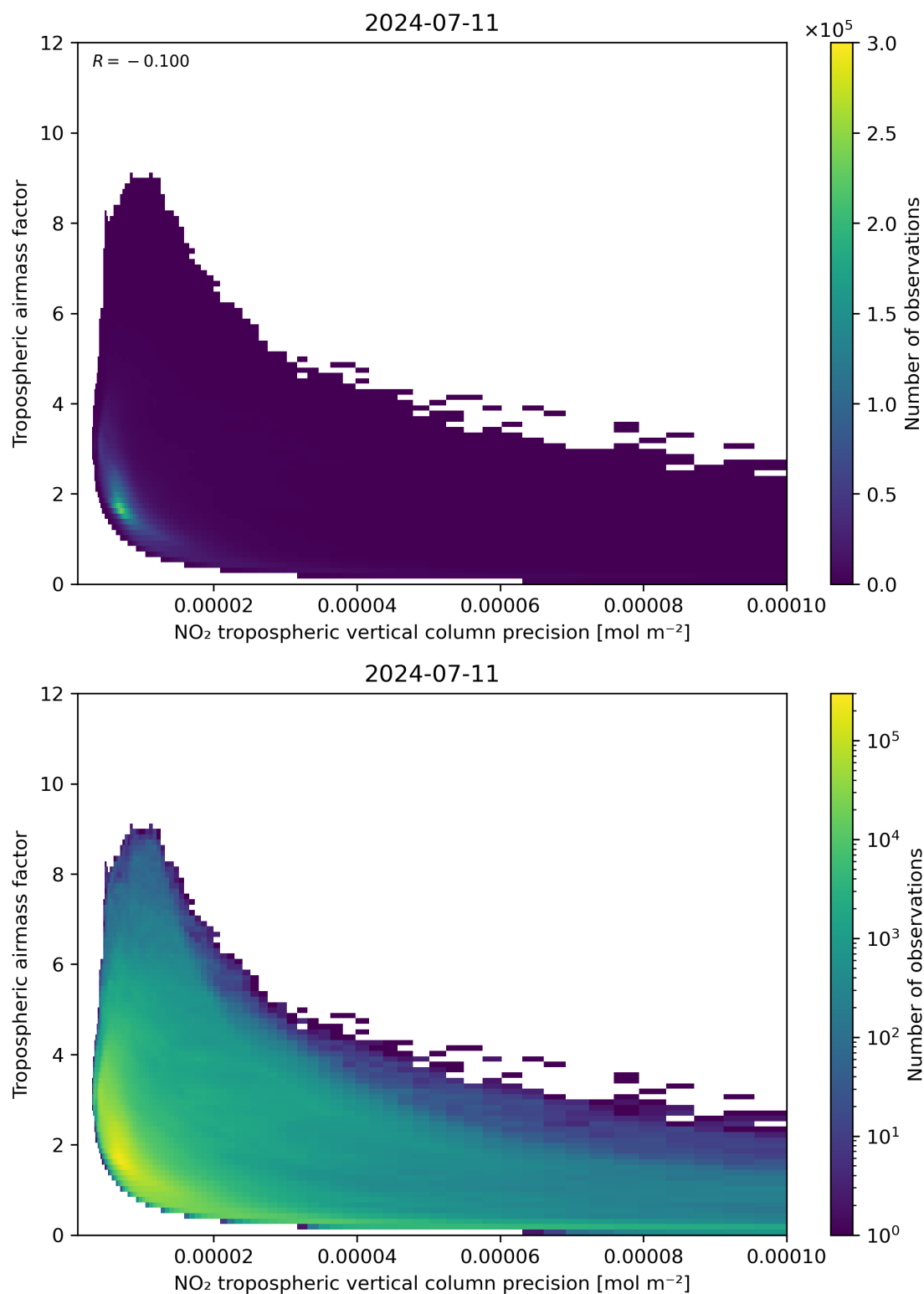
Figure 133: Scatter density plot of “NO 2 tropospheric vertical column precision” against “Tropospheric airmass factor” for 2024-07-10 to 2024-07-12.
