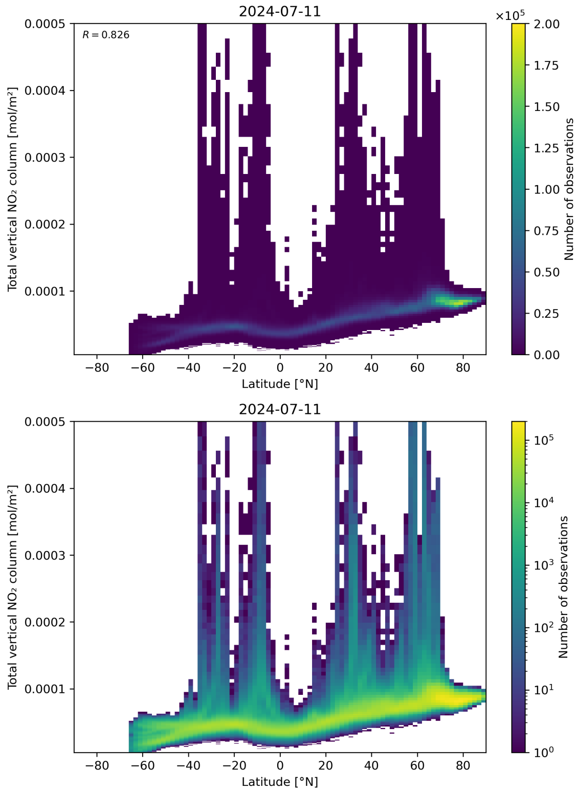
Figure 90: Scatter density plot of “Latitude” against “Total vertical NO 2 column” for 2024-07-10 to 2024-07-12.
