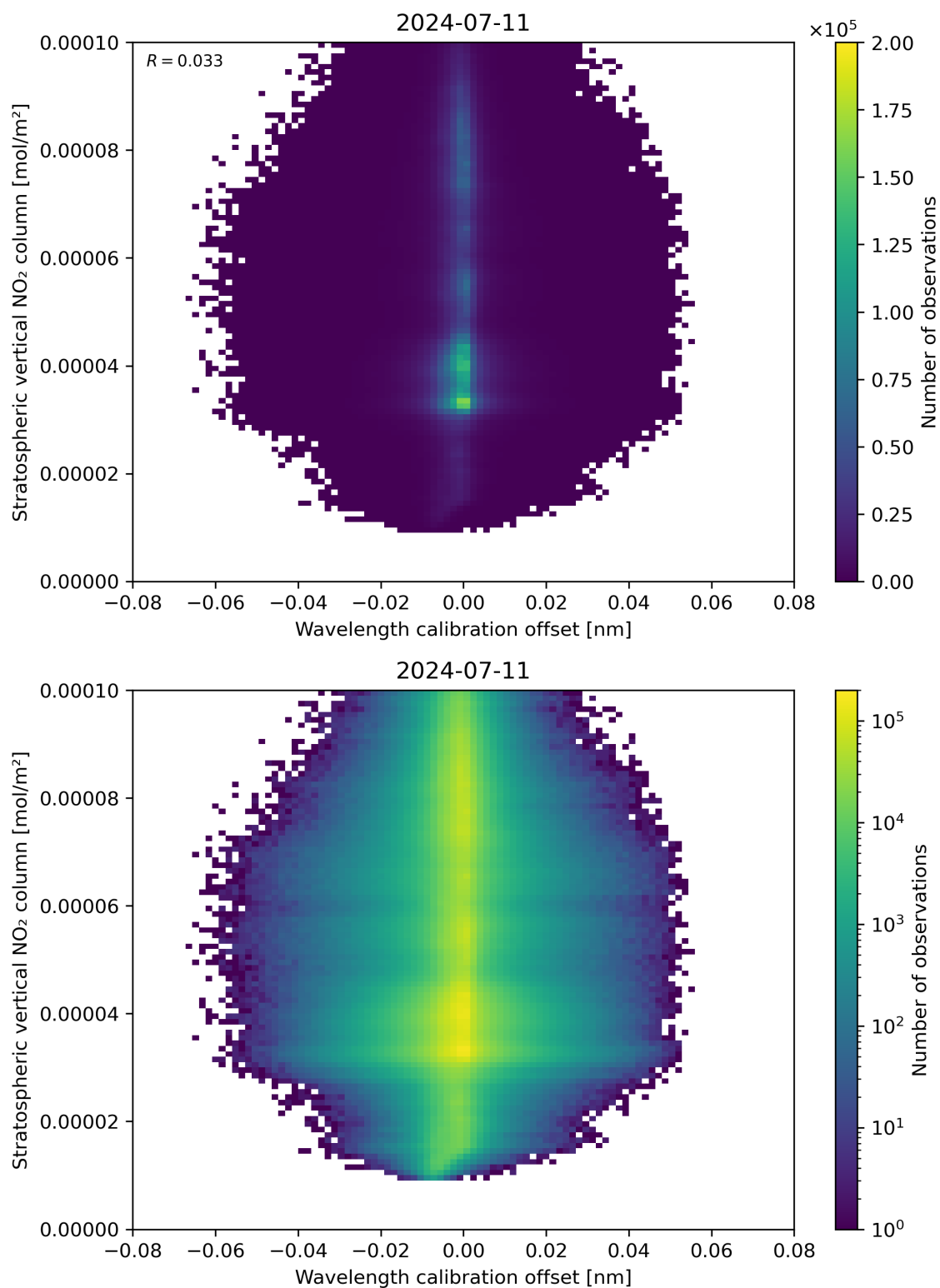
Figure 176: Scatter density plot of “Wavelength calibration offset” against “Stratospheric vertical NO 2 column” for 2024-07-10 to 2024-07-12.
