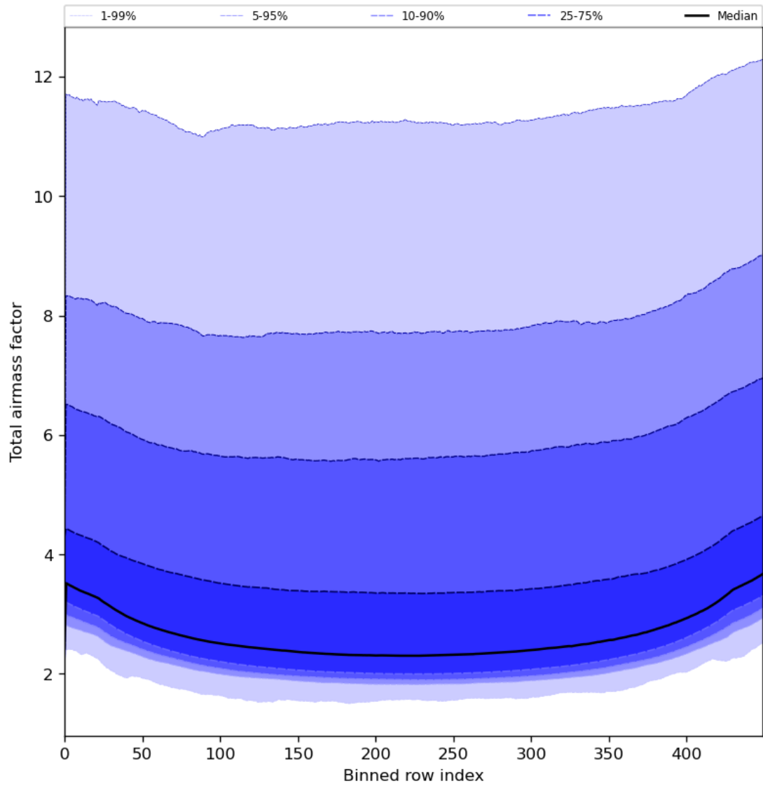
Figure 49: Along track statistics of “Total airmass factor” for 2024-07-10 to 2024-07-12
