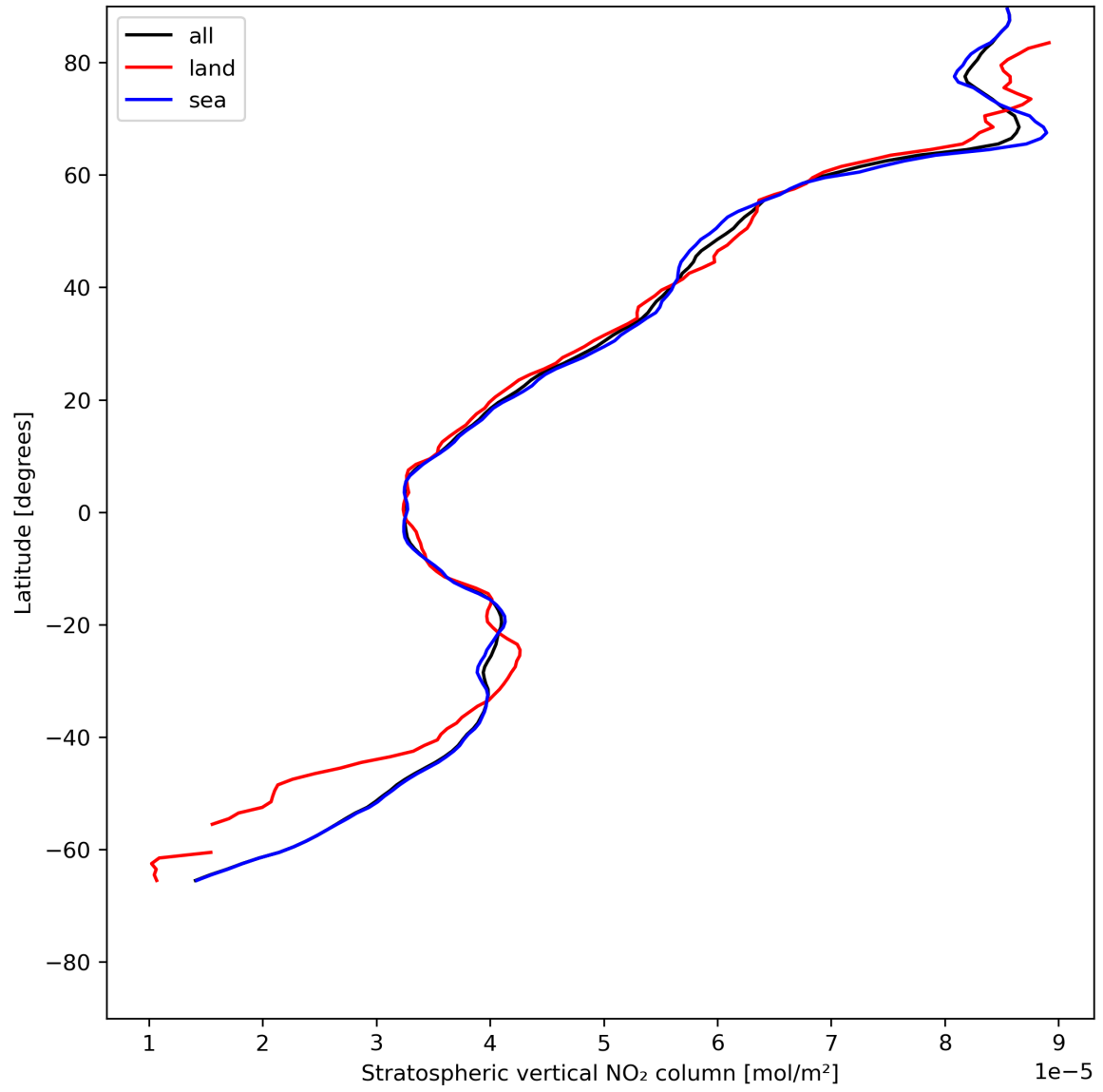
Figure 19: Zonal average of “Stratospheric vertical NO 2 column” for 2024-07-10 to 2024-07-12.
