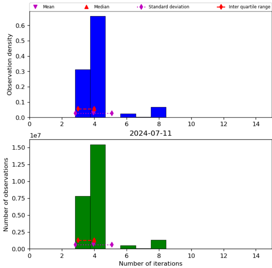
Figure 34: Histogram of “Number of iterations” for 2024-07-10 to 2024-07-12
