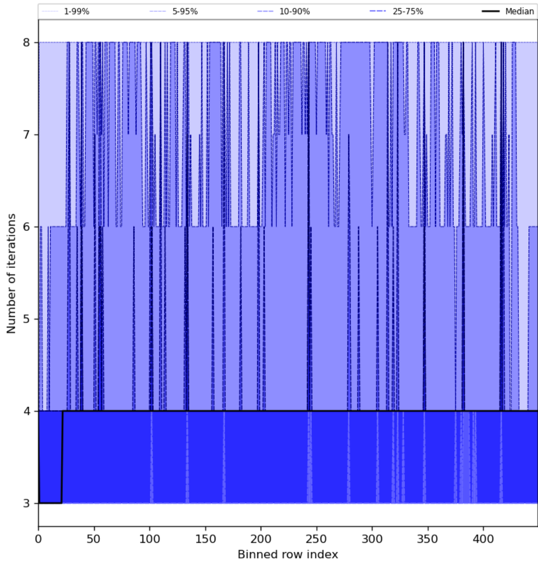
Figure 51: Along track statistics of “Number of iterations” for 2024-07-10 to 2024-07-12
