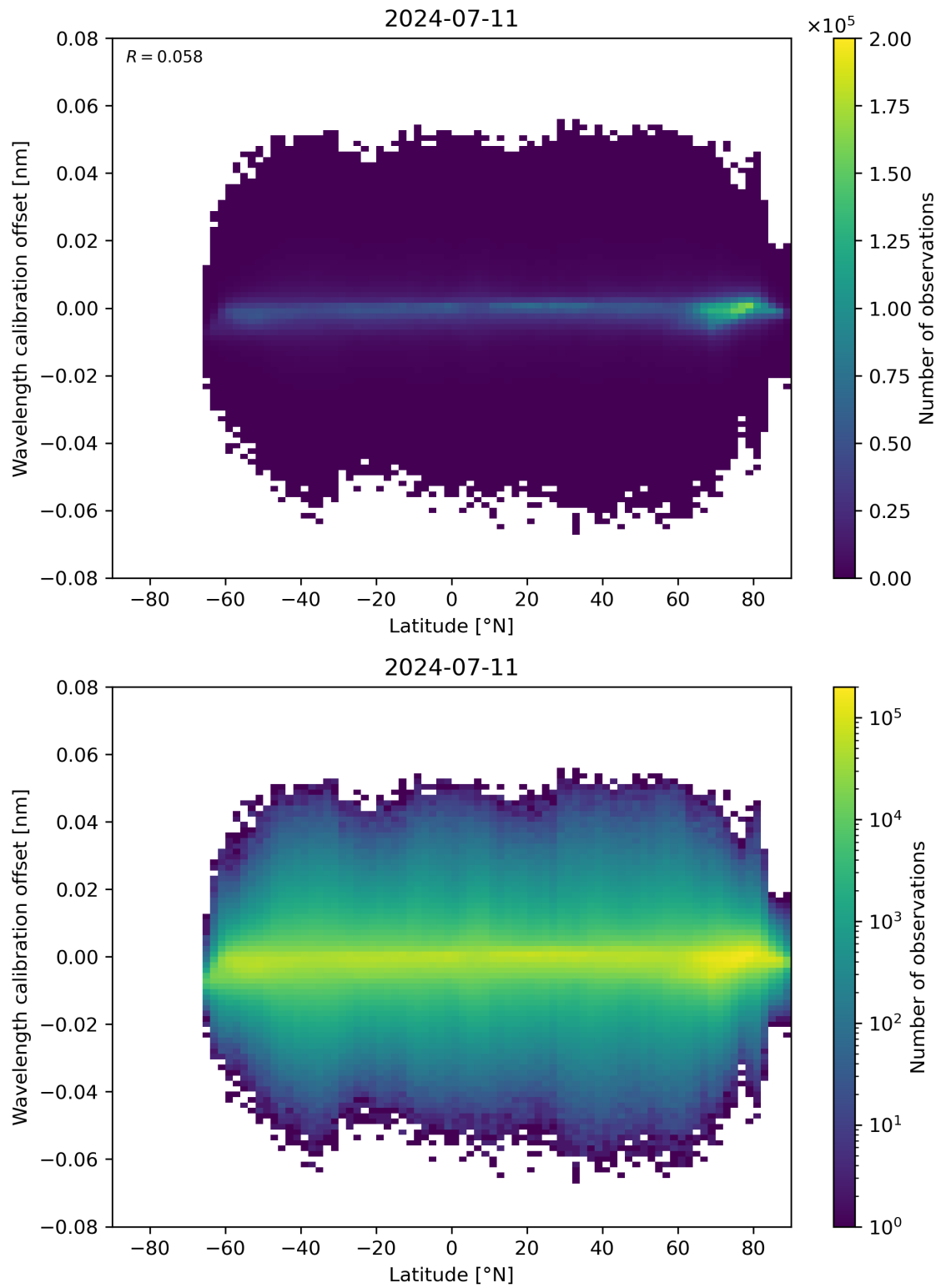
Figure 95: Scatter density plot of “Latitude” against “Wavelength calibration offset” for 2024-07-10 to 2024-07-12.
