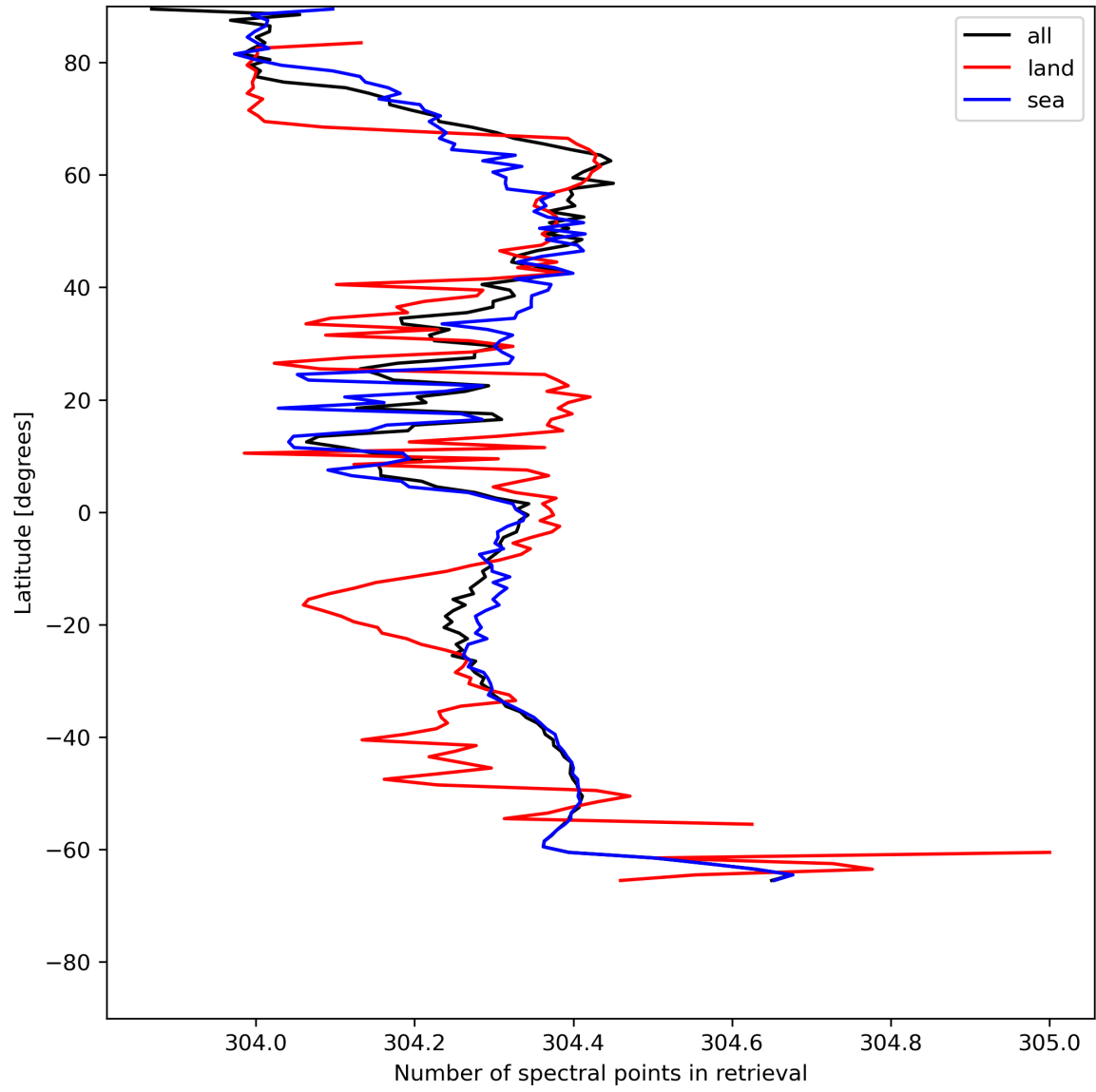
Figure 16: Zonal average of “Number of spectral points in retrieval” for 2024-07-10 to 2024-07-12.
