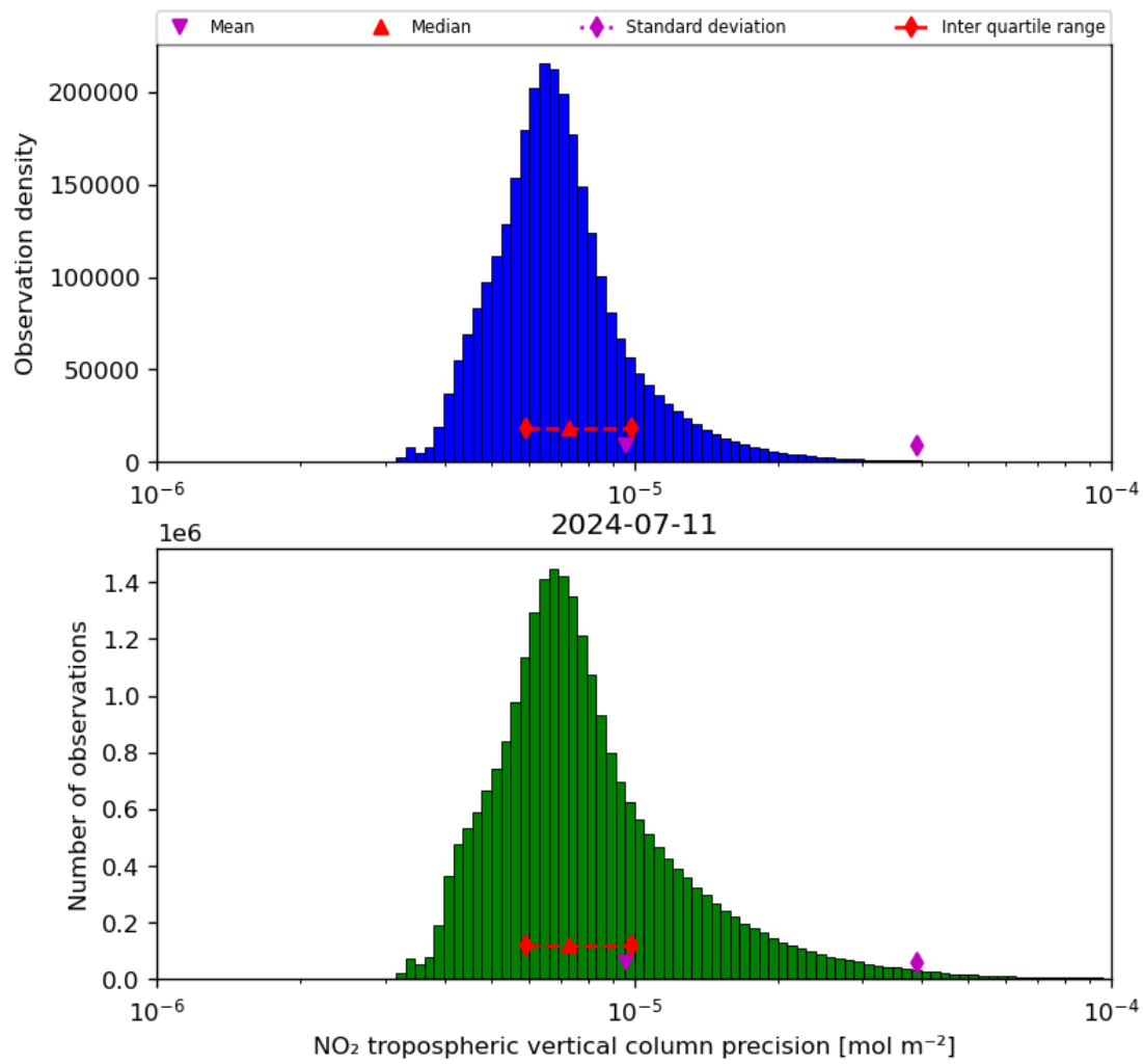
Figure 30: Histogram of “NO 2 tropospheric vertical column precision” for 2024-07-10 to 2024-07-12
