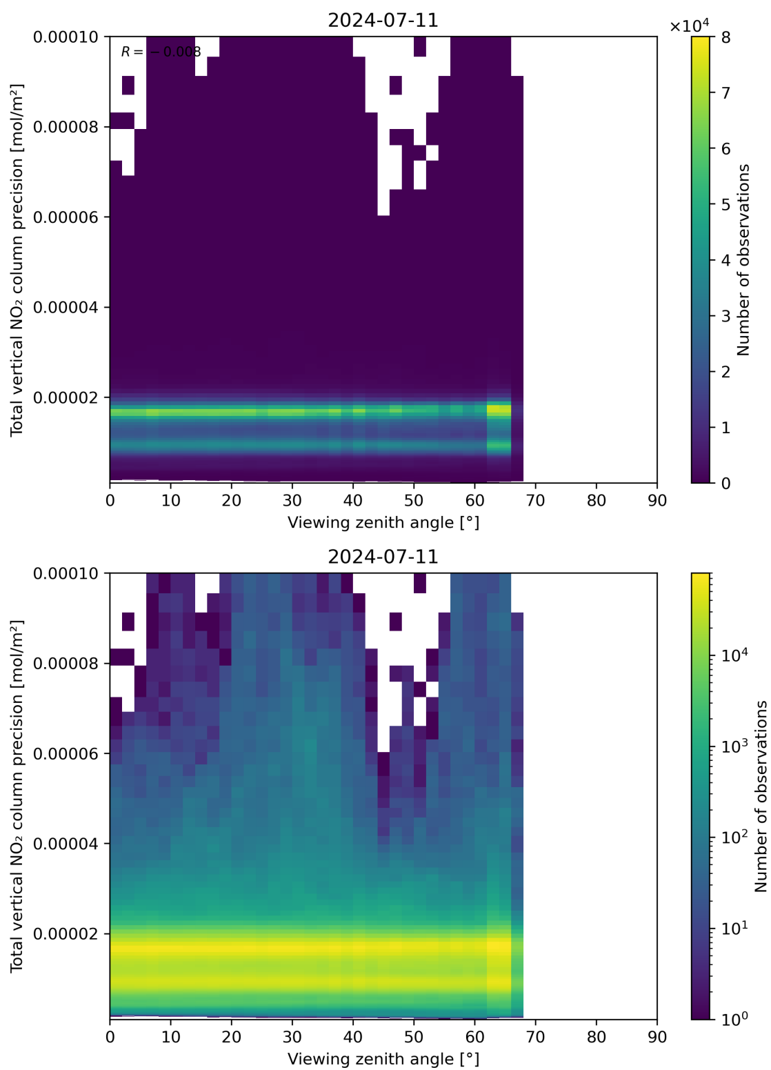
Figure 168: Scatter density plot of “Viewing zenith angle” against “Total vertical NO 2 column precision” for 2024-07-10 to 2024-07-12.
