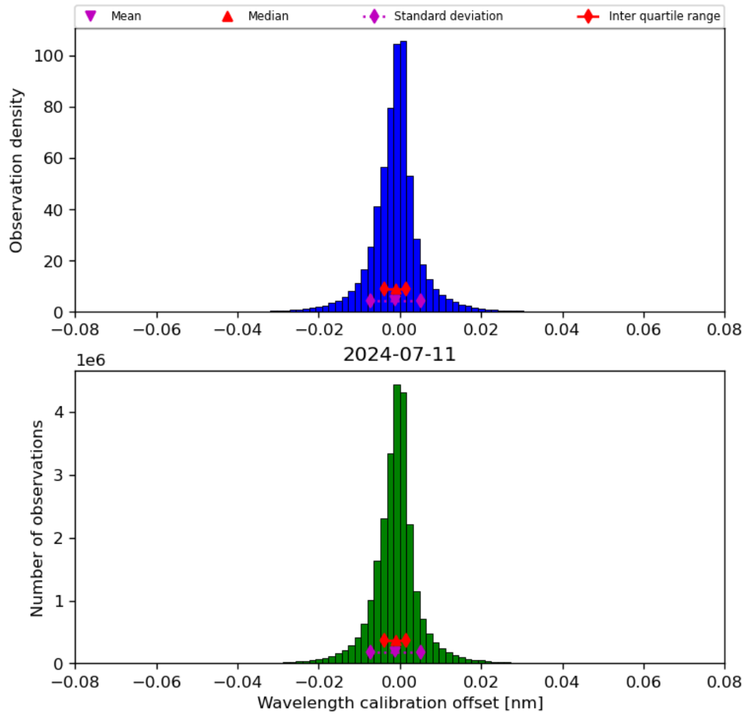
Figure 35: Histogram of “Wavelength calibration offset” for 2024-07-10 to 2024-07-12
