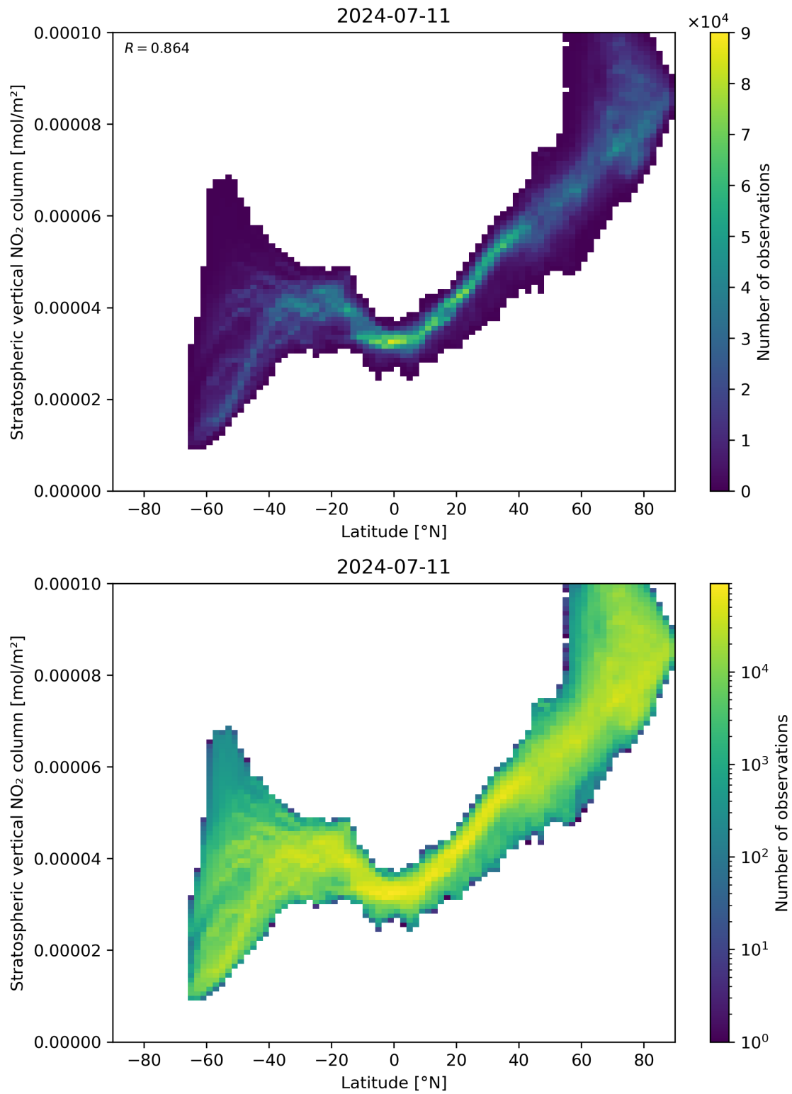
Figure 87: Scatter density plot of “Latitude” against “Stratospheric vertical NO 2 column” for 2024-07-10 to 2024-07-12.
