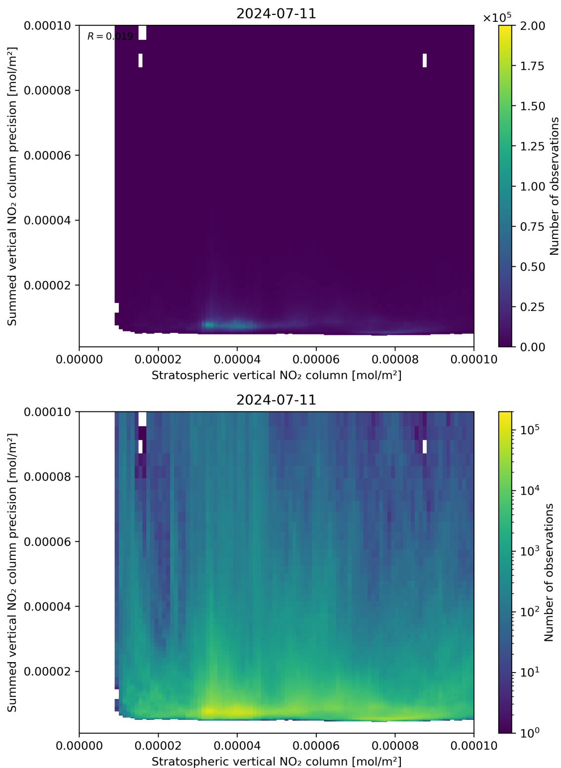
Figure 99: Scatter density plot of “Stratospheric vertical NO 2 column” against “Summed vertical NO 2 column precision” for 2024-07-10 to 2024-07-12.
