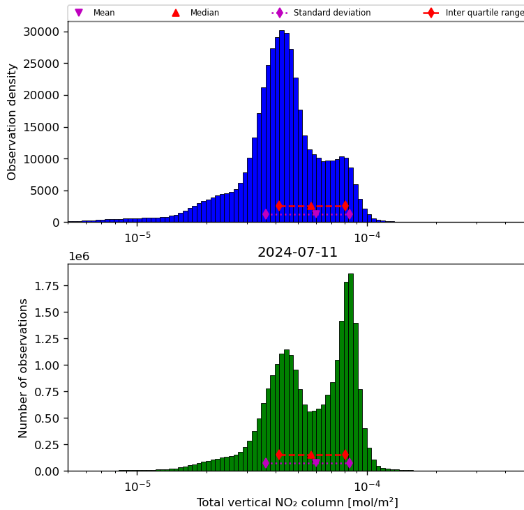
Figure 38: Histogram of “Total vertical NO 2 column” for 2024-07-10 to 2024-07-12
