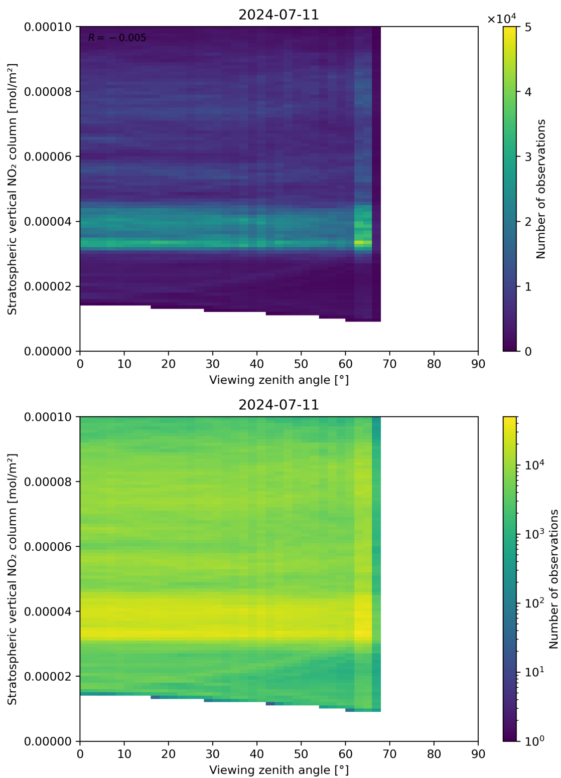
Figure 164: Scatter density plot of “Viewing zenith angle” against “Stratospheric vertical NO 2 column” for 2024-07-10 to 2024-07-12.
