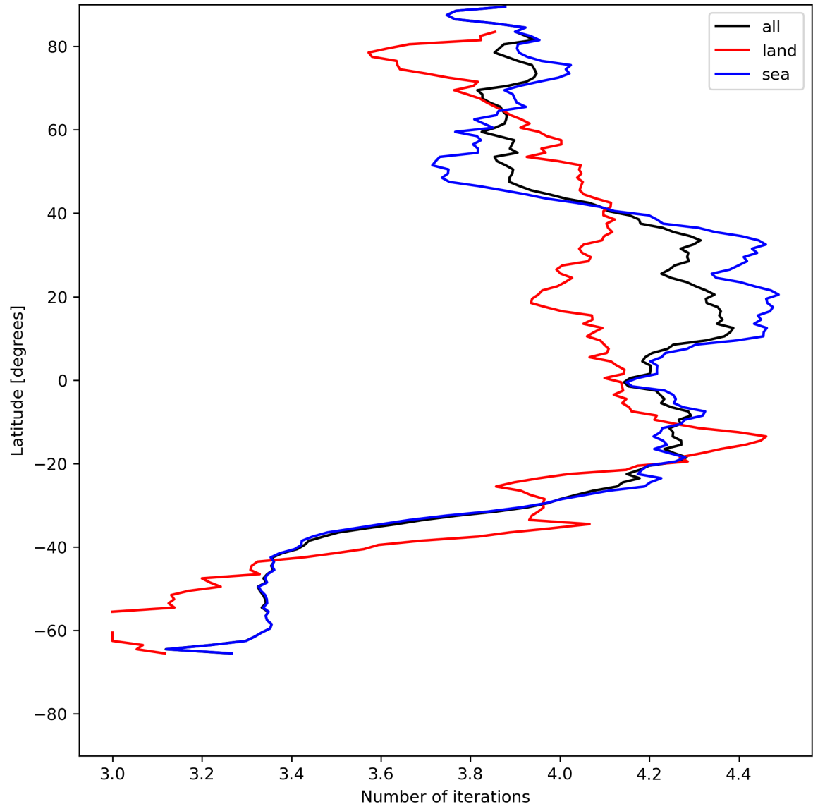
Figure 17: Zonal average of “Number of iterations” for 2024-07-10 to 2024-07-12.
