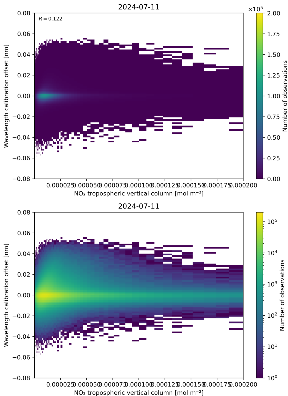
Figure 143: Scatter density plot of “NO 2 tropospheric vertical column” against “Wavelength calibration offset” for 2024-07-10 to 2024-07-12.
