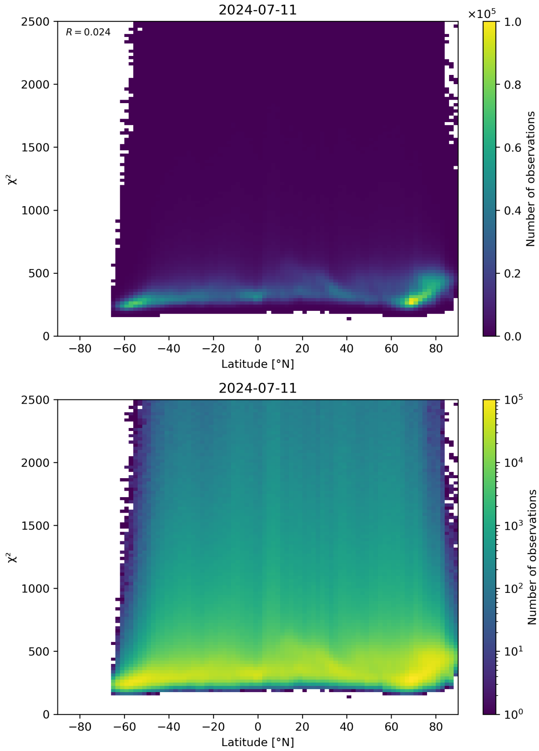
Figure 86: Scatter density plot of “Latitude” against “ \chi^2 ” for 2024-07-10 to 2024-07-12.
