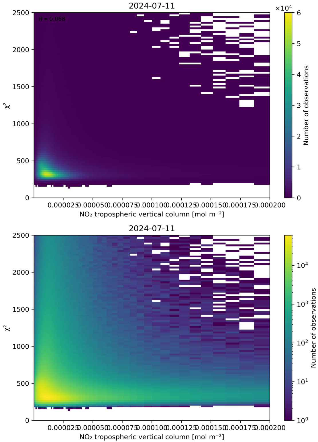
Figure 124: Scatter density plot of “NO 2 tropospheric vertical column” against “ \chi^2 ” for 2024-07-10 to 2024-07-12.
