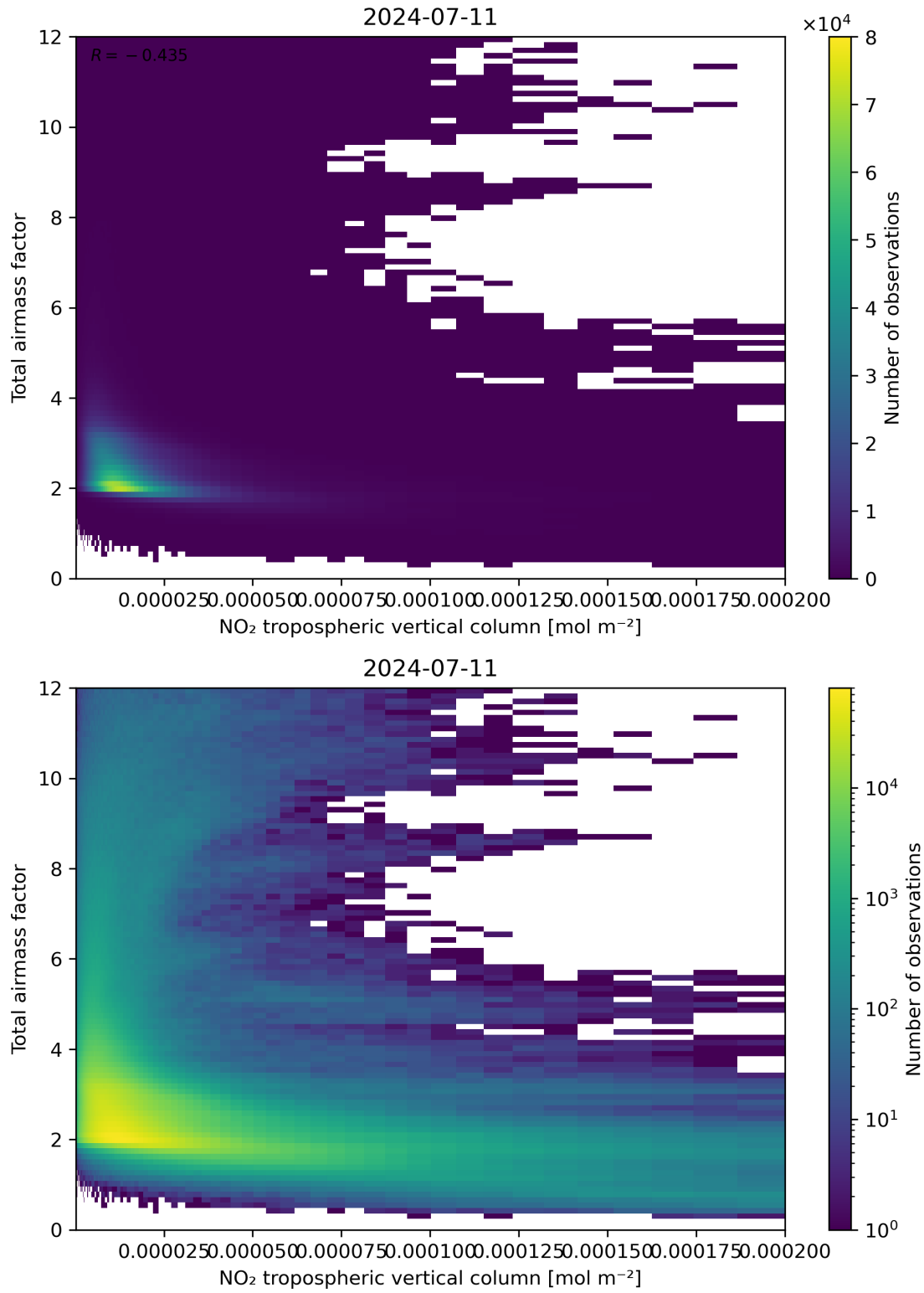
Figure 122: Scatter density plot of “NO 2 tropospheric vertical column” against “Total air mass factor” for 2024-07-10 to 2024-07-12.
