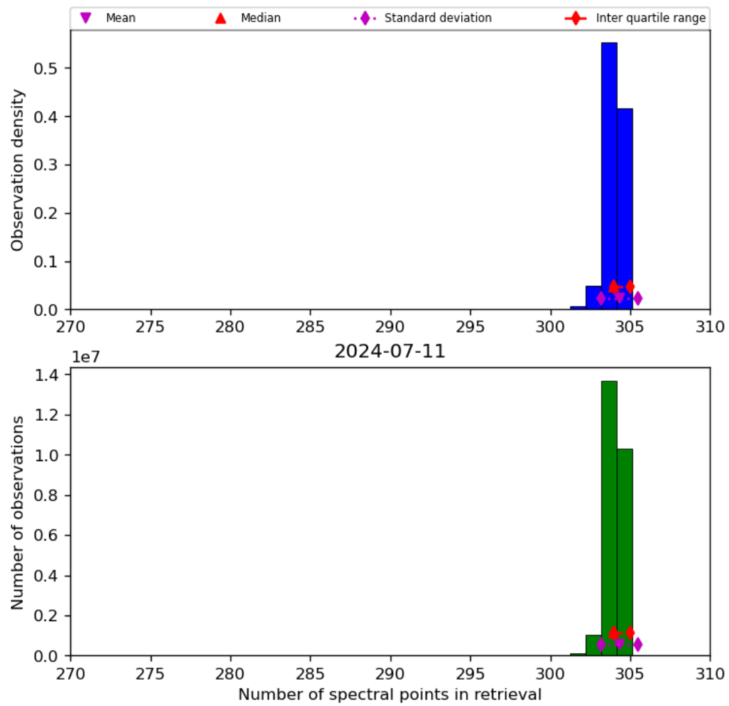
Figure 33: Histogram of “Number of spectral points in retrieval” for 2024-07-10 to 2024-07-12
