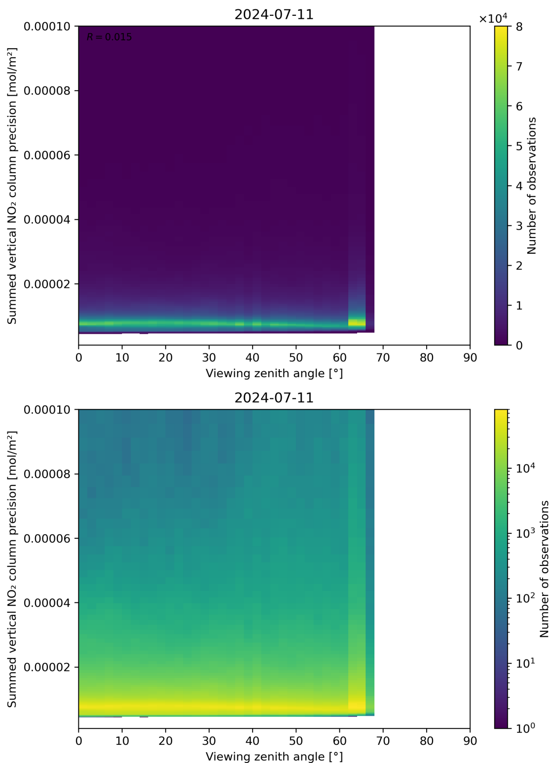
Figure 166: Scatter density plot of “Viewing zenith angle” against “Summed vertical NO 2 column precision” for 2024-07-10 to 2024-07-12.
