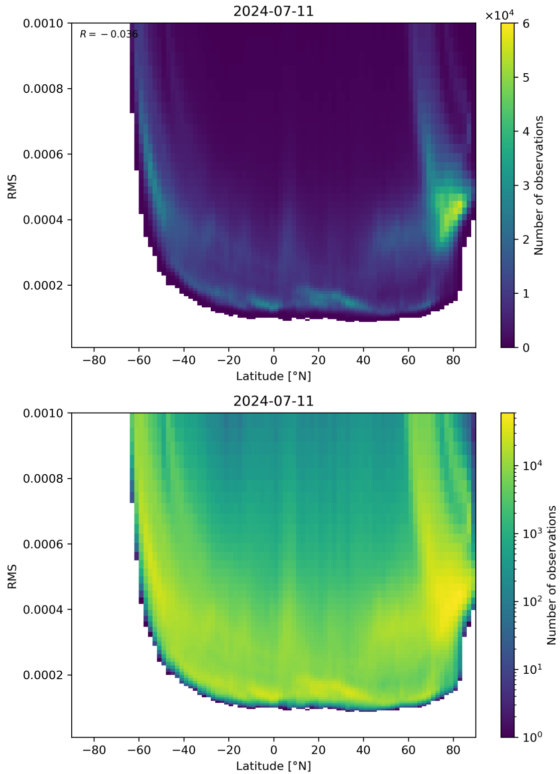
Figure 94: Scatter density plot of “Latitude” against “RMS” for 2024-07-10 to 2024-07-12.
