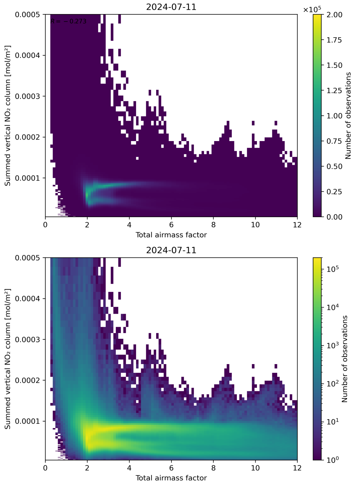
Figure 65: Scatter density plot of “Total airmass factor” against “Summed vertical NO 2 column” for 2024-07-10 to 2024-07-12.
