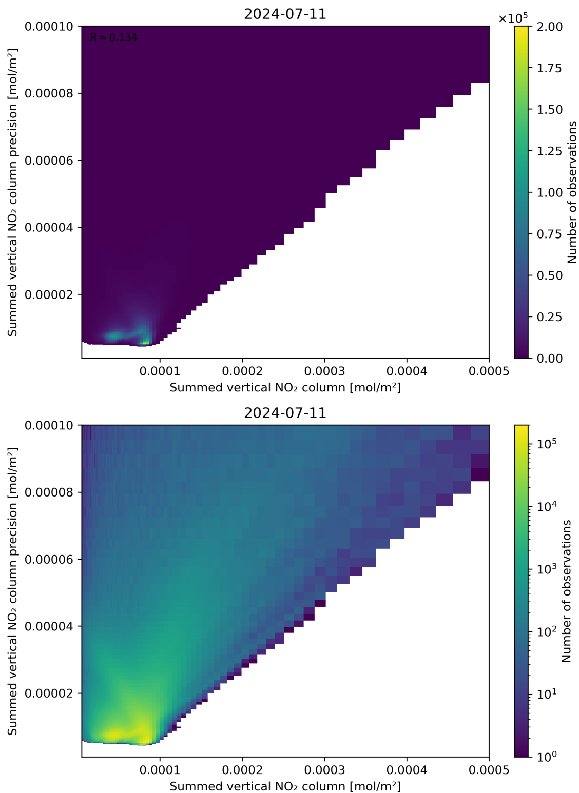
Figure 105: Scatter density plot of “Summed vertical NO 2 column” against “Summed vertical NO 2 column precision” for 2024-07-10 to 2024-07-12.
