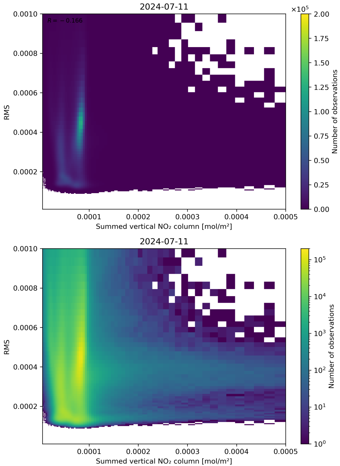
Figure 109: Scatter density plot of “Summed vertical NO 2 column” against “RMS” for 2024-07-10 to 2024-07-12.
