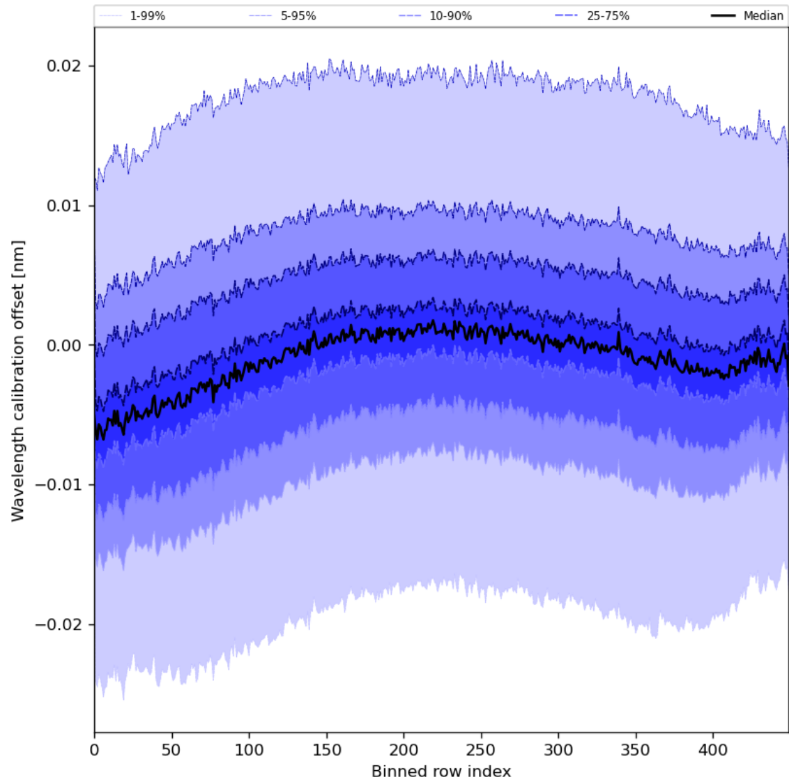
Figure 52: Along track statistics of “Wavelength calibration offset” for 2024-07-10 to 2024-07-12
