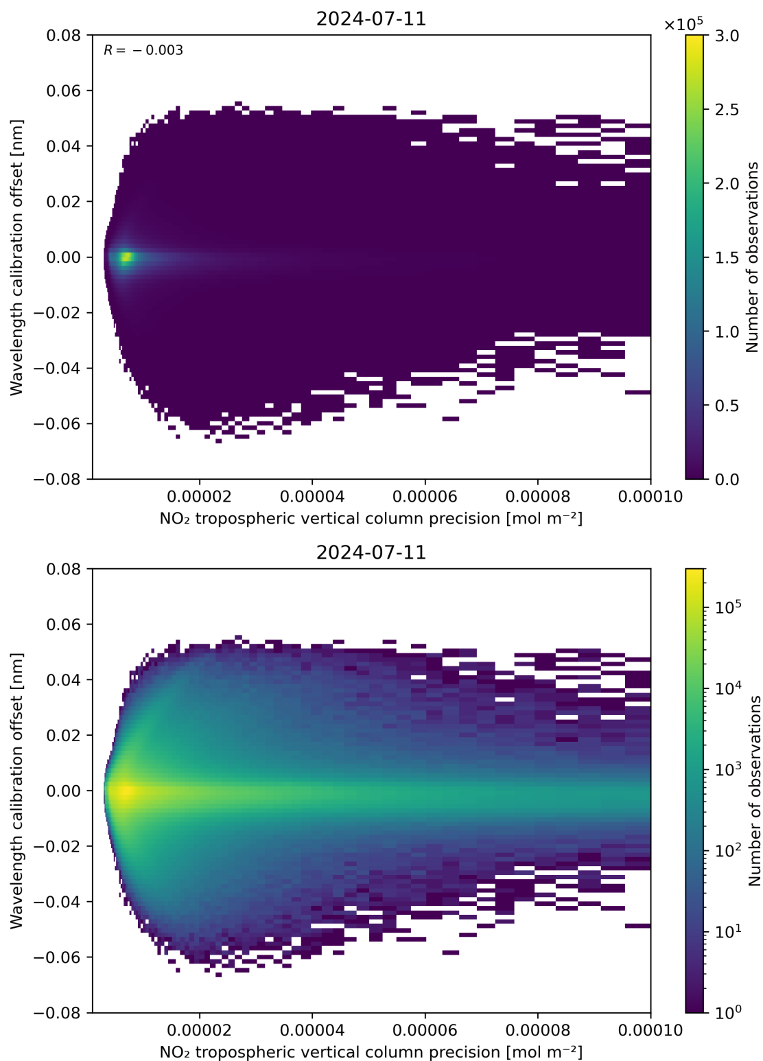
Figure 141: Scatter density plot of “NO 2 tropospheric vertical column precision” against “Wavelength calibration offset” for 2024-07-10 to 2024-07-12.
