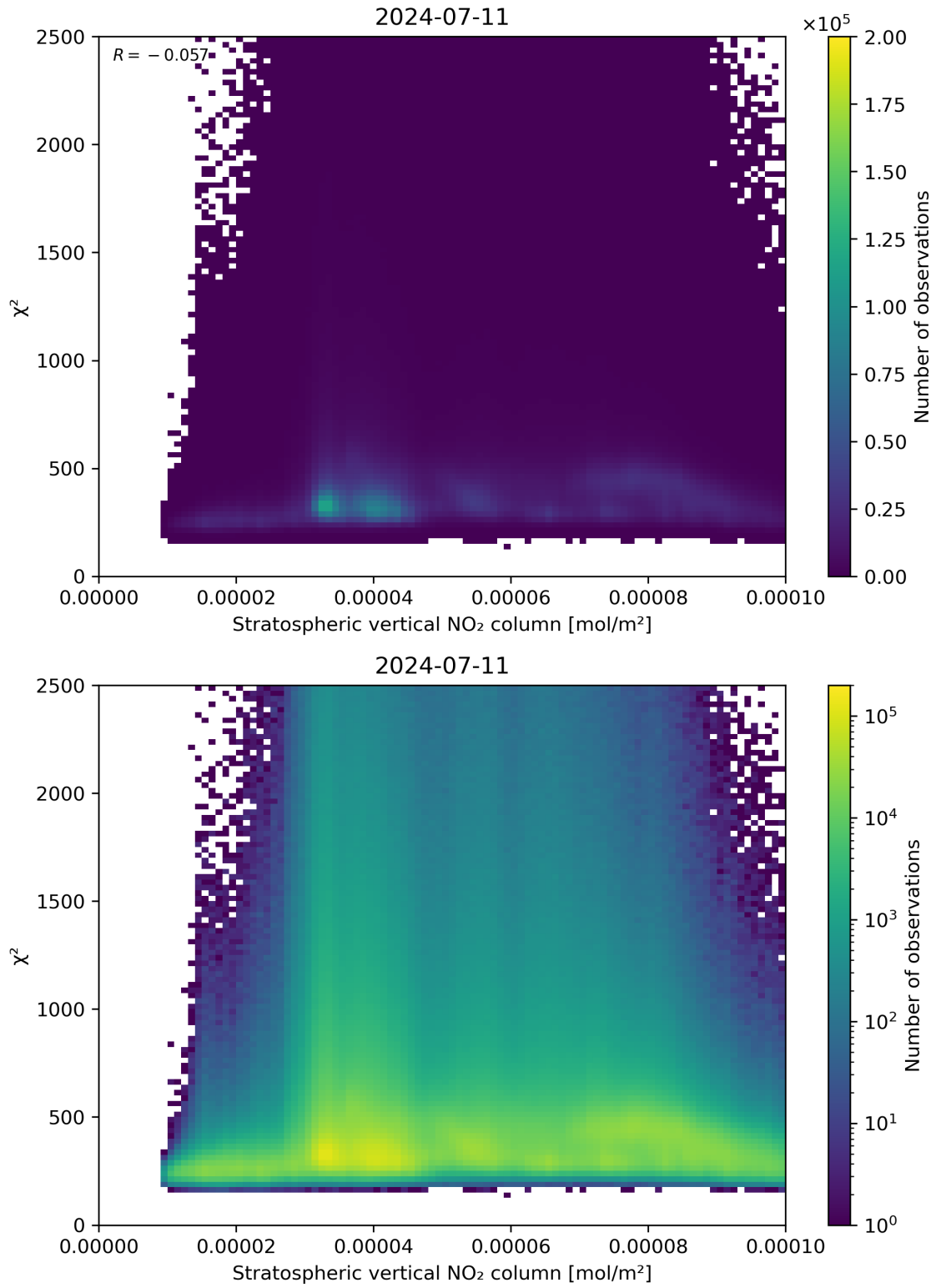
Figure 97: Scatter density plot of “Stratospheric vertical NO 2 column” against “ \chi^2 ” for 2024-07-10 to 2024-07-12.
