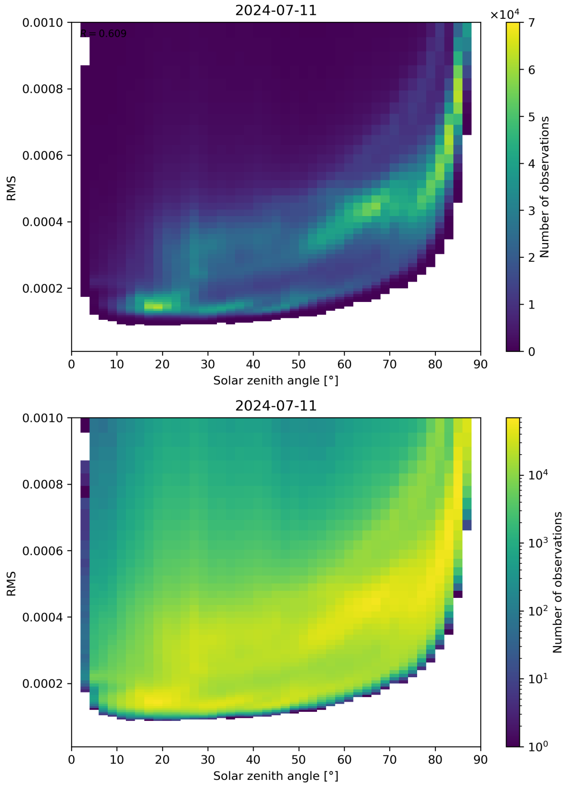
Figure 157: Scatter density plot of “Solar zenith angle” against “RMS” for 2024-07-10 to 2024-07-12.
