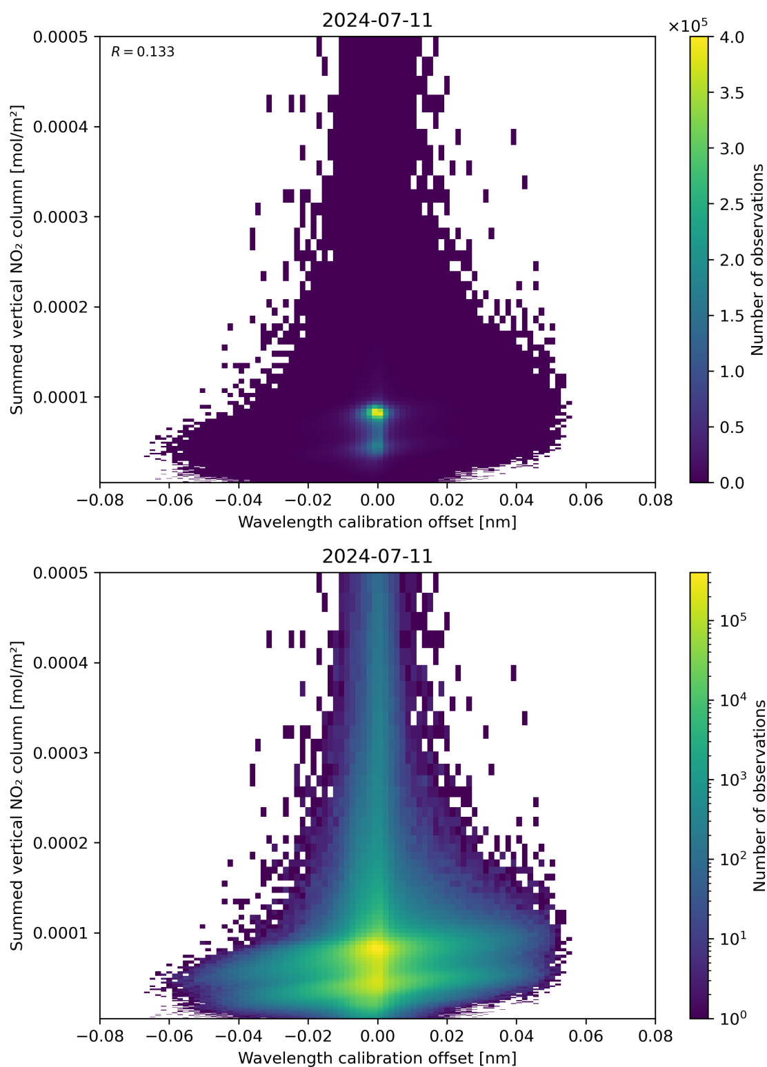
Figure 177: Scatter density plot of “Wavelength calibration offset” against “Summed vertical NO 2 column” for 2024-07-10 to 2024-07-12.
