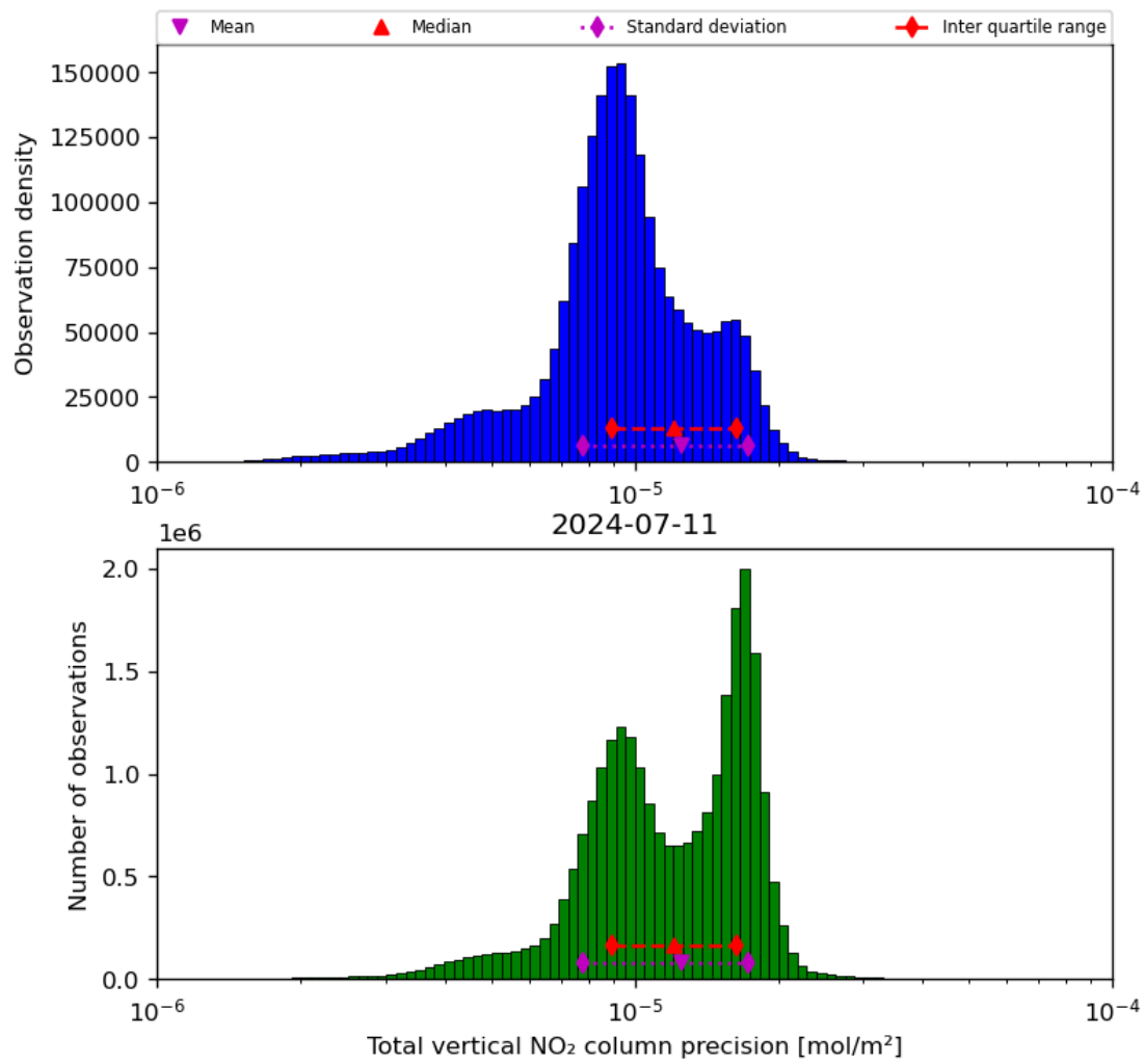
Figure 39: Histogram of “Total vertical NO 2 column precision” for 2024-07-10 to 2024-07-12
