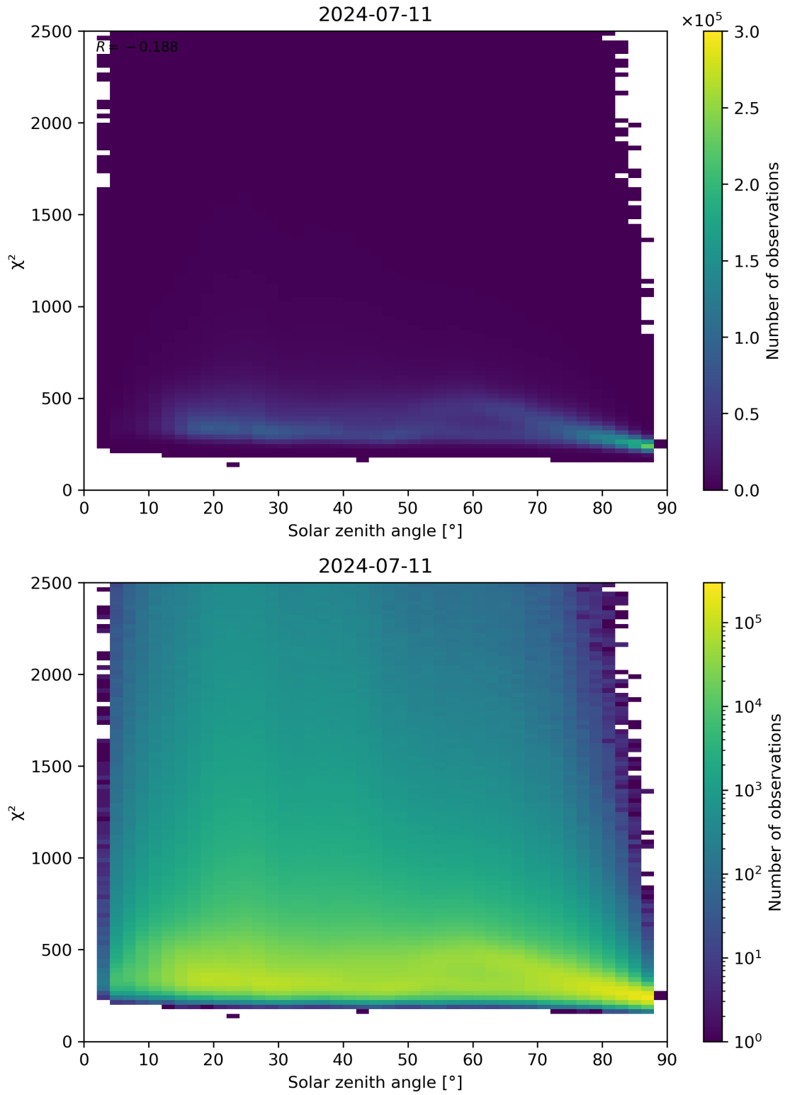
Figure 148: Scatter density plot of “Solar zenith angle” against “ \chi^2 ” for 2024-07-10 to 2024-07-12.
