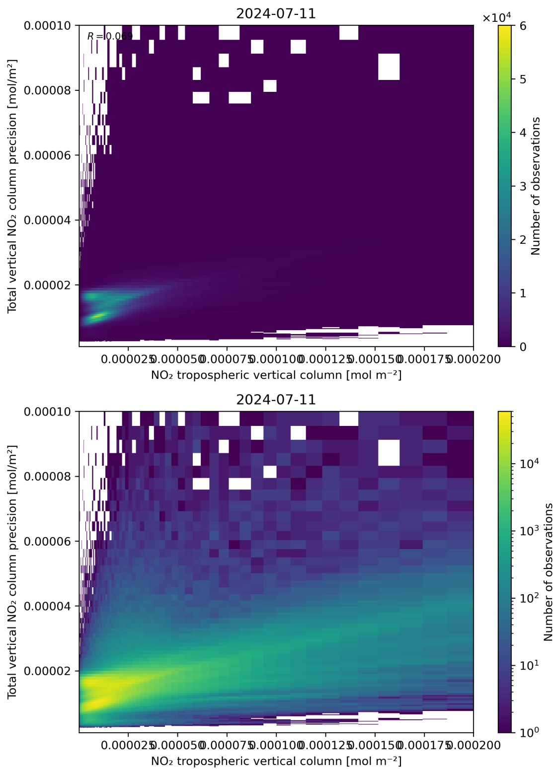
Figure 129: Scatter density plot of “NO 2 tropospheric vertical column” against “Total vertical NO 2 column precision” for 2024-07-10 to 2024-07-12.
