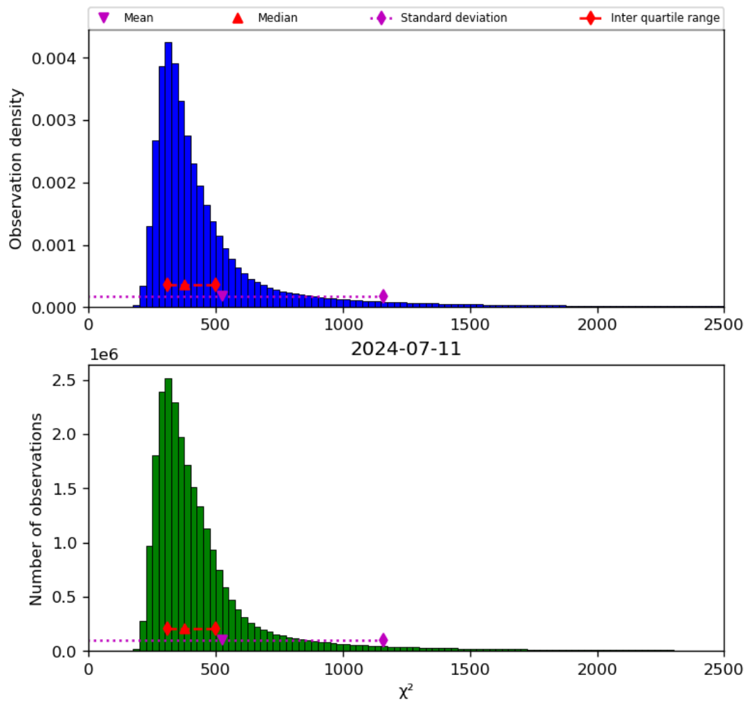
Figure 42: Histogram of “ \chi^2 ” for 2024-07-10 to 2024-07-12
