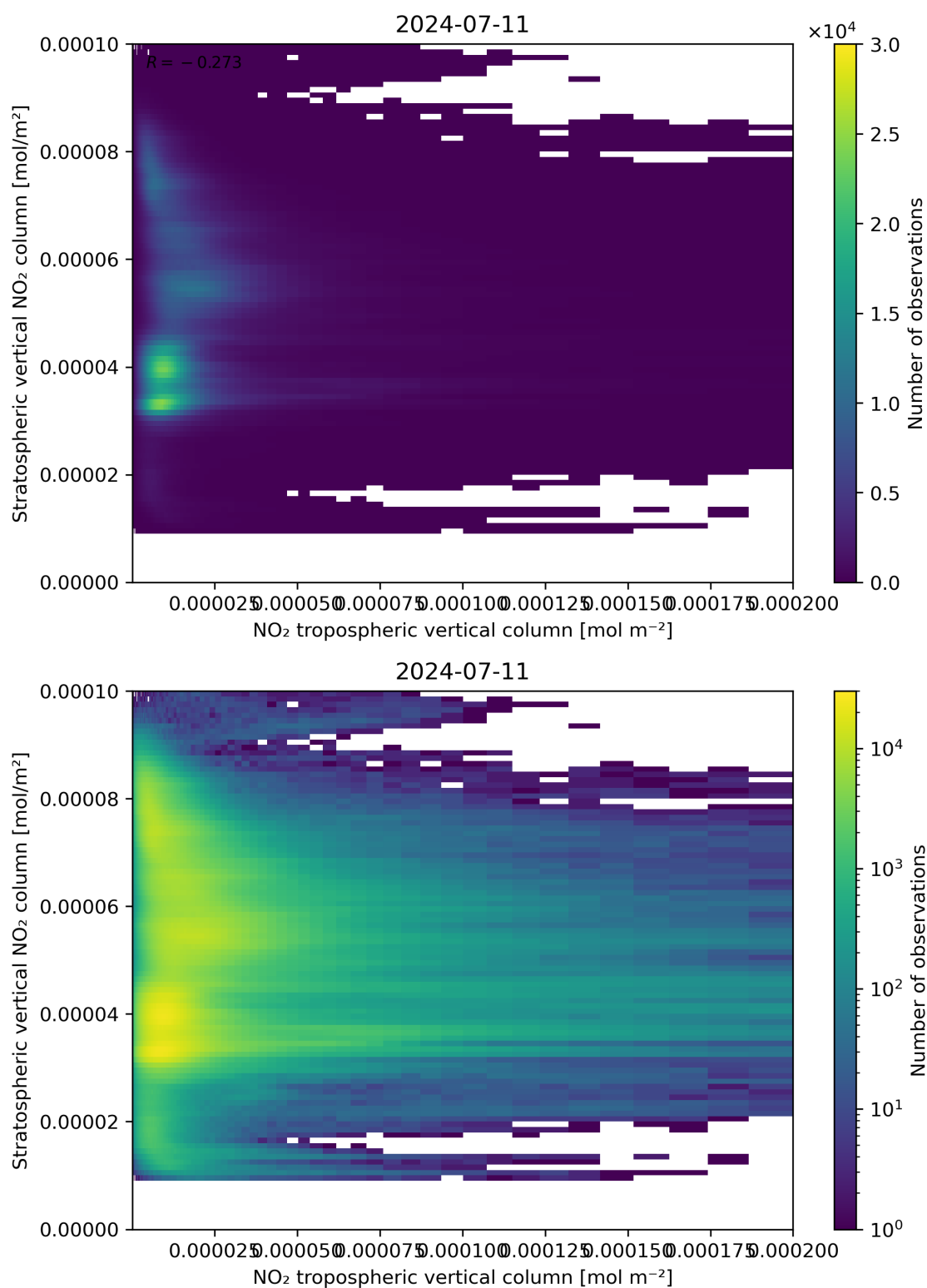
Figure 125: Scatter density plot of “NO 2 tropospheric vertical column” against “Stratospheric vertical NO 2 column” for 2024-07-10 to 2024-07-12.
