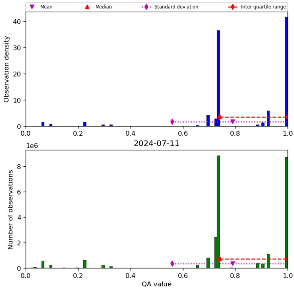
Figure 28: Histogram of “QA value” for 2024-07-10 to 2024-07-12
