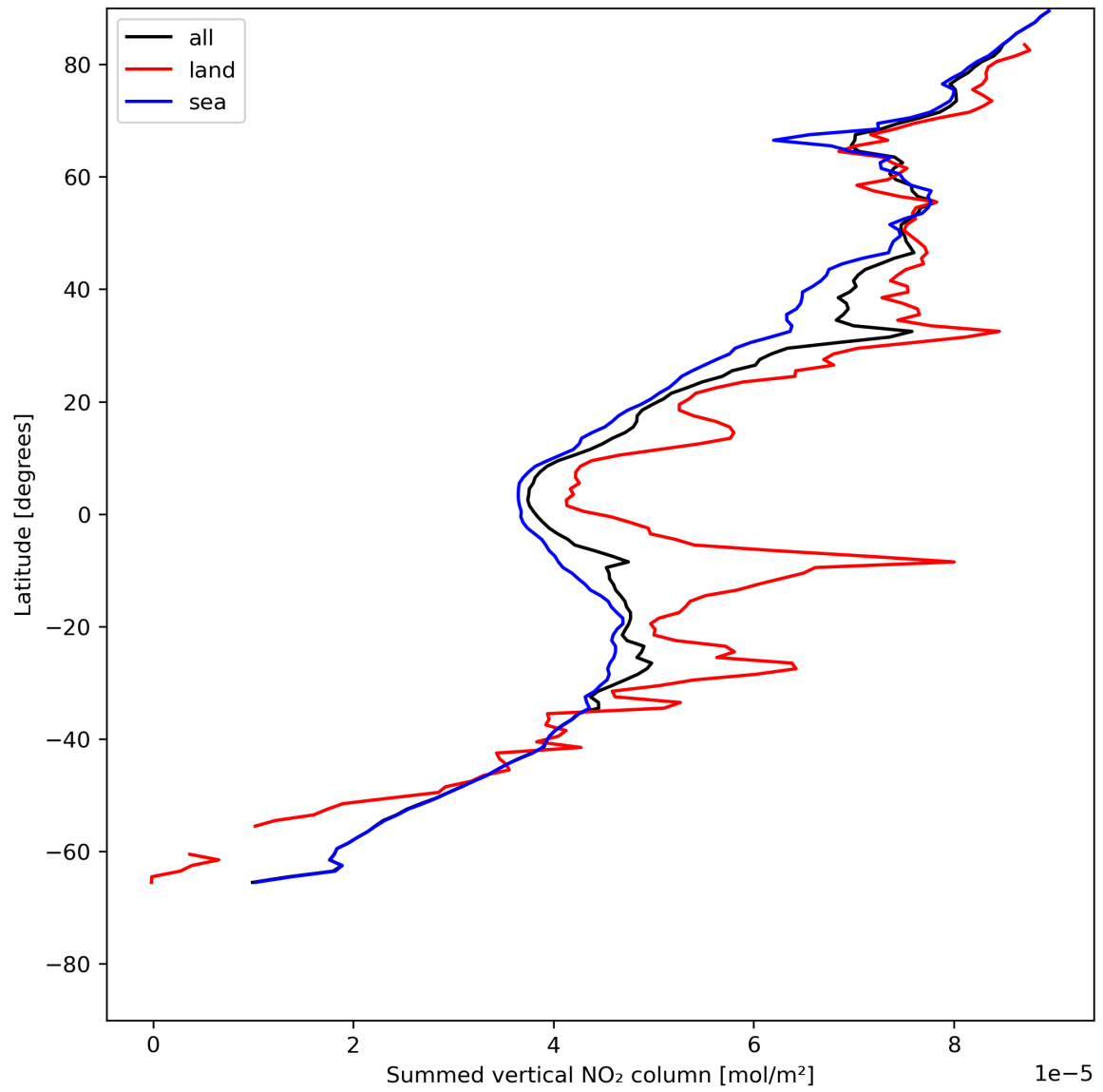
Figure 23: Zonal average of “Summed vertical NO 2 column” for 2024-07-10 to 2024-07-12.
