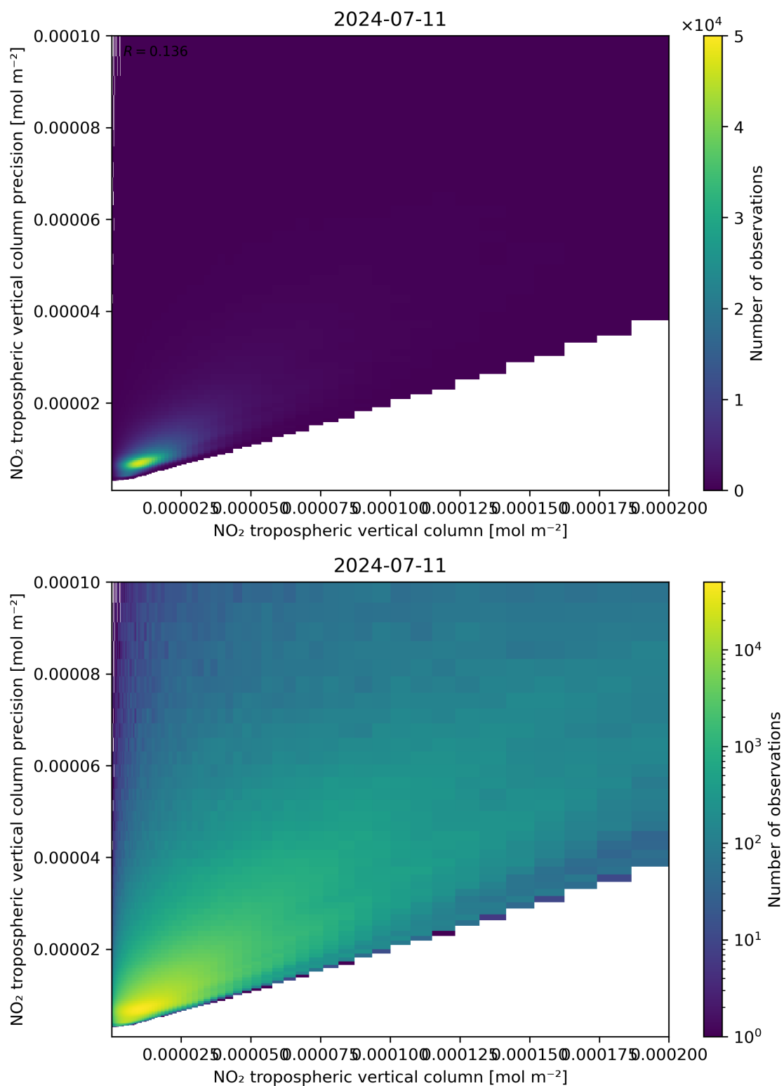
Figure 130: Scatter density plot of “NO 2 tropospheric vertical column” against “NO 2 tropospheric vertical column precision” for 2024-07-10 to 2024-07-12.
