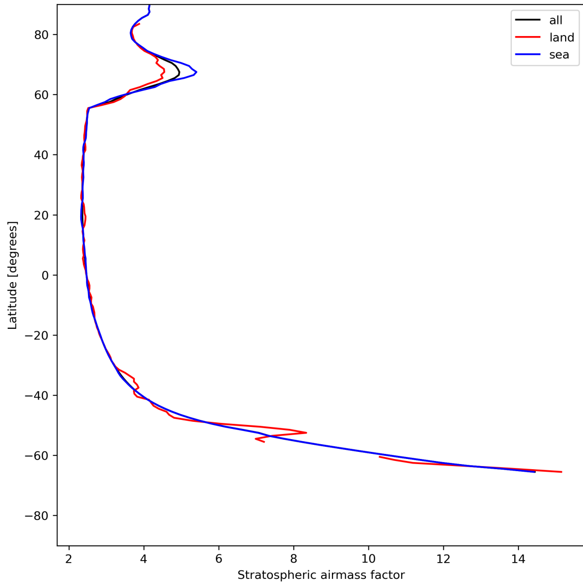
Figure 27: Zonal average of “Stratospheric airmass factor” for 2024-07-10 to 2024-07-12.
