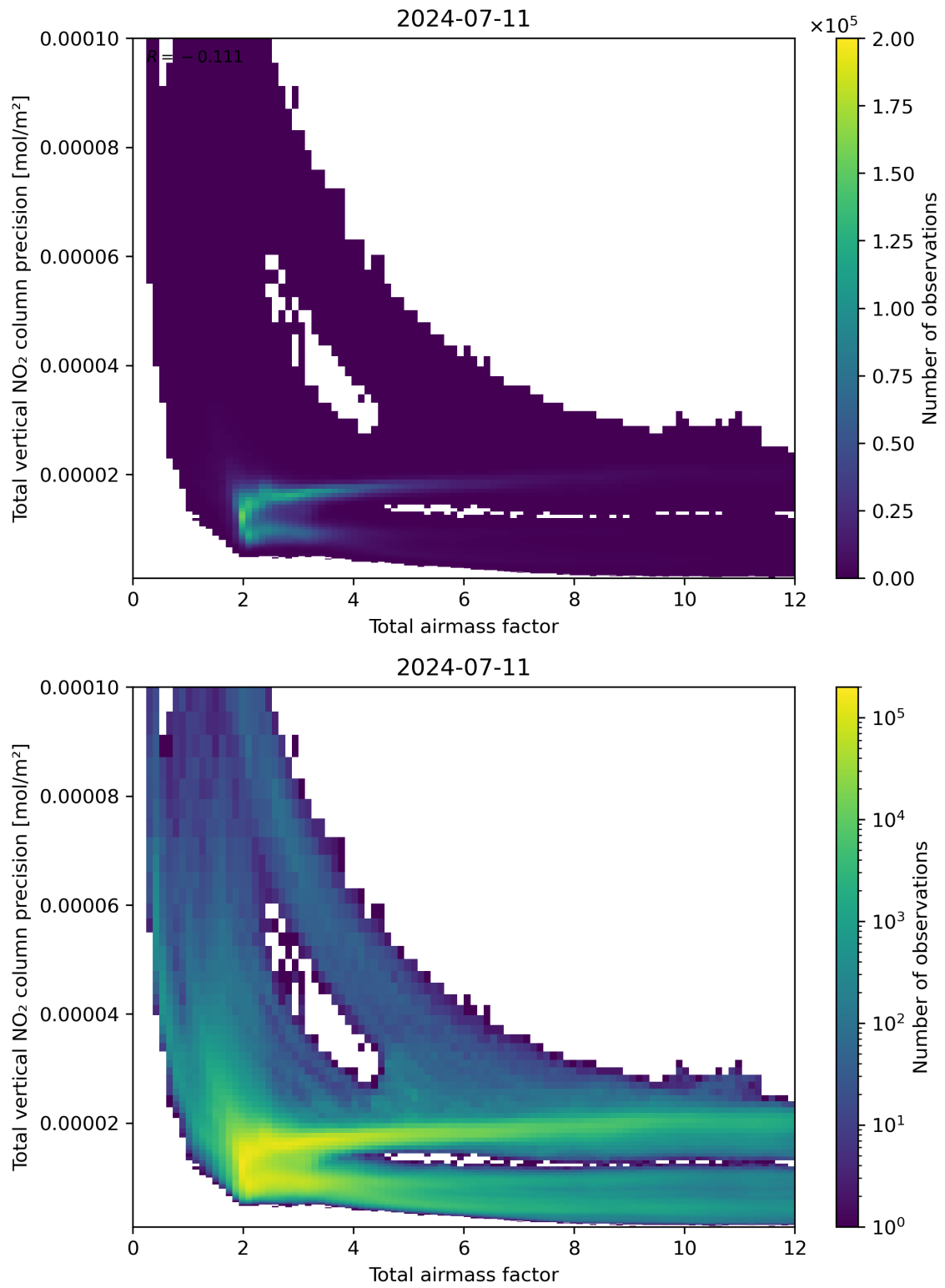
Figure 68: Scatter density plot of “Total airmass factor” against “Total vertical NO 2 column precision” for 2024-07-10 to 2024-07-12.
