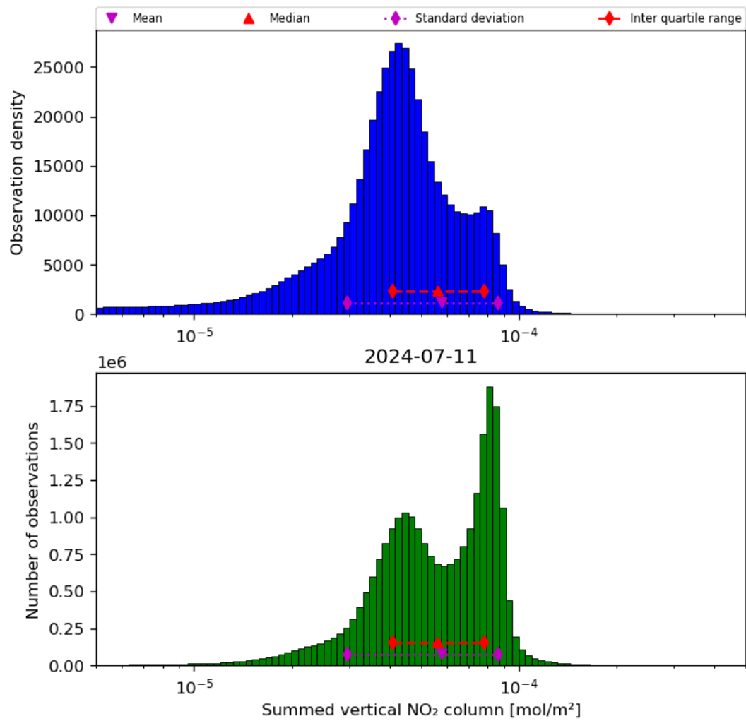
Figure 40: Histogram of “Summed vertical NO 2 column” for 2024-07-10 to 2024-07-12
