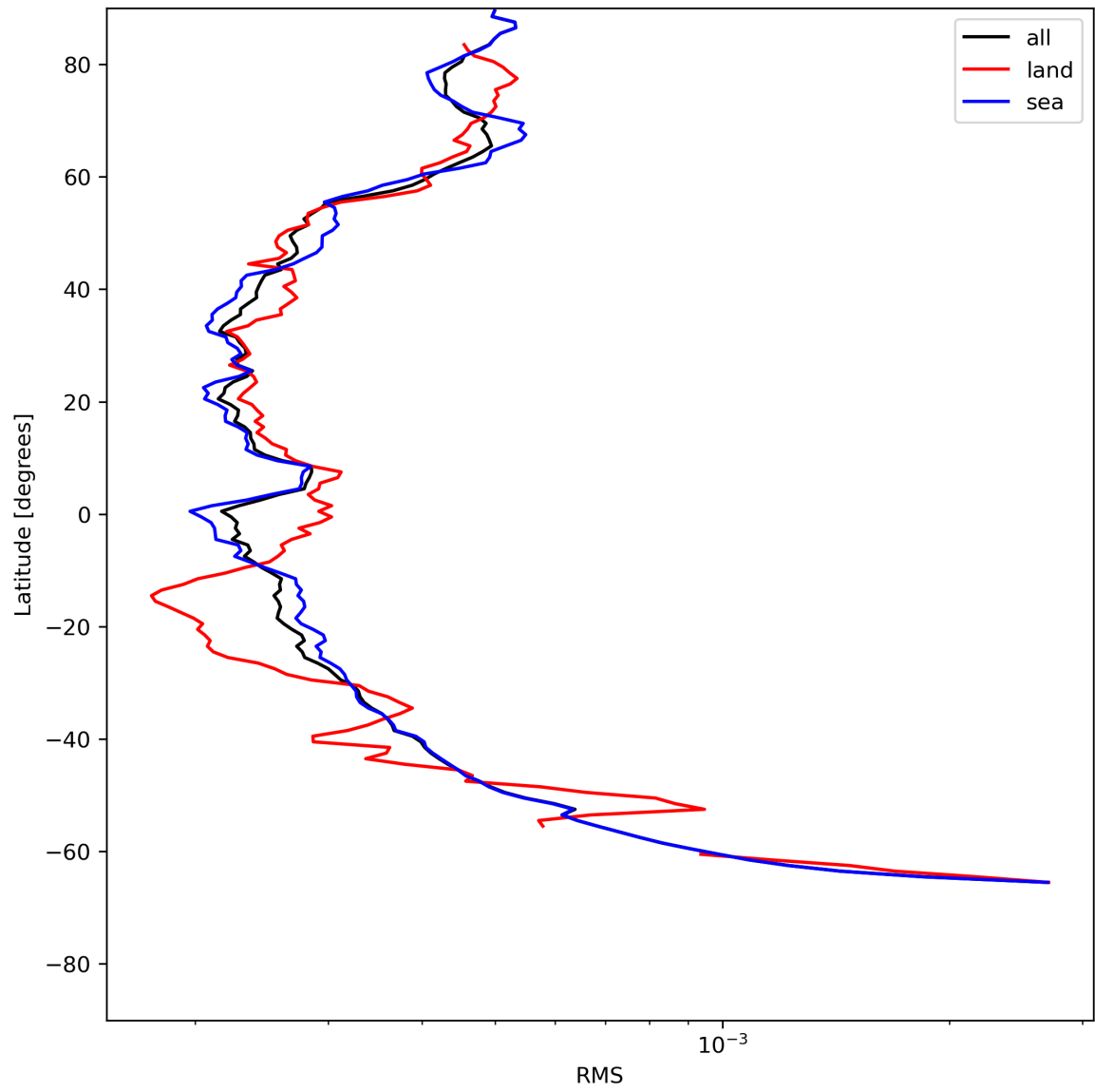
Figure 26: Zonal average of “RMS” for 2024-07-10 to 2024-07-12.
