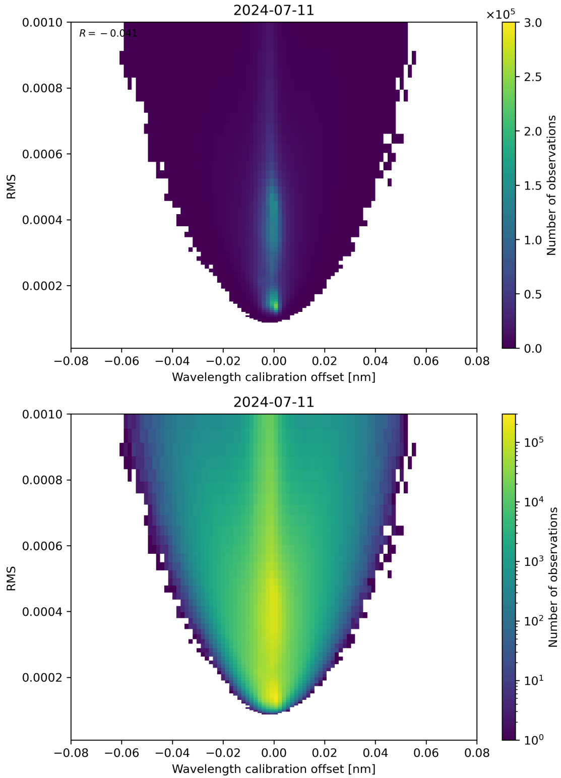
Figure 181: Scatter density plot of “Wavelength calibration offset” against “RMS” for 2024-07-10 to 2024-07-12.
