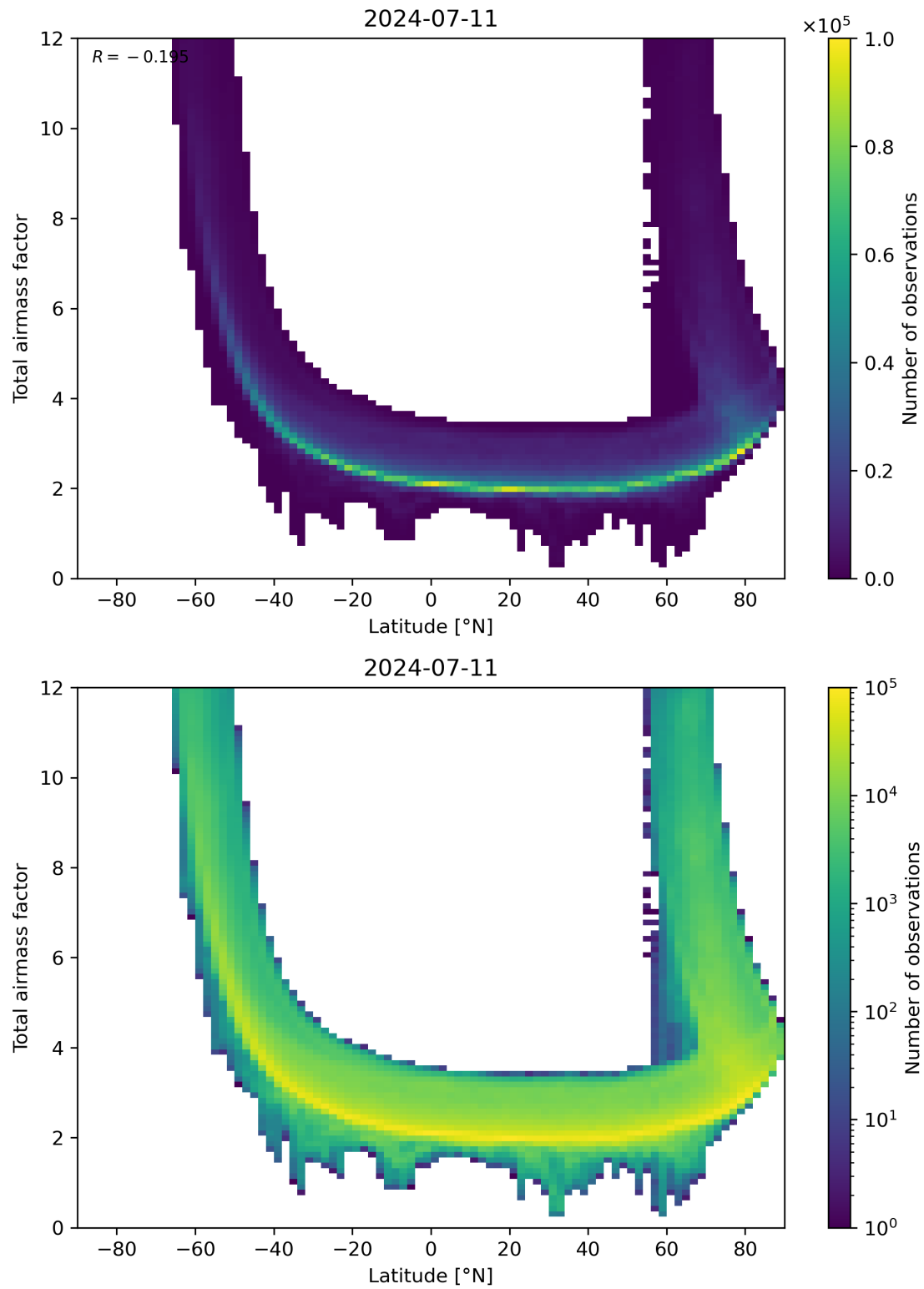
Figure 84: Scatter density plot of “Latitude” against “Total airmass factor” for 2024-07-10 to 2024-07-12.
