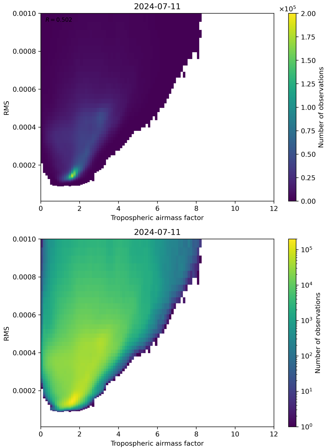
Figure 79: Scatter density plot of “Tropospheric airmass factor” against “RMS” for 2024-07-10 to 2024-07-12.
