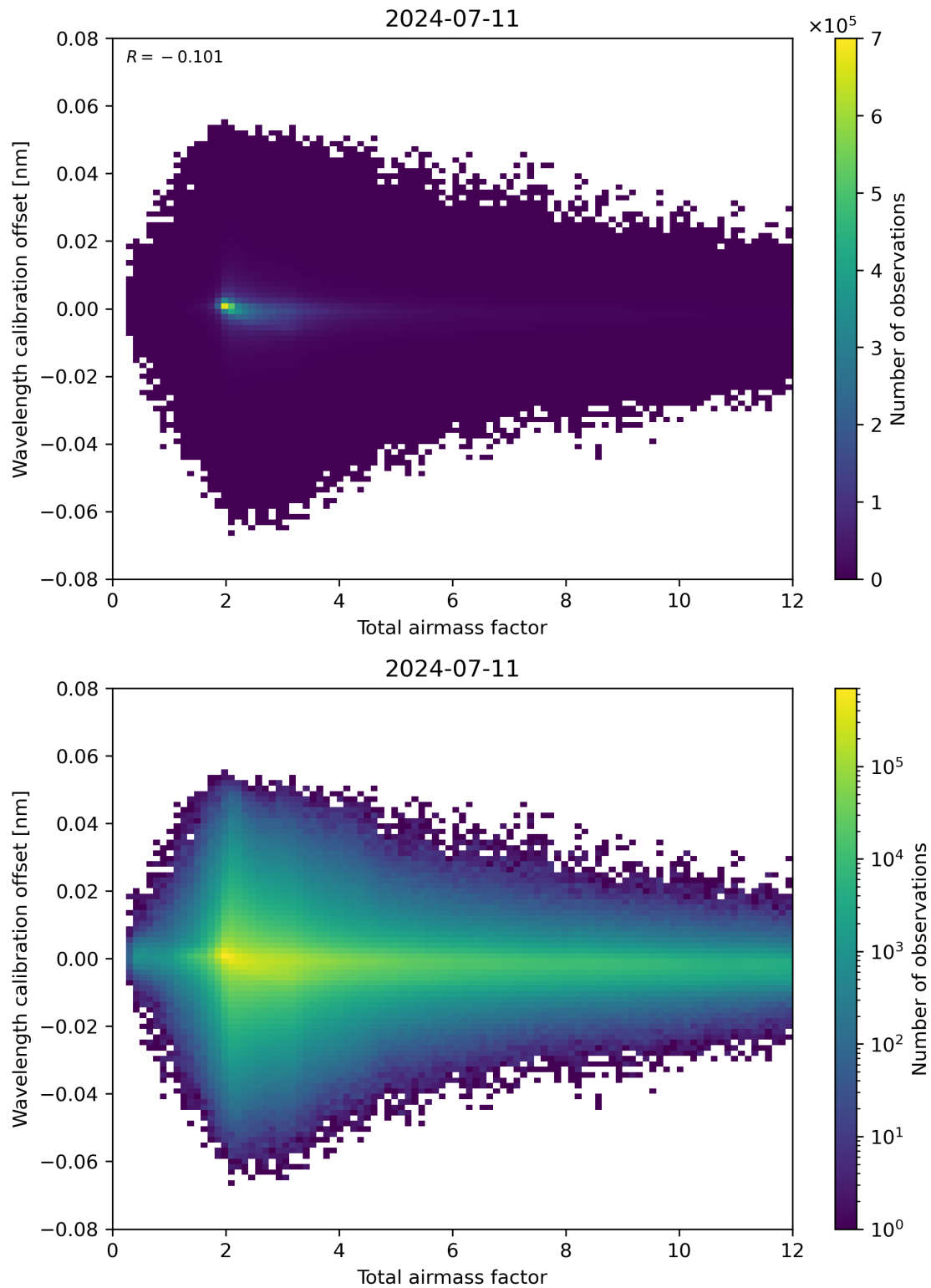
Figure 70: Scatter density plot of “Total airmass factor” against “Wavelength calibration offset” for 2024-07-10 to 2024-07-12.
