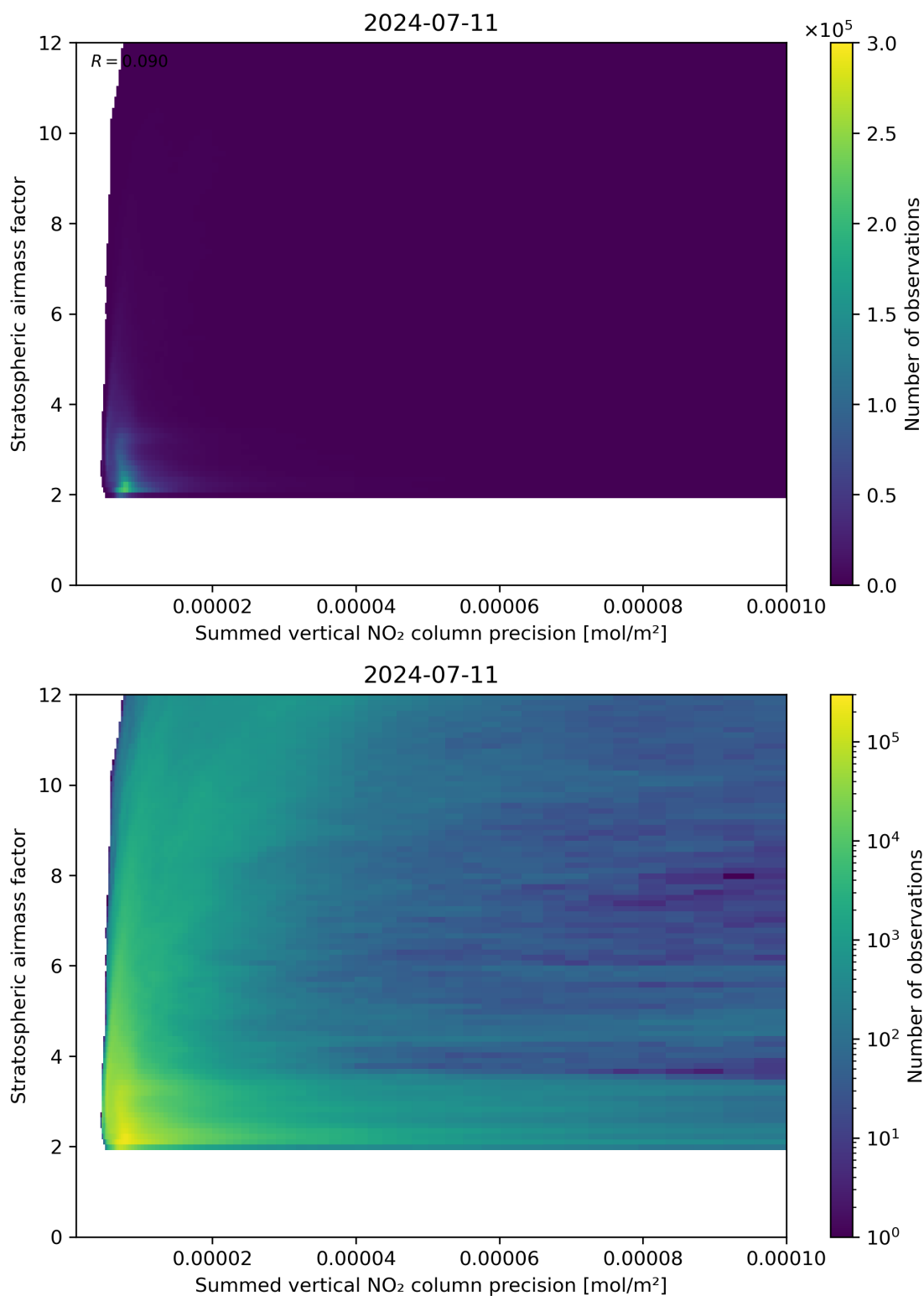
Figure 106: Scatter density plot of “Summed vertical NO 2 column precision” against “Stratospheric airmass factor” for 2024-07-10 to 2024-07-12.
