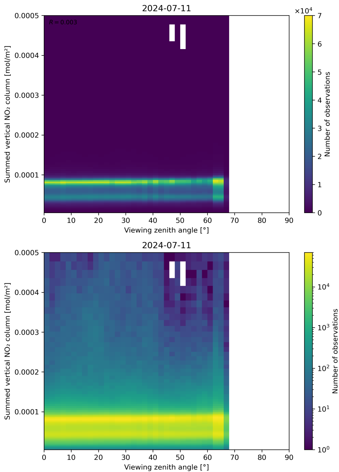
Figure 165: Scatter density plot of “Viewing zenith angle” against “Summed vertical NO 2 column” for 2024-07-10 to 2024-07-12.
