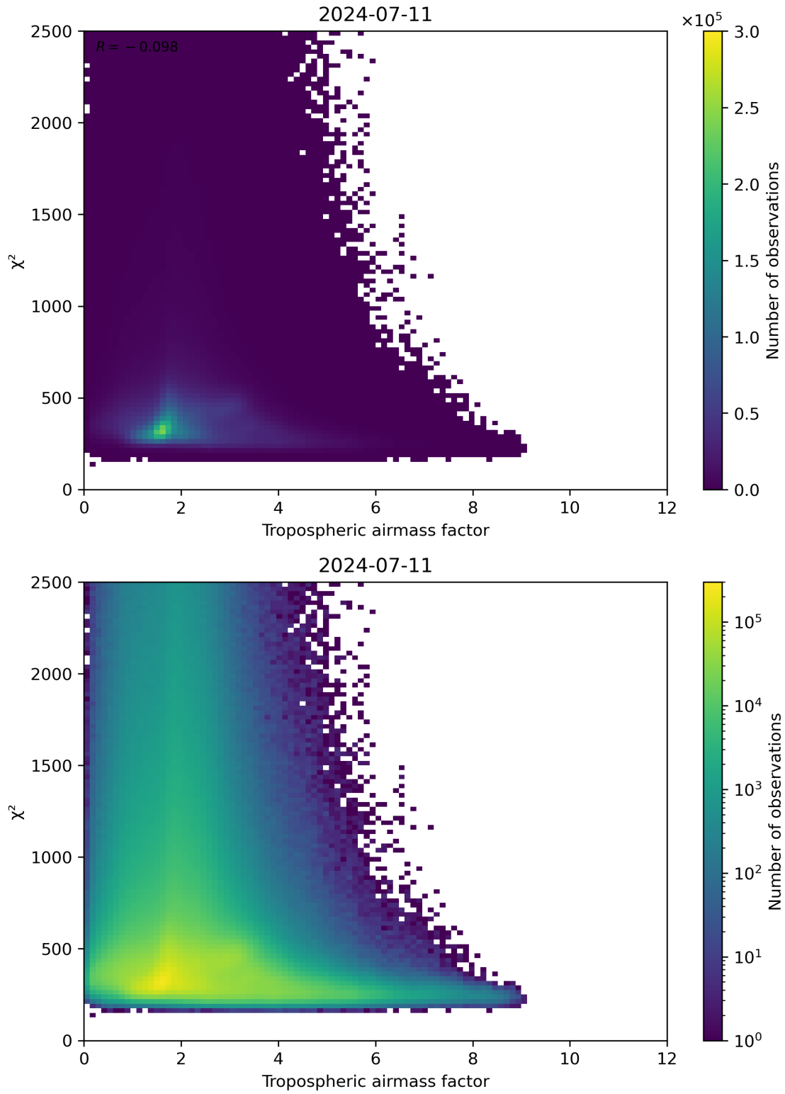
Figure 73: Scatter density plot of “Tropospheric airmass factor” against “ \chi^2 ” for 2024-07-10 to 2024-07-12.
