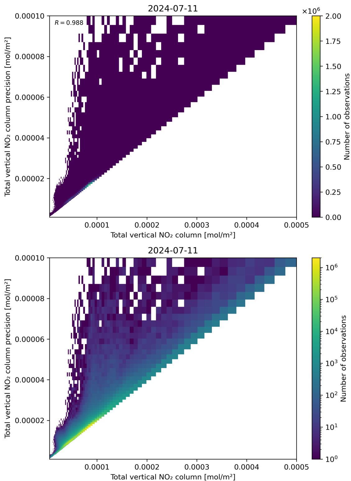
Figure 114: Scatter density plot of “Total vertical NO 2 column” against “Total vertical NO 2 column precision” for 2024-07-10 to 2024-07-12.
