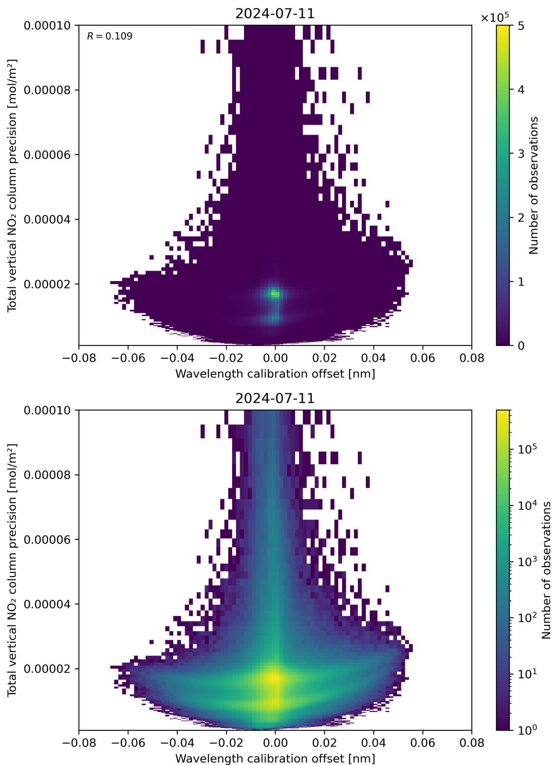
Figure 180: Scatter density plot of “Wavelength calibration offset” against “Total vertical NO 2 column precision” for 2024-07-10 to 2024-07-12.
