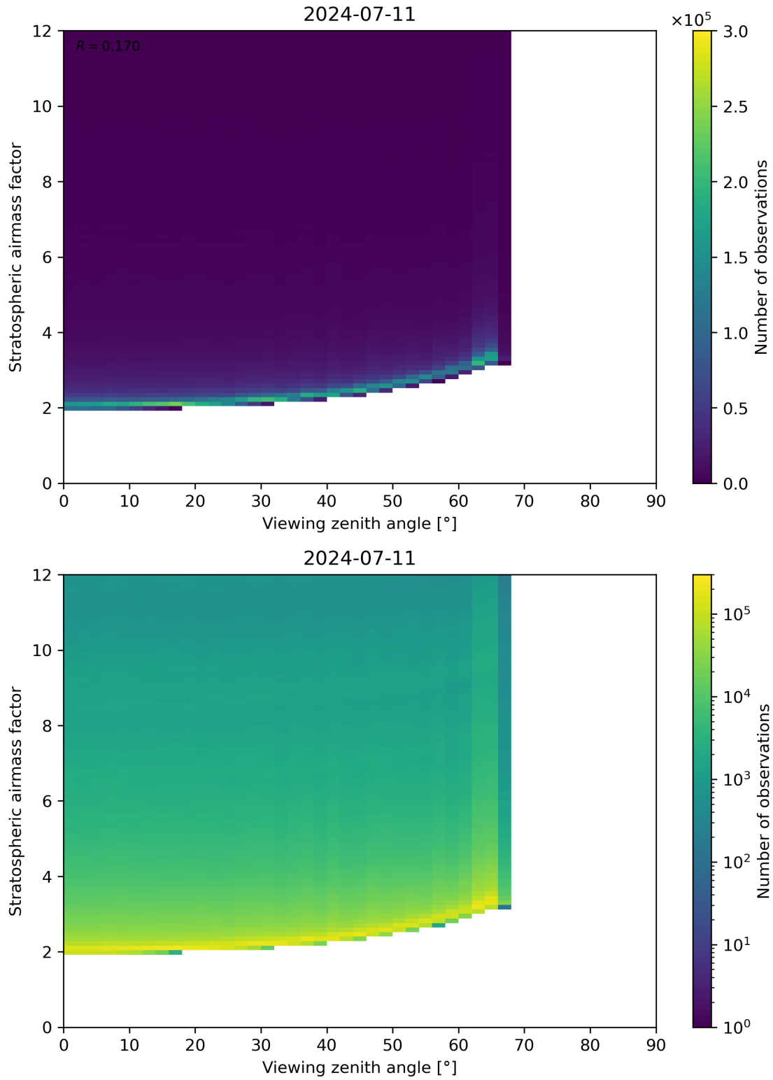
Figure 159: Scatter density plot of “Viewing zenith angle” against “Stratospheric airmass factor” for 2024-07-10 to 2024-07-12.
