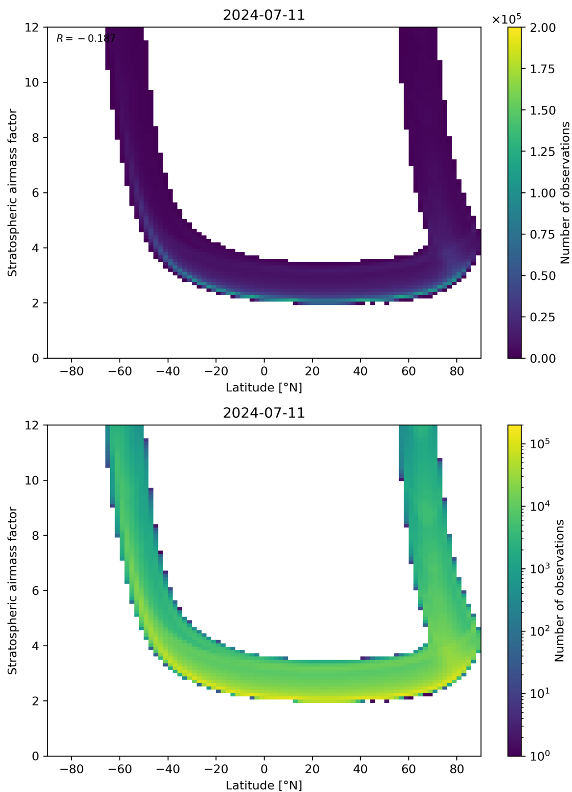
Figure 83: Scatter density plot of “Latitude” against “Stratospheric air mass factor” for 2024-07-10 to 2024-07-12.
