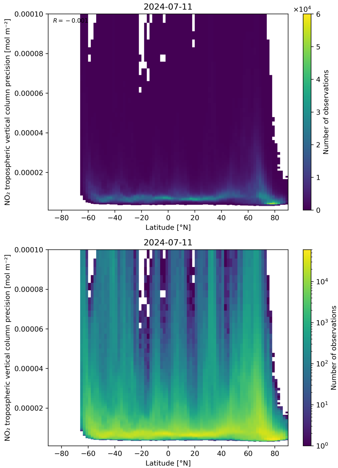
Figure 93: Scatter density plot of “Latitude” against “NO 2 tropospheric vertical column precision” for 2024-07-10 to 2024-07-12.
