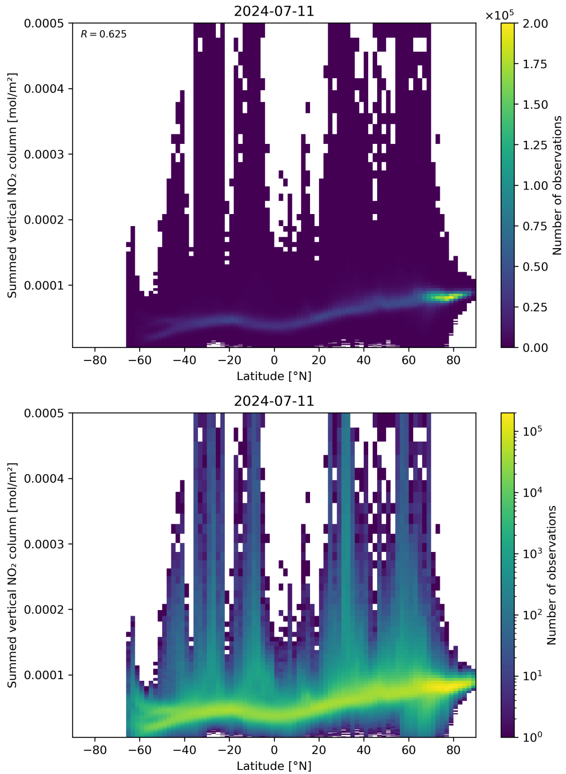
Figure 88: Scatter density plot of “Latitude” against “Summed vertical NO 2 column” for 2024-07-10 to 2024-07-12.
