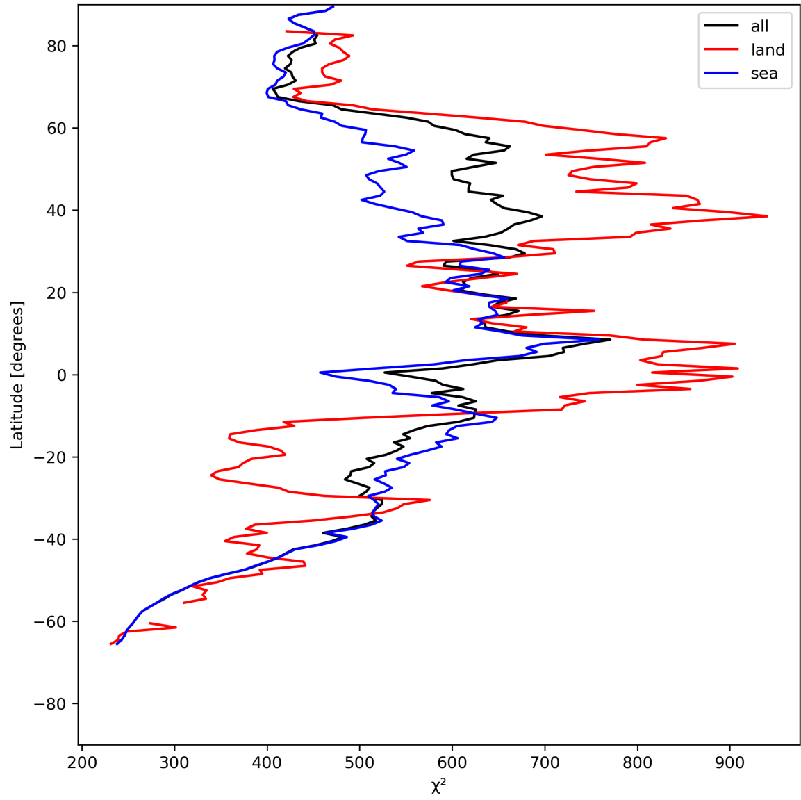
Figure 25: Zonal average of “ \chi^2 ” for 2024-07-10 to 2024-07-12.
