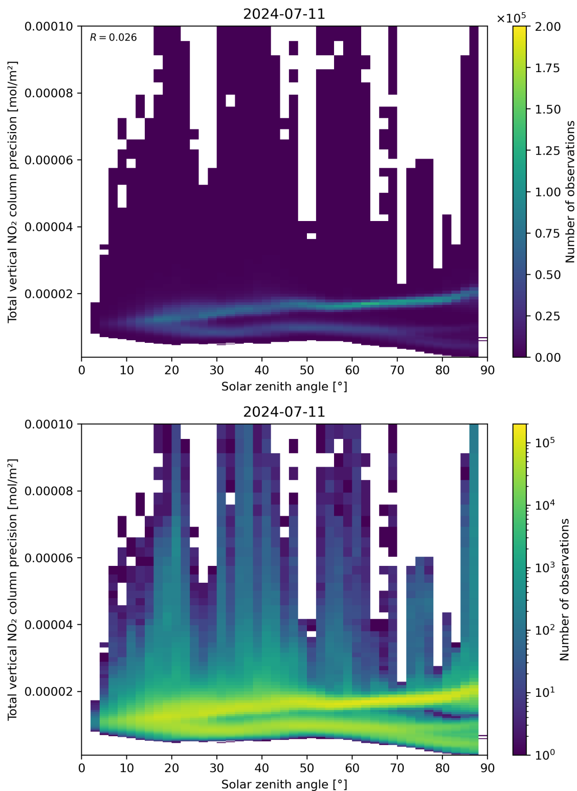
Figure 154: Scatter density plot of “Solar zenith angle” against “Total vertical NO 2 column precision” for 2024-07-10 to 2024-07-12.
