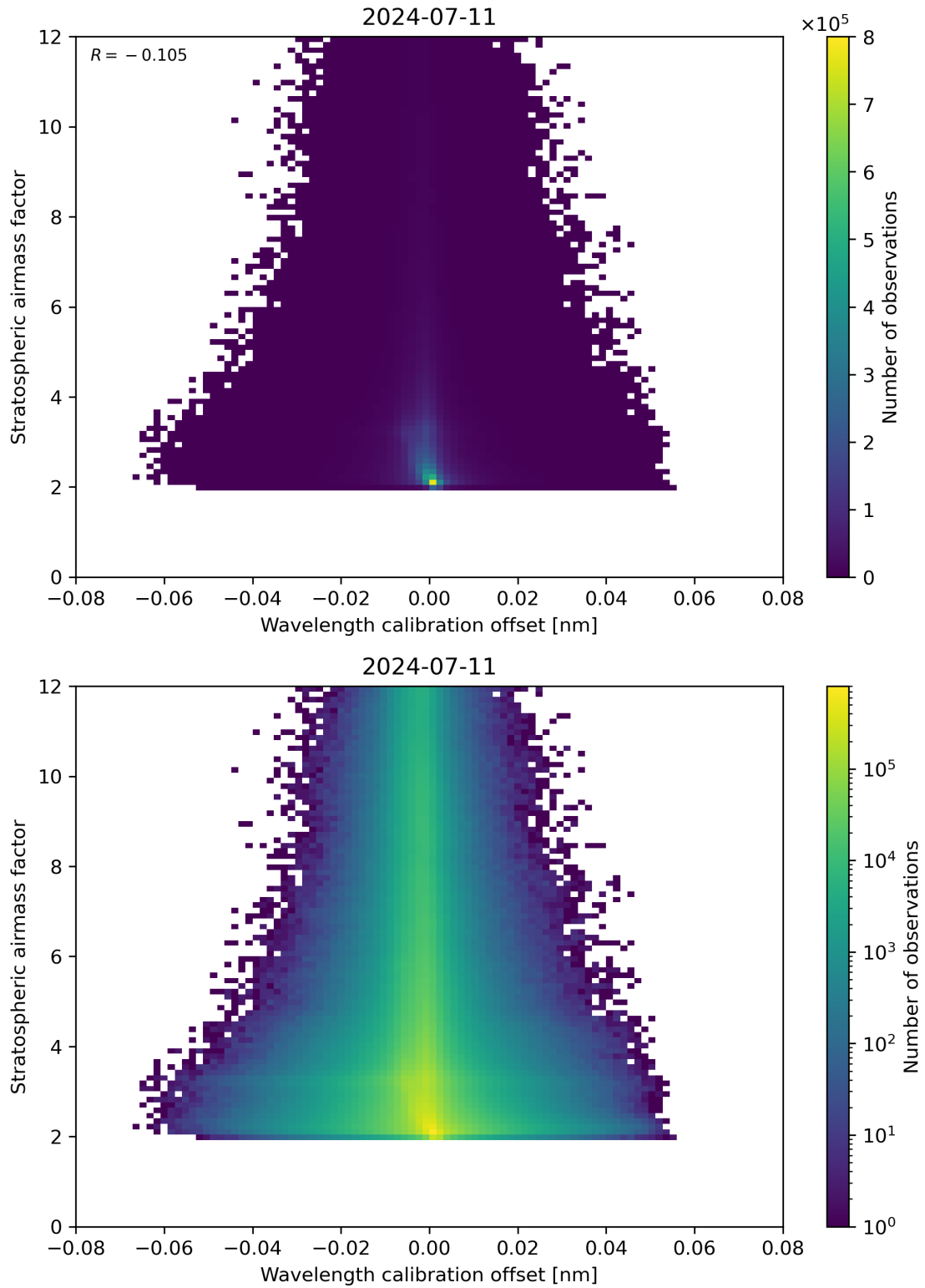
Figure 174: Scatter density plot of “Wavelength calibration offset” against “Stratospheric air mass factor” for 2024-07-10 to 2024-07-12.
