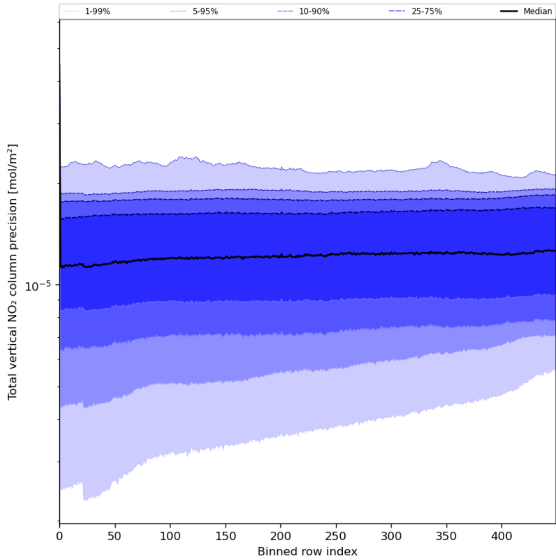
Figure 56: Along track statistics of “Total vertical NO 2 column precision” for 2024-07-10 to 2024-07-12
