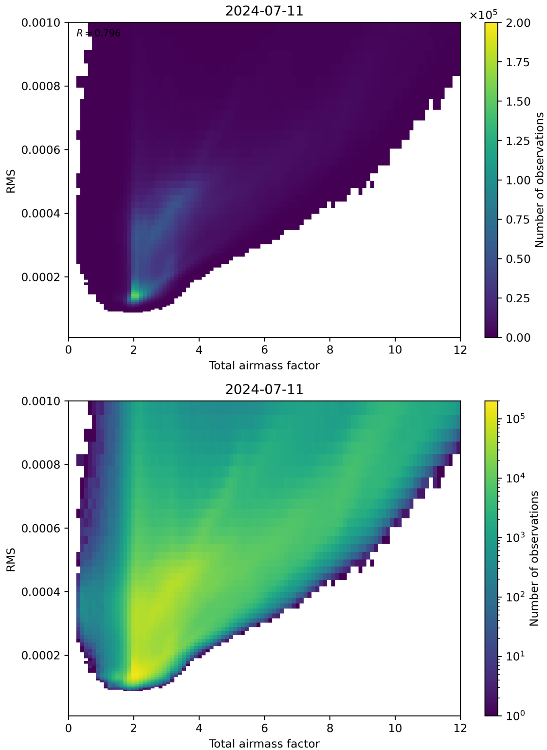
Figure 69: Scatter density plot of “Total airmass factor” against “RMS” for 2024-07-10 to 2024-07-12.
