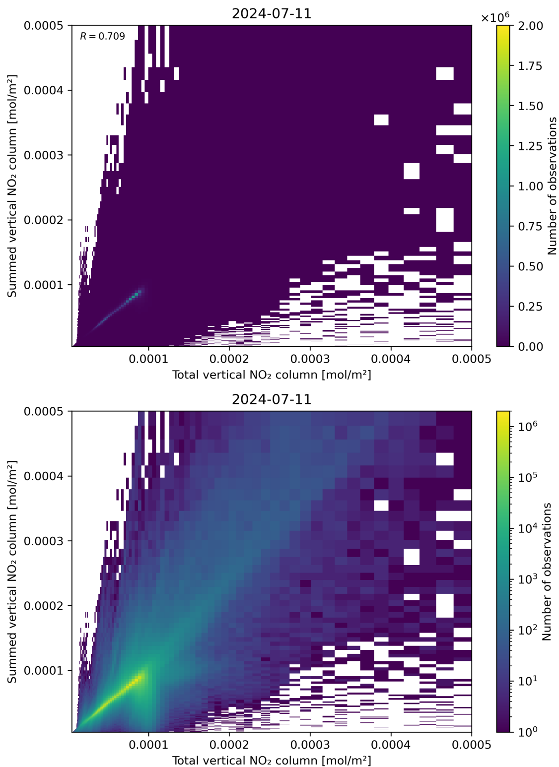
Figure 112: Scatter density plot of “Total vertical NO 2 column” against “Summed vertical NO 2 column” for 2024-07-10 to 2024-07-12.
