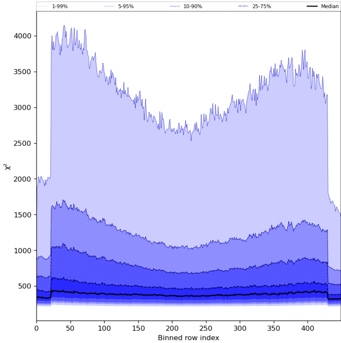
Figure 59: Along track statistics of “ \chi^2 ” for 2024-07-10 to 2024-07-12
