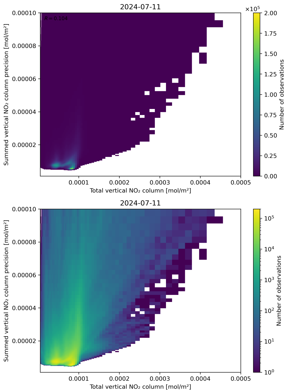
Figure 113: Scatter density plot of “Total vertical NO 2 column” against “Summed vertical NO 2 column precision” for 2024-07-10 to 2024-07-12.
