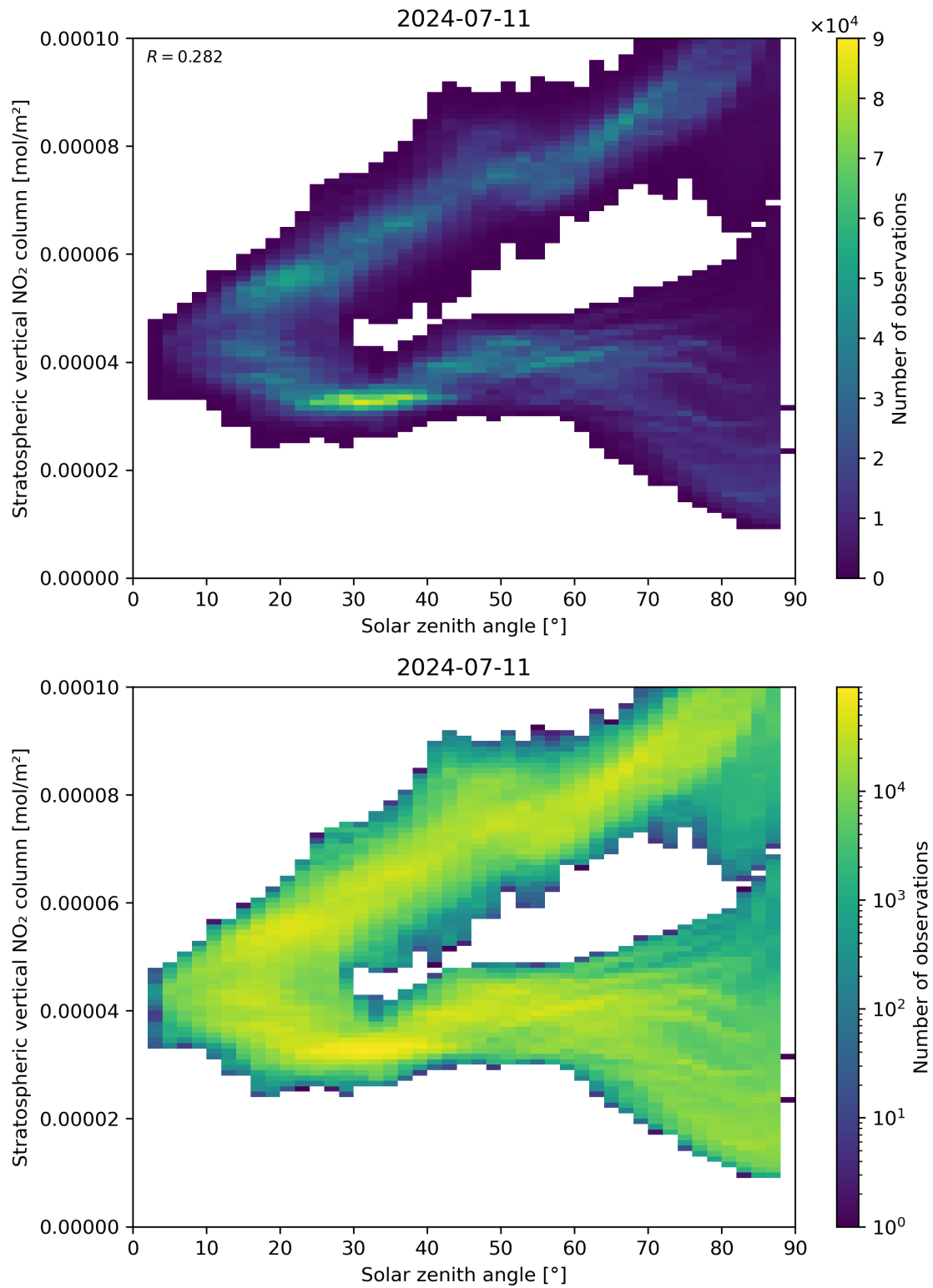
Figure 150: Scatter density plot of “Solar zenith angle” against “Stratospheric vertical NO 2 column” for 2024-07-10 to 2024-07-12.
