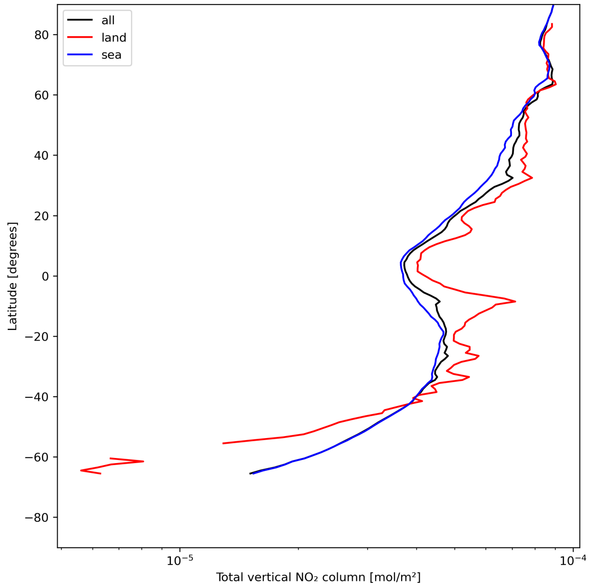
Figure 21: Zonal average of “Total vertical NO 2 column” for 2024-07-10 to 2024-07-12.
