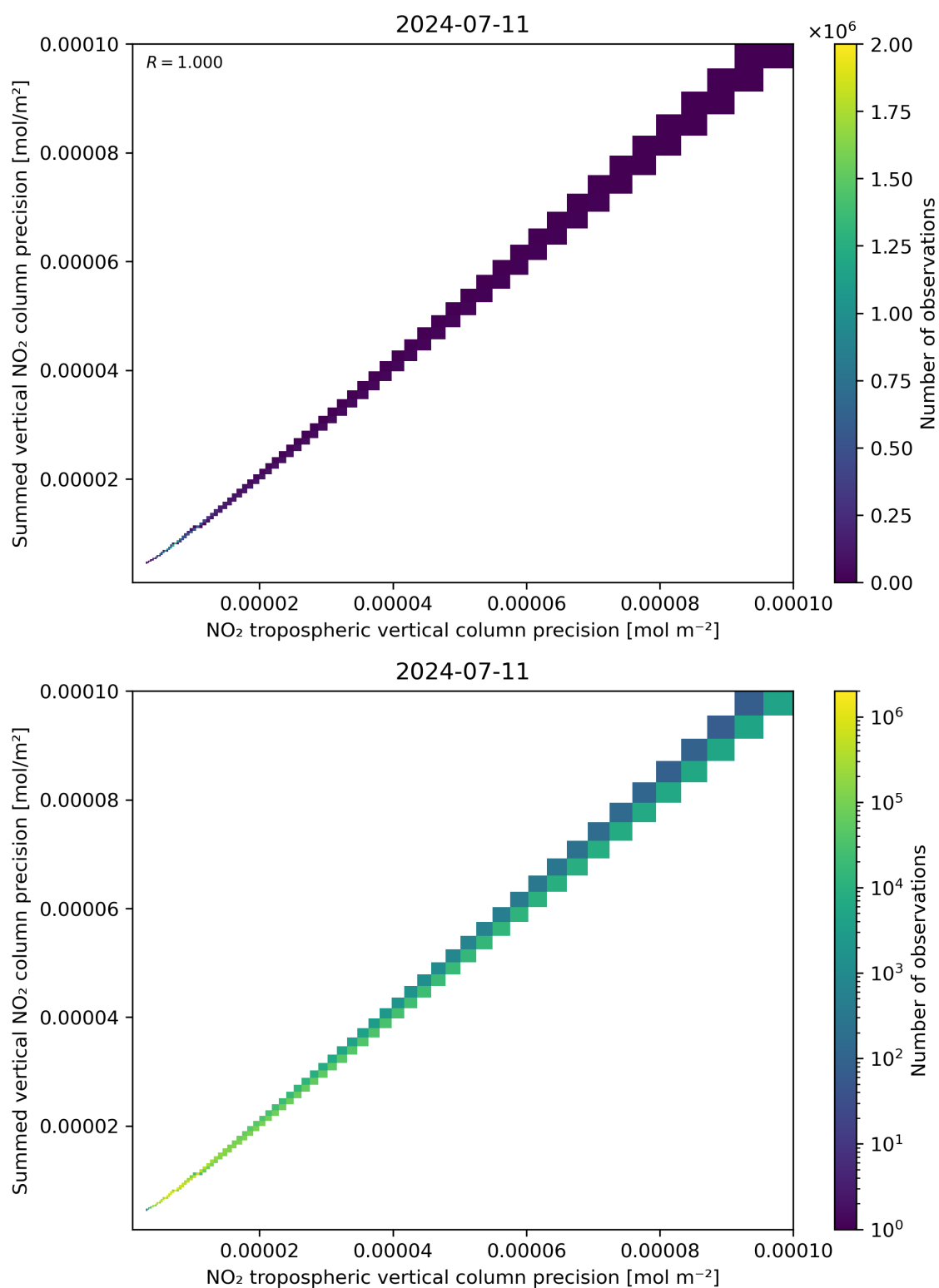
Figure 137: Scatter density plot of “NO 2 tropospheric vertical column precision” against “Summed vertical NO 2 column precision” for 2024-07-10 to 2024-07-12.
