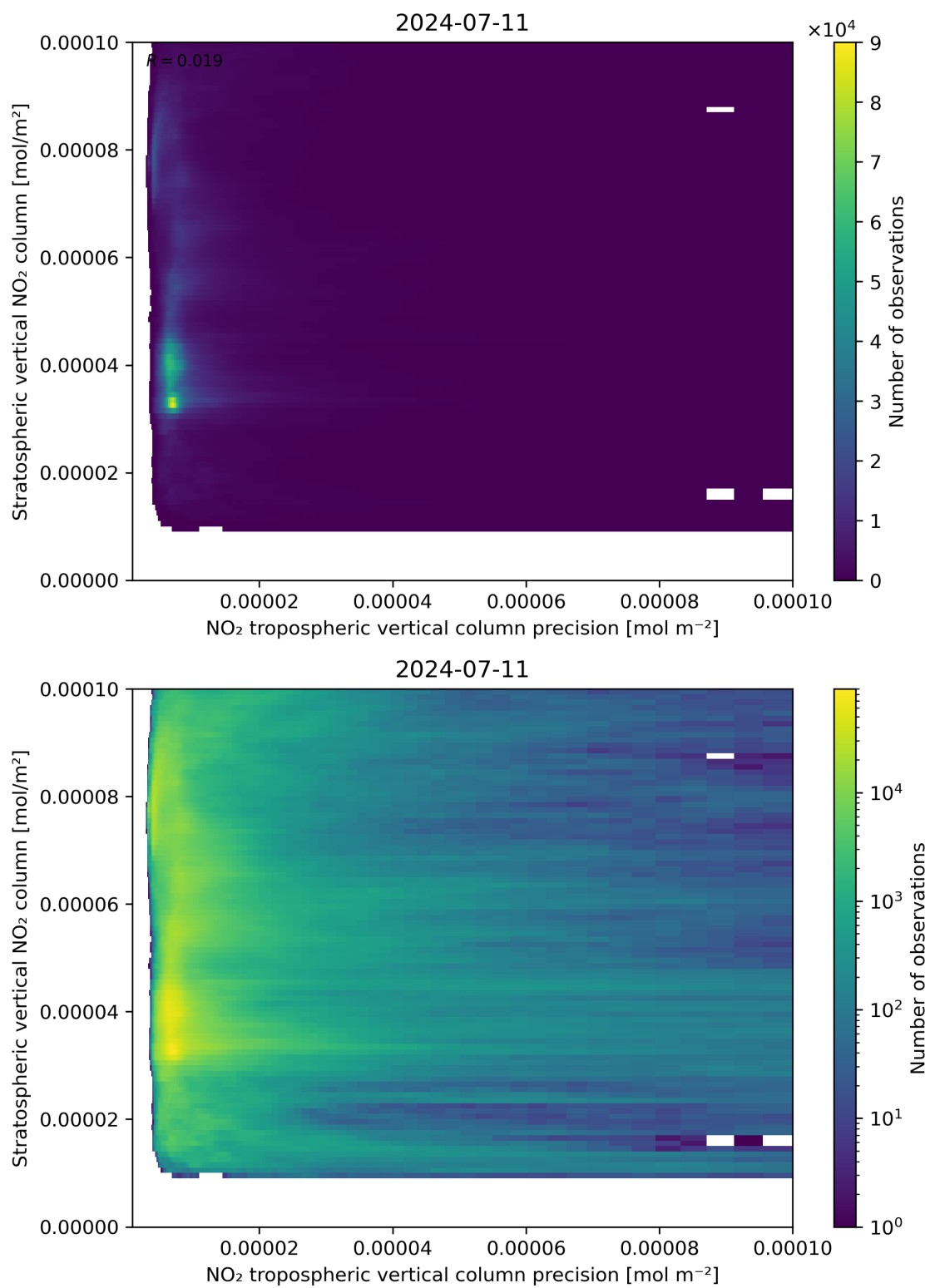
Figure 135: Scatter density plot of “NO 2 tropospheric vertical column precision” against “Stratospheric vertical NO 2 column” for 2024-07-10 to 2024-07-12.
