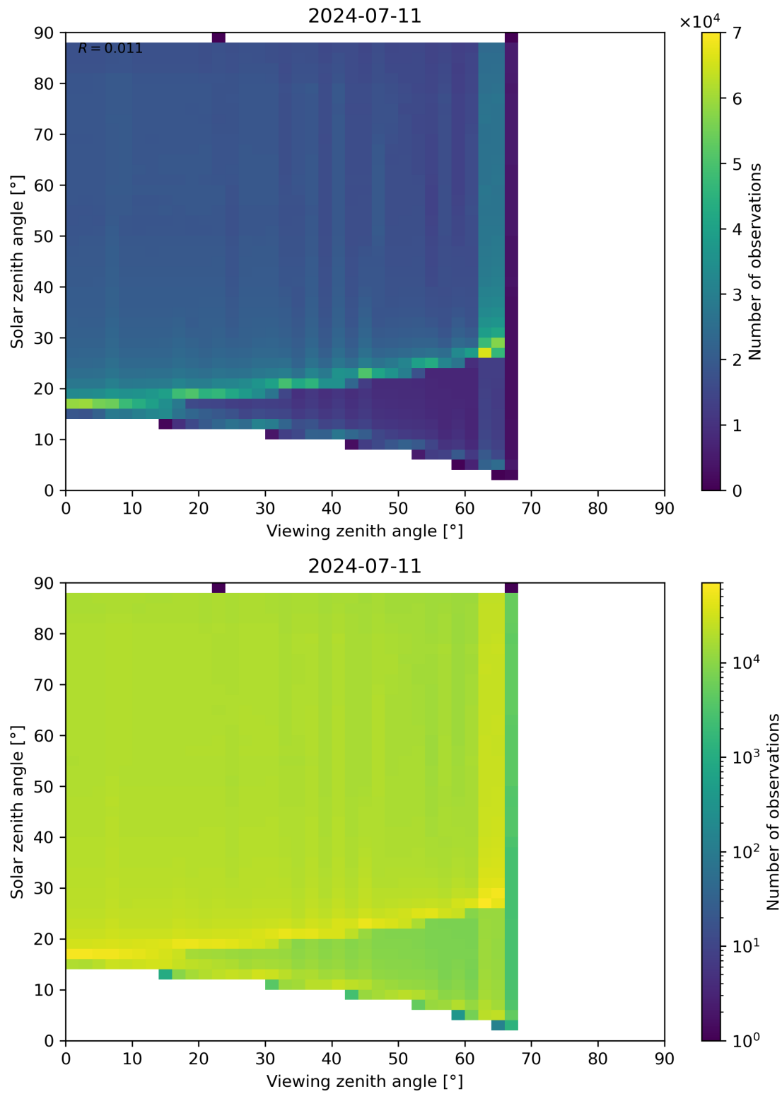
Figure 172: Scatter density plot of “Viewing zenith angle” against “Solar zenith angle” for 2024-07-10 to 2024-07-12.
