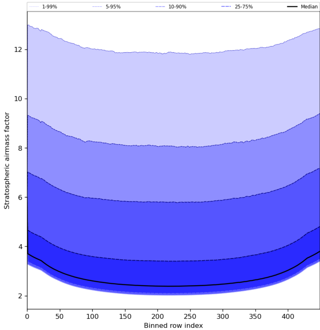
Figure 61: Along track statistics of “Stratospheric airmass factor” for 2024-07-10 to 2024-07-12
