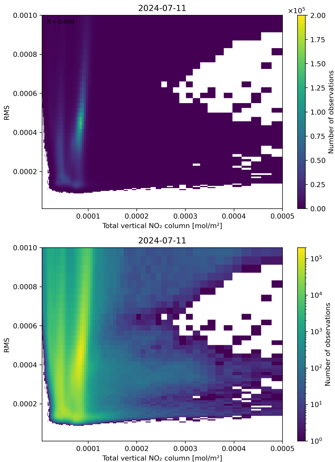
Figure 120: Scatter density plot of “Total vertical NO 2 column” against “RMS” for 2024-07-10 to 2024-07-12.
