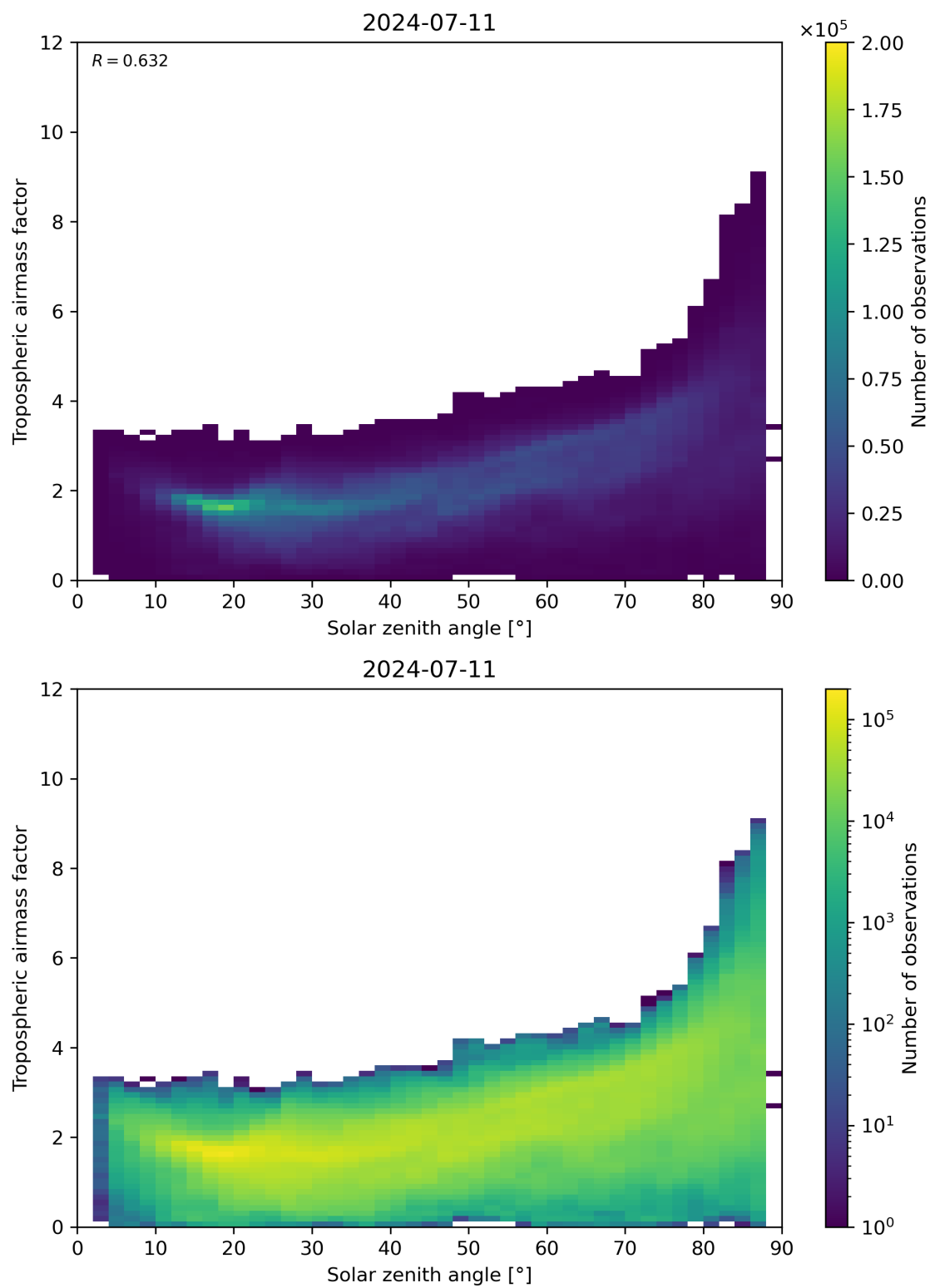
Figure 147: Scatter density plot of “Solar zenith angle” against “Tropospheric airmass factor” for 2024-07-10 to 2024-07-12.
