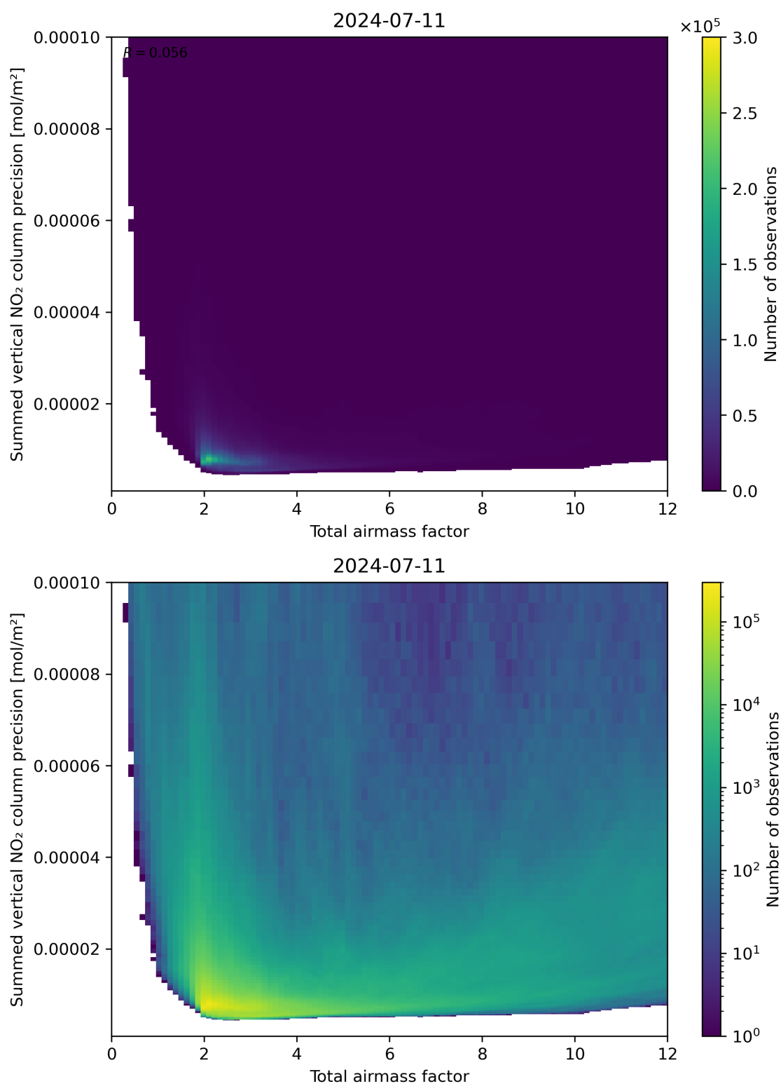
Figure 66: Scatter density plot of “Total airmass factor” against “Summed vertical NO 2 column precision” for 2024-07-10 to 2024-07-12.
