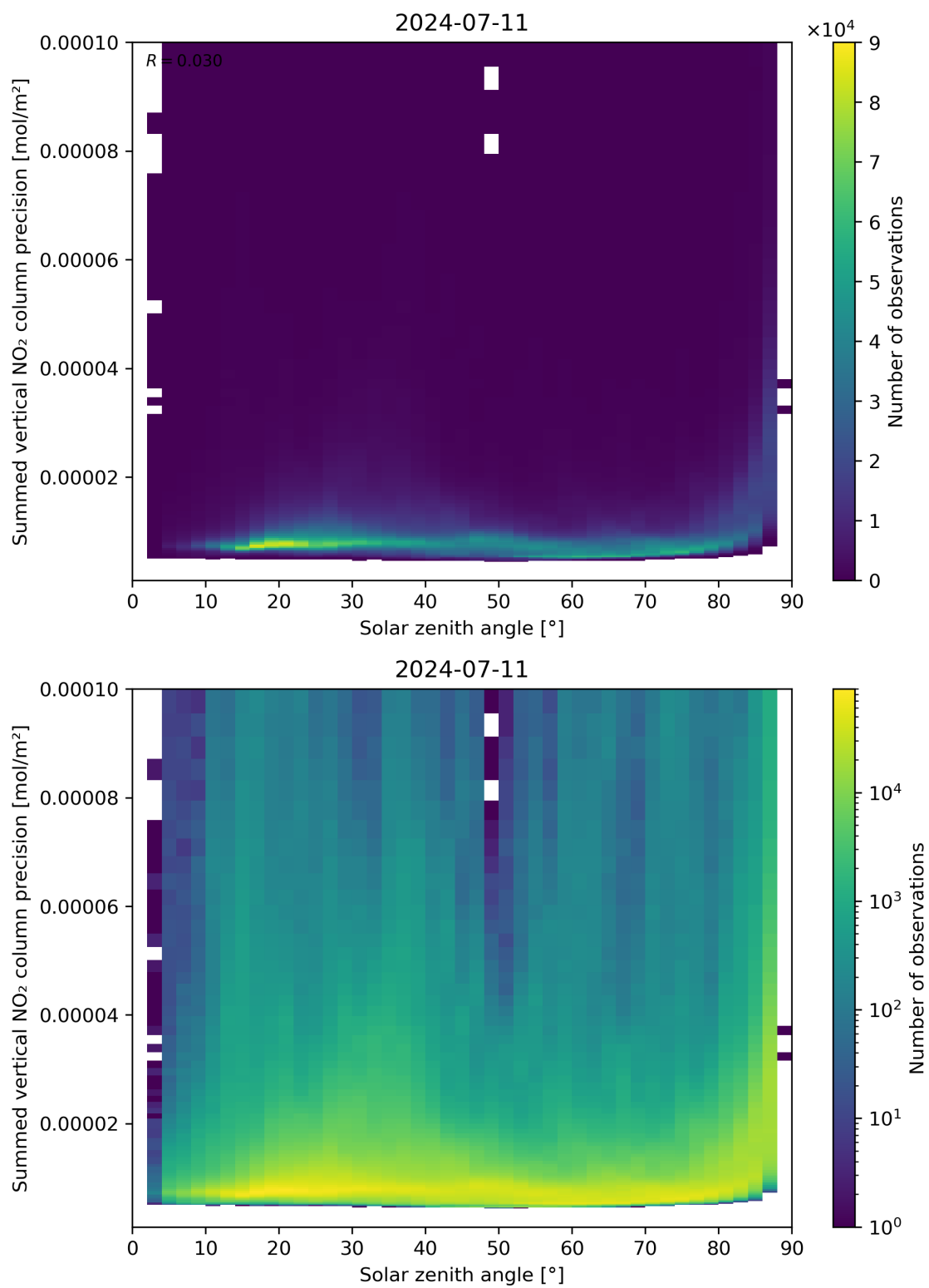
Figure 152: Scatter density plot of “Solar zenith angle” against “Summed vertical NO 2 column precision” for 2024-07-10 to 2024-07-12.
