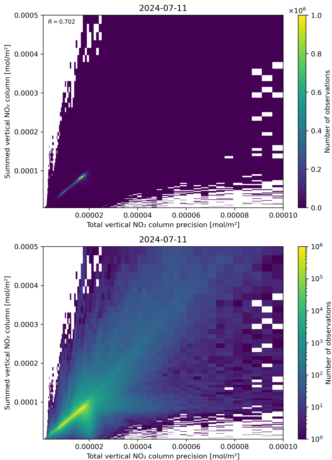
Figure 117: Scatter density plot of “Total vertical NO 2 column precision” against “Summed vertical NO 2 column” for 2024-07-10 to 2024-07-12.
