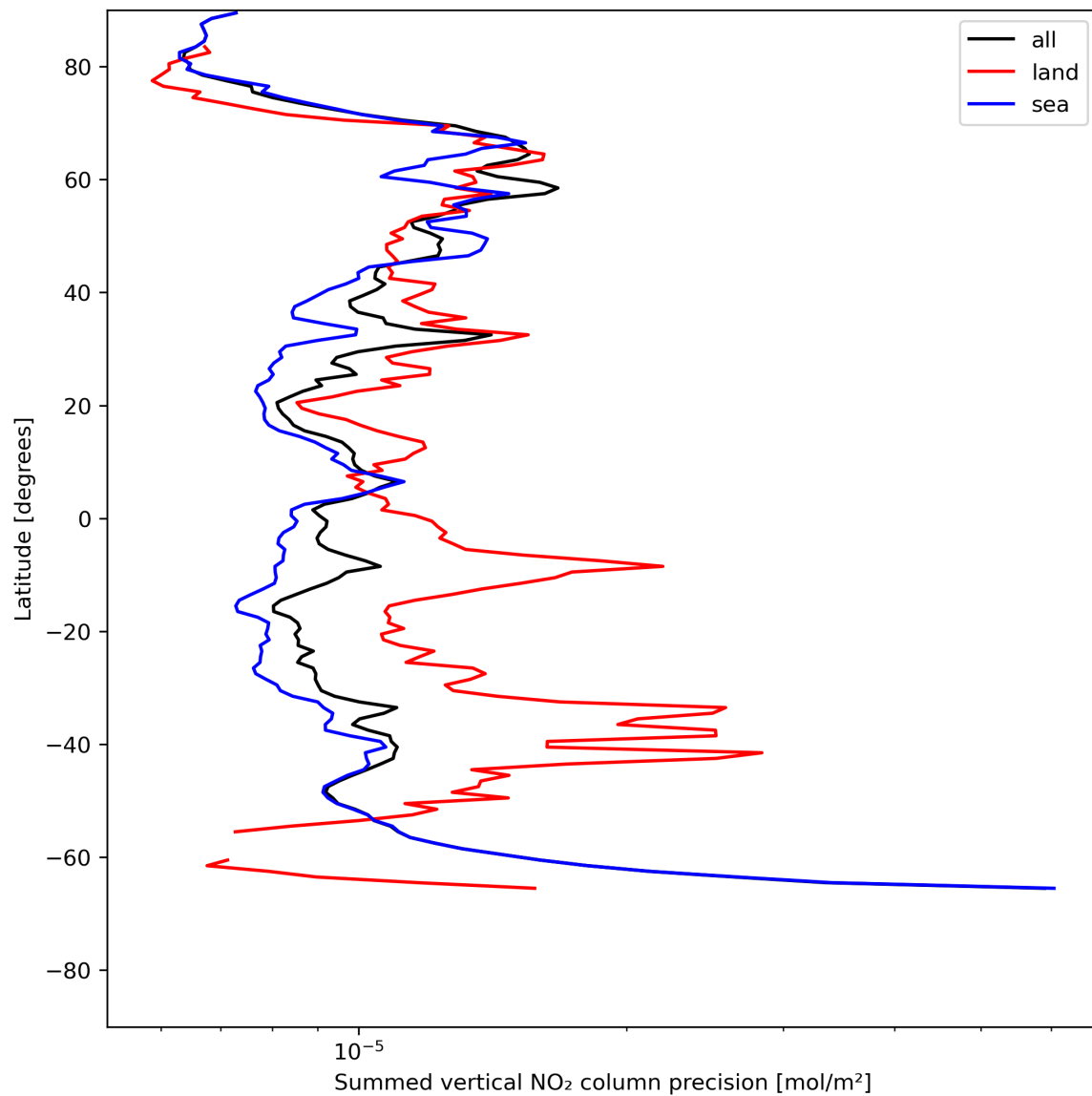
Figure 24: Zonal average of “Summed vertical NO 2 column precision” for 2024-07-10 to 2024-07-12.
