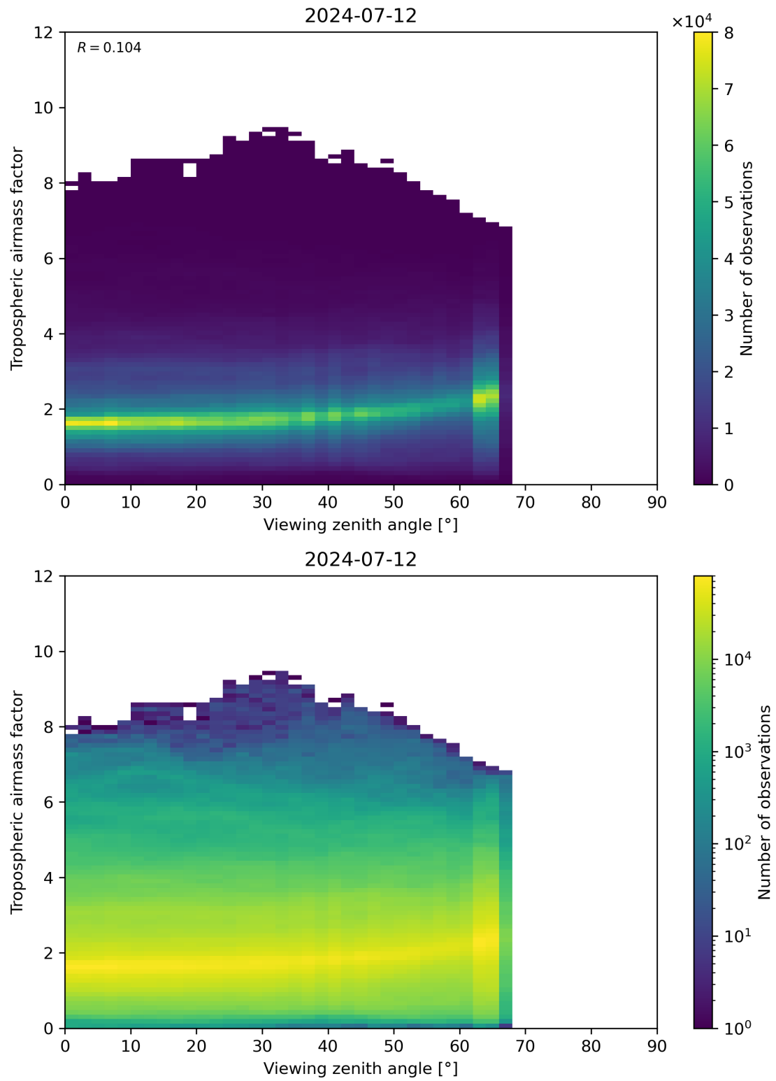
Figure 161: Scatter density plot of “Viewing zenith angle” against “Tropospheric airmass factor” for 2024-07-11 to 2024-07-13.
