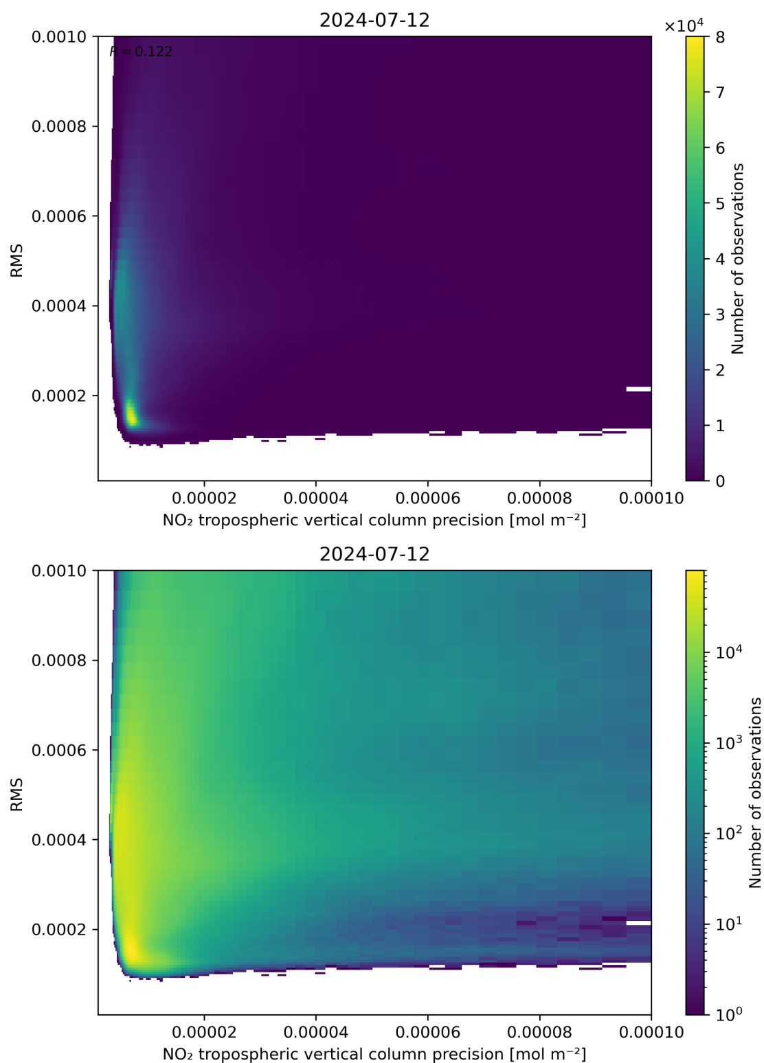
Figure 140: Scatter density plot of “NO 2 tropospheric vertical column precision” against “RMS” for 2024-07-11 to 2024-07-13.
