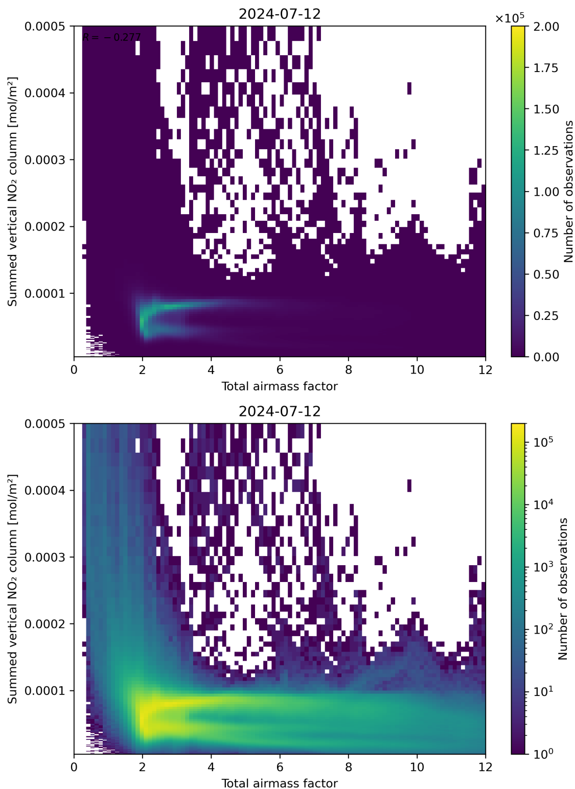
Figure 65: Scatter density plot of “Total airmass factor” against “Summed vertical NO 2 column” for 2024-07-11 to 2024-07-13.
