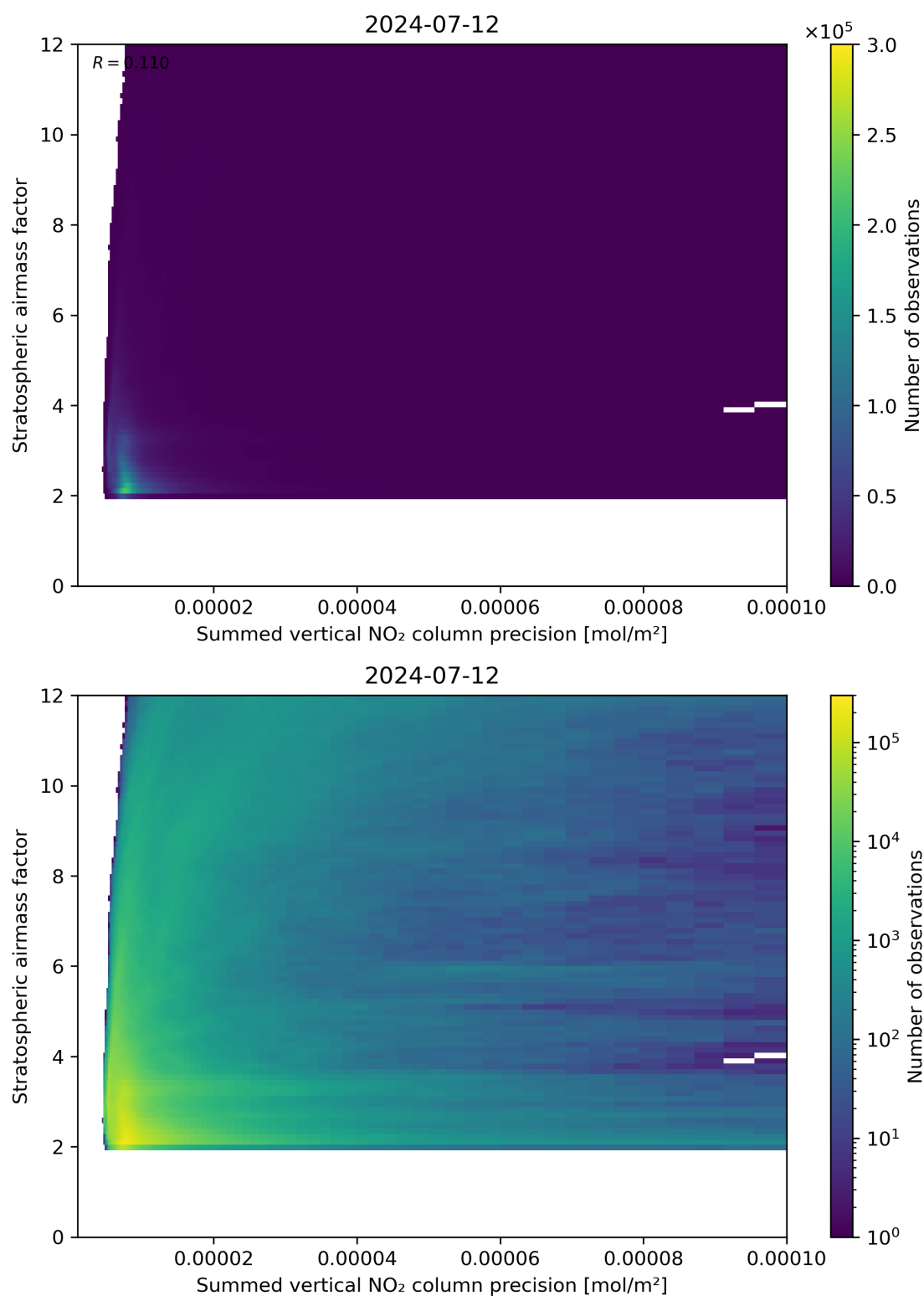
Figure 106: Scatter density plot of “Summed vertical NO 2 column precision” against “Stratospheric airmass factor” for 2024-07-11 to 2024-07-13.
