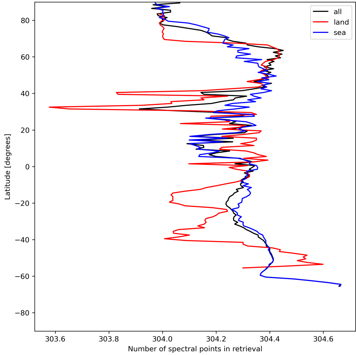
Figure 16: Zonal average of “Number of spectral points in retrieval” for 2024-07-11 to 2024-07-13.
