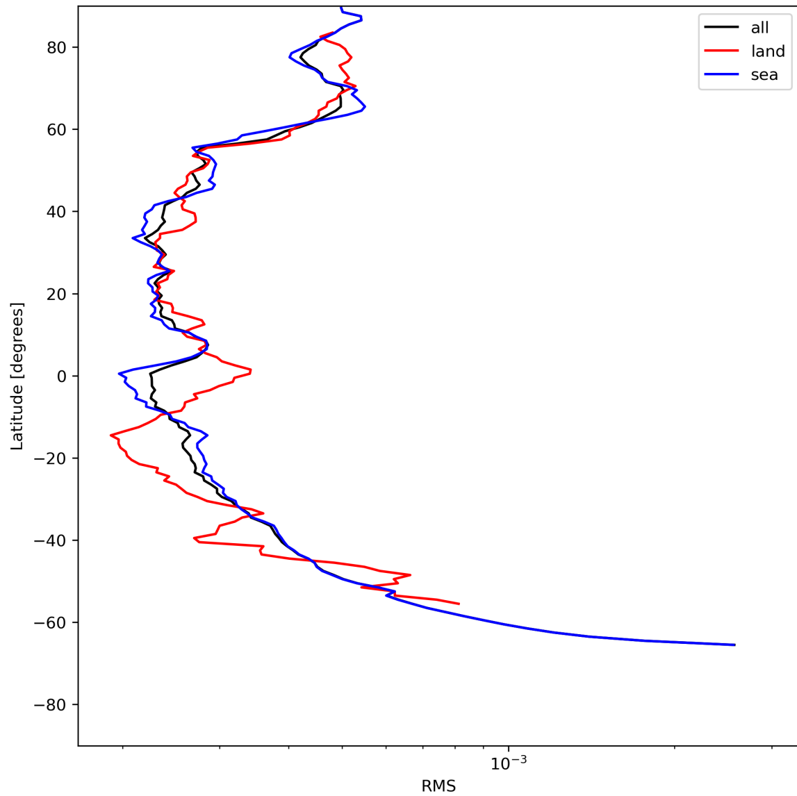
Figure 26: Zonal average of “RMS” for 2024-07-11 to 2024-07-13.
