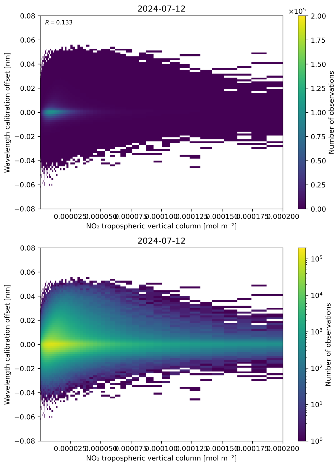
Figure 143: Scatter density plot of “NO 2 tropospheric vertical column” against “Wavelength calibration offset” for 2024-07-11 to 2024-07-13.
