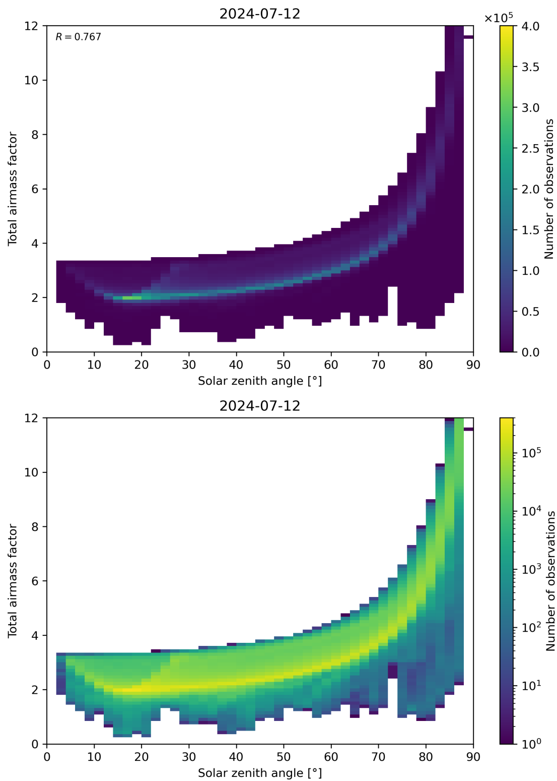
Figure 146: Scatter density plot of “Solar zenith angle” against “Total air mass factor” for 2024-07-11 to 2024-07-13.
