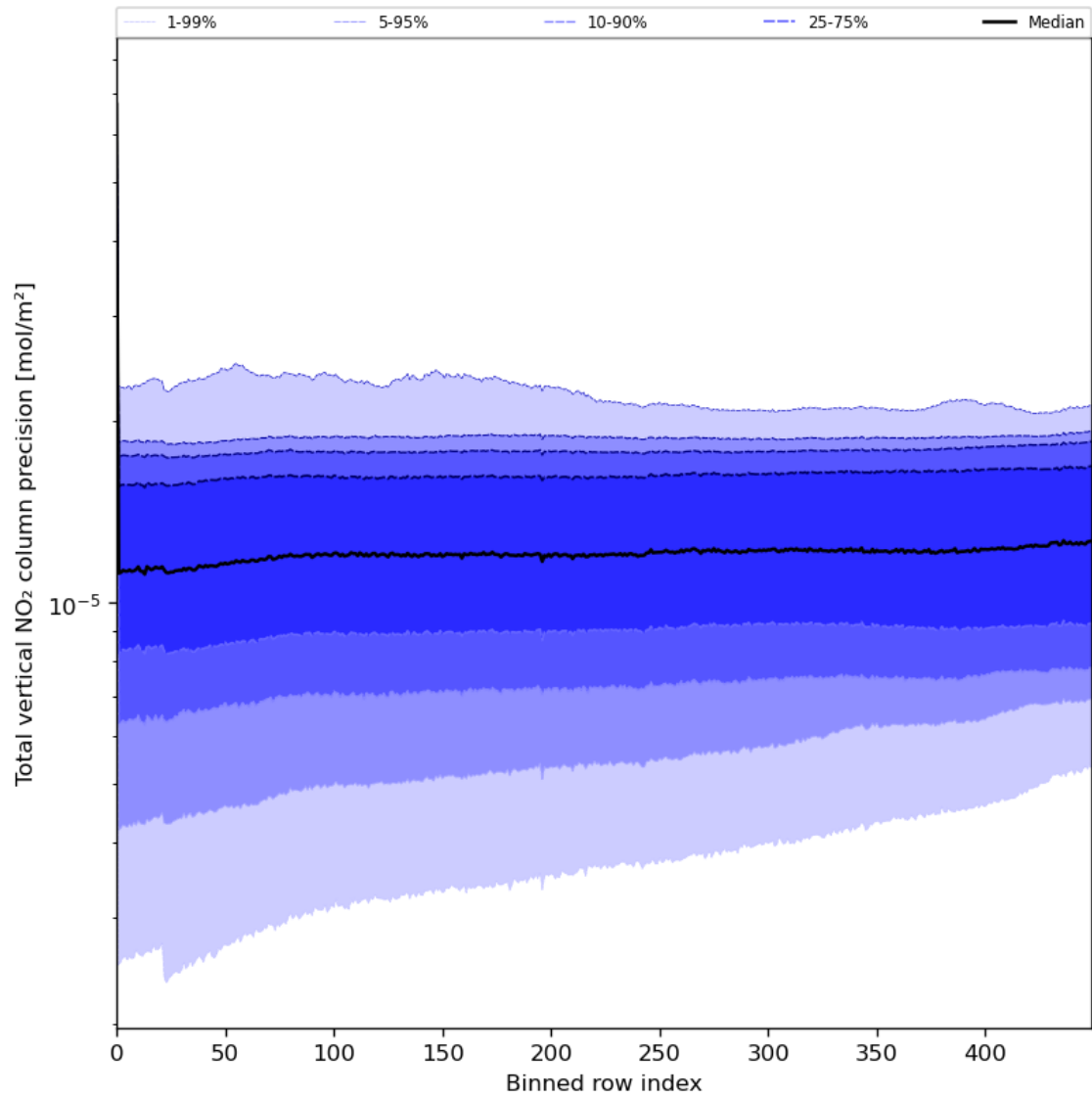
Figure 56: Along track statistics of “Total vertical NO 2 column precision” for 2024-07-11 to 2024-07-13
