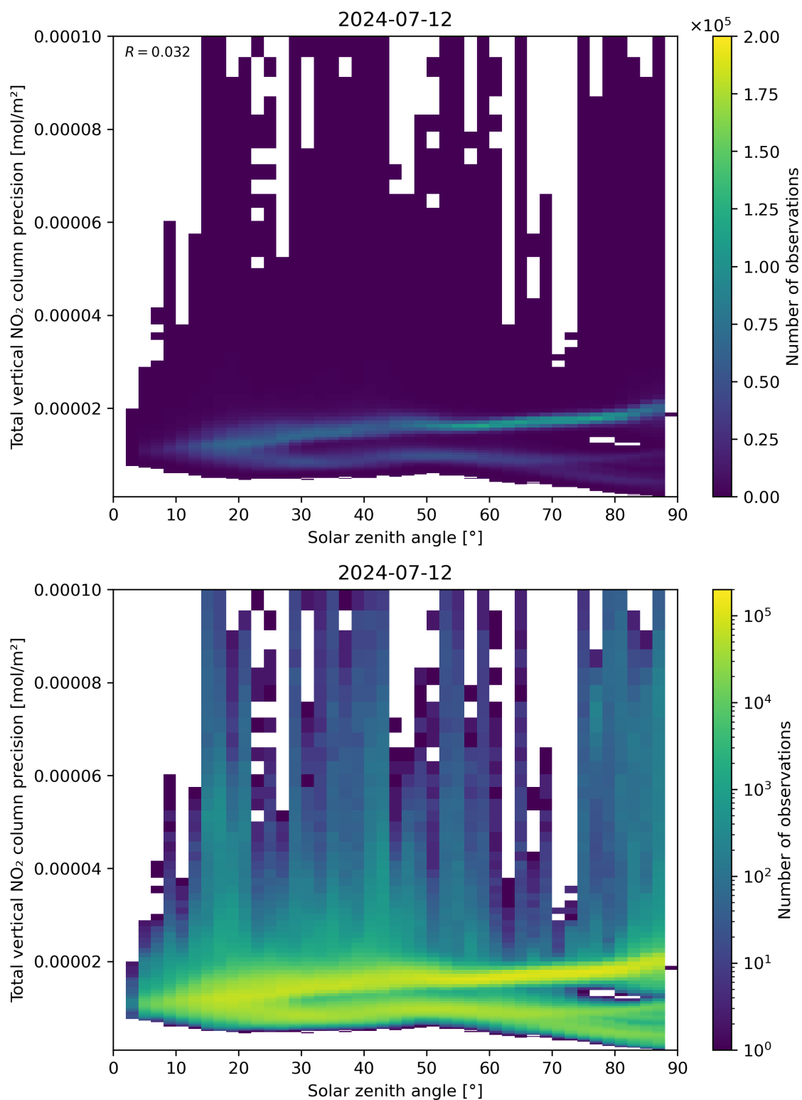
Figure 154: Scatter density plot of “Solar zenith angle” against “Total vertical NO 2 column precision” for 2024-07-11 to 2024-07-13.
