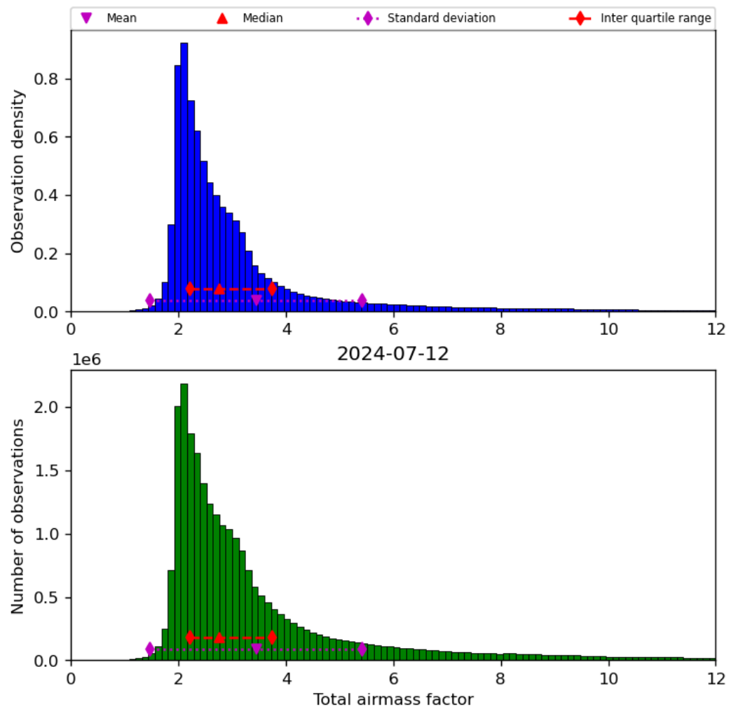
Figure 32: Histogram of “Total airmass factor” for 2024-07-11 to 2024-07-13
