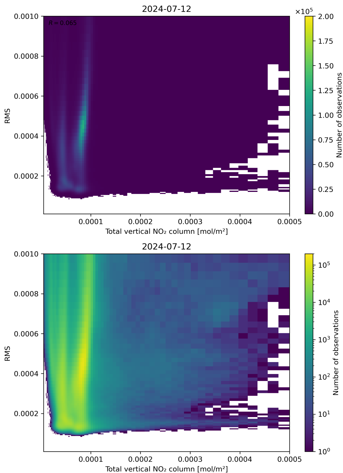
Figure 120: Scatter density plot of “Total vertical NO 2 column” against “RMS” for 2024-07-11 to 2024-07-13.
