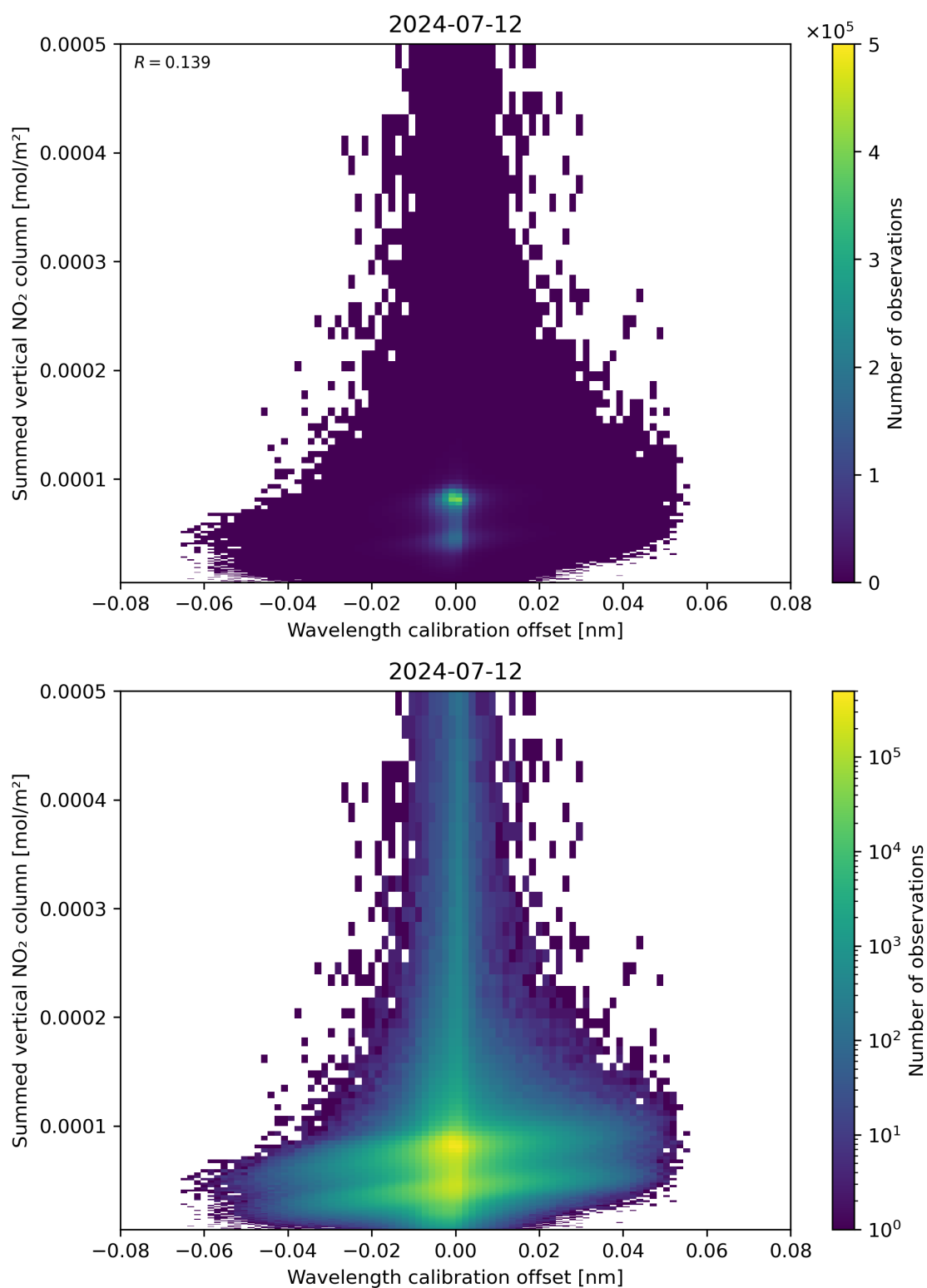
Figure 177: Scatter density plot of “Wavelength calibration offset” against “Summed vertical NO 2 column” for 2024-07-11 to 2024-07-13.
