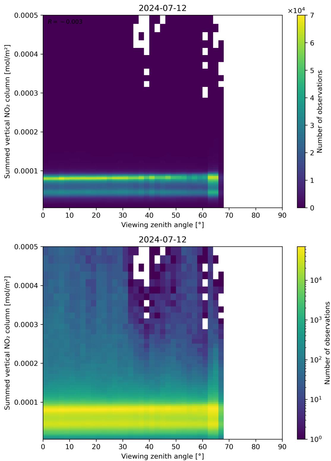
Figure 165: Scatter density plot of “Viewing zenith angle” against “Summed vertical NO 2 column” for 2024-07-11 to 2024-07-13.
