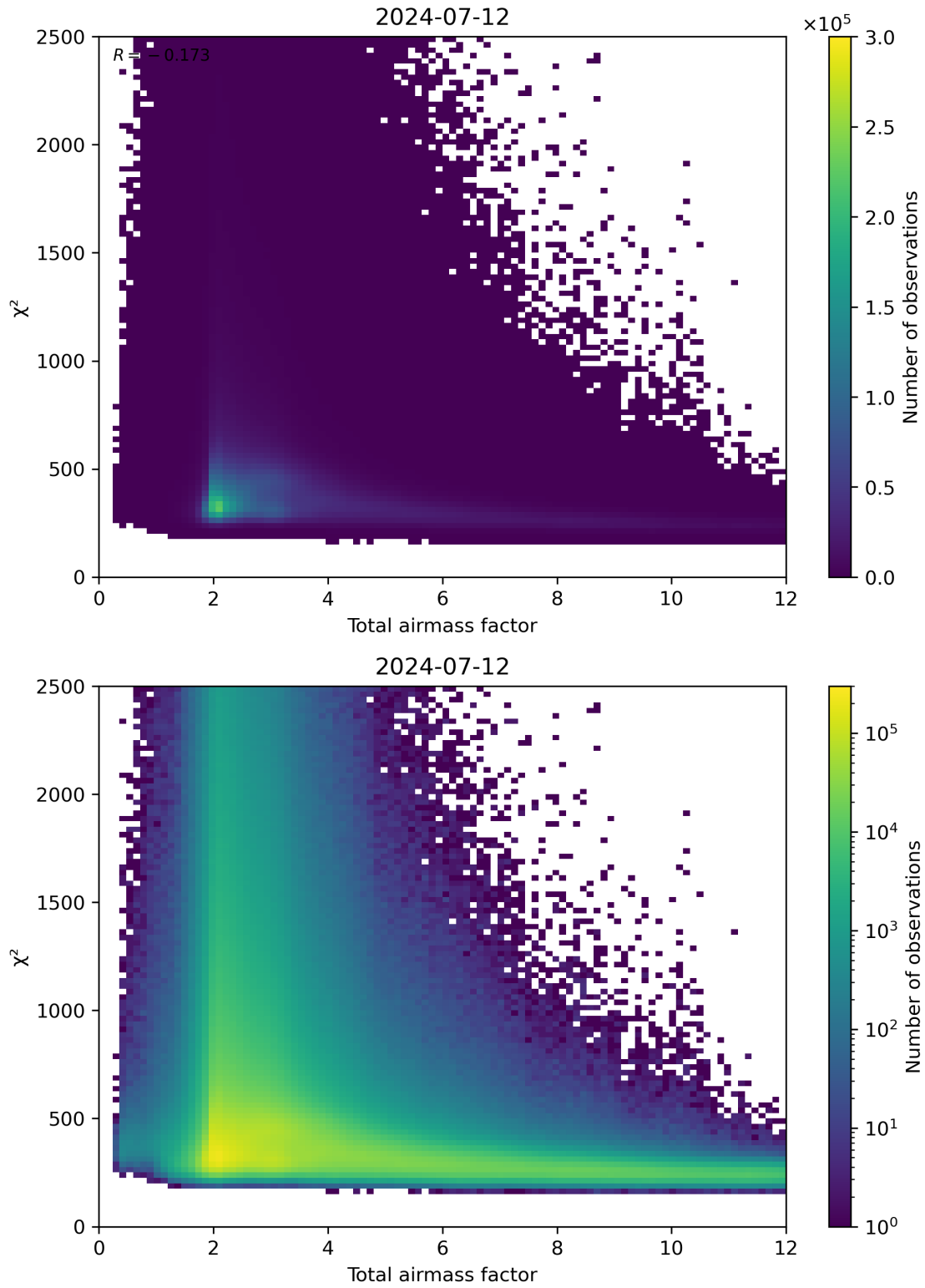
Figure 63: Scatter density plot of “Total airmass factor” against “ \chi^2 ” for 2024-07-11 to 2024-07-13.
