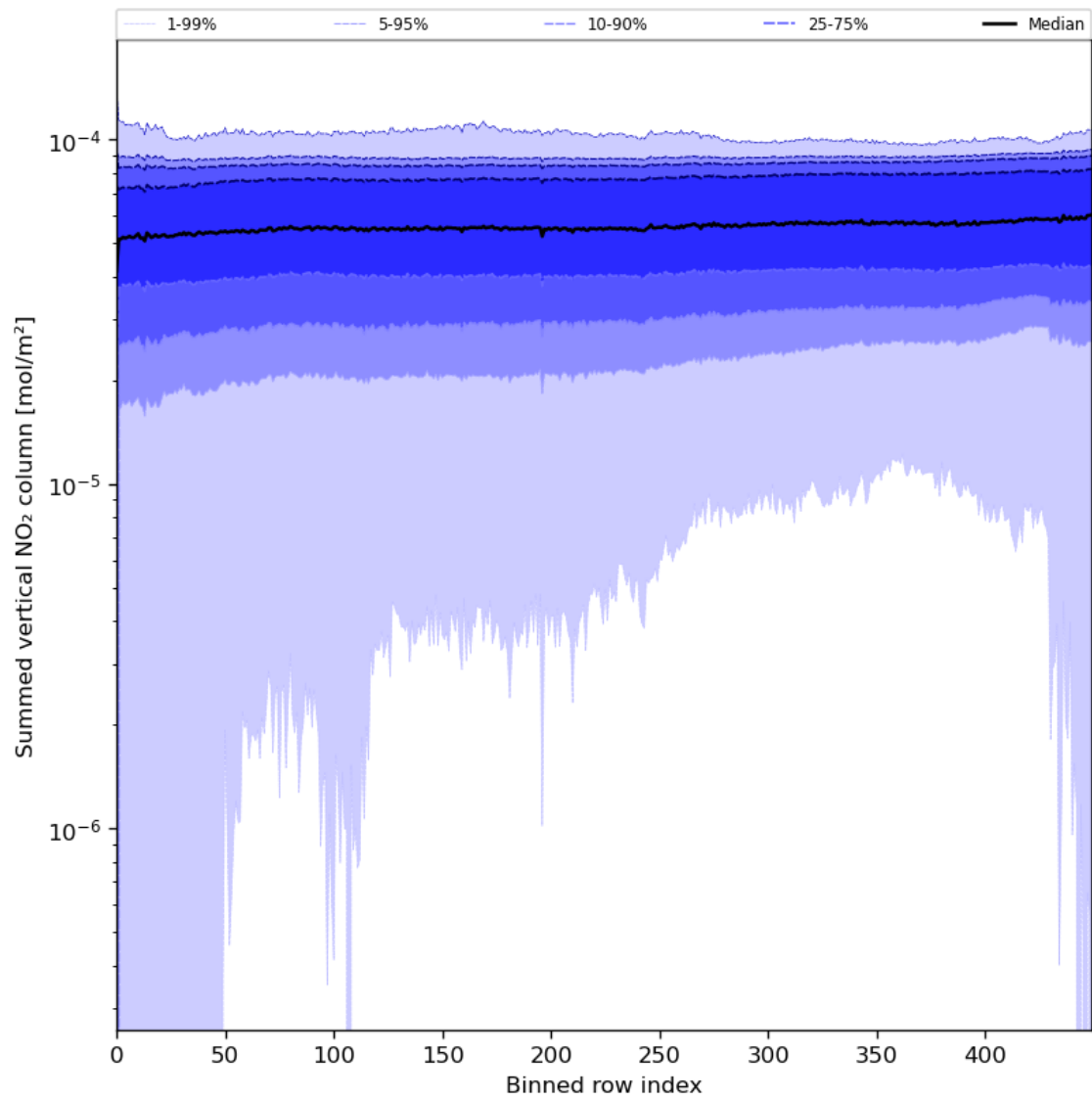
Figure 57: Along track statistics of “Summed vertical NO 2 column” for 2024-07-11 to 2024-07-13
