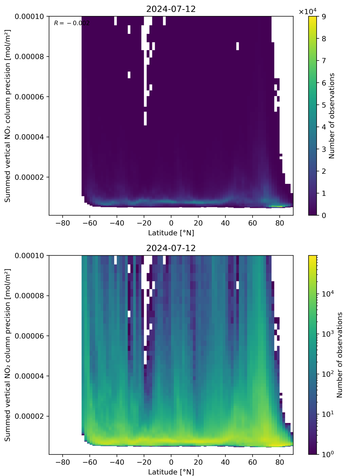
Figure 89: Scatter density plot of “Latitude” against “Summed vertical NO 2 column precision” for 2024-07-11 to 2024-07-13.
