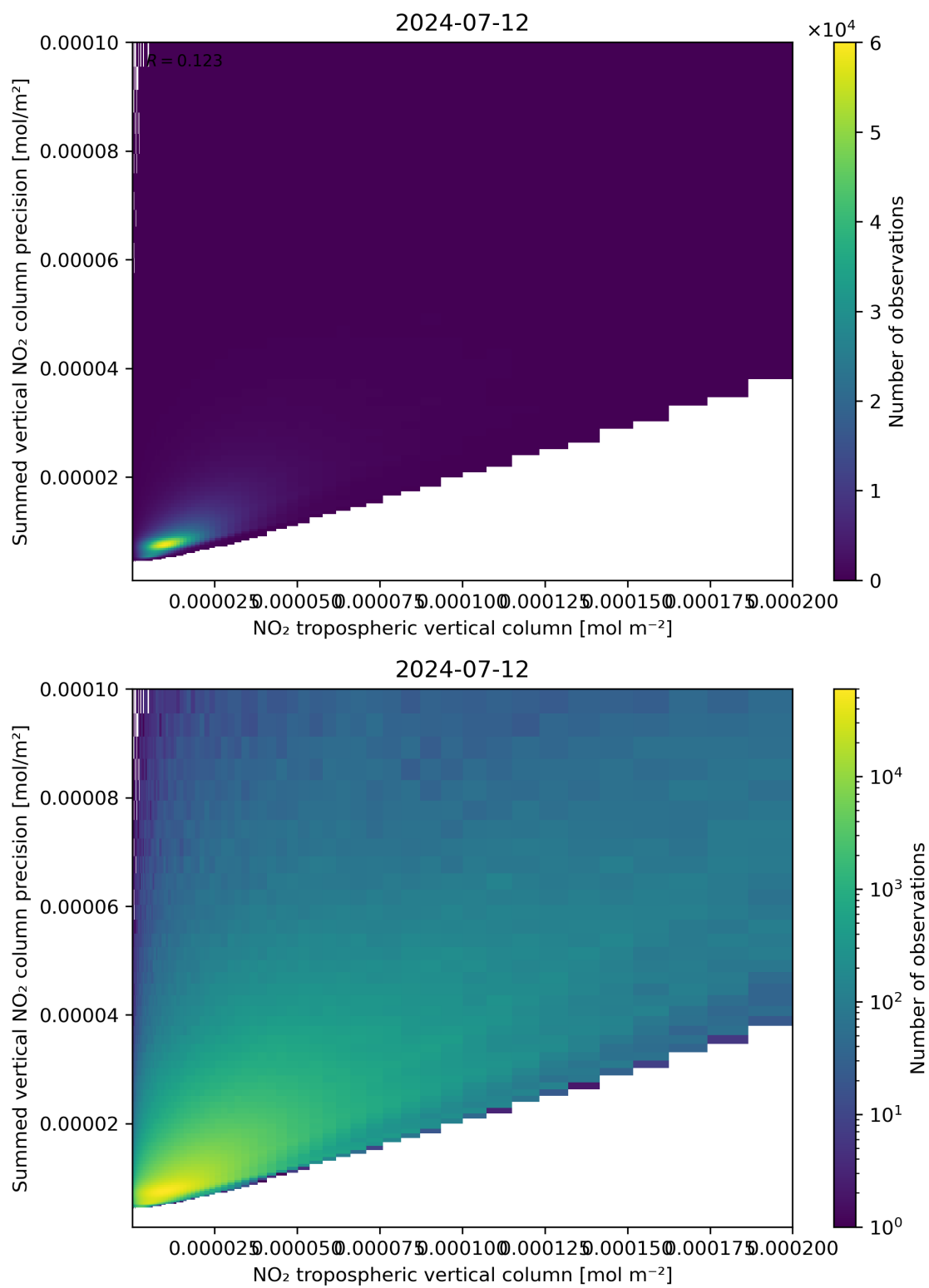
Figure 127: Scatter density plot of “NO 2 tropospheric vertical column” against “Summed vertical NO 2 column precision” for 2024-07-11 to 2024-07-13.
