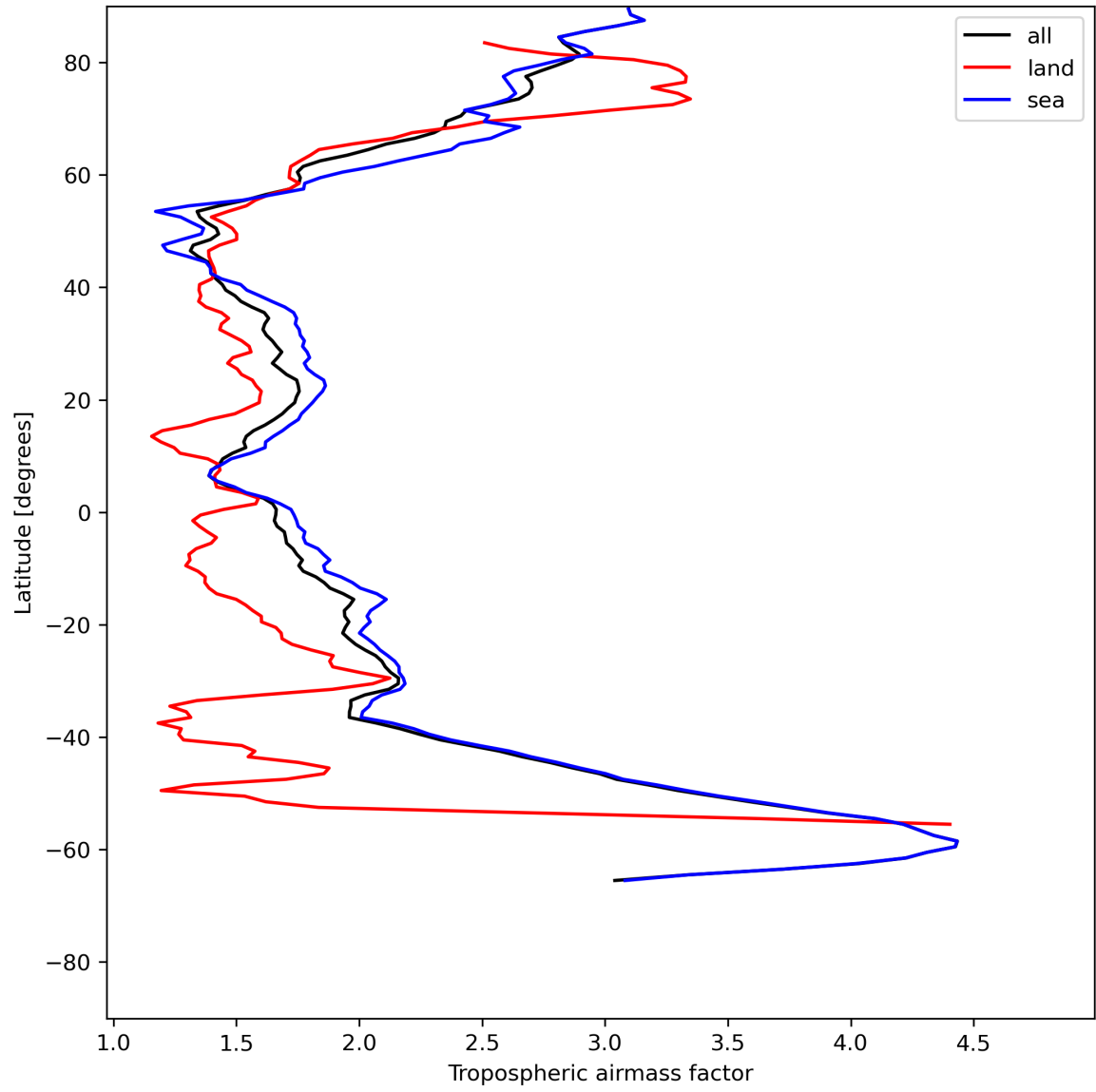
Figure 14: Zonal average of “Tropospheric airmass factor” for 2024-07-11 to 2024-07-13.
