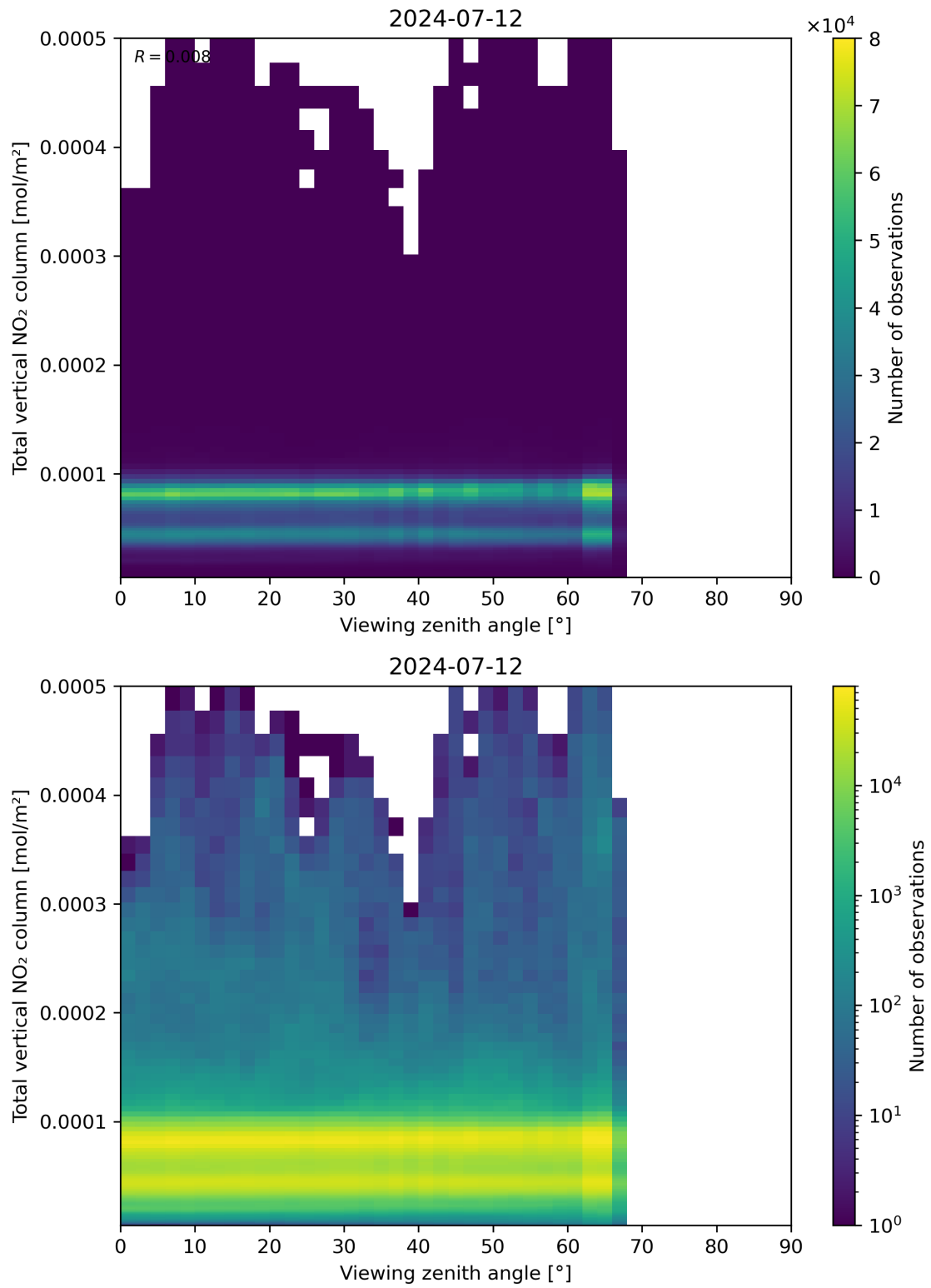
Figure 167: Scatter density plot of “Viewing zenith angle” against “Total vertical NO 2 column” for 2024-07-11 to 2024-07-13.
