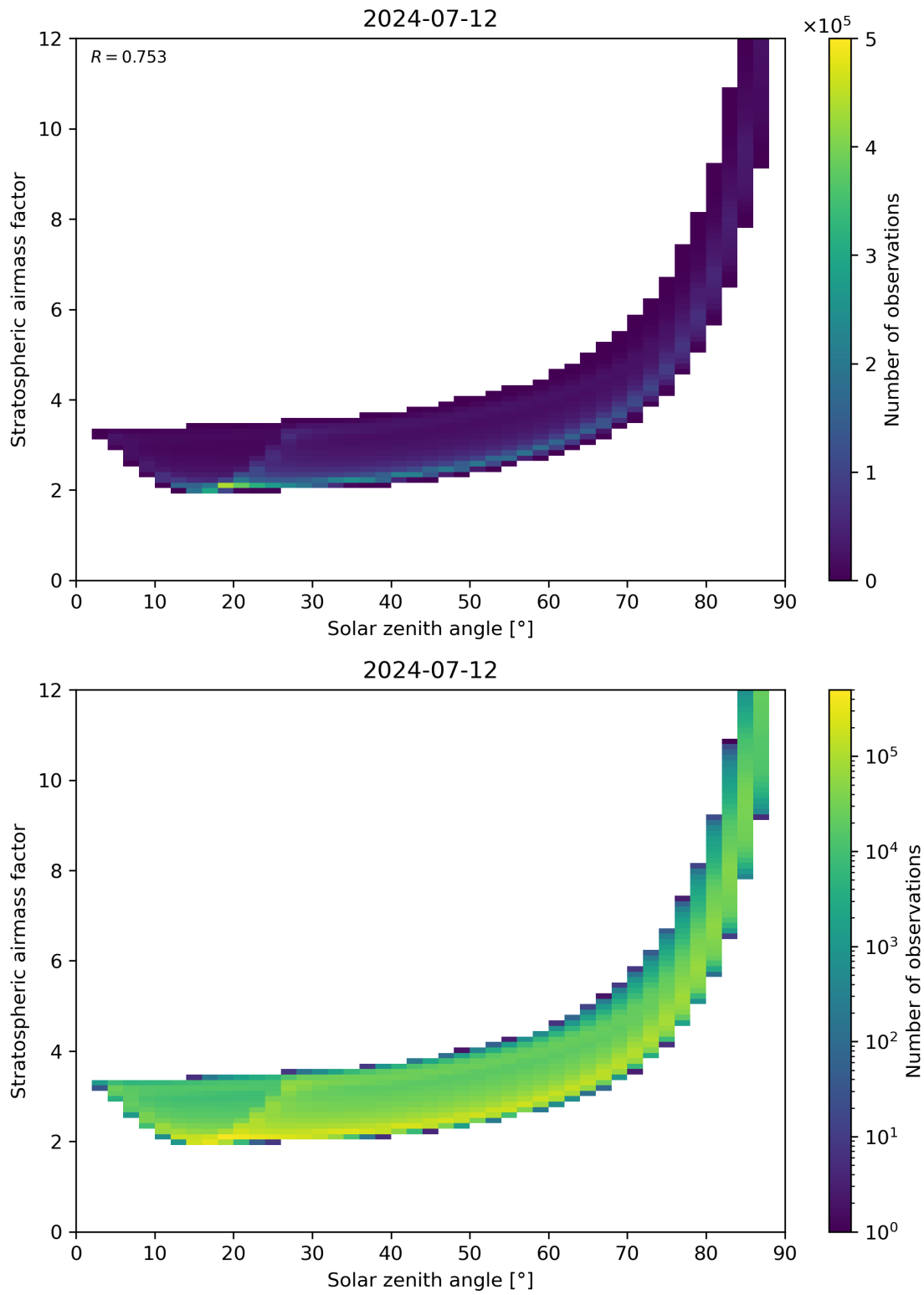
Figure 145: Scatter density plot of “Solar zenith angle” against “Stratospheric airmass factor” for 2024-07-11 to 2024-07-13.
