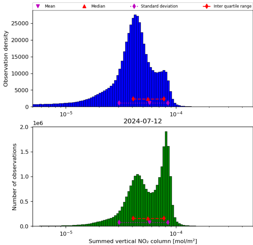
Figure 40: Histogram of “Summed vertical NO 2 column” for 2024-07-11 to 2024-07-13
