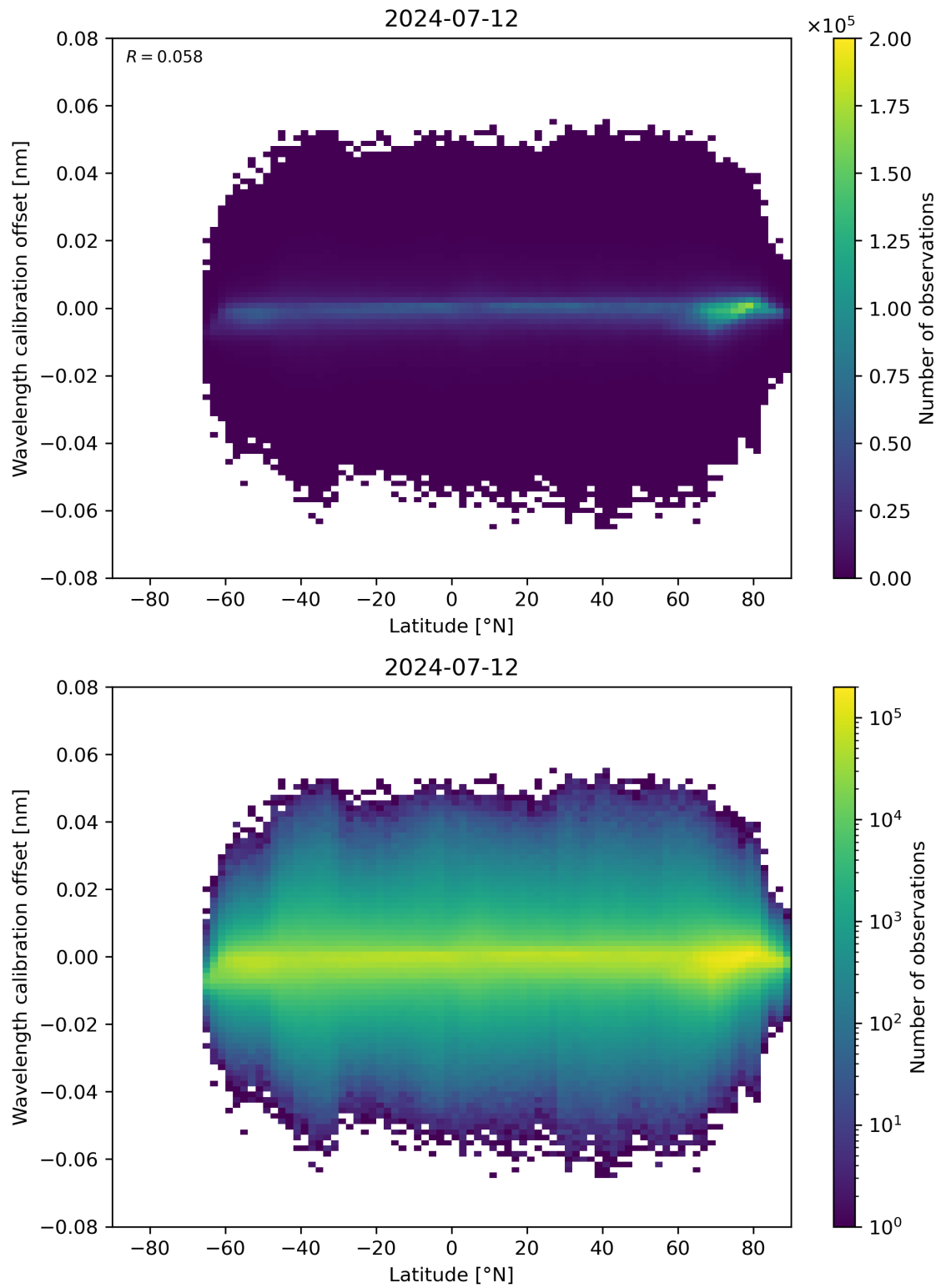
Figure 95: Scatter density plot of “Latitude” against “Wavelength calibration offset” for 2024-07-11 to 2024-07-13.
