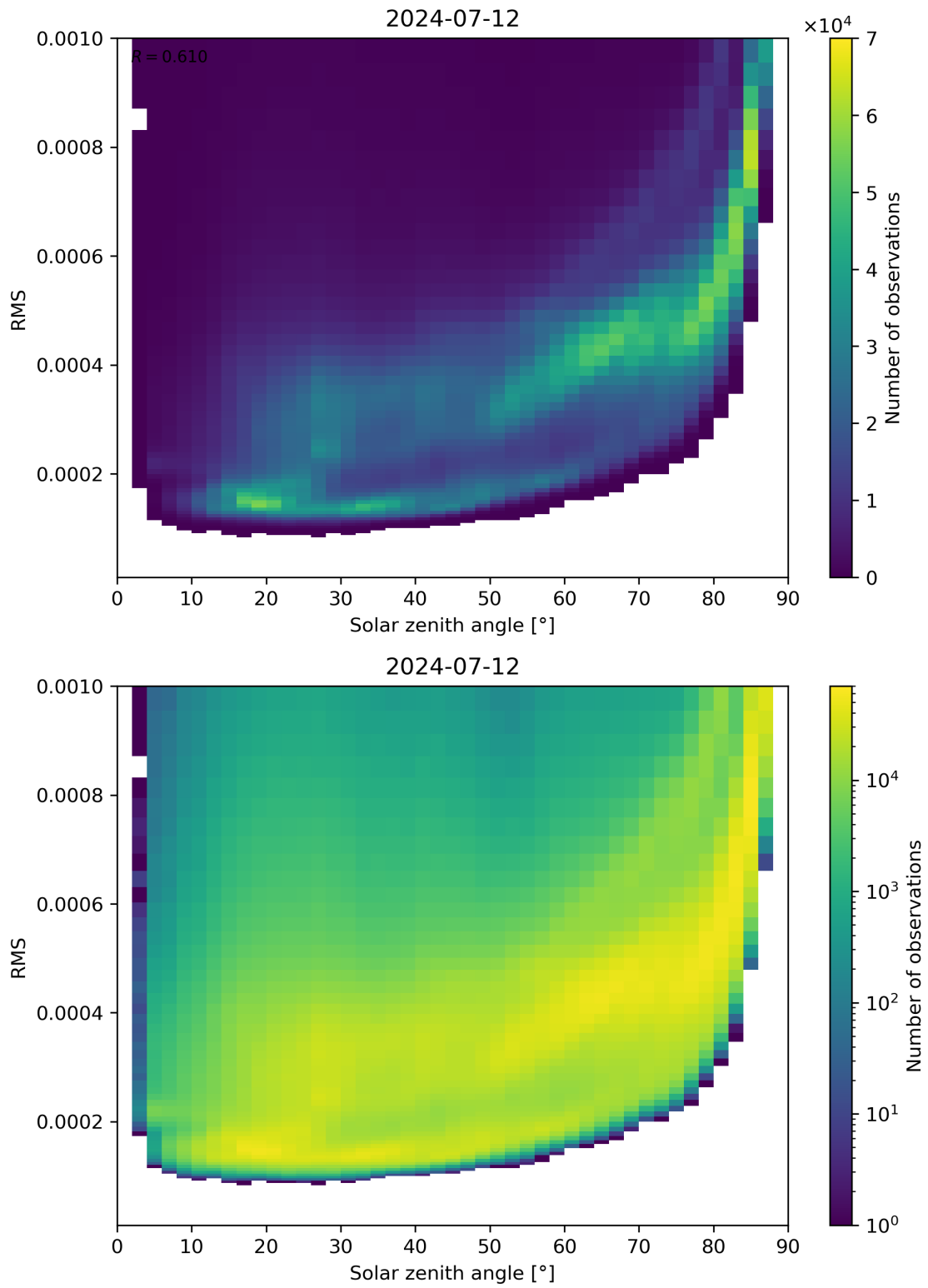
Figure 157: Scatter density plot of “Solar zenith angle” against “RMS” for 2024-07-11 to 2024-07-13.
