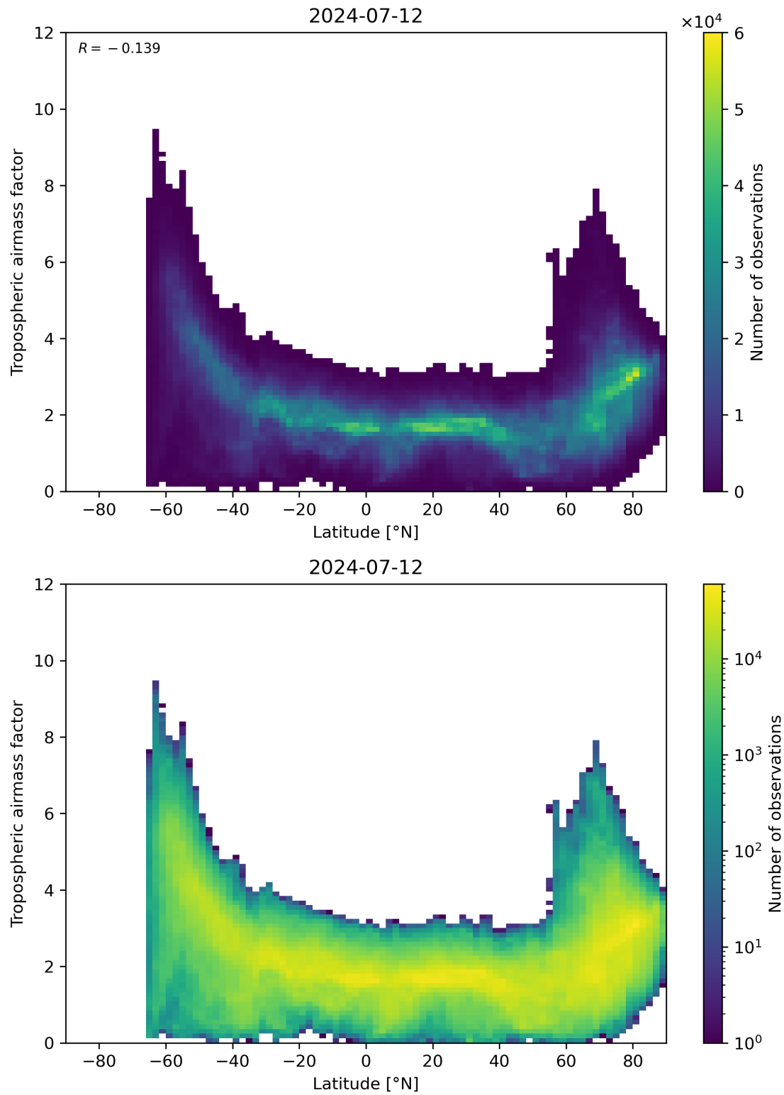
Figure 85: Scatter density plot of “Latitude” against “Tropospheric airmass factor” for 2024-07-11 to 2024-07-13.
