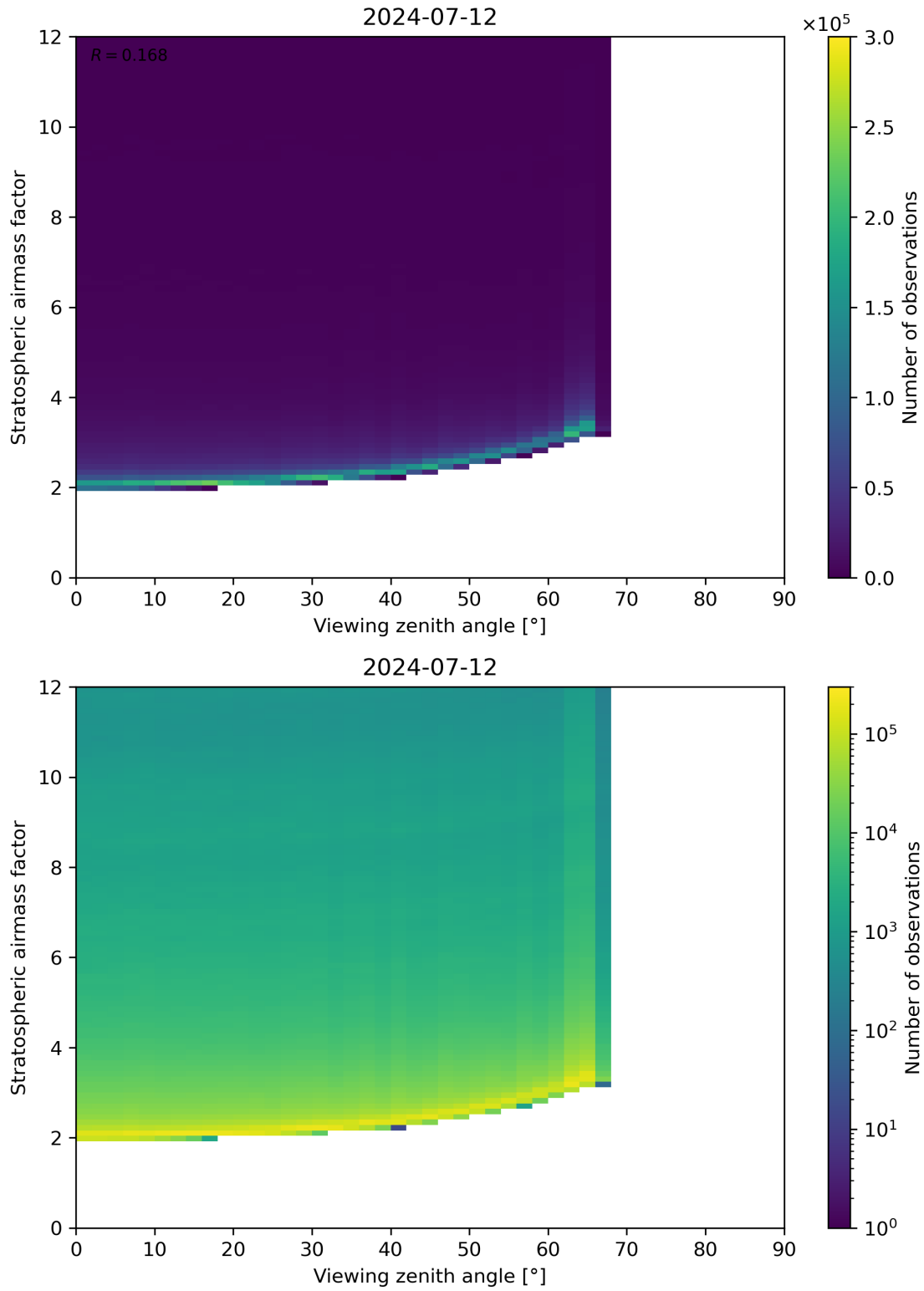
Figure 159: Scatter density plot of “Viewing zenith angle” against “Stratospheric airmass factor” for 2024-07-11 to 2024-07-13.
