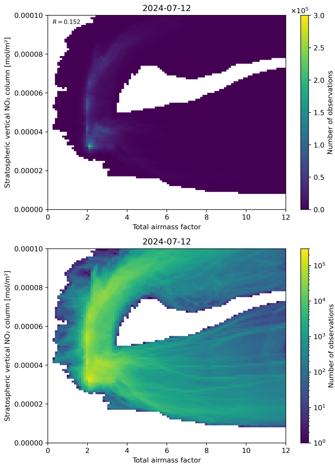
Figure 64: Scatter density plot of “Total airmass factor” against “Stratospheric vertical NO 2 column” for 2024-07-11 to 2024-07-13.
