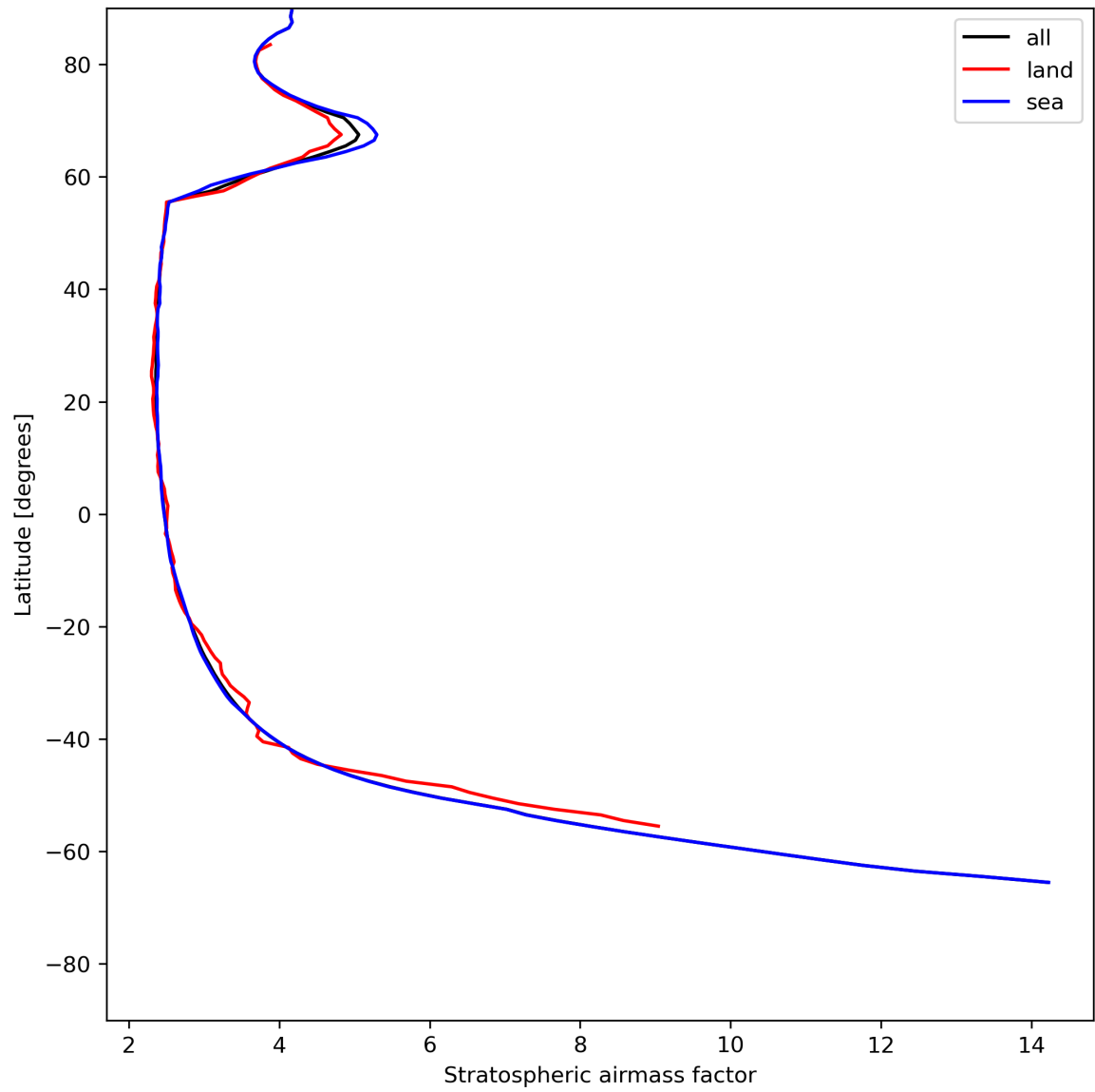
Figure 27: Zonal average of “Stratospheric airmass factor” for 2024-07-11 to 2024-07-13.
