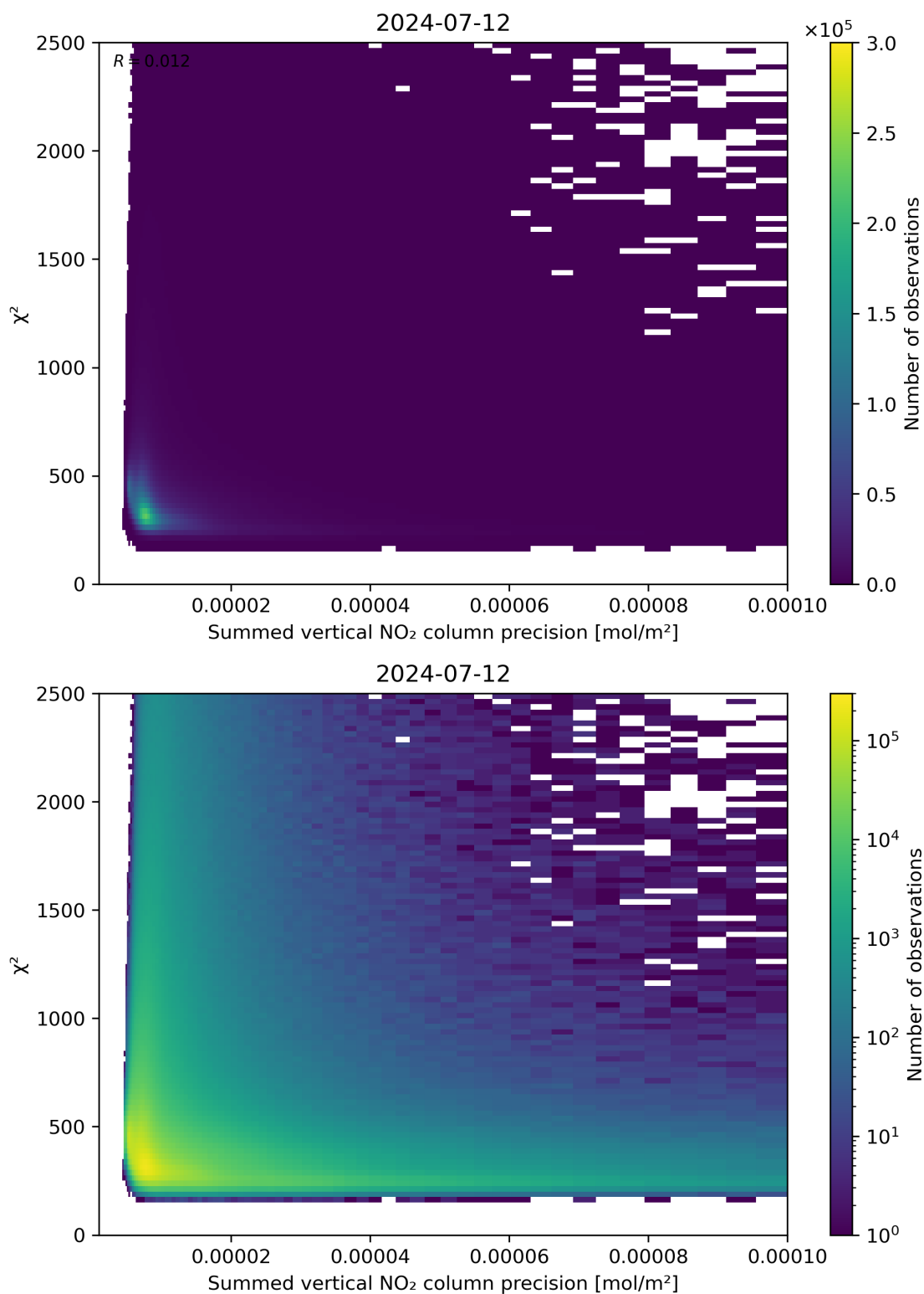
Figure 107: Scatter density plot of “Summed vertical NO 2 column precision” against “ \chi^2 ” for 2024-07-11 to 2024-07-13.
