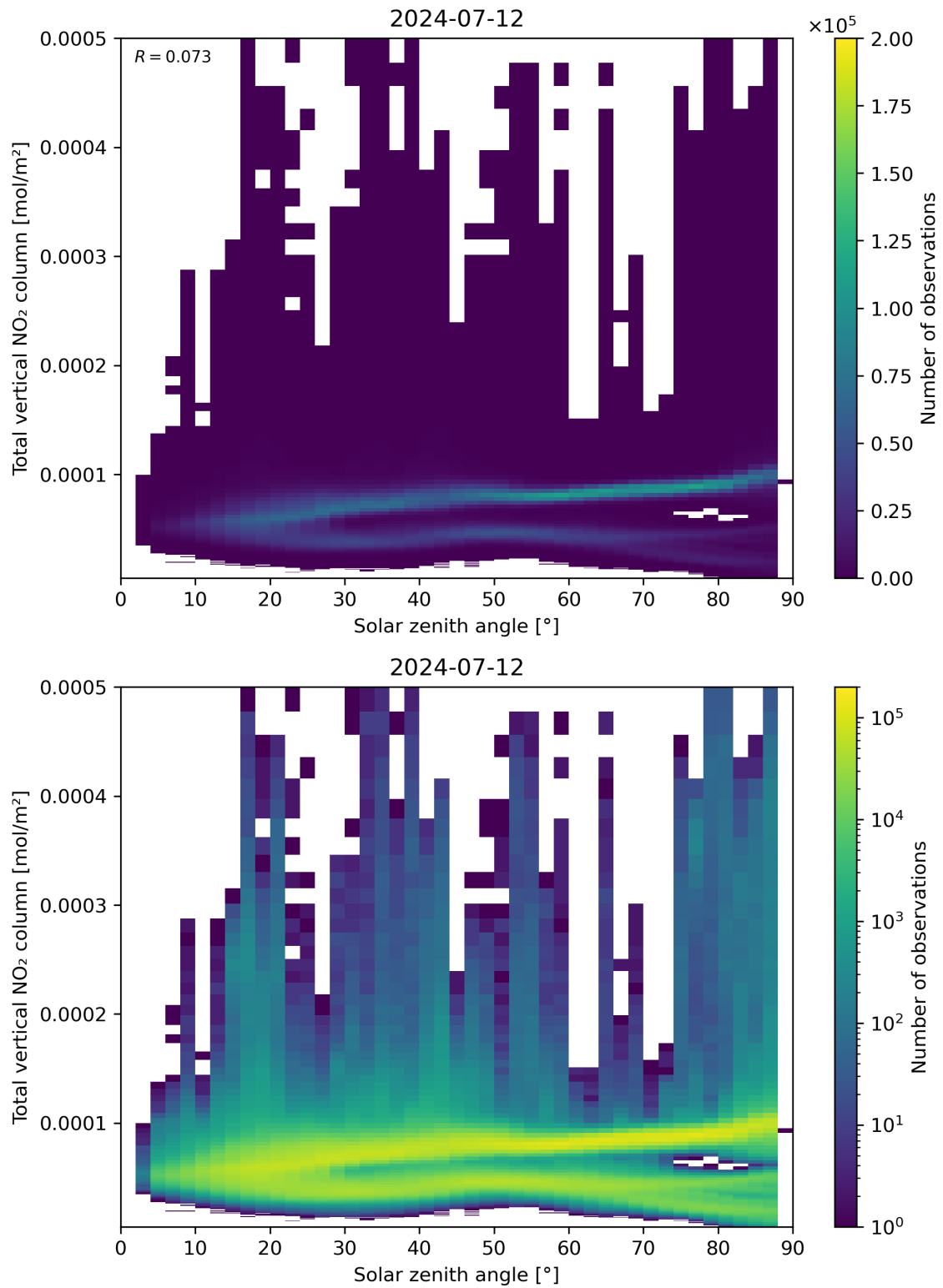
Figure 153: Scatter density plot of “Solar zenith angle” against “Total vertical NO 2 column” for 2024-07-11 to 2024-07-13.
