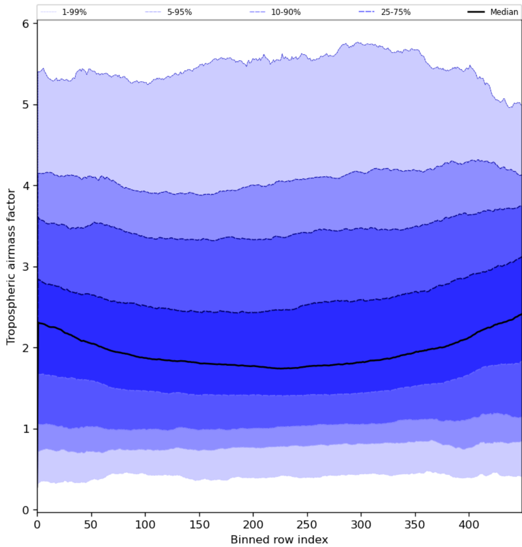
Figure 48: Along track statistics of “Tropospheric airmass factor” for 2024-07-11 to 2024-07-13
