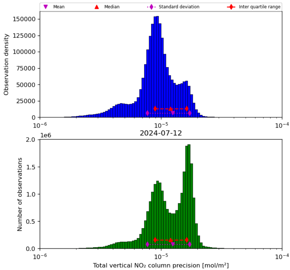
Figure 39: Histogram of "Total vertical NO 2 column precision" for 2024-07-11 to 2024-07-13
