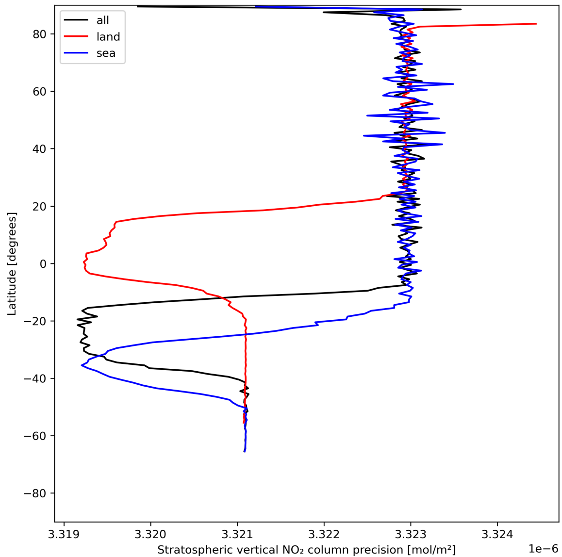
Figure 20: Zonal average of “Stratospheric vertical NO 2 column precision” for 2024-07-11 to 2024-07-13.
