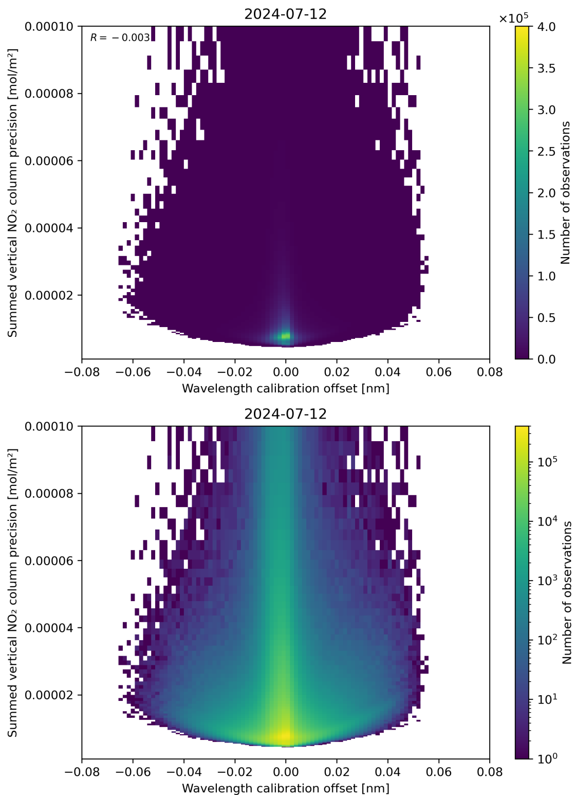
Figure 178: Scatter density plot of “Wavelength calibration offset” against “Summed vertical NO 2 column precision” for 2024-07-11 to 2024-07-13.
