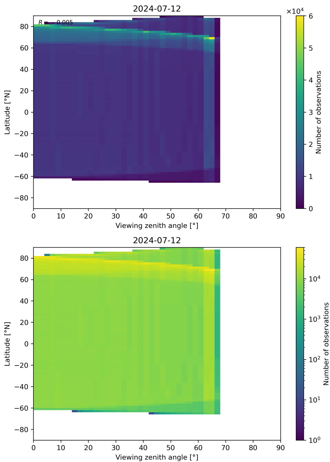
Figure 163: Scatter density plot of “Viewing zenith angle” against “Latitude” for 2024-07-11 to 2024-07-13.
