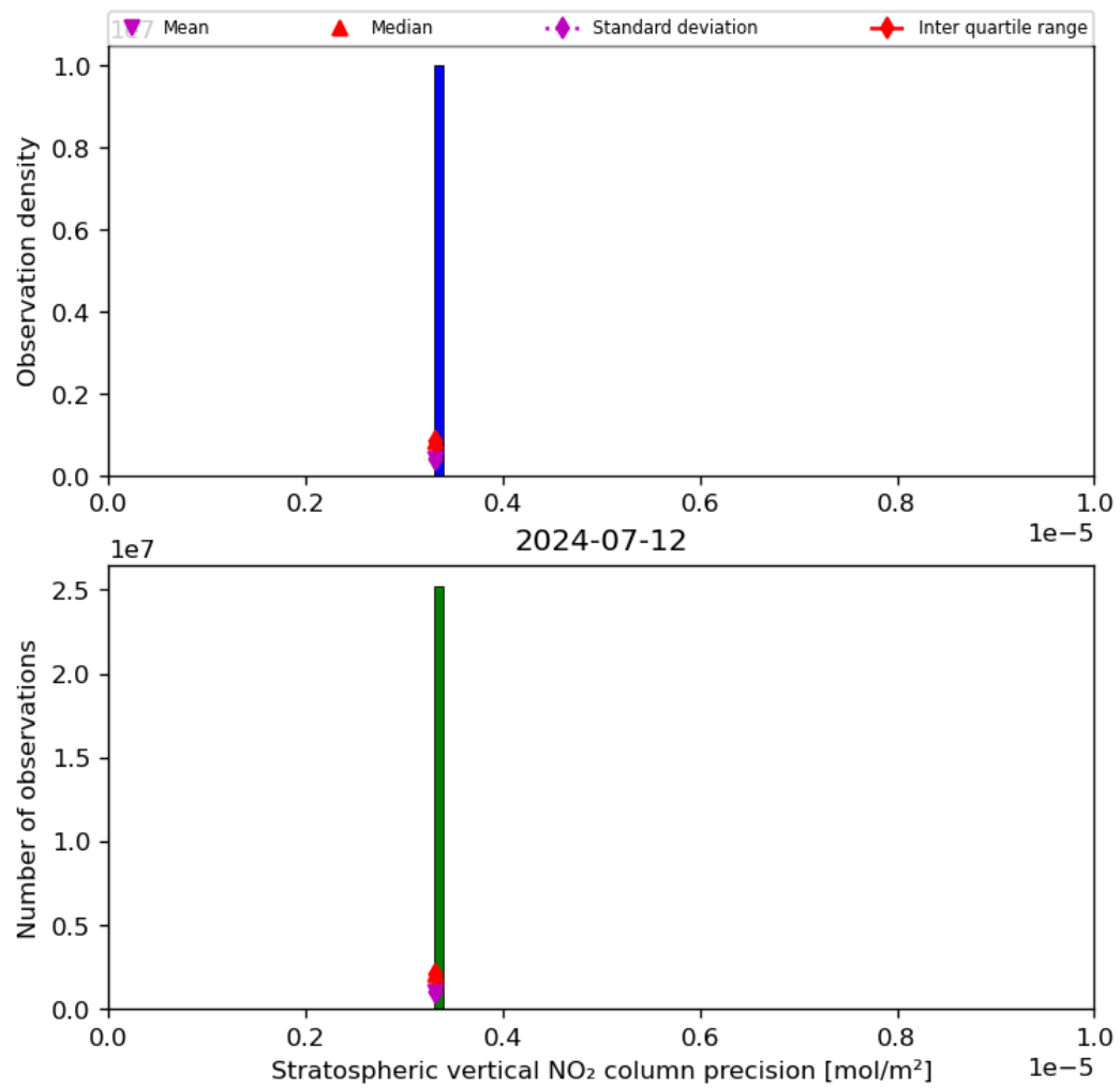
Figure 37: Histogram of “Stratospheric vertical NO 2 column precision” for 2024-07-11 to 2024-07-13
