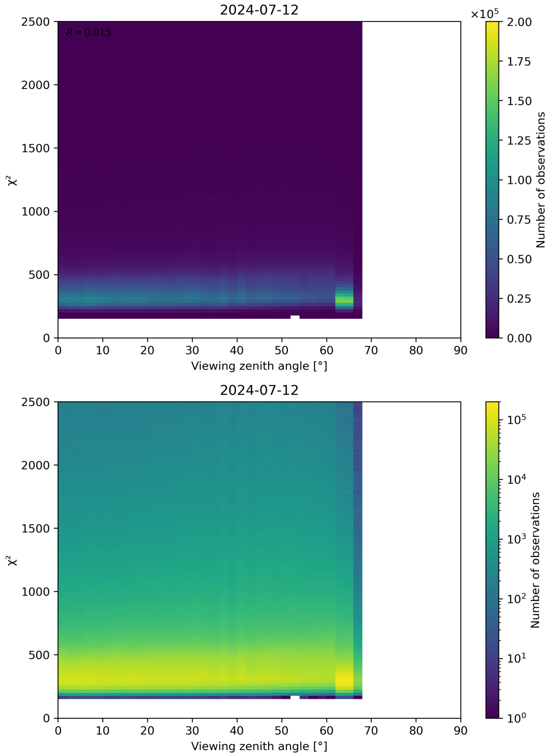
Figure 162: Scatter density plot of “Viewing zenith angle” against “ \chi^2 ” for 2024-07-11 to 2024-07-13.
