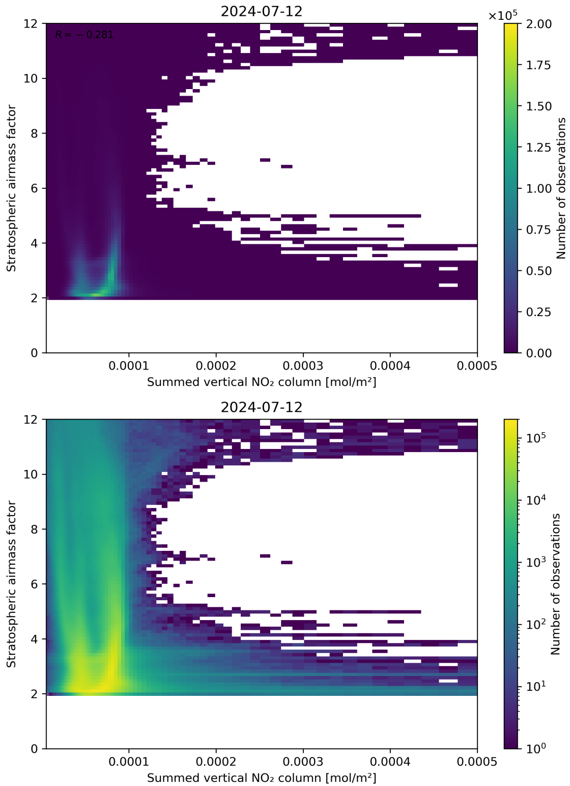
Figure 103: Scatter density plot of “Summed vertical NO 2 column” against “Stratospheric air mass factor” for 2024-07-11 to 2024-07-13.
