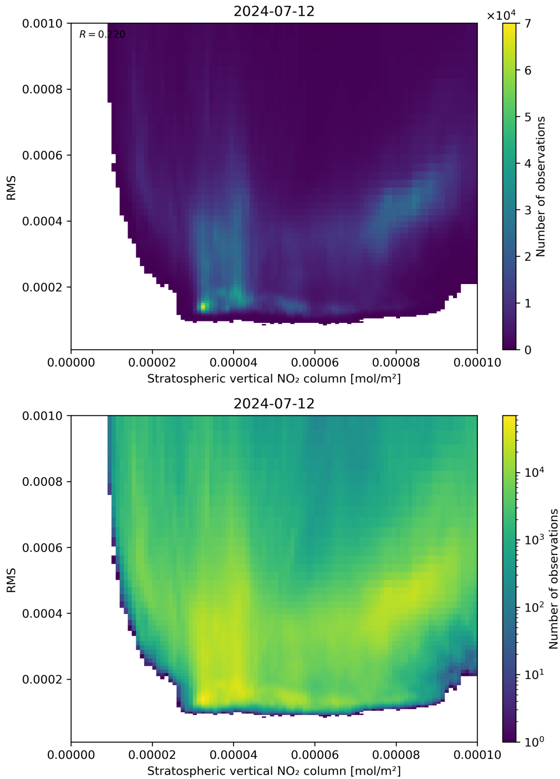
Figure 102: Scatter density plot of “Stratospheric vertical NO 2 column” against “RMS” for 2024-07-11 to 2024-07-13.
