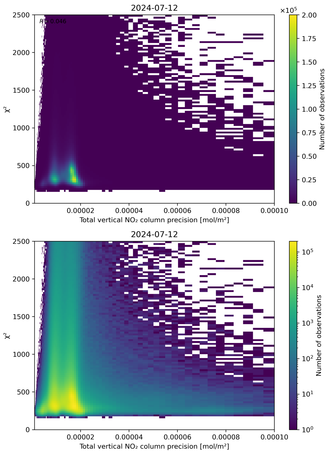
Figure 116: Scatter density plot of “Total vertical NO 2 column precision” against “ \chi^2 ” for 2024-07-11 to 2024-07-13.
