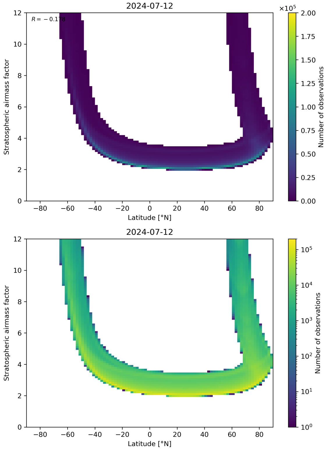
Figure 83: Scatter density plot of “Latitude” against “Stratospheric air mass factor” for 2024-07-11 to 2024-07-13.
