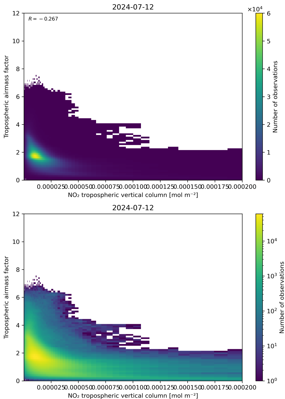
Figure 123: Scatter density plot of “NO 2 tropospheric vertical column” against “Tropospheric airmass factor” for 2024-07-11 to 2024-07-13.
