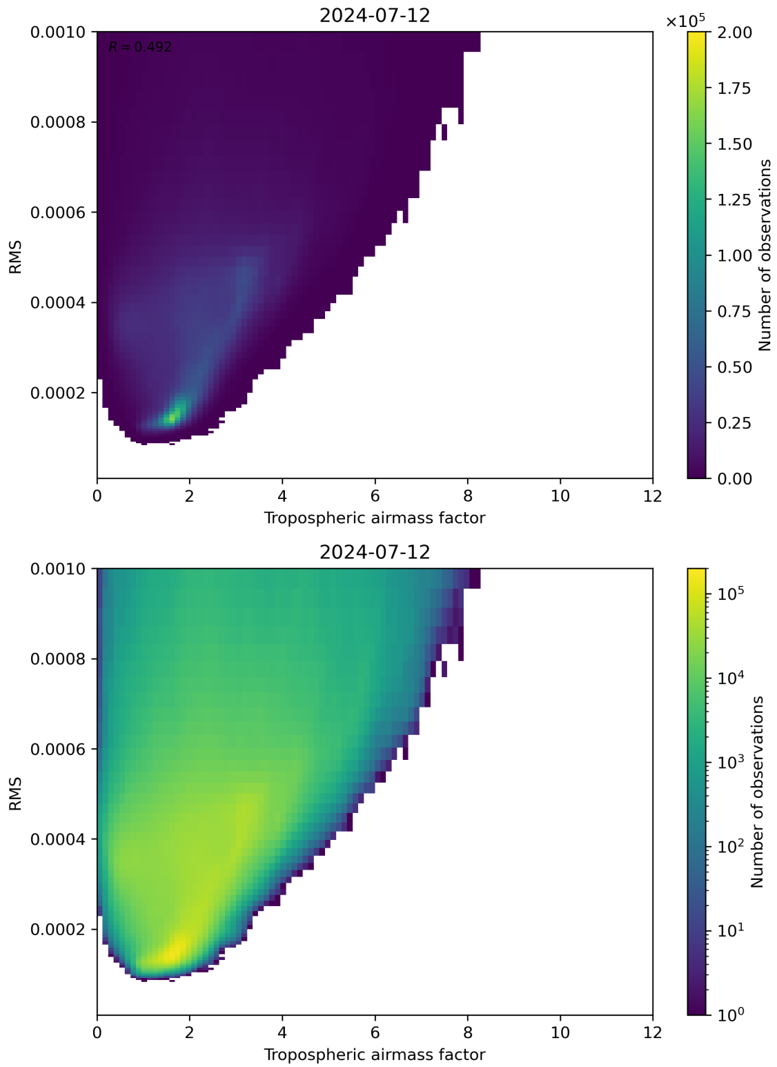
Figure 79: Scatter density plot of “Tropospheric airmass factor” against “RMS” for 2024-07-11 to 2024-07-13.
