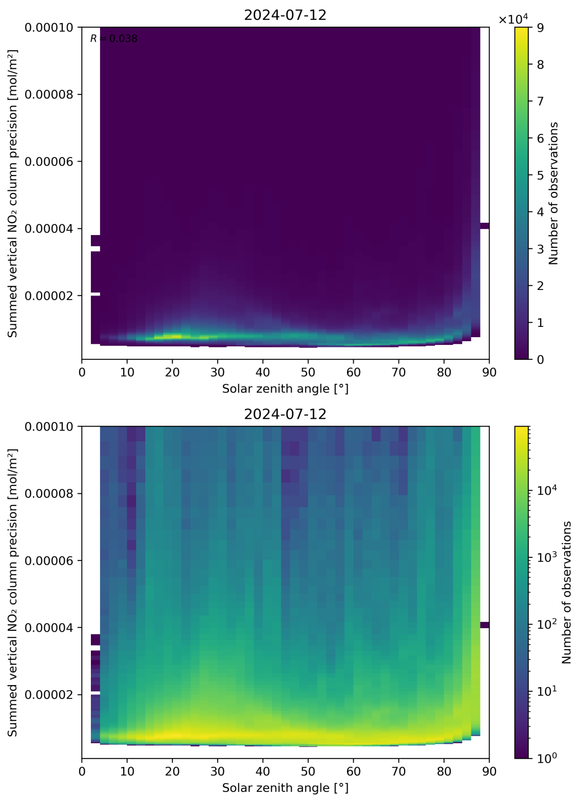
Figure 152: Scatter density plot of “Solar zenith angle” against “Summed vertical NO 2 column precision” for 2024-07-11 to 2024-07-13.
