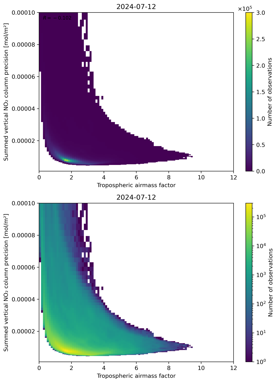
Figure 76: Scatter density plot of “Tropospheric air mass factor” against “Summed vertical NO 2 column precision” for 2024-07-11 to 2024-07-13.
