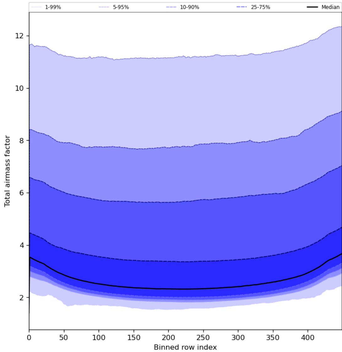
Figure 49: Along track statistics of “Total airmass factor” for 2024-07-11 to 2024-07-13
