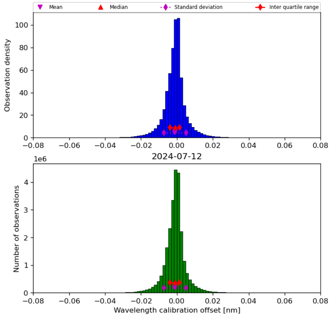
Figure 35: Histogram of “Wavelength calibration offset” for 2024-07-11 to 2024-07-13
