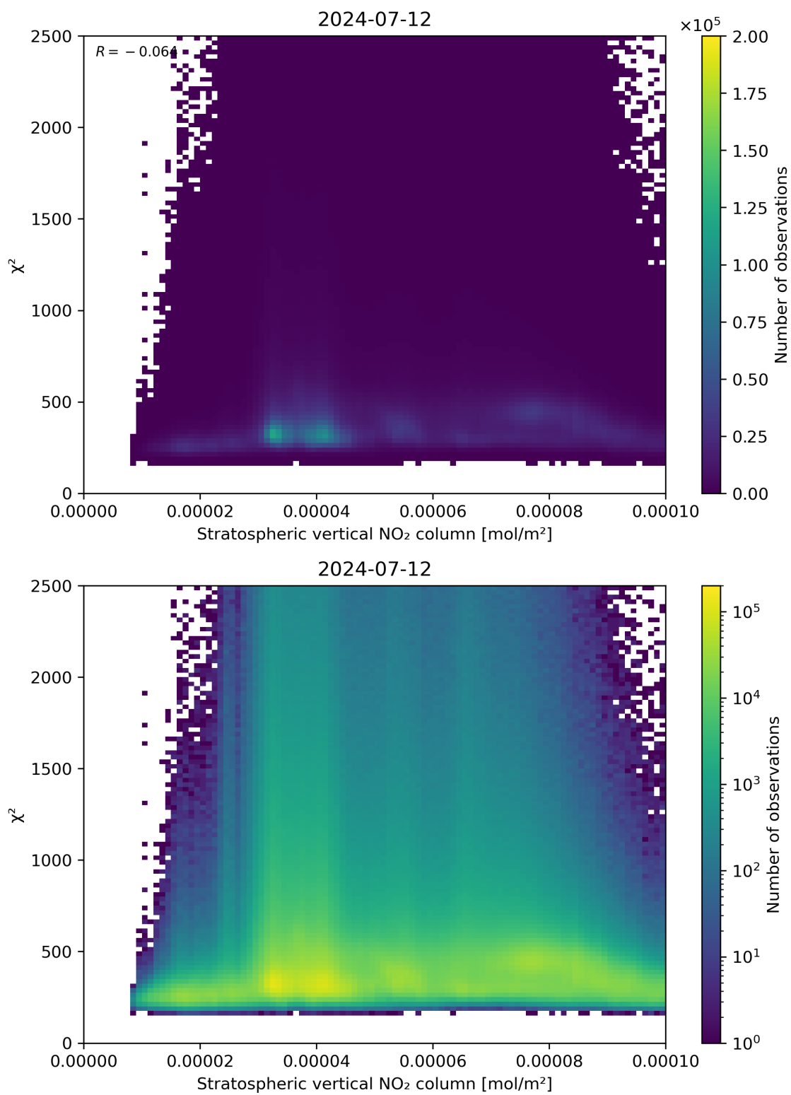
Figure 97: Scatter density plot of “Stratospheric vertical NO 2 column” against “ \chi^2 ” for 2024-07-11 to 2024-07-13.
