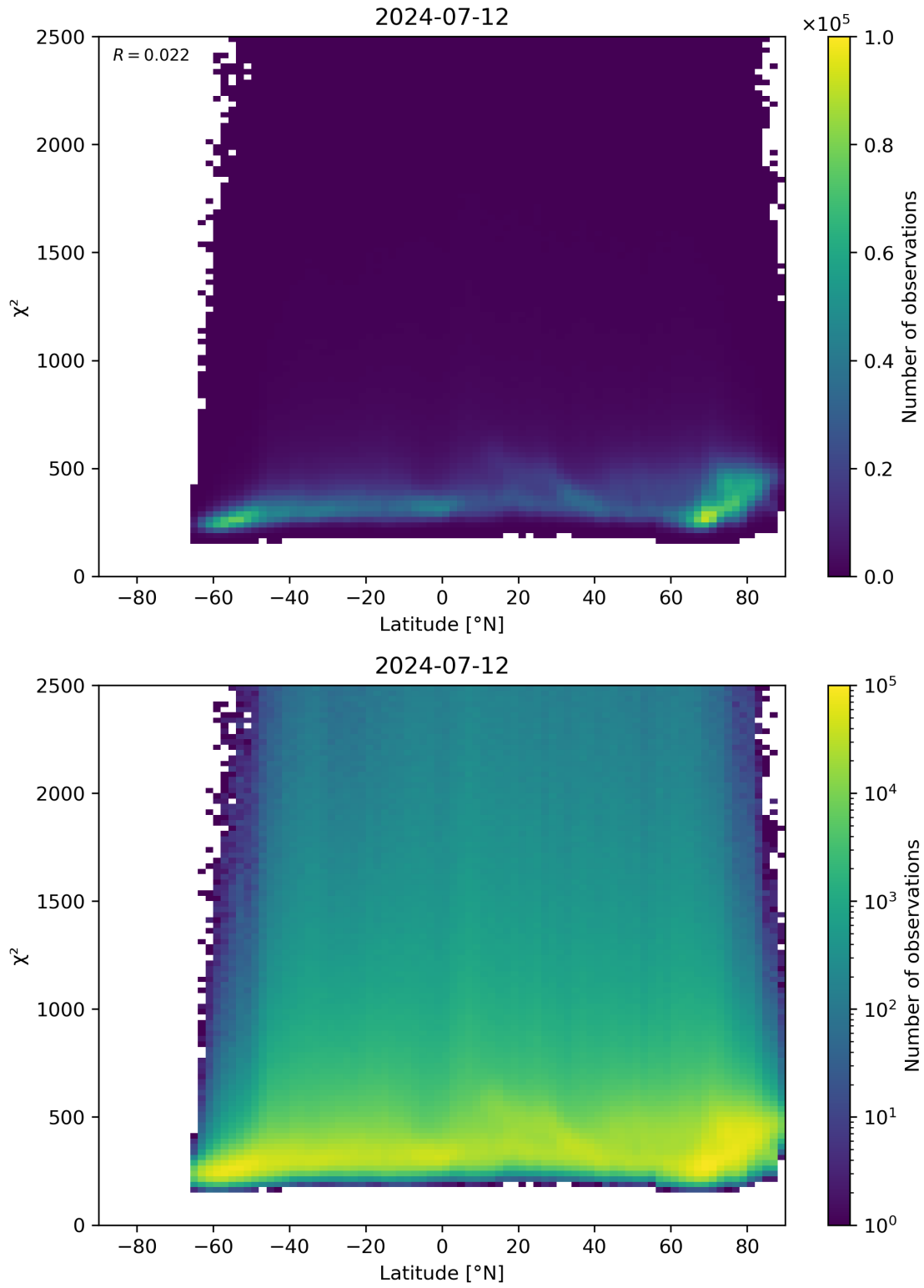
Figure 86: Scatter density plot of “Latitude” against “ \chi^2 ” for 2024-07-11 to 2024-07-13.
