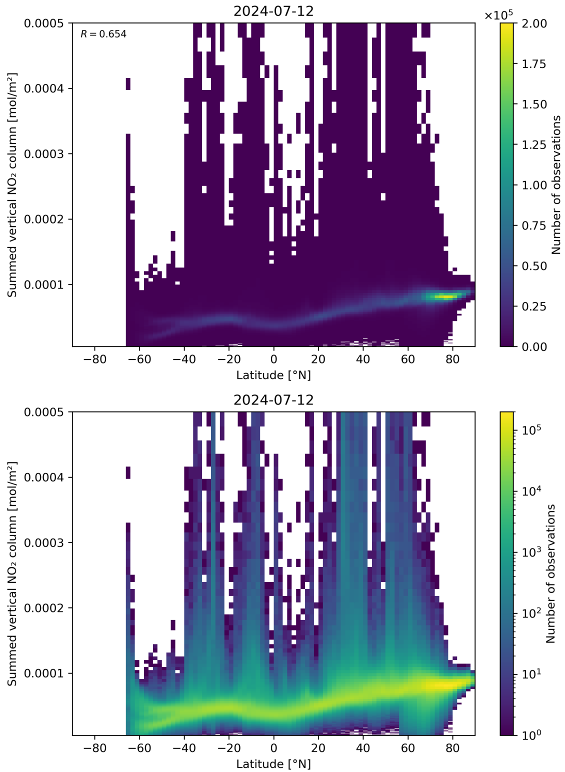
Figure 88: Scatter density plot of “Latitude” against “Summed vertical NO 2 column” for 2024-07-11 to 2024-07-13.
