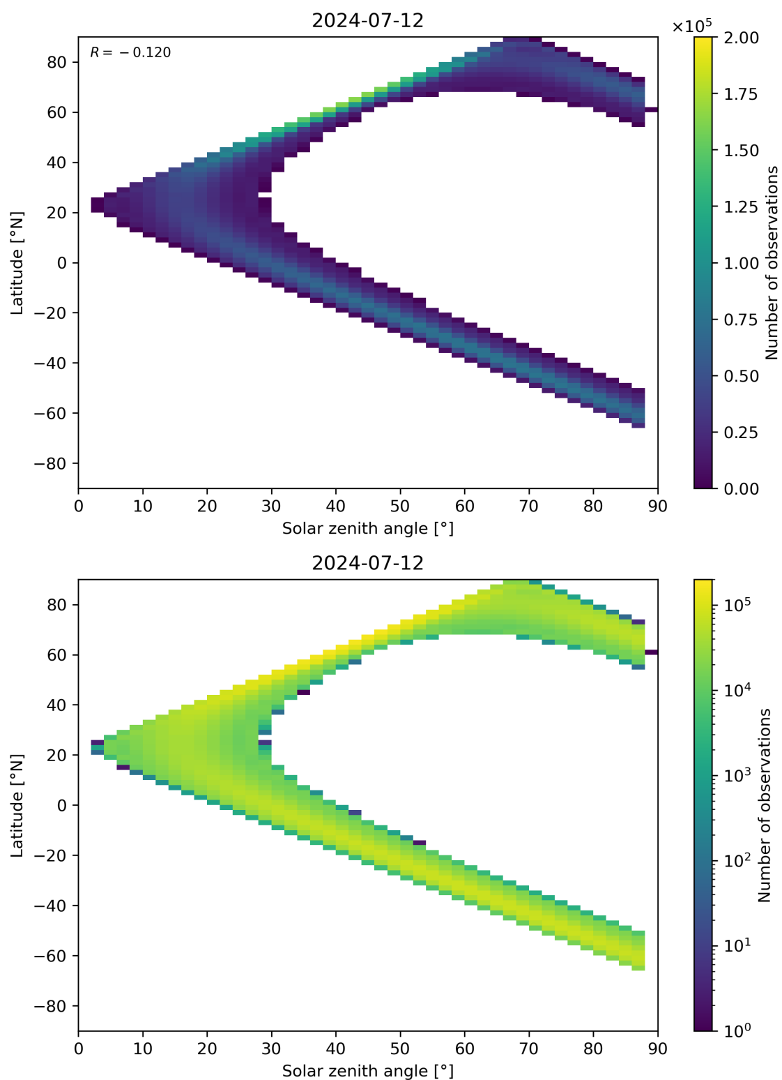
Figure 149: Scatter density plot of “Solar zenith angle” against “Latitude” for 2024-07-11 to 2024-07-13.
