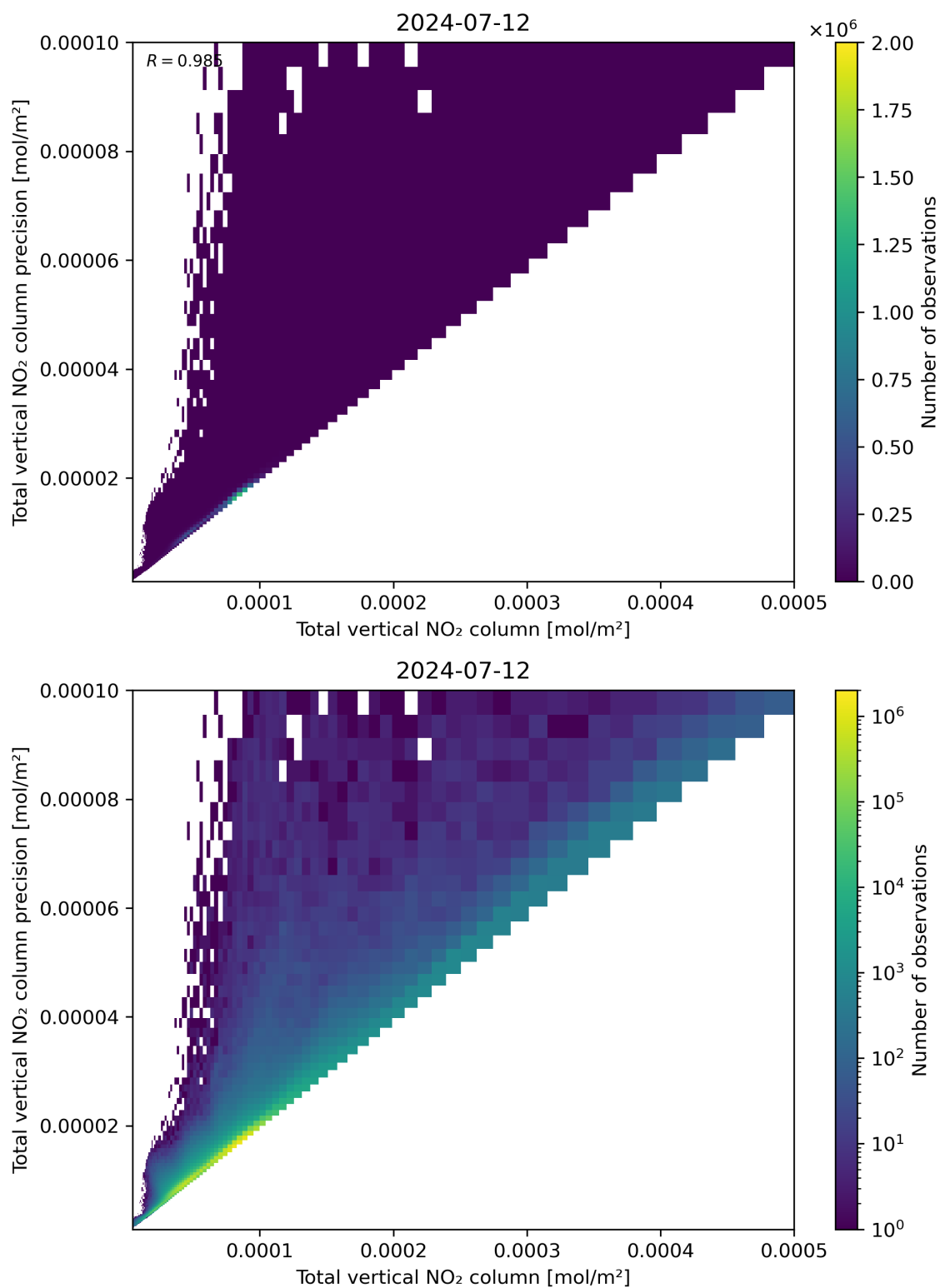
Figure 114: Scatter density plot of “Total vertical NO 2 column” against “Total vertical NO 2 column precision” for 2024-07-11 to 2024-07-13.
