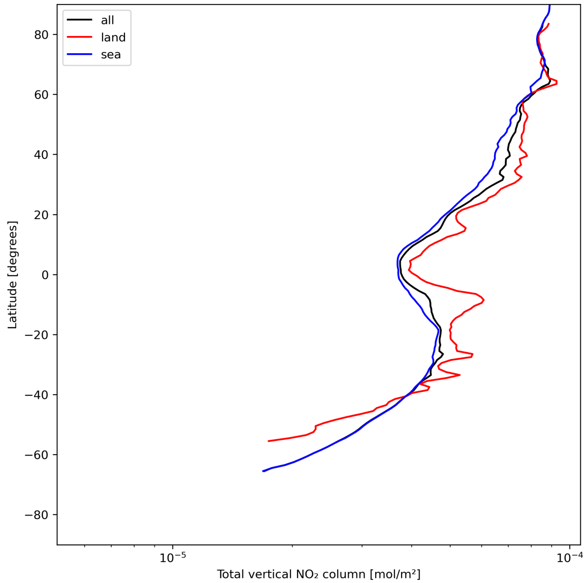
Figure 21: Zonal average of “Total vertical NO 2 column” for 2024-07-11 to 2024-07-13.
