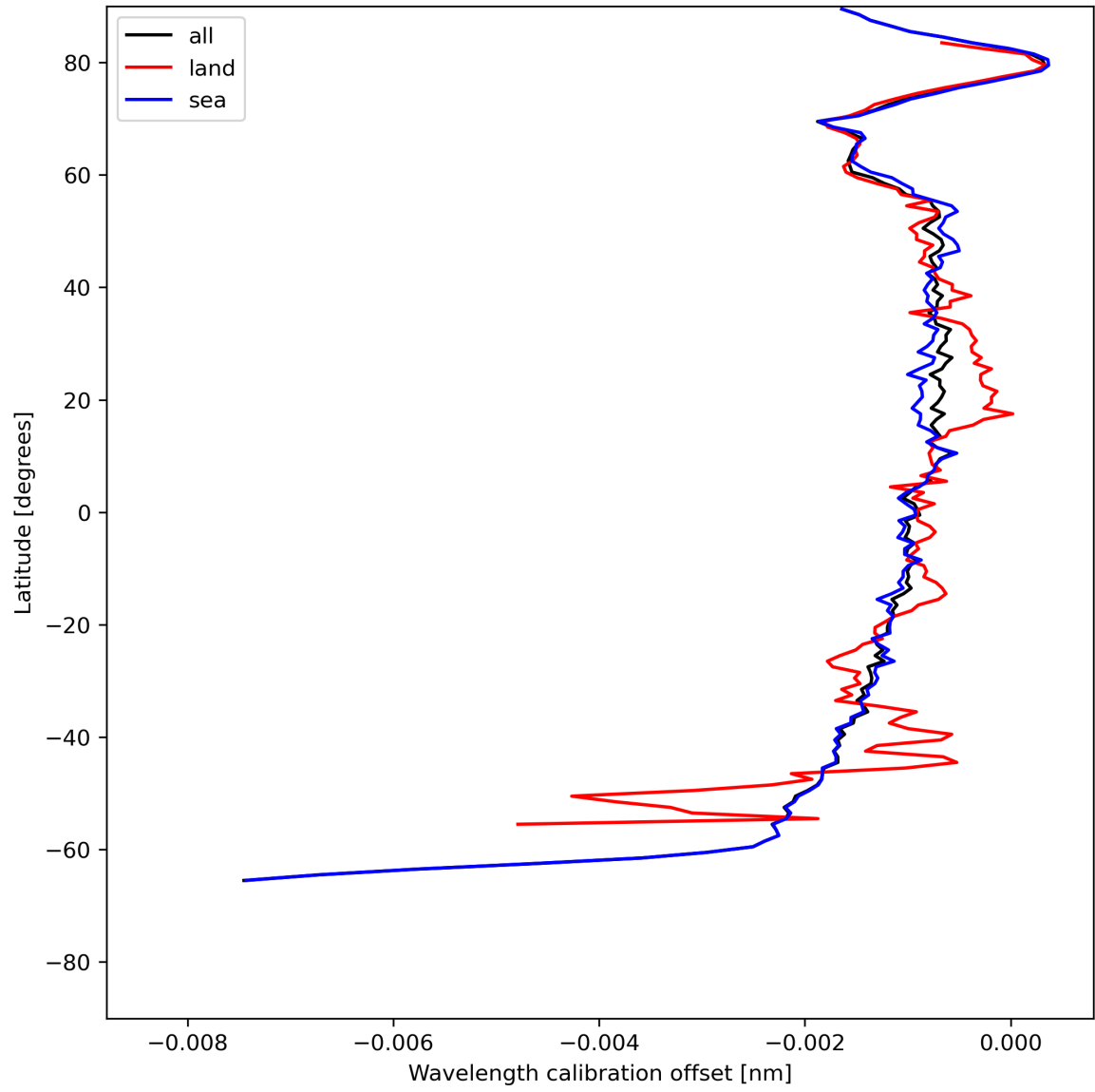
Figure 18: Zonal average of “Wavelength calibration offset” for 2024-07-11 to 2024-07-13.
