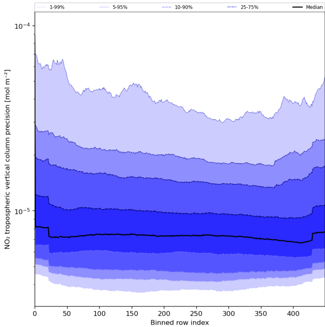
Figure 47: Along track statistics of “NO 2 tropospheric vertical column precision” for 2024-07-11 to 2024-07-13
