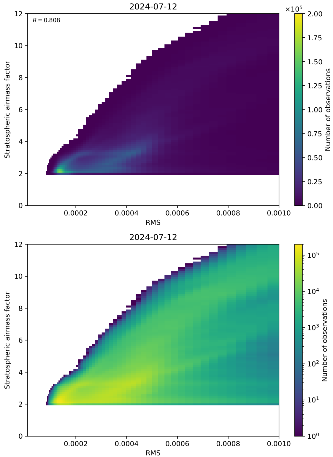
Figure 144: Scatter density plot of “RMS” against “Stratospheric airmass factor” for 2024-07-11 to 2024-07-13.
