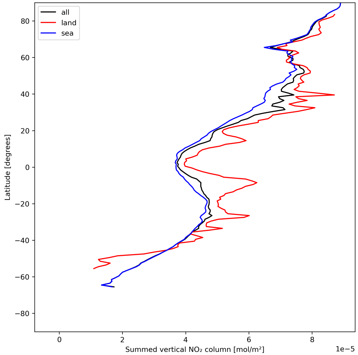
Figure 23: Zonal average of “Summed vertical NO 2 column” for 2024-07-11 to 2024-07-13.
