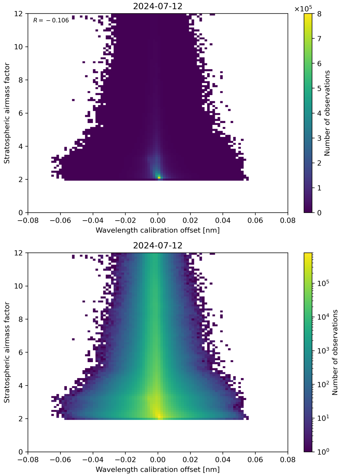
Figure 174: Scatter density plot of “Wavelength calibration offset” against “Stratospheric air mass factor” for 2024-07-11 to 2024-07-13.
