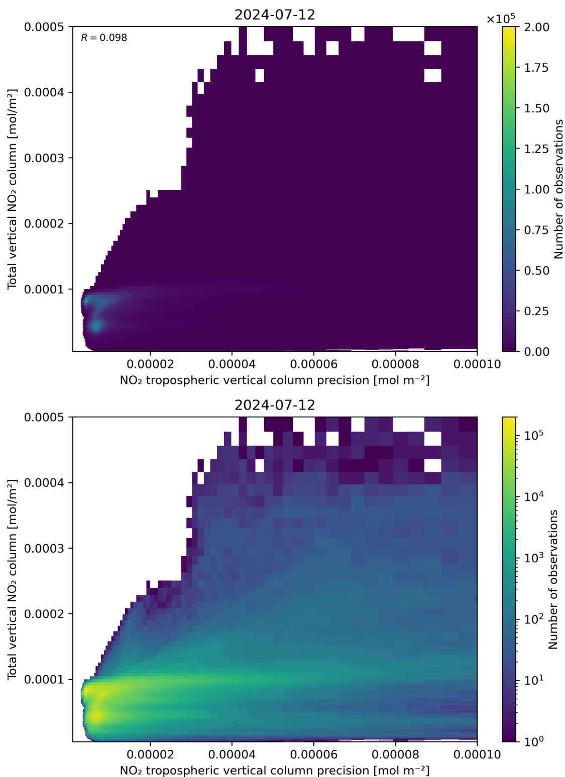
Figure 138: Scatter density plot of “NO 2 tropospheric vertical column precision” against “Total vertical NO 2 column” for 2024-07-11 to 2024-07-13.
