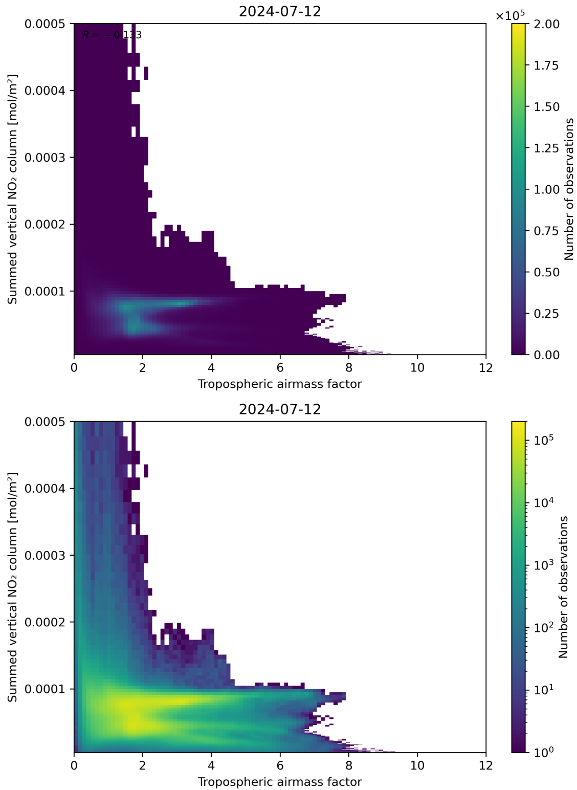
Figure 75: Scatter density plot of “Tropospheric airmass factor” against “Summed vertical NO 2 column” for 2024-07-11 to 2024-07-13.
