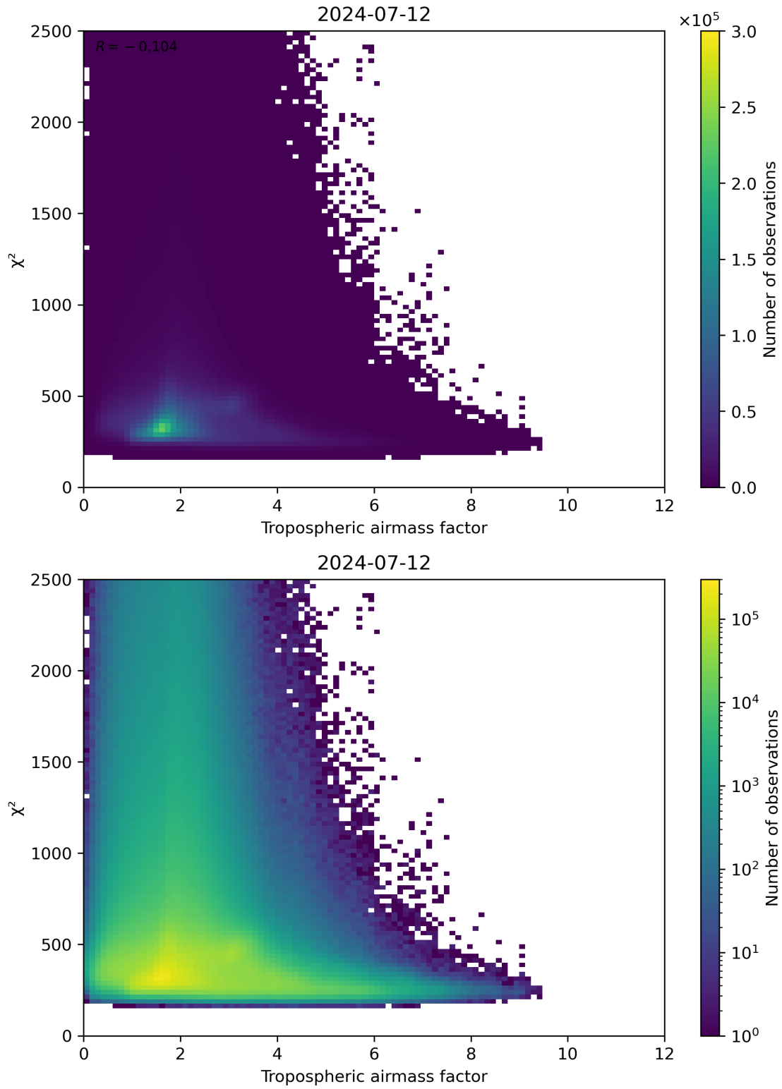
Figure 73: Scatter density plot of “Tropospheric airmass factor” against “ \chi^2 ” for 2024-07-11 to 2024-07-13.
