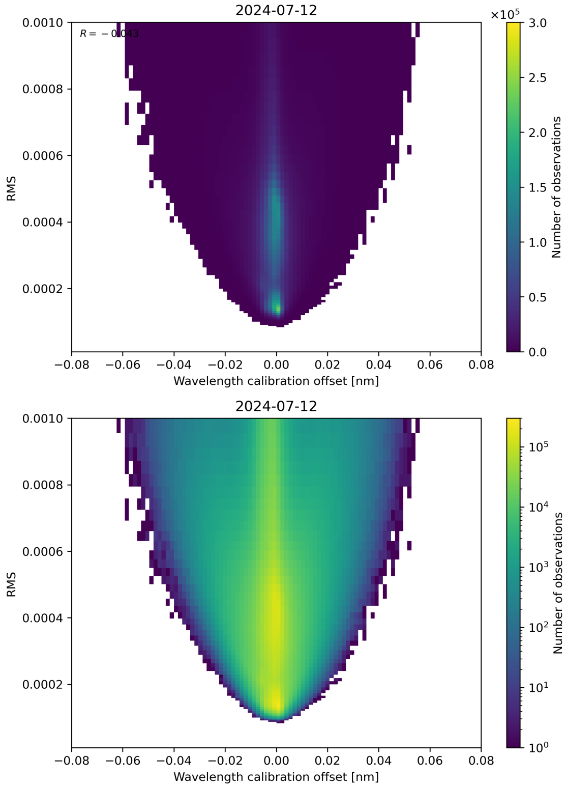
Figure 181: Scatter density plot of “Wavelength calibration offset” against “RMS” for 2024-07-11 to 2024-07-13.
