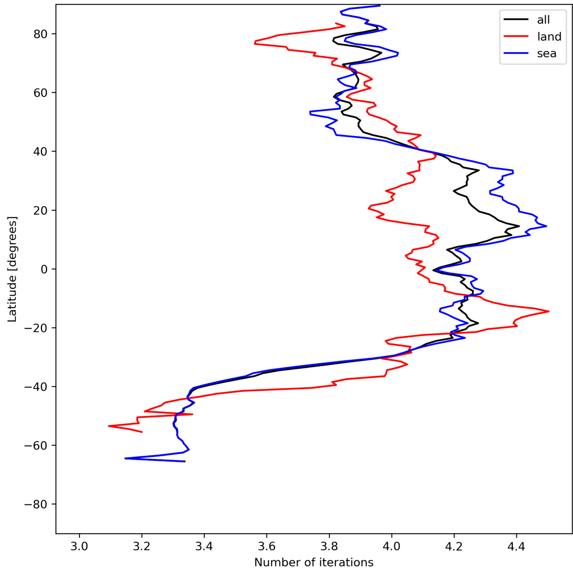
Figure 17: Zonal average of “Number of iterations” for 2024-07-11 to 2024-07-13.
