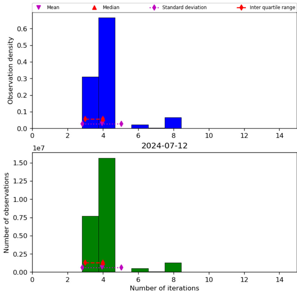
Figure 34: Histogram of “Number of iterations” for 2024-07-11 to 2024-07-13
