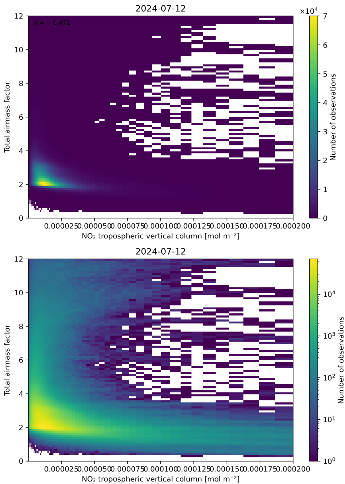
Figure 122: Scatter density plot of “NO 2 tropospheric vertical column” against “Total airmass factor” for 2024-07-11 to 2024-07-13.
