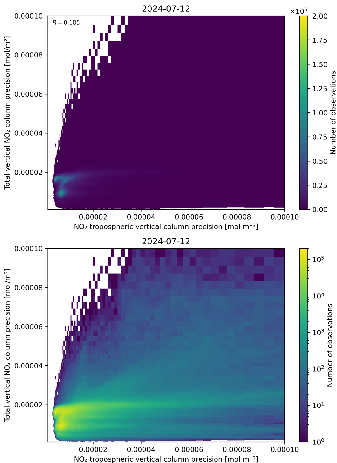
Figure 139: Scatter density plot of “NO 2 tropospheric vertical column precision” against “Total vertical NO 2 column precision” for 2024-07-11 to 2024-07-13.
