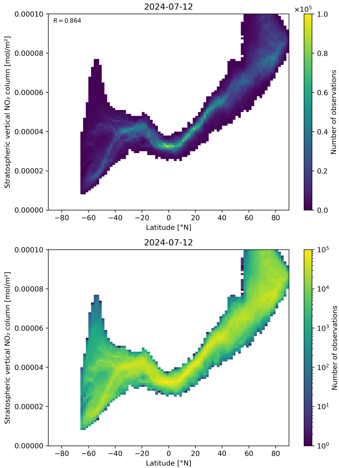
Figure 87: Scatter density plot of “Latitude” against “Stratospheric vertical NO 2 column” for 2024-07-11 to 2024-07-13.
