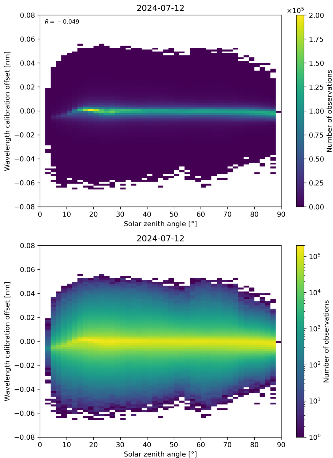
Figure 158: Scatter density plot of “Solar zenith angle” against “Wavelength calibration offset” for 2024-07-11 to 2024-07-13.
