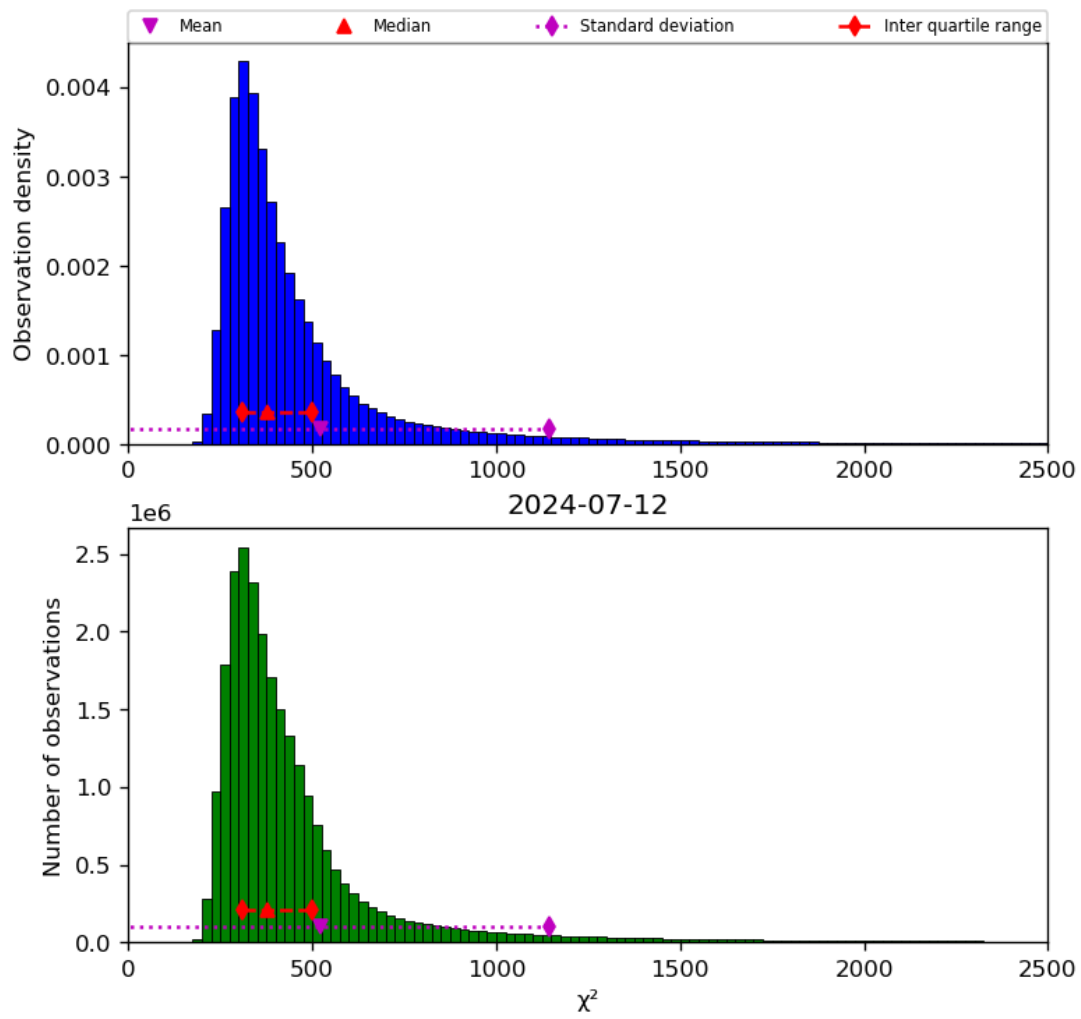
Figure 42: Histogram of “ \chi^2 ” for 2024-07-11 to 2024-07-13
