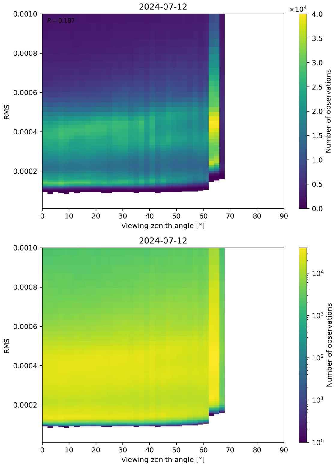
Figure 171: Scatter density plot of “Viewing zenith angle” against “RMS” for 2024-07-11 to 2024-07-13.
