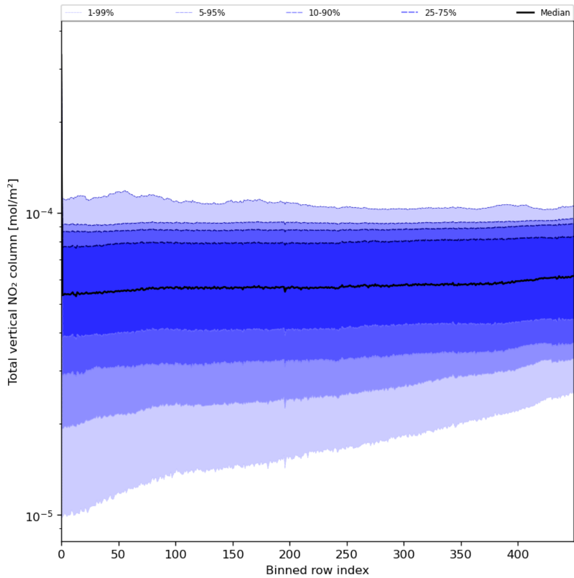
Figure 55: Along track statistics of “Total vertical NO 2 column” for 2024-07-11 to 2024-07-13
