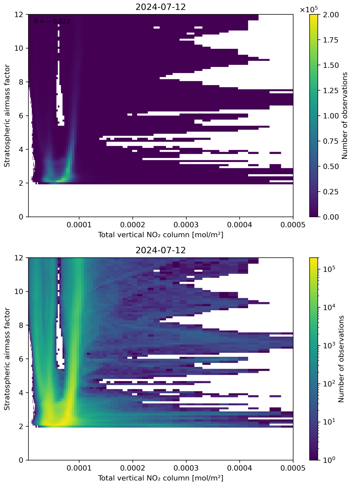
Figure 110: Scatter density plot of “Total vertical NO 2 column” against “Stratospheric airmass factor” for 2024-07-11 to 2024-07-13.
