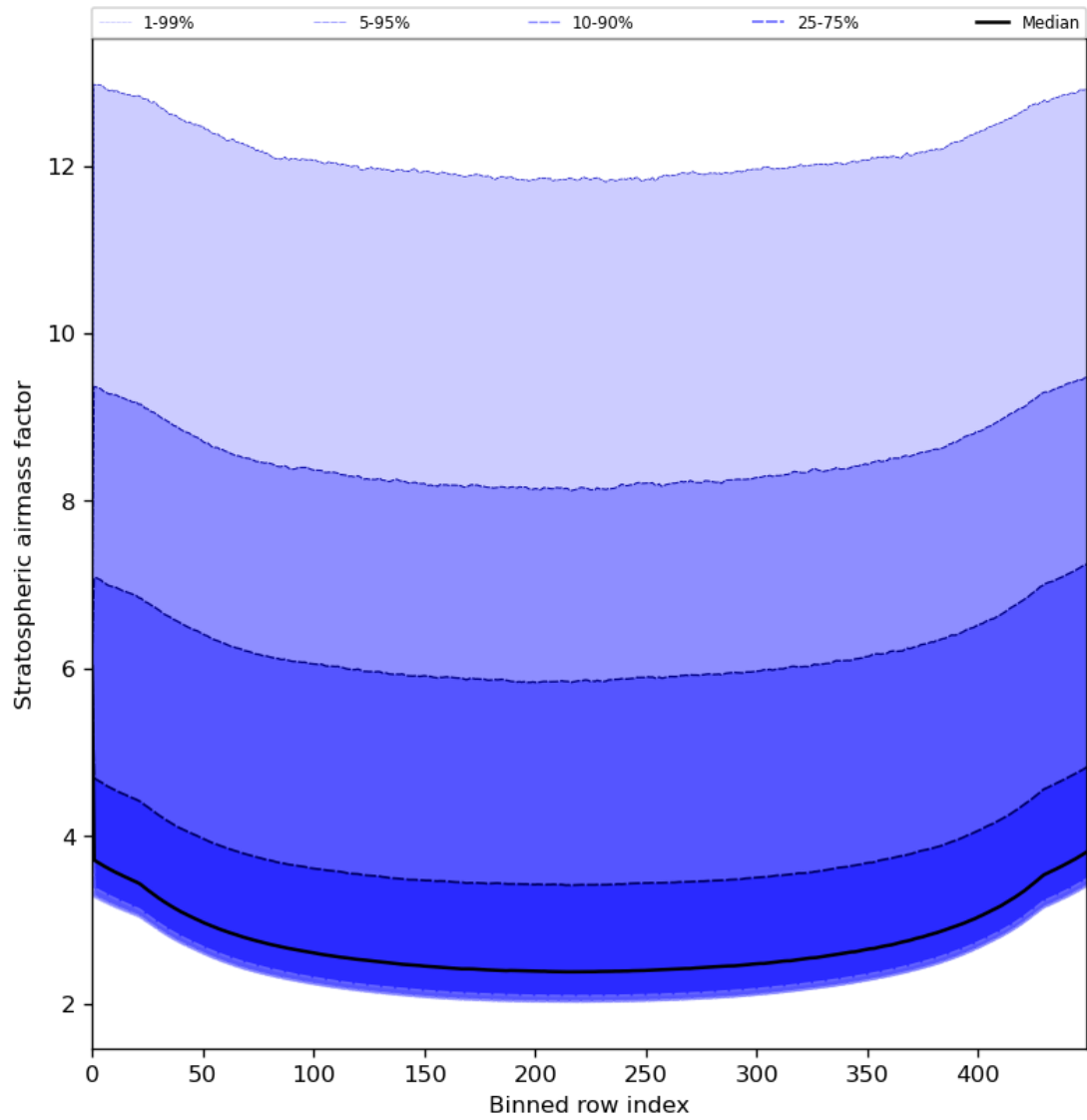
Figure 61: Along track statistics of “Stratospheric airmass factor” for 2024-07-11 to 2024-07-13
