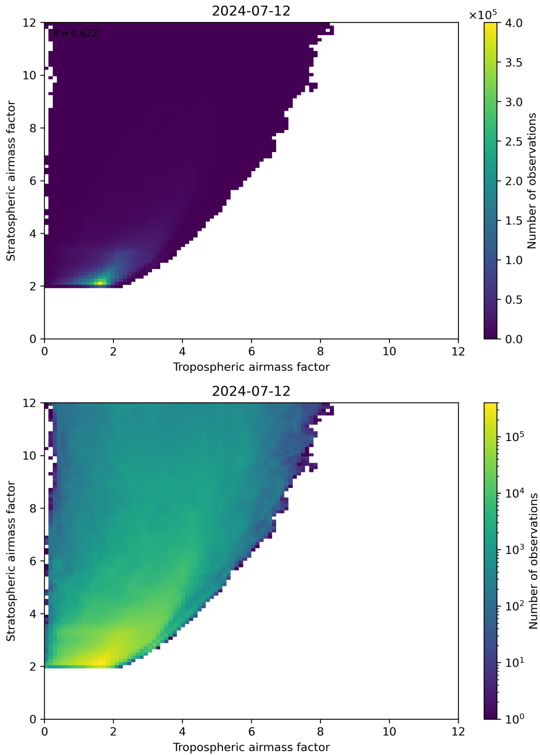
Figure 71: Scatter density plot of “Tropospheric airmass factor” against “Stratospheric airmass factor” for 2024-07-11 to 2024-07-13.
