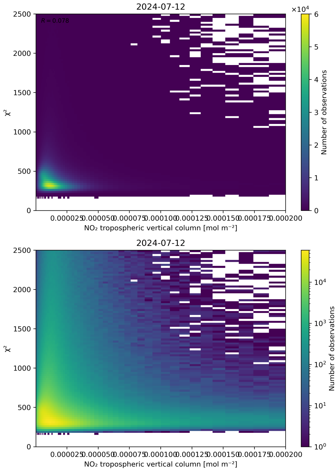
Figure 124: Scatter density plot of “NO 2 tropospheric vertical column” against “ \chi^2 ” for 2024-07-11 to 2024-07-13.
