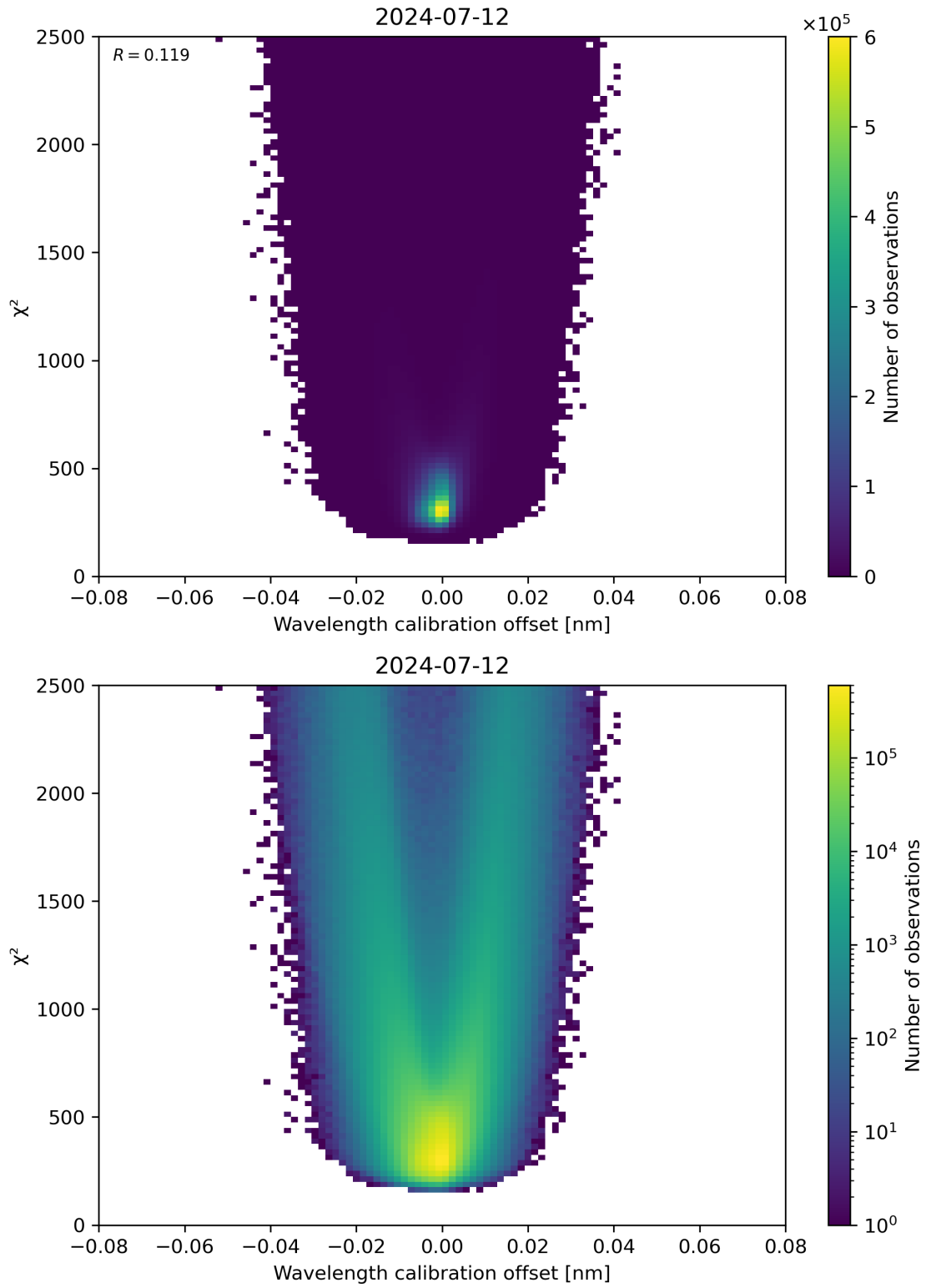
Figure 175: Scatter density plot of “Wavelength calibration offset” against “ \chi^2 ” for 2024-07-11 to 2024-07-13.
