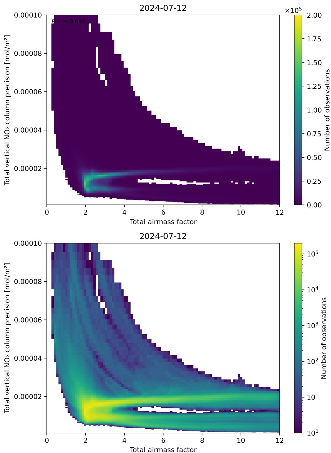
Figure 68: Scatter density plot of “Total airmass factor” against “Total vertical NO 2 column precision” for 2024-07-11 to 2024-07-13.
