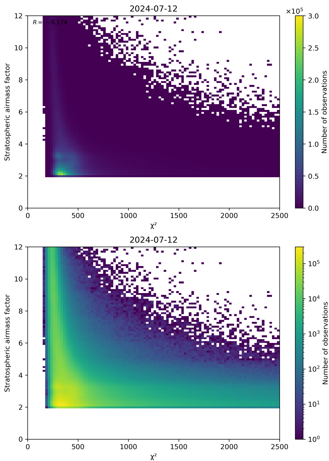
Figure 81: Scatter density plot of “ \chi^2 ” against “Stratospheric airmass factor” for 2024-07-11 to 2024-07-13.
