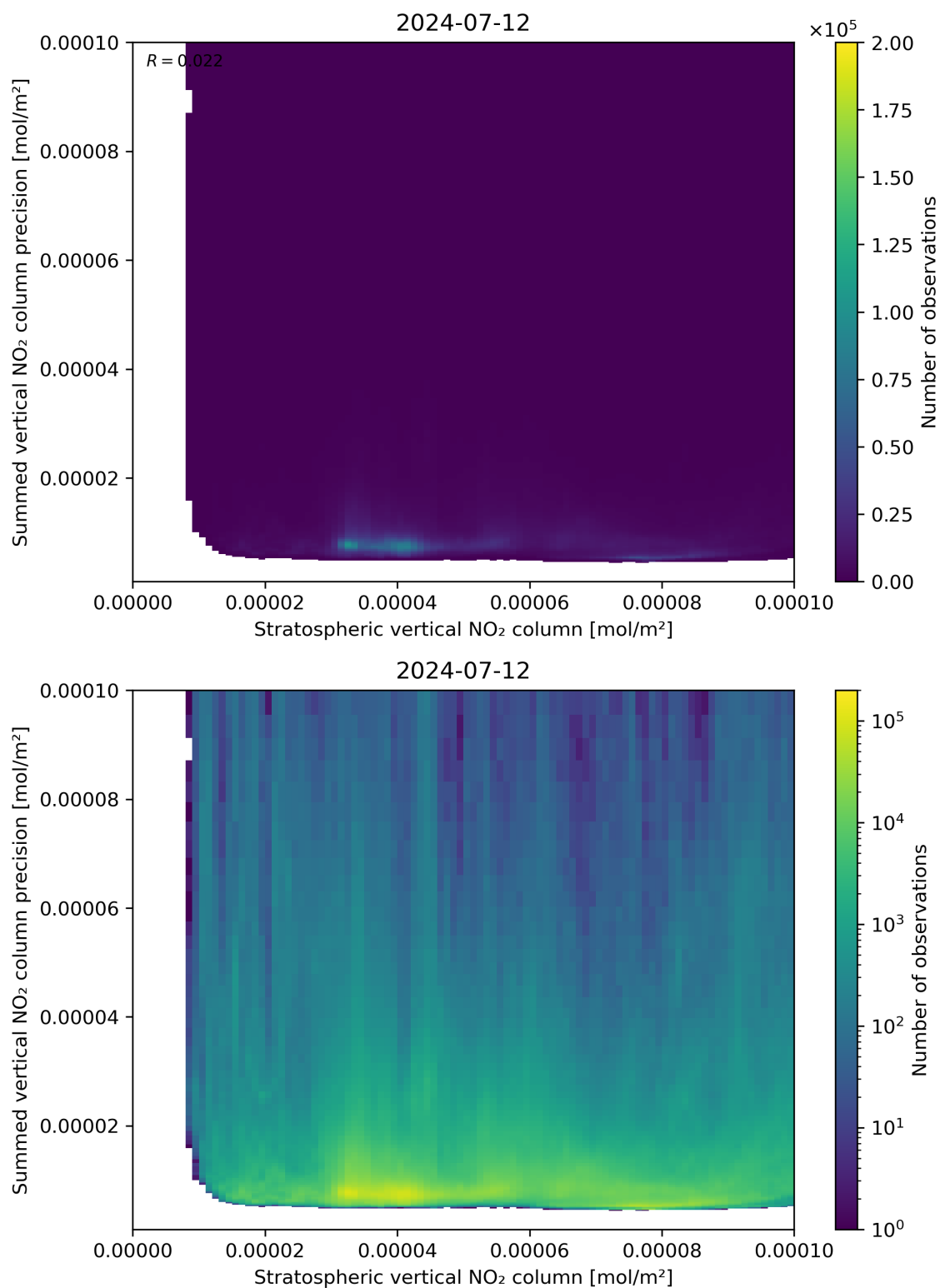
Figure 99: Scatter density plot of “Stratospheric vertical NO 2 column” against “Summed vertical NO 2 column precision” for 2024-07-11 to 2024-07-13.
