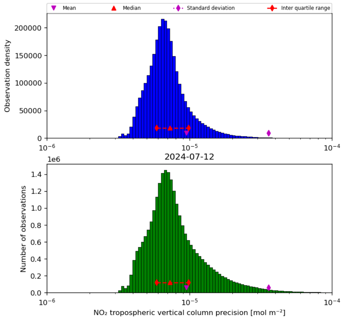
Figure 30: Histogram of “NO 2 tropospheric vertical column precision” for 2024-07-11 to 2024-07-13
