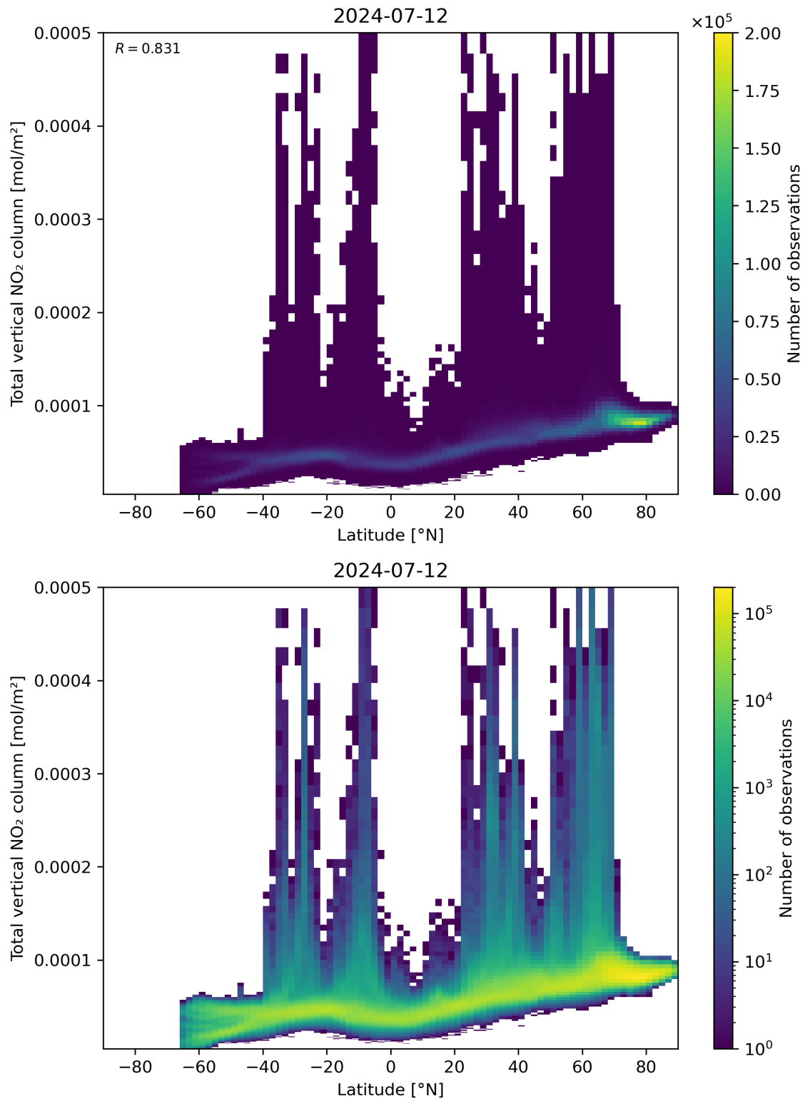
Figure 90: Scatter density plot of “Latitude” against “Total vertical NO 2 column” for 2024-07-11 to 2024-07-13.
