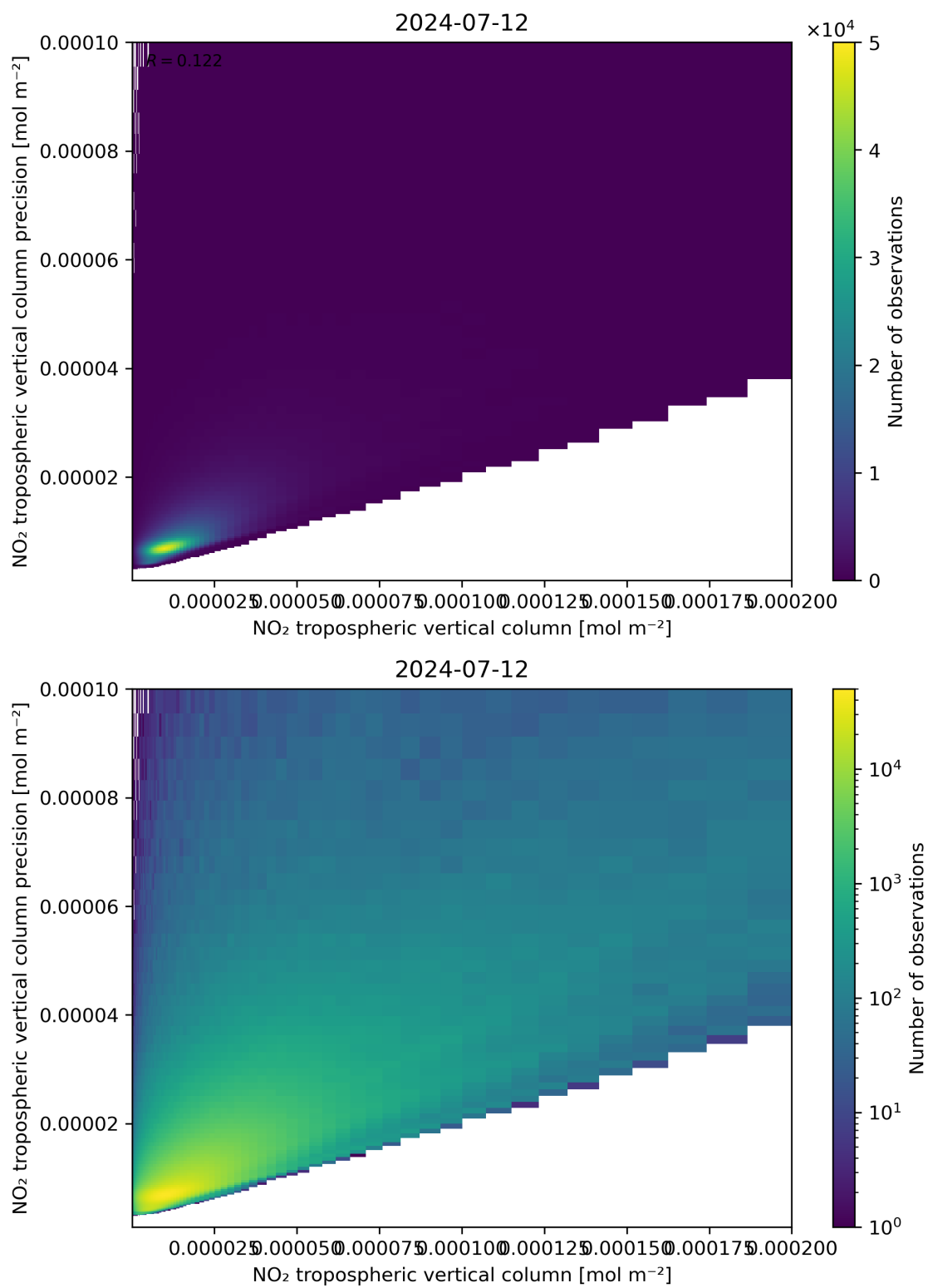
Figure 130: Scatter density plot of “NO 2 tropospheric vertical column” against “NO 2 tropospheric vertical column precision” for 2024-07-11 to 2024-07-13.
