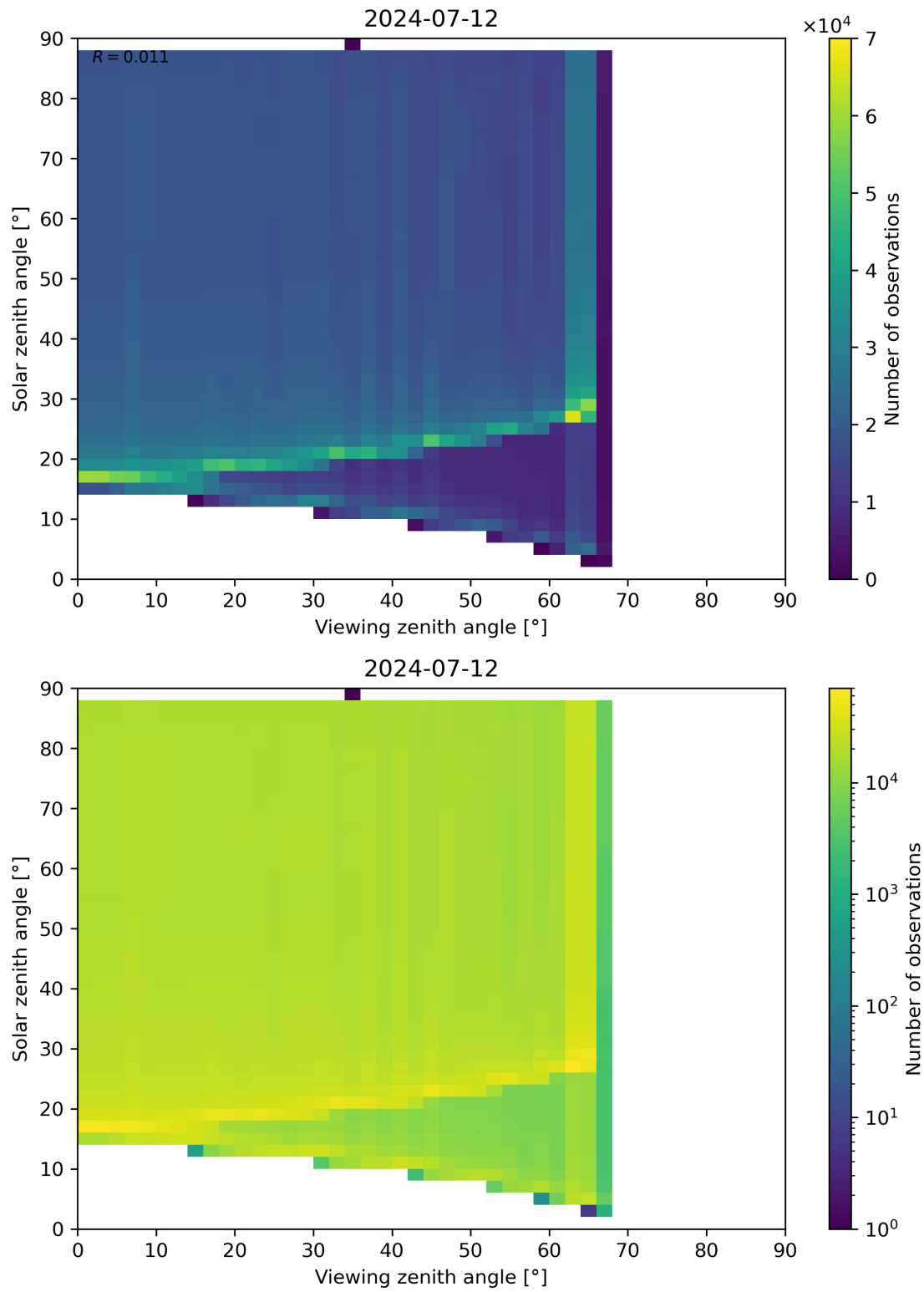
Figure 172: Scatter density plot of “Viewing zenith angle” against “Solar zenith angle” for 2024-07-11 to 2024-07-13.
