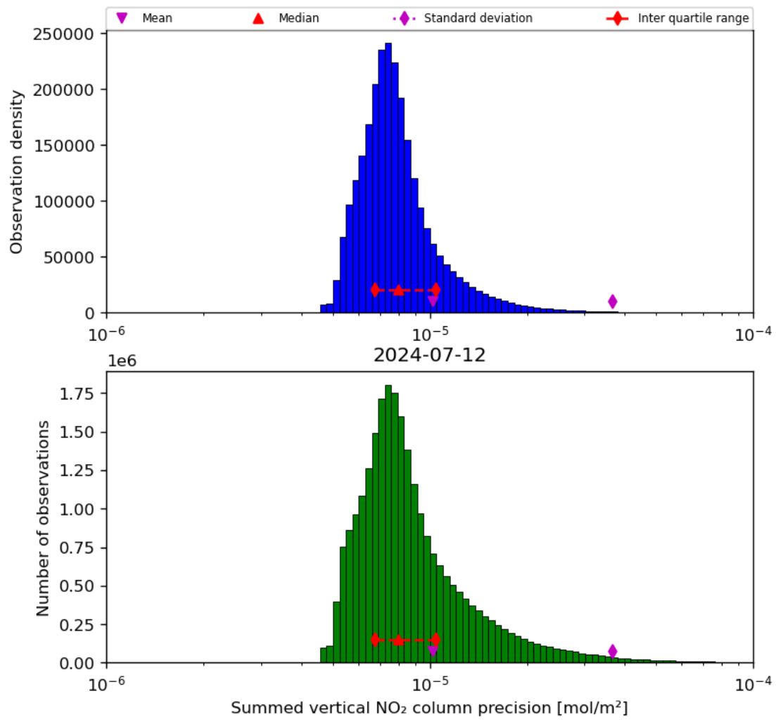
Figure 41: Histogram of "Summed vertical NO 2 column precision" for 2024-07-11 to 2024-07-13
