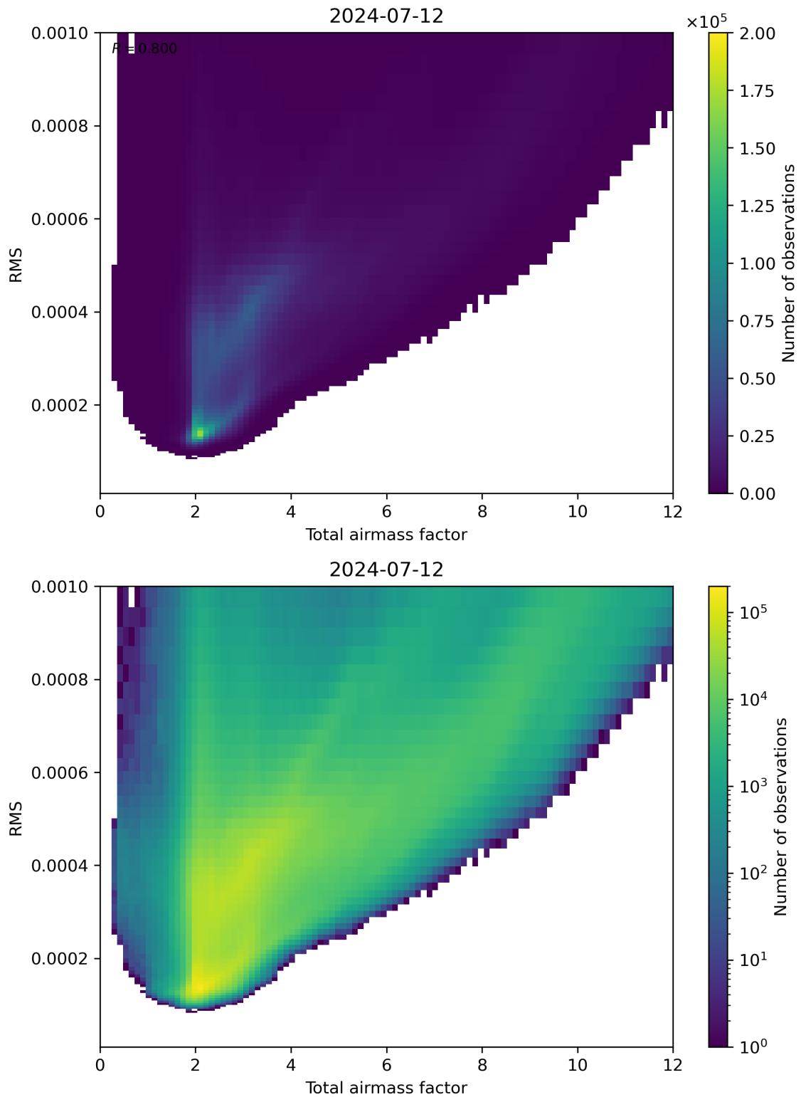
Figure 69: Scatter density plot of “Total airmass factor” against “RMS” for 2024-07-11 to 2024-07-13.
