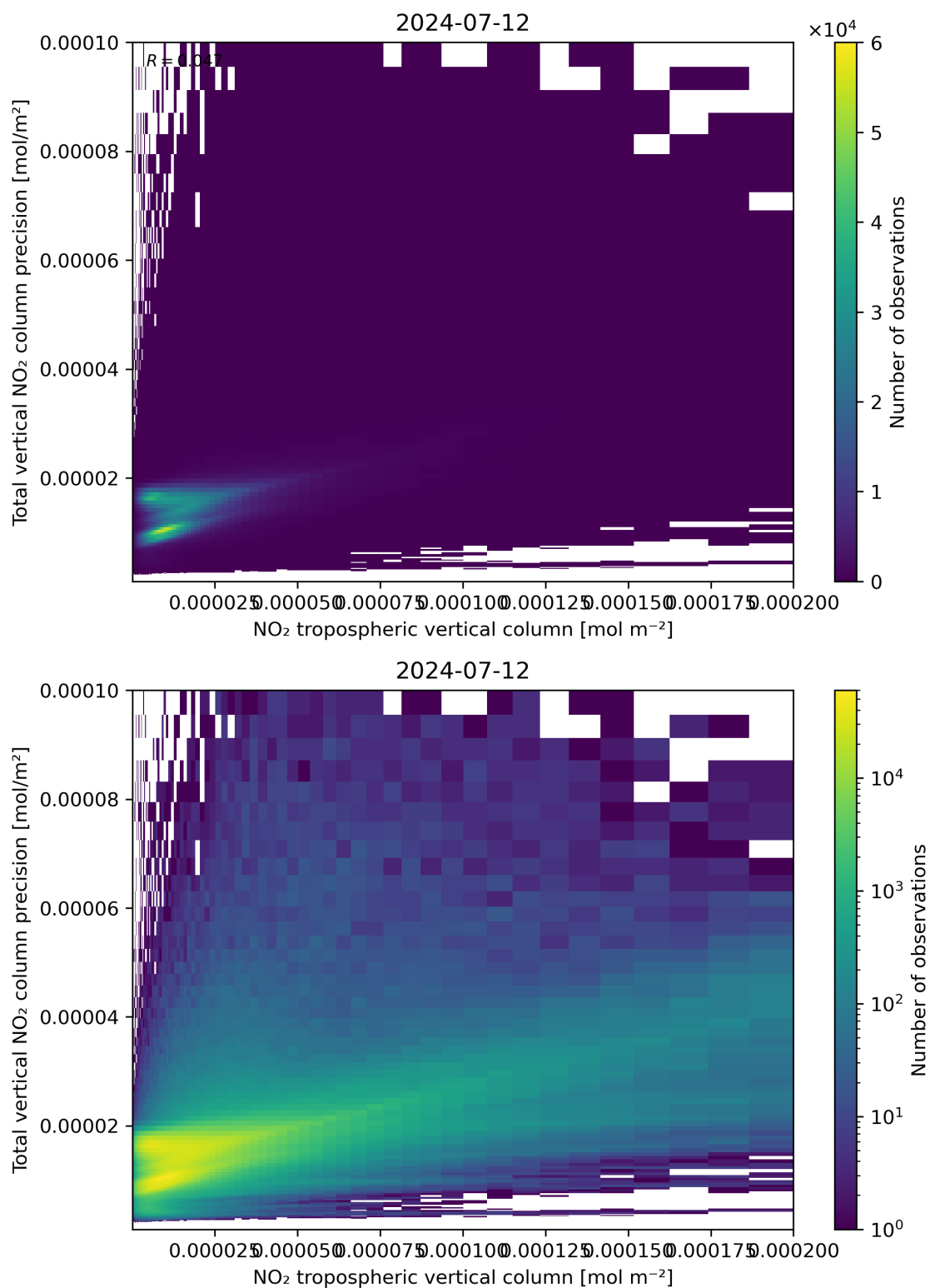
Figure 129: Scatter density plot of “NO 2 tropospheric vertical column” against “Total vertical NO 2 column precision” for 2024-07-11 to 2024-07-13.
