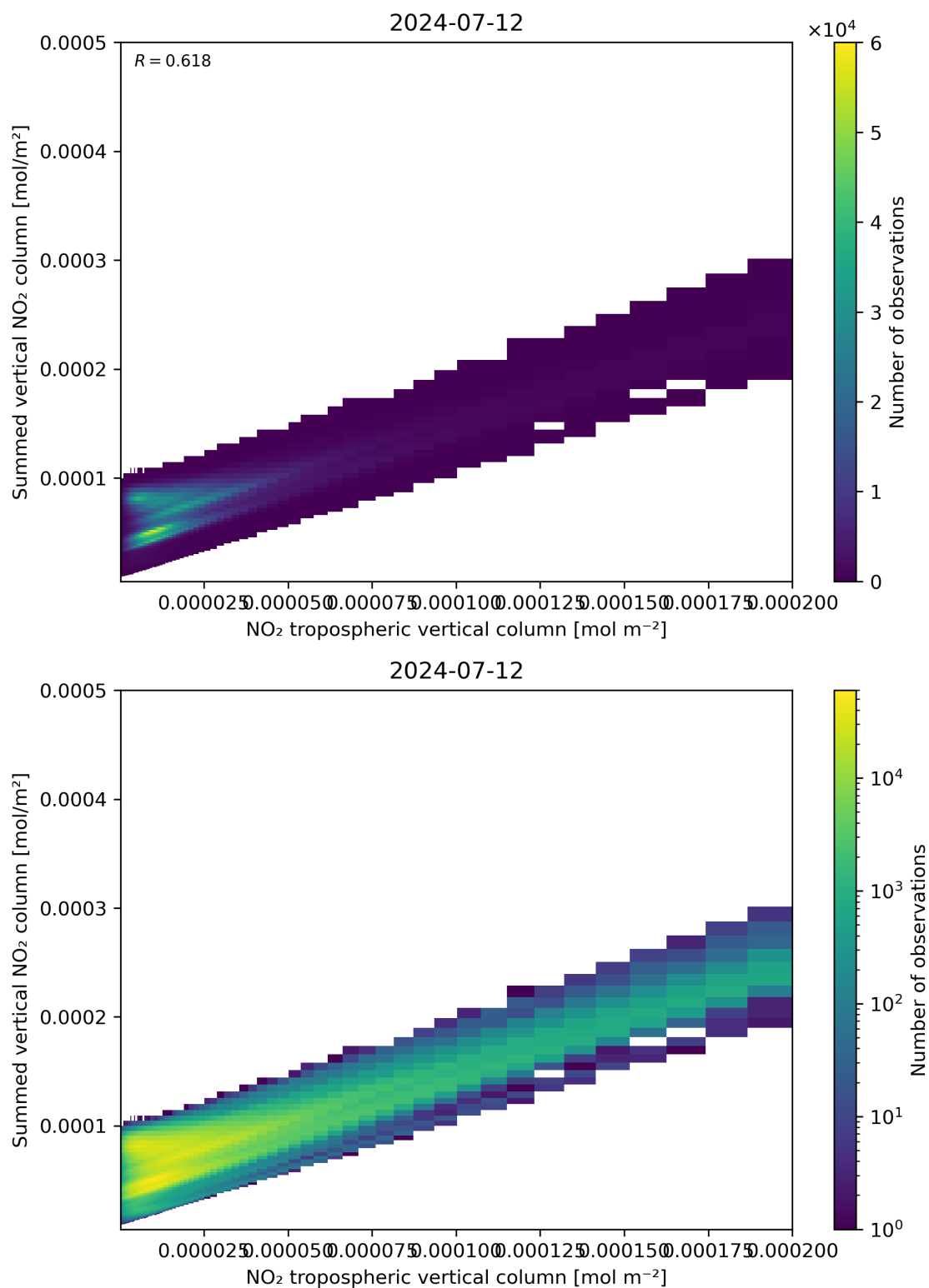
Figure 126: Scatter density plot of “NO 2 tropospheric vertical column” against “Summed vertical NO 2 column” for 2024-07-11 to 2024-07-13.
