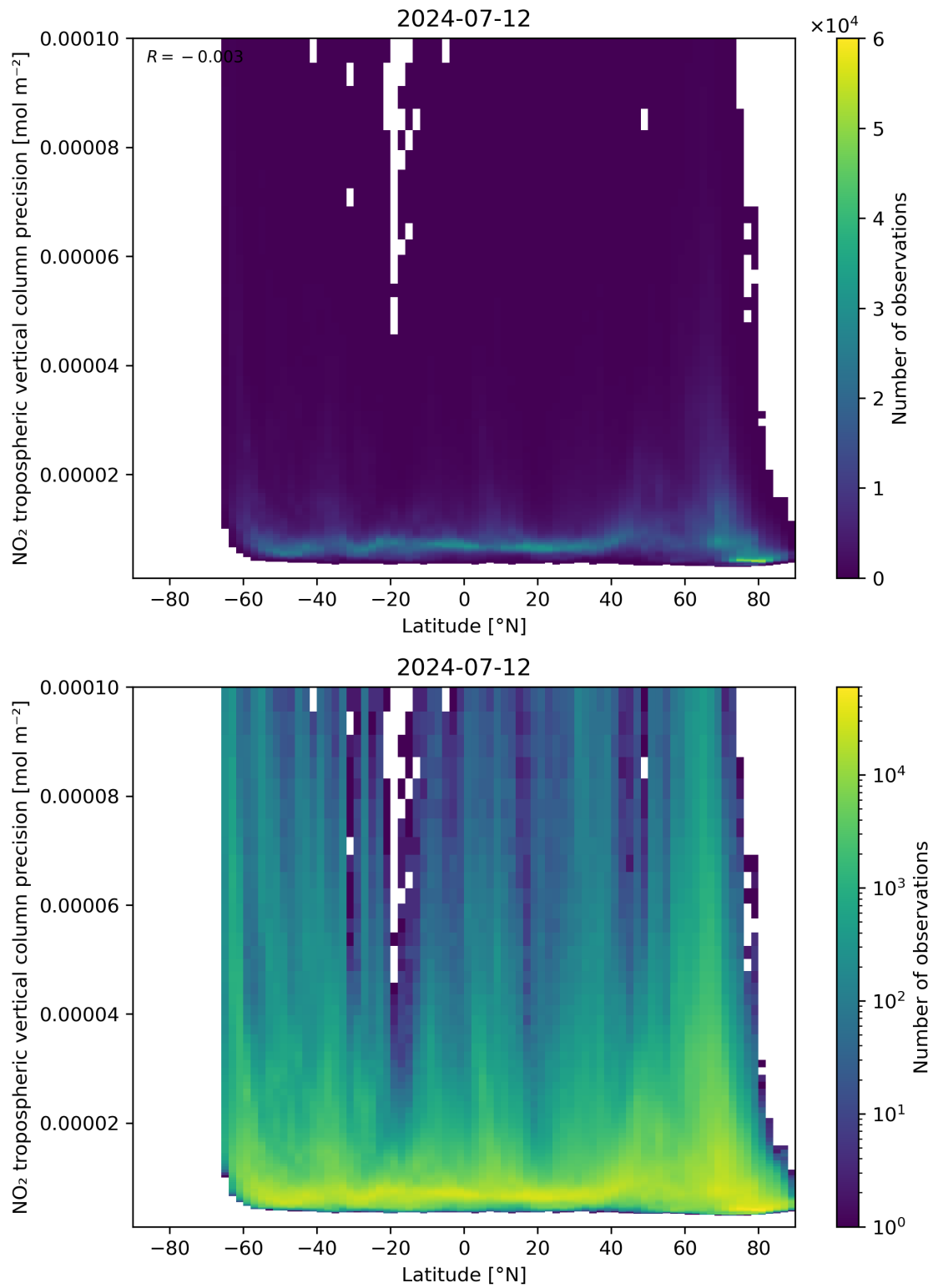
Figure 93: Scatter density plot of “Latitude” against “NO 2 tropospheric vertical column precision” for 2024-07-11 to 2024-07-13.
