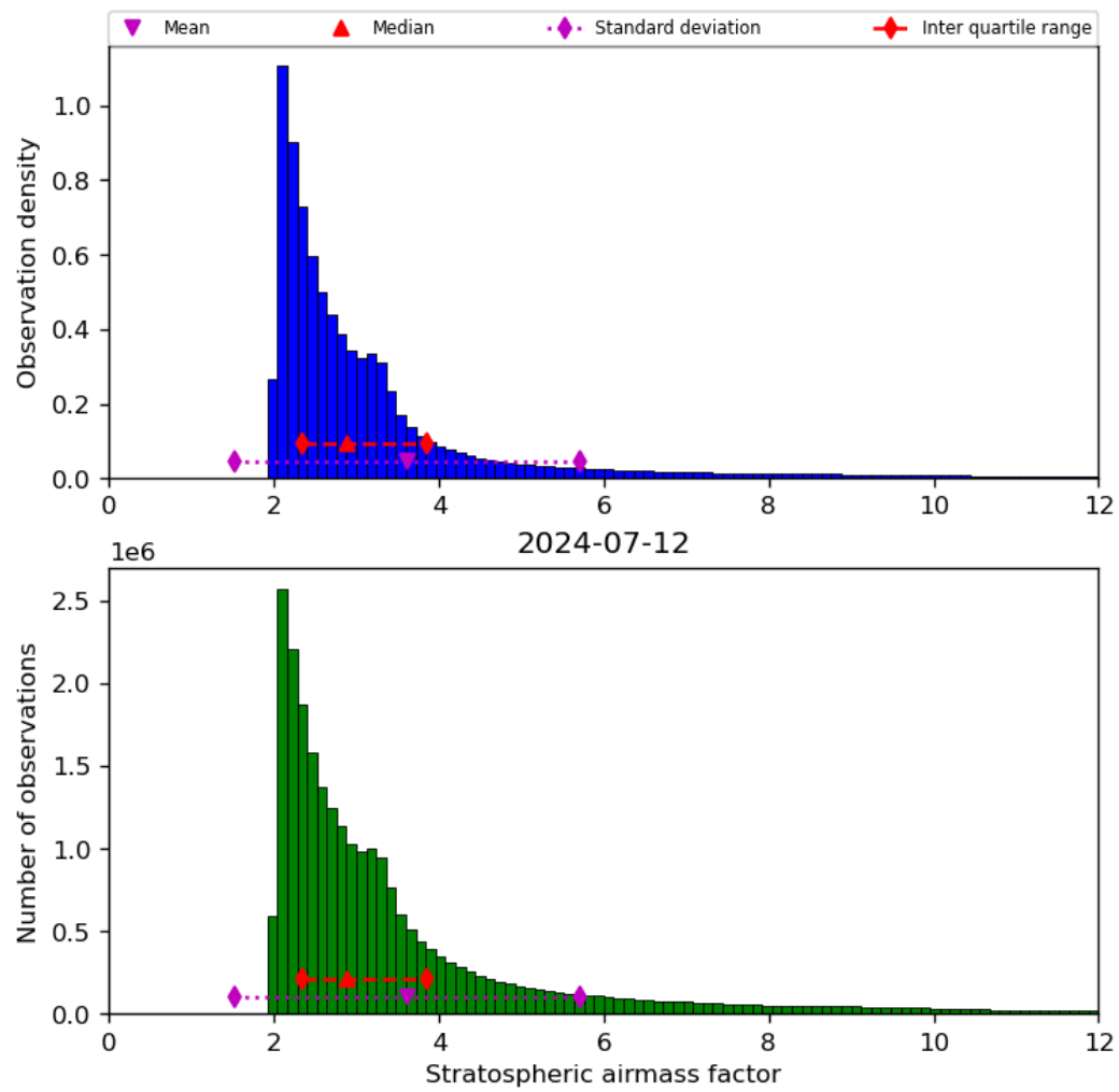
Figure 44: Histogram of “Stratospheric airmass factor” for 2024-07-11 to 2024-07-13
