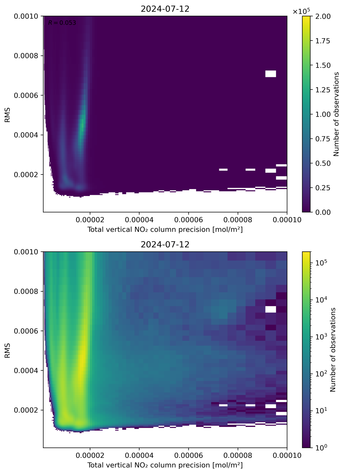
Figure 119: Scatter density plot of “Total vertical NO 2 column precision” against “RMS” for 2024-07-11 to 2024-07-13.
