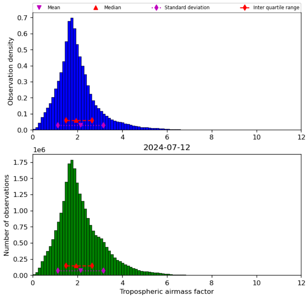
Figure 31: Histogram of “Tropospheric airmass factor” for 2024-07-11 to 2024-07-13
