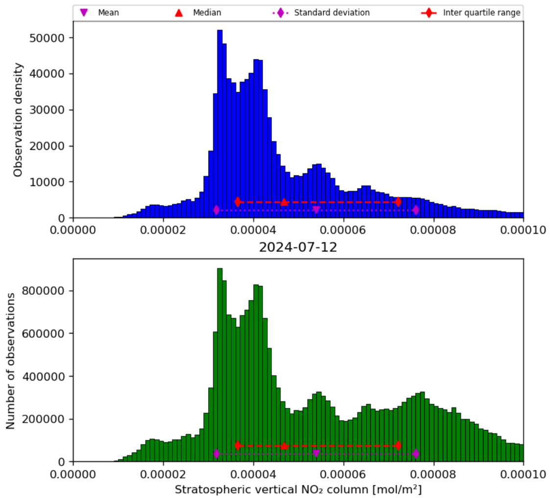
Figure 36: Histogram of “Stratospheric vertical NO 2 column” for 2024-07-11 to 2024-07-13
