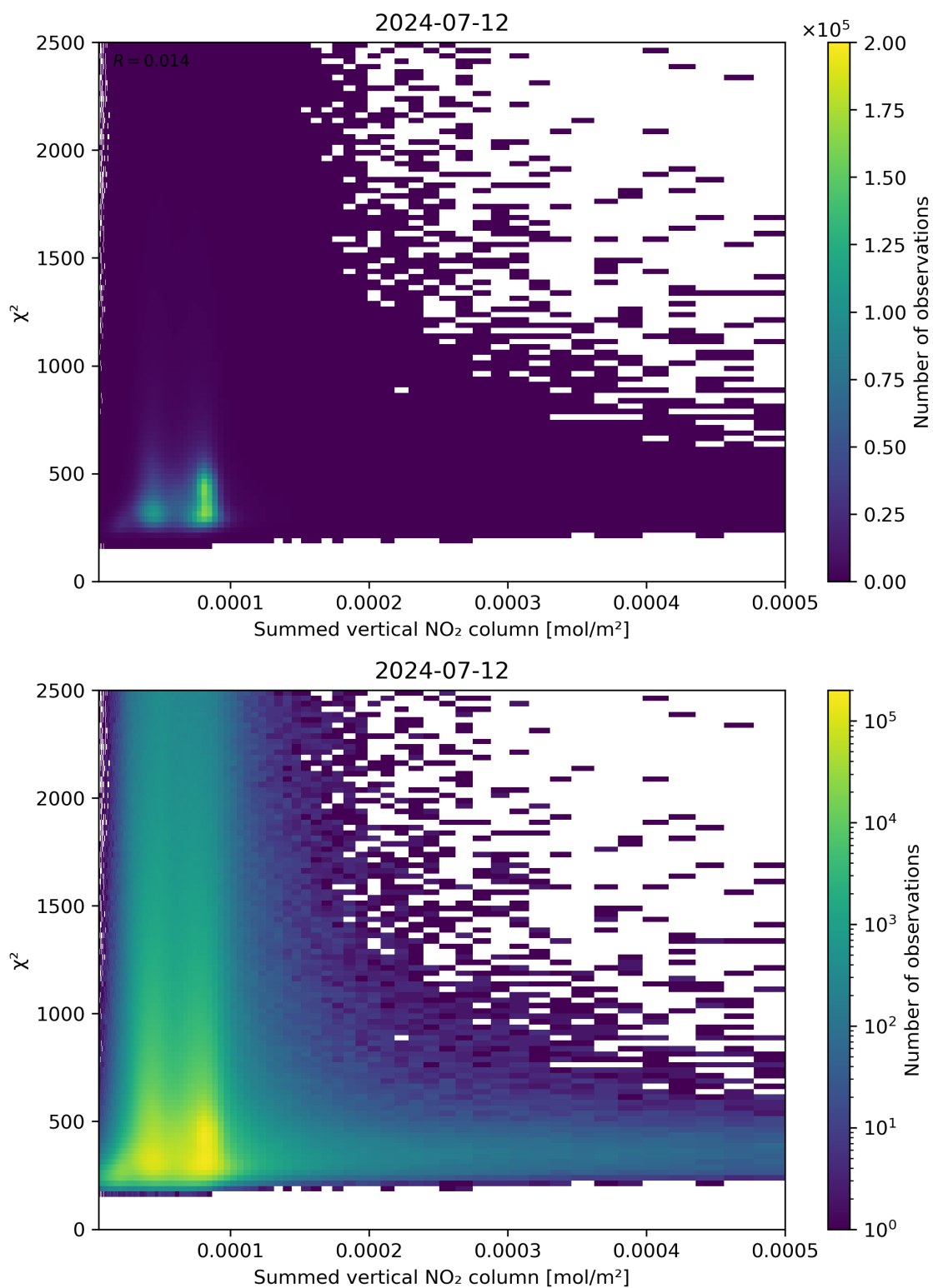
Figure 104: Scatter density plot of “Summed vertical NO 2 column” against “ \chi^2 ” for 2024-07-11 to 2024-07-13.
