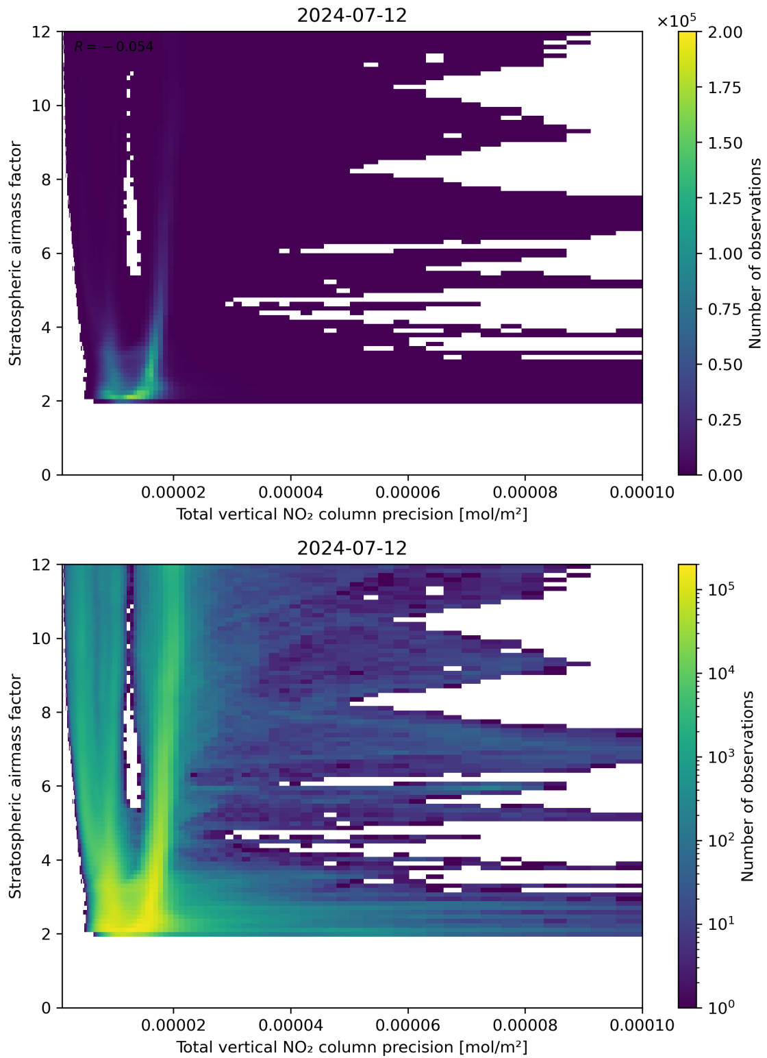
Figure 115: Scatter density plot of “Total vertical NO 2 column precision” against “Stratospheric air mass factor” for 2024-07-11 to 2024-07-13.
