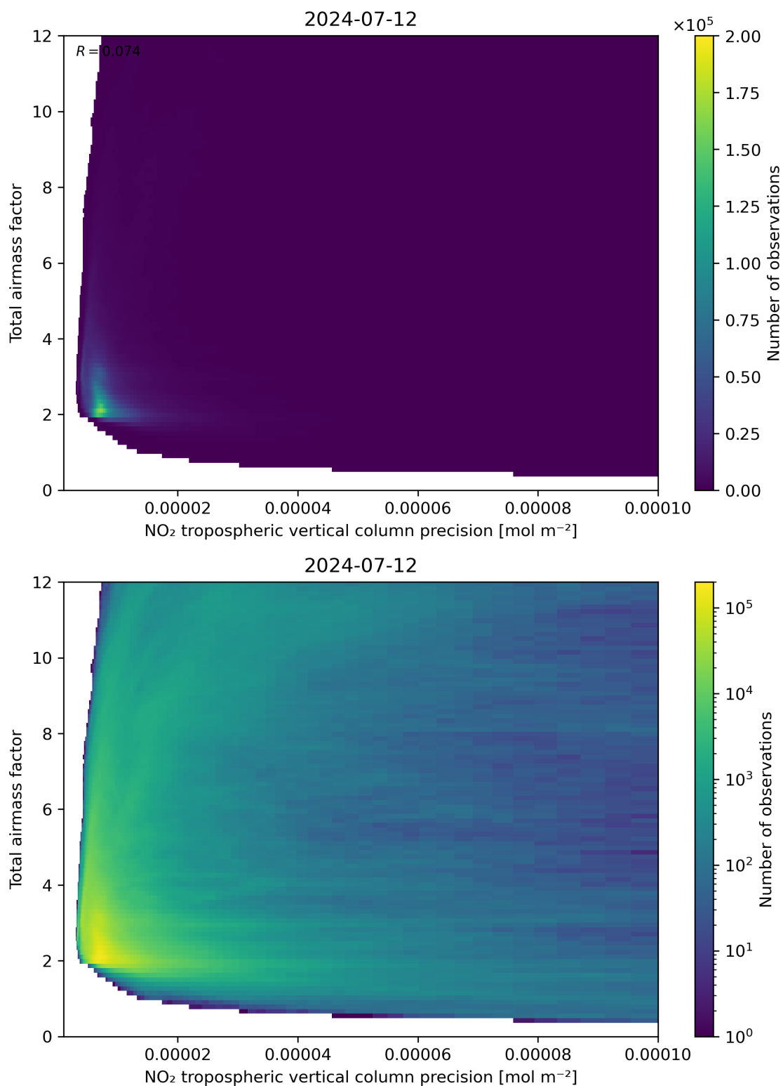
Figure 132: Scatter density plot of “NO 2 tropospheric vertical column precision” against “Total air mass factor” for 2024-07-11 to 2024-07-13.
