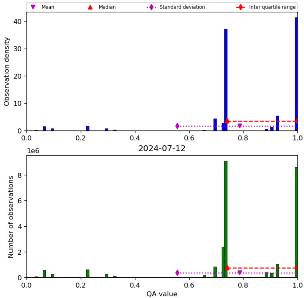
Figure 28: Histogram of “QA value” for 2024-07-11 to 2024-07-13
