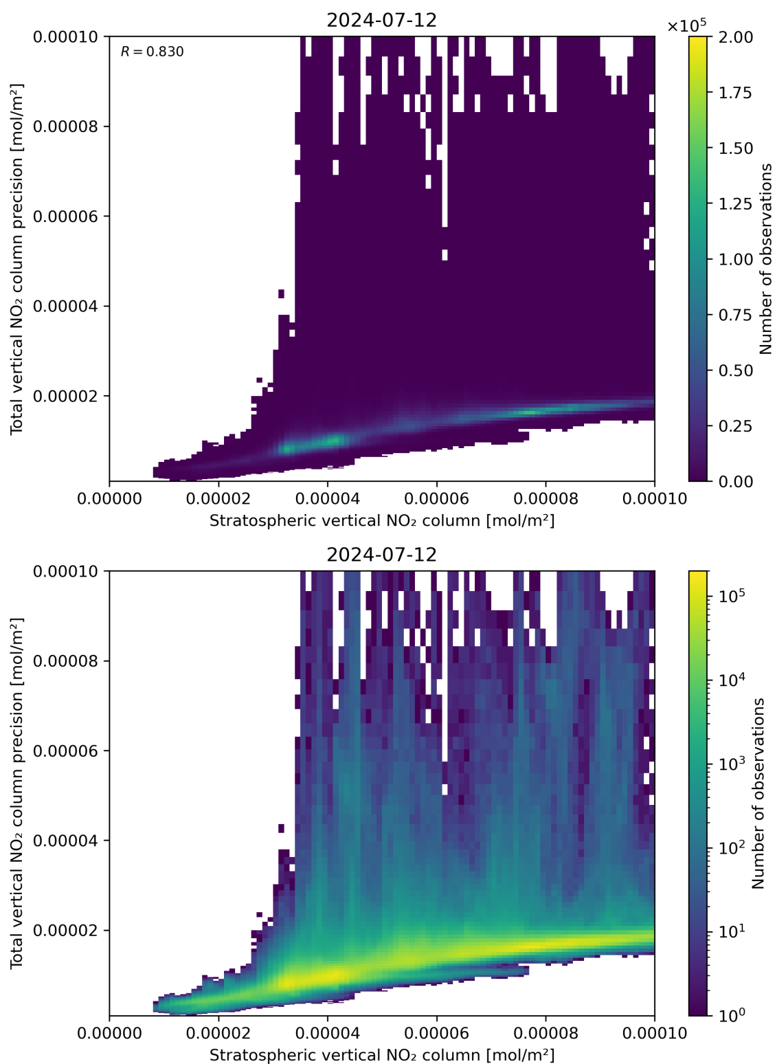
Figure 101: Scatter density plot of “Stratospheric vertical NO 2 column” against “Total vertical NO 2 column precision” for 2024-07-11 to 2024-07-13.
