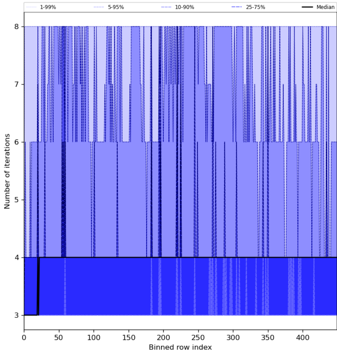
Figure 51: Along track statistics of “Number of iterations” for 2024-07-11 to 2024-07-13
