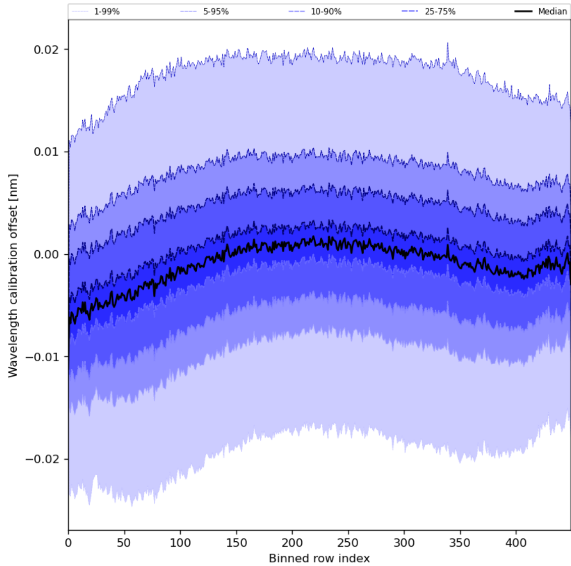
Figure 52: Along track statistics of “Wavelength calibration offset” for 2024-07-11 to 2024-07-13
