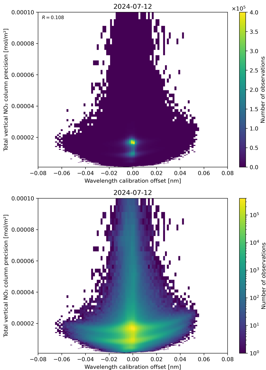
Figure 180: Scatter density plot of “Wavelength calibration offset” against “Total vertical NO 2 column precision” for 2024-07-11 to 2024-07-13.
