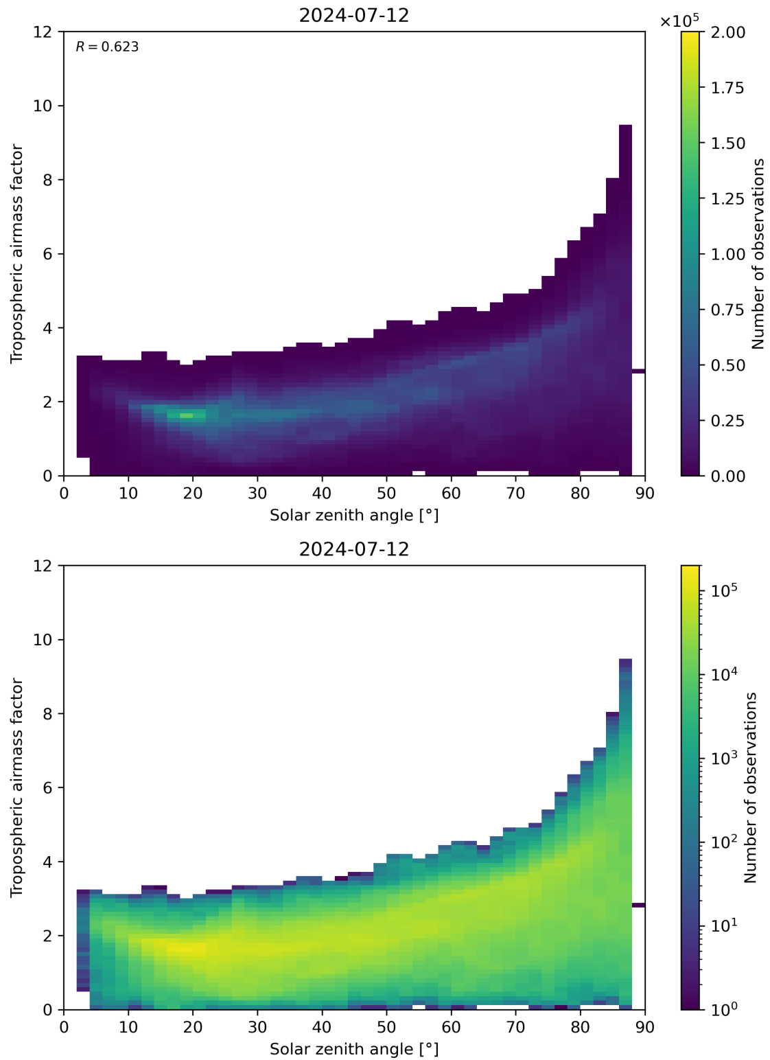
Figure 147: Scatter density plot of “Solar zenith angle” against “Tropospheric airmass factor” for 2024-07-11 to 2024-07-13.
