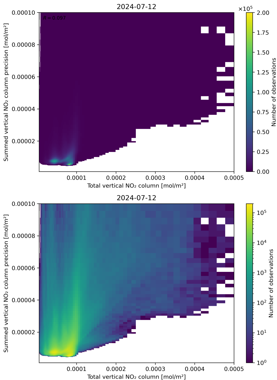
Figure 113: Scatter density plot of “Total vertical NO 2 column” against “Summed vertical NO 2 column precision” for 2024-07-11 to 2024-07-13.
