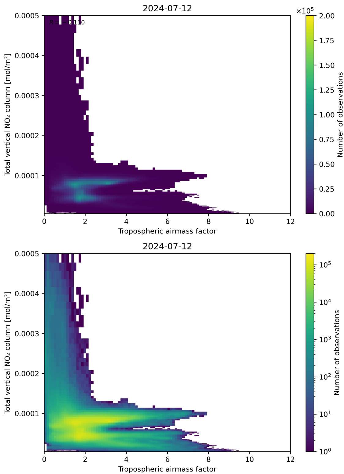
Figure 77: Scatter density plot of “Tropospheric airmass factor” against “Total vertical NO 2 column” for 2024-07-11 to 2024-07-13.
