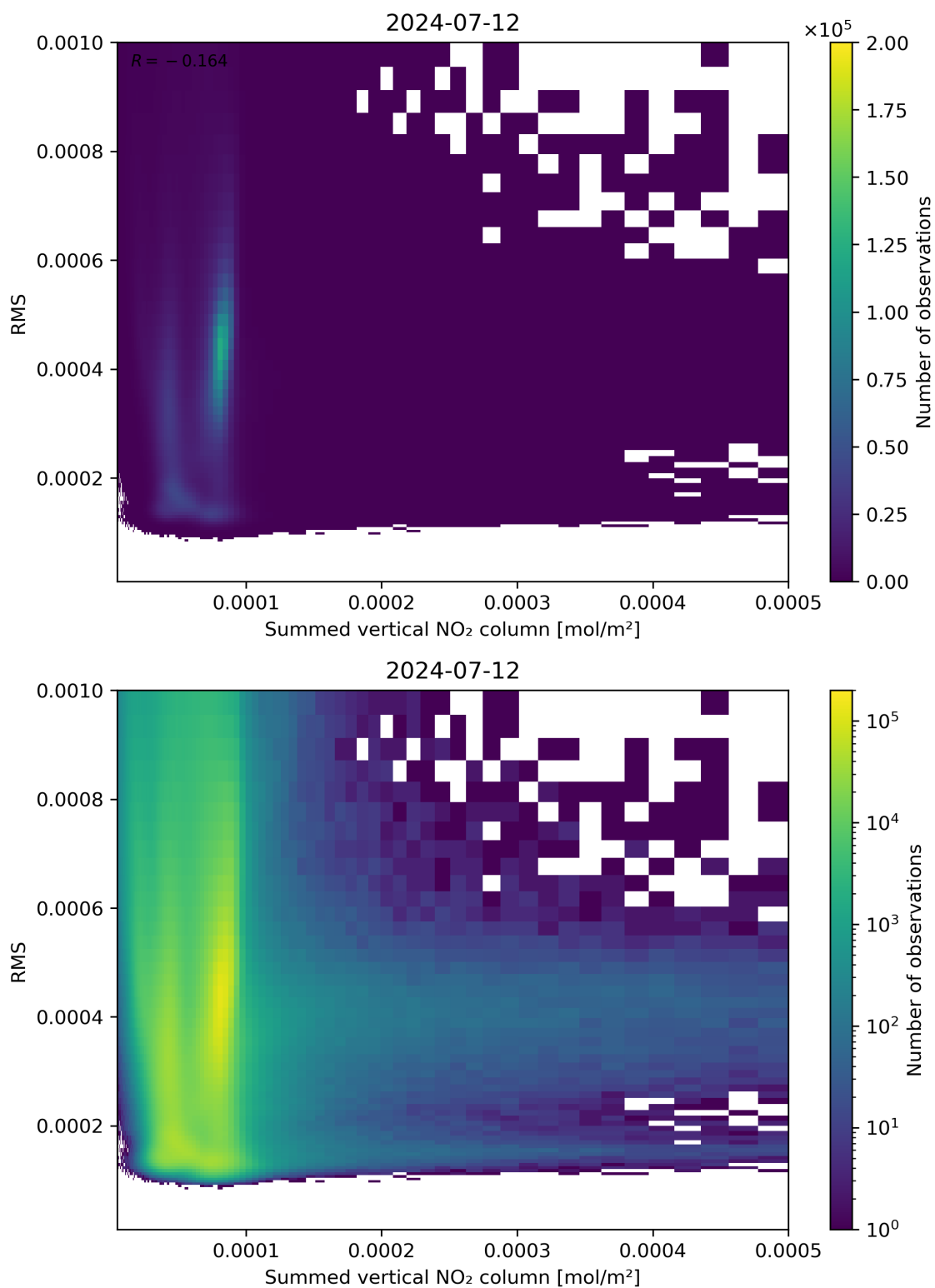
Figure 109: Scatter density plot of “Summed vertical NO 2 column” against “RMS” for 2024-07-11 to 2024-07-13.
