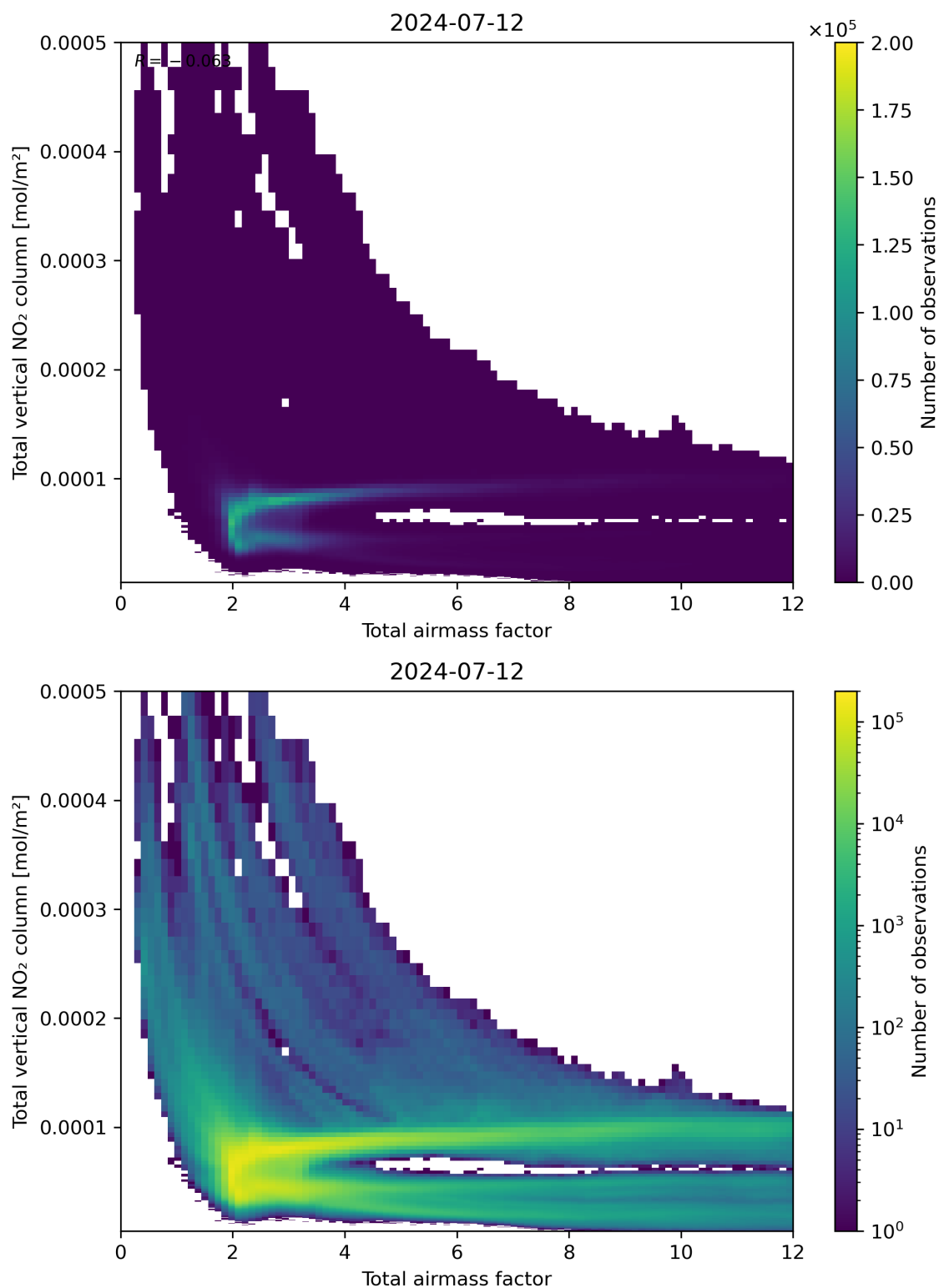
Figure 67: Scatter density plot of “Total airmass factor” against “Total vertical NO 2 column” for 2024-07-11 to 2024-07-13.
