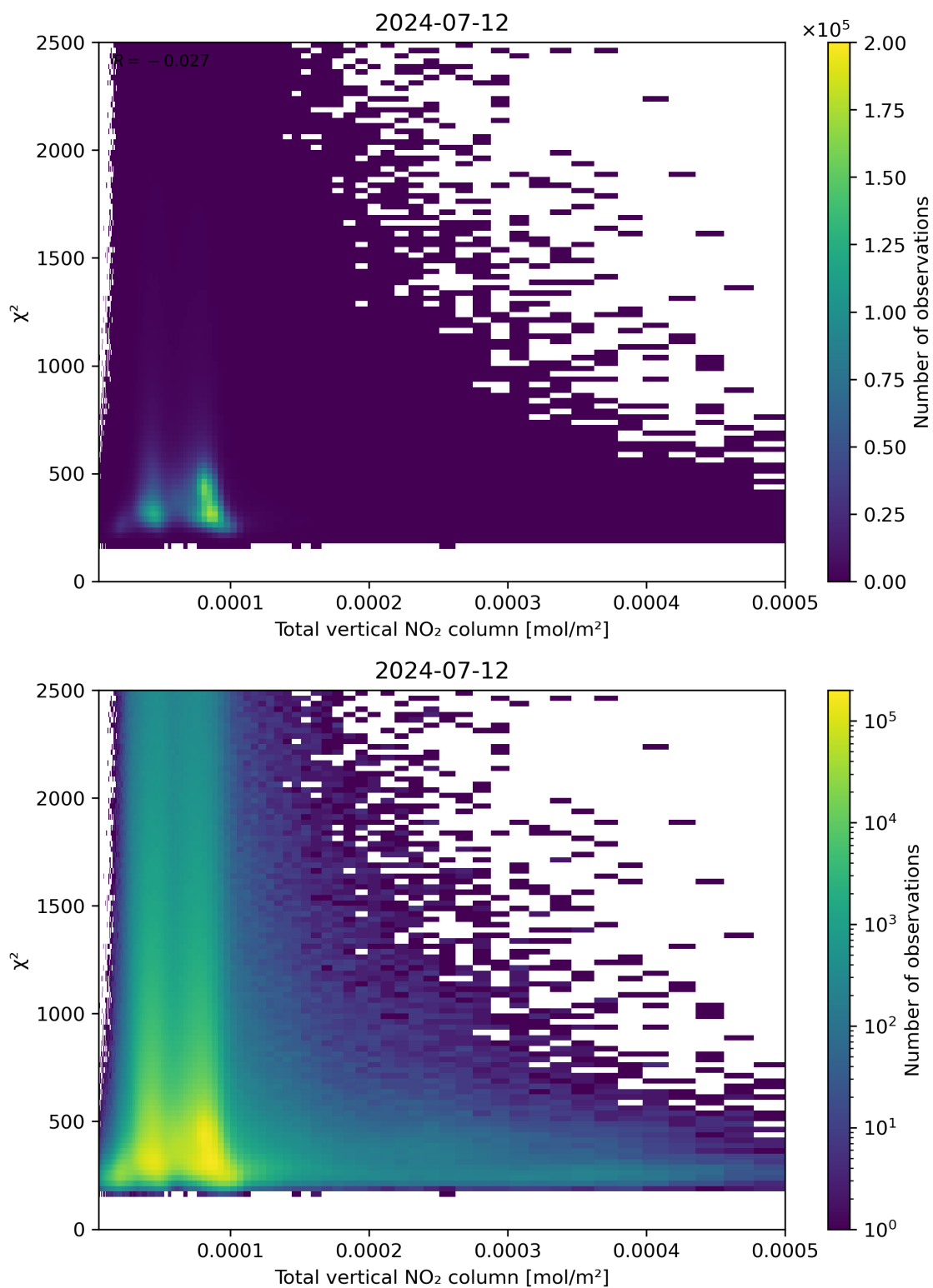
Figure 111: Scatter density plot of “Total vertical NO 2 column” against “ \chi^2 ” for 2024-07-11 to 2024-07-13.
