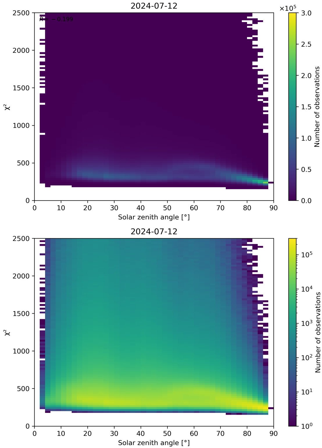
Figure 148: Scatter density plot of “Solar zenith angle” against “ \chi^2 ” for 2024-07-11 to 2024-07-13.
