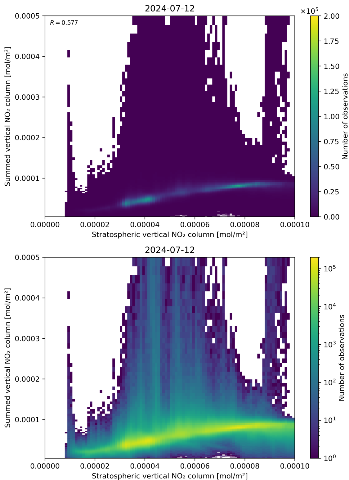
Figure 98: Scatter density plot of “Stratospheric vertical NO 2 column” against “Summed vertical NO 2 column” for 2024-07-11 to 2024-07-13.
