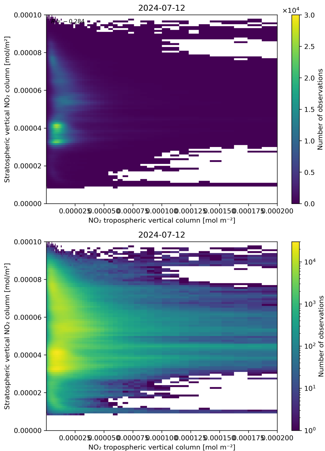
Figure 125: Scatter density plot of “NO 2 tropospheric vertical column” against “Stratospheric vertical NO 2 column” for 2024-07-11 to 2024-07-13.
