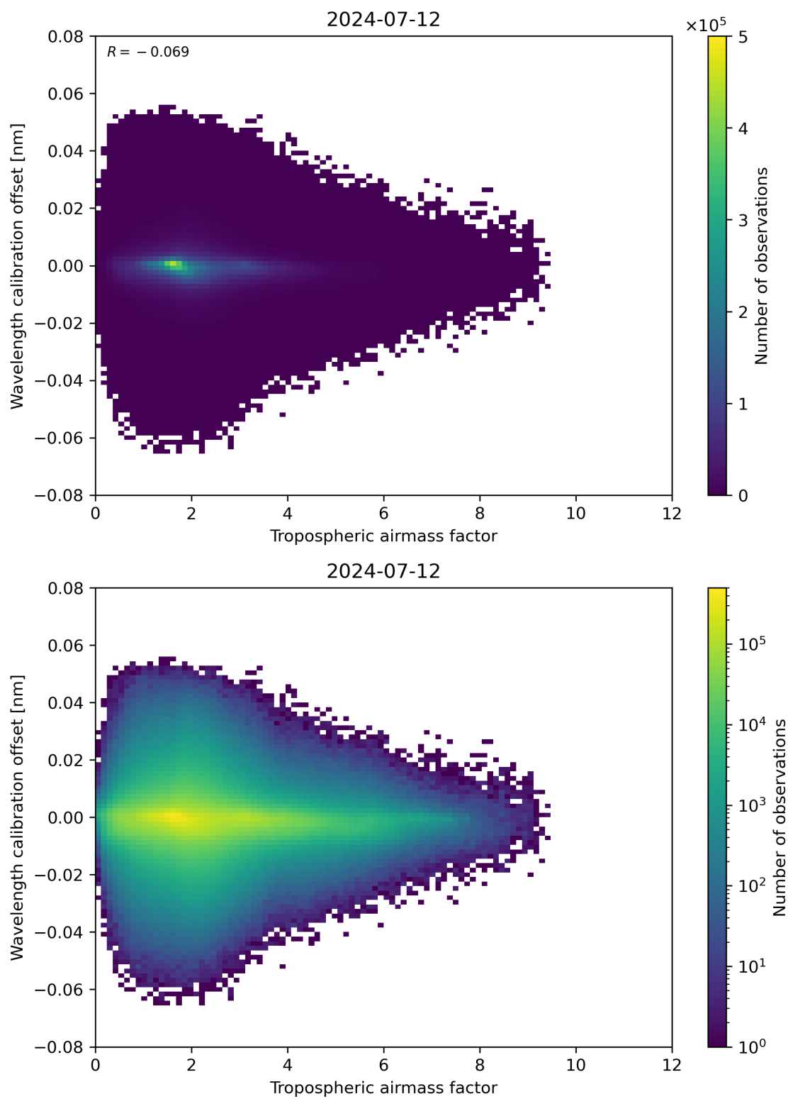
Figure 80: Scatter density plot of “Tropospheric airmass factor” against “Wavelength calibration offset” for 2024-07-11 to 2024-07-13.
