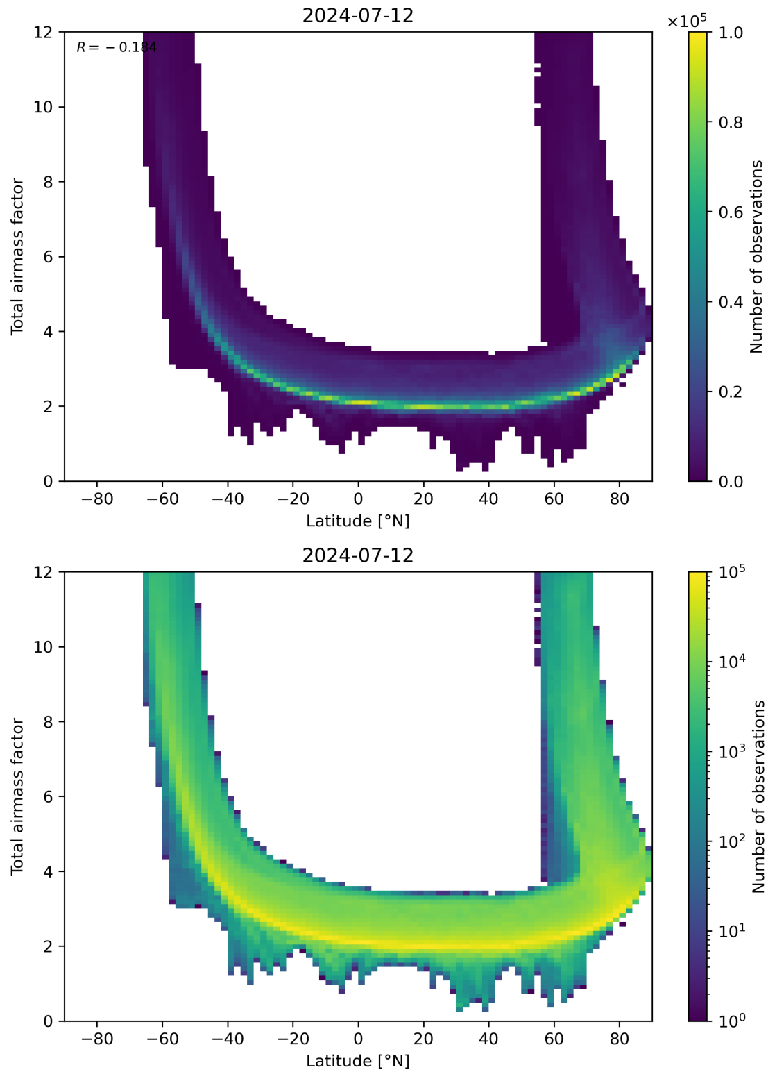
Figure 84: Scatter density plot of “Latitude” against “Total airmass factor” for 2024-07-11 to 2024-07-13.
