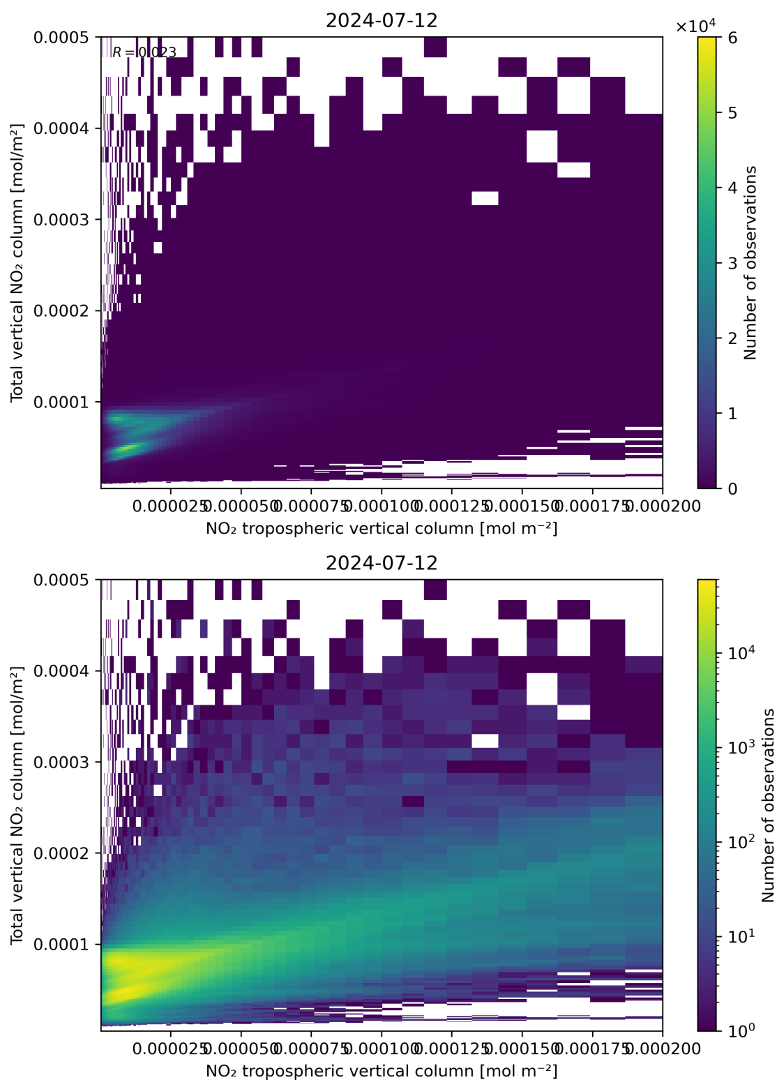
Figure 128: Scatter density plot of “NO 2 tropospheric vertical column” against “Total vertical NO 2 column” for 2024-07-11 to 2024-07-13.
