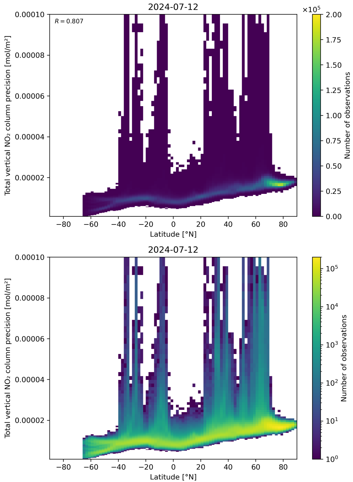
Figure 91: Scatter density plot of “Latitude” against “Total vertical NO 2 column precision” for 2024-07-11 to 2024-07-13.
