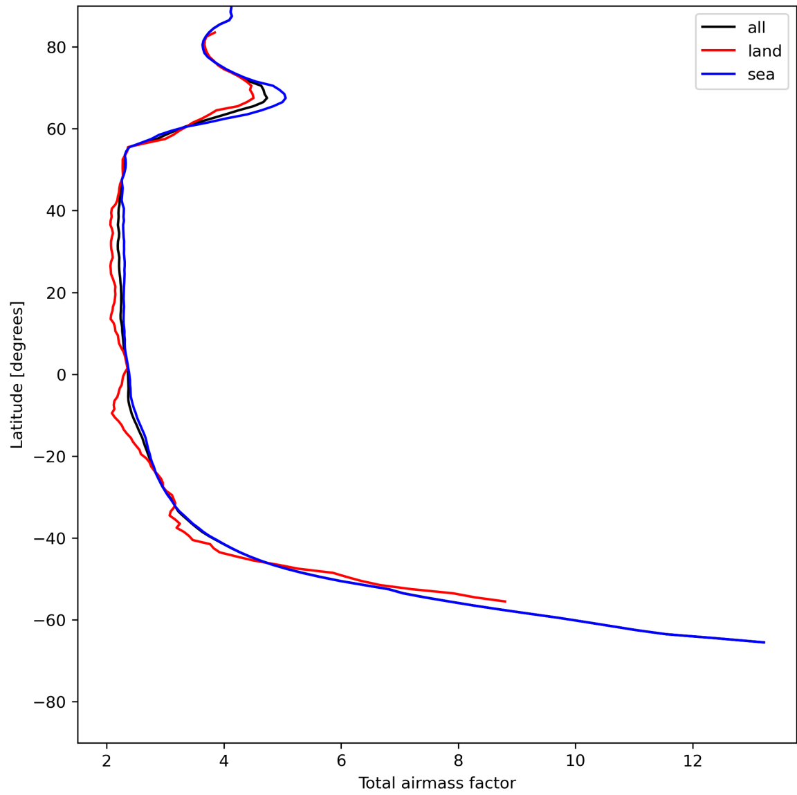
Figure 15: Zonal average of “Total airmass factor” for 2024-07-11 to 2024-07-13.
