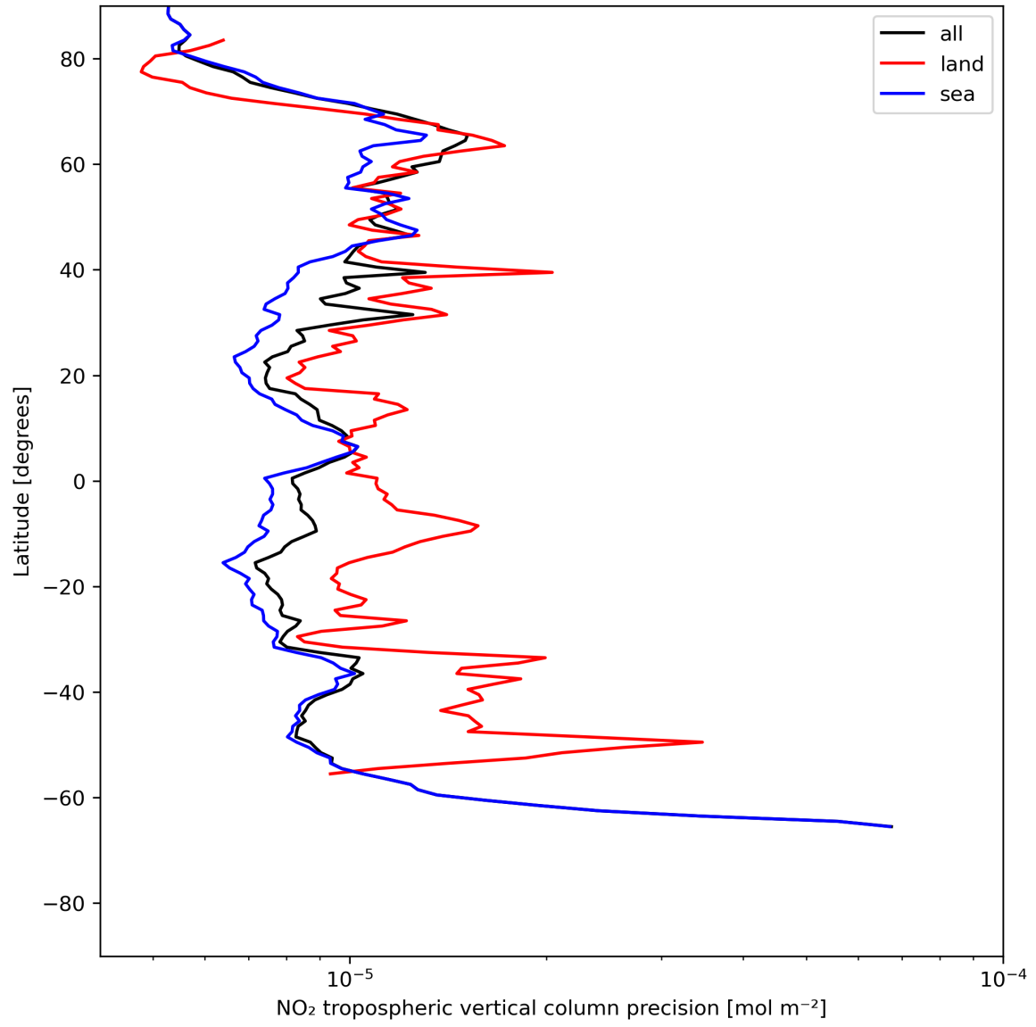
Figure 13: Zonal average of "NO 2 tropospheric vertical column precision" for 2024-07-11 to 2024-07-13.
