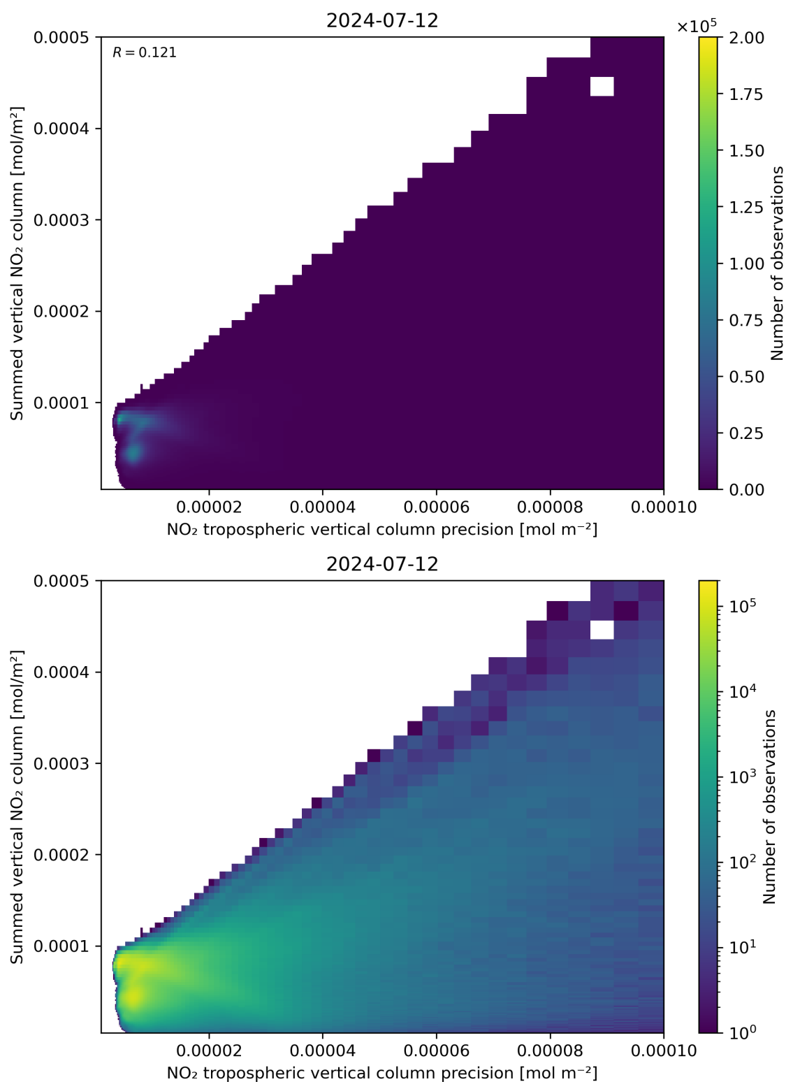
Figure 136: Scatter density plot of “NO 2 tropospheric vertical column precision” against “Summed vertical NO 2 column” for 2024-07-11 to 2024-07-13.
