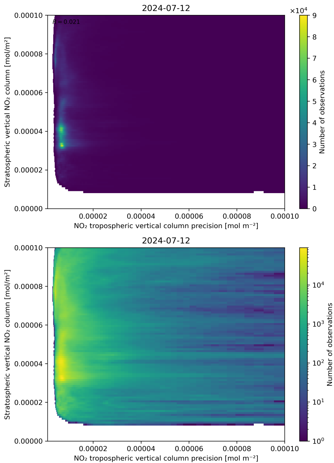
Figure 135: Scatter density plot of “NO 2 tropospheric vertical column precision” against “Stratospheric vertical NO 2 column” for 2024-07-11 to 2024-07-13.
