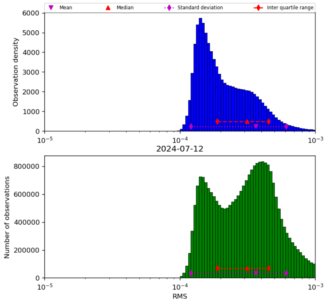
Figure 43: Histogram of “RMS” for 2024-07-11 to 2024-07-13
