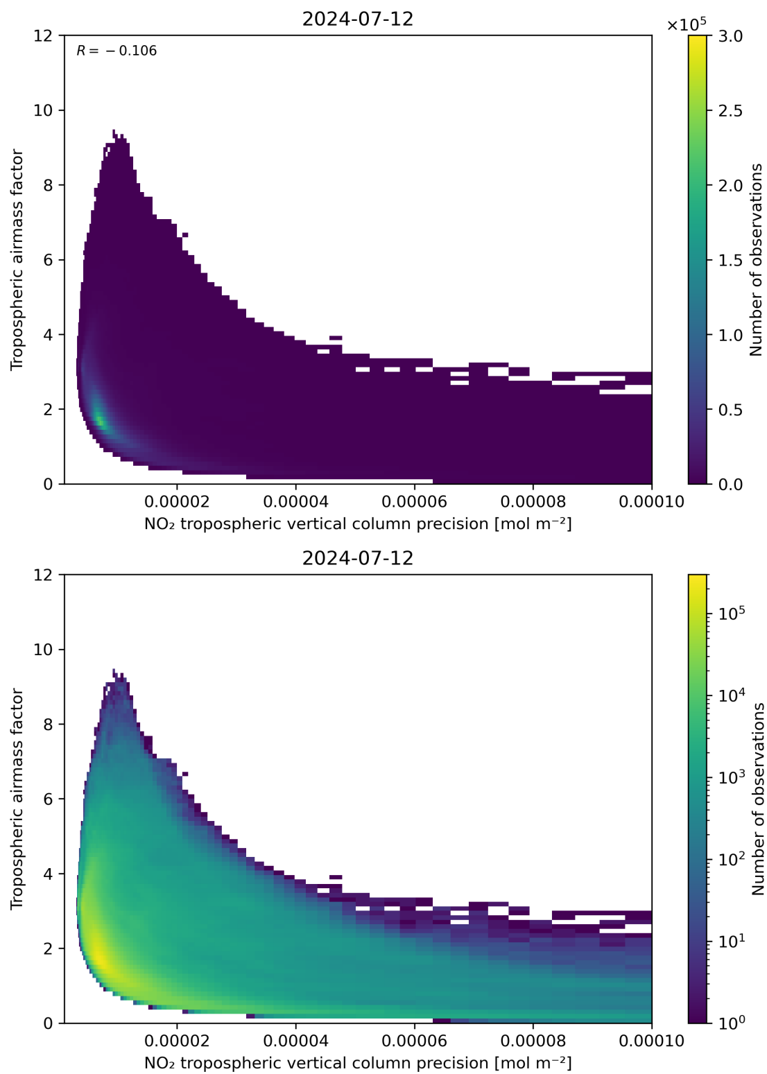
Figure 133: Scatter density plot of “NO 2 tropospheric vertical column precision” against “Tropospheric airmass factor” for 2024-07-11 to 2024-07-13.
