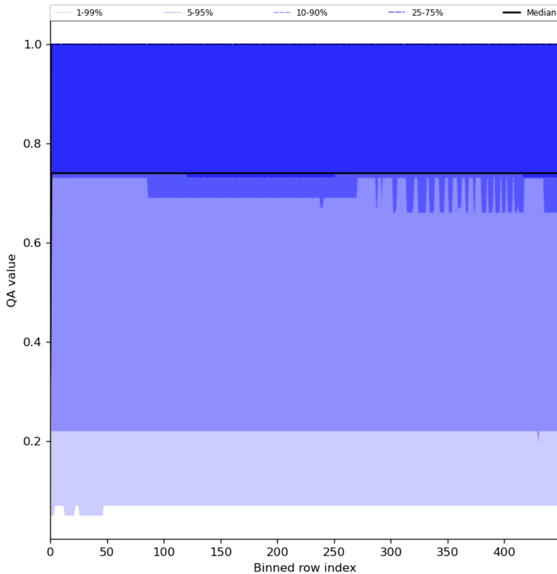
Figure 45: Along track statistics of “QA value” for 2024-07-11 to 2024-07-13
