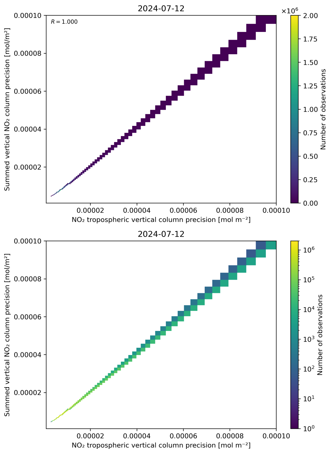
Figure 137: Scatter density plot of “NO 2 tropospheric vertical column precision” against “Summed vertical NO 2 column precision” for 2024-07-11 to 2024-07-13.
