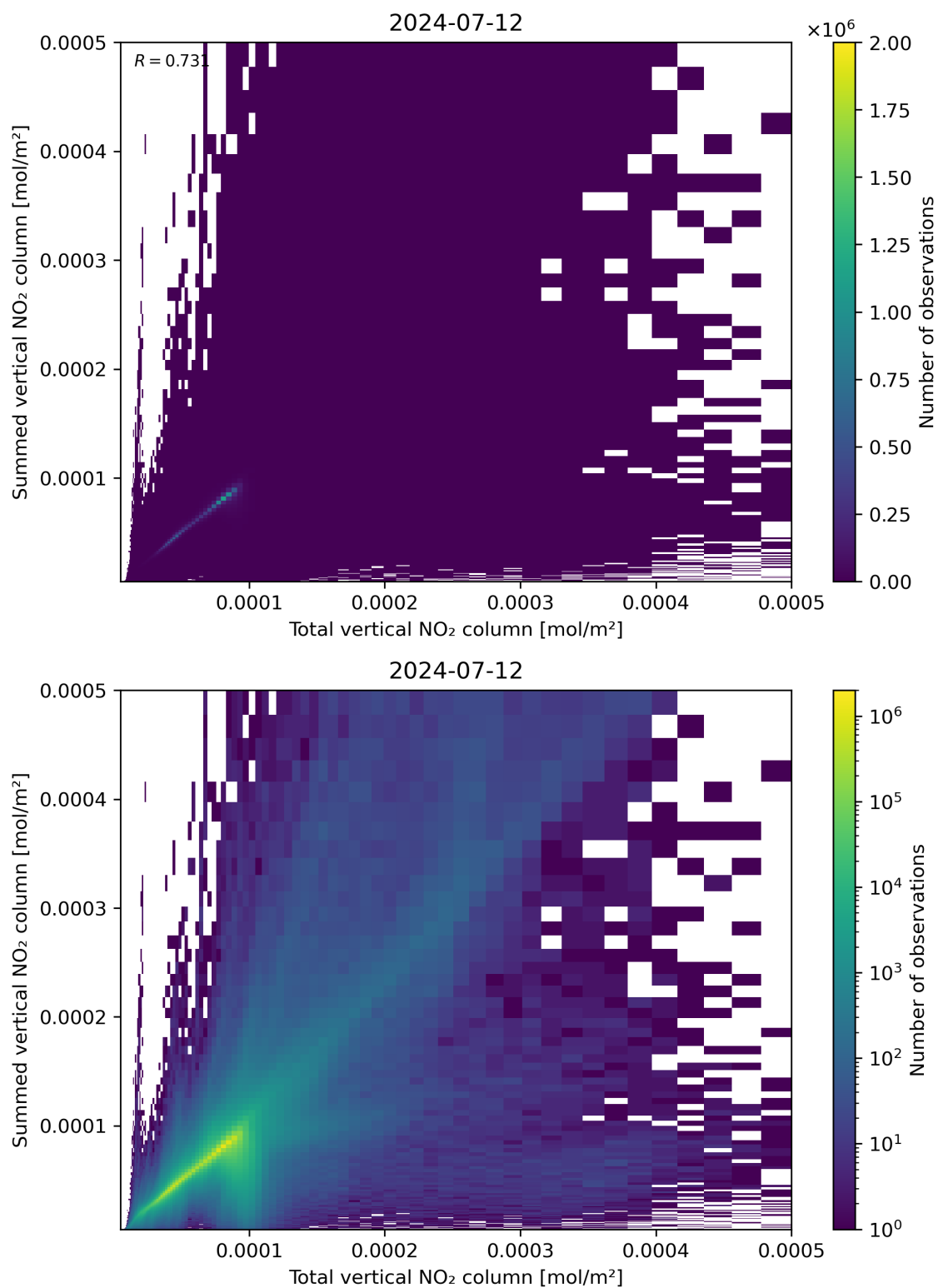
Figure 112: Scatter density plot of “Total vertical NO 2 column” against “Summed vertical NO 2 column” for 2024-07-11 to 2024-07-13.
