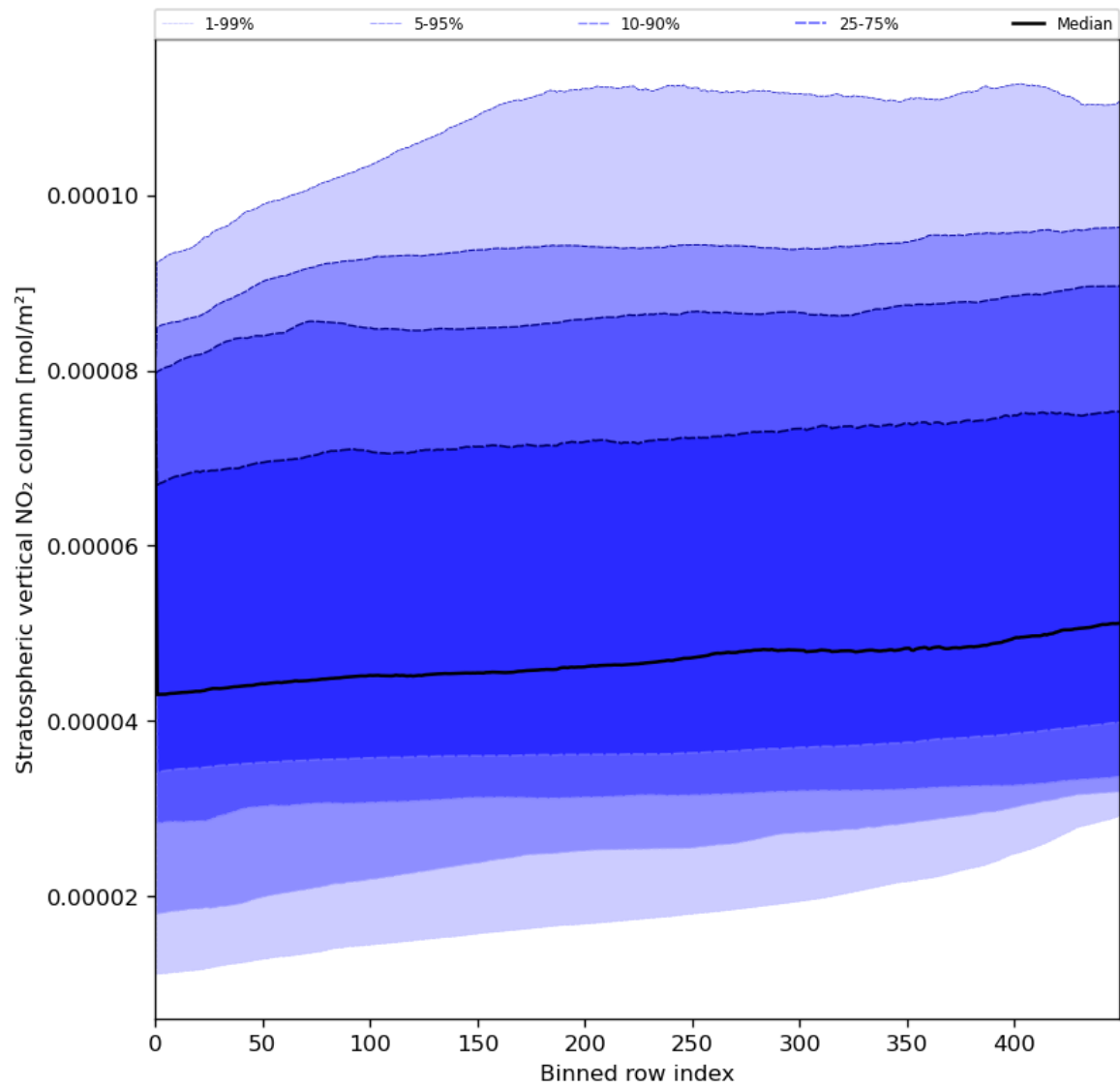
Figure 53: Along track statistics of “Stratospheric vertical NO 2 column” for 2024-07-11 to 2024-07-13
