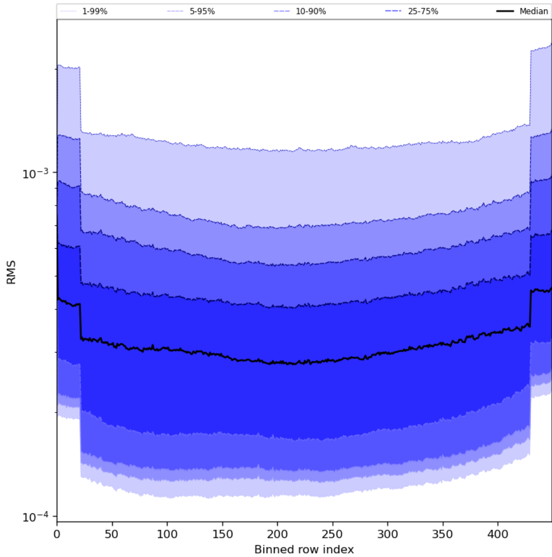
Figure 60: Along track statistics of “RMS” for 2024-07-11 to 2024-07-13
