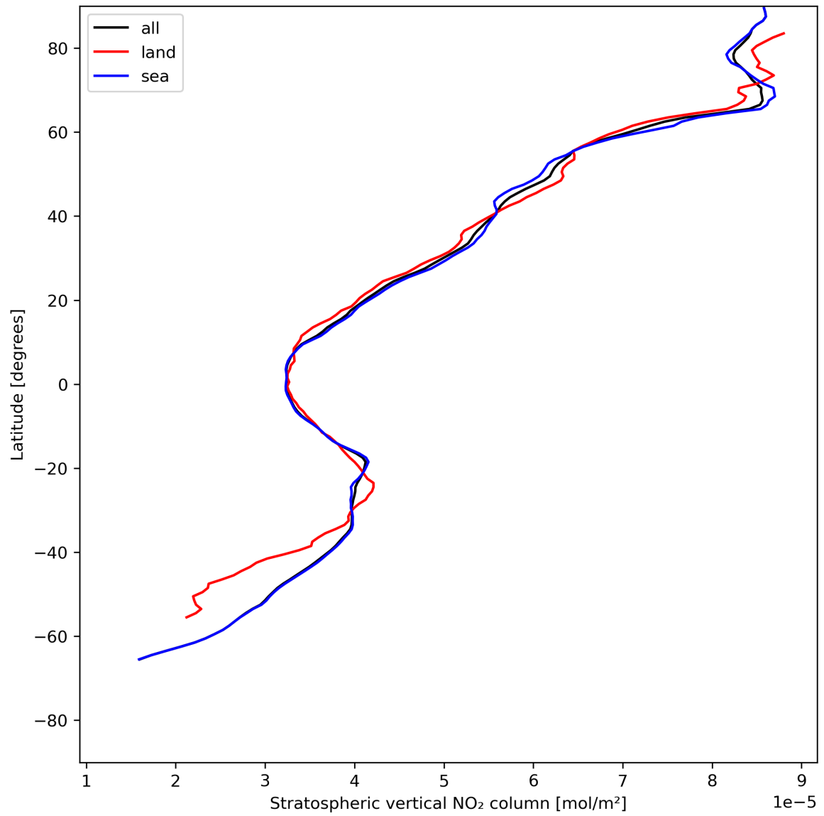
Figure 19: Zonal average of “Stratospheric vertical NO 2 column” for 2024-07-11 to 2024-07-13.
