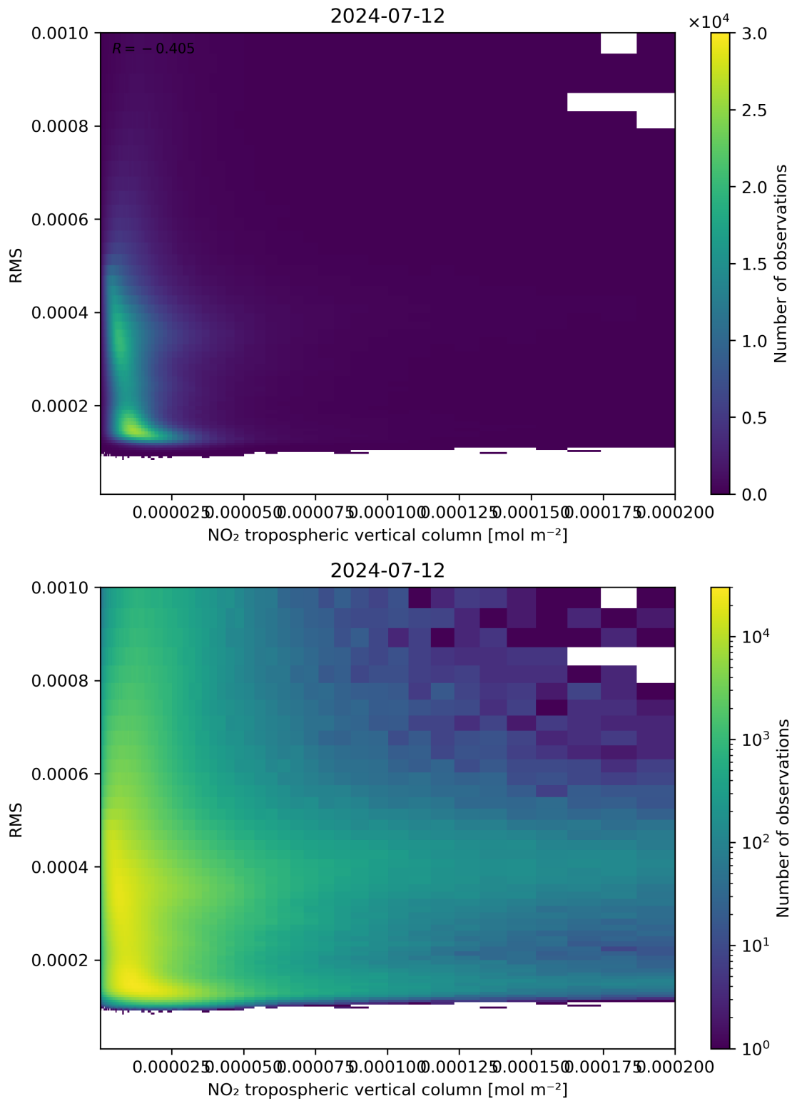
Figure 142: Scatter density plot of “NO 2 tropospheric vertical column” against “RMS” for 2024-07-11 to 2024-07-13.
