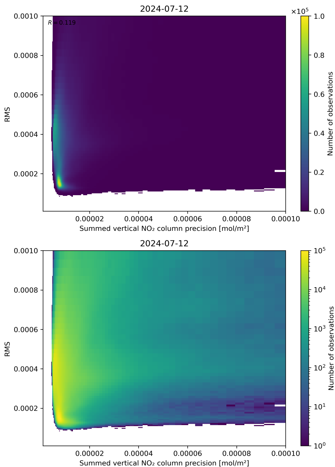
Figure 108: Scatter density plot of “Summed vertical NO 2 column precision” against “RMS” for 2024-07-11 to 2024-07-13.
