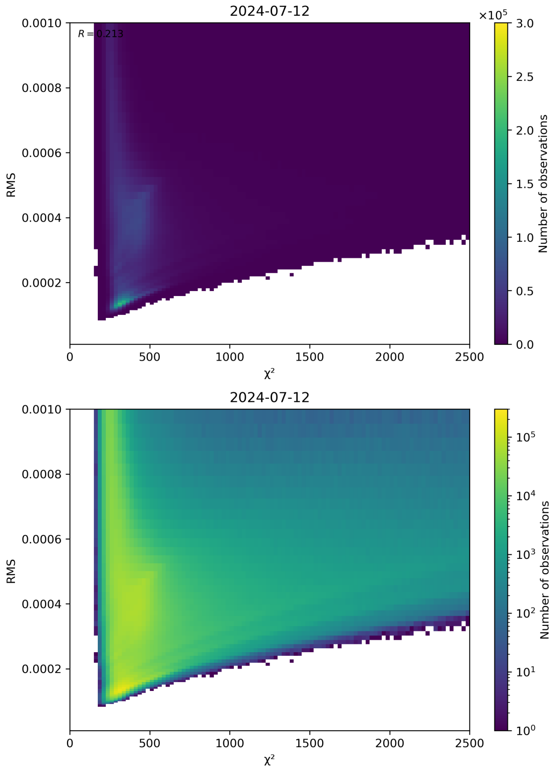
Figure 82: Scatter density plot of “ \chi^2 ” against “RMS” for 2024-07-11 to 2024-07-13.
