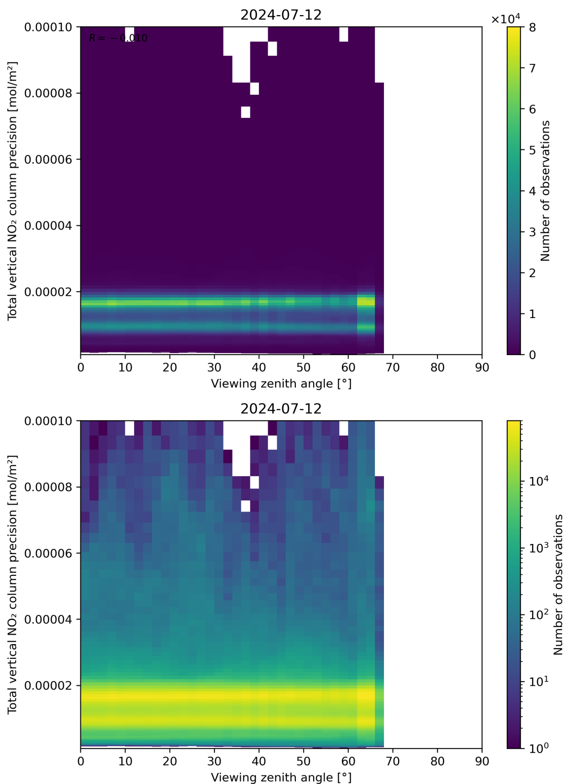
Figure 168: Scatter density plot of “Viewing zenith angle” against “Total vertical NO 2 column precision” for 2024-07-11 to 2024-07-13.
