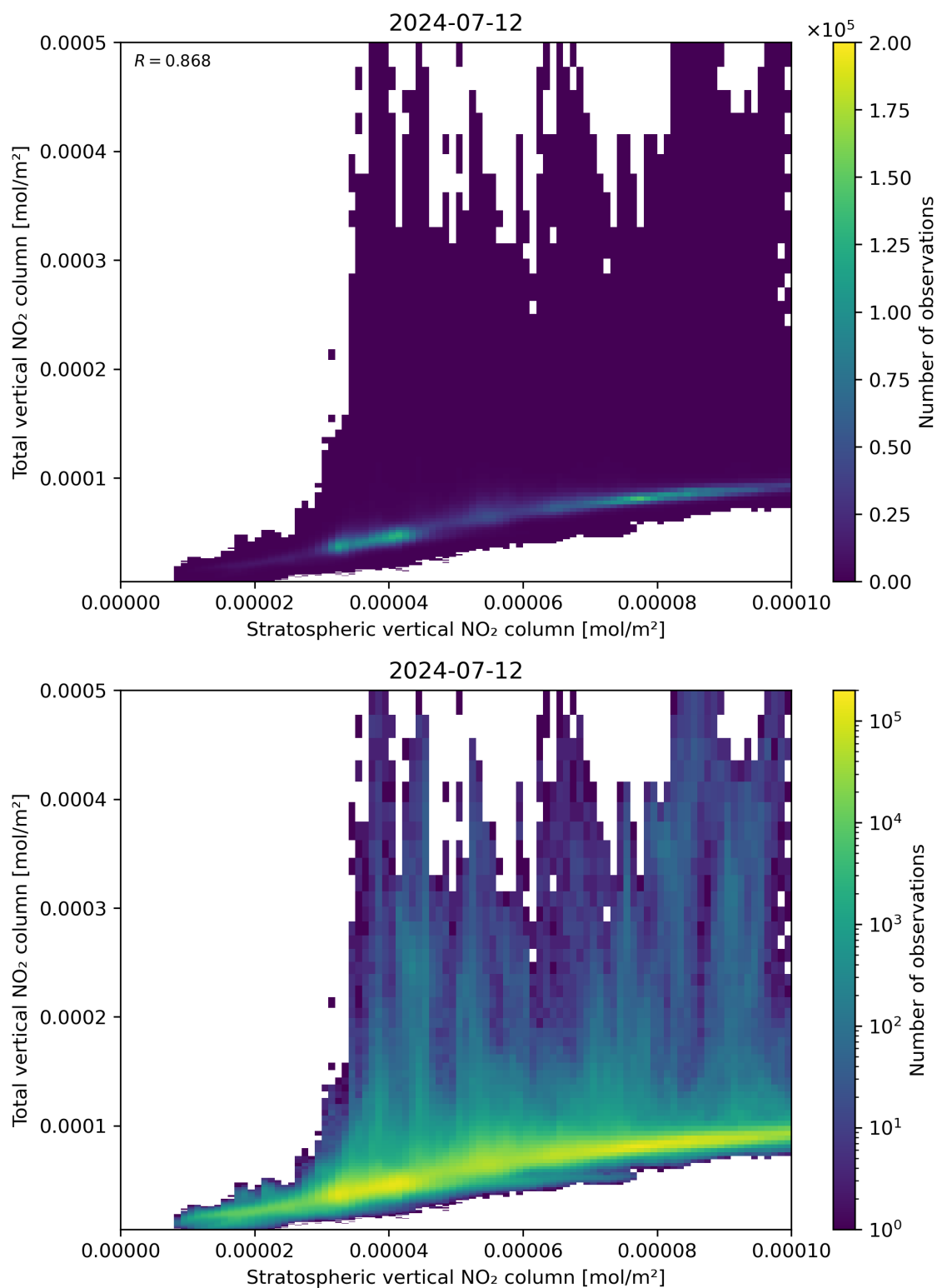
Figure 100: Scatter density plot of “Stratospheric vertical NO 2 column” against “Total vertical NO 2 column” for 2024-07-11 to 2024-07-13.
