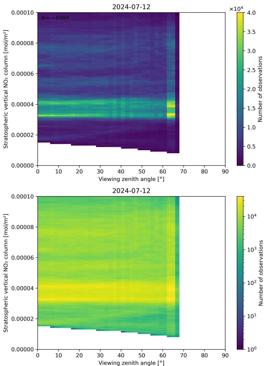
Figure 164: Scatter density plot of “Viewing zenith angle” against “Stratospheric vertical NO 2 column” for 2024-07-11 to 2024-07-13.
