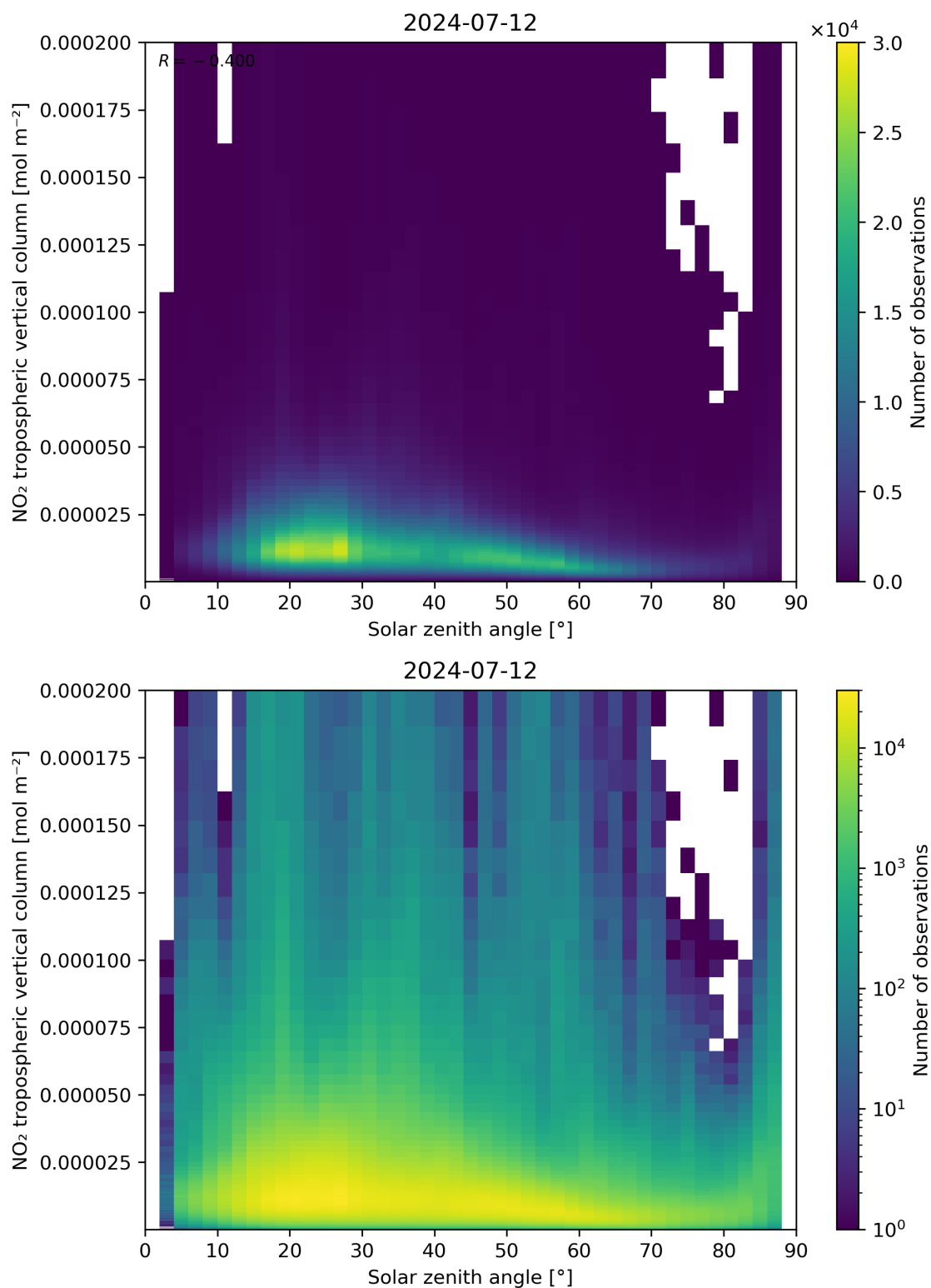
Figure 155: Scatter density plot of “Solar zenith angle” against “NO 2 tropospheric vertical column” for 2024-07-11 to 2024-07-13.
