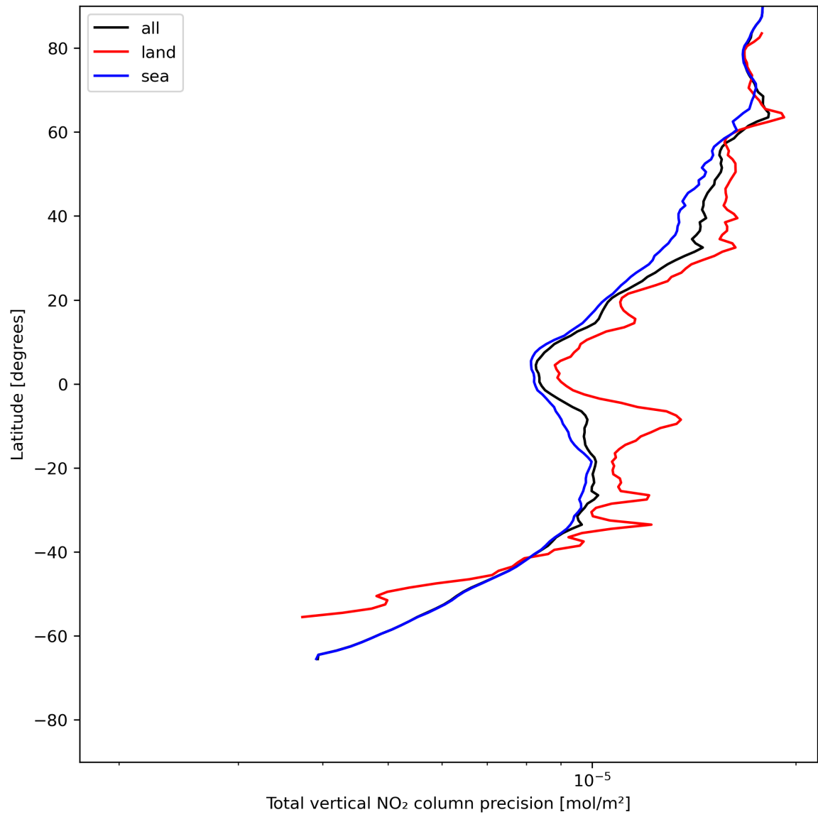
Figure 22: Zonal average of “Total vertical NO 2 column precision” for 2024-07-11 to 2024-07-13.
