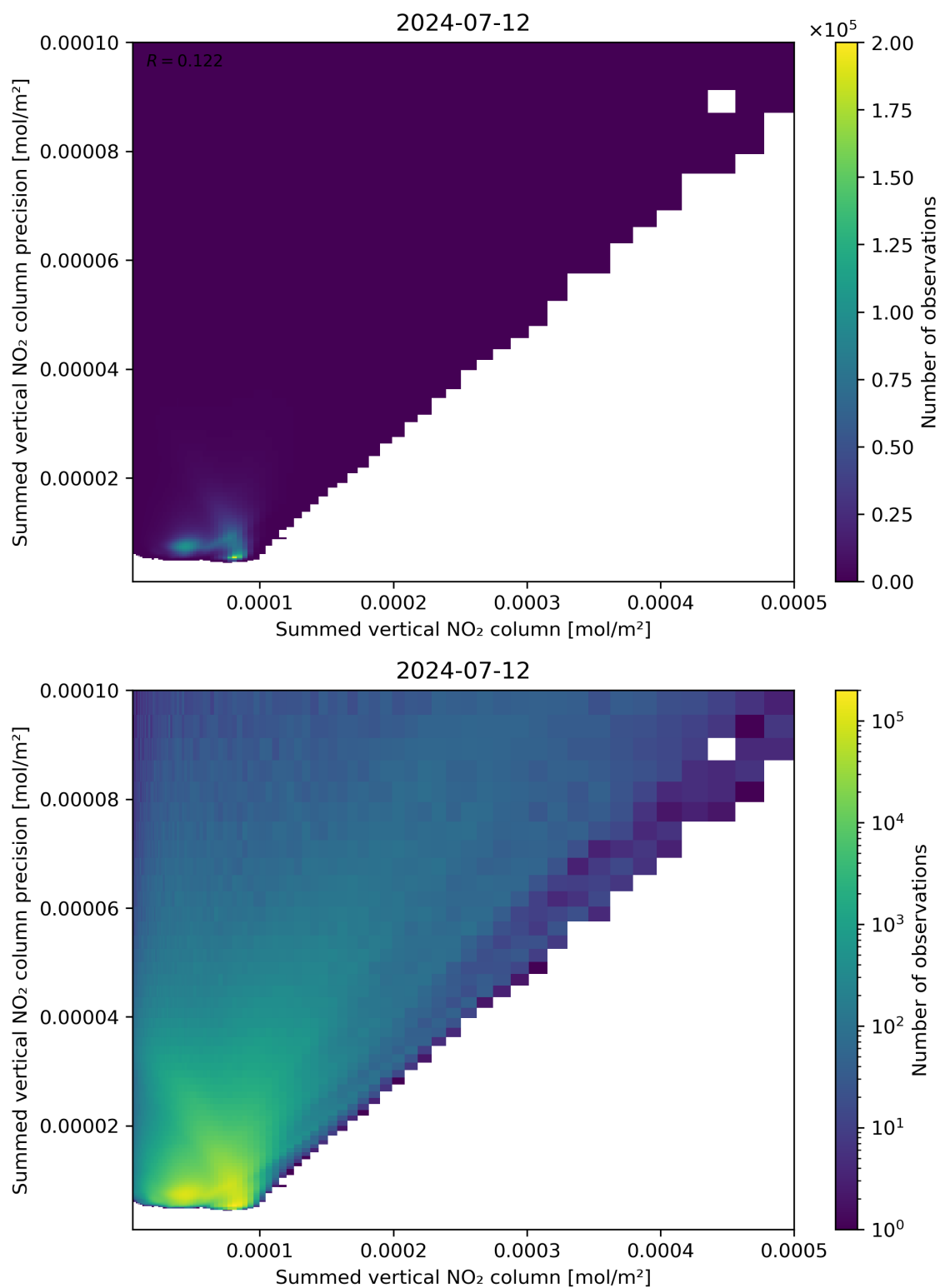
Figure 105: Scatter density plot of “Summed vertical NO 2 column” against “Summed vertical NO 2 column precision” for 2024-07-11 to 2024-07-13.
