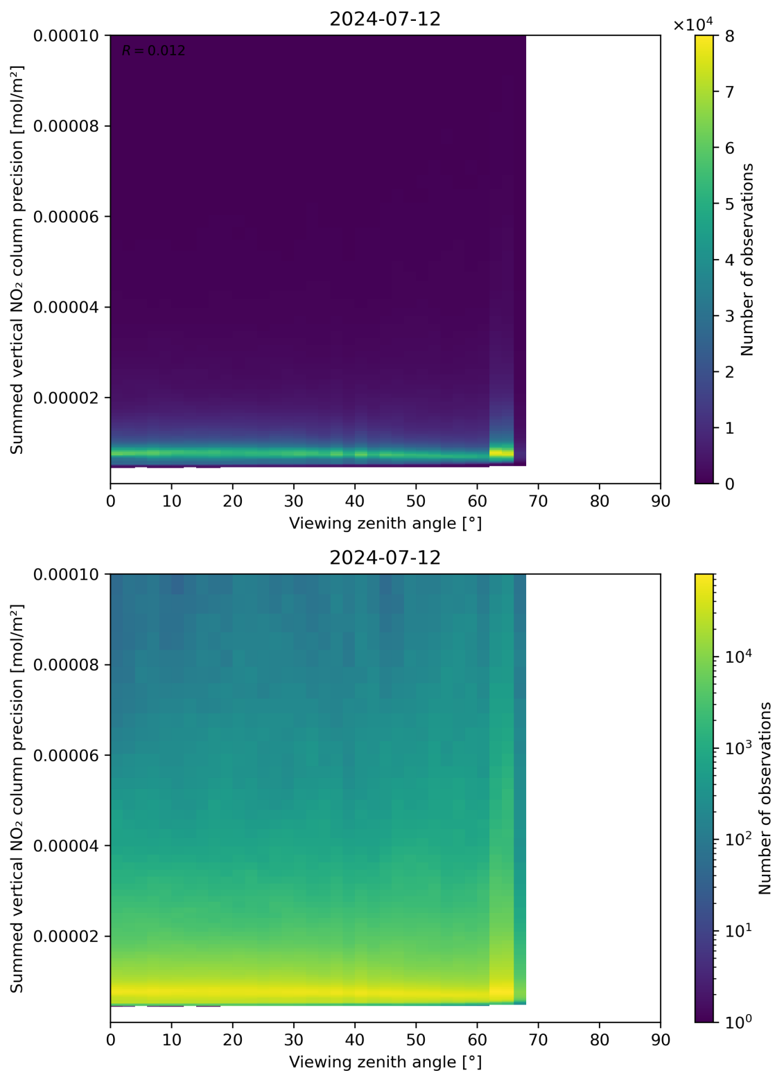
Figure 166: Scatter density plot of “Viewing zenith angle” against “Summed vertical NO 2 column precision” for 2024-07-11 to 2024-07-13.
