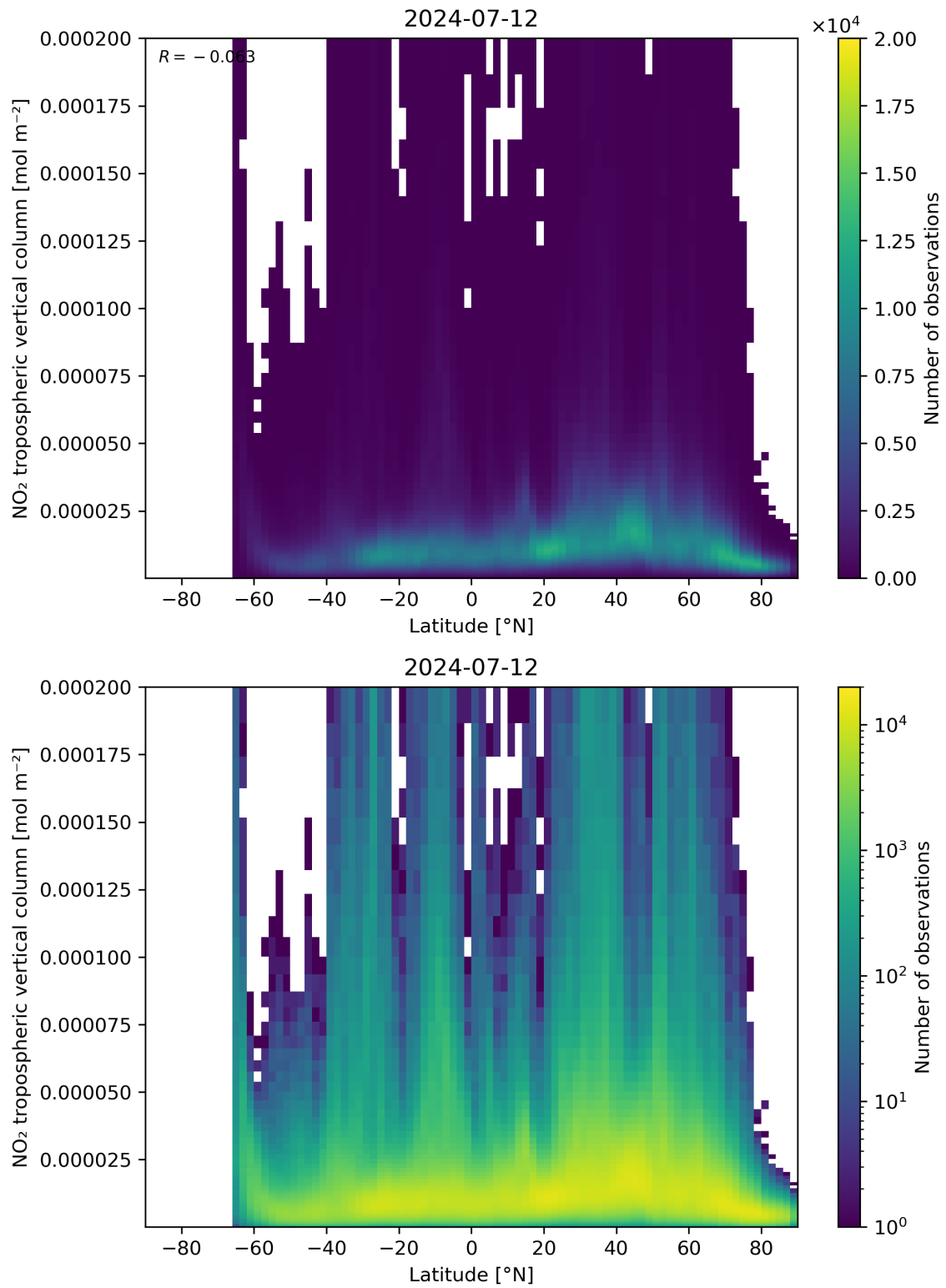
Figure 92: Scatter density plot of “Latitude” against “NO 2 tropospheric vertical column” for 2024-07-11 to 2024-07-13.
