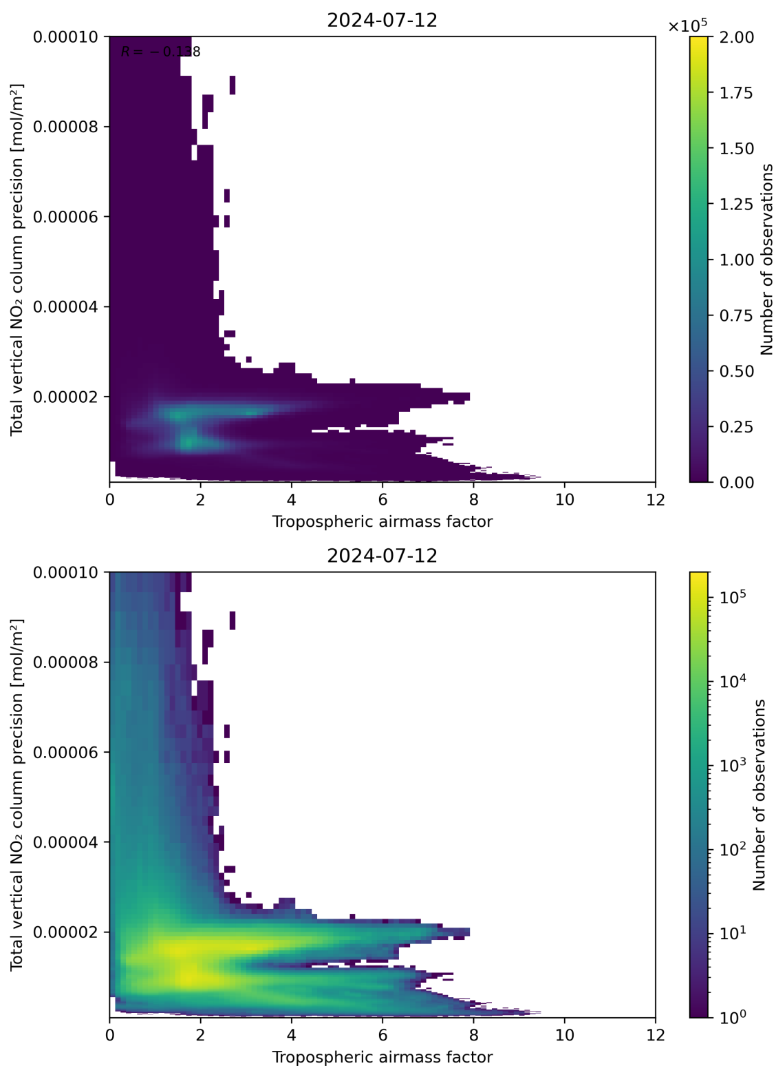
Figure 78: Scatter density plot of “Tropospheric air mass factor” against “Total vertical NO 2 column precision” for 2024-07-11 to 2024-07-13.
