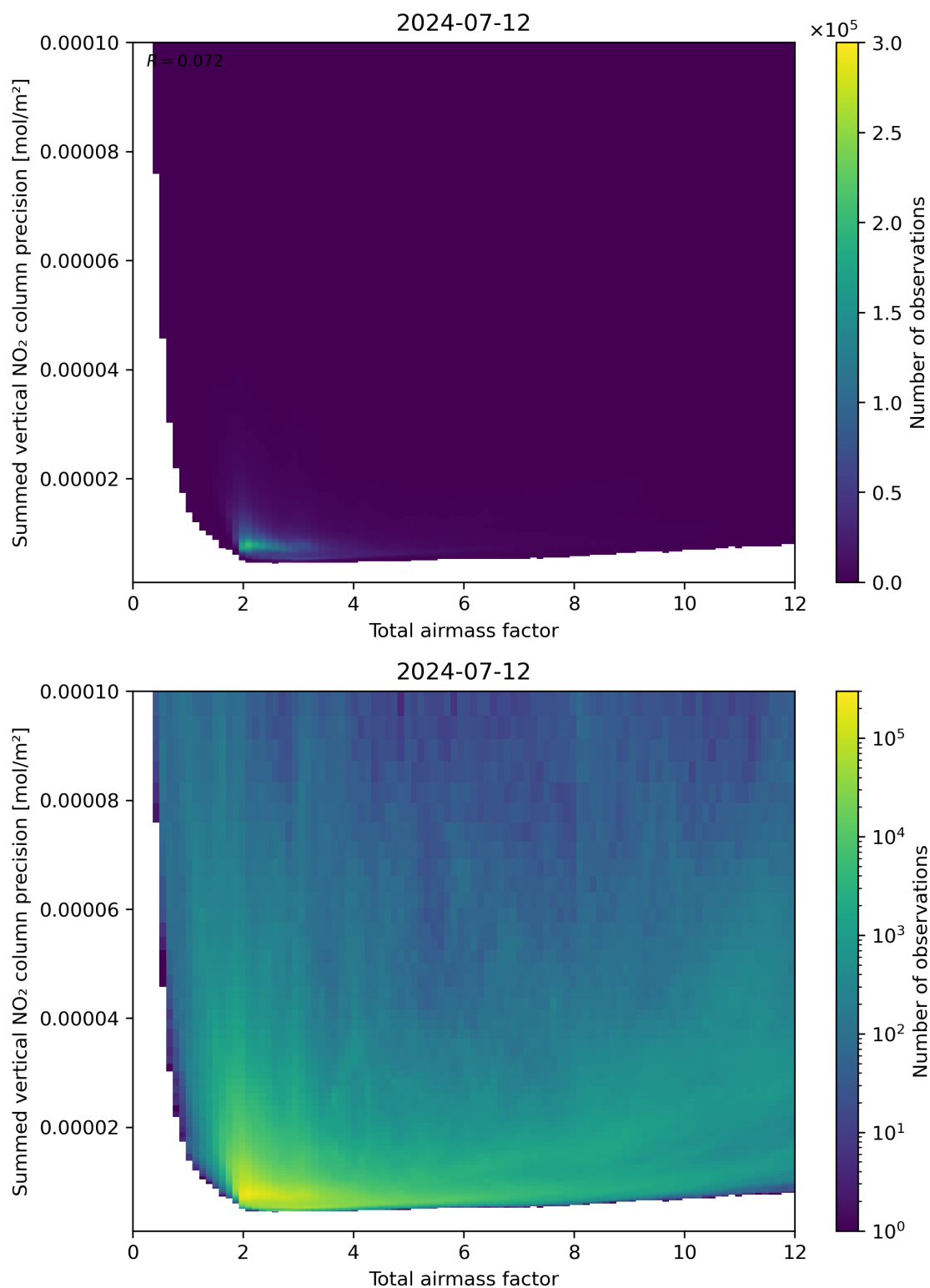
Figure 66: Scatter density plot of “Total airmass factor” against “Summed vertical NO 2 column precision” for 2024-07-11 to 2024-07-13.
