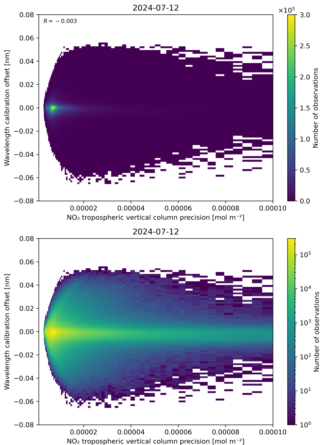
Figure 141: Scatter density plot of “NO 2 tropospheric vertical column precision” against “Wavelength calibration offset” for 2024-07-11 to 2024-07-13.
