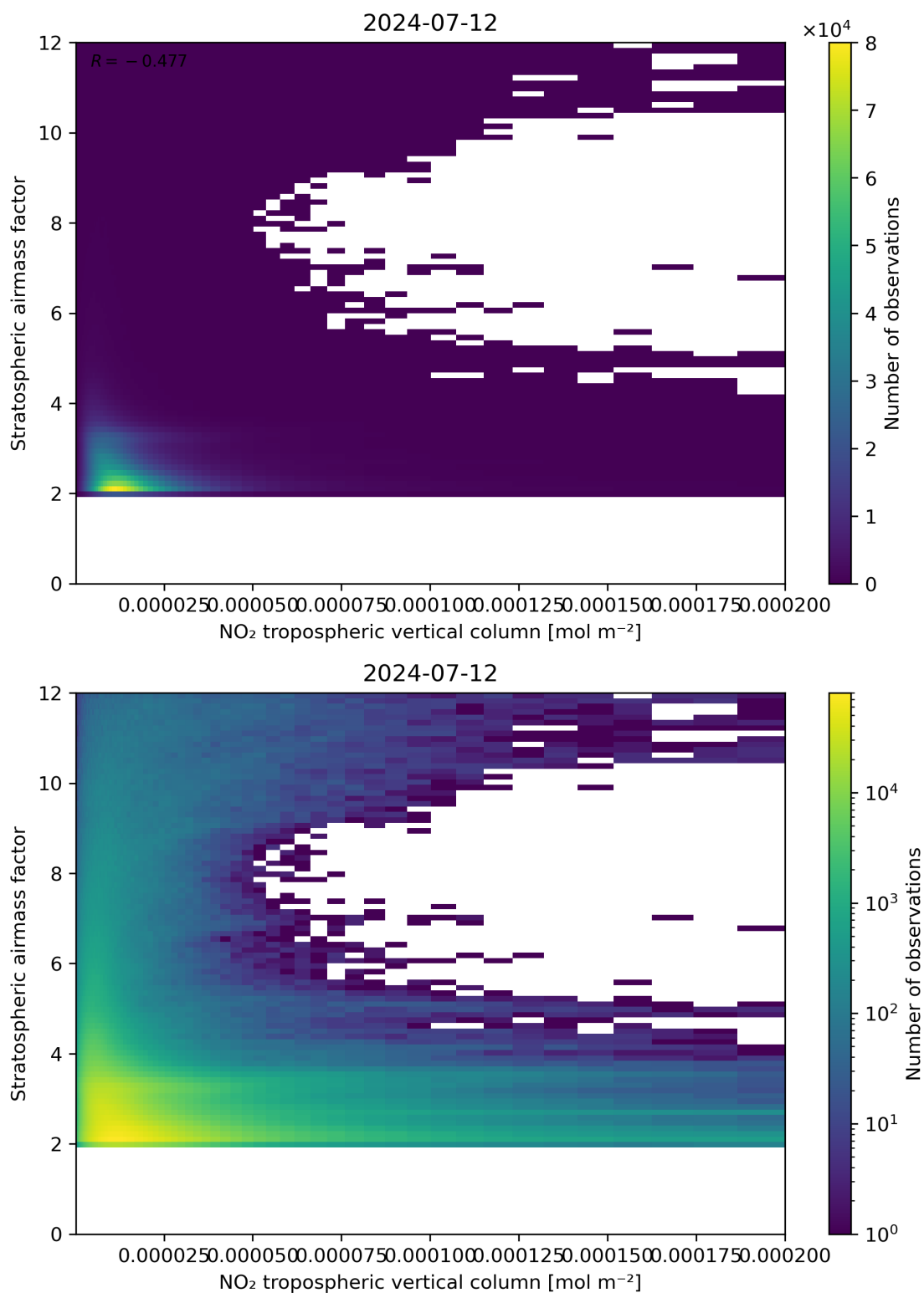
Figure 121: Scatter density plot of “NO 2 tropospheric vertical column” against “Stratospheric air mass factor” for 2024-07-11 to 2024-07-13.
