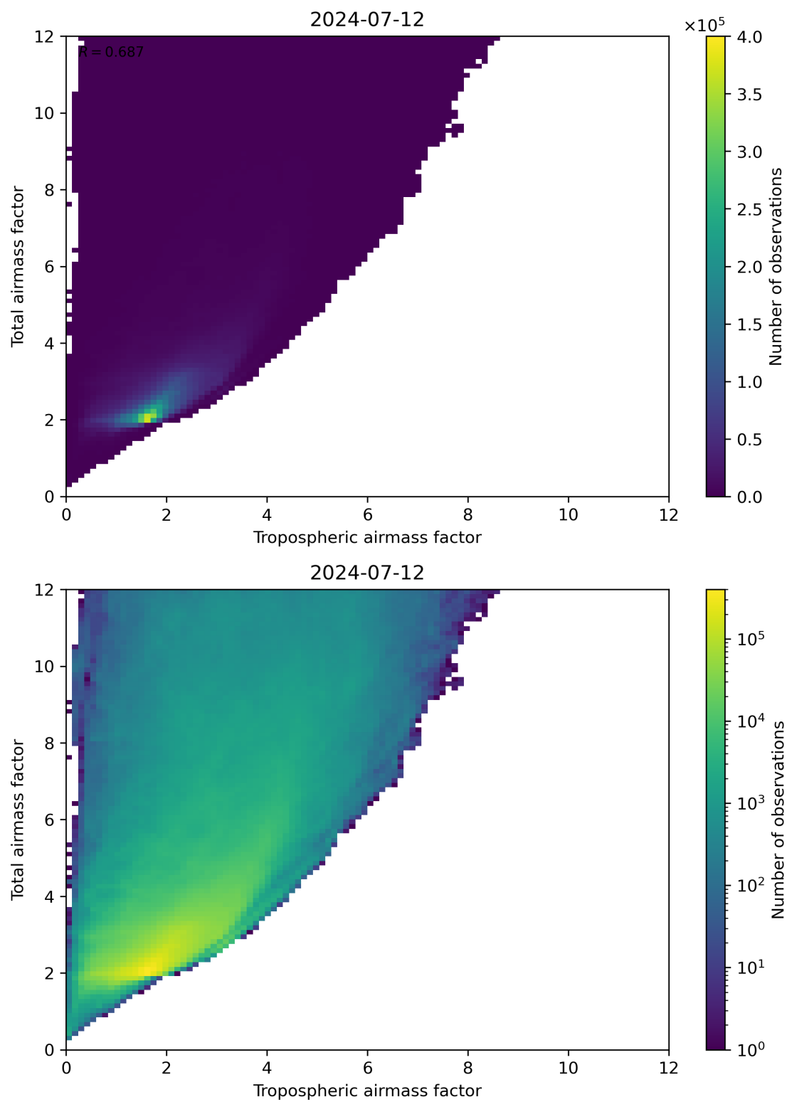
Figure 72: Scatter density plot of “Tropospheric airmass factor” against “Total airmass factor” for 2024-07-11 to 2024-07-13.
