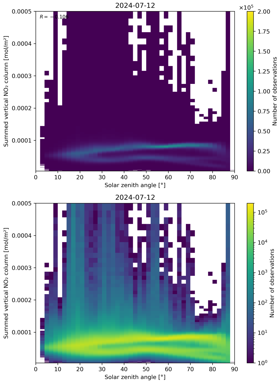
Figure 151: Scatter density plot of “Solar zenith angle” against “Summed vertical NO 2 column” for 2024-07-11 to 2024-07-13.
