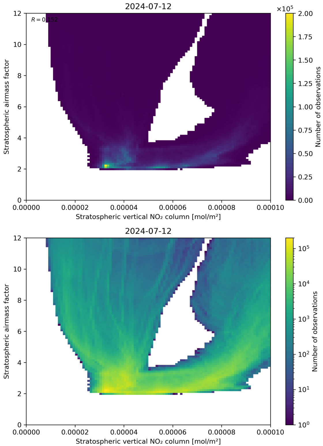
Figure 96: Scatter density plot of “Stratospheric vertical NO 2 column” against “Stratospheric airmass factor” for 2024-07-11 to 2024-07-13.
