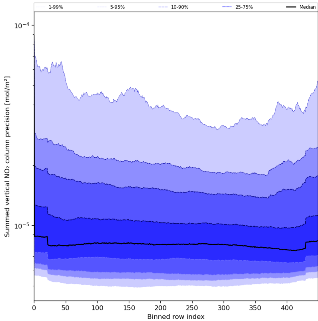
Figure 58: Along track statistics of “Summed vertical NO 2 column precision” for 2024-07-11 to 2024-07-13
