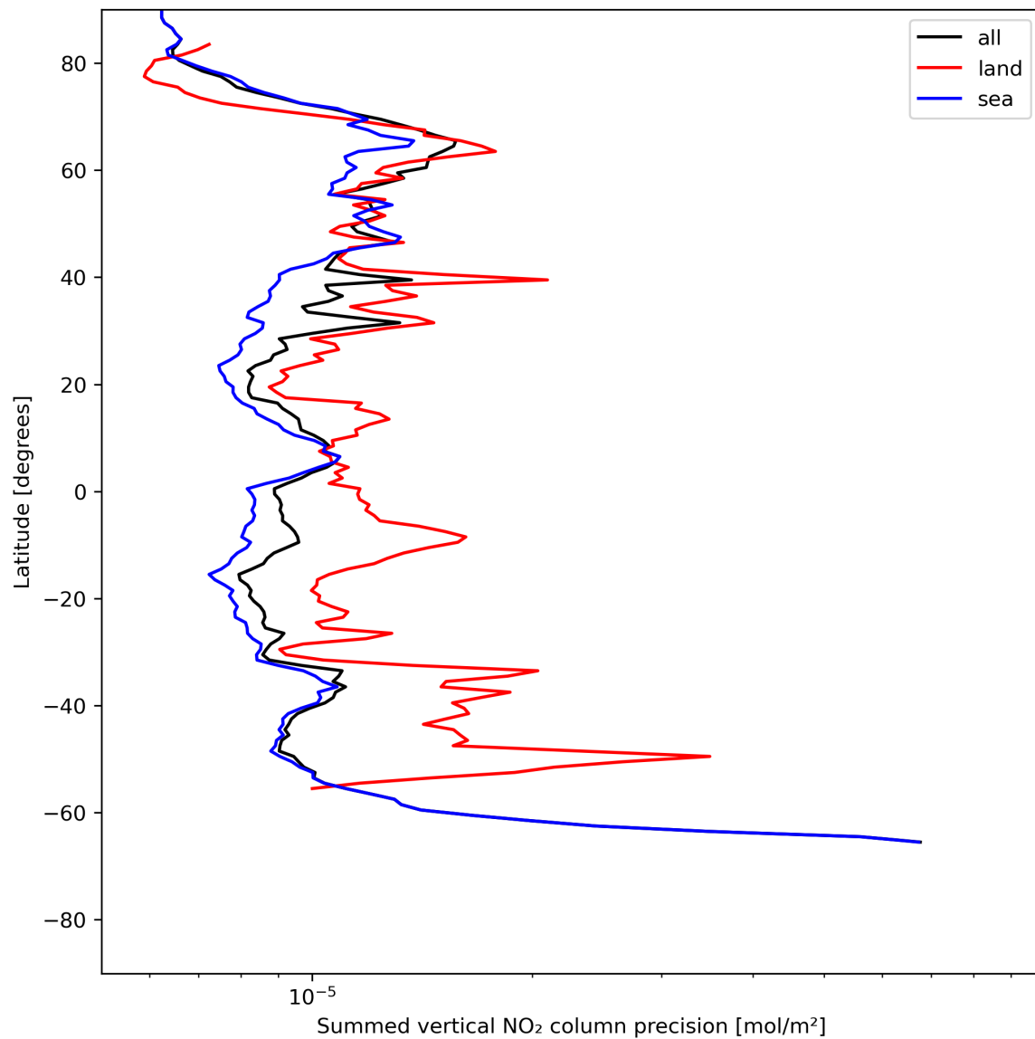
Figure 24: Zonal average of “Summed vertical NO 2 column precision” for 2024-07-11 to 2024-07-13.
