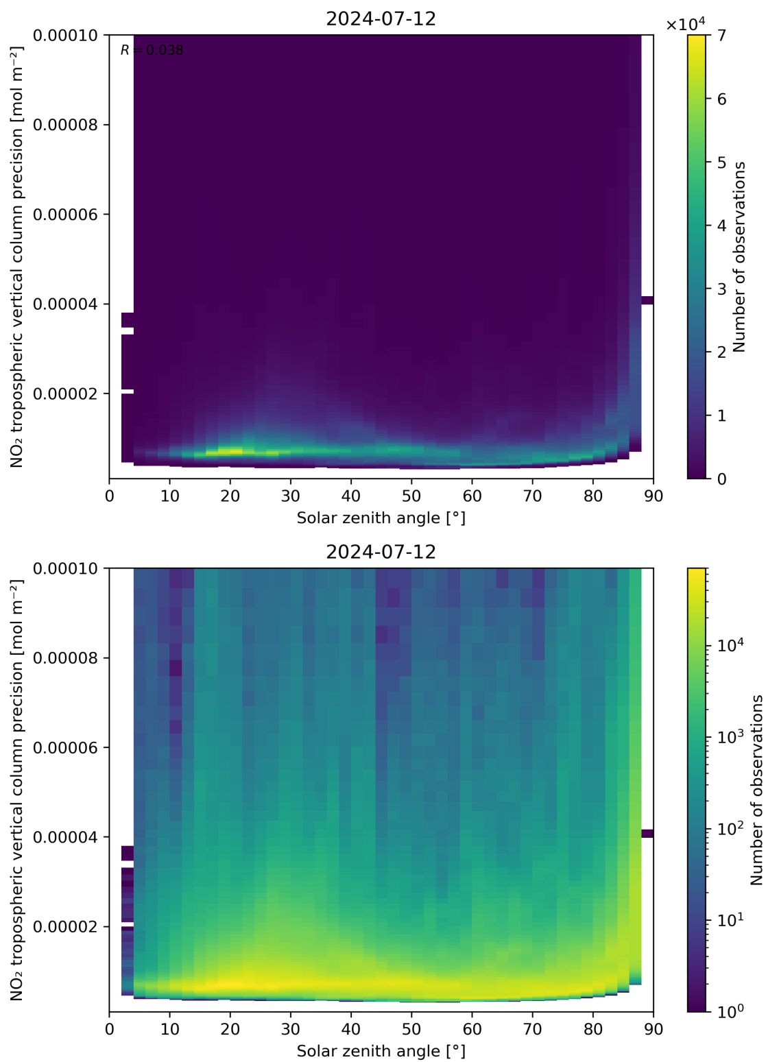
Figure 156: Scatter density plot of “Solar zenith angle” against “NO 2 tropospheric vertical column precision” for 2024-07-11 to 2024-07-13.
