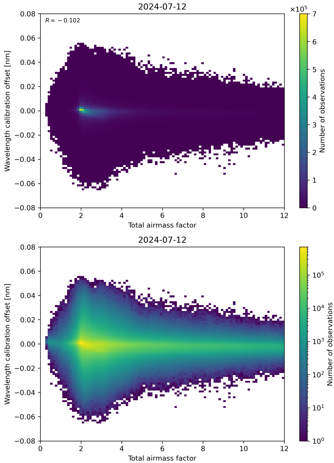
Figure 70: Scatter density plot of “Total airmass factor” against “Wavelength calibration offset” for 2024-07-11 to 2024-07-13.
