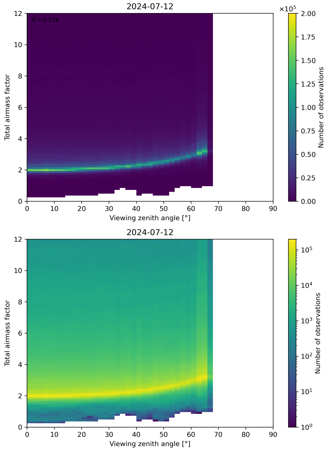
Figure 160: Scatter density plot of “Viewing zenith angle” against “Total airmass factor” for 2024-07-11 to 2024-07-13.
