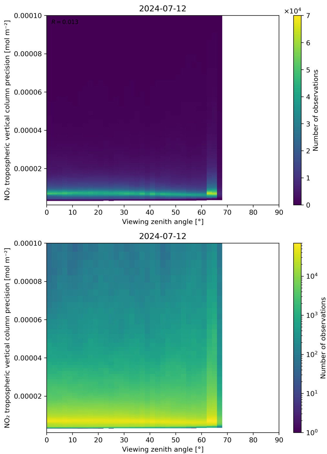
Figure 170: Scatter density plot of “Viewing zenith angle” against “NO 2 tropospheric vertical column precision” for 2024-07-11 to 2024-07-13.
