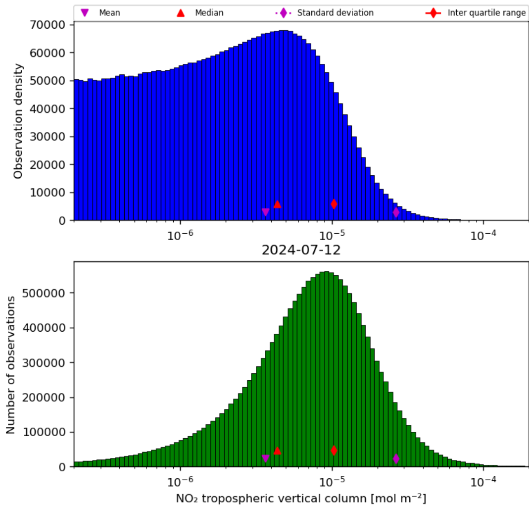
Figure 29: Histogram of “NO 2 tropospheric vertical column” for 2024-07-11 to 2024-07-13
