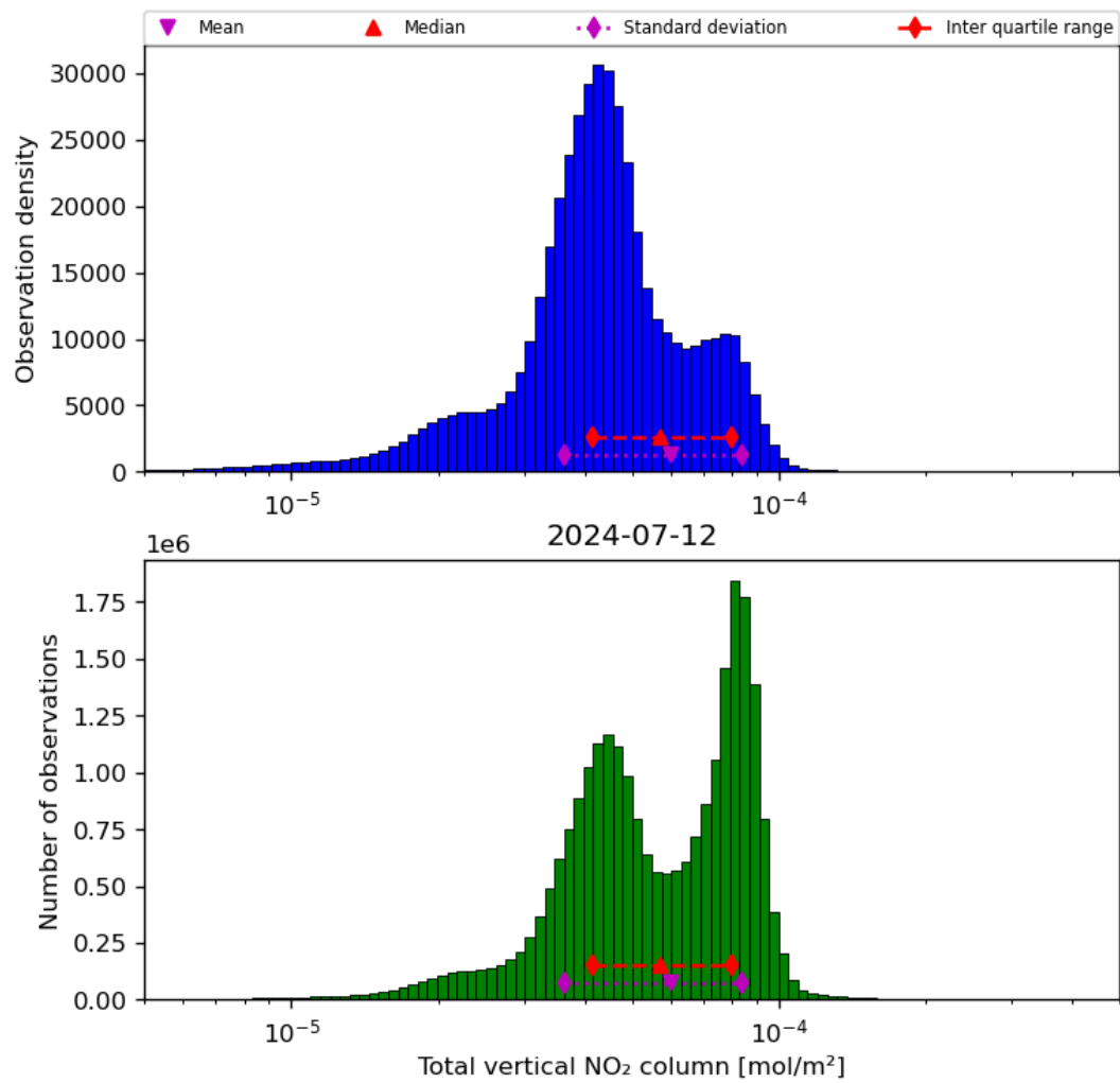
Figure 38: Histogram of "Total vertical NO 2 column" for 2024-07-11 to 2024-07-13
