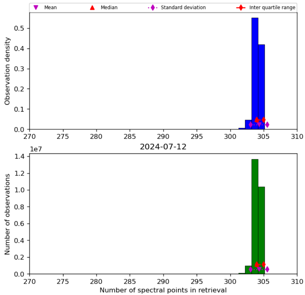
Figure 33: Histogram of “Number of spectral points in retrieval” for 2024-07-11 to 2024-07-13
