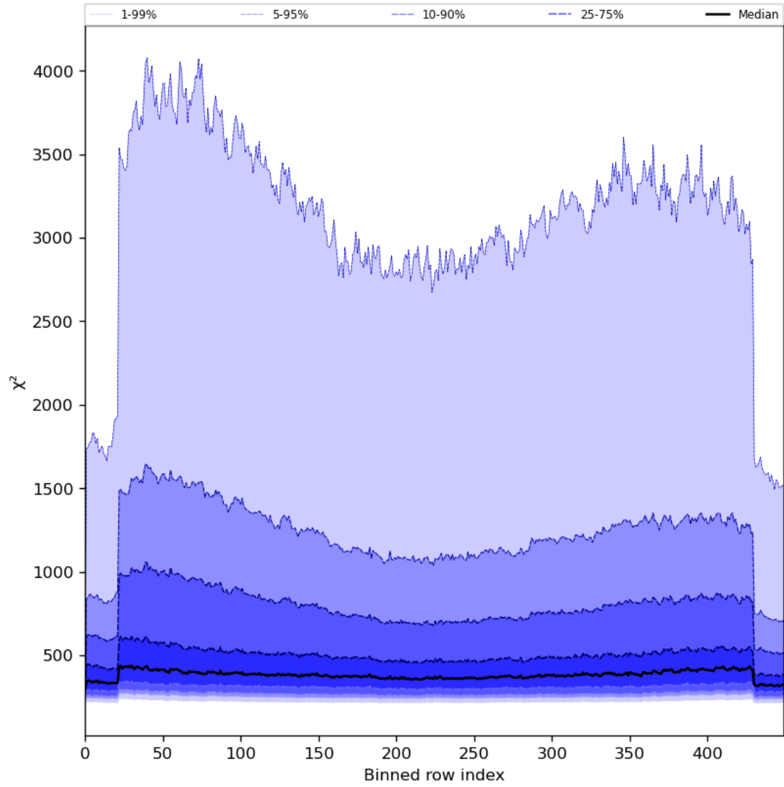
Figure 59: Along track statistics of “ \chi^2 ” for 2024-07-11 to 2024-07-13
