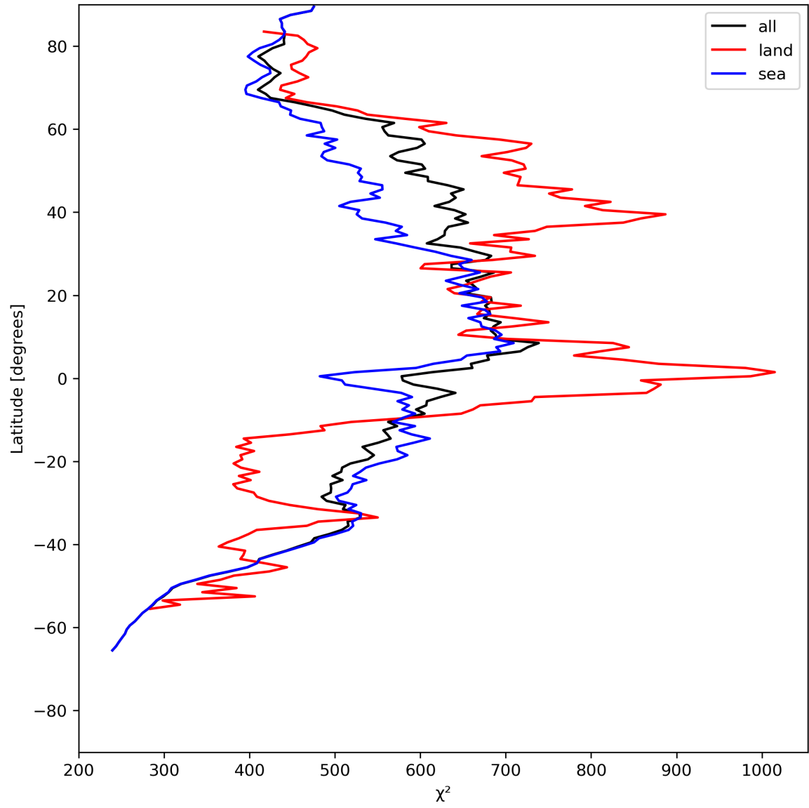
Figure 25: Zonal average of “ \chi^2 ” for 2024-07-11 to 2024-07-13.
