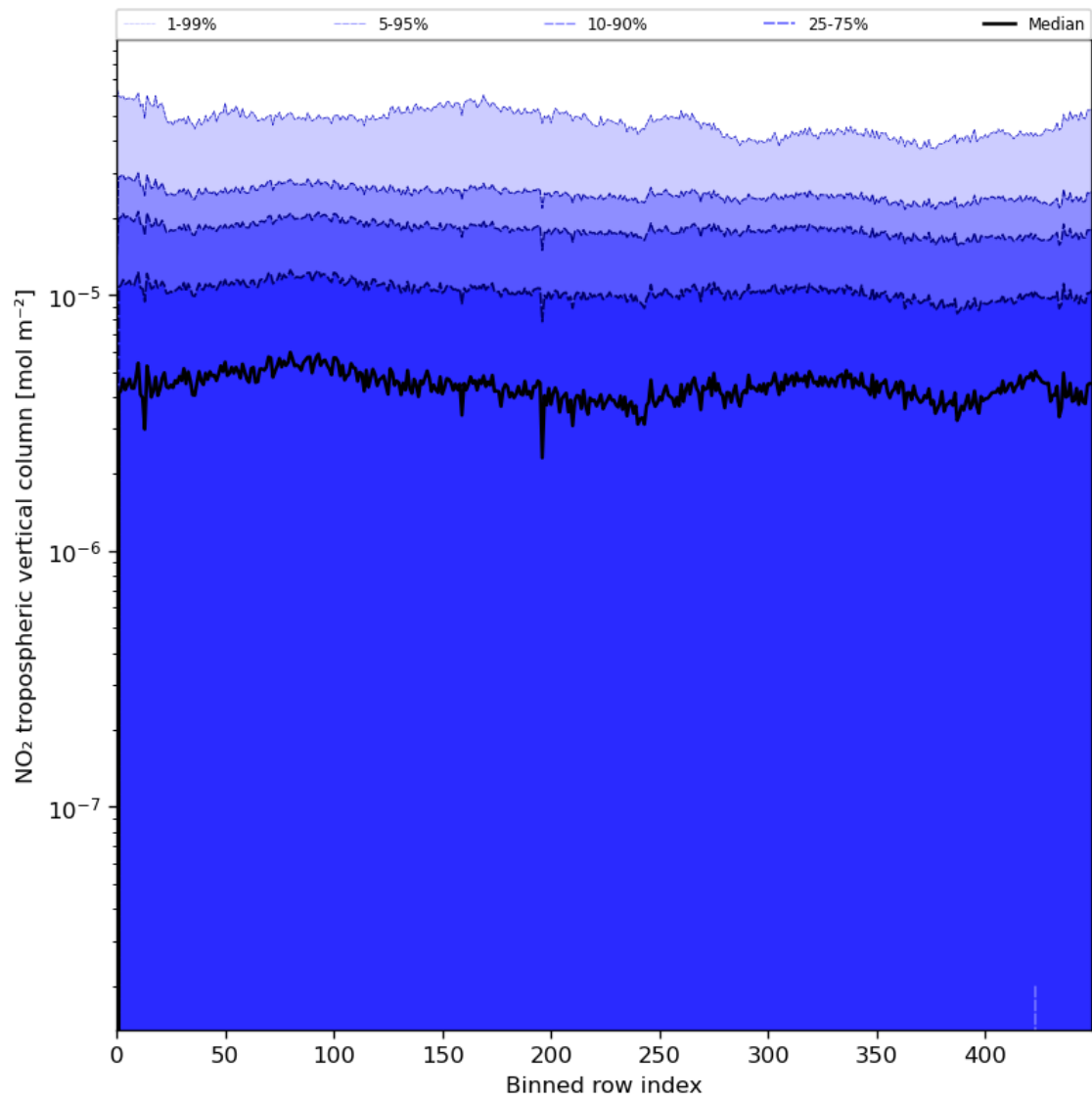
Figure 46: Along track statistics of “NO 2 tropospheric vertical column” for 2024-07-11 to 2024-07-13
