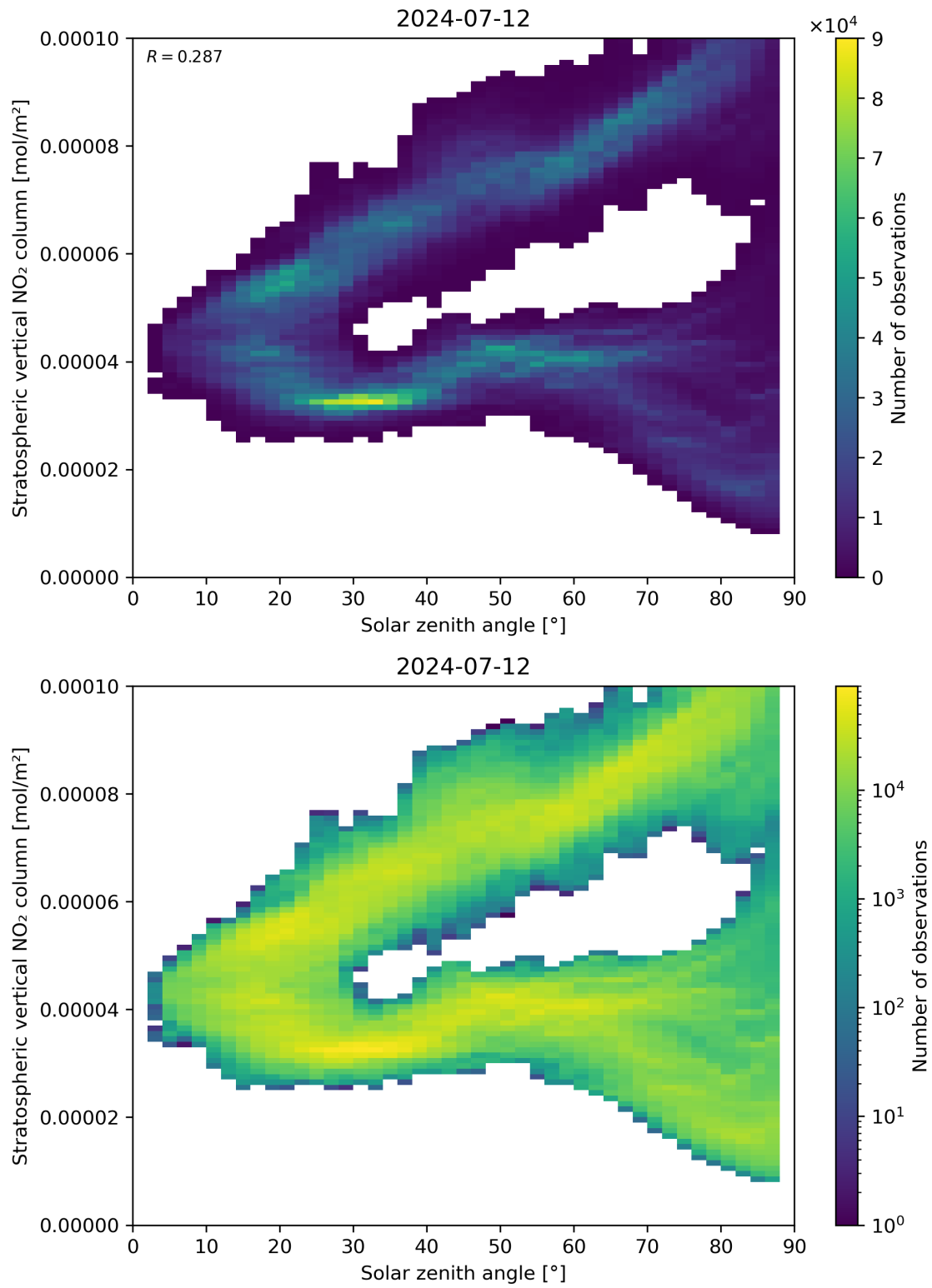
Figure 150: Scatter density plot of “Solar zenith angle” against “Stratospheric vertical NO 2 column” for 2024-07-11 to 2024-07-13.
