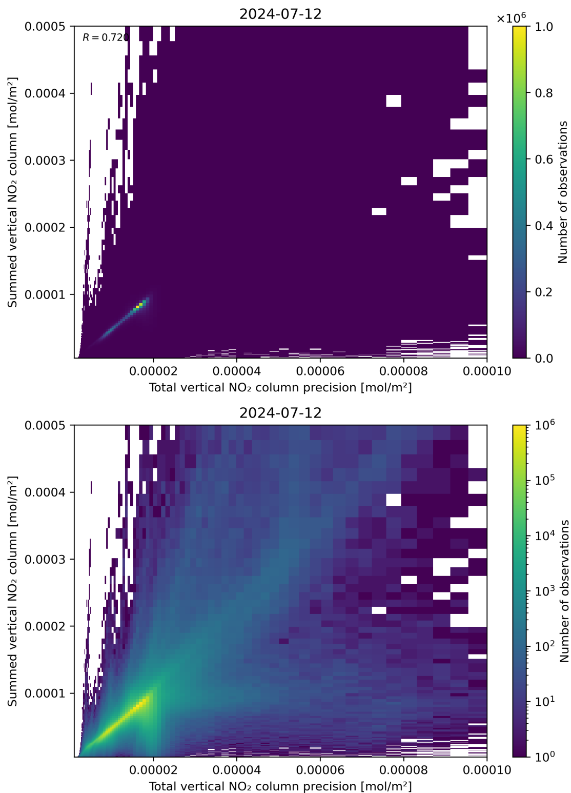
Figure 117: Scatter density plot of “Total vertical NO 2 column precision” against “Summed vertical NO 2 column” for 2024-07-11 to 2024-07-13.
