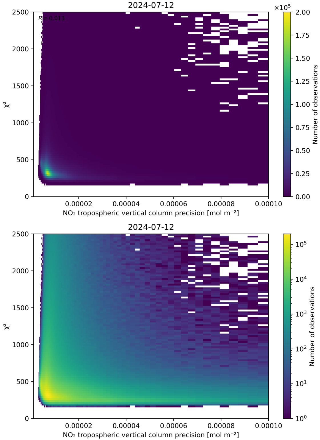
Figure 134: Scatter density plot of “NO 2 tropospheric vertical column precision” against “ \chi^2 ” for 2024-07-11 to 2024-07-13.
