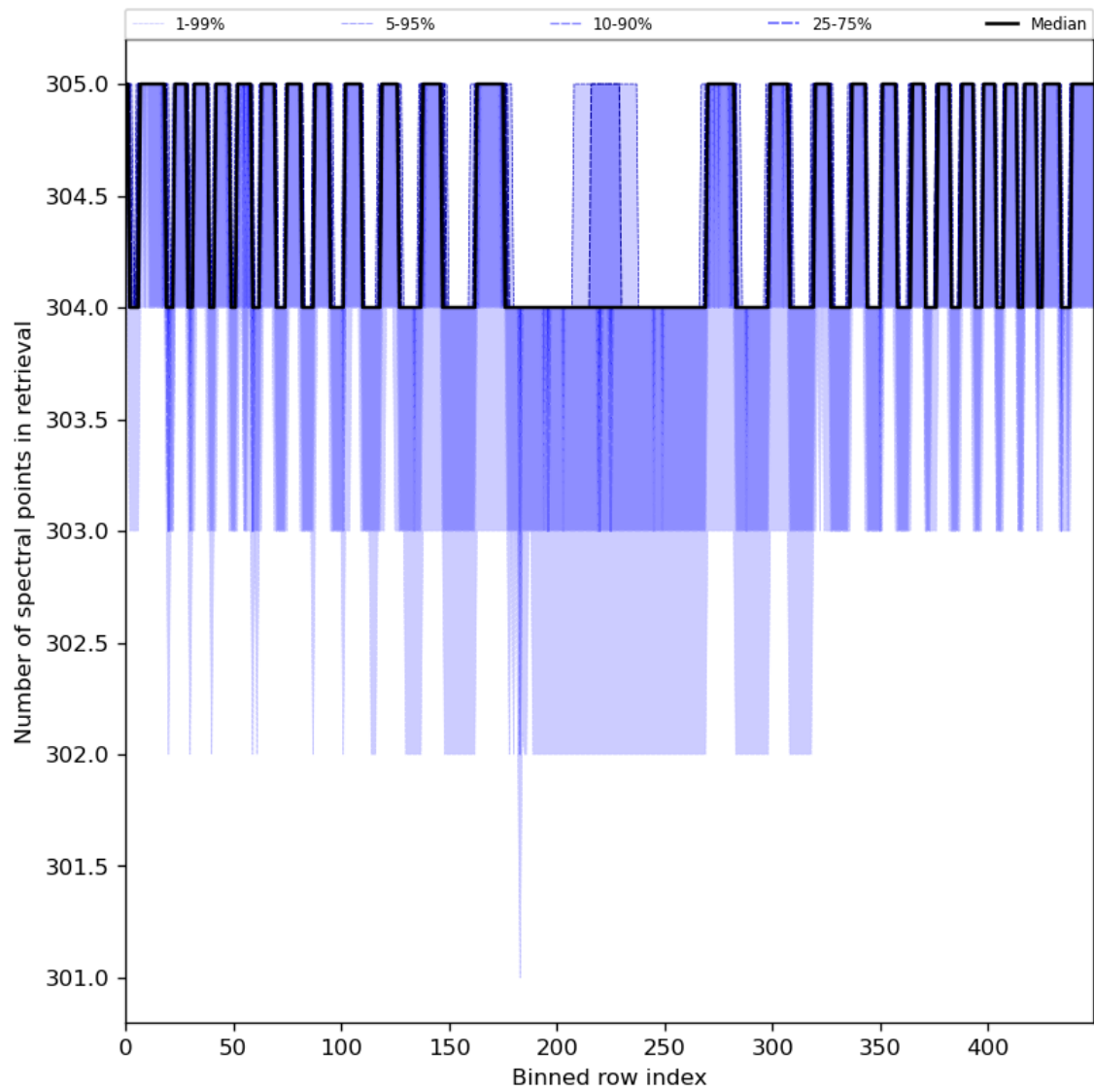
Figure 50: Along track statistics of “Number of spectral points in retrieval” for 2024-07-11 to 2024-07-13
