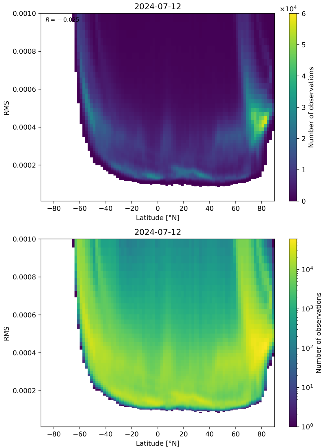
Figure 94: Scatter density plot of “Latitude” against “RMS” for 2024-07-11 to 2024-07-13.
