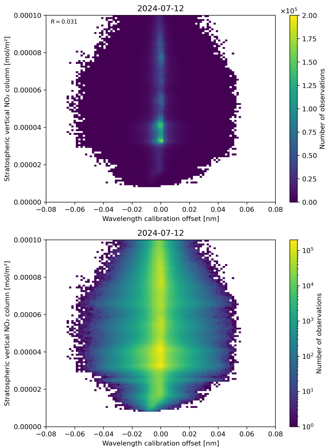
Figure 176: Scatter density plot of “Wavelength calibration offset” against “Stratospheric vertical NO 2 column” for 2024-07-11 to 2024-07-13.
