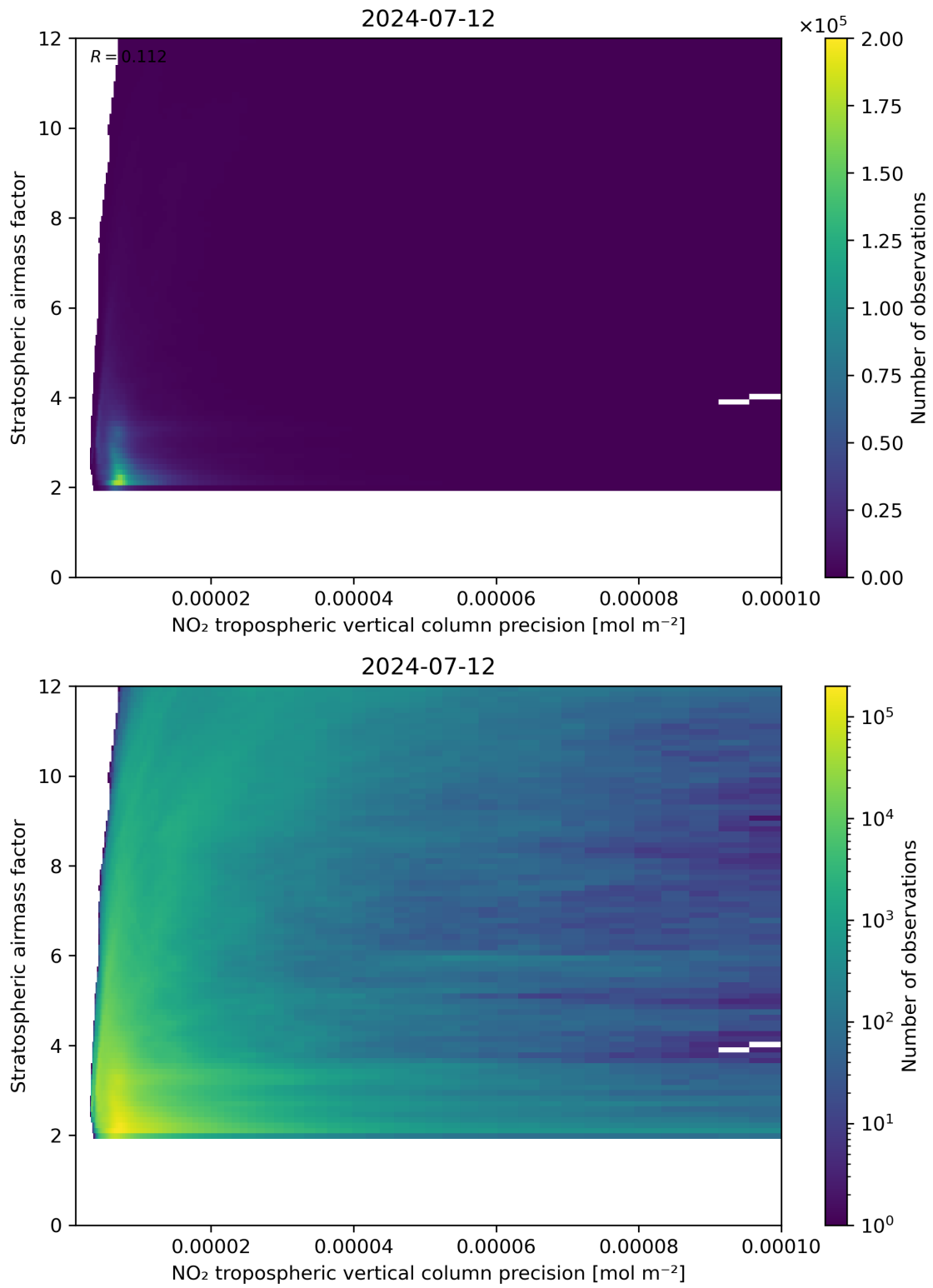
Figure 131: Scatter density plot of “NO 2 tropospheric vertical column precision” against “Stratospheric airmass factor” for 2024-07-11 to 2024-07-13.
