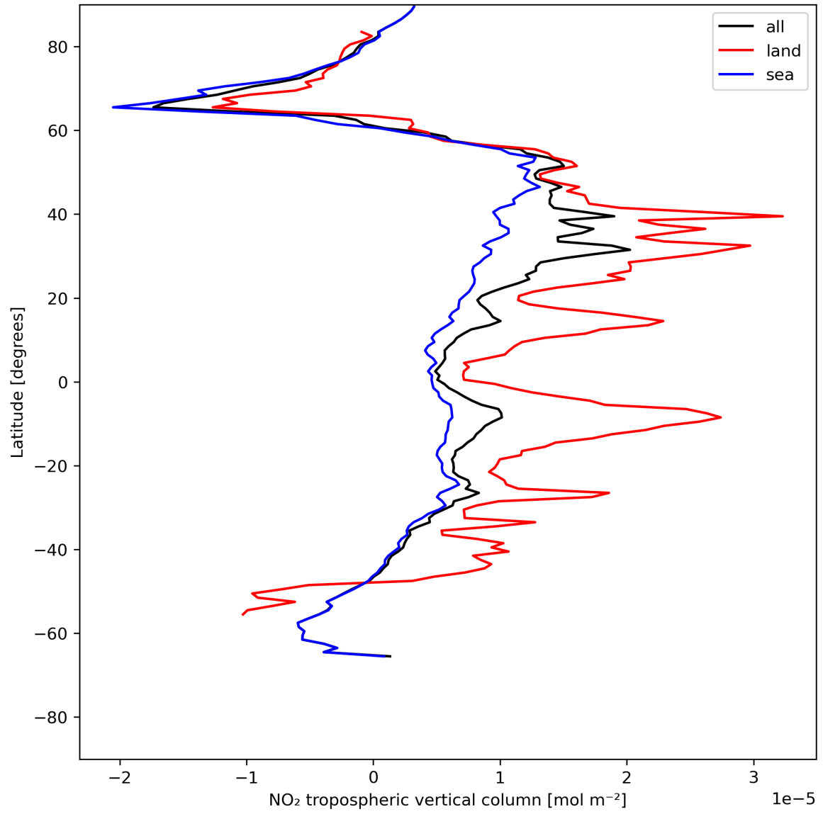
Figure 12: Zonal average of “NO 2 tropospheric vertical column” for 2024-07-11 to 2024-07-13.
