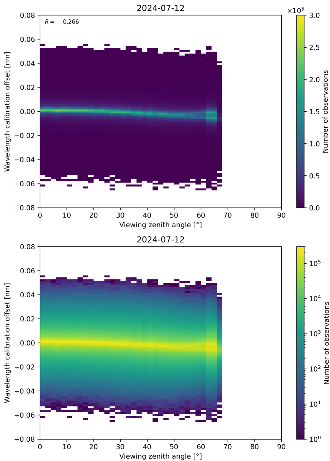
Figure 173: Scatter density plot of “Viewing zenith angle” against “Wavelength calibration offset” for 2024-07-11 to 2024-07-13.
