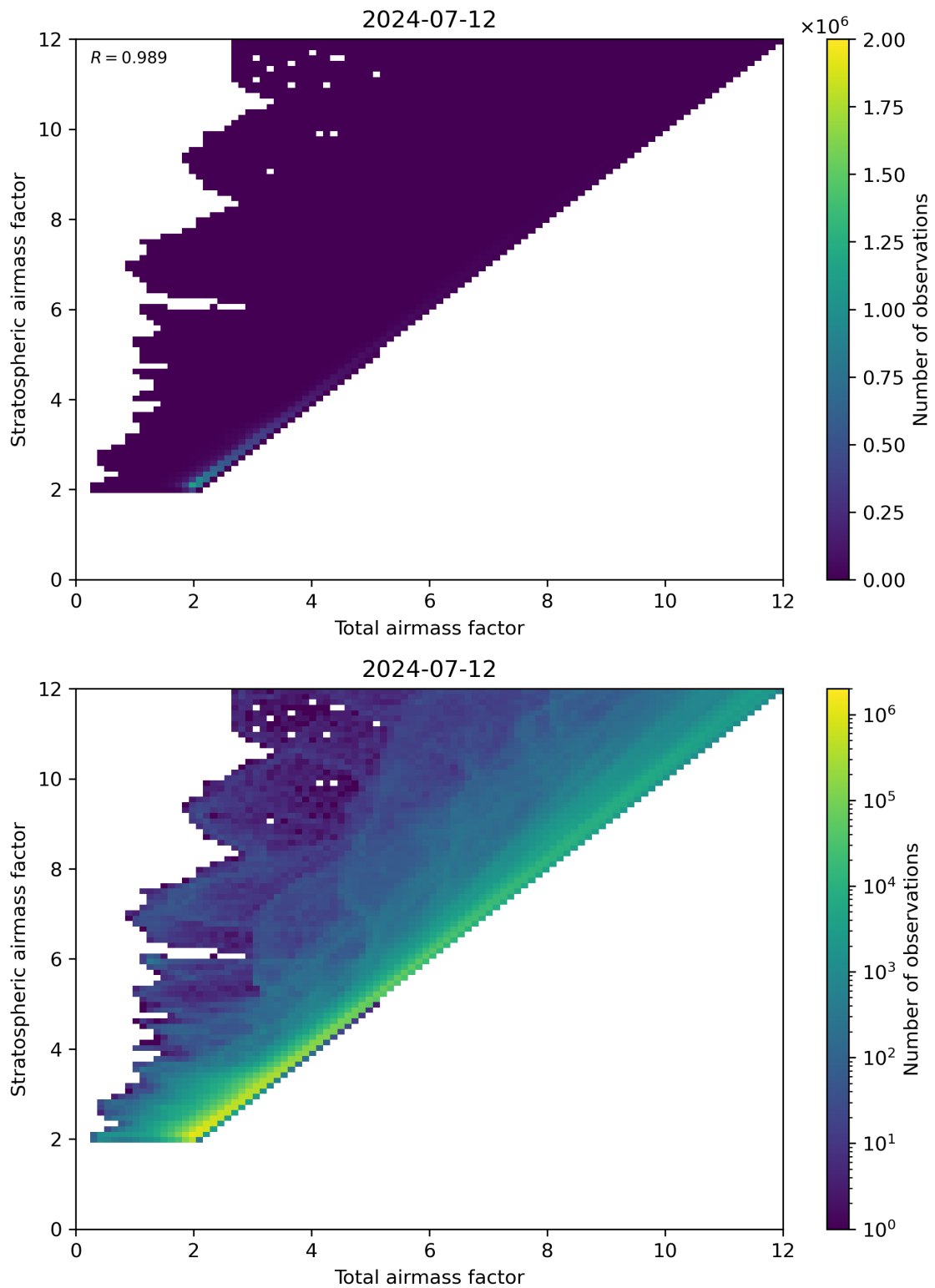
Figure 62: Scatter density plot of “Total airmass factor” against “Stratospheric airmass factor” for 2024-07-11 to 2024-07-13.
