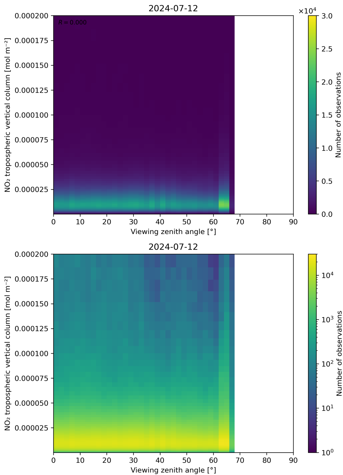
Figure 169: Scatter density plot of “Viewing zenith angle” against “NO 2 tropospheric vertical column” for 2024-07-11 to 2024-07-13.
