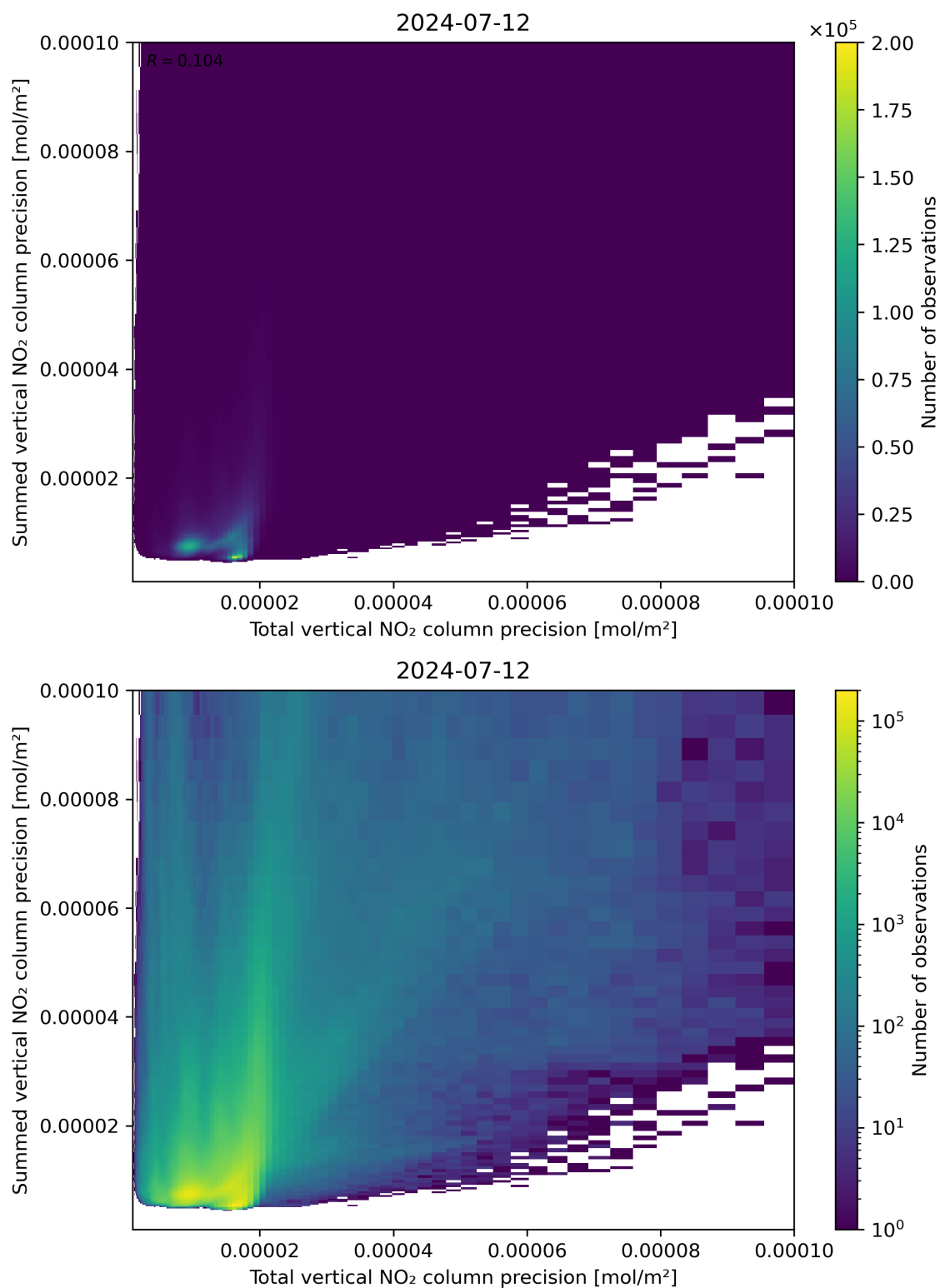
Figure 118: Scatter density plot of “Total vertical NO 2 column precision” against “Summed vertical NO 2 column precision” for 2024-07-11 to 2024-07-13.
