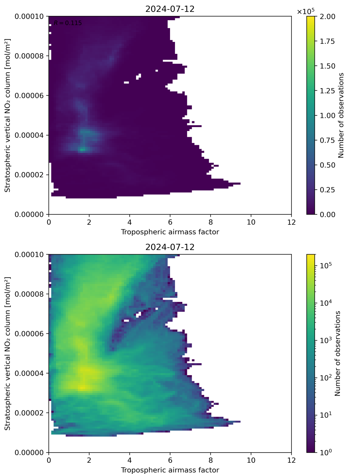
Figure 74: Scatter density plot of “Tropospheric air mass factor” against “Stratospheric vertical NO 2 column” for 2024-07-11 to 2024-07-13.
