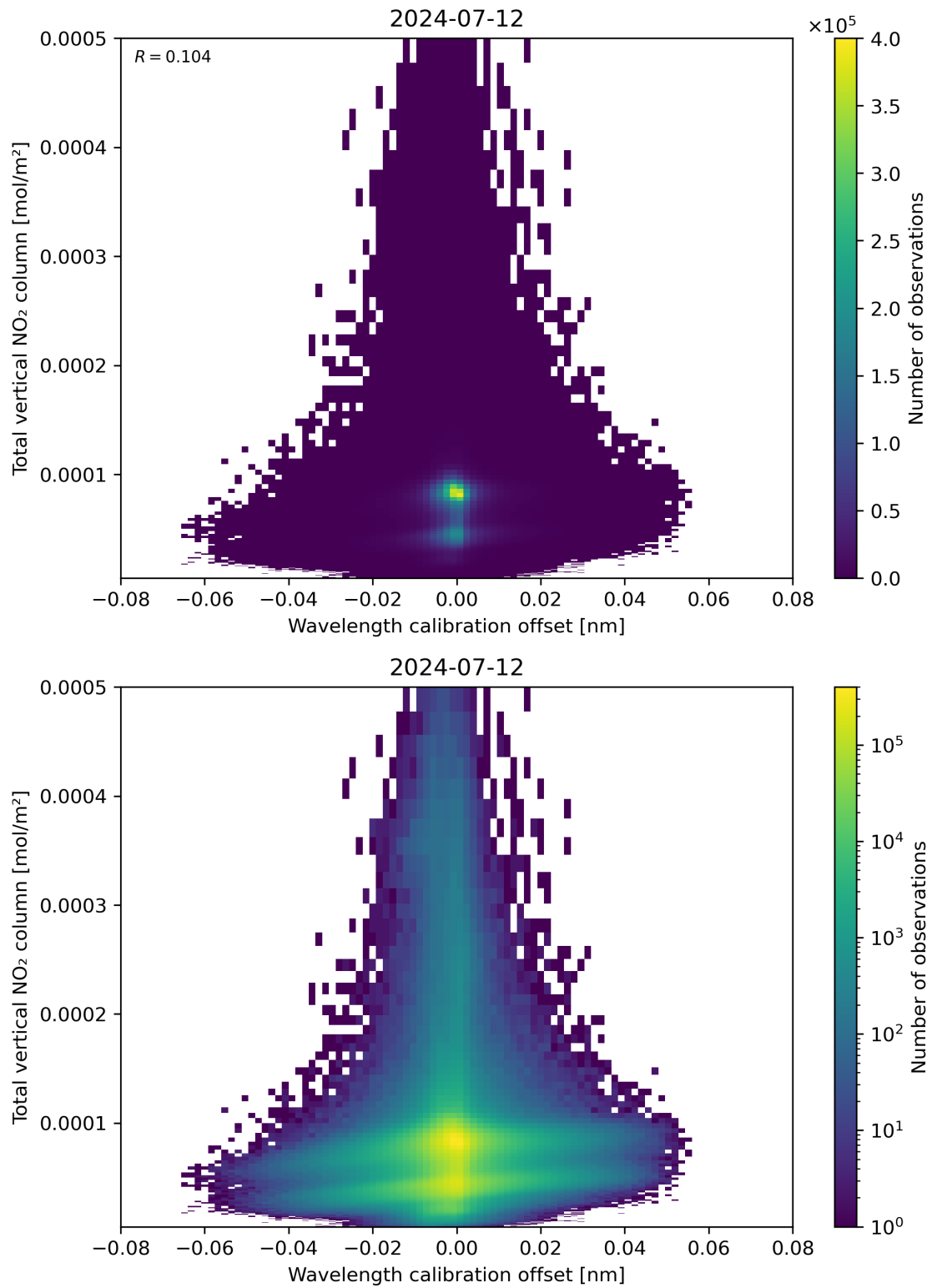
Figure 179: Scatter density plot of “Wavelength calibration offset” against “Total vertical NO 2 column” for 2024-07-11 to 2024-07-13.
