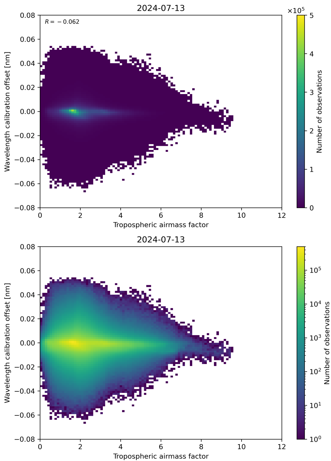
Figure 80: Scatter density plot of “Tropospheric air mass factor” against “Wavelength calibration offset” for 2024-07-12 to 2024-07-14.
