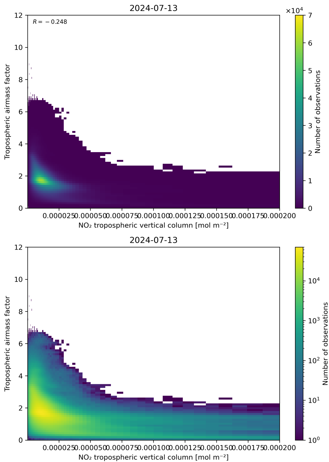
Figure 123: Scatter density plot of “NO 2 tropospheric vertical column” against “Tropospheric airmass factor” for 2024-07-12 to 2024-07-14.
