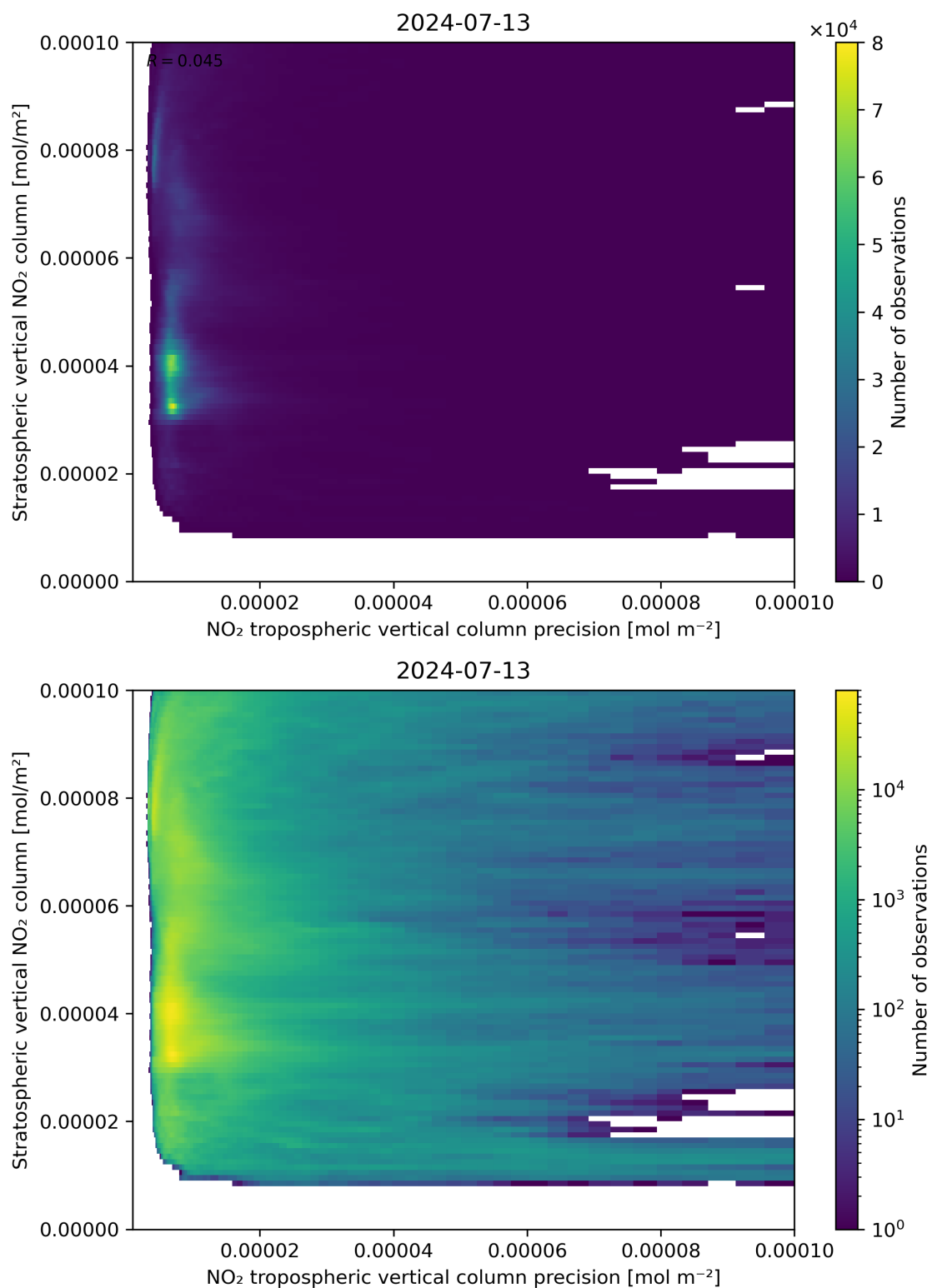
Figure 135: Scatter density plot of “NO 2 tropospheric vertical column precision” against “Stratospheric vertical NO 2 column” for 2024-07-12 to 2024-07-14.
