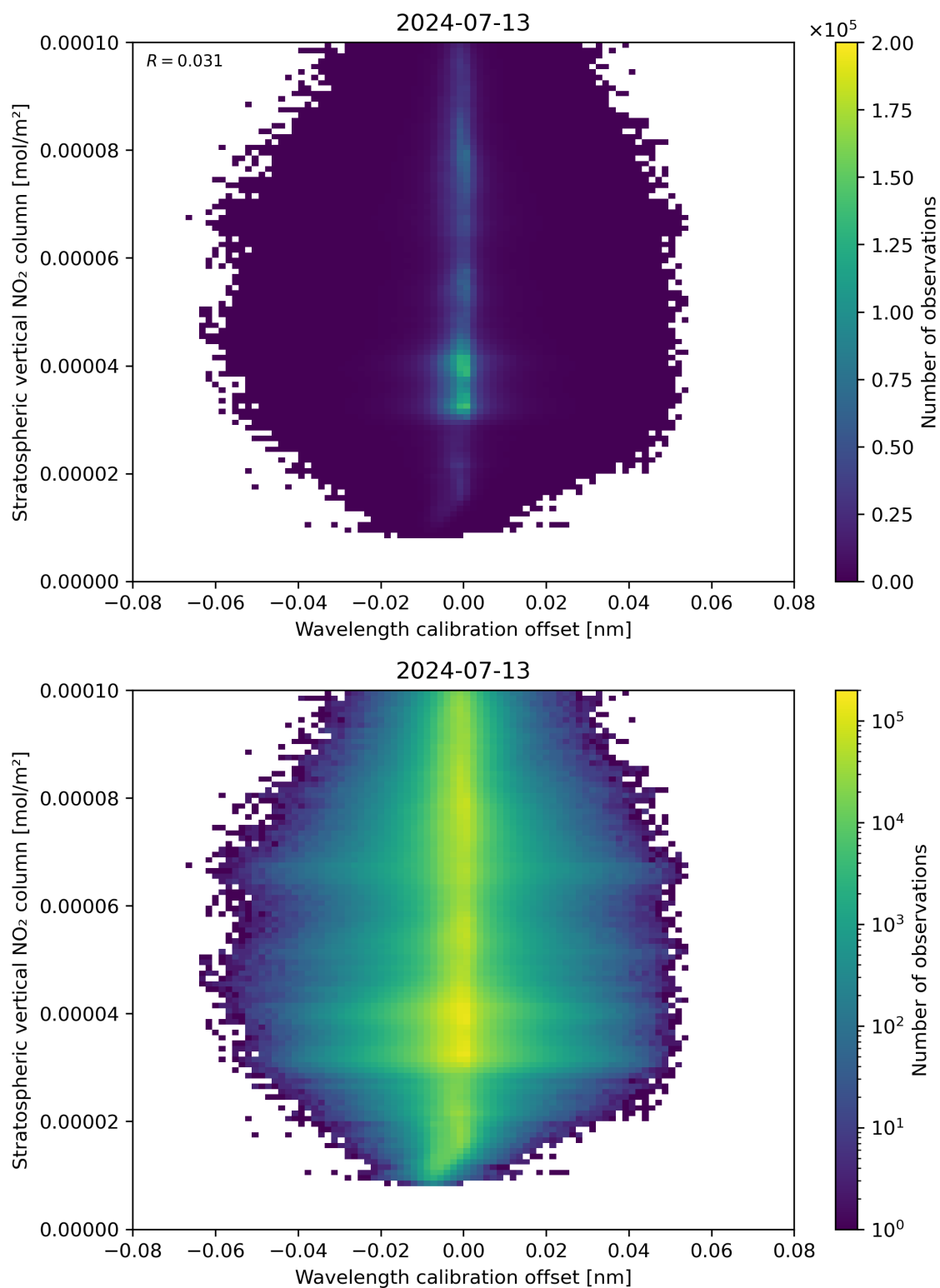
Figure 176: Scatter density plot of “Wavelength calibration offset” against “Stratospheric vertical NO 2 column” for 2024-07-12 to 2024-07-14.
