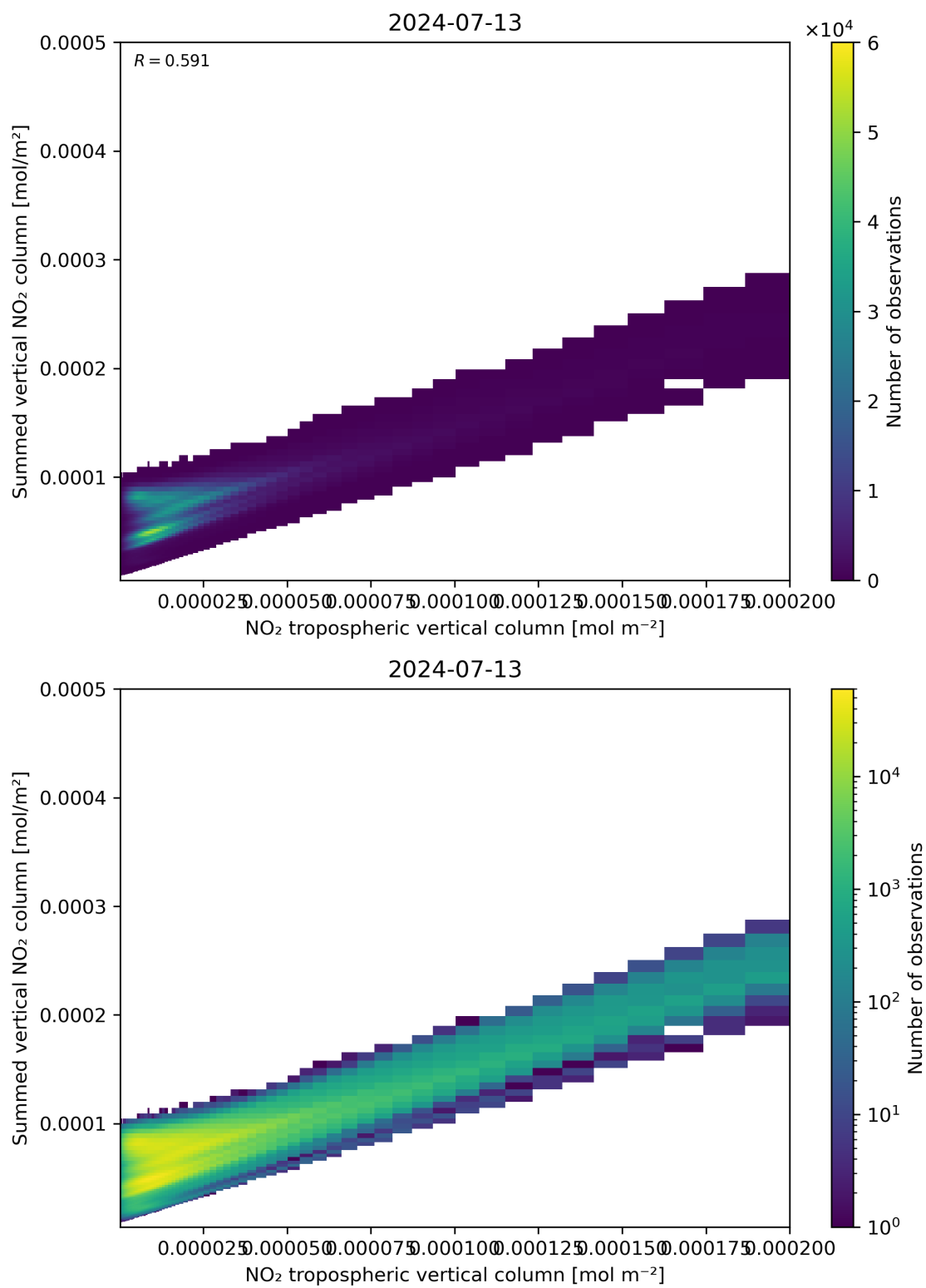
Figure 126: Scatter density plot of “NO 2 tropospheric vertical column” against “Summed vertical NO 2 column” for 2024-07-12 to 2024-07-14.
