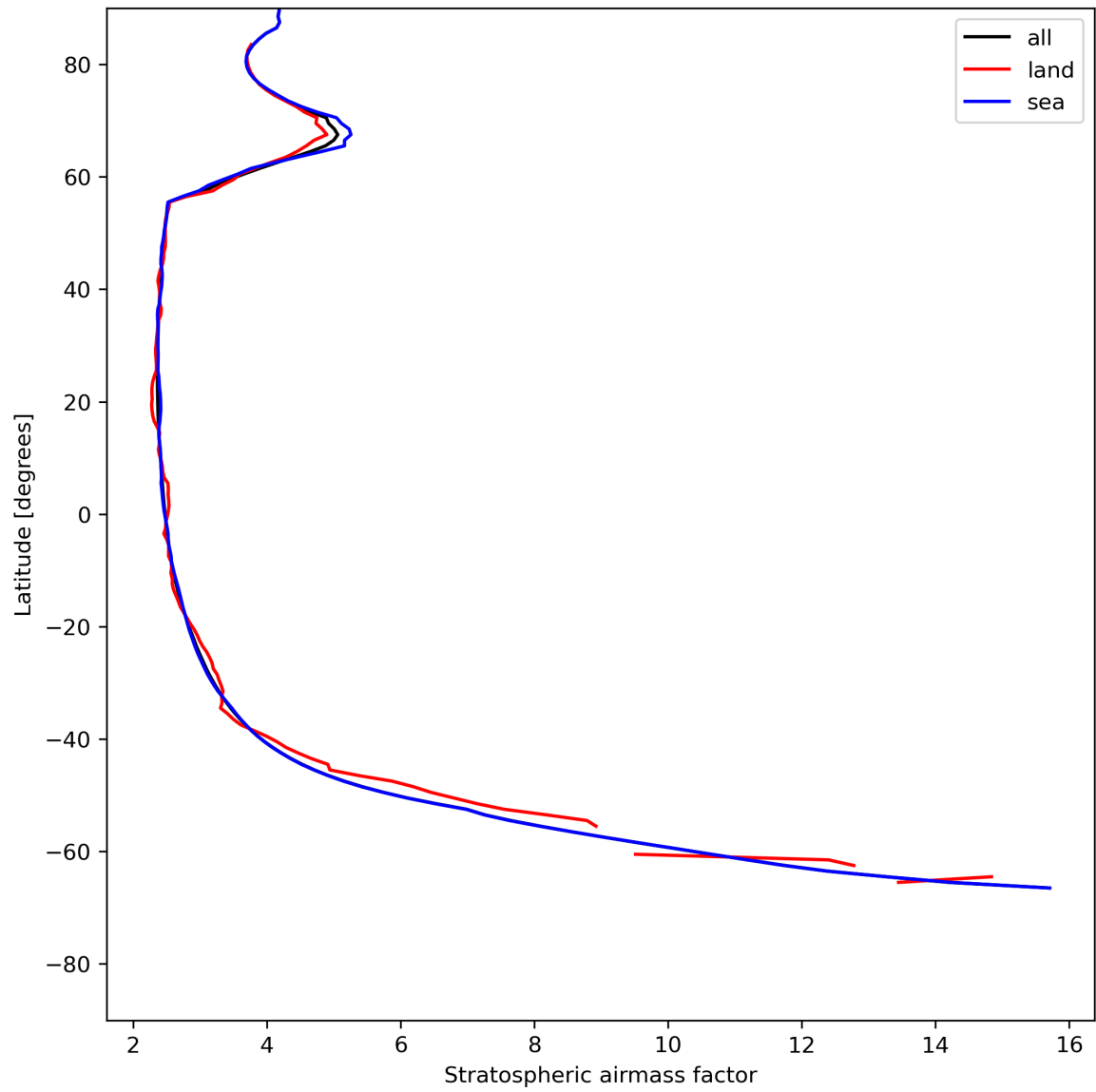
Figure 27: Zonal average of “Stratospheric airmass factor” for 2024-07-12 to 2024-07-14.
