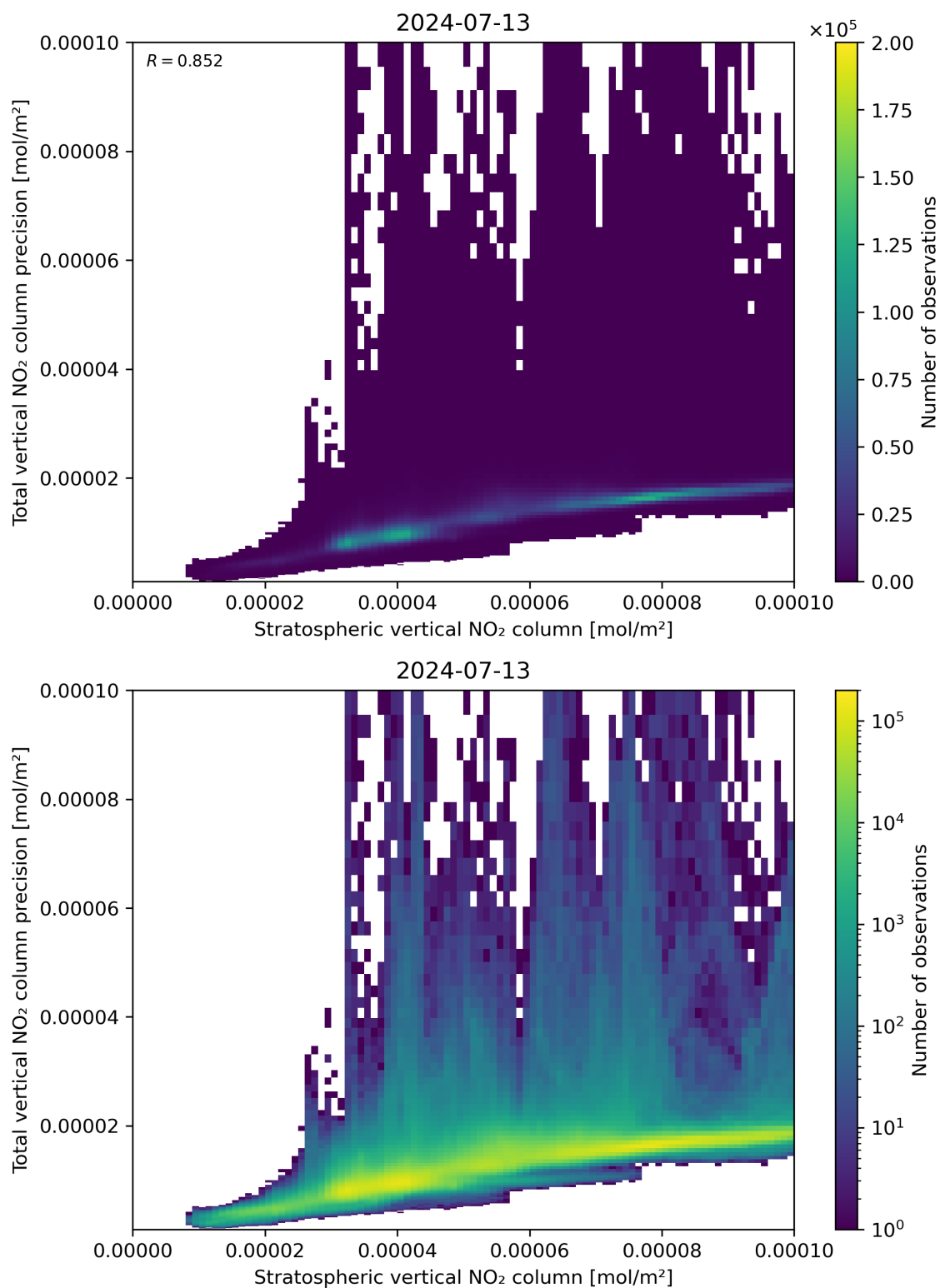
Figure 101: Scatter density plot of “Stratospheric vertical NO 2 column” against “Total vertical NO 2 column precision” for 2024-07-12 to 2024-07-14.
