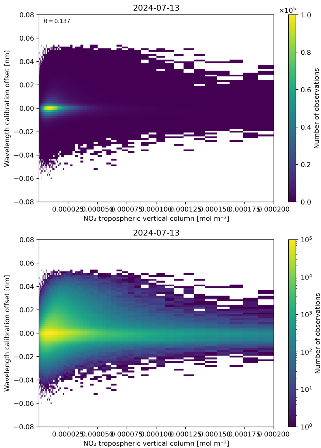
Figure 143: Scatter density plot of “NO 2 tropospheric vertical column” against “Wavelength calibration offset” for 2024-07-12 to 2024-07-14.
