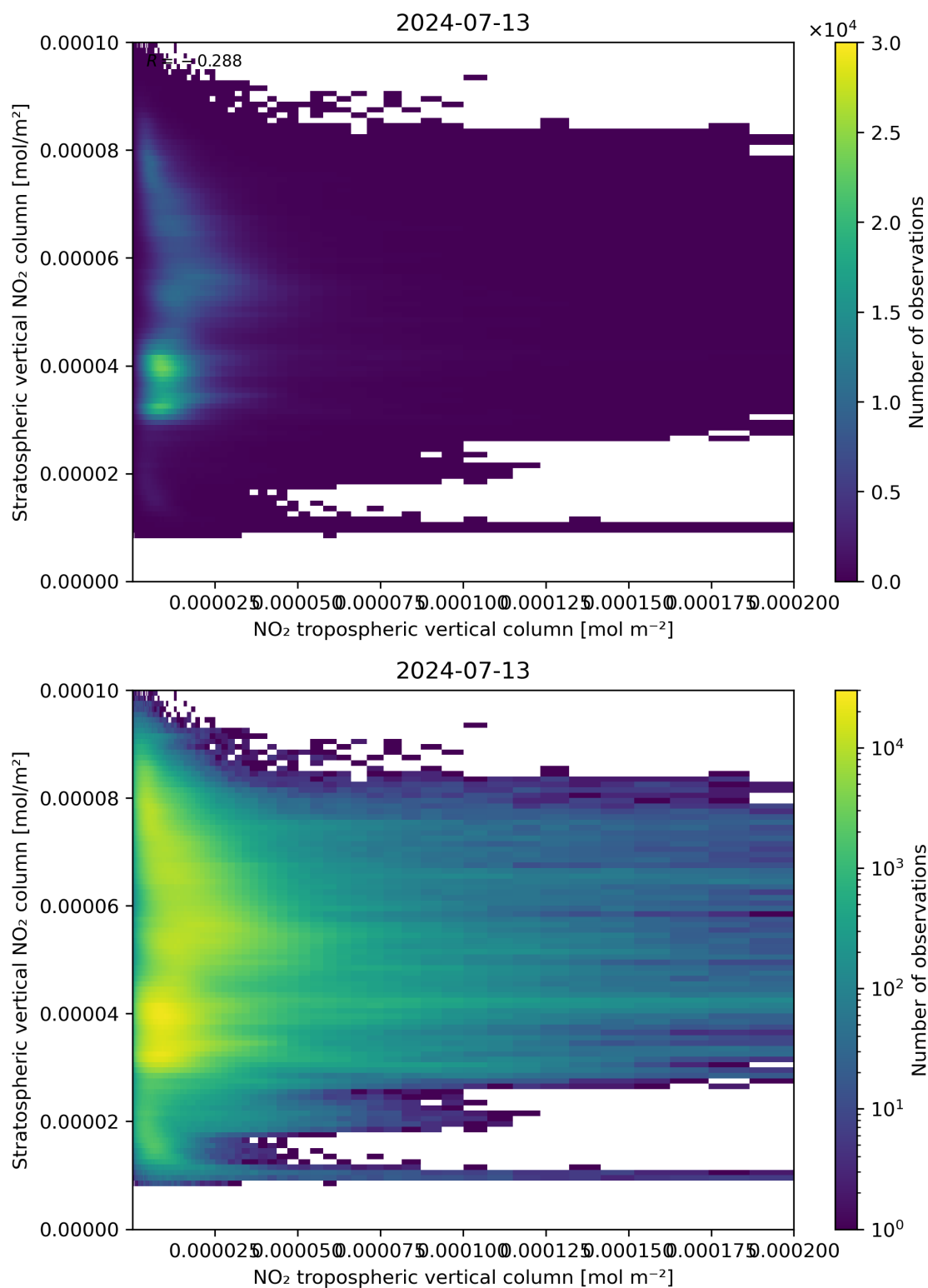
Figure 125: Scatter density plot of “NO 2 tropospheric vertical column” against “Stratospheric vertical NO 2 column” for 2024-07-12 to 2024-07-14.
