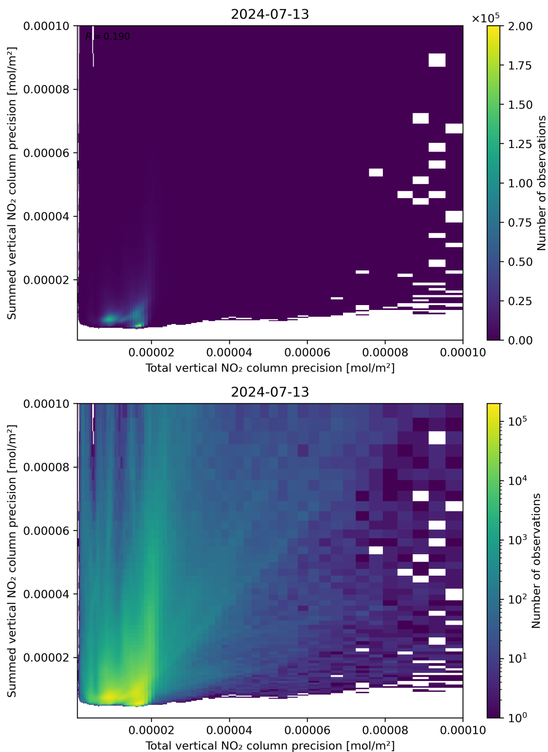
Figure 118: Scatter density plot of “Total vertical NO 2 column precision” against “Summed vertical NO 2 column precision” for 2024-07-12 to 2024-07-14.
