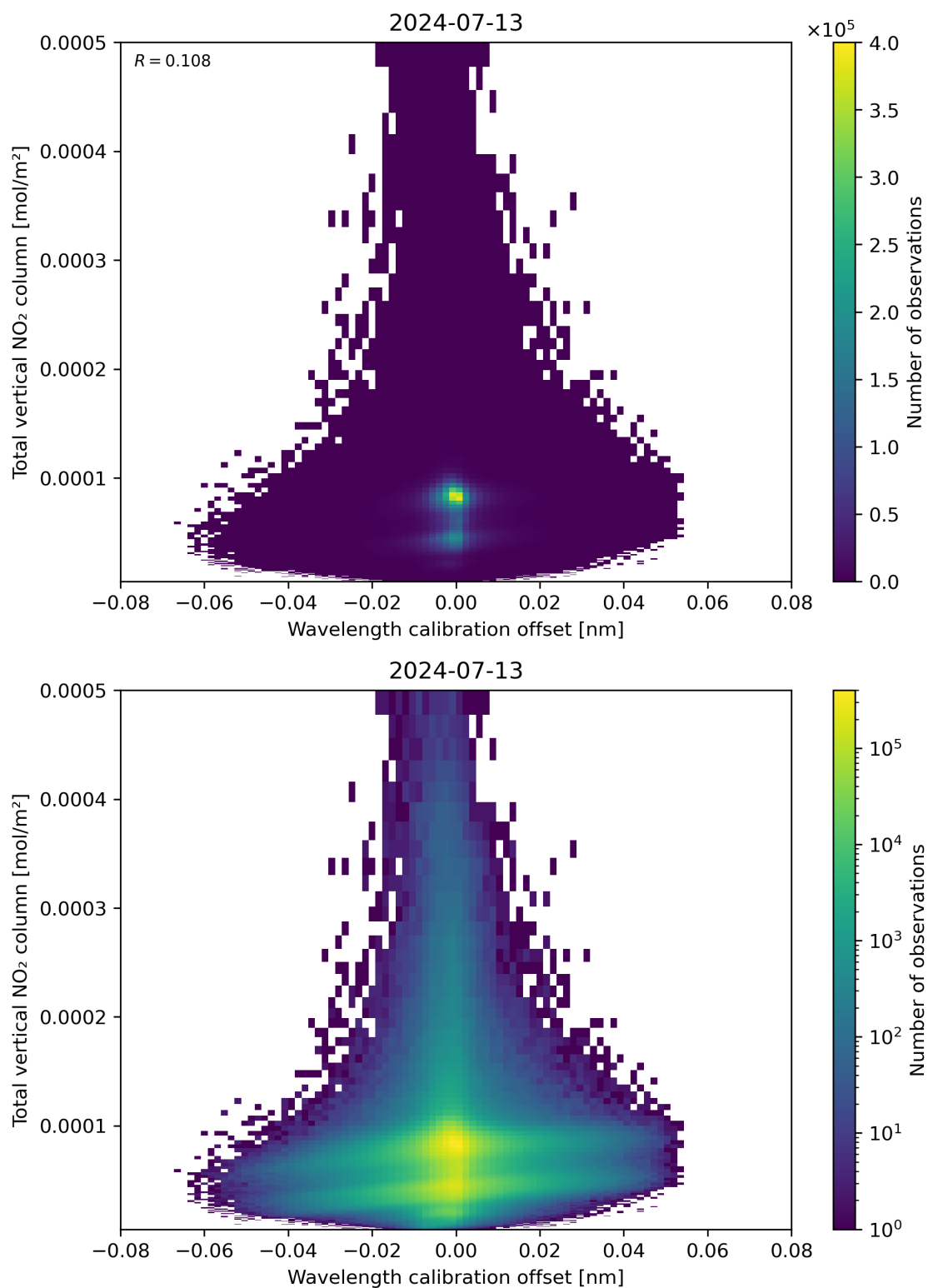
Figure 179: Scatter density plot of “Wavelength calibration offset” against “Total vertical NO 2 column” for 2024-07-12 to 2024-07-14.
