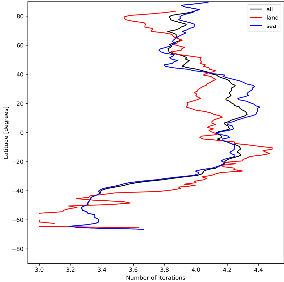
Figure 17: Zonal average of “Number of iterations” for 2024-07-12 to 2024-07-14.
