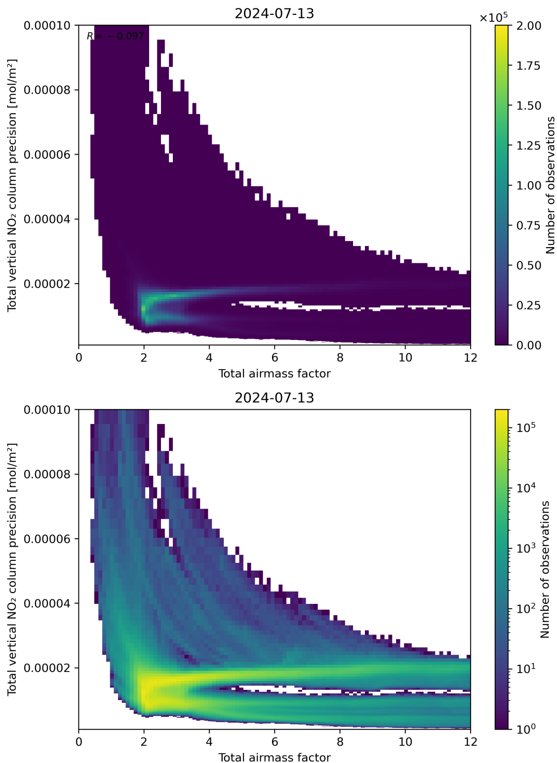
Figure 68: Scatter density plot of “Total airmass factor” against “Total vertical NO 2 column precision” for 2024-07-12 to 2024-07-14.
