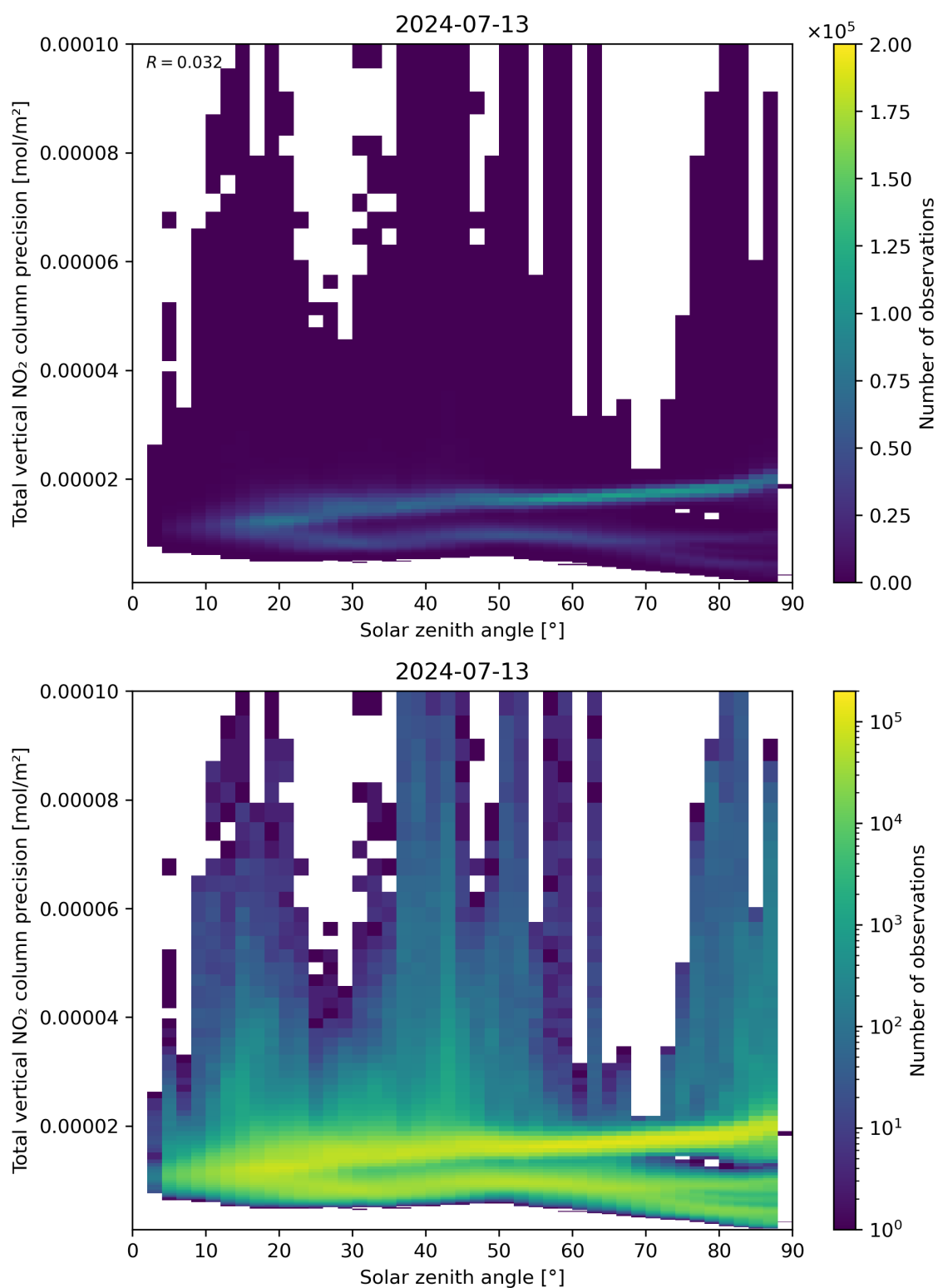
Figure 154: Scatter density plot of “Solar zenith angle” against “Total vertical NO 2 column precision” for 2024-07-12 to 2024-07-14.
