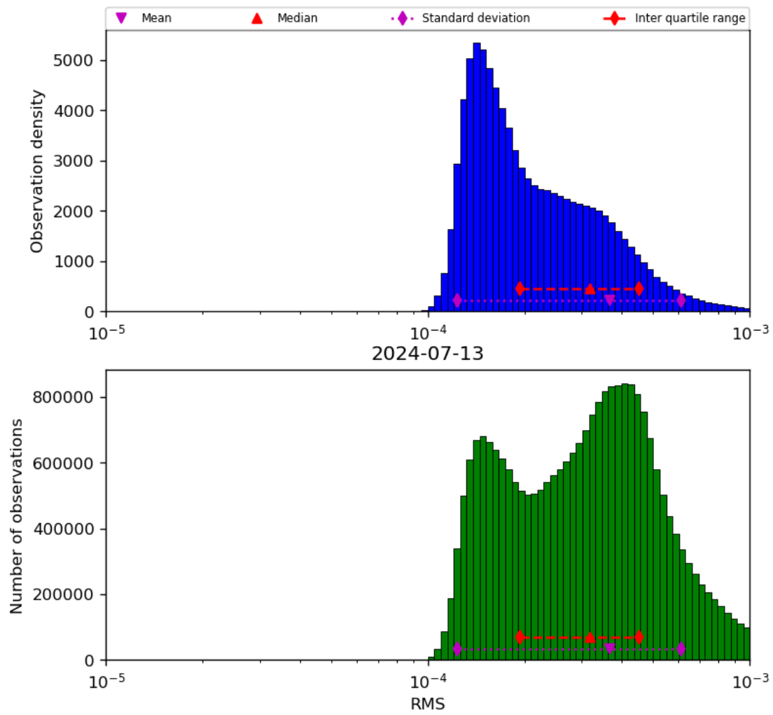
Figure 43: Histogram of “RMS” for 2024-07-12 to 2024-07-14
