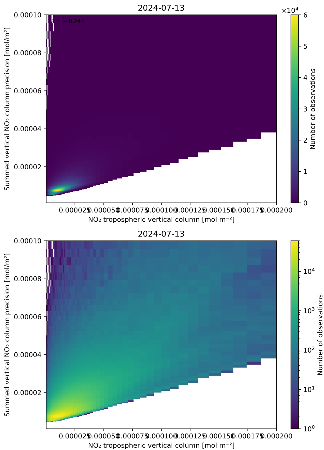
Figure 127: Scatter density plot of “NO 2 tropospheric vertical column” against “Summed vertical NO 2 column precision” for 2024-07-12 to 2024-07-14.
