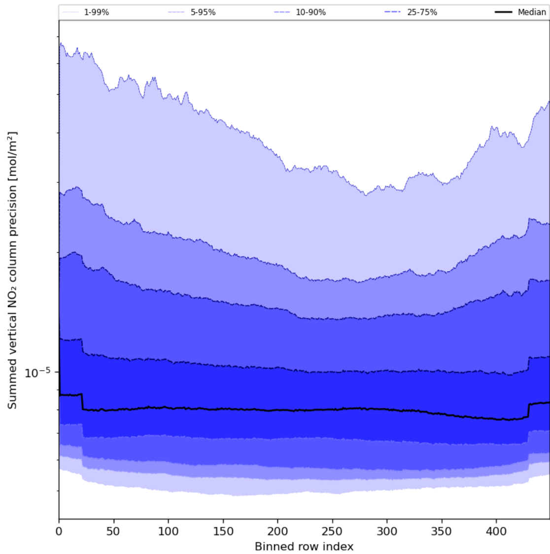
Figure 58: Along track statistics of “Summed vertical NO 2 column precision” for 2024-07-12 to 2024-07-14
