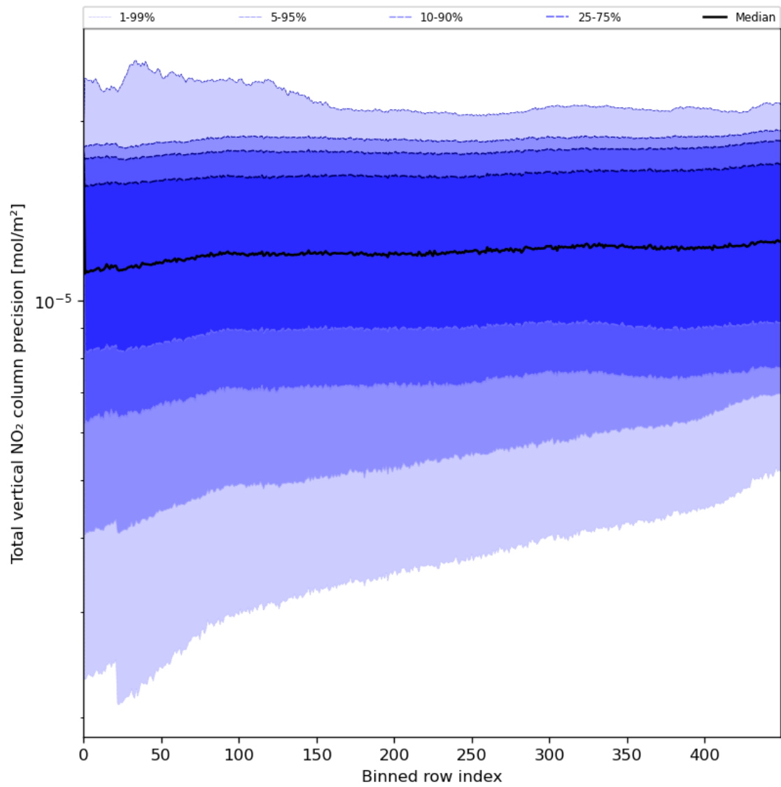
Figure 56: Along track statistics of “Total vertical NO 2 column precision” for 2024-07-12 to 2024-07-14
