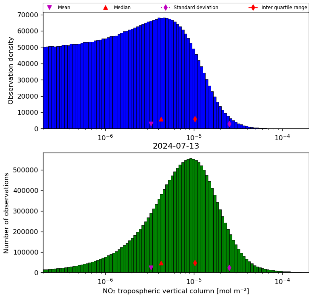
Figure 29: Histogram of “NO 2 tropospheric vertical column” for 2024-07-12 to 2024-07-14
