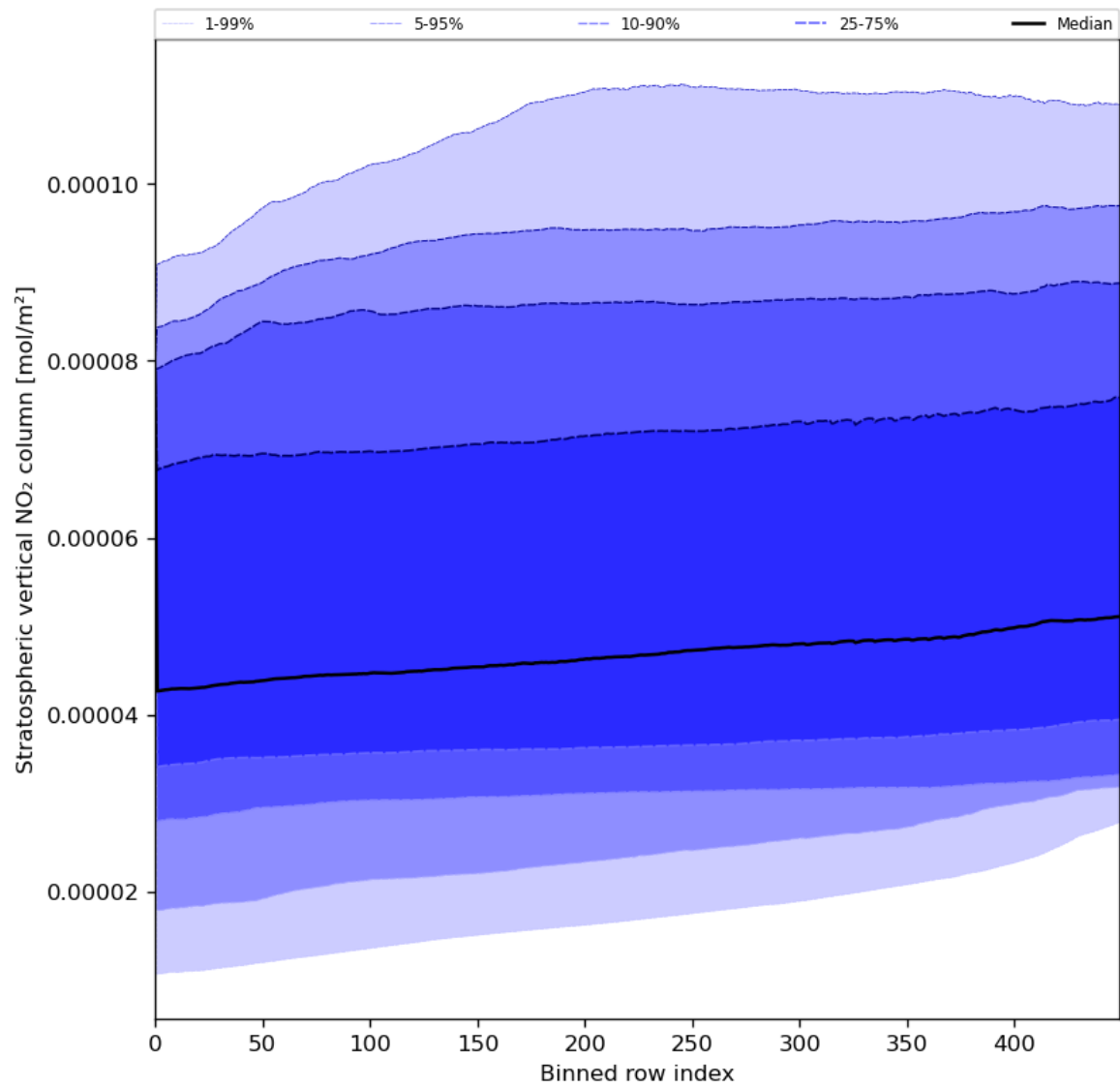
Figure 53: Along track statistics of “Stratospheric vertical NO 2 column” for 2024-07-12 to 2024-07-14
