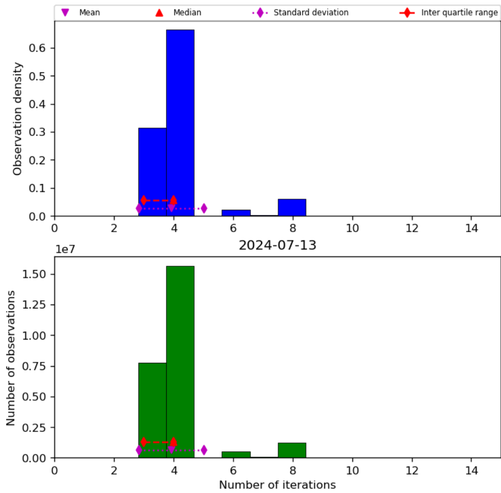
Figure 34: Histogram of “Number of iterations” for 2024-07-12 to 2024-07-14
