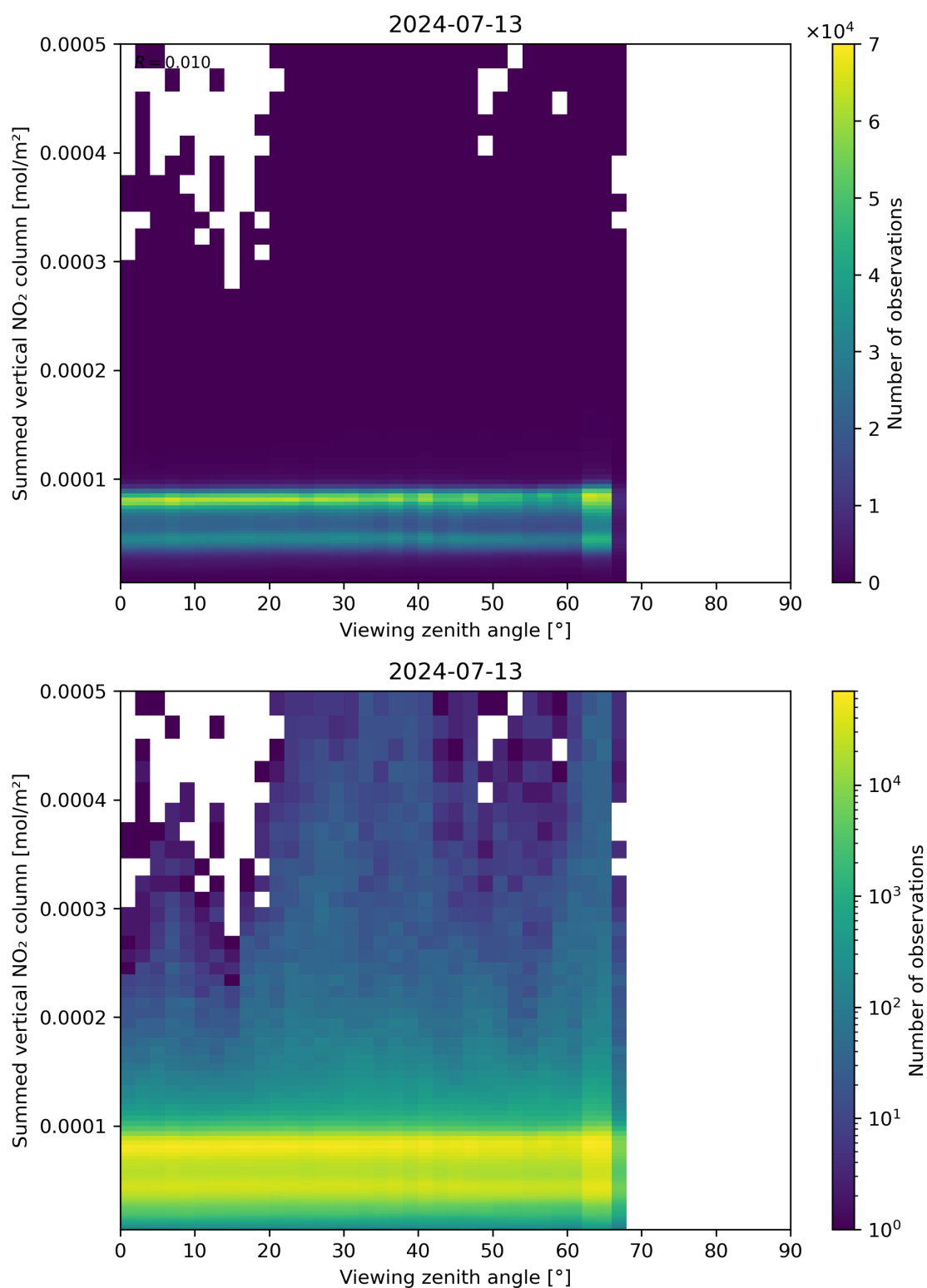
Figure 165: Scatter density plot of “Viewing zenith angle” against “Summed vertical NO 2 column” for 2024-07-12 to 2024-07-14.
