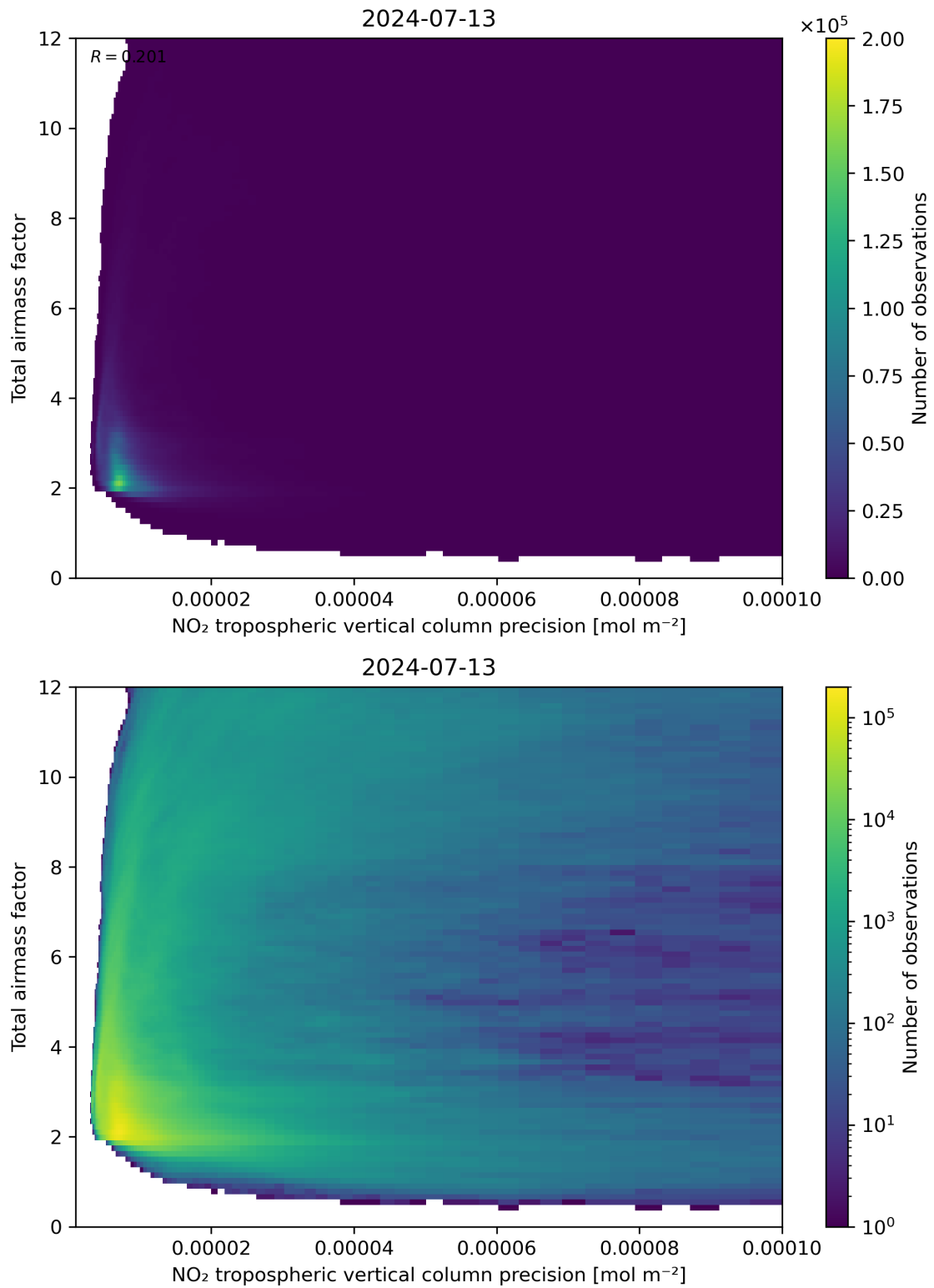
Figure 132: Scatter density plot of “NO 2 tropospheric vertical column precision” against “Total air mass factor” for 2024-07-12 to 2024-07-14.
