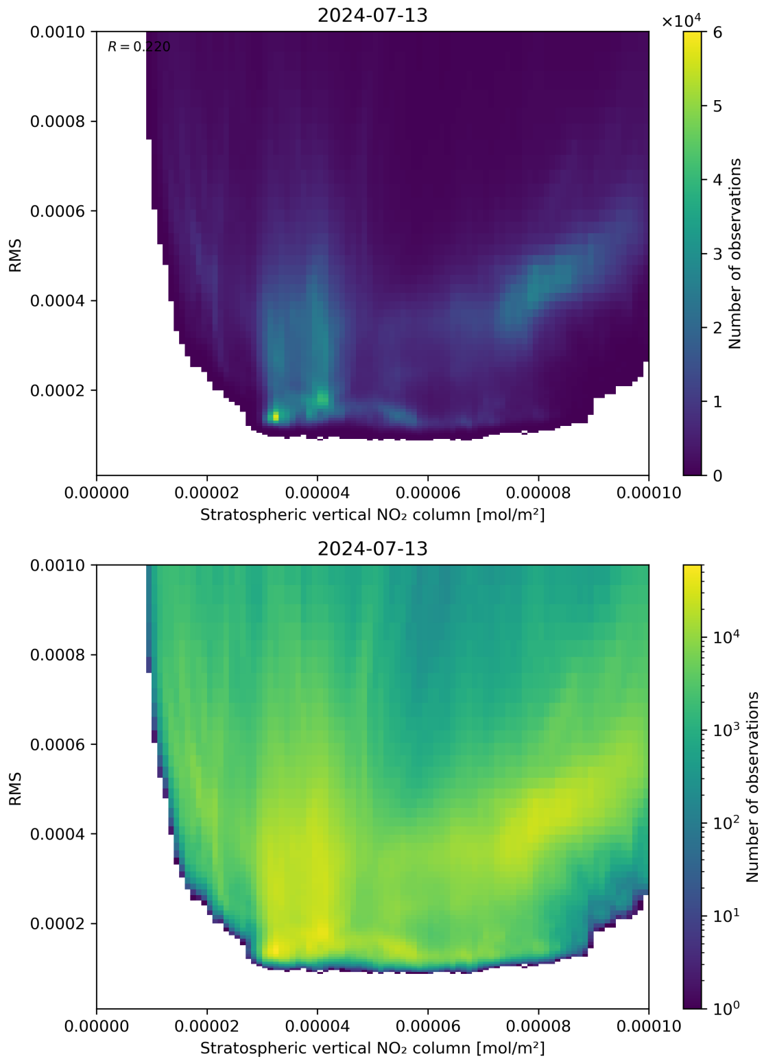
Figure 102: Scatter density plot of “Stratospheric vertical NO 2 column” against “RMS” for 2024-07-12 to 2024-07-14.
