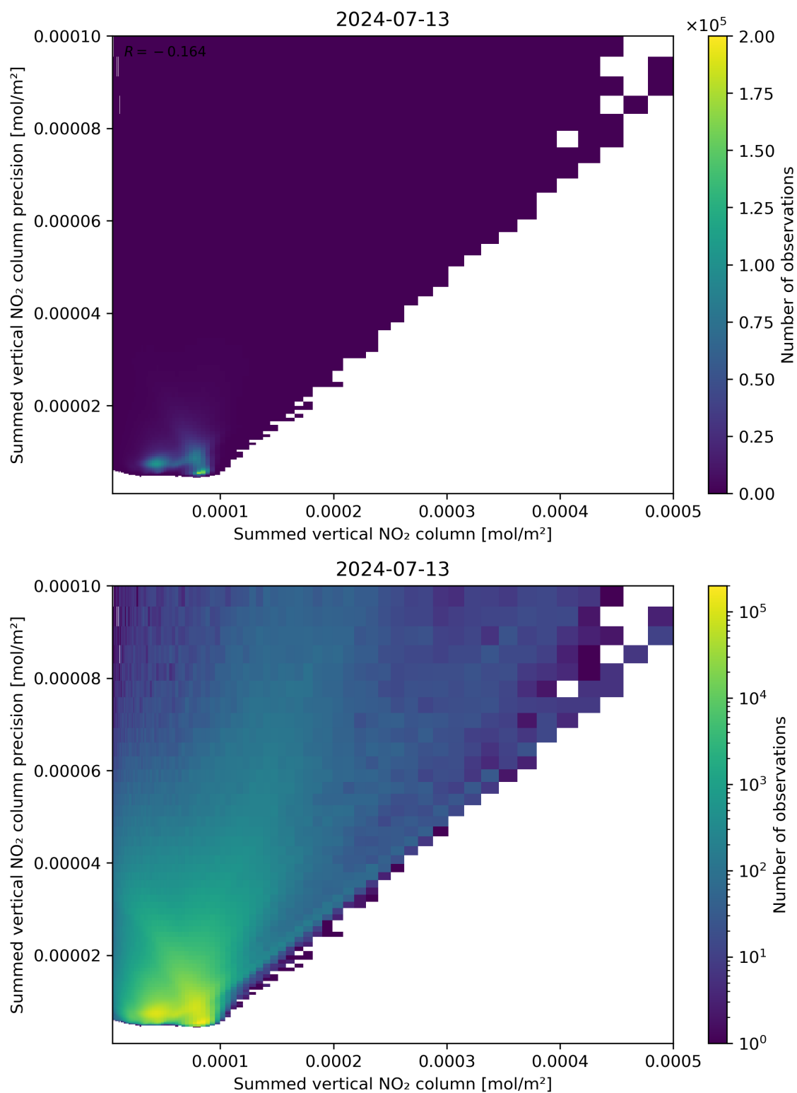
Figure 105: Scatter density plot of “Summed vertical NO 2 column” against “Summed vertical NO 2 column precision” for 2024-07-12 to 2024-07-14.
