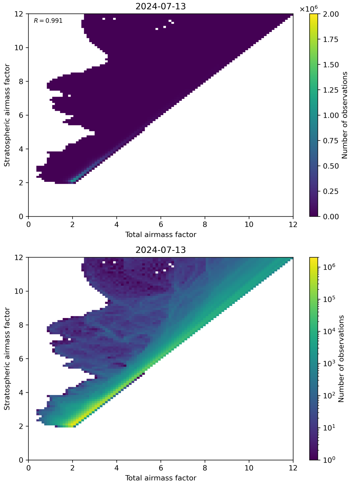
Figure 62: Scatter density plot of “Total airmass factor” against “Stratospheric airmass factor” for 2024-07-12 to 2024-07-14.
