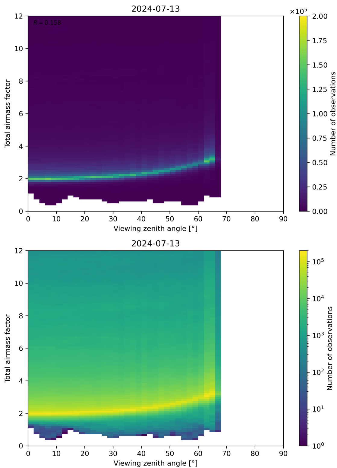
Figure 160: Scatter density plot of “Viewing zenith angle” against “Total airmass factor” for 2024-07-12 to 2024-07-14.
