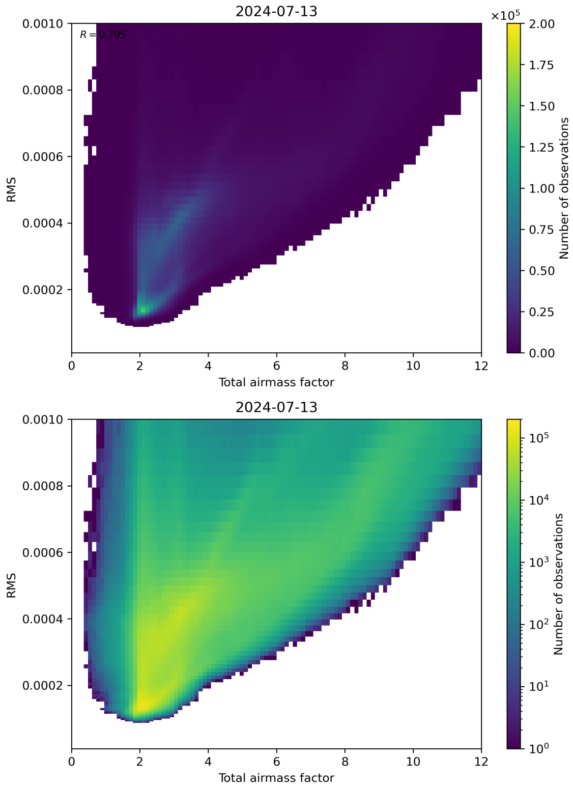
Figure 69: Scatter density plot of “Total airmass factor” against “RMS” for 2024-07-12 to 2024-07-14.
