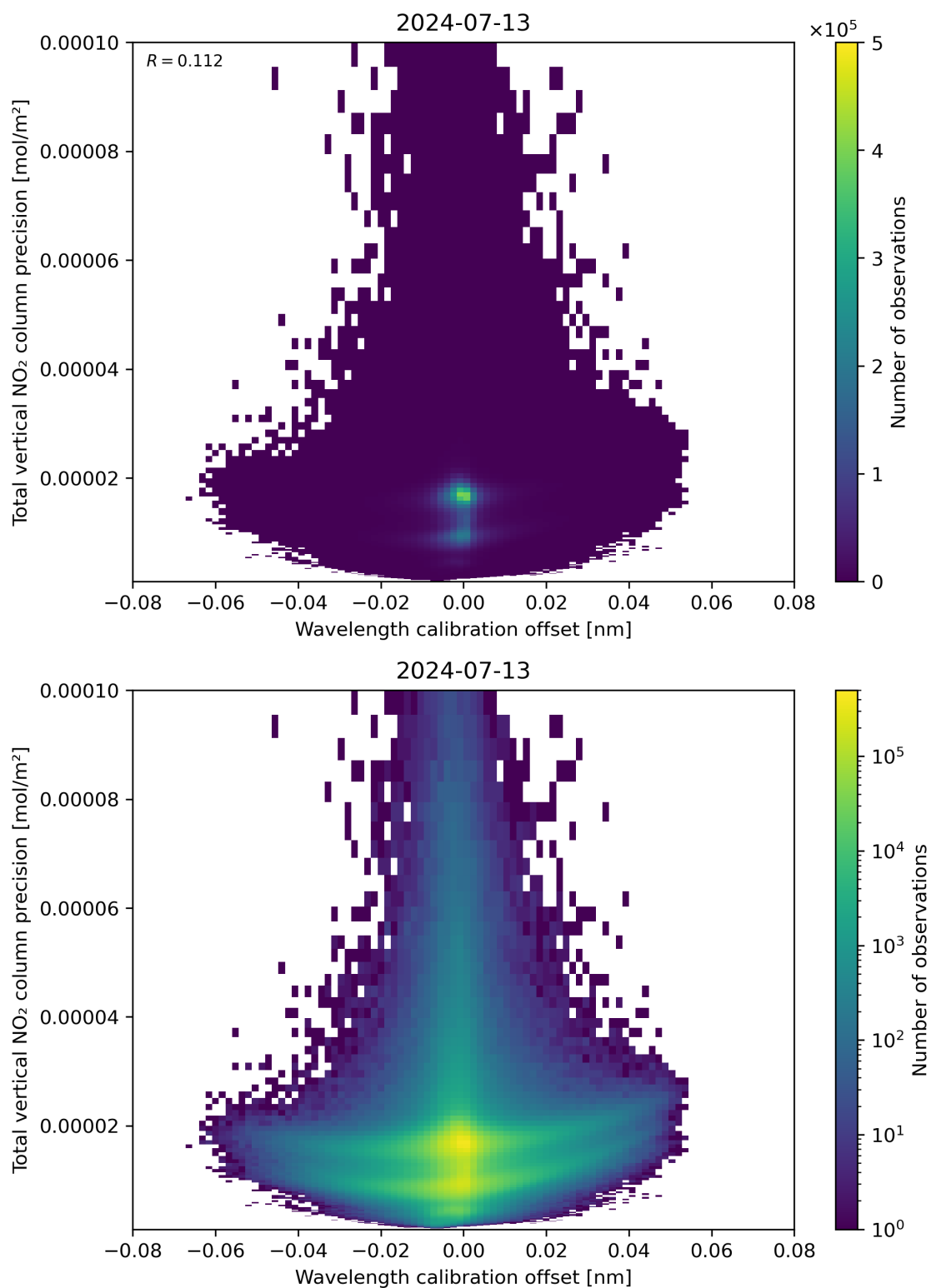
Figure 180: Scatter density plot of “Wavelength calibration offset” against “Total vertical NO 2 column precision” for 2024-07-12 to 2024-07-14.
