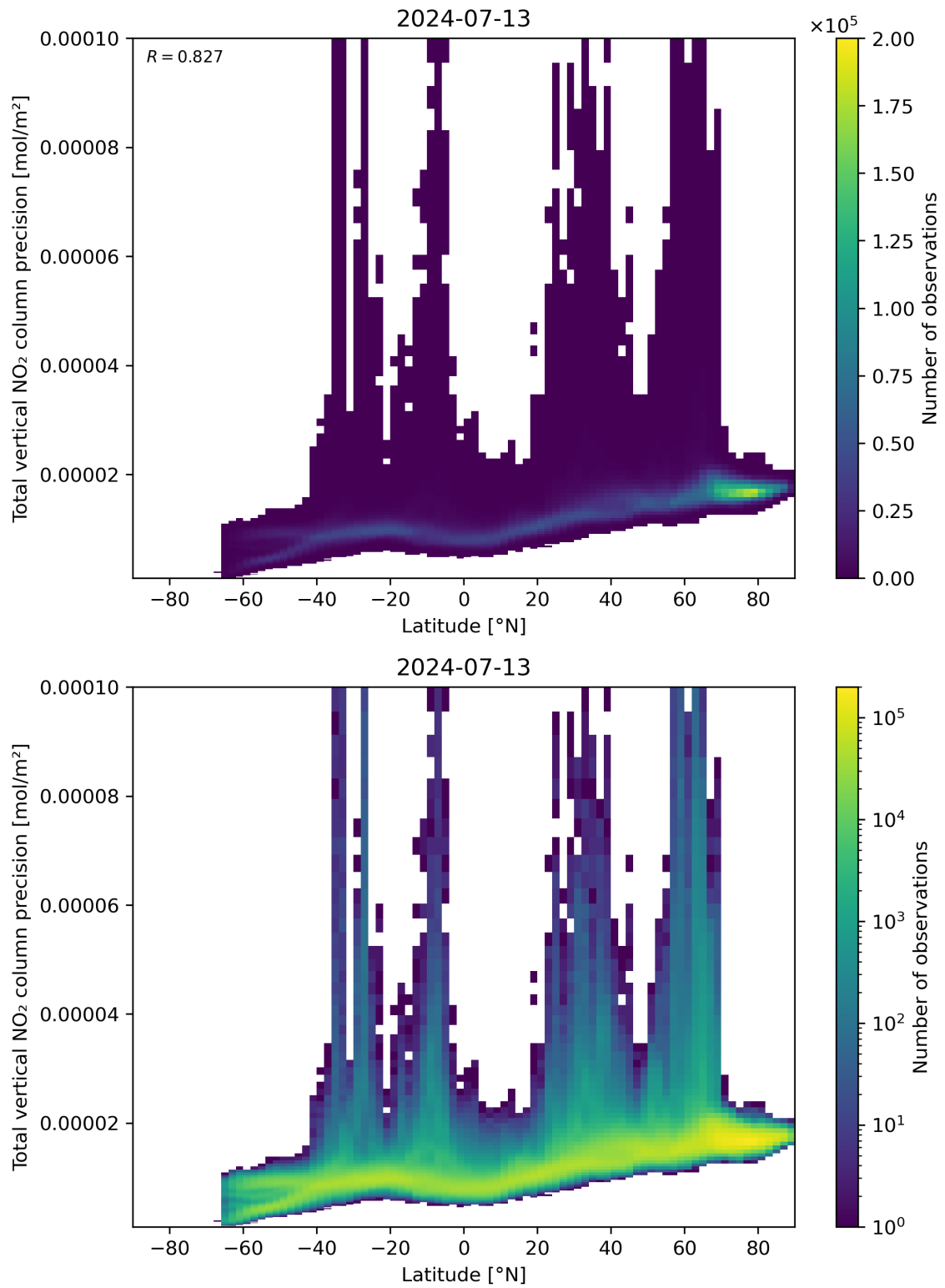
Figure 91: Scatter density plot of “Latitude” against “Total vertical NO 2 column precision” for 2024-07-12 to 2024-07-14.
