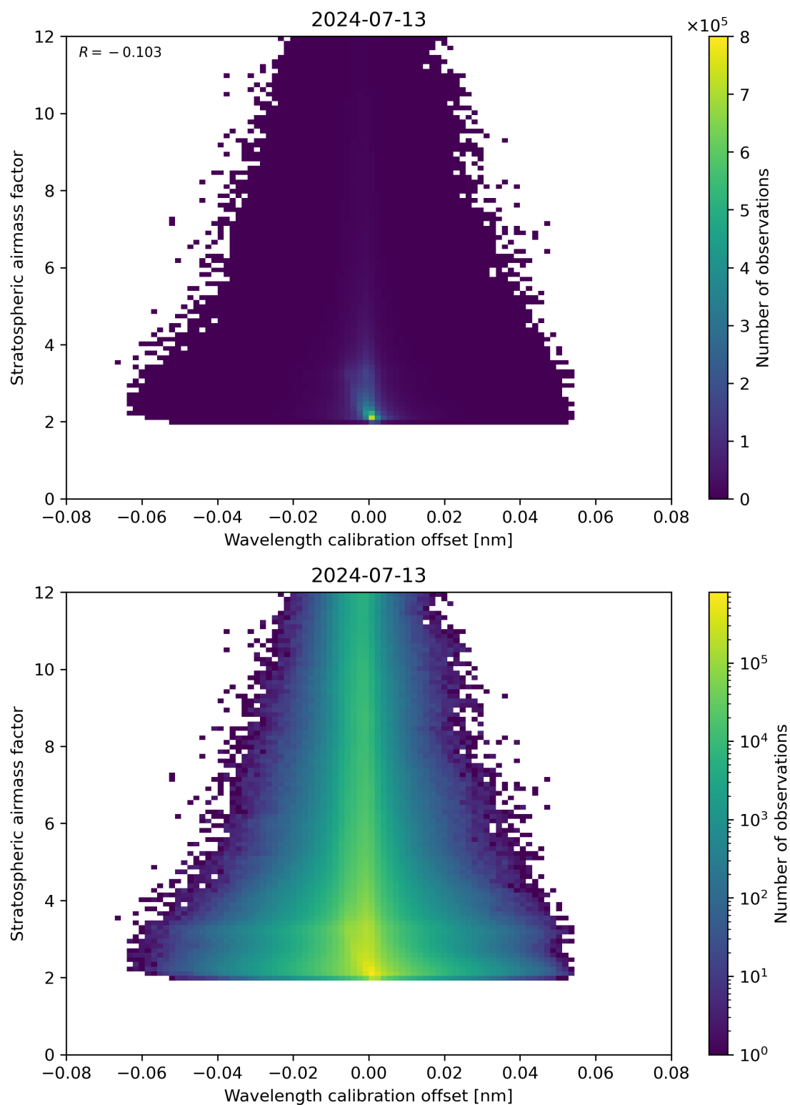
Figure 174: Scatter density plot of “Wavelength calibration offset” against “Stratospheric airmass factor” for 2024-07-12 to 2024-07-14.
