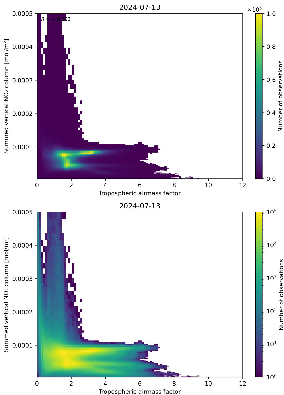
Figure 75: Scatter density plot of “Tropospheric air mass factor” against “Summed vertical NO 2 column” for 2024-07-12 to 2024-07-14.
