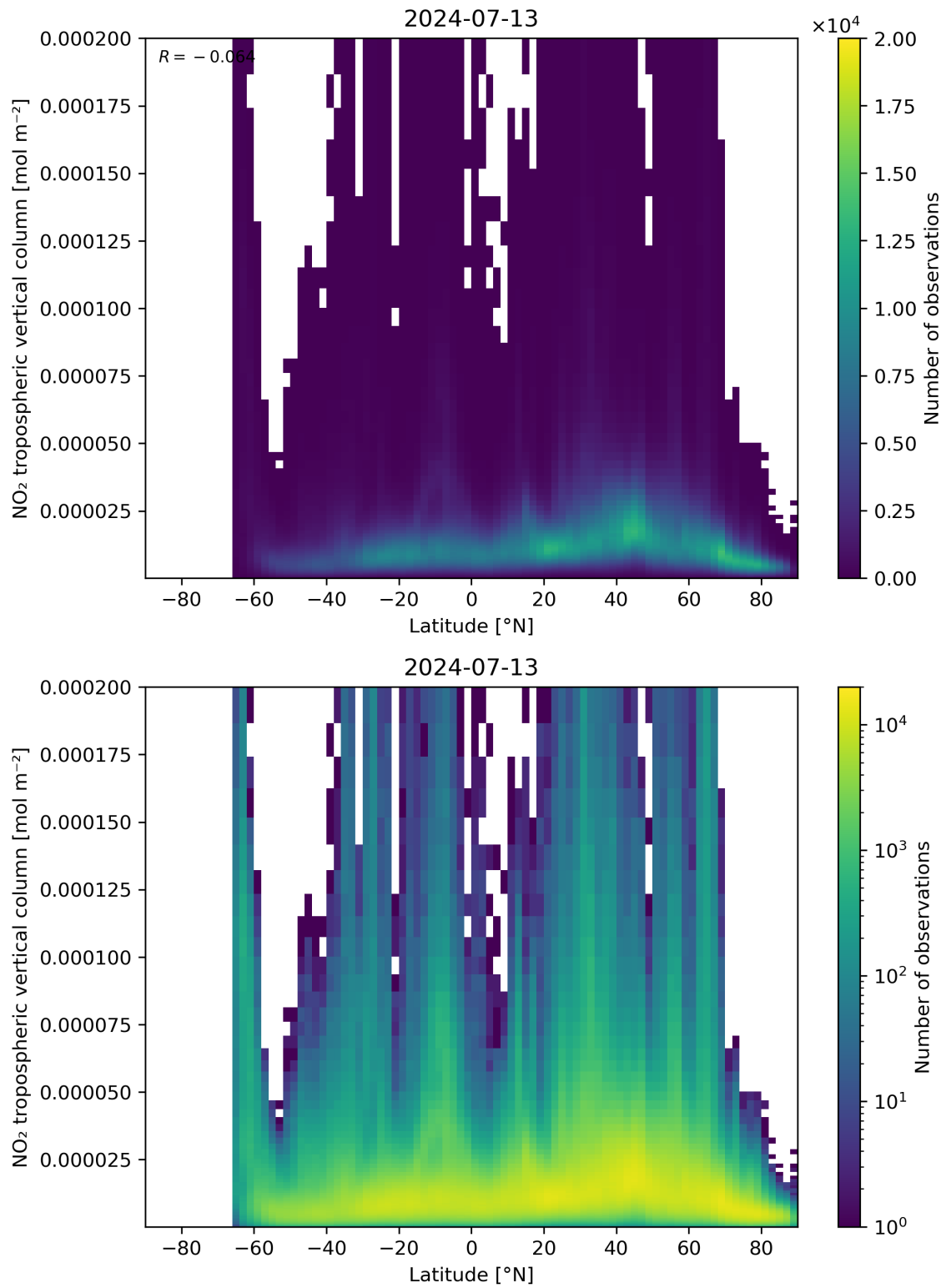
Figure 92: Scatter density plot of “Latitude” against “NO 2 tropospheric vertical column” for 2024-07-12 to 2024-07-14.
