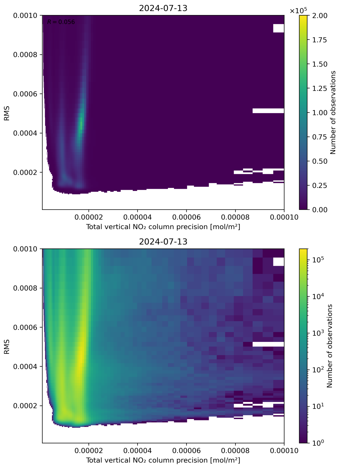
Figure 119: Scatter density plot of “Total vertical NO 2 column precision” against “RMS” for 2024-07-12 to 2024-07-14.
