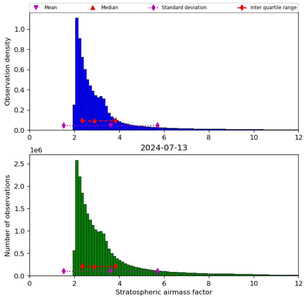
Figure 44: Histogram of “Stratospheric airmass factor” for 2024-07-12 to 2024-07-14
