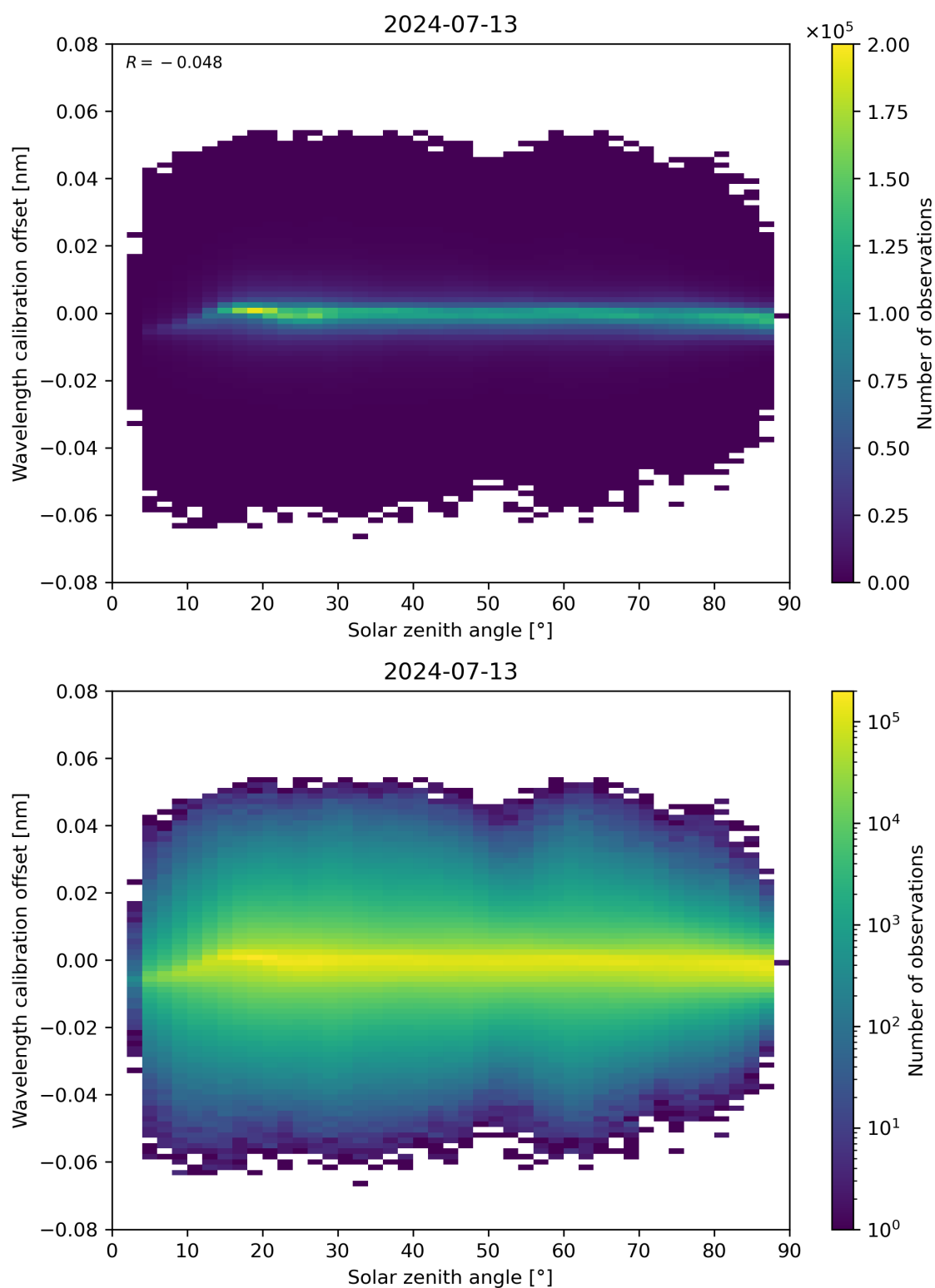
Figure 158: Scatter density plot of “Solar zenith angle” against “Wavelength calibration offset” for 2024-07-12 to 2024-07-14.
