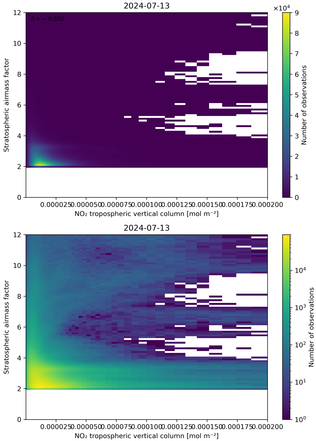
Figure 121: Scatter density plot of “NO 2 tropospheric vertical column” against “Stratospheric air mass factor” for 2024-07-12 to 2024-07-14.
