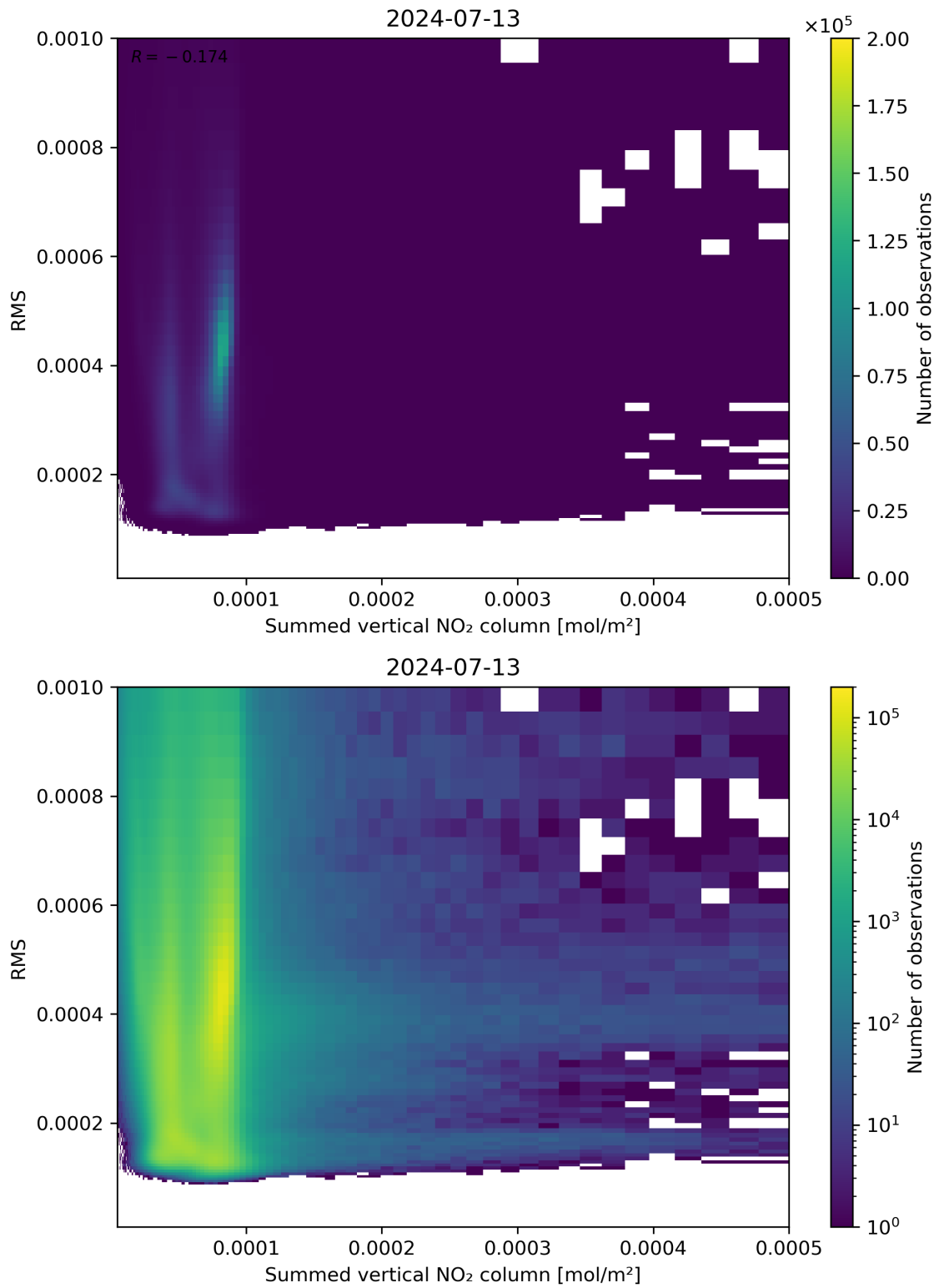
Figure 109: Scatter density plot of “Summed vertical NO 2 column” against “RMS” for 2024-07-12 to 2024-07-14.
