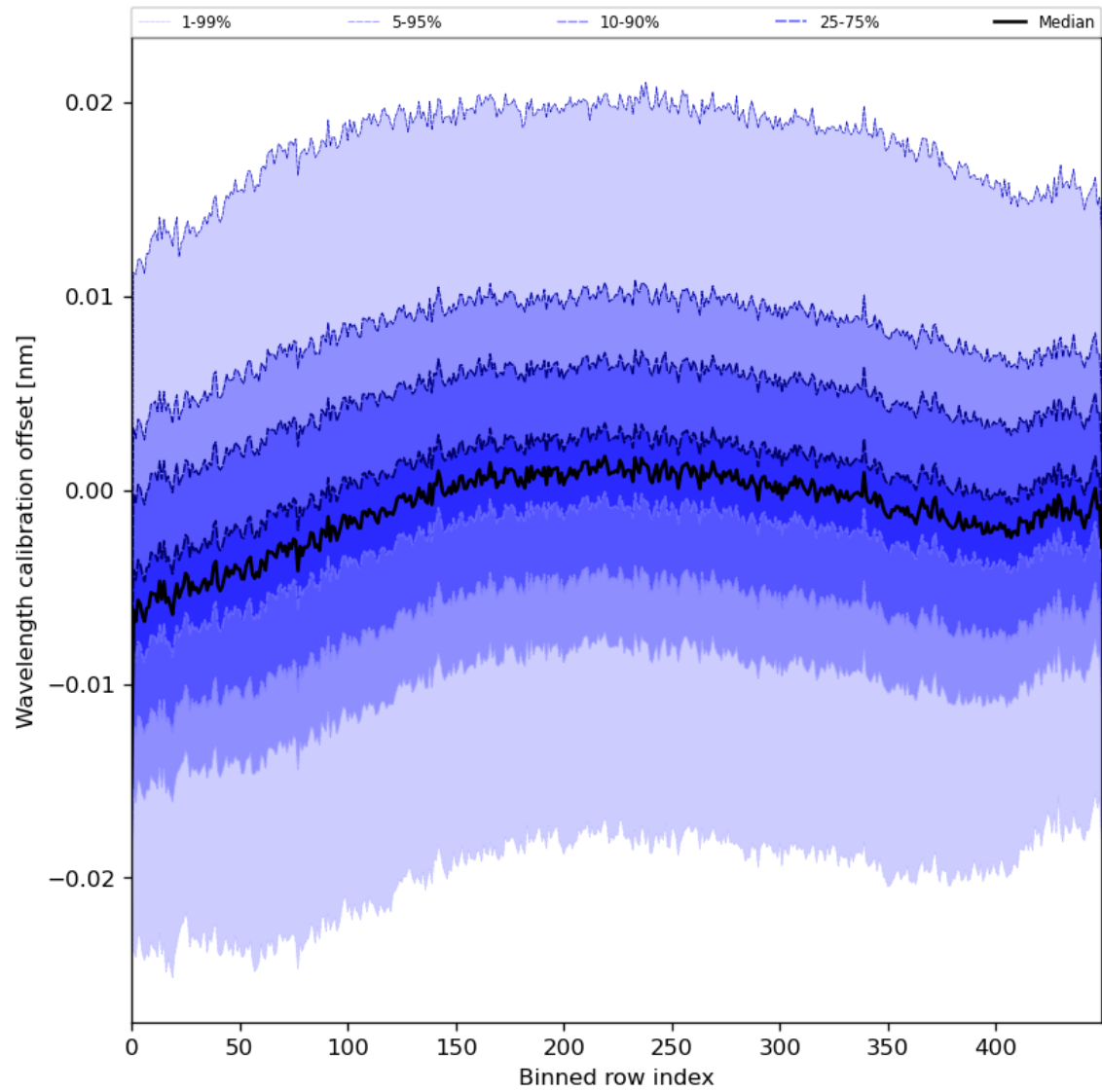
Figure 52: Along track statistics of “Wavelength calibration offset” for 2024-07-12 to 2024-07-14
