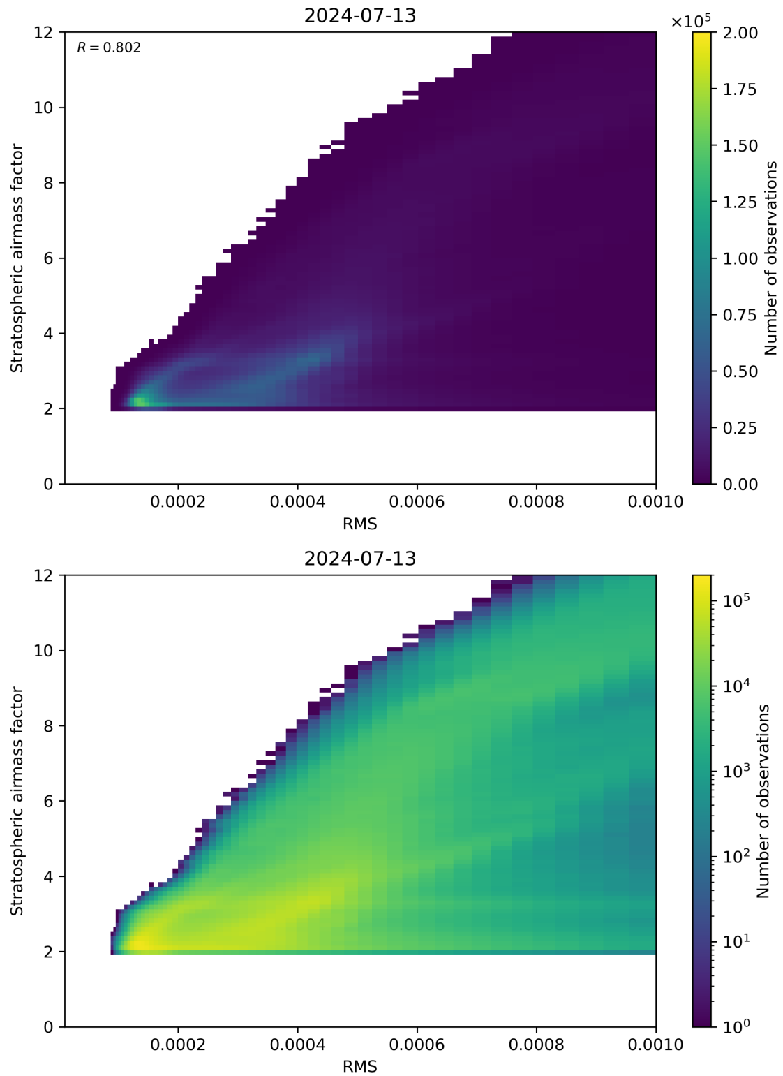
Figure 144: Scatter density plot of “RMS” against “Stratospheric airmass factor” for 2024-07-12 to 2024-07-14.
