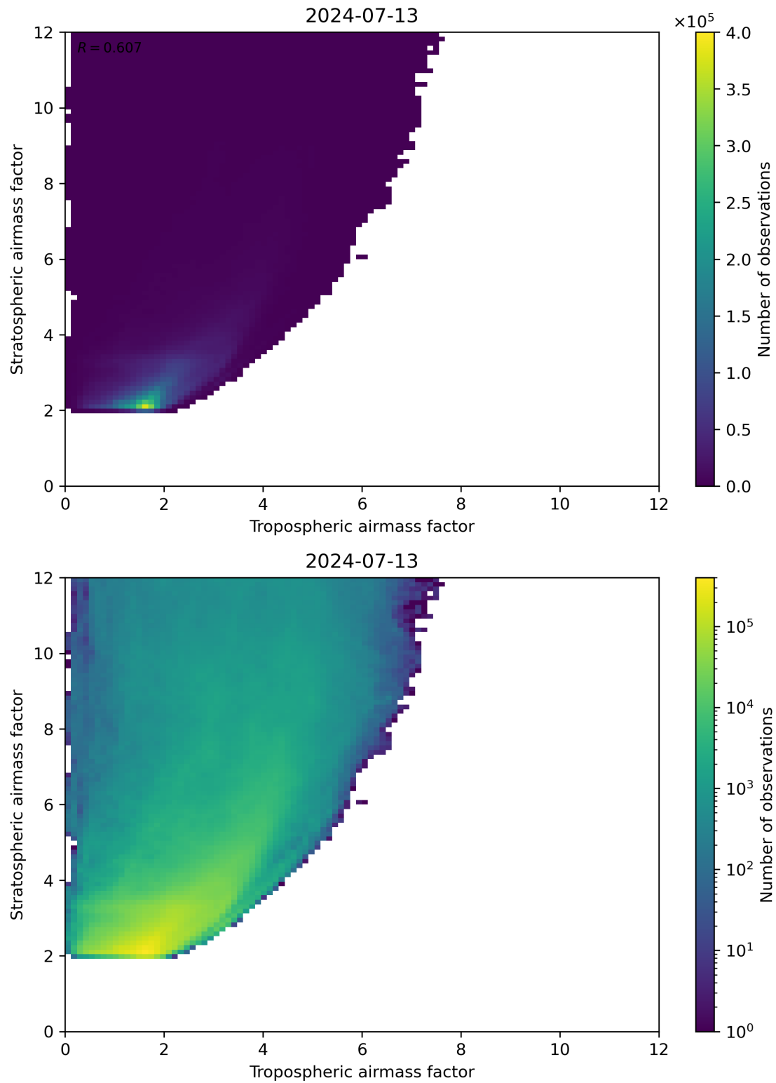
Figure 71: Scatter density plot of “Tropospheric airmass factor” against “Stratospheric airmass factor” for 2024-07-12 to 2024-07-14.
