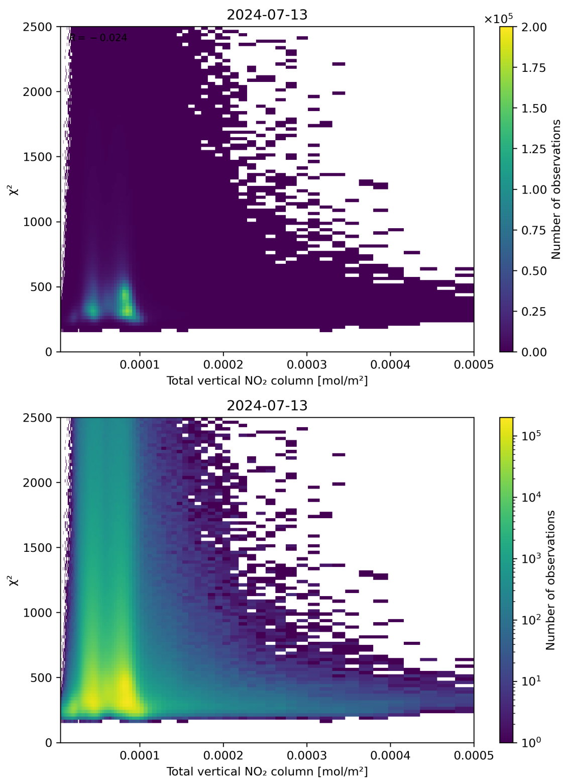
Figure 111: Scatter density plot of “Total vertical NO 2 column” against “ \chi^2 ” for 2024-07-12 to 2024-07-14.
