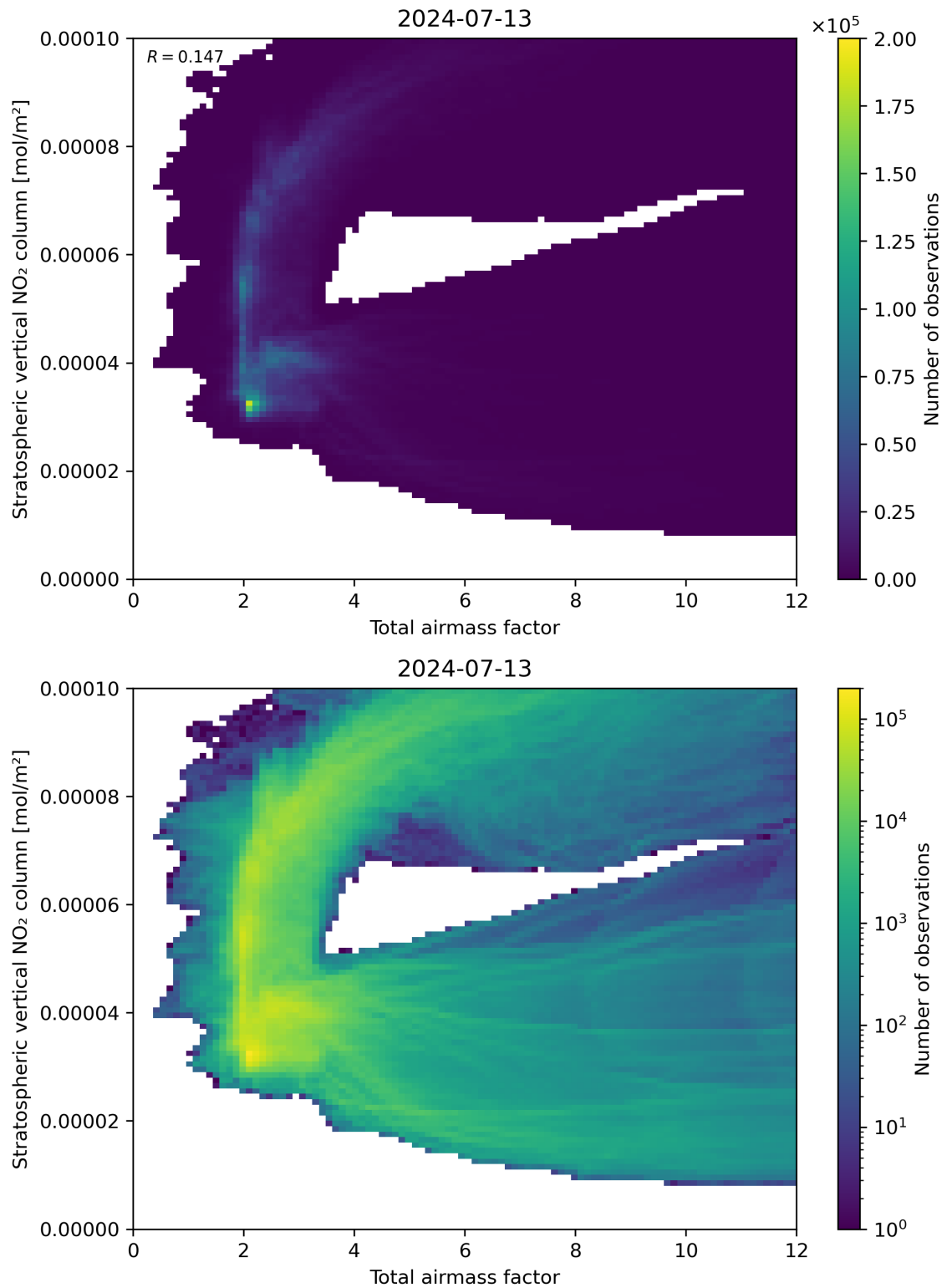
Figure 64: Scatter density plot of “Total airmass factor” against “Stratospheric vertical NO 2 column” for 2024-07-12 to 2024-07-14.
