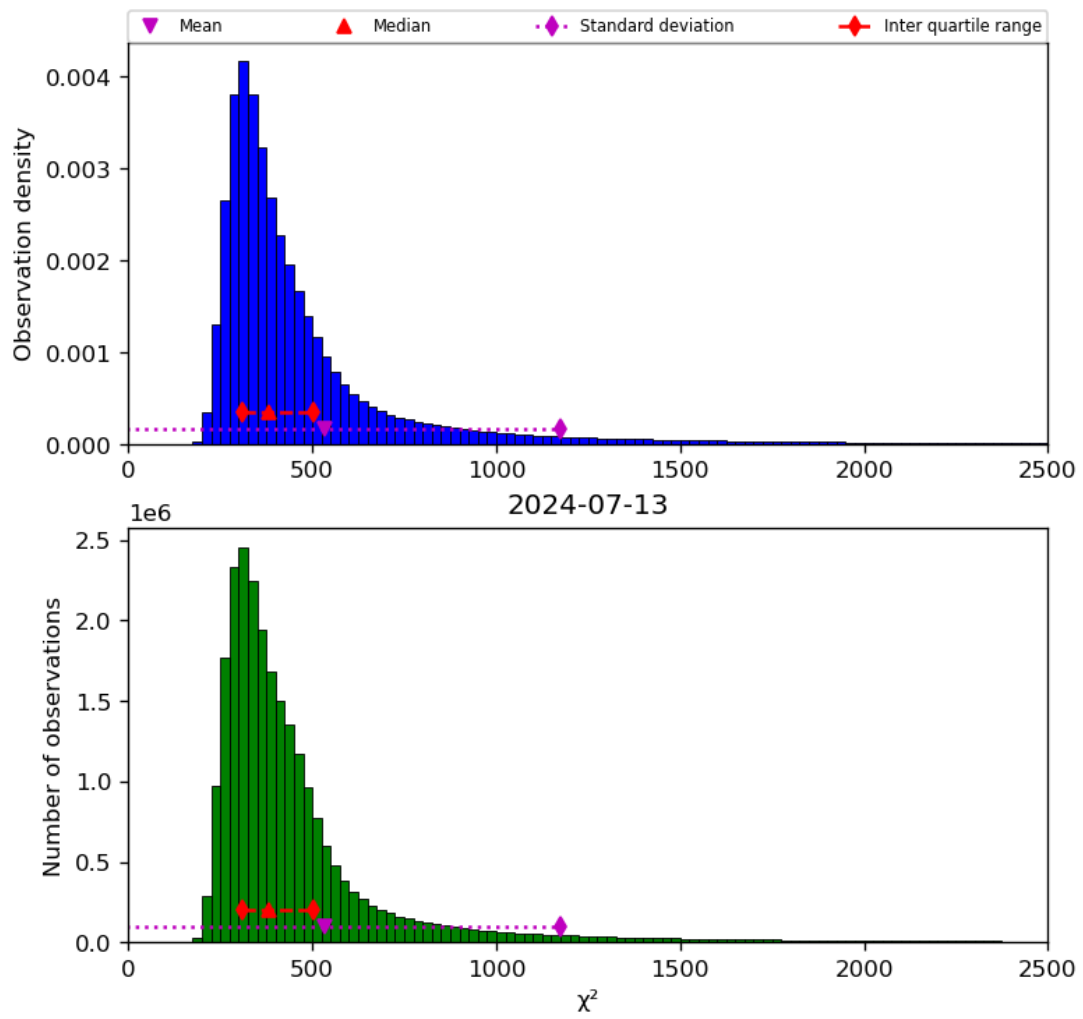
Figure 42: Histogram of “ \chi^2 ” for 2024-07-12 to 2024-07-14
