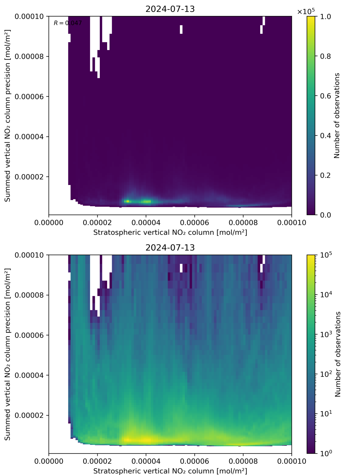
Figure 99: Scatter density plot of “Stratospheric vertical NO 2 column” against “Summed vertical NO 2 column precision” for 2024-07-12 to 2024-07-14.
