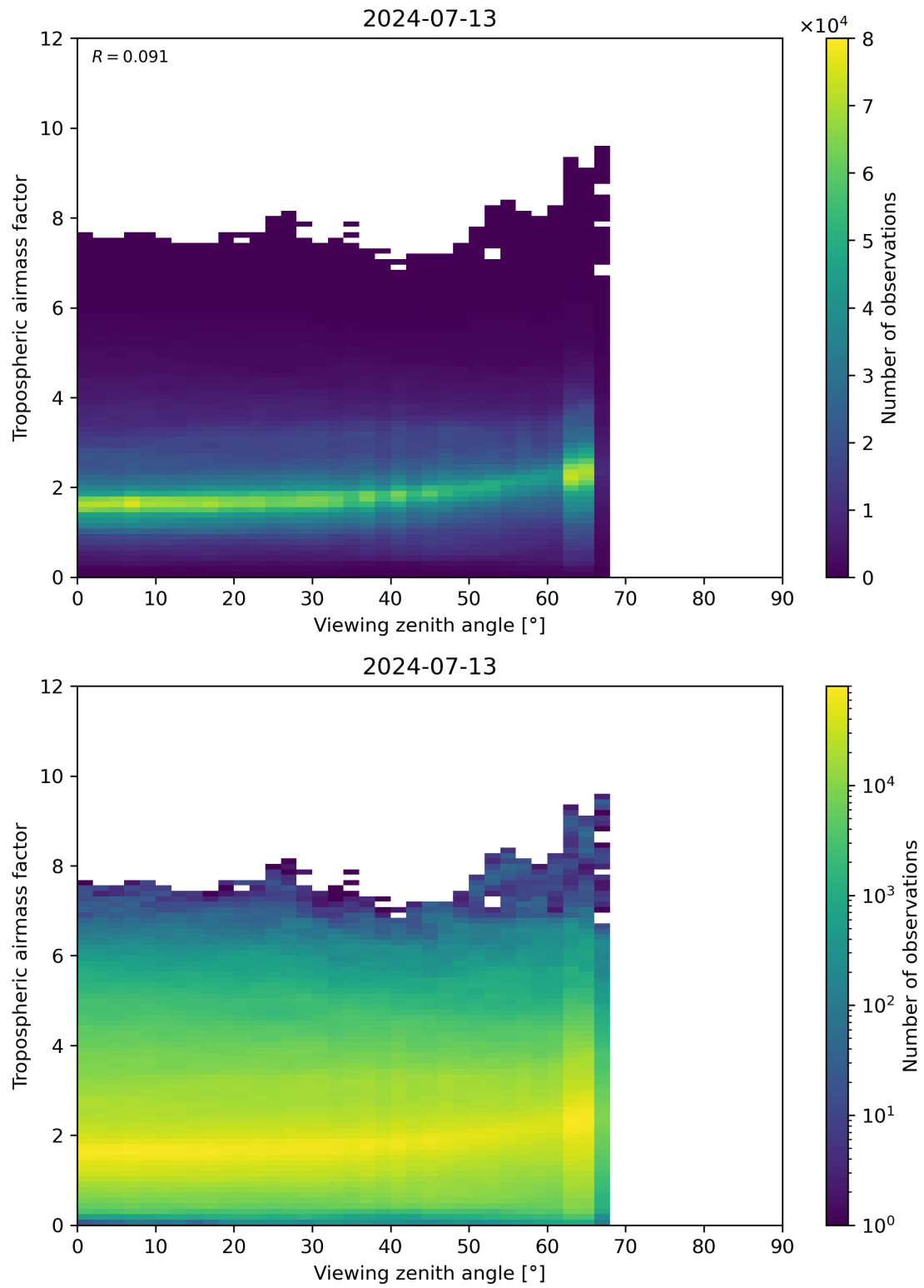
Figure 161: Scatter density plot of “Viewing zenith angle” against “Tropospheric airmass factor” for 2024-07-12 to 2024-07-14.
