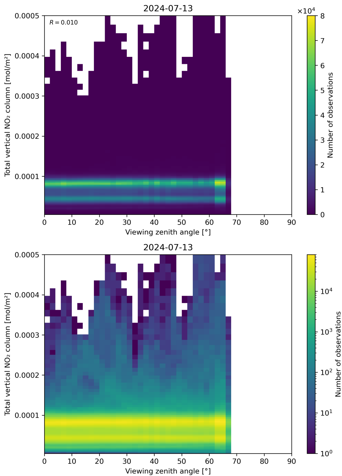
Figure 167: Scatter density plot of “Viewing zenith angle” against “Total vertical NO 2 column” for 2024-07-12 to 2024-07-14.
