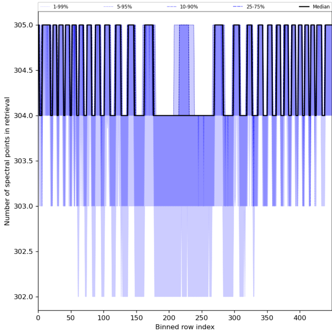
Figure 50: Along track statistics of “Number of spectral points in retrieval” for 2024-07-12 to 2024-07-14
