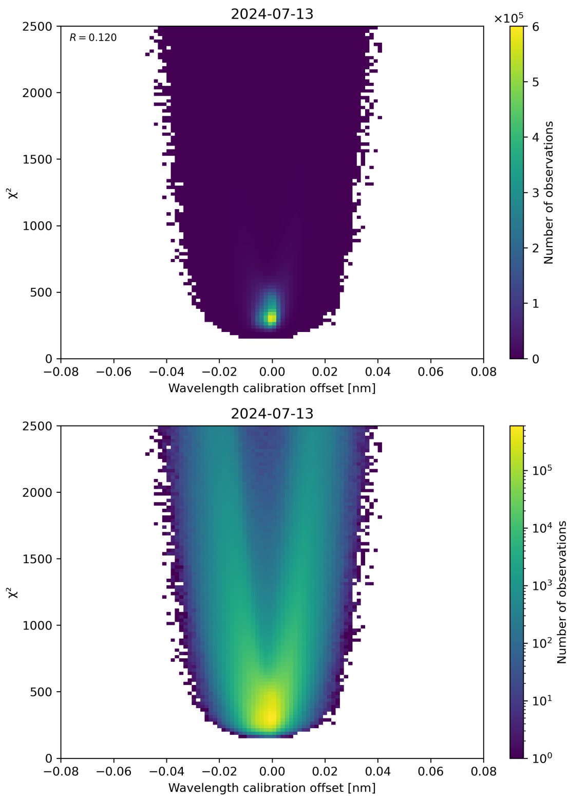
Figure 175: Scatter density plot of “Wavelength calibration offset” against “ \chi^2 ” for 2024-07-12 to 2024-07-14.
