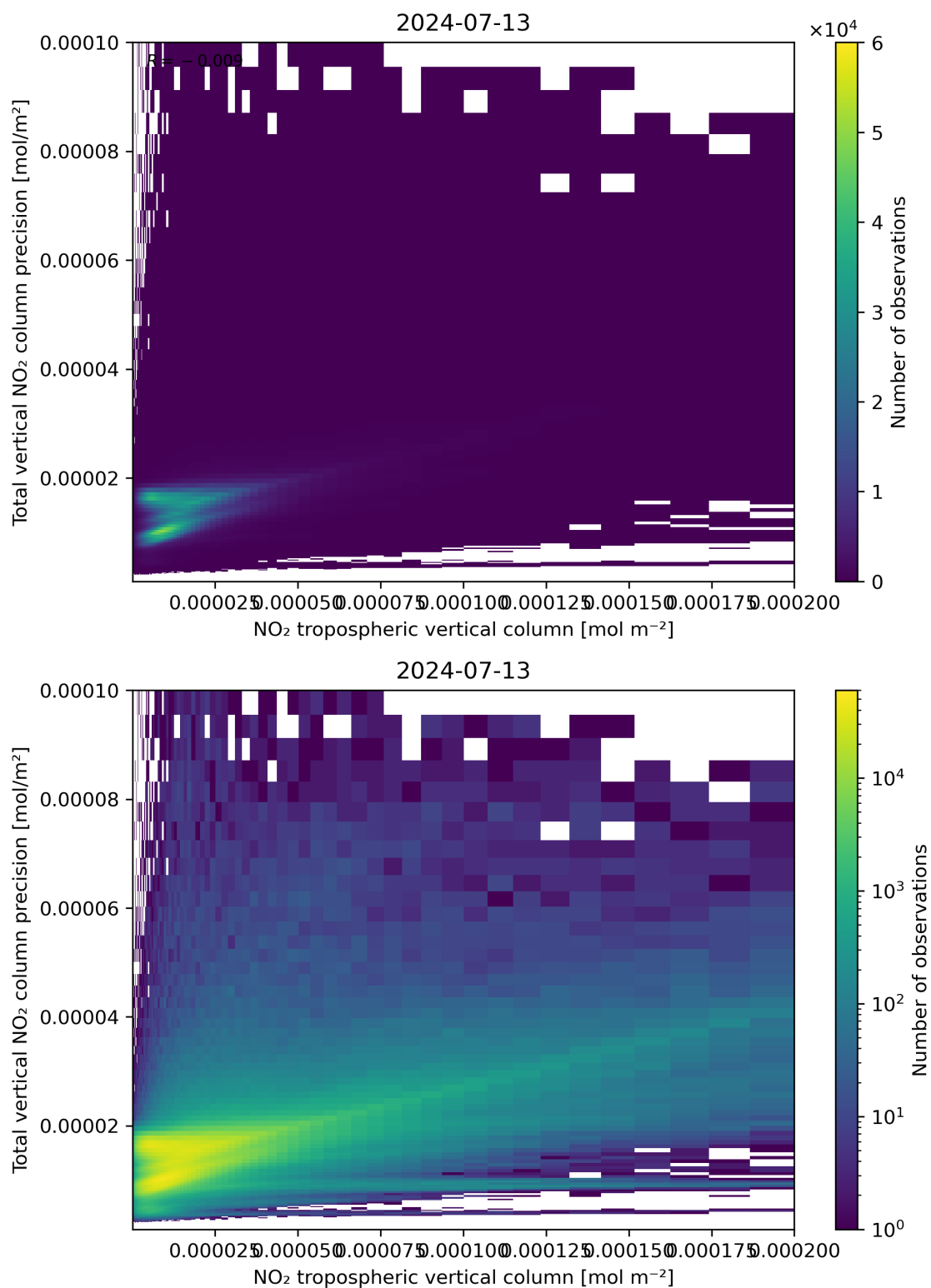
Figure 129: Scatter density plot of “NO 2 tropospheric vertical column” against “Total vertical NO 2 column precision” for 2024-07-12 to 2024-07-14.
