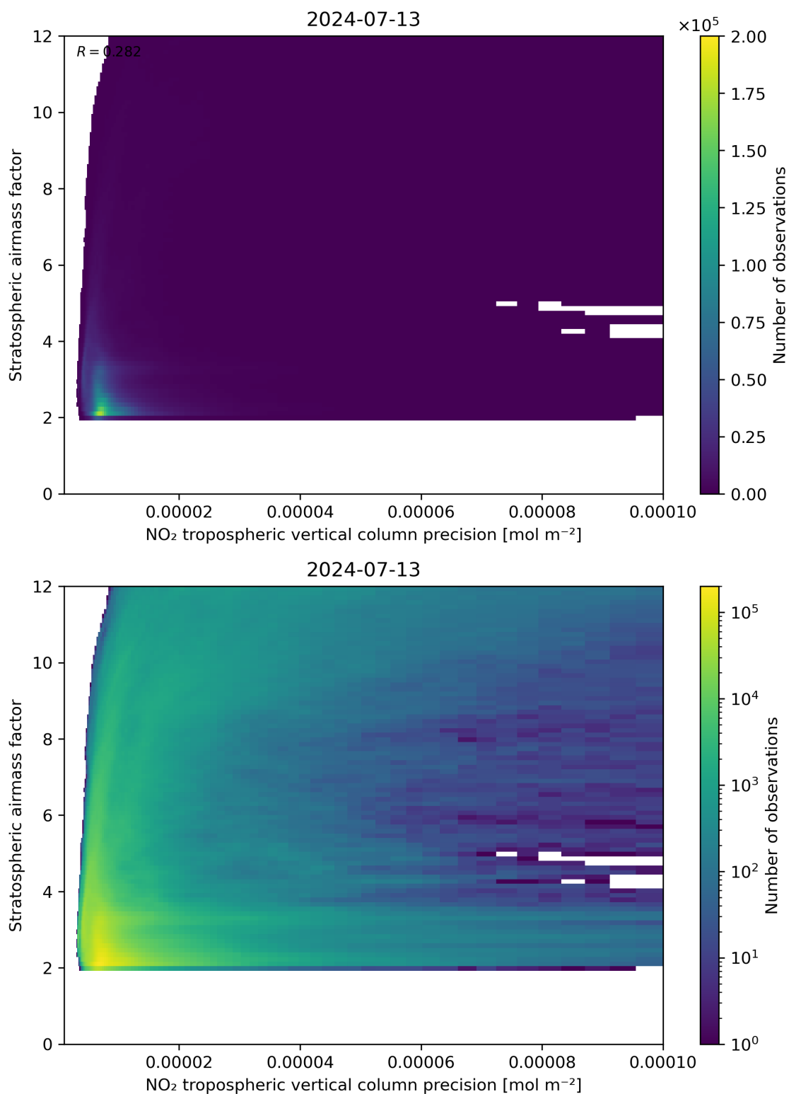
Figure 131: Scatter density plot of “NO 2 tropospheric vertical column precision” against “Stratospheric airmass factor” for 2024-07-12 to 2024-07-14.
