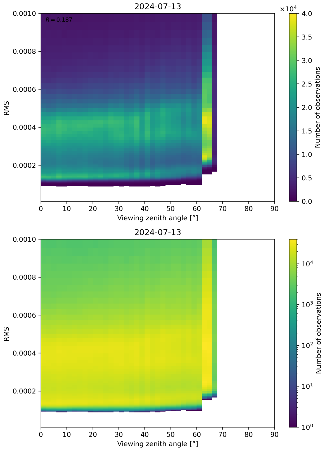
Figure 171: Scatter density plot of “Viewing zenith angle” against “RMS” for 2024-07-12 to 2024-07-14.
