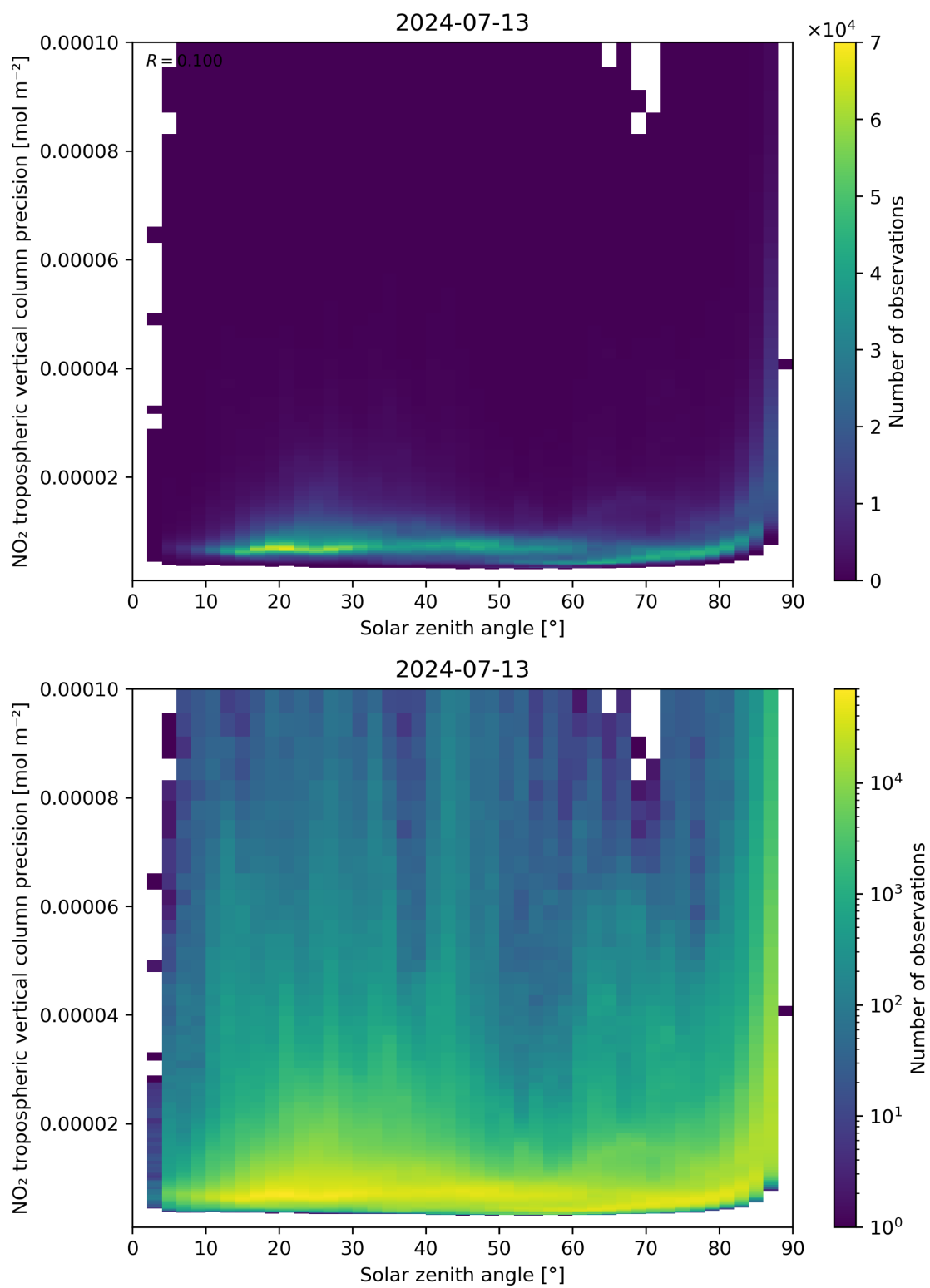
Figure 156: Scatter density plot of “Solar zenith angle” against “NO 2 tropospheric vertical column precision” for 2024-07-12 to 2024-07-14.
