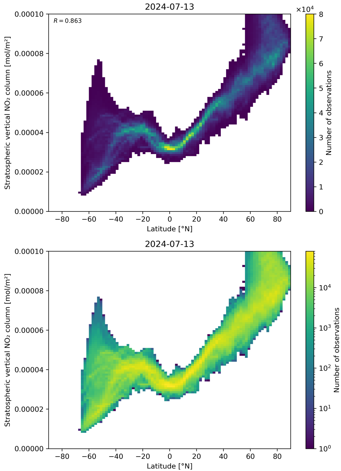
Figure 87: Scatter density plot of “Latitude” against “Stratospheric vertical NO 2 column” for 2024-07-12 to 2024-07-14.
