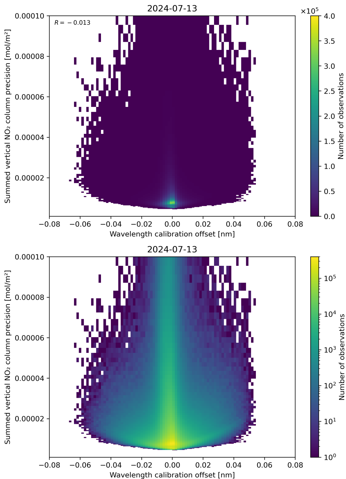
Figure 178: Scatter density plot of “Wavelength calibration offset” against “Summed vertical NO 2 column precision” for 2024-07-12 to 2024-07-14.
