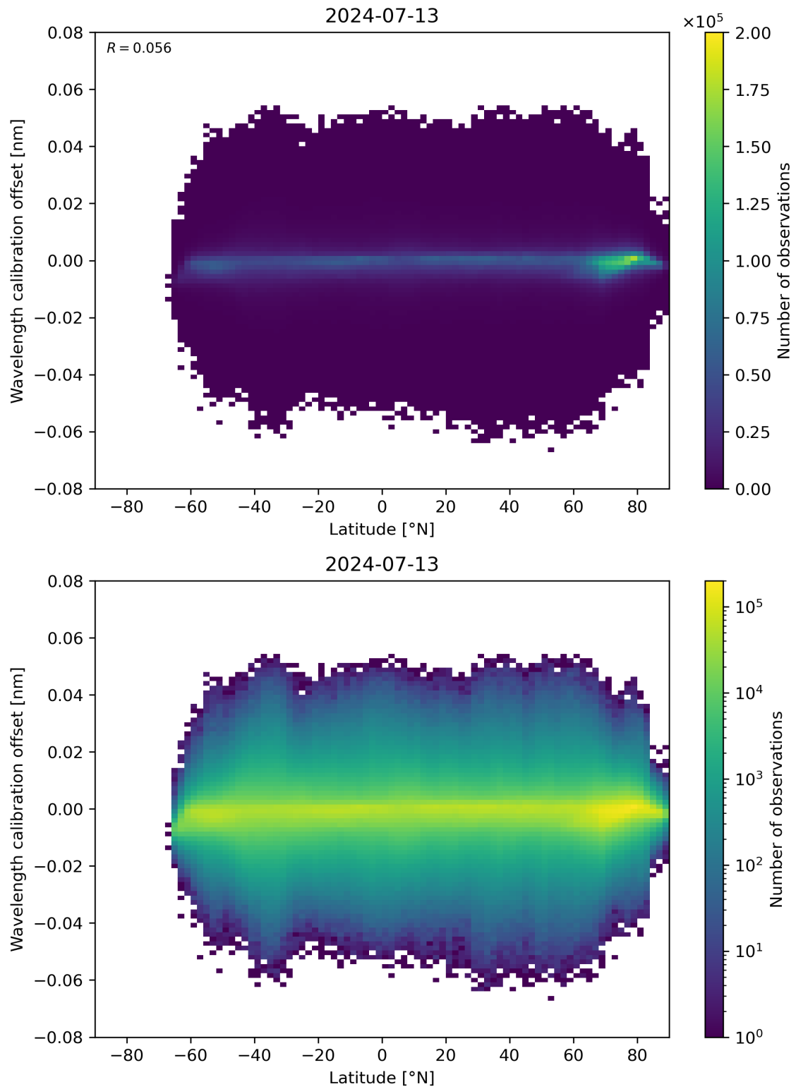
Figure 95: Scatter density plot of “Latitude” against “Wavelength calibration offset” for 2024-07-12 to 2024-07-14.
