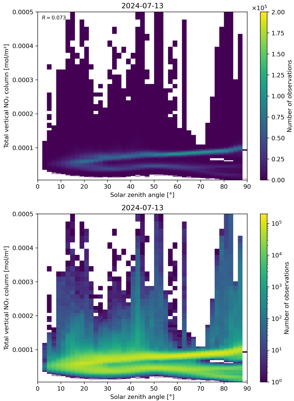
Figure 153: Scatter density plot of “Solar zenith angle” against “Total vertical NO 2 column” for 2024-07-12 to 2024-07-14.
