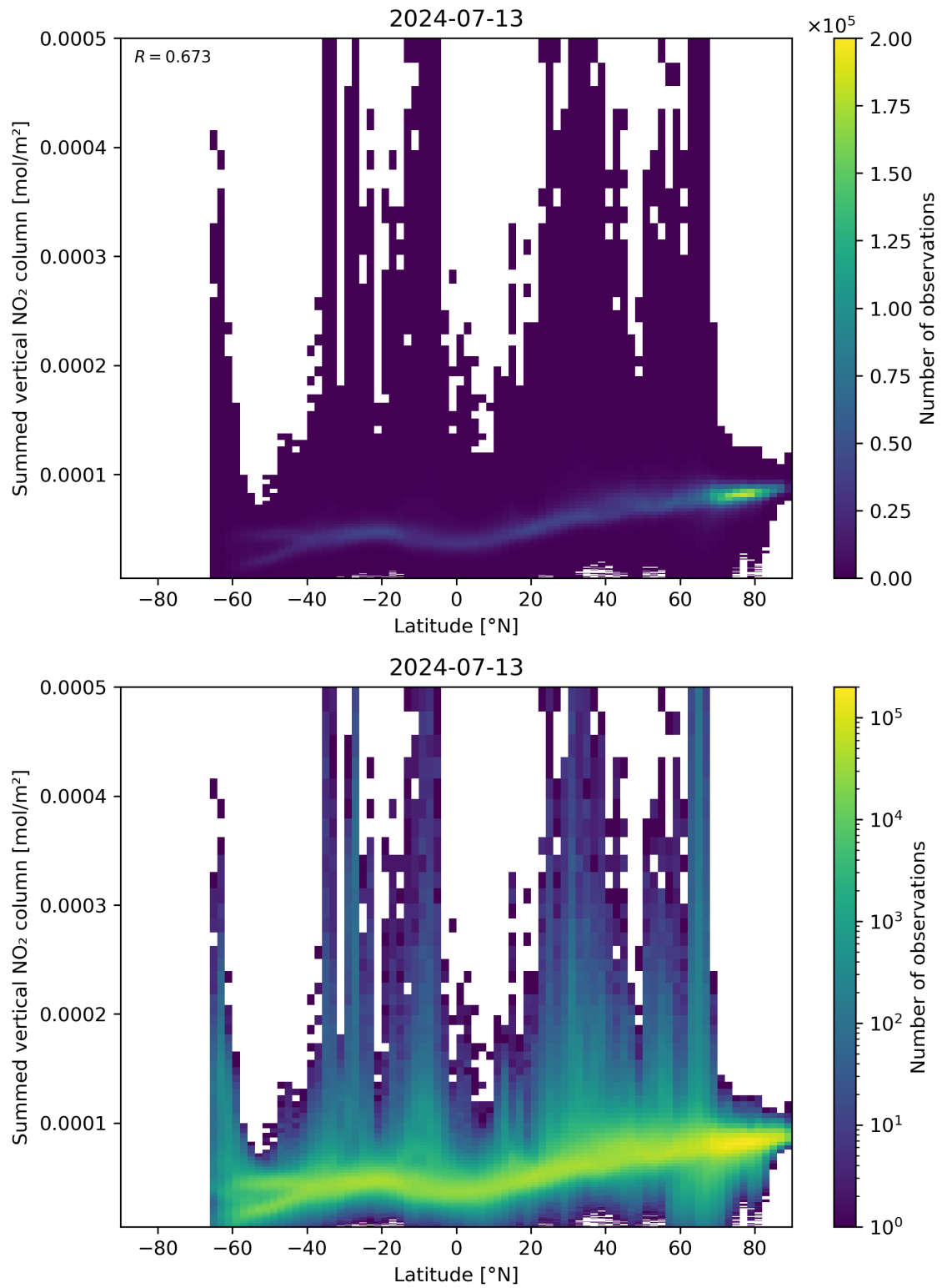
Figure 88: Scatter density plot of “Latitude” against “Summed vertical NO 2 column” for 2024-07-12 to 2024-07-14.
