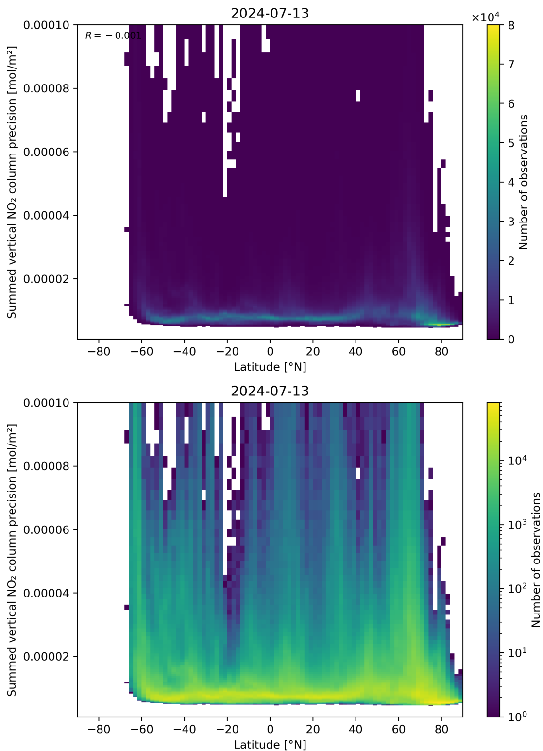
Figure 89: Scatter density plot of “Latitude” against “Summed vertical NO 2 column precision” for 2024-07-12 to 2024-07-14.
