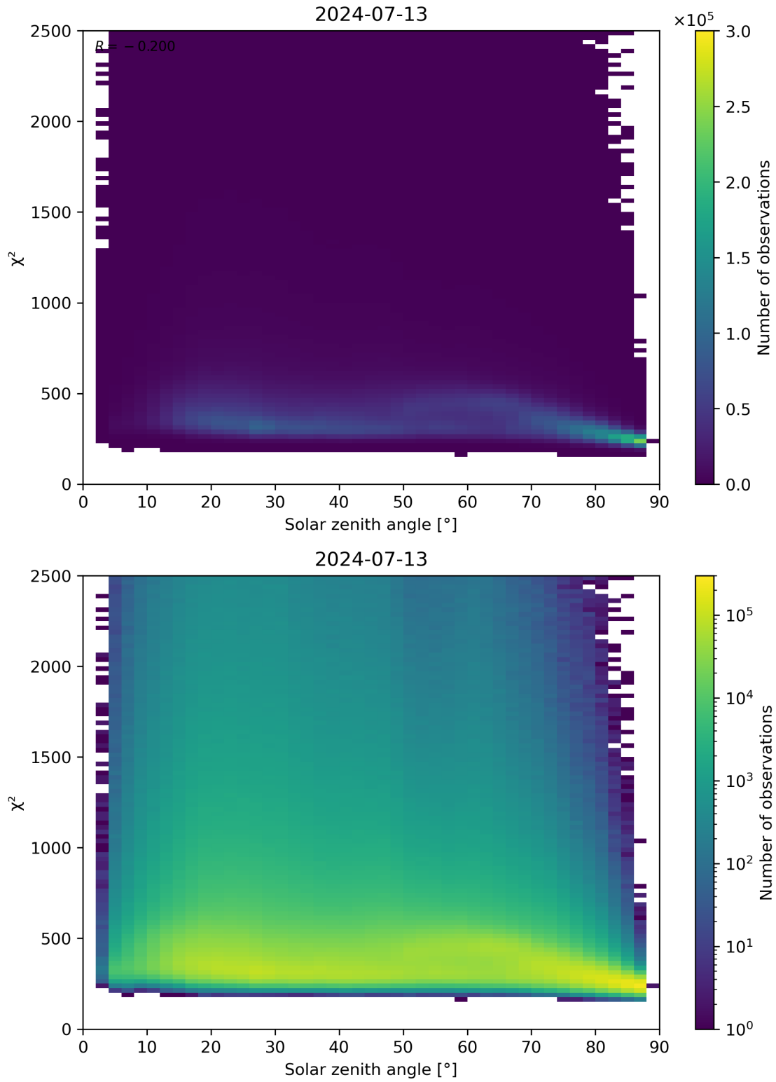
Figure 148: Scatter density plot of “Solar zenith angle” against “ \chi^2 ” for 2024-07-12 to 2024-07-14.
