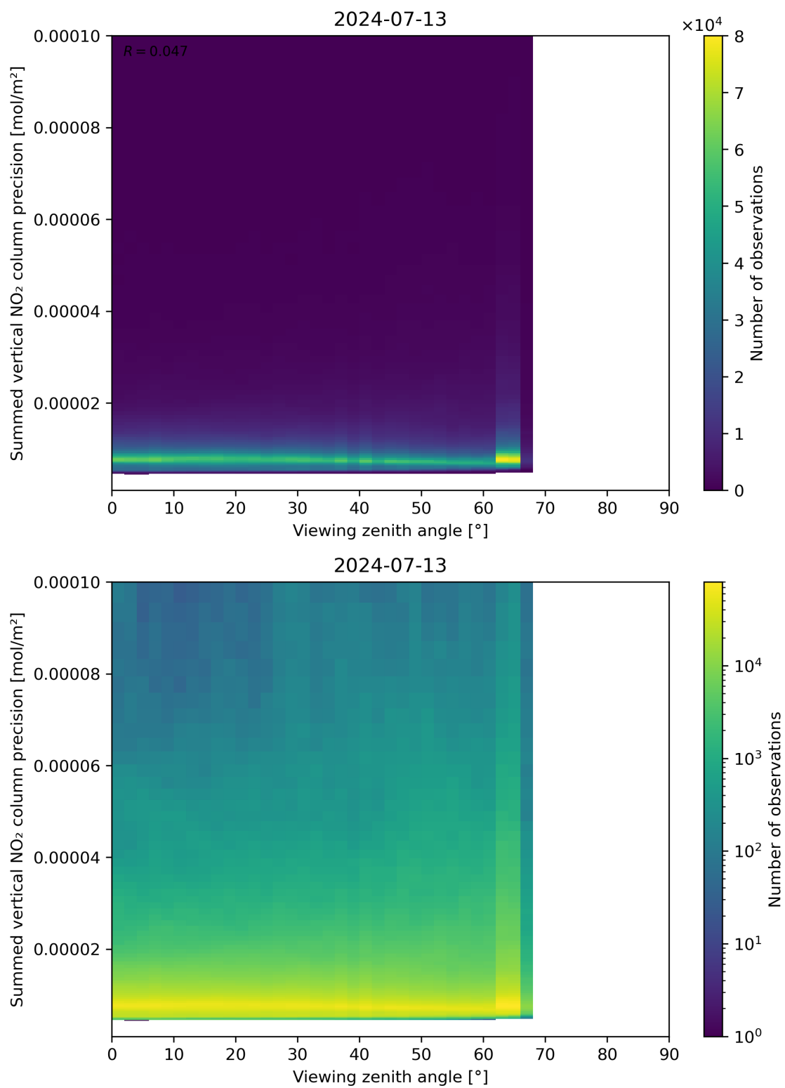
Figure 166: Scatter density plot of “Viewing zenith angle” against “Summed vertical NO 2 column precision” for 2024-07-12 to 2024-07-14.
