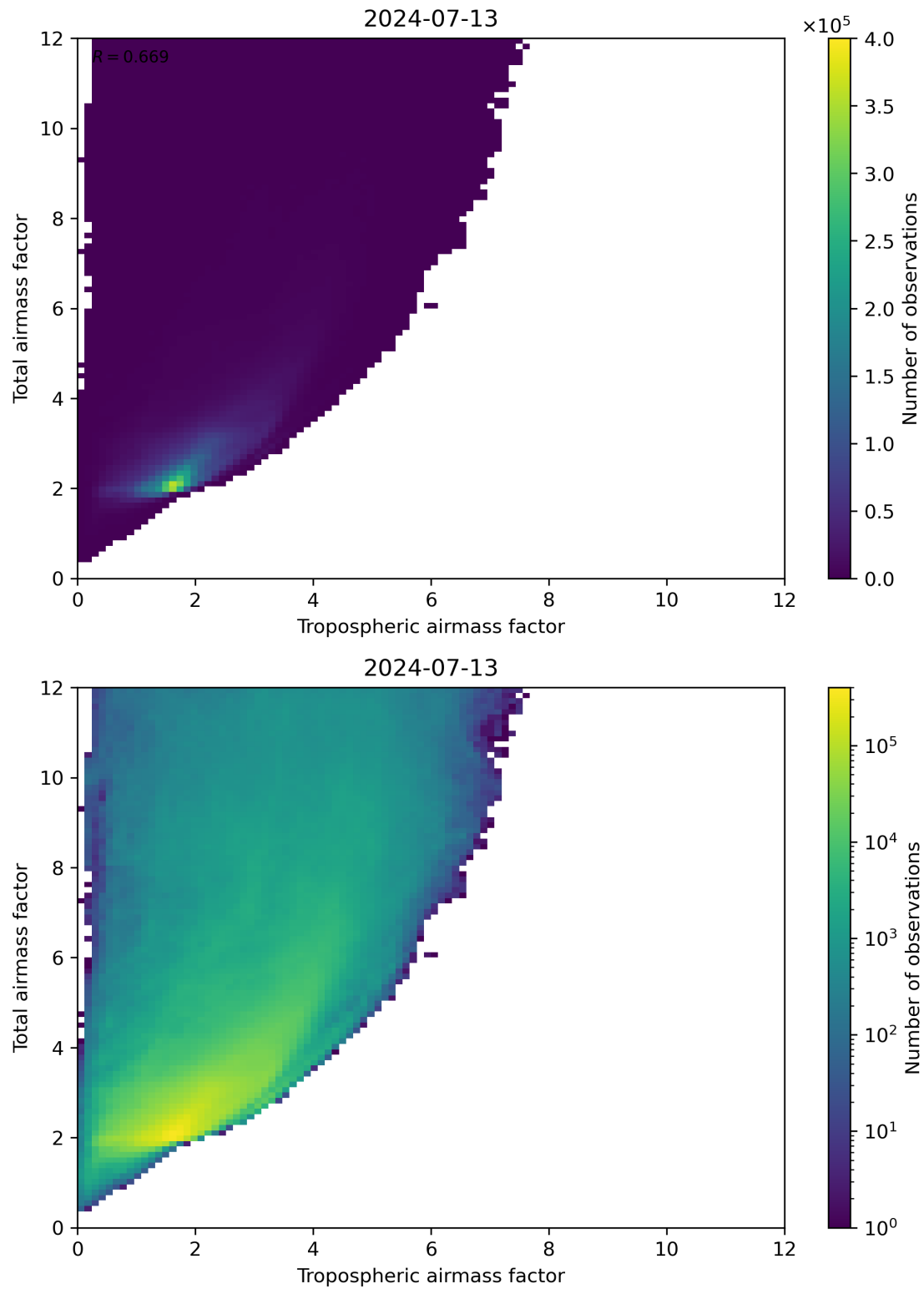
Figure 72: Scatter density plot of “Tropospheric airmass factor” against “Total airmass factor” for 2024-07-12 to 2024-07-14.
