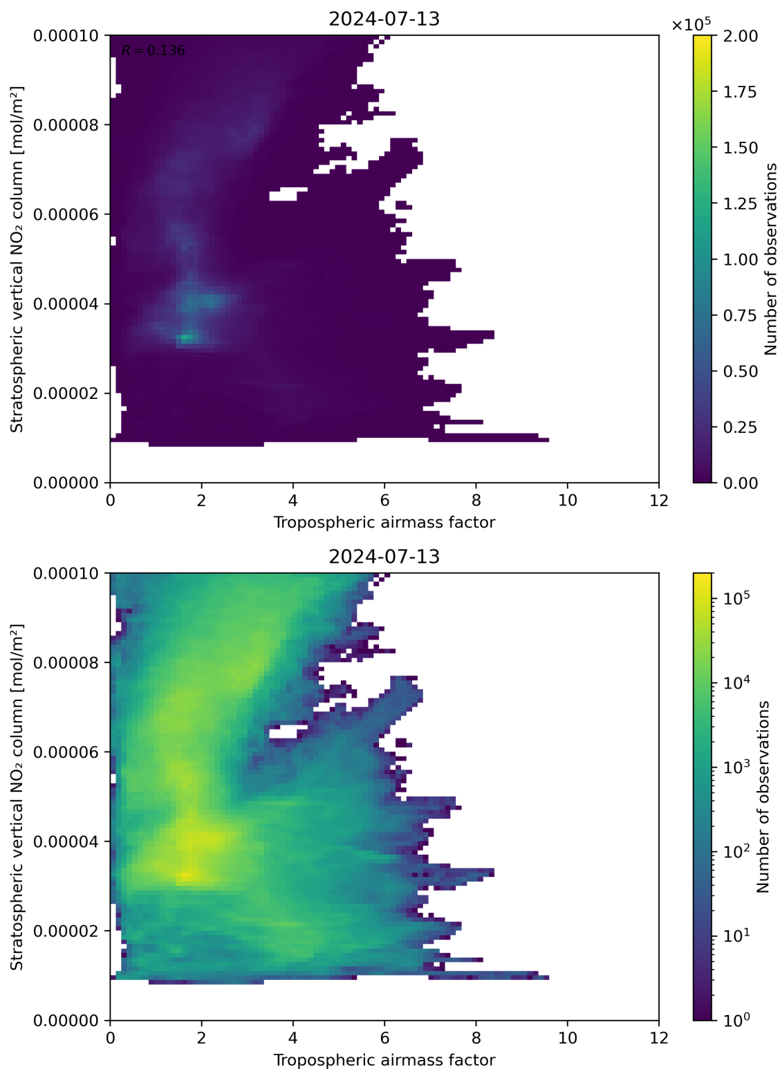
Figure 74: Scatter density plot of “Tropospheric air mass factor” against “Stratospheric vertical NO 2 column” for 2024-07-12 to 2024-07-14.
