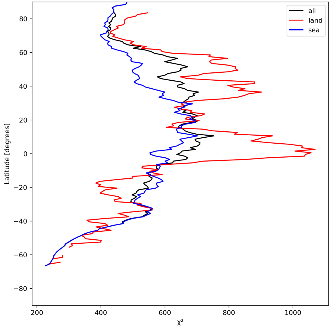
Figure 25: Zonal average of “ \chi^2 ” for 2024-07-12 to 2024-07-14.
