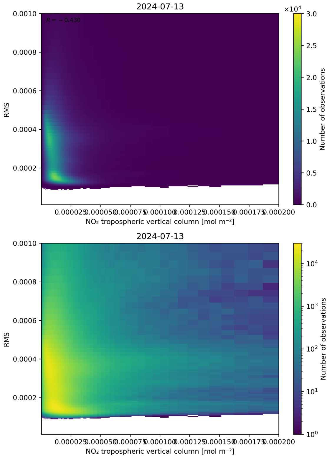
Figure 142: Scatter density plot of “NO 2 tropospheric vertical column” against “RMS” for 2024-07-12 to 2024-07-14.
