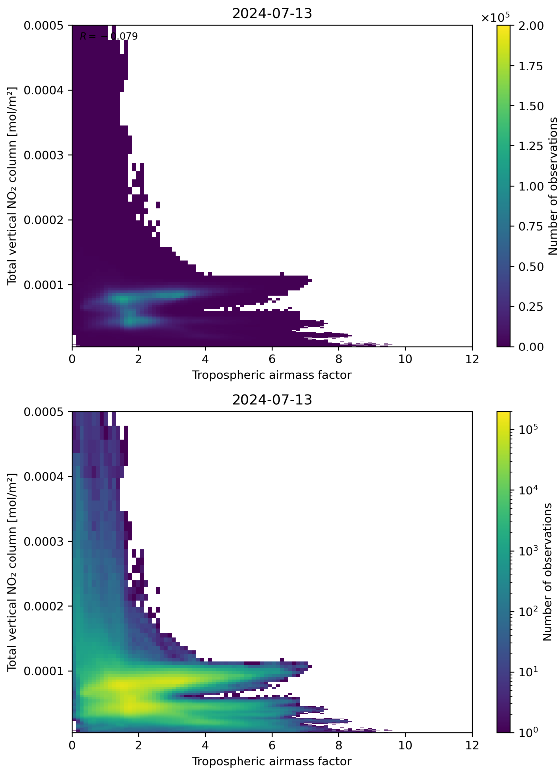
Figure 77: Scatter density plot of “Tropospheric airmass factor” against “Total vertical NO 2 column” for 2024-07-12 to 2024-07-14.
