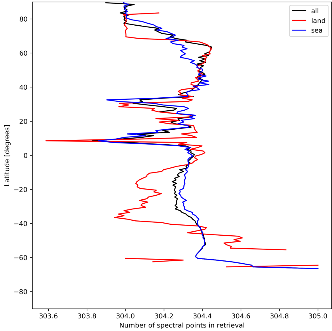
Figure 16: Zonal average of “Number of spectral points in retrieval” for 2024-07-12 to 2024-07-14.
