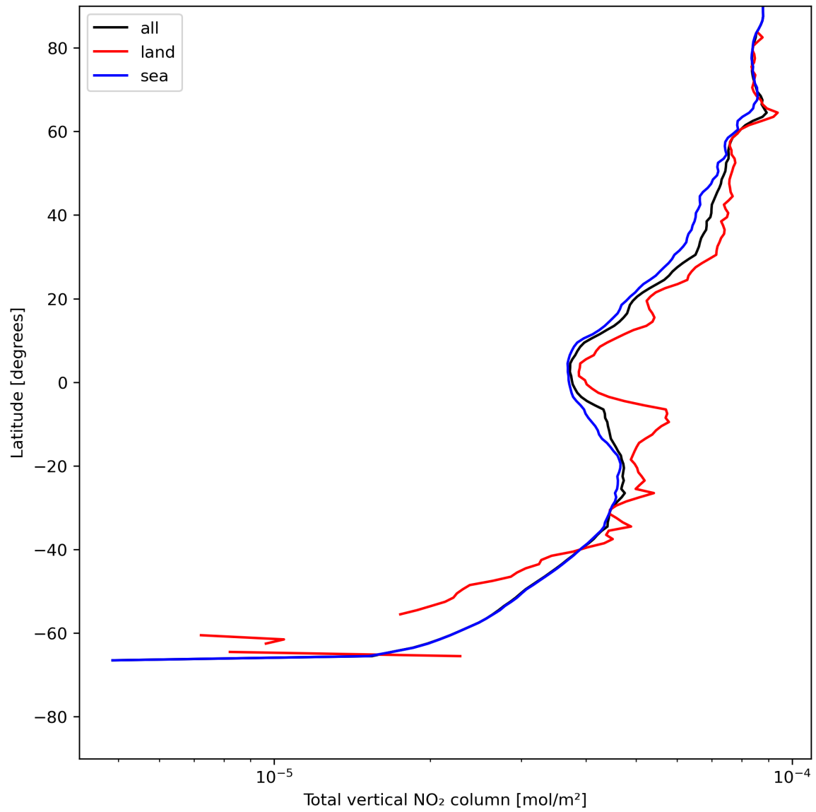
Figure 21: Zonal average of “Total vertical NO 2 column” for 2024-07-12 to 2024-07-14.
