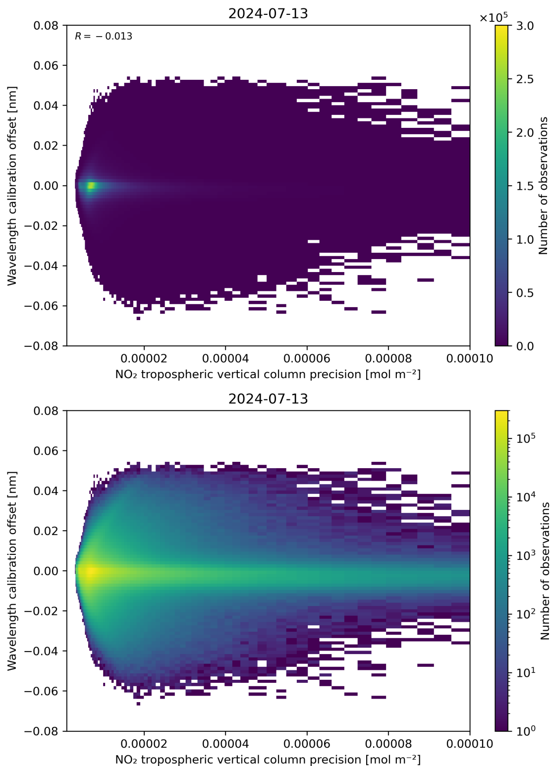
Figure 141: Scatter density plot of “NO 2 tropospheric vertical column precision” against “Wavelength calibration offset” for 2024-07-12 to 2024-07-14.
