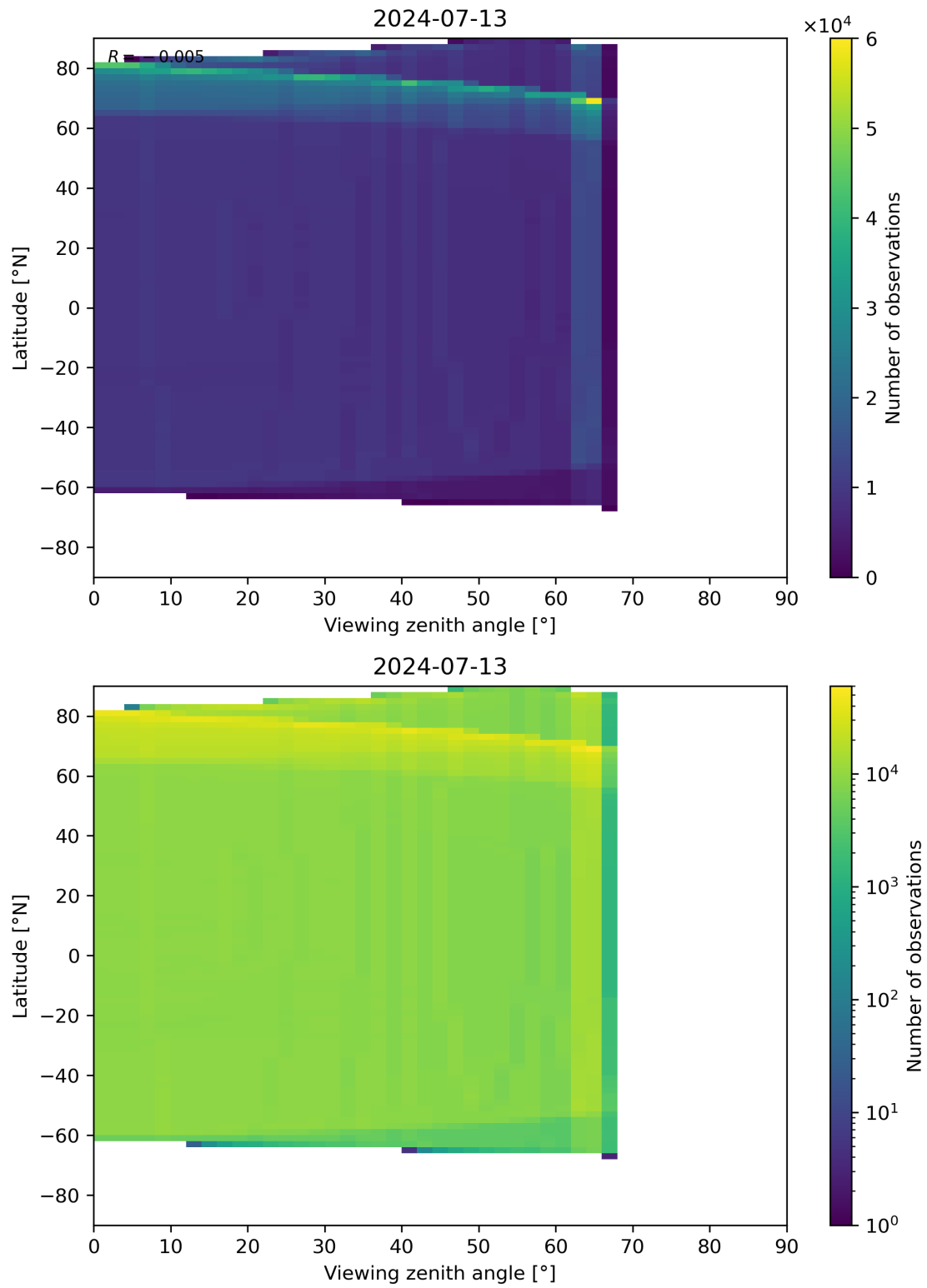
Figure 163: Scatter density plot of “Viewing zenith angle” against “Latitude” for 2024-07-12 to 2024-07-14.
