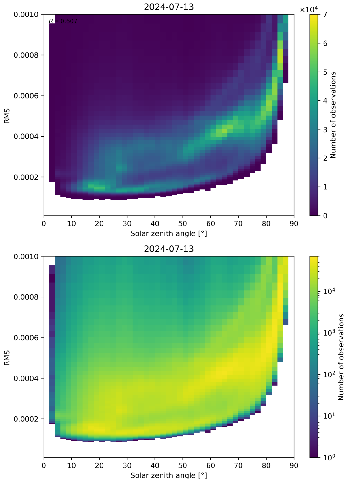
Figure 157: Scatter density plot of “Solar zenith angle” against “RMS” for 2024-07-12 to 2024-07-14.
