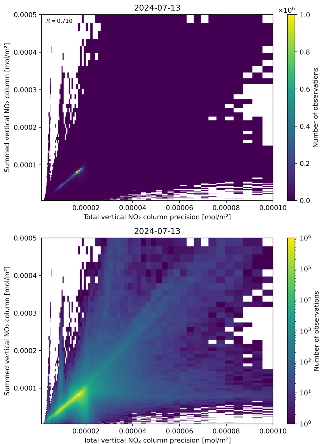
Figure 117: Scatter density plot of “Total vertical NO 2 column precision” against “Summed vertical NO 2 column” for 2024-07-12 to 2024-07-14.
