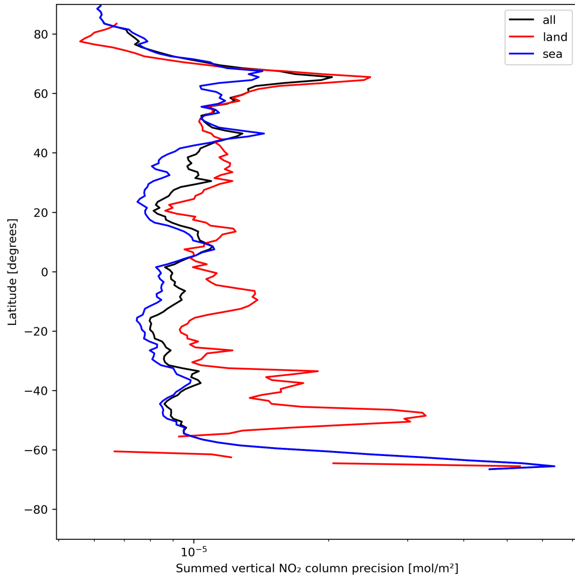
Figure 24: Zonal average of “Summed vertical NO 2 column precision” for 2024-07-12 to 2024-07-14.
