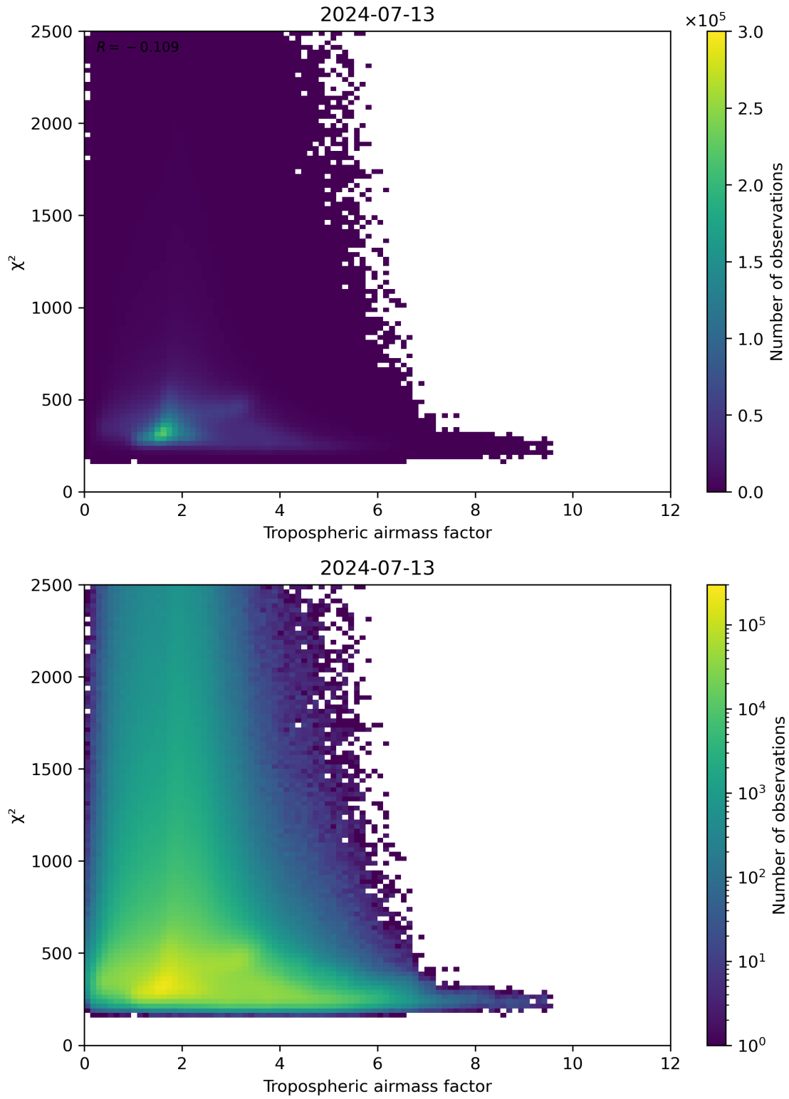
Figure 73: Scatter density plot of “Tropospheric airmass factor” against “ \chi^2 ” for 2024-07-12 to 2024-07-14.
