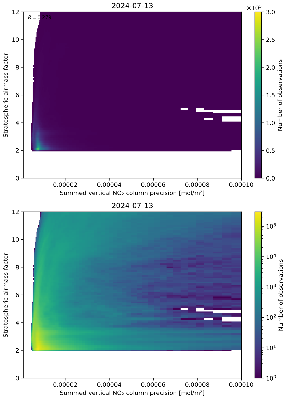
Figure 106: Scatter density plot of “Summed vertical NO 2 column precision” against “Stratospheric airmass factor” for 2024-07-12 to 2024-07-14.
