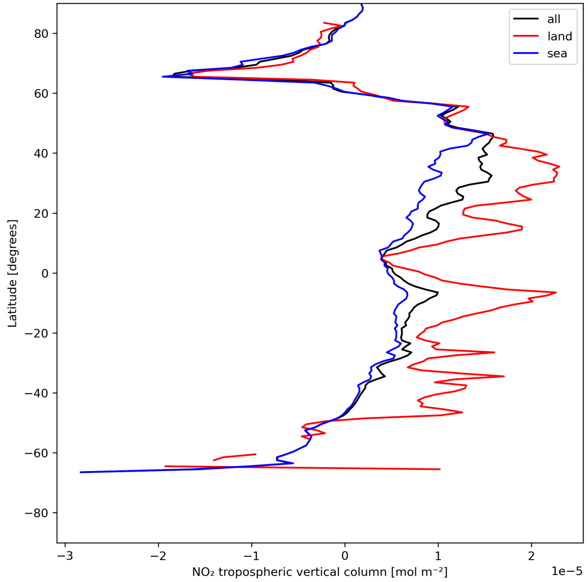
Figure 12: Zonal average of “NO 2 tropospheric vertical column” for 2024-07-12 to 2024-07-14.
