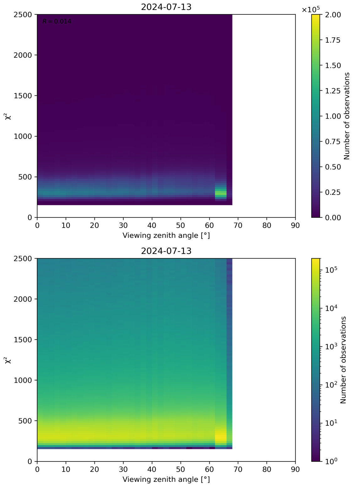
Figure 162: Scatter density plot of “Viewing zenith angle” against “ \chi^2 ” for 2024-07-12 to 2024-07-14.
