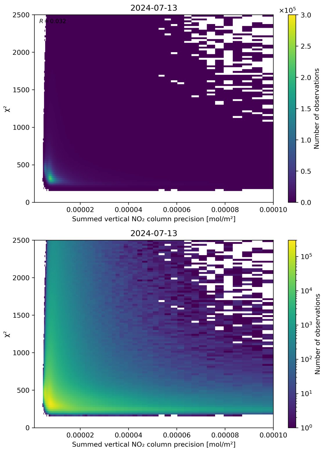
Figure 107: Scatter density plot of “Summed vertical NO 2 column precision” against “ \chi^2 ” for 2024-07-12 to 2024-07-14.
