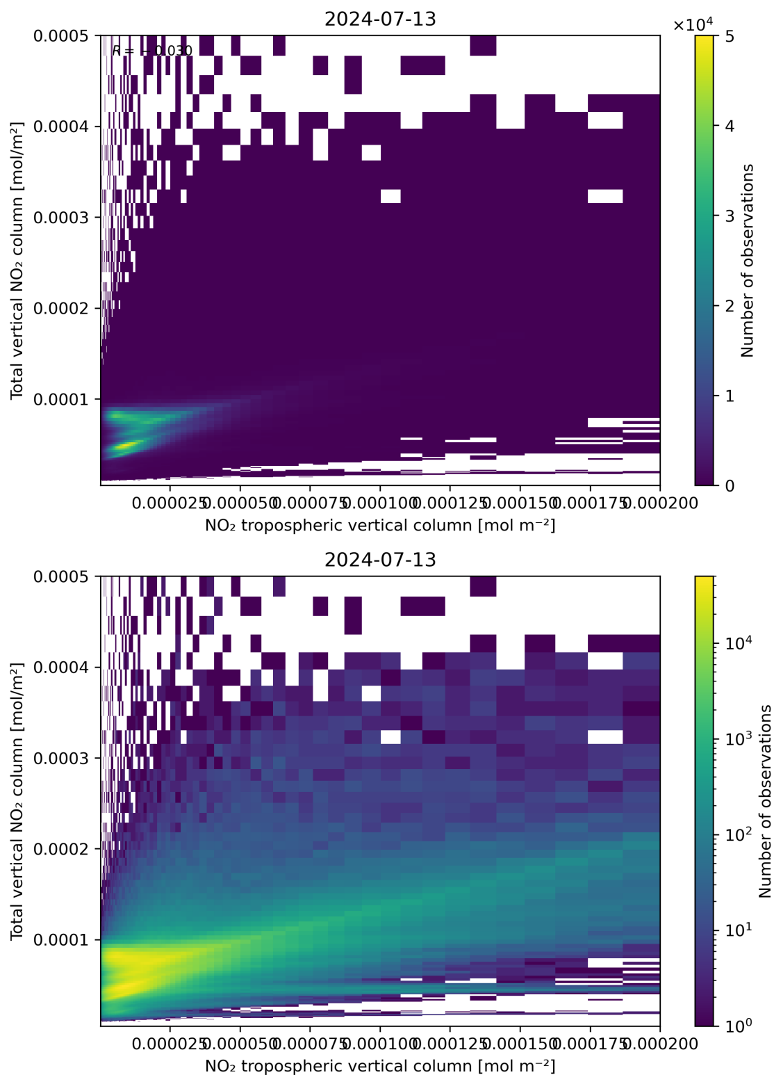
Figure 128: Scatter density plot of “NO 2 tropospheric vertical column” against “Total vertical NO 2 column” for 2024-07-12 to 2024-07-14.
