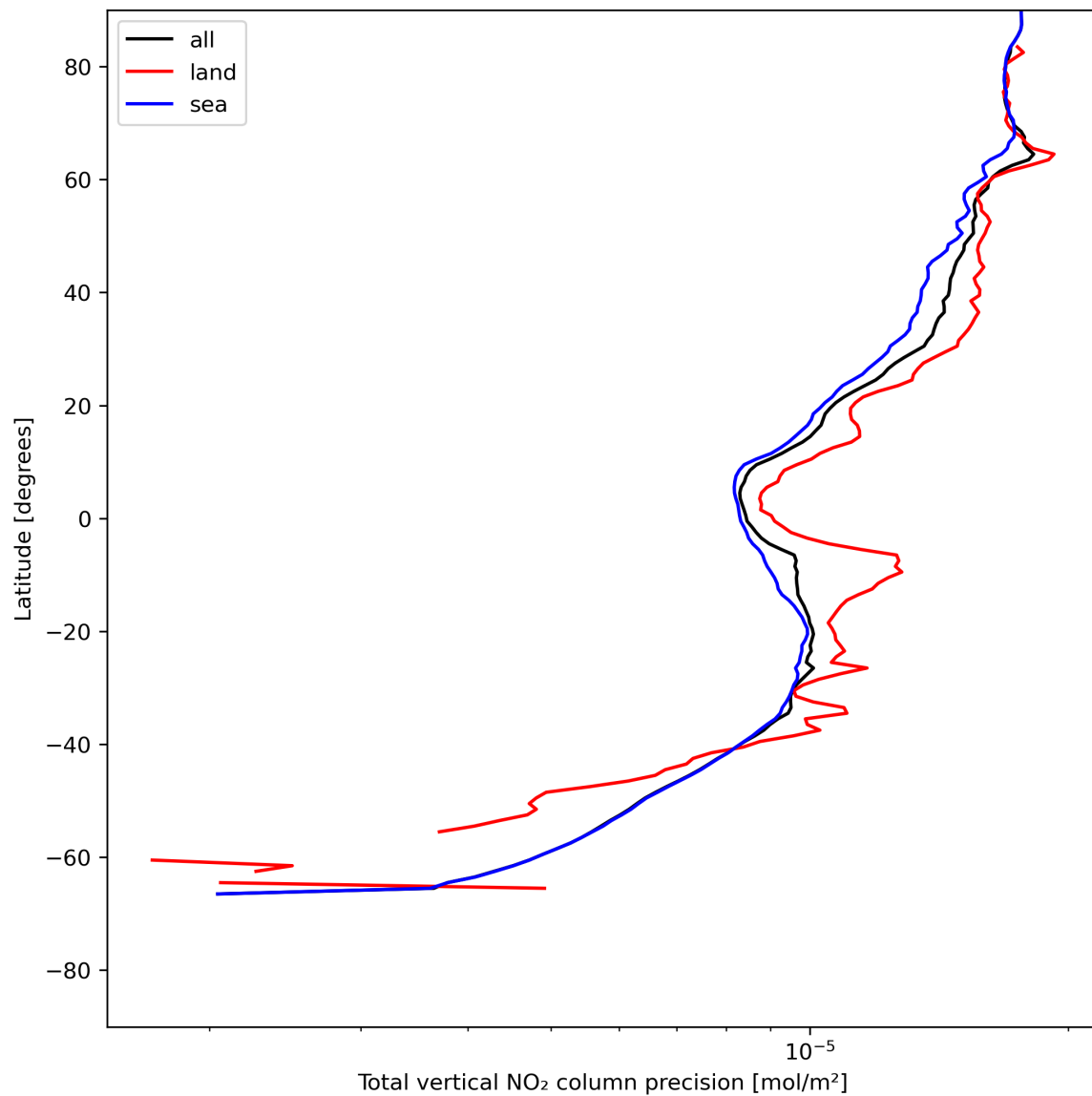
Figure 22: Zonal average of “Total vertical NO 2 column precision” for 2024-07-12 to 2024-07-14.
