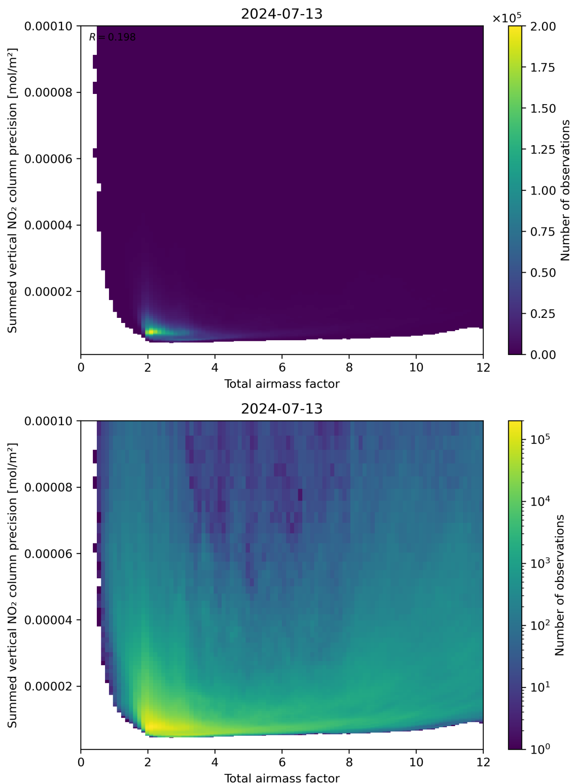
Figure 66: Scatter density plot of “Total airmass factor” against “Summed vertical NO 2 column precision” for 2024-07-12 to 2024-07-14.
