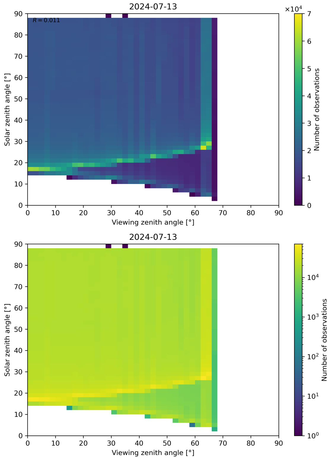
Figure 172: Scatter density plot of “Viewing zenith angle” against “Solar zenith angle” for 2024-07-12 to 2024-07-14.
