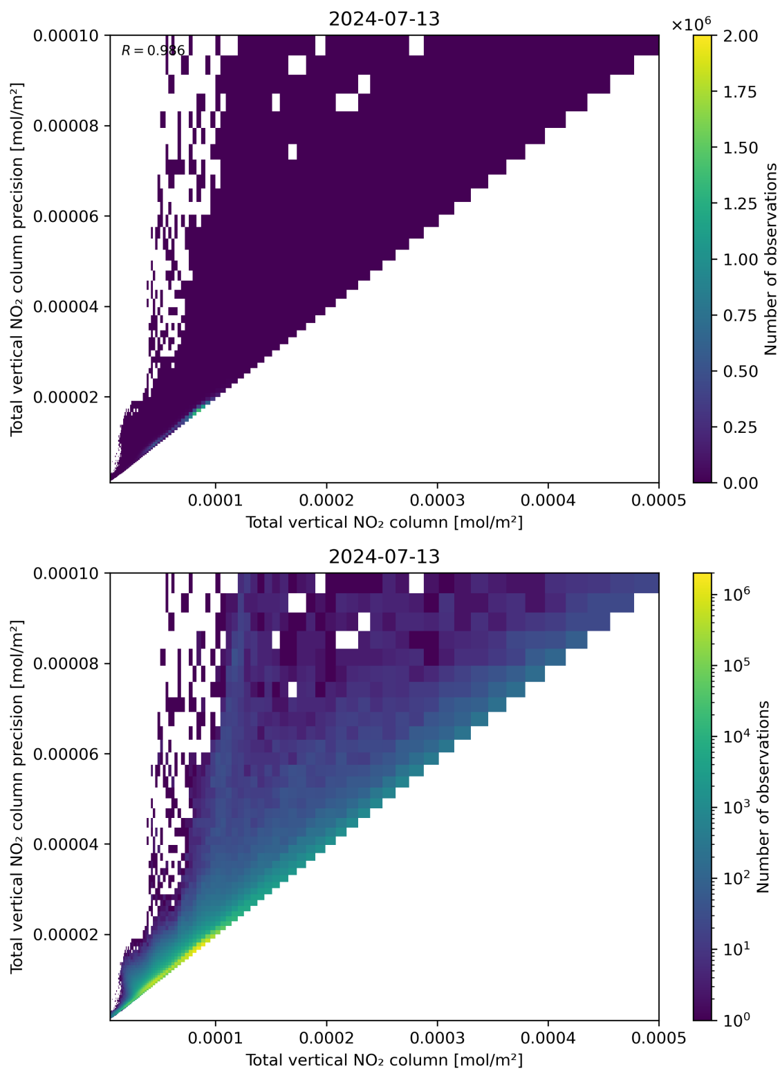
Figure 114: Scatter density plot of “Total vertical NO 2 column” against “Total vertical NO 2 column precision” for 2024-07-12 to 2024-07-14.
