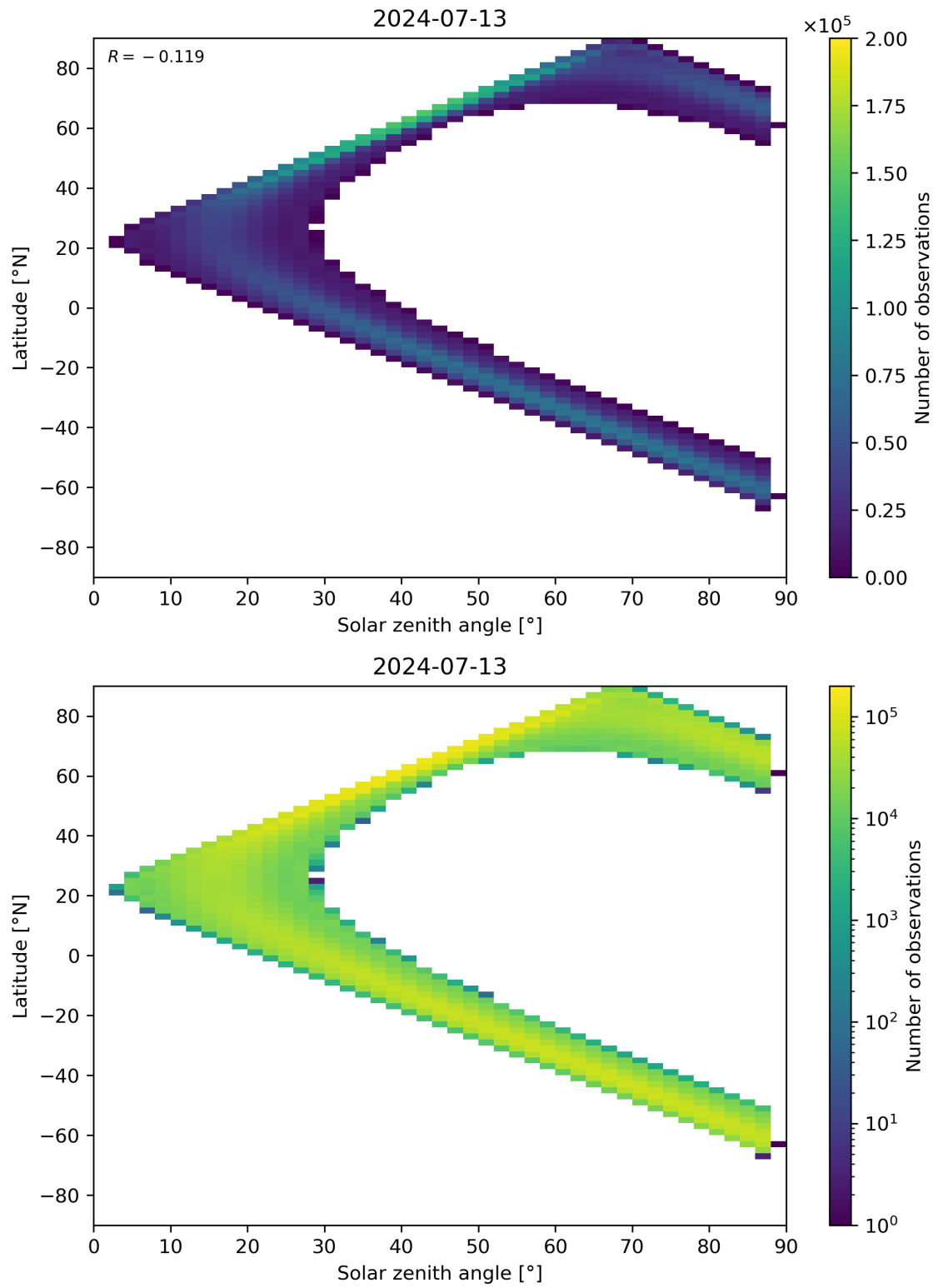
Figure 149: Scatter density plot of “Solar zenith angle” against “Latitude” for 2024-07-12 to 2024-07-14.
