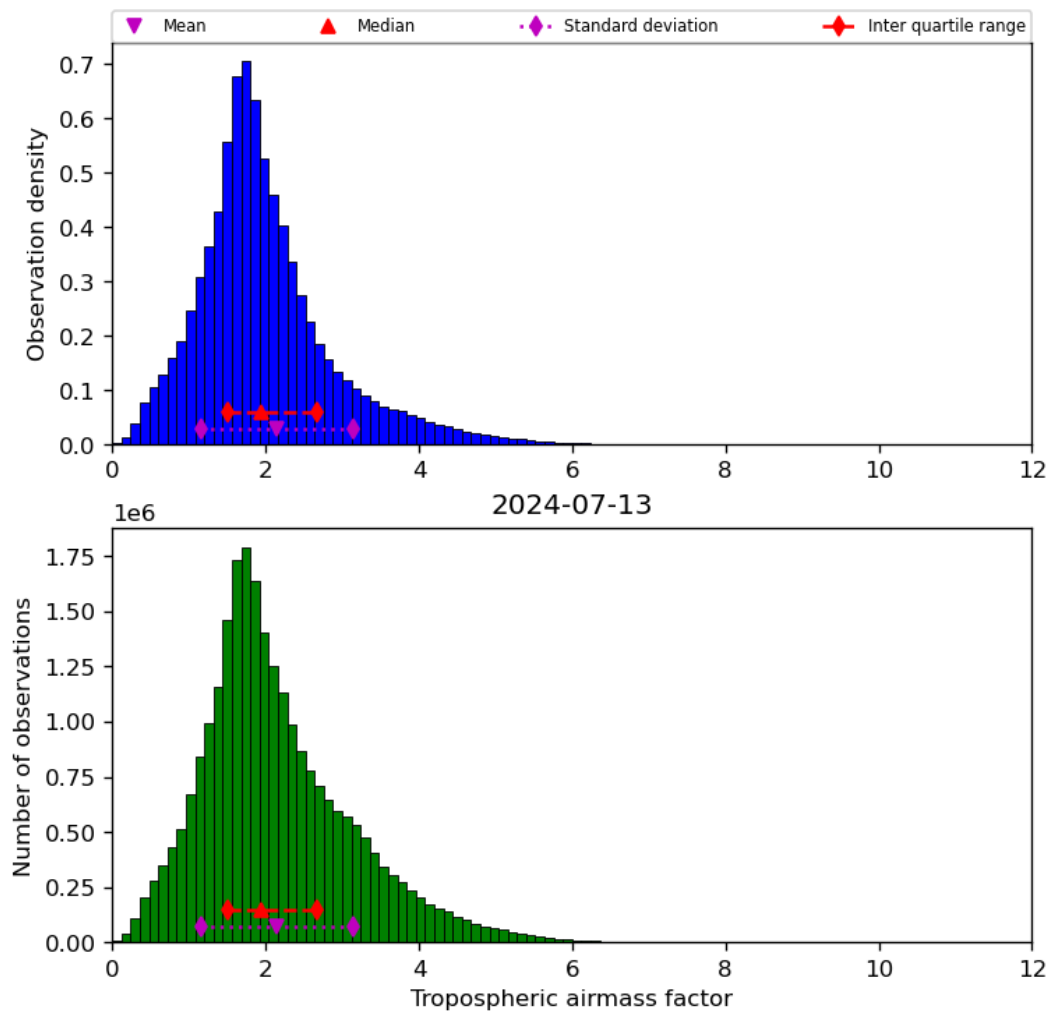
Figure 31: Histogram of “Tropospheric airmass factor” for 2024-07-12 to 2024-07-14
