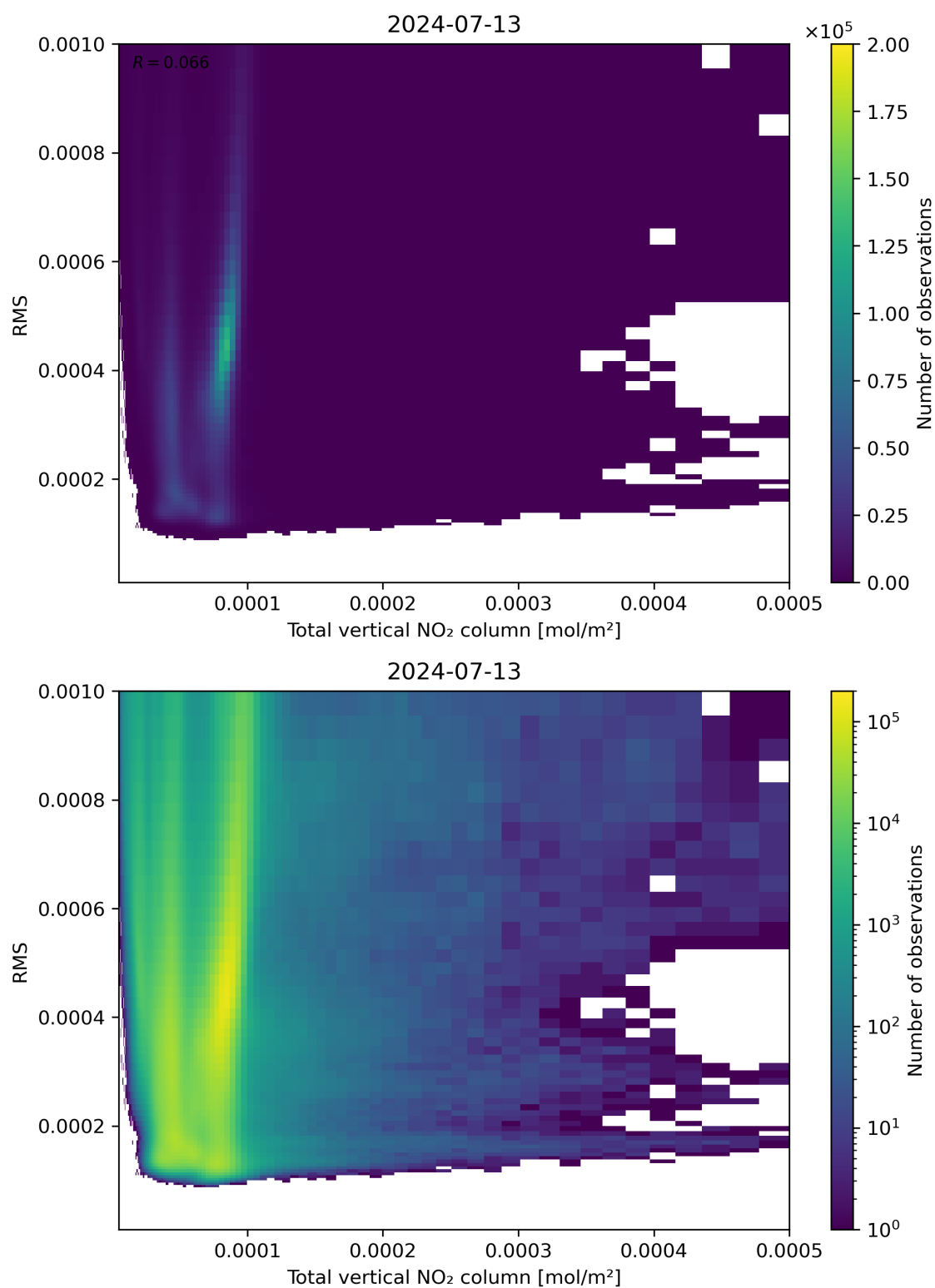
Figure 120: Scatter density plot of “Total vertical NO 2 column” against “RMS” for 2024-07-12 to 2024-07-14.
