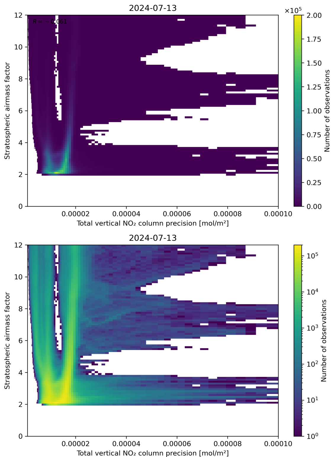
Figure 115: Scatter density plot of “Total vertical NO 2 column precision” against “Stratospheric air mass factor” for 2024-07-12 to 2024-07-14.
