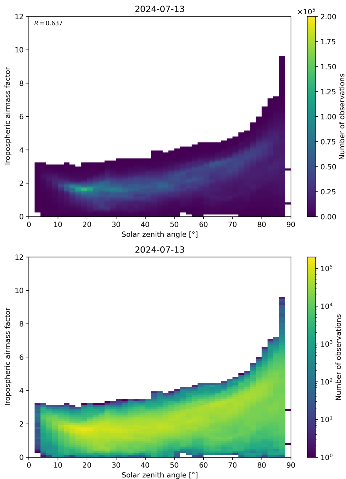
Figure 147: Scatter density plot of “Solar zenith angle” against “Tropospheric airmass factor” for 2024-07-12 to 2024-07-14.
