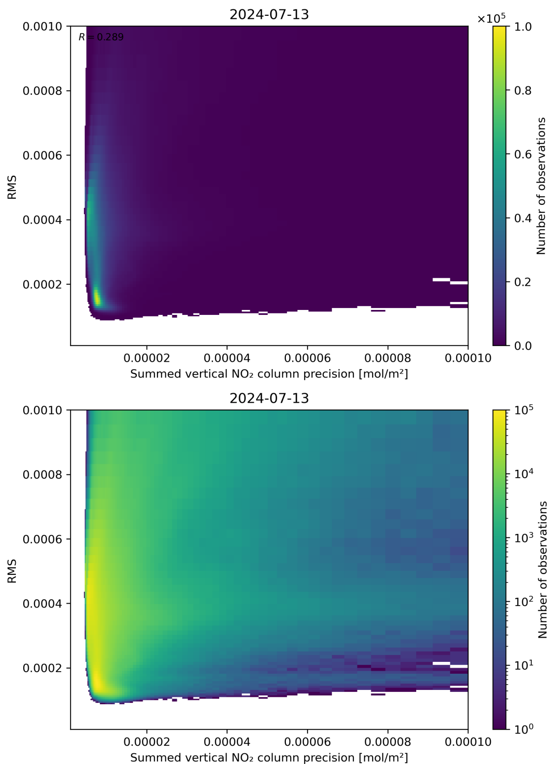
Figure 108: Scatter density plot of “Summed vertical NO 2 column precision” against “RMS” for 2024-07-12 to 2024-07-14.
