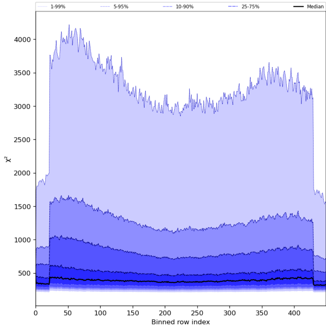
Figure 59: Along track statistics of “ \chi^2 ” for 2024-07-12 to 2024-07-14
