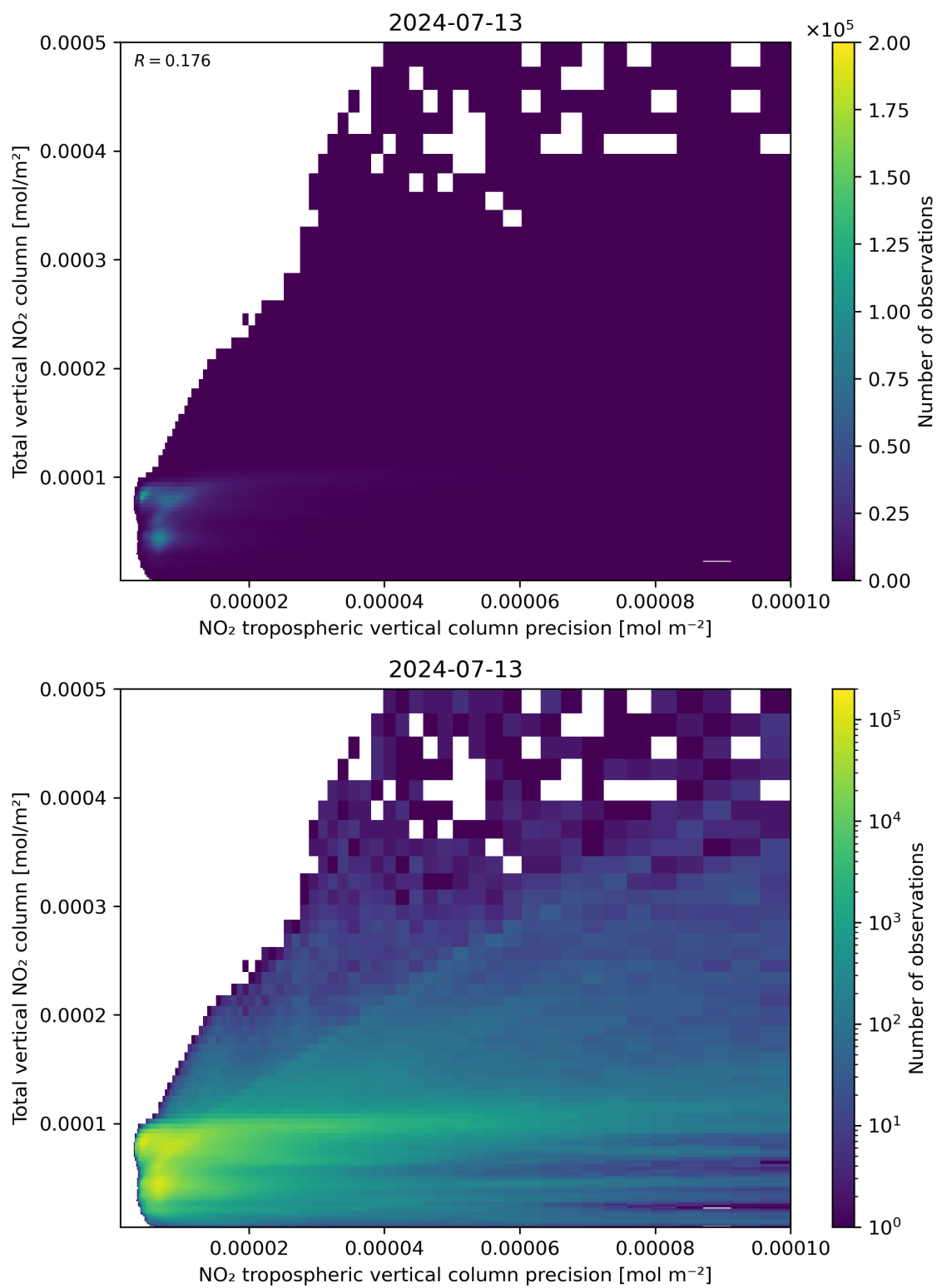
Figure 138: Scatter density plot of “NO 2 tropospheric vertical column precision” against “Total vertical NO 2 column” for 2024-07-12 to 2024-07-14.
