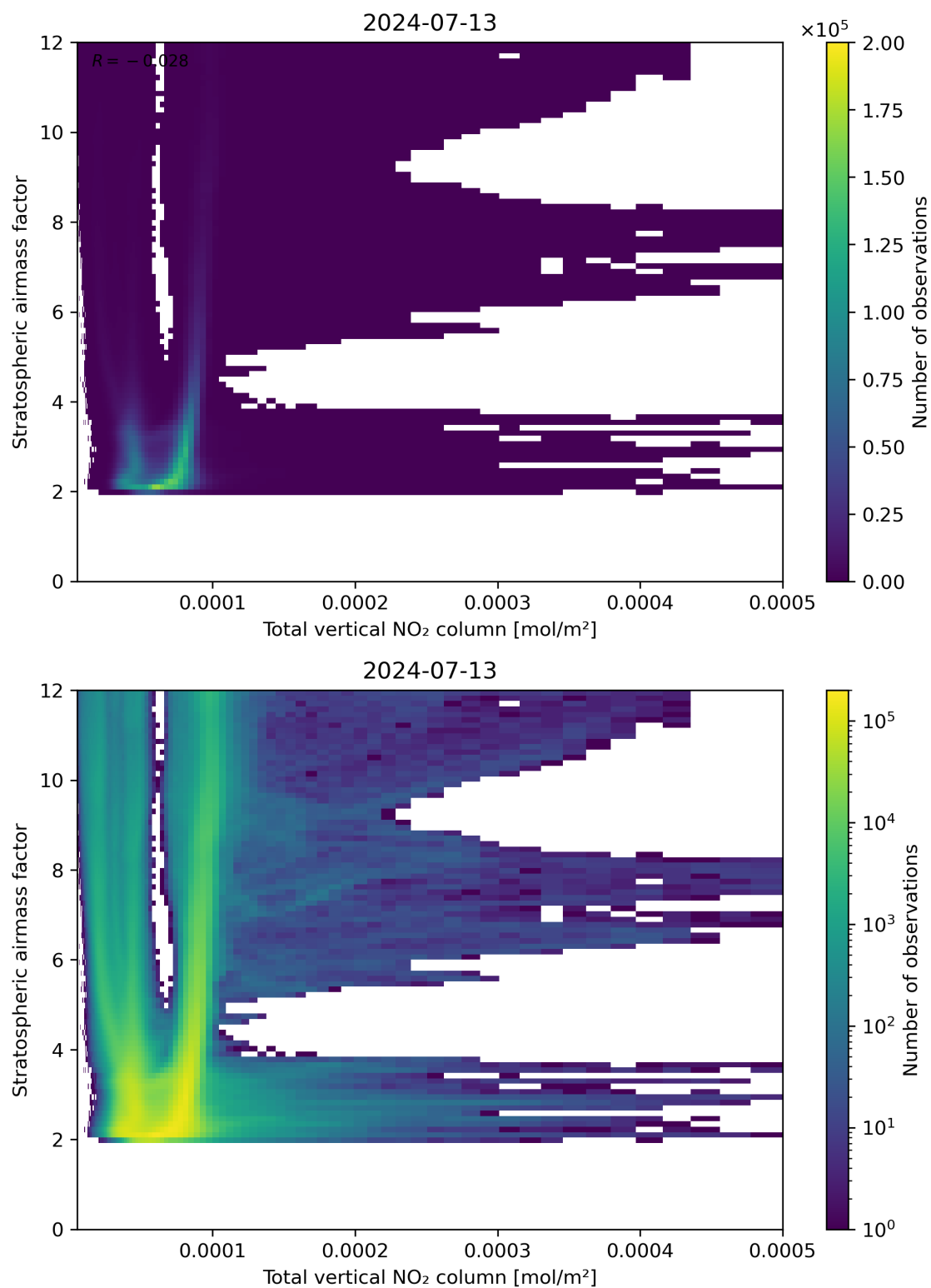
Figure 110: Scatter density plot of “Total vertical NO 2 column” against “Stratospheric airmass factor” for 2024-07-12 to 2024-07-14.
