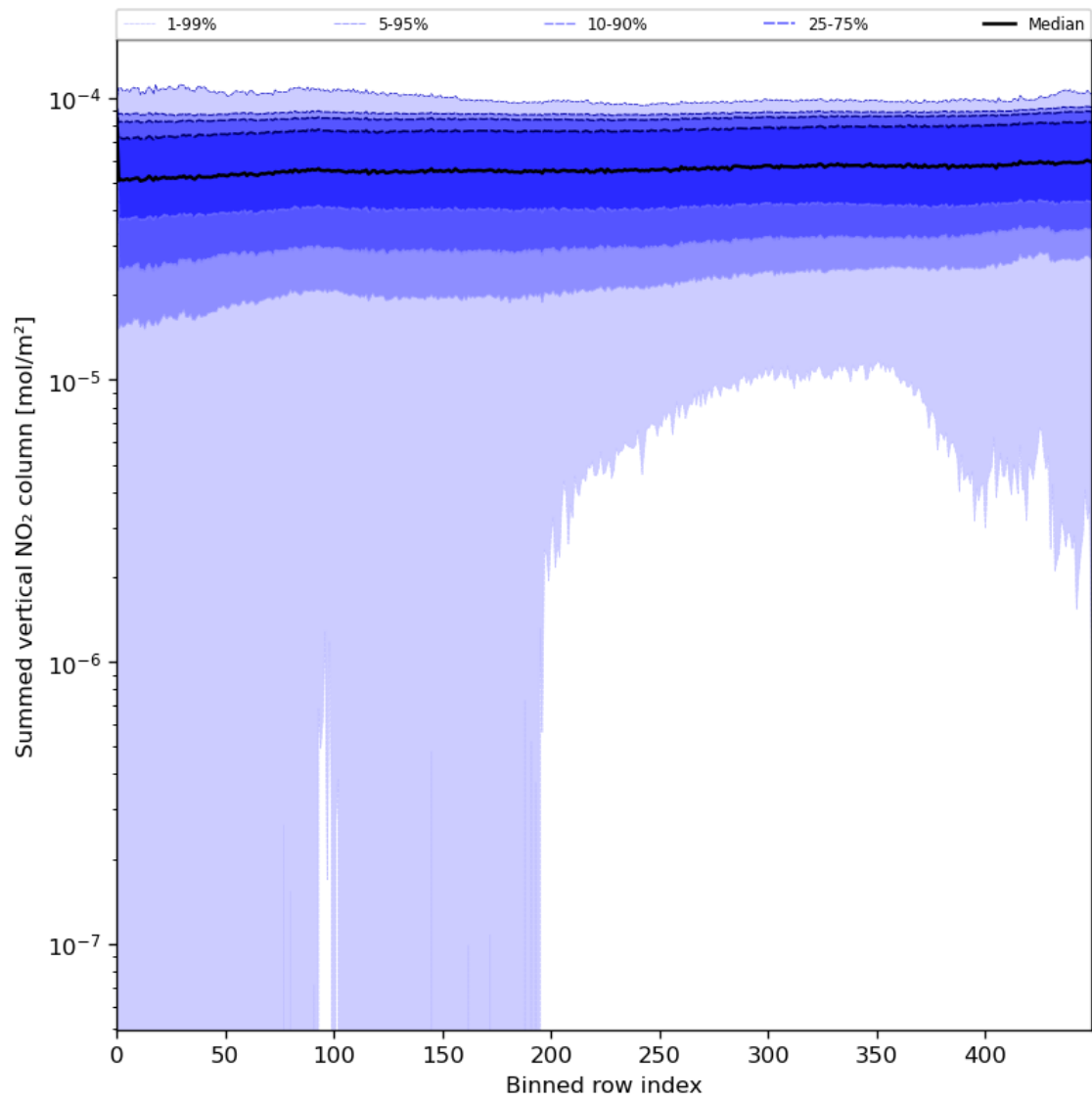
Figure 57: Along track statistics of “Summed vertical NO 2 column” for 2024-07-12 to 2024-07-14
