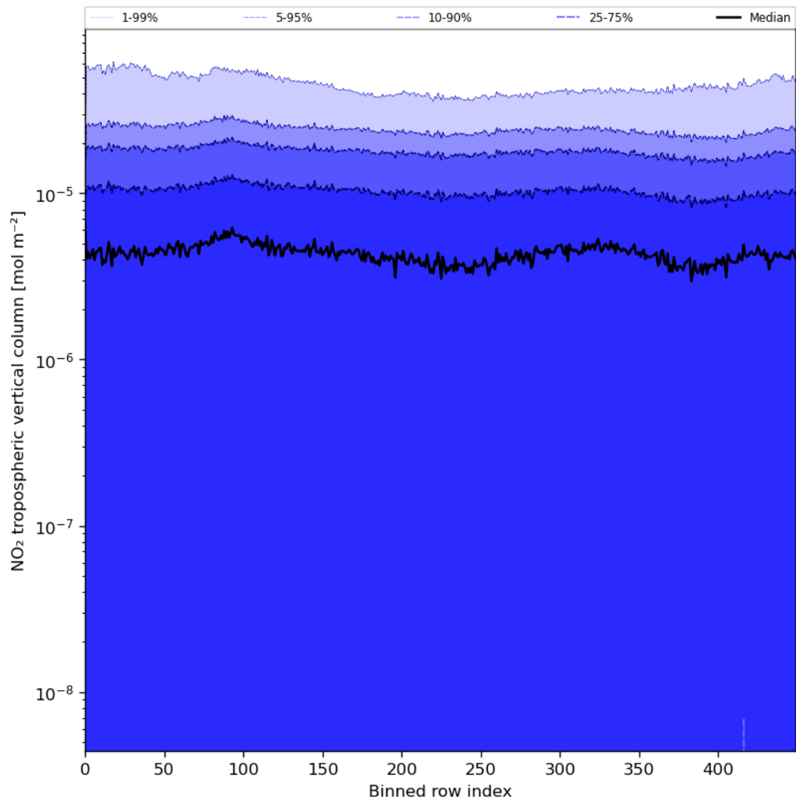
Figure 46: Along track statistics of “NO 2 tropospheric vertical column” for 2024-07-12 to 2024-07-14
