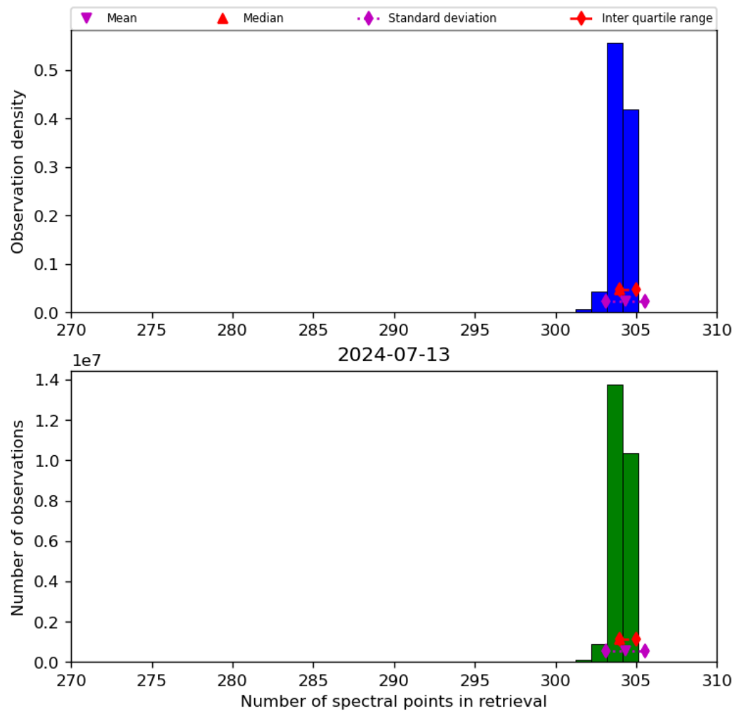
Figure 33: Histogram of “Number of spectral points in retrieval” for 2024-07-12 to 2024-07-14
