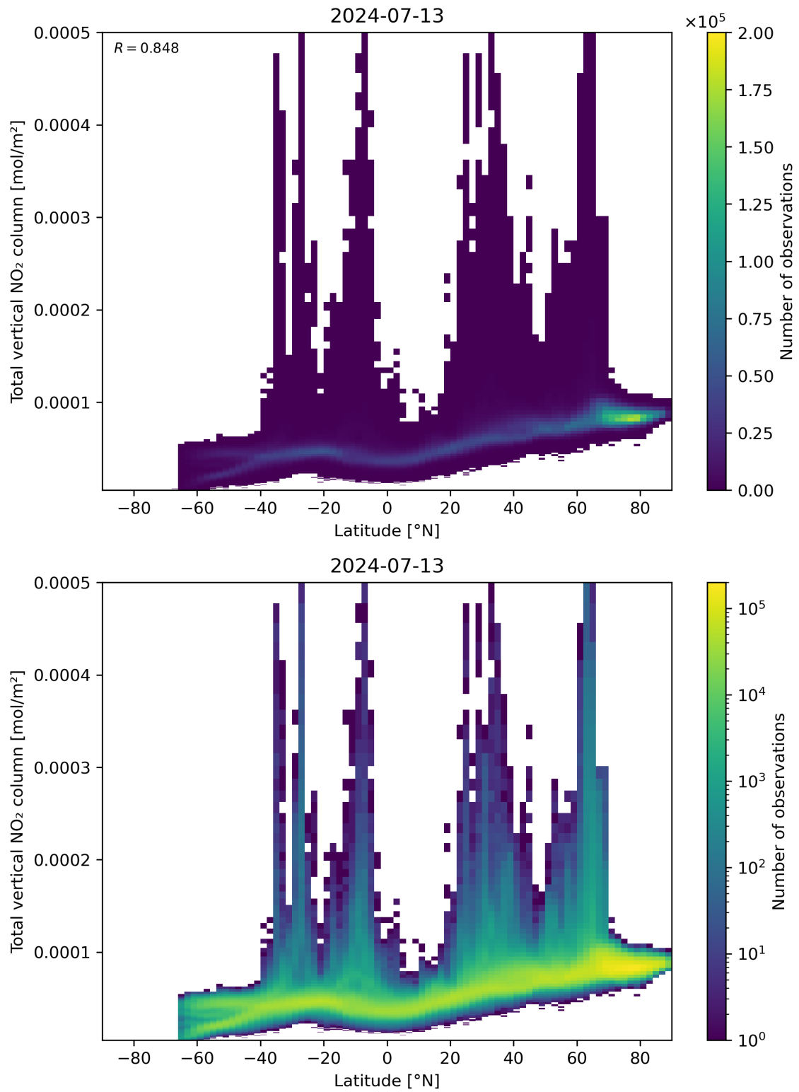
Figure 90: Scatter density plot of “Latitude” against “Total vertical NO 2 column” for 2024-07-12 to 2024-07-14.
