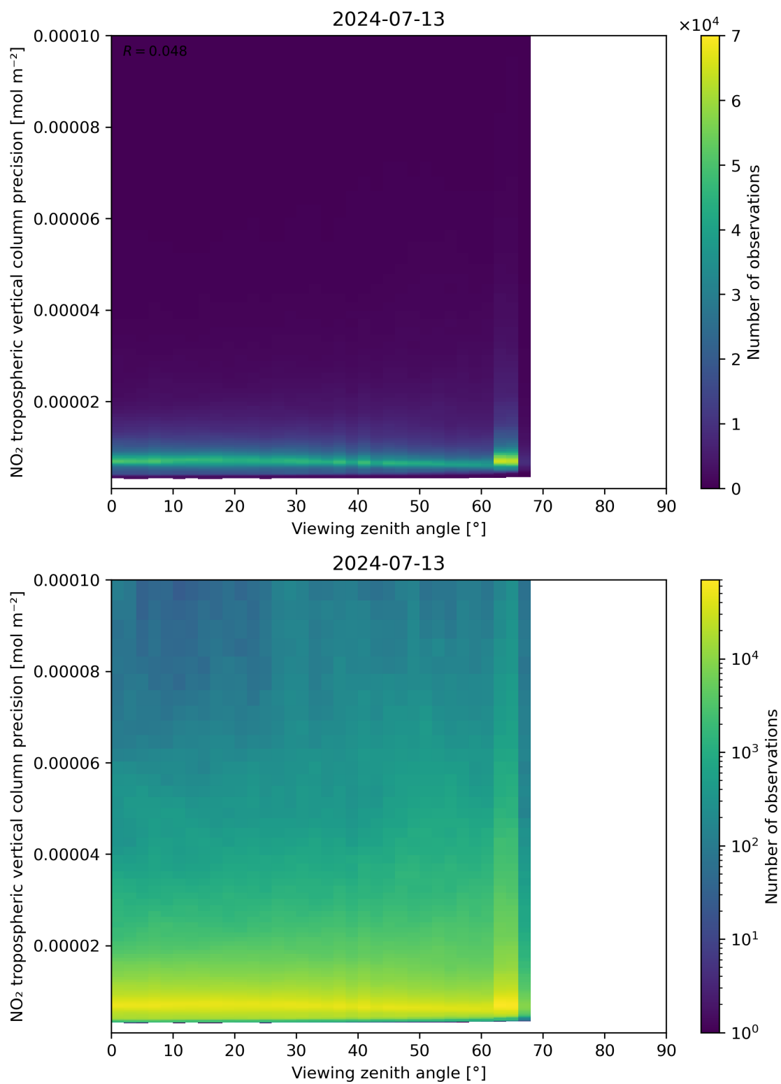
Figure 170: Scatter density plot of “Viewing zenith angle” against “NO 2 tropospheric vertical column precision” for 2024-07-12 to 2024-07-14.
