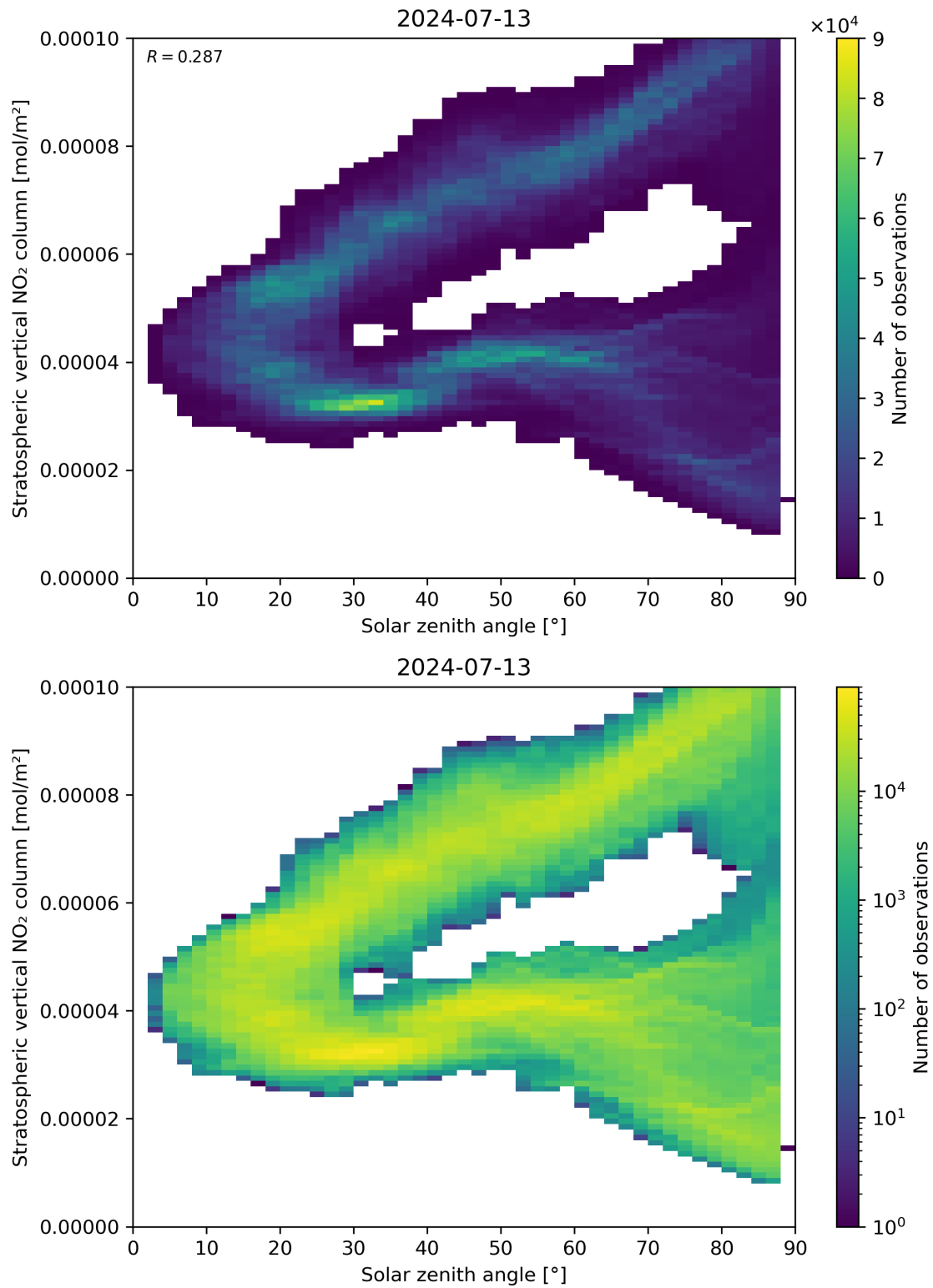
Figure 150: Scatter density plot of “Solar zenith angle” against “Stratospheric vertical NO 2 column” for 2024-07-12 to 2024-07-14.
