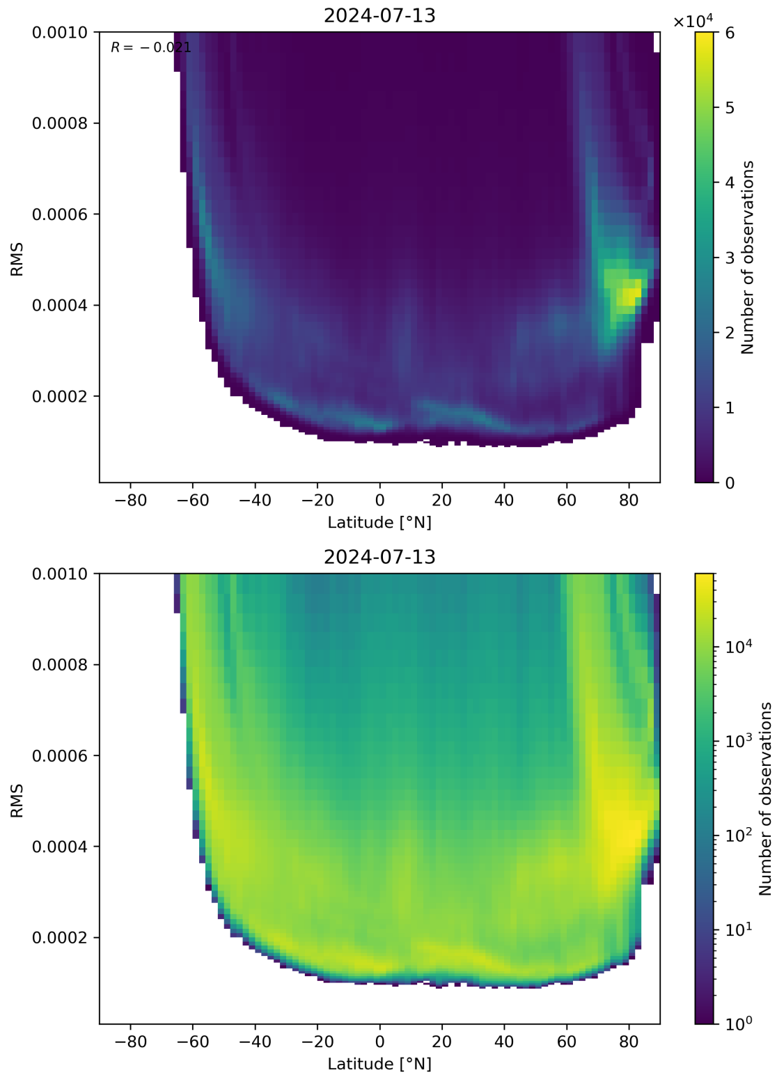
Figure 94: Scatter density plot of “Latitude” against “RMS” for 2024-07-12 to 2024-07-14.
