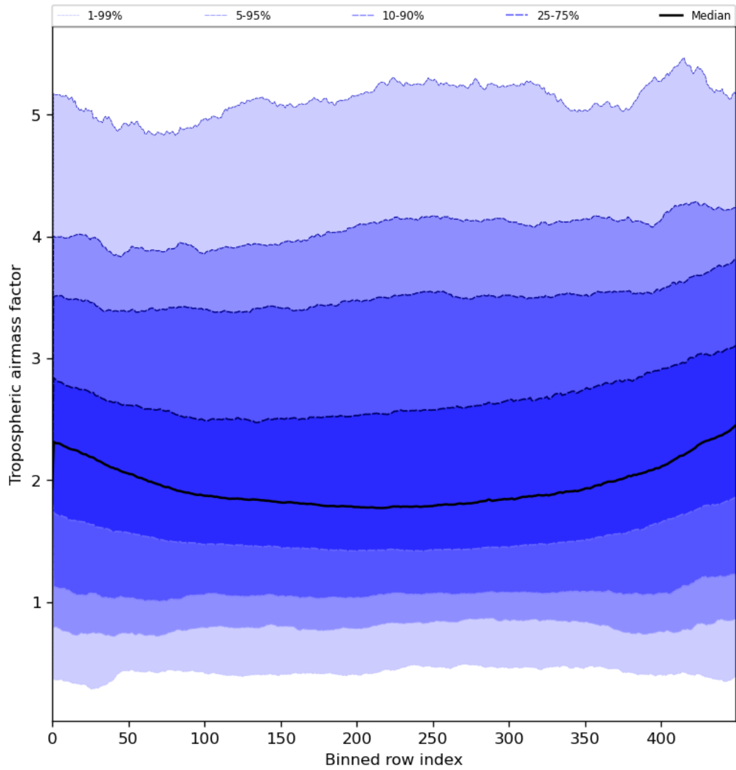
Figure 48: Along track statistics of “Tropospheric air mass factor” for 2024-07-12 to 2024-07-14
