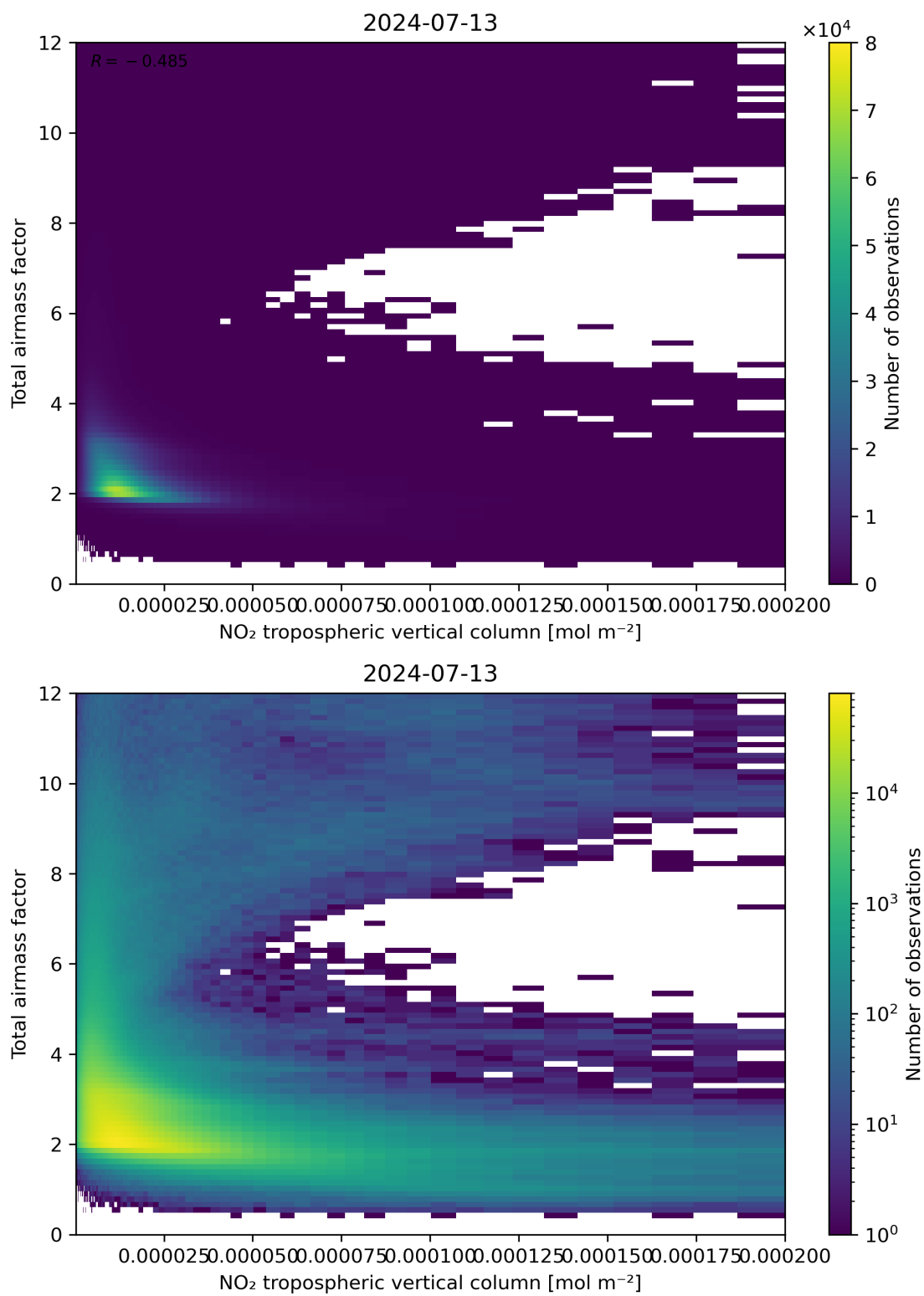
Figure 122: Scatter density plot of “NO 2 tropospheric vertical column” against “Total air mass factor” for 2024-07-12 to 2024-07-14.
