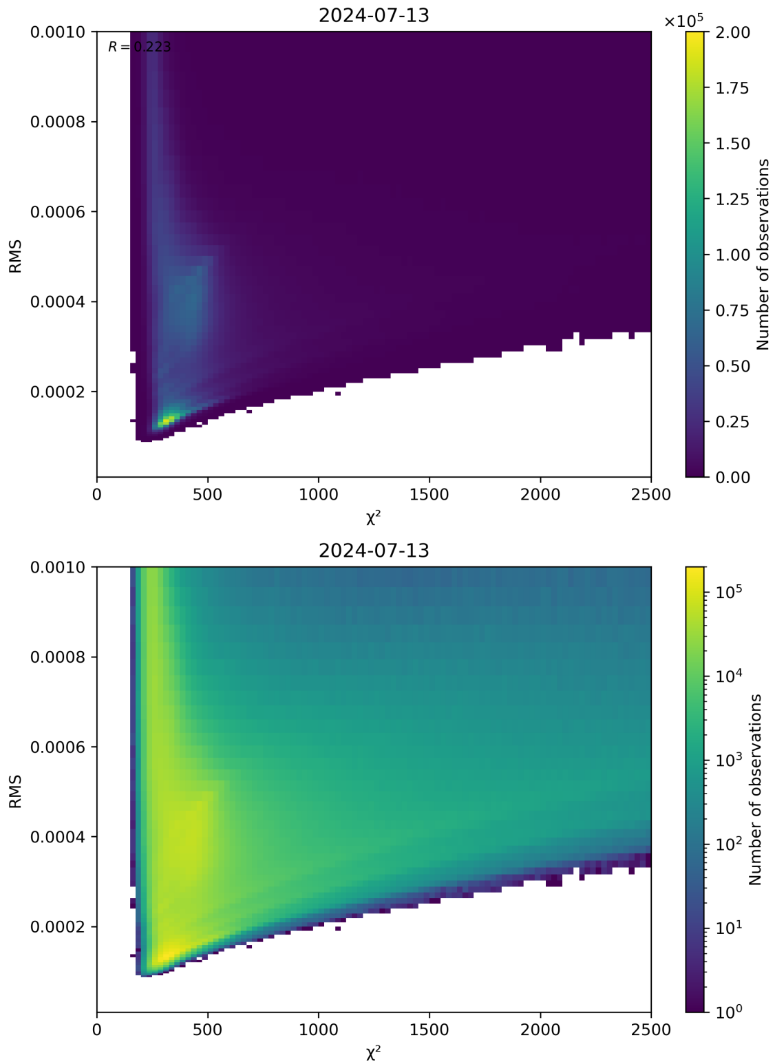
Figure 82: Scatter density plot of “ \chi^2 ” against “RMS” for 2024-07-12 to 2024-07-14.
