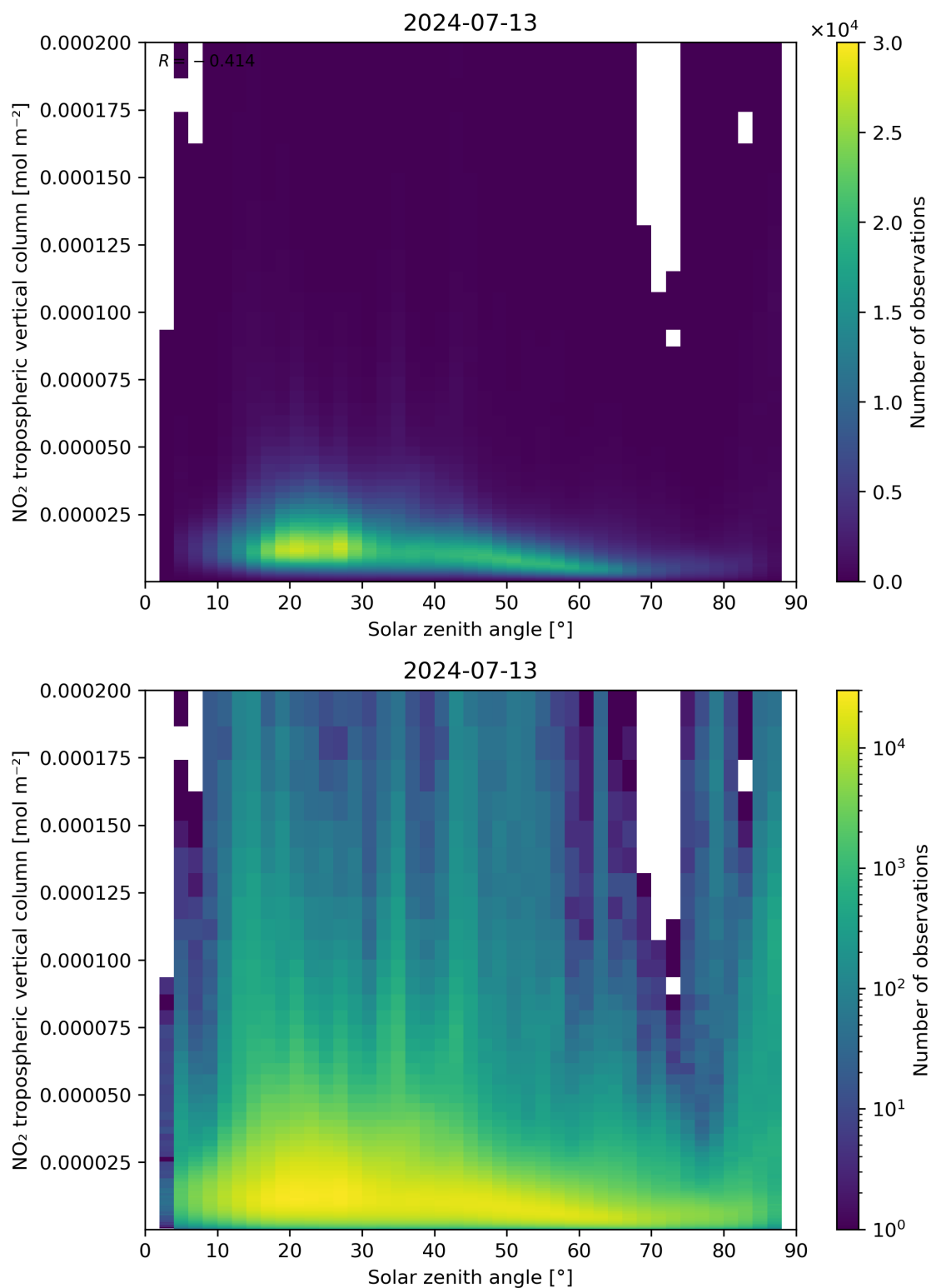
Figure 155: Scatter density plot of “Solar zenith angle” against “NO 2 tropospheric vertical column” for 2024-07-12 to 2024-07-14.
