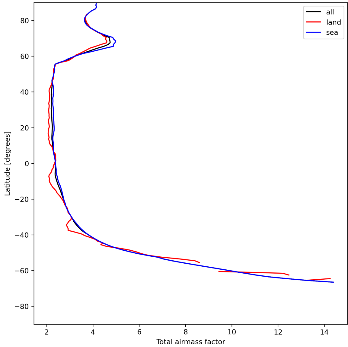
Figure 15: Zonal average of “Total airmass factor” for 2024-07-12 to 2024-07-14.
