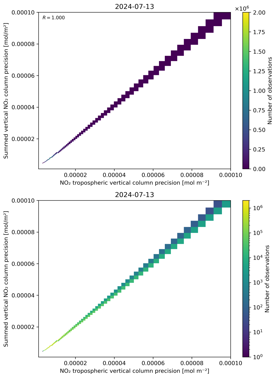
Figure 137: Scatter density plot of “NO 2 tropospheric vertical column precision” against “Summed vertical NO 2 column precision” for 2024-07-12 to 2024-07-14.
