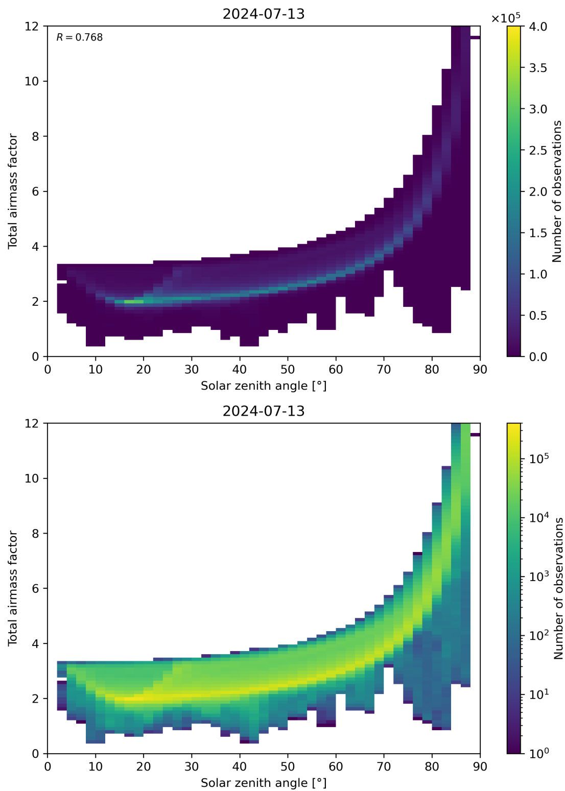
Figure 146: Scatter density plot of “Solar zenith angle” against “Total air mass factor” for 2024-07-12 to 2024-07-14.
