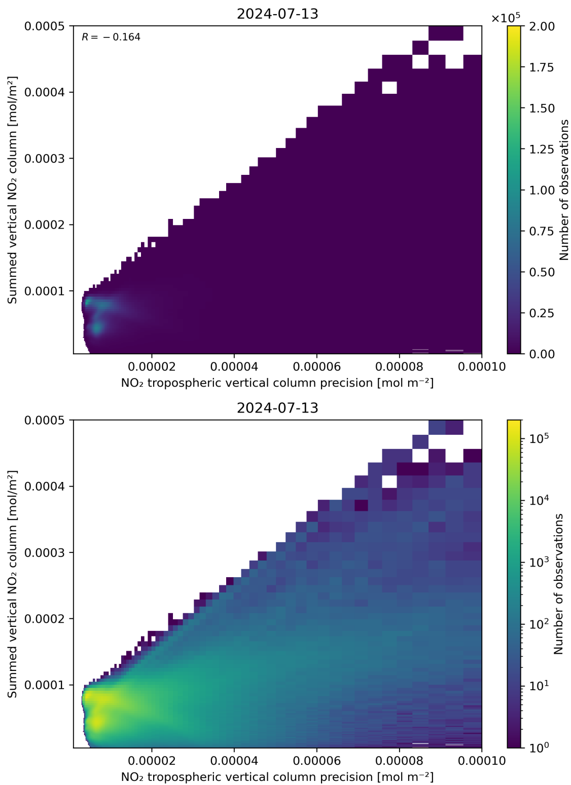
Figure 136: Scatter density plot of “NO 2 tropospheric vertical column precision” against “Summed vertical NO 2 column” for 2024-07-12 to 2024-07-14.
