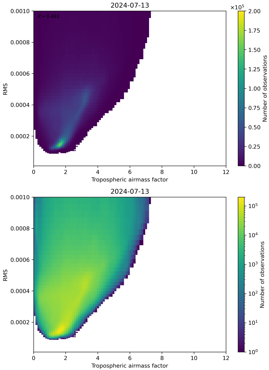
Figure 79: Scatter density plot of “Tropospheric airmass factor” against “RMS” for 2024-07-12 to 2024-07-14.
