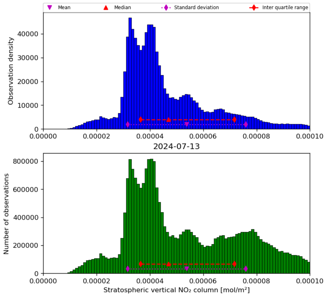
Figure 36: Histogram of “Stratospheric vertical NO 2 column” for 2024-07-12 to 2024-07-14
