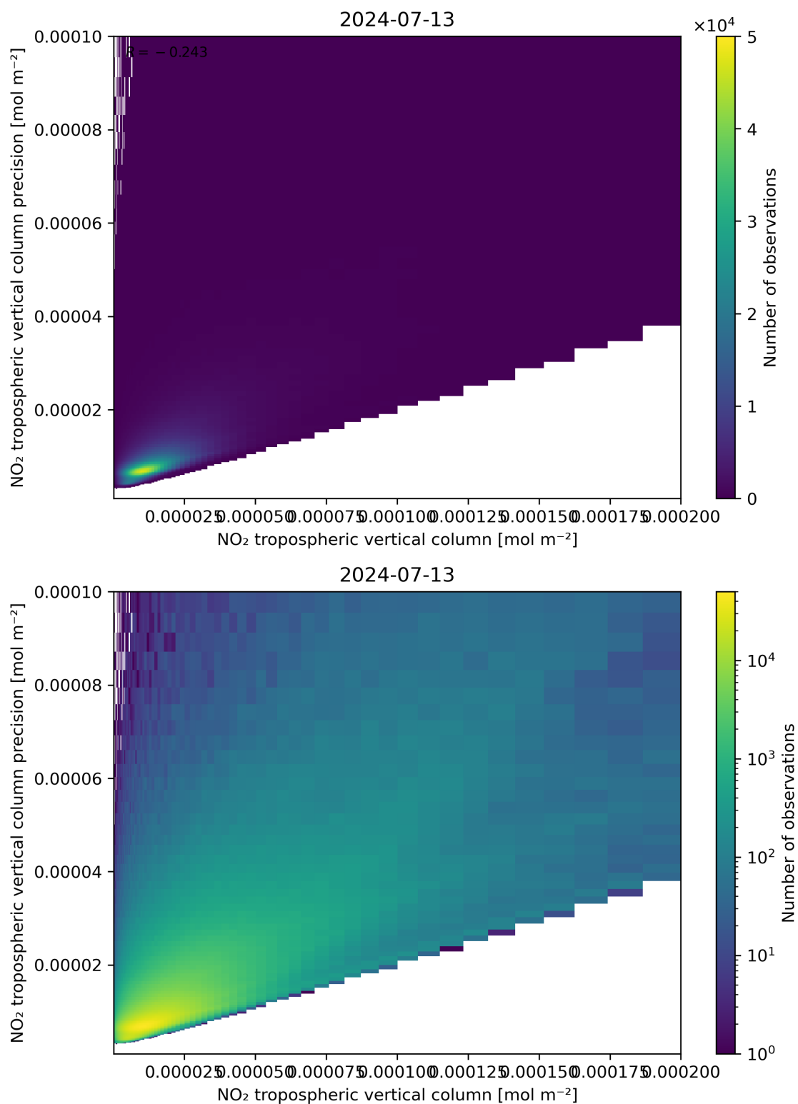
Figure 130: Scatter density plot of “NO 2 tropospheric vertical column” against “NO 2 tropospheric vertical column precision” for 2024-07-12 to 2024-07-14.
