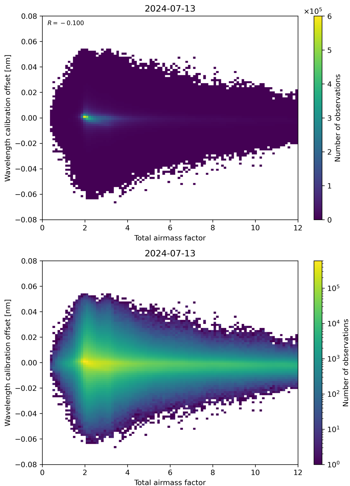
Figure 70: Scatter density plot of “Total airmass factor” against “Wavelength calibration offset” for 2024-07-12 to 2024-07-14.
