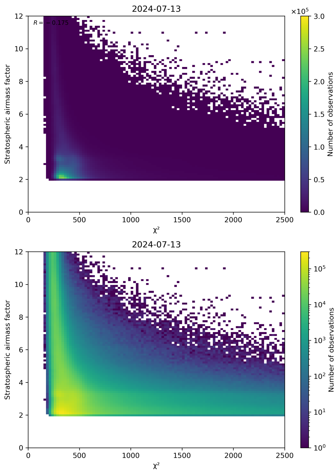
Figure 81: Scatter density plot of “ \chi^2 ” against “Stratospheric airmass factor” for 2024-07-12 to 2024-07-14.
