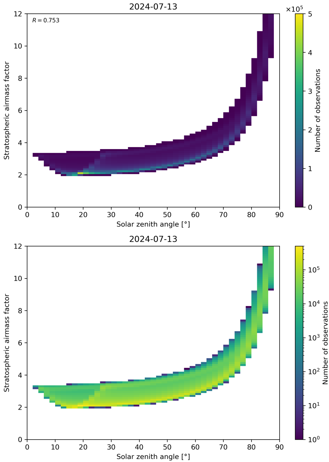
Figure 145: Scatter density plot of “Solar zenith angle” against “Stratospheric airmass factor” for 2024-07-12 to 2024-07-14.
