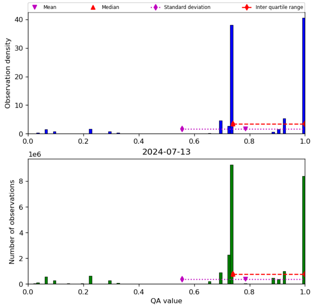
Figure 28: Histogram of “QA value” for 2024-07-12 to 2024-07-14
