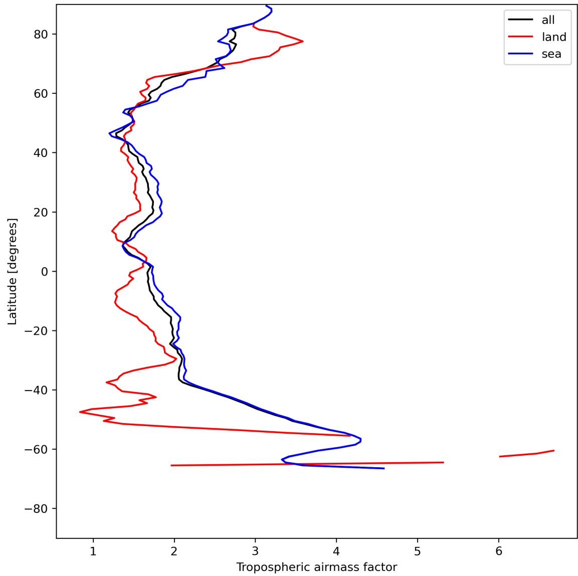
Figure 14: Zonal average of “Tropospheric airmass factor” for 2024-07-12 to 2024-07-14.
