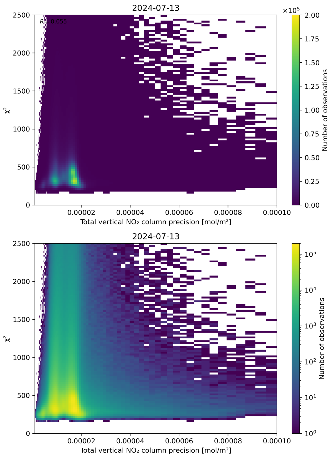
Figure 116: Scatter density plot of “Total vertical NO 2 column precision” against “ \chi^2 ” for 2024-07-12 to 2024-07-14.
