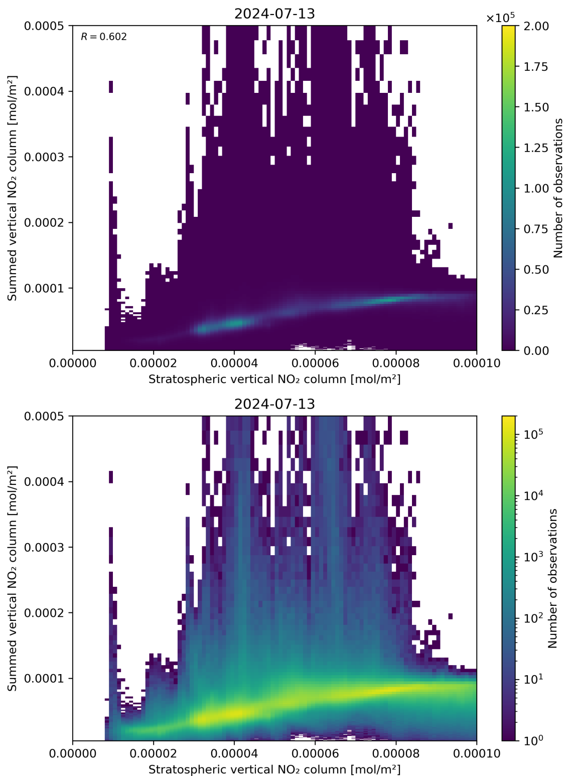
Figure 98: Scatter density plot of “Stratospheric vertical NO 2 column” against “Summed vertical NO 2 column” for 2024-07-12 to 2024-07-14.
