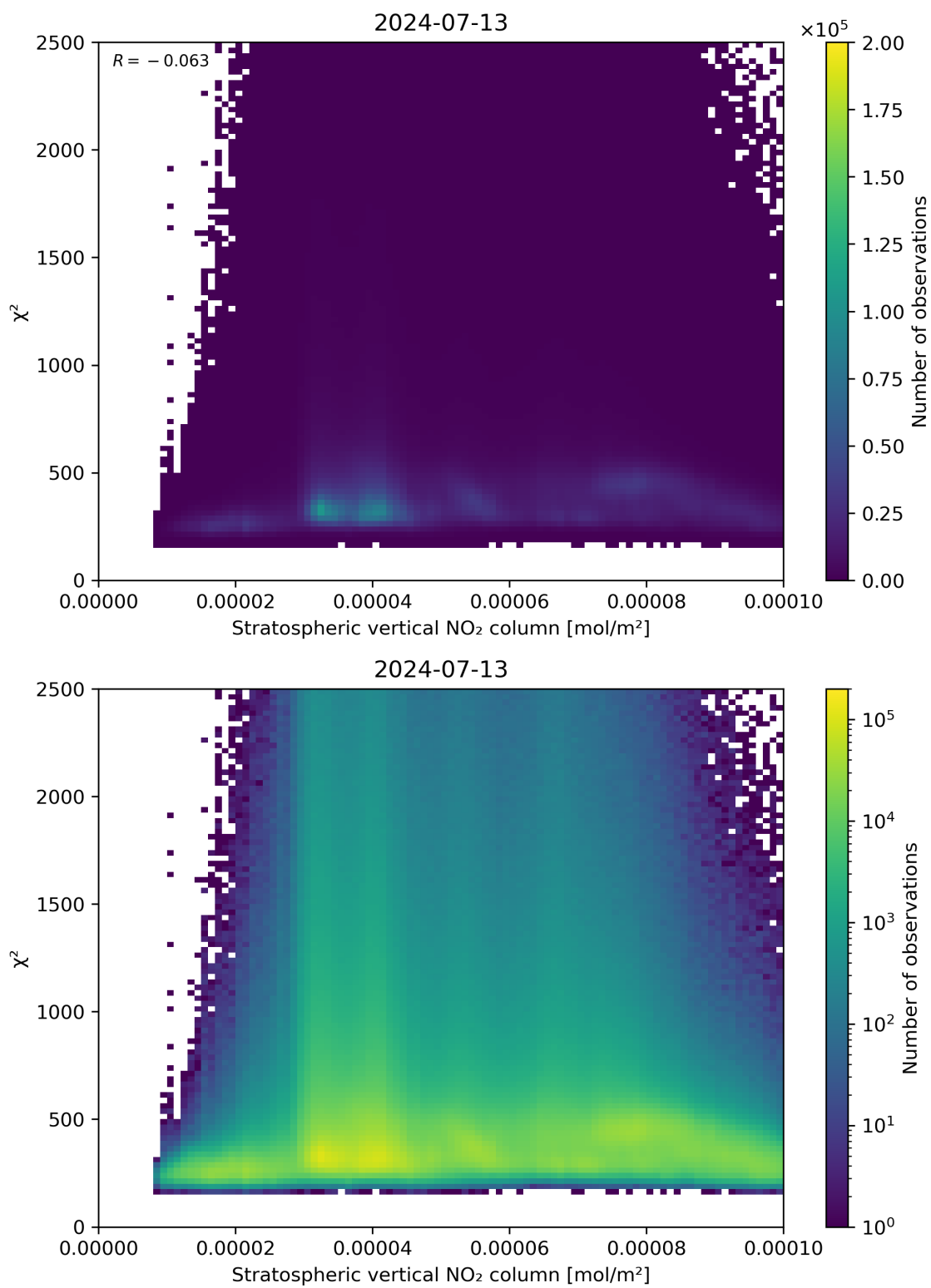
Figure 97: Scatter density plot of “Stratospheric vertical NO 2 column” against “ \chi^2 ” for 2024-07-12 to 2024-07-14.
