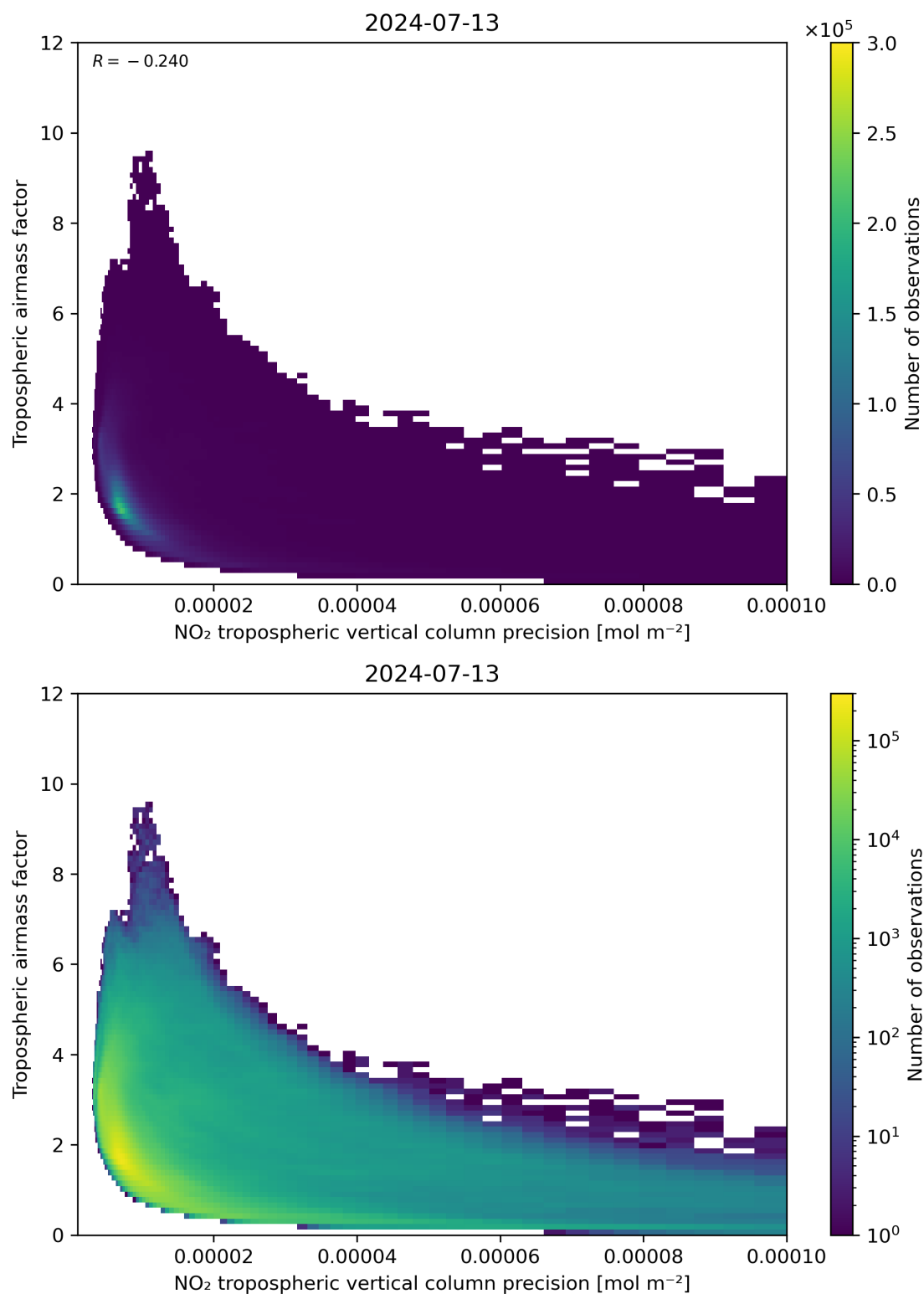
Figure 133: Scatter density plot of “NO 2 tropospheric vertical column precision” against “Tropospheric airmass factor” for 2024-07-12 to 2024-07-14.
