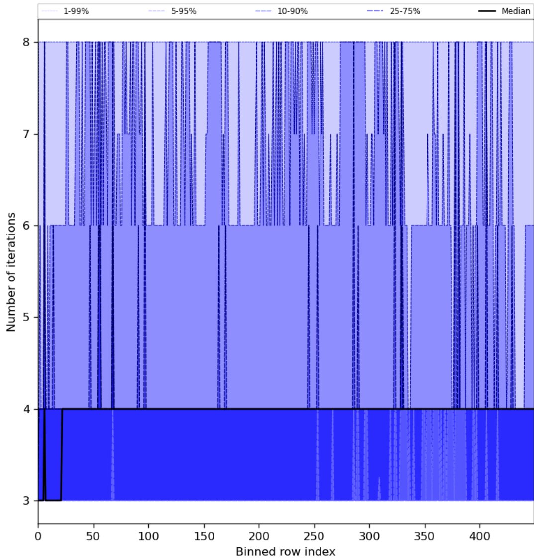
Figure 51: Along track statistics of “Number of iterations” for 2024-07-12 to 2024-07-14
