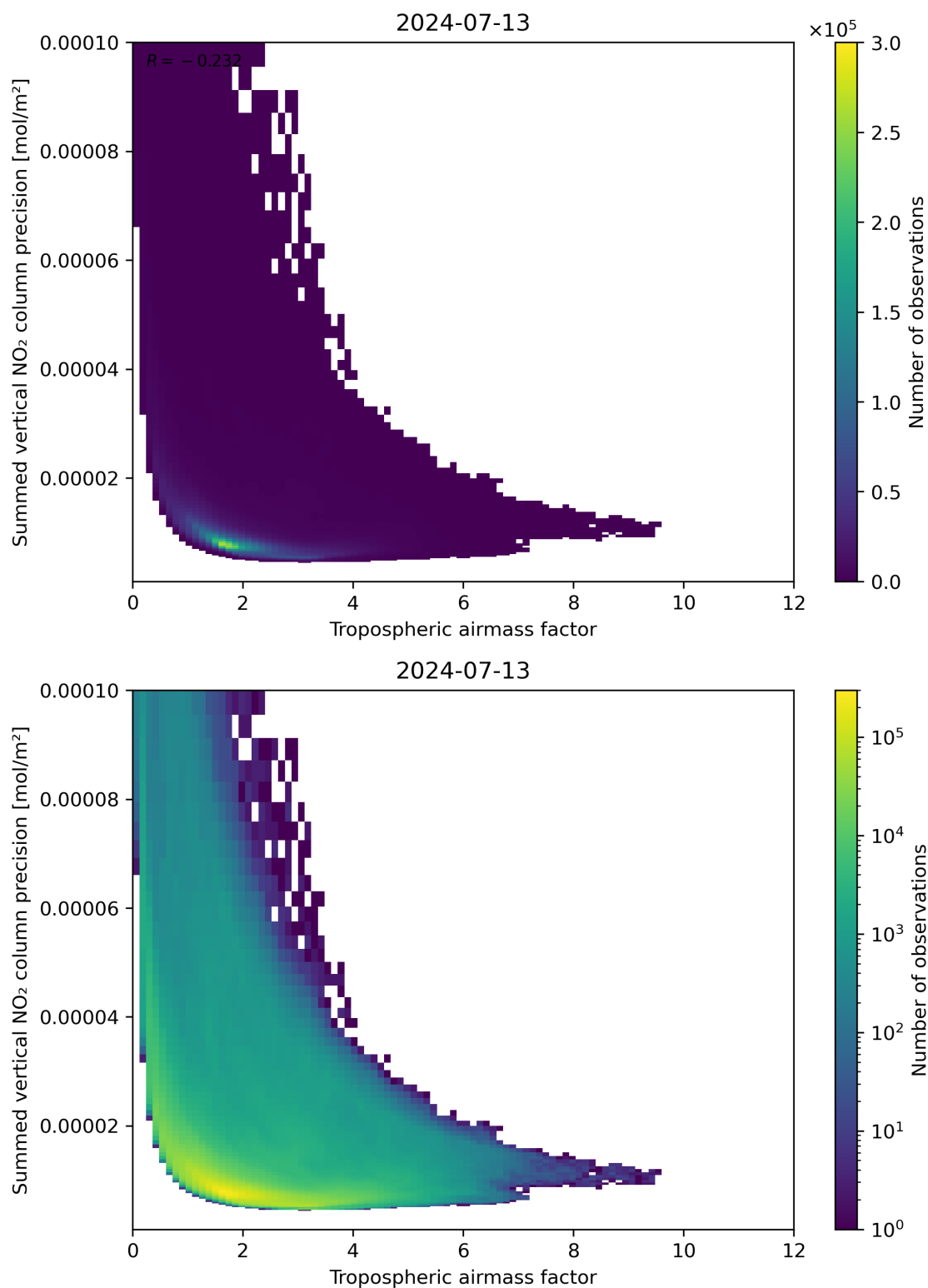
Figure 76: Scatter density plot of “Tropospheric air mass factor” against “Summed vertical NO 2 column precision” for 2024-07-12 to 2024-07-14.
