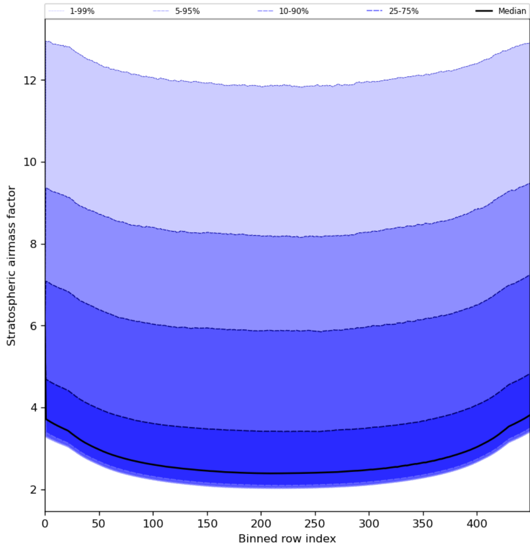
Figure 61: Along track statistics of “Stratospheric airmass factor” for 2024-07-12 to 2024-07-14
