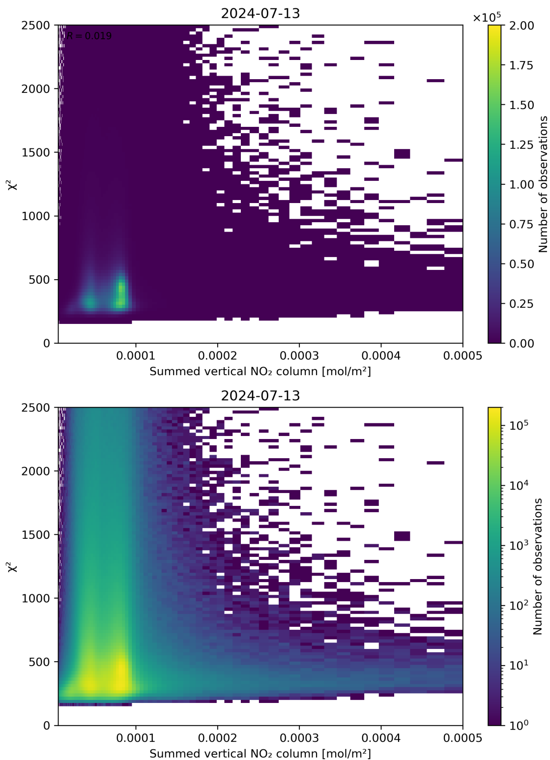
Figure 104: Scatter density plot of “Summed vertical NO 2 column” against “ \chi^2 ” for 2024-07-12 to 2024-07-14.
