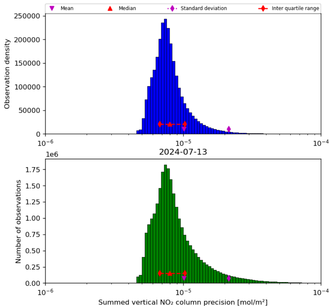
Figure 41: Histogram of “Summed vertical NO 2 column precision” for 2024-07-12 to 2024-07-14
