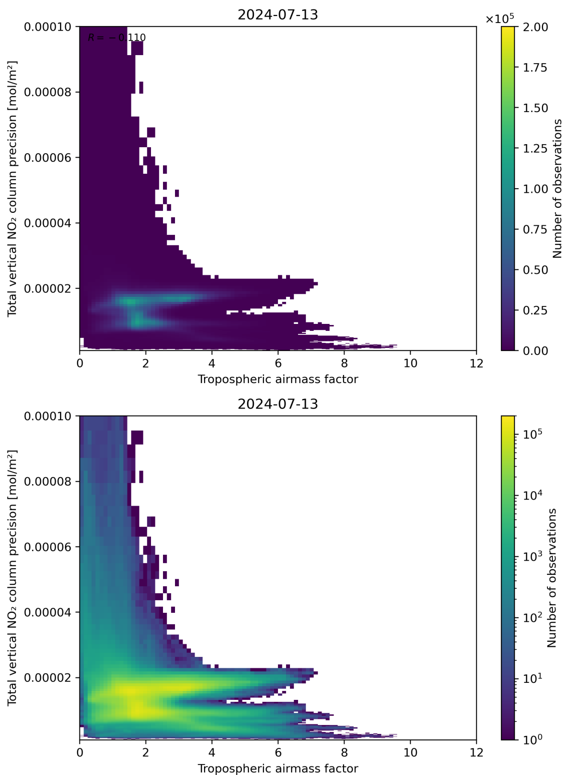
Figure 78: Scatter density plot of “Tropospheric air mass factor” against “Total vertical NO 2 column precision” for 2024-07-12 to 2024-07-14.
