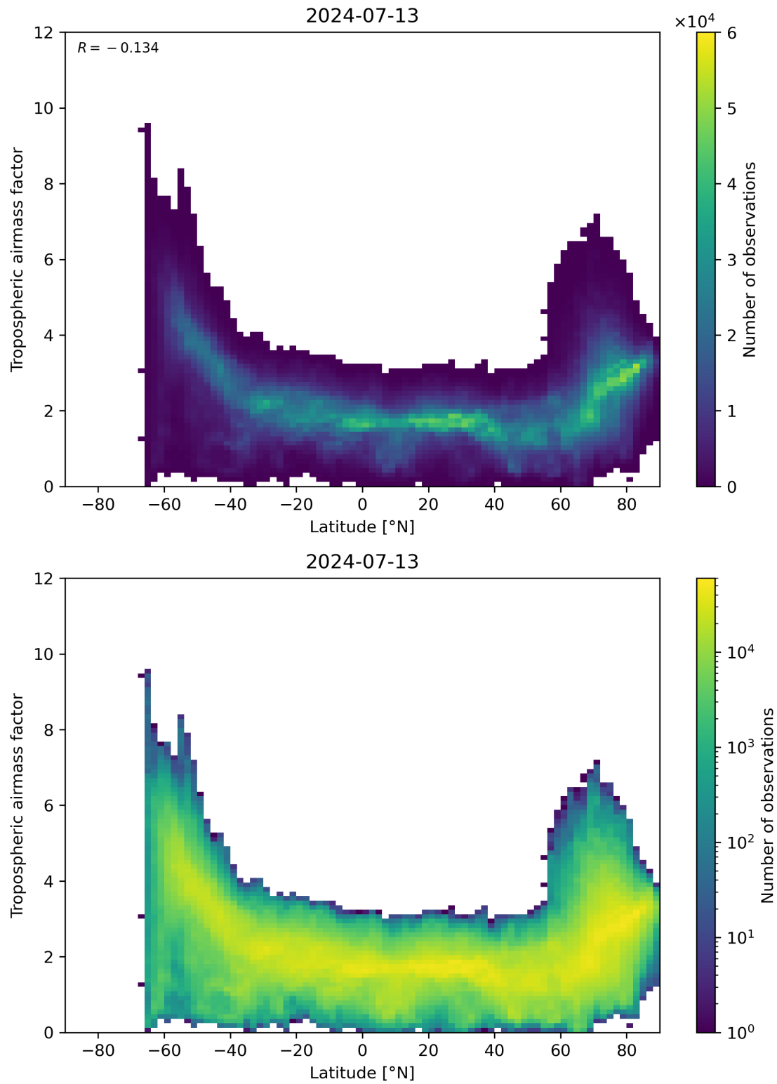
Figure 85: Scatter density plot of “Latitude” against “Tropospheric airmass factor” for 2024-07-12 to 2024-07-14.
