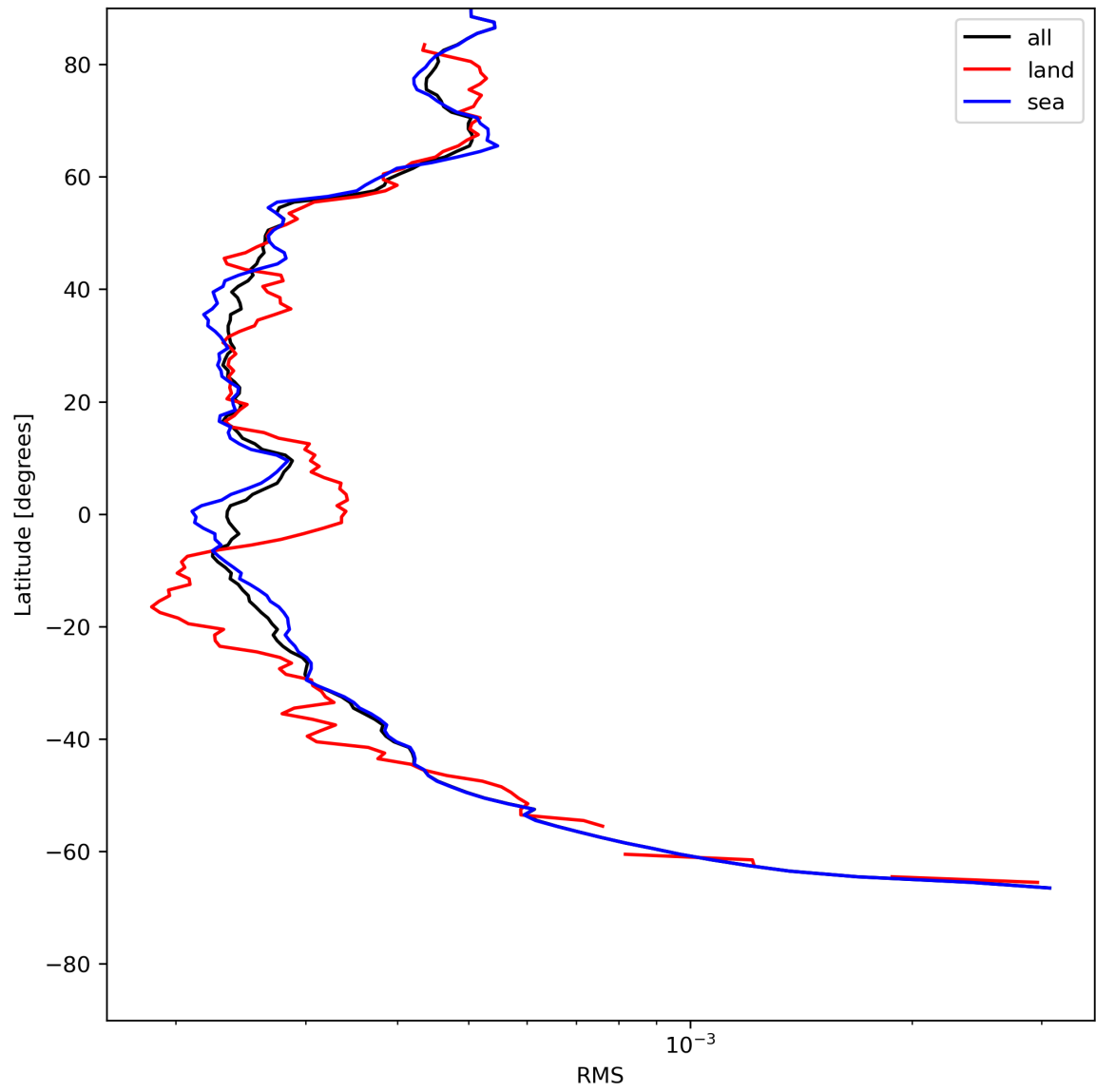
Figure 26: Zonal average of “RMS” for 2024-07-12 to 2024-07-14.
