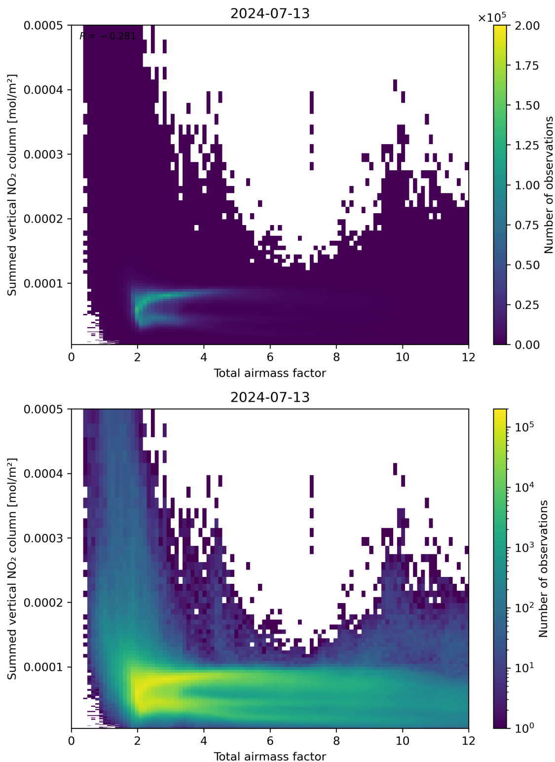
Figure 65: Scatter density plot of “Total airmass factor” against “Summed vertical NO 2 column” for 2024-07-12 to 2024-07-14.
