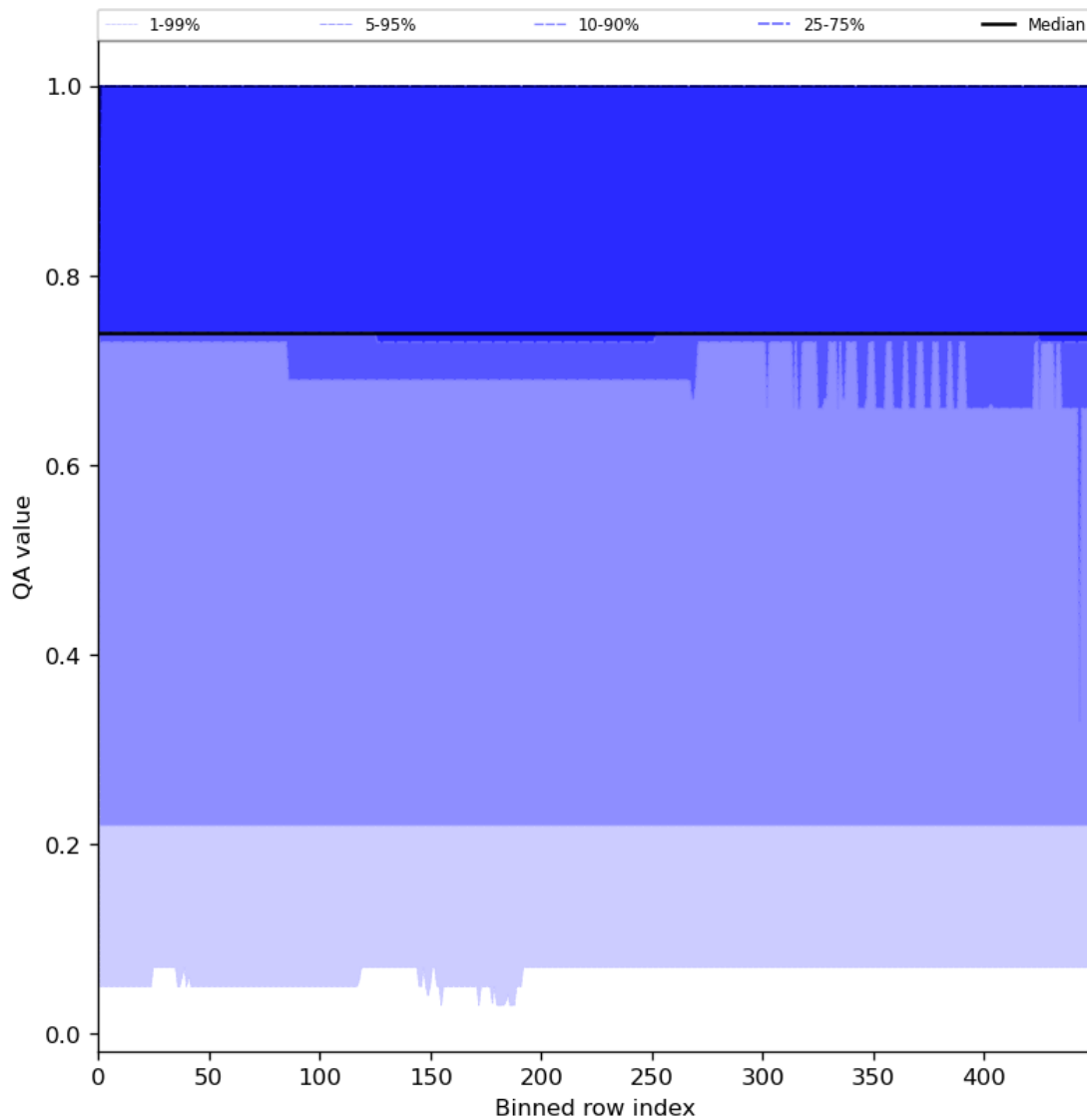
Figure 45: Along track statistics of “QA value” for 2024-07-12 to 2024-07-14
