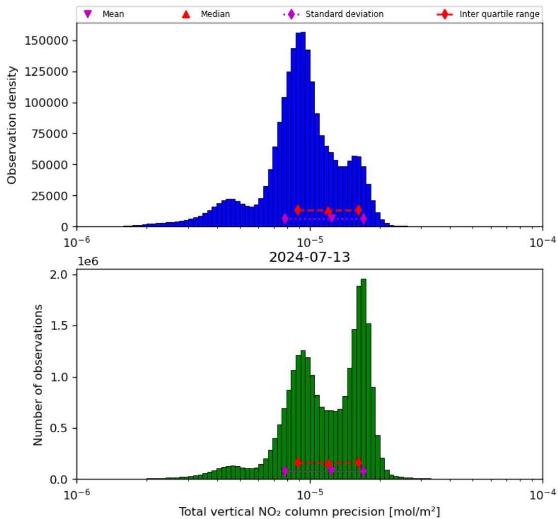
Figure 39: Histogram of “Total vertical NO 2 column precision” for 2024-07-12 to 2024-07-14
