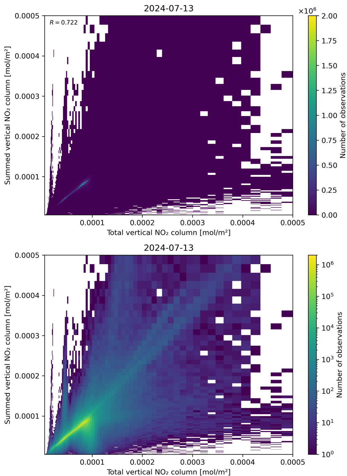
Figure 112: Scatter density plot of “Total vertical NO 2 column” against “Summed vertical NO 2 column” for 2024-07-12 to 2024-07-14.
