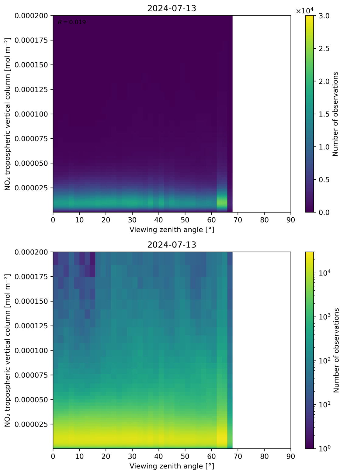
Figure 169: Scatter density plot of “Viewing zenith angle” against “NO 2 tropospheric vertical column” for 2024-07-12 to 2024-07-14.
