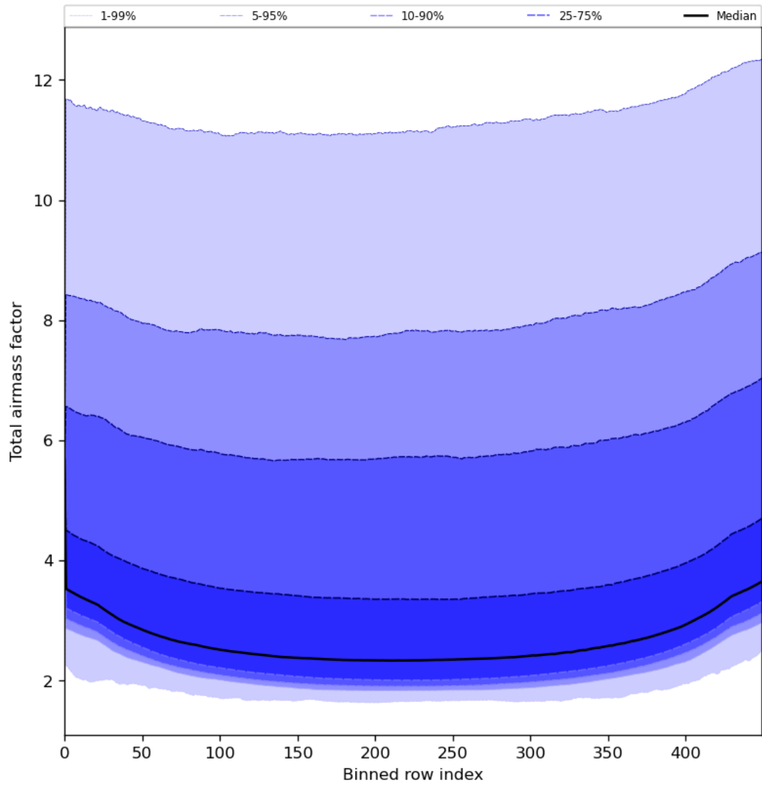
Figure 49: Along track statistics of “Total airmass factor” for 2024-07-12 to 2024-07-14
