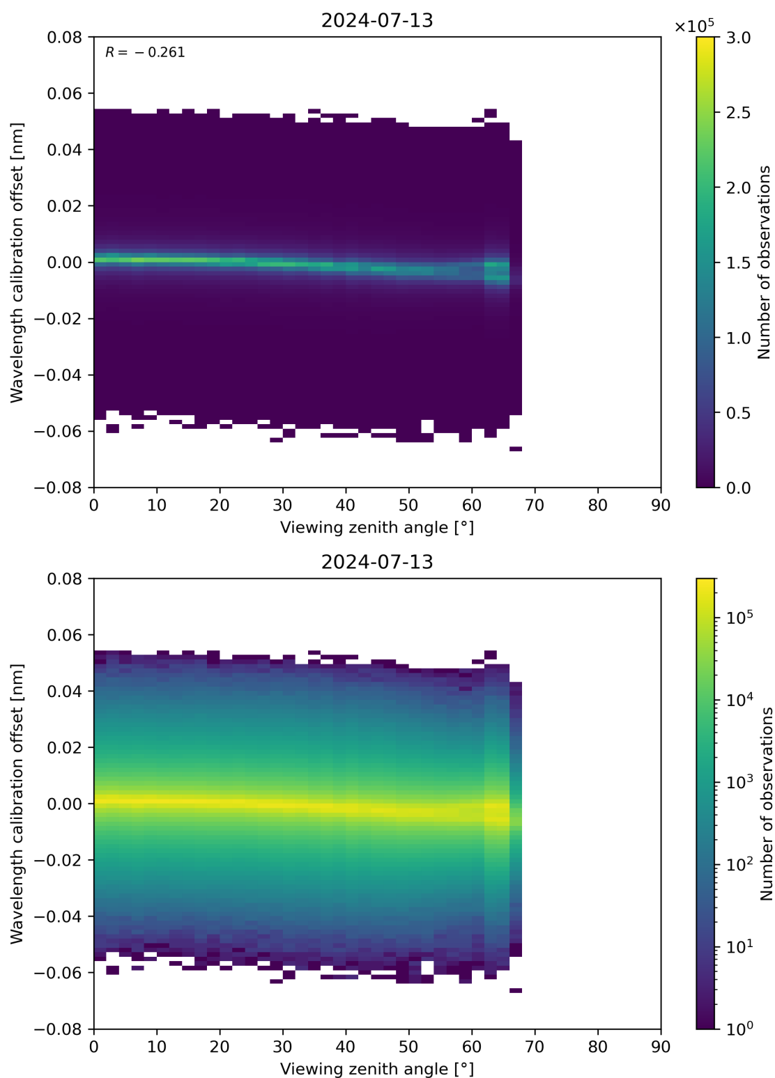
Figure 173: Scatter density plot of “Viewing zenith angle” against “Wavelength calibration offset” for 2024-07-12 to 2024-07-14.
