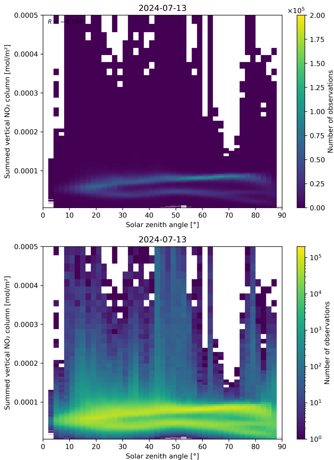
Figure 151: Scatter density plot of “Solar zenith angle” against “Summed vertical NO 2 column” for 2024-07-12 to 2024-07-14.
