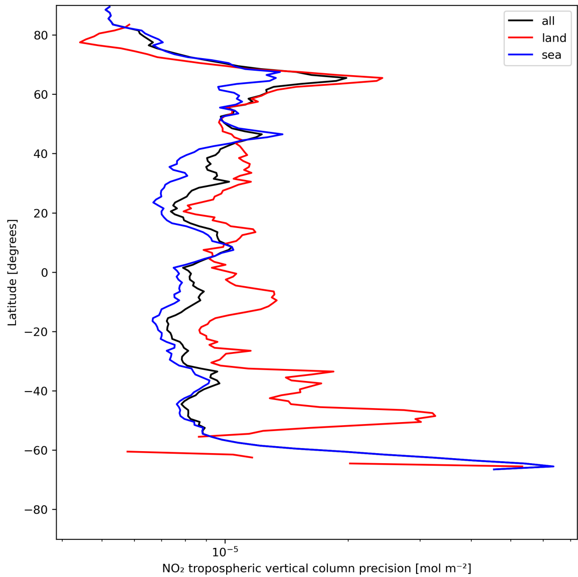
Figure 13: Zonal average of “NO 2 tropospheric vertical column precision” for 2024-07-12 to 2024-07-14.
