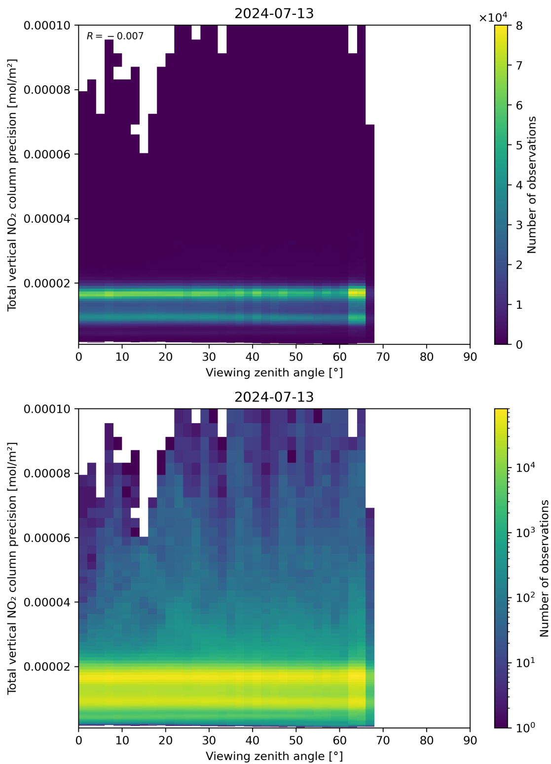
Figure 168: Scatter density plot of “Viewing zenith angle” against “Total vertical NO 2 column precision” for 2024-07-12 to 2024-07-14.
