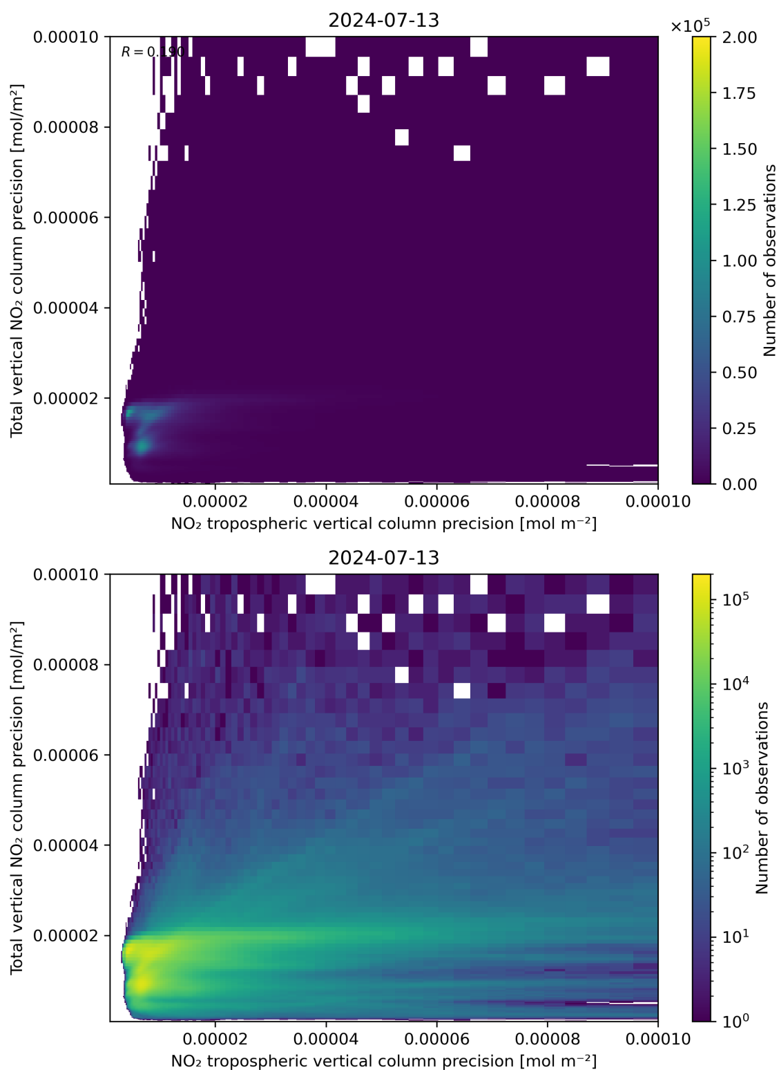
Figure 139: Scatter density plot of “NO 2 tropospheric vertical column precision” against “Total vertical NO 2 column precision” for 2024-07-12 to 2024-07-14.
