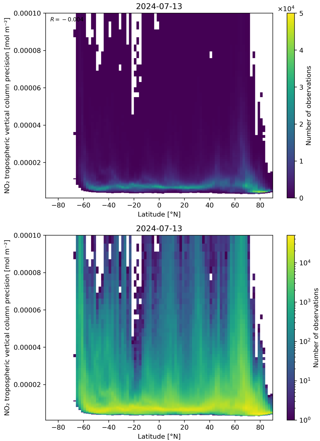
Figure 93: Scatter density plot of “Latitude” against “NO 2 tropospheric vertical column precision” for 2024-07-12 to 2024-07-14.
