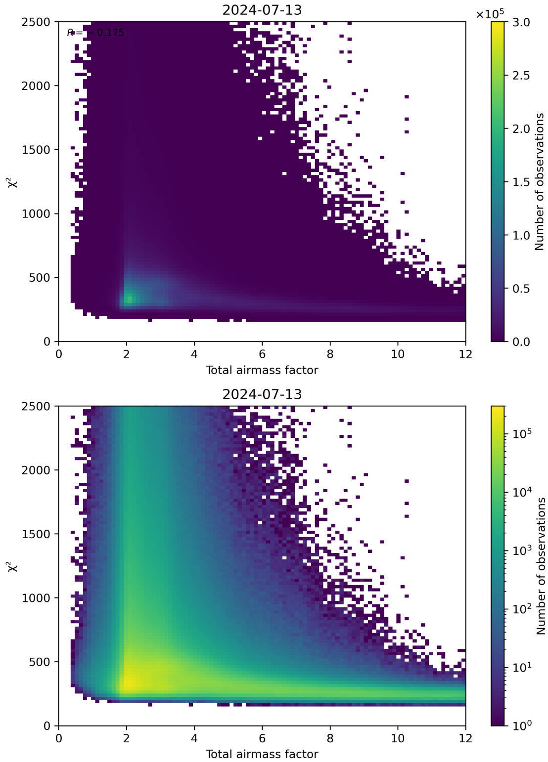
Figure 63: Scatter density plot of “Total airmass factor” against “ \chi^2 ” for 2024-07-12 to 2024-07-14.
