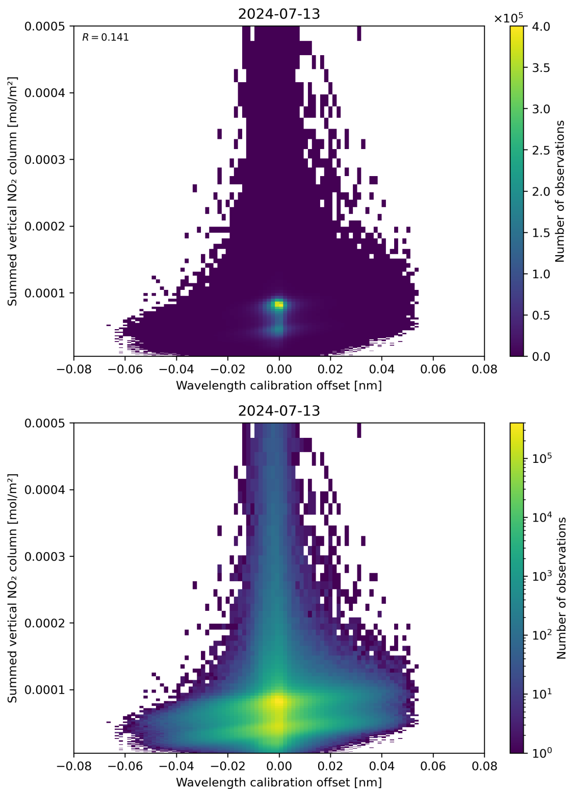
Figure 177: Scatter density plot of “Wavelength calibration offset” against “Summed vertical NO 2 column” for 2024-07-12 to 2024-07-14.
