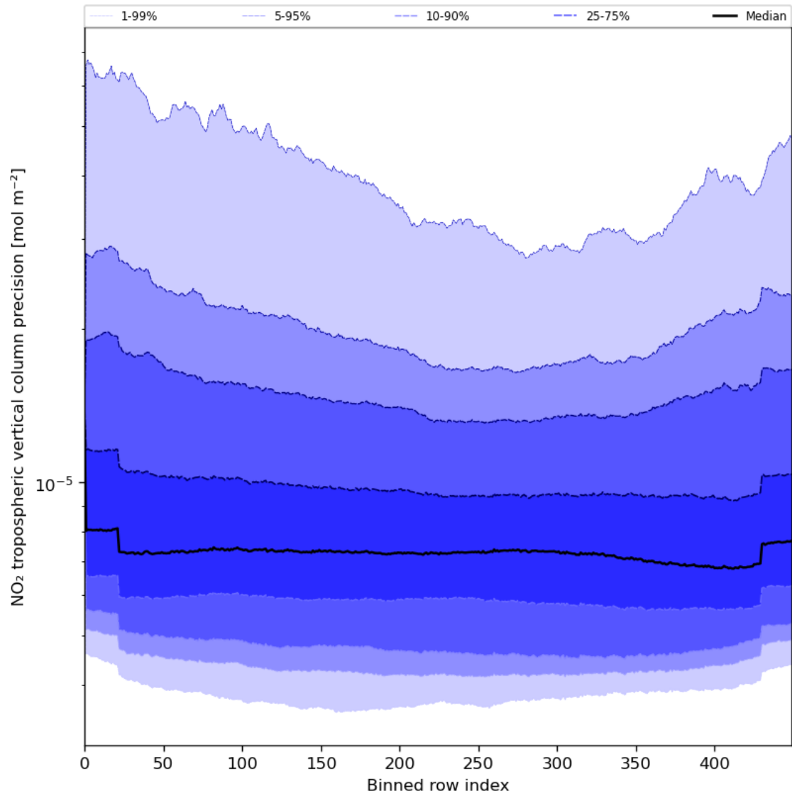
Figure 47: Along track statistics of “NO 2 tropospheric vertical column precision” for 2024-07-12 to 2024-07-14
