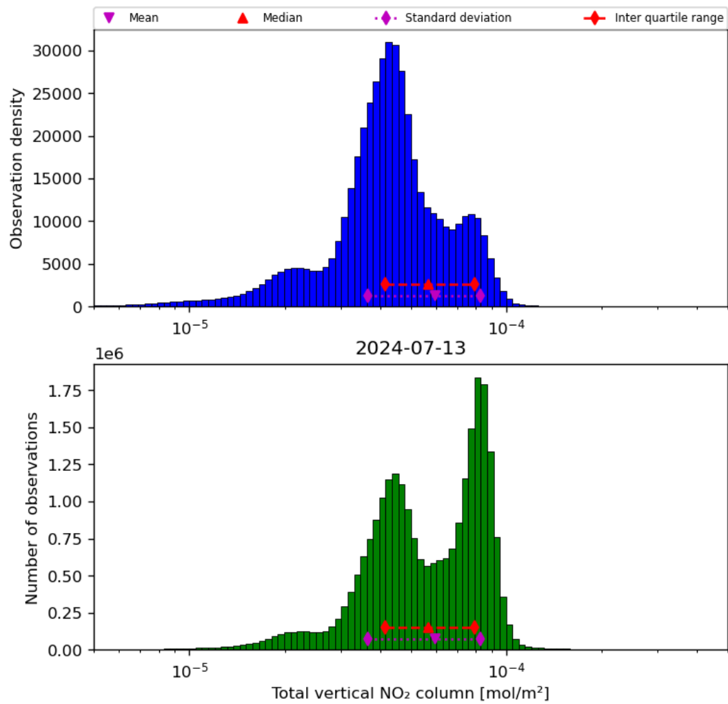
Figure 38: Histogram of “Total vertical NO 2 column” for 2024-07-12 to 2024-07-14
