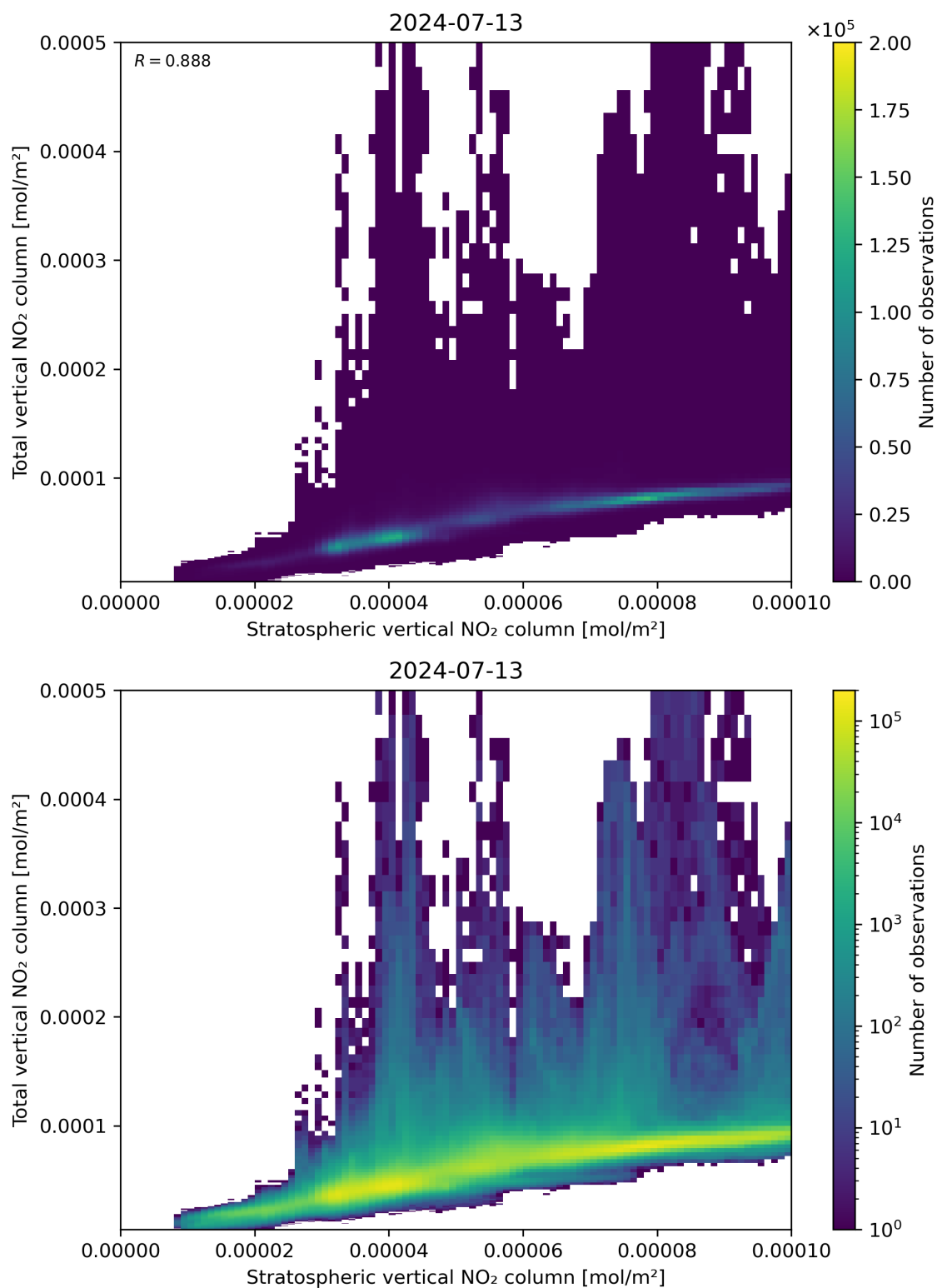
Figure 100: Scatter density plot of “Stratospheric vertical NO 2 column” against “Total vertical NO 2 column” for 2024-07-12 to 2024-07-14.
