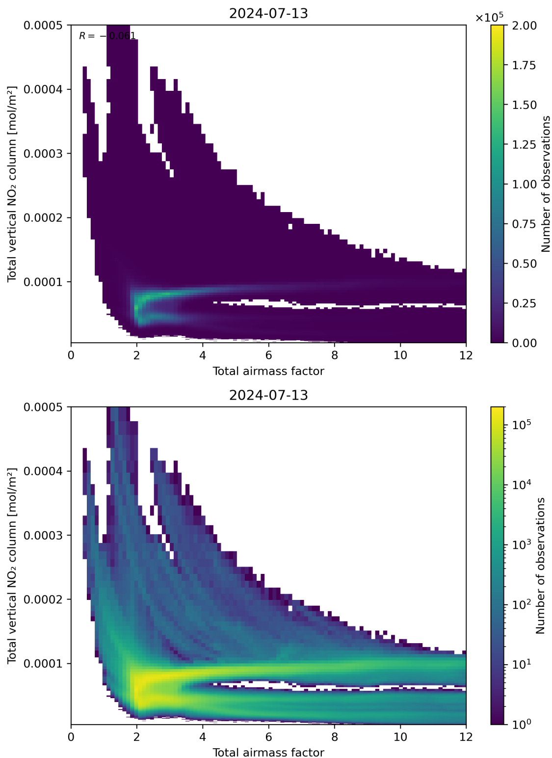
Figure 67: Scatter density plot of “Total airmass factor” against “Total vertical NO 2 column” for 2024-07-12 to 2024-07-14.
