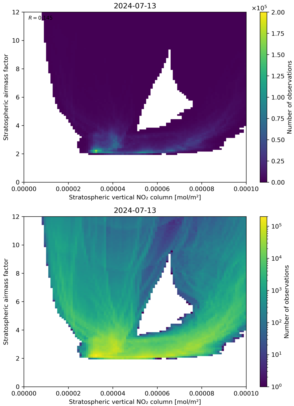
Figure 96: Scatter density plot of “Stratospheric vertical NO 2 column” against “Stratospheric airmass factor” for 2024-07-12 to 2024-07-14.
