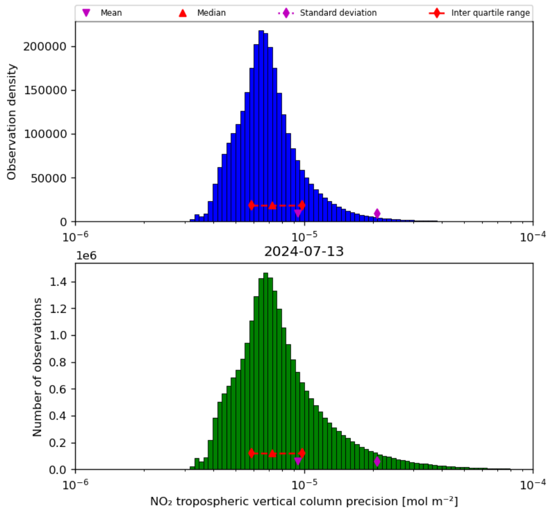
Figure 30: Histogram of “NO 2 tropospheric vertical column precision” for 2024-07-12 to 2024-07-14
