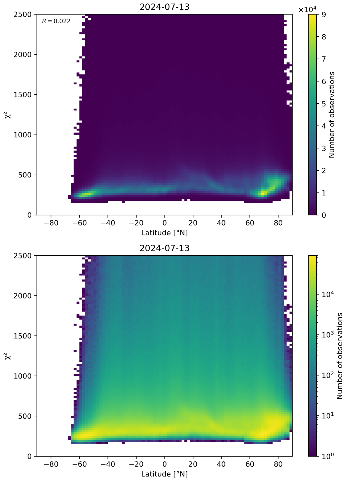
Figure 86: Scatter density plot of “Latitude” against “ \chi^2 ” for 2024-07-12 to 2024-07-14.
