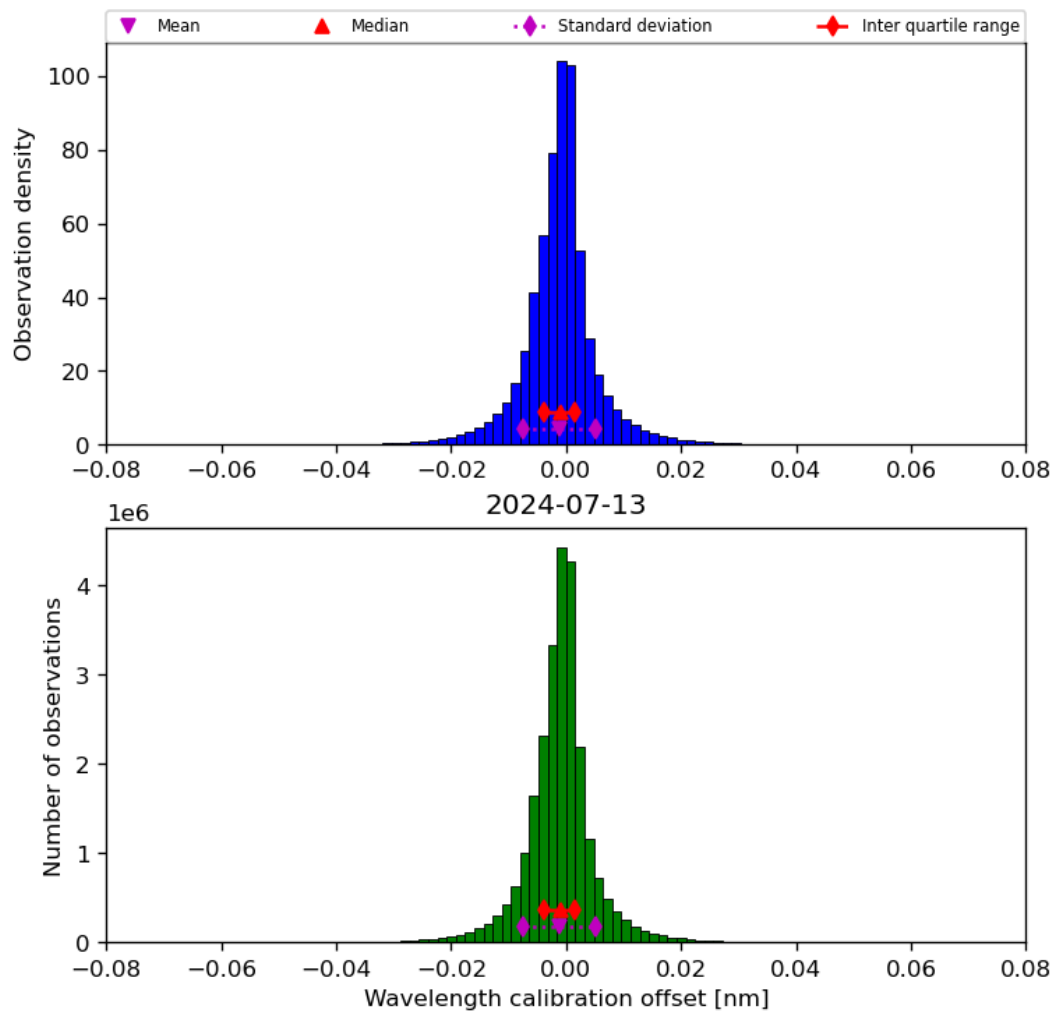
Figure 35: Histogram of “Wavelength calibration offset” for 2024-07-12 to 2024-07-14
