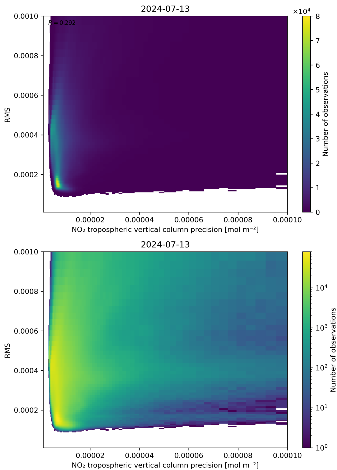
Figure 140: Scatter density plot of “NO 2 tropospheric vertical column precision” against “RMS” for 2024-07-12 to 2024-07-14.
