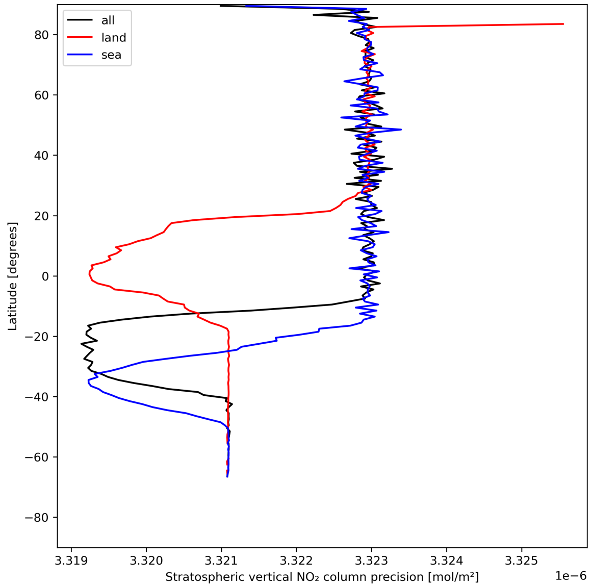
Figure 20: Zonal average of “Stratospheric vertical NO 2 column precision” for 2024-07-12 to 2024-07-14.
