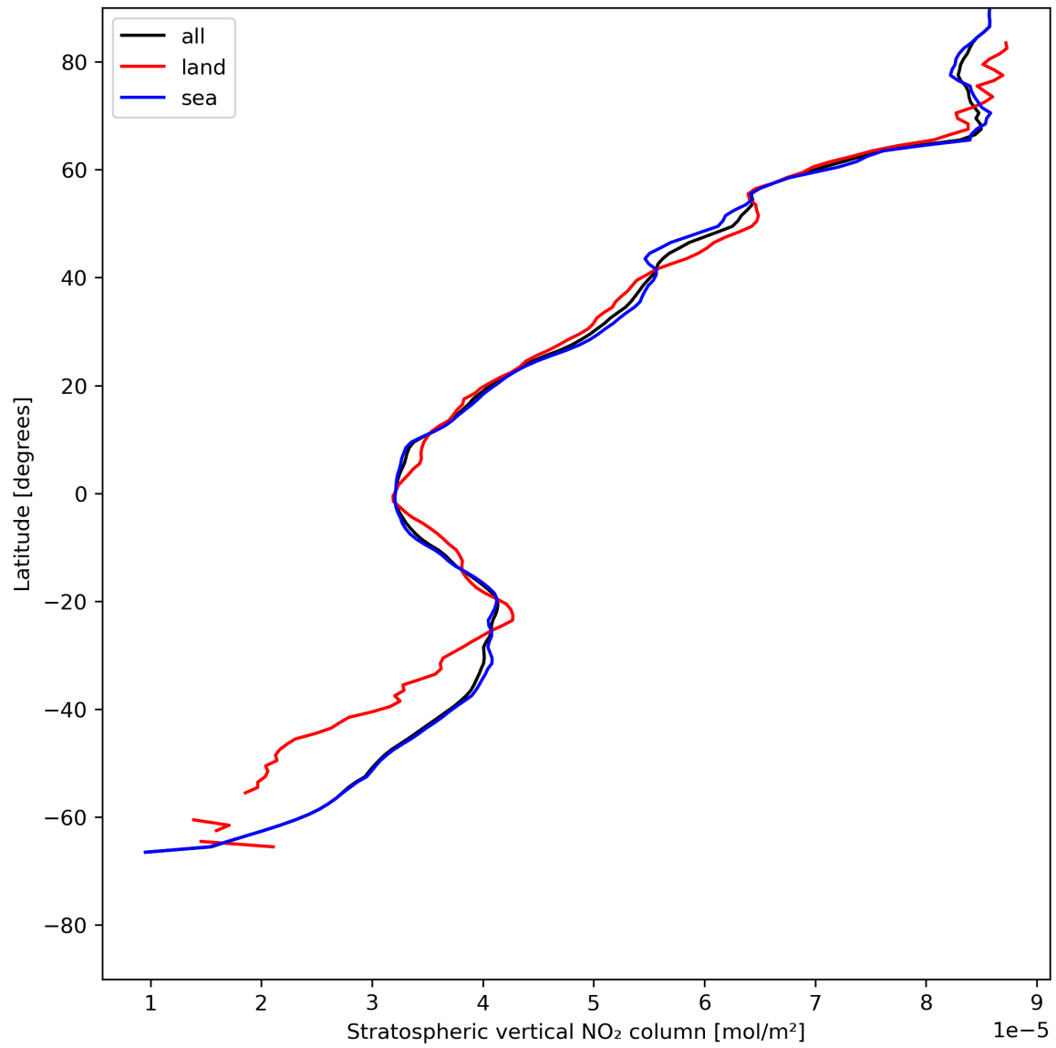
Figure 19: Zonal average of “Stratospheric vertical NO 2 column” for 2024-07-12 to 2024-07-14.
