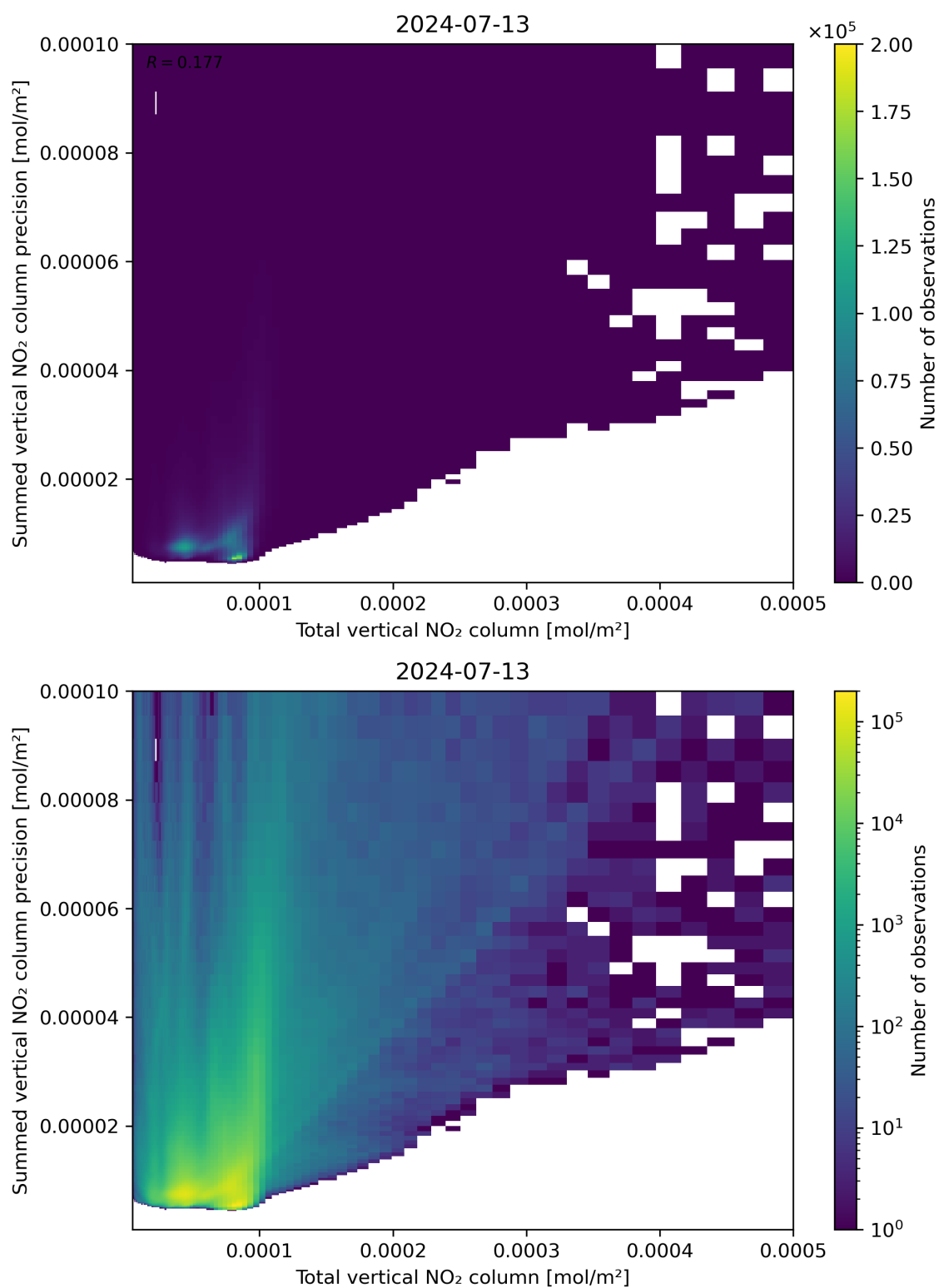
Figure 113: Scatter density plot of “Total vertical NO 2 column” against “Summed vertical NO 2 column precision” for 2024-07-12 to 2024-07-14.
