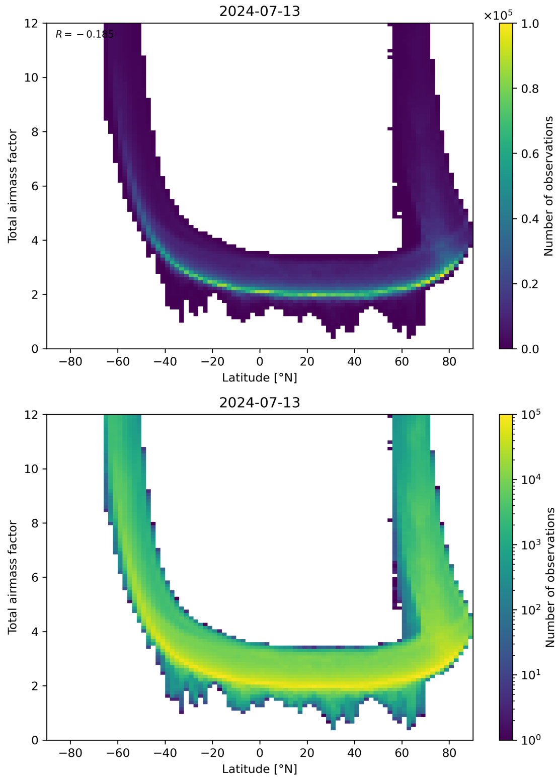
Figure 84: Scatter density plot of “Latitude” against “Total airmass factor” for 2024-07-12 to 2024-07-14.
