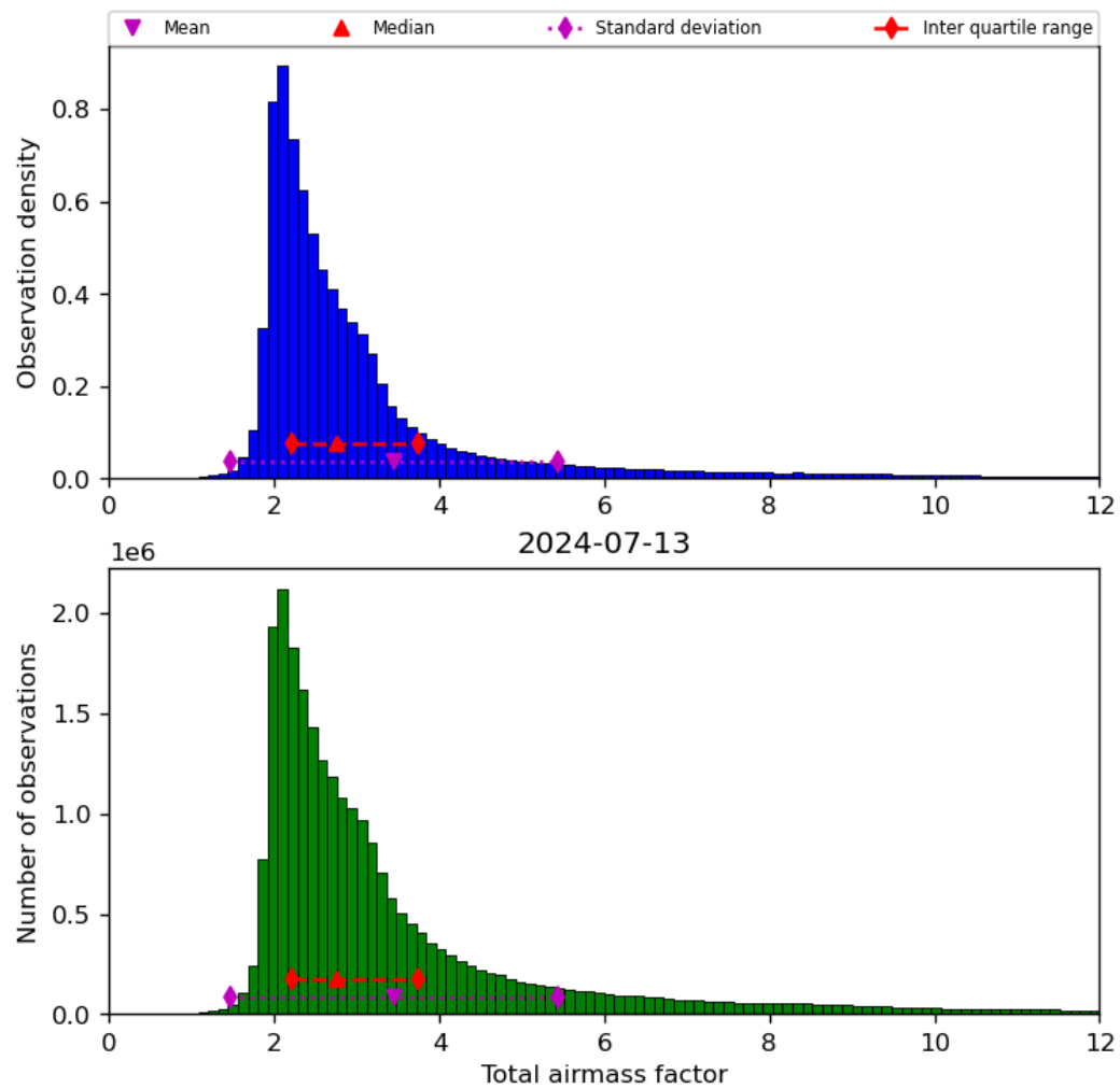
Figure 32: Histogram of “Total airmass factor” for 2024-07-12 to 2024-07-14
