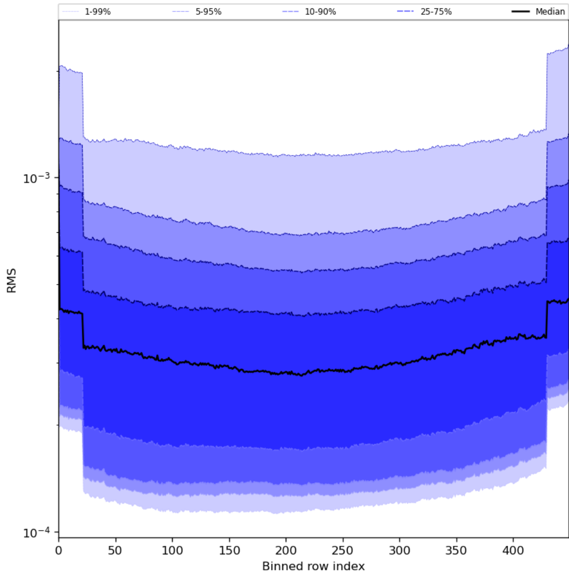
Figure 60: Along track statistics of “RMS” for 2024-07-12 to 2024-07-14
