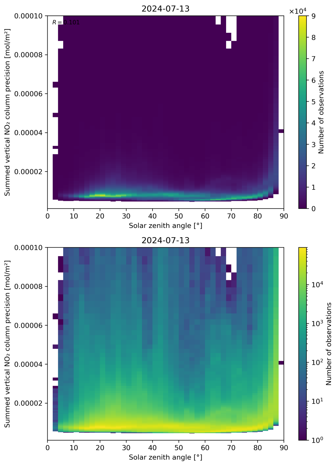
Figure 152: Scatter density plot of “Solar zenith angle” against “Summed vertical NO 2 column precision” for 2024-07-12 to 2024-07-14.
