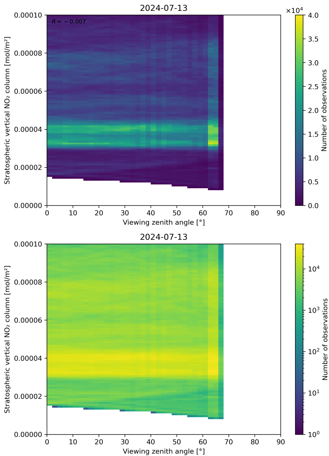
Figure 164: Scatter density plot of “Viewing zenith angle” against “Stratospheric vertical NO 2 column” for 2024-07-12 to 2024-07-14.
