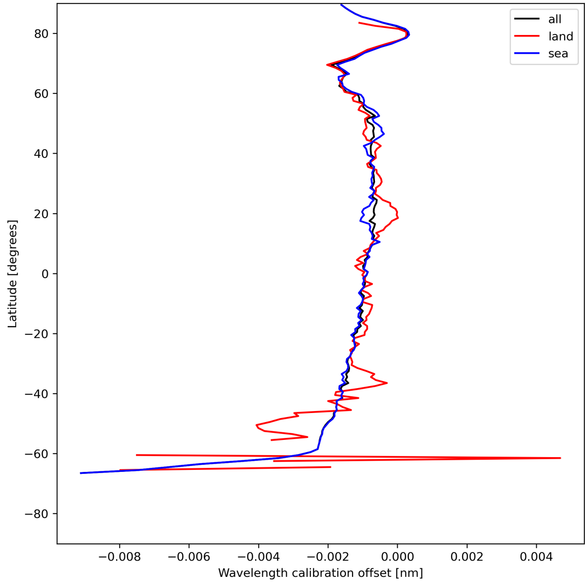
Figure 18: Zonal average of “Wavelength calibration offset” for 2024-07-12 to 2024-07-14.
