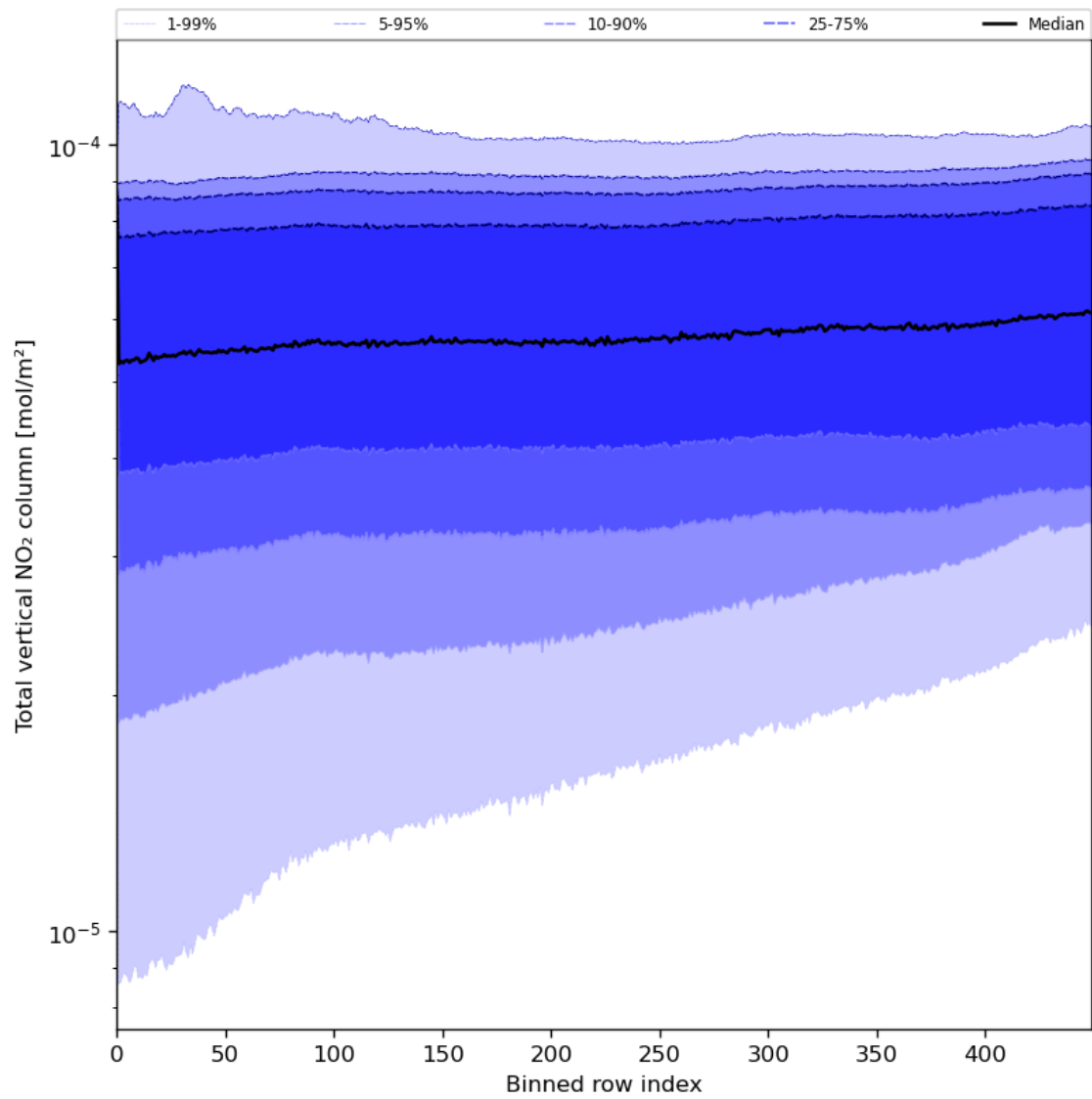
Figure 55: Along track statistics of “Total vertical NO 2 column” for 2024-07-12 to 2024-07-14
