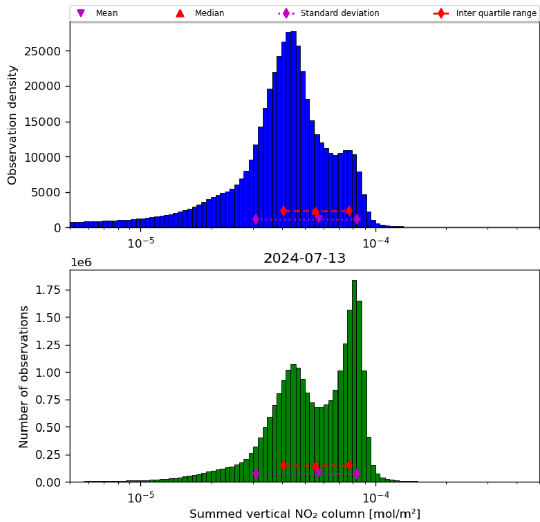
Figure 40: Histogram of “Summed vertical NO 2 column” for 2024-07-12 to 2024-07-14
