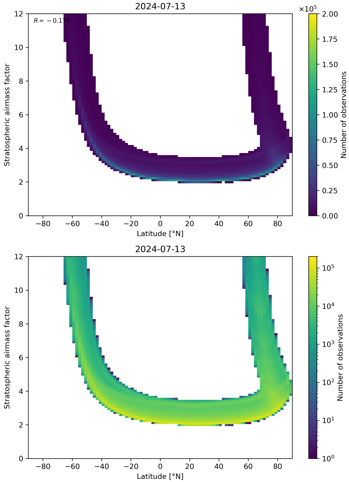
Figure 83: Scatter density plot of “Latitude” against “Stratospheric air mass factor” for 2024-07-12 to 2024-07-14.
