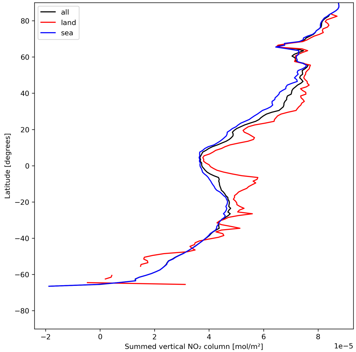
Figure 23: Zonal average of “Summed vertical NO 2 column” for 2024-07-12 to 2024-07-14.
