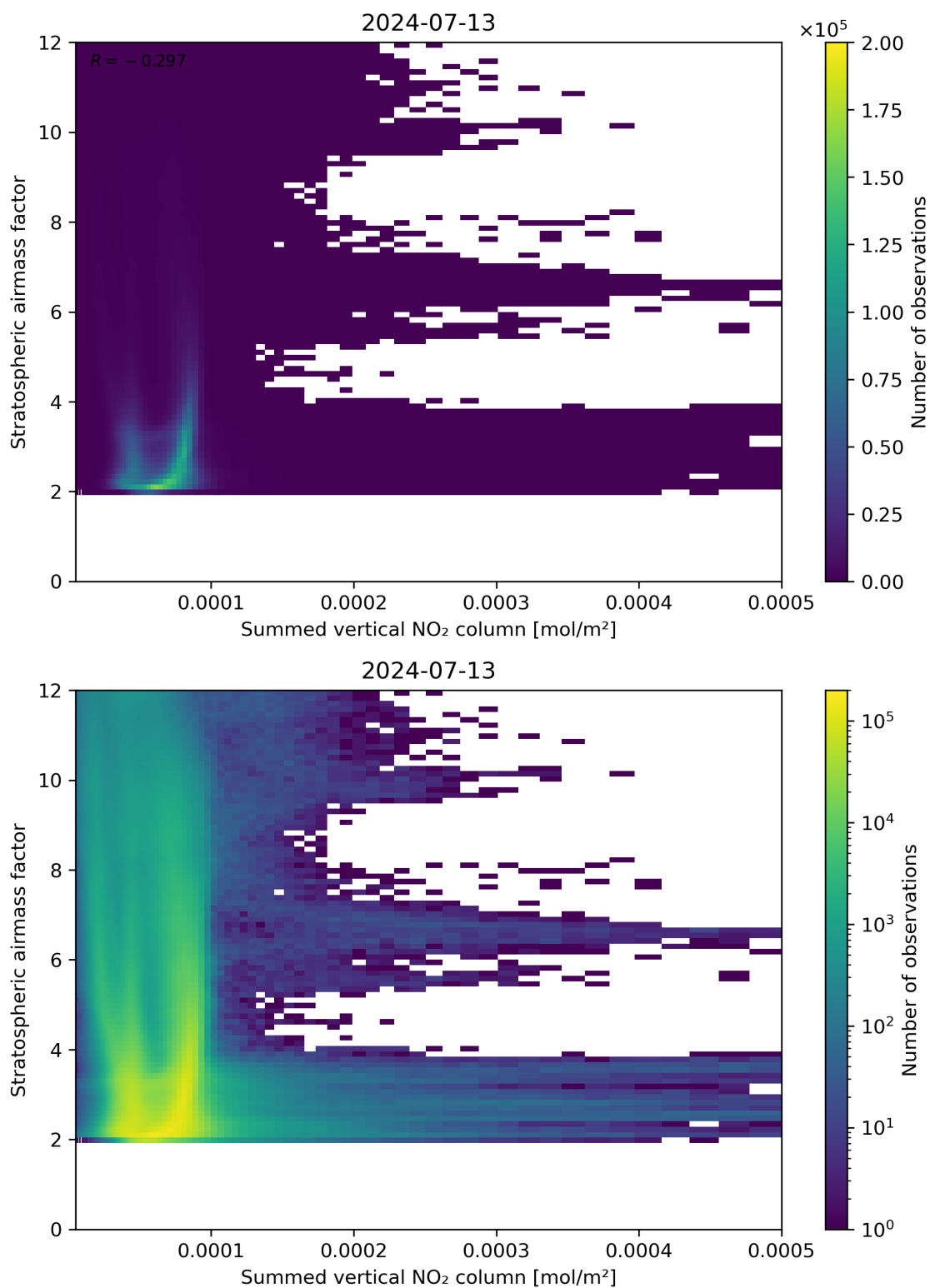
Figure 103: Scatter density plot of “Summed vertical NO 2 column” against “Stratospheric air mass factor” for 2024-07-12 to 2024-07-14.
