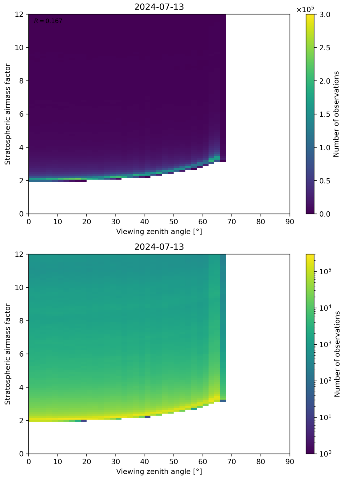
Figure 159: Scatter density plot of “Viewing zenith angle” against “Stratospheric airmass factor” for 2024-07-12 to 2024-07-14.
