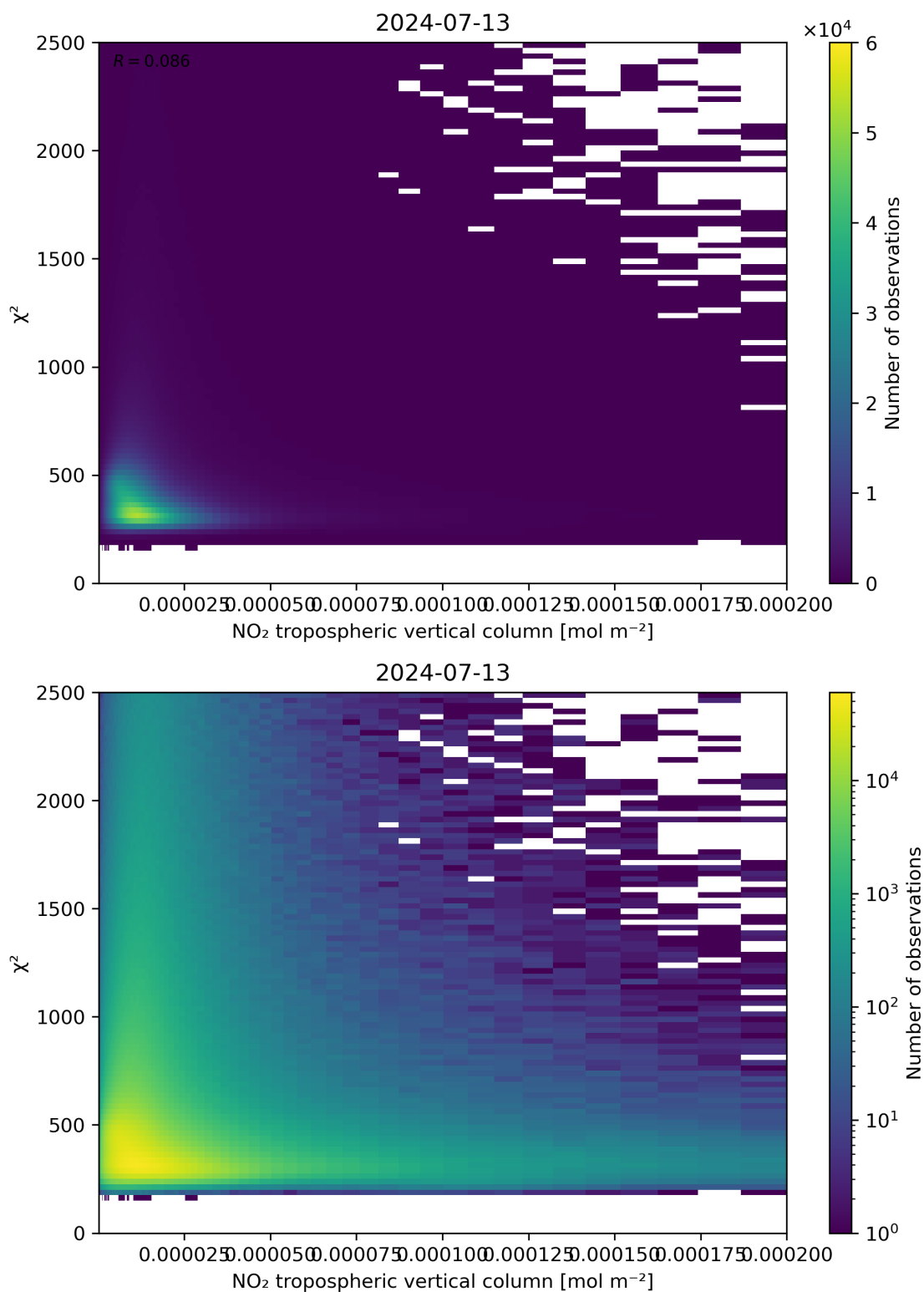
Figure 124: Scatter density plot of “NO 2 tropospheric vertical column” against “ \chi^2 ” for 2024-07-12 to 2024-07-14.
