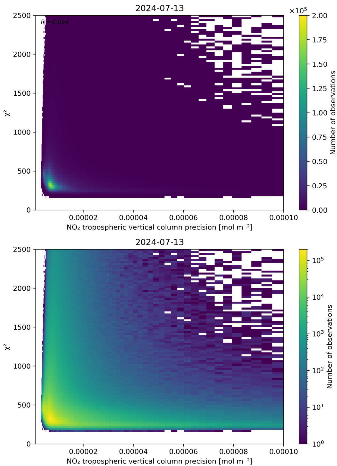
Figure 134: Scatter density plot of “NO 2 tropospheric vertical column precision” against “ \chi^2 ” for 2024-07-12 to 2024-07-14.
