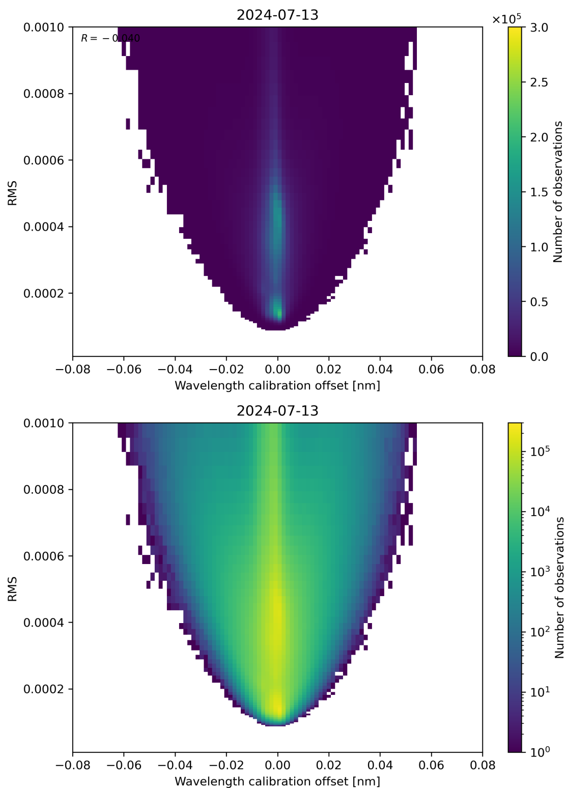
Figure 181: Scatter density plot of “Wavelength calibration offset” against “RMS” for 2024-07-12 to 2024-07-14.
