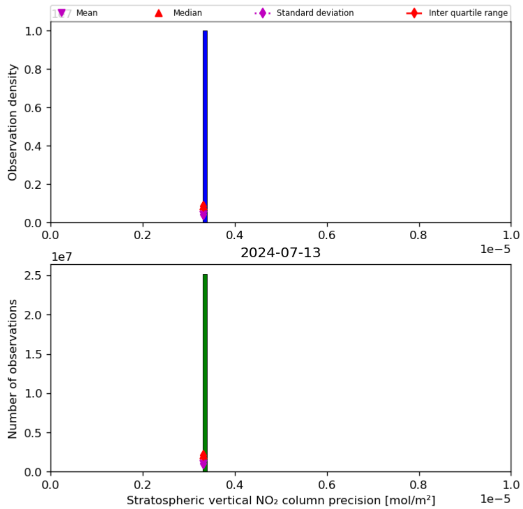
Figure 37: Histogram of “Stratospheric vertical NO 2 column precision” for 2024-07-12 to 2024-07-14
