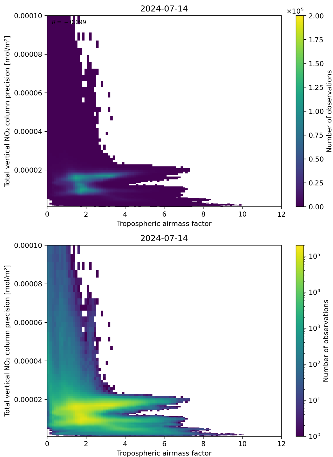
Figure 78: Scatter density plot of “Tropospheric air mass factor” against “Total vertical NO 2 column precision” for 2024-07-13 to 2024-07-15.
