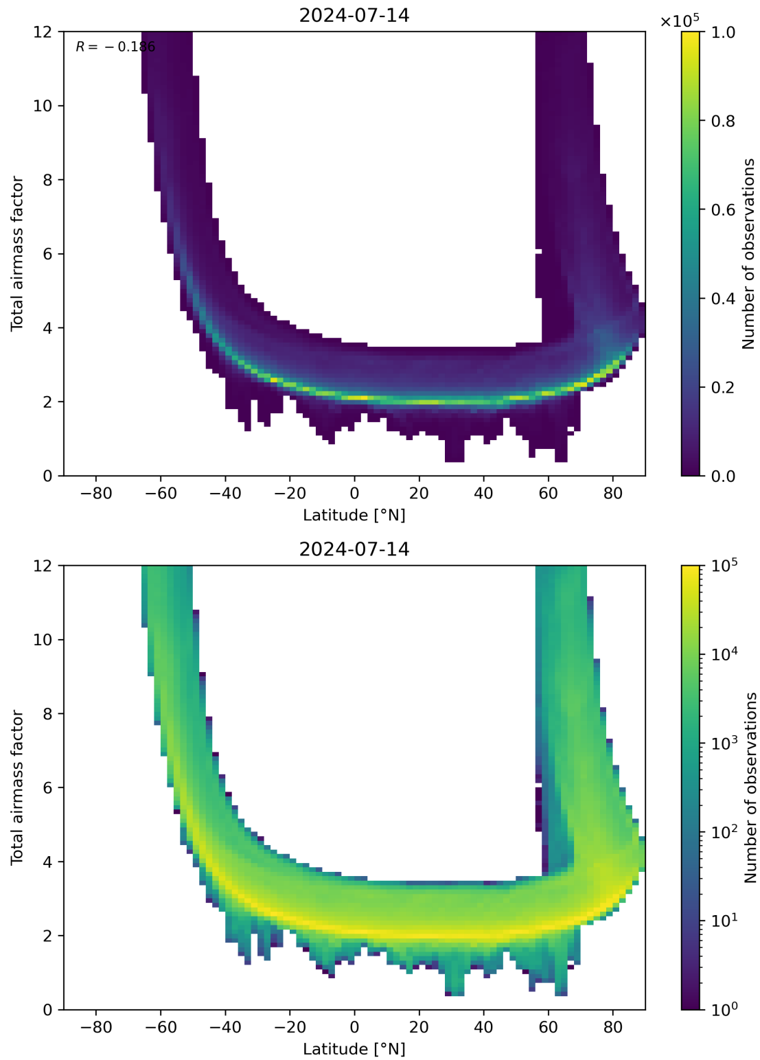
Figure 84: Scatter density plot of “Latitude” against “Total airmass factor” for 2024-07-13 to 2024-07-15.
