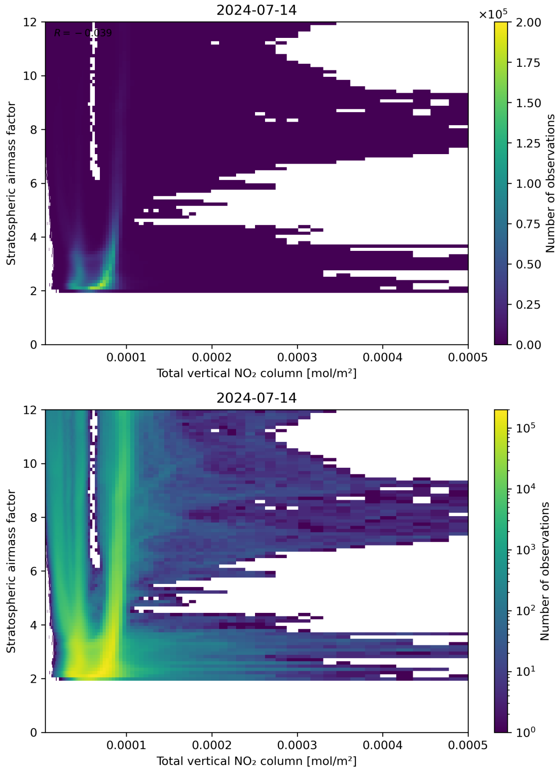
Figure 110: Scatter density plot of “Total vertical NO 2 column” against “Stratospheric airmass factor” for 2024-07-13 to 2024-07-15.
