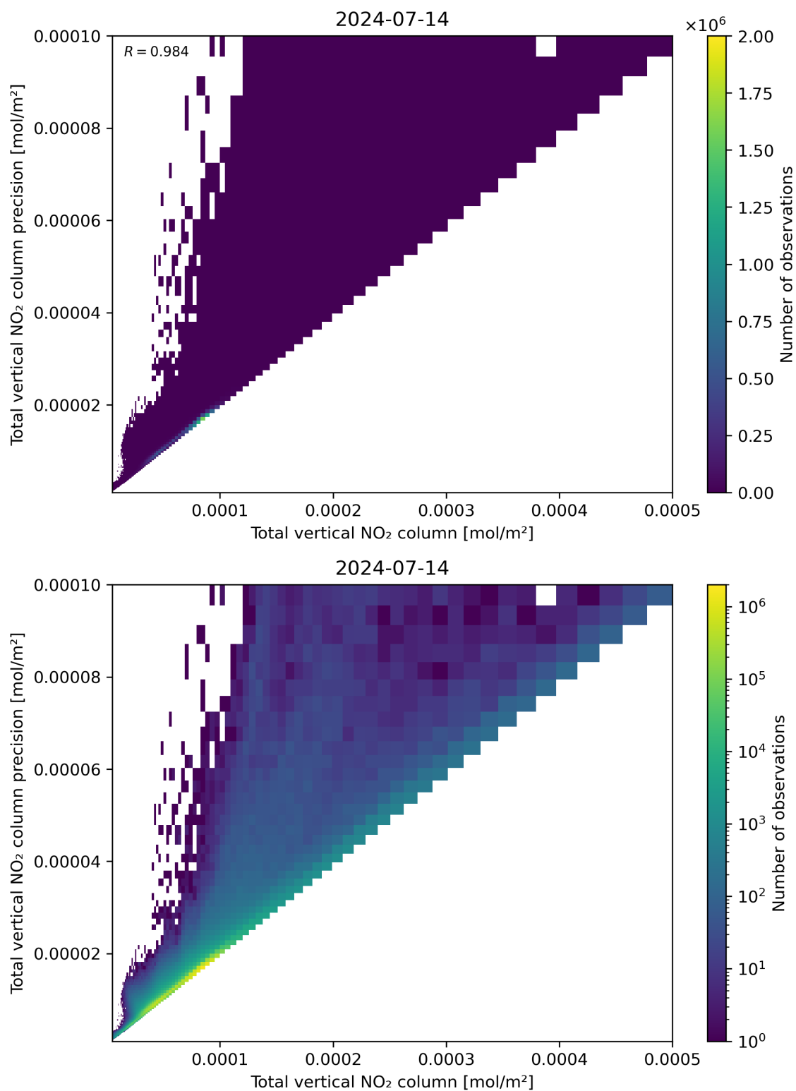
Figure 114: Scatter density plot of “Total vertical NO 2 column” against “Total vertical NO 2 column precision” for 2024-07-13 to 2024-07-15.
