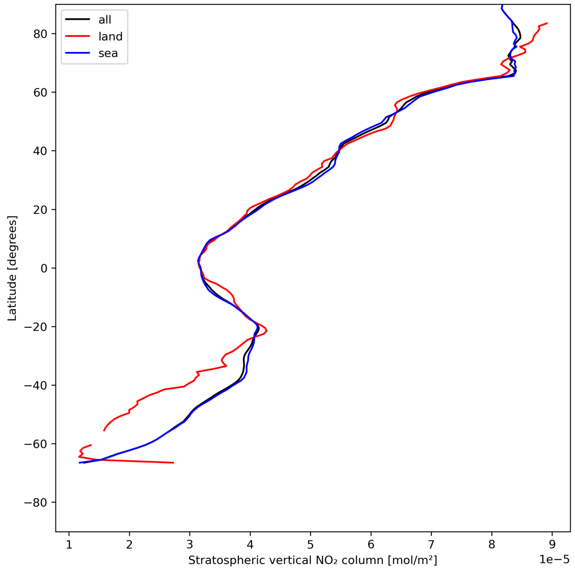
Figure 19: Zonal average of “Stratospheric vertical NO 2 column” for 2024-07-13 to 2024-07-15.
