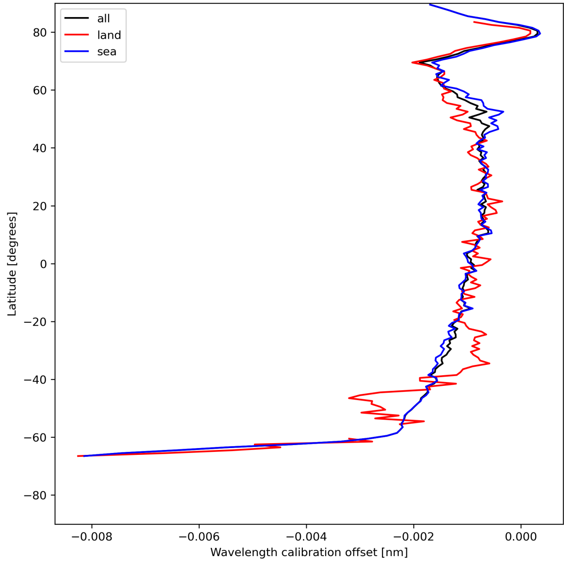
Figure 18: Zonal average of “Wavelength calibration offset” for 2024-07-13 to 2024-07-15.
