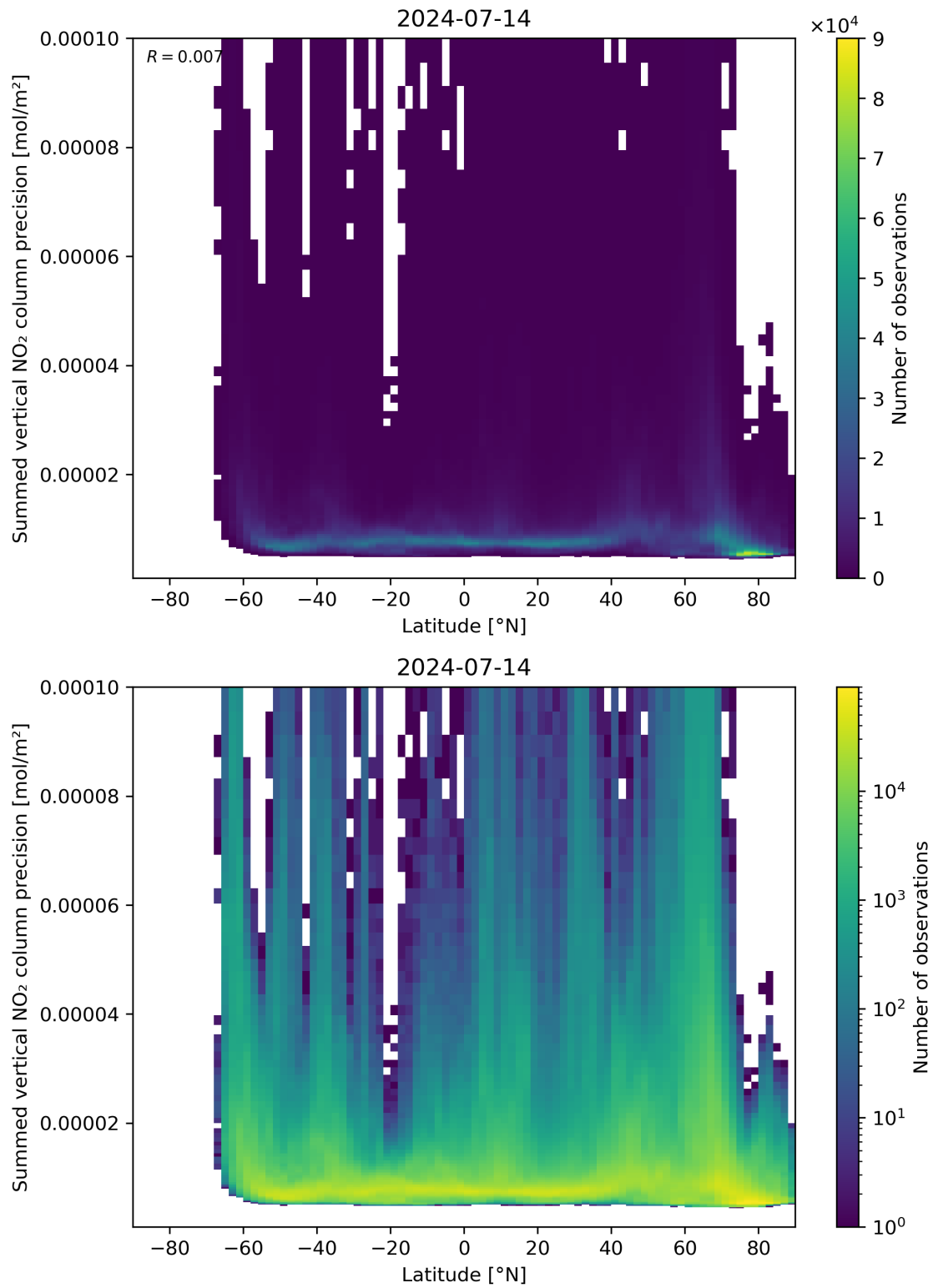
Figure 89: Scatter density plot of “Latitude” against “Summed vertical NO 2 column precision” for 2024-07-13 to 2024-07-15.
