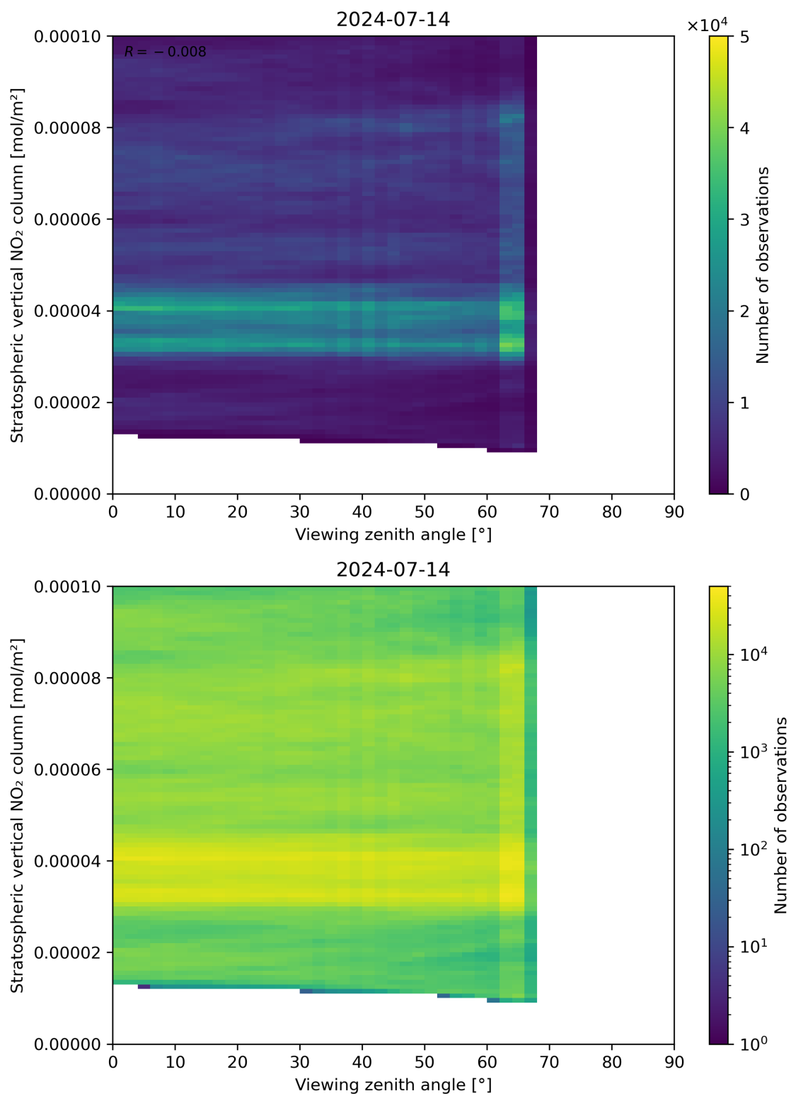
Figure 164: Scatter density plot of “Viewing zenith angle” against “Stratospheric vertical NO 2 column” for 2024-07-13 to 2024-07-15.
