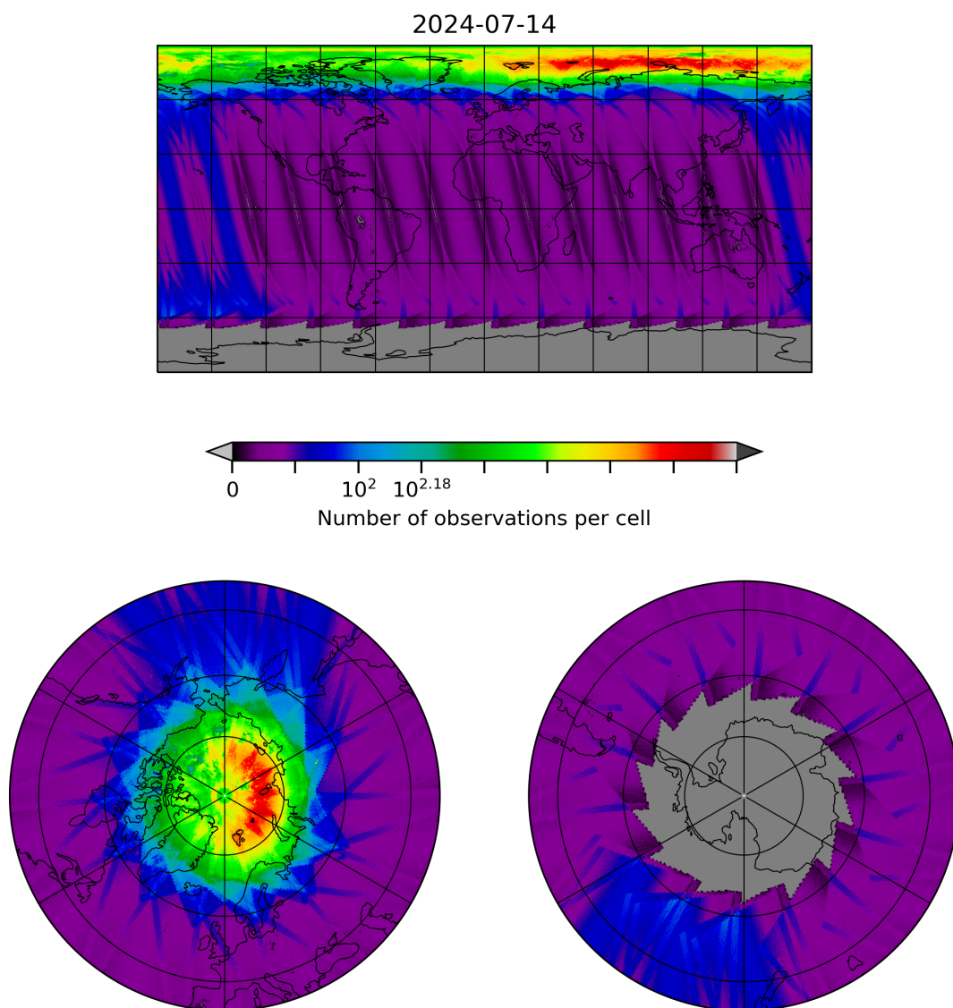
Figure 10: Map of the number of observations for 2024-07-13 to 2024-07-15
