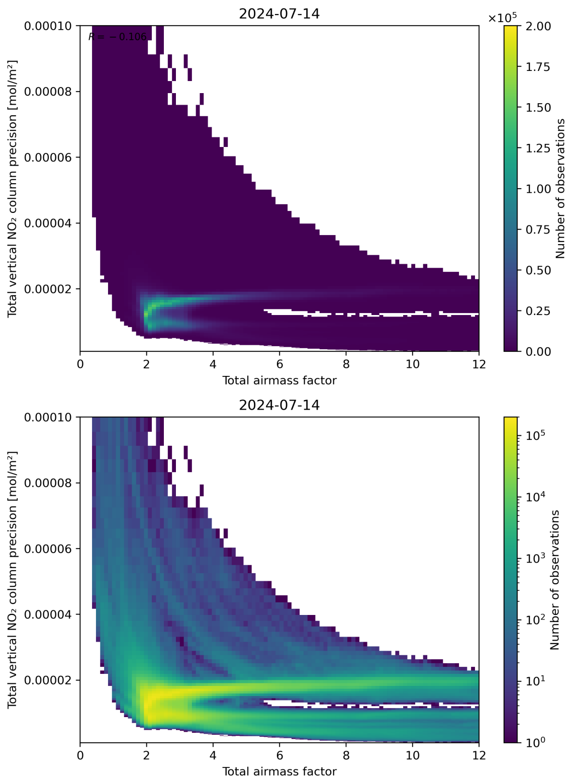
Figure 68: Scatter density plot of “Total airmass factor” against “Total vertical NO 2 column precision” for 2024-07-13 to 2024-07-15.
