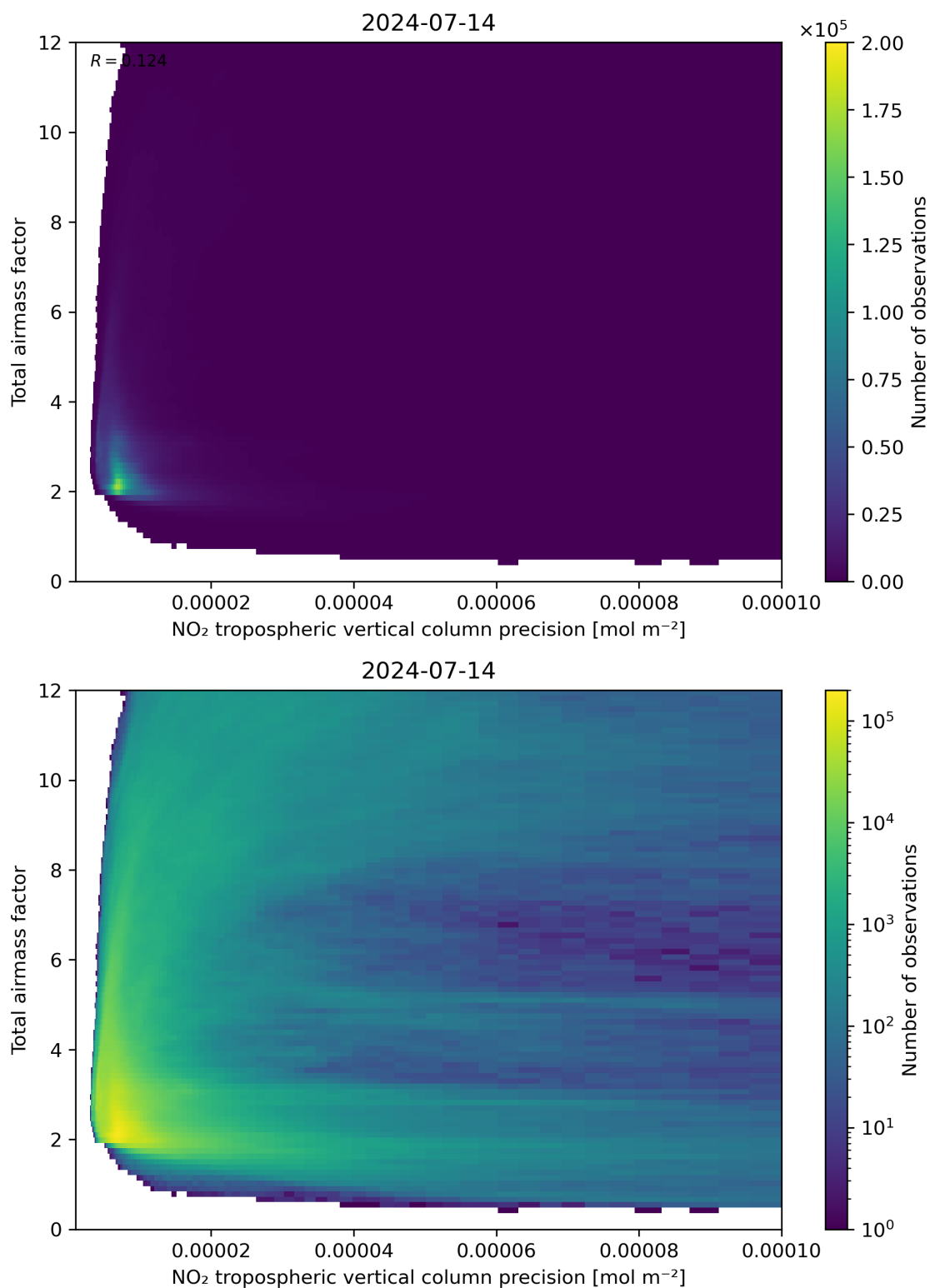
Figure 132: Scatter density plot of “NO 2 tropospheric vertical column precision” against “Total air mass factor” for 2024-07-13 to 2024-07-15.
