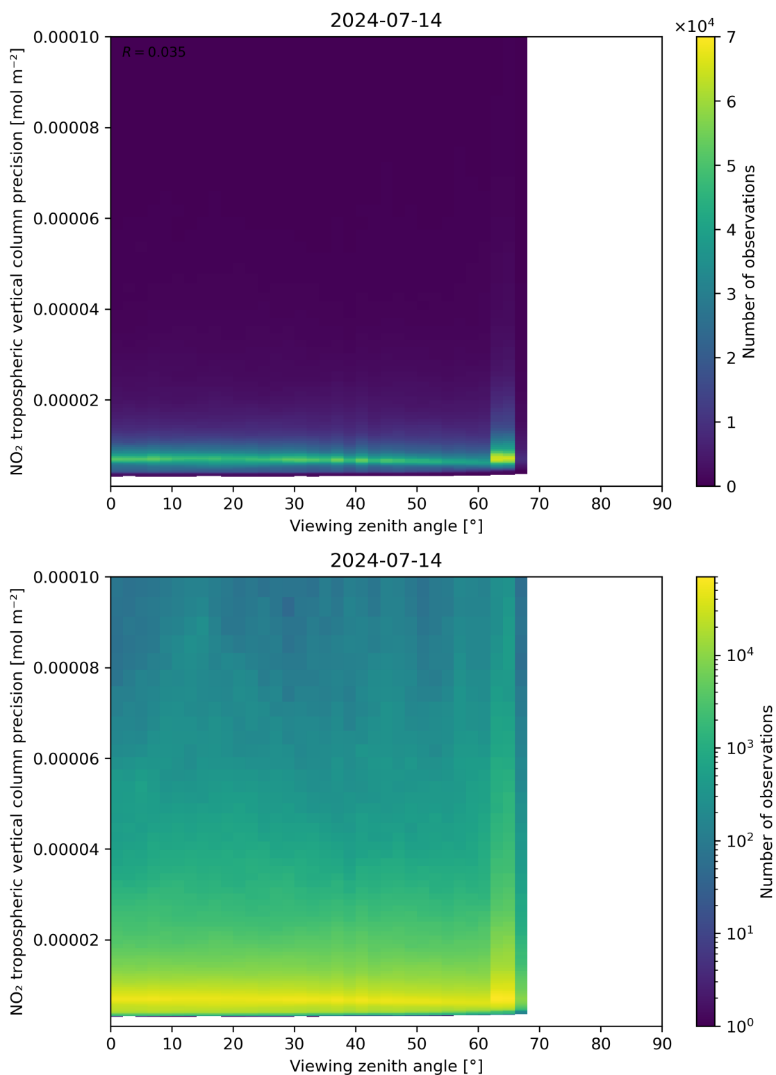
Figure 170: Scatter density plot of “Viewing zenith angle” against “NO 2 tropospheric vertical column precision” for 2024-07-13 to 2024-07-15.
