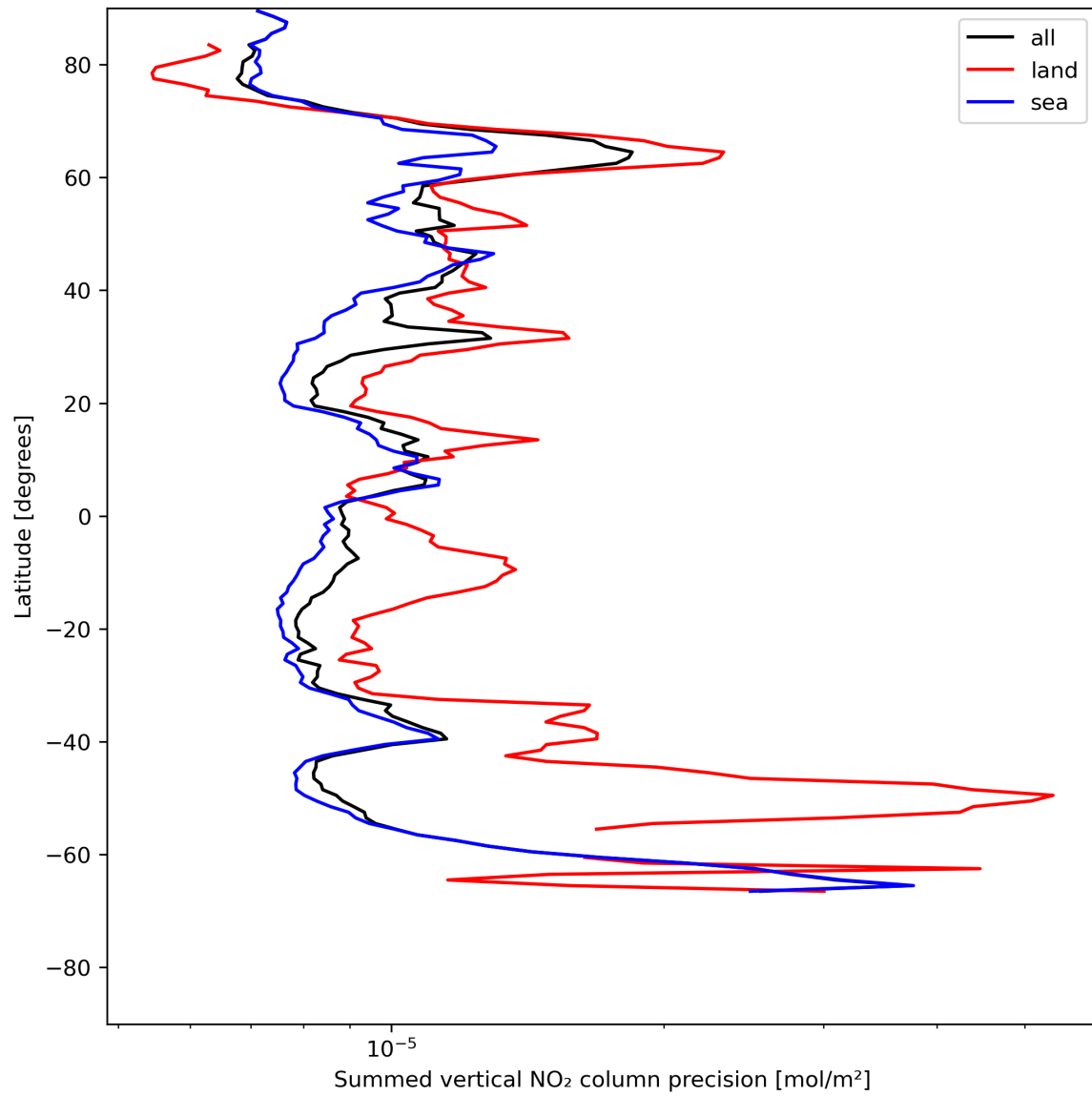
Figure 24: Zonal average of “Summed vertical NO 2 column precision” for 2024-07-13 to 2024-07-15.
