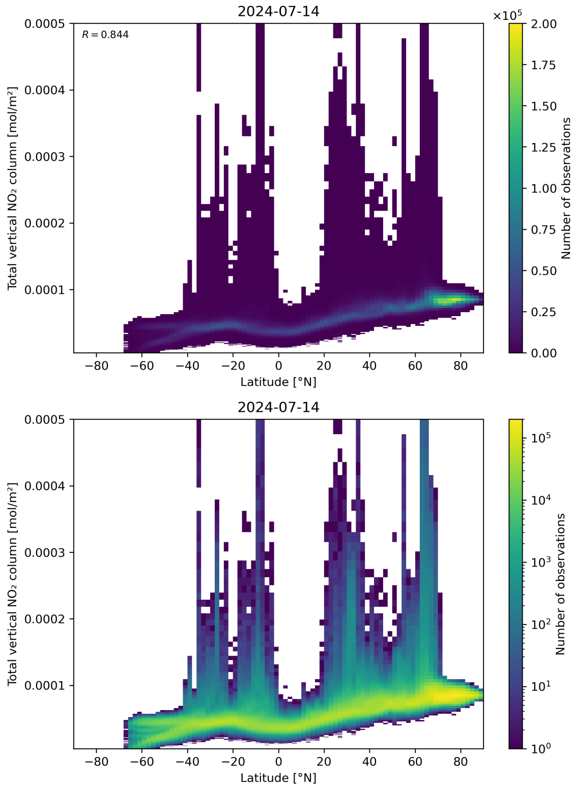
Figure 90: Scatter density plot of “Latitude” against “Total vertical NO 2 column” for 2024-07-13 to 2024-07-15.
