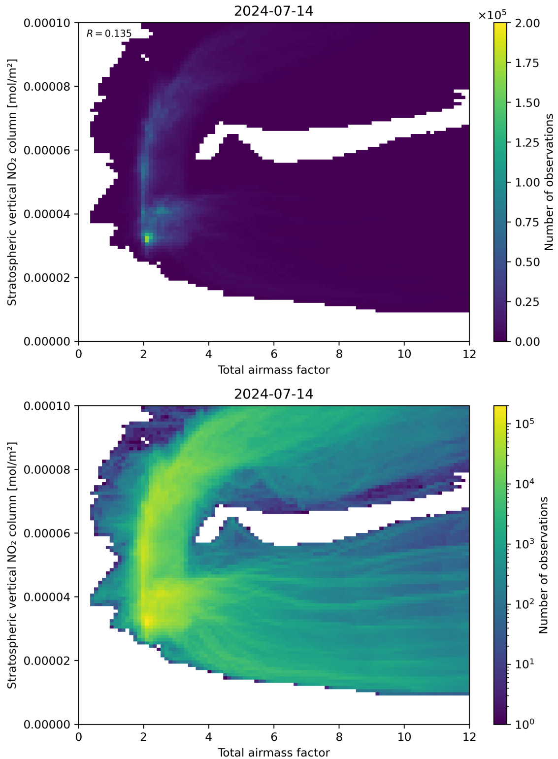
Figure 64: Scatter density plot of “Total airmass factor” against “Stratospheric vertical \text{NO}_2 column” for 2024-07-13 to 2024-07-15.
