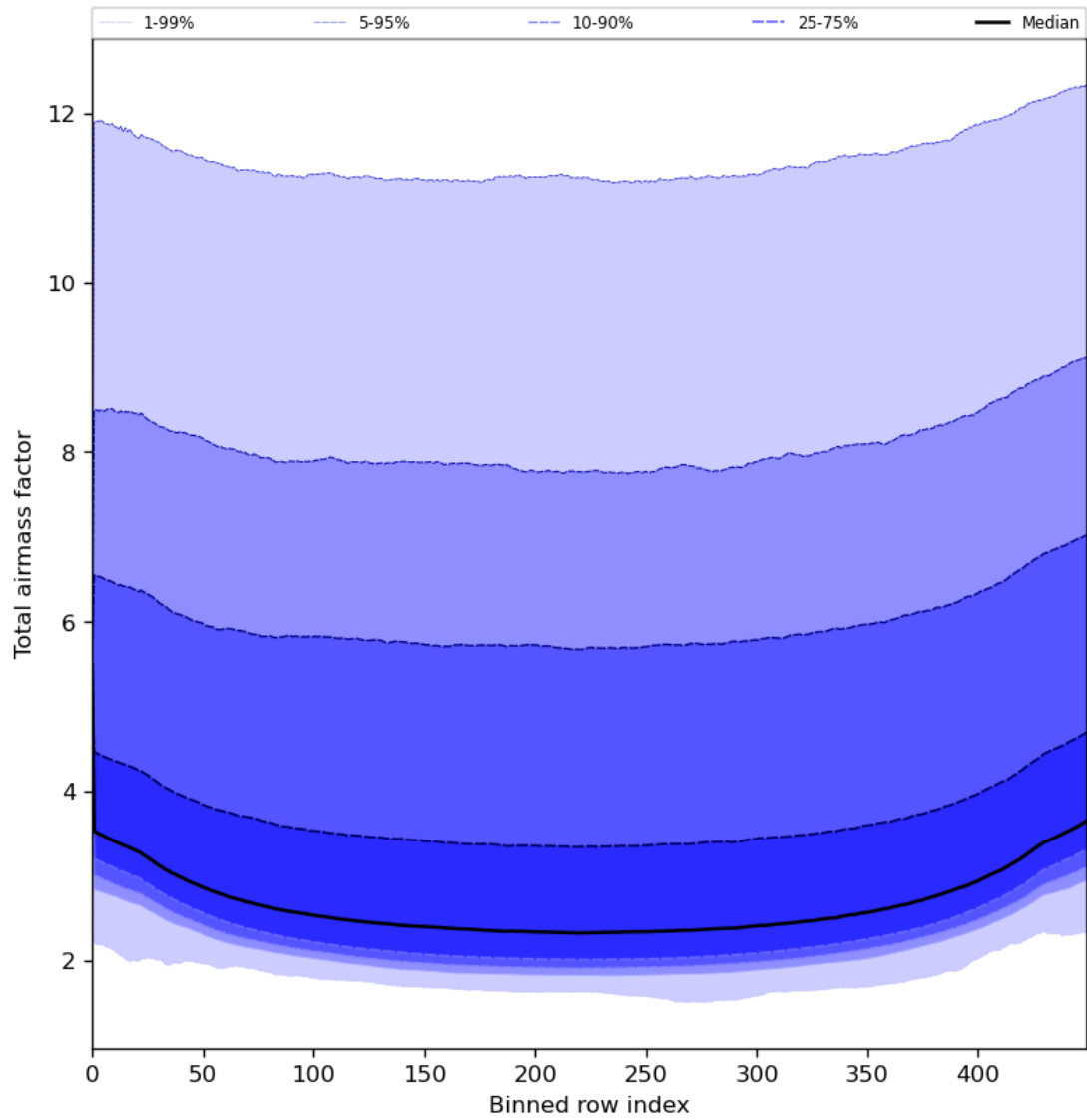
Figure 49: Along track statistics of “Total airmass factor” for 2024-07-13 to 2024-07-15
