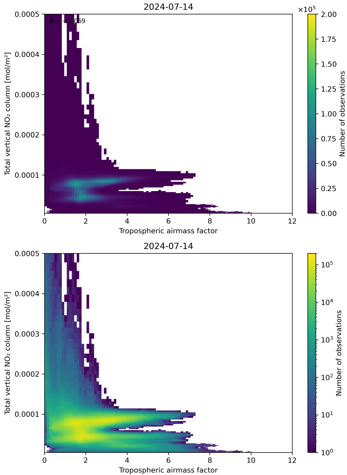
Figure 77: Scatter density plot of “Tropospheric airmass factor” against “Total vertical NO 2 column” for 2024-07-13 to 2024-07-15.
