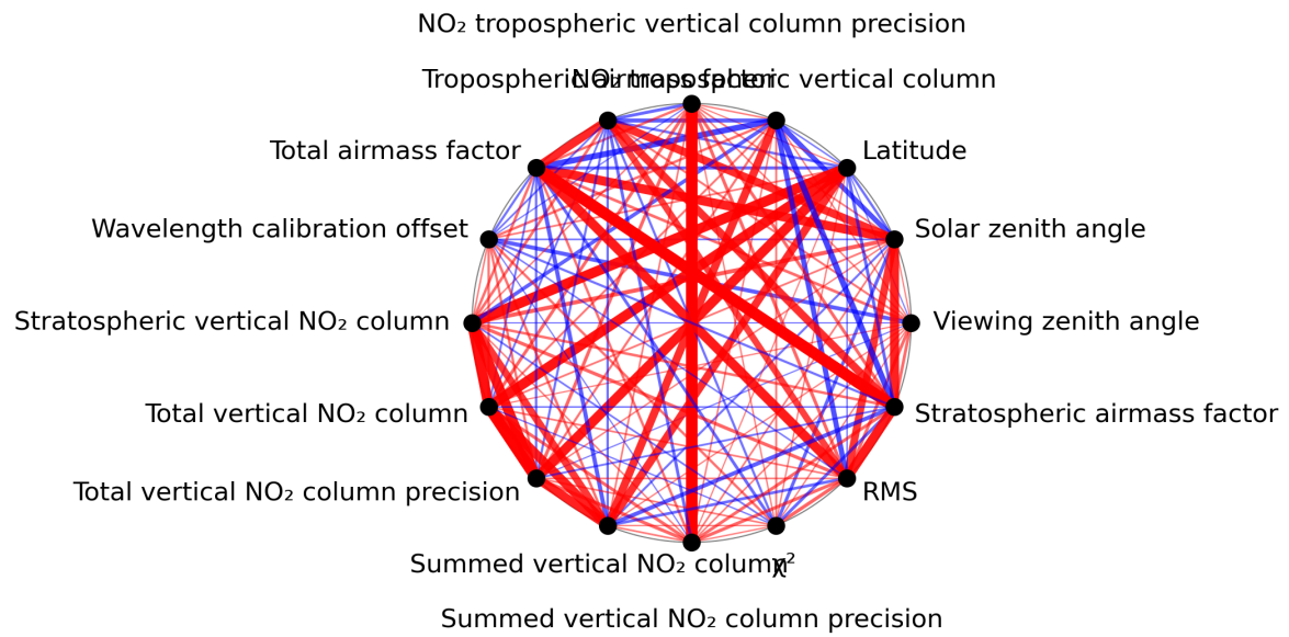
Figure 1: Map of correlation graph for 2024-07-13 to 2024-07-15.
