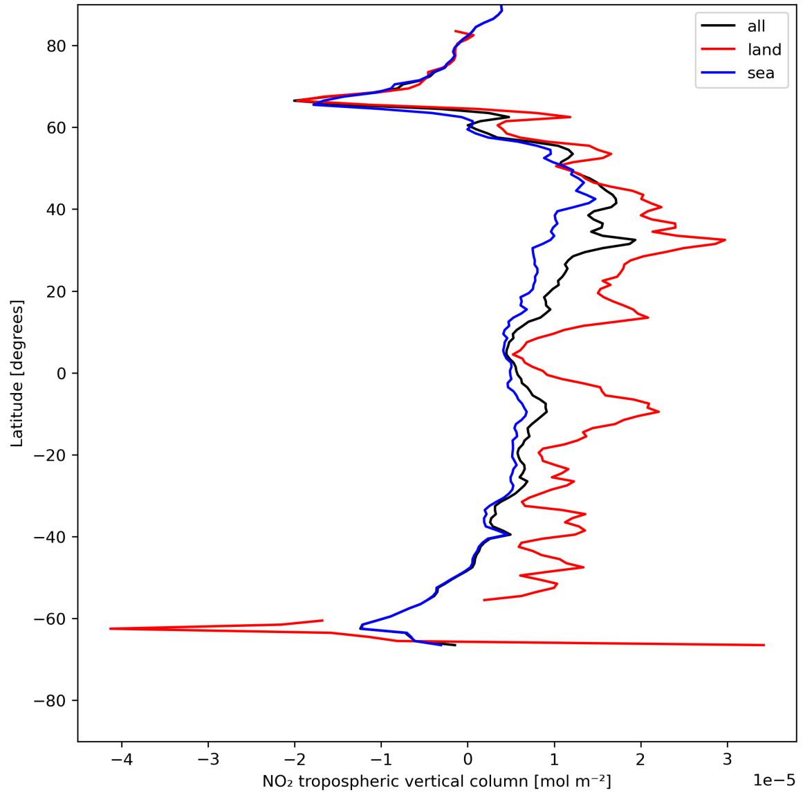
Figure 12: Zonal average of “NO 2 tropospheric vertical column” for 2024-07-13 to 2024-07-15.
