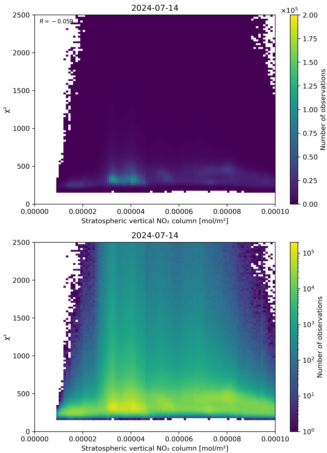
Figure 97: Scatter density plot of “Stratospheric vertical NO 2 column” against “ \chi^2 ” for 2024-07-13 to 2024-07-15.
