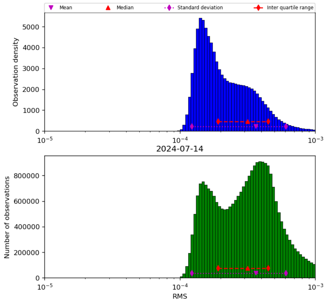
Figure 43: Histogram of “RMS” for 2024-07-13 to 2024-07-15
