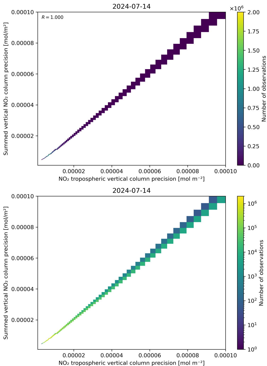
Figure 137: Scatter density plot of “NO 2 tropospheric vertical column precision” against “Summed vertical NO 2 column precision” for 2024-07-13 to 2024-07-15.
