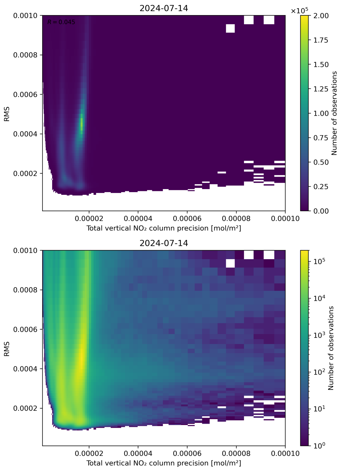
Figure 119: Scatter density plot of “Total vertical NO 2 column precision” against “RMS” for 2024-07-13 to 2024-07-15.
