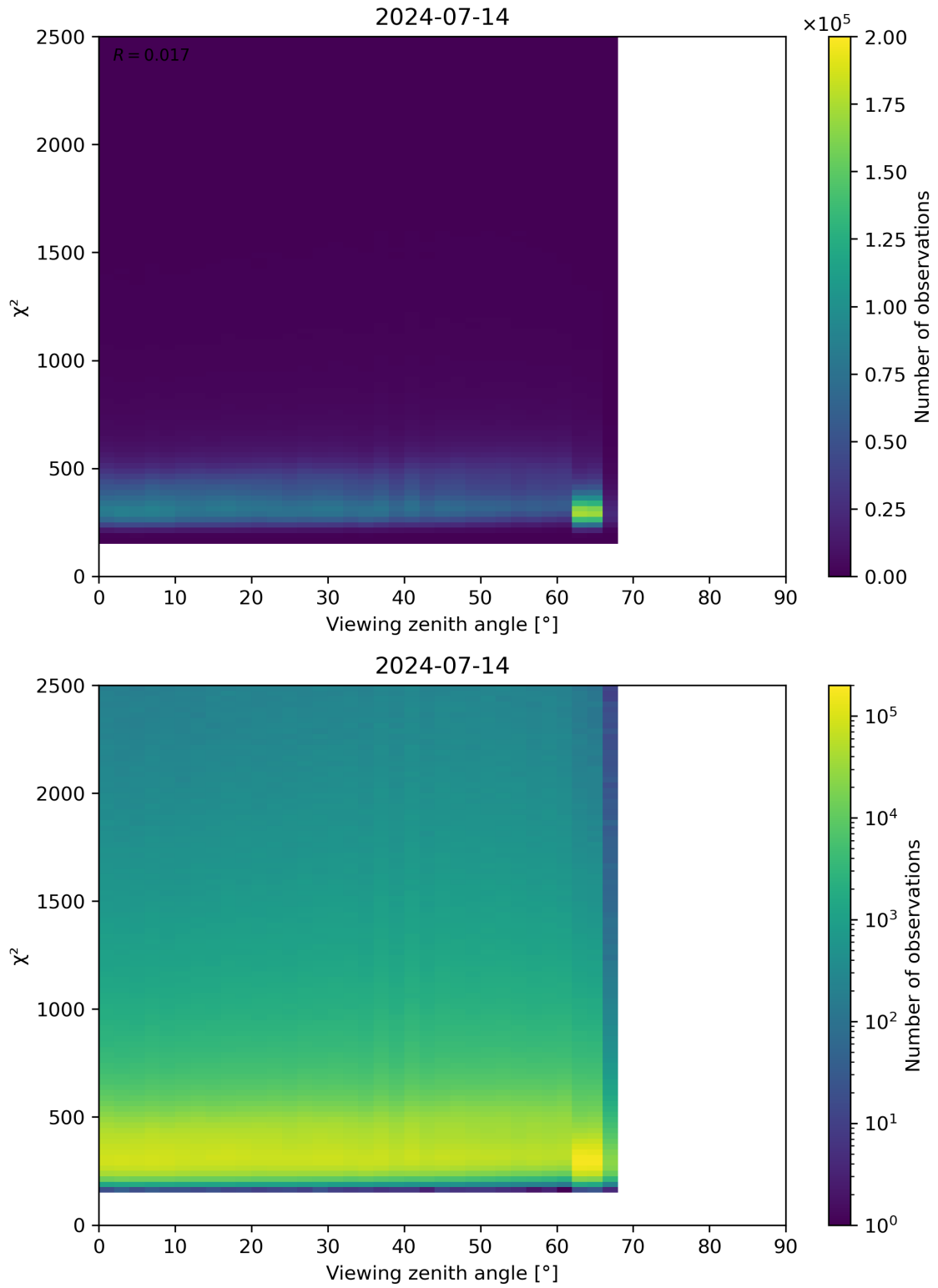
Figure 162: Scatter density plot of “Viewing zenith angle” against “ \chi^2 ” for 2024-07-13 to 2024-07-15.
