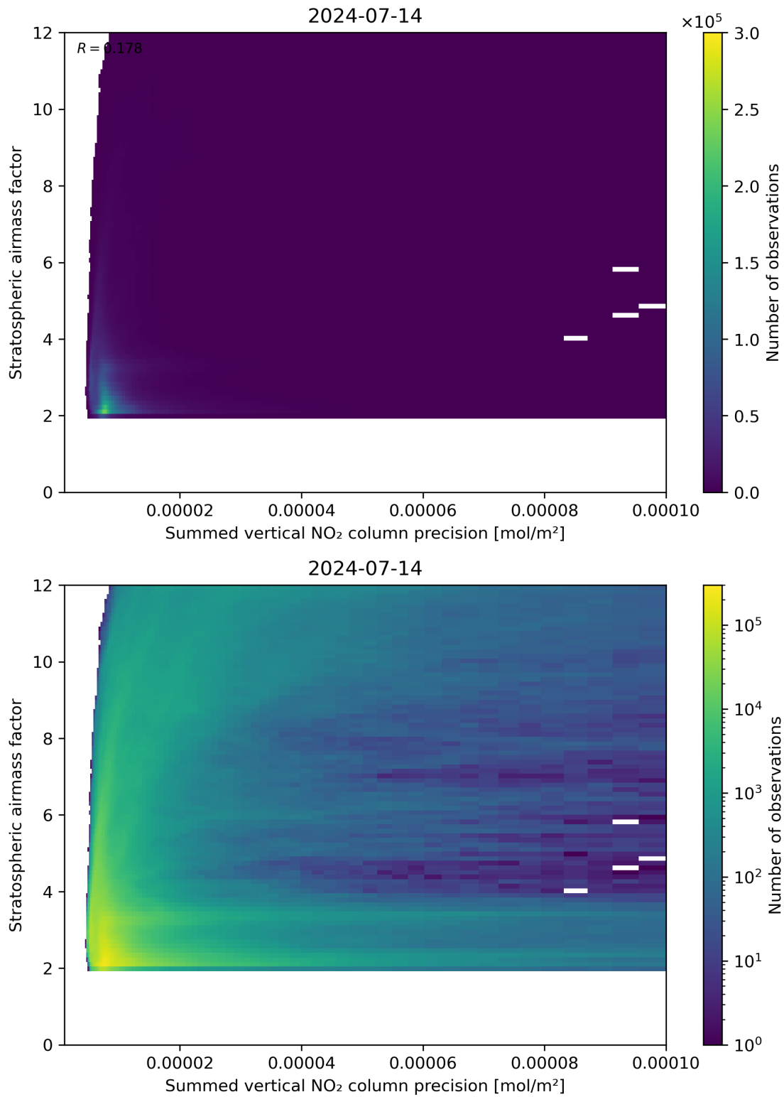
Figure 106: Scatter density plot of “Summed vertical NO 2 column precision” against “Stratospheric airmass factor” for 2024-07-13 to 2024-07-15.
