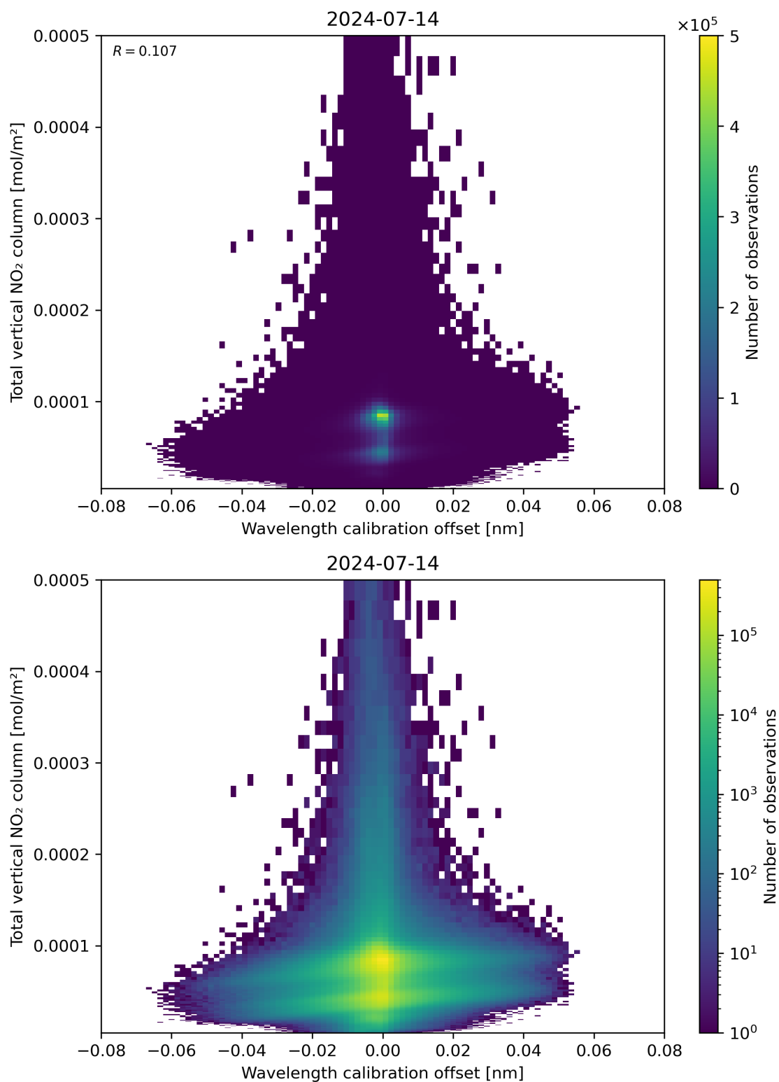
Figure 179: Scatter density plot of “Wavelength calibration offset” against “Total vertical NO 2 column” for 2024-07-13 to 2024-07-15.
