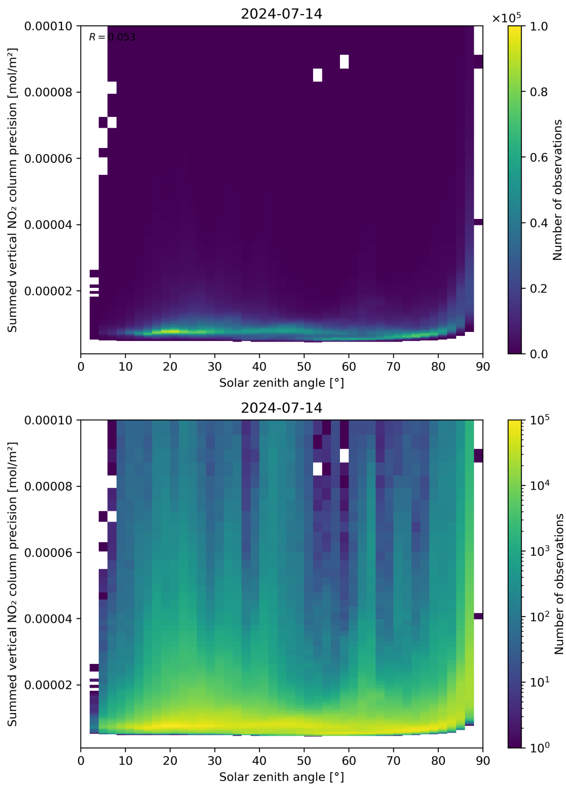
Figure 152: Scatter density plot of “Solar zenith angle” against “Summed vertical NO 2 column precision” for 2024-07-13 to 2024-07-15.
