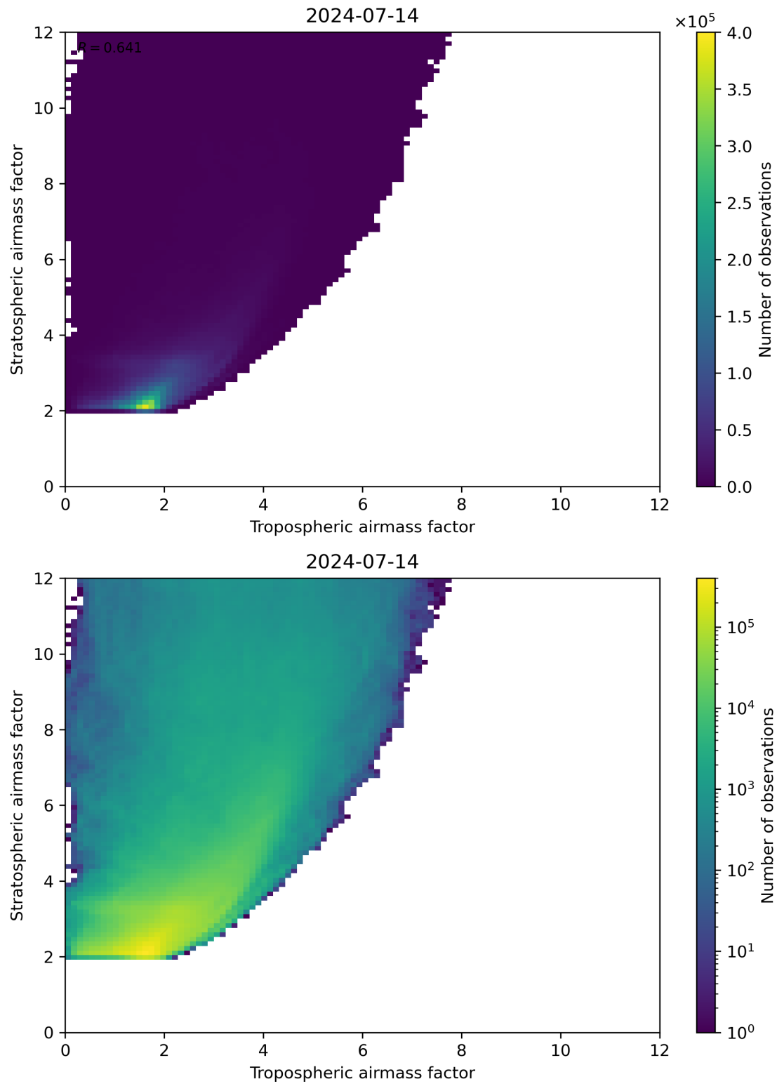
Figure 71: Scatter density plot of “Tropospheric airmass factor” against “Stratospheric airmass factor” for 2024-07-13 to 2024-07-15.
