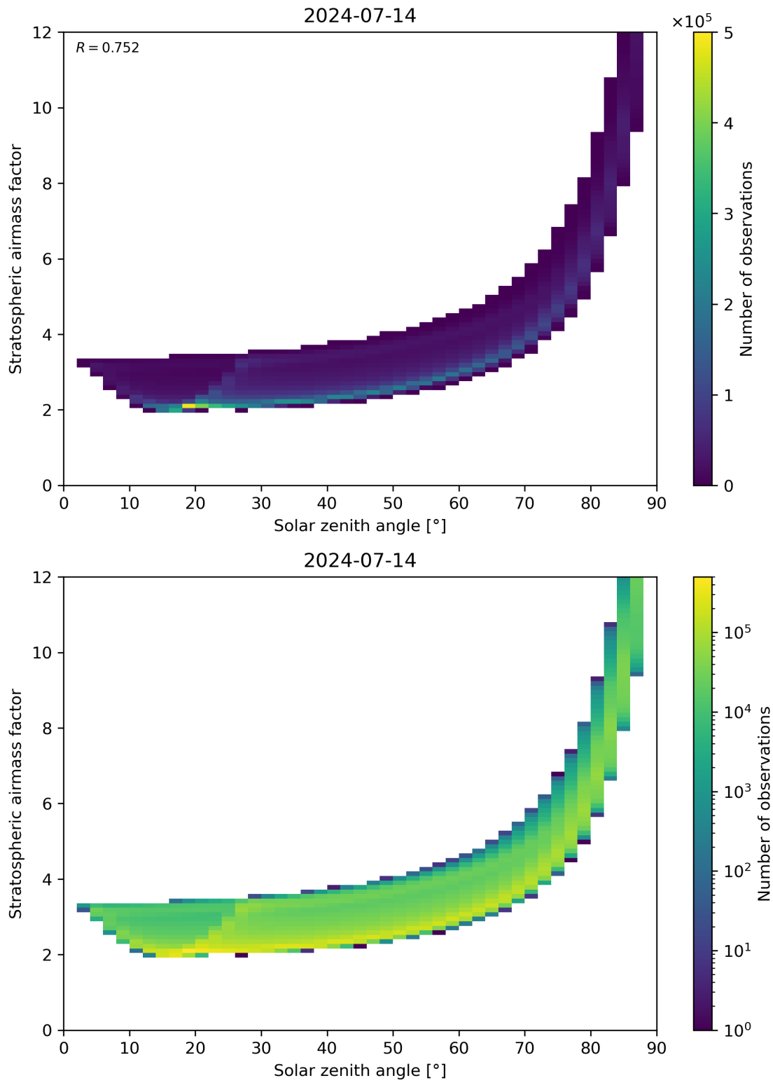
Figure 145: Scatter density plot of “Solar zenith angle” against “Stratospheric airmass factor” for 2024-07-13 to 2024-07-15.
