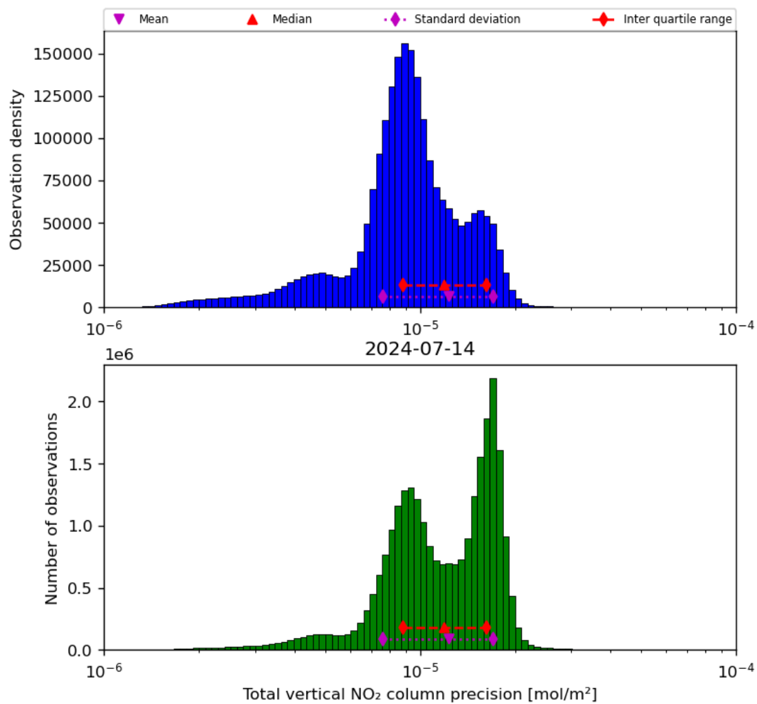
Figure 39: Histogram of “Total vertical NO 2 column precision” for 2024-07-13 to 2024-07-15
