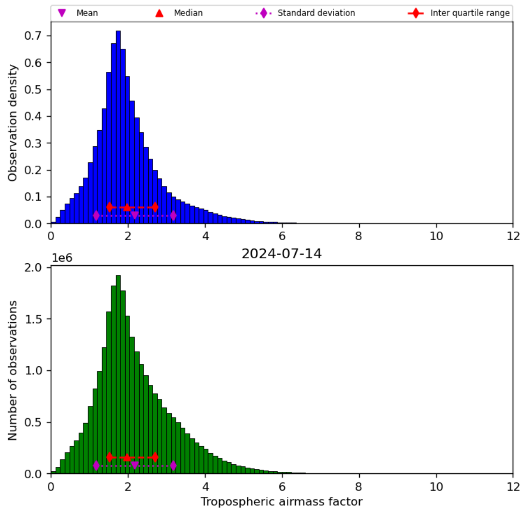
Figure 31: Histogram of “Tropospheric airmass factor” for 2024-07-13 to 2024-07-15
