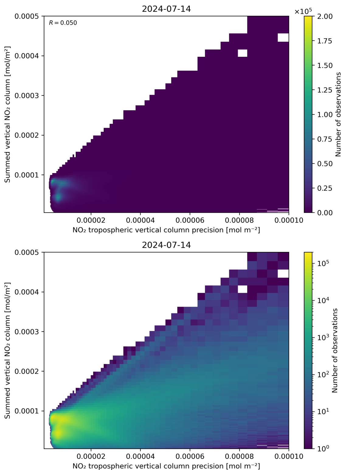
Figure 136: Scatter density plot of “NO 2 tropospheric vertical column precision” against “Summed vertical NO 2 column” for 2024-07-13 to 2024-07-15.
