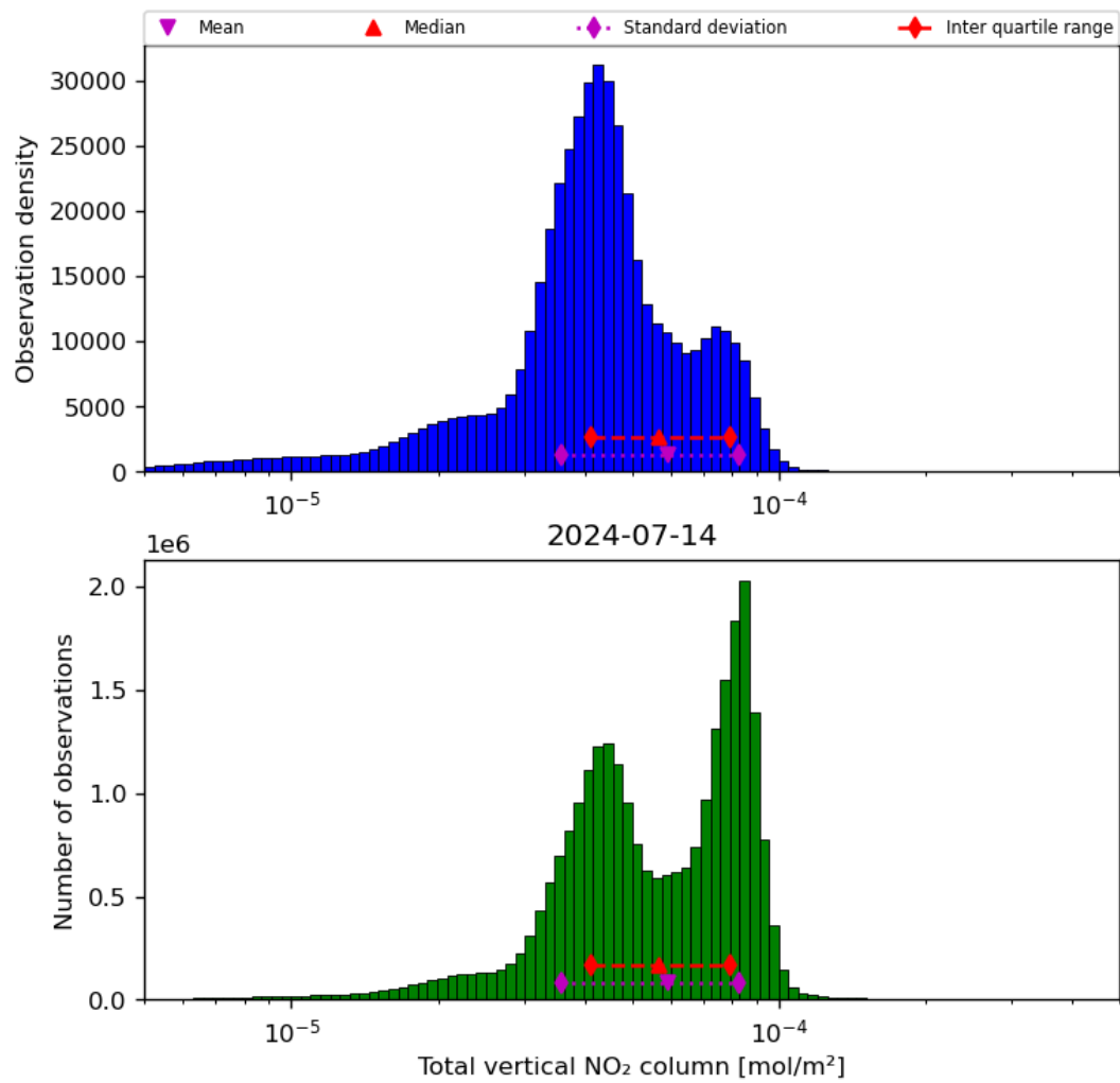
Figure 38: Histogram of “Total vertical NO 2 column” for 2024-07-13 to 2024-07-15
