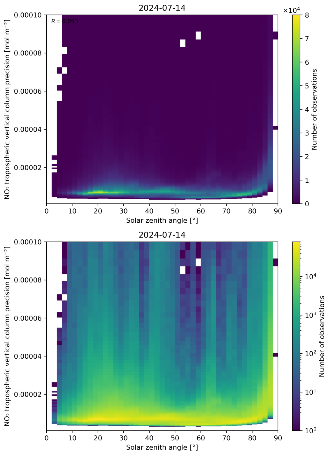
Figure 156: Scatter density plot of “Solar zenith angle” against “NO 2 tropospheric vertical column precision” for 2024-07-13 to 2024-07-15.
