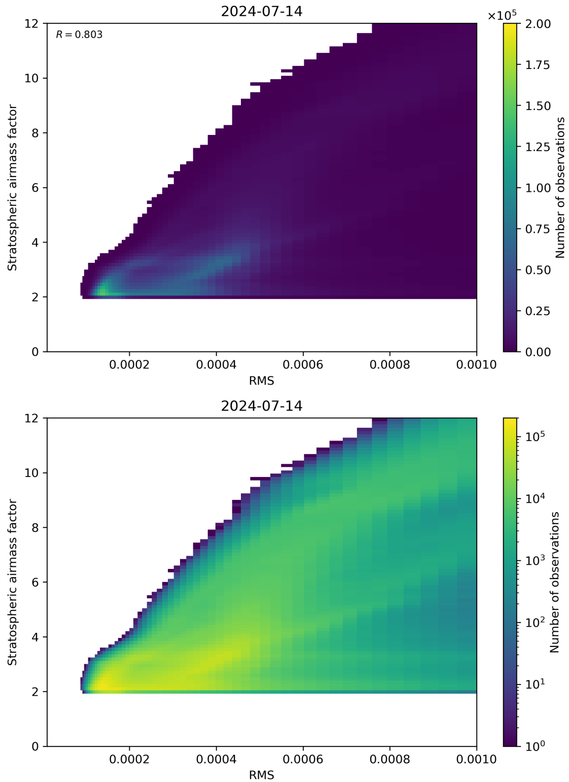
Figure 144: Scatter density plot of “RMS” against “Stratospheric airmass factor” for 2024-07-13 to 2024-07-15.
