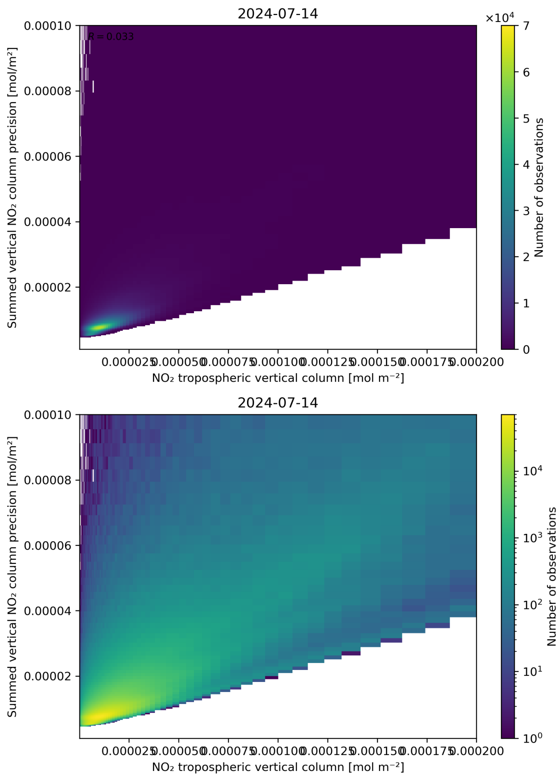
Figure 127: Scatter density plot of “NO 2 tropospheric vertical column” against “Summed vertical NO 2 column precision” for 2024-07-13 to 2024-07-15.
