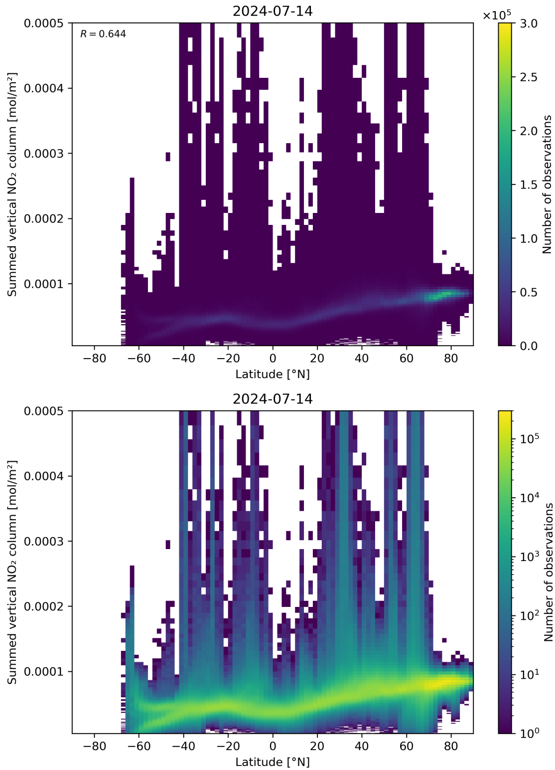
Figure 88: Scatter density plot of “Latitude” against “Summed vertical NO 2 column” for 2024-07-13 to 2024-07-15.
