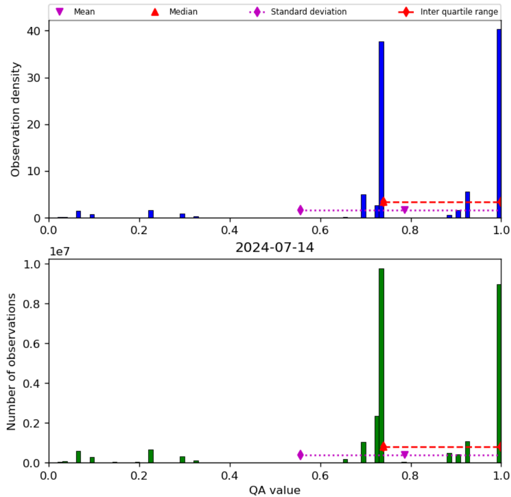
Figure 28: Histogram of “QA value” for 2024-07-13 to 2024-07-15
