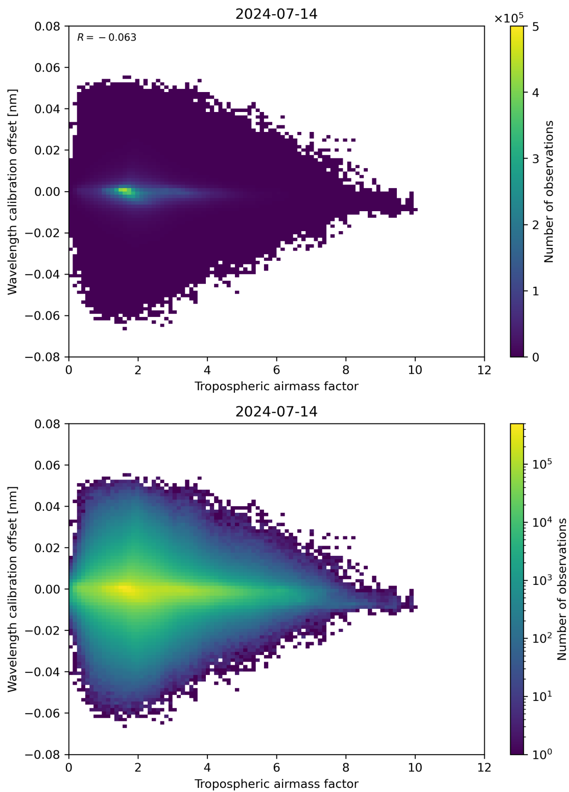
Figure 80: Scatter density plot of “Tropospheric airmass factor” against “Wavelength calibration offset” for 2024-07-13 to 2024-07-15.
