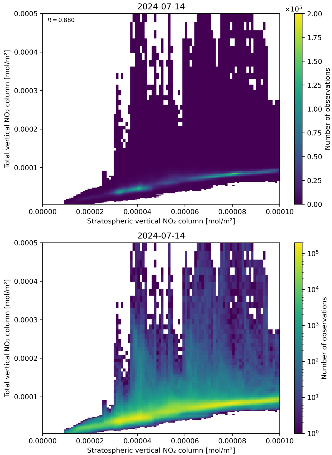
Figure 100: Scatter density plot of “Stratospheric vertical NO 2 column” against “Total vertical NO 2 column” for 2024-07-13 to 2024-07-15.
