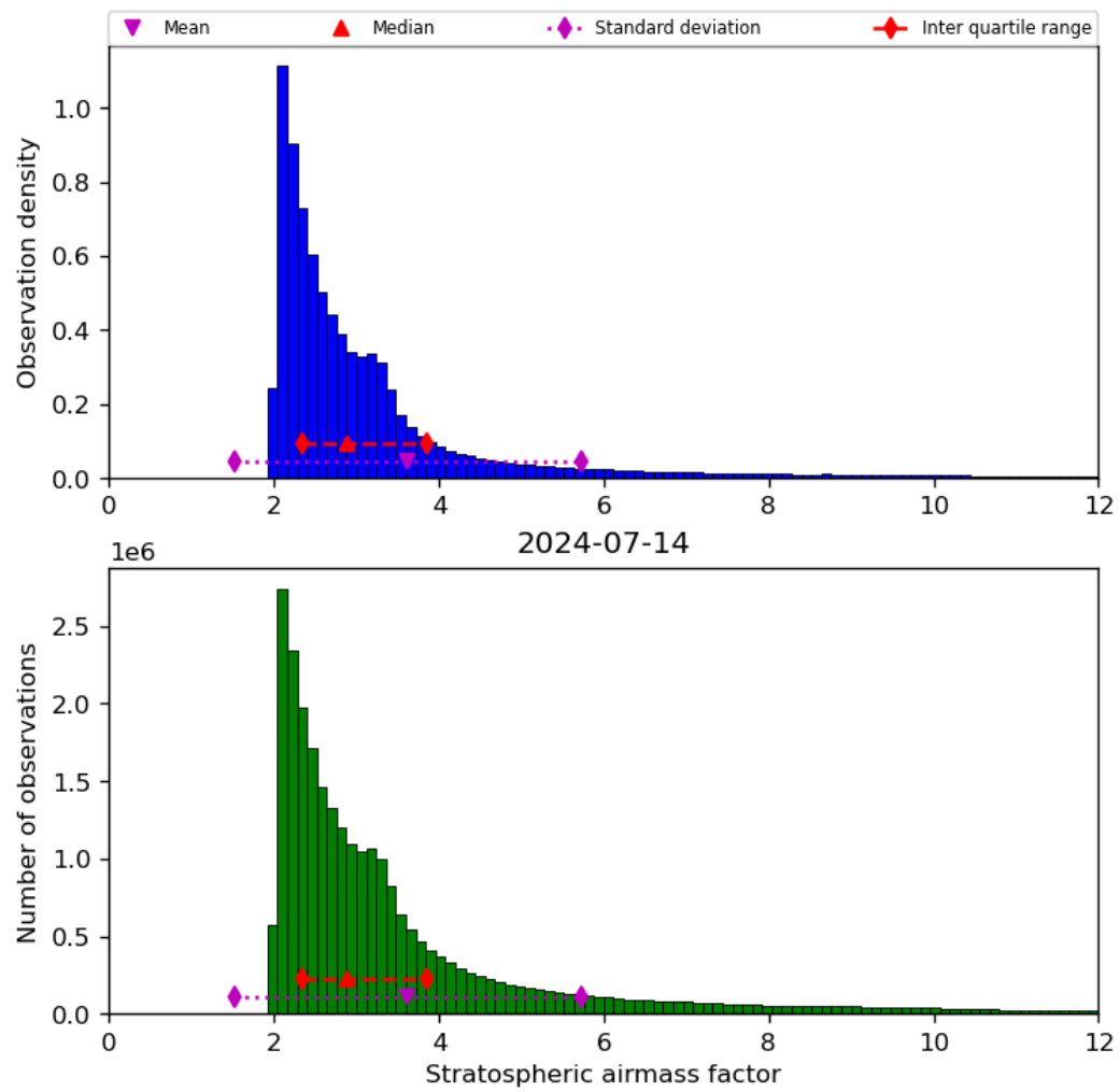
Figure 44: Histogram of “Stratospheric airmass factor” for 2024-07-13 to 2024-07-15
