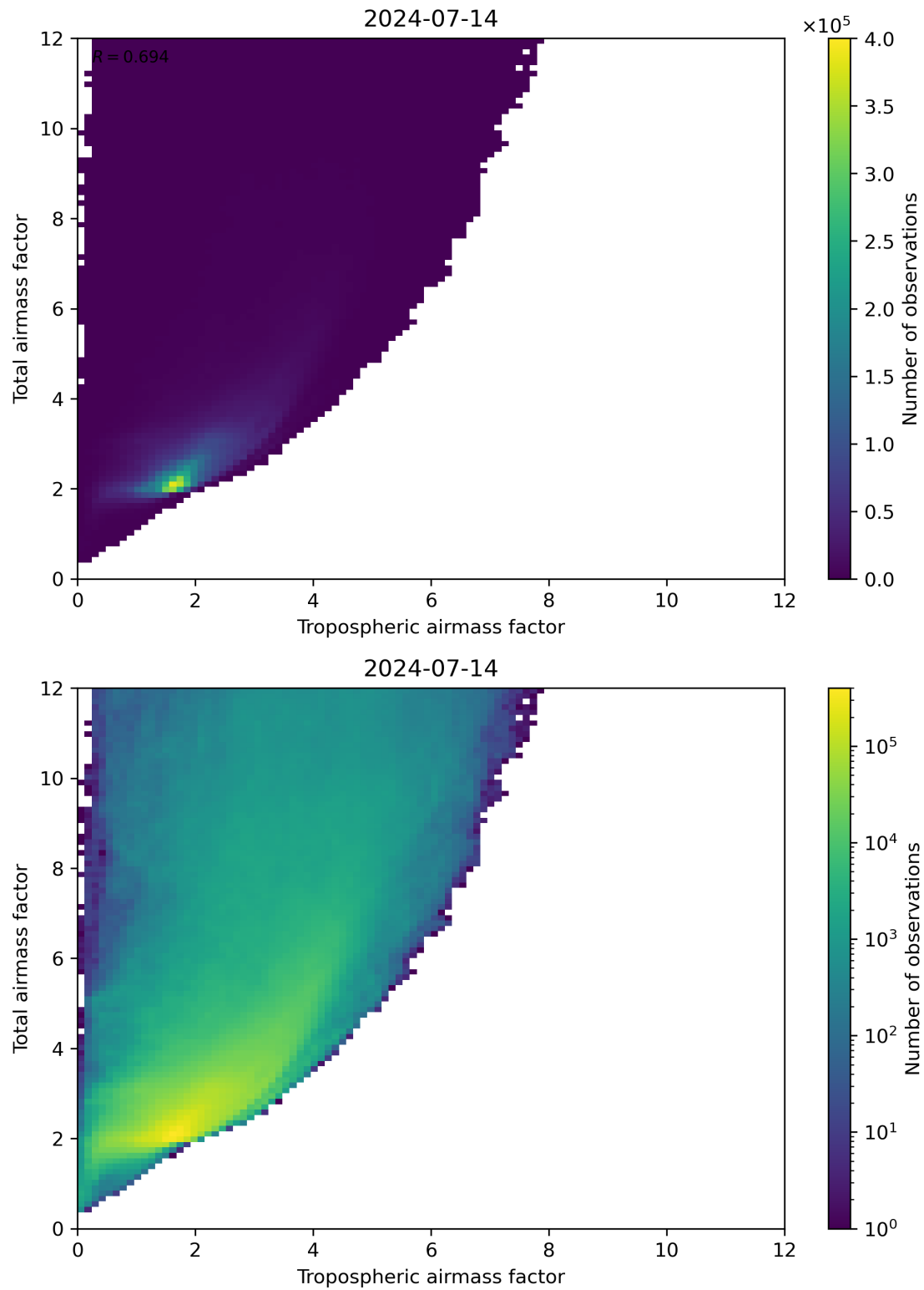
Figure 72: Scatter density plot of “Tropospheric airmass factor” against “Total airmass factor” for 2024-07-13 to 2024-07-15.
