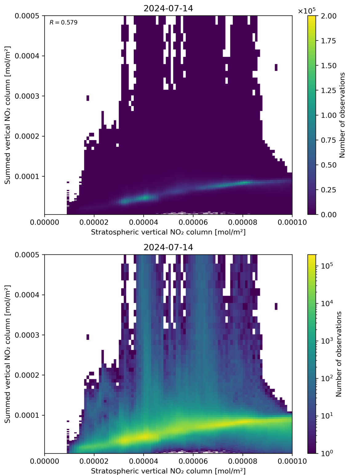
Figure 98: Scatter density plot of “Stratospheric vertical NO 2 column” against “Summed vertical NO 2 column” for 2024-07-13 to 2024-07-15.
