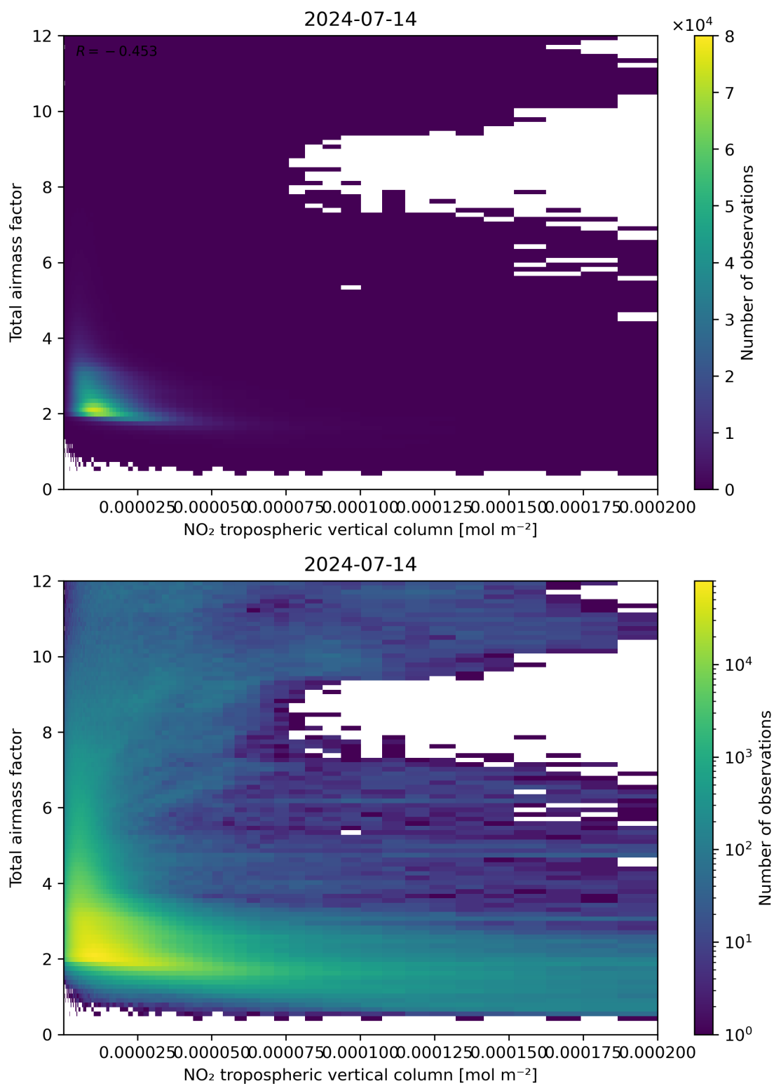
Figure 122: Scatter density plot of “NO 2 tropospheric vertical column” against “Total air mass factor” for 2024-07-13 to 2024-07-15.
