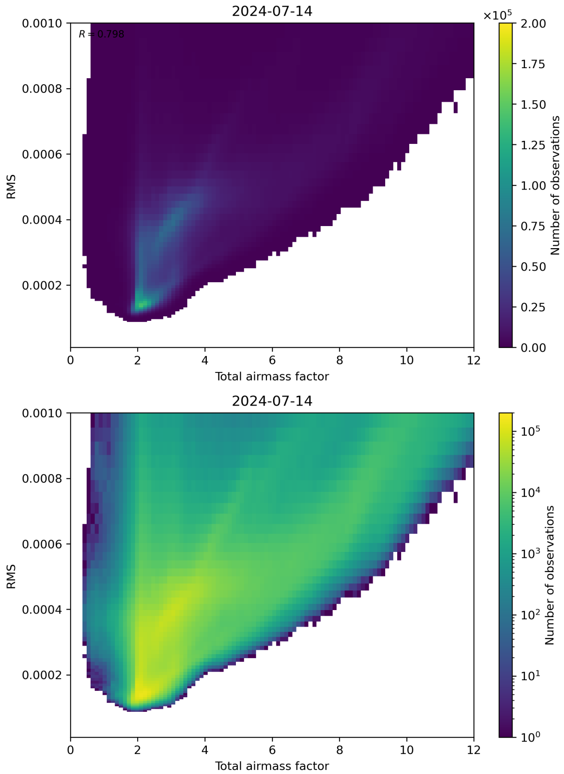
Figure 69: Scatter density plot of “Total airmass factor” against “RMS” for 2024-07-13 to 2024-07-15.
