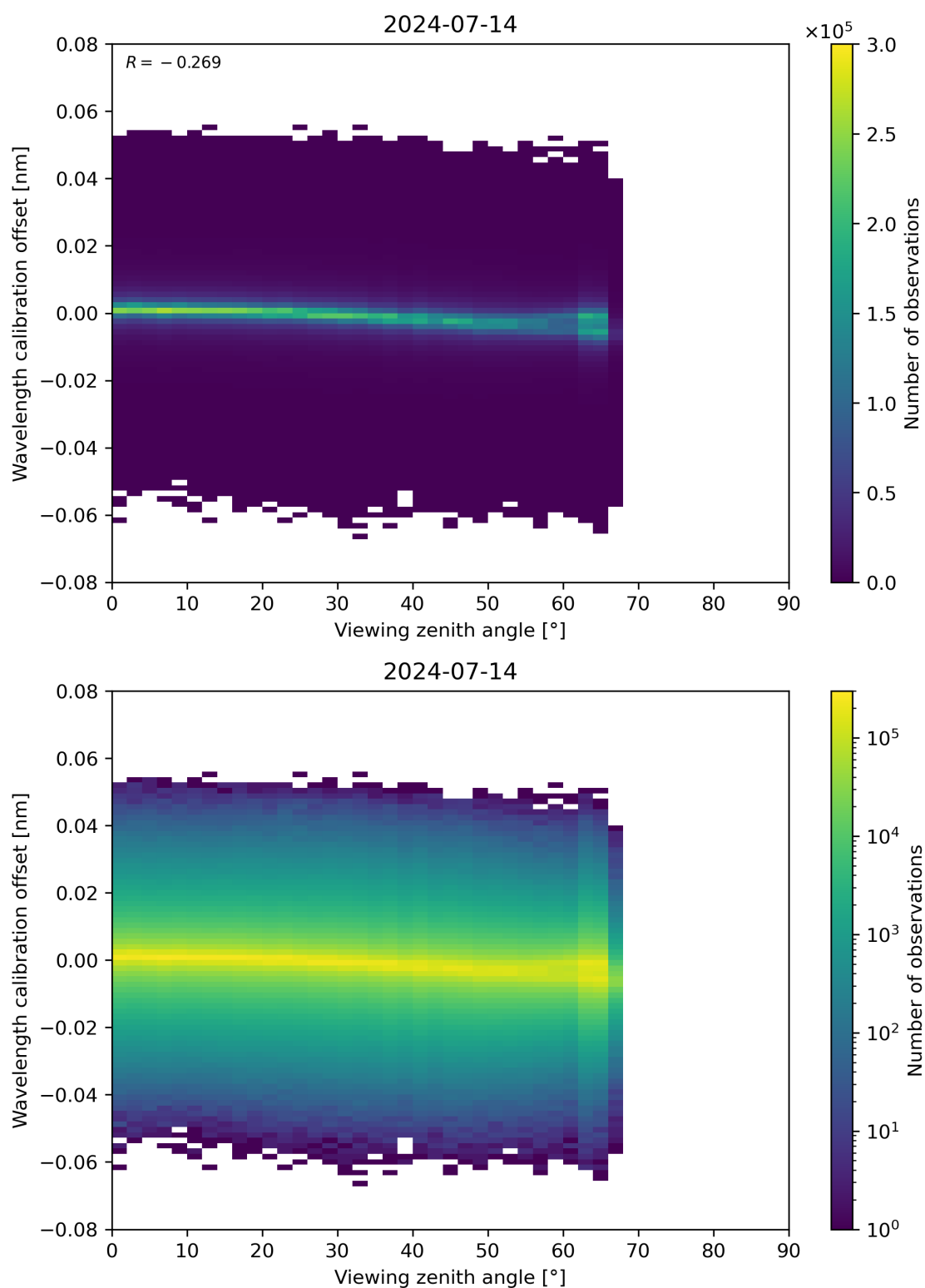
Figure 173: Scatter density plot of “Viewing zenith angle” against “Wavelength calibration offset” for 2024-07-13 to 2024-07-15.
