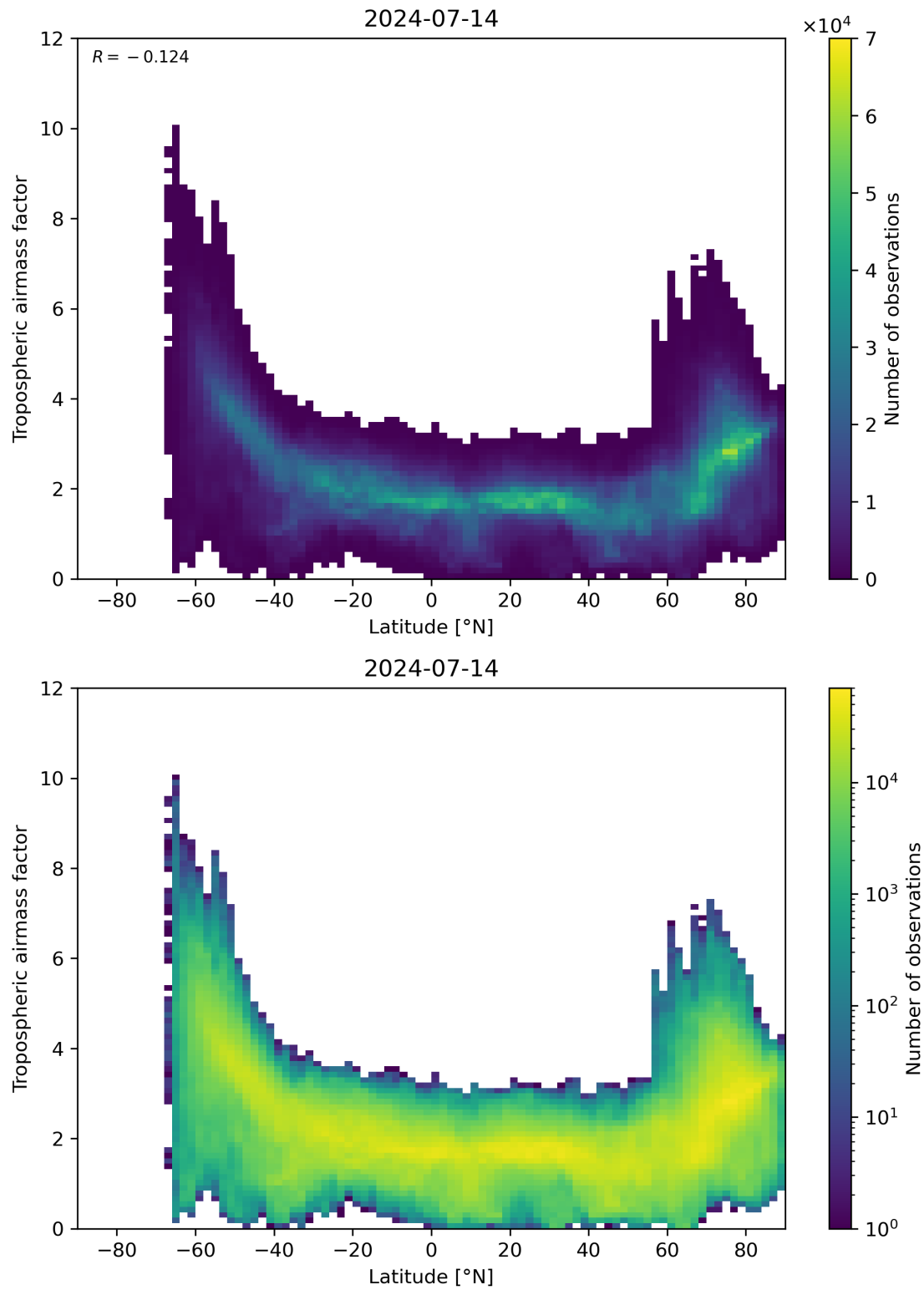
Figure 85: Scatter density plot of “Latitude” against “Tropospheric airmass factor” for 2024-07-13 to 2024-07-15.
