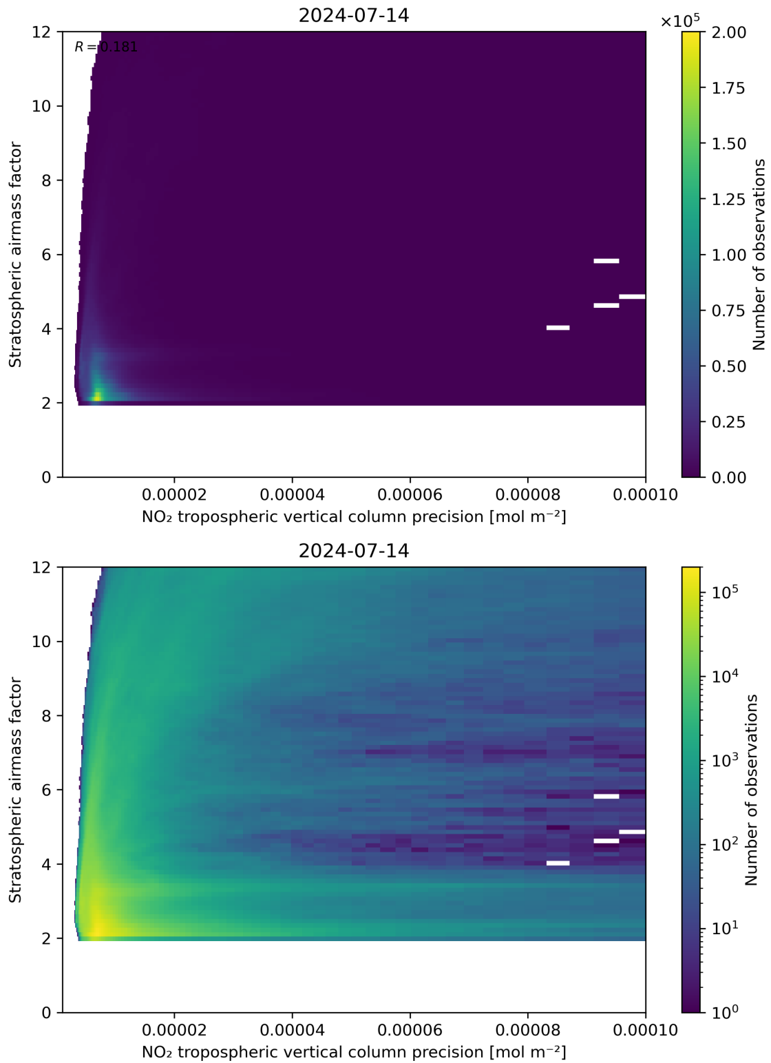
Figure 131: Scatter density plot of “NO 2 tropospheric vertical column precision” against “Stratospheric airmass factor” for 2024-07-13 to 2024-07-15.
