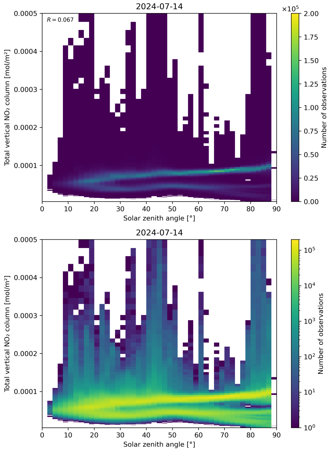
Figure 153: Scatter density plot of “Solar zenith angle” against “Total vertical NO 2 column” for 2024-07-13 to 2024-07-15.
