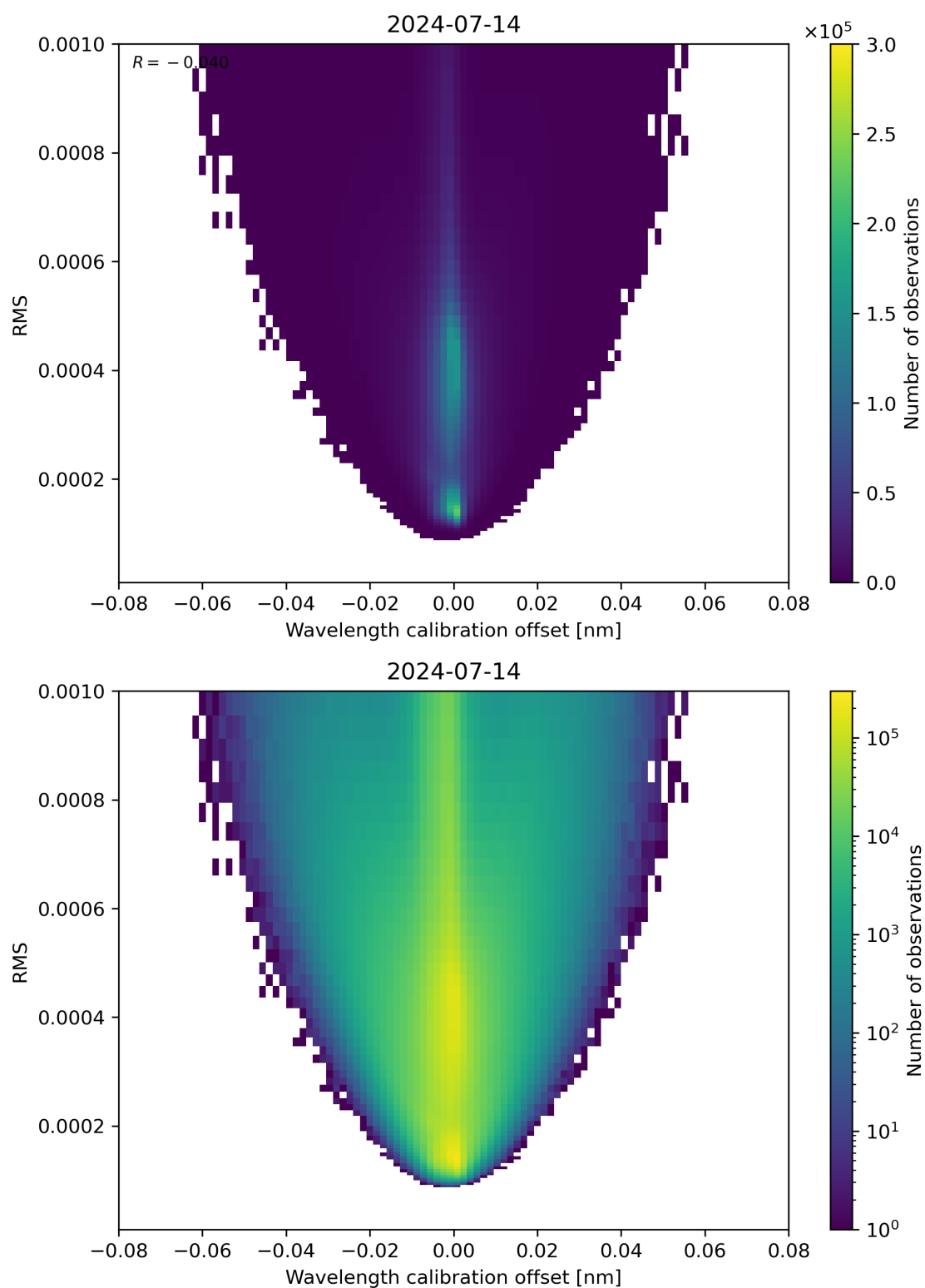
Figure 181: Scatter density plot of “Wavelength calibration offset” against “RMS” for 2024-07-13 to 2024-07-15.
