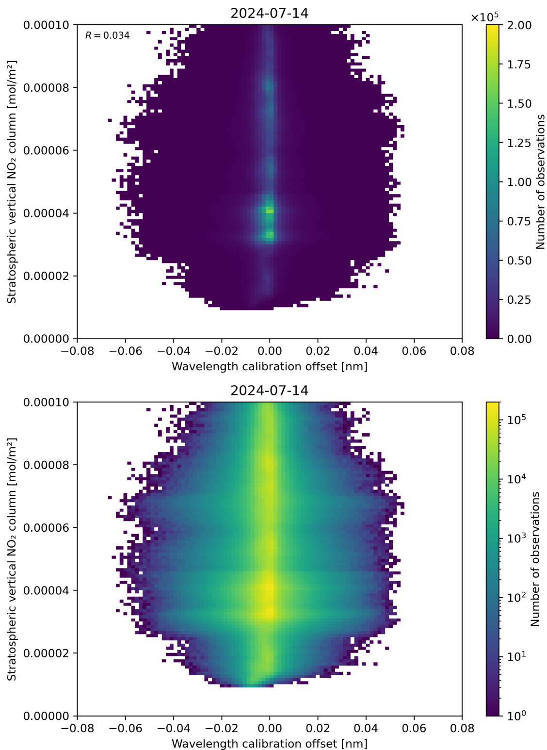
Figure 176: Scatter density plot of “Wavelength calibration offset” against “Stratospheric vertical NO 2 column” for 2024-07-13 to 2024-07-15.
