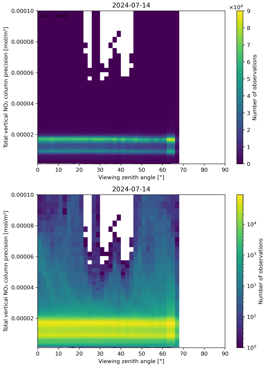
Figure 168: Scatter density plot of “Viewing zenith angle” against “Total vertical NO 2 column precision” for 2024-07-13 to 2024-07-15.
