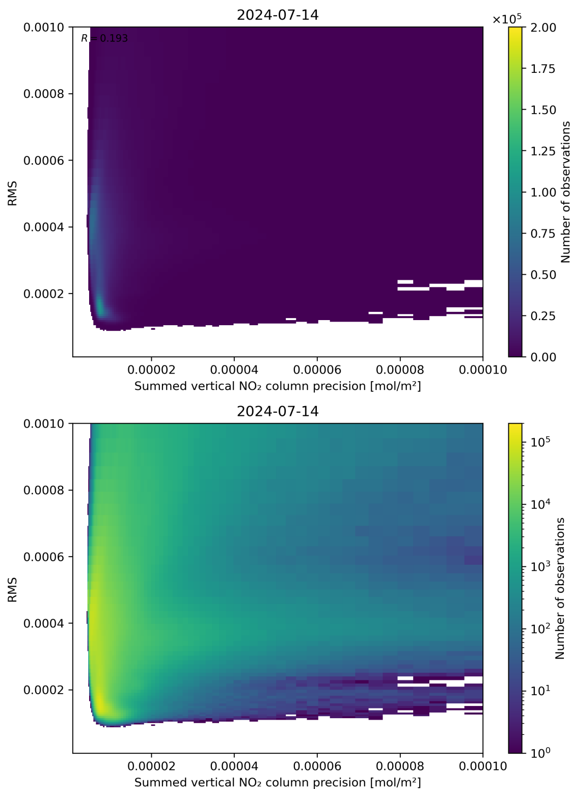
Figure 108: Scatter density plot of “Summed vertical NO 2 column precision” against “RMS” for 2024-07-13 to 2024-07-15.
