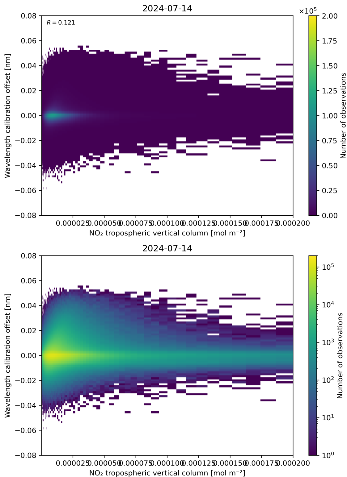
Figure 143: Scatter density plot of “NO 2 tropospheric vertical column” against “Wavelength calibration offset” for 2024-07-13 to 2024-07-15.
