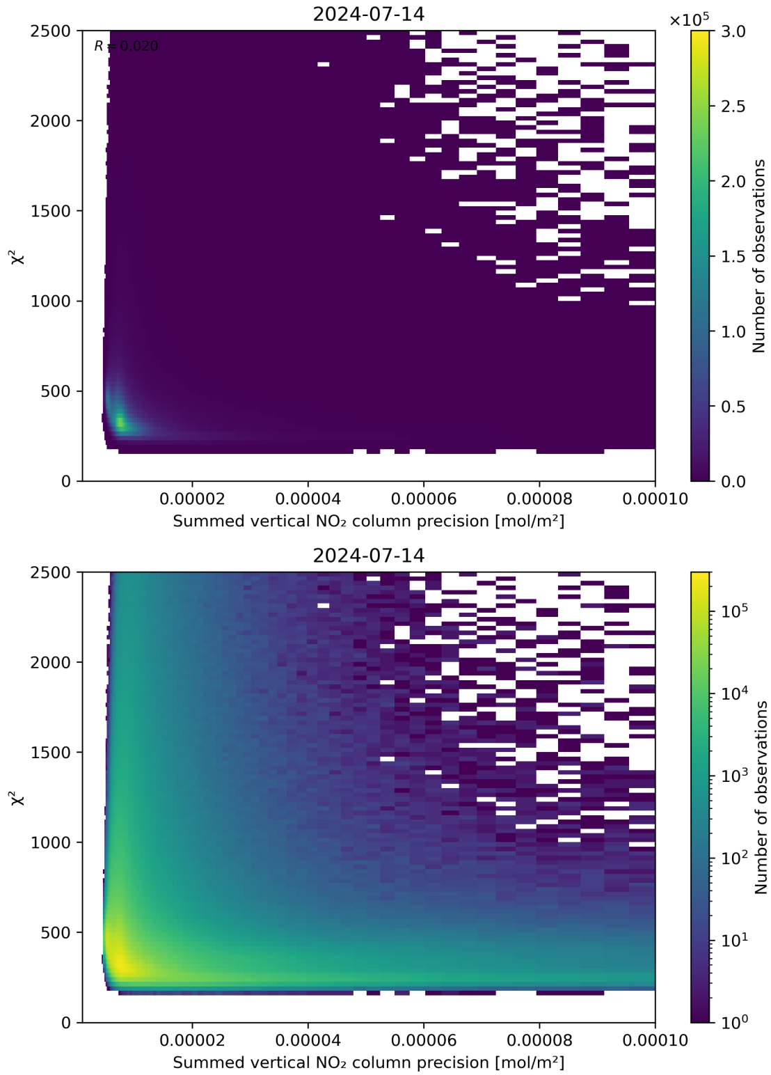
Figure 107: Scatter density plot of “Summed vertical NO 2 column precision” against “ \chi^2 ” for 2024-07-13 to 2024-07-15.
