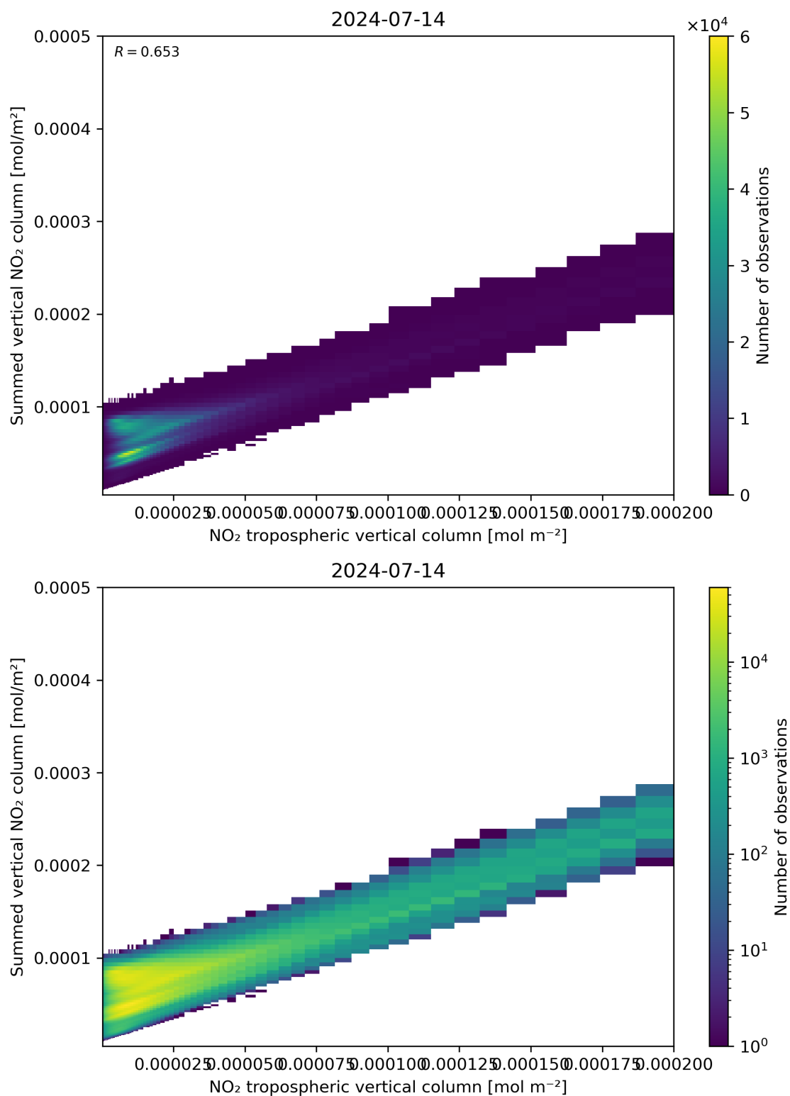
Figure 126: Scatter density plot of “NO 2 tropospheric vertical column” against “Summed vertical NO 2 column” for 2024-07-13 to 2024-07-15.
