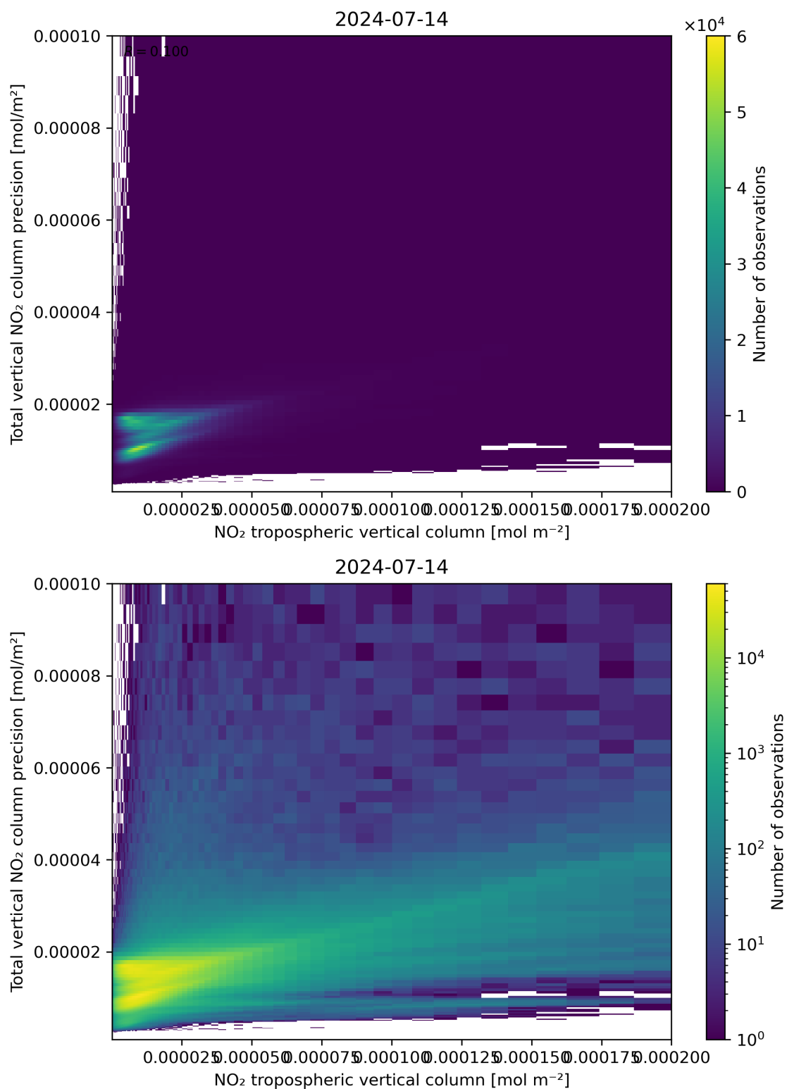
Figure 129: Scatter density plot of “NO 2 tropospheric vertical column” against “Total vertical NO 2 column precision” for 2024-07-13 to 2024-07-15.
