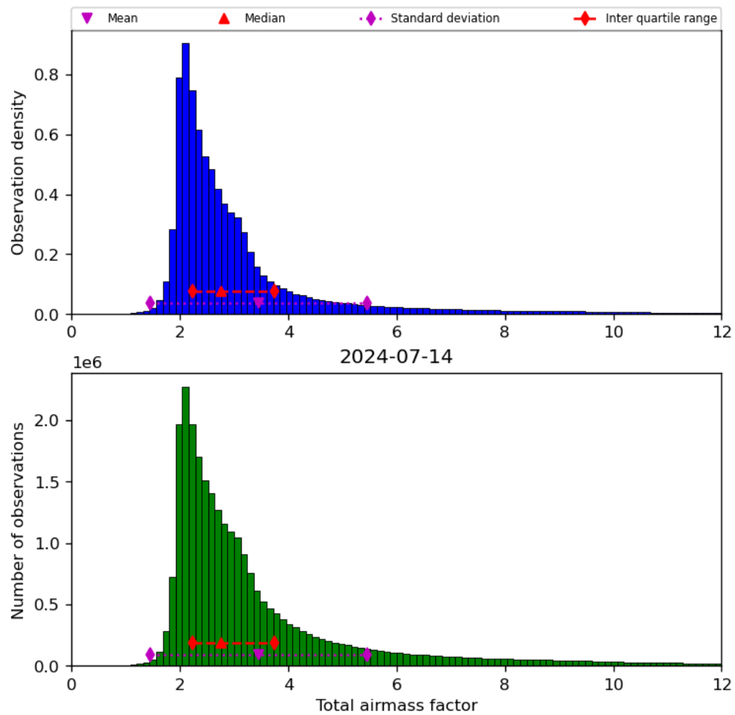
Figure 32: Histogram of “Total airmass factor” for 2024-07-13 to 2024-07-15
