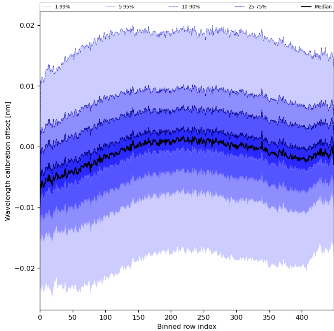
Figure 52: Along track statistics of “Wavelength calibration offset” for 2024-07-13 to 2024-07-15
