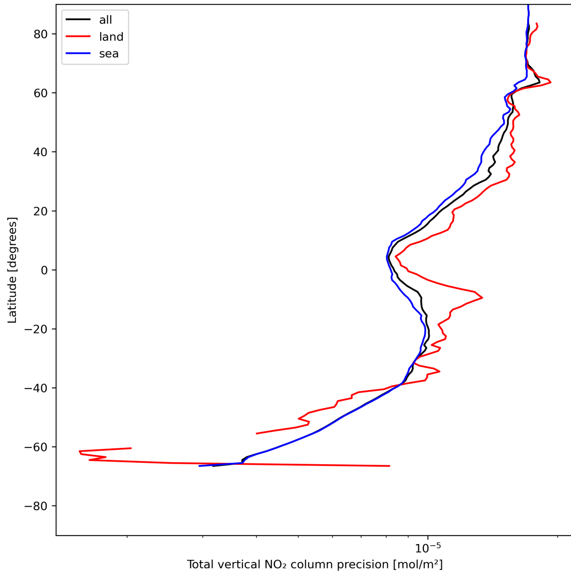
Figure 22: Zonal average of “Total vertical NO 2 column precision” for 2024-07-13 to 2024-07-15.
