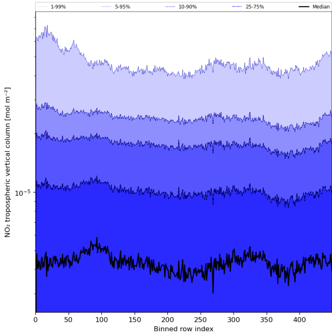
Figure 46: Along track statistics of “NO 2 tropospheric vertical column” for 2024-07-13 to 2024-07-15
