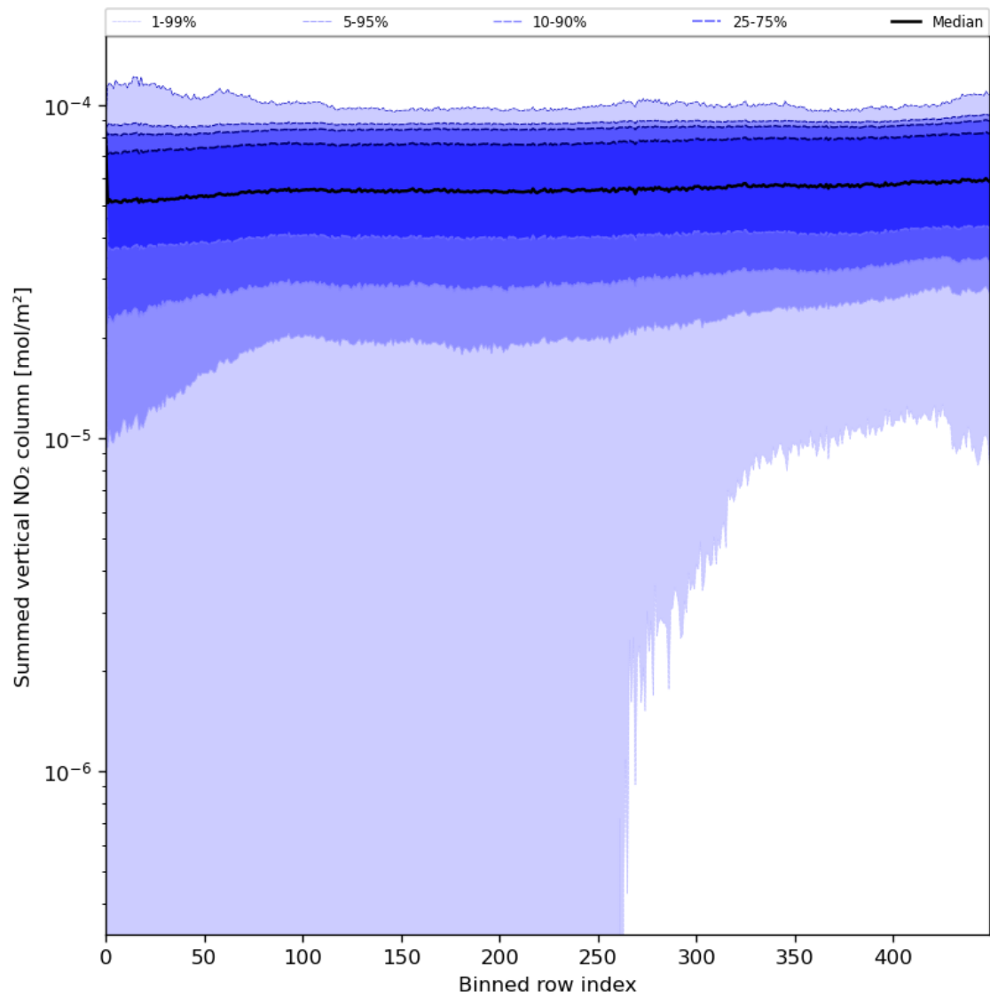
Figure 57: Along track statistics of “Summed vertical NO 2 column” for 2024-07-13 to 2024-07-15
