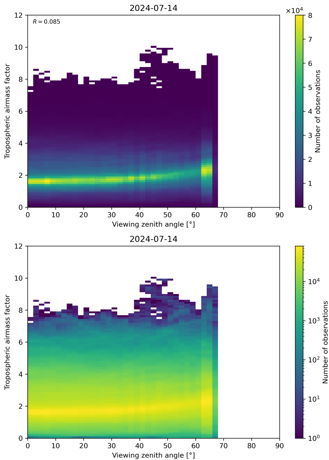
Figure 161: Scatter density plot of “Viewing zenith angle” against “Tropospheric airmass factor” for 2024-07-13 to 2024-07-15.
