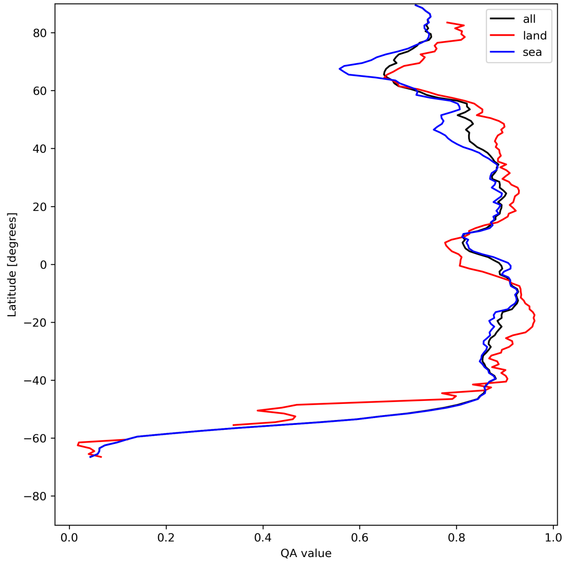
Figure 11: Zonal average of “QA value” for 2024-07-13 to 2024-07-15.
