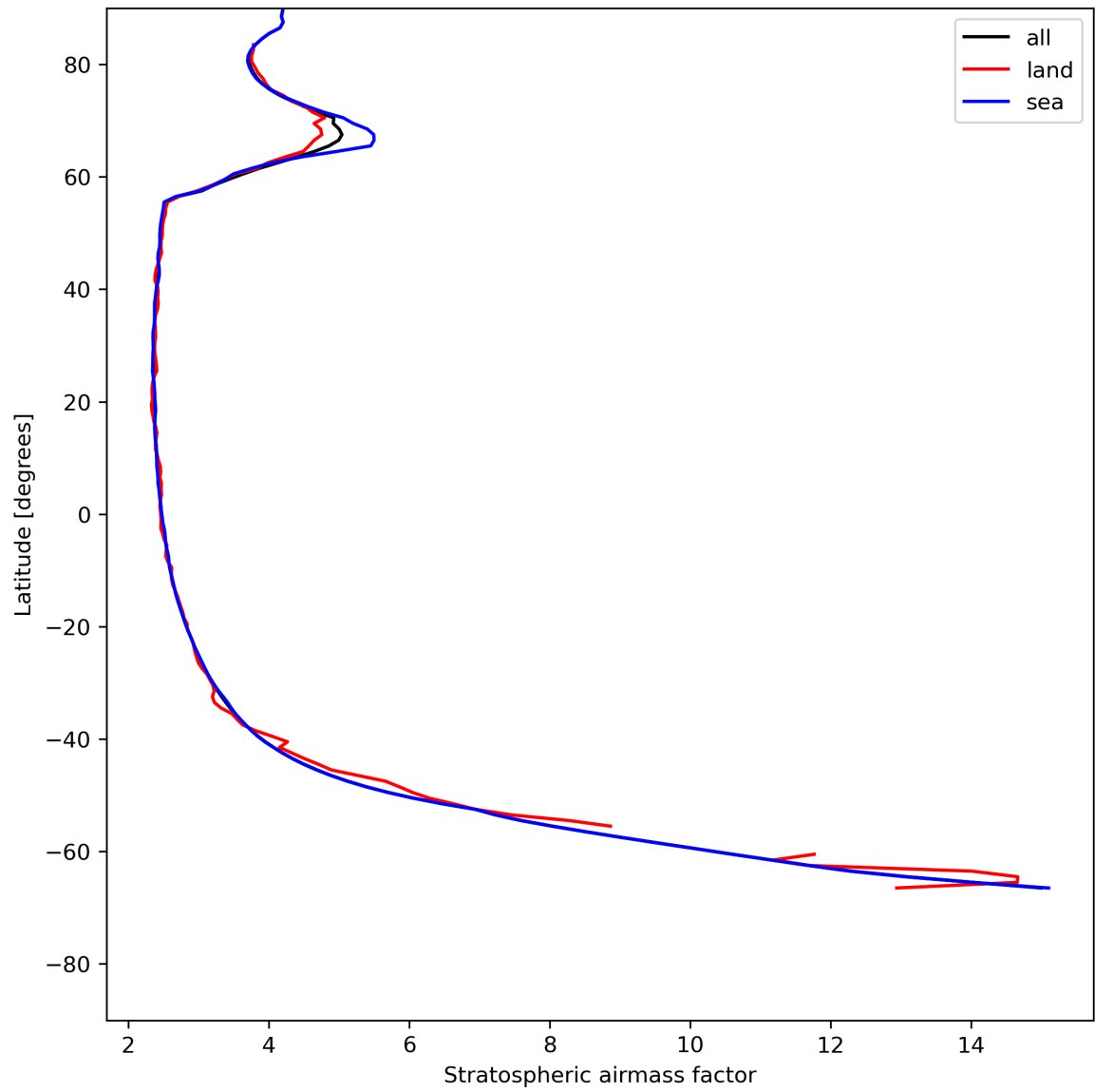
Figure 27: Zonal average of “Stratospheric air mass factor” for 2024-07-13 to 2024-07-15.
