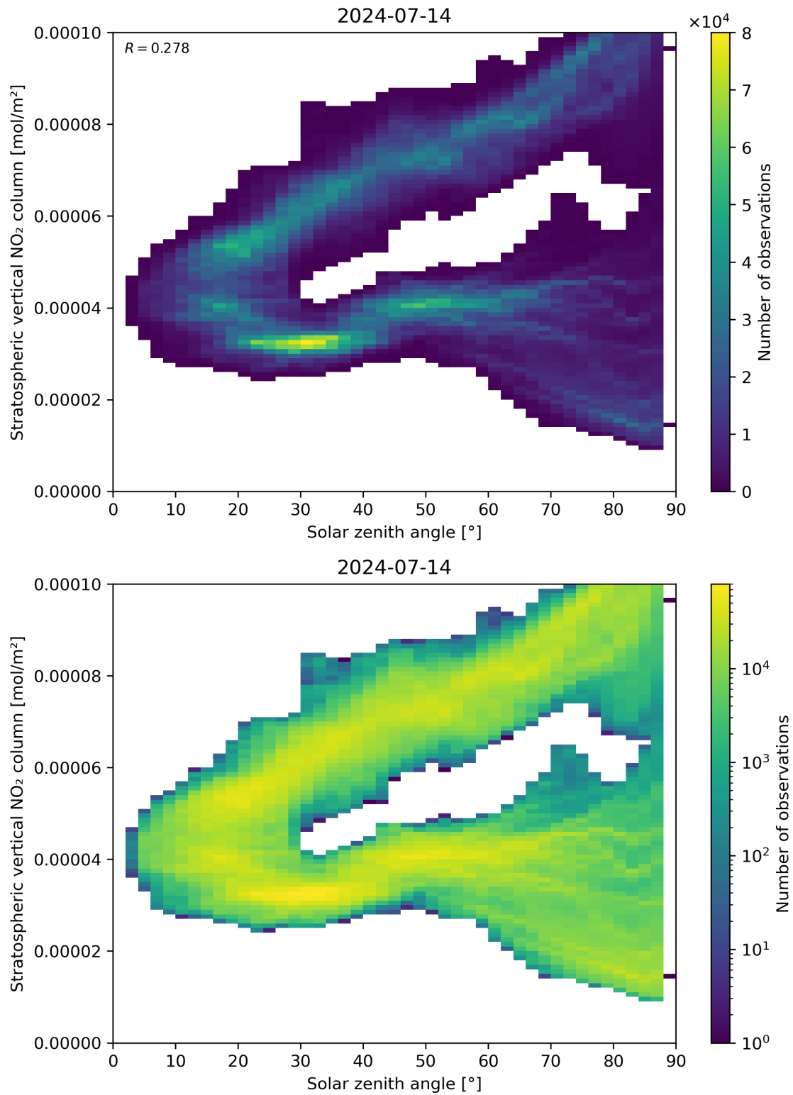
Figure 150: Scatter density plot of “Solar zenith angle” against “Stratospheric vertical NO 2 column” for 2024-07-13 to 2024-07-15.
