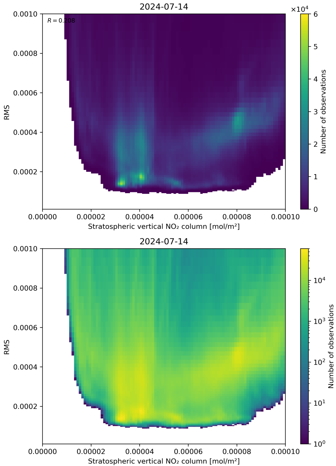
Figure 102: Scatter density plot of “Stratospheric vertical NO 2 column” against “RMS” for 2024-07-13 to 2024-07-15.
