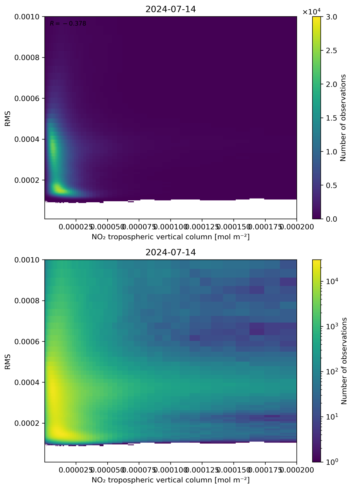
Figure 142: Scatter density plot of “NO 2 tropospheric vertical column” against “RMS” for 2024-07-13 to 2024-07-15.
