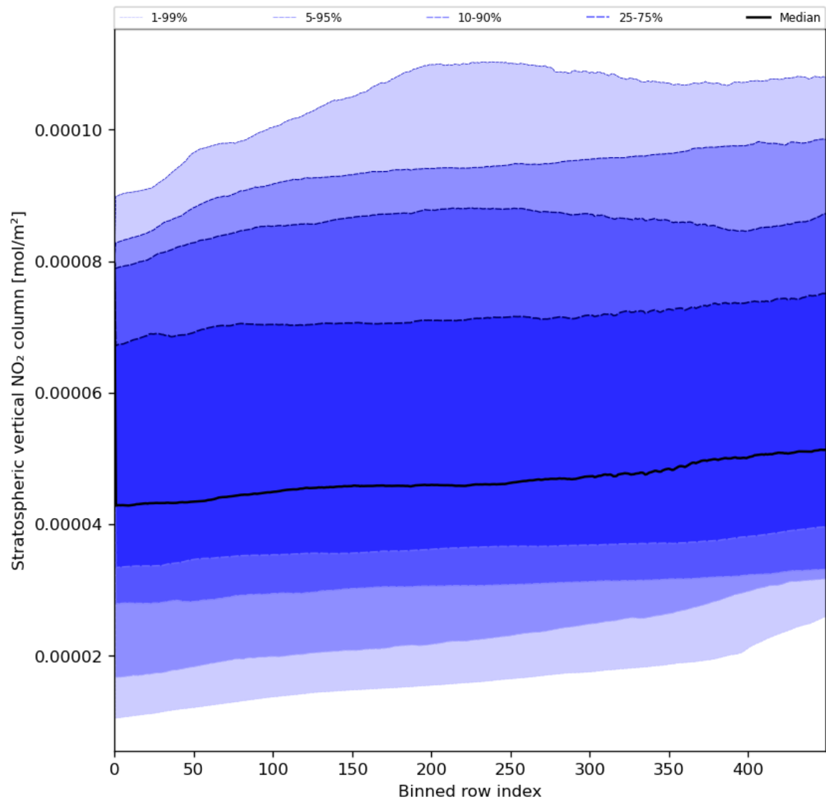
Figure 53: Along track statistics of “Stratospheric vertical NO 2 column” for 2024-07-13 to 2024-07-15
