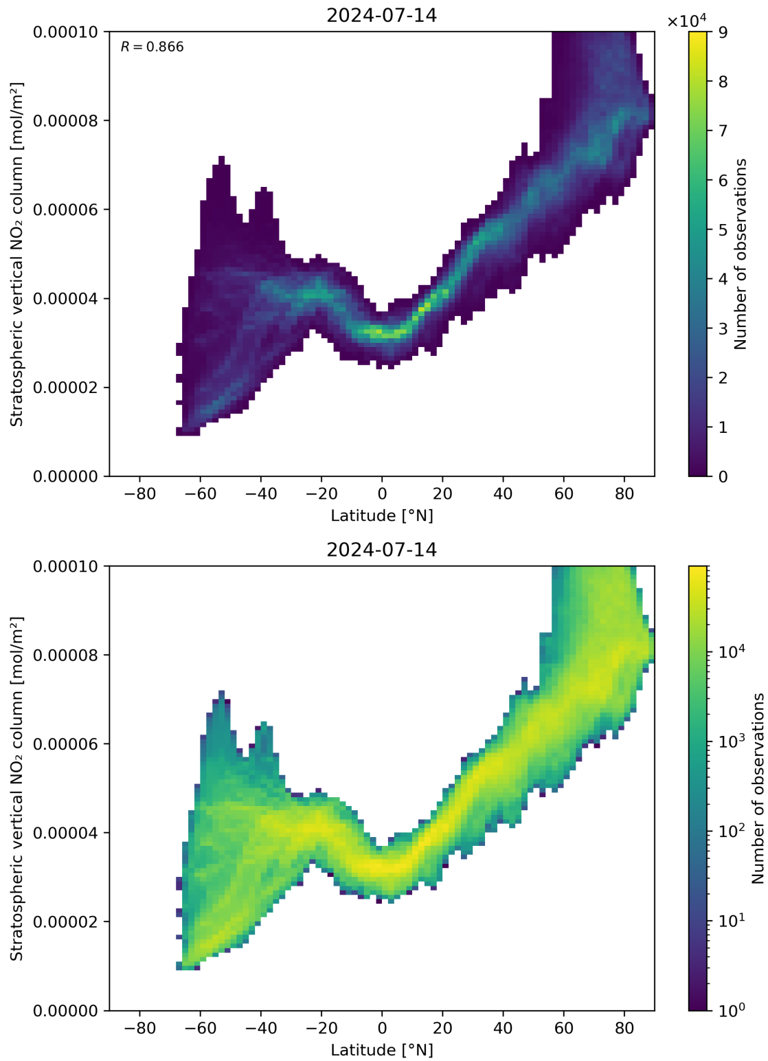
Figure 87: Scatter density plot of “Latitude” against “Stratospheric vertical NO 2 column” for 2024-07-13 to 2024-07-15.
