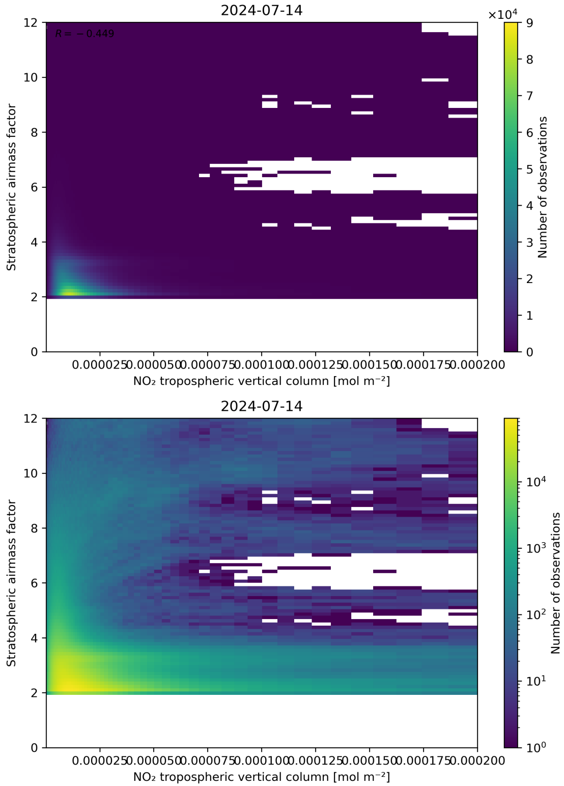
Figure 121: Scatter density plot of “NO 2 tropospheric vertical column” against “Stratospheric air mass factor” for 2024-07-13 to 2024-07-15.
