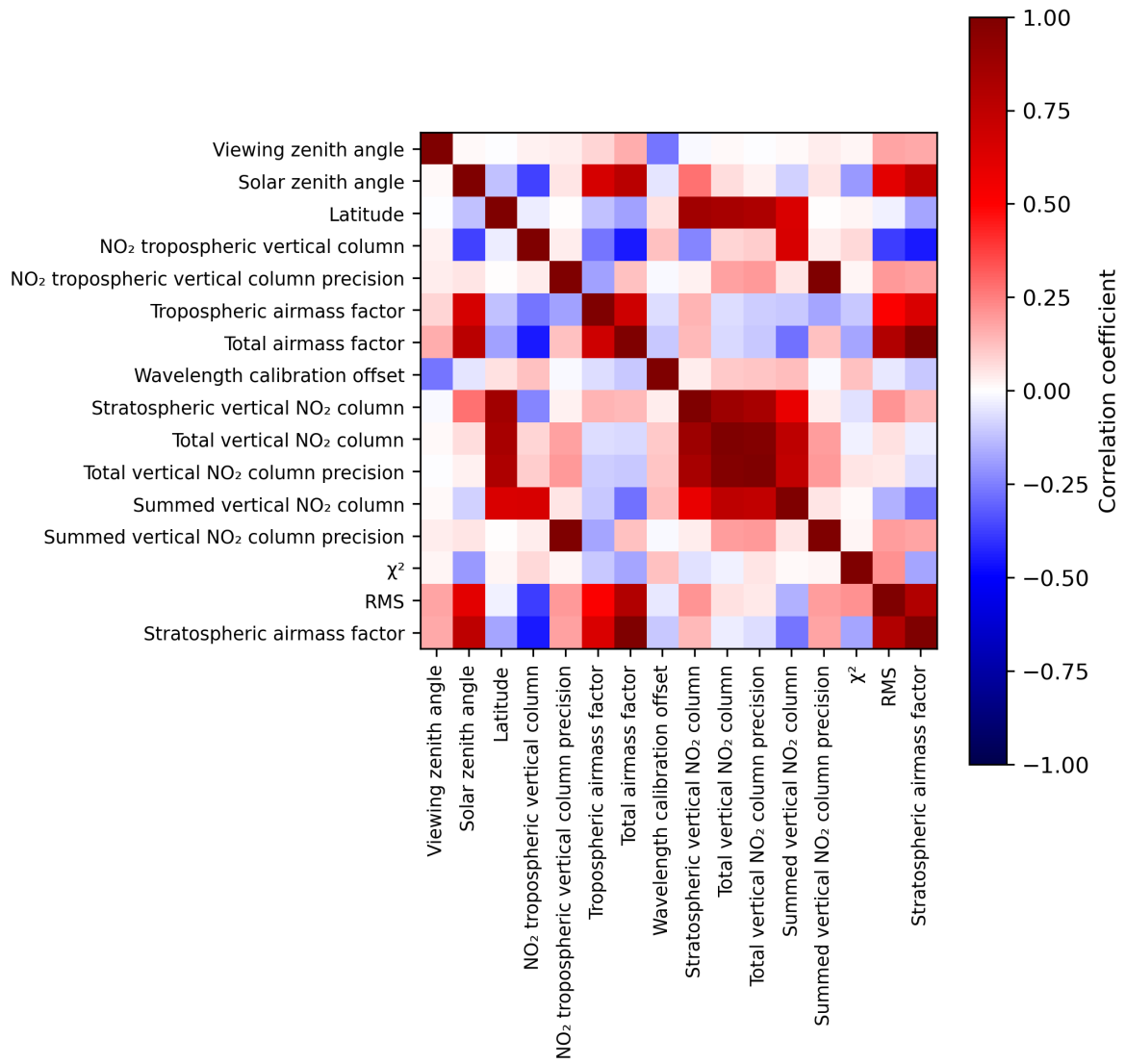
Figure 2: Map of correlation matrix for 2024-07-13 to 2024-07-15.
