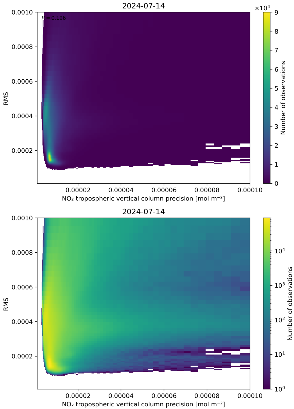
Figure 140: Scatter density plot of “NO 2 tropospheric vertical column precision” against “RMS” for 2024-07-13 to 2024-07-15.
