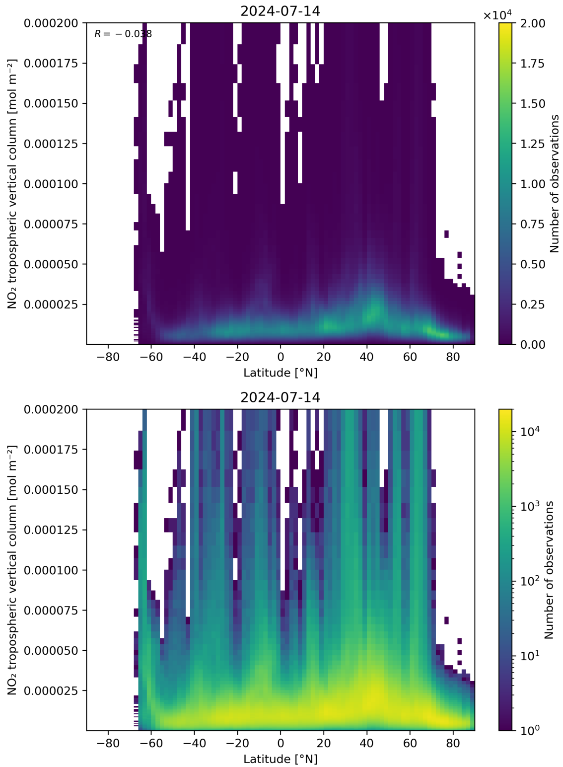
Figure 92: Scatter density plot of “Latitude” against “NO 2 tropospheric vertical column” for 2024-07-13 to 2024-07-15.
