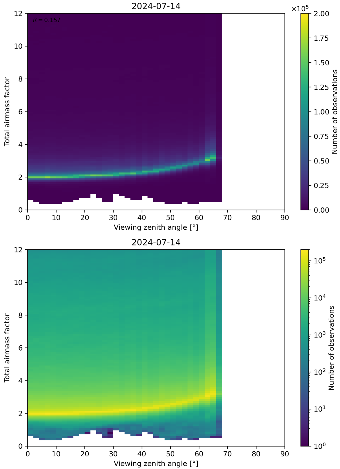
Figure 160: Scatter density plot of “Viewing zenith angle” against “Total airmass factor” for 2024-07-13 to 2024-07-15.
