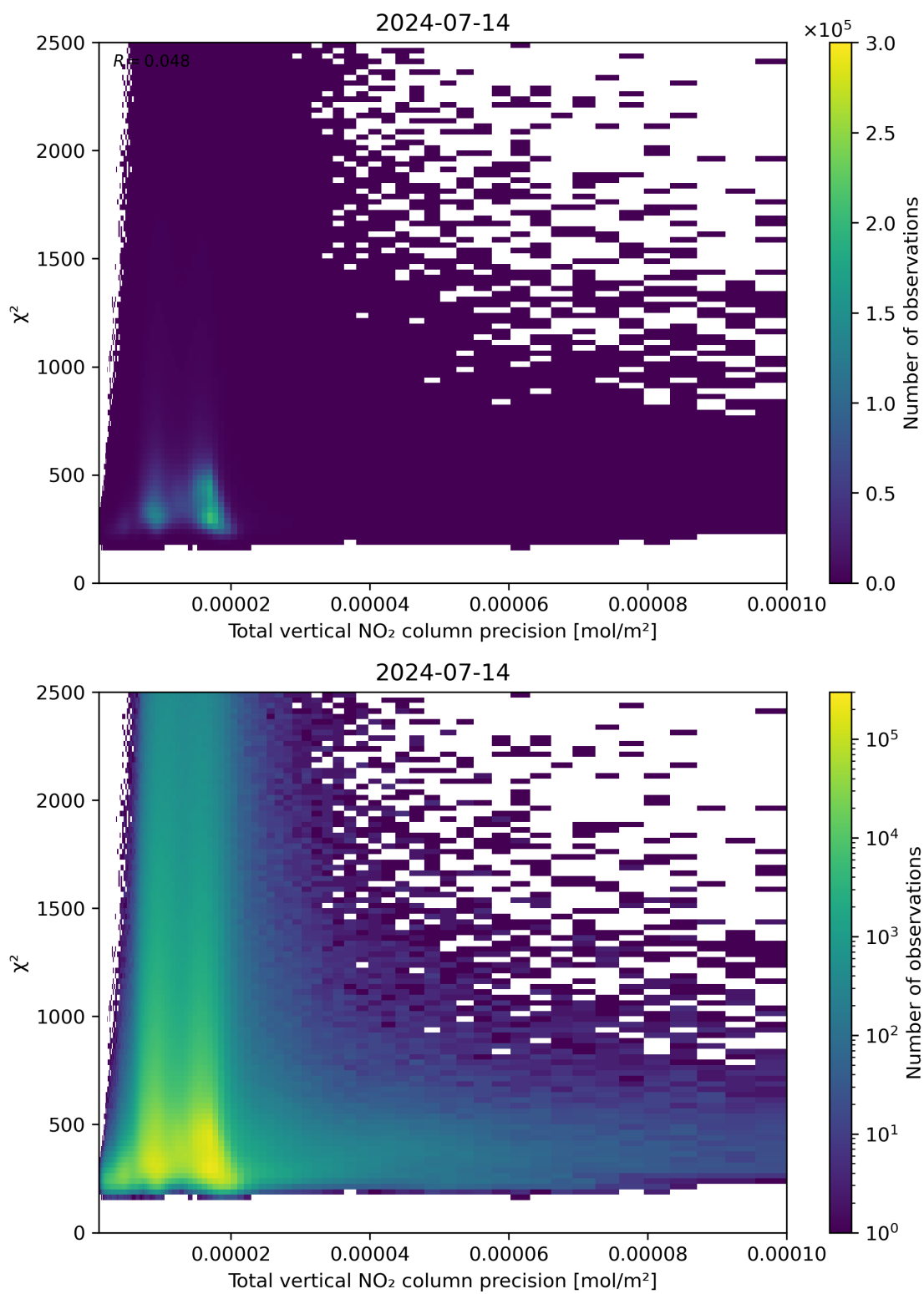
Figure 116: Scatter density plot of “Total vertical NO 2 column precision” against “ \chi^2 ” for 2024-07-13 to 2024-07-15.
