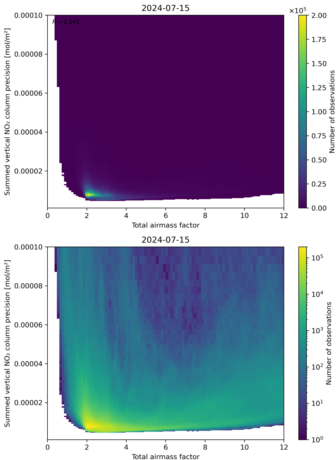
Figure 66: Scatter density plot of “Total airmass factor” against “Summed vertical NO 2 column precision” for 2024-07-15 to 2024-07-16.
