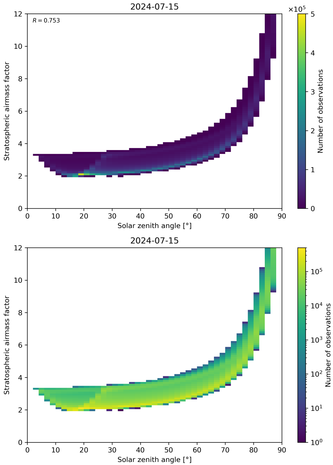
Figure 145: Scatter density plot of “Solar zenith angle” against “Stratospheric airmass factor” for 2024-07-15 to 2024-07-16.
