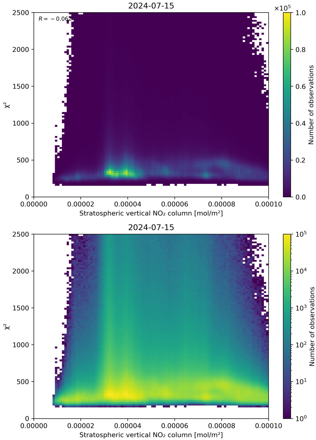
Figure 97: Scatter density plot of “Stratospheric vertical NO 2 column” against “ \chi^2 ” for 2024-07-15 to 2024-07-16.
