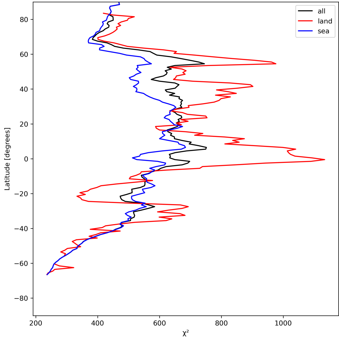
Figure 25: Zonal average of “ \chi^2 ” for 2024-07-15 to 2024-07-16.
