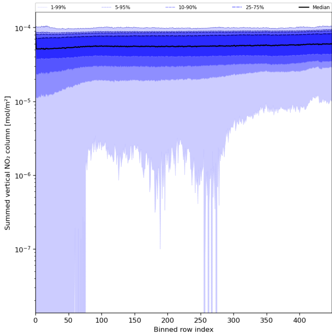
Figure 57: Along track statistics of “Summed vertical NO 2 column” for 2024-07-15 to 2024-07-16
