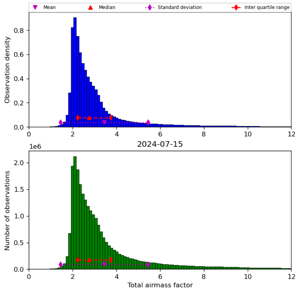
Figure 32: Histogram of “Total airmass factor” for 2024-07-15 to 2024-07-16
