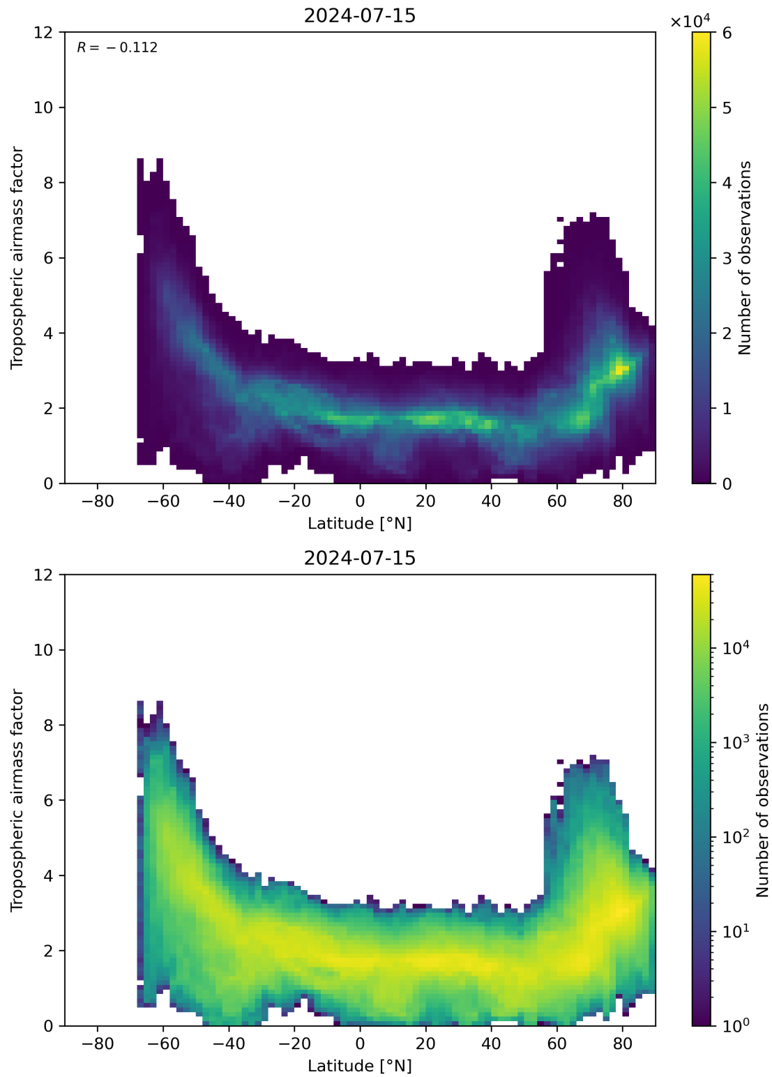
Figure 85: Scatter density plot of “Latitude” against “Tropospheric airmass factor” for 2024-07-15 to 2024-07-16.
