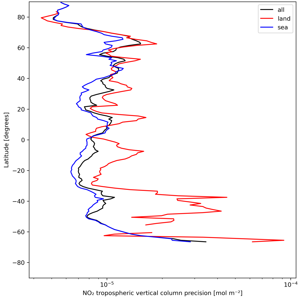
Figure 13: Zonal average of “NO 2 tropospheric vertical column precision” for 2024-07-15 to 2024-07-16.
