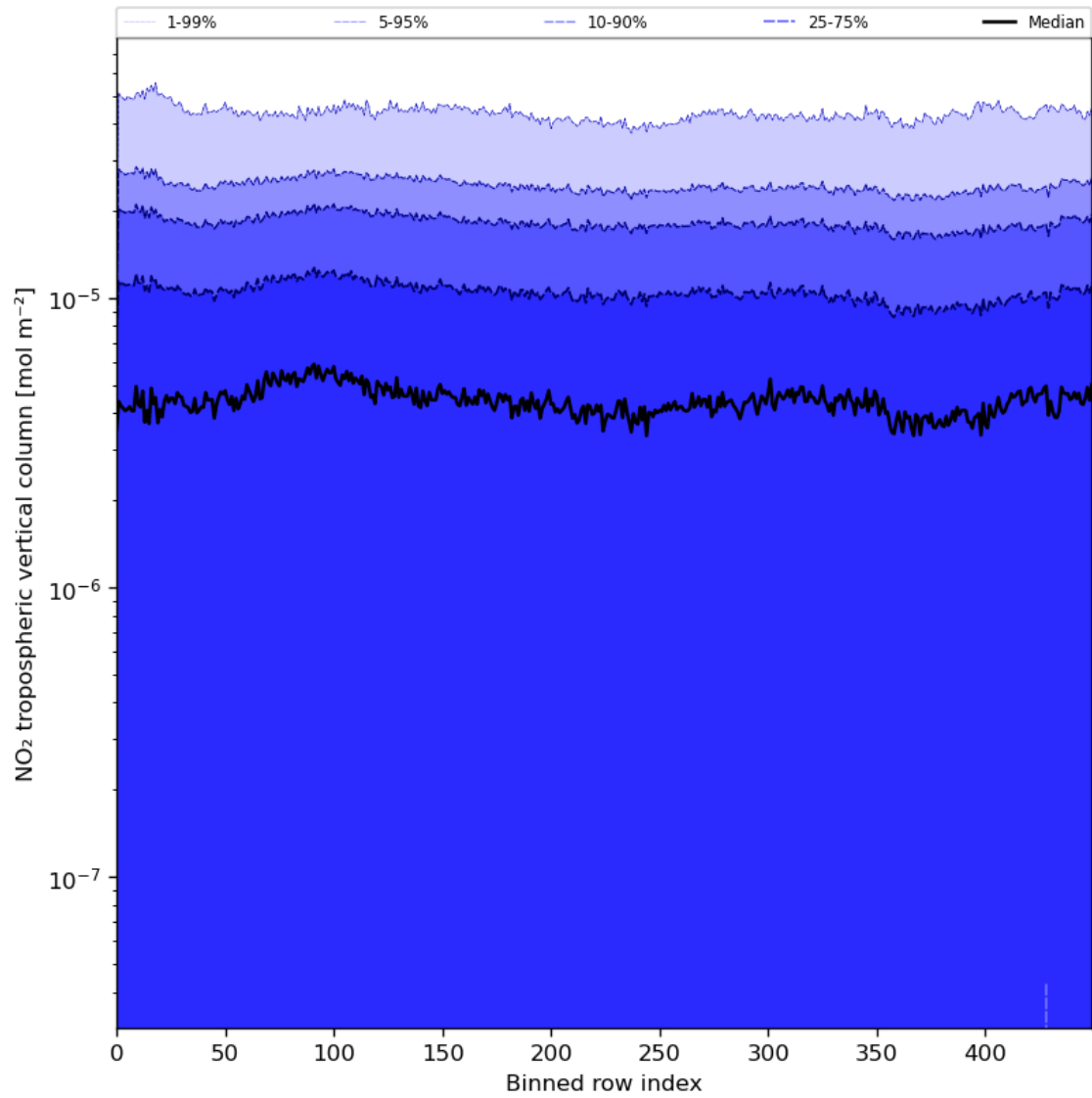
Figure 46: Along track statistics of “NO 2 tropospheric vertical column” for 2024-07-15 to 2024-07-16
