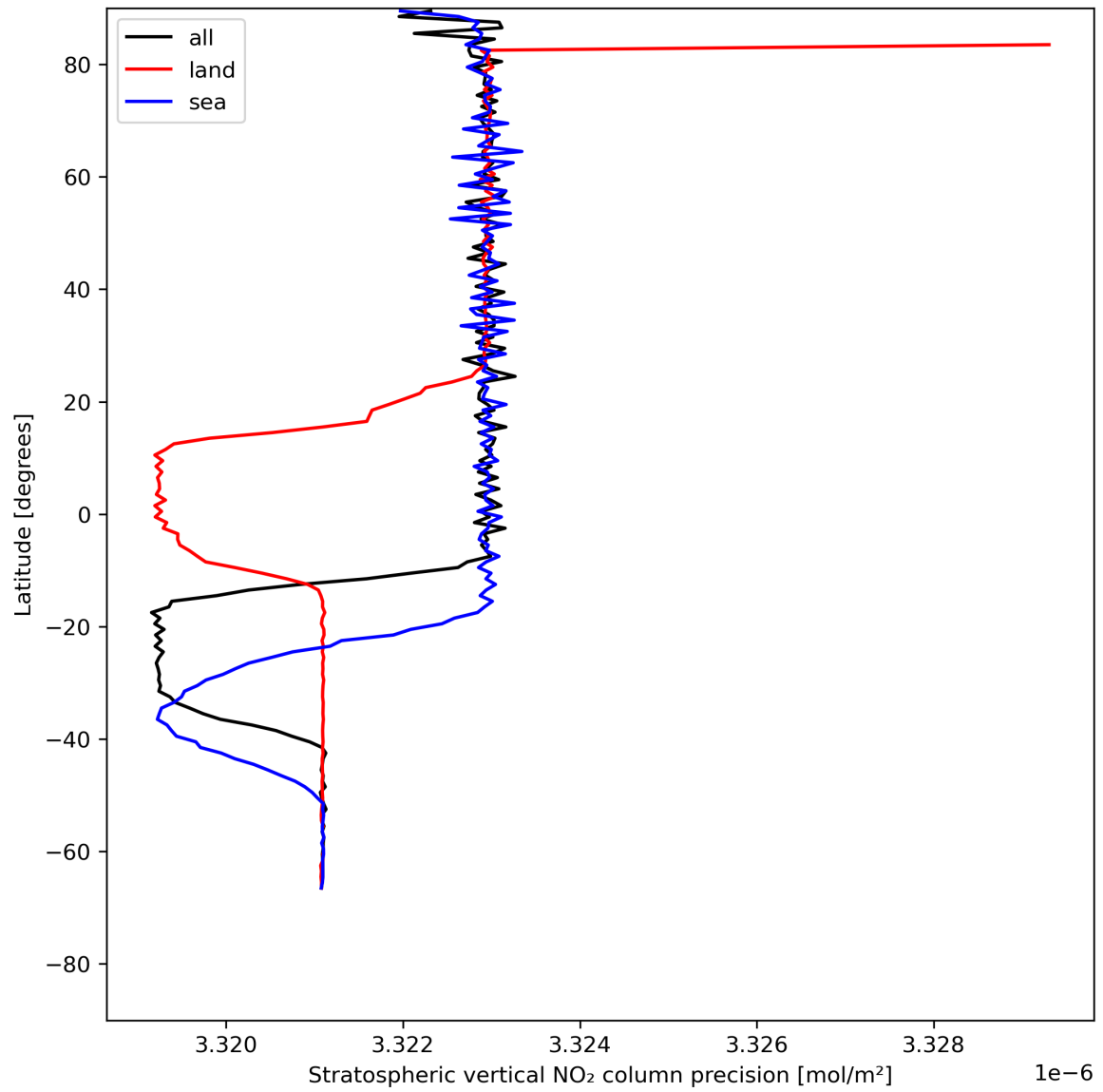
Figure 20: Zonal average of “Stratospheric vertical NO 2 column precision” for 2024-07-15 to 2024-07-16.
