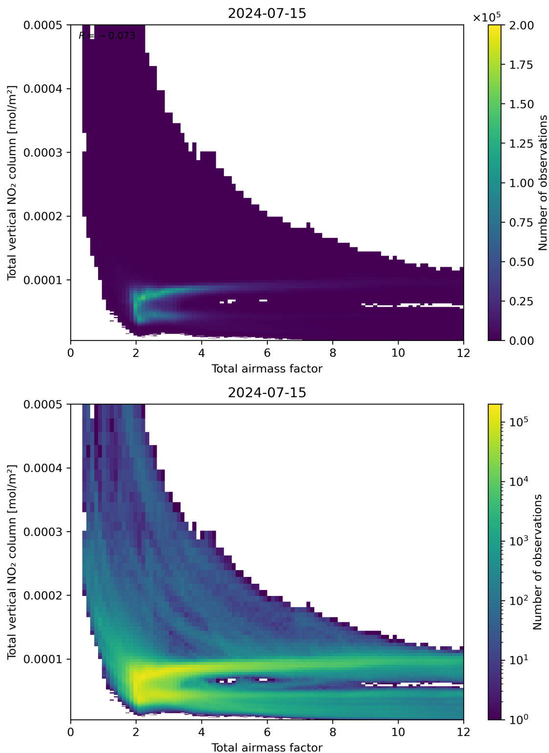
Figure 67: Scatter density plot of “Total airmass factor” against “Total vertical NO 2 column” for 2024-07-15 to 2024-07-16.
