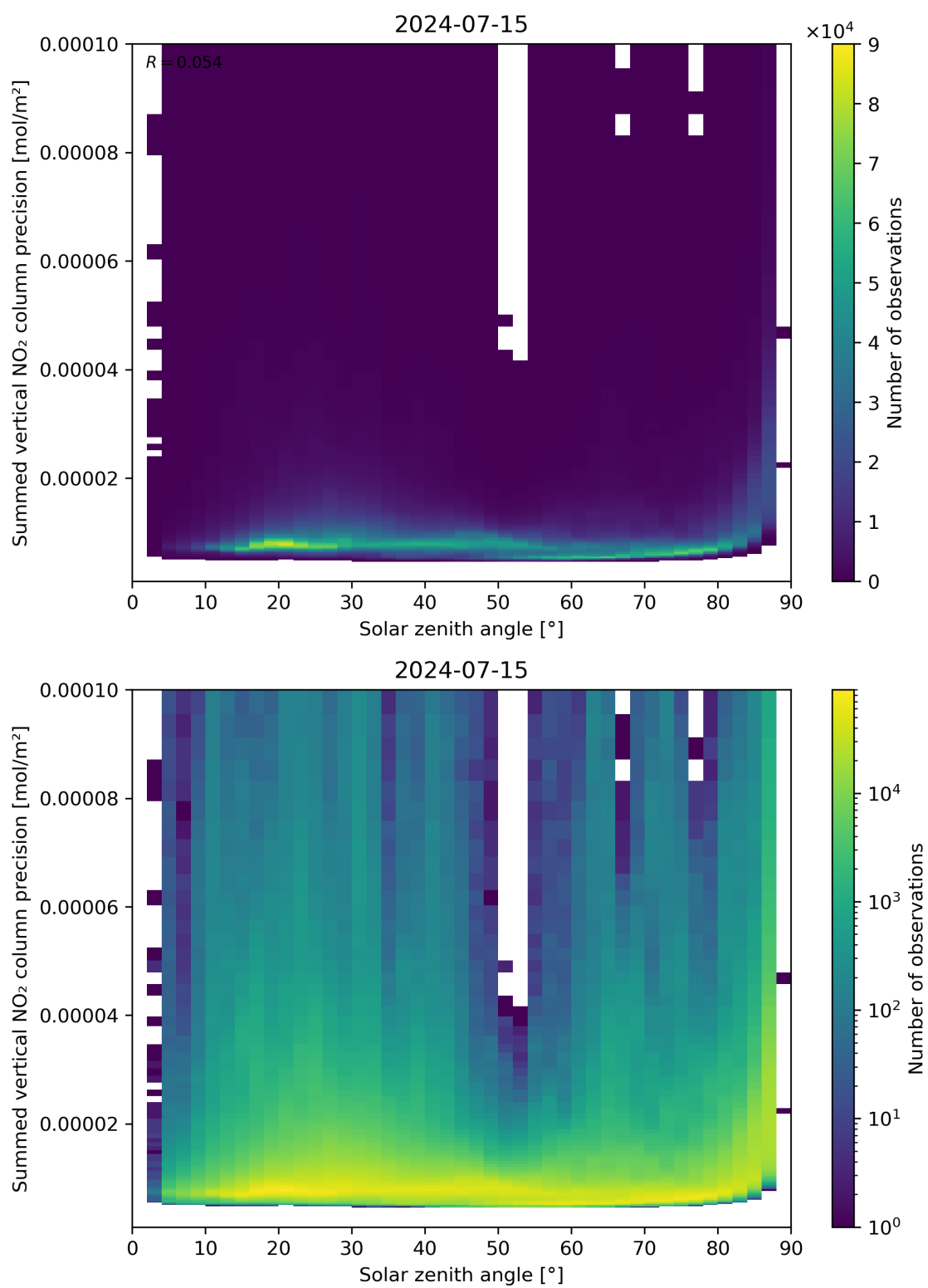
Figure 152: Scatter density plot of “Solar zenith angle” against “Summed vertical NO 2 column precision” for 2024-07-15 to 2024-07-16.
