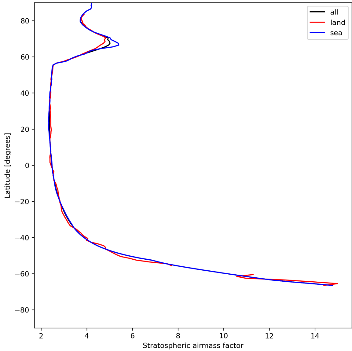
Figure 27: Zonal average of “Stratospheric air mass factor” for 2024-07-15 to 2024-07-16.
