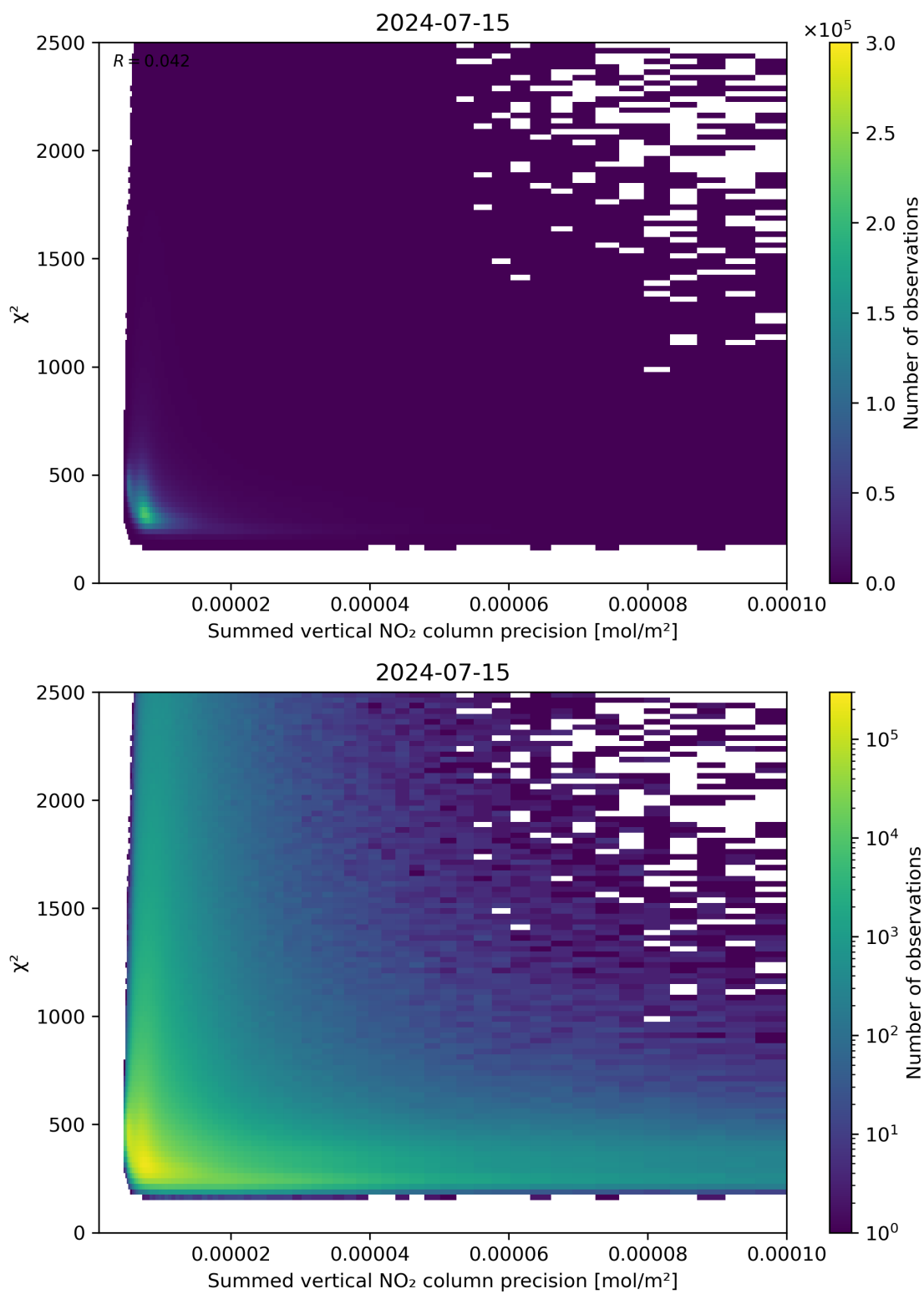
Figure 107: Scatter density plot of “Summed vertical NO 2 column precision” against “ \chi^2 ” for 2024-07-15 to 2024-07-16.
