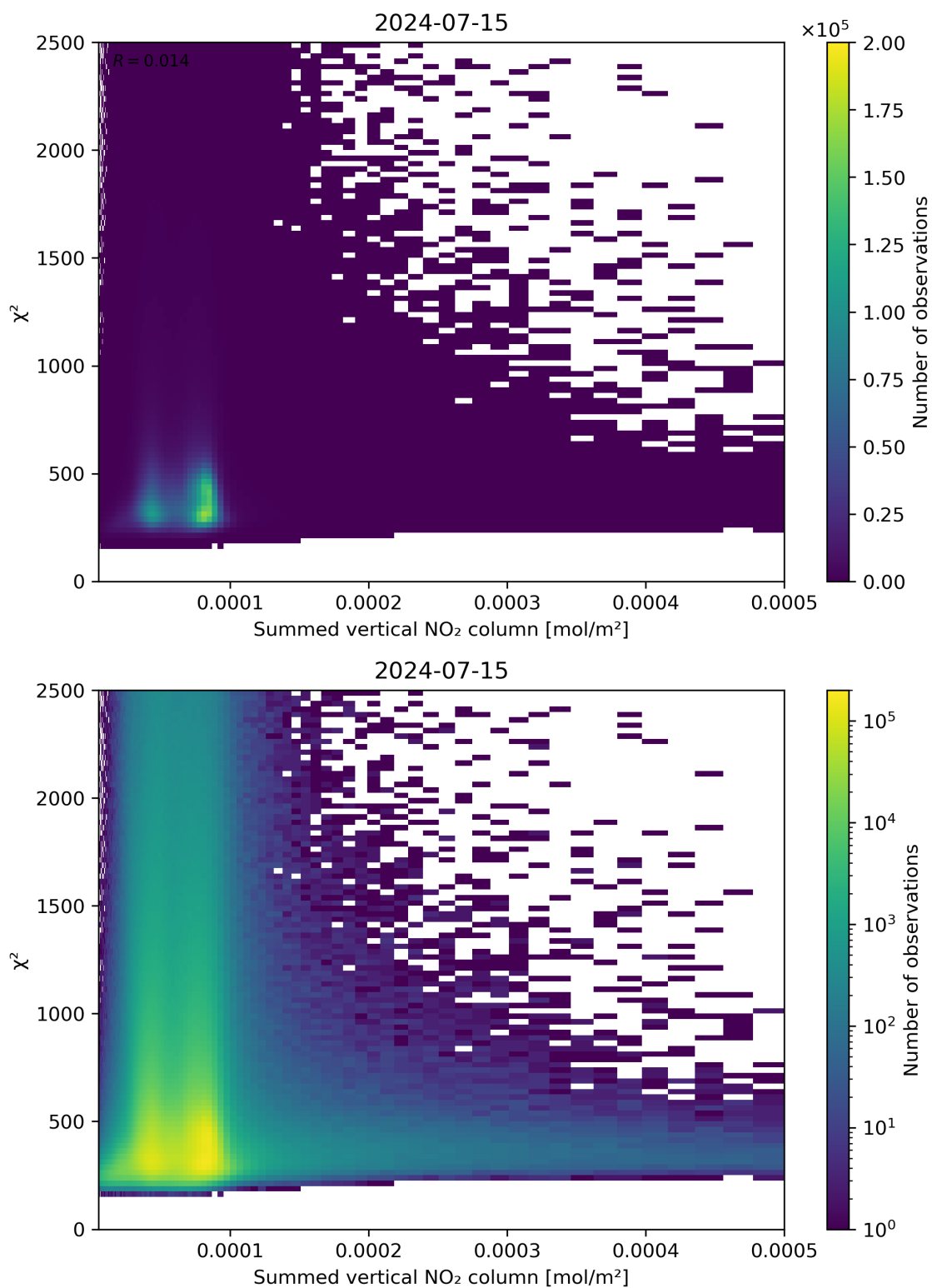
Figure 104: Scatter density plot of “Summed vertical NO 2 column” against “ \chi^2 ” for 2024-07-15 to 2024-07-16.
