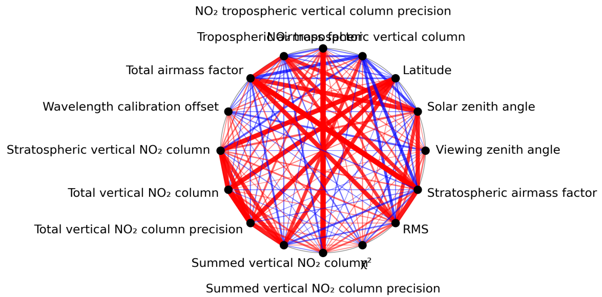
Figure 1: Map of correlation graph for 2024-07-15 to 2024-07-16.
