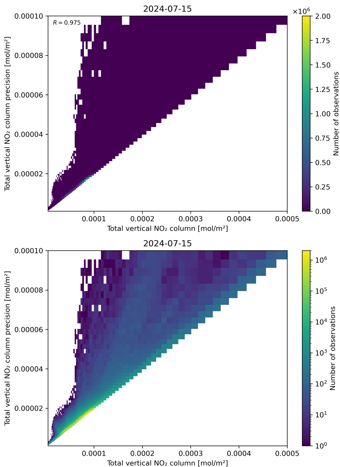
Figure 114: Scatter density plot of “Total vertical NO 2 column” against “Total vertical NO 2 column precision” for 2024-07-15 to 2024-07-16.
