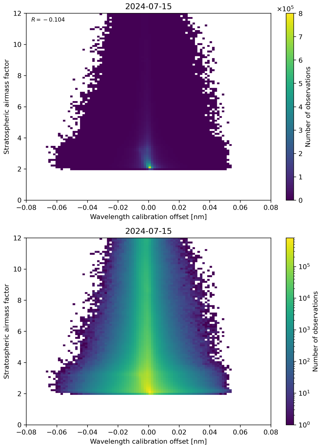
Figure 174: Scatter density plot of “Wavelength calibration offset” against “Stratospheric air mass factor” for 2024-07-15 to 2024-07-16.
