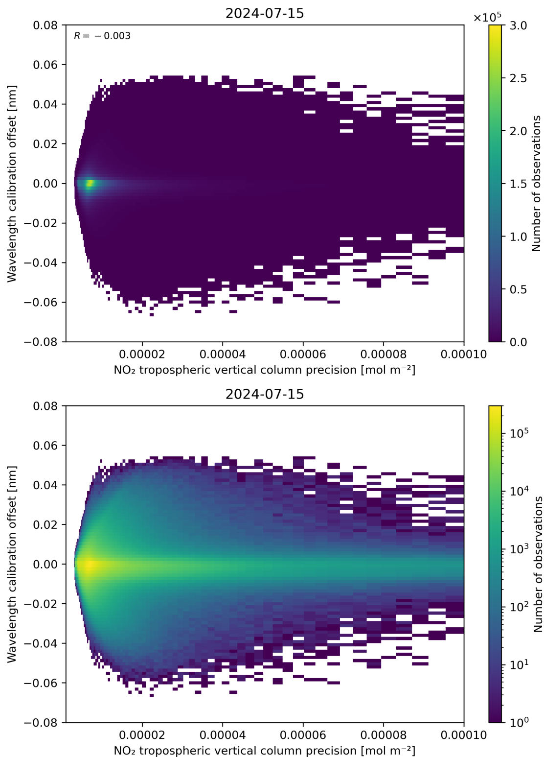
Figure 141: Scatter density plot of “NO 2 tropospheric vertical column precision” against “Wavelength calibration offset” for 2024-07-15 to 2024-07-16.
