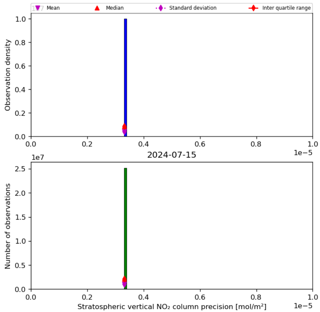
Figure 37: Histogram of “Stratospheric vertical NO 2 column precision” for 2024-07-15 to 2024-07-16
