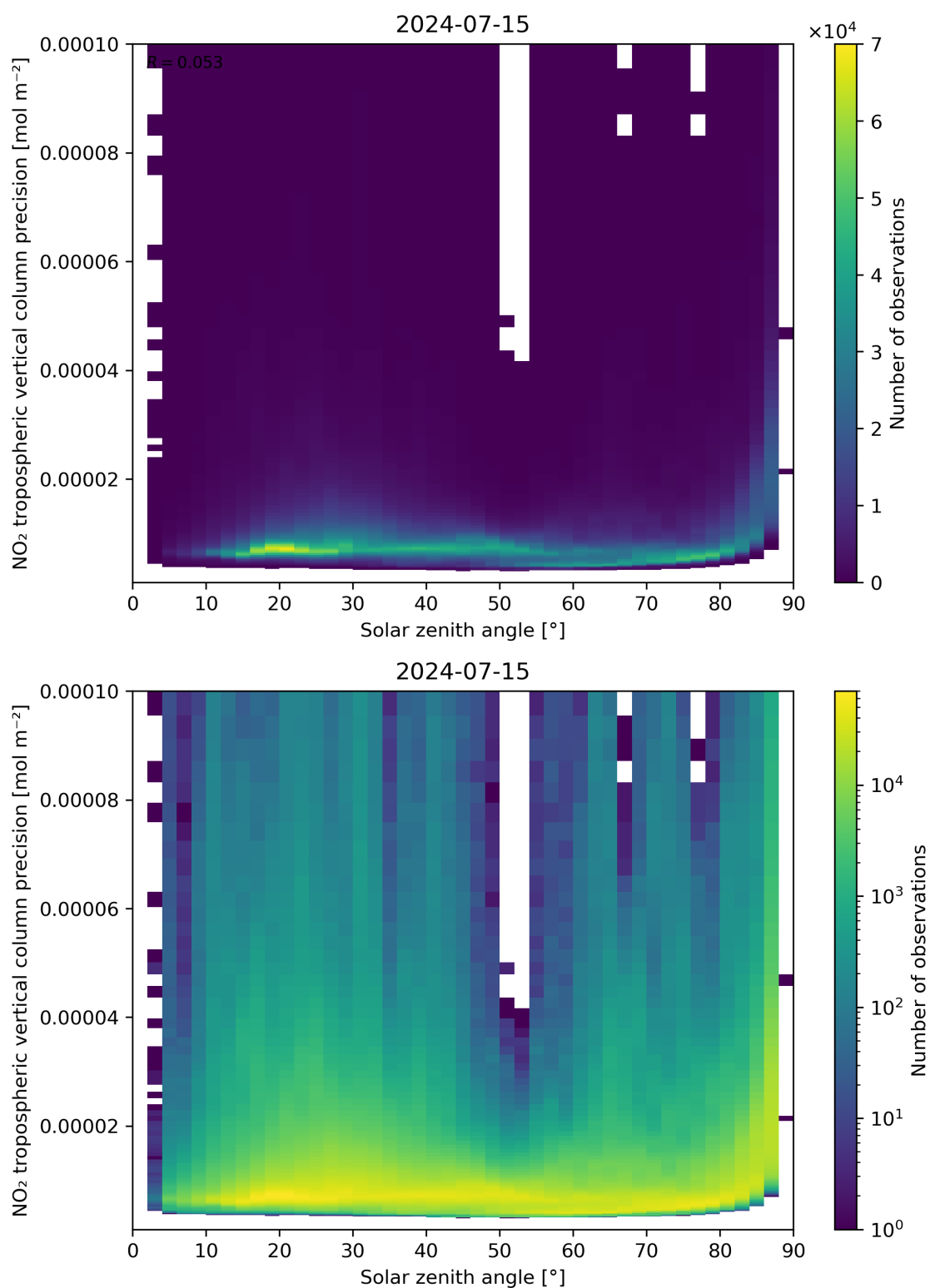
Figure 156: Scatter density plot of “Solar zenith angle” against “NO 2 tropospheric vertical column precision” for 2024-07-15 to 2024-07-16.
