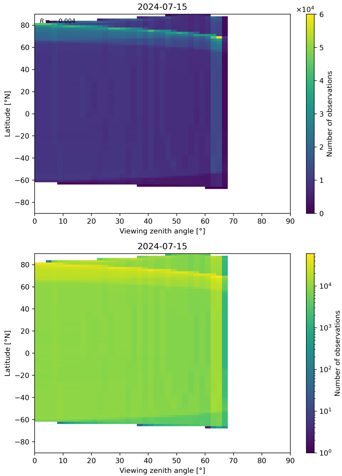
Figure 163: Scatter density plot of “Viewing zenith angle” against “Latitude” for 2024-07-15 to 2024-07-16.
