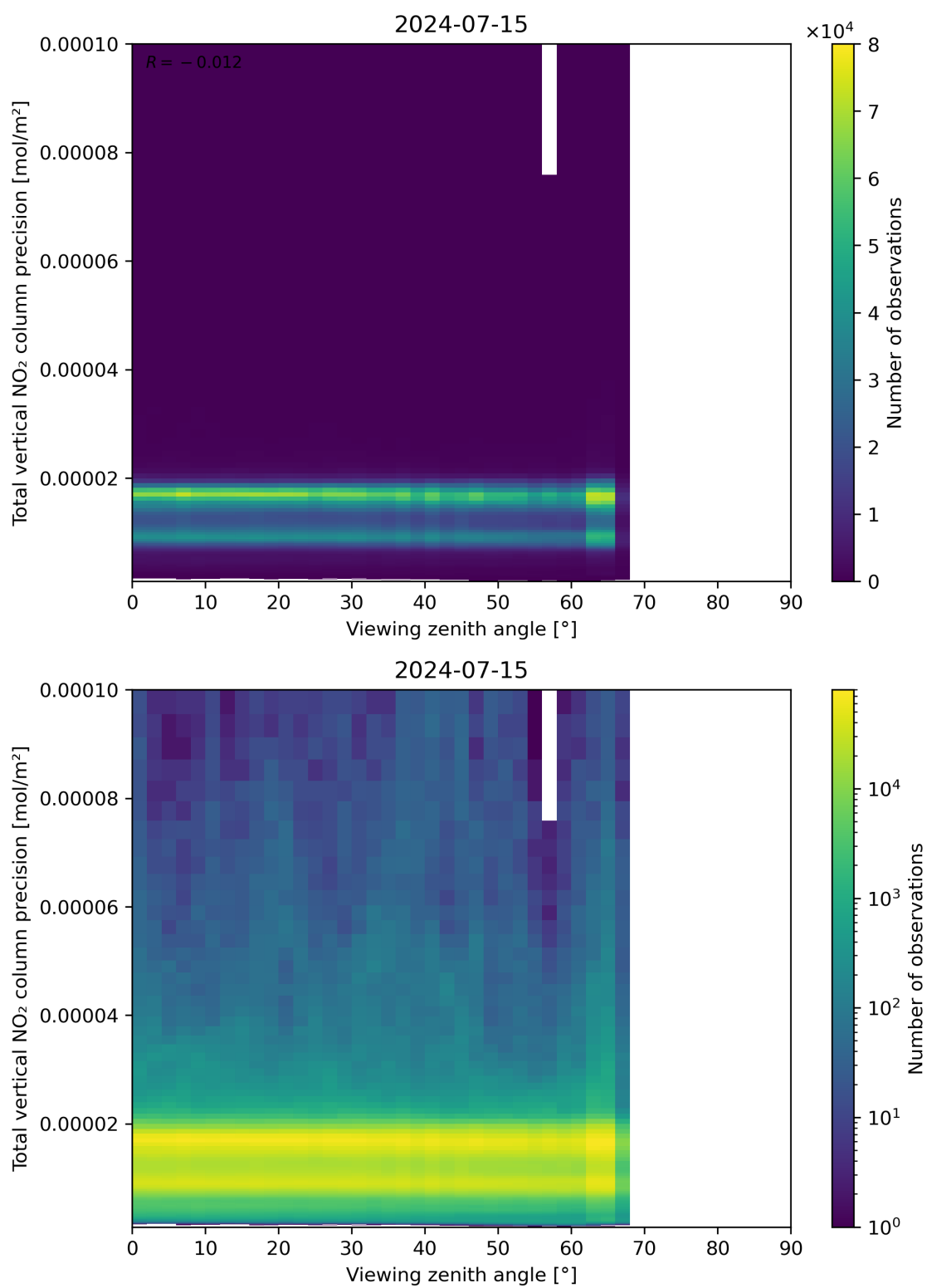
Figure 168: Scatter density plot of “Viewing zenith angle” against “Total vertical NO 2 column precision” for 2024-07-15 to 2024-07-16.
