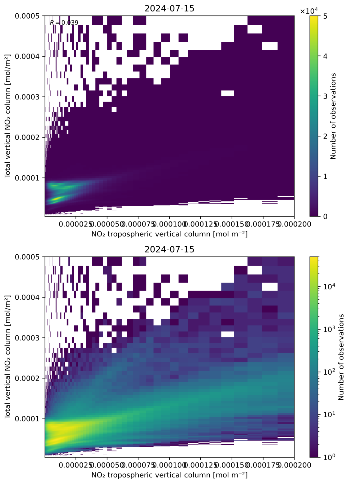
Figure 128: Scatter density plot of “NO 2 tropospheric vertical column” against “Total vertical NO 2 column” for 2024-07-15 to 2024-07-16.
