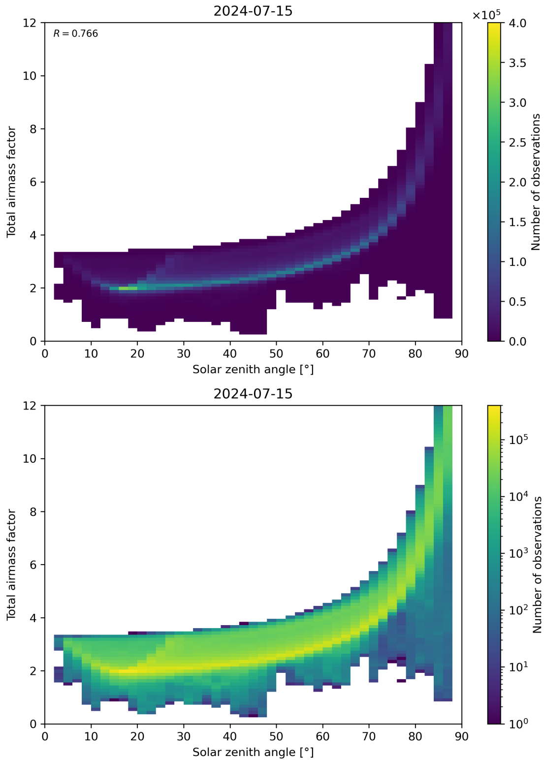
Figure 146: Scatter density plot of “Solar zenith angle” against “Total air mass factor” for 2024-07-15 to 2024-07-16.
