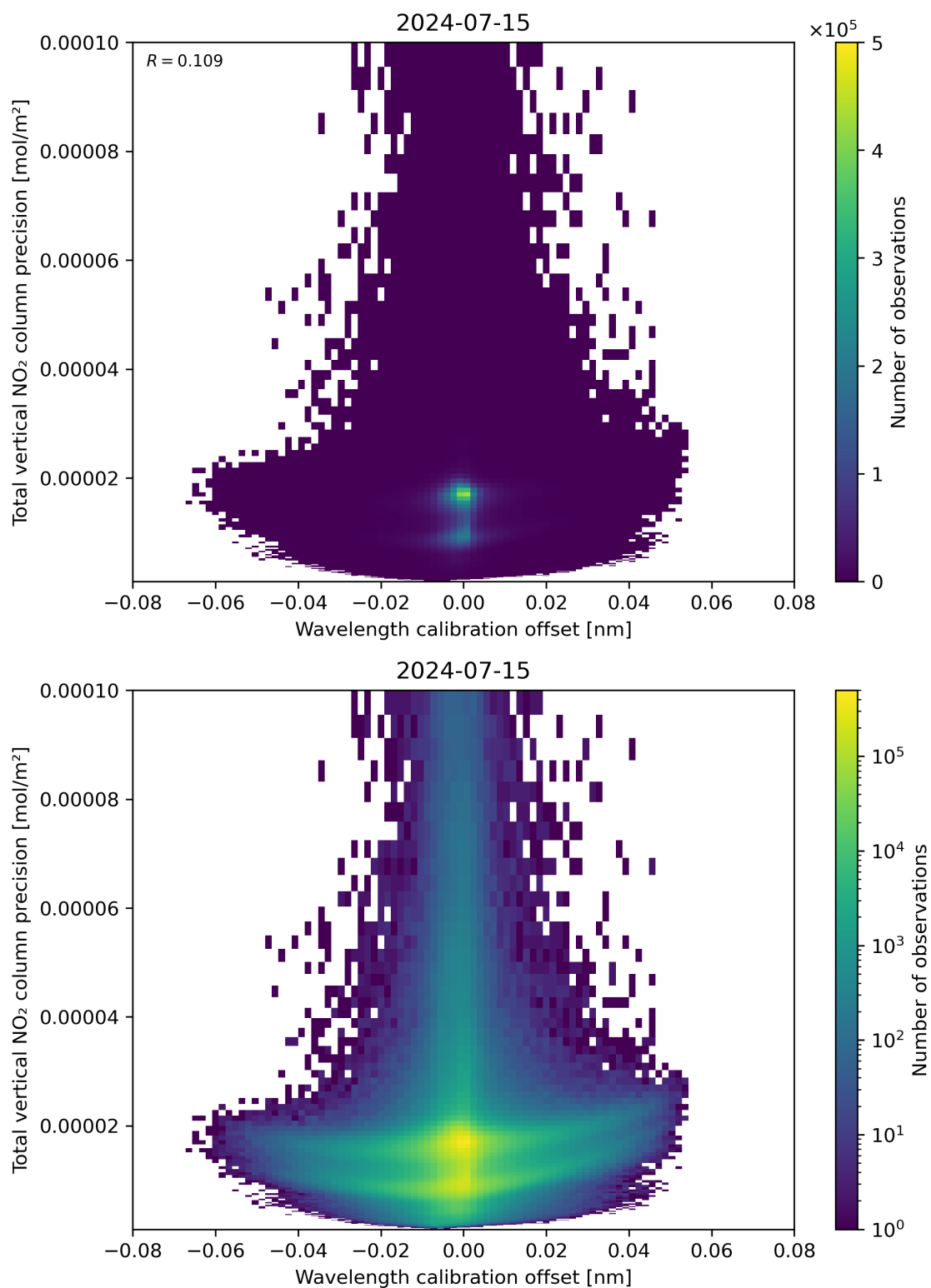
Figure 180: Scatter density plot of “Wavelength calibration offset” against “Total vertical NO 2 column precision” for 2024-07-15 to 2024-07-16.
