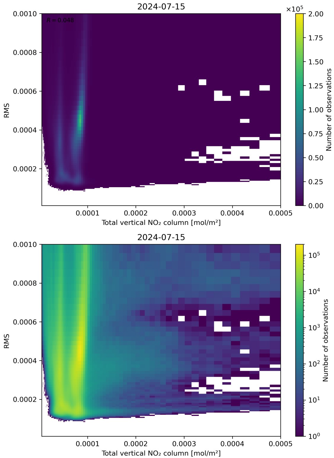
Figure 120: Scatter density plot of “Total vertical NO 2 column” against “RMS” for 2024-07-15 to 2024-07-16.
