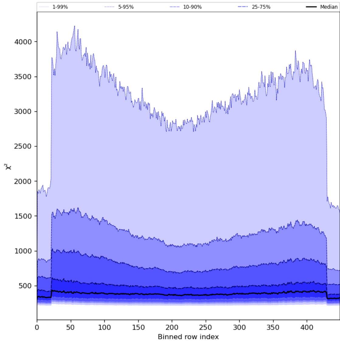
Figure 59: Along track statistics of “ \chi^2 ” for 2024-07-15 to 2024-07-16
