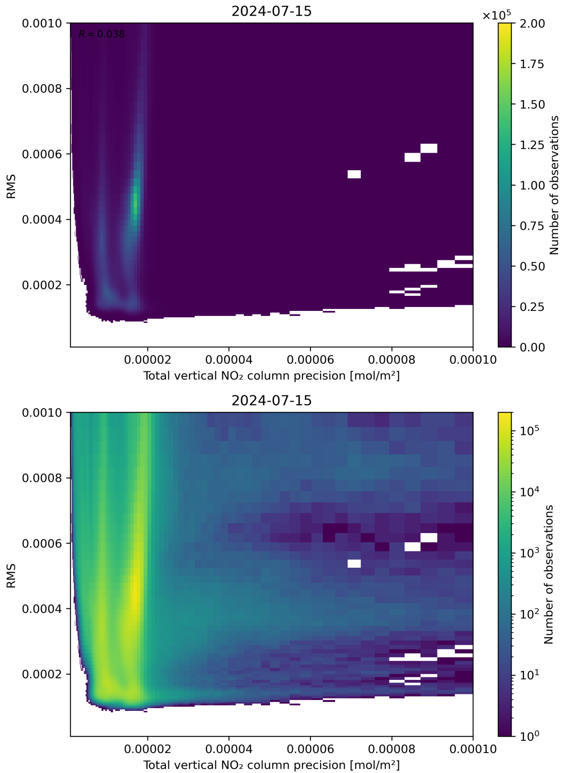
Figure 119: Scatter density plot of “Total vertical NO 2 column precision” against “RMS” for 2024-07-15 to 2024-07-16.
