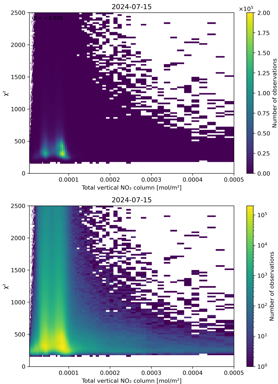
Figure 111: Scatter density plot of “Total vertical NO 2 column” against “ \chi^2 ” for 2024-07-15 to 2024-07-16.
