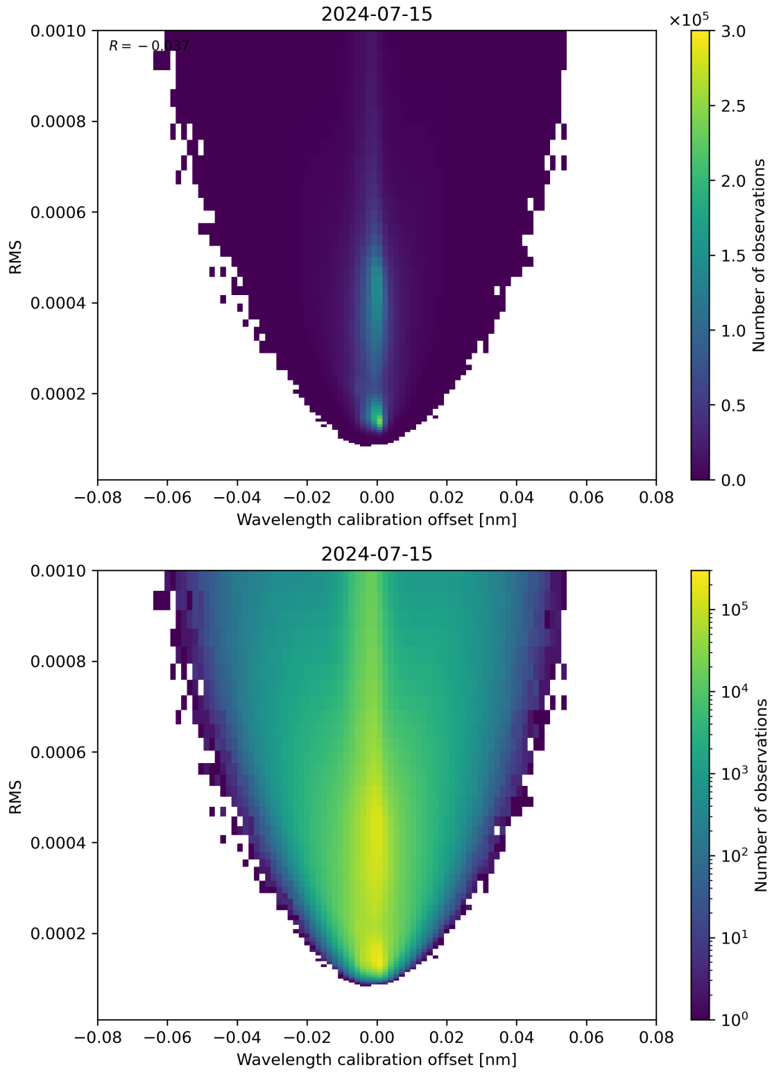
Figure 181: Scatter density plot of “Wavelength calibration offset” against “RMS” for 2024-07-15 to 2024-07-16.
