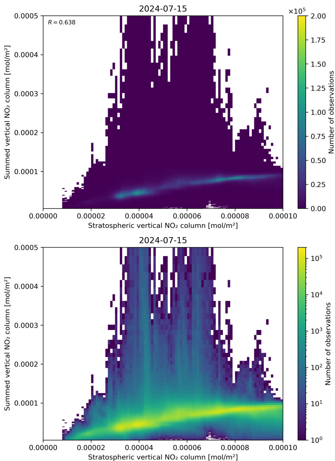
Figure 98: Scatter density plot of “Stratospheric vertical NO 2 column” against “Summed vertical NO 2 column” for 2024-07-15 to 2024-07-16.
