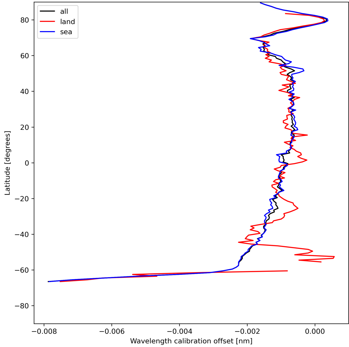
Figure 18: Zonal average of “Wavelength calibration offset” for 2024-07-15 to 2024-07-16.
