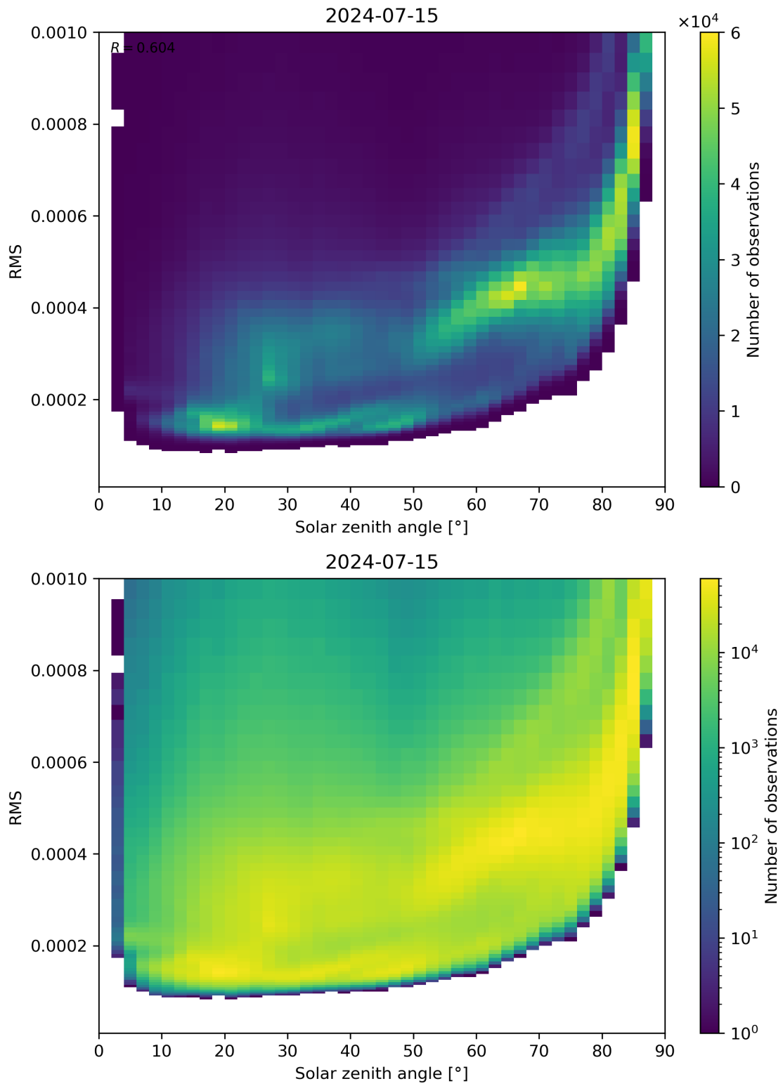
Figure 157: Scatter density plot of “Solar zenith angle” against “RMS” for 2024-07-15 to 2024-07-16.
