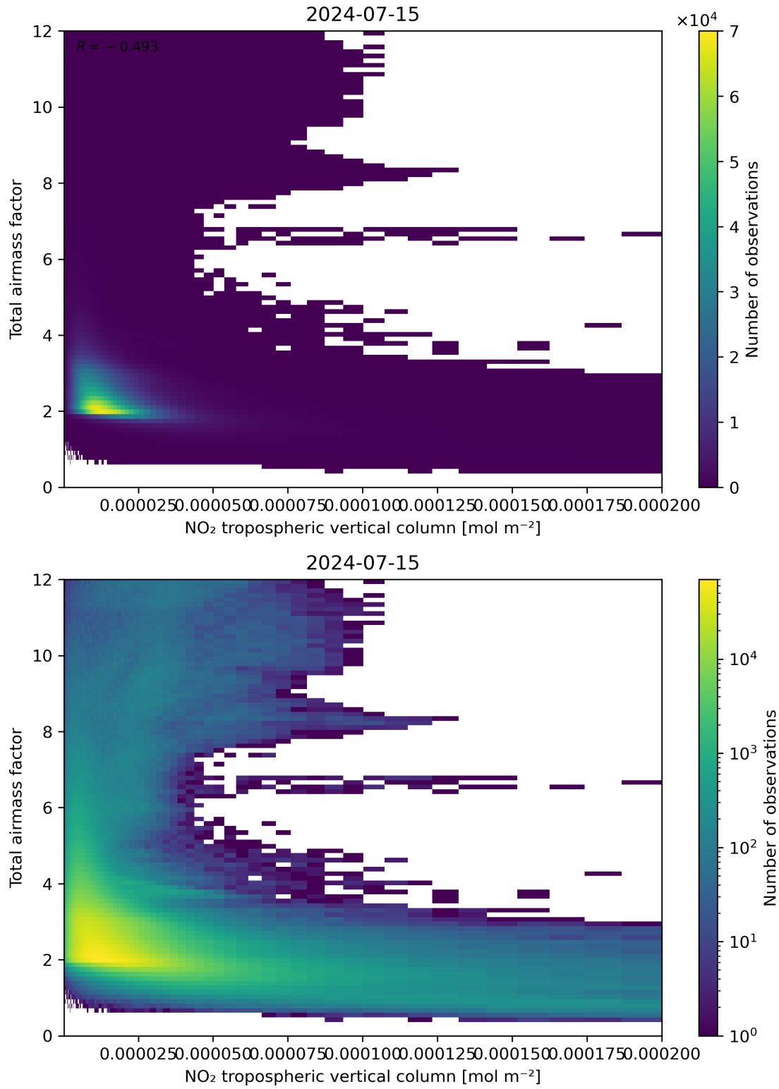
Figure 122: Scatter density plot of “NO 2 tropospheric vertical column” against “Total air mass factor” for 2024-07-15 to 2024-07-16.
