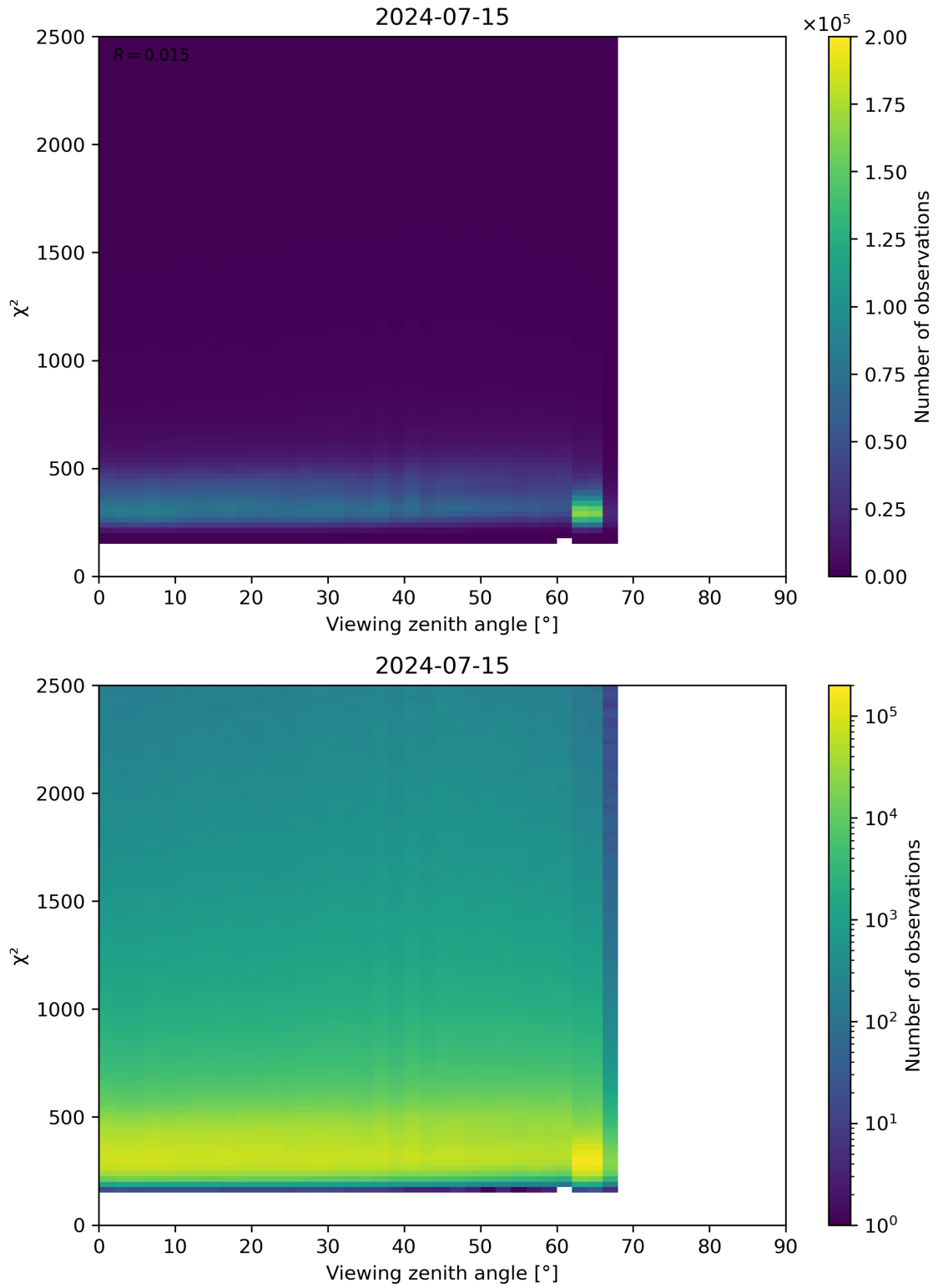
Figure 162: Scatter density plot of “Viewing zenith angle” against “ \chi^2 ” for 2024-07-15 to 2024-07-16.
