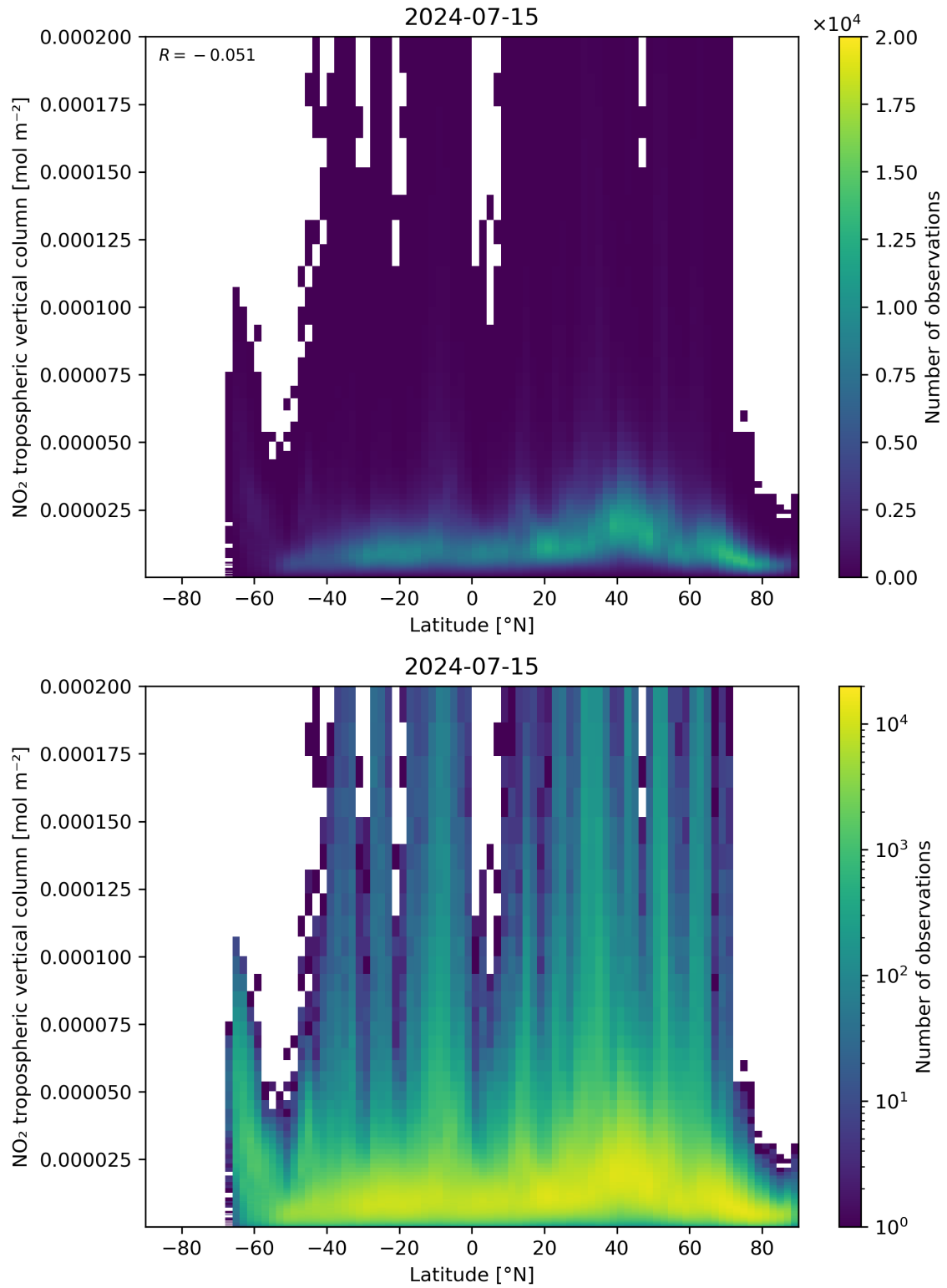
Figure 92: Scatter density plot of “Latitude” against “NO 2 tropospheric vertical column” for 2024-07-15 to 2024-07-16.
