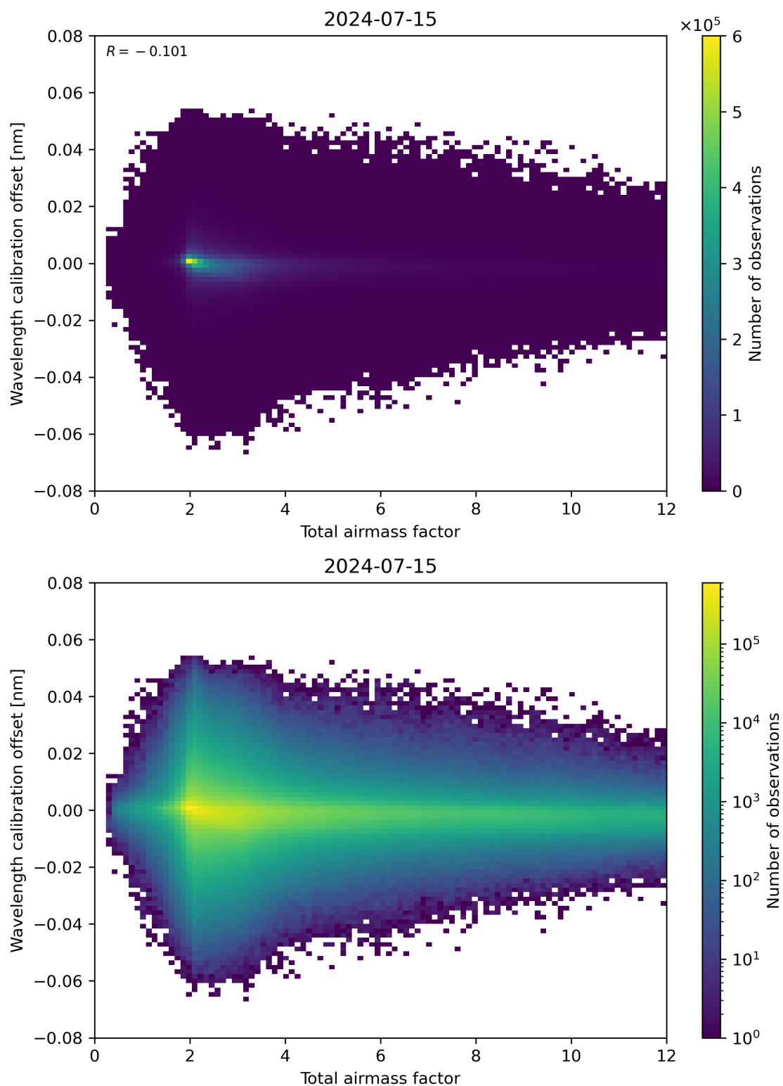
Figure 70: Scatter density plot of “Total airmass factor” against “Wavelength calibration offset” for 2024-07-15 to 2024-07-16.
