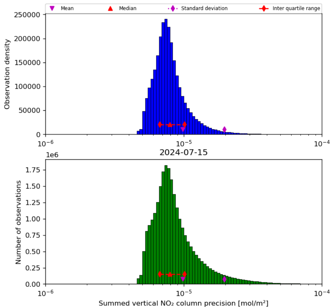
Figure 41: Histogram of "Summed vertical NO 2 column precision" for 2024-07-15 to 2024-07-16
