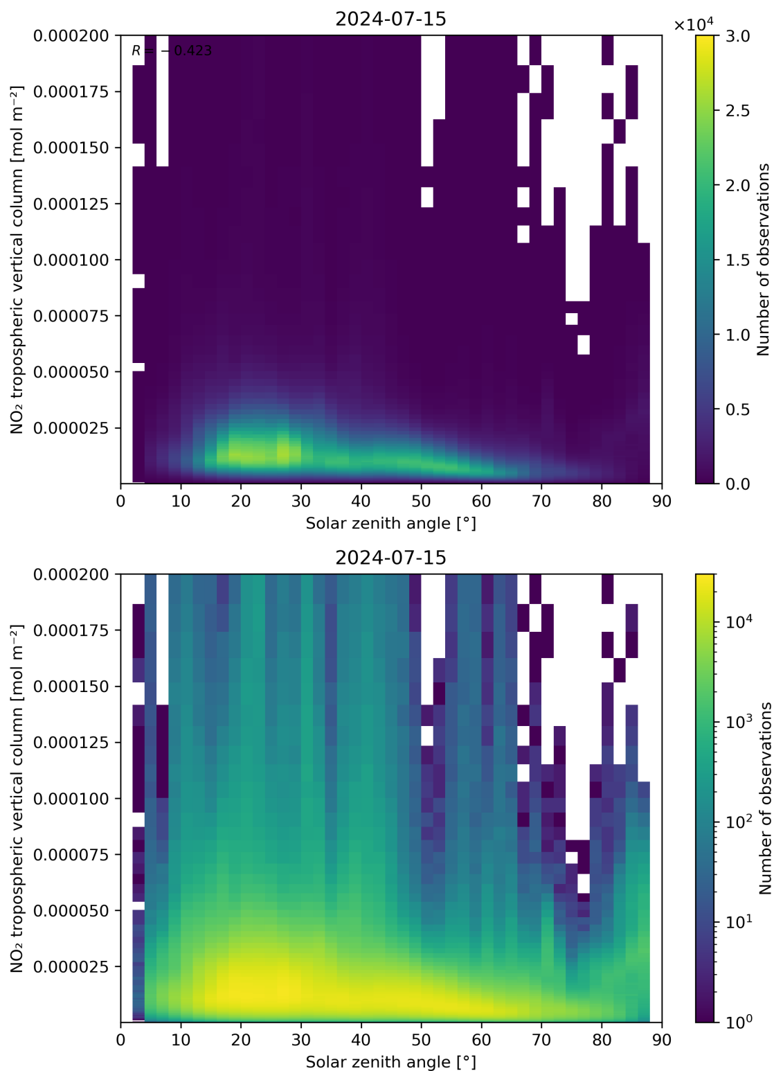
Figure 155: Scatter density plot of “Solar zenith angle” against “NO 2 tropospheric vertical column” for 2024-07-15 to 2024-07-16.
