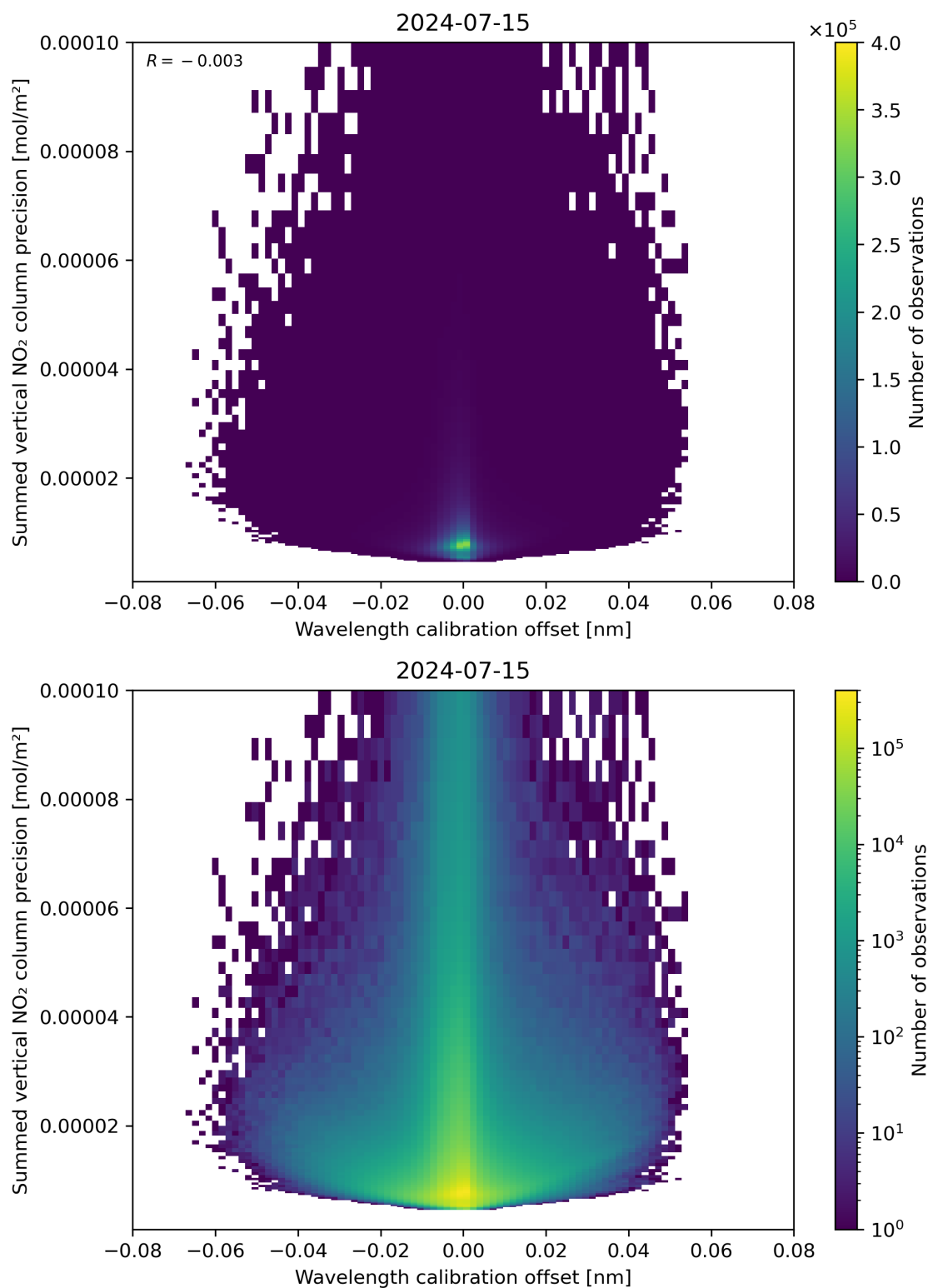
Figure 178: Scatter density plot of “Wavelength calibration offset” against “Summed vertical NO 2 column precision” for 2024-07-15 to 2024-07-16.
