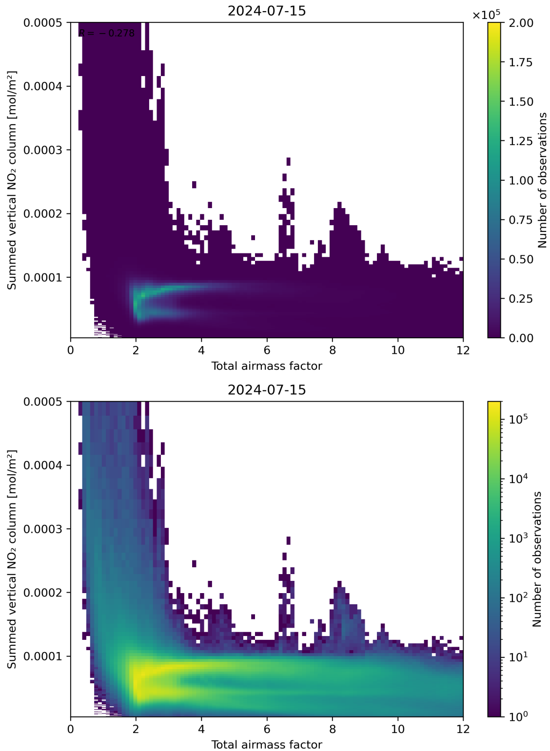
Figure 65: Scatter density plot of “Total airmass factor” against “Summed vertical NO 2 column” for 2024-07-15 to 2024-07-16.
