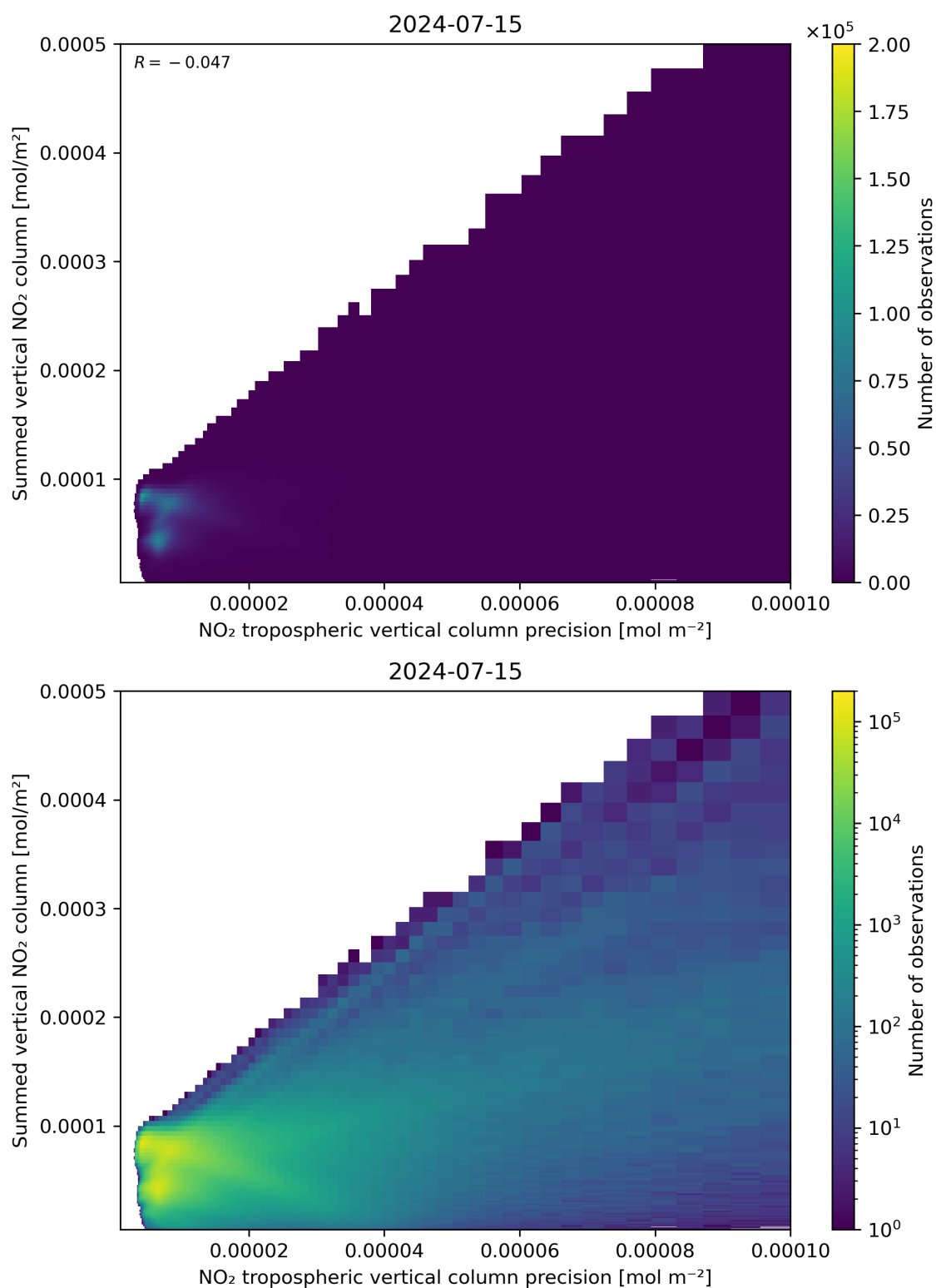
Figure 136: Scatter density plot of “NO 2 tropospheric vertical column precision” against “Summed vertical NO 2 column” for 2024-07-15 to 2024-07-16.
