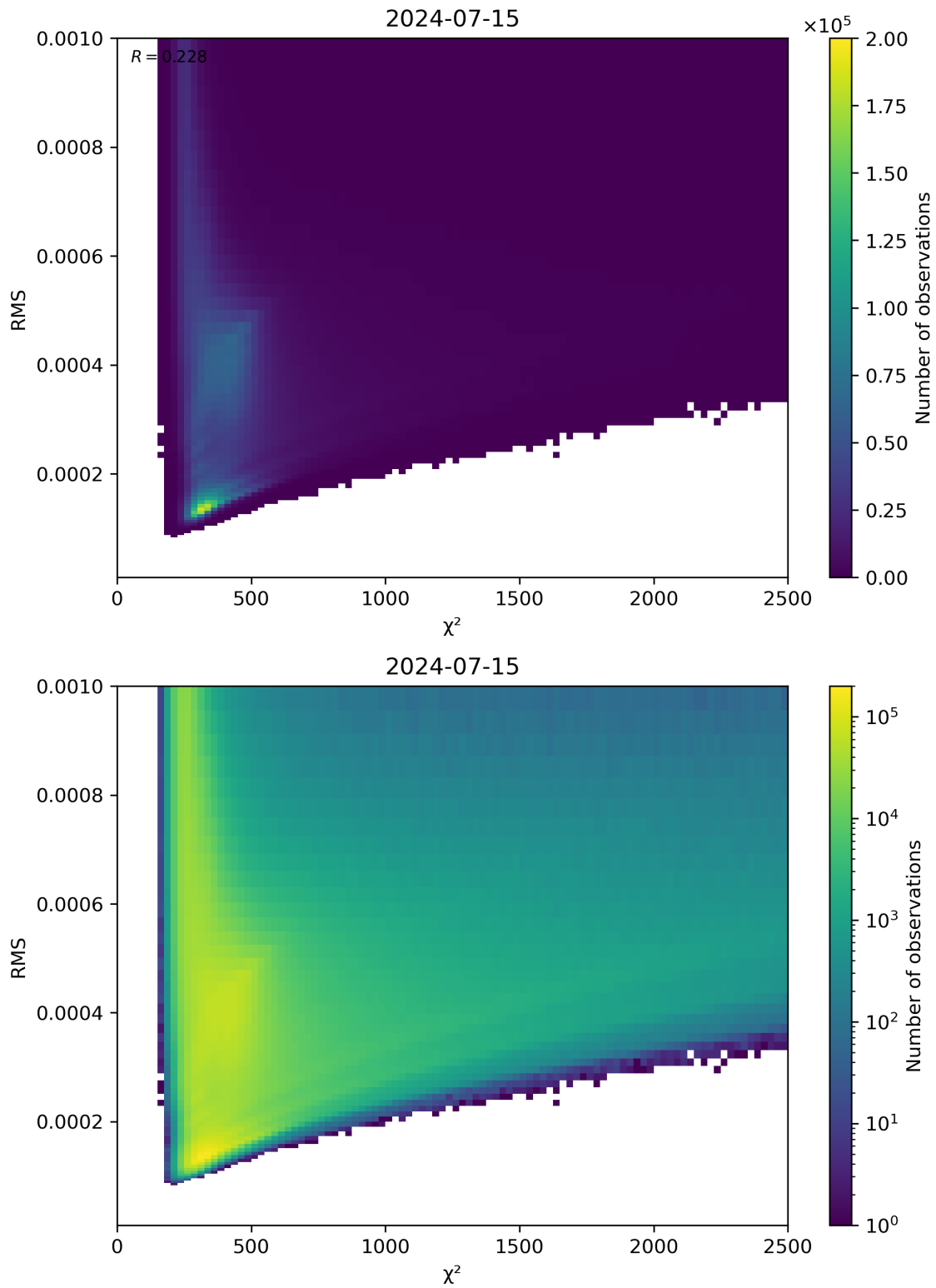
Figure 82: Scatter density plot of “ \chi^2 ” against “RMS” for 2024-07-15 to 2024-07-16.
