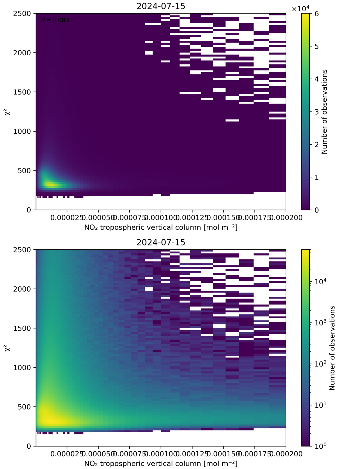
Figure 124: Scatter density plot of “NO 2 tropospheric vertical column” against “ \chi^2 ” for 2024-07-15 to 2024-07-16.
