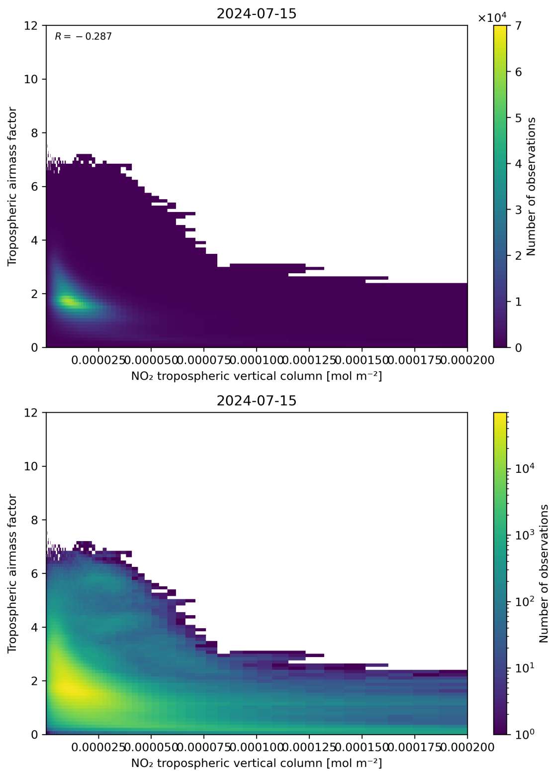
Figure 123: Scatter density plot of “NO 2 tropospheric vertical column” against “Tropospheric air mass factor” for 2024-07-15 to 2024-07-16.
