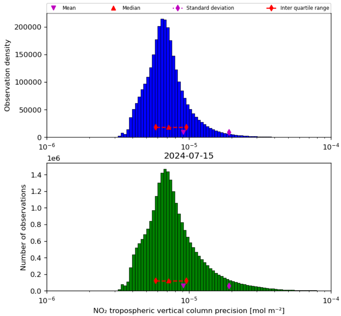
Figure 30: Histogram of “NO 2 tropospheric vertical column precision” for 2024-07-15 to 2024-07-16
