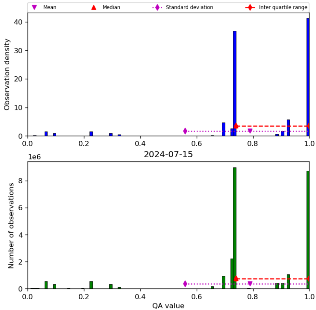
Figure 28: Histogram of “QA value” for 2024-07-15 to 2024-07-16
