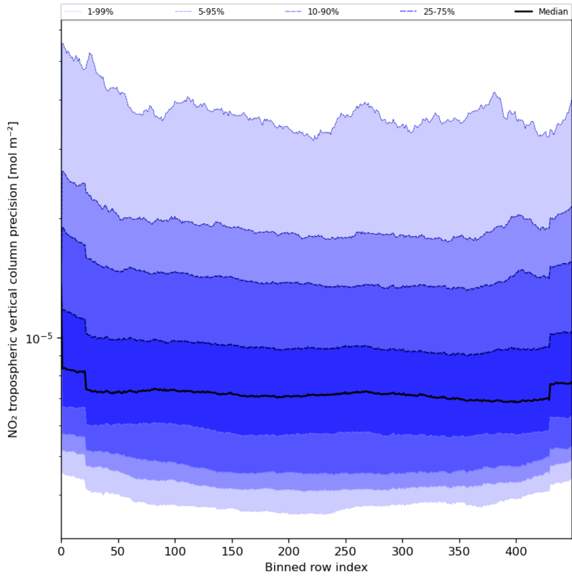
Figure 47: Along track statistics of “NO 2 tropospheric vertical column precision” for 2024-07-15 to 2024-07-16
