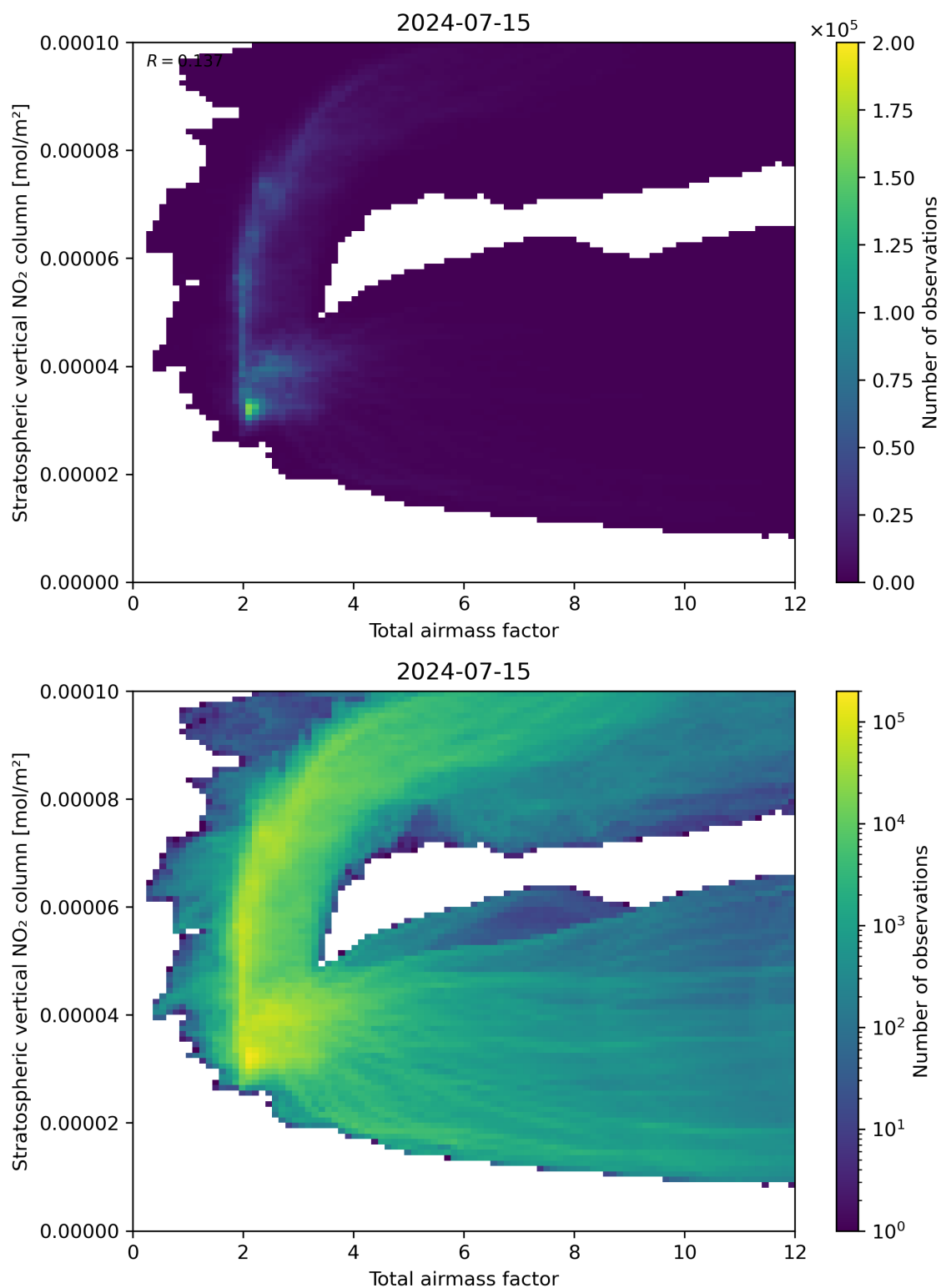
Figure 64: Scatter density plot of “Total airmass factor” against “Stratospheric vertical NO 2 column” for 2024-07-15 to 2024-07-16.
