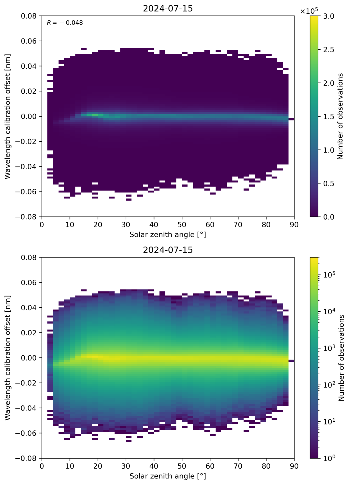
Figure 158: Scatter density plot of “Solar zenith angle” against “Wavelength calibration offset” for 2024-07-15 to 2024-07-16.
