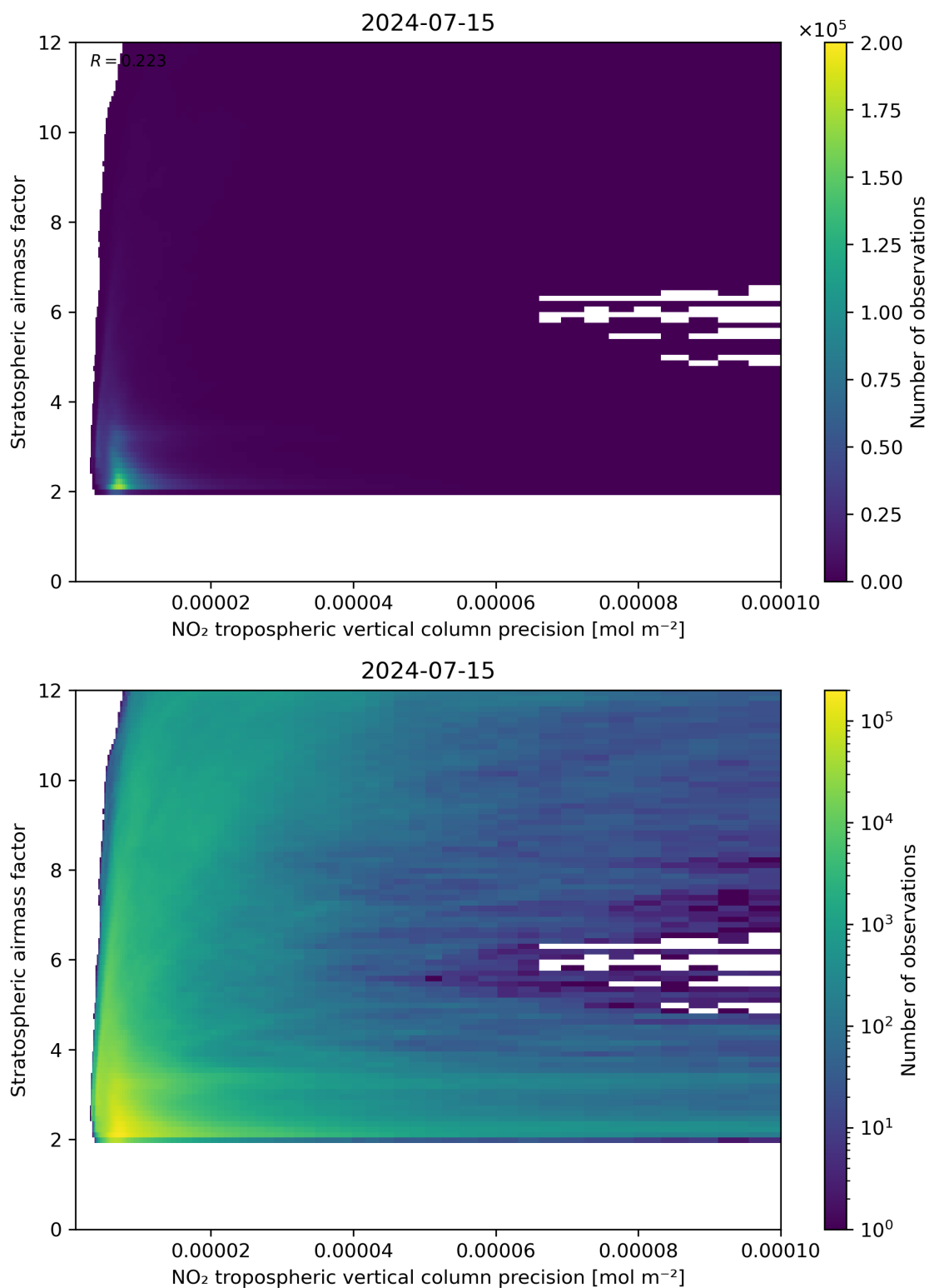
Figure 131: Scatter density plot of “NO 2 tropospheric vertical column precision” against “Stratospheric airmass factor” for 2024-07-15 to 2024-07-16.
