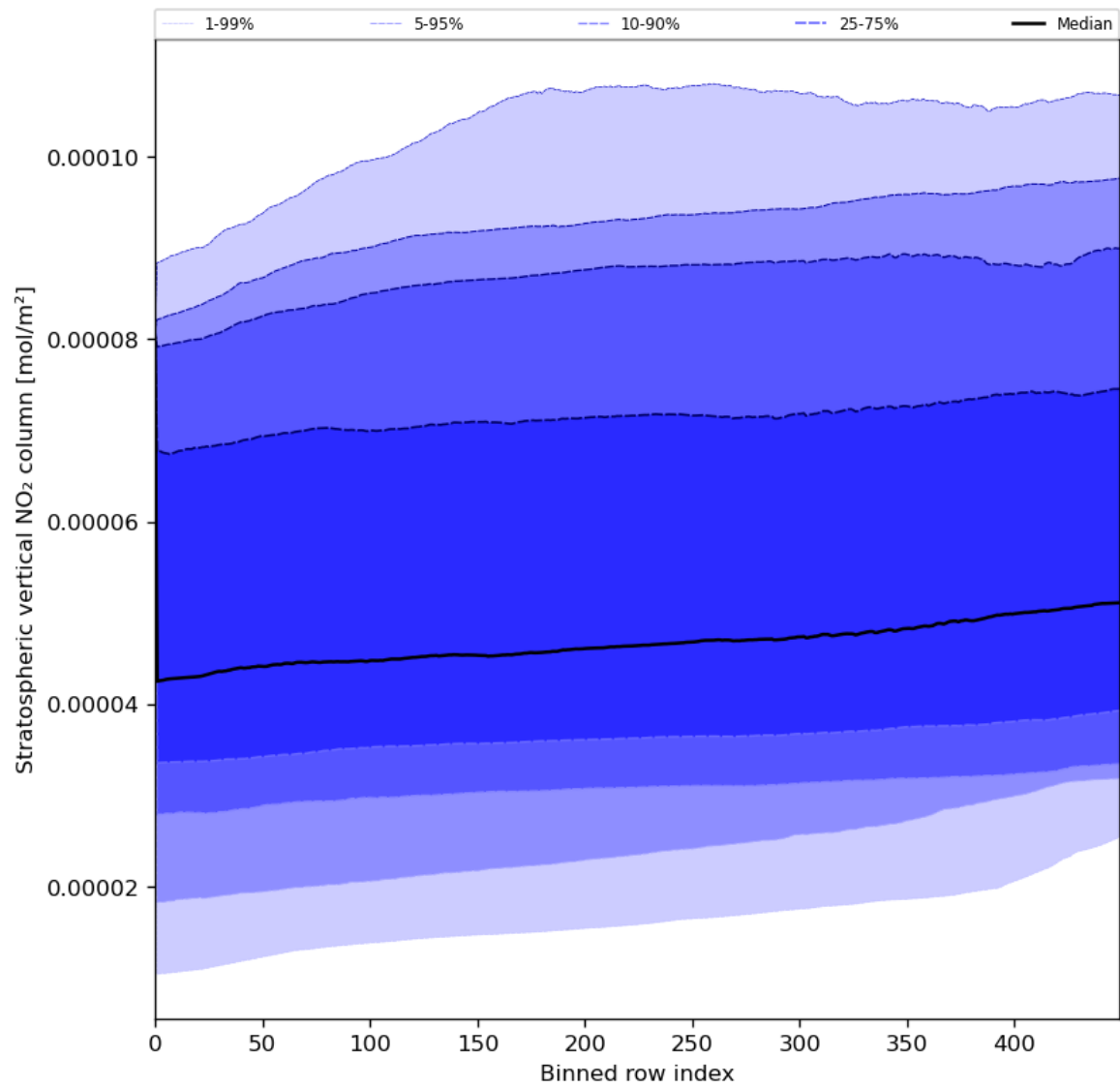
Figure 53: Along track statistics of “Stratospheric vertical NO 2 column” for 2024-07-15 to 2024-07-16
