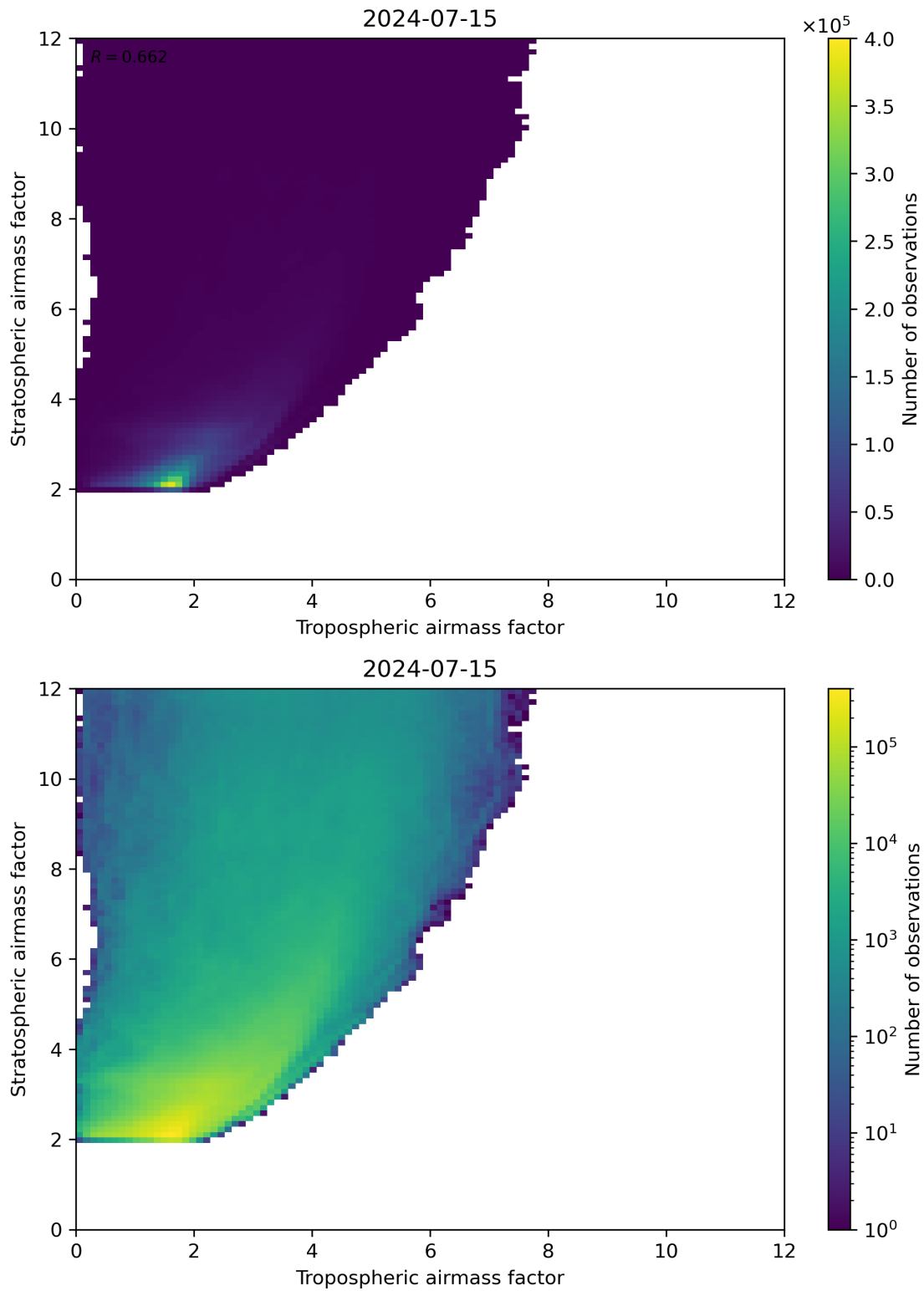
Figure 71: Scatter density plot of “Tropospheric airmass factor” against “Stratospheric airmass factor” for 2024-07-15 to 2024-07-16.
