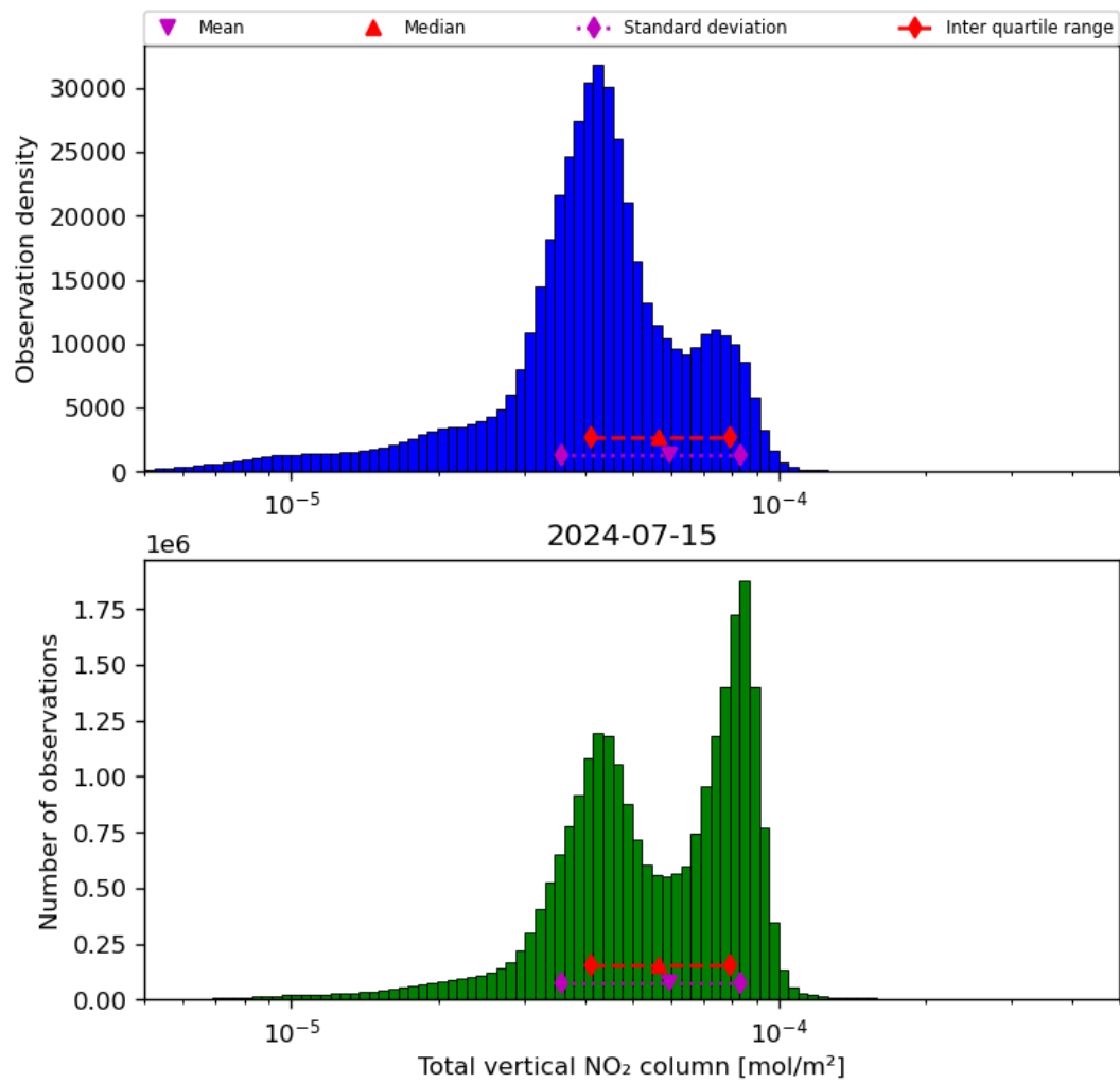
Figure 38: Histogram of “Total vertical NO 2 column” for 2024-07-15 to 2024-07-16
