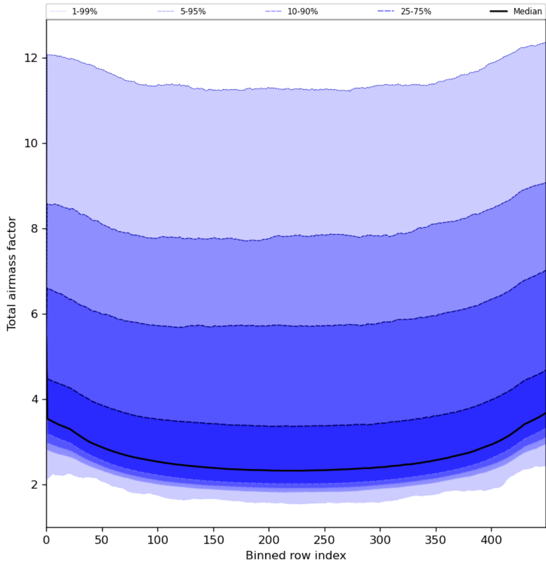
Figure 49: Along track statistics of “Total airmass factor” for 2024-07-15 to 2024-07-16
