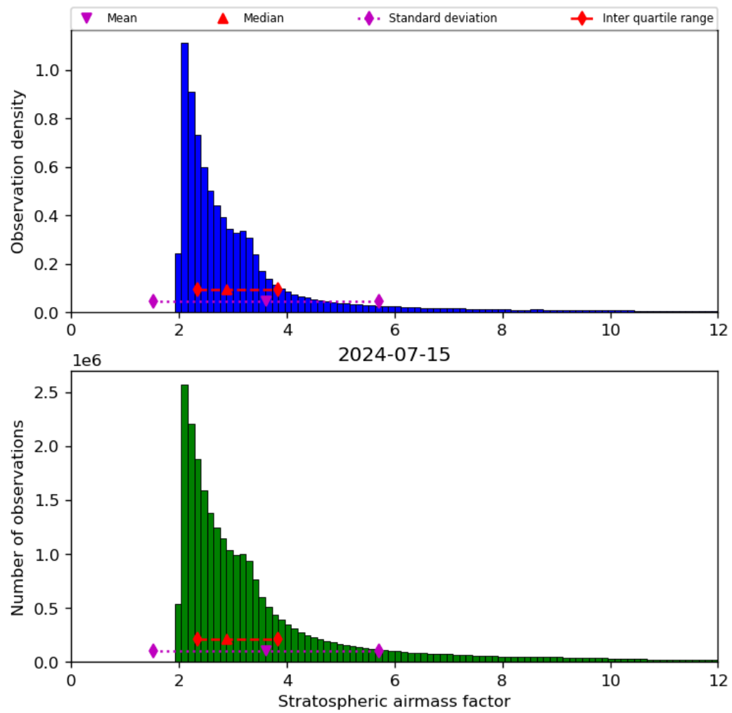
Figure 44: Histogram of “Stratospheric airmass factor” for 2024-07-15 to 2024-07-16
