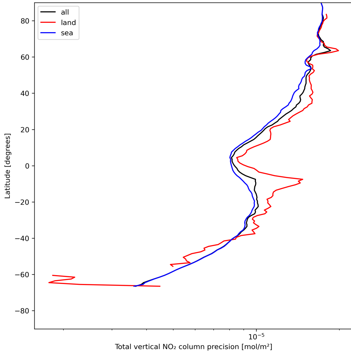
Figure 22: Zonal average of “Total vertical NO 2 column precision” for 2024-07-15 to 2024-07-16.
