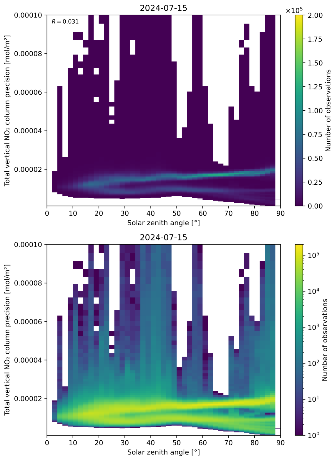
Figure 154: Scatter density plot of “Solar zenith angle” against “Total vertical NO 2 column precision” for 2024-07-15 to 2024-07-16.
