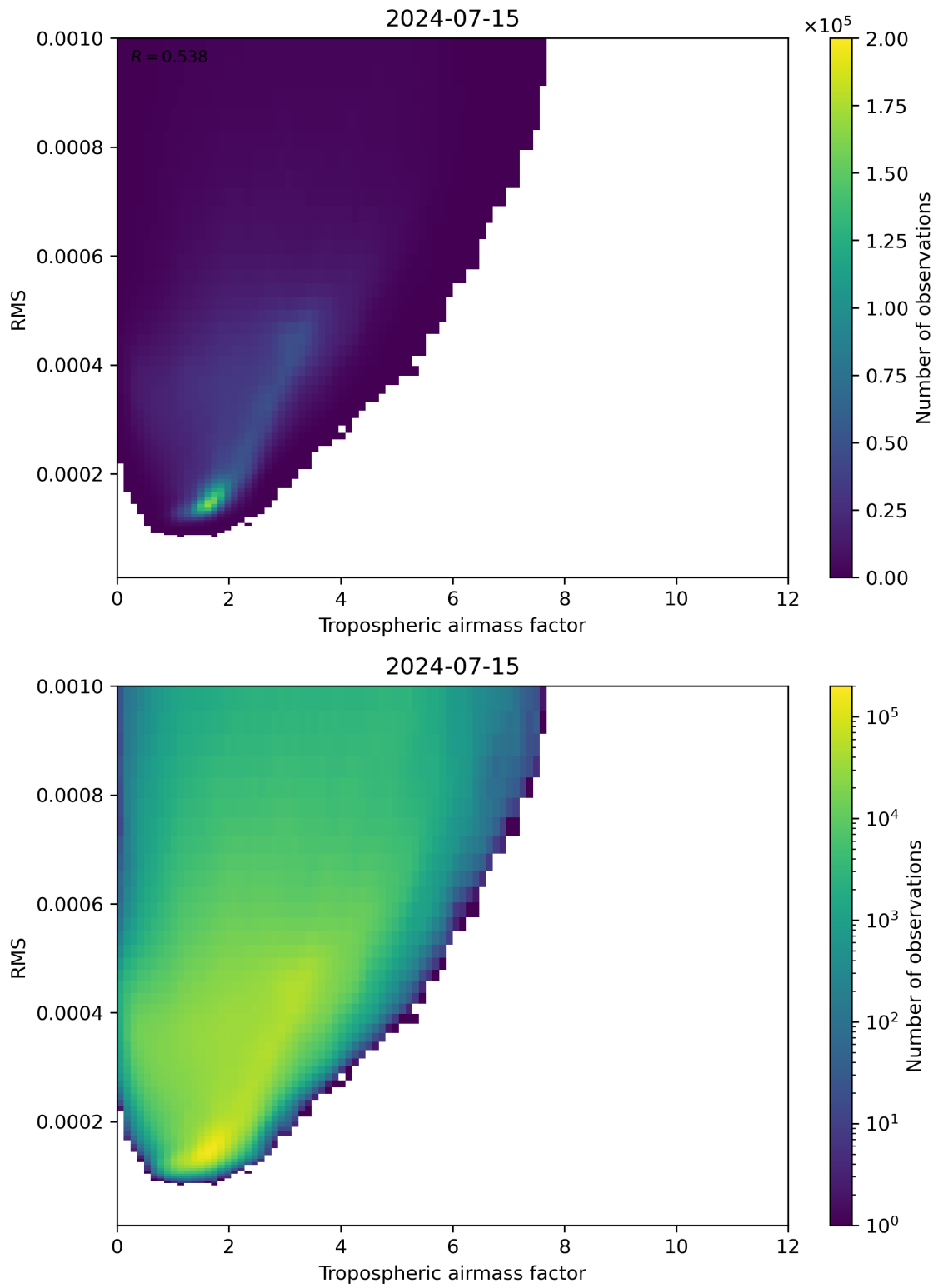
Figure 79: Scatter density plot of “Tropospheric airmass factor” against “RMS” for 2024-07-15 to 2024-07-16.
