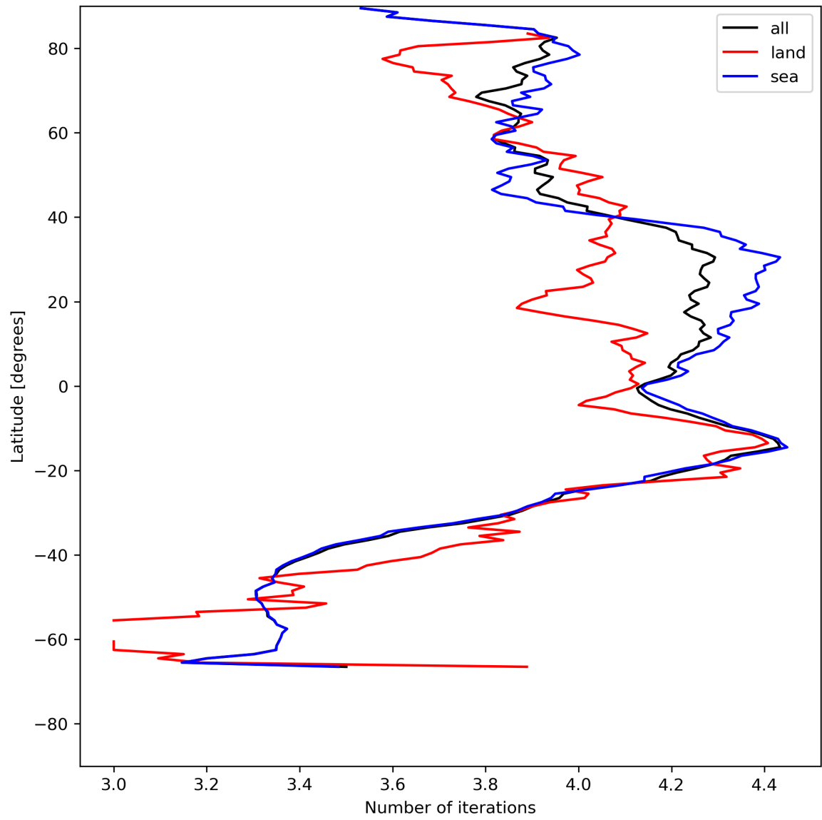
Figure 17: Zonal average of “Number of iterations” for 2024-07-15 to 2024-07-16.
