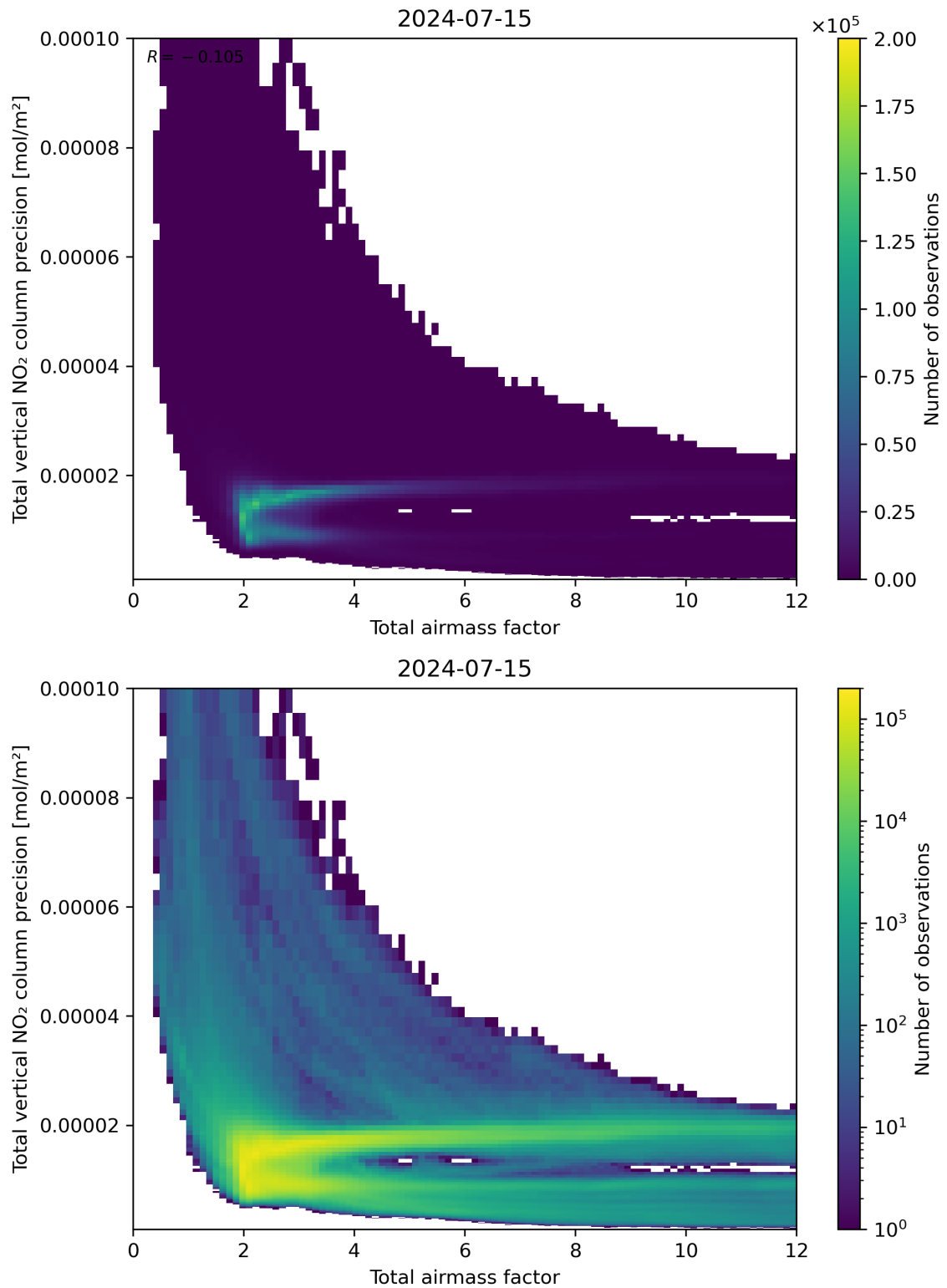
Figure 68: Scatter density plot of “Total airmass factor” against “Total vertical NO 2 column precision” for 2024-07-15 to 2024-07-16.
