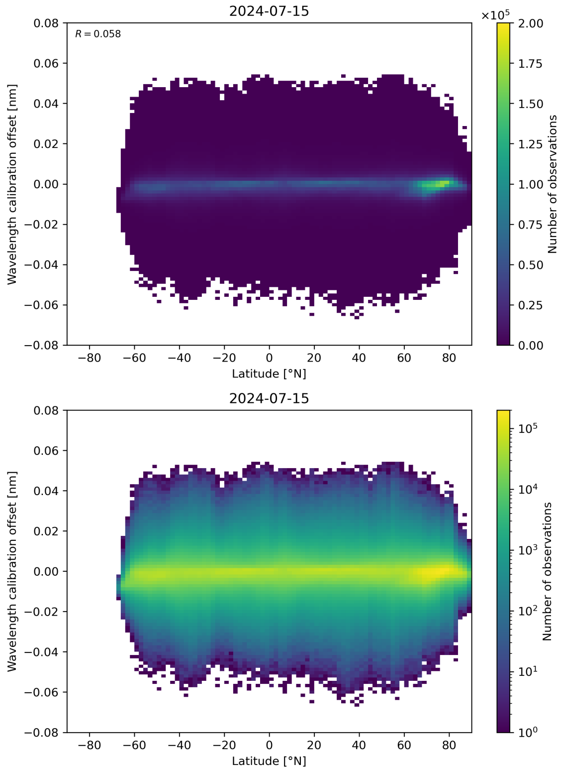
Figure 95: Scatter density plot of “Latitude” against “Wavelength calibration offset” for 2024-07-15 to 2024-07-16.
