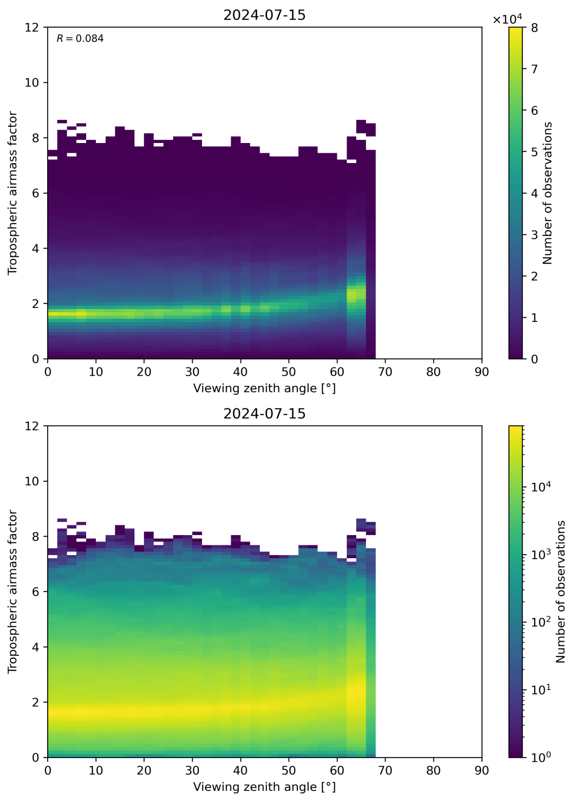
Figure 161: Scatter density plot of “Viewing zenith angle” against “Tropospheric airmass factor” for 2024-07-15 to 2024-07-16.
