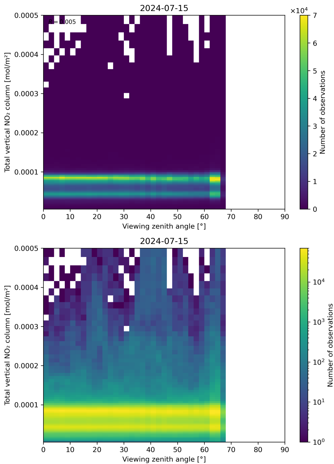
Figure 167: Scatter density plot of “Viewing zenith angle” against “Total vertical NO 2 column” for 2024-07-15 to 2024-07-16.
