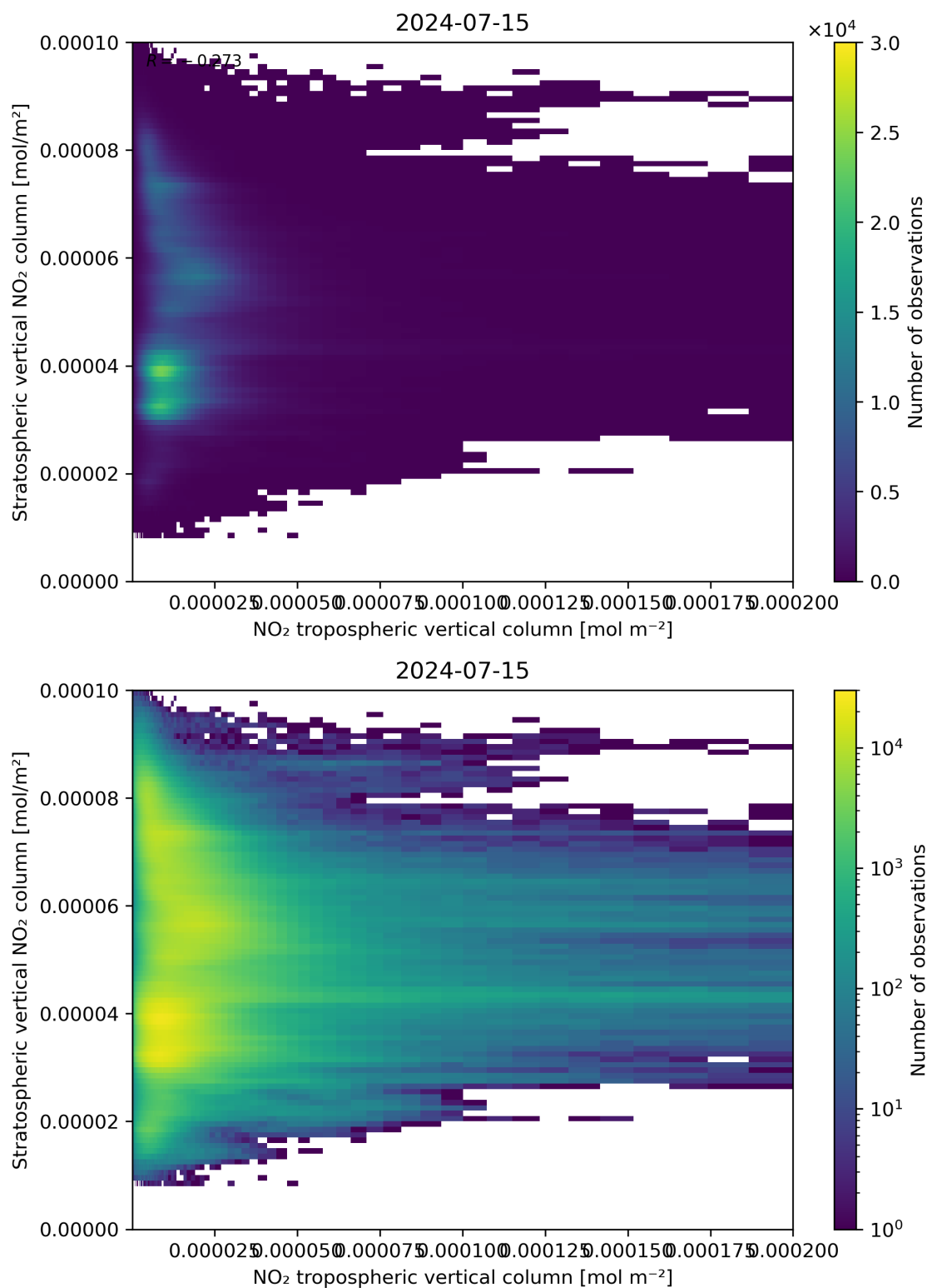
Figure 125: Scatter density plot of “NO 2 tropospheric vertical column” against “Stratospheric vertical NO 2 column” for 2024-07-15 to 2024-07-16.
