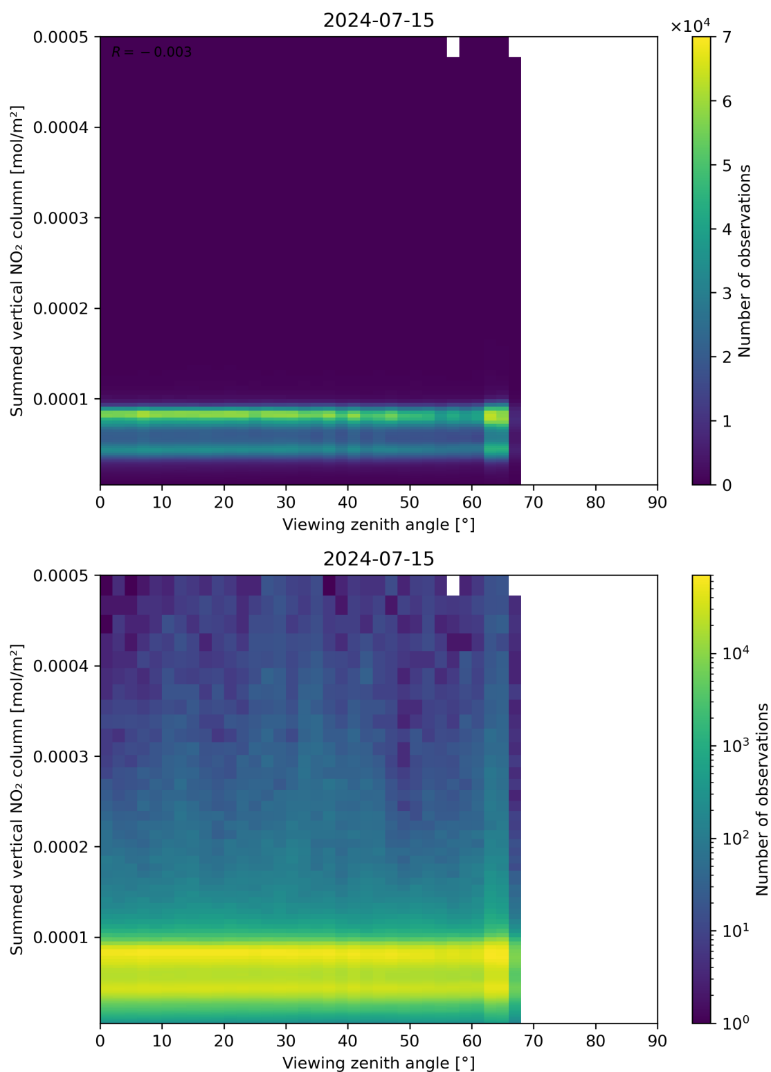
Figure 165: Scatter density plot of “Viewing zenith angle” against “Summed vertical NO 2 column” for 2024-07-15 to 2024-07-16.
