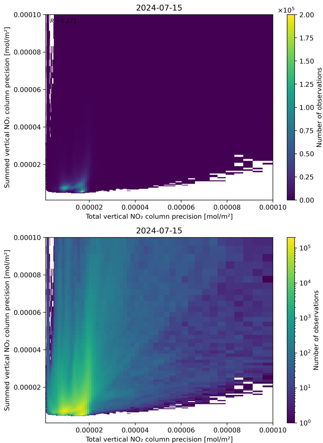
Figure 118: Scatter density plot of “Total vertical NO 2 column precision” against “Summed vertical NO 2 column precision” for 2024-07-15 to 2024-07-16.
