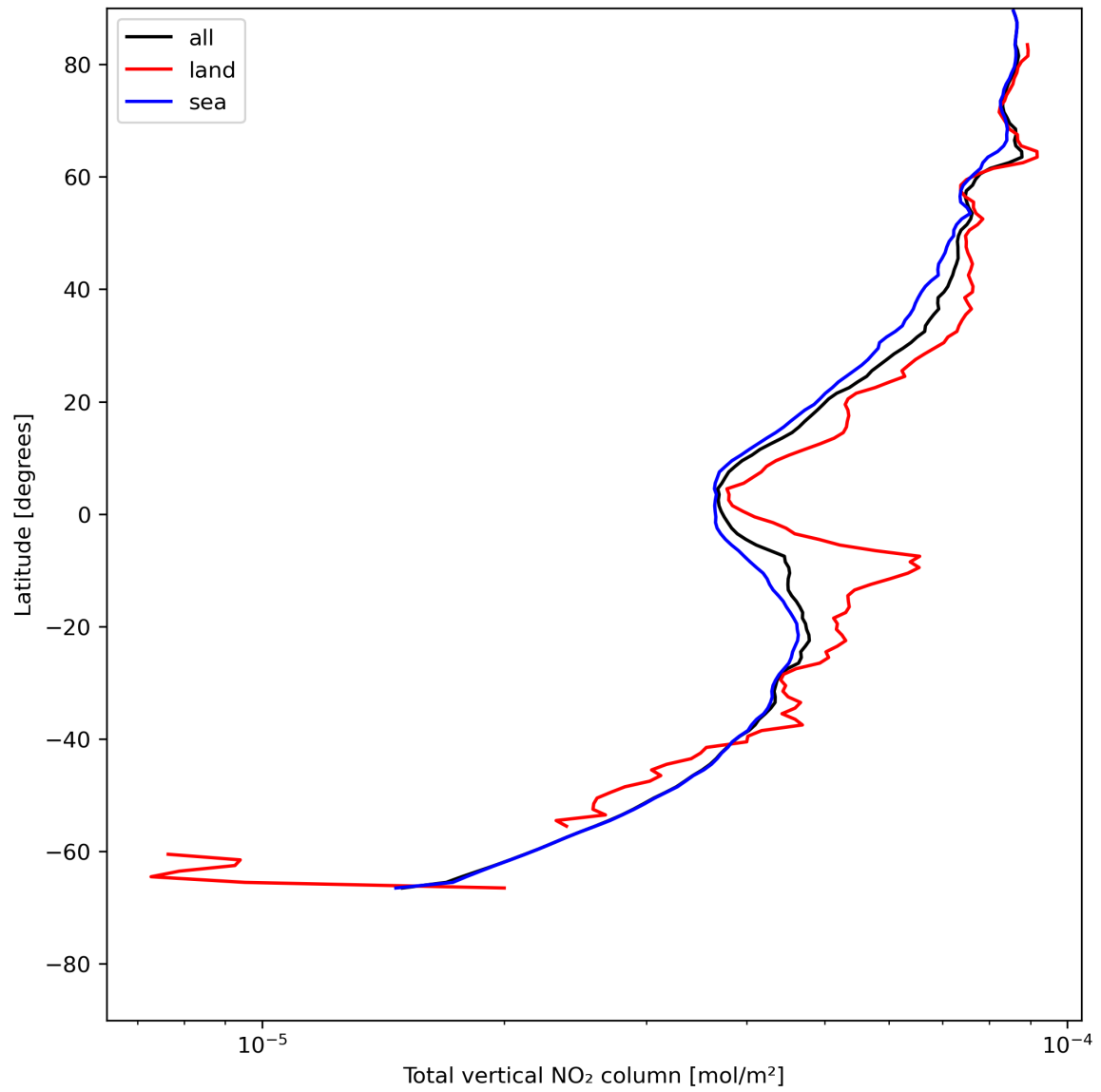
Figure 21: Zonal average of “Total vertical NO 2 column” for 2024-07-15 to 2024-07-16.
