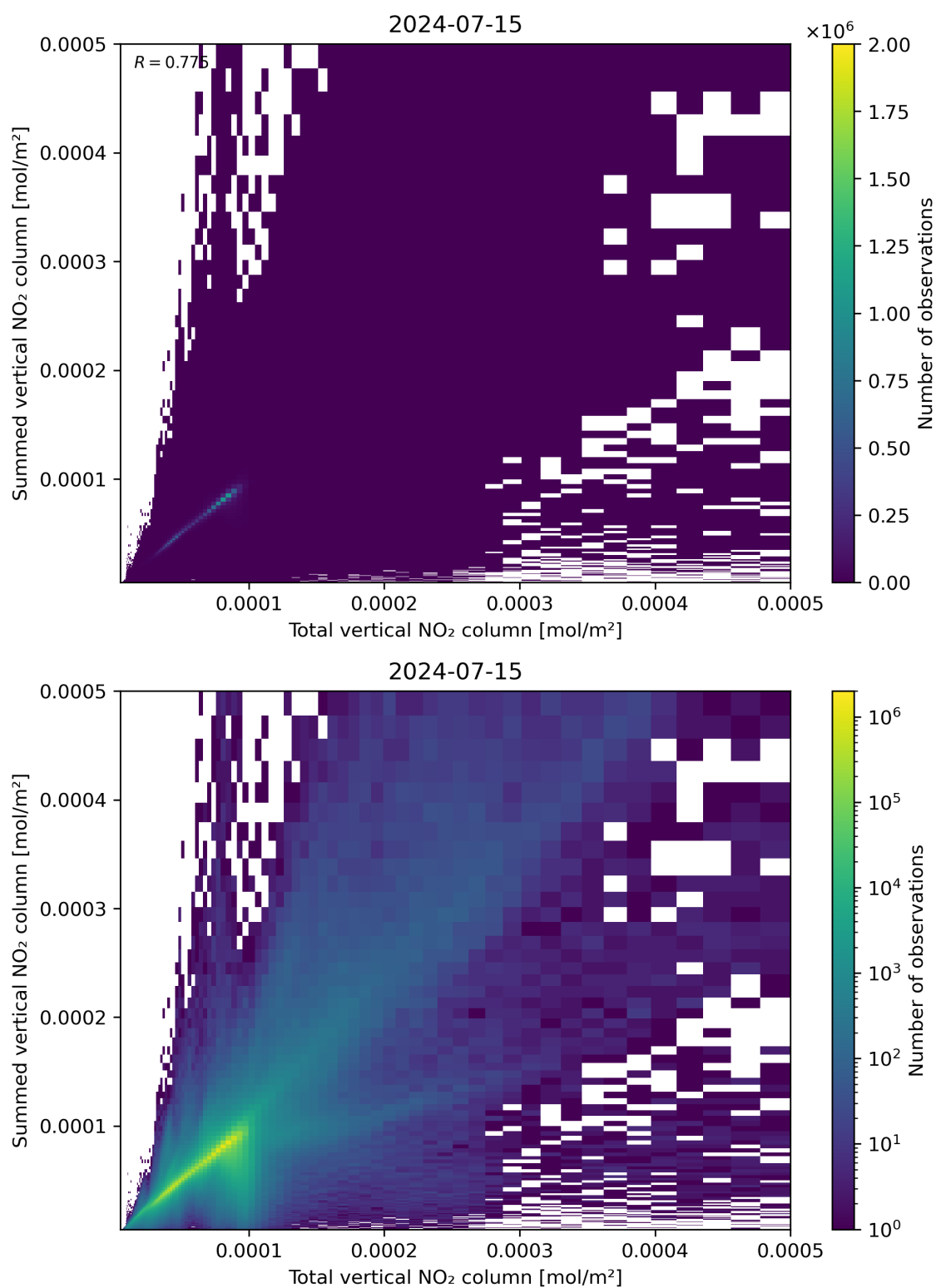
Figure 112: Scatter density plot of “Total vertical NO 2 column” against “Summed vertical NO 2 column” for 2024-07-15 to 2024-07-16.
