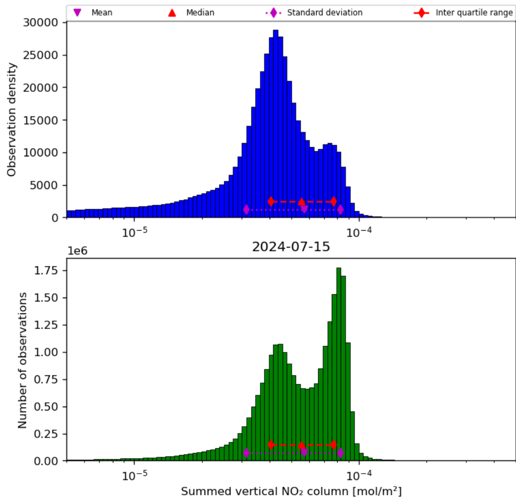
Figure 40: Histogram of "Summed vertical NO 2 column" for 2024-07-15 to 2024-07-16
