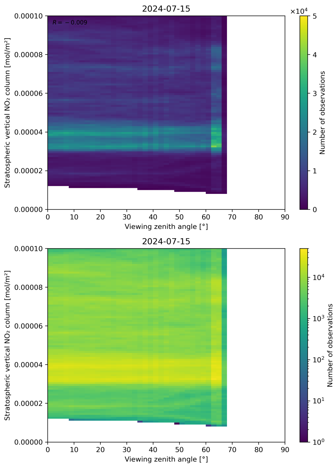
Figure 164: Scatter density plot of “Viewing zenith angle” against “Stratospheric vertical NO 2 column” for 2024-07-15 to 2024-07-16.
