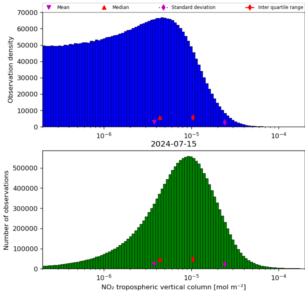
Figure 29: Histogram of “NO 2 tropospheric vertical column” for 2024-07-15 to 2024-07-16
