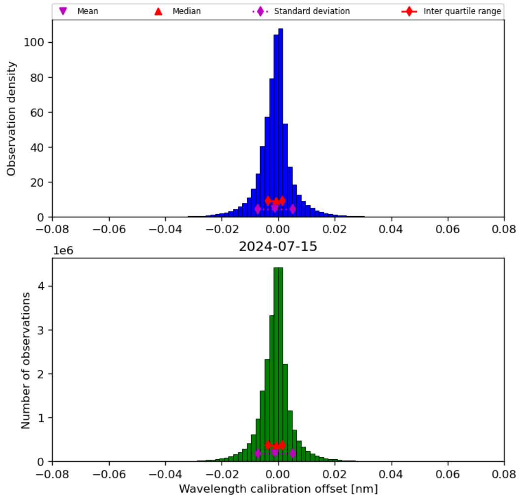
Figure 35: Histogram of “Wavelength calibration offset” for 2024-07-15 to 2024-07-16
