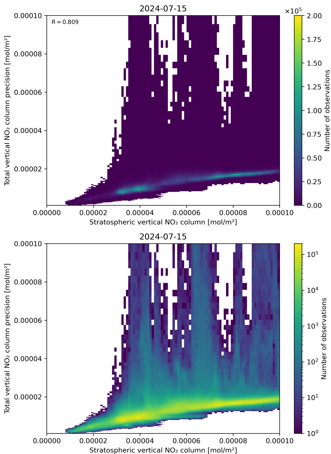
Figure 101: Scatter density plot of “Stratospheric vertical NO 2 column” against “Total vertical NO 2 column precision” for 2024-07-15 to 2024-07-16.
