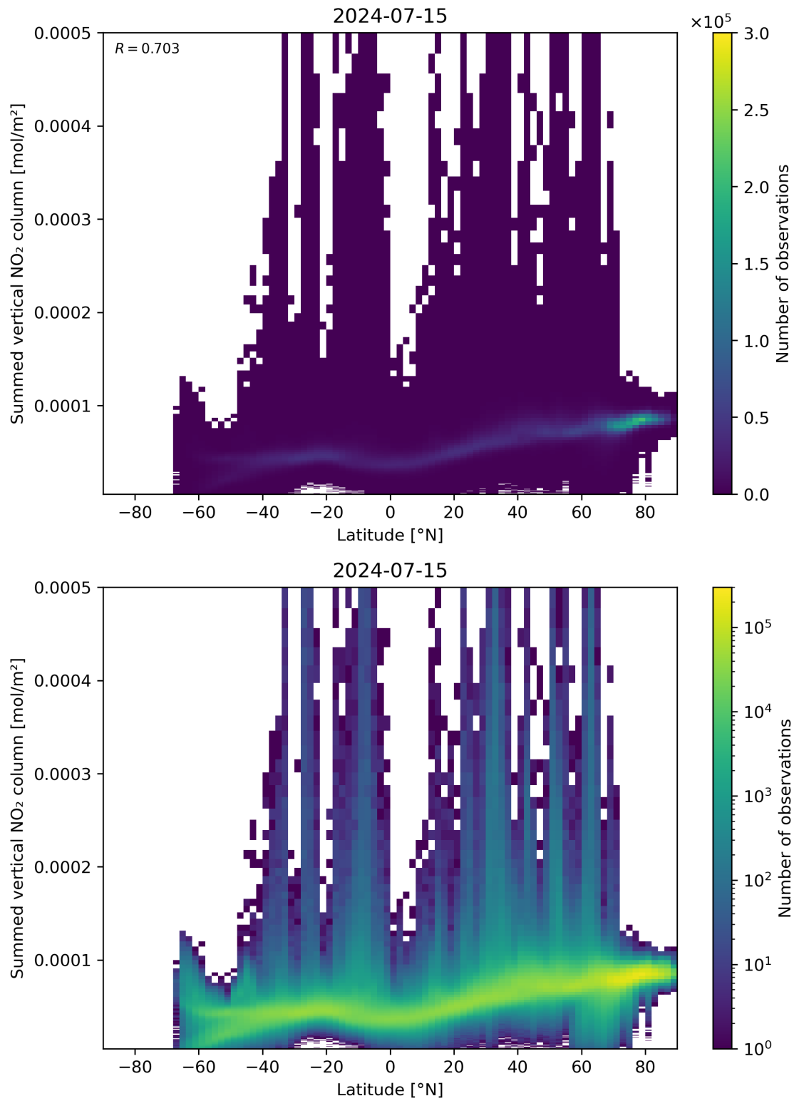
Figure 88: Scatter density plot of “Latitude” against “Summed vertical NO 2 column” for 2024-07-15 to 2024-07-16.
