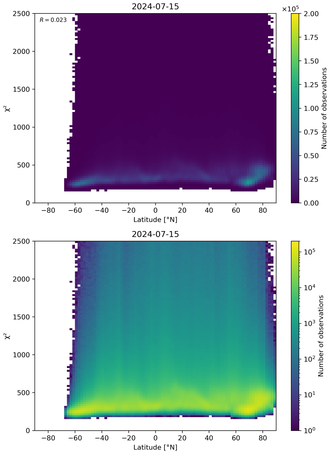
Figure 86: Scatter density plot of “Latitude” against “ \chi^2 ” for 2024-07-15 to 2024-07-16.
