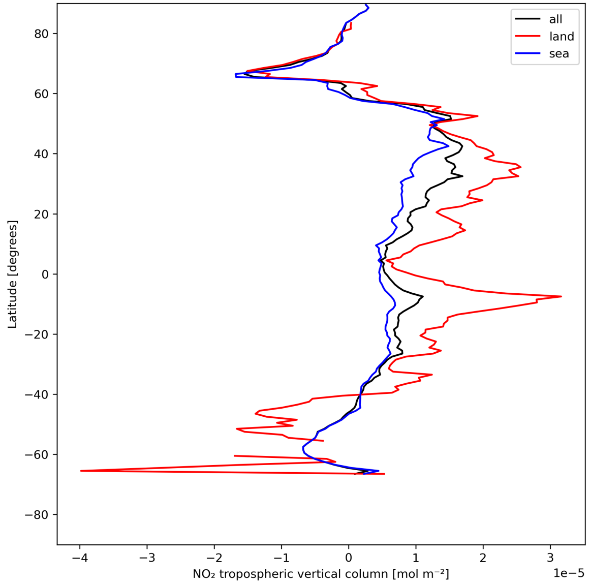
Figure 12: Zonal average of “NO 2 tropospheric vertical column” for 2024-07-15 to 2024-07-16.
