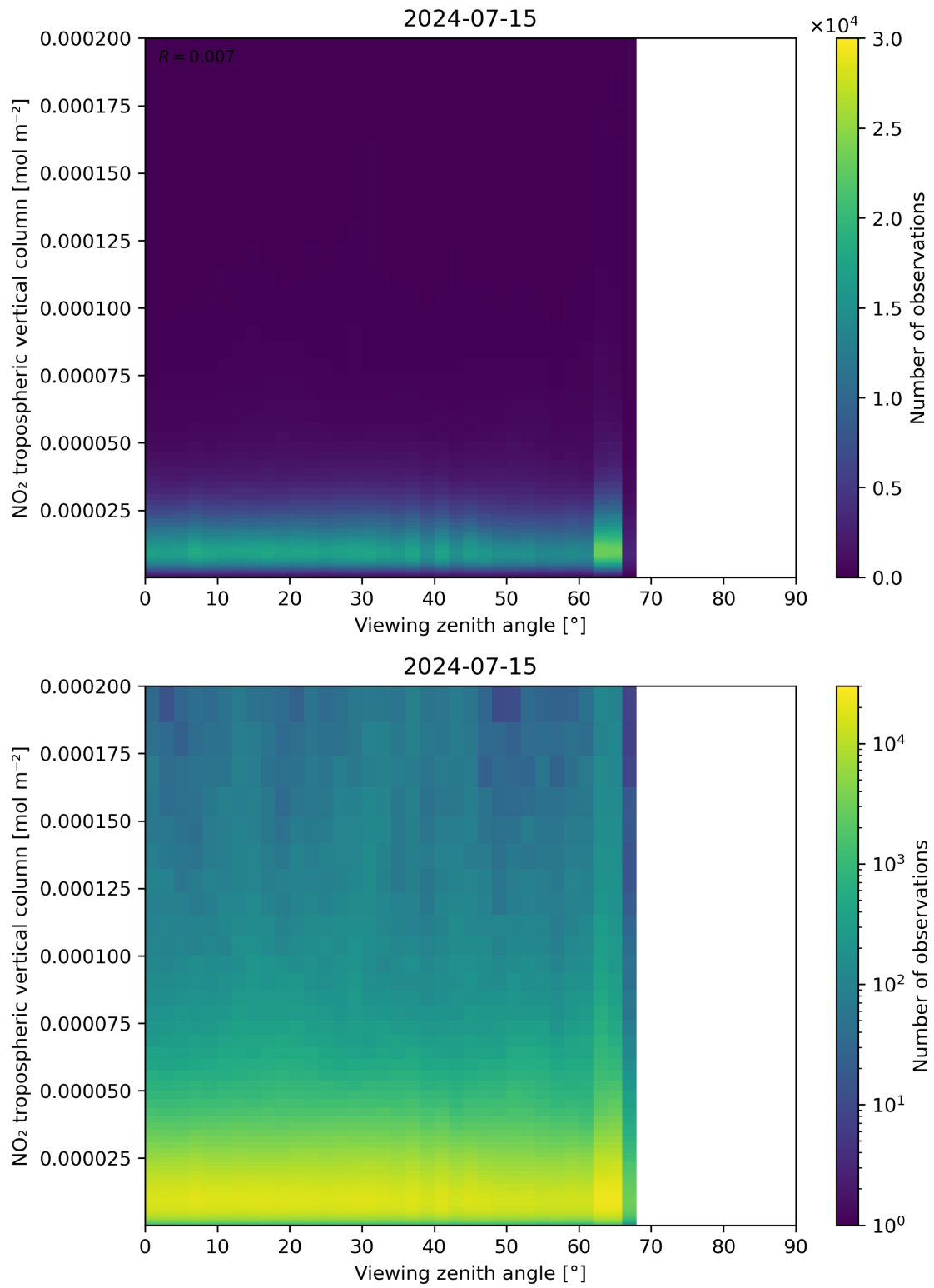
Figure 169: Scatter density plot of “Viewing zenith angle” against “NO 2 tropospheric vertical column” for 2024-07-15 to 2024-07-16.
