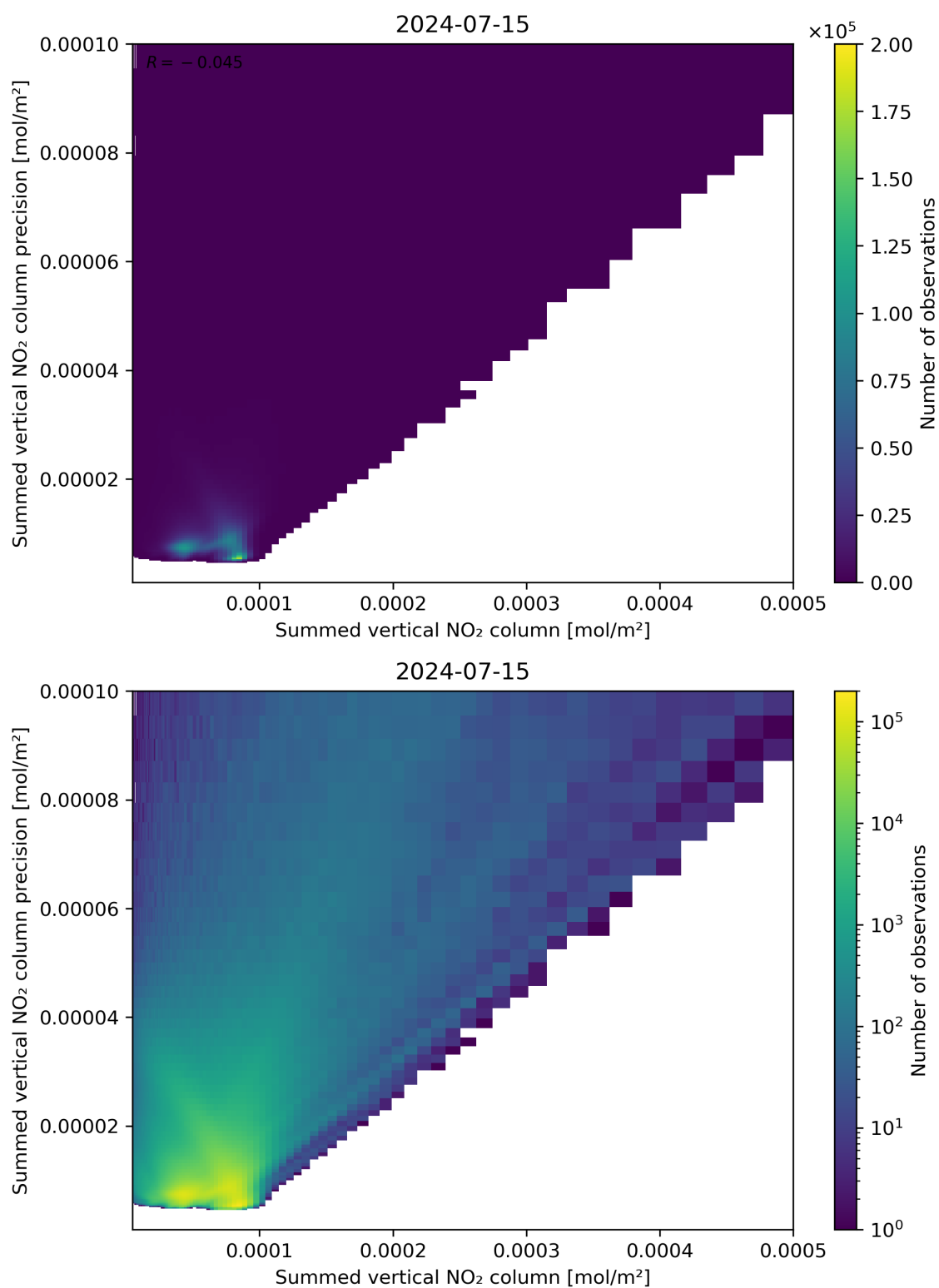
Figure 105: Scatter density plot of “Summed vertical NO 2 column” against “Summed vertical NO 2 column precision” for 2024-07-15 to 2024-07-16.
