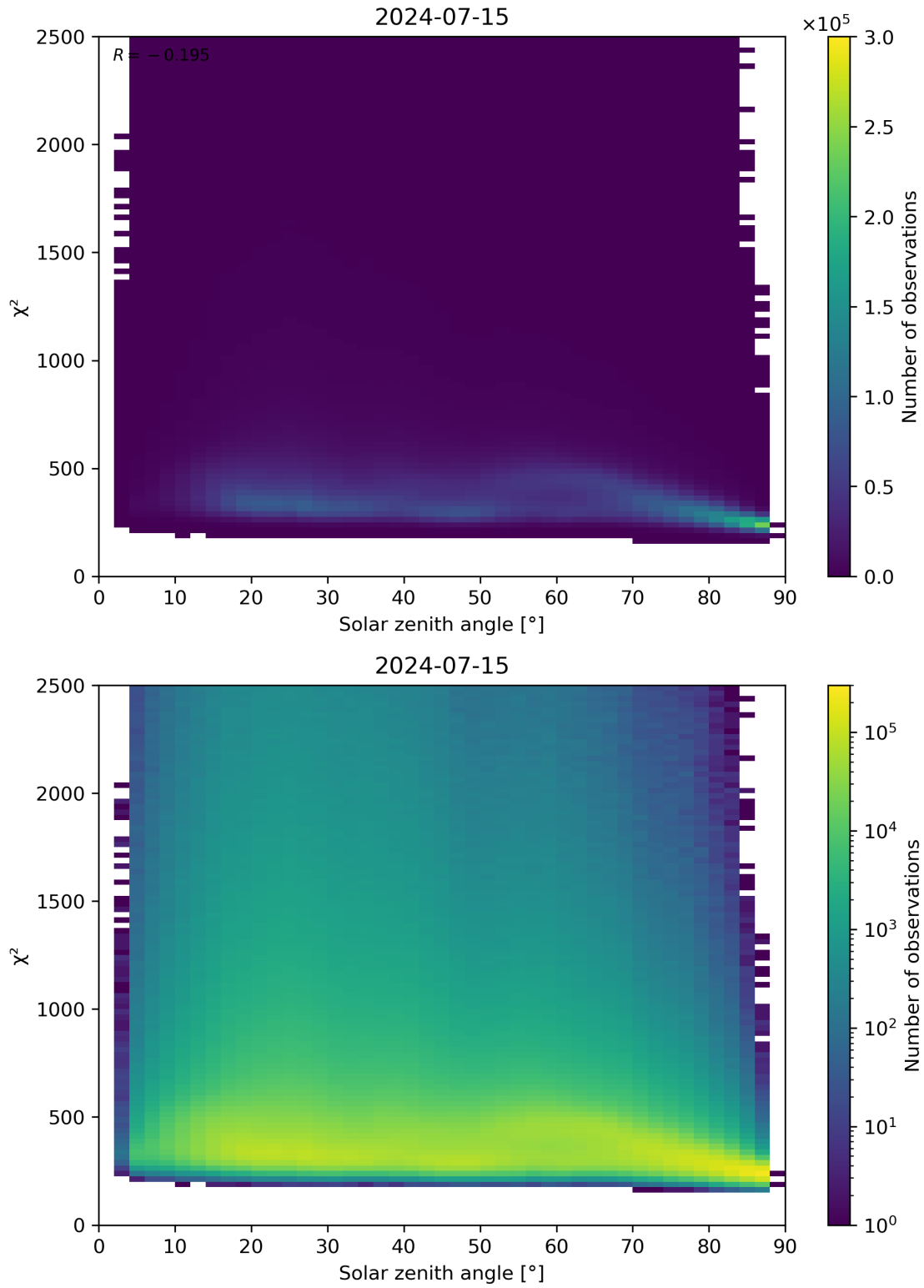
Figure 148: Scatter density plot of “Solar zenith angle” against “ \chi^2 ” for 2024-07-15 to 2024-07-16.
