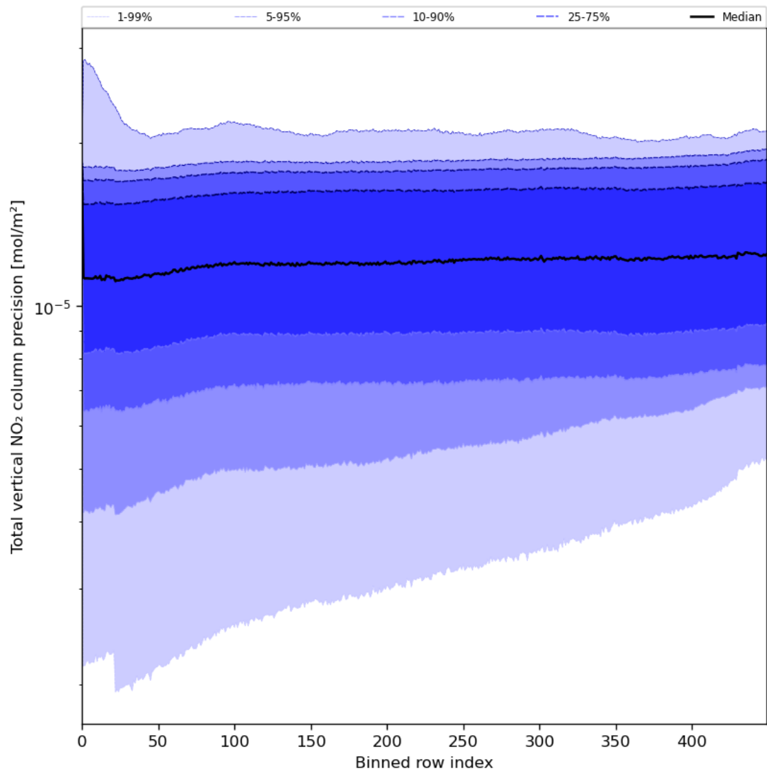
Figure 56: Along track statistics of “Total vertical NO 2 column precision” for 2024-07-15 to 2024-07-16
