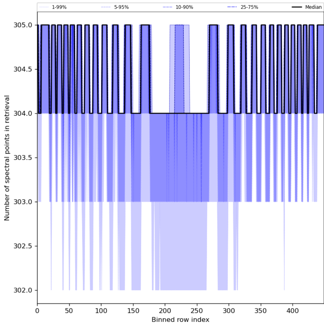
Figure 50: Along track statistics of “Number of spectral points in retrieval” for 2024-07-15 to 2024-07-16
