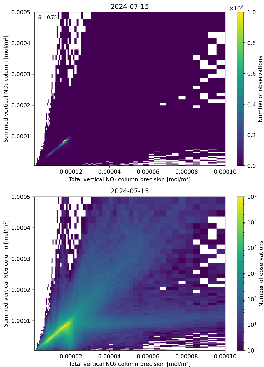
Figure 117: Scatter density plot of “Total vertical NO 2 column precision” against “Summed vertical NO 2 column” for 2024-07-15 to 2024-07-16.
