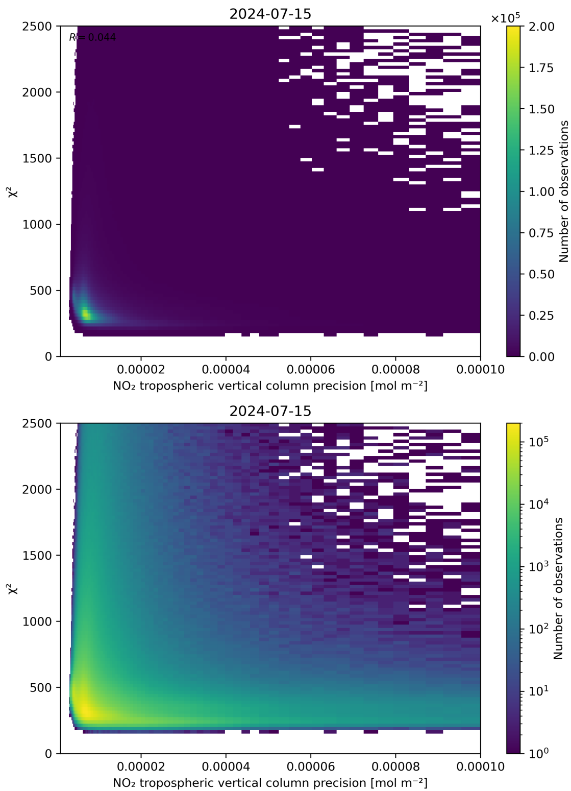
Figure 134: Scatter density plot of “NO 2 tropospheric vertical column precision” against “ \chi^2 ” for 2024-07-15 to 2024-07-16.
