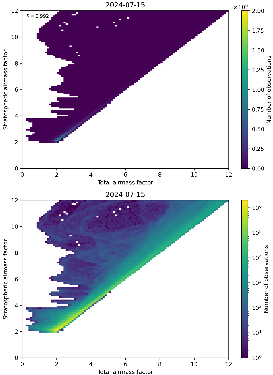
Figure 62: Scatter density plot of “Total airmass factor” against “Stratospheric airmass factor” for 2024-07-15 to 2024-07-16.
