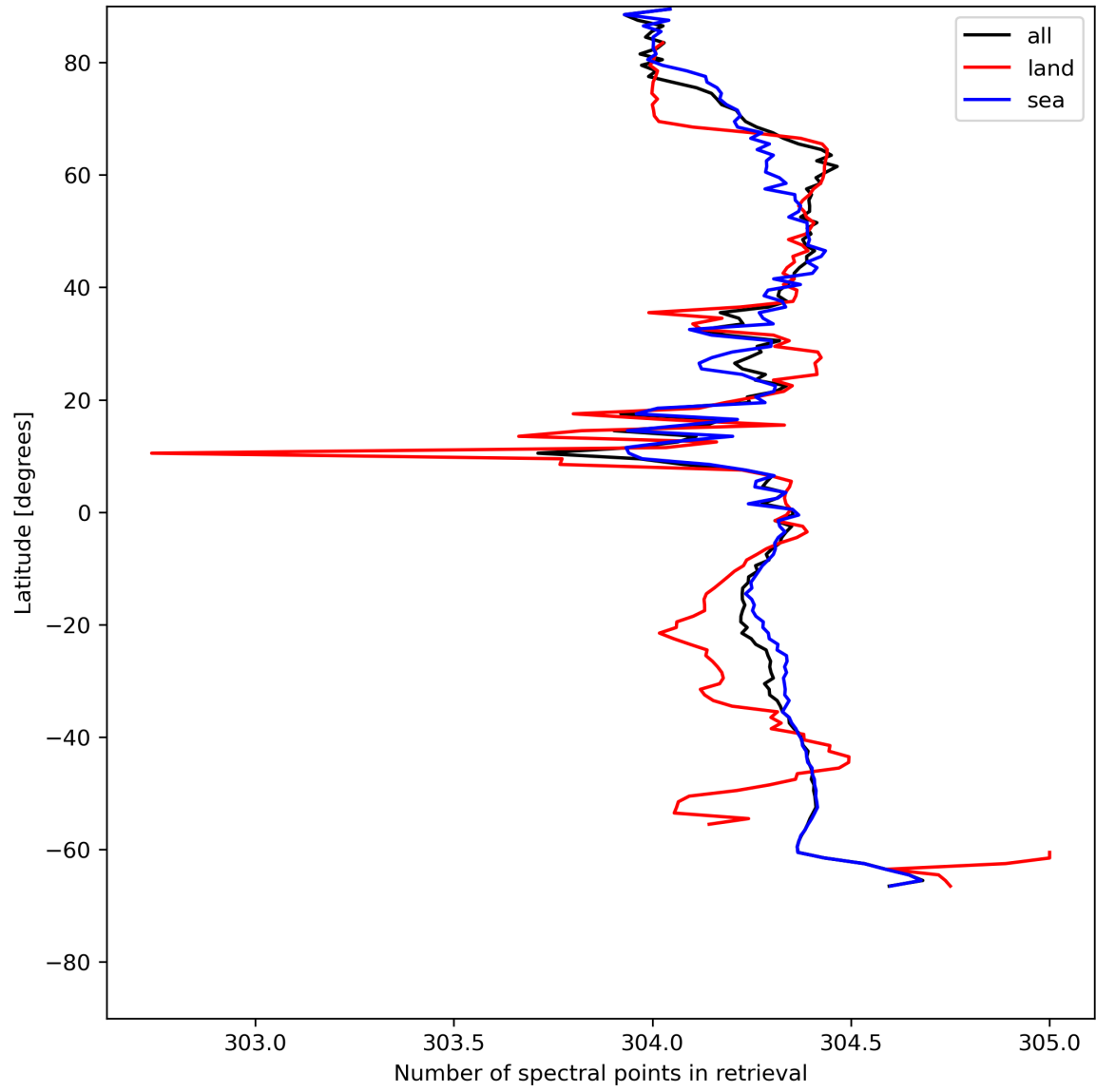
Figure 16: Zonal average of “Number of spectral points in retrieval” for 2024-07-15 to 2024-07-16.
