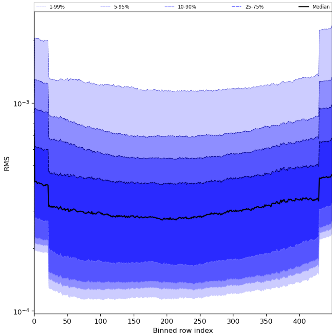
Figure 60: Along track statistics of “RMS” for 2024-07-15 to 2024-07-16
