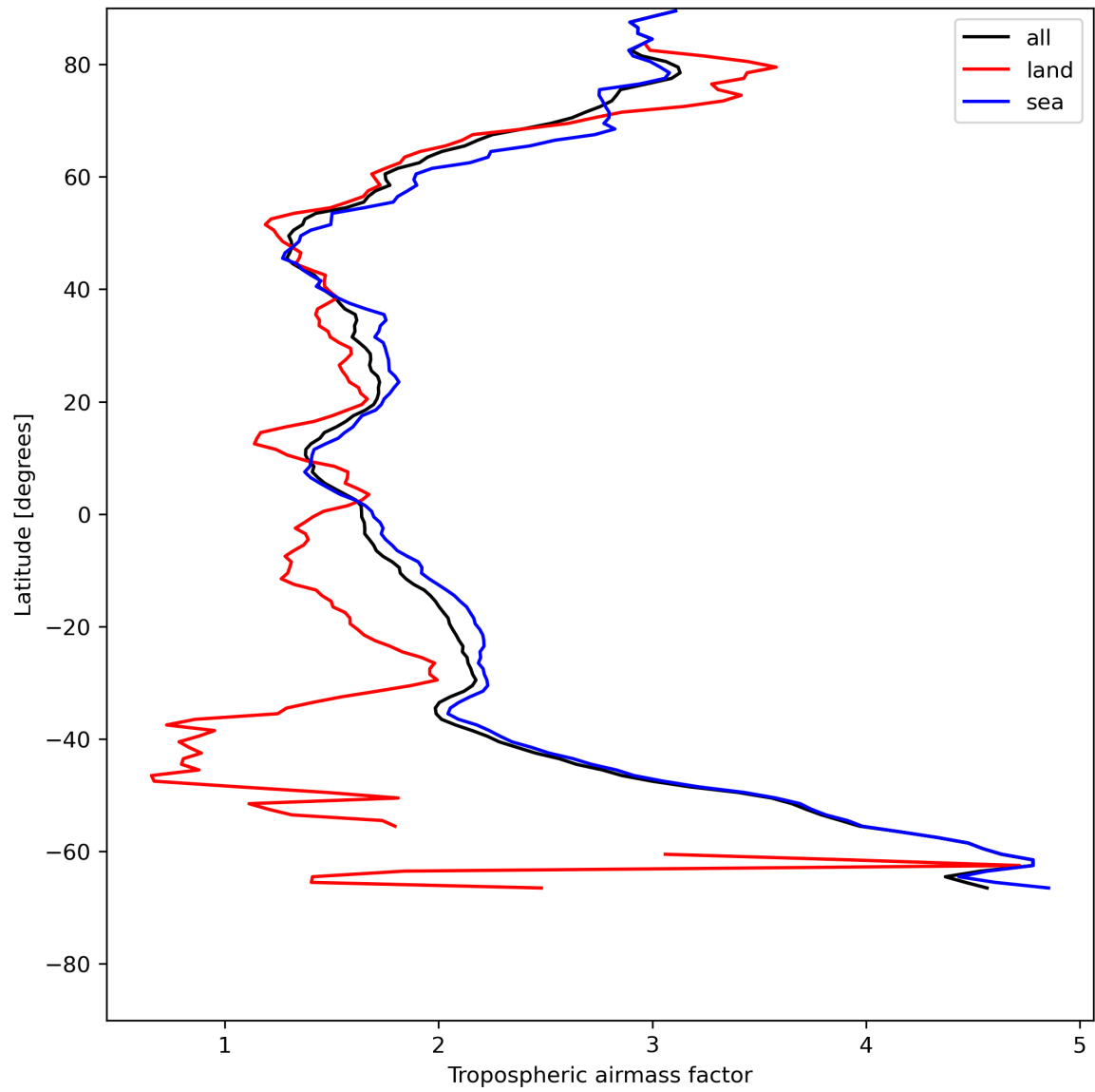
Figure 14: Zonal average of “Tropospheric air mass factor” for 2024-07-15 to 2024-07-16.
