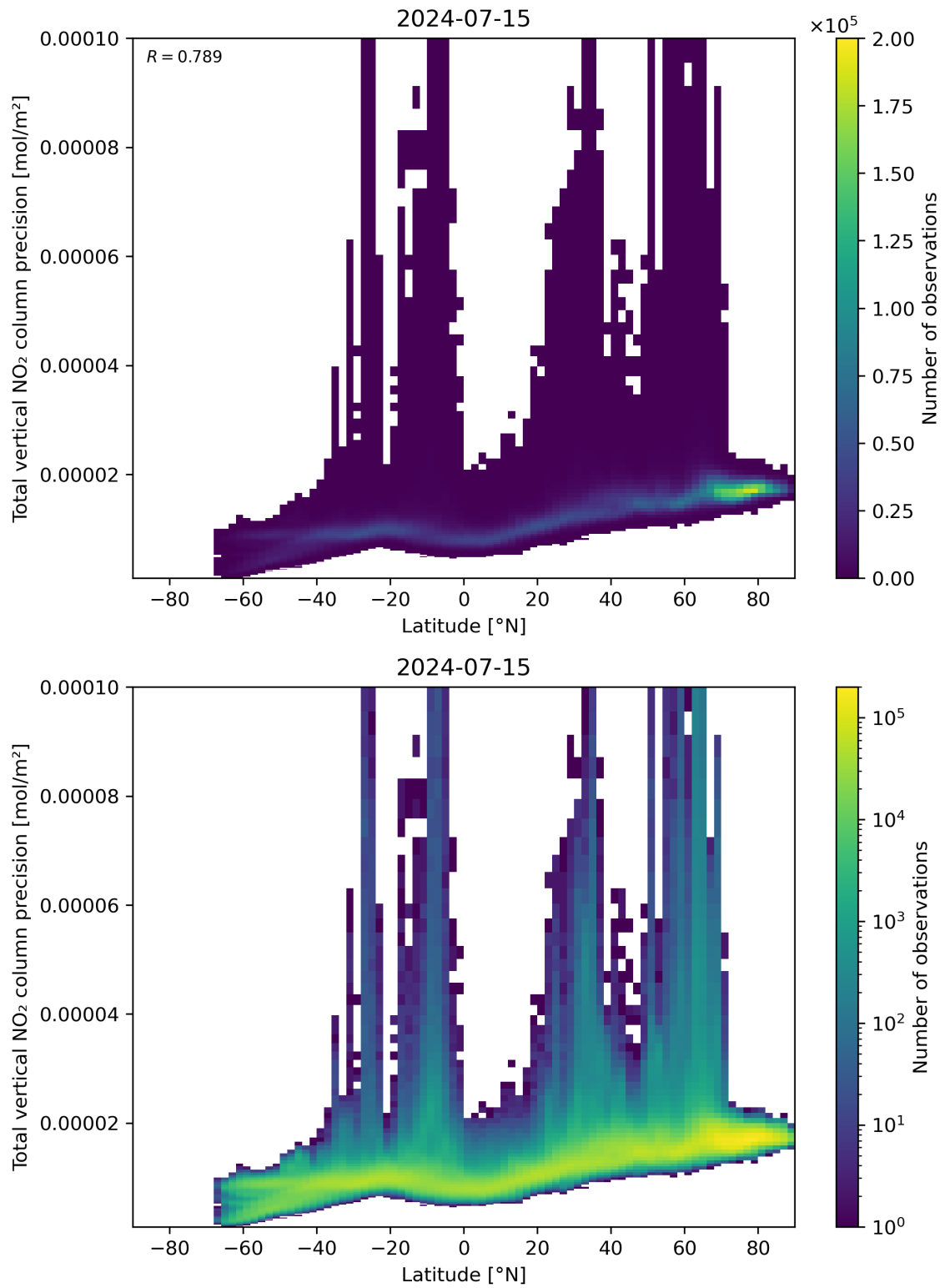
Figure 91: Scatter density plot of “Latitude” against “Total vertical NO 2 column precision” for 2024-07-15 to 2024-07-16.
