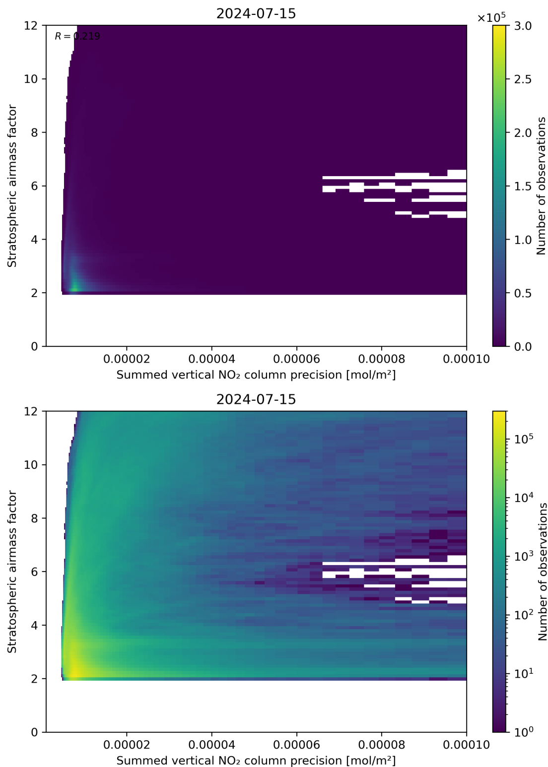
Figure 106: Scatter density plot of “Summed vertical NO 2 column precision” against “Stratospheric airmass factor” for 2024-07-15 to 2024-07-16.
