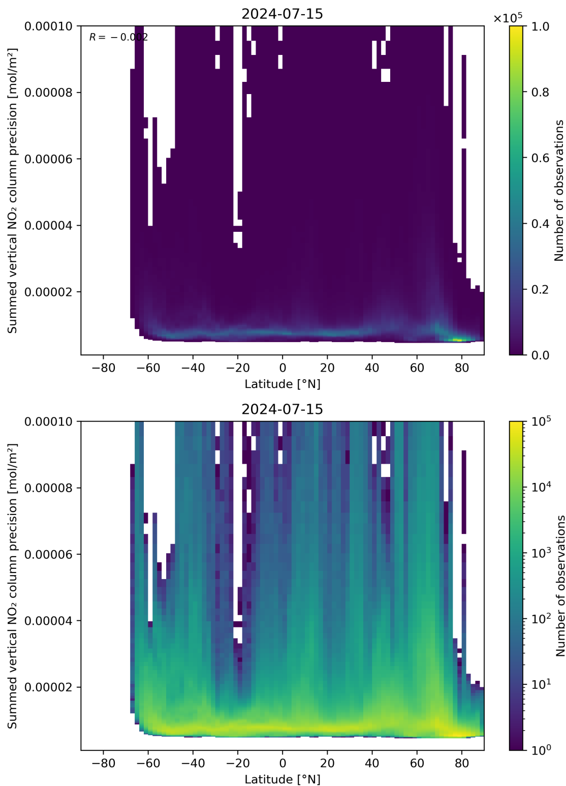
Figure 89: Scatter density plot of “Latitude” against “Summed vertical NO 2 column precision” for 2024-07-15 to 2024-07-16.
