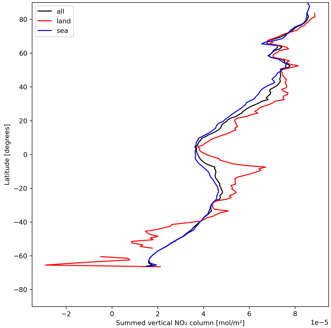
Figure 23: Zonal average of “Summed vertical NO 2 column” for 2024-07-15 to 2024-07-16.
