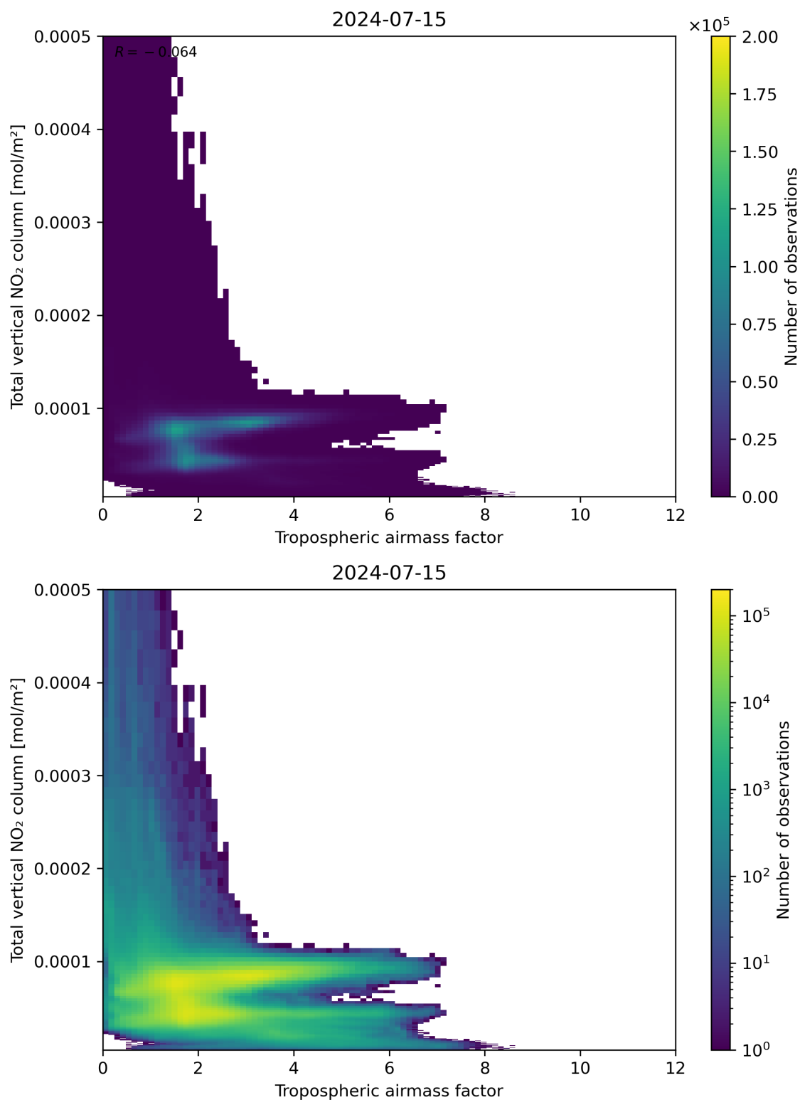
Figure 77: Scatter density plot of “Tropospheric airmass factor” against “Total vertical NO 2 column” for 2024-07-15 to 2024-07-16.
