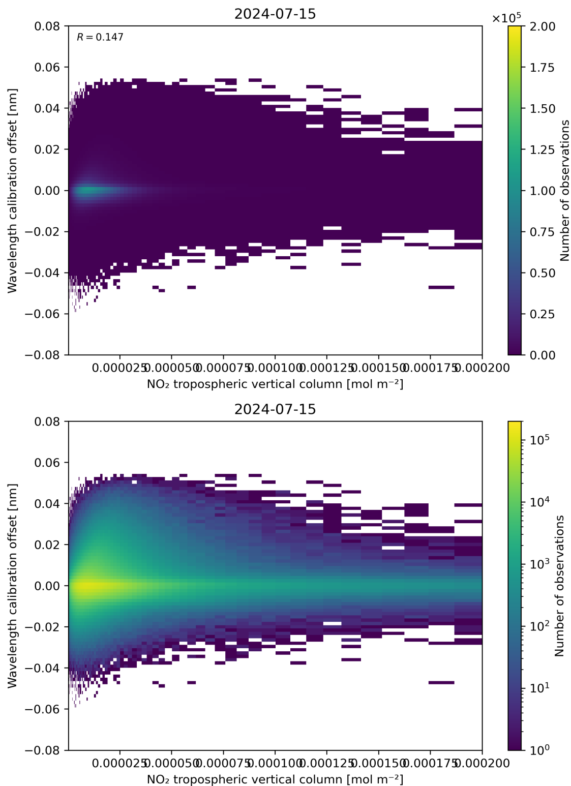
Figure 143: Scatter density plot of “NO 2 tropospheric vertical column” against “Wavelength calibration offset” for 2024-07-15 to 2024-07-16.
