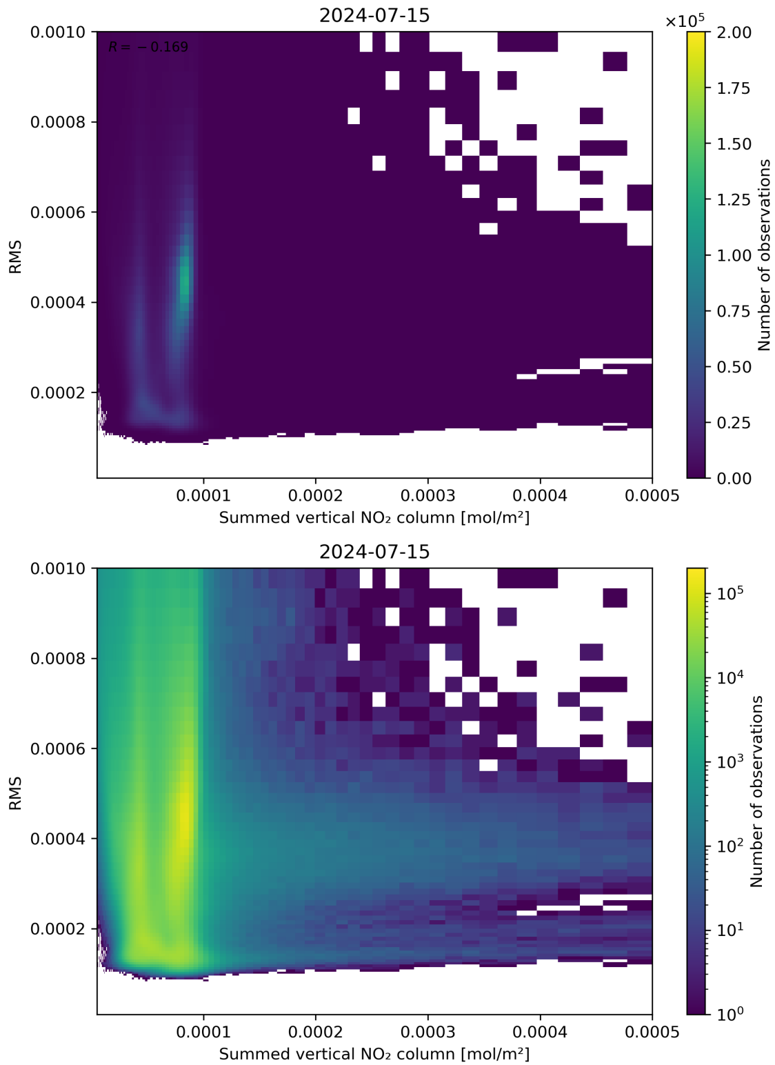
Figure 109: Scatter density plot of “Summed vertical NO 2 column” against “RMS” for 2024-07-15 to 2024-07-16.
