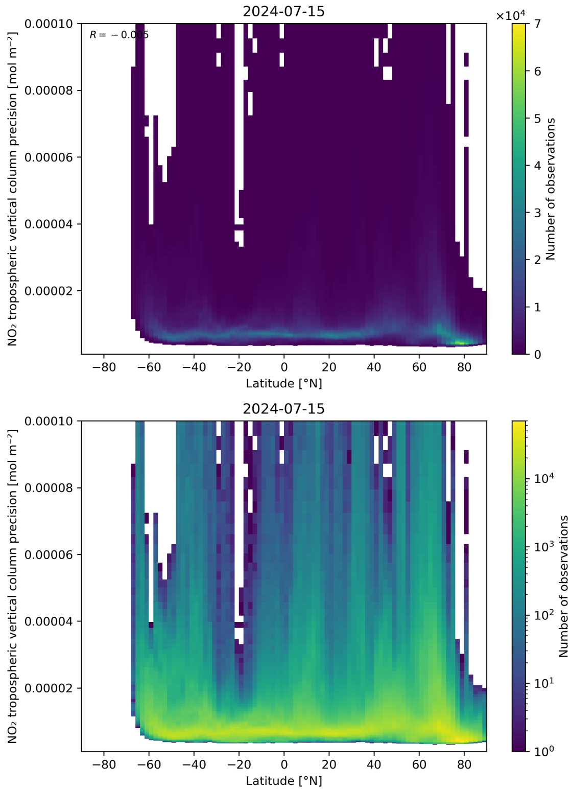
Figure 93: Scatter density plot of “Latitude” against “NO 2 tropospheric vertical column precision” for 2024-07-15 to 2024-07-16.
