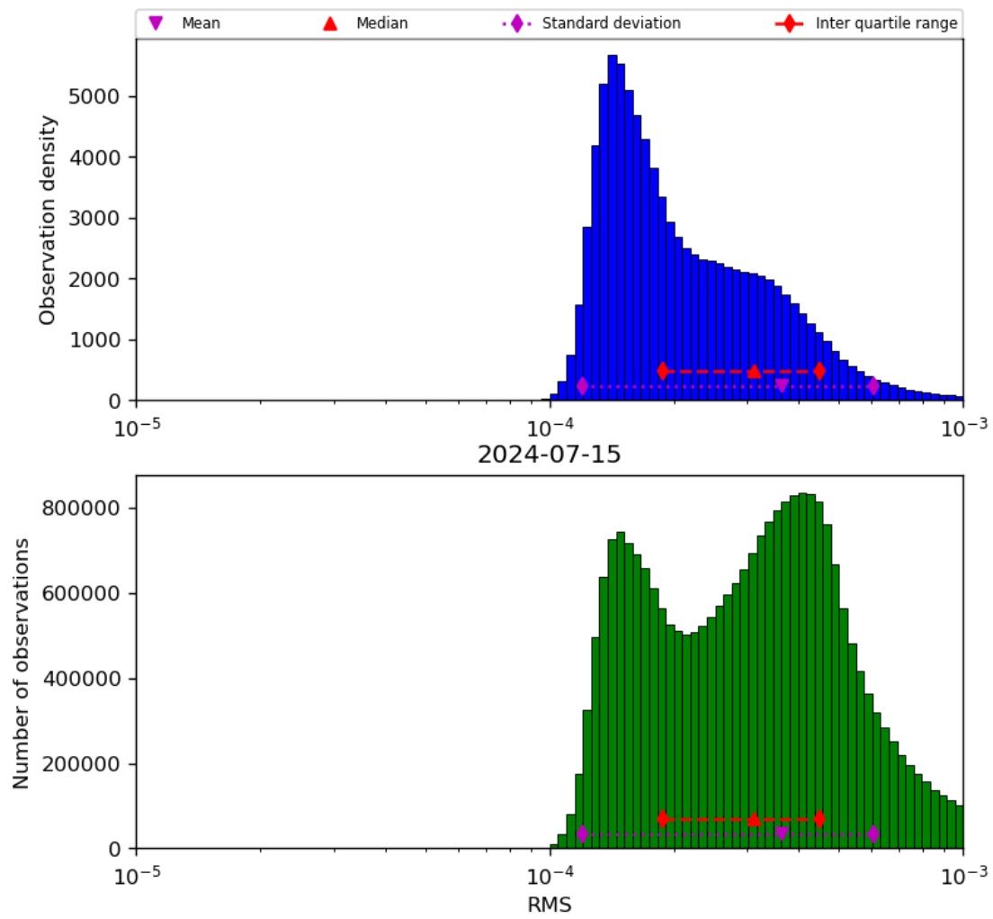
Figure 43: Histogram of “RMS” for 2024-07-15 to 2024-07-16
