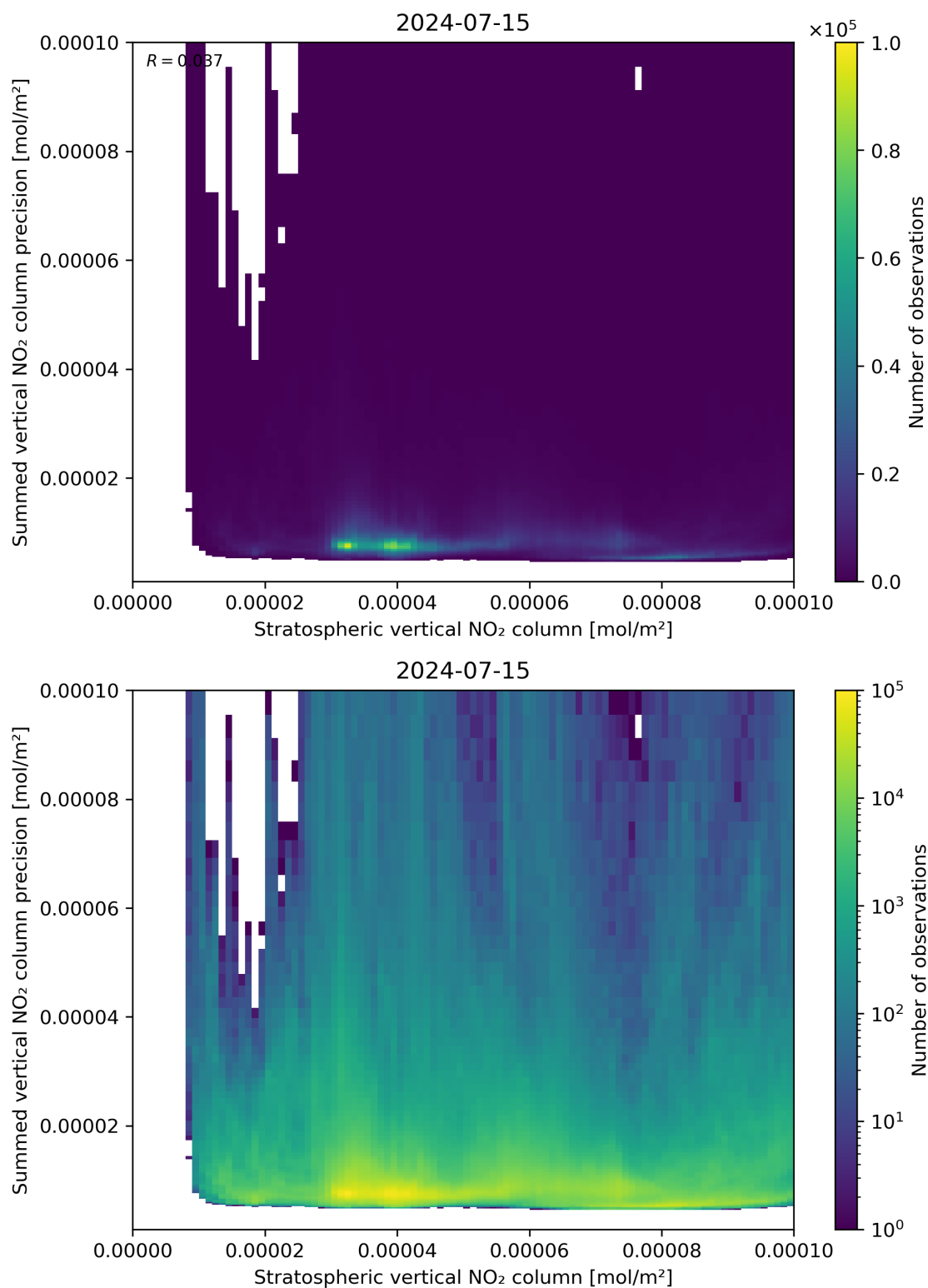
Figure 99: Scatter density plot of “Stratospheric vertical NO 2 column” against “Summed vertical NO 2 column precision” for 2024-07-15 to 2024-07-16.
