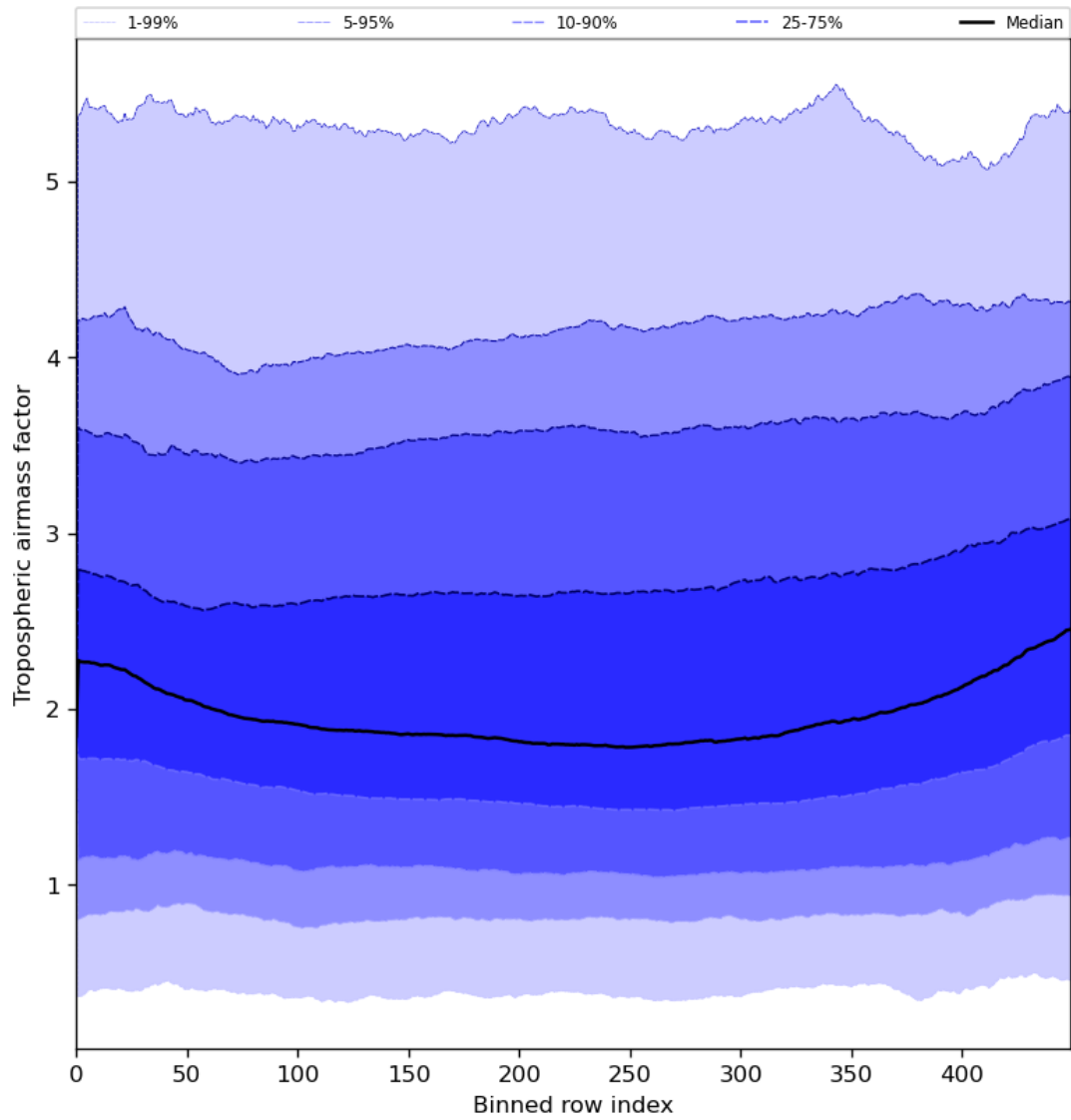
Figure 48: Along track statistics of “Tropospheric airmass factor” for 2024-07-15 to 2024-07-16
