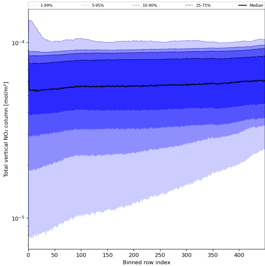
Figure 55: Along track statistics of “Total vertical NO 2 column” for 2024-07-15 to 2024-07-16
