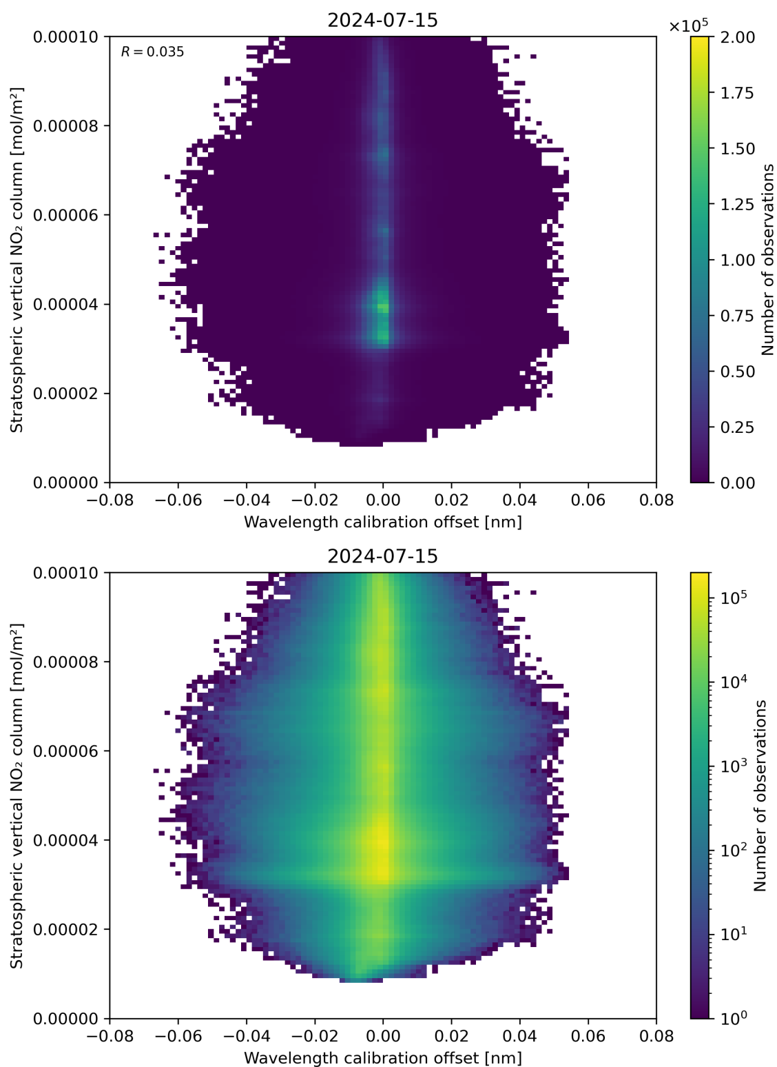
Figure 176: Scatter density plot of “Wavelength calibration offset” against “Stratospheric vertical NO 2 column” for 2024-07-15 to 2024-07-16.
