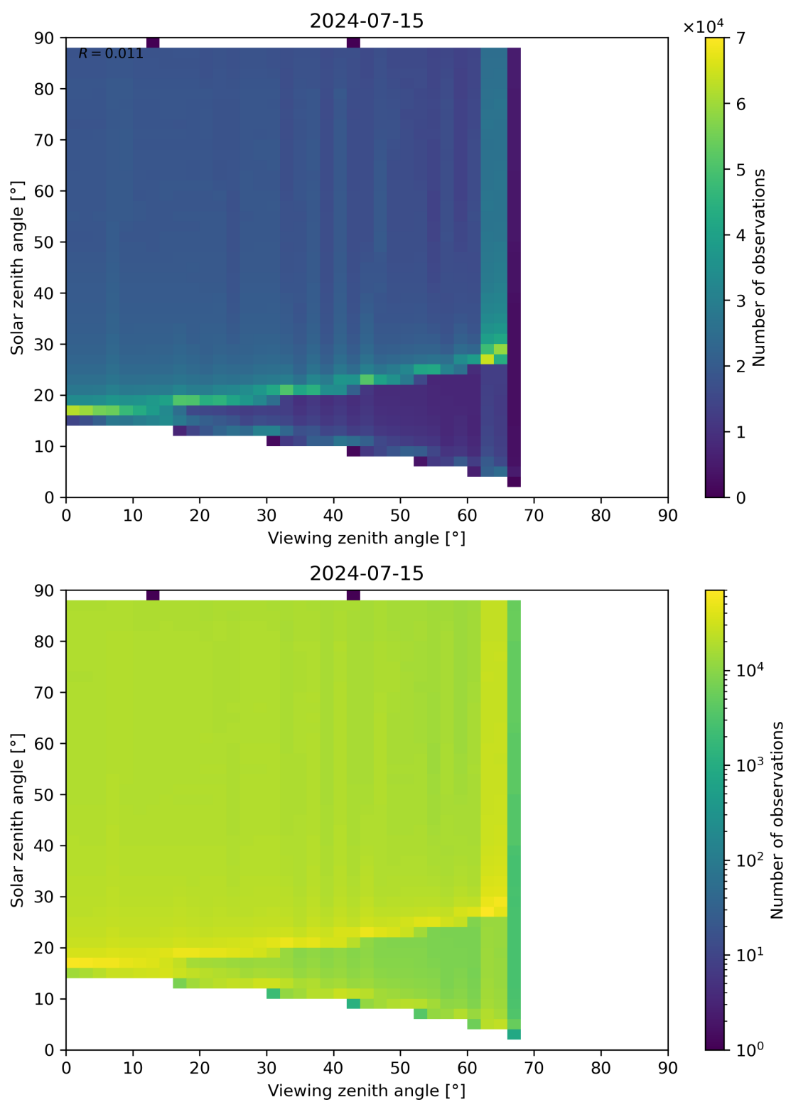
Figure 172: Scatter density plot of “Viewing zenith angle” against “Solar zenith angle” for 2024-07-15 to 2024-07-16.
