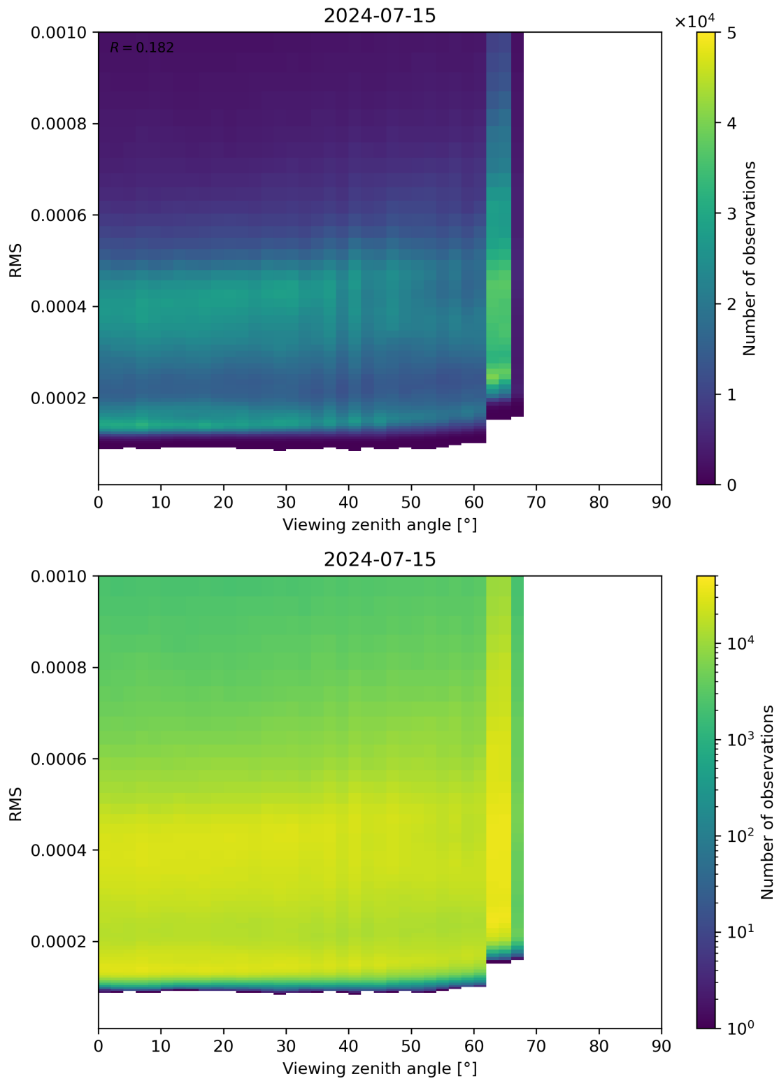
Figure 171: Scatter density plot of “Viewing zenith angle” against “RMS” for 2024-07-15 to 2024-07-16.
