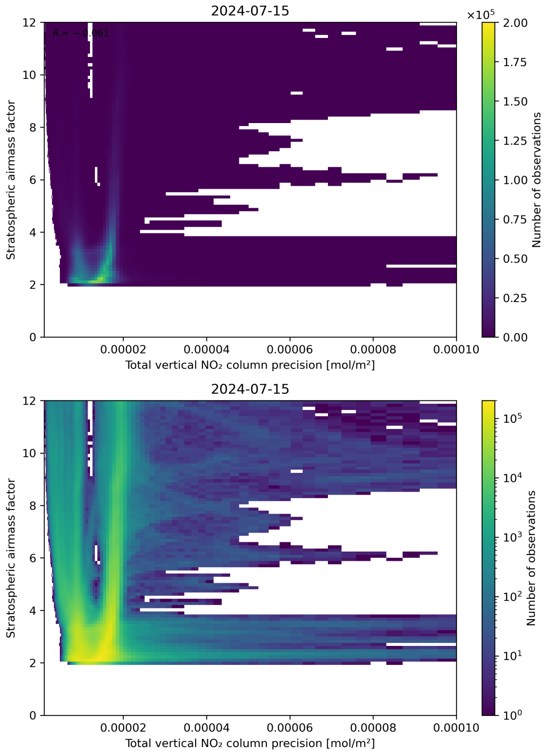
Figure 115: Scatter density plot of “Total vertical NO 2 column precision” against “Stratospheric air mass factor” for 2024-07-15 to 2024-07-16.
