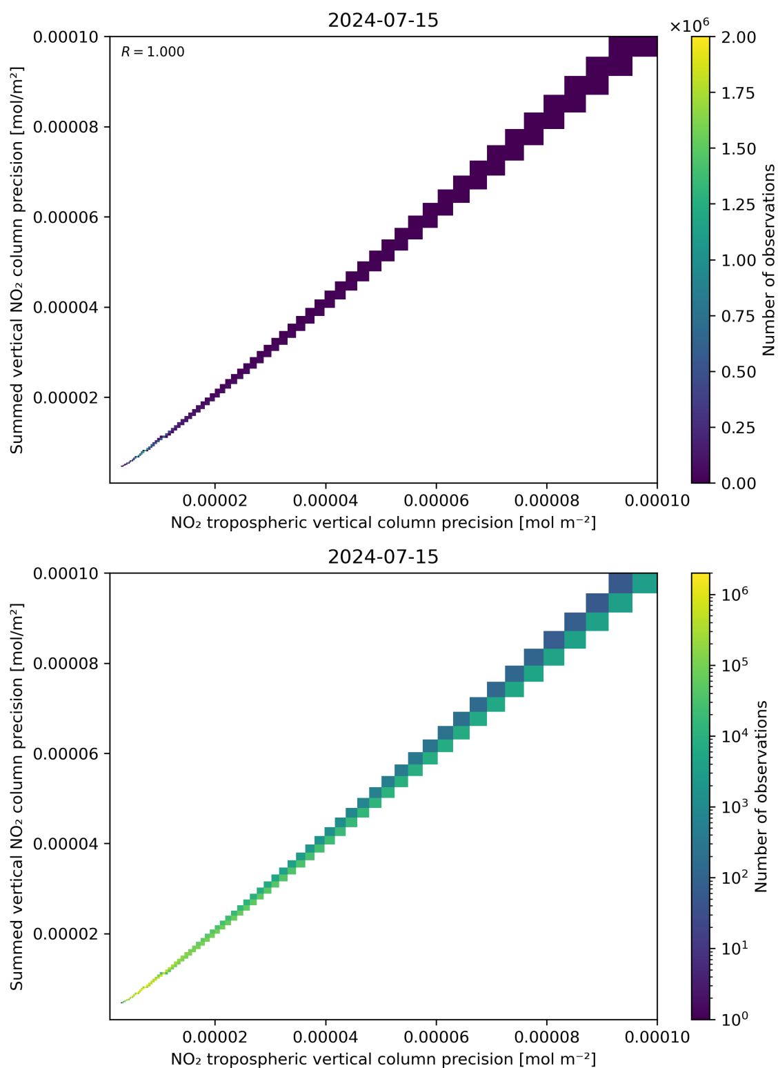
Figure 137: Scatter density plot of “NO 2 tropospheric vertical column precision” against “Summed vertical NO 2 column precision” for 2024-07-15 to 2024-07-16.
