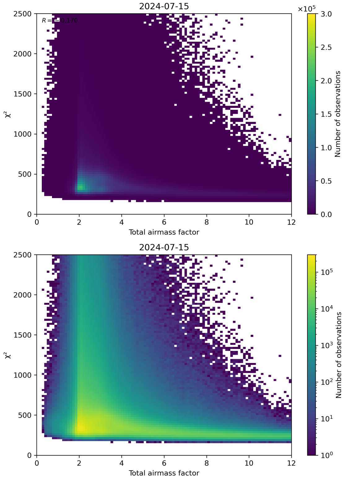
Figure 63: Scatter density plot of “Total airmass factor” against “ \chi^2 ” for 2024-07-15 to 2024-07-16.
