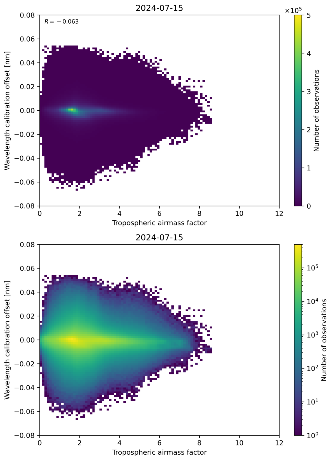
Figure 80: Scatter density plot of “Tropospheric airmass factor” against “Wavelength calibration offset” for 2024-07-15 to 2024-07-16.
