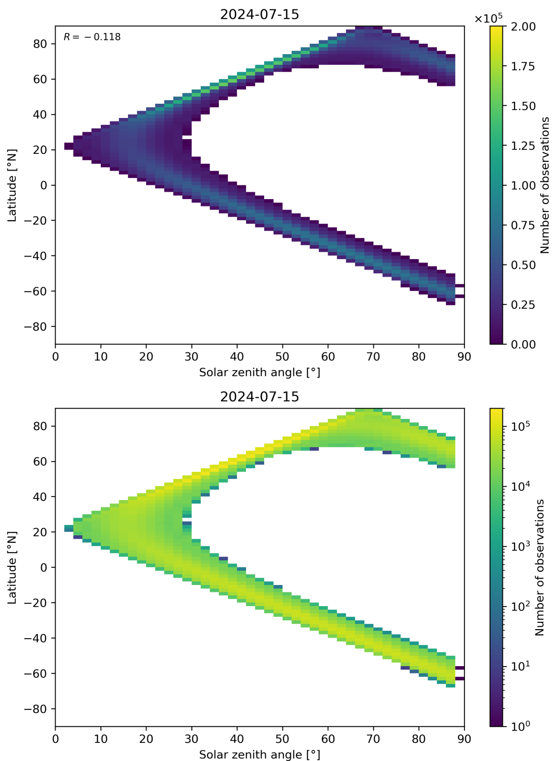
Figure 149: Scatter density plot of “Solar zenith angle” against “Latitude” for 2024-07-15 to 2024-07-16.
