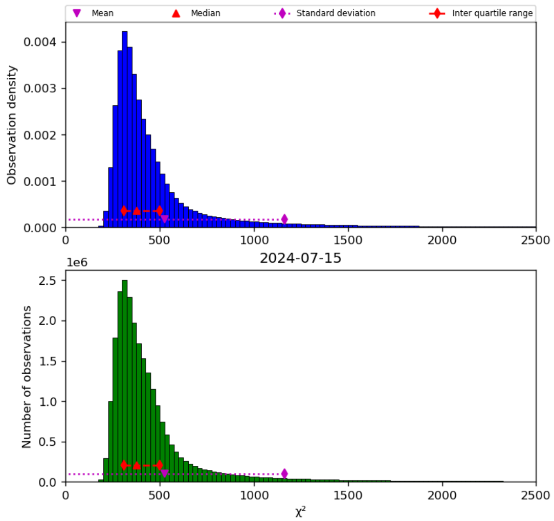
Figure 42: Histogram of " \chi^2 " for 2024-07-15 to 2024-07-16
