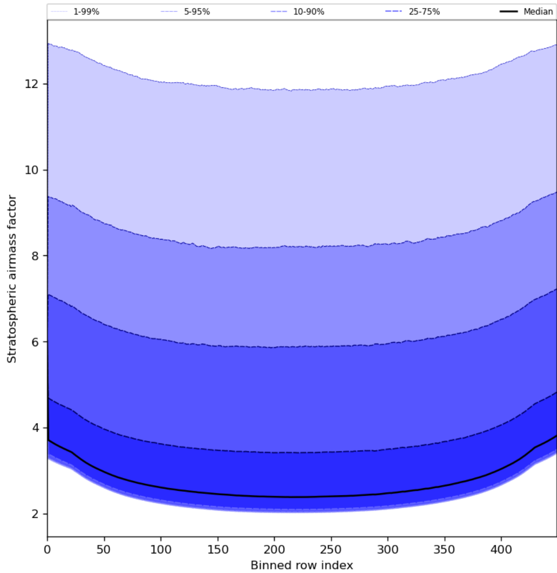
Figure 61: Along track statistics of “Stratospheric airmass factor” for 2024-07-15 to 2024-07-16
