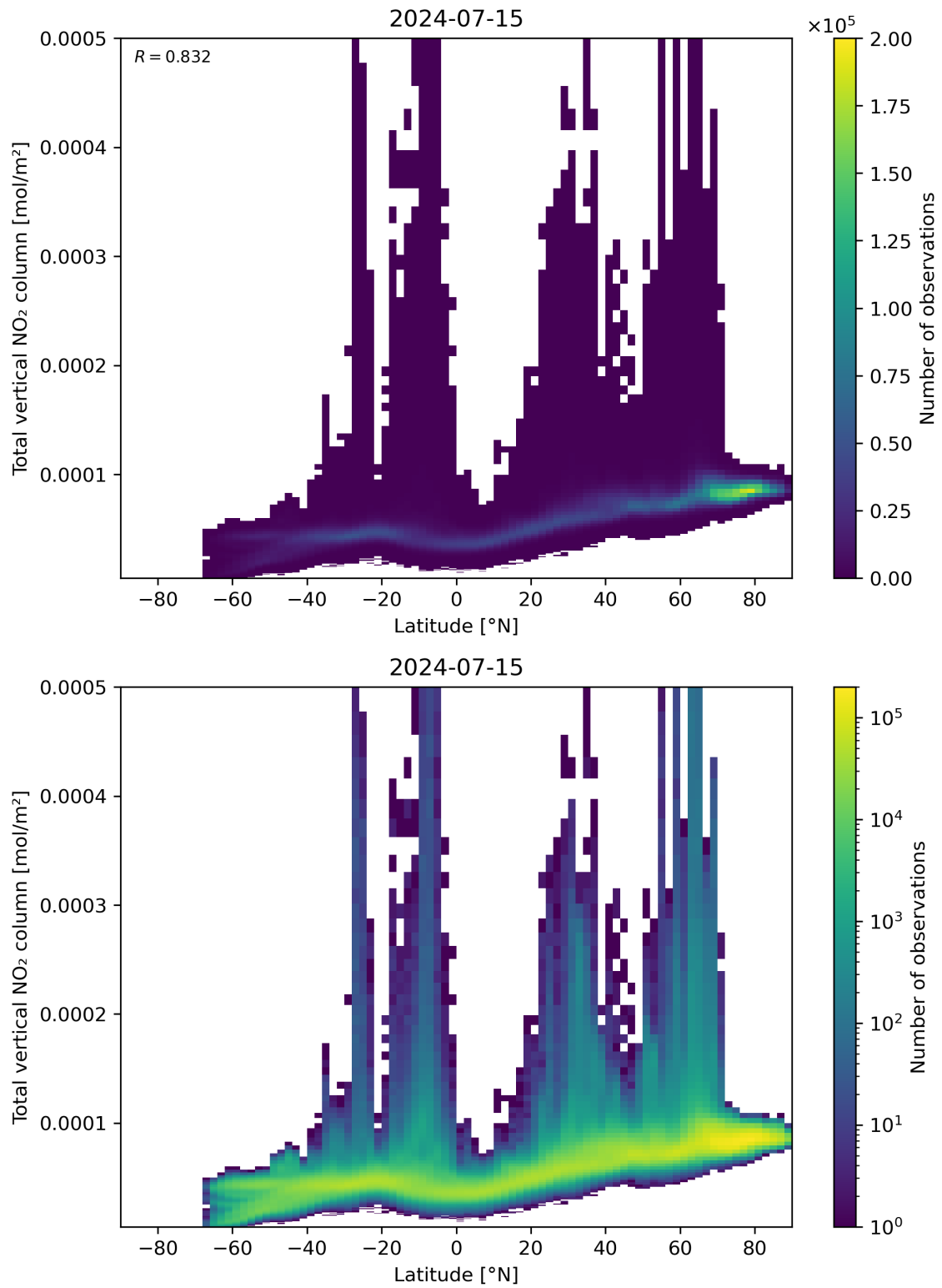
Figure 90: Scatter density plot of “Latitude” against “Total vertical NO 2 column” for 2024-07-15 to 2024-07-16.
