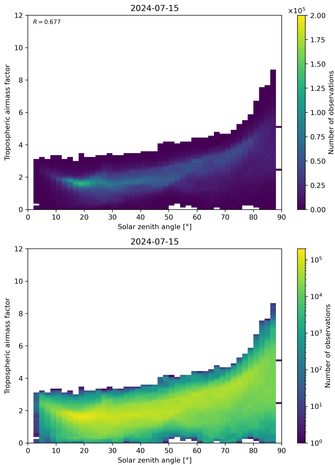
Figure 147: Scatter density plot of “Solar zenith angle” against “Tropospheric airmass factor” for 2024-07-15 to 2024-07-16.
