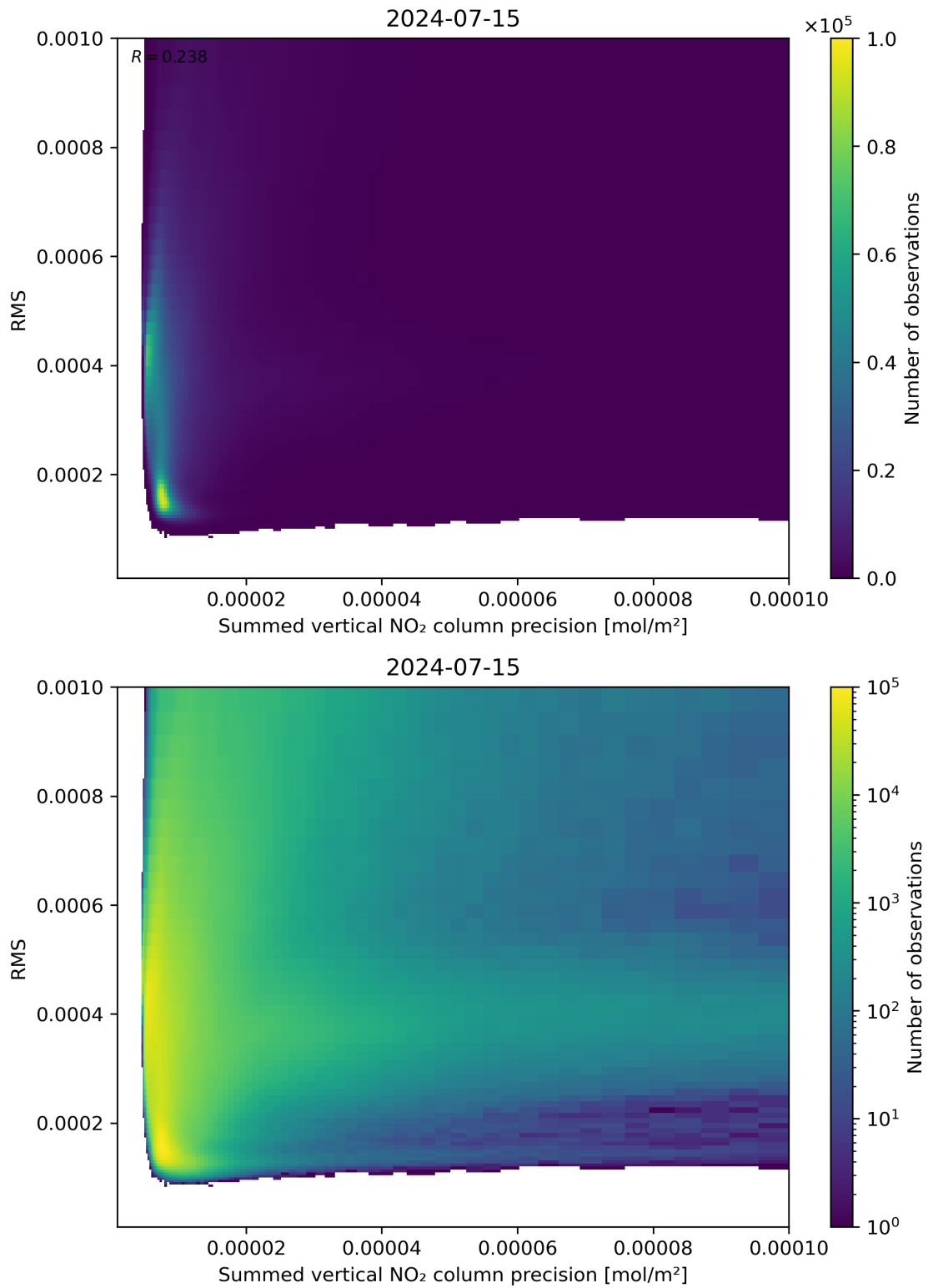
Figure 108: Scatter density plot of “Summed vertical NO 2 column precision” against “RMS” for 2024-07-15 to 2024-07-16.
