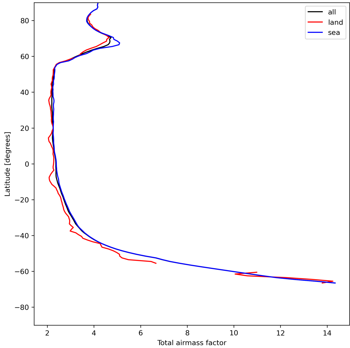
Figure 15: Zonal average of “Total airmass factor” for 2024-07-15 to 2024-07-16.
