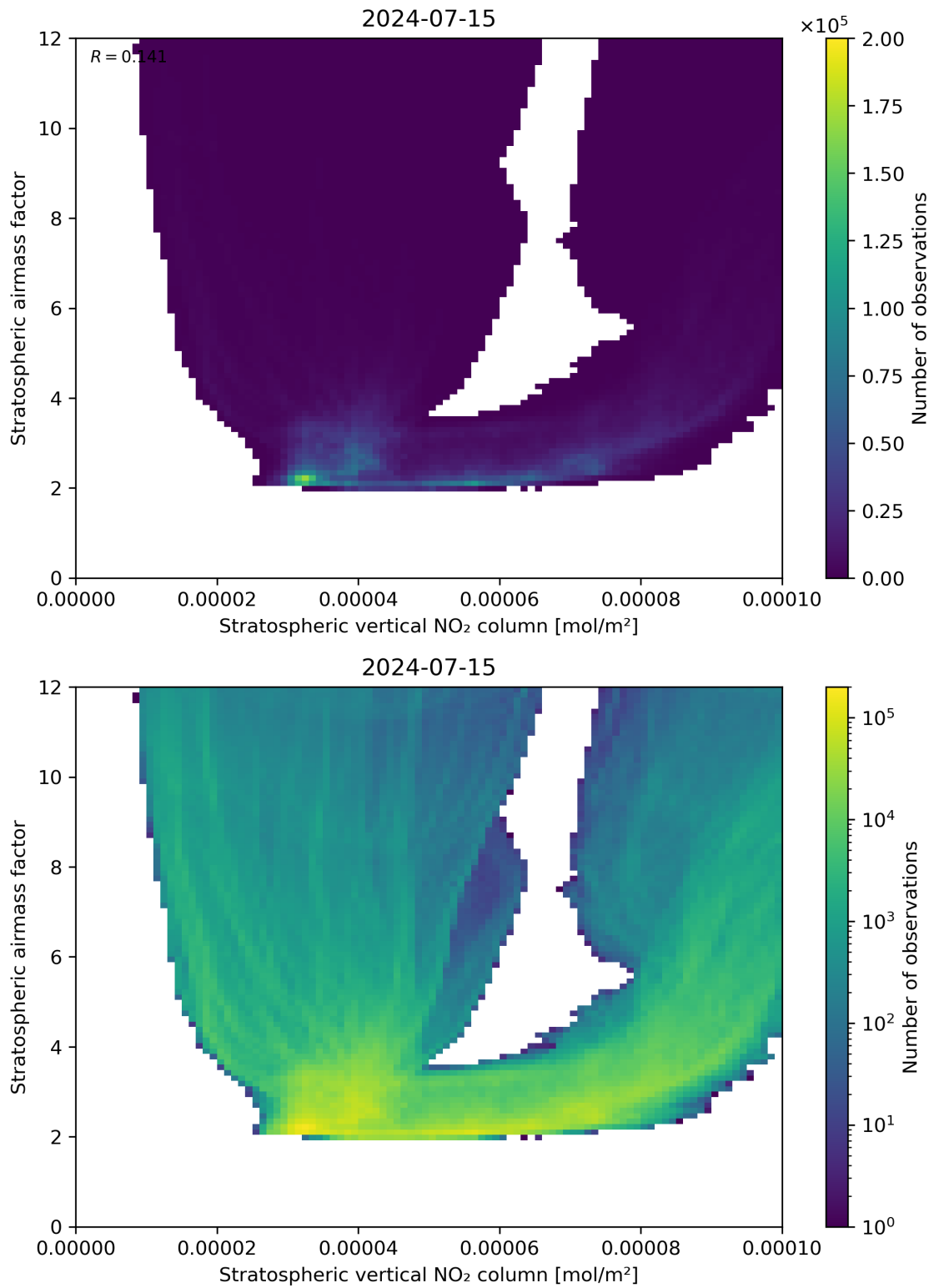
Figure 96: Scatter density plot of “Stratospheric vertical NO 2 column” against “Stratospheric airmass factor” for 2024-07-15 to 2024-07-16.
