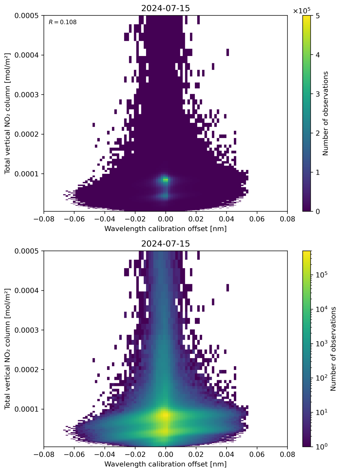
Figure 179: Scatter density plot of “Wavelength calibration offset” against “Total vertical NO 2 column” for 2024-07-15 to 2024-07-16.
