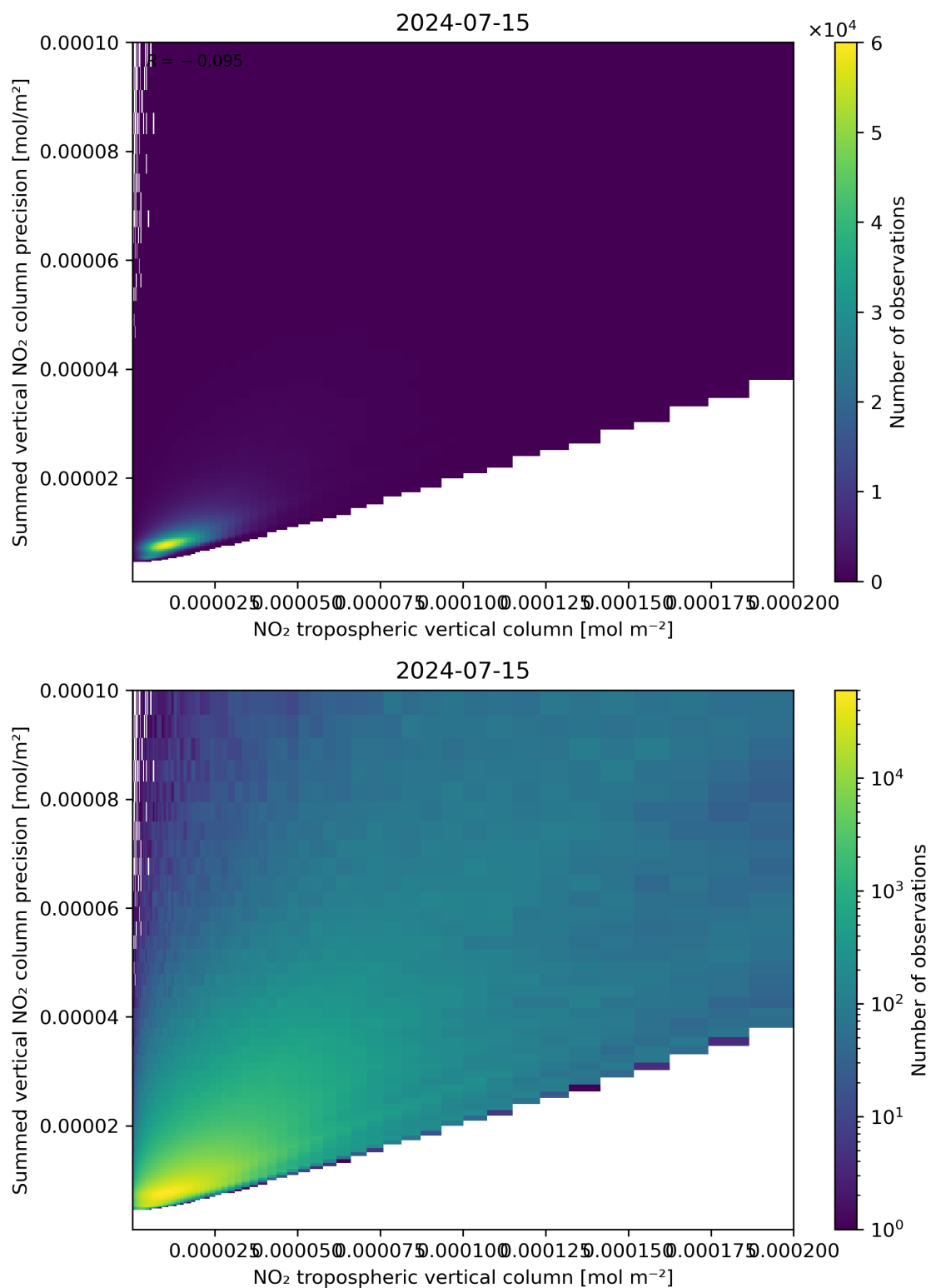
Figure 127: Scatter density plot of “NO 2 tropospheric vertical column” against “Summed vertical NO 2 column precision” for 2024-07-15 to 2024-07-16.
