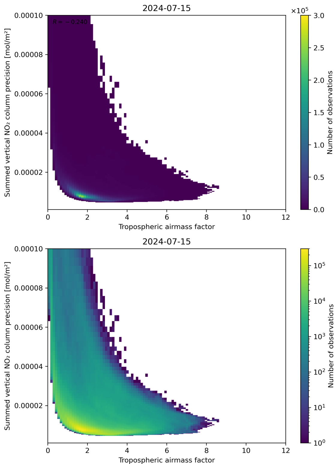
Figure 76: Scatter density plot of “Tropospheric air mass factor” against “Summed vertical NO 2 column precision” for 2024-07-15 to 2024-07-16.
