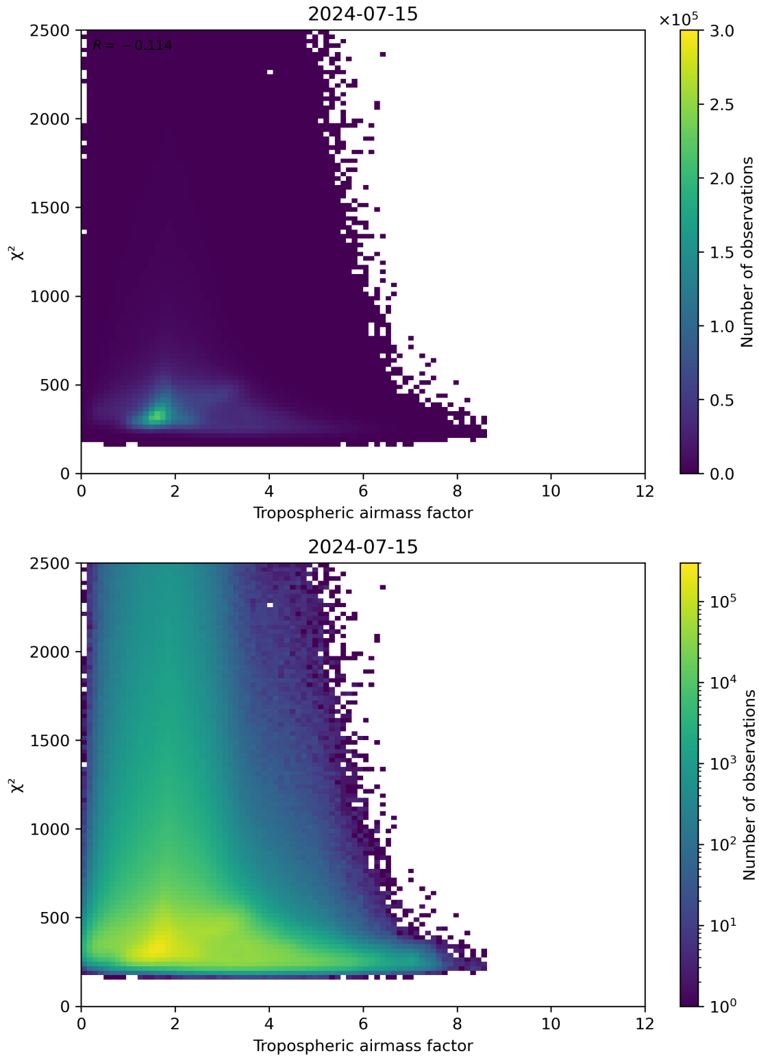
Figure 73: Scatter density plot of “Tropospheric airmass factor” against “ \chi^2 ” for 2024-07-15 to 2024-07-16.
