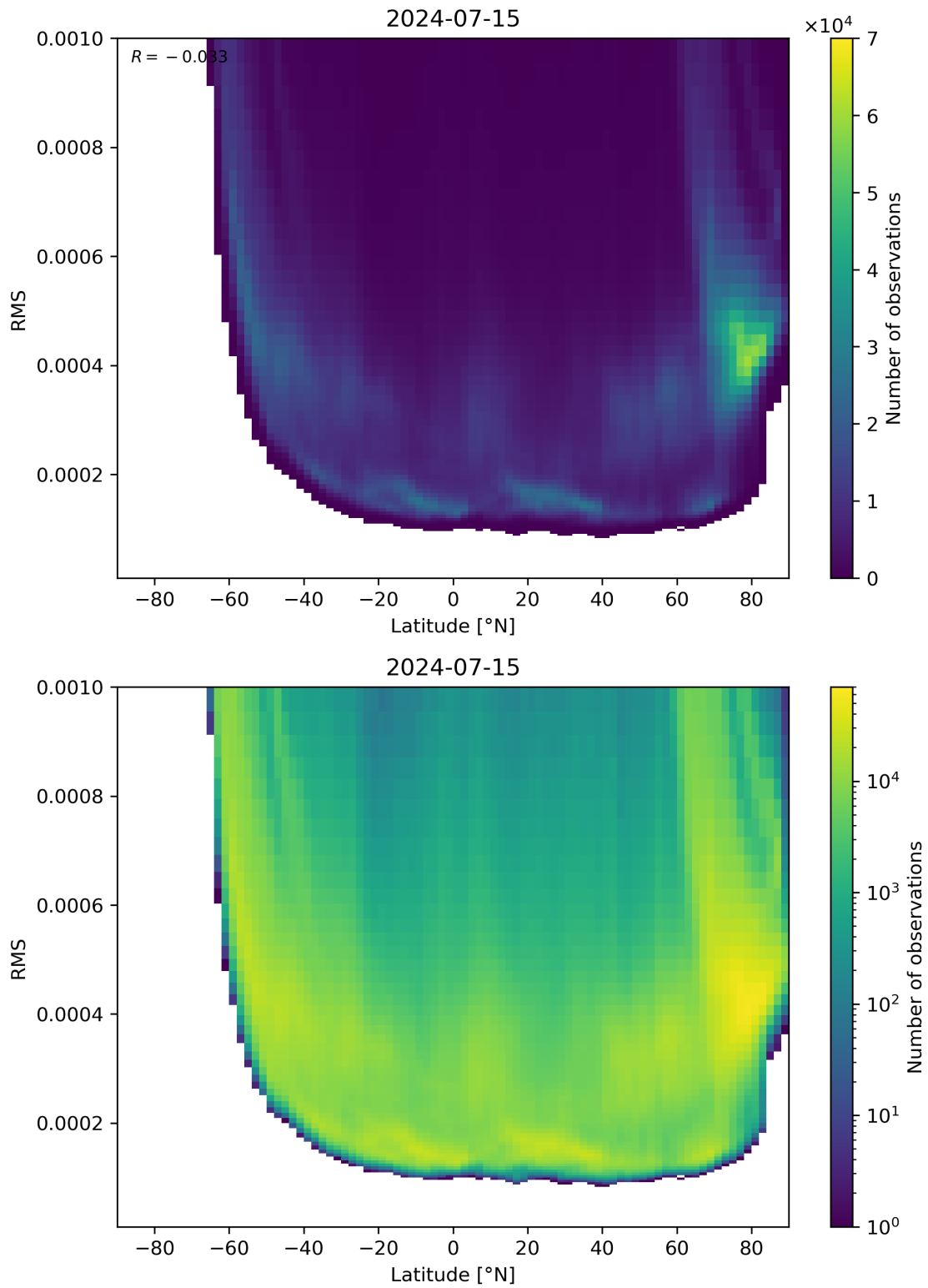
Figure 94: Scatter density plot of “Latitude” against “RMS” for 2024-07-15 to 2024-07-16.
