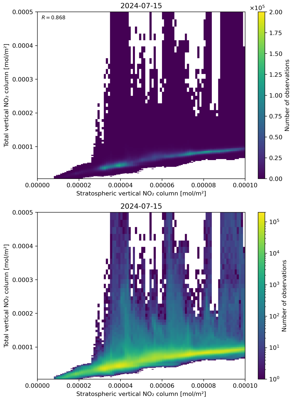
Figure 100: Scatter density plot of “Stratospheric vertical NO 2 column” against “Total vertical NO 2 column” for 2024-07-15 to 2024-07-16.
