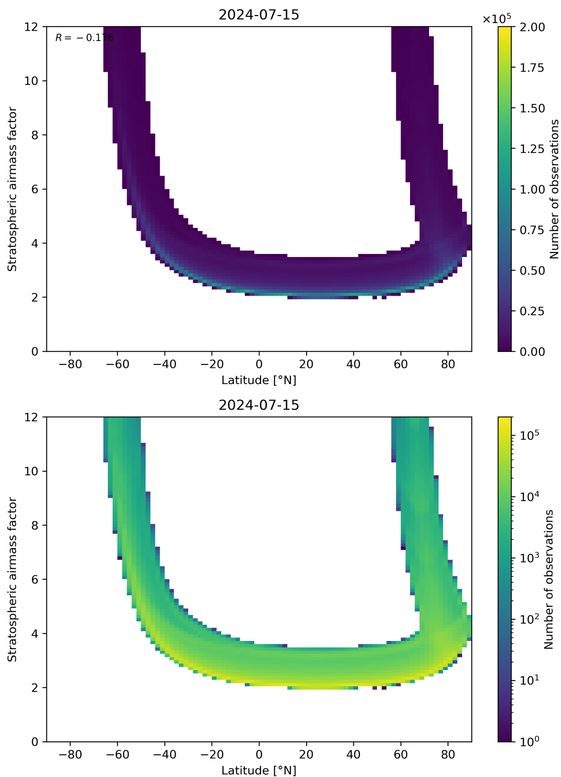
Figure 83: Scatter density plot of “Latitude” against “Stratospheric air mass factor” for 2024-07-15 to 2024-07-16.
