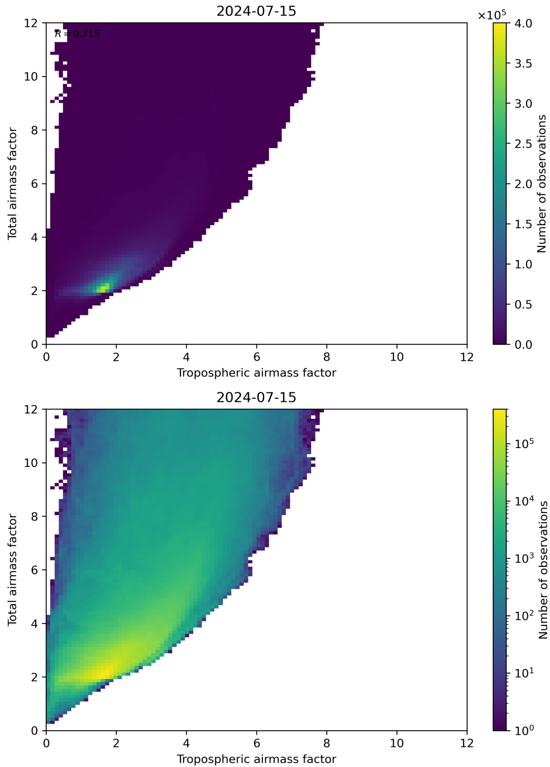
Figure 72: Scatter density plot of “Tropospheric airmass factor” against “Total airmass factor” for 2024-07-15 to 2024-07-16.
