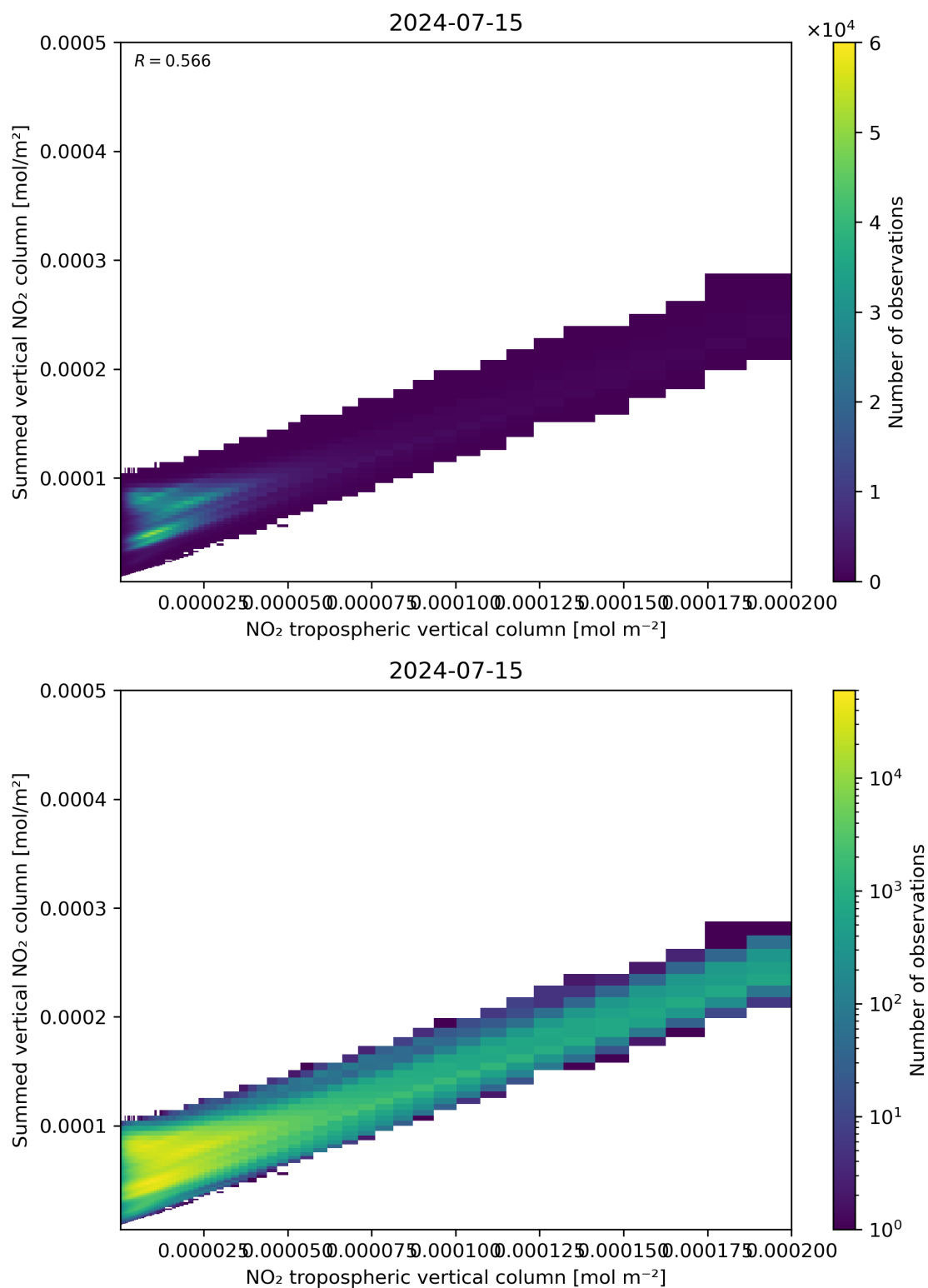
Figure 126: Scatter density plot of “NO 2 tropospheric vertical column” against “Summed vertical NO 2 column” for 2024-07-15 to 2024-07-16.
