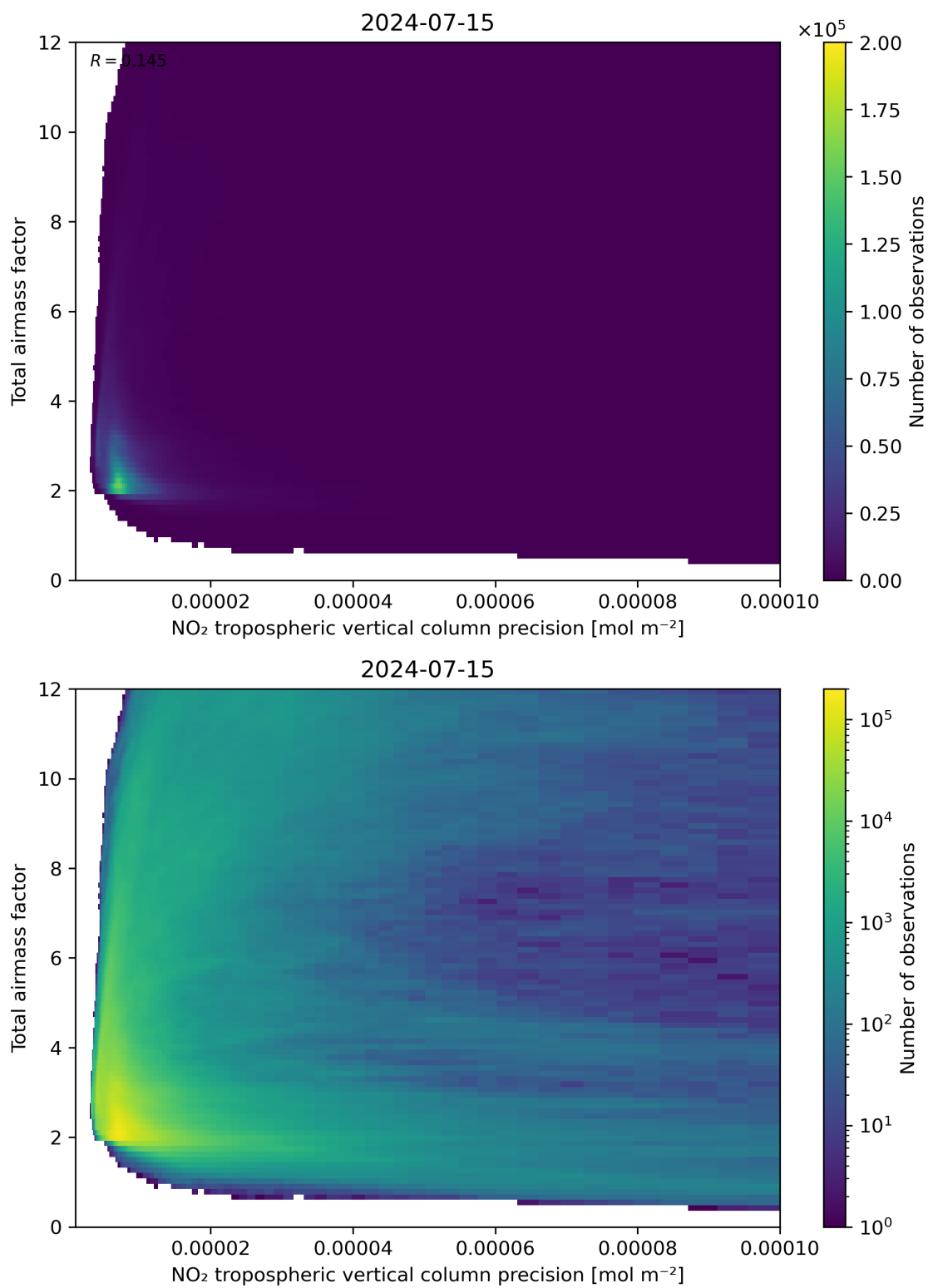
Figure 132: Scatter density plot of “NO 2 tropospheric vertical column precision” against “Total air mass factor” for 2024-07-15 to 2024-07-16.
