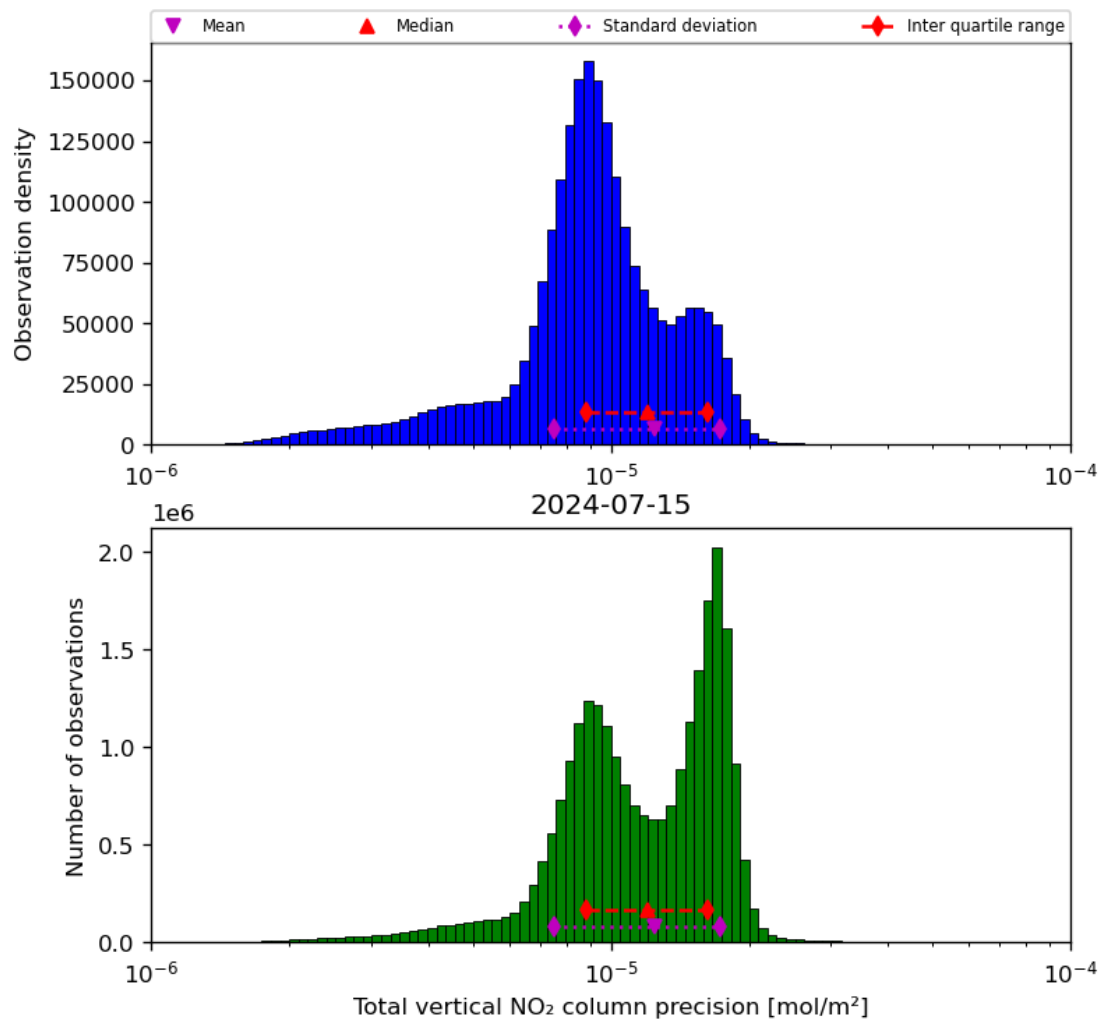
Figure 39: Histogram of “Total vertical NO 2 column precision” for 2024-07-15 to 2024-07-16
