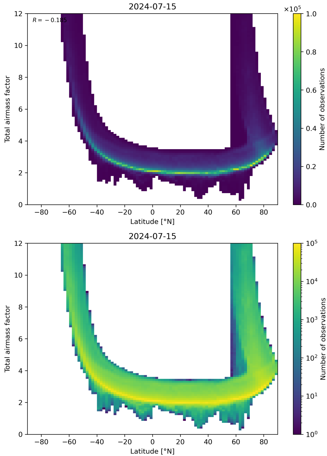
Figure 84: Scatter density plot of “Latitude” against “Total airmass factor” for 2024-07-15 to 2024-07-16.
