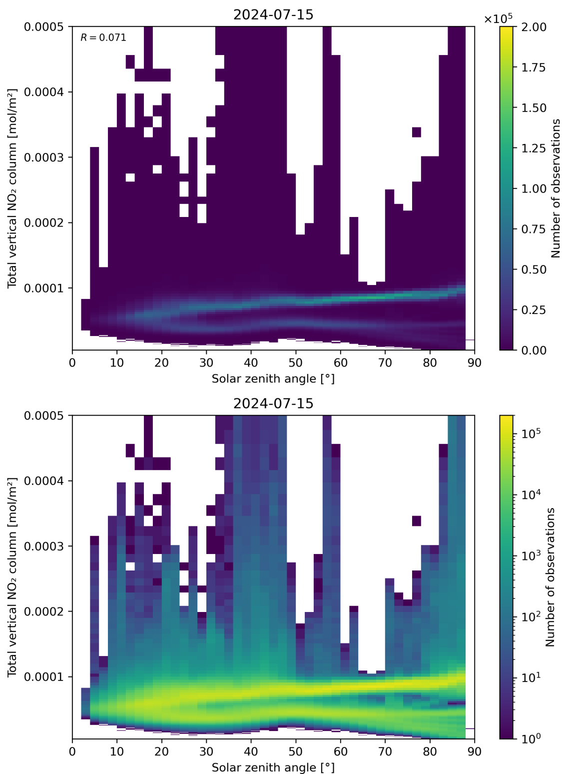
Figure 153: Scatter density plot of “Solar zenith angle” against “Total vertical NO 2 column” for 2024-07-15 to 2024-07-16.
