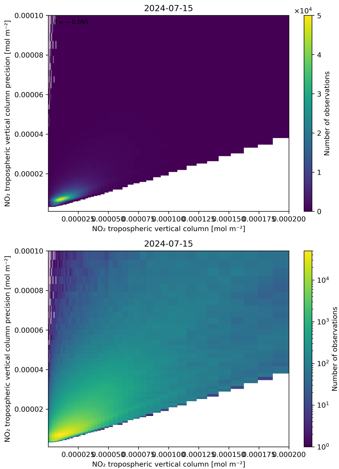
Figure 130: Scatter density plot of “NO 2 tropospheric vertical column” against “NO 2 tropospheric vertical column precision” for 2024-07-15 to 2024-07-16.
