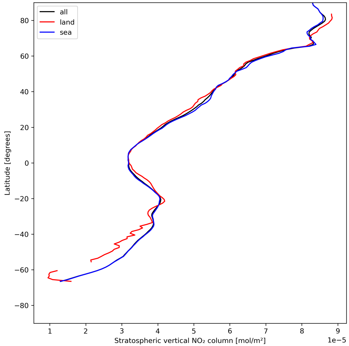
Figure 19: Zonal average of “Stratospheric vertical NO 2 column” for 2024-07-15 to 2024-07-16.
