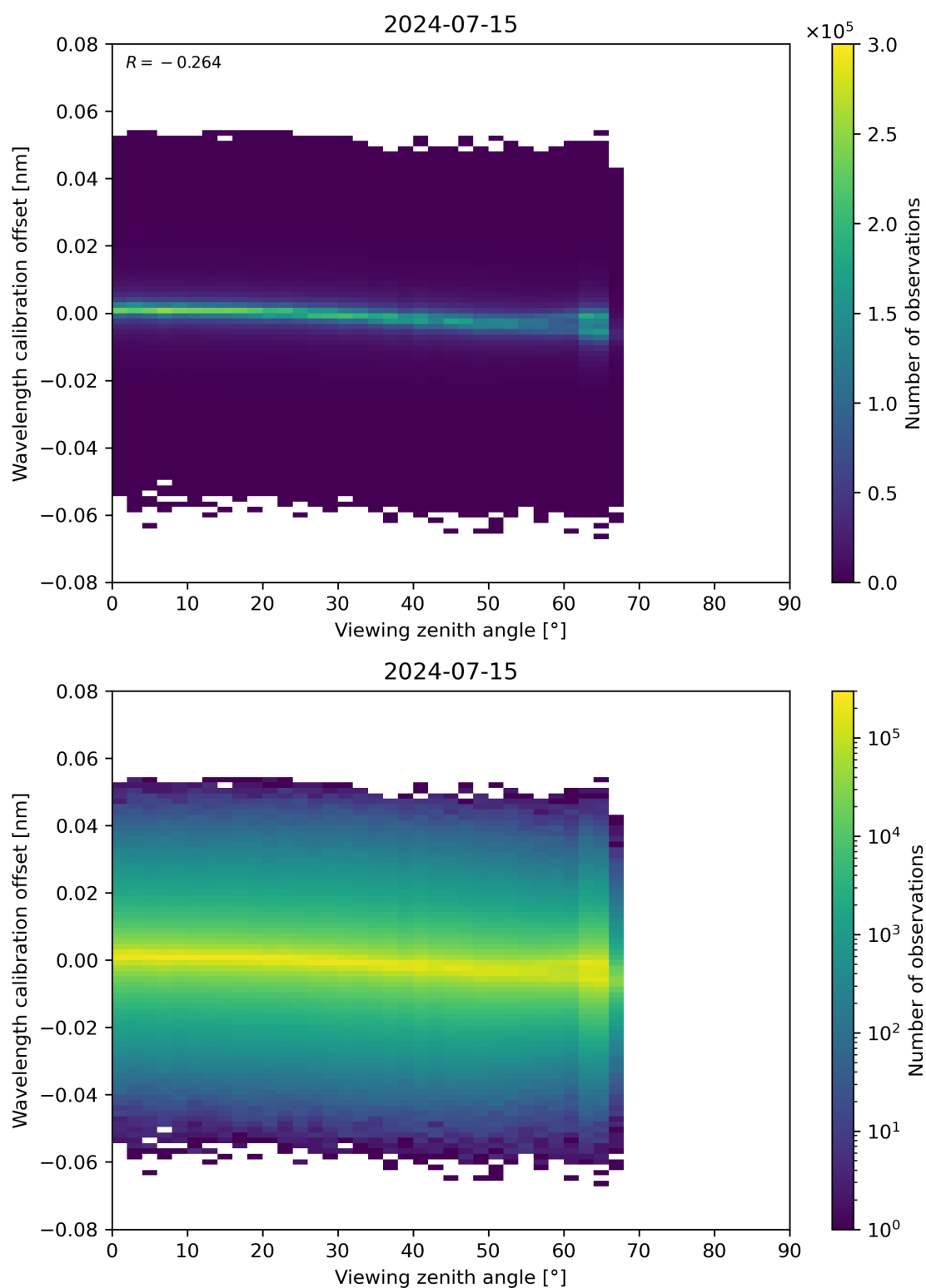
Figure 173: Scatter density plot of “Viewing zenith angle” against “Wavelength calibration offset” for 2024-07-15 to 2024-07-16.
