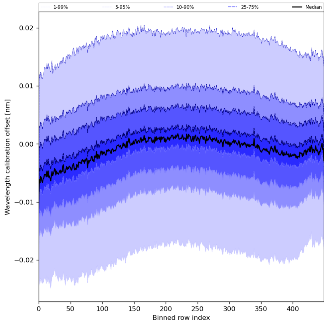
Figure 52: Along track statistics of “Wavelength calibration offset” for 2024-07-15 to 2024-07-16
