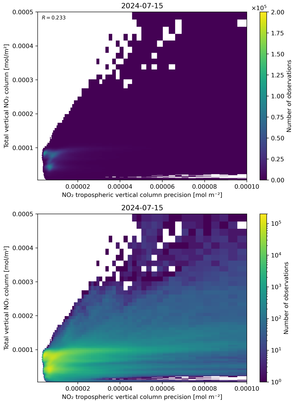
Figure 138: Scatter density plot of “NO 2 tropospheric vertical column precision” against “Total vertical NO 2 column” for 2024-07-15 to 2024-07-16.
