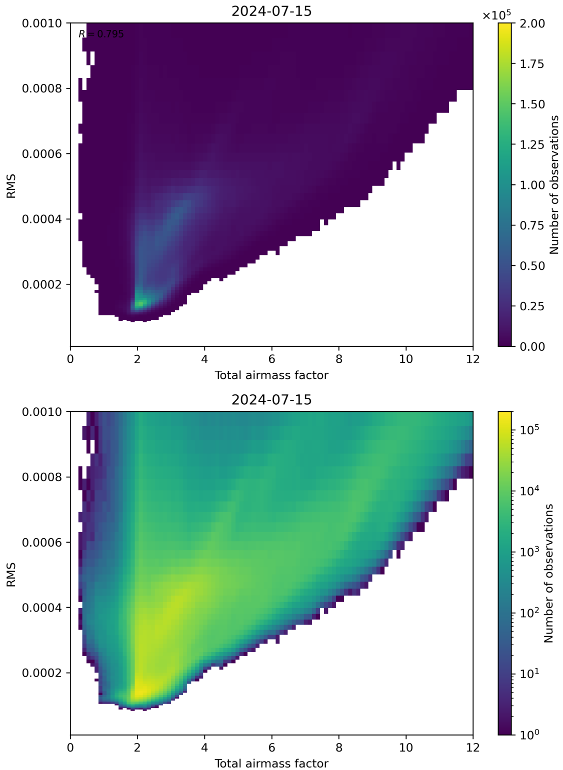
Figure 69: Scatter density plot of “Total airmass factor” against “RMS” for 2024-07-15 to 2024-07-16.
