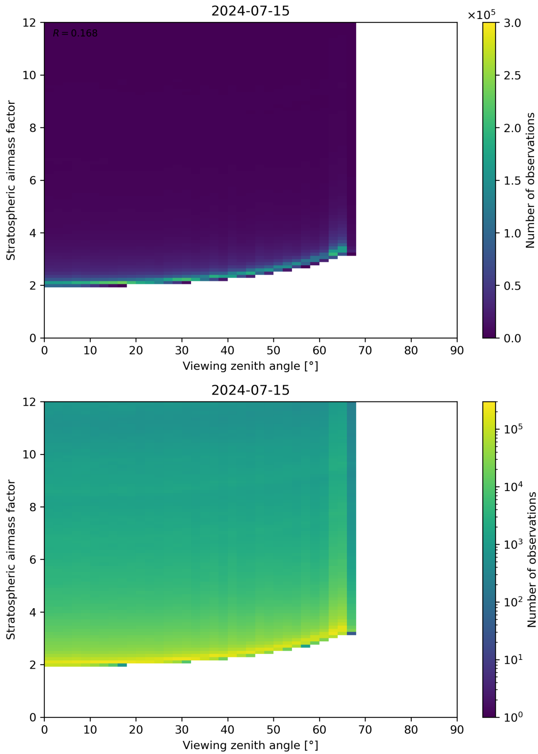
Figure 159: Scatter density plot of “Viewing zenith angle” against “Stratospheric airmass factor” for 2024-07-15 to 2024-07-16.
