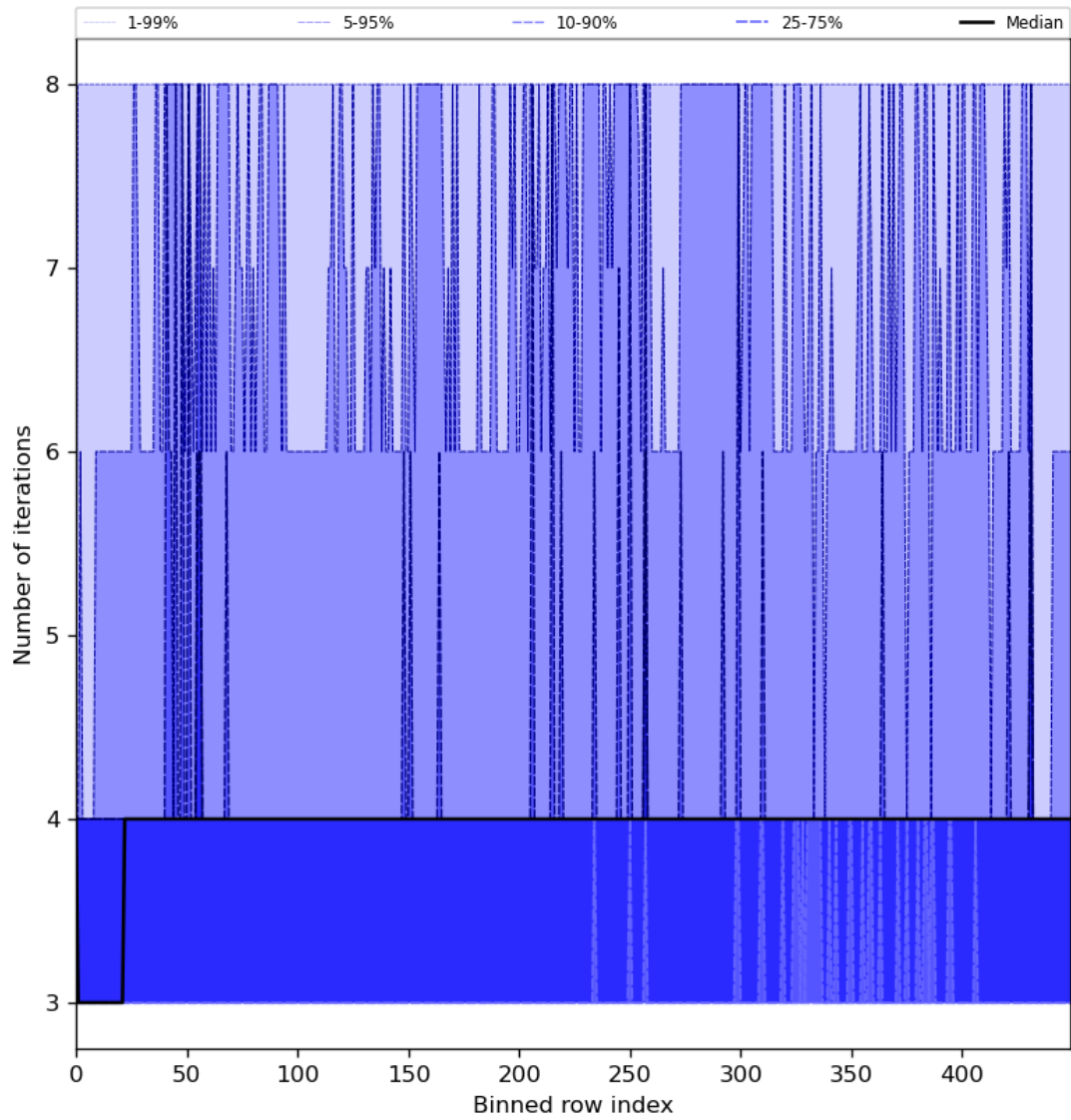
Figure 51: Along track statistics of “Number of iterations” for 2024-07-15 to 2024-07-16
