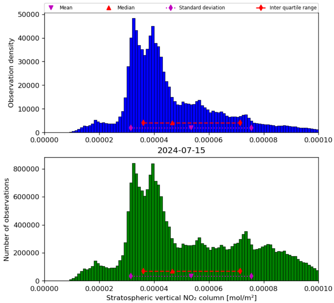
Figure 36: Histogram of “Stratospheric vertical NO 2 column” for 2024-07-15 to 2024-07-16
