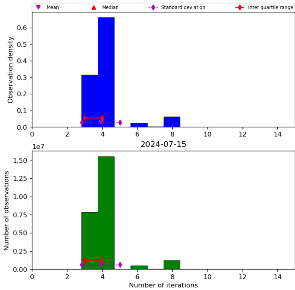
Figure 34: Histogram of “Number of iterations” for 2024-07-15 to 2024-07-16
