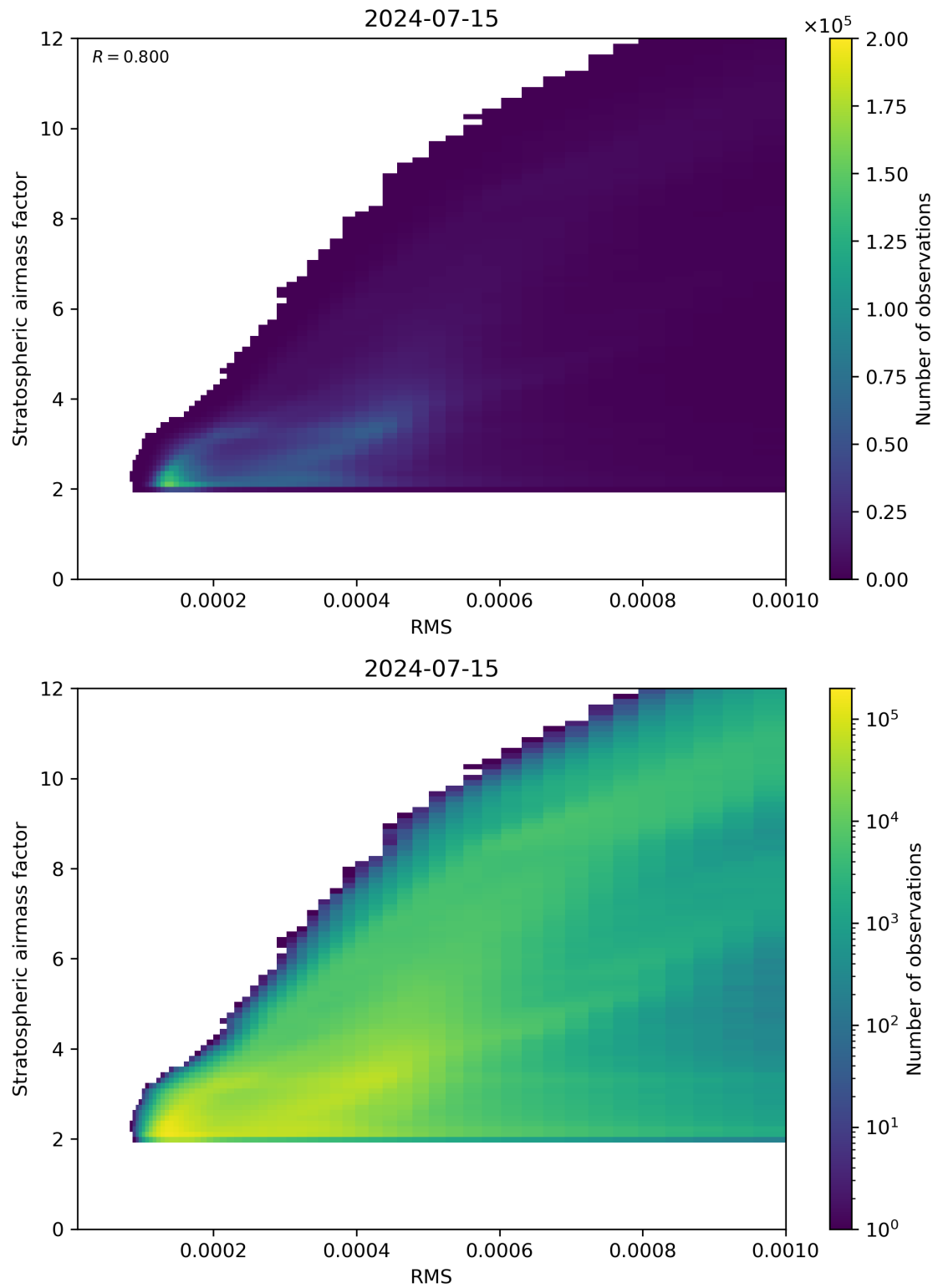
Figure 144: Scatter density plot of “RMS” against “Stratospheric airmass factor” for 2024-07-15 to 2024-07-16.
