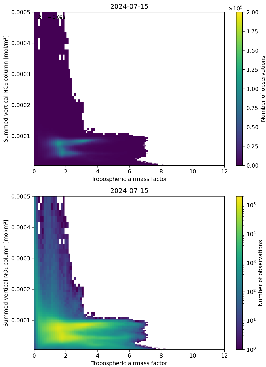
Figure 75: Scatter density plot of “Tropospheric airmass factor” against “Summed vertical NO 2 column” for 2024-07-15 to 2024-07-16.
