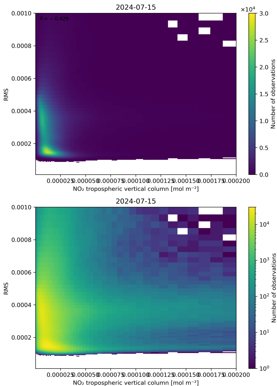
Figure 142: Scatter density plot of “NO 2 tropospheric vertical column” against “RMS” for 2024-07-15 to 2024-07-16.
