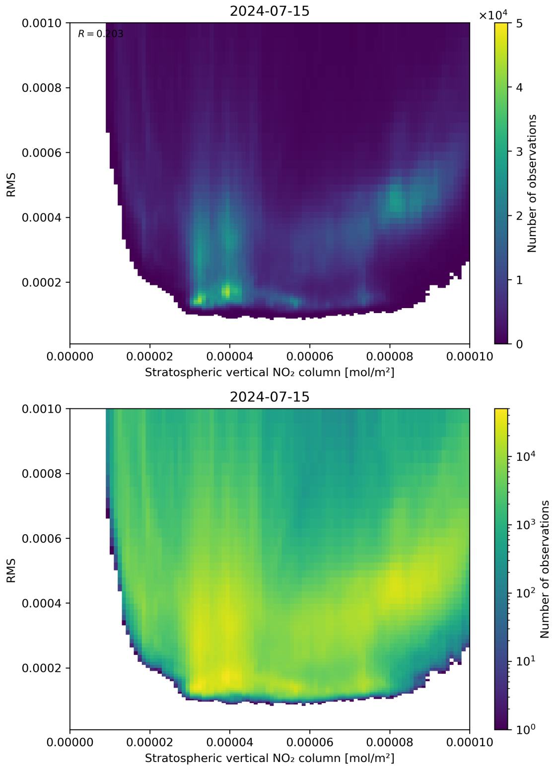
Figure 102: Scatter density plot of “Stratospheric vertical NO 2 column” against “RMS” for 2024-07-15 to 2024-07-16.
