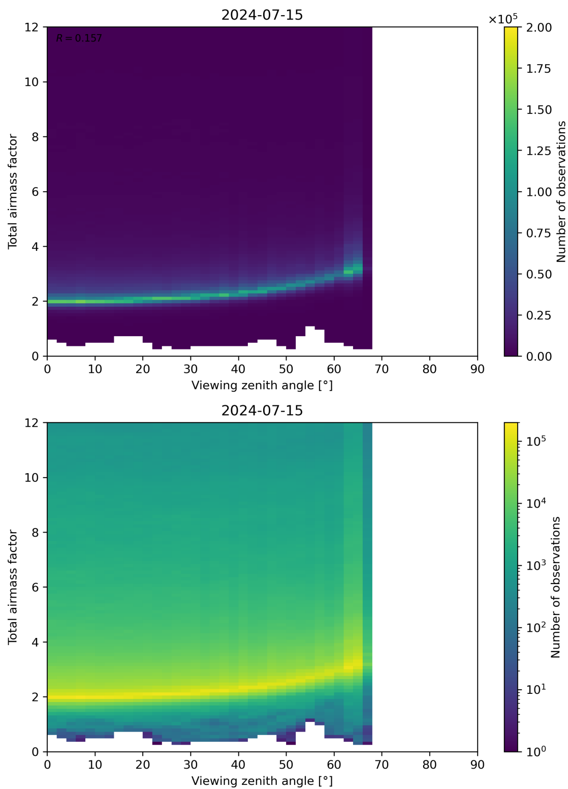
Figure 160: Scatter density plot of “Viewing zenith angle” against “Total airmass factor” for 2024-07-15 to 2024-07-16.
