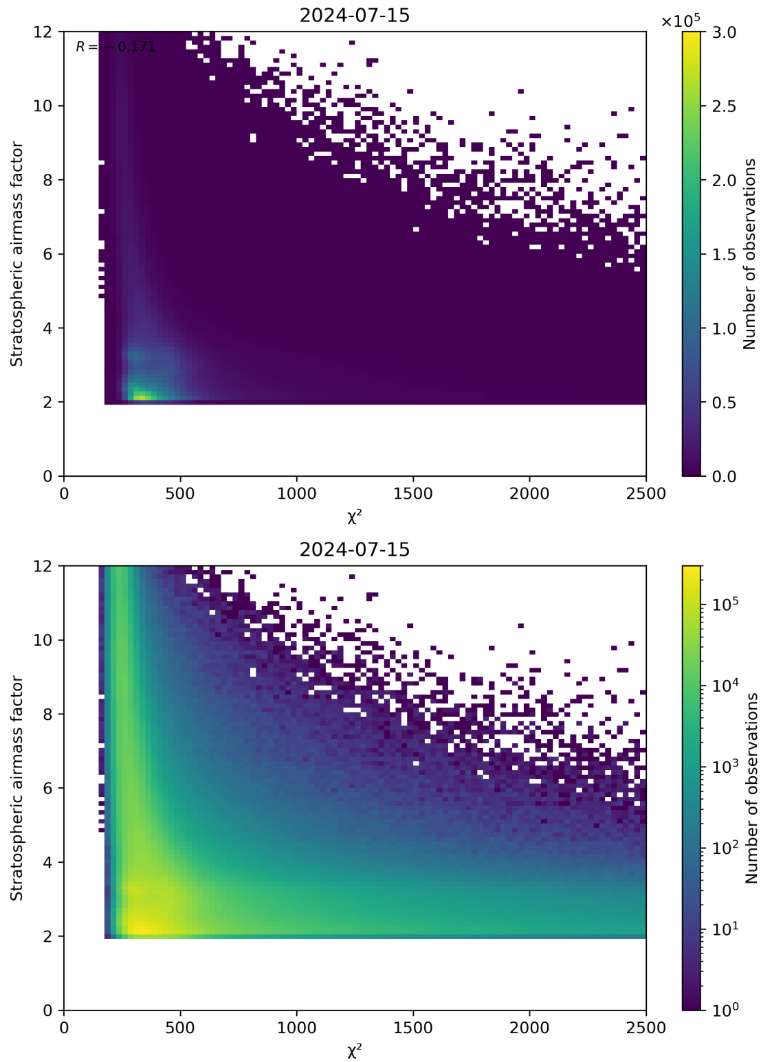
Figure 81: Scatter density plot of “ \chi^2 ” against “Stratospheric airmass factor” for 2024-07-15 to 2024-07-16.
