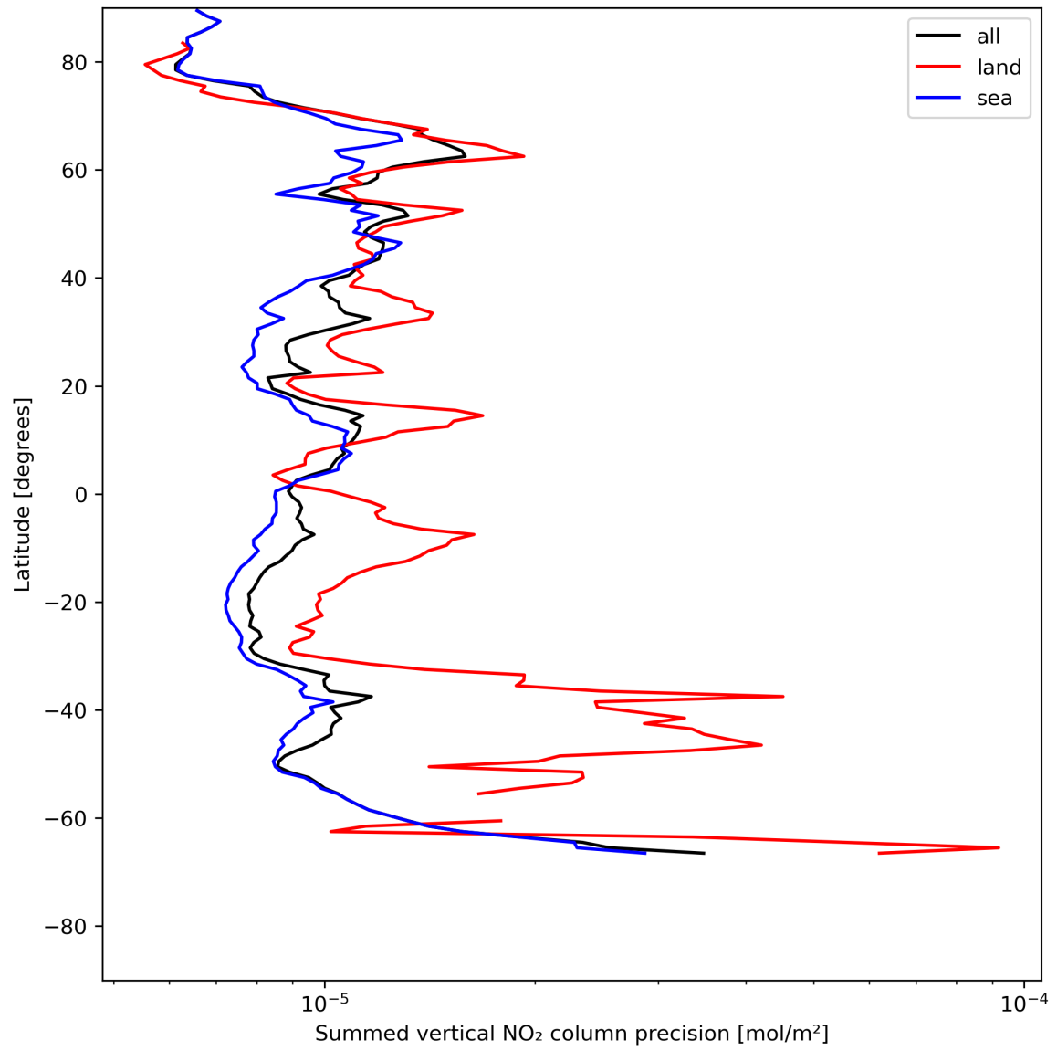
Figure 24: Zonal average of “Summed vertical NO 2 column precision” for 2024-07-15 to 2024-07-16.
