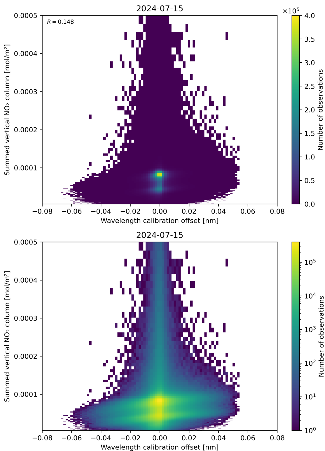
Figure 177: Scatter density plot of “Wavelength calibration offset” against “Summed vertical NO 2 column” for 2024-07-15 to 2024-07-16.
