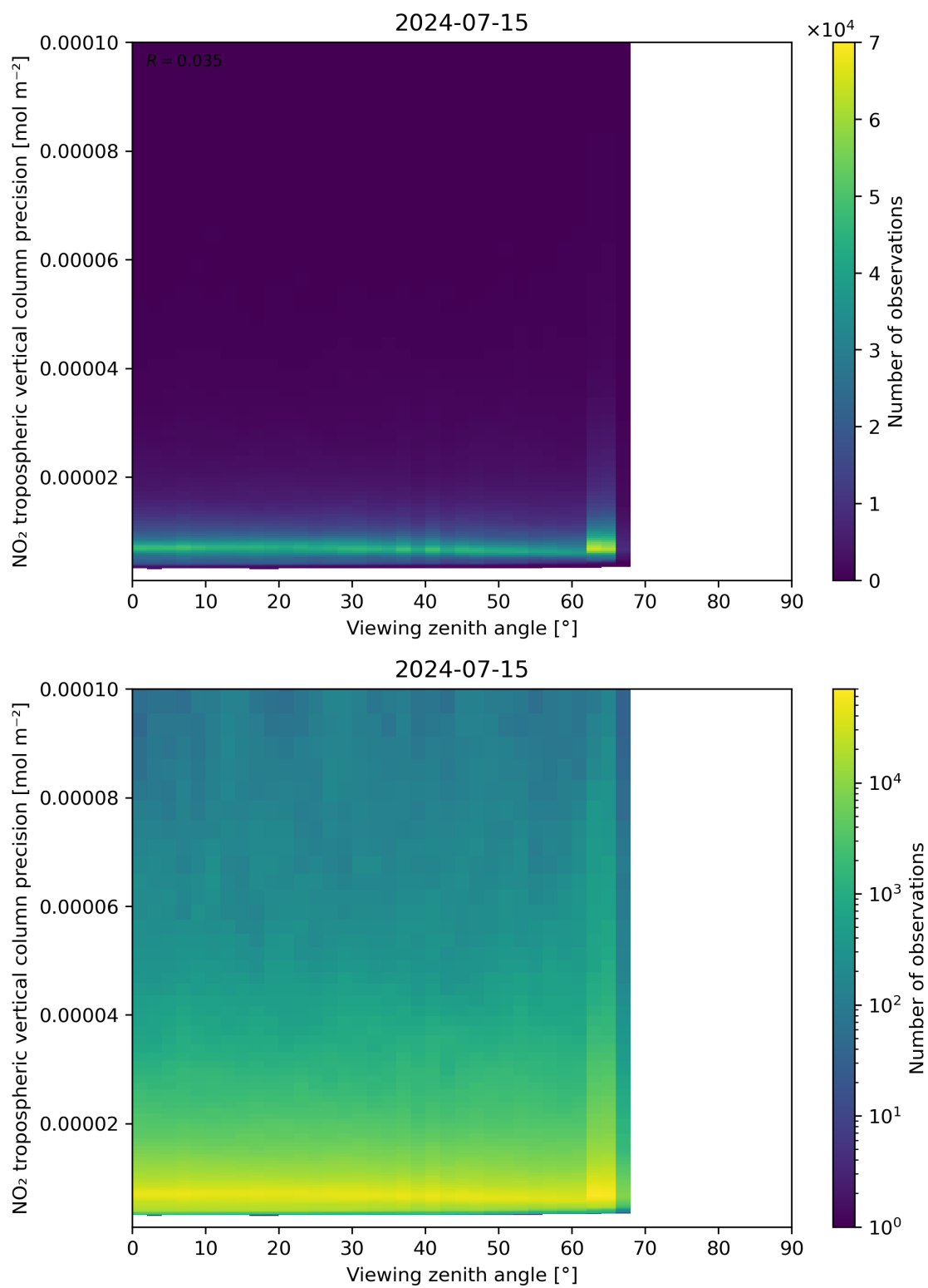
Figure 170: Scatter density plot of “Viewing zenith angle” against “NO 2 tropospheric vertical column precision” for 2024-07-15 to 2024-07-16.
