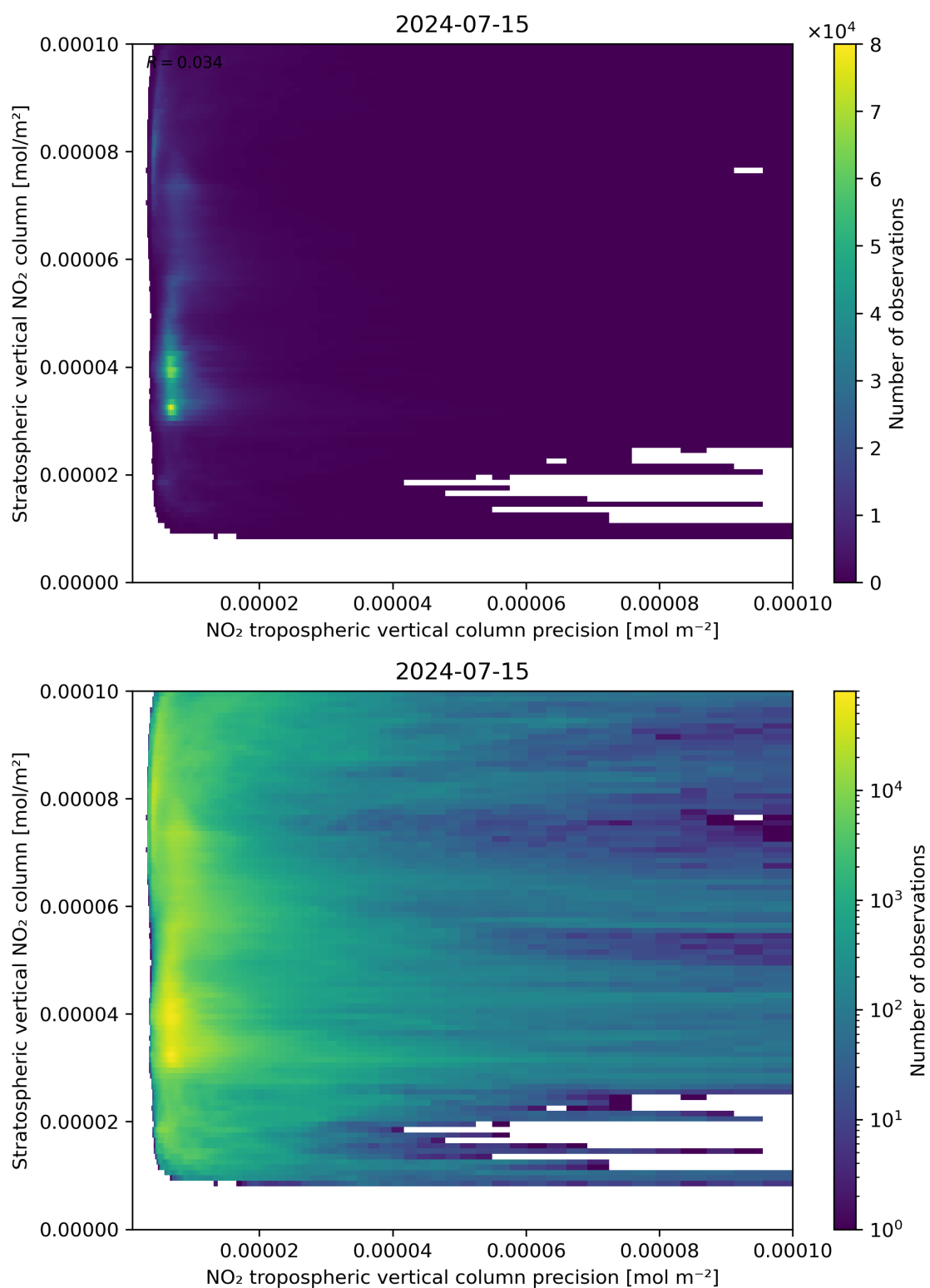
Figure 135: Scatter density plot of “NO 2 tropospheric vertical column precision” against “Stratospheric vertical NO 2 column” for 2024-07-15 to 2024-07-16.
