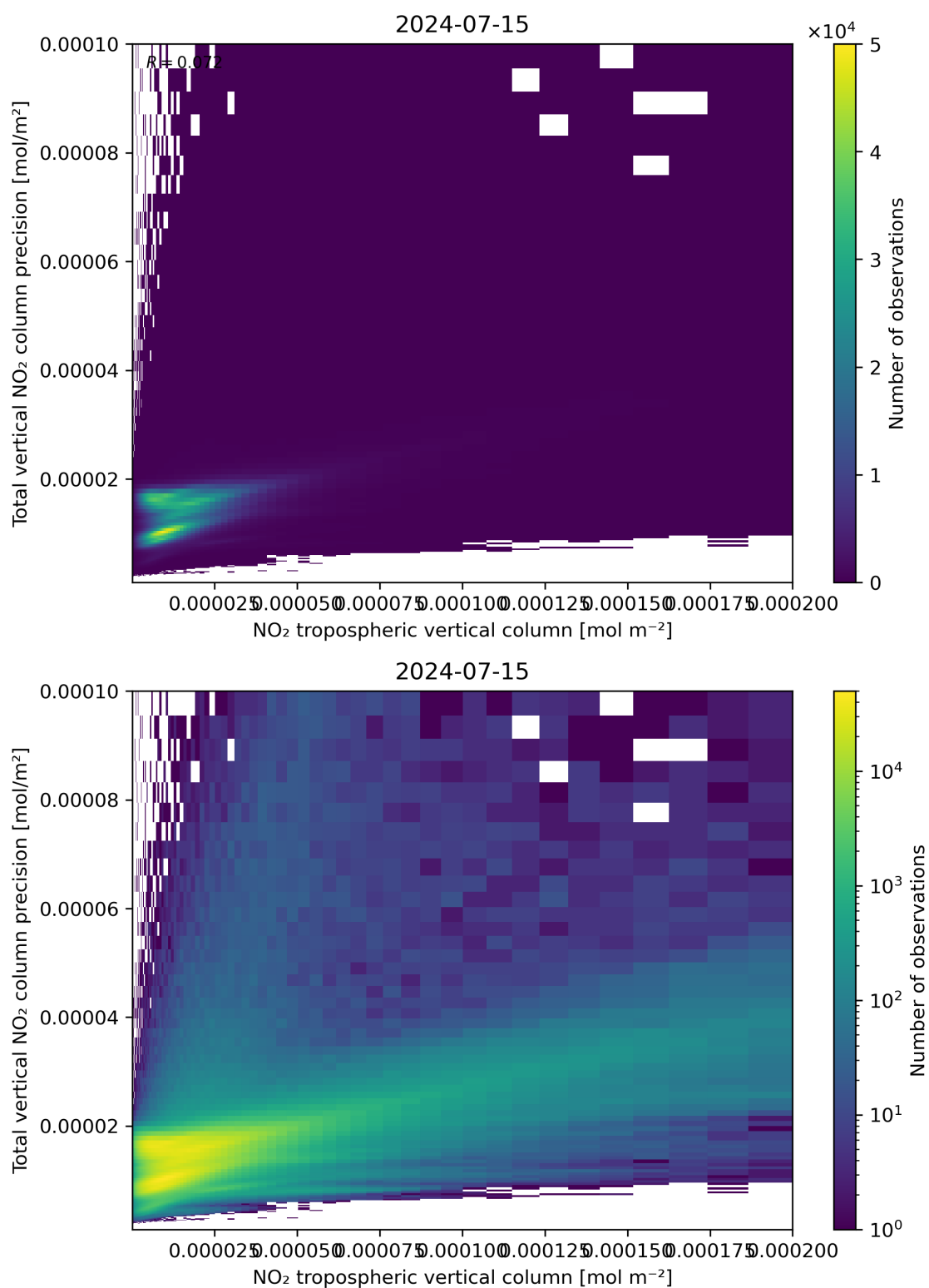
Figure 129: Scatter density plot of “NO 2 tropospheric vertical column” against “Total vertical NO 2 column precision” for 2024-07-15 to 2024-07-16.
