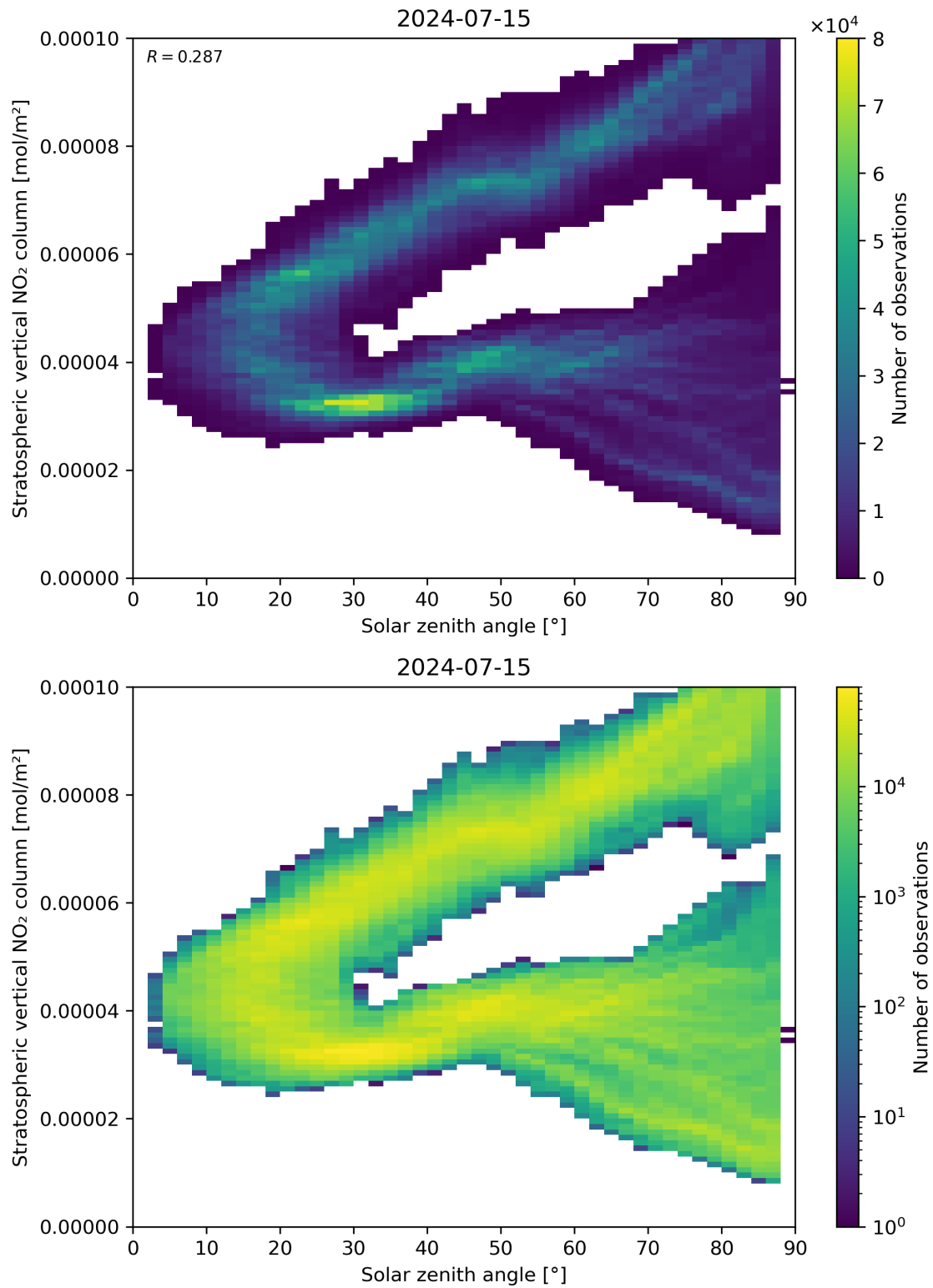
Figure 150: Scatter density plot of “Solar zenith angle” against “Stratospheric vertical NO 2 column” for 2024-07-15 to 2024-07-16.
