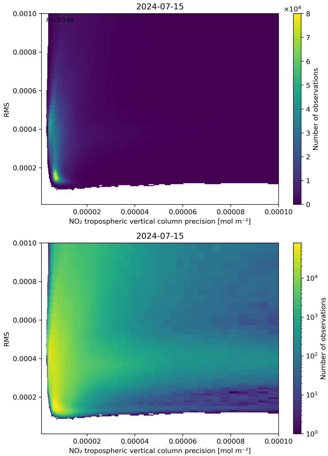
Figure 140: Scatter density plot of “NO 2 tropospheric vertical column precision” against “RMS” for 2024-07-15 to 2024-07-16.
