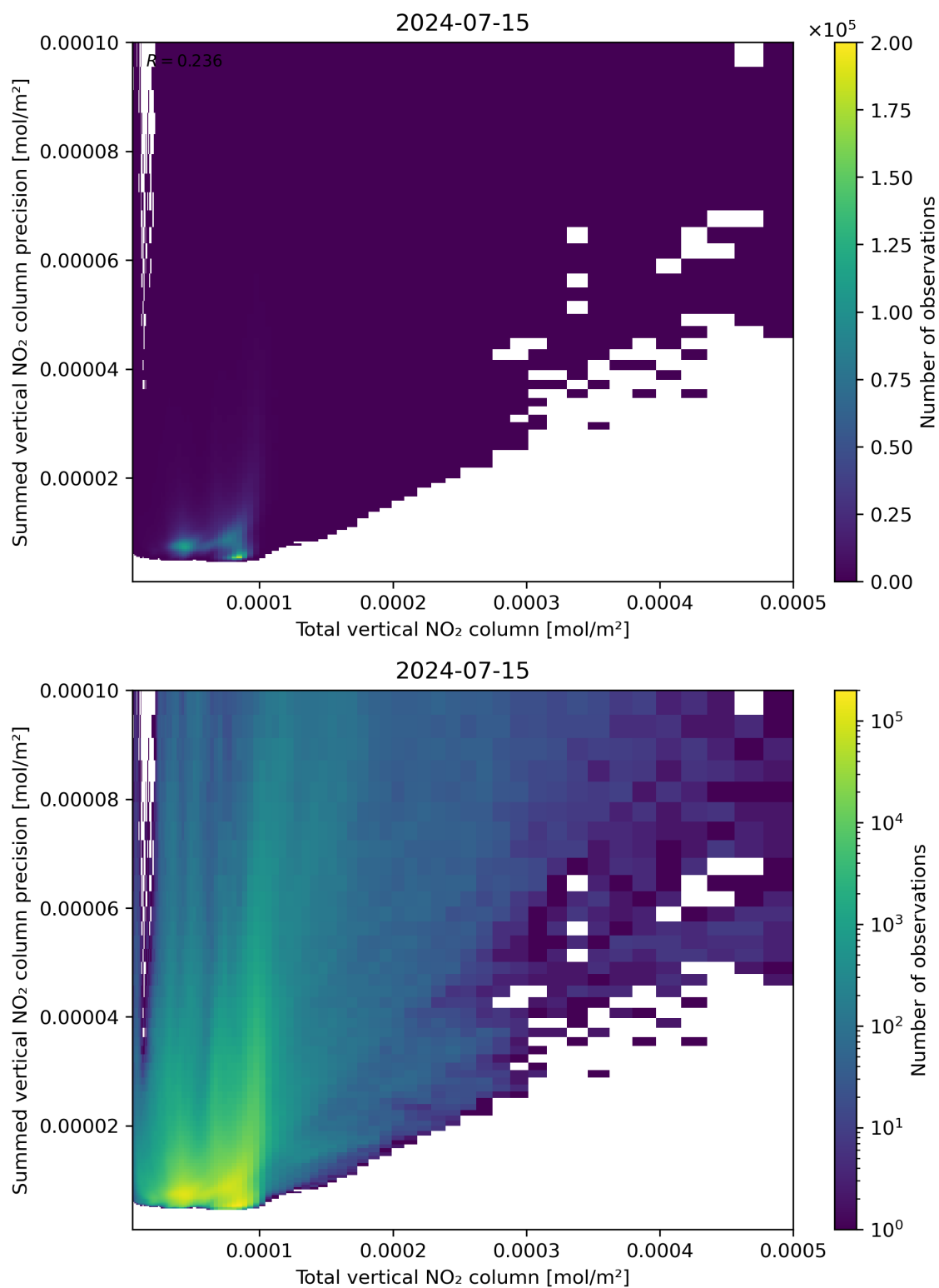
Figure 113: Scatter density plot of “Total vertical NO 2 column” against “Summed vertical NO 2 column precision” for 2024-07-15 to 2024-07-16.
