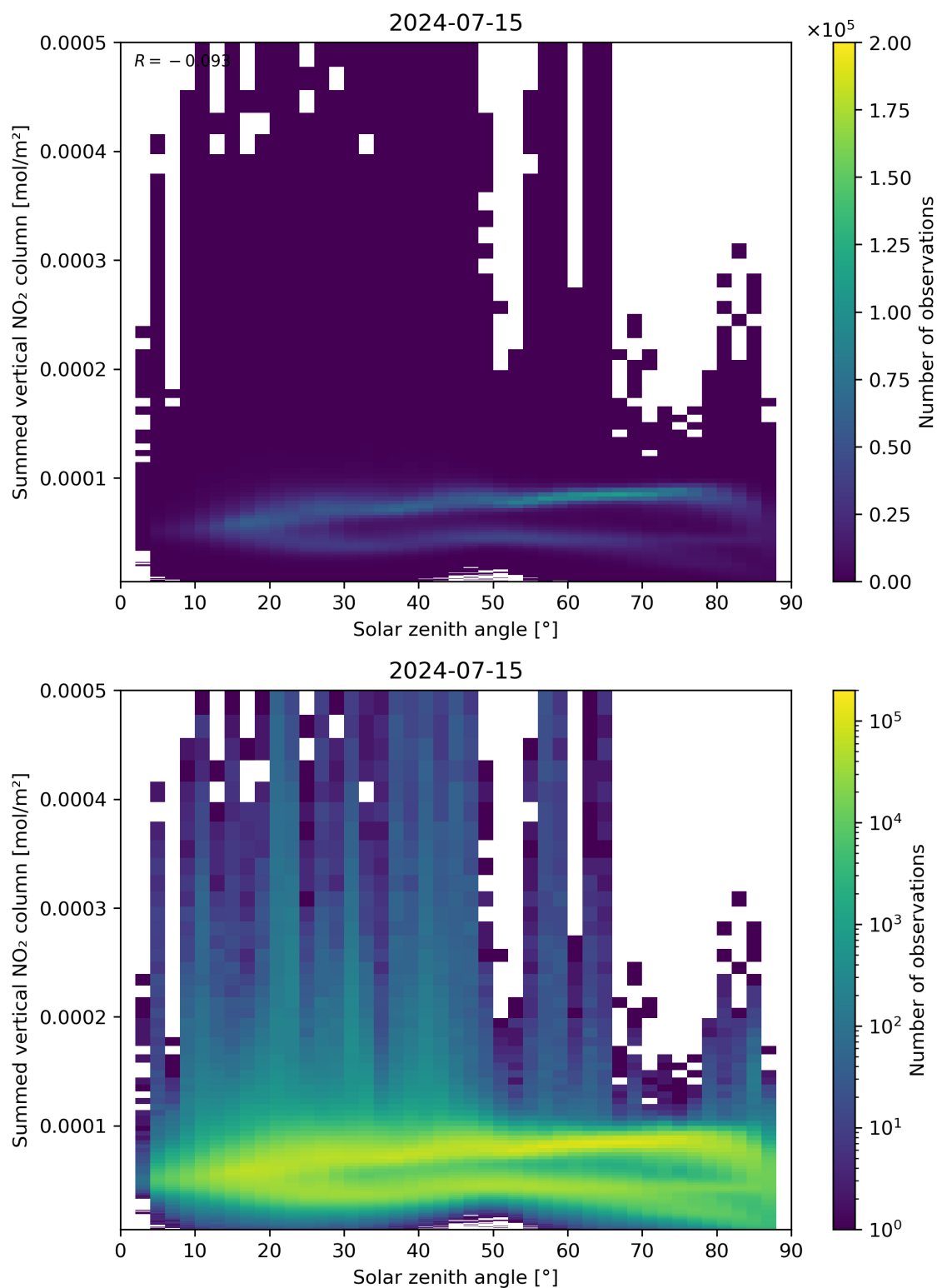
Figure 151: Scatter density plot of “Solar zenith angle” against “Summed vertical NO 2 column” for 2024-07-15 to 2024-07-16.
