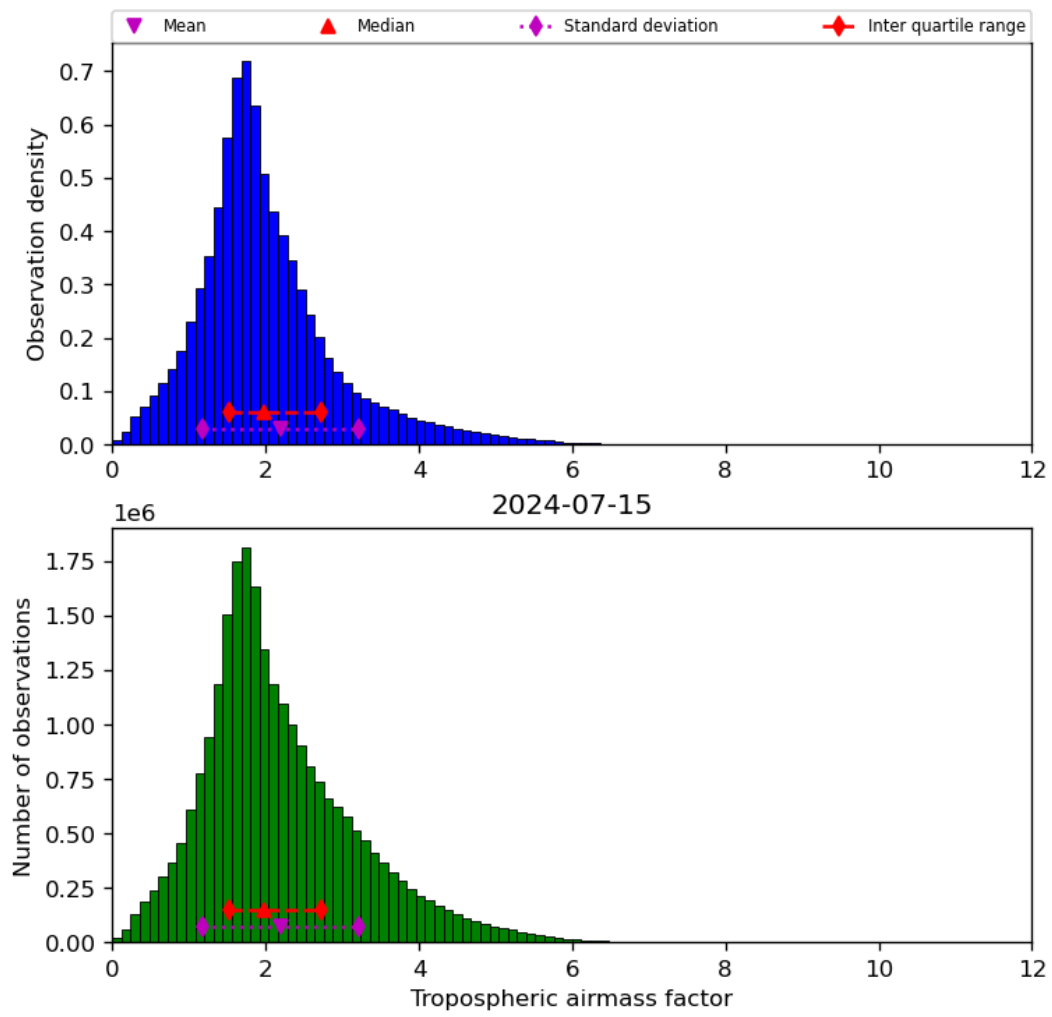
Figure 31: Histogram of “Tropospheric airmass factor” for 2024-07-15 to 2024-07-16
