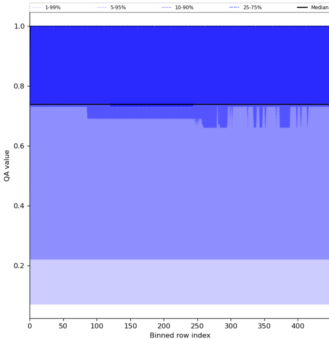
Figure 45: Along track statistics of “QA value” for 2024-07-15 to 2024-07-16
