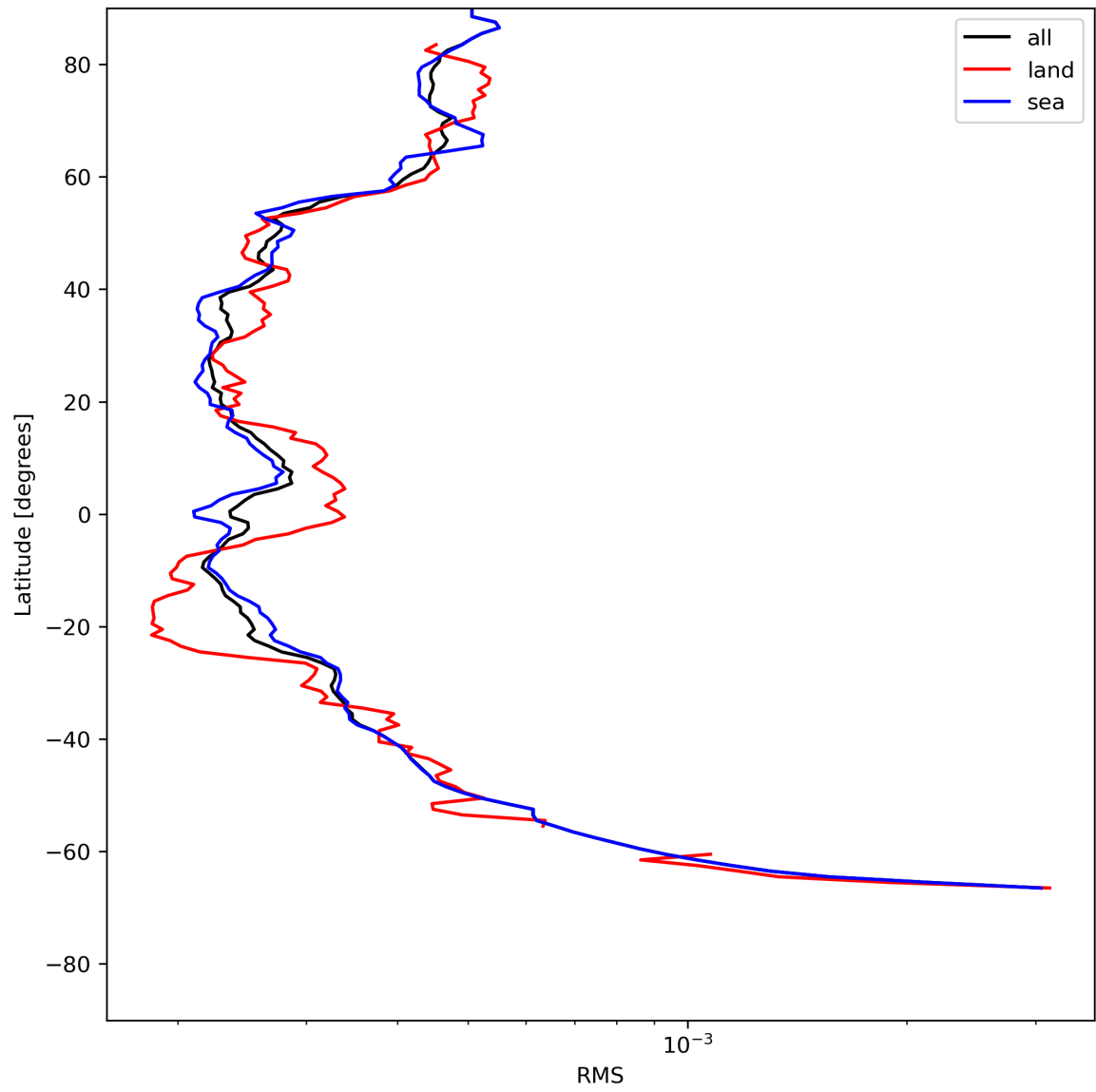
Figure 26: Zonal average of “RMS” for 2024-07-15 to 2024-07-16.
