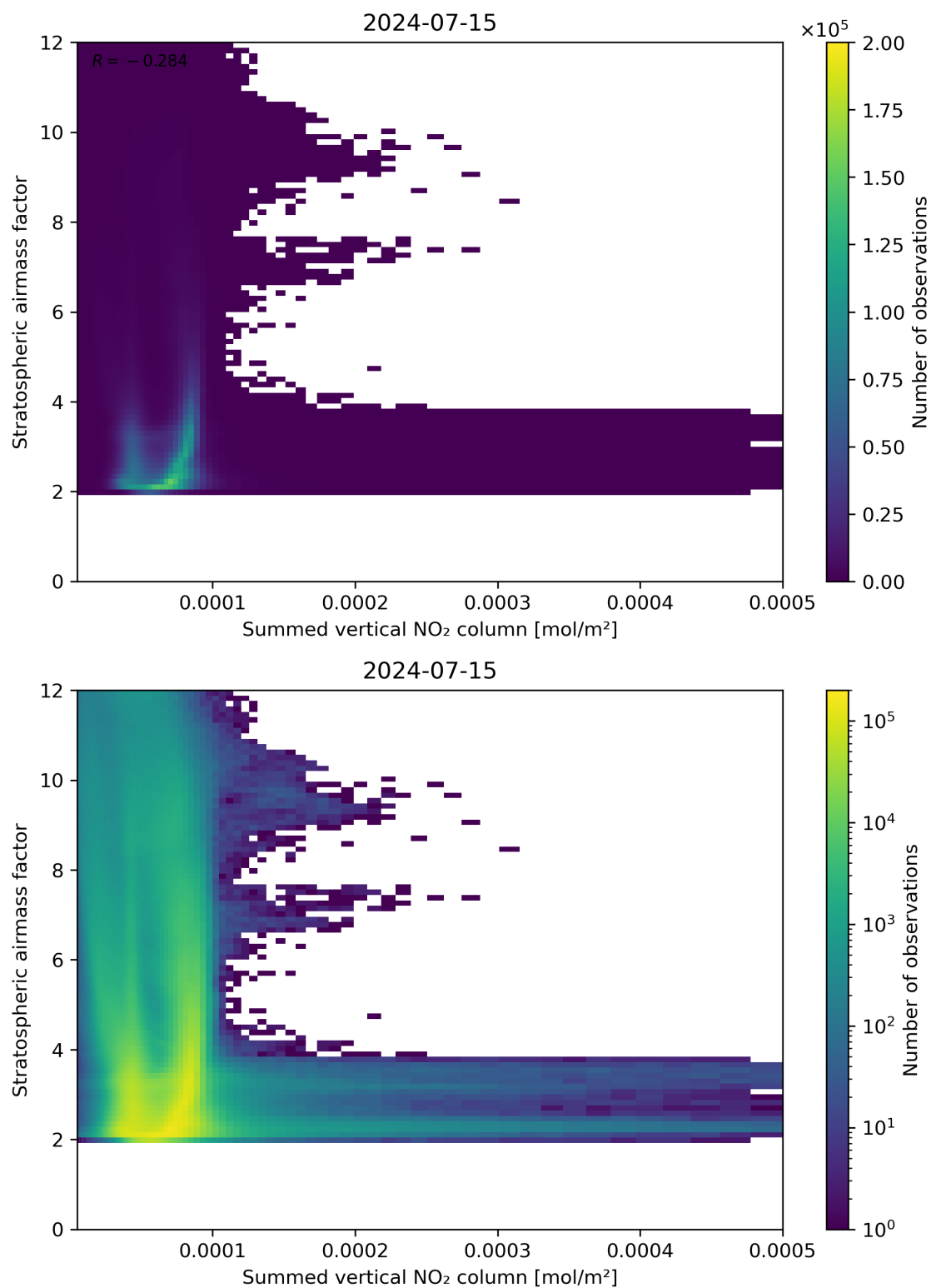
Figure 103: Scatter density plot of “Summed vertical NO 2 column” against “Stratospheric air mass factor” for 2024-07-15 to 2024-07-16.
