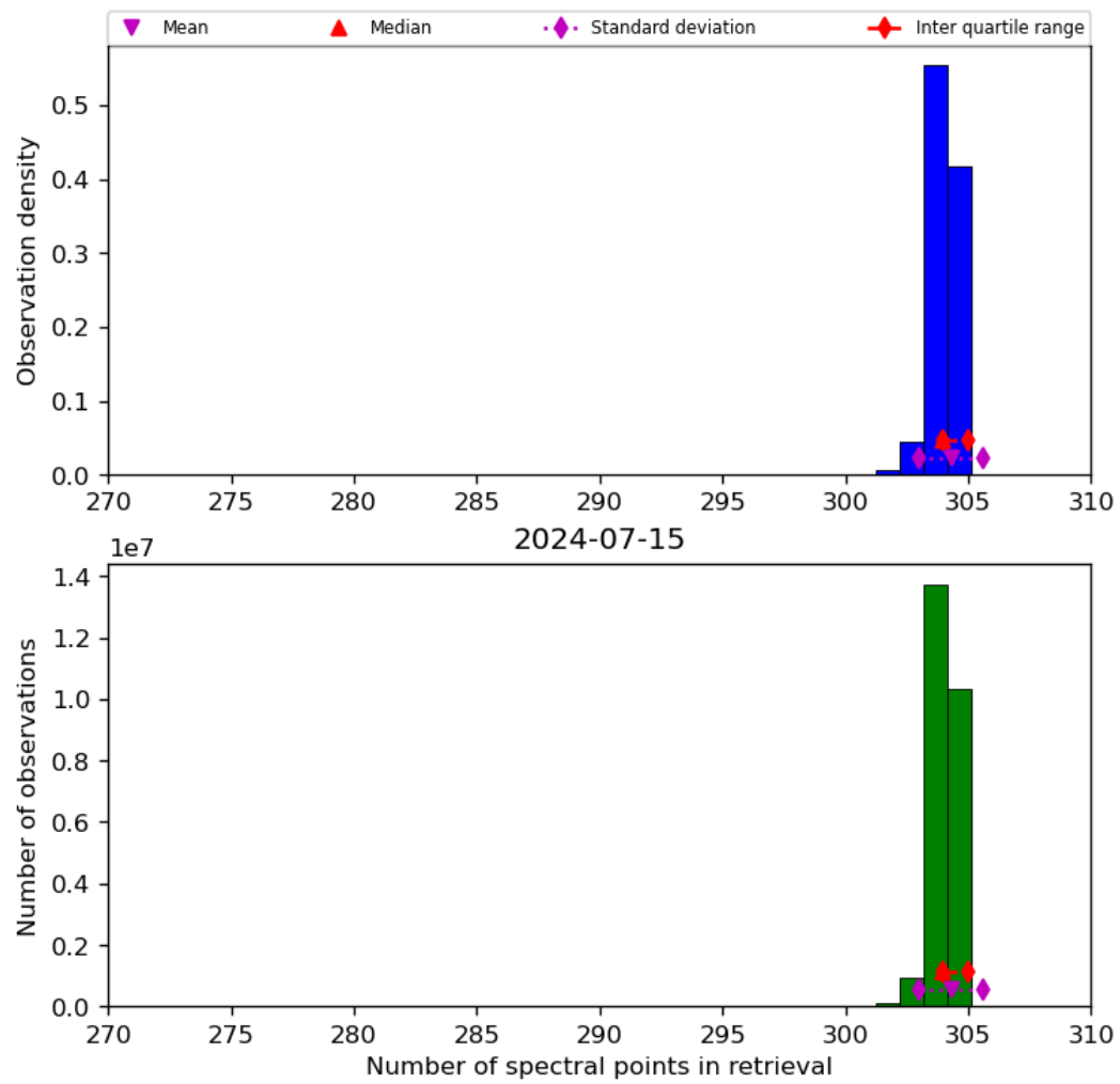
Figure 33: Histogram of “Number of spectral points in retrieval” for 2024-07-15 to 2024-07-16
