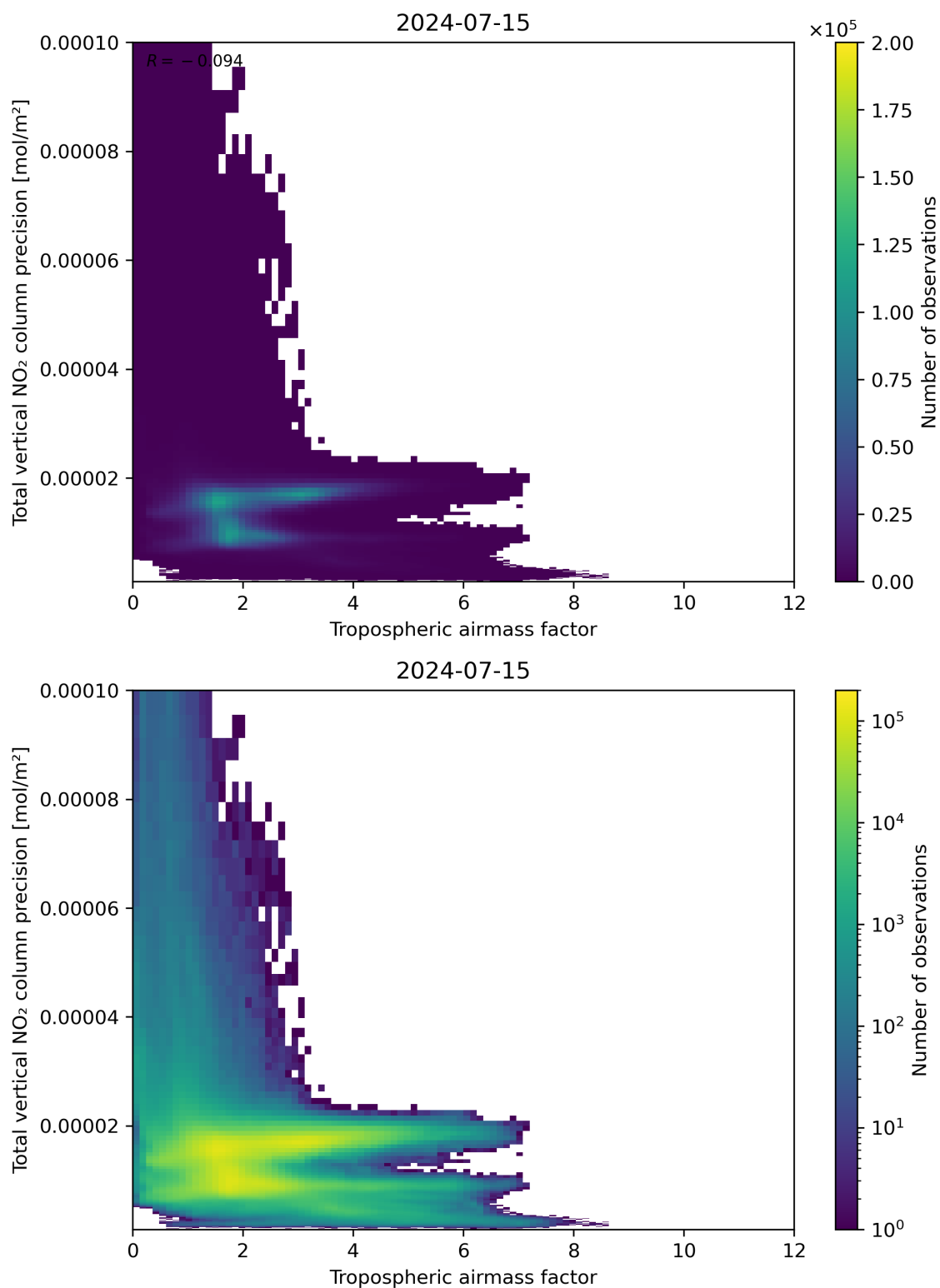
Figure 78: Scatter density plot of “Tropospheric air mass factor” against “Total vertical NO 2 column precision” for 2024-07-15 to 2024-07-16.
