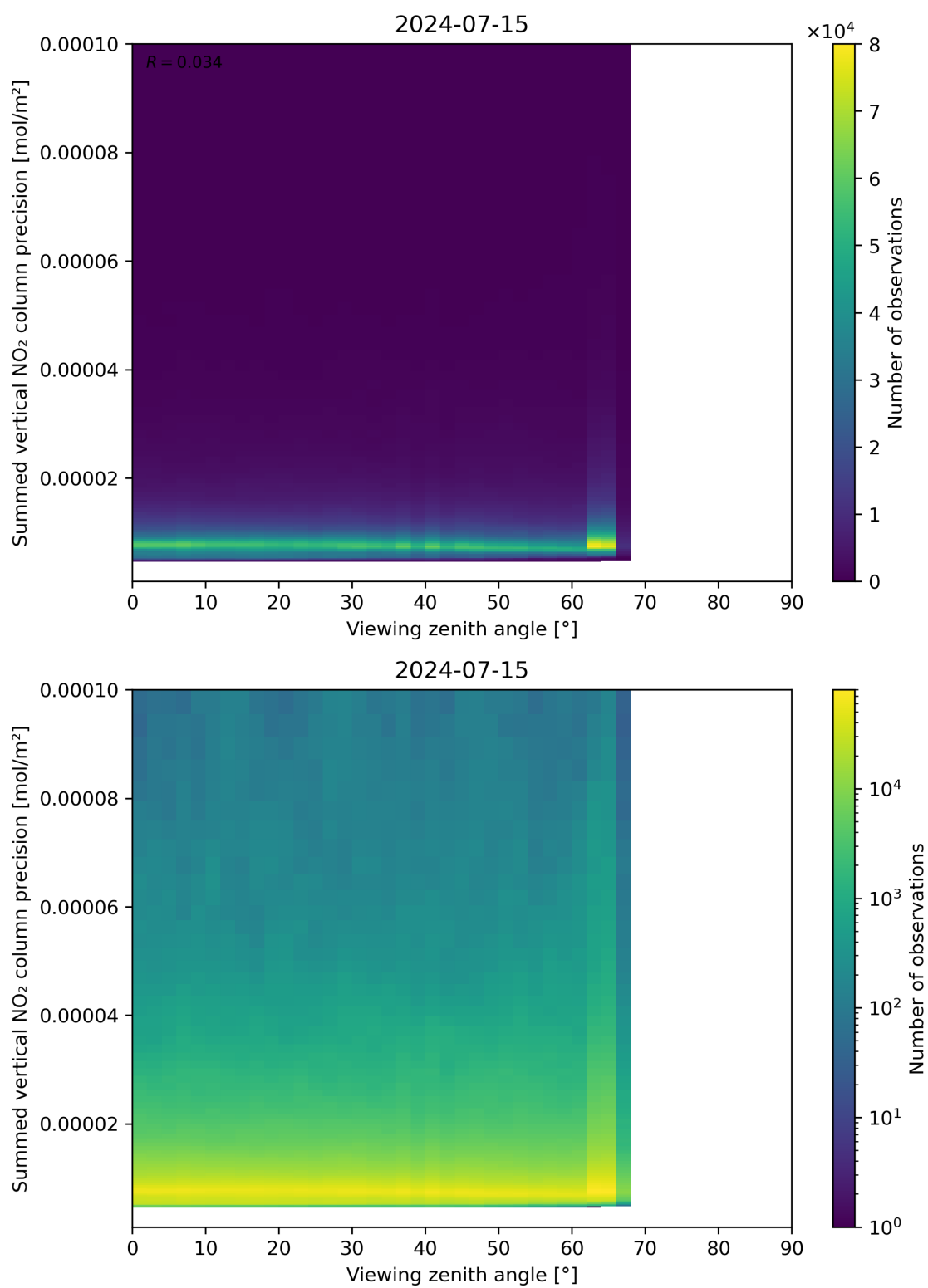
Figure 166: Scatter density plot of “Viewing zenith angle” against “Summed vertical NO 2 column precision” for 2024-07-15 to 2024-07-16.
