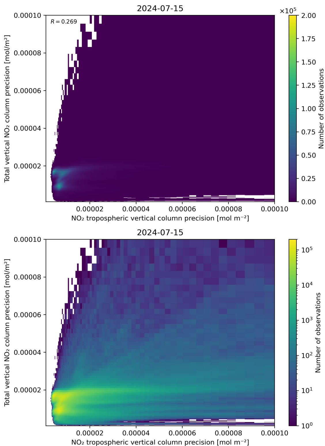
Figure 139: Scatter density plot of “NO 2 tropospheric vertical column precision” against “Total vertical NO 2 column precision” for 2024-07-15 to 2024-07-16.
