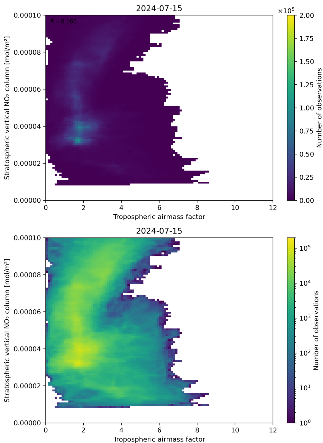
Figure 74: Scatter density plot of “Tropospheric air mass factor” against “Stratospheric vertical NO 2 column” for 2024-07-15 to 2024-07-16.
