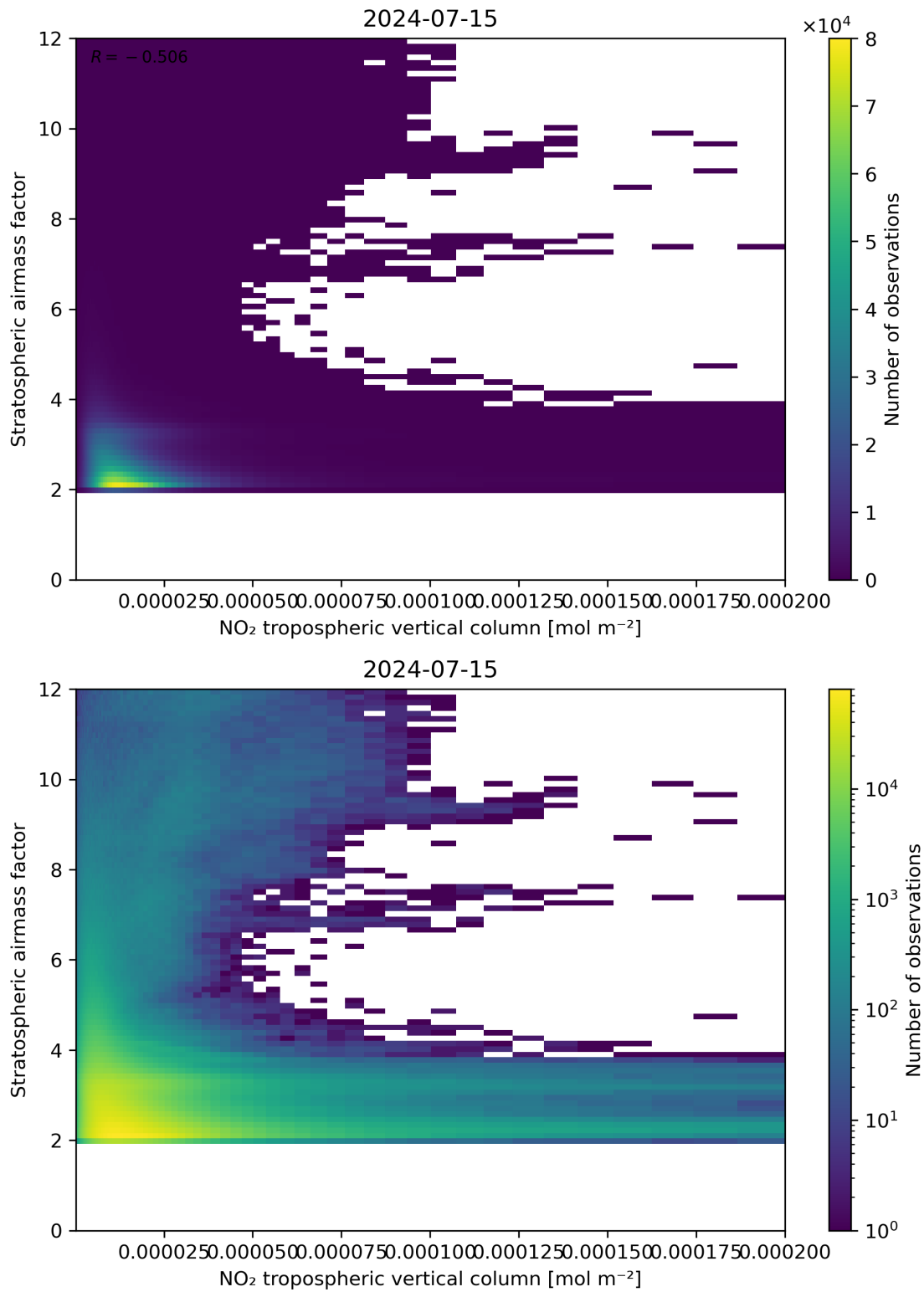
Figure 121: Scatter density plot of “NO 2 tropospheric vertical column” against “Stratospheric air mass factor” for 2024-07-15 to 2024-07-16.
