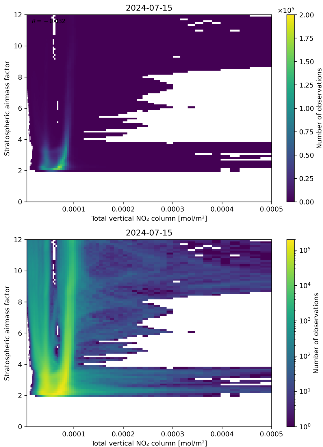
Figure 110: Scatter density plot of “Total vertical NO 2 column” against “Stratospheric airmass factor” for 2024-07-15 to 2024-07-16.
