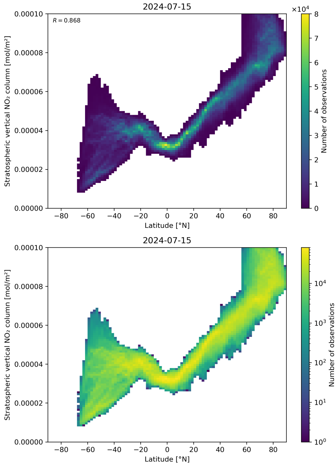
Figure 87: Scatter density plot of “Latitude” against “Stratospheric vertical NO 2 column” for 2024-07-15 to 2024-07-16.
