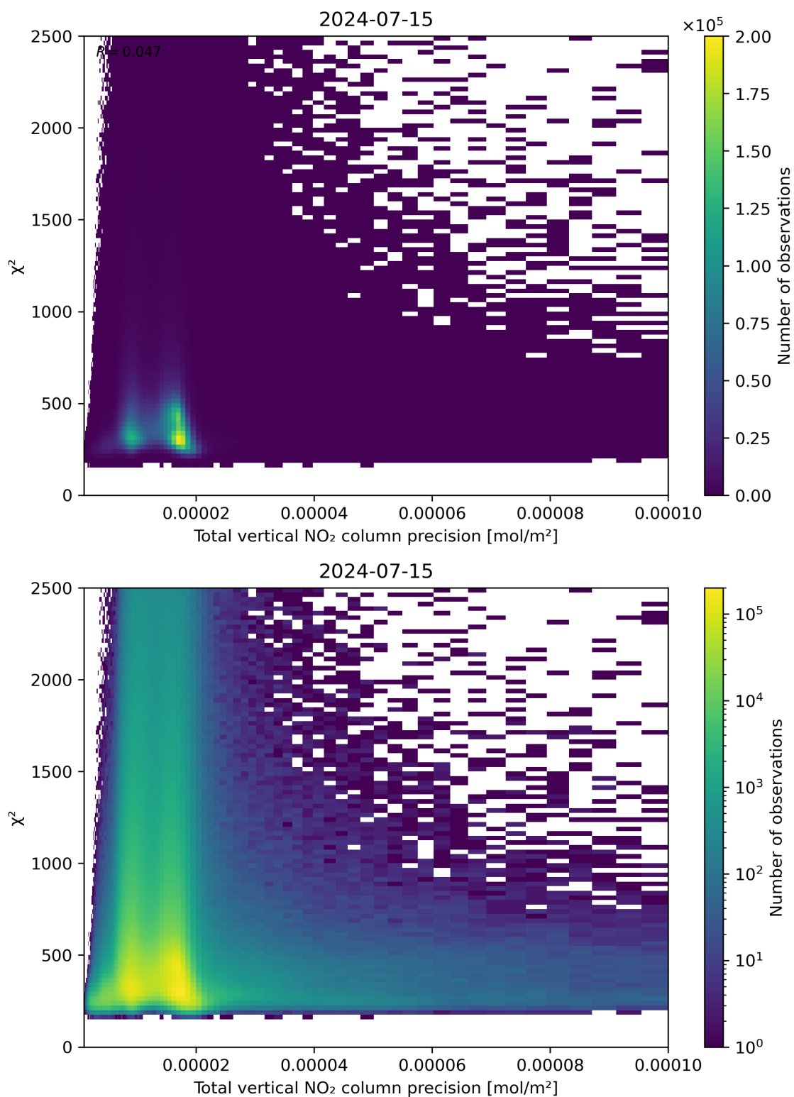
Figure 116: Scatter density plot of “Total vertical NO 2 column precision” against “ \chi^2 ” for 2024-07-15 to 2024-07-16.
