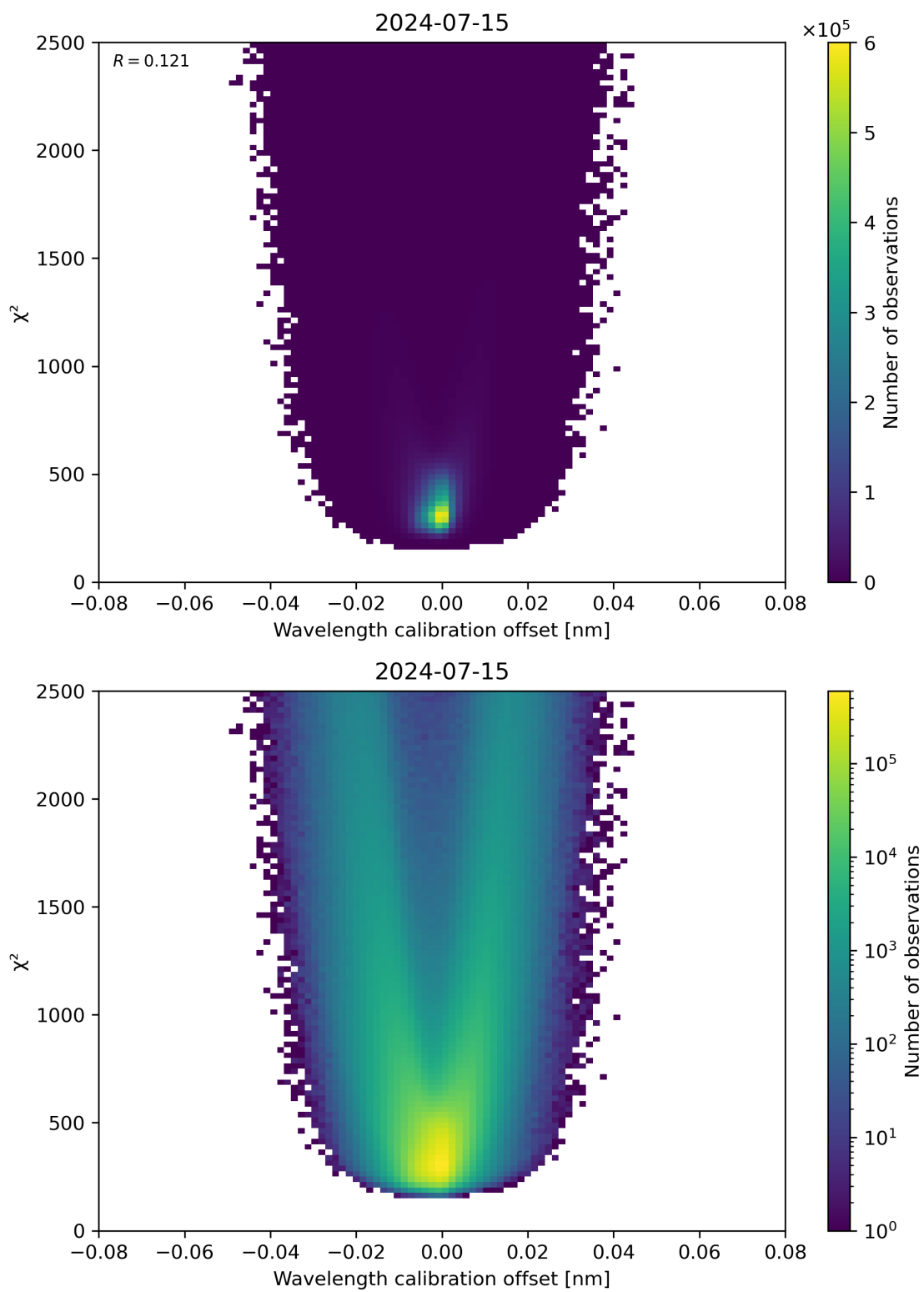
Figure 175: Scatter density plot of “Wavelength calibration offset” against “ \chi^2 ” for 2024-07-15 to 2024-07-16.
