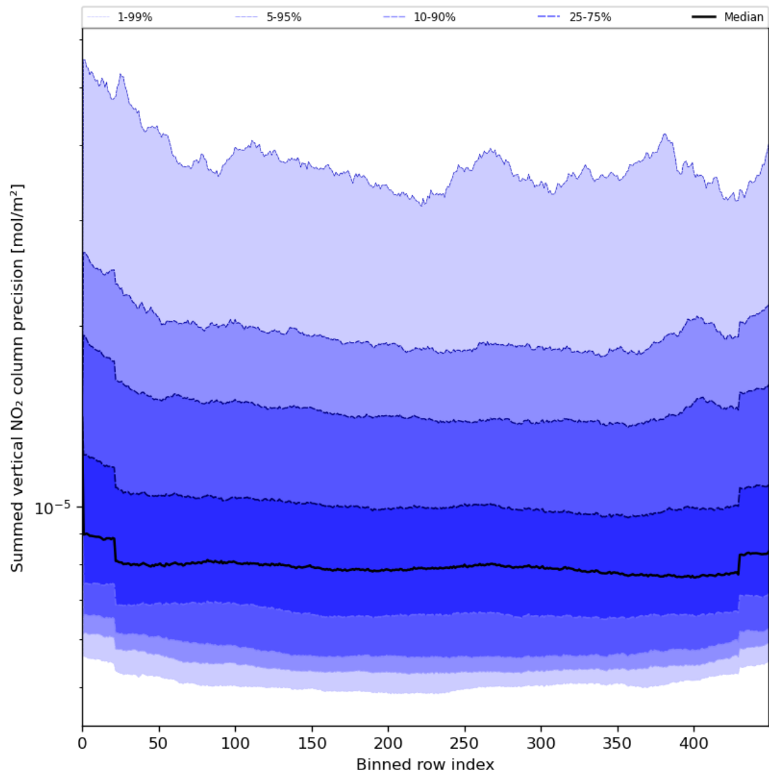
Figure 58: Along track statistics of “Summed vertical NO 2 column precision” for 2024-07-15 to 2024-07-16
