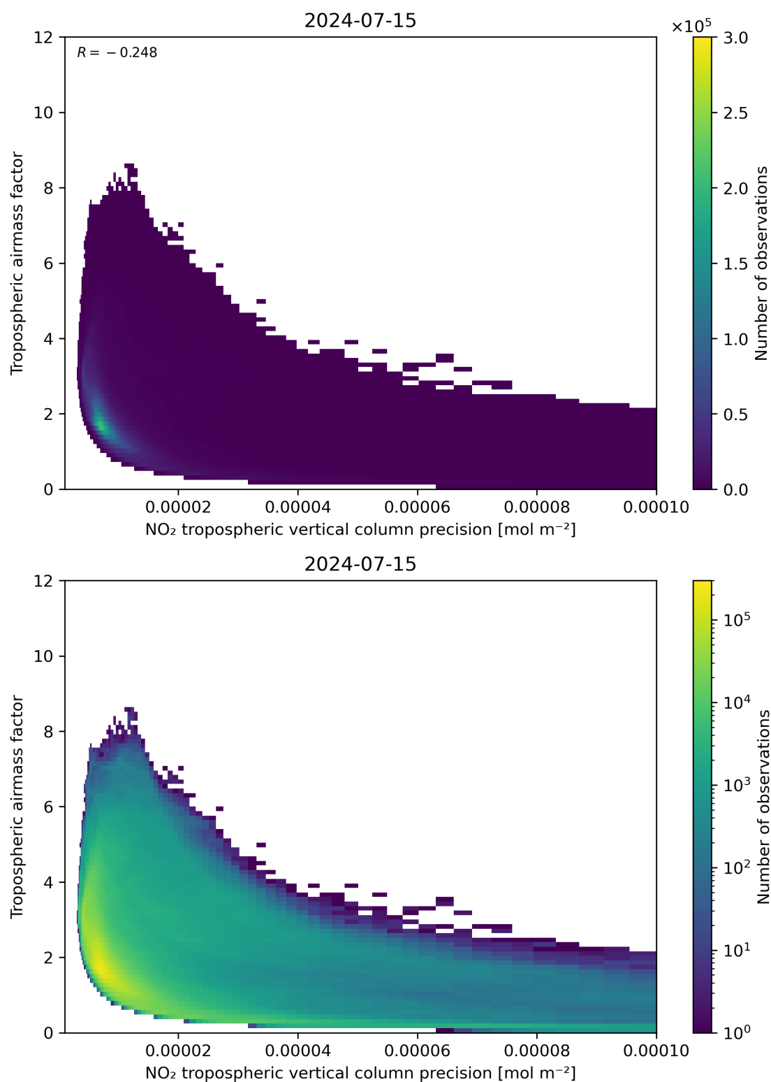
Figure 133: Scatter density plot of “NO 2 tropospheric vertical column precision” against “Tropospheric airmass factor” for 2024-07-15 to 2024-07-16.
