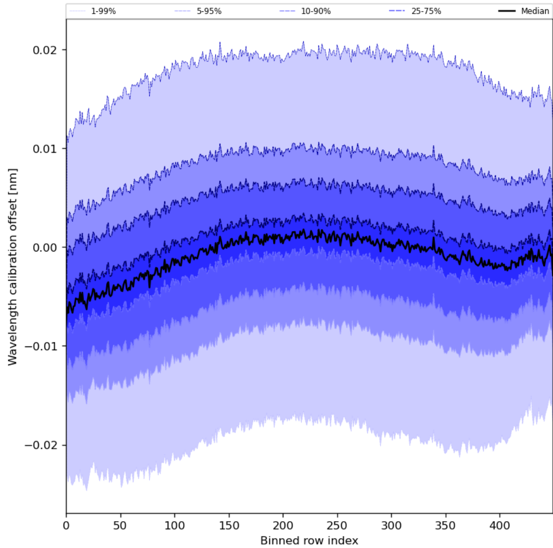
Figure 52: Along track statistics of “Wavelength calibration offset” for 2024-07-15 to 2024-07-17
