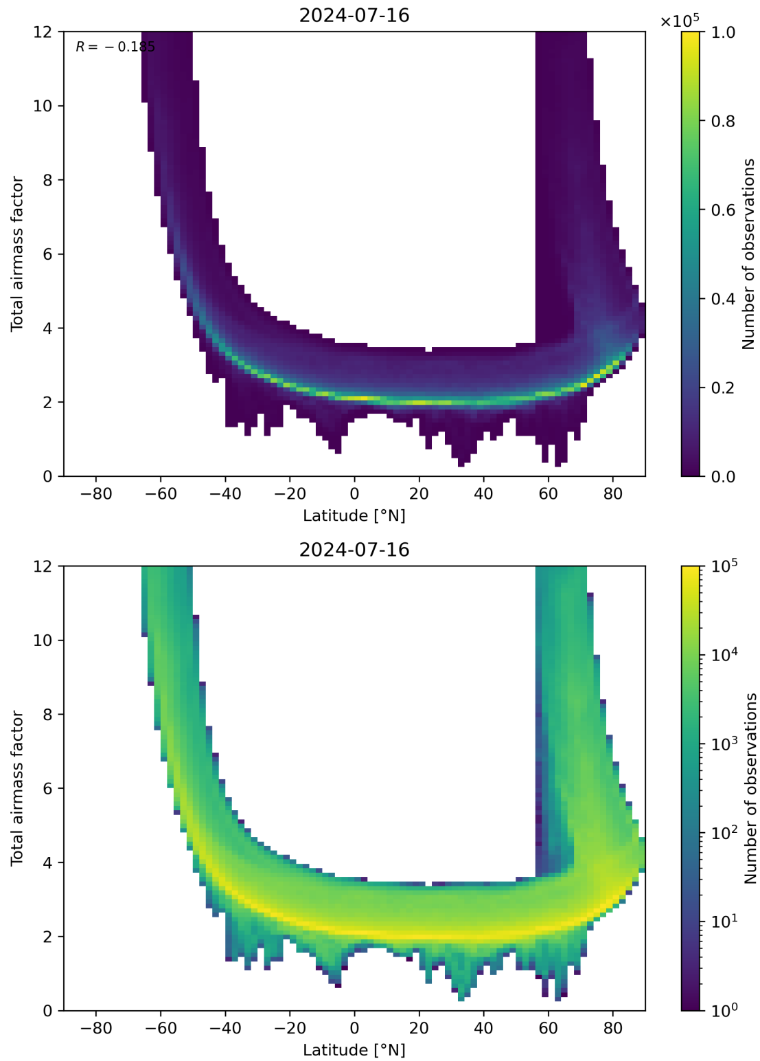
Figure 84: Scatter density plot of “Latitude” against “Total airmass factor” for 2024-07-15 to 2024-07-17.
