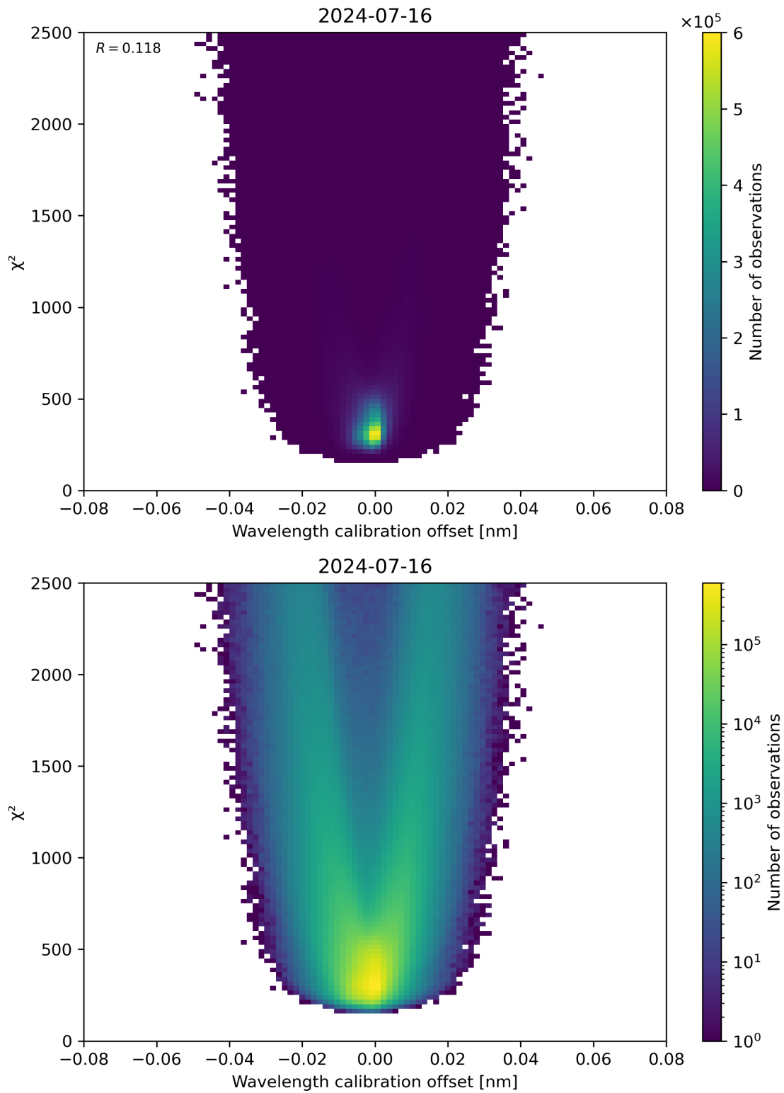
Figure 175: Scatter density plot of “Wavelength calibration offset” against “ \chi^2 ” for 2024-07-15 to 2024-07-17.
