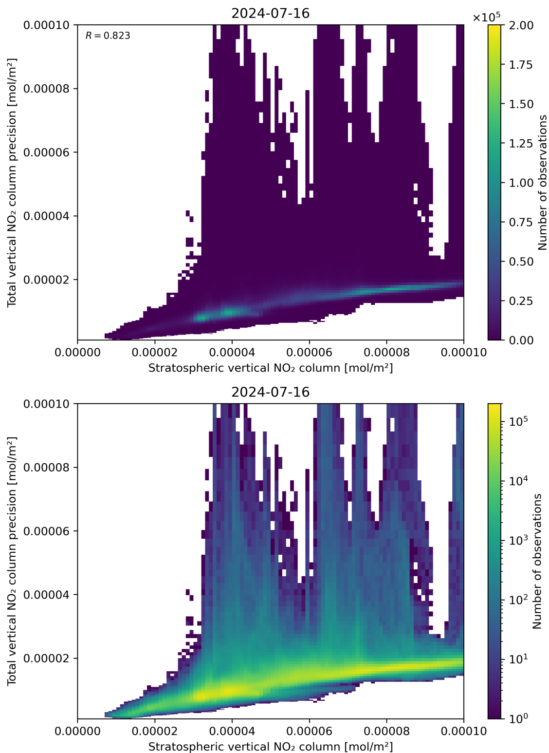
Figure 101: Scatter density plot of “Stratospheric vertical NO 2 column” against “Total vertical NO 2 column precision” for 2024-07-15 to 2024-07-17.
