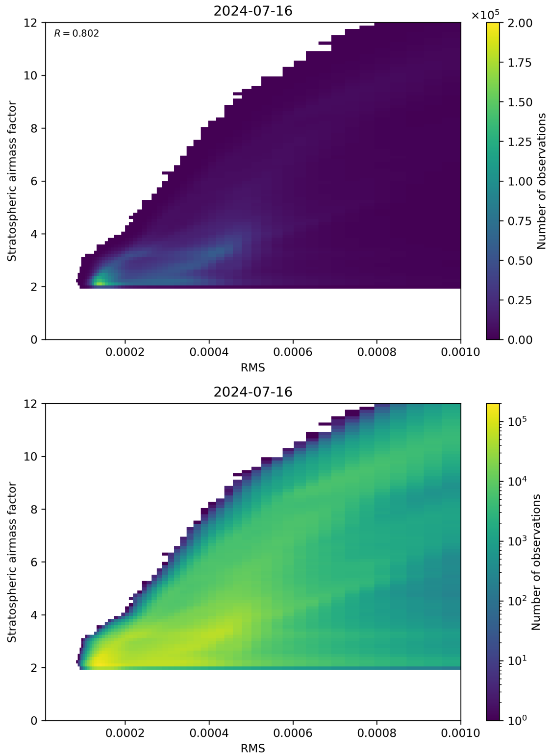
Figure 144: Scatter density plot of “RMS” against “Stratospheric airmass factor” for 2024-07-15 to 2024-07-17.
