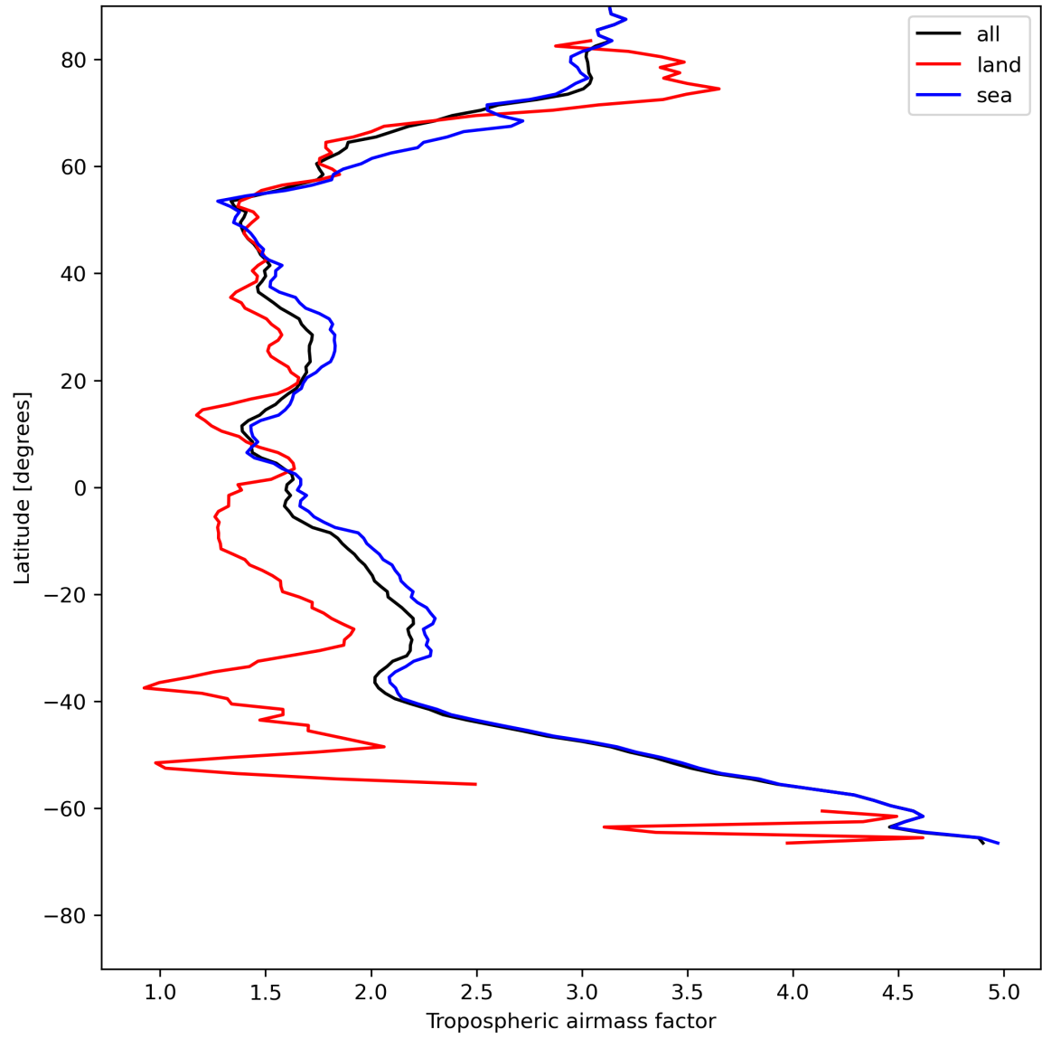
Figure 14: Zonal average of “Tropospheric airmass factor” for 2024-07-15 to 2024-07-17.
