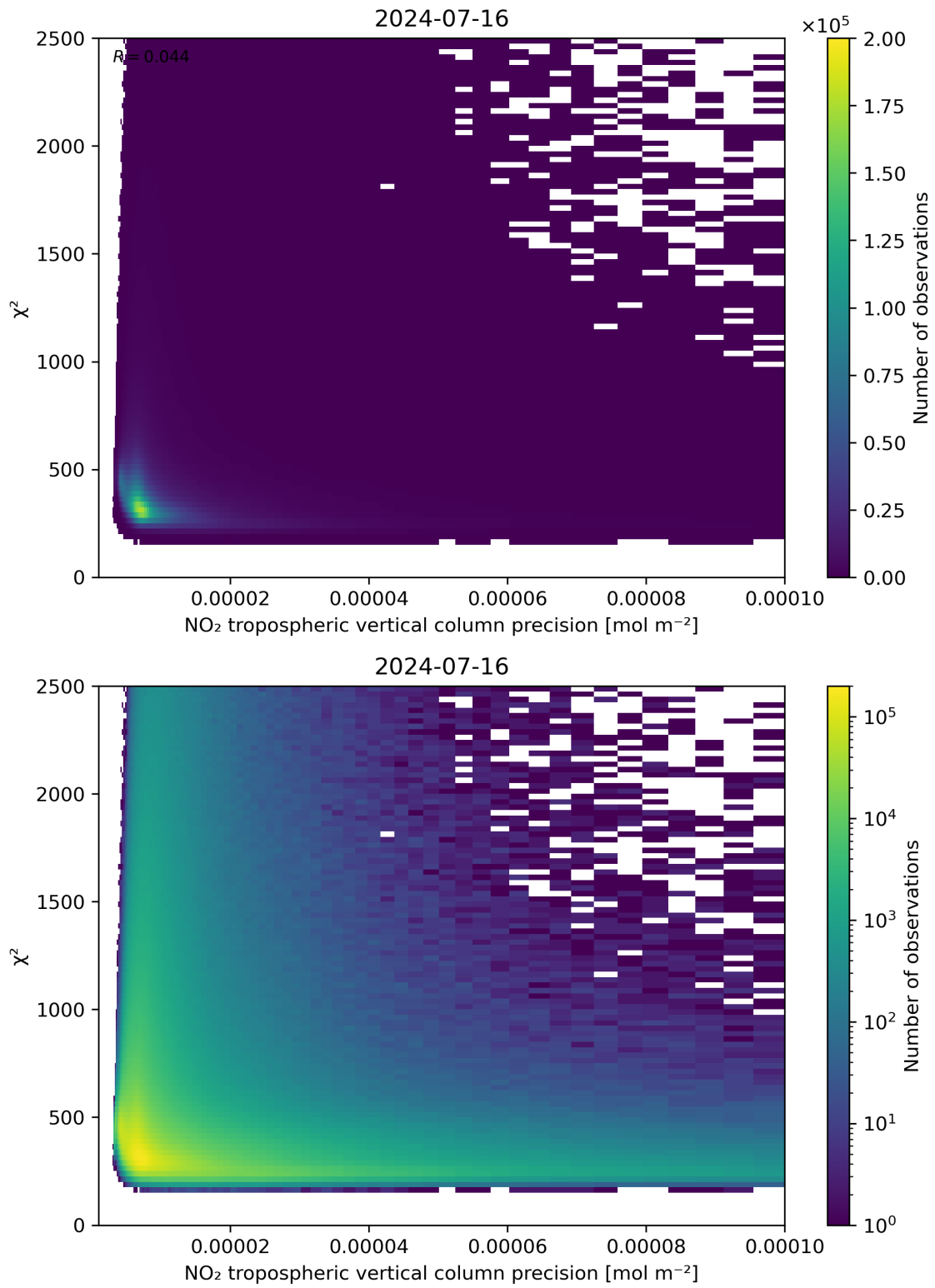
Figure 134: Scatter density plot of “NO 2 tropospheric vertical column precision” against “ \chi^2 ” for 2024-07-15 to 2024-07-17.
