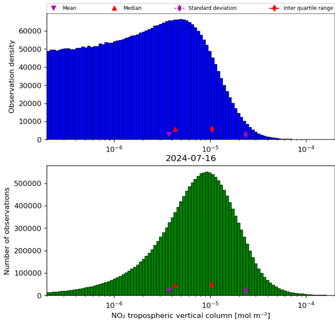
Figure 29: Histogram of “NO 2 tropospheric vertical column” for 2024-07-15 to 2024-07-17
