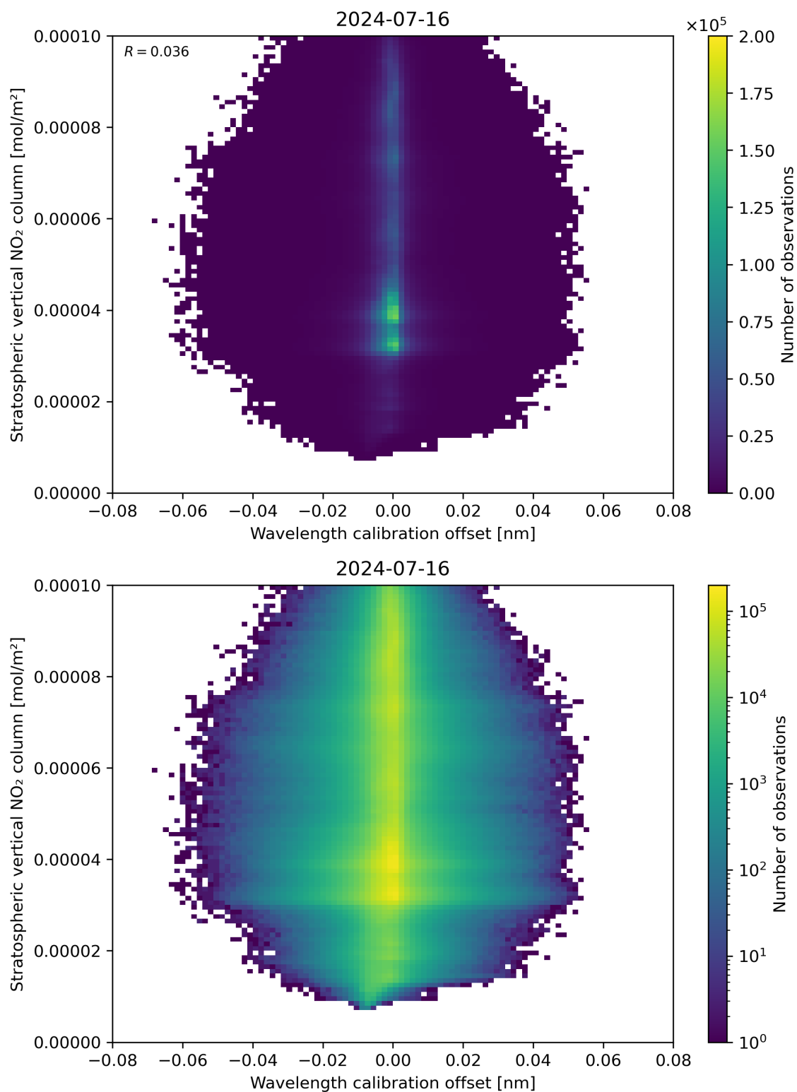
Figure 176: Scatter density plot of “Wavelength calibration offset” against “Stratospheric vertical NO 2 column” for 2024-07-15 to 2024-07-17.
