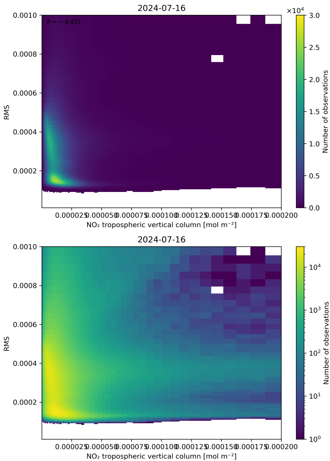
Figure 142: Scatter density plot of “NO 2 tropospheric vertical column” against “RMS” for 2024-07-15 to 2024-07-17.
