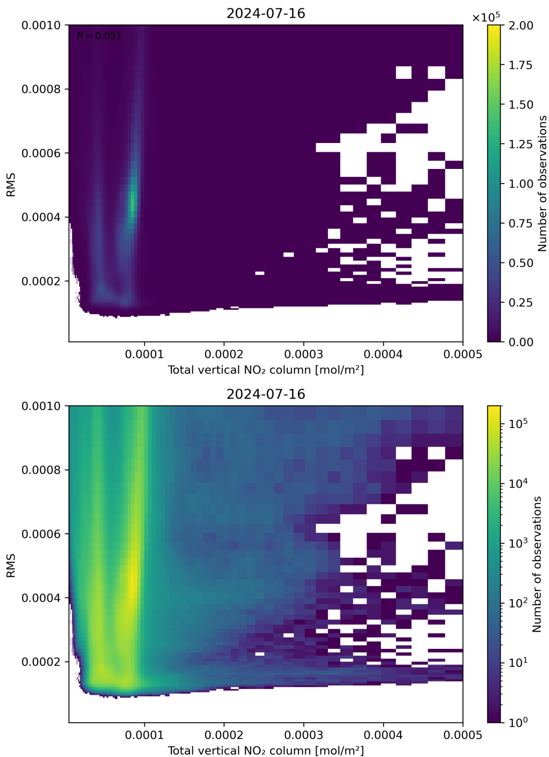
Figure 120: Scatter density plot of “Total vertical NO 2 column” against “RMS” for 2024-07-15 to 2024-07-17.
