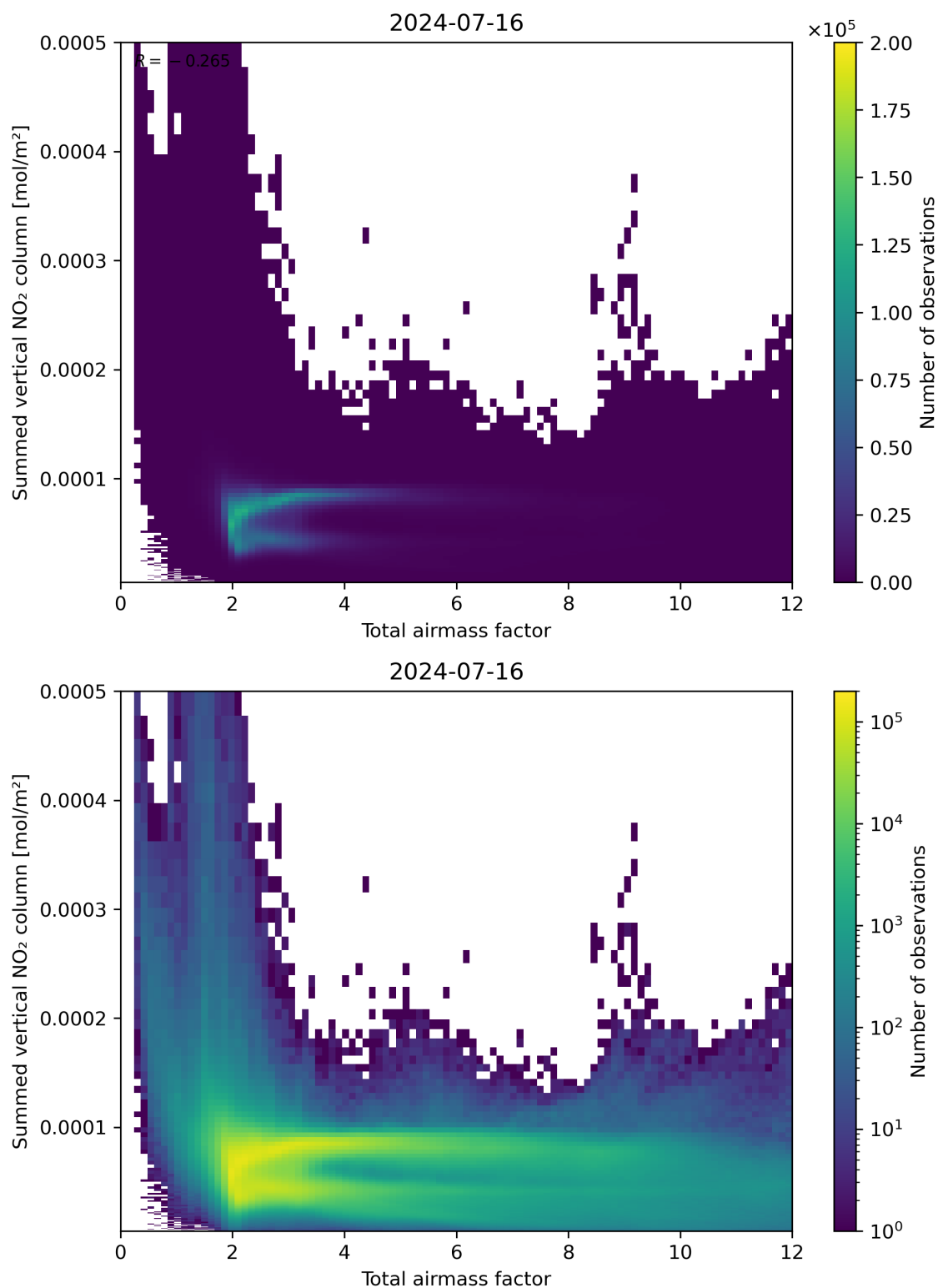
Figure 65: Scatter density plot of “Total airmass factor” against “Summed vertical NO 2 column” for 2024-07-15 to 2024-07-17.
