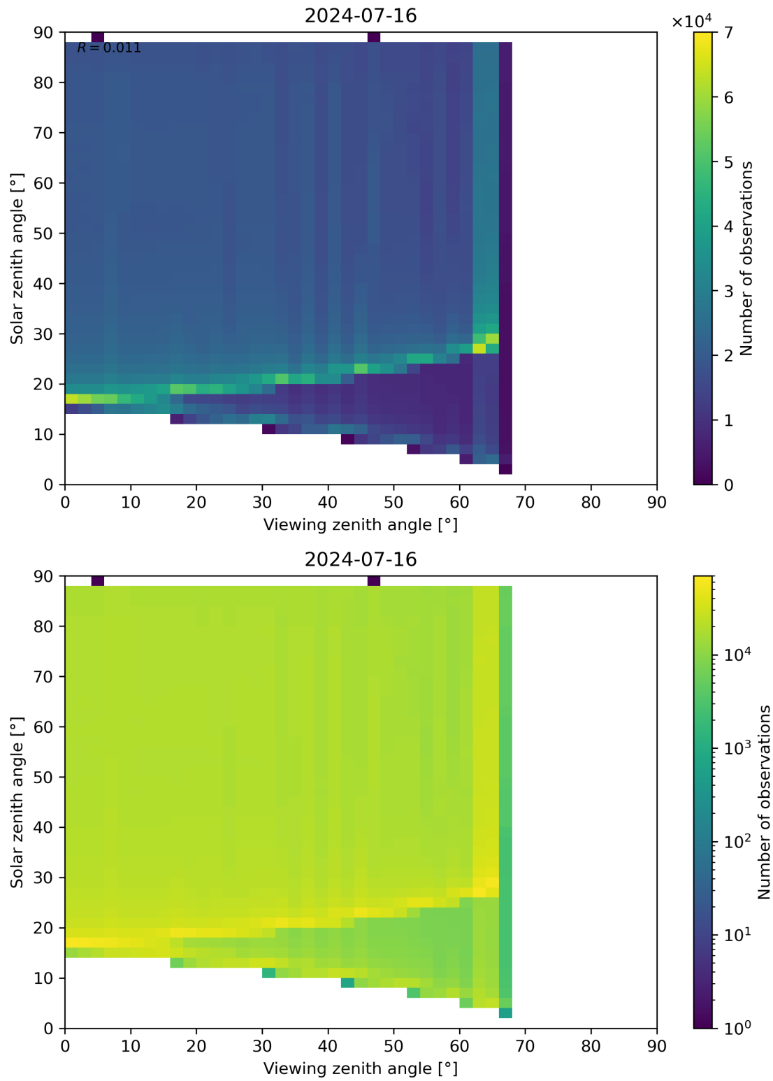
Figure 172: Scatter density plot of “Viewing zenith angle” against “Solar zenith angle” for 2024-07-15 to 2024-07-17.
