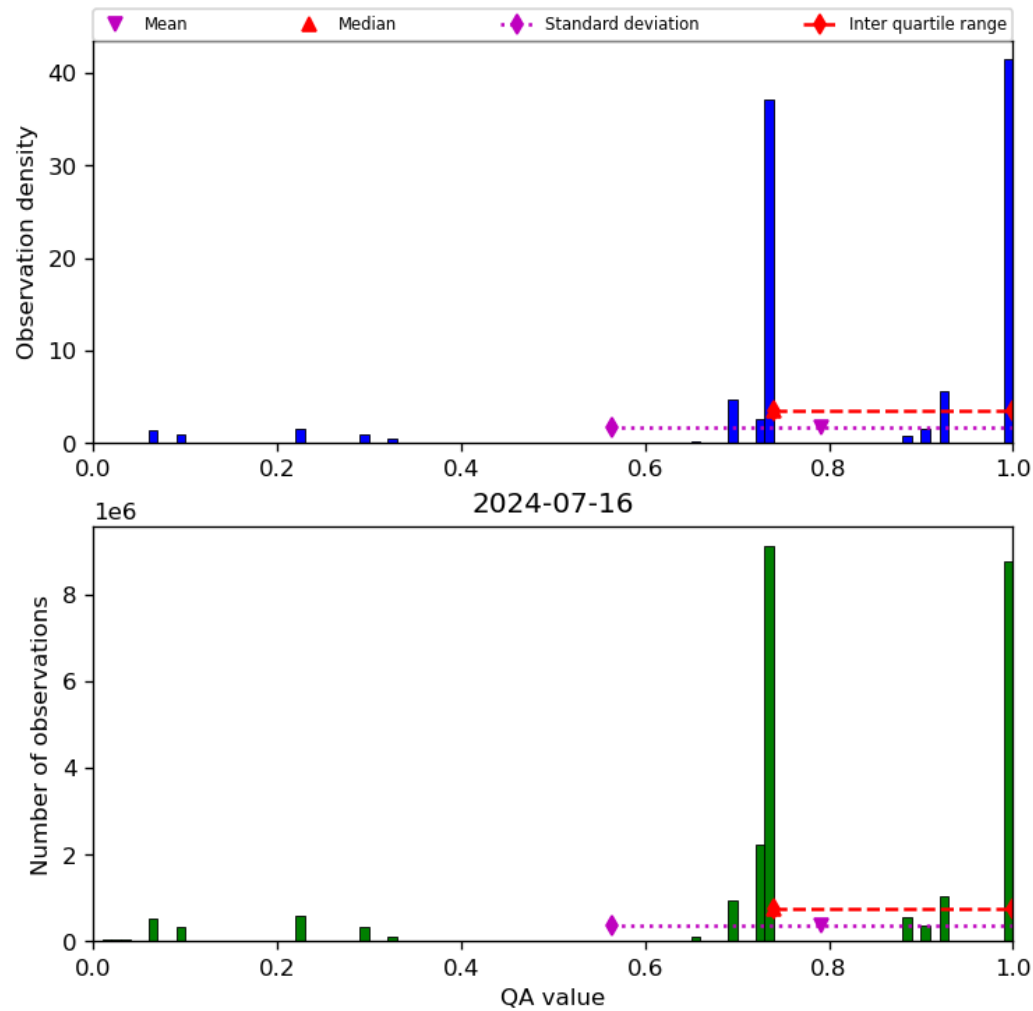
Figure 28: Histogram of “QA value” for 2024-07-15 to 2024-07-17
