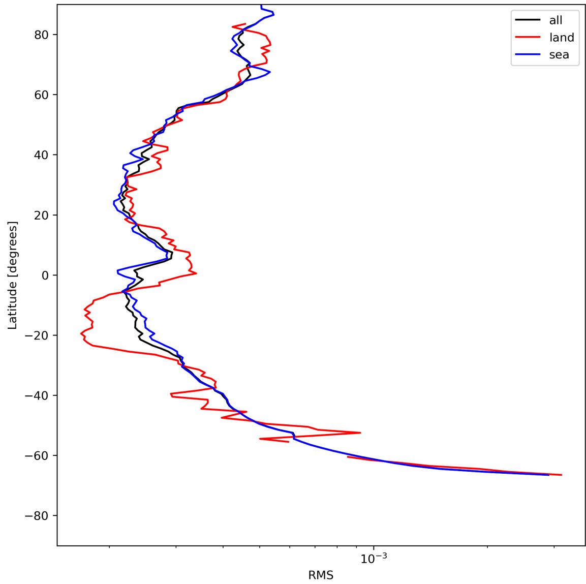
Figure 26: Zonal average of “RMS” for 2024-07-15 to 2024-07-17.
