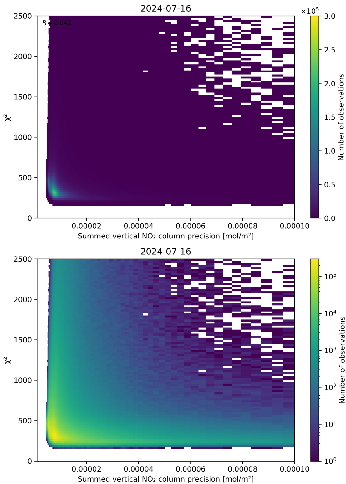
Figure 107: Scatter density plot of “Summed vertical NO 2 column precision” against “ \chi^2 ” for 2024-07-15 to 2024-07-17.
