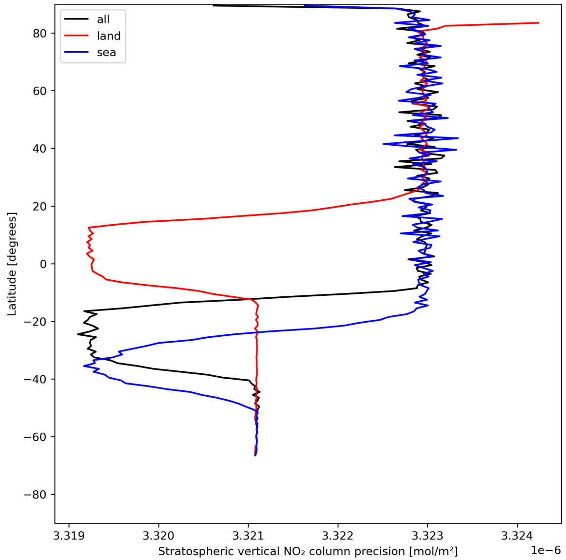
Figure 20: Zonal average of “Stratospheric vertical NO 2 column precision” for 2024-07-15 to 2024-07-17.
