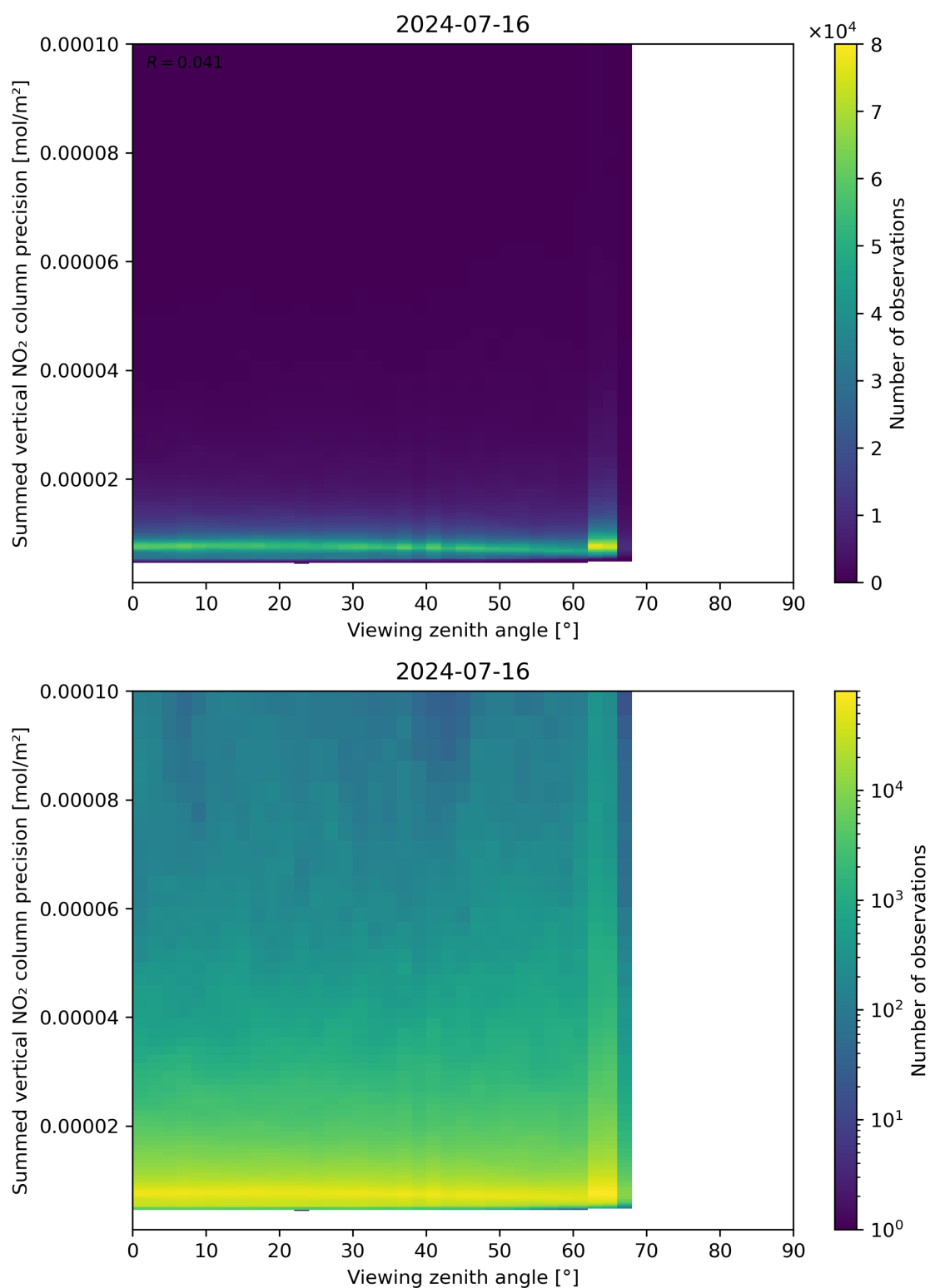
Figure 166: Scatter density plot of “Viewing zenith angle” against “Summed vertical NO 2 column precision” for 2024-07-15 to 2024-07-17.
