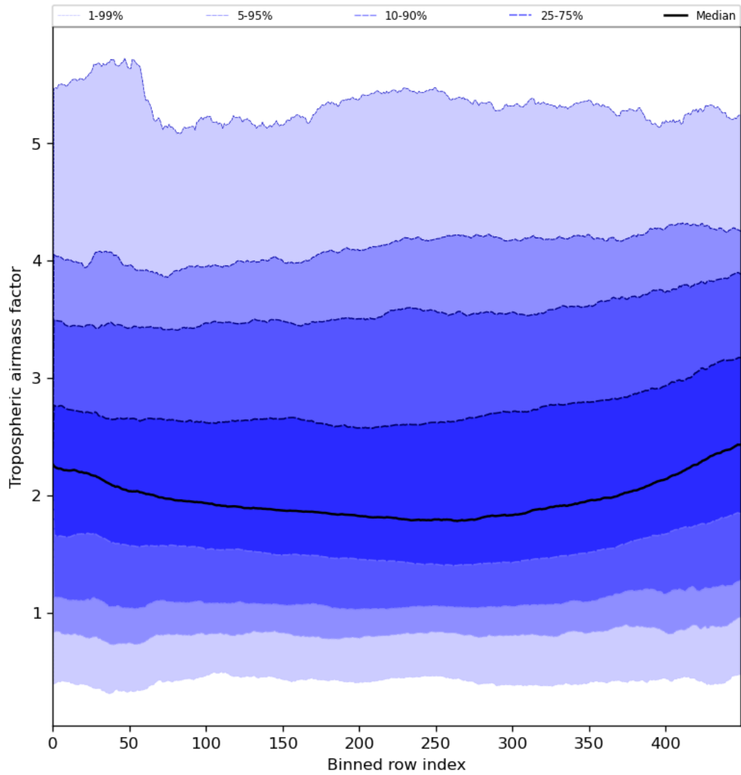
Figure 48: Along track statistics of “Tropospheric airmass factor” for 2024-07-15 to 2024-07-17
