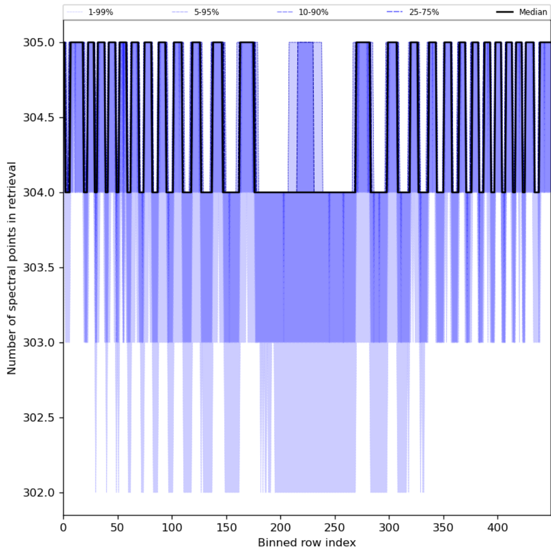
Figure 50: Along track statistics of “Number of spectral points in retrieval” for 2024-07-15 to 2024-07-17
