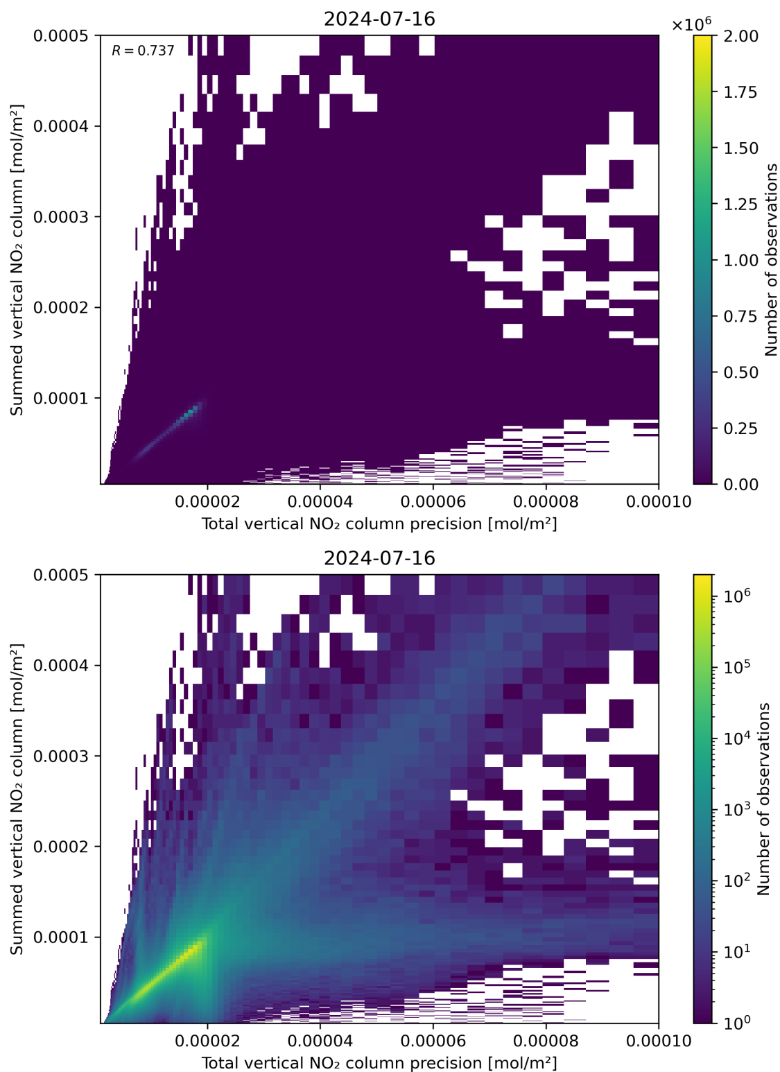
Figure 117: Scatter density plot of “Total vertical NO 2 column precision” against “Summed vertical NO 2 column” for 2024-07-15 to 2024-07-17.
