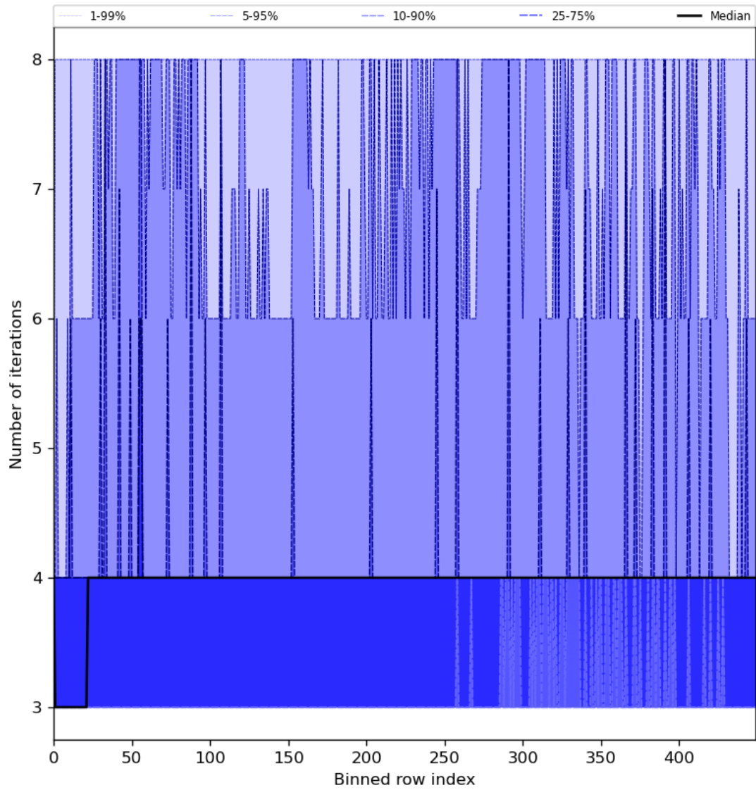
Figure 51: Along track statistics of “Number of iterations” for 2024-07-15 to 2024-07-17
