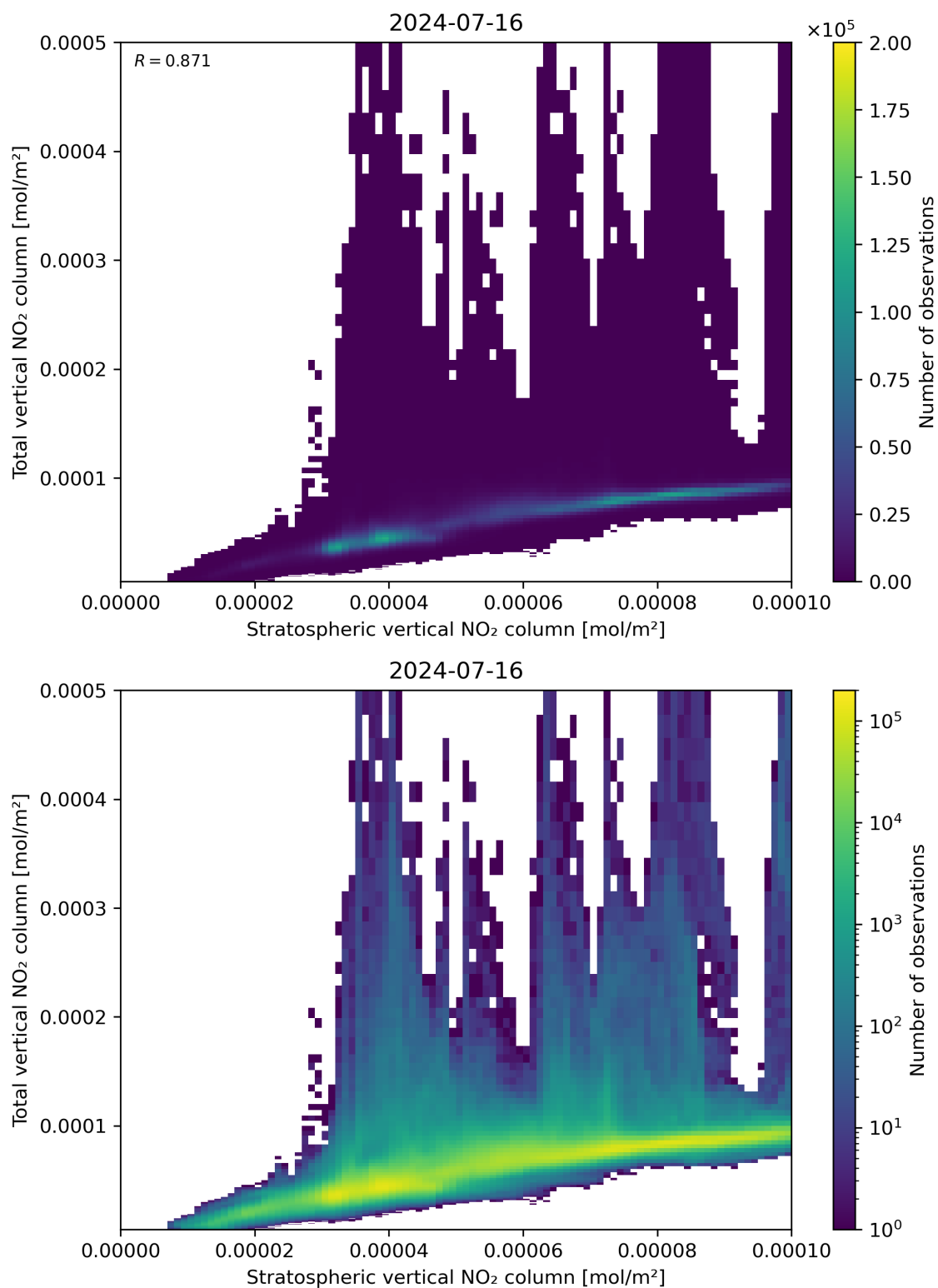
Figure 100: Scatter density plot of “Stratospheric vertical NO 2 column” against “Total vertical NO 2 column” for 2024-07-15 to 2024-07-17.
