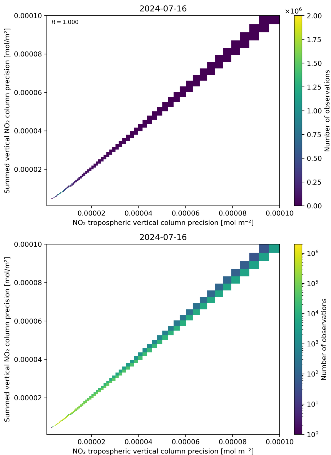
Figure 137: Scatter density plot of “NO 2 tropospheric vertical column precision” against “Summed vertical NO 2 column precision” for 2024-07-15 to 2024-07-17.
