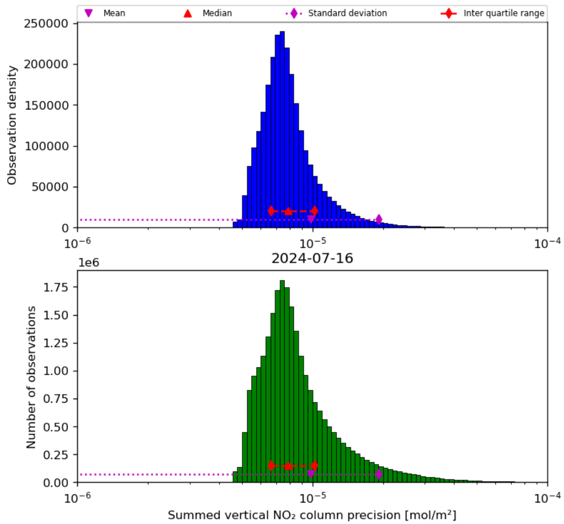
Figure 41: Histogram of “Summed vertical NO 2 column precision” for 2024-07-15 to 2024-07-17
