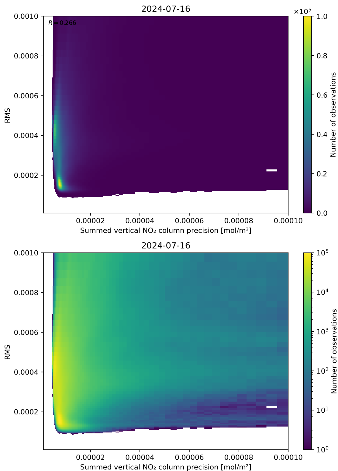
Figure 108: Scatter density plot of “Summed vertical NO 2 column precision” against “RMS” for 2024-07-15 to 2024-07-17.
