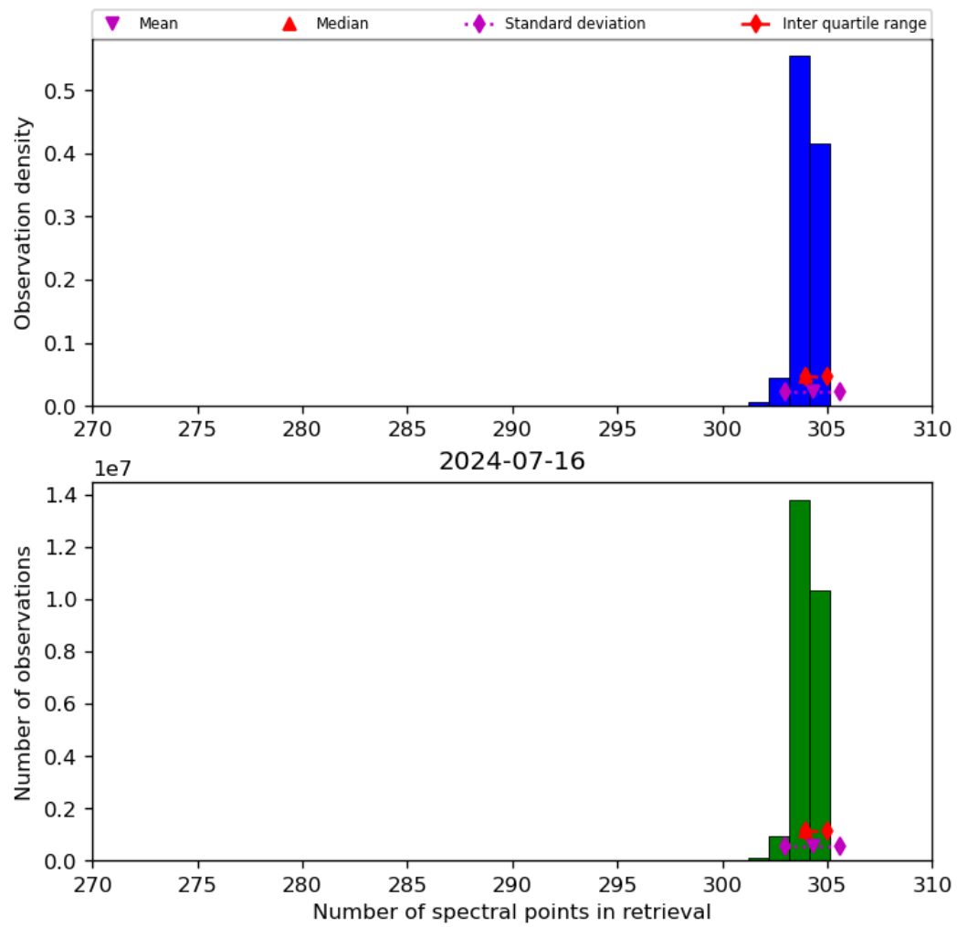
Figure 33: Histogram of “Number of spectral points in retrieval” for 2024-07-15 to 2024-07-17
