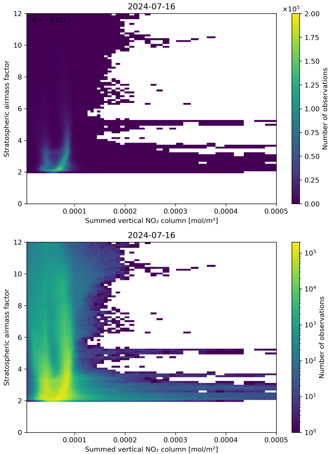
Figure 103: Scatter density plot of “Summed vertical NO 2 column” against “Stratospheric air mass factor” for 2024-07-15 to 2024-07-17.
