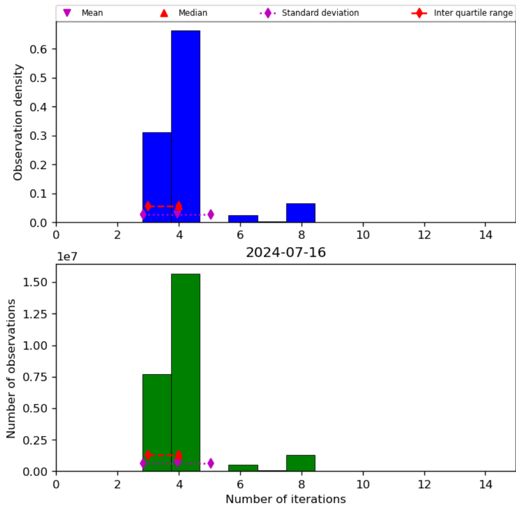
Figure 34: Histogram of “Number of iterations” for 2024-07-15 to 2024-07-17
