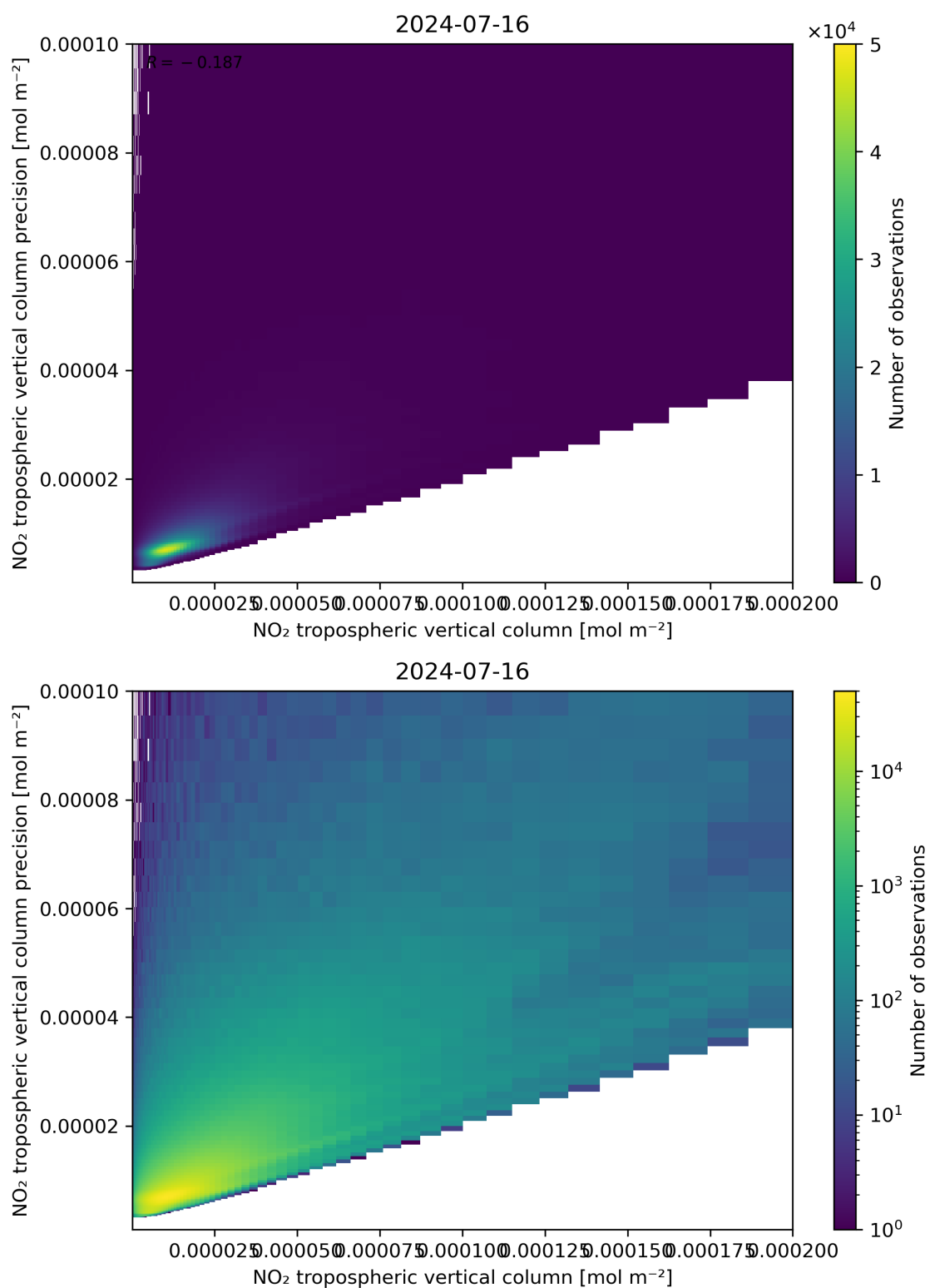
Figure 130: Scatter density plot of “NO 2 tropospheric vertical column” against “NO 2 tropospheric vertical column precision” for 2024-07-15 to 2024-07-17.
