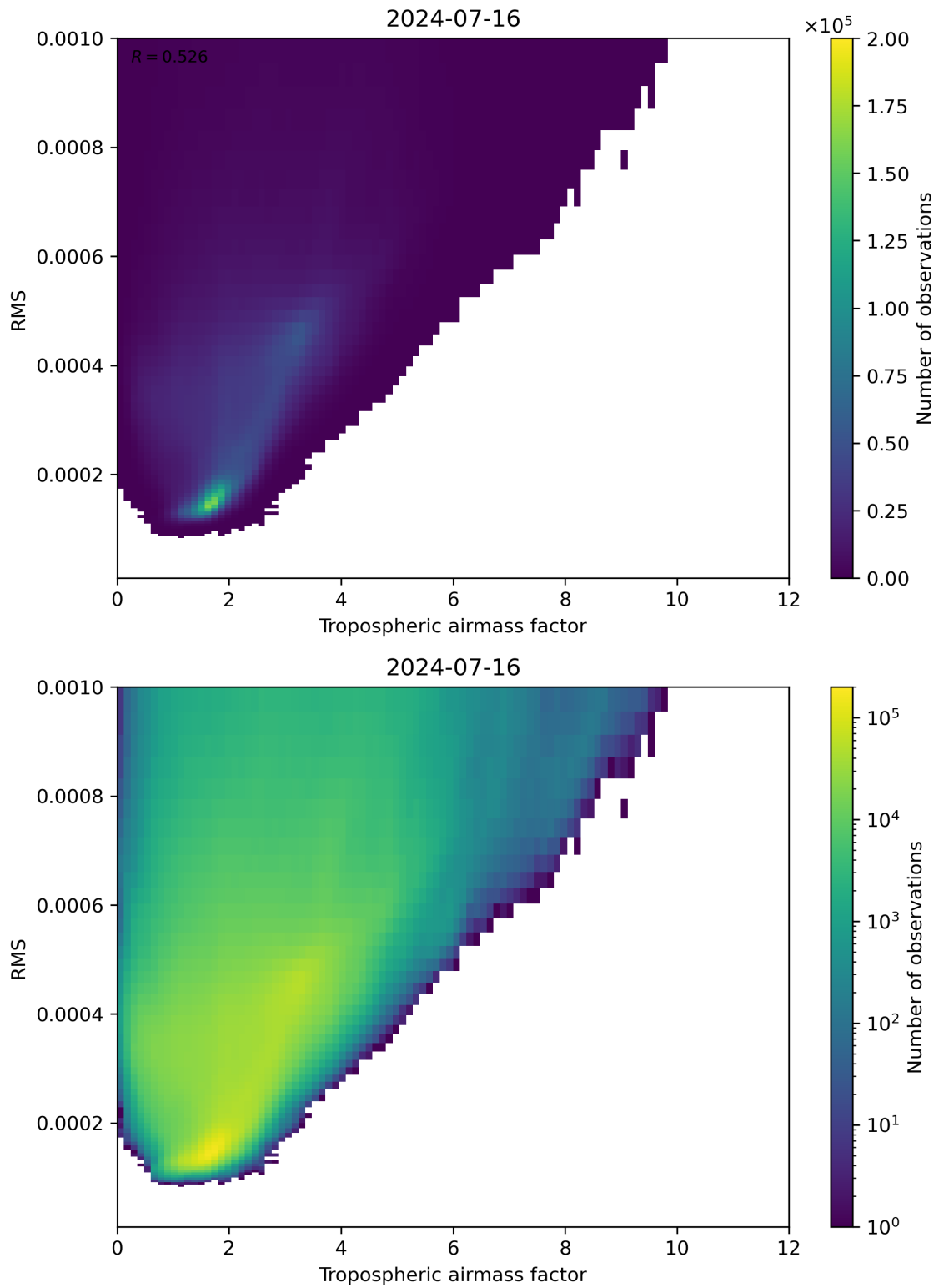
Figure 79: Scatter density plot of “Tropospheric airmass factor” against “RMS” for 2024-07-15 to 2024-07-17.
