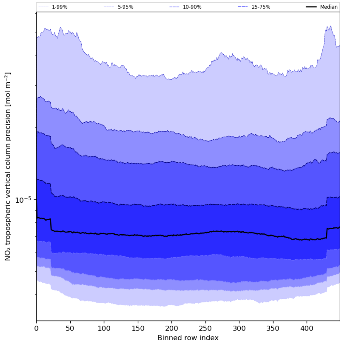
Figure 47: Along track statistics of “NO 2 tropospheric vertical column precision” for 2024-07-15 to 2024-07-17
