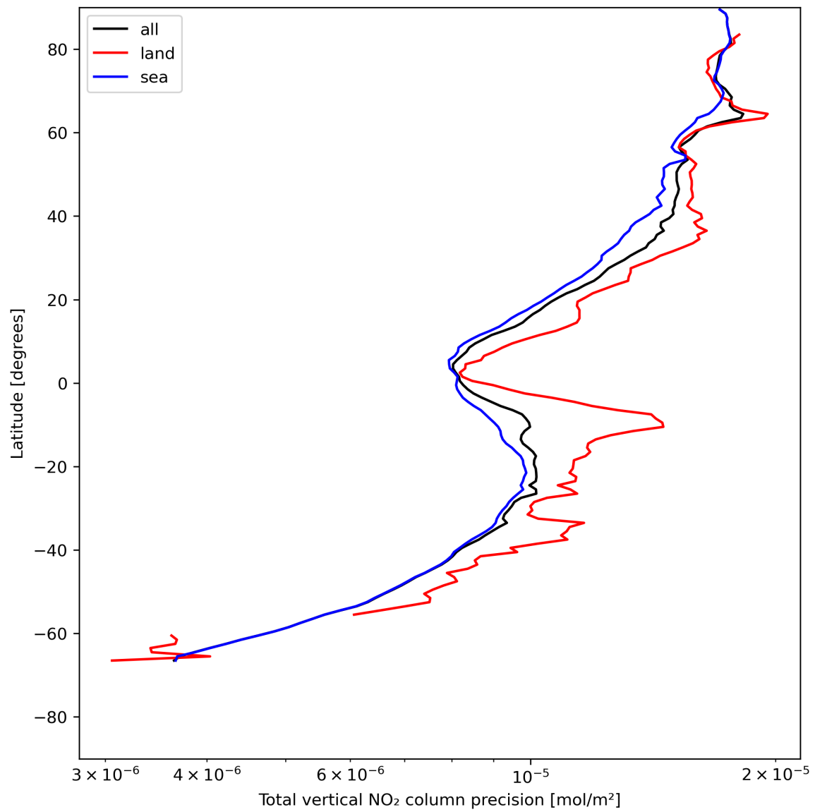
Figure 22: Zonal average of “Total vertical NO 2 column precision” for 2024-07-15 to 2024-07-17.
