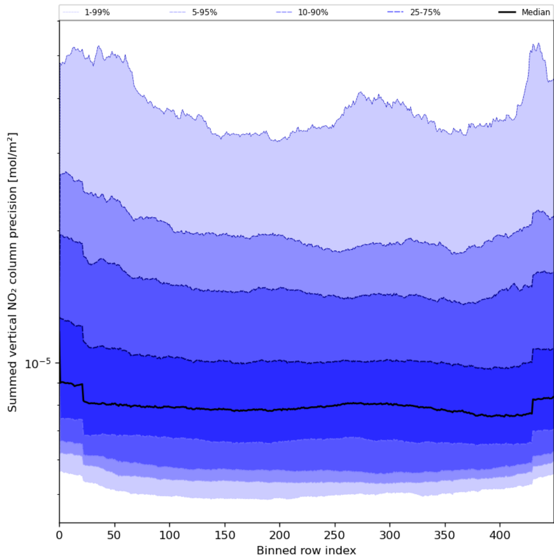
Figure 58: Along track statistics of “Summed vertical NO 2 column precision” for 2024-07-15 to 2024-07-17
