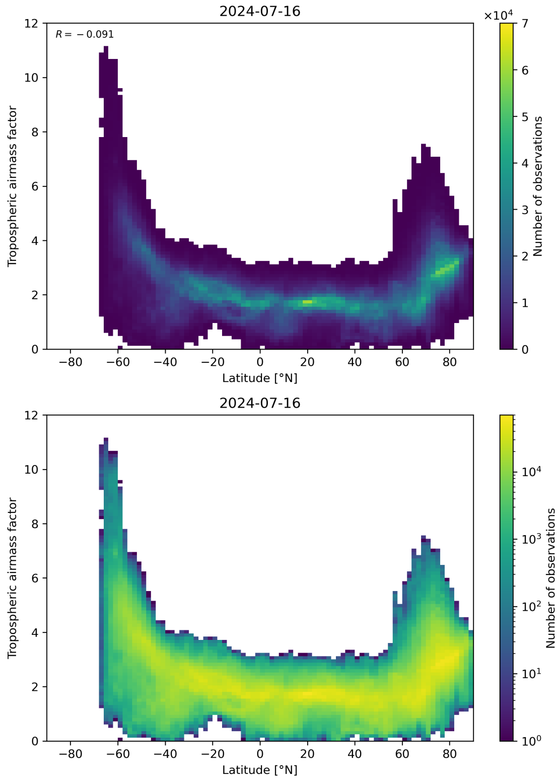
Figure 85: Scatter density plot of “Latitude” against “Tropospheric airmass factor” for 2024-07-15 to 2024-07-17.
