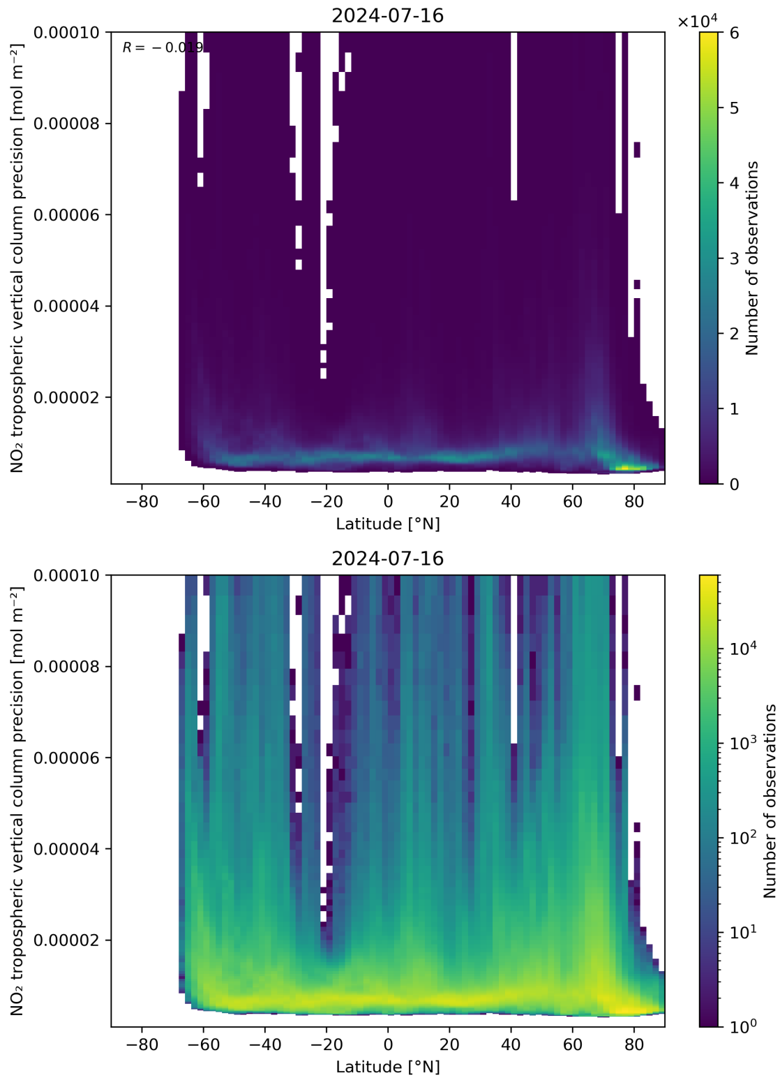
Figure 93: Scatter density plot of “Latitude” against “NO 2 tropospheric vertical column precision” for 2024-07-15 to 2024-07-17.
