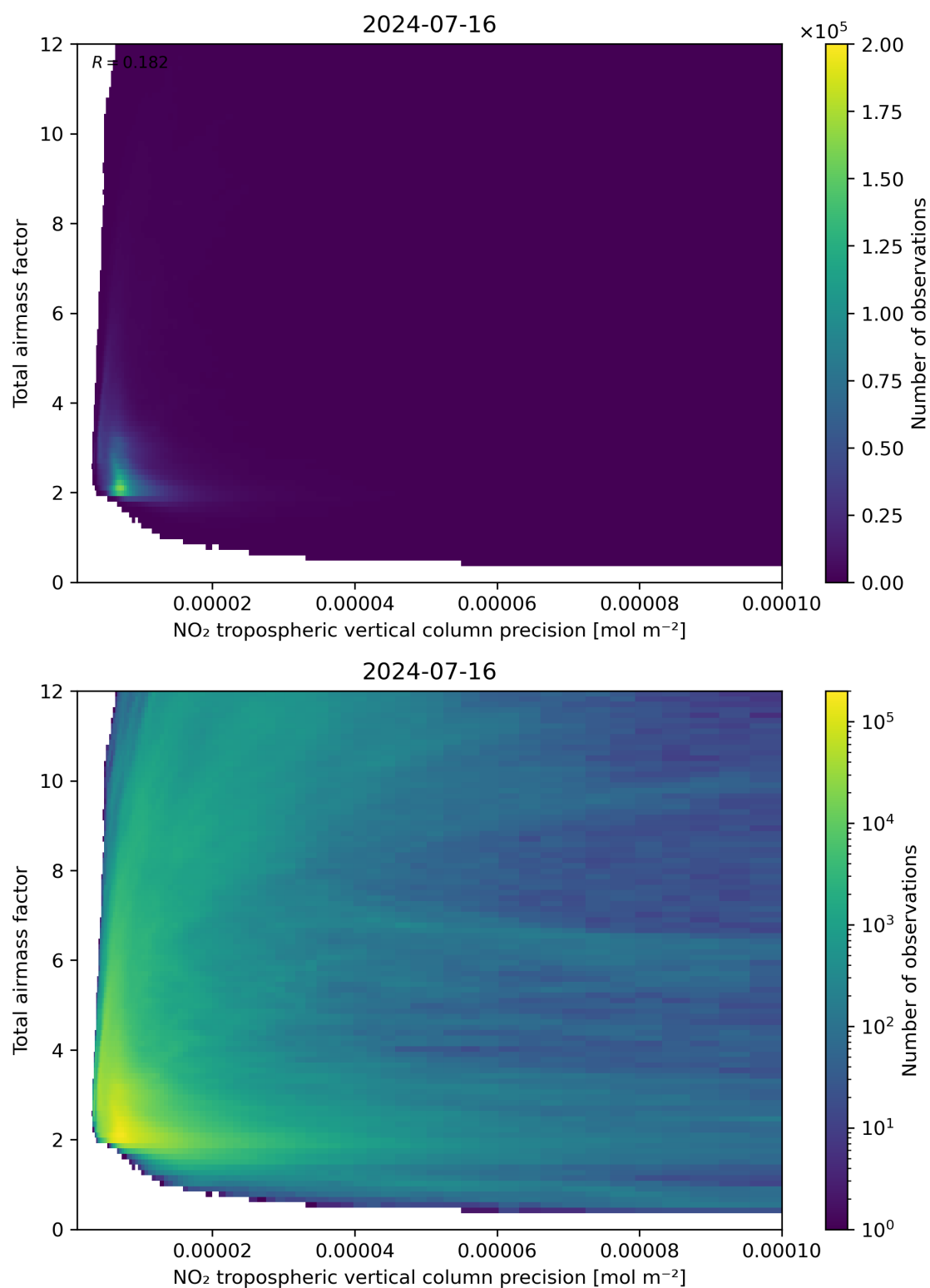
Figure 132: Scatter density plot of “NO 2 tropospheric vertical column precision” against “Total air mass factor” for 2024-07-15 to 2024-07-17.
