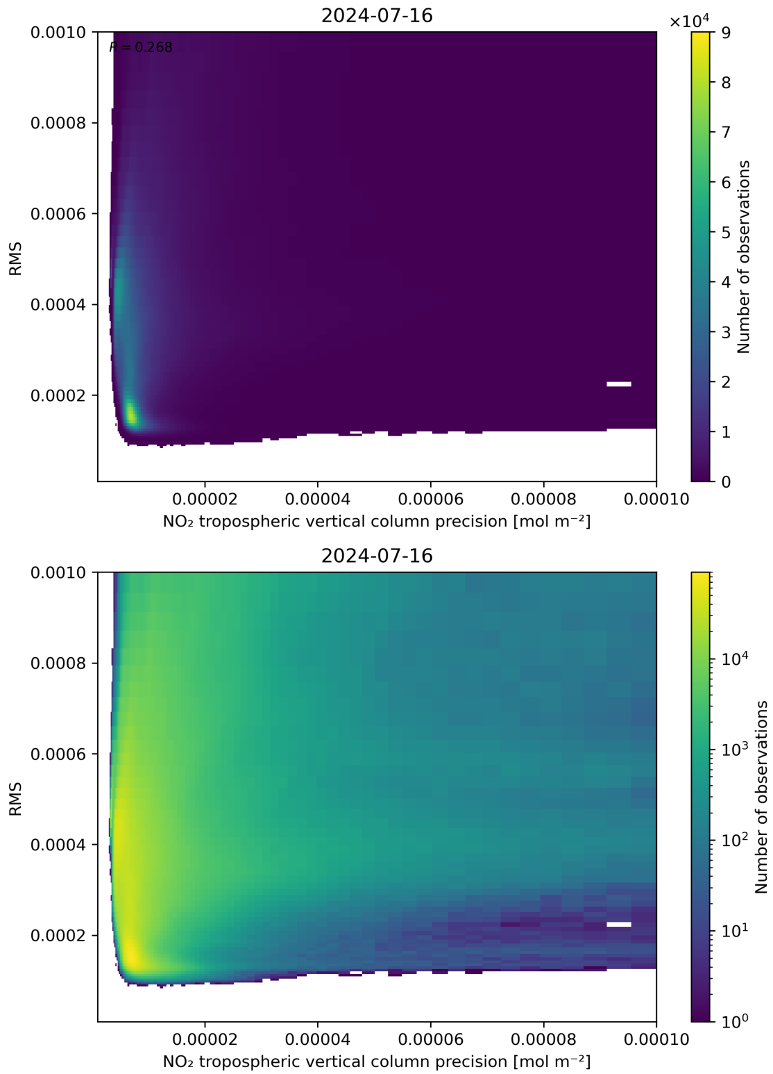
Figure 140: Scatter density plot of “NO 2 tropospheric vertical column precision” against “RMS” for 2024-07-15 to 2024-07-17.
