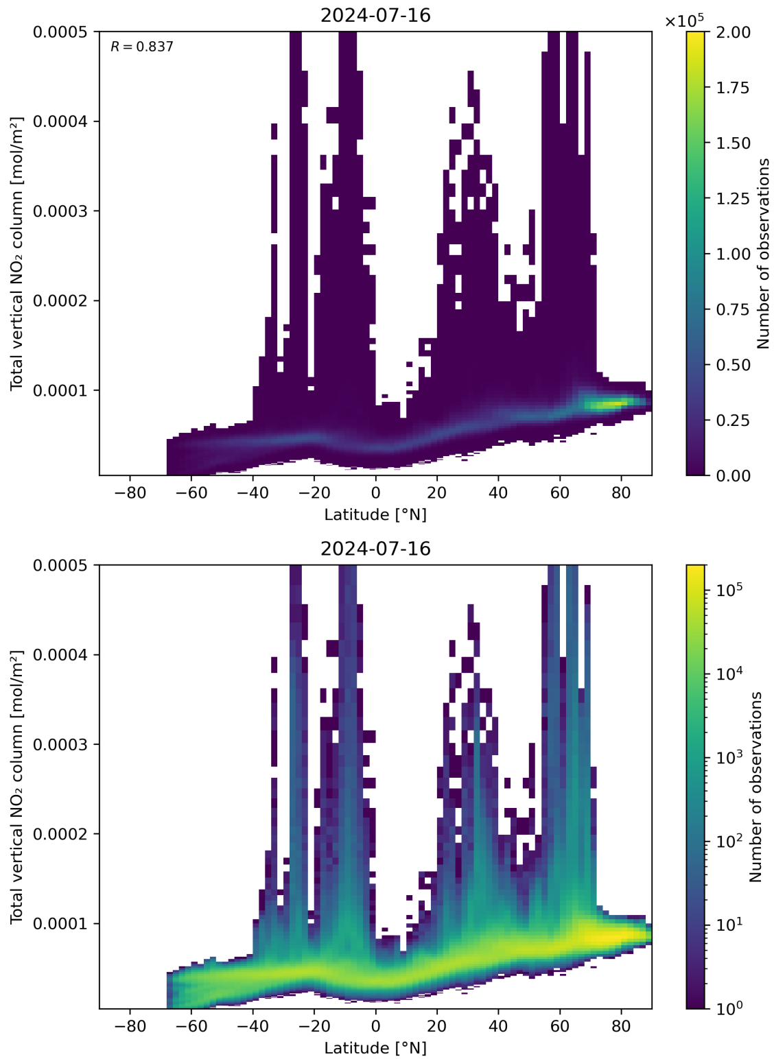
Figure 90: Scatter density plot of “Latitude” against “Total vertical NO 2 column” for 2024-07-15 to 2024-07-17.
