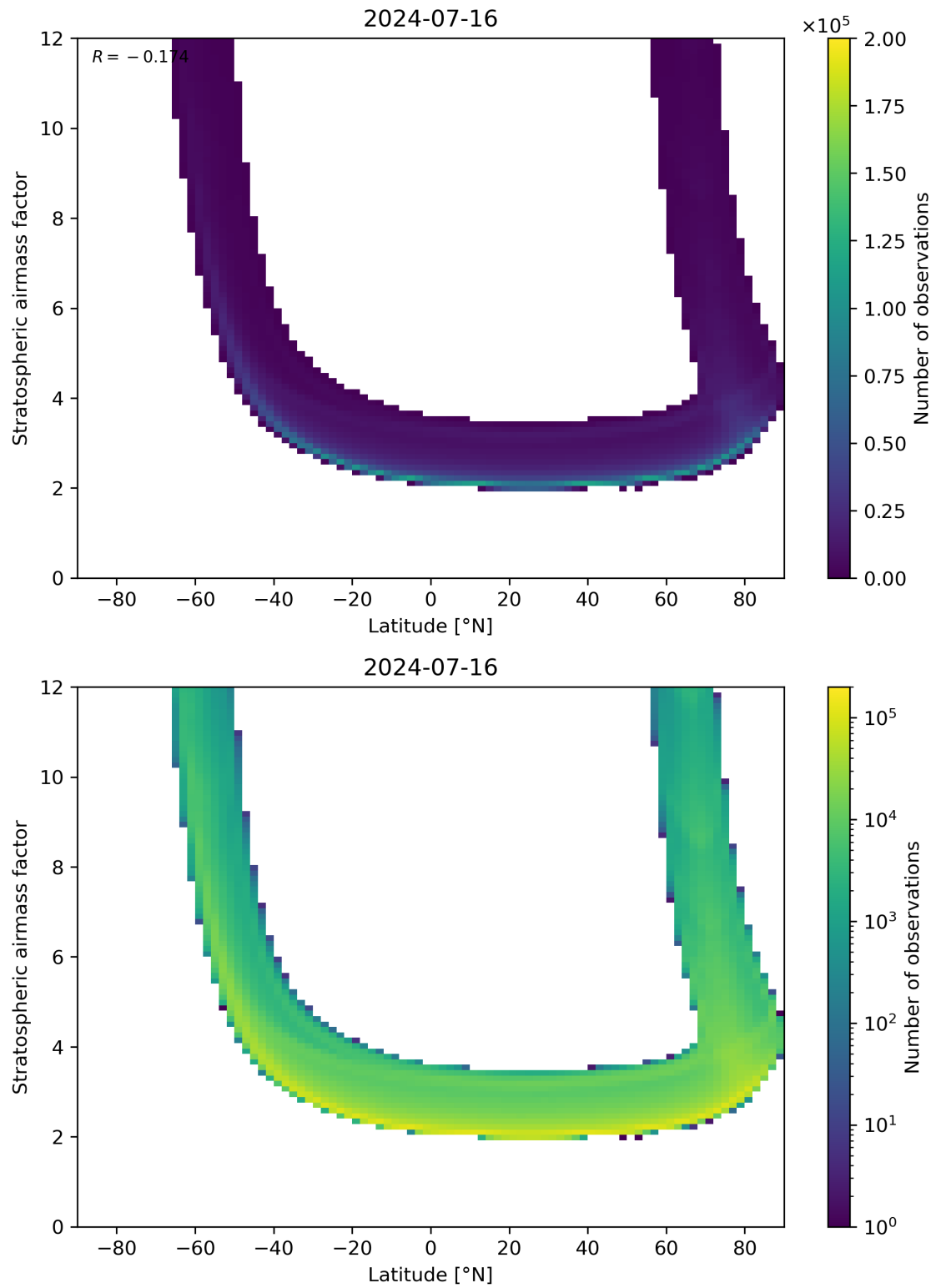
Figure 83: Scatter density plot of “Latitude” against “Stratospheric air mass factor” for 2024-07-15 to 2024-07-17.
