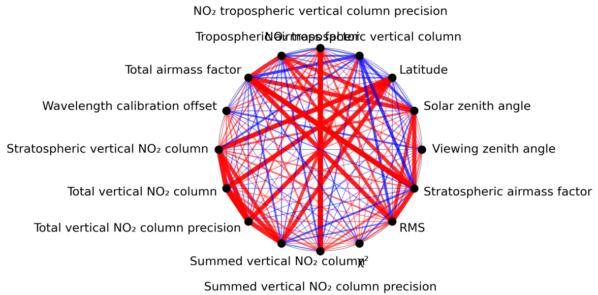
Figure 1: Map of correlation graph for 2024-07-15 to 2024-07-17.
