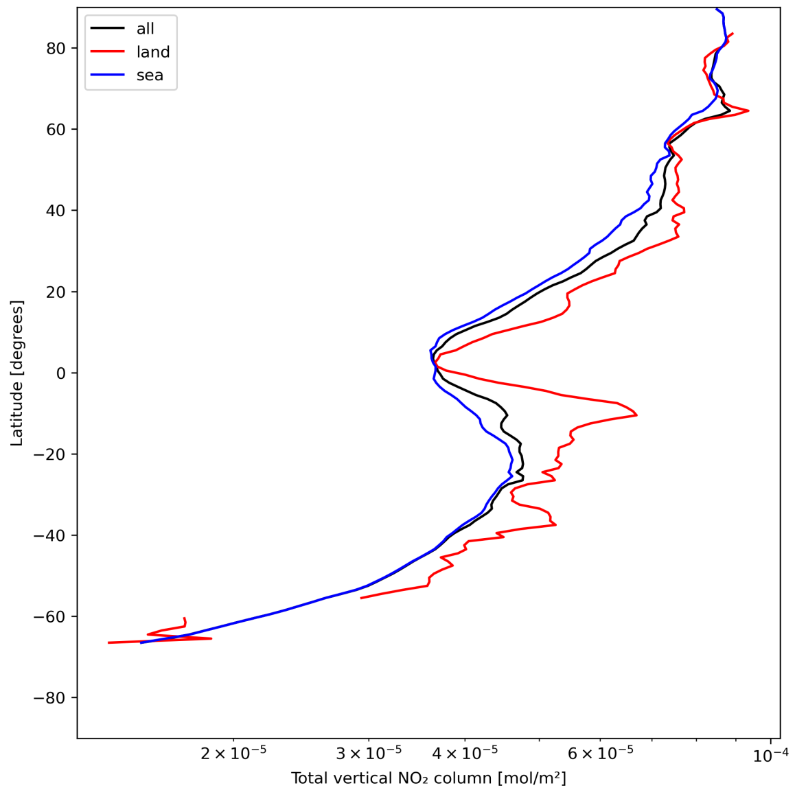
Figure 21: Zonal average of “Total vertical NO 2 column” for 2024-07-15 to 2024-07-17.
