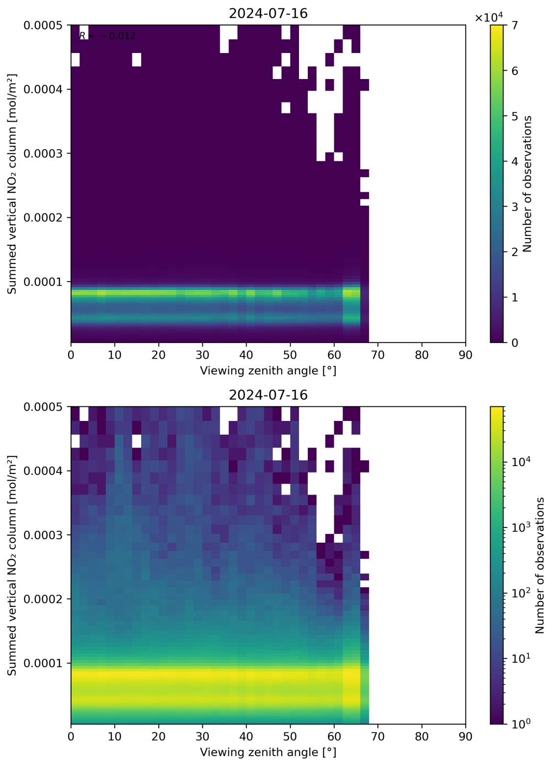
Figure 165: Scatter density plot of “Viewing zenith angle” against “Summed vertical NO 2 column” for 2024-07-15 to 2024-07-17.
