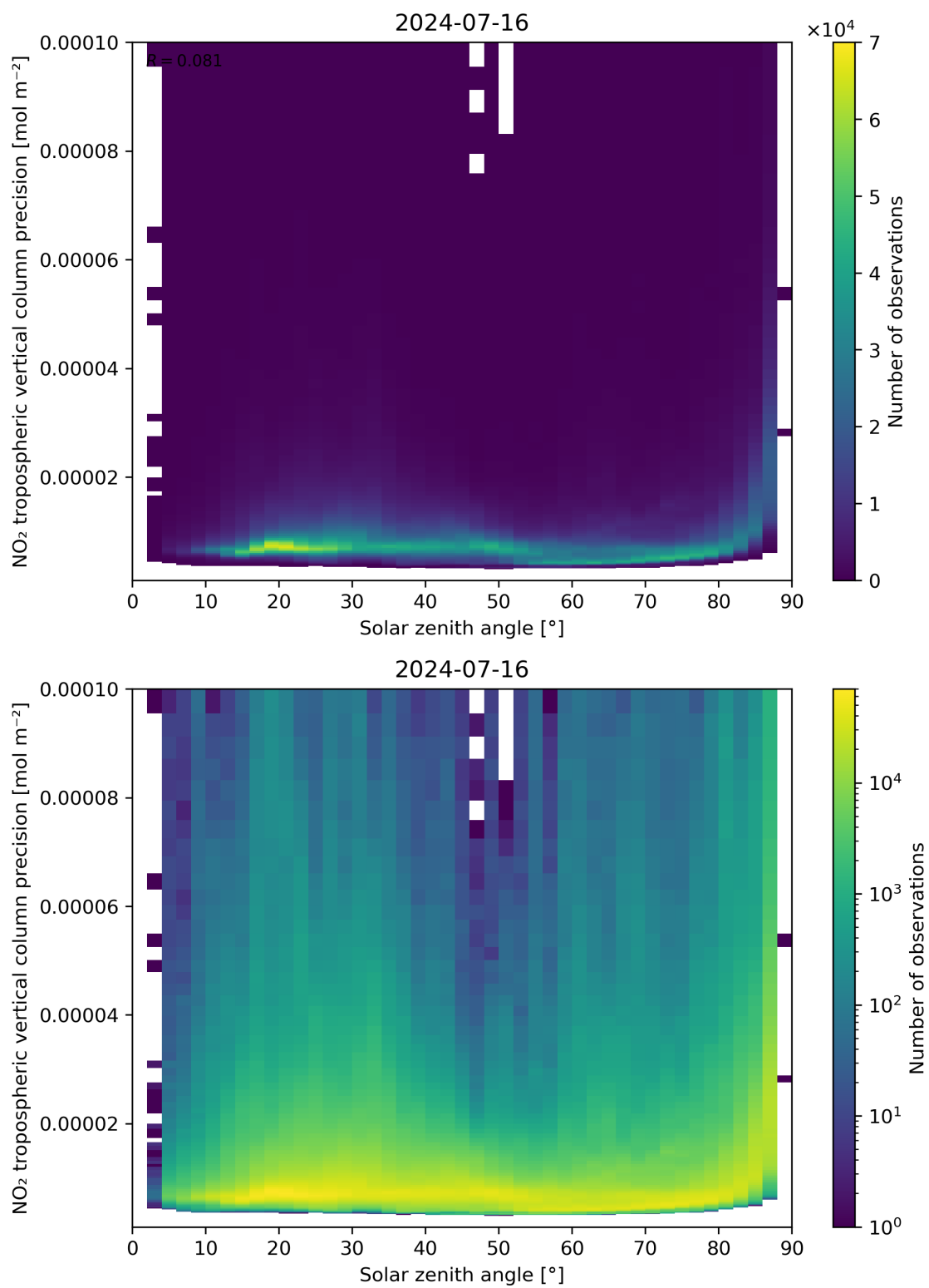
Figure 156: Scatter density plot of “Solar zenith angle” against “NO 2 tropospheric vertical column precision” for 2024-07-15 to 2024-07-17.
