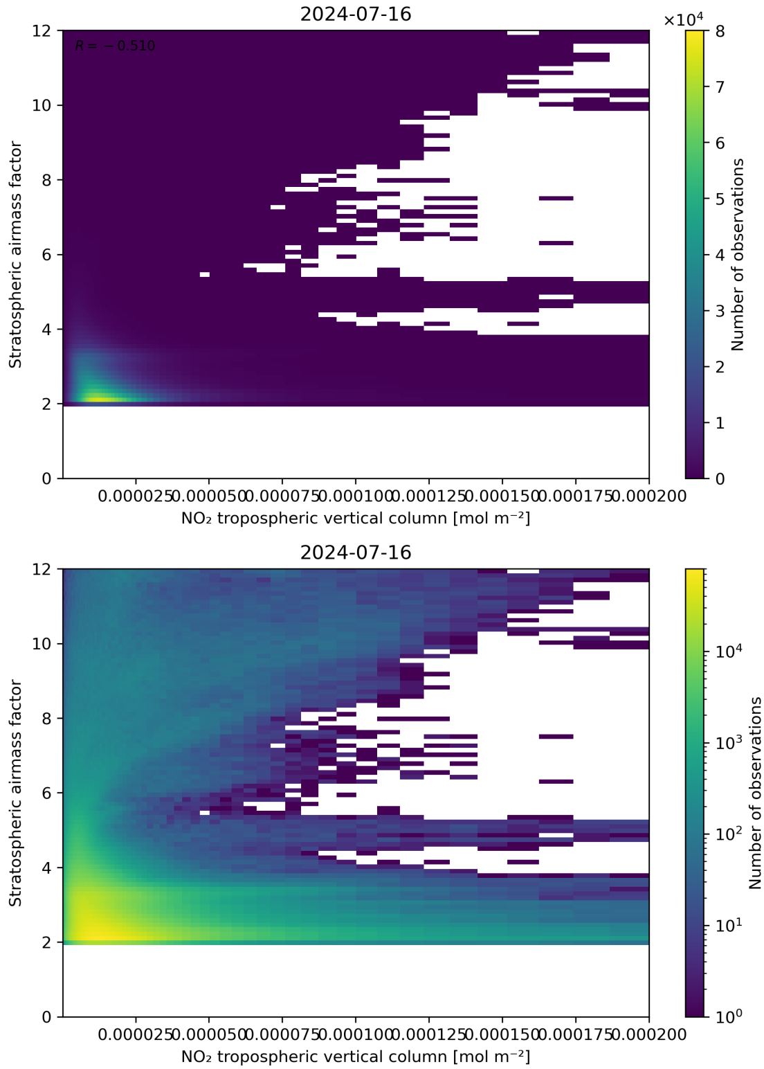
Figure 121: Scatter density plot of “NO 2 tropospheric vertical column” against “Stratospheric air mass factor” for 2024-07-15 to 2024-07-17.
