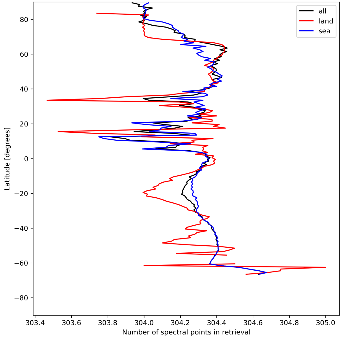
Figure 16: Zonal average of “Number of spectral points in retrieval” for 2024-07-15 to 2024-07-17.
