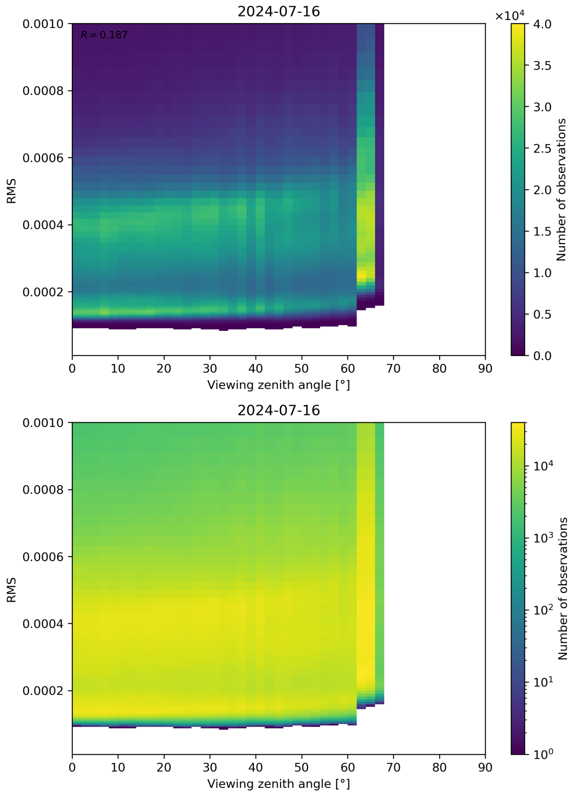
Figure 171: Scatter density plot of “Viewing zenith angle” against “RMS” for 2024-07-15 to 2024-07-17.
