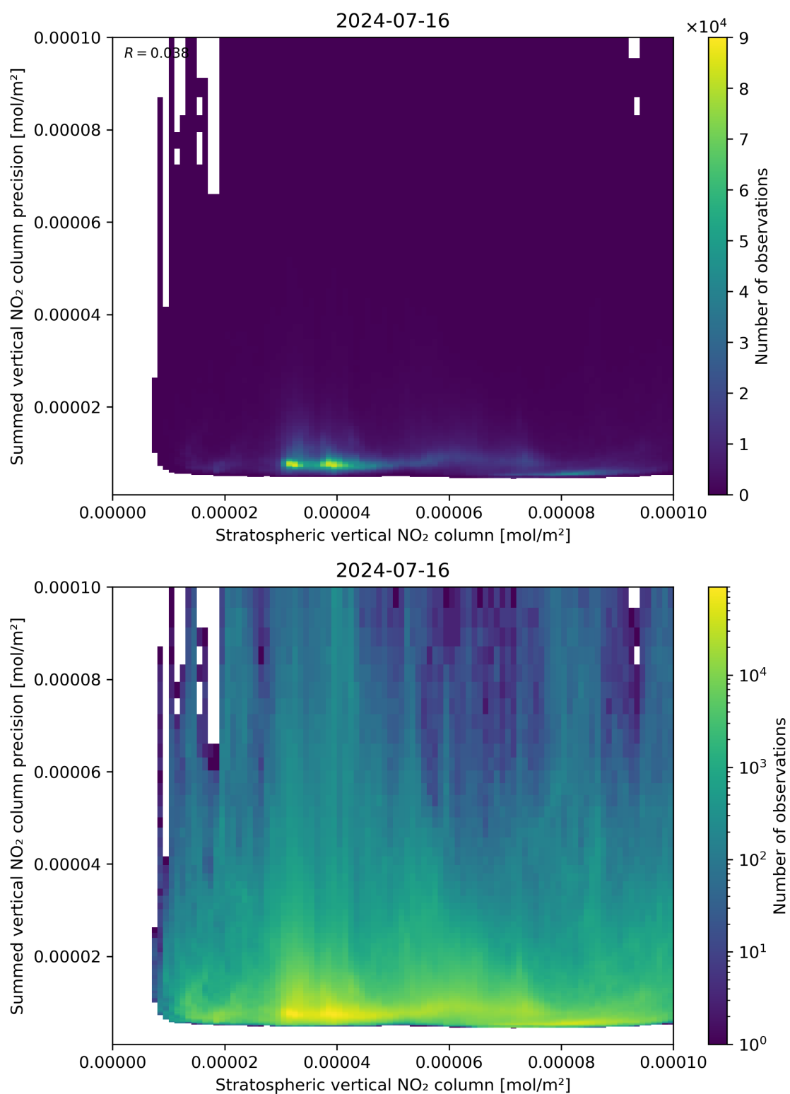
Figure 99: Scatter density plot of “Stratospheric vertical NO 2 column” against “Summed vertical NO 2 column precision” for 2024-07-15 to 2024-07-17.
