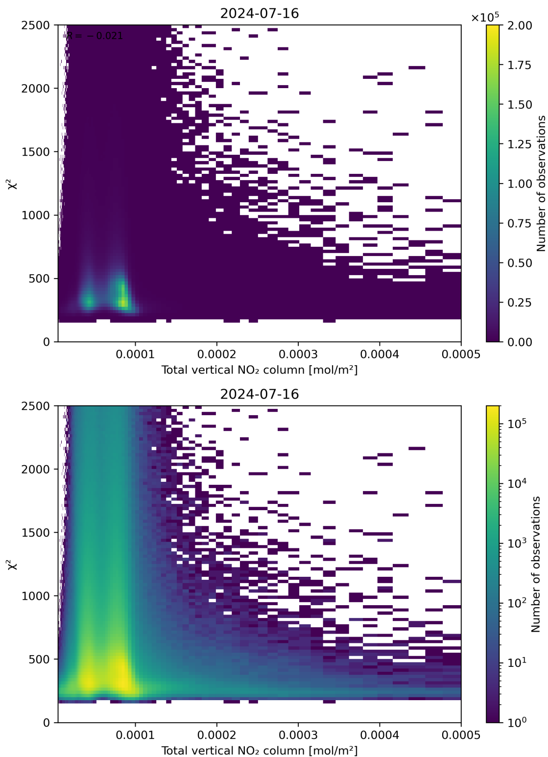
Figure 111: Scatter density plot of “Total vertical NO 2 column” against “ \chi^2 ” for 2024-07-15 to 2024-07-17.
