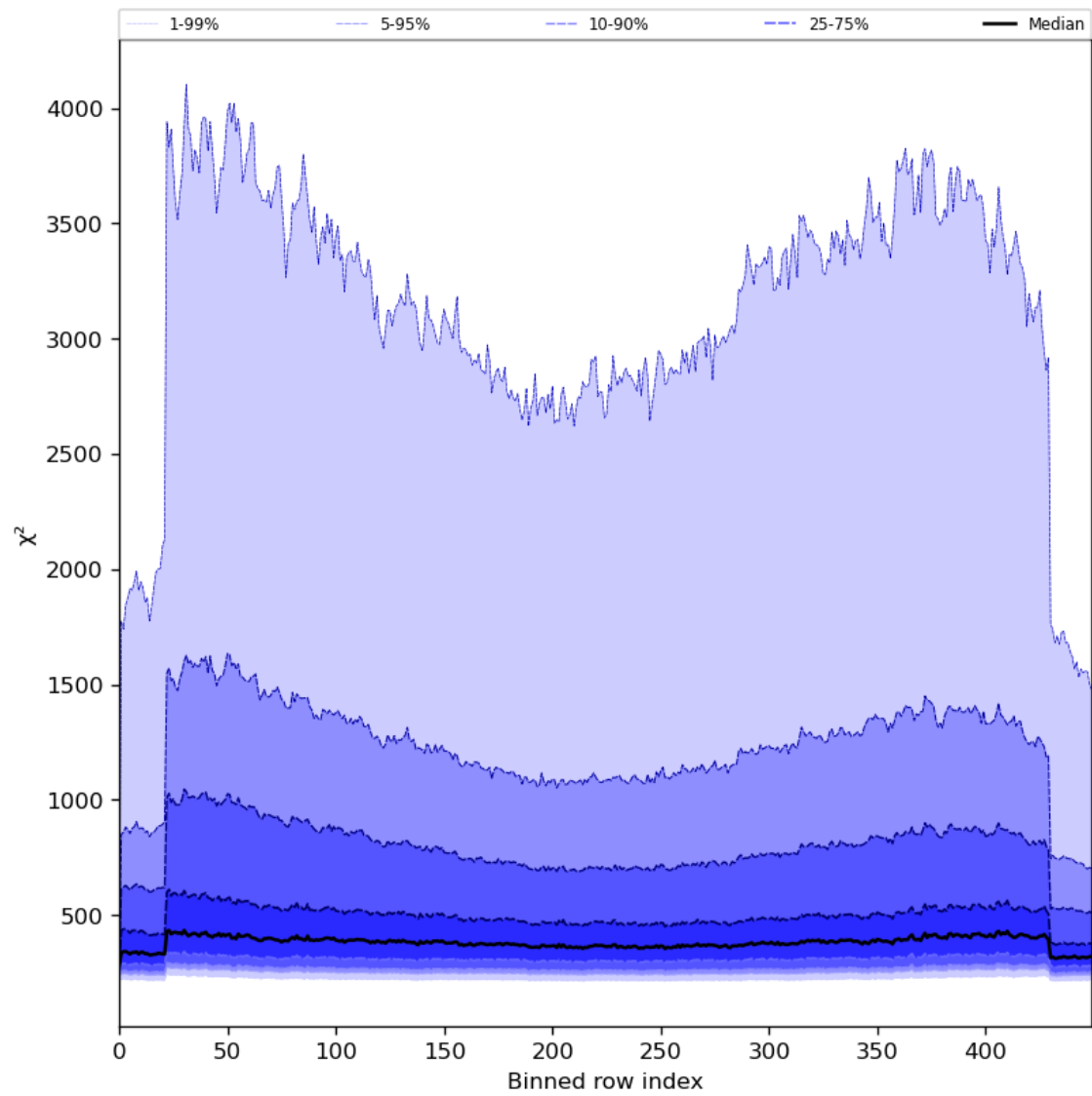
Figure 59: Along track statistics of “ \chi^2 ” for 2024-07-15 to 2024-07-17
