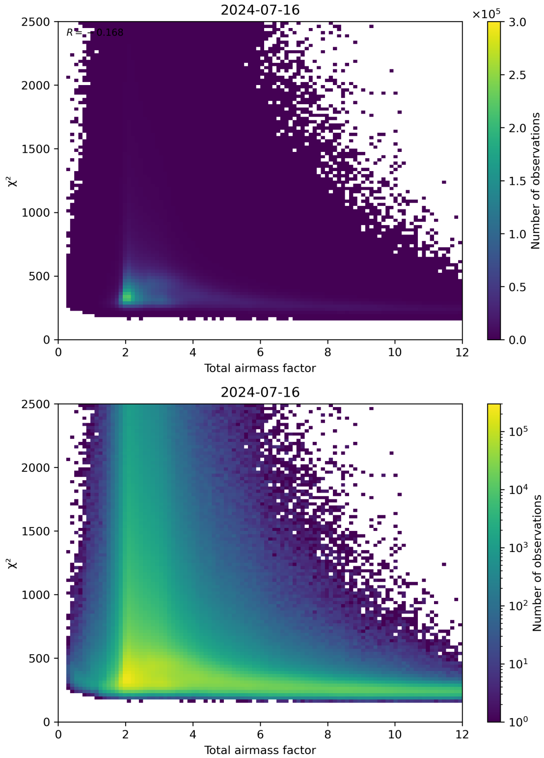
Figure 63: Scatter density plot of “Total airmass factor” against “ \chi^2 ” for 2024-07-15 to 2024-07-17.
