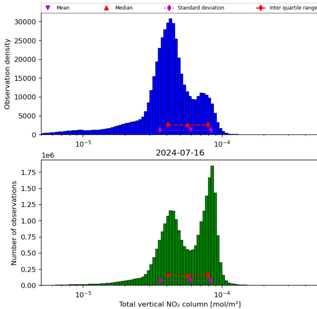
Figure 38: Histogram of “Total vertical NO 2 column” for 2024-07-15 to 2024-07-17
