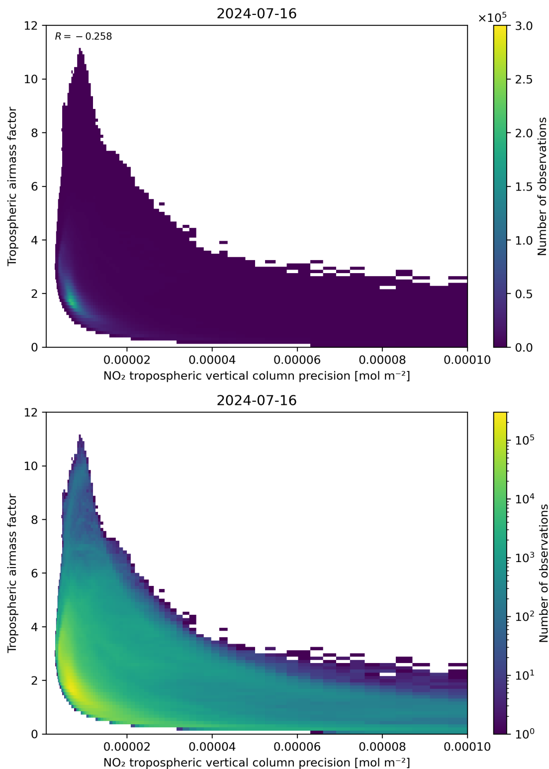
Figure 133: Scatter density plot of “NO 2 tropospheric vertical column precision” against “Tropospheric airmass factor” for 2024-07-15 to 2024-07-17.
