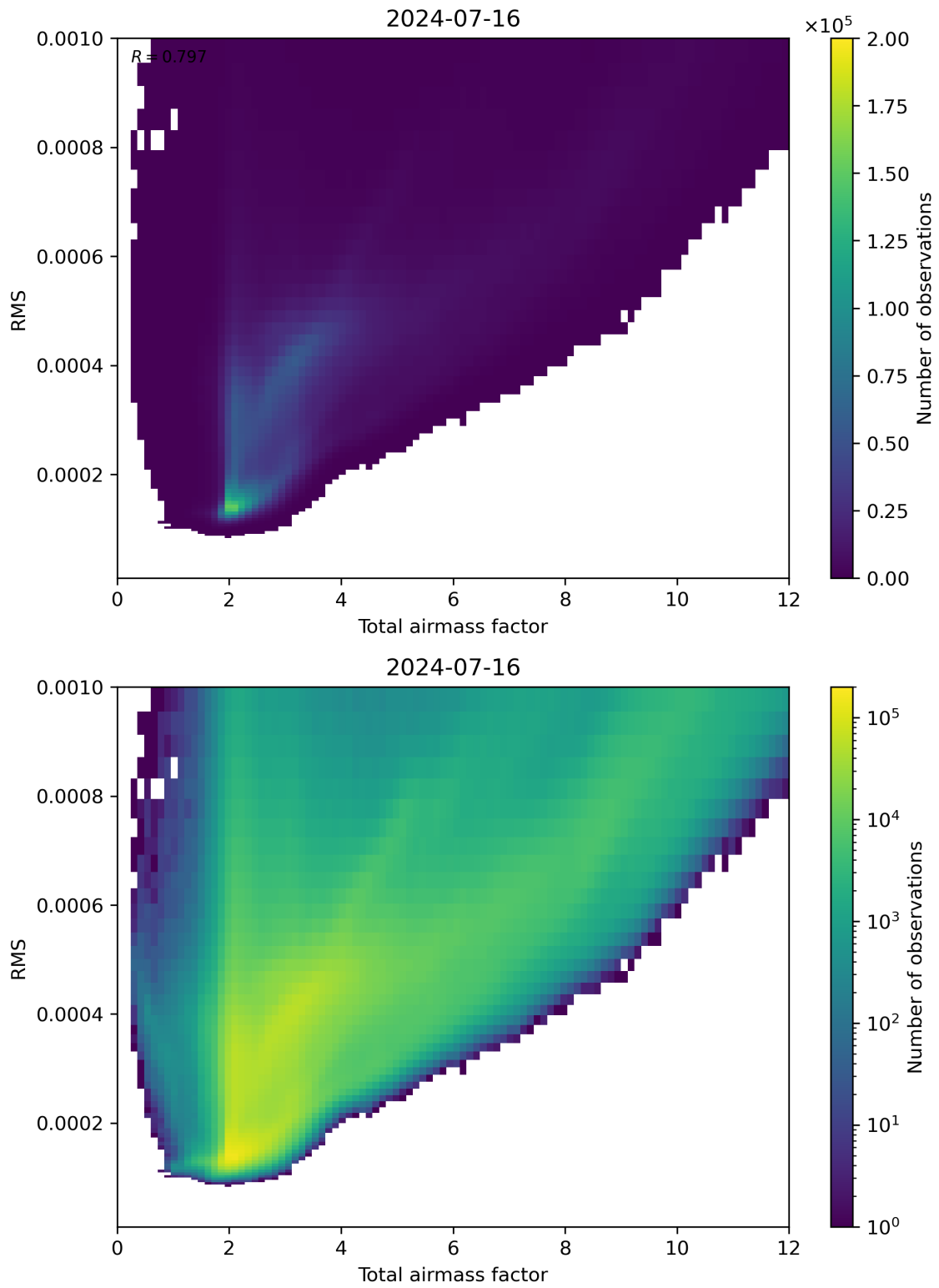
Figure 69: Scatter density plot of “Total airmass factor” against “RMS” for 2024-07-15 to 2024-07-17.
