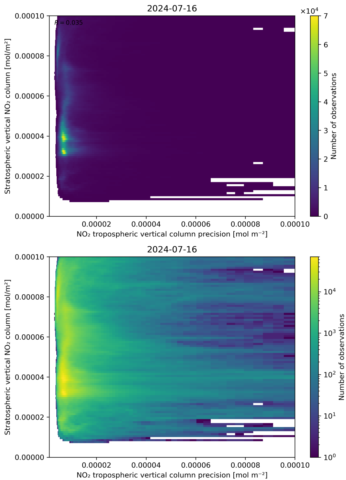
Figure 135: Scatter density plot of “NO 2 tropospheric vertical column precision” against “Stratospheric vertical NO 2 column” for 2024-07-15 to 2024-07-17.
