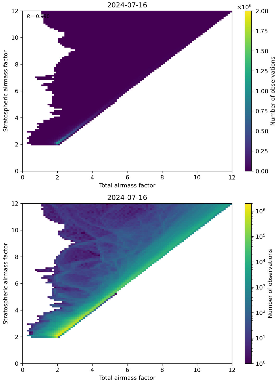
Figure 62: Scatter density plot of “Total airmass factor” against “Stratospheric airmass factor” for 2024-07-15 to 2024-07-17.
