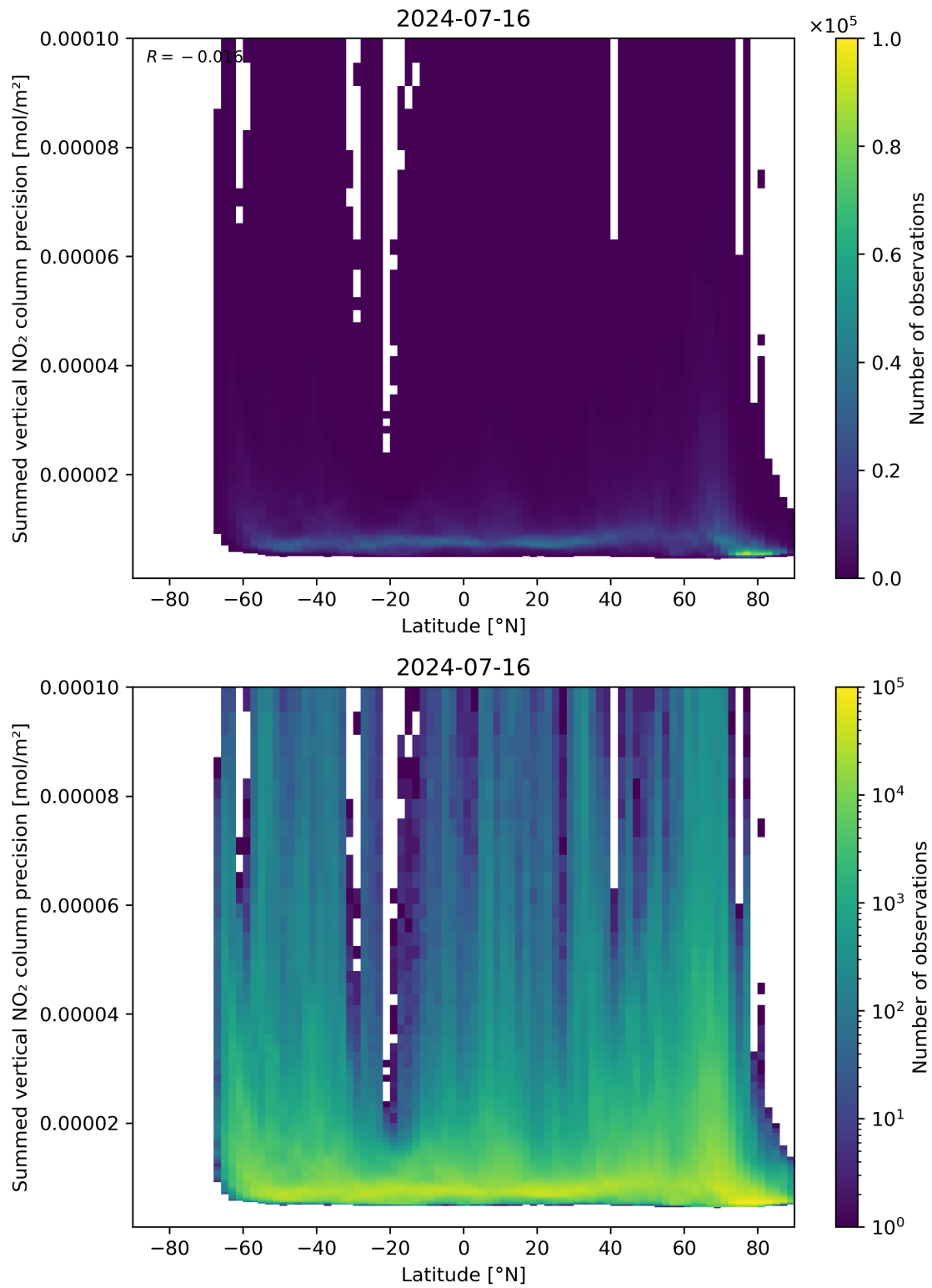
Figure 89: Scatter density plot of “Latitude” against “Summed vertical NO 2 column precision” for 2024-07-15 to 2024-07-17.
