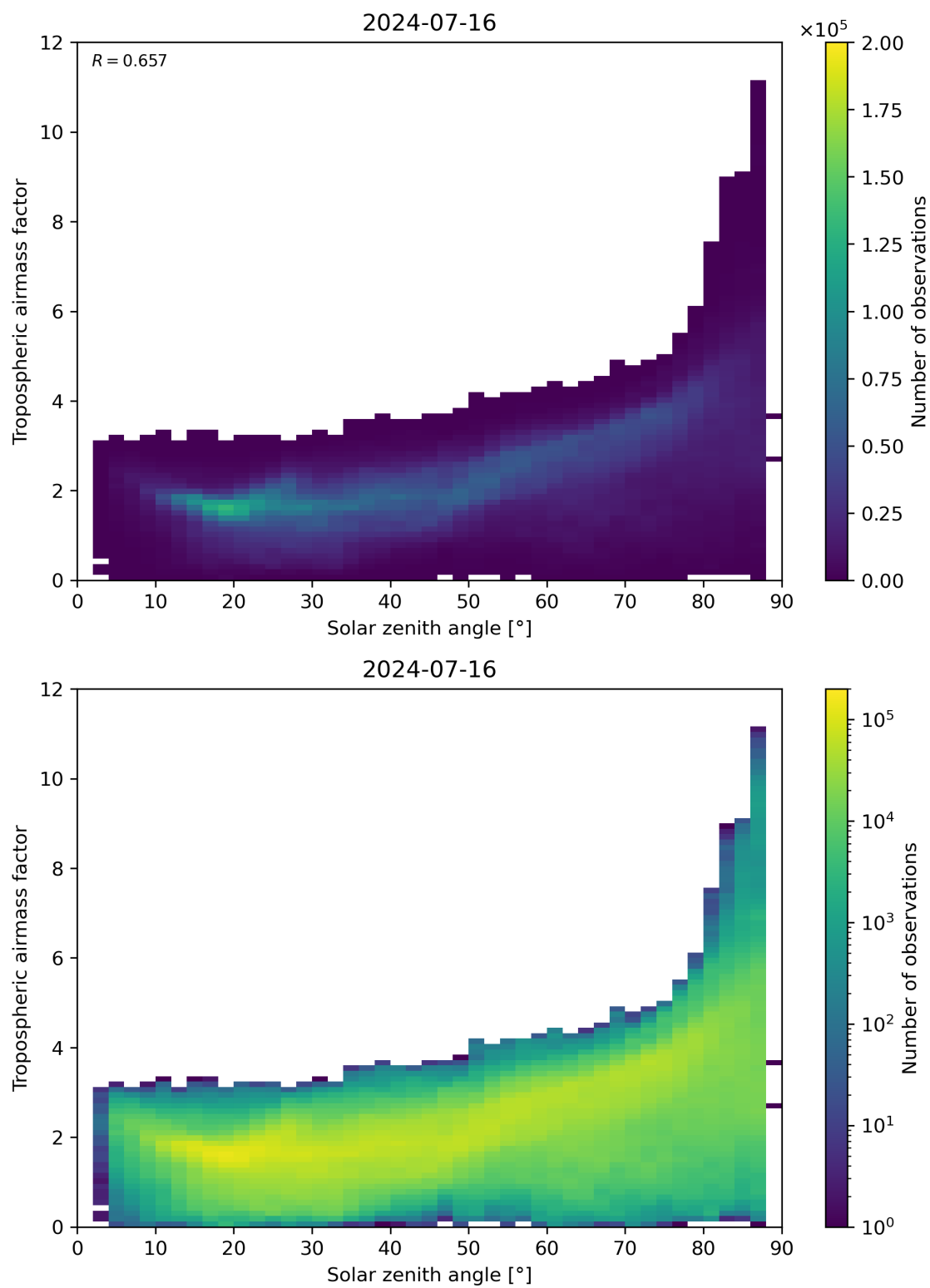
Figure 147: Scatter density plot of “Solar zenith angle” against “Tropospheric airmass factor” for 2024-07-15 to 2024-07-17.
