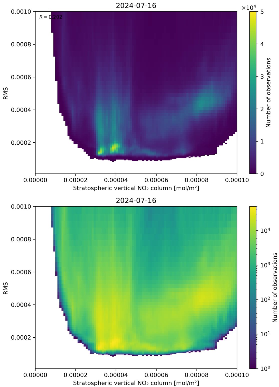
Figure 102: Scatter density plot of “Stratospheric vertical NO 2 column” against “RMS” for 2024-07-15 to 2024-07-17.
