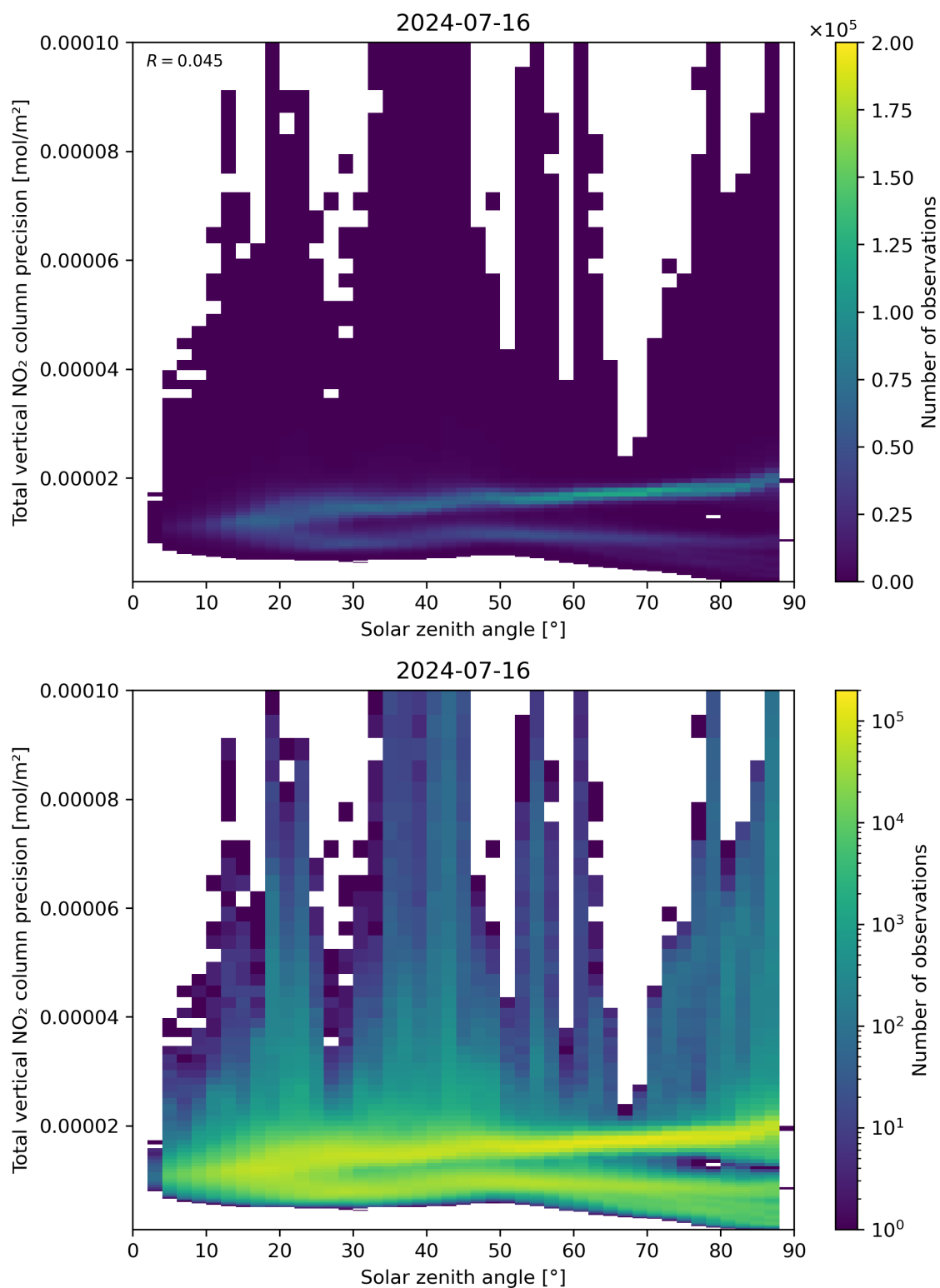
Figure 154: Scatter density plot of “Solar zenith angle” against “Total vertical NO 2 column precision” for 2024-07-15 to 2024-07-17.
