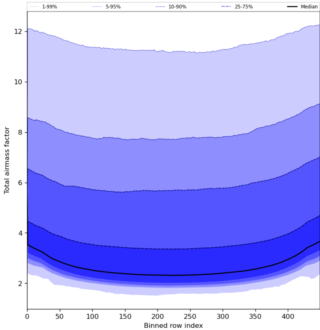
Figure 49: Along track statistics of “Total airmass factor” for 2024-07-15 to 2024-07-17
