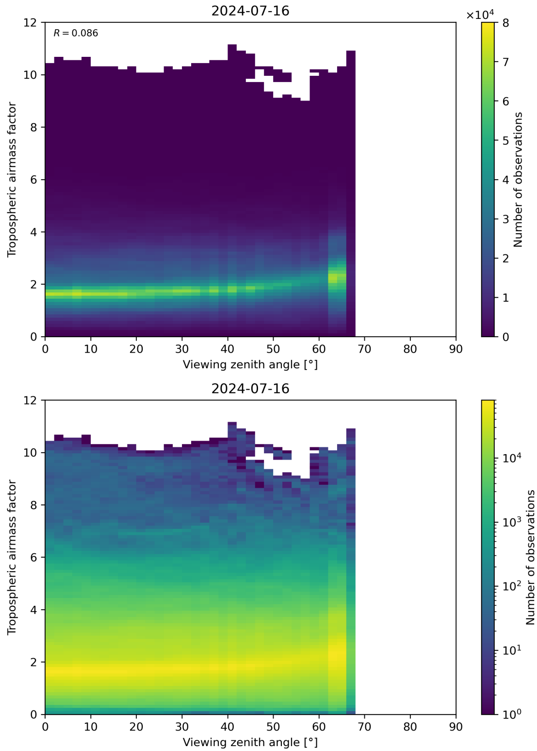
Figure 161: Scatter density plot of “Viewing zenith angle” against “Tropospheric airmass factor” for 2024-07-15 to 2024-07-17.
