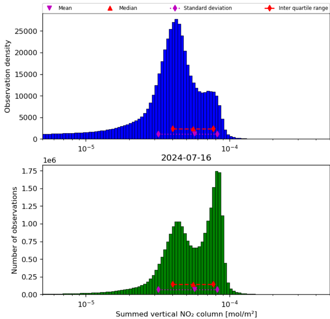
Figure 40: Histogram of “Summed vertical NO 2 column” for 2024-07-15 to 2024-07-17
