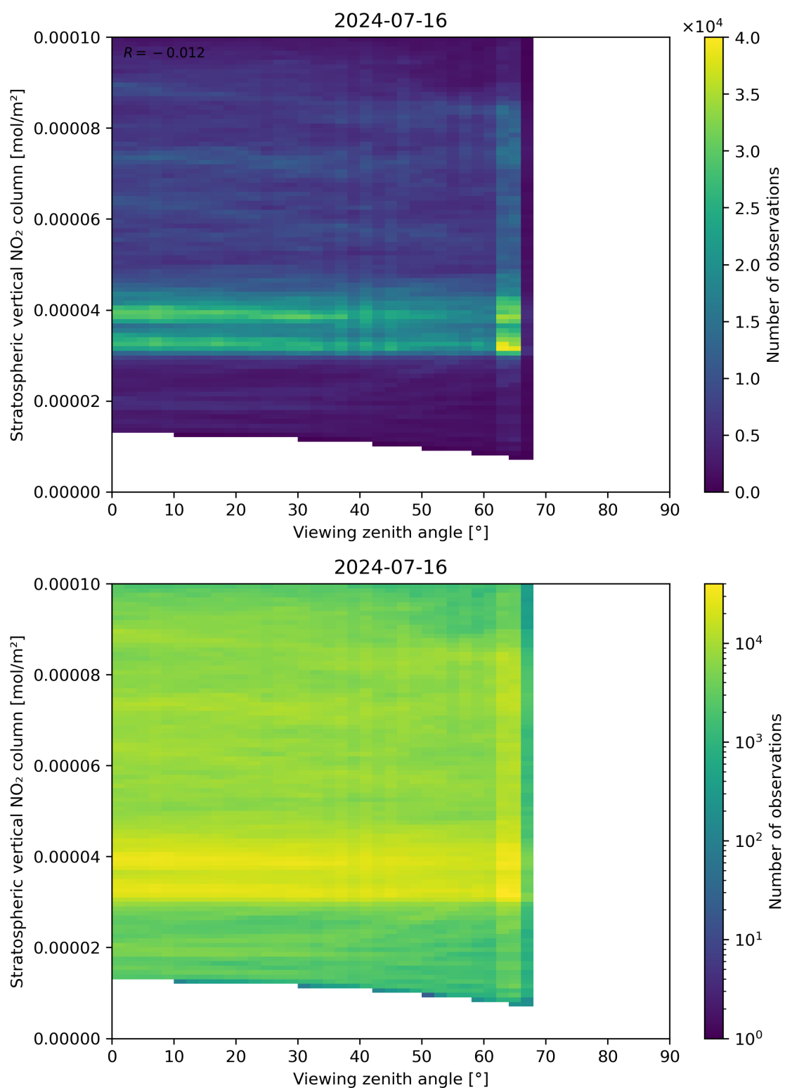
Figure 164: Scatter density plot of “Viewing zenith angle” against “Stratospheric vertical NO 2 column” for 2024-07-15 to 2024-07-17.
