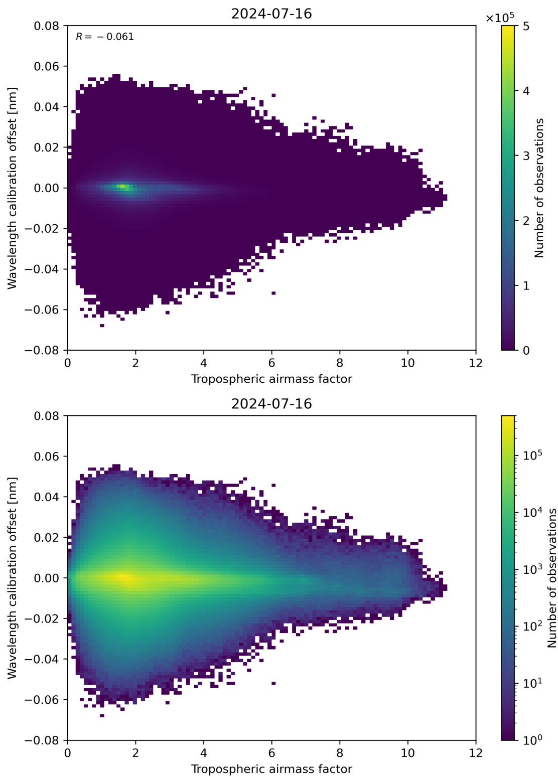
Figure 80: Scatter density plot of “Tropospheric airmass factor” against “Wavelength calibration offset” for 2024-07-15 to 2024-07-17.
