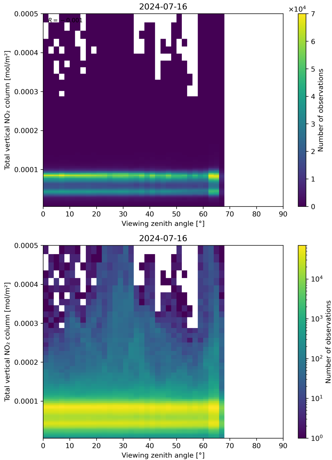
Figure 167: Scatter density plot of “Viewing zenith angle” against “Total vertical NO 2 column” for 2024-07-15 to 2024-07-17.
