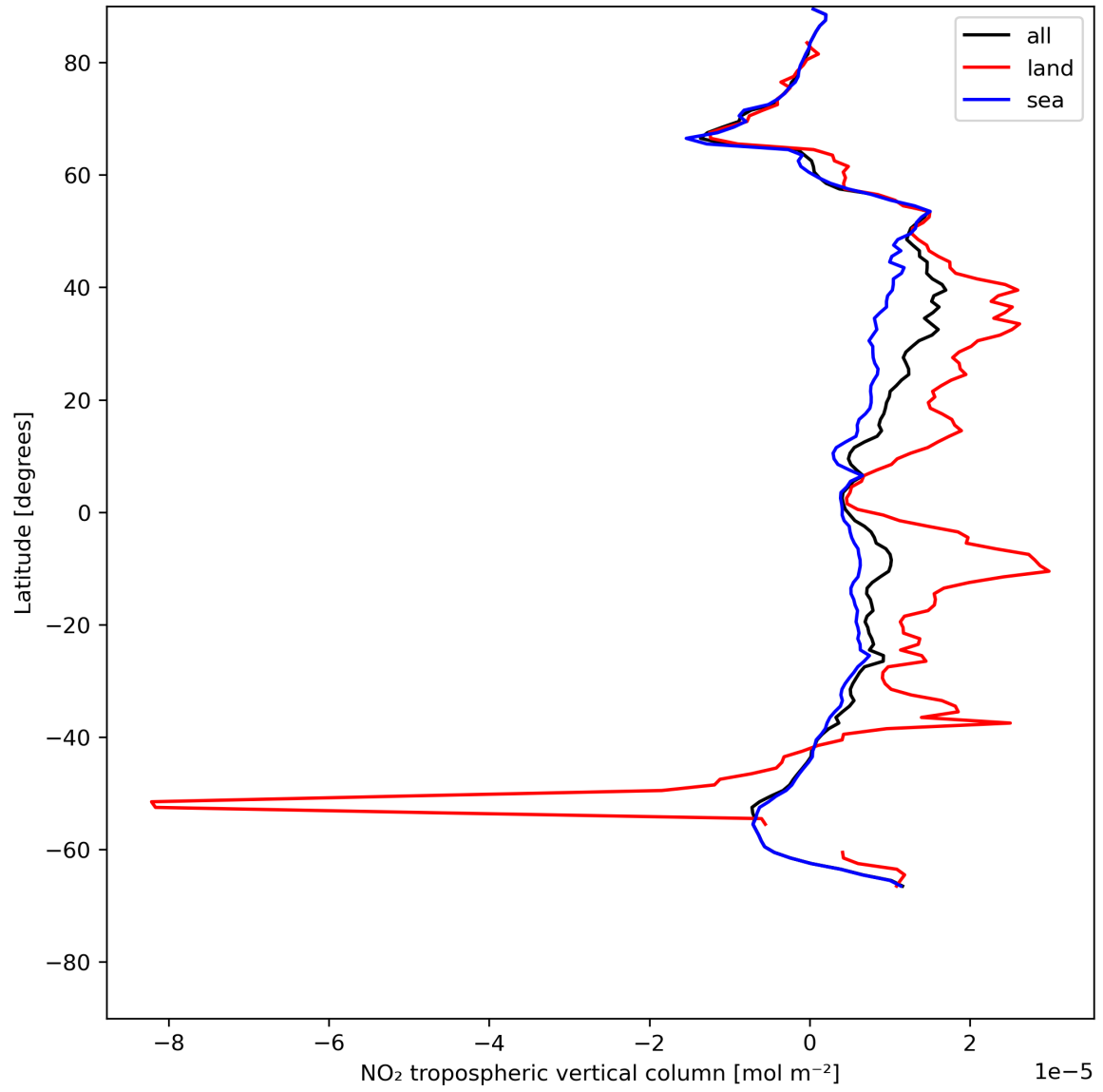
Figure 12: Zonal average of “NO 2 tropospheric vertical column” for 2024-07-15 to 2024-07-17.
