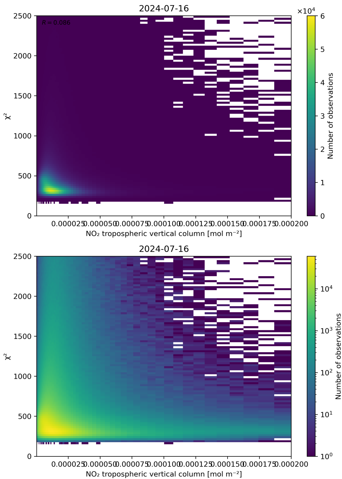
Figure 124: Scatter density plot of “NO 2 tropospheric vertical column” against “ \chi^2 ” for 2024-07-15 to 2024-07-17.
