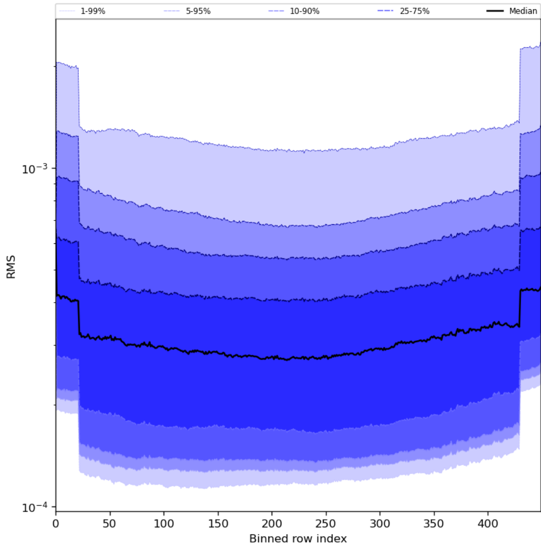
Figure 60: Along track statistics of “RMS” for 2024-07-15 to 2024-07-17
