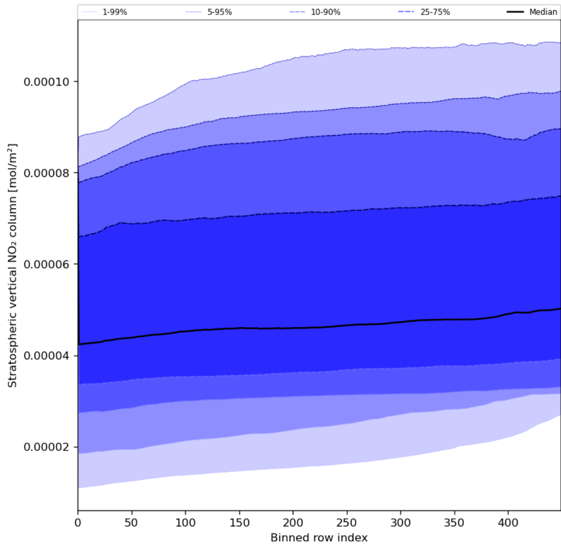
Figure 53: Along track statistics of “Stratospheric vertical NO 2 column” for 2024-07-15 to 2024-07-17
