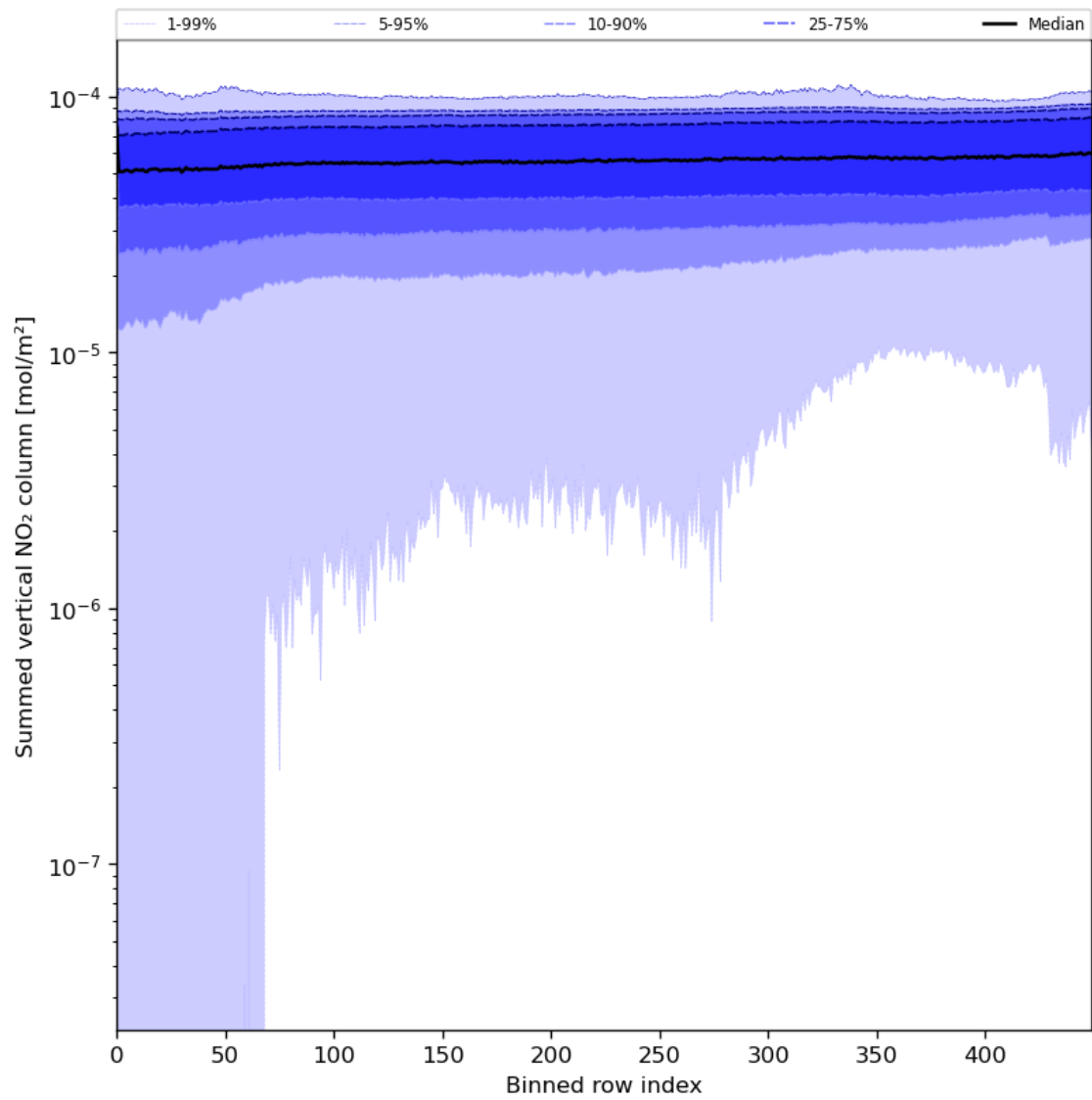
Figure 57: Along track statistics of “Summed vertical NO 2 column” for 2024-07-15 to 2024-07-17
