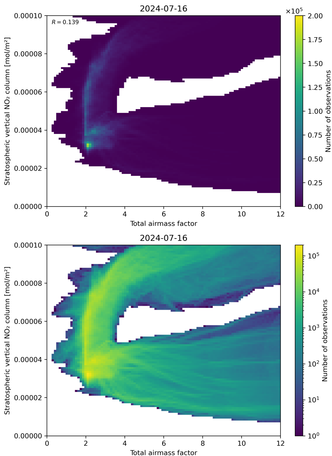
Figure 64: Scatter density plot of “Total airmass factor” against “Stratospheric vertical NO 2 column” for 2024-07-15 to 2024-07-17.
