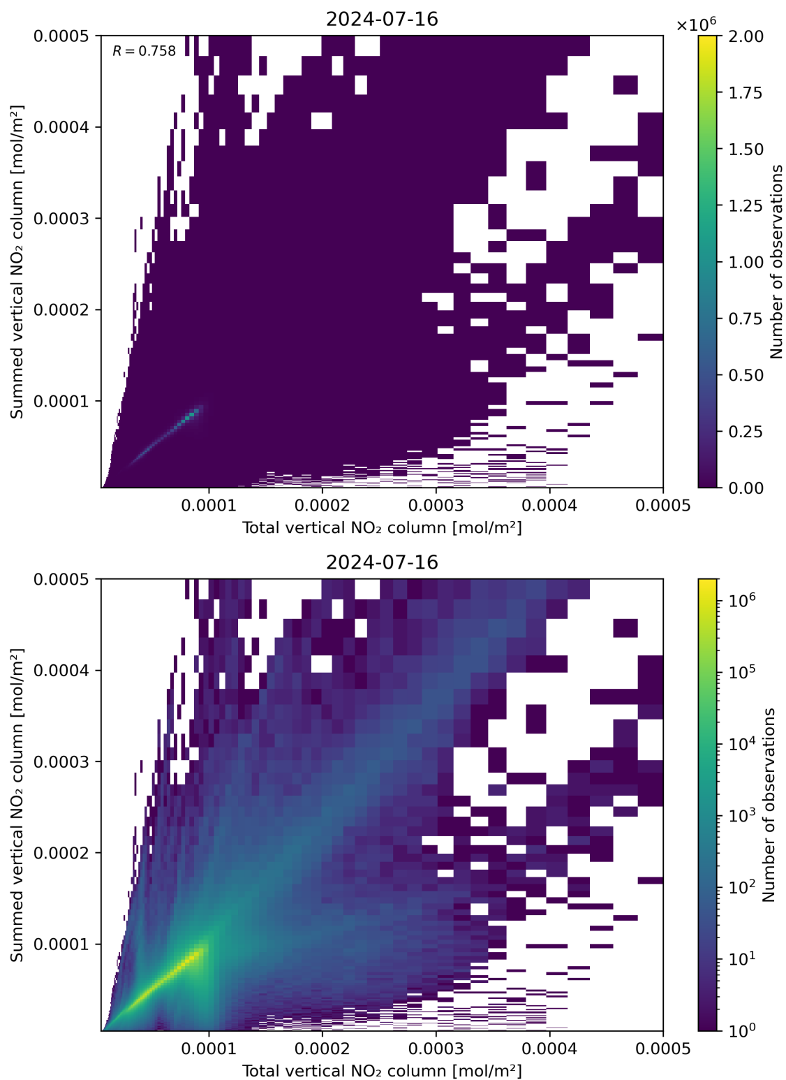
Figure 112: Scatter density plot of “Total vertical NO 2 column” against “Summed vertical NO 2 column” for 2024-07-15 to 2024-07-17.
