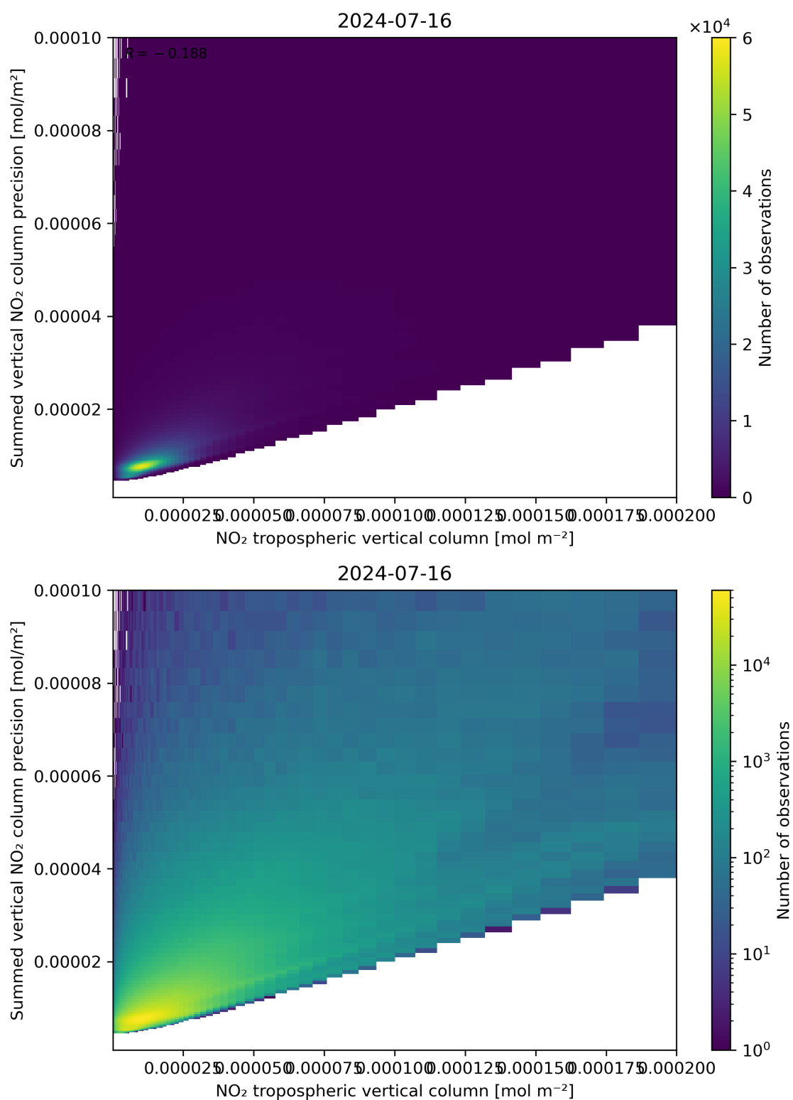
Figure 127: Scatter density plot of “NO 2 tropospheric vertical column” against “Summed vertical NO 2 column precision” for 2024-07-15 to 2024-07-17.
