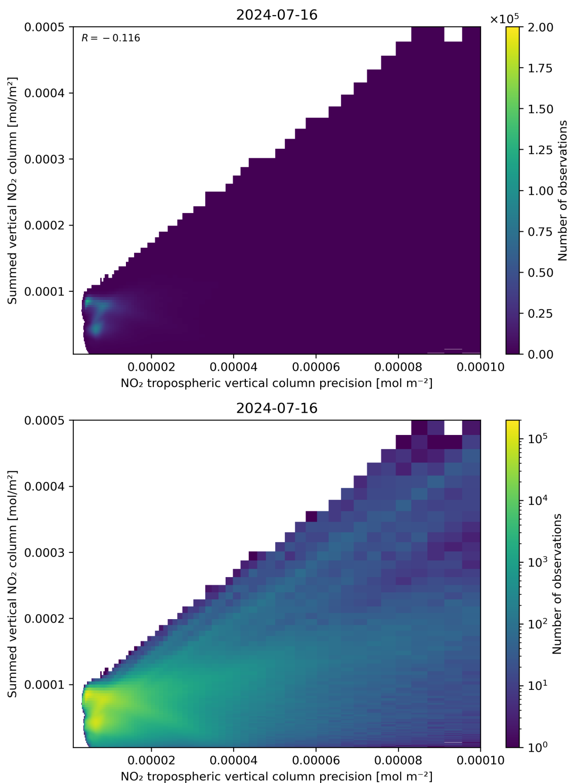
Figure 136: Scatter density plot of “NO 2 tropospheric vertical column precision” against “Summed vertical NO 2 column” for 2024-07-15 to 2024-07-17.
