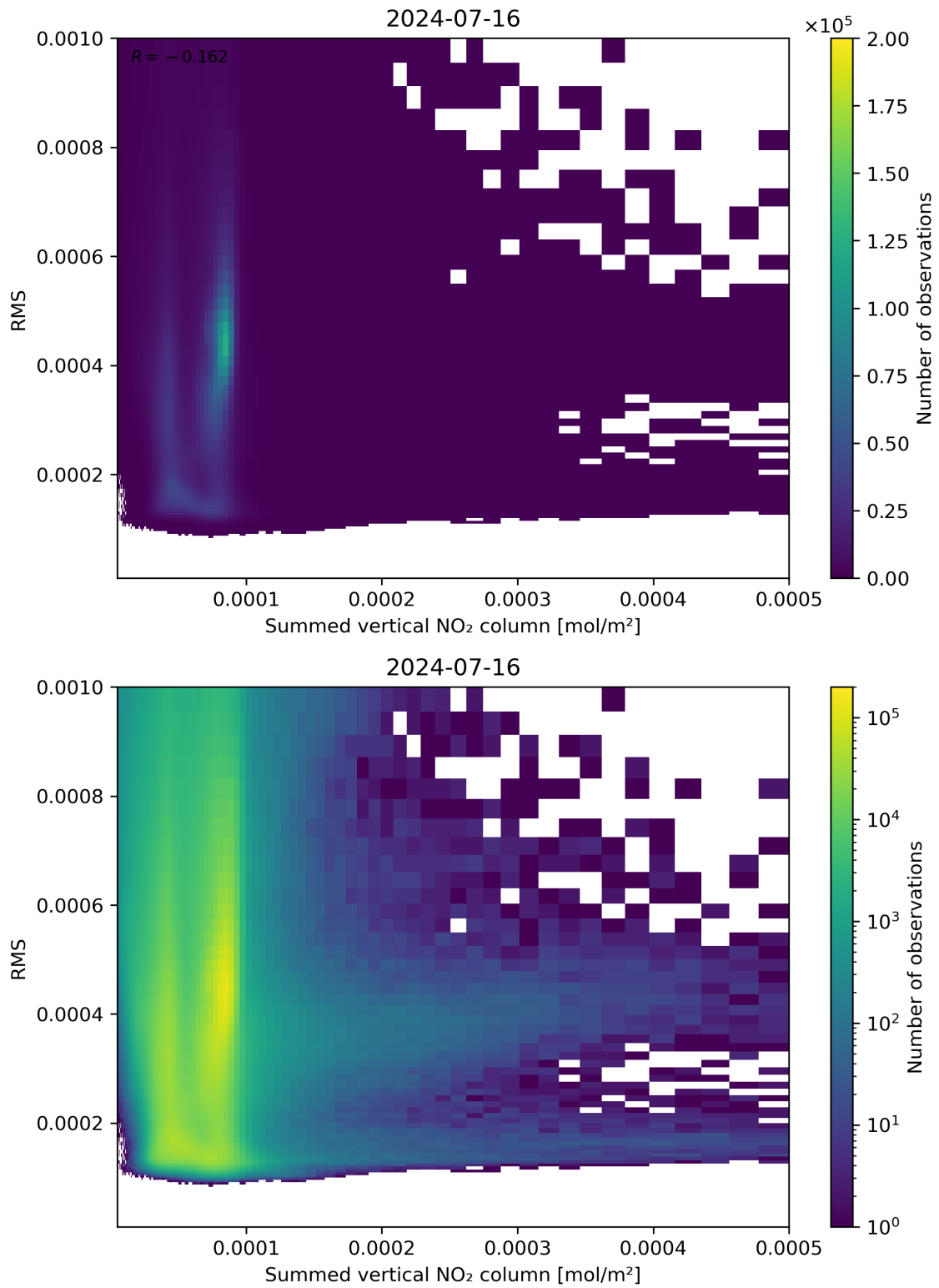
Figure 109: Scatter density plot of “Summed vertical NO 2 column” against “RMS” for 2024-07-15 to 2024-07-17.
