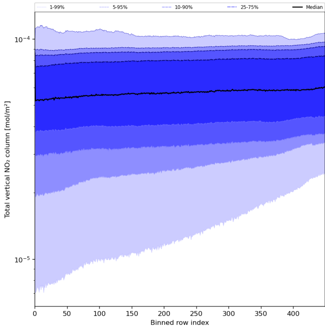
Figure 55: Along track statistics of “Total vertical NO 2 column” for 2024-07-15 to 2024-07-17
