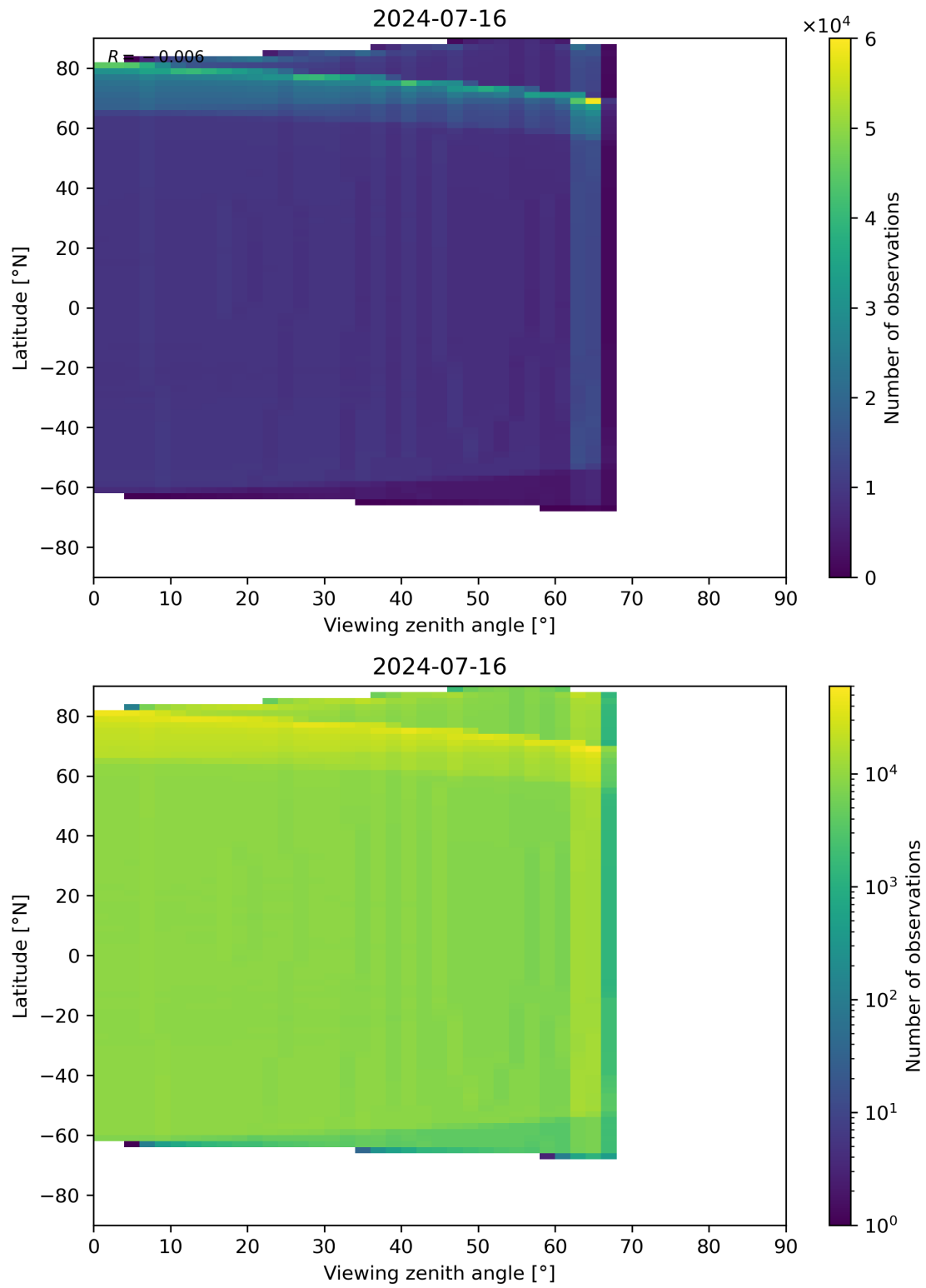
Figure 163: Scatter density plot of “Viewing zenith angle” against “Latitude” for 2024-07-15 to 2024-07-17.
