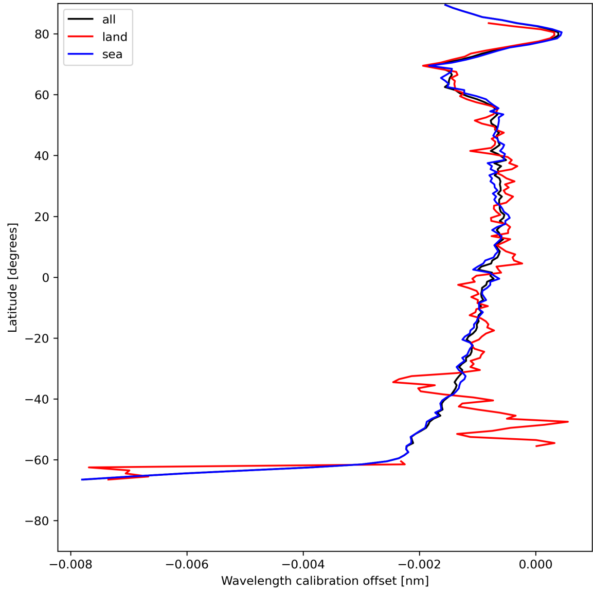
Figure 18: Zonal average of “Wavelength calibration offset” for 2024-07-15 to 2024-07-17.
