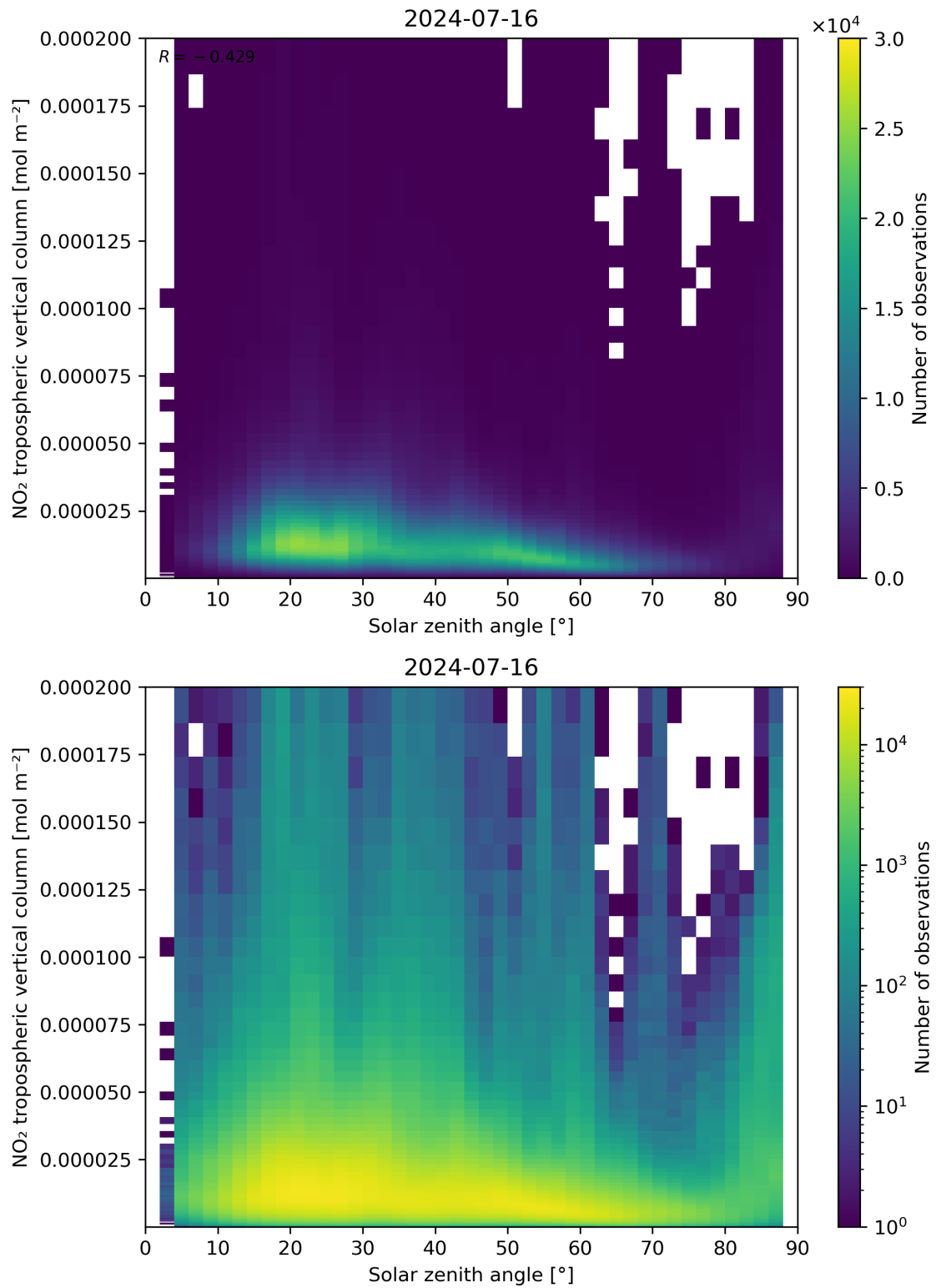
Figure 155: Scatter density plot of “Solar zenith angle” against “NO 2 tropospheric vertical column” for 2024-07-15 to 2024-07-17.
