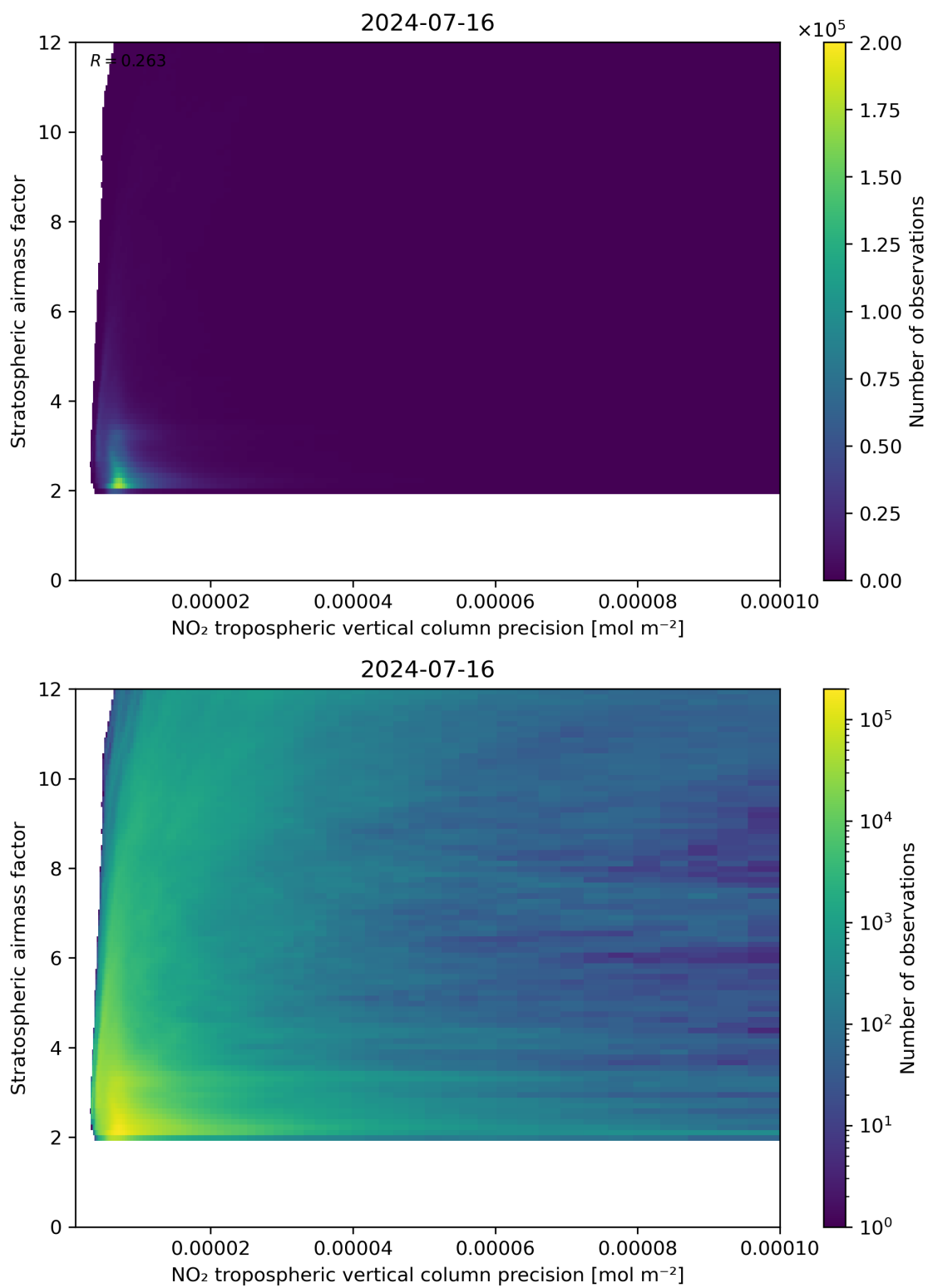
Figure 131: Scatter density plot of “NO 2 tropospheric vertical column precision” against “Stratospheric airmass factor” for 2024-07-15 to 2024-07-17.
