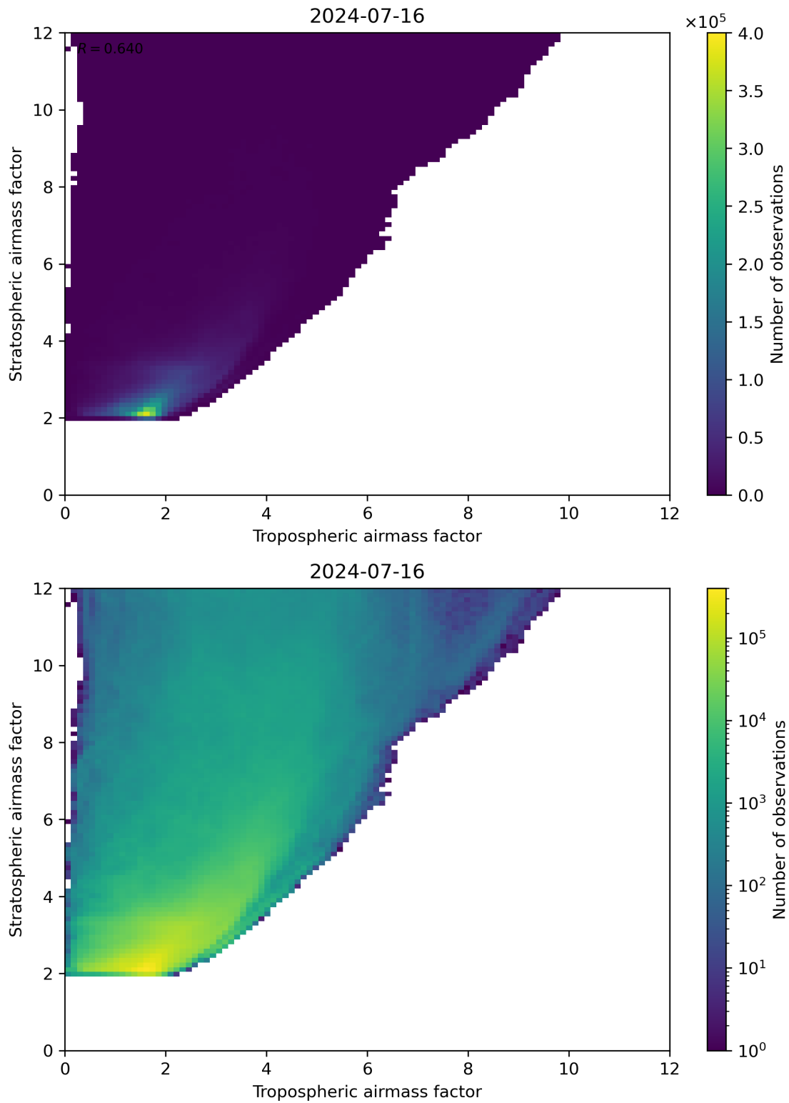
Figure 71: Scatter density plot of “Tropospheric airmass factor” against “Stratospheric airmass factor” for 2024-07-15 to 2024-07-17.
