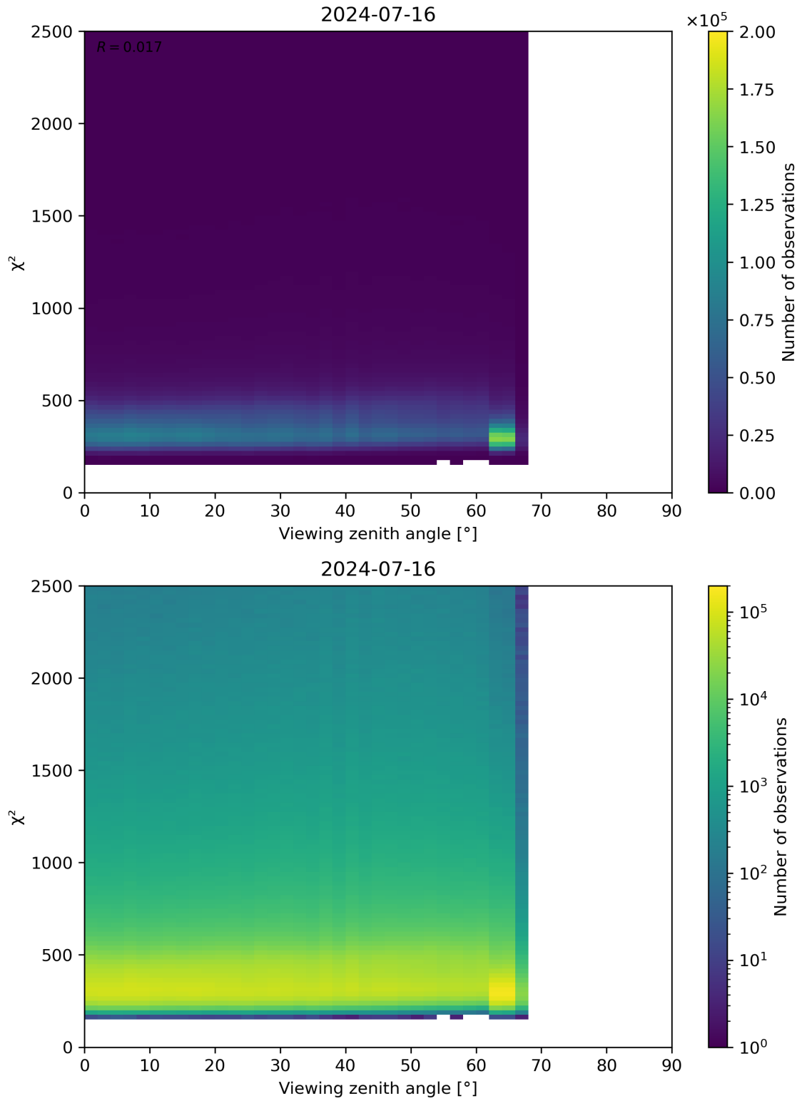
Figure 162: Scatter density plot of “Viewing zenith angle” against “ \chi^2 ” for 2024-07-15 to 2024-07-17.
