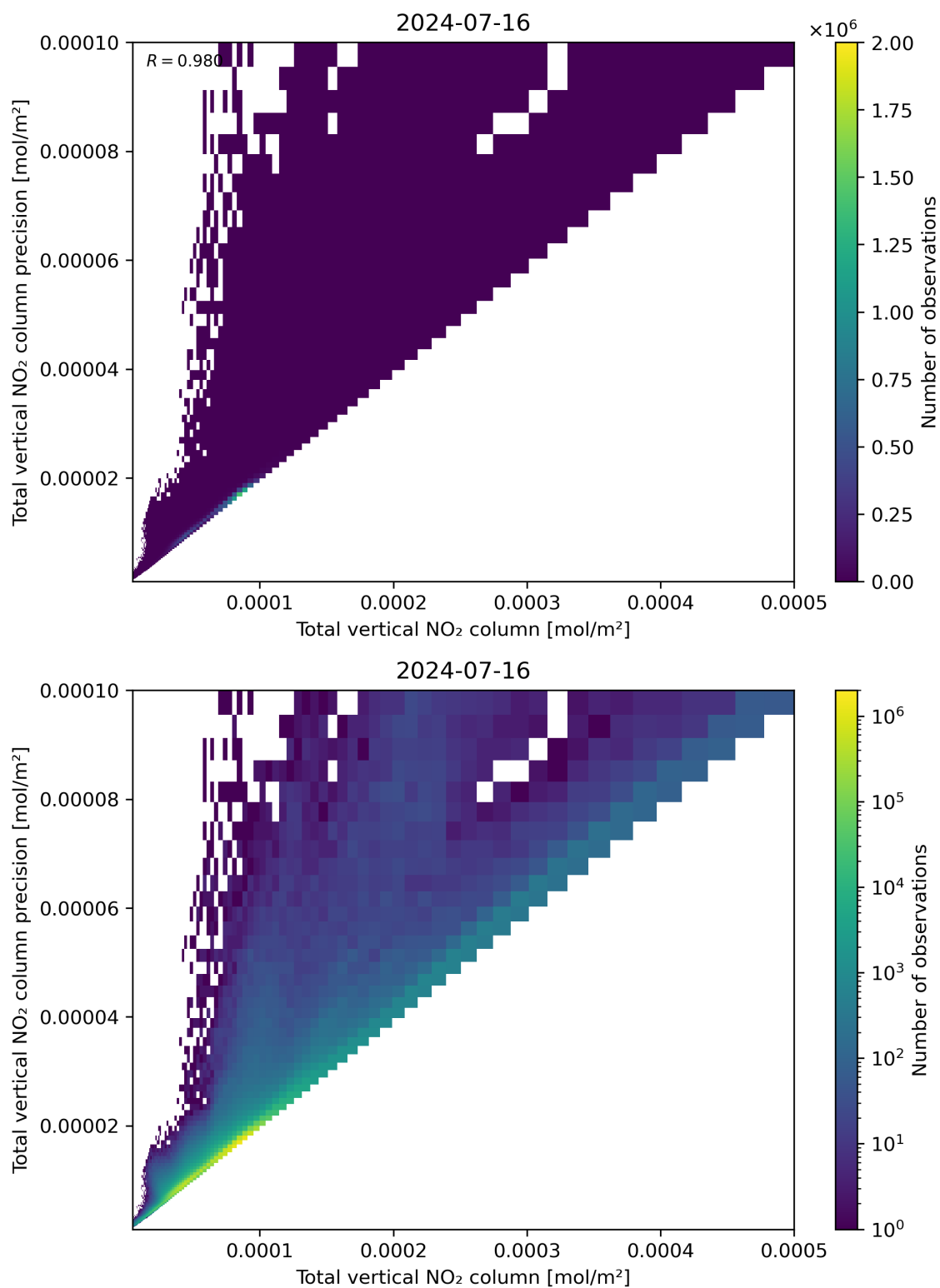
Figure 114: Scatter density plot of “Total vertical NO 2 column” against “Total vertical NO 2 column precision” for 2024-07-15 to 2024-07-17.
