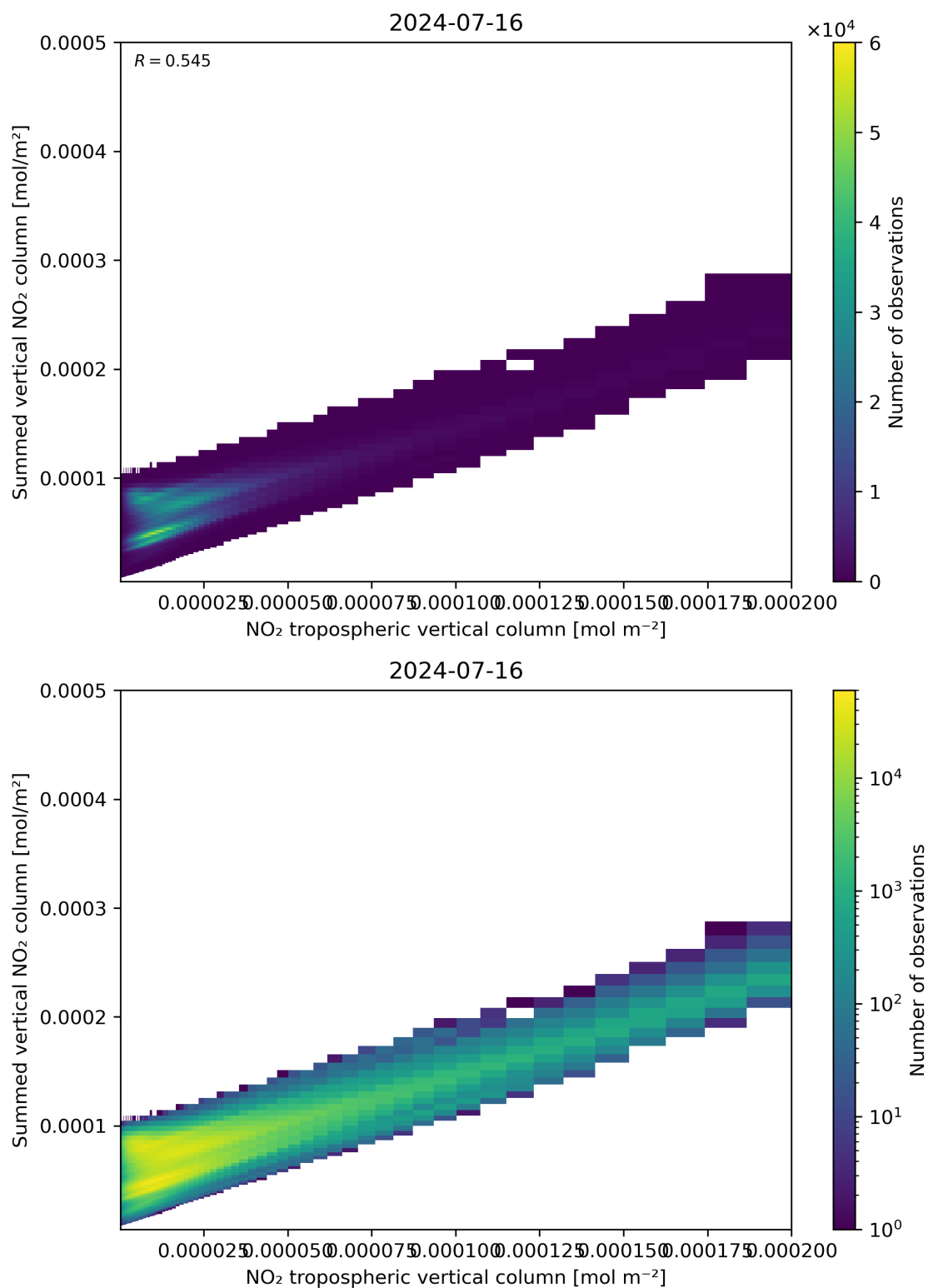
Figure 126: Scatter density plot of “NO 2 tropospheric vertical column” against “Summed vertical NO 2 column” for 2024-07-15 to 2024-07-17.
