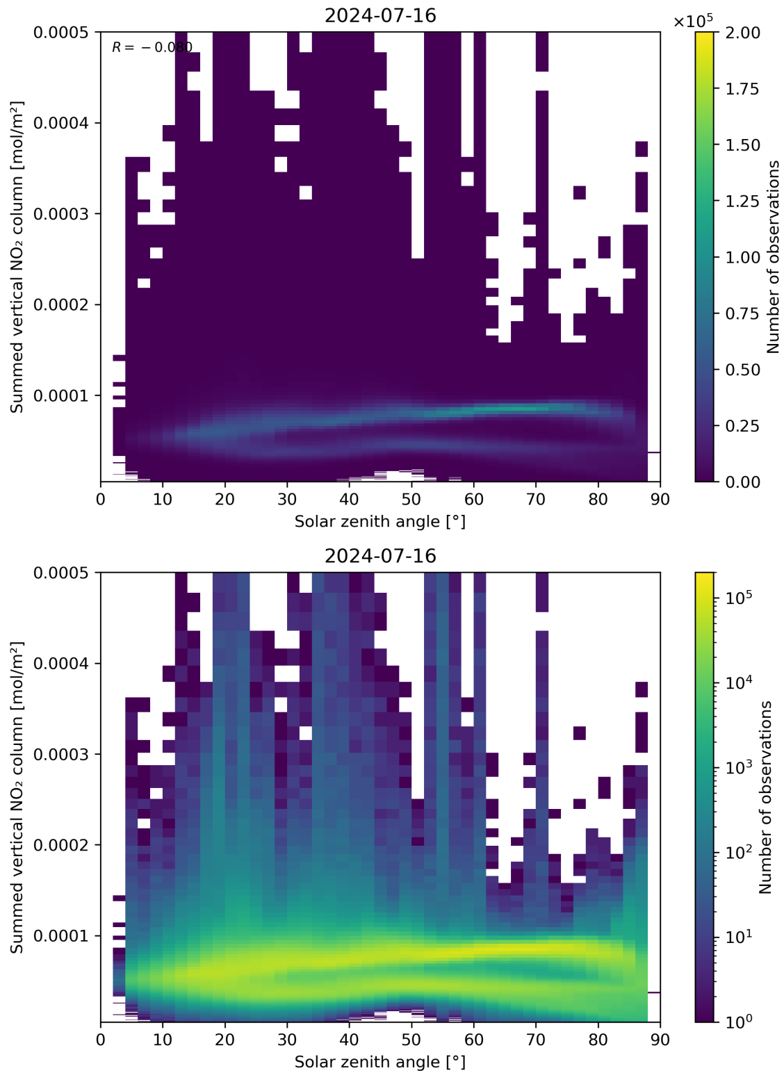
Figure 151: Scatter density plot of “Solar zenith angle” against “Summed vertical NO 2 column” for 2024-07-15 to 2024-07-17.
