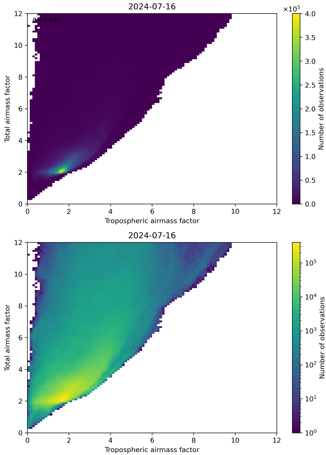
Figure 72: Scatter density plot of “Tropospheric airmass factor” against “Total airmass factor” for 2024-07-15 to 2024-07-17.
