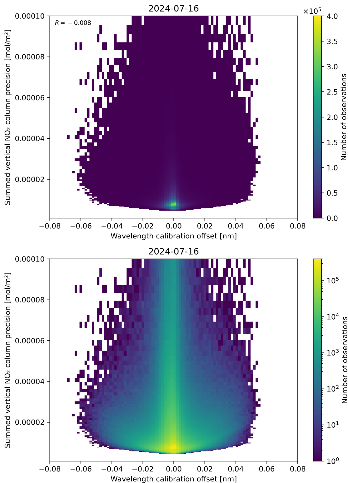
Figure 178: Scatter density plot of “Wavelength calibration offset” against “Summed vertical NO 2 column precision” for 2024-07-15 to 2024-07-17.
