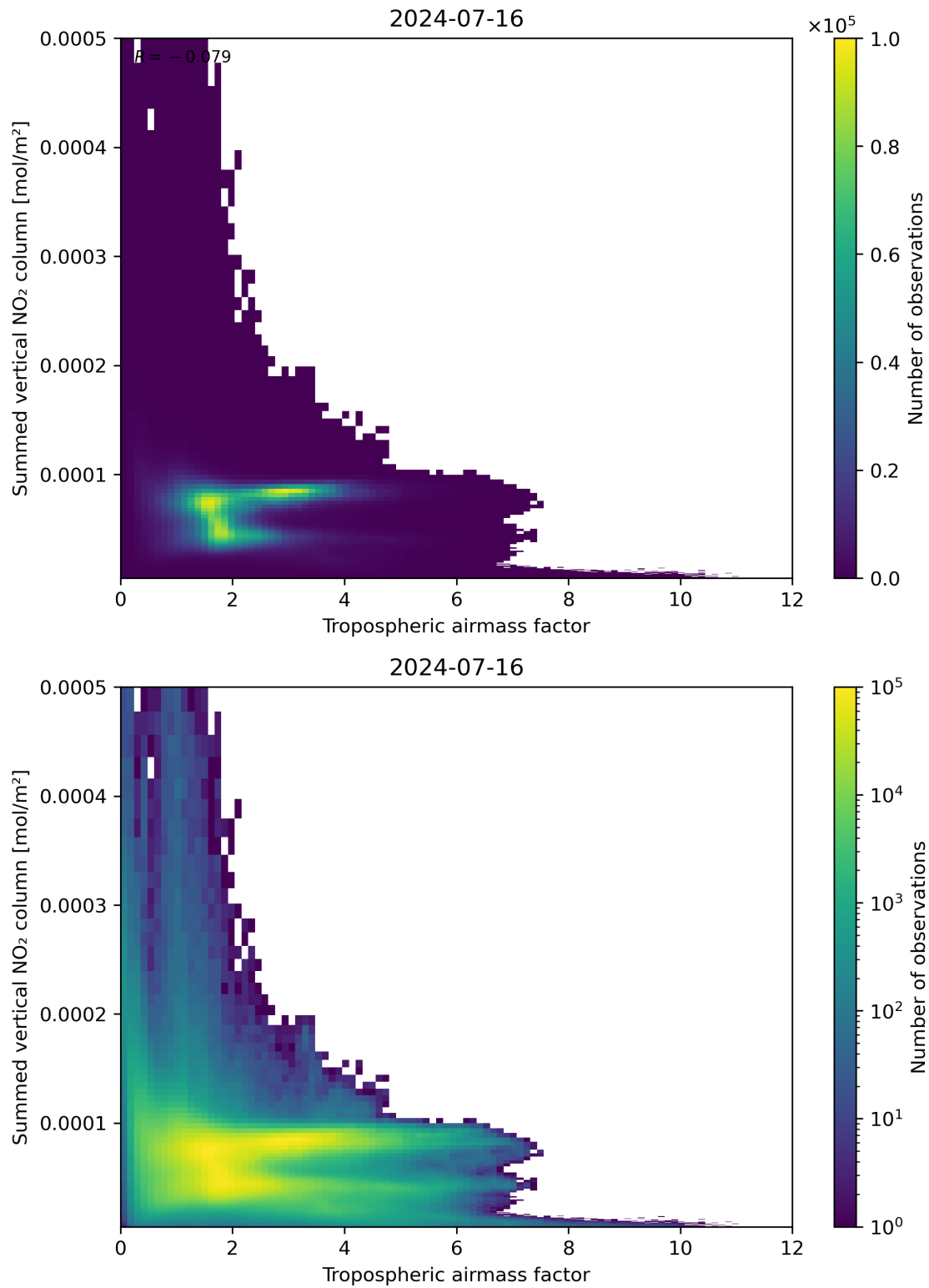
Figure 75: Scatter density plot of “Tropospheric airmass factor” against “Summed vertical NO 2 column” for 2024-07-15 to 2024-07-17.
