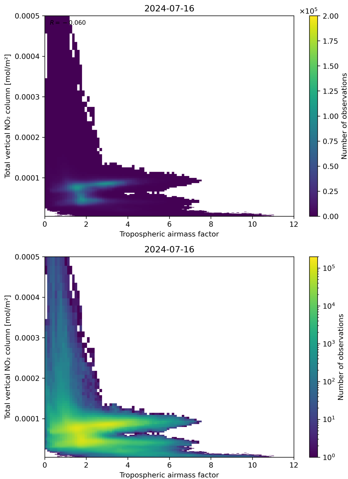
Figure 77: Scatter density plot of “Tropospheric airmass factor” against “Total vertical NO 2 column” for 2024-07-15 to 2024-07-17.
