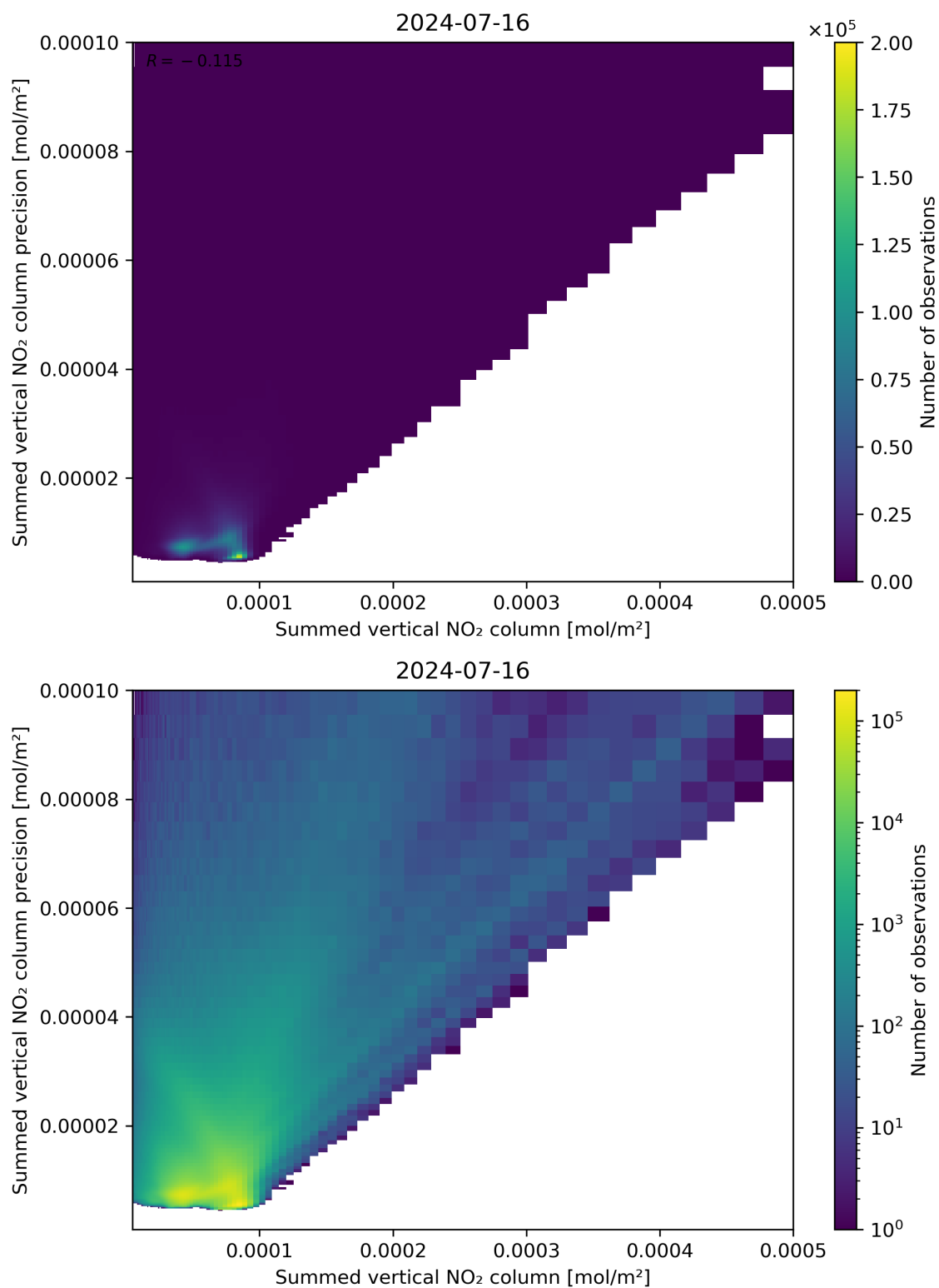
Figure 105: Scatter density plot of “Summed vertical NO 2 column” against “Summed vertical NO 2 column precision” for 2024-07-15 to 2024-07-17.
