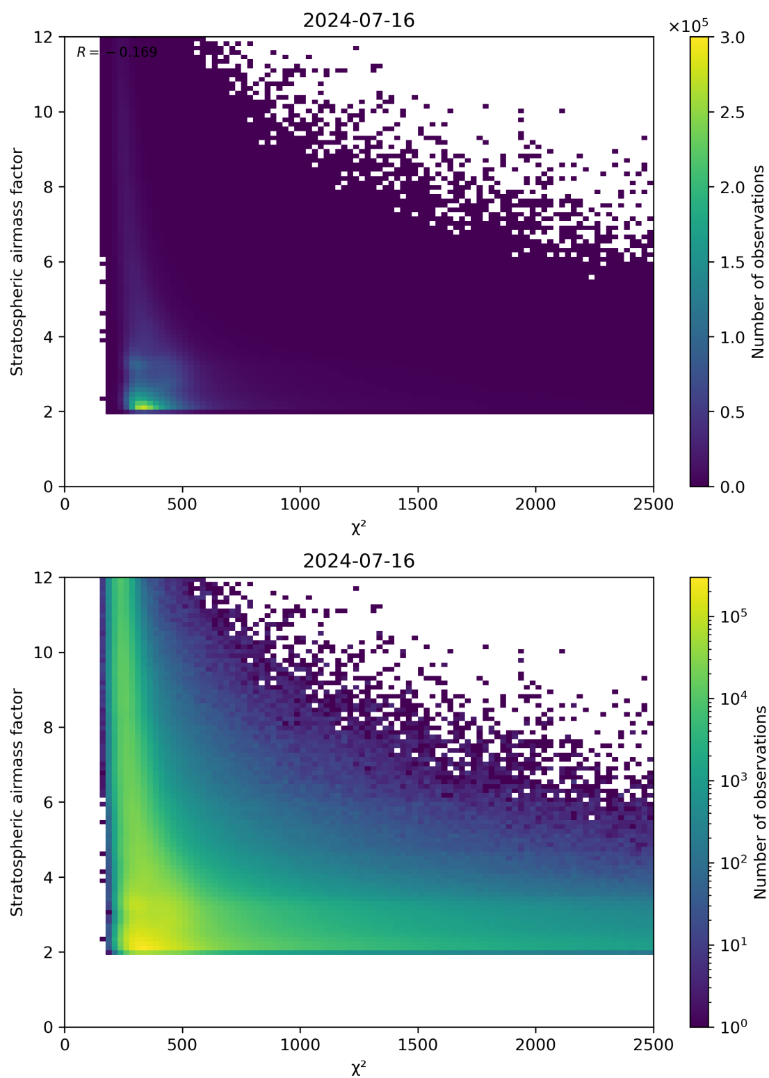
Figure 81: Scatter density plot of “ \chi^2 ” against “Stratospheric airmass factor” for 2024-07-15 to 2024-07-17.
