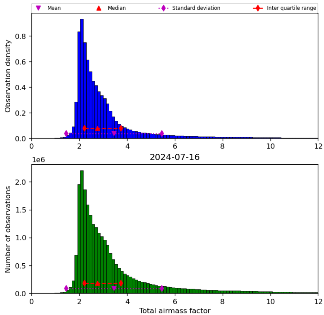
Figure 32: Histogram of “Total airmass factor” for 2024-07-15 to 2024-07-17
