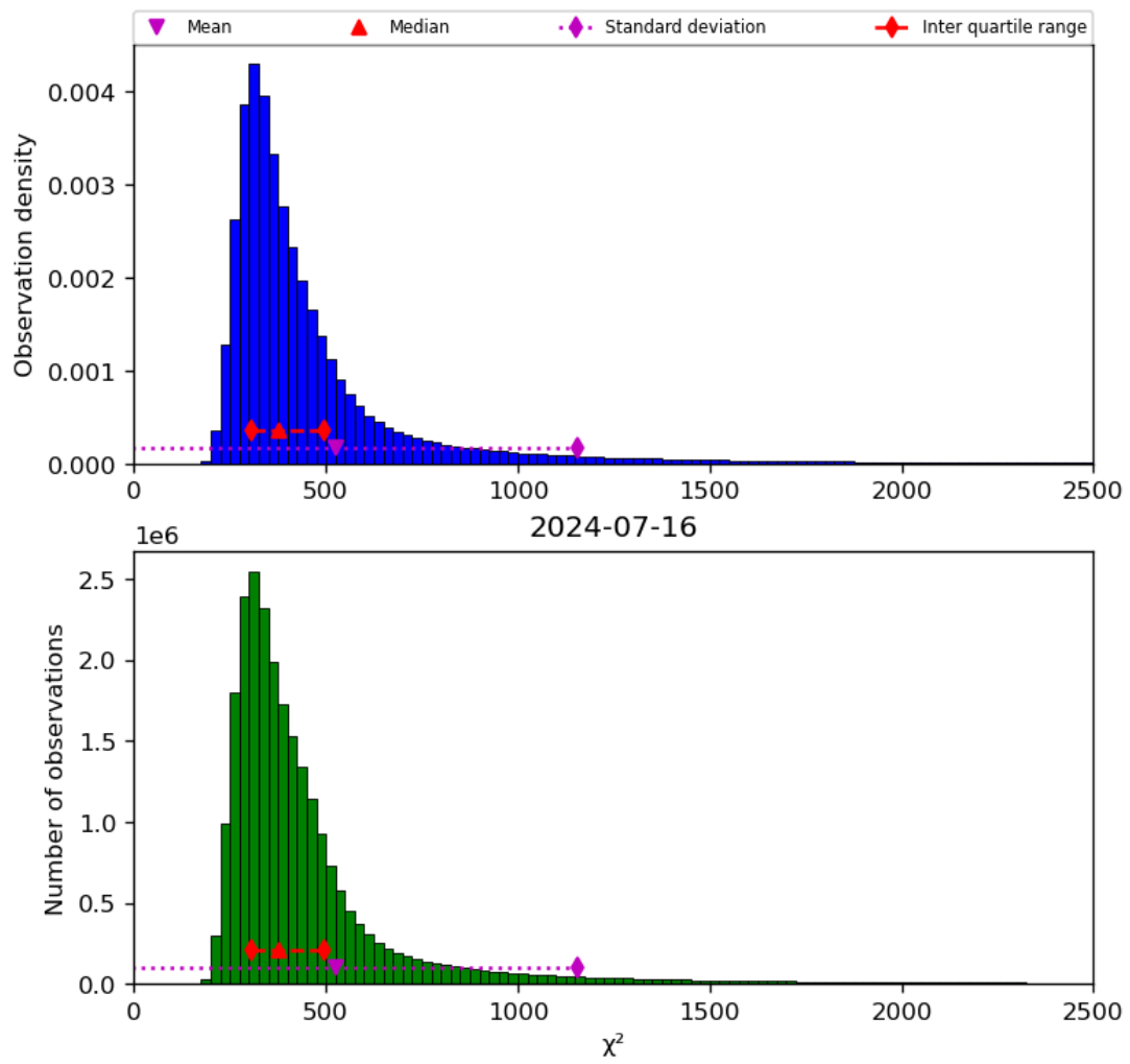
Figure 42: Histogram of " \chi^2 " for 2024-07-15 to 2024-07-17
