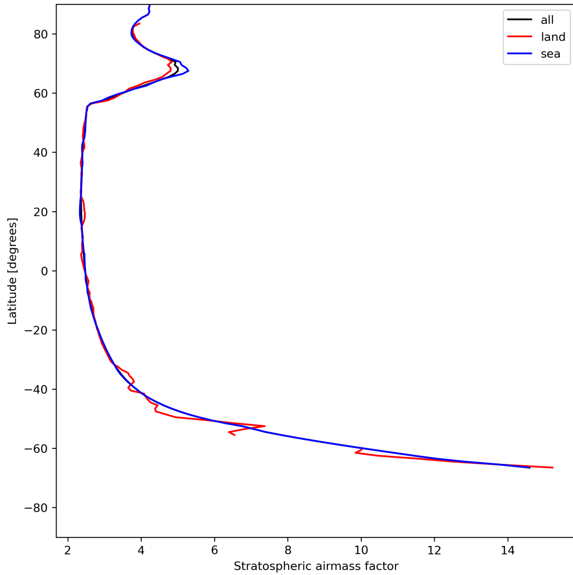
Figure 27: Zonal average of “Stratospheric airmass factor” for 2024-07-15 to 2024-07-17.
