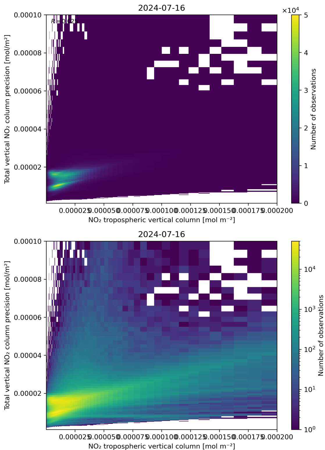
Figure 129: Scatter density plot of “NO 2 tropospheric vertical column” against “Total vertical NO 2 column precision” for 2024-07-15 to 2024-07-17.
