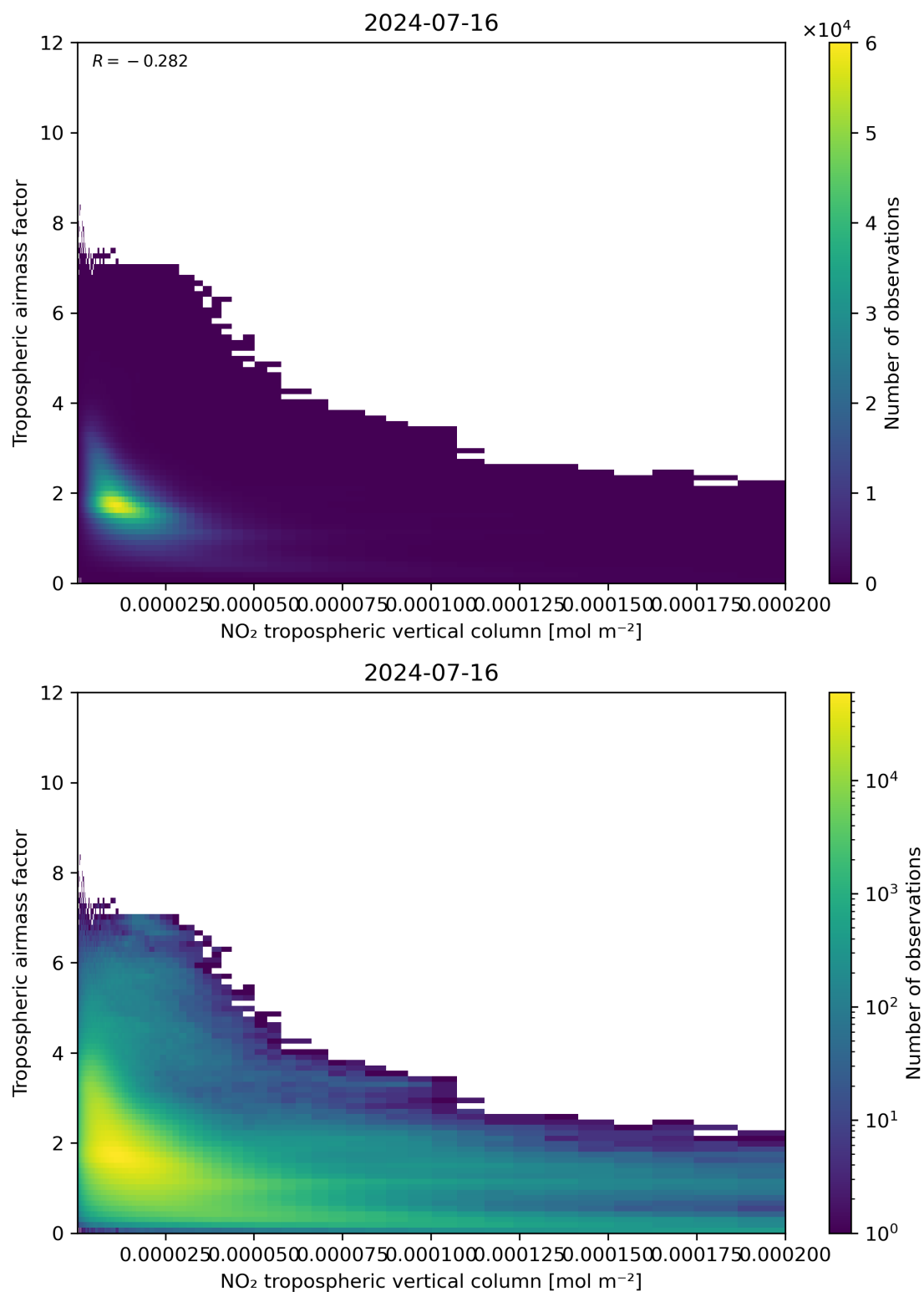
Figure 123: Scatter density plot of “NO 2 tropospheric vertical column” against “Tropospheric airmass factor” for 2024-07-15 to 2024-07-17.
