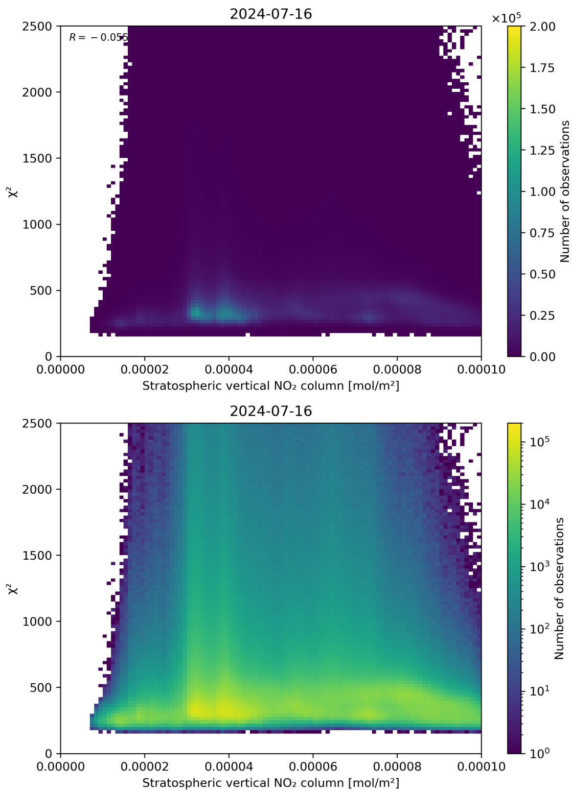
Figure 97: Scatter density plot of “Stratospheric vertical NO 2 column” against “ \chi^2 ” for 2024-07-15 to 2024-07-17.
