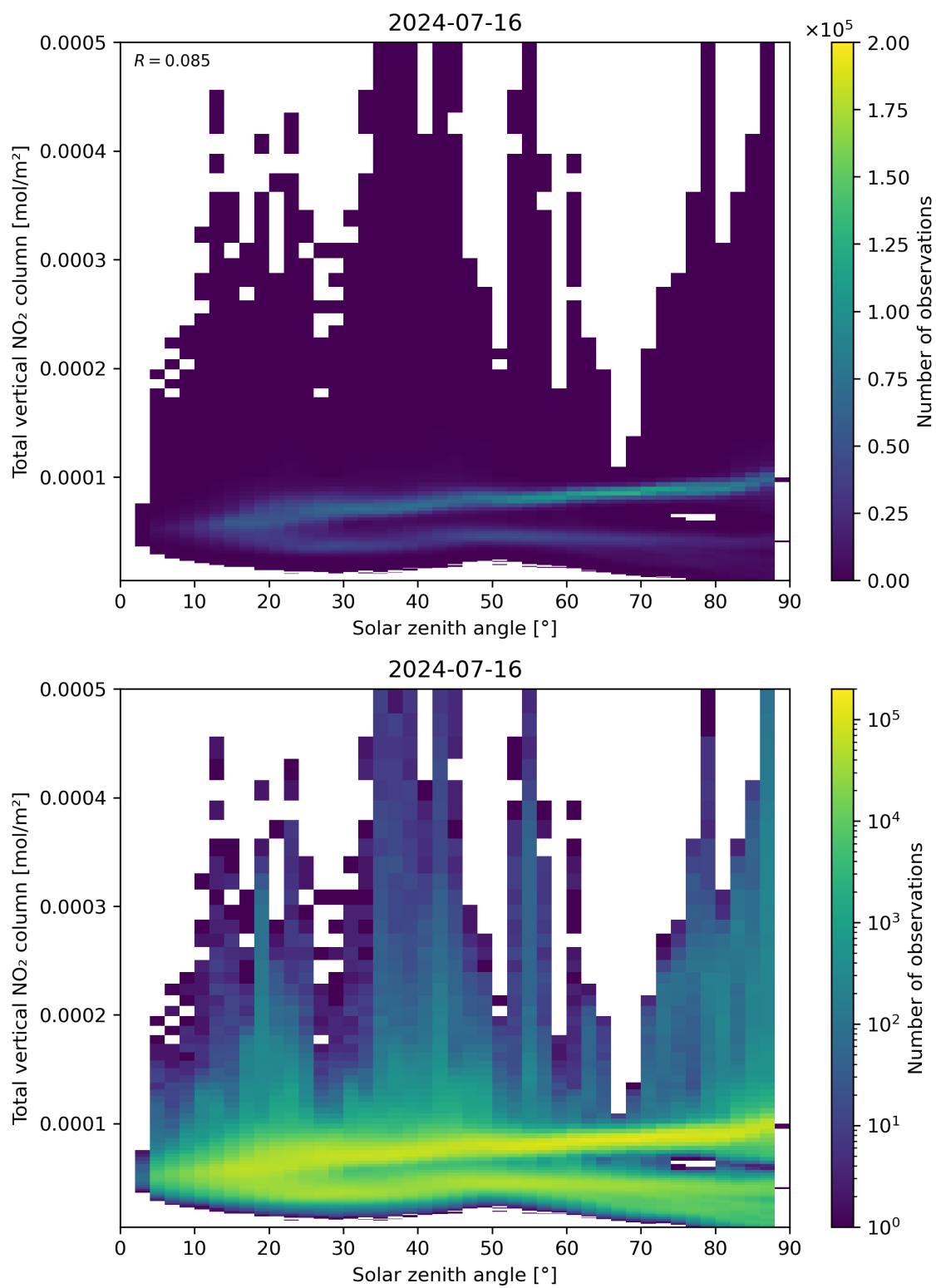
Figure 153: Scatter density plot of “Solar zenith angle” against “Total vertical \text{NO}_2 column” for 2024-07-15 to 2024-07-17.
