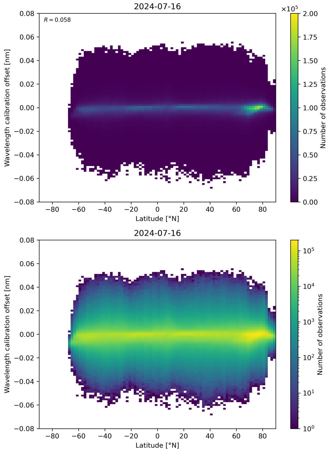
Figure 95: Scatter density plot of “Latitude” against “Wavelength calibration offset” for 2024-07-15 to 2024-07-17.
