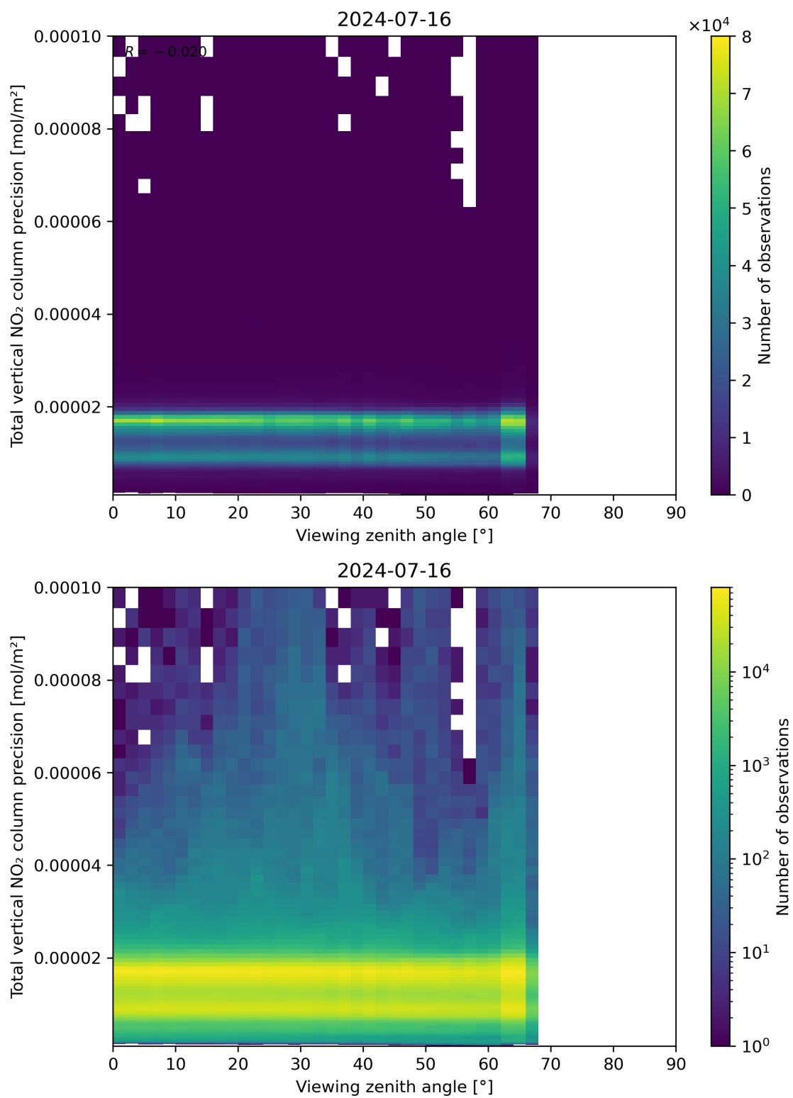
Figure 168: Scatter density plot of “Viewing zenith angle” against “Total vertical NO 2 column precision” for 2024-07-15 to 2024-07-17.
