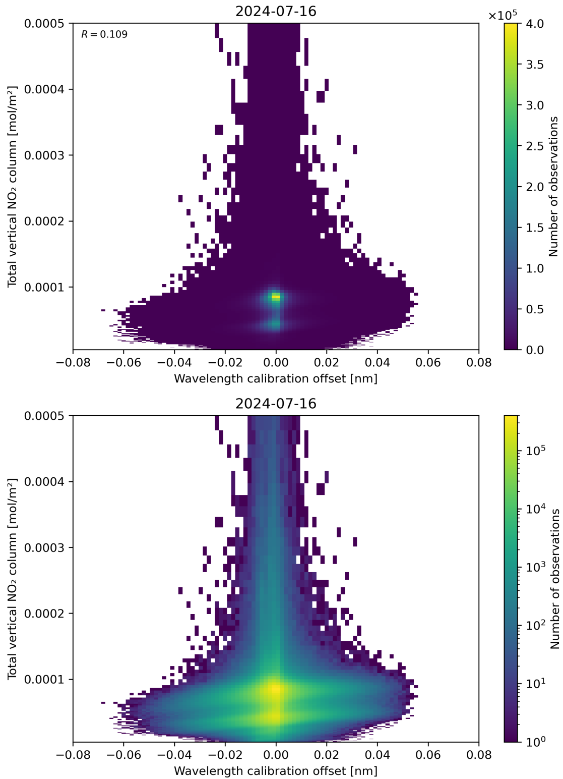
Figure 179: Scatter density plot of “Wavelength calibration offset” against “Total vertical NO 2 column” for 2024-07-15 to 2024-07-17.
