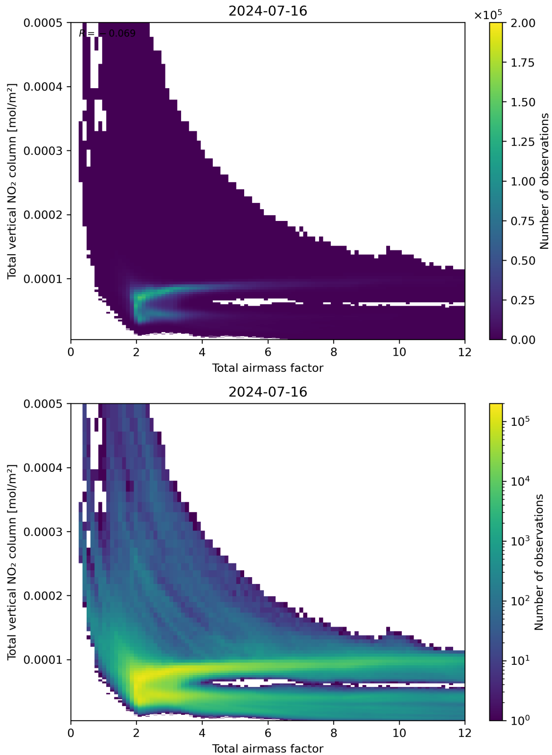
Figure 67: Scatter density plot of “Total airmass factor” against “Total vertical NO 2 column” for 2024-07-15 to 2024-07-17.
