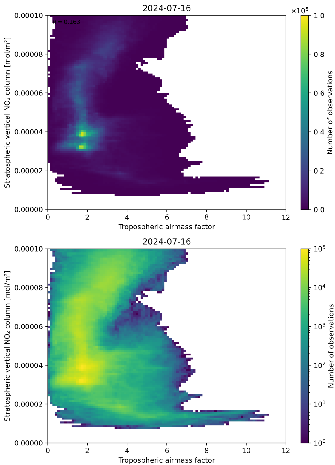
Figure 74: Scatter density plot of “Tropospheric air mass factor” against “Stratospheric vertical NO 2 column” for 2024-07-15 to 2024-07-17.
