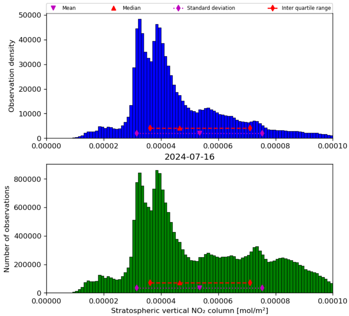
Figure 36: Histogram of “Stratospheric vertical NO 2 column” for 2024-07-15 to 2024-07-17
