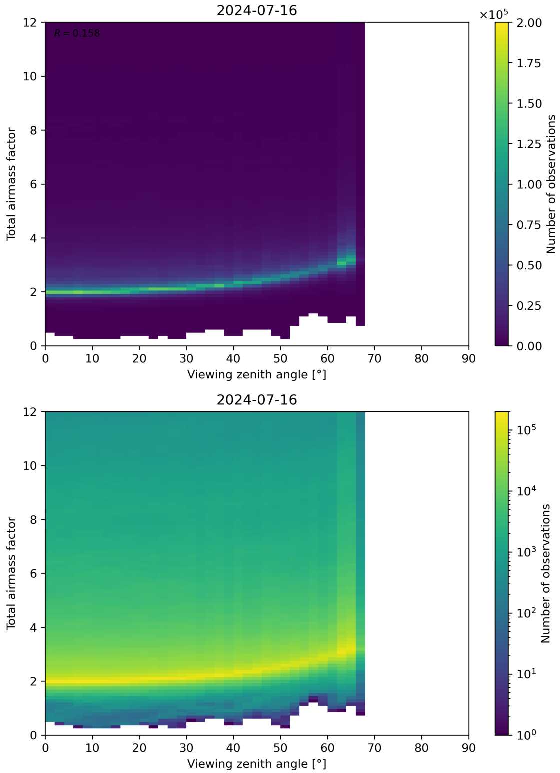
Figure 160: Scatter density plot of “Viewing zenith angle” against “Total airmass factor” for 2024-07-15 to 2024-07-17.
