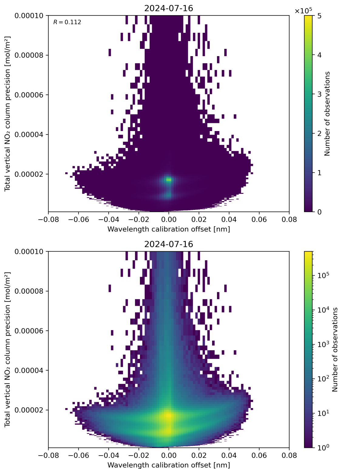
Figure 180: Scatter density plot of “Wavelength calibration offset” against “Total vertical NO 2 column precision” for 2024-07-15 to 2024-07-17.
