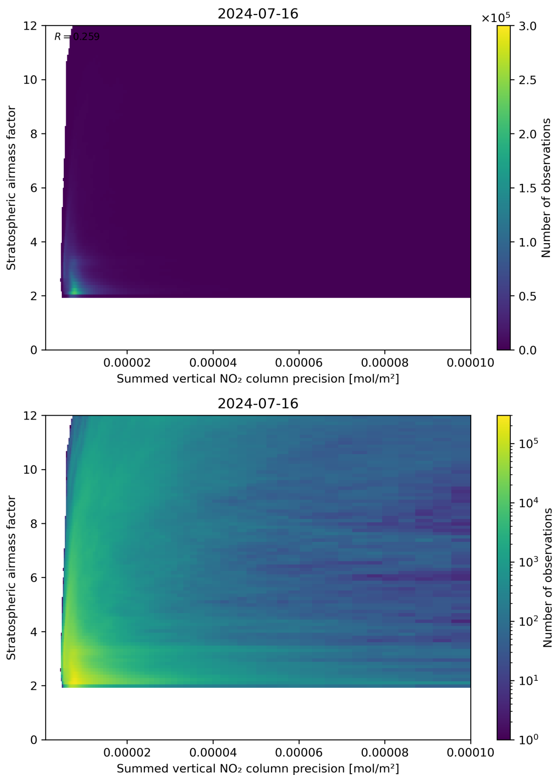
Figure 106: Scatter density plot of “Summed vertical NO 2 column precision” against “Stratospheric airmass factor” for 2024-07-15 to 2024-07-17.
