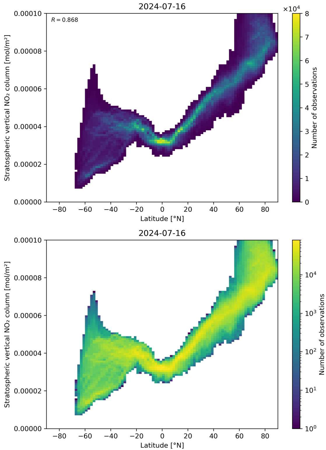
Figure 87: Scatter density plot of “Latitude” against “Stratospheric vertical NO 2 column” for 2024-07-15 to 2024-07-17.
