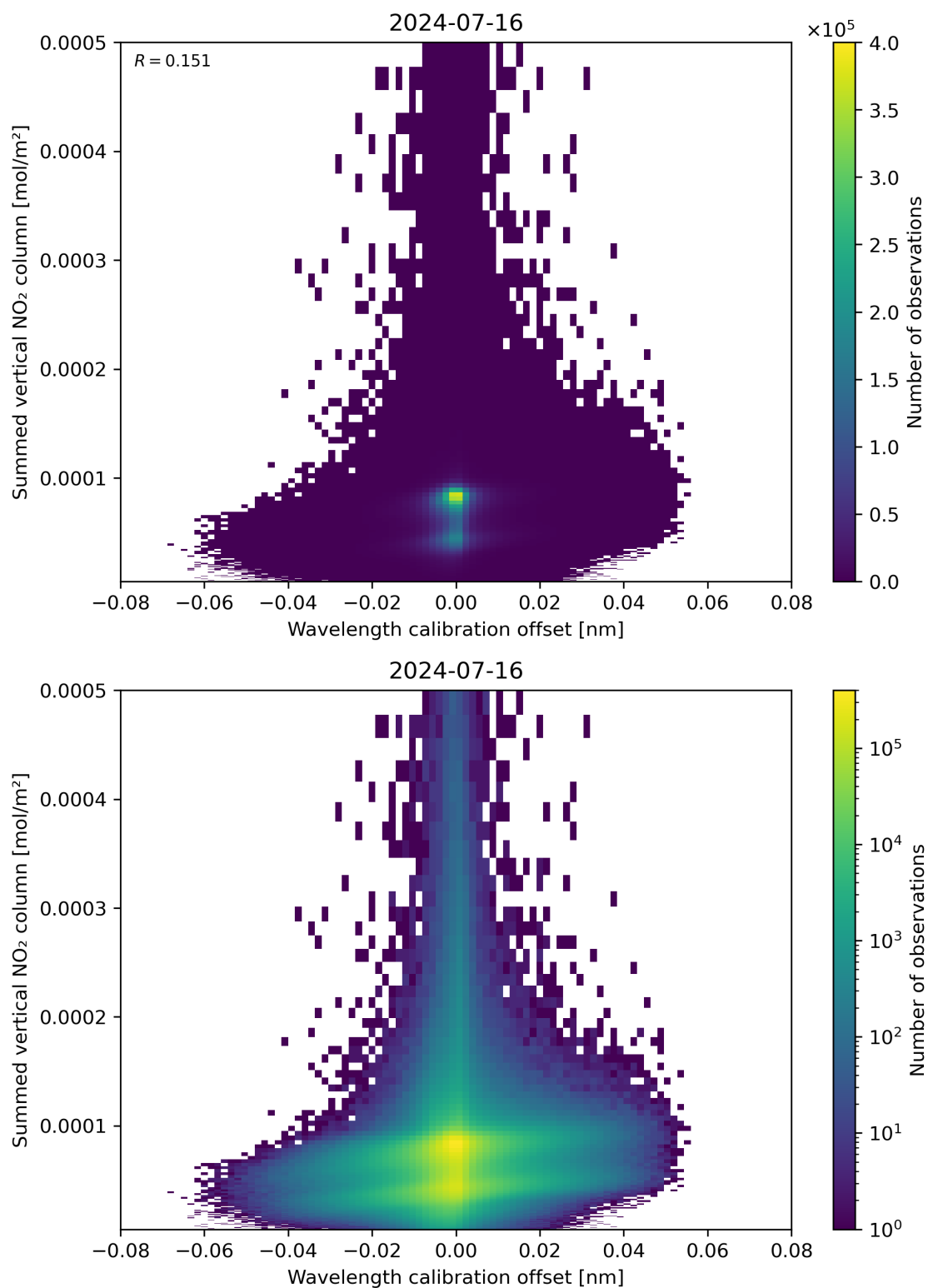
Figure 177: Scatter density plot of “Wavelength calibration offset” against “Summed vertical NO 2 column” for 2024-07-15 to 2024-07-17.
