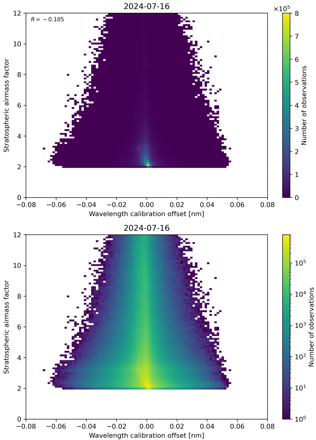
Figure 174: Scatter density plot of “Wavelength calibration offset” against “Stratospheric airmass factor” for 2024-07-15 to 2024-07-17.
