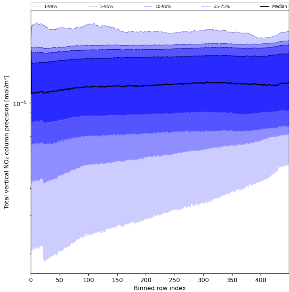
Figure 56: Along track statistics of “Total vertical NO 2 column precision” for 2024-07-15 to 2024-07-17
