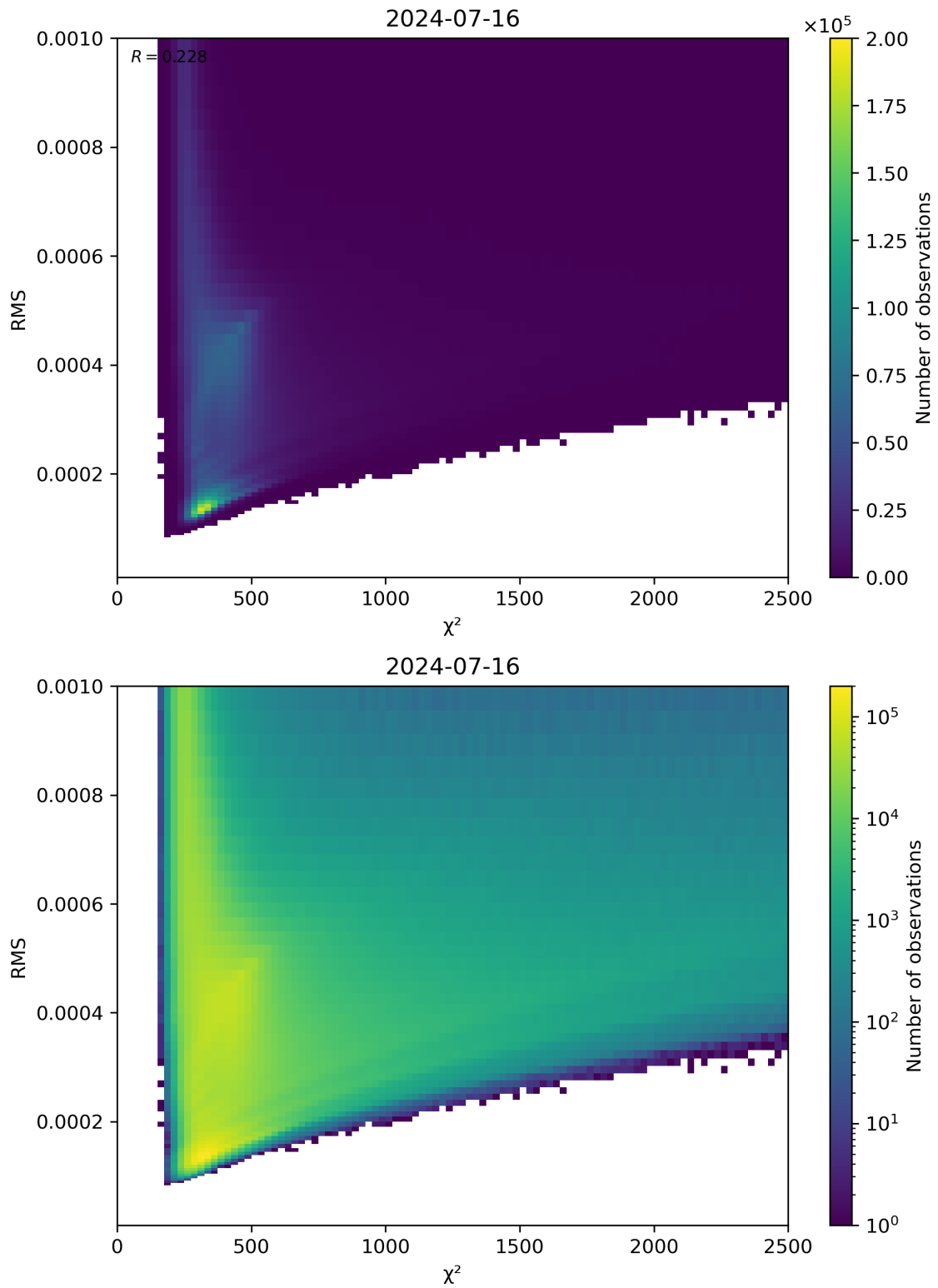
Figure 82: Scatter density plot of “ \chi^2 ” against “RMS” for 2024-07-15 to 2024-07-17.
