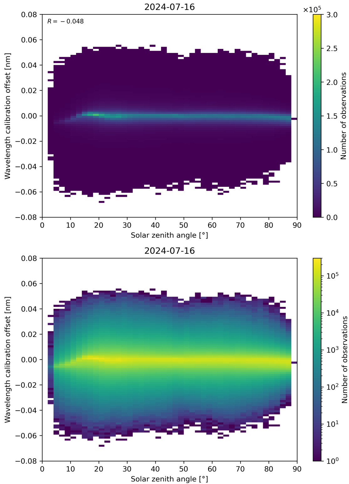
Figure 158: Scatter density plot of “Solar zenith angle” against “Wavelength calibration offset” for 2024-07-15 to 2024-07-17.
