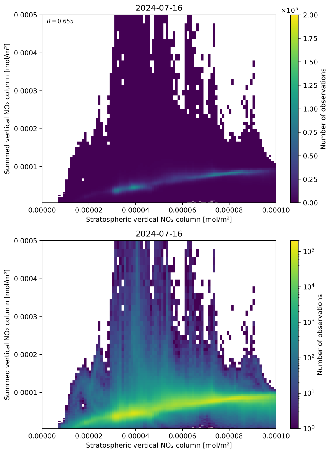
Figure 98: Scatter density plot of “Stratospheric vertical NO 2 column” against “Summed vertical NO 2 column” for 2024-07-15 to 2024-07-17.
