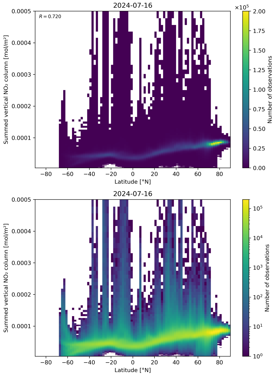
Figure 88: Scatter density plot of “Latitude” against “Summed vertical NO 2 column” for 2024-07-15 to 2024-07-17.
