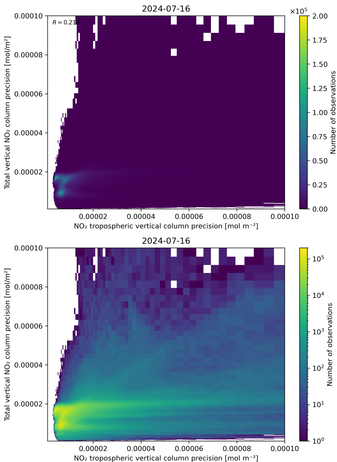
Figure 139: Scatter density plot of “NO 2 tropospheric vertical column precision” against “Total vertical NO 2 column precision” for 2024-07-15 to 2024-07-17.
