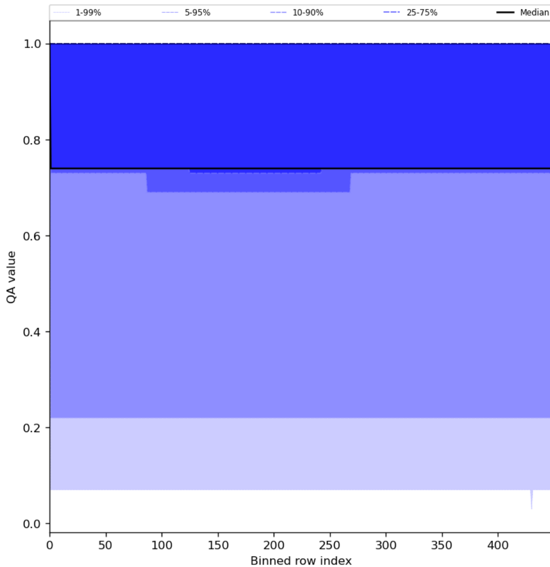
Figure 45: Along track statistics of “QA value” for 2024-07-15 to 2024-07-17
