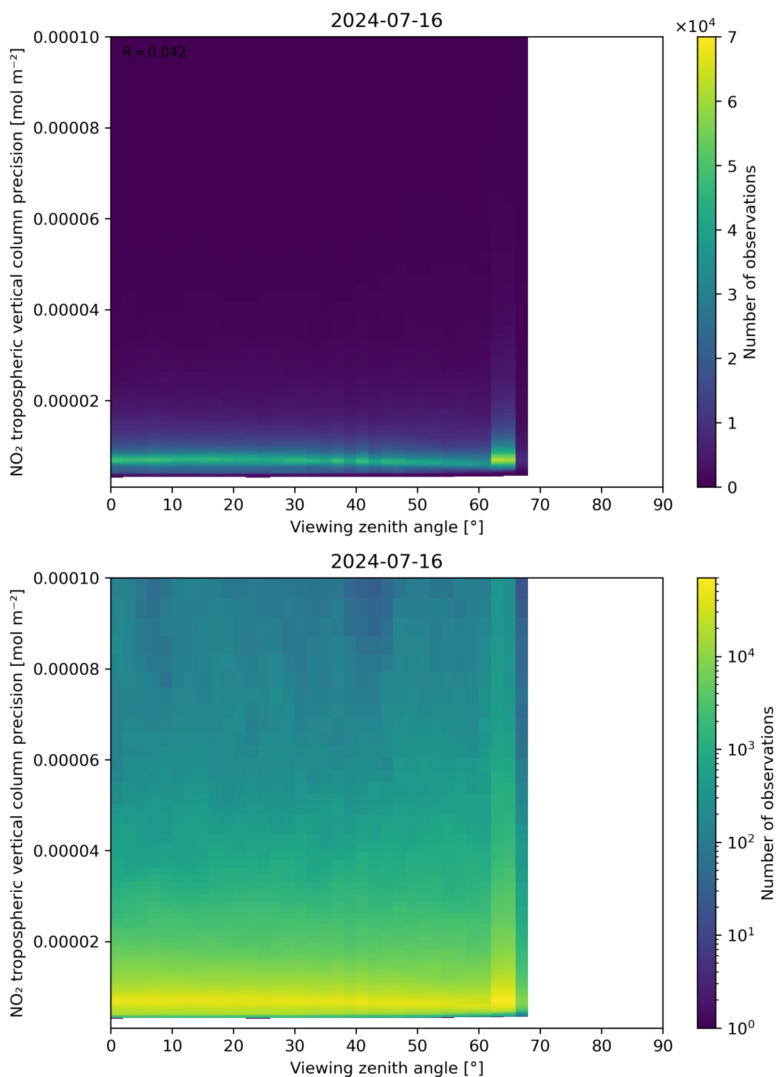
Figure 170: Scatter density plot of “Viewing zenith angle” against “NO 2 tropospheric vertical column precision” for 2024-07-15 to 2024-07-17.
