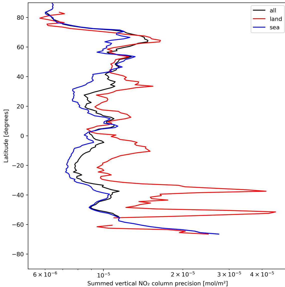
Figure 24: Zonal average of “Summed vertical NO 2 column precision” for 2024-07-15 to 2024-07-17.
