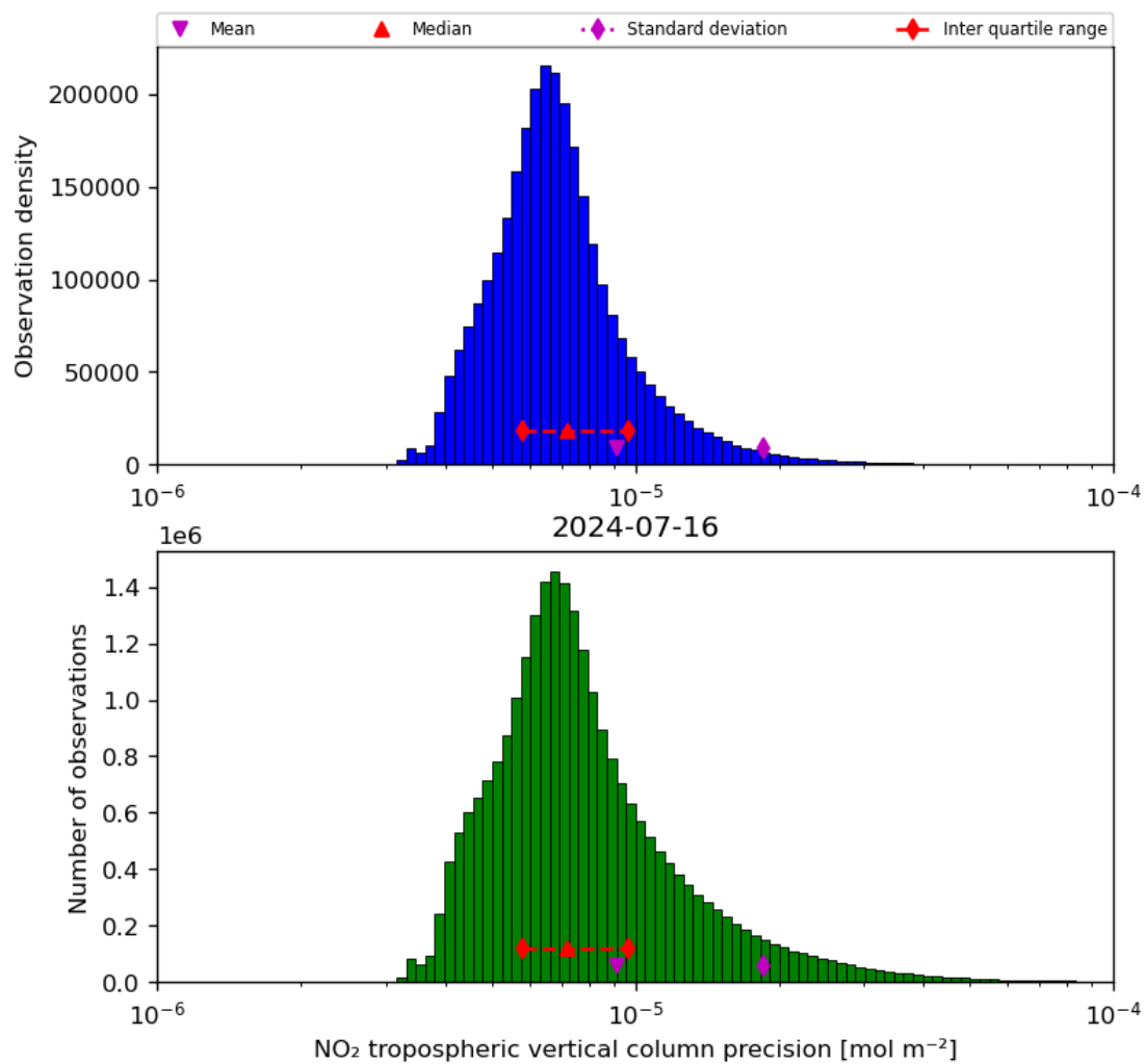
Figure 30: Histogram of “NO 2 tropospheric vertical column precision” for 2024-07-15 to 2024-07-17
