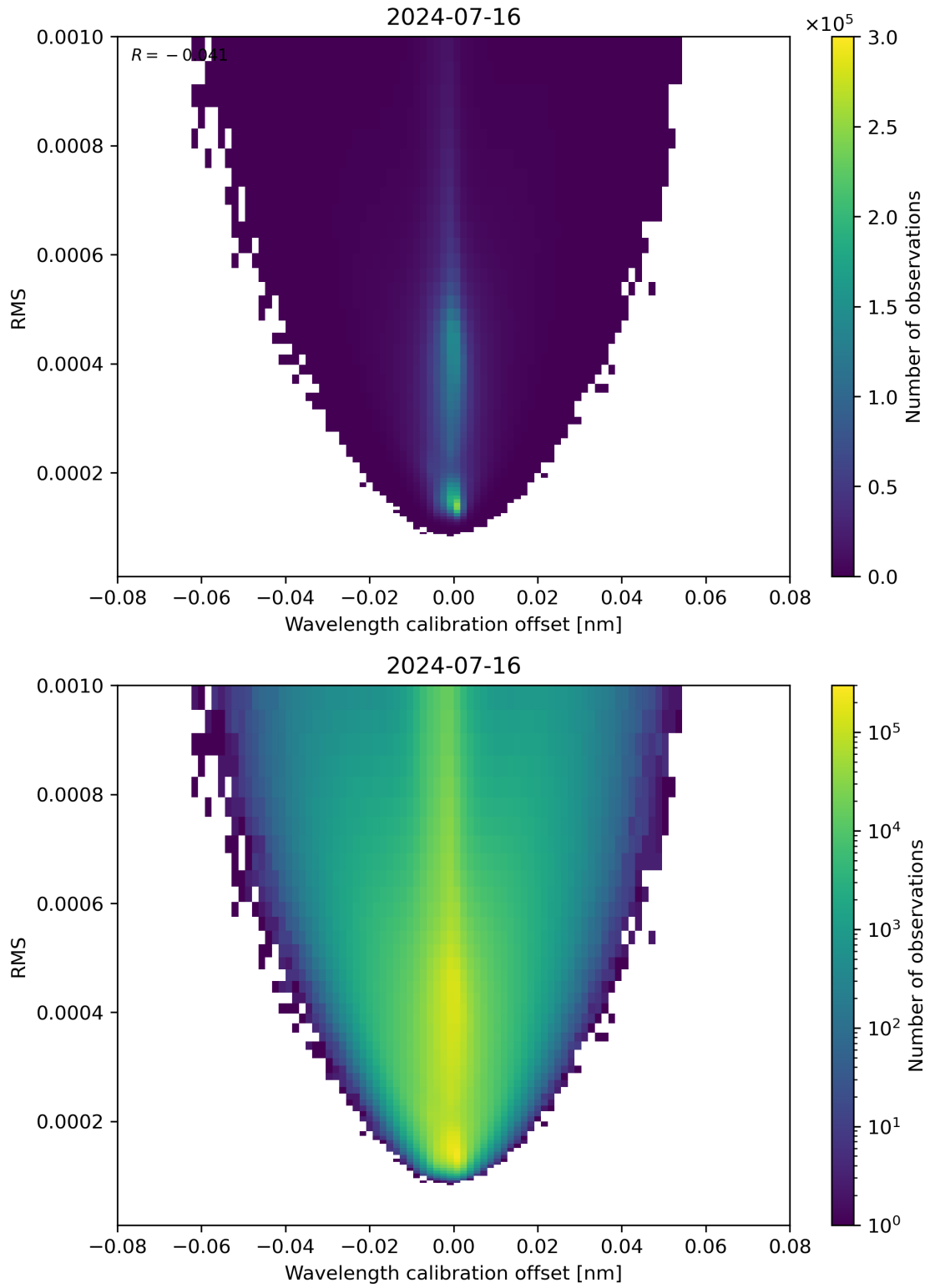
Figure 181: Scatter density plot of “Wavelength calibration offset” against “RMS” for 2024-07-15 to 2024-07-17.
