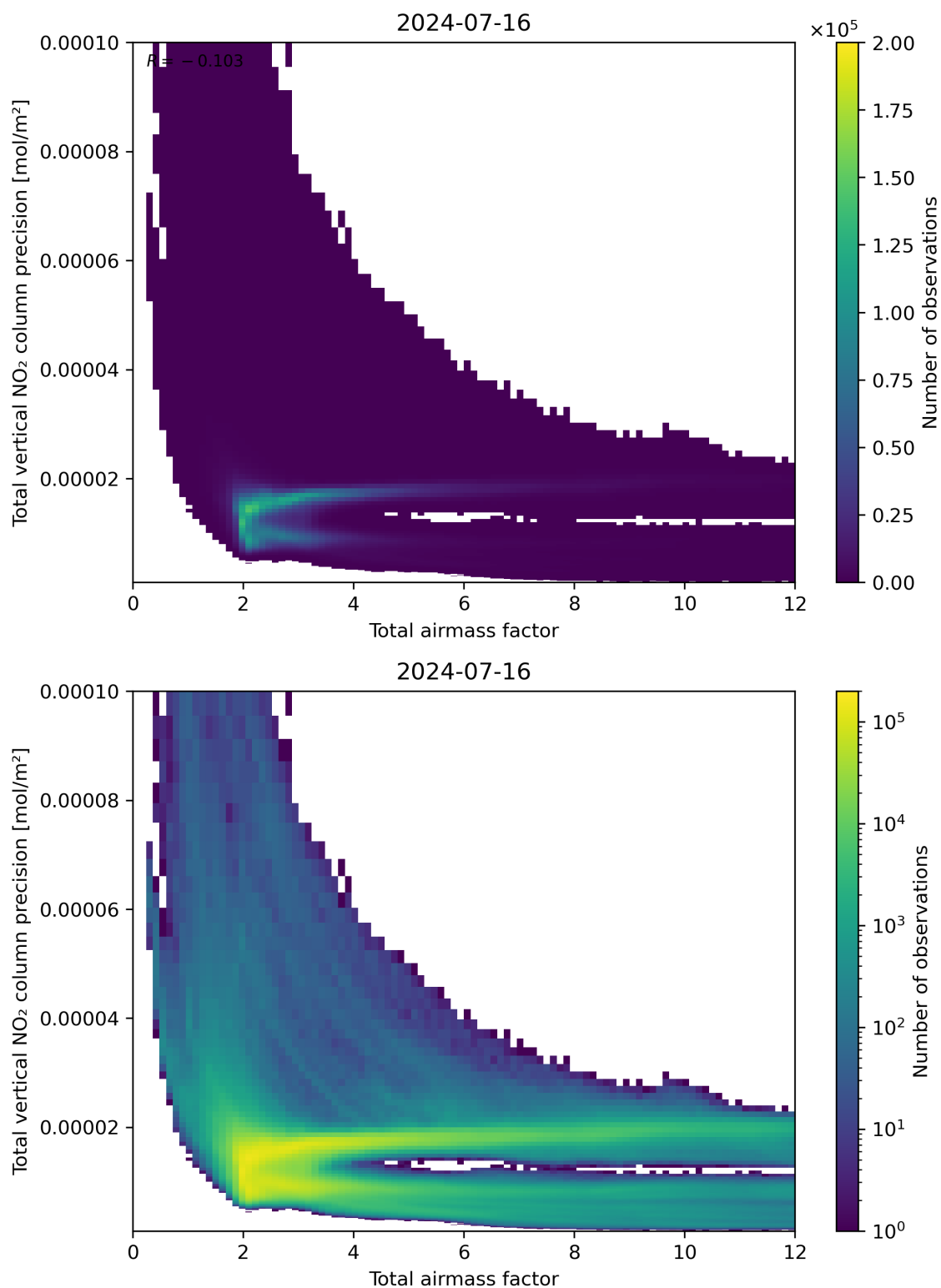
Figure 68: Scatter density plot of “Total airmass factor” against “Total vertical NO 2 column precision” for 2024-07-15 to 2024-07-17.
