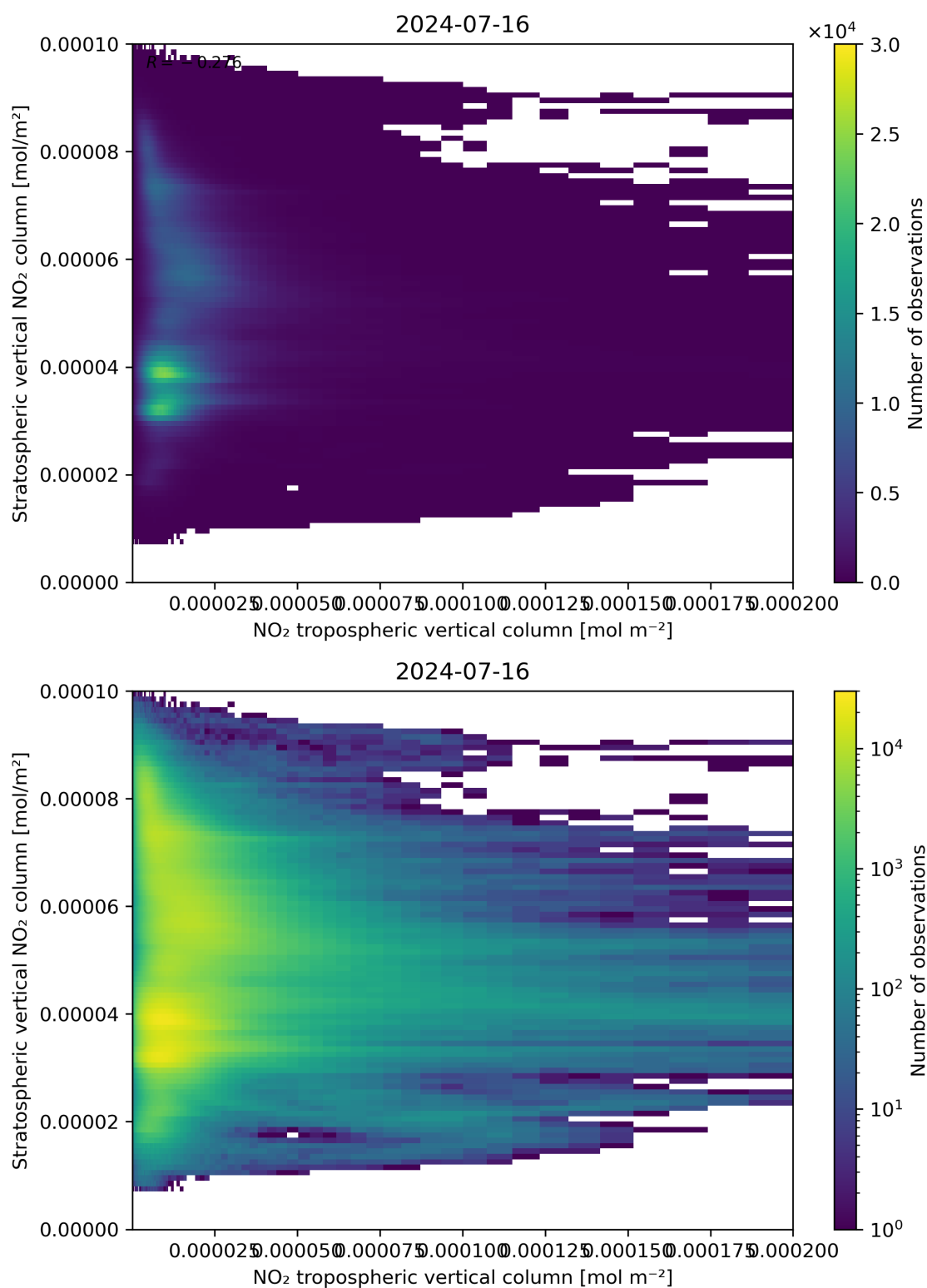
Figure 125: Scatter density plot of “NO 2 tropospheric vertical column” against “Stratospheric vertical NO 2 column” for 2024-07-15 to 2024-07-17.
