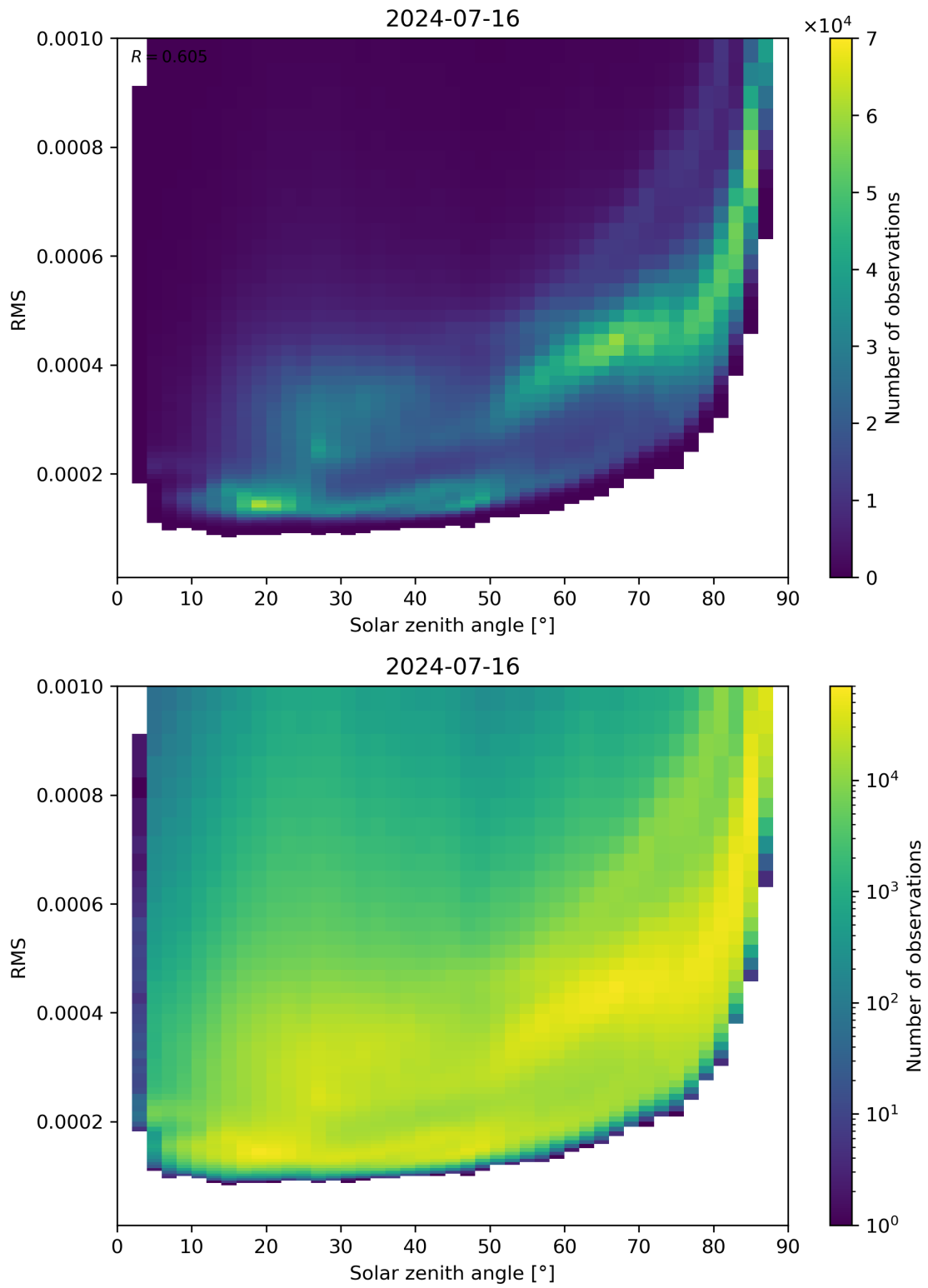
Figure 157: Scatter density plot of “Solar zenith angle” against “RMS” for 2024-07-15 to 2024-07-17.
