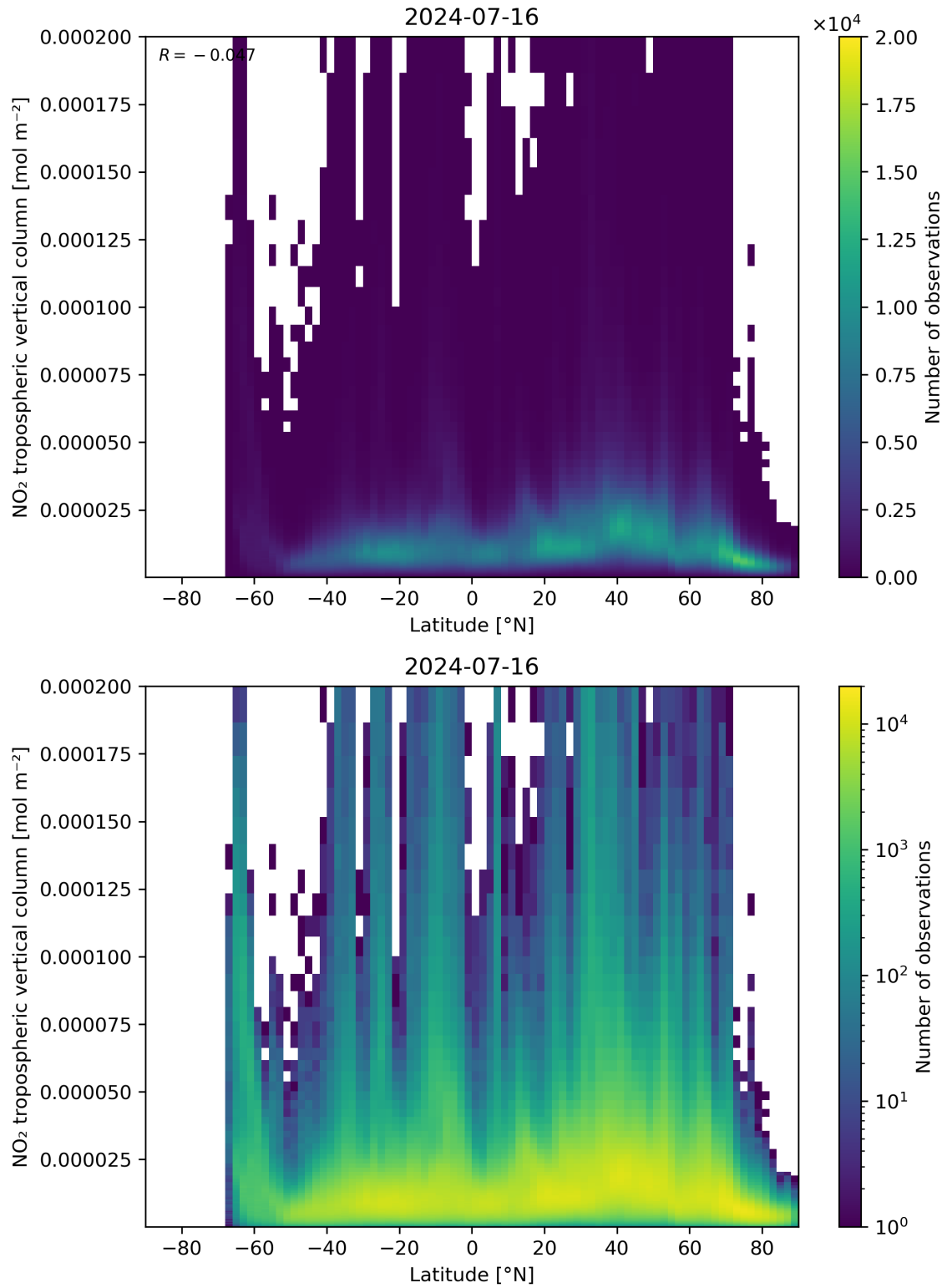
Figure 92: Scatter density plot of “Latitude” against “NO 2 tropospheric vertical column” for 2024-07-15 to 2024-07-17.
