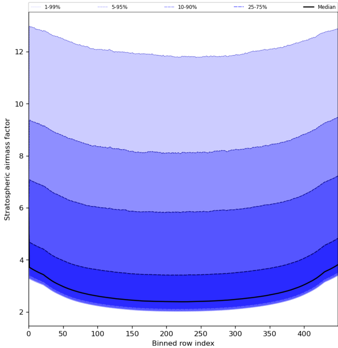
Figure 61: Along track statistics of “Stratospheric airmass factor” for 2024-07-15 to 2024-07-17
