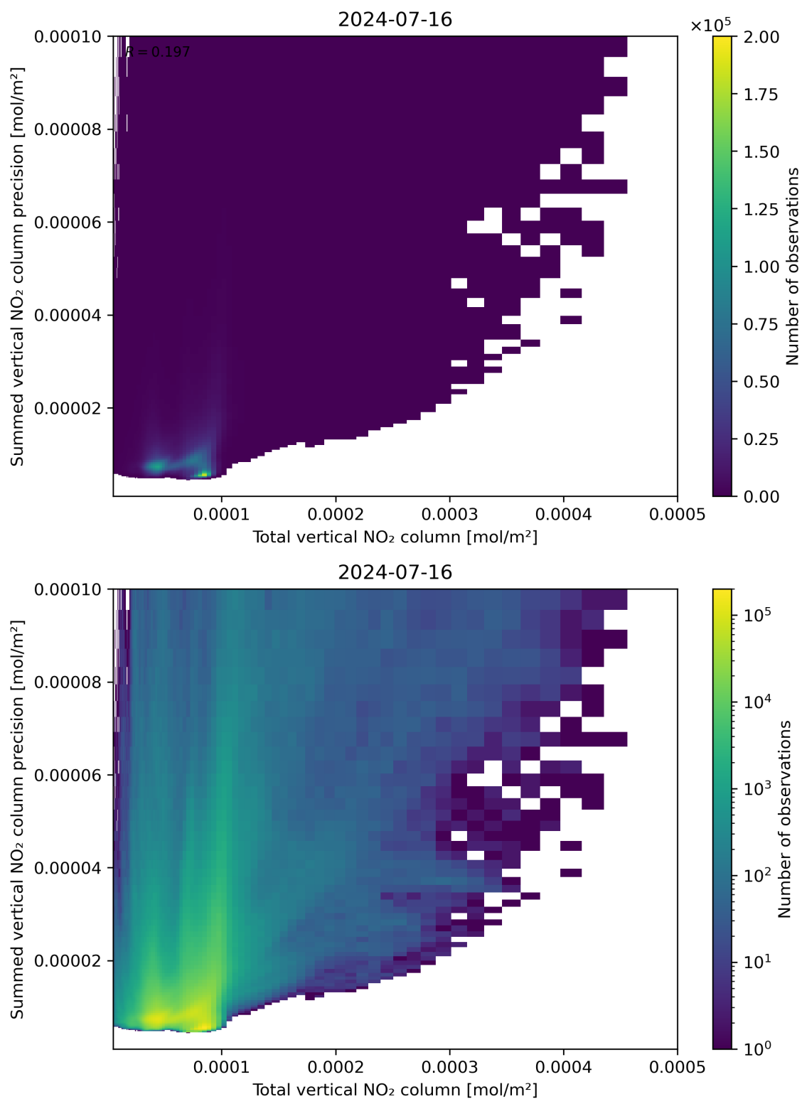
Figure 113: Scatter density plot of “Total vertical NO 2 column” against “Summed vertical NO 2 column precision” for 2024-07-15 to 2024-07-17.
