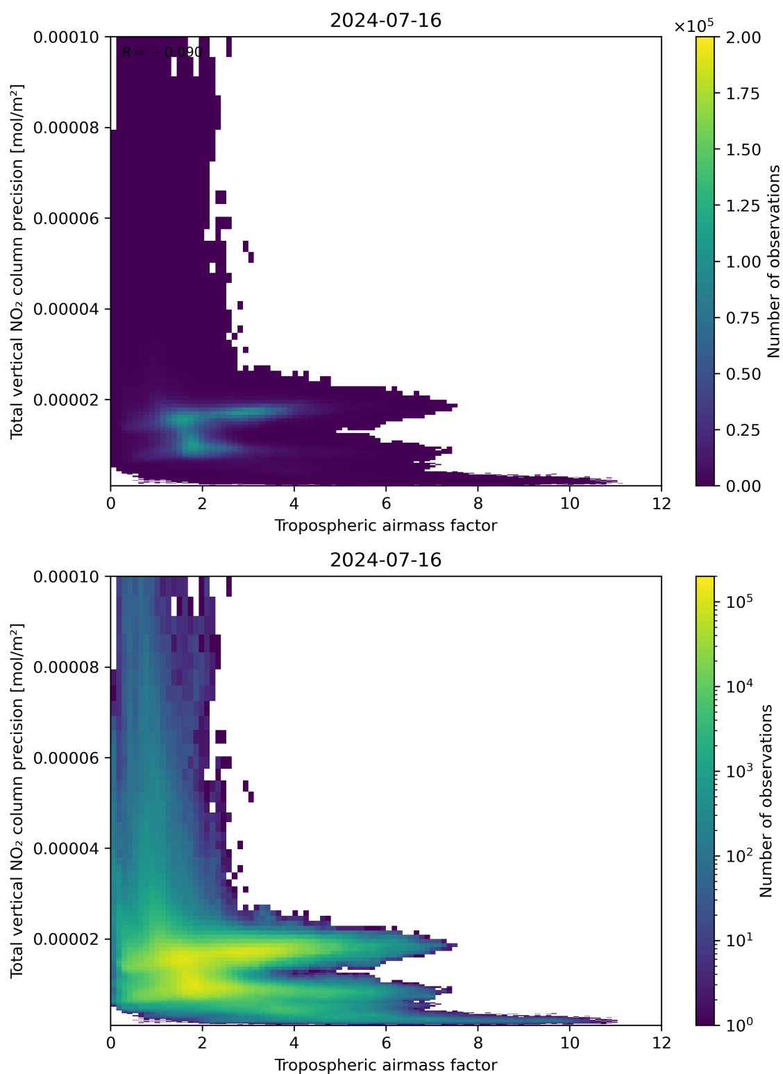
Figure 78: Scatter density plot of “Tropospheric air mass factor” against “Total vertical NO 2 column precision” for 2024-07-15 to 2024-07-17.
