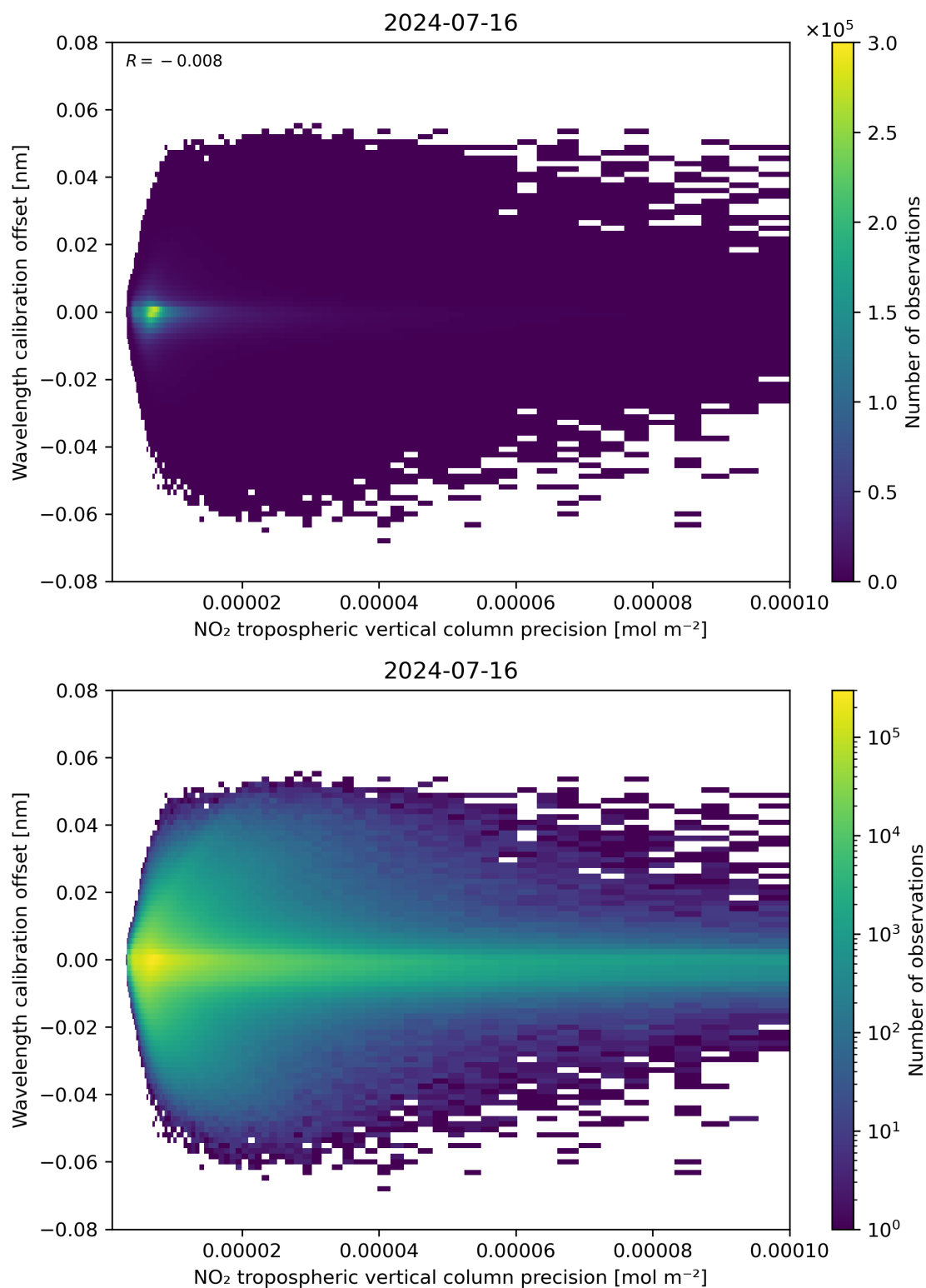
Figure 141: Scatter density plot of “NO 2 tropospheric vertical column precision” against “Wavelength calibration offset” for 2024-07-15 to 2024-07-17.
