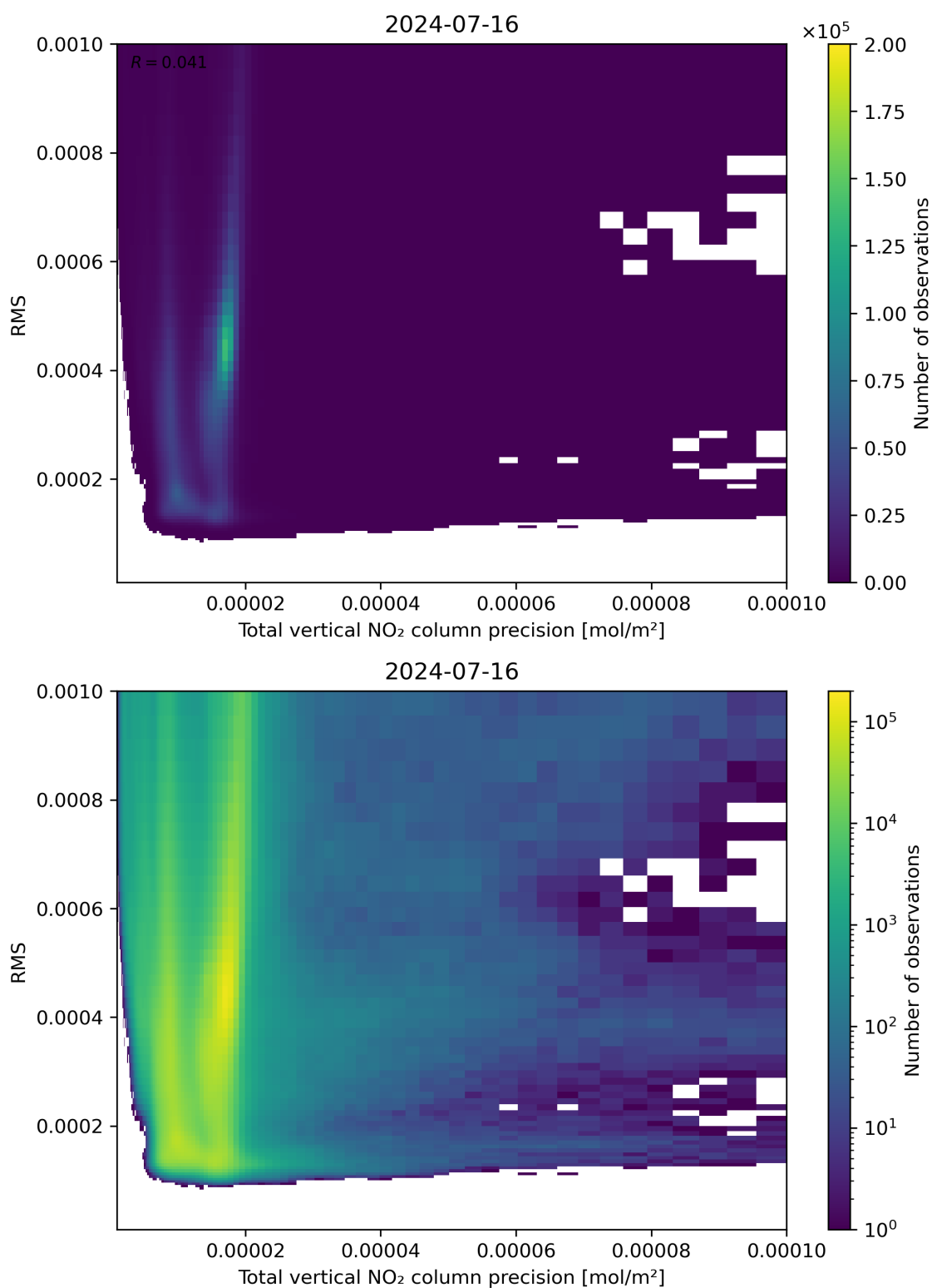
Figure 119: Scatter density plot of “Total vertical NO 2 column precision” against “RMS” for 2024-07-15 to 2024-07-17.
