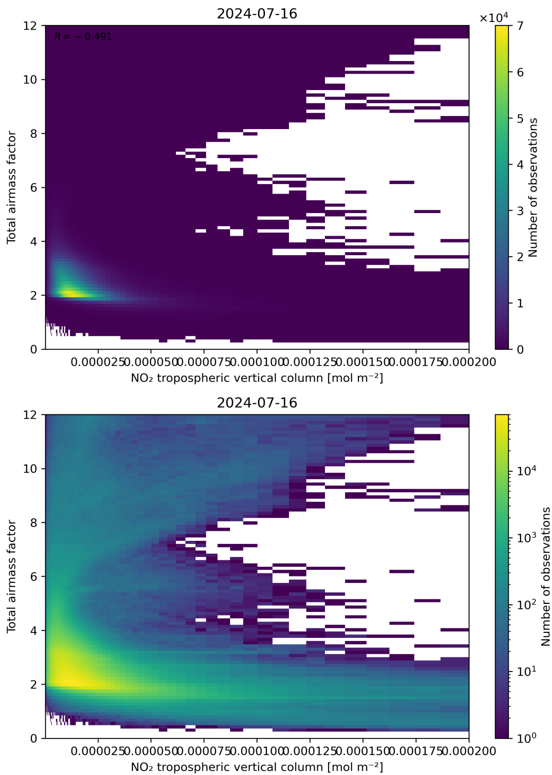
Figure 122: Scatter density plot of “NO 2 tropospheric vertical column” against “Total air mass factor” for 2024-07-15 to 2024-07-17.
