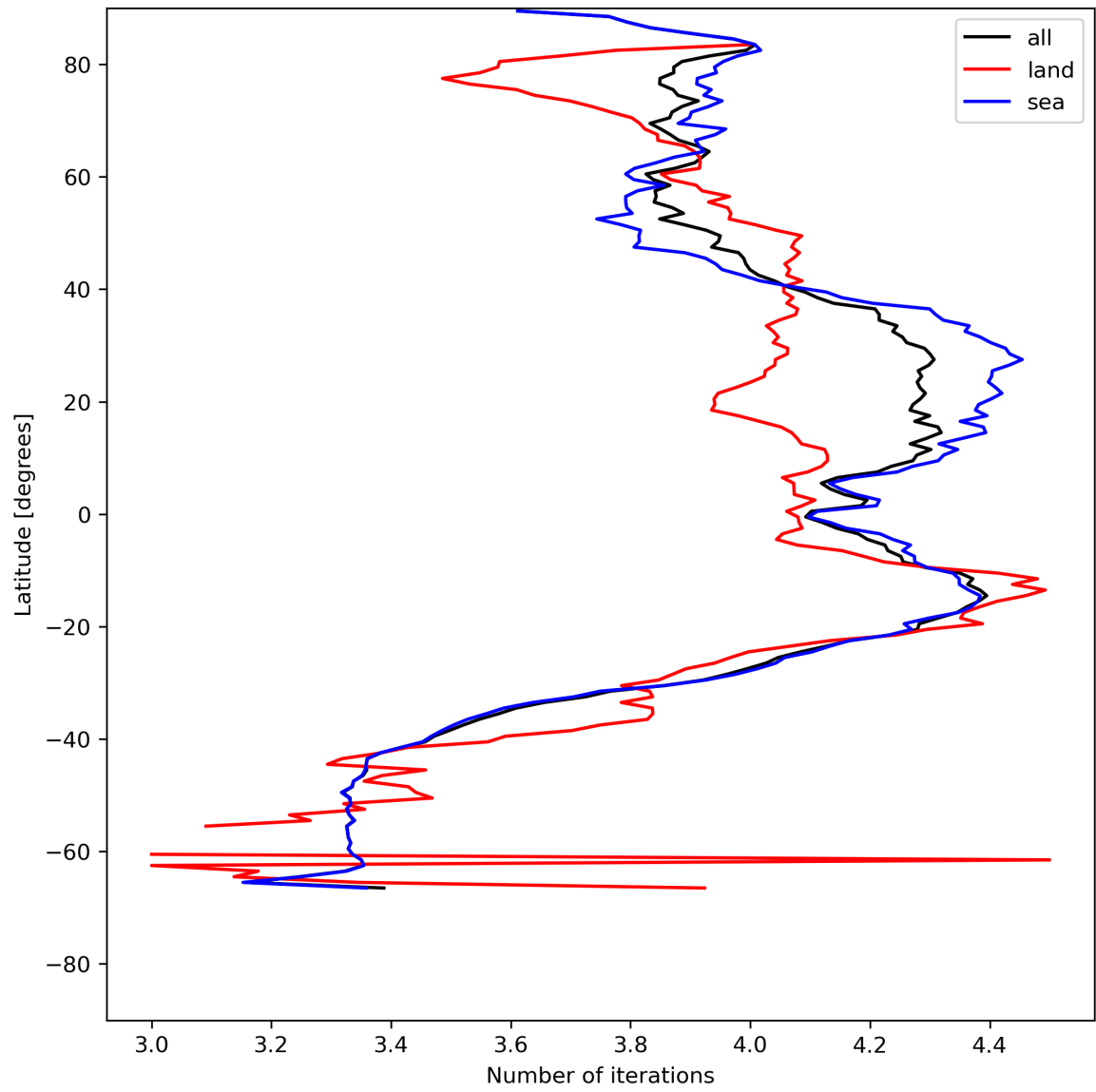
Figure 17: Zonal average of “Number of iterations” for 2024-07-15 to 2024-07-17.
