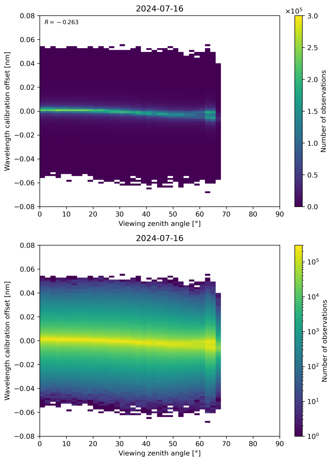
Figure 173: Scatter density plot of “Viewing zenith angle” against “Wavelength calibration offset” for 2024-07-15 to 2024-07-17.
