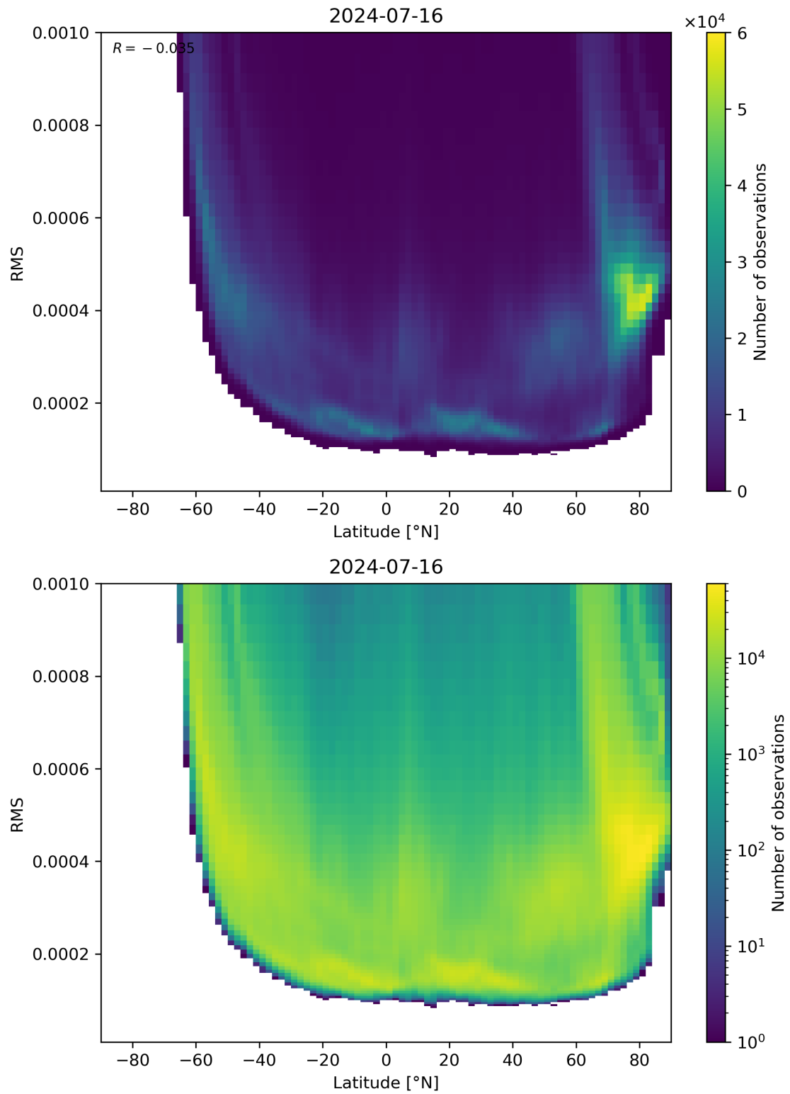
Figure 94: Scatter density plot of “Latitude” against “RMS” for 2024-07-15 to 2024-07-17.
