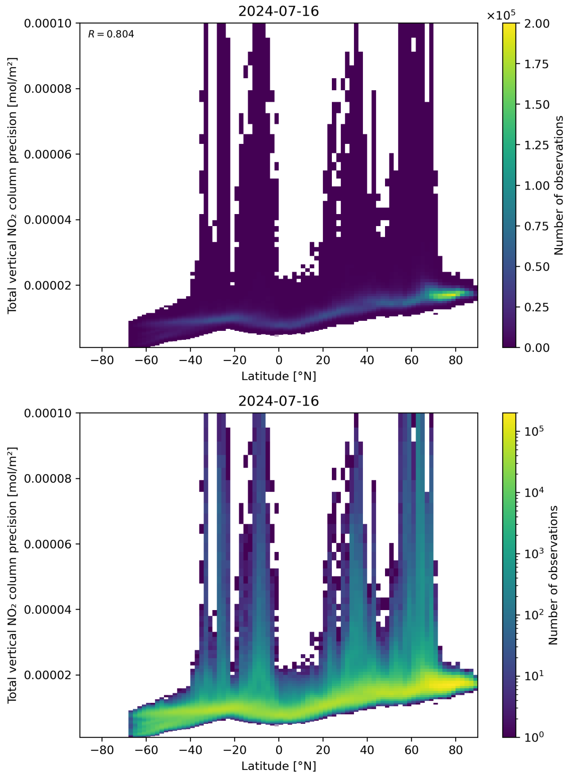
Figure 91: Scatter density plot of “Latitude” against “Total vertical NO 2 column precision” for 2024-07-15 to 2024-07-17.
