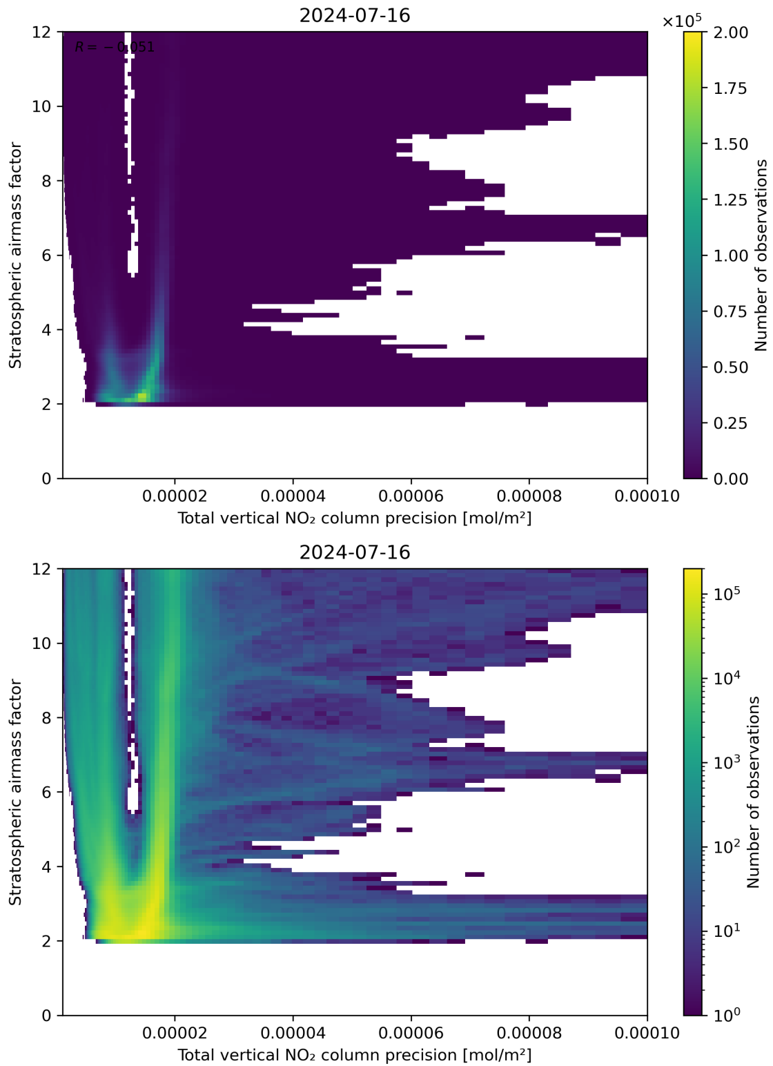
Figure 115: Scatter density plot of “Total vertical NO 2 column precision” against “Stratospheric air mass factor” for 2024-07-15 to 2024-07-17.
