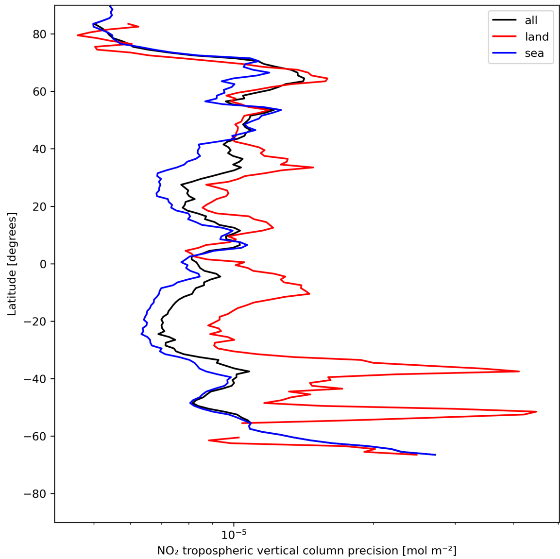
Figure 13: Zonal average of “NO 2 tropospheric vertical column precision” for 2024-07-15 to 2024-07-17.
