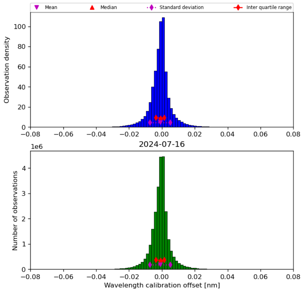
Figure 35: Histogram of “Wavelength calibration offset” for 2024-07-15 to 2024-07-17
