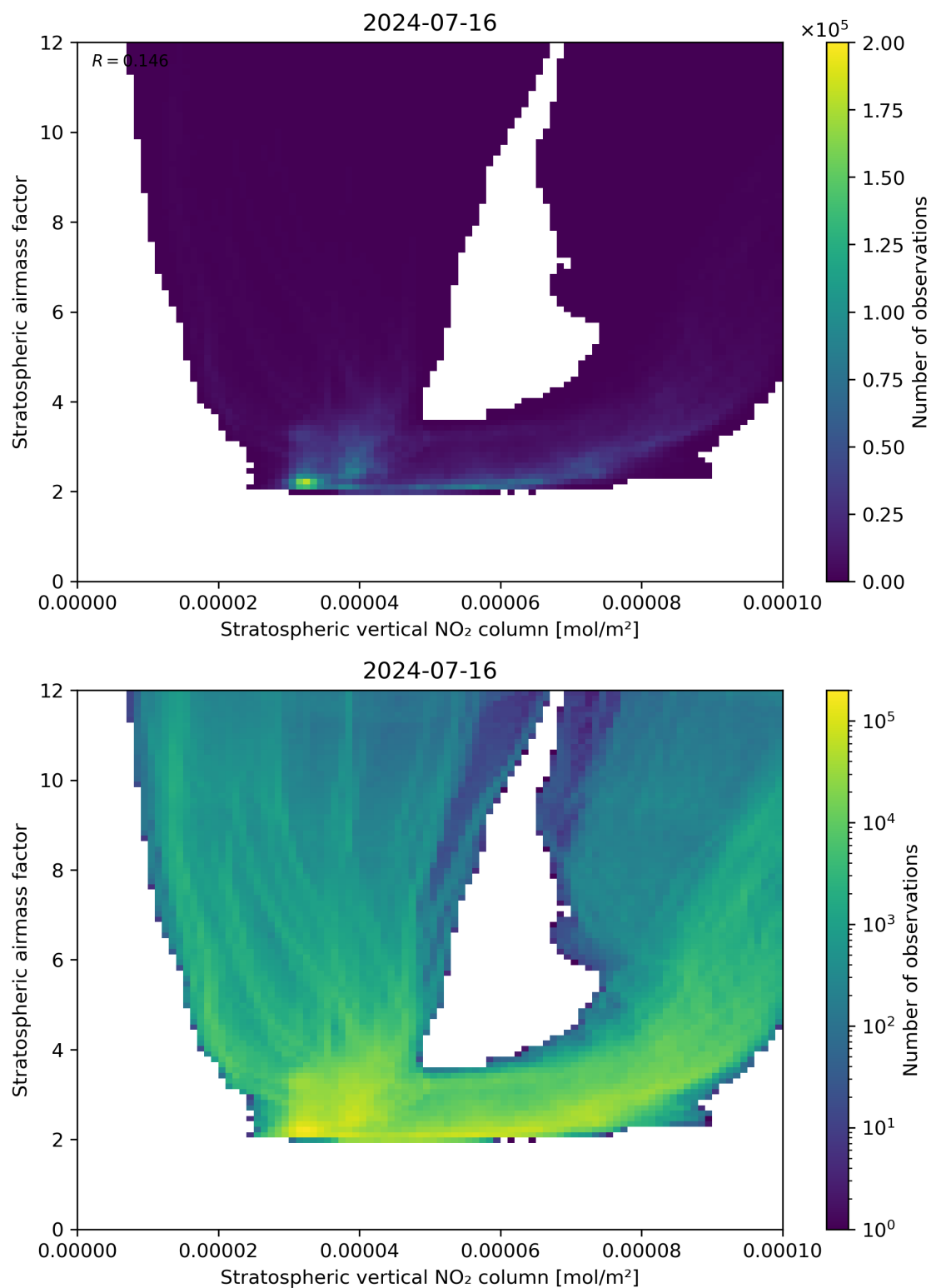
Figure 96: Scatter density plot of “Stratospheric vertical NO 2 column” against “Stratospheric airmass factor” for 2024-07-15 to 2024-07-17.
