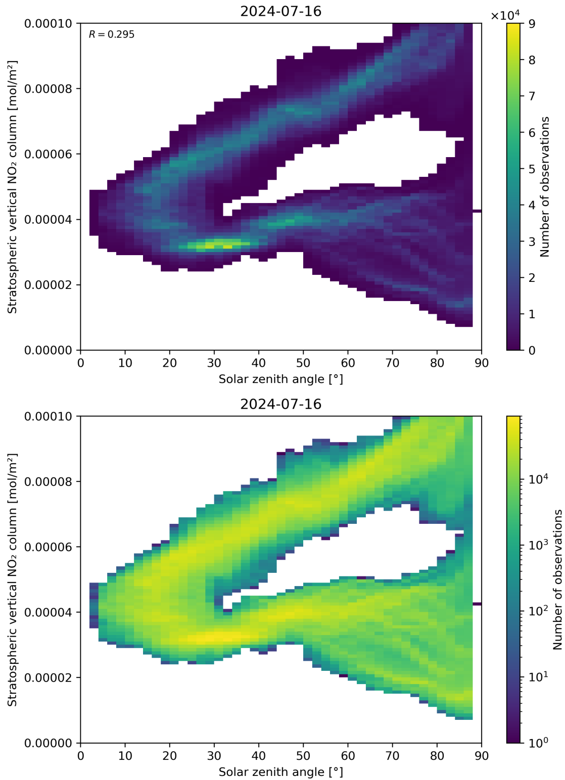
Figure 150: Scatter density plot of “Solar zenith angle” against “Stratospheric vertical NO 2 column” for 2024-07-15 to 2024-07-17.
