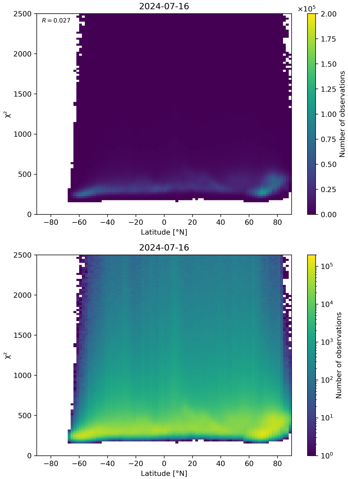
Figure 86: Scatter density plot of “Latitude” against “ \chi^2 ” for 2024-07-15 to 2024-07-17.
