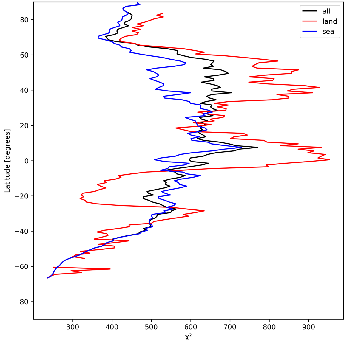
Figure 25: Zonal average of “ \chi^2 ” for 2024-07-15 to 2024-07-17.
