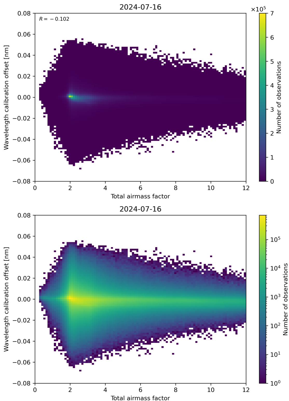
Figure 70: Scatter density plot of “Total airmass factor” against “Wavelength calibration offset” for 2024-07-15 to 2024-07-17.
