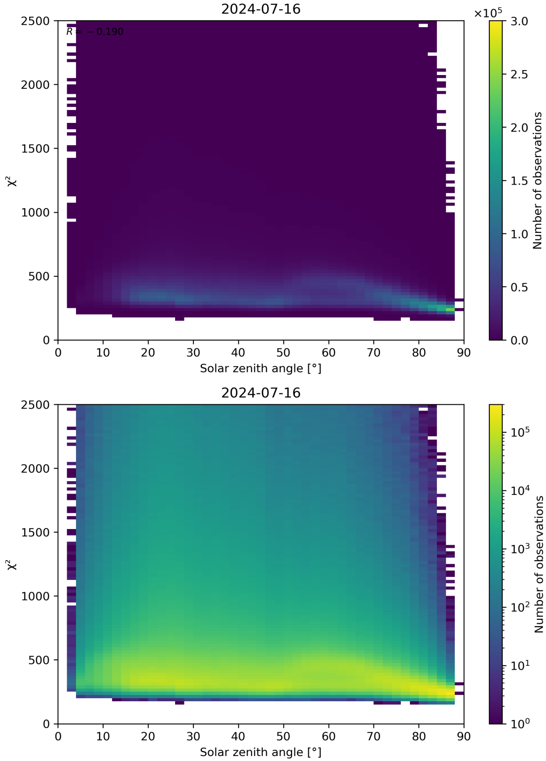
Figure 148: Scatter density plot of “Solar zenith angle” against “ \chi^2 ” for 2024-07-15 to 2024-07-17.
