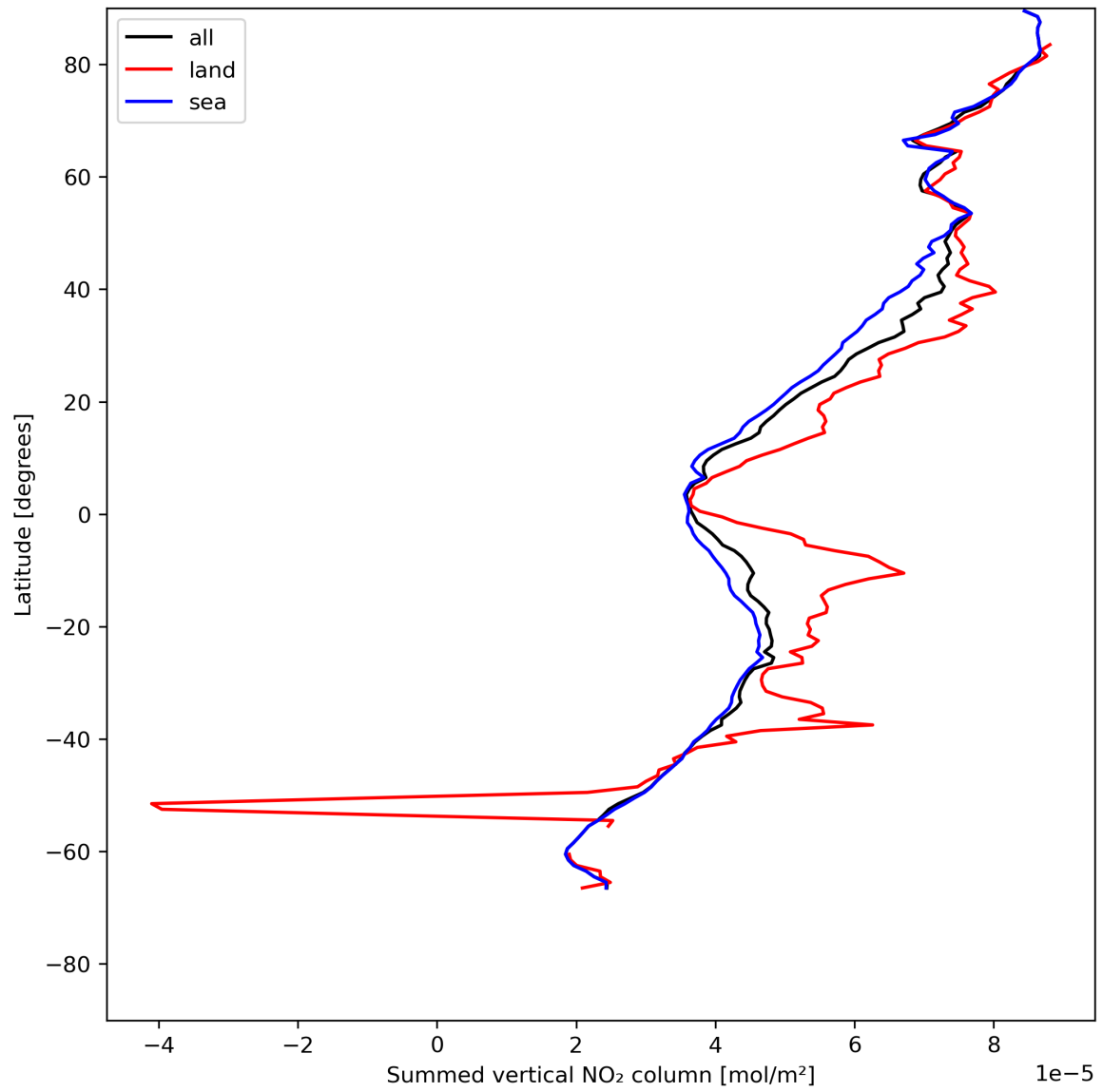
Figure 23: Zonal average of “Summed vertical NO 2 column” for 2024-07-15 to 2024-07-17.
