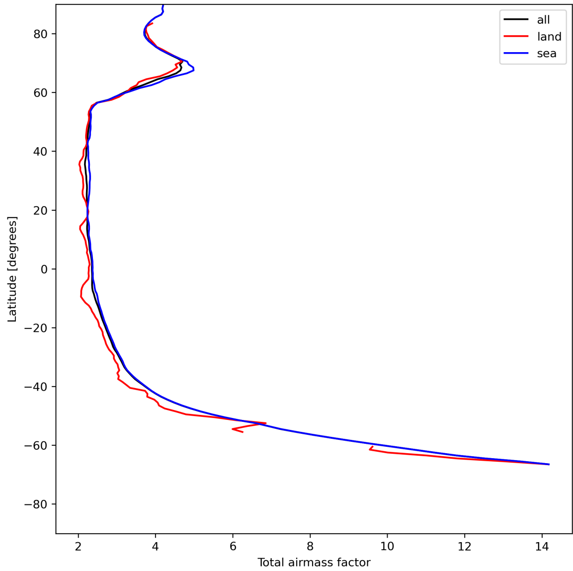
Figure 15: Zonal average of “Total airmass factor” for 2024-07-15 to 2024-07-17.
