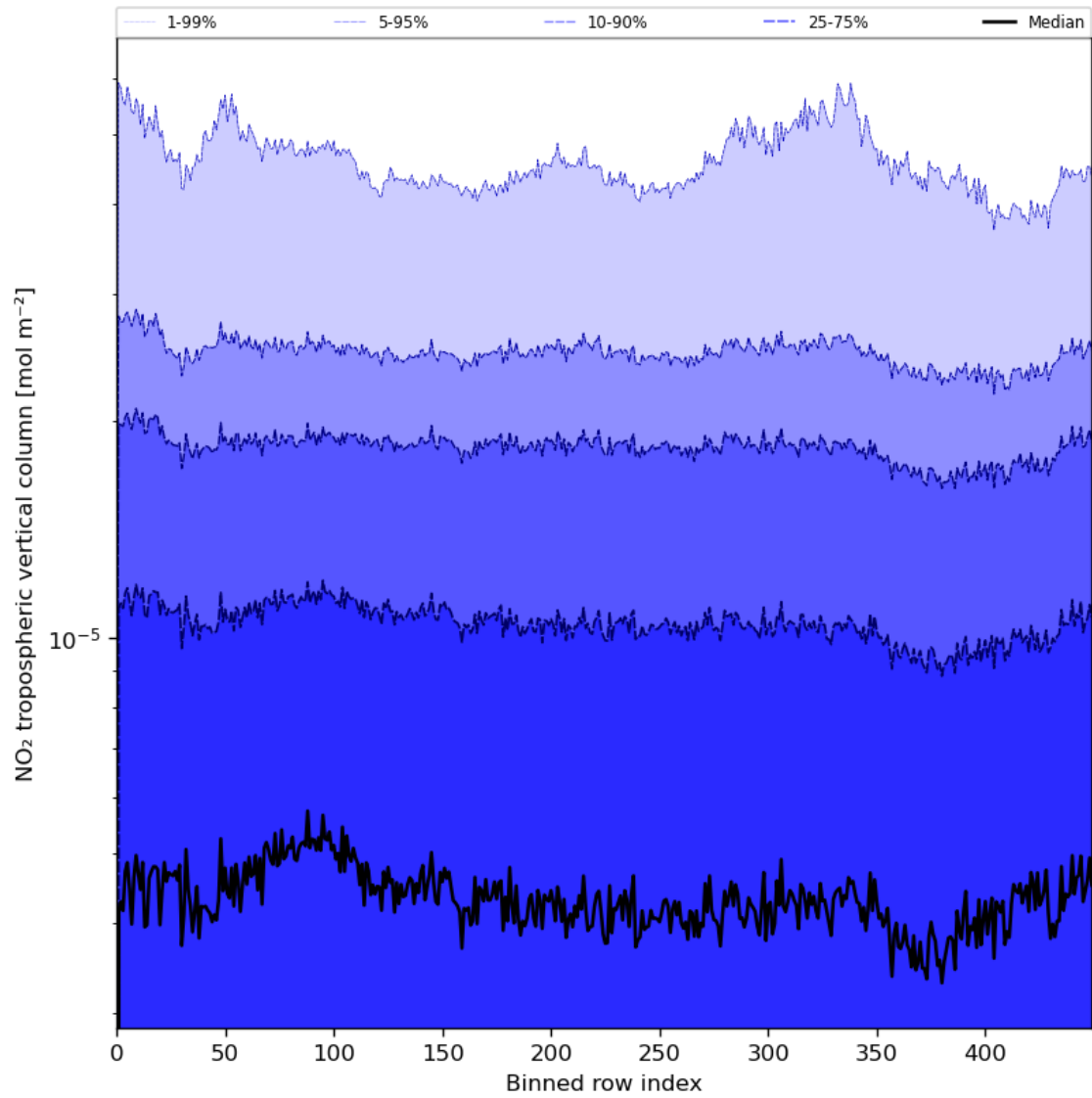
Figure 46: Along track statistics of “NO 2 tropospheric vertical column” for 2024-07-15 to 2024-07-17
