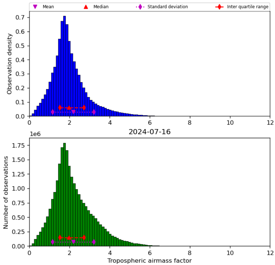
Figure 31: Histogram of “Tropospheric airmass factor” for 2024-07-15 to 2024-07-17
