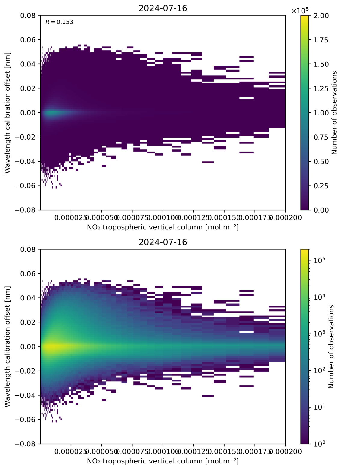
Figure 143: Scatter density plot of “NO 2 tropospheric vertical column” against “Wavelength calibration offset” for 2024-07-15 to 2024-07-17.
