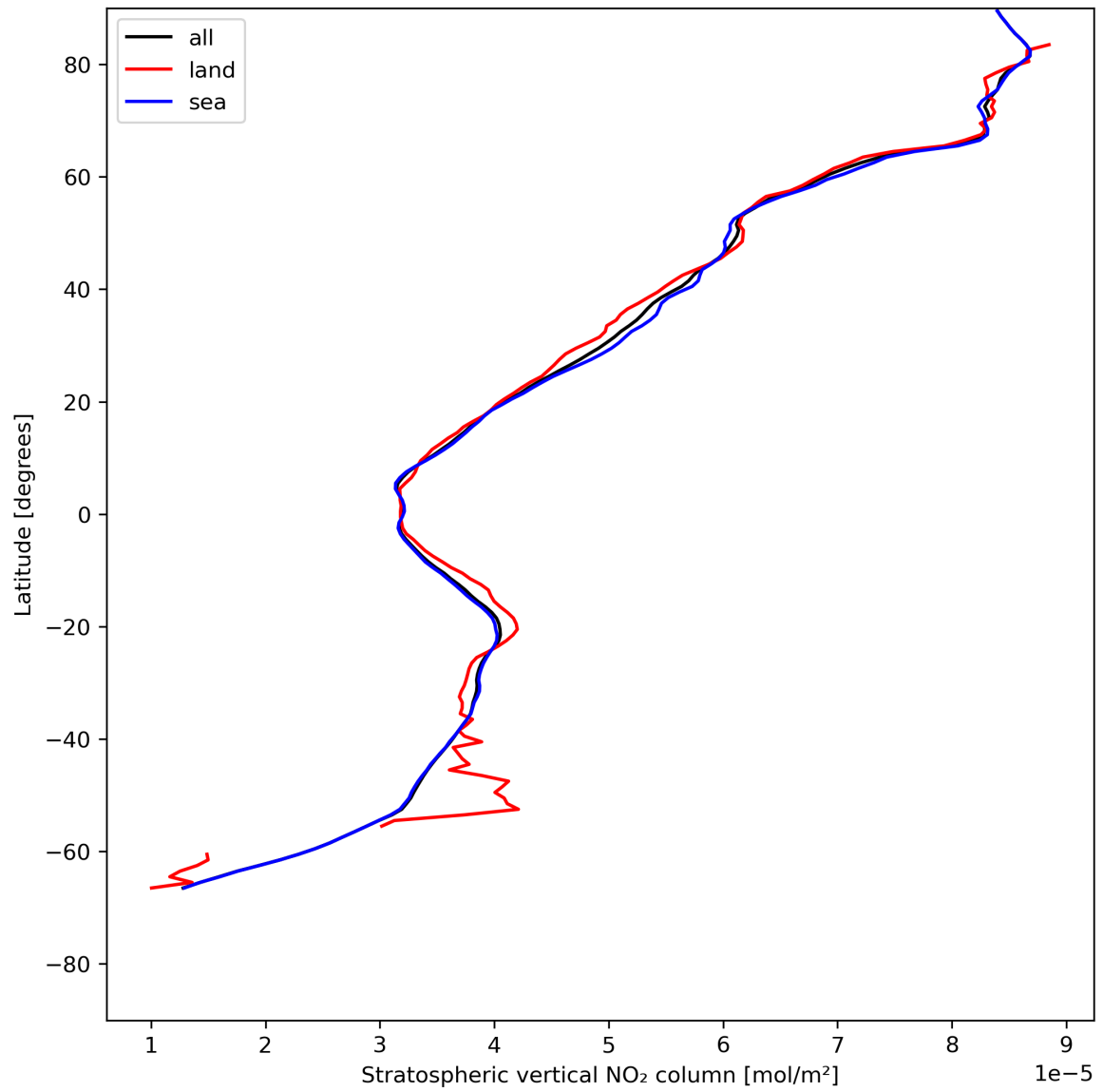
Figure 19: Zonal average of “Stratospheric vertical NO 2 column” for 2024-07-15 to 2024-07-17.
