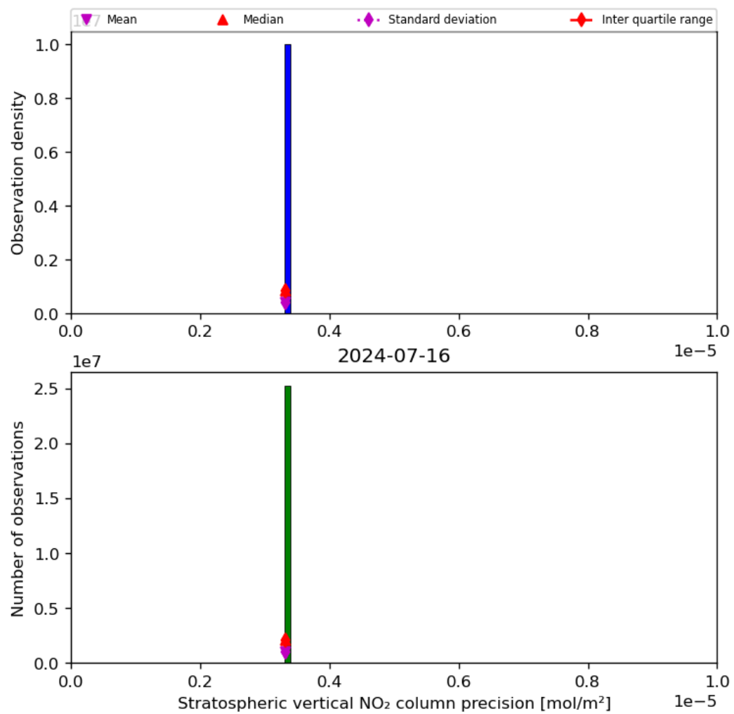
Figure 37: Histogram of “Stratospheric vertical NO 2 column precision” for 2024-07-15 to 2024-07-17
