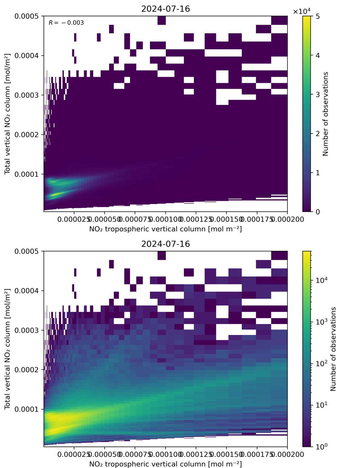
Figure 128: Scatter density plot of “NO 2 tropospheric vertical column” against “Total vertical NO 2 column” for 2024-07-15 to 2024-07-17.
