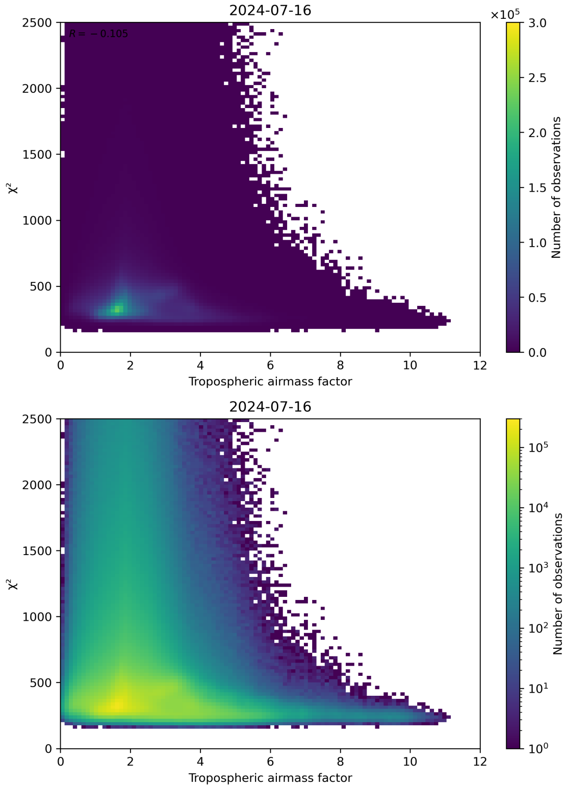
Figure 73: Scatter density plot of “Tropospheric airmass factor” against “ \chi^2 ” for 2024-07-15 to 2024-07-17.
