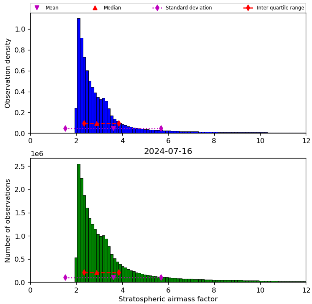
Figure 44: Histogram of “Stratospheric airmass factor” for 2024-07-15 to 2024-07-17
