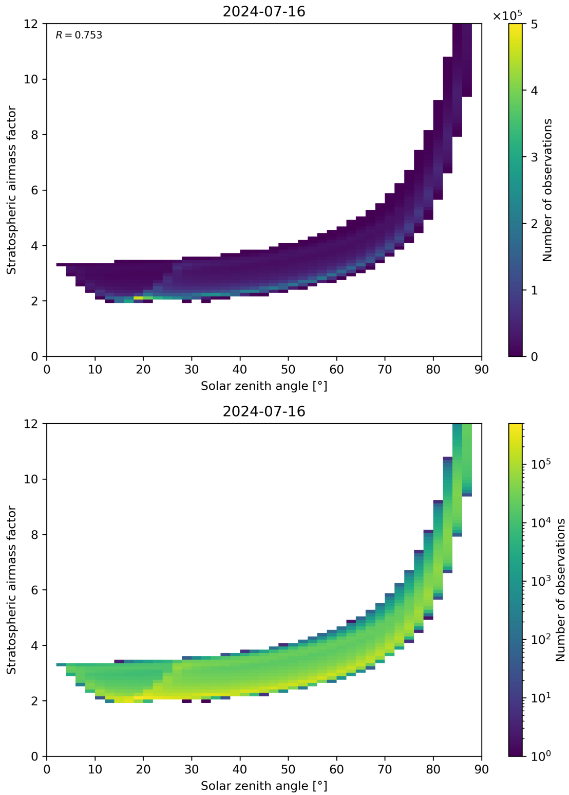
Figure 145: Scatter density plot of “Solar zenith angle” against “Stratospheric airmass factor” for 2024-07-15 to 2024-07-17.
