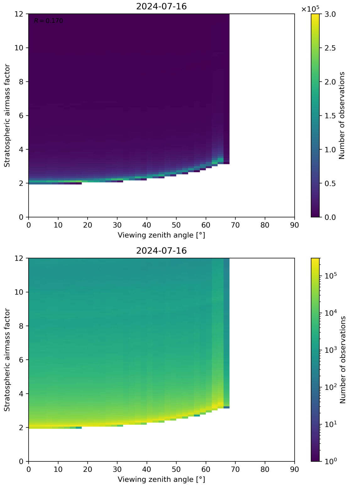
Figure 159: Scatter density plot of “Viewing zenith angle” against “Stratospheric airmass factor” for 2024-07-15 to 2024-07-17.
