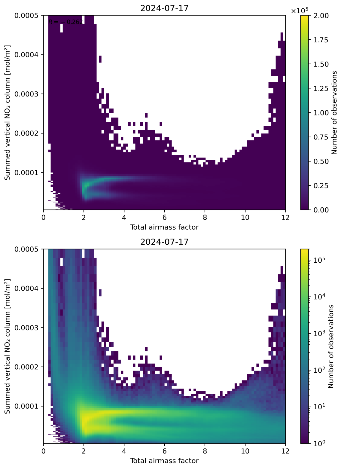
Figure 65: Scatter density plot of “Total airmass factor” against “Summed vertical NO 2 column” for 2024-07-16 to 2024-07-18.
