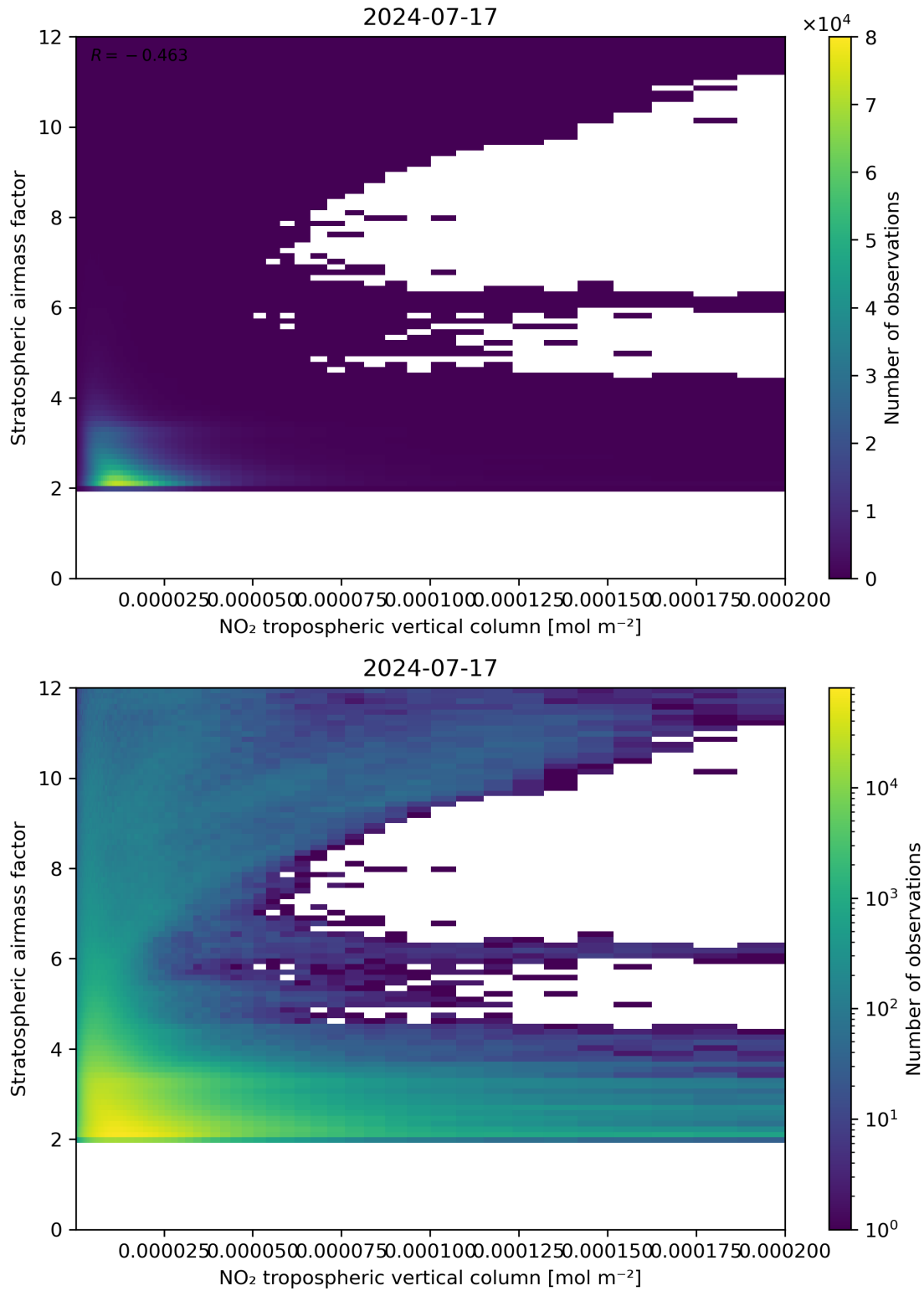
Figure 121: Scatter density plot of “NO 2 tropospheric vertical column” against “Stratospheric air mass factor” for 2024-07-16 to 2024-07-18.
