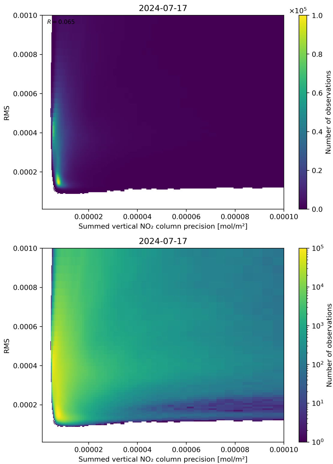
Figure 108: Scatter density plot of “Summed vertical NO 2 column precision” against “RMS” for 2024-07-16 to 2024-07-18.
