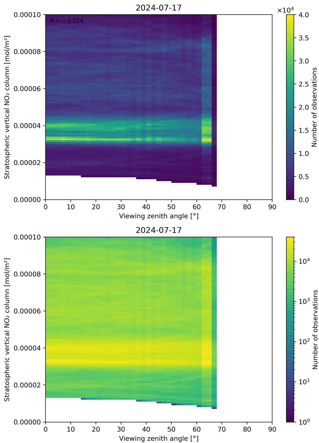
Figure 164: Scatter density plot of “Viewing zenith angle” against “Stratospheric vertical NO 2 column” for 2024-07-16 to 2024-07-18.
