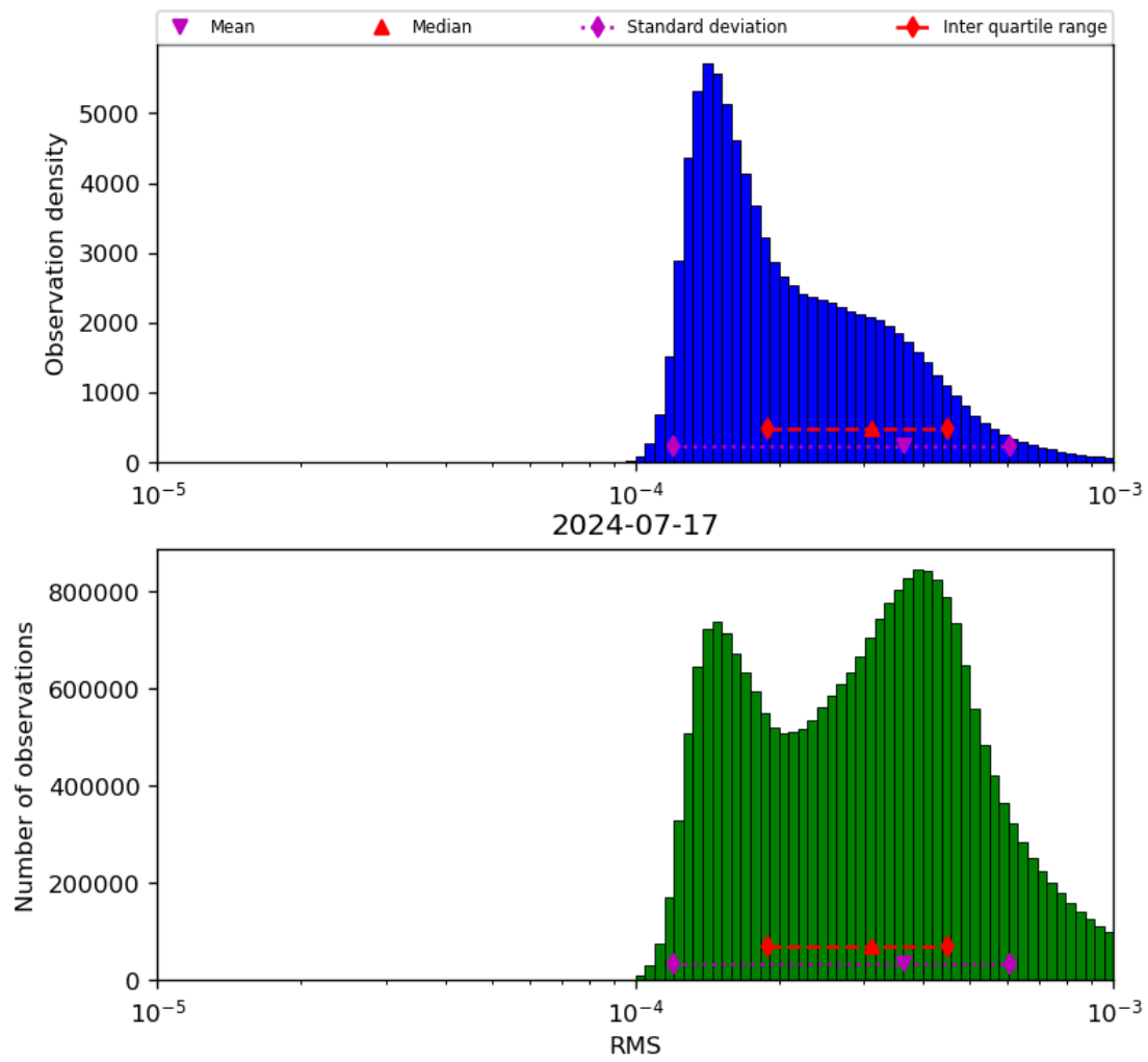
Figure 43: Histogram of “RMS” for 2024-07-16 to 2024-07-18
