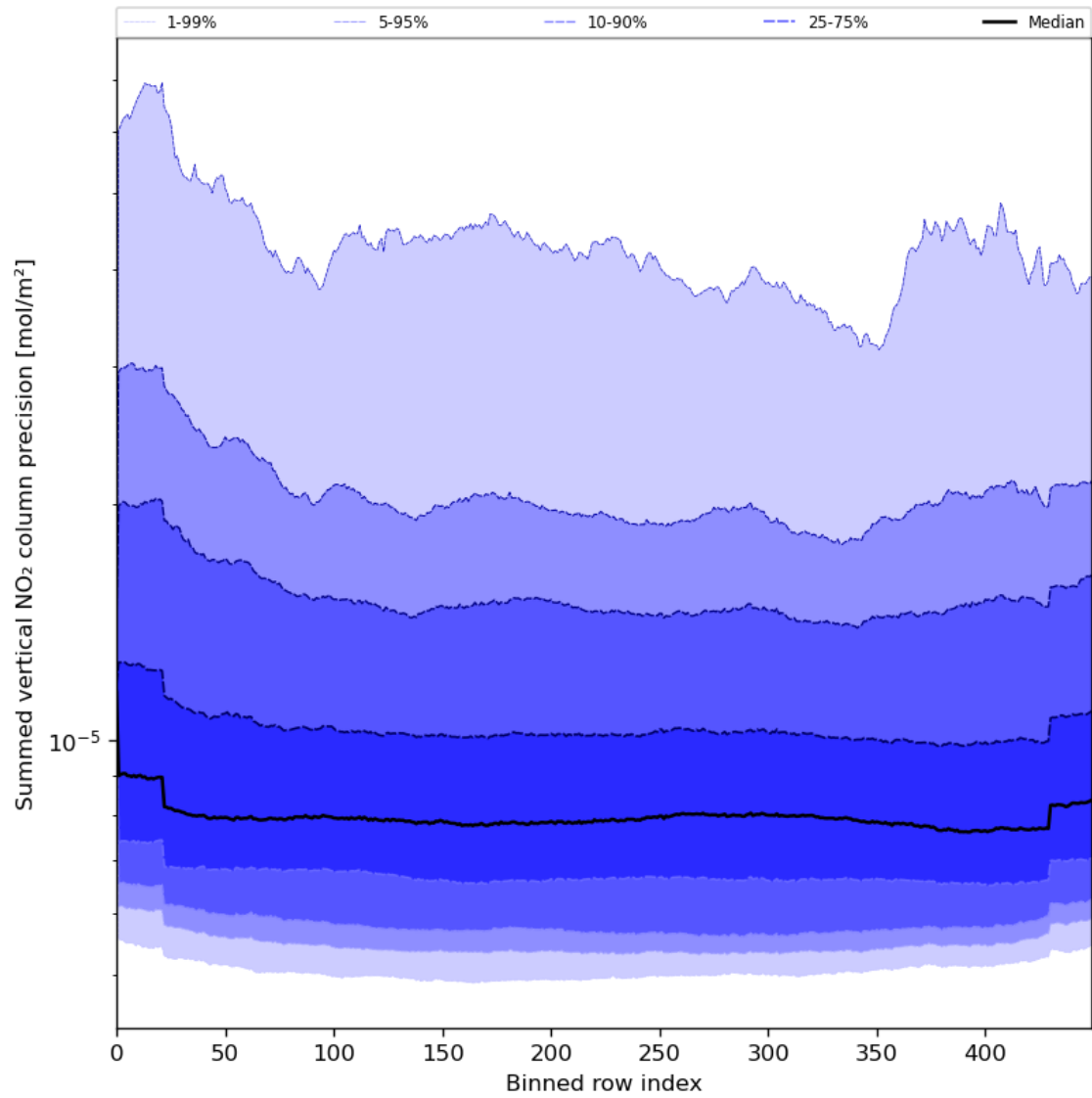
Figure 58: Along track statistics of “Summed vertical NO 2 column precision” for 2024-07-16 to 2024-07-18
