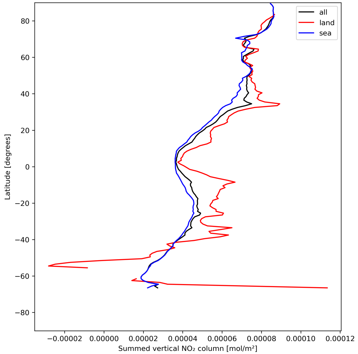
Figure 23: Zonal average of “Summed vertical NO 2 column” for 2024-07-16 to 2024-07-18.
