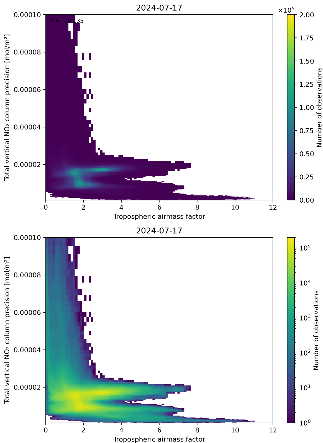
Figure 78: Scatter density plot of “Tropospheric air mass factor” against “Total vertical NO 2 column precision” for 2024-07-16 to 2024-07-18.
