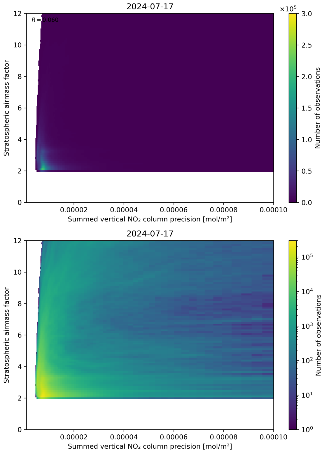
Figure 106: Scatter density plot of “Summed vertical NO 2 column precision” against “Stratospheric airmass factor” for 2024-07-16 to 2024-07-18.
