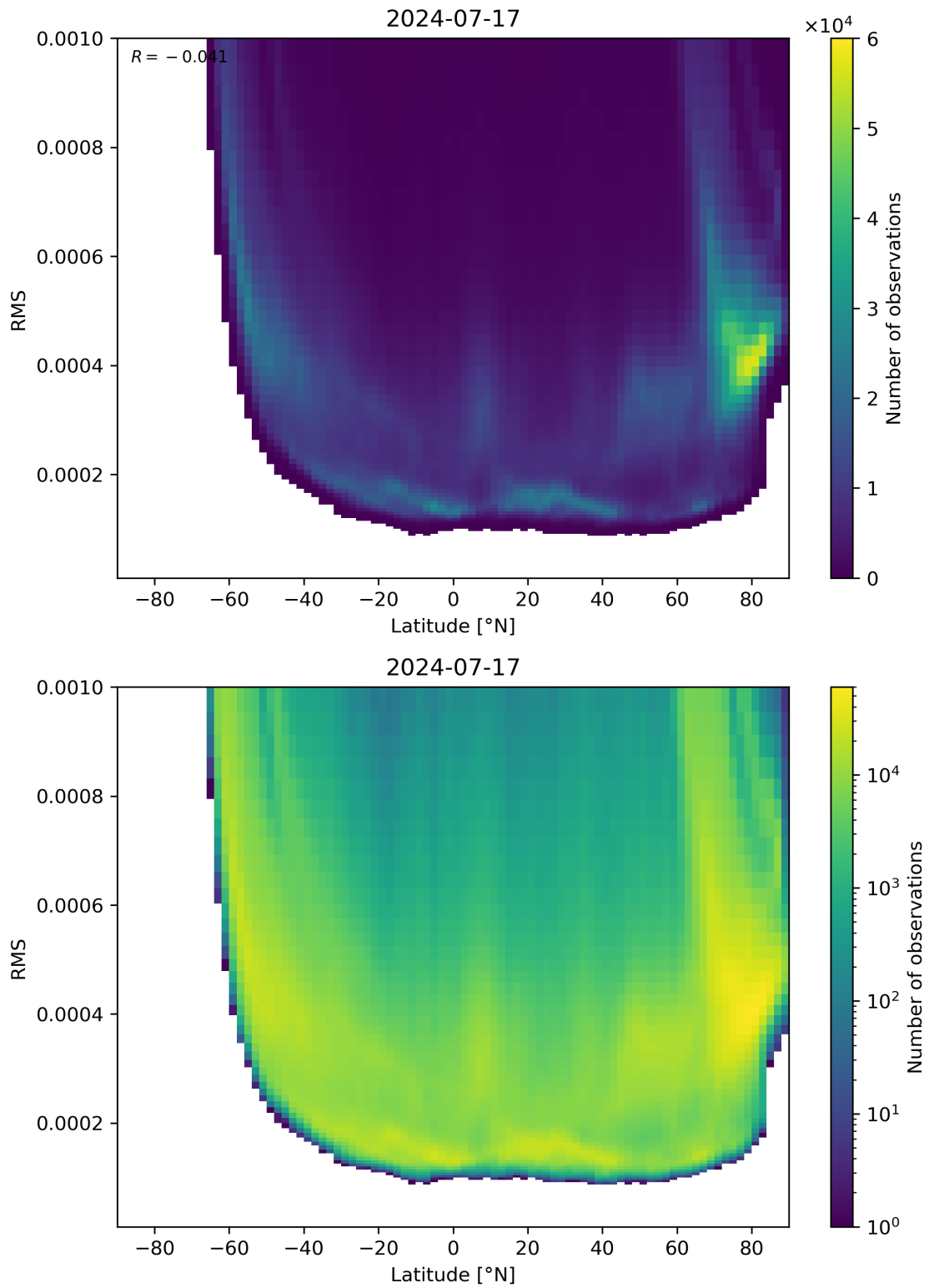
Figure 94: Scatter density plot of “Latitude” against “RMS” for 2024-07-16 to 2024-07-18.
