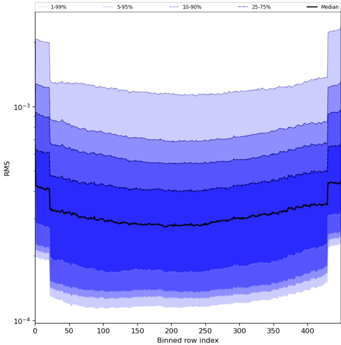
Figure 60: Along track statistics of “RMS” for 2024-07-16 to 2024-07-18
