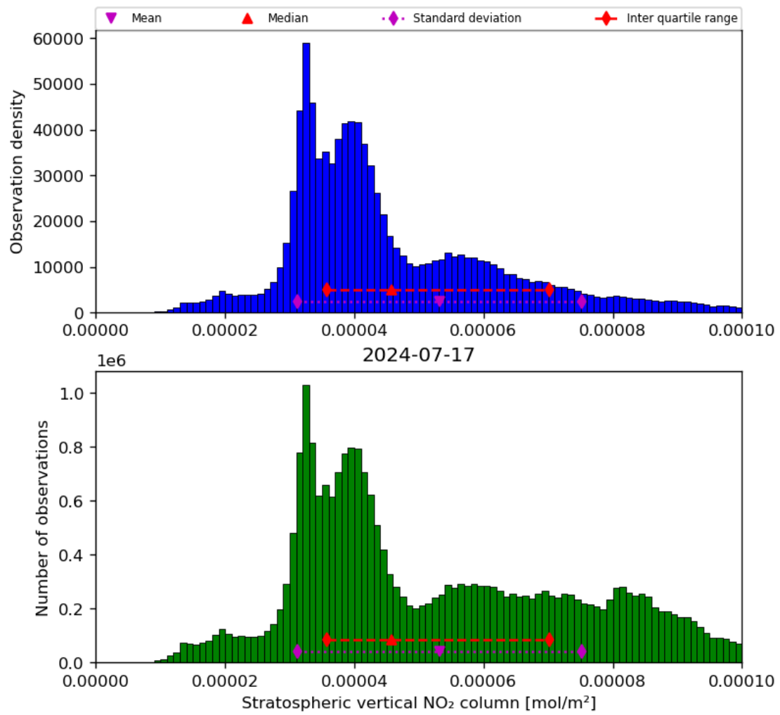
Figure 36: Histogram of “Stratospheric vertical NO 2 column” for 2024-07-16 to 2024-07-18
