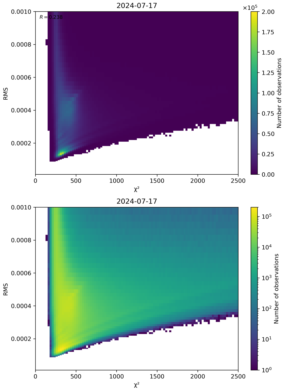
Figure 82: Scatter density plot of “ \chi^2 ” against “RMS” for 2024-07-16 to 2024-07-18.
