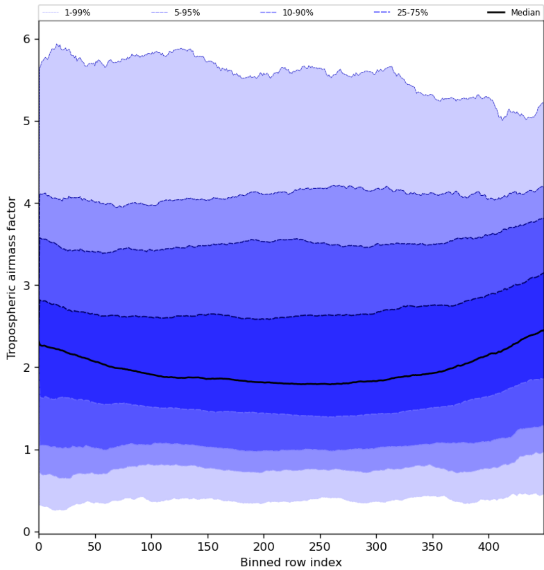
Figure 48: Along track statistics of “Tropospheric airmass factor” for 2024-07-16 to 2024-07-18
