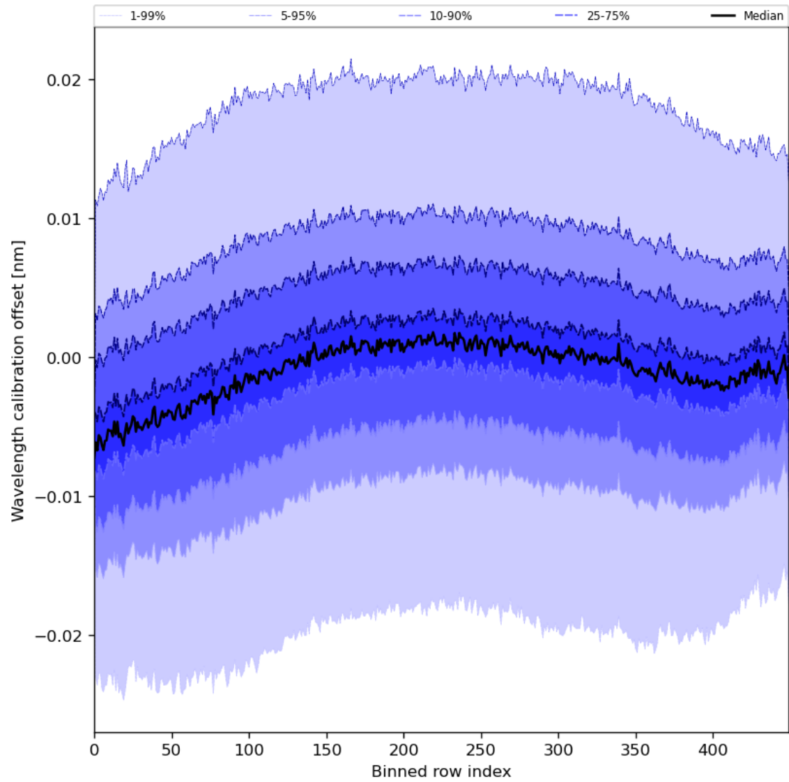
Figure 52: Along track statistics of “Wavelength calibration offset” for 2024-07-16 to 2024-07-18
