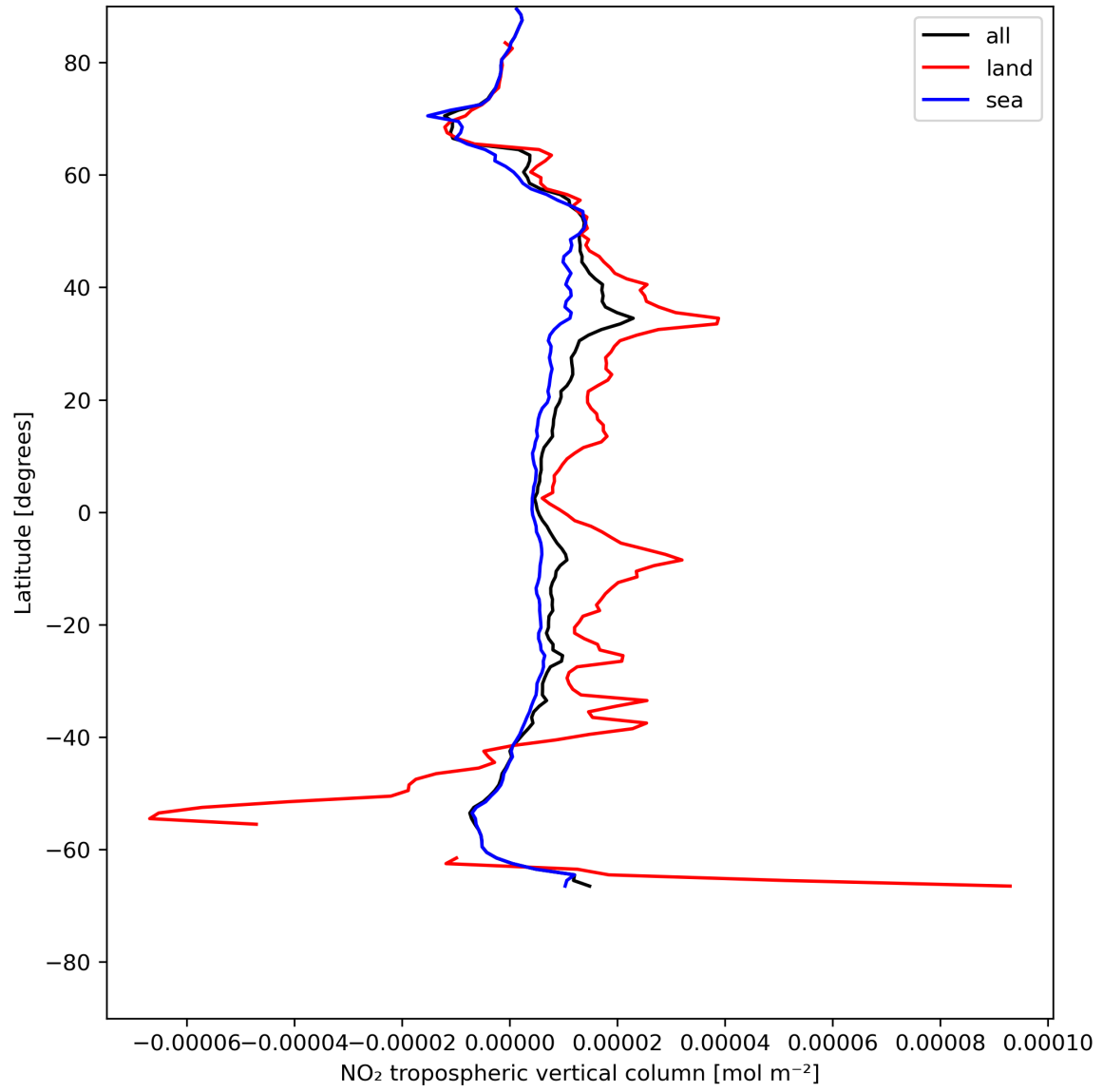
Figure 12: Zonal average of “NO 2 tropospheric vertical column” for 2024-07-16 to 2024-07-18.
