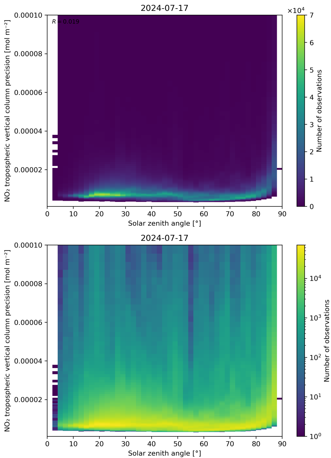
Figure 156: Scatter density plot of “Solar zenith angle” against “NO 2 tropospheric vertical column precision” for 2024-07-16 to 2024-07-18.
