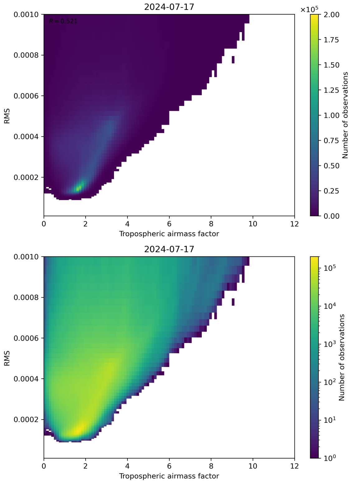
Figure 79: Scatter density plot of “Tropospheric airmass factor” against “RMS” for 2024-07-16 to 2024-07-18.
