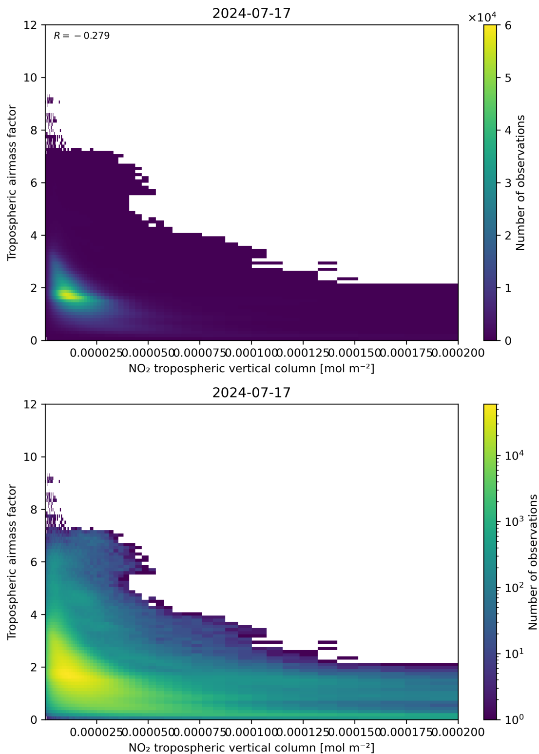
Figure 123: Scatter density plot of “NO 2 tropospheric vertical column” against “Tropospheric airmass factor” for 2024-07-16 to 2024-07-18.
