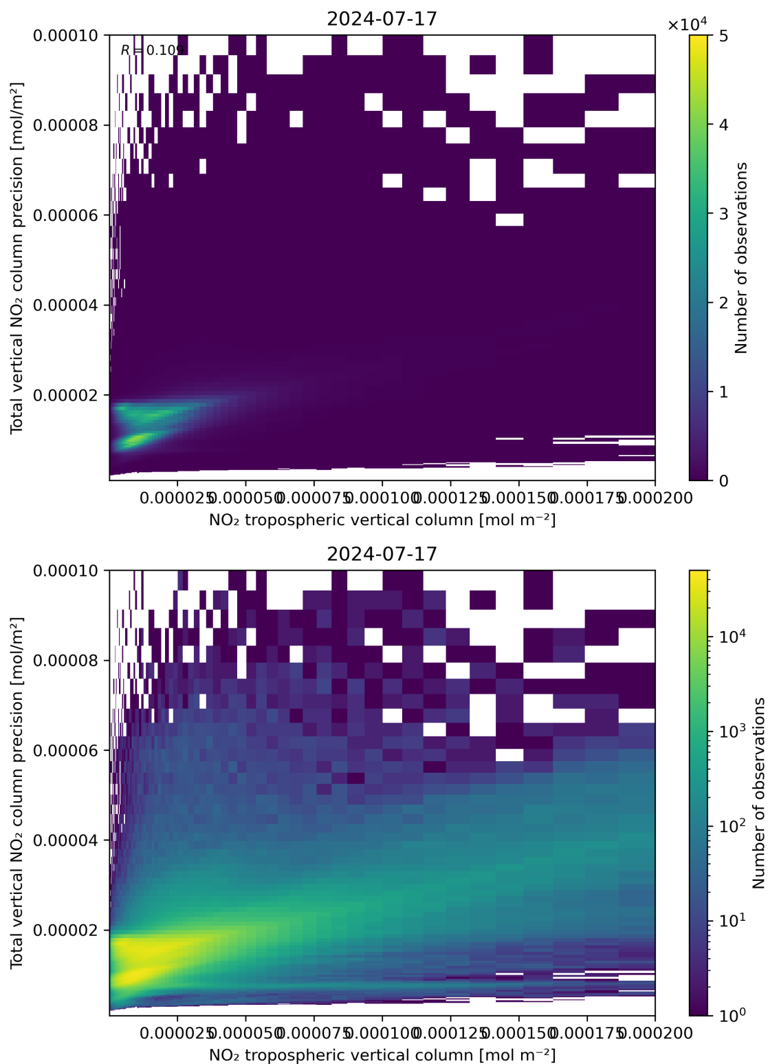
Figure 129: Scatter density plot of “NO 2 tropospheric vertical column” against “Total vertical NO 2 column precision” for 2024-07-16 to 2024-07-18.
