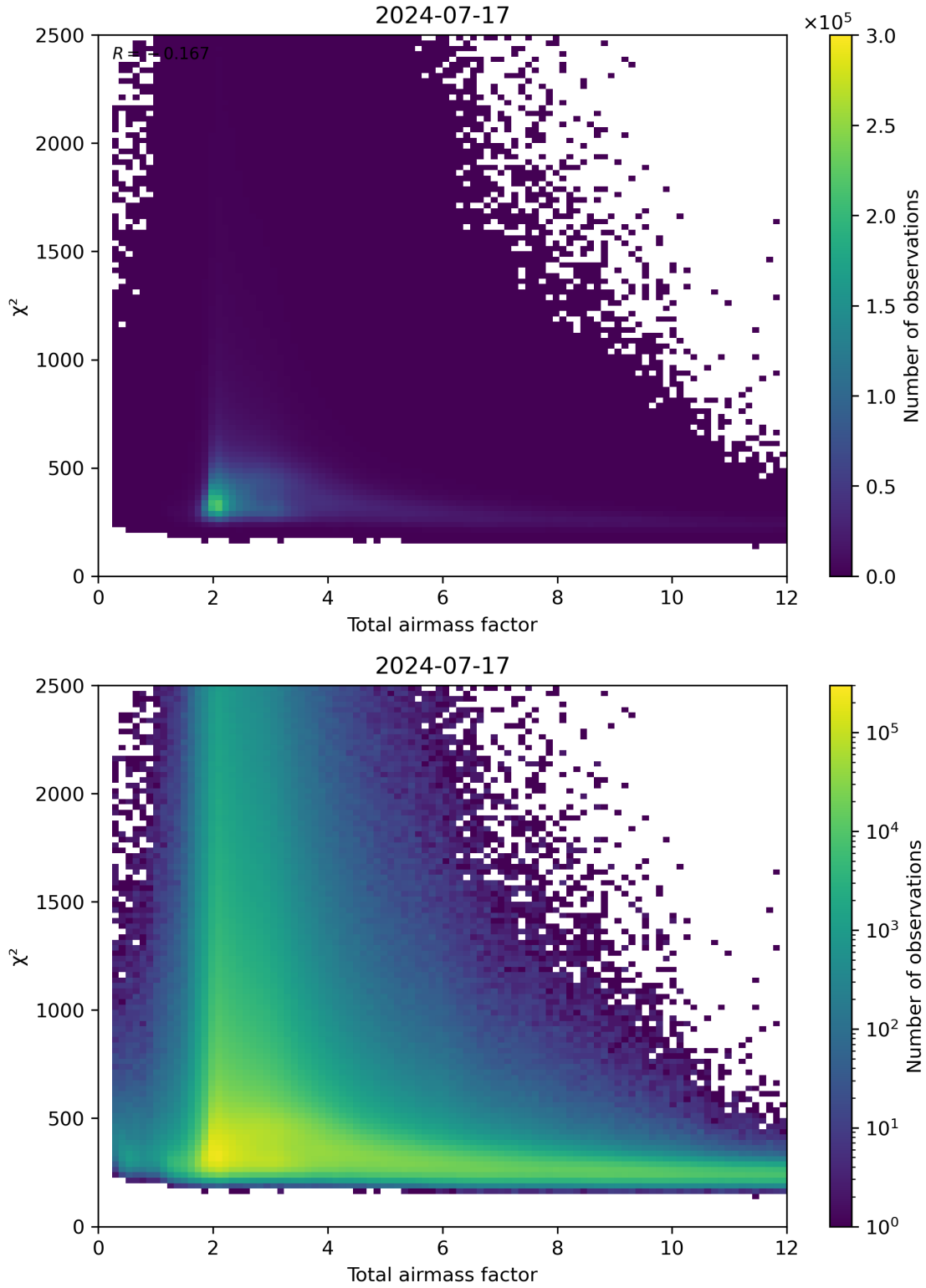
Figure 63: Scatter density plot of “Total airmass factor” against “ \chi^2 ” for 2024-07-16 to 2024-07-18.
