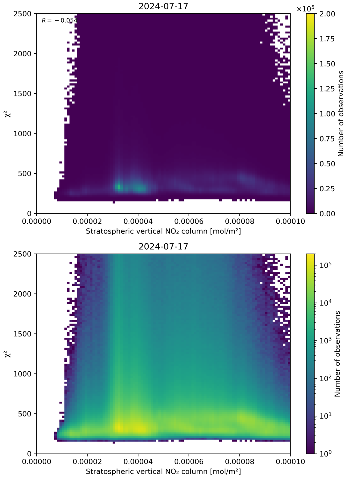
Figure 97: Scatter density plot of “Stratospheric vertical NO 2 column” against “ \chi^2 ” for 2024-07-16 to 2024-07-18.
