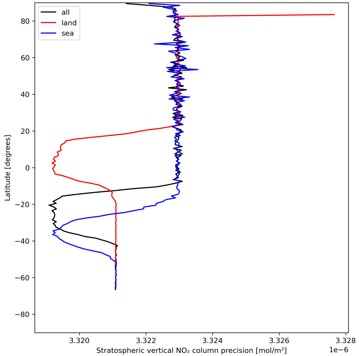
Figure 20: Zonal average of “Stratospheric vertical NO 2 column precision” for 2024-07-16 to 2024-07-18.
