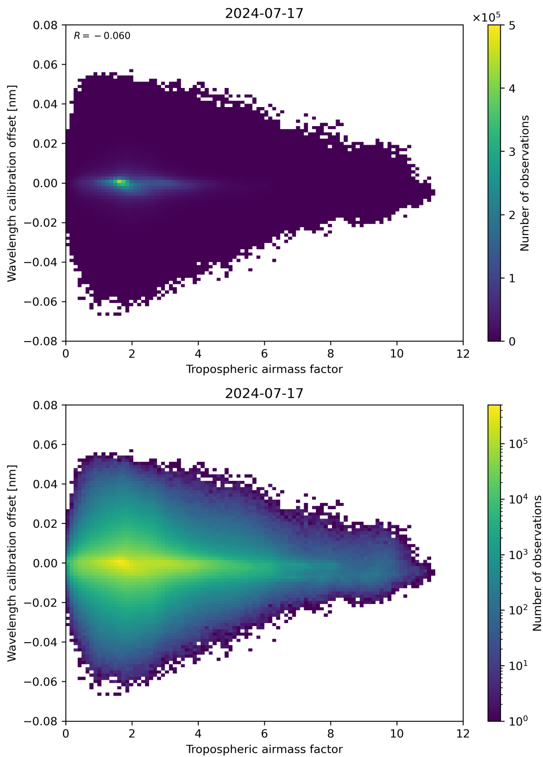
Figure 80: Scatter density plot of “Tropospheric air mass factor” against “Wavelength calibration offset” for 2024-07-16 to 2024-07-18.
