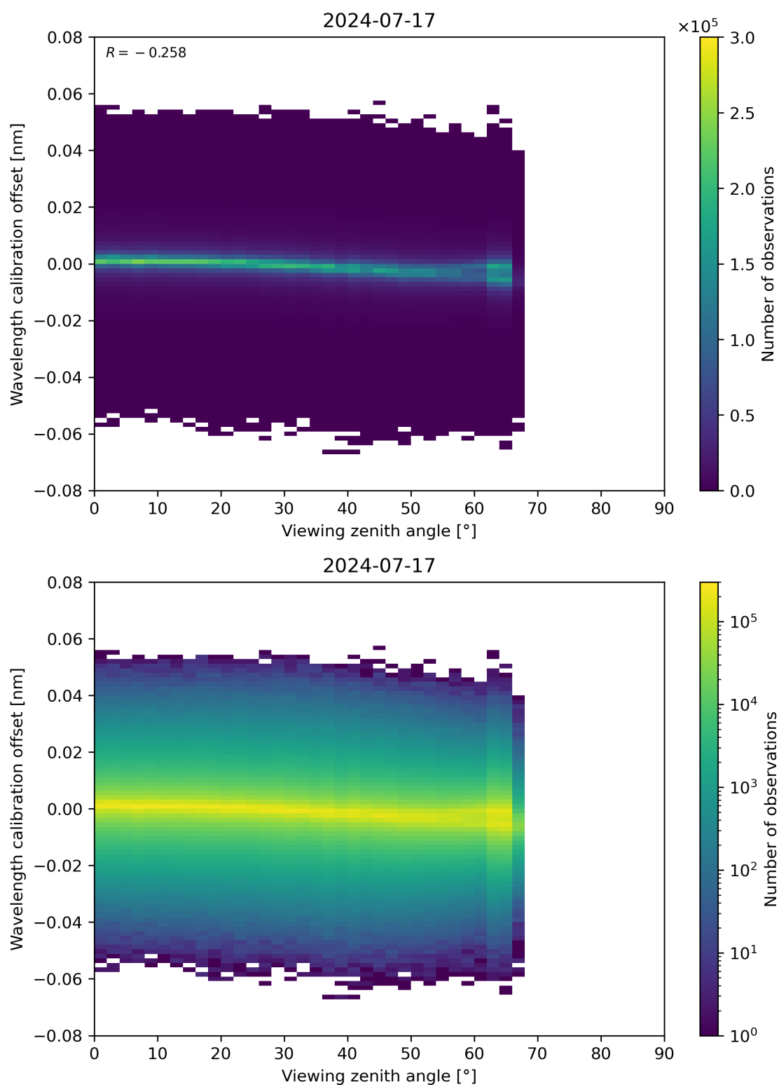
Figure 173: Scatter density plot of “Viewing zenith angle” against “Wavelength calibration offset” for 2024-07-16 to 2024-07-18.
