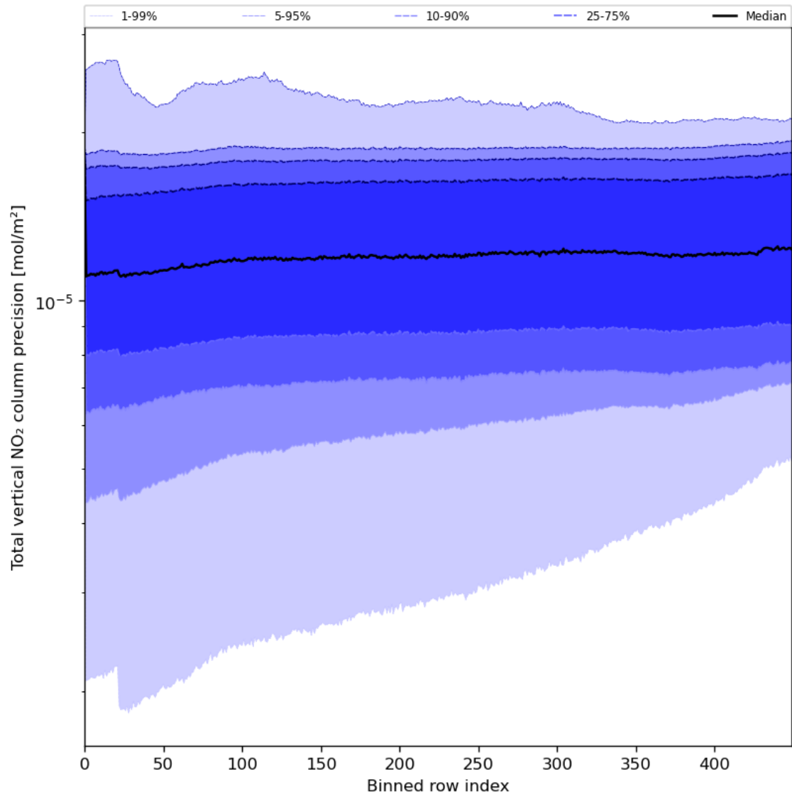
Figure 56: Along track statistics of “Total vertical NO 2 column precision” for 2024-07-16 to 2024-07-18
