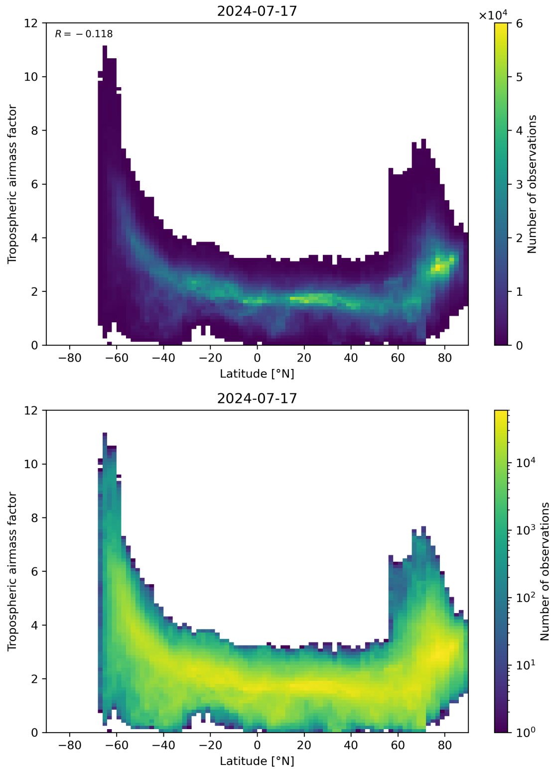
Figure 85: Scatter density plot of “Latitude” against “Tropospheric air mass factor” for 2024-07-16 to 2024-07-18.
