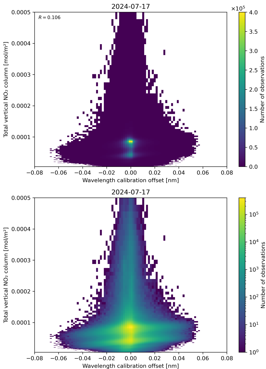
Figure 179: Scatter density plot of “Wavelength calibration offset” against “Total vertical NO 2 column” for 2024-07-16 to 2024-07-18.
