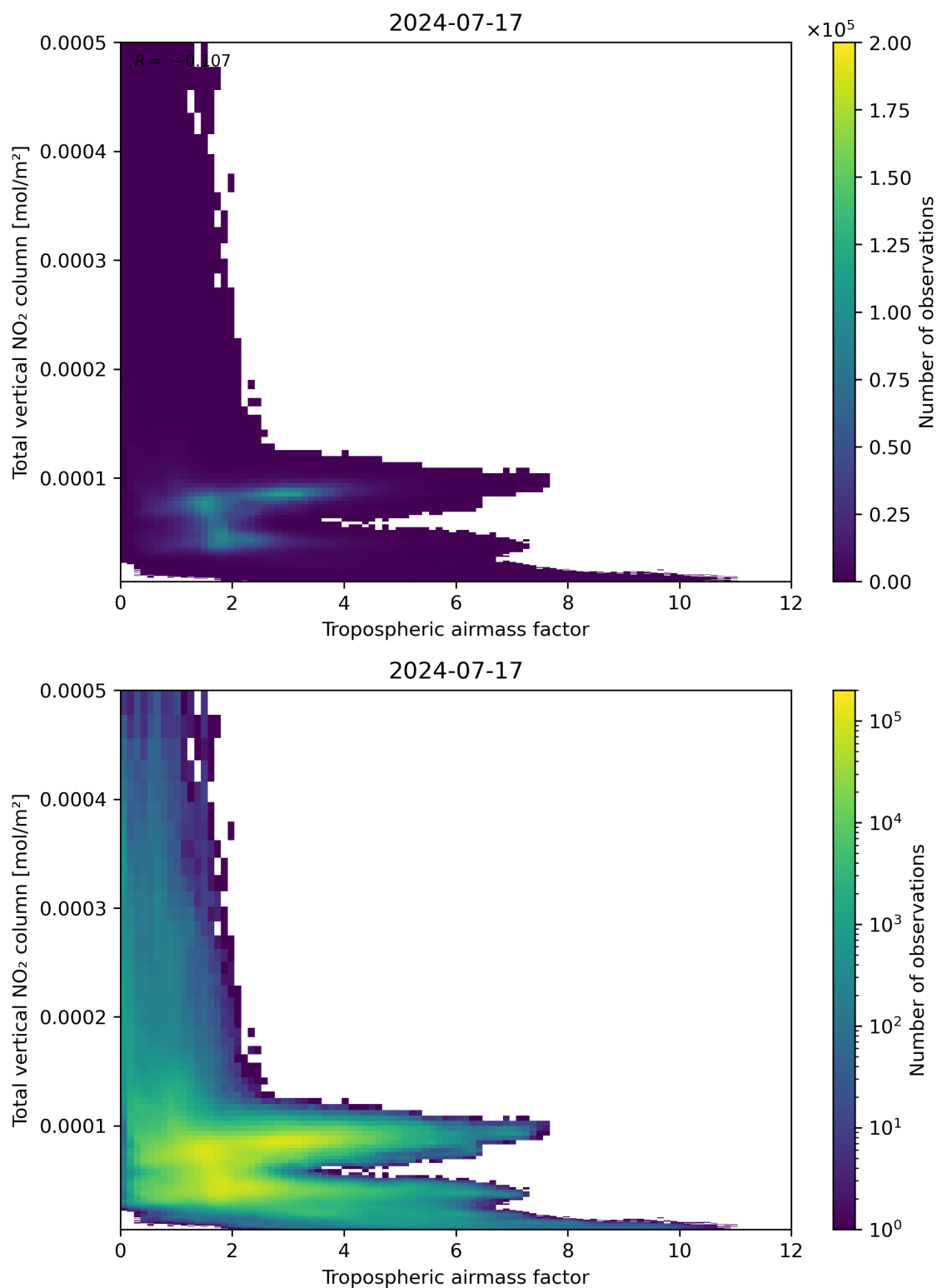
Figure 77: Scatter density plot of “Tropospheric airmass factor” against “Total vertical NO 2 column” for 2024-07-16 to 2024-07-18.
