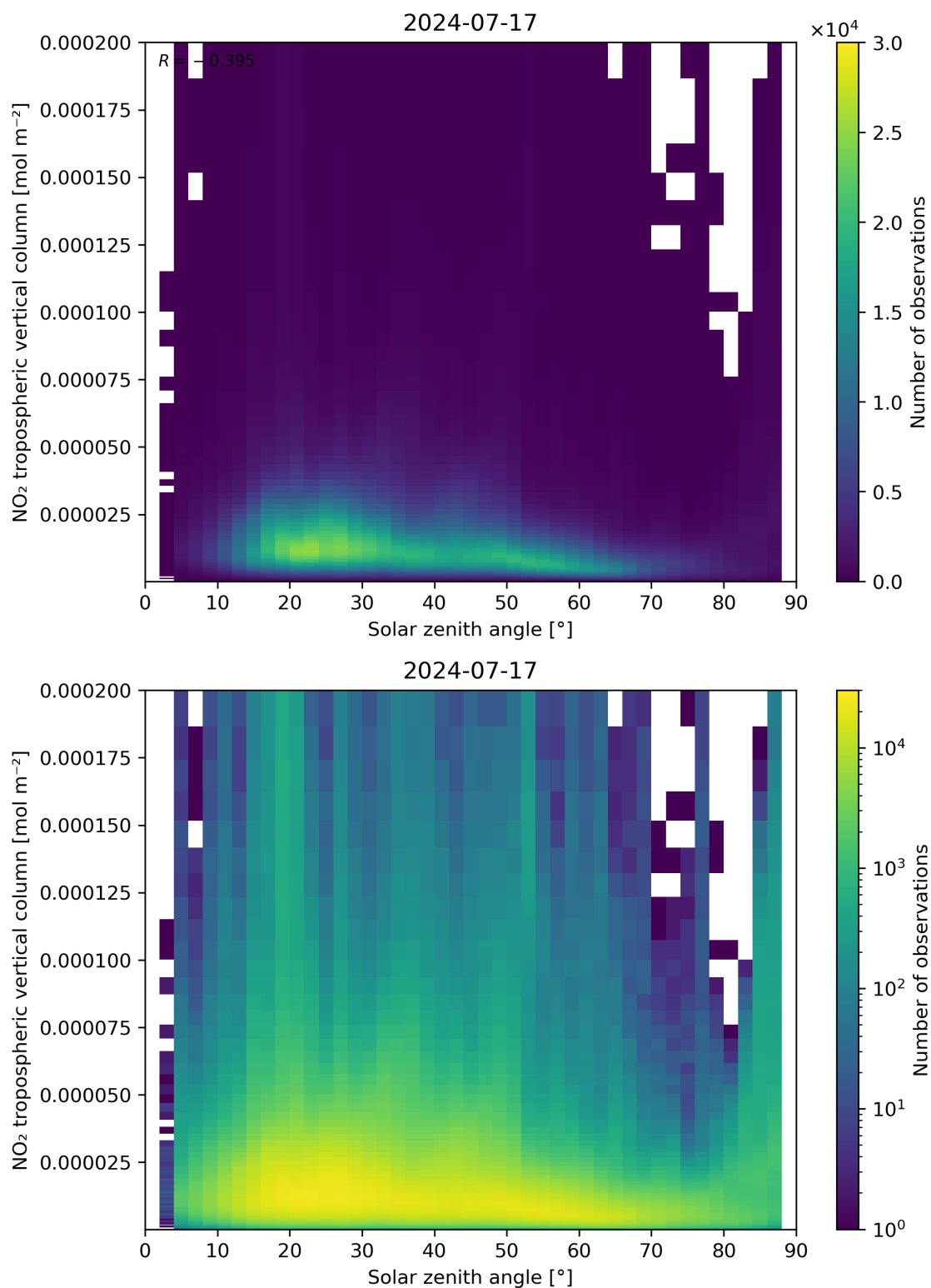
Figure 155: Scatter density plot of “Solar zenith angle” against “NO 2 tropospheric vertical column” for 2024-07-16 to 2024-07-18.
