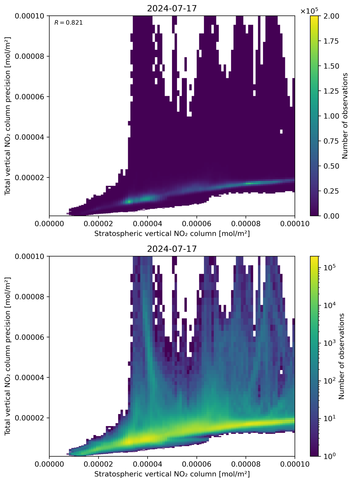
Figure 101: Scatter density plot of “Stratospheric vertical NO 2 column” against “Total vertical NO 2 column precision” for 2024-07-16 to 2024-07-18.
