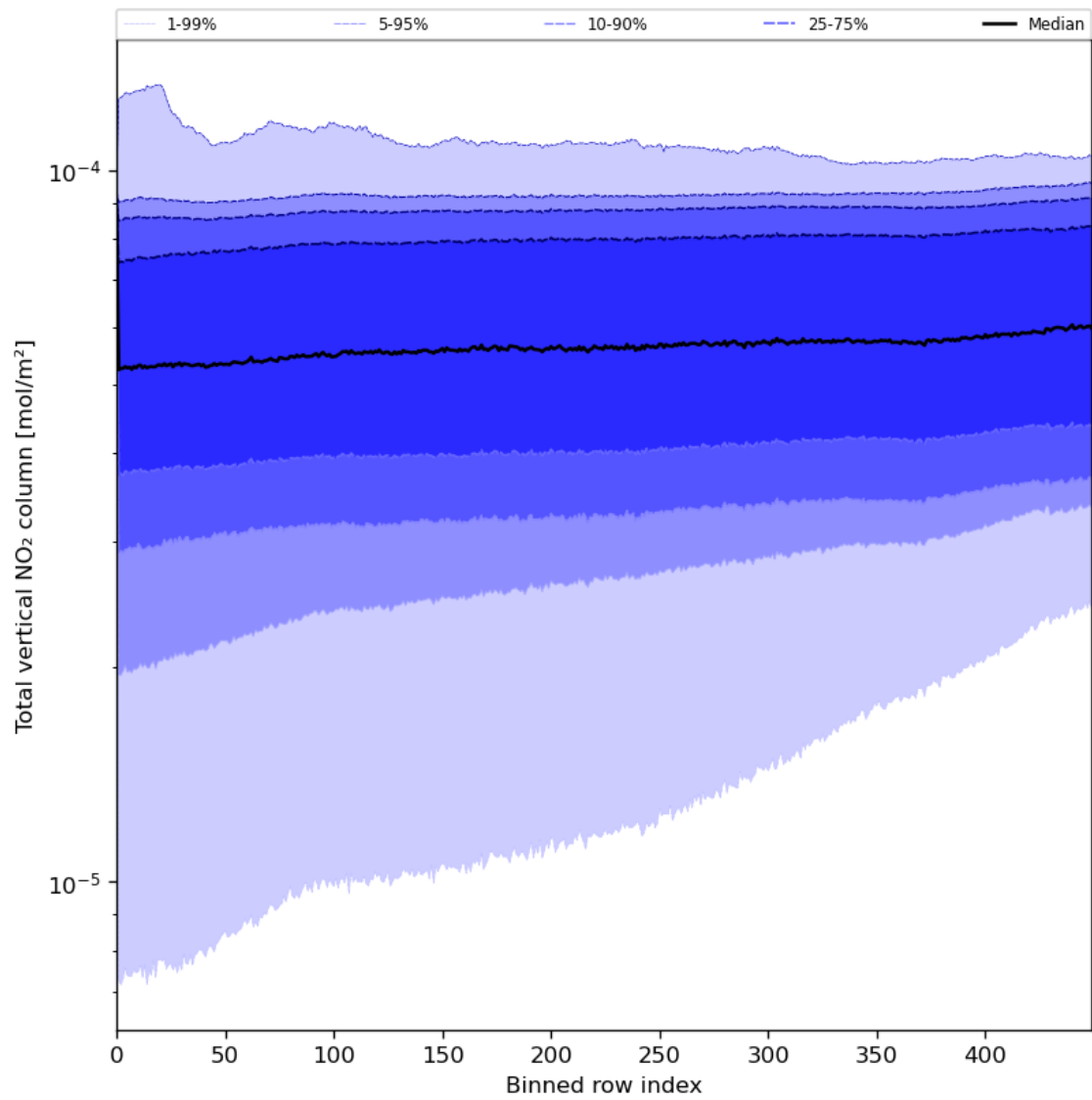
Figure 55: Along track statistics of “Total vertical NO 2 column” for 2024-07-16 to 2024-07-18
