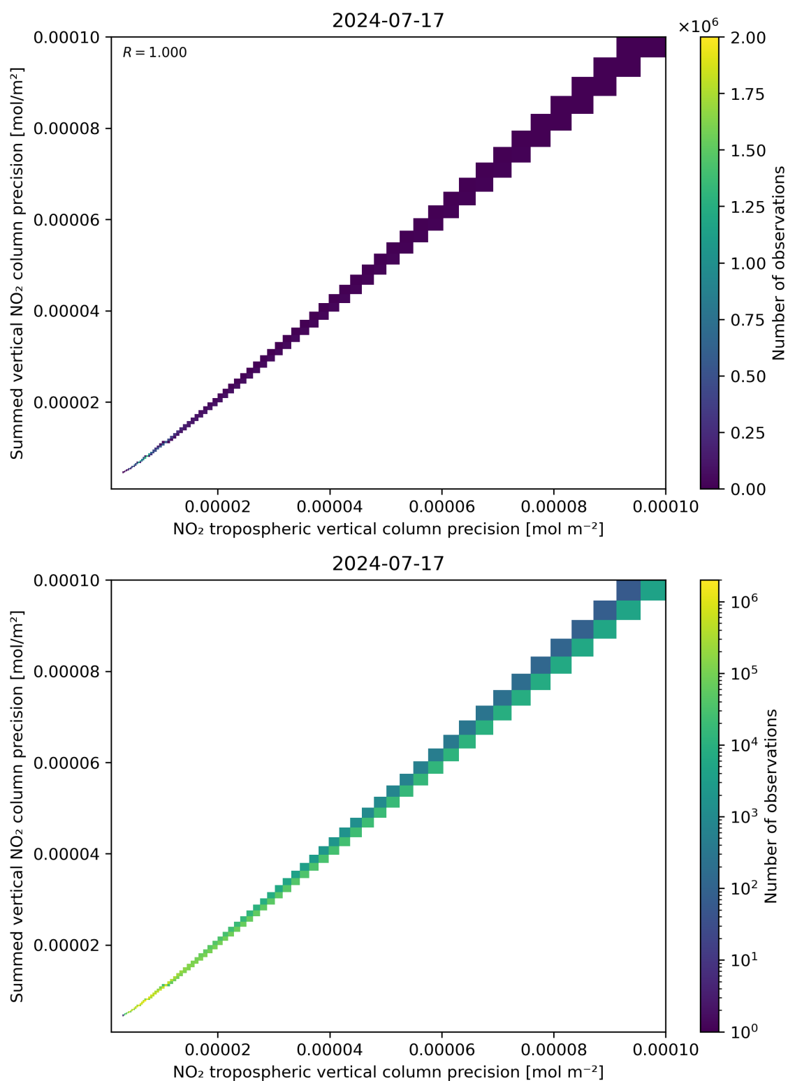
Figure 137: Scatter density plot of “NO 2 tropospheric vertical column precision” against “Summed vertical NO 2 column precision” for 2024-07-16 to 2024-07-18.
