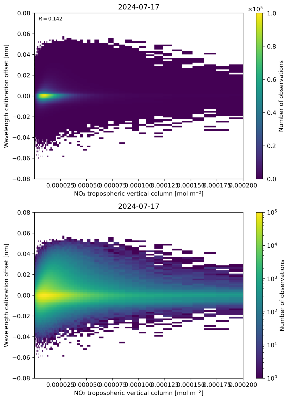
Figure 143: Scatter density plot of “NO 2 tropospheric vertical column” against “Wavelength calibration offset” for 2024-07-16 to 2024-07-18.
