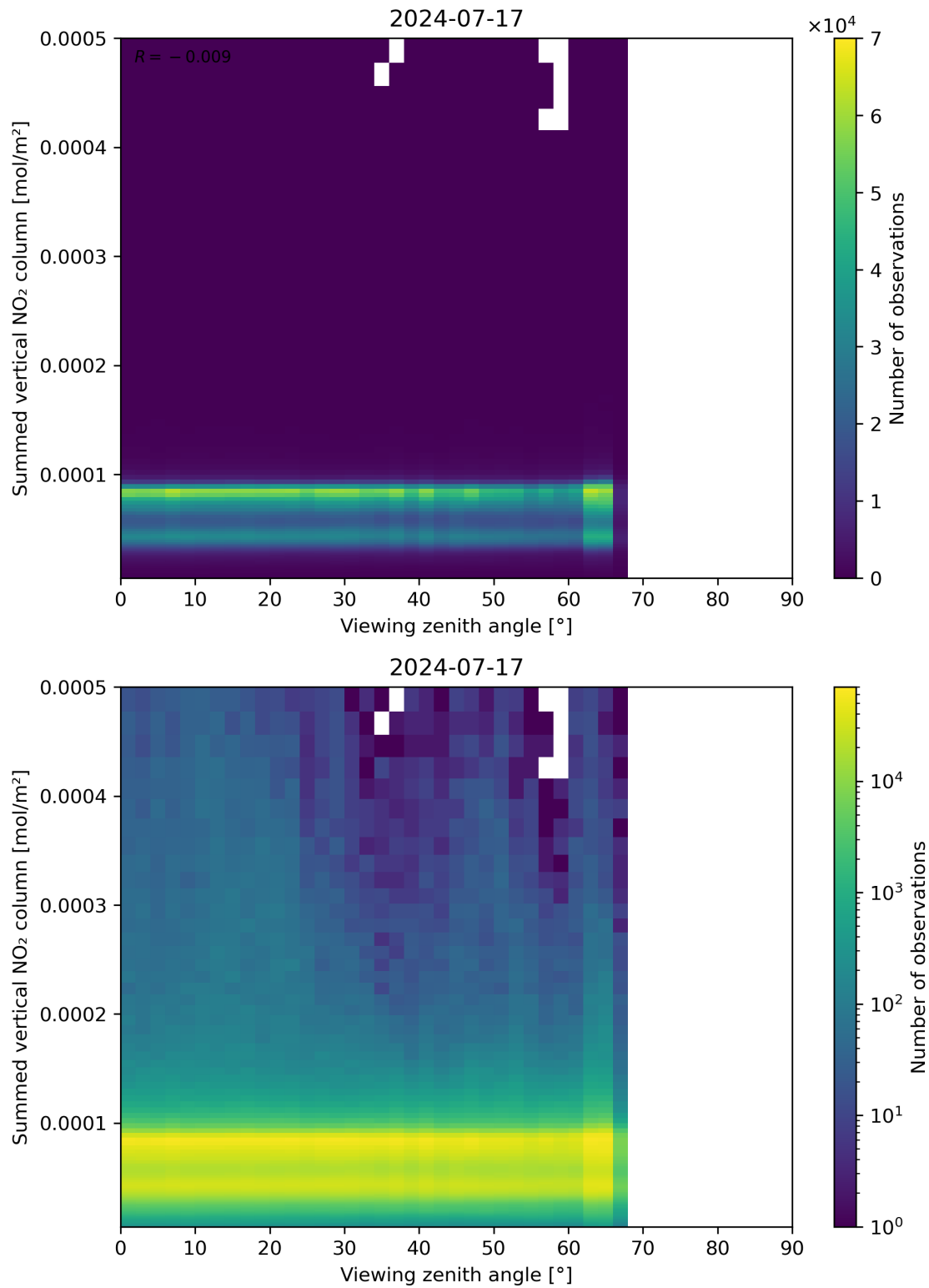
Figure 165: Scatter density plot of “Viewing zenith angle” against “Summed vertical NO 2 column” for 2024-07-16 to 2024-07-18.
