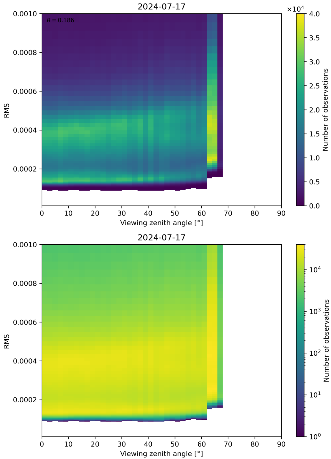
Figure 171: Scatter density plot of “Viewing zenith angle” against “RMS” for 2024-07-16 to 2024-07-18.
