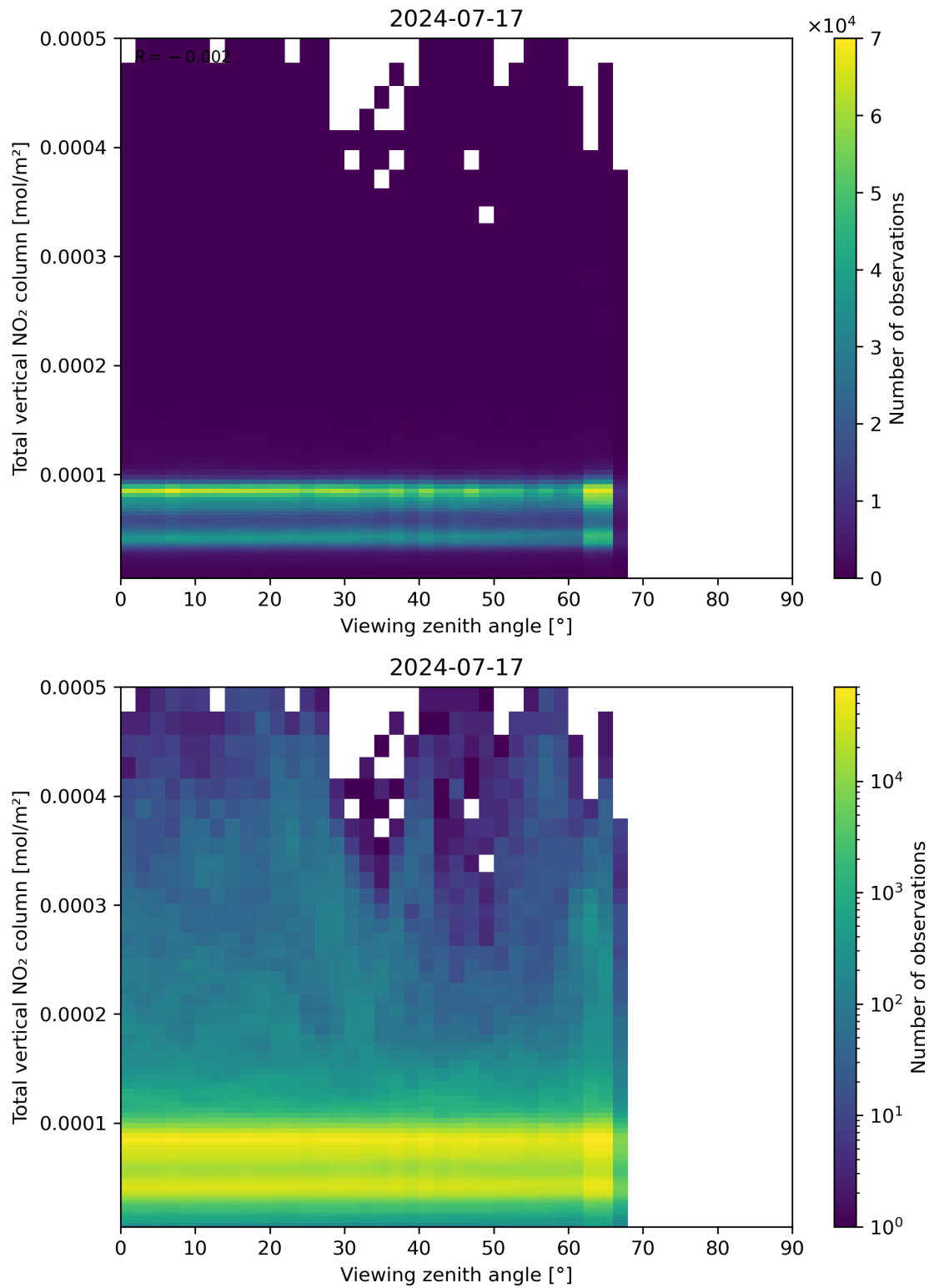
Figure 167: Scatter density plot of “Viewing zenith angle” against “Total vertical NO 2 column” for 2024-07-16 to 2024-07-18.
