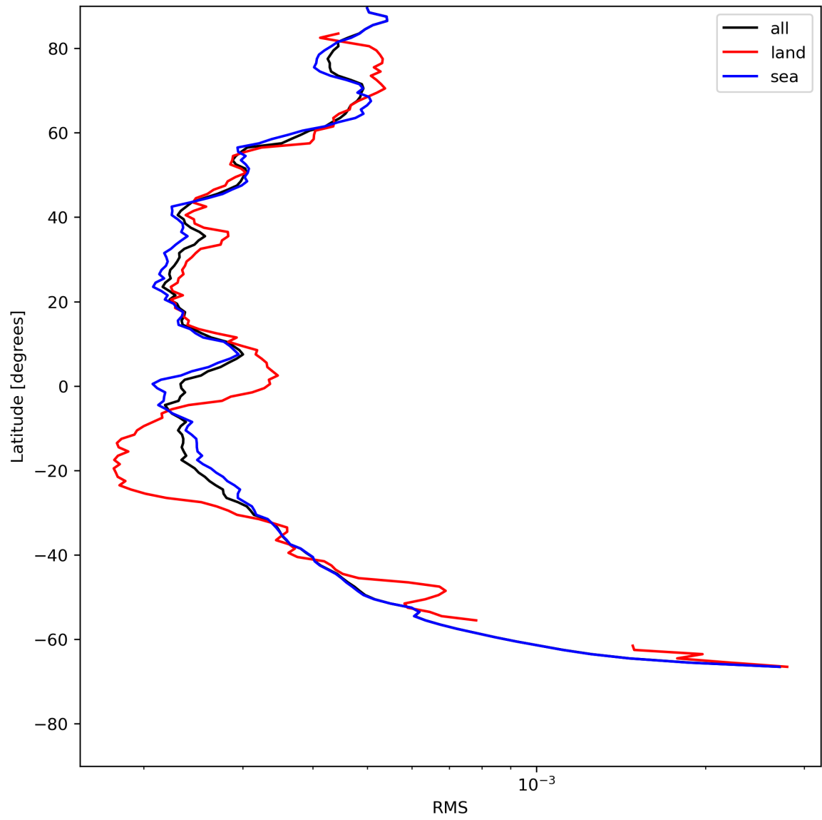
Figure 26: Zonal average of “RMS” for 2024-07-16 to 2024-07-18.
