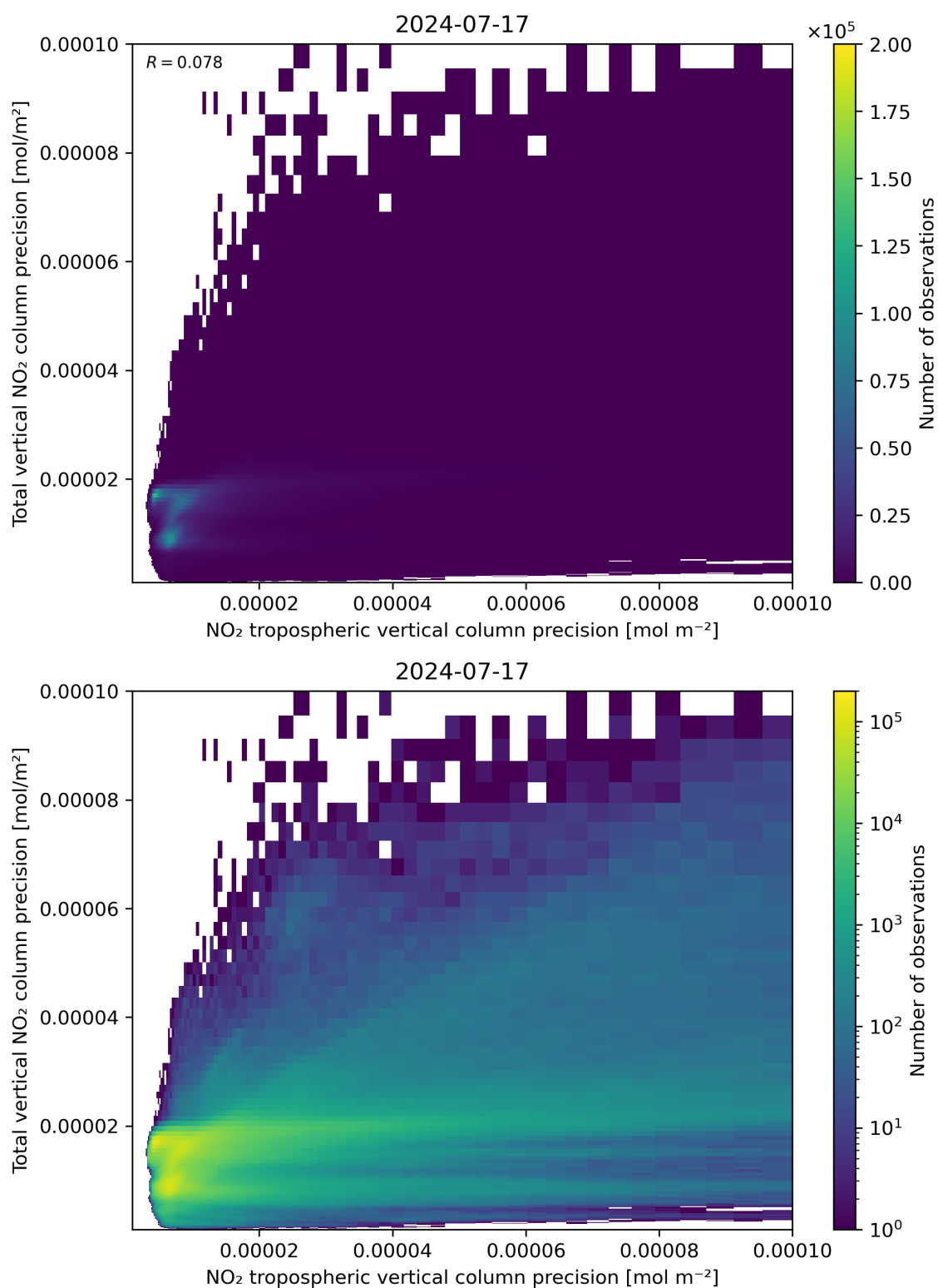
Figure 139: Scatter density plot of “NO 2 tropospheric vertical column precision” against “Total vertical NO 2 column precision” for 2024-07-16 to 2024-07-18.
