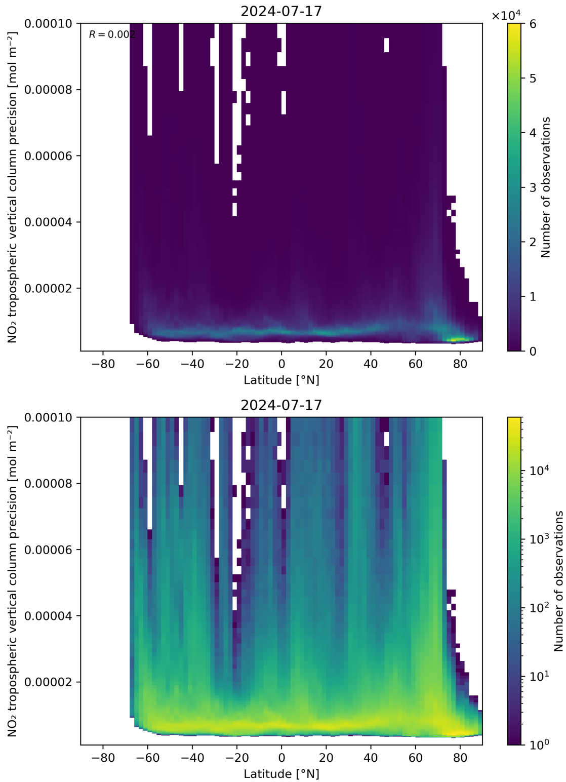
Figure 93: Scatter density plot of “Latitude” against “NO 2 tropospheric vertical column precision” for 2024-07-16 to 2024-07-18.
