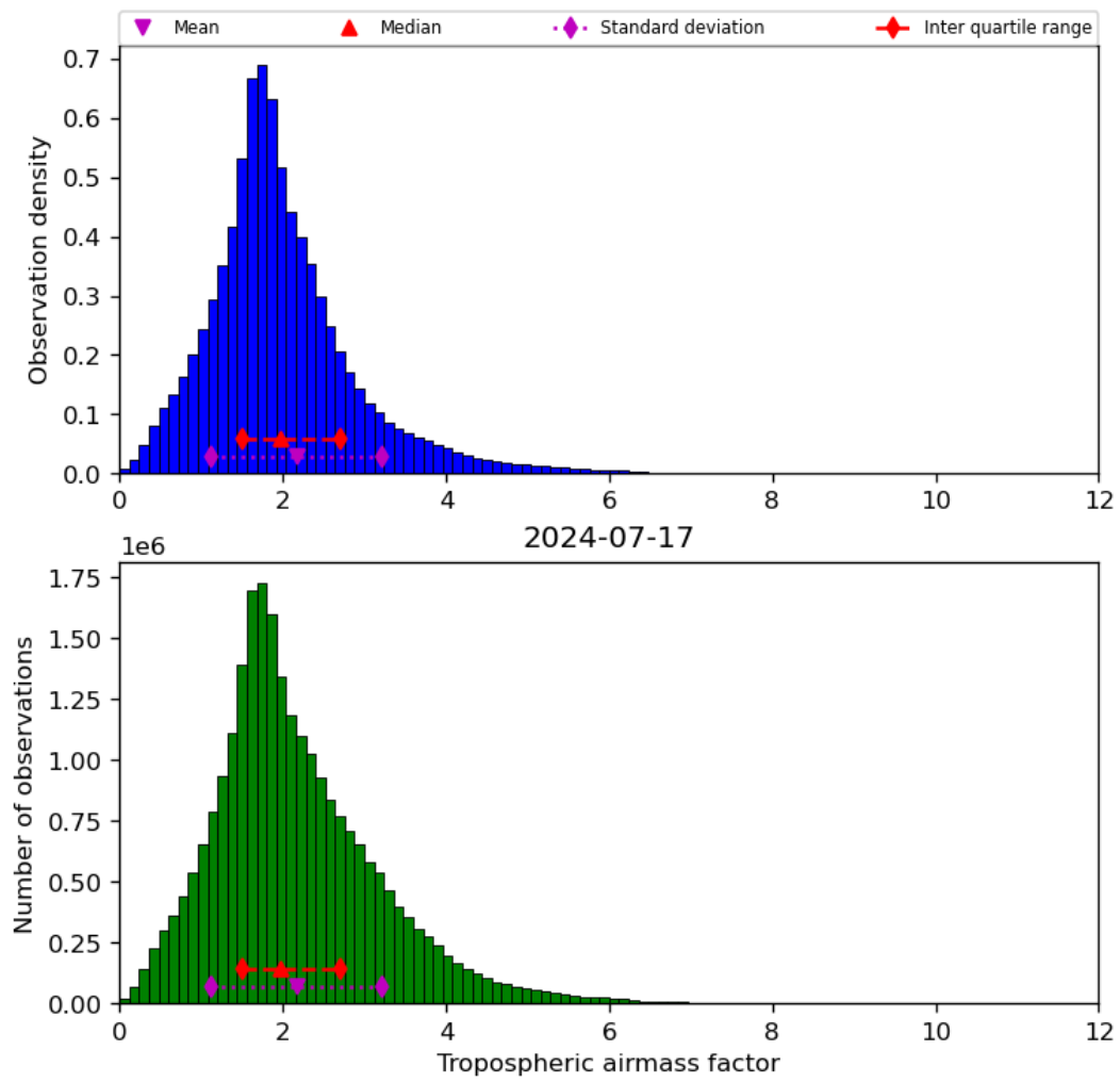
Figure 31: Histogram of “Tropospheric airmass factor” for 2024-07-16 to 2024-07-18
