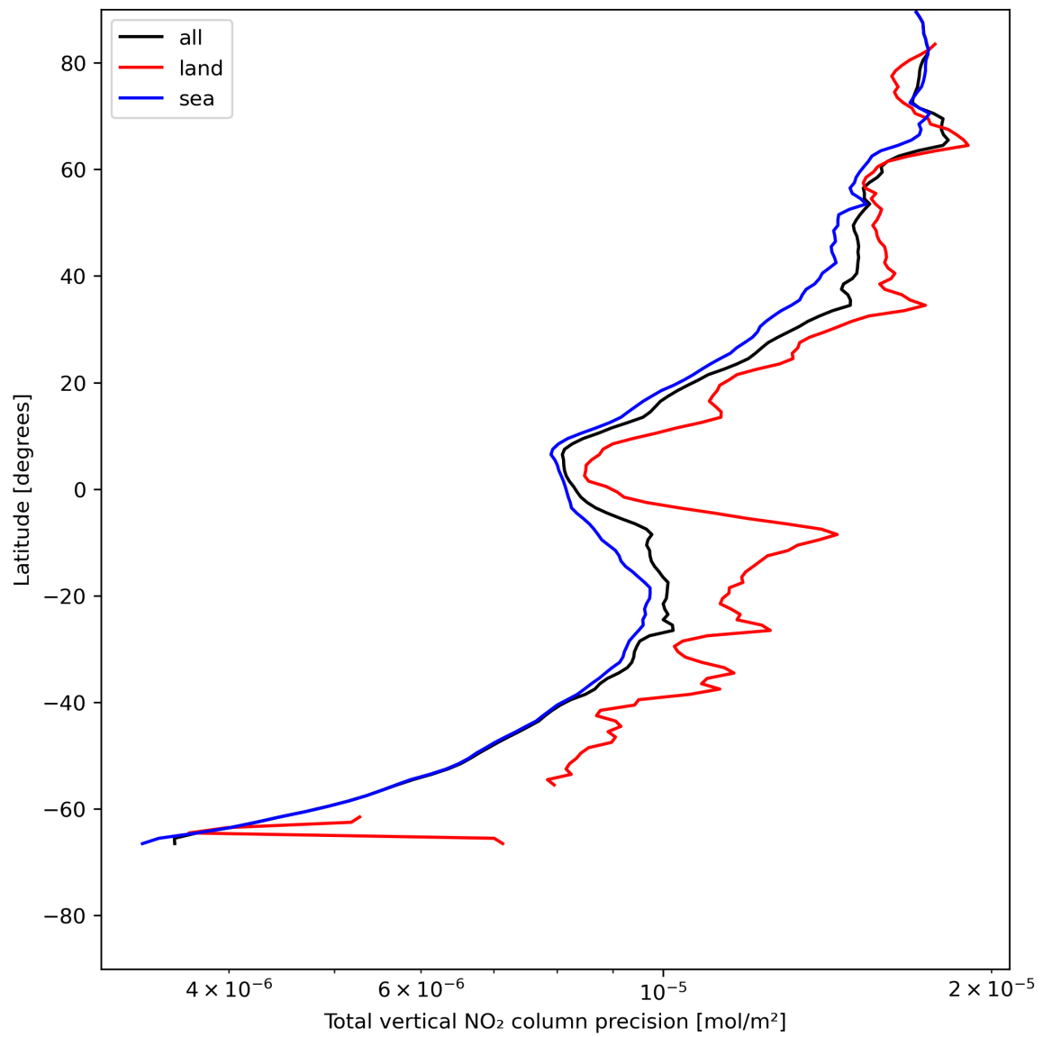
Figure 22: Zonal average of “Total vertical NO 2 column precision” for 2024-07-16 to 2024-07-18.
