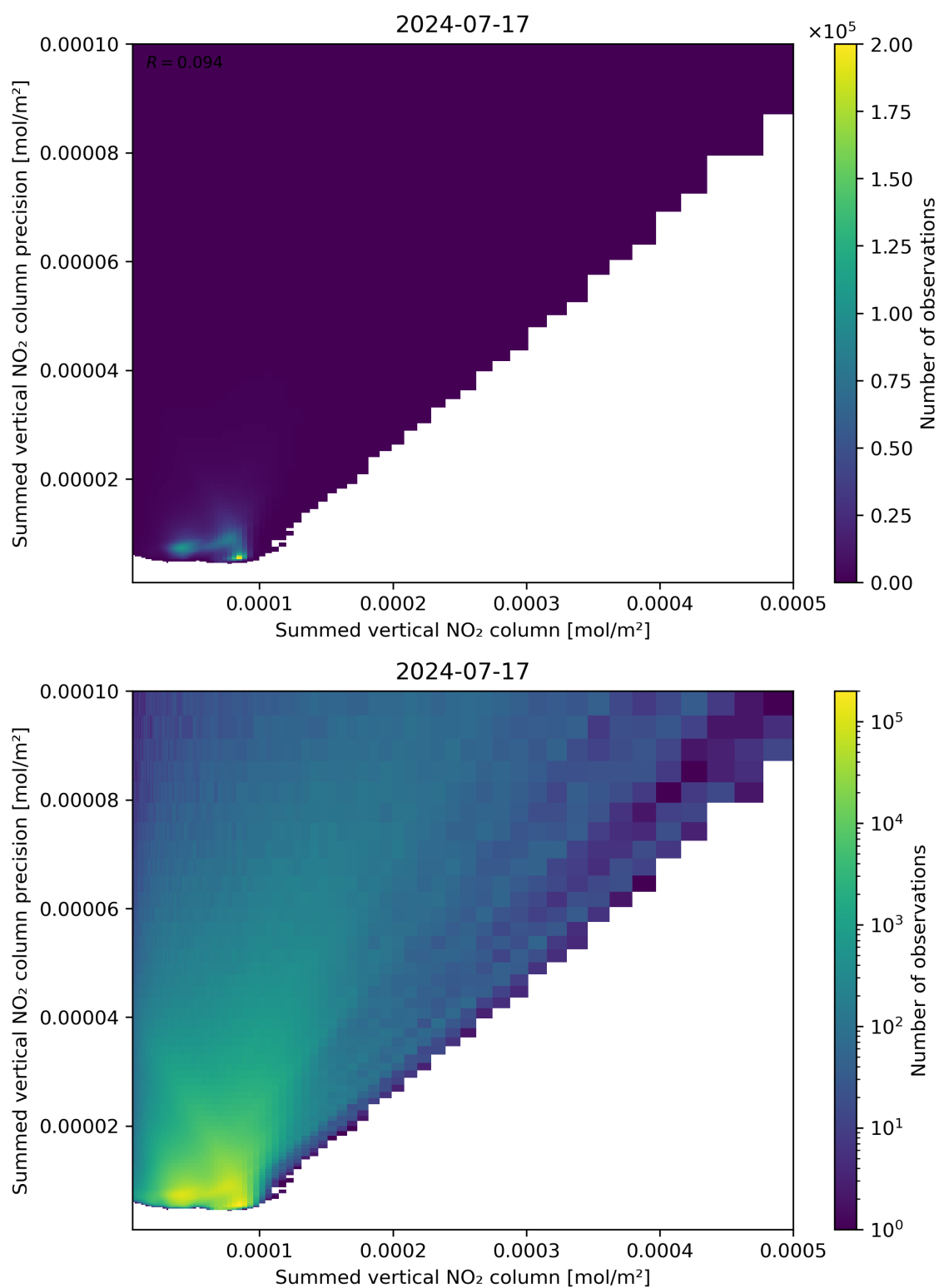
Figure 105: Scatter density plot of “Summed vertical NO 2 column” against “Summed vertical NO 2 column precision” for 2024-07-16 to 2024-07-18.
