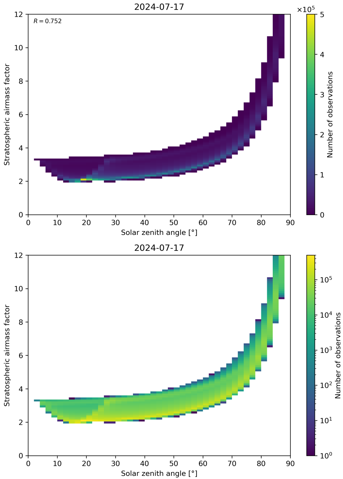
Figure 145: Scatter density plot of “Solar zenith angle” against “Stratospheric airmass factor” for 2024-07-16 to 2024-07-18.
