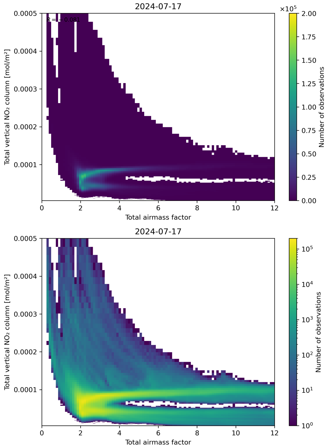
Figure 67: Scatter density plot of “Total airmass factor” against “Total vertical NO 2 column” for 2024-07-16 to 2024-07-18.
