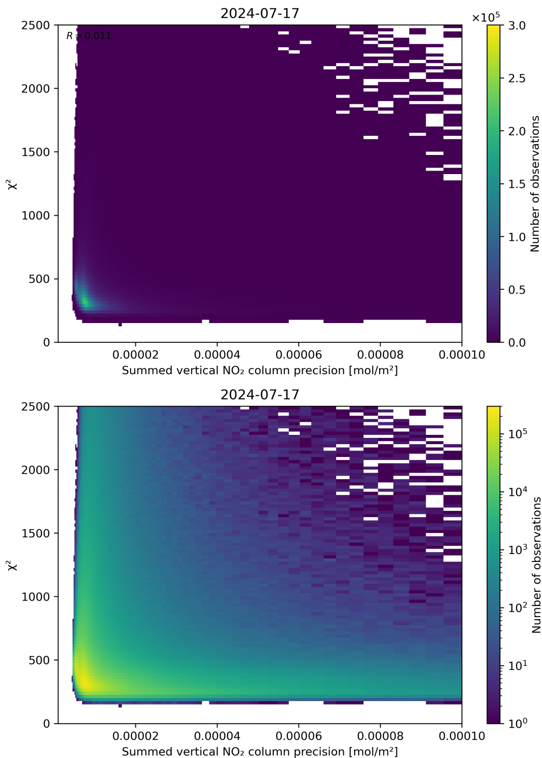
Figure 107: Scatter density plot of “Summed vertical NO 2 column precision” against “ \chi^2 ” for 2024-07-16 to 2024-07-18.
