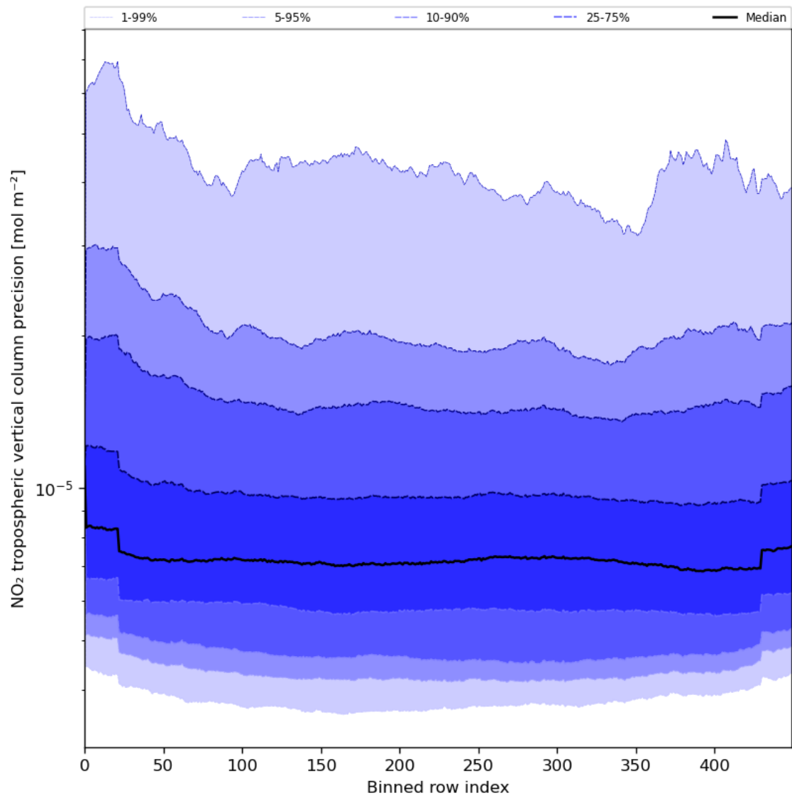
Figure 47: Along track statistics of “NO 2 tropospheric vertical column precision” for 2024-07-16 to 2024-07-18
