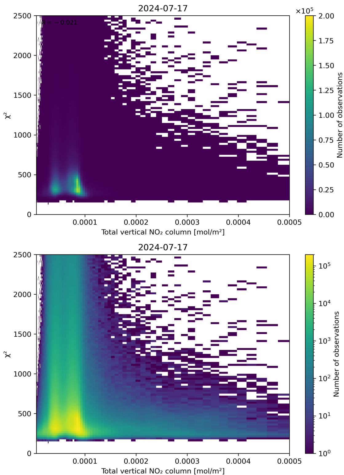
Figure 111: Scatter density plot of “Total vertical NO 2 column” against “ \chi^2 ” for 2024-07-16 to 2024-07-18.
