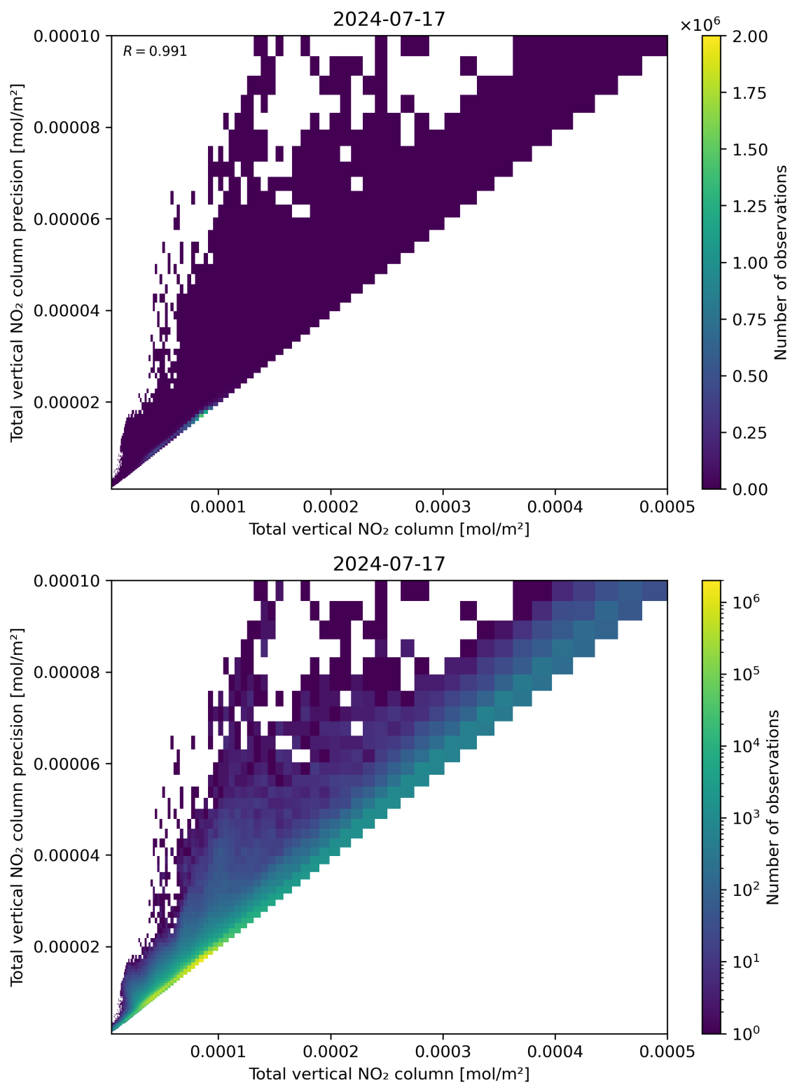
Figure 114: Scatter density plot of “Total vertical NO 2 column” against “Total vertical NO 2 column precision” for 2024-07-16 to 2024-07-18.
