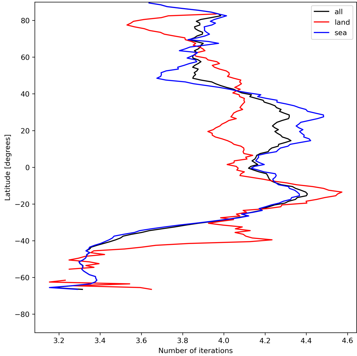
Figure 17: Zonal average of “Number of iterations” for 2024-07-16 to 2024-07-18.
