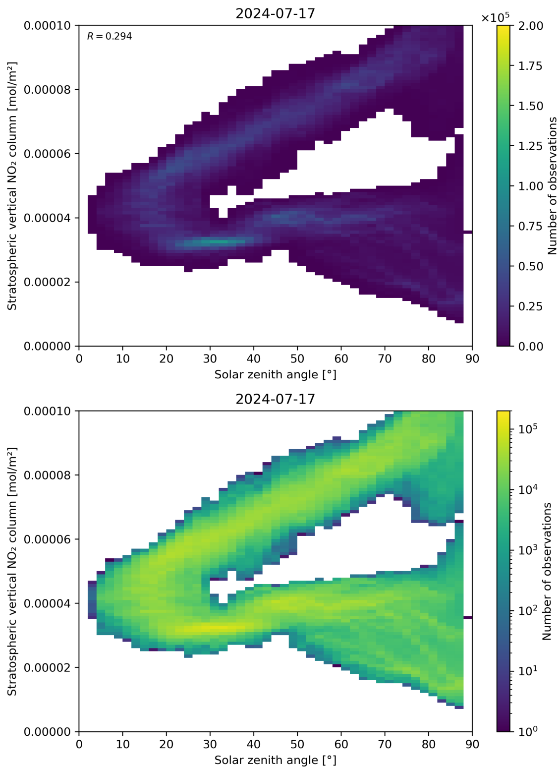
Figure 150: Scatter density plot of “Solar zenith angle” against “Stratospheric vertical NO 2 column” for 2024-07-16 to 2024-07-18.
