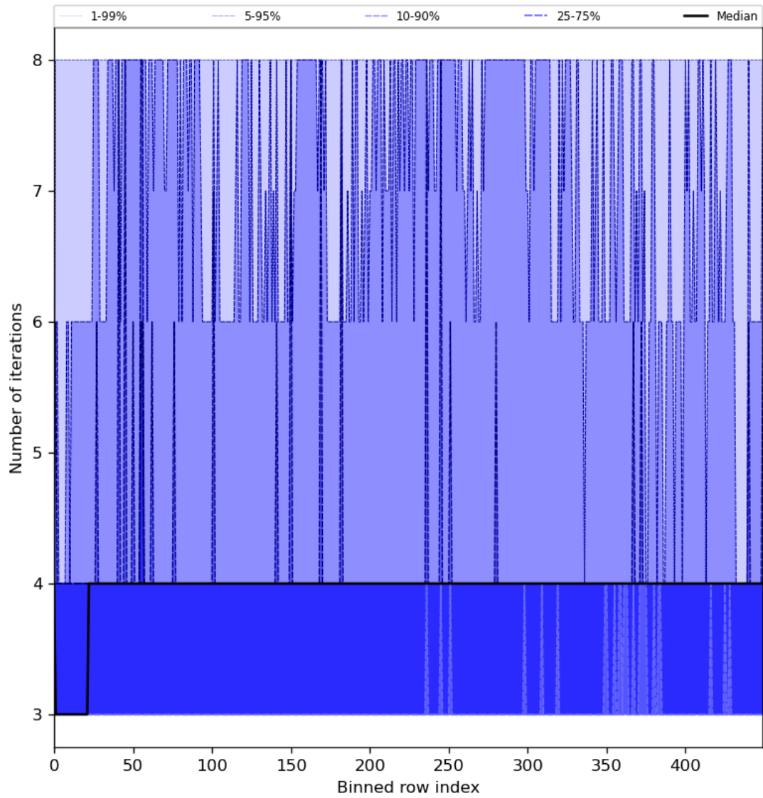
Figure 51: Along track statistics of “Number of iterations” for 2024-07-16 to 2024-07-18
