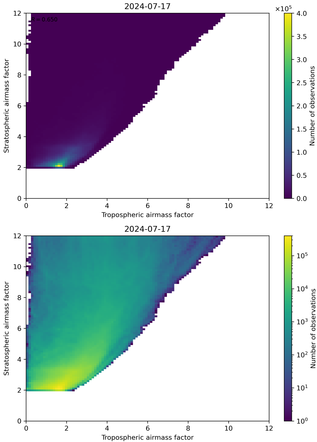
Figure 71: Scatter density plot of “Tropospheric airmass factor” against “Stratospheric airmass factor” for 2024-07-16 to 2024-07-18.
