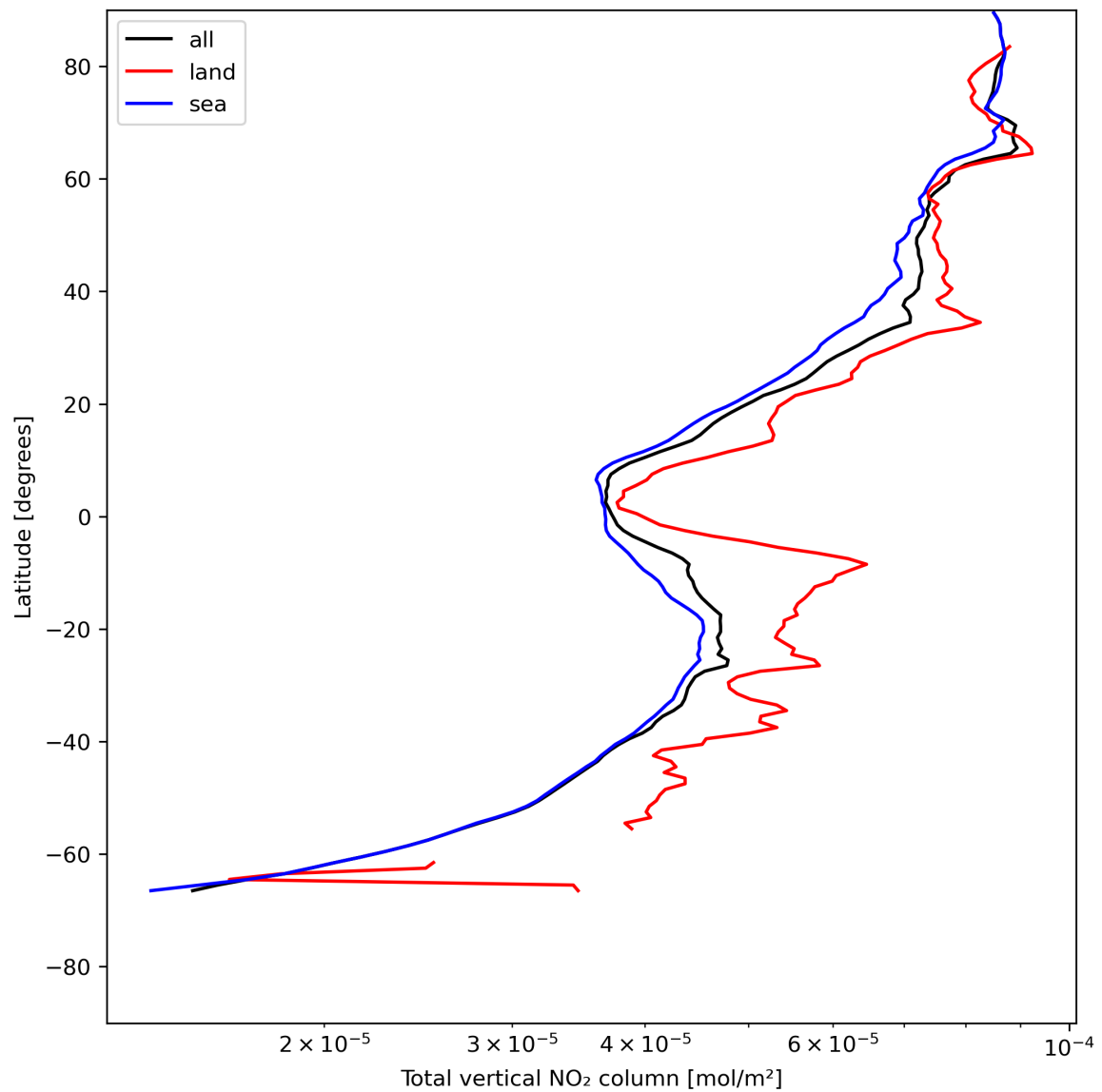
Figure 21: Zonal average of “Total vertical NO 2 column” for 2024-07-16 to 2024-07-18.
