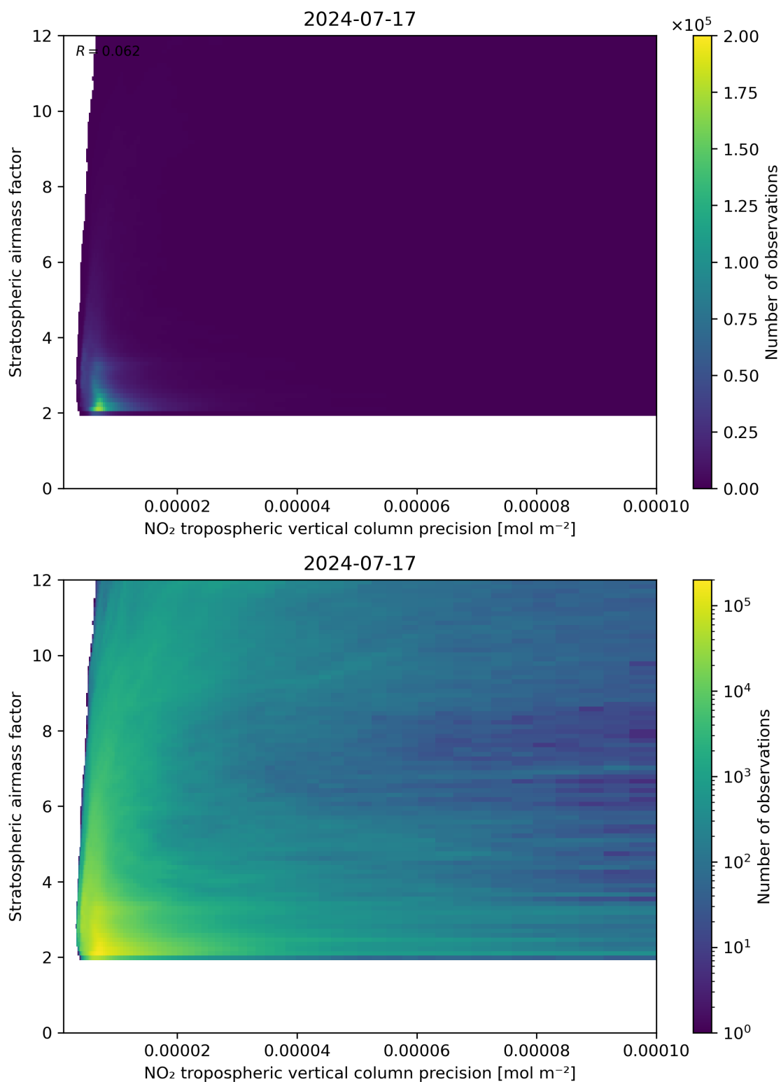
Figure 131: Scatter density plot of “NO 2 tropospheric vertical column precision” against “Stratospheric airmass factor” for 2024-07-16 to 2024-07-18.
