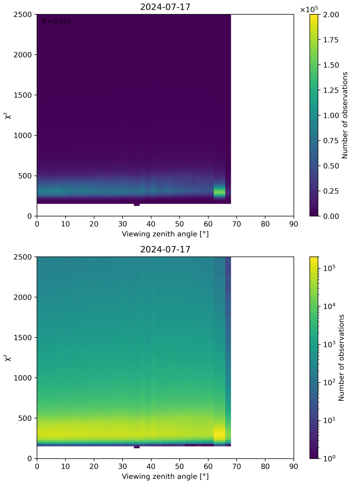
Figure 162: Scatter density plot of “Viewing zenith angle” against “ \chi^2 ” for 2024-07-16 to 2024-07-18.
