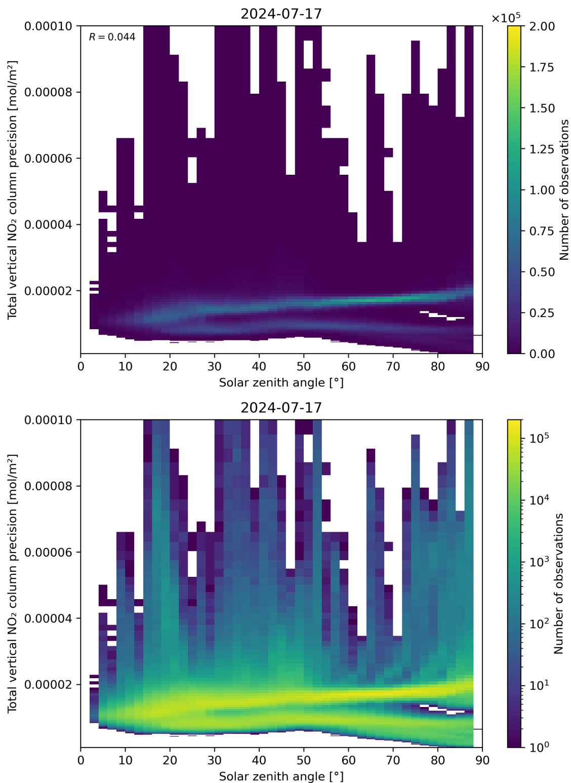
Figure 154: Scatter density plot of “Solar zenith angle” against “Total vertical NO 2 column precision” for 2024-07-16 to 2024-07-18.
