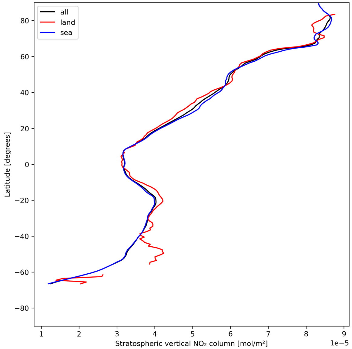
Figure 19: Zonal average of “Stratospheric vertical NO 2 column” for 2024-07-16 to 2024-07-18.
