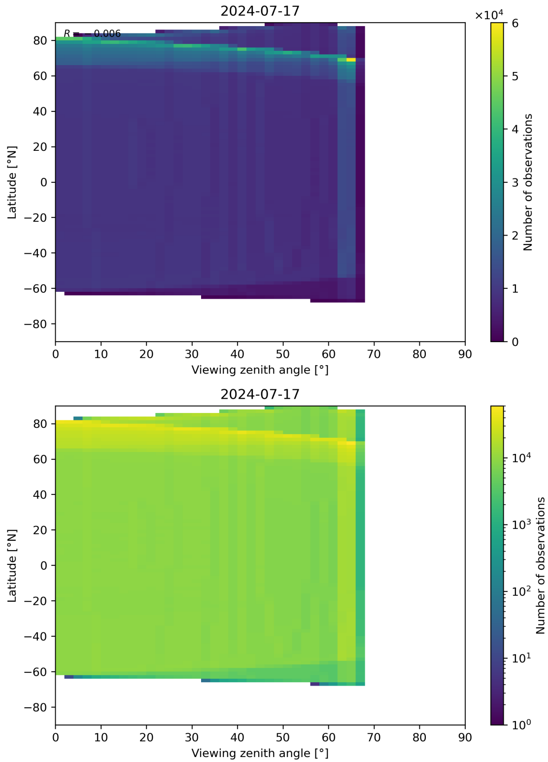
Figure 163: Scatter density plot of “Viewing zenith angle” against “Latitude” for 2024-07-16 to 2024-07-18.
