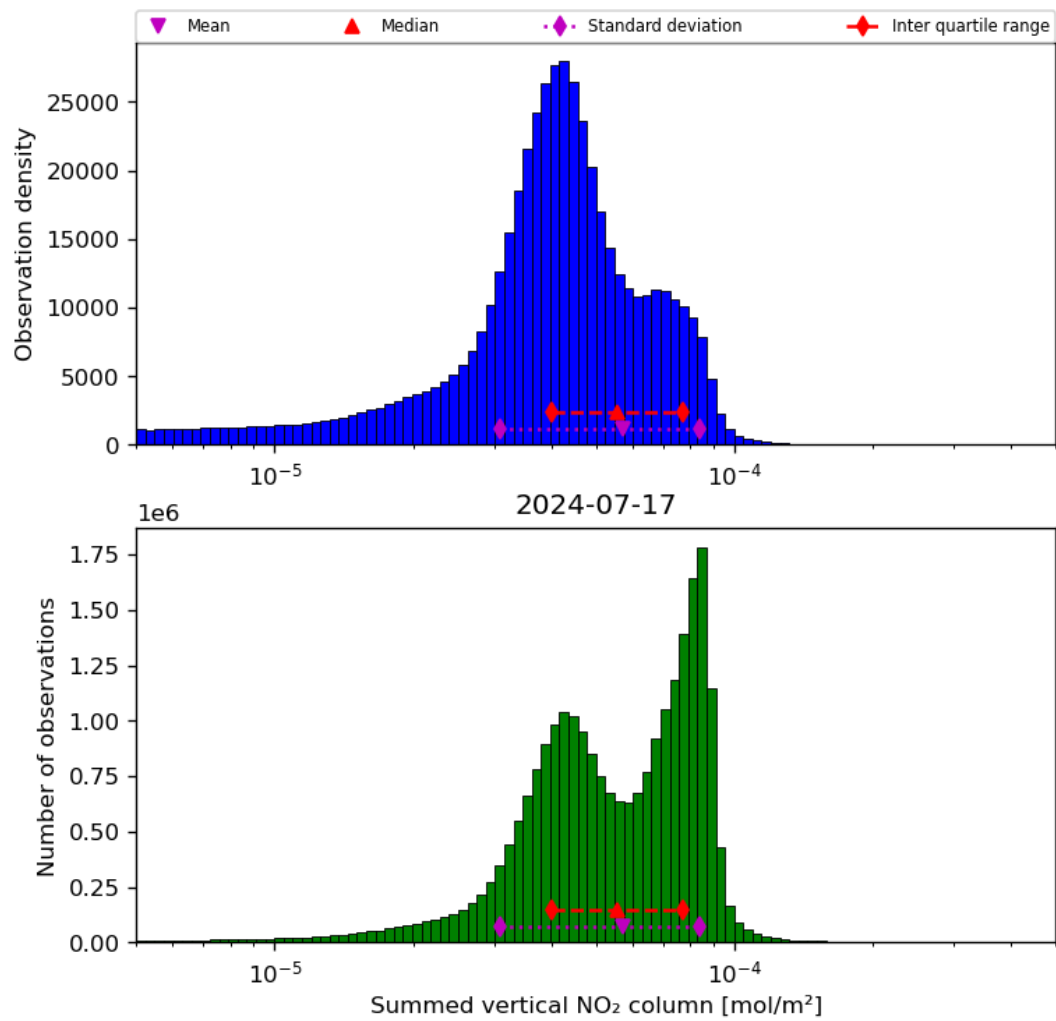
Figure 40: Histogram of “Summed vertical NO 2 column” for 2024-07-16 to 2024-07-18
