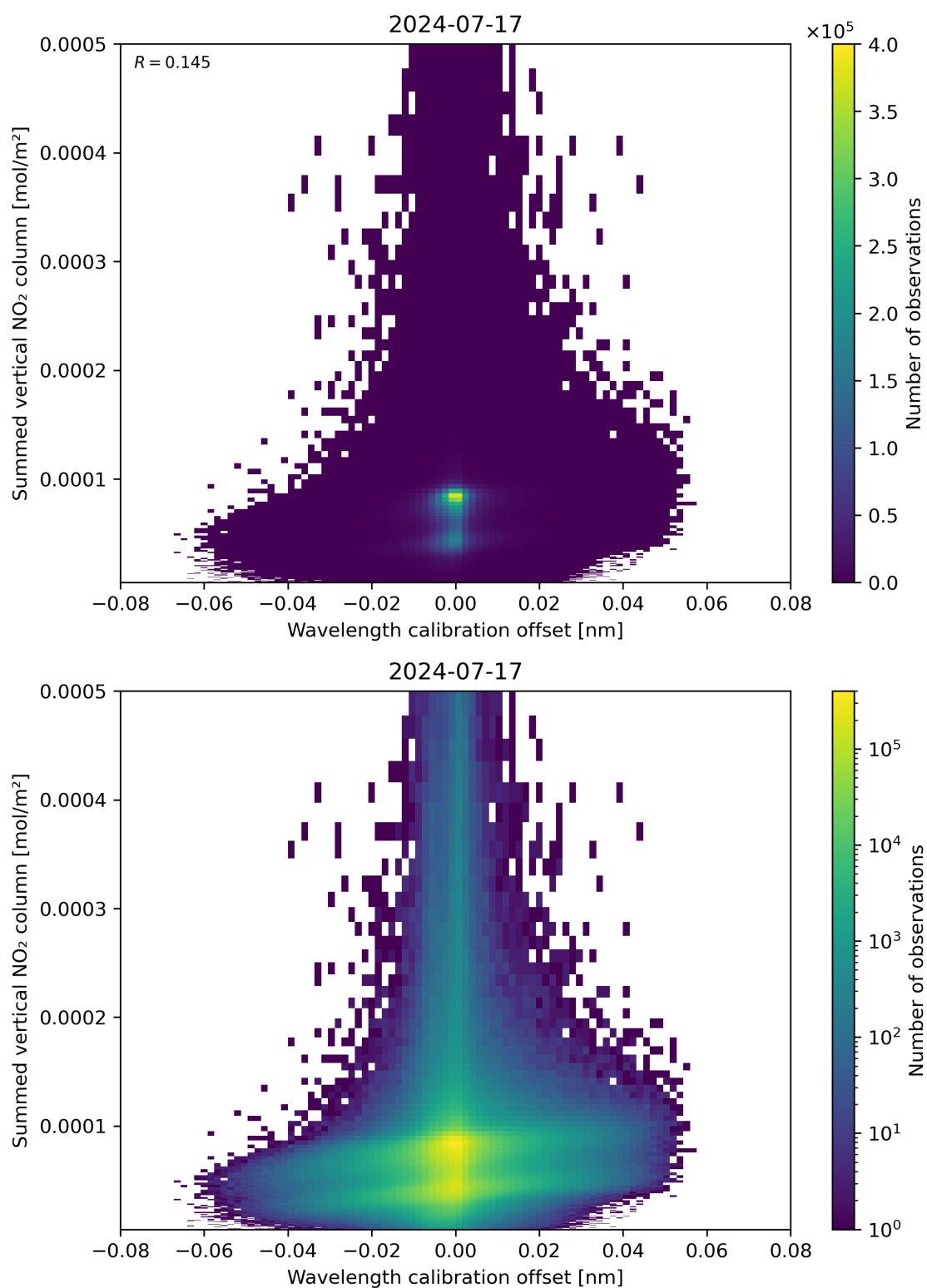
Figure 177: Scatter density plot of “Wavelength calibration offset” against “Summed vertical NO 2 column” for 2024-07-16 to 2024-07-18.
