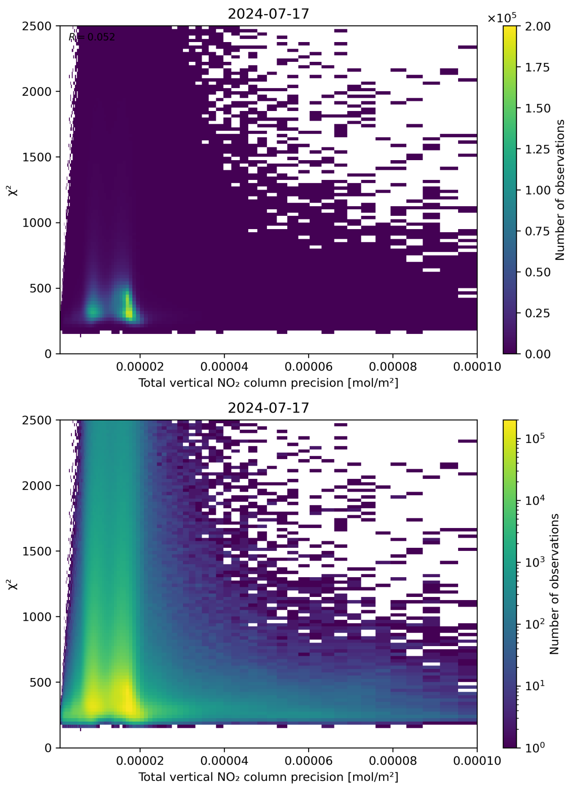
Figure 116: Scatter density plot of “Total vertical NO 2 column precision” against “ \chi^2 ” for 2024-07-16 to 2024-07-18.
