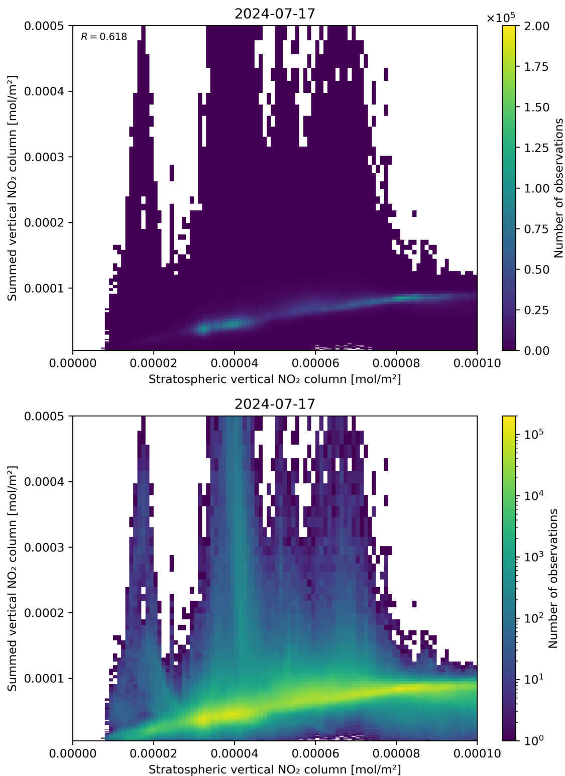
Figure 98: Scatter density plot of “Stratospheric vertical NO 2 column” against “Summed vertical NO 2 column” for 2024-07-16 to 2024-07-18.
