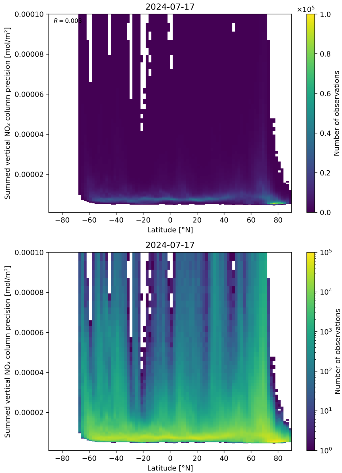
Figure 89: Scatter density plot of “Latitude” against “Summed vertical NO 2 column precision” for 2024-07-16 to 2024-07-18.
