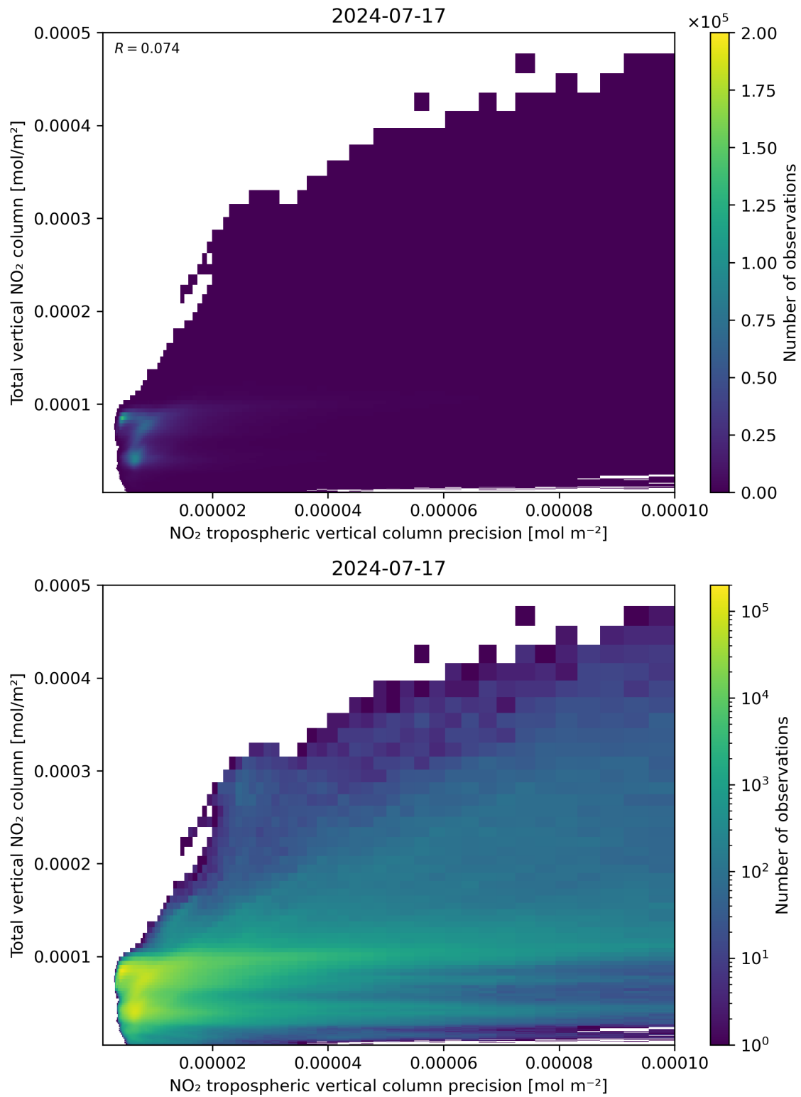
Figure 138: Scatter density plot of “NO 2 tropospheric vertical column precision” against “Total vertical NO 2 column” for 2024-07-16 to 2024-07-18.
