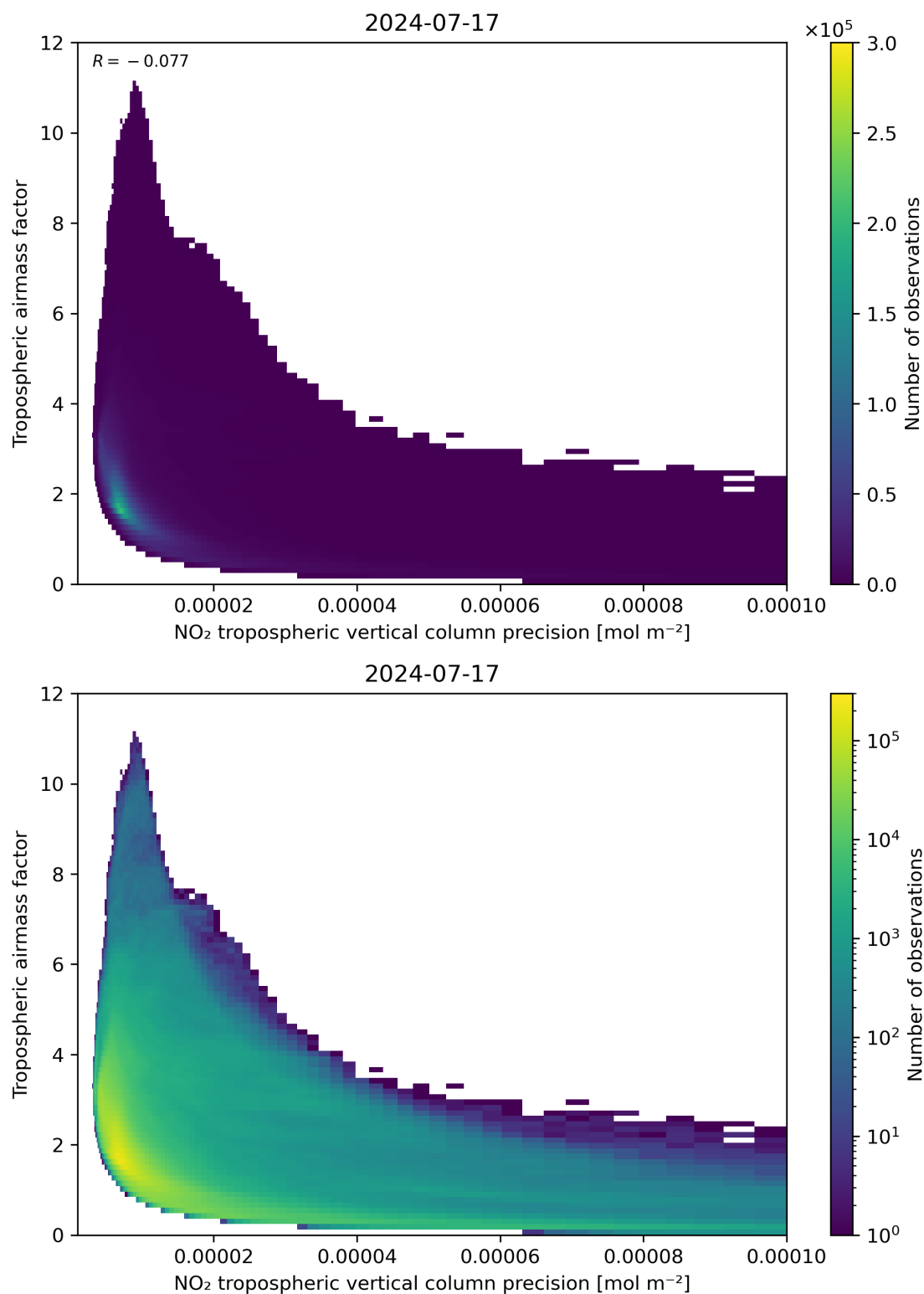
Figure 133: Scatter density plot of “NO 2 tropospheric vertical column precision” against “Tropospheric airmass factor” for 2024-07-16 to 2024-07-18.
