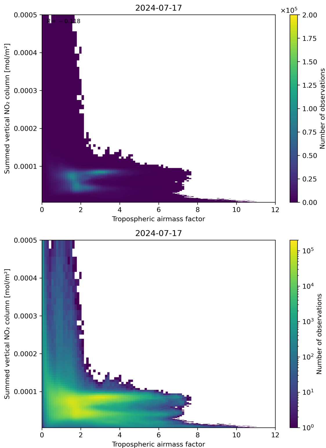
Figure 75: Scatter density plot of “Tropospheric airmass factor” against “Summed vertical NO 2 column” for 2024-07-16 to 2024-07-18.
