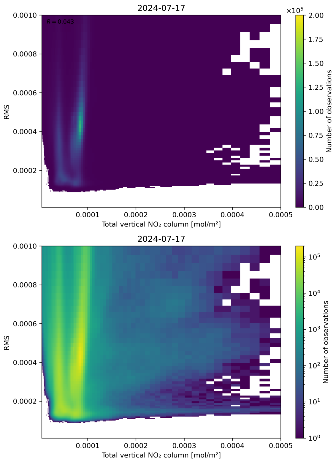
Figure 120: Scatter density plot of “Total vertical NO 2 column” against “RMS” for 2024-07-16 to 2024-07-18.
