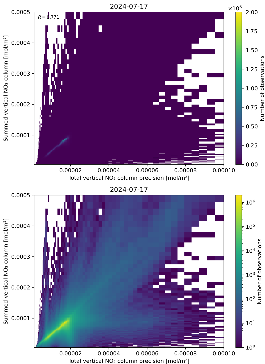
Figure 117: Scatter density plot of “Total vertical NO 2 column precision” against “Summed vertical NO 2 column” for 2024-07-16 to 2024-07-18.
