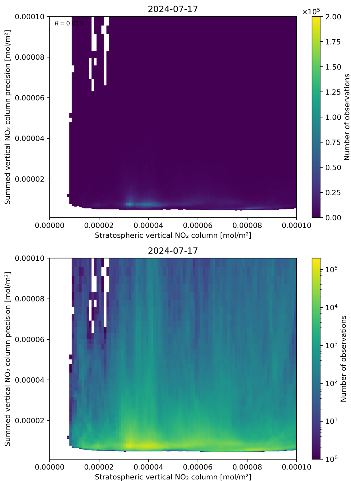
Figure 99: Scatter density plot of “Stratospheric vertical NO 2 column” against “Summed vertical NO 2 column precision” for 2024-07-16 to 2024-07-18.
