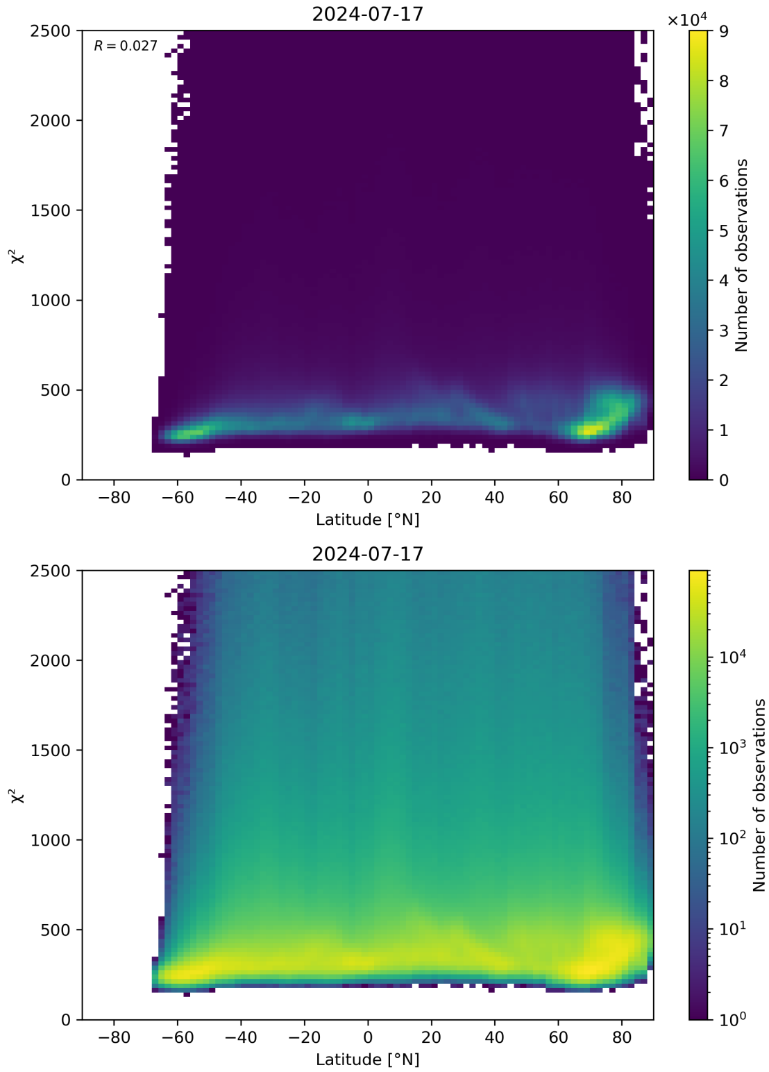
Figure 86: Scatter density plot of “Latitude” against “ \chi^2 ” for 2024-07-16 to 2024-07-18.
