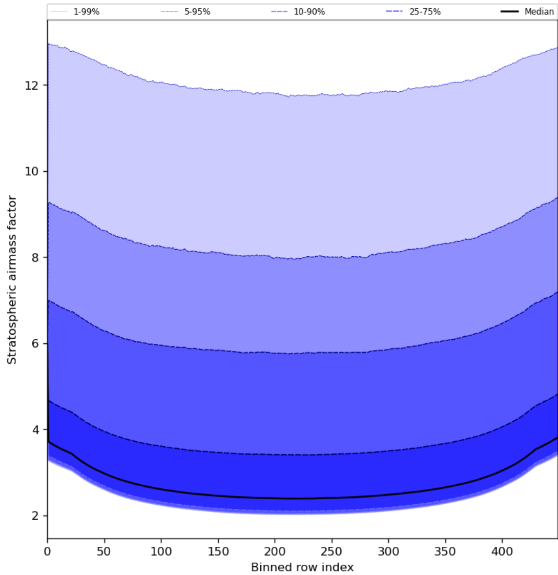
Figure 61: Along track statistics of “Stratospheric airmass factor” for 2024-07-16 to 2024-07-18
