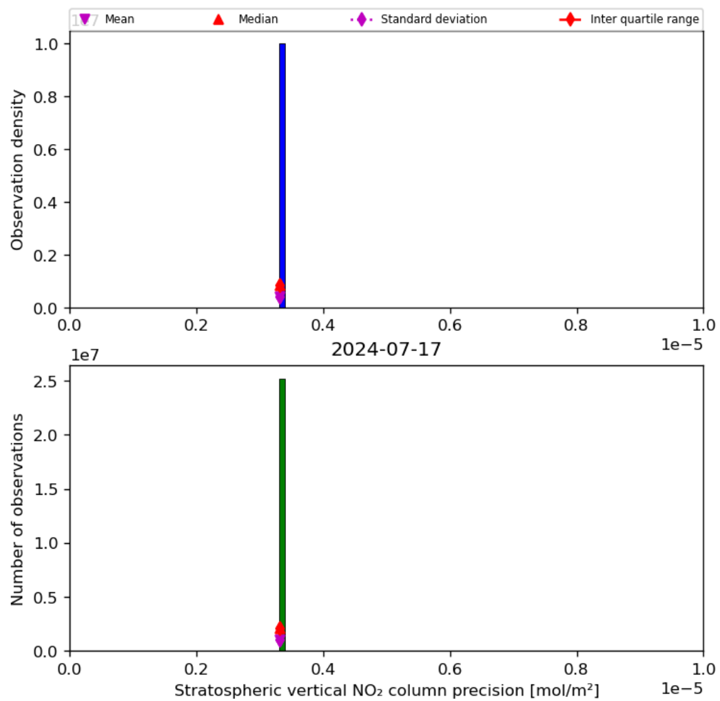
Figure 37: Histogram of “Stratospheric vertical NO 2 column precision” for 2024-07-16 to 2024-07-18
