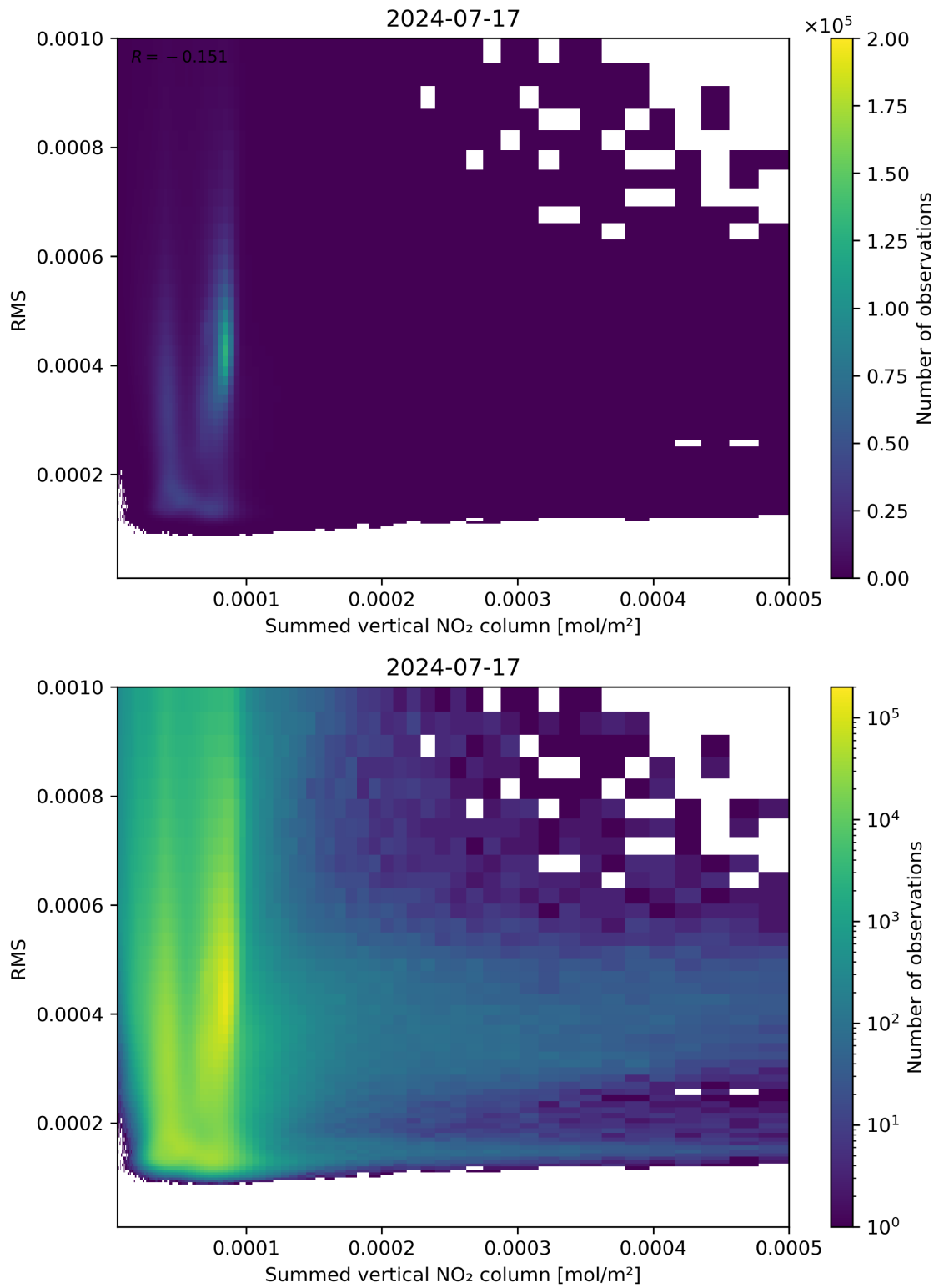
Figure 109: Scatter density plot of “Summed vertical NO 2 column” against “RMS” for 2024-07-16 to 2024-07-18.
