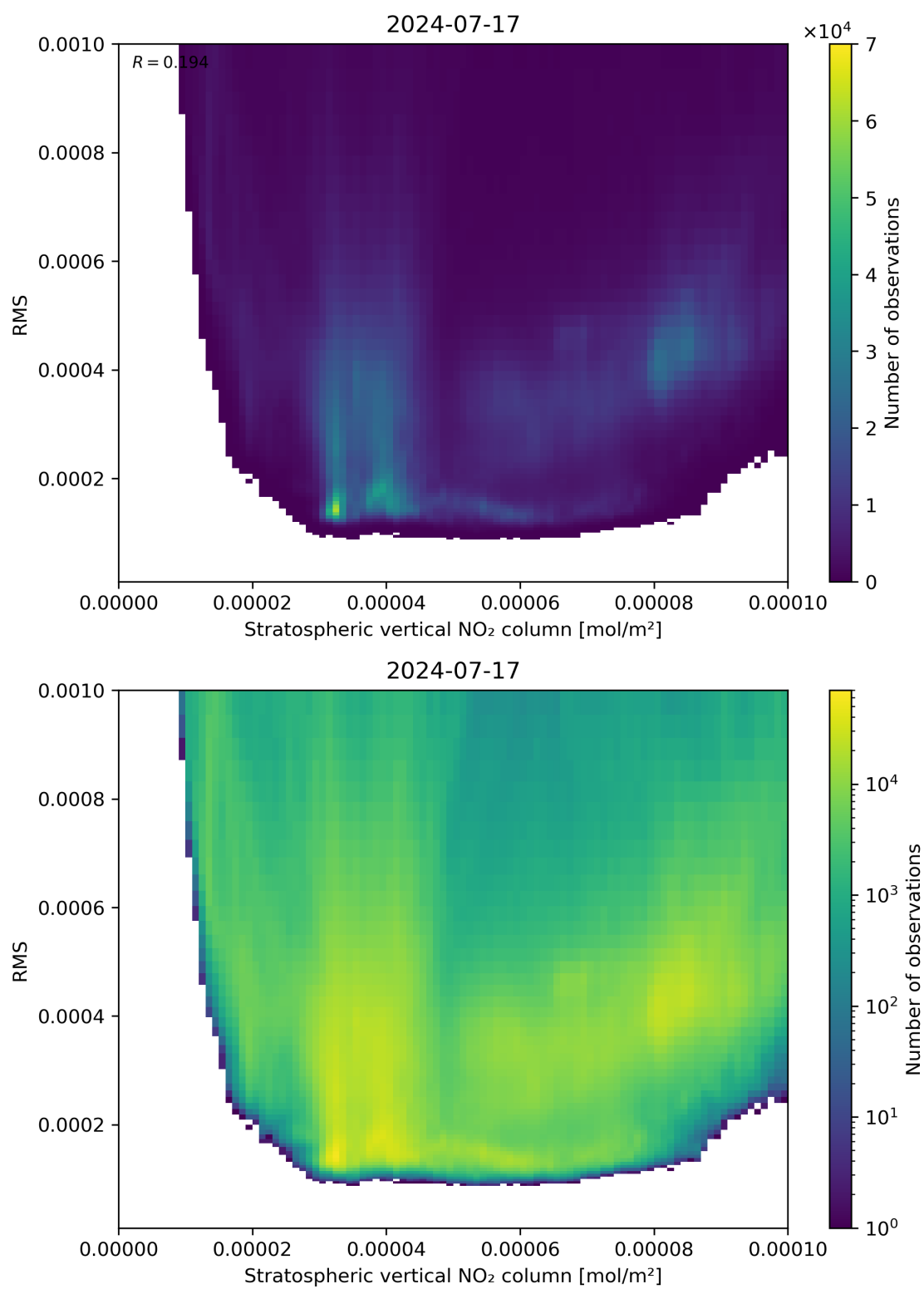
Figure 102: Scatter density plot of “Stratospheric vertical NO 2 column” against “RMS” for 2024-07-16 to 2024-07-18.
