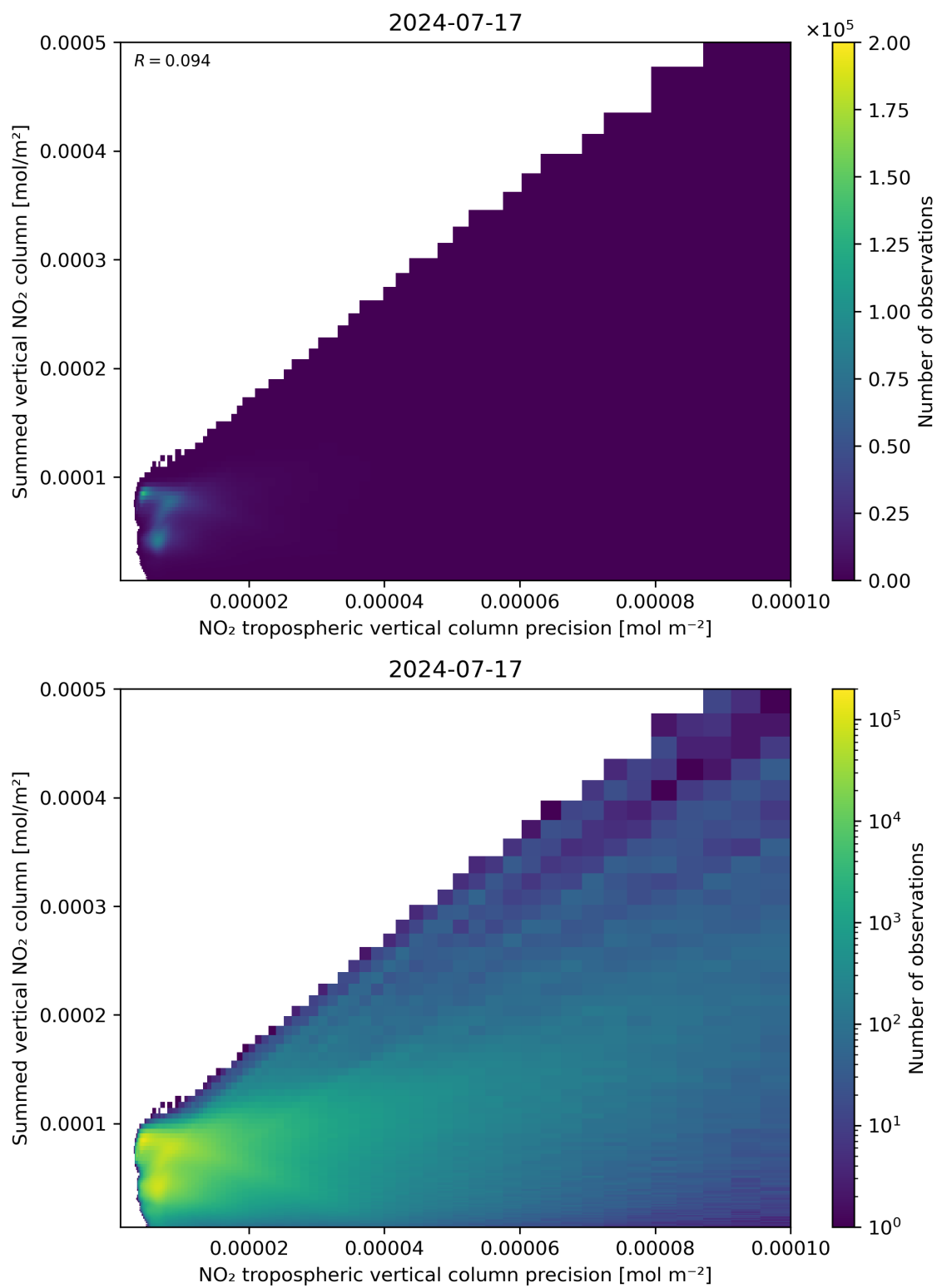
Figure 136: Scatter density plot of “NO 2 tropospheric vertical column precision” against “Summed vertical NO 2 column” for 2024-07-16 to 2024-07-18.
