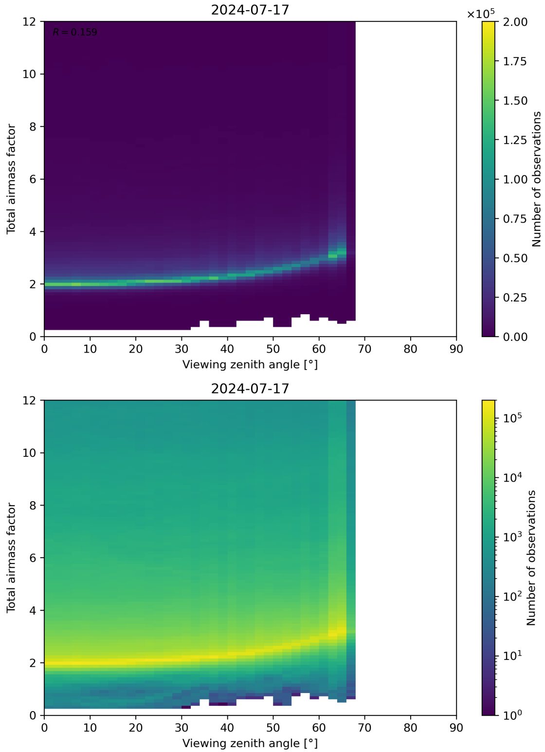
Figure 160: Scatter density plot of “Viewing zenith angle” against “Total airmass factor” for 2024-07-16 to 2024-07-18.
