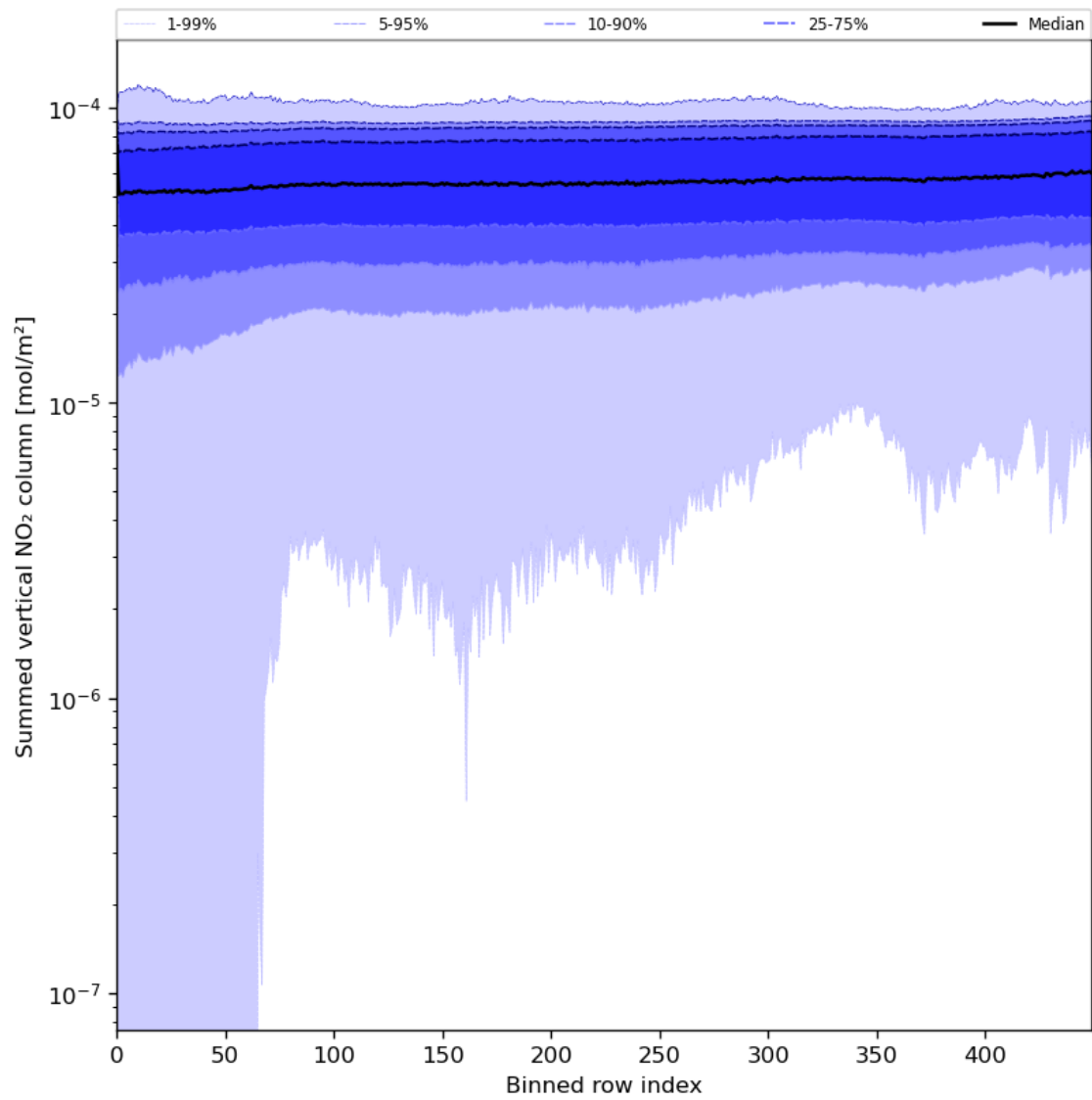
Figure 57: Along track statistics of “Summed vertical NO 2 column” for 2024-07-16 to 2024-07-18
