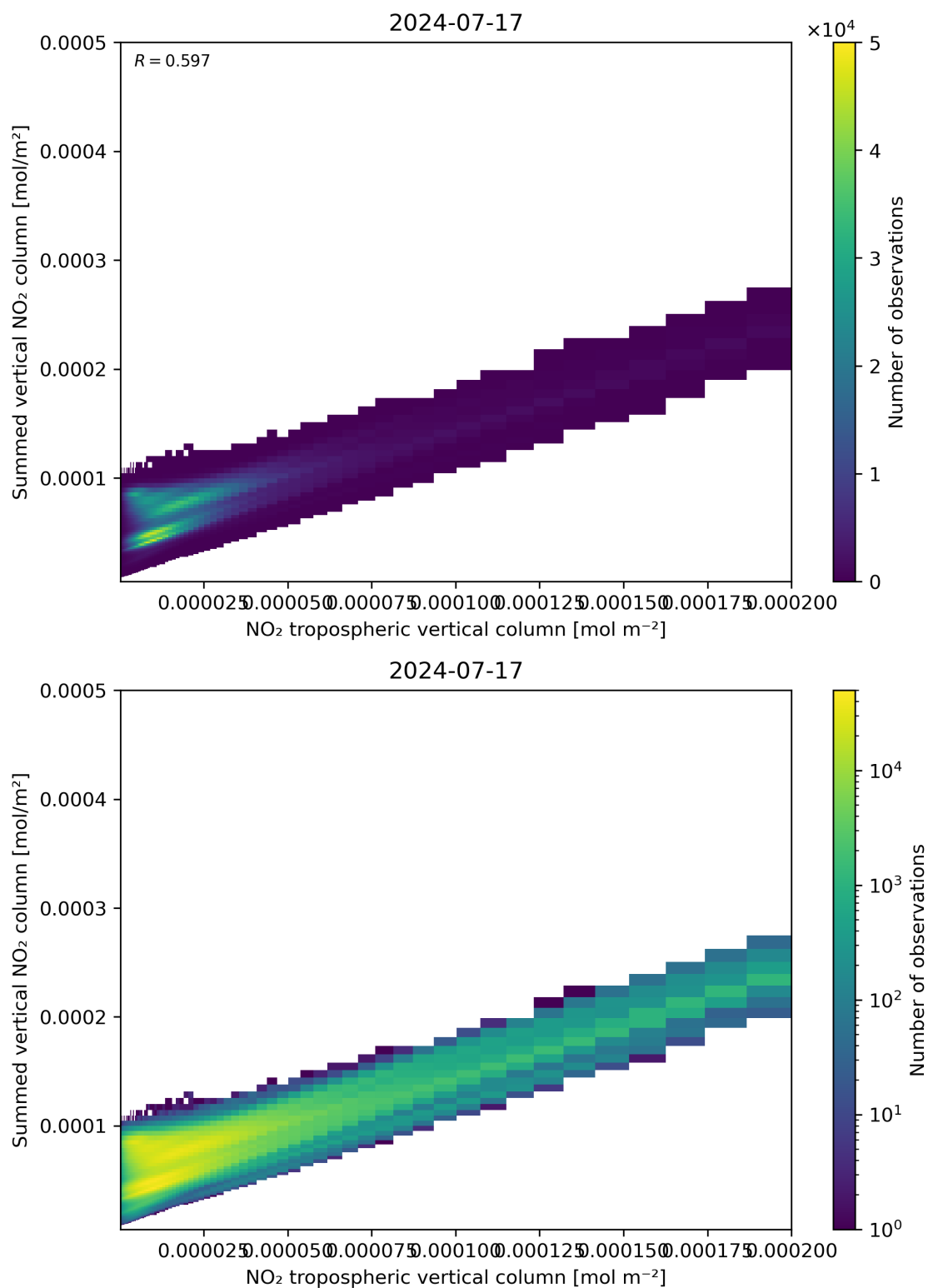
Figure 126: Scatter density plot of “NO 2 tropospheric vertical column” against “Summed vertical NO 2 column” for 2024-07-16 to 2024-07-18.
