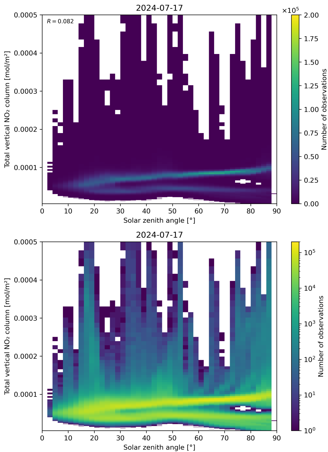
Figure 153: Scatter density plot of “Solar zenith angle” against “Total vertical NO 2 column” for 2024-07-16 to 2024-07-18.
