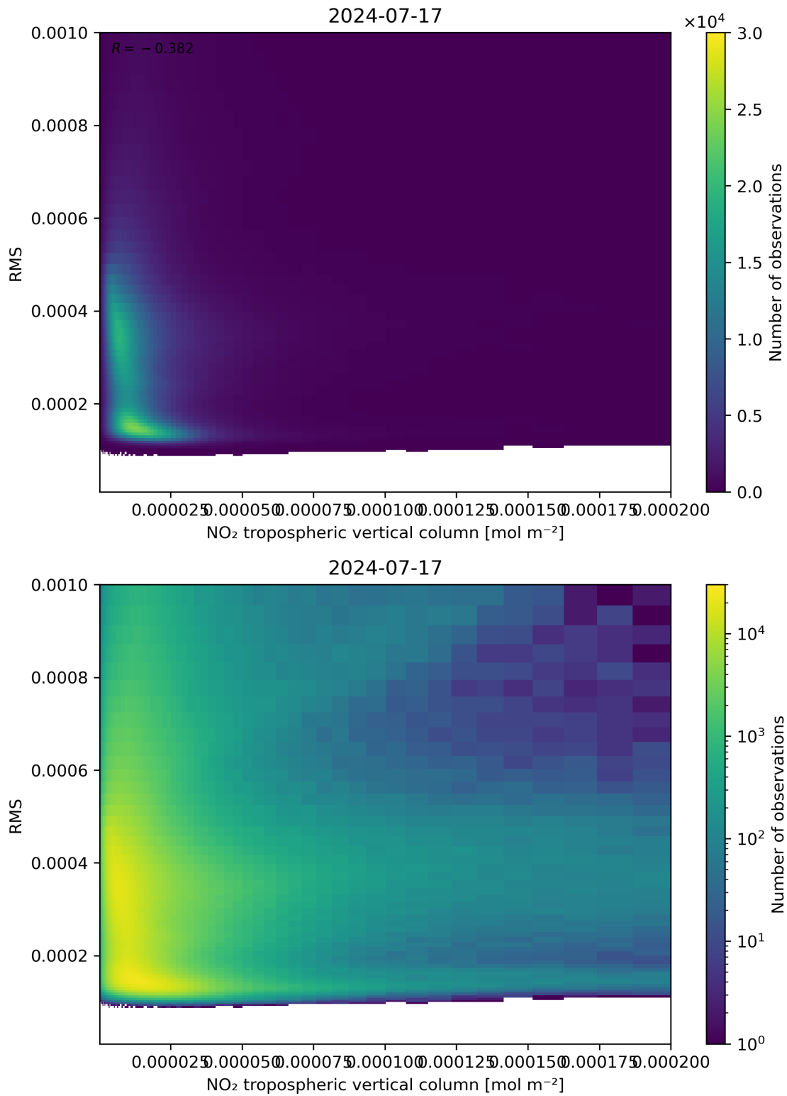
Figure 142: Scatter density plot of “NO 2 tropospheric vertical column” against “RMS” for 2024-07-16 to 2024-07-18.
