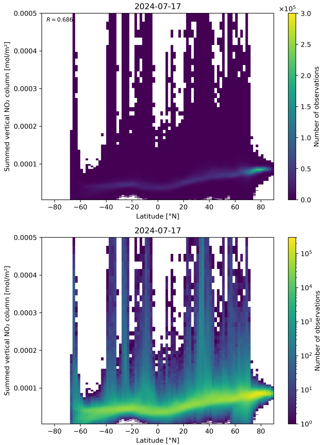
Figure 88: Scatter density plot of “Latitude” against “Summed vertical NO 2 column” for 2024-07-16 to 2024-07-18.
