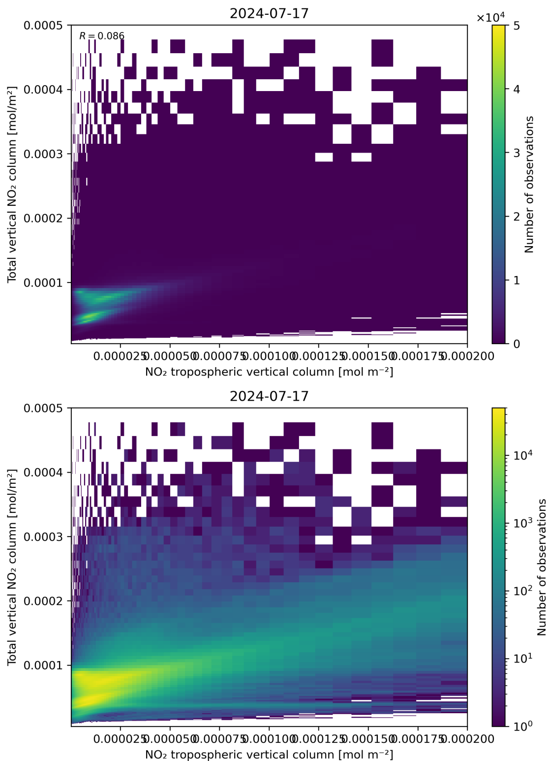
Figure 128: Scatter density plot of “NO 2 tropospheric vertical column” against “Total vertical NO 2 column” for 2024-07-16 to 2024-07-18.
