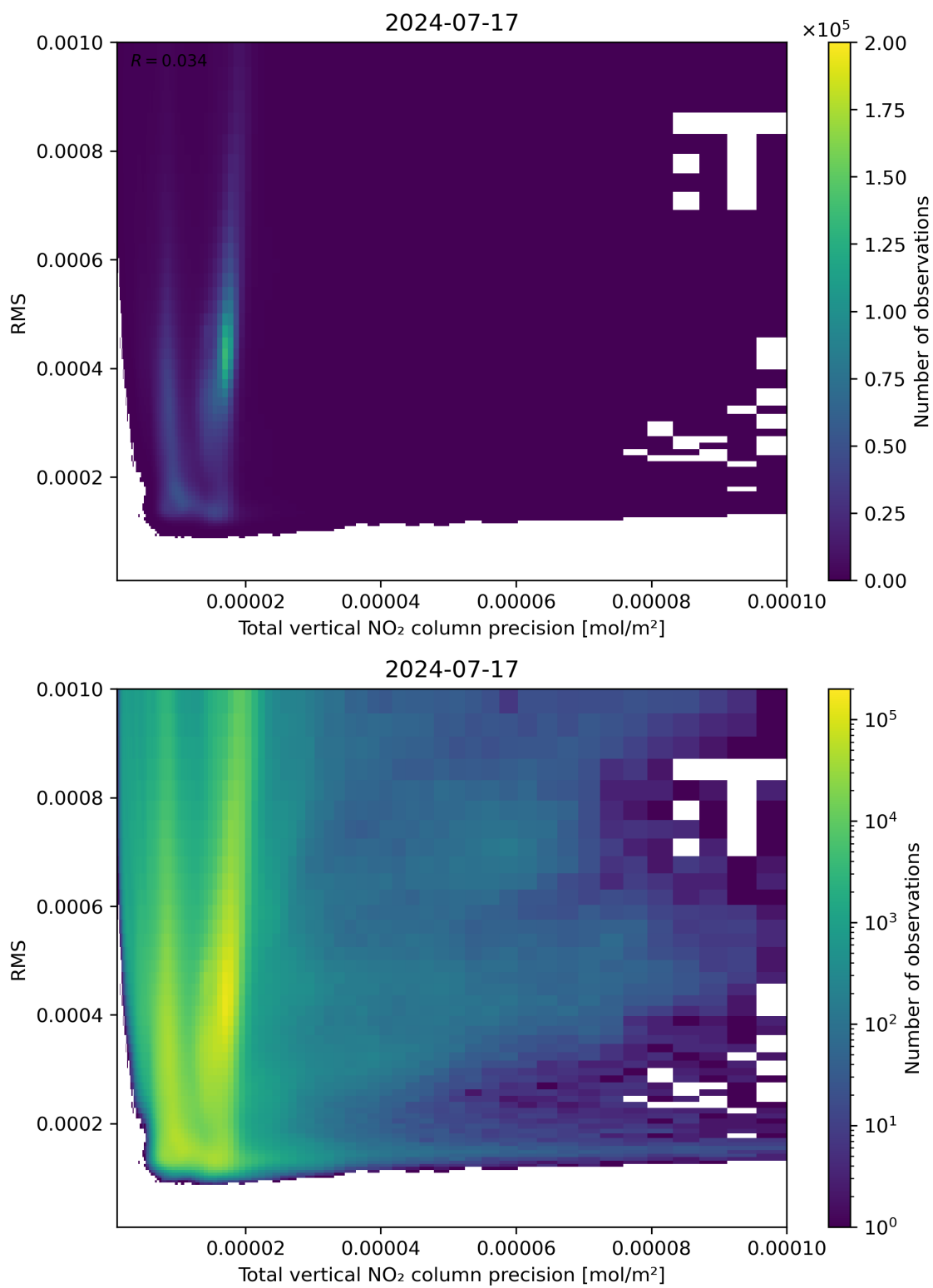
Figure 119: Scatter density plot of “Total vertical NO 2 column precision” against “RMS” for 2024-07-16 to 2024-07-18.
