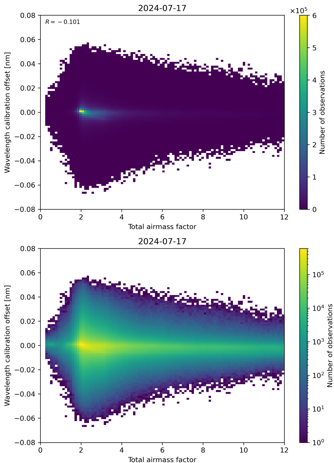
Figure 70: Scatter density plot of “Total airmass factor” against “Wavelength calibration offset” for 2024-07-16 to 2024-07-18.
