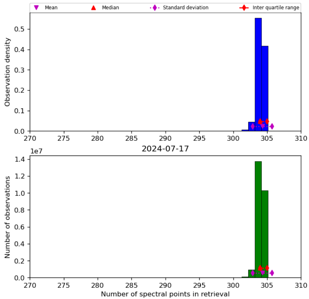
Figure 33: Histogram of “Number of spectral points in retrieval” for 2024-07-16 to 2024-07-18
