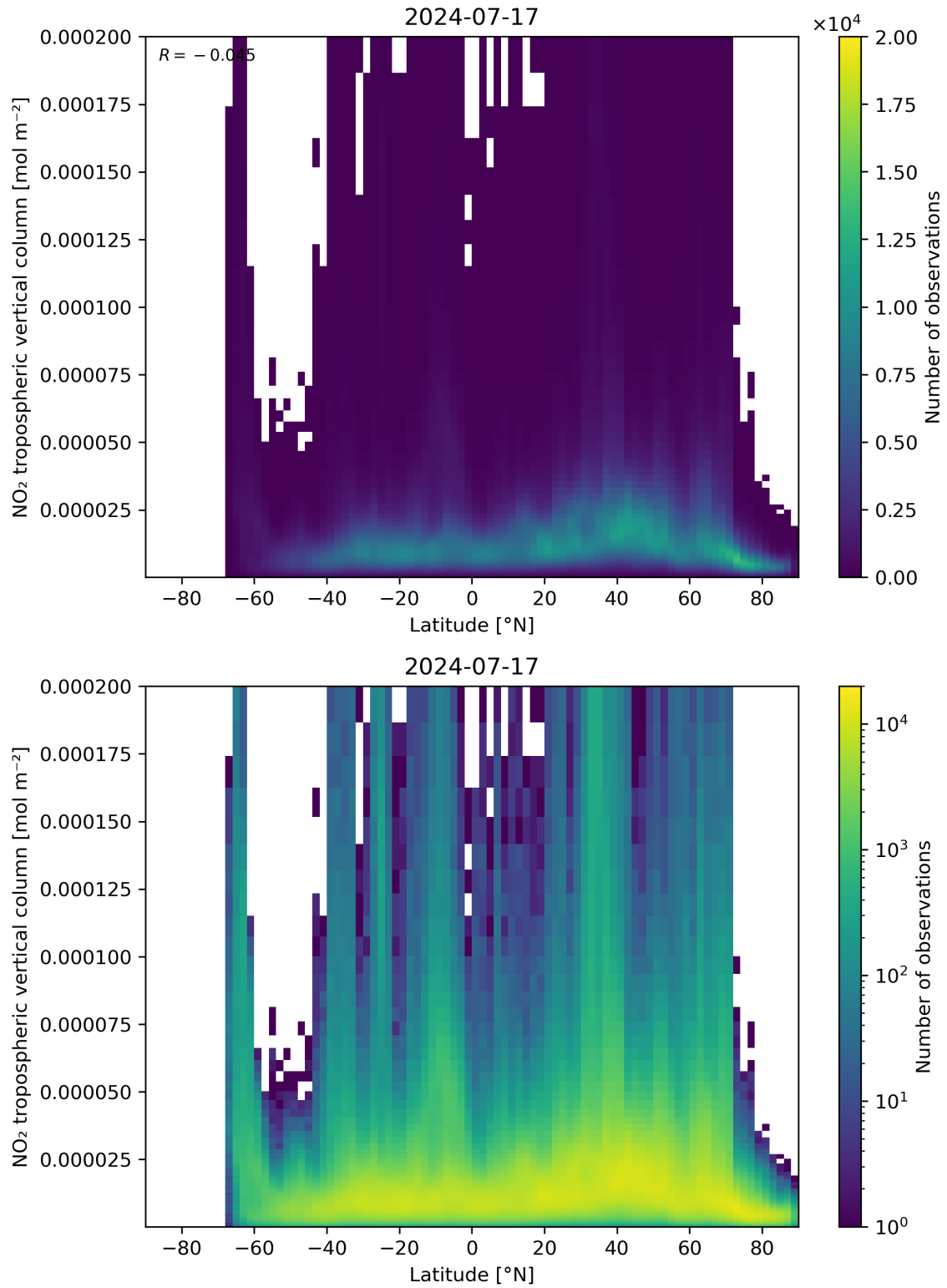
Figure 92: Scatter density plot of “Latitude” against “NO 2 tropospheric vertical column” for 2024-07-16 to 2024-07-18.
