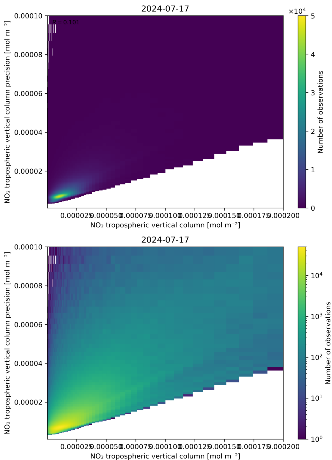
Figure 130: Scatter density plot of “NO 2 tropospheric vertical column” against “NO 2 tropospheric vertical column precision” for 2024-07-16 to 2024-07-18.
