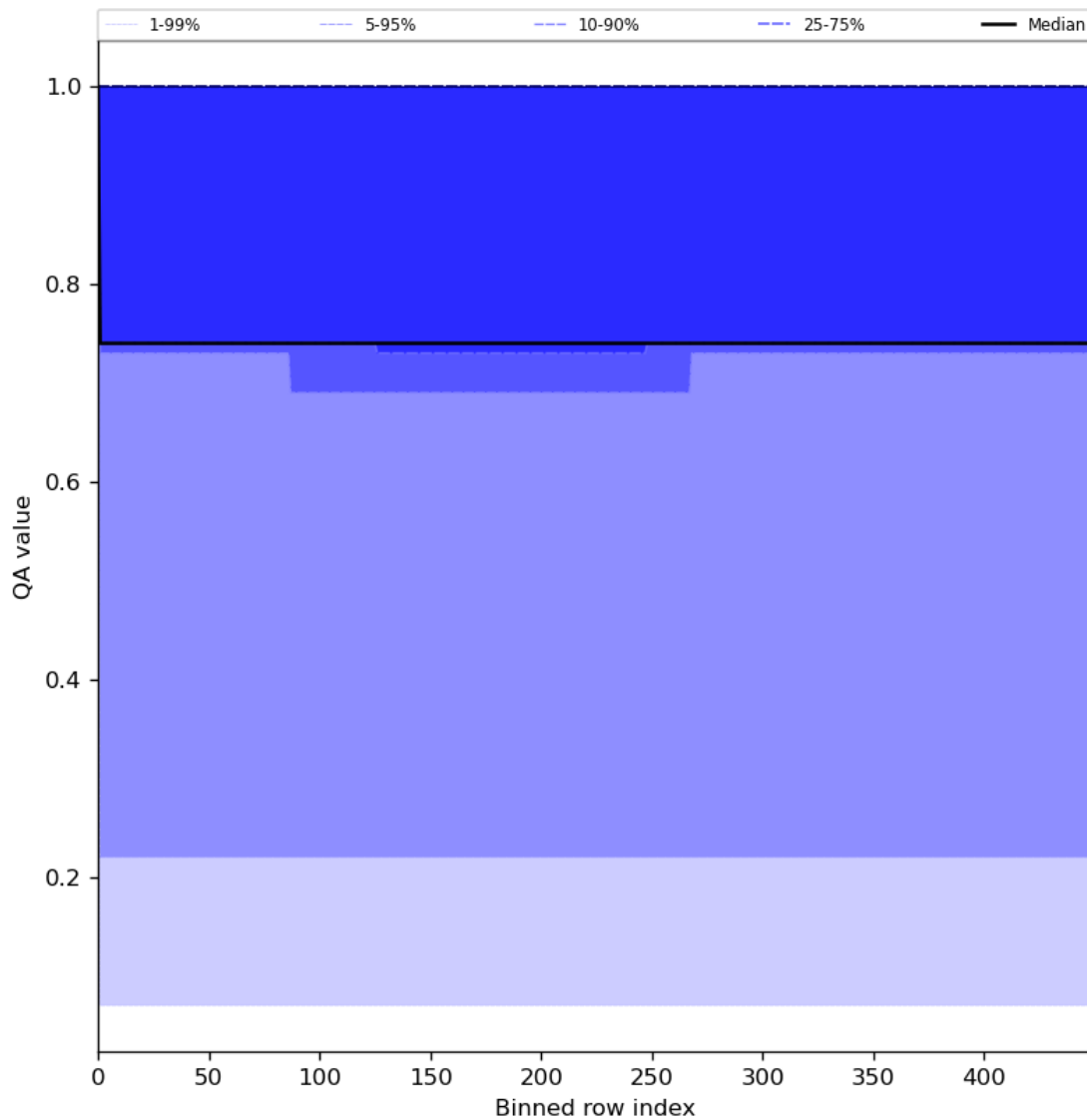
Figure 45: Along track statistics of “QA value” for 2024-07-16 to 2024-07-18
