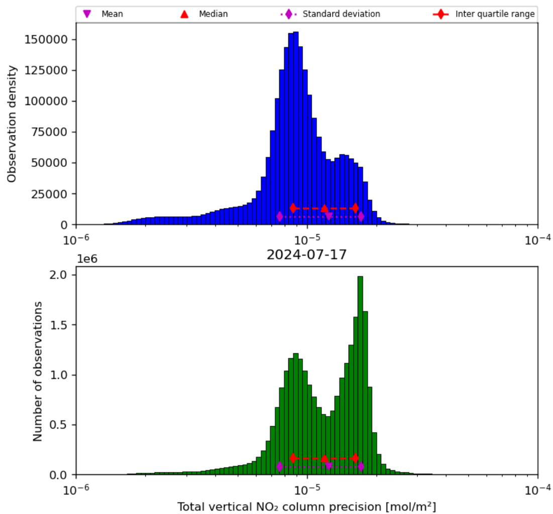
Figure 39: Histogram of “Total vertical NO 2 column precision” for 2024-07-16 to 2024-07-18
