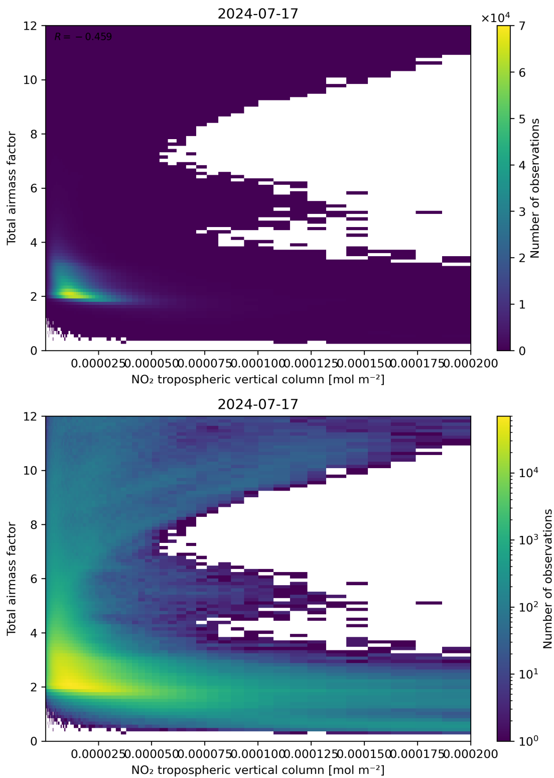
Figure 122: Scatter density plot of “NO 2 tropospheric vertical column” against “Total air mass factor” for 2024-07-16 to 2024-07-18.
