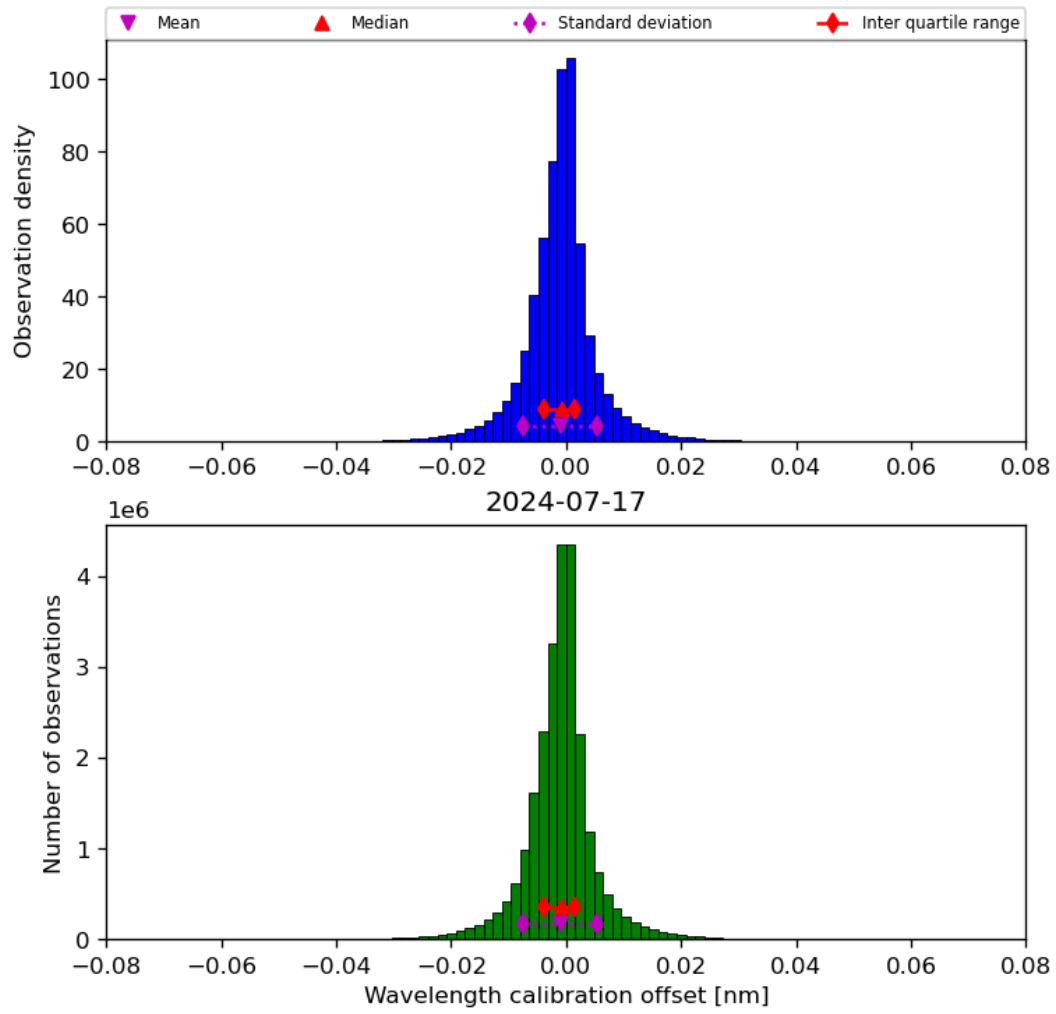
Figure 35: Histogram of “Wavelength calibration offset” for 2024-07-16 to 2024-07-18
