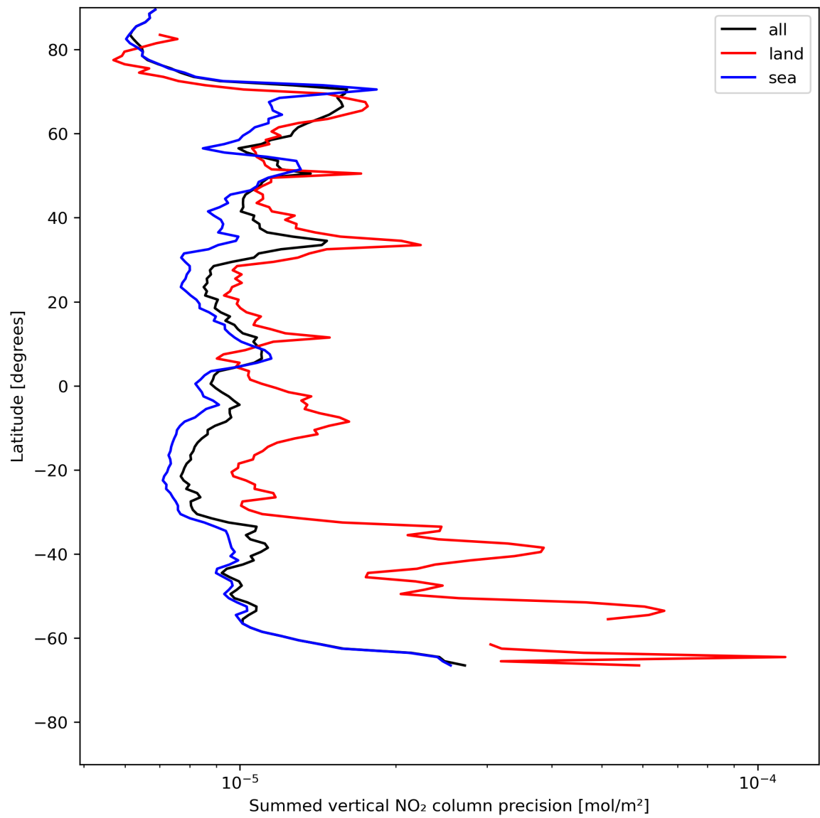
Figure 24: Zonal average of “Summed vertical NO 2 column precision” for 2024-07-16 to 2024-07-18.
