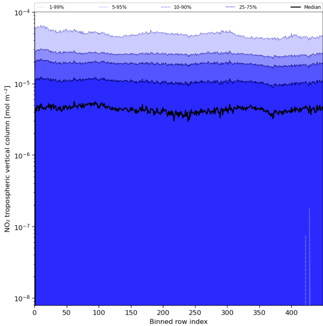
Figure 46: Along track statistics of “NO 2 tropospheric vertical column” for 2024-07-16 to 2024-07-18
