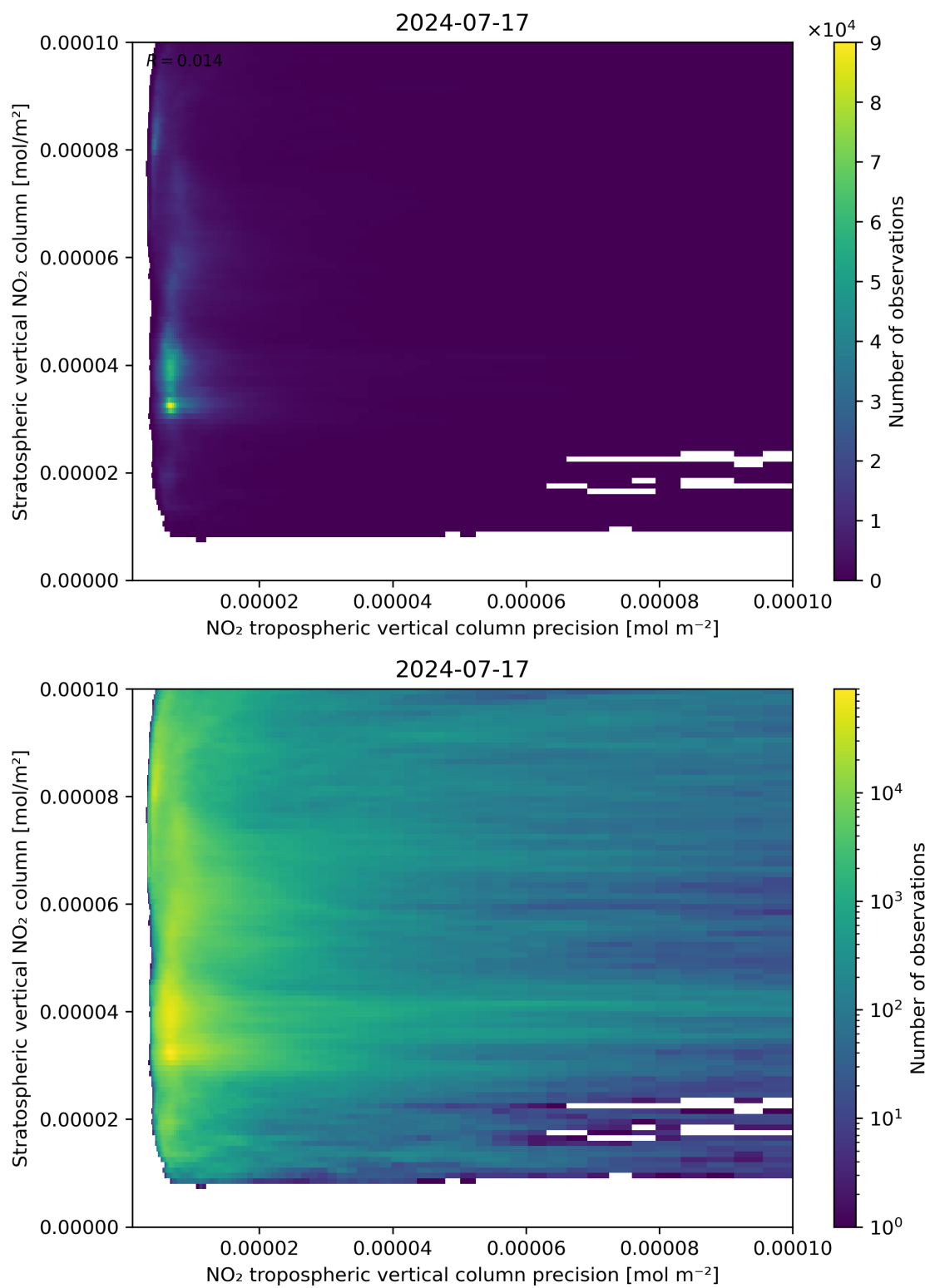
Figure 135: Scatter density plot of “NO 2 tropospheric vertical column precision” against “Stratospheric vertical NO 2 column” for 2024-07-16 to 2024-07-18.
