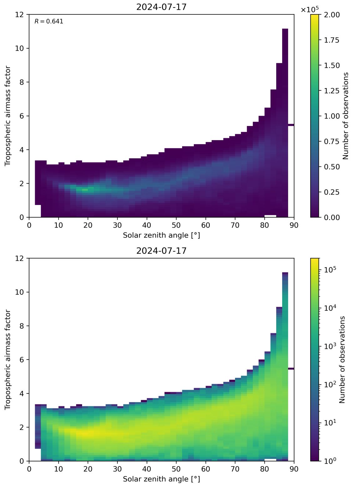
Figure 147: Scatter density plot of “Solar zenith angle” against “Tropospheric airmass factor” for 2024-07-16 to 2024-07-18.
