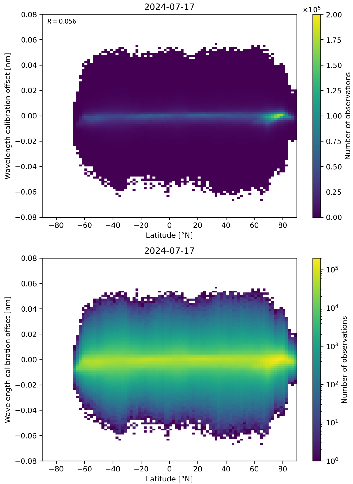
Figure 95: Scatter density plot of “Latitude” against “Wavelength calibration offset” for 2024-07-16 to 2024-07-18.
