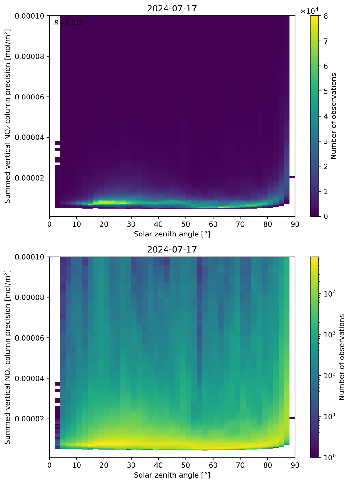
Figure 152: Scatter density plot of “Solar zenith angle” against “Summed vertical NO 2 column precision” for 2024-07-16 to 2024-07-18.
