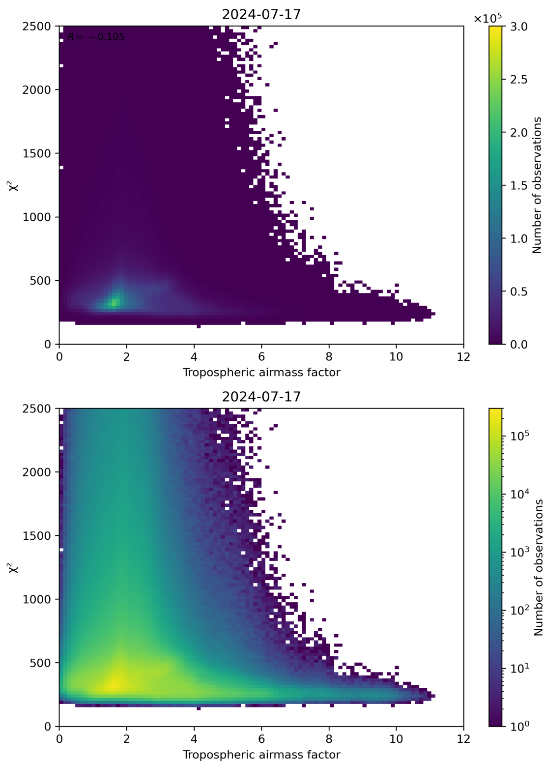
Figure 73: Scatter density plot of “Tropospheric airmass factor” against “ \chi^2 ” for 2024-07-16 to 2024-07-18.
