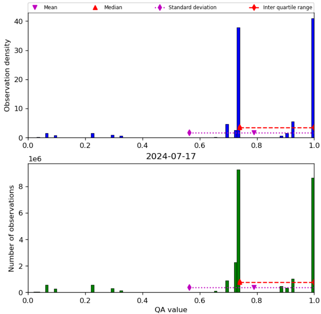
Figure 28: Histogram of “QA value” for 2024-07-16 to 2024-07-18
