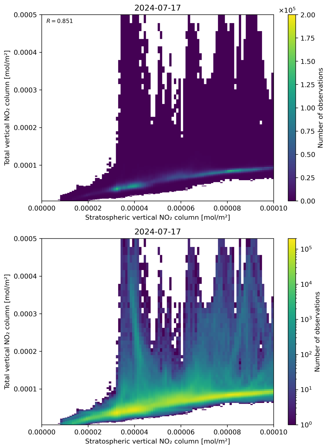
Figure 100: Scatter density plot of “Stratospheric vertical NO 2 column” against “Total vertical NO 2 column” for 2024-07-16 to 2024-07-18.
