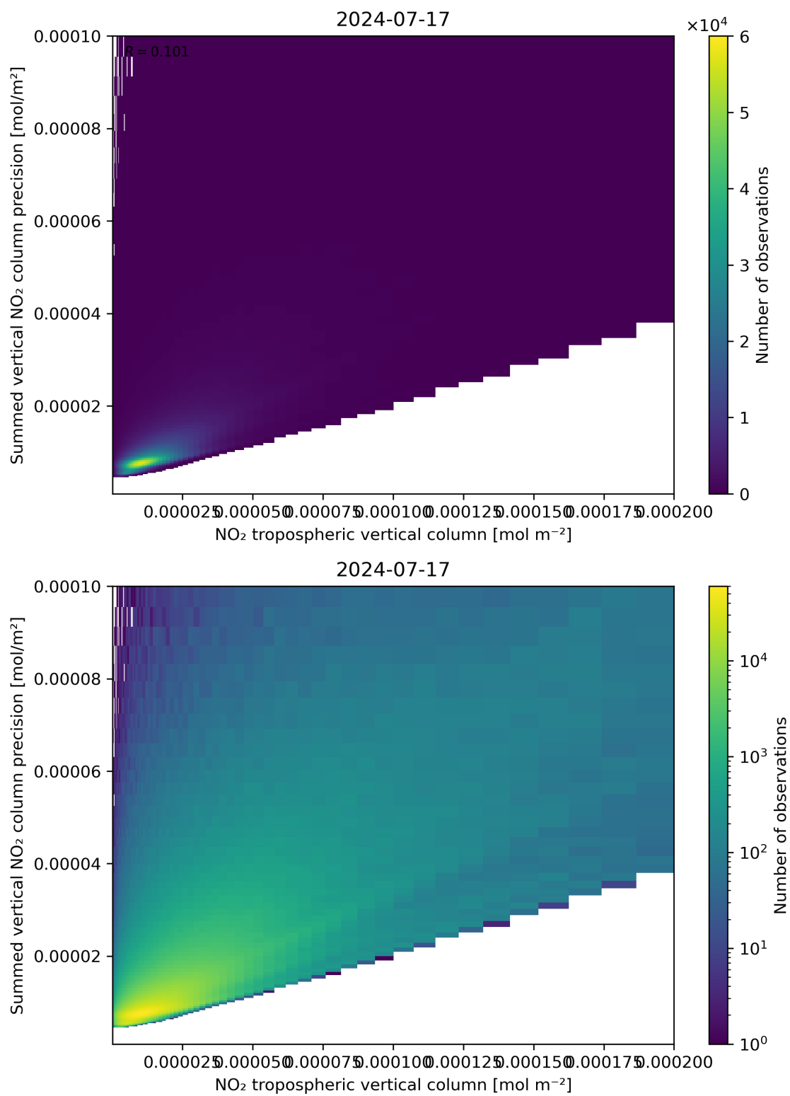
Figure 127: Scatter density plot of “NO 2 tropospheric vertical column” against “Summed vertical NO 2 column precision” for 2024-07-16 to 2024-07-18.
