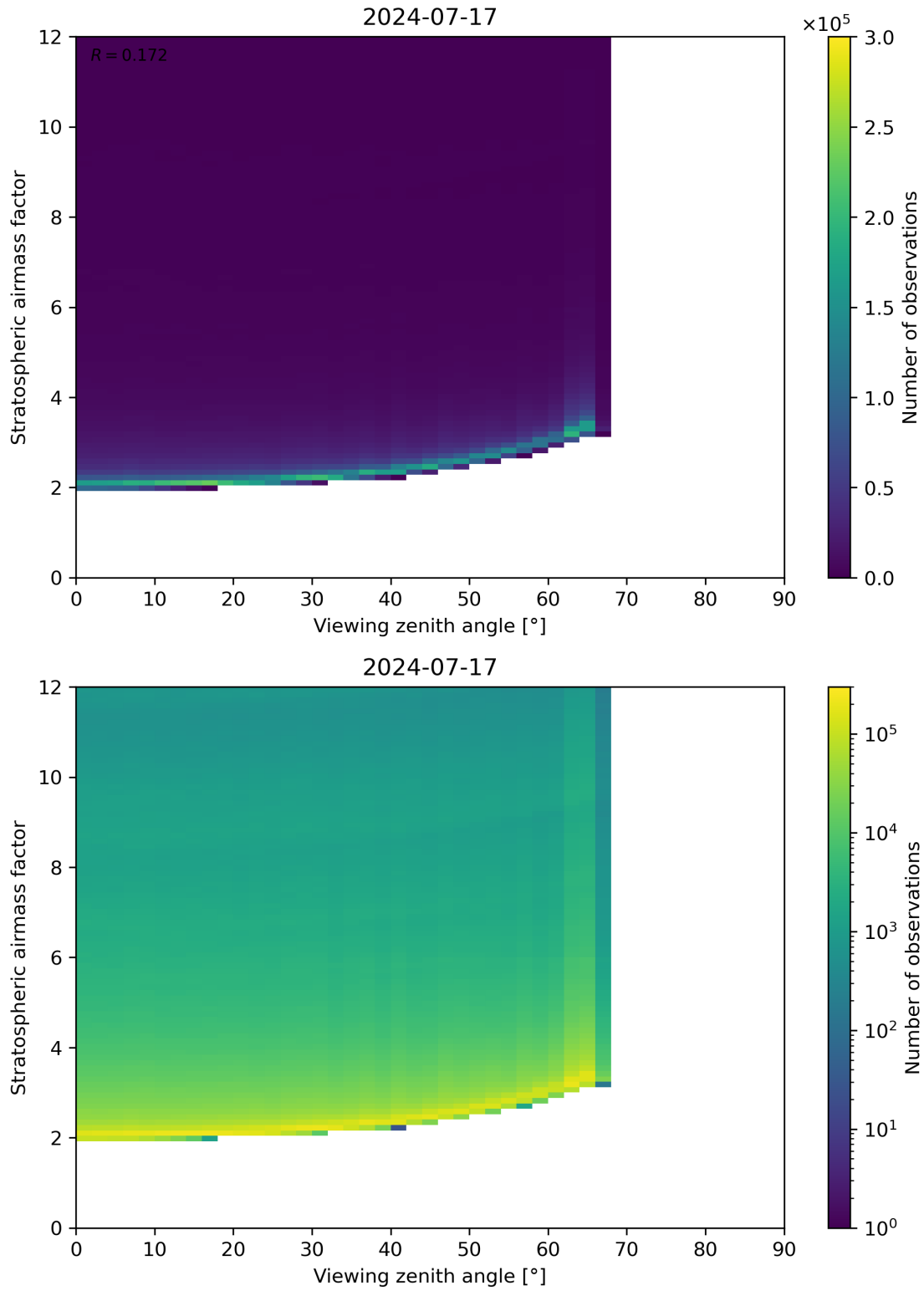
Figure 159: Scatter density plot of “Viewing zenith angle” against “Stratospheric airmass factor” for 2024-07-16 to 2024-07-18.
