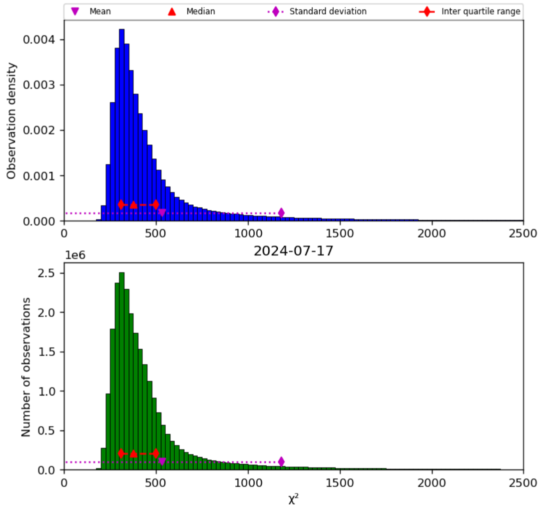
Figure 42: Histogram of “ \chi^2 ” for 2024-07-16 to 2024-07-18
