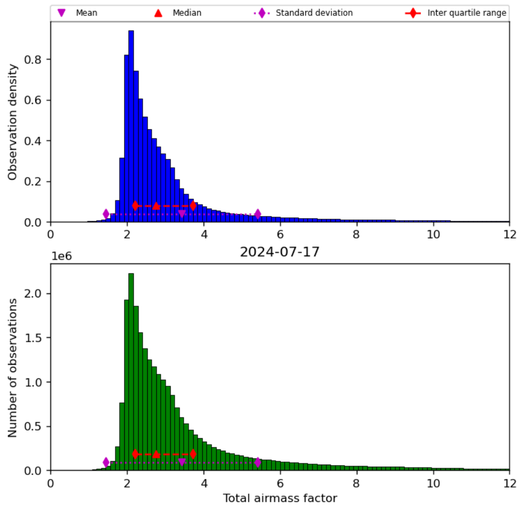
Figure 32: Histogram of “Total airmass factor” for 2024-07-16 to 2024-07-18
