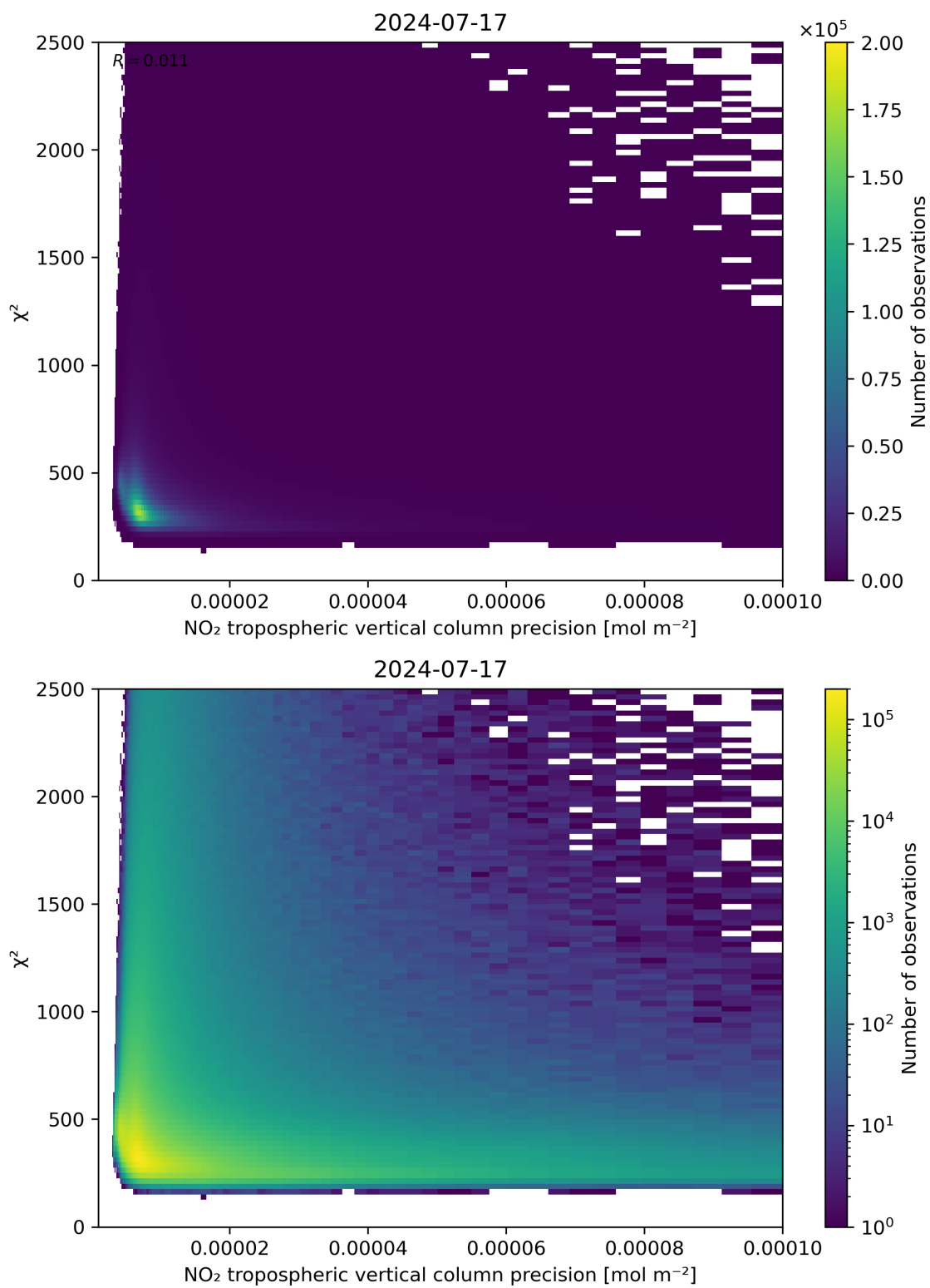
Figure 134: Scatter density plot of “NO 2 tropospheric vertical column precision” against “ \chi^2 ” for 2024-07-16 to 2024-07-18.
