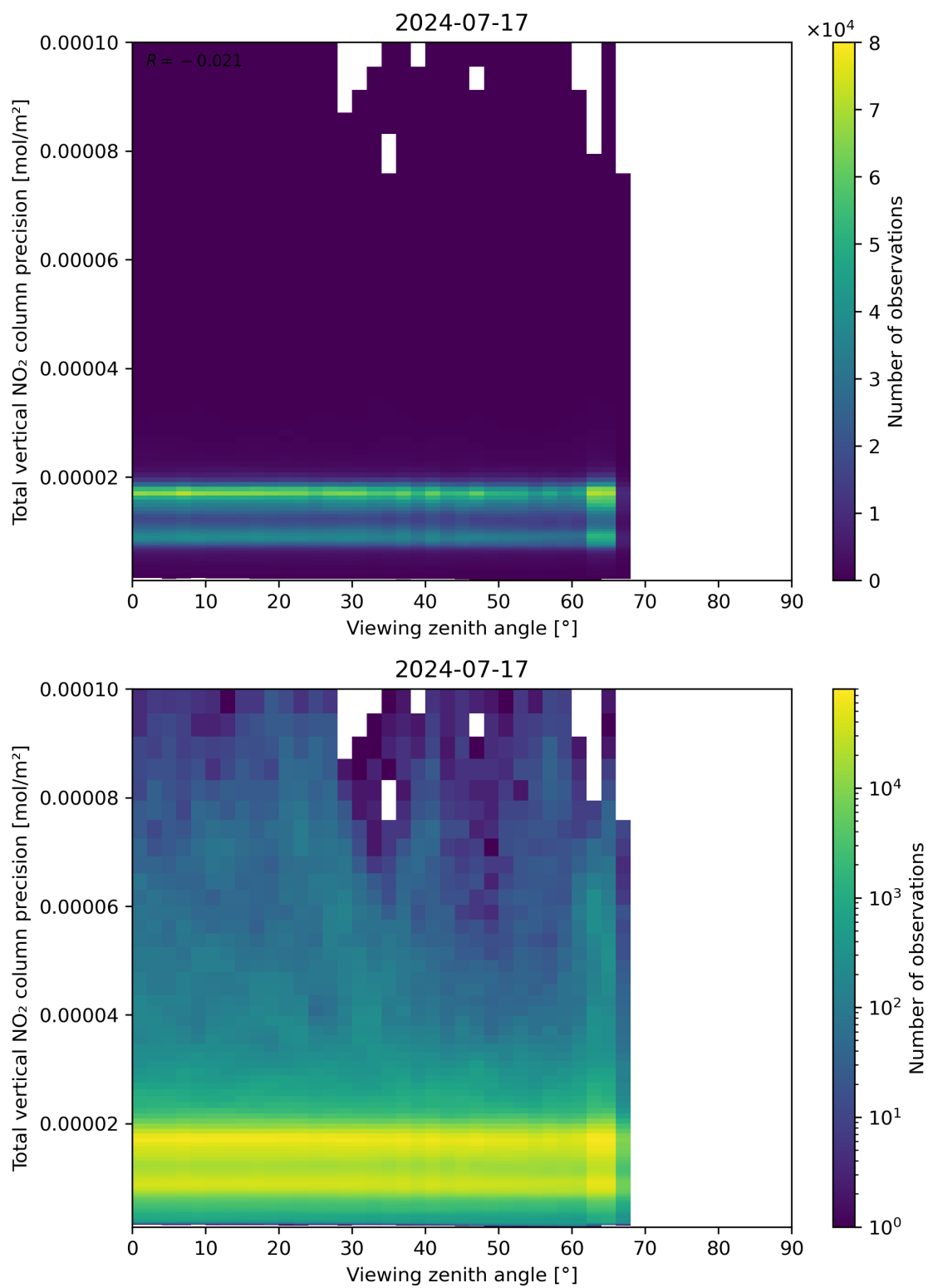
Figure 168: Scatter density plot of “Viewing zenith angle” against “Total vertical NO 2 column precision” for 2024-07-16 to 2024-07-18.
