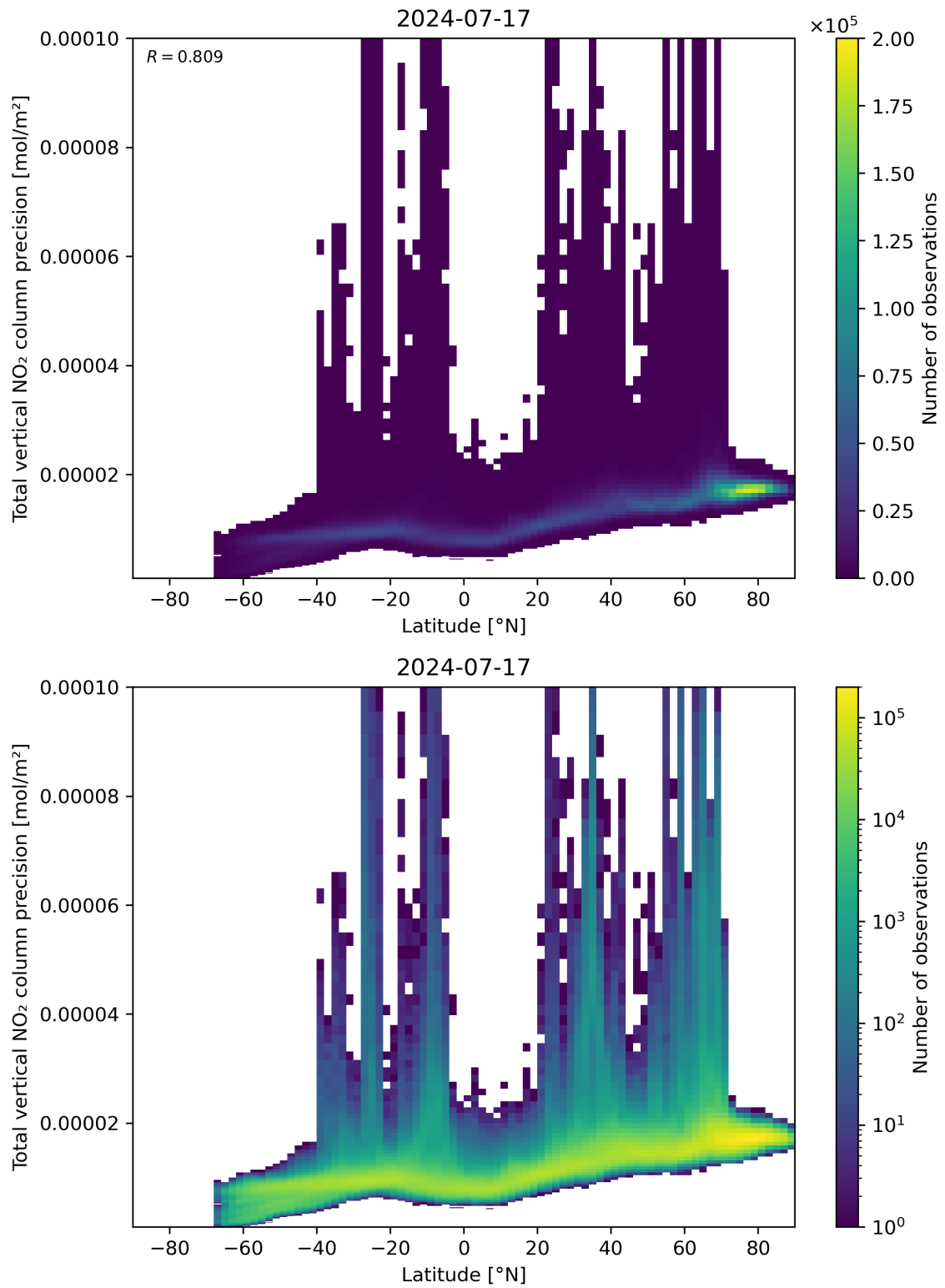
Figure 91: Scatter density plot of “Latitude” against “Total vertical NO 2 column precision” for 2024-07-16 to 2024-07-18.
