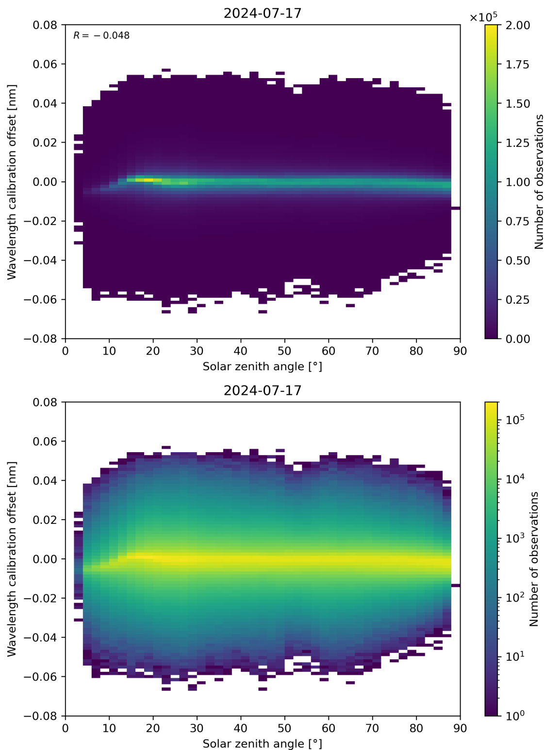
Figure 158: Scatter density plot of “Solar zenith angle” against “Wavelength calibration offset” for 2024-07-16 to 2024-07-18.
