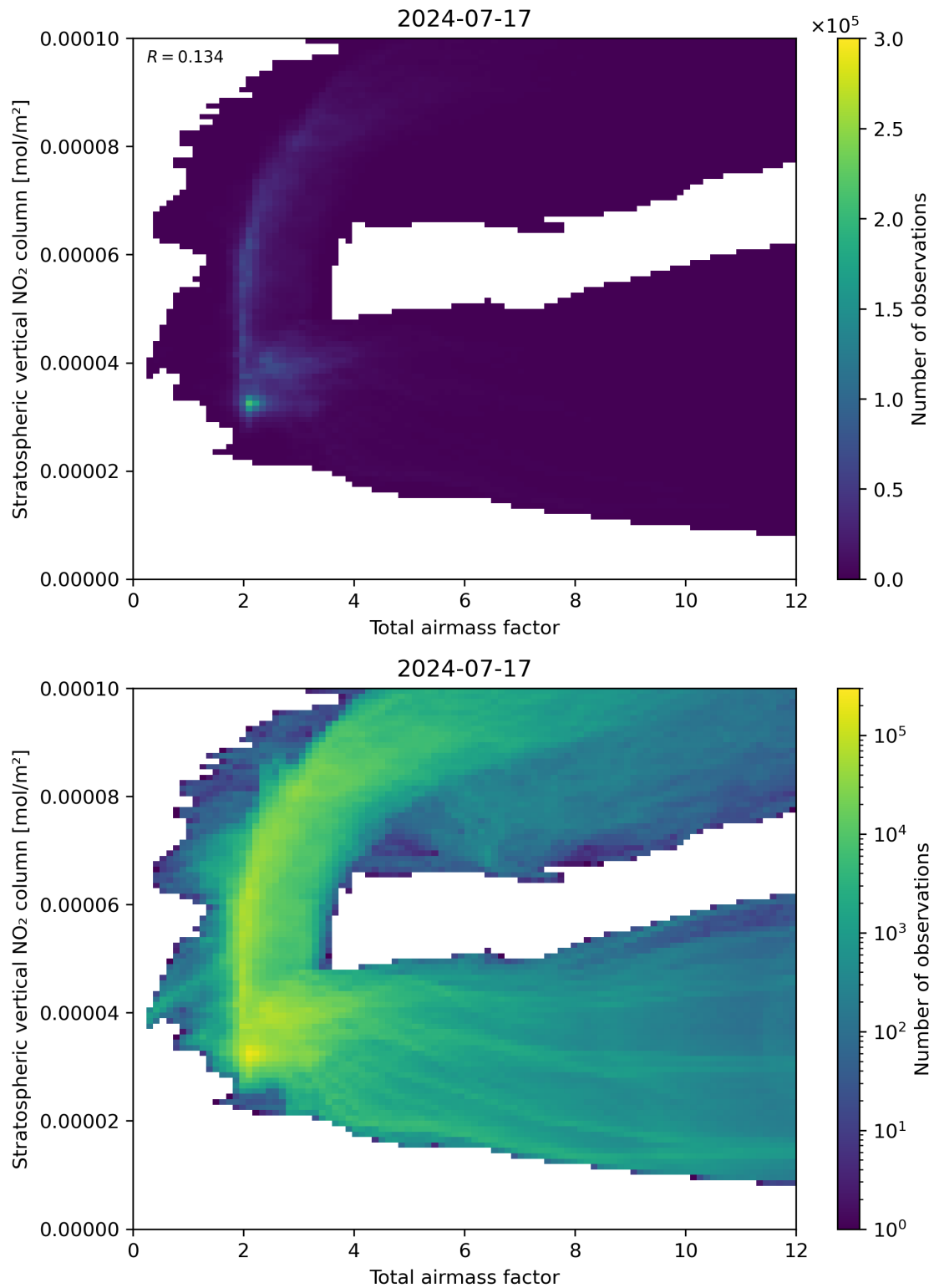
Figure 64: Scatter density plot of “Total airmass factor” against “Stratospheric vertical NO 2 column” for 2024-07-16 to 2024-07-18.
