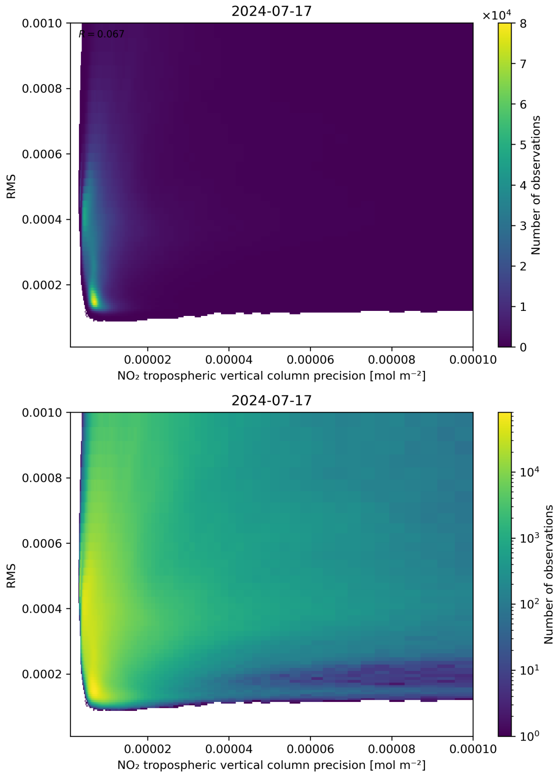
Figure 140: Scatter density plot of “NO 2 tropospheric vertical column precision” against “RMS” for 2024-07-16 to 2024-07-18.
