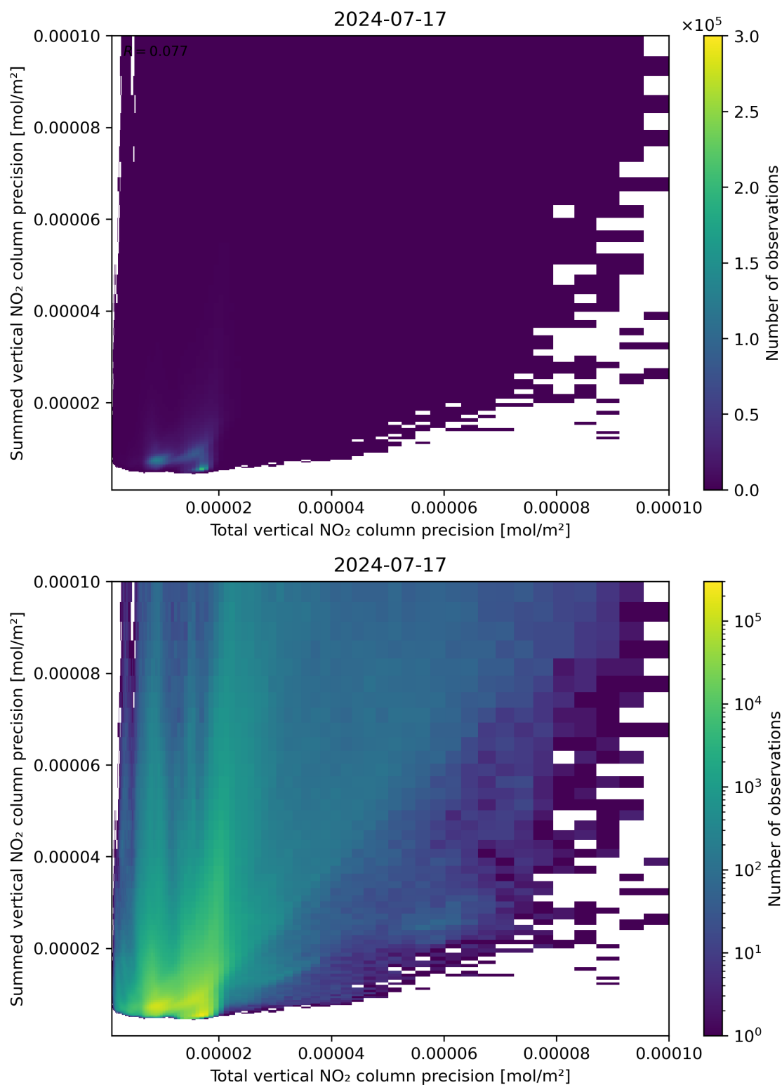
Figure 118: Scatter density plot of “Total vertical NO 2 column precision” against “Summed vertical NO 2 column precision” for 2024-07-16 to 2024-07-18.
