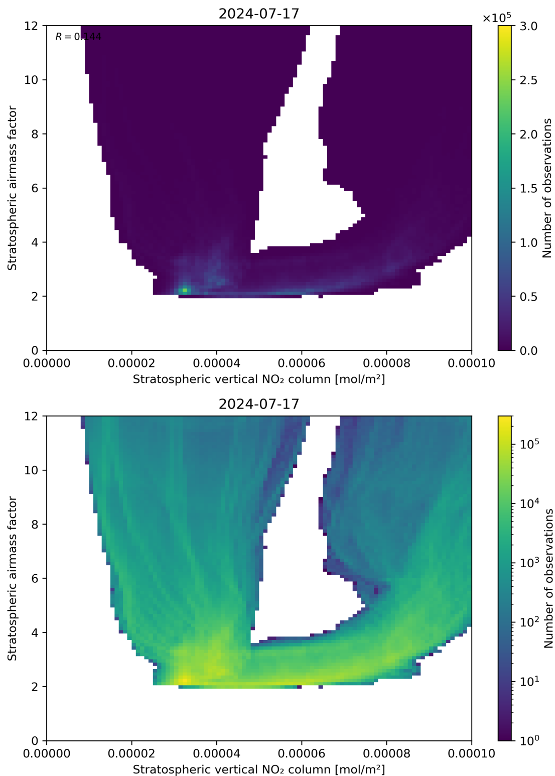
Figure 96: Scatter density plot of “Stratospheric vertical NO 2 column” against “Stratospheric airmass factor” for 2024-07-16 to 2024-07-18.
