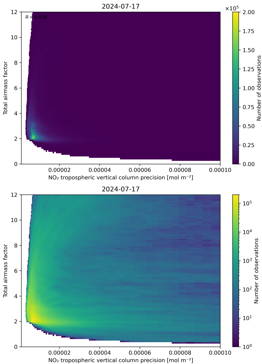
Figure 132: Scatter density plot of “NO 2 tropospheric vertical column precision” against “Total air mass factor” for 2024-07-16 to 2024-07-18.
