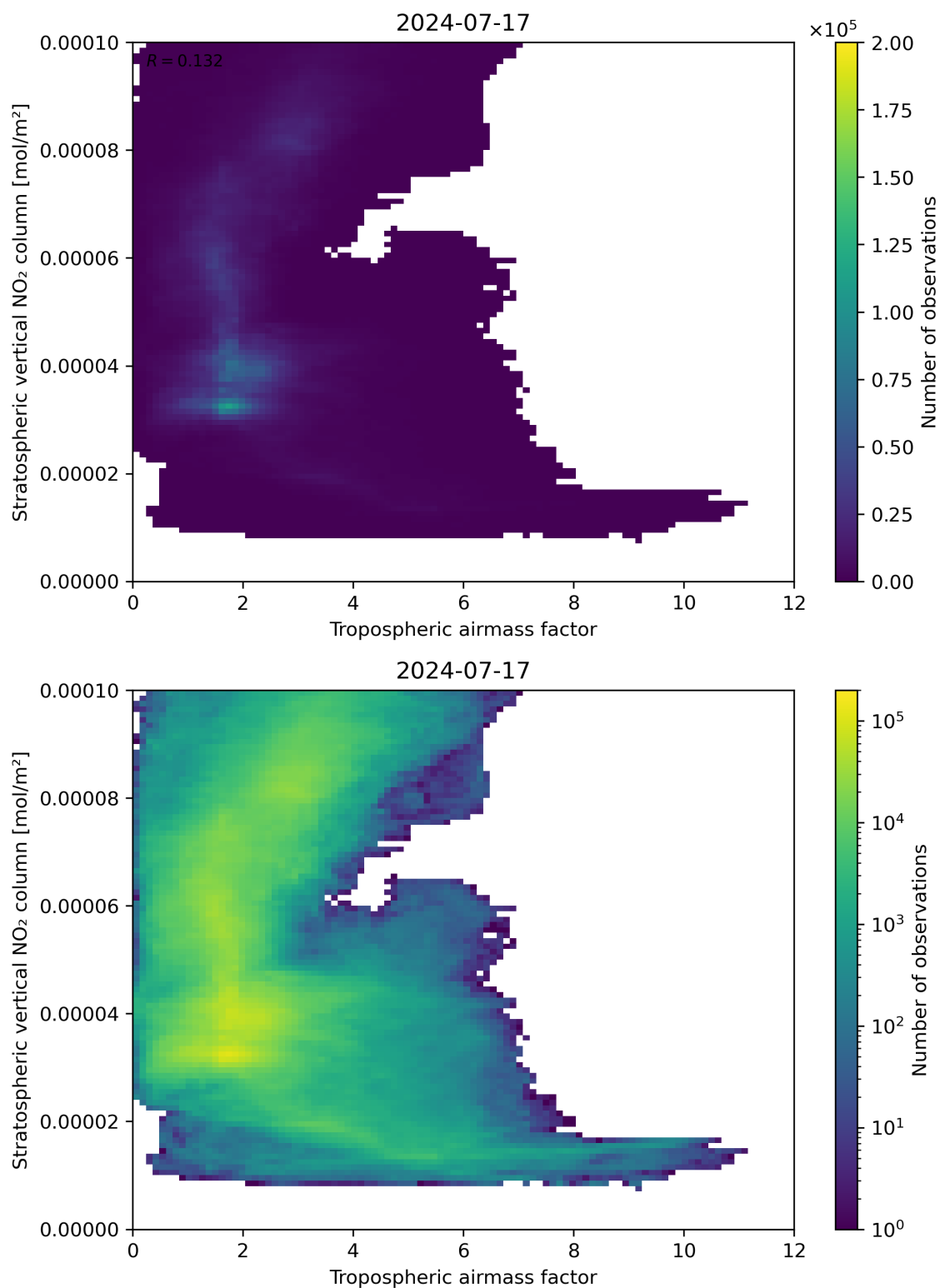
Figure 74: Scatter density plot of “Tropospheric air mass factor” against “Stratospheric vertical NO 2 column” for 2024-07-16 to 2024-07-18.
