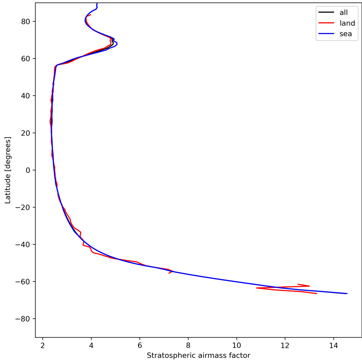
Figure 27: Zonal average of “Stratospheric airmass factor” for 2024-07-16 to 2024-07-18.
