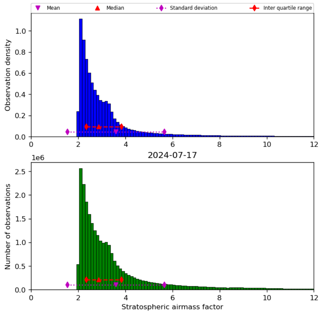
Figure 44: Histogram of “Stratospheric airmass factor” for 2024-07-16 to 2024-07-18
