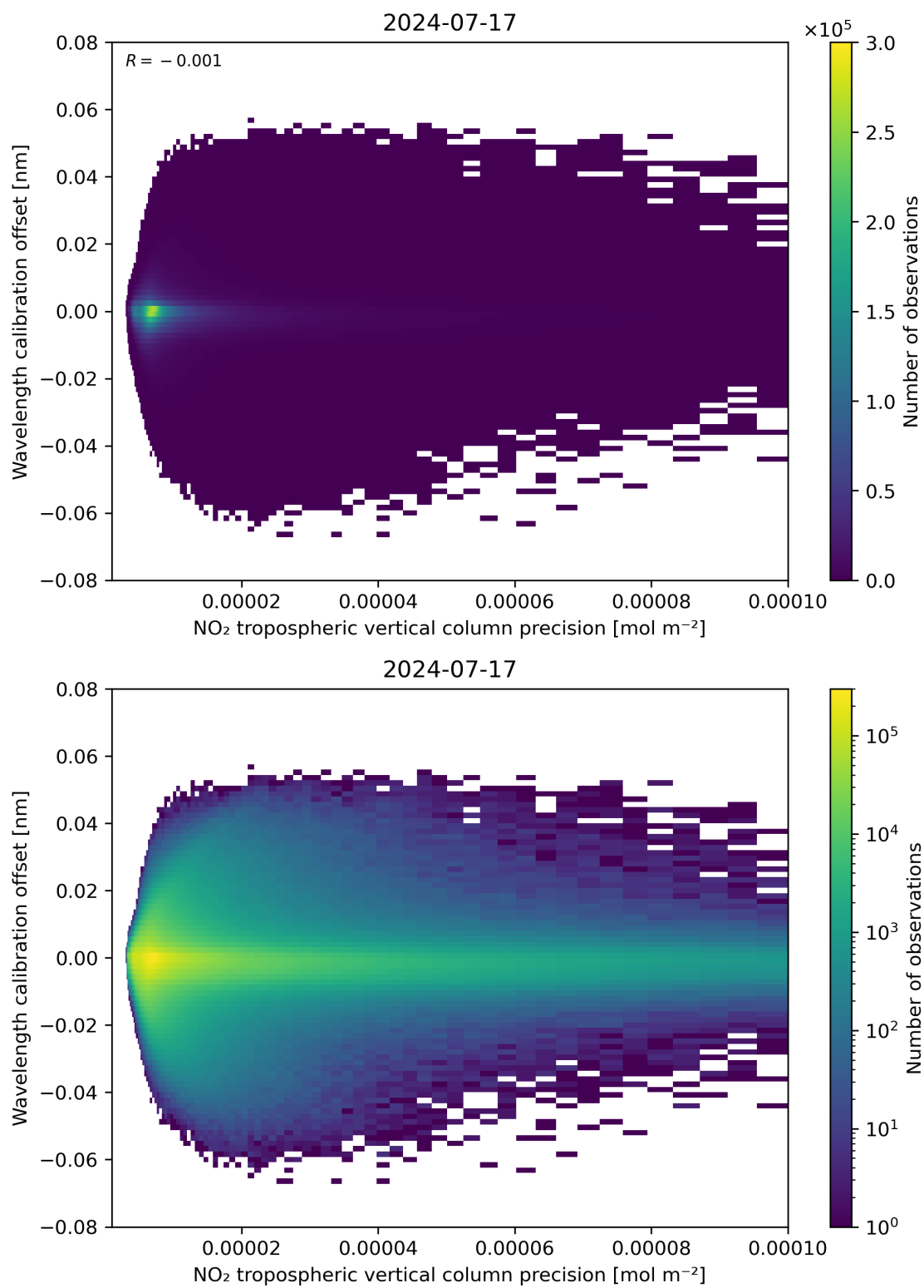
Figure 141: Scatter density plot of “NO 2 tropospheric vertical column precision” against “Wavelength calibration offset” for 2024-07-16 to 2024-07-18.
