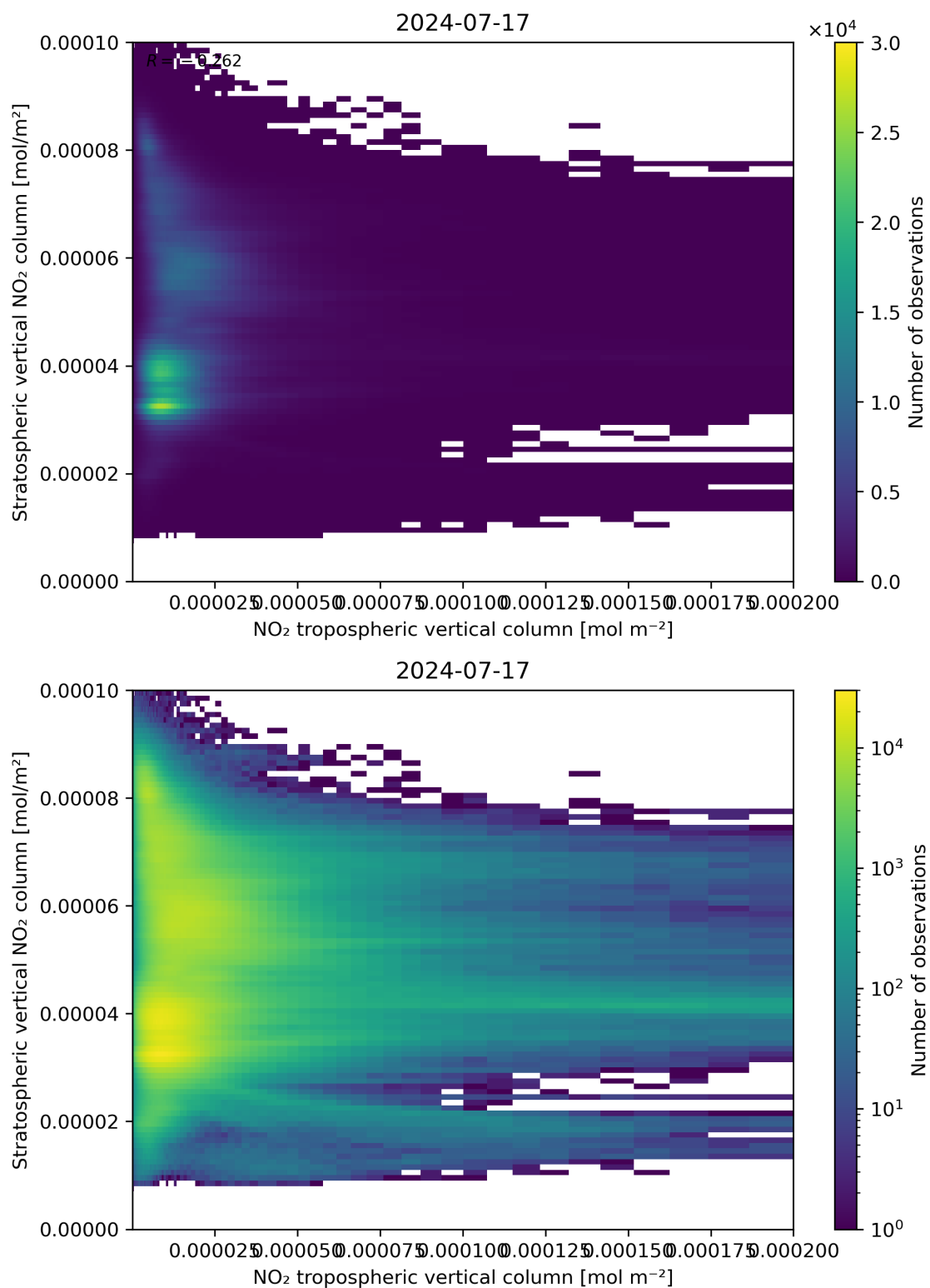
Figure 125: Scatter density plot of “NO 2 tropospheric vertical column” against “Stratospheric vertical NO 2 column” for 2024-07-16 to 2024-07-18.
