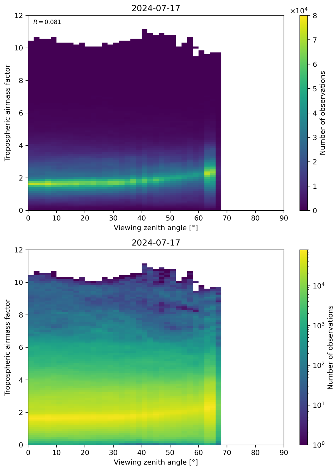
Figure 161: Scatter density plot of “Viewing zenith angle” against “Tropospheric airmass factor” for 2024-07-16 to 2024-07-18.
