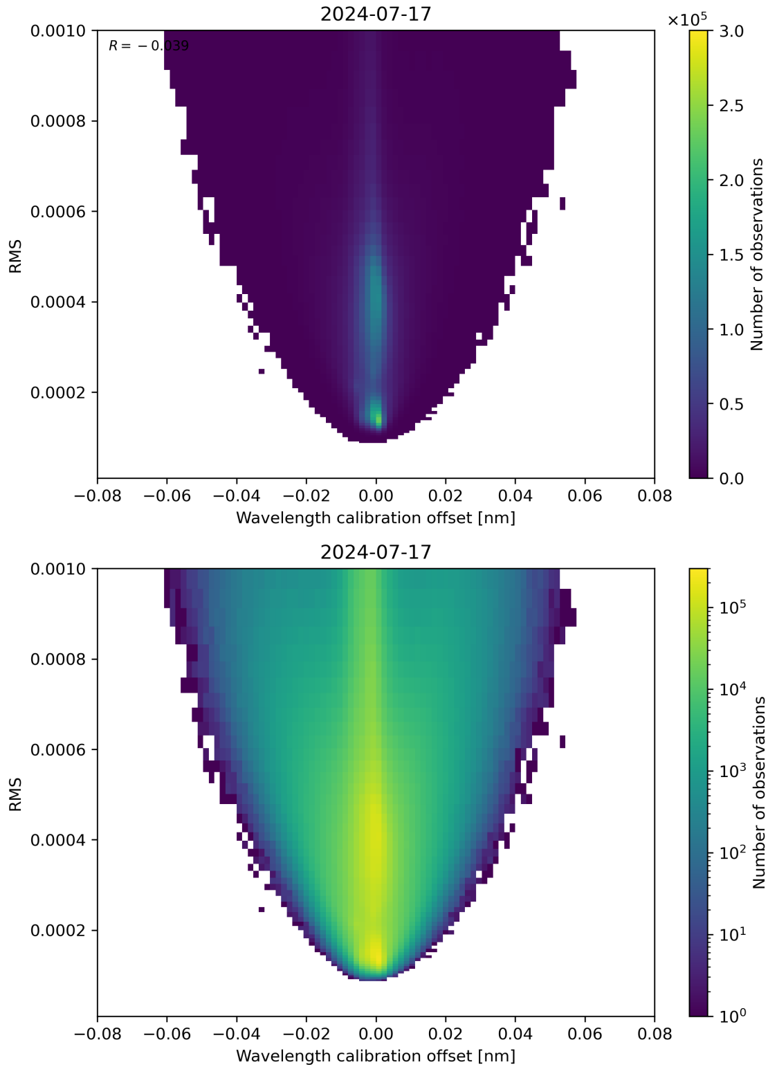
Figure 181: Scatter density plot of “Wavelength calibration offset” against “RMS” for 2024-07-16 to 2024-07-18.
