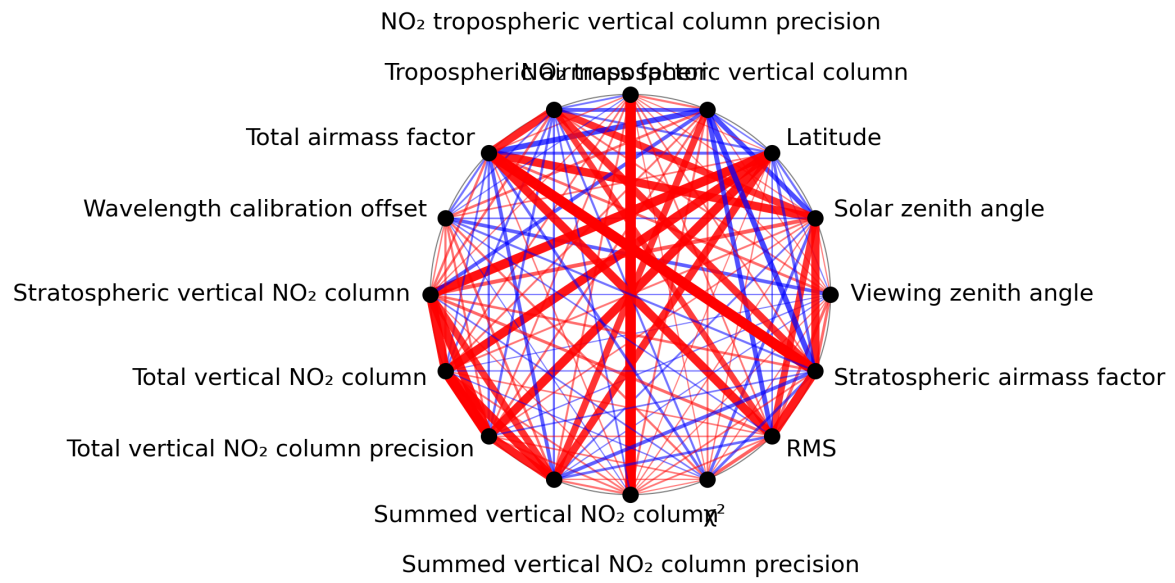
Figure 1: Map of correlation graph for 2024-07-16 to 2024-07-18.
