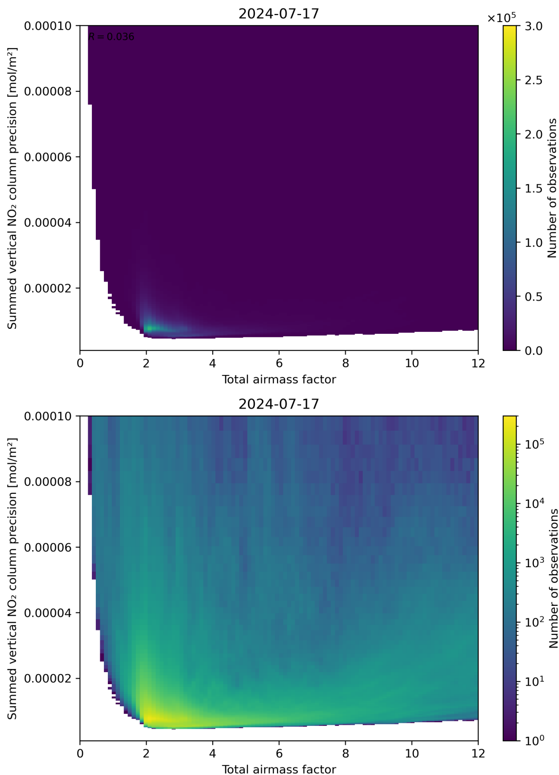
Figure 66: Scatter density plot of “Total airmass factor” against “Summed vertical NO 2 column precision” for 2024-07-16 to 2024-07-18.
