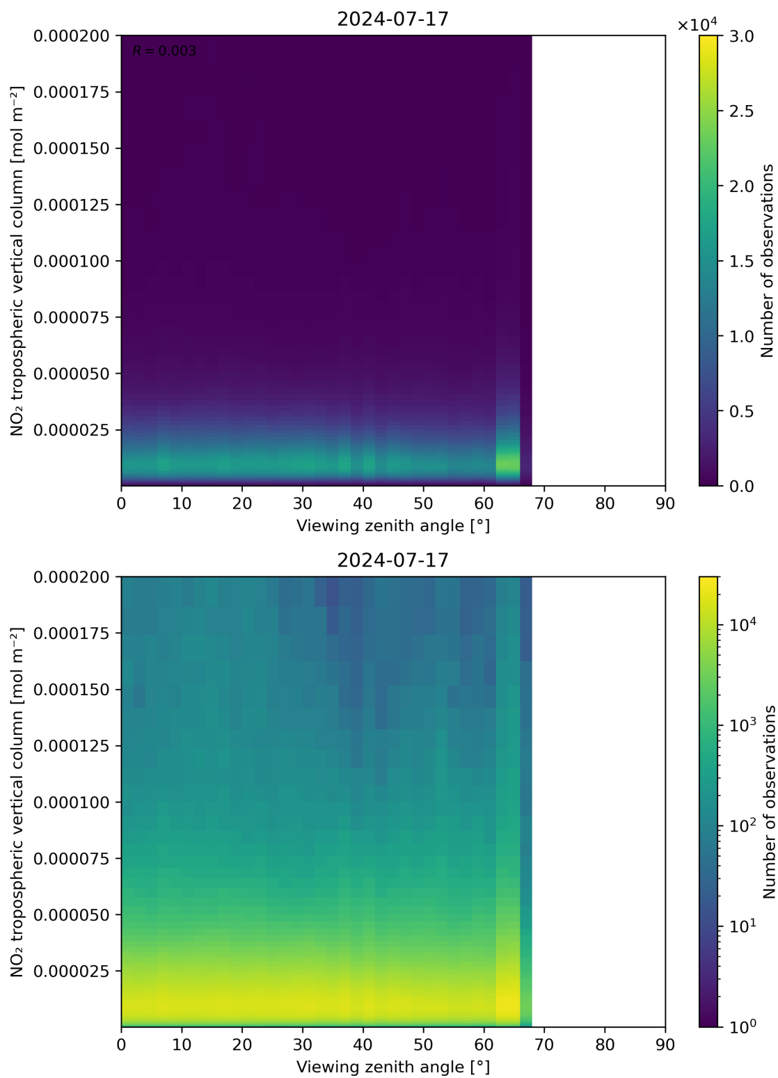
Figure 169: Scatter density plot of “Viewing zenith angle” against “NO 2 tropospheric vertical column” for 2024-07-16 to 2024-07-18.
