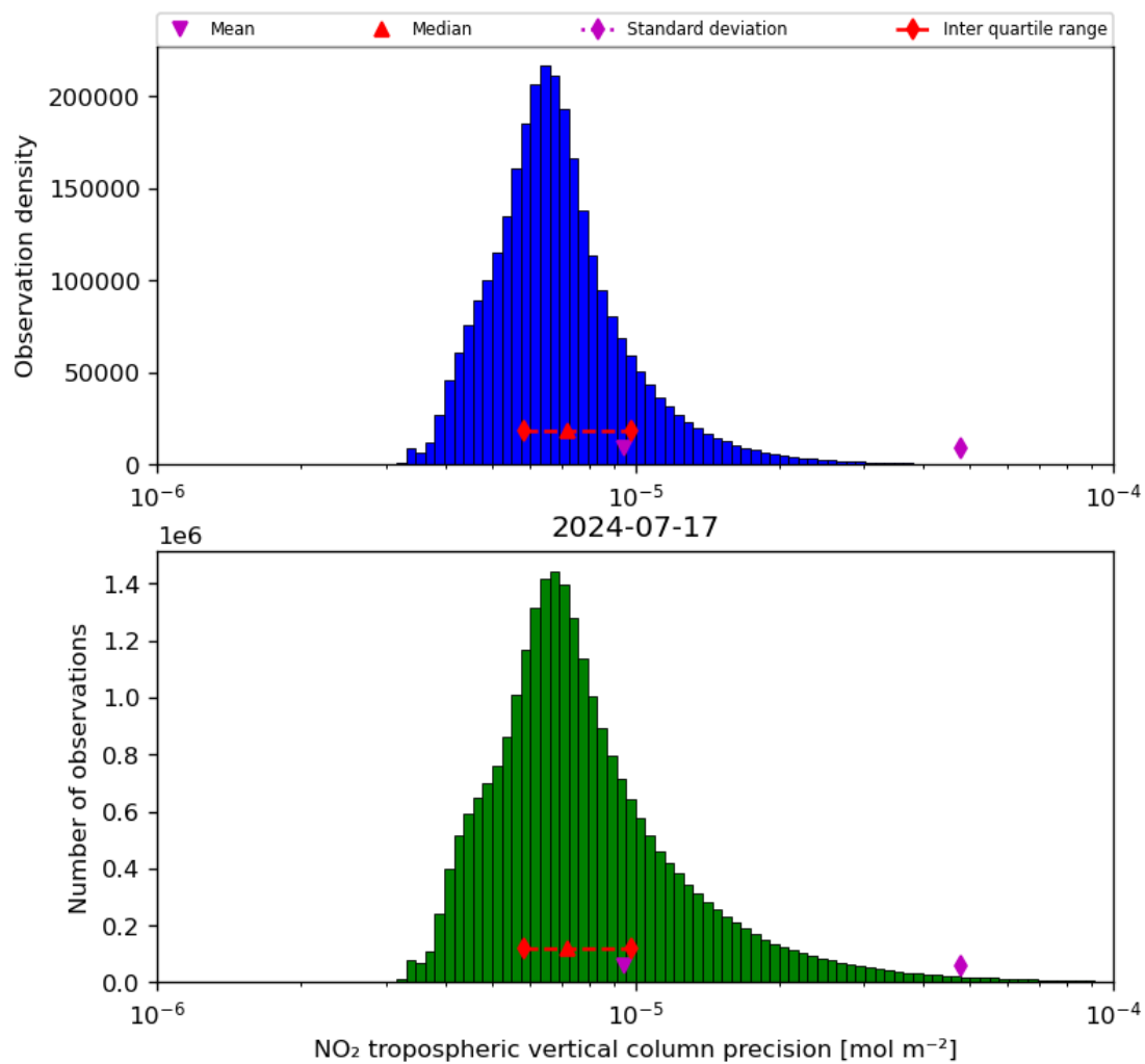
Figure 30: Histogram of “NO 2 tropospheric vertical column precision” for 2024-07-16 to 2024-07-18
