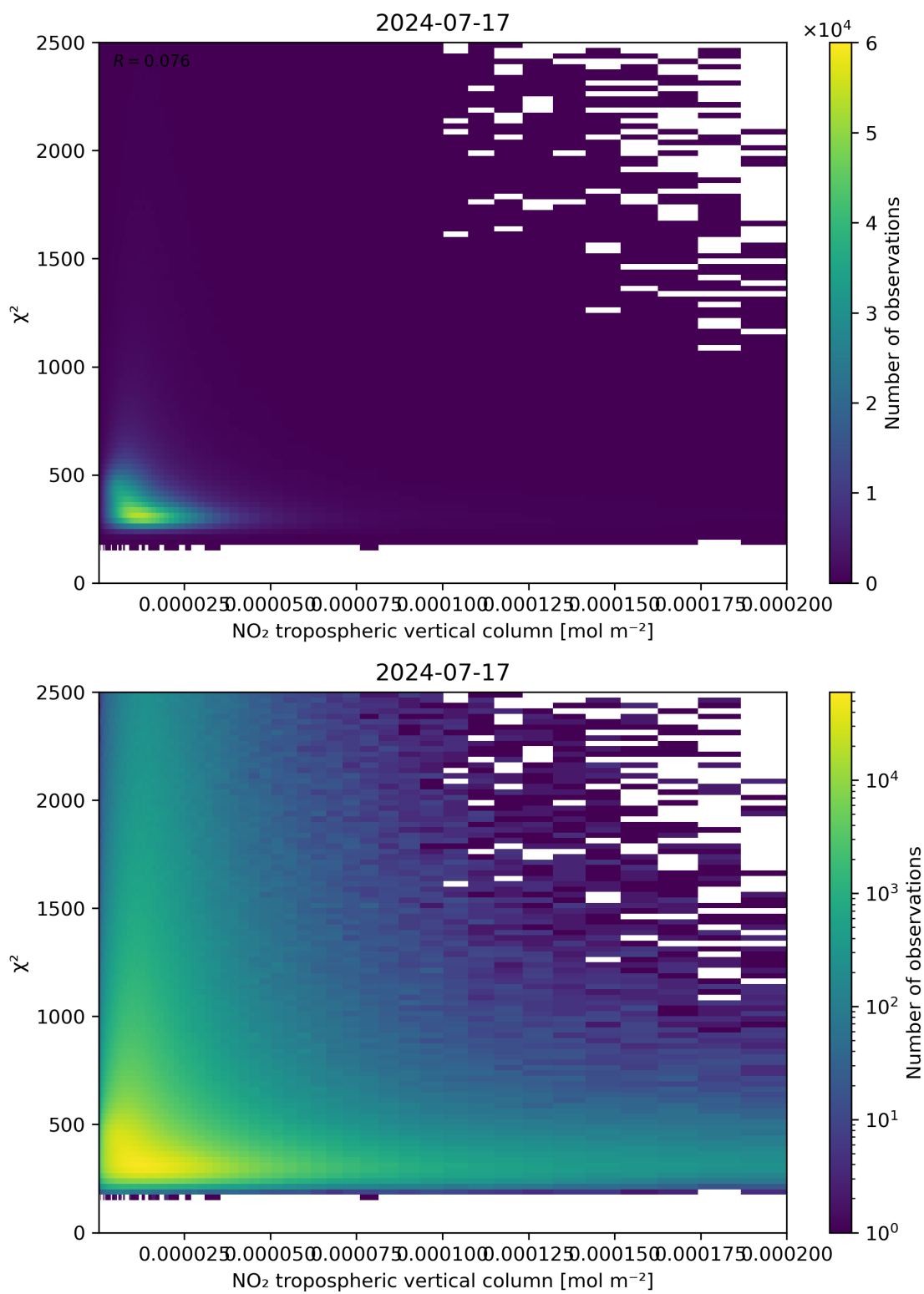
Figure 124: Scatter density plot of “NO 2 tropospheric vertical column” against “ \chi^2 ” for 2024-07-16 to 2024-07-18.
