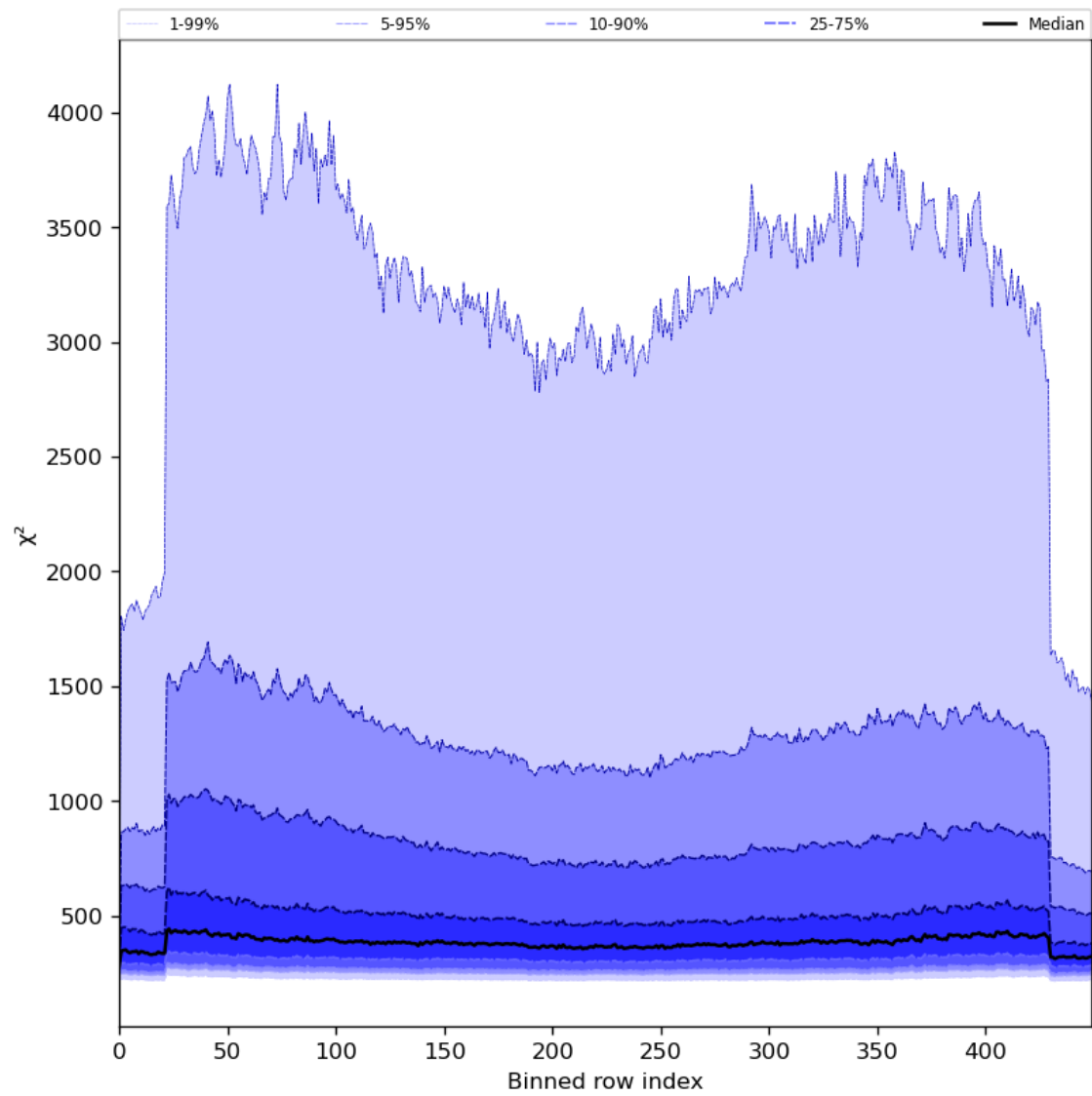
Figure 59: Along track statistics of “ \chi^2 ” for 2024-07-16 to 2024-07-18
