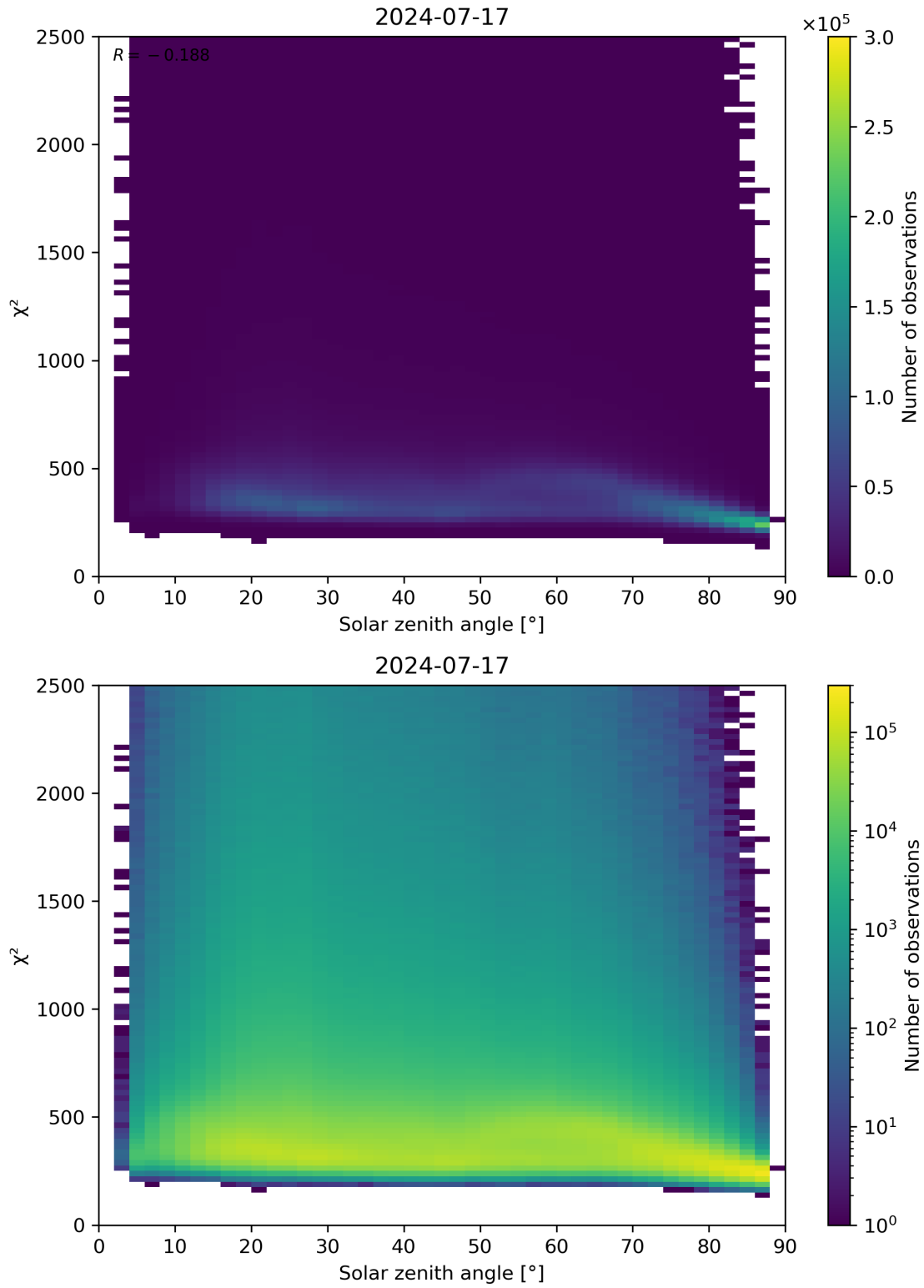
Figure 148: Scatter density plot of “Solar zenith angle” against “ \chi^2 ” for 2024-07-16 to 2024-07-18.
