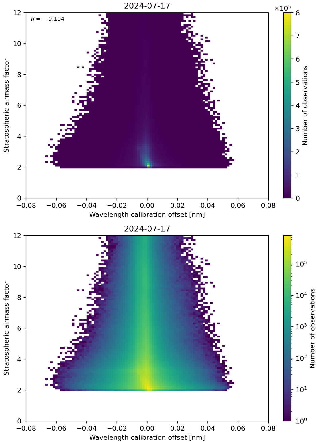
Figure 174: Scatter density plot of “Wavelength calibration offset” against “Stratospheric airmass factor” for 2024-07-16 to 2024-07-18.
