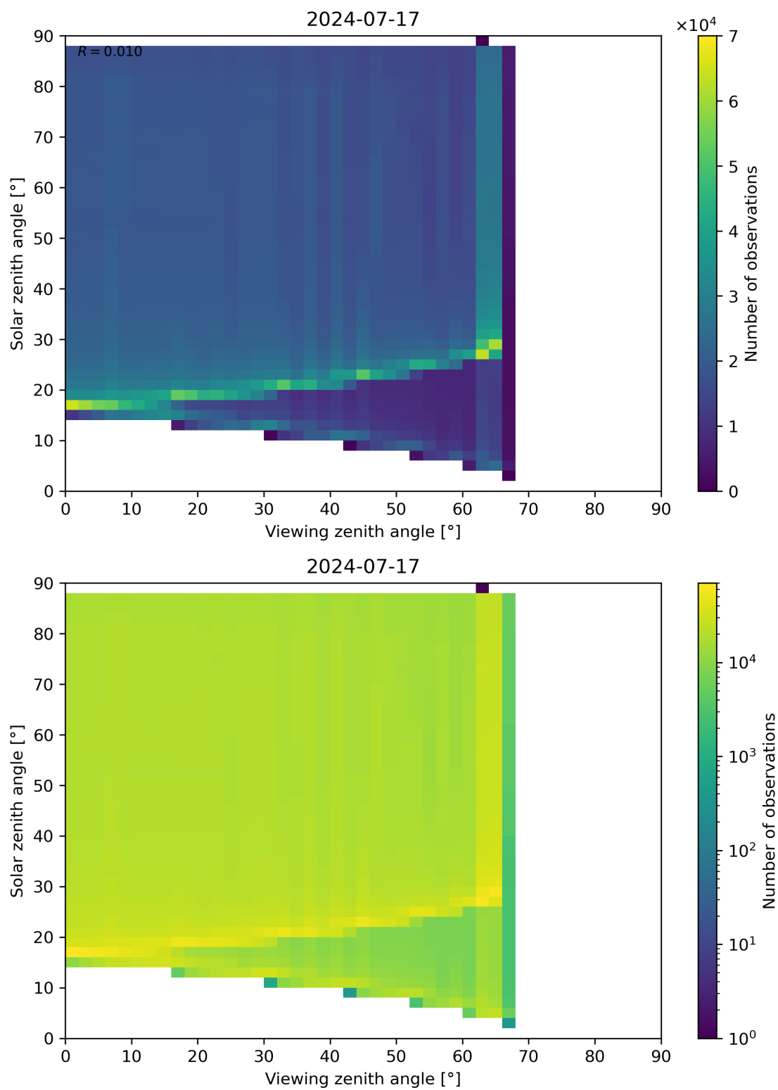
Figure 172: Scatter density plot of “Viewing zenith angle” against “Solar zenith angle” for 2024-07-16 to 2024-07-18.
