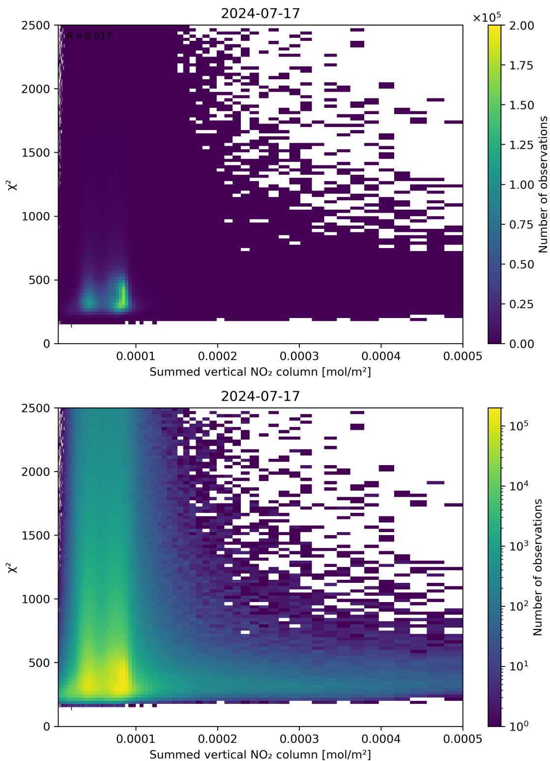
Figure 104: Scatter density plot of “Summed vertical NO 2 column” against “ \chi^2 ” for 2024-07-16 to 2024-07-18.
