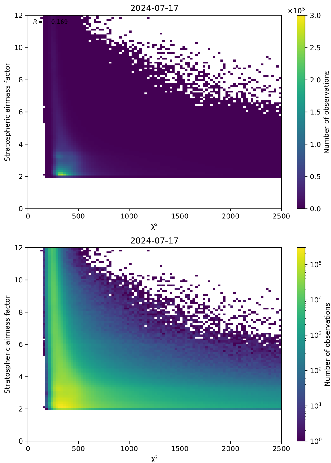
Figure 81: Scatter density plot of “ \chi^2 ” against “Stratospheric airmass factor” for 2024-07-16 to 2024-07-18.
