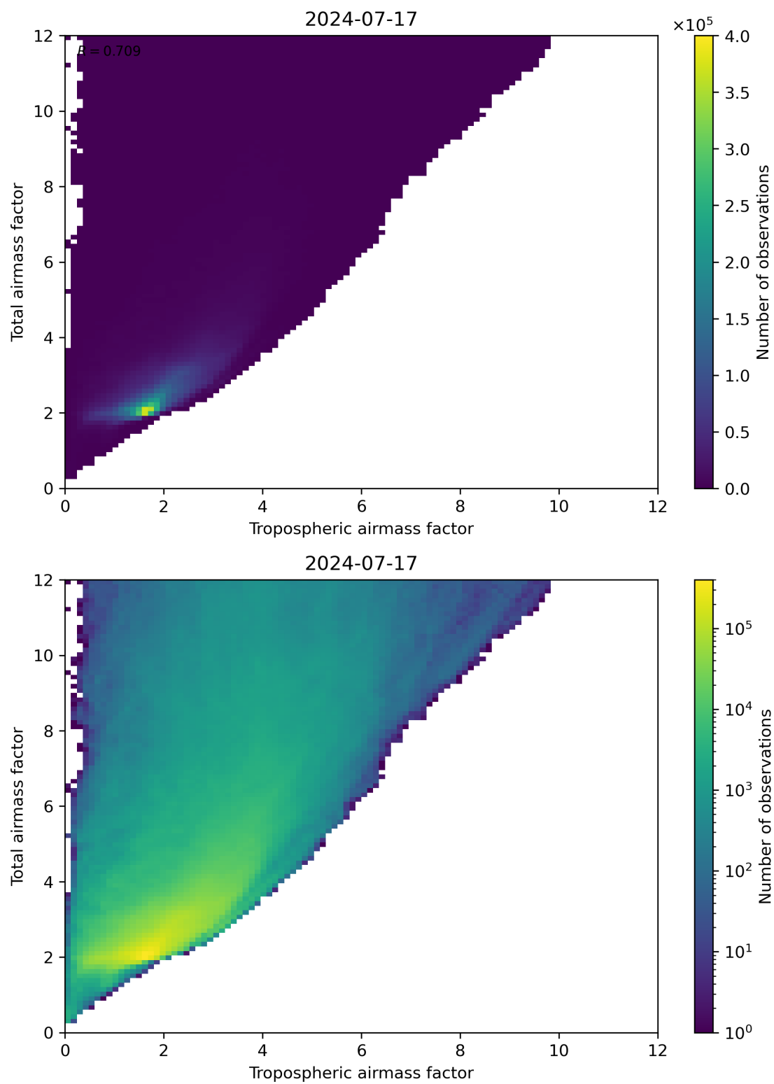
Figure 72: Scatter density plot of “Tropospheric airmass factor” against “Total airmass factor” for 2024-07-16 to 2024-07-18.
