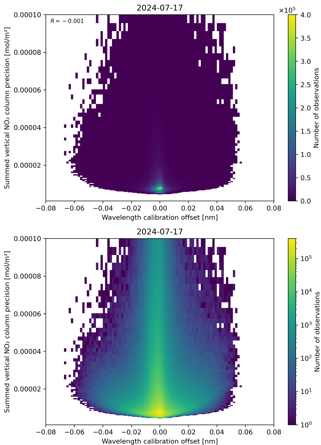
Figure 178: Scatter density plot of “Wavelength calibration offset” against “Summed vertical NO 2 column precision” for 2024-07-16 to 2024-07-18.
