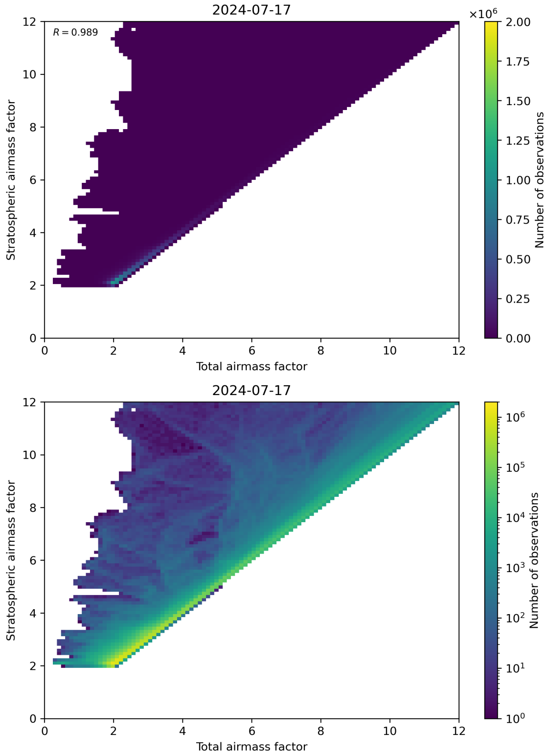
Figure 62: Scatter density plot of “Total airmass factor” against “Stratospheric airmass factor” for 2024-07-16 to 2024-07-18.
