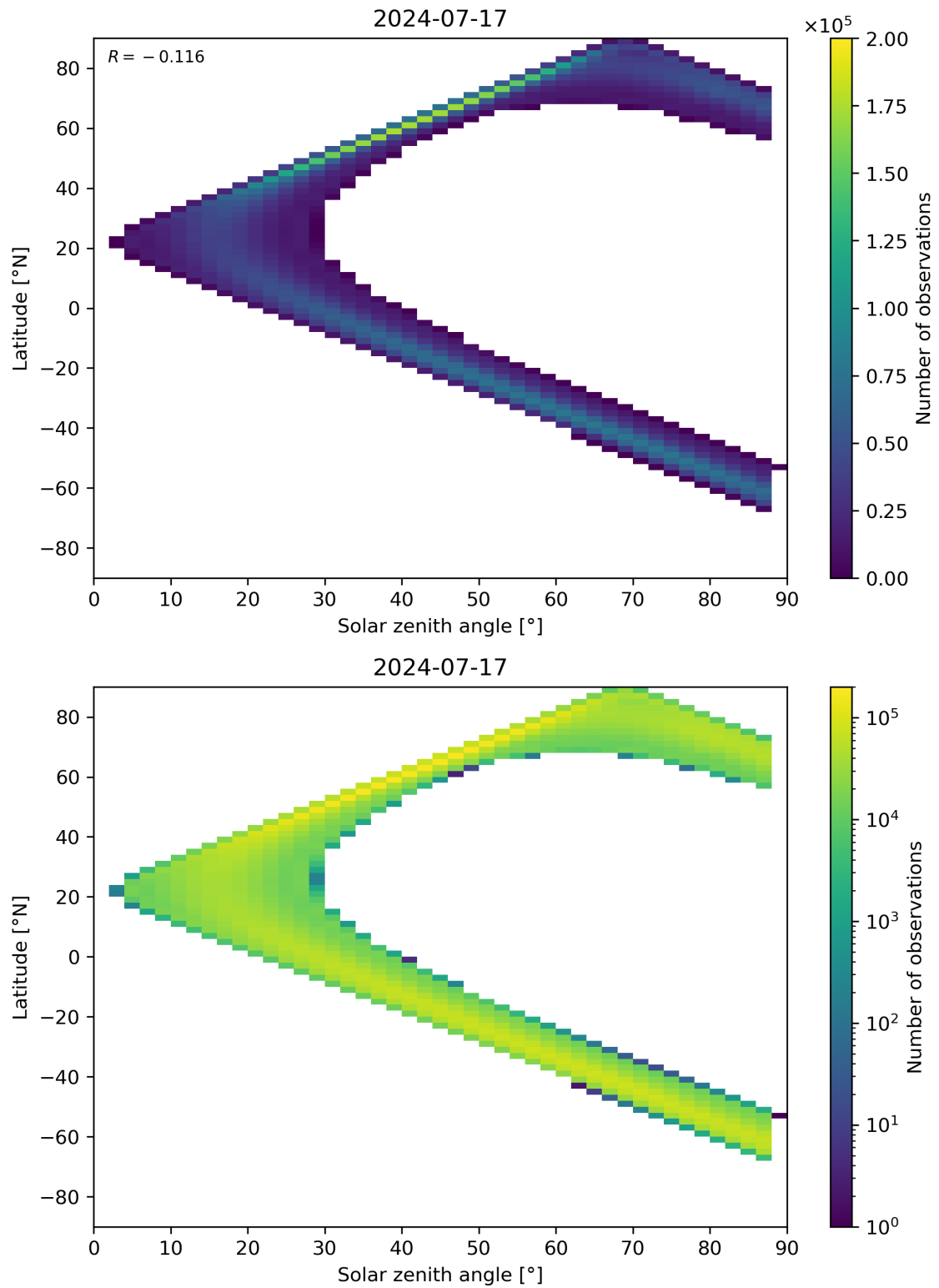
Figure 149: Scatter density plot of “Solar zenith angle” against “Latitude” for 2024-07-16 to 2024-07-18.
