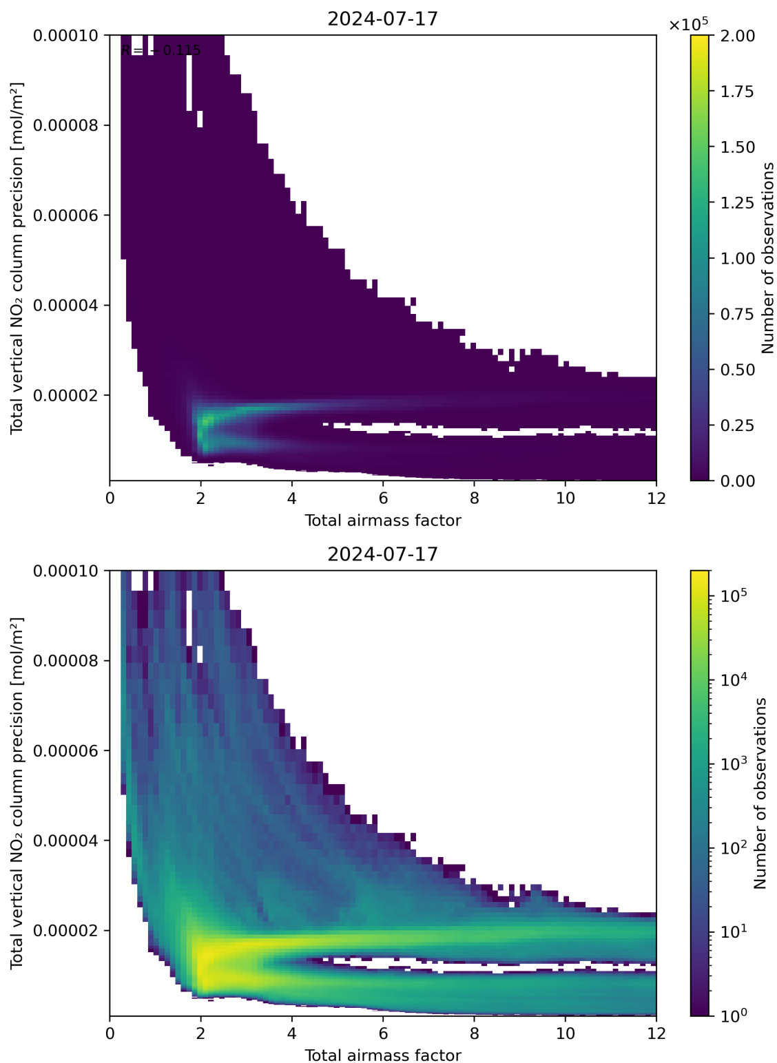
Figure 68: Scatter density plot of “Total airmass factor” against “Total vertical NO 2 column precision” for 2024-07-16 to 2024-07-18.
