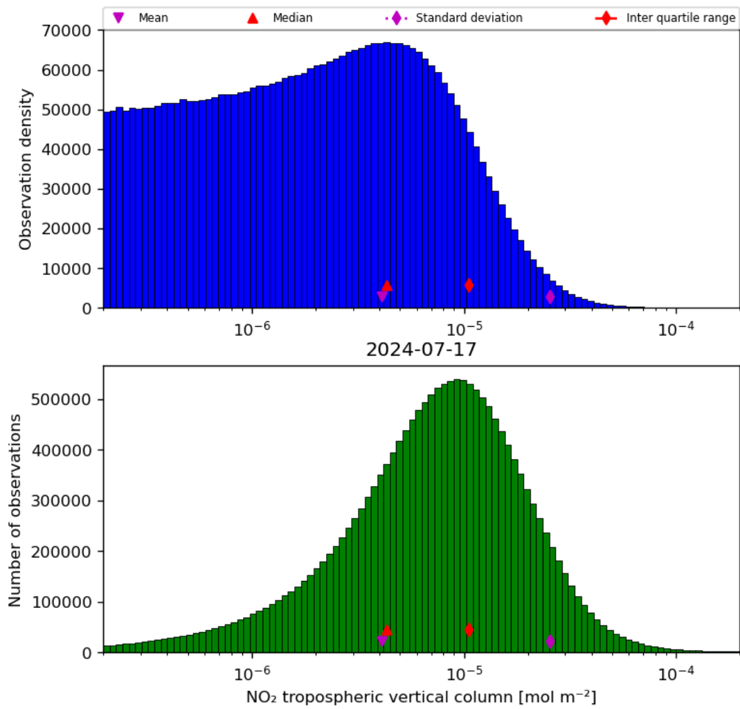
Figure 29: Histogram of “ \text{NO}_2 tropospheric vertical column” for 2024-07-16 to 2024-07-18
