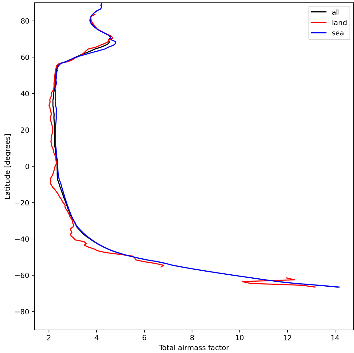
Figure 15: Zonal average of “Total airmass factor” for 2024-07-16 to 2024-07-18.
