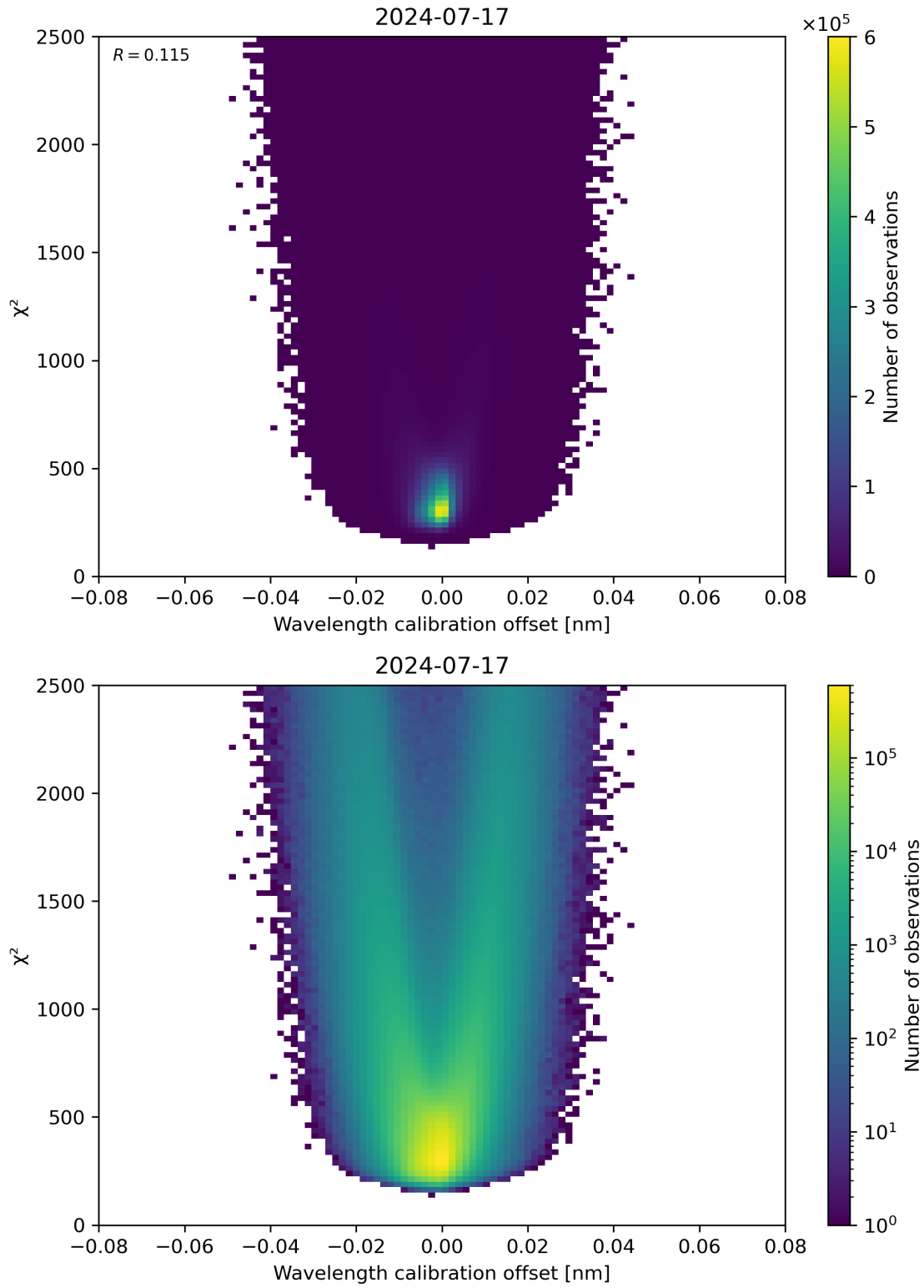
Figure 175: Scatter density plot of “Wavelength calibration offset” against “ \chi^2 ” for 2024-07-16 to 2024-07-18.
