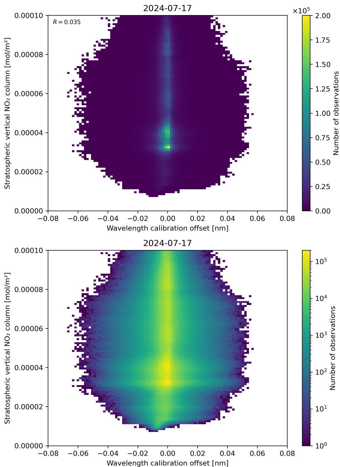
Figure 176: Scatter density plot of “Wavelength calibration offset” against “Stratospheric vertical NO 2 column” for 2024-07-16 to 2024-07-18.
