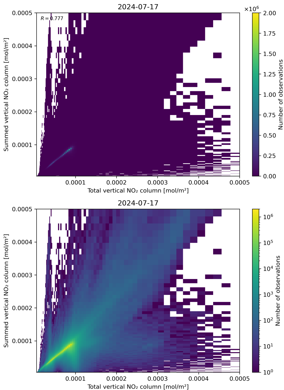
Figure 112: Scatter density plot of “Total vertical NO 2 column” against “Summed vertical NO 2 column” for 2024-07-16 to 2024-07-18.
