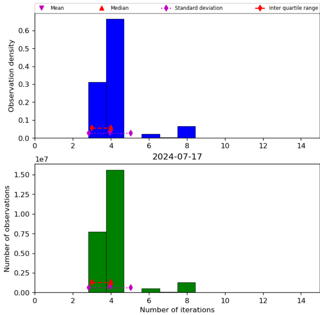
Figure 34: Histogram of “Number of iterations” for 2024-07-16 to 2024-07-18
