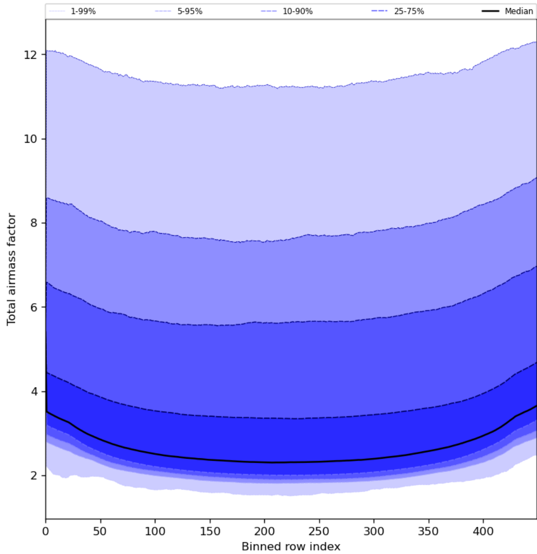
Figure 49: Along track statistics of “Total airmass factor” for 2024-07-16 to 2024-07-18
