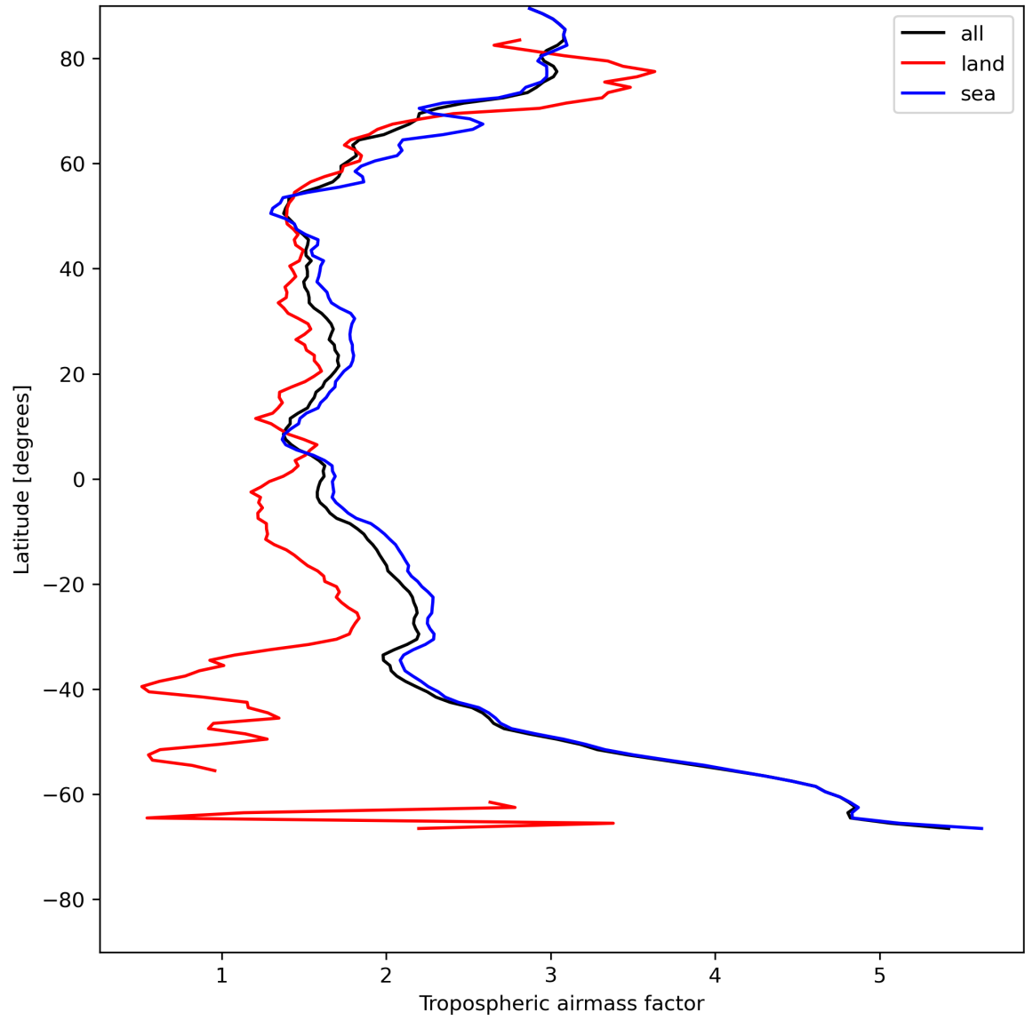
Figure 14: Zonal average of “Tropospheric airmass factor” for 2024-07-16 to 2024-07-18.
