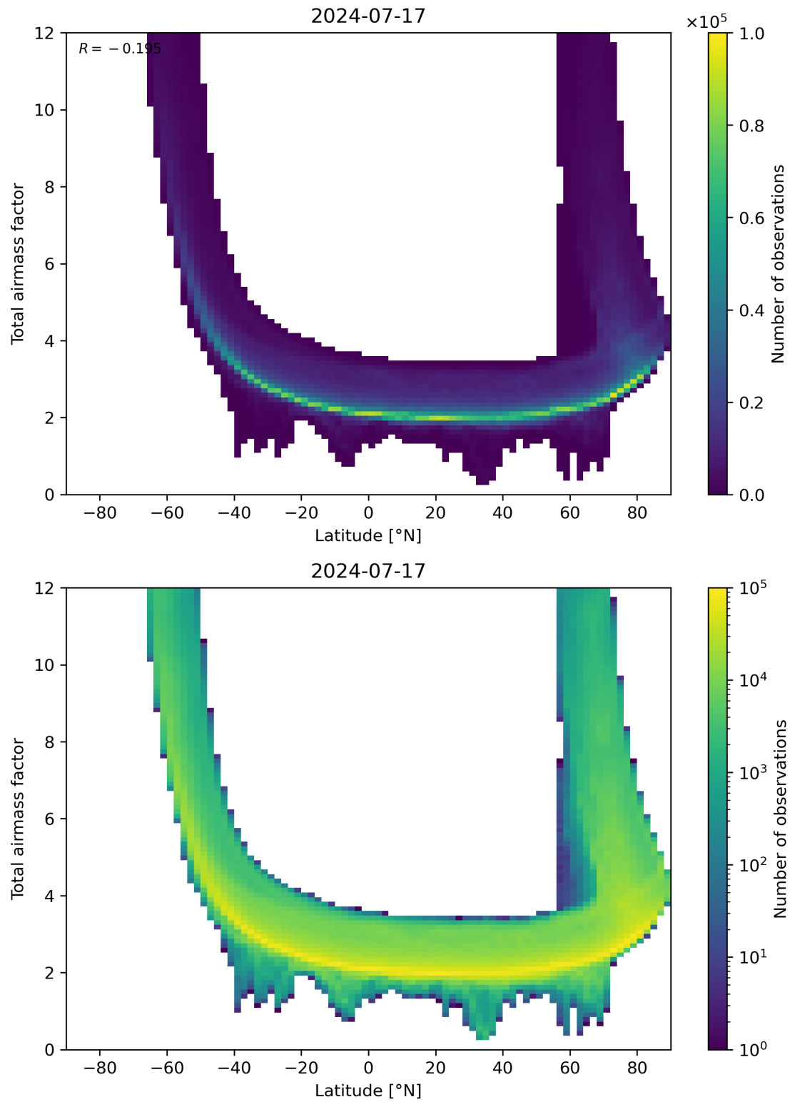
Figure 84: Scatter density plot of “Latitude” against “Total airmass factor” for 2024-07-16 to 2024-07-18.
