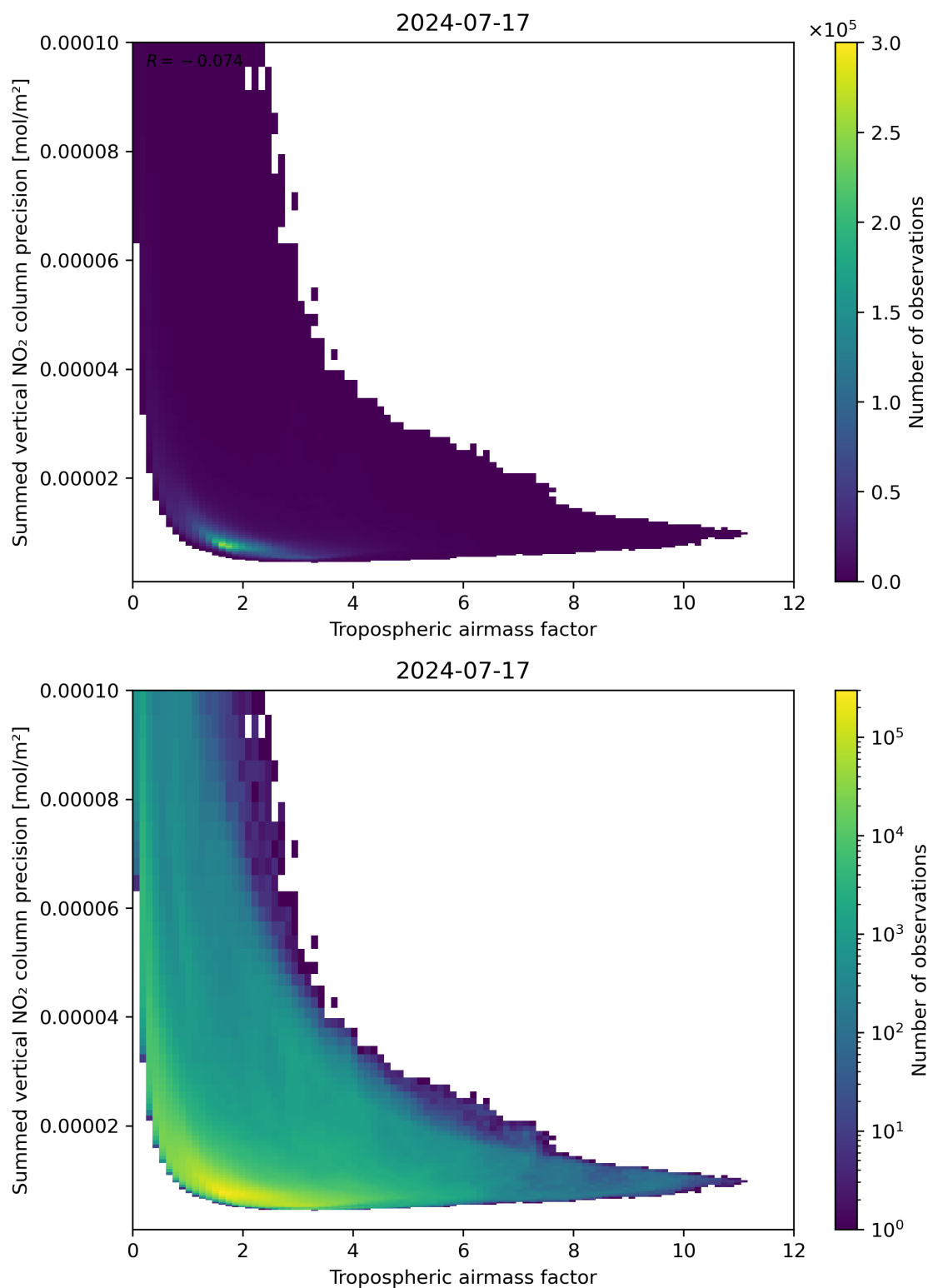
Figure 76: Scatter density plot of “Tropospheric air mass factor” against “Summed vertical NO 2 column precision” for 2024-07-16 to 2024-07-18.
