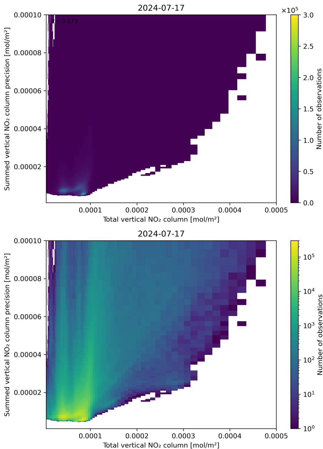
Figure 113: Scatter density plot of “Total vertical NO 2 column” against “Summed vertical NO 2 column precision” for 2024-07-16 to 2024-07-18.
