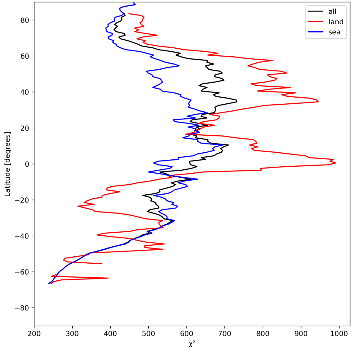
Figure 25: Zonal average of “ \chi^2 ” for 2024-07-16 to 2024-07-18.
