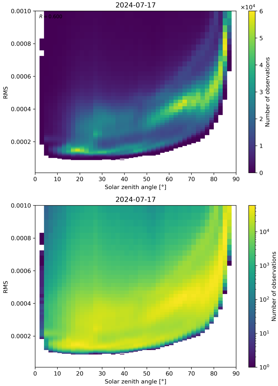
Figure 157: Scatter density plot of “Solar zenith angle” against “RMS” for 2024-07-16 to 2024-07-18.
