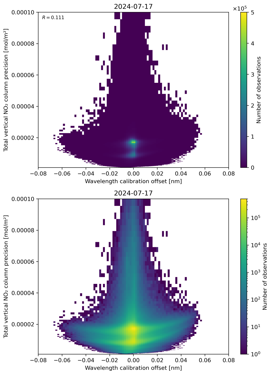
Figure 180: Scatter density plot of “Wavelength calibration offset” against “Total vertical NO 2 column precision” for 2024-07-16 to 2024-07-18.
