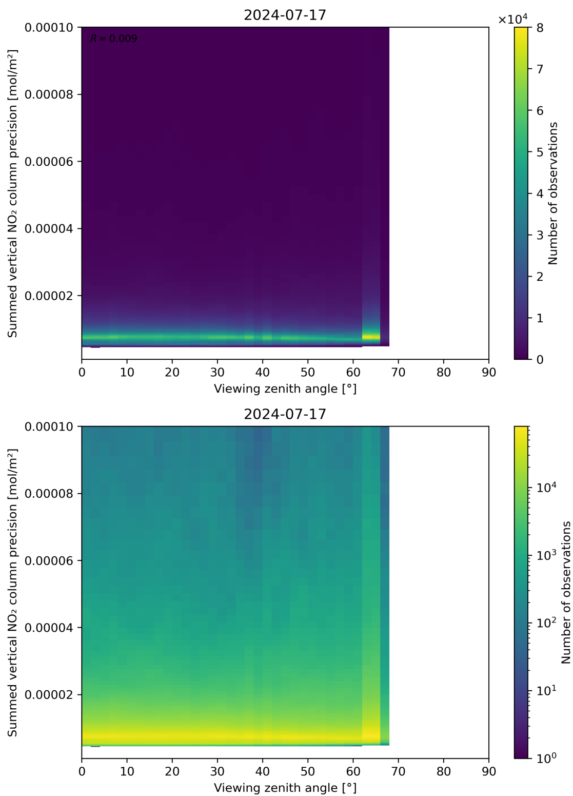
Figure 166: Scatter density plot of “Viewing zenith angle” against “Summed vertical NO 2 column precision” for 2024-07-16 to 2024-07-18.
