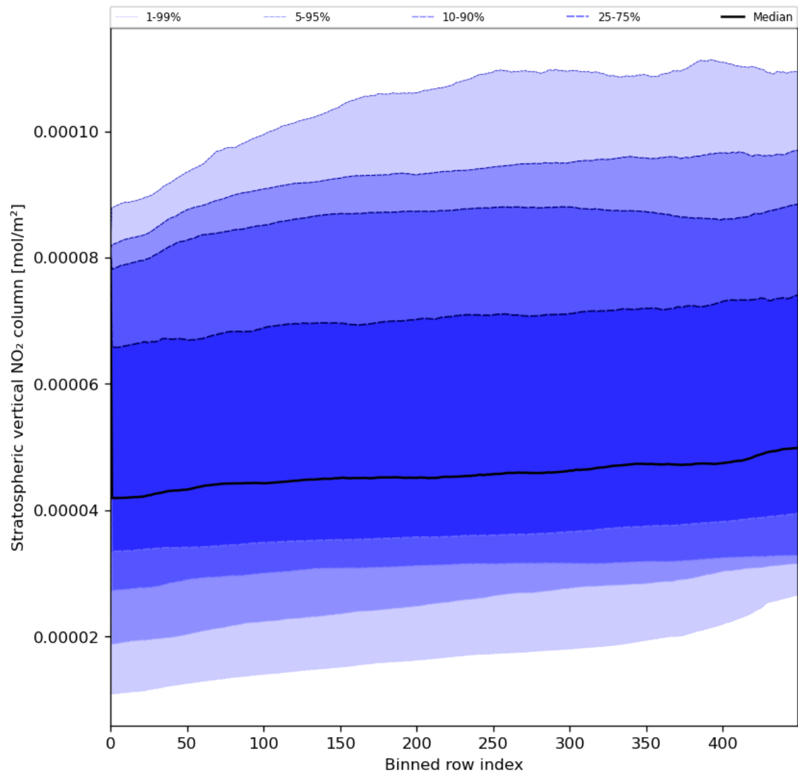
Figure 53: Along track statistics of “Stratospheric vertical NO 2 column” for 2024-07-16 to 2024-07-18
