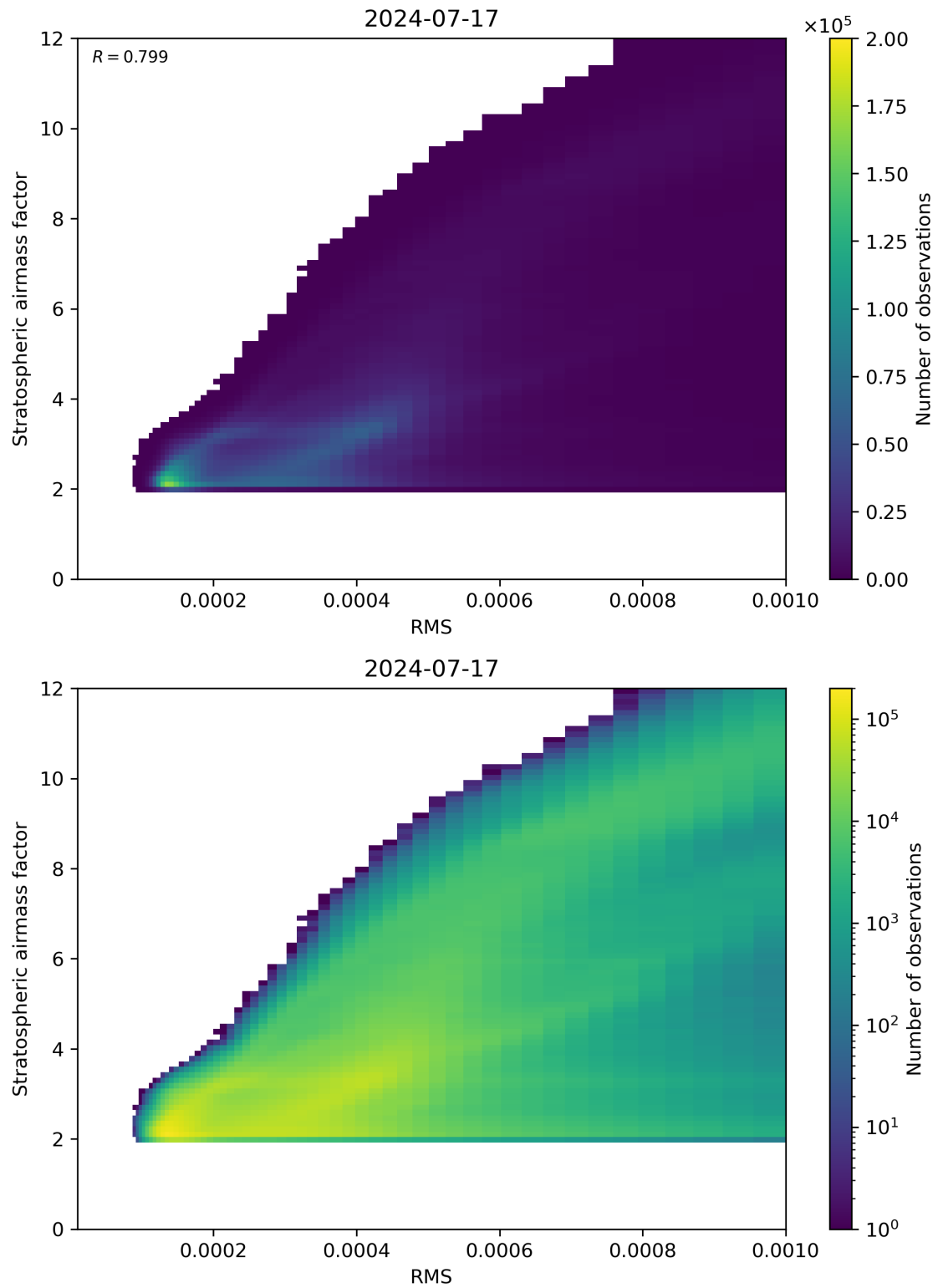
Figure 144: Scatter density plot of “RMS” against “Stratospheric airmass factor” for 2024-07-16 to 2024-07-18.
