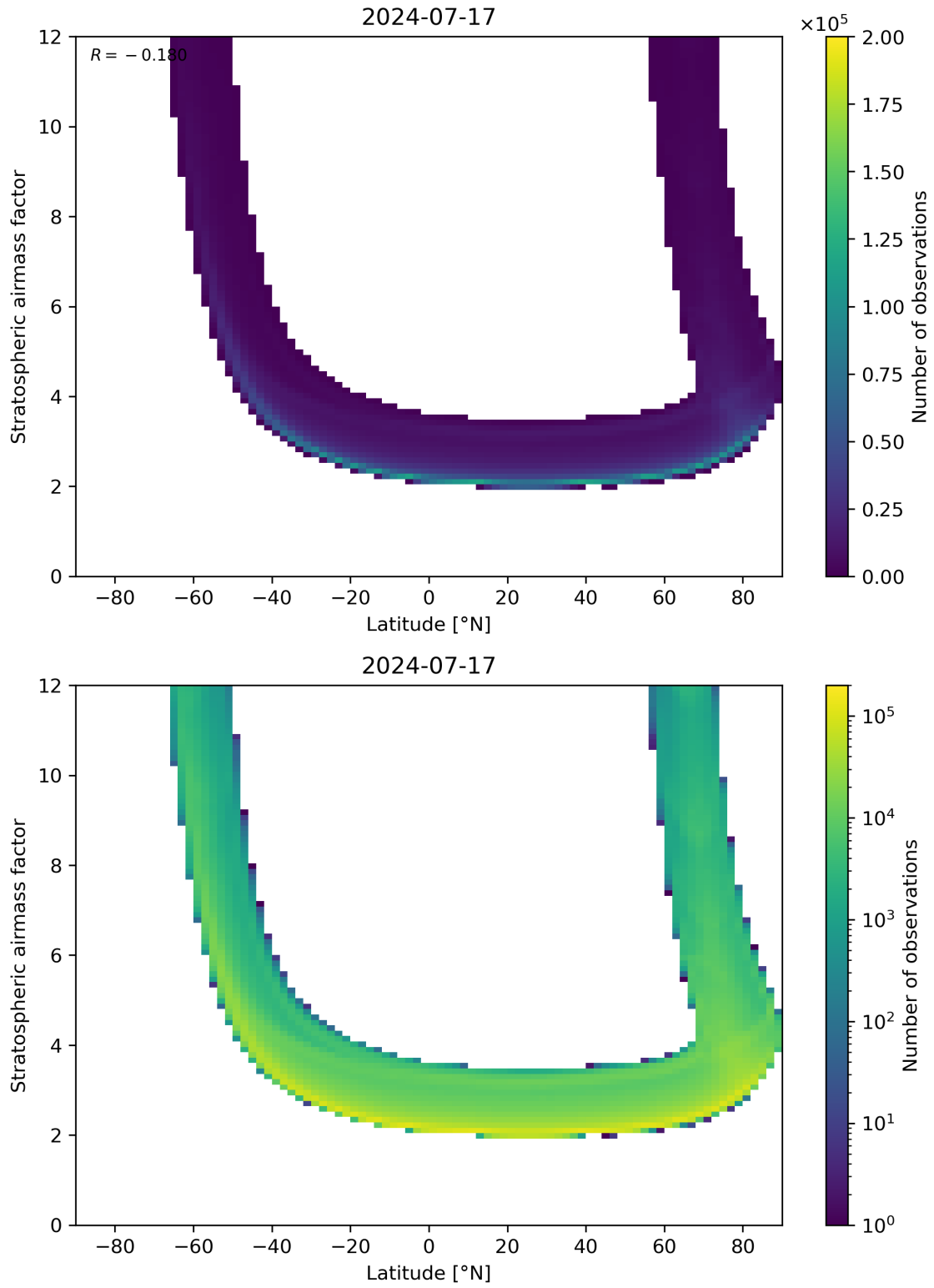
Figure 83: Scatter density plot of “Latitude” against “Stratospheric air mass factor” for 2024-07-16 to 2024-07-18.
