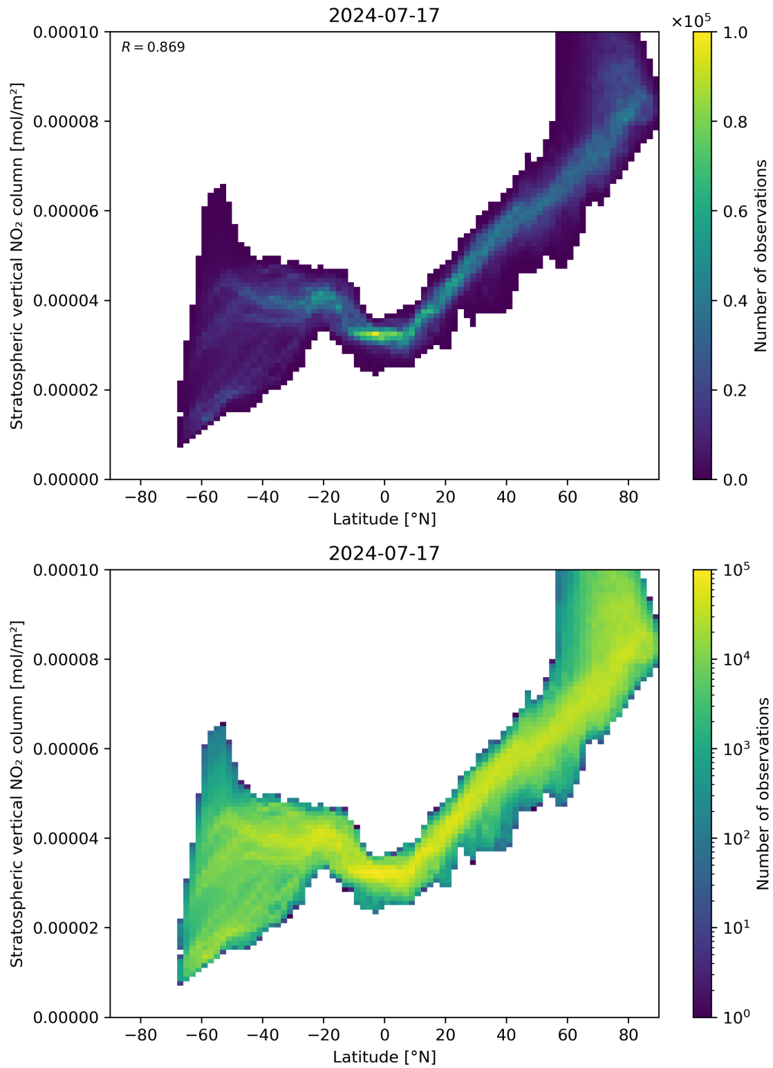
Figure 87: Scatter density plot of “Latitude” against “Stratospheric vertical NO 2 column” for 2024-07-16 to 2024-07-18.
