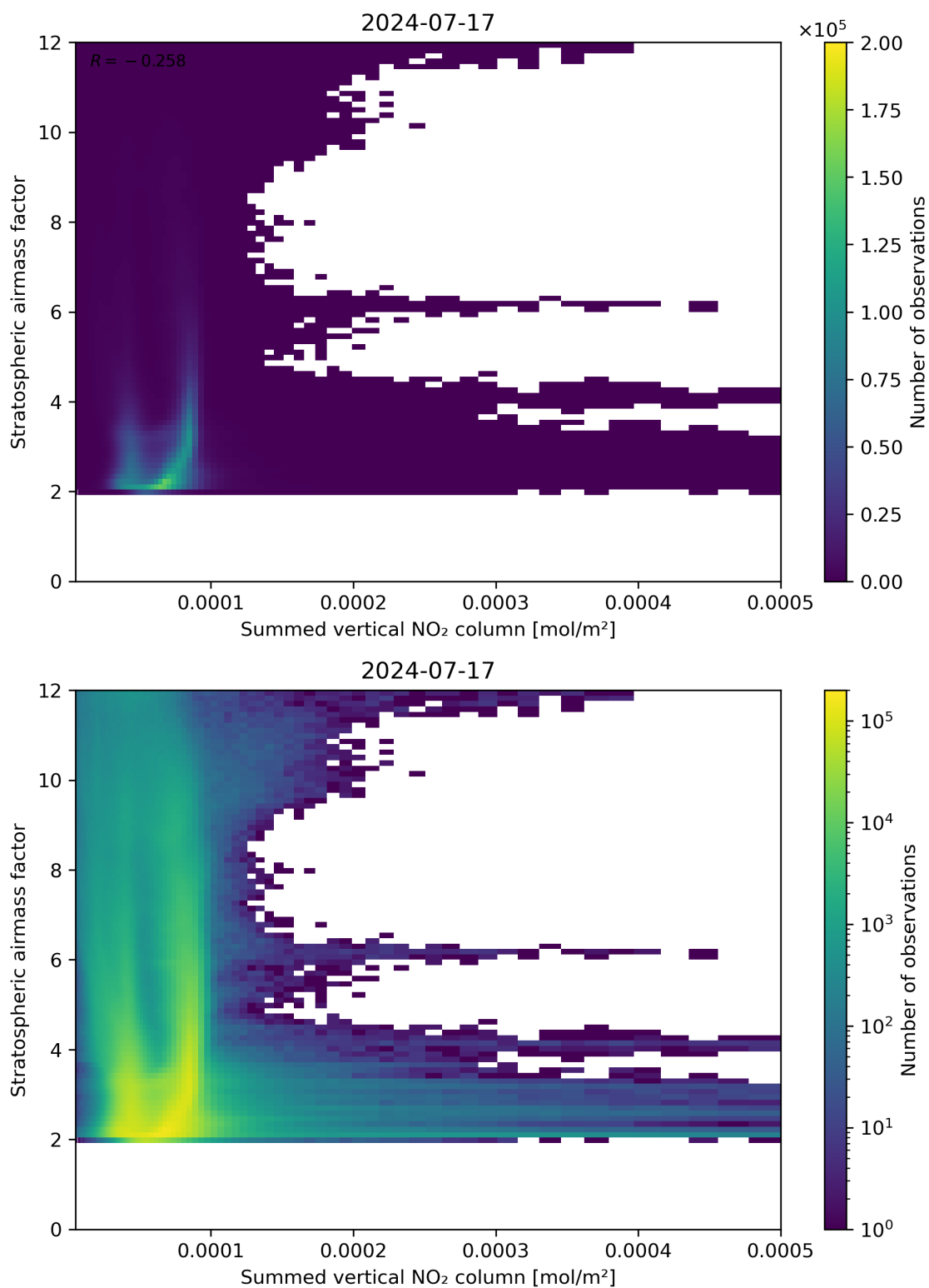
Figure 103: Scatter density plot of “Summed vertical NO 2 column” against “Stratospheric air mass factor” for 2024-07-16 to 2024-07-18.
