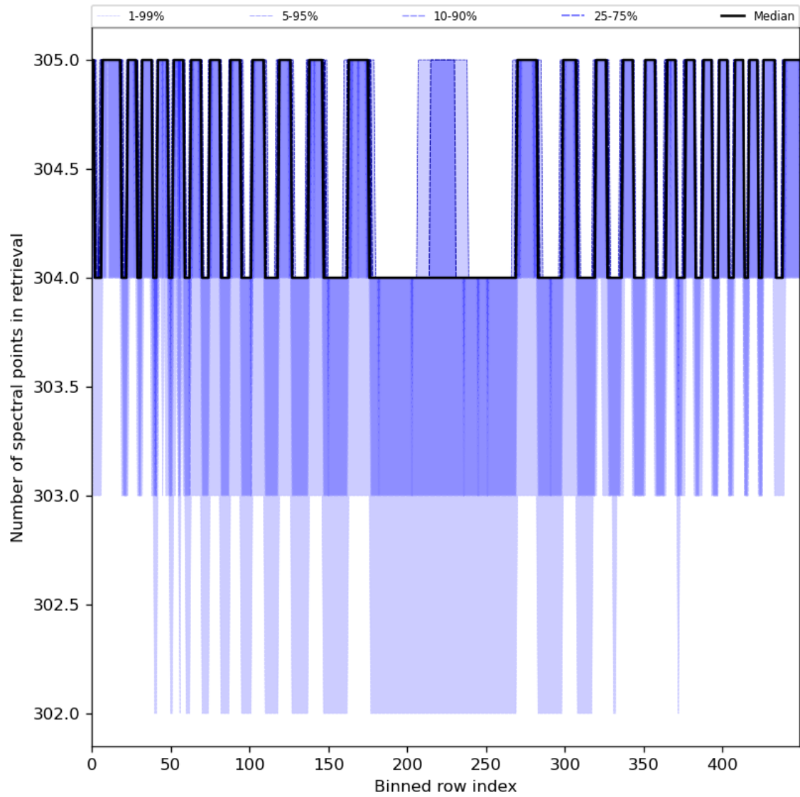
Figure 50: Along track statistics of “Number of spectral points in retrieval” for 2024-07-16 to 2024-07-18
