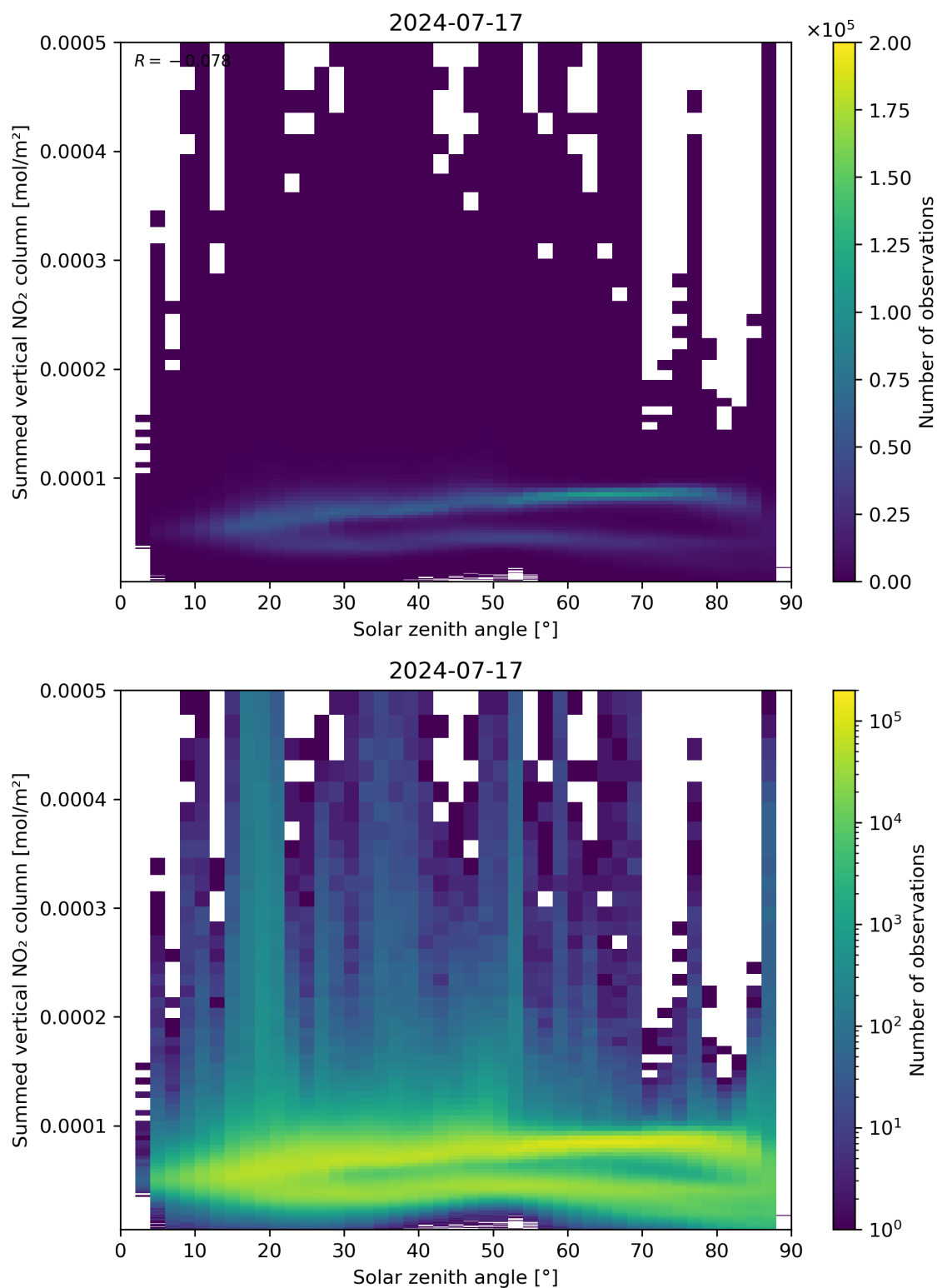
Figure 151: Scatter density plot of “Solar zenith angle” against “Summed vertical NO 2 column” for 2024-07-16 to 2024-07-18.
