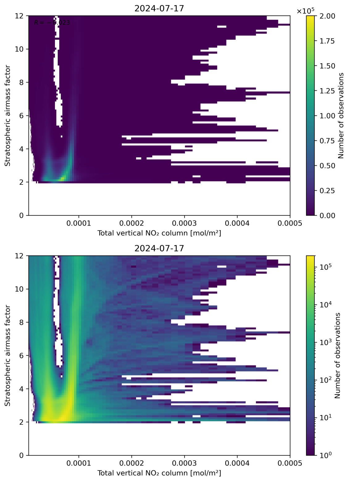
Figure 110: Scatter density plot of “Total vertical NO 2 column” against “Stratospheric airmass factor” for 2024-07-16 to 2024-07-18.
