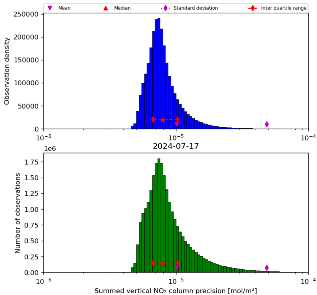
Figure 41: Histogram of “Summed vertical NO 2 column precision” for 2024-07-16 to 2024-07-18
