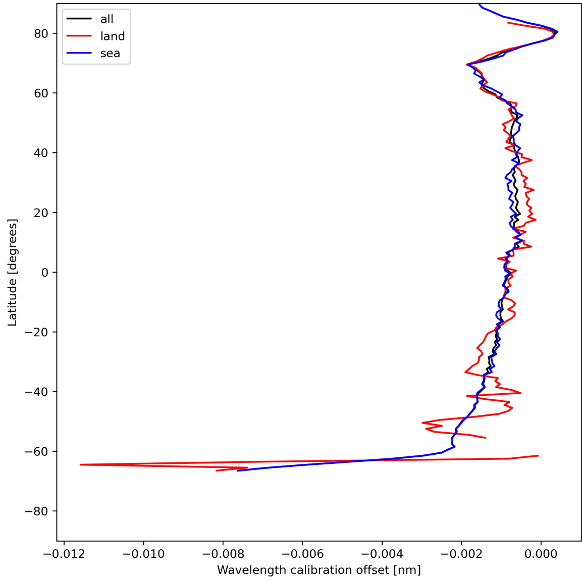
Figure 18: Zonal average of “Wavelength calibration offset” for 2024-07-16 to 2024-07-18.
