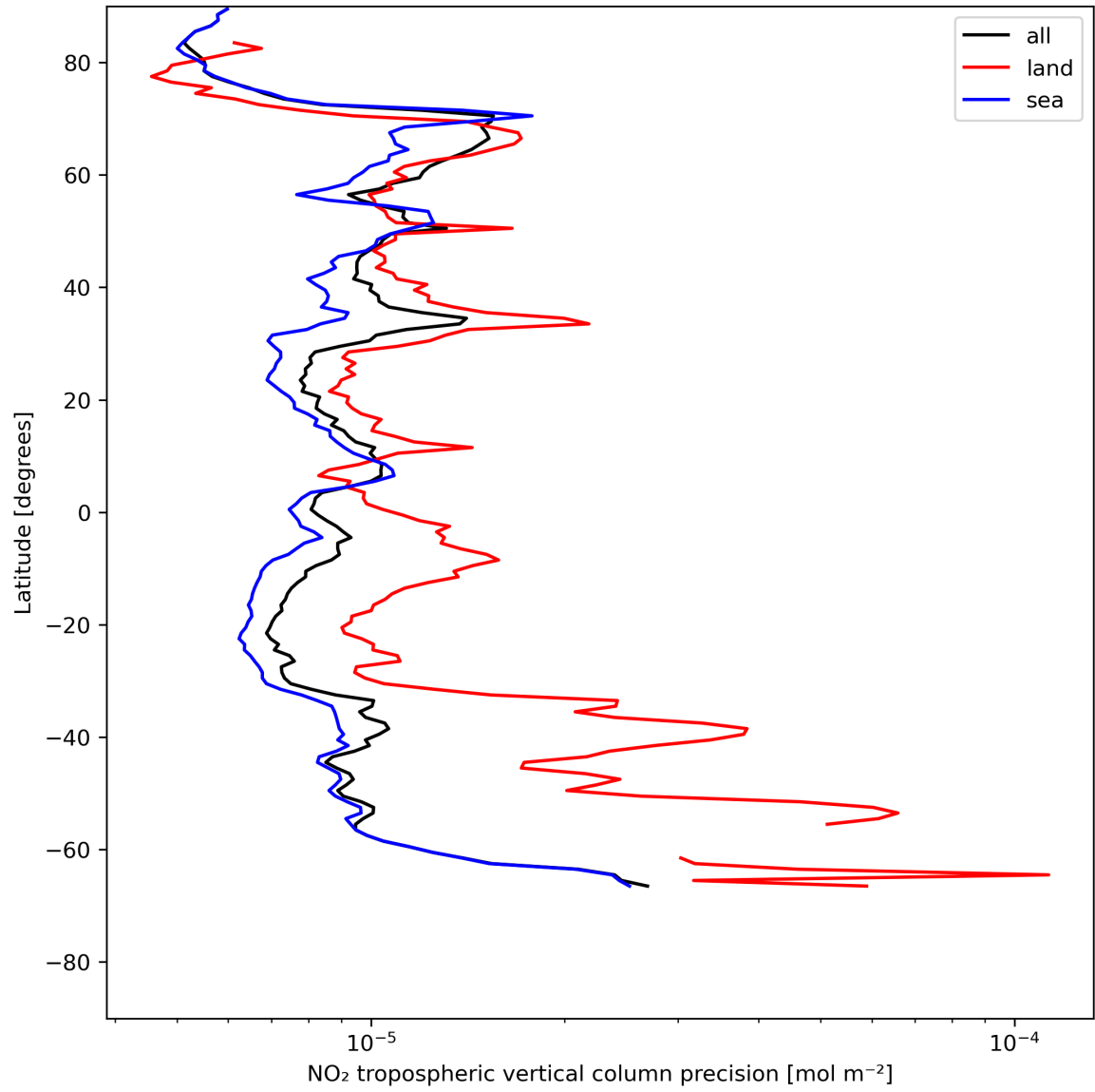
Figure 13: Zonal average of “NO 2 tropospheric vertical column precision” for 2024-07-16 to 2024-07-18.
