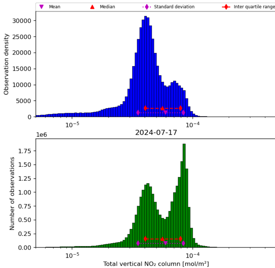
Figure 38: Histogram of “Total vertical NO 2 column” for 2024-07-16 to 2024-07-18
