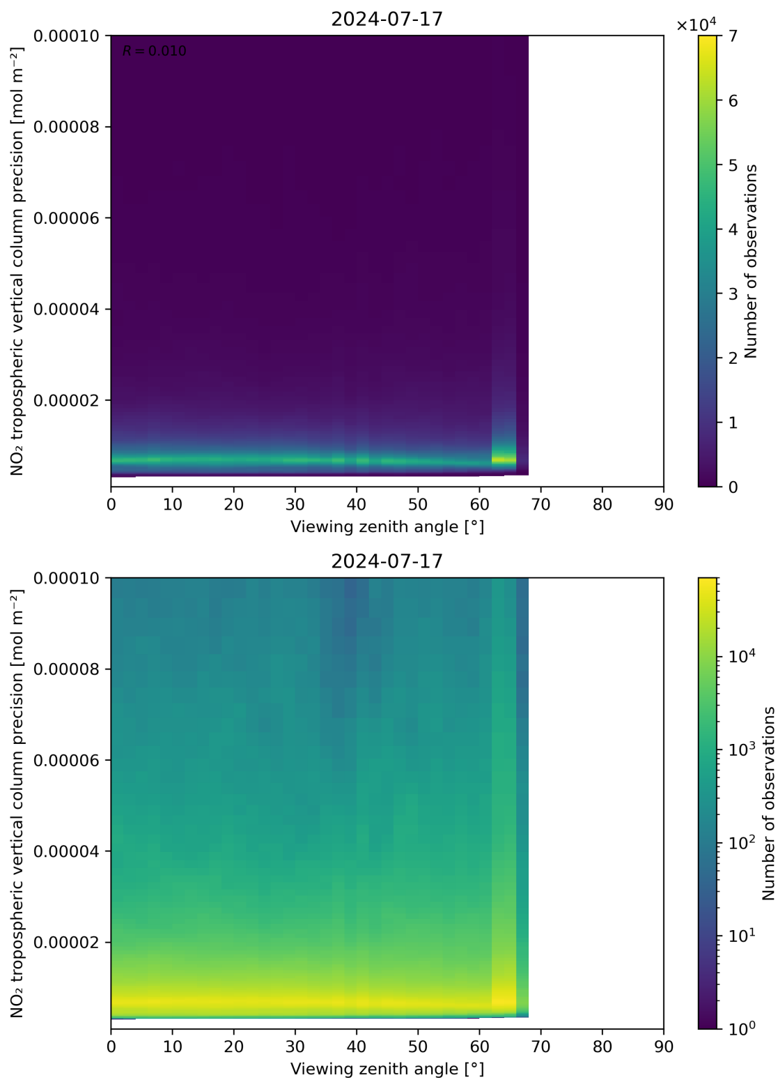
Figure 170: Scatter density plot of “Viewing zenith angle” against “NO 2 tropospheric vertical column precision” for 2024-07-16 to 2024-07-18.
