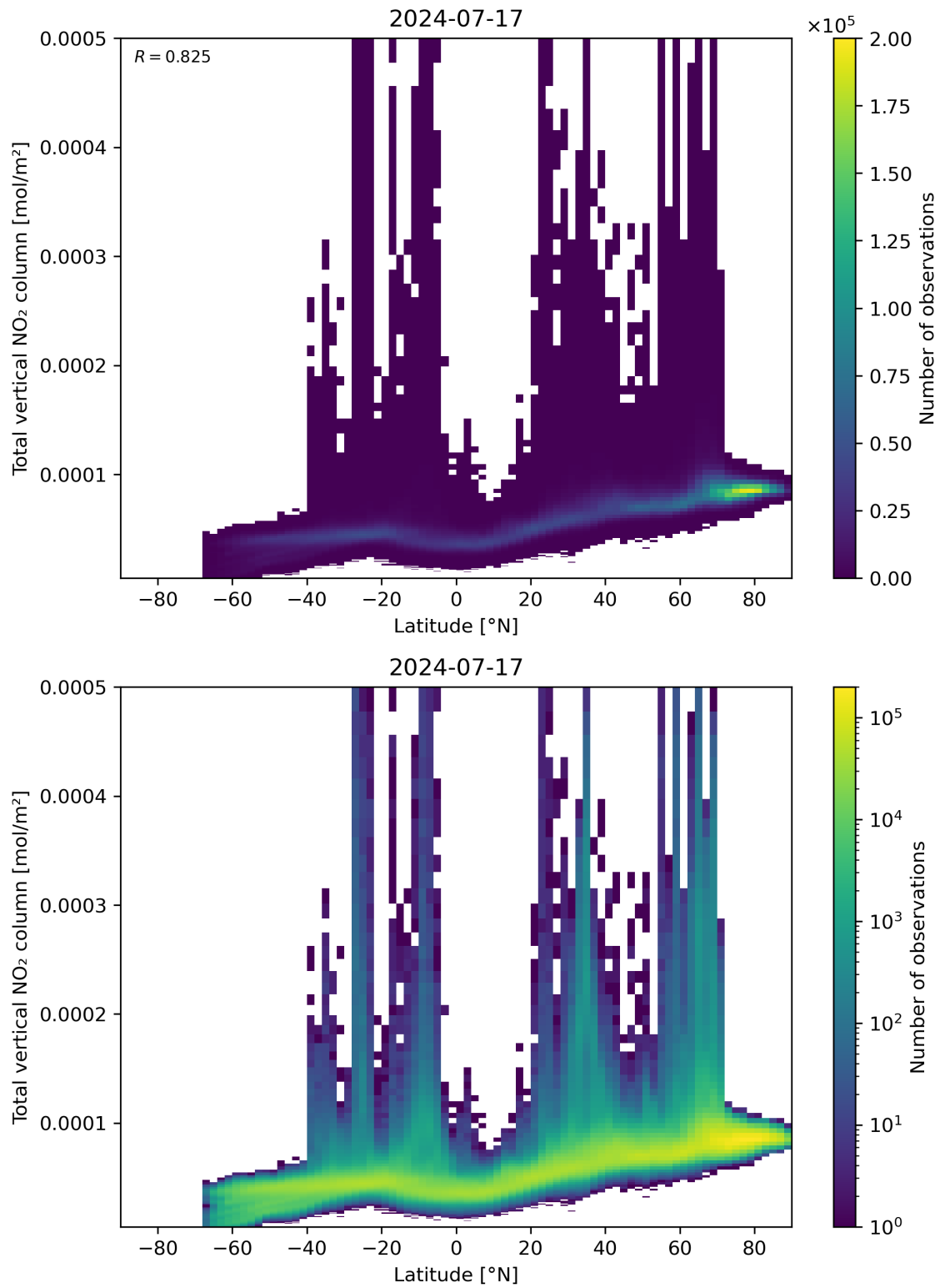
Figure 90: Scatter density plot of “Latitude” against “Total vertical NO 2 column” for 2024-07-16 to 2024-07-18.
