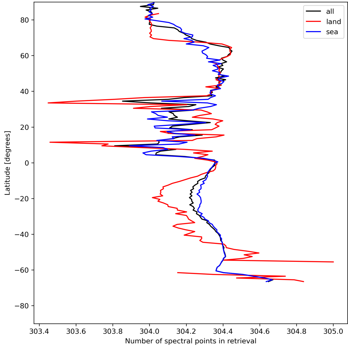
Figure 16: Zonal average of “Number of spectral points in retrieval” for 2024-07-16 to 2024-07-18.
