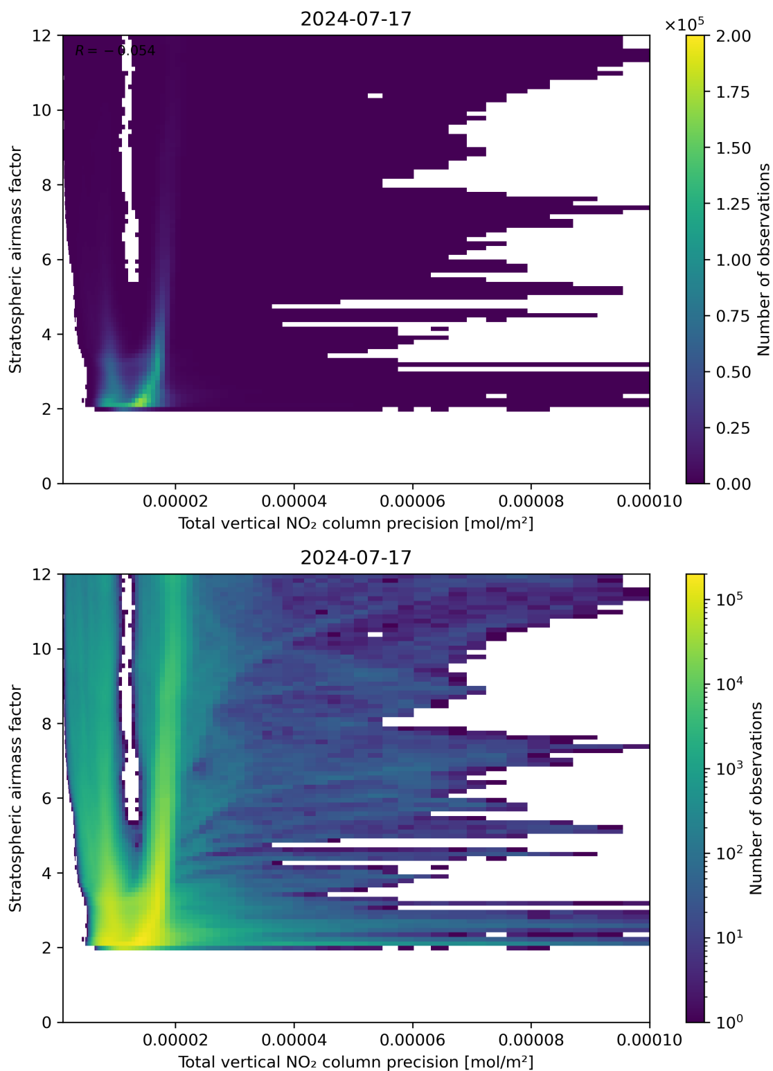
Figure 115: Scatter density plot of “Total vertical NO 2 column precision” against “Stratospheric air mass factor” for 2024-07-16 to 2024-07-18.
