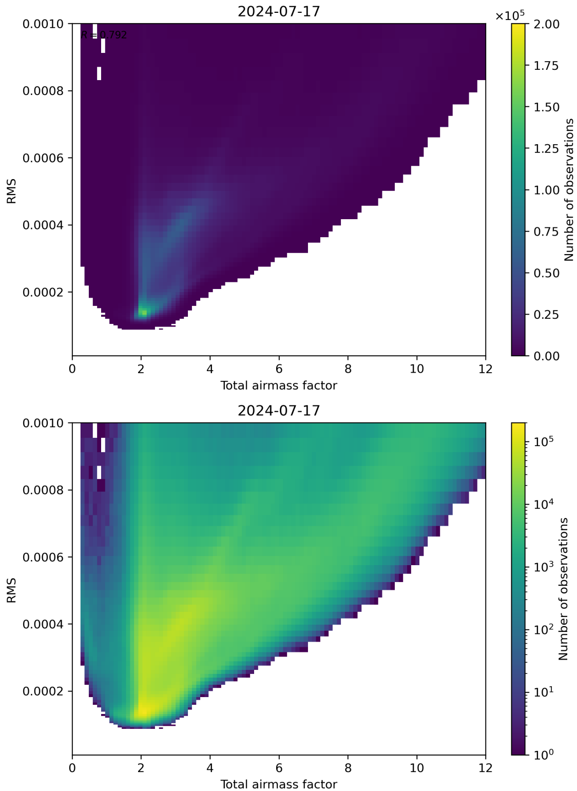
Figure 69: Scatter density plot of “Total airmass factor” against “RMS” for 2024-07-16 to 2024-07-18.
