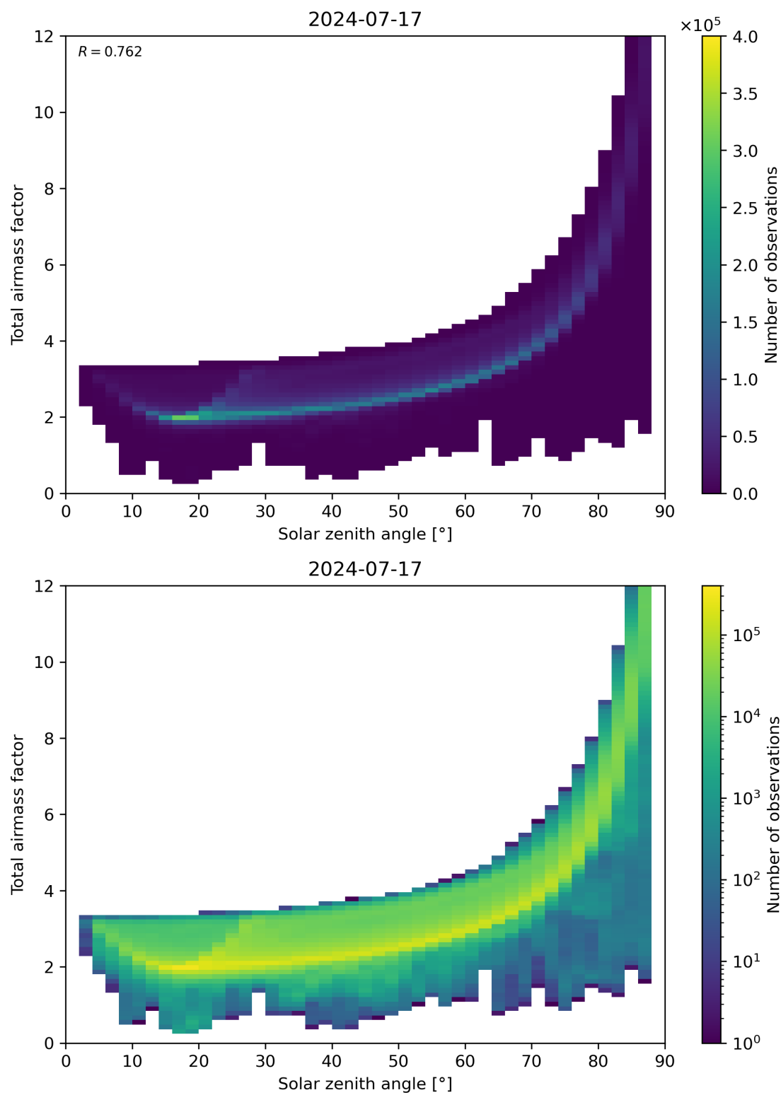
Figure 146: Scatter density plot of “Solar zenith angle” against “Total air mass factor” for 2024-07-16 to 2024-07-18.
