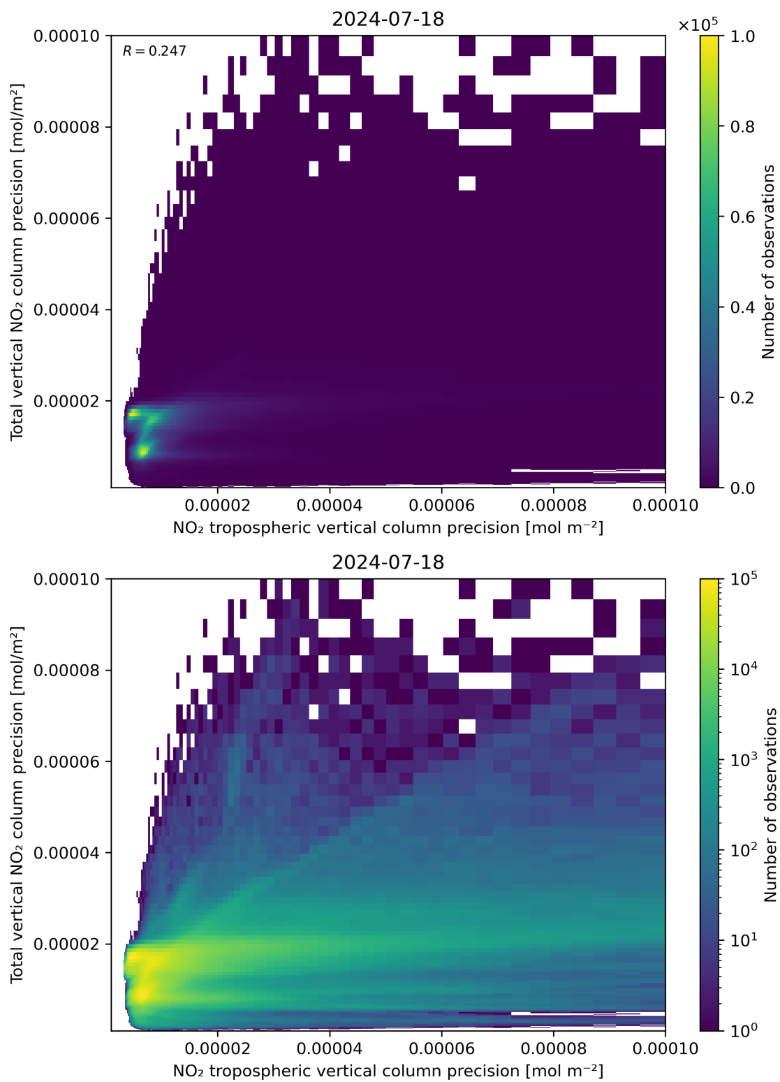
Figure 139: Scatter density plot of “NO 2 tropospheric vertical column precision” against “Total vertical NO 2 column precision” for 2024-07-17 to 2024-07-19.
