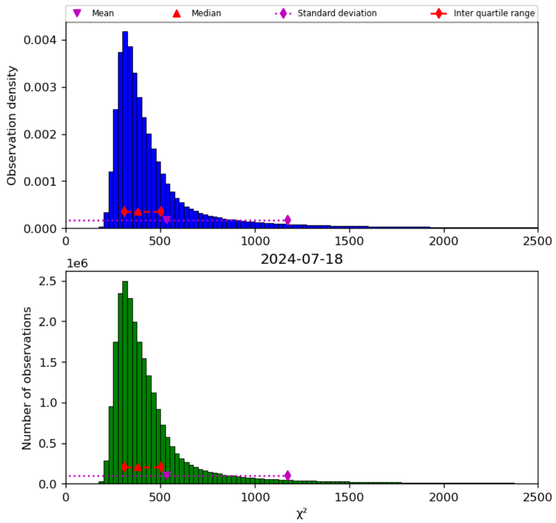
Figure 42: Histogram of " \chi^2 " for 2024-07-17 to 2024-07-19
