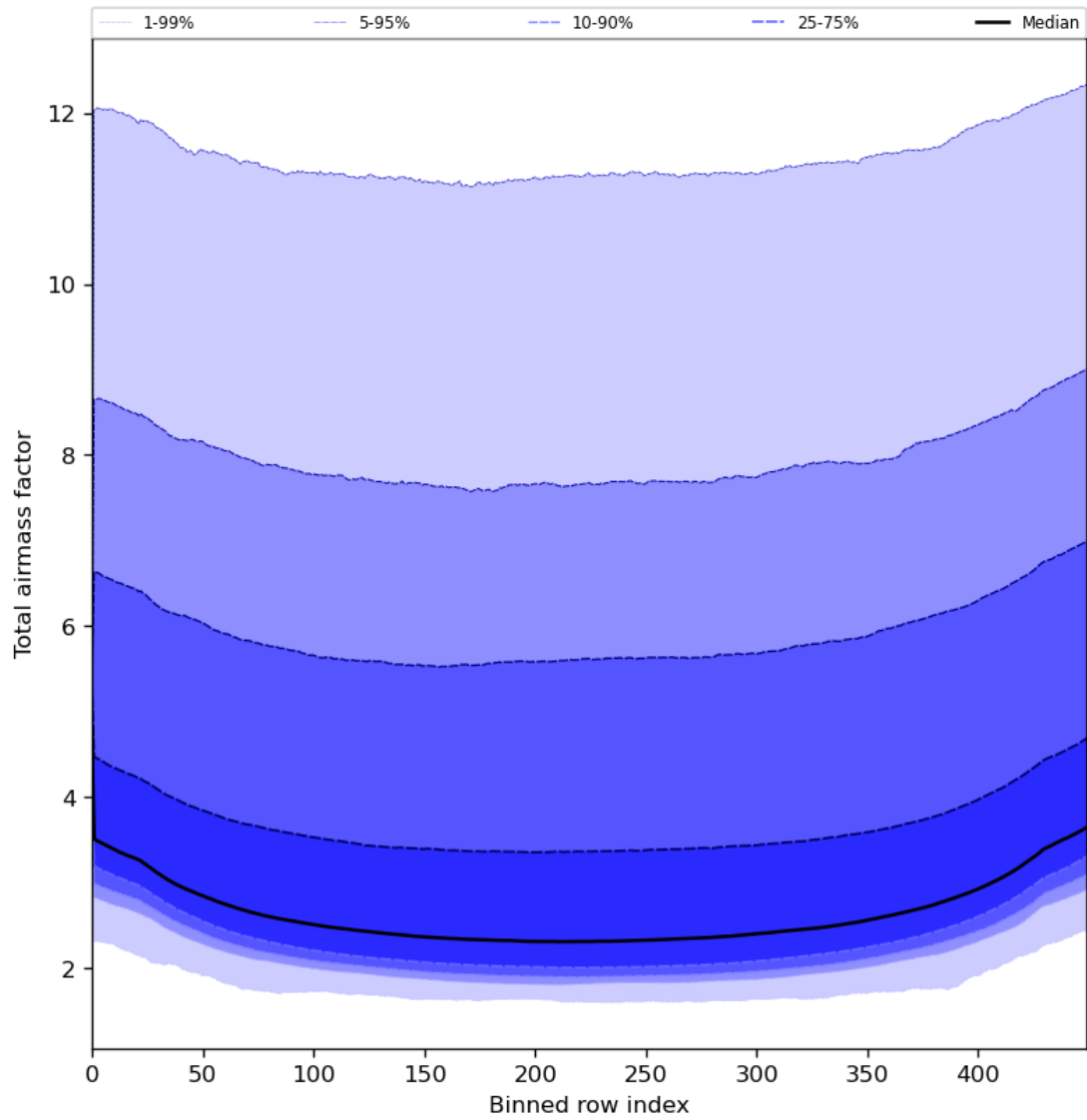
Figure 49: Along track statistics of “Total airmass factor” for 2024-07-17 to 2024-07-19
