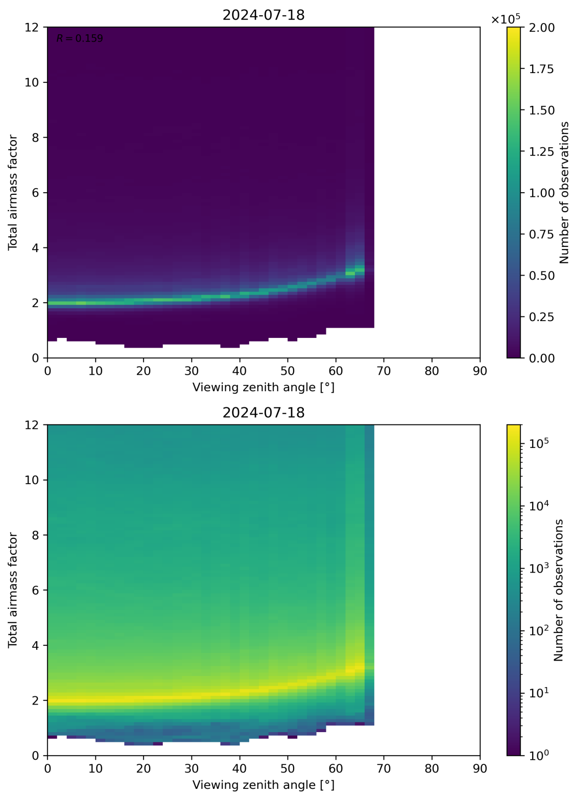
Figure 160: Scatter density plot of “Viewing zenith angle” against “Total airmass factor” for 2024-07-17 to 2024-07-19.
