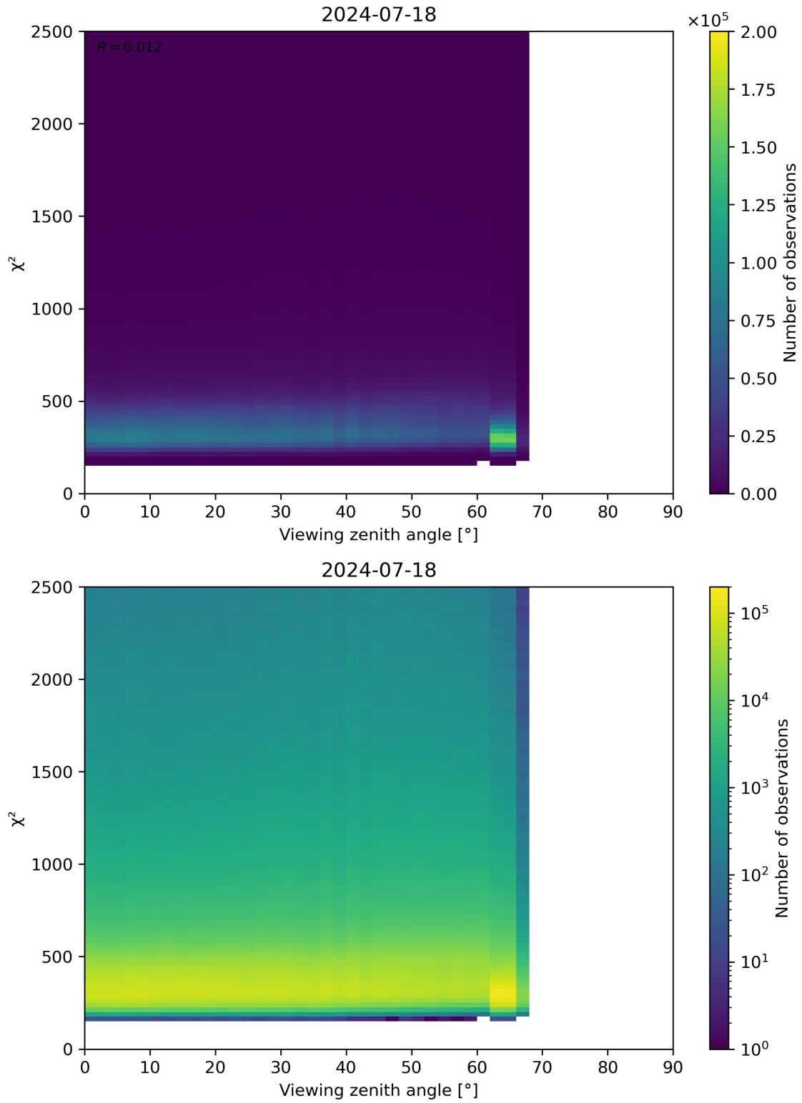
Figure 162: Scatter density plot of “Viewing zenith angle” against “ \chi^2 ” for 2024-07-17 to 2024-07-19.
