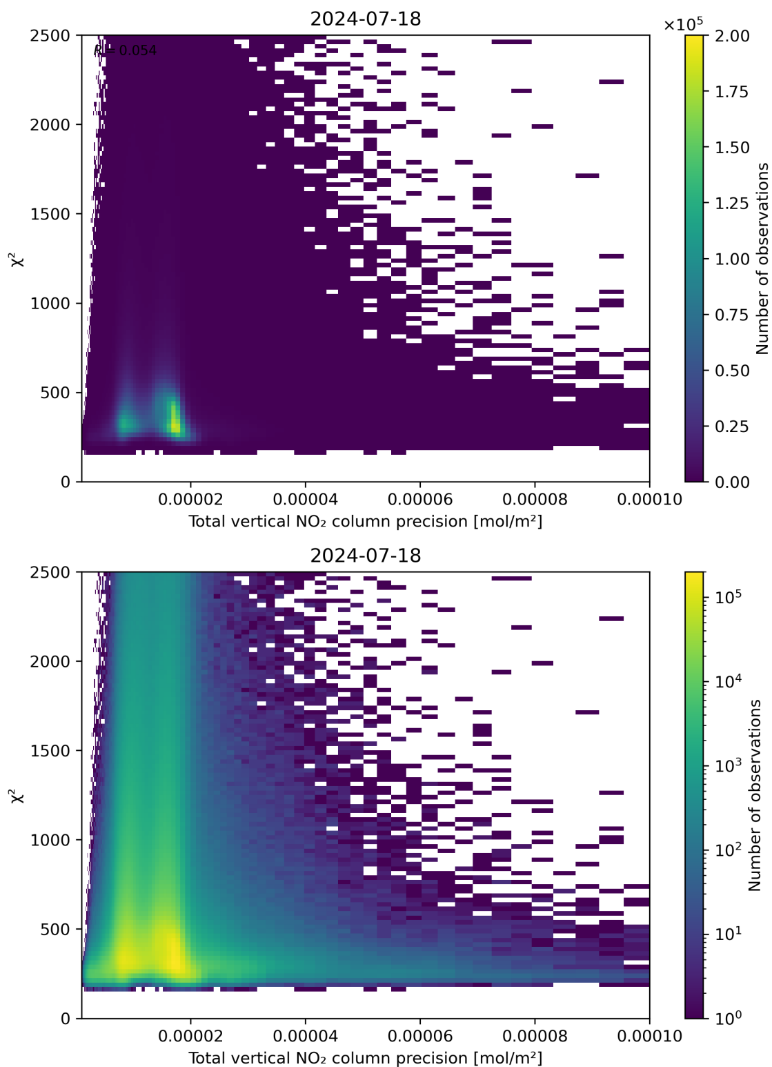
Figure 116: Scatter density plot of “Total vertical NO 2 column precision” against “ \chi^2 ” for 2024-07-17 to 2024-07-19.
