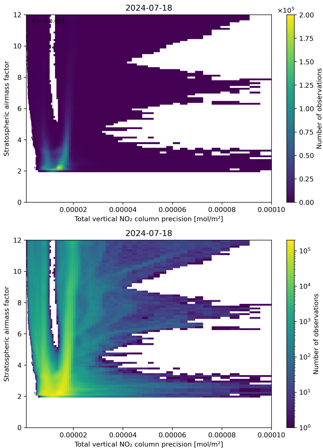
Figure 115: Scatter density plot of “Total vertical NO 2 column precision” against “Stratospheric air mass factor” for 2024-07-17 to 2024-07-19.
