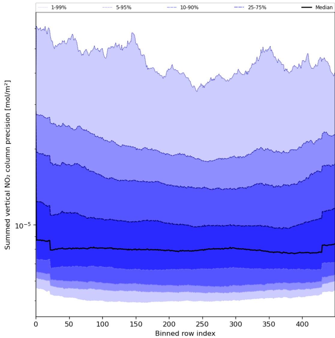
Figure 58: Along track statistics of “Summed vertical NO 2 column precision” for 2024-07-17 to 2024-07-19
