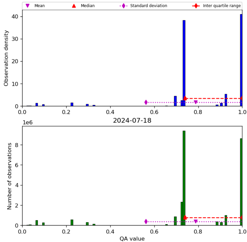
Figure 28: Histogram of “QA value” for 2024-07-17 to 2024-07-19
