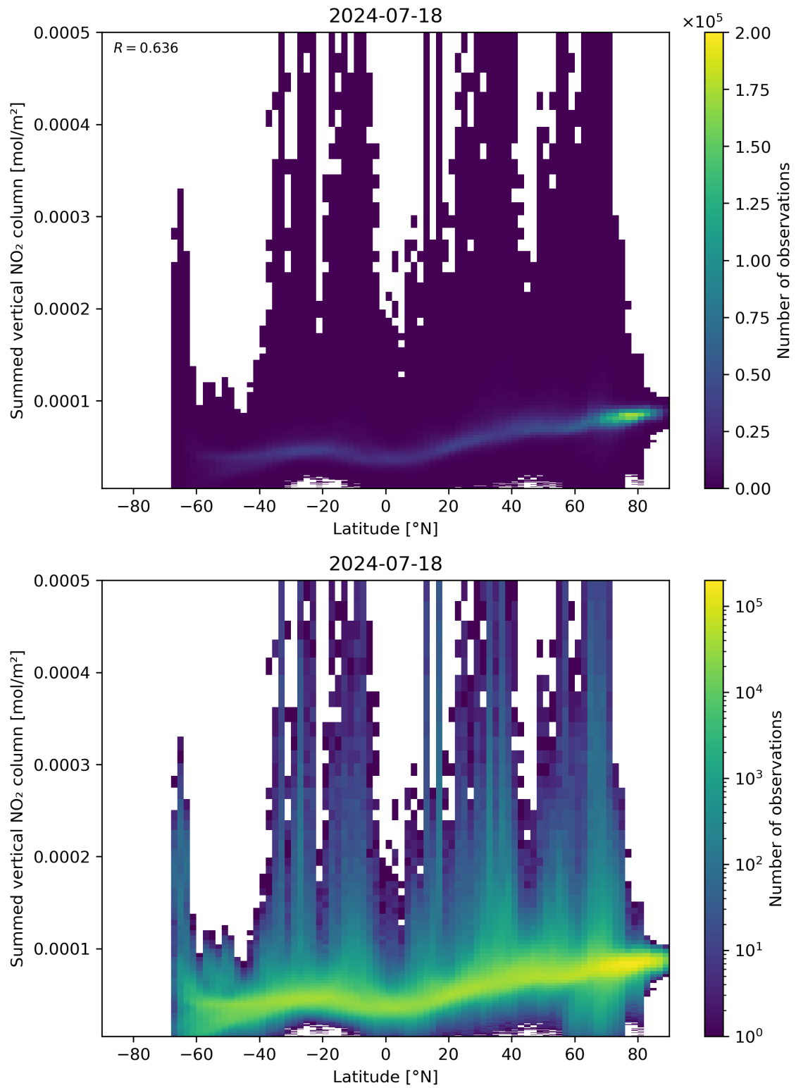
Figure 88: Scatter density plot of “Latitude” against “Summed vertical NO 2 column” for 2024-07-17 to 2024-07-19.
