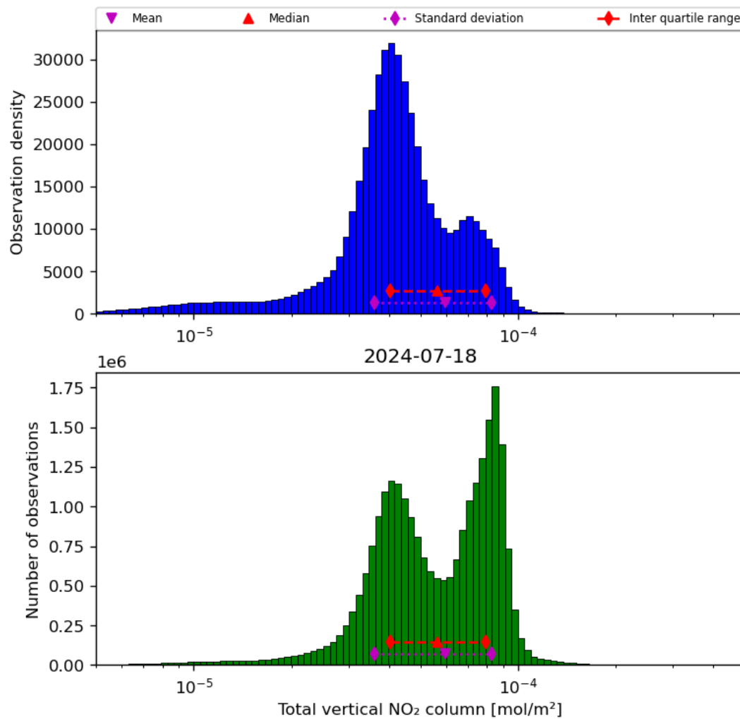
Figure 38: Histogram of “Total vertical NO 2 column” for 2024-07-17 to 2024-07-19
