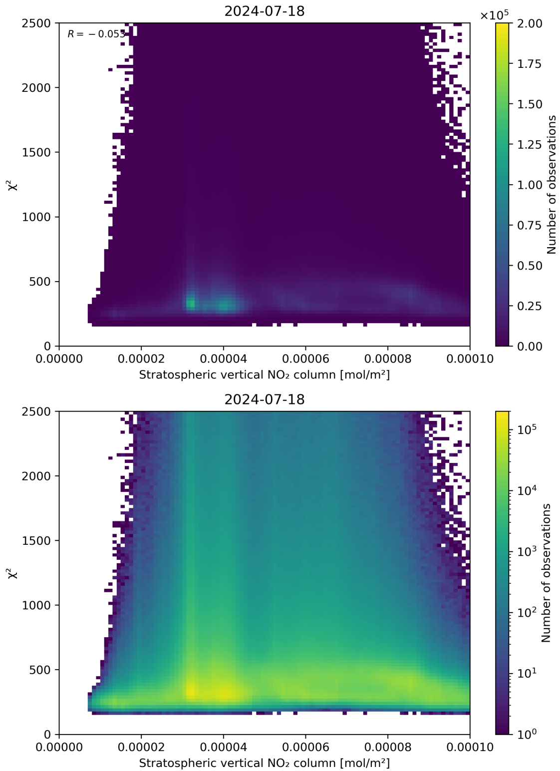
Figure 97: Scatter density plot of “Stratospheric vertical NO 2 column” against “ \chi^2 ” for 2024-07-17 to 2024-07-19.
