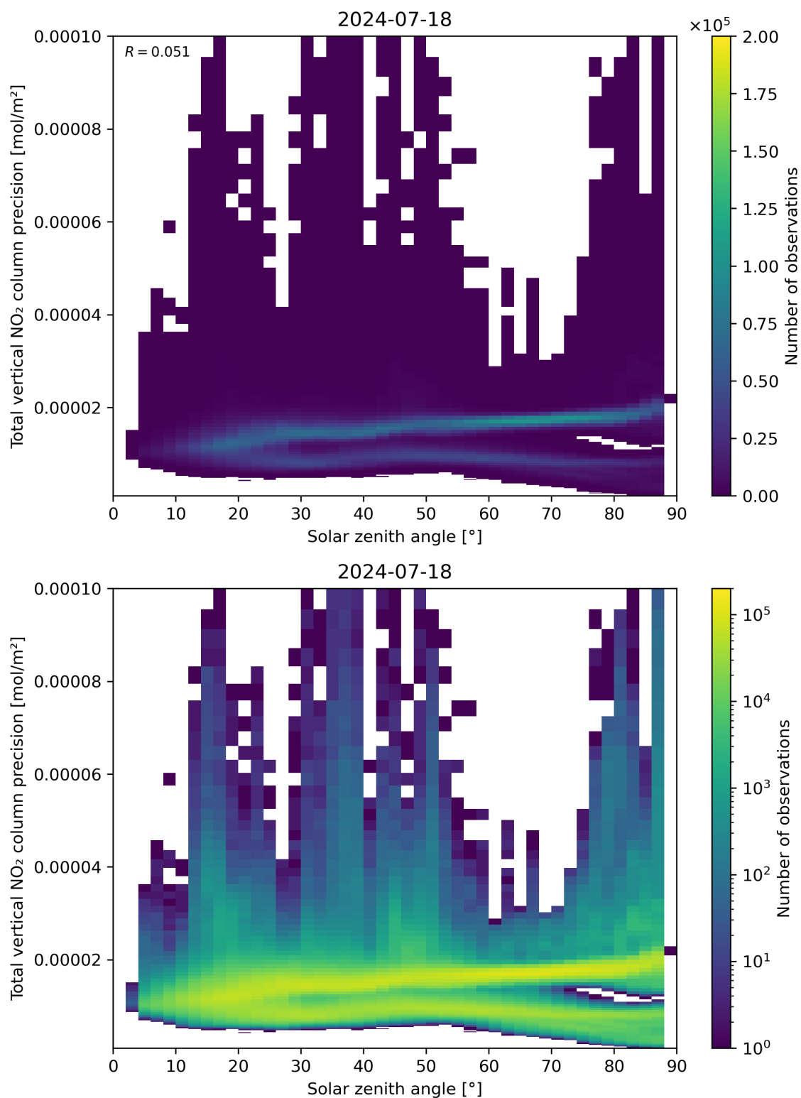
Figure 154: Scatter density plot of “Solar zenith angle” against “Total vertical NO 2 column precision” for 2024-07-17 to 2024-07-19.
