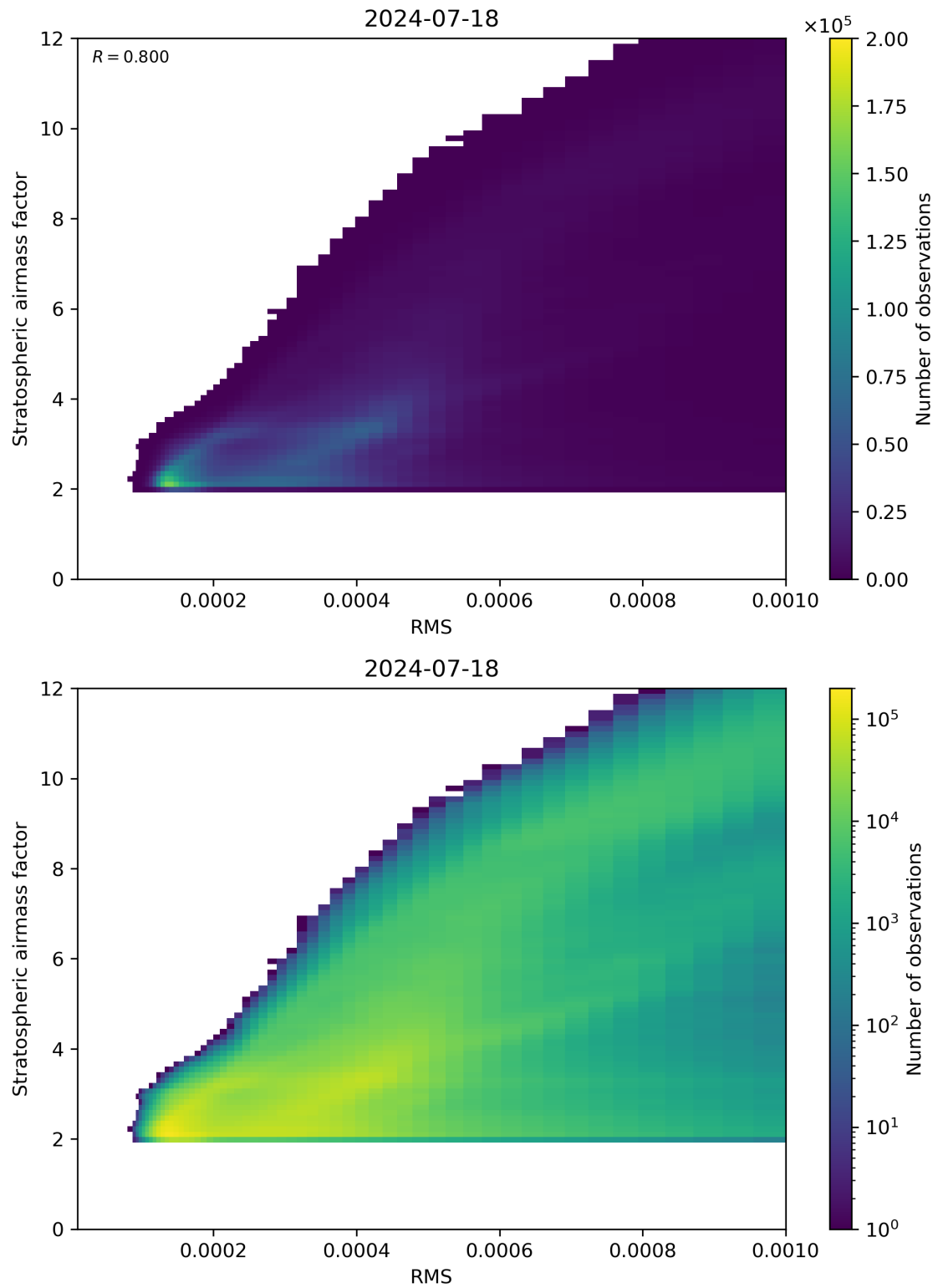
Figure 144: Scatter density plot of “RMS” against “Stratospheric airmass factor” for 2024-07-17 to 2024-07-19.
