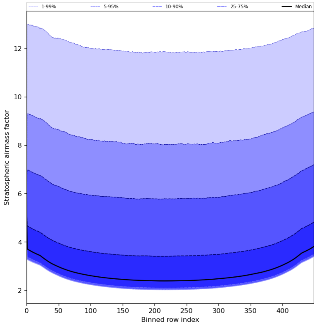
Figure 61: Along track statistics of “Stratospheric air mass factor” for 2024-07-17 to 2024-07-19
