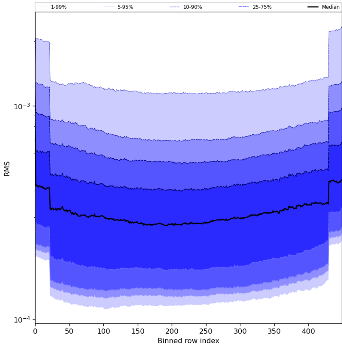
Figure 60: Along track statistics of “RMS” for 2024-07-17 to 2024-07-19
