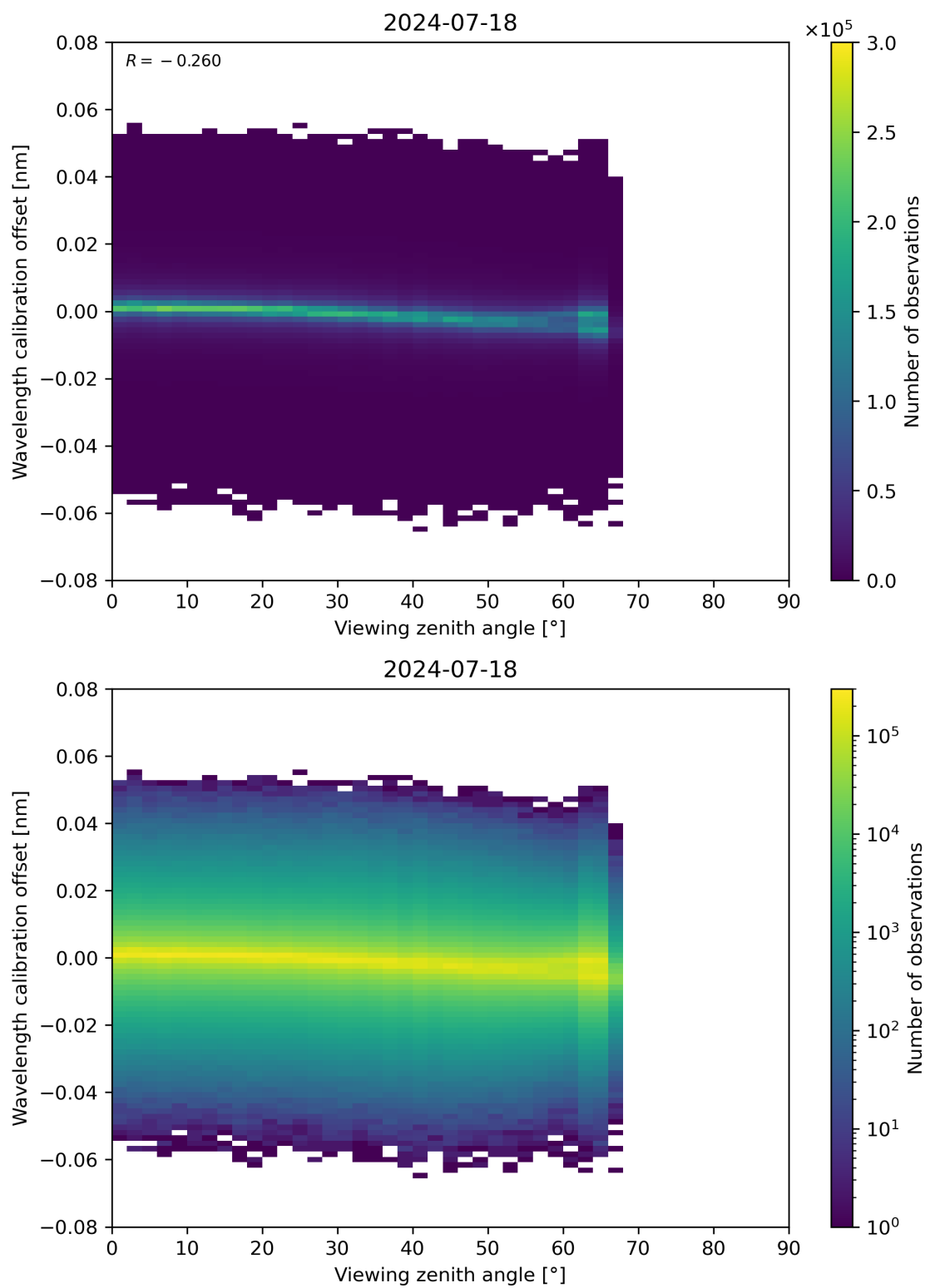
Figure 173: Scatter density plot of “Viewing zenith angle” against “Wavelength calibration offset” for 2024-07-17 to 2024-07-19.
