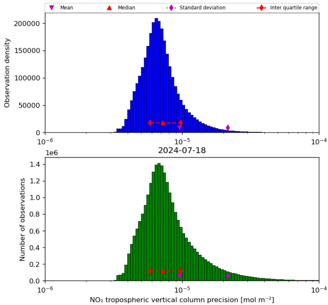
Figure 30: Histogram of “NO 2 tropospheric vertical column precision” for 2024-07-17 to 2024-07-19
