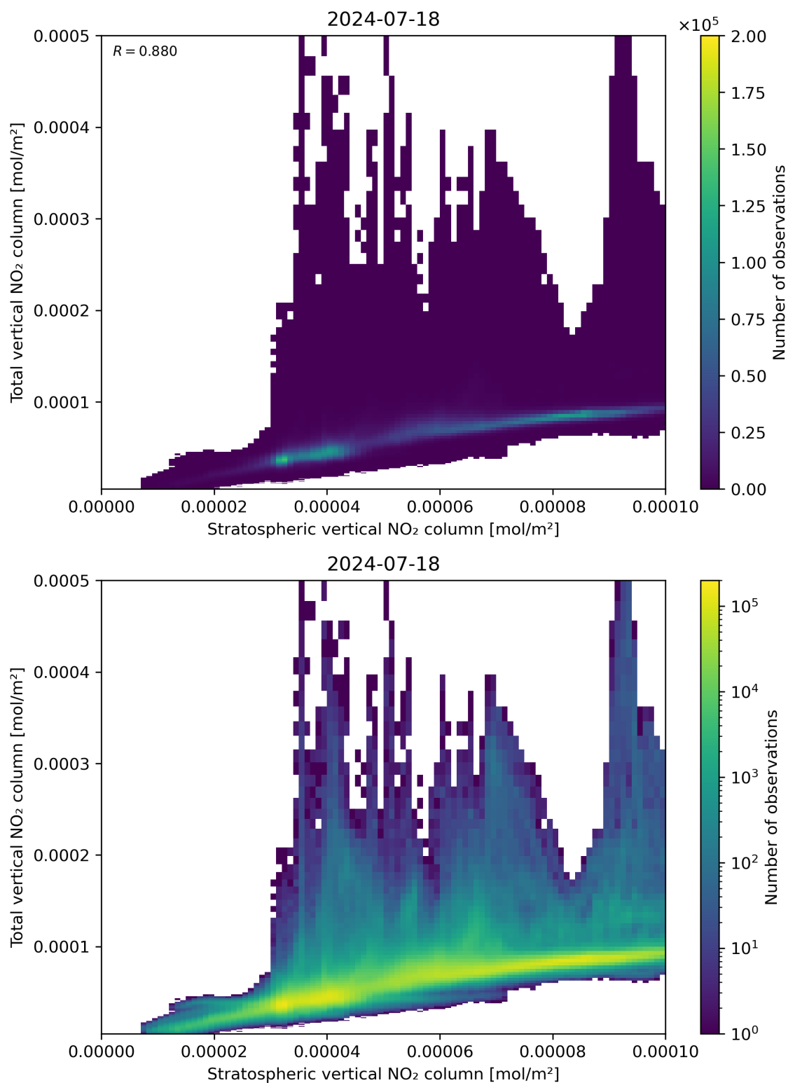
Figure 100: Scatter density plot of “Stratospheric vertical NO 2 column” against “Total vertical NO 2 column” for 2024-07-17 to 2024-07-19.
