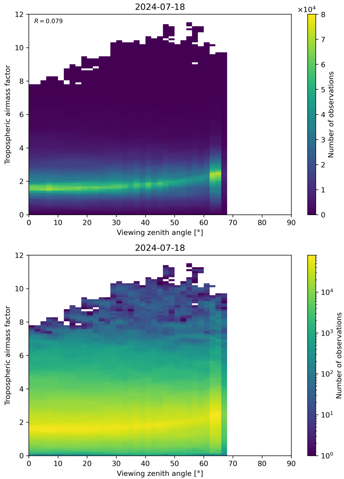
Figure 161: Scatter density plot of “Viewing zenith angle” against “Tropospheric airmass factor” for 2024-07-17 to 2024-07-19.
