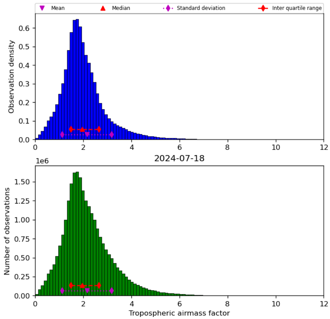
Figure 31: Histogram of “Tropospheric airmass factor” for 2024-07-17 to 2024-07-19
