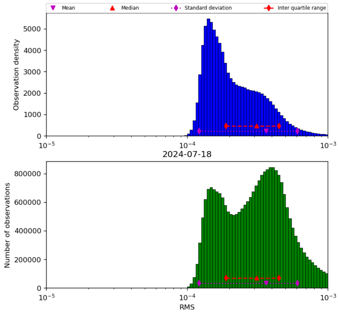
Figure 43: Histogram of “RMS” for 2024-07-17 to 2024-07-19
