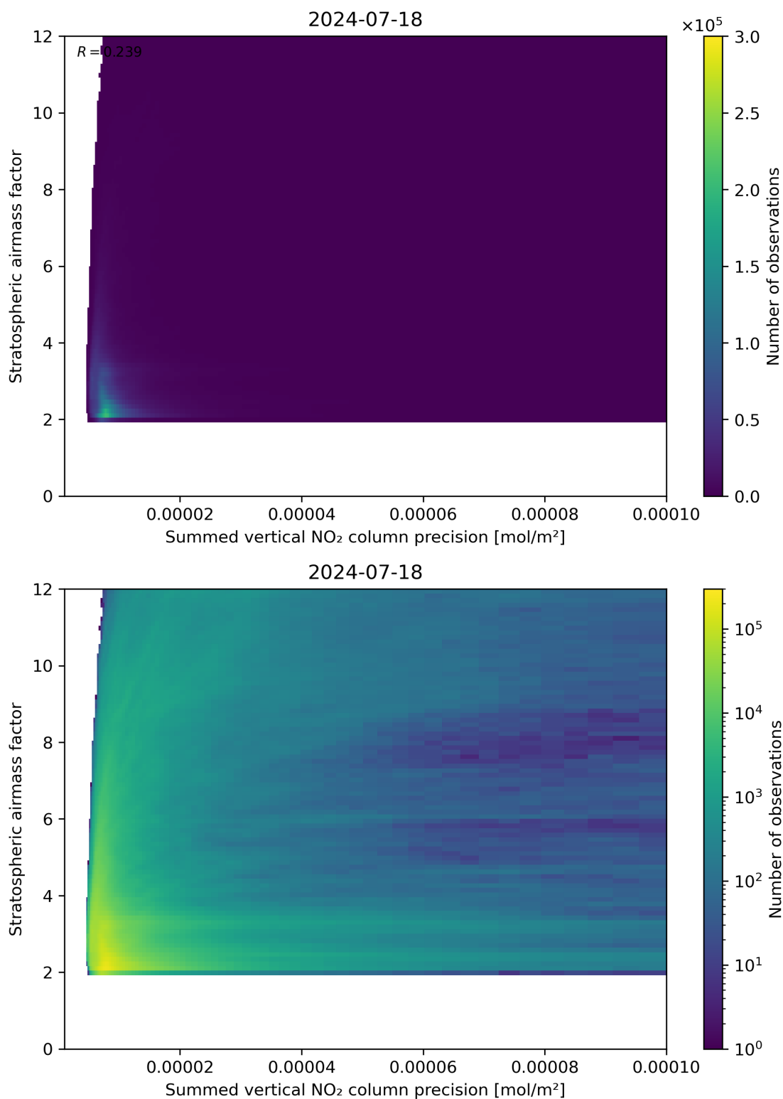
Figure 106: Scatter density plot of “Summed vertical NO 2 column precision” against “Stratospheric airmass factor” for 2024-07-17 to 2024-07-19.
