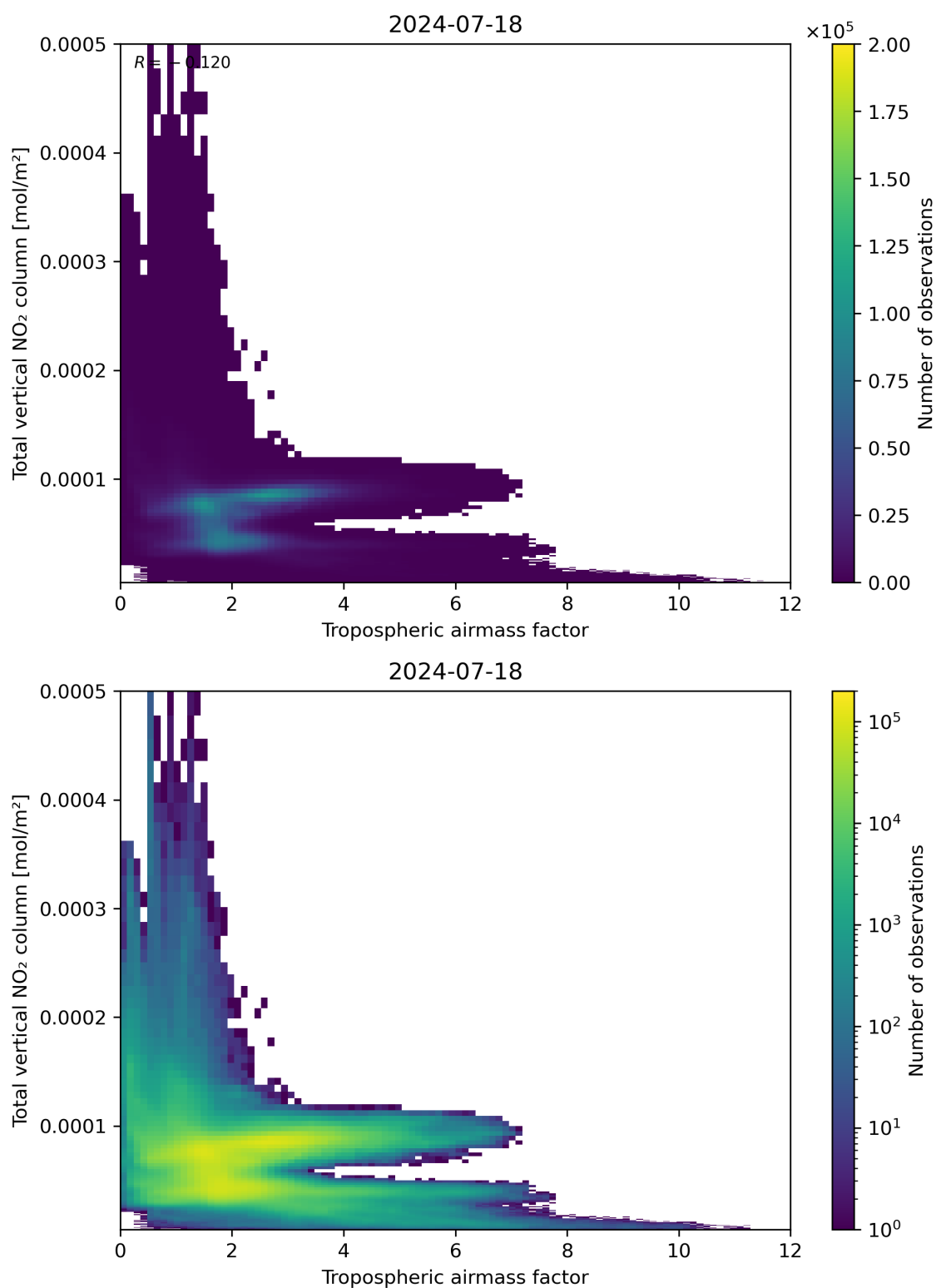
Figure 77: Scatter density plot of “Tropospheric airmass factor” against “Total vertical NO 2 column” for 2024-07-17 to 2024-07-19.
