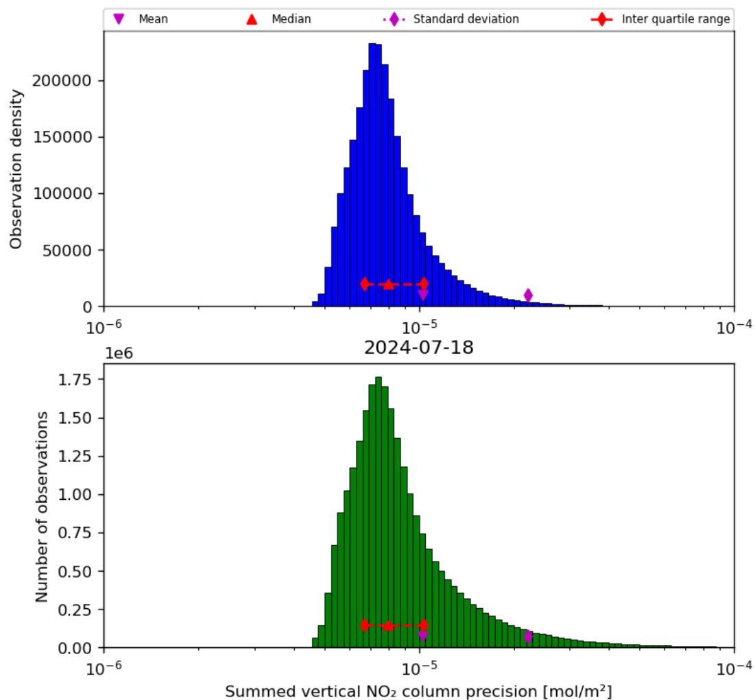
Figure 41: Histogram of "Summed vertical NO 2 column precision" for 2024-07-17 to 2024-07-19
