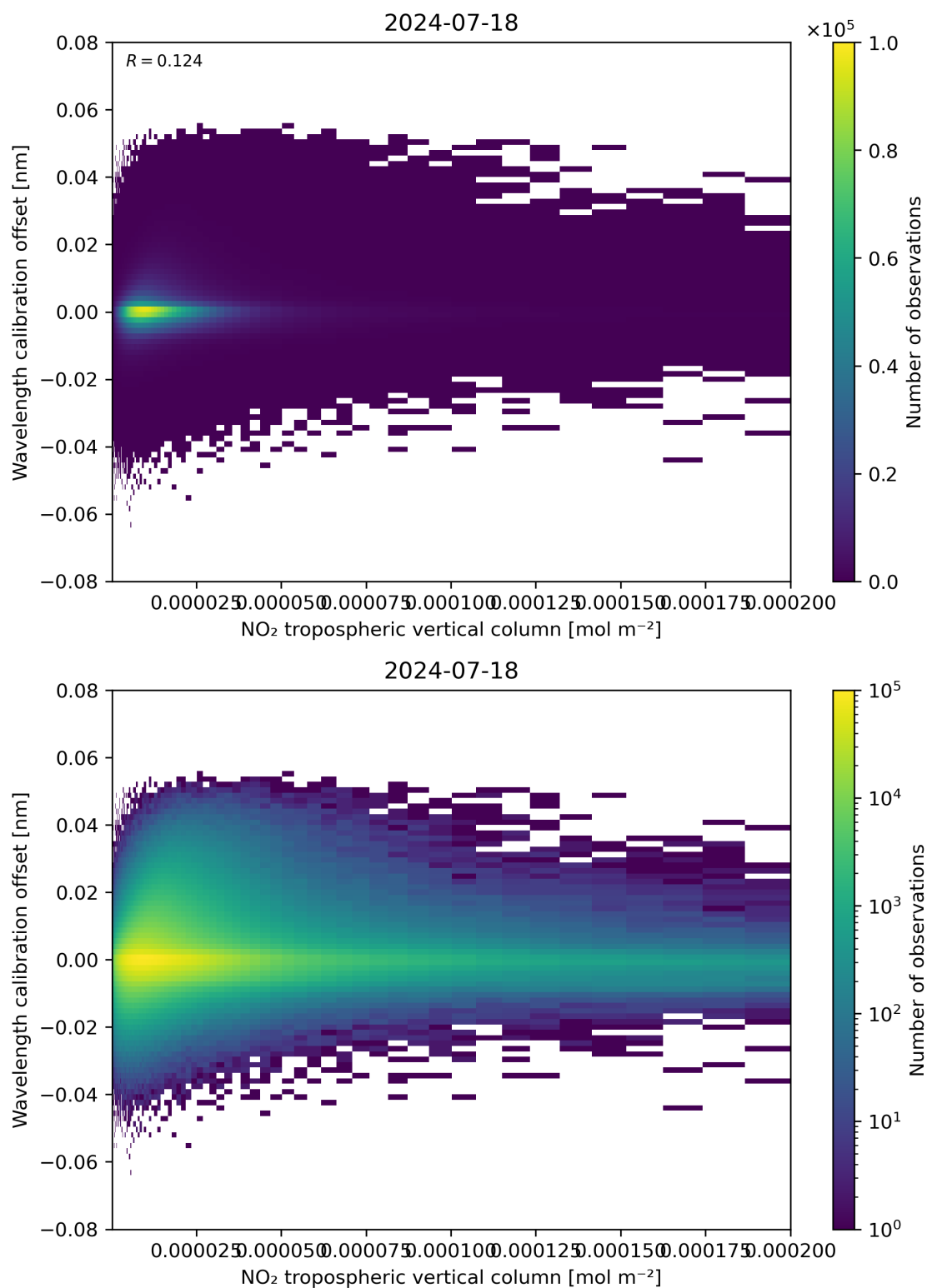
Figure 143: Scatter density plot of “NO 2 tropospheric vertical column” against “Wavelength calibration offset” for 2024-07-17 to 2024-07-19.
