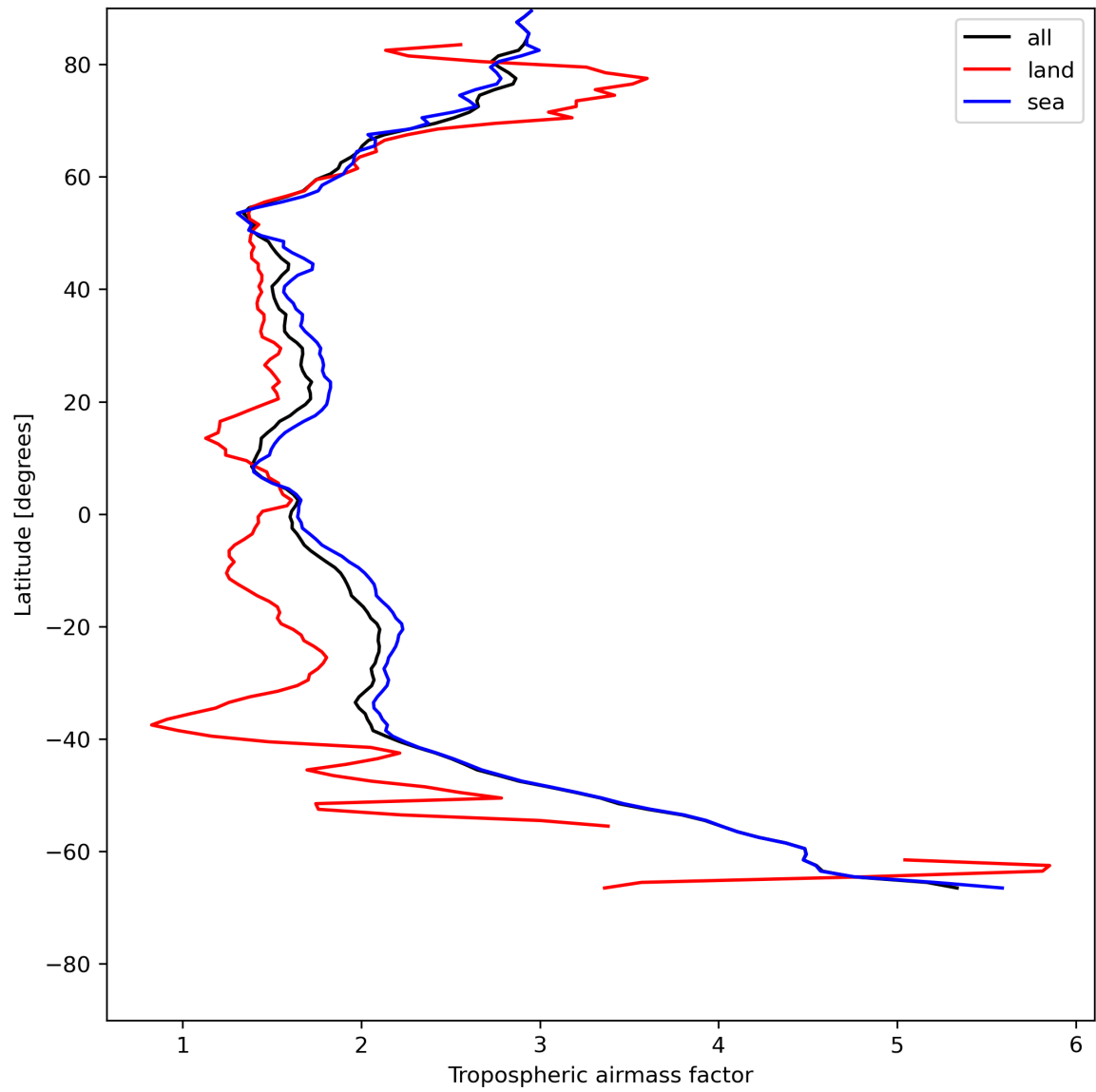
Figure 14: Zonal average of “Tropospheric airmass factor” for 2024-07-17 to 2024-07-19.
