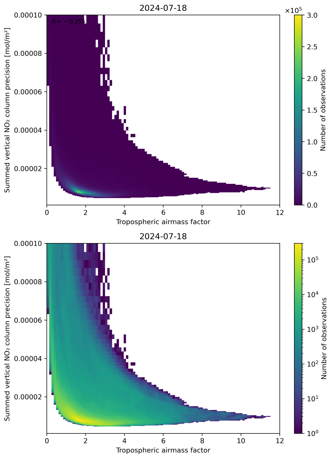
Figure 76: Scatter density plot of “Tropospheric air mass factor” against “Summed vertical NO 2 column precision” for 2024-07-17 to 2024-07-19.
