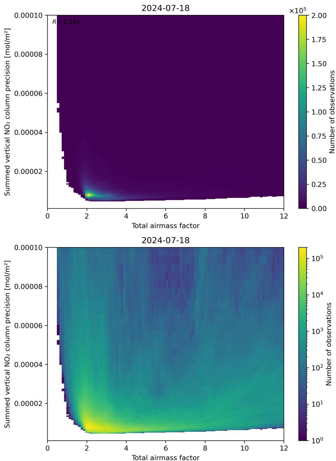
Figure 66: Scatter density plot of “Total airmass factor” against “Summed vertical NO 2 column precision” for 2024-07-17 to 2024-07-19.
