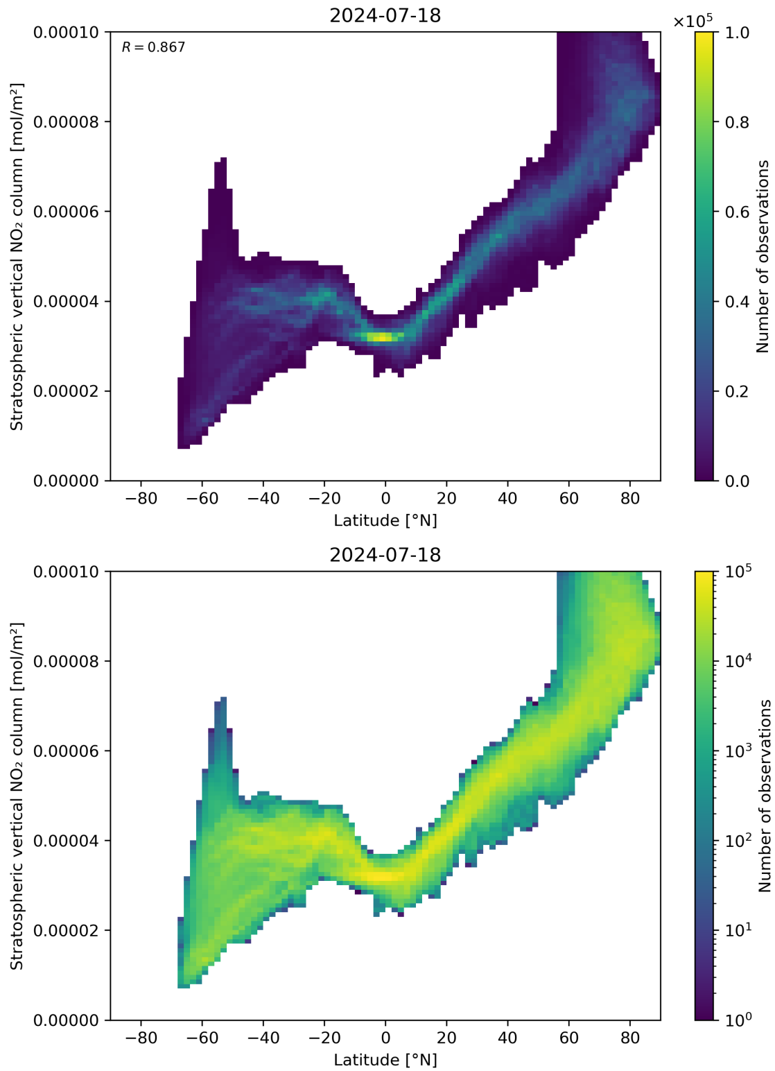
Figure 87: Scatter density plot of “Latitude” against “Stratospheric vertical NO 2 column” for 2024-07-17 to 2024-07-19.
