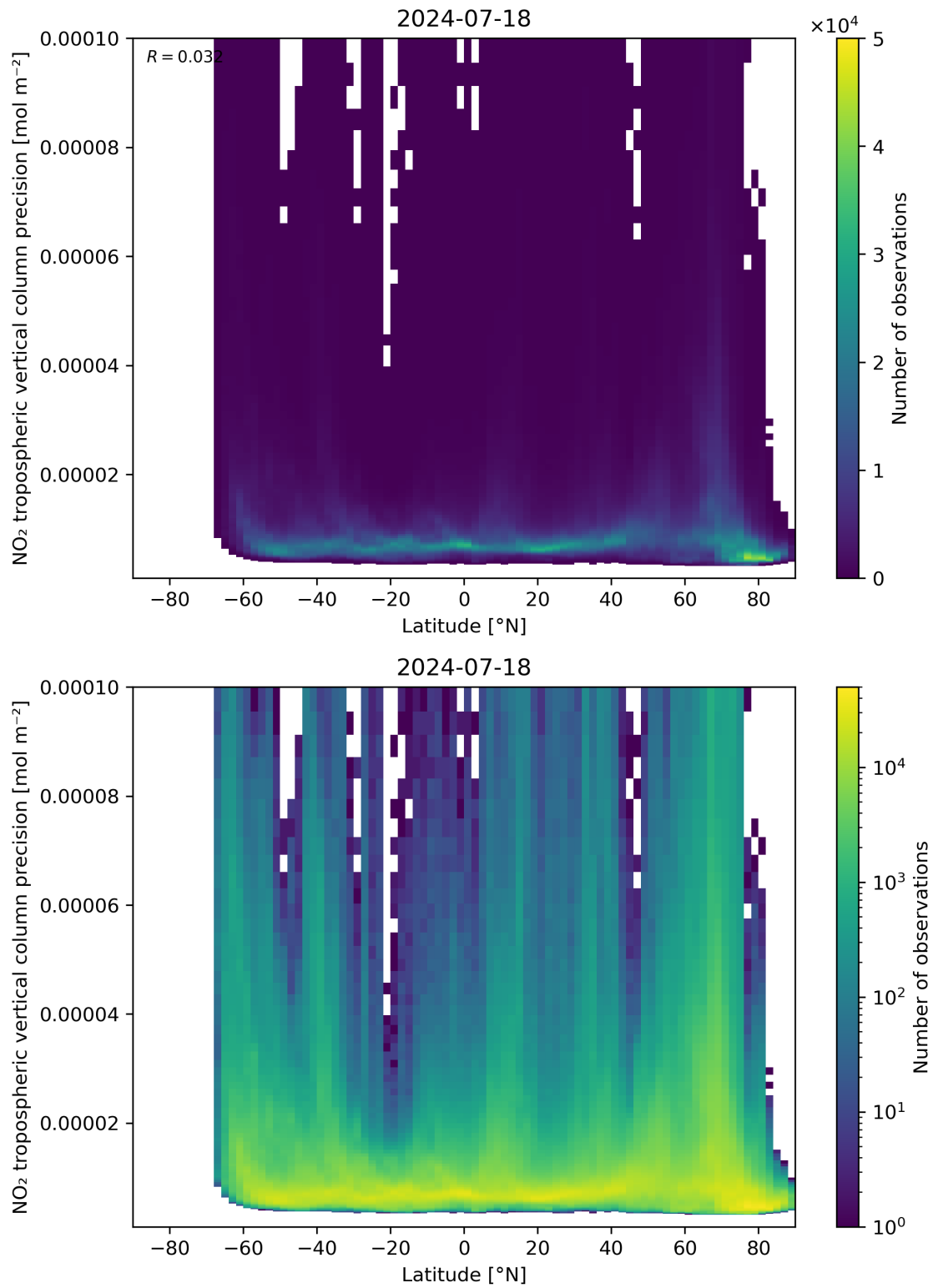
Figure 93: Scatter density plot of “Latitude” against “NO 2 tropospheric vertical column precision” for 2024-07-17 to 2024-07-19.
