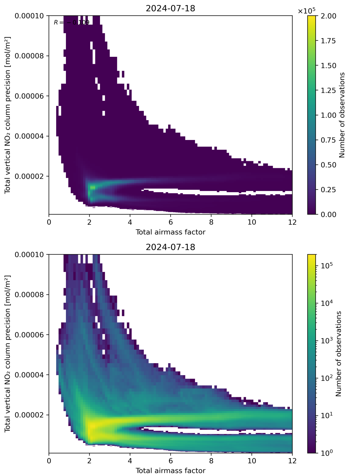
Figure 68: Scatter density plot of “Total airmass factor” against “Total vertical NO 2 column precision” for 2024-07-17 to 2024-07-19.
