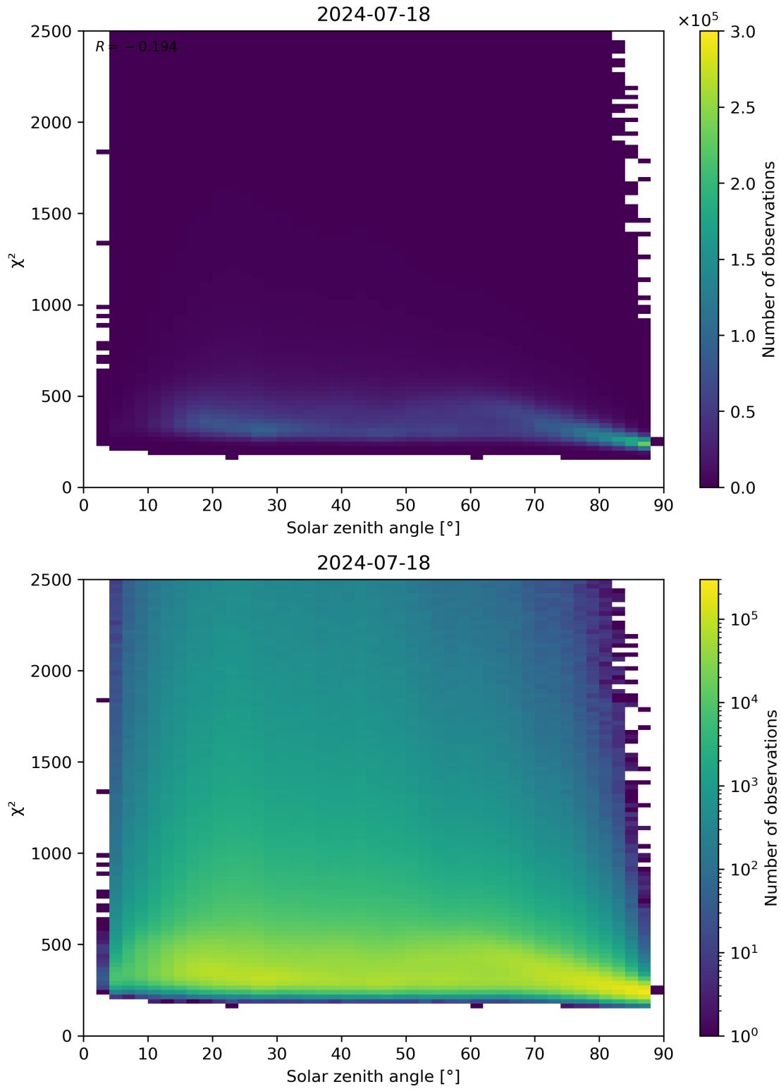
Figure 148: Scatter density plot of “Solar zenith angle” against “ \chi^2 ” for 2024-07-17 to 2024-07-19.
