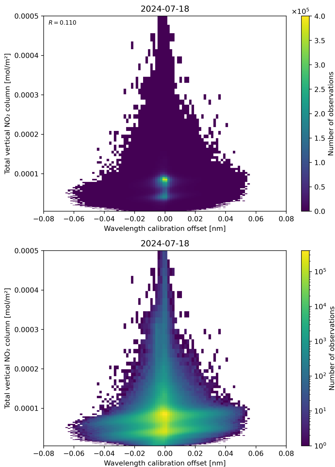
Figure 179: Scatter density plot of “Wavelength calibration offset” against “Total vertical NO 2 column” for 2024-07-17 to 2024-07-19.
