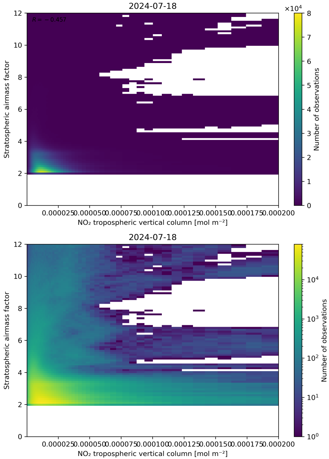
Figure 121: Scatter density plot of “NO 2 tropospheric vertical column” against “Stratospheric air mass factor” for 2024-07-17 to 2024-07-19.
