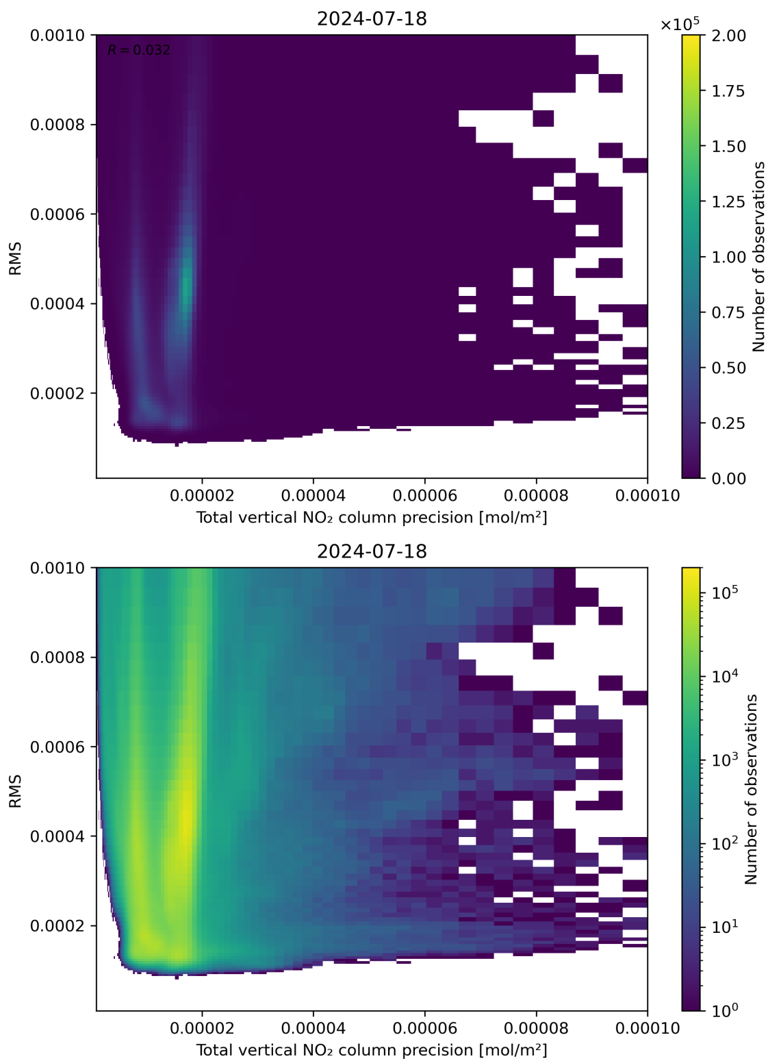
Figure 119: Scatter density plot of “Total vertical NO 2 column precision” against “RMS” for 2024-07-17 to 2024-07-19.
