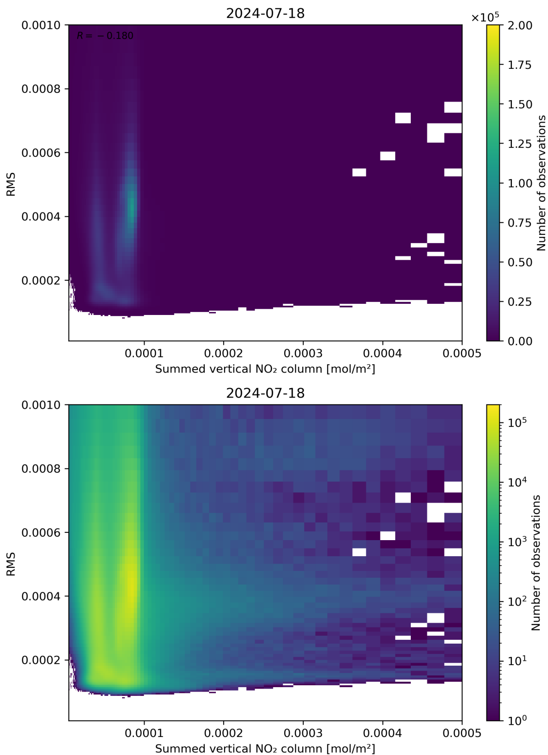
Figure 109: Scatter density plot of “Summed vertical NO 2 column” against “RMS” for 2024-07-17 to 2024-07-19.
