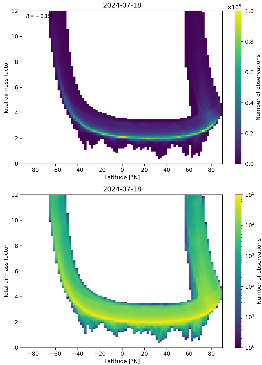
Figure 84: Scatter density plot of “Latitude” against “Total airmass factor” for 2024-07-17 to 2024-07-19.
