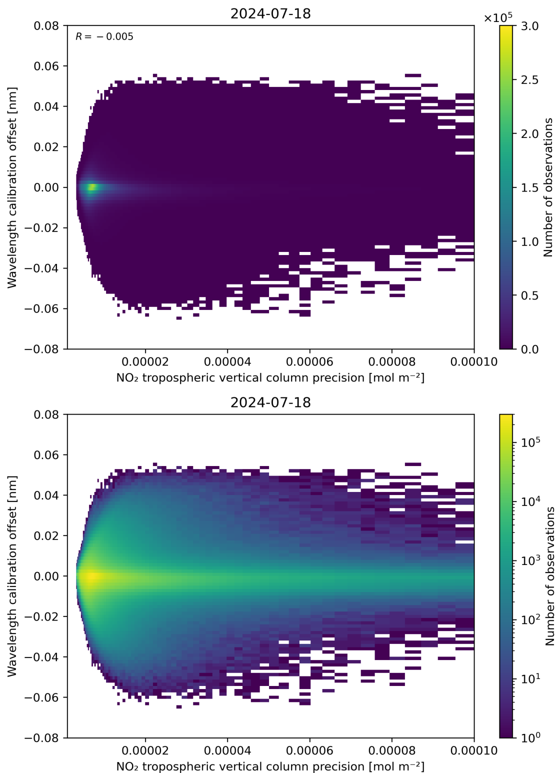
Figure 141: Scatter density plot of “NO 2 tropospheric vertical column precision” against “Wavelength calibration offset” for 2024-07-17 to 2024-07-19.
