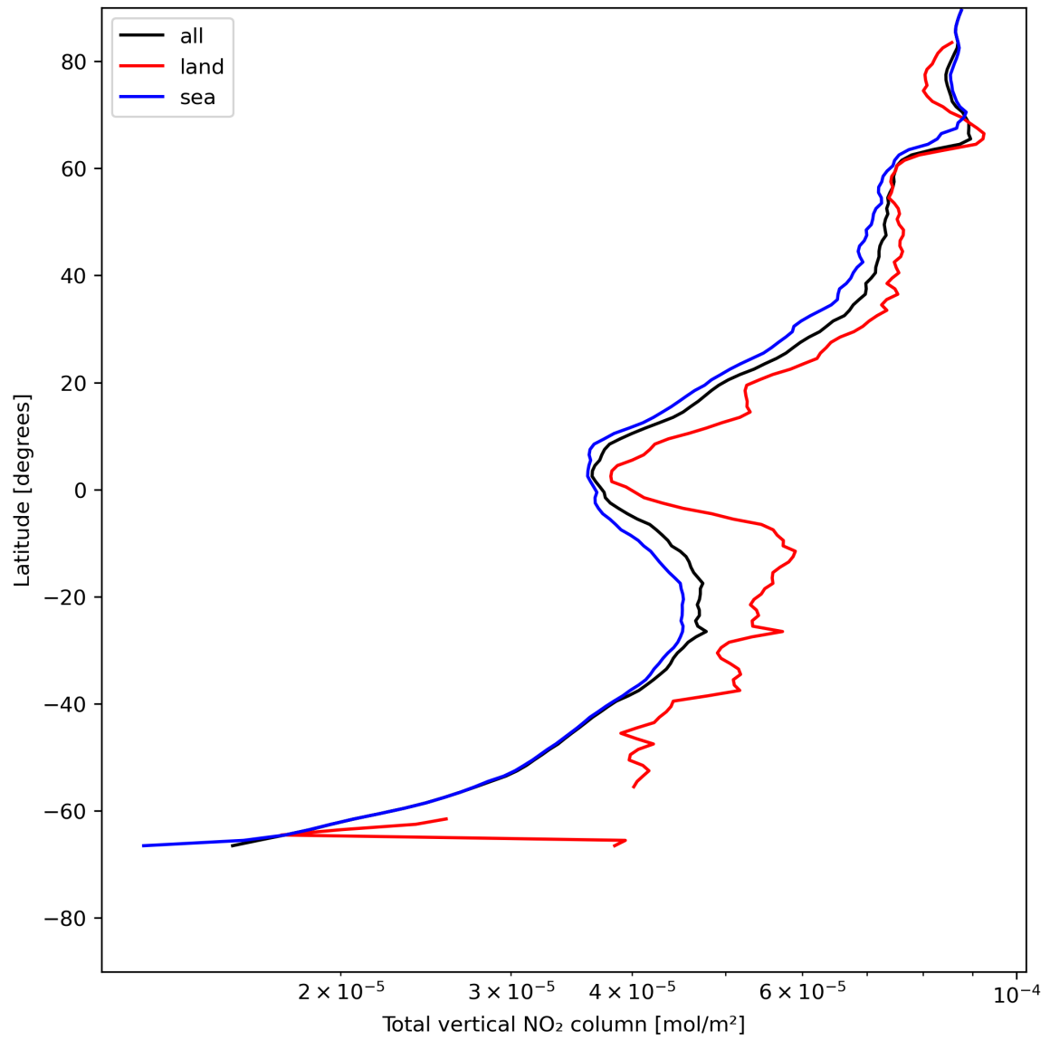
Figure 21: Zonal average of “Total vertical NO 2 column” for 2024-07-17 to 2024-07-19.
