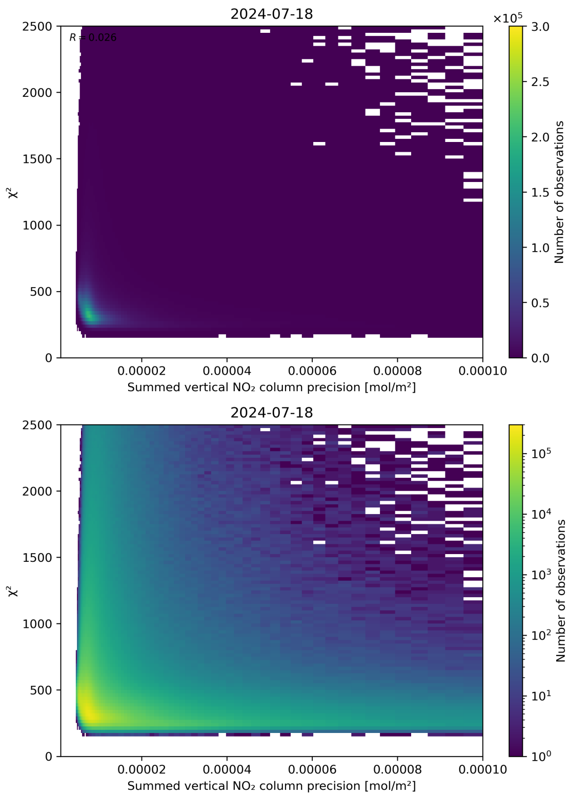
Figure 107: Scatter density plot of “Summed vertical NO 2 column precision” against “ \chi^2 ” for 2024-07-17 to 2024-07-19.
