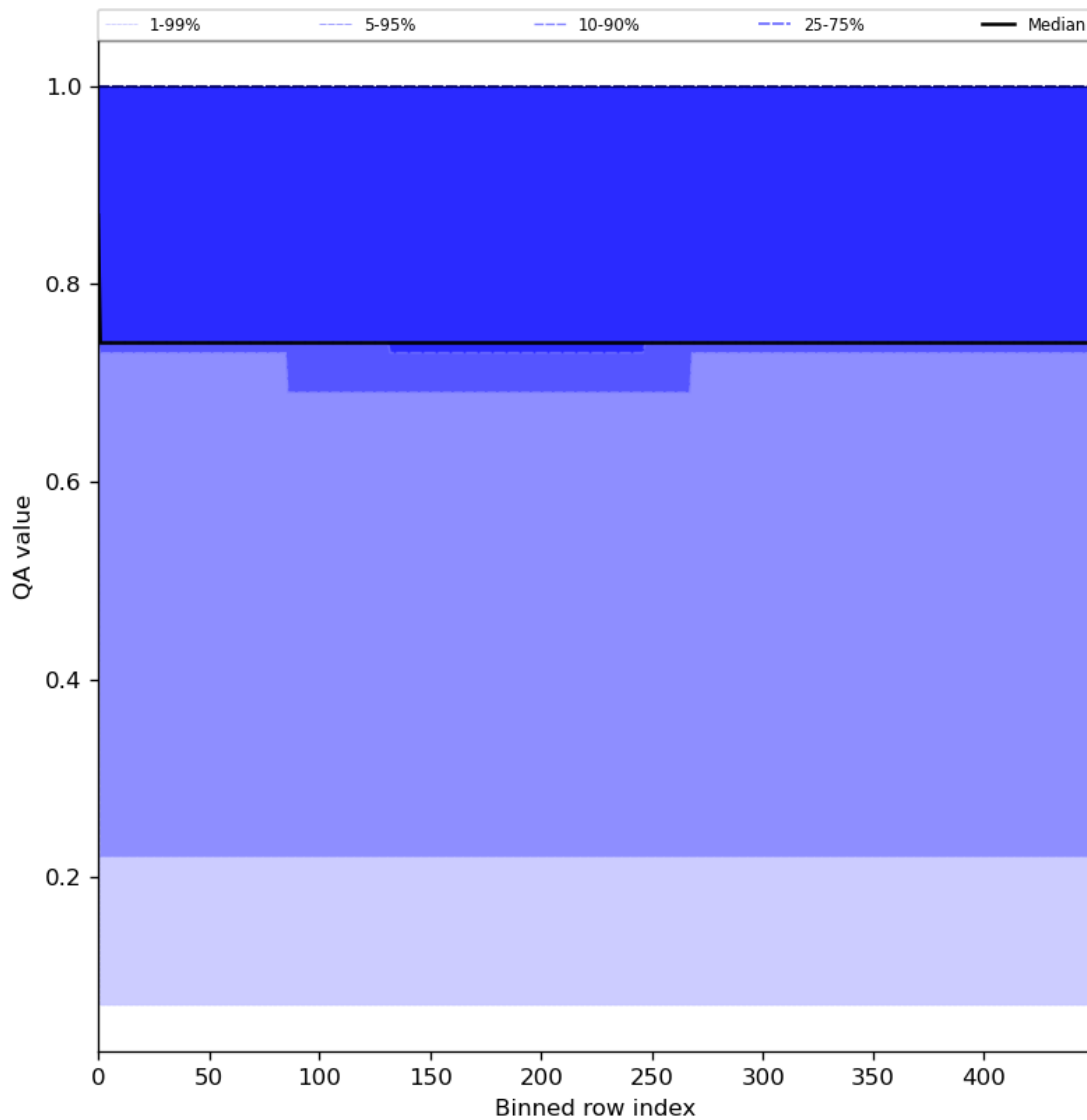
Figure 45: Along track statistics of “QA value” for 2024-07-17 to 2024-07-19
