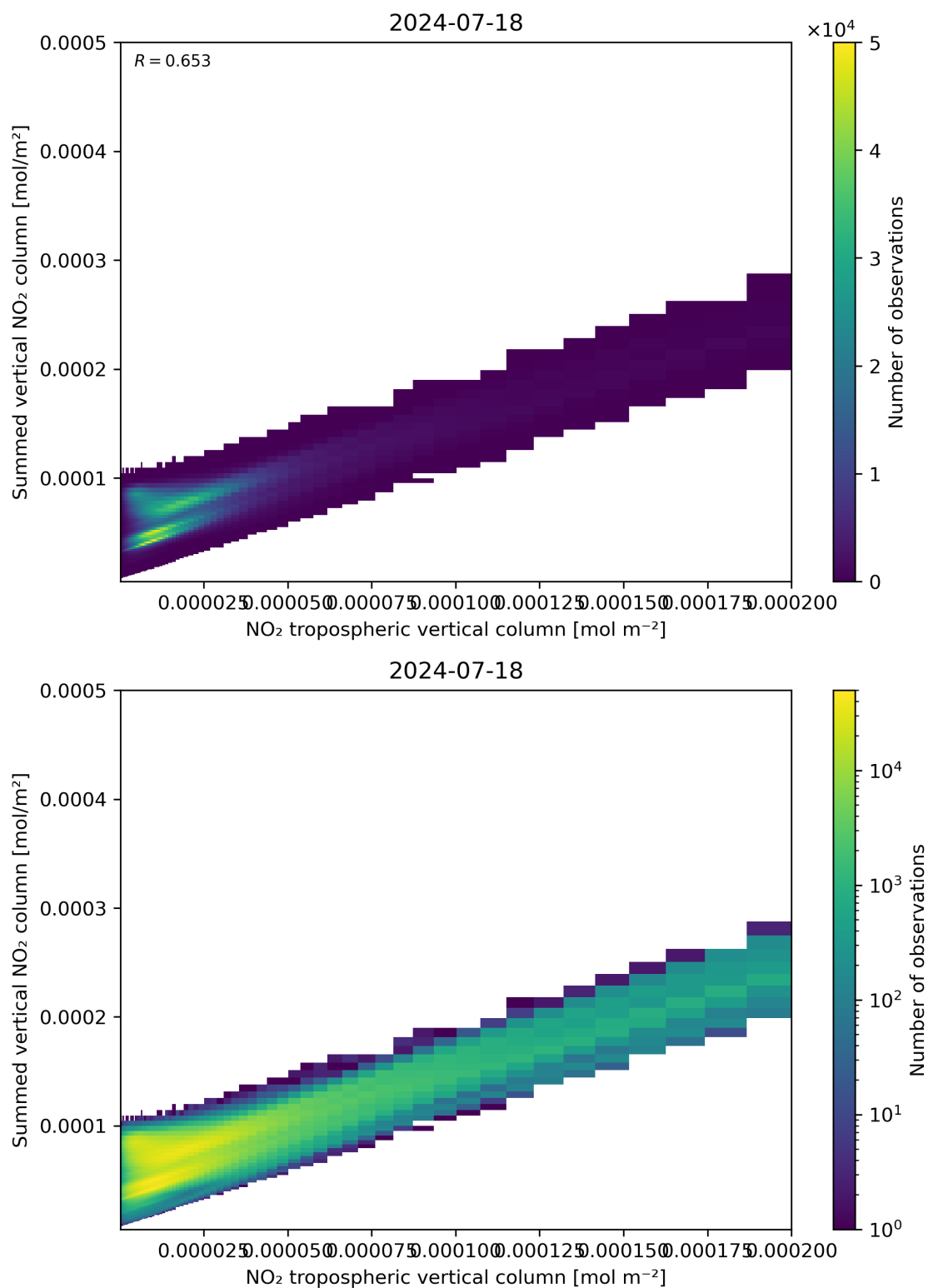
Figure 126: Scatter density plot of “NO 2 tropospheric vertical column” against “Summed vertical NO 2 column” for 2024-07-17 to 2024-07-19.
