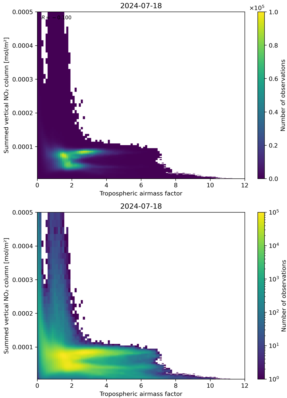
Figure 75: Scatter density plot of “Tropospheric airmass factor” against “Summed vertical NO 2 column” for 2024-07-17 to 2024-07-19.
