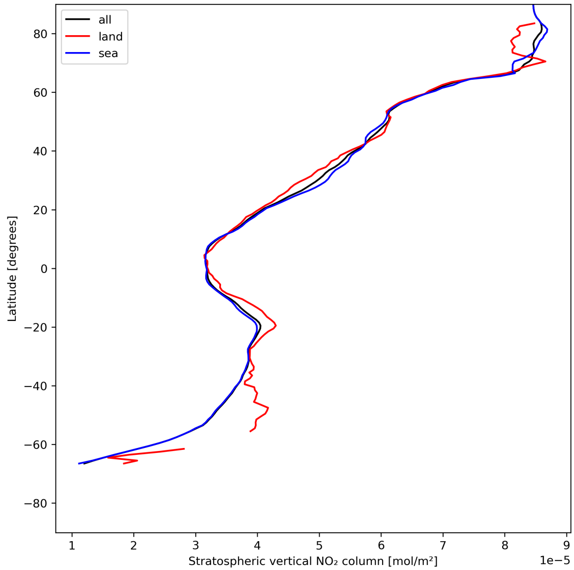
Figure 19: Zonal average of “Stratospheric vertical NO 2 column” for 2024-07-17 to 2024-07-19.
