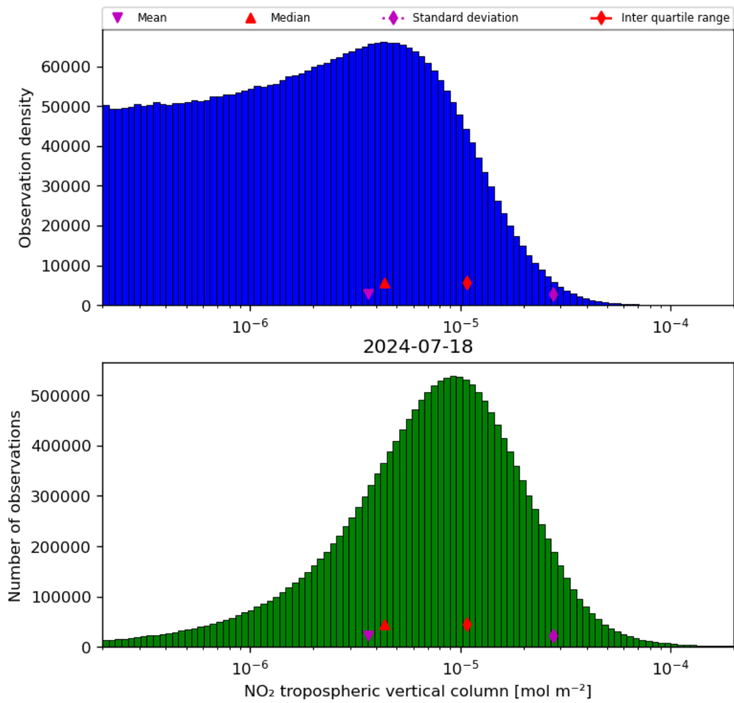
Figure 29: Histogram of “NO 2 tropospheric vertical column” for 2024-07-17 to 2024-07-19
