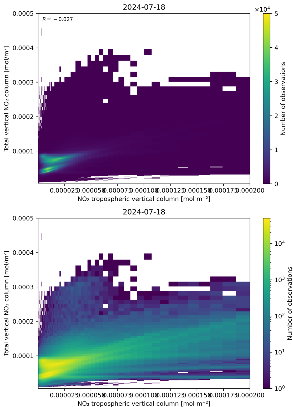
Figure 128: Scatter density plot of “NO 2 tropospheric vertical column” against “Total vertical NO 2 column” for 2024-07-17 to 2024-07-19.
