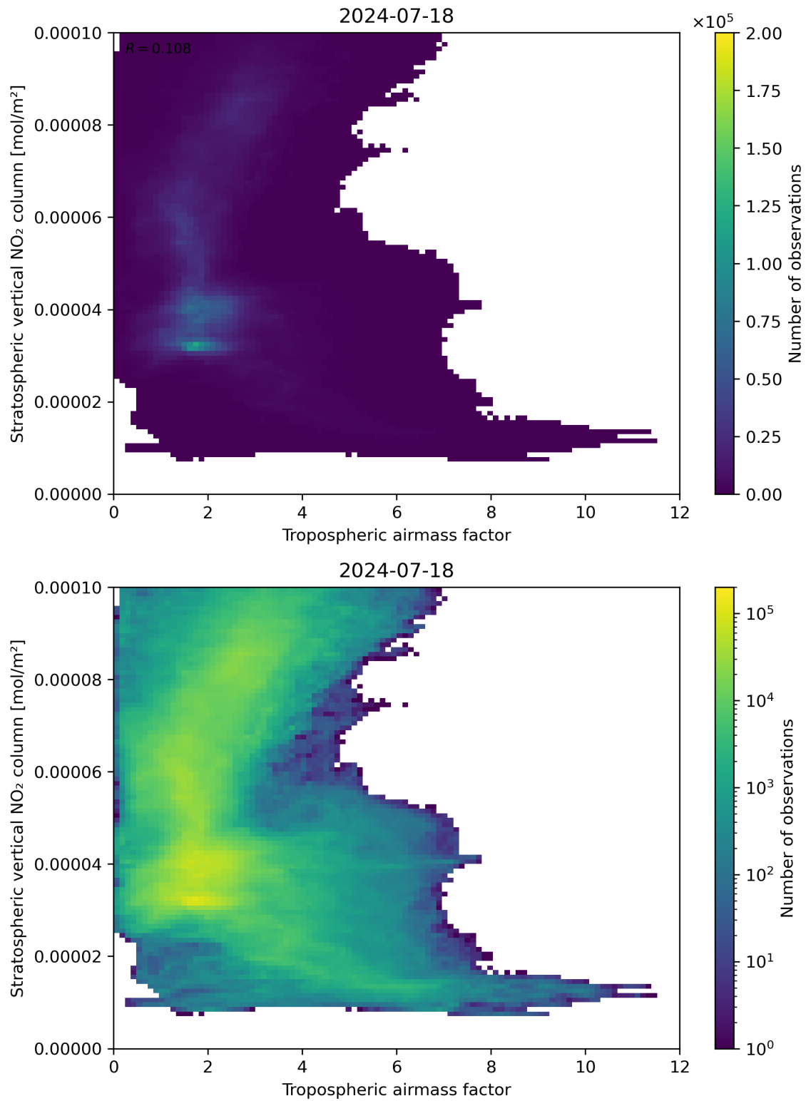
Figure 74: Scatter density plot of “Tropospheric airmass factor” against “Stratospheric vertical NO 2 column” for 2024-07-17 to 2024-07-19.
