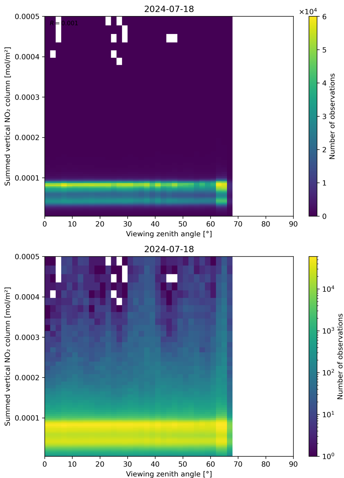
Figure 165: Scatter density plot of “Viewing zenith angle” against “Summed vertical NO 2 column” for 2024-07-17 to 2024-07-19.
