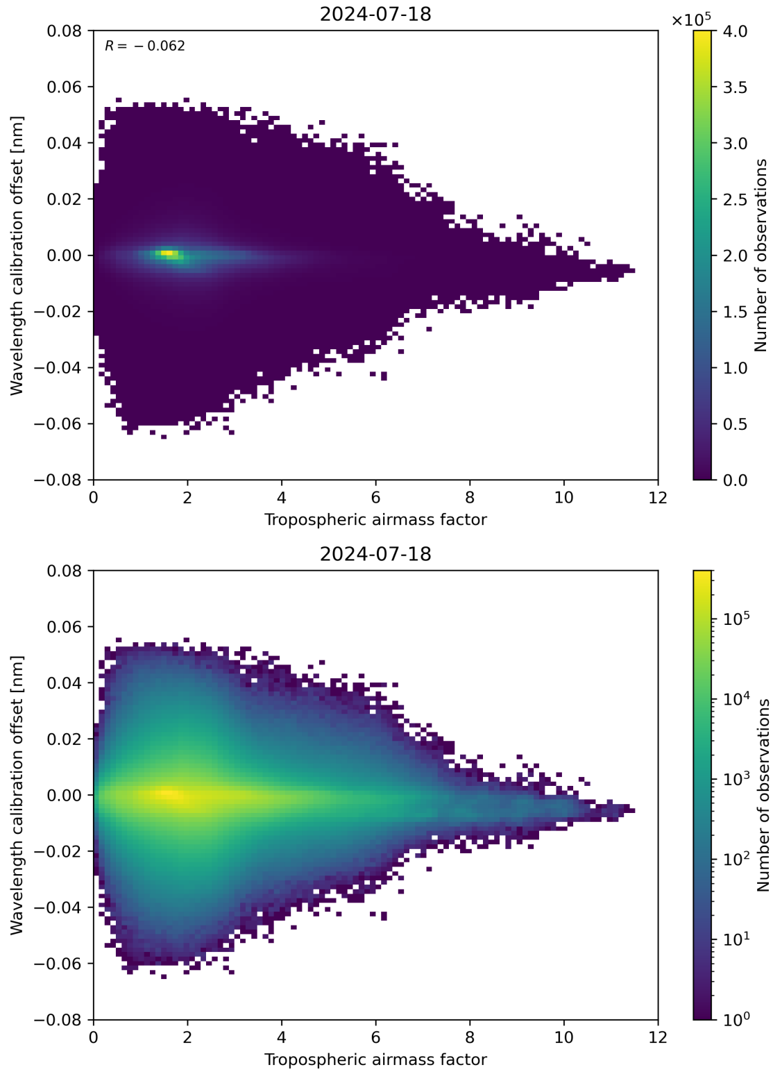
Figure 80: Scatter density plot of “Tropospheric airmass factor” against “Wavelength calibration offset” for 2024-07-17 to 2024-07-19.
