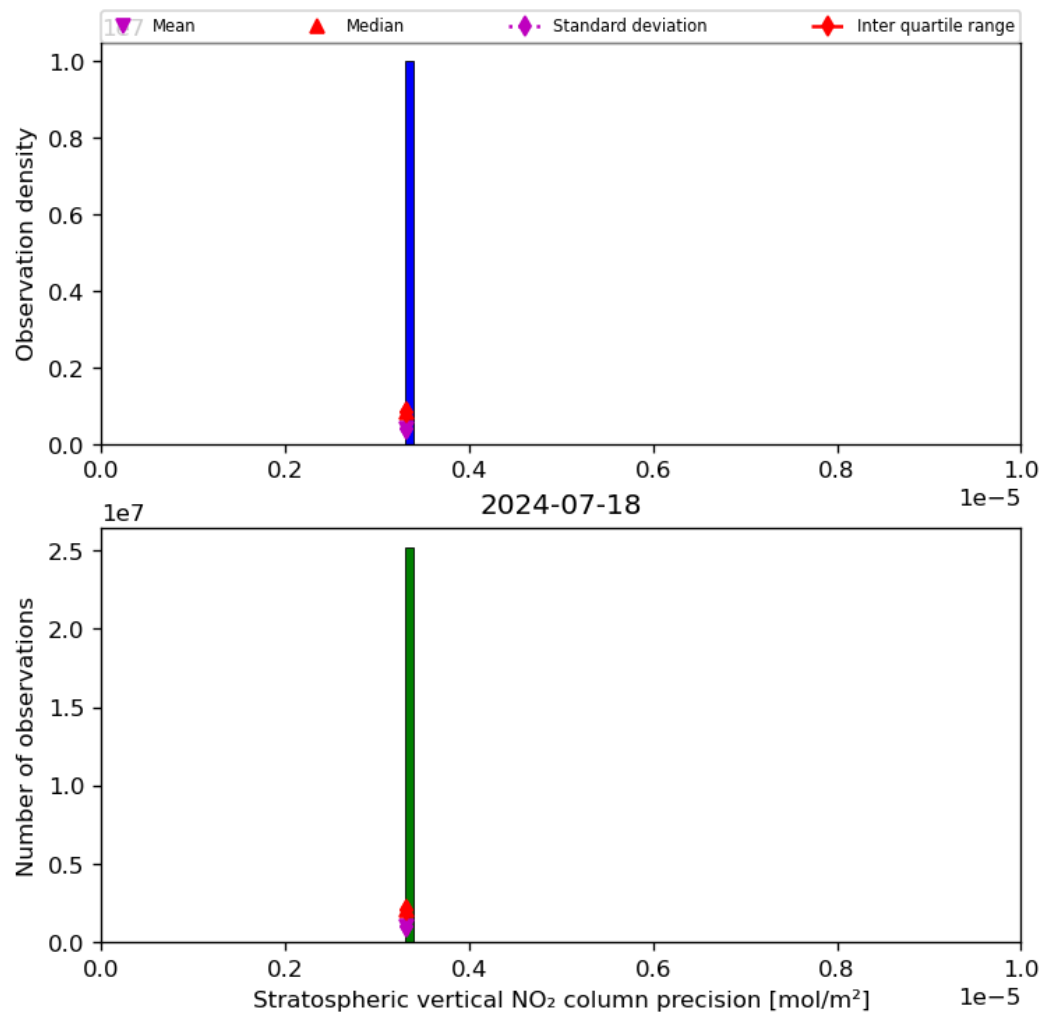
Figure 37: Histogram of “Stratospheric vertical NO 2 column precision” for 2024-07-17 to 2024-07-19
