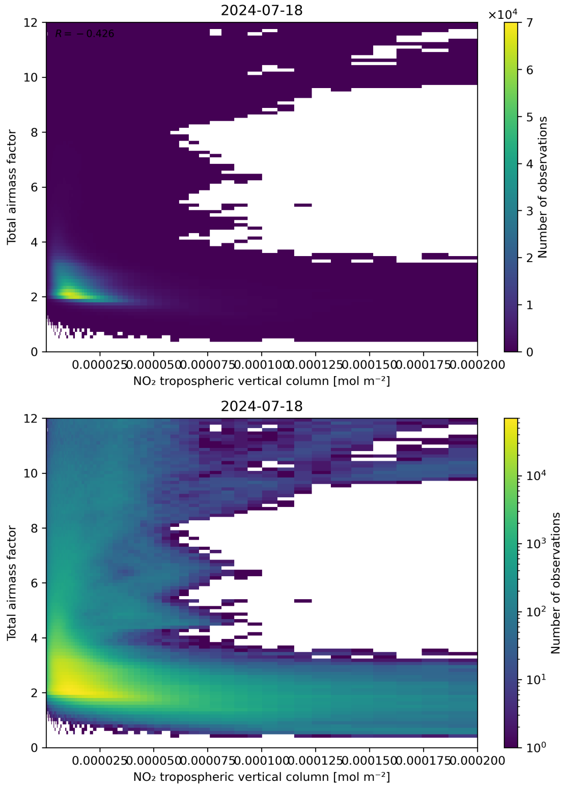
Figure 122: Scatter density plot of “NO 2 tropospheric vertical column” against “Total air mass factor” for 2024-07-17 to 2024-07-19.
