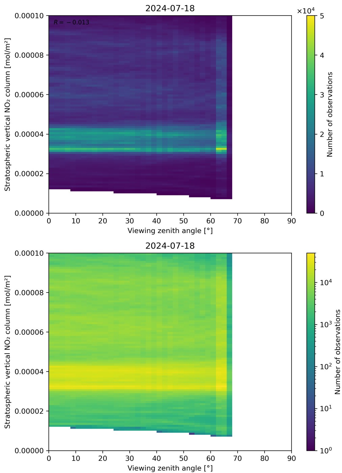
Figure 164: Scatter density plot of “Viewing zenith angle” against “Stratospheric vertical NO 2 column” for 2024-07-17 to 2024-07-19.
