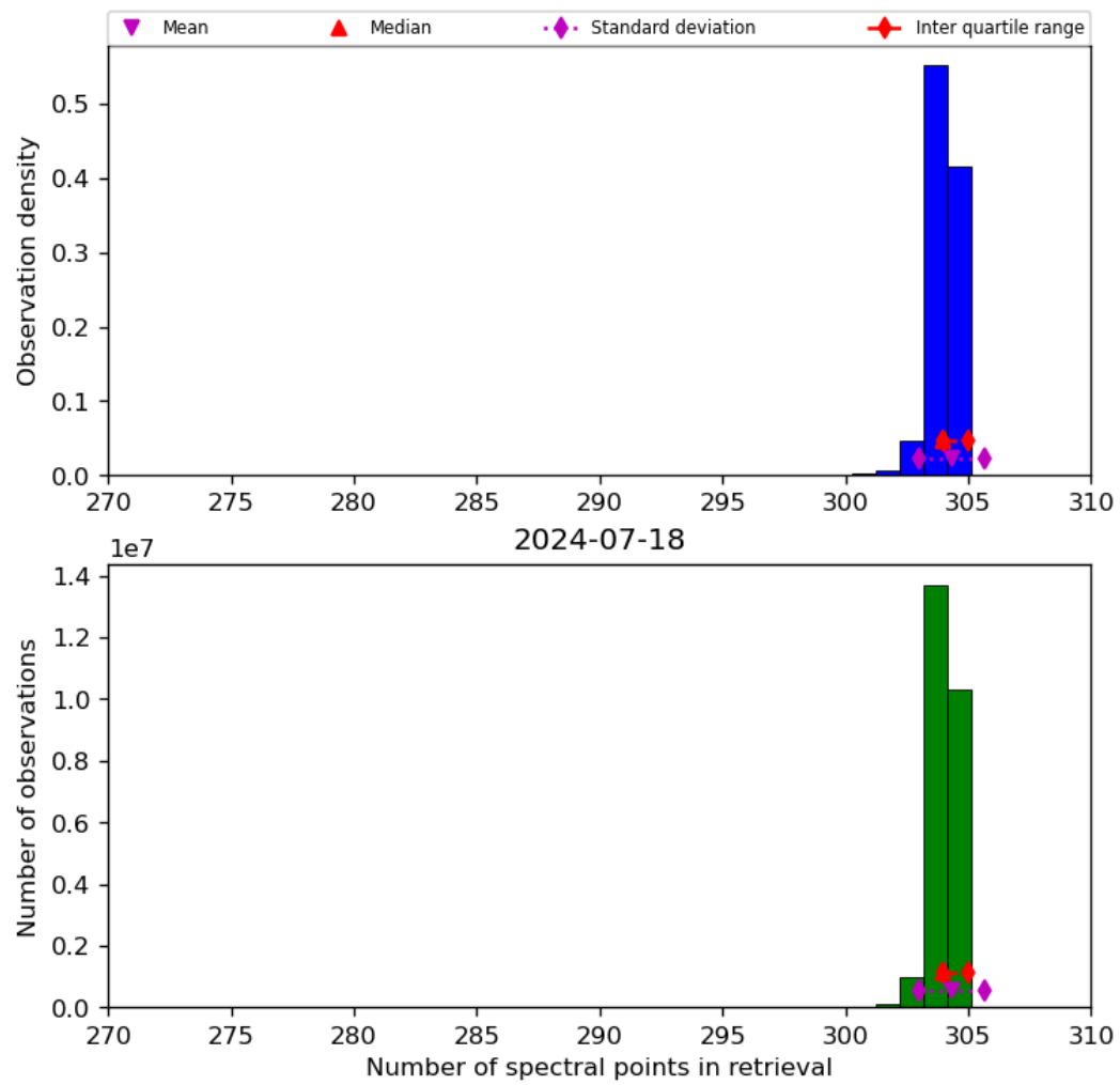
Figure 33: Histogram of “Number of spectral points in retrieval” for 2024-07-17 to 2024-07-19
