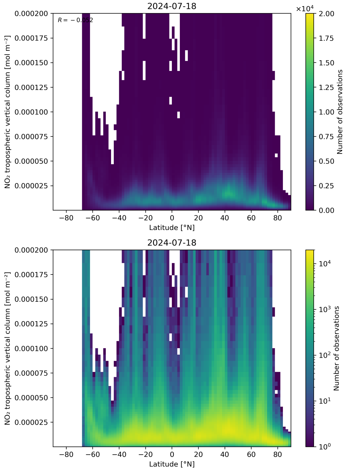
Figure 92: Scatter density plot of “Latitude” against “NO 2 tropospheric vertical column” for 2024-07-17 to 2024-07-19.
