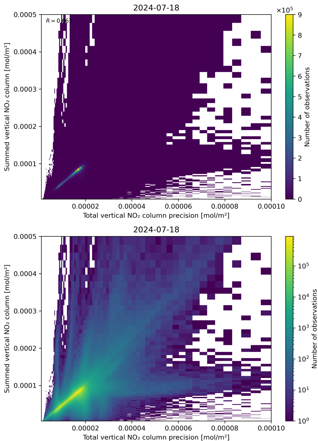
Figure 117: Scatter density plot of “Total vertical NO 2 column precision” against “Summed vertical NO 2 column” for 2024-07-17 to 2024-07-19.
