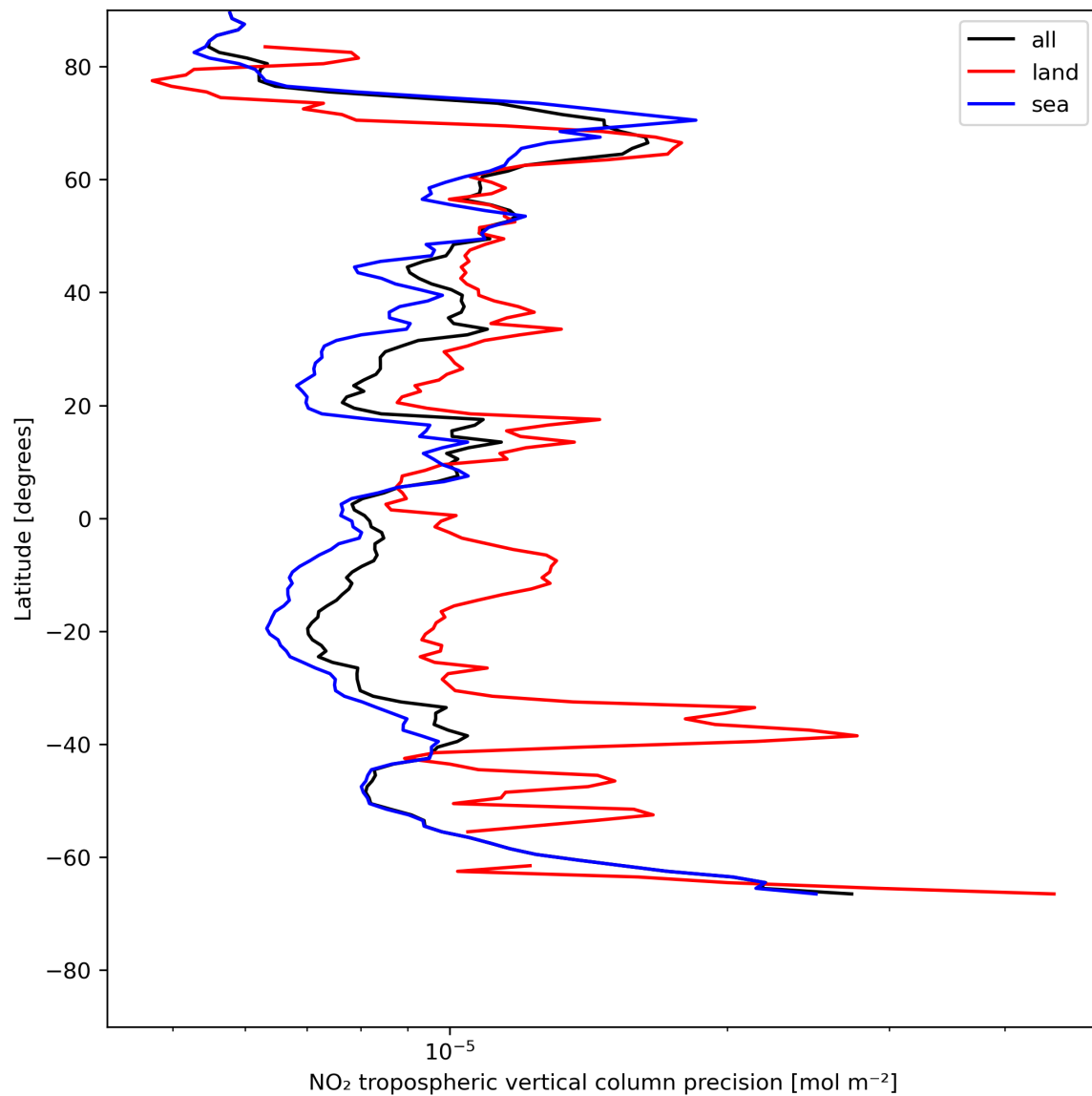
Figure 13: Zonal average of “NO 2 tropospheric vertical column precision” for 2024-07-17 to 2024-07-19.
