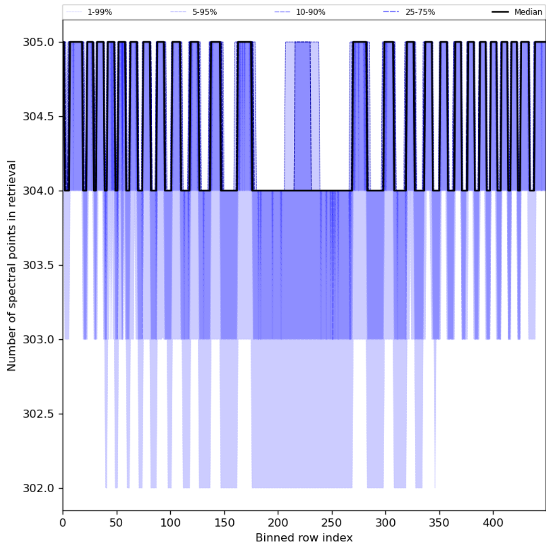
Figure 50: Along track statistics of “Number of spectral points in retrieval” for 2024-07-17 to 2024-07-19
