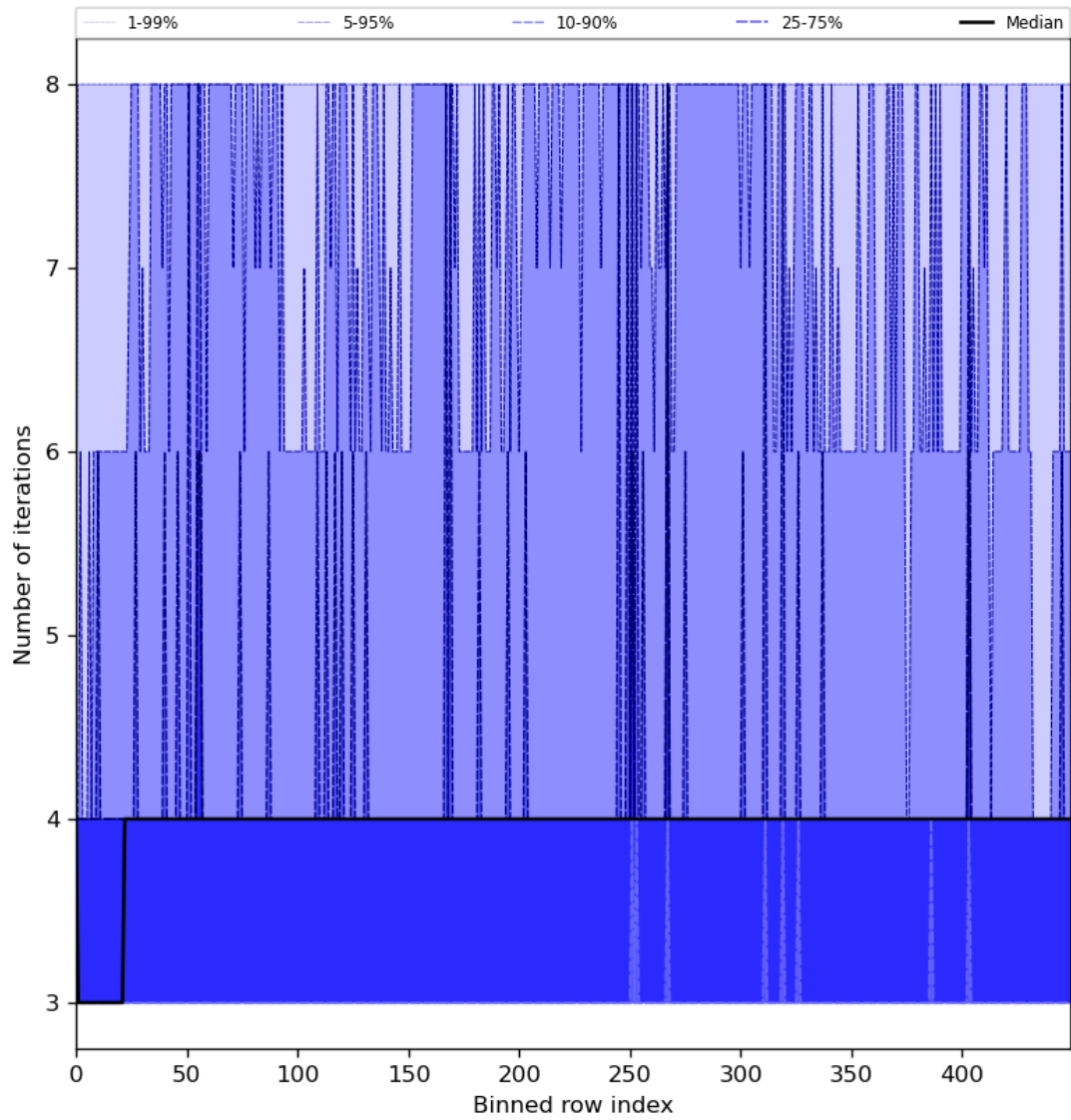
Figure 51: Along track statistics of “Number of iterations” for 2024-07-17 to 2024-07-19
