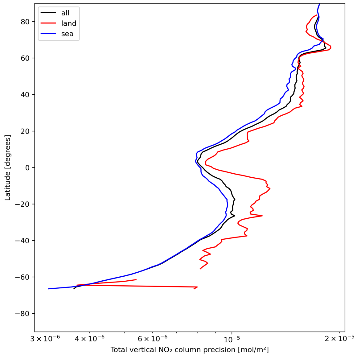
Figure 22: Zonal average of “Total vertical NO 2 column precision” for 2024-07-17 to 2024-07-19.
