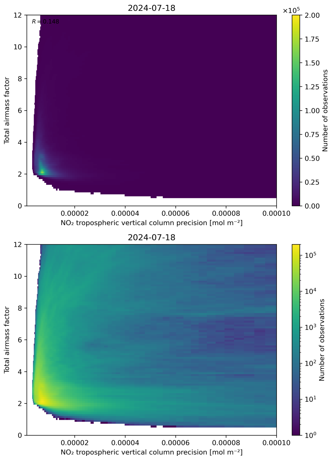
Figure 132: Scatter density plot of “NO 2 tropospheric vertical column precision” against “Total air mass factor” for 2024-07-17 to 2024-07-19.
