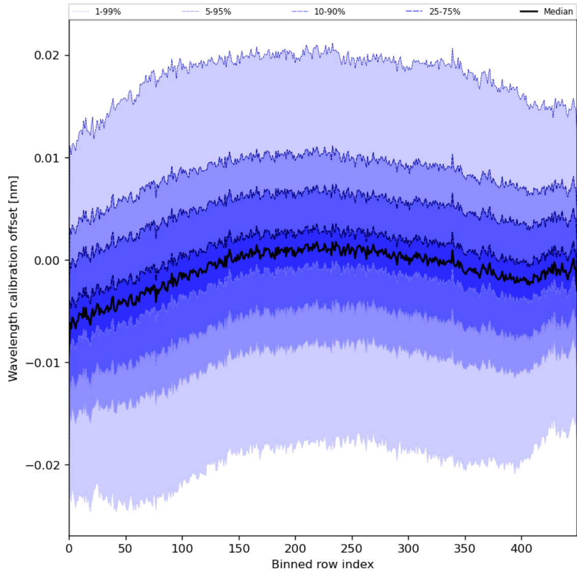
Figure 52: Along track statistics of “Wavelength calibration offset” for 2024-07-17 to 2024-07-19
