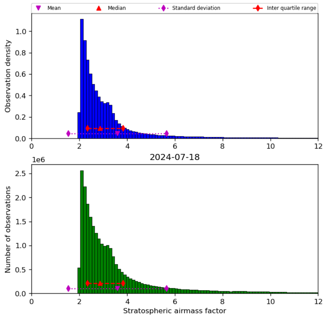
Figure 44: Histogram of “Stratospheric airmass factor” for 2024-07-17 to 2024-07-19
