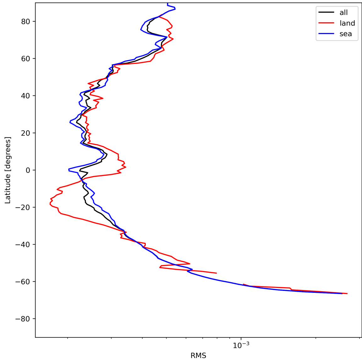
Figure 26: Zonal average of “RMS” for 2024-07-17 to 2024-07-19.
