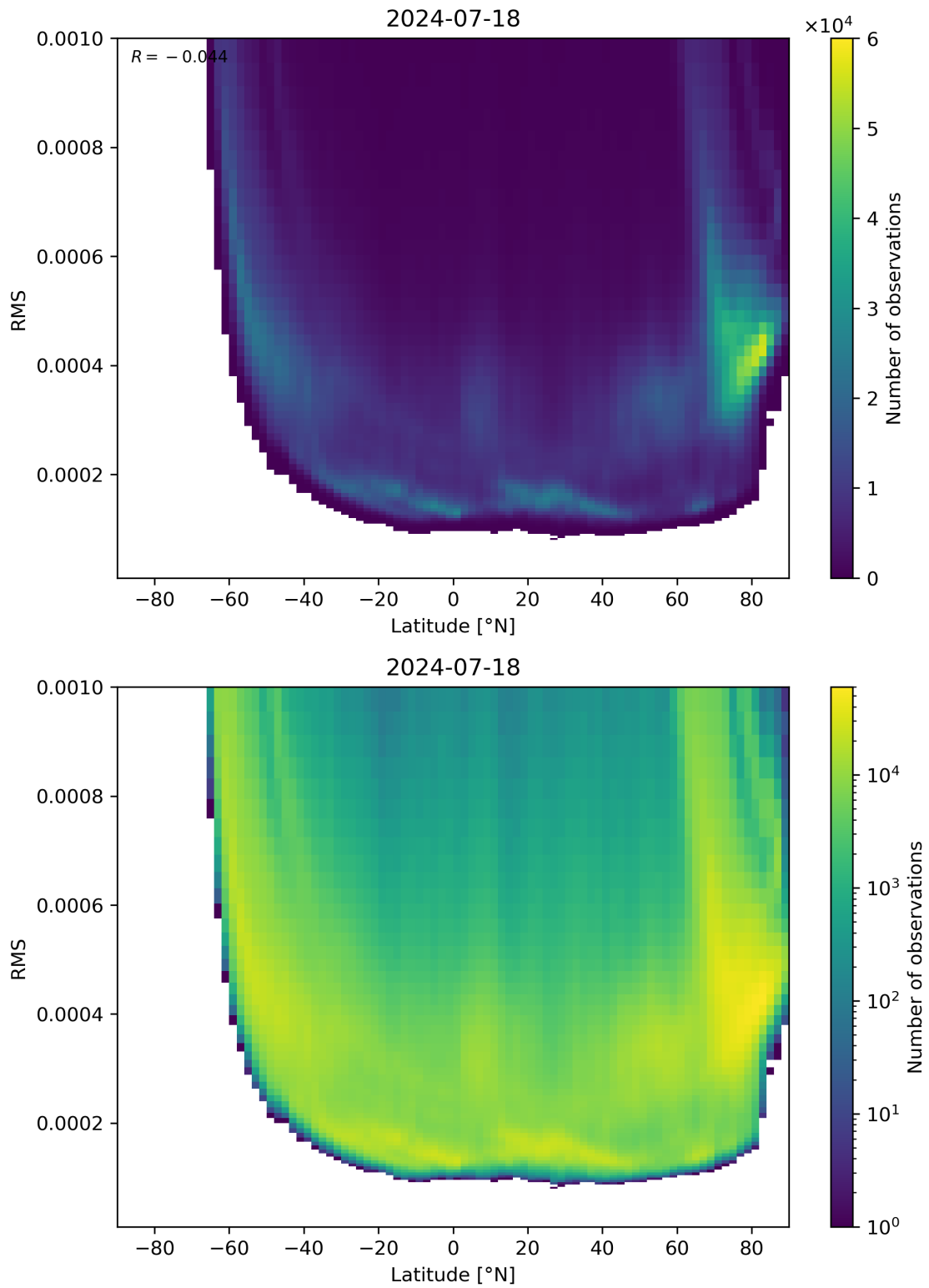
Figure 94: Scatter density plot of “Latitude” against “RMS” for 2024-07-17 to 2024-07-19.
