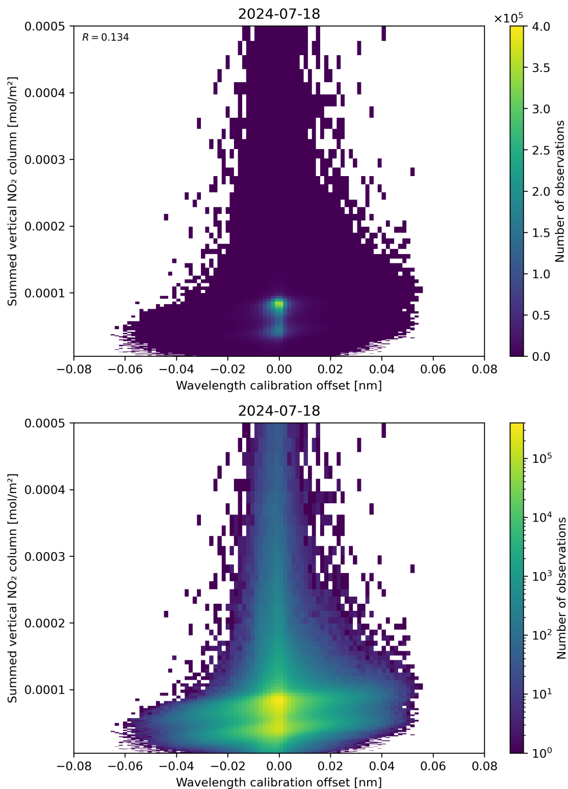
Figure 177: Scatter density plot of “Wavelength calibration offset” against “Summed vertical NO 2 column” for 2024-07-17 to 2024-07-19.
