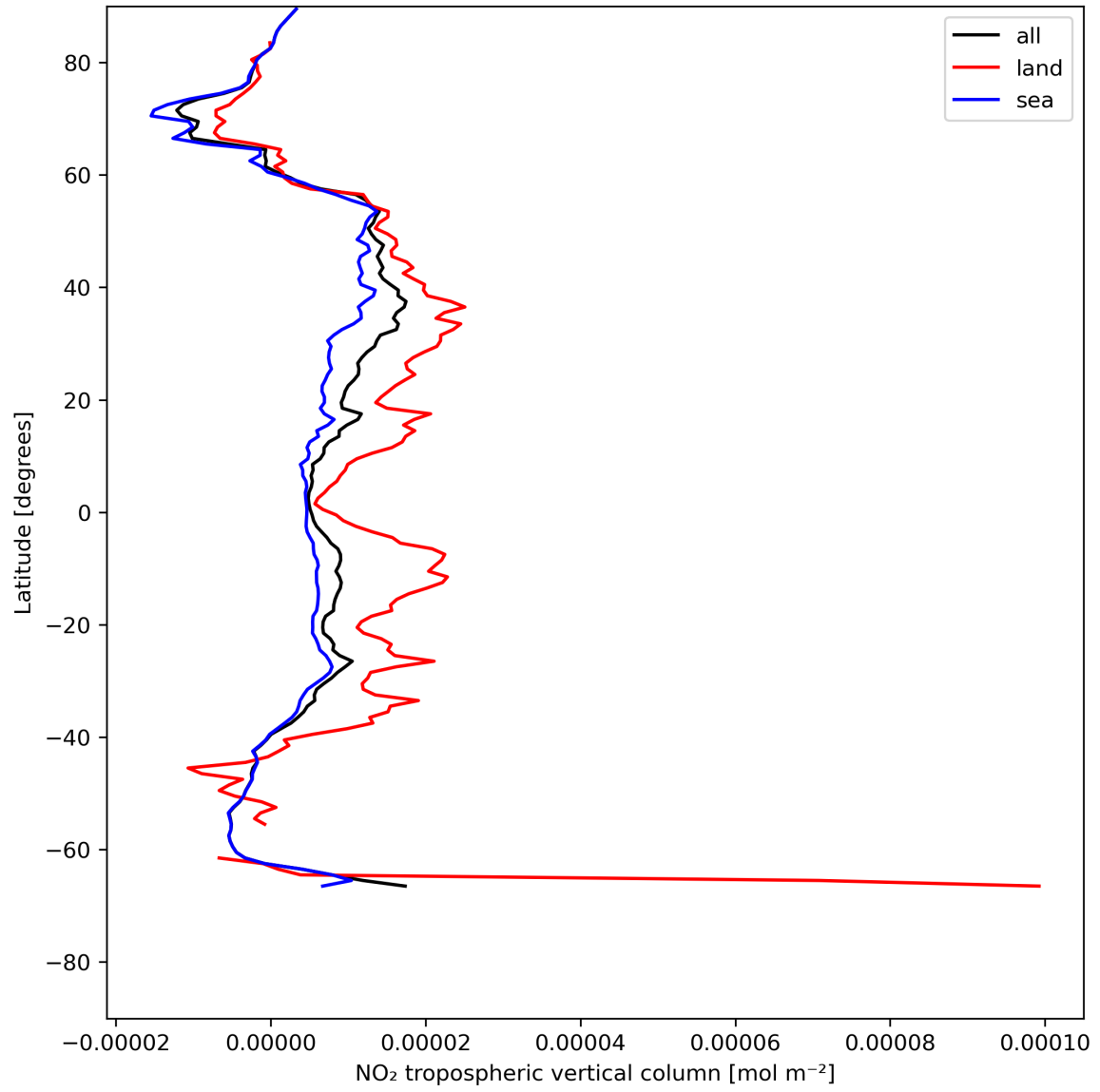
Figure 12: Zonal average of “NO 2 tropospheric vertical column” for 2024-07-17 to 2024-07-19.
