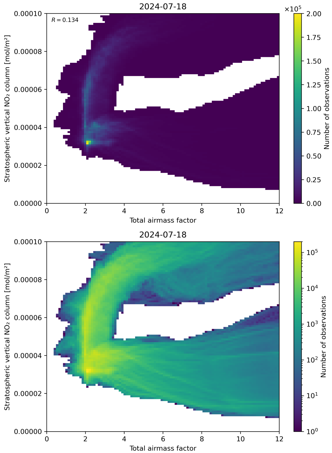
Figure 64: Scatter density plot of “Total airmass factor” against “Stratospheric vertical \text{NO}_2 column” for 2024-07-17 to 2024-07-19.
