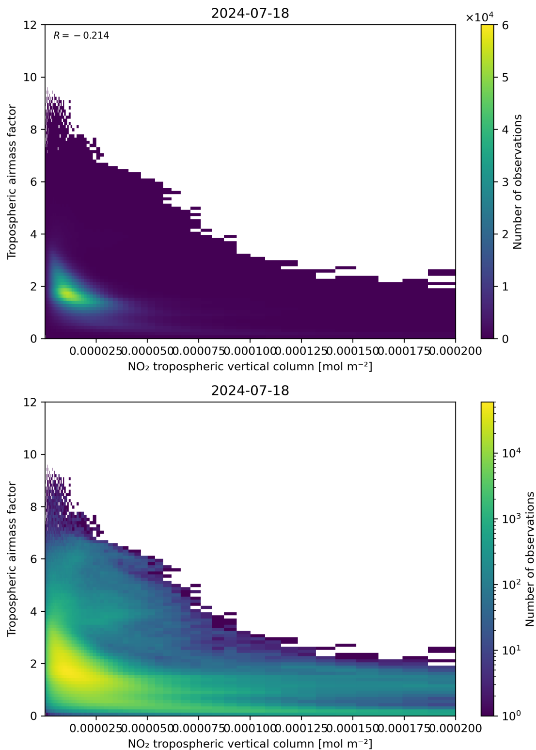
Figure 123: Scatter density plot of “NO 2 tropospheric vertical column” against “Tropospheric air mass factor” for 2024-07-17 to 2024-07-19.
