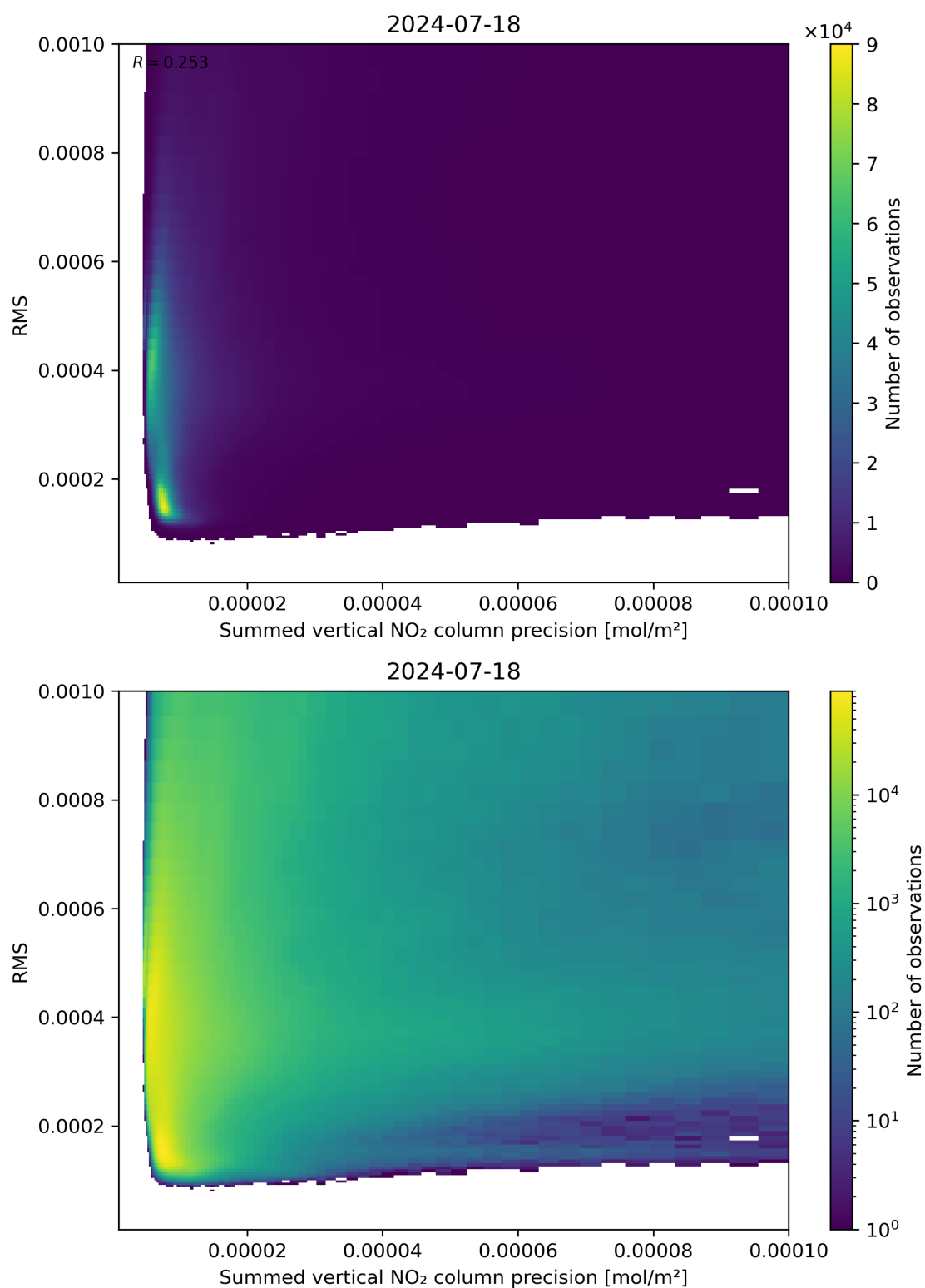
Figure 108: Scatter density plot of “Summed vertical NO 2 column precision” against “RMS” for 2024-07-17 to 2024-07-19.
