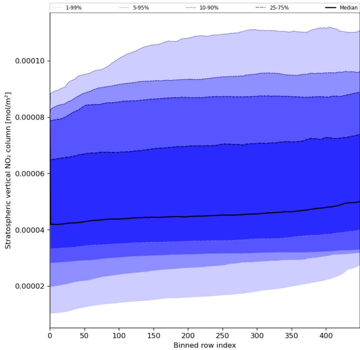
Figure 53: Along track statistics of “Stratospheric vertical NO 2 column” for 2024-07-17 to 2024-07-19
