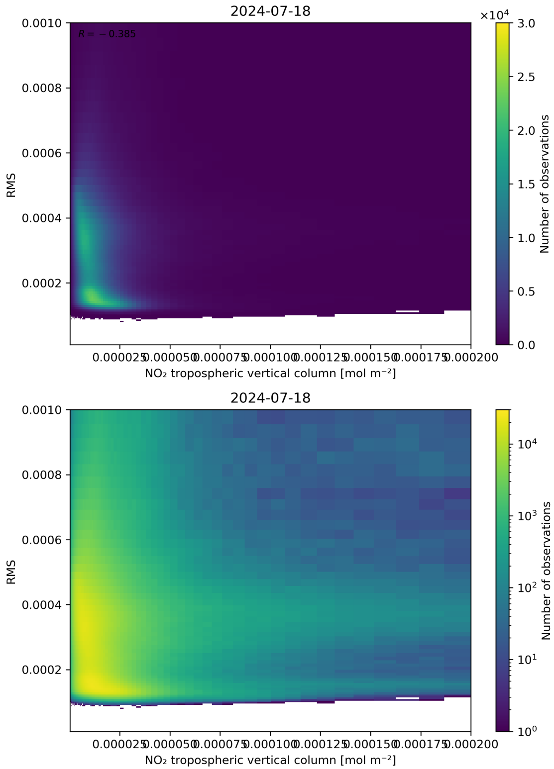
Figure 142: Scatter density plot of “NO 2 tropospheric vertical column” against “RMS” for 2024-07-17 to 2024-07-19.
