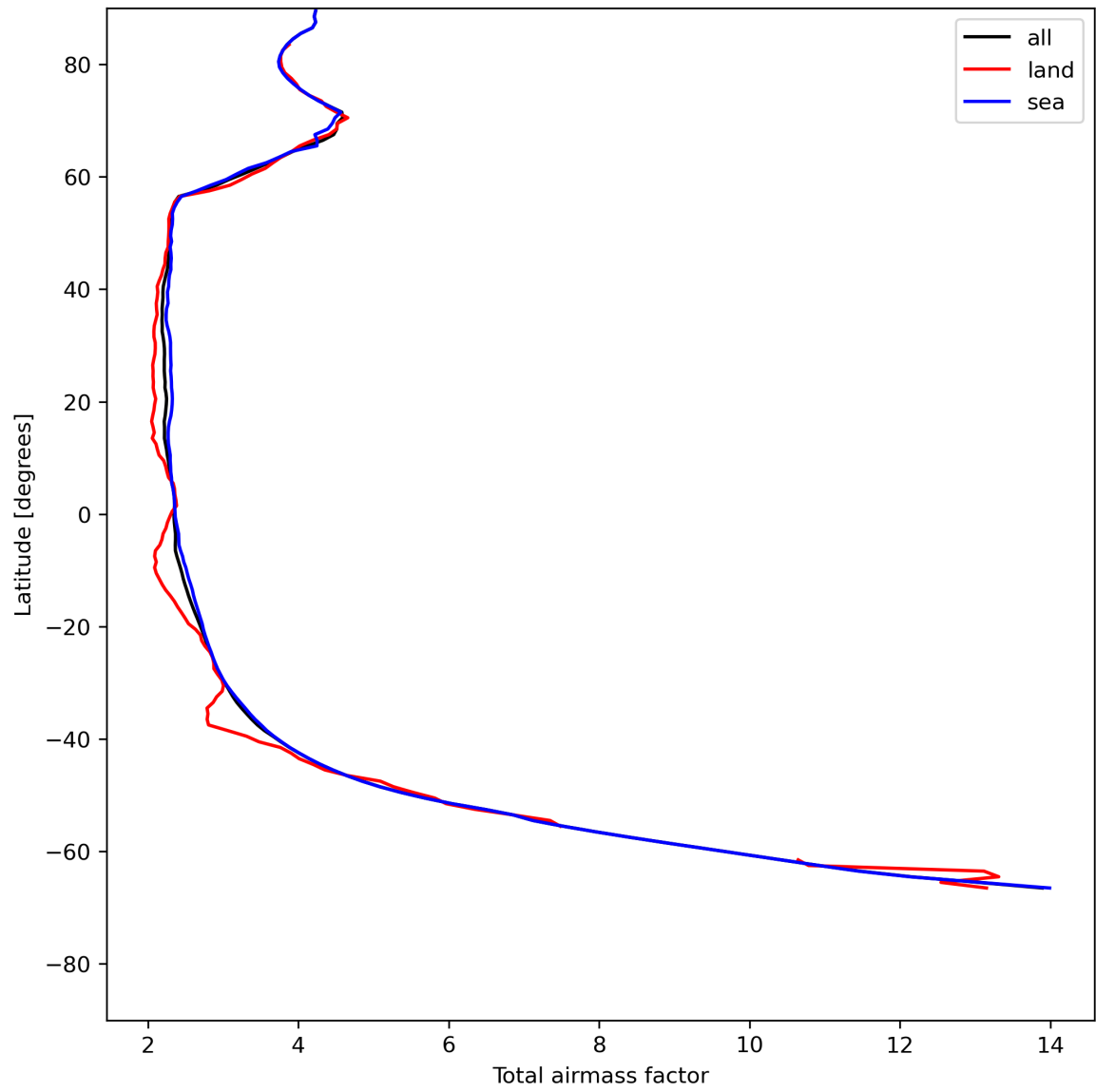
Figure 15: Zonal average of “Total airmass factor” for 2024-07-17 to 2024-07-19.
