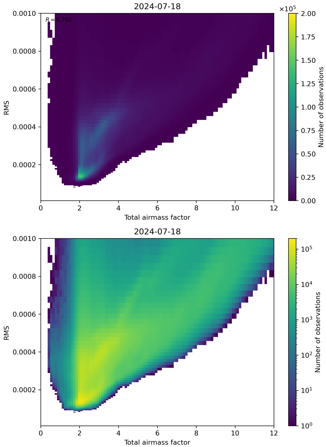
Figure 69: Scatter density plot of “Total airmass factor” against “RMS” for 2024-07-17 to 2024-07-19.
