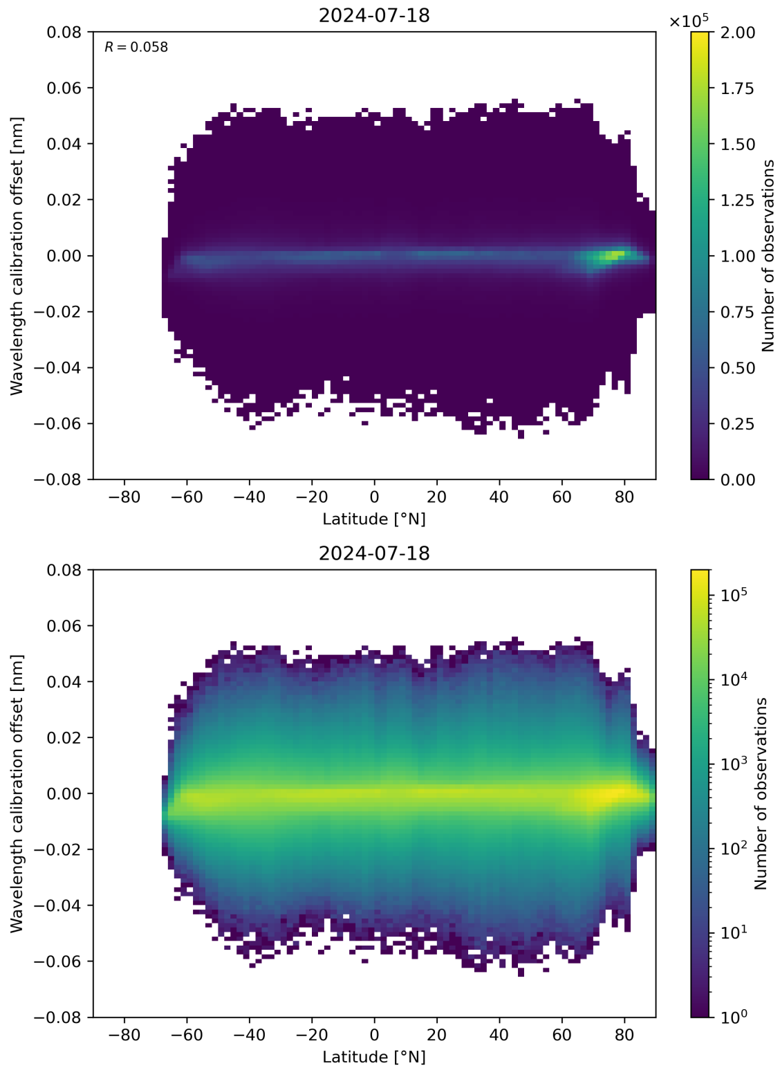
Figure 95: Scatter density plot of “Latitude” against “Wavelength calibration offset” for 2024-07-17 to 2024-07-19.
