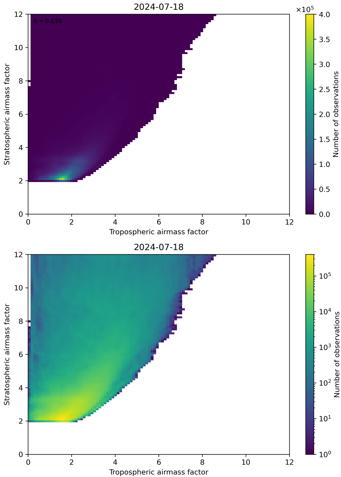
Figure 71: Scatter density plot of “Tropospheric airmass factor” against “Stratospheric airmass factor” for 2024-07-17 to 2024-07-19.
