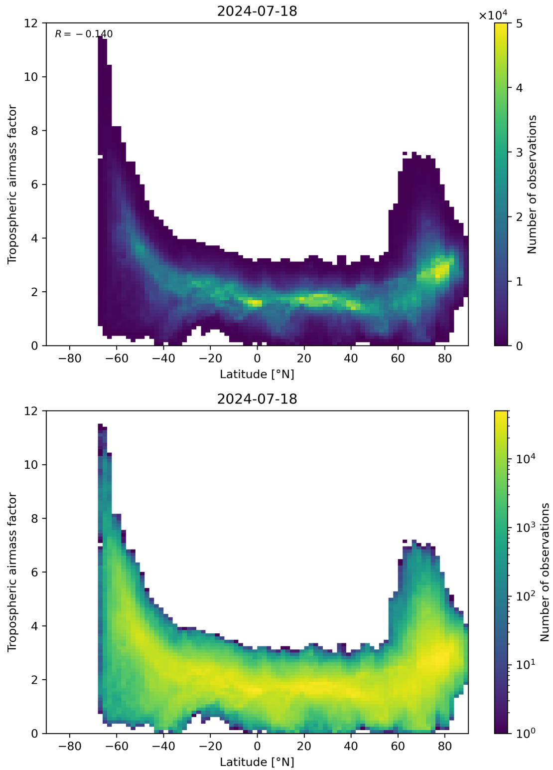
Figure 85: Scatter density plot of “Latitude” against “Tropospheric airmass factor” for 2024-07-17 to 2024-07-19.
