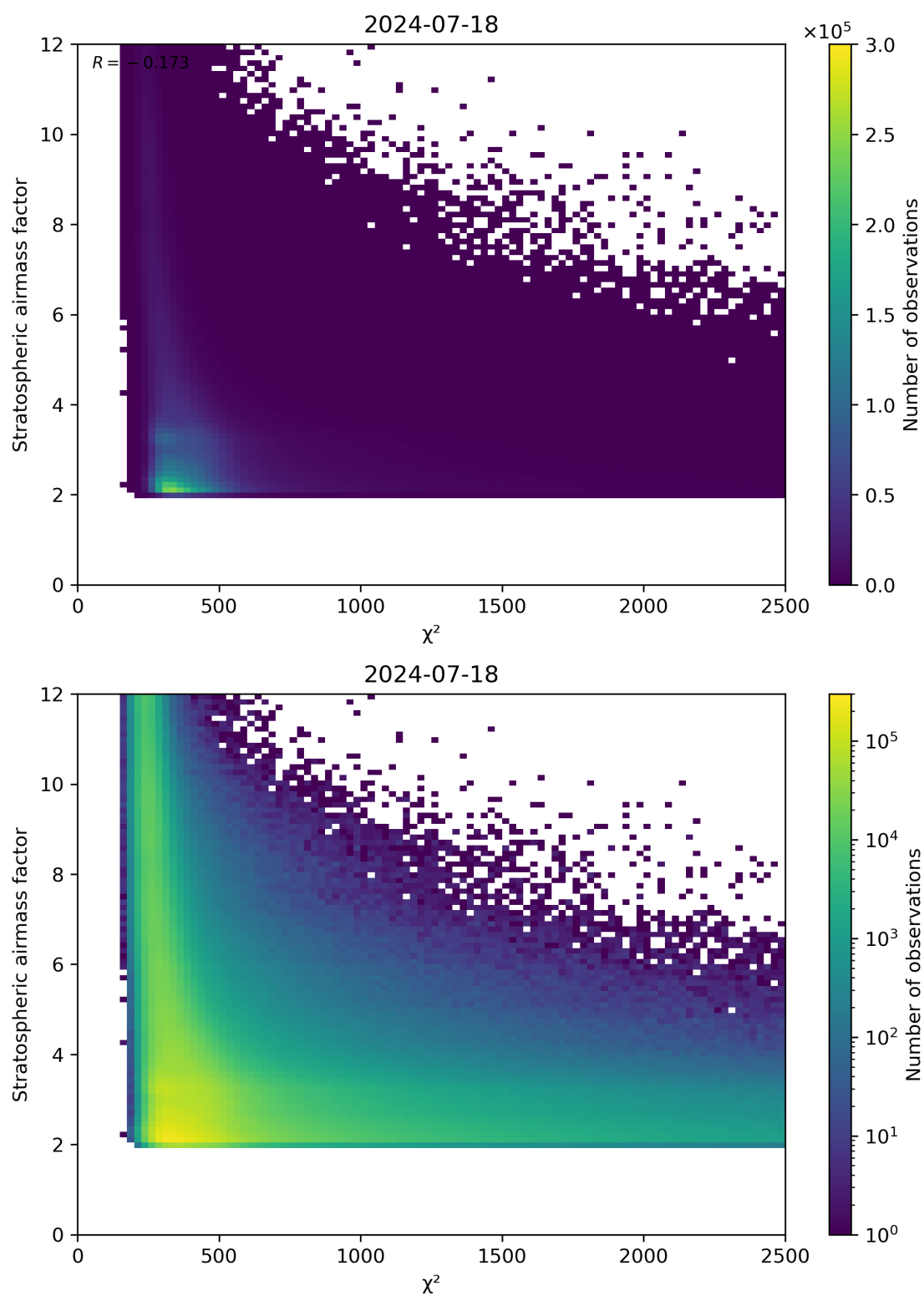
Figure 81: Scatter density plot of “ \chi^2 ” against “Stratospheric airmass factor” for 2024-07-17 to 2024-07-19.
