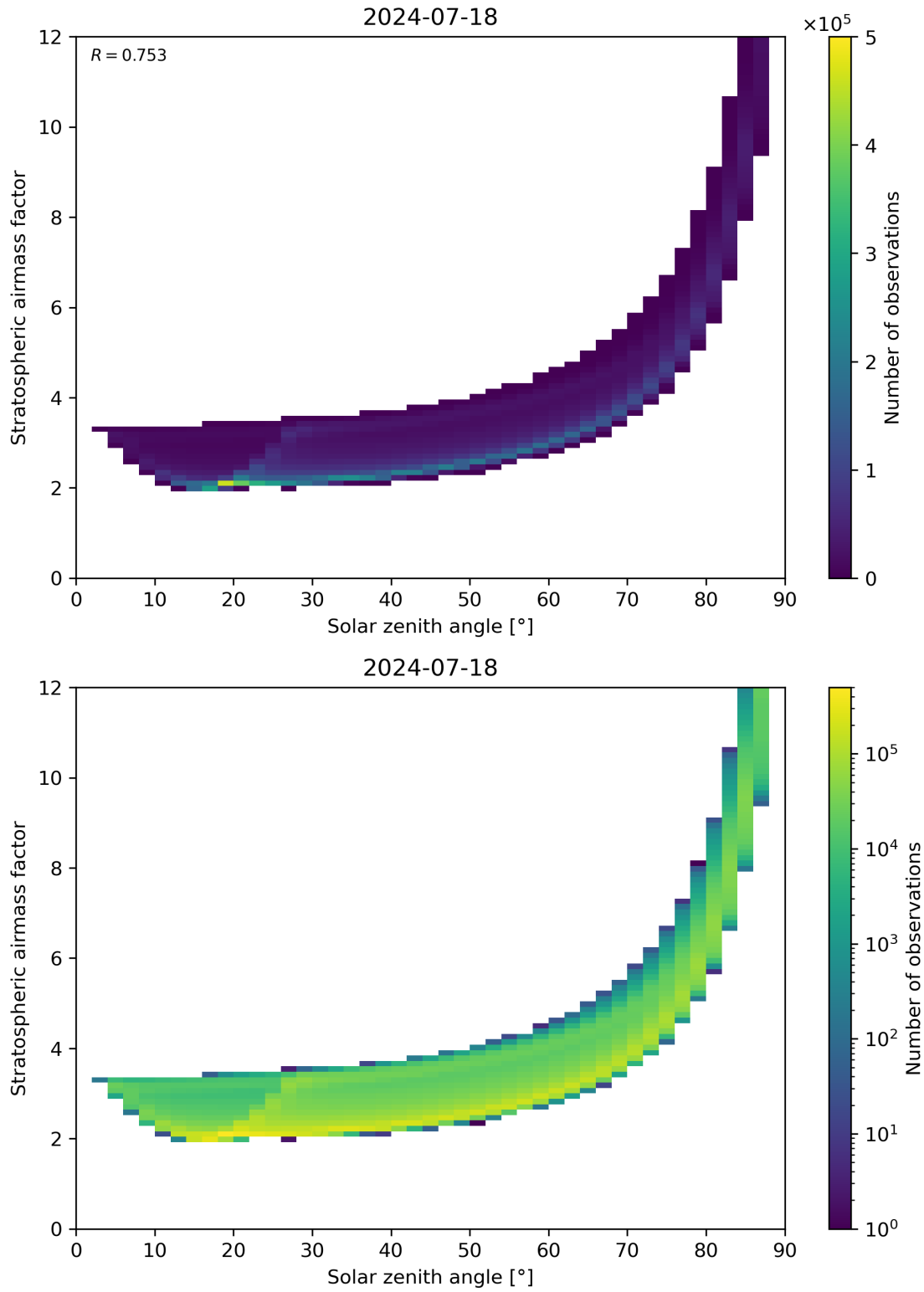
Figure 145: Scatter density plot of “Solar zenith angle” against “Stratospheric airmass factor” for 2024-07-17 to 2024-07-19.
