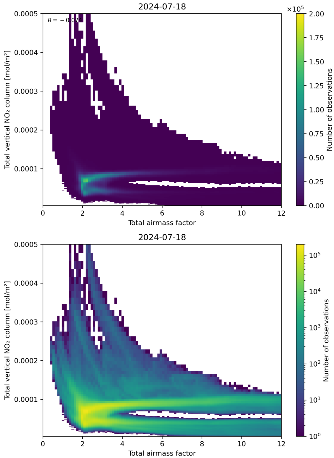
Figure 67: Scatter density plot of “Total airmass factor” against “Total vertical NO 2 column” for 2024-07-17 to 2024-07-19.
