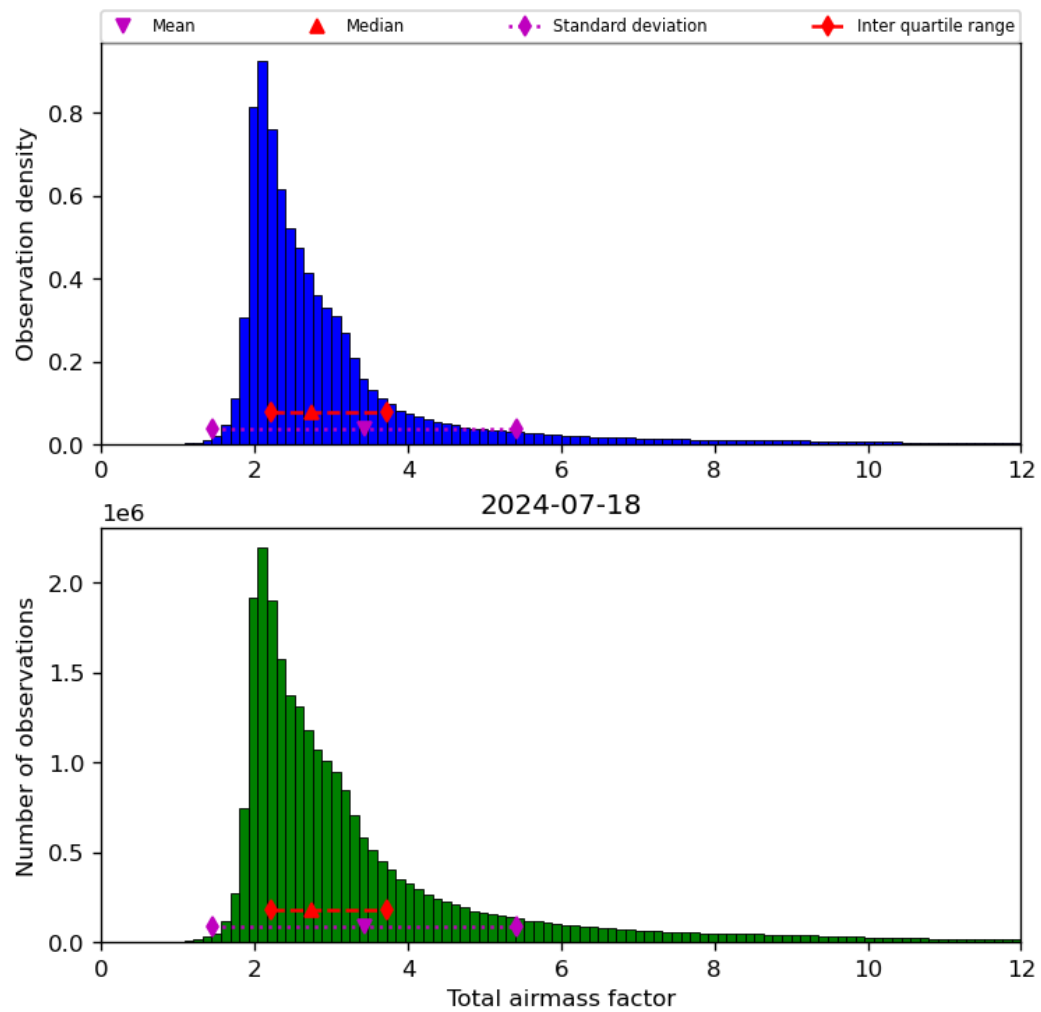
Figure 32: Histogram of “Total airmass factor” for 2024-07-17 to 2024-07-19
