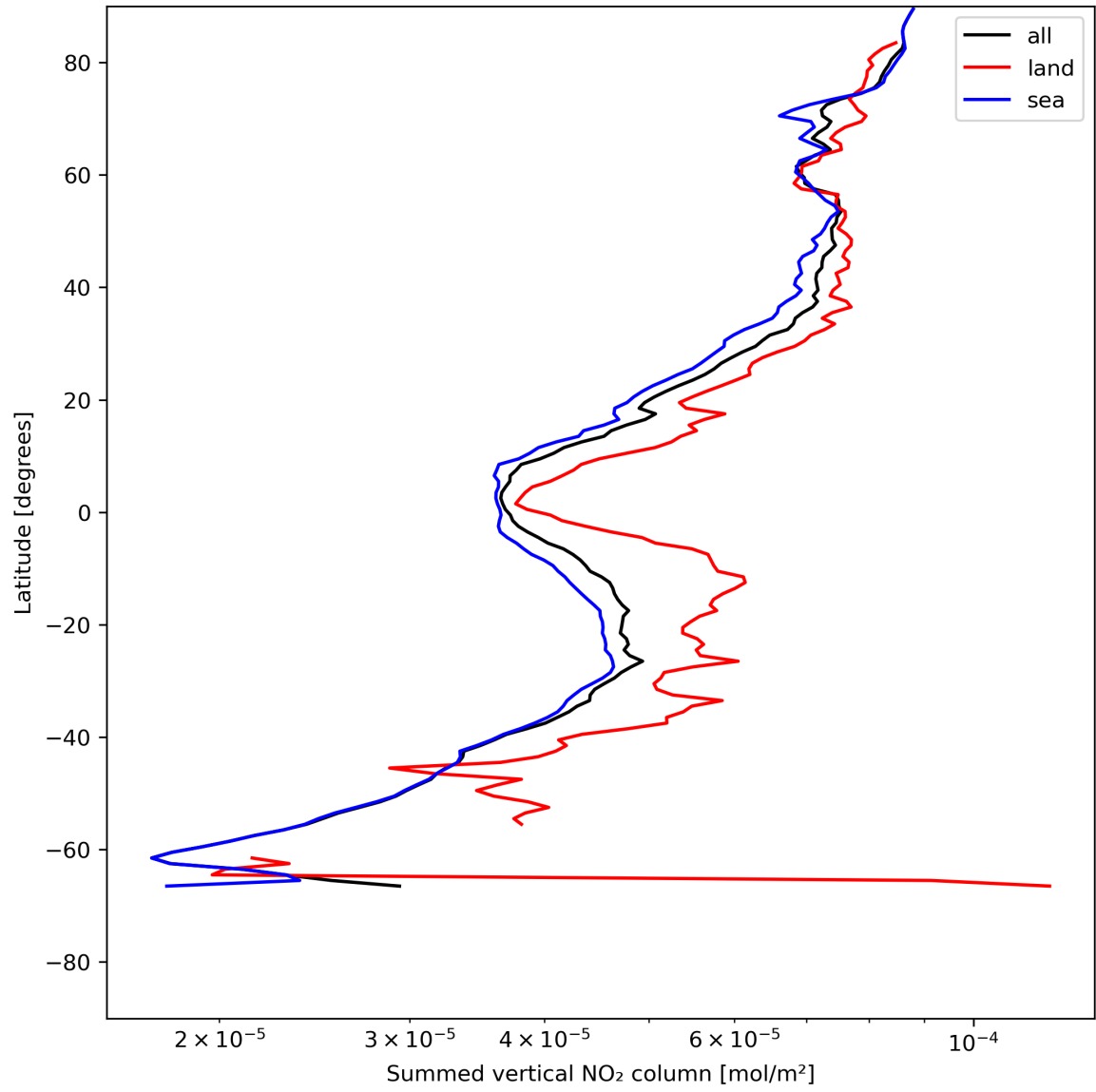
Figure 23: Zonal average of “Summed vertical NO 2 column” for 2024-07-17 to 2024-07-19.
