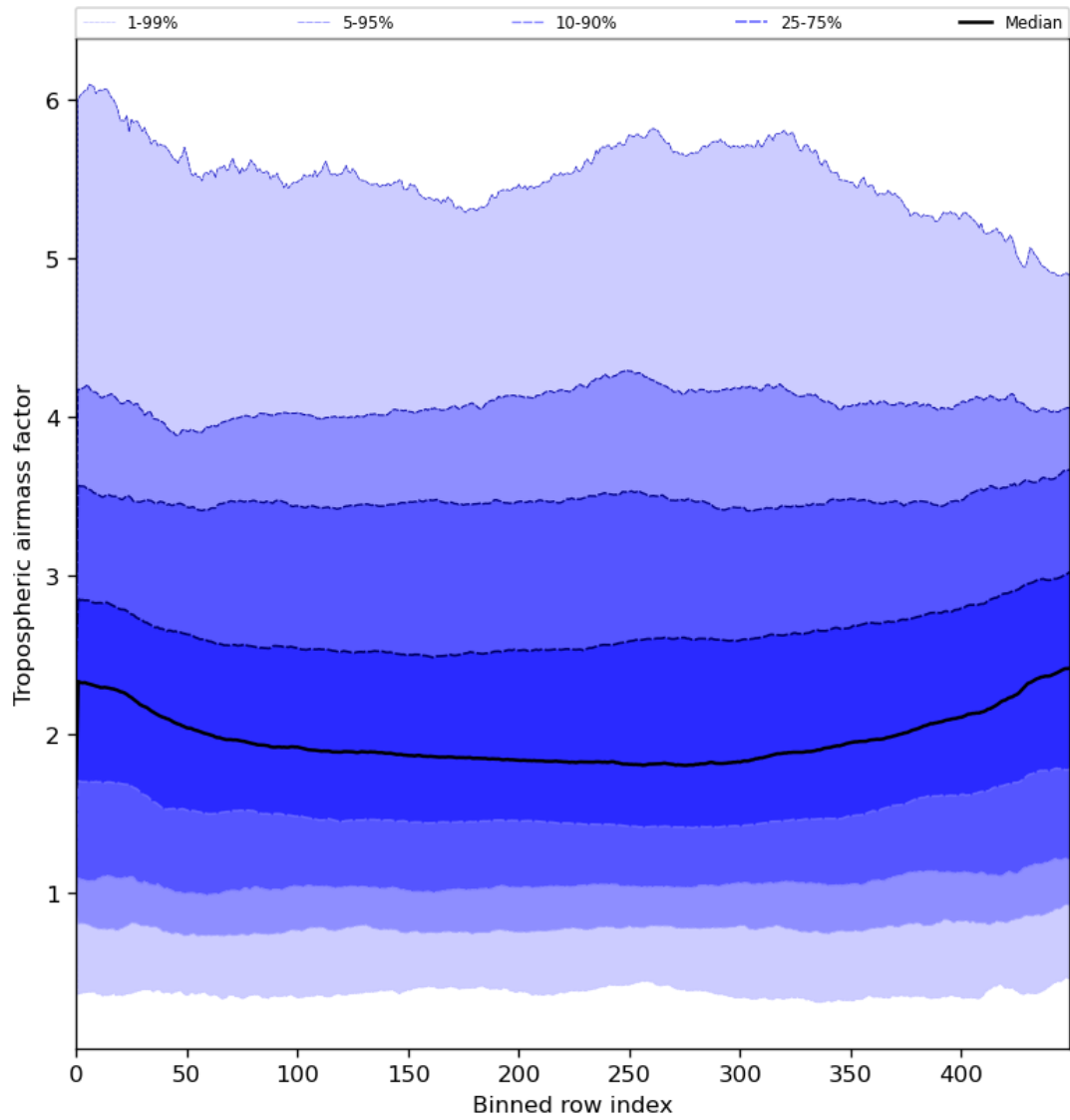
Figure 48: Along track statistics of “Tropospheric airmass factor” for 2024-07-17 to 2024-07-19
