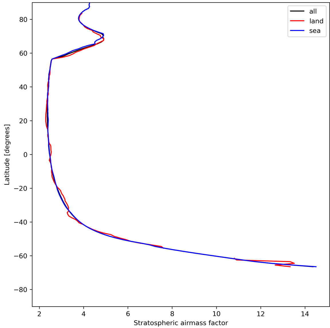
Figure 27: Zonal average of “Stratospheric airmass factor” for 2024-07-17 to 2024-07-19.
