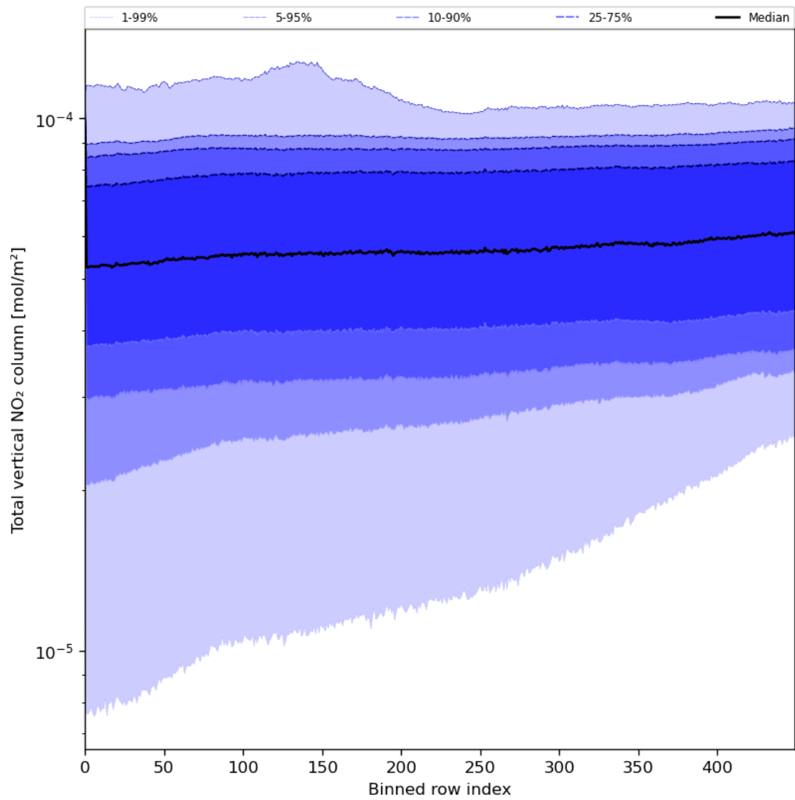
Figure 55: Along track statistics of “Total vertical NO 2 column” for 2024-07-17 to 2024-07-19
