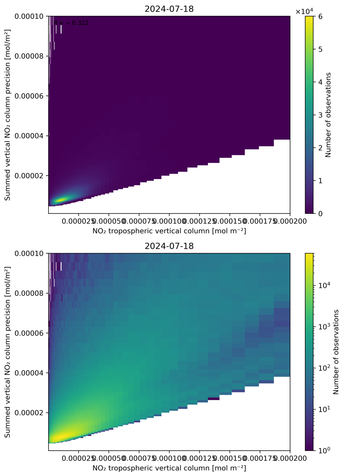
Figure 127: Scatter density plot of “NO 2 tropospheric vertical column” against “Summed vertical NO 2 column precision” for 2024-07-17 to 2024-07-19.
