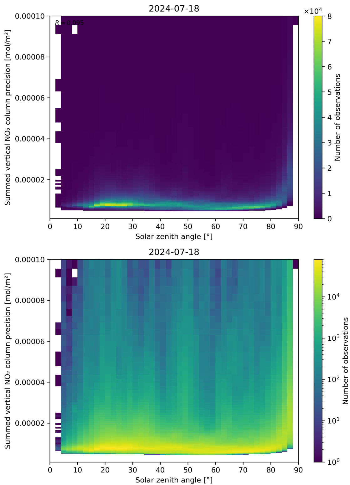
Figure 152: Scatter density plot of “Solar zenith angle” against “Summed vertical NO 2 column precision” for 2024-07-17 to 2024-07-19.
