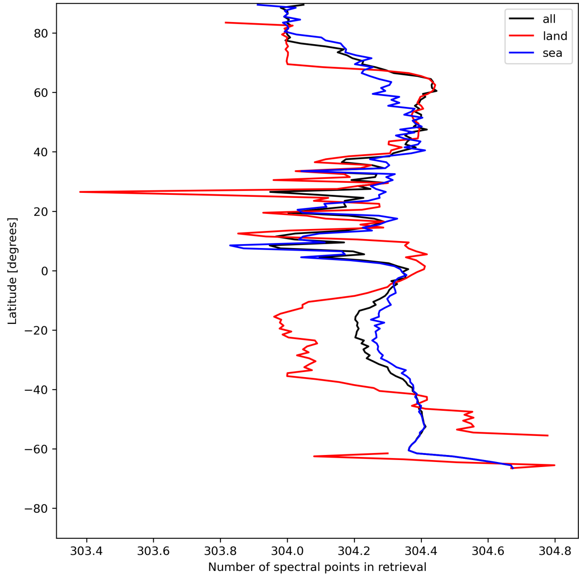
Figure 16: Zonal average of “Number of spectral points in retrieval” for 2024-07-17 to 2024-07-19.
