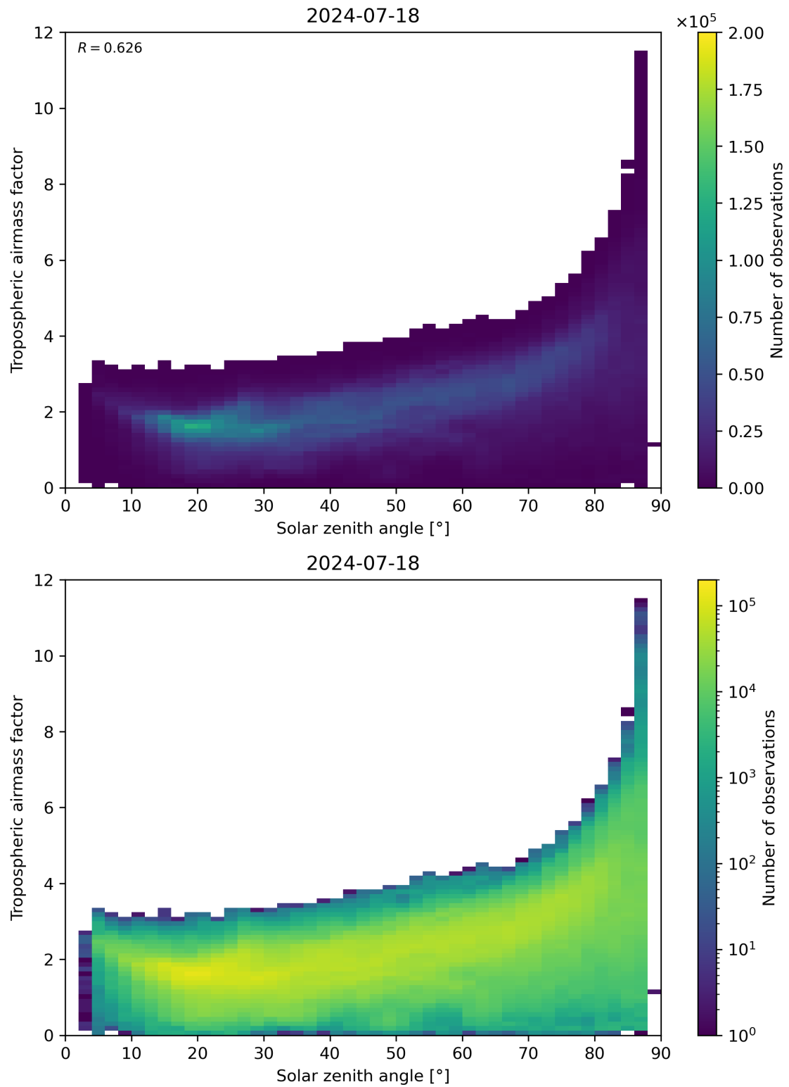
Figure 147: Scatter density plot of “Solar zenith angle” against “Tropospheric airmass factor” for 2024-07-17 to 2024-07-19.
