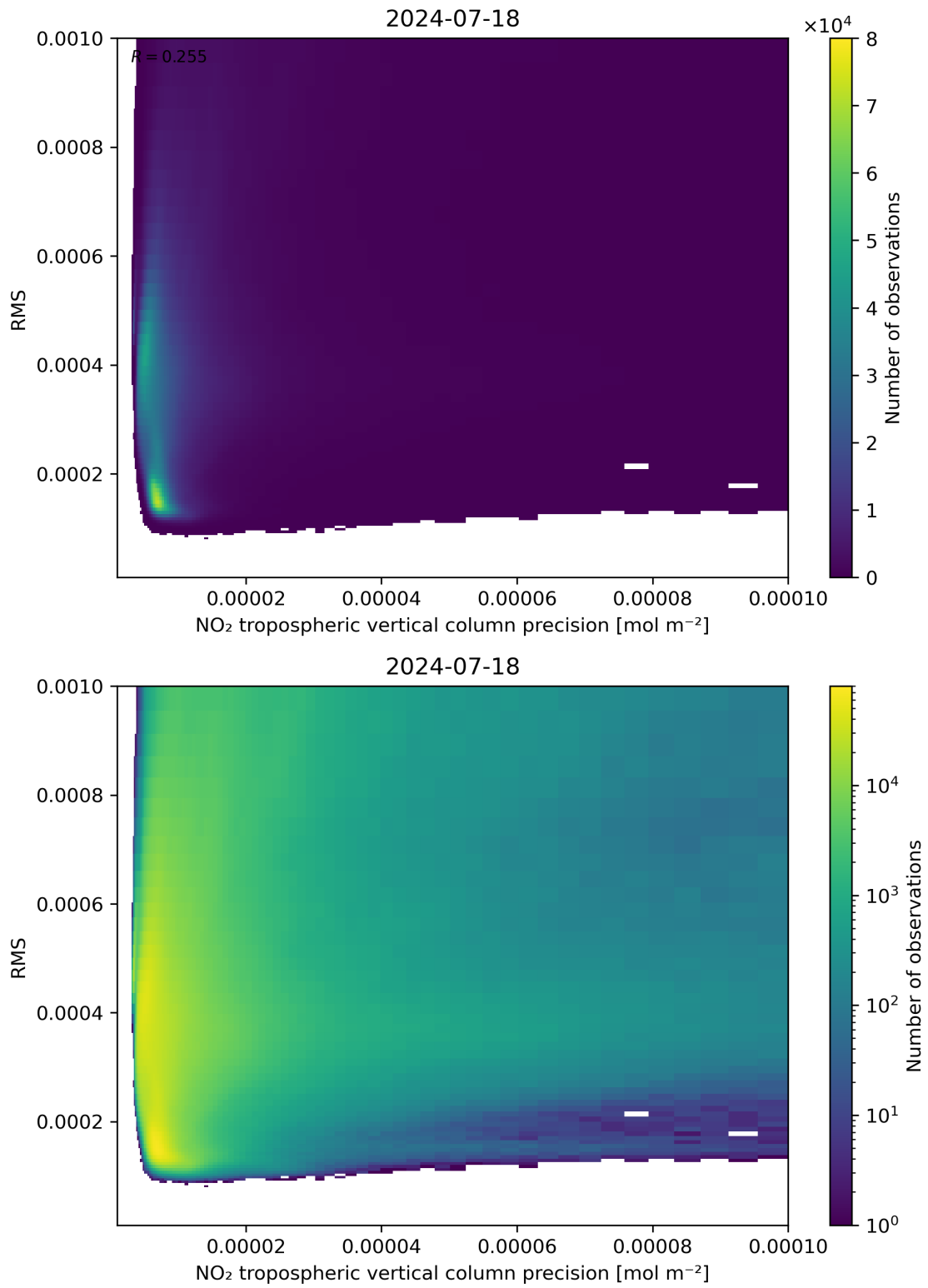
Figure 140: Scatter density plot of “NO 2 tropospheric vertical column precision” against “RMS” for 2024-07-17 to 2024-07-19.
