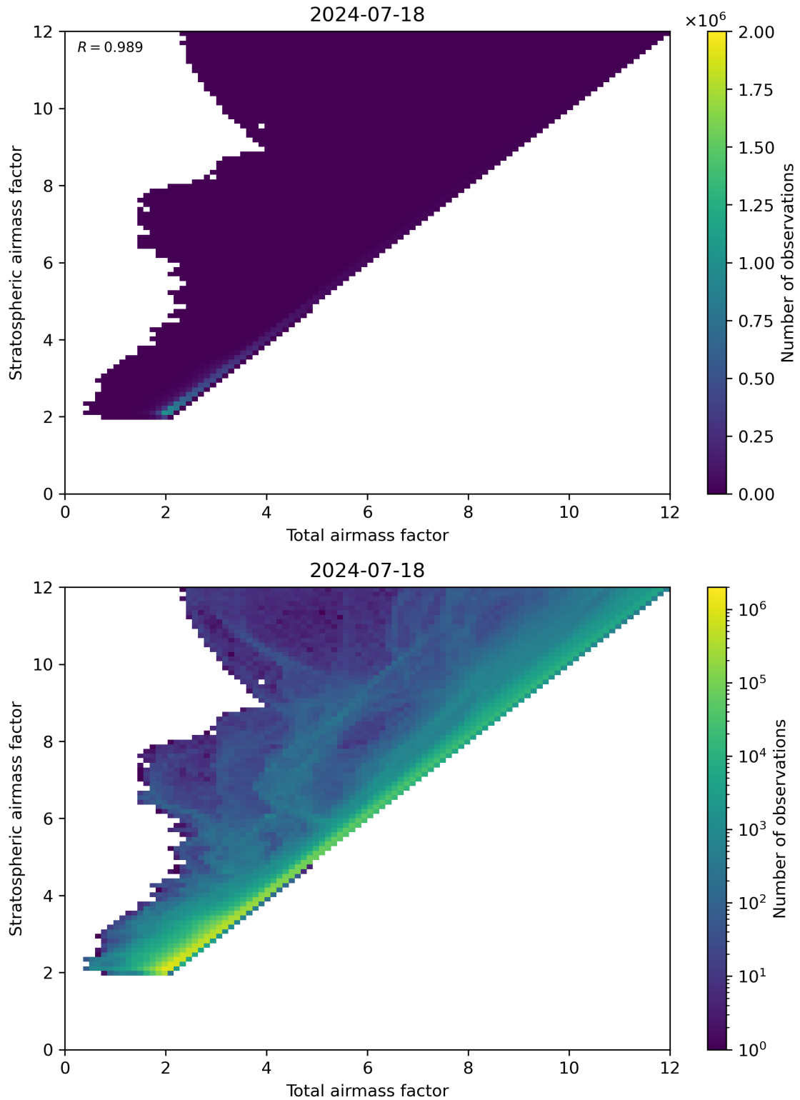
Figure 62: Scatter density plot of “Total airmass factor” against “Stratospheric airmass factor” for 2024-07-17 to 2024-07-19.
