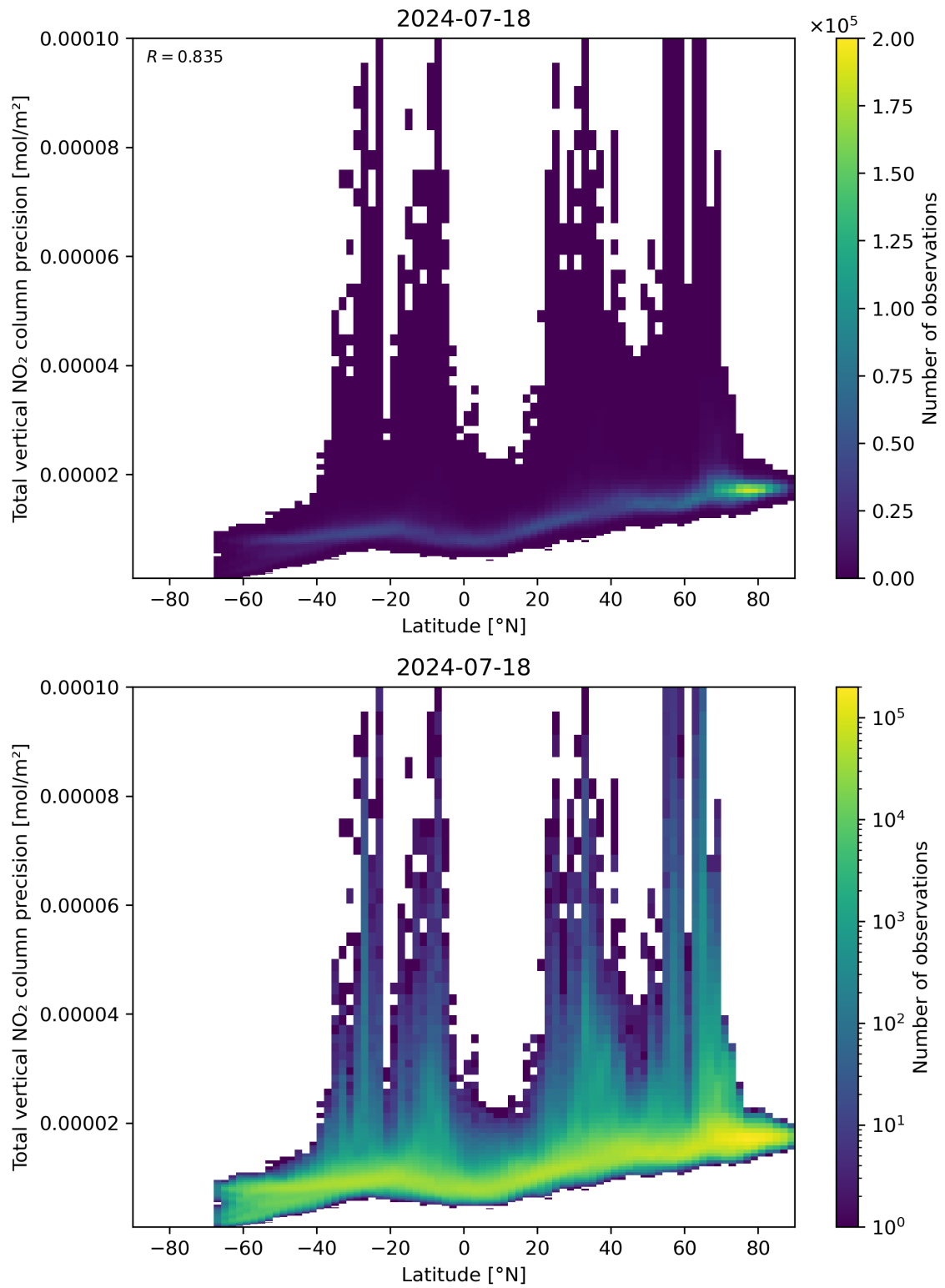
Figure 91: Scatter density plot of “Latitude” against “Total vertical NO 2 column precision” for 2024-07-17 to 2024-07-19.
