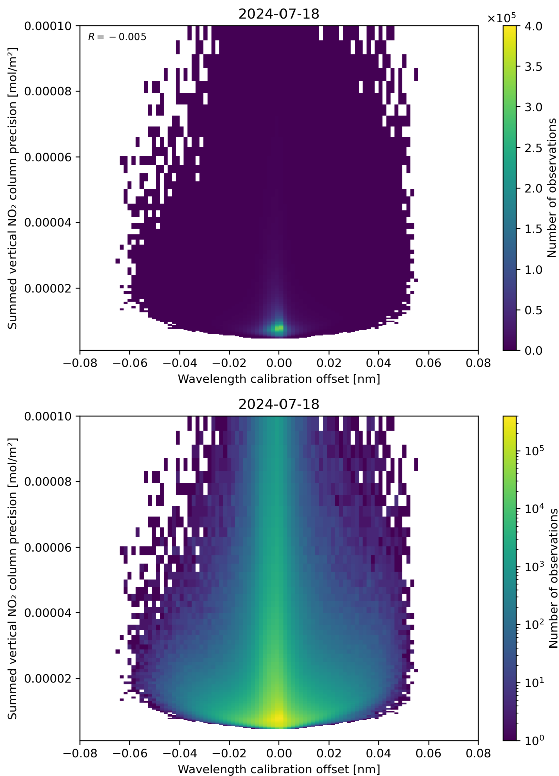
Figure 178: Scatter density plot of “Wavelength calibration offset” against “Summed vertical NO 2 column precision” for 2024-07-17 to 2024-07-19.
