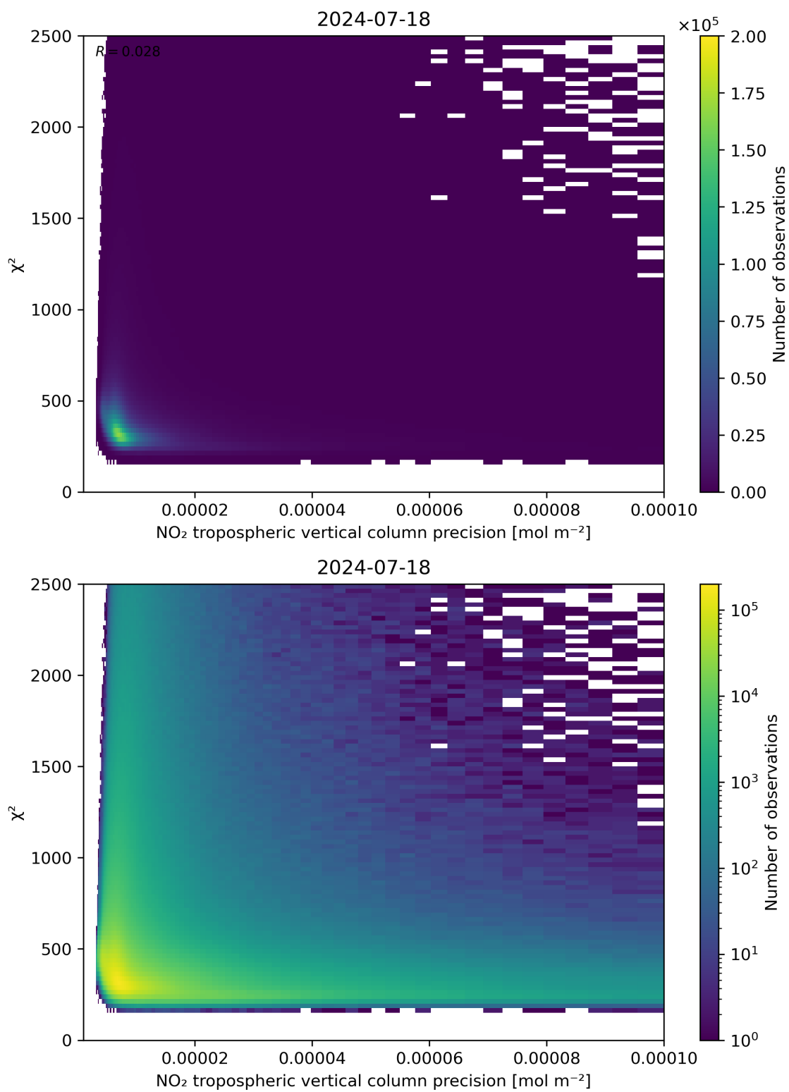
Figure 134: Scatter density plot of “NO 2 tropospheric vertical column precision” against “ \chi^2 ” for 2024-07-17 to 2024-07-19.
