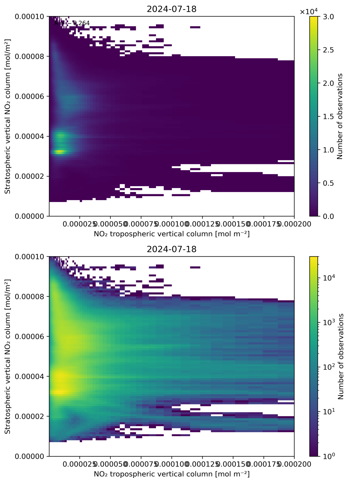
Figure 125: Scatter density plot of “NO 2 tropospheric vertical column” against “Stratospheric vertical NO 2 column” for 2024-07-17 to 2024-07-19.
