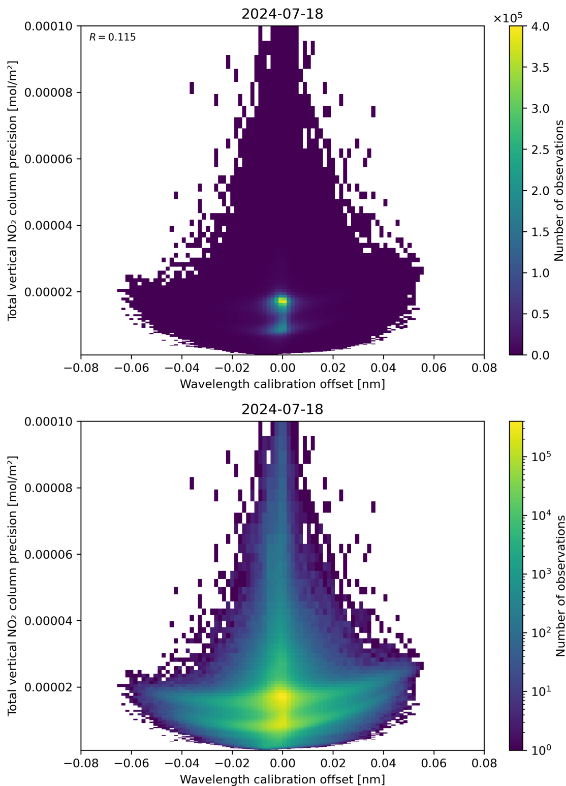
Figure 180: Scatter density plot of “Wavelength calibration offset” against “Total vertical NO 2 column precision” for 2024-07-17 to 2024-07-19.
