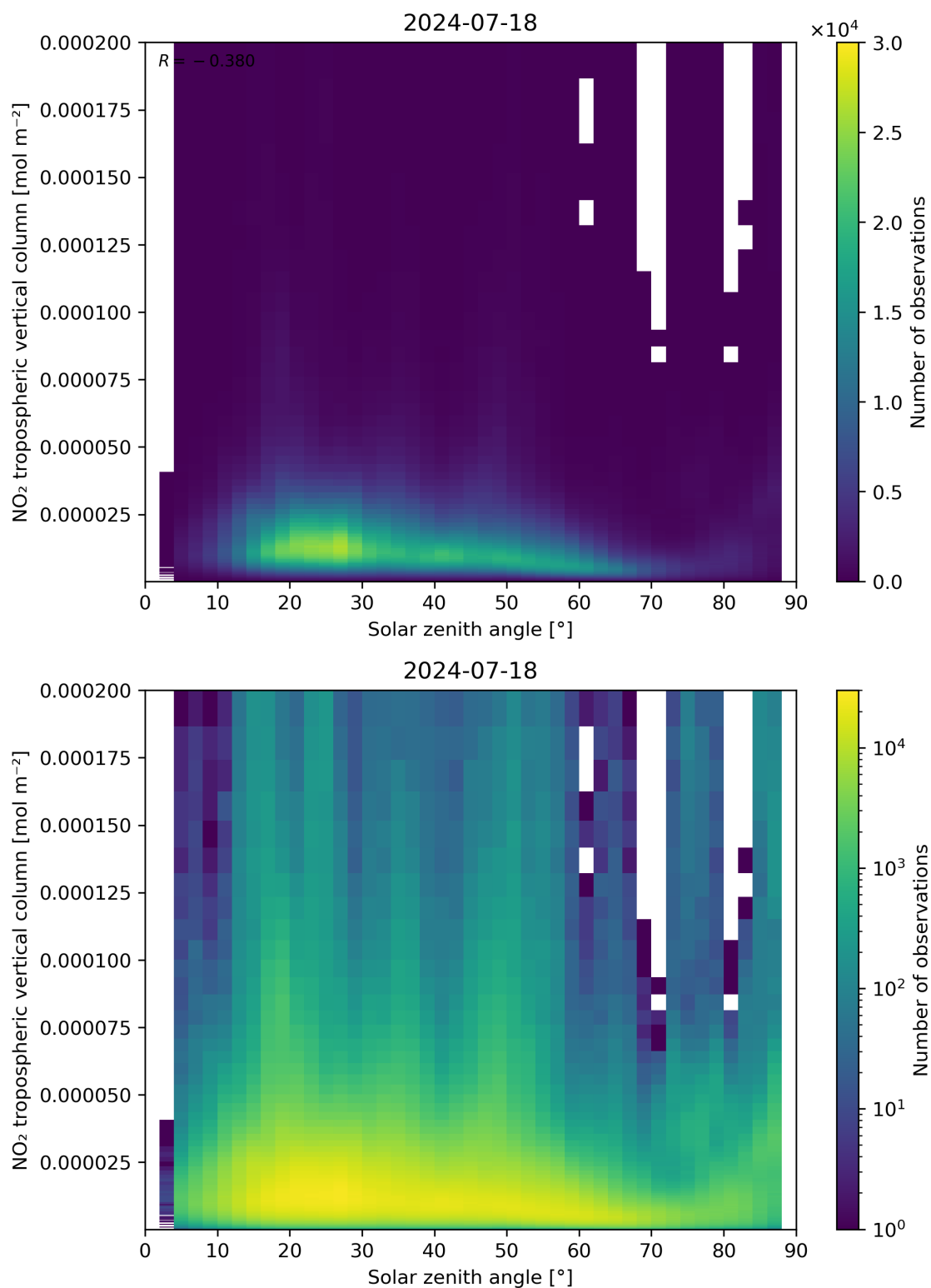
Figure 155: Scatter density plot of “Solar zenith angle” against “NO 2 tropospheric vertical column” for 2024-07-17 to 2024-07-19.
