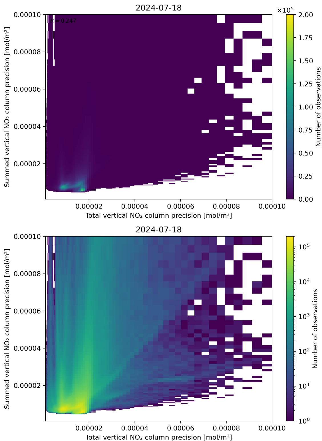
Figure 118: Scatter density plot of “Total vertical NO 2 column precision” against “Summed vertical NO 2 column precision” for 2024-07-17 to 2024-07-19.
