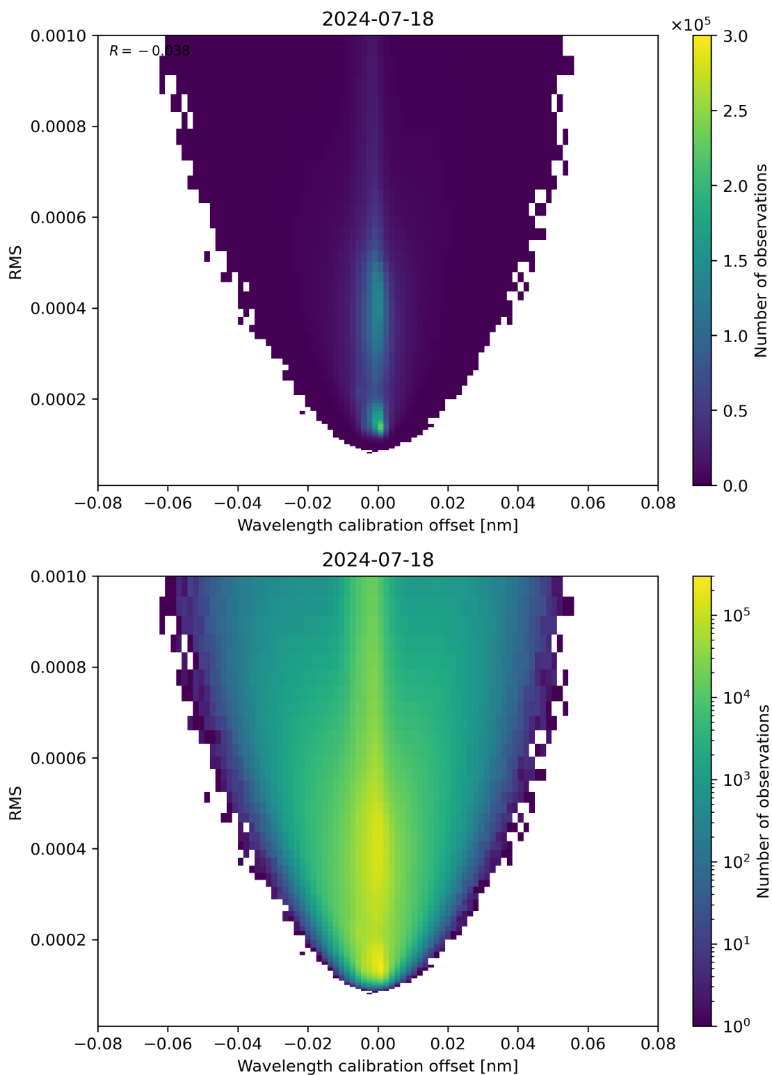
Figure 181: Scatter density plot of “Wavelength calibration offset” against “RMS” for 2024-07-17 to 2024-07-19.
