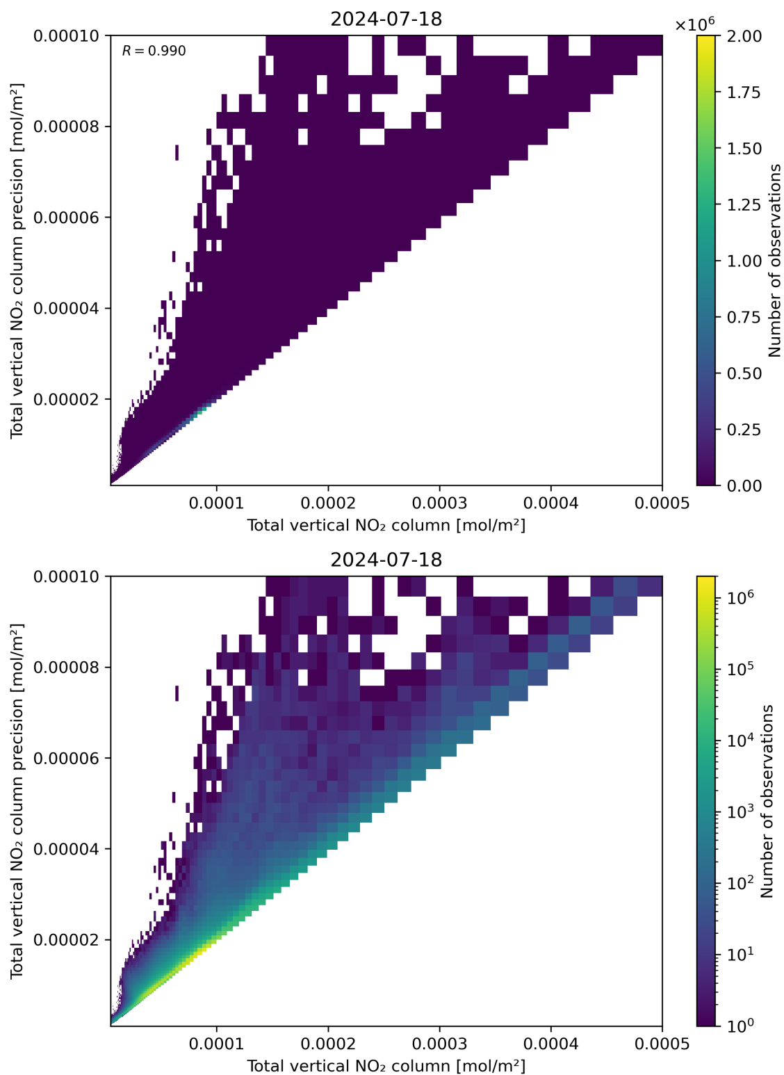
Figure 114: Scatter density plot of “Total vertical NO 2 column” against “Total vertical NO 2 column precision” for 2024-07-17 to 2024-07-19.
