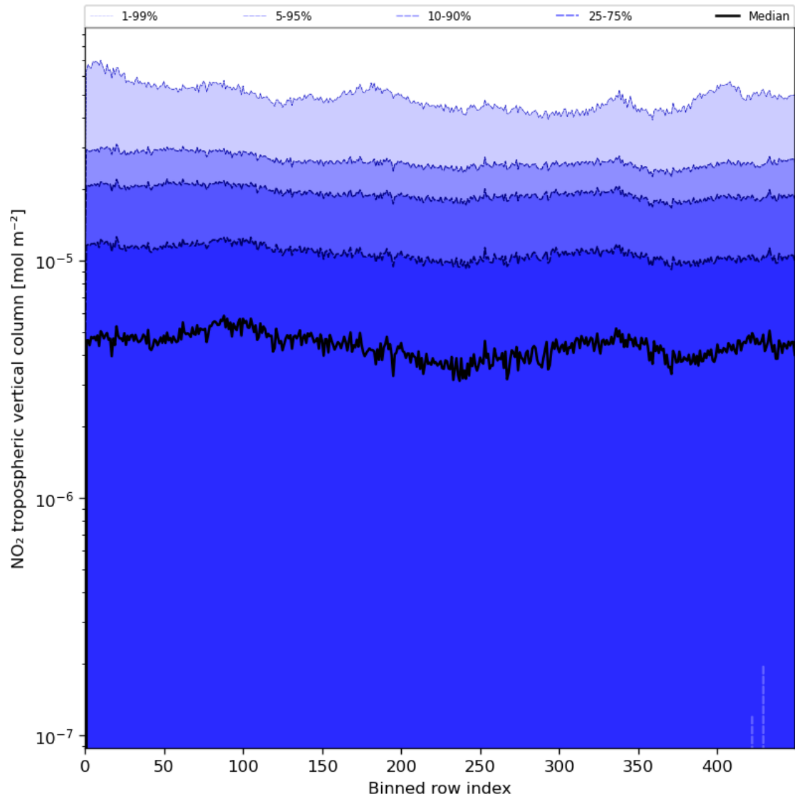
Figure 46: Along track statistics of “NO 2 tropospheric vertical column” for 2024-07-17 to 2024-07-19
