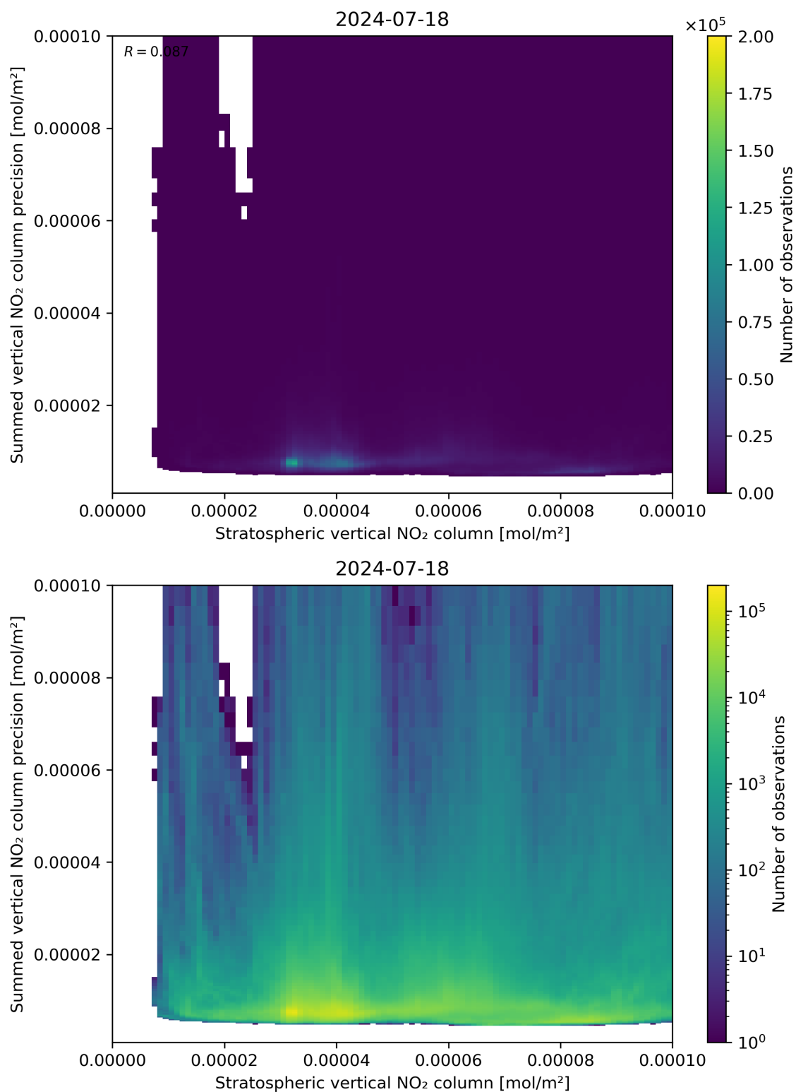
Figure 99: Scatter density plot of “Stratospheric vertical NO 2 column” against “Summed vertical NO 2 column precision” for 2024-07-17 to 2024-07-19.
