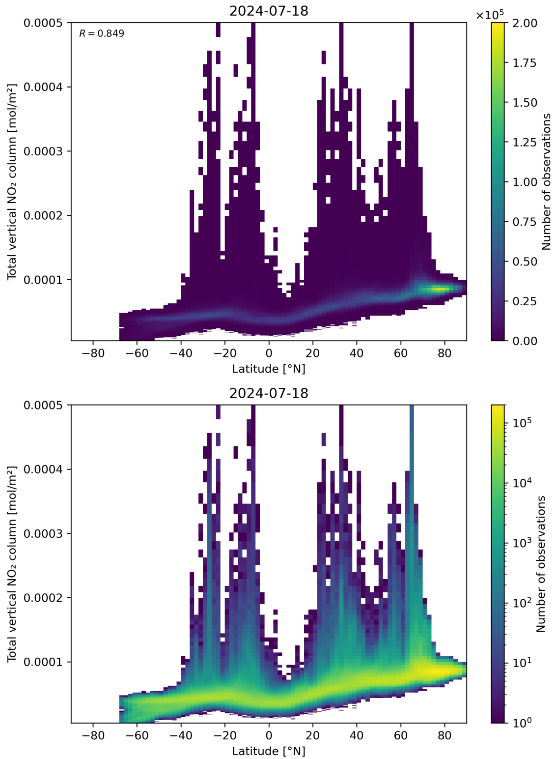
Figure 90: Scatter density plot of “Latitude” against “Total vertical NO 2 column” for 2024-07-17 to 2024-07-19.
