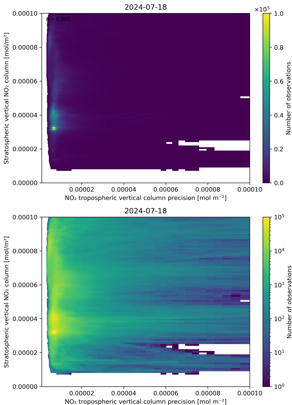
Figure 135: Scatter density plot of “NO 2 tropospheric vertical column precision” against “Stratospheric vertical NO 2 column” for 2024-07-17 to 2024-07-19.
