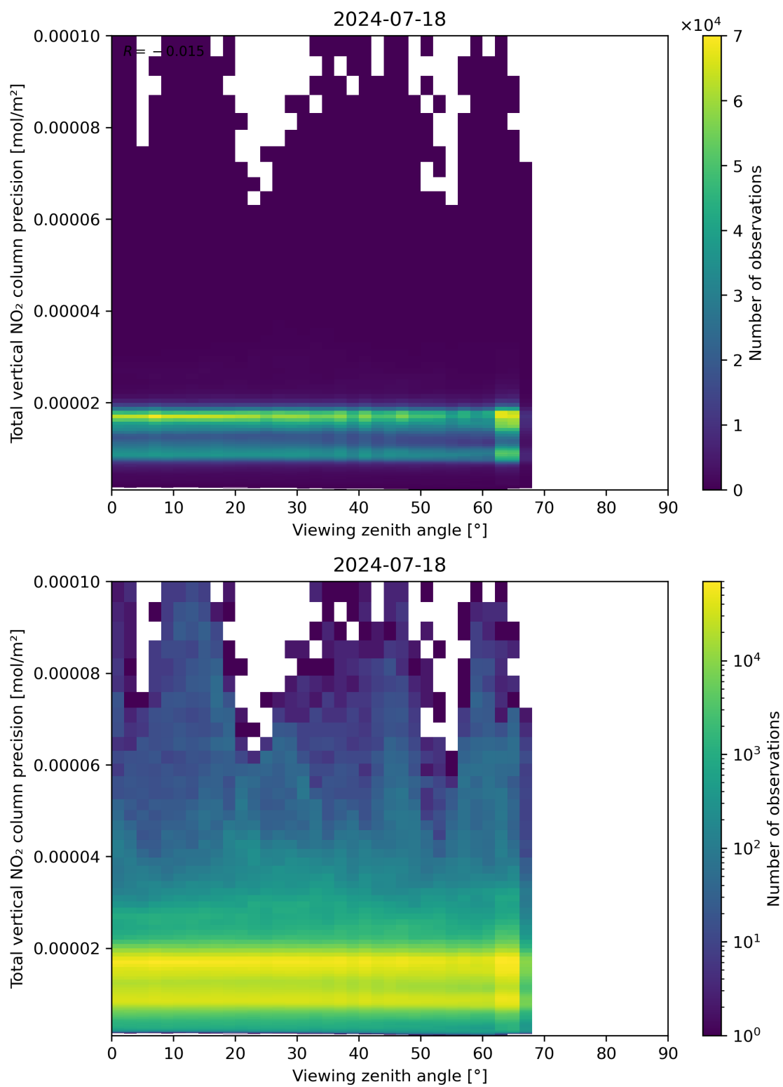
Figure 168: Scatter density plot of “Viewing zenith angle” against “Total vertical NO 2 column precision” for 2024-07-17 to 2024-07-19.
