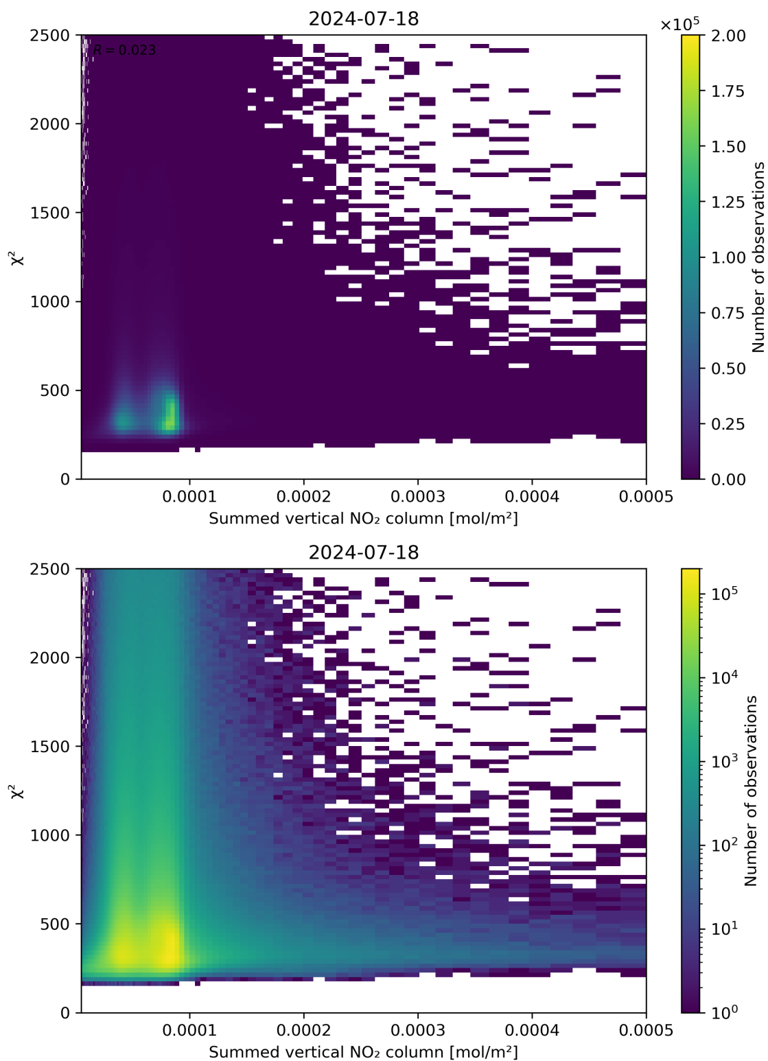
Figure 104: Scatter density plot of “Summed vertical NO 2 column” against “ \chi^2 ” for 2024-07-17 to 2024-07-19.
