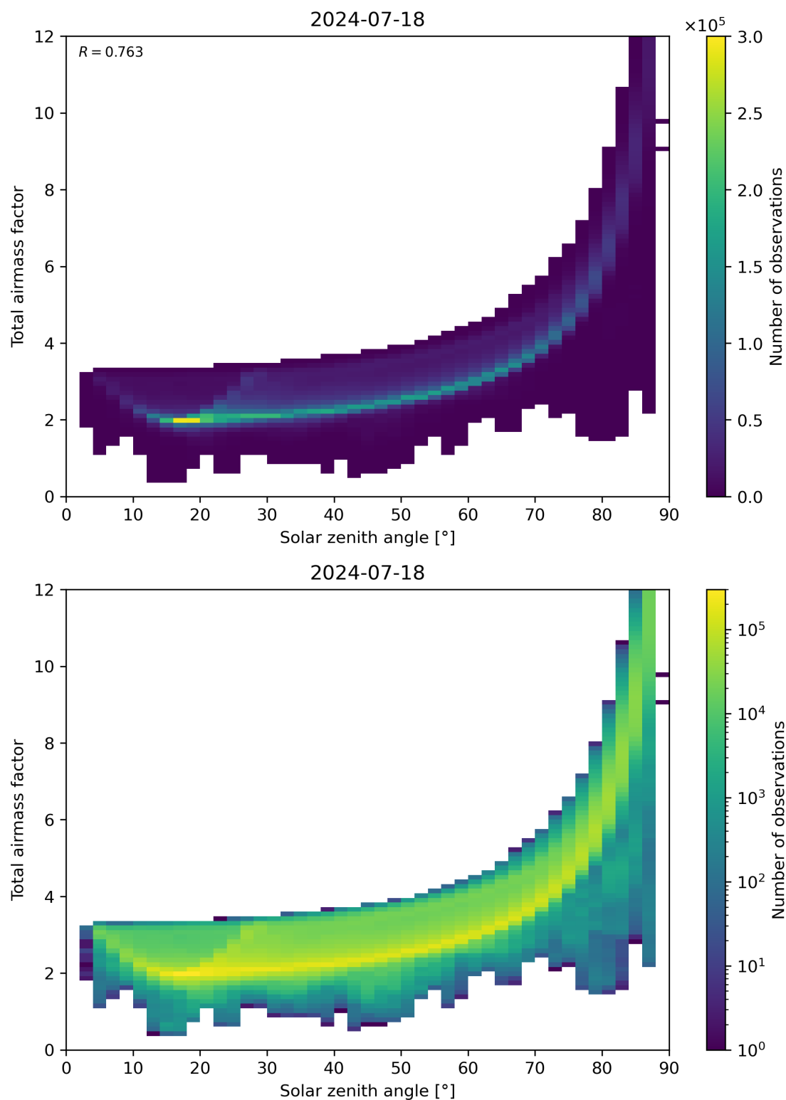
Figure 146: Scatter density plot of “Solar zenith angle” against “Total air mass factor” for 2024-07-17 to 2024-07-19.
