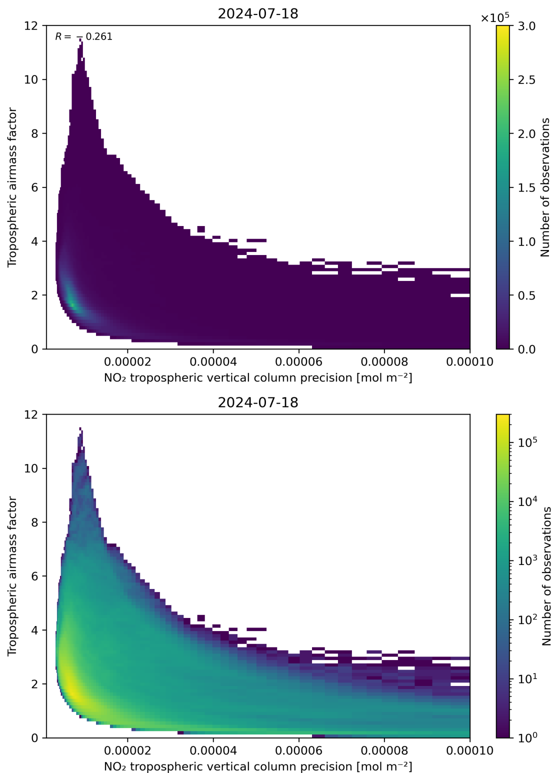
Figure 133: Scatter density plot of “NO 2 tropospheric vertical column precision” against “Tropospheric airmass factor” for 2024-07-17 to 2024-07-19.
