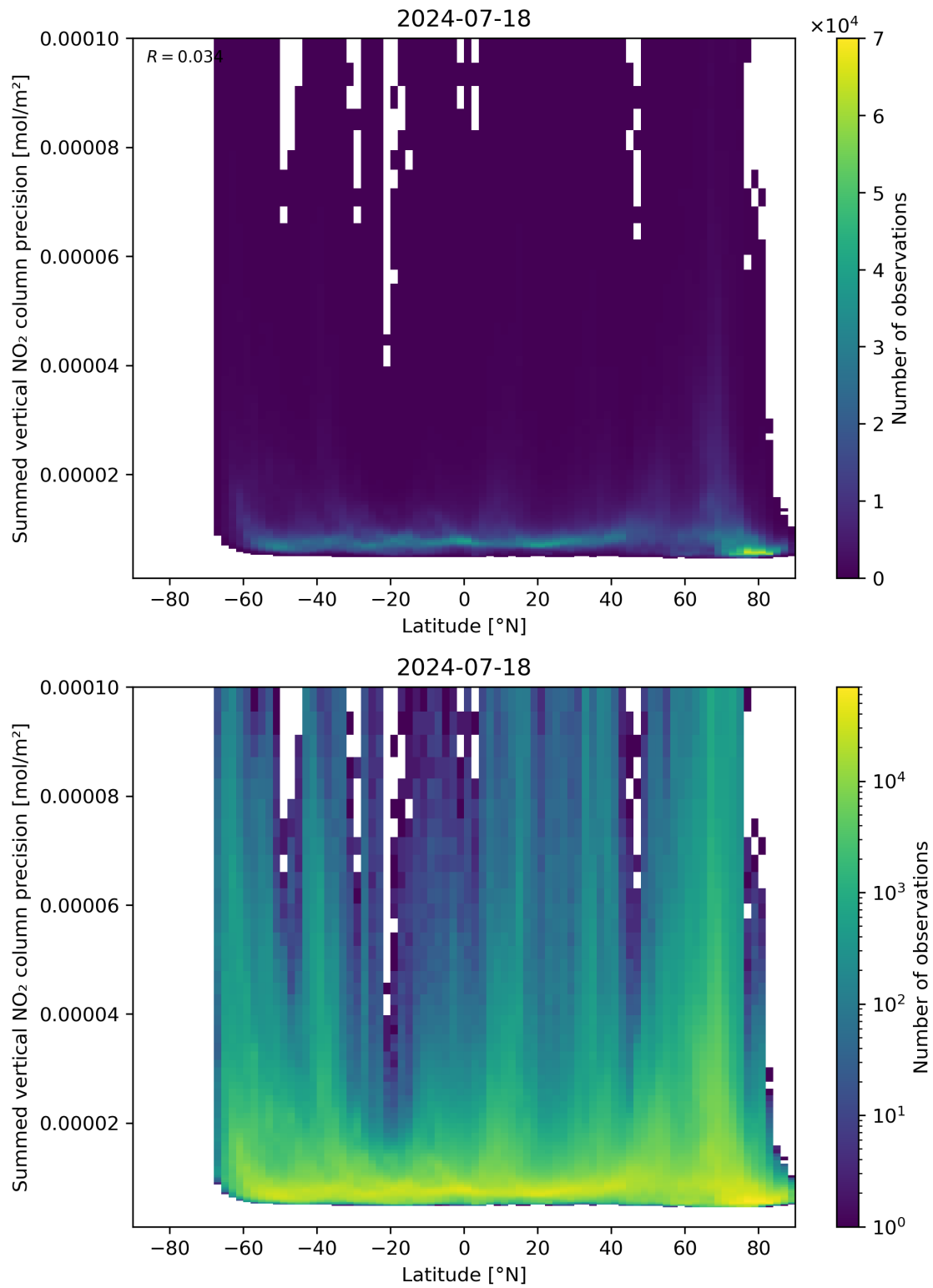
Figure 89: Scatter density plot of “Latitude” against “Summed vertical NO 2 column precision” for 2024-07-17 to 2024-07-19.
