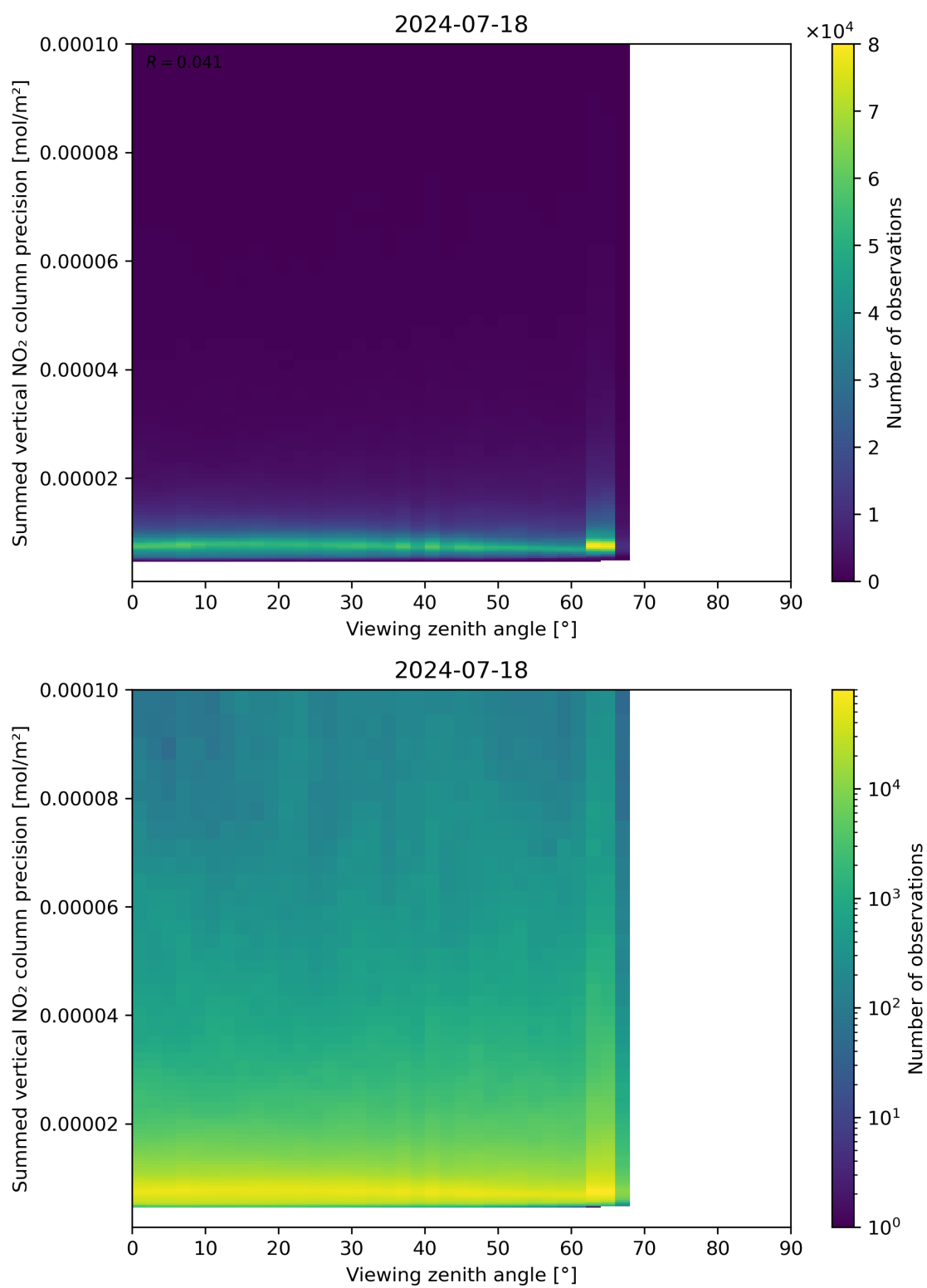
Figure 166: Scatter density plot of “Viewing zenith angle” against “Summed vertical NO 2 column precision” for 2024-07-17 to 2024-07-19.
