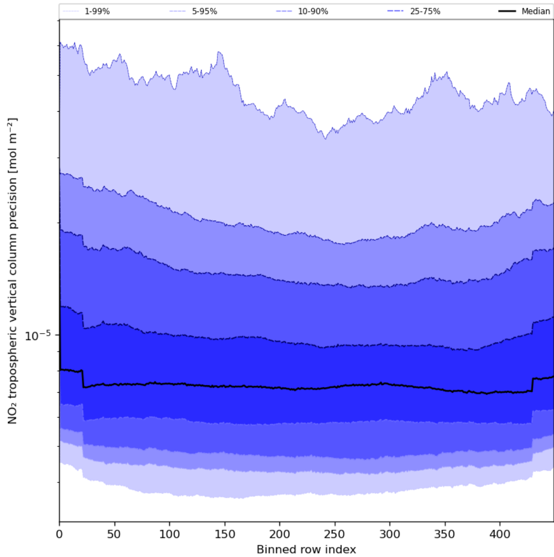
Figure 47: Along track statistics of “NO 2 tropospheric vertical column precision” for 2024-07-17 to 2024-07-19
