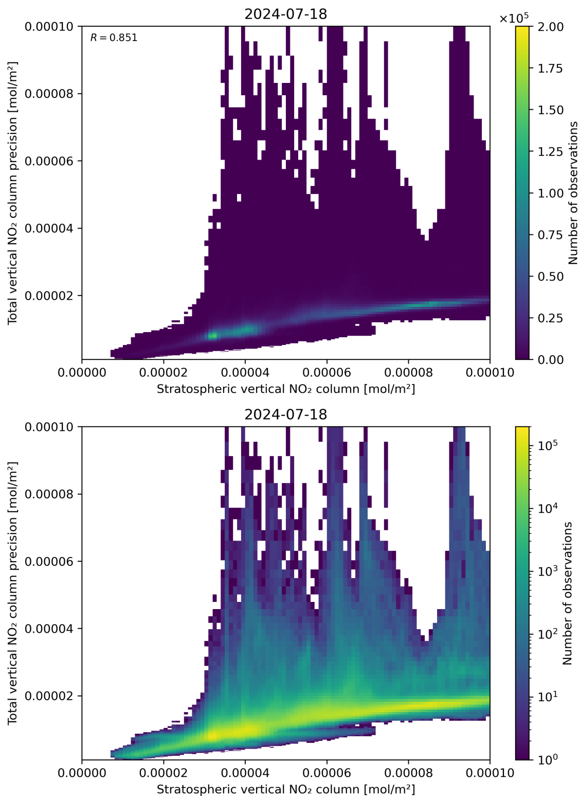
Figure 101: Scatter density plot of “Stratospheric vertical NO 2 column” against “Total vertical NO 2 column precision” for 2024-07-17 to 2024-07-19.
