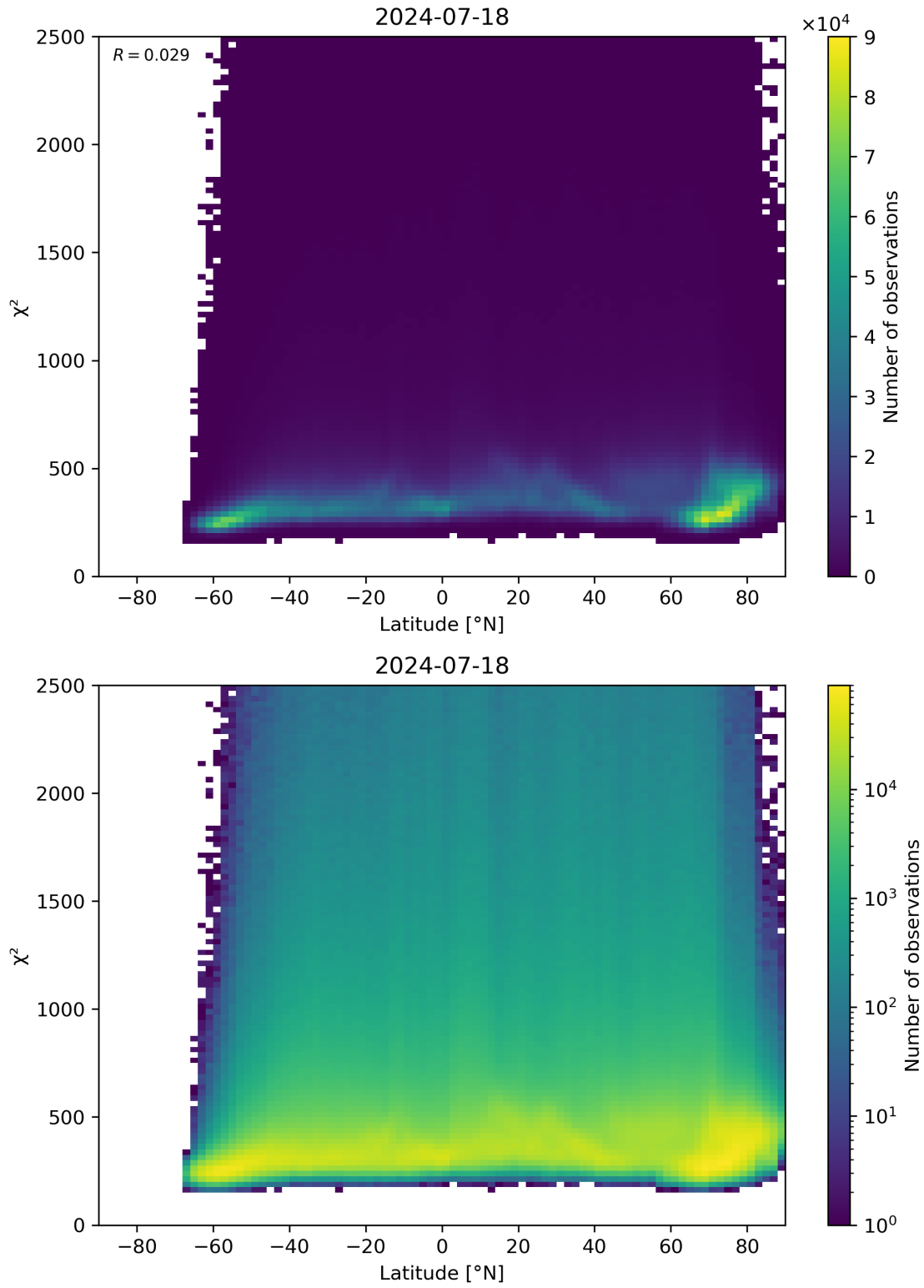
Figure 86: Scatter density plot of “Latitude” against “ \chi^2 ” for 2024-07-17 to 2024-07-19.
