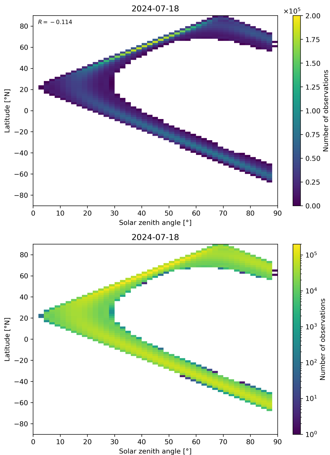
Figure 149: Scatter density plot of “Solar zenith angle” against “Latitude” for 2024-07-17 to 2024-07-19.
