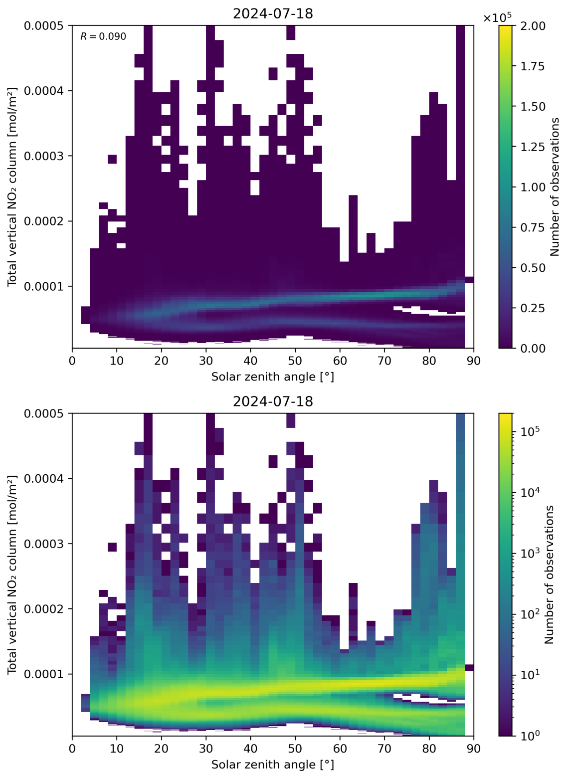
Figure 153: Scatter density plot of “Solar zenith angle” against “Total vertical NO 2 column” for 2024-07-17 to 2024-07-19.
