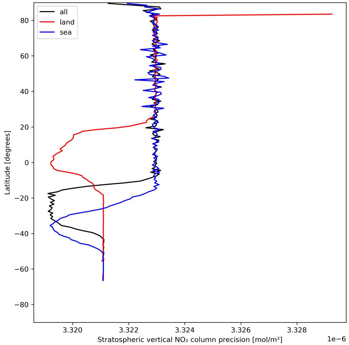
Figure 20: Zonal average of “Stratospheric vertical NO 2 column precision” for 2024-07-17 to 2024-07-19.
