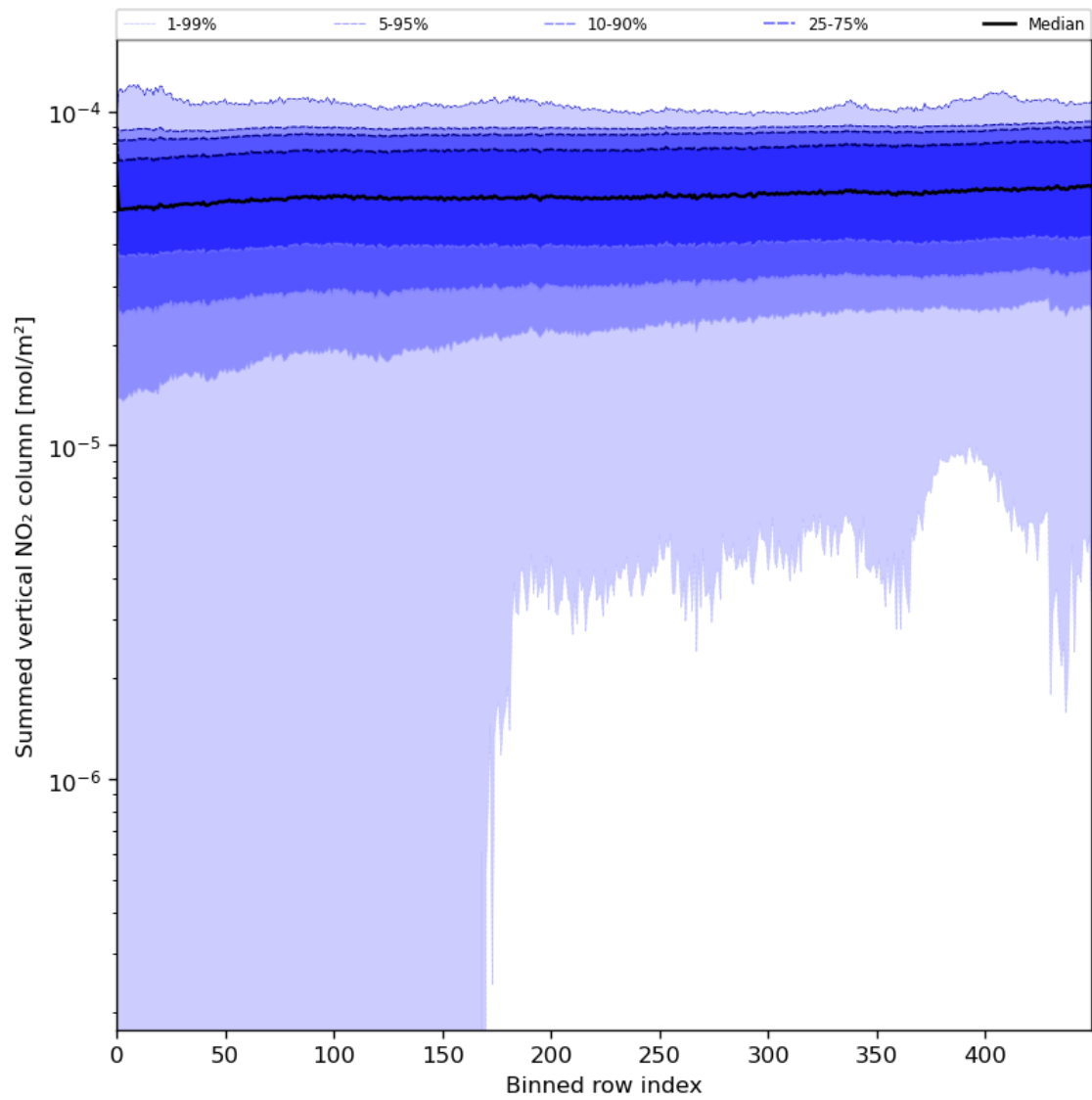
Figure 57: Along track statistics of “Summed vertical NO 2 column” for 2024-07-17 to 2024-07-19
