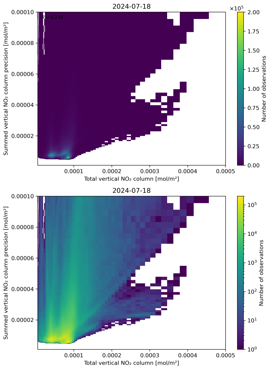
Figure 113: Scatter density plot of “Total vertical NO 2 column” against “Summed vertical NO 2 column precision” for 2024-07-17 to 2024-07-19.
