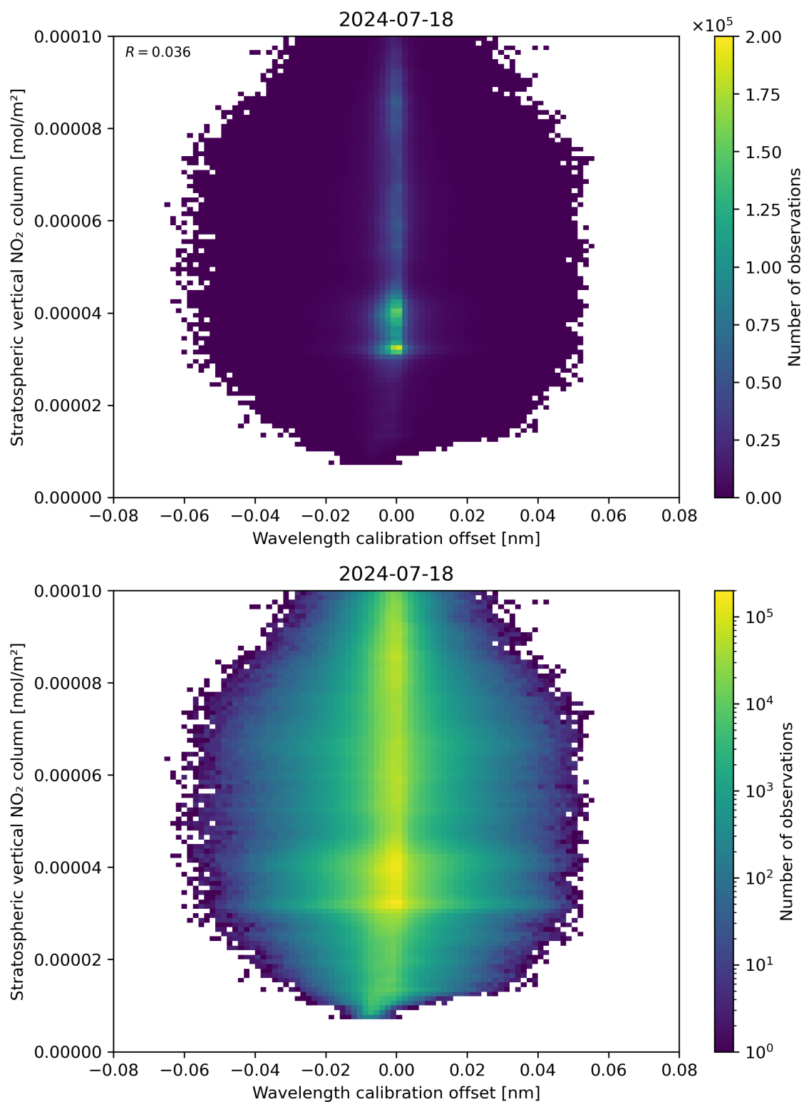
Figure 176: Scatter density plot of “Wavelength calibration offset” against “Stratospheric vertical NO 2 column” for 2024-07-17 to 2024-07-19.
