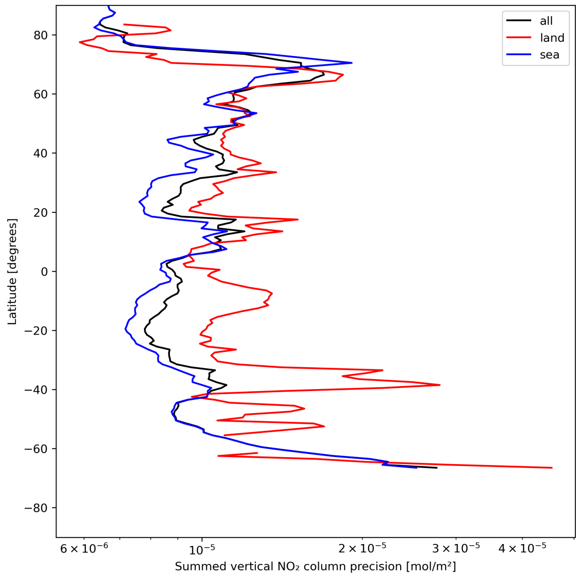
Figure 24: Zonal average of “Summed vertical NO 2 column precision” for 2024-07-17 to 2024-07-19.
