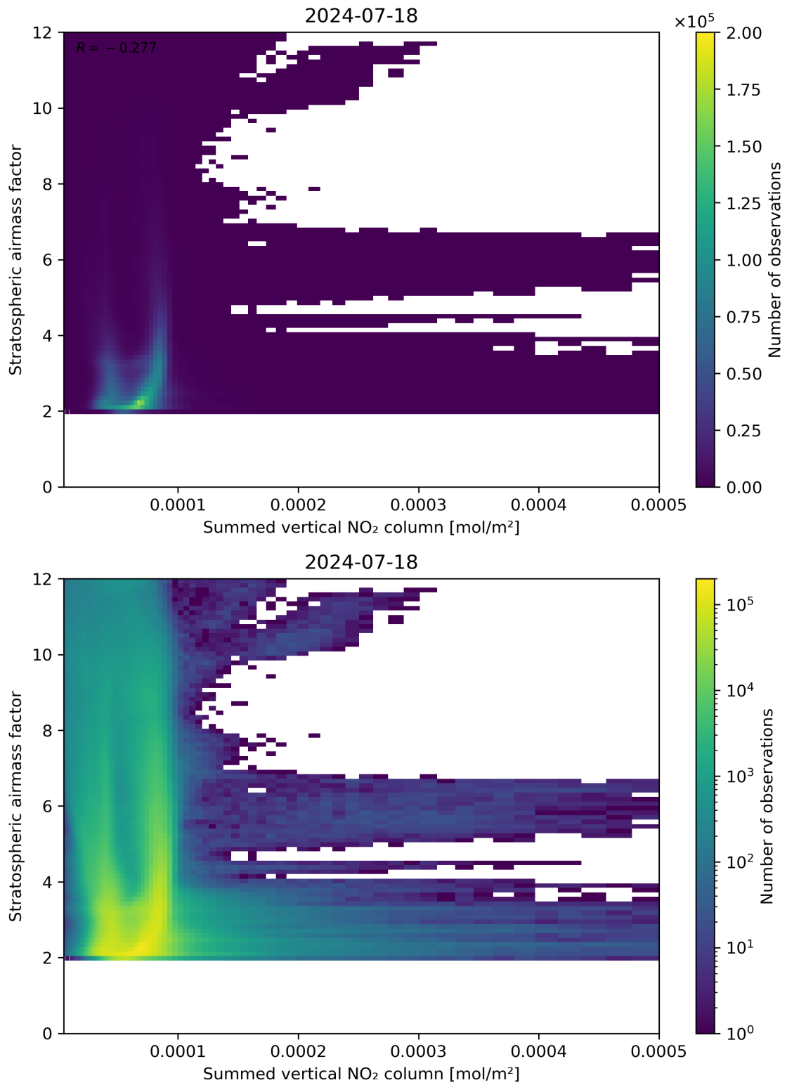
Figure 103: Scatter density plot of “Summed vertical NO 2 column” against “Stratospheric air mass factor” for 2024-07-17 to 2024-07-19.
