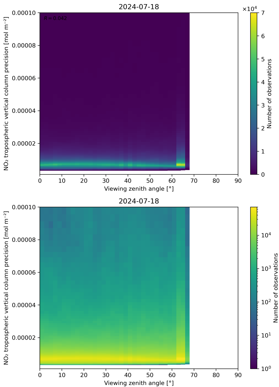
Figure 170: Scatter density plot of “Viewing zenith angle” against “NO 2 tropospheric vertical column precision” for 2024-07-17 to 2024-07-19.
