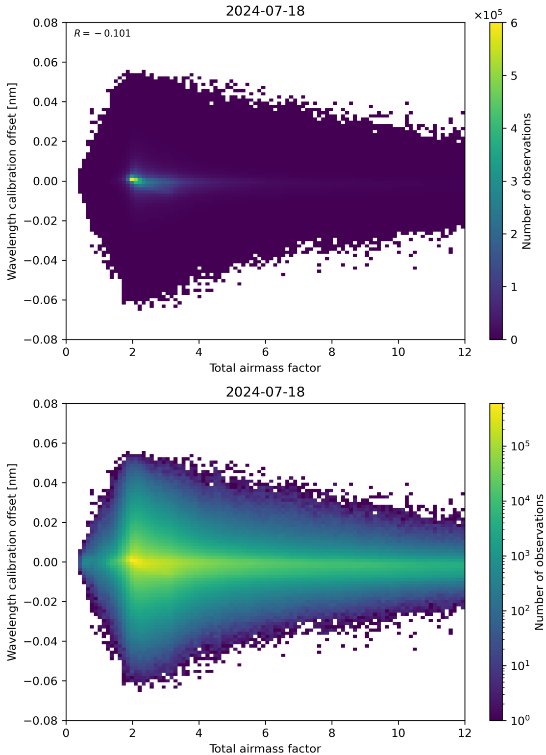
Figure 70: Scatter density plot of “Total airmass factor” against “Wavelength calibration offset” for 2024-07-17 to 2024-07-19.
