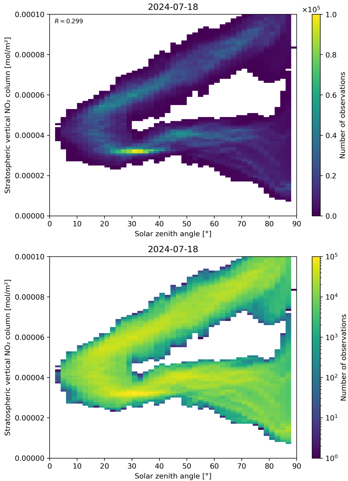
Figure 150: Scatter density plot of “Solar zenith angle” against “Stratospheric vertical NO 2 column” for 2024-07-17 to 2024-07-19.
