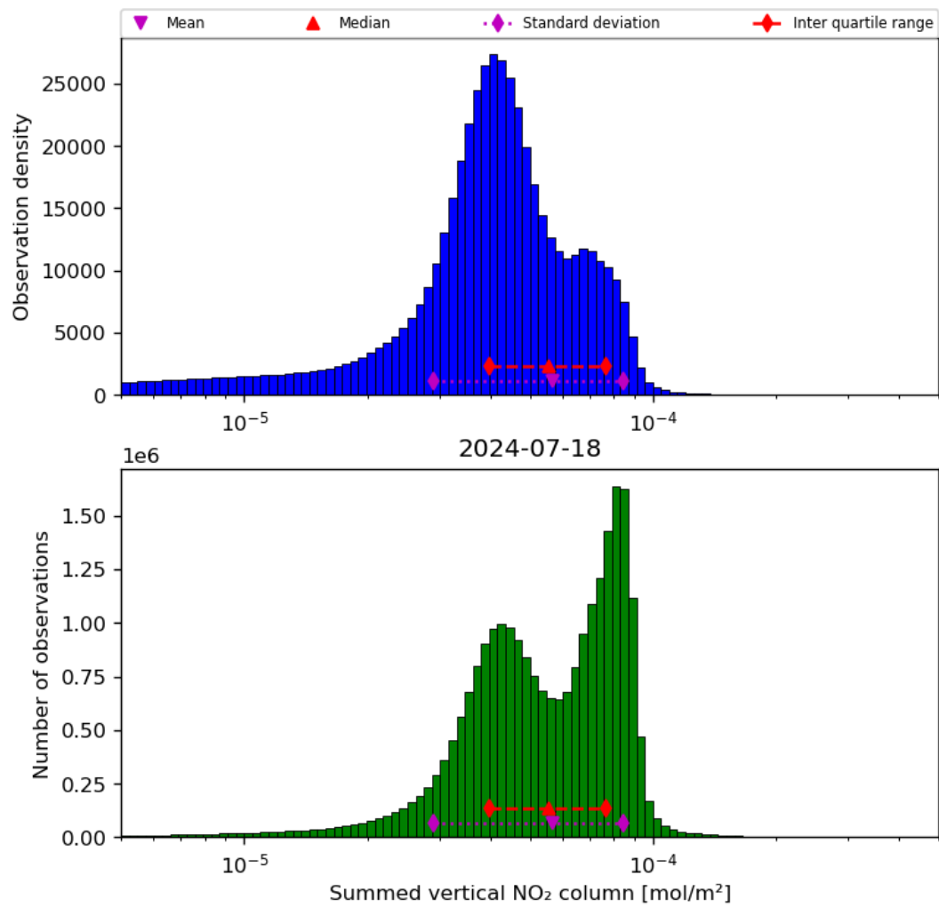
Figure 40: Histogram of “Summed vertical NO 2 column” for 2024-07-17 to 2024-07-19
