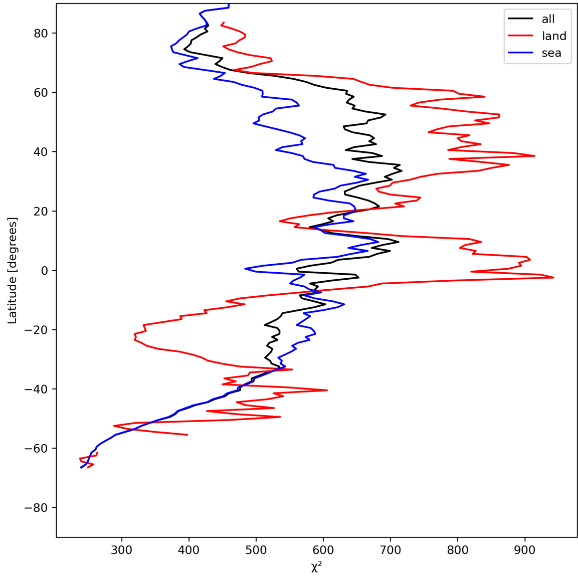
Figure 25: Zonal average of “ \chi^2 ” for 2024-07-17 to 2024-07-19.
