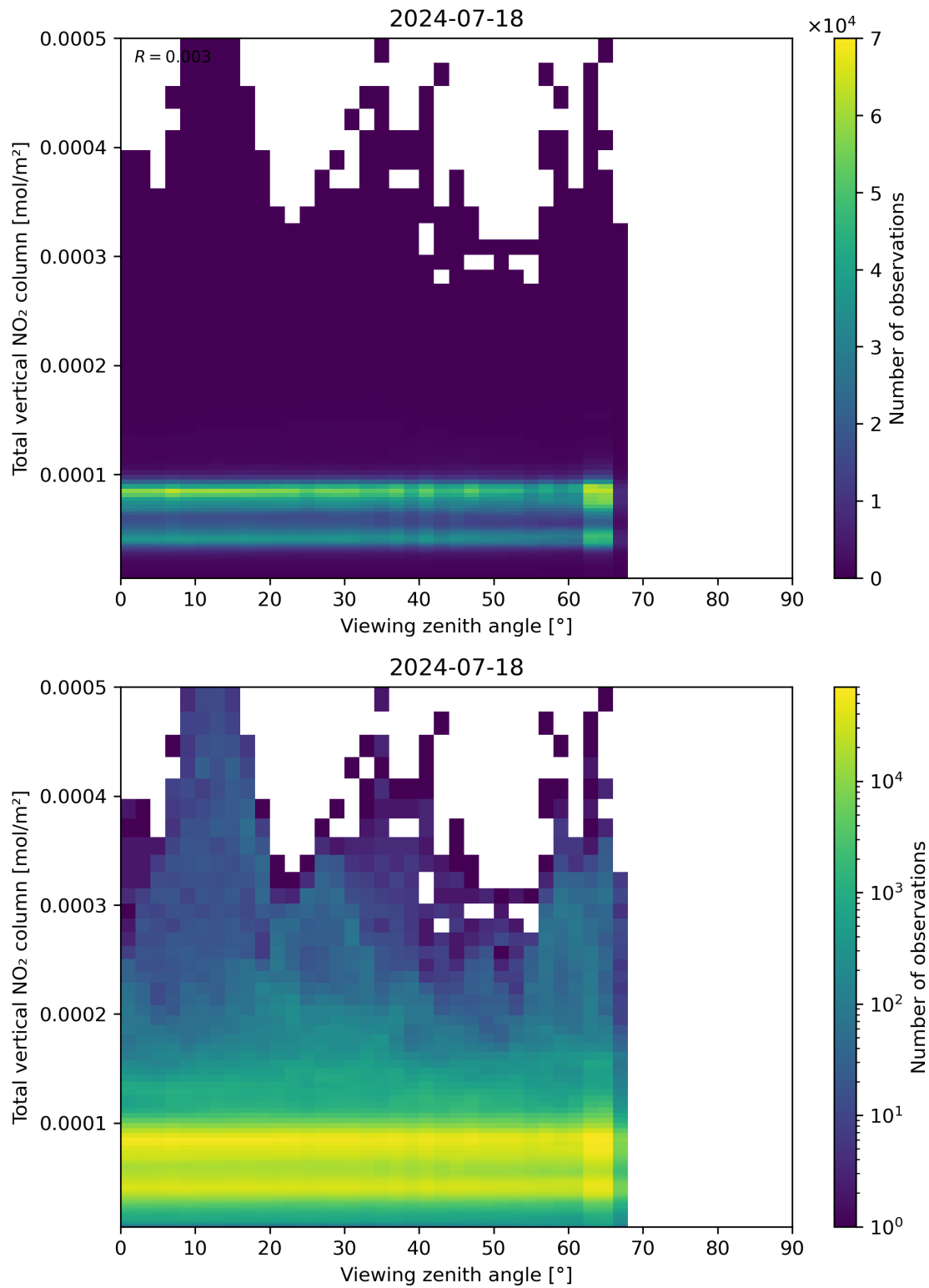
Figure 167: Scatter density plot of “Viewing zenith angle” against “Total vertical NO 2 column” for 2024-07-17 to 2024-07-19.
