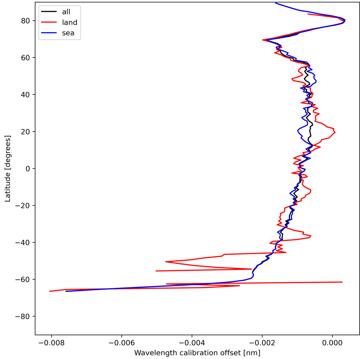
Figure 18: Zonal average of “Wavelength calibration offset” for 2024-07-17 to 2024-07-19.
