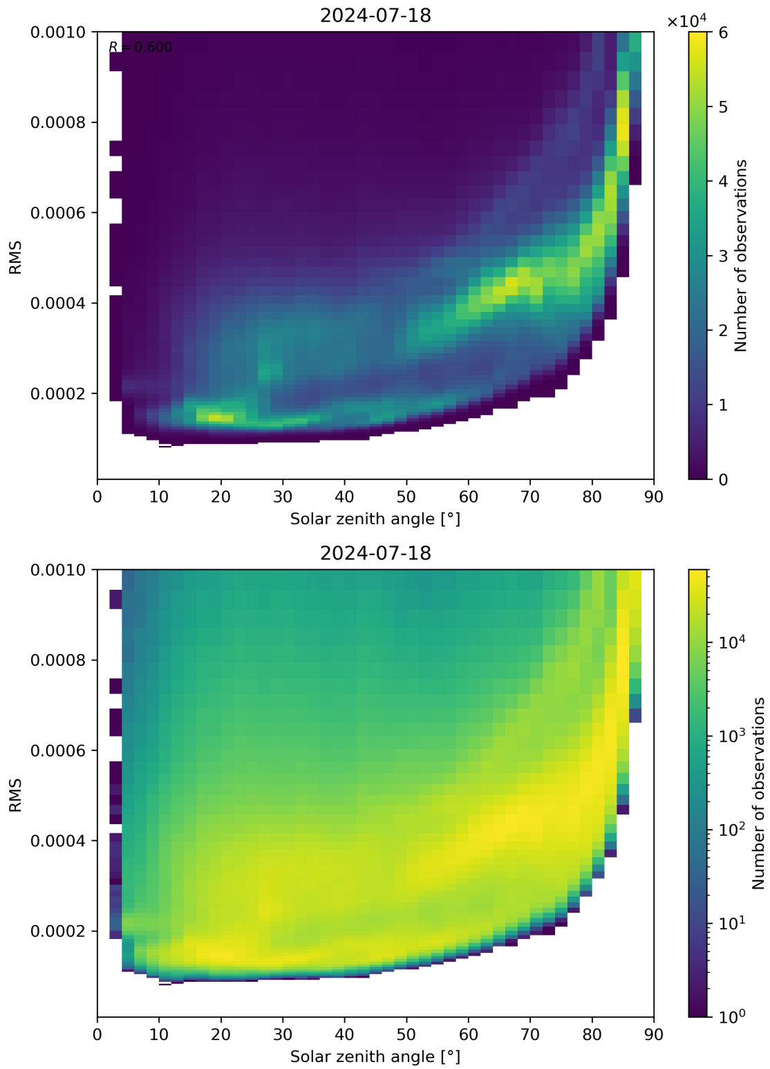
Figure 157: Scatter density plot of “Solar zenith angle” against “RMS” for 2024-07-17 to 2024-07-19.
