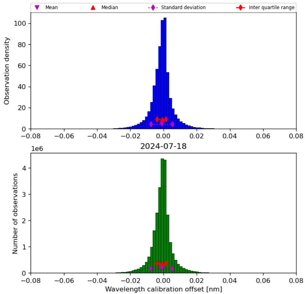
Figure 35: Histogram of “Wavelength calibration offset” for 2024-07-17 to 2024-07-19
