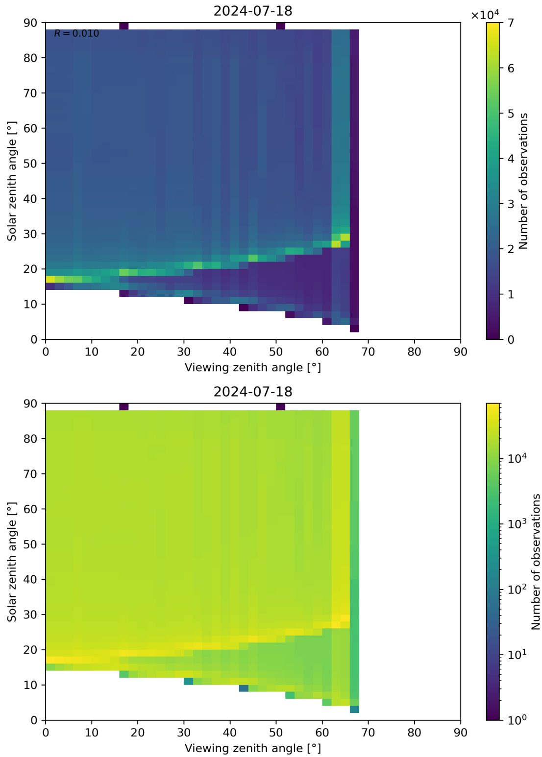
Figure 172: Scatter density plot of “Viewing zenith angle” against “Solar zenith angle” for 2024-07-17 to 2024-07-19.
