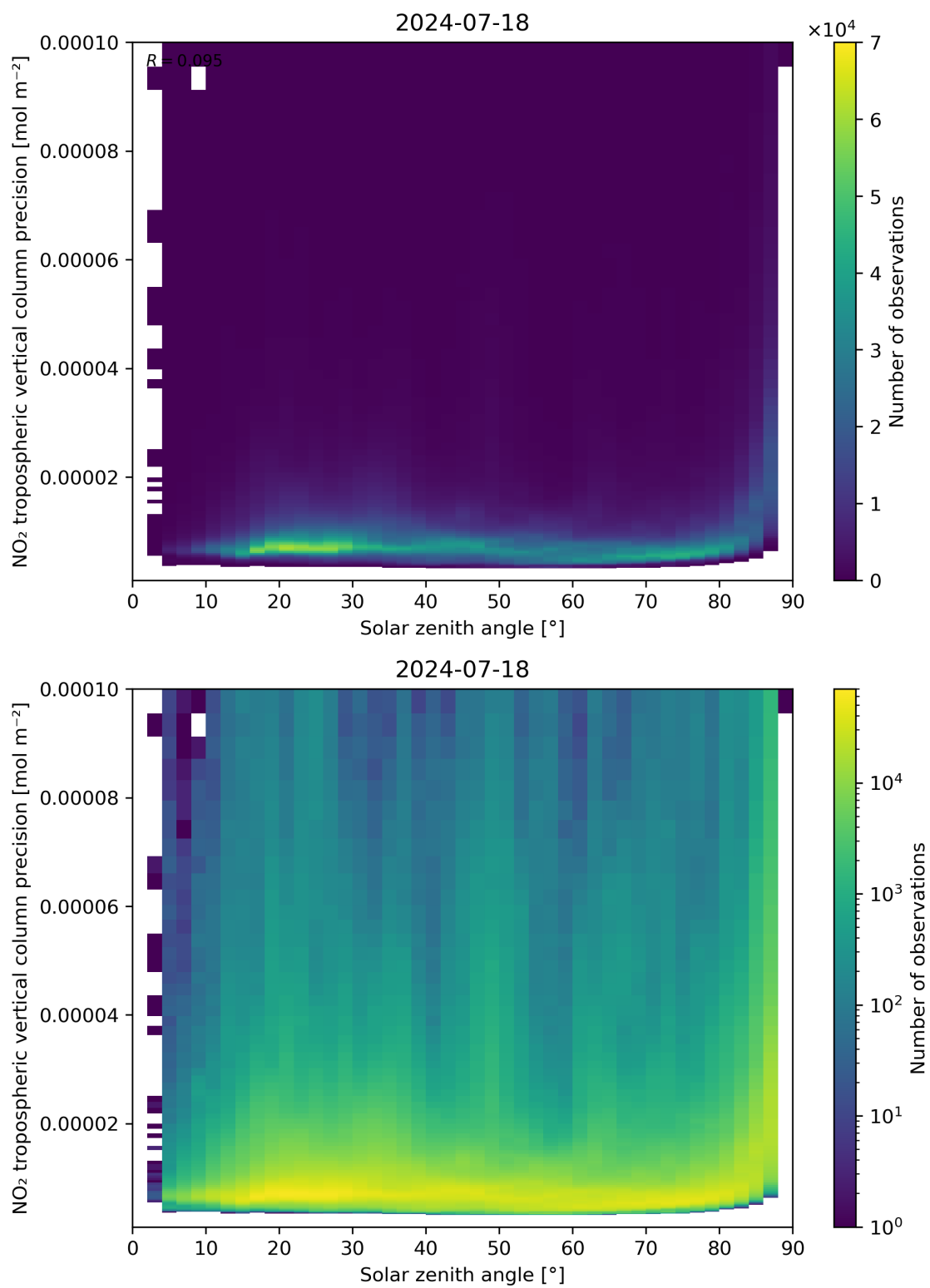
Figure 156: Scatter density plot of “Solar zenith angle” against “NO 2 tropospheric vertical column precision” for 2024-07-17 to 2024-07-19.
