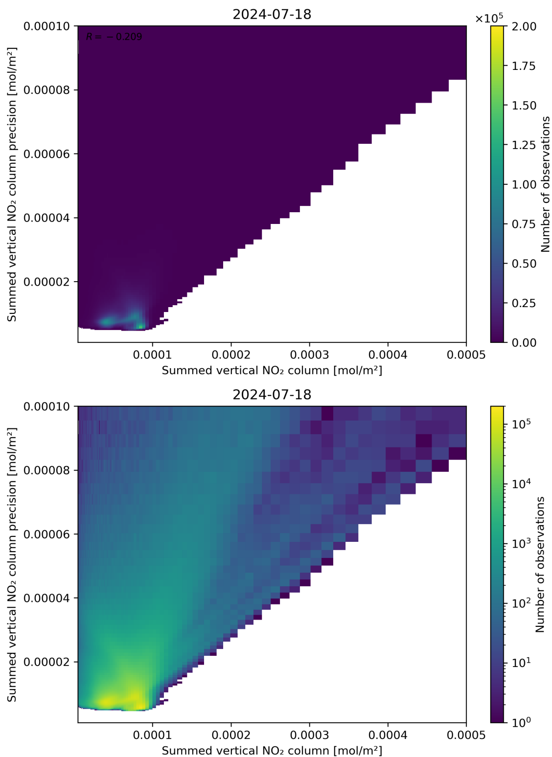
Figure 105: Scatter density plot of “Summed vertical NO 2 column” against “Summed vertical NO 2 column precision” for 2024-07-17 to 2024-07-19.
