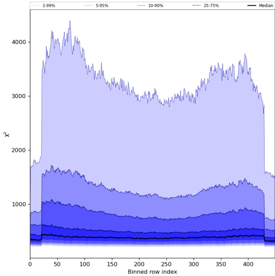
Figure 59: Along track statistics of “ \chi^2 ” for 2024-07-17 to 2024-07-19
