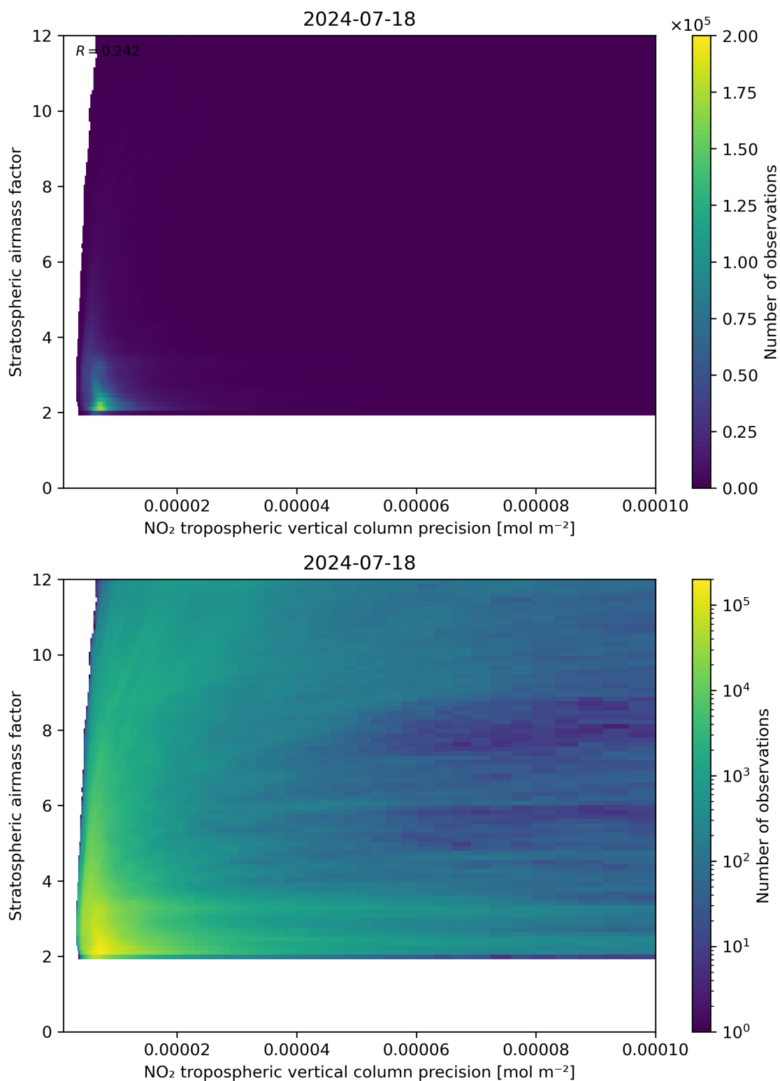
Figure 131: Scatter density plot of “NO 2 tropospheric vertical column precision” against “Stratospheric airmass factor” for 2024-07-17 to 2024-07-19.
