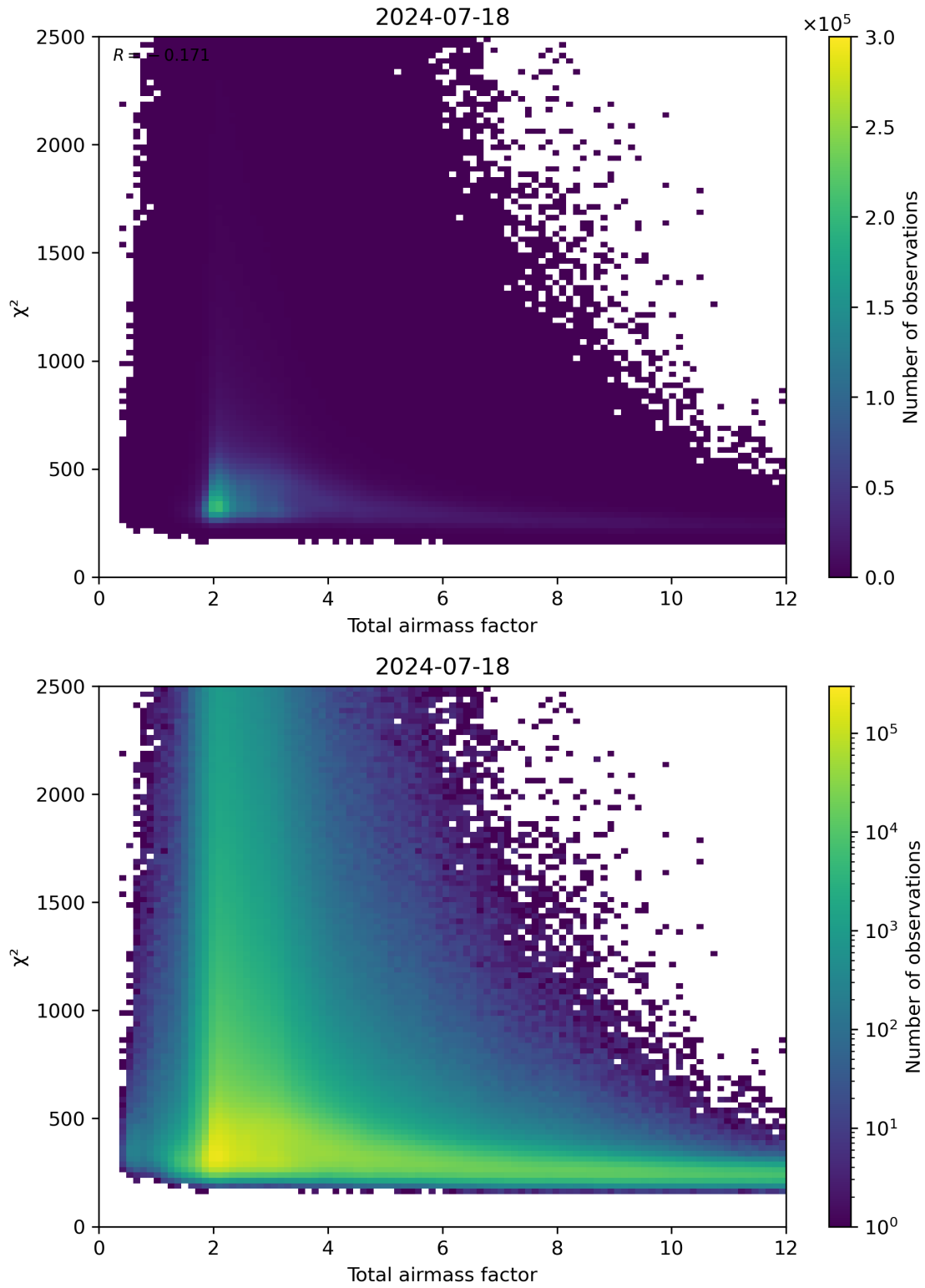
Figure 63: Scatter density plot of “Total airmass factor” against “ \chi^2 ” for 2024-07-17 to 2024-07-19.
