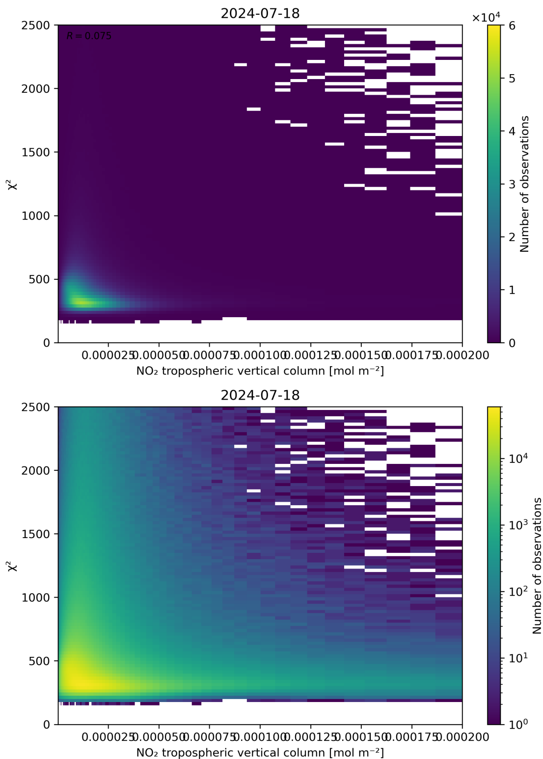
Figure 124: Scatter density plot of “NO 2 tropospheric vertical column” against “ \chi^2 ” for 2024-07-17 to 2024-07-19.
