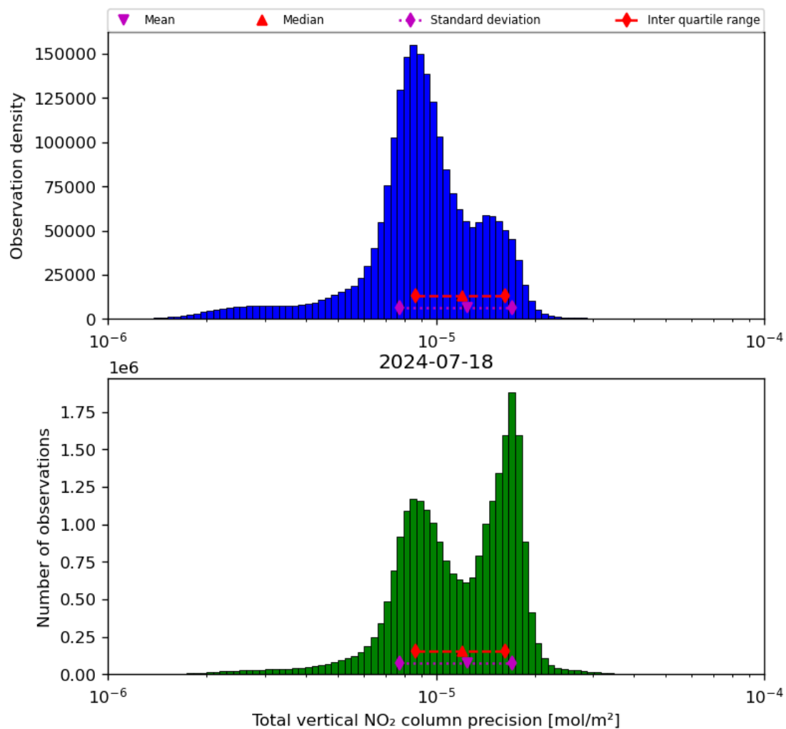
Figure 39: Histogram of “Total vertical NO 2 column precision” for 2024-07-17 to 2024-07-19
