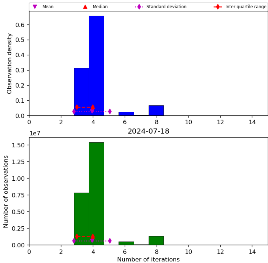
Figure 34: Histogram of “Number of iterations” for 2024-07-17 to 2024-07-19
