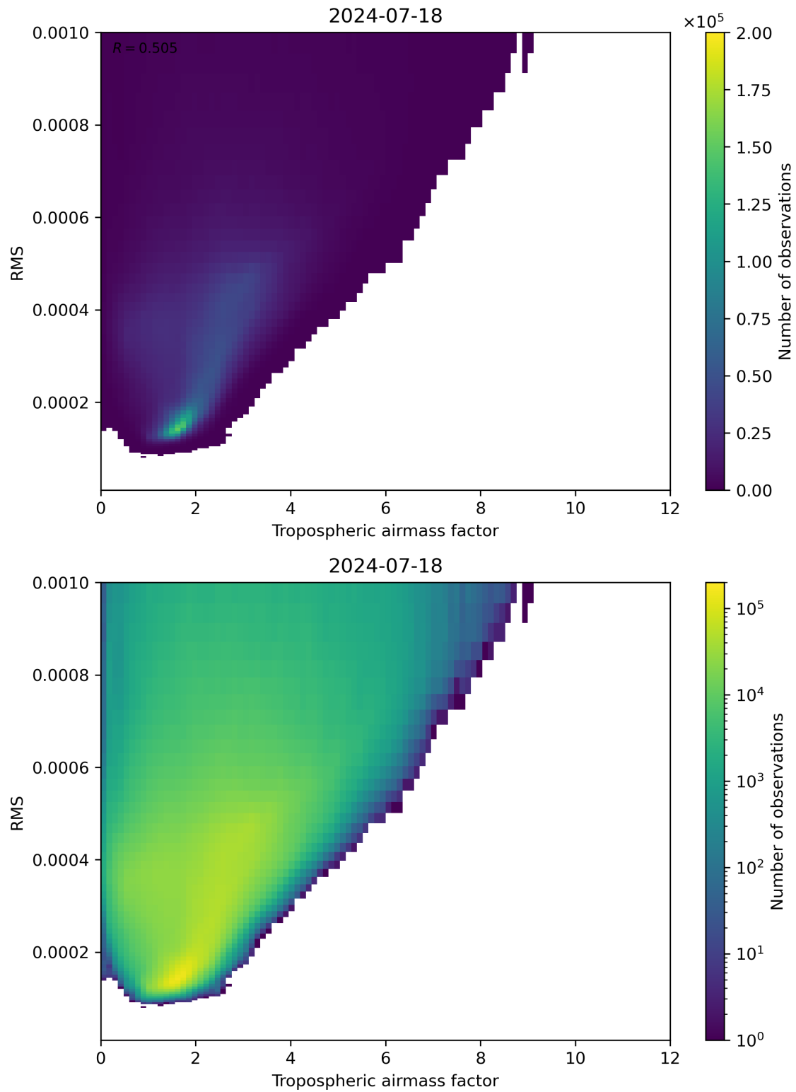
Figure 79: Scatter density plot of “Tropospheric airmass factor” against “RMS” for 2024-07-17 to 2024-07-19.
