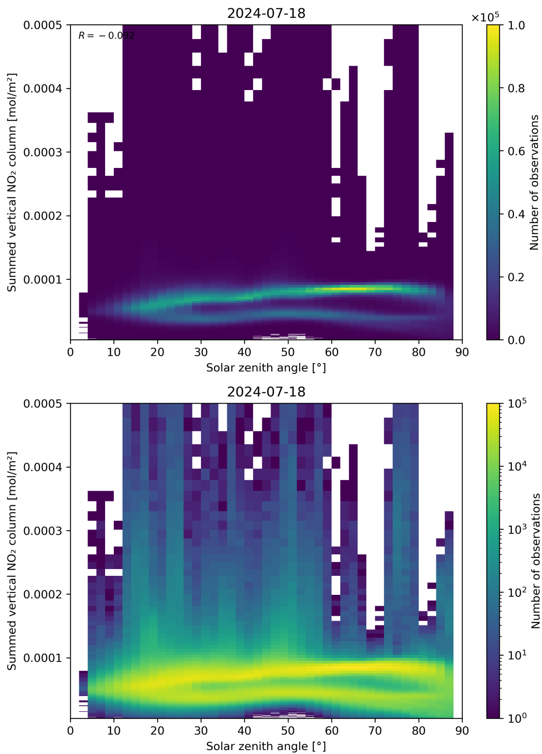
Figure 151: Scatter density plot of “Solar zenith angle” against “Summed vertical NO 2 column” for 2024-07-17 to 2024-07-19.
