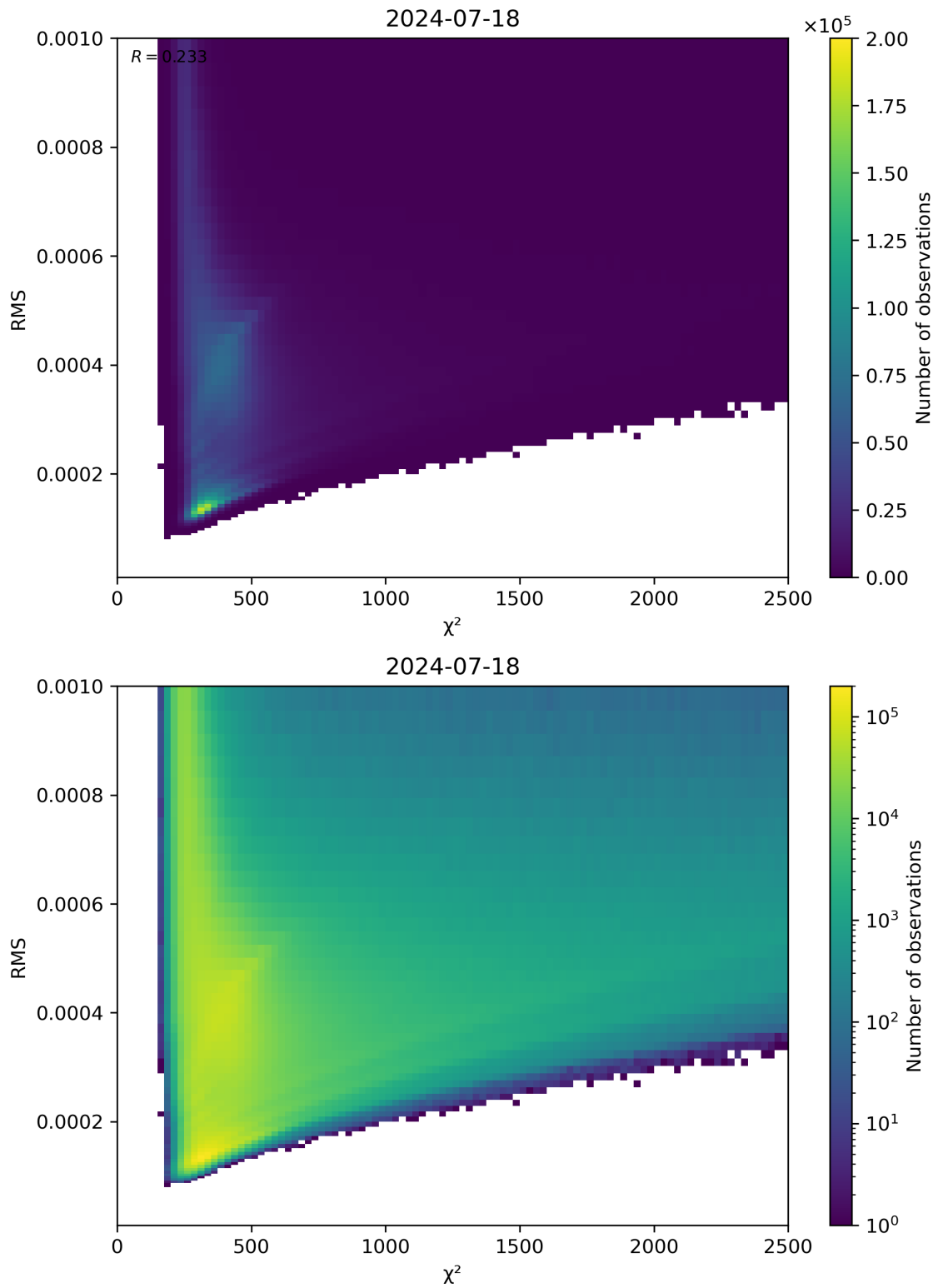
Figure 82: Scatter density plot of “ \chi^2 ” against “RMS” for 2024-07-17 to 2024-07-19.
