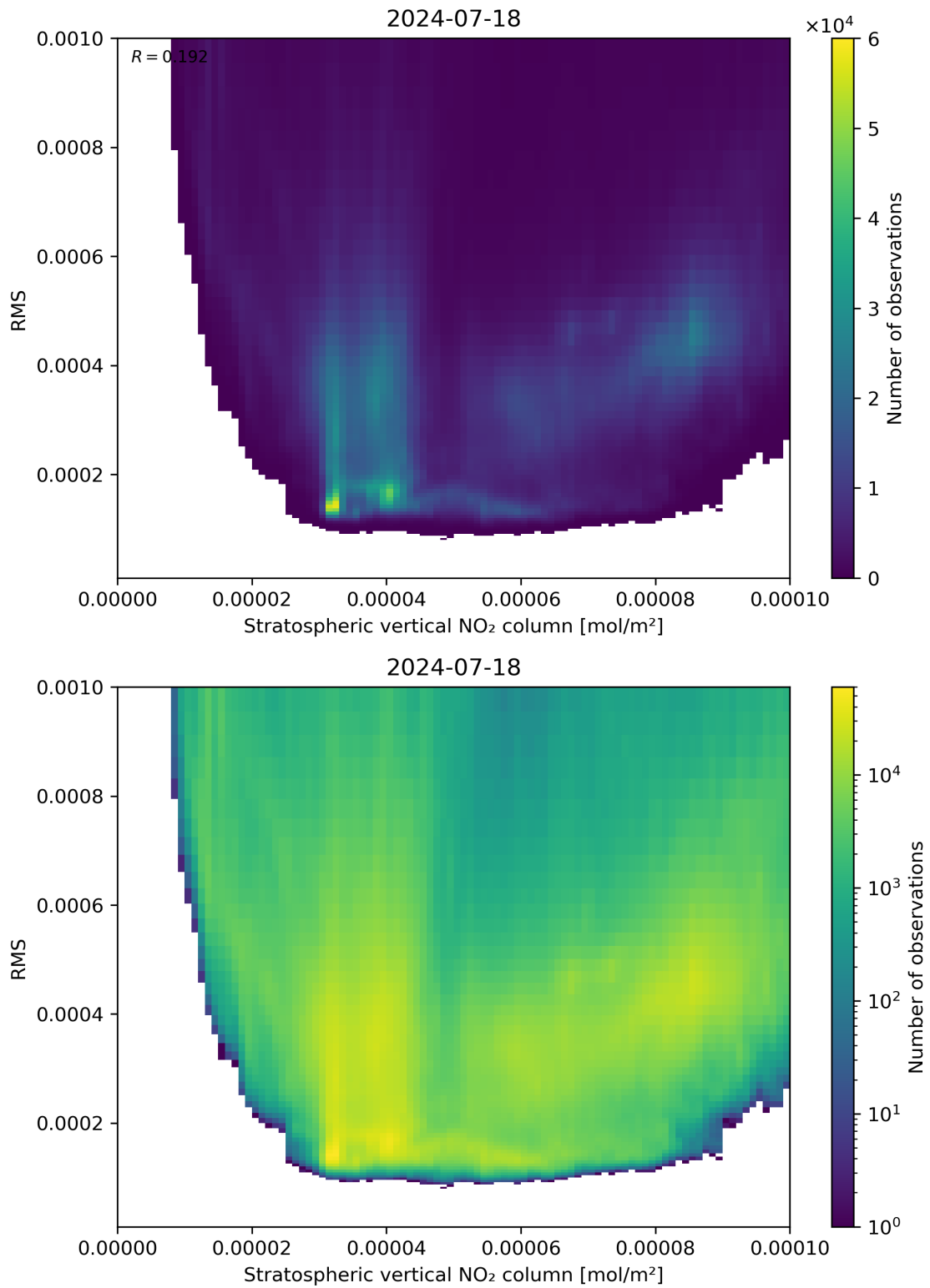
Figure 102: Scatter density plot of “Stratospheric vertical NO 2 column” against “RMS” for 2024-07-17 to 2024-07-19.
