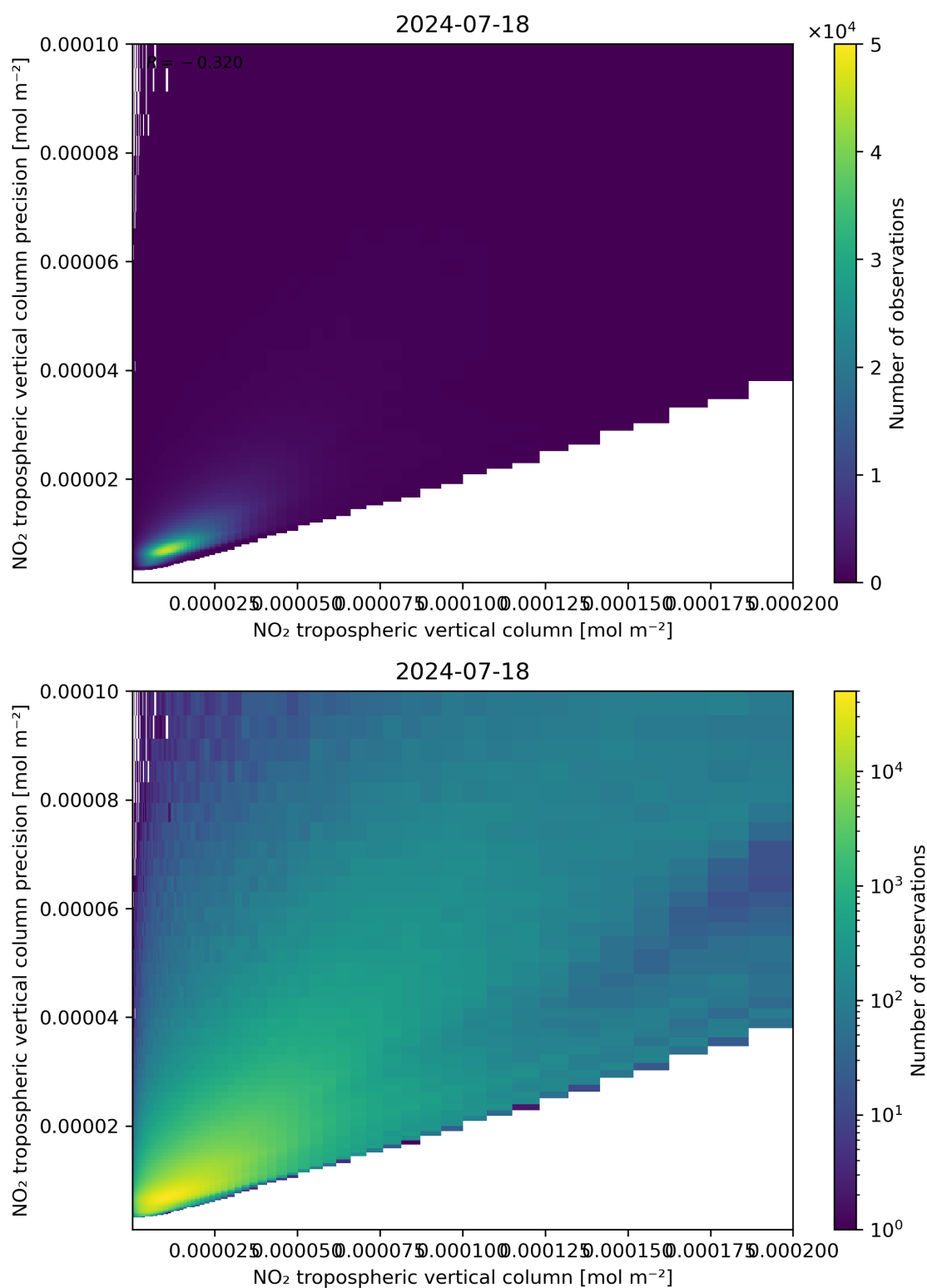
Figure 130: Scatter density plot of “NO 2 tropospheric vertical column” against “NO 2 tropospheric vertical column precision” for 2024-07-17 to 2024-07-19.
