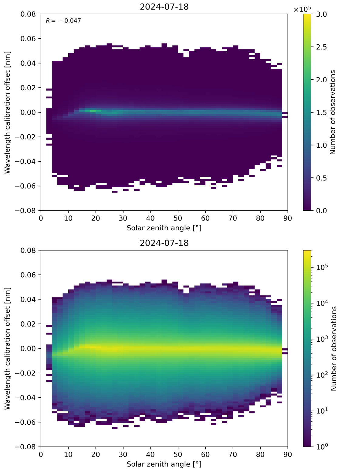
Figure 158: Scatter density plot of “Solar zenith angle” against “Wavelength calibration offset” for 2024-07-17 to 2024-07-19.
