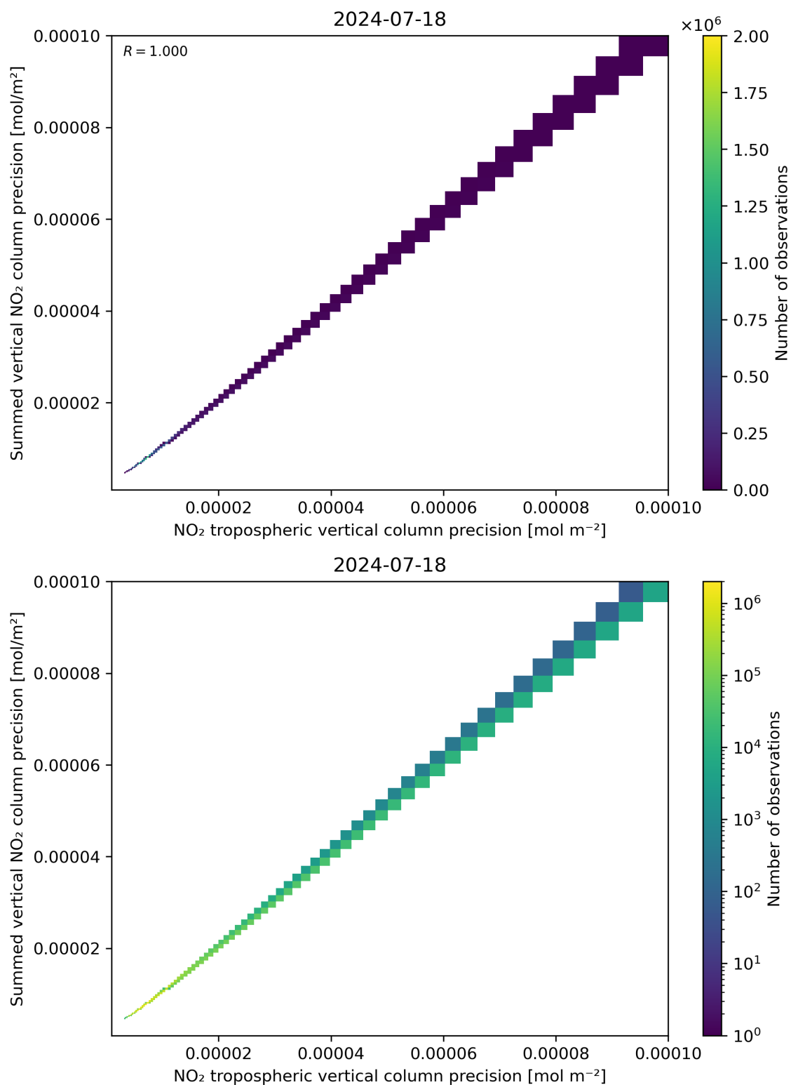
Figure 137: Scatter density plot of “NO 2 tropospheric vertical column precision” against “Summed vertical NO 2 column precision” for 2024-07-17 to 2024-07-19.
