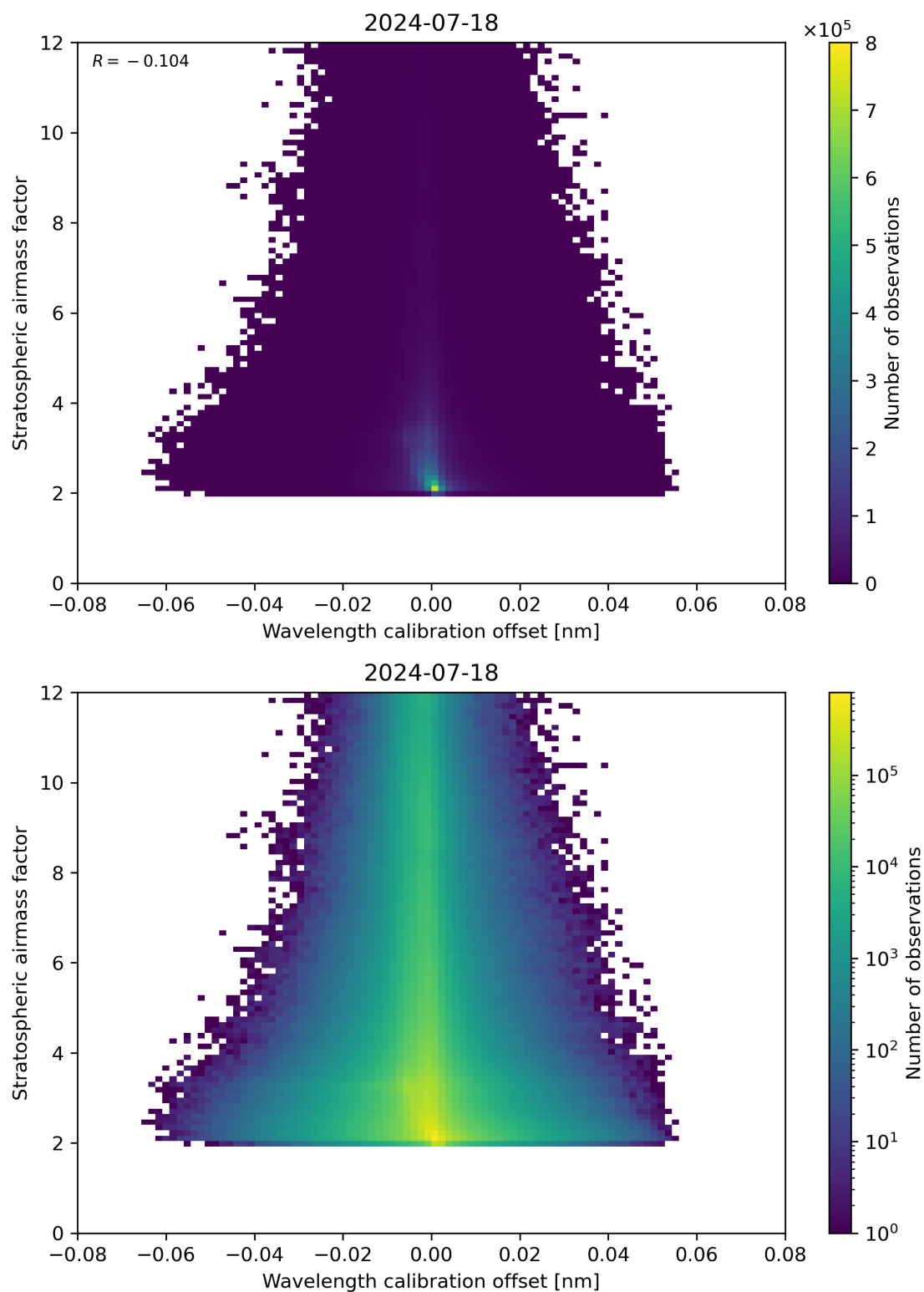
Figure 174: Scatter density plot of “Wavelength calibration offset” against “Stratospheric air mass factor” for 2024-07-17 to 2024-07-19.
