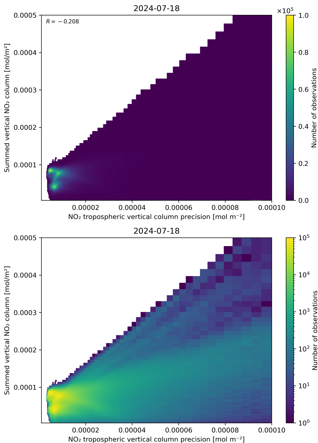
Figure 136: Scatter density plot of “NO 2 tropospheric vertical column precision” against “Summed vertical NO 2 column” for 2024-07-17 to 2024-07-19.
