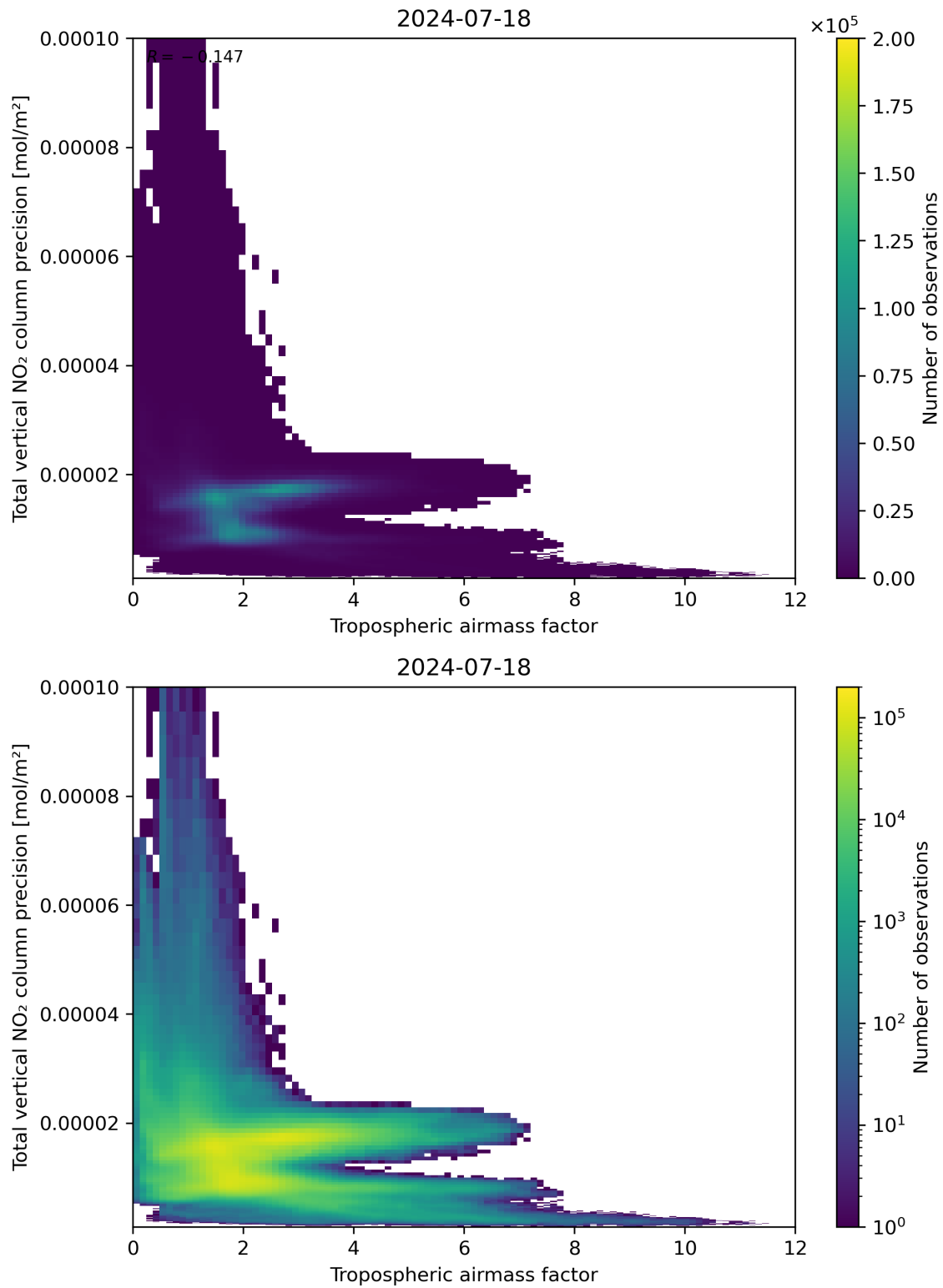
Figure 78: Scatter density plot of “Tropospheric air mass factor” against “Total vertical NO 2 column precision” for 2024-07-17 to 2024-07-19.
