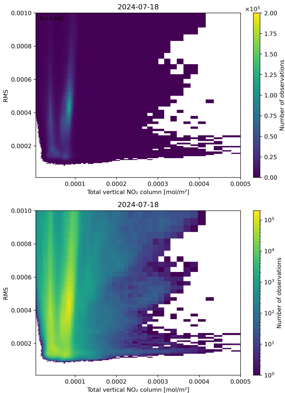
Figure 120: Scatter density plot of “Total vertical NO 2 column” against “RMS” for 2024-07-17 to 2024-07-19.
