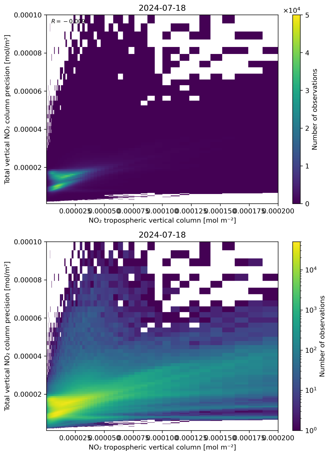
Figure 129: Scatter density plot of “NO 2 tropospheric vertical column” against “Total vertical NO 2 column precision” for 2024-07-17 to 2024-07-19.
