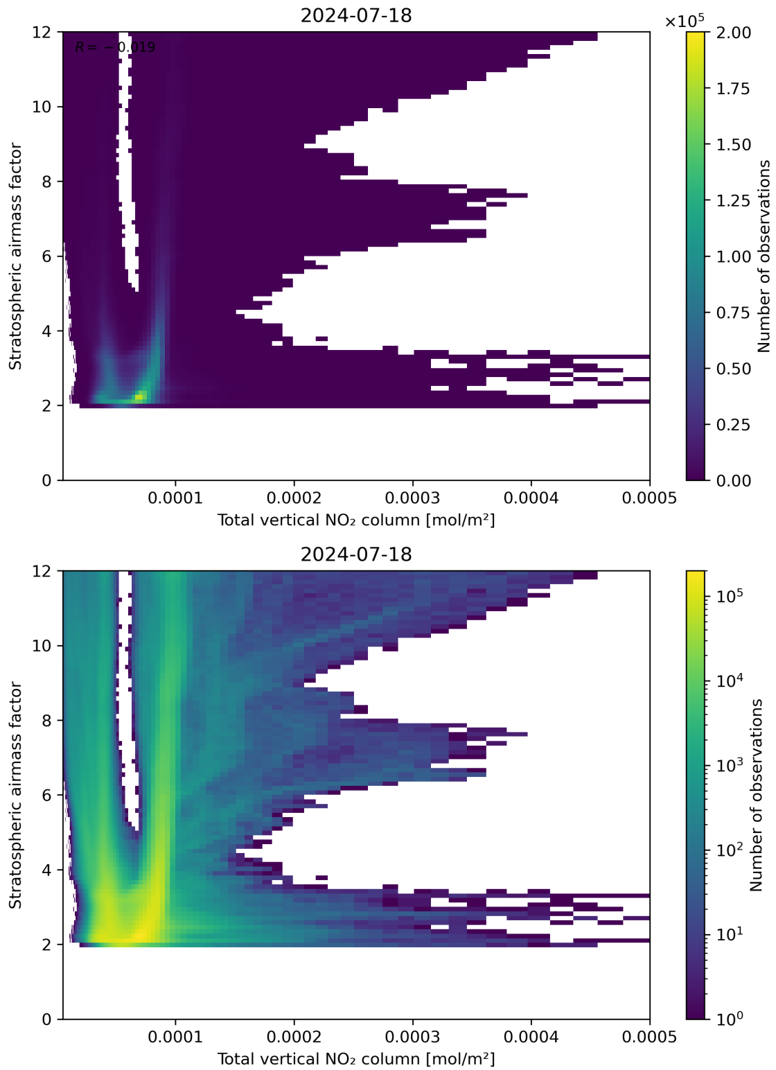
Figure 110: Scatter density plot of “Total vertical NO 2 column” against “Stratospheric airmass factor” for 2024-07-17 to 2024-07-19.
