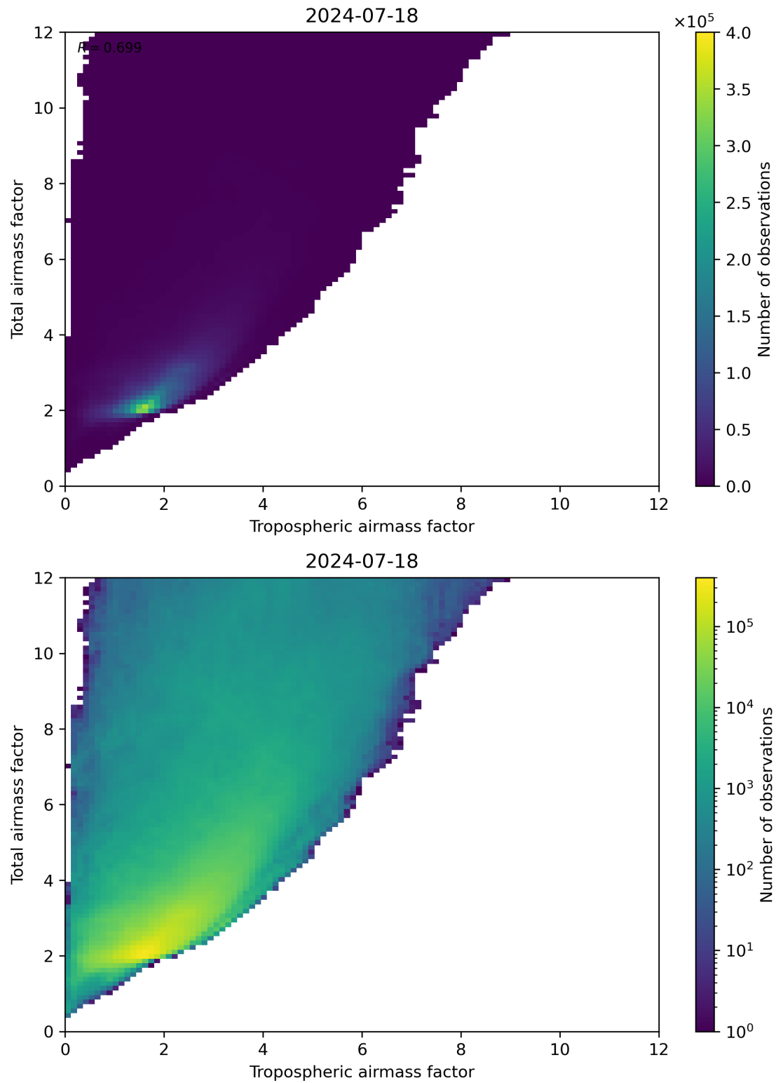
Figure 72: Scatter density plot of “Tropospheric airmass factor” against “Total airmass factor” for 2024-07-17 to 2024-07-19.
