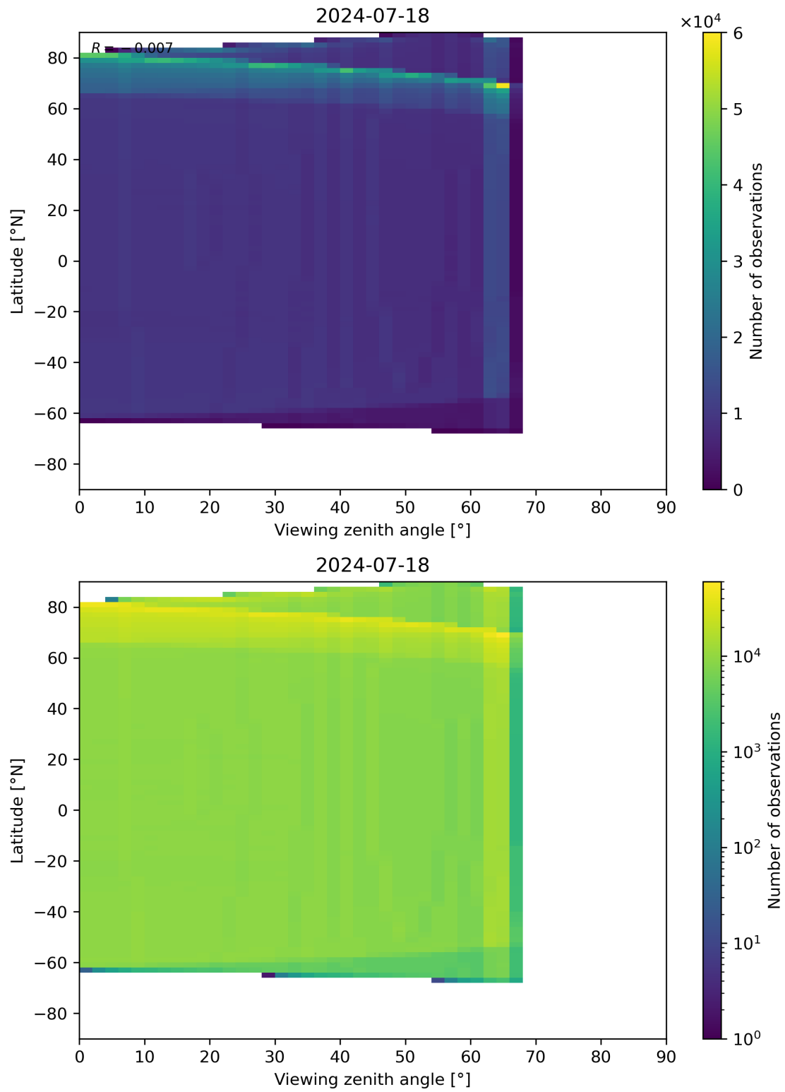
Figure 163: Scatter density plot of “Viewing zenith angle” against “Latitude” for 2024-07-17 to 2024-07-19.
