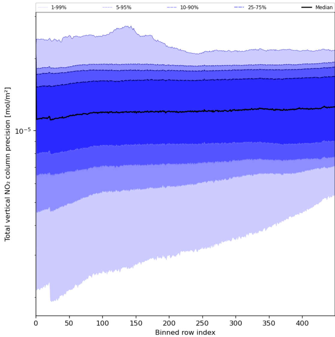
Figure 56: Along track statistics of “Total vertical NO 2 column precision” for 2024-07-17 to 2024-07-19
