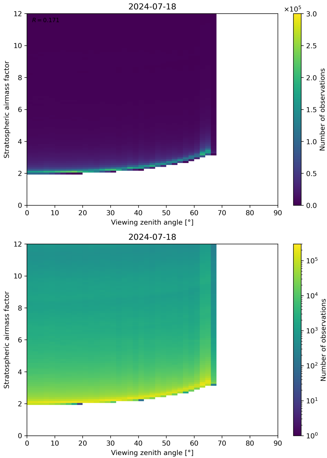
Figure 159: Scatter density plot of “Viewing zenith angle” against “Stratospheric airmass factor” for 2024-07-17 to 2024-07-19.
