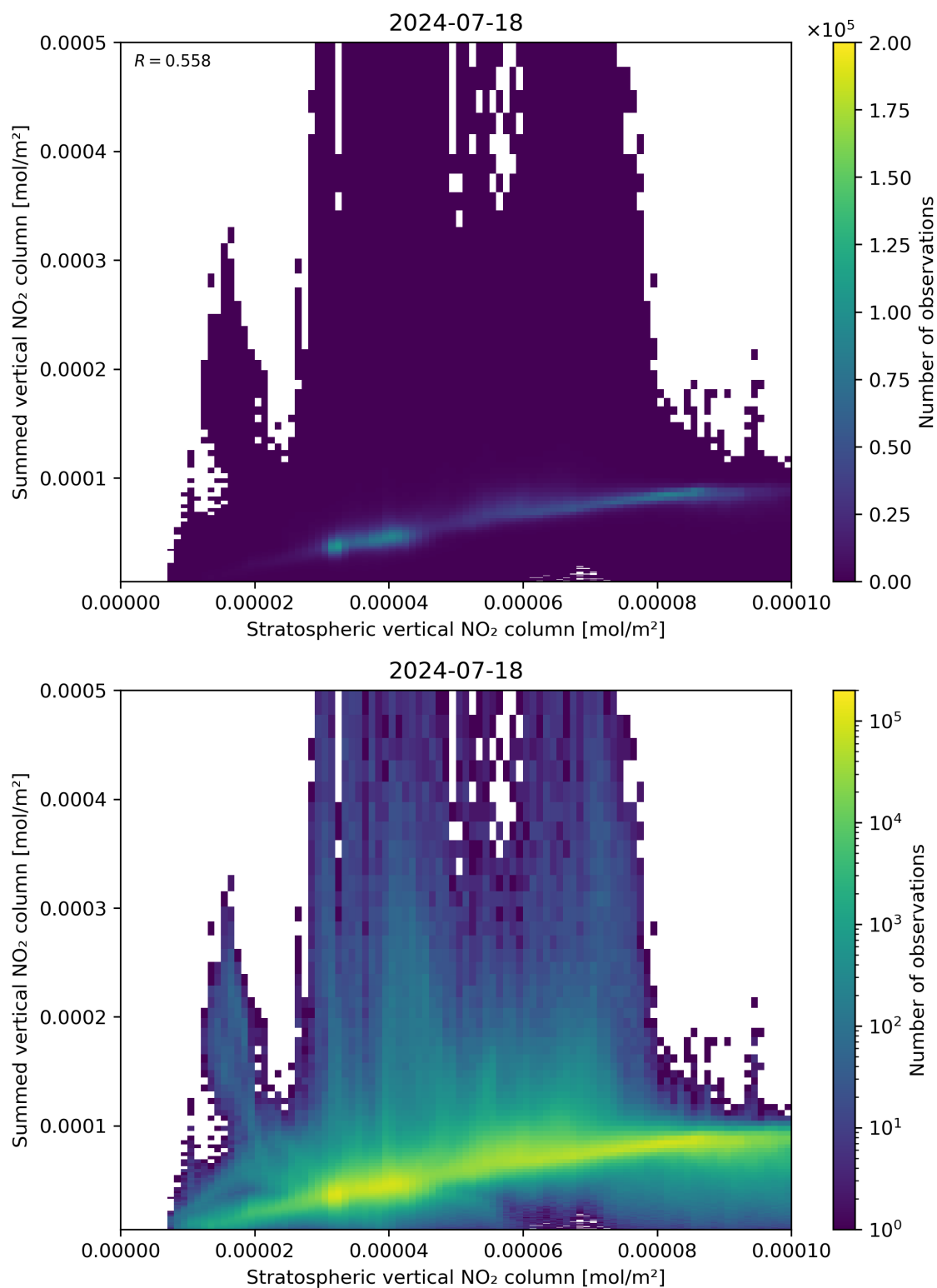
Figure 98: Scatter density plot of “Stratospheric vertical NO 2 column” against “Summed vertical NO 2 column” for 2024-07-17 to 2024-07-19.
