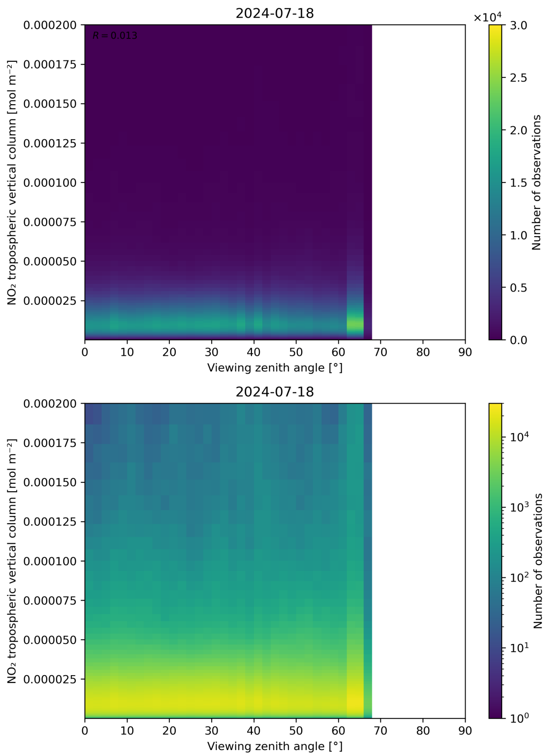
Figure 169: Scatter density plot of “Viewing zenith angle” against “NO 2 tropospheric vertical column” for 2024-07-17 to 2024-07-19.
