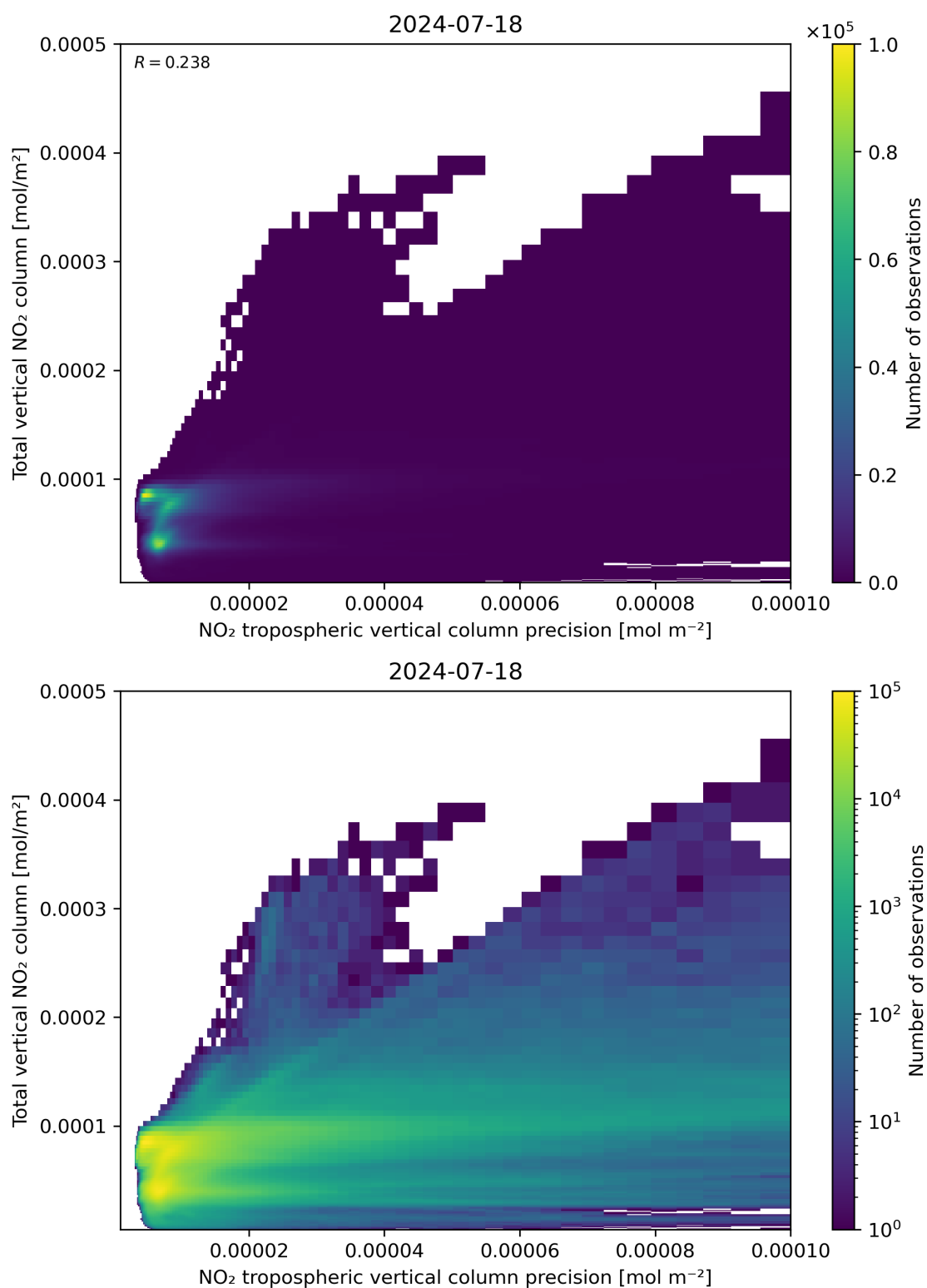
Figure 138: Scatter density plot of “NO 2 tropospheric vertical column precision” against “Total vertical NO 2 column” for 2024-07-17 to 2024-07-19.
