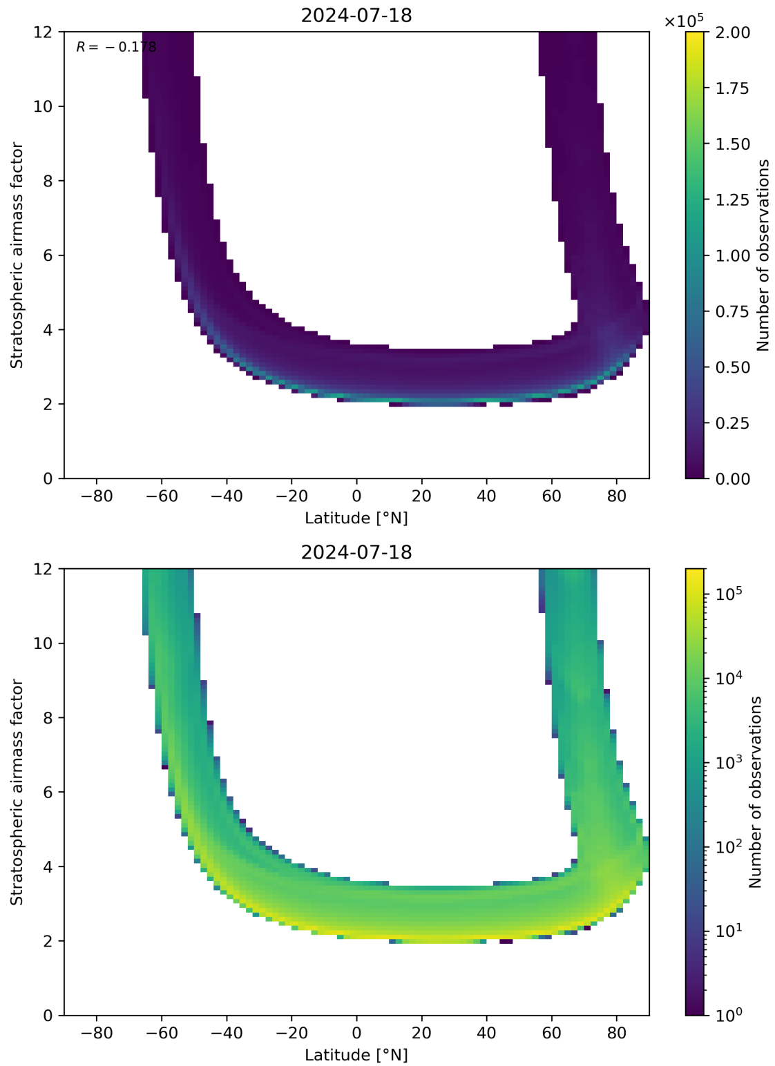
Figure 83: Scatter density plot of “Latitude” against “Stratospheric air mass factor” for 2024-07-17 to 2024-07-19.
