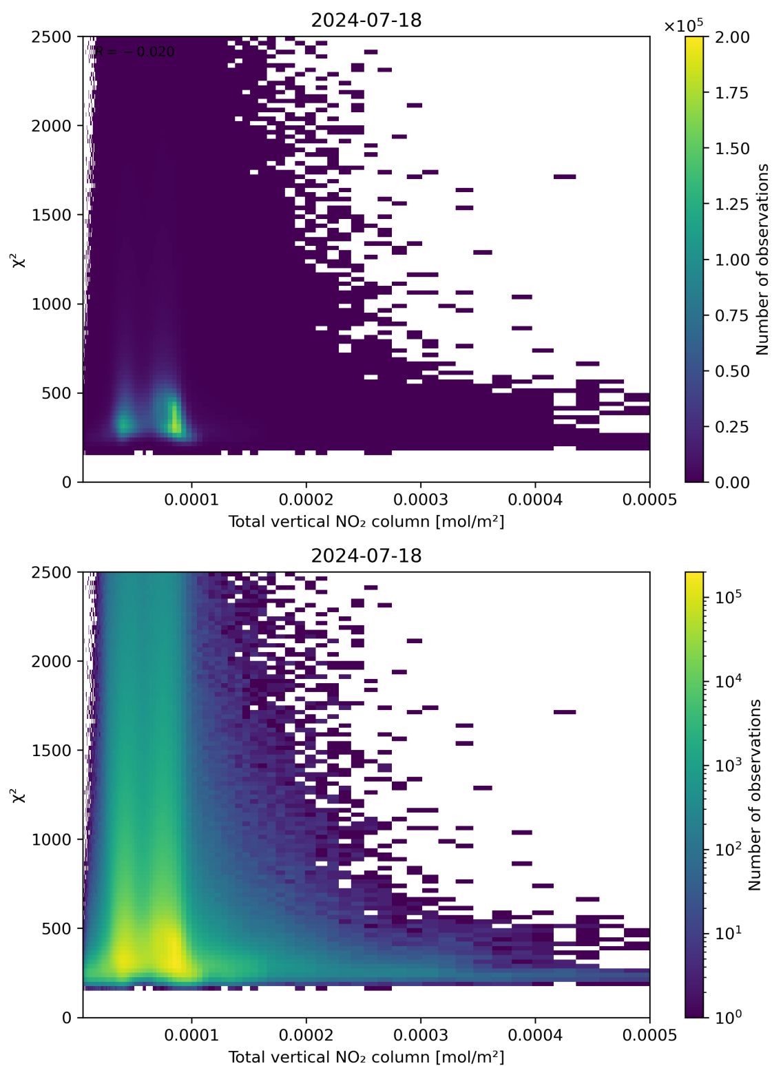
Figure 111: Scatter density plot of “Total vertical NO 2 column” against “ \chi^2 ” for 2024-07-17 to 2024-07-19.
