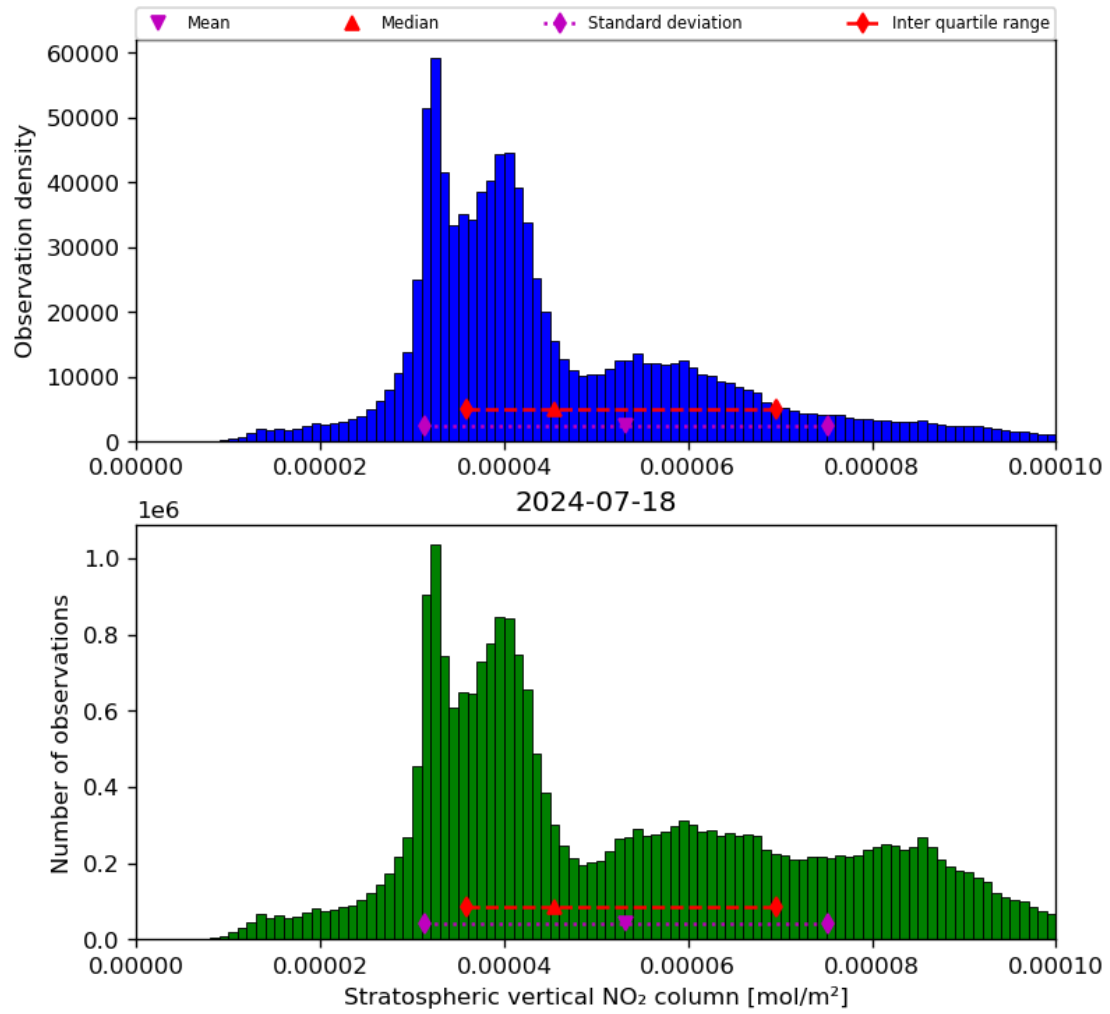
Figure 36: Histogram of “Stratospheric vertical NO 2 column” for 2024-07-17 to 2024-07-19
