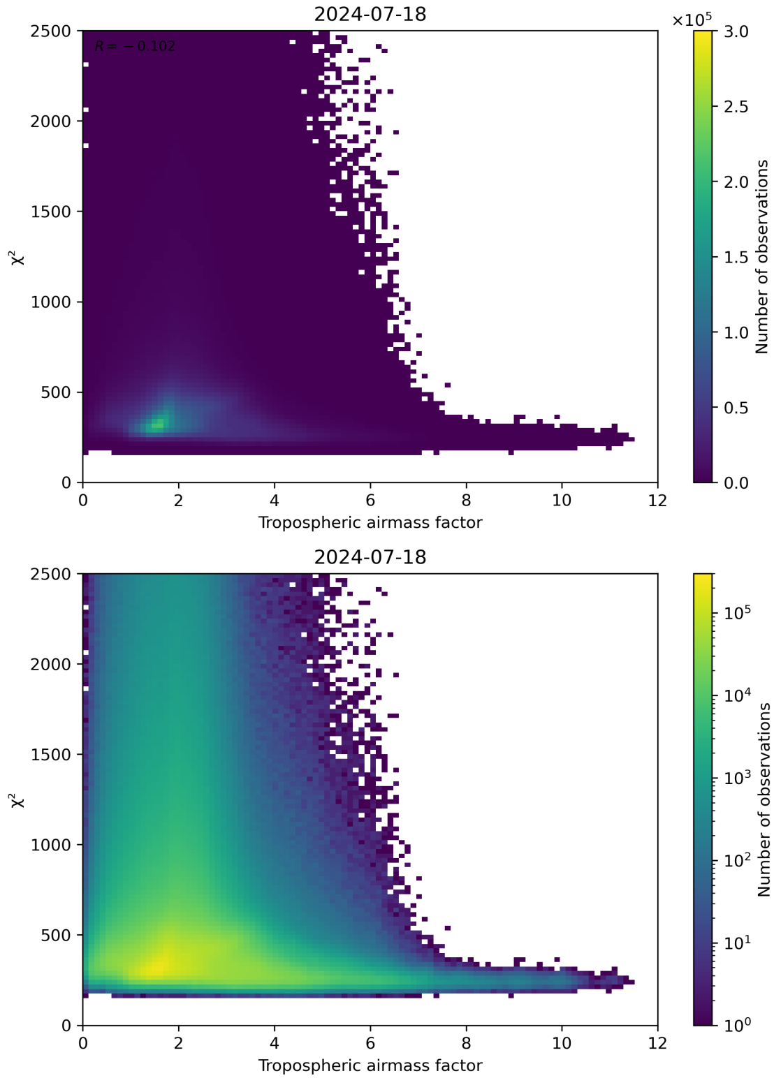
Figure 73: Scatter density plot of “Tropospheric airmass factor” against “ \chi^2 ” for 2024-07-17 to 2024-07-19.
