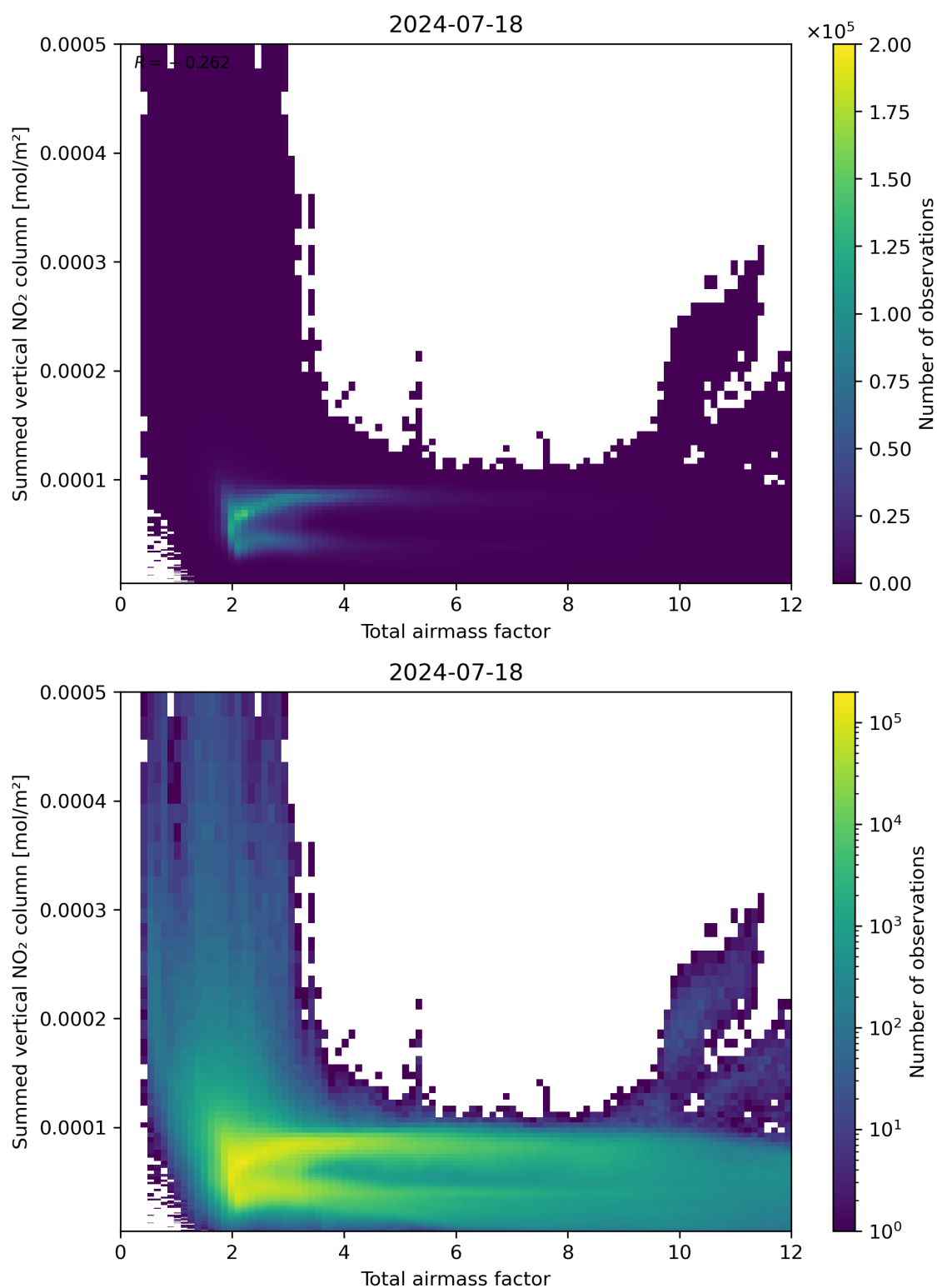
Figure 65: Scatter density plot of “Total airmass factor” against “Summed vertical NO 2 column” for 2024-07-17 to 2024-07-19.
