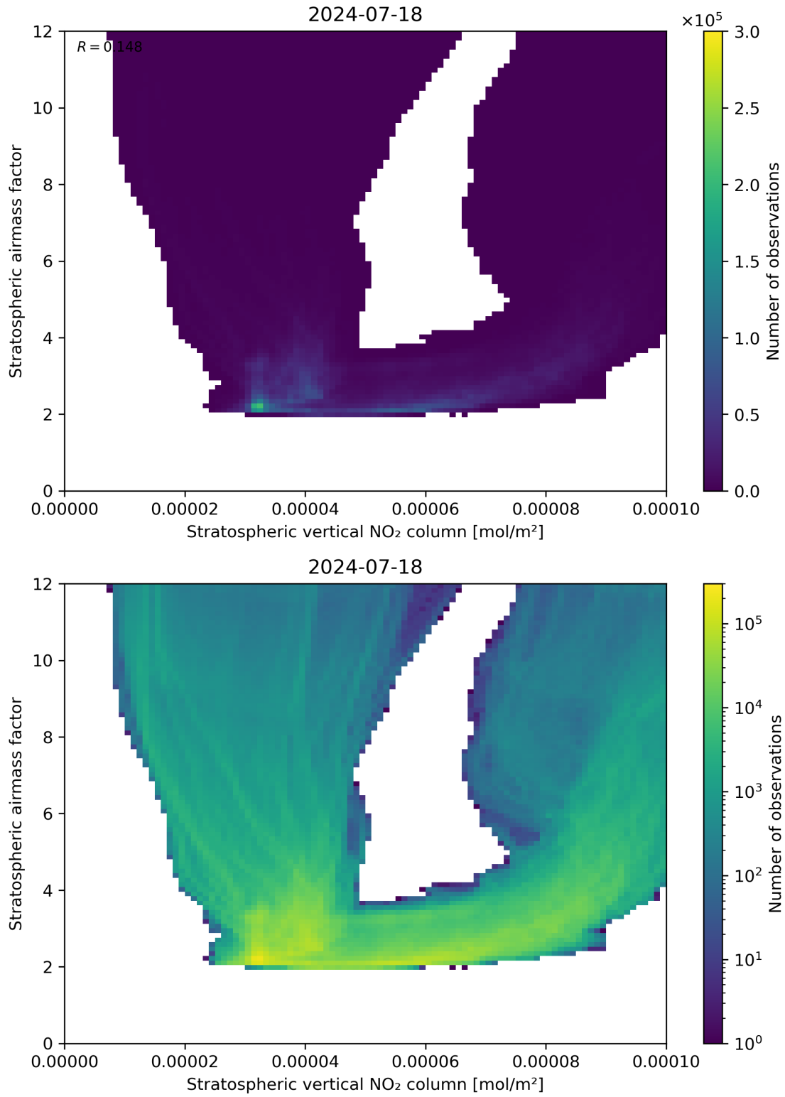
Figure 96: Scatter density plot of “Stratospheric vertical NO 2 column” against “Stratospheric airmass factor” for 2024-07-17 to 2024-07-19.
