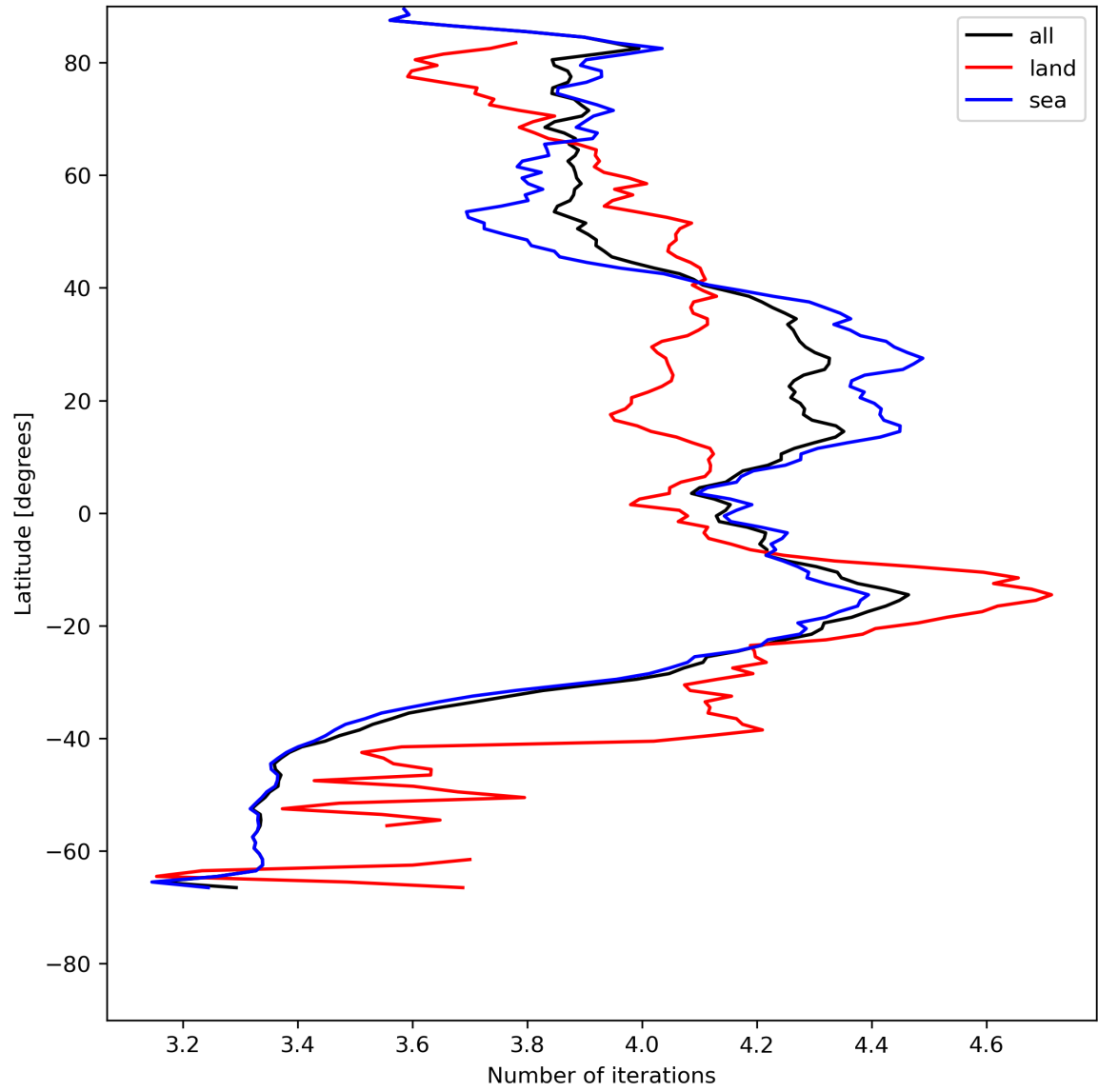
Figure 17: Zonal average of “Number of iterations” for 2024-07-17 to 2024-07-19.
