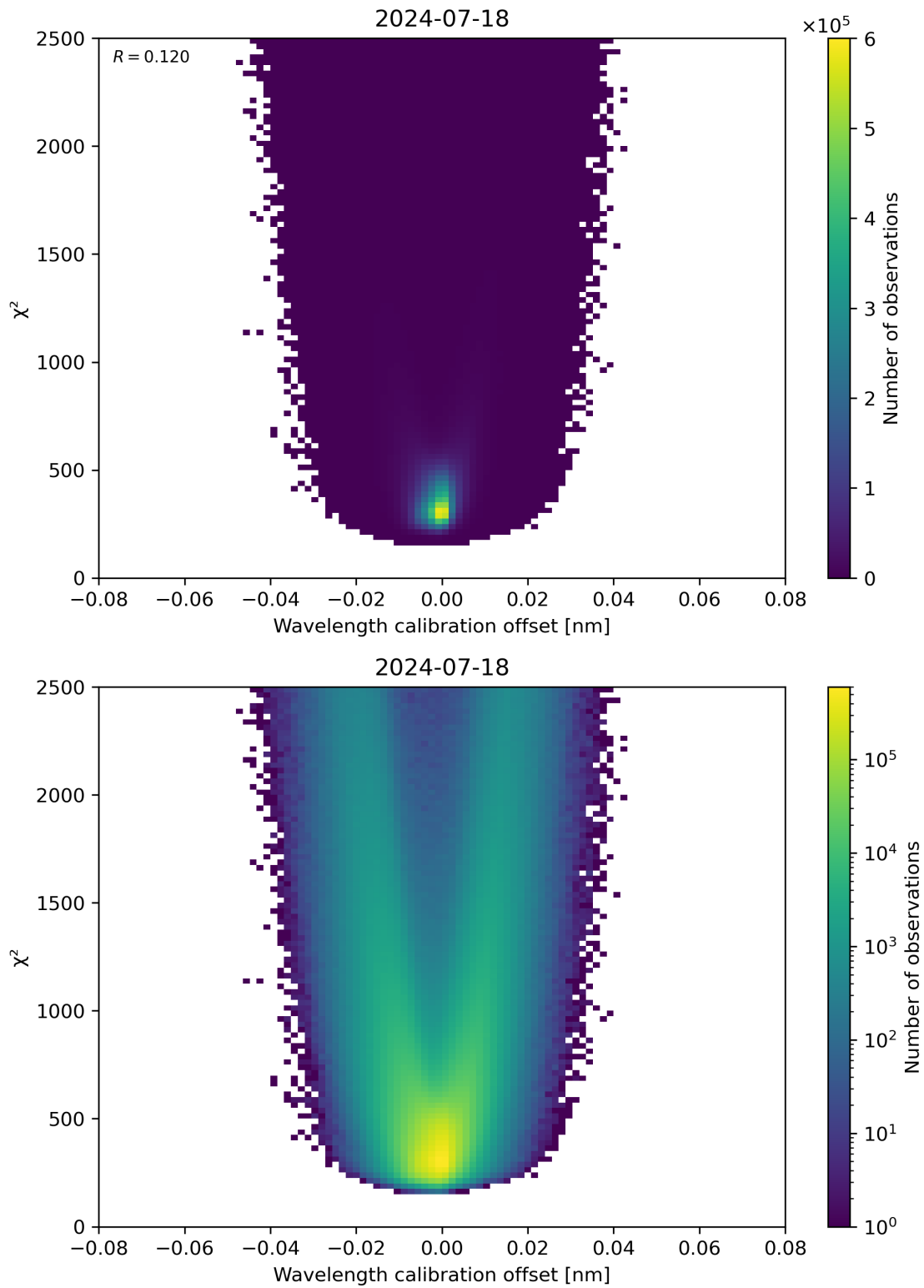
Figure 175: Scatter density plot of “Wavelength calibration offset” against “ \chi^2 ” for 2024-07-17 to 2024-07-19.
