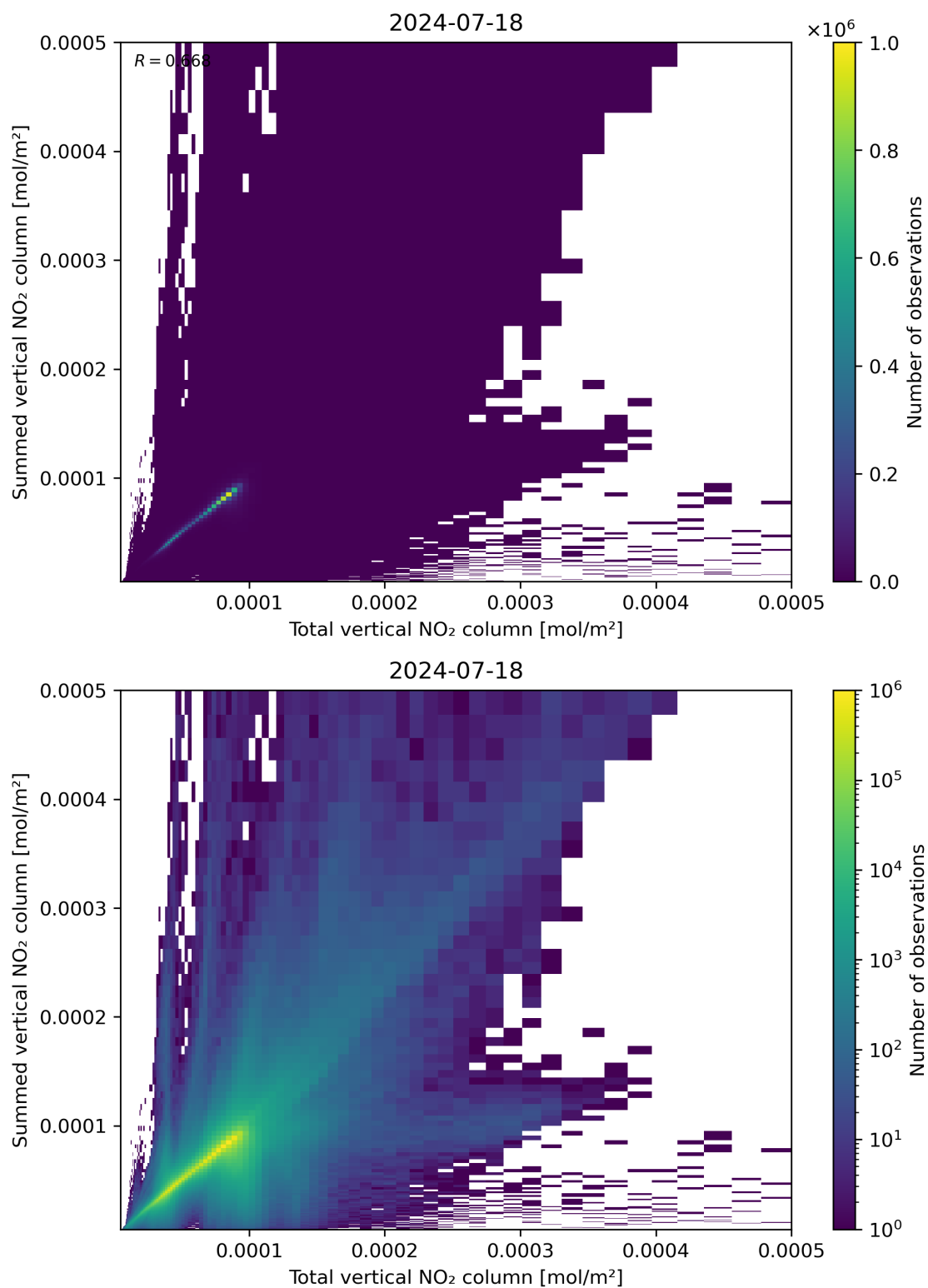
Figure 112: Scatter density plot of “Total vertical NO 2 column” against “Summed vertical NO 2 column” for 2024-07-17 to 2024-07-19.
