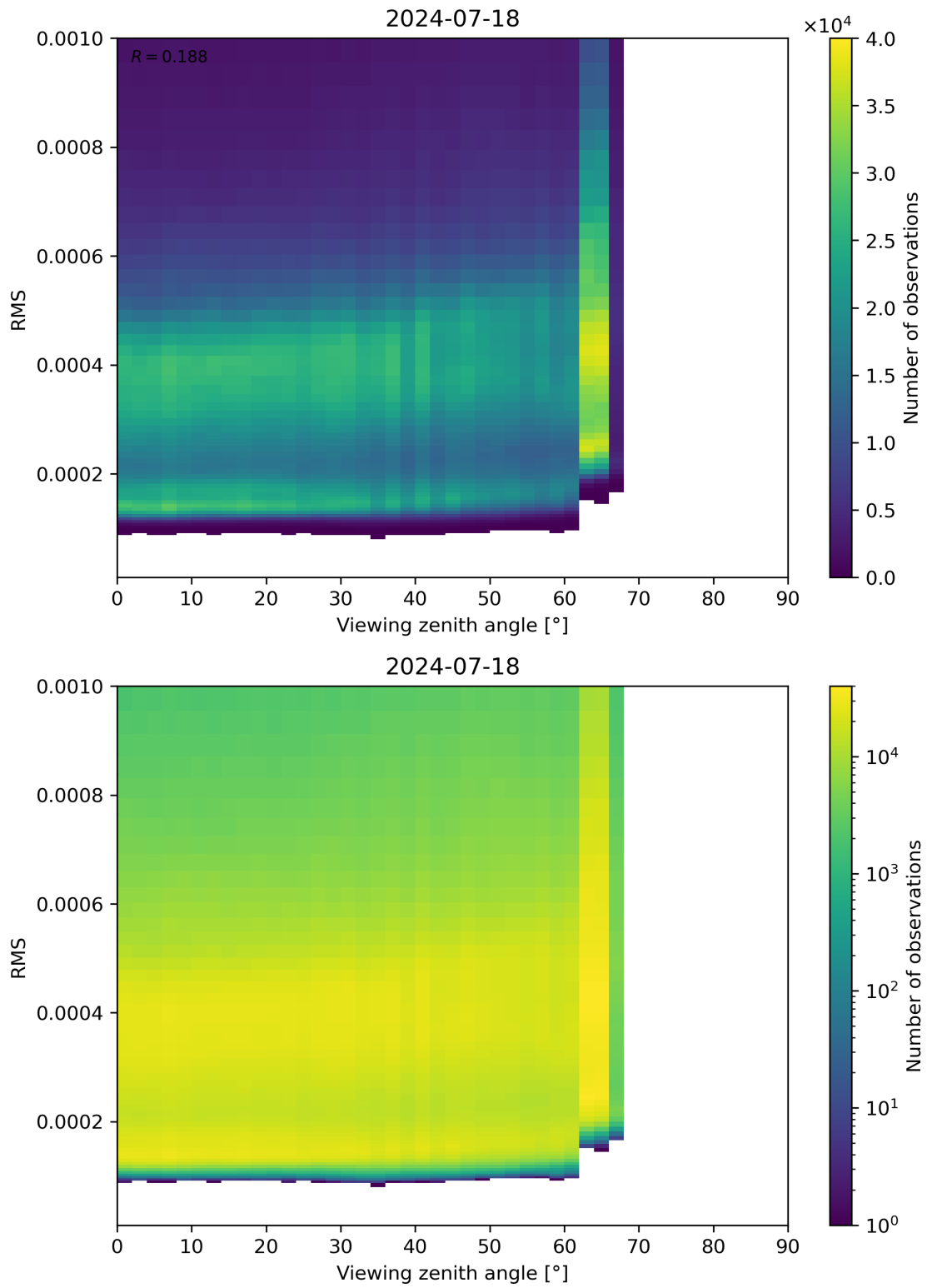
Figure 171: Scatter density plot of “Viewing zenith angle” against “RMS” for 2024-07-17 to 2024-07-19.
