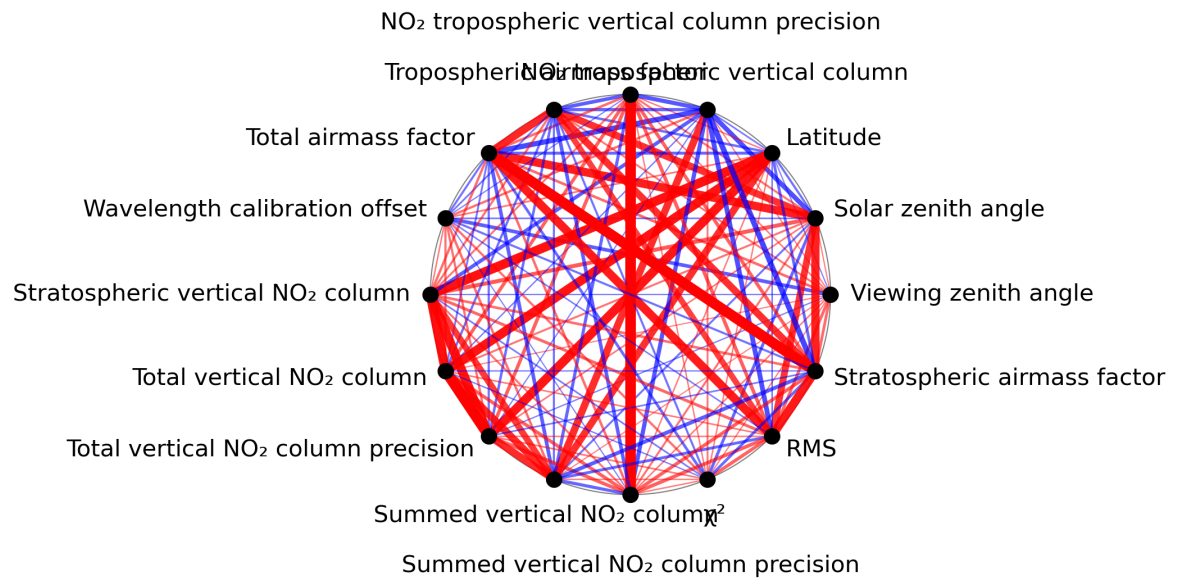
Figure 1: Map of correlation graph for 2024-07-17 to 2024-07-19.
