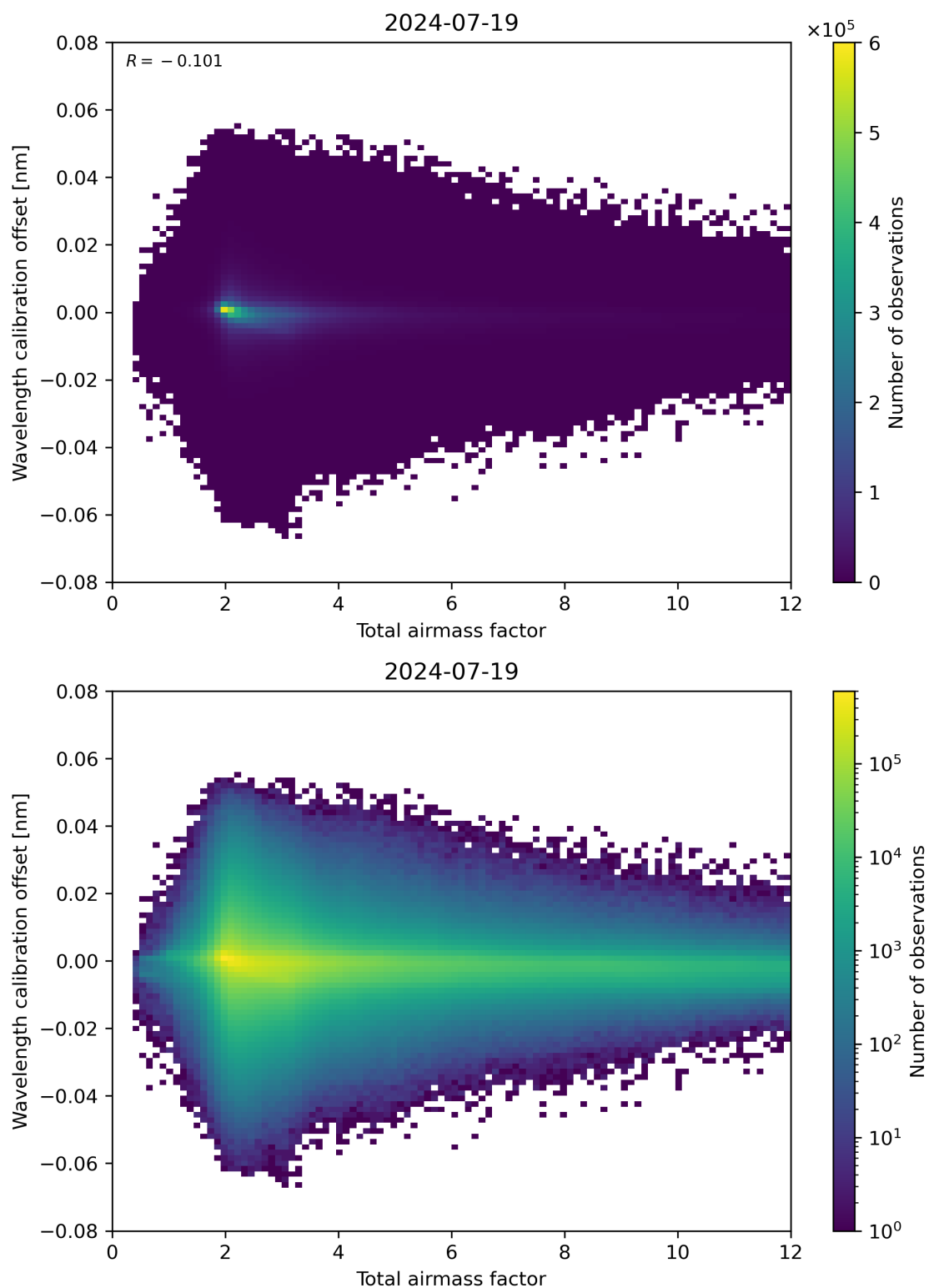
Figure 70: Scatter density plot of “Total airmass factor” against “Wavelength calibration offset” for 2024-07-18 to 2024-07-20.
