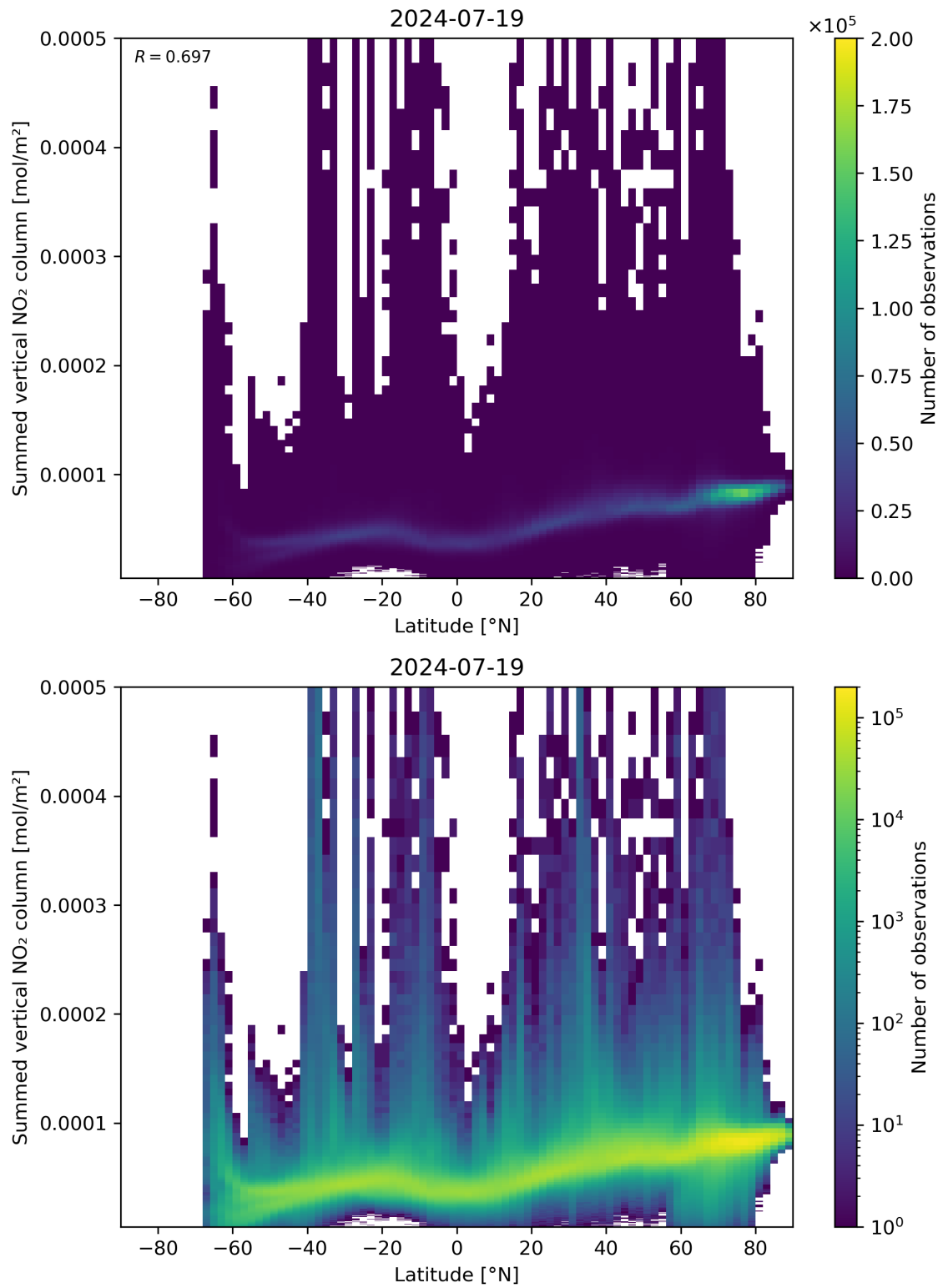
Figure 88: Scatter density plot of “Latitude” against “Summed vertical NO 2 column” for 2024-07-18 to 2024-07-20.
