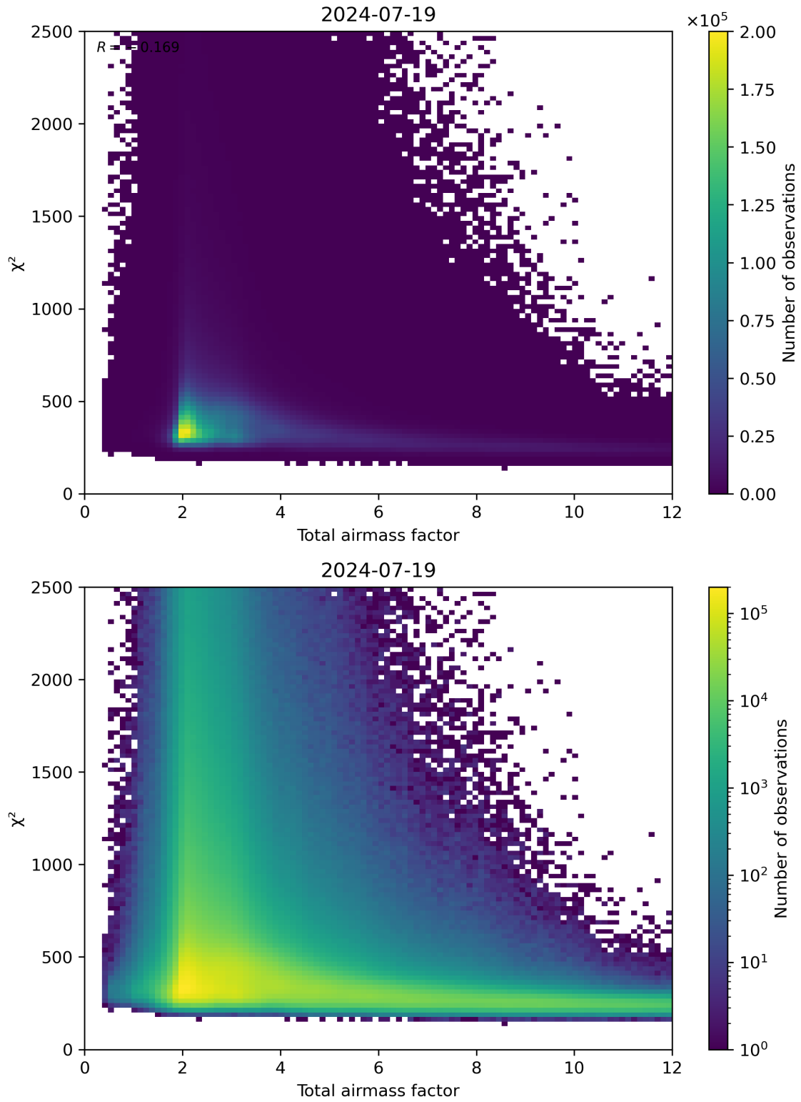
Figure 63: Scatter density plot of “Total airmass factor” against “ \chi^2 ” for 2024-07-18 to 2024-07-20.
