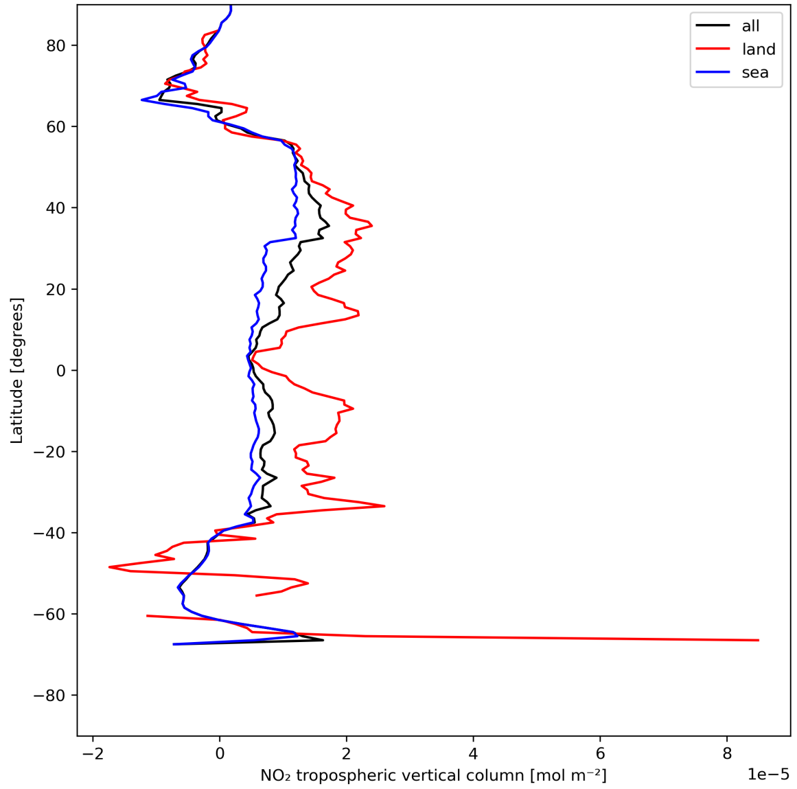
Figure 12: Zonal average of “NO 2 tropospheric vertical column” for 2024-07-18 to 2024-07-20.
