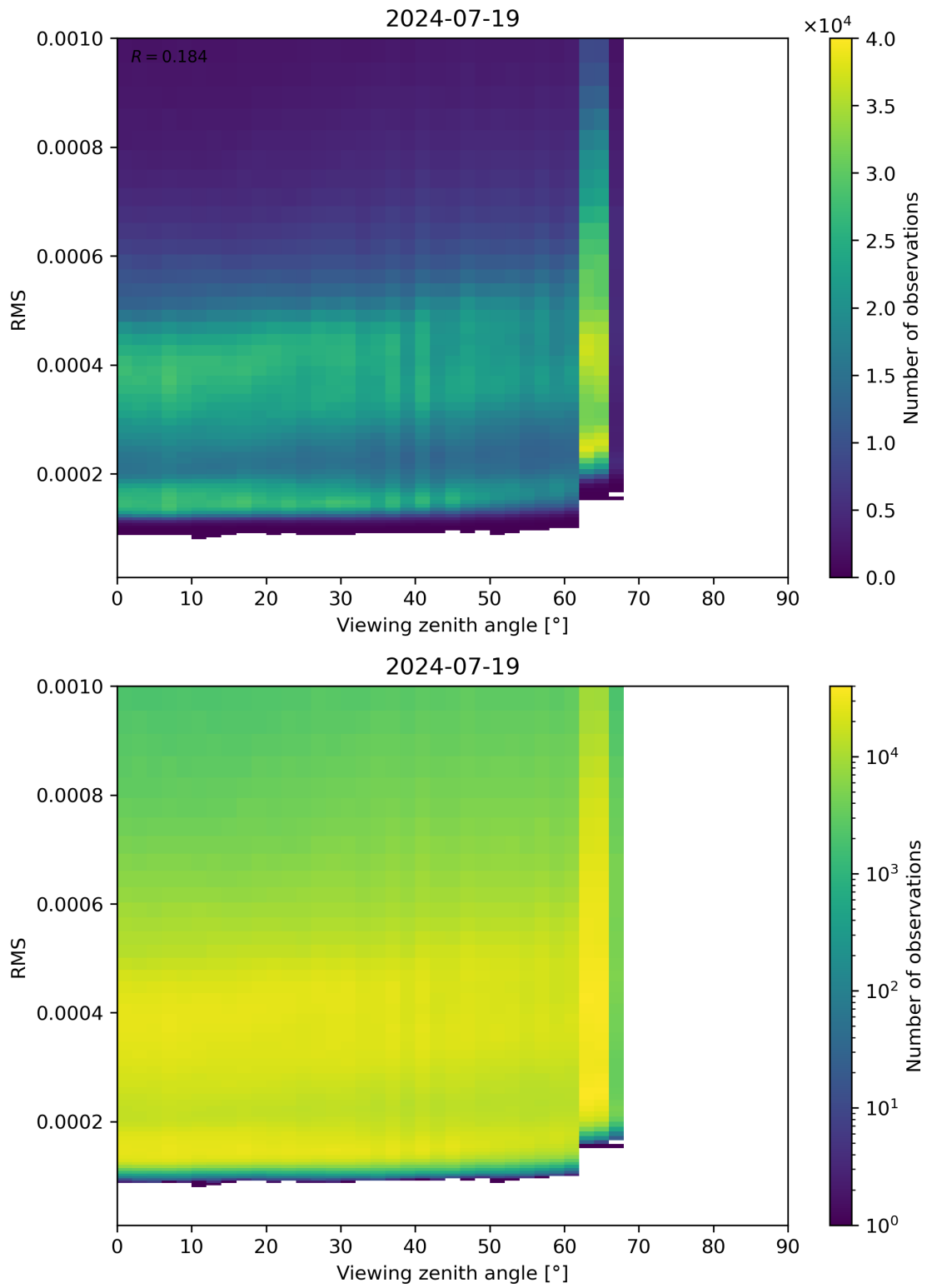
Figure 171: Scatter density plot of “Viewing zenith angle” against “RMS” for 2024-07-18 to 2024-07-20.
