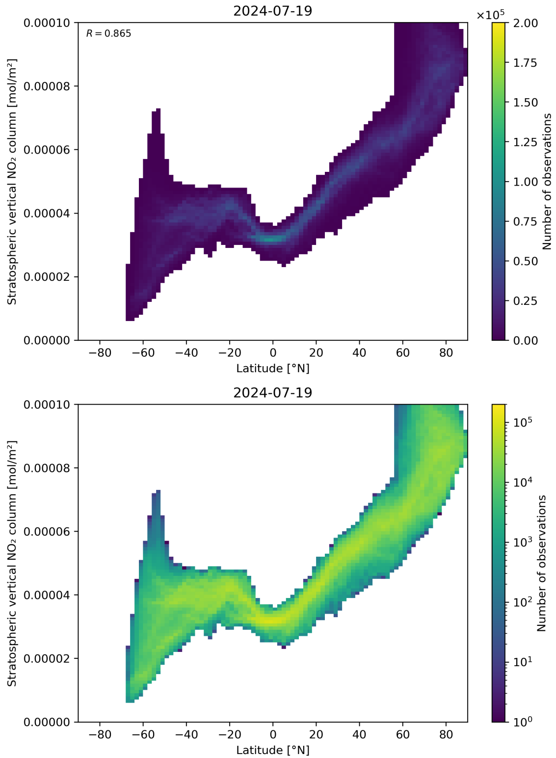
Figure 87: Scatter density plot of “Latitude” against “Stratospheric vertical NO 2 column” for 2024-07-18 to 2024-07-20.
