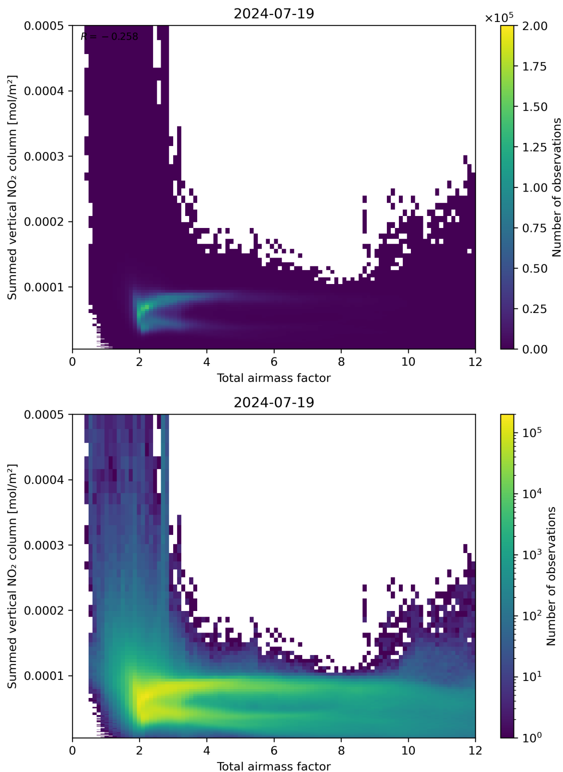
Figure 65: Scatter density plot of “Total airmass factor” against “Summed vertical NO 2 column” for 2024-07-18 to 2024-07-20.
