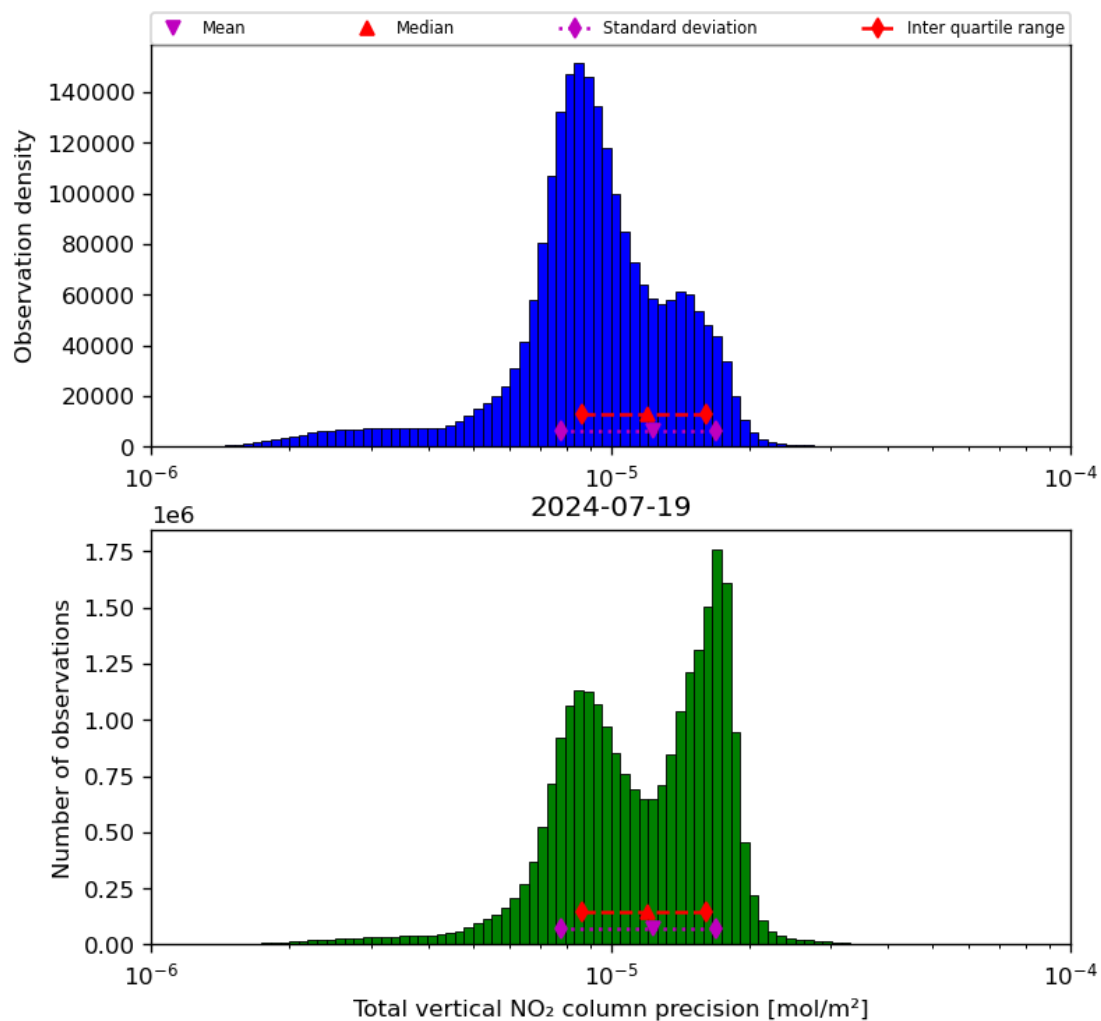
Figure 39: Histogram of “Total vertical NO 2 column precision” for 2024-07-18 to 2024-07-20
