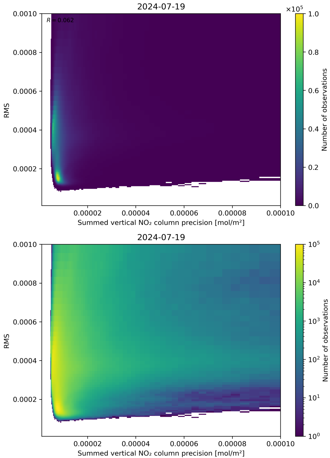
Figure 108: Scatter density plot of “Summed vertical NO 2 column precision” against “RMS” for 2024-07-18 to 2024-07-20.
