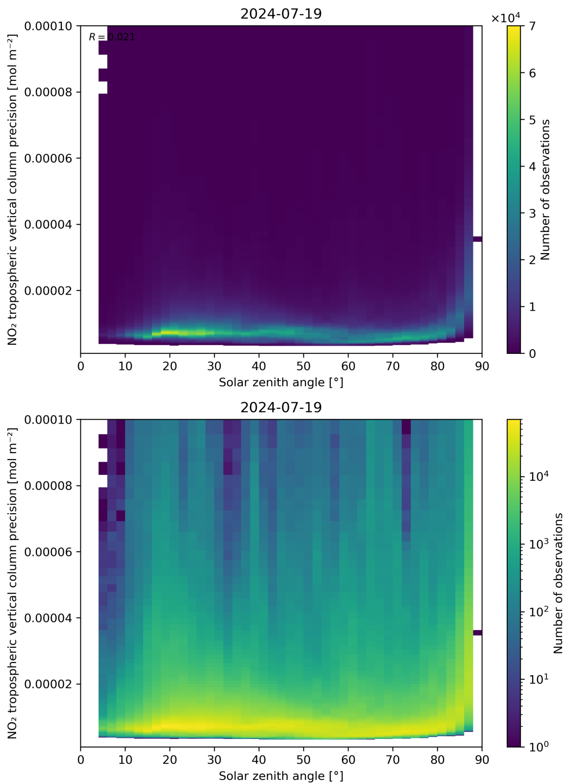
Figure 156: Scatter density plot of “Solar zenith angle” against “NO 2 tropospheric vertical column precision” for 2024-07-18 to 2024-07-20.
