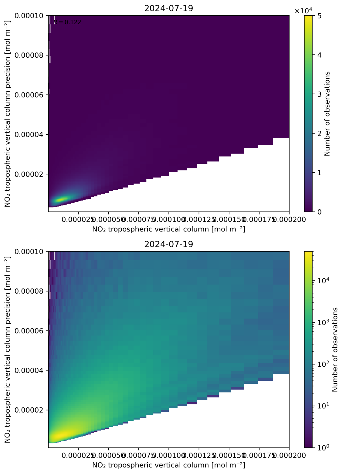
Figure 130: Scatter density plot of “NO 2 tropospheric vertical column” against “NO 2 tropospheric vertical column precision” for 2024-07-18 to 2024-07-20.
