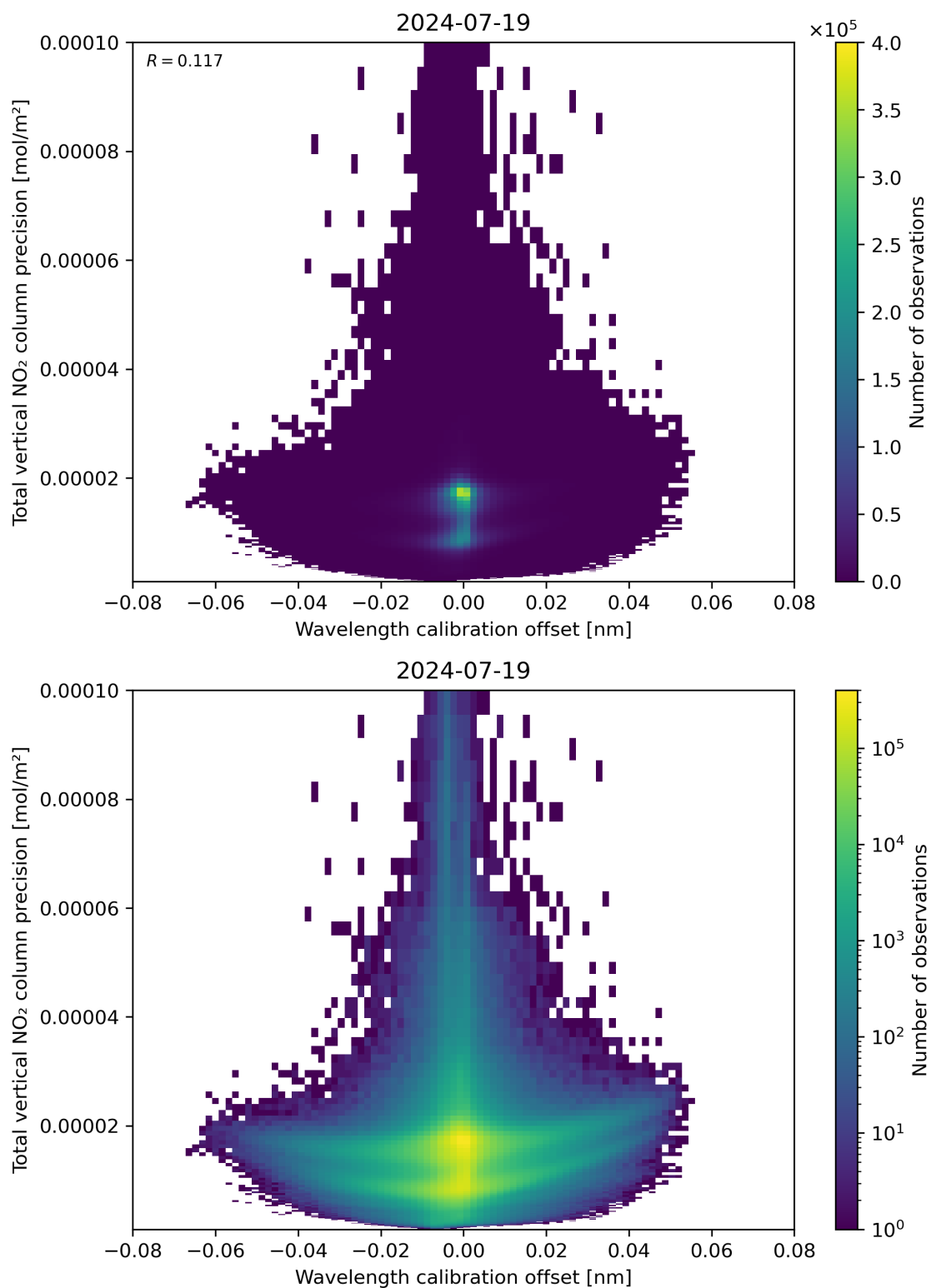
Figure 180: Scatter density plot of “Wavelength calibration offset” against “Total vertical NO 2 column precision” for 2024-07-18 to 2024-07-20.
