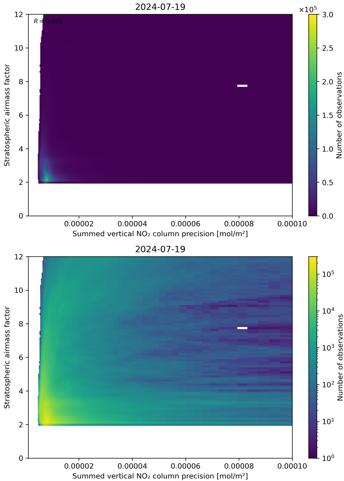
Figure 106: Scatter density plot of “Summed vertical NO 2 column precision” against “Stratospheric airmass factor” for 2024-07-18 to 2024-07-20.
