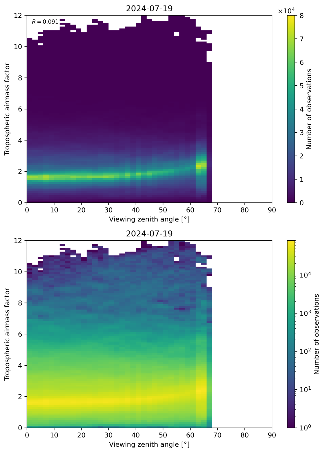
Figure 161: Scatter density plot of “Viewing zenith angle” against “Tropospheric airmass factor” for 2024-07-18 to 2024-07-20.
