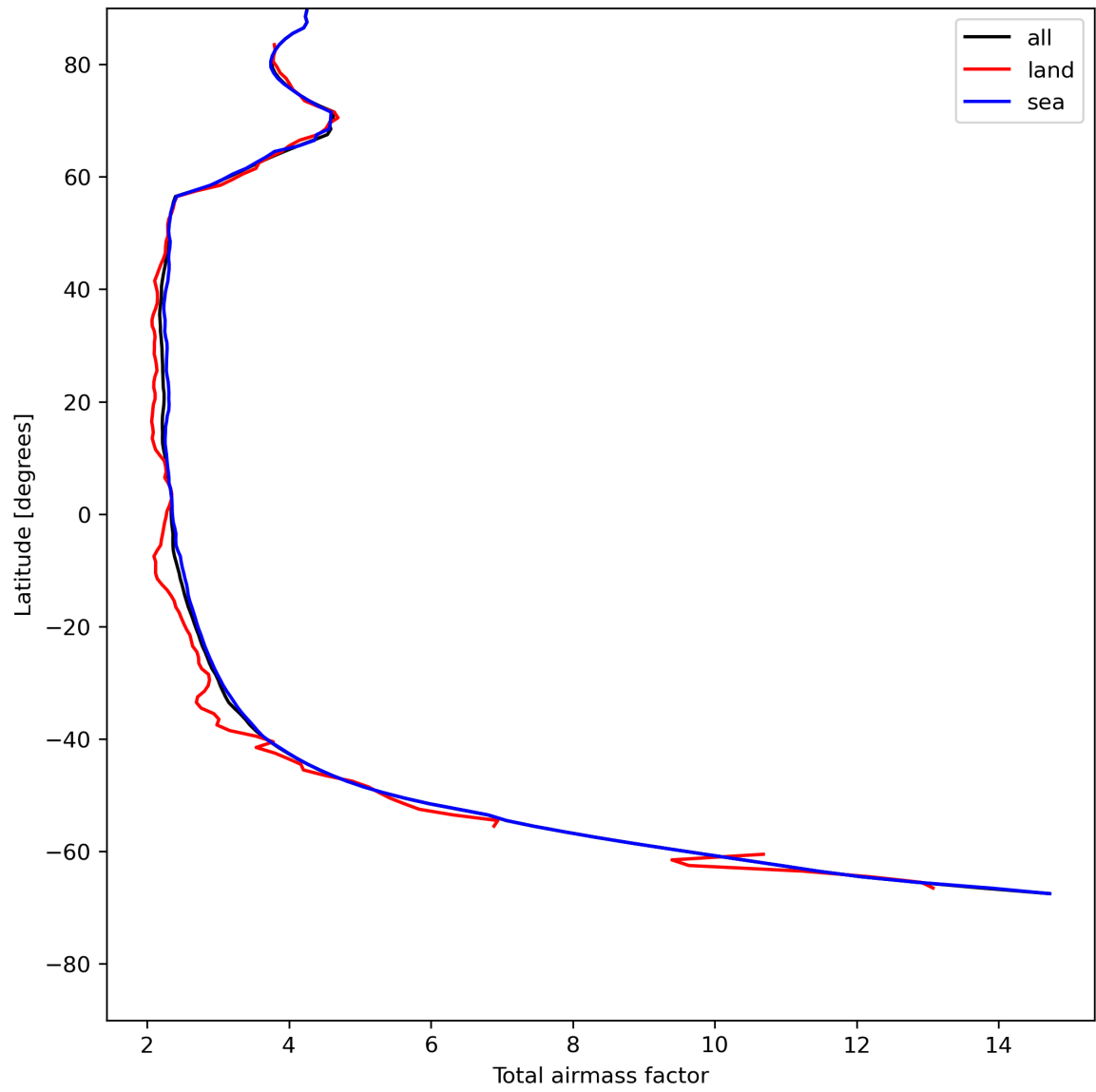
Figure 15: Zonal average of “Total airmass factor” for 2024-07-18 to 2024-07-20.
