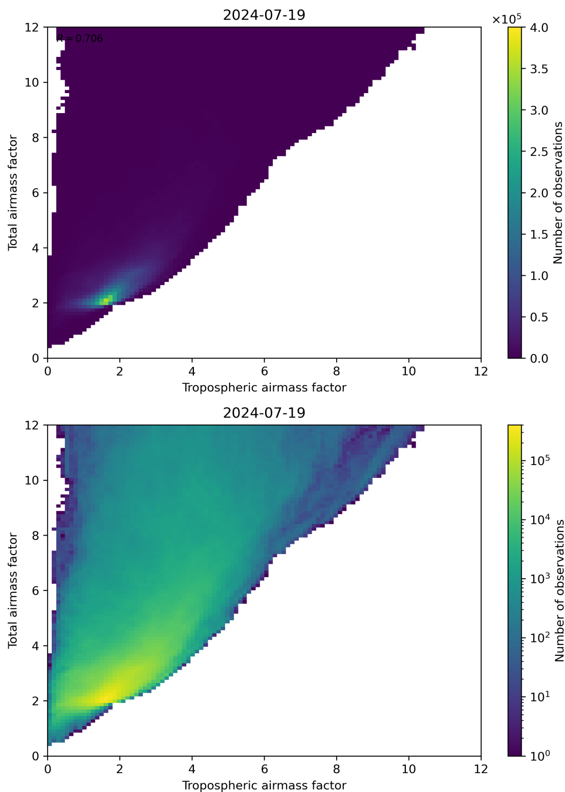
Figure 72: Scatter density plot of “Tropospheric airmass factor” against “Total airmass factor” for 2024-07-18 to 2024-07-20.
