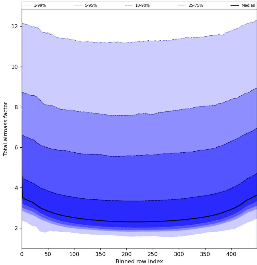
Figure 49: Along track statistics of “Total airmass factor” for 2024-07-18 to 2024-07-20
