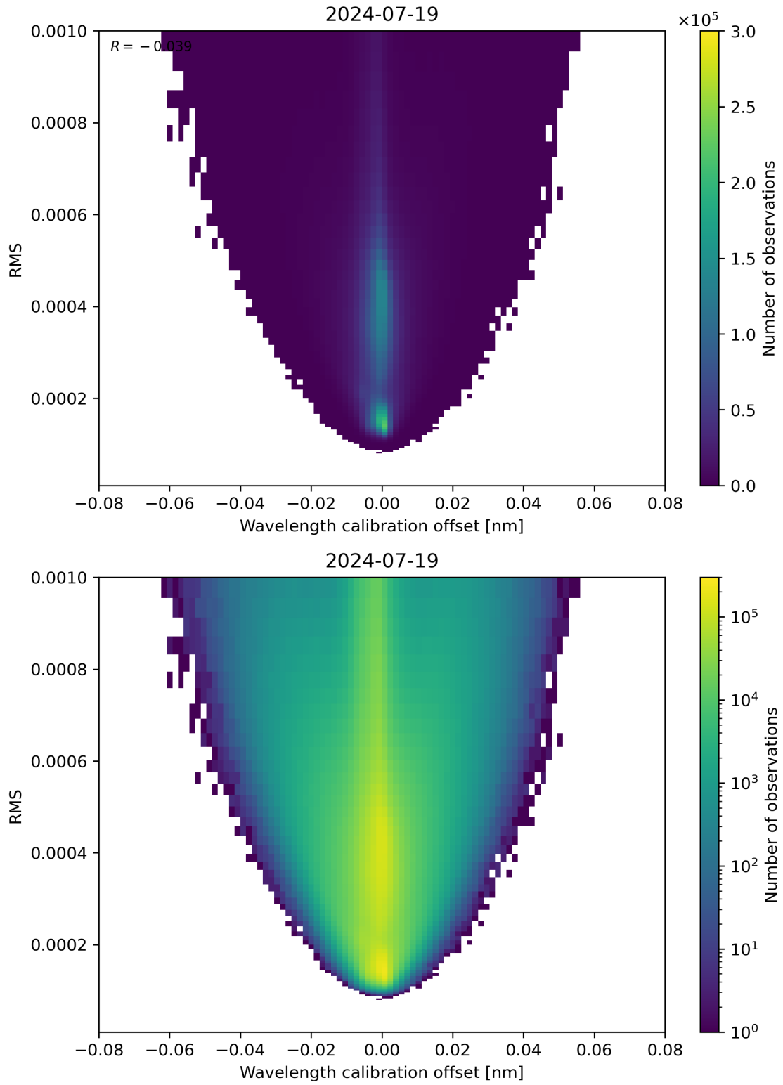
Figure 181: Scatter density plot of “Wavelength calibration offset” against “RMS” for 2024-07-18 to 2024-07-20.
