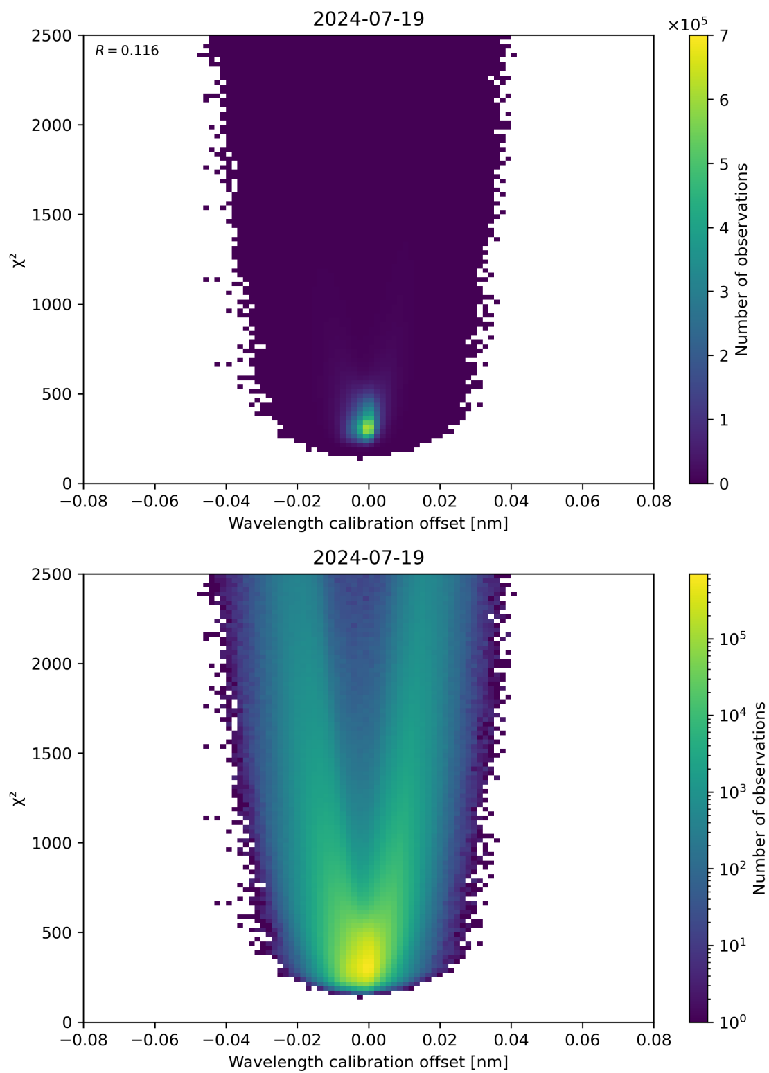
Figure 175: Scatter density plot of “Wavelength calibration offset” against “ \chi^2 ” for 2024-07-18 to 2024-07-20.
