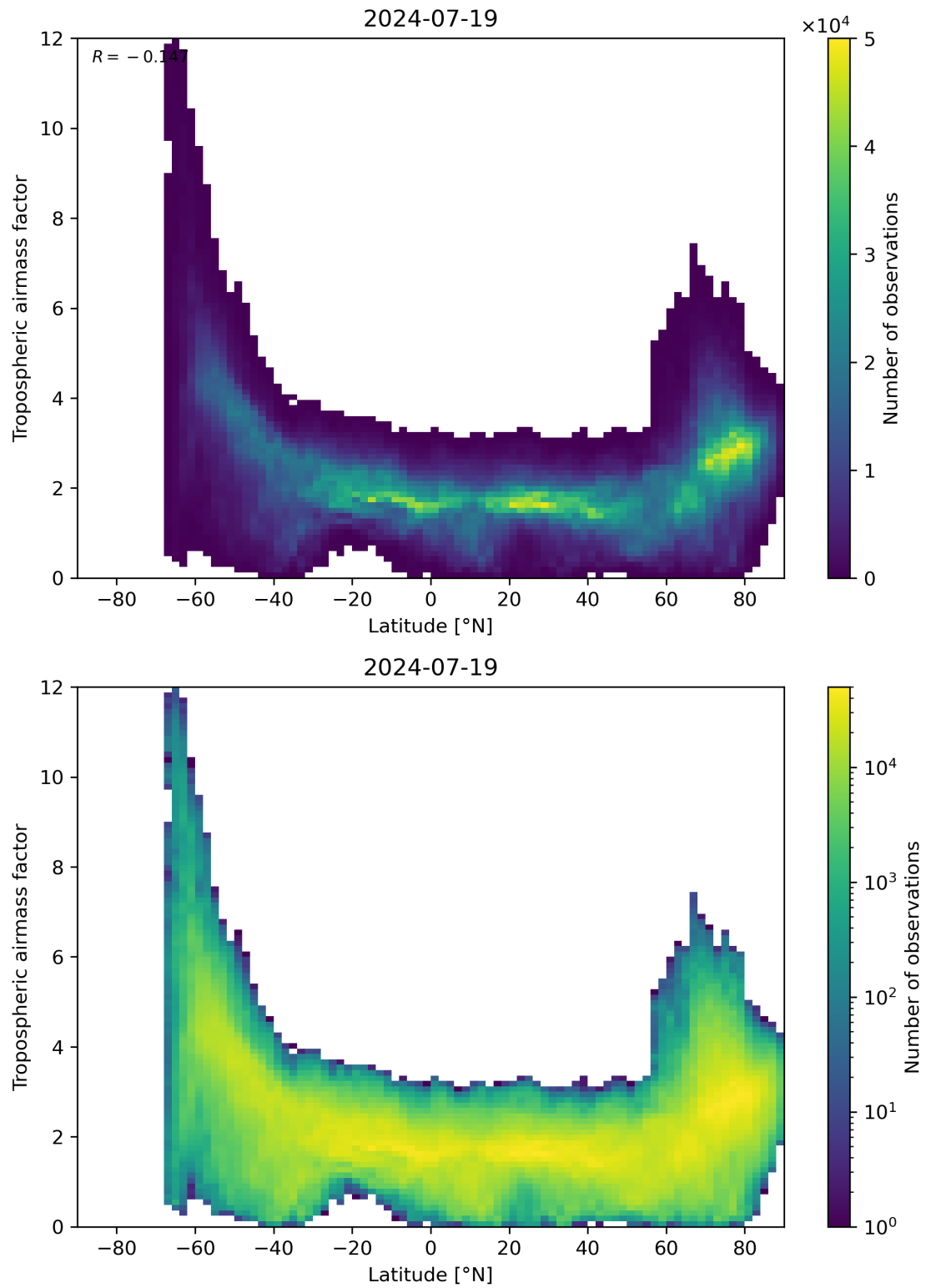
Figure 85: Scatter density plot of “Latitude” against “Tropospheric air mass factor” for 2024-07-18 to 2024-07-20.
