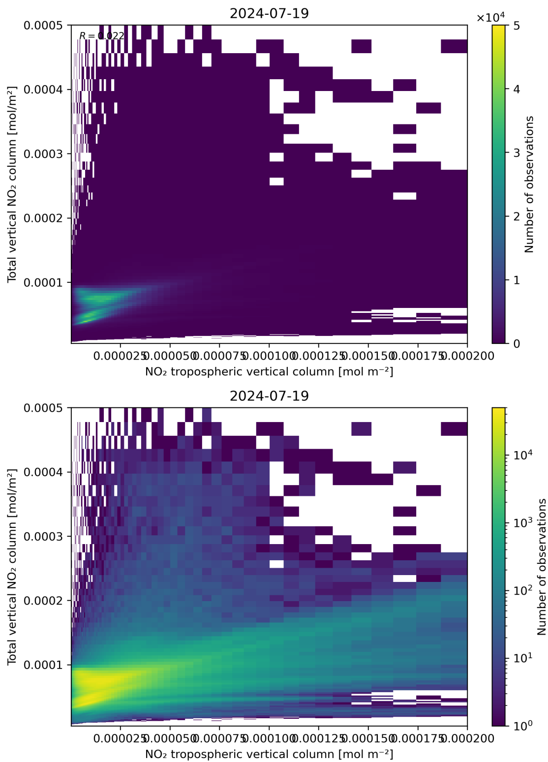
Figure 128: Scatter density plot of “NO 2 tropospheric vertical column” against “Total vertical NO 2 column” for 2024-07-18 to 2024-07-20.
