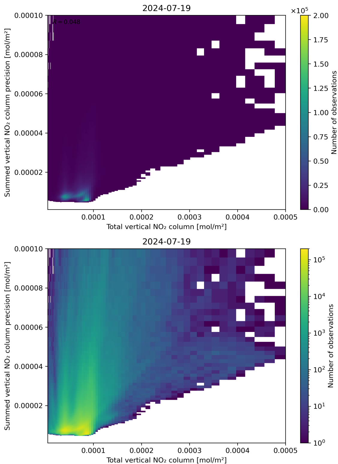
Figure 113: Scatter density plot of “Total vertical NO 2 column” against “Summed vertical NO 2 column precision” for 2024-07-18 to 2024-07-20.
