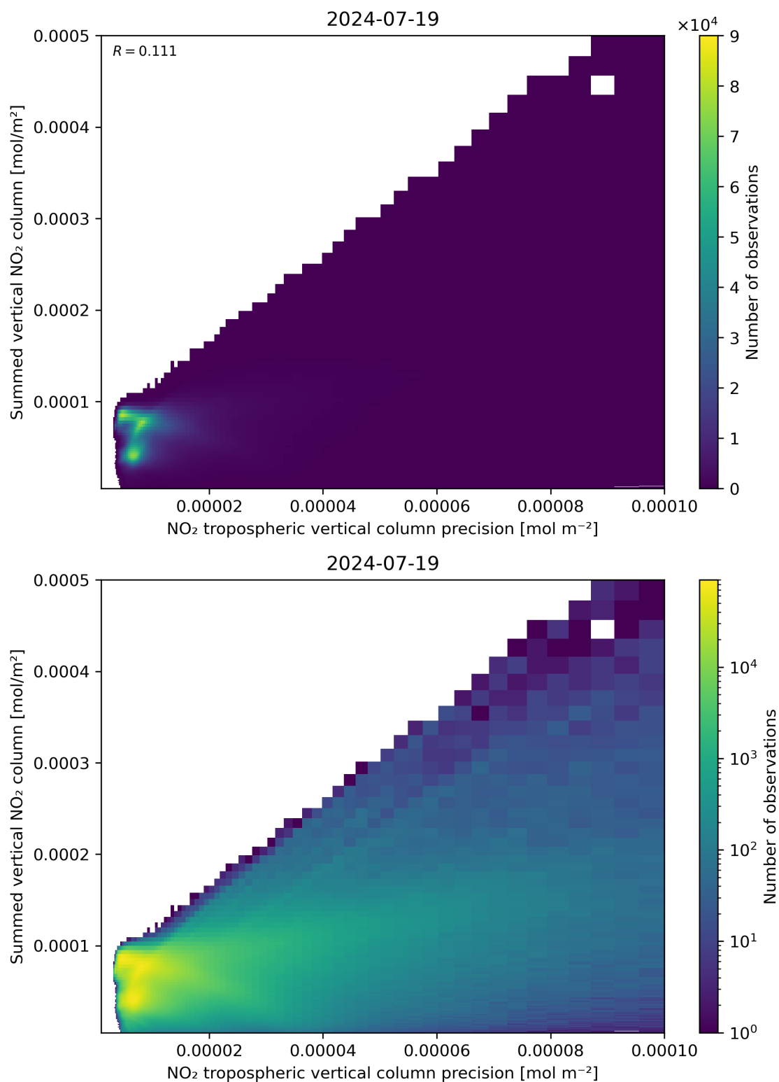
Figure 136: Scatter density plot of “NO 2 tropospheric vertical column precision” against “Summed vertical NO 2 column” for 2024-07-18 to 2024-07-20.
