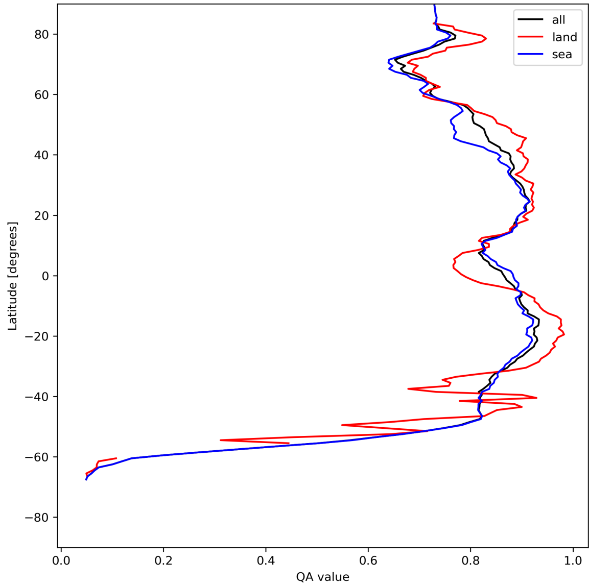
Figure 11: Zonal average of “QA value” for 2024-07-18 to 2024-07-20.
