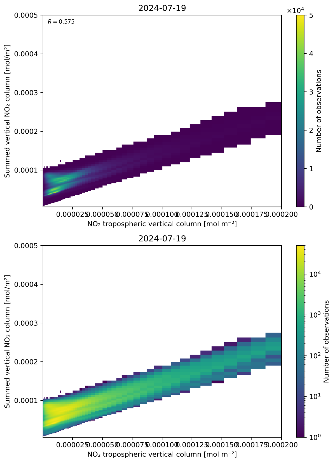
Figure 126: Scatter density plot of “NO 2 tropospheric vertical column” against “Summed vertical NO 2 column” for 2024-07-18 to 2024-07-20.
