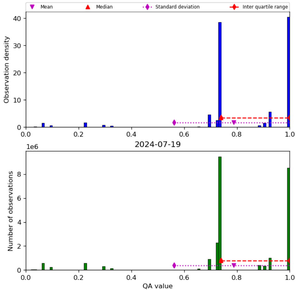
Figure 28: Histogram of “QA value” for 2024-07-18 to 2024-07-20
