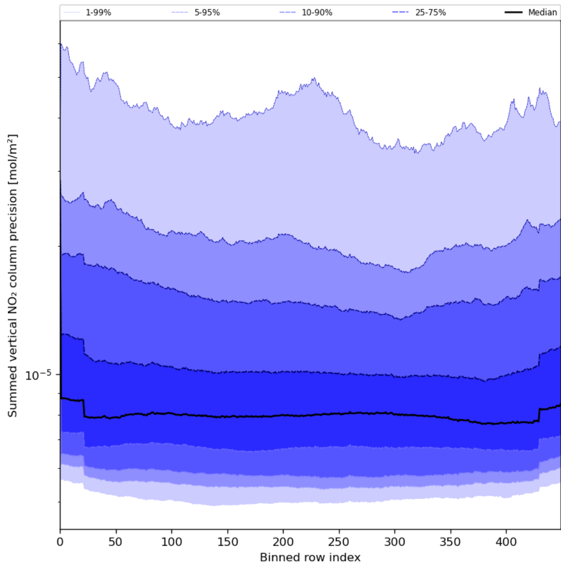
Figure 58: Along track statistics of “Summed vertical NO 2 column precision” for 2024-07-18 to 2024-07-20
