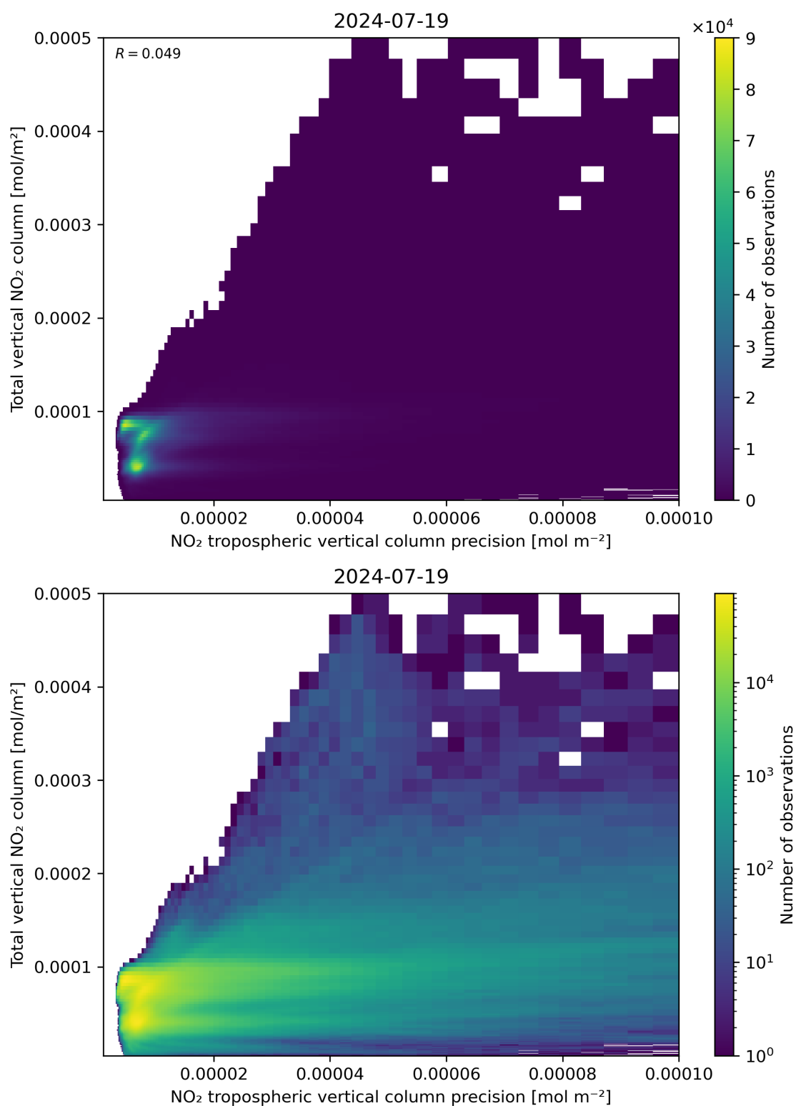
Figure 138: Scatter density plot of “NO 2 tropospheric vertical column precision” against “Total vertical NO 2 column” for 2024-07-18 to 2024-07-20.
