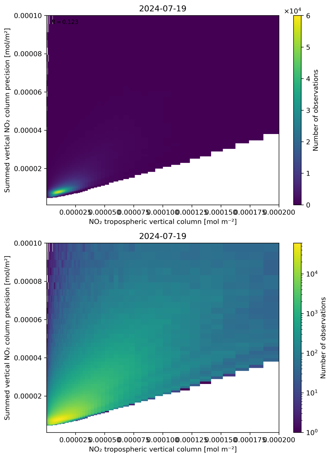
Figure 127: Scatter density plot of “NO 2 tropospheric vertical column” against “Summed vertical NO 2 column precision” for 2024-07-18 to 2024-07-20.
