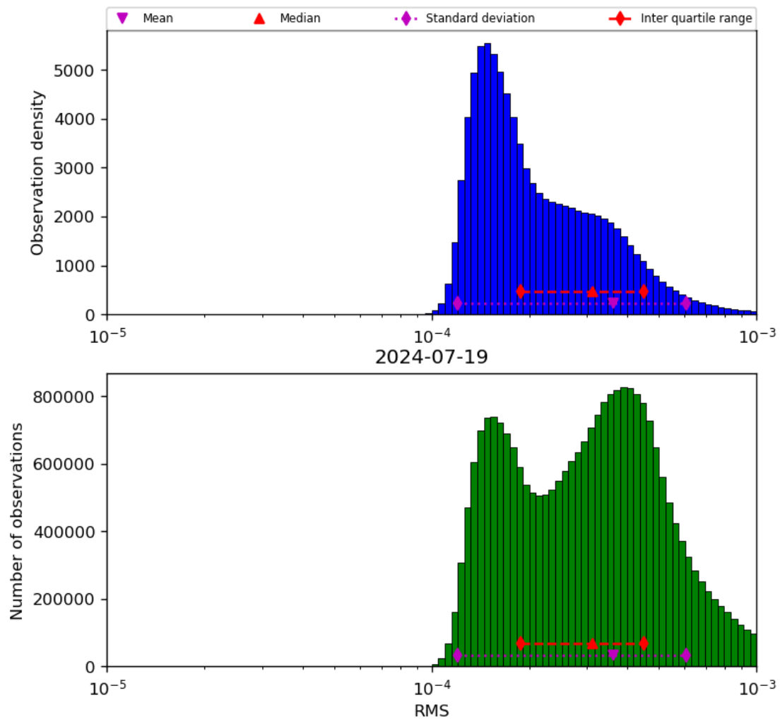
Figure 43: Histogram of “RMS” for 2024-07-18 to 2024-07-20
