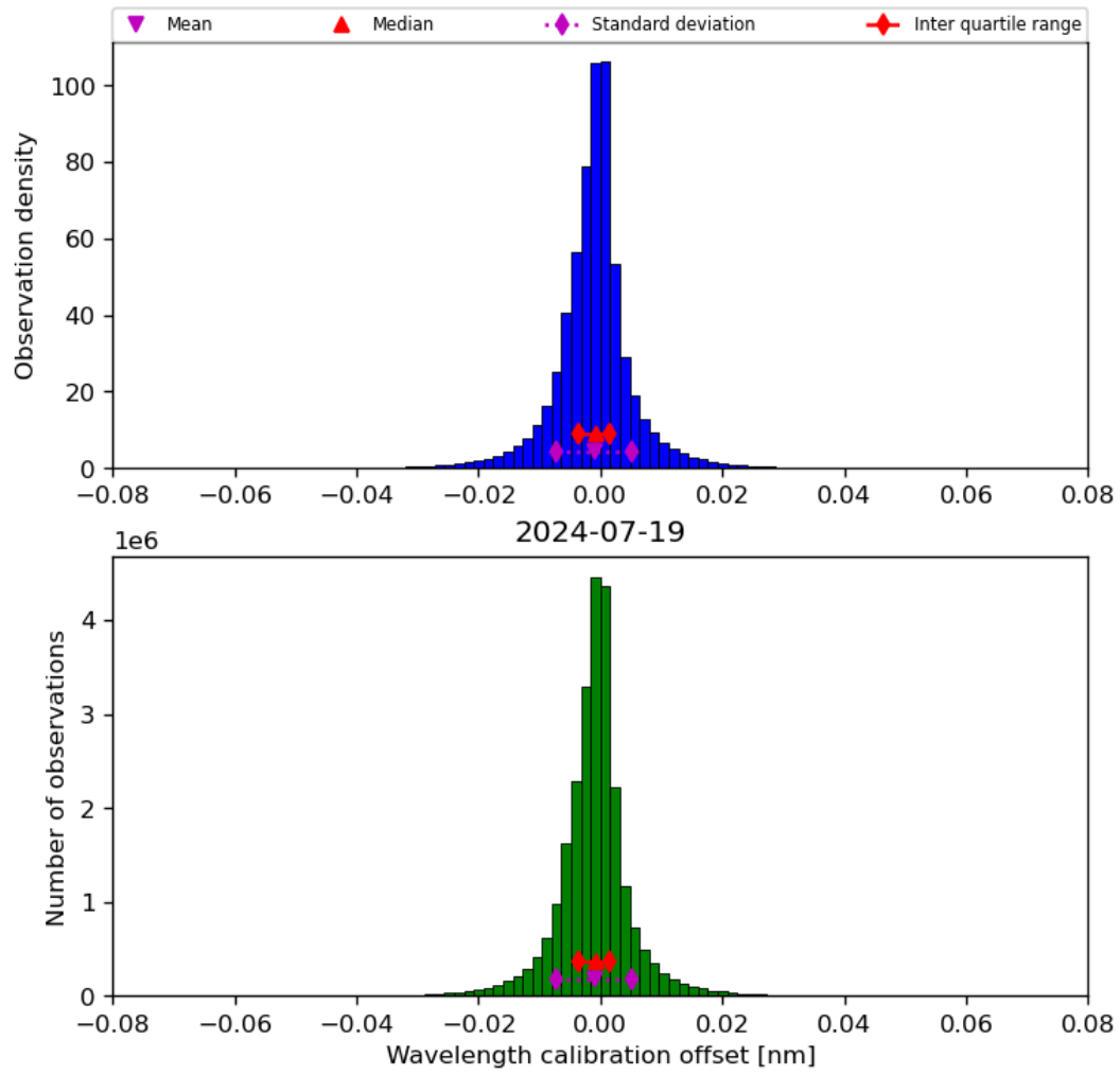
Figure 35: Histogram of “Wavelength calibration offset” for 2024-07-18 to 2024-07-20
