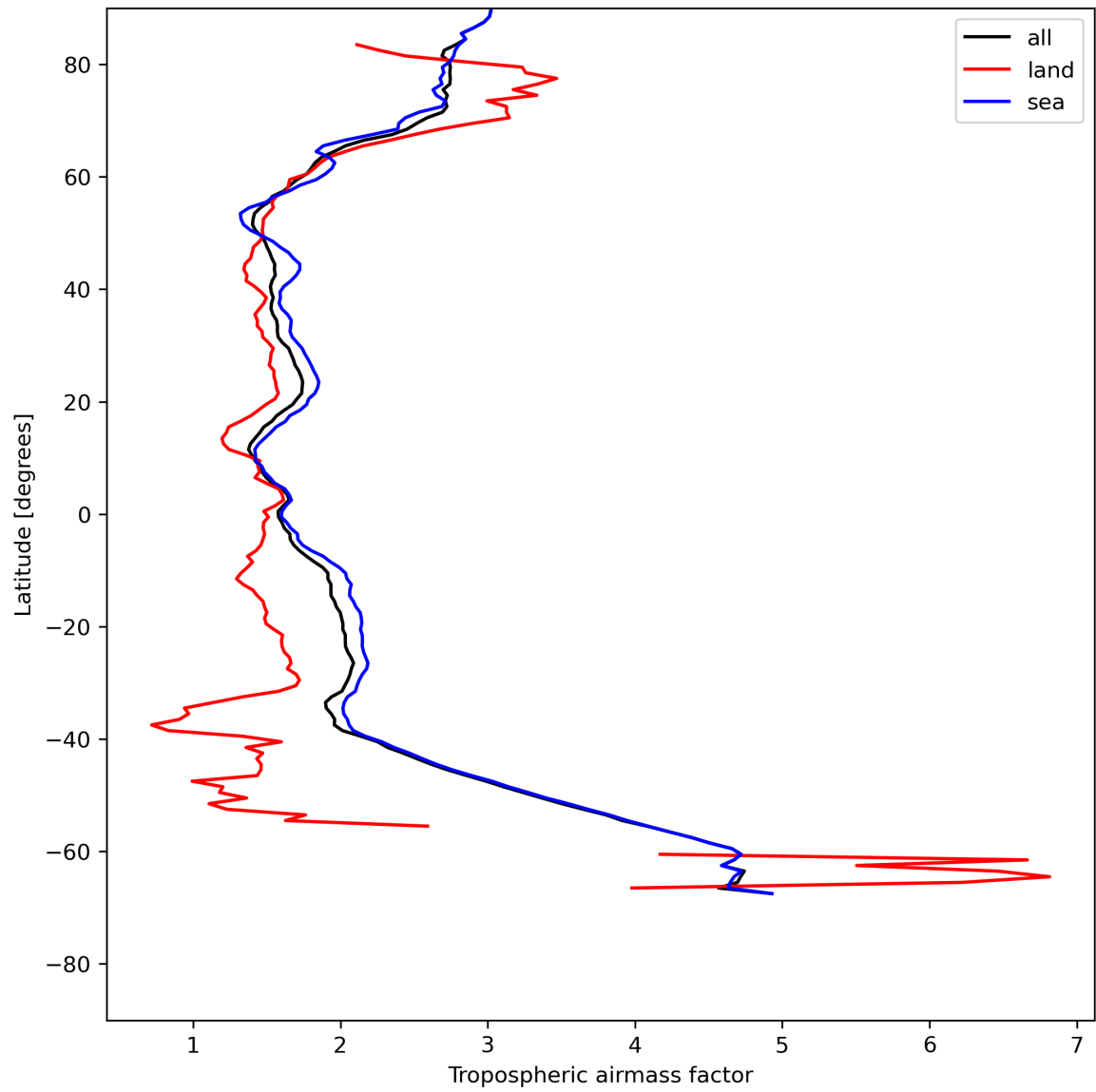
Figure 14: Zonal average of “Tropospheric airmass factor” for 2024-07-18 to 2024-07-20.
