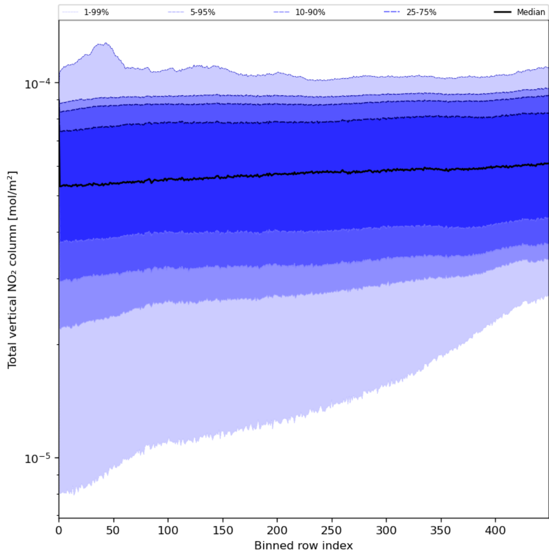
Figure 55: Along track statistics of “Total vertical NO 2 column” for 2024-07-18 to 2024-07-20
