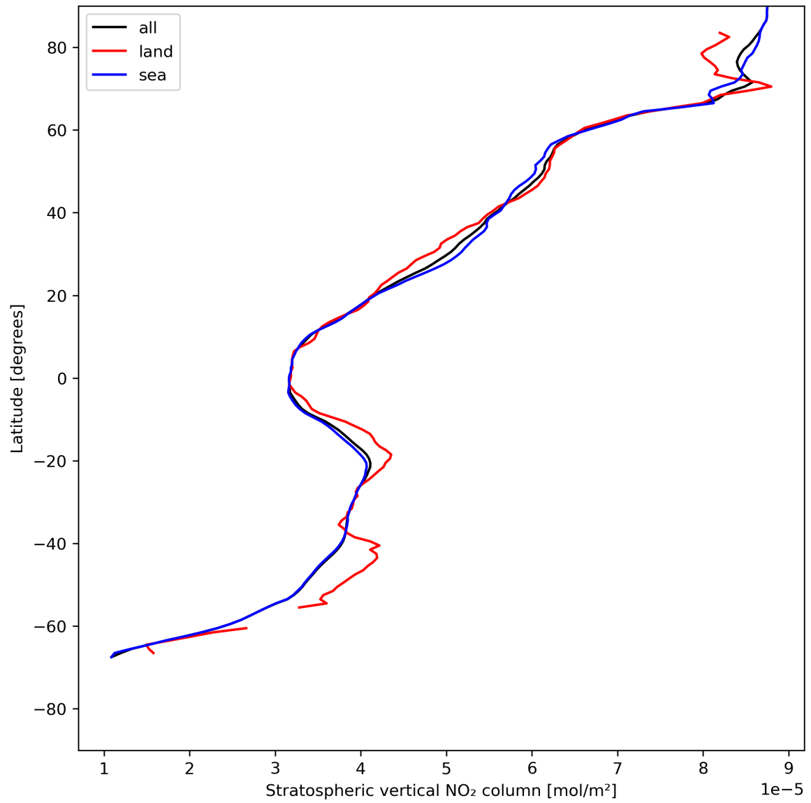
Figure 19: Zonal average of “Stratospheric vertical NO 2 column” for 2024-07-18 to 2024-07-20.
