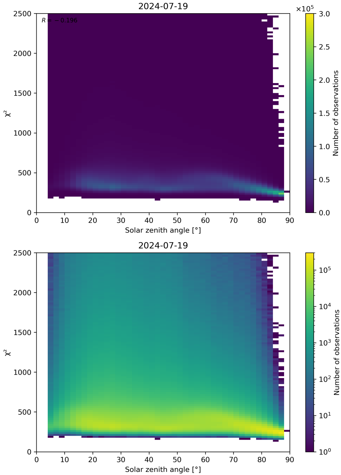
Figure 148: Scatter density plot of “Solar zenith angle” against “ \chi^2 ” for 2024-07-18 to 2024-07-20.
