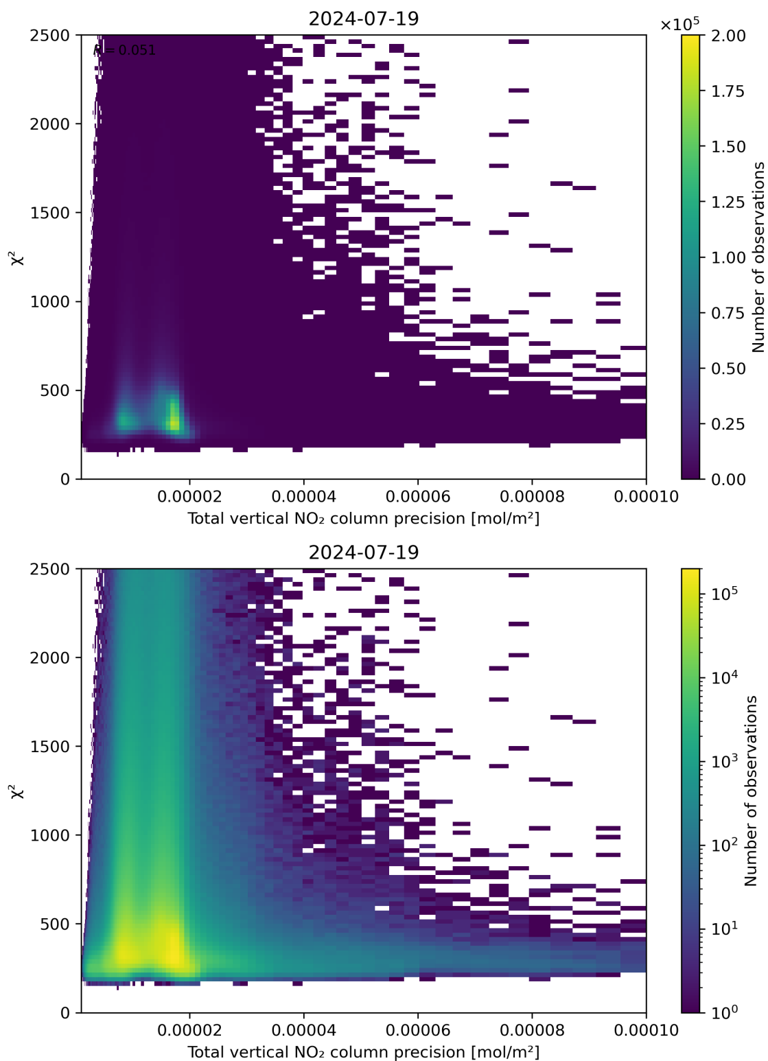
Figure 116: Scatter density plot of “Total vertical NO 2 column precision” against “ \chi^2 ” for 2024-07-18 to 2024-07-20.
