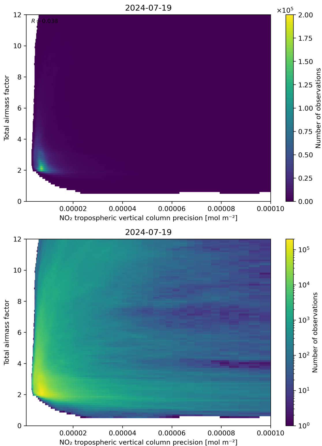
Figure 132: Scatter density plot of “NO 2 tropospheric vertical column precision” against “Total air mass factor” for 2024-07-18 to 2024-07-20.
