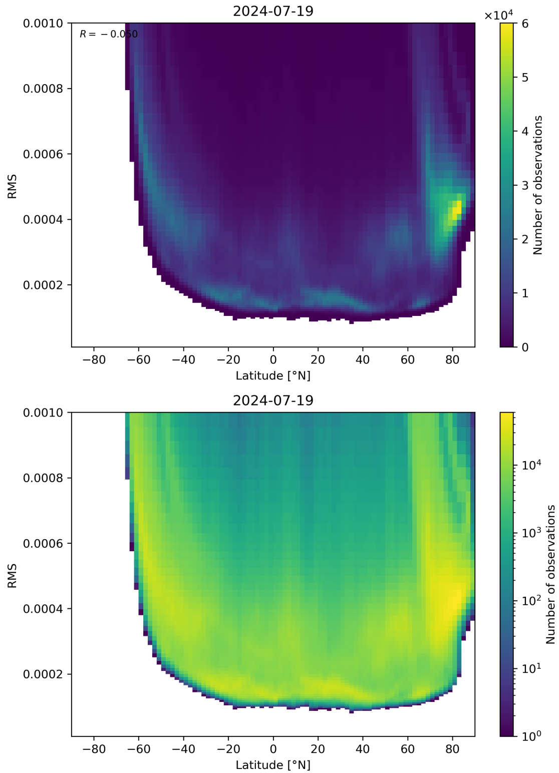
Figure 94: Scatter density plot of “Latitude” against “RMS” for 2024-07-18 to 2024-07-20.
