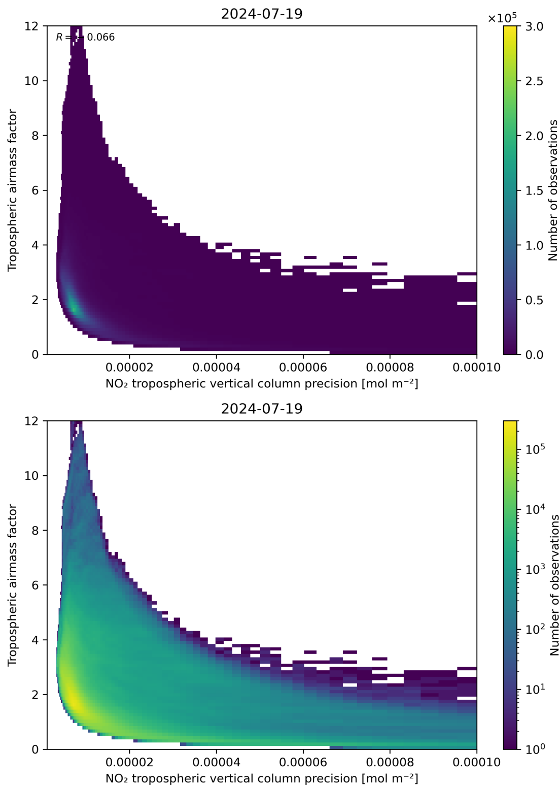
Figure 133: Scatter density plot of “NO 2 tropospheric vertical column precision” against “Tropospheric airmass factor” for 2024-07-18 to 2024-07-20.
