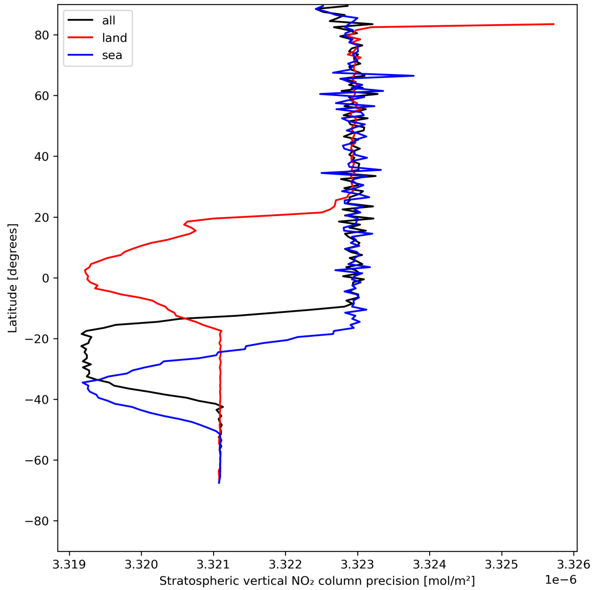
Figure 20: Zonal average of “Stratospheric vertical NO 2 column precision” for 2024-07-18 to 2024-07-20.
