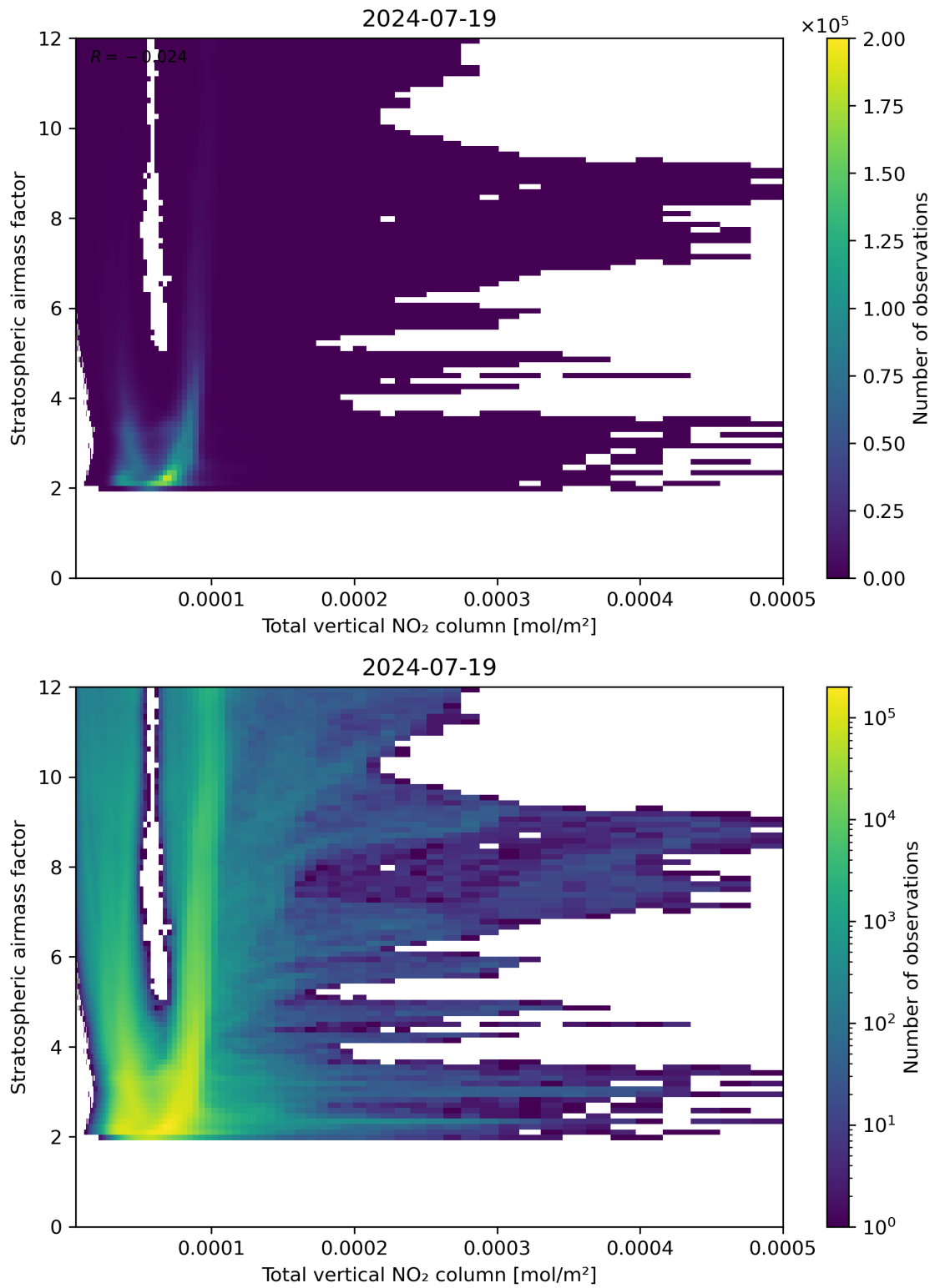
Figure 110: Scatter density plot of “Total vertical NO 2 column” against “Stratospheric airmass factor” for 2024-07-18 to 2024-07-20.
