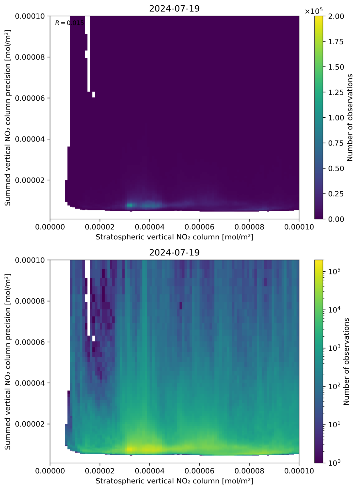
Figure 99: Scatter density plot of “Stratospheric vertical NO 2 column” against “Summed vertical NO 2 column precision” for 2024-07-18 to 2024-07-20.
