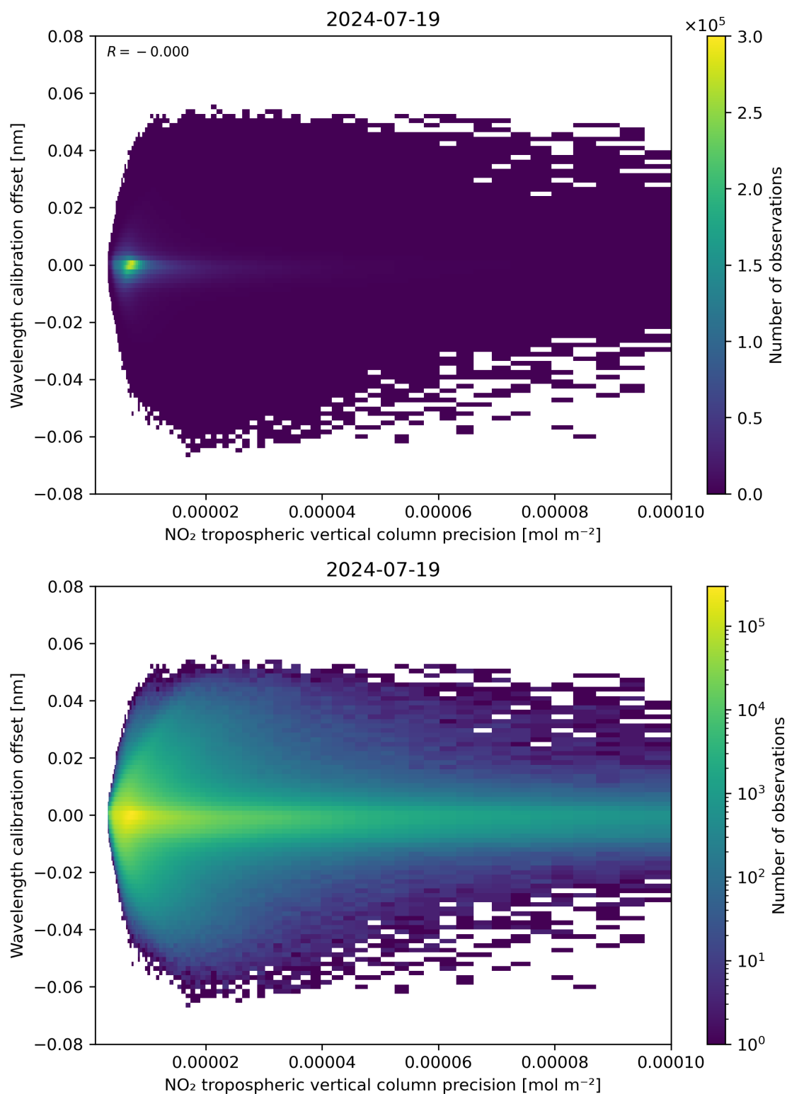
Figure 141: Scatter density plot of “NO 2 tropospheric vertical column precision” against “Wavelength calibration offset” for 2024-07-18 to 2024-07-20.
