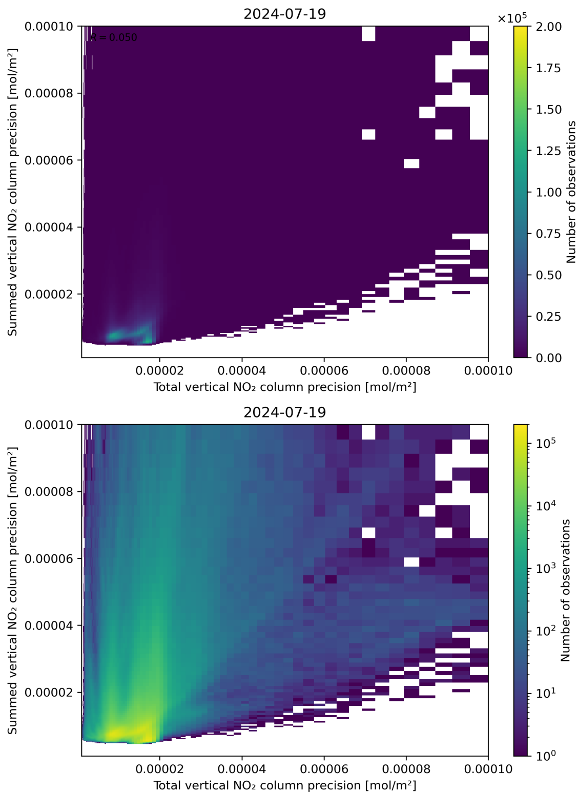
Figure 118: Scatter density plot of “Total vertical NO 2 column precision” against “Summed vertical NO 2 column precision” for 2024-07-18 to 2024-07-20.
