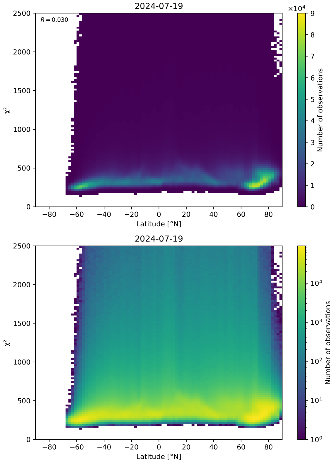
Figure 86: Scatter density plot of “Latitude” against “ \chi^2 ” for 2024-07-18 to 2024-07-20.
