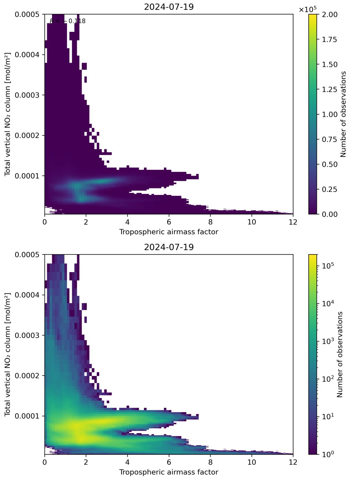
Figure 77: Scatter density plot of “Tropospheric airmass factor” against “Total vertical NO 2 column” for 2024-07-18 to 2024-07-20.
