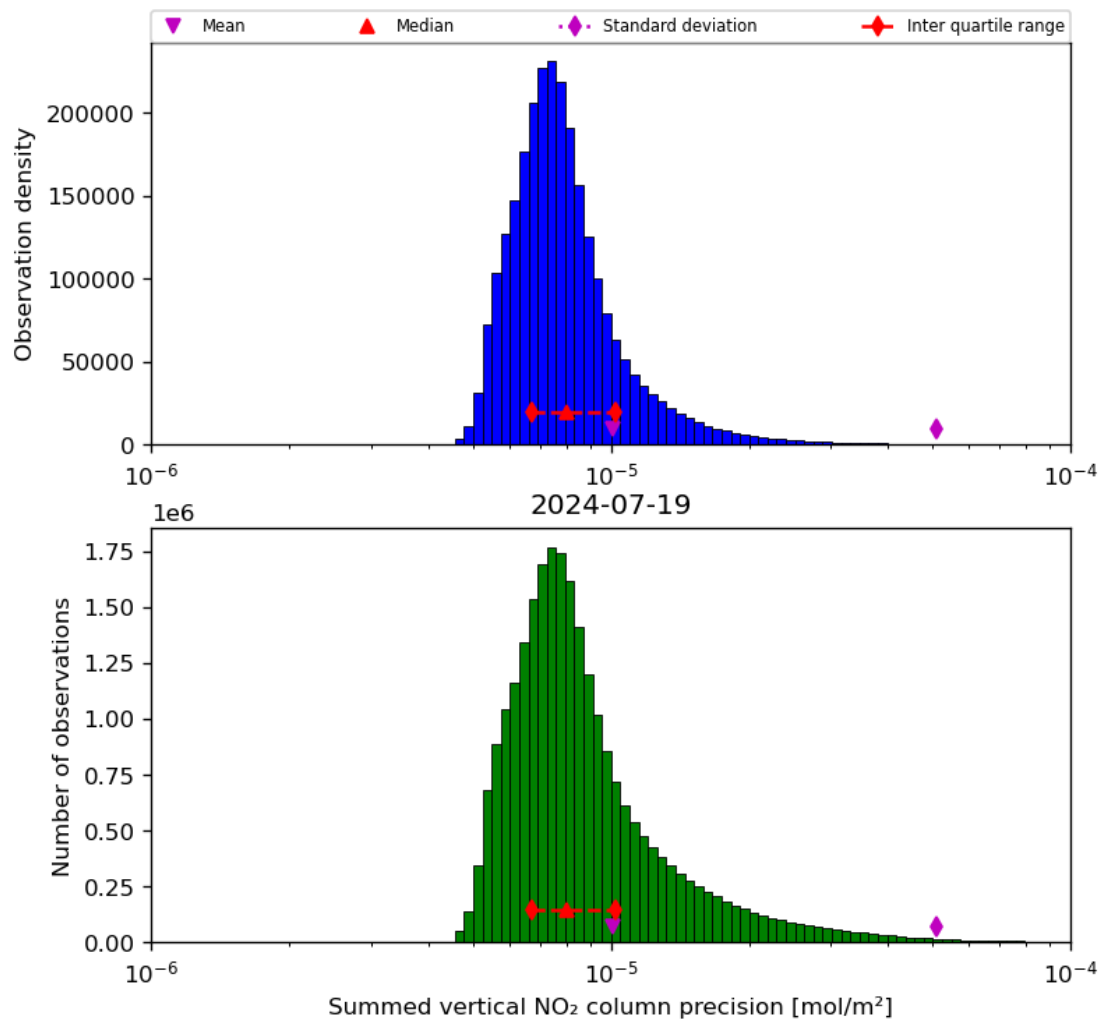
Figure 41: Histogram of “Summed vertical NO 2 column precision” for 2024-07-18 to 2024-07-20
