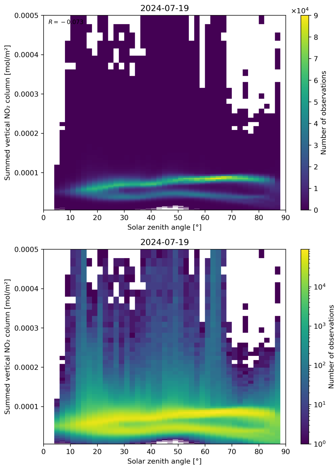
Figure 151: Scatter density plot of “Solar zenith angle” against “Summed vertical NO 2 column” for 2024-07-18 to 2024-07-20.
