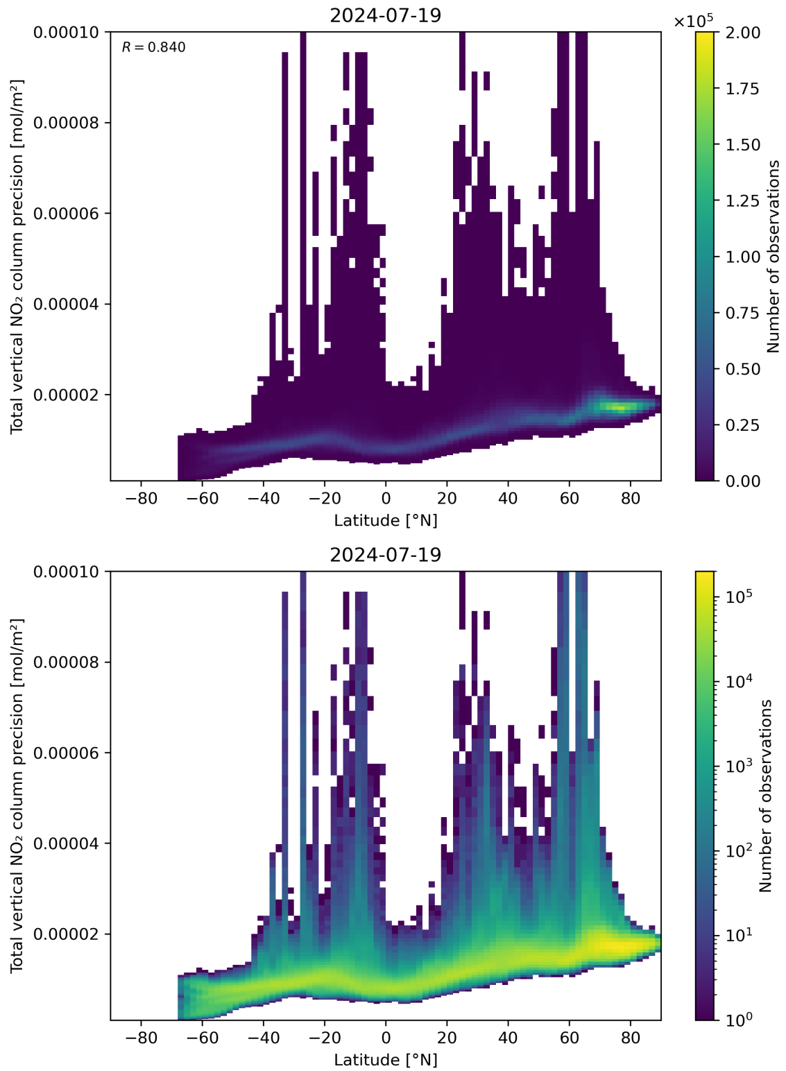
Figure 91: Scatter density plot of “Latitude” against “Total vertical NO 2 column precision” for 2024-07-18 to 2024-07-20.
