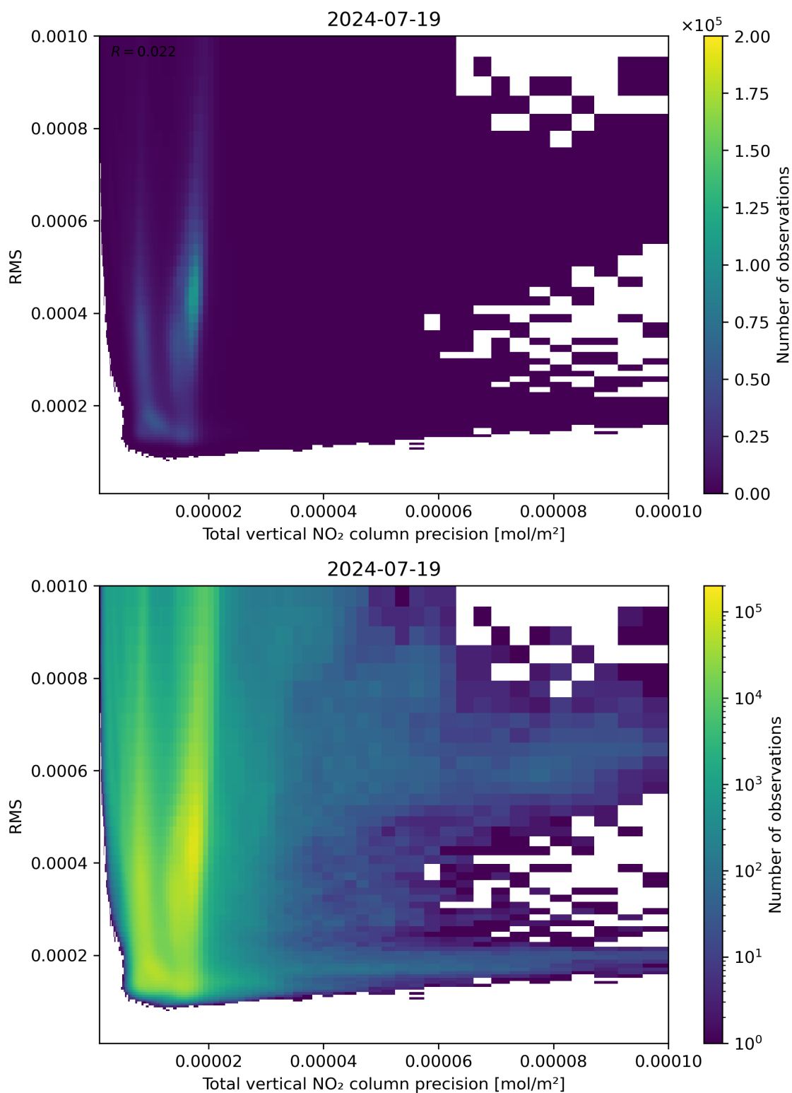
Figure 119: Scatter density plot of “Total vertical NO 2 column precision” against “RMS” for 2024-07-18 to 2024-07-20.
