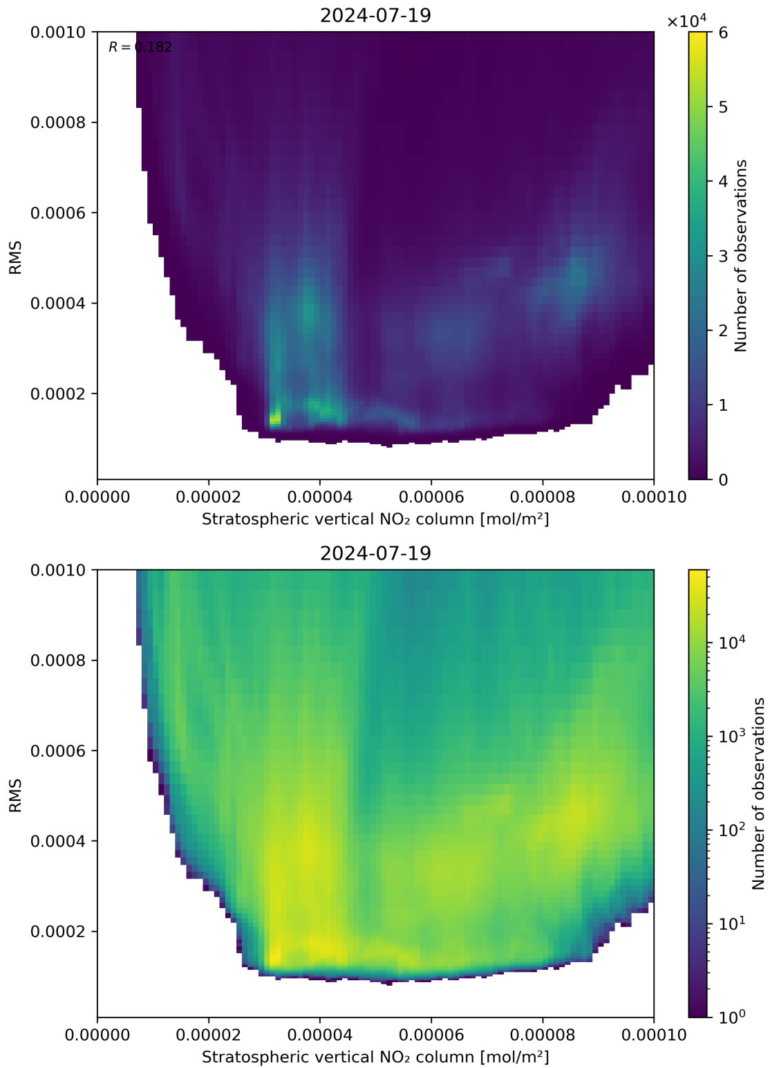
Figure 102: Scatter density plot of “Stratospheric vertical NO 2 column” against “RMS” for 2024-07-18 to 2024-07-20.
