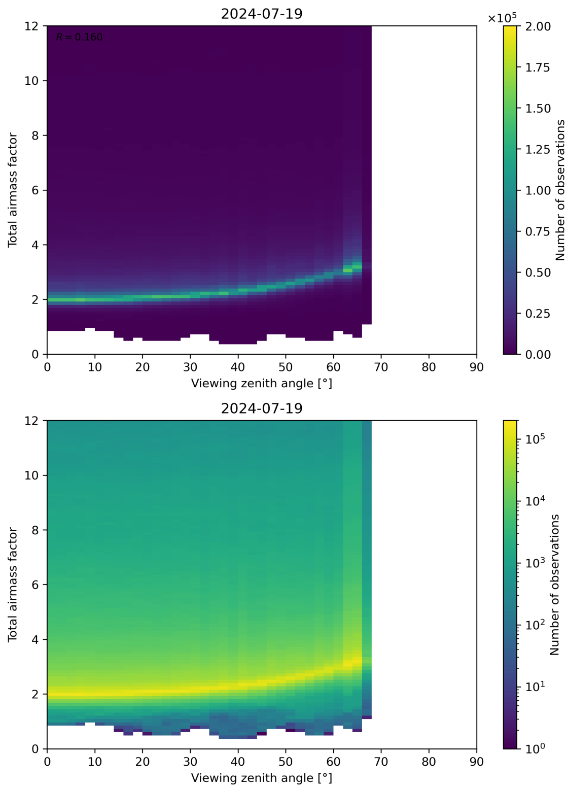
Figure 160: Scatter density plot of “Viewing zenith angle” against “Total airmass factor” for 2024-07-18 to 2024-07-20.
