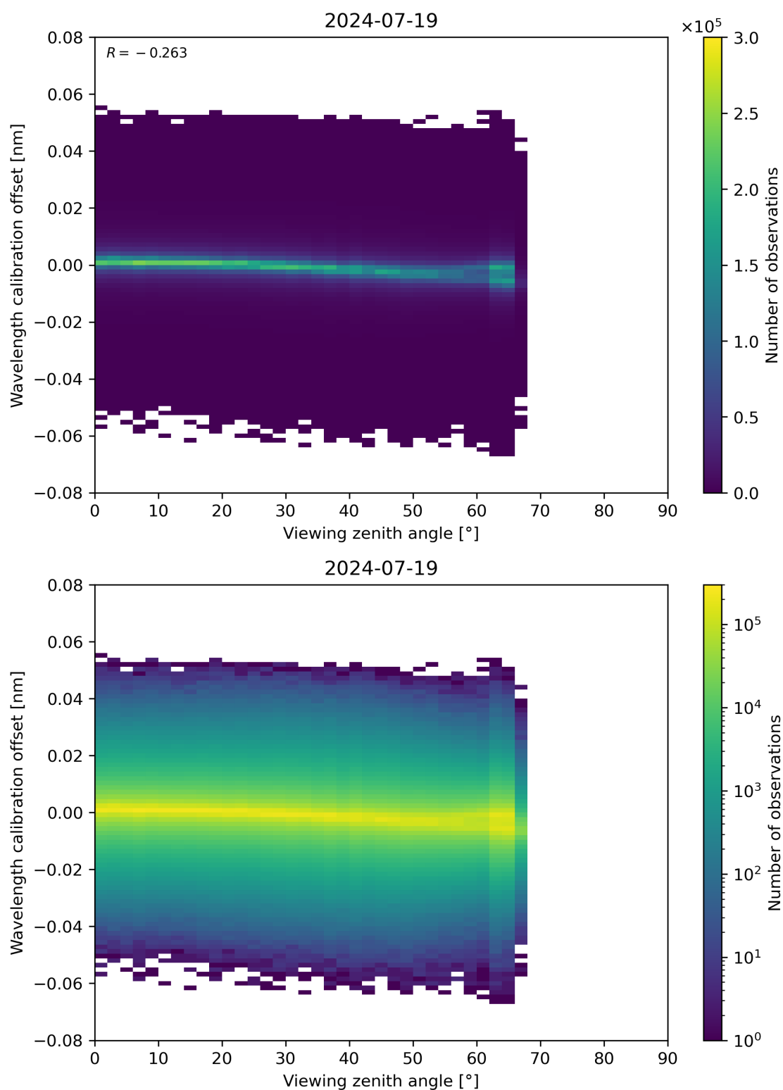
Figure 173: Scatter density plot of “Viewing zenith angle” against “Wavelength calibration offset” for 2024-07-18 to 2024-07-20.
