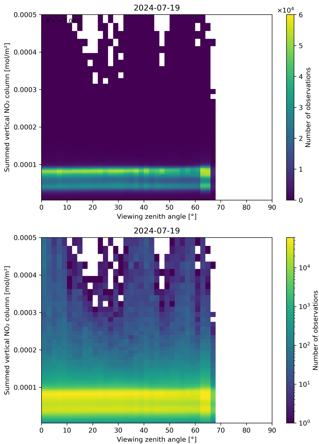
Figure 165: Scatter density plot of “Viewing zenith angle” against “Summed vertical NO 2 column” for 2024-07-18 to 2024-07-20.
