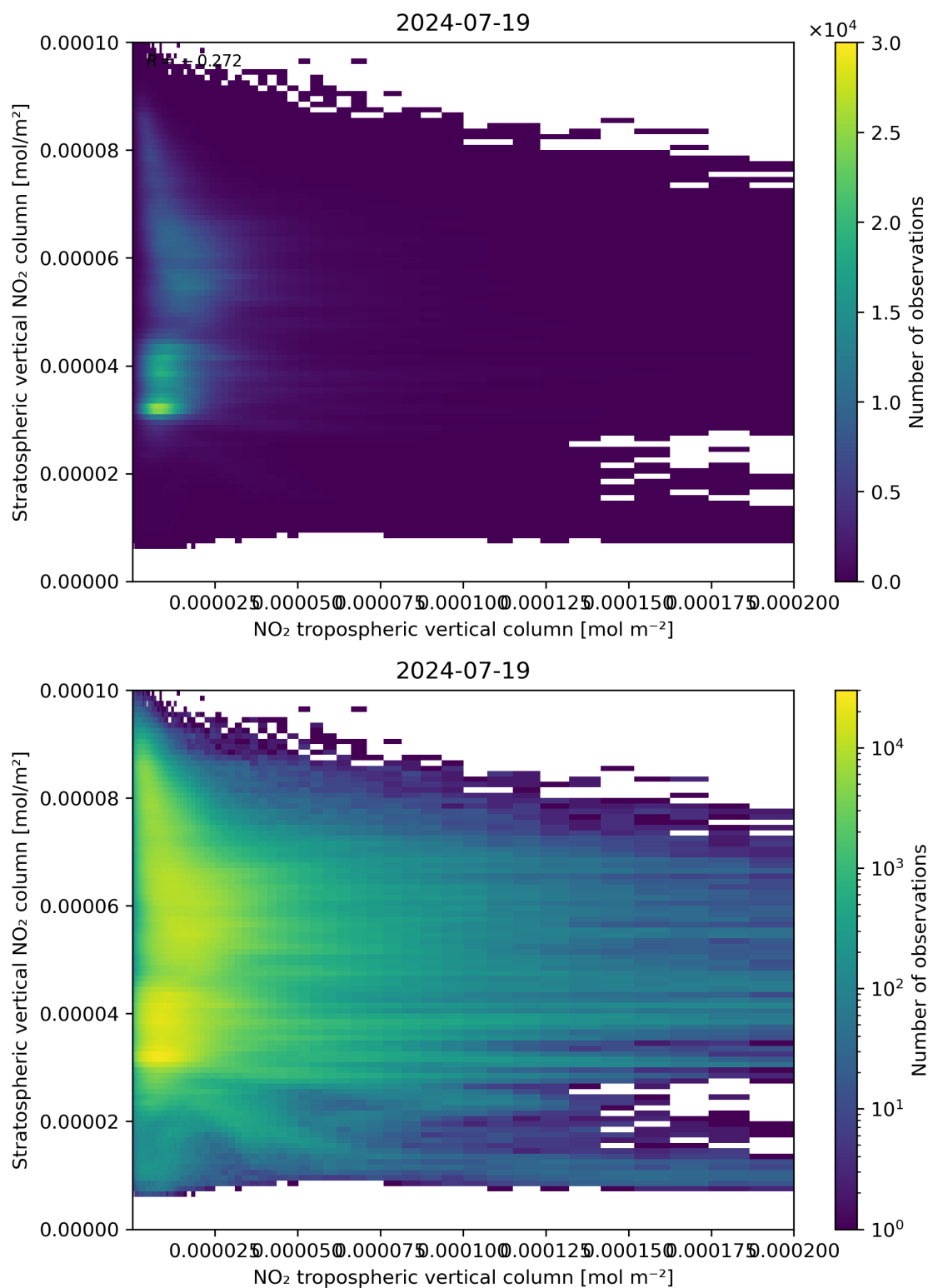
Figure 125: Scatter density plot of “NO 2 tropospheric vertical column” against “Stratospheric vertical NO 2 column” for 2024-07-18 to 2024-07-20.
