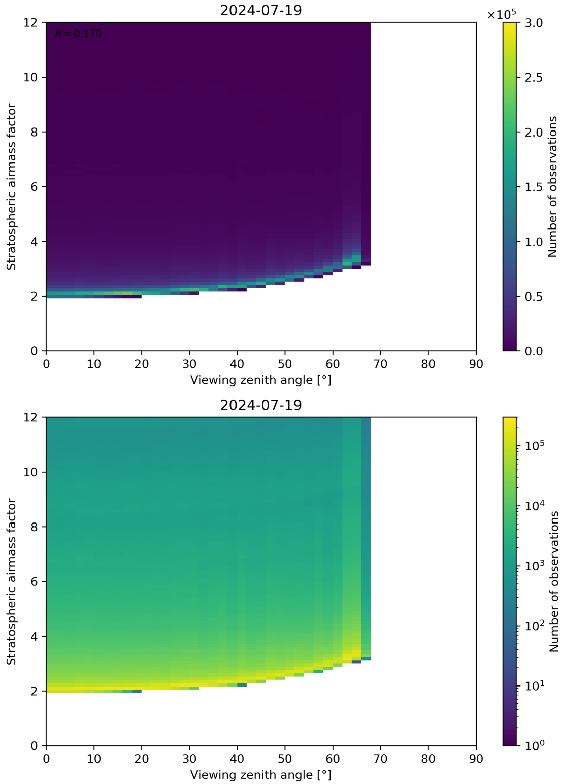
Figure 159: Scatter density plot of “Viewing zenith angle” against “Stratospheric airmass factor” for 2024-07-18 to 2024-07-20.
