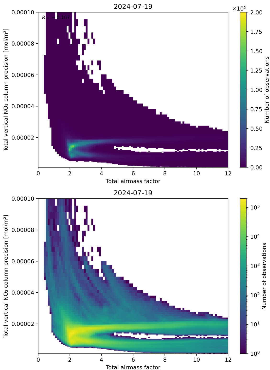
Figure 68: Scatter density plot of “Total airmass factor” against “Total vertical NO 2 column precision” for 2024-07-18 to 2024-07-20.
