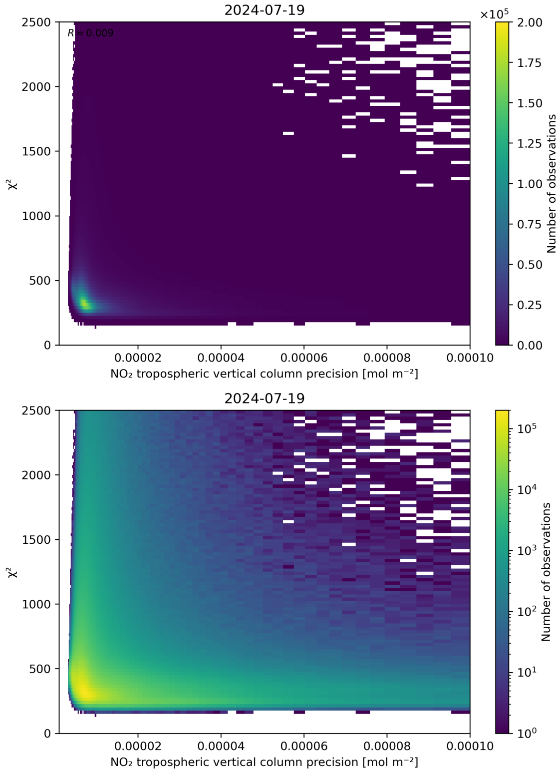
Figure 134: Scatter density plot of “NO 2 tropospheric vertical column precision” against “ \chi^2 ” for 2024-07-18 to 2024-07-20.
