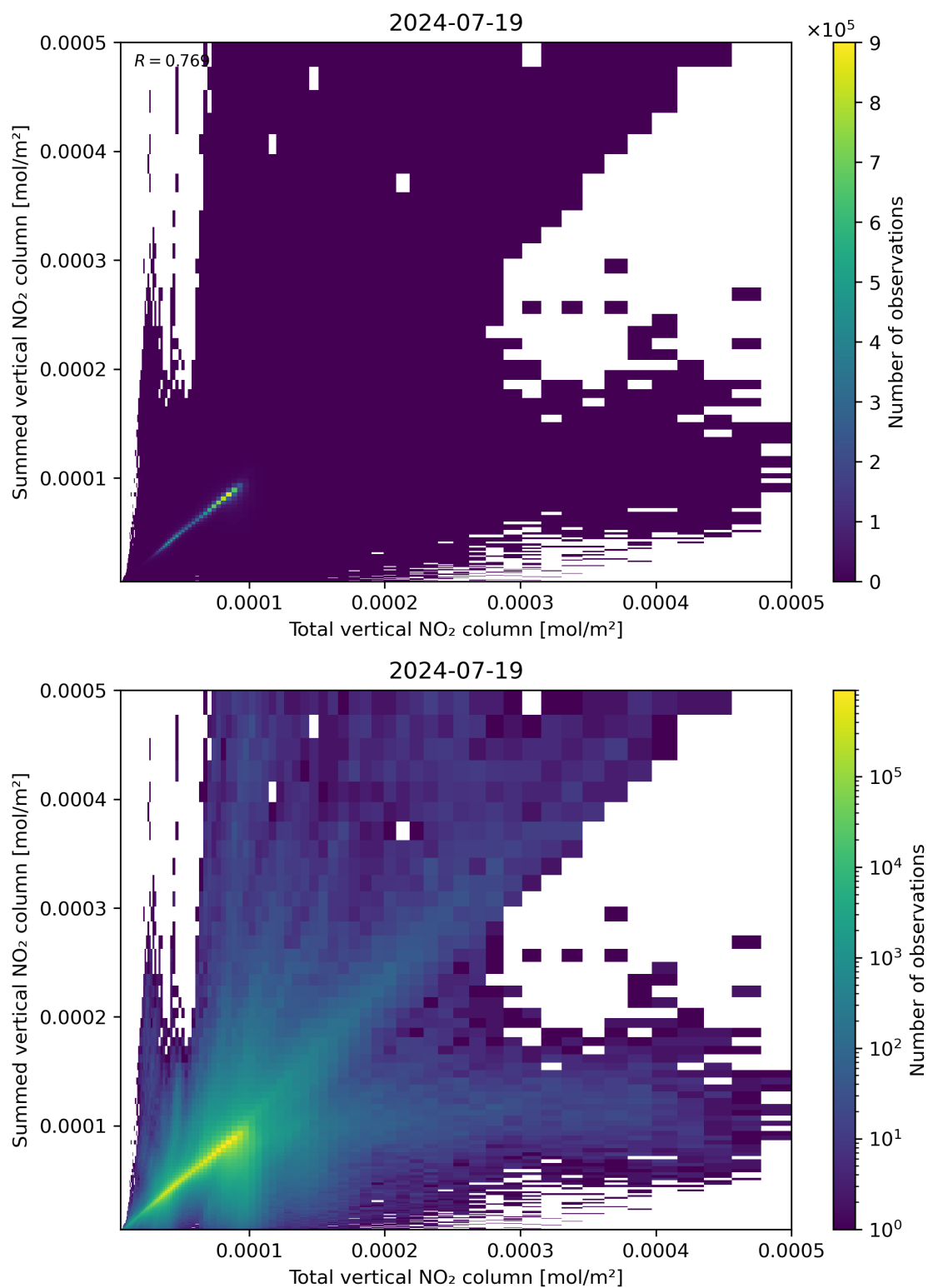
Figure 112: Scatter density plot of “Total vertical NO 2 column” against “Summed vertical NO 2 column” for 2024-07-18 to 2024-07-20.
