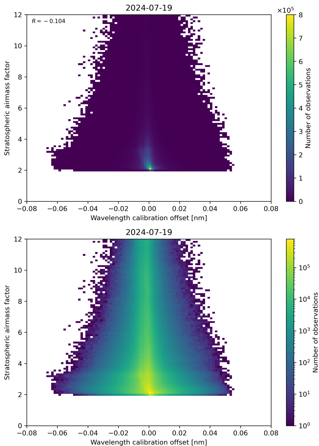
Figure 174: Scatter density plot of “Wavelength calibration offset” against “Stratospheric air mass factor” for 2024-07-18 to 2024-07-20.
