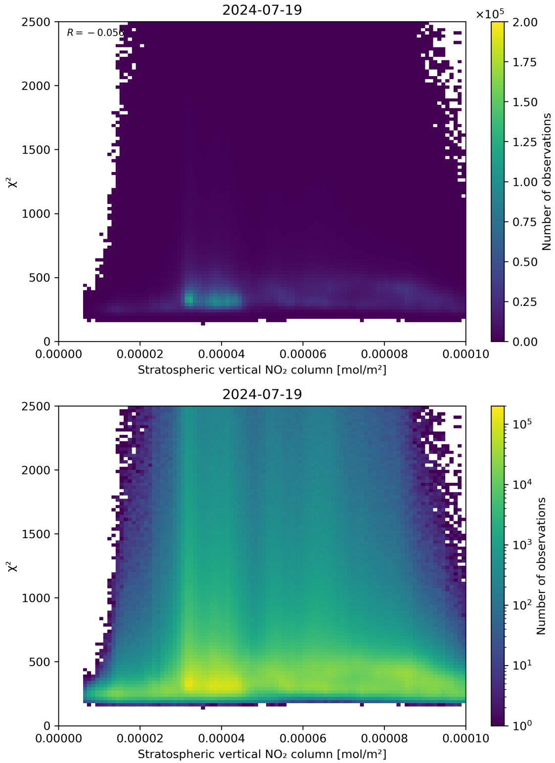
Figure 97: Scatter density plot of “Stratospheric vertical NO 2 column” against “ \chi^2 ” for 2024-07-18 to 2024-07-20.
