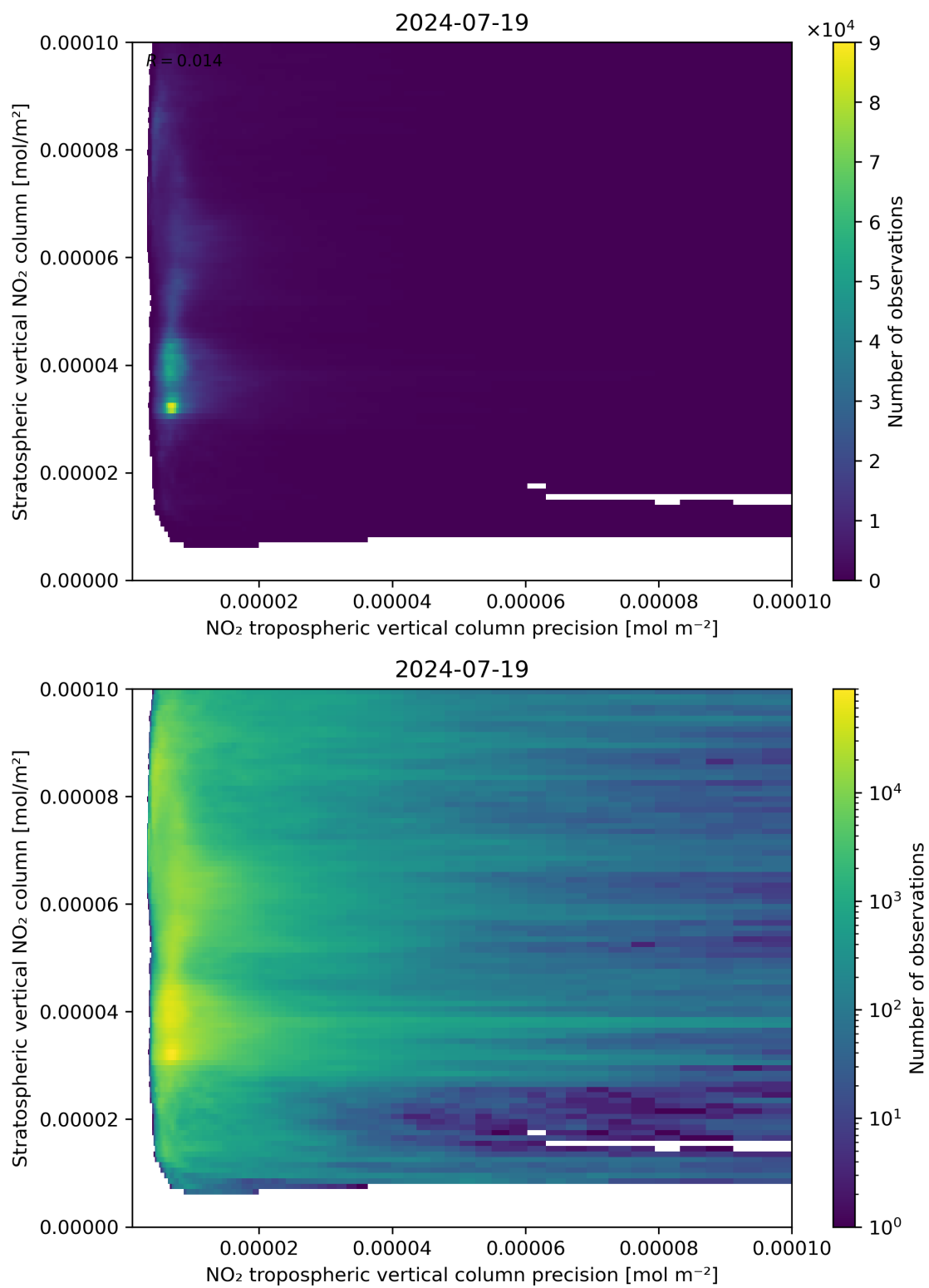
Figure 135: Scatter density plot of “NO 2 tropospheric vertical column precision” against “Stratospheric vertical NO 2 column” for 2024-07-18 to 2024-07-20.
