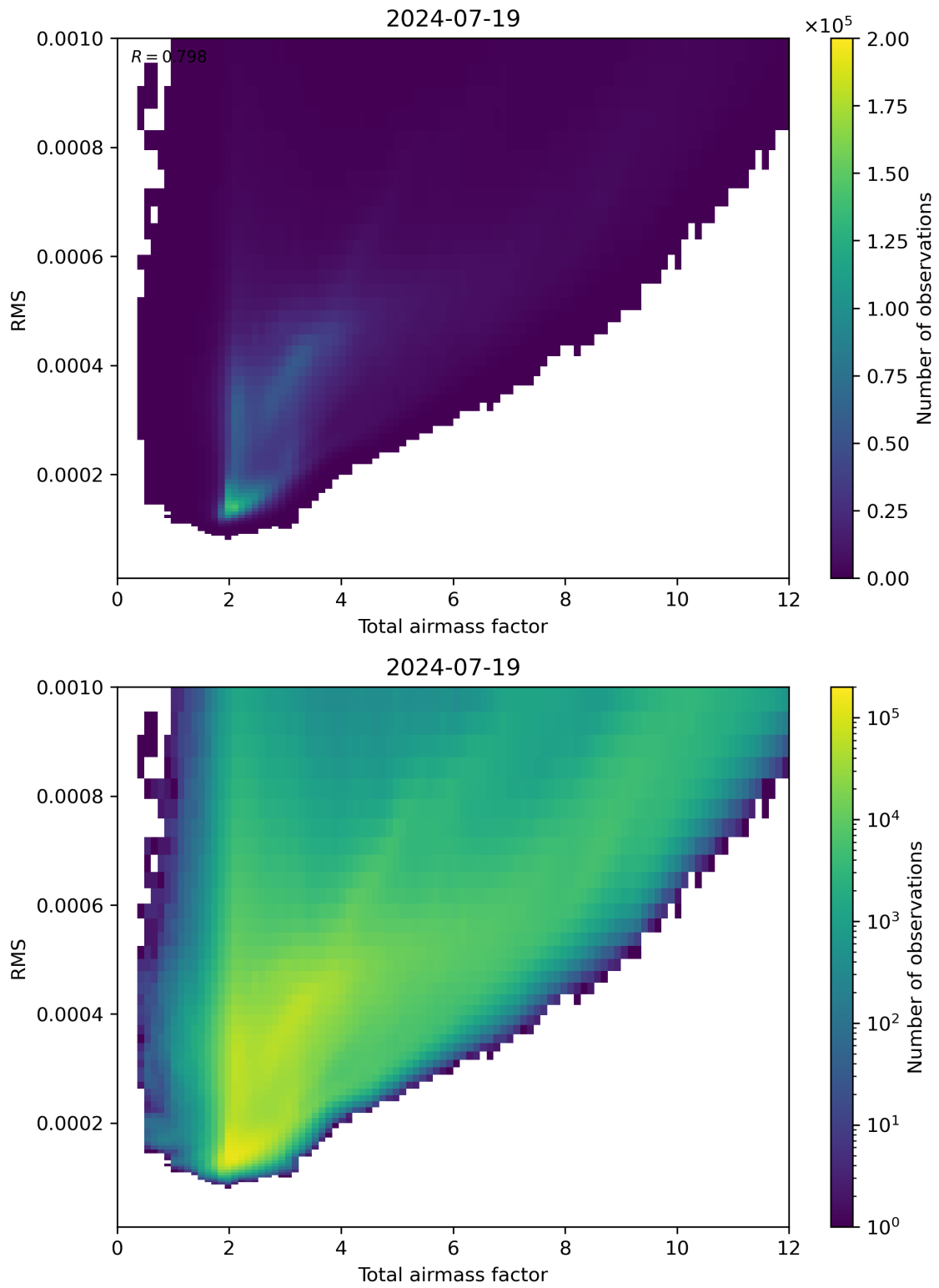
Figure 69: Scatter density plot of “Total airmass factor” against “RMS” for 2024-07-18 to 2024-07-20.
