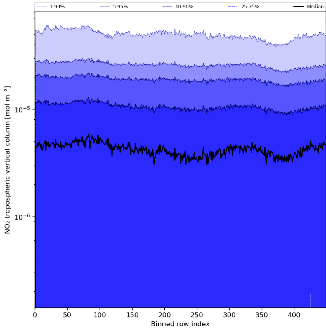
Figure 46: Along track statistics of “NO 2 tropospheric vertical column” for 2024-07-18 to 2024-07-20
