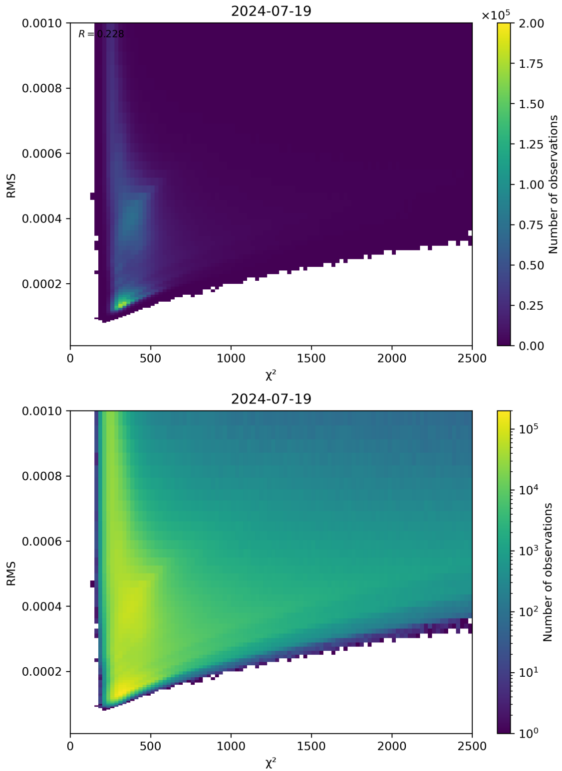
Figure 82: Scatter density plot of “ \chi^2 ” against “RMS” for 2024-07-18 to 2024-07-20.
