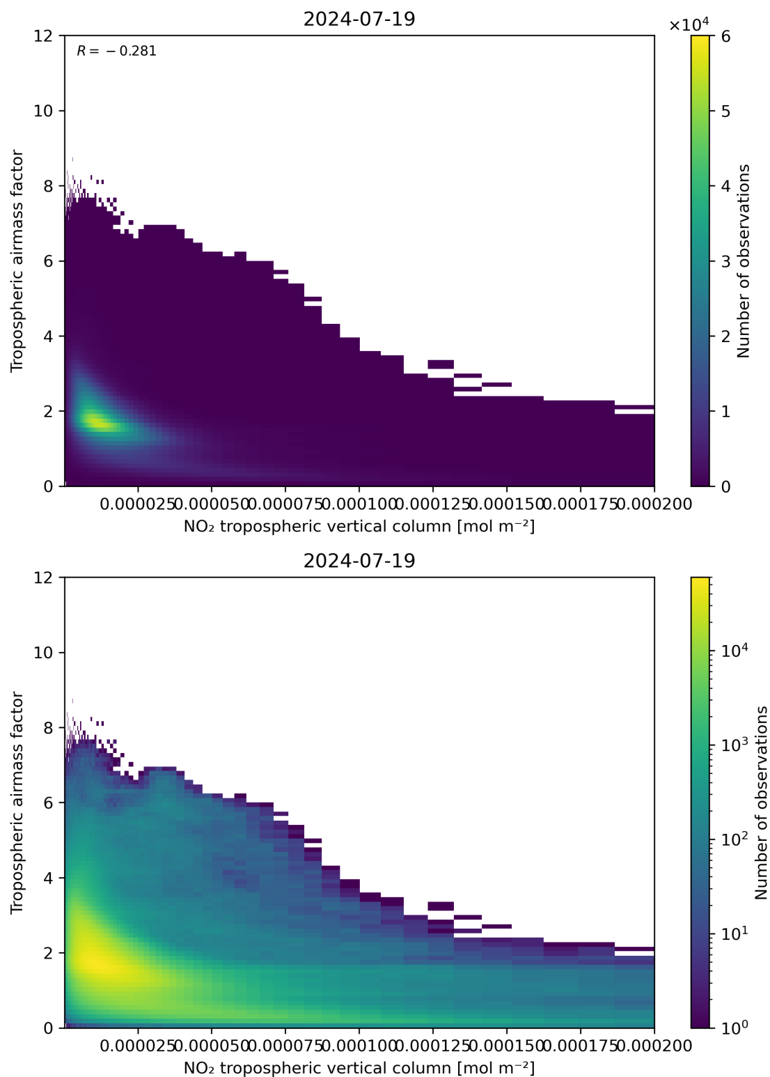
Figure 123: Scatter density plot of “NO 2 tropospheric vertical column” against “Tropospheric air mass factor” for 2024-07-18 to 2024-07-20.
