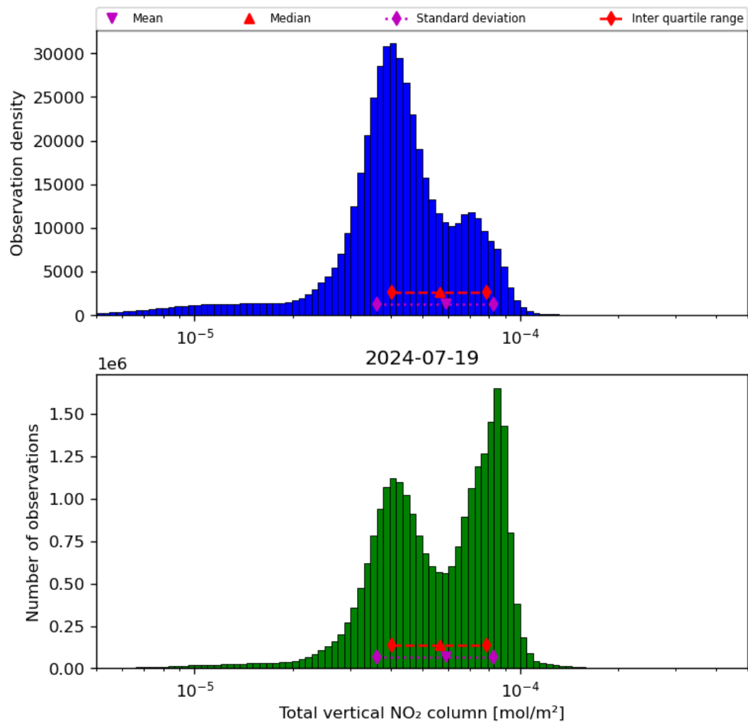
Figure 38: Histogram of “Total vertical NO 2 column” for 2024-07-18 to 2024-07-20
