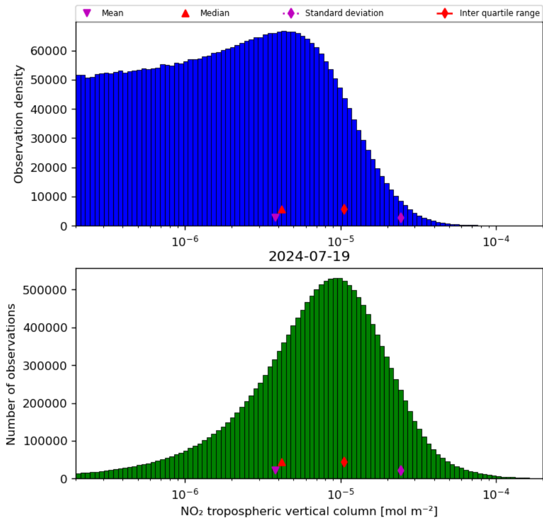
Figure 29: Histogram of “NO 2 tropospheric vertical column” for 2024-07-18 to 2024-07-20
