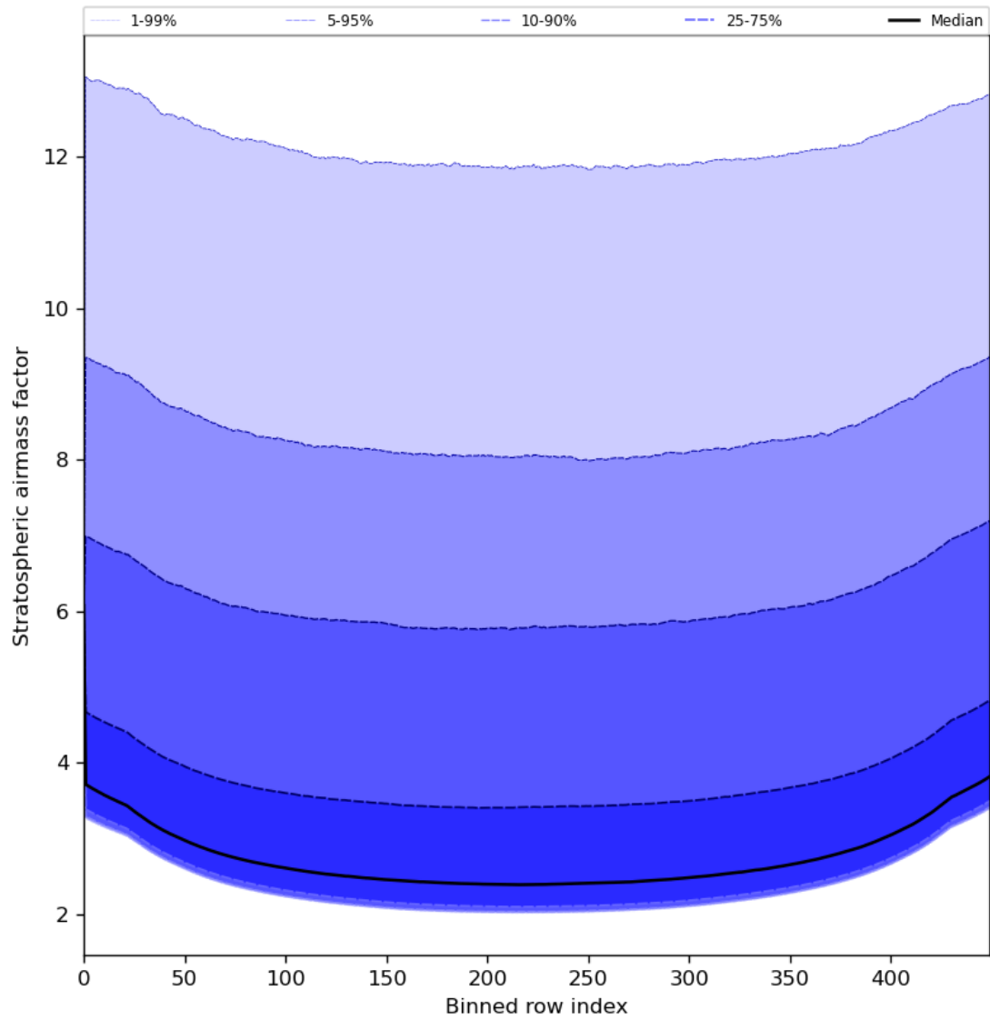
Figure 61: Along track statistics of “Stratospheric airmass factor” for 2024-07-18 to 2024-07-20
