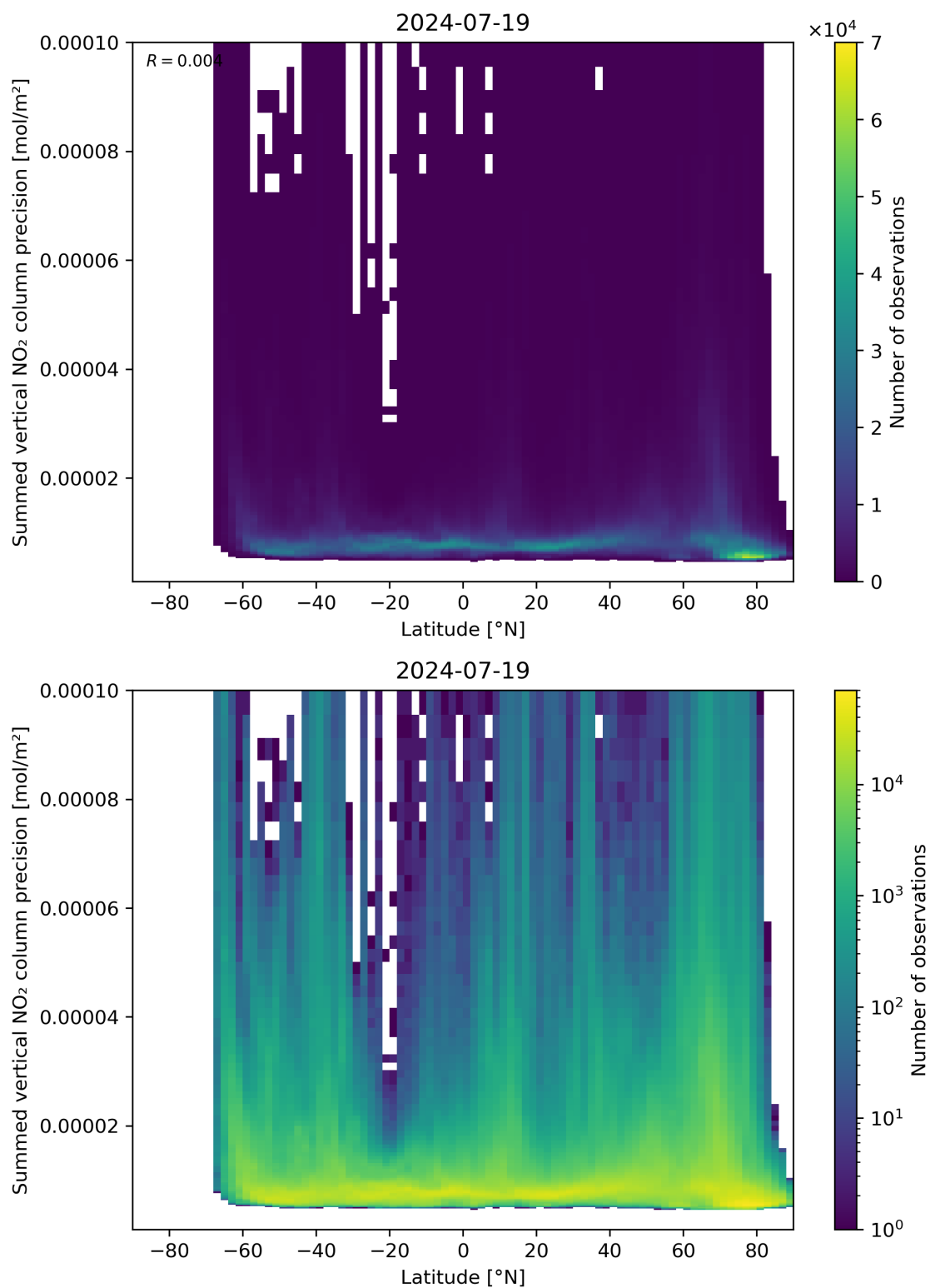
Figure 89: Scatter density plot of “Latitude” against “Summed vertical NO 2 column precision” for 2024-07-18 to 2024-07-20.
