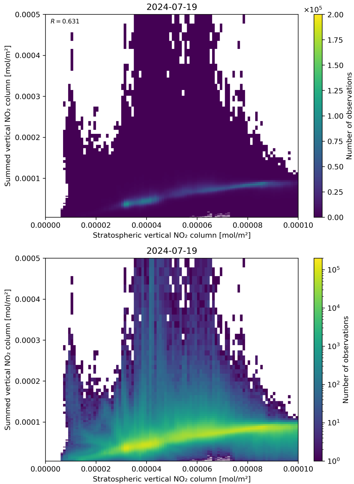
Figure 98: Scatter density plot of “Stratospheric vertical NO 2 column” against “Summed vertical NO 2 column” for 2024-07-18 to 2024-07-20.
