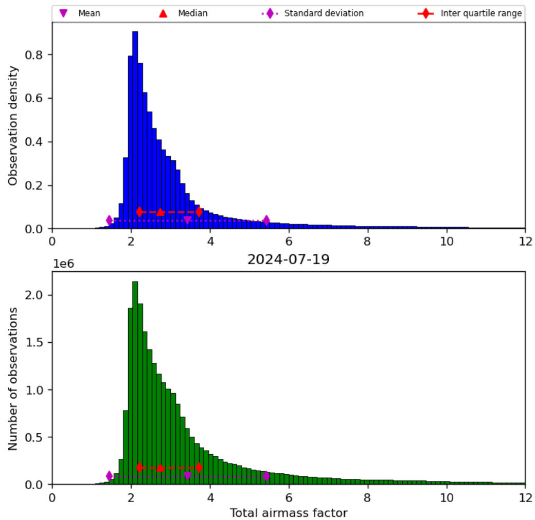
Figure 32: Histogram of “Total airmass factor” for 2024-07-18 to 2024-07-20
