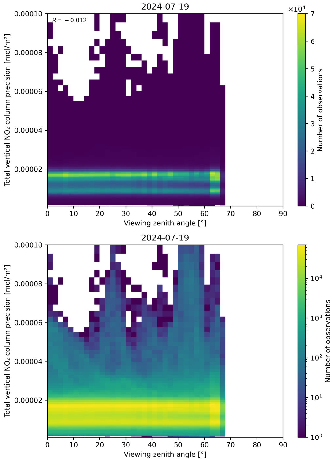
Figure 168: Scatter density plot of “Viewing zenith angle” against “Total vertical NO 2 column precision” for 2024-07-18 to 2024-07-20.
