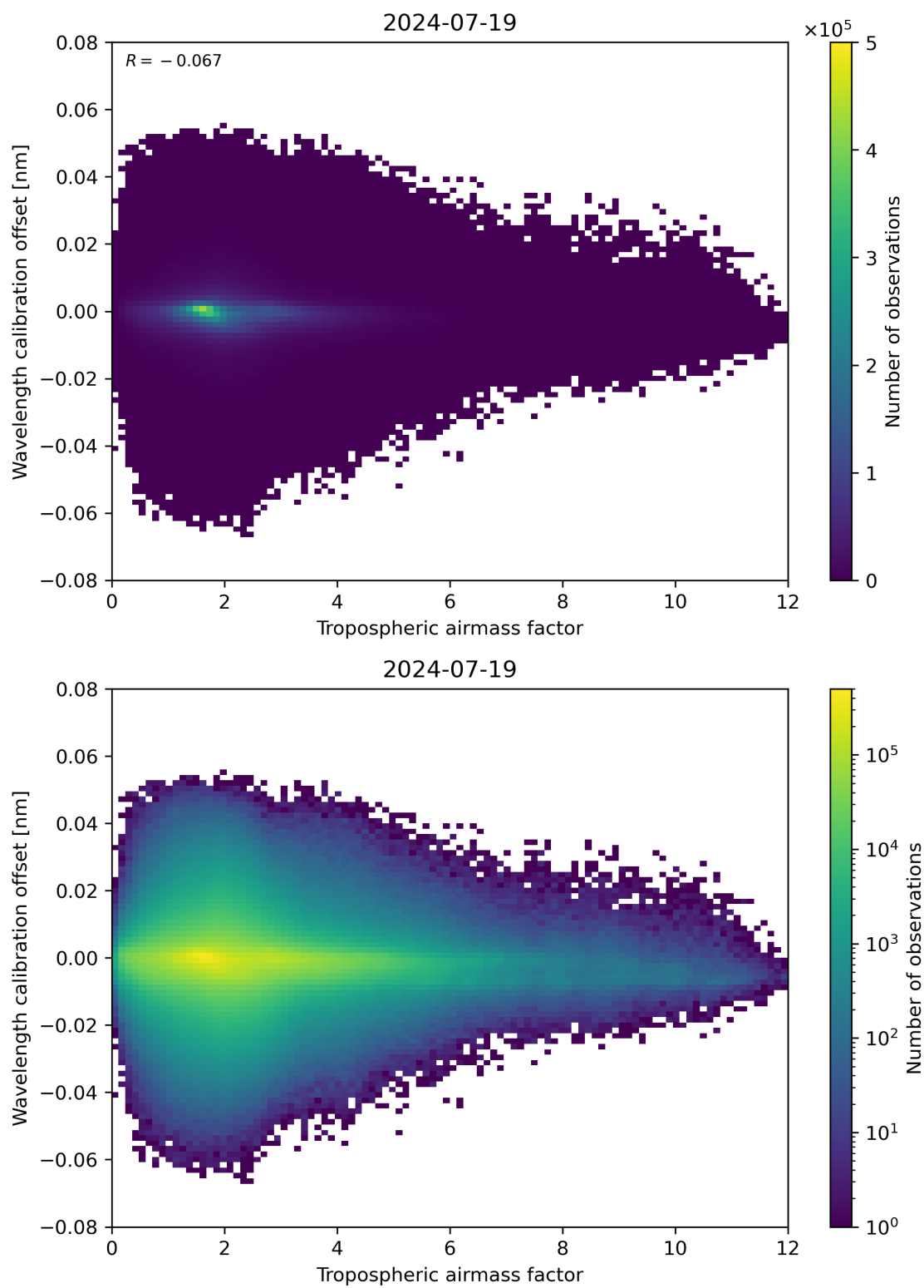
Figure 80: Scatter density plot of “Tropospheric airmass factor” against “Wavelength calibration offset” for 2024-07-18 to 2024-07-20.
