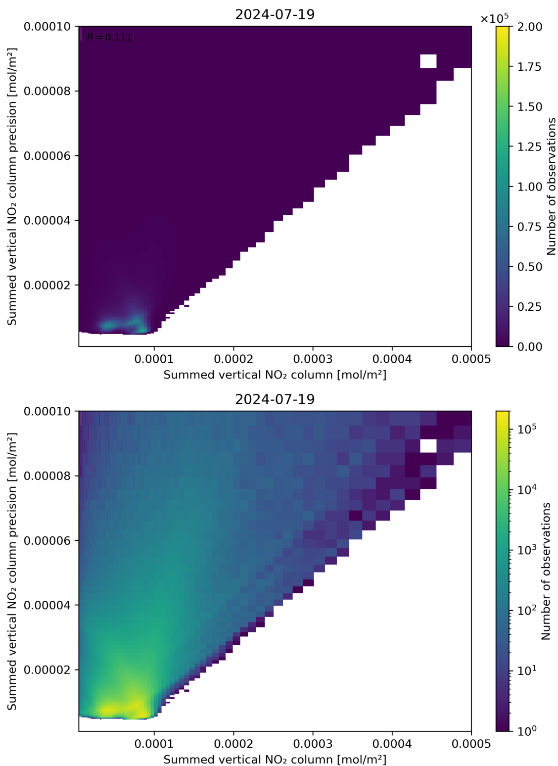
Figure 105: Scatter density plot of “Summed vertical NO 2 column” against “Summed vertical NO 2 column precision” for 2024-07-18 to 2024-07-20.
