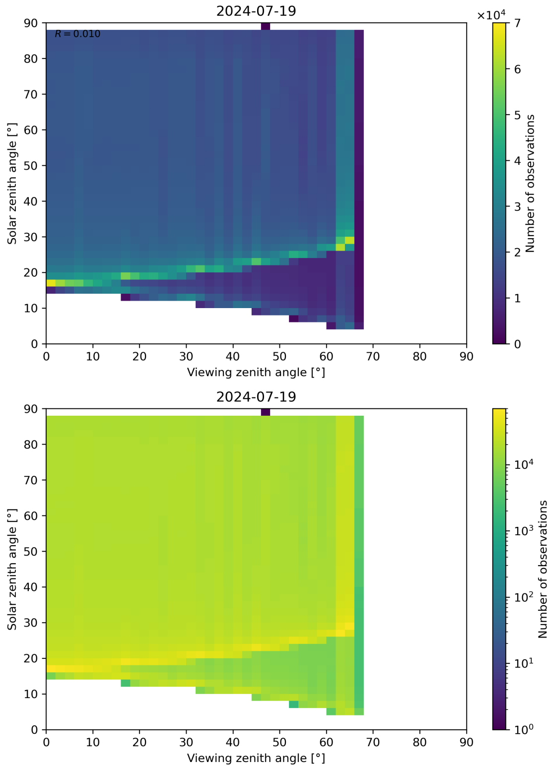
Figure 172: Scatter density plot of “Viewing zenith angle” against “Solar zenith angle” for 2024-07-18 to 2024-07-20.
