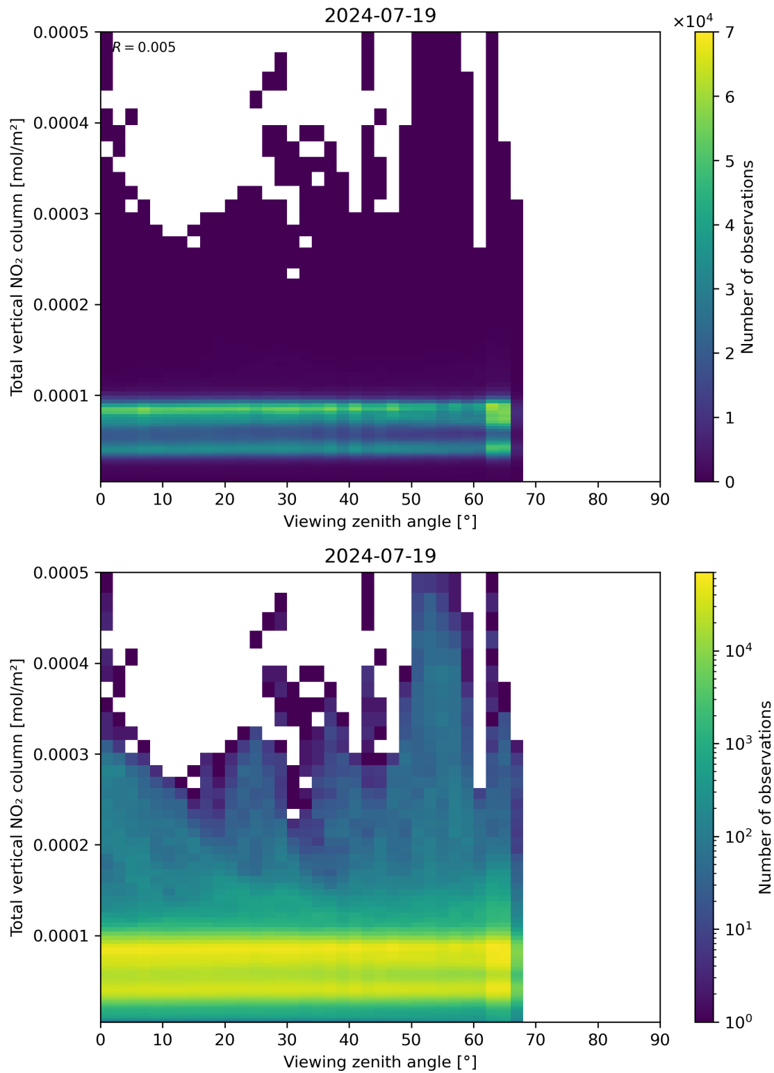
Figure 167: Scatter density plot of “Viewing zenith angle” against “Total vertical NO 2 column” for 2024-07-18 to 2024-07-20.
