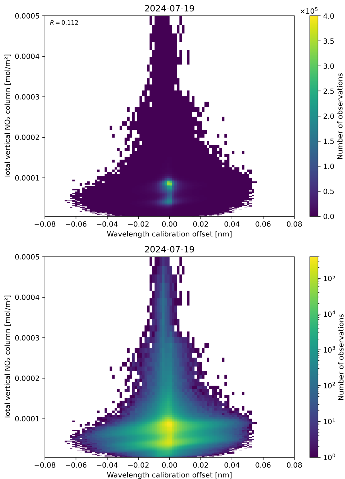
Figure 179: Scatter density plot of “Wavelength calibration offset” against “Total vertical NO 2 column” for 2024-07-18 to 2024-07-20.
