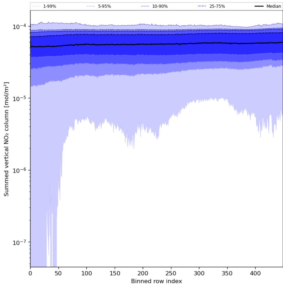
Figure 57: Along track statistics of “Summed vertical NO 2 column” for 2024-07-18 to 2024-07-20
