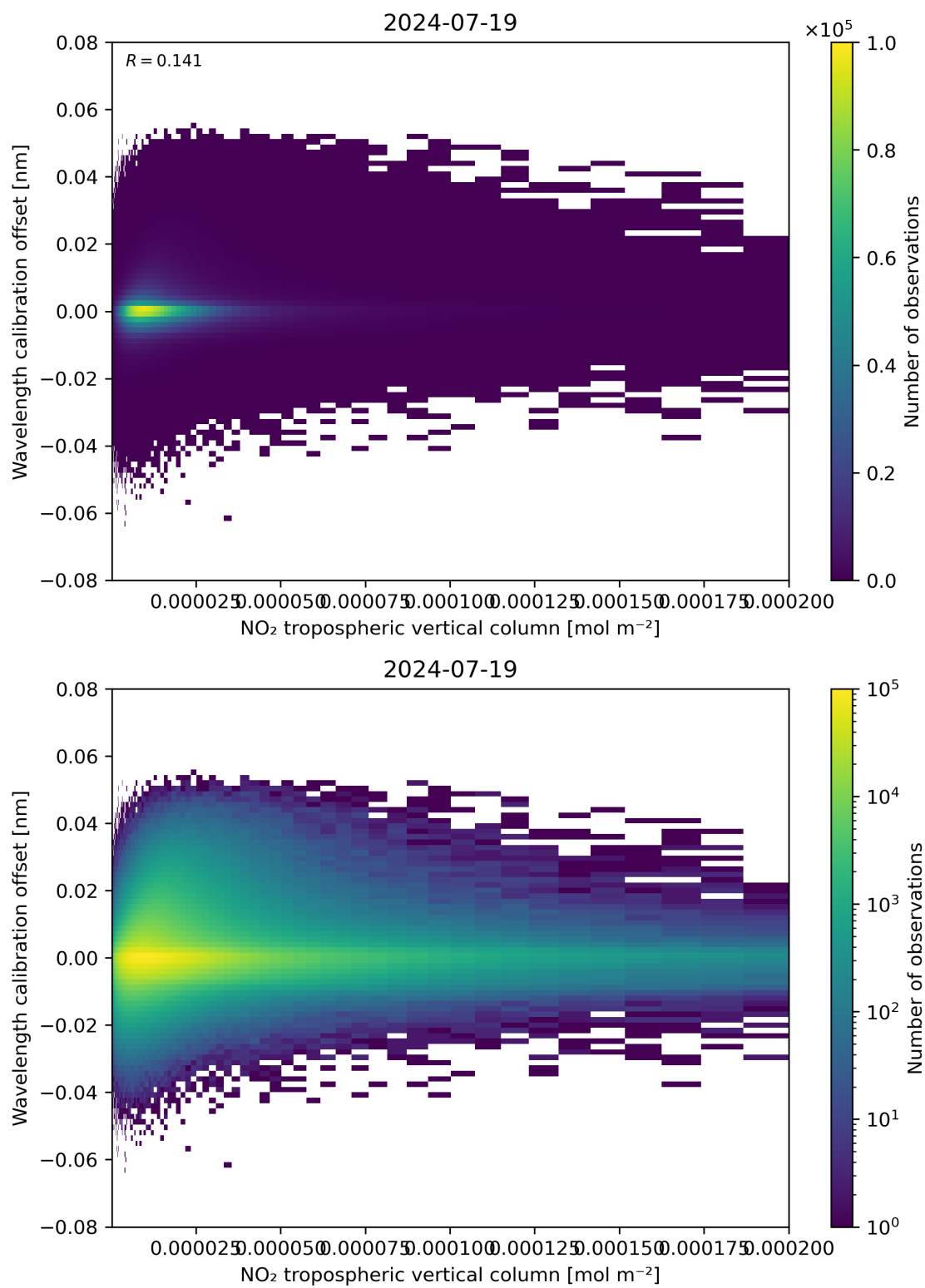
Figure 143: Scatter density plot of “NO 2 tropospheric vertical column” against “Wavelength calibration offset” for 2024-07-18 to 2024-07-20.
