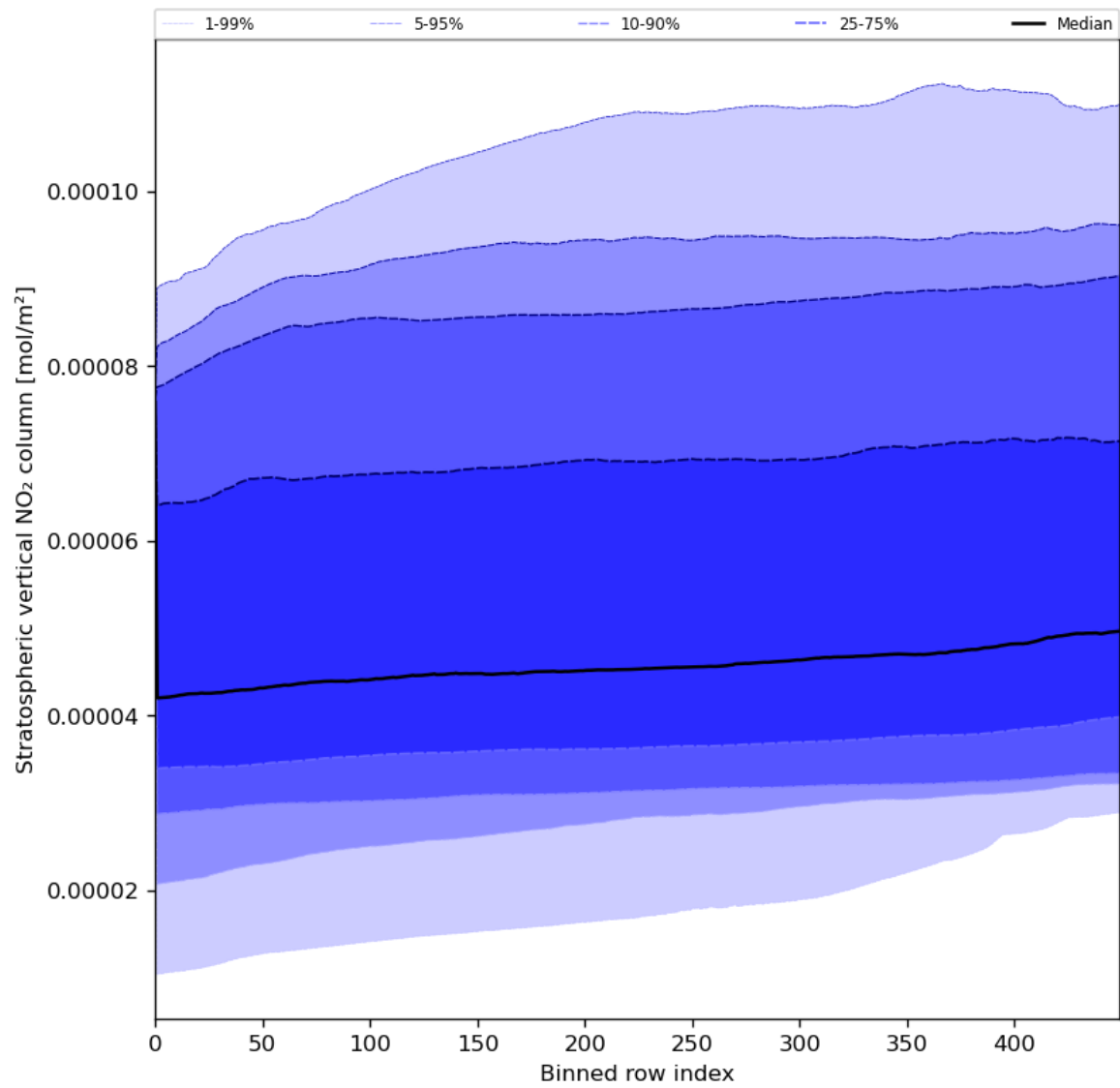
Figure 53: Along track statistics of “Stratospheric vertical NO 2 column” for 2024-07-18 to 2024-07-20
