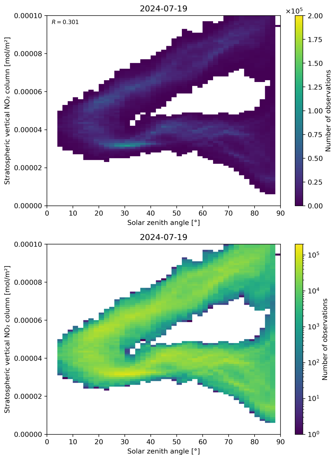
Figure 150: Scatter density plot of “Solar zenith angle” against “Stratospheric vertical NO 2 column” for 2024-07-18 to 2024-07-20.
