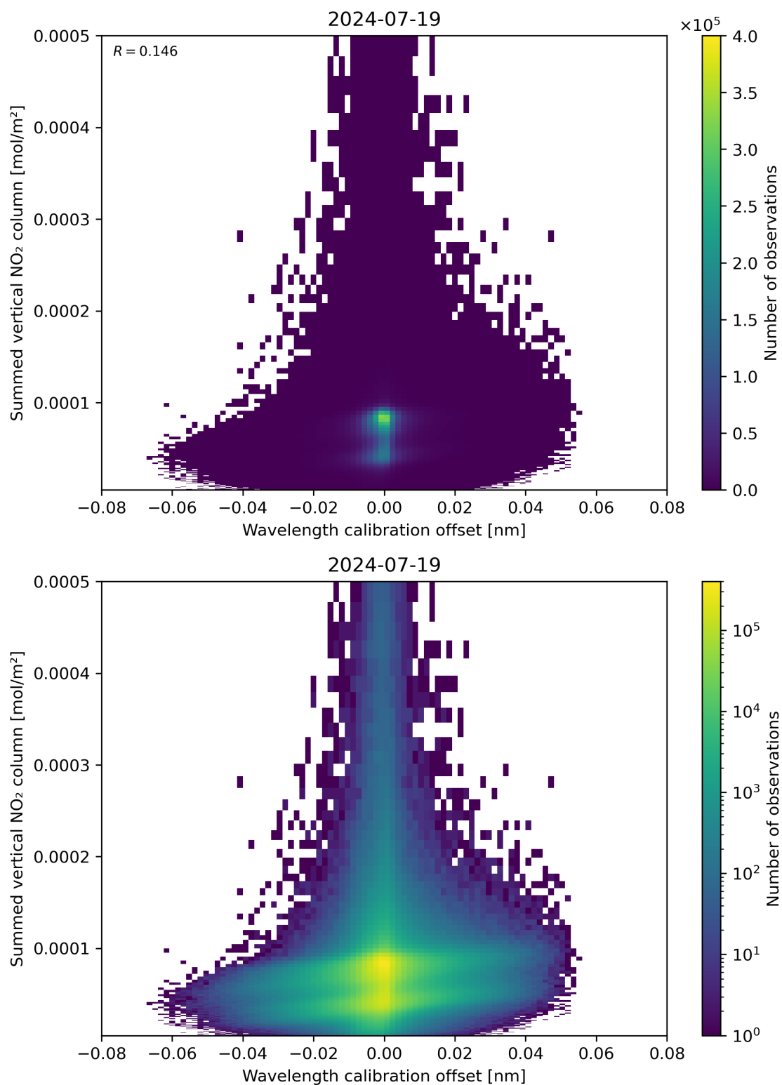
Figure 177: Scatter density plot of “Wavelength calibration offset” against “Summed vertical NO 2 column” for 2024-07-18 to 2024-07-20.
