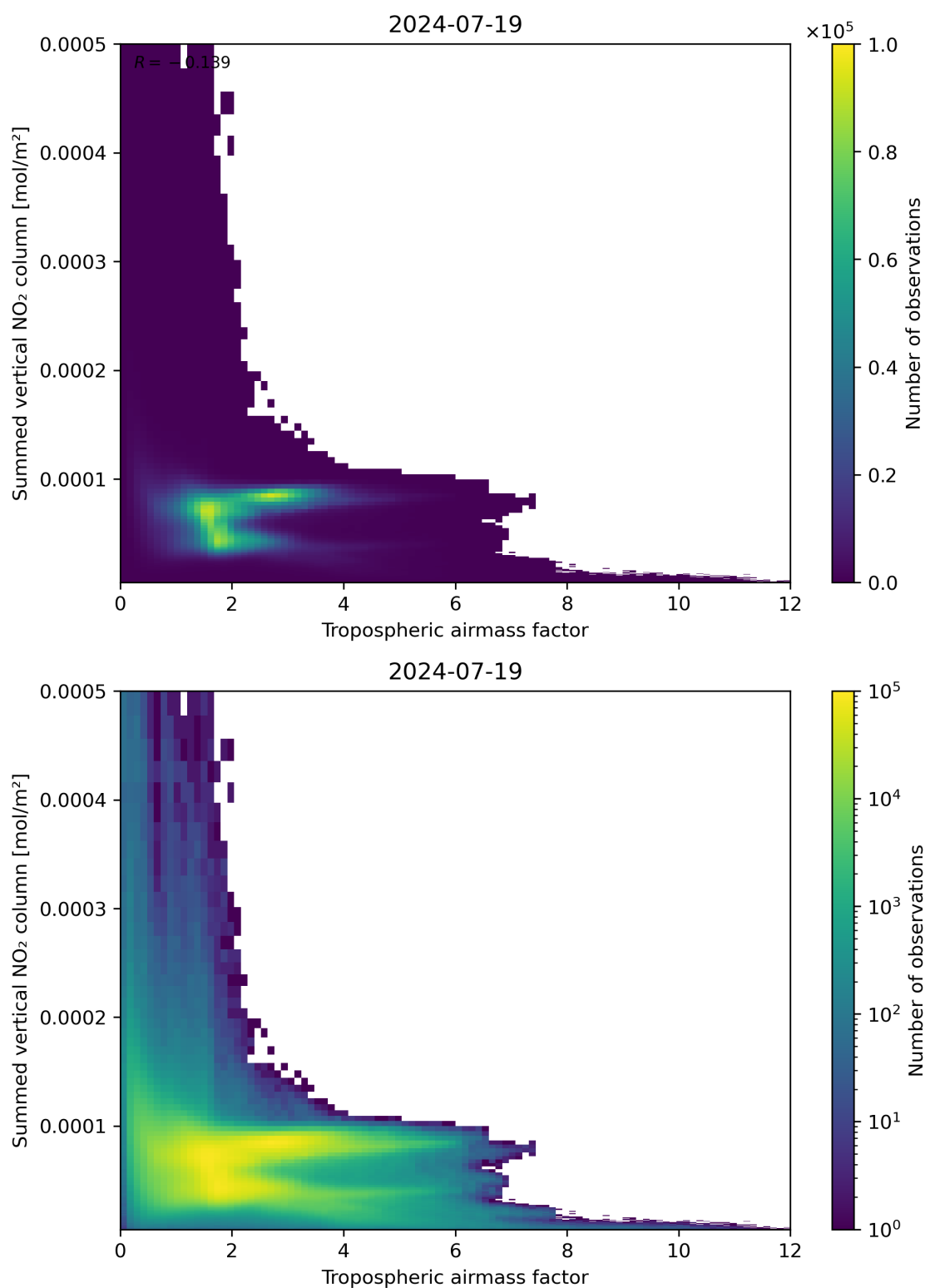
Figure 75: Scatter density plot of “Tropospheric airmass factor” against “Summed vertical NO 2 column” for 2024-07-18 to 2024-07-20.
