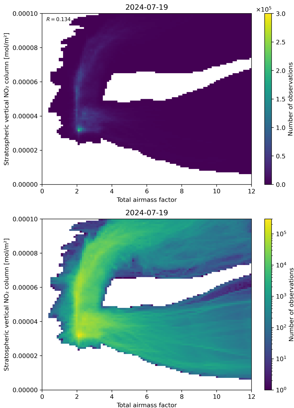
Figure 64: Scatter density plot of “Total airmass factor” against “Stratospheric vertical NO 2 column” for 2024-07-18 to 2024-07-20.
