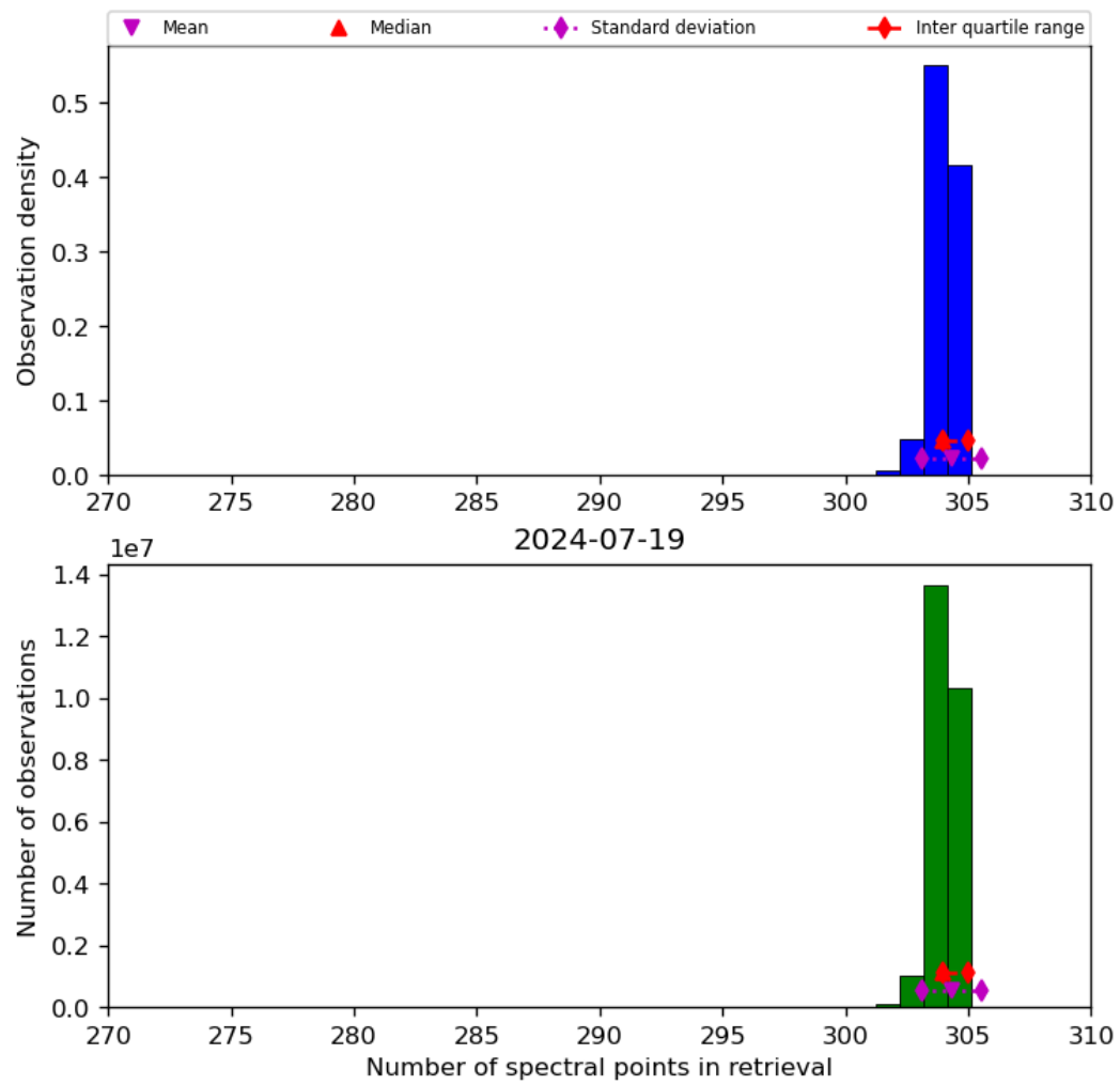
Figure 33: Histogram of “Number of spectral points in retrieval” for 2024-07-18 to 2024-07-20
