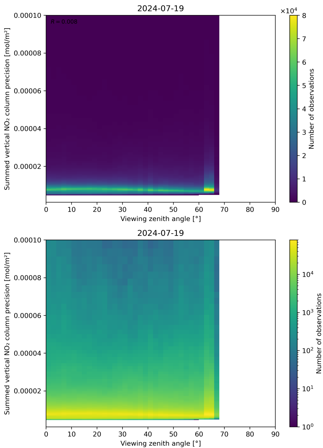
Figure 166: Scatter density plot of “Viewing zenith angle” against “Summed vertical NO 2 column precision” for 2024-07-18 to 2024-07-20.
