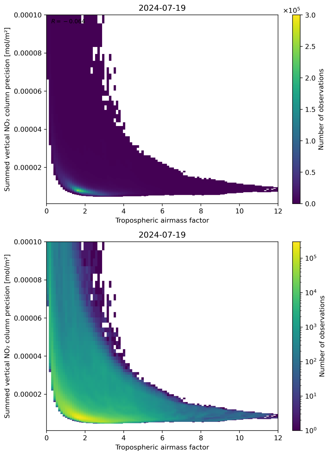
Figure 76: Scatter density plot of “Tropospheric air mass factor” against “Summed vertical NO 2 column precision” for 2024-07-18 to 2024-07-20.
