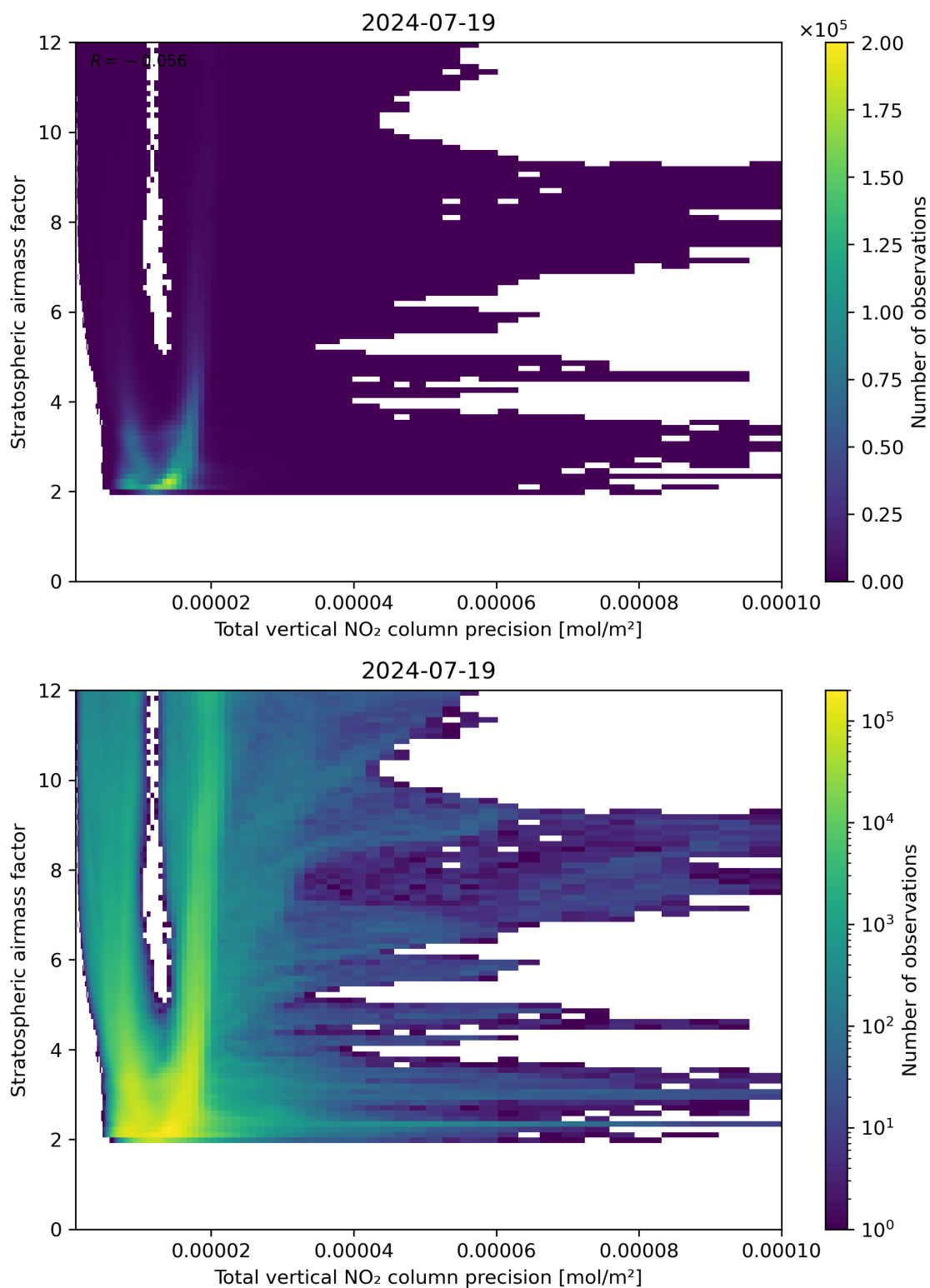
Figure 115: Scatter density plot of “Total vertical NO 2 column precision” against “Stratospheric air mass factor” for 2024-07-18 to 2024-07-20.
