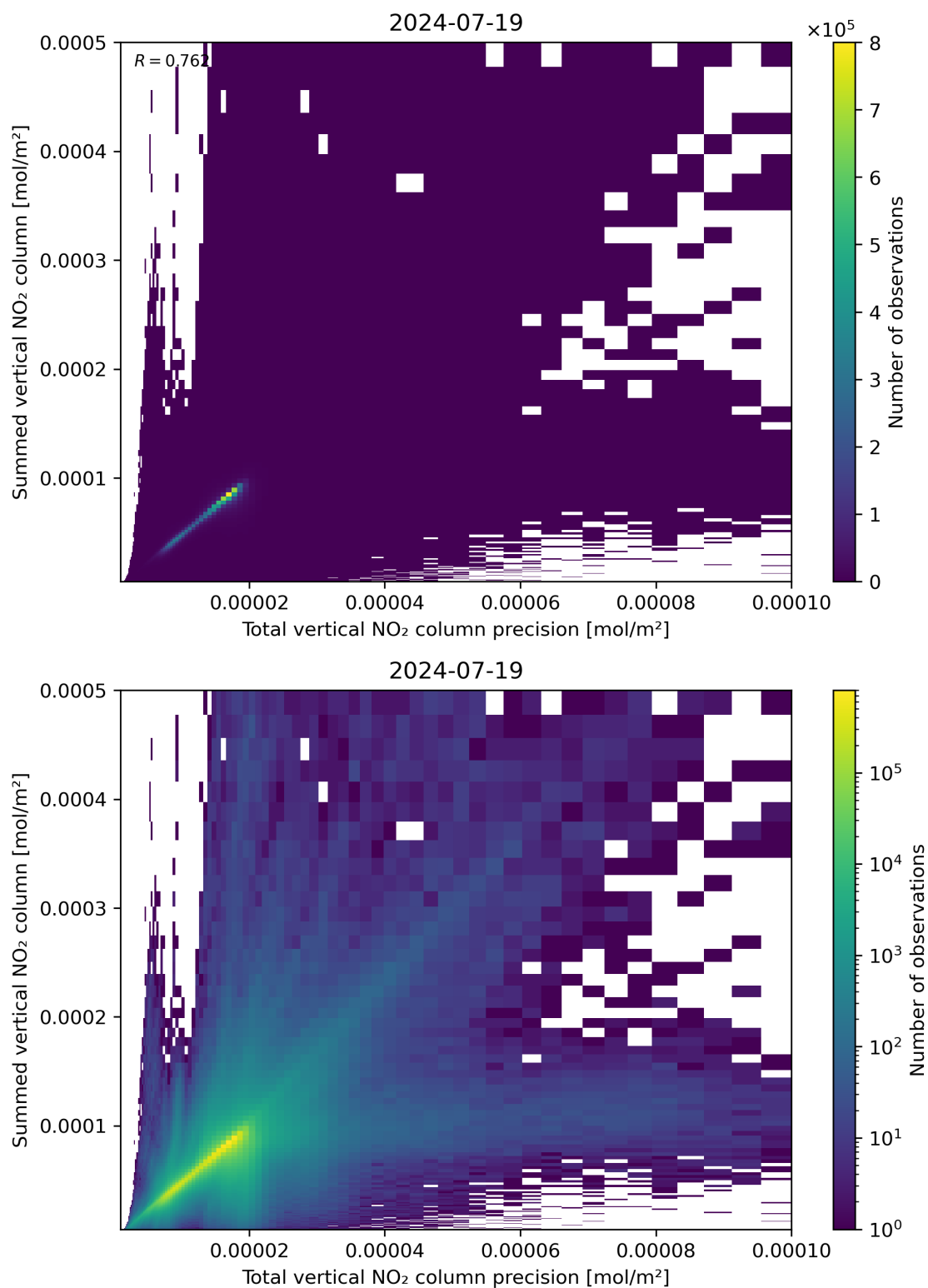
Figure 117: Scatter density plot of “Total vertical NO 2 column precision” against “Summed vertical NO 2 column” for 2024-07-18 to 2024-07-20.
