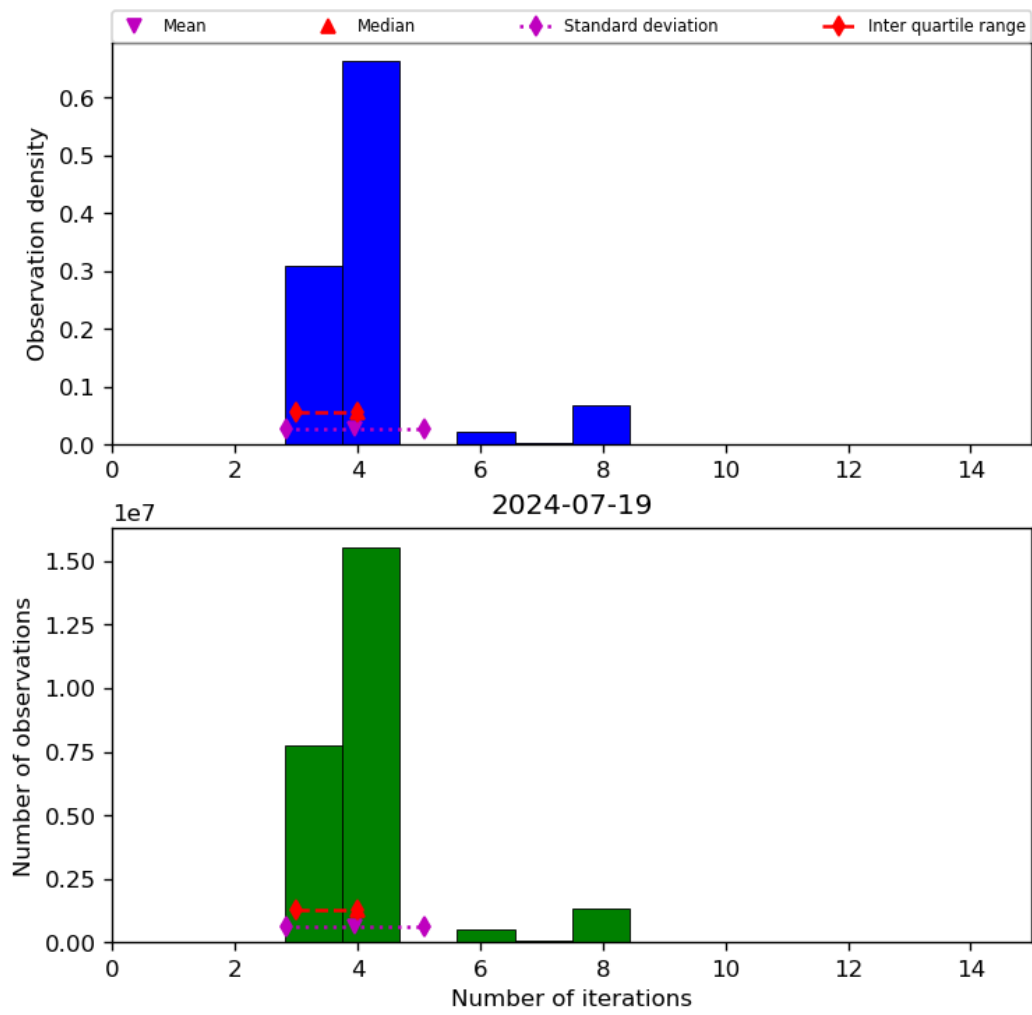
Figure 34: Histogram of “Number of iterations” for 2024-07-18 to 2024-07-20
