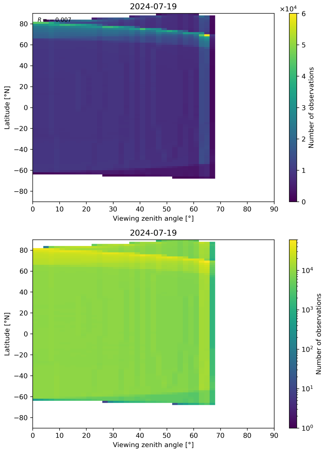
Figure 163: Scatter density plot of “Viewing zenith angle” against “Latitude” for 2024-07-18 to 2024-07-20.
