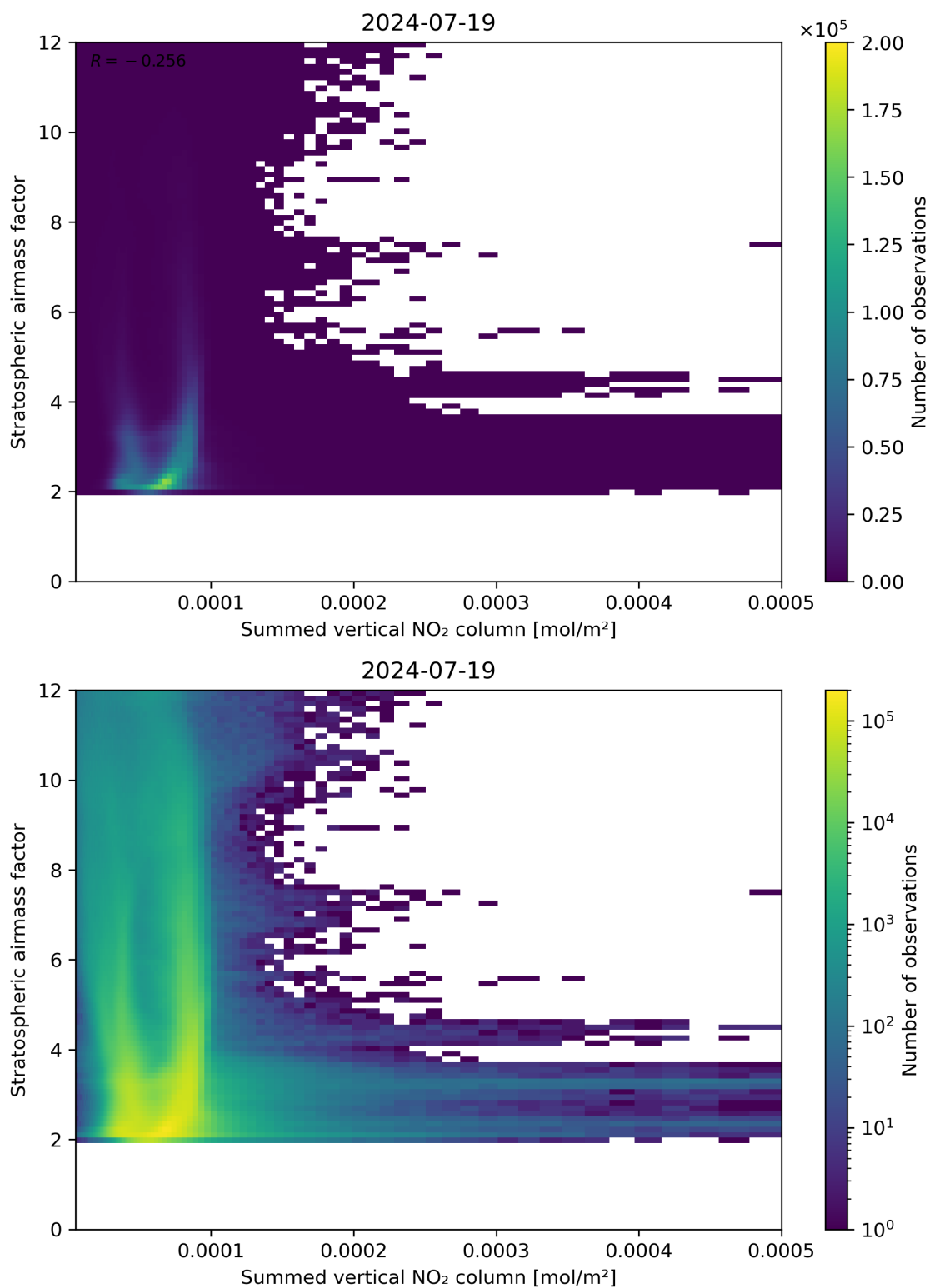
Figure 103: Scatter density plot of “Summed vertical NO 2 column” against “Stratospheric air mass factor” for 2024-07-18 to 2024-07-20.
