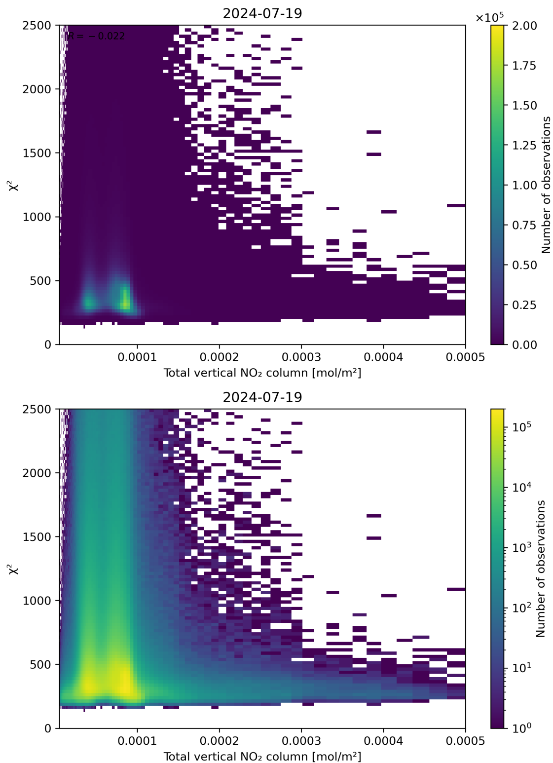
Figure 111: Scatter density plot of “Total vertical NO 2 column” against “ \chi^2 ” for 2024-07-18 to 2024-07-20.
