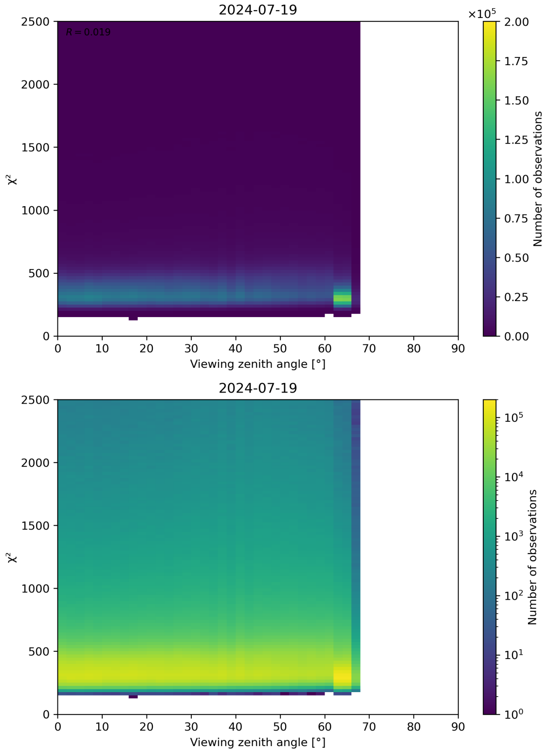
Figure 162: Scatter density plot of “Viewing zenith angle” against “ \chi^2 ” for 2024-07-18 to 2024-07-20.
