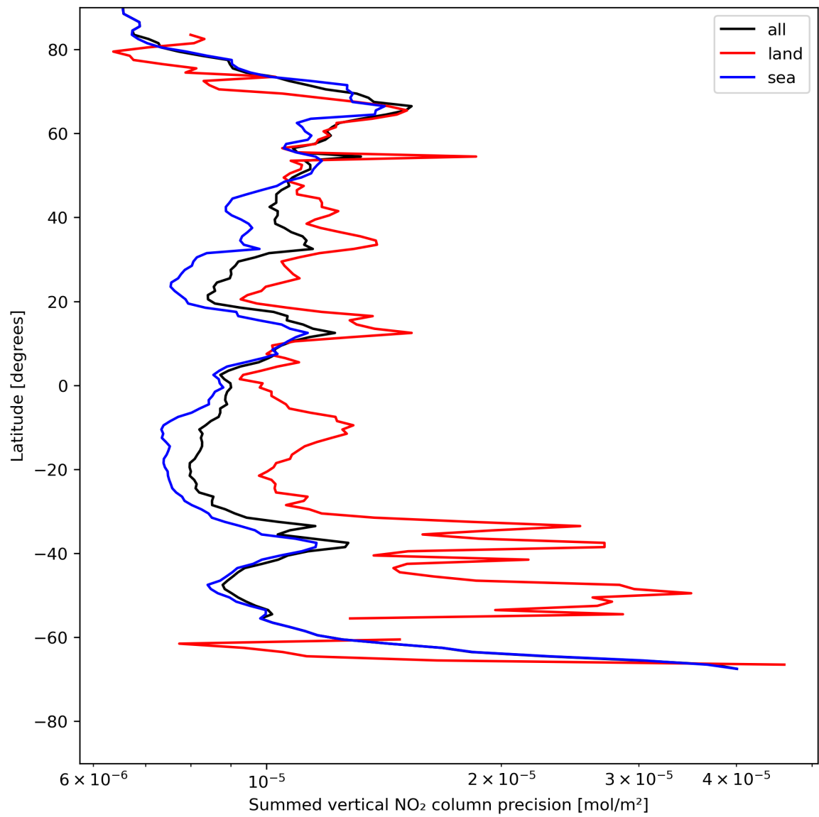
Figure 24: Zonal average of “Summed vertical NO 2 column precision” for 2024-07-18 to 2024-07-20.
