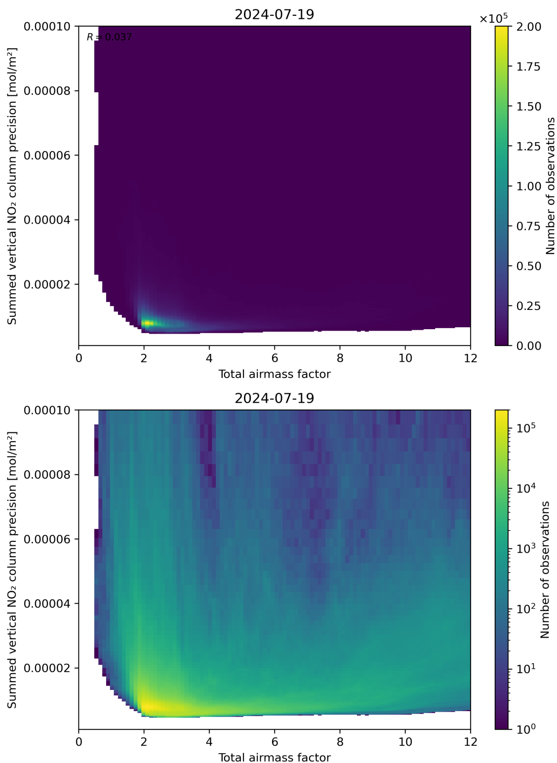
Figure 66: Scatter density plot of “Total airmass factor” against “Summed vertical NO 2 column precision” for 2024-07-18 to 2024-07-20.
