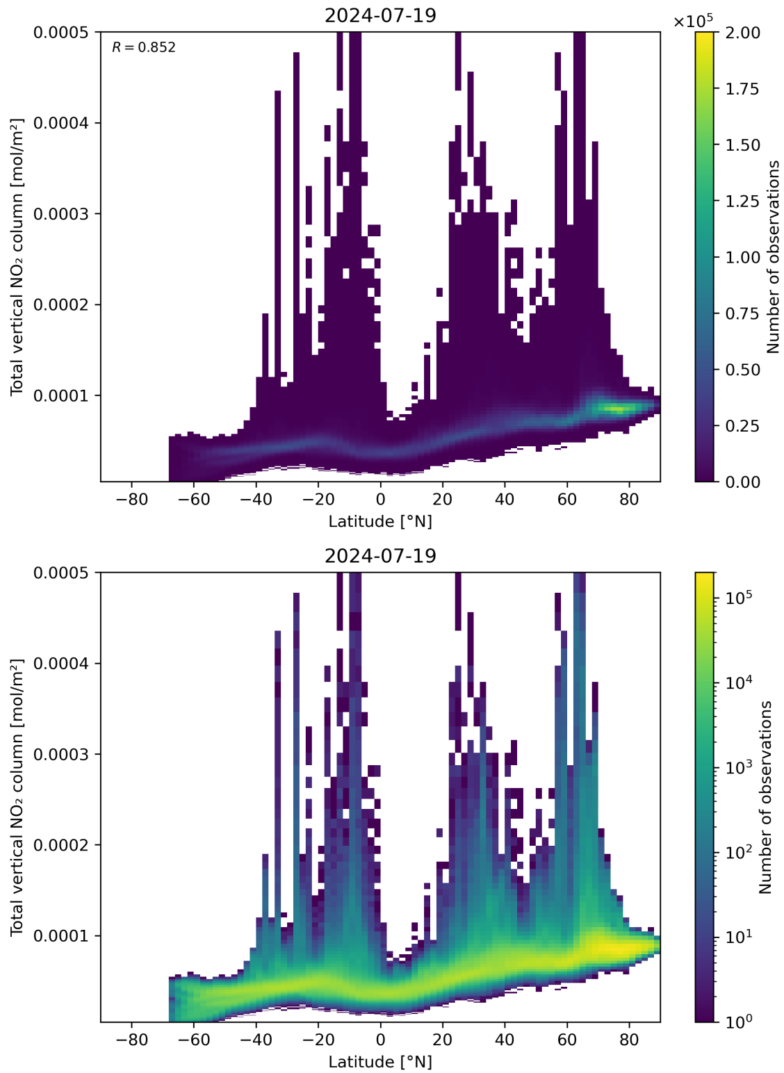
Figure 90: Scatter density plot of “Latitude” against “Total vertical NO 2 column” for 2024-07-18 to 2024-07-20.
