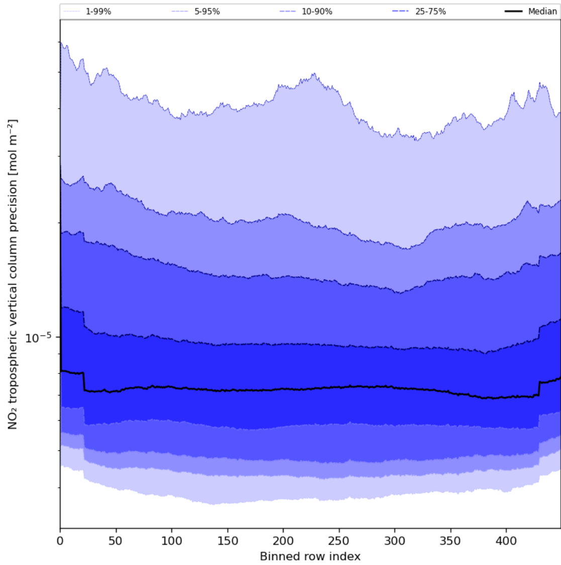
Figure 47: Along track statistics of “NO 2 tropospheric vertical column precision” for 2024-07-18 to 2024-07-20
