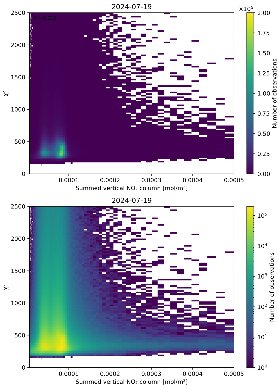
Figure 104: Scatter density plot of “Summed vertical NO 2 column” against “ \chi^2 ” for 2024-07-18 to 2024-07-20.
