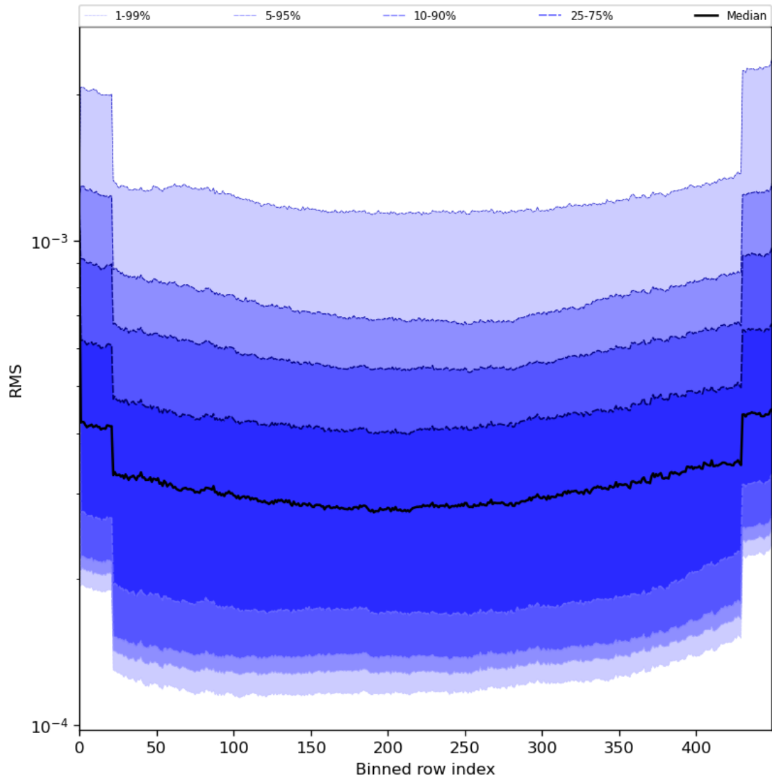
Figure 60: Along track statistics of “RMS” for 2024-07-18 to 2024-07-20
