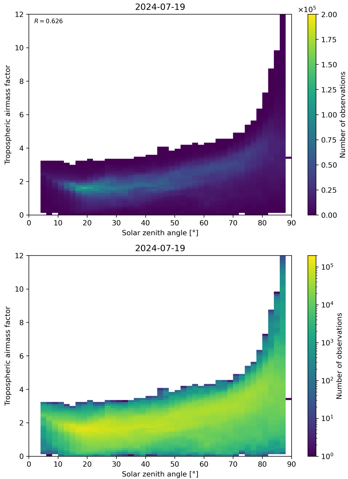
Figure 147: Scatter density plot of “Solar zenith angle” against “Tropospheric airmass factor” for 2024-07-18 to 2024-07-20.
