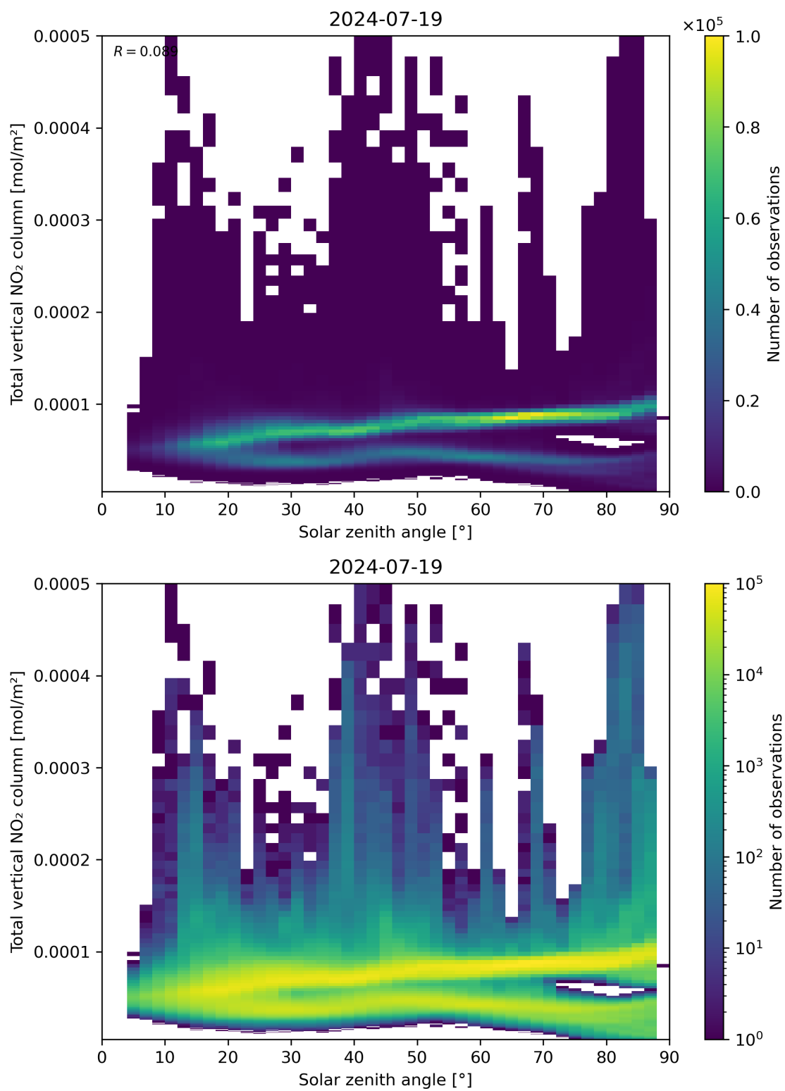
Figure 153: Scatter density plot of “Solar zenith angle” against “Total vertical NO 2 column” for 2024-07-18 to 2024-07-20.
