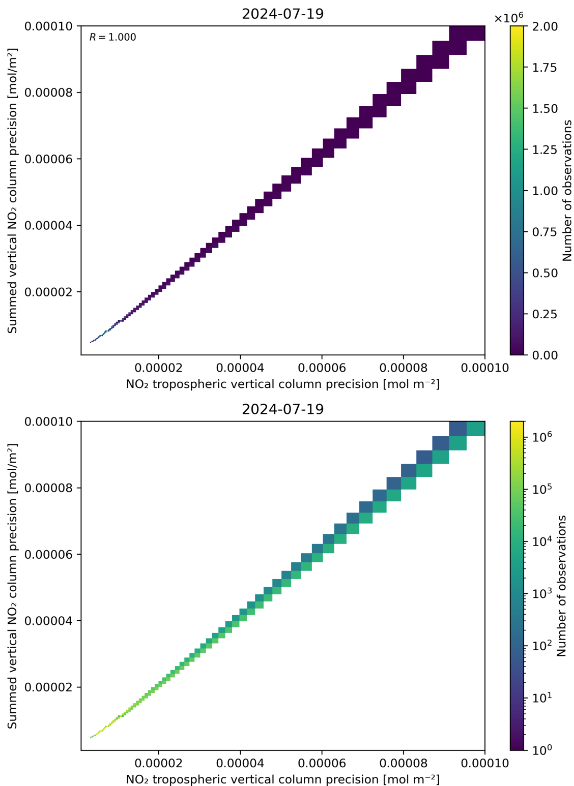
Figure 137: Scatter density plot of “NO 2 tropospheric vertical column precision” against “Summed vertical NO 2 column precision” for 2024-07-18 to 2024-07-20.
