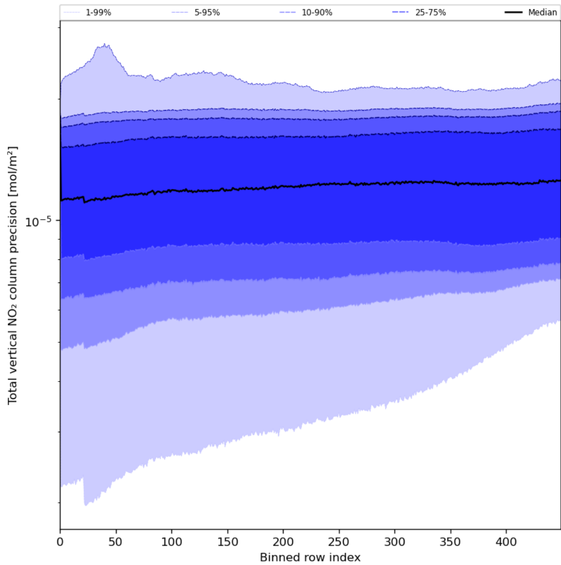
Figure 56: Along track statistics of “Total vertical NO 2 column precision” for 2024-07-18 to 2024-07-20
