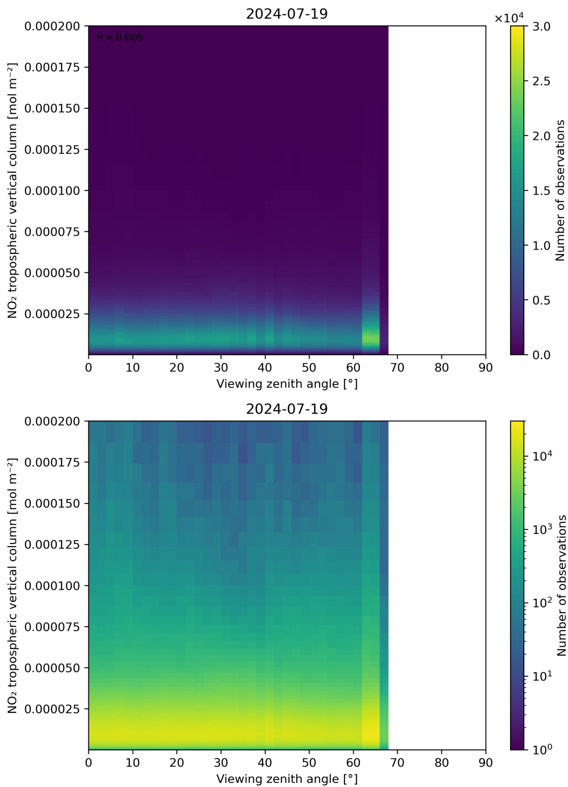
Figure 169: Scatter density plot of “Viewing zenith angle” against “NO 2 tropospheric vertical column” for 2024-07-18 to 2024-07-20.
