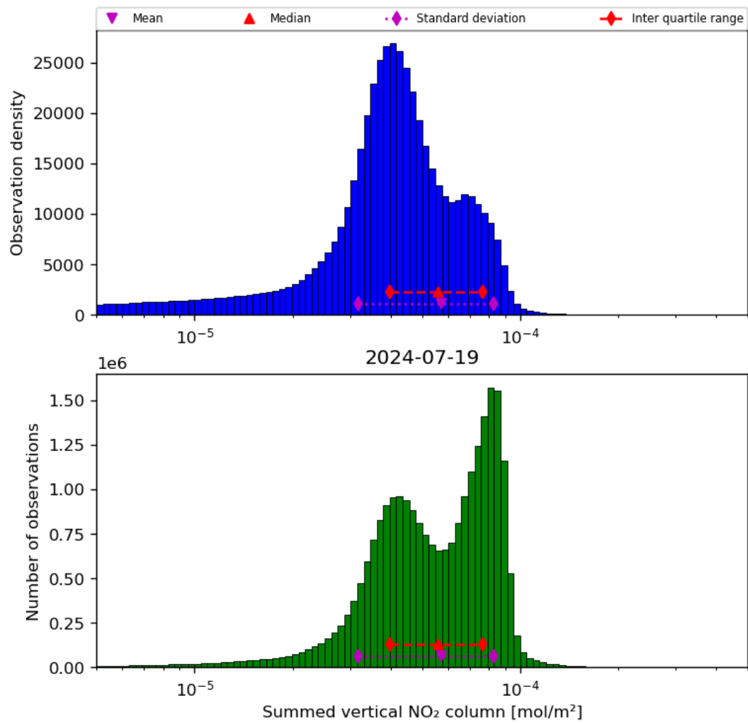
Figure 40: Histogram of “Summed vertical NO 2 column” for 2024-07-18 to 2024-07-20
