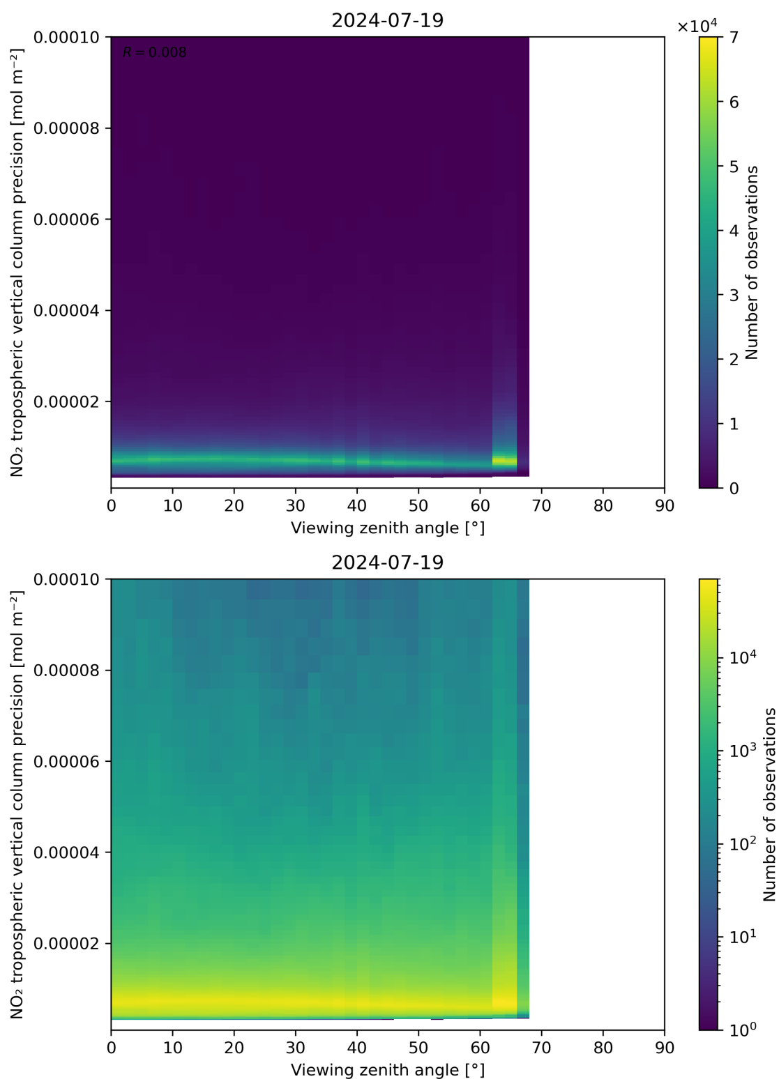
Figure 170: Scatter density plot of “Viewing zenith angle” against “NO 2 tropospheric vertical column precision” for 2024-07-18 to 2024-07-20.
