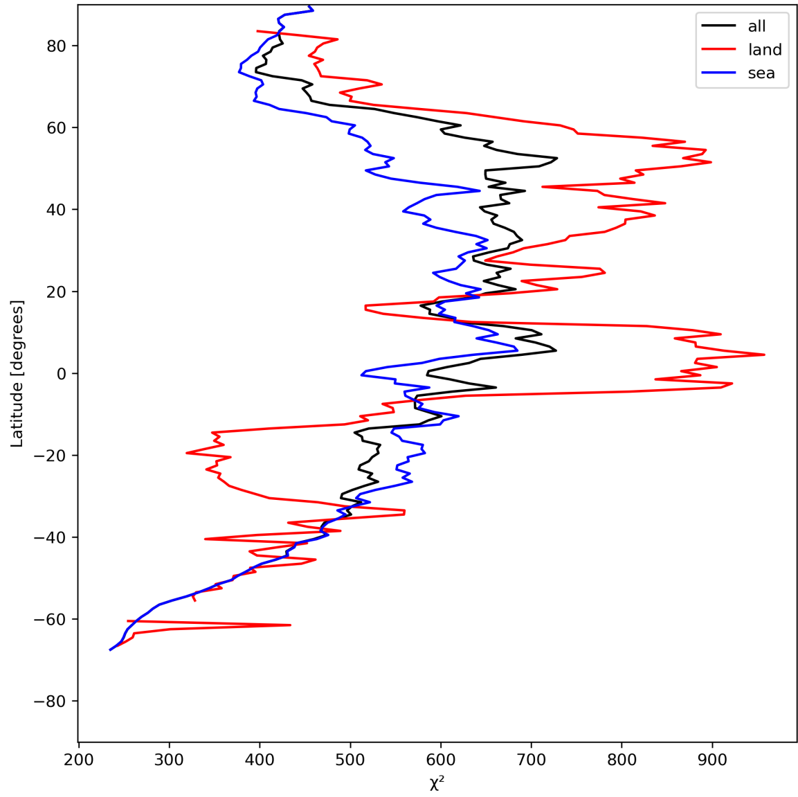
Figure 25: Zonal average of “ \chi^2 ” for 2024-07-18 to 2024-07-20.
