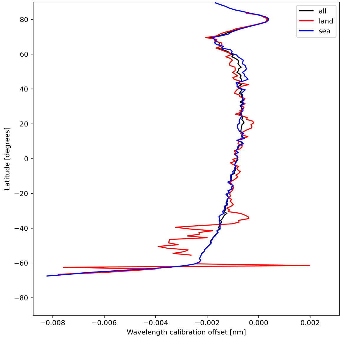
Figure 18: Zonal average of “Wavelength calibration offset” for 2024-07-18 to 2024-07-20.
