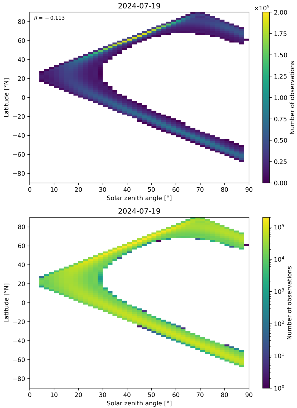
Figure 149: Scatter density plot of “Solar zenith angle” against “Latitude” for 2024-07-18 to 2024-07-20.
