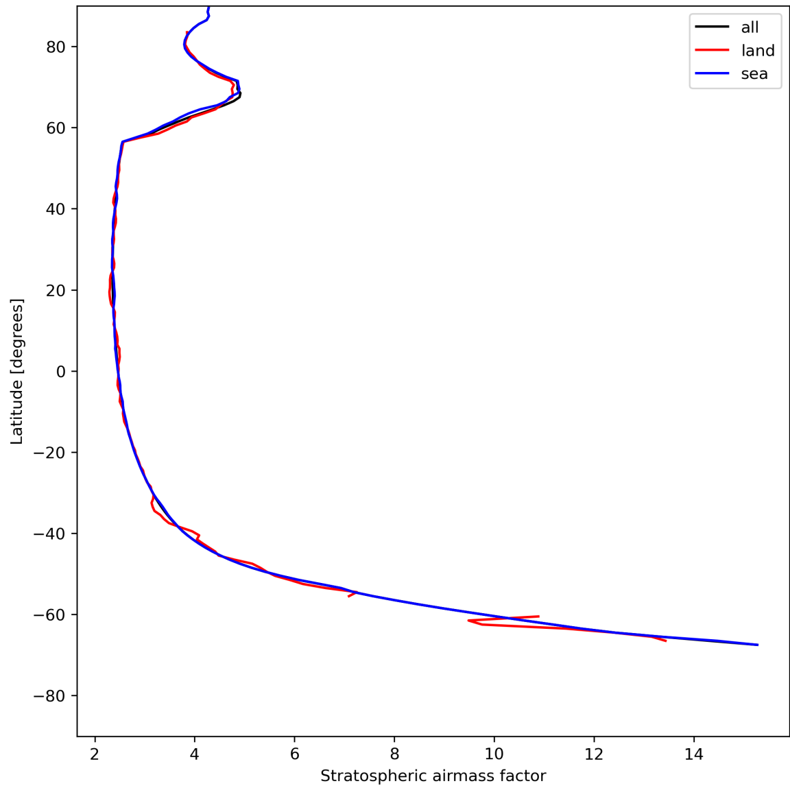
Figure 27: Zonal average of “Stratospheric airmass factor” for 2024-07-18 to 2024-07-20.
