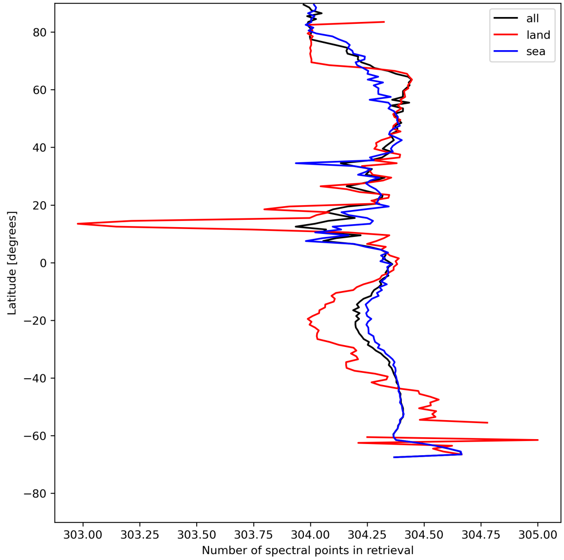
Figure 16: Zonal average of “Number of spectral points in retrieval” for 2024-07-18 to 2024-07-20.
