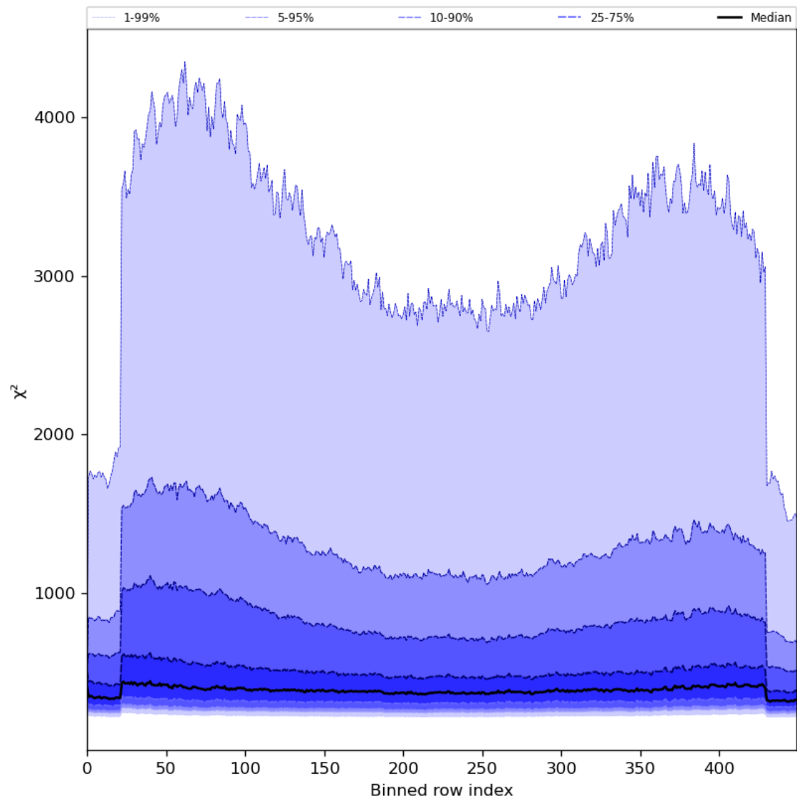
Figure 59: Along track statistics of “ \chi^2 ” for 2024-07-18 to 2024-07-20
