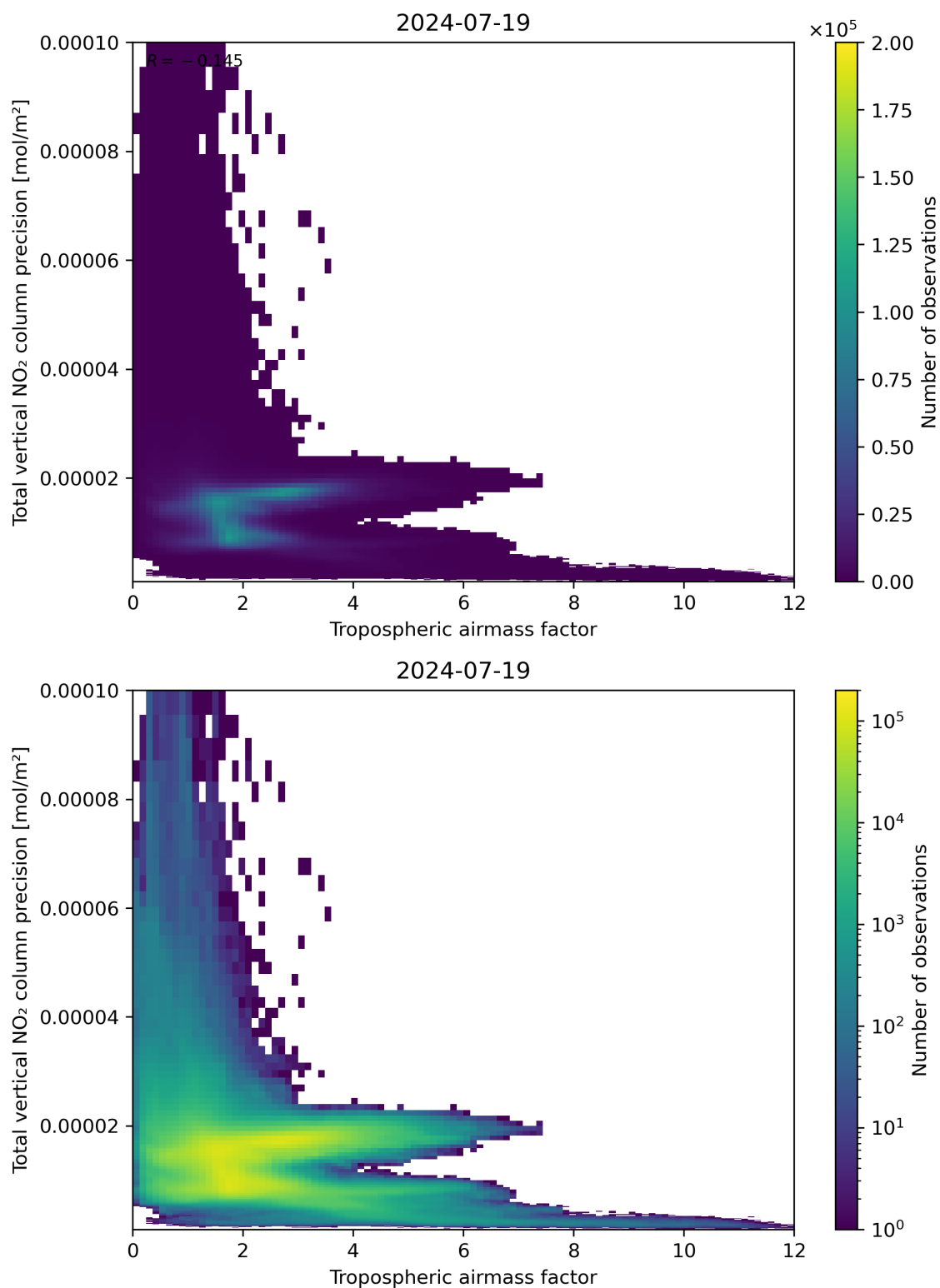
Figure 78: Scatter density plot of “Tropospheric air mass factor” against “Total vertical NO 2 column precision” for 2024-07-18 to 2024-07-20.
