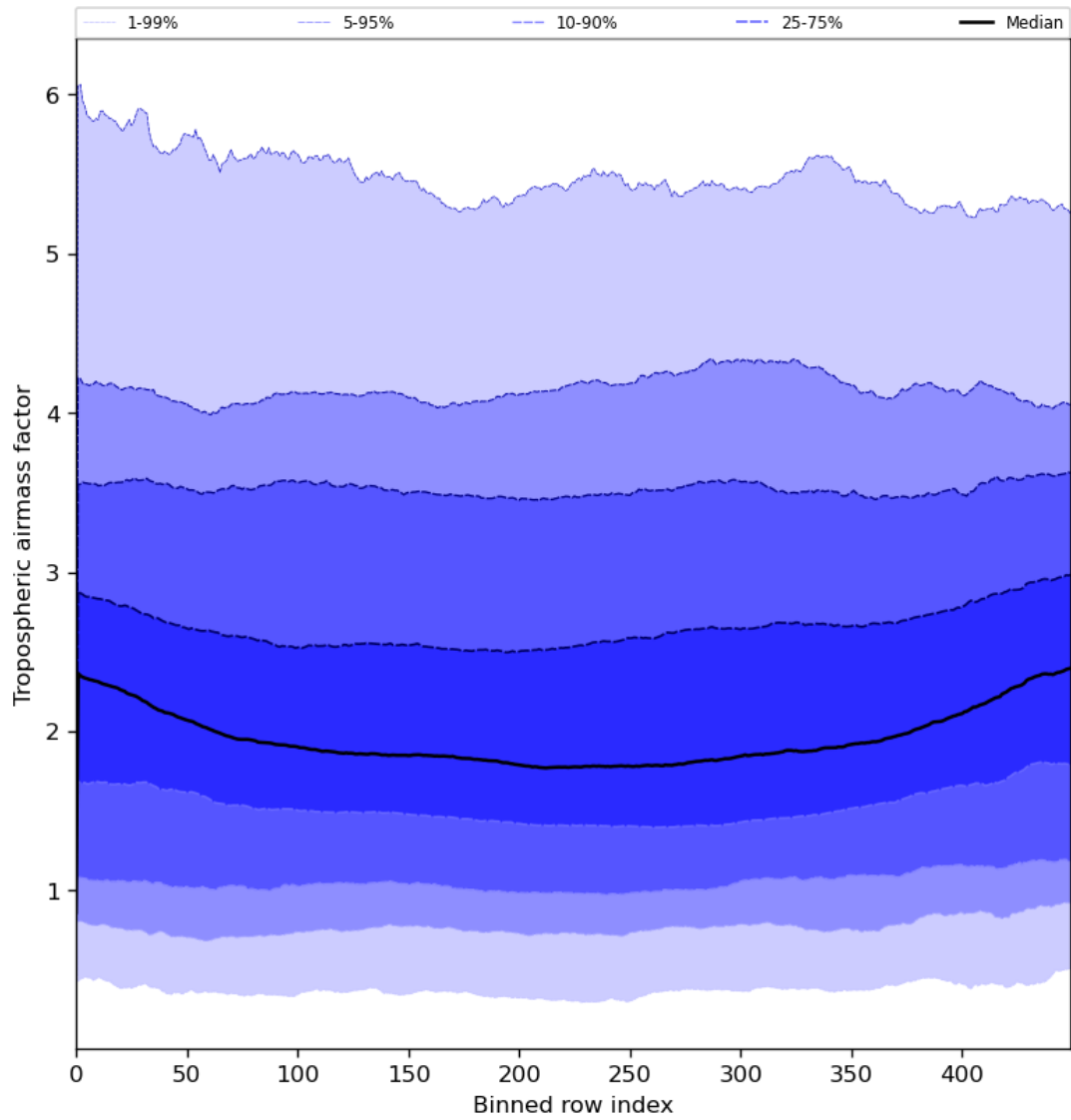
Figure 48: Along track statistics of “Tropospheric airmass factor” for 2024-07-18 to 2024-07-20
