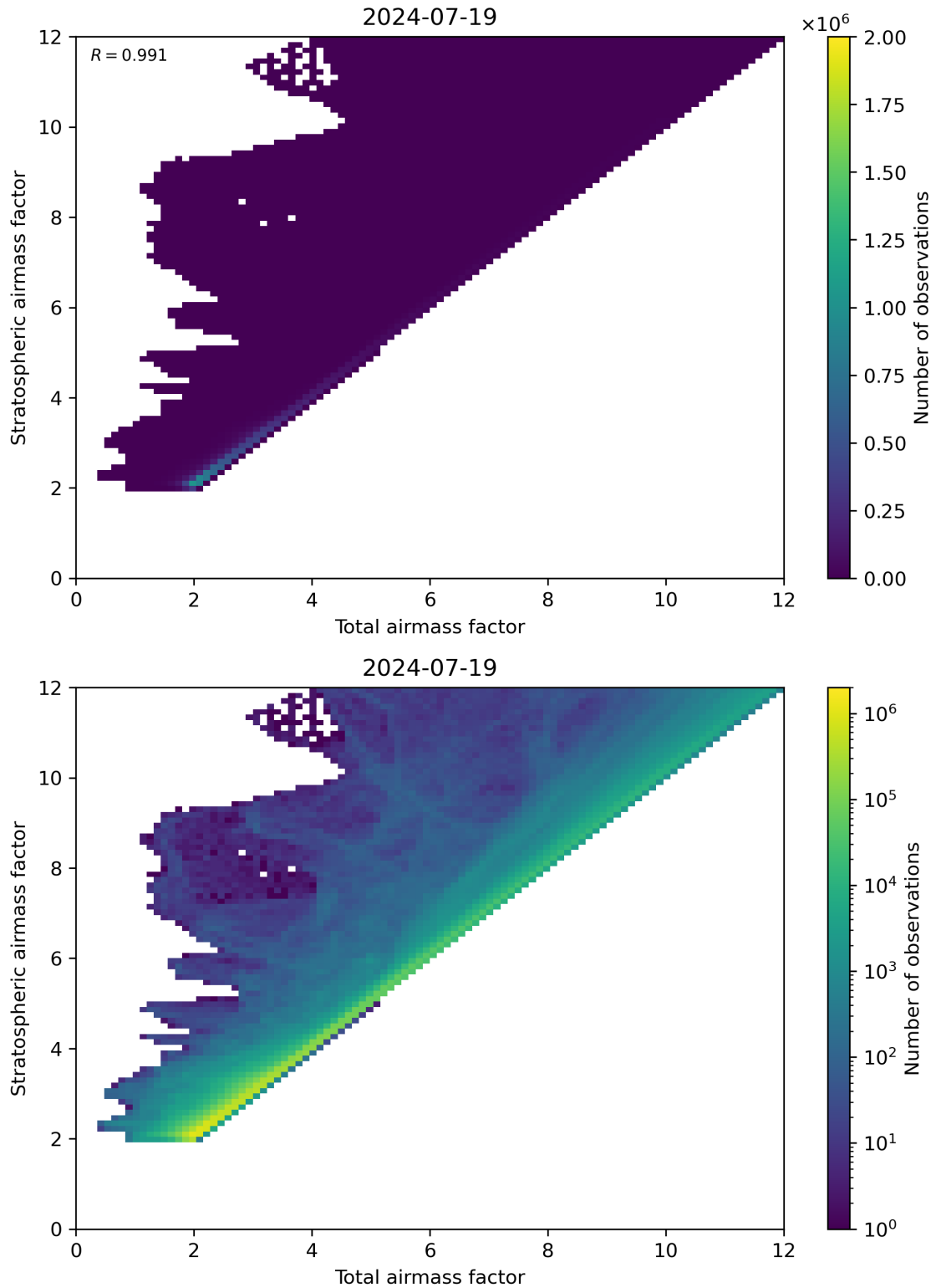
Figure 62: Scatter density plot of “Total airmass factor” against “Stratospheric airmass factor” for 2024-07-18 to 2024-07-20.
