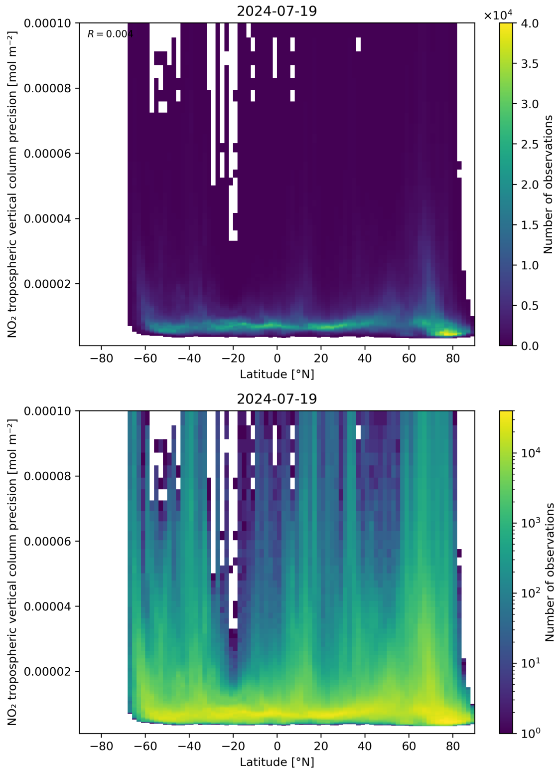
Figure 93: Scatter density plot of “Latitude” against “NO 2 tropospheric vertical column precision” for 2024-07-18 to 2024-07-20.
