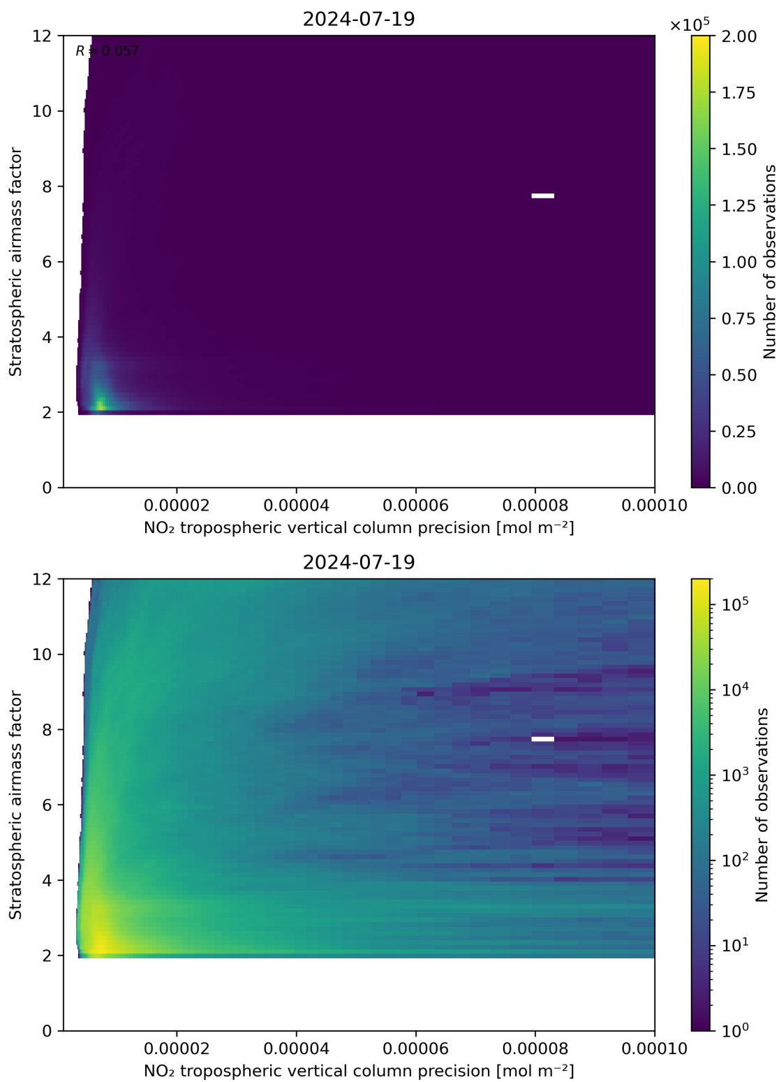
Figure 131: Scatter density plot of “NO 2 tropospheric vertical column precision” against “Stratospheric airmass factor” for 2024-07-18 to 2024-07-20.
