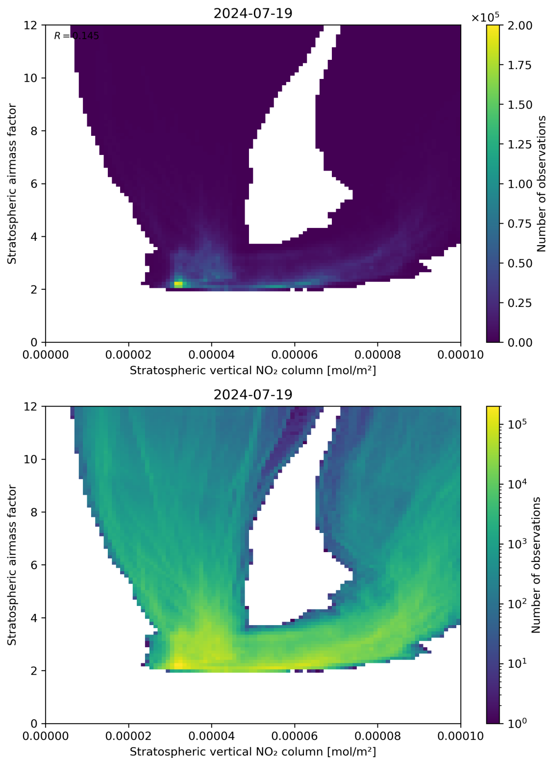
Figure 96: Scatter density plot of “Stratospheric vertical NO 2 column” against “Stratospheric airmass factor” for 2024-07-18 to 2024-07-20.
