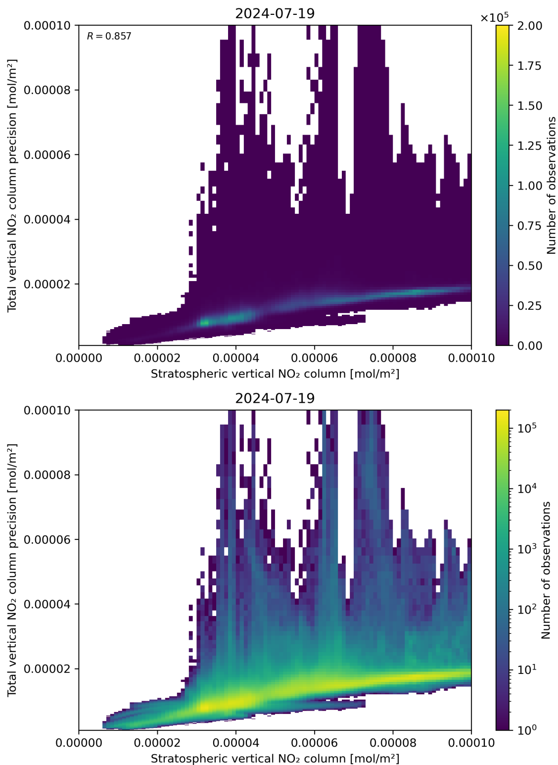
Figure 101: Scatter density plot of “Stratospheric vertical NO 2 column” against “Total vertical NO 2 column precision” for 2024-07-18 to 2024-07-20.
