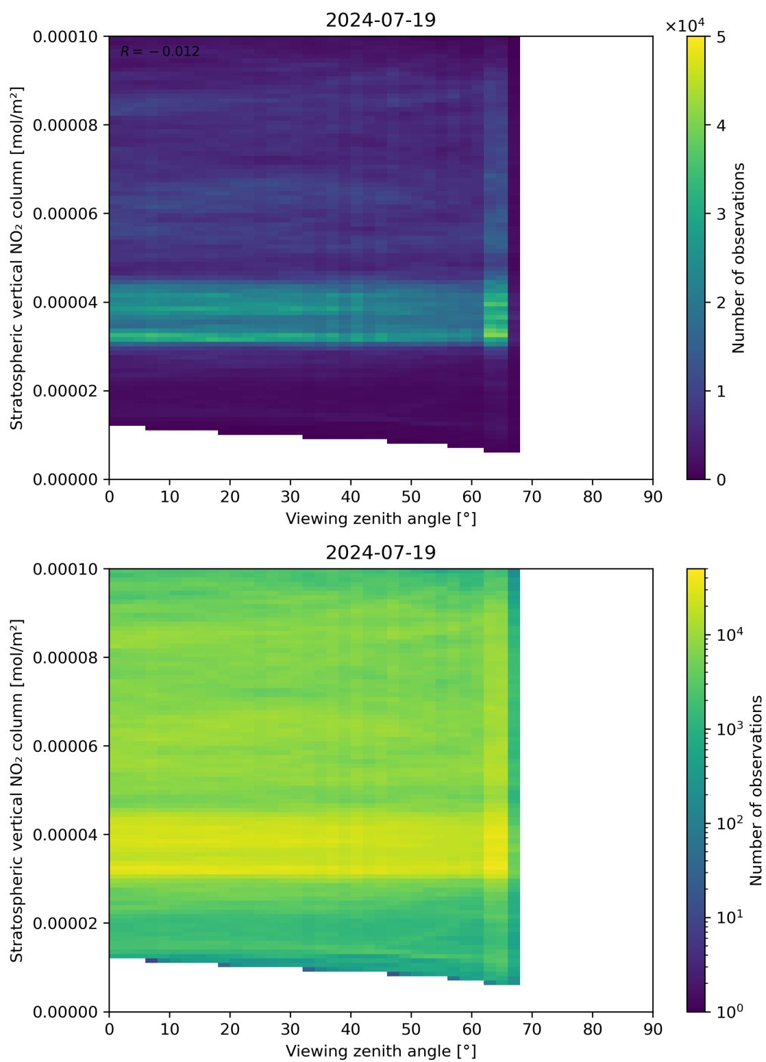
Figure 164: Scatter density plot of “Viewing zenith angle” against “Stratospheric vertical NO 2 column” for 2024-07-18 to 2024-07-20.
