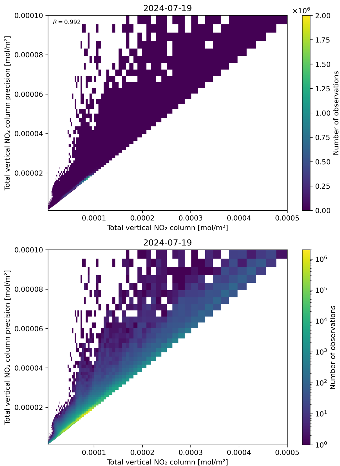
Figure 114: Scatter density plot of “Total vertical NO 2 column” against “Total vertical NO 2 column precision” for 2024-07-18 to 2024-07-20.
