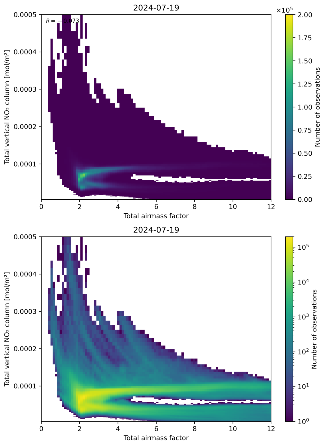
Figure 67: Scatter density plot of “Total airmass factor” against “Total vertical NO 2 column” for 2024-07-18 to 2024-07-20.
