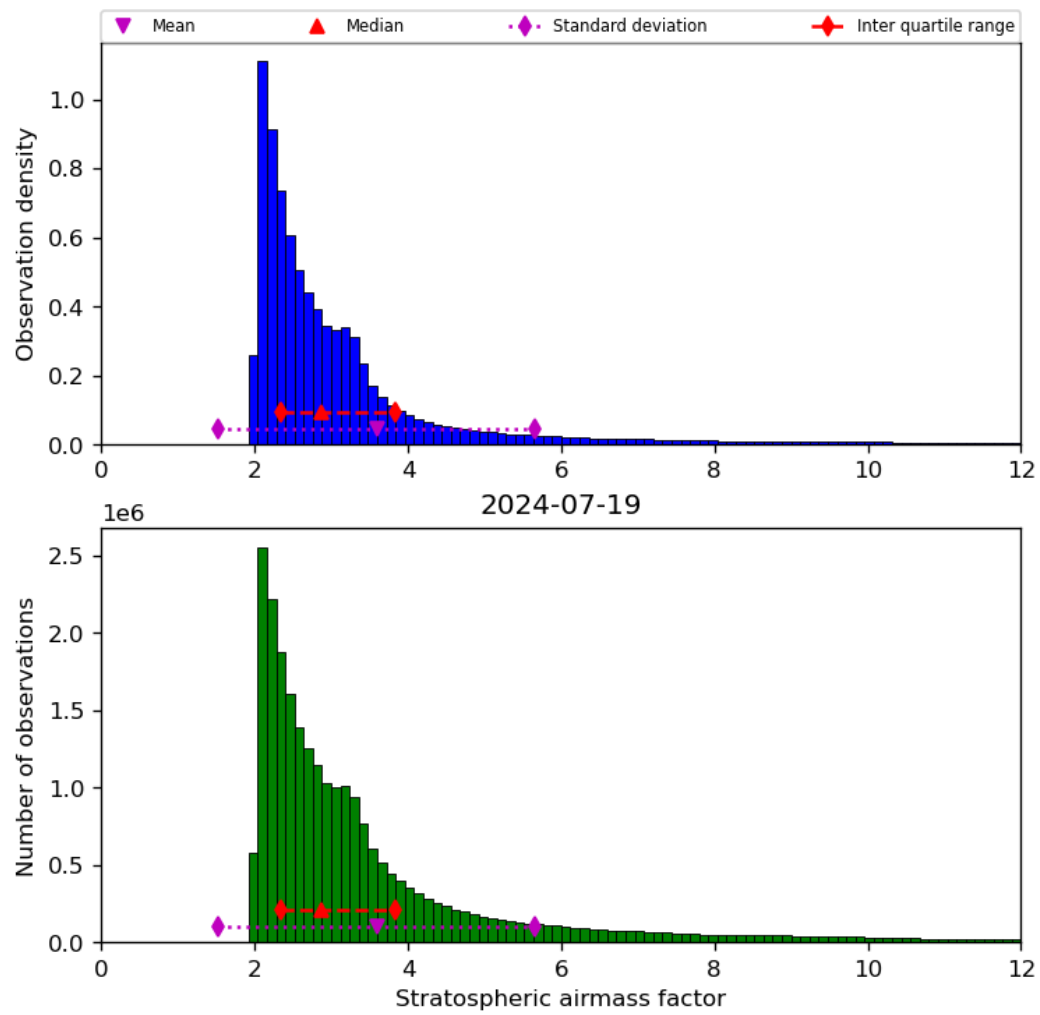
Figure 44: Histogram of “Stratospheric airmass factor” for 2024-07-18 to 2024-07-20
