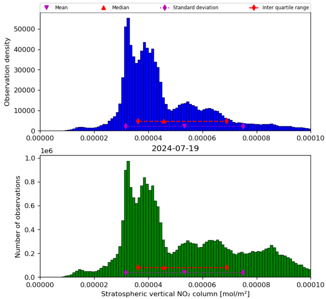
Figure 36: Histogram of “Stratospheric vertical NO 2 column” for 2024-07-18 to 2024-07-20
