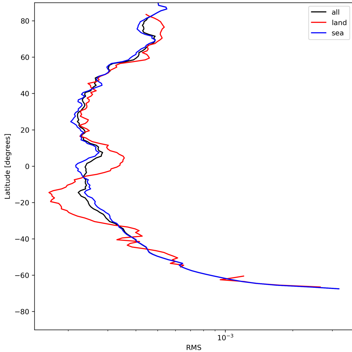
Figure 26: Zonal average of “RMS” for 2024-07-18 to 2024-07-20.
