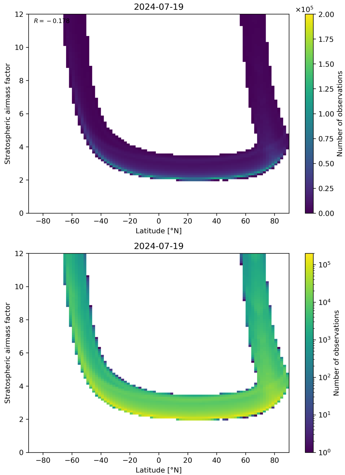
Figure 83: Scatter density plot of “Latitude” against “Stratospheric air mass factor” for 2024-07-18 to 2024-07-20.
