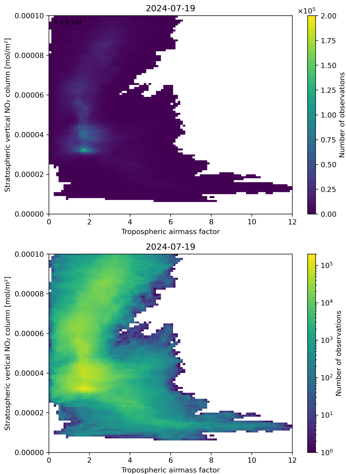
Figure 74: Scatter density plot of “Tropospheric air mass factor” against “Stratospheric vertical NO 2 column” for 2024-07-18 to 2024-07-20.
