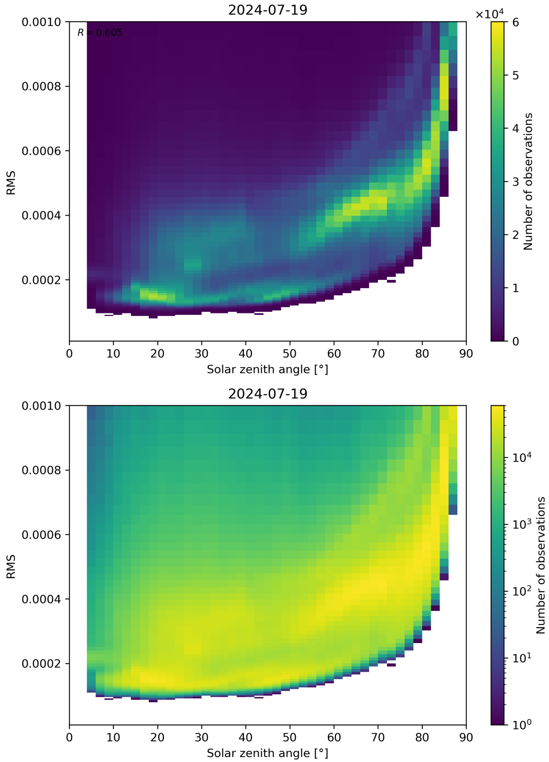
Figure 157: Scatter density plot of “Solar zenith angle” against “RMS” for 2024-07-18 to 2024-07-20.
