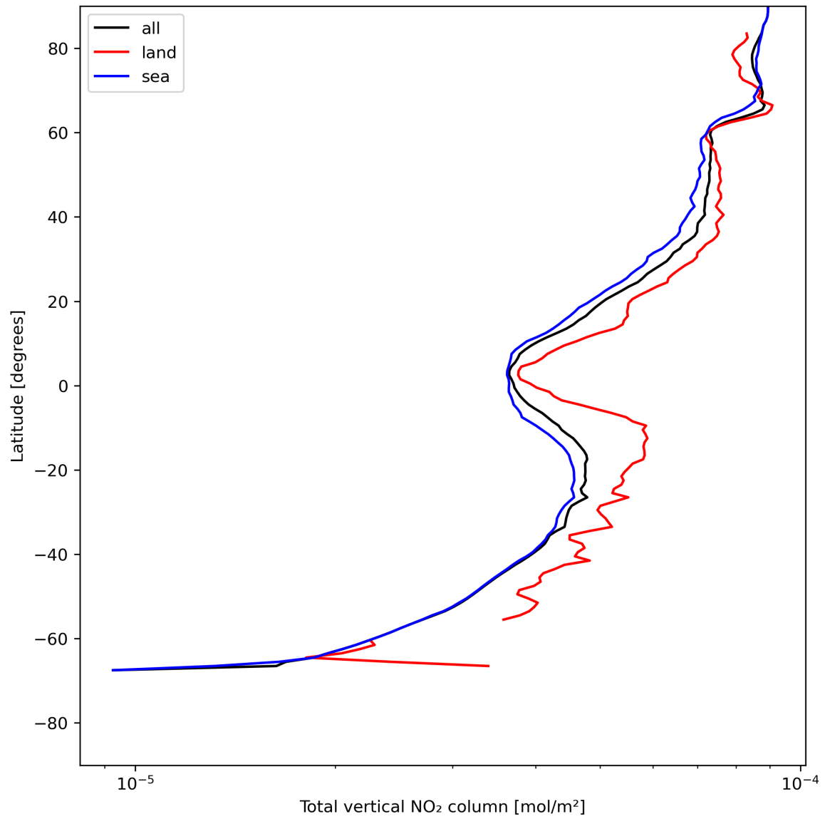
Figure 21: Zonal average of “Total vertical NO 2 column” for 2024-07-18 to 2024-07-20.
