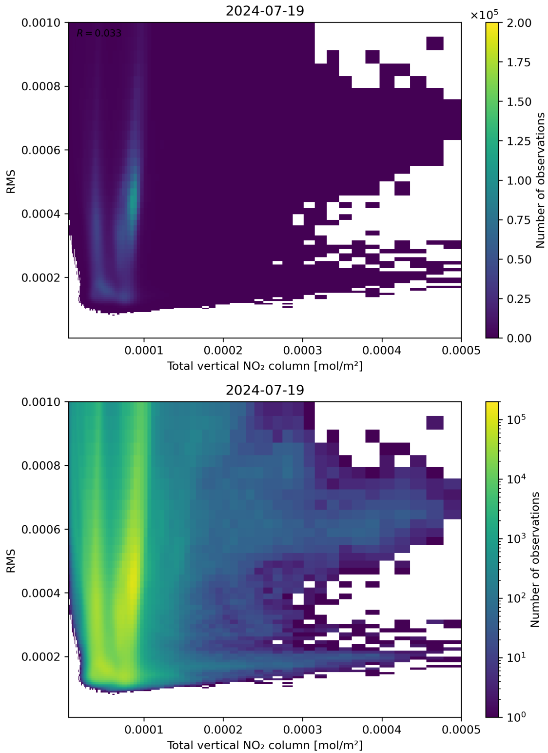
Figure 120: Scatter density plot of “Total vertical NO 2 column” against “RMS” for 2024-07-18 to 2024-07-20.
