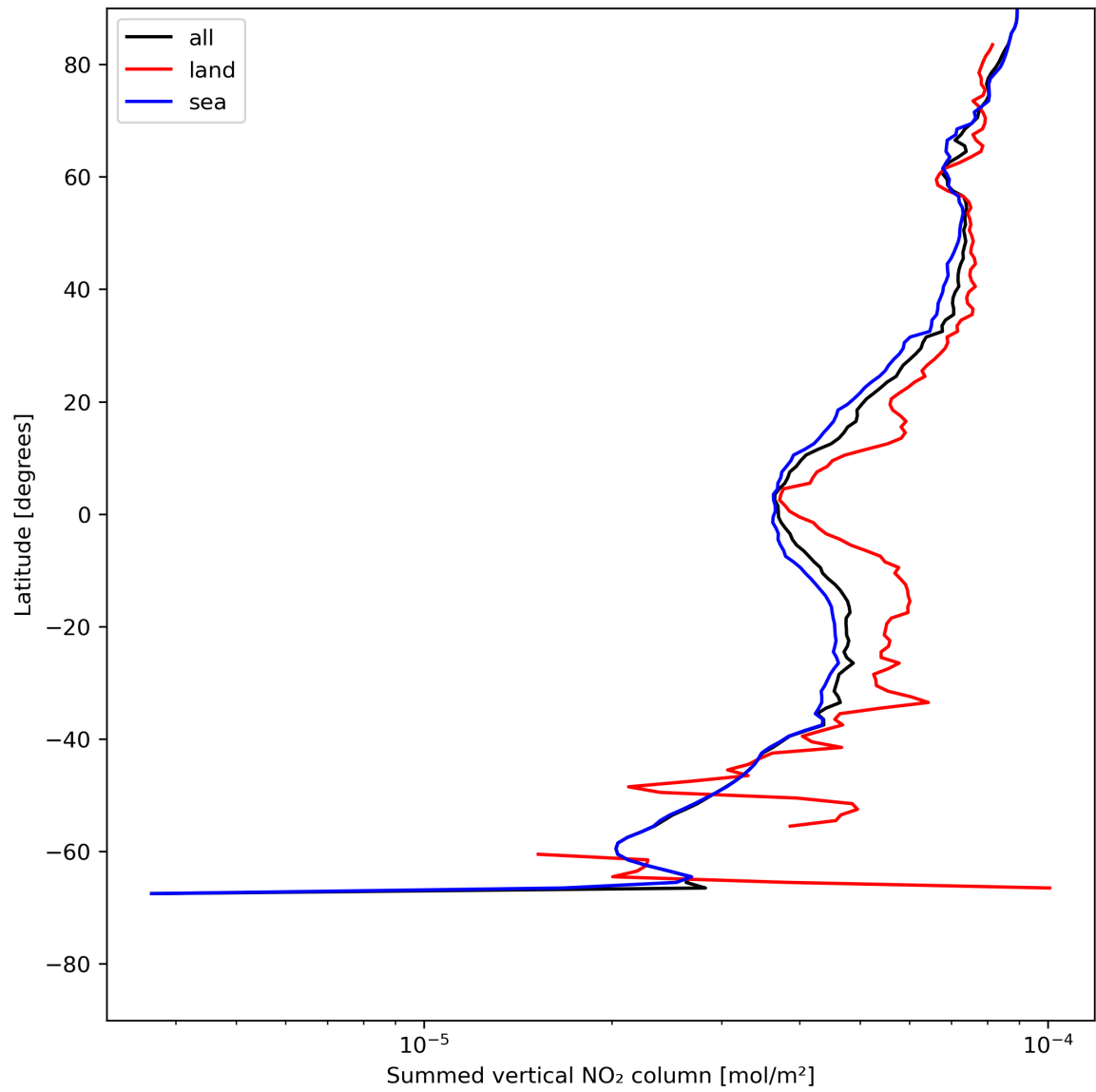
Figure 23: Zonal average of “Summed vertical NO 2 column” for 2024-07-18 to 2024-07-20.
