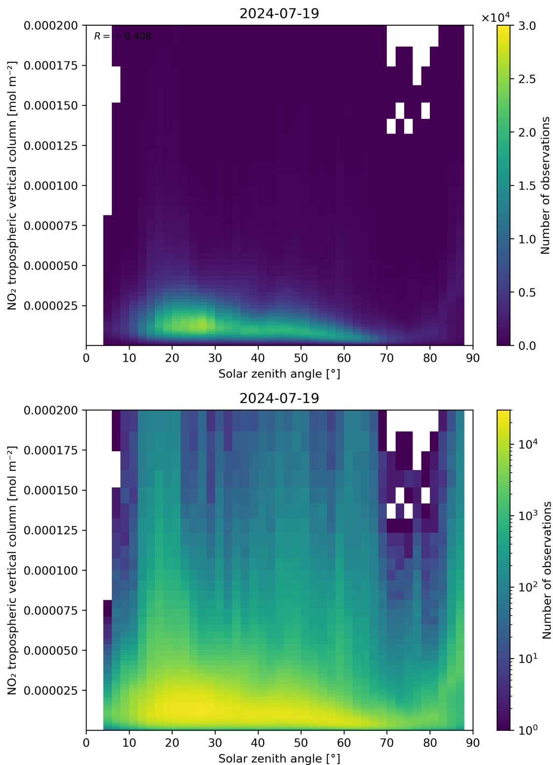
Figure 155: Scatter density plot of “Solar zenith angle” against “NO 2 tropospheric vertical column” for 2024-07-18 to 2024-07-20.
