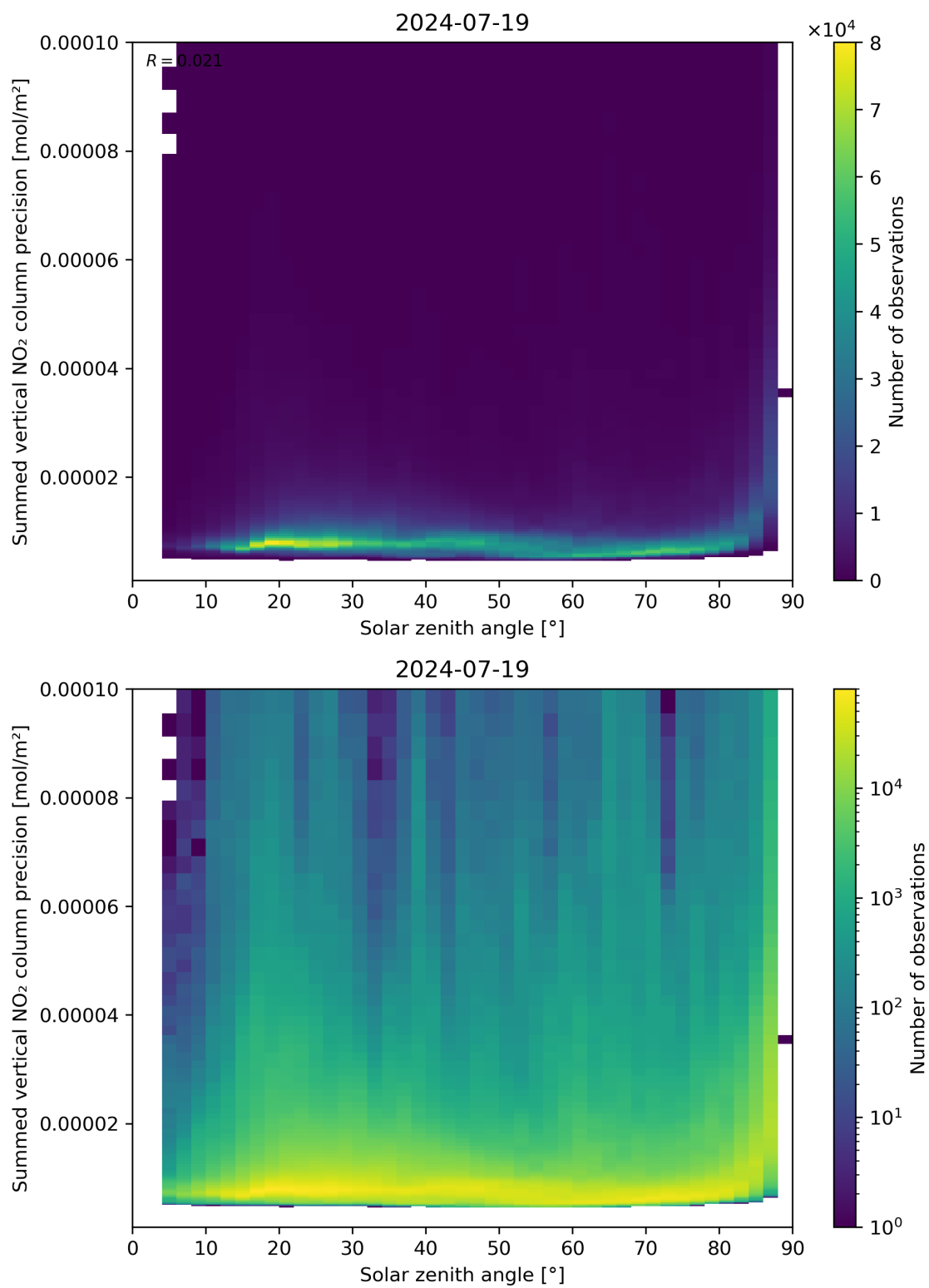
Figure 152: Scatter density plot of “Solar zenith angle” against “Summed vertical NO 2 column precision” for 2024-07-18 to 2024-07-20.
