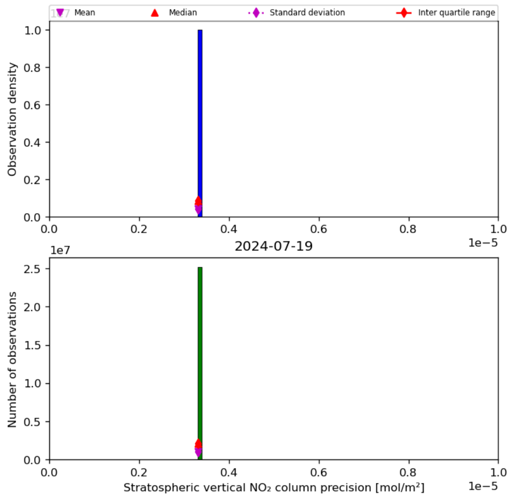
Figure 37: Histogram of “Stratospheric vertical NO 2 column precision” for 2024-07-18 to 2024-07-20
