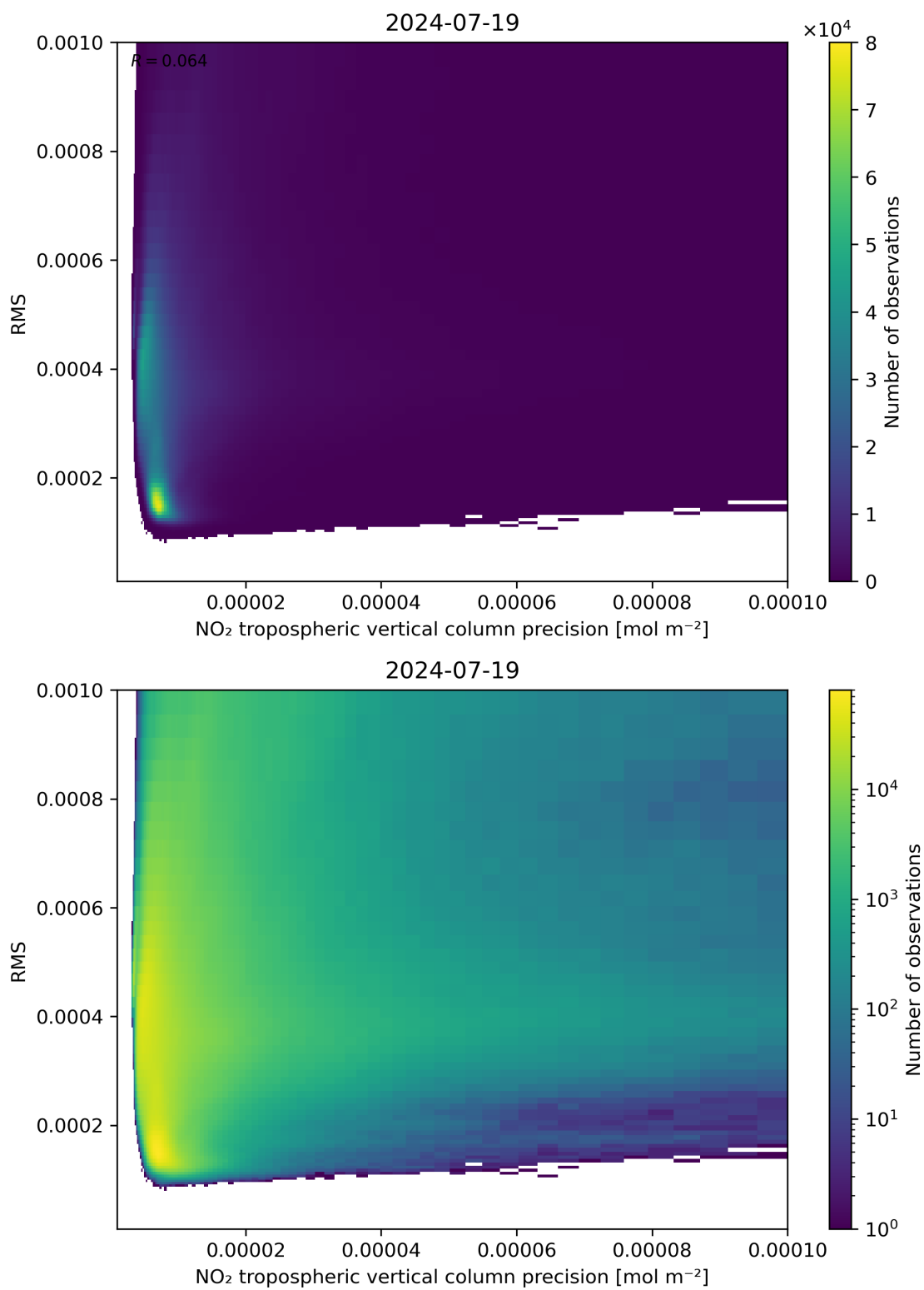
Figure 140: Scatter density plot of “NO 2 tropospheric vertical column precision” against “RMS” for 2024-07-18 to 2024-07-20.
