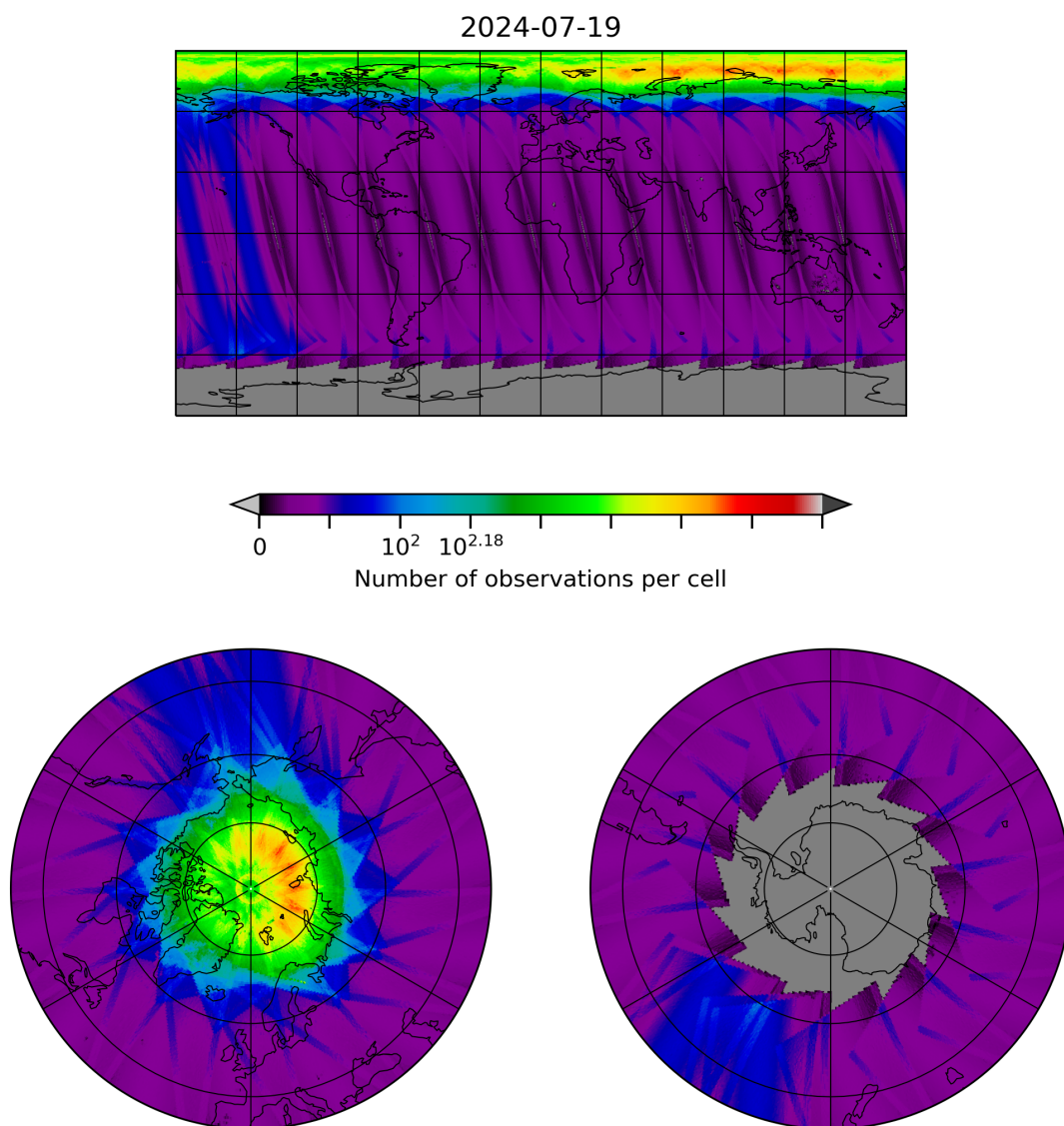
Figure 10: Map of the number of observations for 2024-07-18 to 2024-07-20
