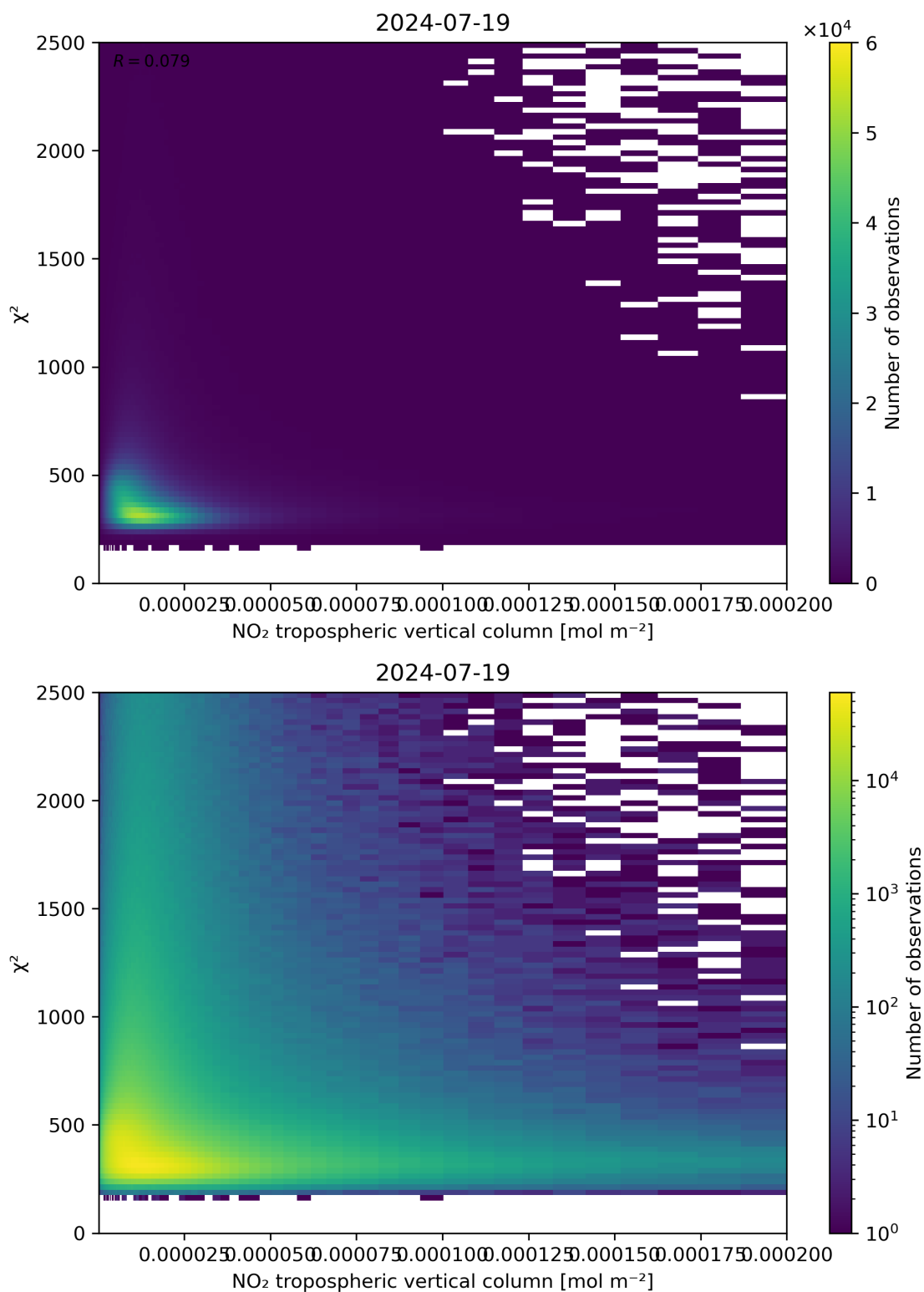
Figure 124: Scatter density plot of “NO 2 tropospheric vertical column” against “ \chi^2 ” for 2024-07-18 to 2024-07-20.
