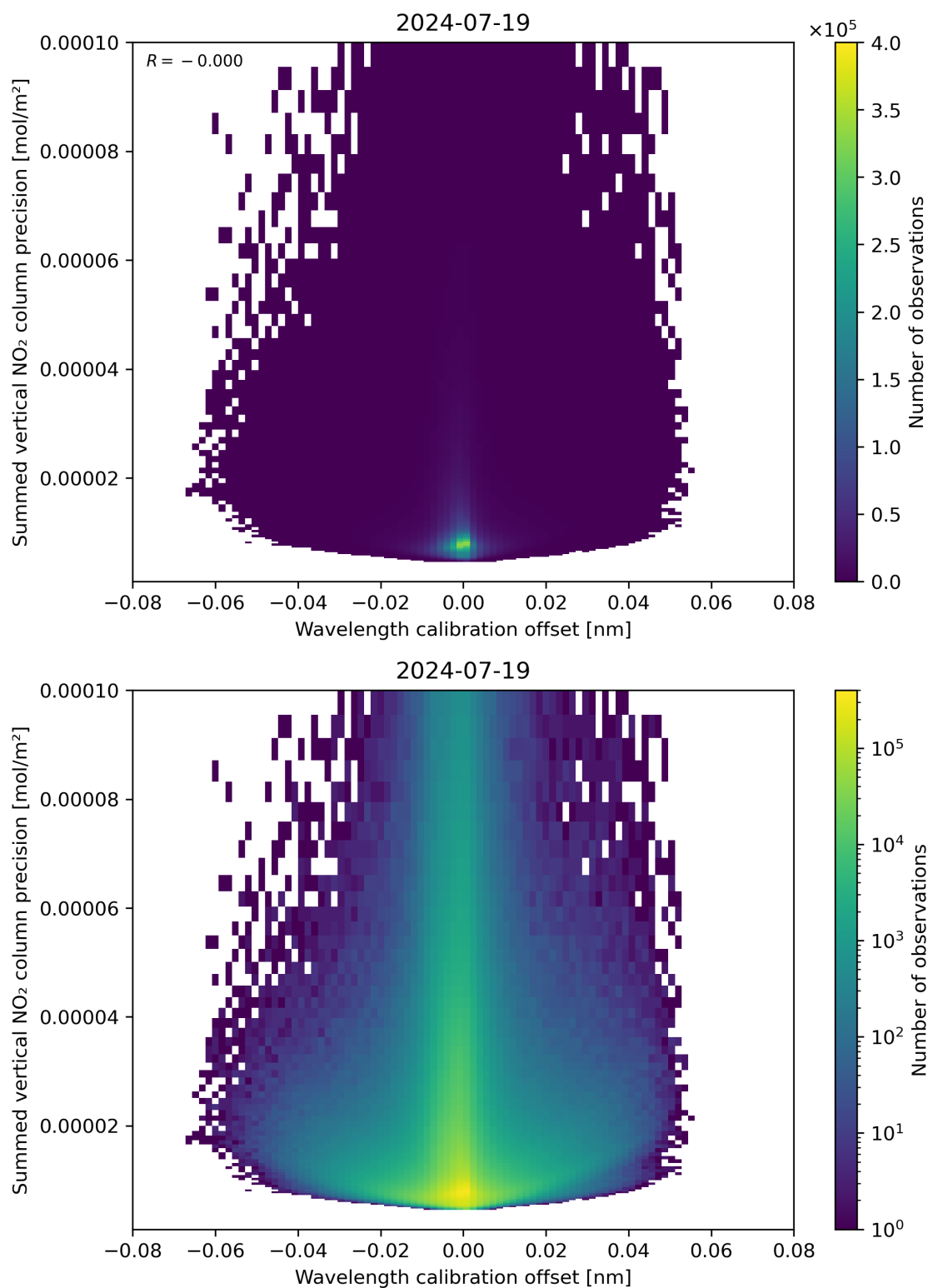
Figure 178: Scatter density plot of “Wavelength calibration offset” against “Summed vertical NO 2 column precision” for 2024-07-18 to 2024-07-20.
