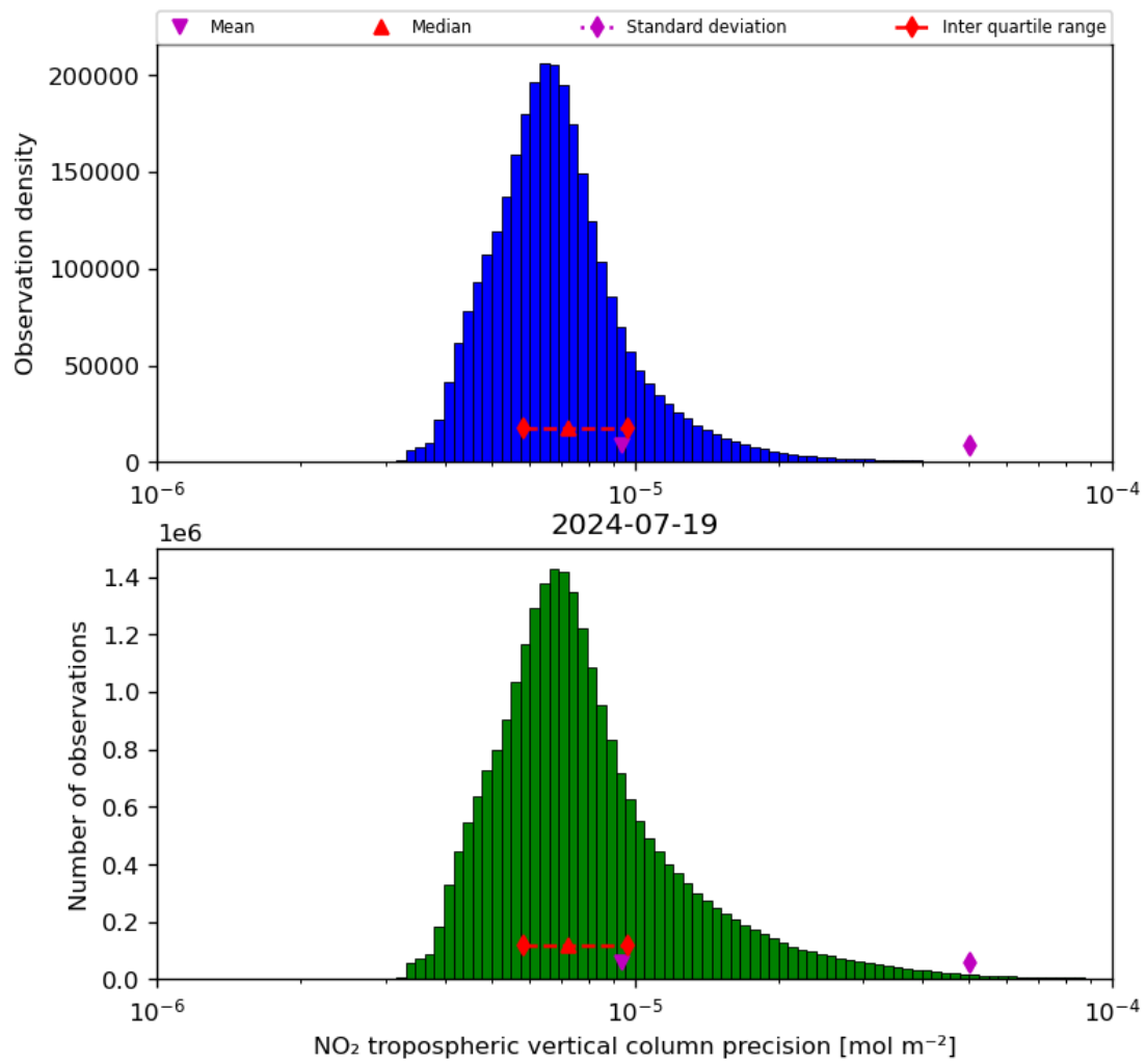
Figure 30: Histogram of “NO 2 tropospheric vertical column precision” for 2024-07-18 to 2024-07-20
