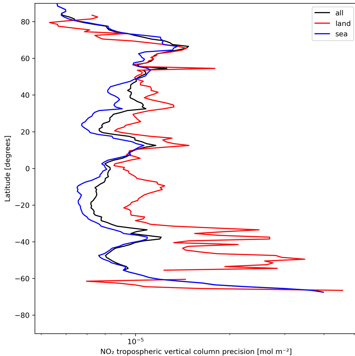
Figure 13: Zonal average of “NO 2 tropospheric vertical column precision” for 2024-07-18 to 2024-07-20.
