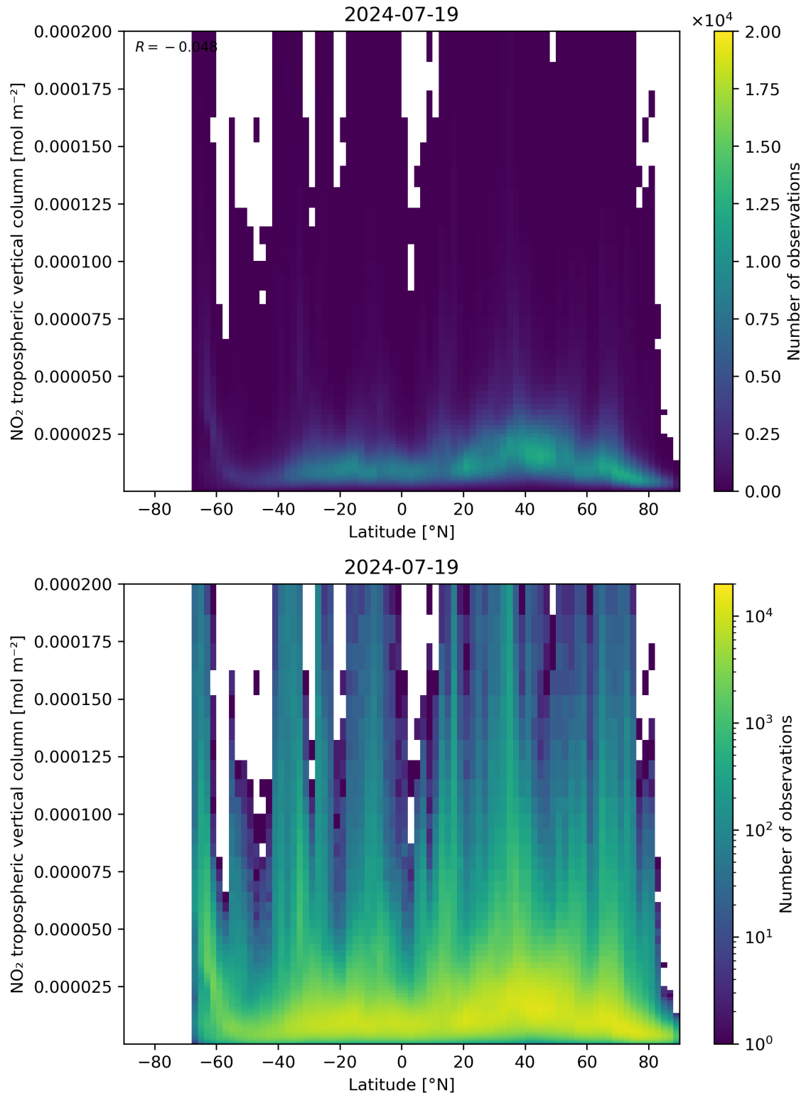
Figure 92: Scatter density plot of “Latitude” against “NO 2 tropospheric vertical column” for 2024-07-18 to 2024-07-20.
