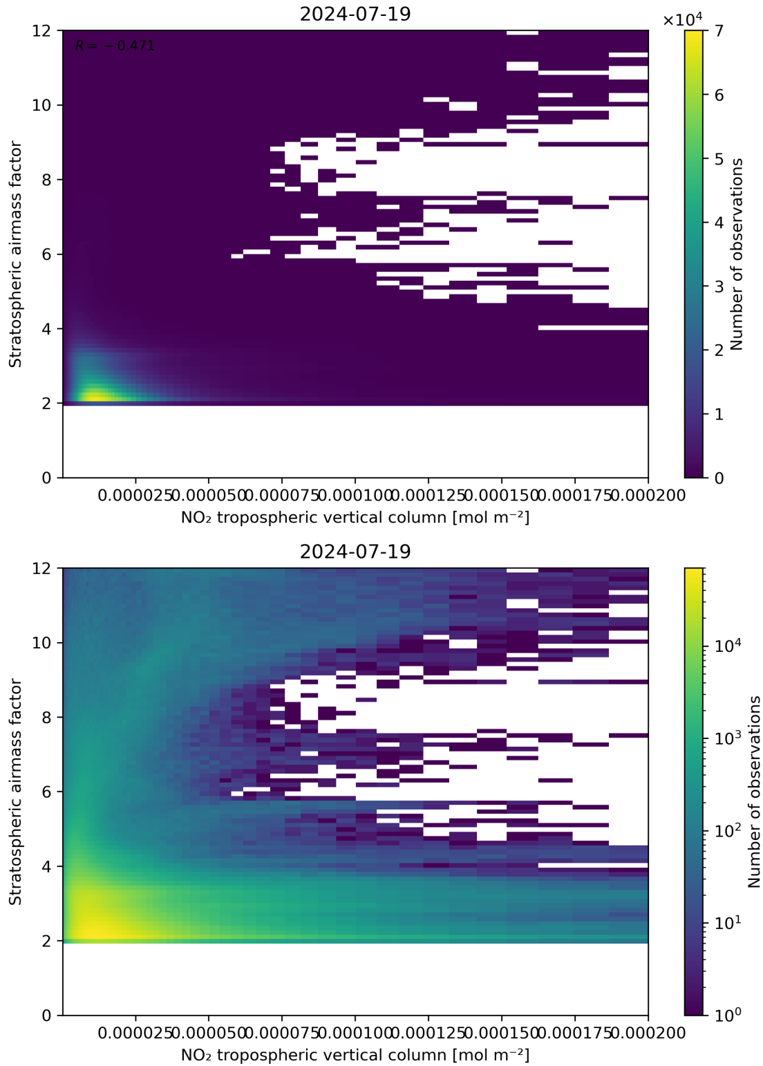
Figure 121: Scatter density plot of “NO 2 tropospheric vertical column” against “Stratospheric air mass factor” for 2024-07-18 to 2024-07-20.
