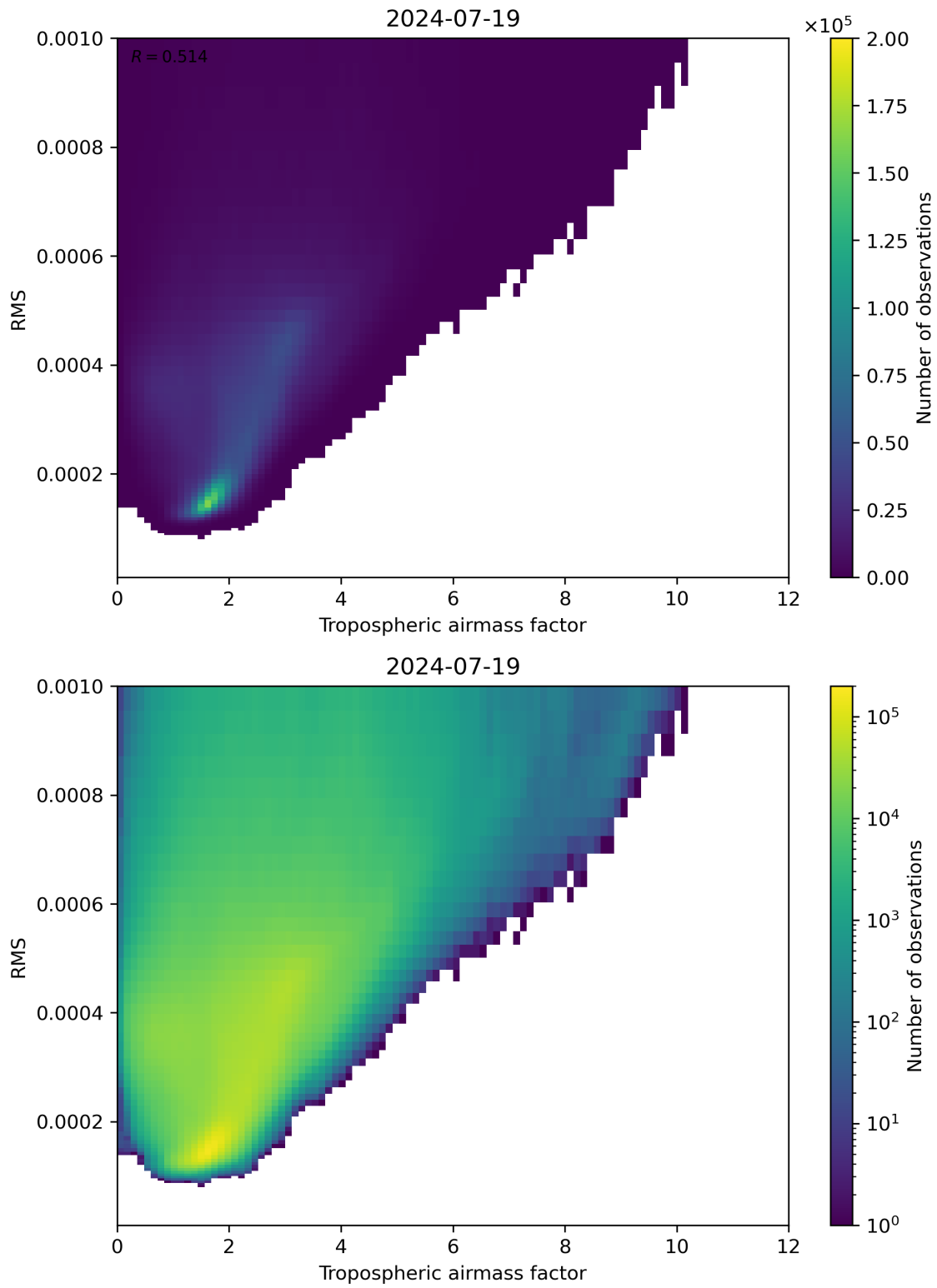
Figure 79: Scatter density plot of “Tropospheric airmass factor” against “RMS” for 2024-07-18 to 2024-07-20.
