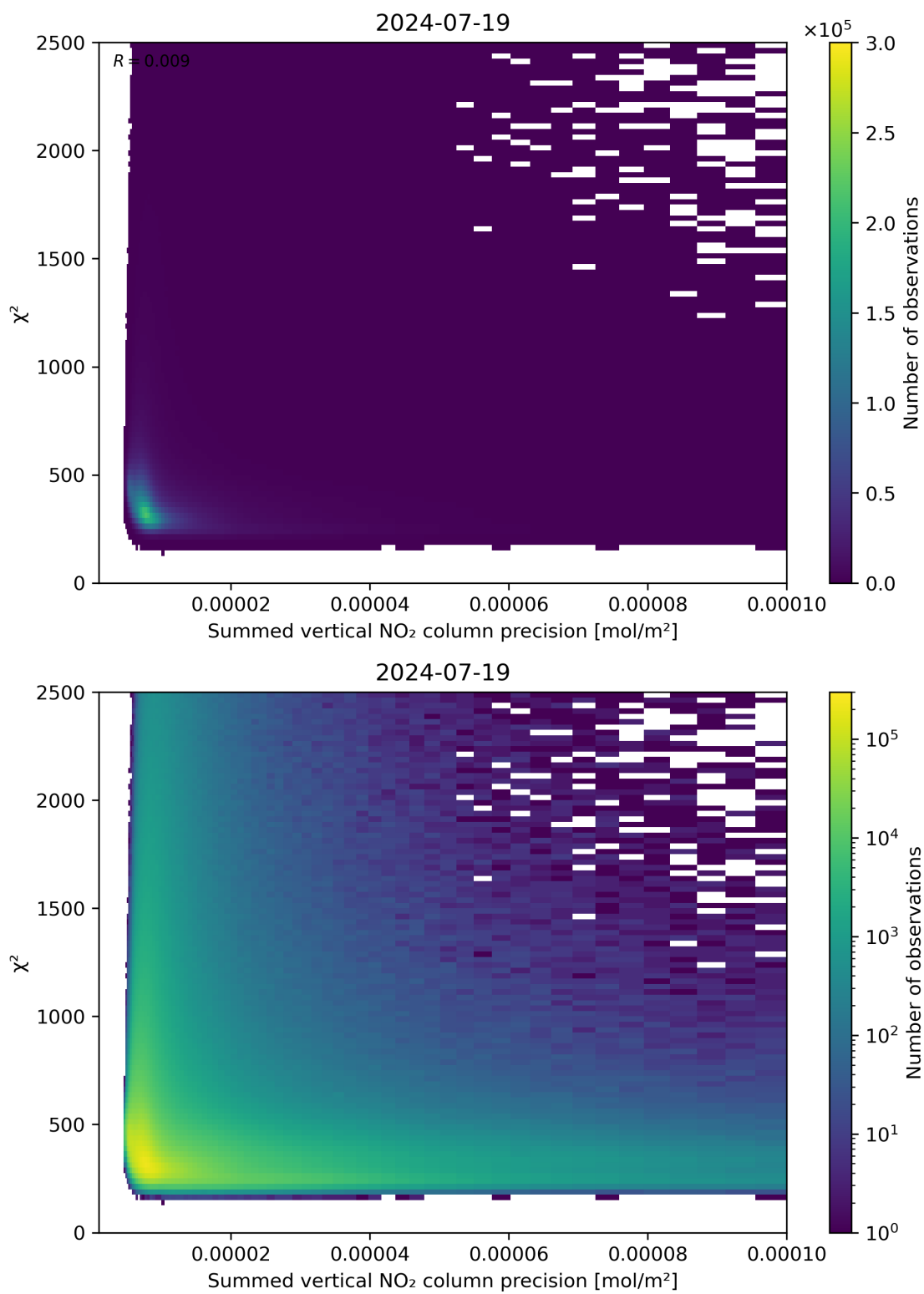
Figure 107: Scatter density plot of “Summed vertical NO 2 column precision” against “ \chi^2 ” for 2024-07-18 to 2024-07-20.
