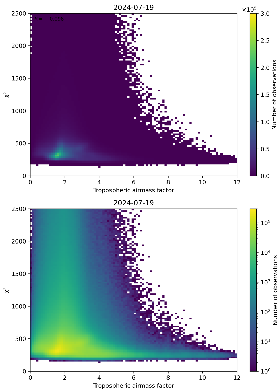
Figure 73: Scatter density plot of “Tropospheric airmass factor” against “ \chi^2 ” for 2024-07-18 to 2024-07-20.
