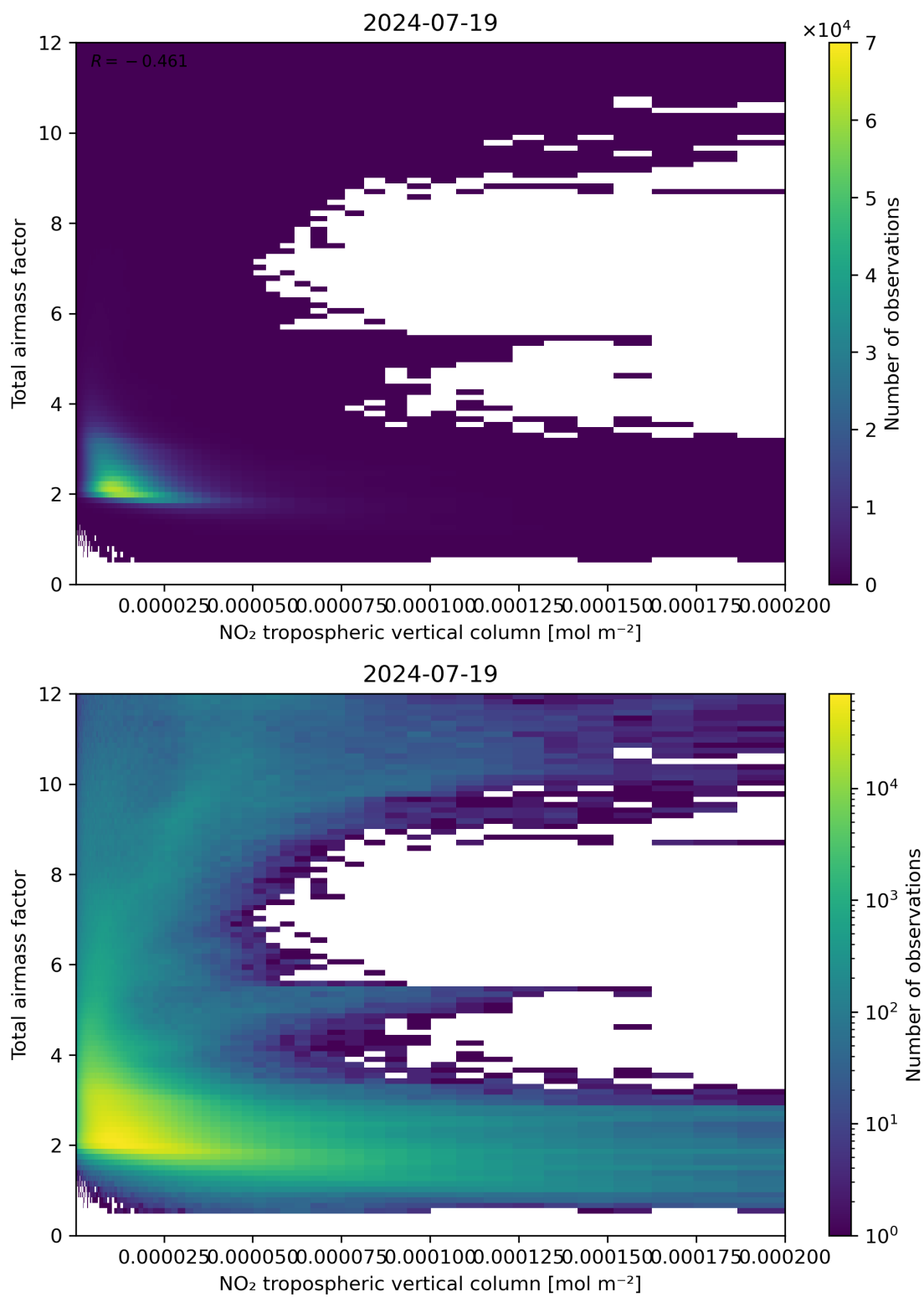
Figure 122: Scatter density plot of “NO 2 tropospheric vertical column” against “Total air mass factor” for 2024-07-18 to 2024-07-20.
