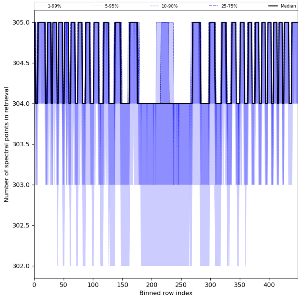
Figure 50: Along track statistics of “Number of spectral points in retrieval” for 2024-07-18 to 2024-07-20
