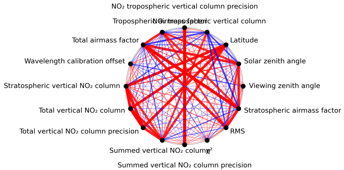
Figure 1: Map of correlation graph for 2024-07-18 to 2024-07-20.
