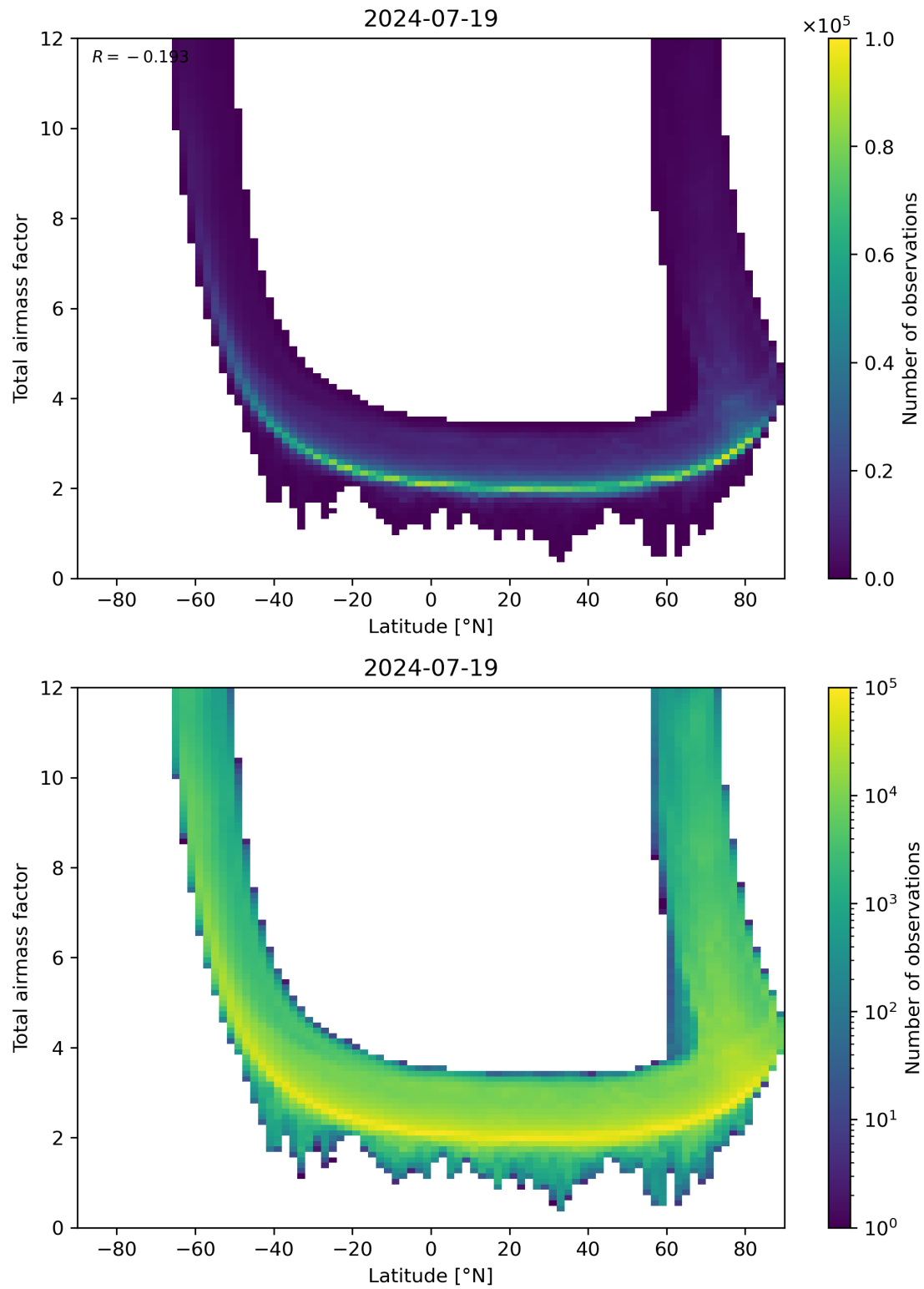
Figure 84: Scatter density plot of “Latitude” against “Total airmass factor” for 2024-07-18 to 2024-07-20.
