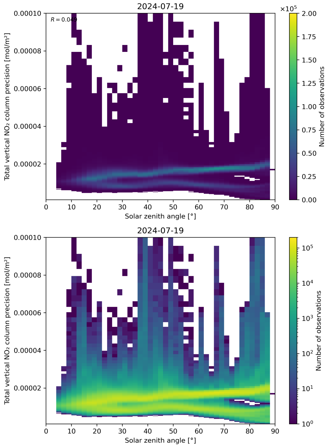
Figure 154: Scatter density plot of “Solar zenith angle” against “Total vertical NO 2 column precision” for 2024-07-18 to 2024-07-20.
