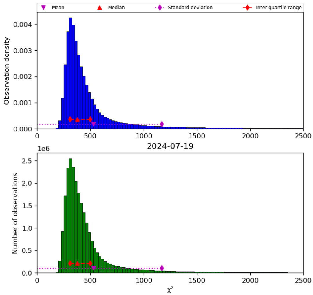
Figure 42: Histogram of “ \chi^2 ” for 2024-07-18 to 2024-07-20
