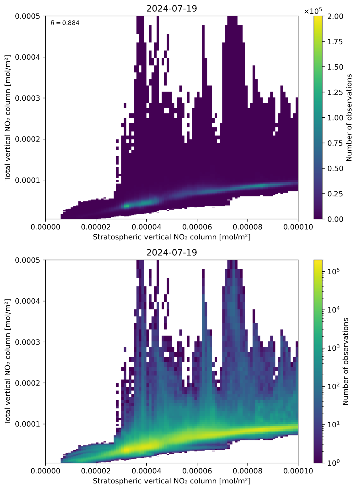
Figure 100: Scatter density plot of “Stratospheric vertical NO 2 column” against “Total vertical NO 2 column” for 2024-07-18 to 2024-07-20.
