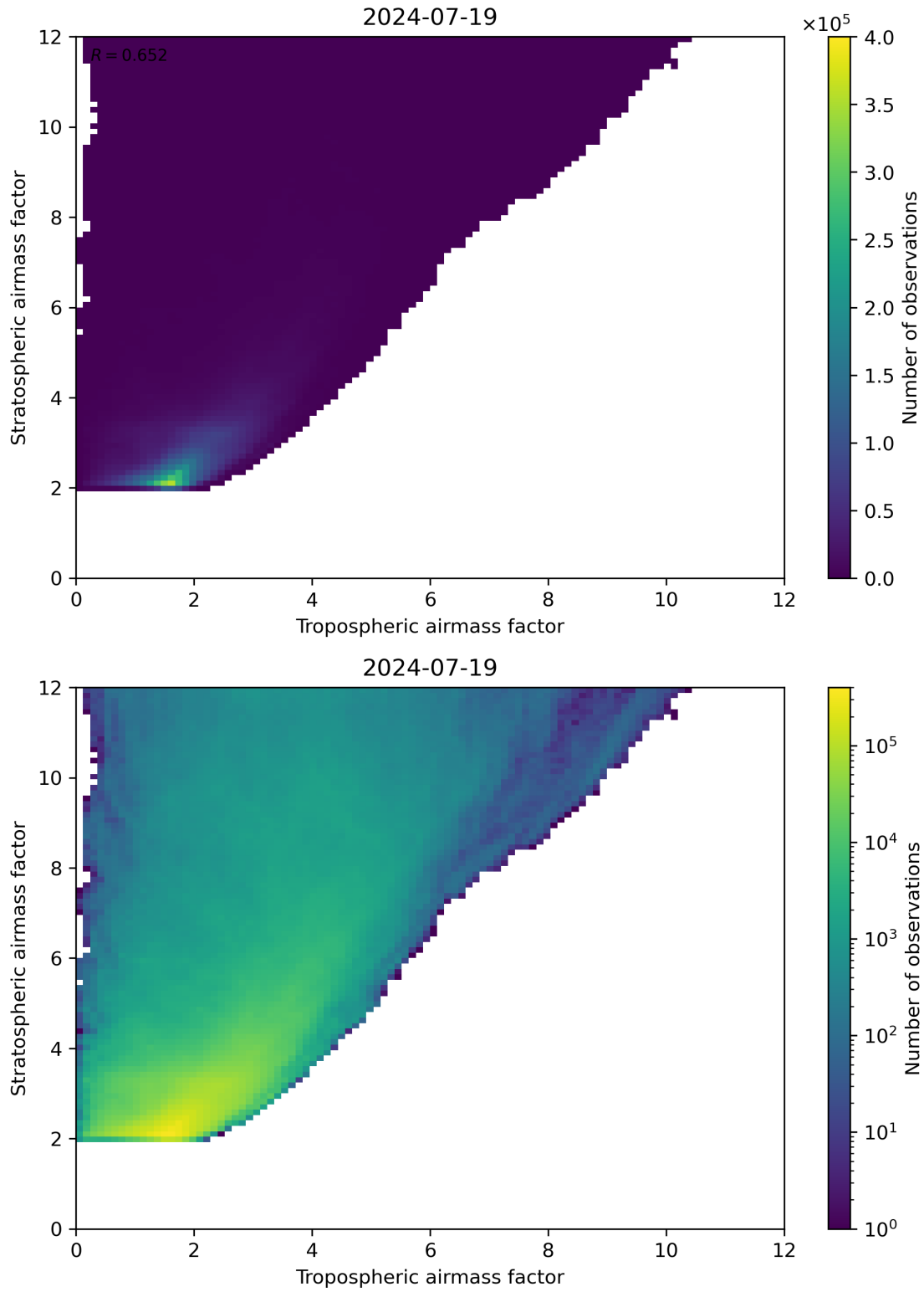
Figure 71: Scatter density plot of “Tropospheric airmass factor” against “Stratospheric airmass factor” for 2024-07-18 to 2024-07-20.
