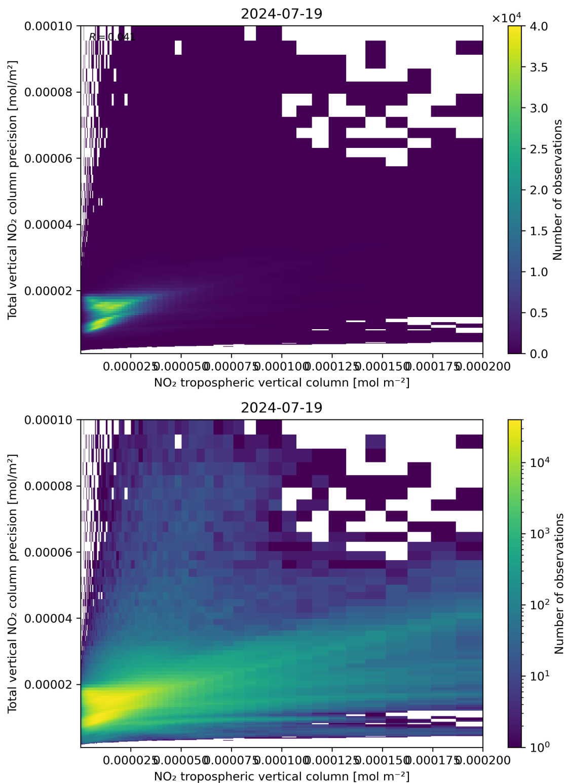
Figure 129: Scatter density plot of “NO 2 tropospheric vertical column” against “Total vertical NO 2 column precision” for 2024-07-18 to 2024-07-20.
