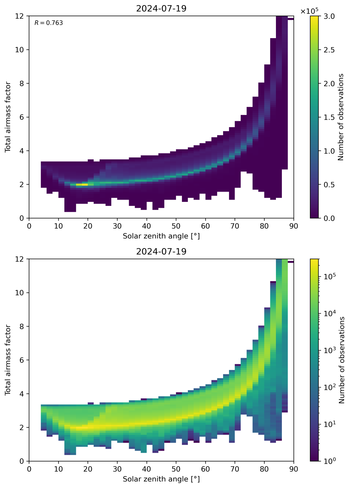
Figure 146: Scatter density plot of “Solar zenith angle” against “Total air mass factor” for 2024-07-18 to 2024-07-20.
