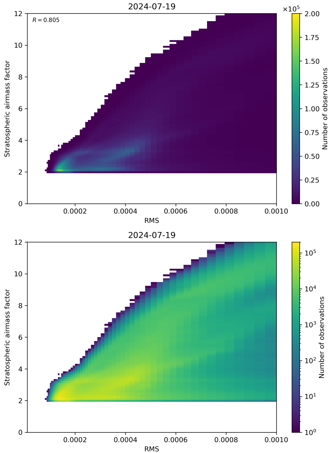
Figure 144: Scatter density plot of “RMS” against “Stratospheric airmass factor” for 2024-07-18 to 2024-07-20.
