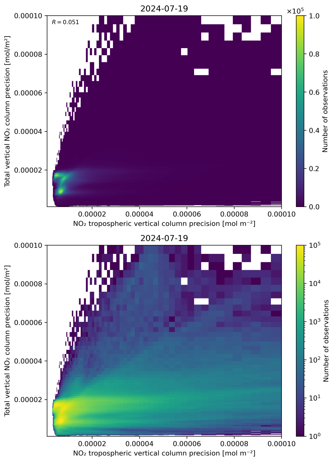
Figure 139: Scatter density plot of “NO 2 tropospheric vertical column precision” against “Total vertical NO 2 column precision” for 2024-07-18 to 2024-07-20.
