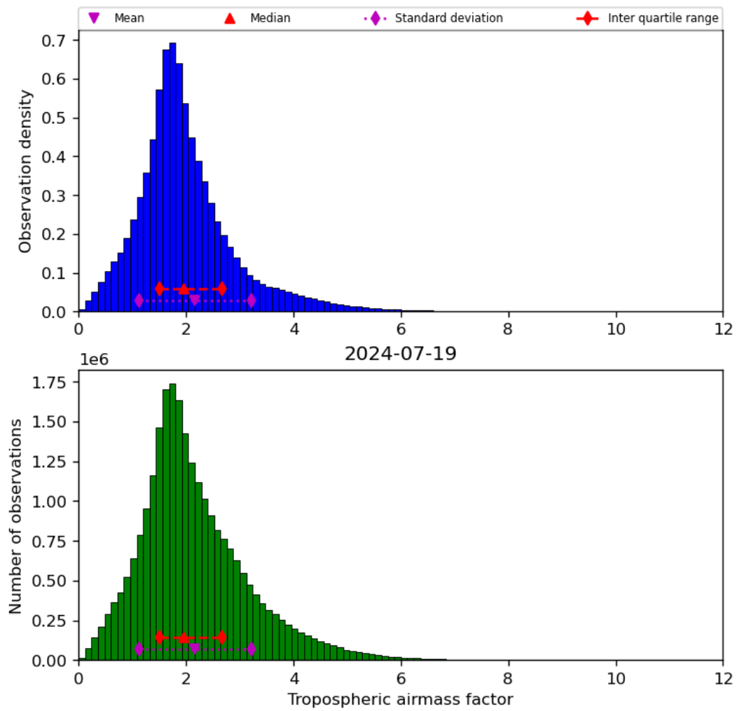
Figure 31: Histogram of “Tropospheric airmass factor” for 2024-07-18 to 2024-07-20
