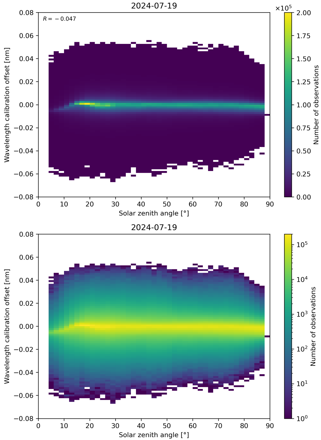
Figure 158: Scatter density plot of “Solar zenith angle” against “Wavelength calibration offset” for 2024-07-18 to 2024-07-20.
