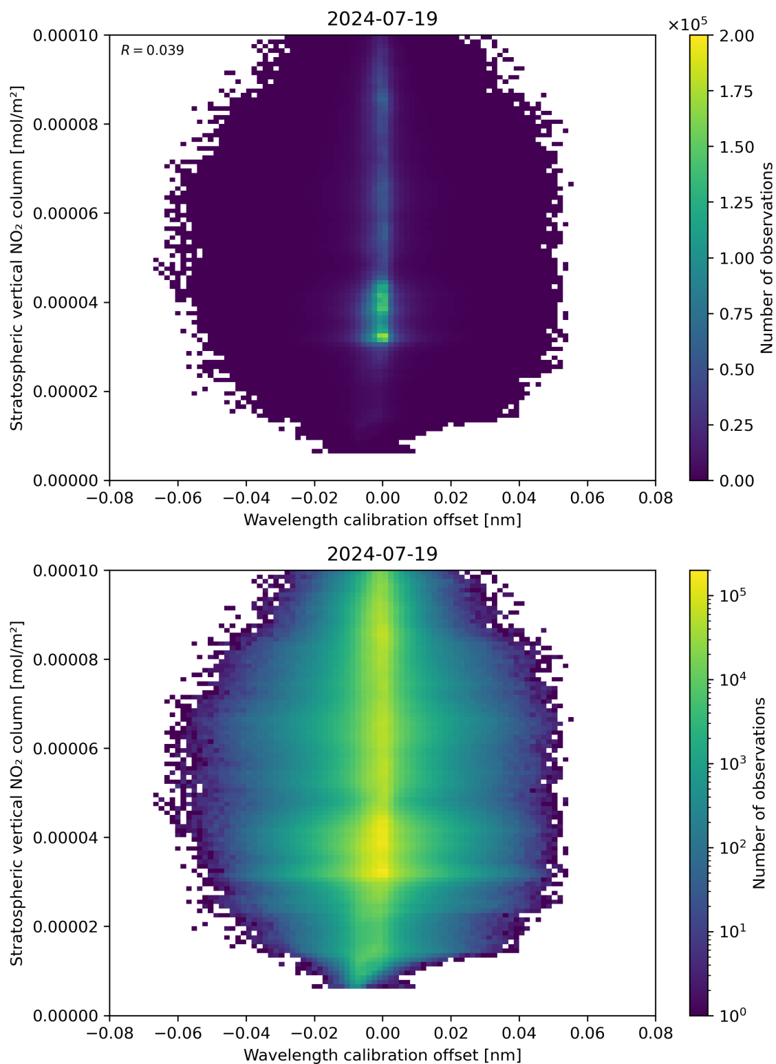
Figure 176: Scatter density plot of “Wavelength calibration offset” against “Stratospheric vertical NO 2 column” for 2024-07-18 to 2024-07-20.
