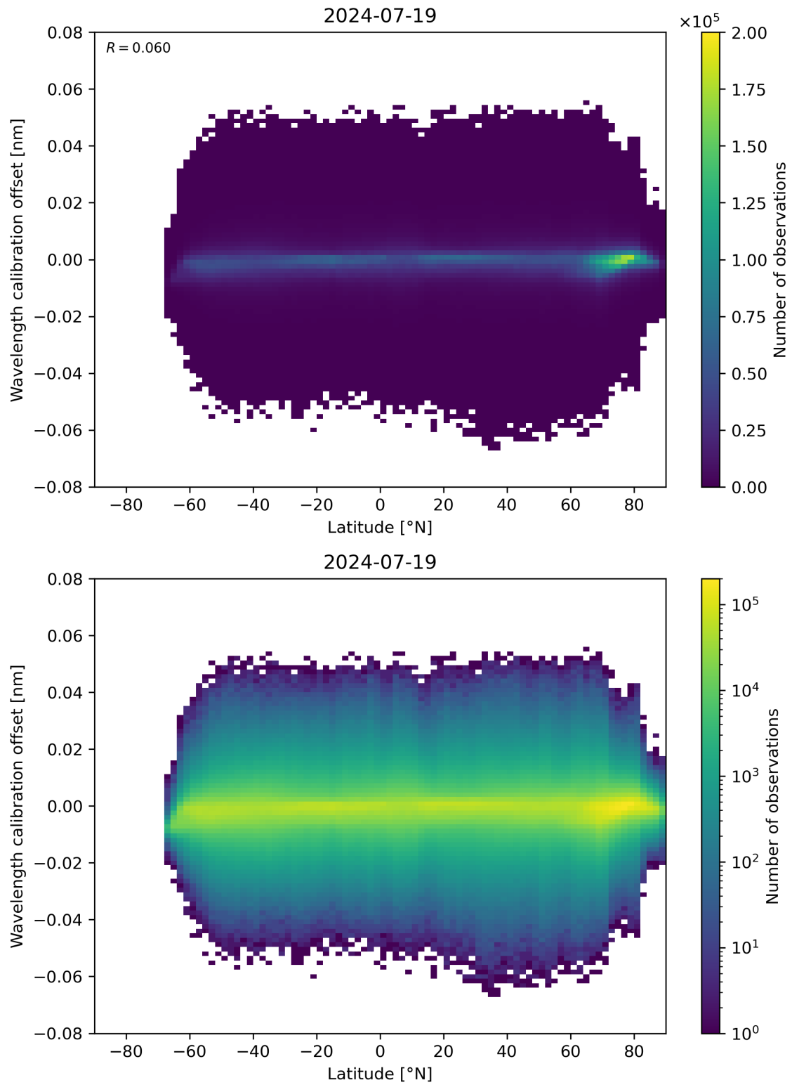
Figure 95: Scatter density plot of “Latitude” against “Wavelength calibration offset” for 2024-07-18 to 2024-07-20.
