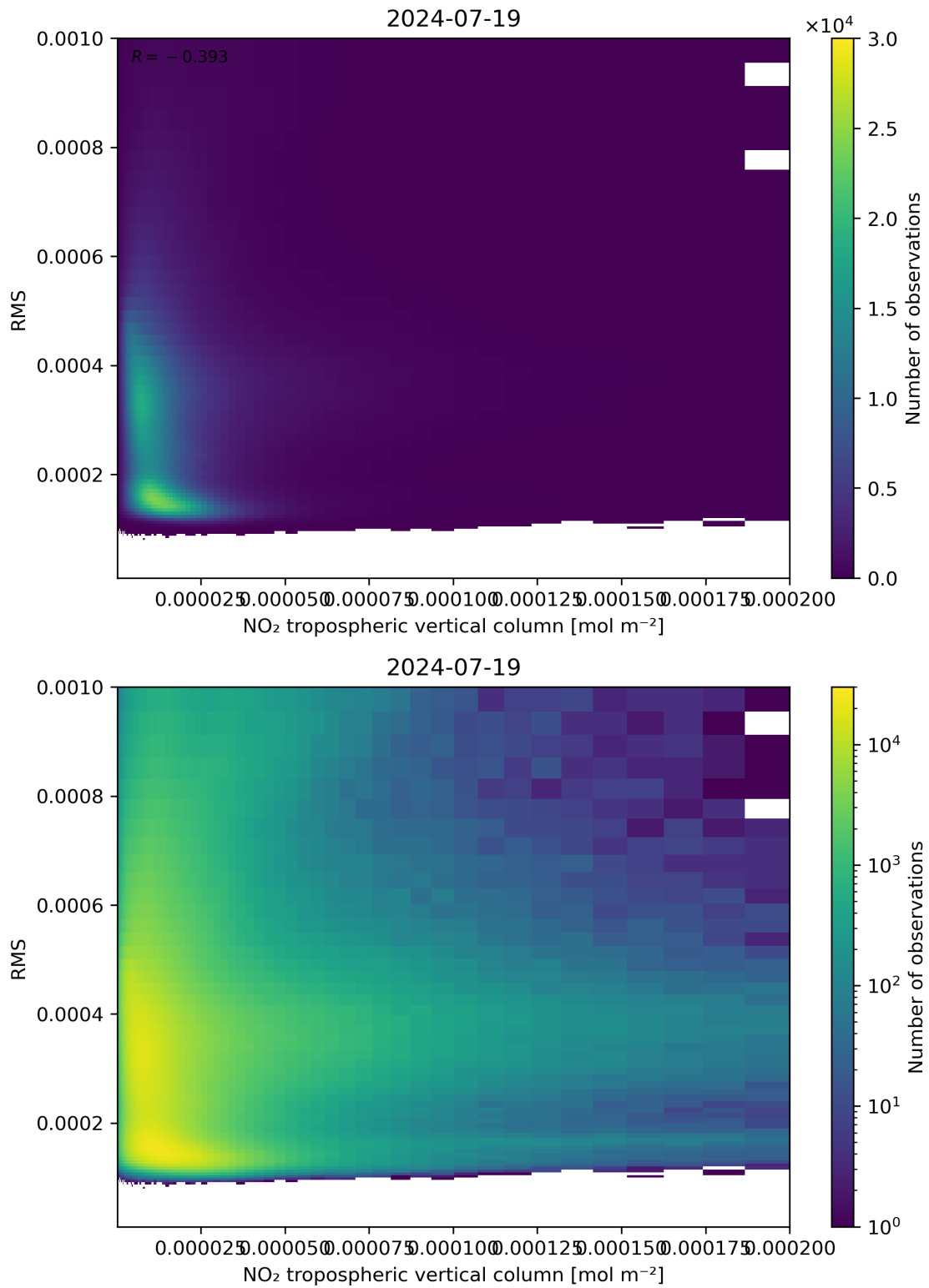
Figure 142: Scatter density plot of “NO 2 tropospheric vertical column” against “RMS” for 2024-07-18 to 2024-07-20.
