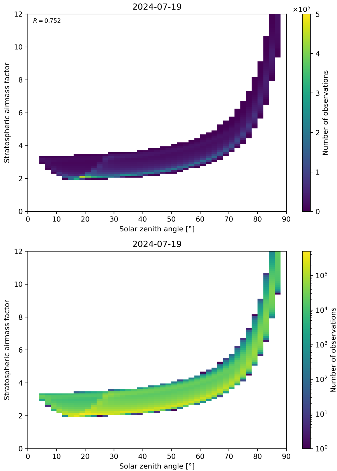
Figure 145: Scatter density plot of “Solar zenith angle” against “Stratospheric airmass factor” for 2024-07-18 to 2024-07-20.
