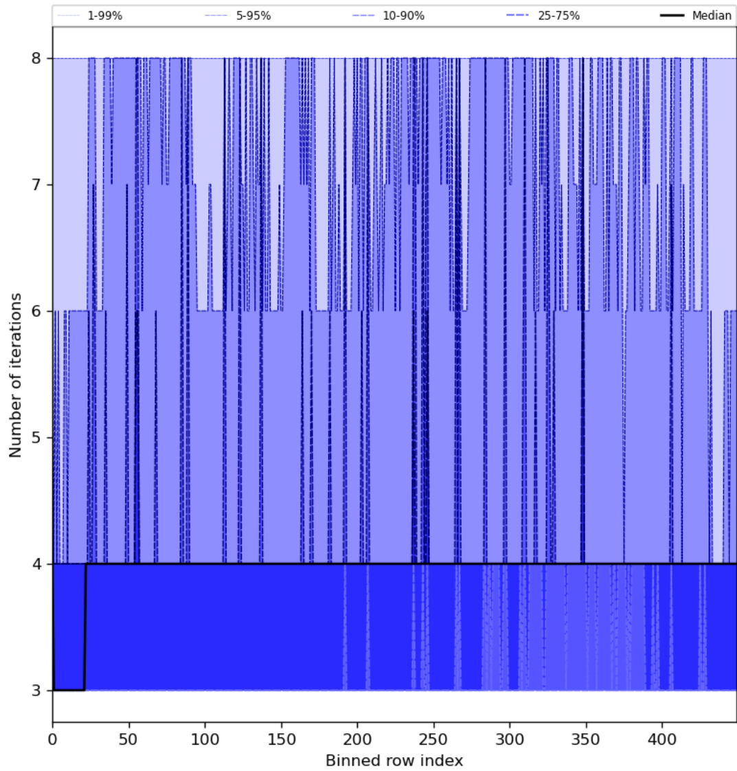
Figure 51: Along track statistics of “Number of iterations” for 2024-07-18 to 2024-07-20
