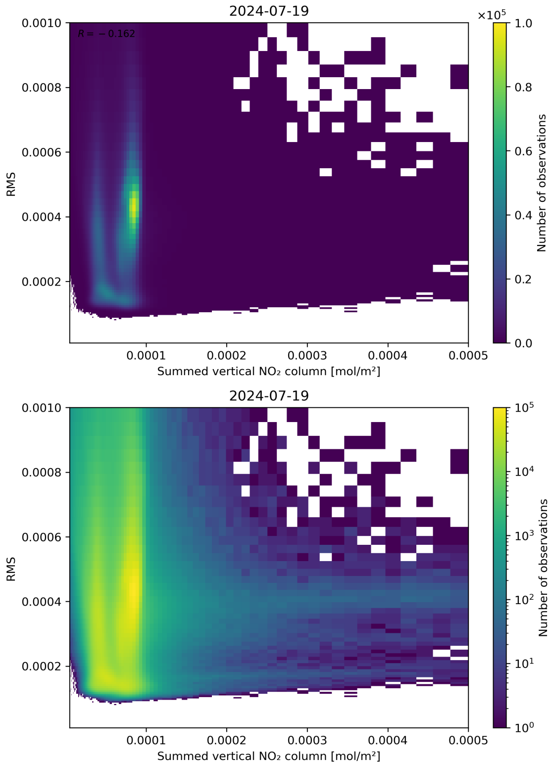
Figure 109: Scatter density plot of “Summed vertical NO 2 column” against “RMS” for 2024-07-18 to 2024-07-20.
