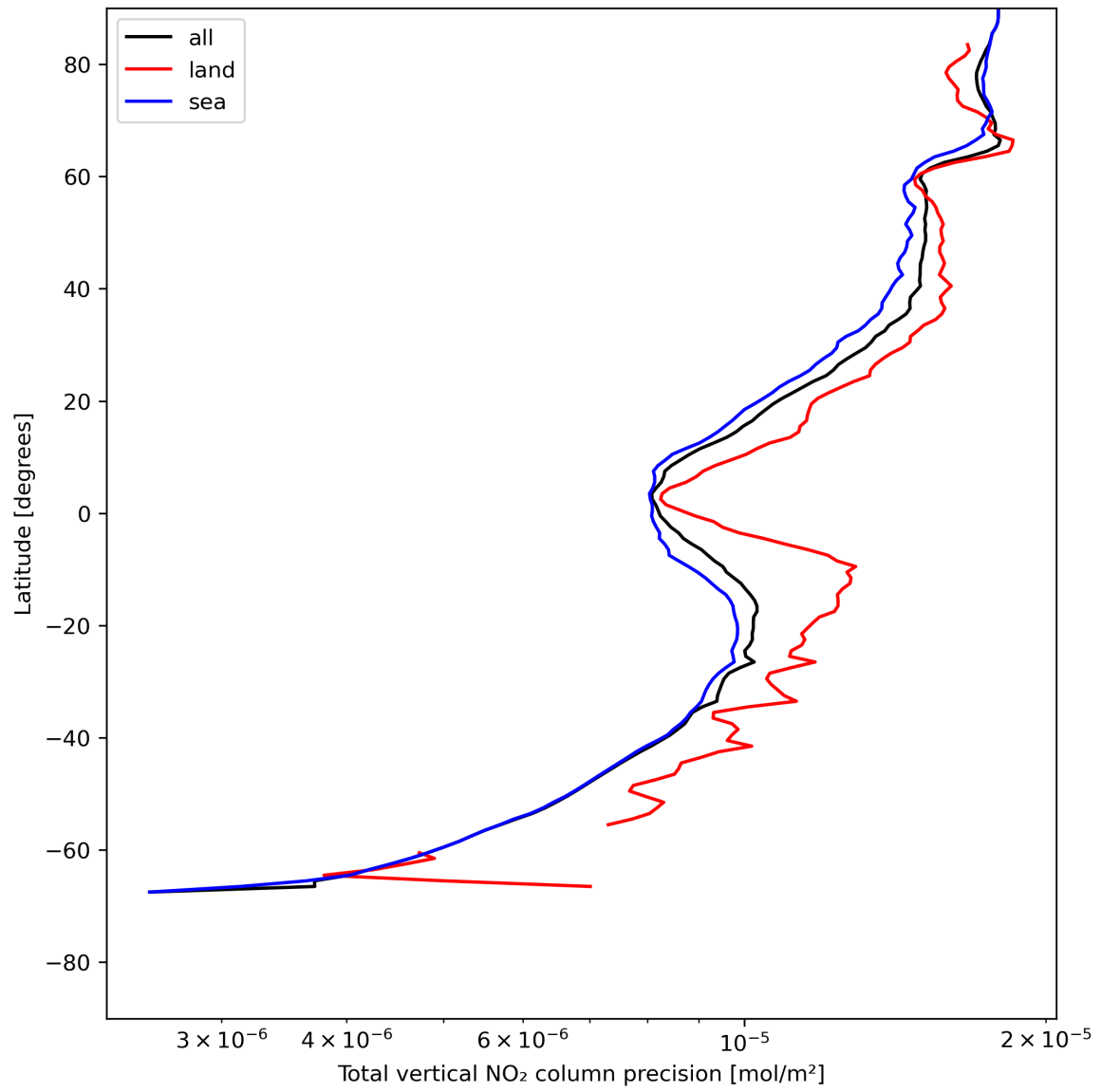
Figure 22: Zonal average of “Total vertical NO 2 column precision” for 2024-07-18 to 2024-07-20.
