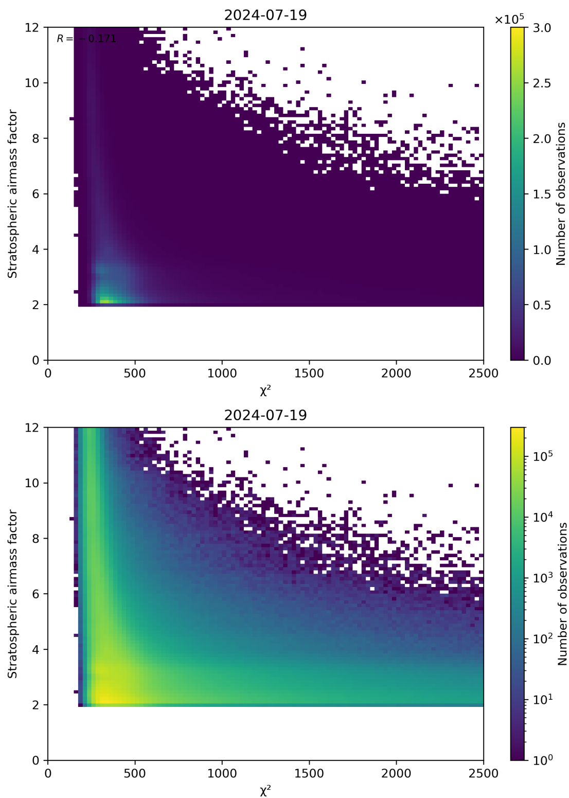
Figure 81: Scatter density plot of “ \chi^2 ” against “Stratospheric air mass factor” for 2024-07-18 to 2024-07-20.
