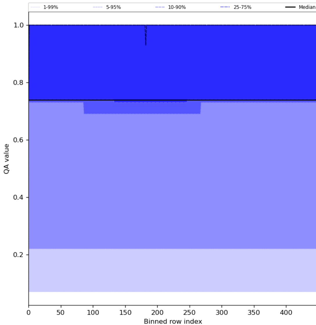
Figure 45: Along track statistics of “QA value” for 2024-07-18 to 2024-07-20
