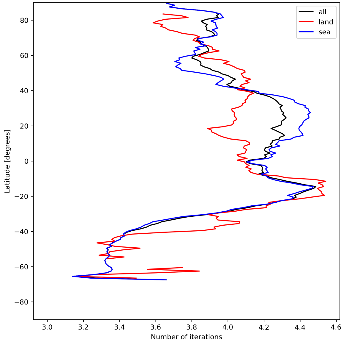
Figure 17: Zonal average of “Number of iterations” for 2024-07-18 to 2024-07-20.
