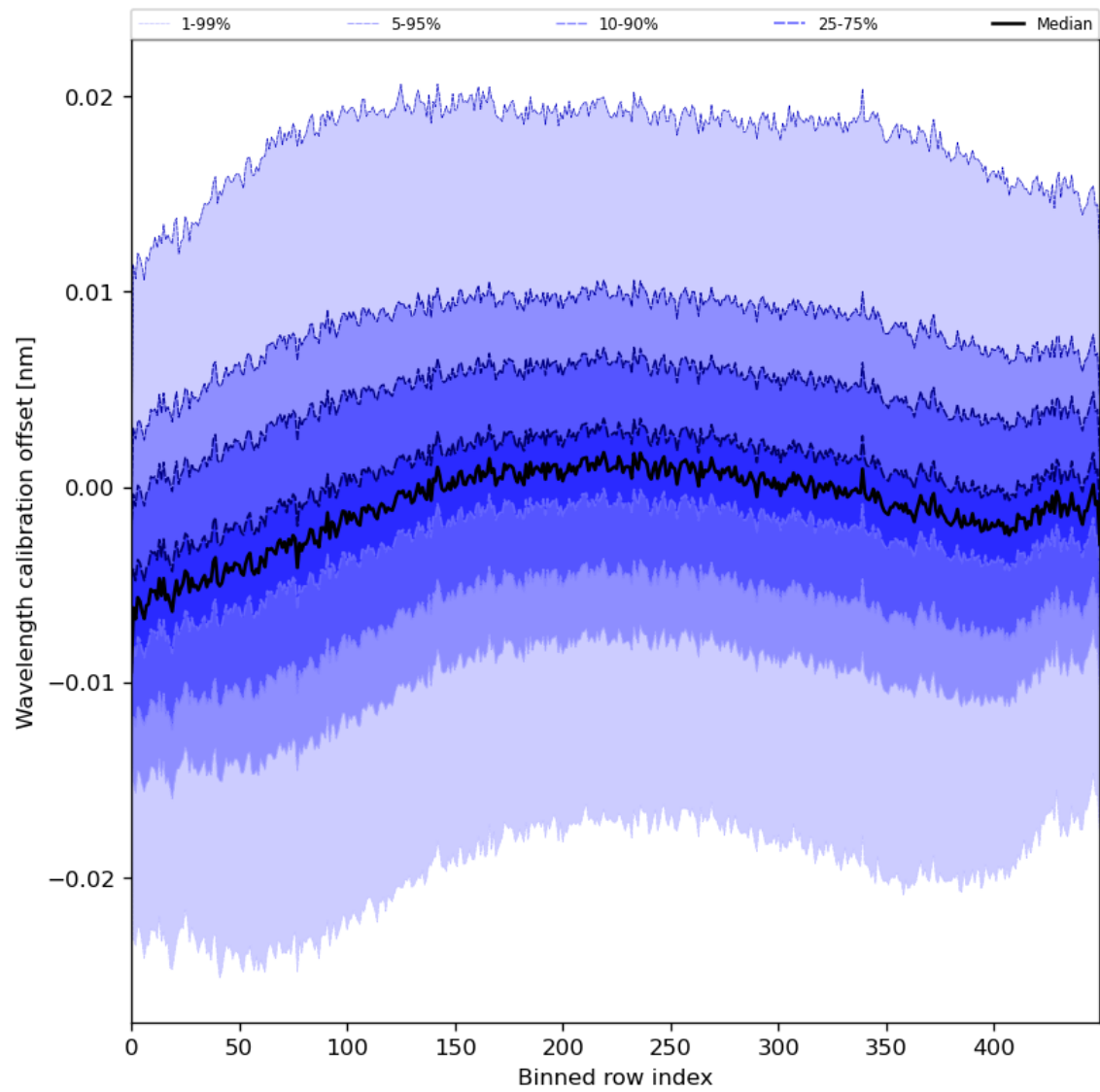
Figure 52: Along track statistics of “Wavelength calibration offset” for 2024-07-18 to 2024-07-20
