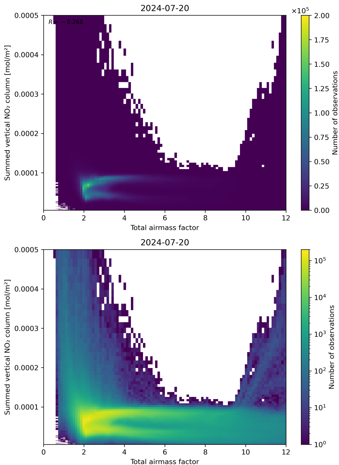
Figure 65: Scatter density plot of “Total airmass factor” against “Summed vertical NO 2 column” for 2024-07-19 to 2024-07-21.
