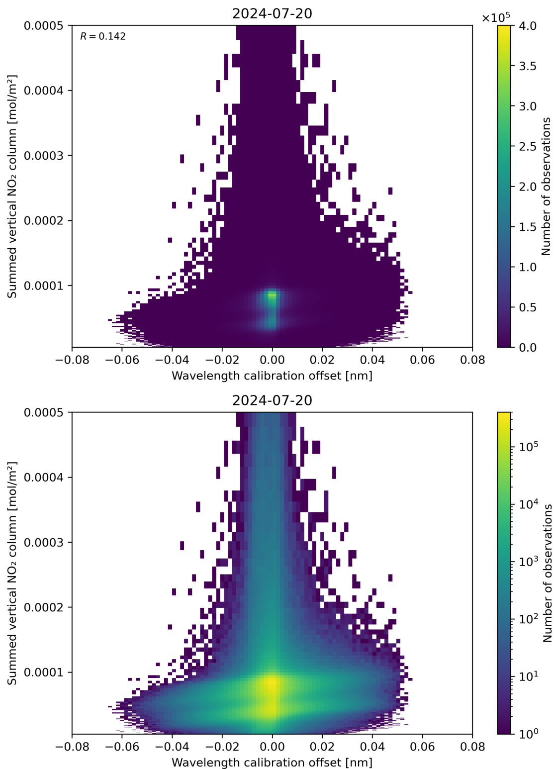
Figure 177: Scatter density plot of “Wavelength calibration offset” against “Summed vertical NO 2 column” for 2024-07-19 to 2024-07-21.
