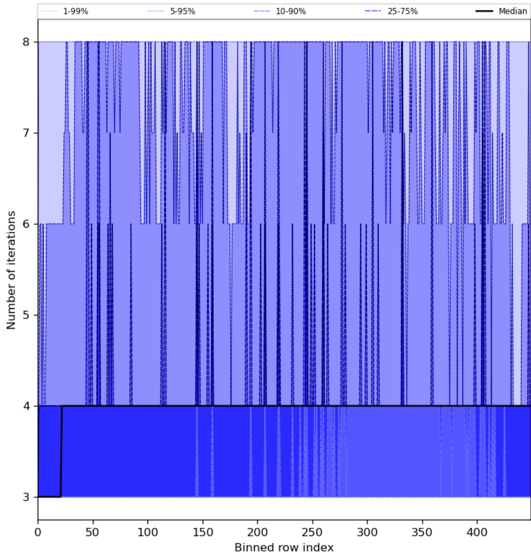
Figure 51: Along track statistics of “Number of iterations” for 2024-07-19 to 2024-07-21
