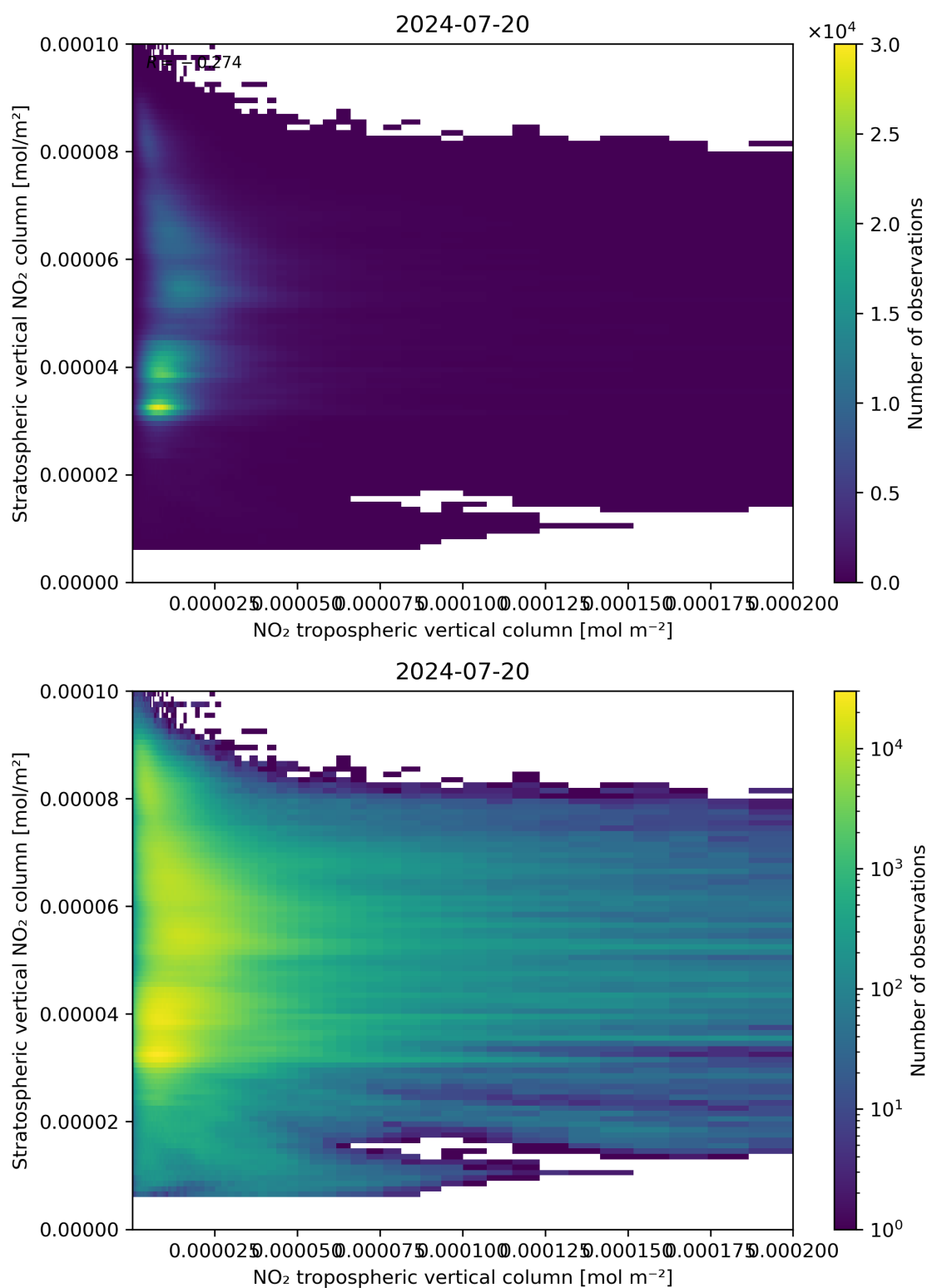
Figure 125: Scatter density plot of “NO 2 tropospheric vertical column” against “Stratospheric vertical NO 2 column” for 2024-07-19 to 2024-07-21.
