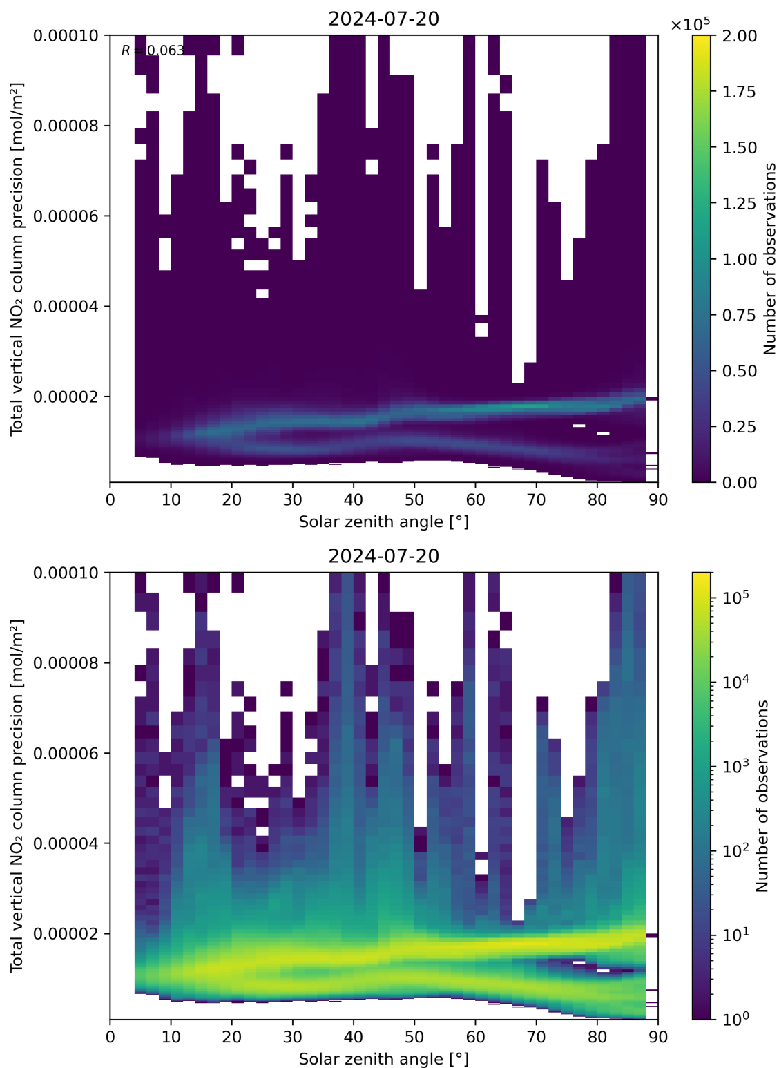
Figure 154: Scatter density plot of “Solar zenith angle” against “Total vertical NO 2 column precision” for 2024-07-19 to 2024-07-21.
