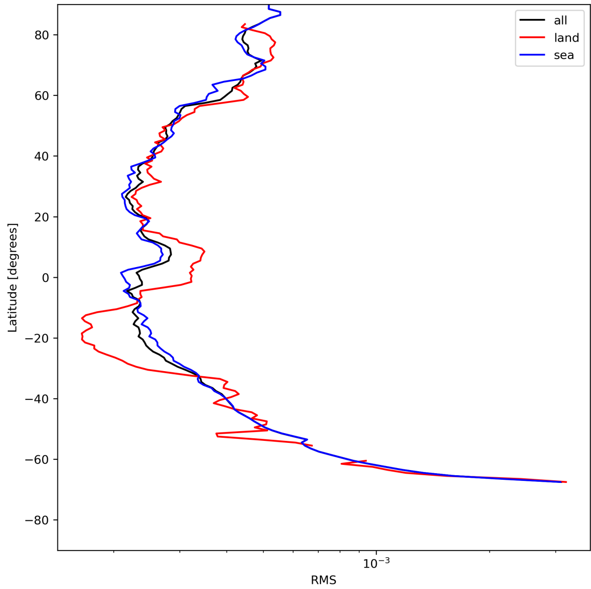
Figure 26: Zonal average of “RMS” for 2024-07-19 to 2024-07-21.
