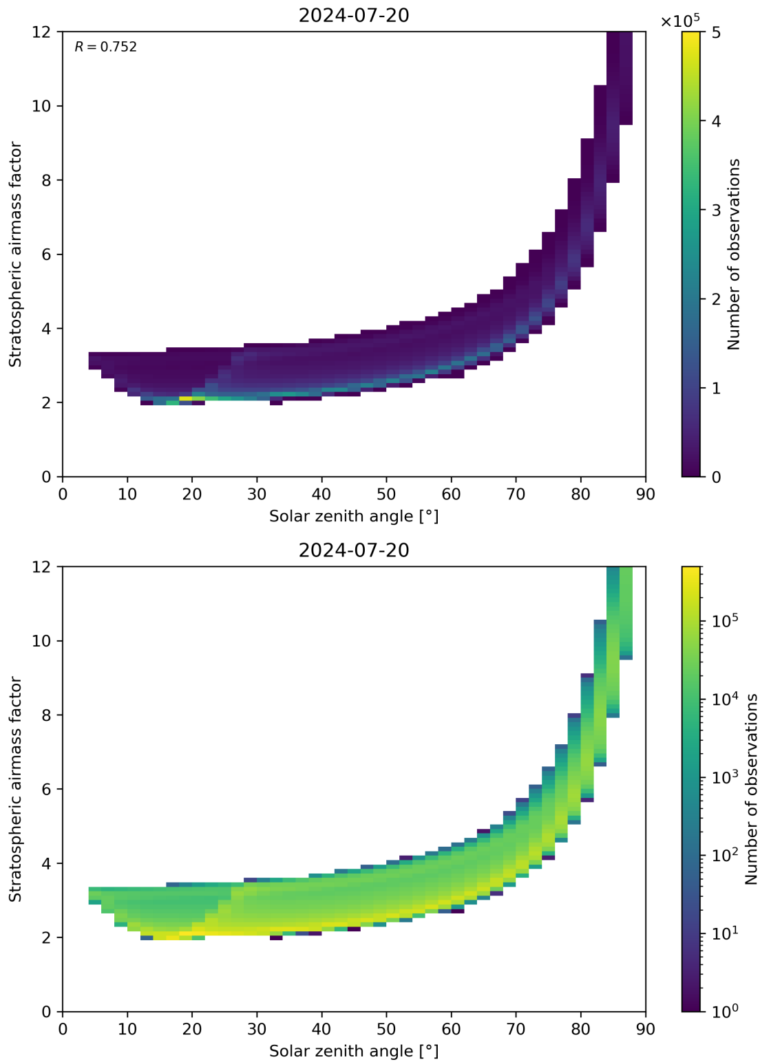
Figure 145: Scatter density plot of “Solar zenith angle” against “Stratospheric airmass factor” for 2024-07-19 to 2024-07-21.
