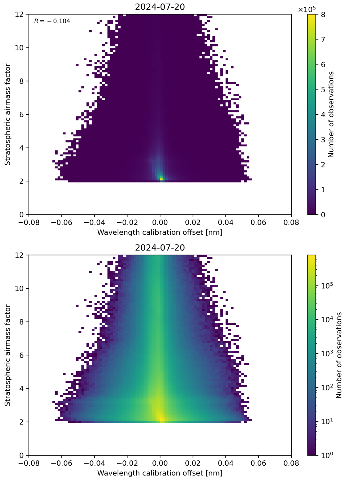
Figure 174: Scatter density plot of “Wavelength calibration offset” against “Stratospheric airmass factor” for 2024-07-19 to 2024-07-21.
