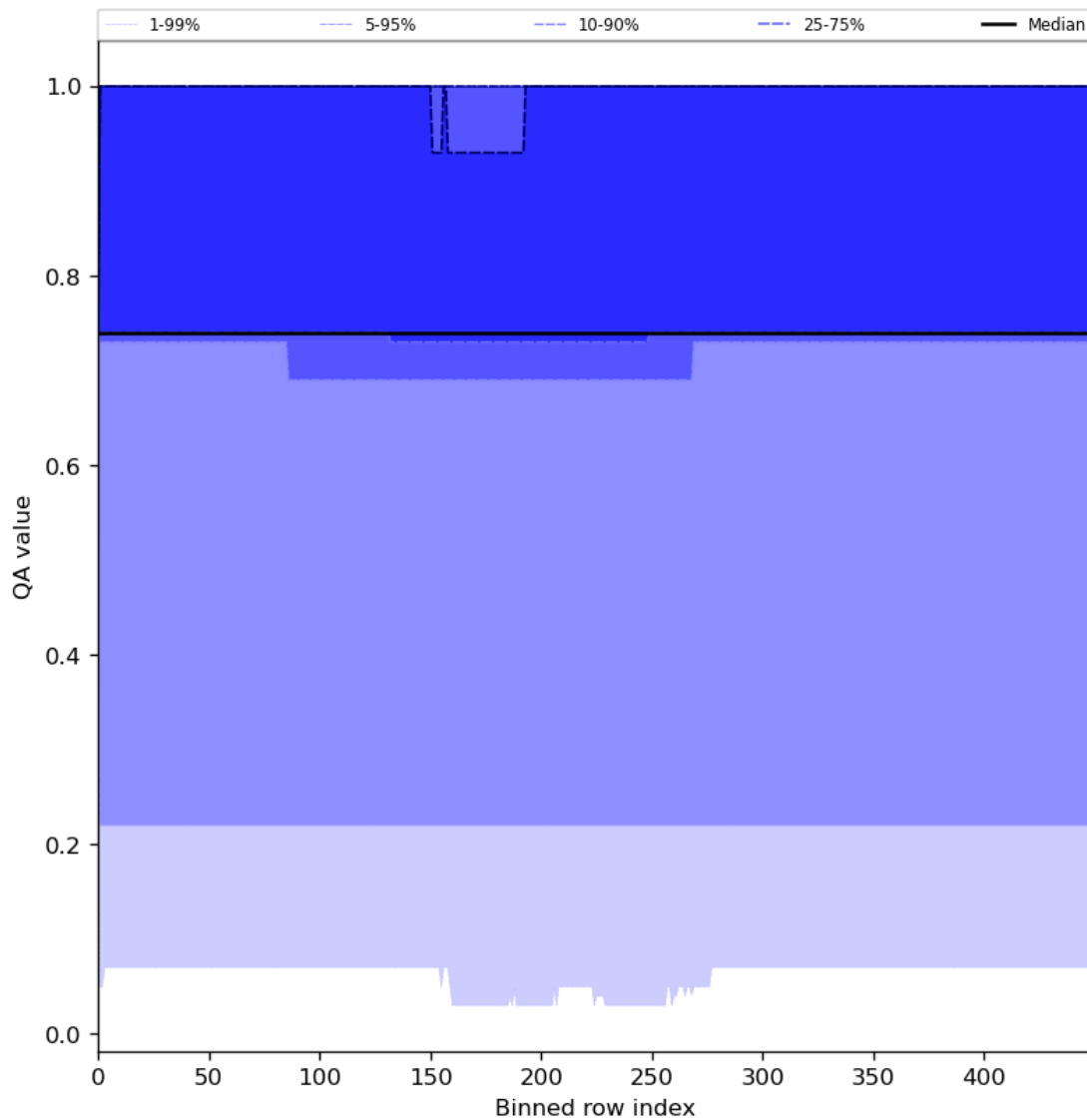
Figure 45: Along track statistics of “QA value” for 2024-07-19 to 2024-07-21
