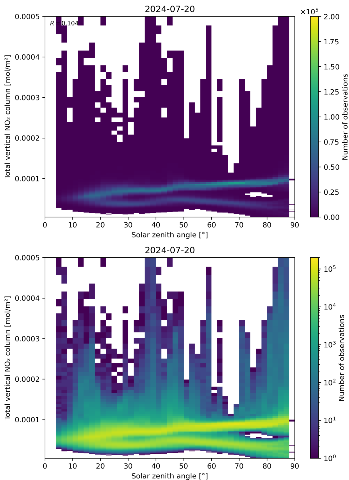
Figure 153: Scatter density plot of “Solar zenith angle” against “Total vertical NO 2 column” for 2024-07-19 to 2024-07-21.
