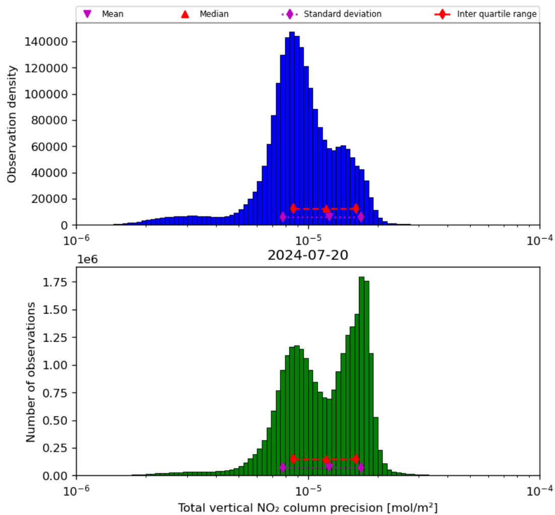
Figure 39: Histogram of "Total vertical NO 2 column precision" for 2024-07-19 to 2024-07-21
