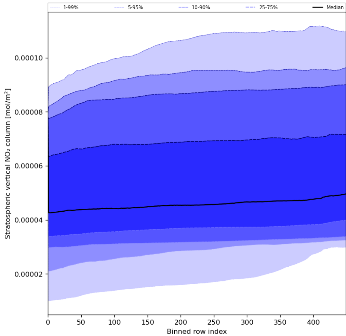
Figure 53: Along track statistics of “Stratospheric vertical NO 2 column” for 2024-07-19 to 2024-07-21
