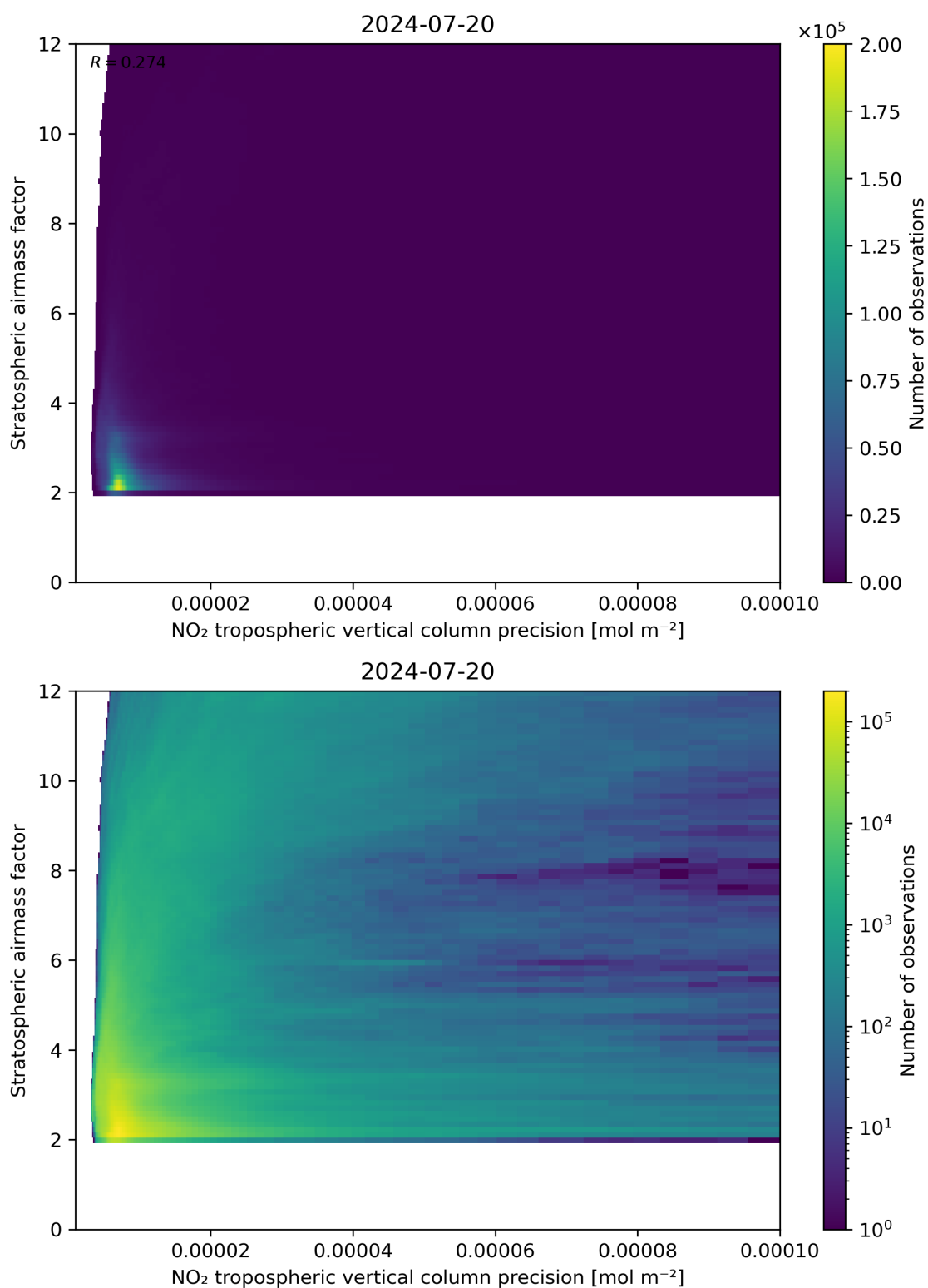
Figure 131: Scatter density plot of “NO 2 tropospheric vertical column precision” against “Stratospheric airmass factor” for 2024-07-19 to 2024-07-21.
