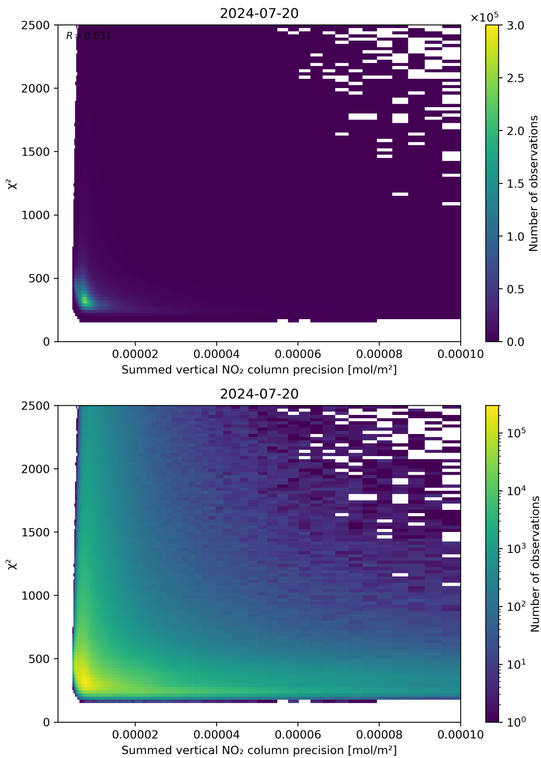
Figure 107: Scatter density plot of “Summed vertical NO 2 column precision” against “ \chi^2 ” for 2024-07-19 to 2024-07-21.
