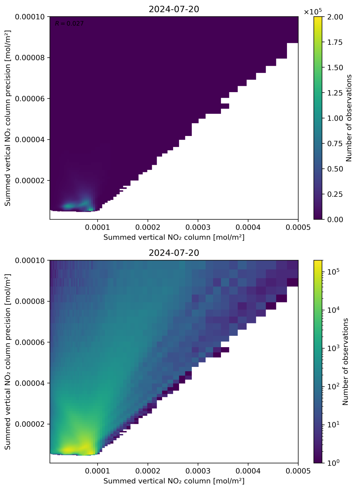
Figure 105: Scatter density plot of “Summed vertical NO 2 column” against “Summed vertical NO 2 column precision” for 2024-07-19 to 2024-07-21.
