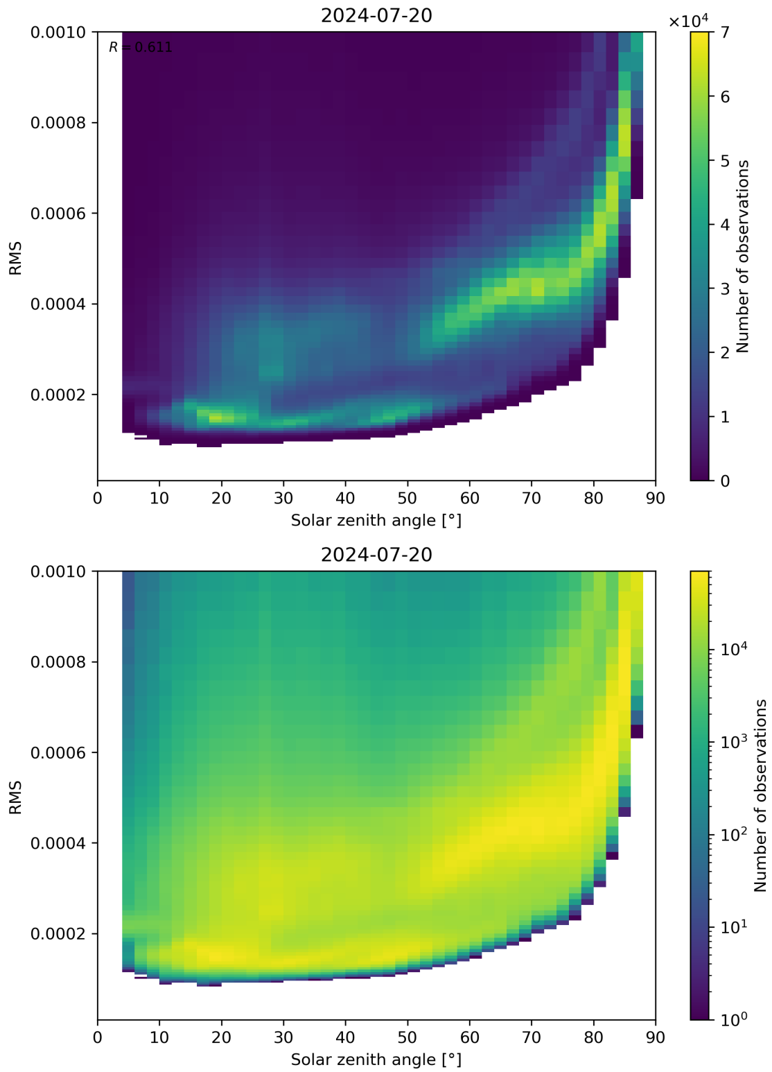
Figure 157: Scatter density plot of “Solar zenith angle” against “RMS” for 2024-07-19 to 2024-07-21.
