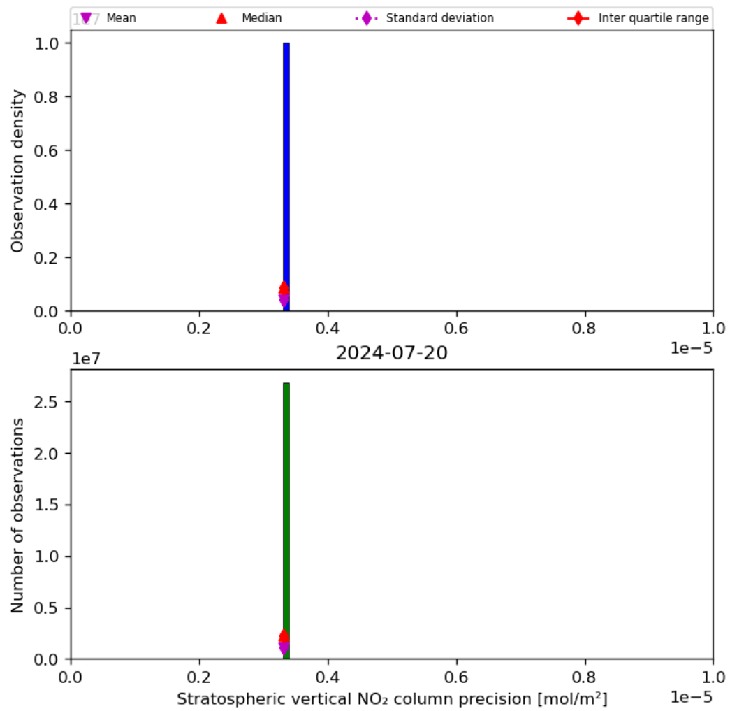
Figure 37: Histogram of “Stratospheric vertical NO 2 column precision” for 2024-07-19 to 2024-07-21
