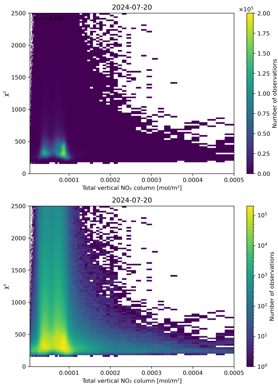
Figure 111: Scatter density plot of “Total vertical NO 2 column” against “ \chi^2 ” for 2024-07-19 to 2024-07-21.
