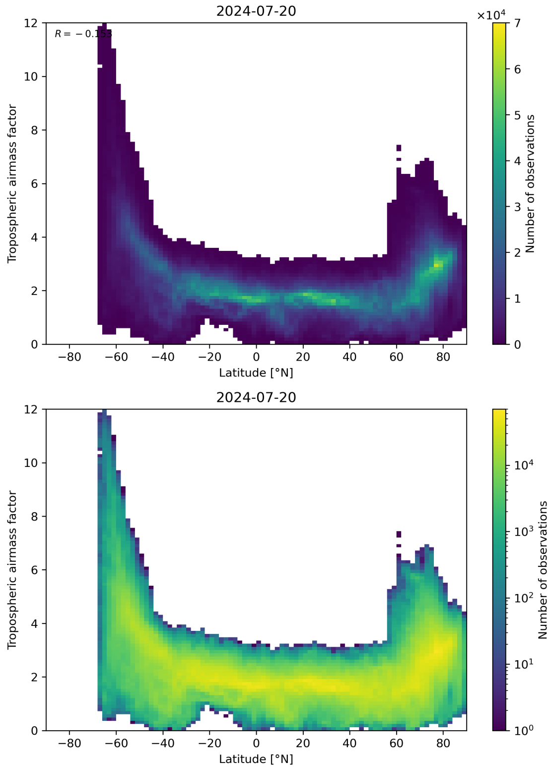
Figure 85: Scatter density plot of “Latitude” against “Tropospheric air mass factor” for 2024-07-19 to 2024-07-21.
