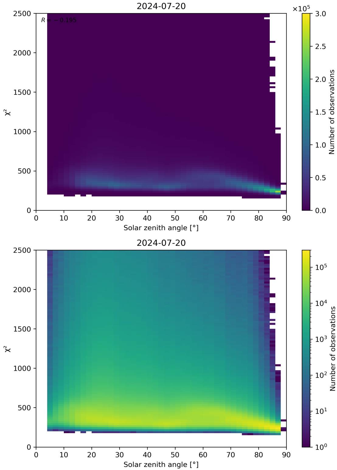
Figure 148: Scatter density plot of “Solar zenith angle” against “ \chi^2 ” for 2024-07-19 to 2024-07-21.
