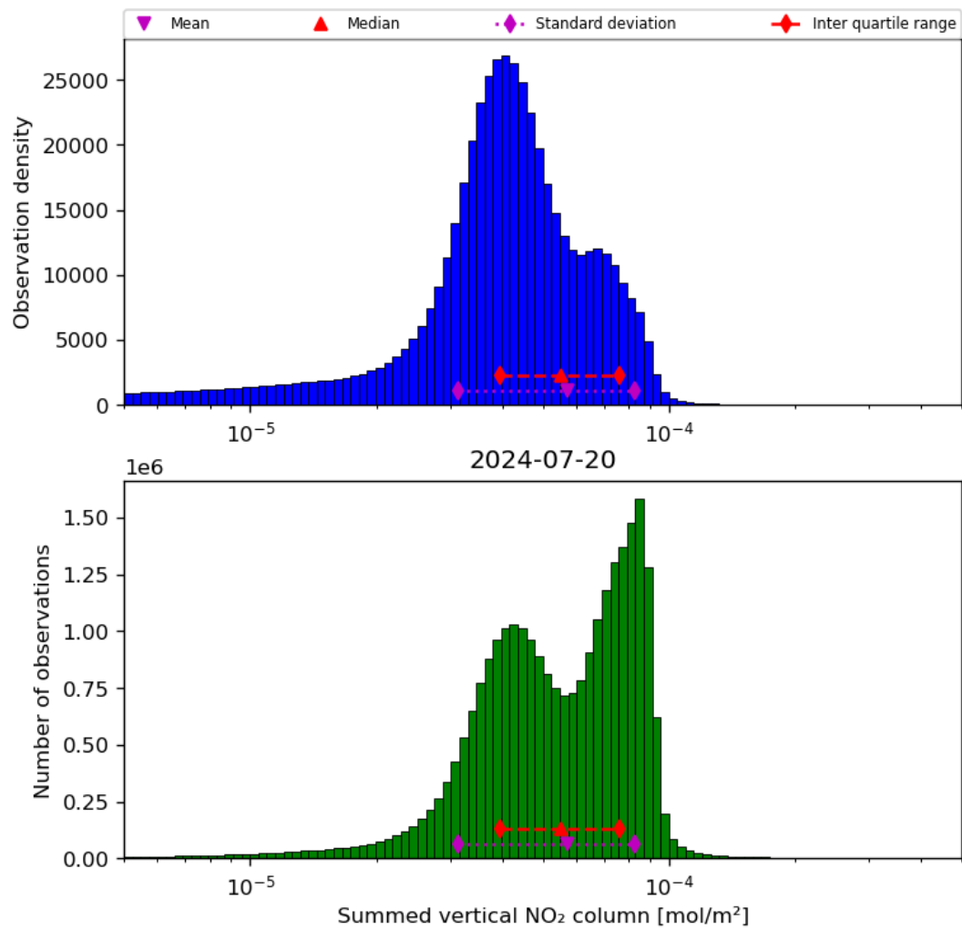
Figure 40: Histogram of “Summed vertical NO 2 column” for 2024-07-19 to 2024-07-21
