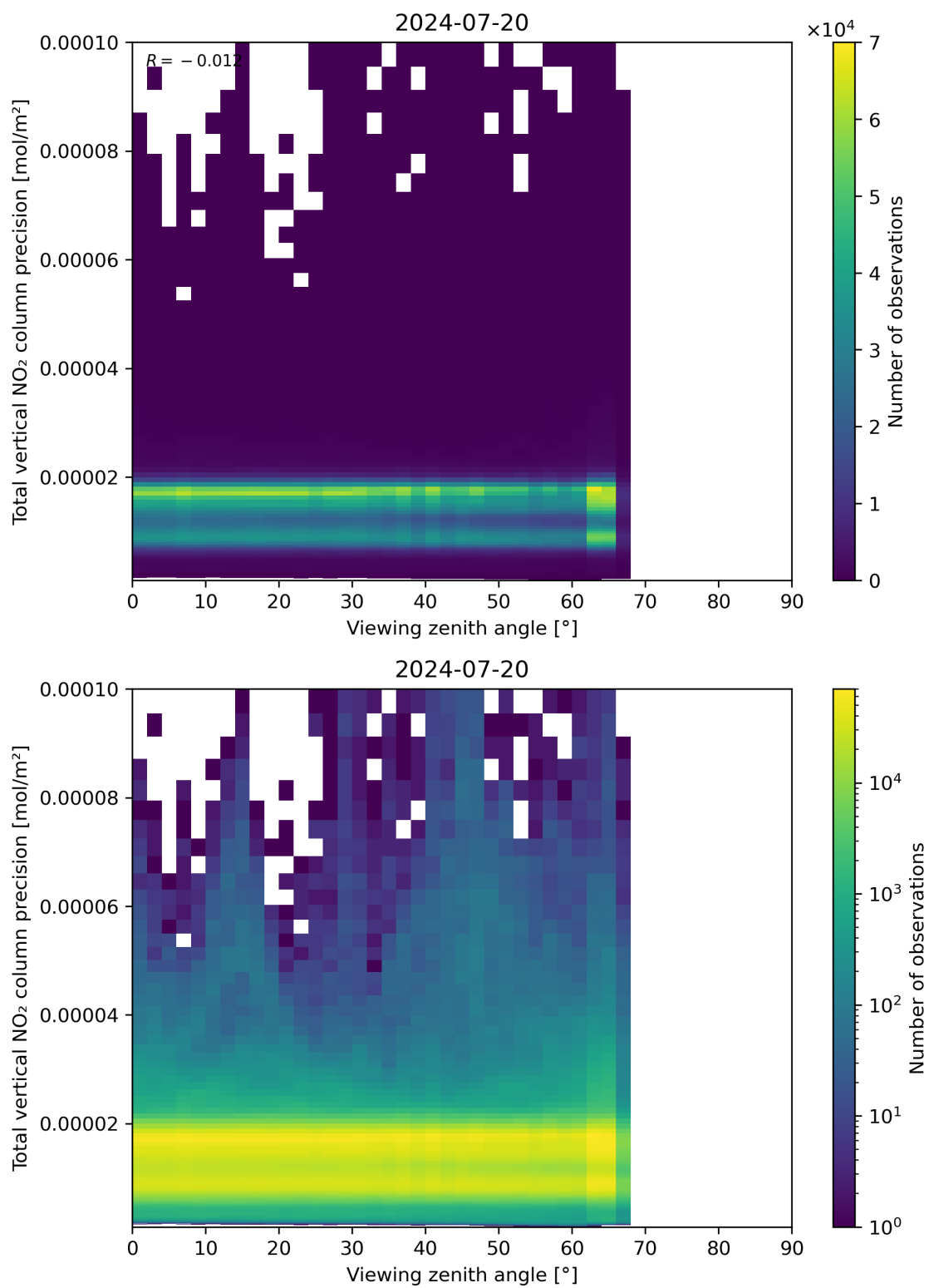
Figure 168: Scatter density plot of “Viewing zenith angle” against “Total vertical NO 2 column precision” for 2024-07-19 to 2024-07-21.
