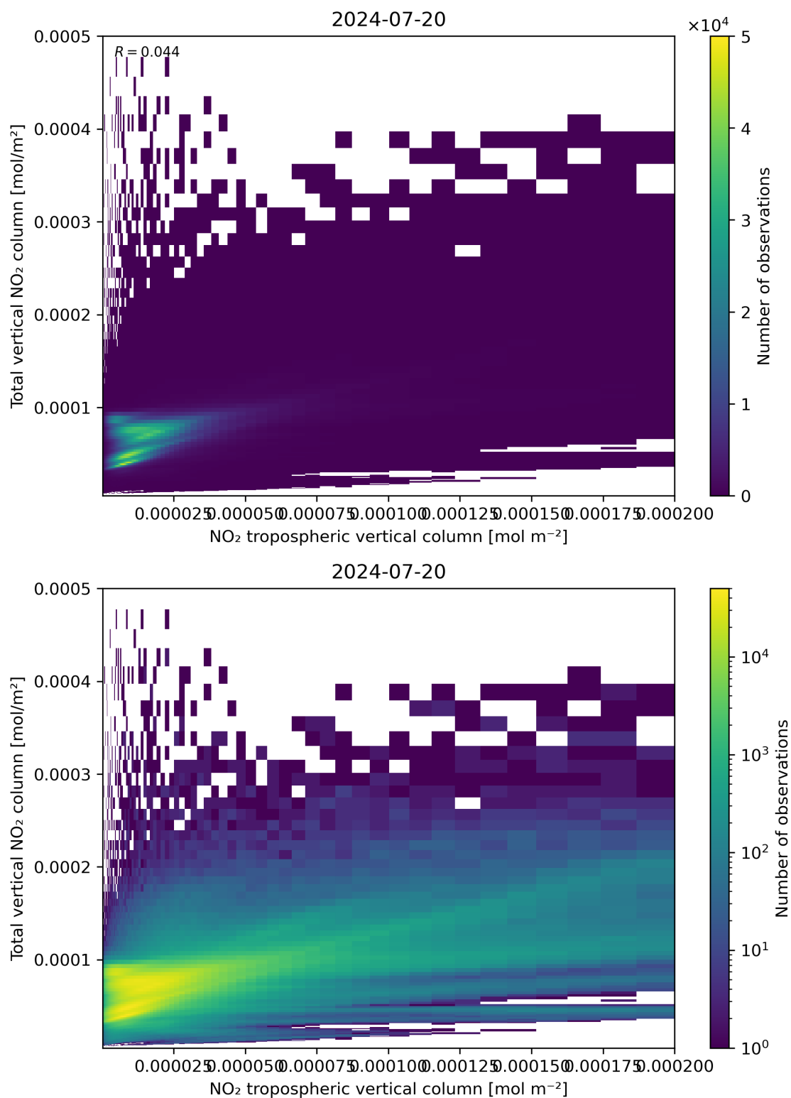
Figure 128: Scatter density plot of “NO 2 tropospheric vertical column” against “Total vertical NO 2 column” for 2024-07-19 to 2024-07-21.
