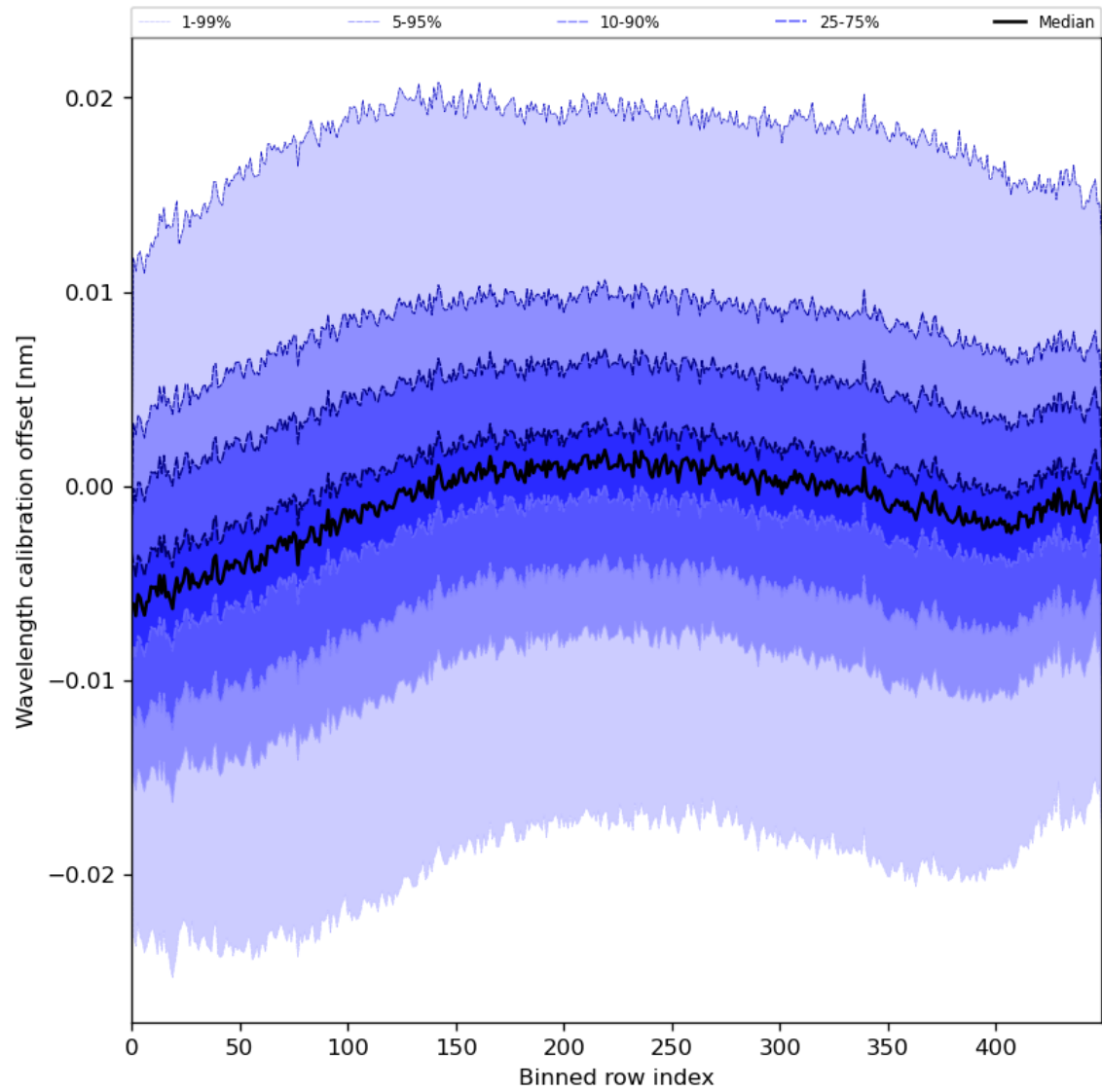
Figure 52: Along track statistics of “Wavelength calibration offset” for 2024-07-19 to 2024-07-21
