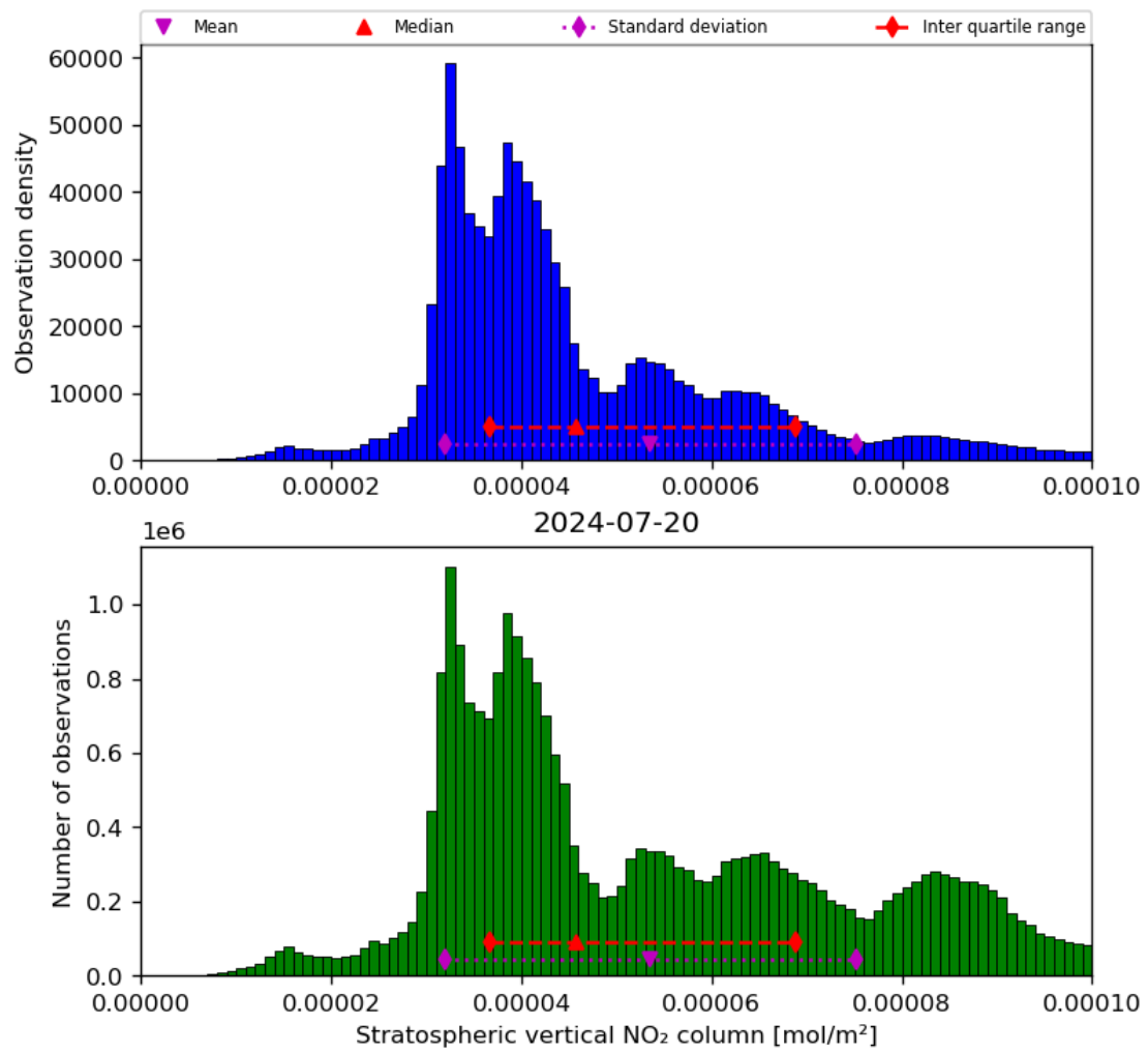
Figure 36: Histogram of “Stratospheric vertical NO 2 column” for 2024-07-19 to 2024-07-21
