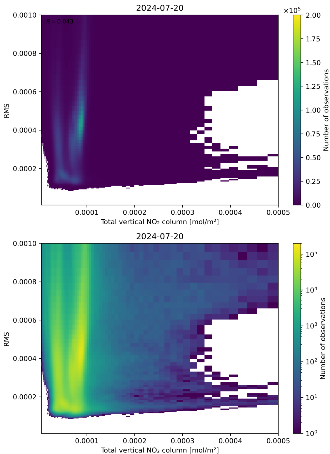
Figure 120: Scatter density plot of “Total vertical NO 2 column” against “RMS” for 2024-07-19 to 2024-07-21.
