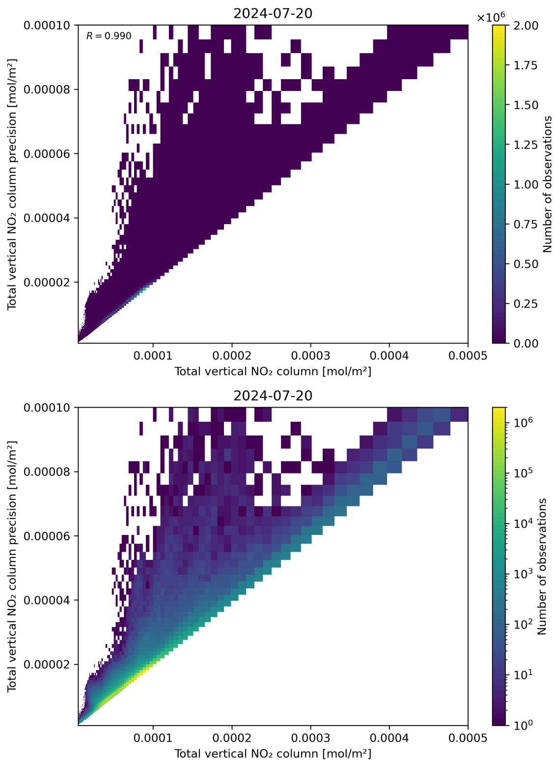
Figure 114: Scatter density plot of “Total vertical NO 2 column” against “Total vertical NO 2 column precision” for 2024-07-19 to 2024-07-21.
