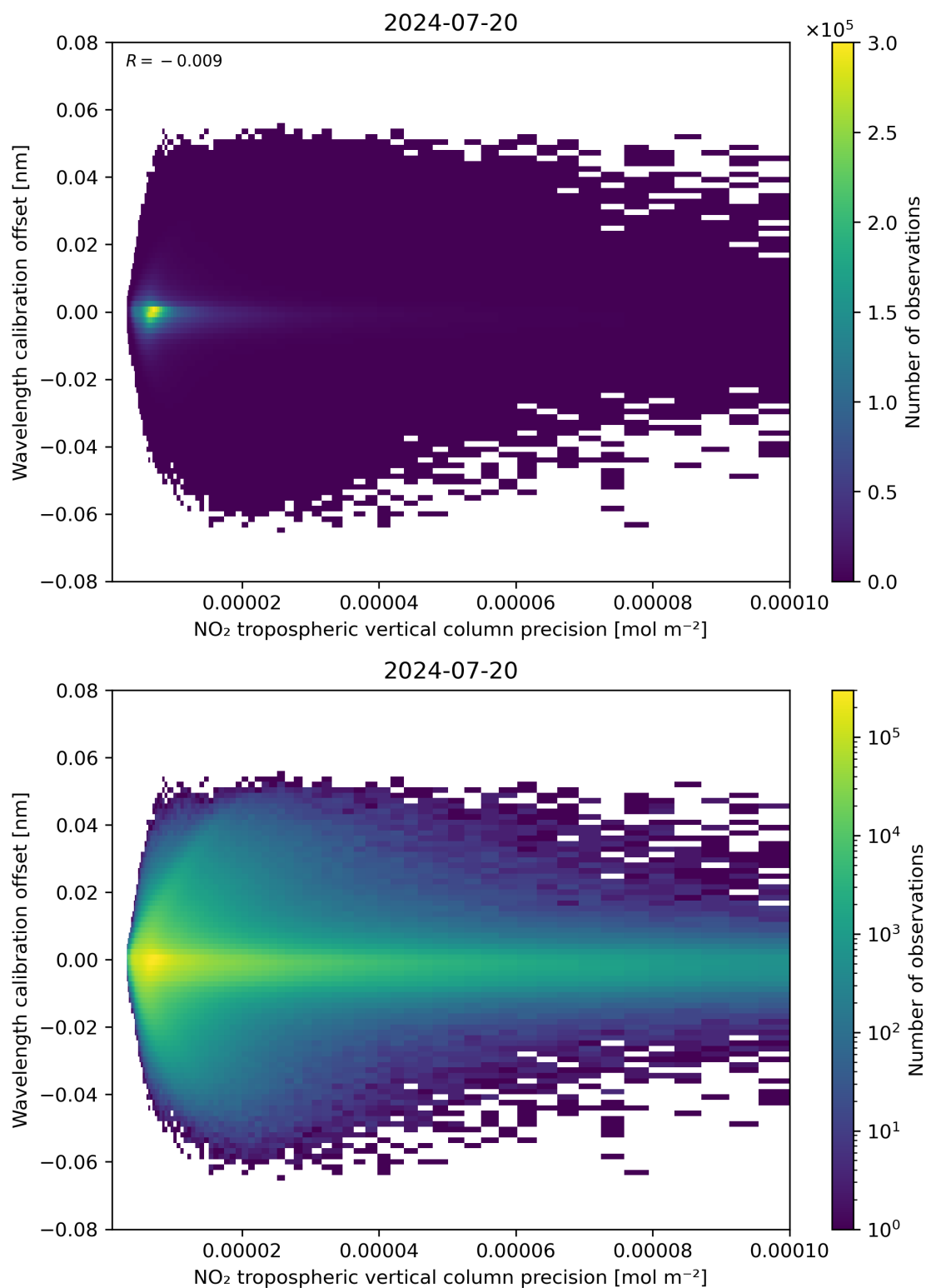
Figure 141: Scatter density plot of “NO 2 tropospheric vertical column precision” against “Wavelength calibration offset” for 2024-07-19 to 2024-07-21.
