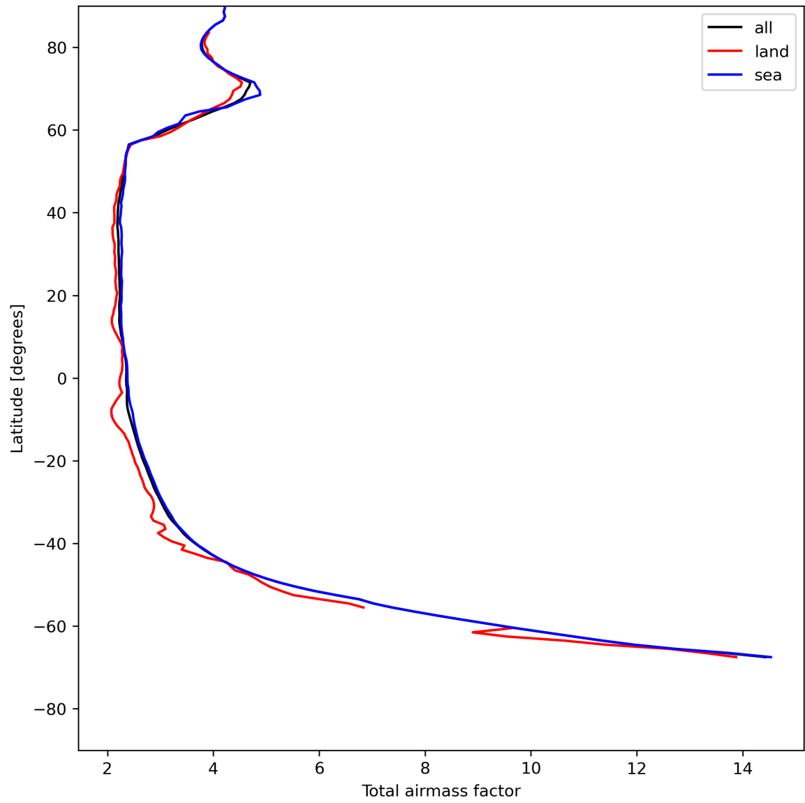
Figure 15: Zonal average of “Total airmass factor” for 2024-07-19 to 2024-07-21.
