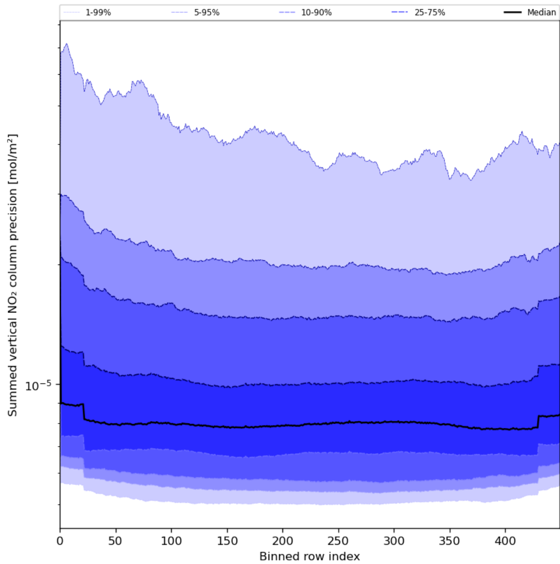
Figure 58: Along track statistics of “Summed vertical NO 2 column precision” for 2024-07-19 to 2024-07-21
