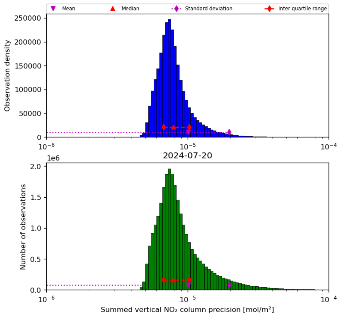
Figure 41: Histogram of "Summed vertical NO 2 column precision" for 2024-07-19 to 2024-07-21
