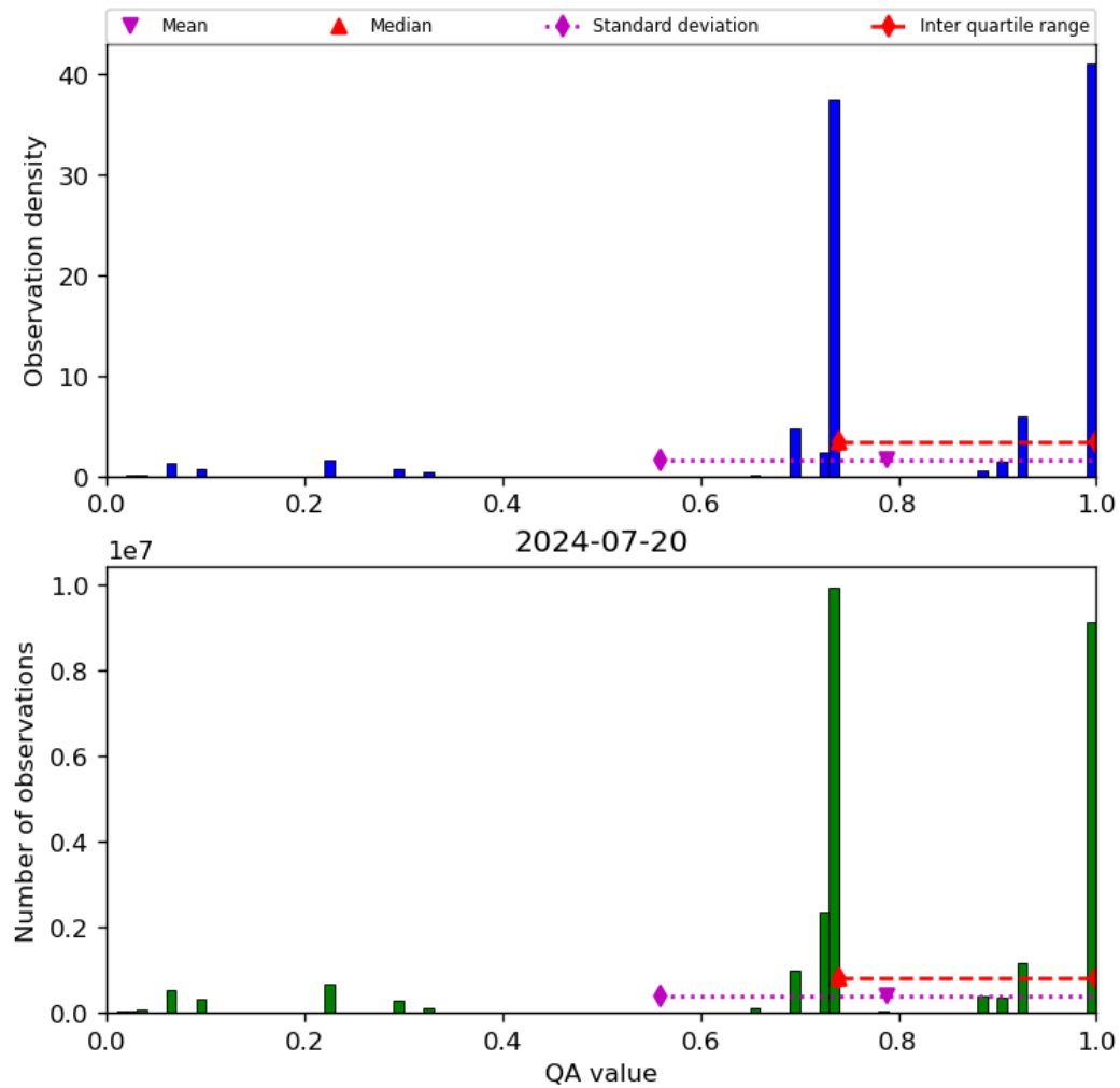
Figure 28: Histogram of “QA value” for 2024-07-19 to 2024-07-21
