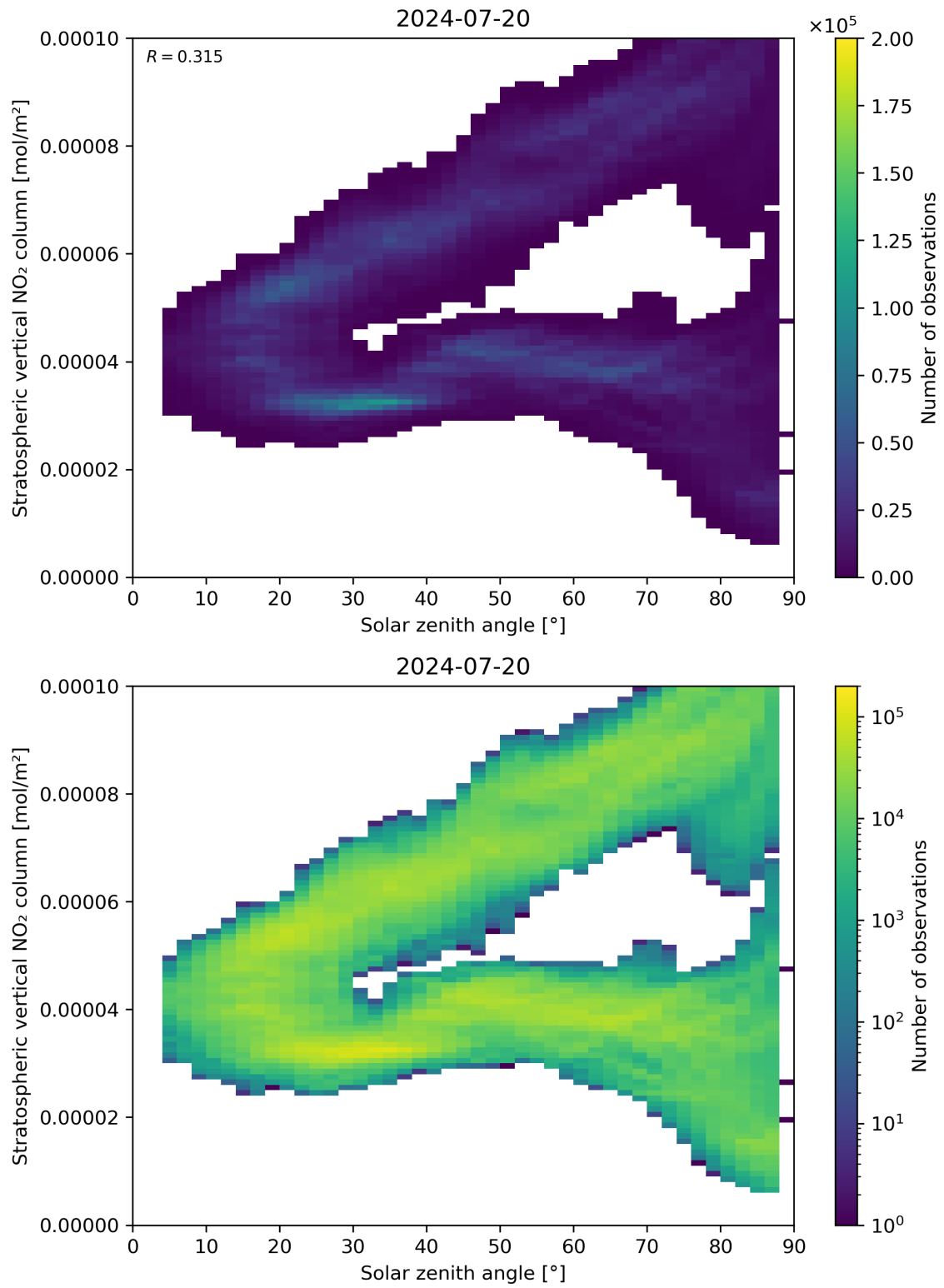
Figure 150: Scatter density plot of “Solar zenith angle” against “Stratospheric vertical NO 2 column” for 2024-07-19 to 2024-07-21.
