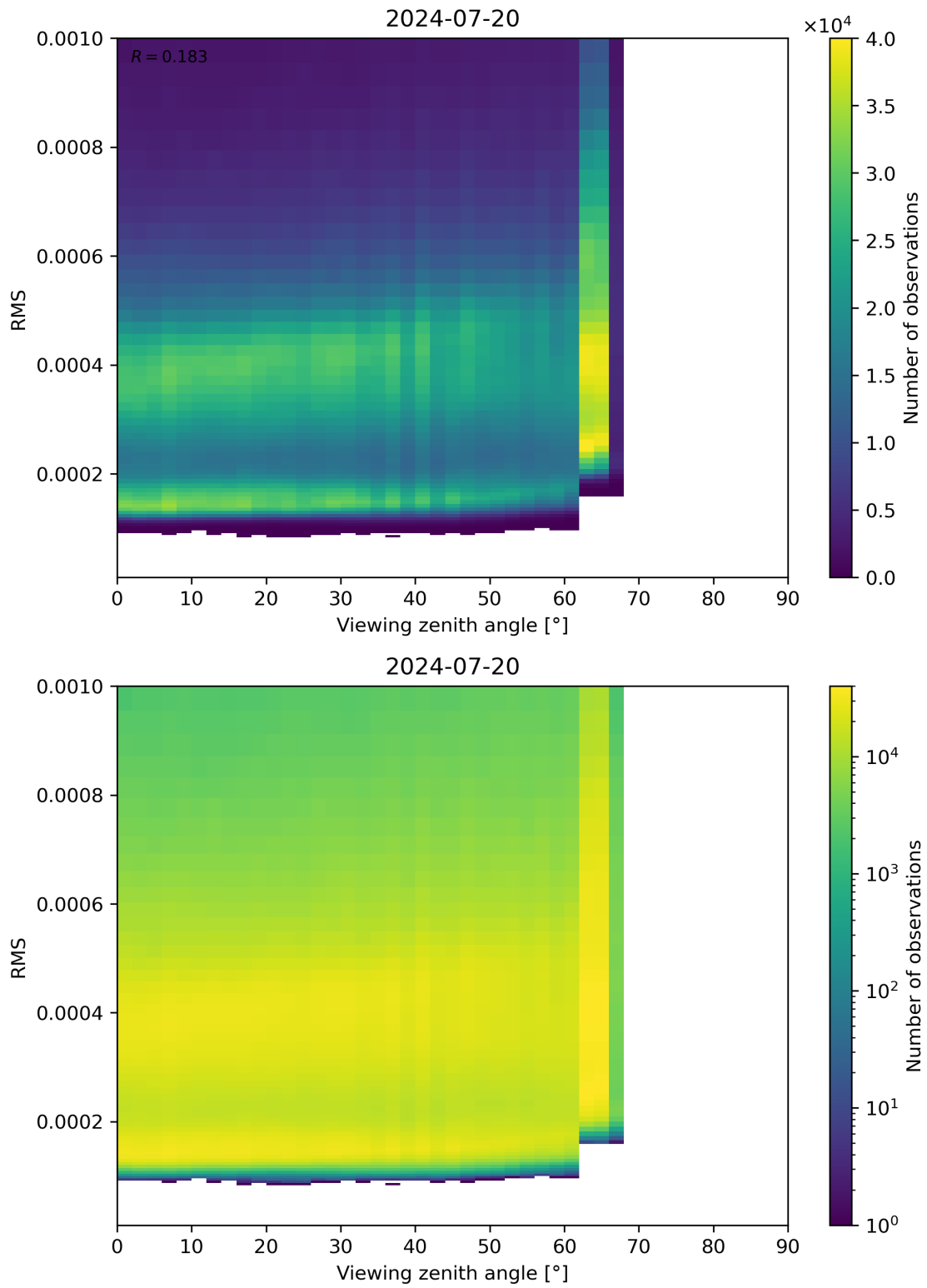
Figure 171: Scatter density plot of “Viewing zenith angle” against “RMS” for 2024-07-19 to 2024-07-21.
