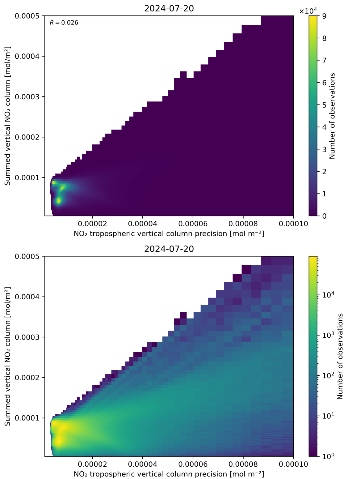
Figure 136: Scatter density plot of “NO 2 tropospheric vertical column precision” against “Summed vertical NO 2 column” for 2024-07-19 to 2024-07-21.
