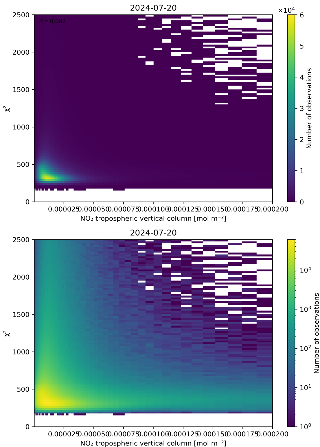
Figure 124: Scatter density plot of “NO 2 tropospheric vertical column” against “ \chi^2 ” for 2024-07-19 to 2024-07-21.
