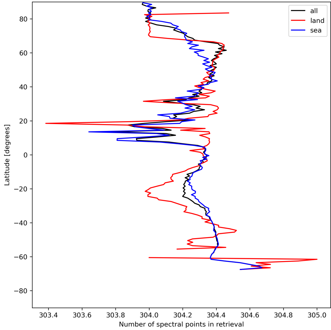
Figure 16: Zonal average of “Number of spectral points in retrieval” for 2024-07-19 to 2024-07-21.
