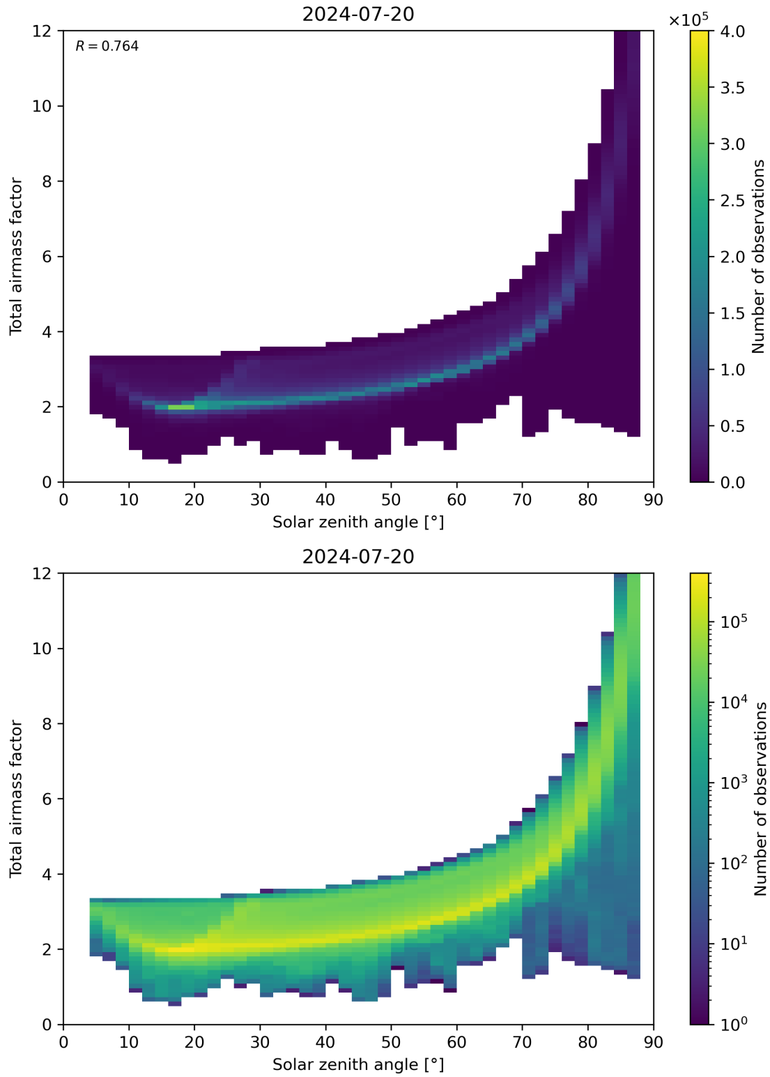
Figure 146: Scatter density plot of “Solar zenith angle” against “Total air mass factor” for 2024-07-19 to 2024-07-21.
