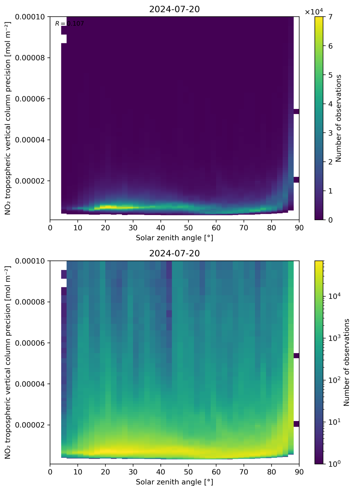
Figure 156: Scatter density plot of “Solar zenith angle” against “NO 2 tropospheric vertical column precision” for 2024-07-19 to 2024-07-21.
