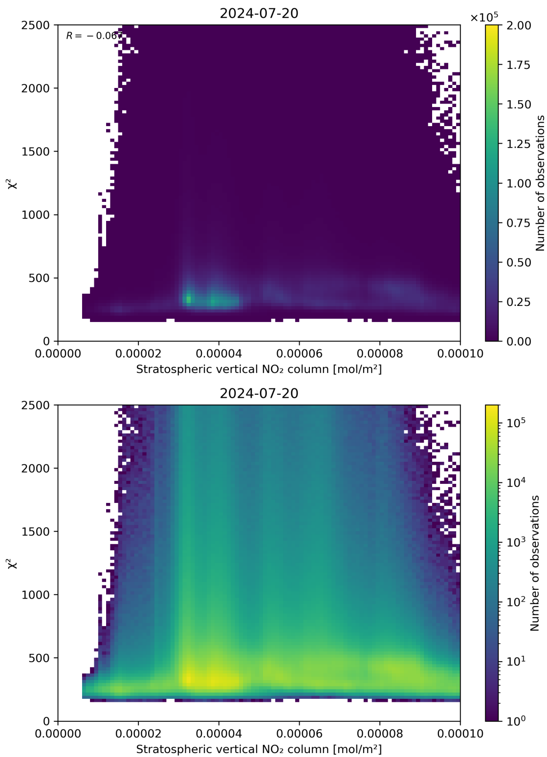
Figure 97: Scatter density plot of “Stratospheric vertical NO 2 column” against “ \chi^2 ” for 2024-07-19 to 2024-07-21.
