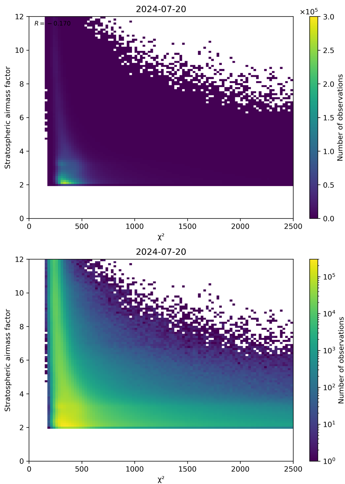
Figure 81: Scatter density plot of “ \chi^2 ” against “Stratospheric airmass factor” for 2024-07-19 to 2024-07-21.
