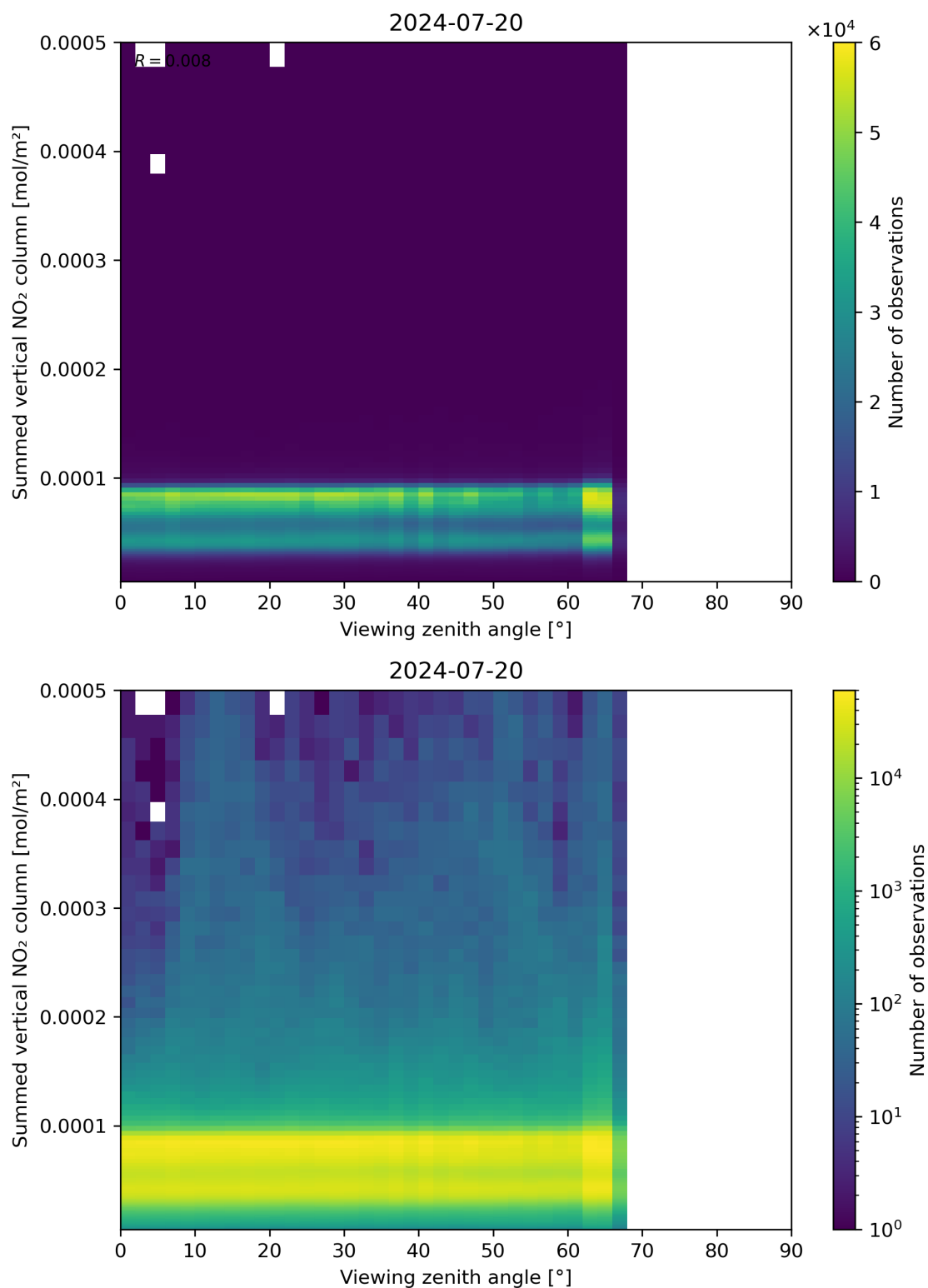
Figure 165: Scatter density plot of “Viewing zenith angle” against “Summed vertical NO 2 column” for 2024-07-19 to 2024-07-21.
