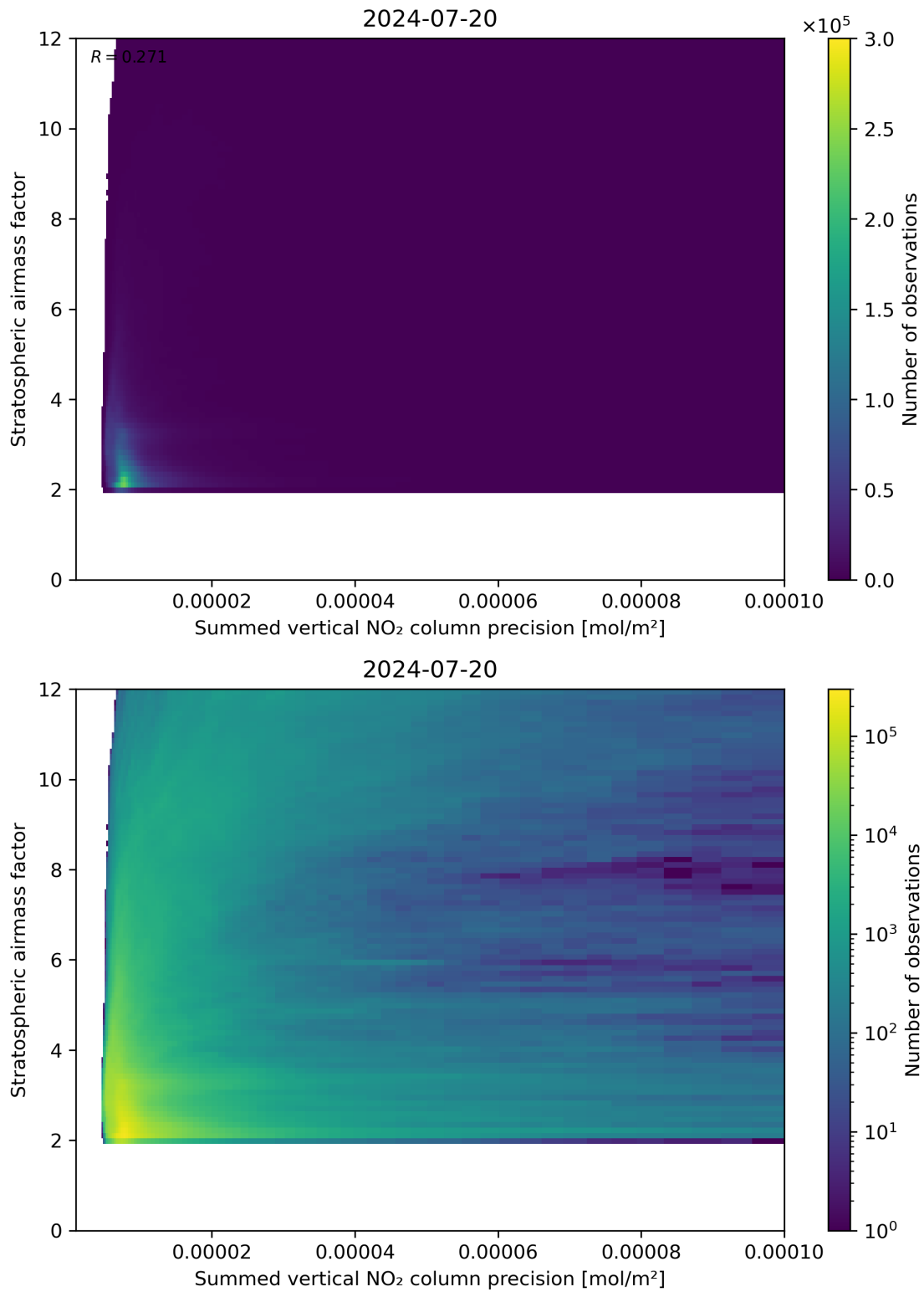
Figure 106: Scatter density plot of “Summed vertical NO 2 column precision” against “Stratospheric airmass factor” for 2024-07-19 to 2024-07-21.
