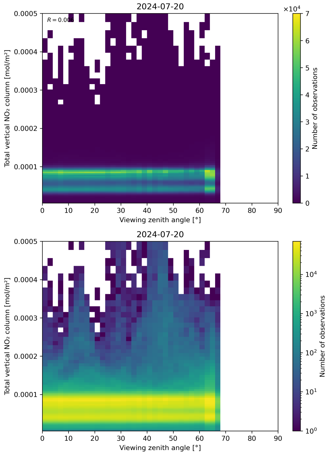
Figure 167: Scatter density plot of “Viewing zenith angle” against “Total vertical NO 2 column” for 2024-07-19 to 2024-07-21.
