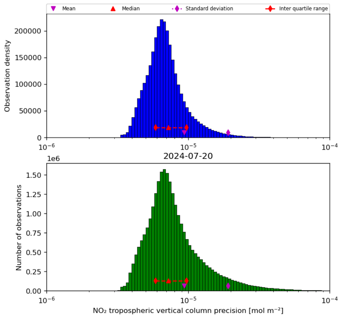
Figure 30: Histogram of “NO 2 tropospheric vertical column precision” for 2024-07-19 to 2024-07-21
