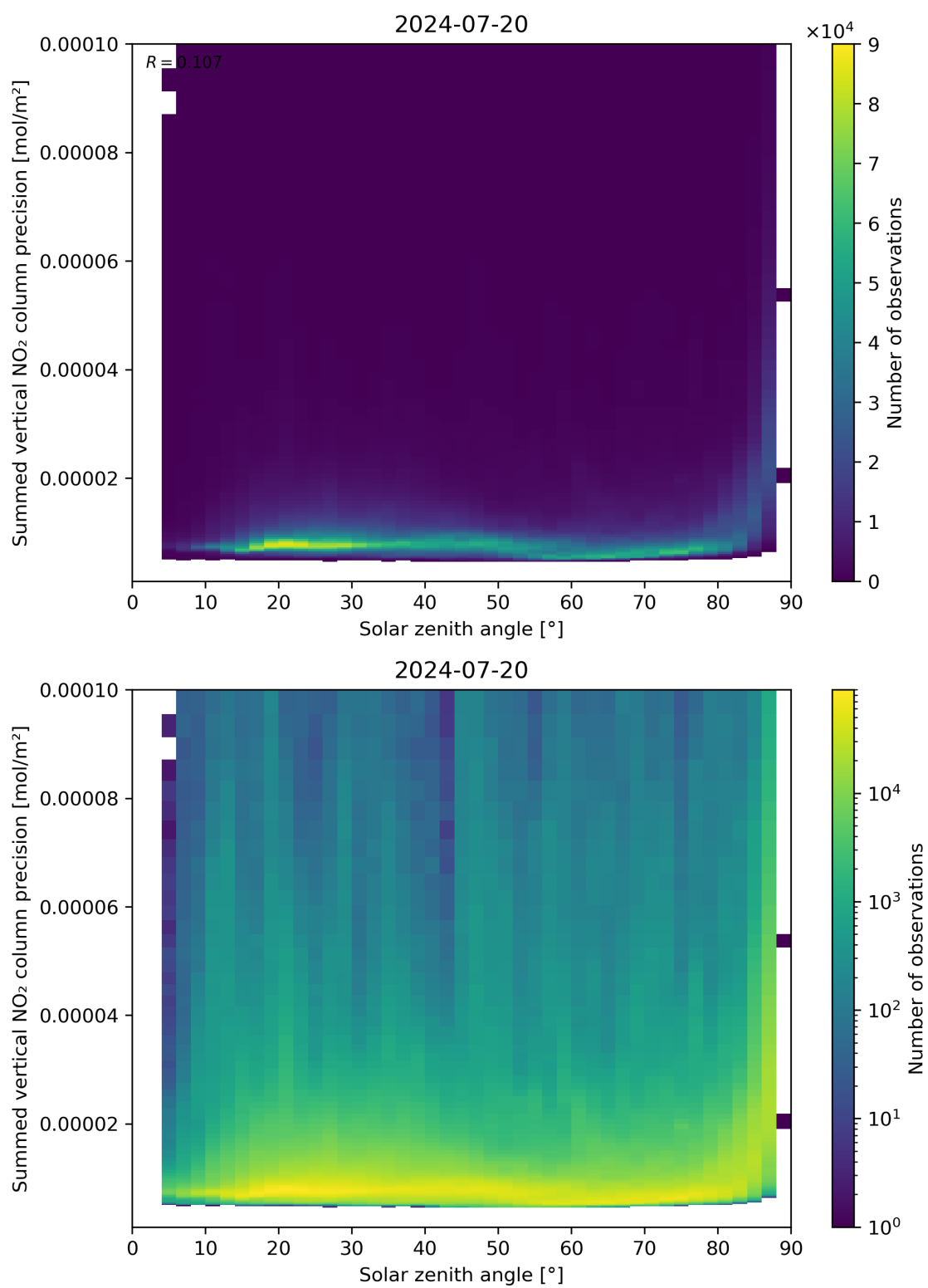
Figure 152: Scatter density plot of “Solar zenith angle” against “Summed vertical NO 2 column precision” for 2024-07-19 to 2024-07-21.
