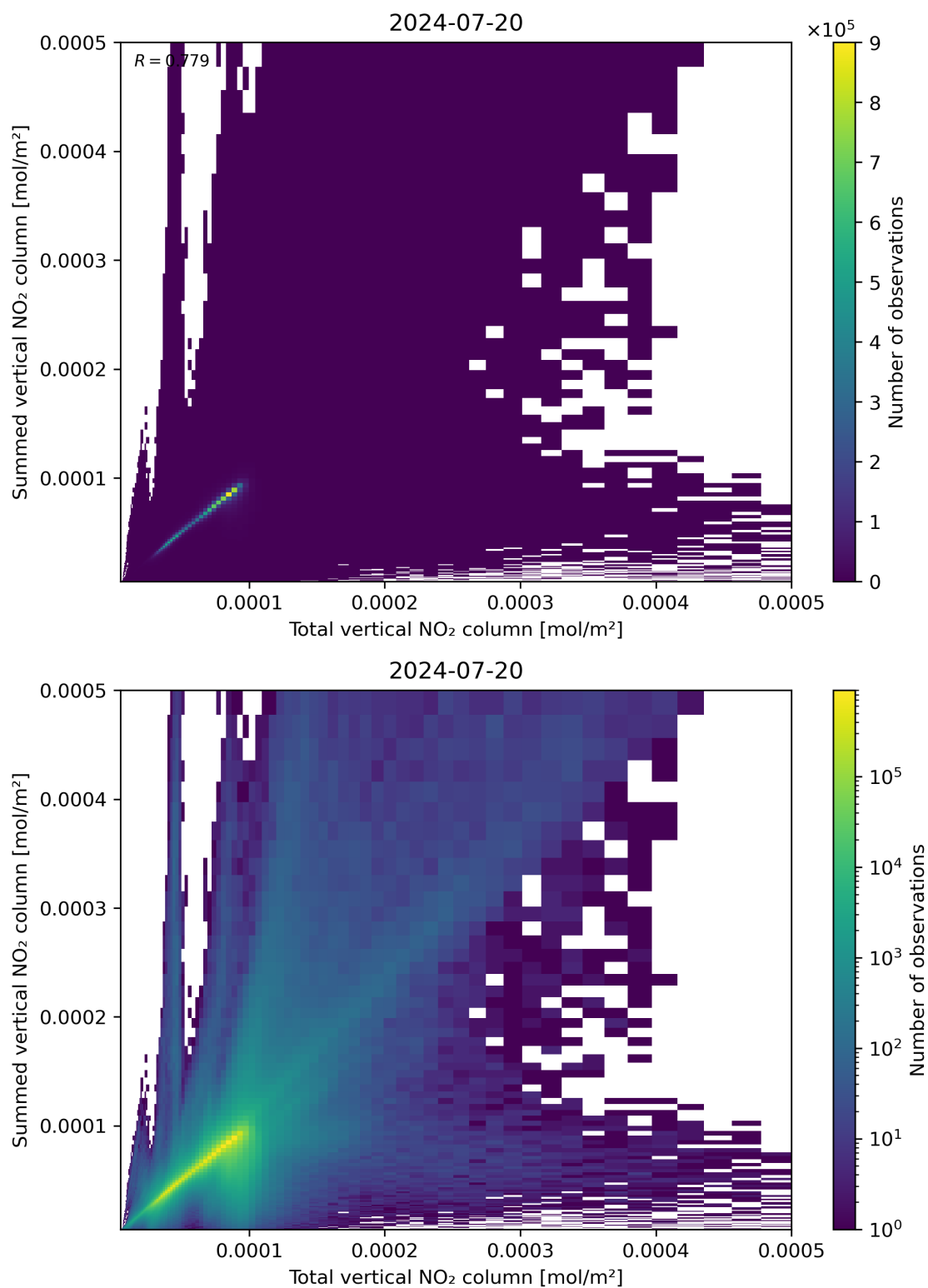
Figure 112: Scatter density plot of “Total vertical NO 2 column” against “Summed vertical NO 2 column” for 2024-07-19 to 2024-07-21.
