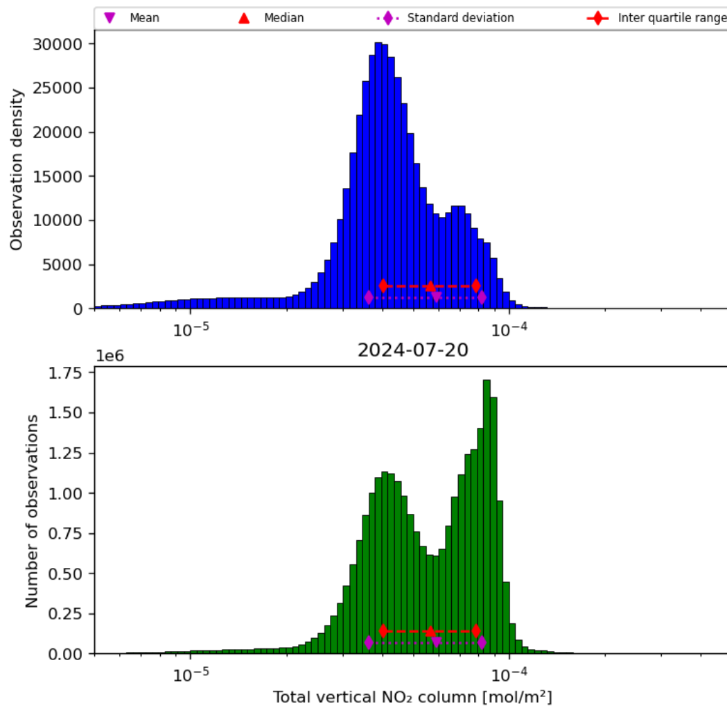
Figure 38: Histogram of “Total vertical NO 2 column” for 2024-07-19 to 2024-07-21
