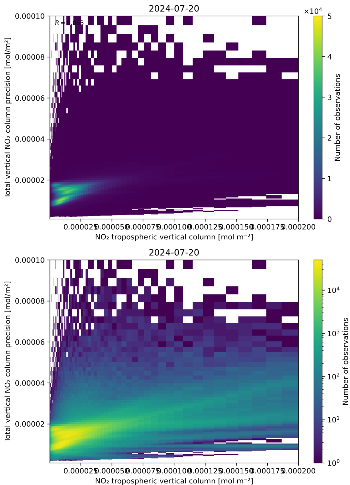
Figure 129: Scatter density plot of “NO 2 tropospheric vertical column” against “Total vertical NO 2 column precision” for 2024-07-19 to 2024-07-21.
