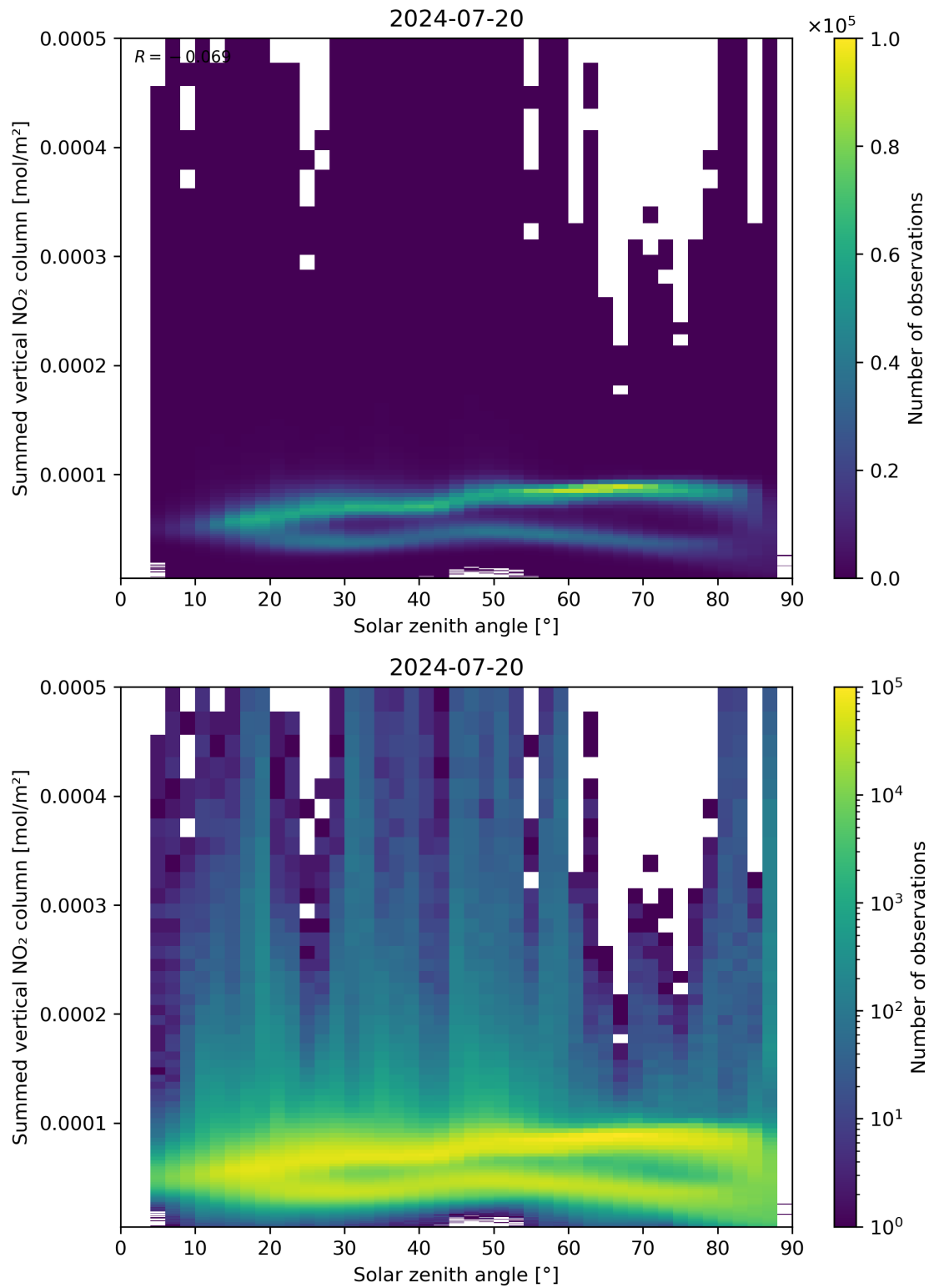
Figure 151: Scatter density plot of “Solar zenith angle” against “Summed vertical NO 2 column” for 2024-07-19 to 2024-07-21.
