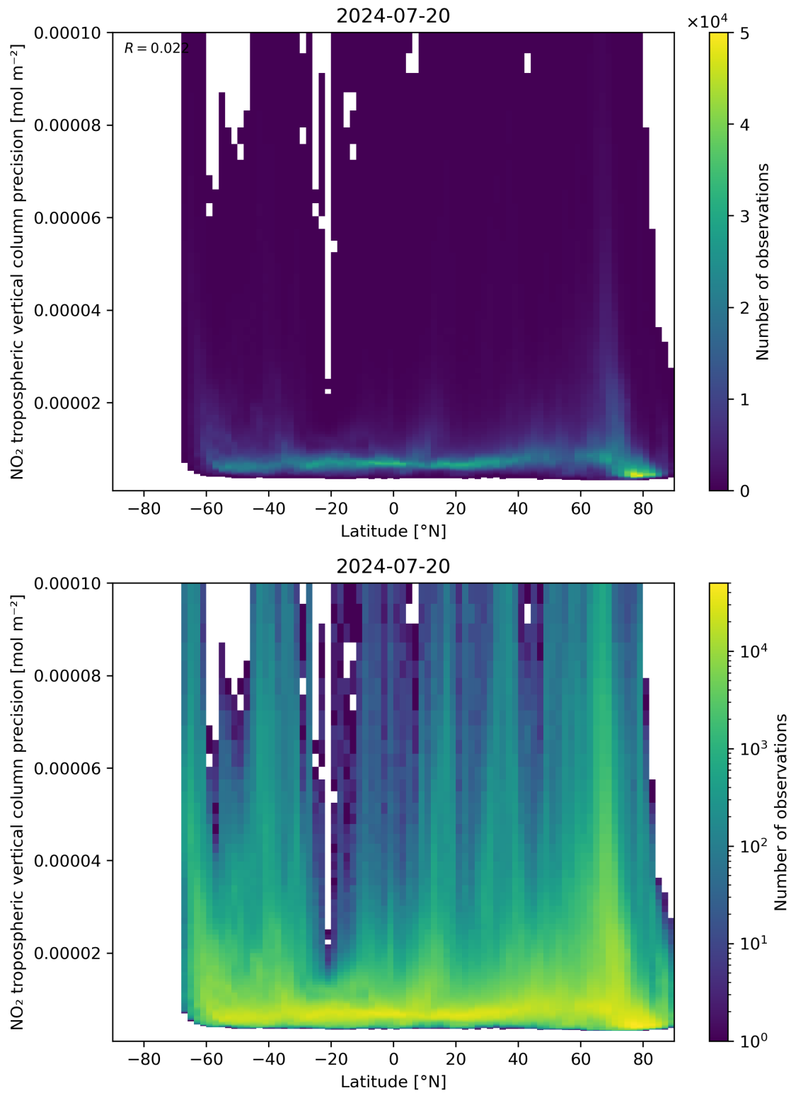
Figure 93: Scatter density plot of “Latitude” against “NO 2 tropospheric vertical column precision” for 2024-07-19 to 2024-07-21.
