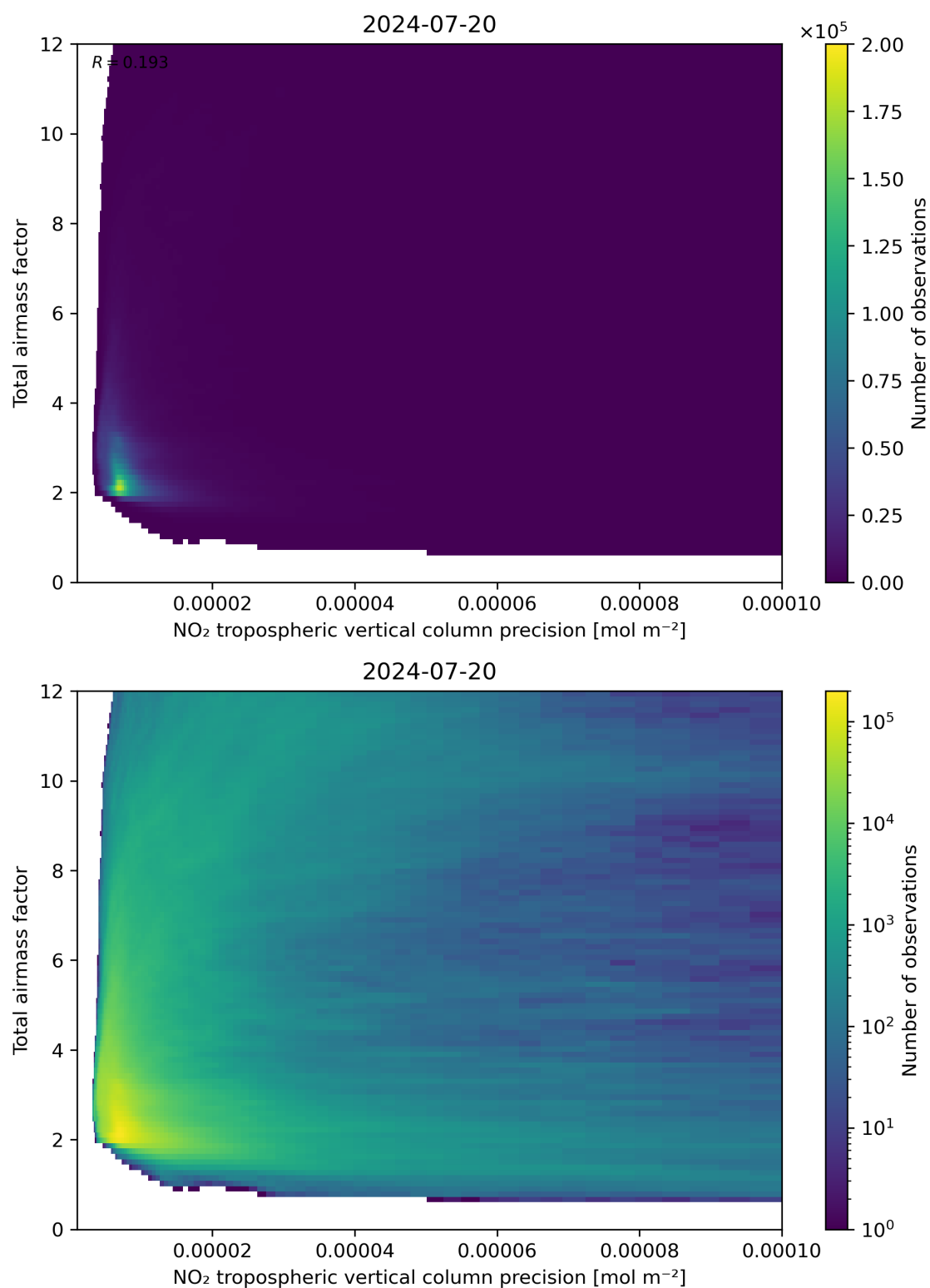
Figure 132: Scatter density plot of “NO 2 tropospheric vertical column precision” against “Total air mass factor” for 2024-07-19 to 2024-07-21.
