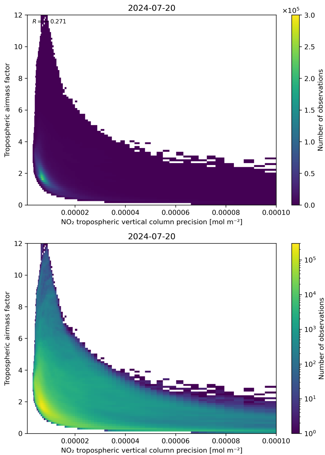
Figure 133: Scatter density plot of “NO 2 tropospheric vertical column precision” against “Tropospheric airmass factor” for 2024-07-19 to 2024-07-21.
