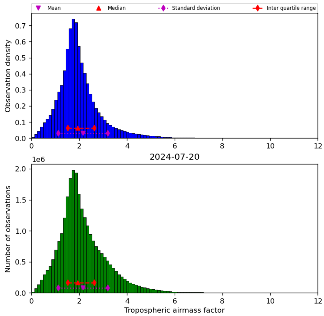
Figure 31: Histogram of “Tropospheric airmass factor” for 2024-07-19 to 2024-07-21
