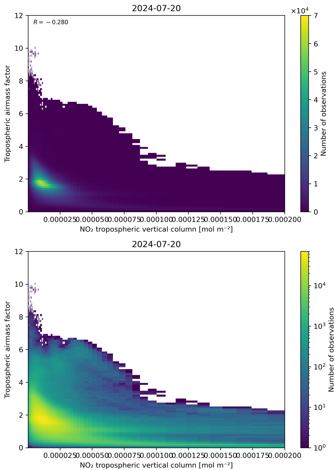
Figure 123: Scatter density plot of “NO 2 tropospheric vertical column” against “Tropospheric airmass factor” for 2024-07-19 to 2024-07-21.
