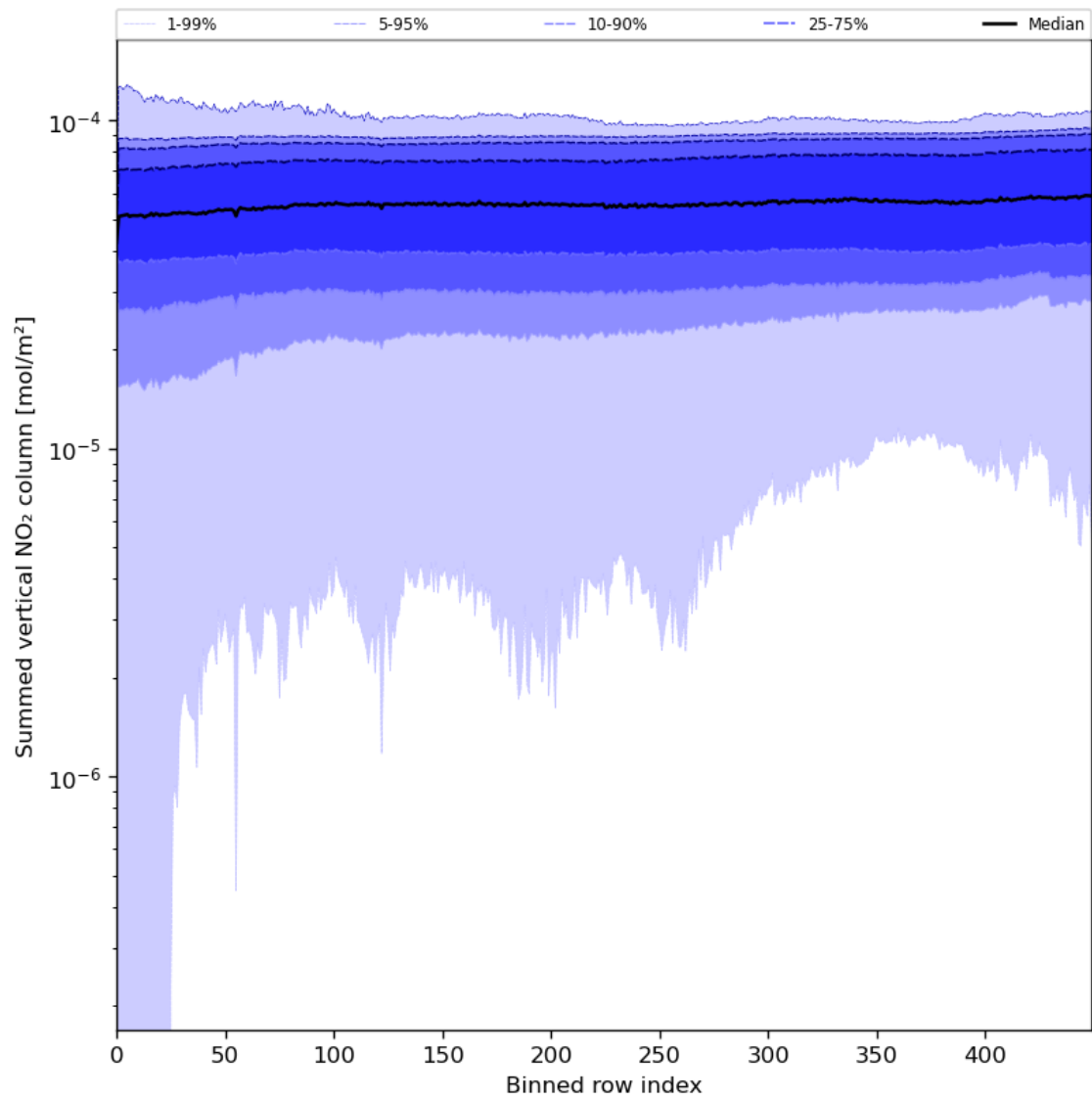
Figure 57: Along track statistics of “Summed vertical NO 2 column” for 2024-07-19 to 2024-07-21
