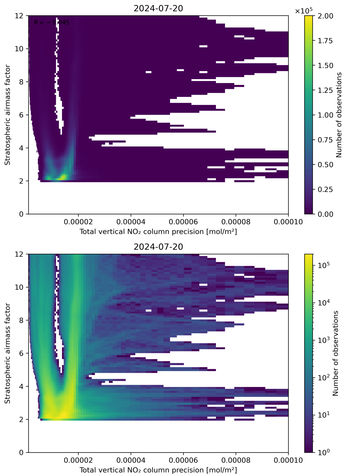
Figure 115: Scatter density plot of “Total vertical NO 2 column precision” against “Stratospheric air mass factor” for 2024-07-19 to 2024-07-21.
