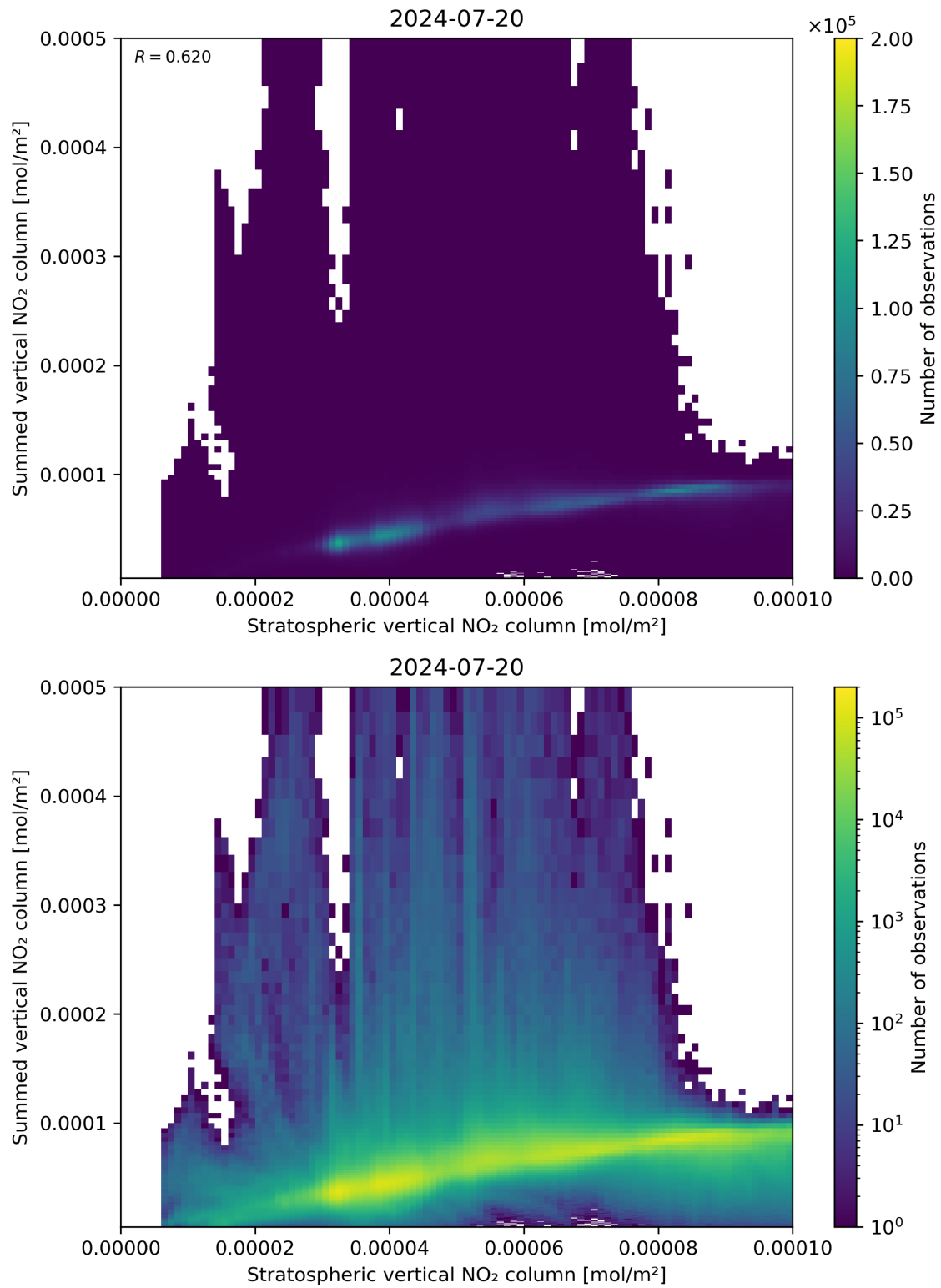
Figure 98: Scatter density plot of “Stratospheric vertical NO 2 column” against “Summed vertical NO 2 column” for 2024-07-19 to 2024-07-21.
