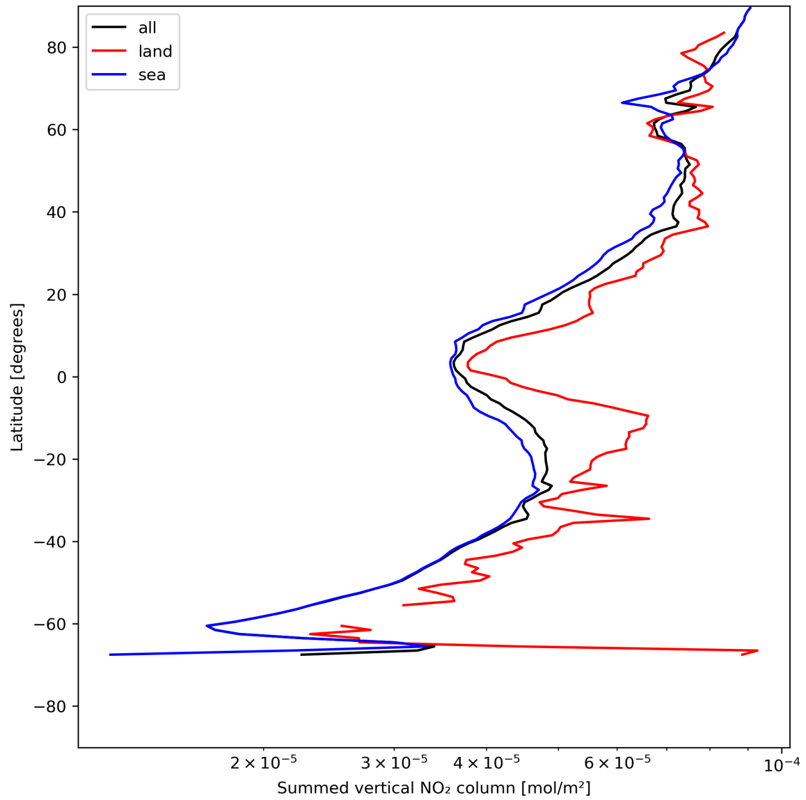
Figure 23: Zonal average of “Summed vertical NO 2 column” for 2024-07-19 to 2024-07-21.
