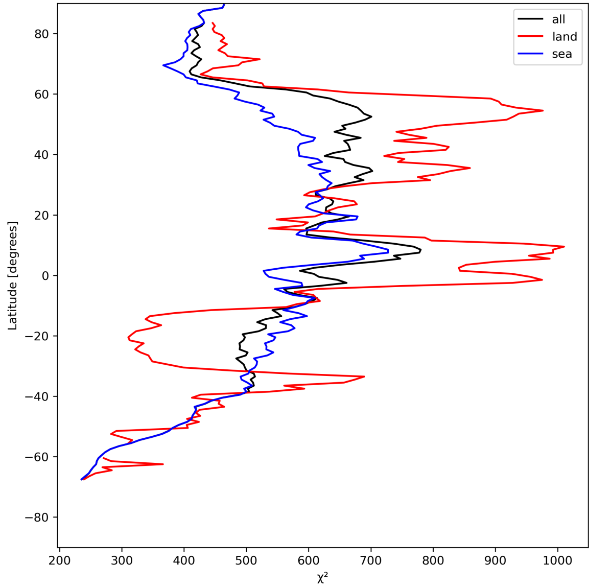
Figure 25: Zonal average of “ \chi^2 ” for 2024-07-19 to 2024-07-21.
