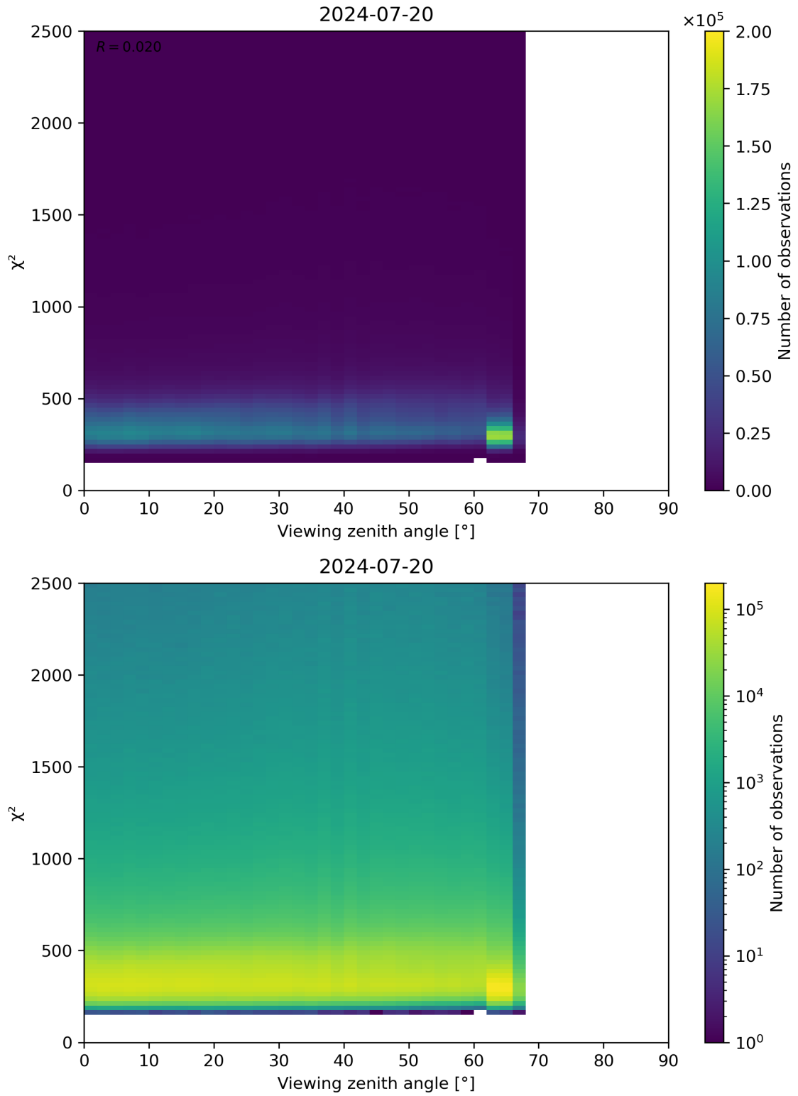
Figure 162: Scatter density plot of “Viewing zenith angle” against “ \chi^2 ” for 2024-07-19 to 2024-07-21.
