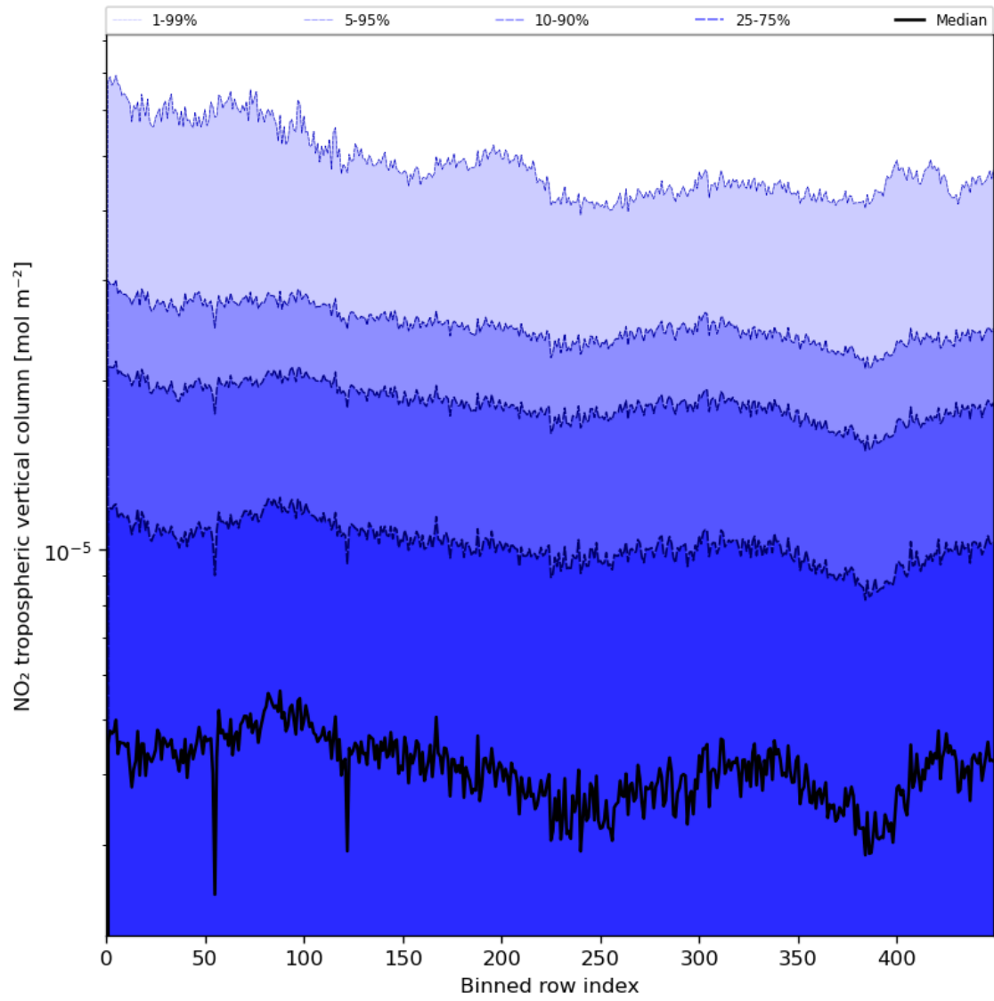
Figure 46: Along track statistics of “NO 2 tropospheric vertical column” for 2024-07-19 to 2024-07-21
