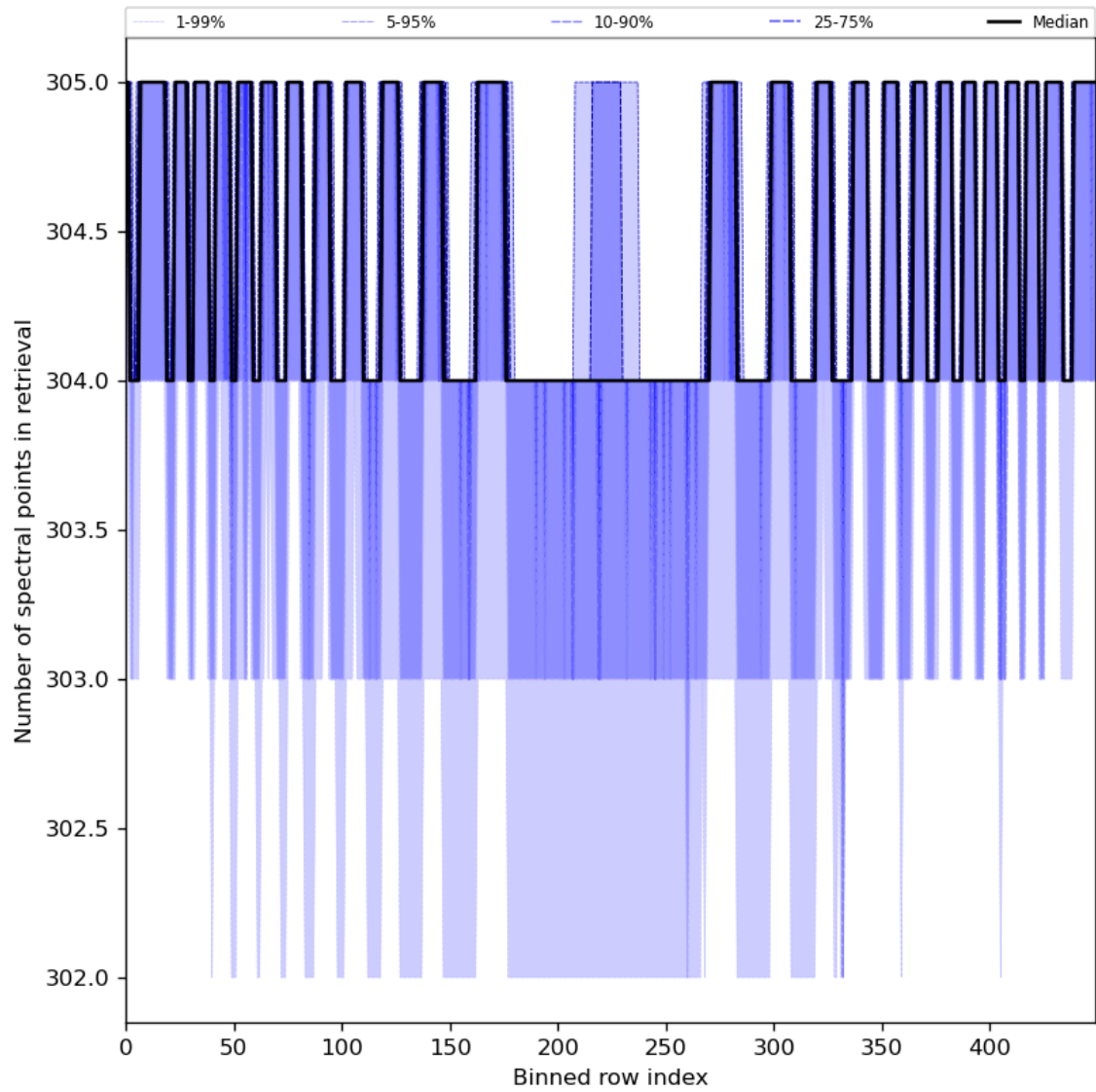
Figure 50: Along track statistics of “Number of spectral points in retrieval” for 2024-07-19 to 2024-07-21
