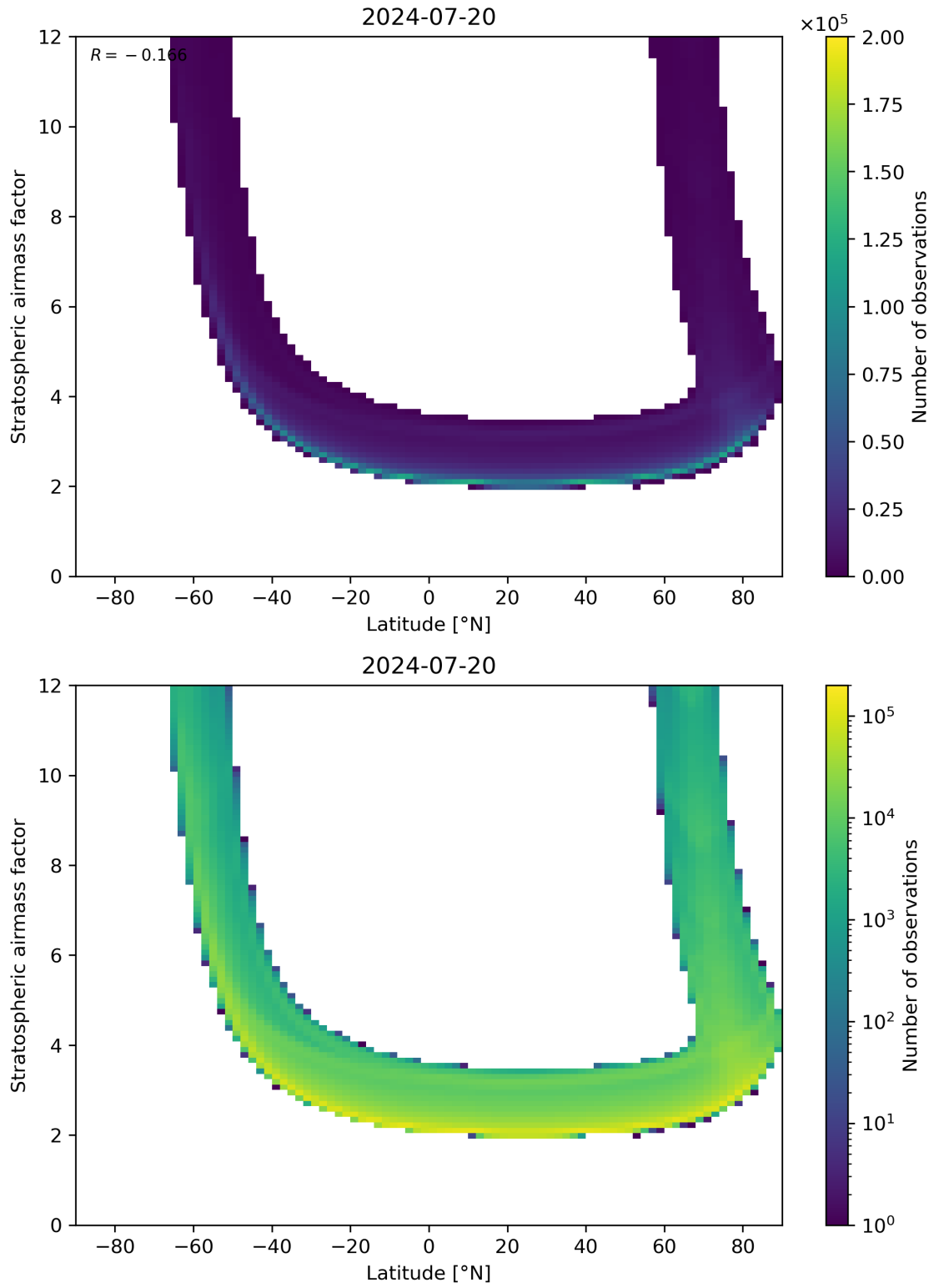
Figure 83: Scatter density plot of “Latitude” against “Stratospheric air mass factor” for 2024-07-19 to 2024-07-21.
