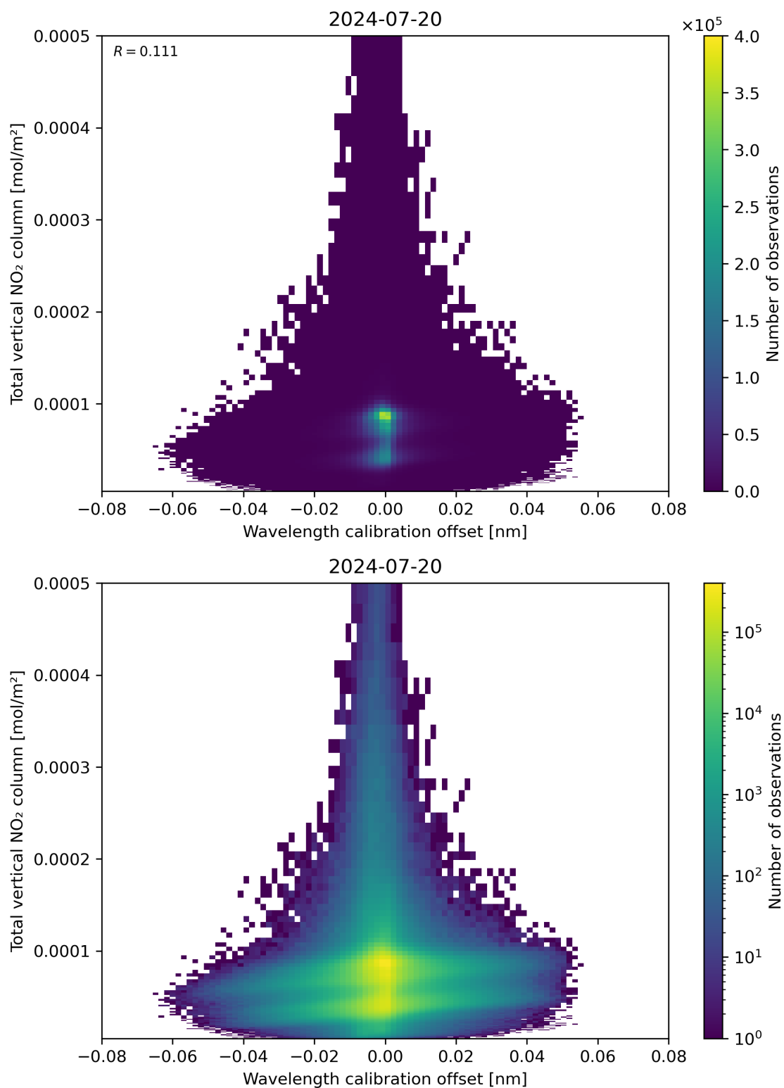
Figure 179: Scatter density plot of “Wavelength calibration offset” against “Total vertical NO 2 column” for 2024-07-19 to 2024-07-21.
