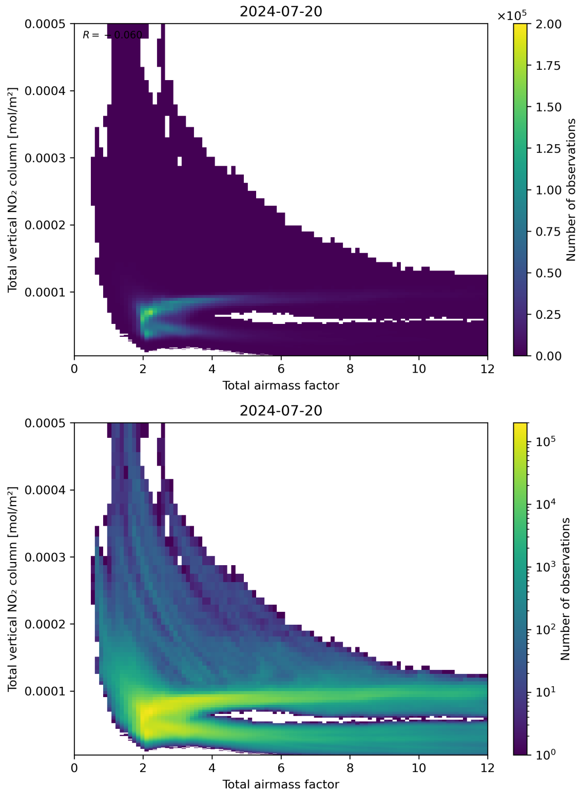
Figure 67: Scatter density plot of “Total airmass factor” against “Total vertical NO 2 column” for 2024-07-19 to 2024-07-21.
