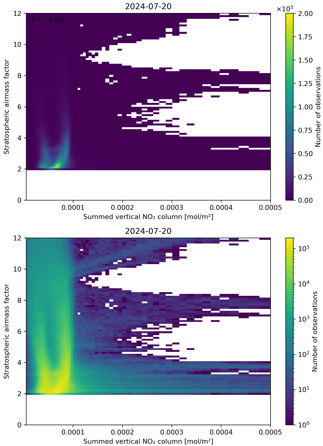
Figure 103: Scatter density plot of “Summed vertical NO 2 column” against “Stratospheric air mass factor” for 2024-07-19 to 2024-07-21.
