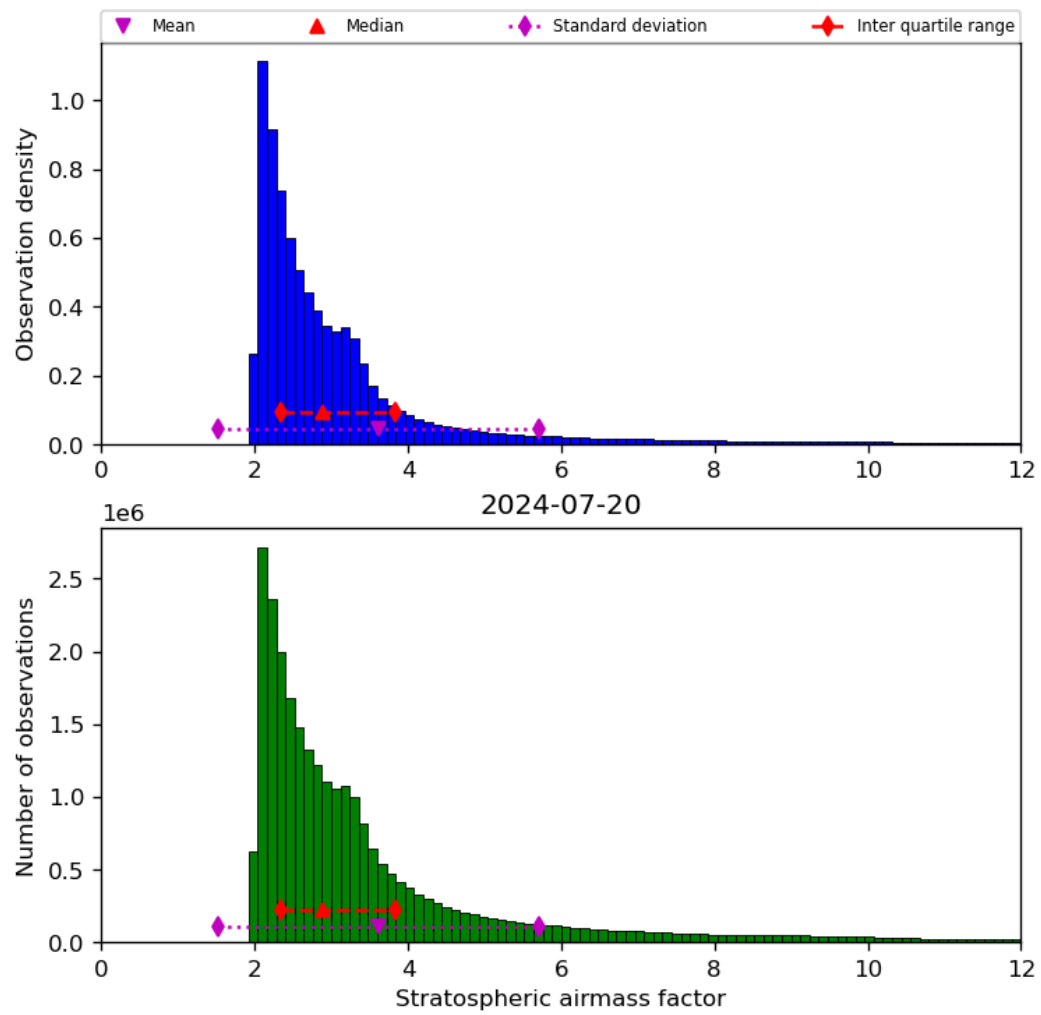
Figure 44: Histogram of “Stratospheric airmass factor” for 2024-07-19 to 2024-07-21
