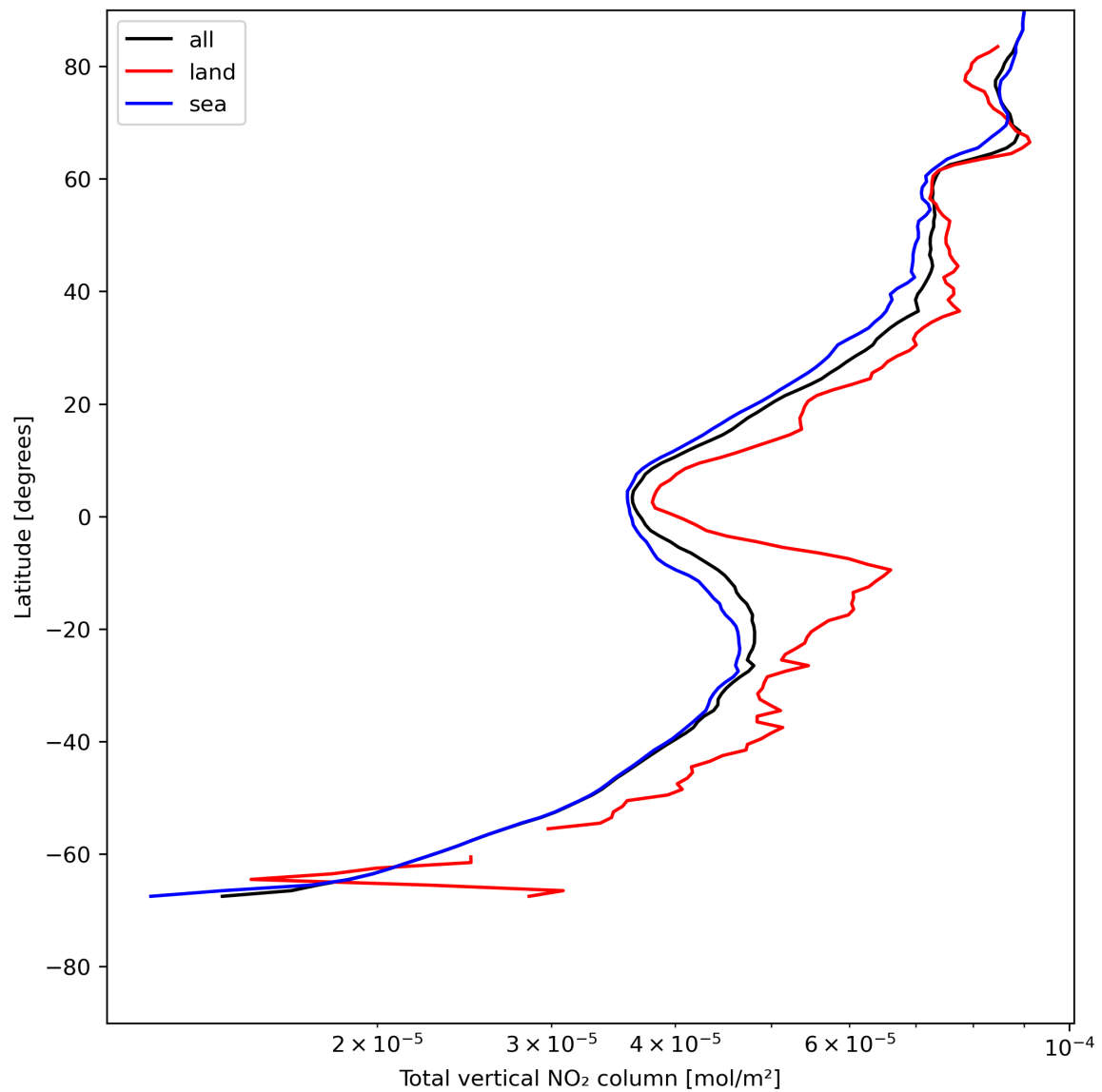
Figure 21: Zonal average of “Total vertical NO 2 column” for 2024-07-19 to 2024-07-21.
