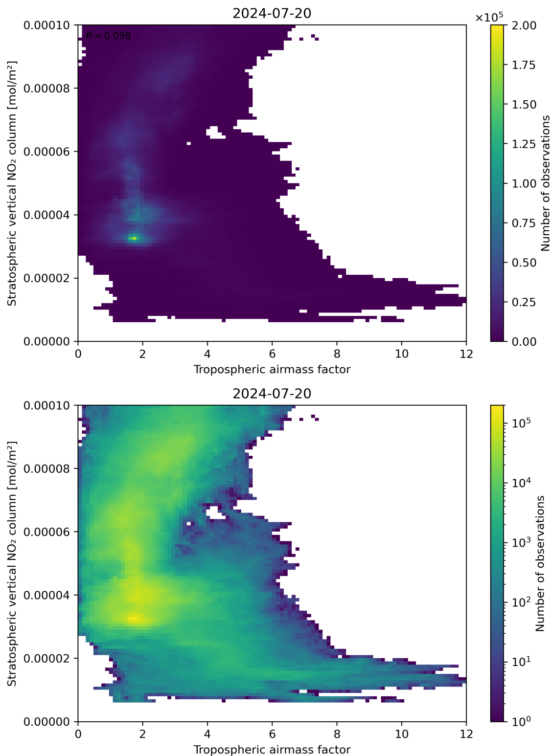
Figure 74: Scatter density plot of “Tropospheric air mass factor” against “Stratospheric vertical NO 2 column” for 2024-07-19 to 2024-07-21.
