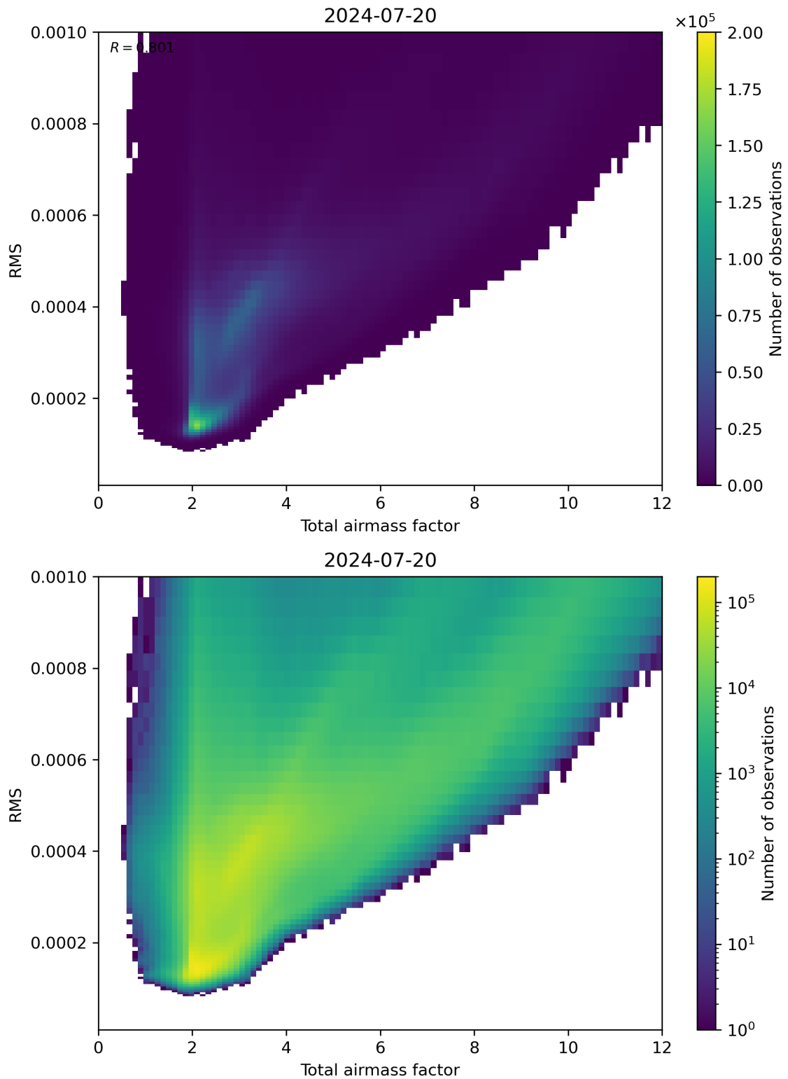
Figure 69: Scatter density plot of “Total airmass factor” against “RMS” for 2024-07-19 to 2024-07-21.
