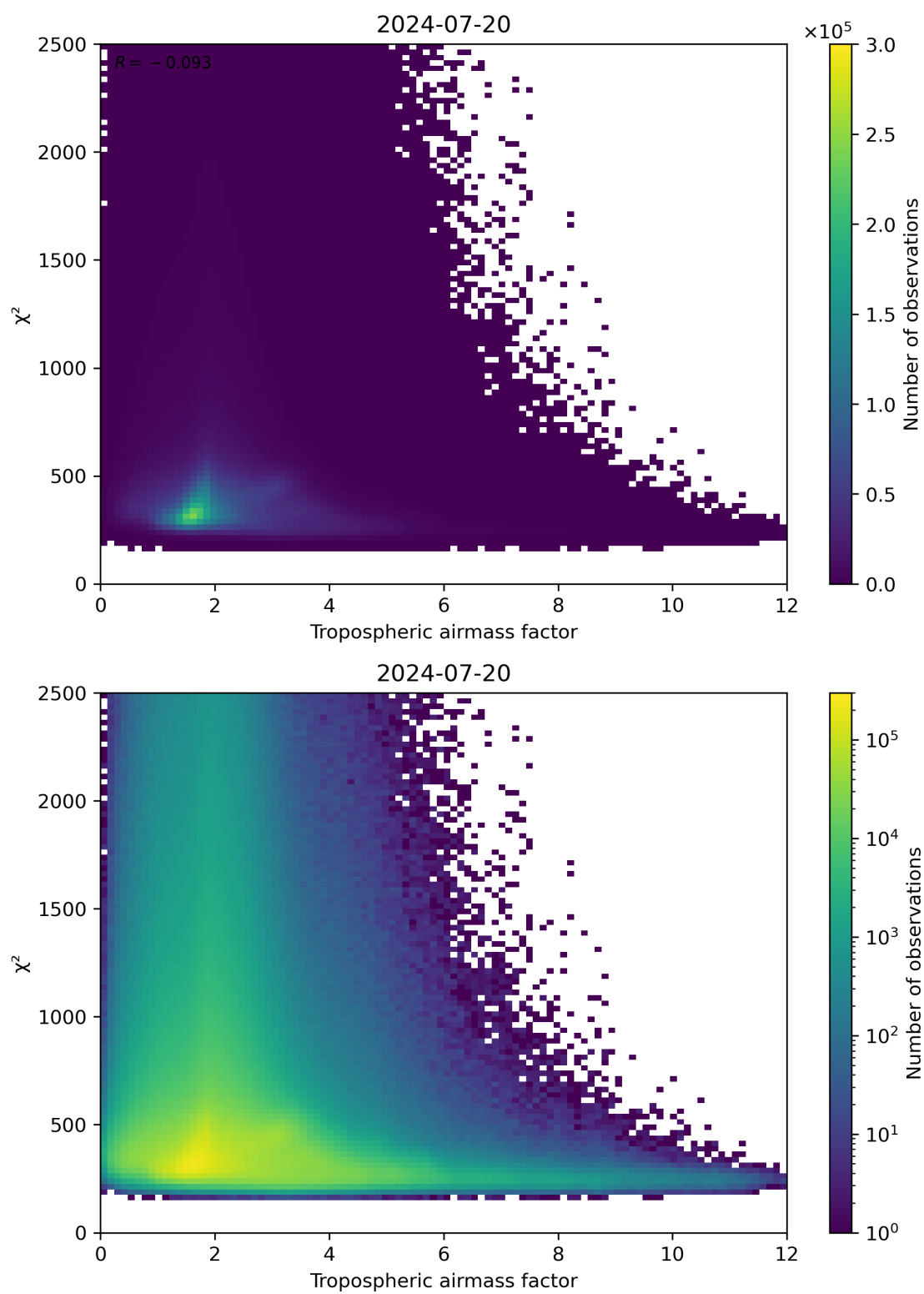
Figure 73: Scatter density plot of “Tropospheric airmass factor” against “ \chi^2 ” for 2024-07-19 to 2024-07-21.
