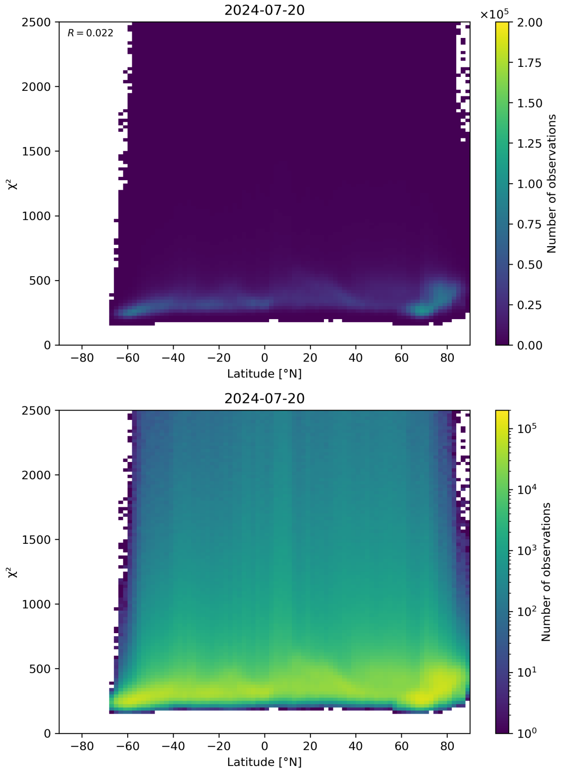
Figure 86: Scatter density plot of “Latitude” against “ \chi^2 ” for 2024-07-19 to 2024-07-21.
