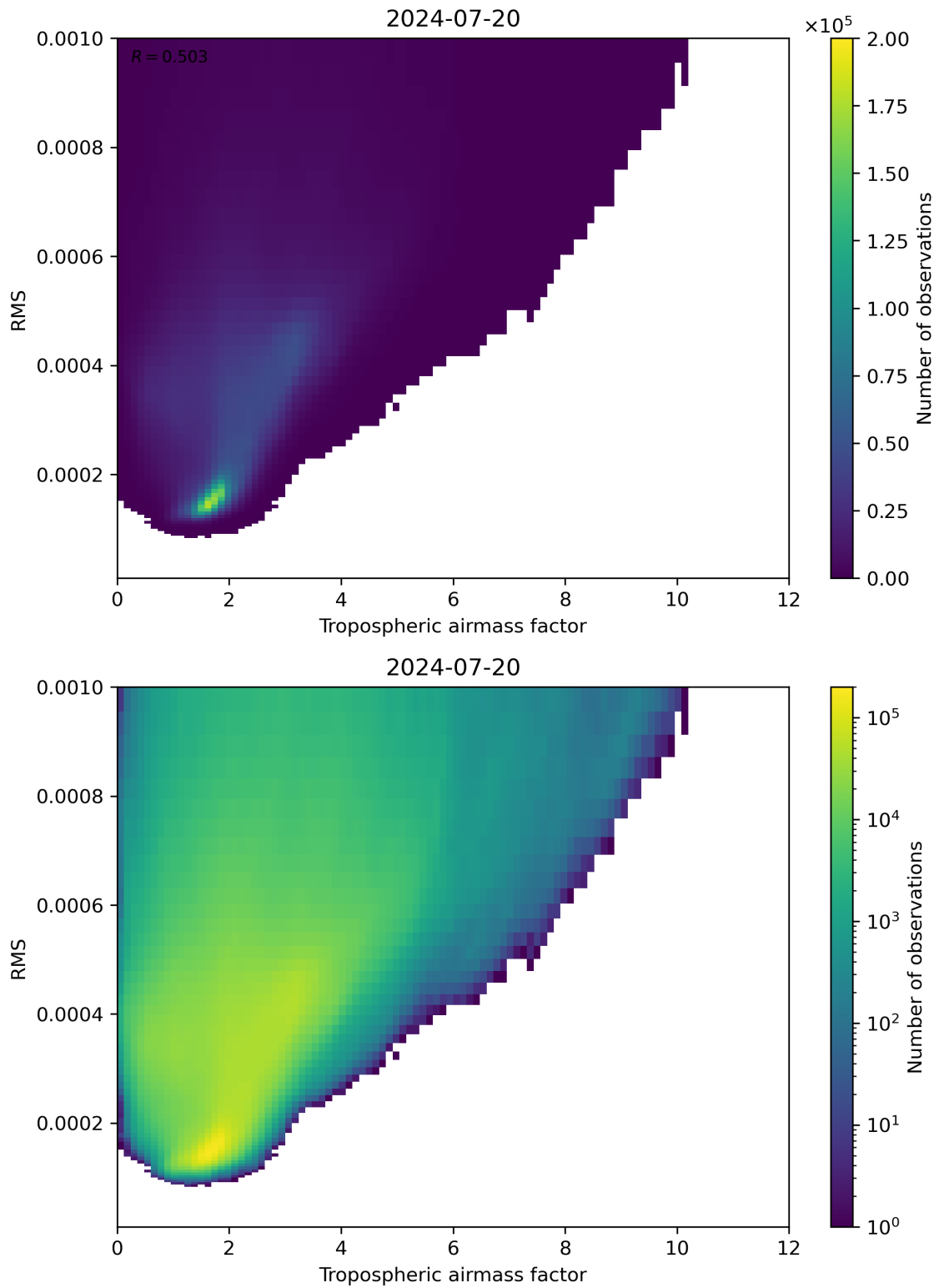
Figure 79: Scatter density plot of “Tropospheric airmass factor” against “RMS” for 2024-07-19 to 2024-07-21.
