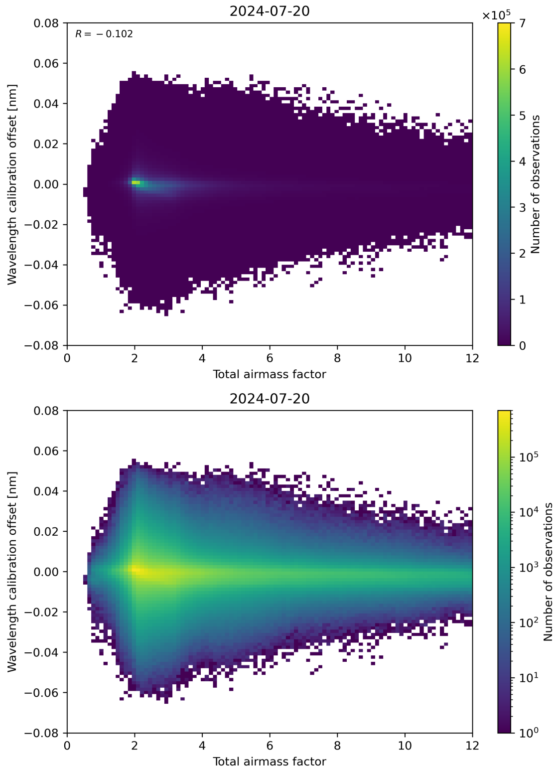
Figure 70: Scatter density plot of “Total airmass factor” against “Wavelength calibration offset” for 2024-07-19 to 2024-07-21.
