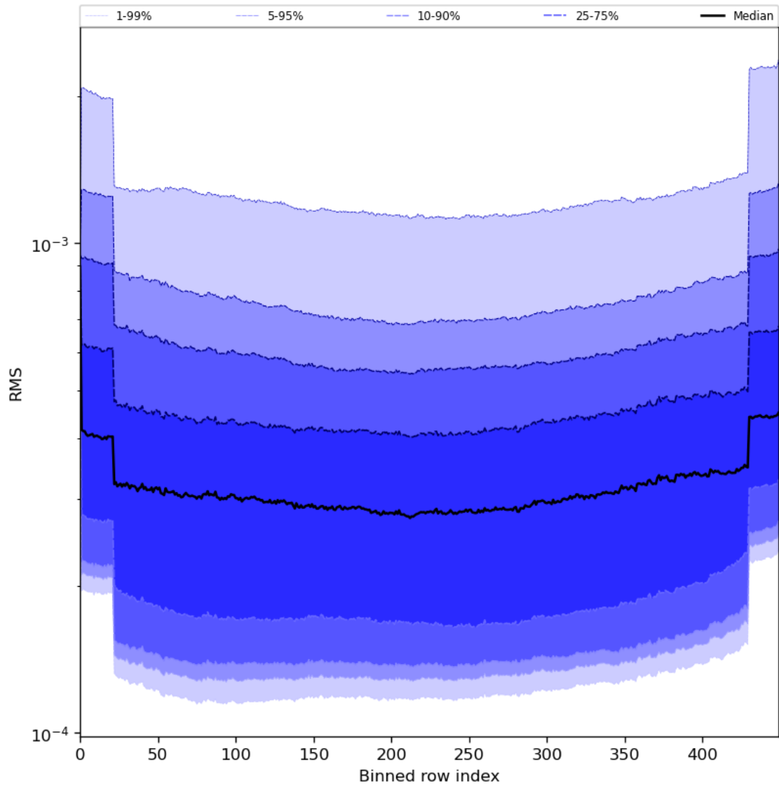
Figure 60: Along track statistics of “RMS” for 2024-07-19 to 2024-07-21
