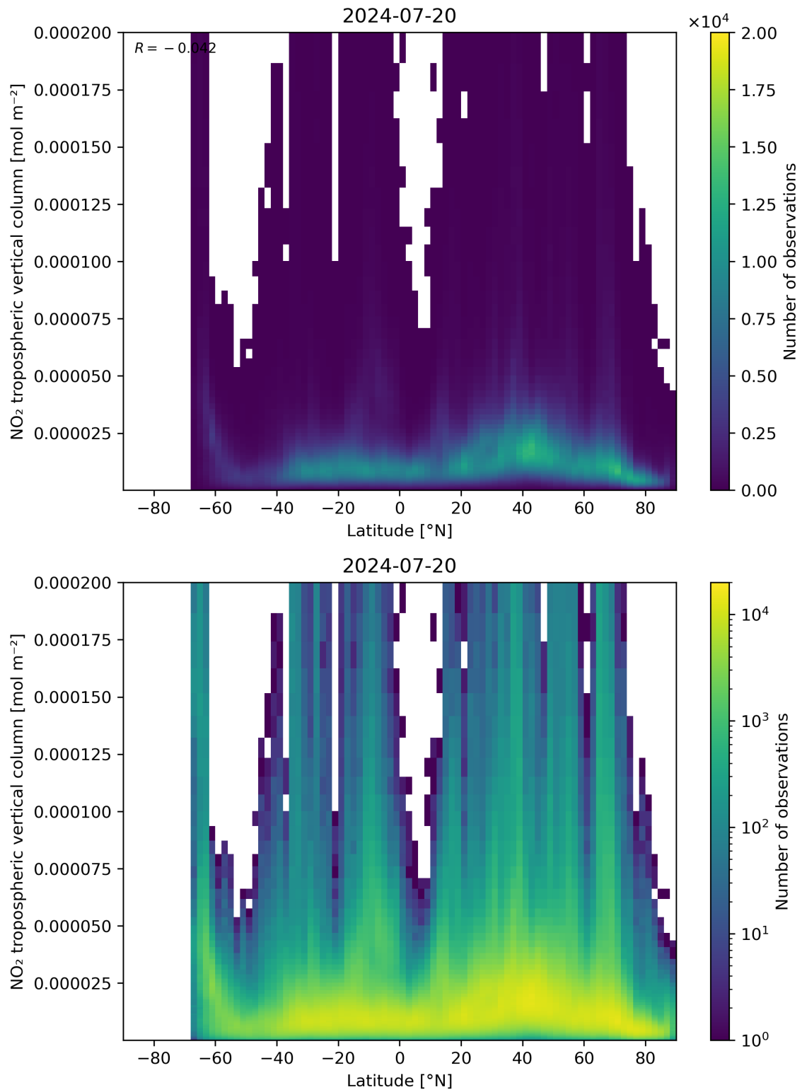
Figure 92: Scatter density plot of “Latitude” against “NO 2 tropospheric vertical column” for 2024-07-19 to 2024-07-21.
