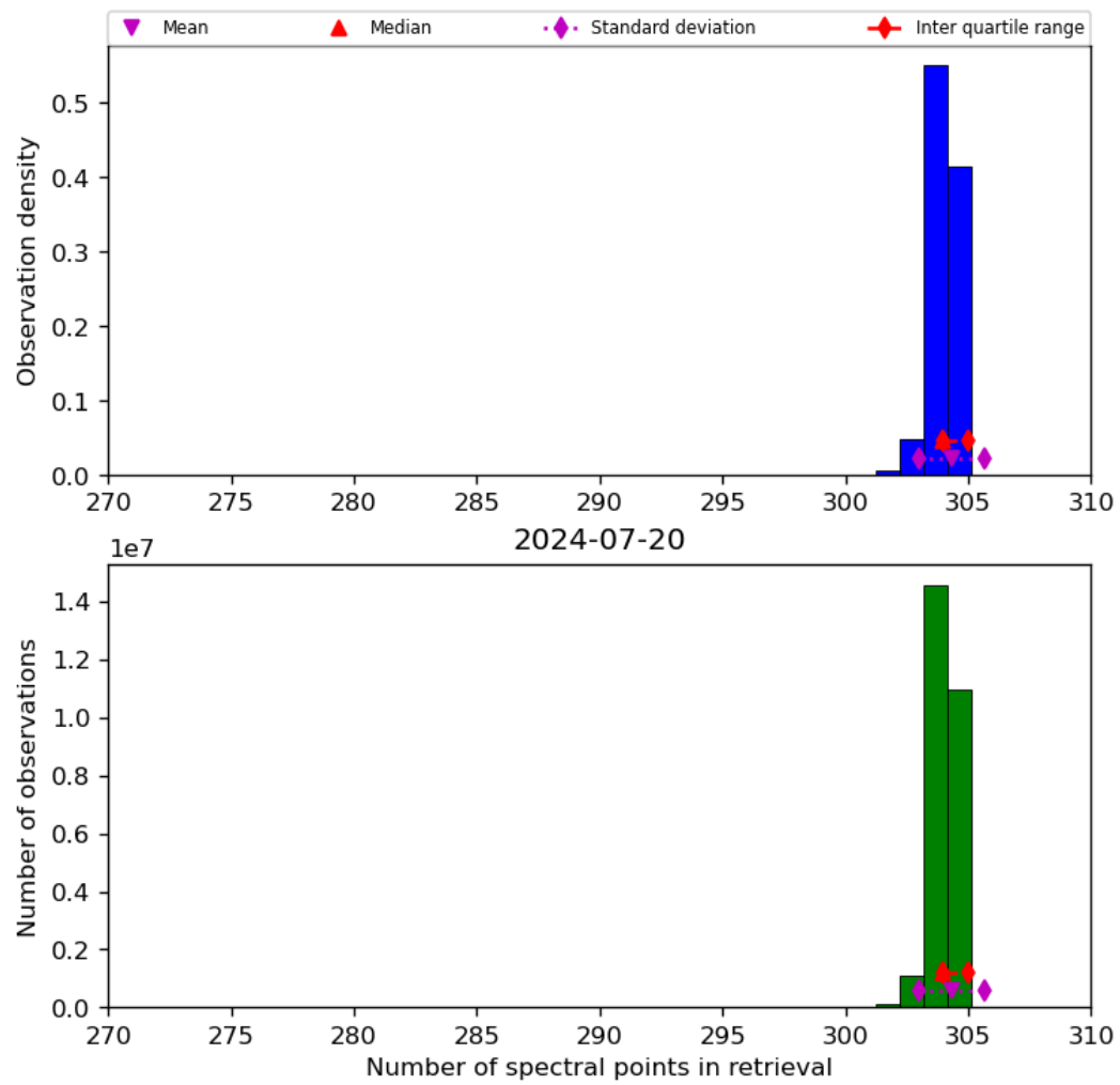
Figure 33: Histogram of “Number of spectral points in retrieval” for 2024-07-19 to 2024-07-21
