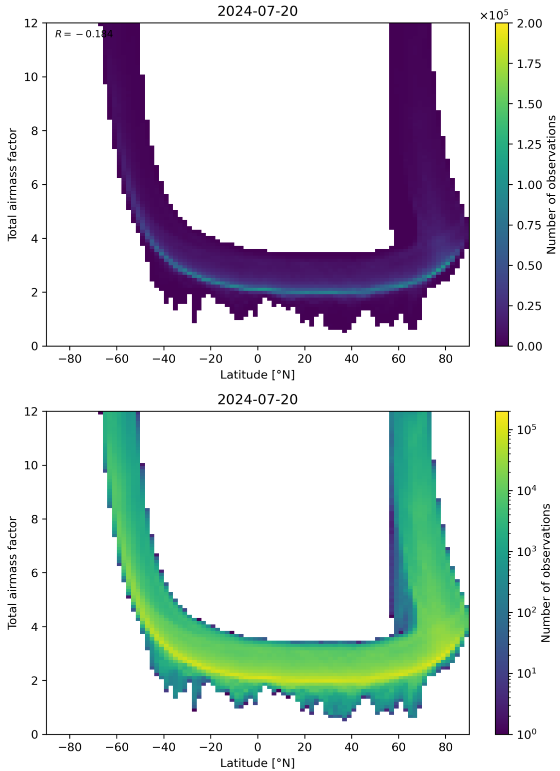
Figure 84: Scatter density plot of “Latitude” against “Total airmass factor” for 2024-07-19 to 2024-07-21.
