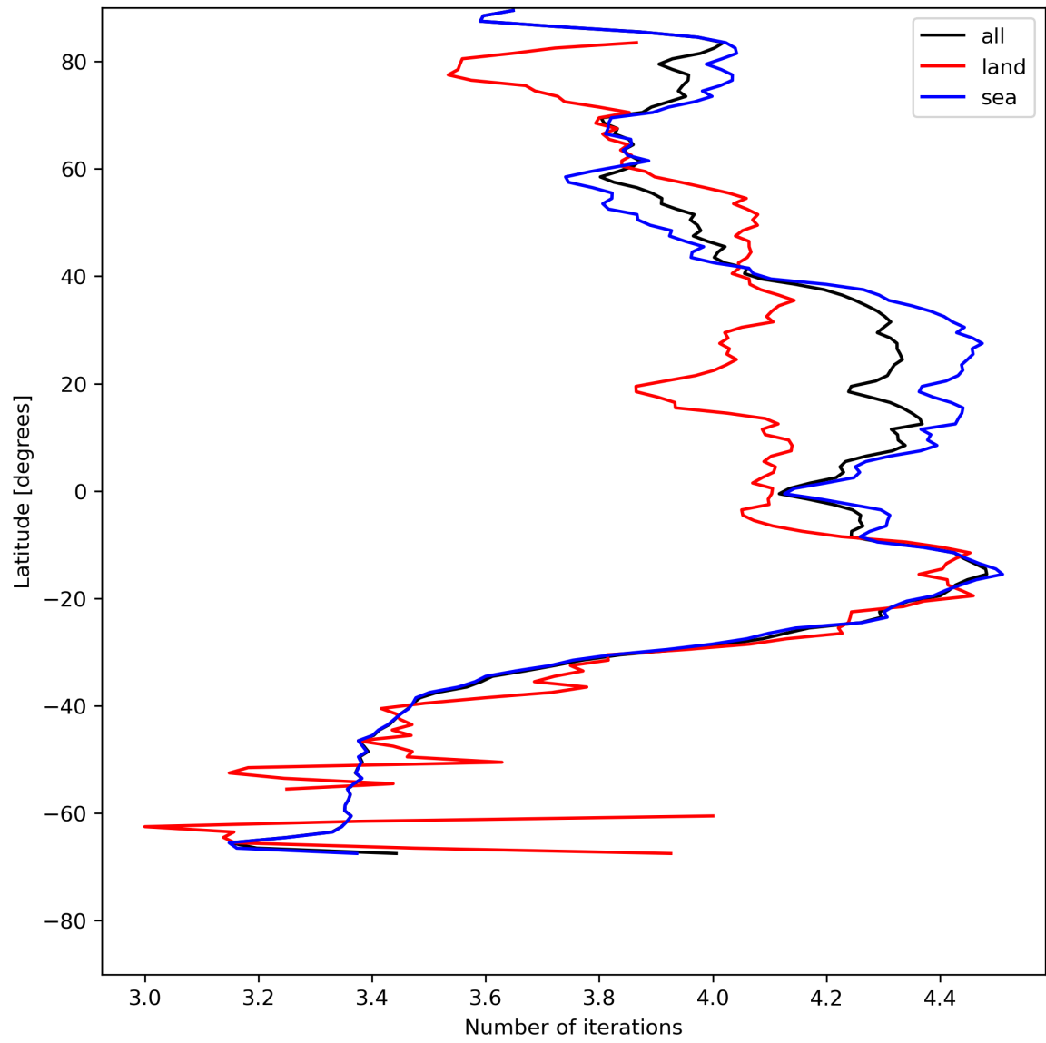
Figure 17: Zonal average of “Number of iterations” for 2024-07-19 to 2024-07-21.
