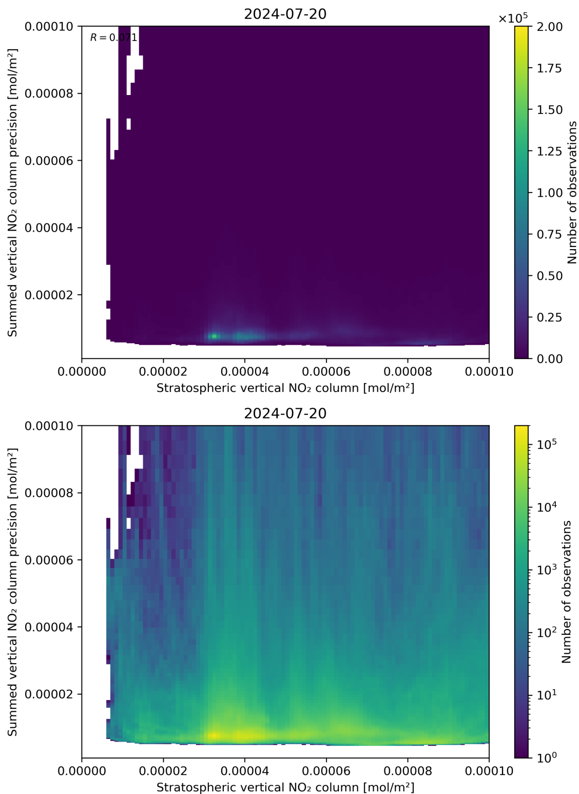
Figure 99: Scatter density plot of “Stratospheric vertical NO 2 column” against “Summed vertical NO 2 column precision” for 2024-07-19 to 2024-07-21.
