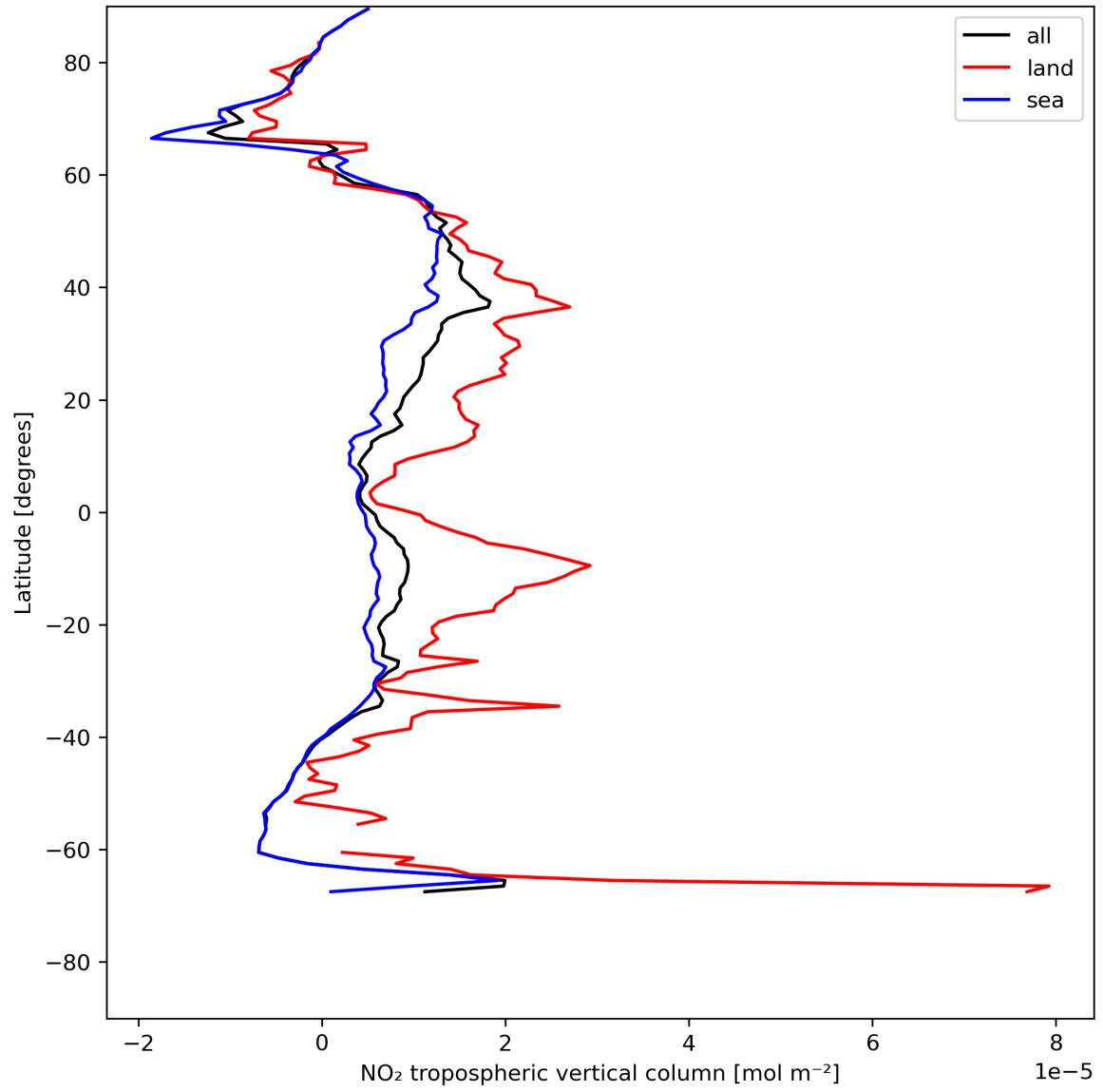
Figure 12: Zonal average of “NO 2 tropospheric vertical column” for 2024-07-19 to 2024-07-21.
