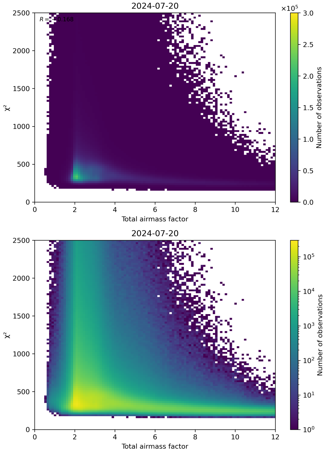
Figure 63: Scatter density plot of “Total airmass factor” against “ \chi^2 ” for 2024-07-19 to 2024-07-21.
