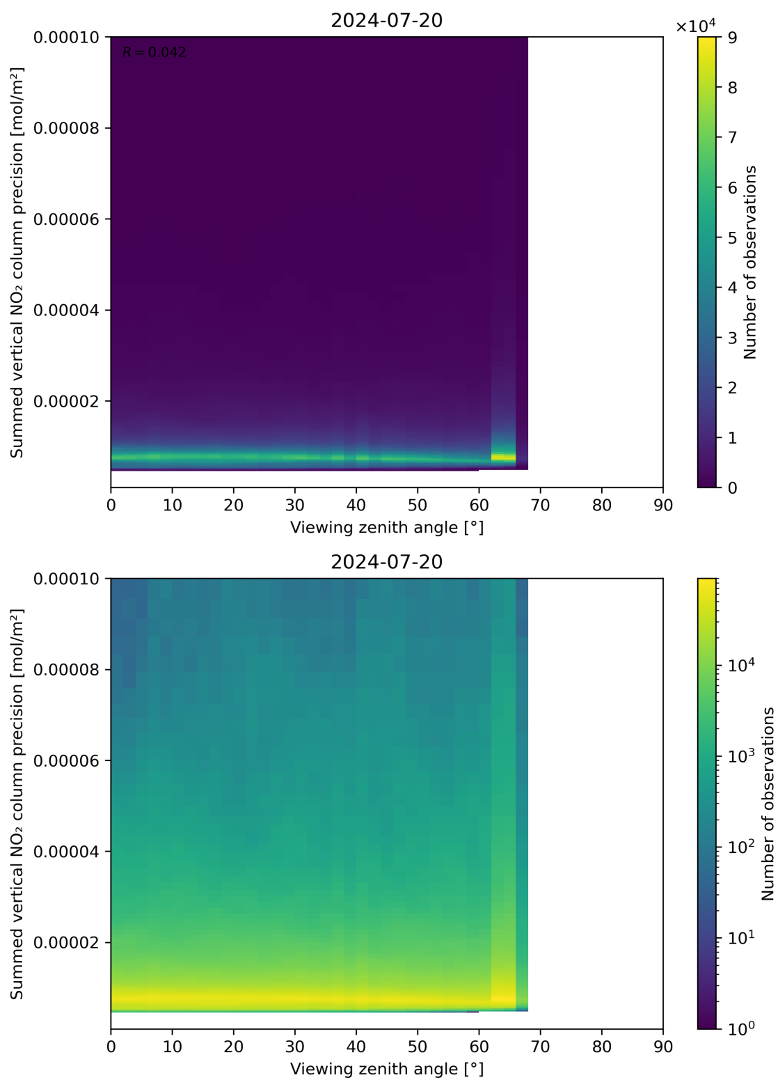
Figure 166: Scatter density plot of “Viewing zenith angle” against “Summed vertical NO 2 column precision” for 2024-07-19 to 2024-07-21.
