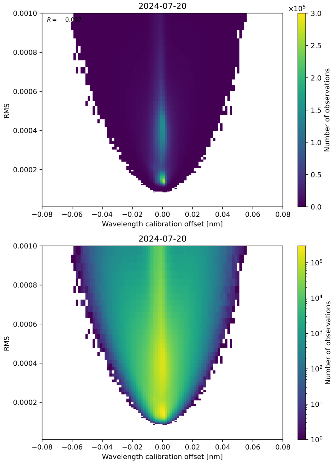
Figure 181: Scatter density plot of “Wavelength calibration offset” against “RMS” for 2024-07-19 to 2024-07-21.
