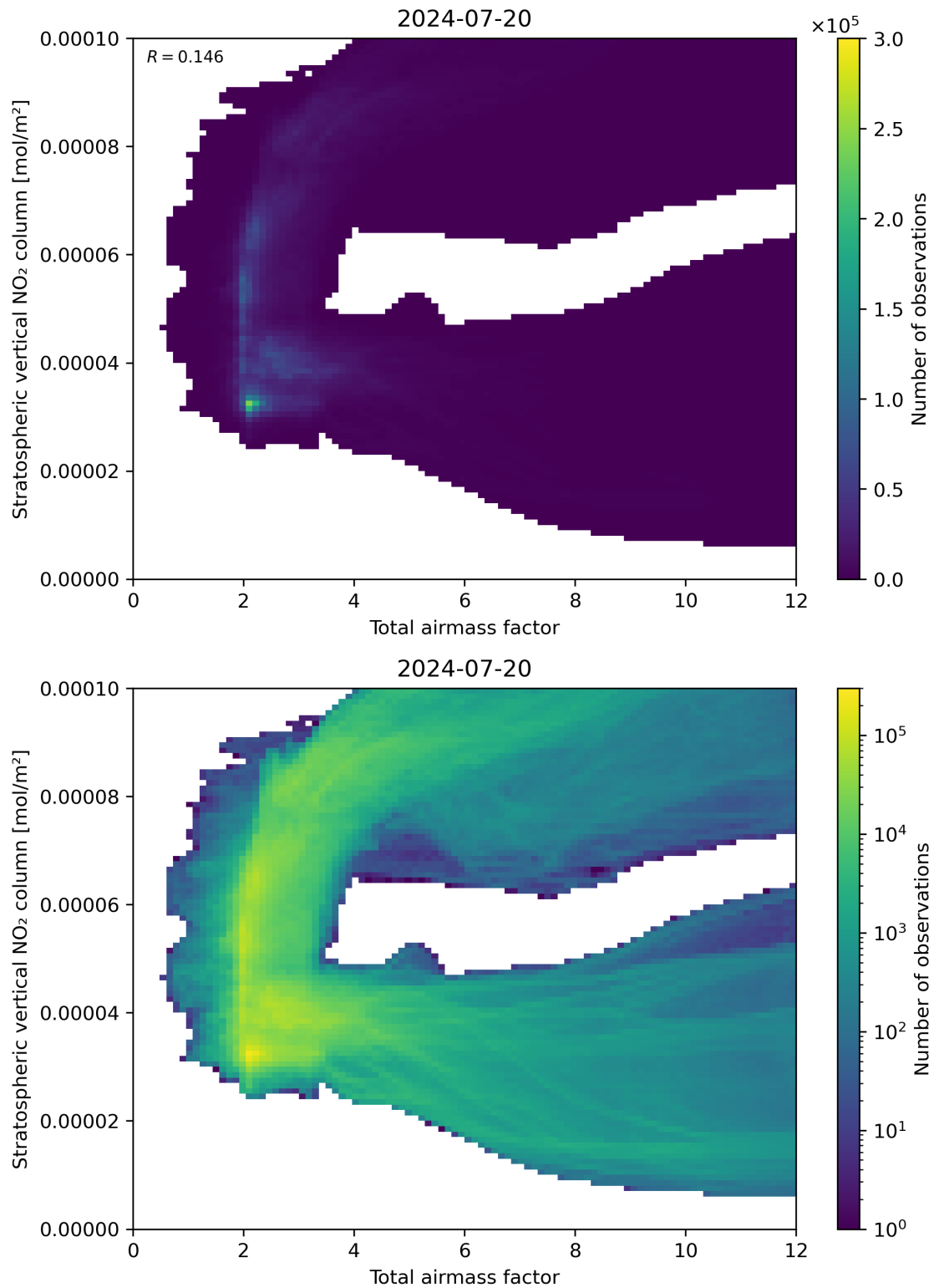
Figure 64: Scatter density plot of “Total airmass factor” against “Stratospheric vertical \text{NO}_2 column” for 2024-07-19 to 2024-07-21.
