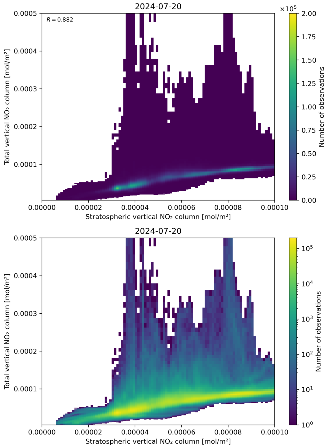
Figure 100: Scatter density plot of “Stratospheric vertical NO 2 column” against “Total vertical NO 2 column” for 2024-07-19 to 2024-07-21.
