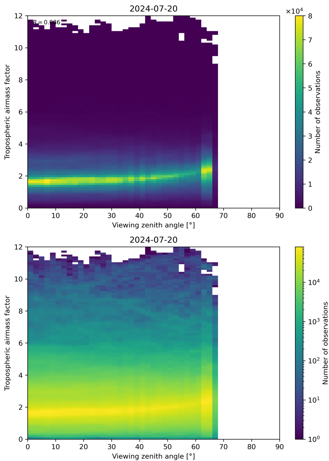
Figure 161: Scatter density plot of “Viewing zenith angle” against “Tropospheric airmass factor” for 2024-07-19 to 2024-07-21.
