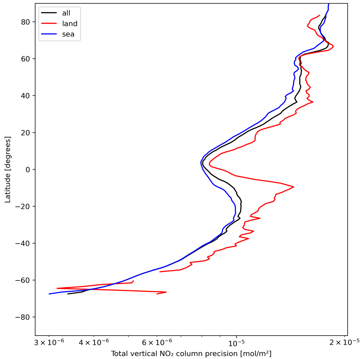
Figure 22: Zonal average of “Total vertical NO 2 column precision” for 2024-07-19 to 2024-07-21.
