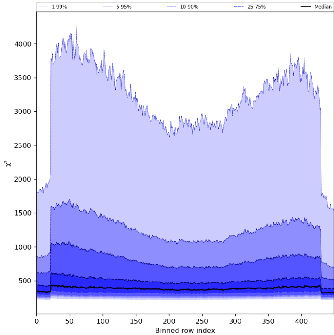
Figure 59: Along track statistics of “ \chi^2 ” for 2024-07-19 to 2024-07-21
