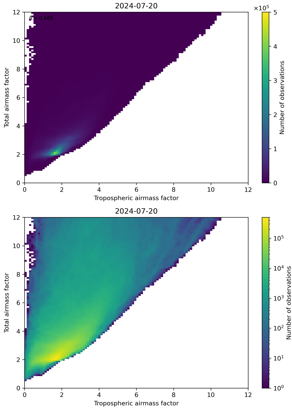
Figure 72: Scatter density plot of “Tropospheric airmass factor” against “Total airmass factor” for 2024-07-19 to 2024-07-21.
