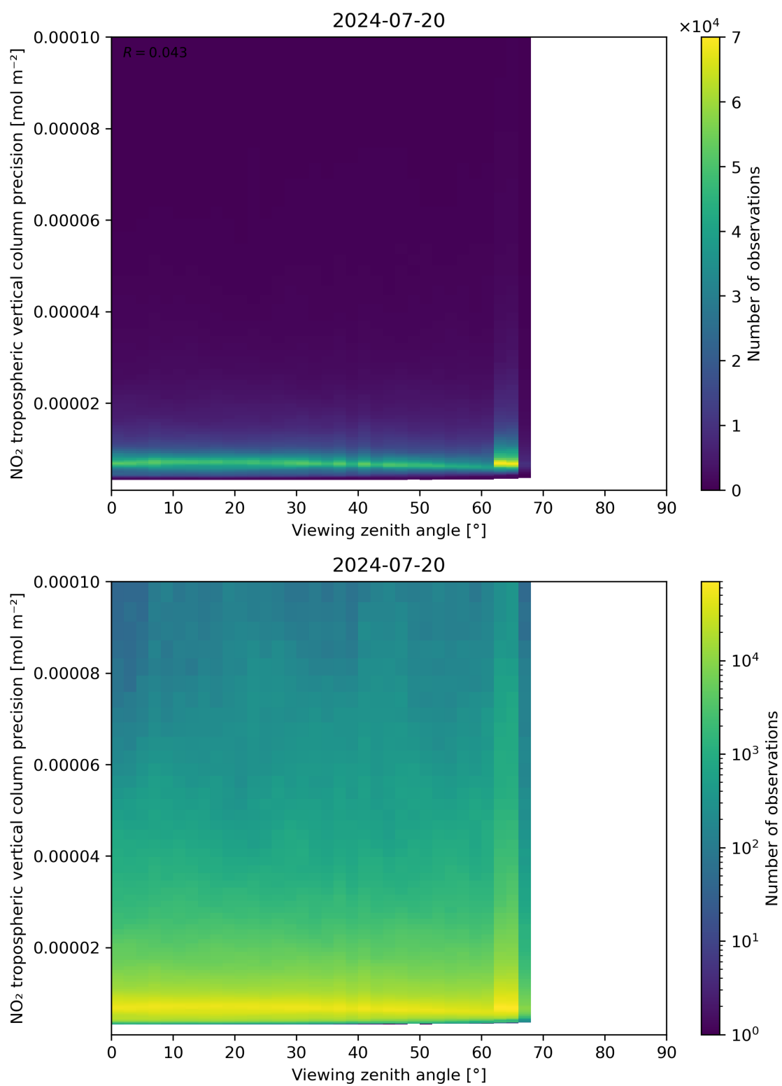
Figure 170: Scatter density plot of “Viewing zenith angle” against “NO 2 tropospheric vertical column precision” for 2024-07-19 to 2024-07-21.
