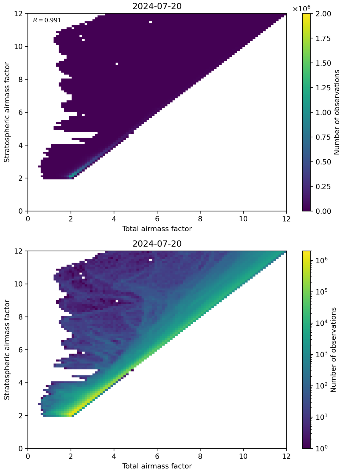
Figure 62: Scatter density plot of “Total airmass factor” against “Stratospheric airmass factor” for 2024-07-19 to 2024-07-21.
