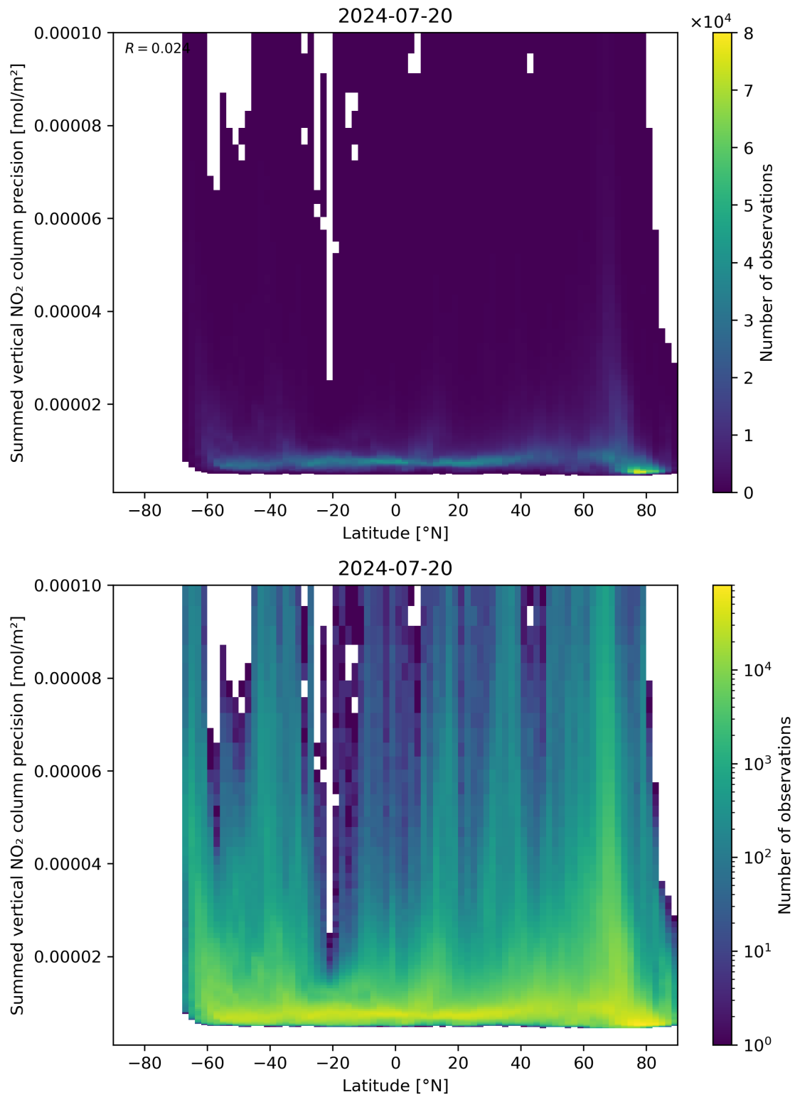
Figure 89: Scatter density plot of “Latitude” against “Summed vertical NO 2 column precision” for 2024-07-19 to 2024-07-21.
