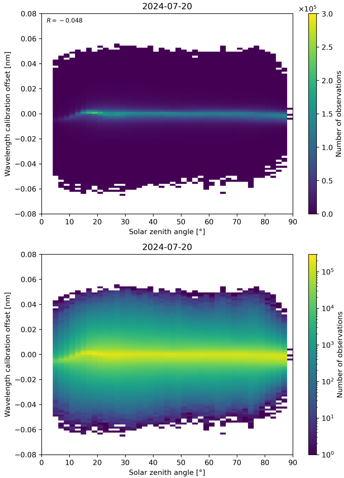
Figure 158: Scatter density plot of “Solar zenith angle” against “Wavelength calibration offset” for 2024-07-19 to 2024-07-21.
