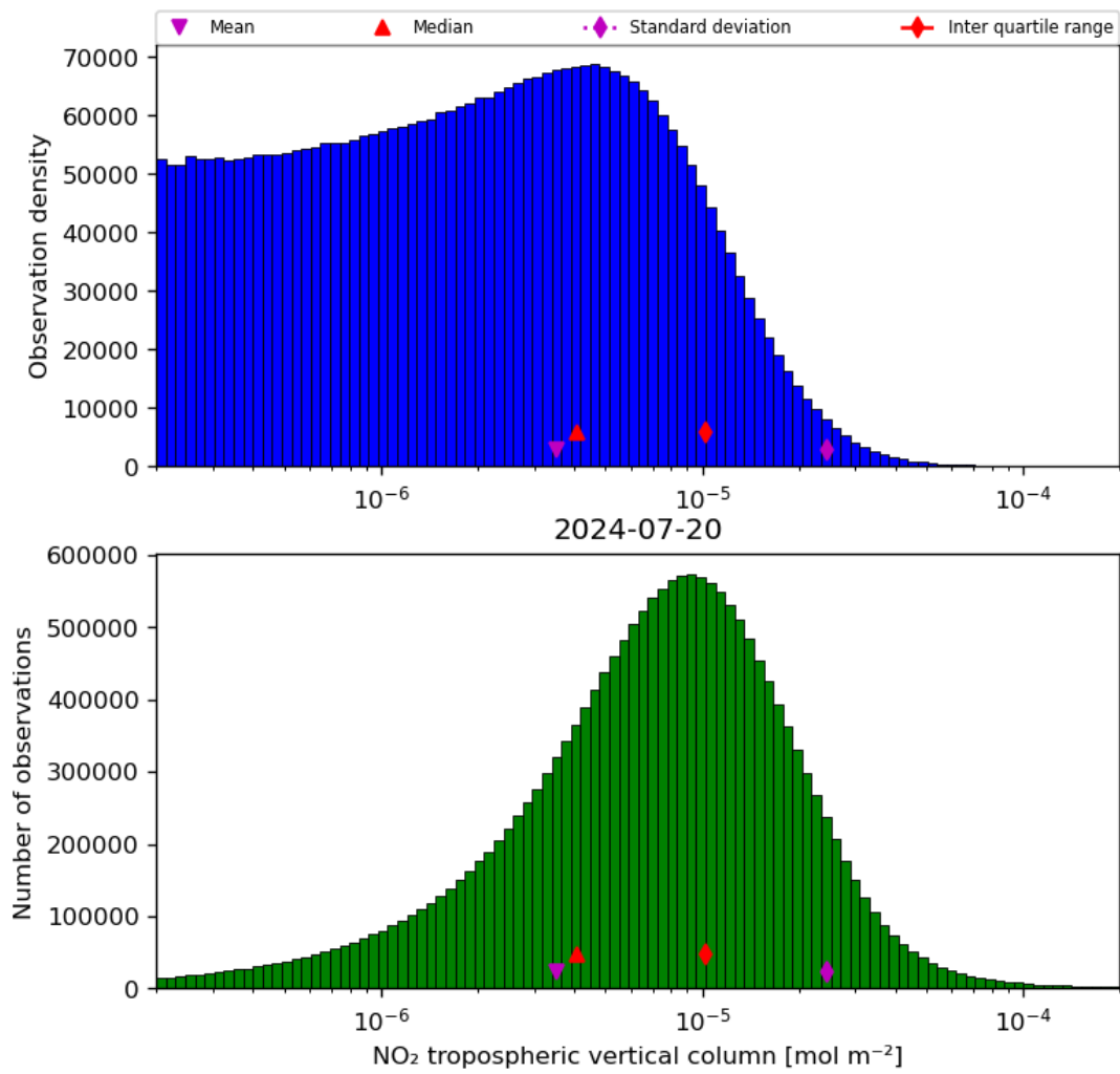
Figure 29: Histogram of “NO 2 tropospheric vertical column” for 2024-07-19 to 2024-07-21
