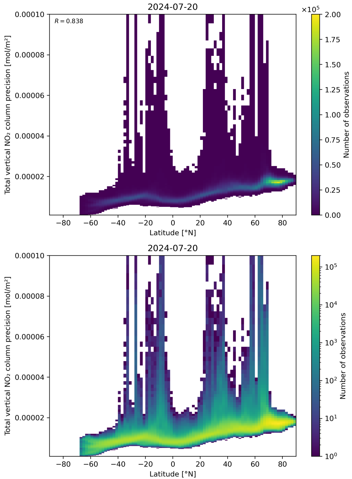
Figure 91: Scatter density plot of “Latitude” against “Total vertical NO 2 column precision” for 2024-07-19 to 2024-07-21.
