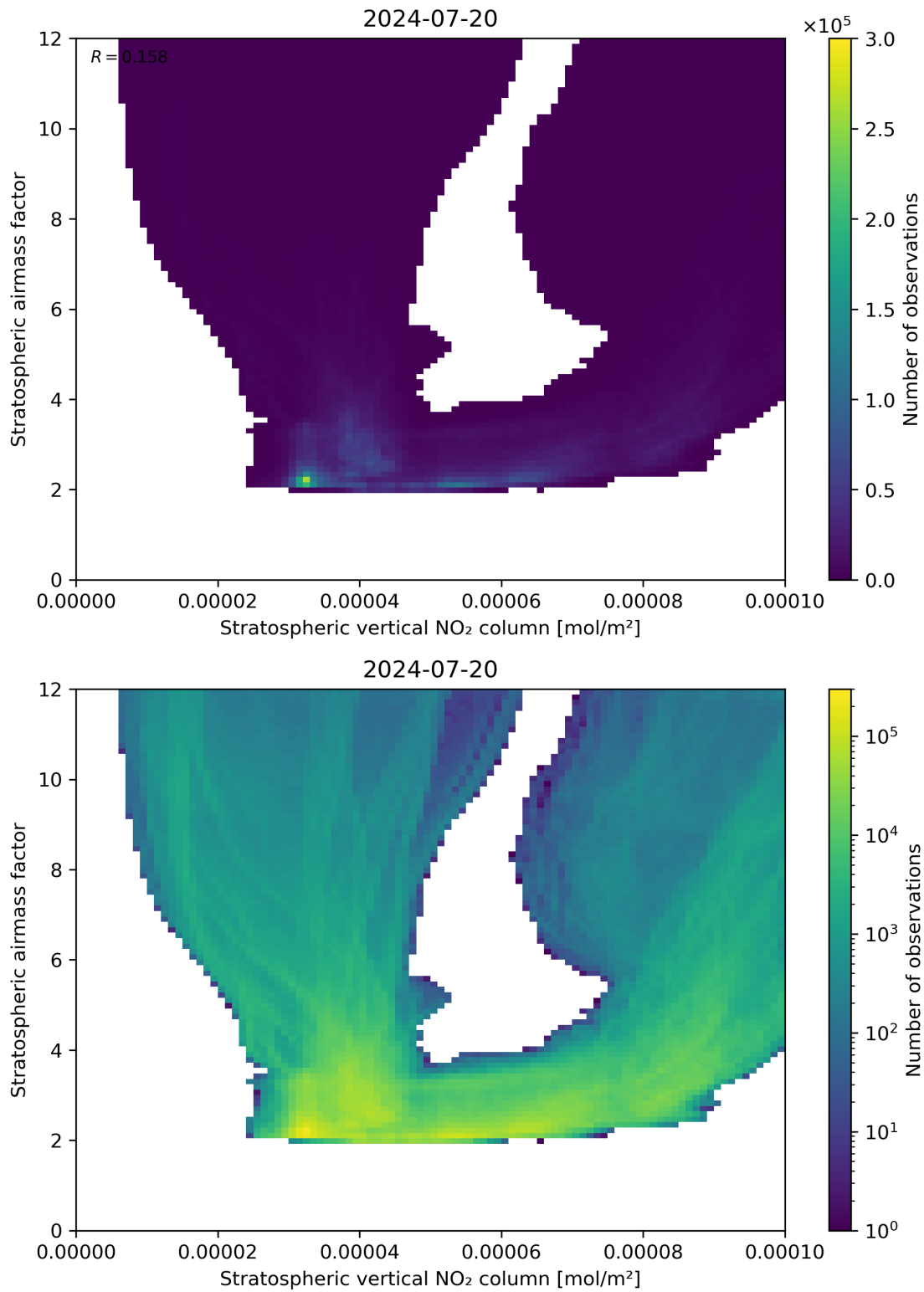
Figure 96: Scatter density plot of “Stratospheric vertical NO 2 column” against “Stratospheric airmass factor” for 2024-07-19 to 2024-07-21.
