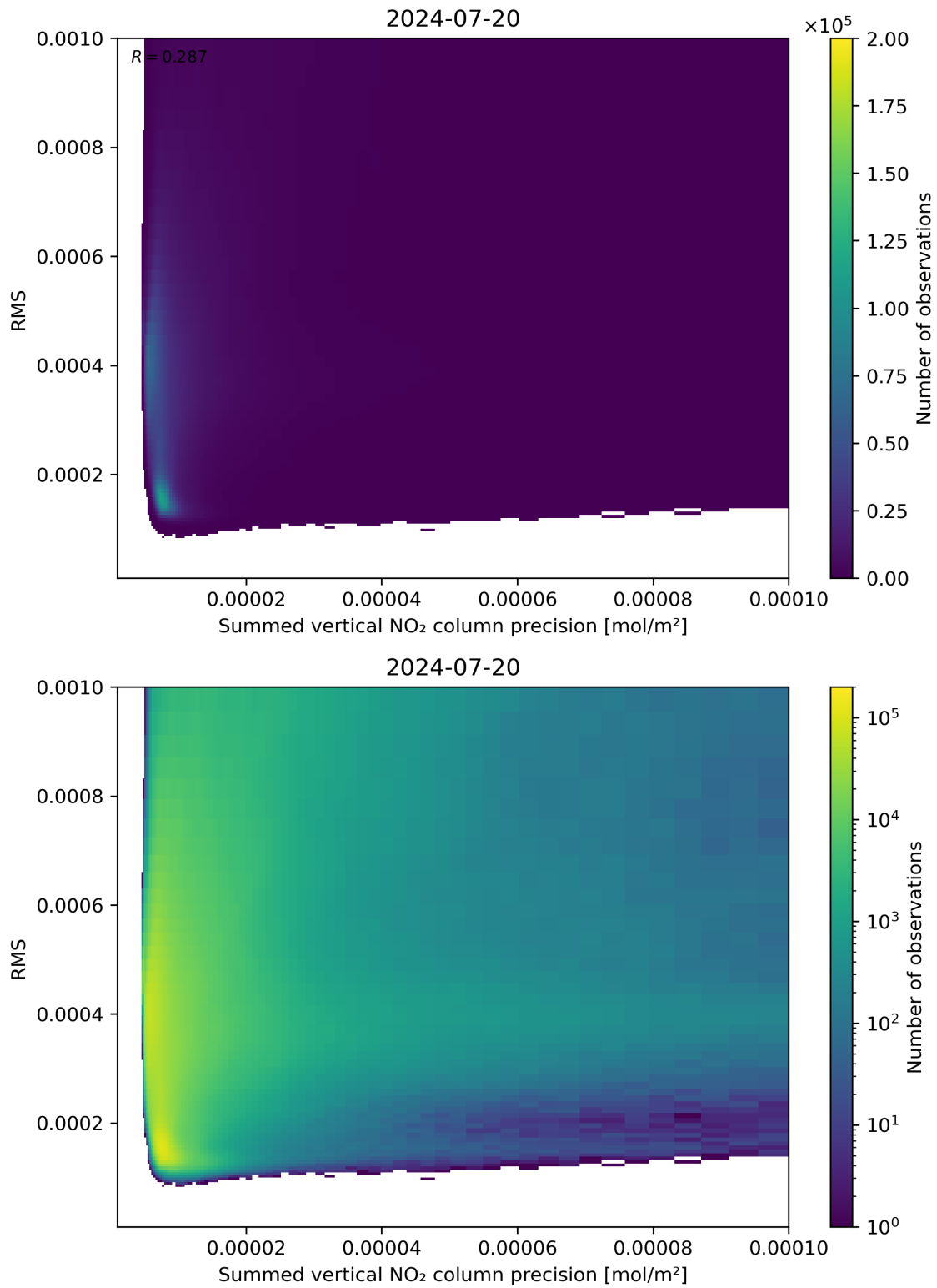
Figure 108: Scatter density plot of “Summed vertical NO 2 column precision” against “RMS” for 2024-07-19 to 2024-07-21.
