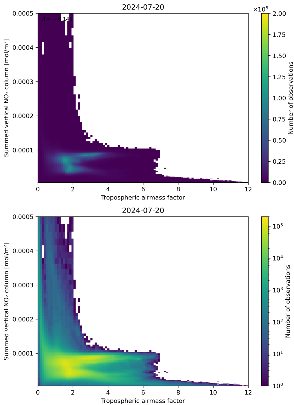
Figure 75: Scatter density plot of “Tropospheric airmass factor” against “Summed vertical NO 2 column” for 2024-07-19 to 2024-07-21.
