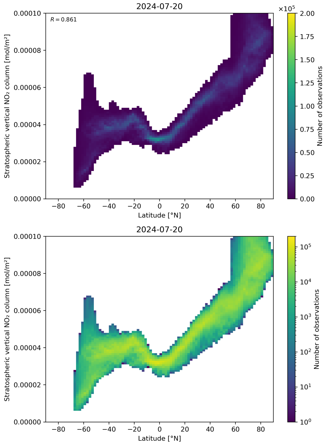
Figure 87: Scatter density plot of “Latitude” against “Stratospheric vertical NO 2 column” for 2024-07-19 to 2024-07-21.
