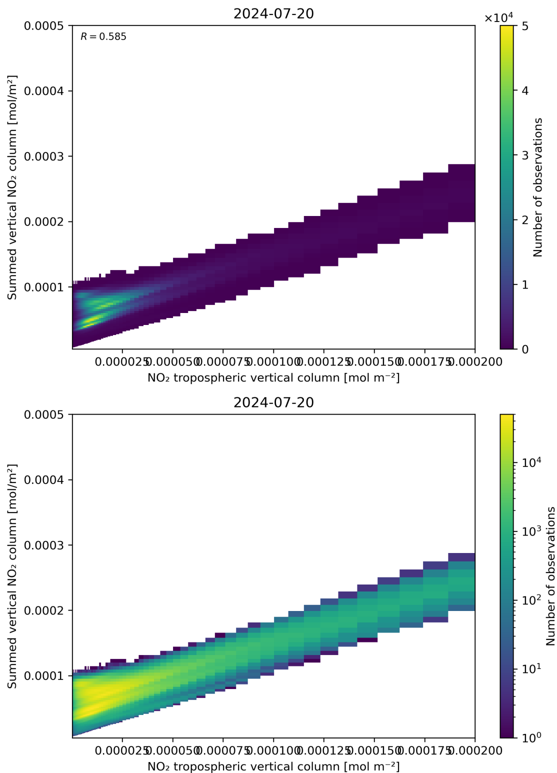
Figure 126: Scatter density plot of “NO 2 tropospheric vertical column” against “Summed vertical NO 2 column” for 2024-07-19 to 2024-07-21.
