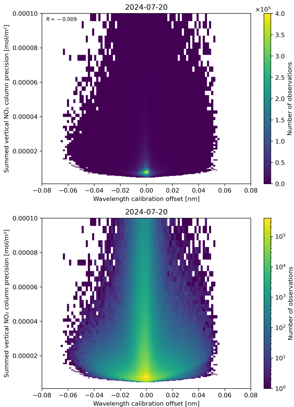
Figure 178: Scatter density plot of “Wavelength calibration offset” against “Summed vertical NO 2 column precision” for 2024-07-19 to 2024-07-21.
