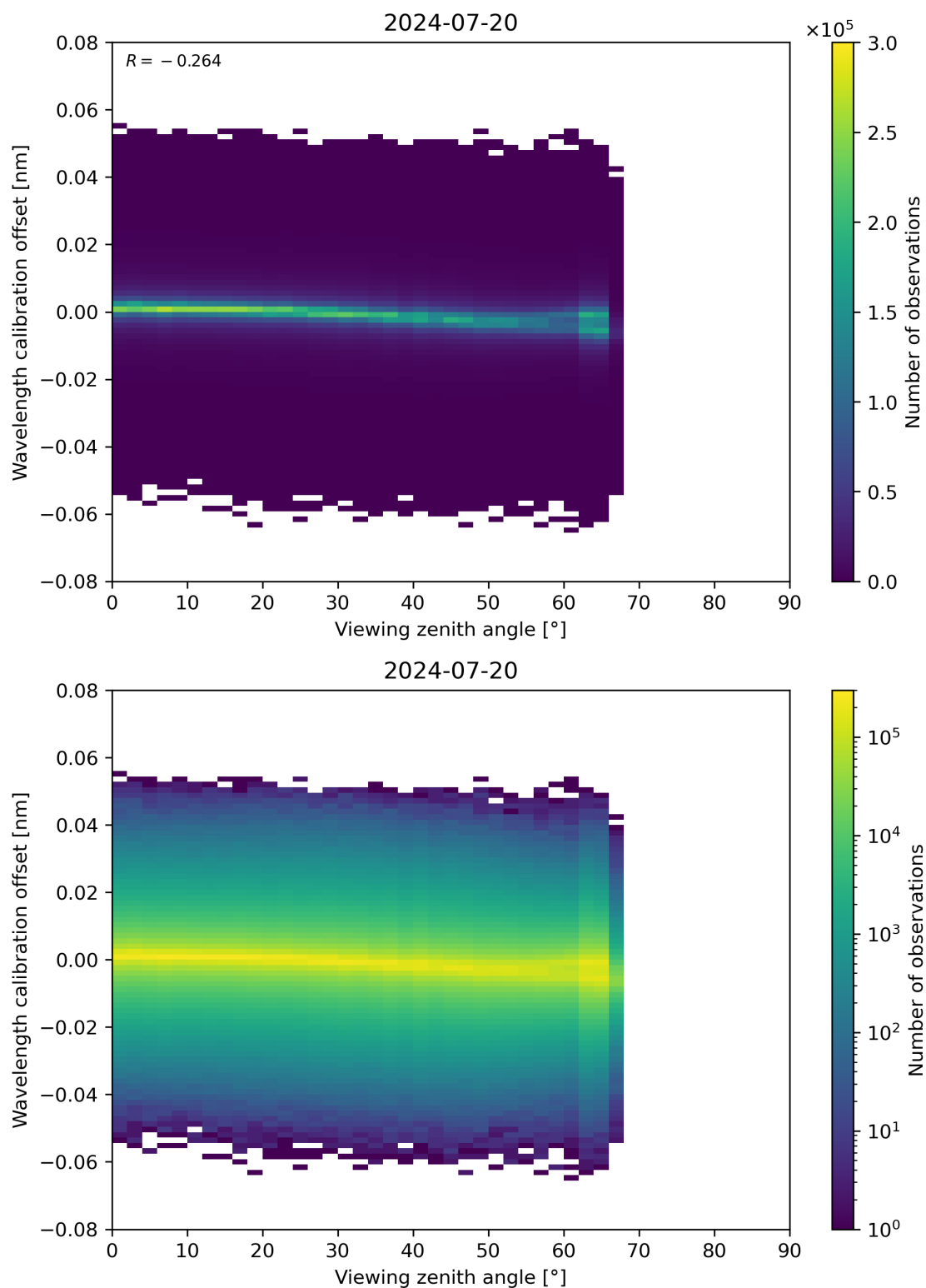
Figure 173: Scatter density plot of “Viewing zenith angle” against “Wavelength calibration offset” for 2024-07-19 to 2024-07-21.
