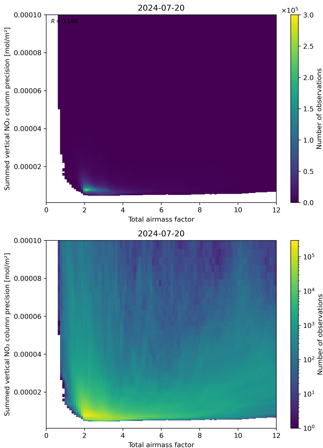
Figure 66: Scatter density plot of “Total airmass factor” against “Summed vertical NO 2 column precision” for 2024-07-19 to 2024-07-21.
