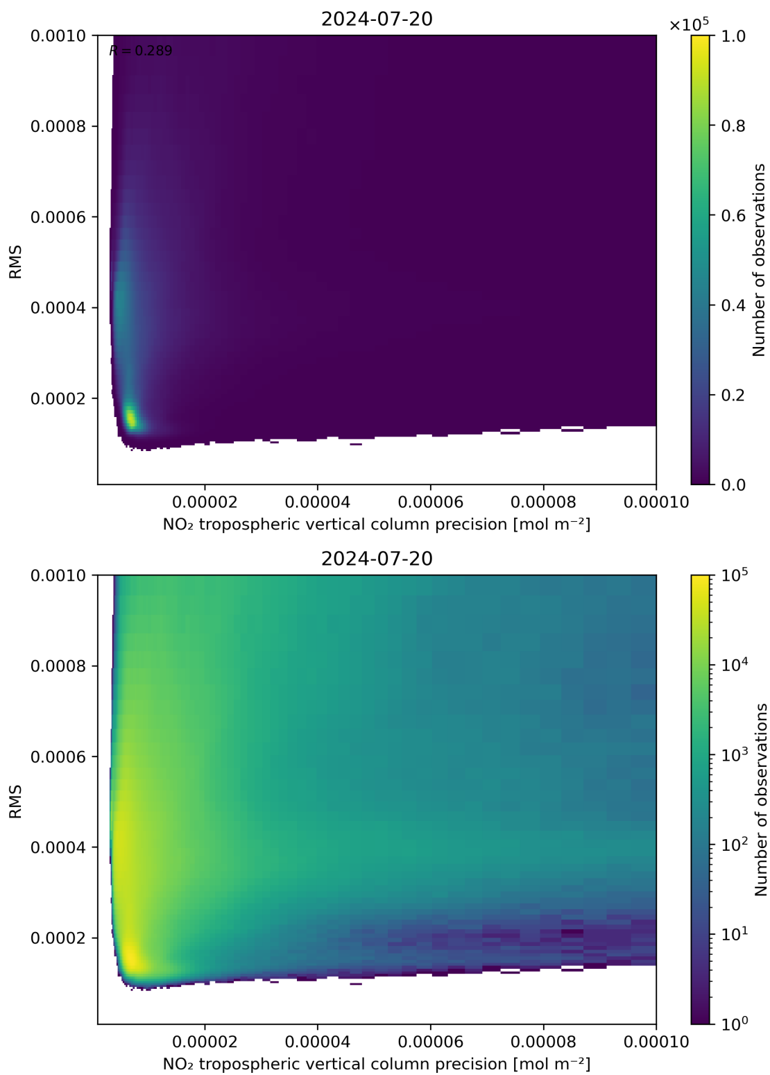
Figure 140: Scatter density plot of “NO 2 tropospheric vertical column precision” against “RMS” for 2024-07-19 to 2024-07-21.
