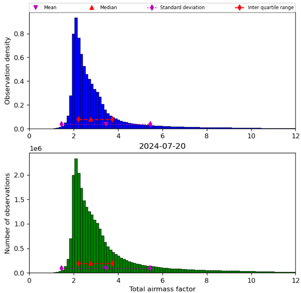
Figure 32: Histogram of “Total airmass factor” for 2024-07-19 to 2024-07-21
