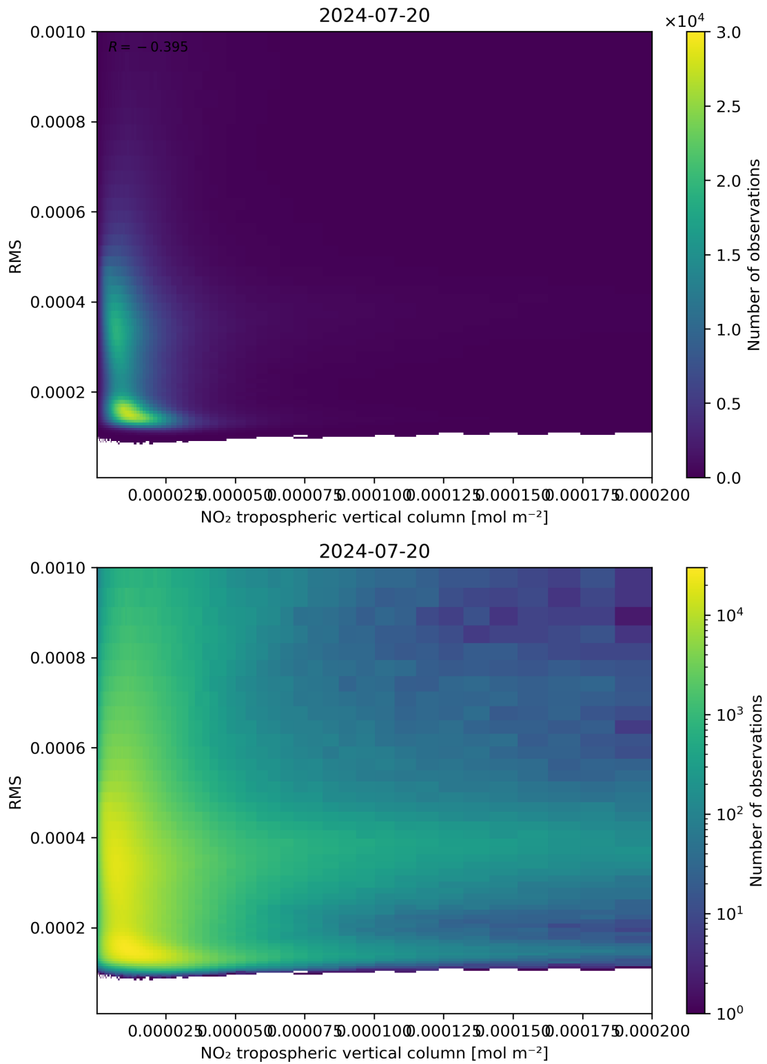
Figure 142: Scatter density plot of “NO 2 tropospheric vertical column” against “RMS” for 2024-07-19 to 2024-07-21.
