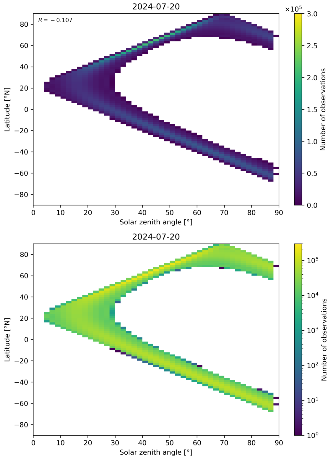
Figure 149: Scatter density plot of “Solar zenith angle” against “Latitude” for 2024-07-19 to 2024-07-21.
