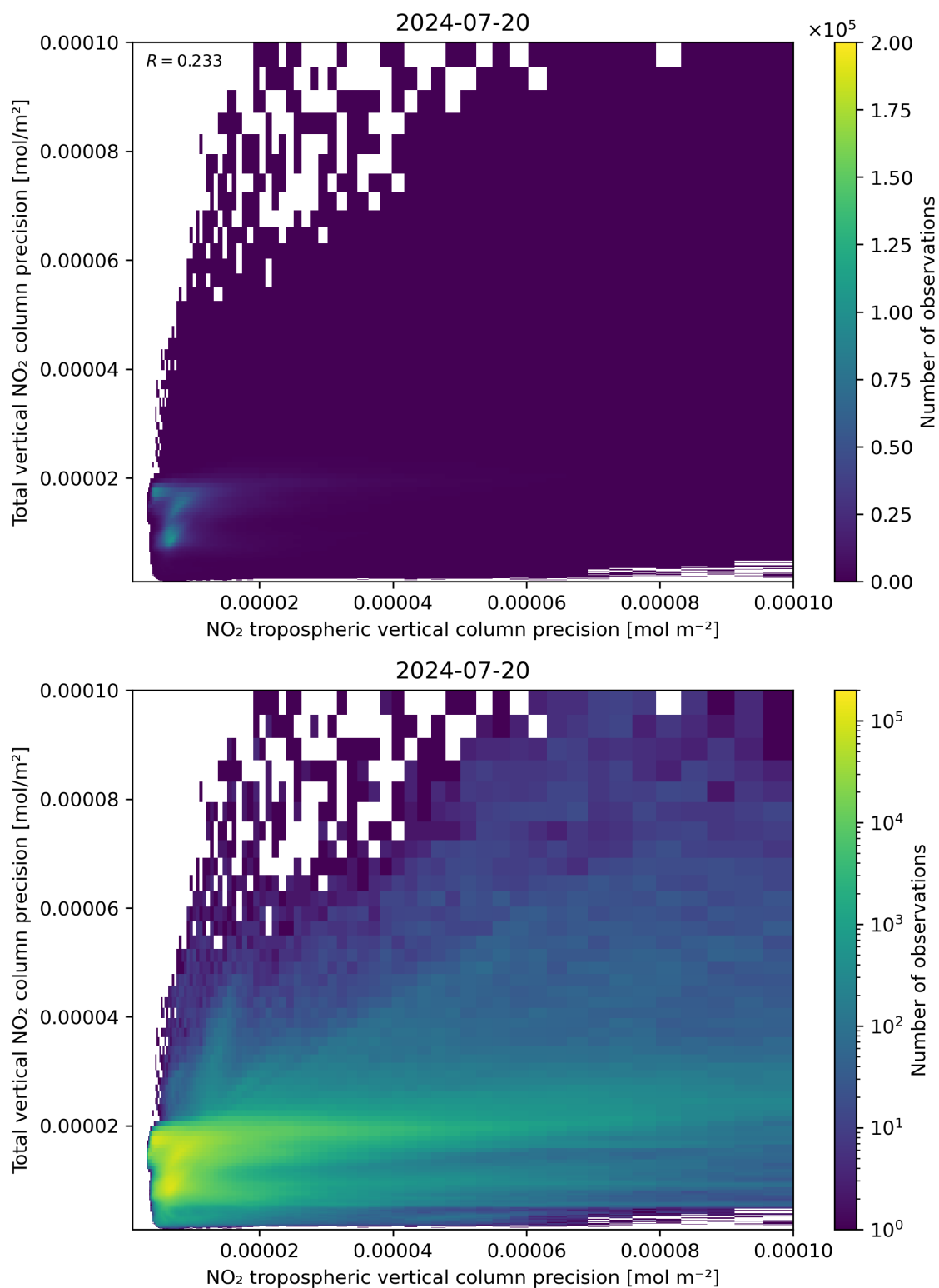
Figure 139: Scatter density plot of “NO 2 tropospheric vertical column precision” against “Total vertical NO 2 column precision” for 2024-07-19 to 2024-07-21.
