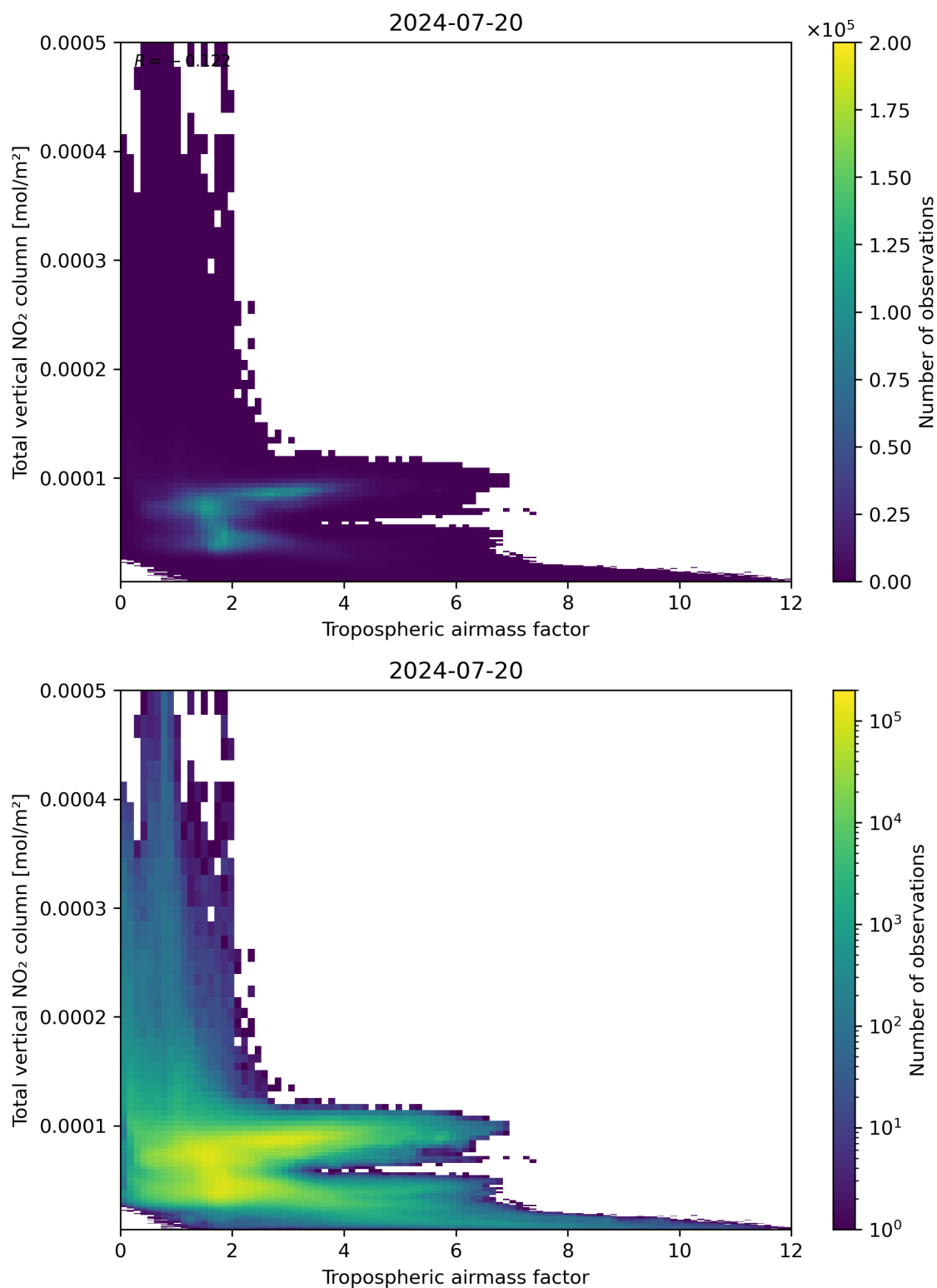
Figure 77: Scatter density plot of “Tropospheric airmass factor” against “Total vertical NO 2 column” for 2024-07-19 to 2024-07-21.
