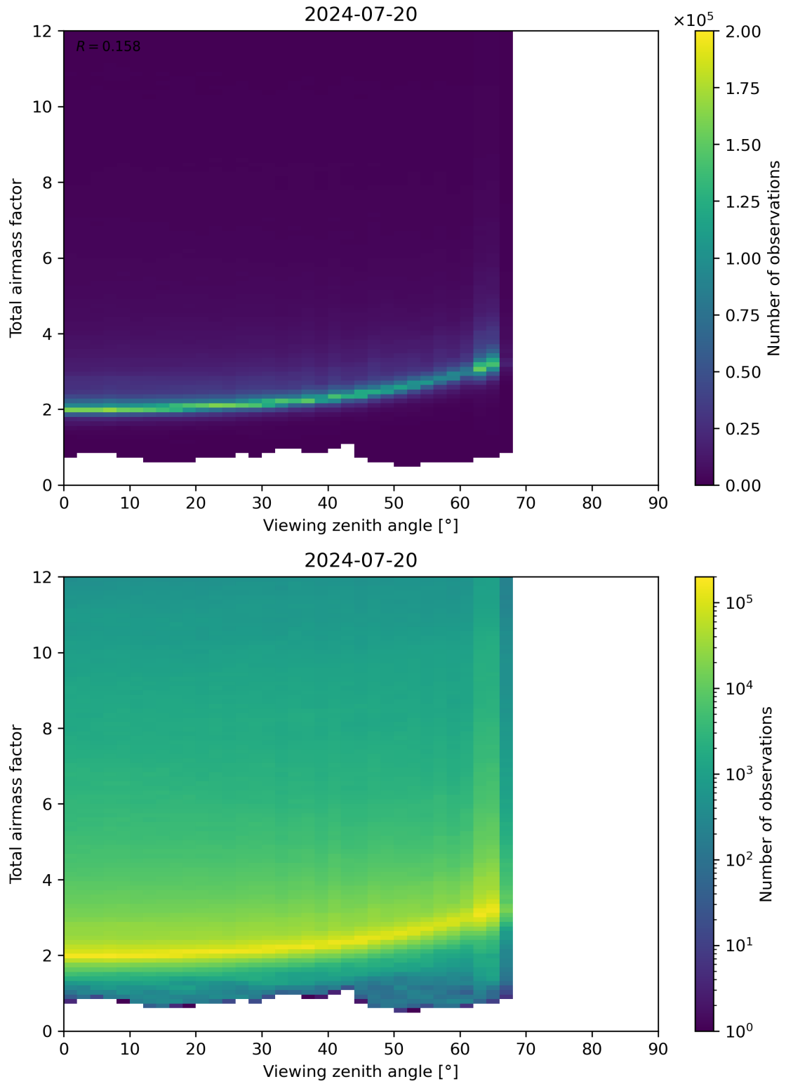
Figure 160: Scatter density plot of “Viewing zenith angle” against “Total airmass factor” for 2024-07-19 to 2024-07-21.
