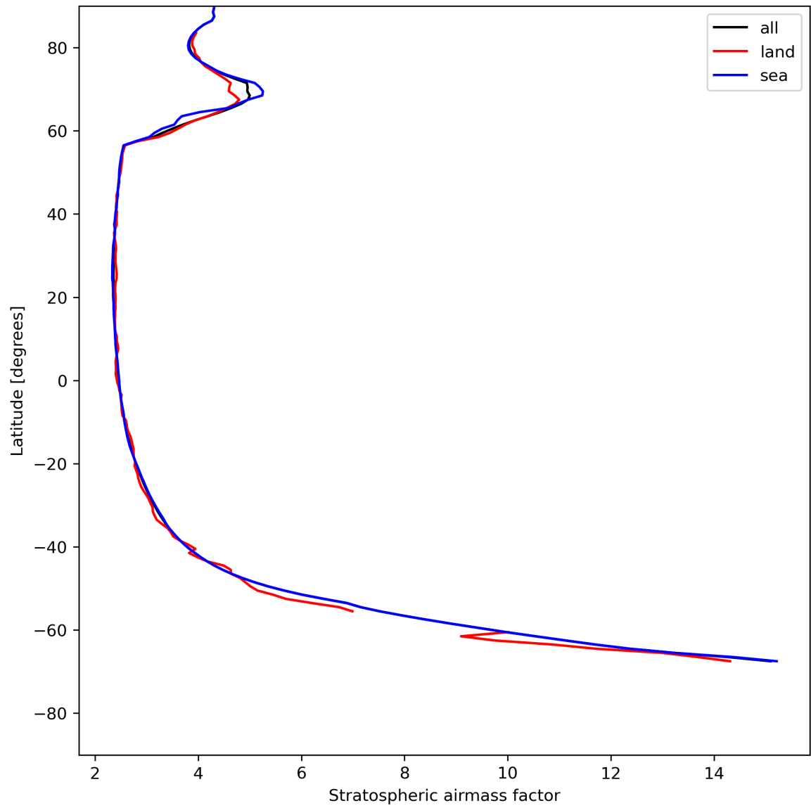
Figure 27: Zonal average of “Stratospheric air mass factor” for 2024-07-19 to 2024-07-21.
