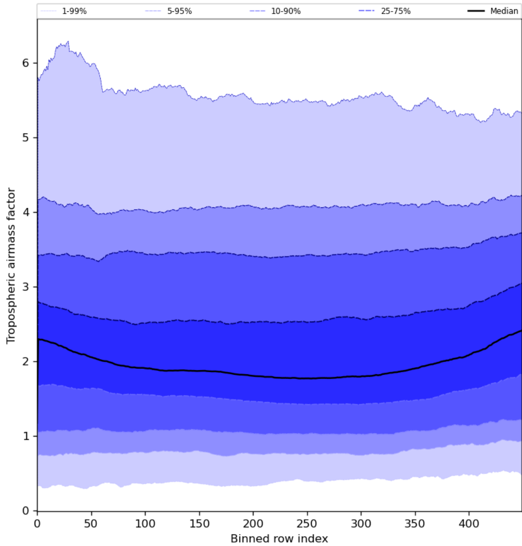
Figure 48: Along track statistics of “Tropospheric airmass factor” for 2024-07-19 to 2024-07-21
