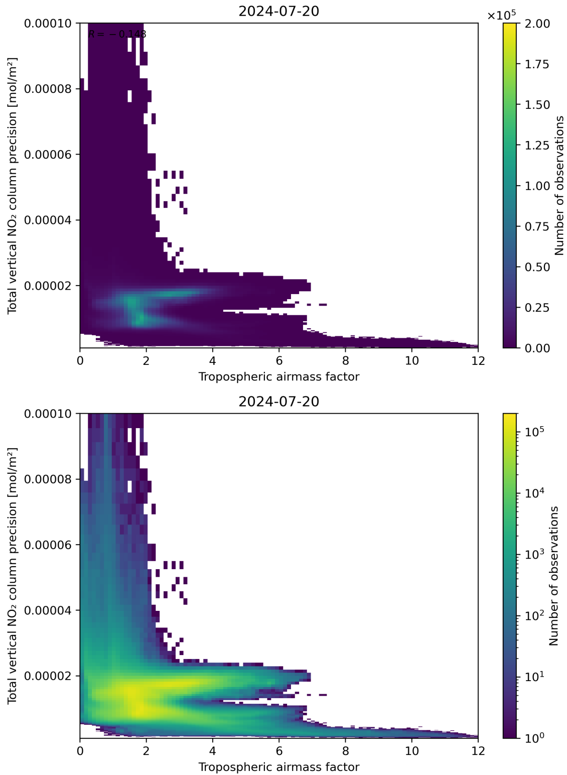
Figure 78: Scatter density plot of “Tropospheric air mass factor” against “Total vertical NO 2 column precision” for 2024-07-19 to 2024-07-21.
