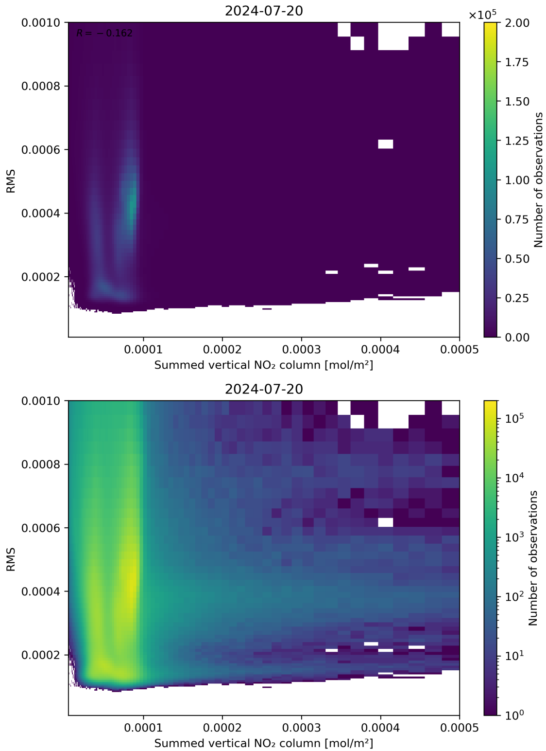
Figure 109: Scatter density plot of “Summed vertical NO 2 column” against “RMS” for 2024-07-19 to 2024-07-21.
