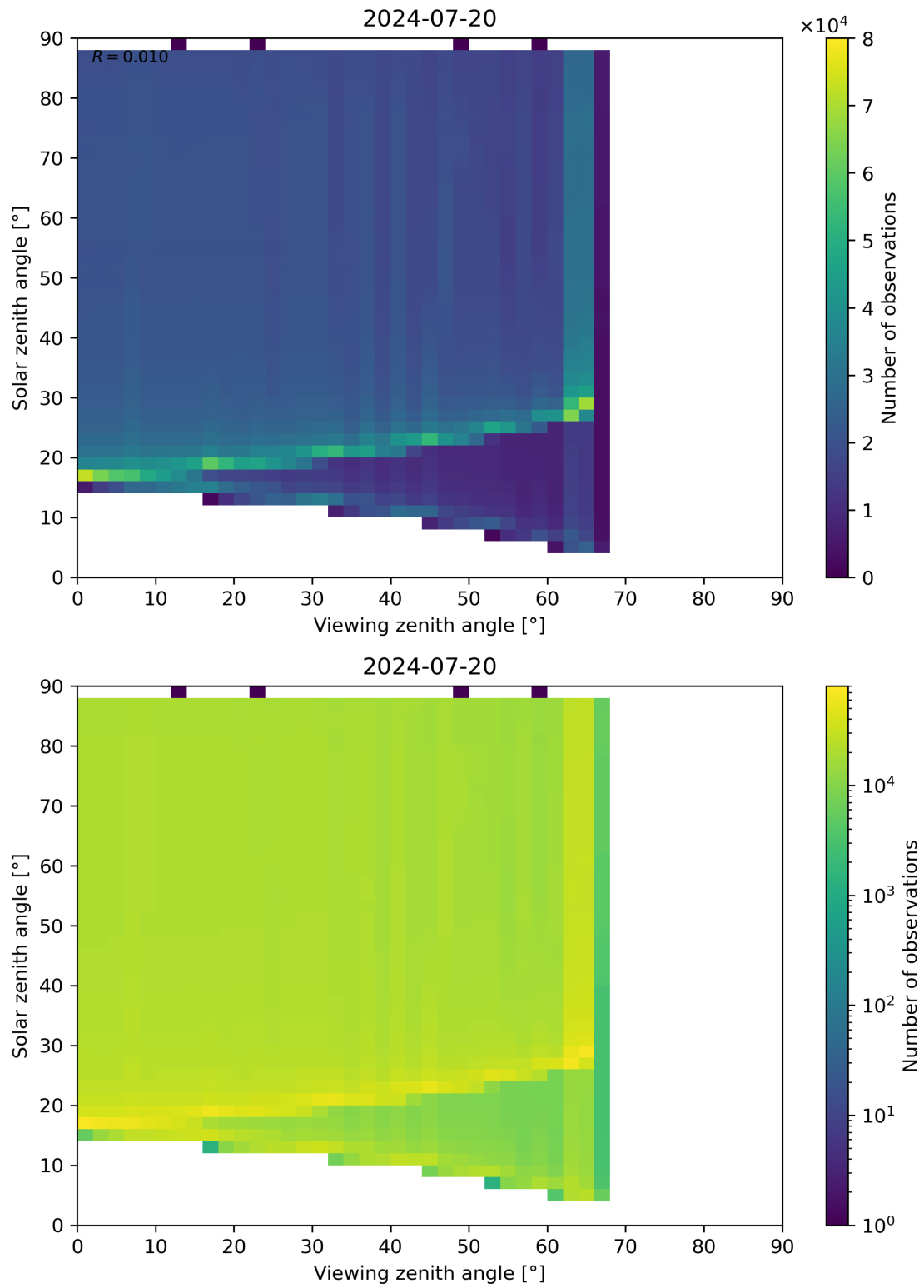
Figure 172: Scatter density plot of “Viewing zenith angle” against “Solar zenith angle” for 2024-07-19 to 2024-07-21.
