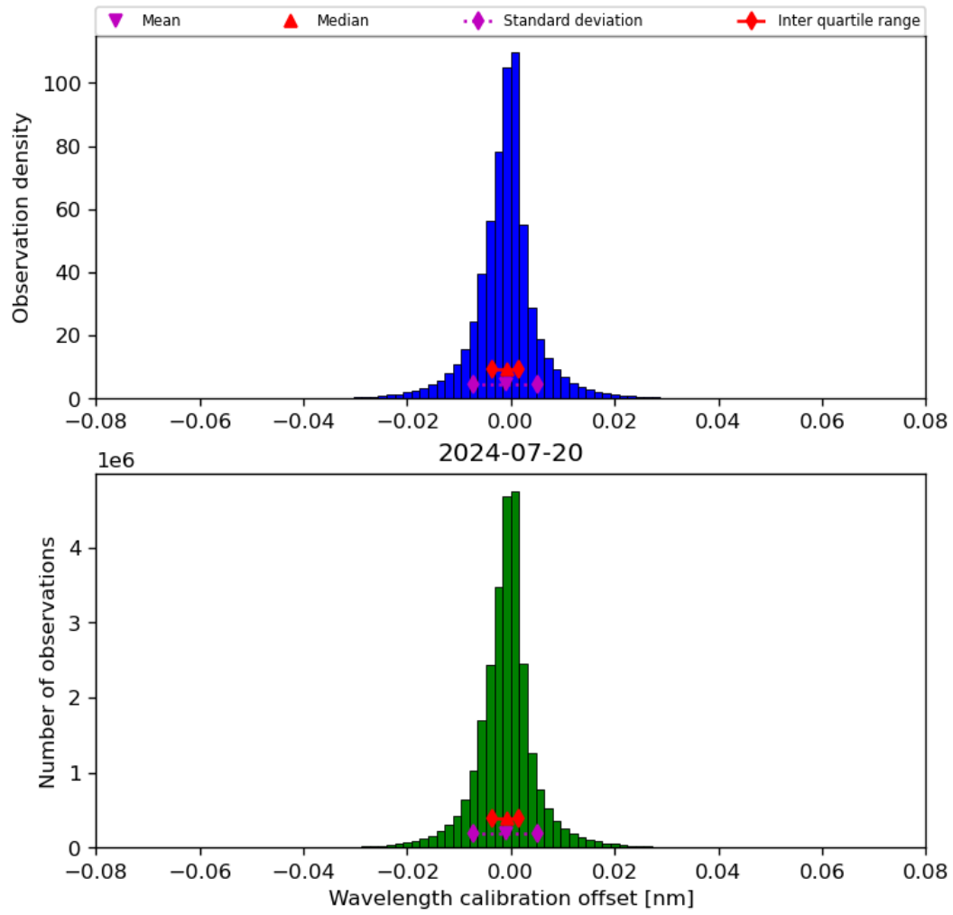
Figure 35: Histogram of “Wavelength calibration offset” for 2024-07-19 to 2024-07-21
