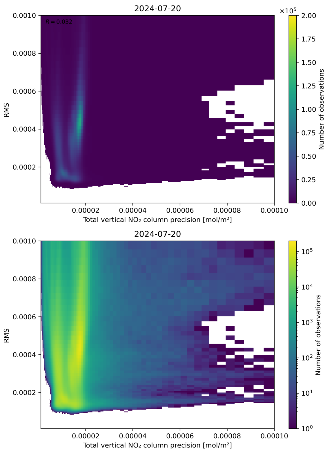
Figure 119: Scatter density plot of “Total vertical NO 2 column precision” against “RMS” for 2024-07-19 to 2024-07-21.
