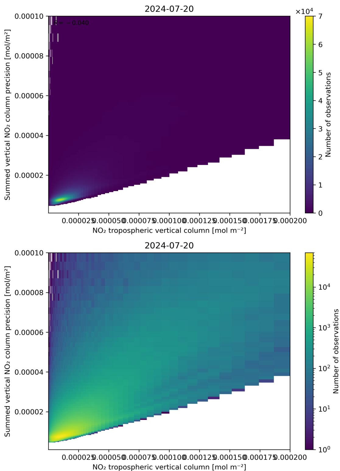
Figure 127: Scatter density plot of “NO 2 tropospheric vertical column” against “Summed vertical NO 2 column precision” for 2024-07-19 to 2024-07-21.
