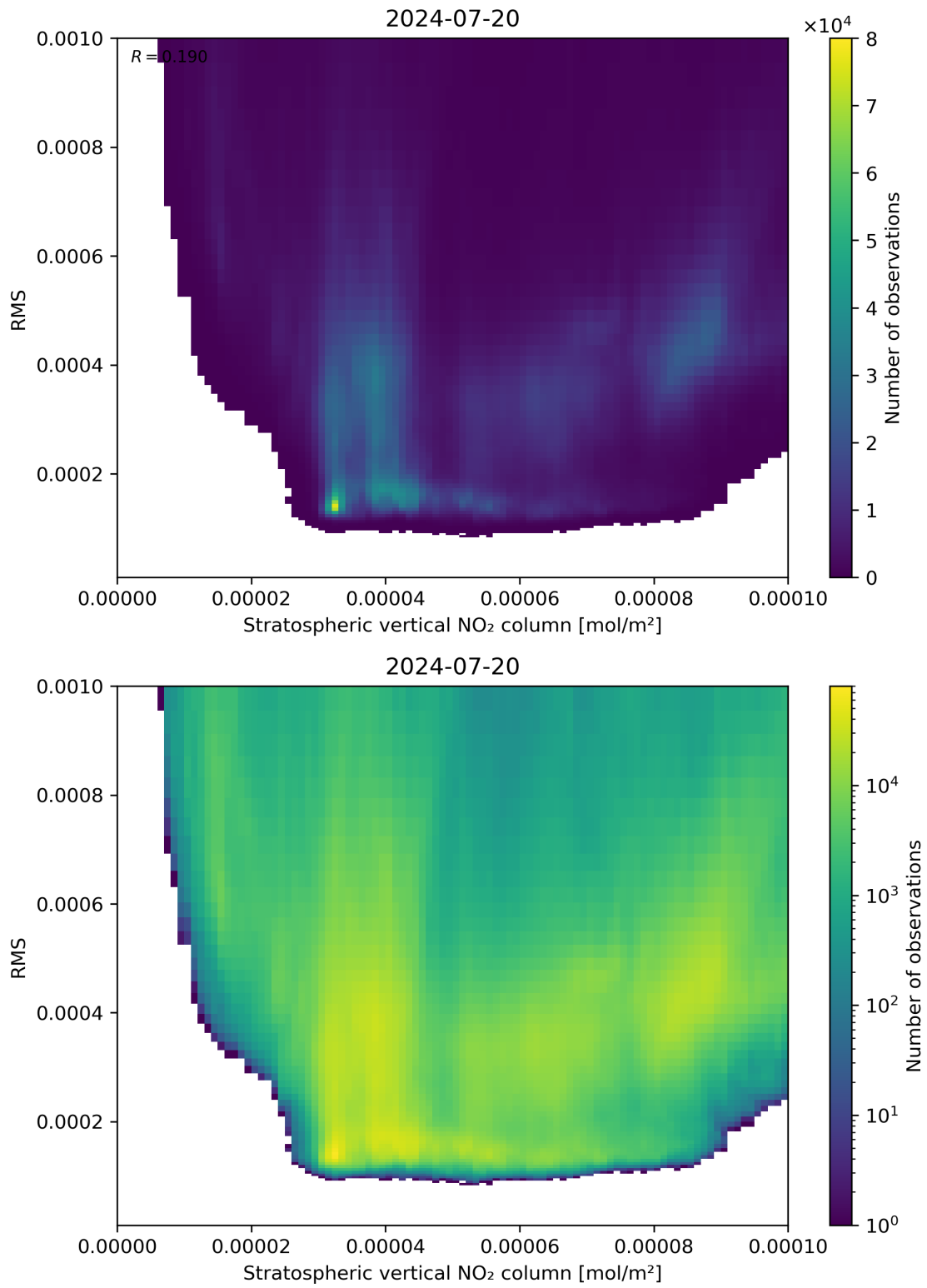
Figure 102: Scatter density plot of “Stratospheric vertical NO 2 column” against “RMS” for 2024-07-19 to 2024-07-21.
