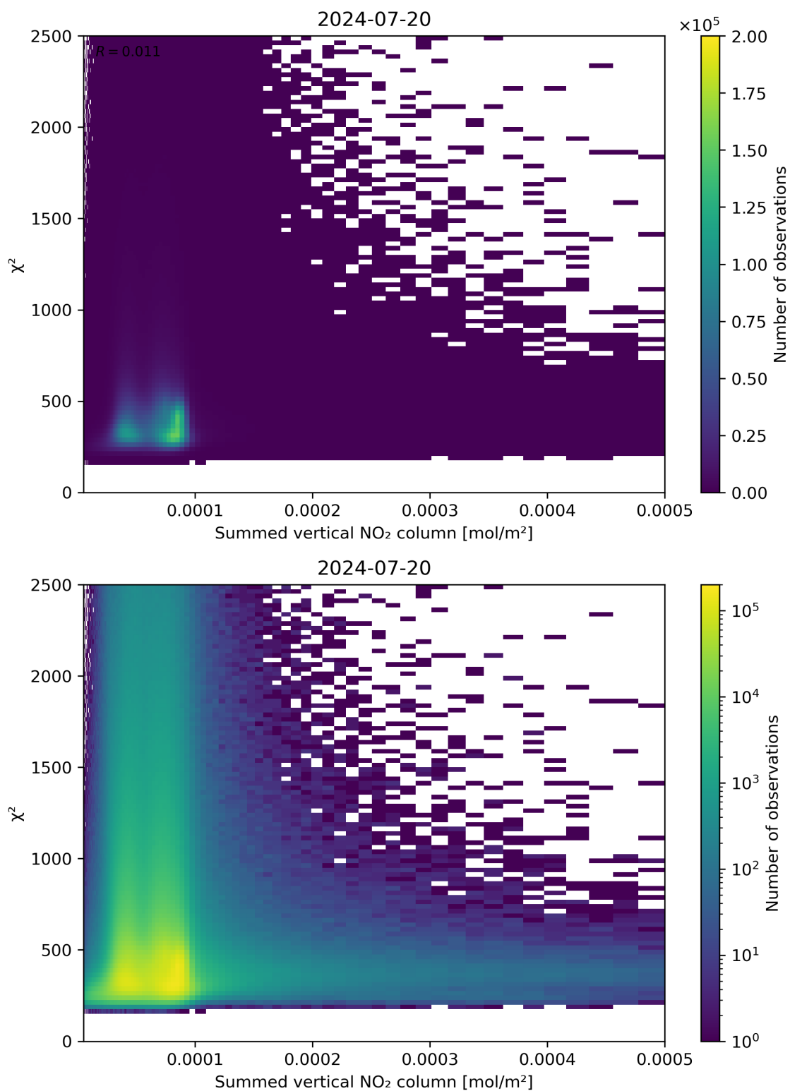
Figure 104: Scatter density plot of “Summed vertical NO 2 column” against “ \chi^2 ” for 2024-07-19 to 2024-07-21.
