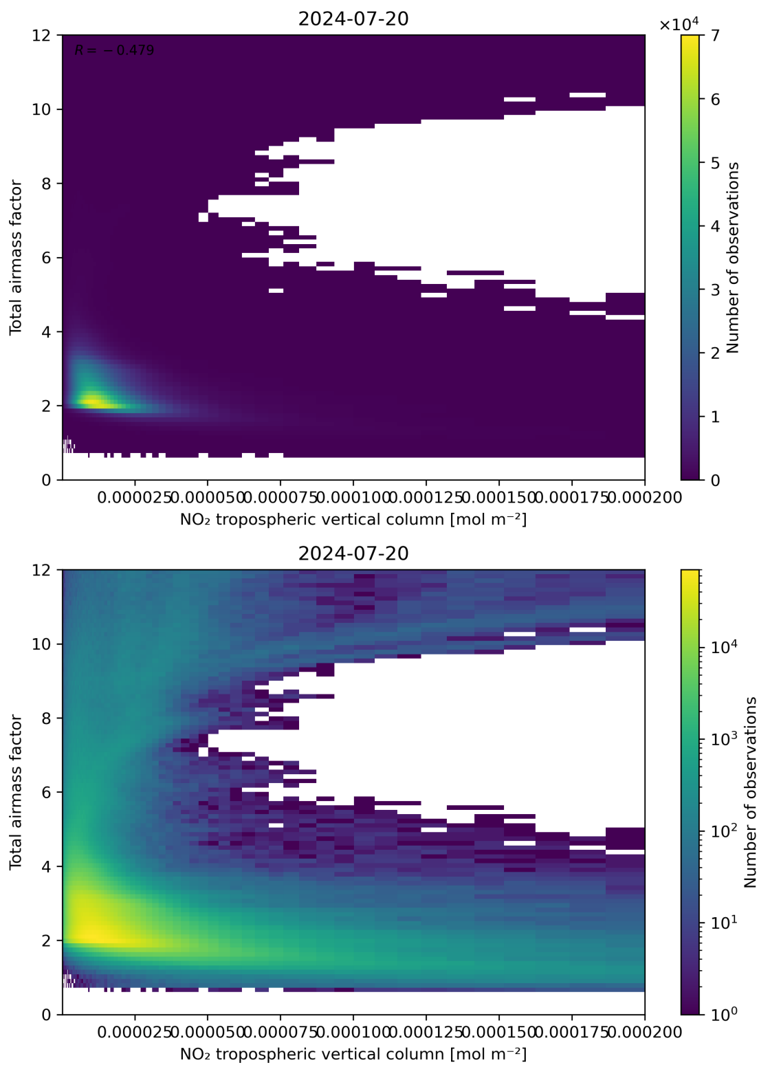
Figure 122: Scatter density plot of “NO 2 tropospheric vertical column” against “Total air mass factor” for 2024-07-19 to 2024-07-21.
