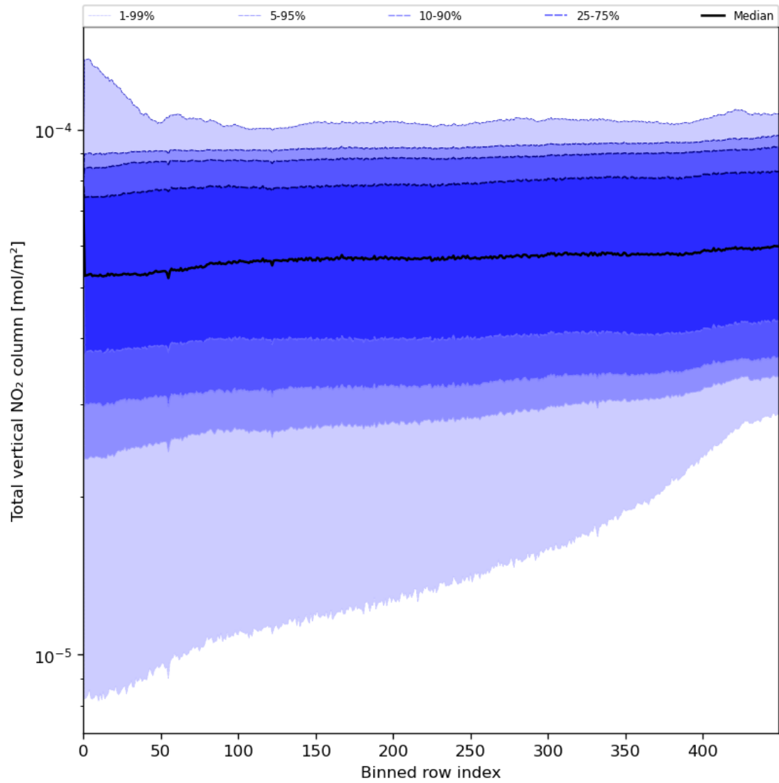
Figure 55: Along track statistics of “Total vertical NO 2 column” for 2024-07-19 to 2024-07-21
