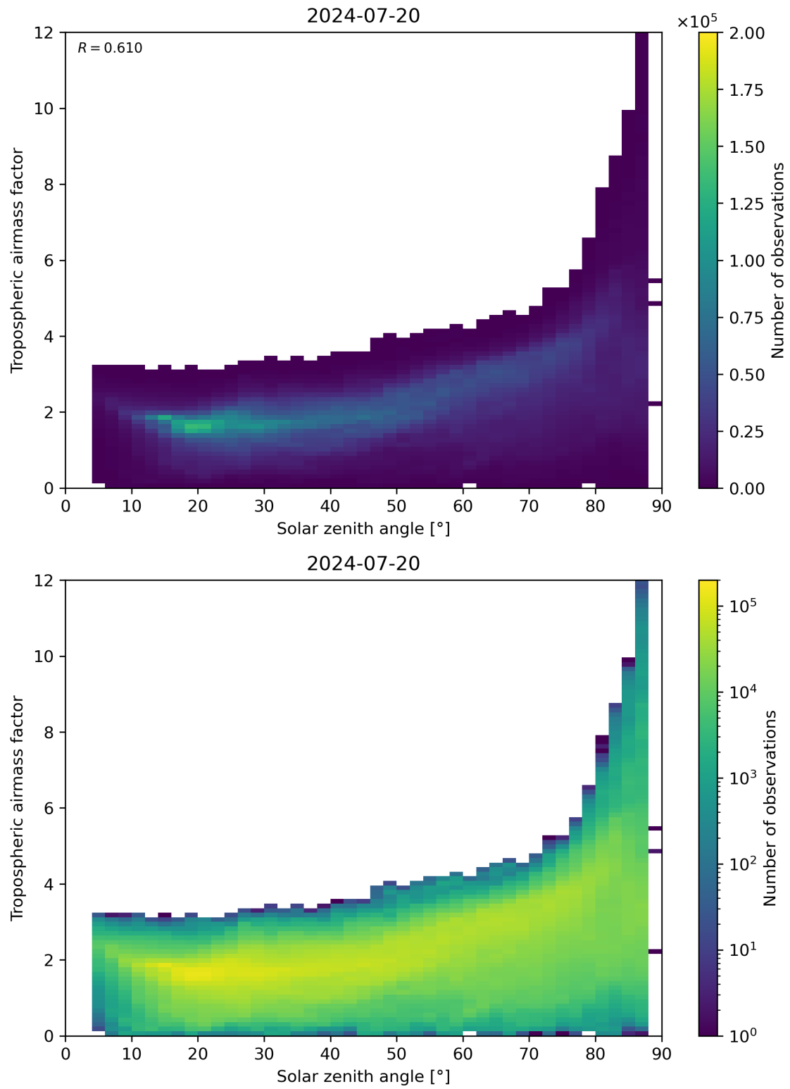
Figure 147: Scatter density plot of “Solar zenith angle” against “Tropospheric airmass factor” for 2024-07-19 to 2024-07-21.
