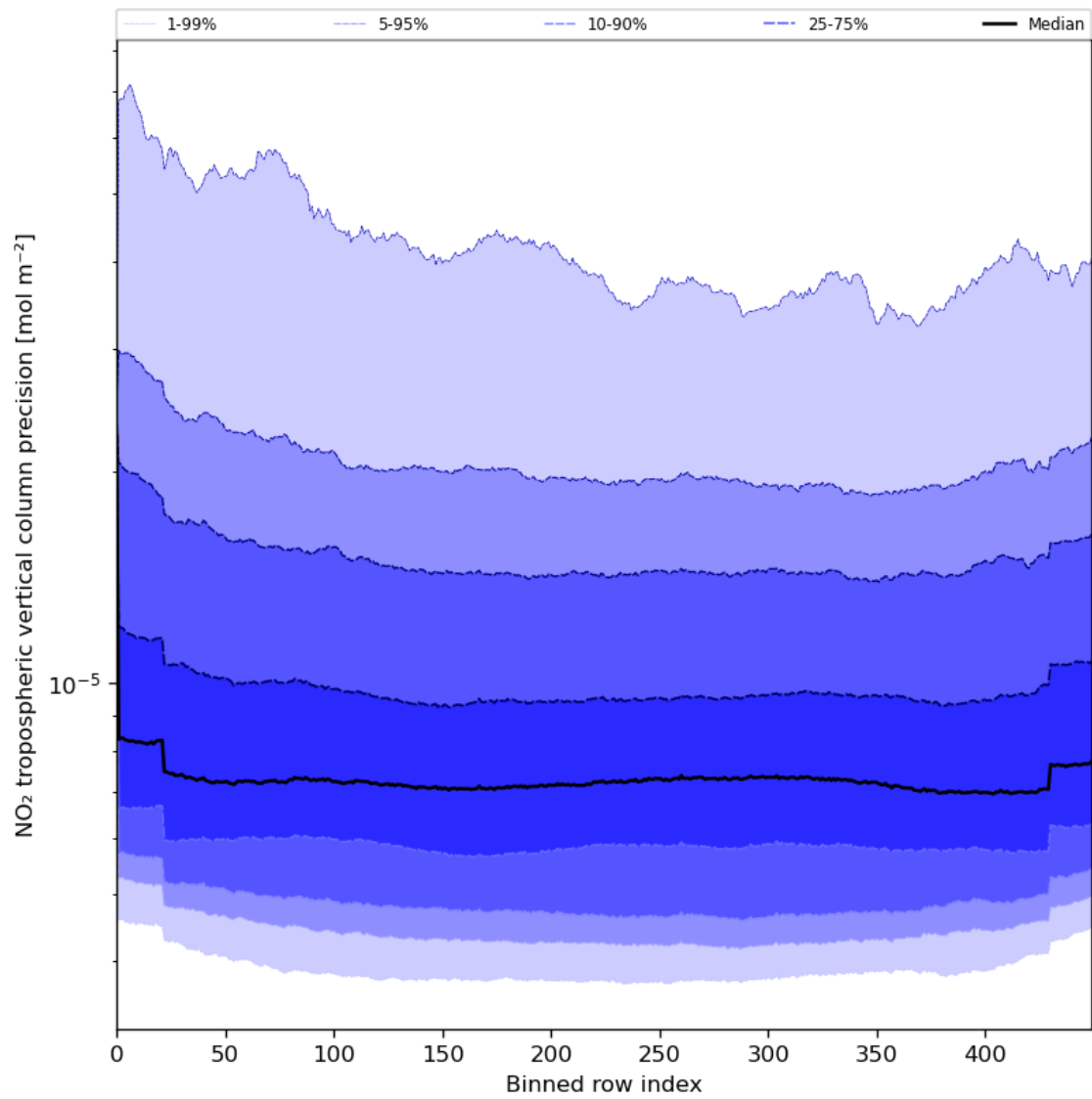
Figure 47: Along track statistics of “NO 2 tropospheric vertical column precision” for 2024-07-19 to 2024-07-21
