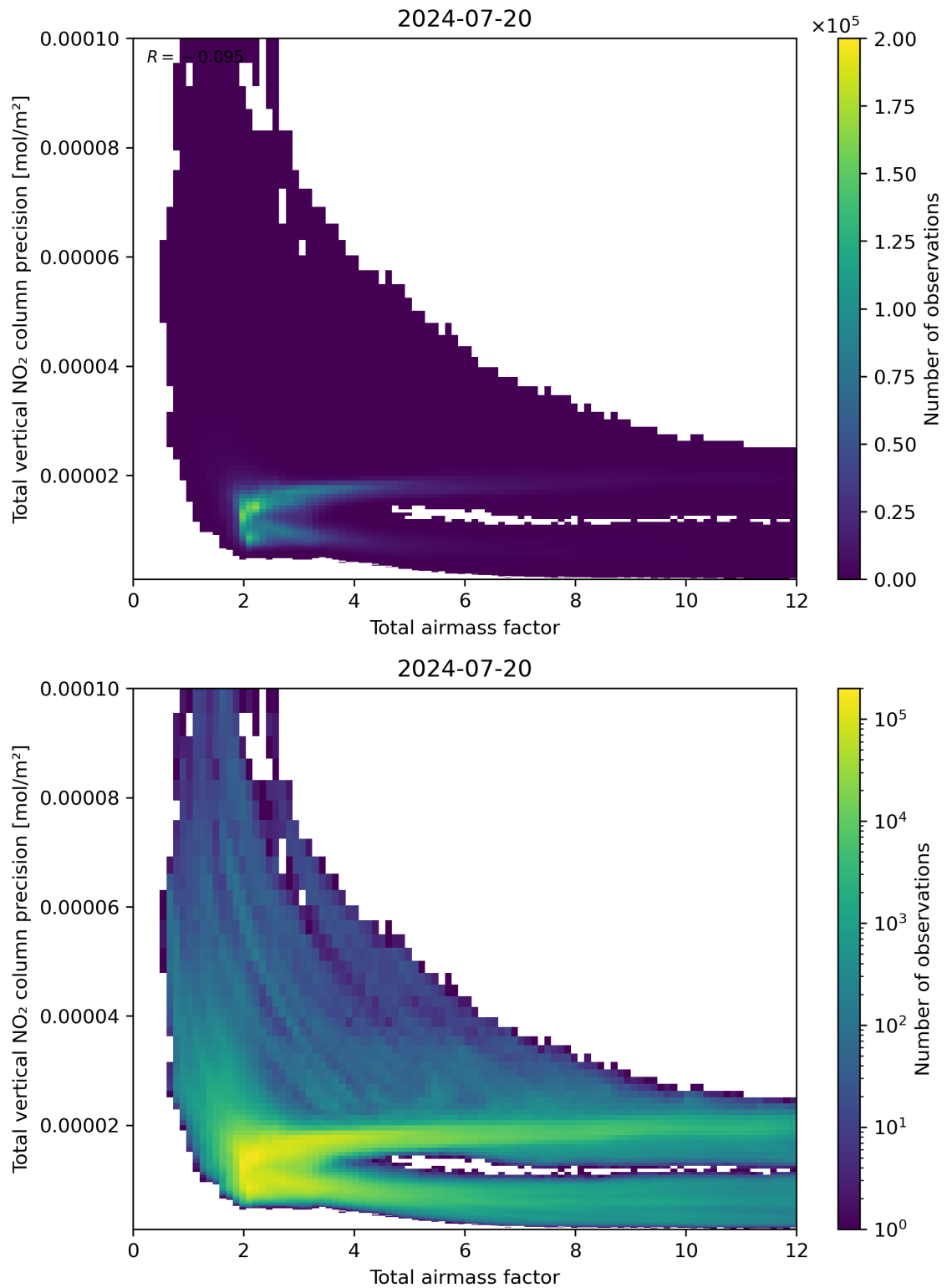
Figure 68: Scatter density plot of “Total airmass factor” against “Total vertical NO 2 column precision” for 2024-07-19 to 2024-07-21.
