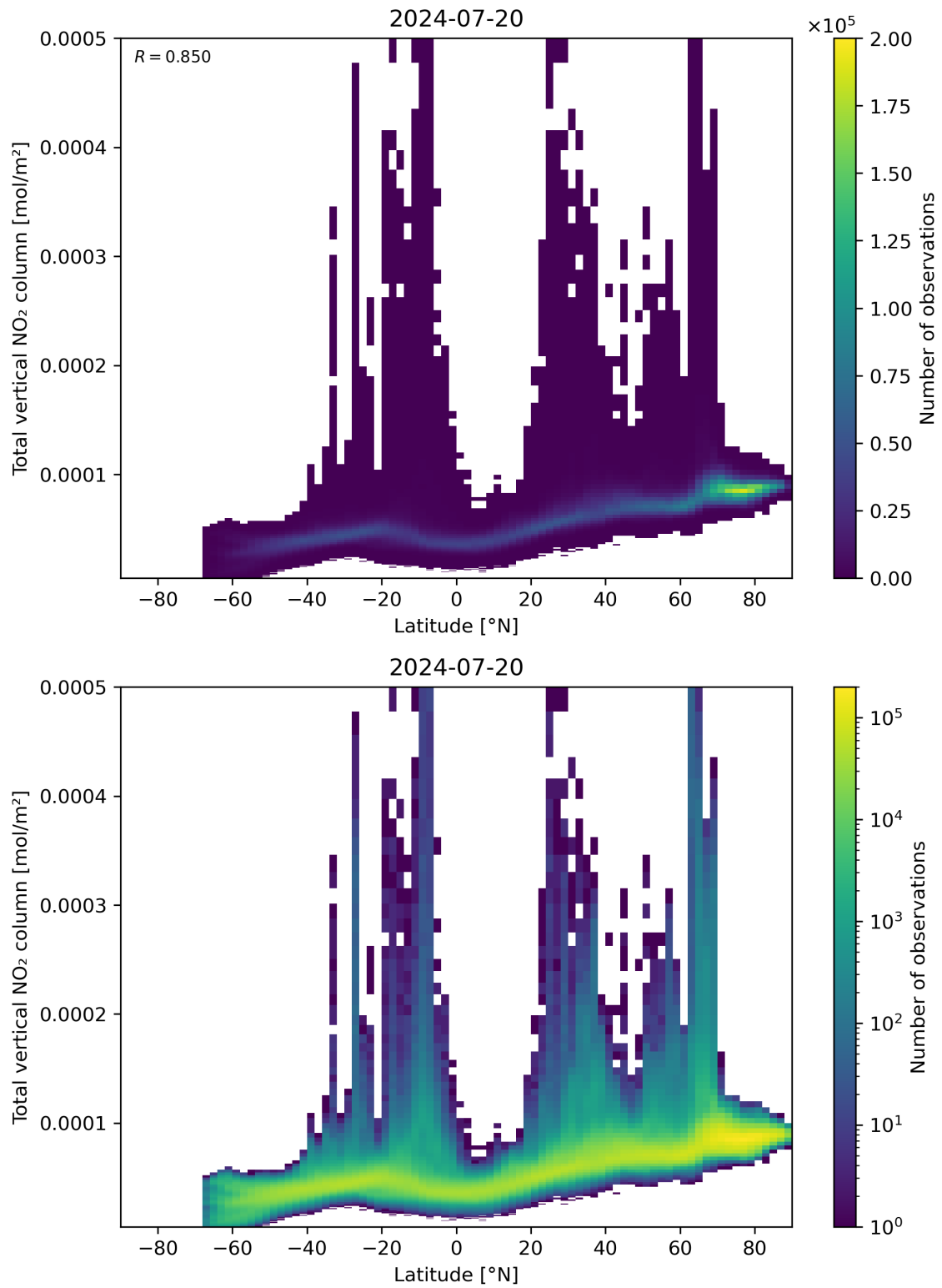
Figure 90: Scatter density plot of “Latitude” against “Total vertical NO 2 column” for 2024-07-19 to 2024-07-21.
