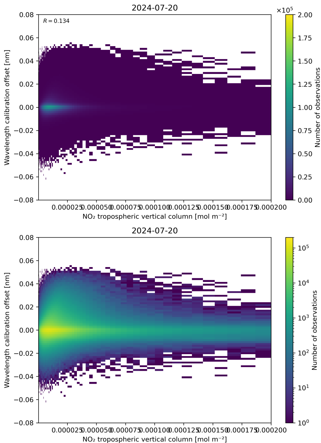
Figure 143: Scatter density plot of “NO 2 tropospheric vertical column” against “Wavelength calibration offset” for 2024-07-19 to 2024-07-21.
