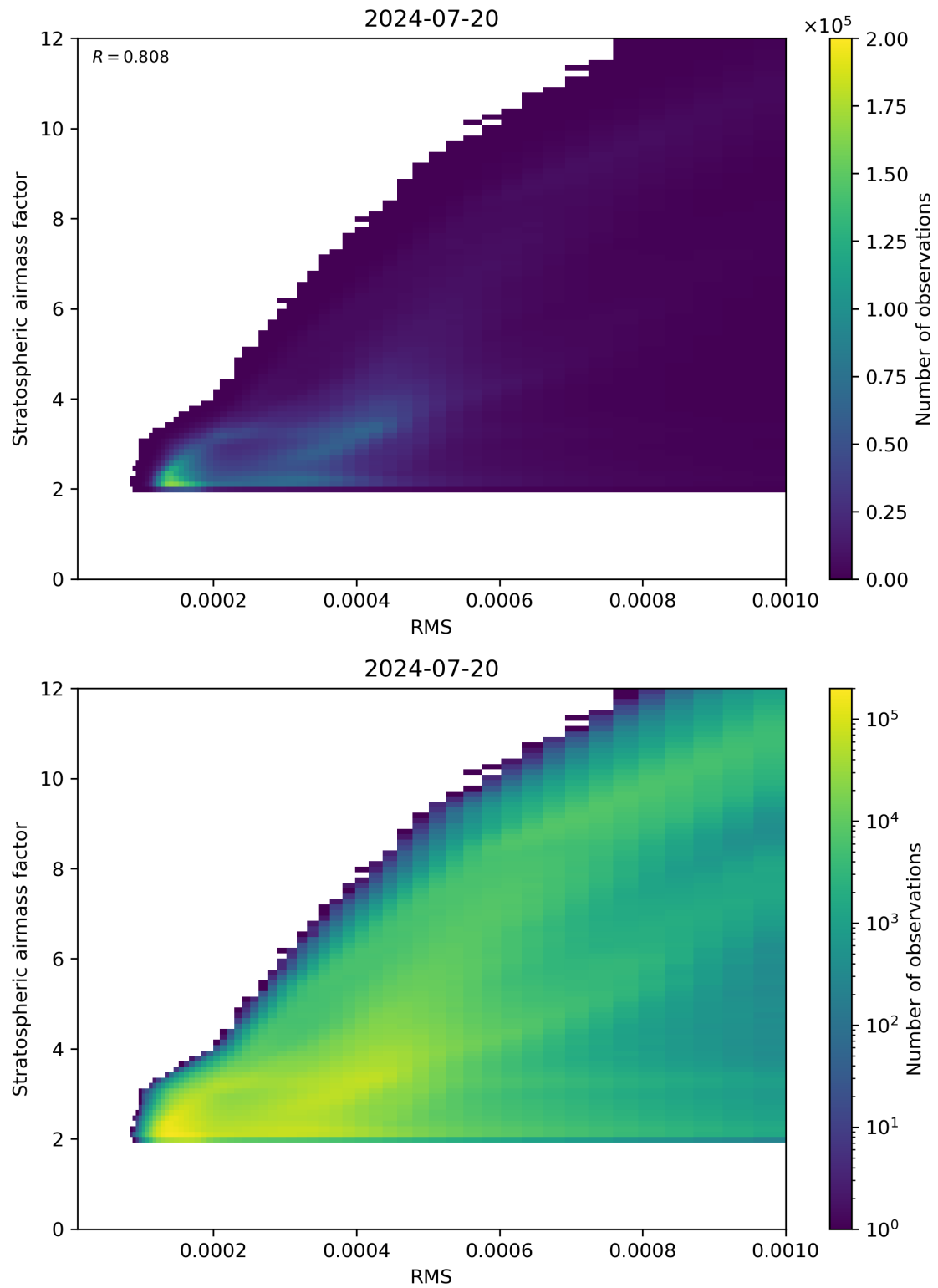
Figure 144: Scatter density plot of “RMS” against “Stratospheric airmass factor” for 2024-07-19 to 2024-07-21.
