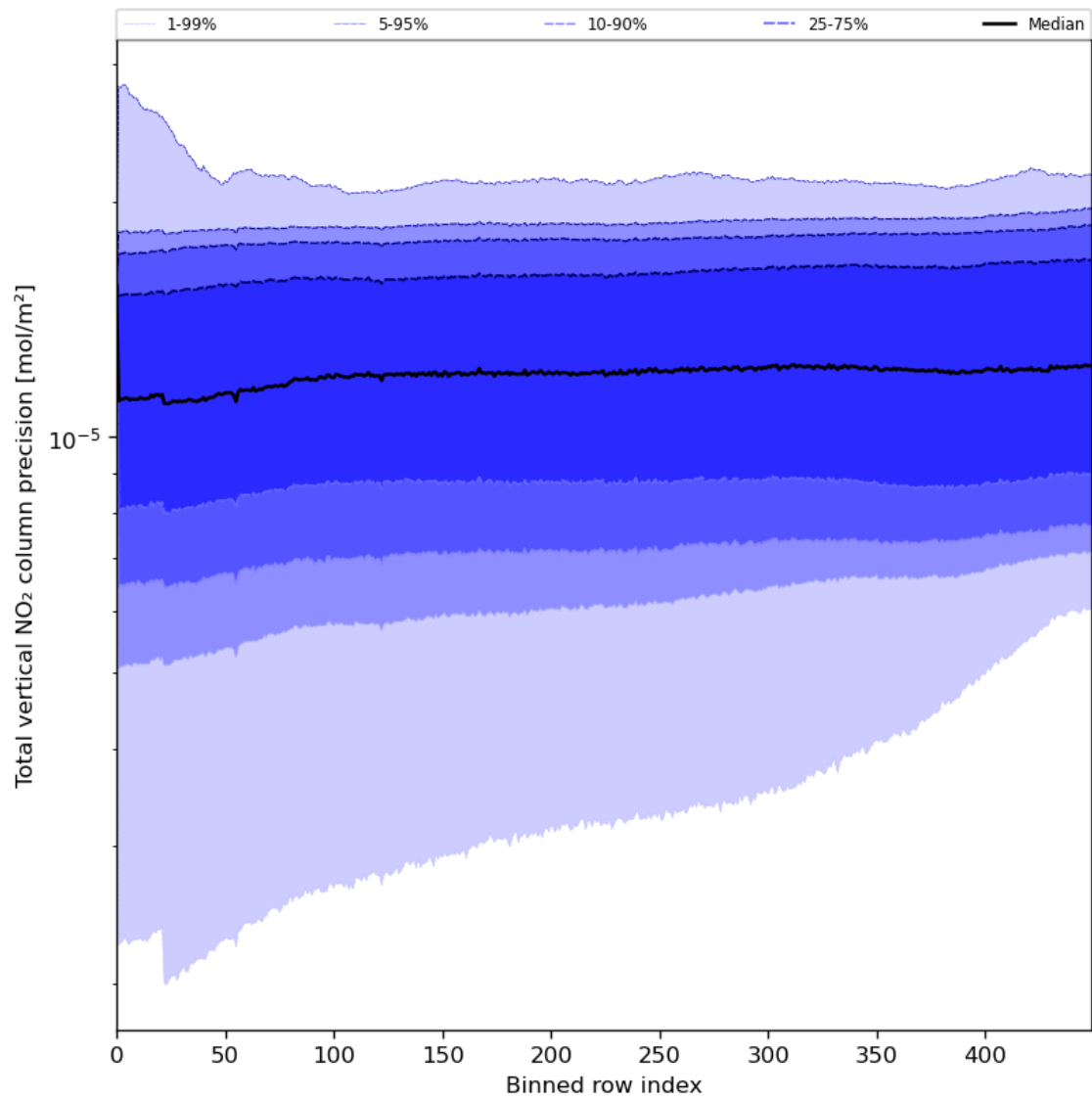
Figure 56: Along track statistics of “Total vertical NO 2 column precision” for 2024-07-19 to 2024-07-21
