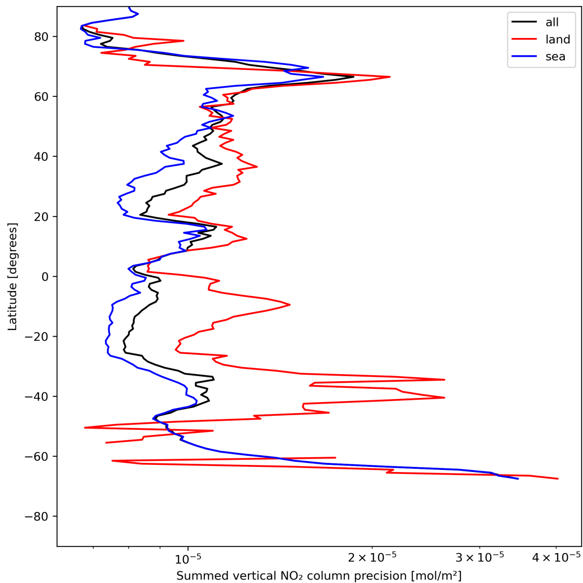
Figure 24: Zonal average of “Summed vertical NO 2 column precision” for 2024-07-19 to 2024-07-21.
