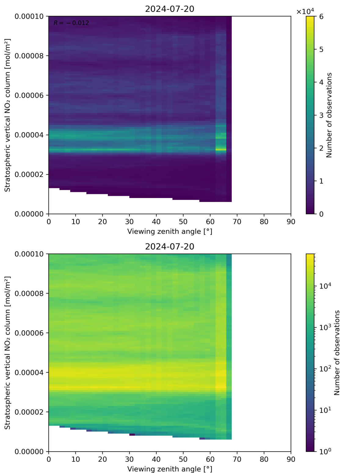
Figure 164: Scatter density plot of “Viewing zenith angle” against “Stratospheric vertical NO 2 column” for 2024-07-19 to 2024-07-21.
