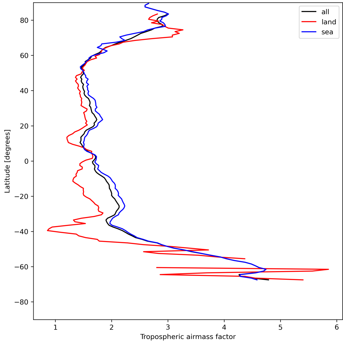
Figure 14: Zonal average of “Tropospheric airmass factor” for 2024-07-19 to 2024-07-21.
