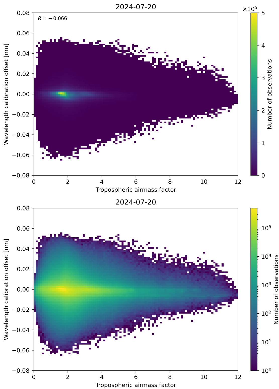
Figure 80: Scatter density plot of “Tropospheric air mass factor” against “Wavelength calibration offset” for 2024-07-19 to 2024-07-21.
