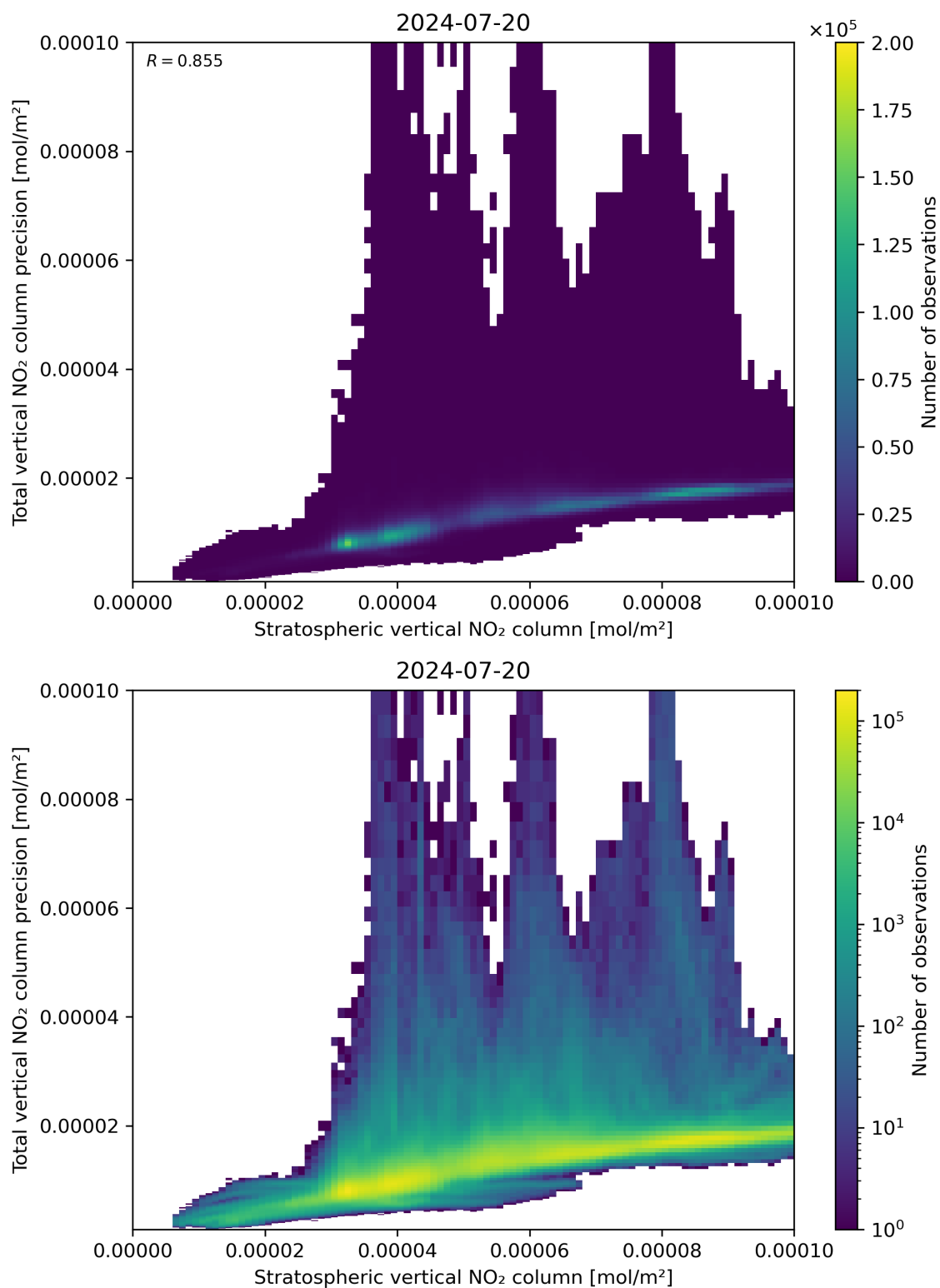
Figure 101: Scatter density plot of “Stratospheric vertical NO 2 column” against “Total vertical NO 2 column precision” for 2024-07-19 to 2024-07-21.
