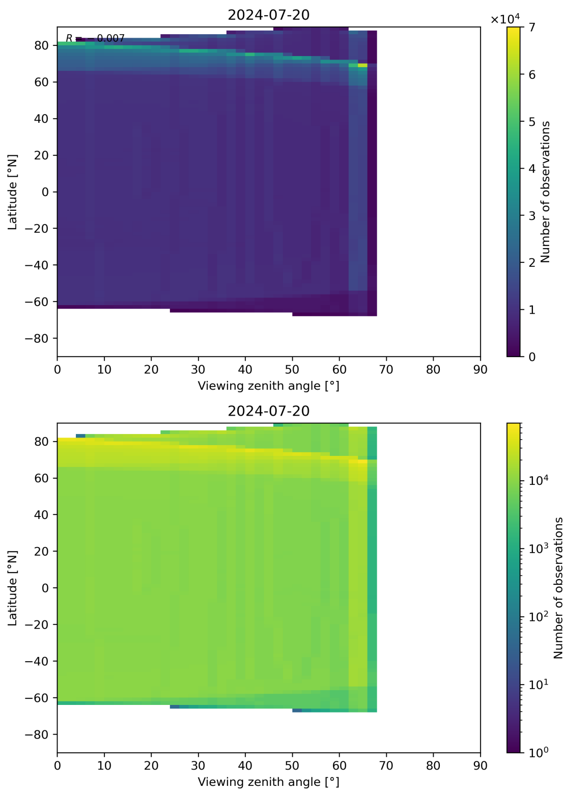
Figure 163: Scatter density plot of “Viewing zenith angle” against “Latitude” for 2024-07-19 to 2024-07-21.
