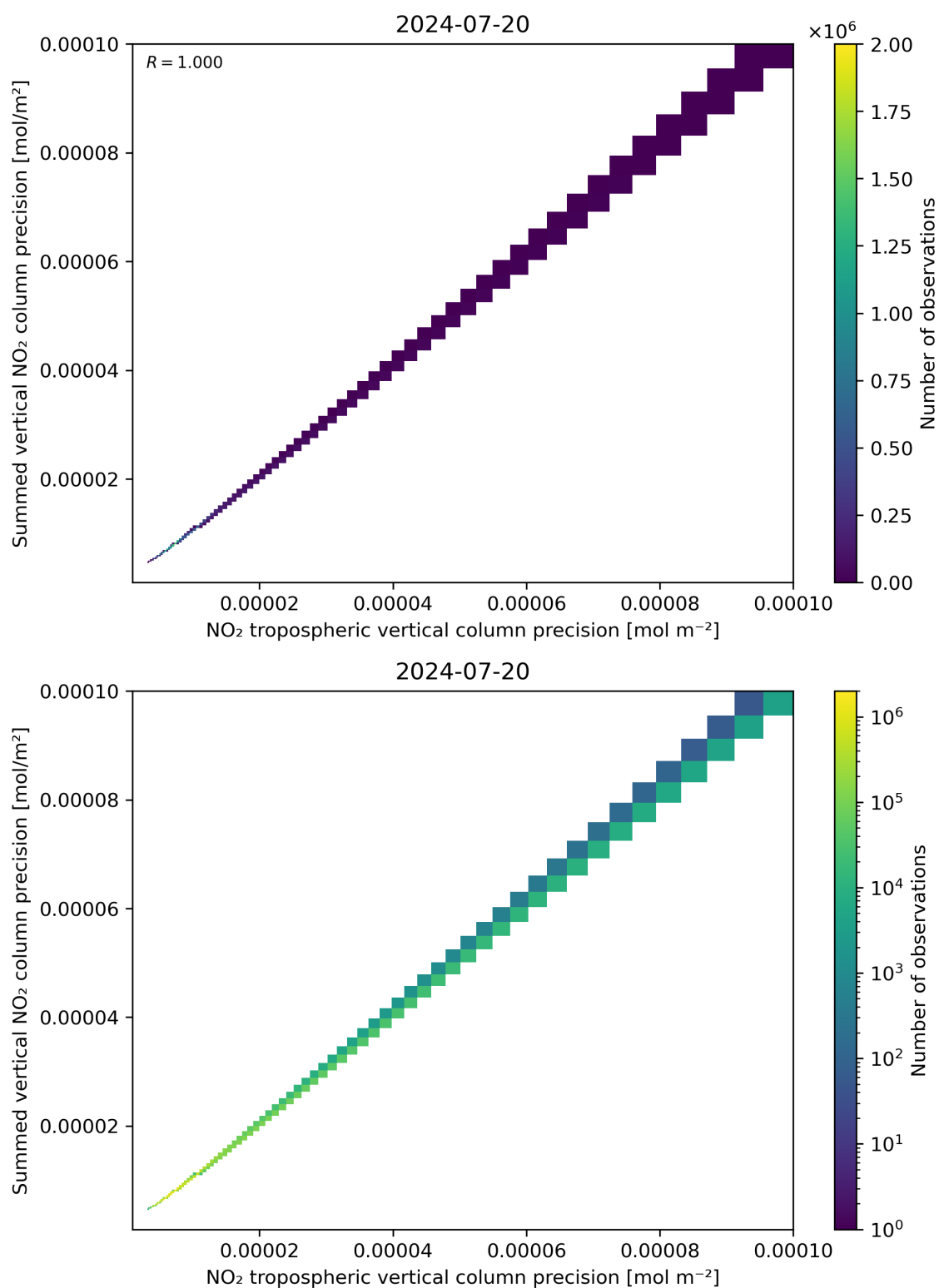
Figure 137: Scatter density plot of “NO 2 tropospheric vertical column precision” against “Summed vertical NO 2 column precision” for 2024-07-19 to 2024-07-21.
