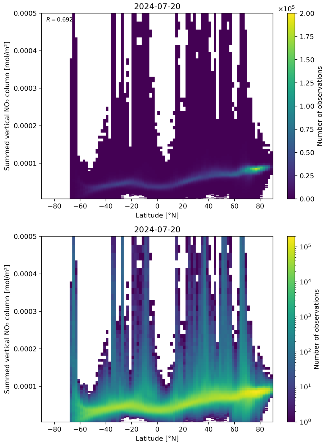
Figure 88: Scatter density plot of “Latitude” against “Summed vertical NO 2 column” for 2024-07-19 to 2024-07-21.
