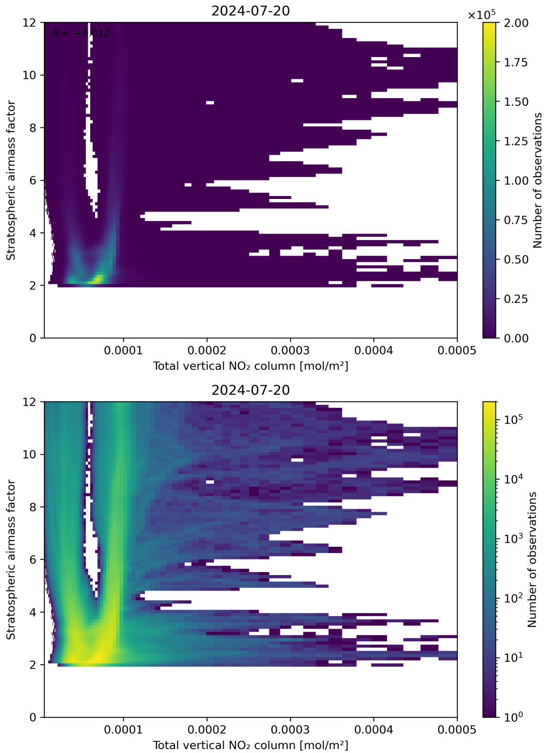
Figure 110: Scatter density plot of “Total vertical NO 2 column” against “Stratospheric airmass factor” for 2024-07-19 to 2024-07-21.
