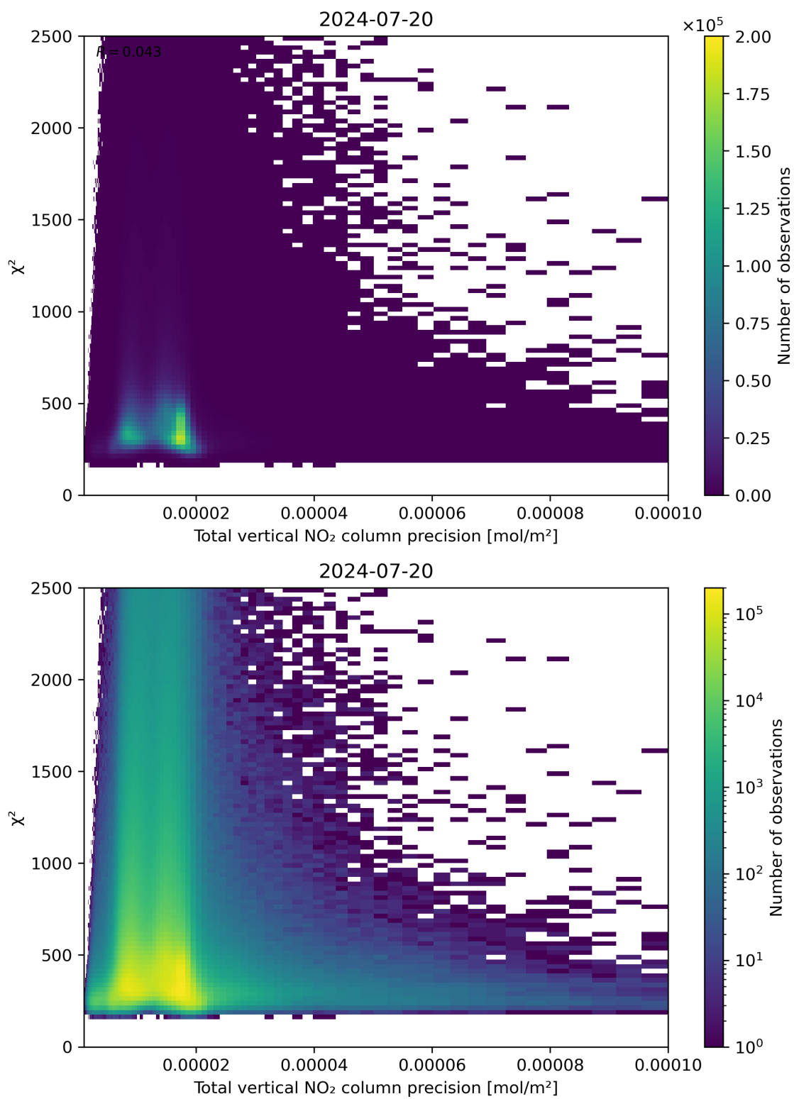
Figure 116: Scatter density plot of “Total vertical NO 2 column precision” against “ \chi^2 ” for 2024-07-19 to 2024-07-21.
