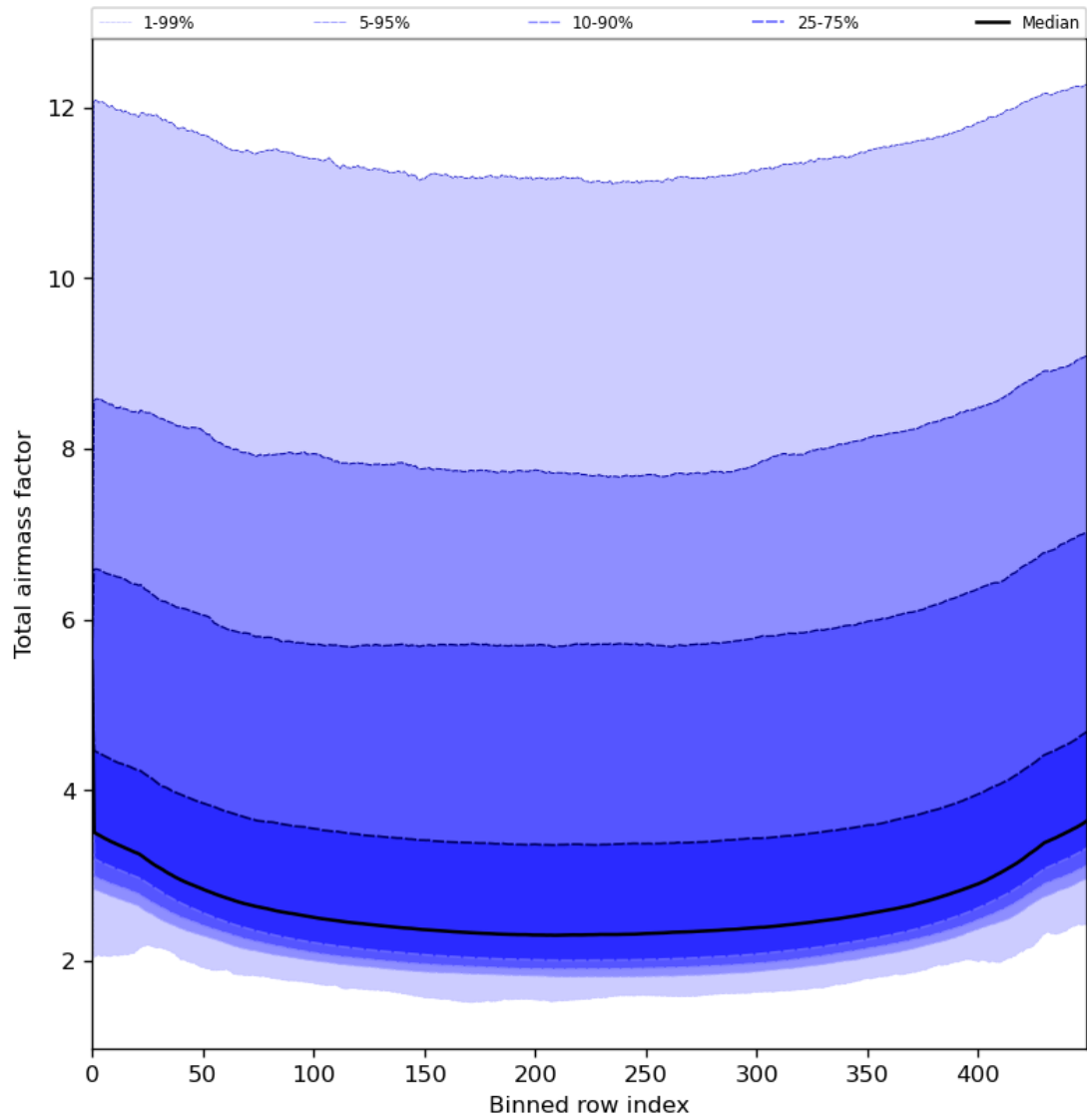
Figure 49: Along track statistics of “Total airmass factor” for 2024-07-19 to 2024-07-21
