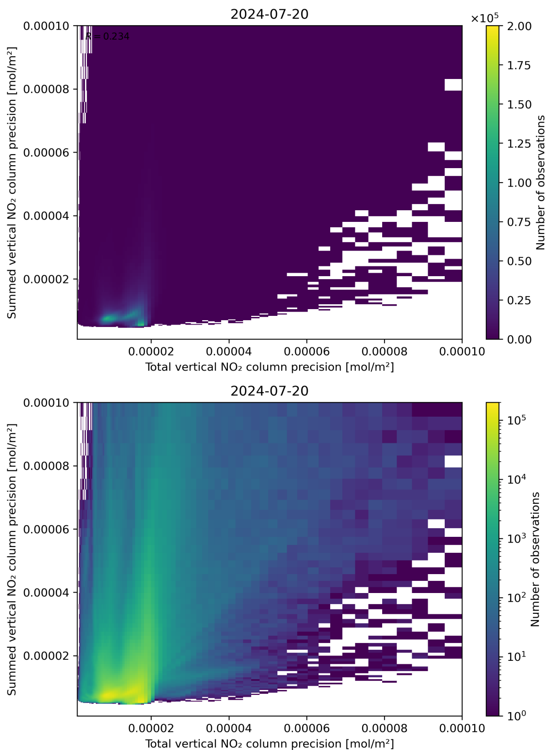
Figure 118: Scatter density plot of “Total vertical NO 2 column precision” against “Summed vertical NO 2 column precision” for 2024-07-19 to 2024-07-21.
