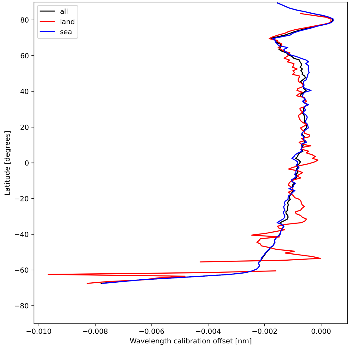
Figure 18: Zonal average of “Wavelength calibration offset” for 2024-07-19 to 2024-07-21.
