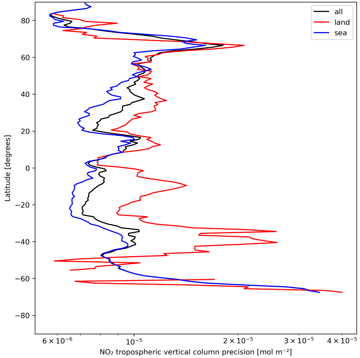
Figure 13: Zonal average of “NO 2 tropospheric vertical column precision” for 2024-07-19 to 2024-07-21.
