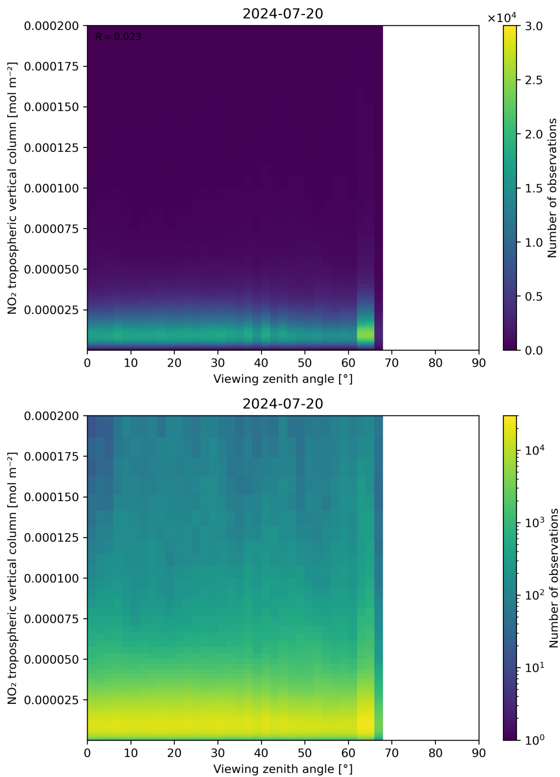
Figure 169: Scatter density plot of “Viewing zenith angle” against “NO 2 tropospheric vertical column” for 2024-07-19 to 2024-07-21.
