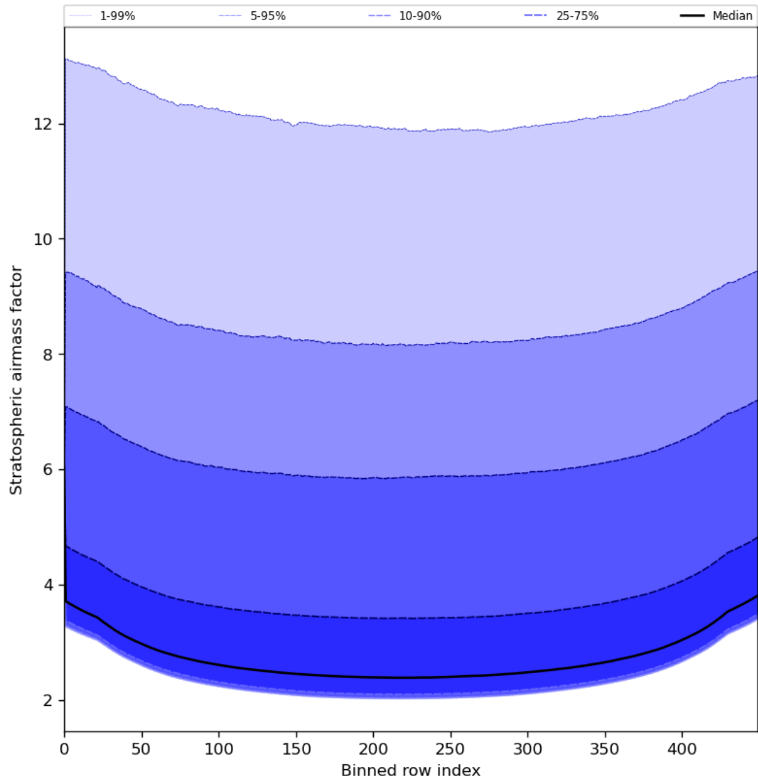
Figure 61: Along track statistics of “Stratospheric airmass factor” for 2024-07-19 to 2024-07-21
