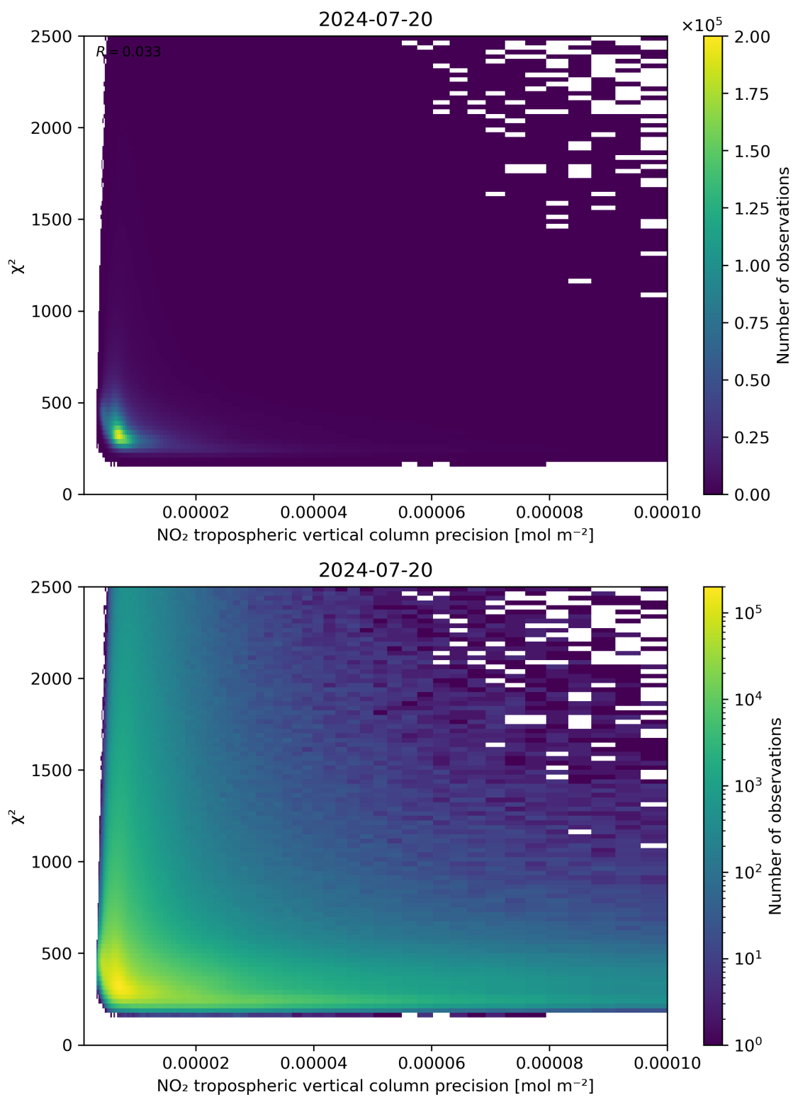
Figure 134: Scatter density plot of “NO 2 tropospheric vertical column precision” against “ \chi^2 ” for 2024-07-19 to 2024-07-21.
