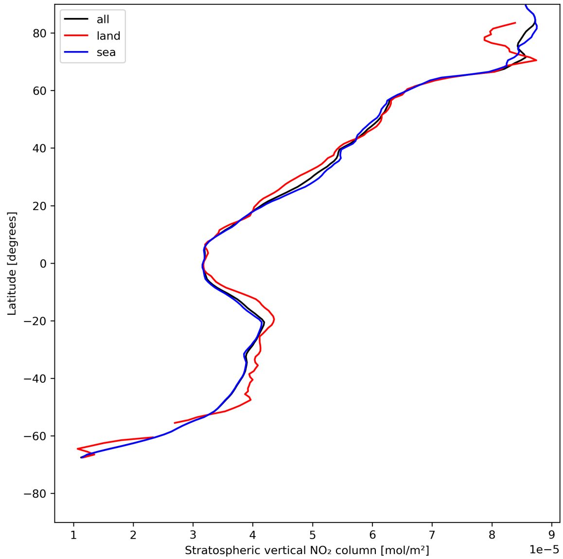
Figure 19: Zonal average of “Stratospheric vertical NO 2 column” for 2024-07-19 to 2024-07-21.
