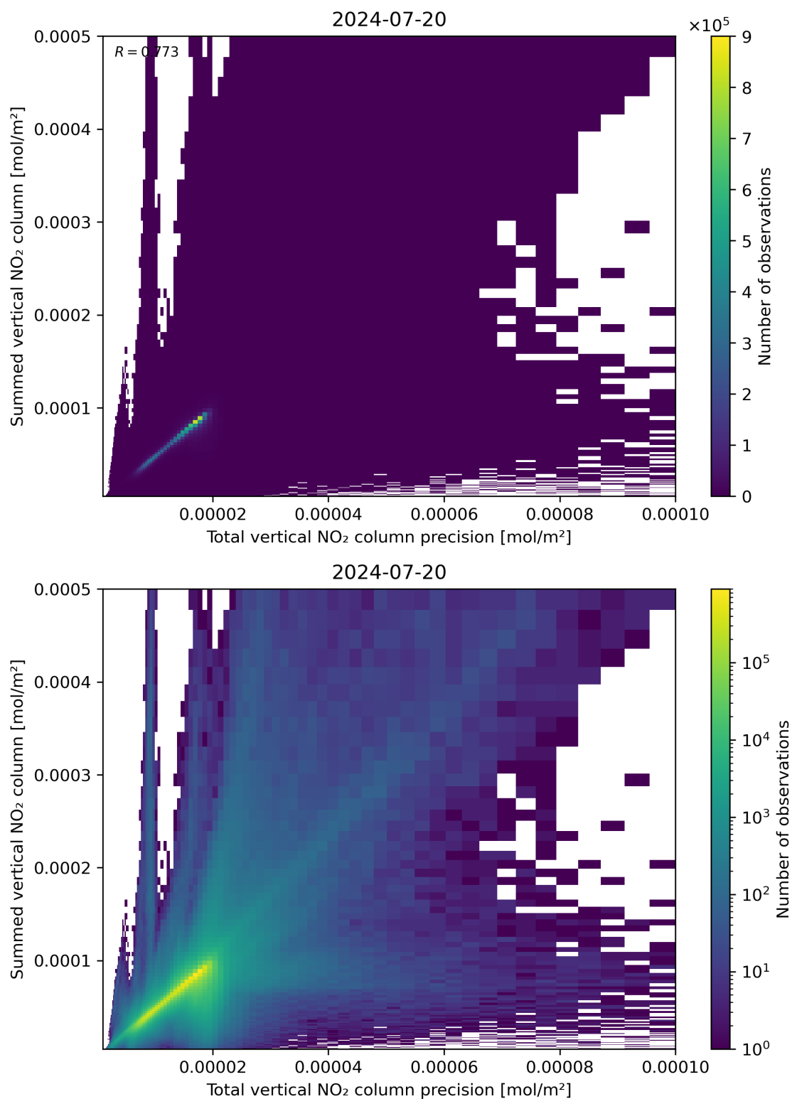
Figure 117: Scatter density plot of “Total vertical NO 2 column precision” against “Summed vertical NO 2 column” for 2024-07-19 to 2024-07-21.
