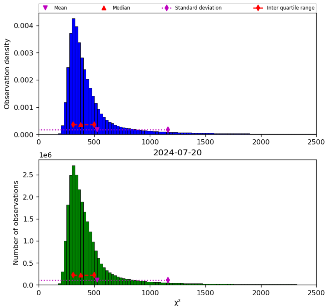
Figure 42: Histogram of “ \chi^2 ” for 2024-07-19 to 2024-07-21
