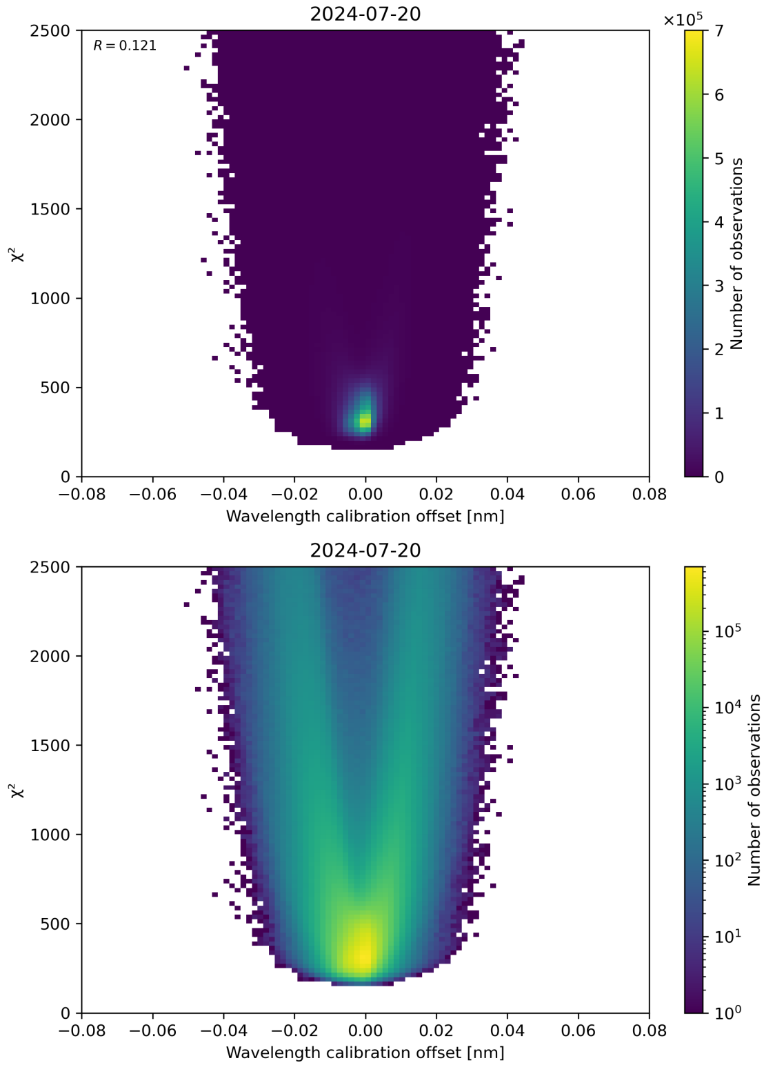
Figure 175: Scatter density plot of “Wavelength calibration offset” against “ \chi^2 ” for 2024-07-19 to 2024-07-21.
