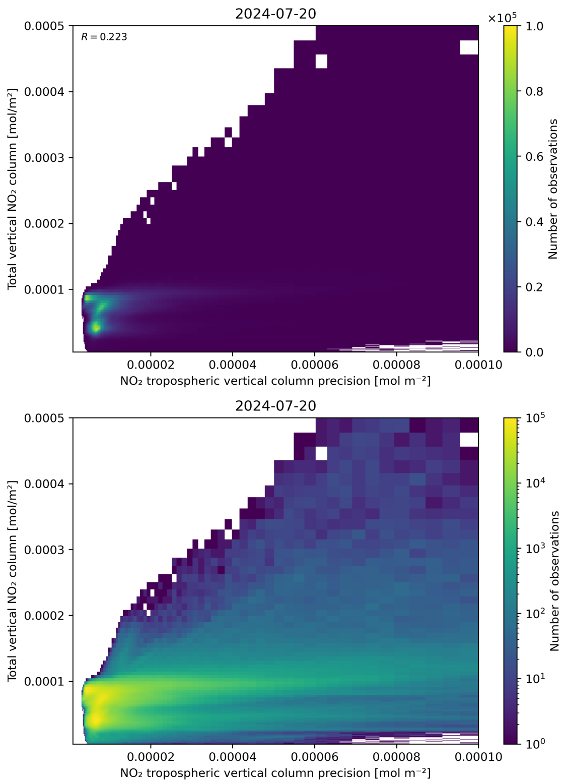
Figure 138: Scatter density plot of “NO 2 tropospheric vertical column precision” against “Total vertical NO 2 column” for 2024-07-19 to 2024-07-21.
