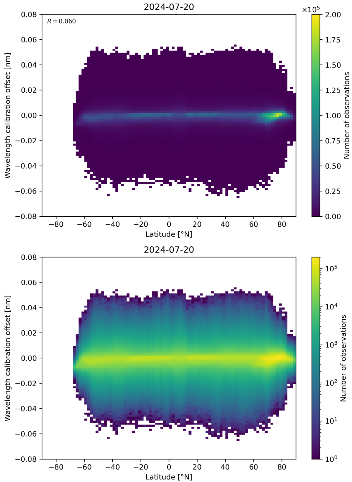
Figure 95: Scatter density plot of “Latitude” against “Wavelength calibration offset” for 2024-07-19 to 2024-07-21.
