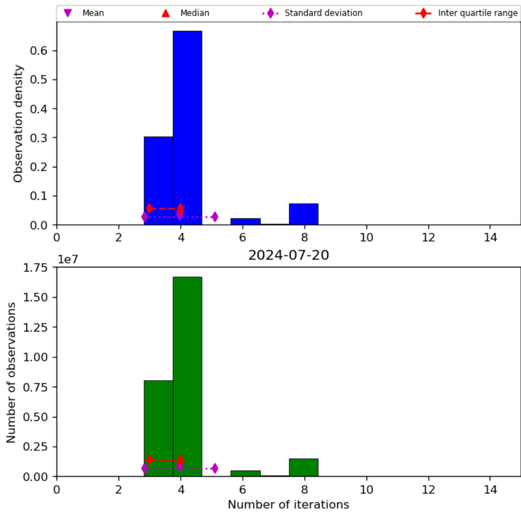
Figure 34: Histogram of “Number of iterations” for 2024-07-19 to 2024-07-21
