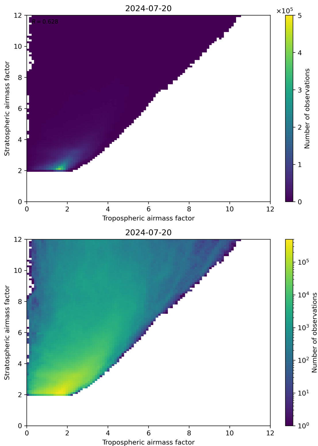
Figure 71: Scatter density plot of “Tropospheric airmass factor” against “Stratospheric airmass factor” for 2024-07-19 to 2024-07-21.
