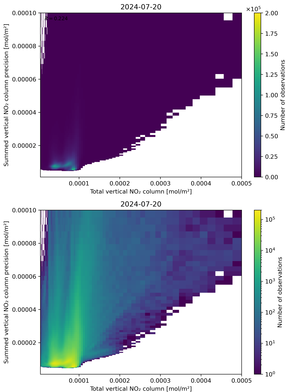
Figure 113: Scatter density plot of “Total vertical NO 2 column” against “Summed vertical NO 2 column precision” for 2024-07-19 to 2024-07-21.
