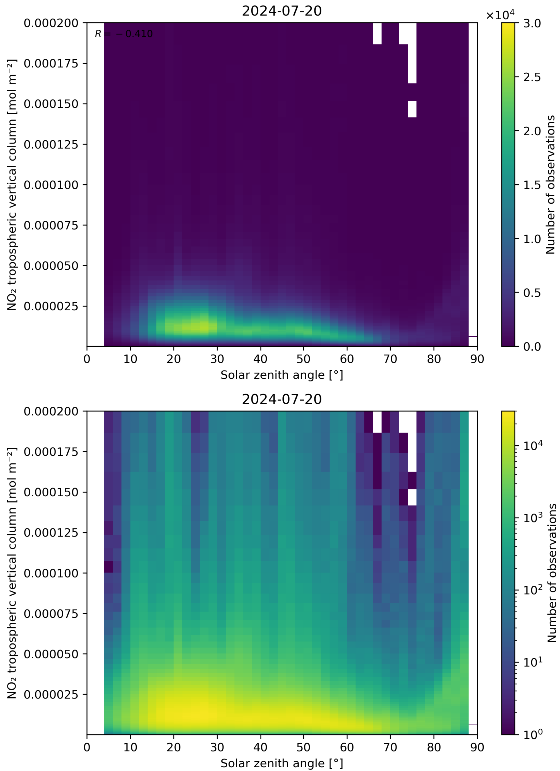
Figure 155: Scatter density plot of “Solar zenith angle” against “NO 2 tropospheric vertical column” for 2024-07-19 to 2024-07-21.
