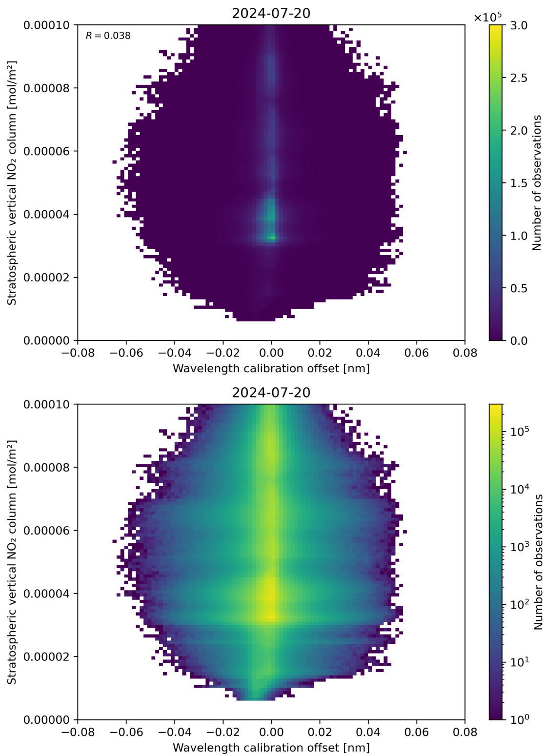
Figure 176: Scatter density plot of “Wavelength calibration offset” against “Stratospheric vertical NO 2 column” for 2024-07-19 to 2024-07-21.
