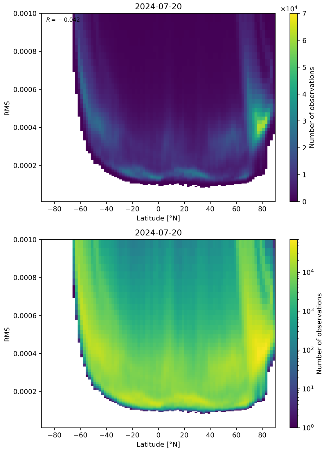
Figure 94: Scatter density plot of “Latitude” against “RMS” for 2024-07-19 to 2024-07-21.
