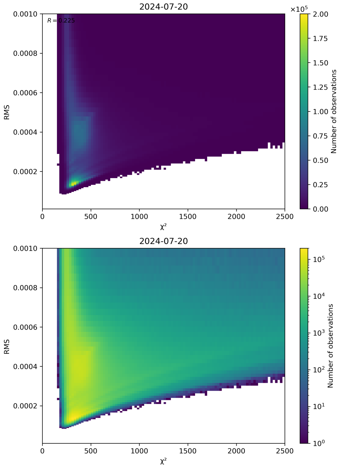
Figure 82: Scatter density plot of “ \chi^2 ” against “RMS” for 2024-07-19 to 2024-07-21.
