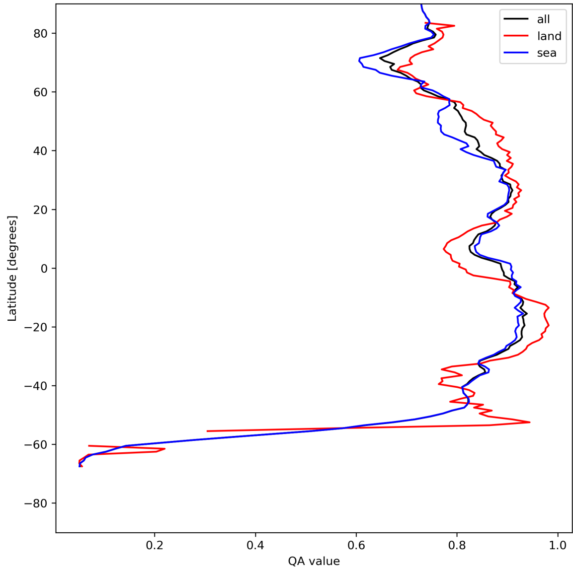
Figure 11: Zonal average of “QA value” for 2024-07-19 to 2024-07-21.
