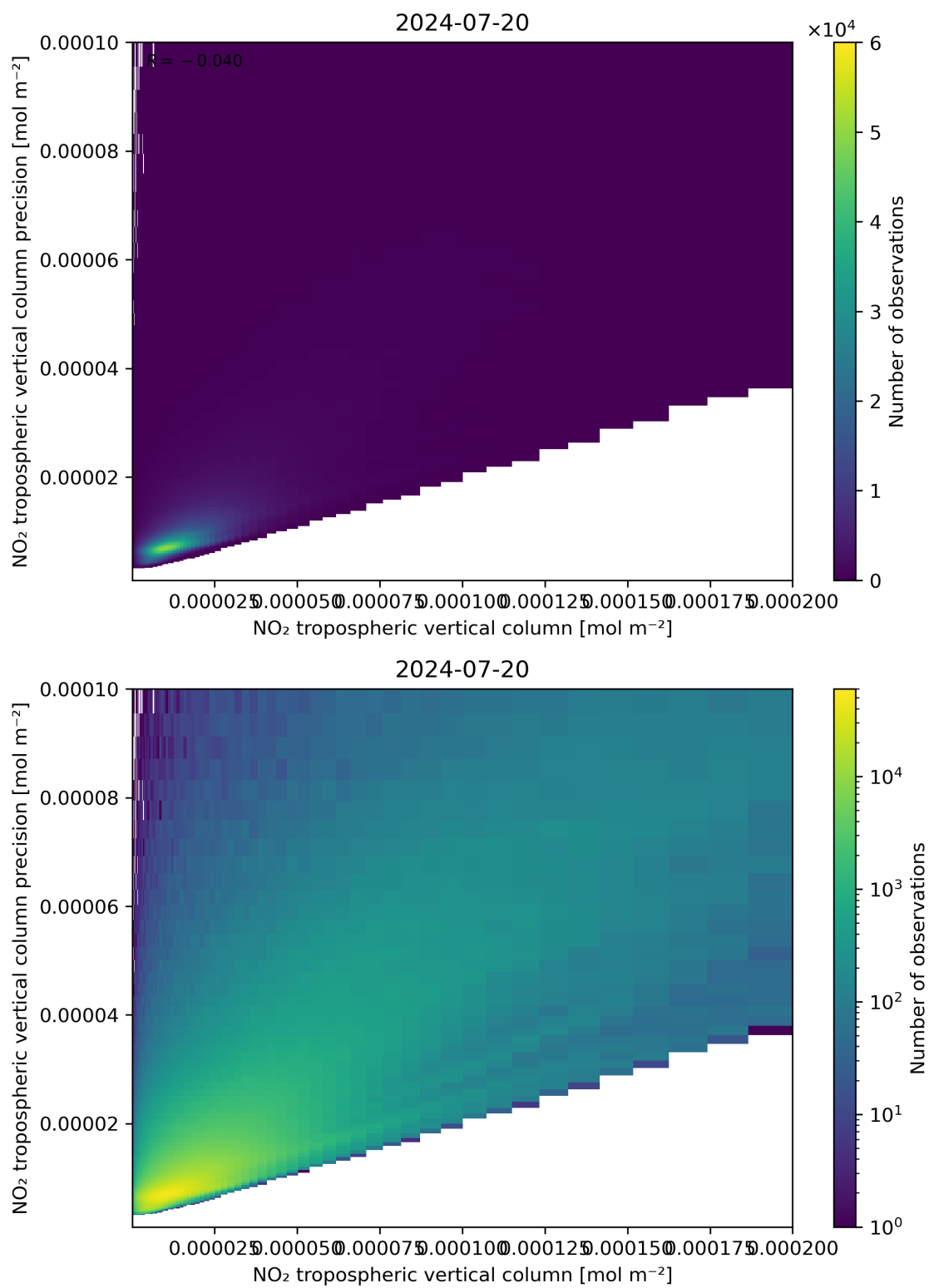
Figure 130: Scatter density plot of “NO 2 tropospheric vertical column” against “NO 2 tropospheric vertical column precision” for 2024-07-19 to 2024-07-21.
