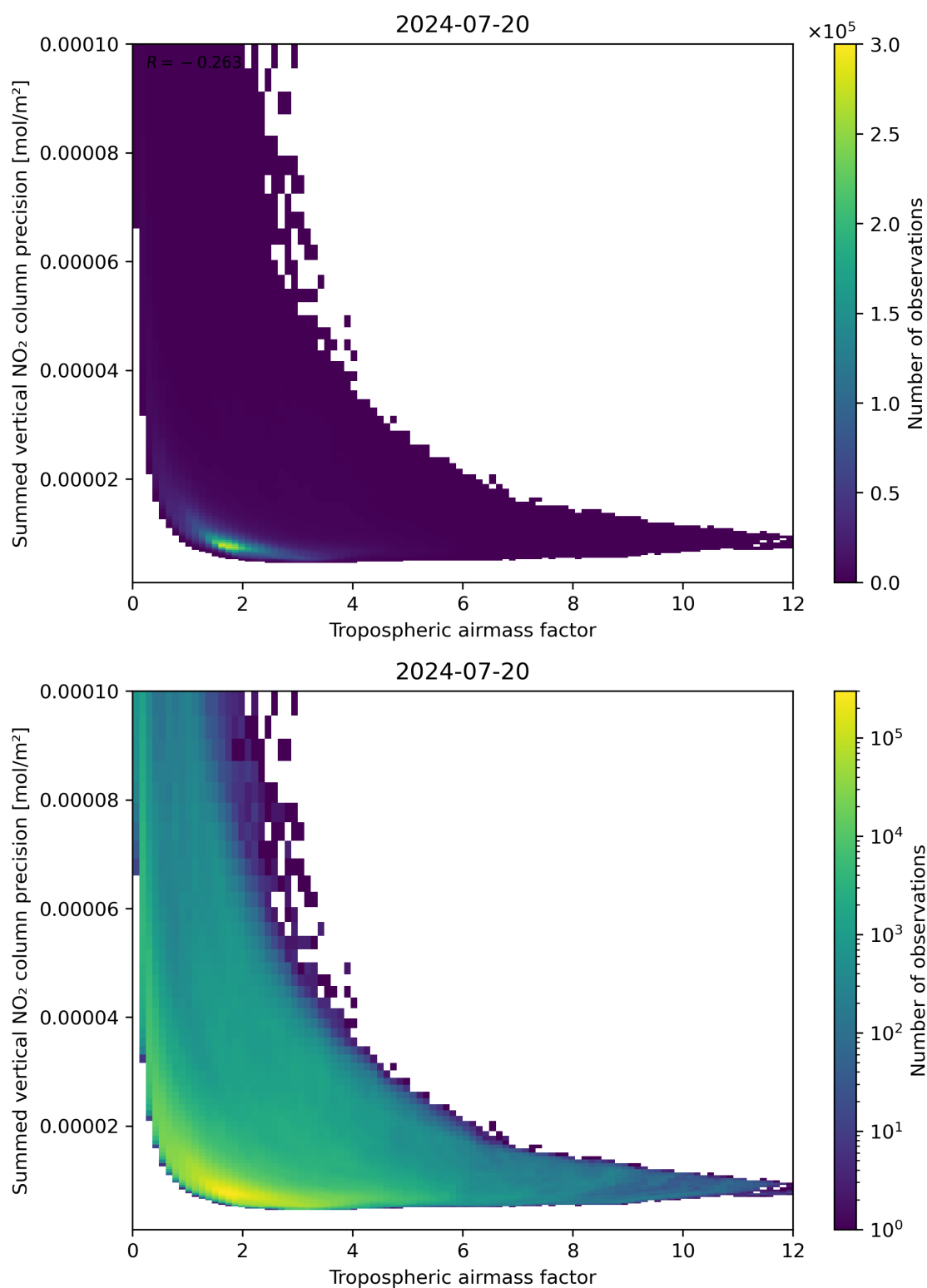
Figure 76: Scatter density plot of “Tropospheric air mass factor” against “Summed vertical NO 2 column precision” for 2024-07-19 to 2024-07-21.
