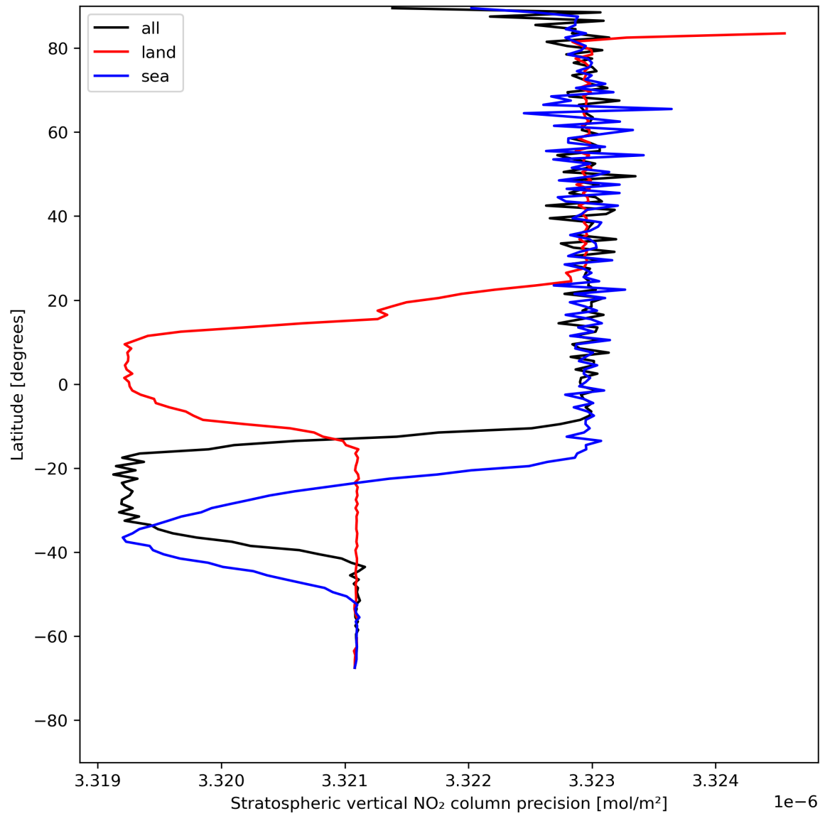
Figure 20: Zonal average of “Stratospheric vertical NO 2 column precision” for 2024-07-19 to 2024-07-21.
