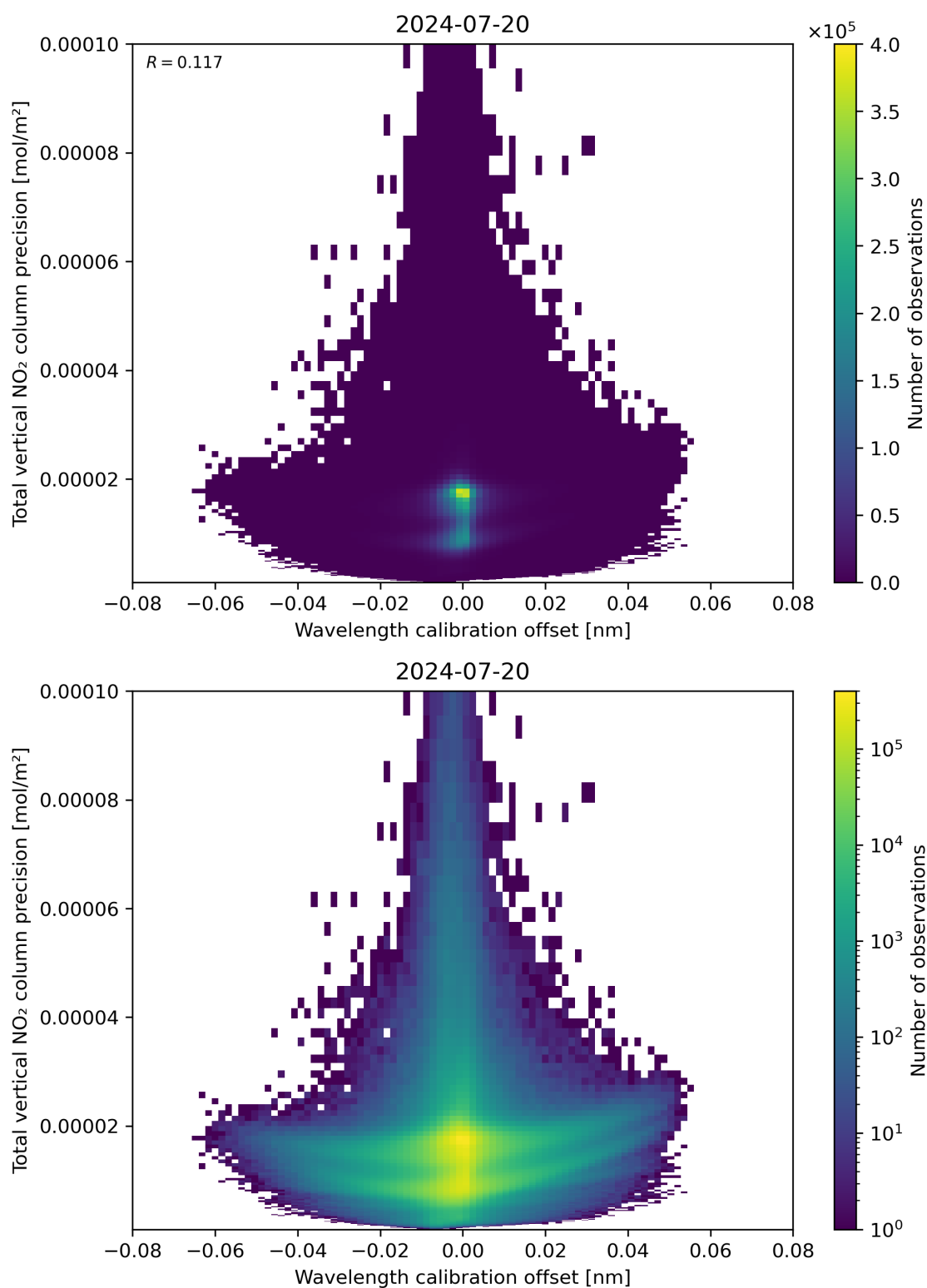
Figure 180: Scatter density plot of “Wavelength calibration offset” against “Total vertical NO 2 column precision” for 2024-07-19 to 2024-07-21.
