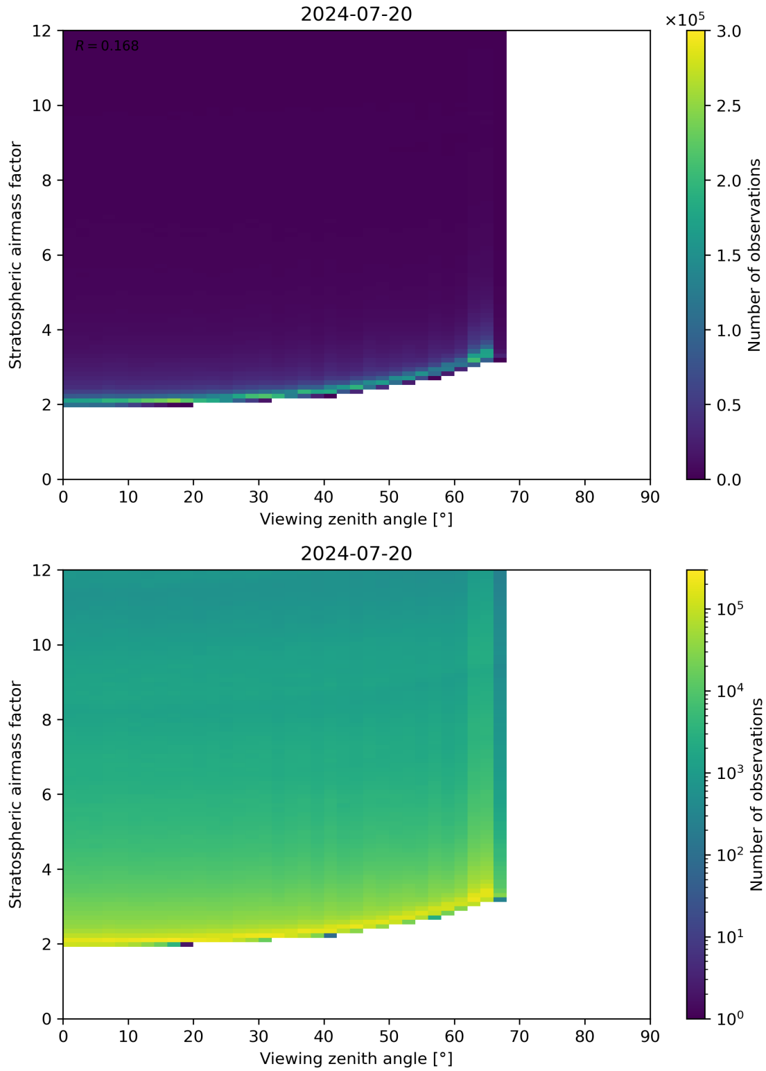
Figure 159: Scatter density plot of “Viewing zenith angle” against “Stratospheric airmass factor” for 2024-07-19 to 2024-07-21.
