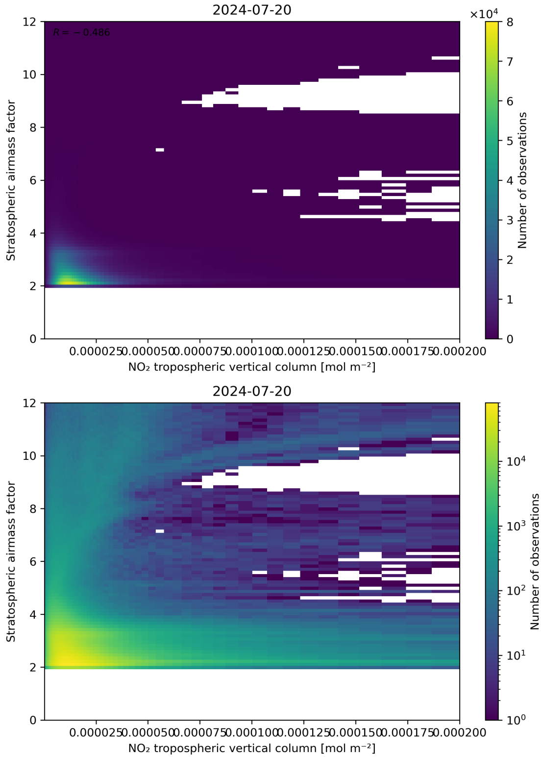
Figure 121: Scatter density plot of “NO 2 tropospheric vertical column” against “Stratospheric air mass factor” for 2024-07-19 to 2024-07-21.
