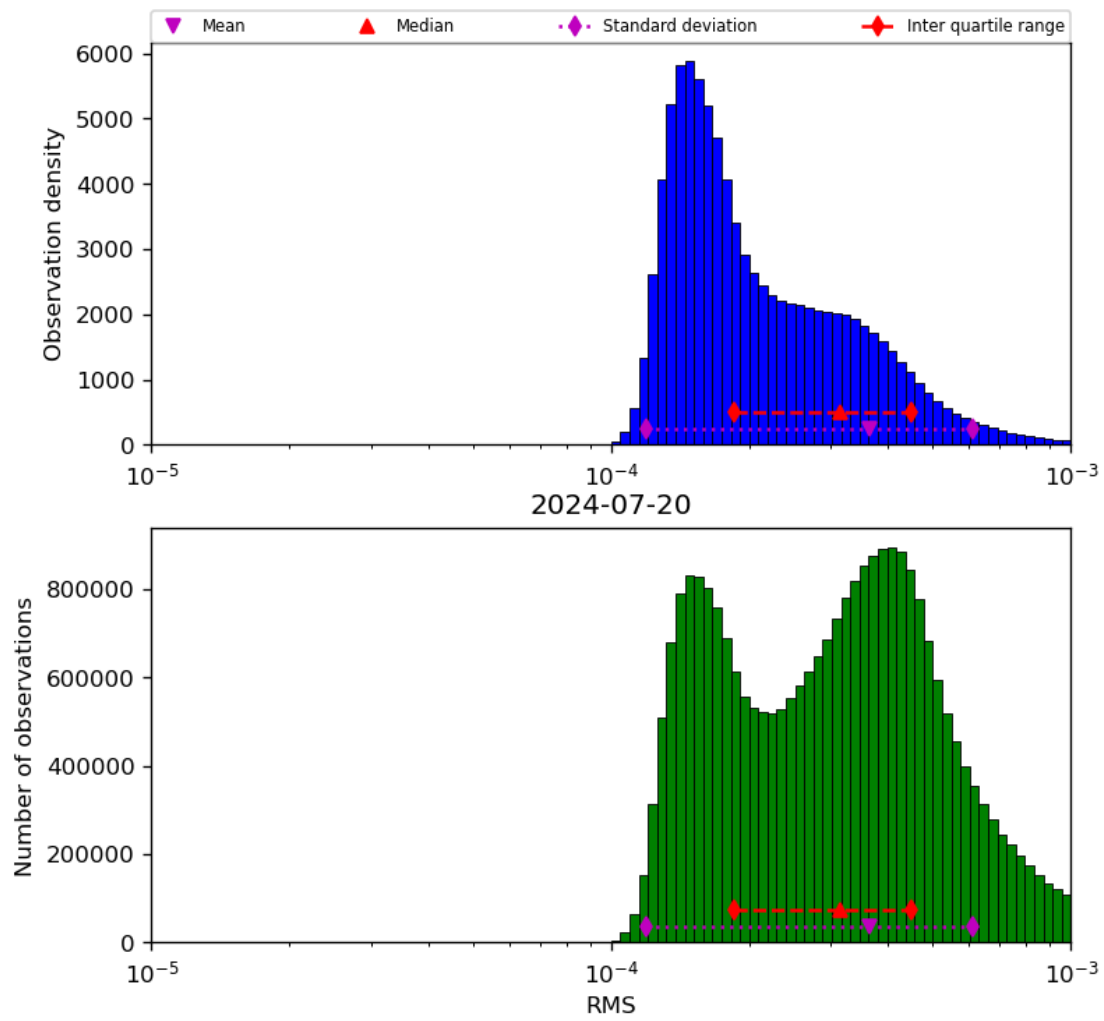
Figure 43: Histogram of “RMS” for 2024-07-19 to 2024-07-21
