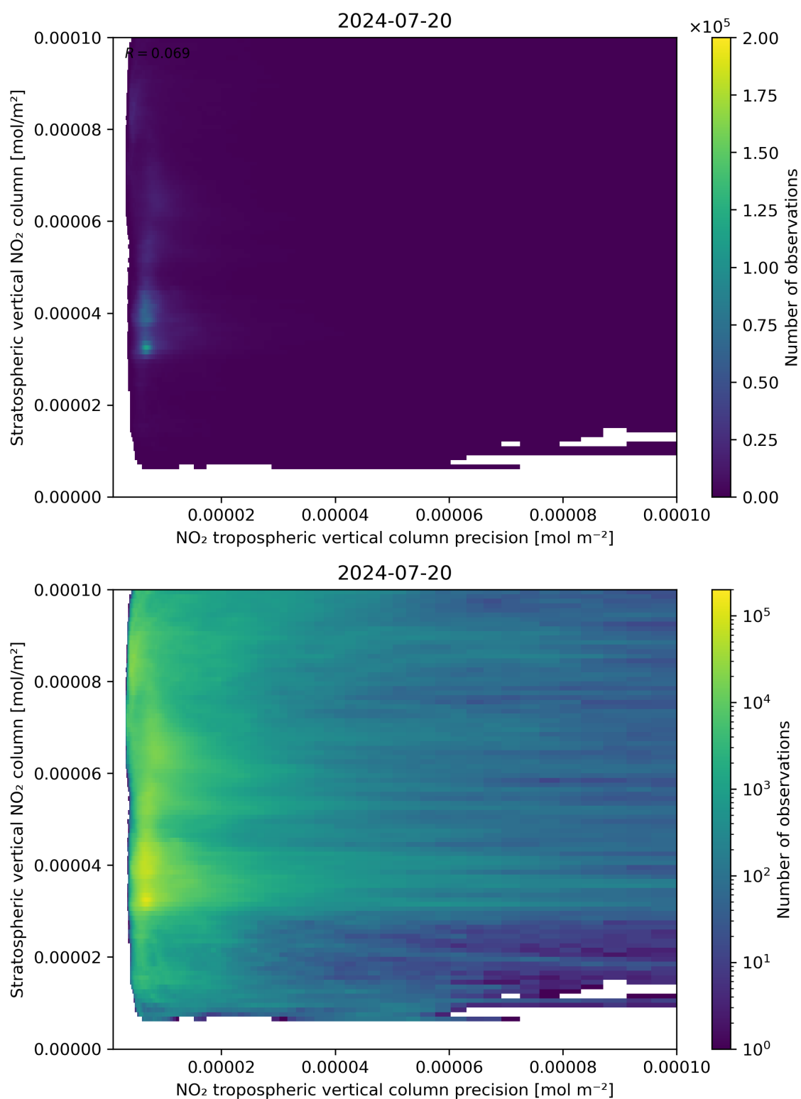
Figure 135: Scatter density plot of “NO 2 tropospheric vertical column precision” against “Stratospheric vertical NO 2 column” for 2024-07-19 to 2024-07-21.
