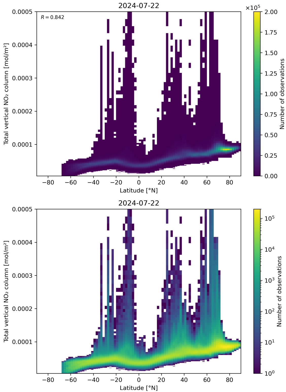
Figure 90: Scatter density plot of “Latitude” against “Total vertical NO 2 column” for 2024-07-21 to 2024-07-23.
