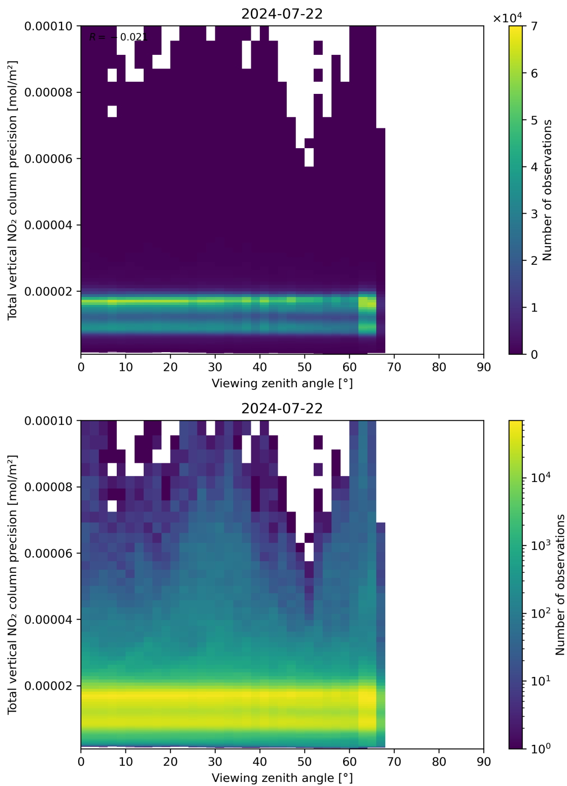
Figure 168: Scatter density plot of “Viewing zenith angle” against “Total vertical NO 2 column precision” for 2024-07-21 to 2024-07-23.
