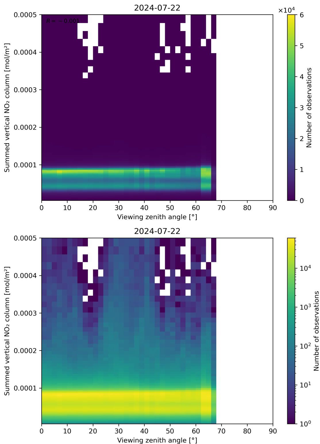
Figure 165: Scatter density plot of “Viewing zenith angle” against “Summed vertical NO 2 column” for 2024-07-21 to 2024-07-23.
