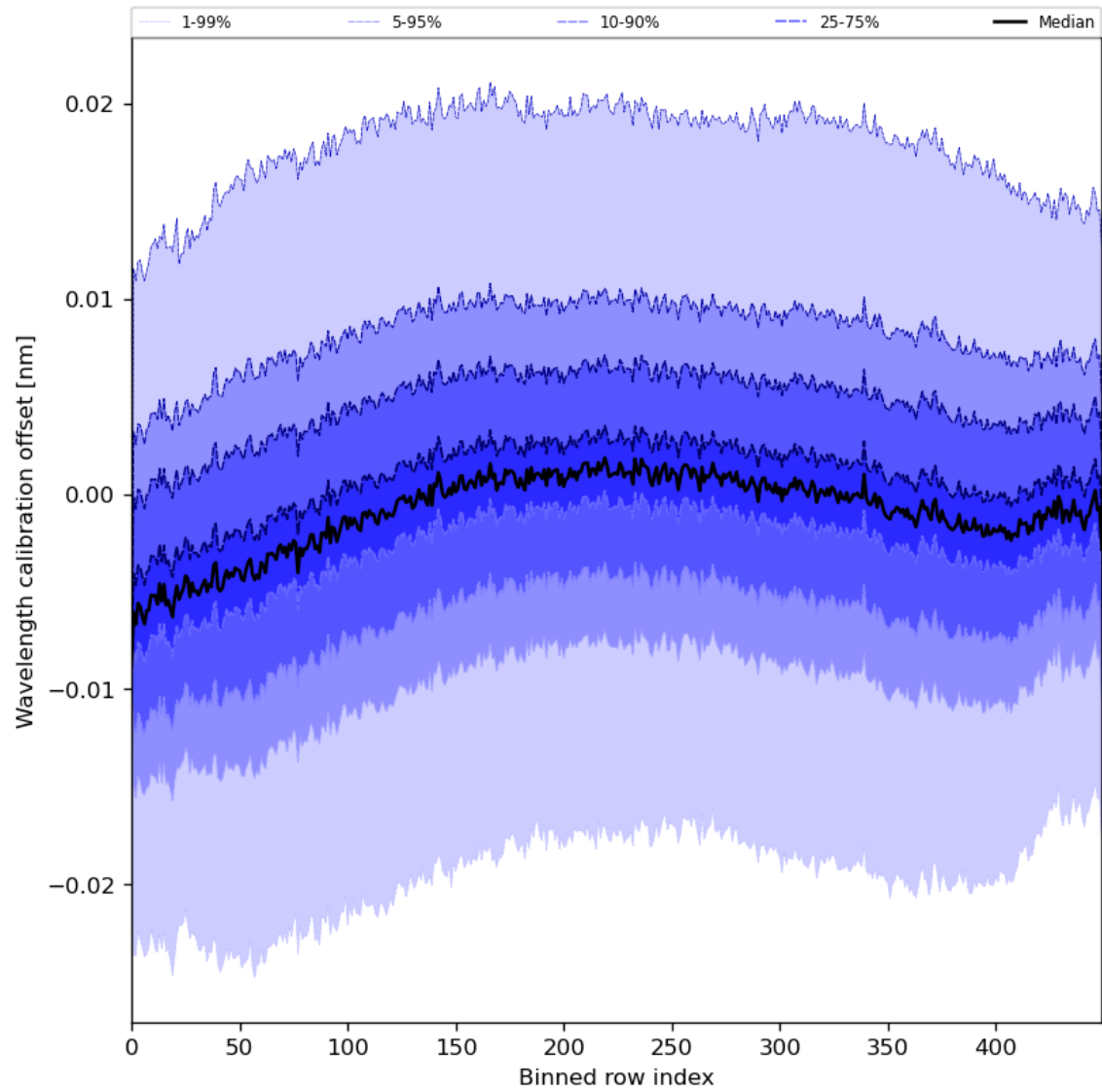
Figure 52: Along track statistics of “Wavelength calibration offset” for 2024-07-21 to 2024-07-23
