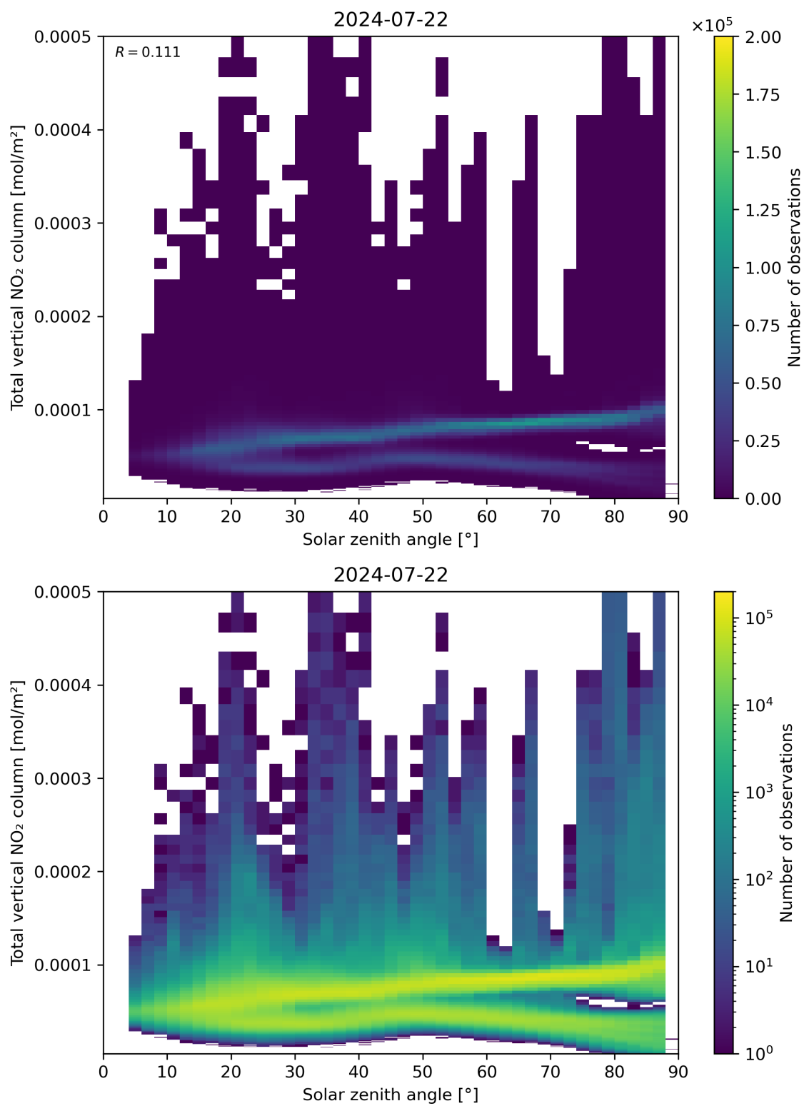
Figure 153: Scatter density plot of “Solar zenith angle” against “Total vertical NO 2 column” for 2024-07-21 to 2024-07-23.
