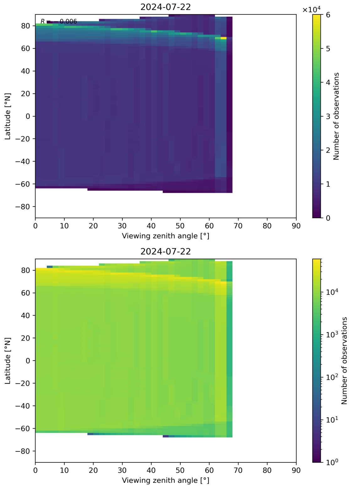
Figure 163: Scatter density plot of “Viewing zenith angle” against “Latitude” for 2024-07-21 to 2024-07-23.
