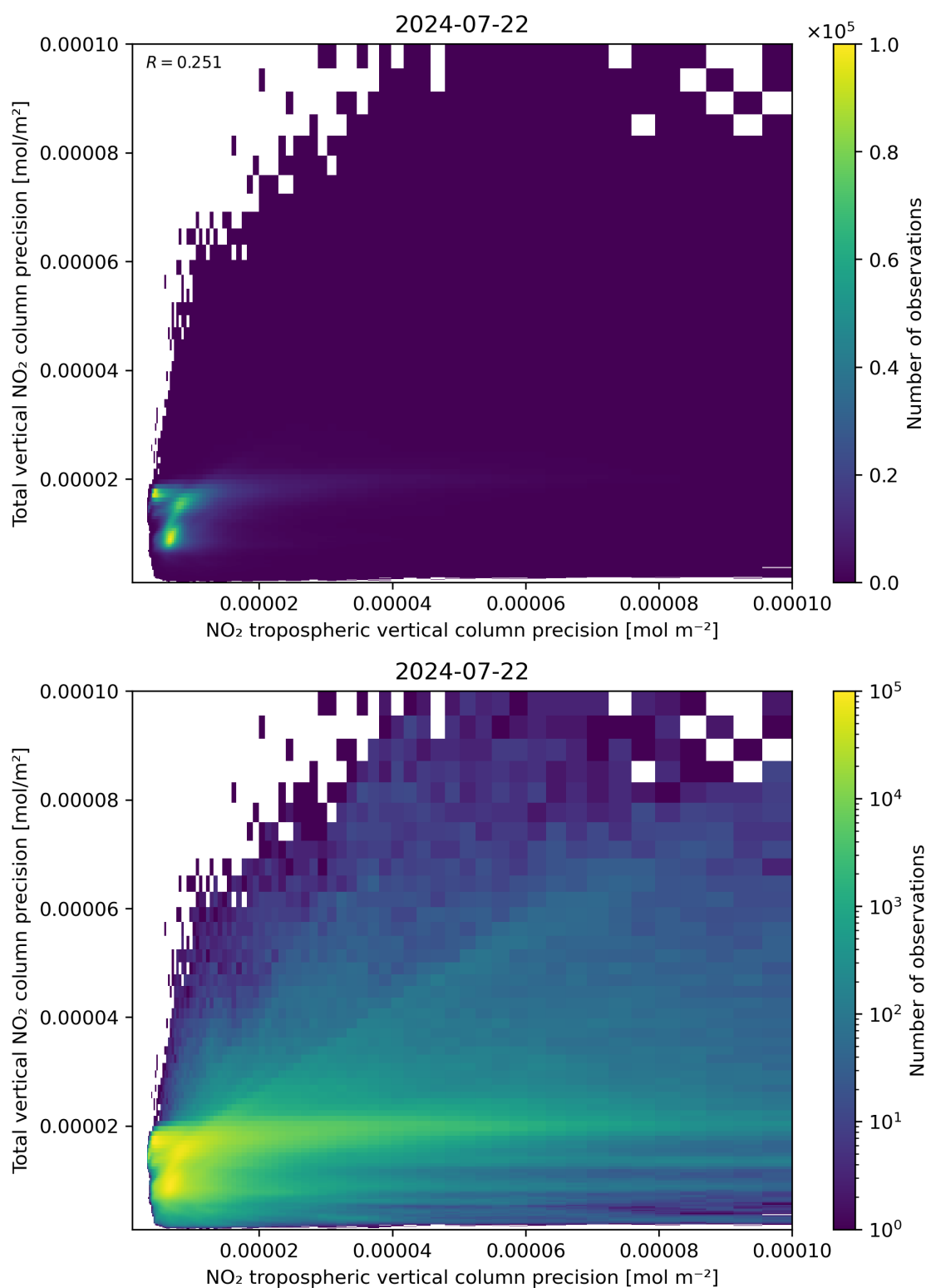
Figure 139: Scatter density plot of “NO 2 tropospheric vertical column precision” against “Total vertical NO 2 column precision” for 2024-07-21 to 2024-07-23.
