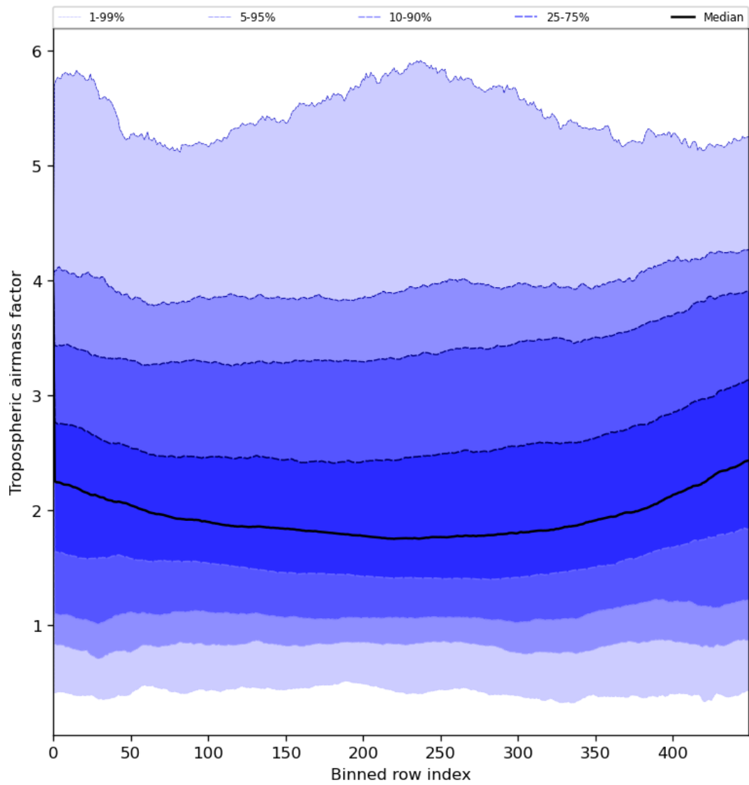
Figure 48: Along track statistics of “Tropospheric airmass factor” for 2024-07-21 to 2024-07-23
