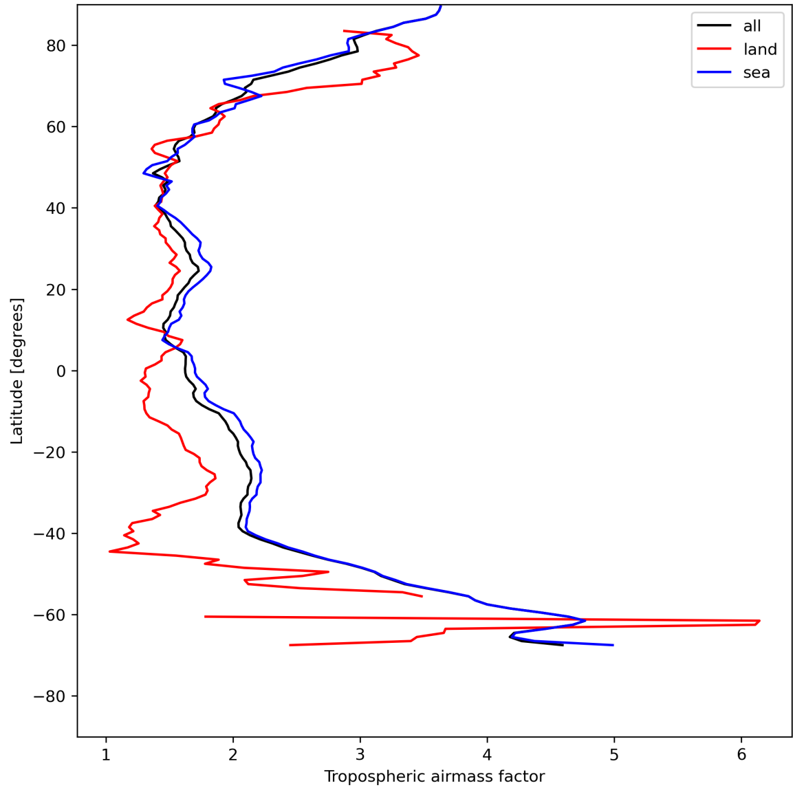
Figure 14: Zonal average of “Tropospheric airmass factor” for 2024-07-21 to 2024-07-23.
