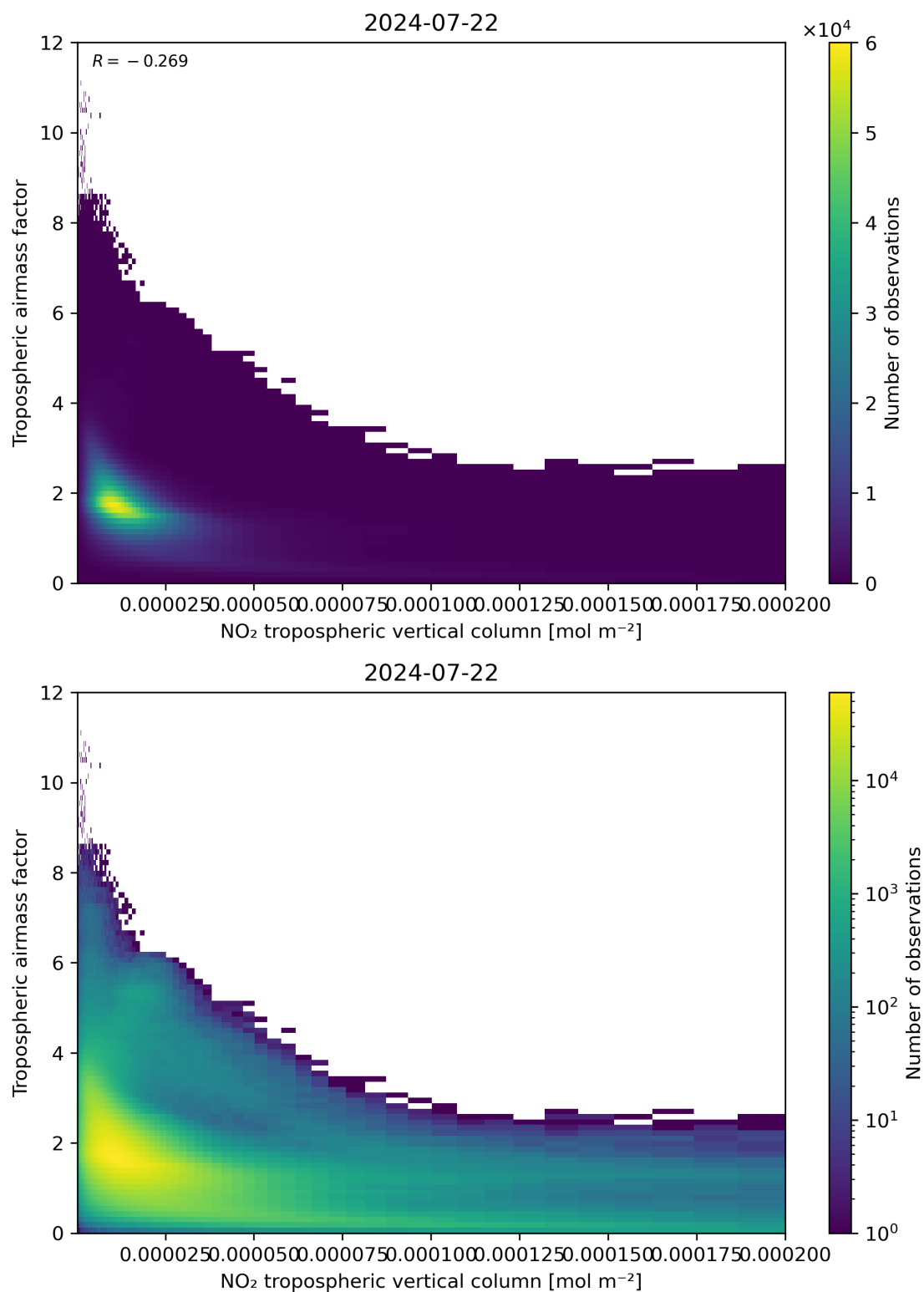
Figure 123: Scatter density plot of “NO 2 tropospheric vertical column” against “Tropospheric airmass factor” for 2024-07-21 to 2024-07-23.
