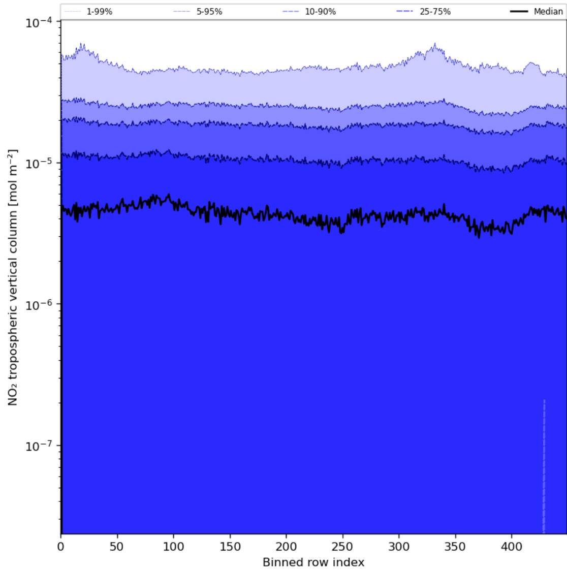
Figure 46: Along track statistics of “NO 2 tropospheric vertical column” for 2024-07-21 to 2024-07-23
