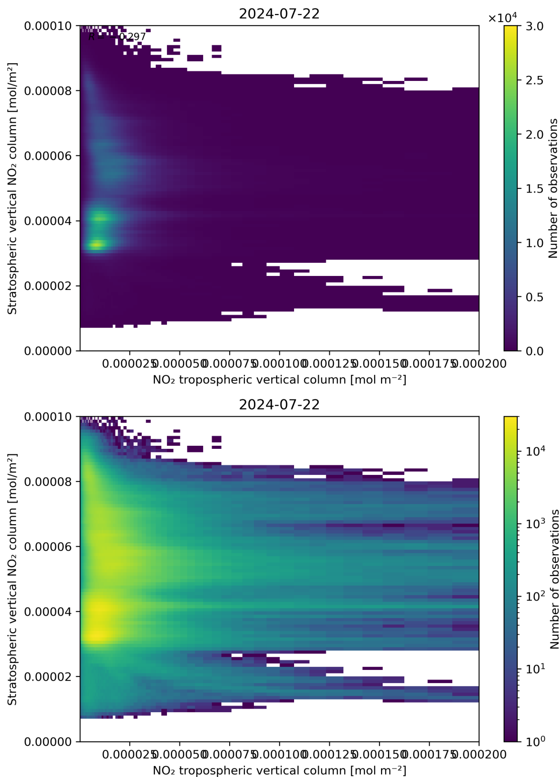
Figure 125: Scatter density plot of “NO 2 tropospheric vertical column” against “Stratospheric vertical NO 2 column” for 2024-07-21 to 2024-07-23.
