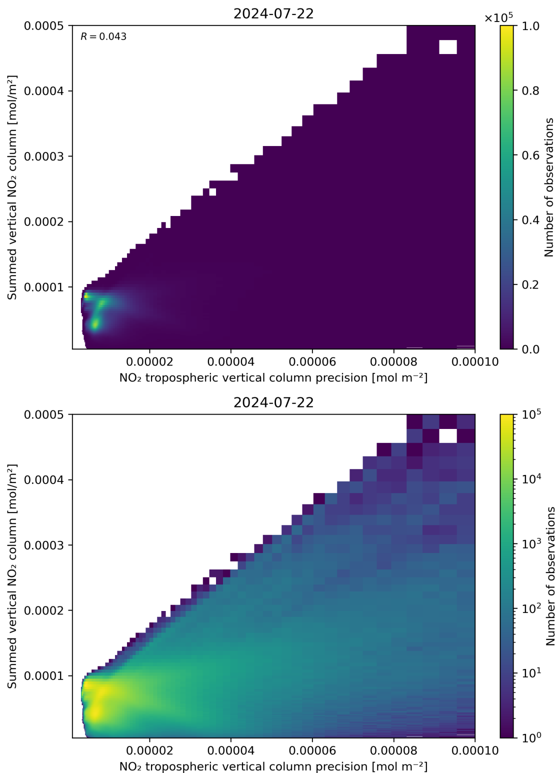
Figure 136: Scatter density plot of “NO 2 tropospheric vertical column precision” against “Summed vertical NO 2 column” for 2024-07-21 to 2024-07-23.
