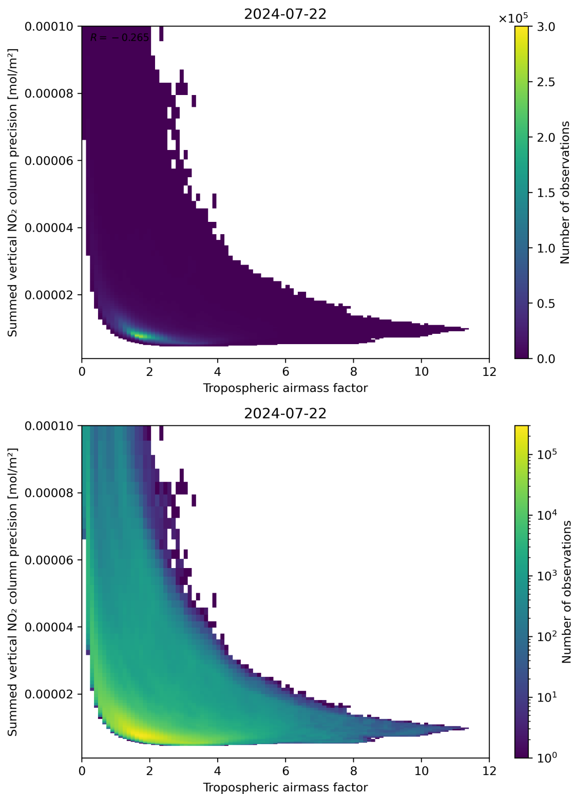
Figure 76: Scatter density plot of “Tropospheric air mass factor” against “Summed vertical NO 2 column precision” for 2024-07-21 to 2024-07-23.
