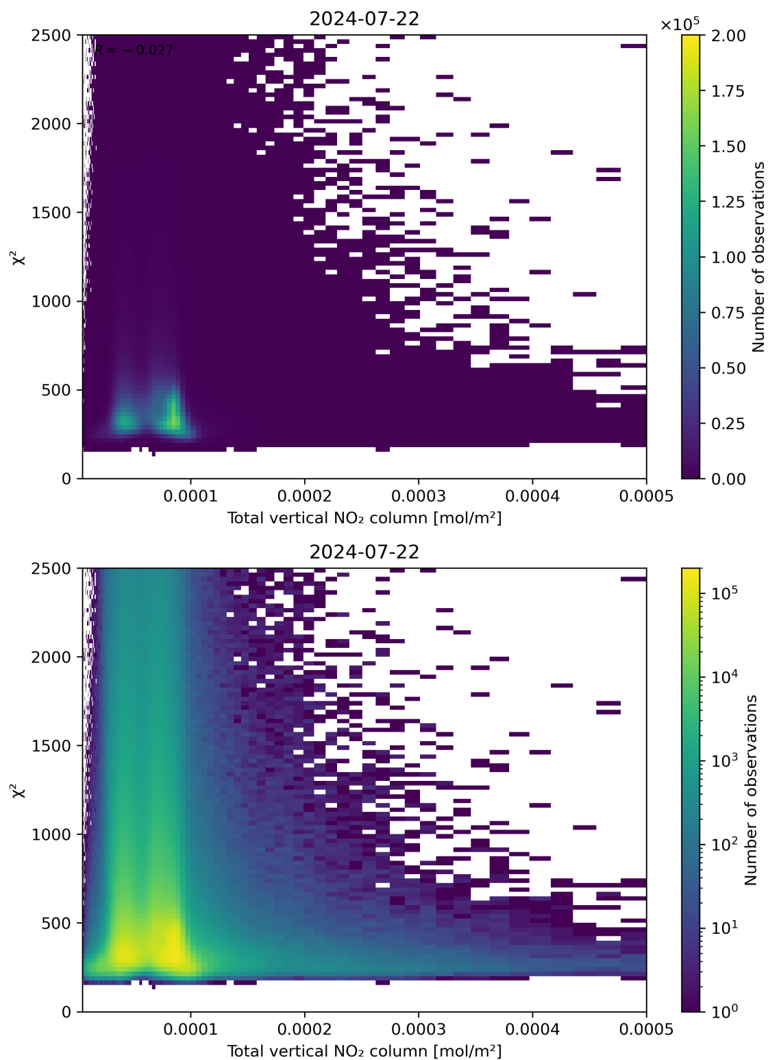
Figure 111: Scatter density plot of “Total vertical NO 2 column” against “ \chi^2 ” for 2024-07-21 to 2024-07-23.
