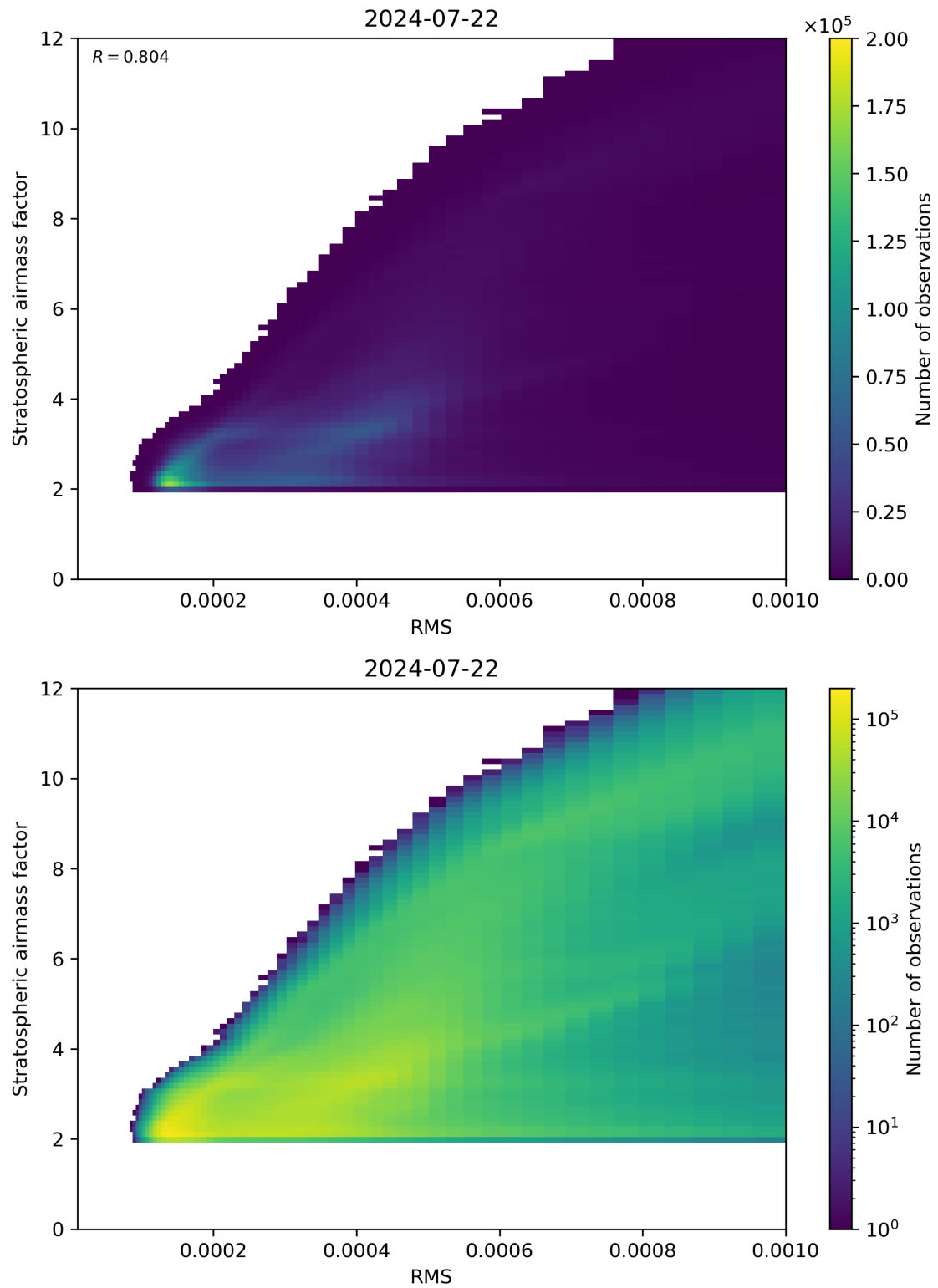
Figure 144: Scatter density plot of “RMS” against “Stratospheric airmass factor” for 2024-07-21 to 2024-07-23.
