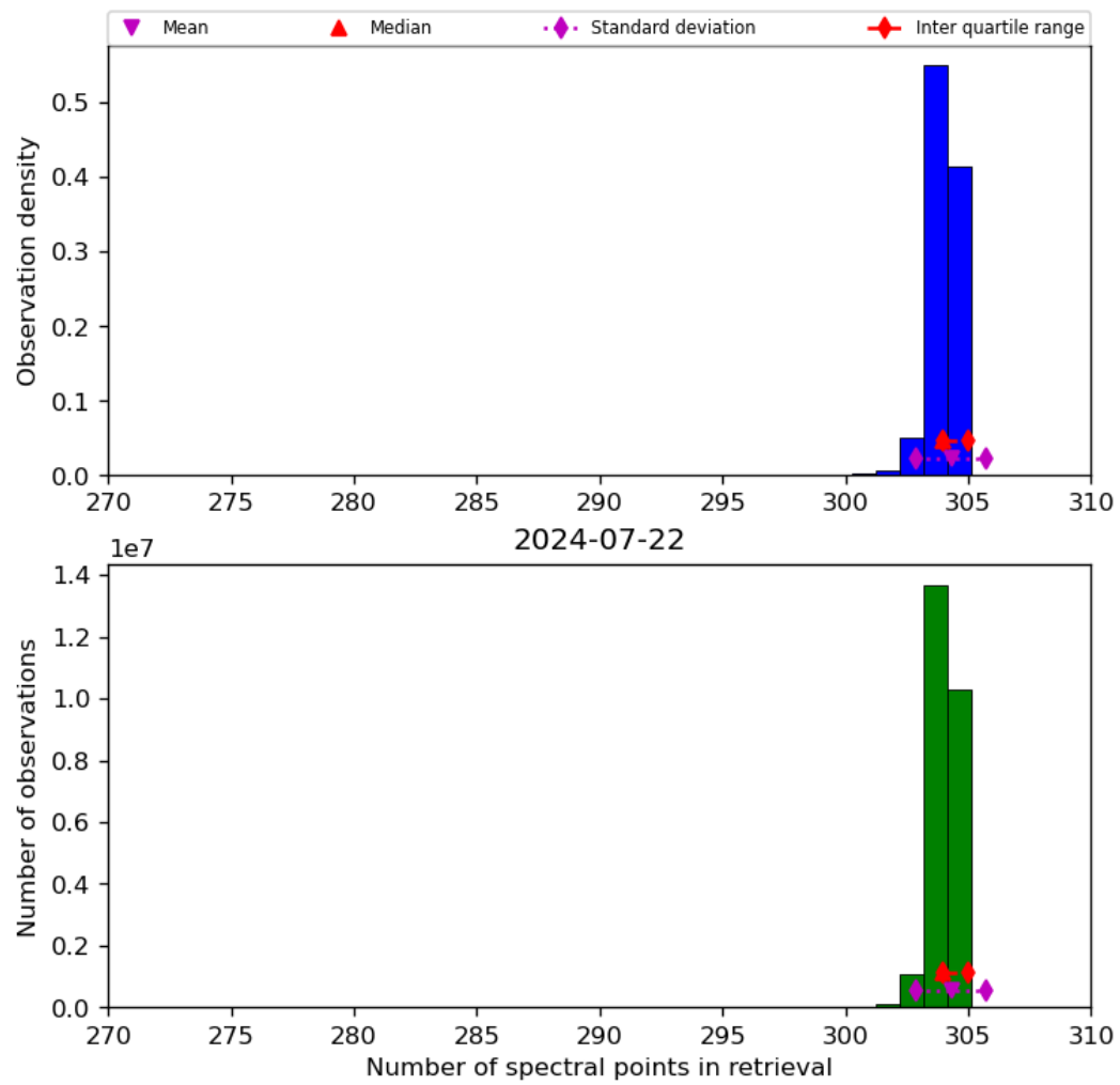
Figure 33: Histogram of “Number of spectral points in retrieval” for 2024-07-21 to 2024-07-23
