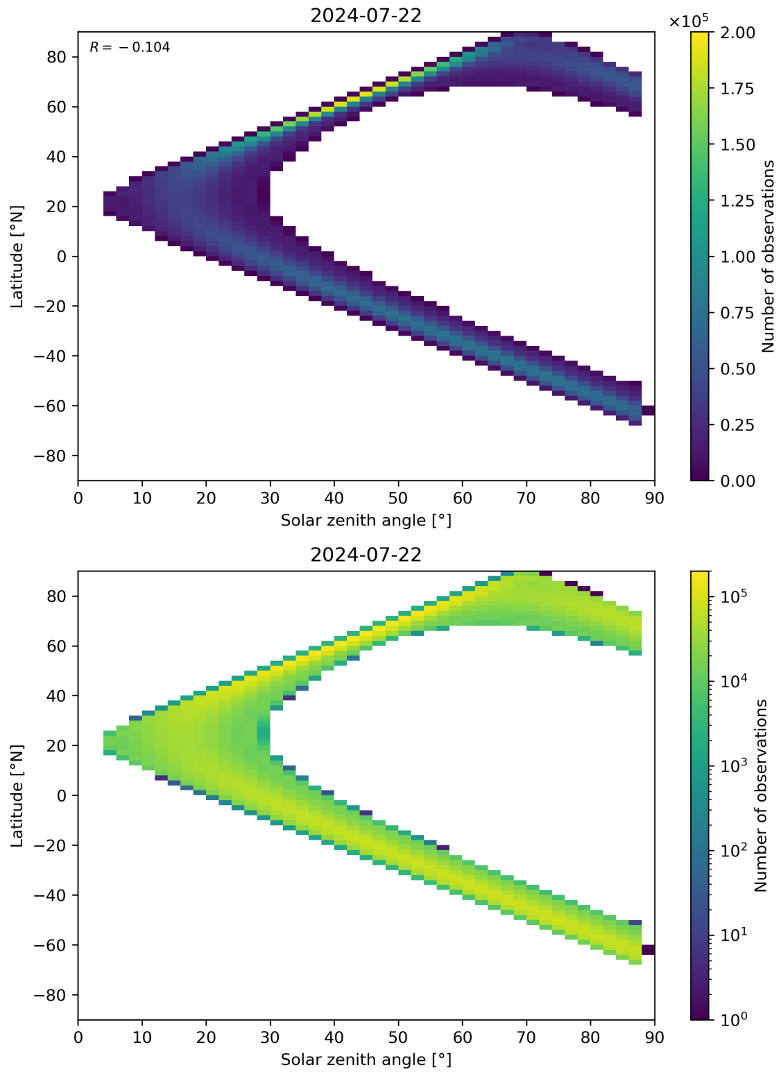
Figure 149: Scatter density plot of “Solar zenith angle” against “Latitude” for 2024-07-21 to 2024-07-23.
