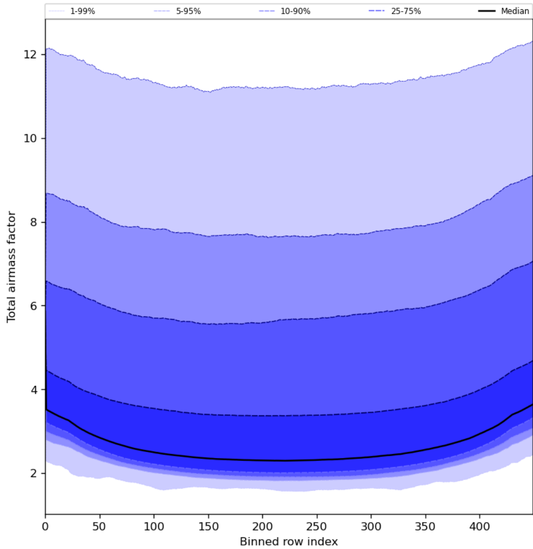
Figure 49: Along track statistics of “Total airmass factor” for 2024-07-21 to 2024-07-23
