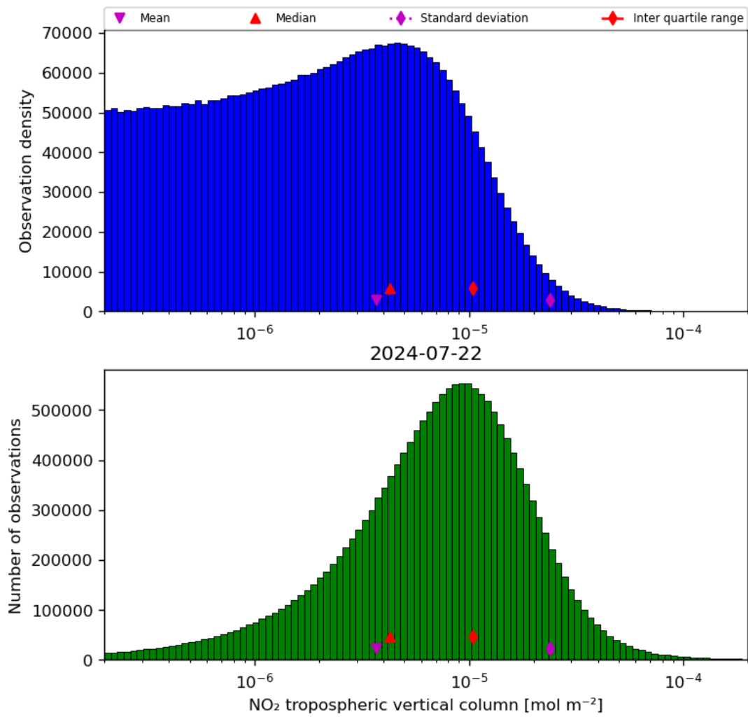
Figure 29: Histogram of “NO 2 tropospheric vertical column” for 2024-07-21 to 2024-07-23
