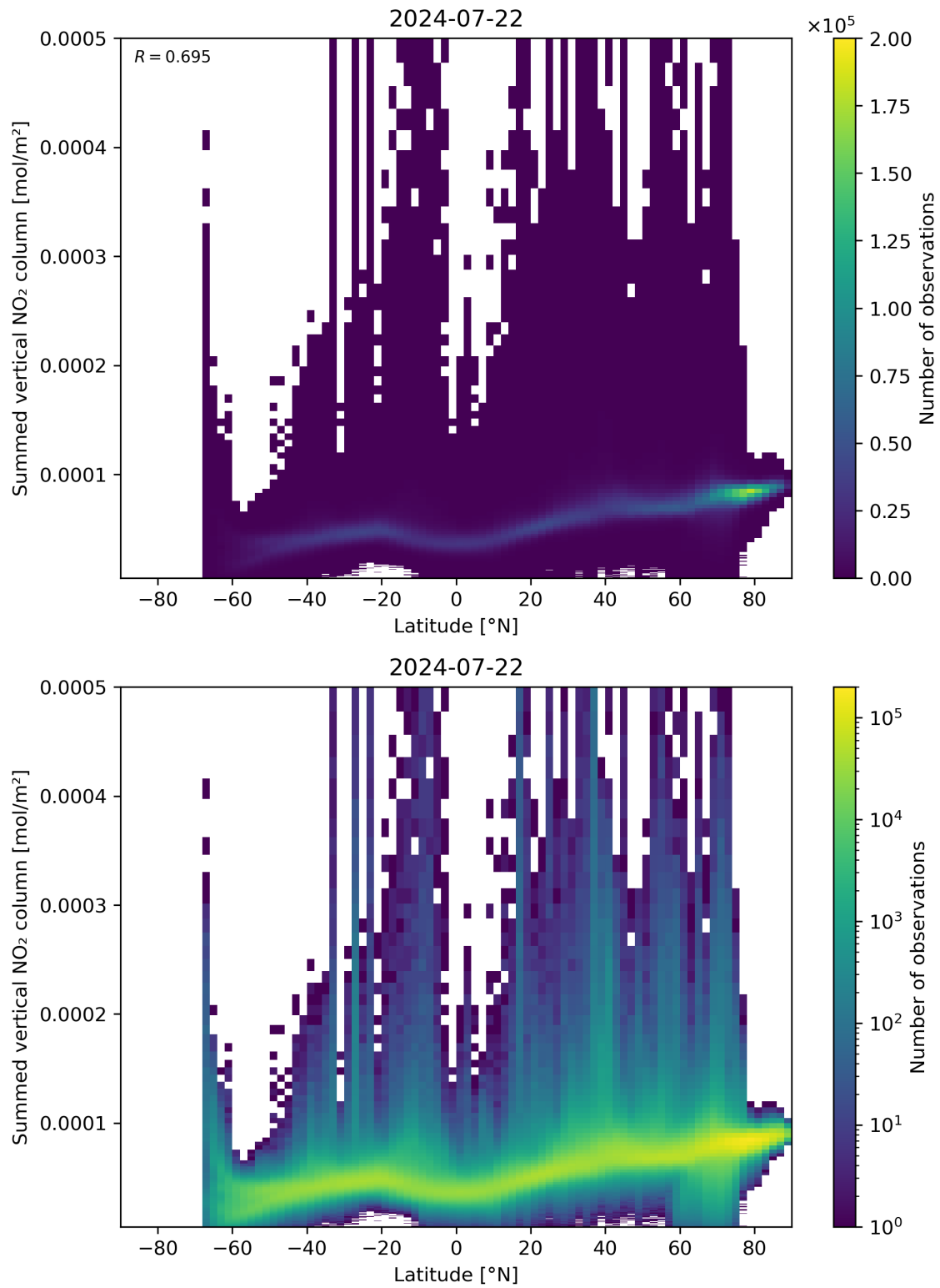
Figure 88: Scatter density plot of “Latitude” against “Summed vertical NO 2 column” for 2024-07-21 to 2024-07-23.
