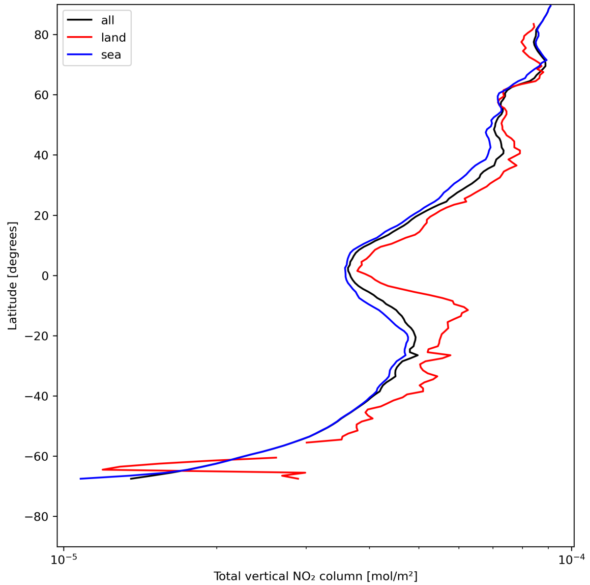
Figure 21: Zonal average of “Total vertical NO 2 column” for 2024-07-21 to 2024-07-23.
