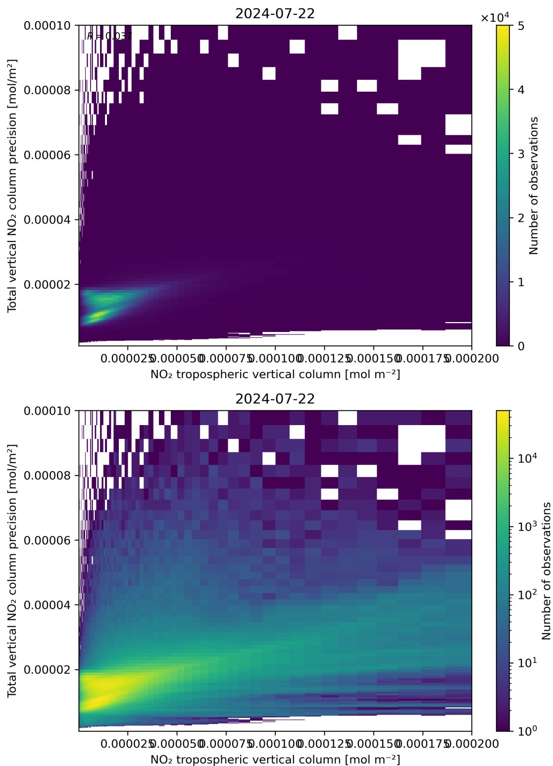
Figure 129: Scatter density plot of “NO 2 tropospheric vertical column” against “Total vertical NO 2 column precision” for 2024-07-21 to 2024-07-23.
