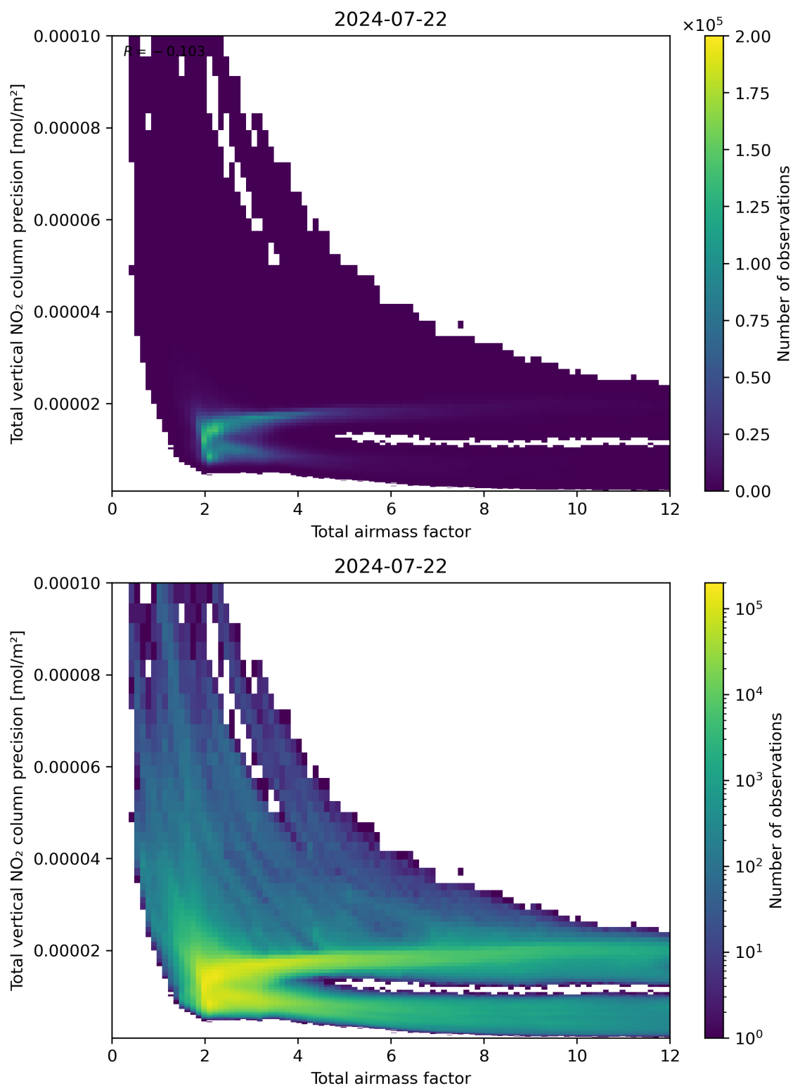
Figure 68: Scatter density plot of “Total airmass factor” against “Total vertical NO 2 column precision” for 2024-07-21 to 2024-07-23.
