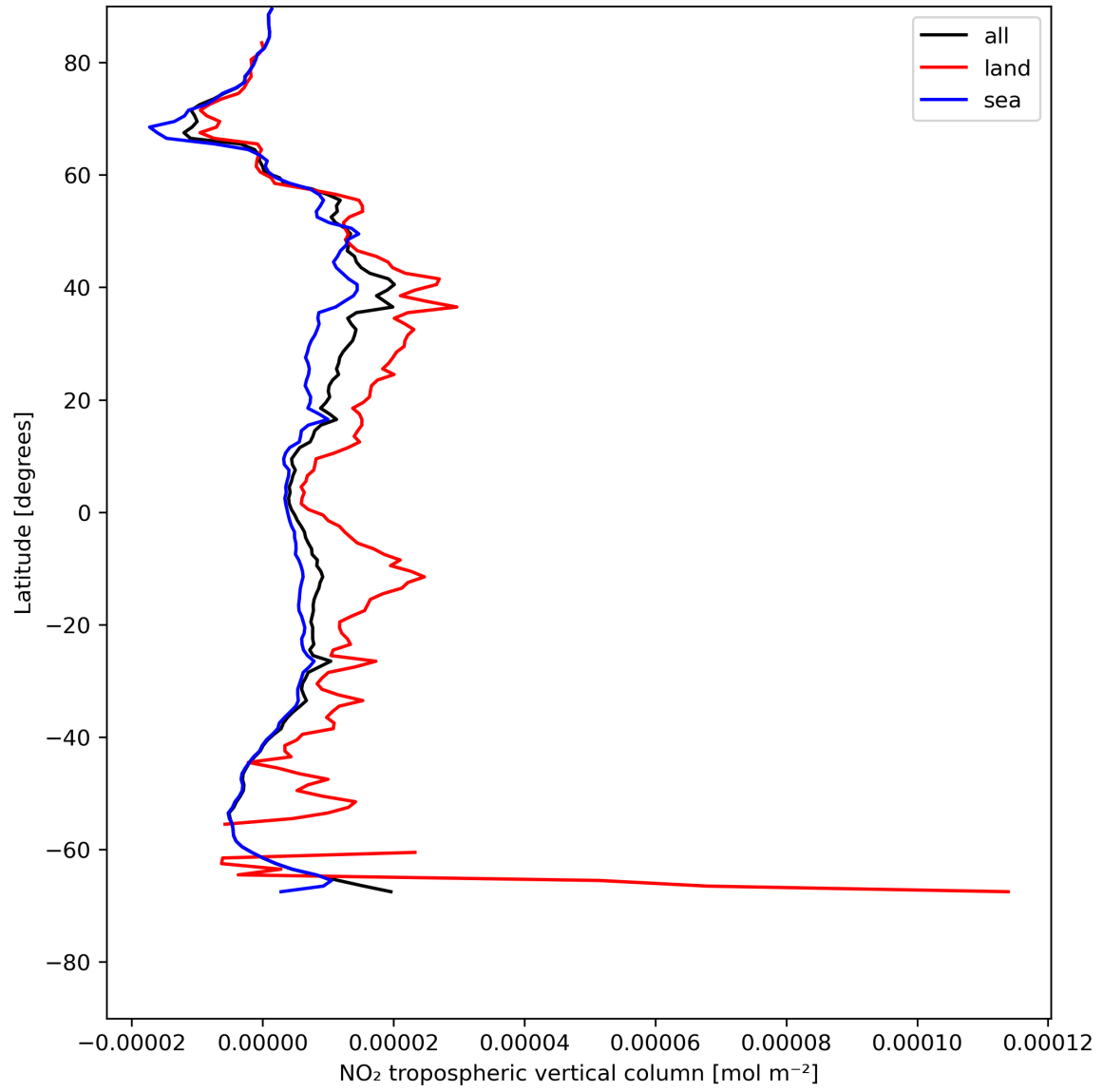
Figure 12: Zonal average of “NO 2 tropospheric vertical column” for 2024-07-21 to 2024-07-23.
