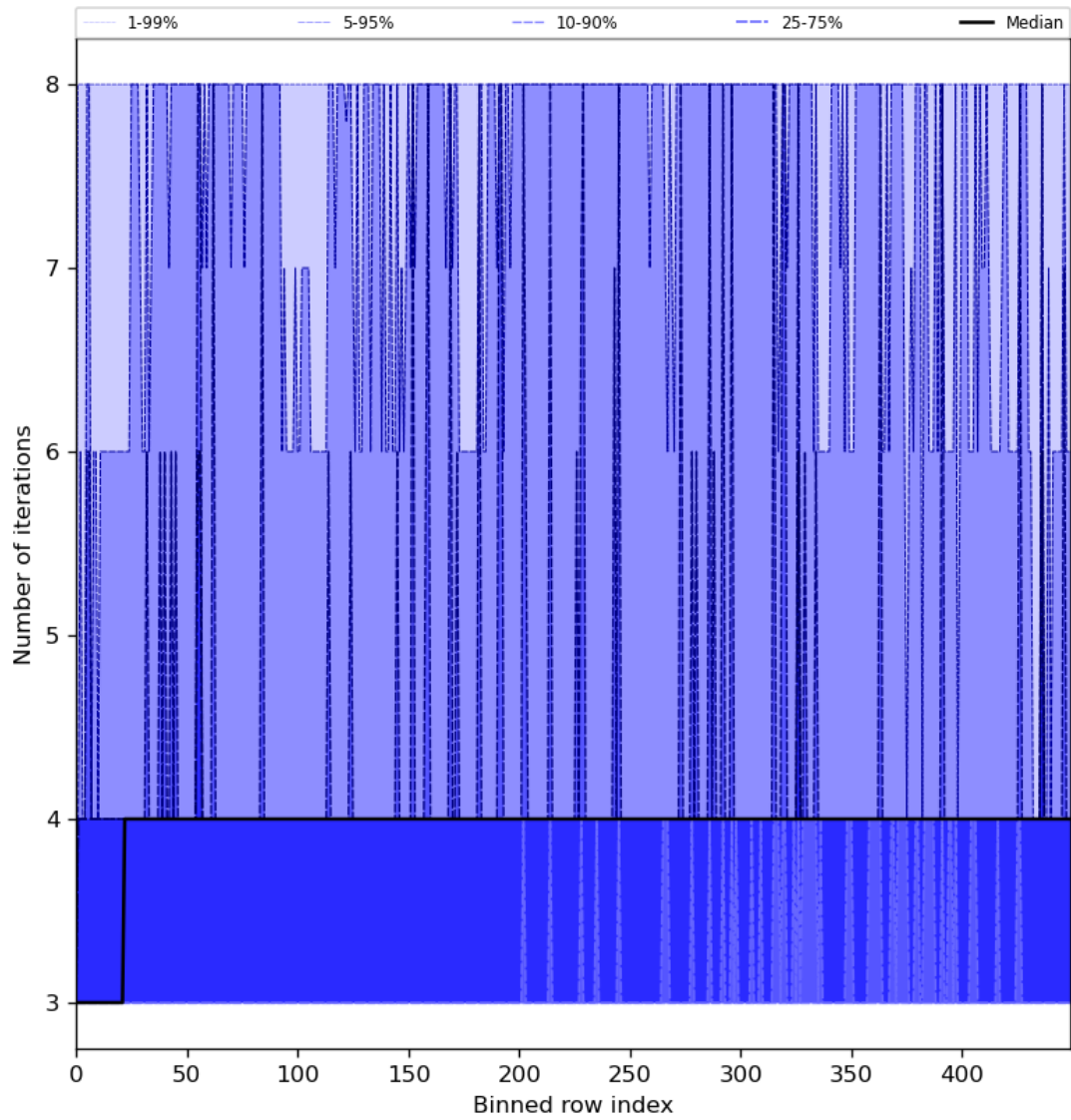
Figure 51: Along track statistics of “Number of iterations” for 2024-07-21 to 2024-07-23
