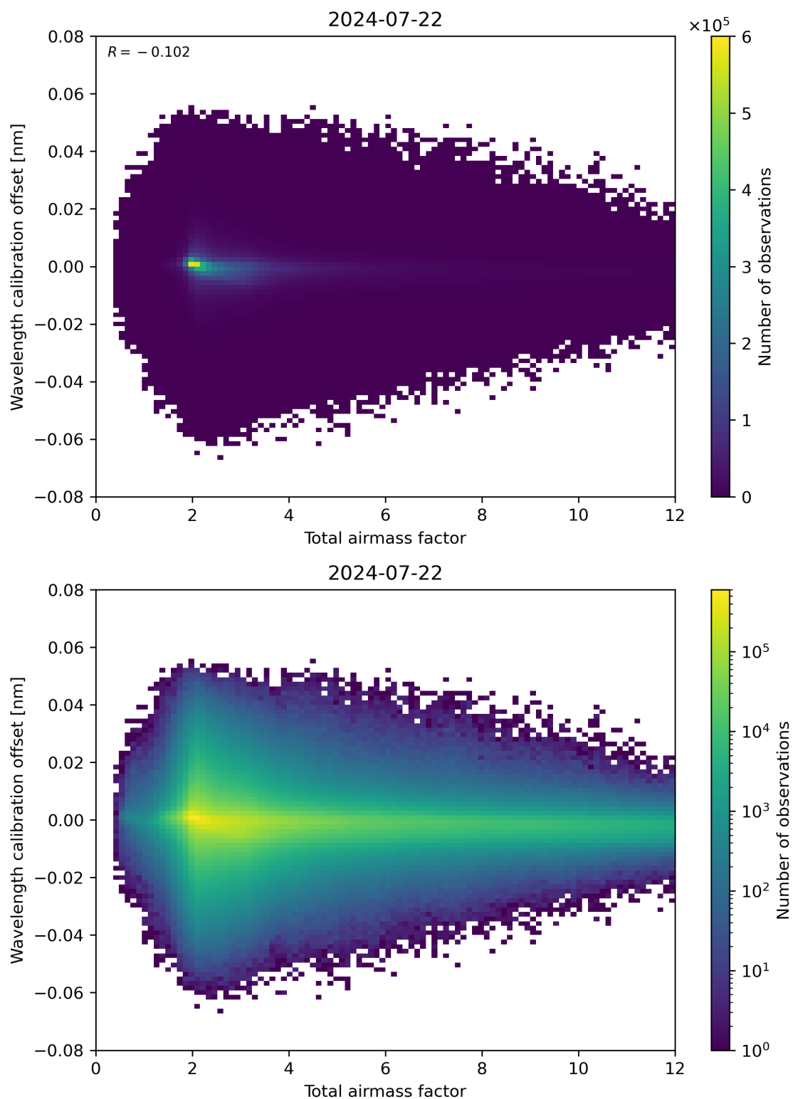
Figure 70: Scatter density plot of “Total airmass factor” against “Wavelength calibration offset” for 2024-07-21 to 2024-07-23.
