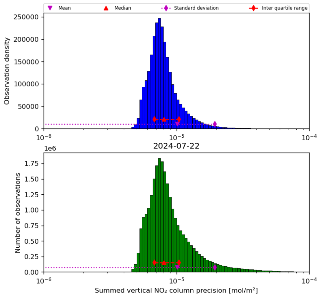
Figure 41: Histogram of “Summed vertical NO 2 column precision” for 2024-07-21 to 2024-07-23
