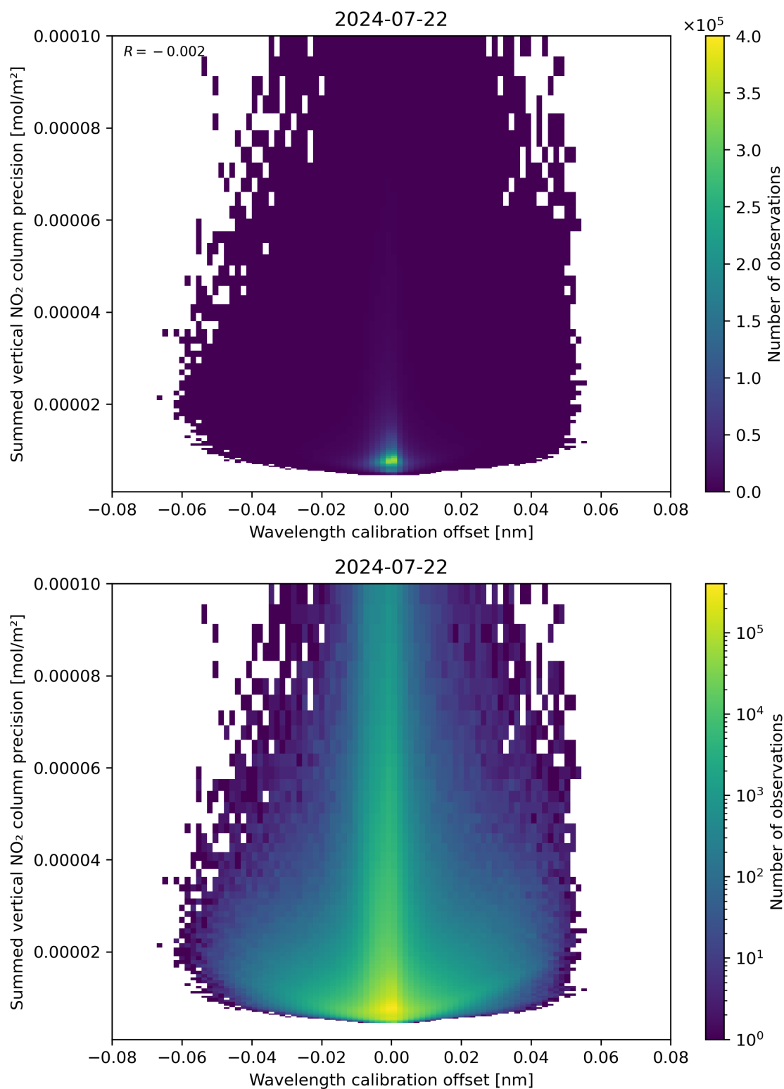
Figure 178: Scatter density plot of “Wavelength calibration offset” against “Summed vertical NO 2 column precision” for 2024-07-21 to 2024-07-23.
