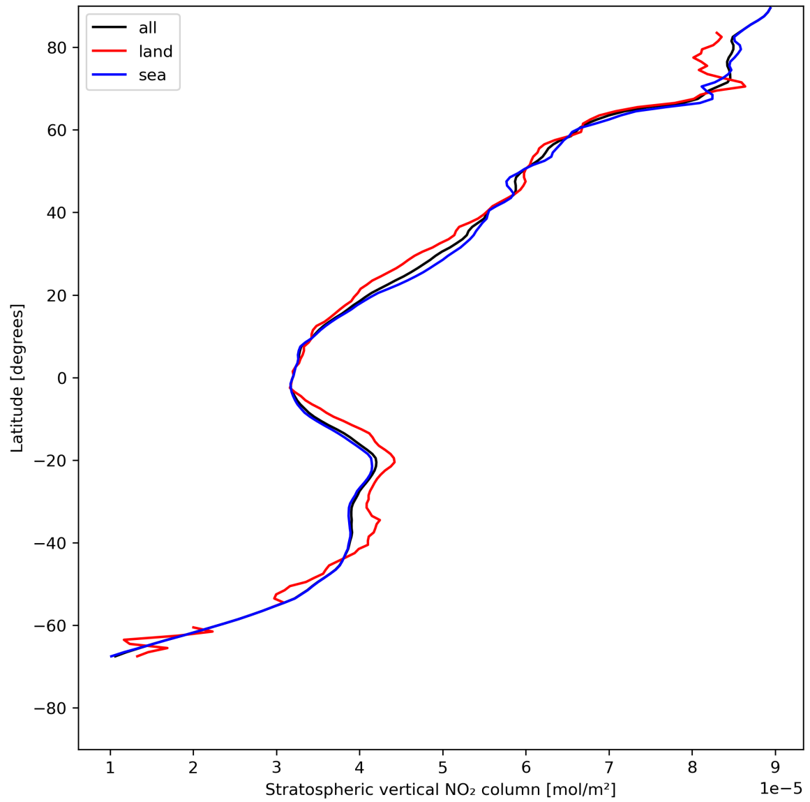
Figure 19: Zonal average of “Stratospheric vertical NO 2 column” for 2024-07-21 to 2024-07-23.
