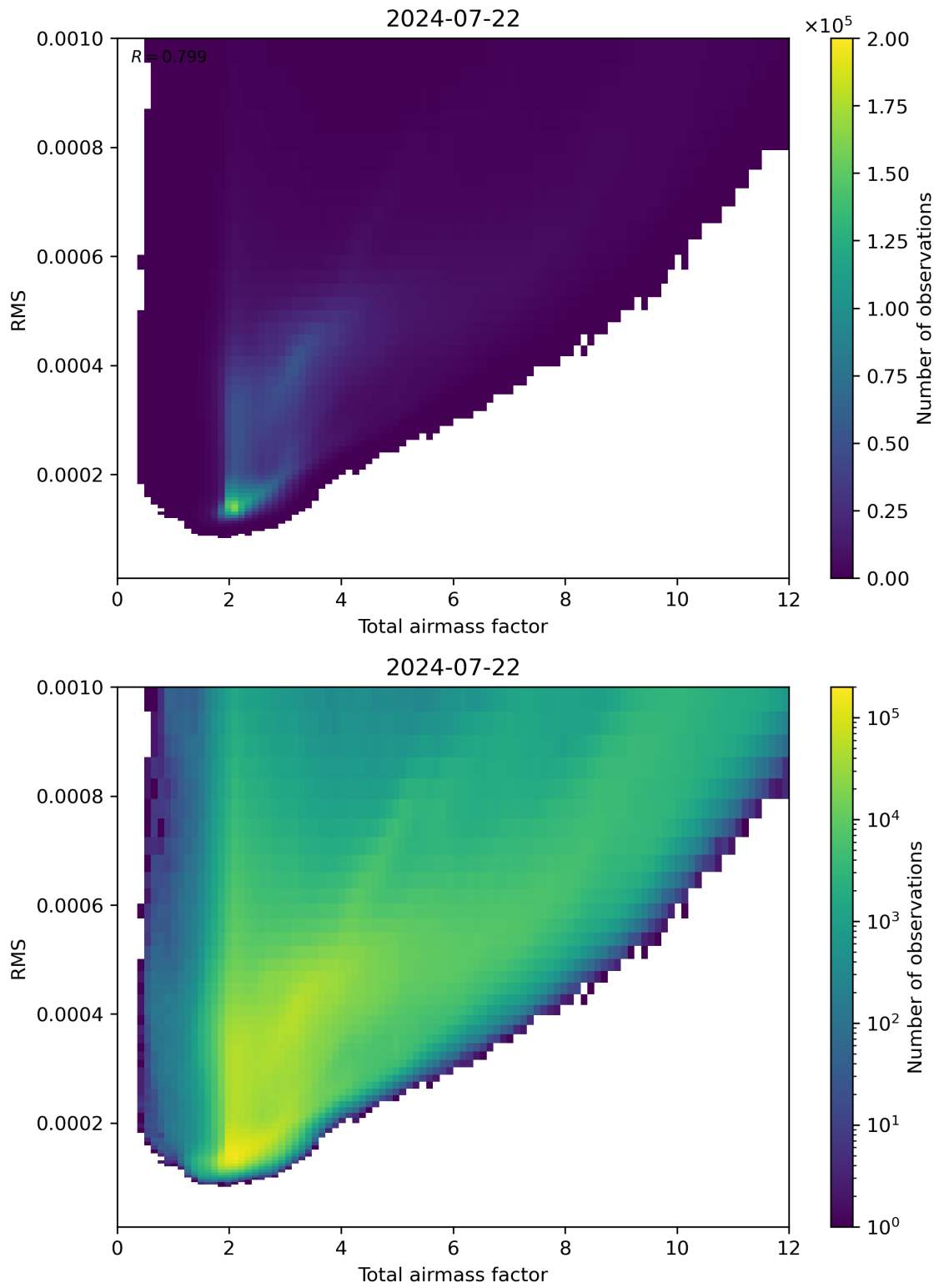
Figure 69: Scatter density plot of “Total airmass factor” against “RMS” for 2024-07-21 to 2024-07-23.
