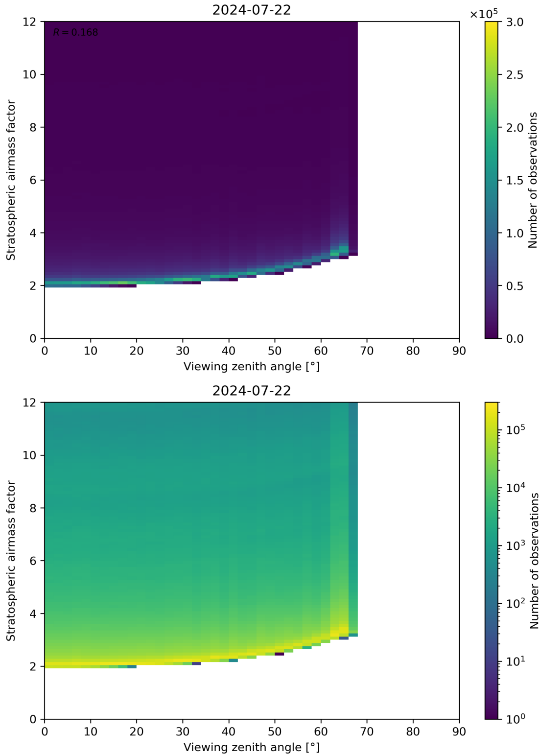
Figure 159: Scatter density plot of “Viewing zenith angle” against “Stratospheric airmass factor” for 2024-07-21 to 2024-07-23.
