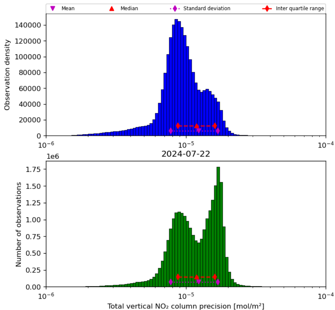
Figure 39: Histogram of “Total vertical NO 2 column precision” for 2024-07-21 to 2024-07-23
