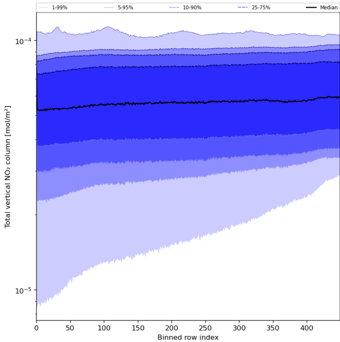
Figure 55: Along track statistics of “Total vertical NO 2 column” for 2024-07-21 to 2024-07-23
