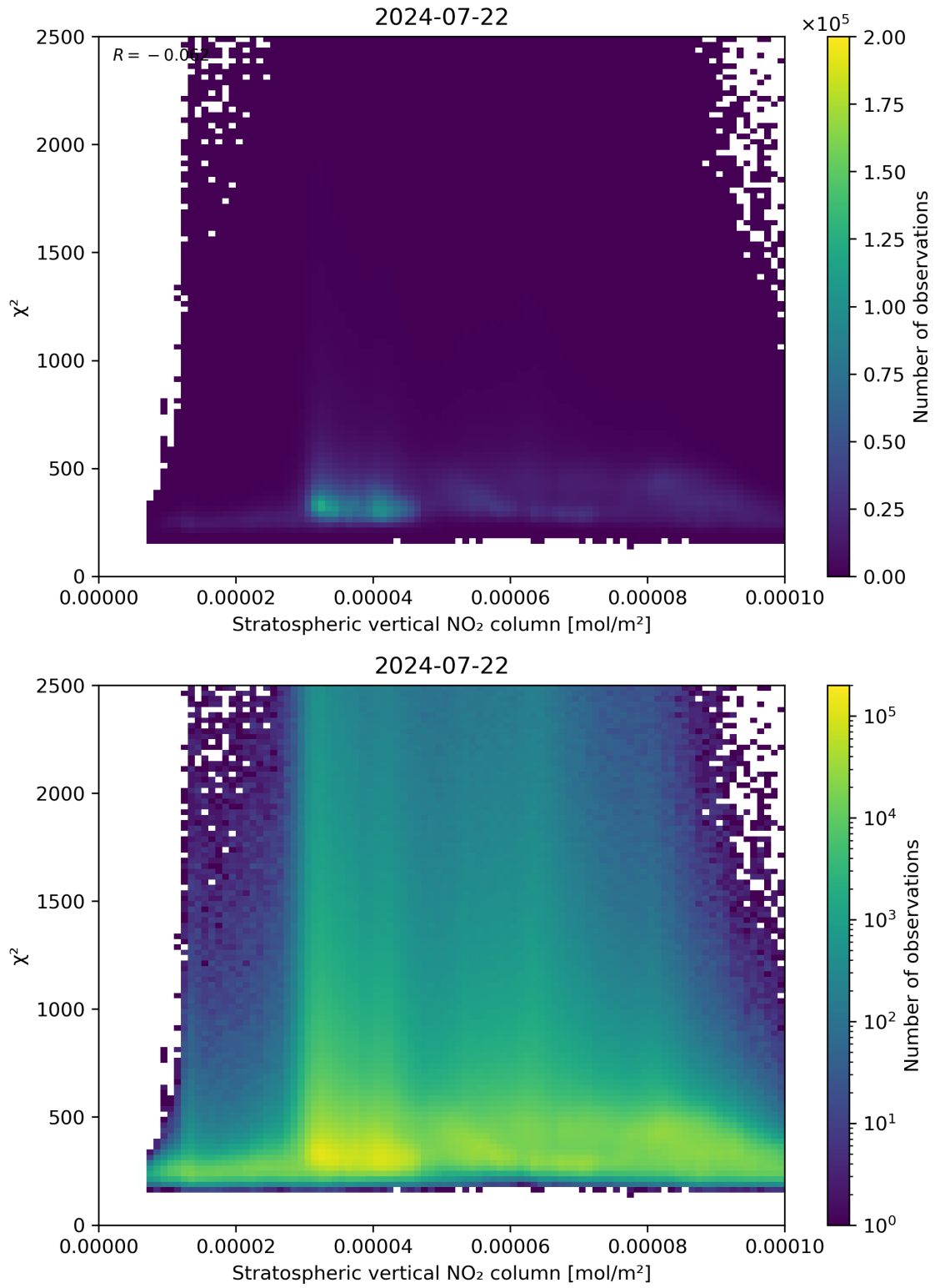
Figure 97: Scatter density plot of “Stratospheric vertical NO 2 column” against “ \chi^2 ” for 2024-07-21 to 2024-07-23.
