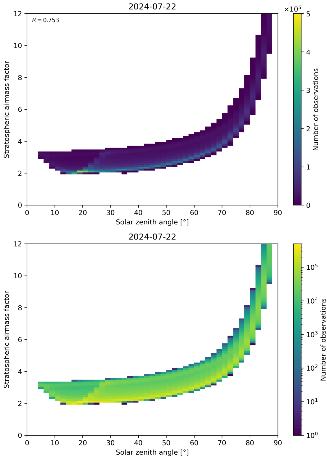
Figure 145: Scatter density plot of “Solar zenith angle” against “Stratospheric airmass factor” for 2024-07-21 to 2024-07-23.
