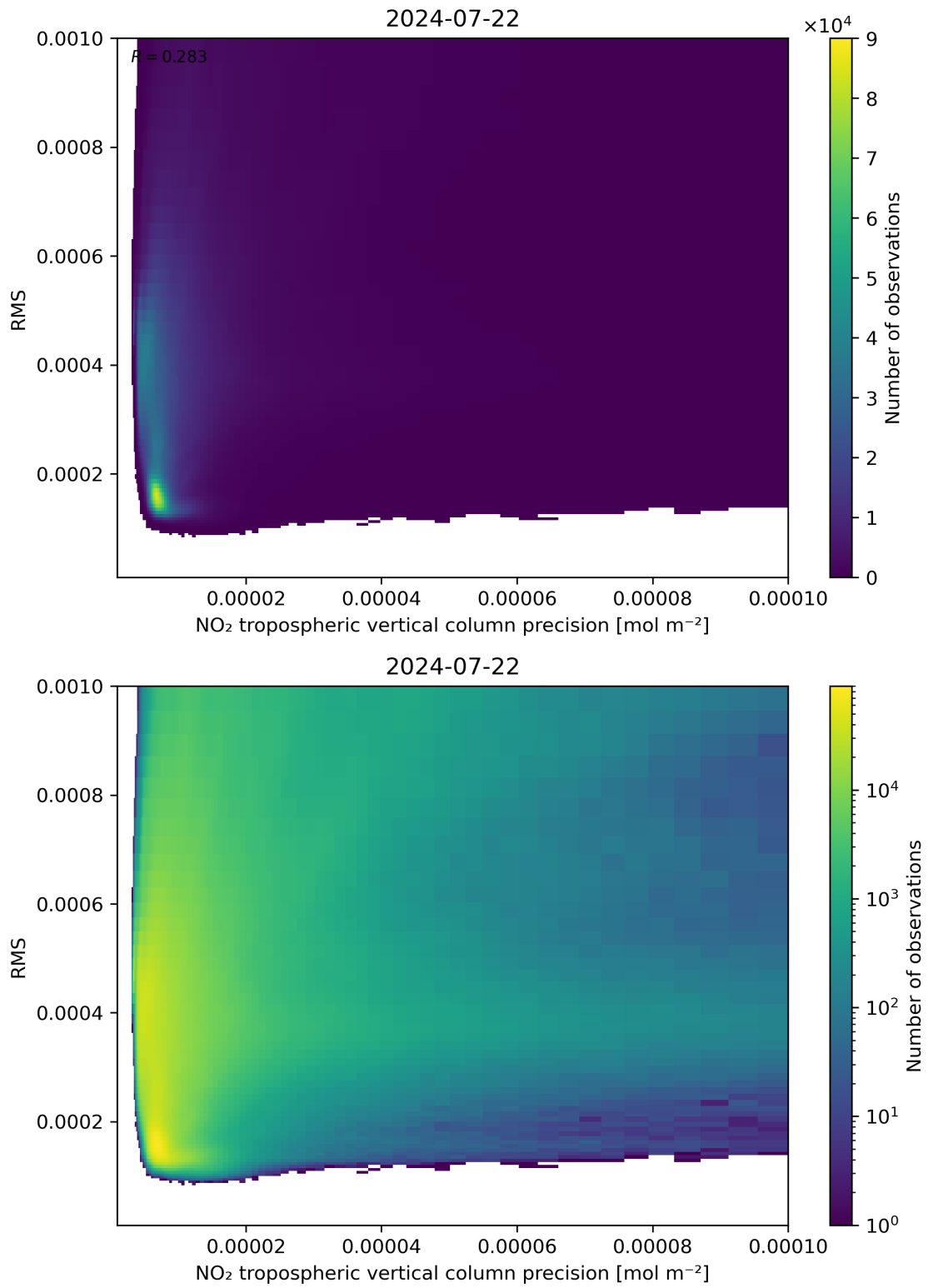
Figure 140: Scatter density plot of “NO 2 tropospheric vertical column precision” against “RMS” for 2024-07-21 to 2024-07-23.
