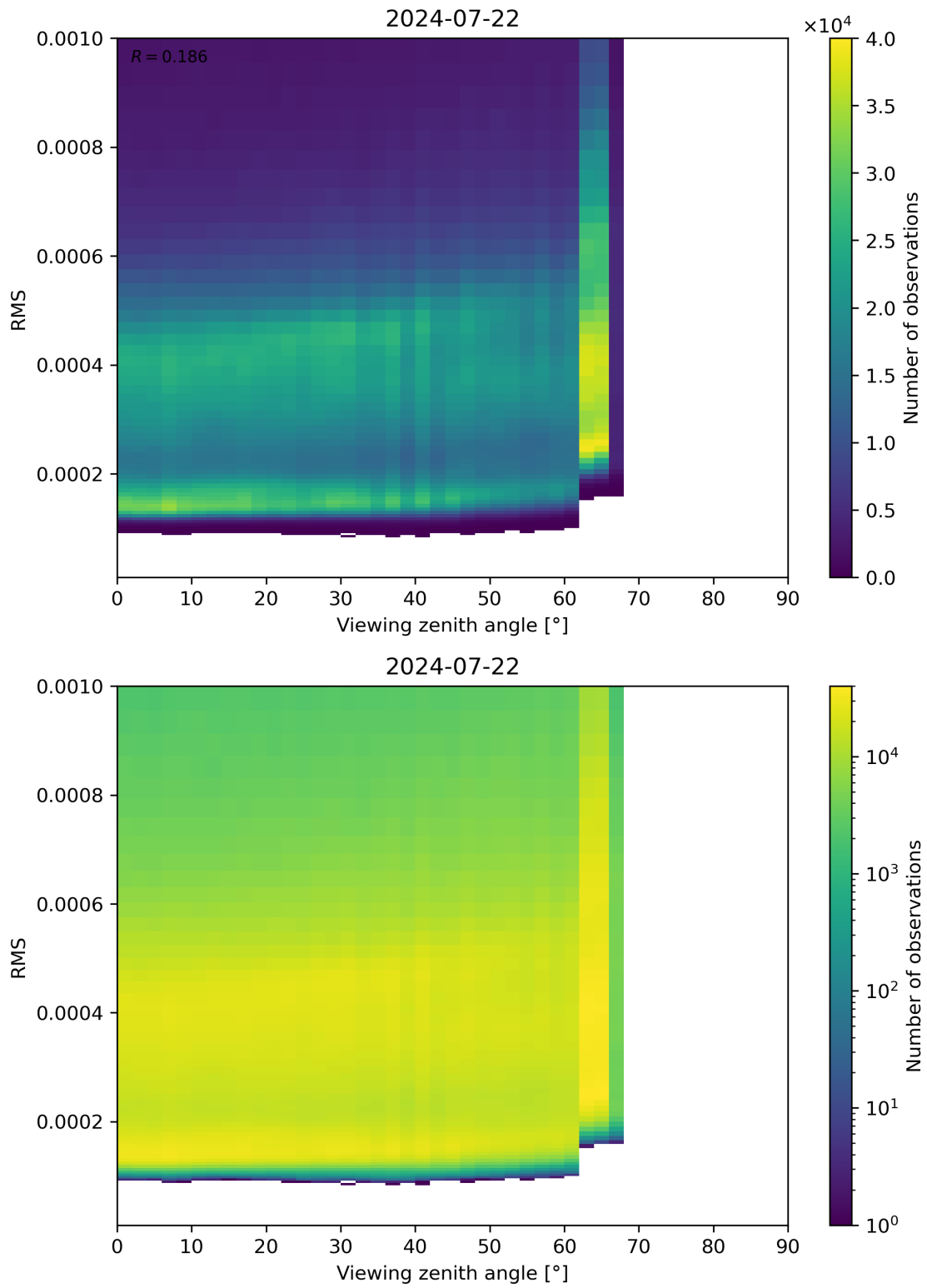
Figure 171: Scatter density plot of “Viewing zenith angle” against “RMS” for 2024-07-21 to 2024-07-23.
