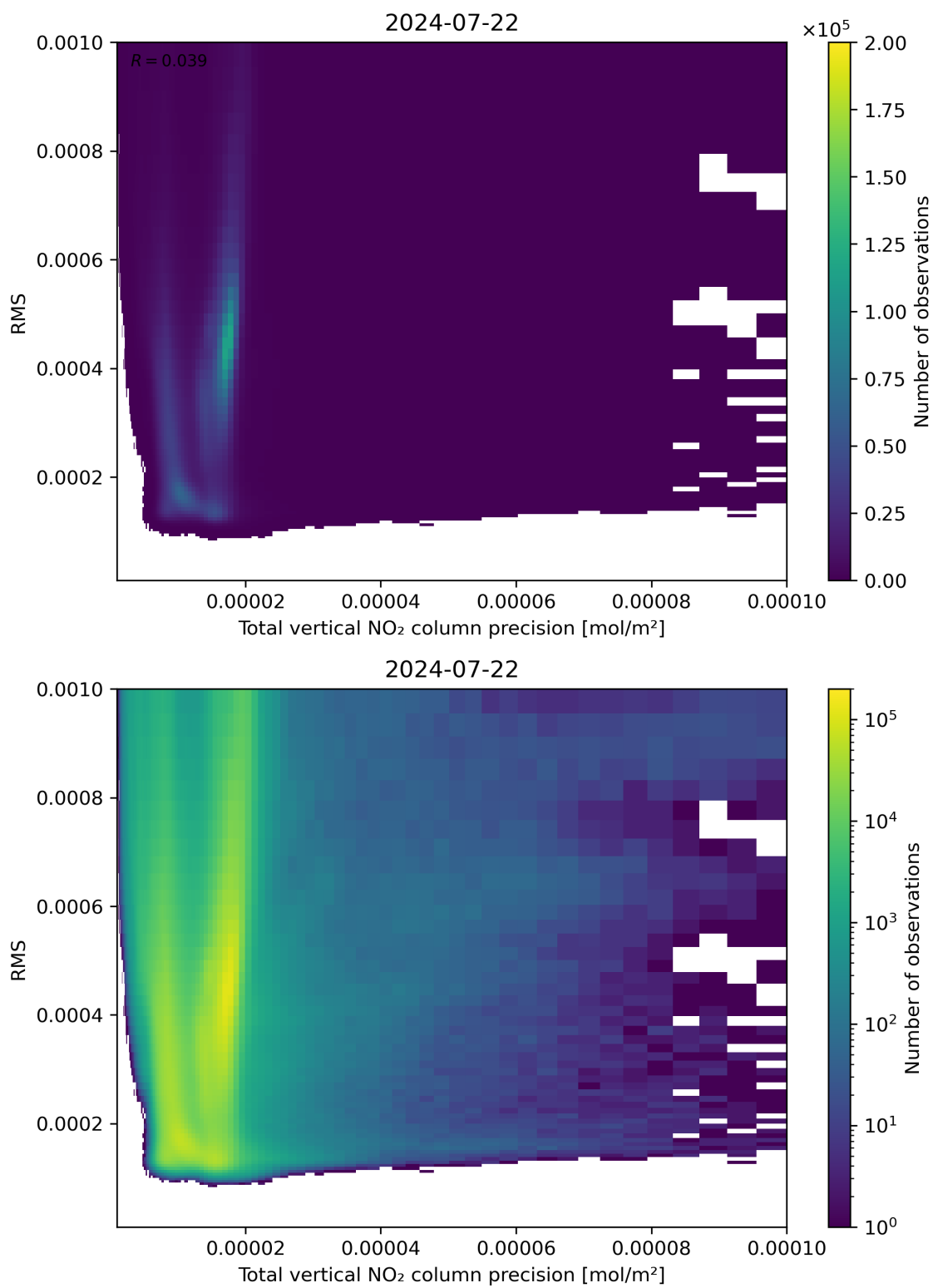
Figure 119: Scatter density plot of “Total vertical NO 2 column precision” against “RMS” for 2024-07-21 to 2024-07-23.
