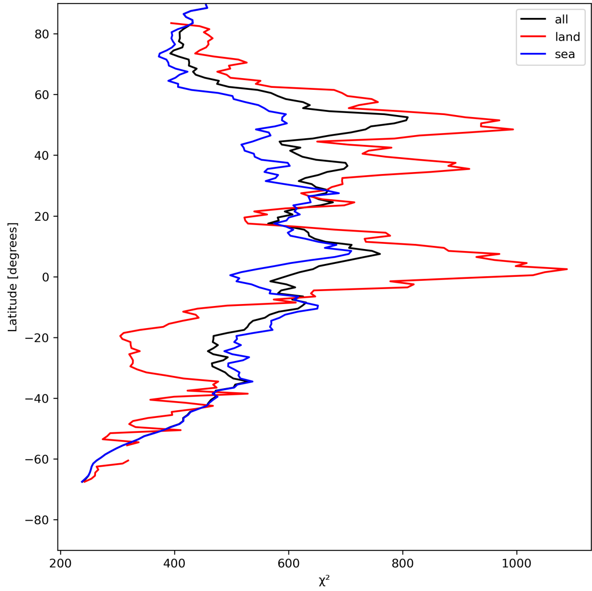
Figure 25: Zonal average of “ \chi^2 ” for 2024-07-21 to 2024-07-23.
