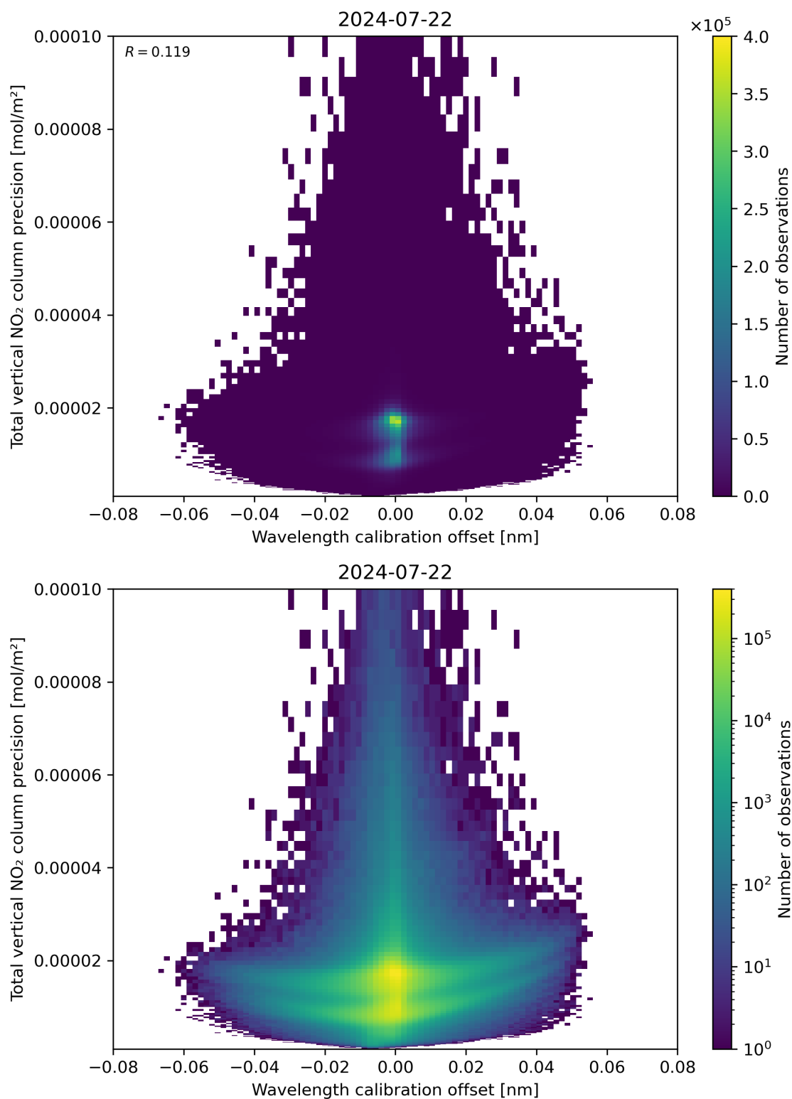
Figure 180: Scatter density plot of “Wavelength calibration offset” against “Total vertical NO 2 column precision” for 2024-07-21 to 2024-07-23.
