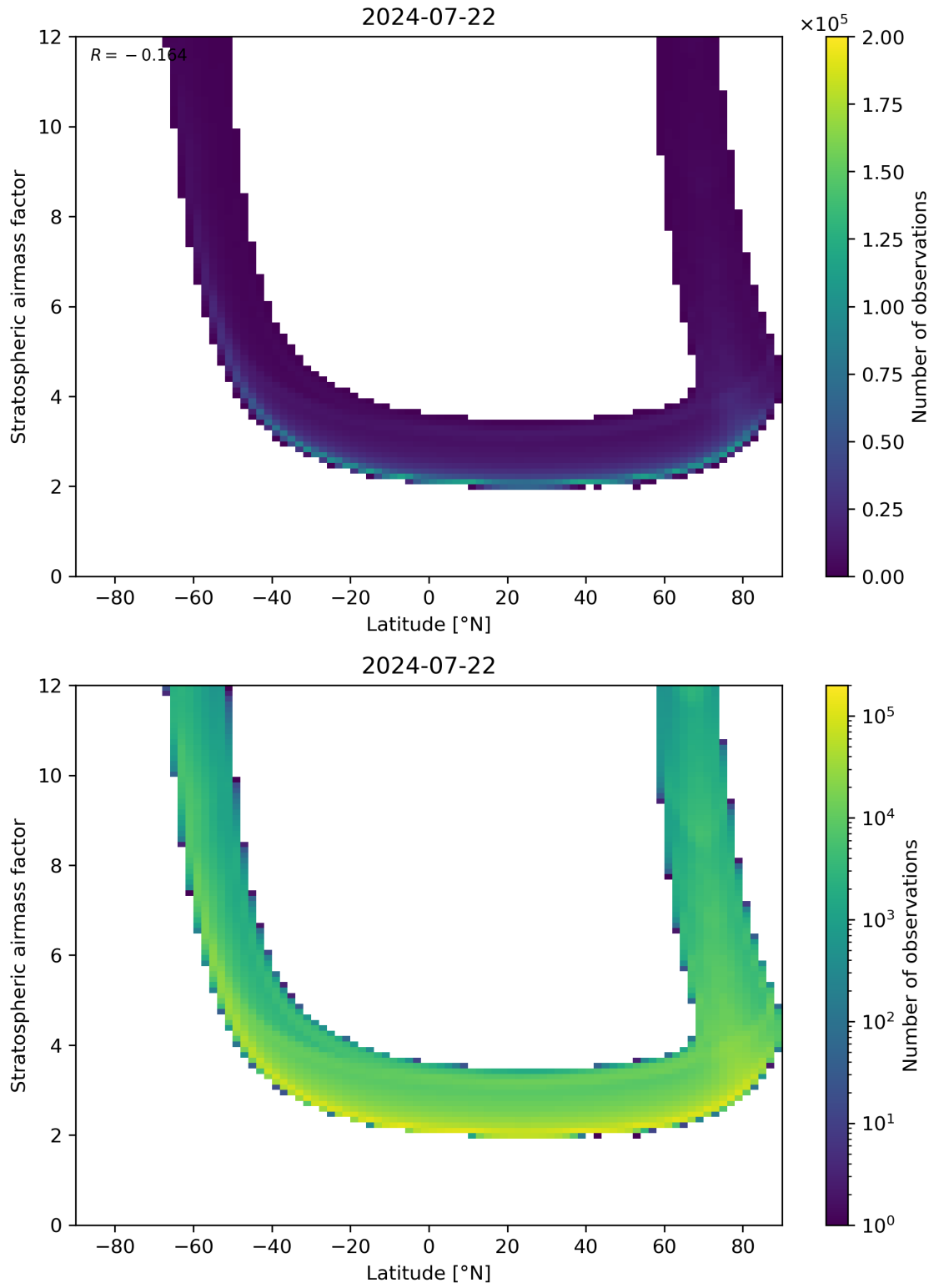
Figure 83: Scatter density plot of “Latitude” against “Stratospheric air mass factor” for 2024-07-21 to 2024-07-23.
