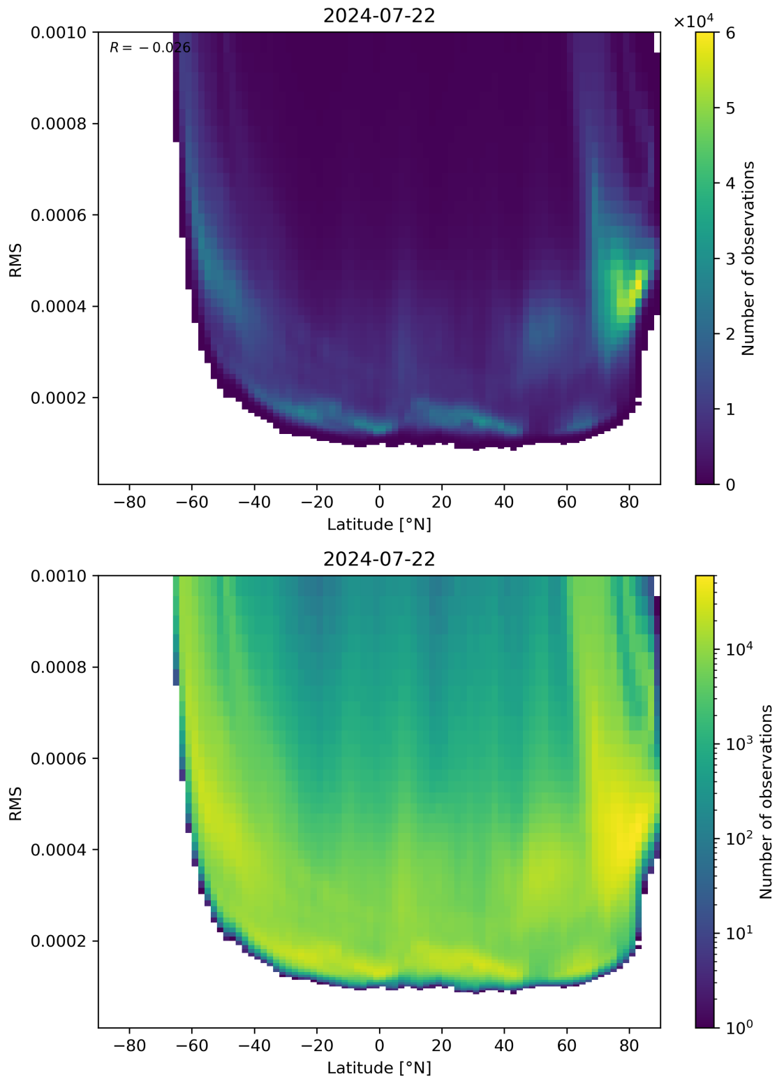
Figure 94: Scatter density plot of “Latitude” against “RMS” for 2024-07-21 to 2024-07-23.
