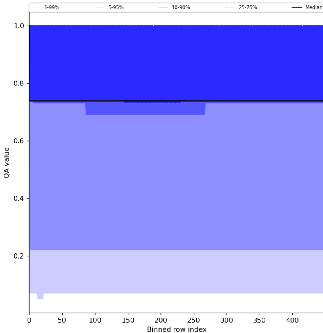
Figure 45: Along track statistics of “QA value” for 2024-07-21 to 2024-07-23
