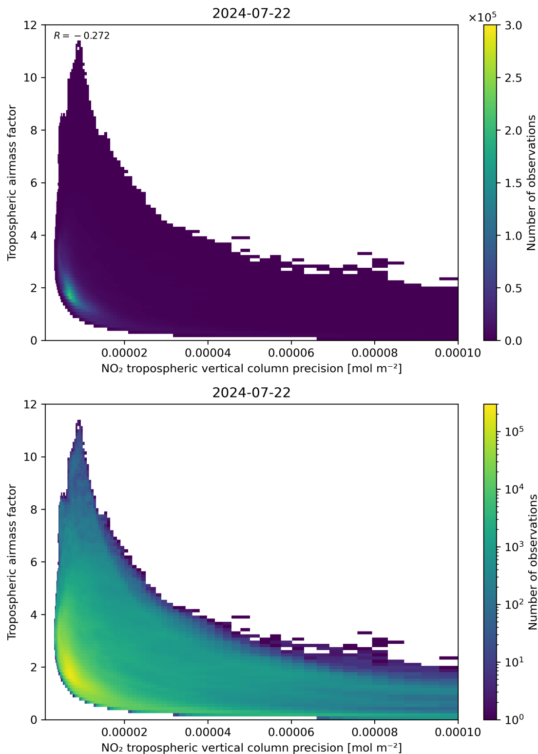
Figure 133: Scatter density plot of “NO 2 tropospheric vertical column precision” against “Tropospheric airmass factor” for 2024-07-21 to 2024-07-23.
