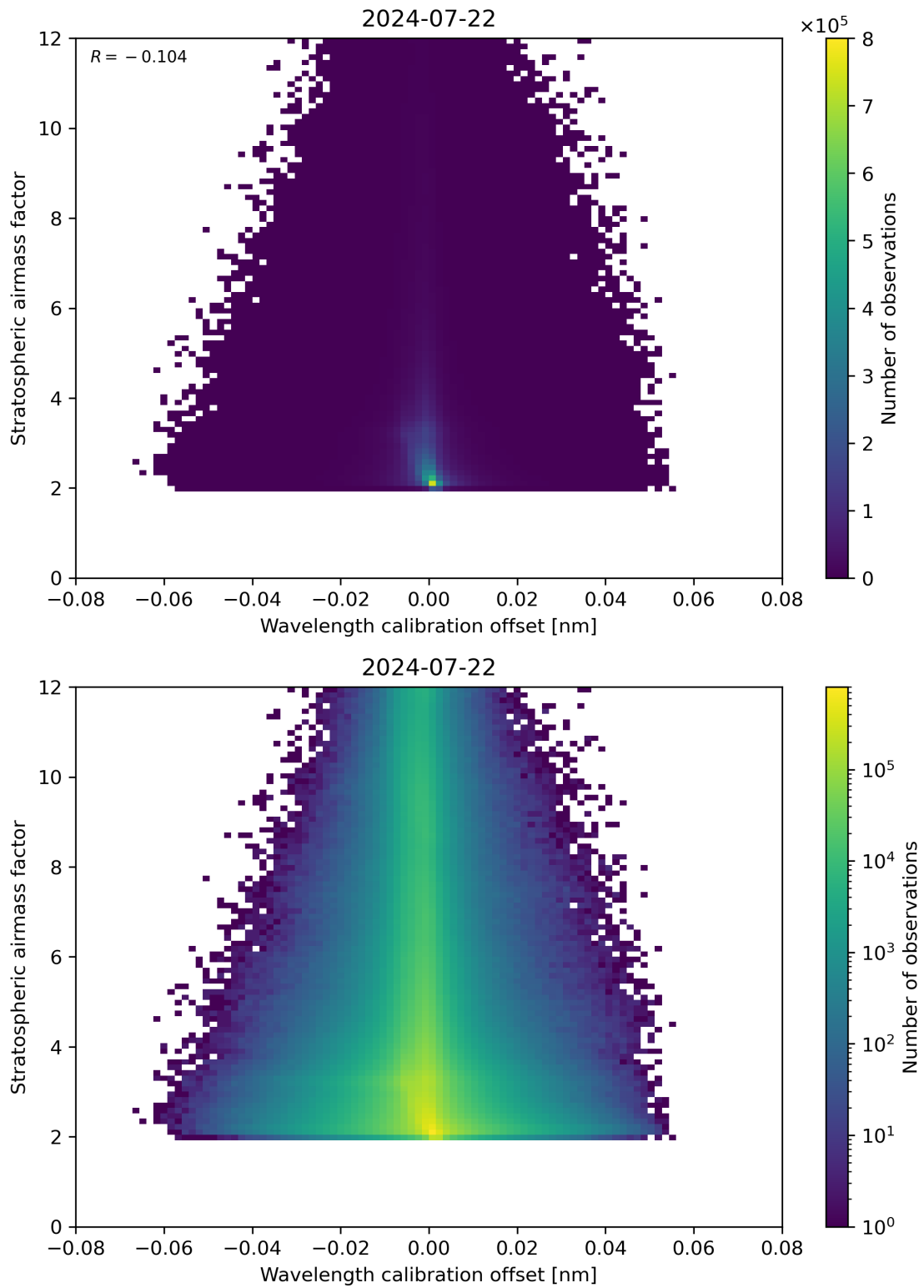
Figure 174: Scatter density plot of “Wavelength calibration offset” against “Stratospheric airmass factor” for 2024-07-21 to 2024-07-23.
