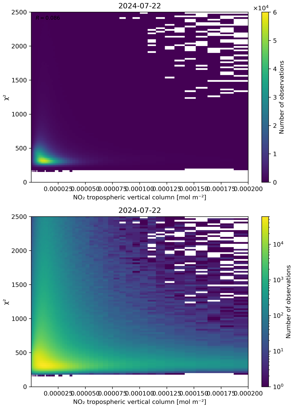
Figure 124: Scatter density plot of “NO 2 tropospheric vertical column” against “ \chi^2 ” for 2024-07-21 to 2024-07-23.
