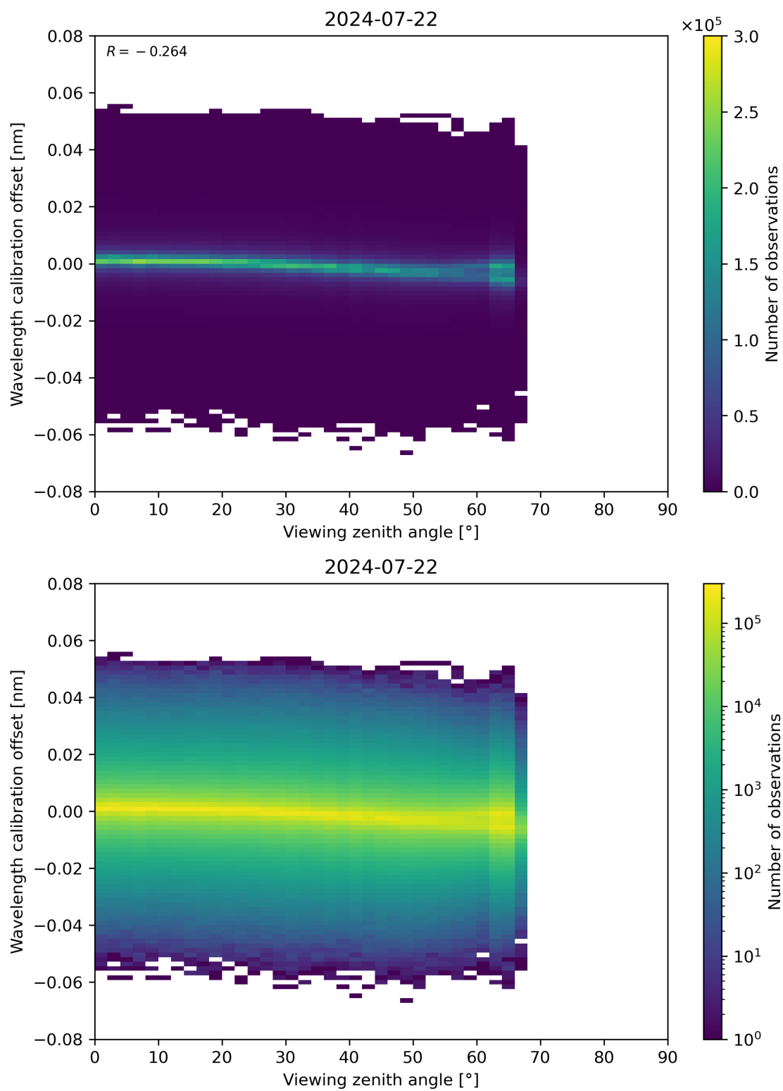
Figure 173: Scatter density plot of “Viewing zenith angle” against “Wavelength calibration offset” for 2024-07-21 to 2024-07-23.
