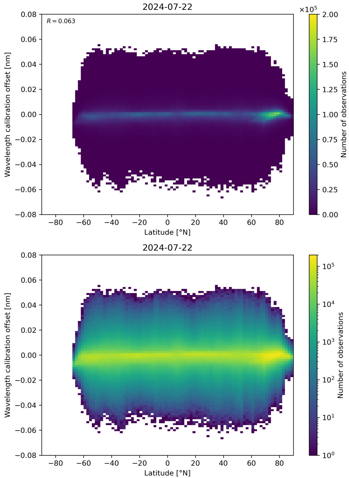
Figure 95: Scatter density plot of “Latitude” against “Wavelength calibration offset” for 2024-07-21 to 2024-07-23.
