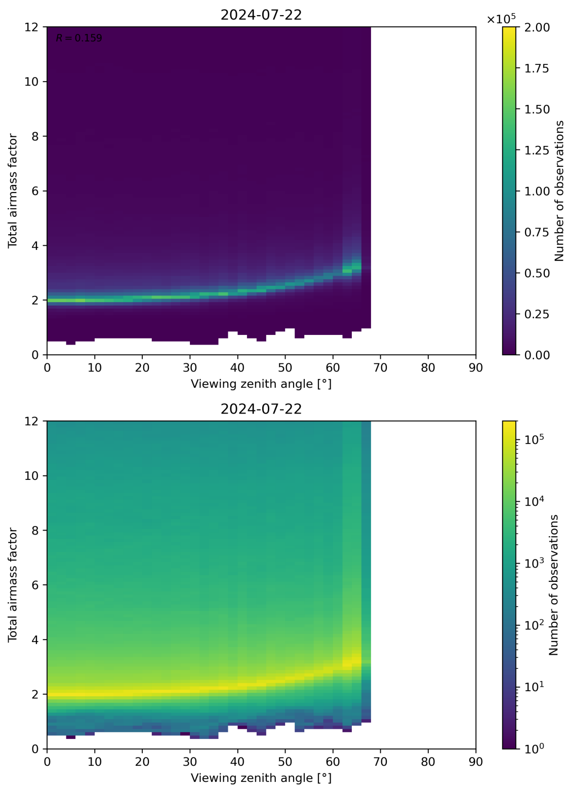
Figure 160: Scatter density plot of “Viewing zenith angle” against “Total airmass factor” for 2024-07-21 to 2024-07-23.
