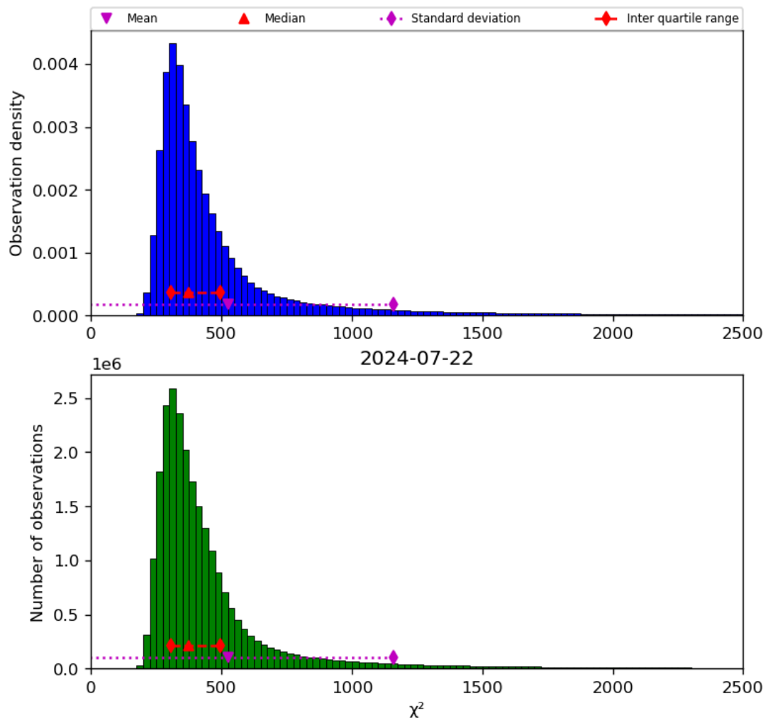
Figure 42: Histogram of " \chi^2 " for 2024-07-21 to 2024-07-23
