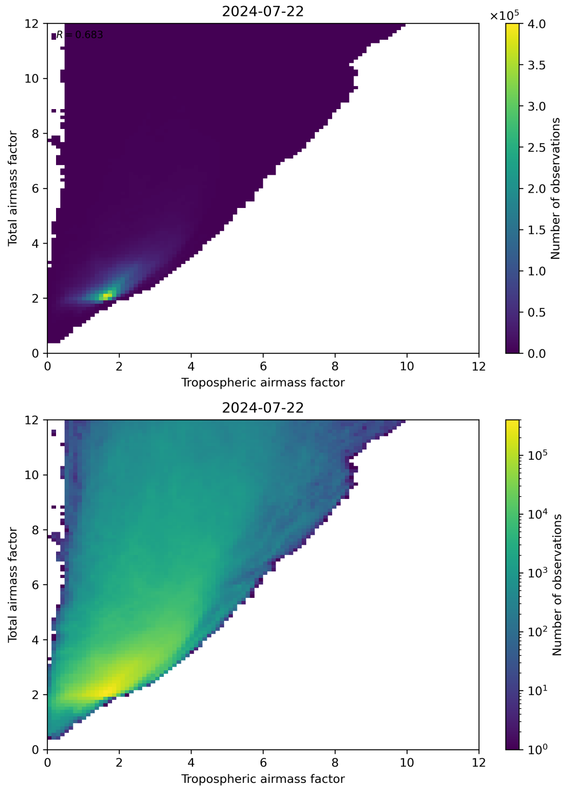
Figure 72: Scatter density plot of “Tropospheric airmass factor” against “Total airmass factor” for 2024-07-21 to 2024-07-23.
