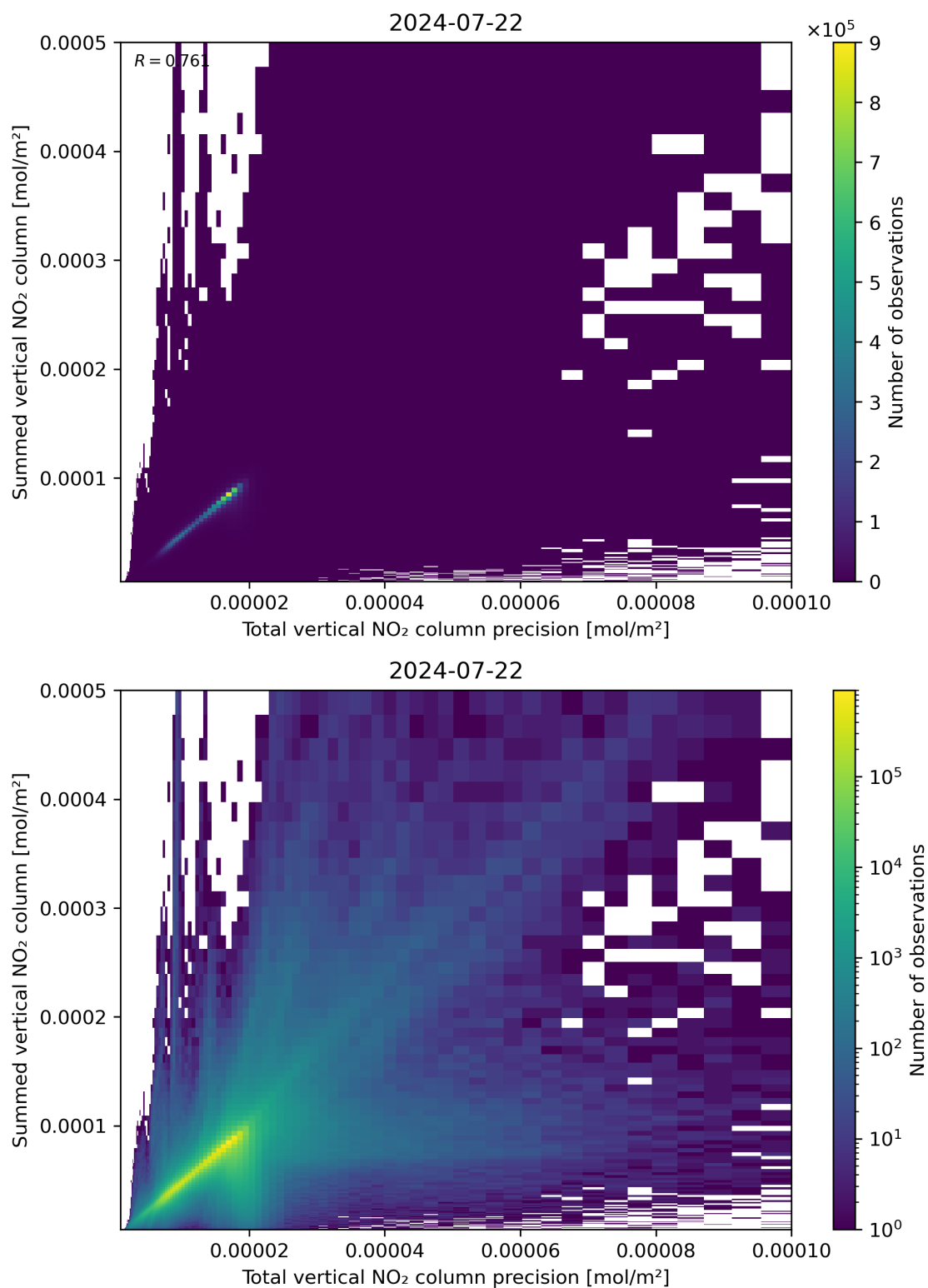
Figure 117: Scatter density plot of “Total vertical NO 2 column precision” against “Summed vertical NO 2 column” for 2024-07-21 to 2024-07-23.
