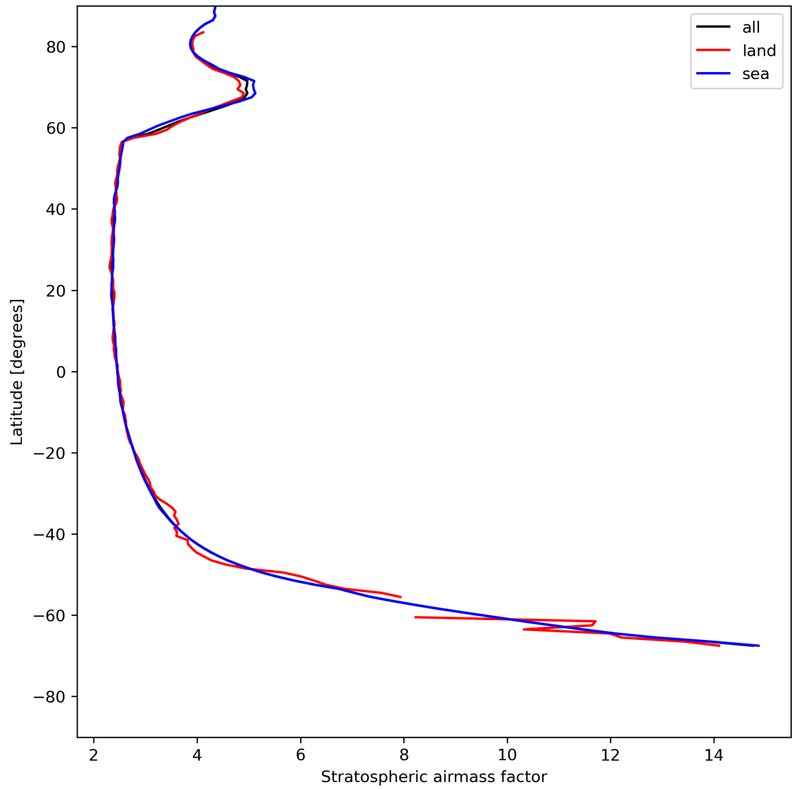
Figure 27: Zonal average of “Stratospheric air mass factor” for 2024-07-21 to 2024-07-23.
