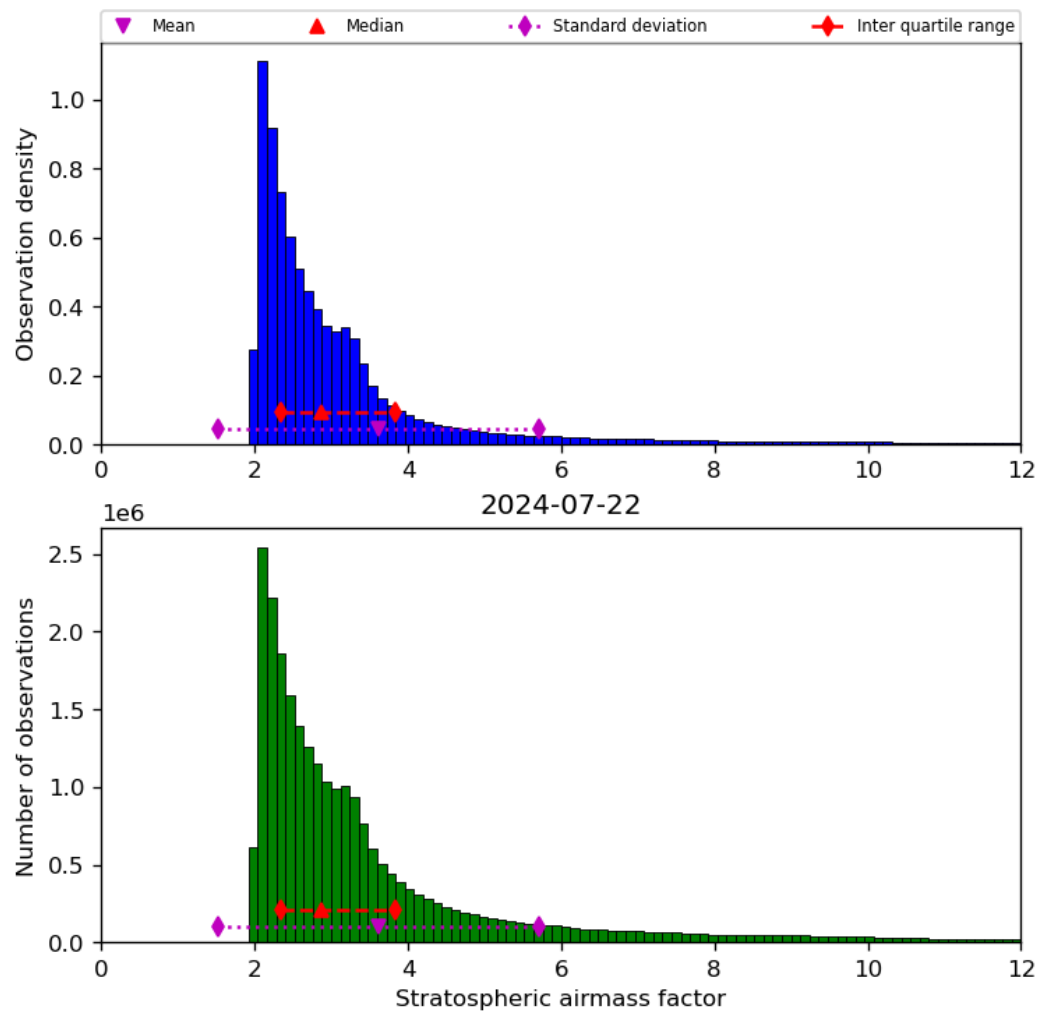
Figure 44: Histogram of “Stratospheric airmass factor” for 2024-07-21 to 2024-07-23
