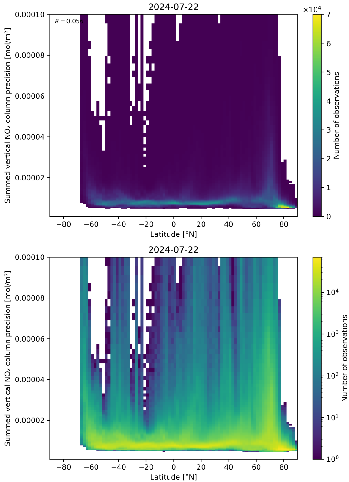
Figure 89: Scatter density plot of “Latitude” against “Summed vertical NO 2 column precision” for 2024-07-21 to 2024-07-23.
