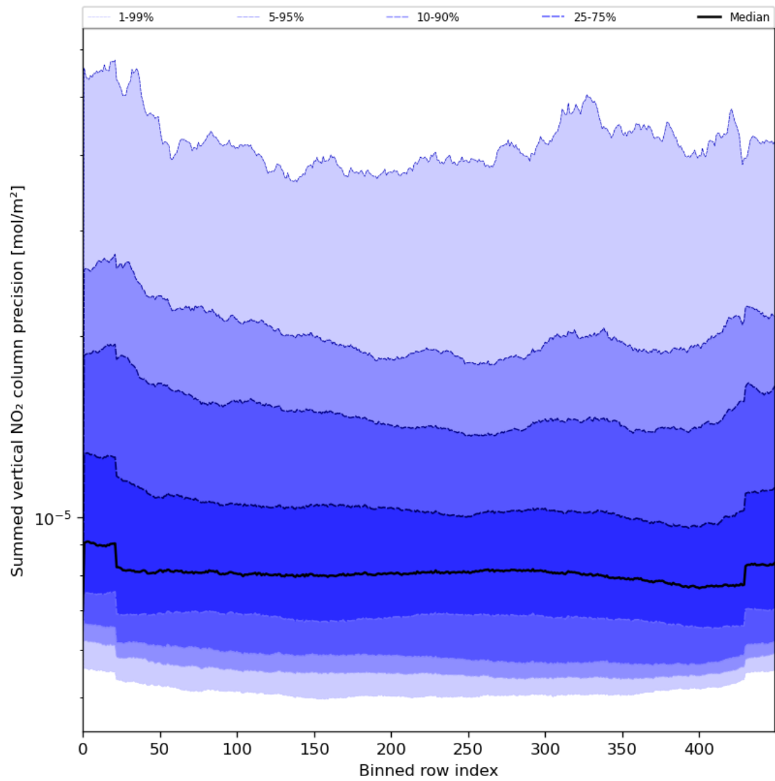
Figure 58: Along track statistics of “Summed vertical NO 2 column precision” for 2024-07-21 to 2024-07-23
