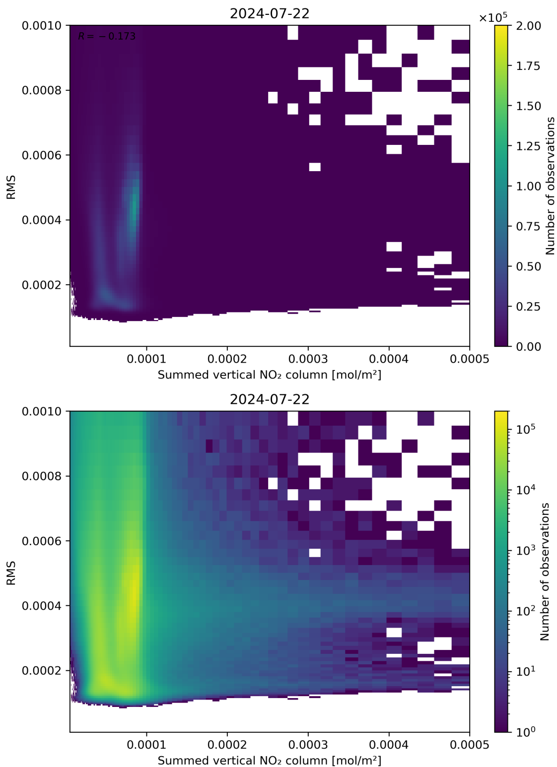
Figure 109: Scatter density plot of “Summed vertical NO 2 column” against “RMS” for 2024-07-21 to 2024-07-23.
