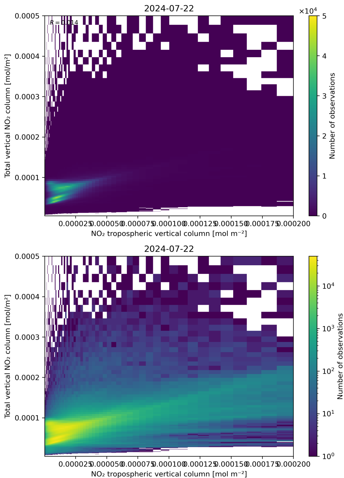
Figure 128: Scatter density plot of “NO 2 tropospheric vertical column” against “Total vertical NO 2 column” for 2024-07-21 to 2024-07-23.
