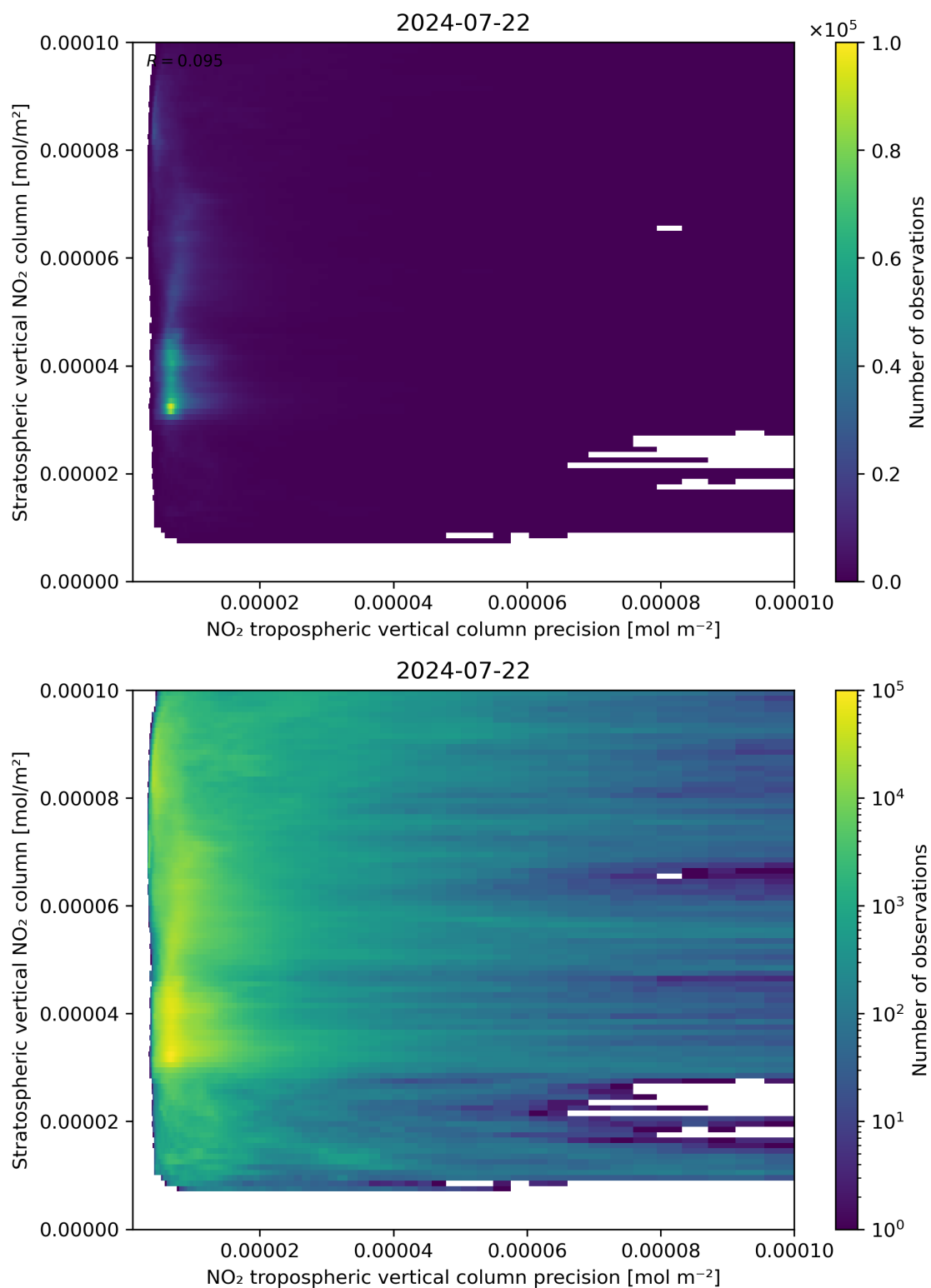
Figure 135: Scatter density plot of “NO 2 tropospheric vertical column precision” against “Stratospheric vertical NO 2 column” for 2024-07-21 to 2024-07-23.
