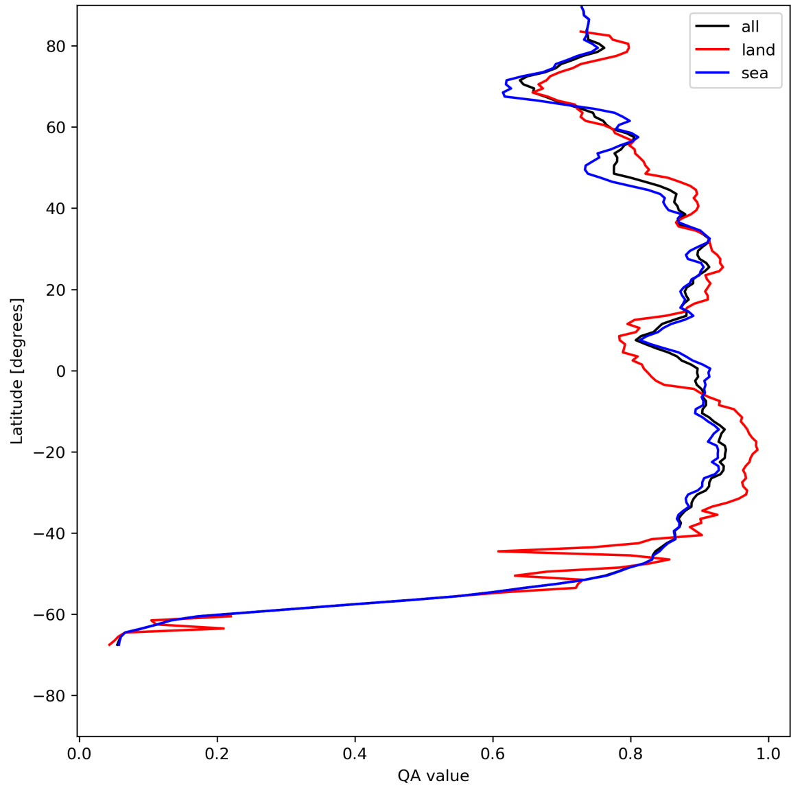
Figure 11: Zonal average of “QA value” for 2024-07-21 to 2024-07-23.
