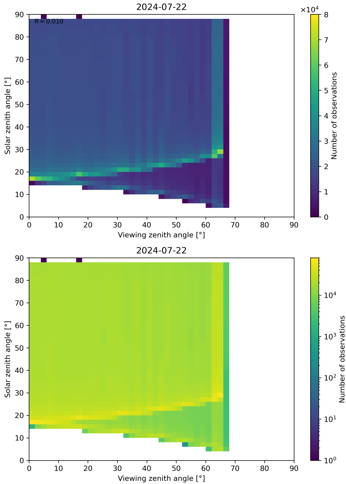
Figure 172: Scatter density plot of “Viewing zenith angle” against “Solar zenith angle” for 2024-07-21 to 2024-07-23.
