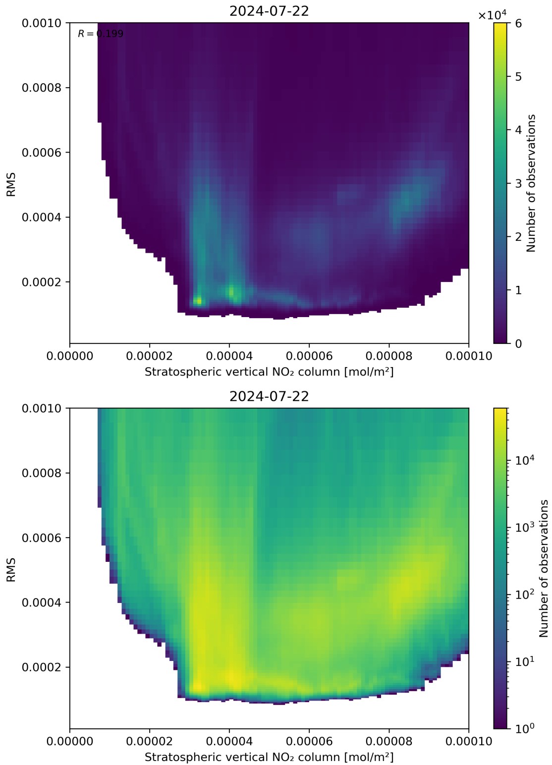
Figure 102: Scatter density plot of “Stratospheric vertical NO 2 column” against “RMS” for 2024-07-21 to 2024-07-23.
