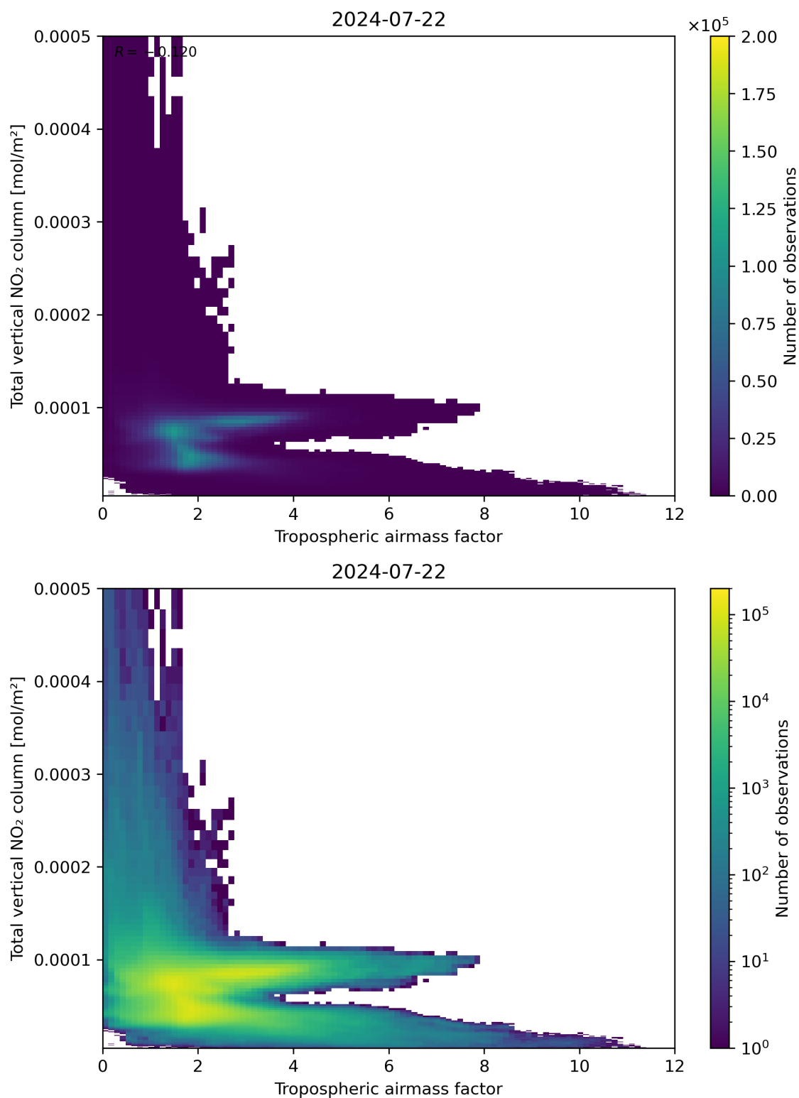
Figure 77: Scatter density plot of “Tropospheric airmass factor” against “Total vertical NO 2 column” for 2024-07-21 to 2024-07-23.
