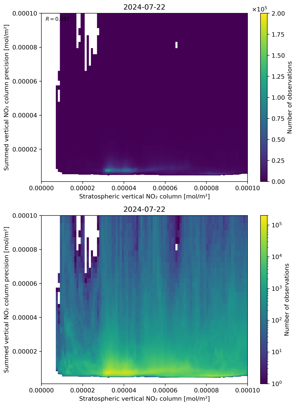
Figure 99: Scatter density plot of “Stratospheric vertical NO 2 column” against “Summed vertical NO 2 column precision” for 2024-07-21 to 2024-07-23.
