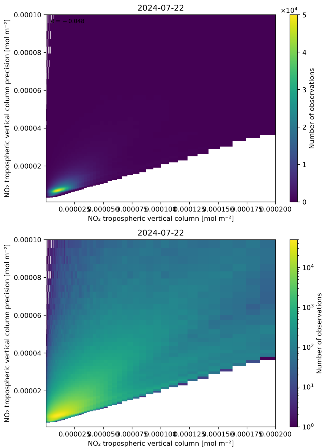
Figure 130: Scatter density plot of “NO 2 tropospheric vertical column” against “NO 2 tropospheric vertical column precision” for 2024-07-21 to 2024-07-23.
