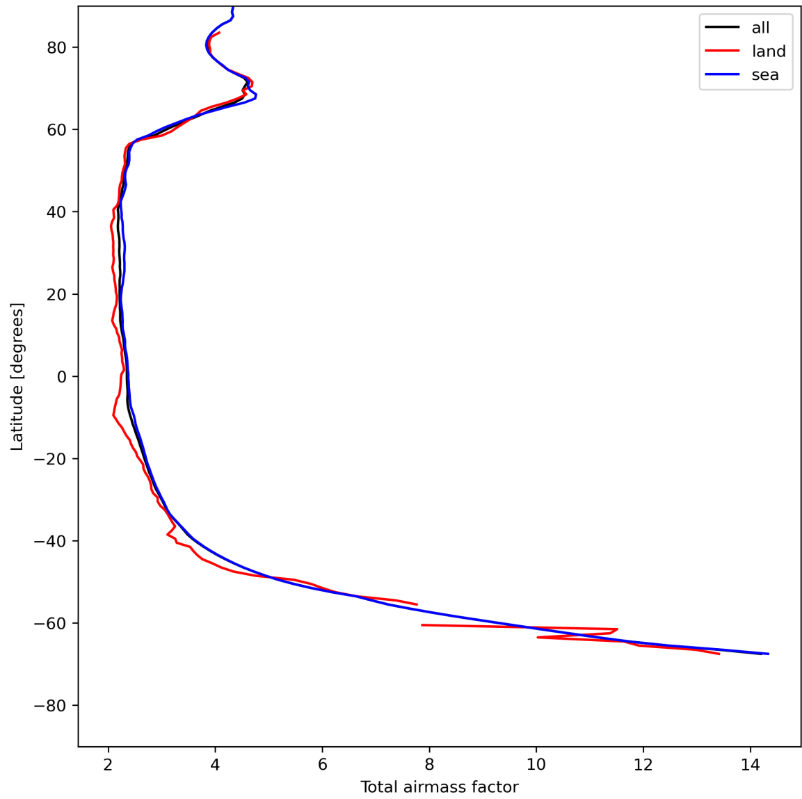
Figure 15: Zonal average of “Total airmass factor” for 2024-07-21 to 2024-07-23.
