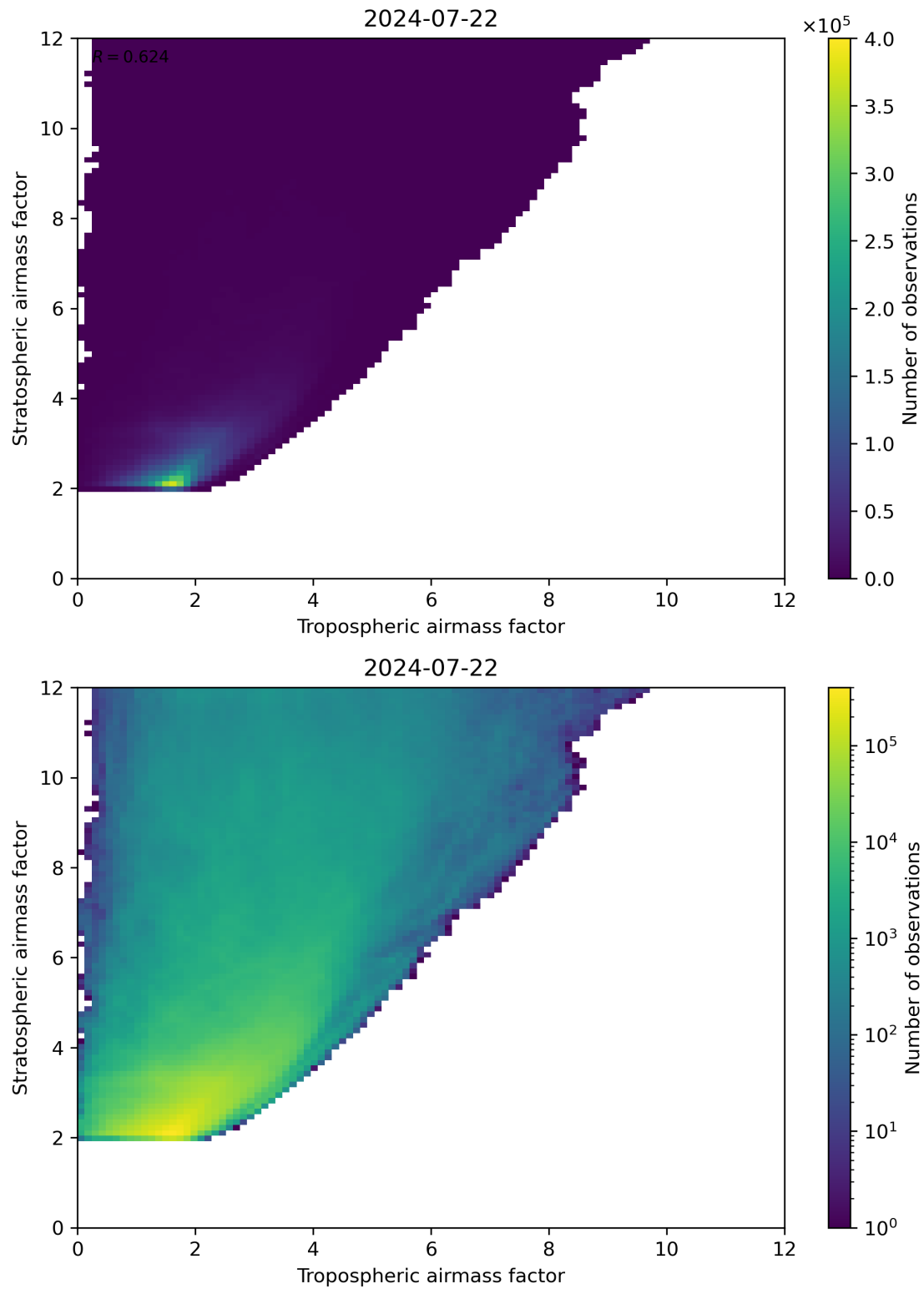
Figure 71: Scatter density plot of “Tropospheric airmass factor” against “Stratospheric airmass factor” for 2024-07-21 to 2024-07-23.
