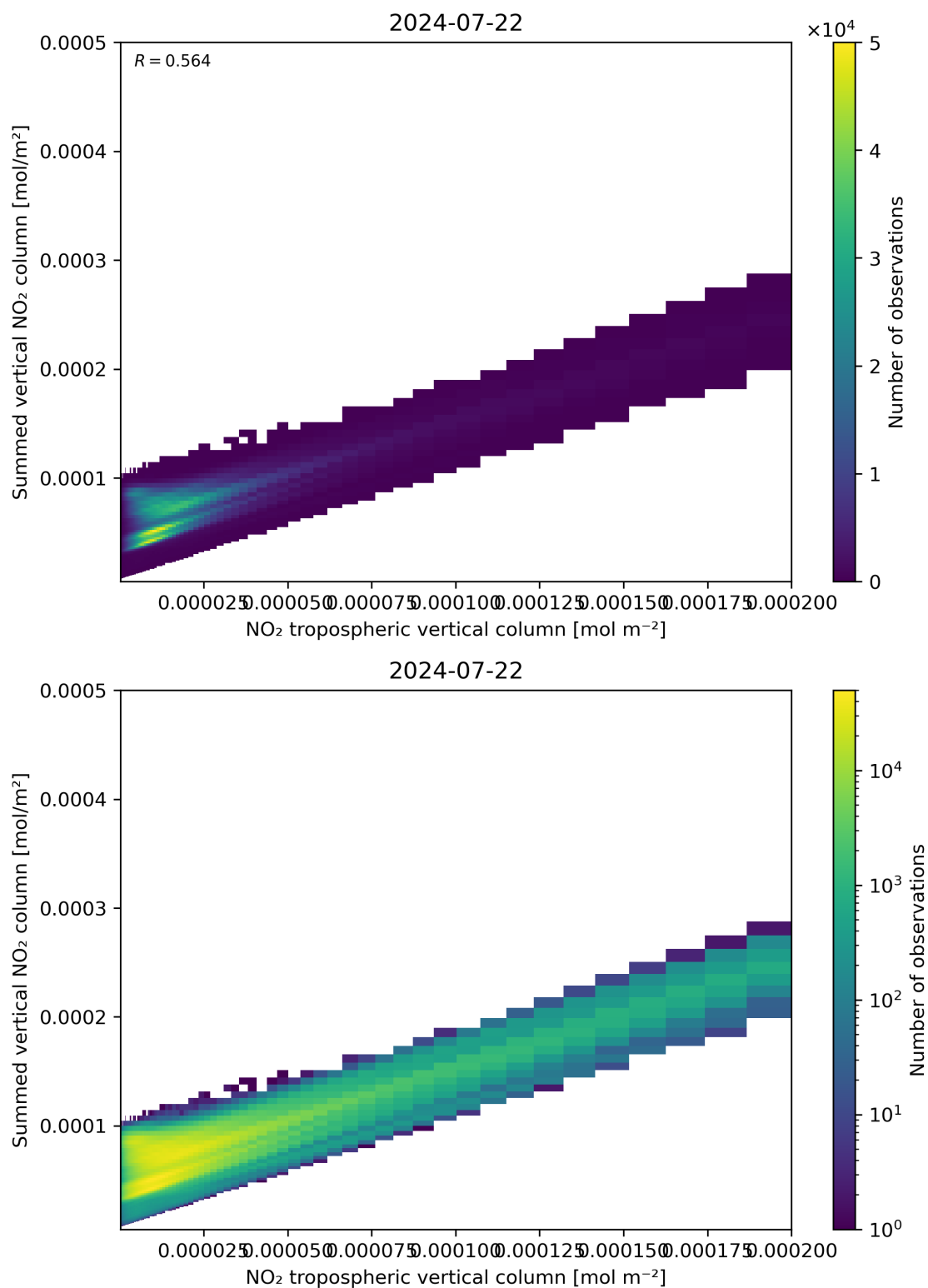
Figure 126: Scatter density plot of “NO 2 tropospheric vertical column” against “Summed vertical NO 2 column” for 2024-07-21 to 2024-07-23.
