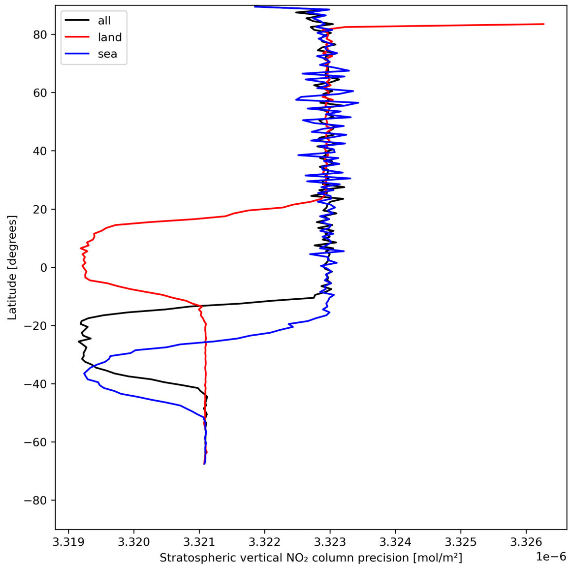
Figure 20: Zonal average of “Stratospheric vertical NO 2 column precision” for 2024-07-21 to 2024-07-23.
