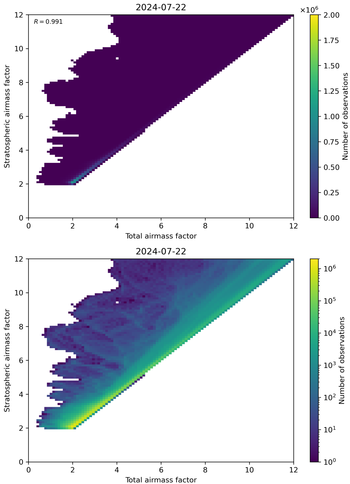
Figure 62: Scatter density plot of “Total airmass factor” against “Stratospheric airmass factor” for 2024-07-21 to 2024-07-23.
