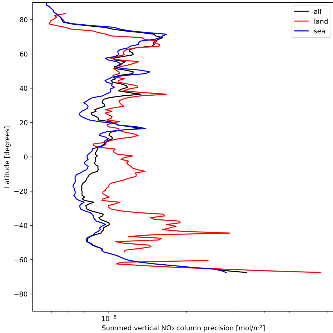
Figure 24: Zonal average of “Summed vertical NO 2 column precision” for 2024-07-21 to 2024-07-23.
