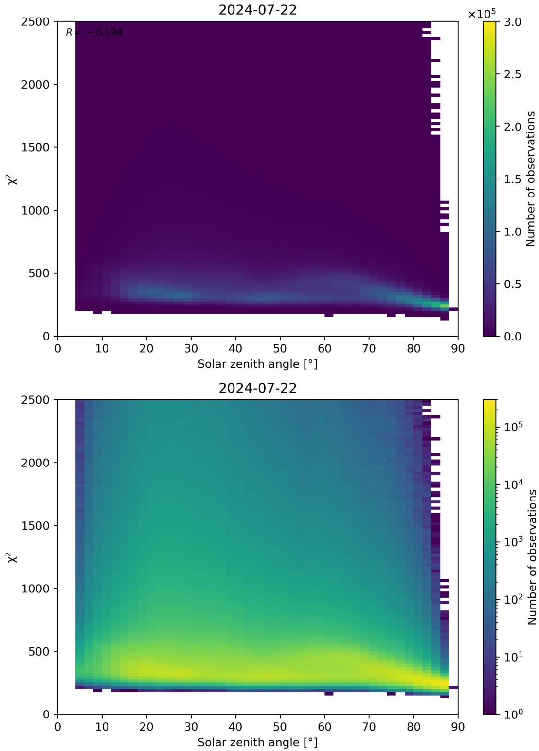
Figure 148: Scatter density plot of “Solar zenith angle” against “ \chi^2 ” for 2024-07-21 to 2024-07-23.
