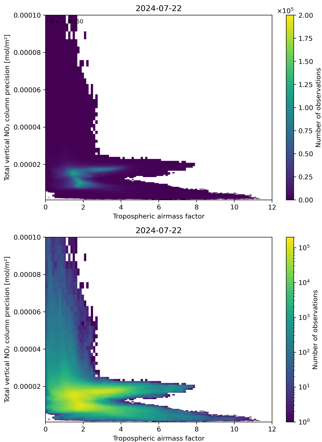
Figure 78: Scatter density plot of “Tropospheric air mass factor” against “Total vertical NO 2 column precision” for 2024-07-21 to 2024-07-23.
