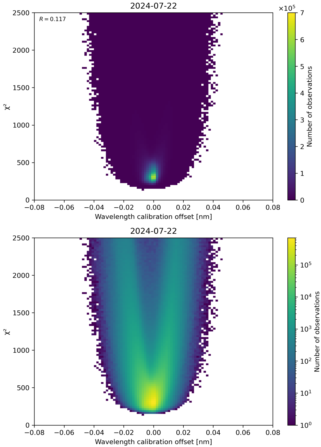
Figure 175: Scatter density plot of “Wavelength calibration offset” against “ \chi^2 ” for 2024-07-21 to 2024-07-23.
