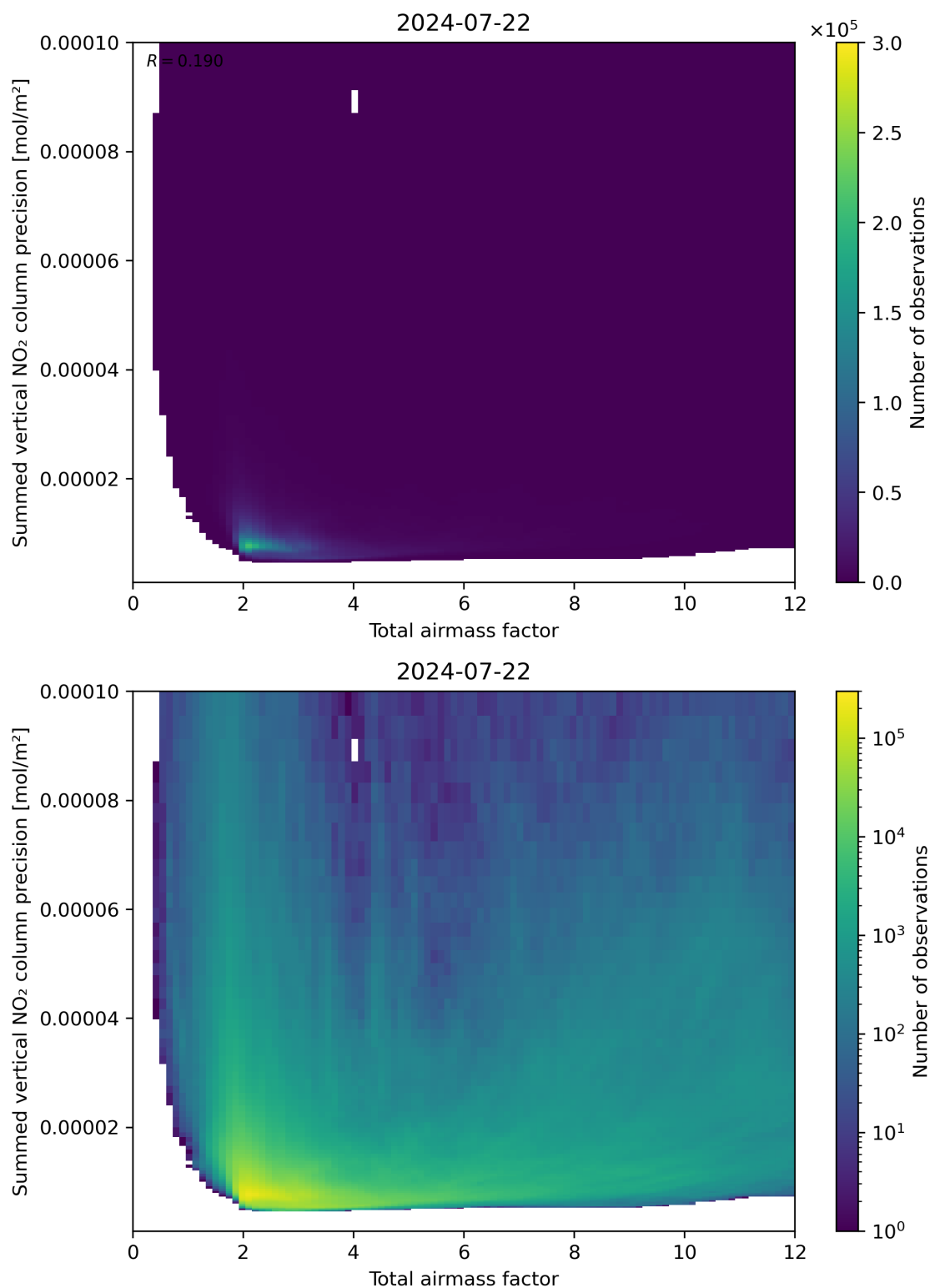
Figure 66: Scatter density plot of “Total airmass factor” against “Summed vertical NO 2 column precision” for 2024-07-21 to 2024-07-23.
