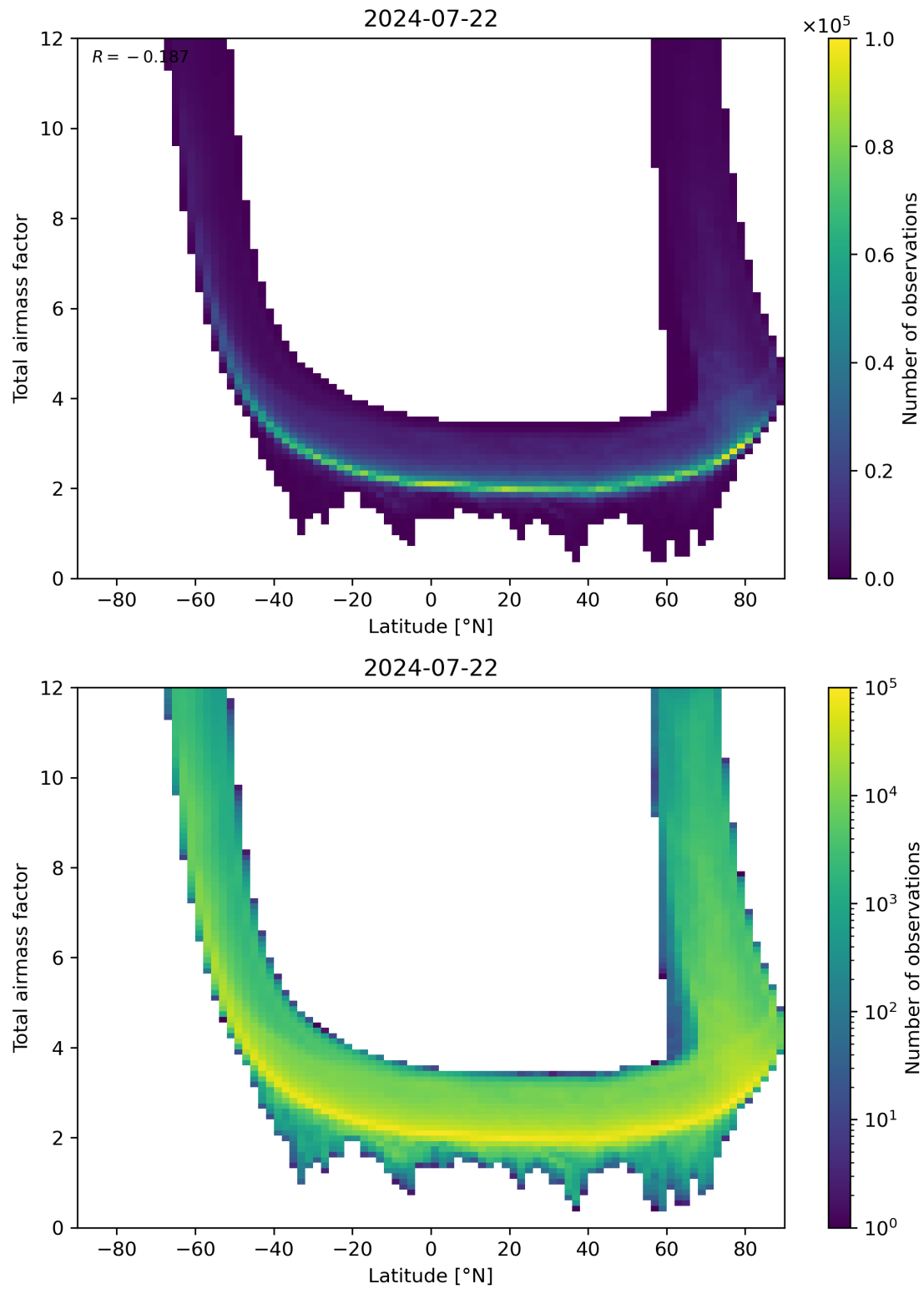
Figure 84: Scatter density plot of “Latitude” against “Total airmass factor” for 2024-07-21 to 2024-07-23.
