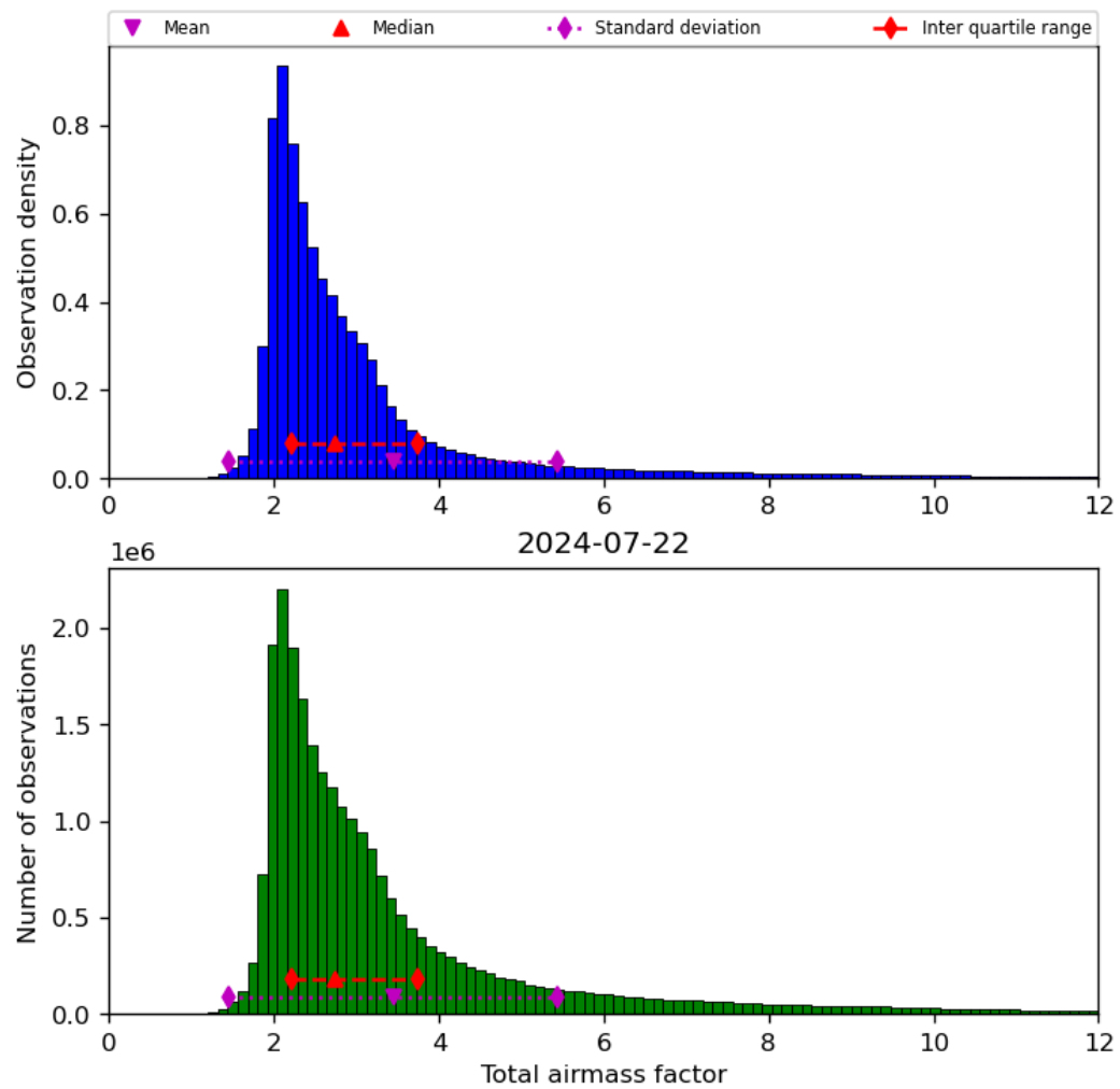
Figure 32: Histogram of “Total airmass factor” for 2024-07-21 to 2024-07-23
