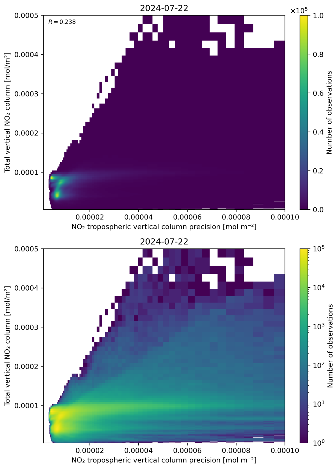
Figure 138: Scatter density plot of “NO 2 tropospheric vertical column precision” against “Total vertical NO 2 column” for 2024-07-21 to 2024-07-23.
