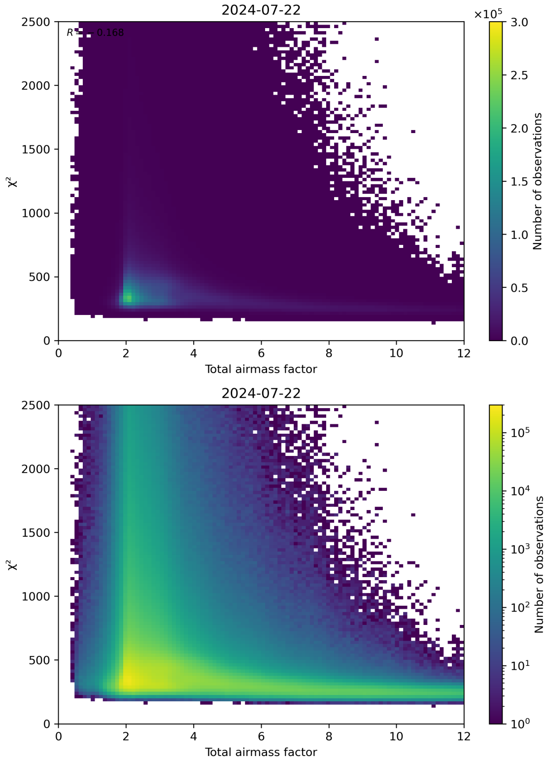
Figure 63: Scatter density plot of “Total airmass factor” against “ \chi^2 ” for 2024-07-21 to 2024-07-23.
