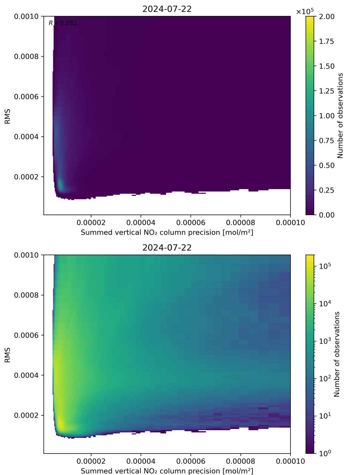
Figure 108: Scatter density plot of “Summed vertical NO 2 column precision” against “RMS” for 2024-07-21 to 2024-07-23.
