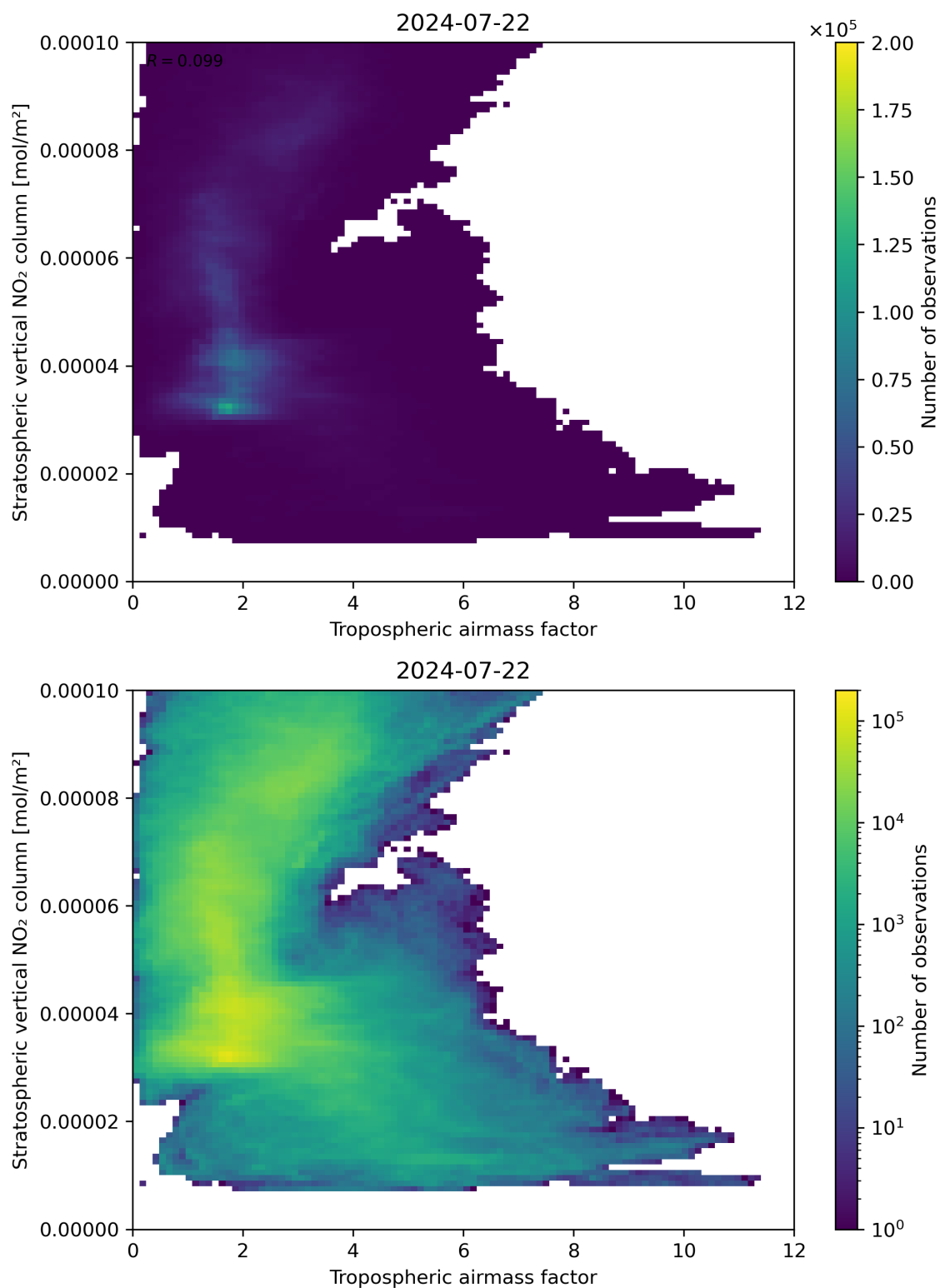
Figure 74: Scatter density plot of “Tropospheric air mass factor” against “Stratospheric vertical NO 2 column” for 2024-07-21 to 2024-07-23.
