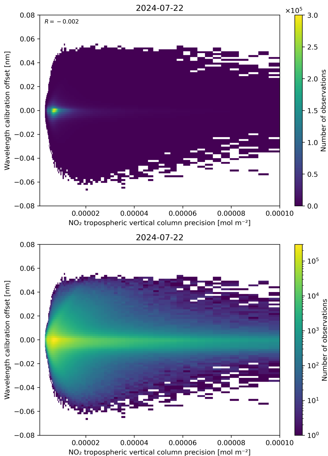
Figure 141: Scatter density plot of “NO 2 tropospheric vertical column precision” against “Wavelength calibration offset” for 2024-07-21 to 2024-07-23.
