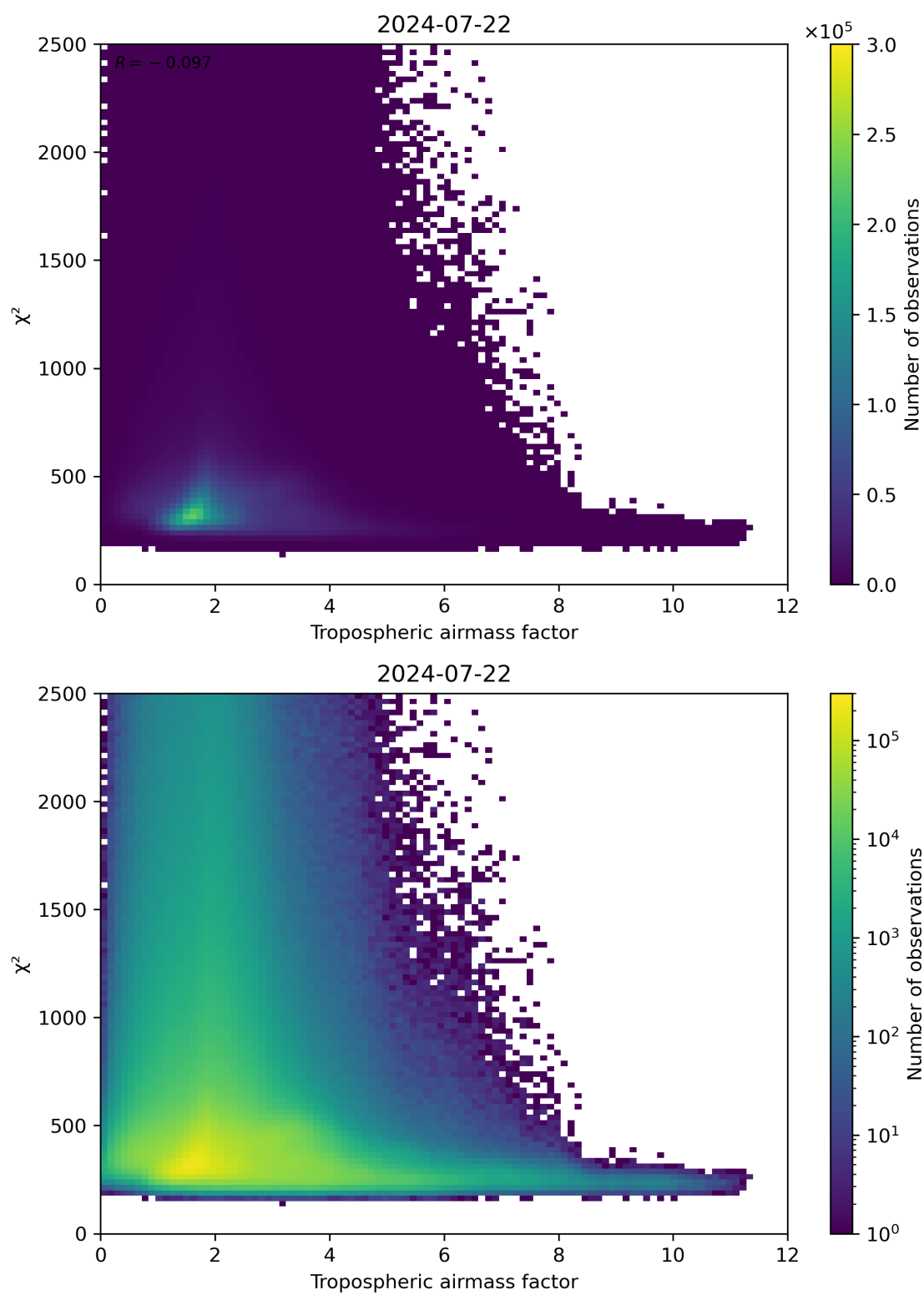
Figure 73: Scatter density plot of “Tropospheric airmass factor” against “ \chi^2 ” for 2024-07-21 to 2024-07-23.
