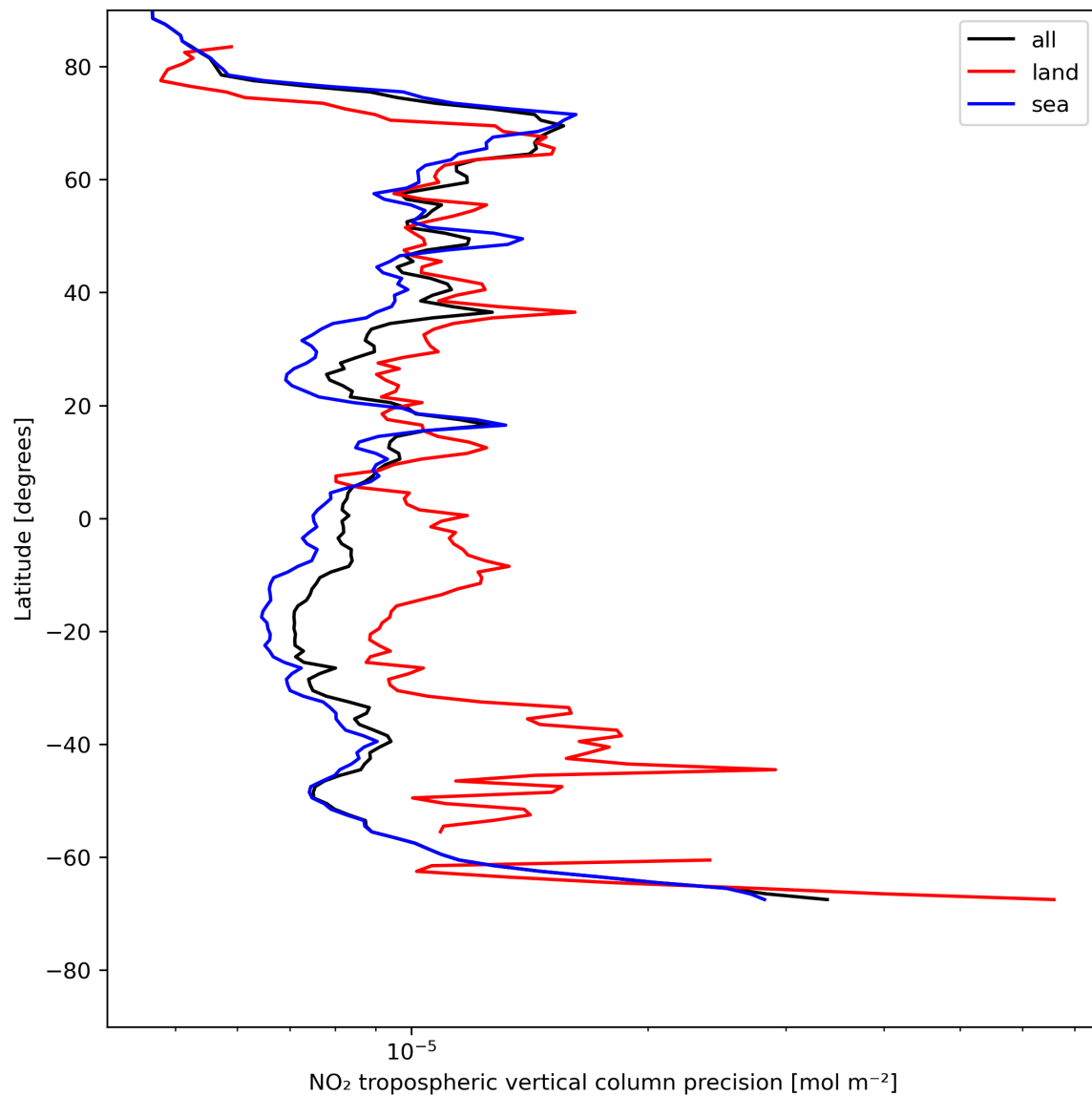
Figure 13: Zonal average of “NO 2 tropospheric vertical column precision” for 2024-07-21 to 2024-07-23.
