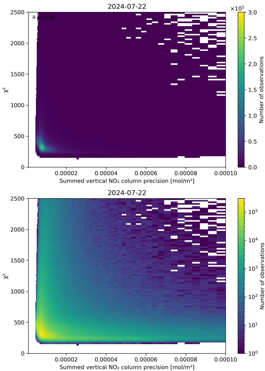
Figure 107: Scatter density plot of “Summed vertical NO 2 column precision” against “ \chi^2 ” for 2024-07-21 to 2024-07-23.
