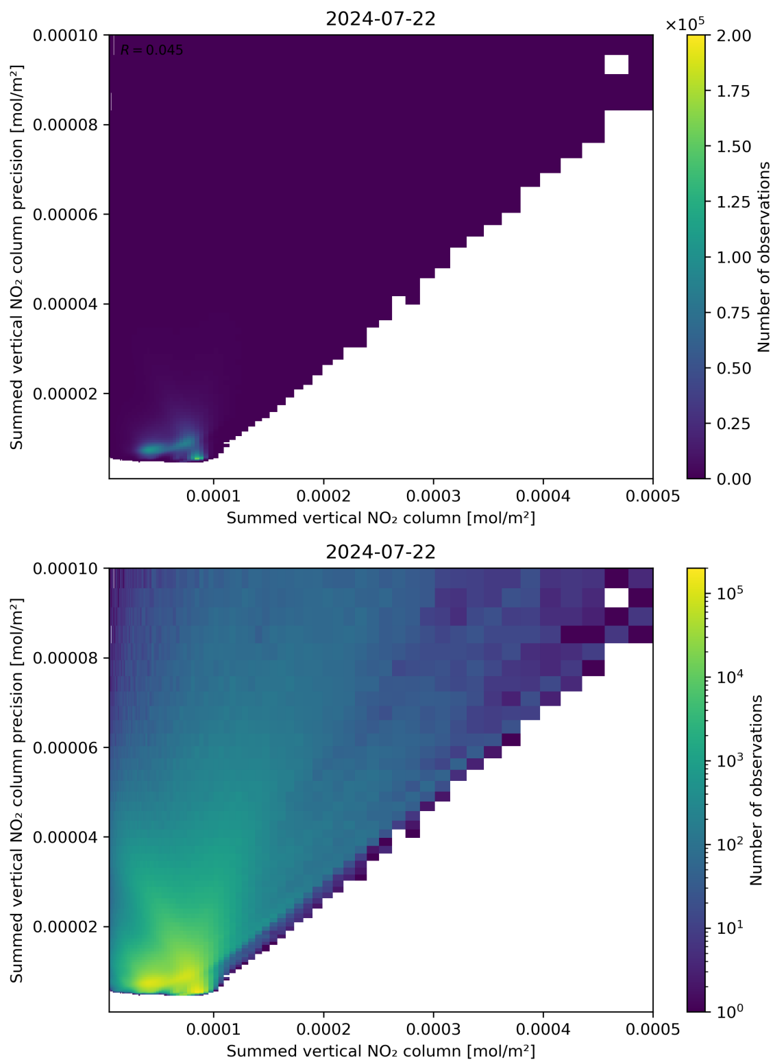
Figure 105: Scatter density plot of “Summed vertical NO 2 column” against “Summed vertical NO 2 column precision” for 2024-07-21 to 2024-07-23.
