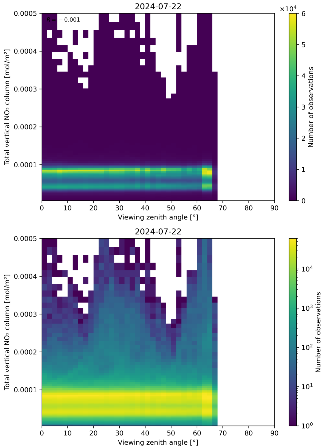
Figure 167: Scatter density plot of “Viewing zenith angle” against “Total vertical NO 2 column” for 2024-07-21 to 2024-07-23.
