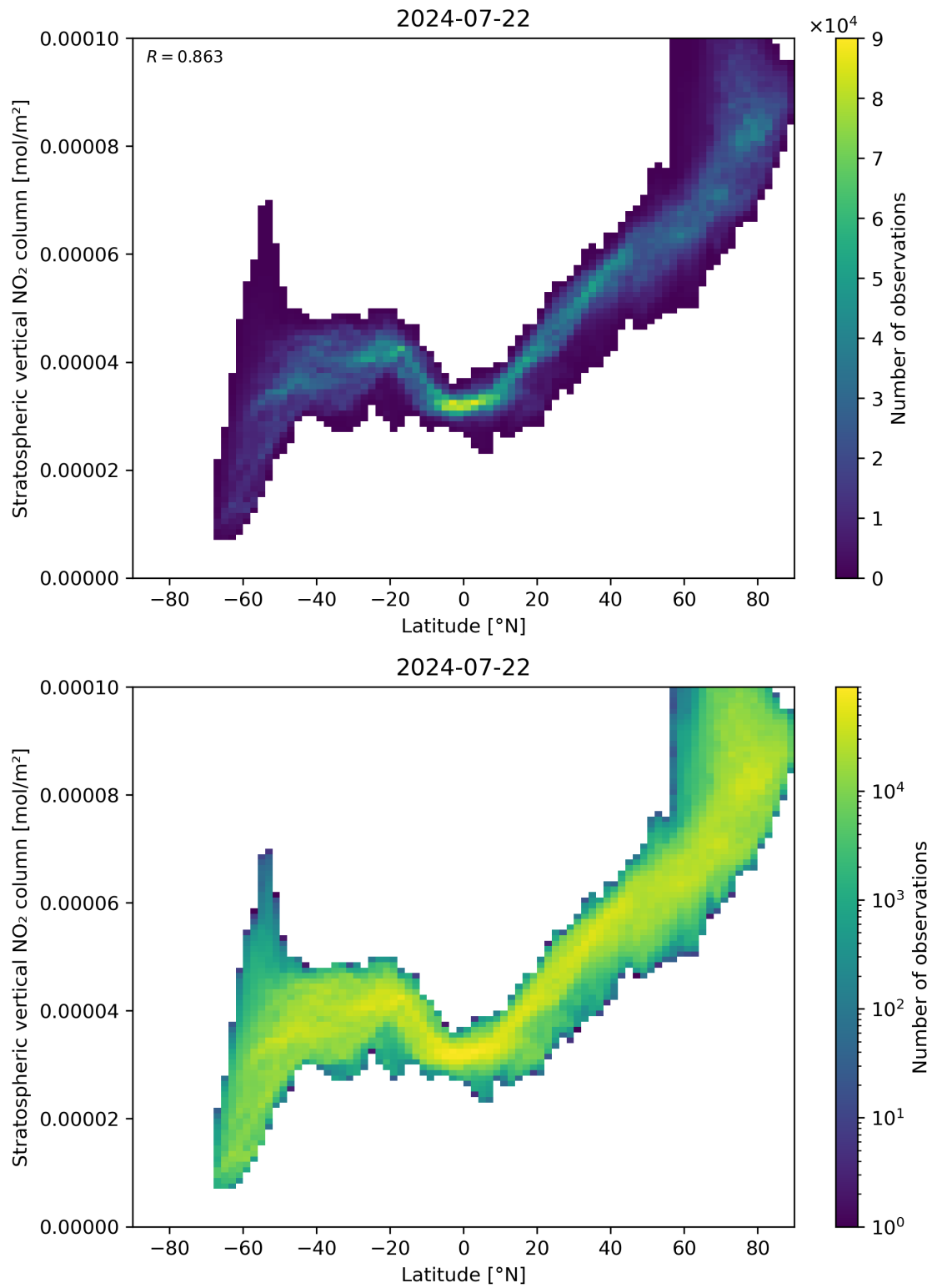
Figure 87: Scatter density plot of “Latitude” against “Stratospheric vertical NO 2 column” for 2024-07-21 to 2024-07-23.
