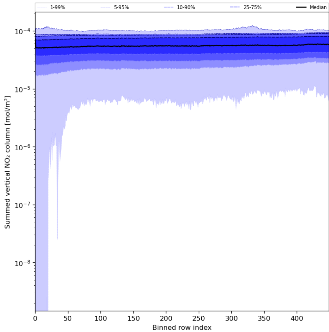
Figure 57: Along track statistics of “Summed vertical NO 2 column” for 2024-07-21 to 2024-07-23
