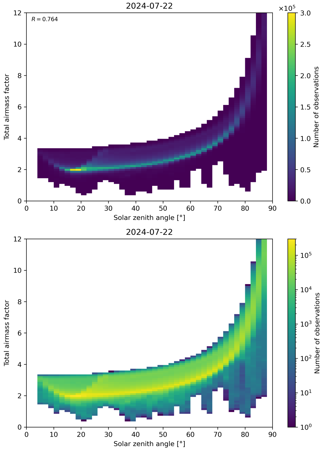
Figure 146: Scatter density plot of “Solar zenith angle” against “Total air mass factor” for 2024-07-21 to 2024-07-23.
