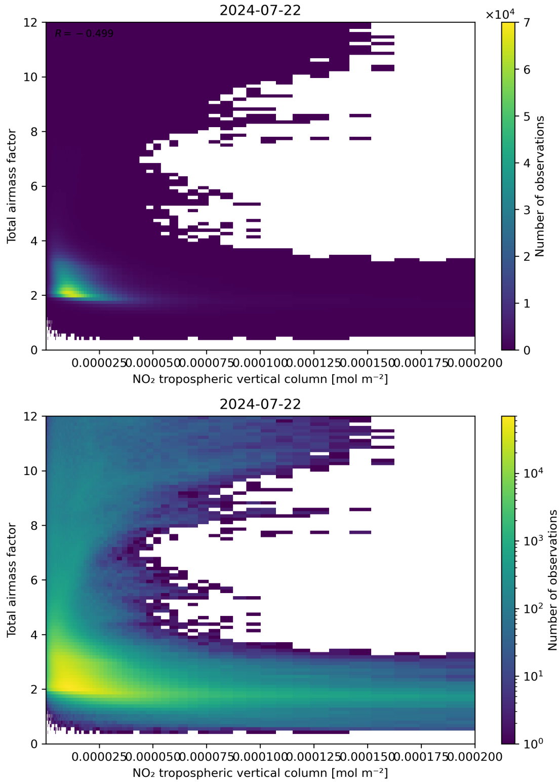
Figure 122: Scatter density plot of “NO 2 tropospheric vertical column” against “Total air mass factor” for 2024-07-21 to 2024-07-23.
