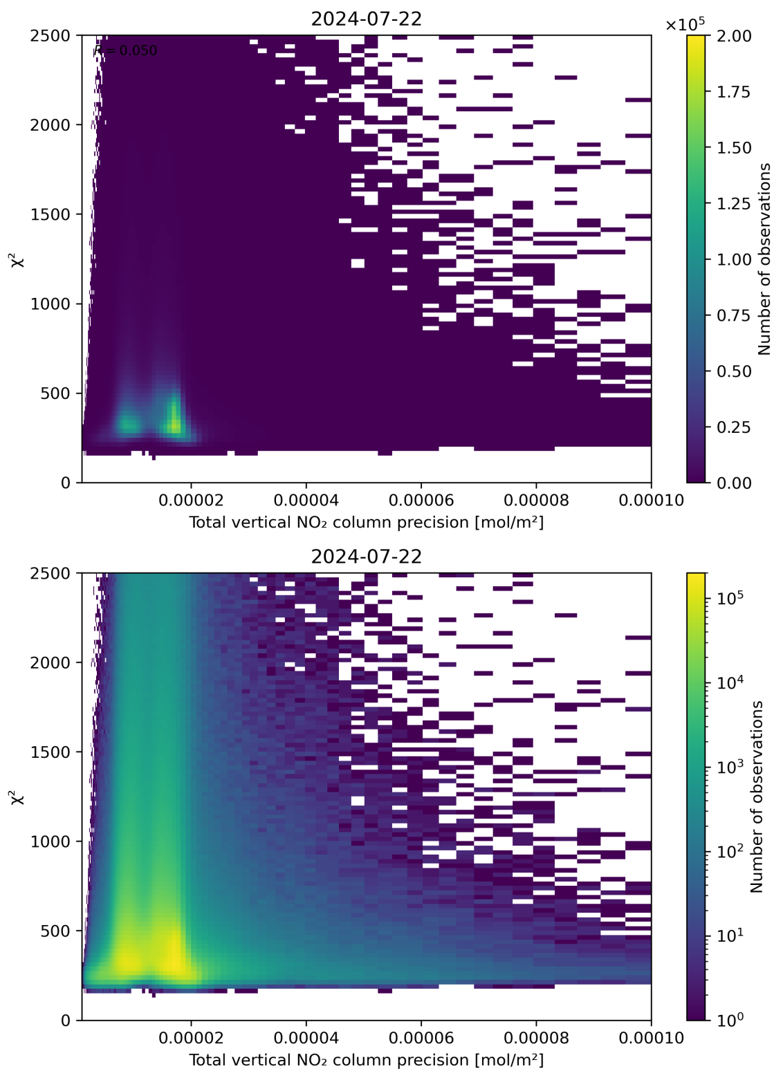
Figure 116: Scatter density plot of “Total vertical NO 2 column precision” against “ \chi^2 ” for 2024-07-21 to 2024-07-23.
