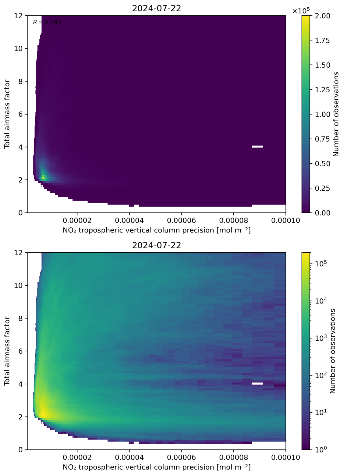
Figure 132: Scatter density plot of “NO 2 tropospheric vertical column precision” against “Total air mass factor” for 2024-07-21 to 2024-07-23.
