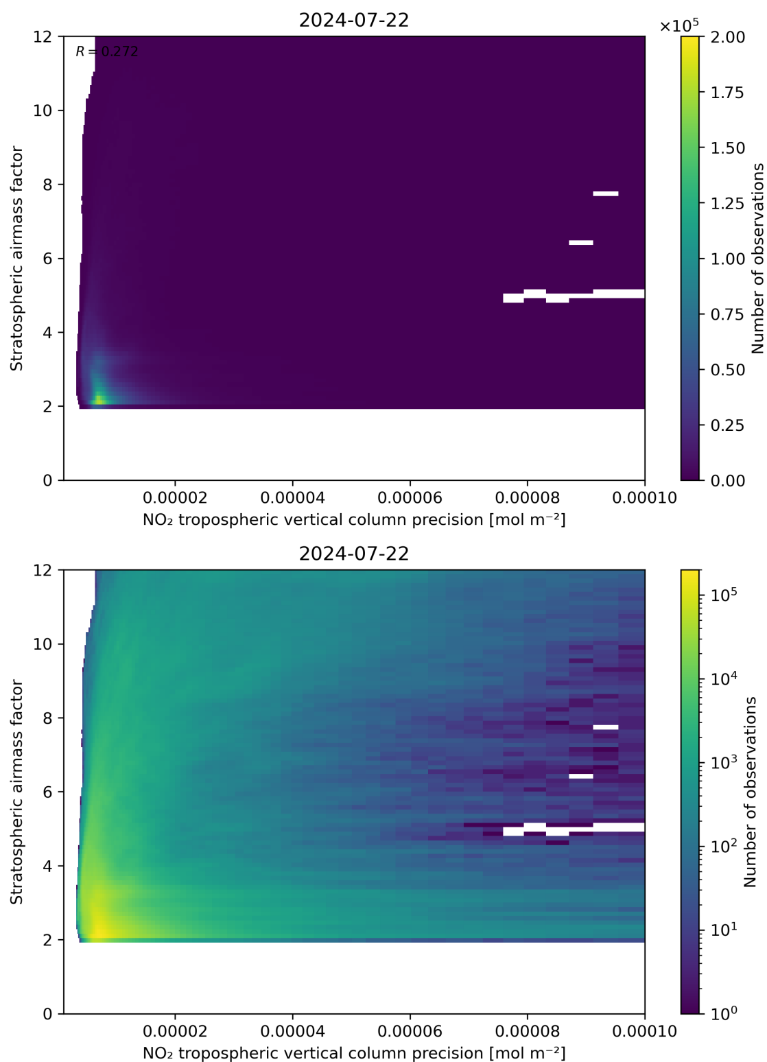
Figure 131: Scatter density plot of “NO 2 tropospheric vertical column precision” against “Stratospheric airmass factor” for 2024-07-21 to 2024-07-23.
