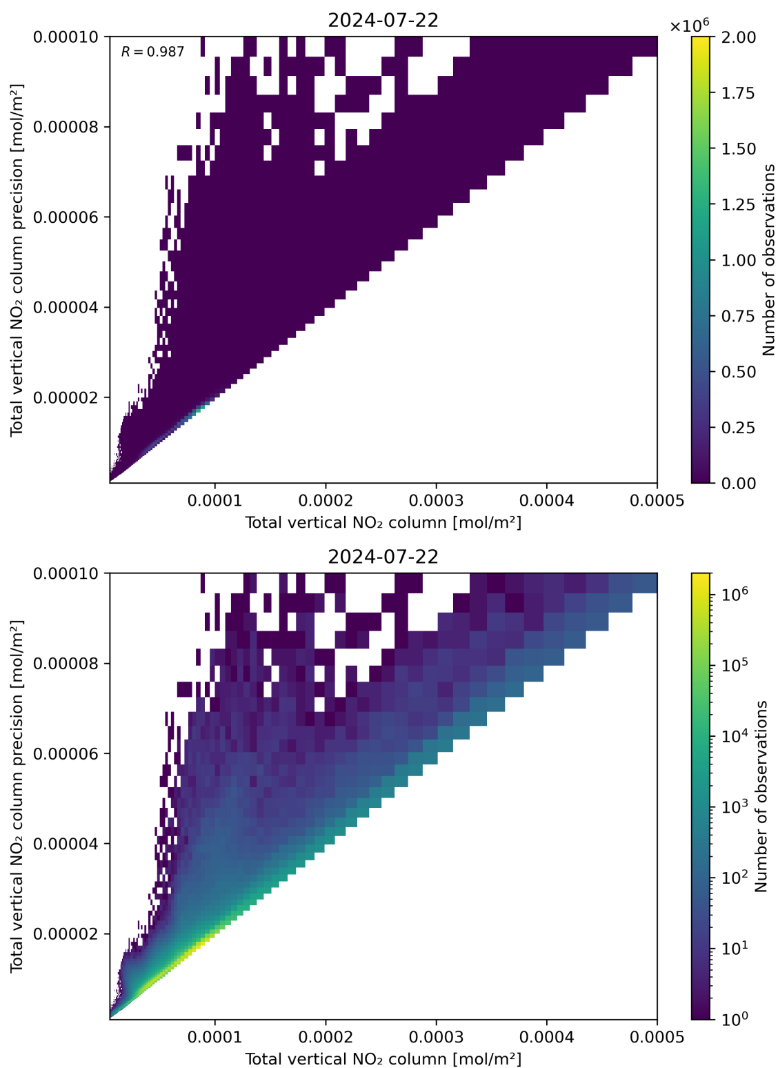
Figure 114: Scatter density plot of “Total vertical NO 2 column” against “Total vertical NO 2 column precision” for 2024-07-21 to 2024-07-23.
