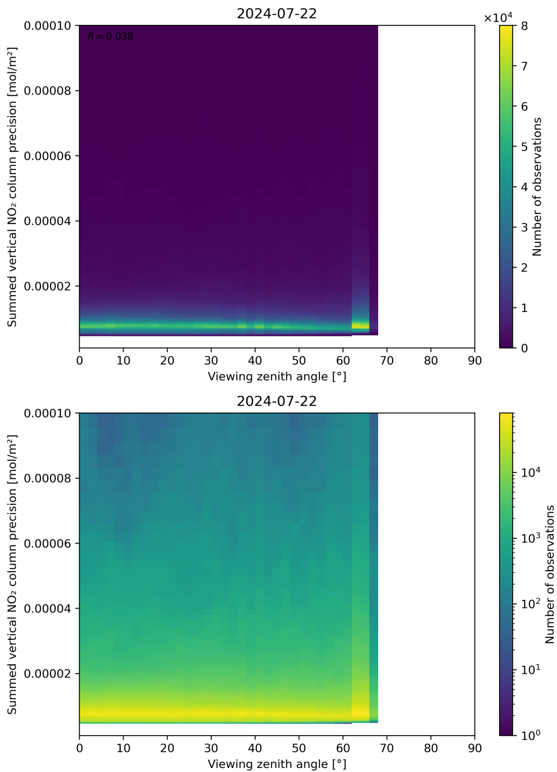
Figure 166: Scatter density plot of “Viewing zenith angle” against “Summed vertical NO 2 column precision” for 2024-07-21 to 2024-07-23.
