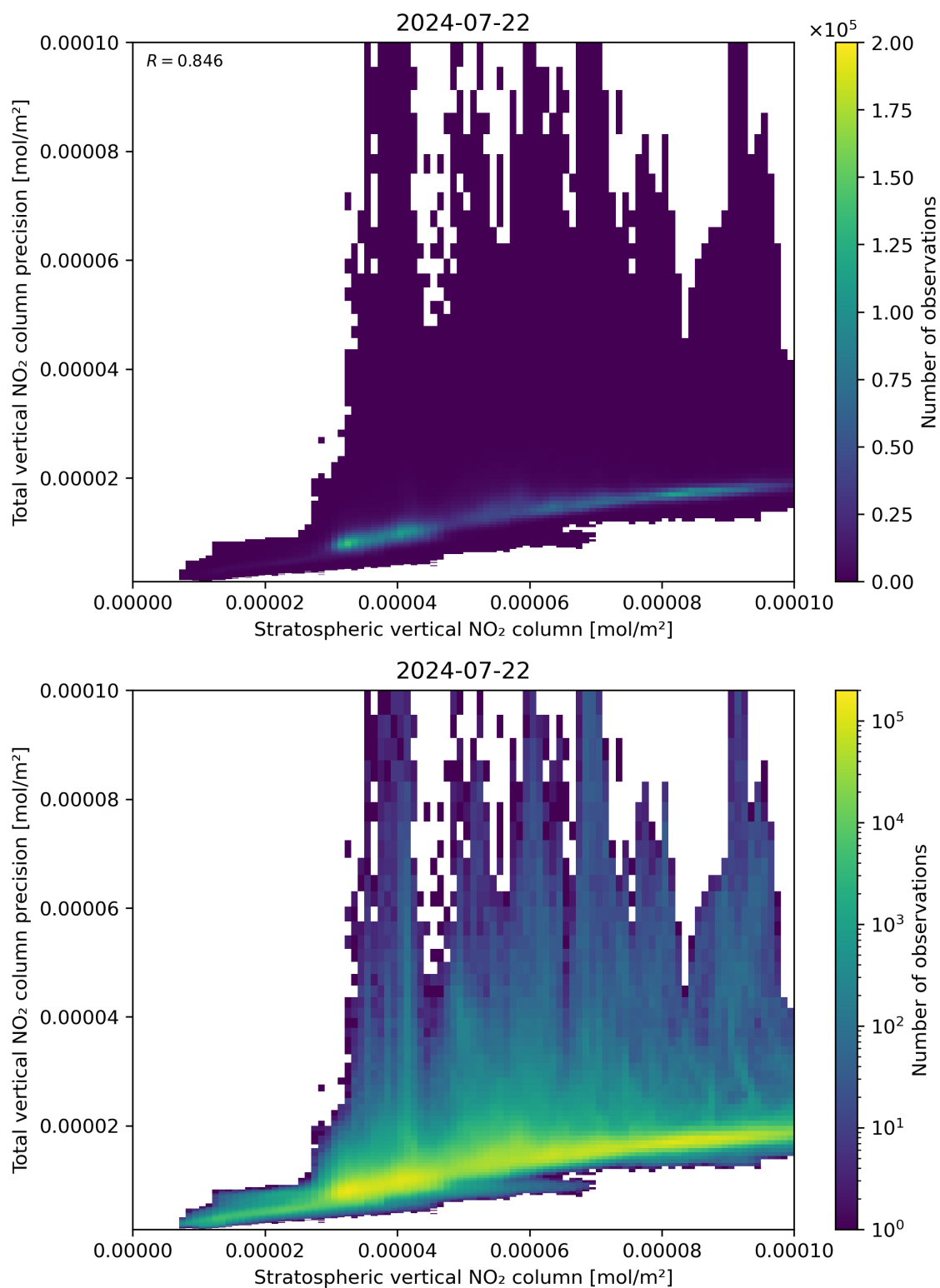
Figure 101: Scatter density plot of “Stratospheric vertical NO 2 column” against “Total vertical NO 2 column precision” for 2024-07-21 to 2024-07-23.
