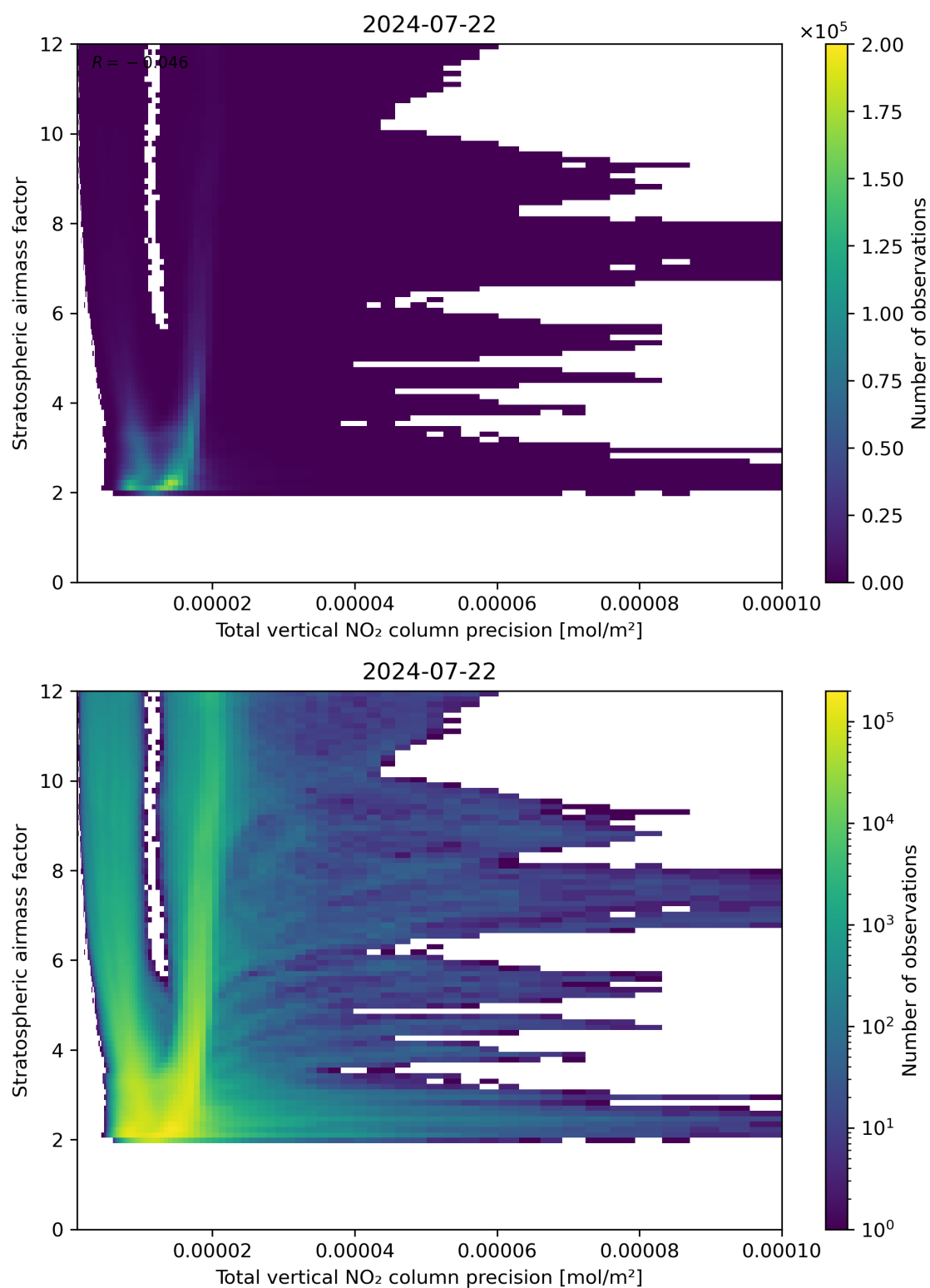
Figure 115: Scatter density plot of “Total vertical NO 2 column precision” against “Stratospheric air mass factor” for 2024-07-21 to 2024-07-23.
