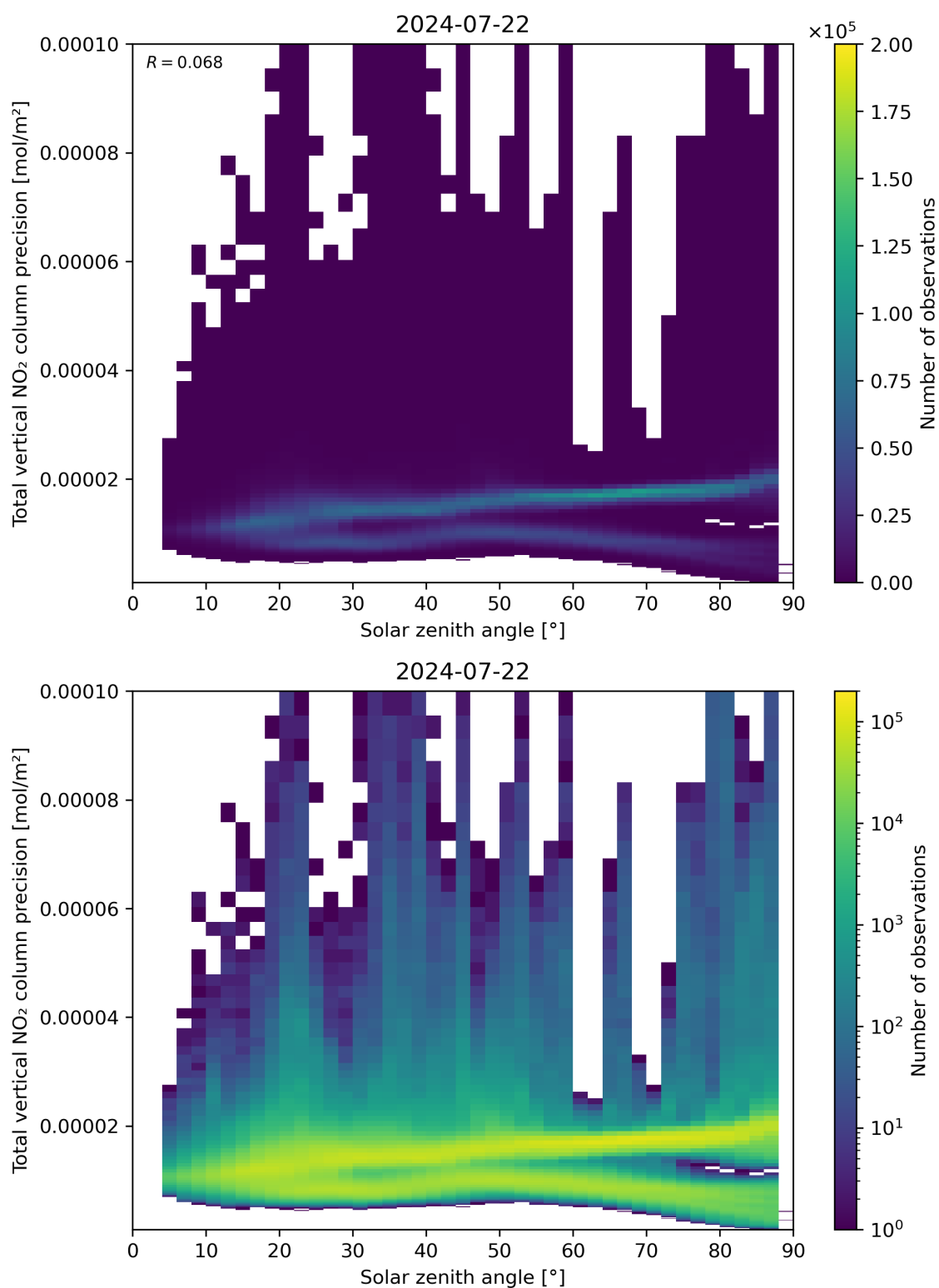
Figure 154: Scatter density plot of “Solar zenith angle” against “Total vertical NO 2 column precision” for 2024-07-21 to 2024-07-23.
