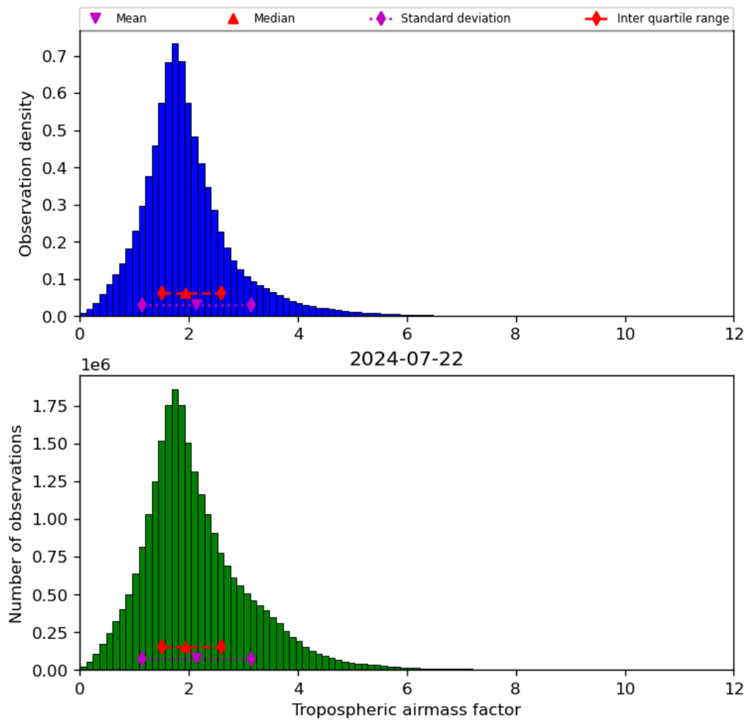
Figure 31: Histogram of “Tropospheric airmass factor” for 2024-07-21 to 2024-07-23
