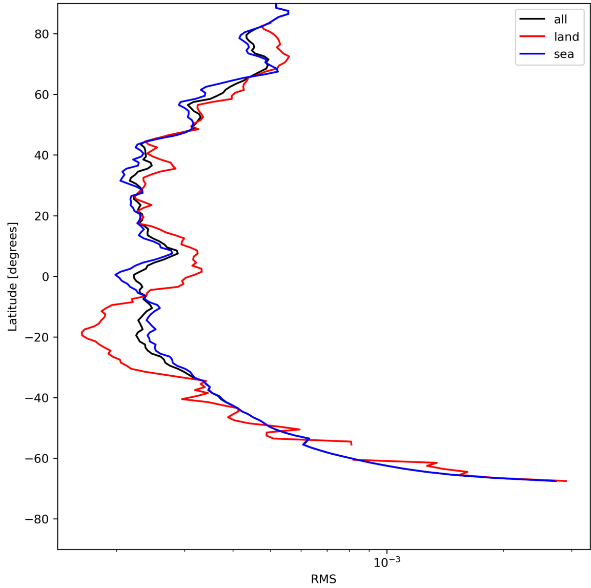
Figure 26: Zonal average of “RMS” for 2024-07-21 to 2024-07-23.
