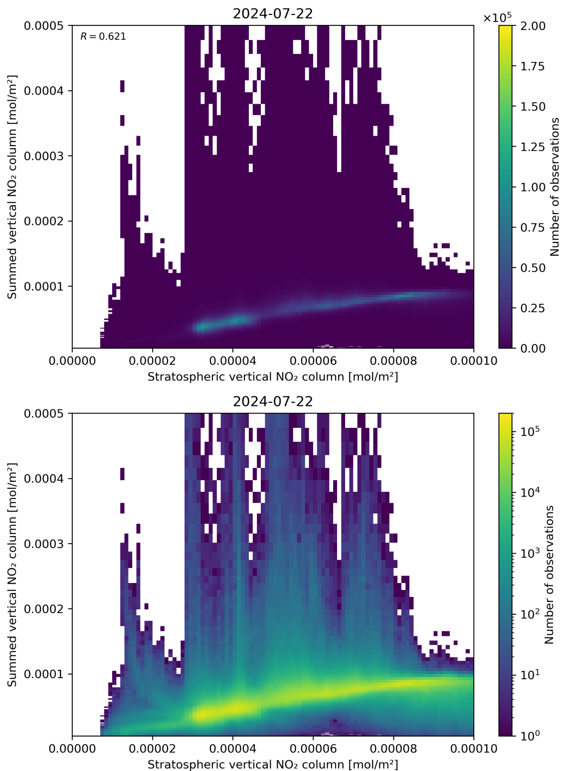
Figure 98: Scatter density plot of “Stratospheric vertical NO 2 column” against “Summed vertical NO 2 column” for 2024-07-21 to 2024-07-23.
