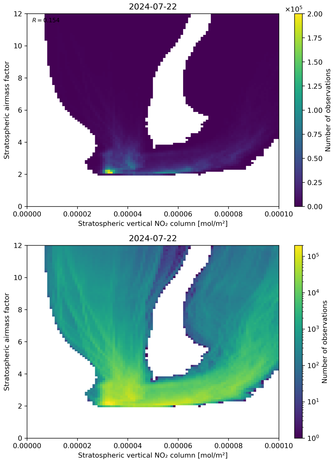
Figure 96: Scatter density plot of “Stratospheric vertical NO 2 column” against “Stratospheric airmass factor” for 2024-07-21 to 2024-07-23.
