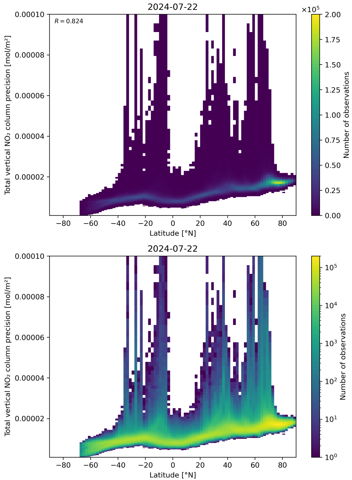
Figure 91: Scatter density plot of “Latitude” against “Total vertical NO 2 column precision” for 2024-07-21 to 2024-07-23.
