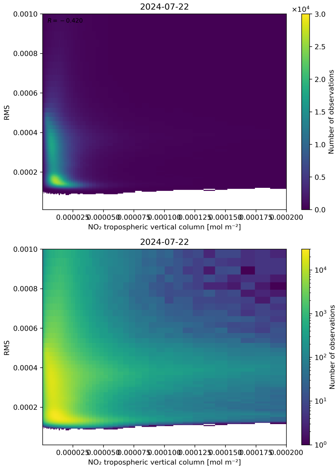
Figure 142: Scatter density plot of “NO 2 tropospheric vertical column” against “RMS” for 2024-07-21 to 2024-07-23.
