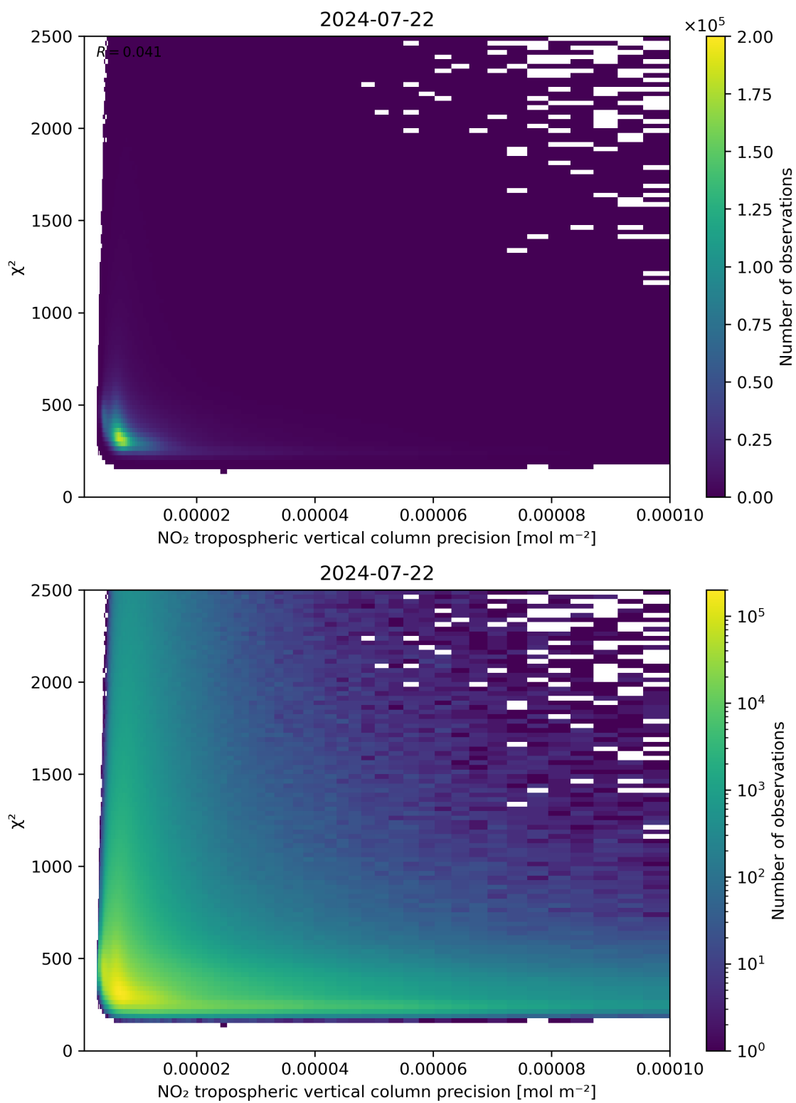
Figure 134: Scatter density plot of “NO 2 tropospheric vertical column precision” against “ \chi^2 ” for 2024-07-21 to 2024-07-23.
