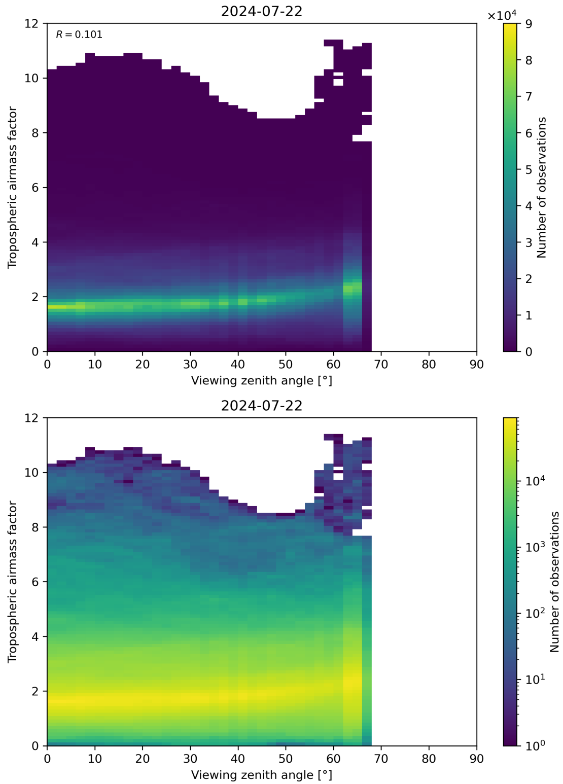
Figure 161: Scatter density plot of “Viewing zenith angle” against “Tropospheric airmass factor” for 2024-07-21 to 2024-07-23.
