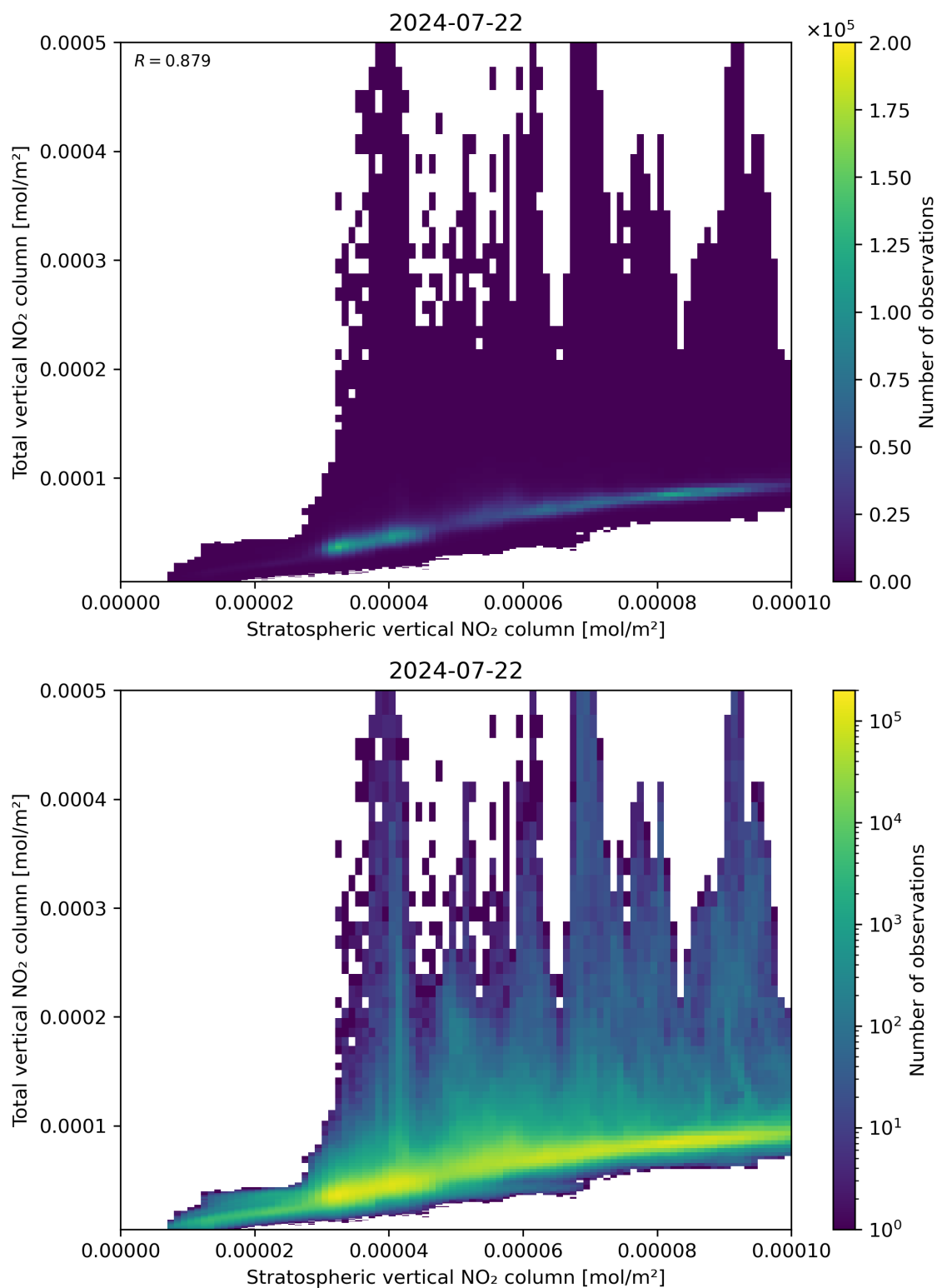
Figure 100: Scatter density plot of “Stratospheric vertical NO 2 column” against “Total vertical NO 2 column” for 2024-07-21 to 2024-07-23.
