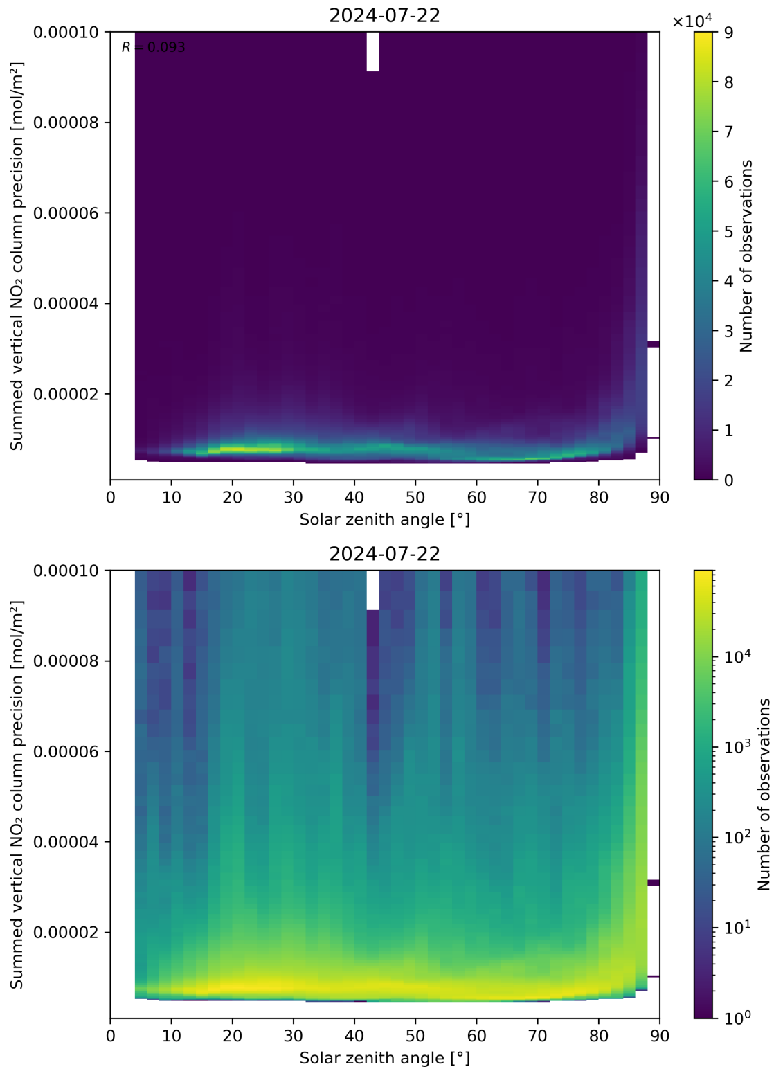
Figure 152: Scatter density plot of “Solar zenith angle” against “Summed vertical NO 2 column precision” for 2024-07-21 to 2024-07-23.
