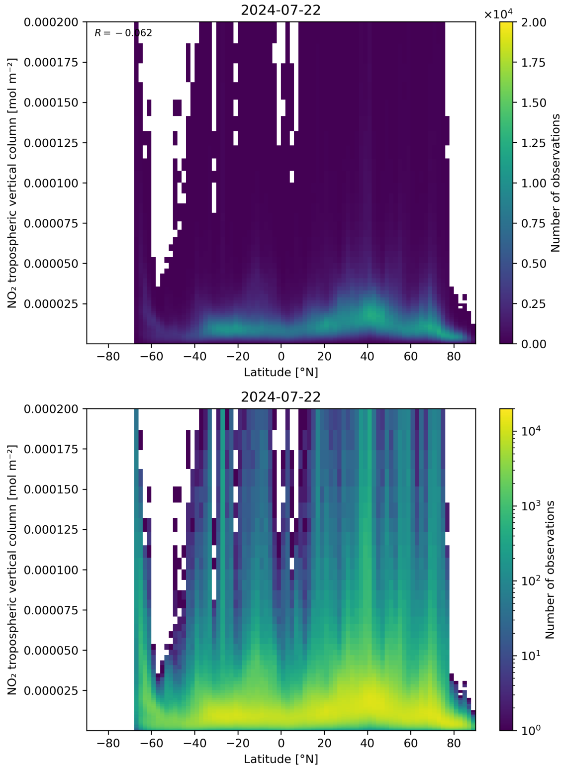
Figure 92: Scatter density plot of “Latitude” against “NO 2 tropospheric vertical column” for 2024-07-21 to 2024-07-23.
