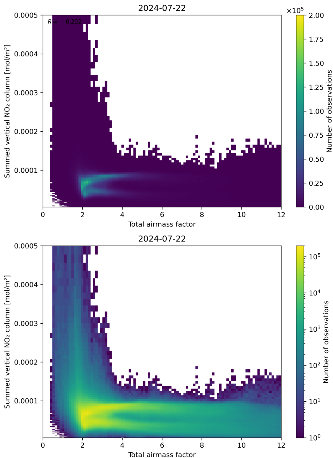
Figure 65: Scatter density plot of “Total airmass factor” against “Summed vertical NO 2 column” for 2024-07-21 to 2024-07-23.
