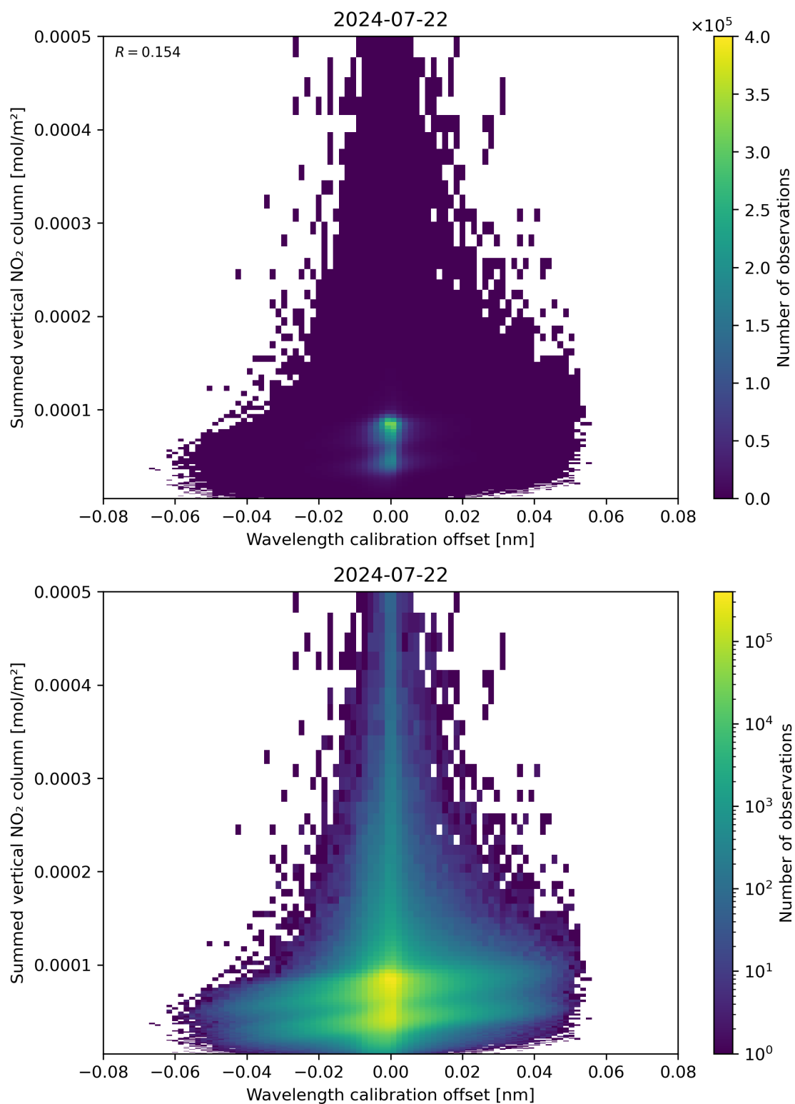
Figure 177: Scatter density plot of “Wavelength calibration offset” against “Summed vertical NO 2 column” for 2024-07-21 to 2024-07-23.
