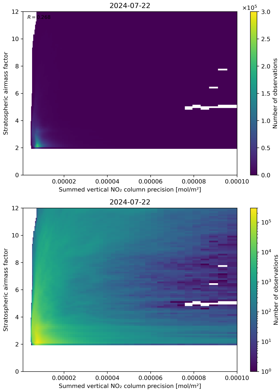
Figure 106: Scatter density plot of “Summed vertical NO 2 column precision” against “Stratospheric airmass factor” for 2024-07-21 to 2024-07-23.
