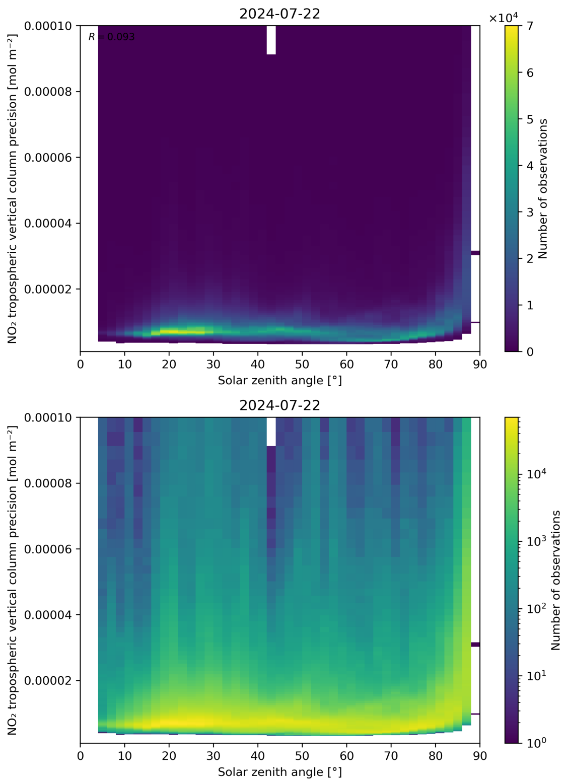
Figure 156: Scatter density plot of “Solar zenith angle” against “NO 2 tropospheric vertical column precision” for 2024-07-21 to 2024-07-23.
