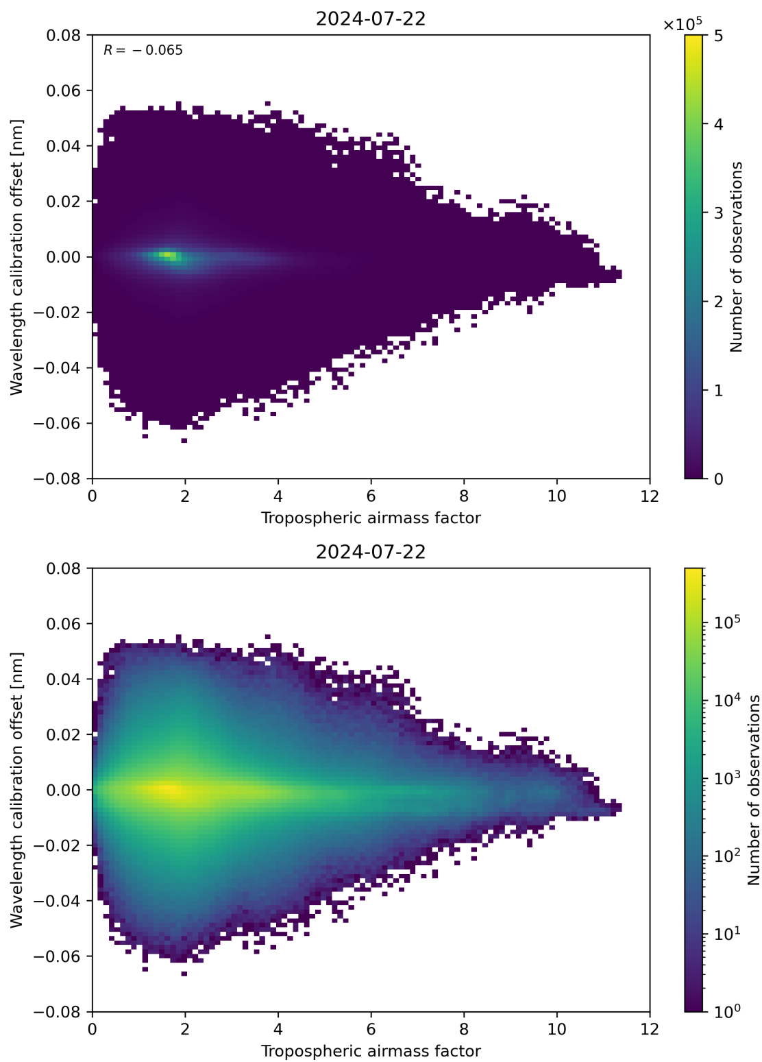
Figure 80: Scatter density plot of “Tropospheric airmass factor” against “Wavelength calibration offset” for 2024-07-21 to 2024-07-23.
