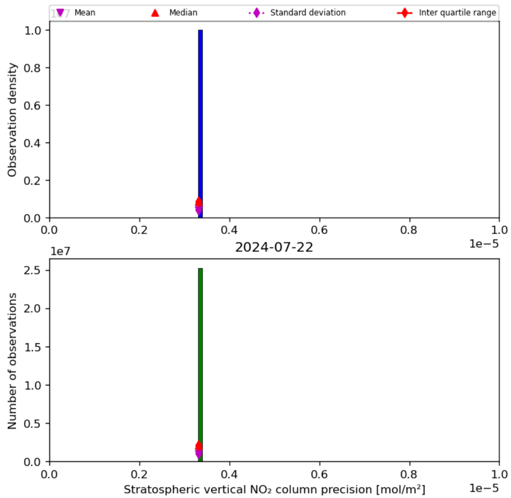
Figure 37: Histogram of “Stratospheric vertical NO 2 column precision” for 2024-07-21 to 2024-07-23
