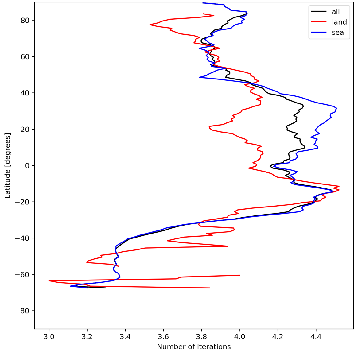
Figure 17: Zonal average of “Number of iterations” for 2024-07-21 to 2024-07-23.
