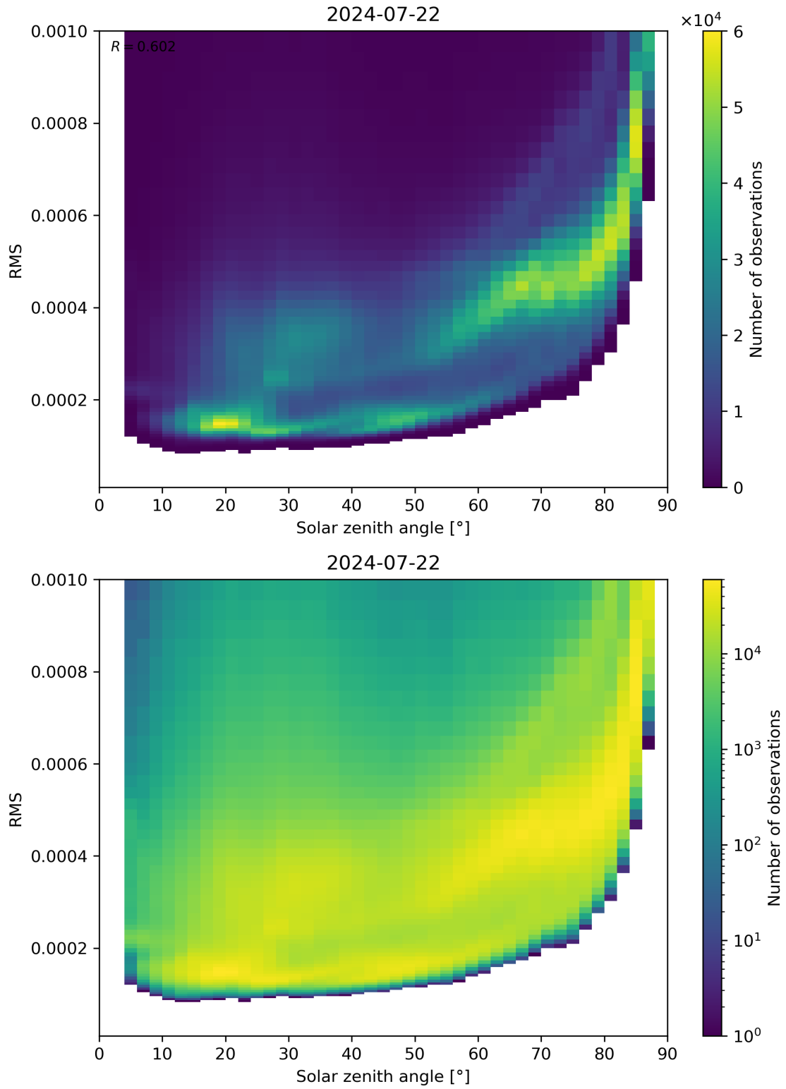
Figure 157: Scatter density plot of “Solar zenith angle” against “RMS” for 2024-07-21 to 2024-07-23.
