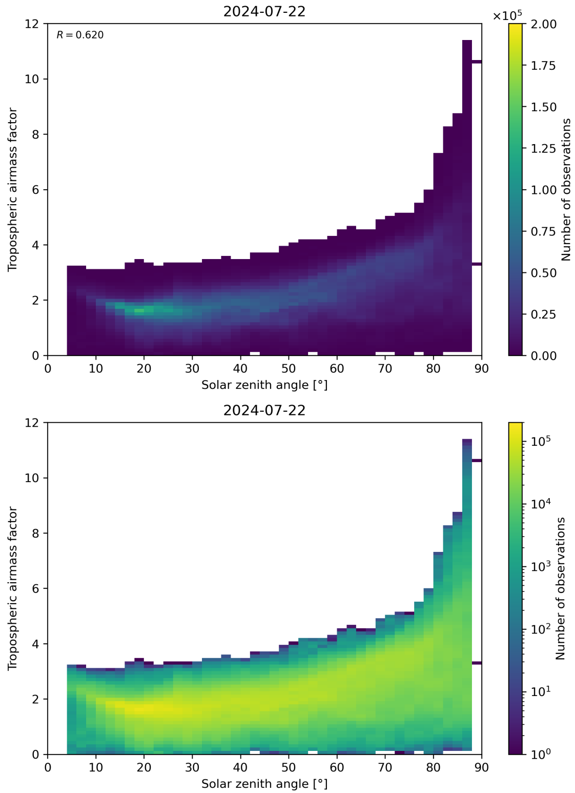
Figure 147: Scatter density plot of “Solar zenith angle” against “Tropospheric airmass factor” for 2024-07-21 to 2024-07-23.
