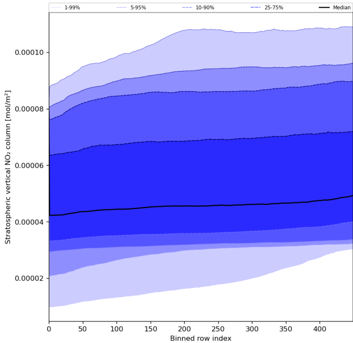
Figure 53: Along track statistics of “Stratospheric vertical NO 2 column” for 2024-07-21 to 2024-07-23
