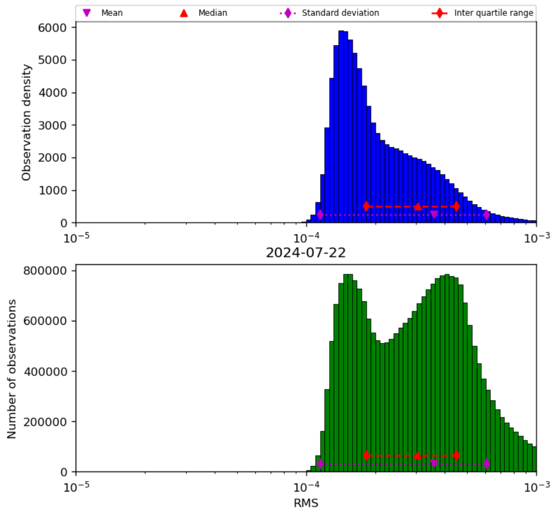
Figure 43: Histogram of “RMS” for 2024-07-21 to 2024-07-23
