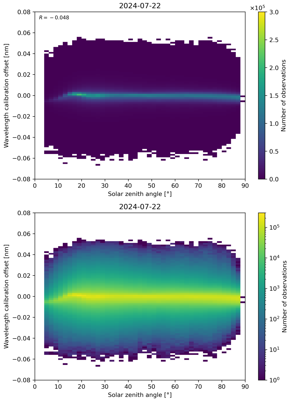
Figure 158: Scatter density plot of “Solar zenith angle” against “Wavelength calibration offset” for 2024-07-21 to 2024-07-23.
