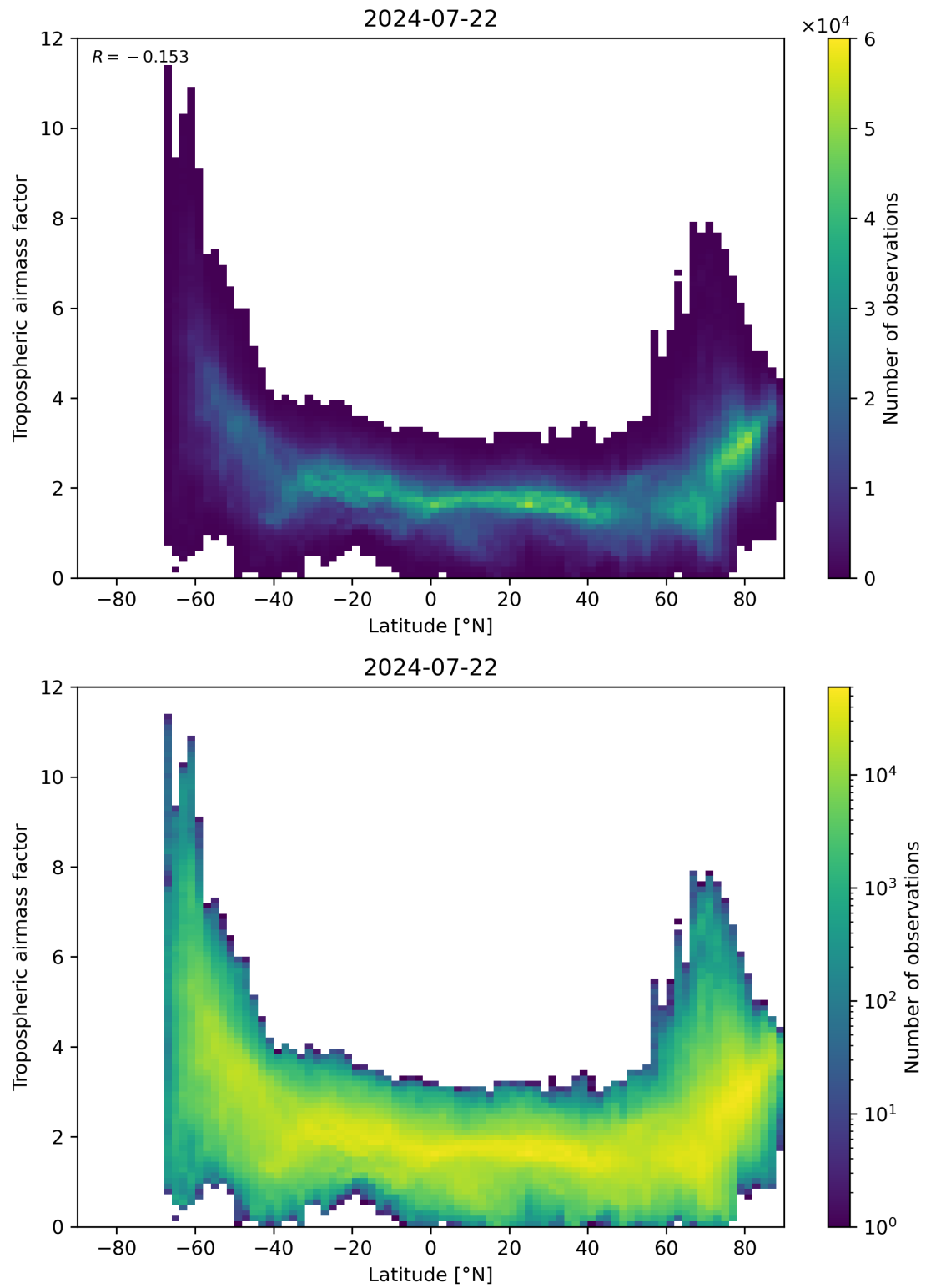
Figure 85: Scatter density plot of “Latitude” against “Tropospheric air mass factor” for 2024-07-21 to 2024-07-23.
