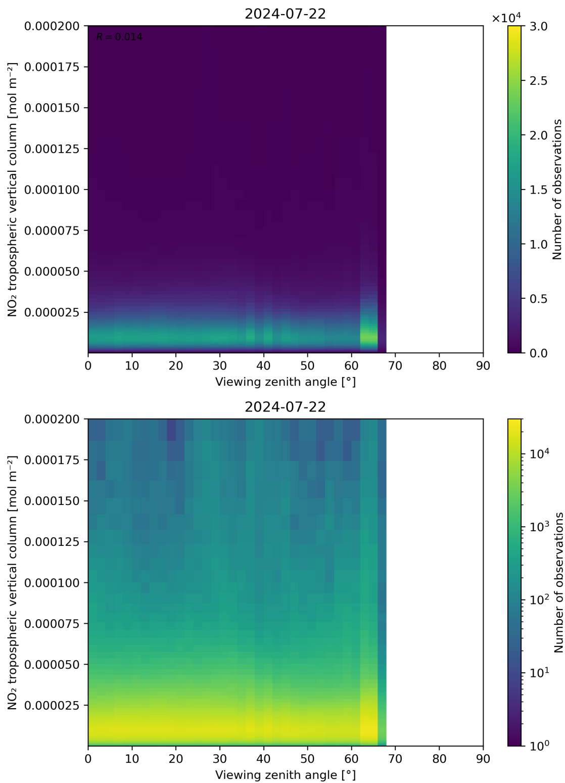
Figure 169: Scatter density plot of “Viewing zenith angle” against “NO 2 tropospheric vertical column” for 2024-07-21 to 2024-07-23.
