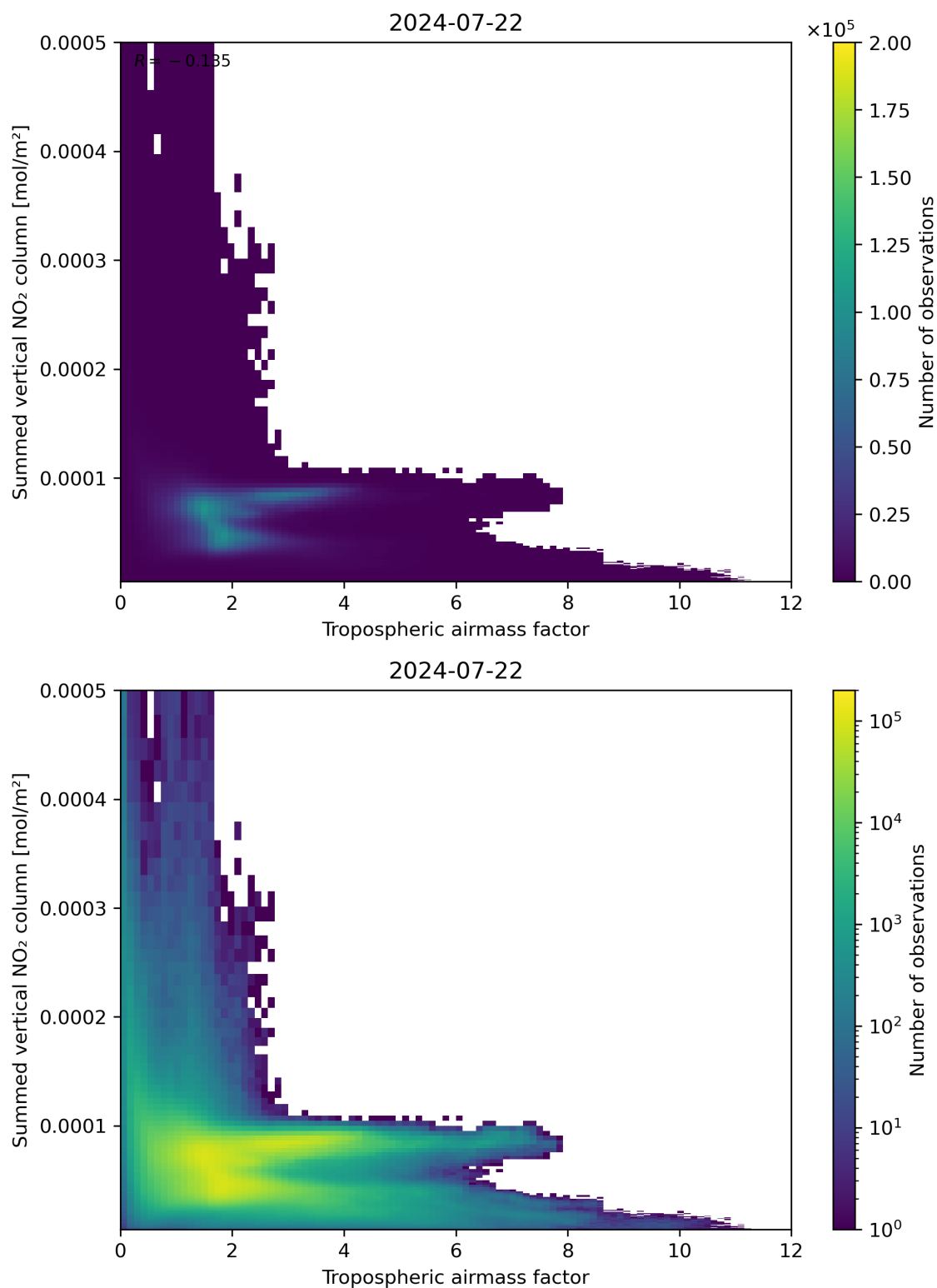
Figure 75: Scatter density plot of “Tropospheric airmass factor” against “Summed vertical NO 2 column” for 2024-07-21 to 2024-07-23.
