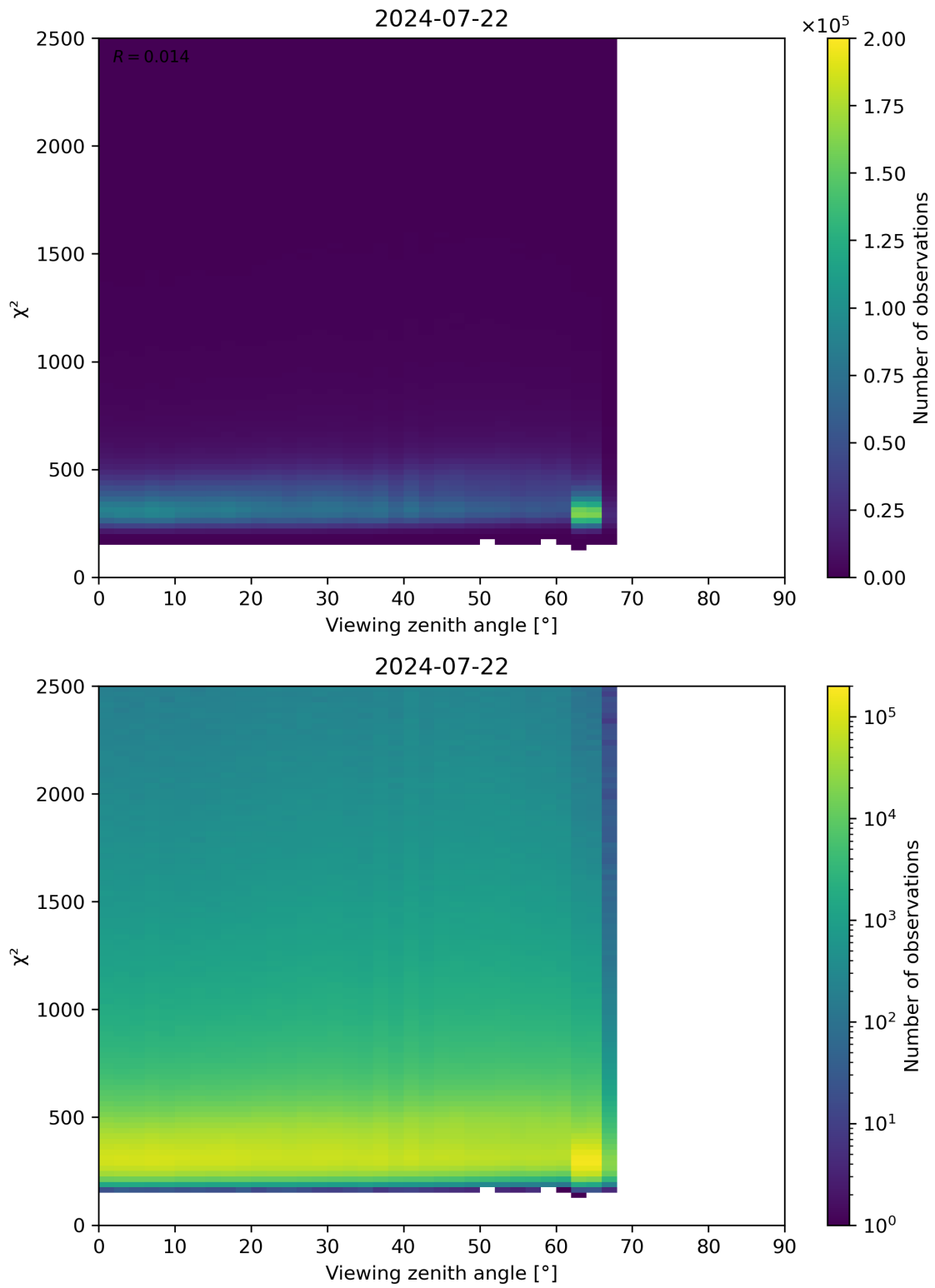
Figure 162: Scatter density plot of “Viewing zenith angle” against “ \chi^2 ” for 2024-07-21 to 2024-07-23.
