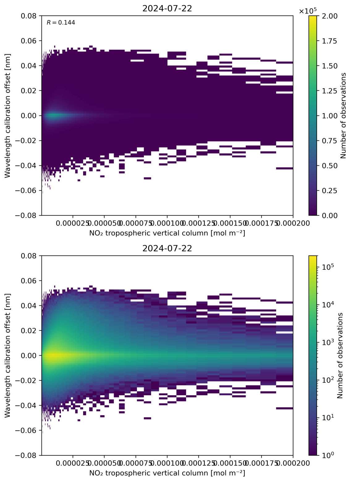
Figure 143: Scatter density plot of “NO 2 tropospheric vertical column” against “Wavelength calibration offset” for 2024-07-21 to 2024-07-23.
