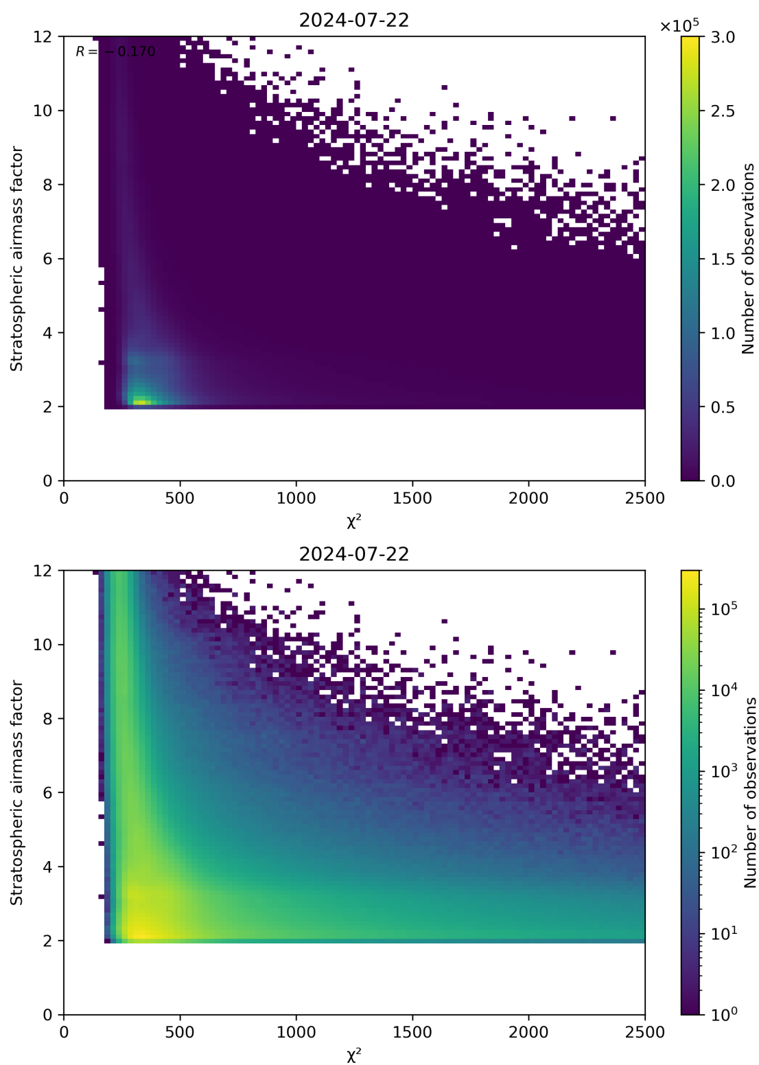
Figure 81: Scatter density plot of “ \chi^2 ” against “Stratospheric airmass factor” for 2024-07-21 to 2024-07-23.
