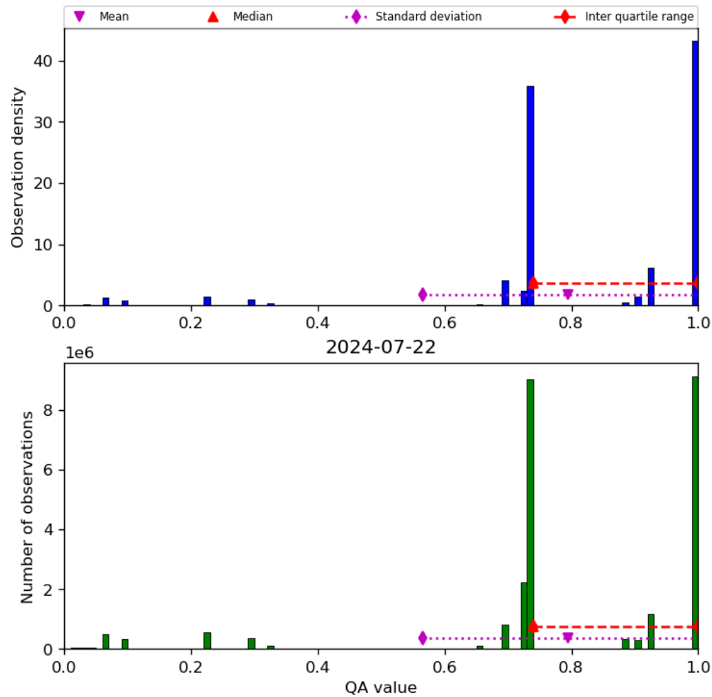
Figure 28: Histogram of “QA value” for 2024-07-21 to 2024-07-23
