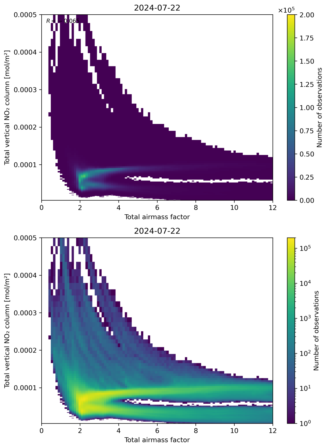
Figure 67: Scatter density plot of “Total airmass factor” against “Total vertical NO 2 column” for 2024-07-21 to 2024-07-23.
