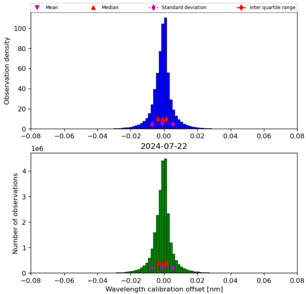
Figure 35: Histogram of “Wavelength calibration offset” for 2024-07-21 to 2024-07-23
