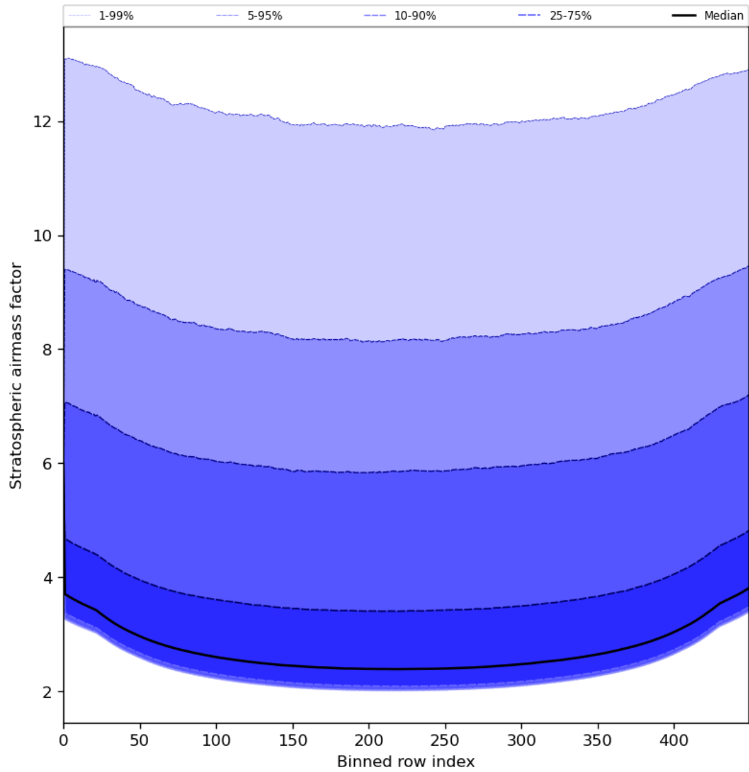
Figure 61: Along track statistics of “Stratospheric airmass factor” for 2024-07-21 to 2024-07-23
