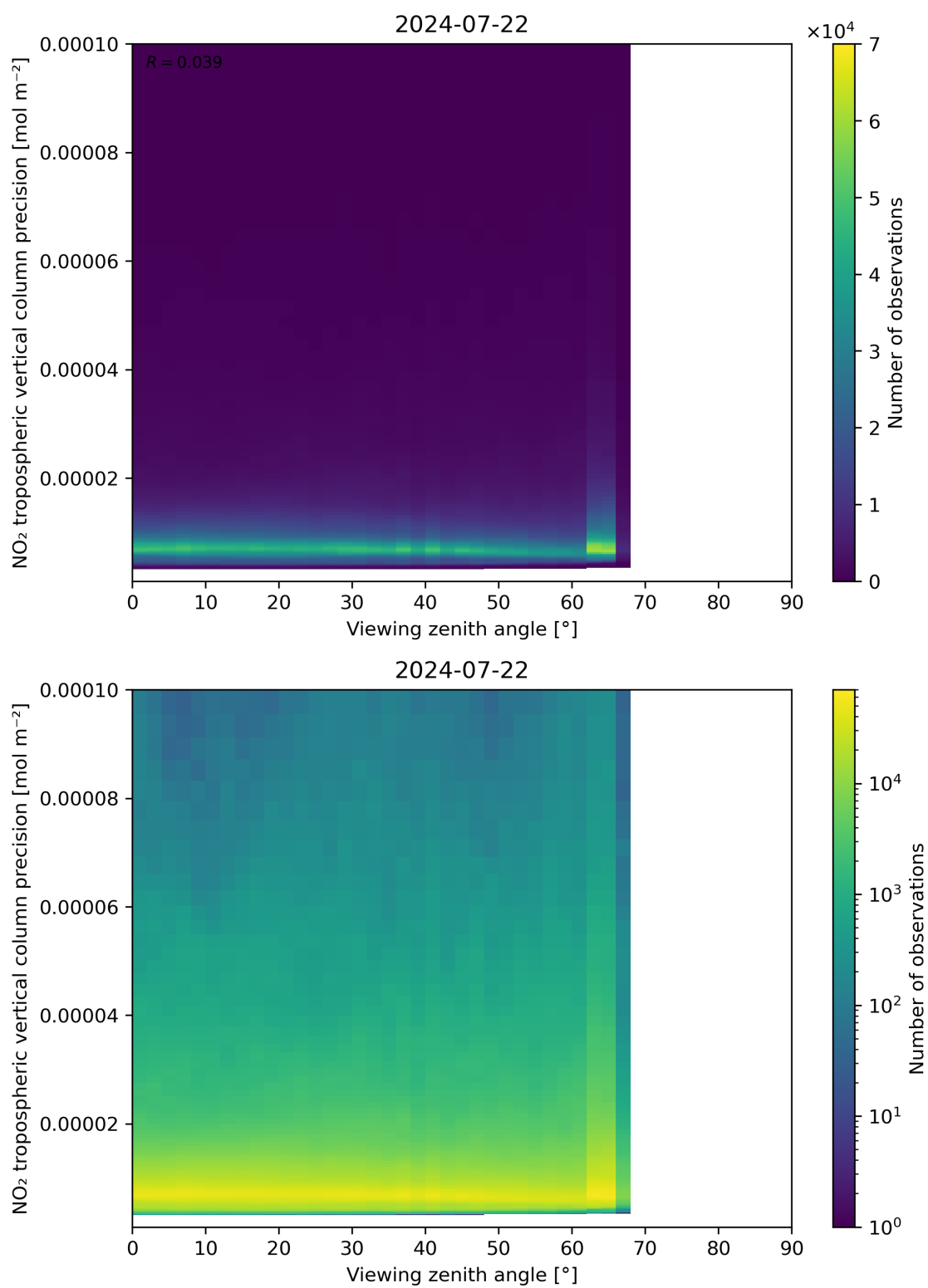
Figure 170: Scatter density plot of “Viewing zenith angle” against “NO 2 tropospheric vertical column precision” for 2024-07-21 to 2024-07-23.
