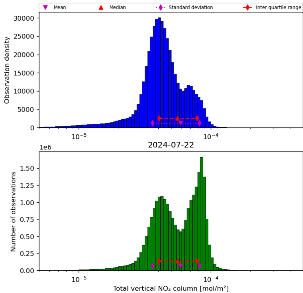
Figure 38: Histogram of “Total vertical NO 2 column” for 2024-07-21 to 2024-07-23
