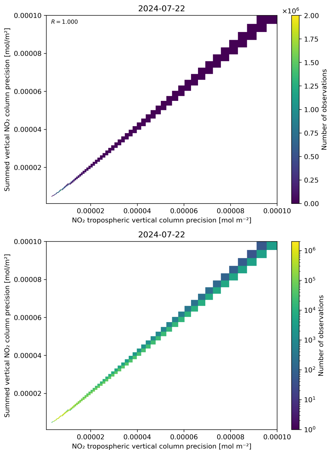
Figure 137: Scatter density plot of “NO 2 tropospheric vertical column precision” against “Summed vertical NO 2 column precision” for 2024-07-21 to 2024-07-23.
