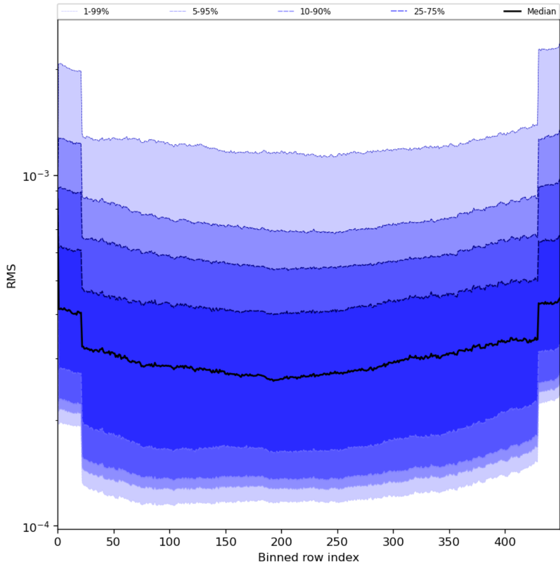
Figure 60: Along track statistics of “RMS” for 2024-07-21 to 2024-07-23
