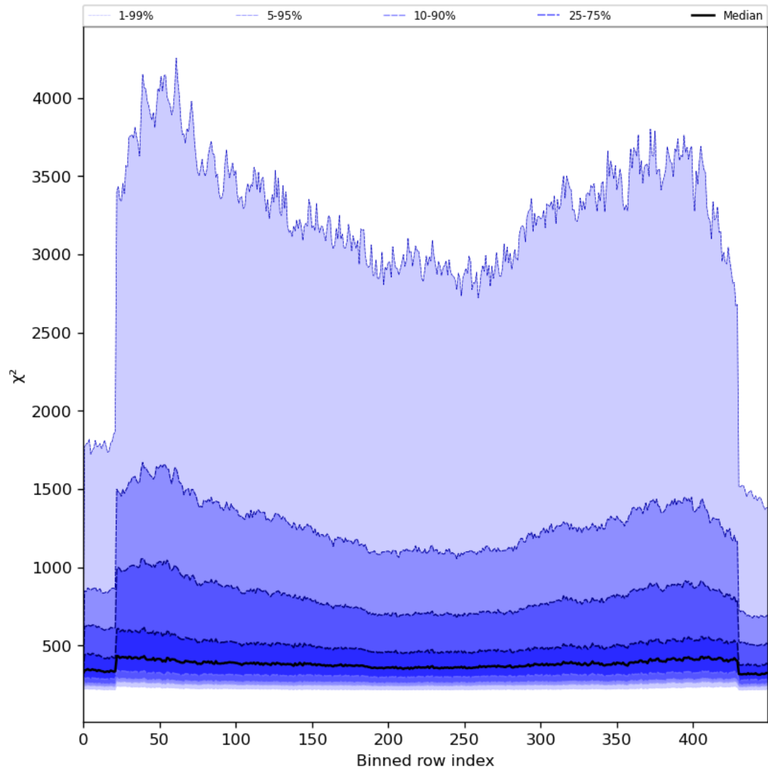
Figure 59: Along track statistics of “ \chi^2 ” for 2024-07-21 to 2024-07-23
