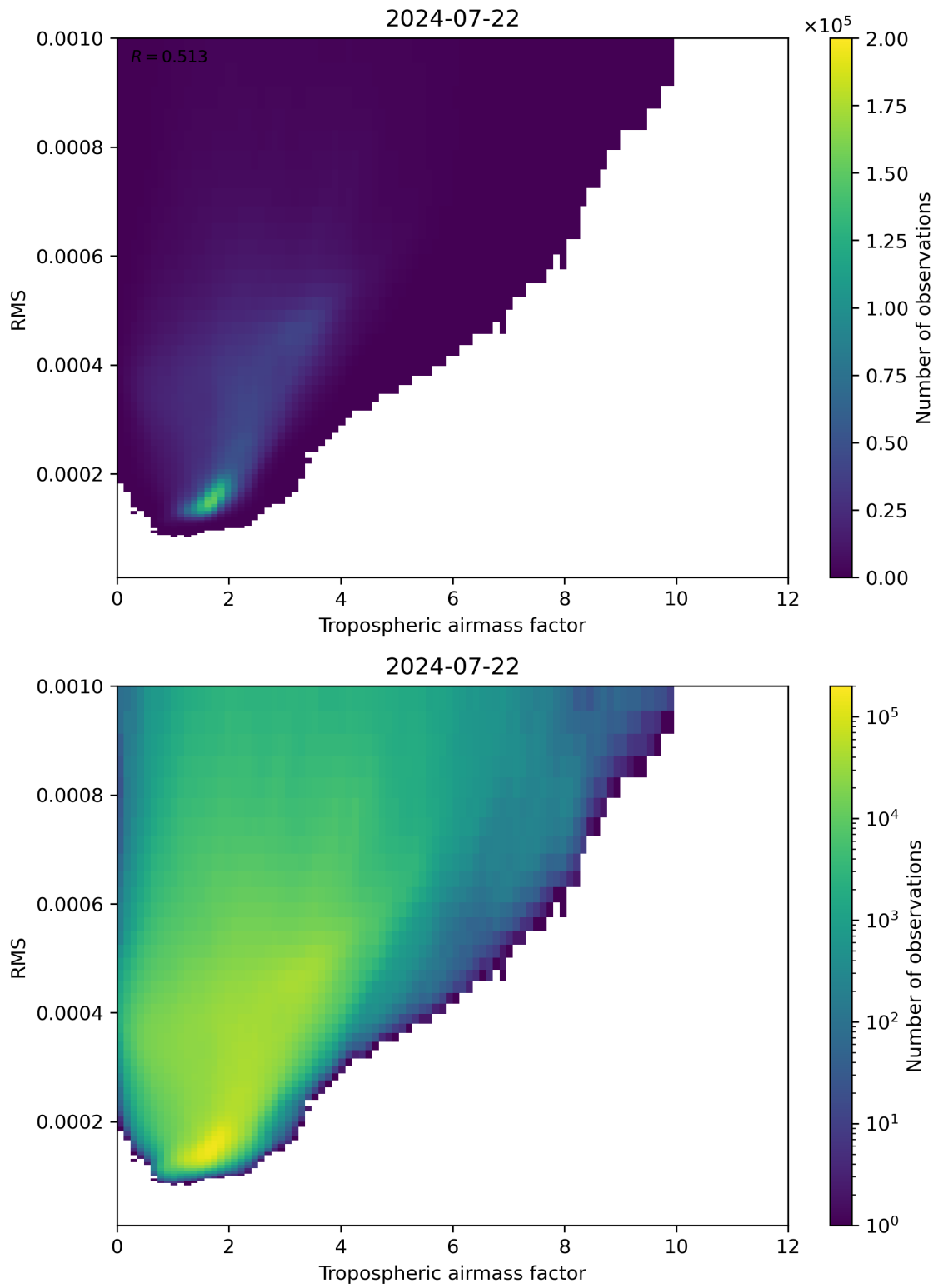
Figure 79: Scatter density plot of “Tropospheric airmass factor” against “RMS” for 2024-07-21 to 2024-07-23.
