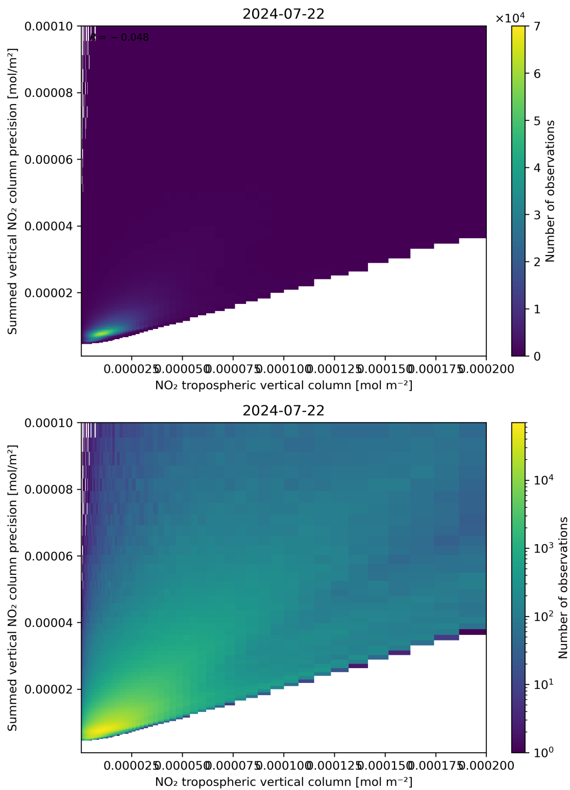
Figure 127: Scatter density plot of “NO 2 tropospheric vertical column” against “Summed vertical NO 2 column precision” for 2024-07-21 to 2024-07-23.
