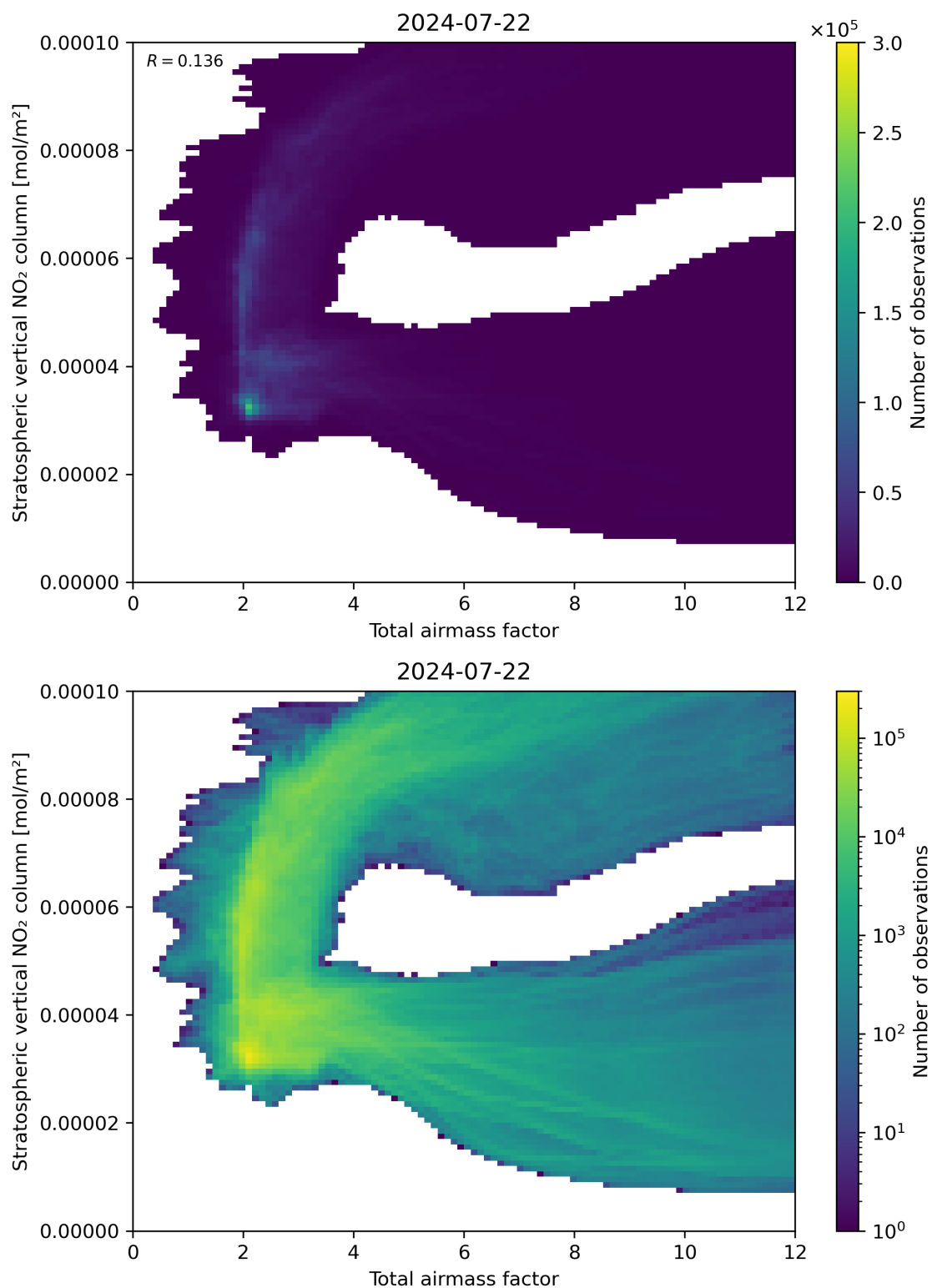
Figure 64: Scatter density plot of “Total airmass factor” against “Stratospheric vertical NO 2 column” for 2024-07-21 to 2024-07-23.
