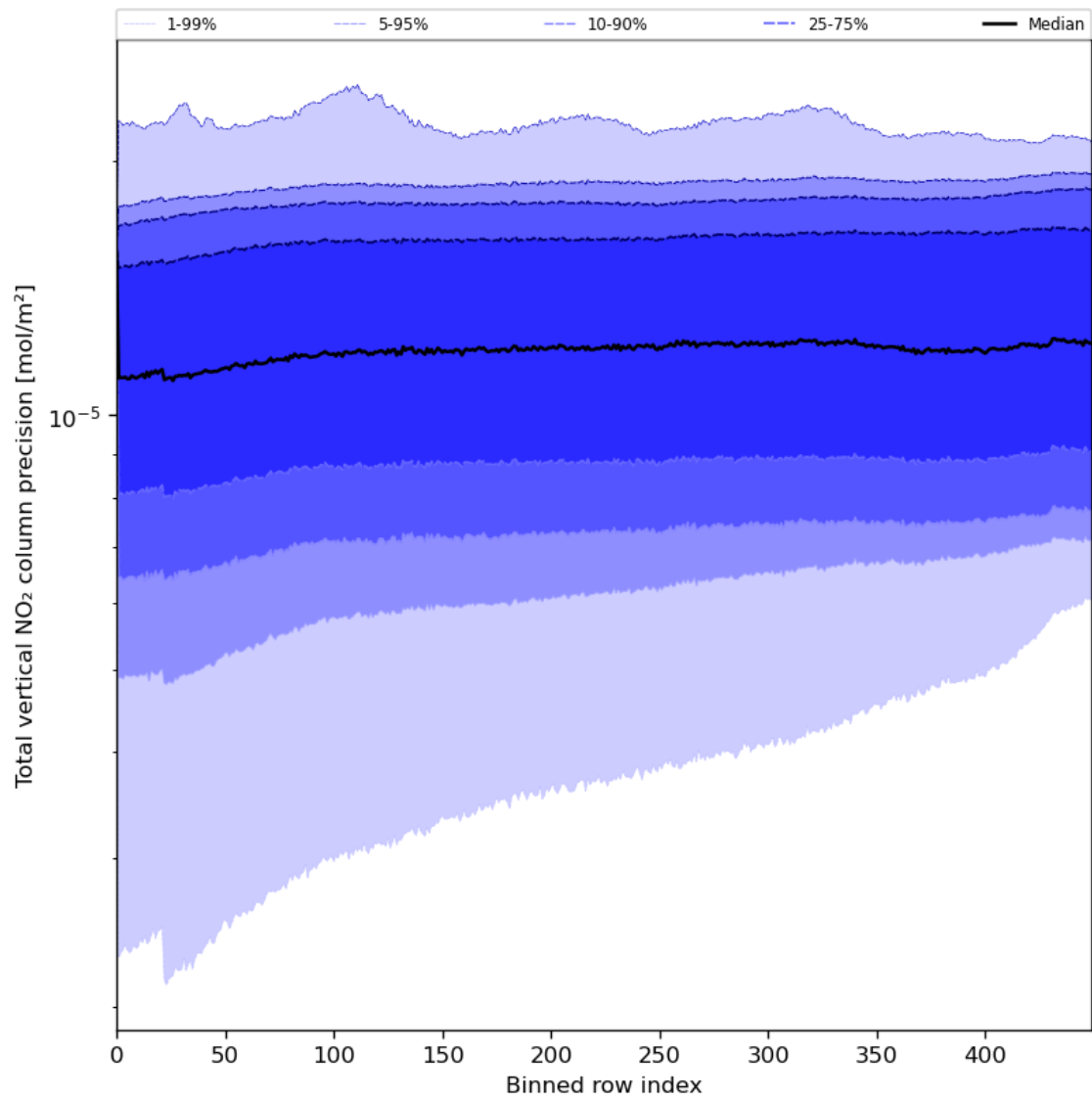
Figure 56: Along track statistics of “Total vertical NO 2 column precision” for 2024-07-21 to 2024-07-23
