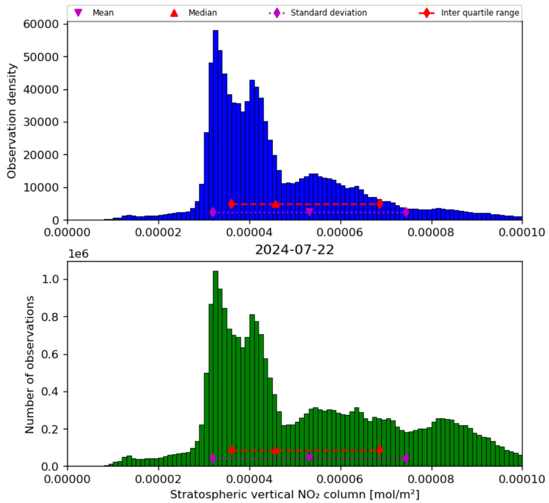
Figure 36: Histogram of “Stratospheric vertical NO 2 column” for 2024-07-21 to 2024-07-23
