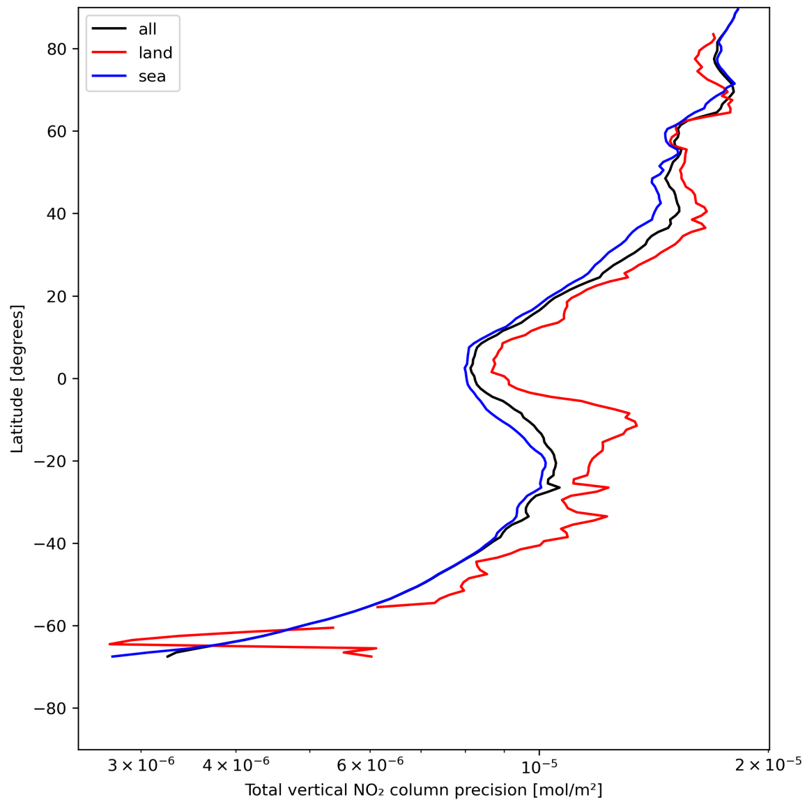
Figure 22: Zonal average of “Total vertical NO 2 column precision” for 2024-07-21 to 2024-07-23.
