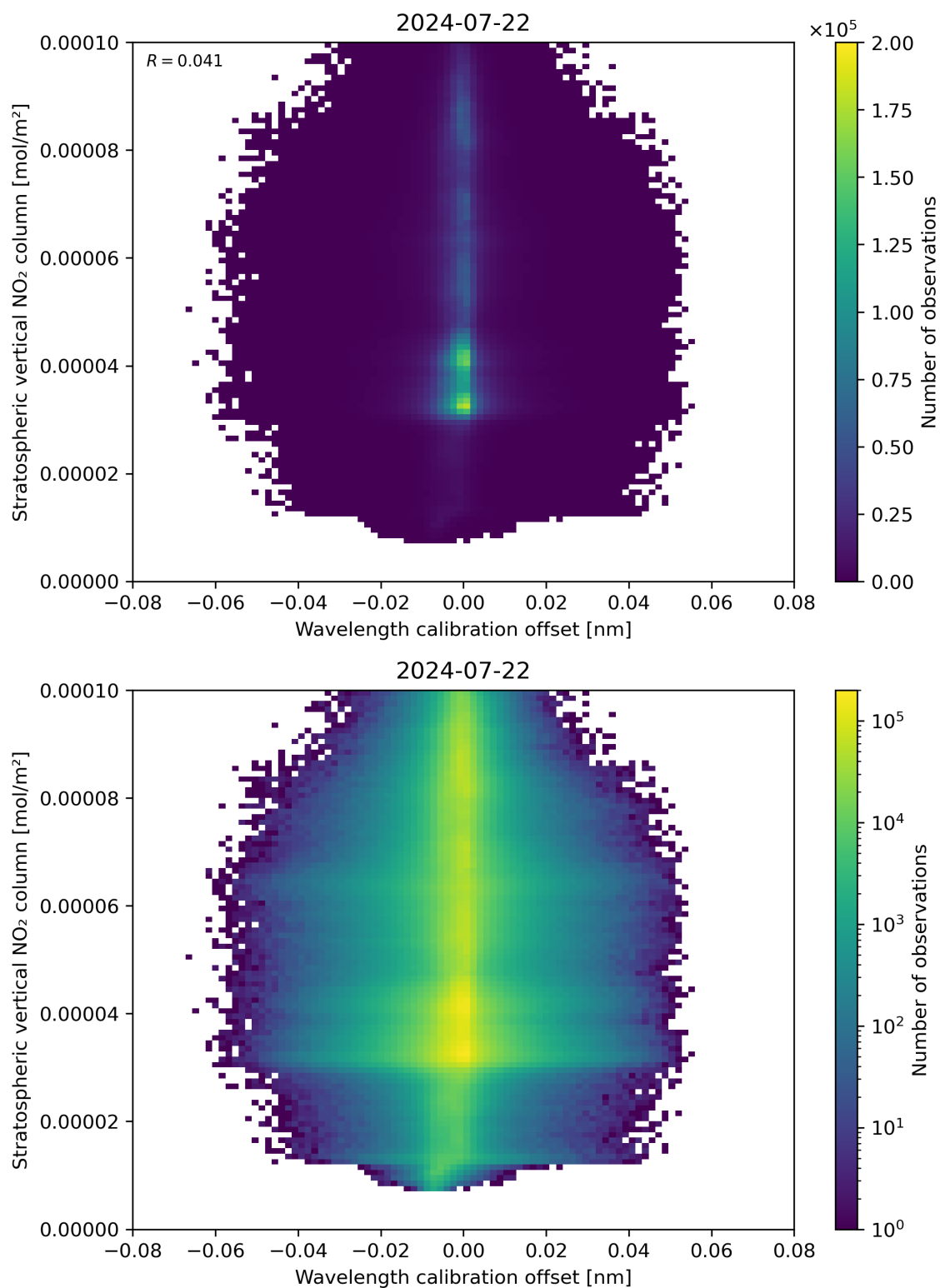
Figure 176: Scatter density plot of “Wavelength calibration offset” against “Stratospheric vertical NO 2 column” for 2024-07-21 to 2024-07-23.
