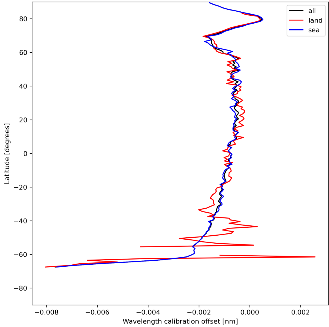
Figure 18: Zonal average of “Wavelength calibration offset” for 2024-07-21 to 2024-07-23.
