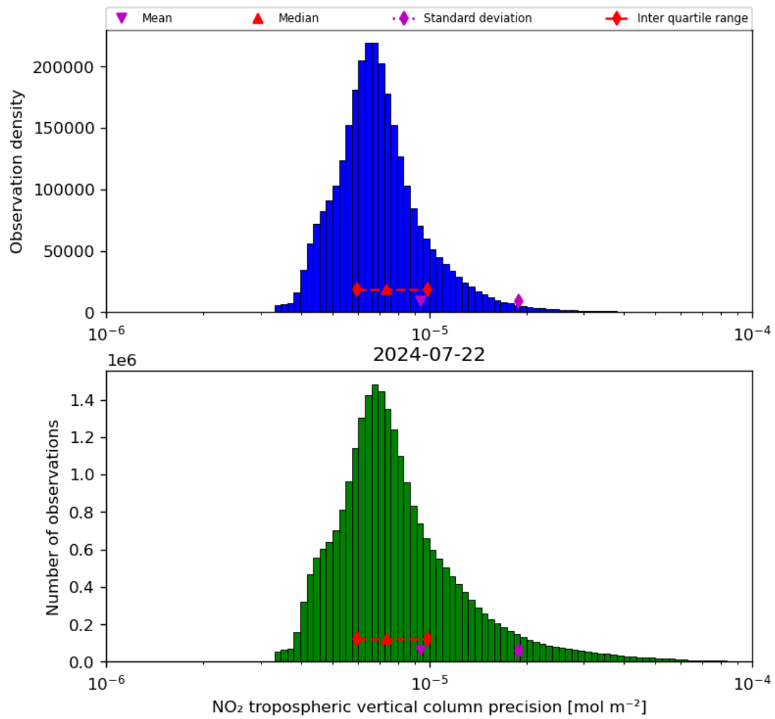
Figure 30: Histogram of “NO 2 tropospheric vertical column precision” for 2024-07-21 to 2024-07-23
