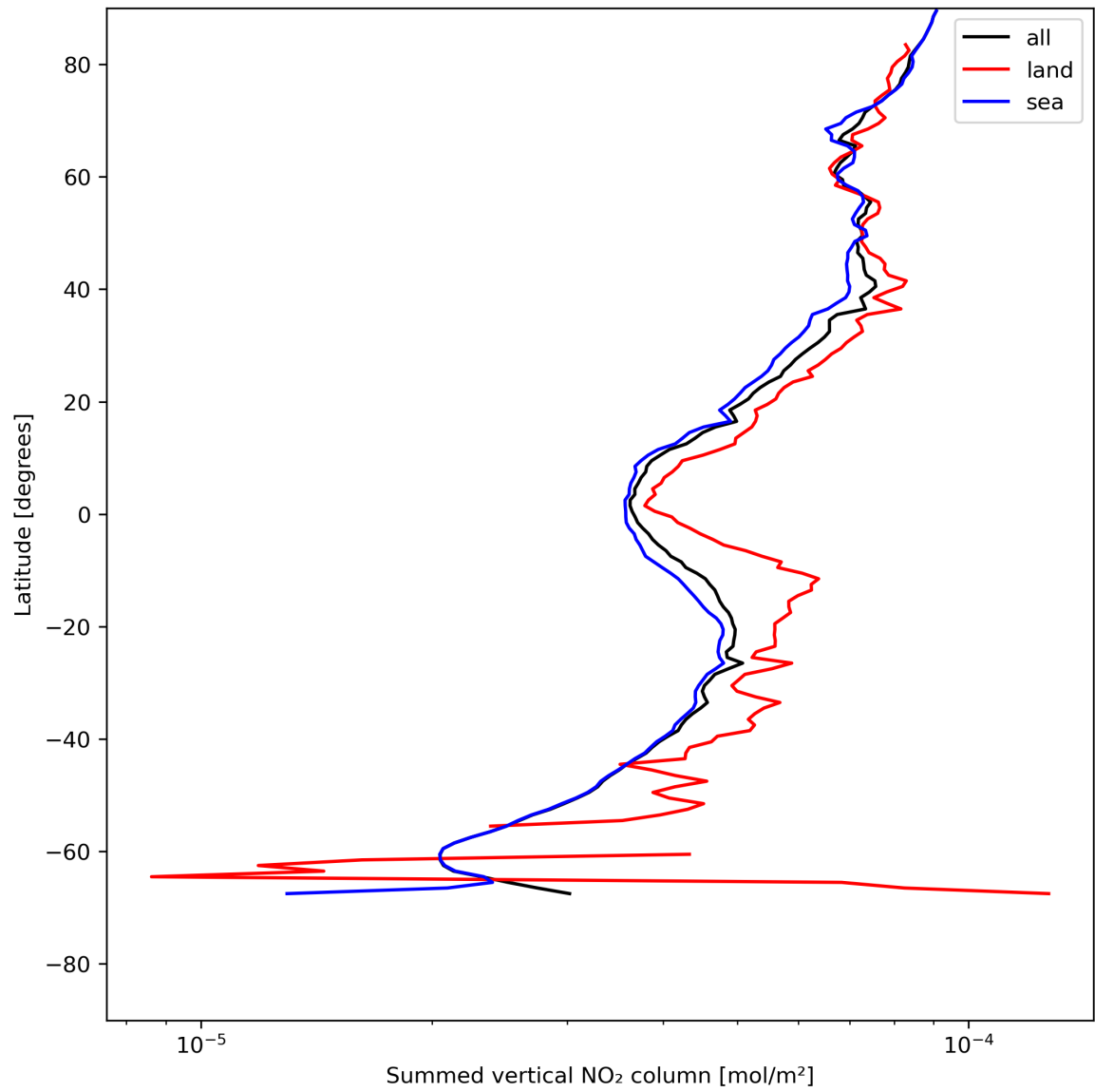
Figure 23: Zonal average of “Summed vertical NO 2 column” for 2024-07-21 to 2024-07-23.
