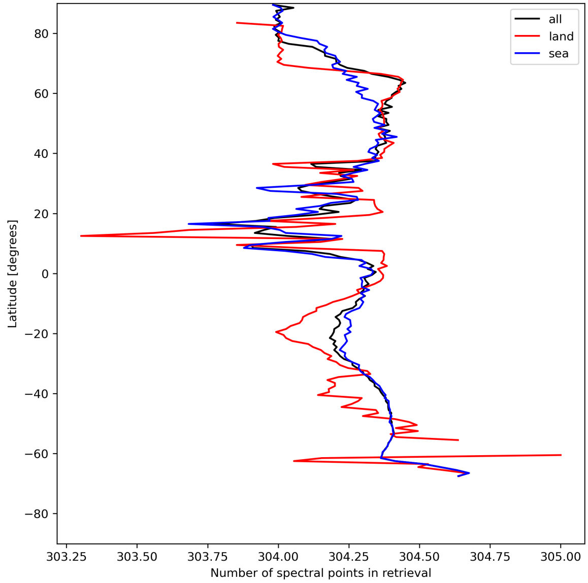
Figure 16: Zonal average of “Number of spectral points in retrieval” for 2024-07-21 to 2024-07-23.
