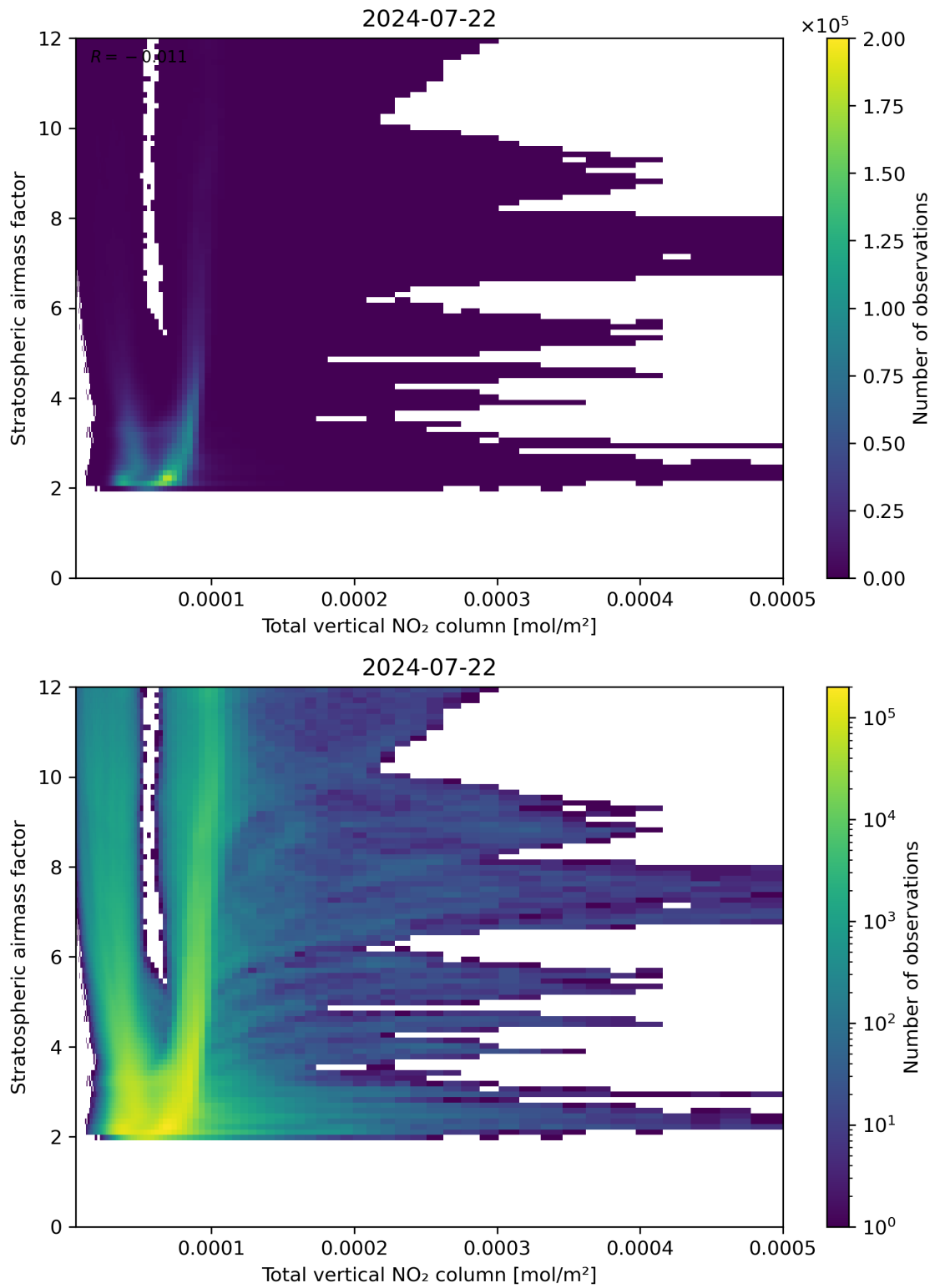
Figure 110: Scatter density plot of “Total vertical NO 2 column” against “Stratospheric airmass factor” for 2024-07-21 to 2024-07-23.
