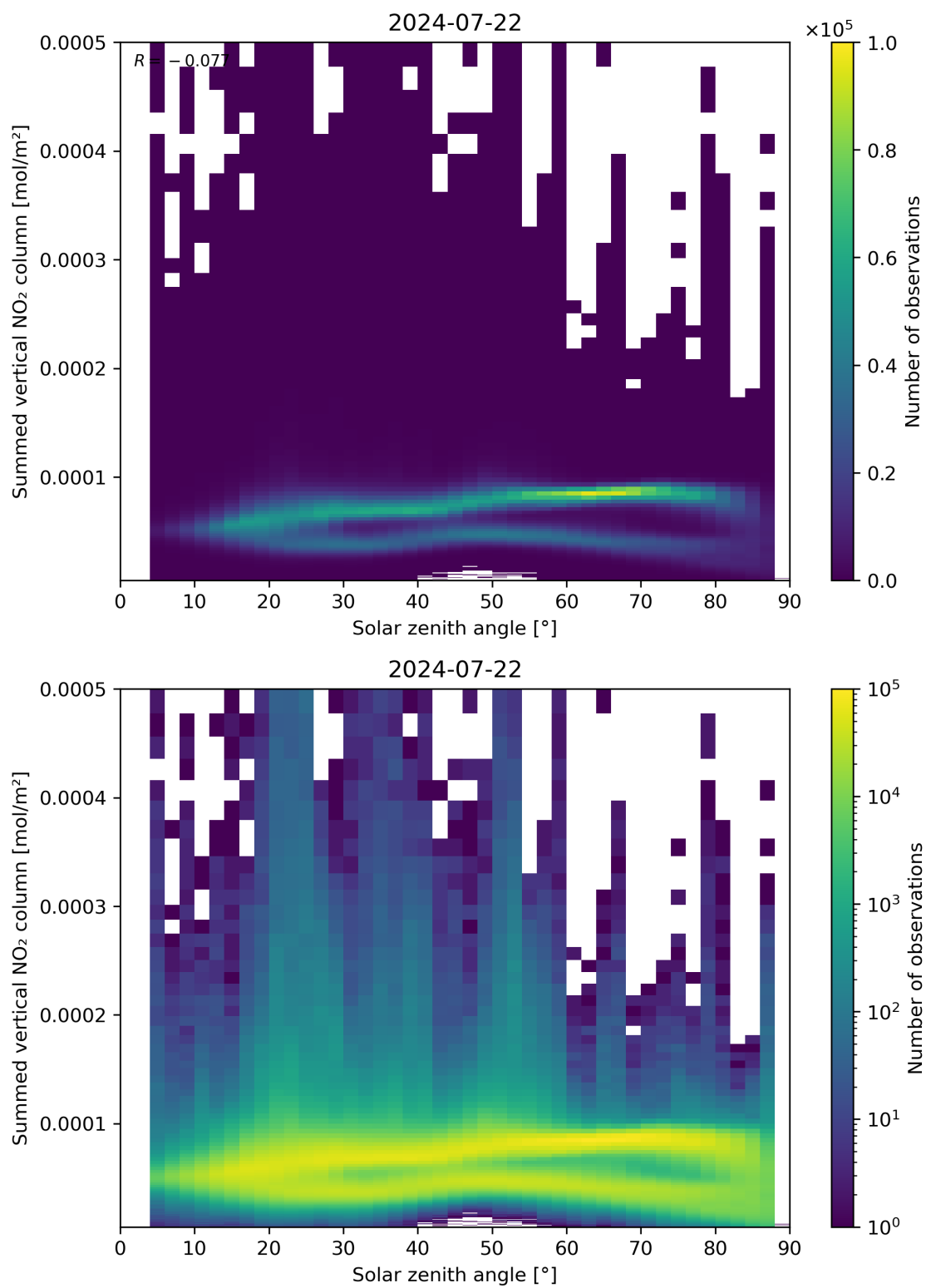
Figure 151: Scatter density plot of “Solar zenith angle” against “Summed vertical NO 2 column” for 2024-07-21 to 2024-07-23.
