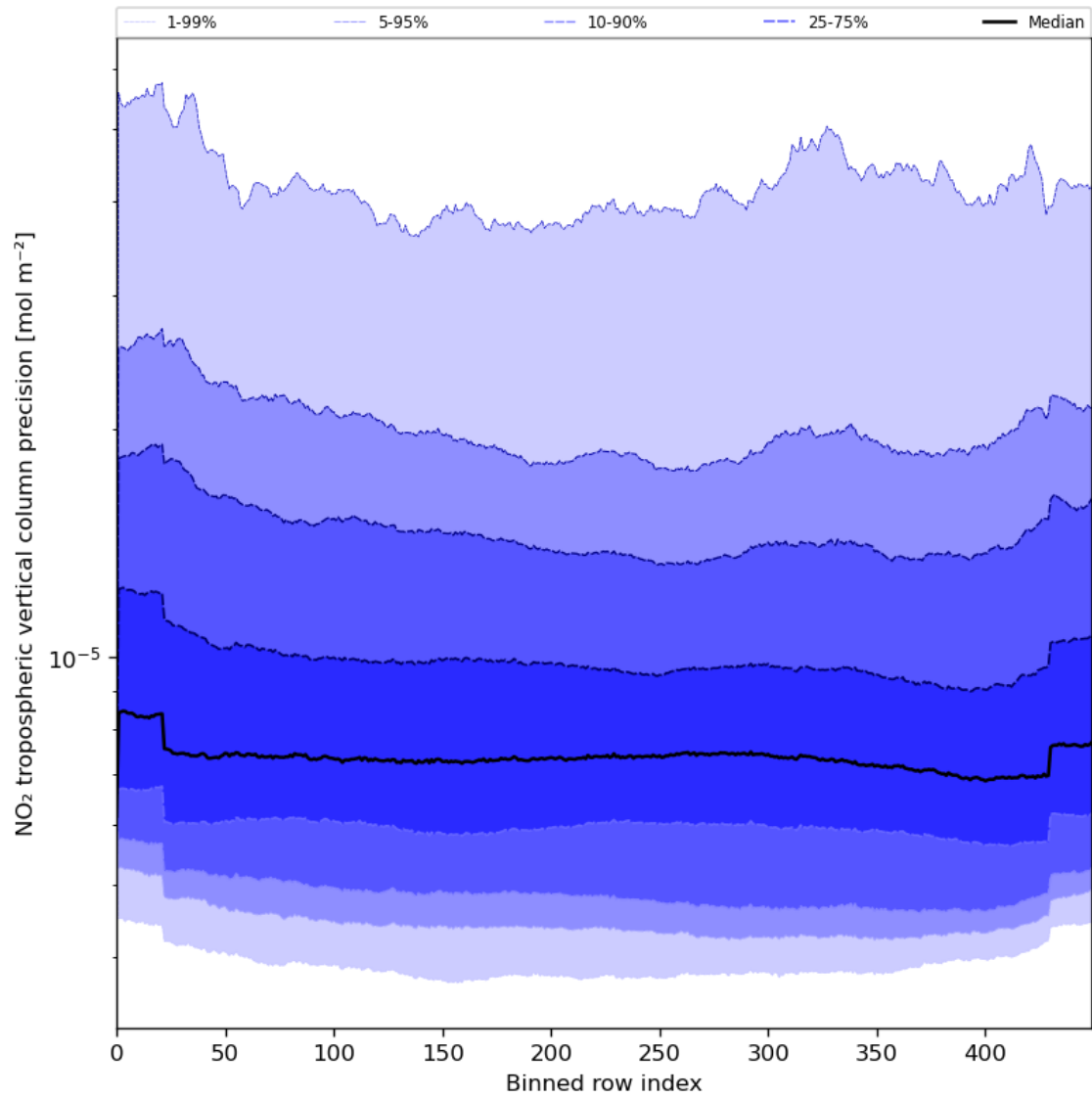
Figure 47: Along track statistics of “NO 2 tropospheric vertical column precision” for 2024-07-21 to 2024-07-23
