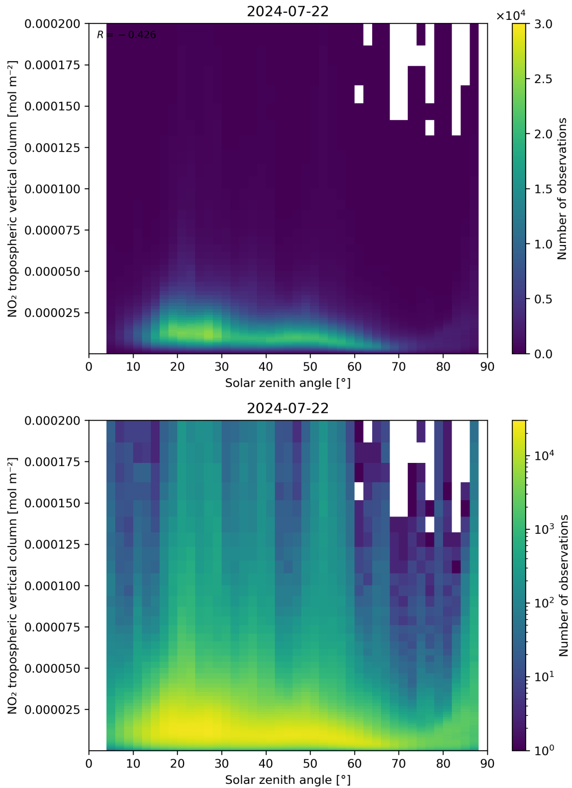
Figure 155: Scatter density plot of “Solar zenith angle” against “NO 2 tropospheric vertical column” for 2024-07-21 to 2024-07-23.
