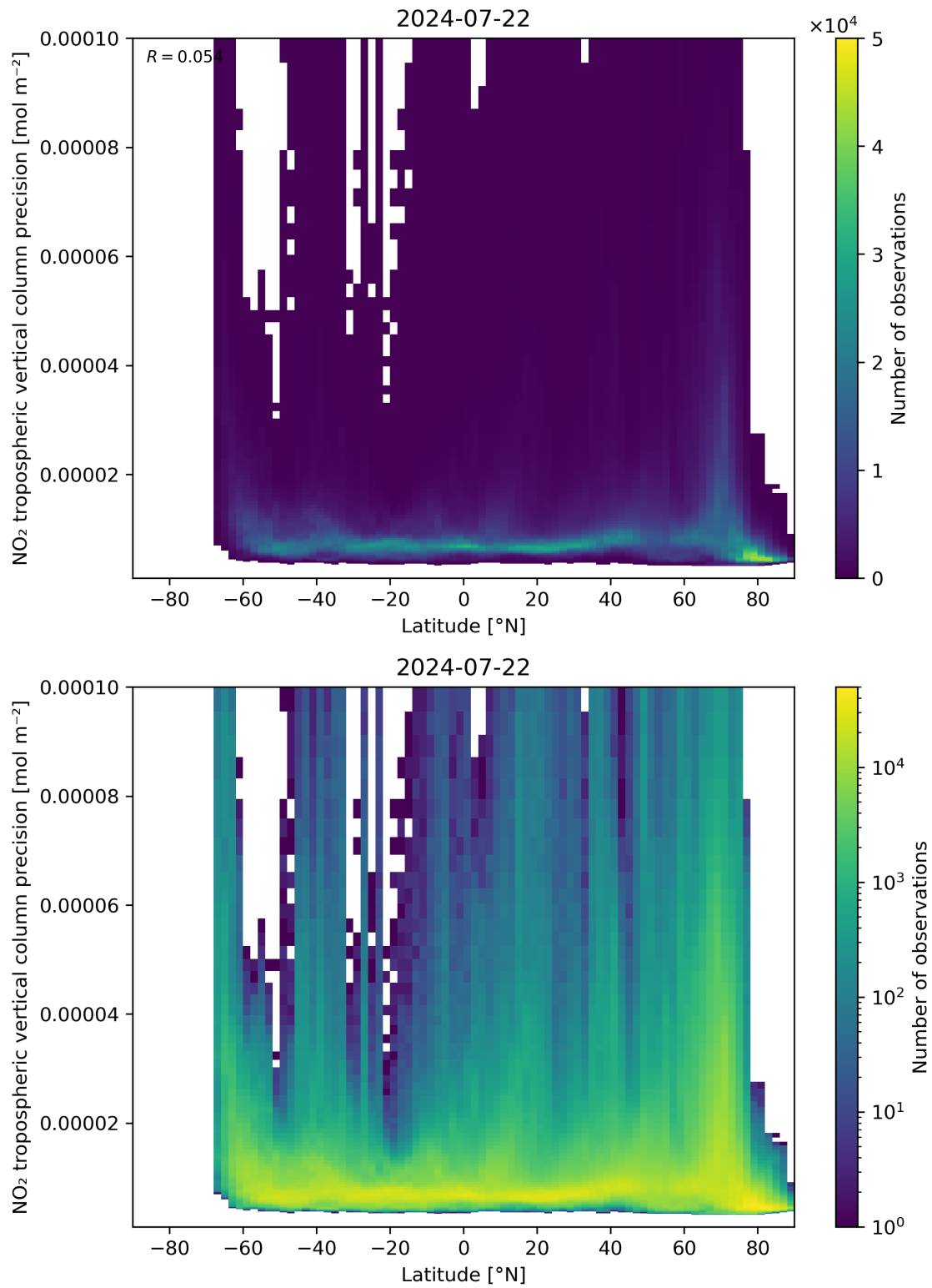
Figure 93: Scatter density plot of “Latitude” against “NO 2 tropospheric vertical column precision” for 2024-07-21 to 2024-07-23.
