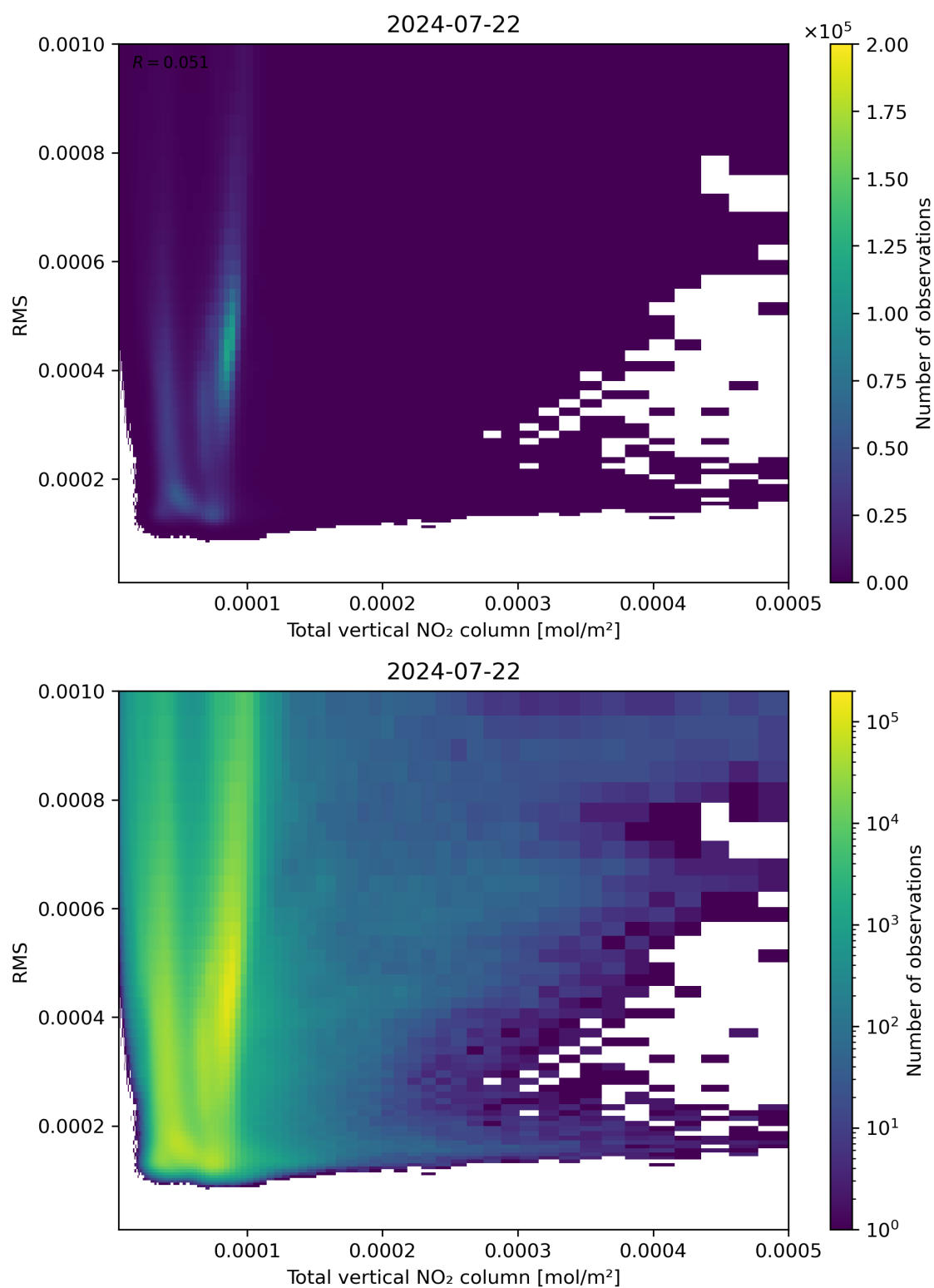
Figure 120: Scatter density plot of “Total vertical NO 2 column” against “RMS” for 2024-07-21 to 2024-07-23.
