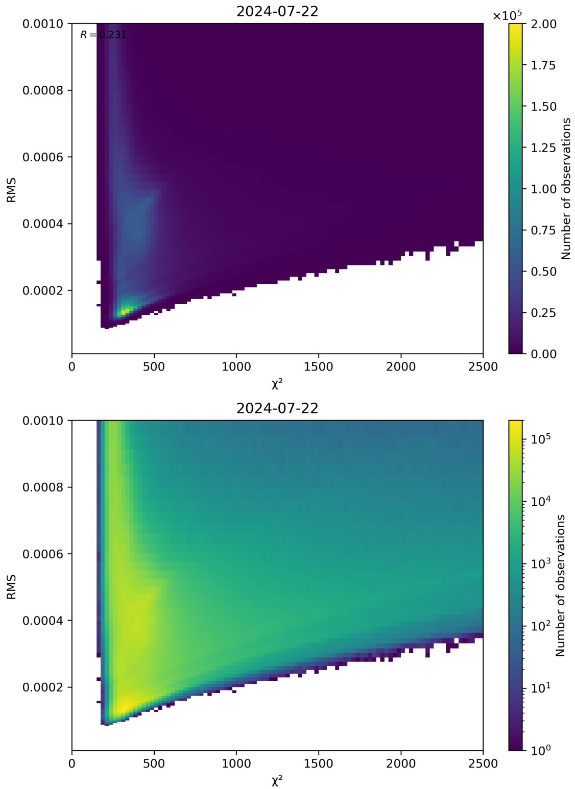
Figure 82: Scatter density plot of “ \chi^2 ” against “RMS” for 2024-07-21 to 2024-07-23.
