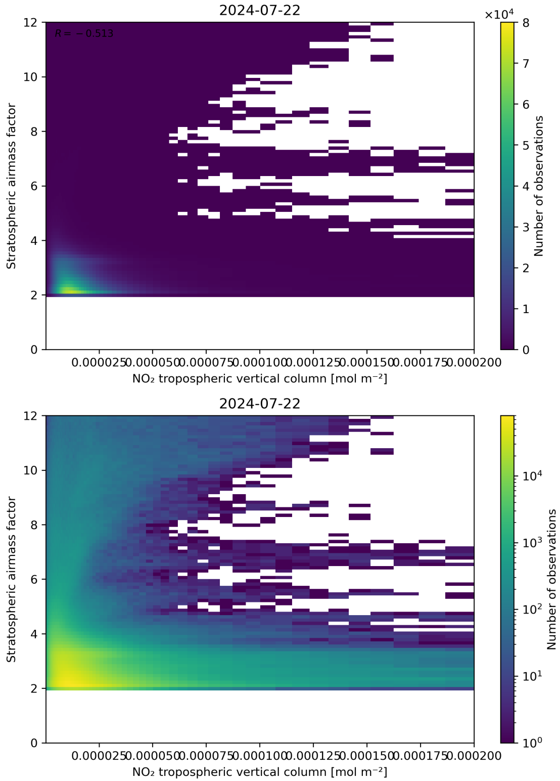
Figure 121: Scatter density plot of “NO 2 tropospheric vertical column” against “Stratospheric air mass factor” for 2024-07-21 to 2024-07-23.
