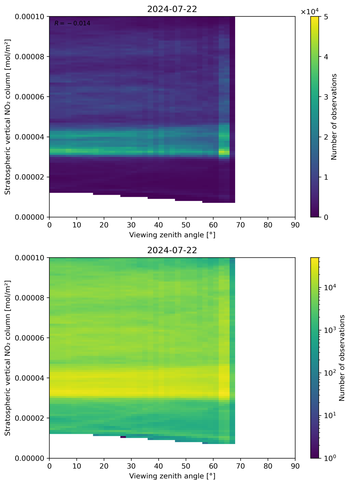
Figure 164: Scatter density plot of “Viewing zenith angle” against “Stratospheric vertical NO 2 column” for 2024-07-21 to 2024-07-23.
