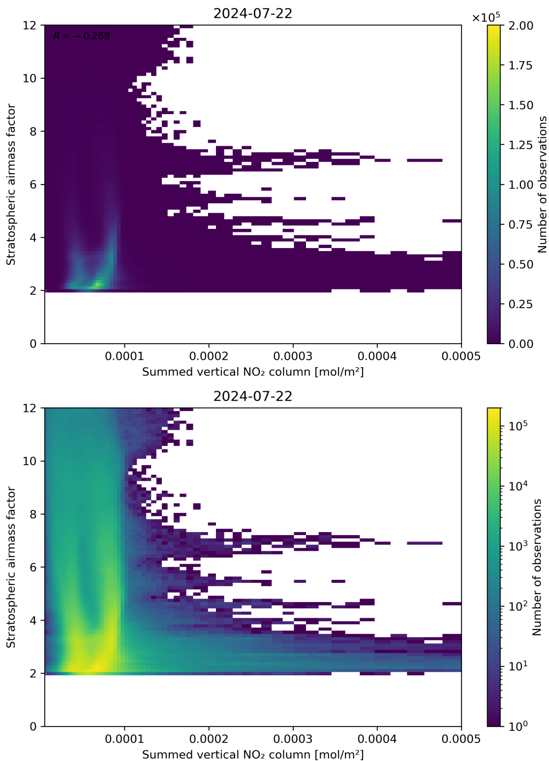
Figure 103: Scatter density plot of “Summed vertical NO 2 column” against “Stratospheric air mass factor” for 2024-07-21 to 2024-07-23.
