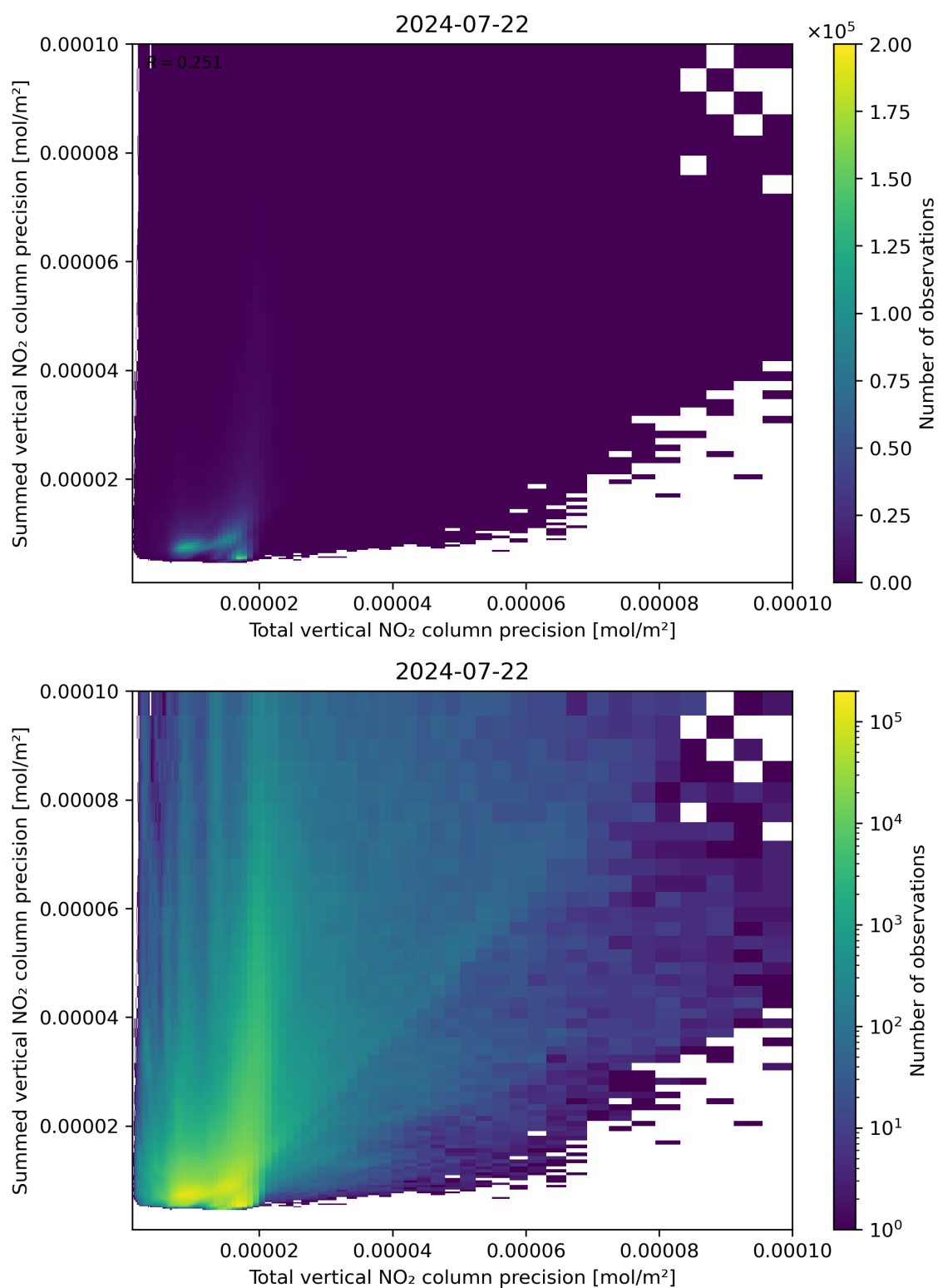
Figure 118: Scatter density plot of “Total vertical NO 2 column precision” against “Summed vertical NO 2 column precision” for 2024-07-21 to 2024-07-23.
