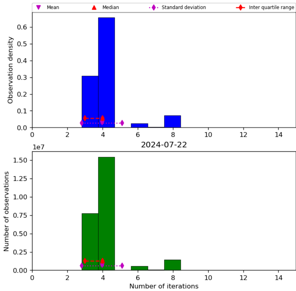
Figure 34: Histogram of “Number of iterations” for 2024-07-21 to 2024-07-23
