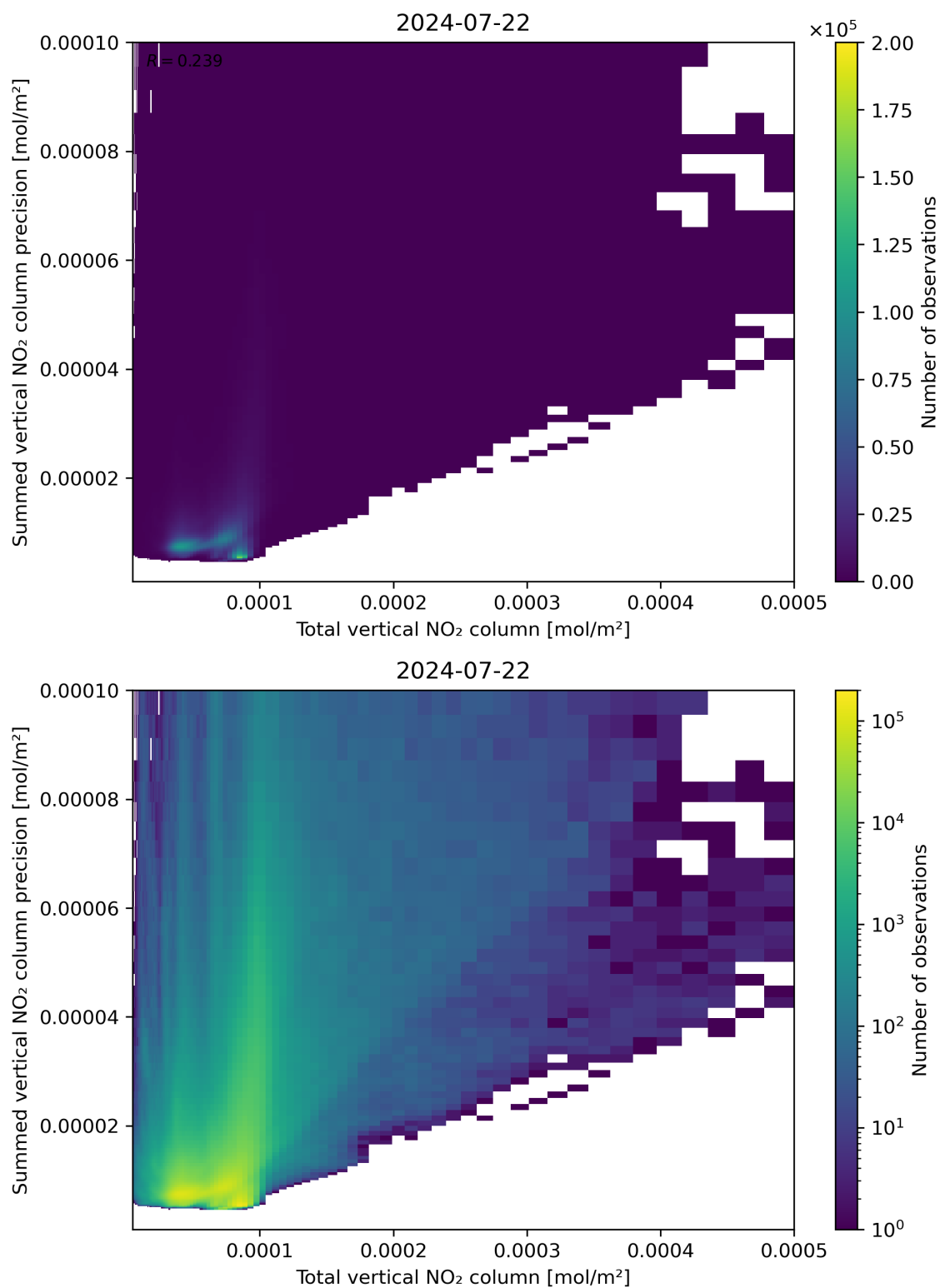
Figure 113: Scatter density plot of “Total vertical NO 2 column” against “Summed vertical NO 2 column precision” for 2024-07-21 to 2024-07-23.
