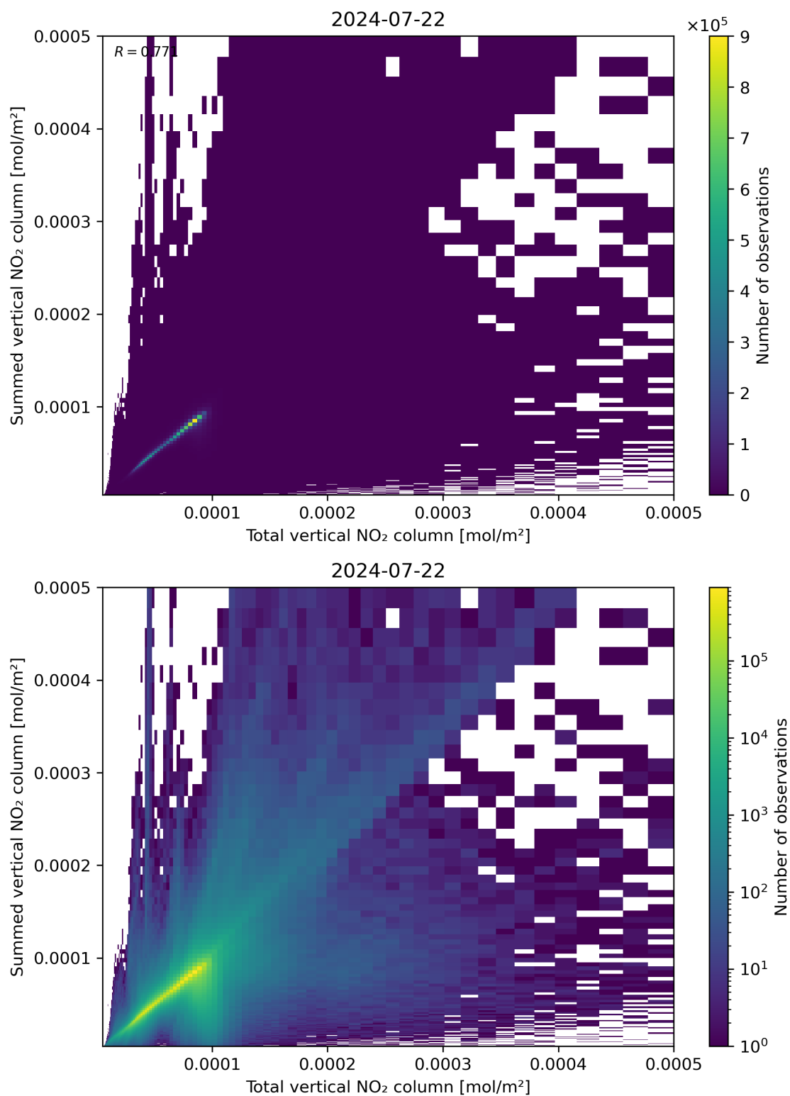
Figure 112: Scatter density plot of “Total vertical NO 2 column” against “Summed vertical NO 2 column” for 2024-07-21 to 2024-07-23.
