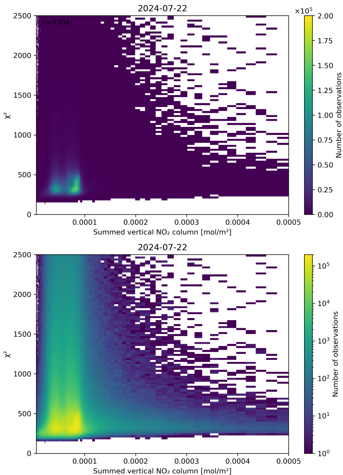
Figure 104: Scatter density plot of “Summed vertical NO 2 column” against “ \chi^2 ” for 2024-07-21 to 2024-07-23.
