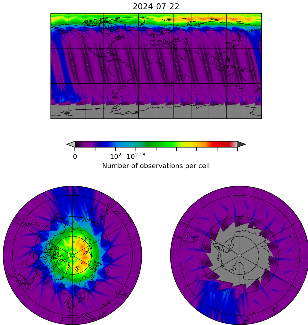
Figure 10: Map of the number of observations for 2024-07-21 to 2024-07-23
