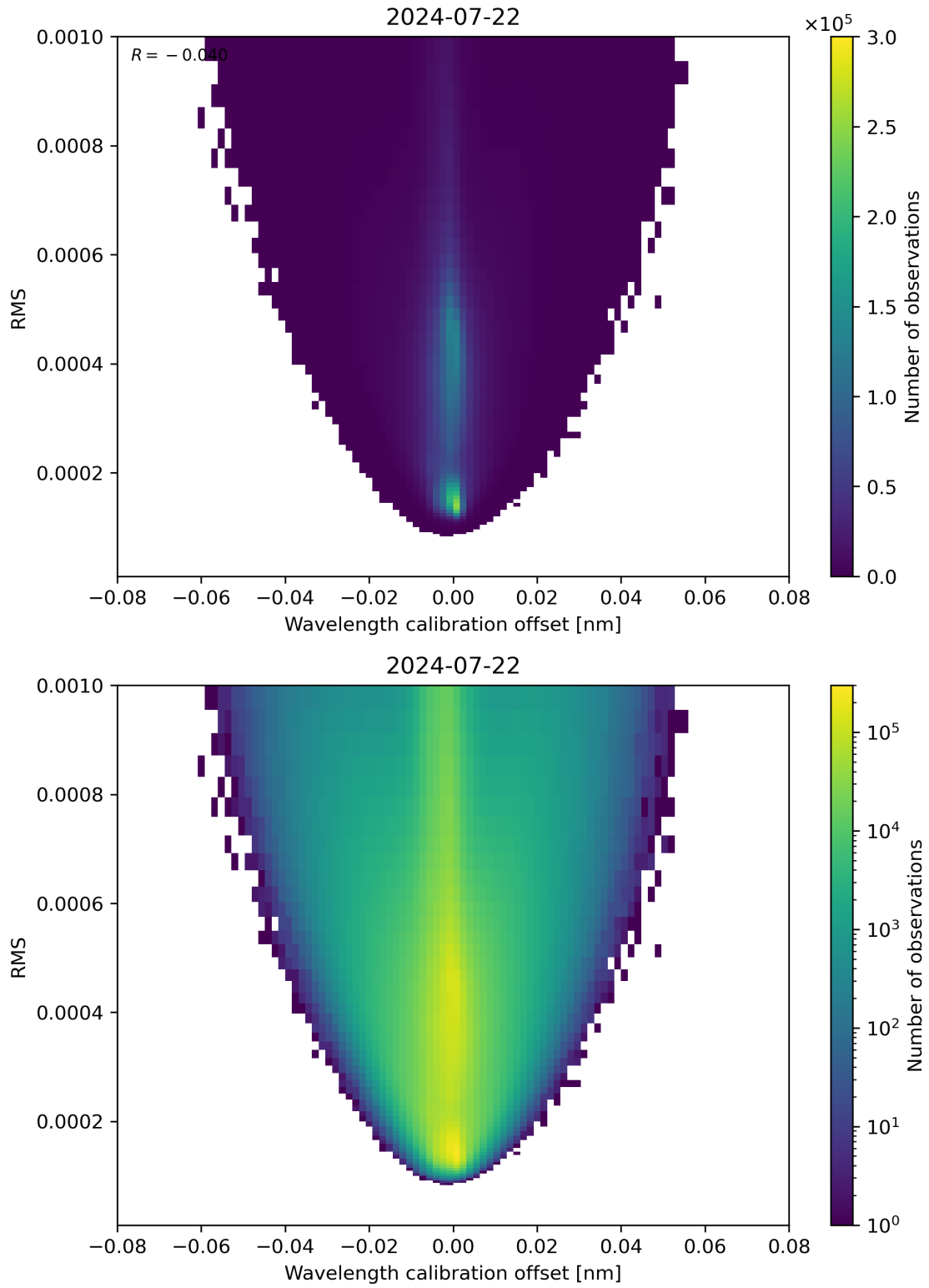
Figure 181: Scatter density plot of “Wavelength calibration offset” against “RMS” for 2024-07-21 to 2024-07-23.
