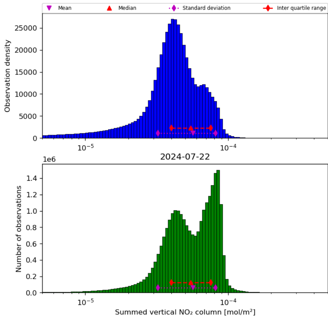
Figure 40: Histogram of “Summed vertical NO 2 column” for 2024-07-21 to 2024-07-23
