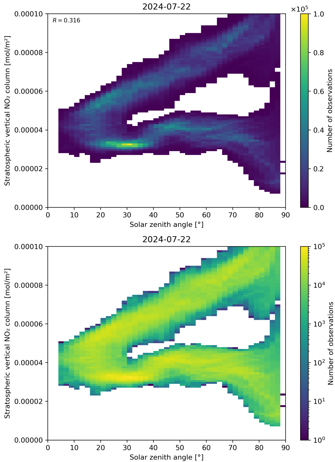
Figure 150: Scatter density plot of “Solar zenith angle” against “Stratospheric vertical NO 2 column” for 2024-07-21 to 2024-07-23.
