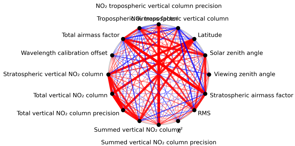
Figure 1: Map of correlation graph for 2024-07-21 to 2024-07-23.
