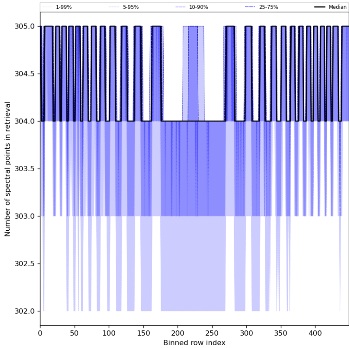
Figure 50: Along track statistics of “Number of spectral points in retrieval” for 2024-07-21 to 2024-07-23
