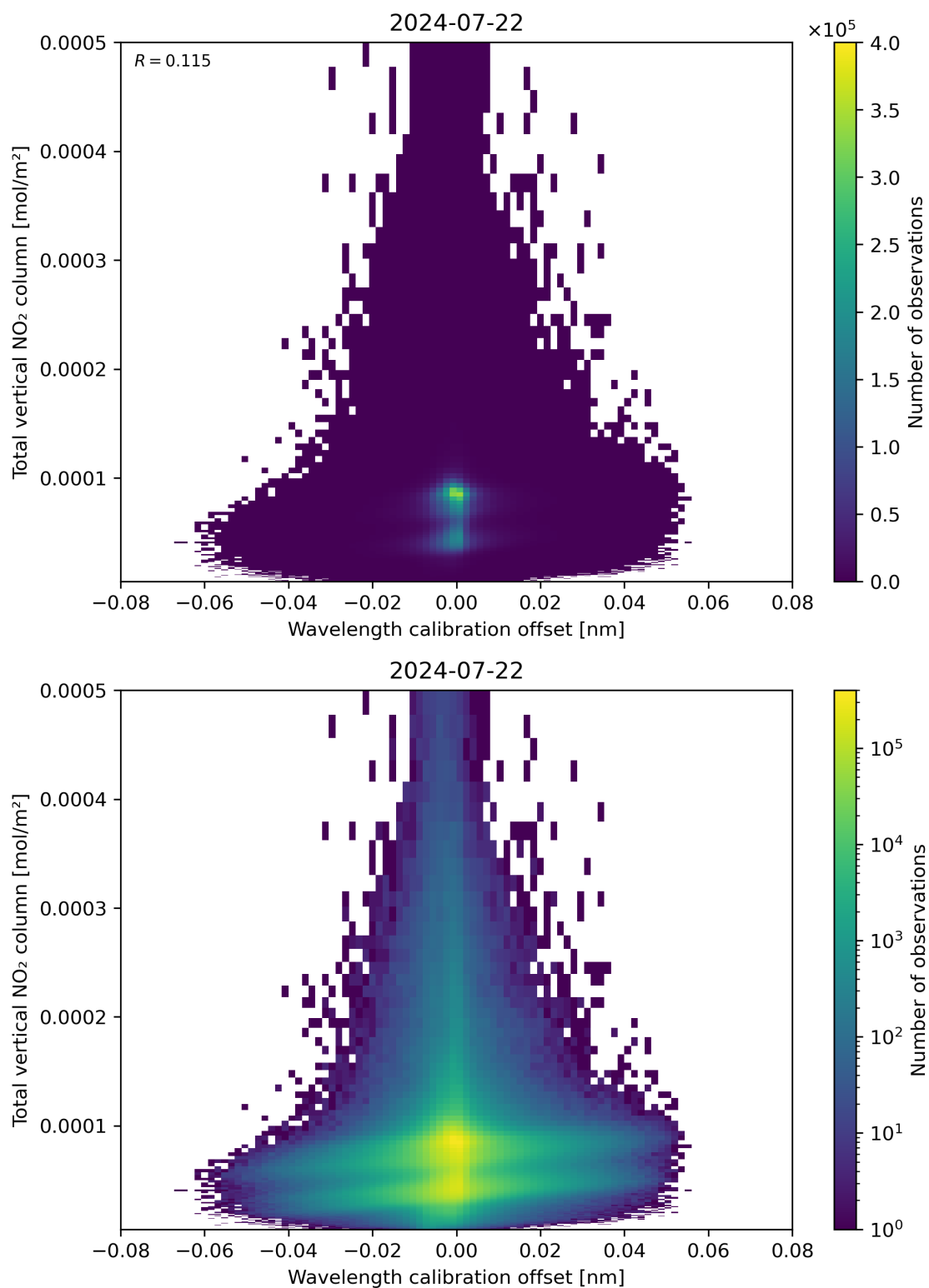
Figure 179: Scatter density plot of “Wavelength calibration offset” against “Total vertical NO 2 column” for 2024-07-21 to 2024-07-23.
