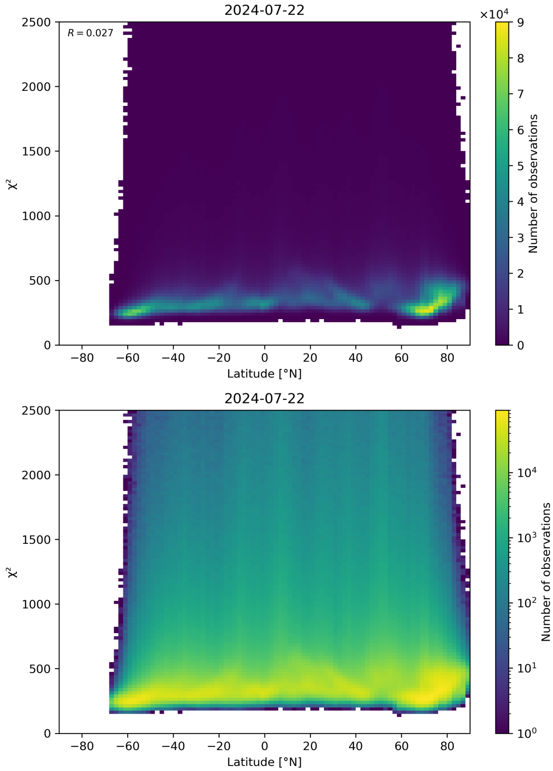
Figure 86: Scatter density plot of “Latitude” against “ \chi^2 ” for 2024-07-21 to 2024-07-23.
