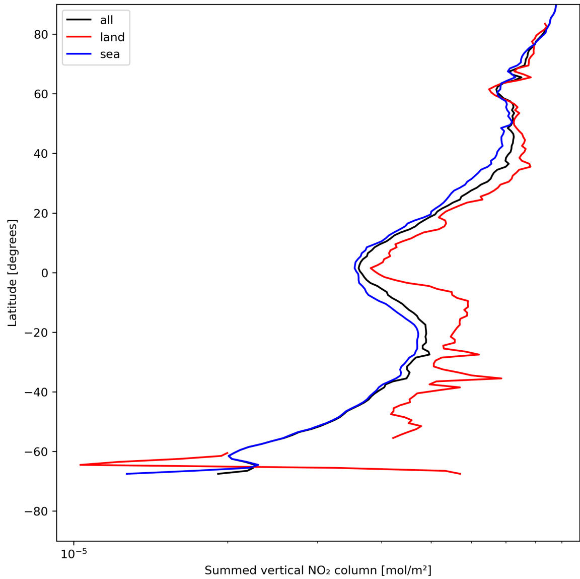
Figure 23: Zonal average of “Summed vertical NO 2 column” for 2024-07-22 to 2024-07-24.
