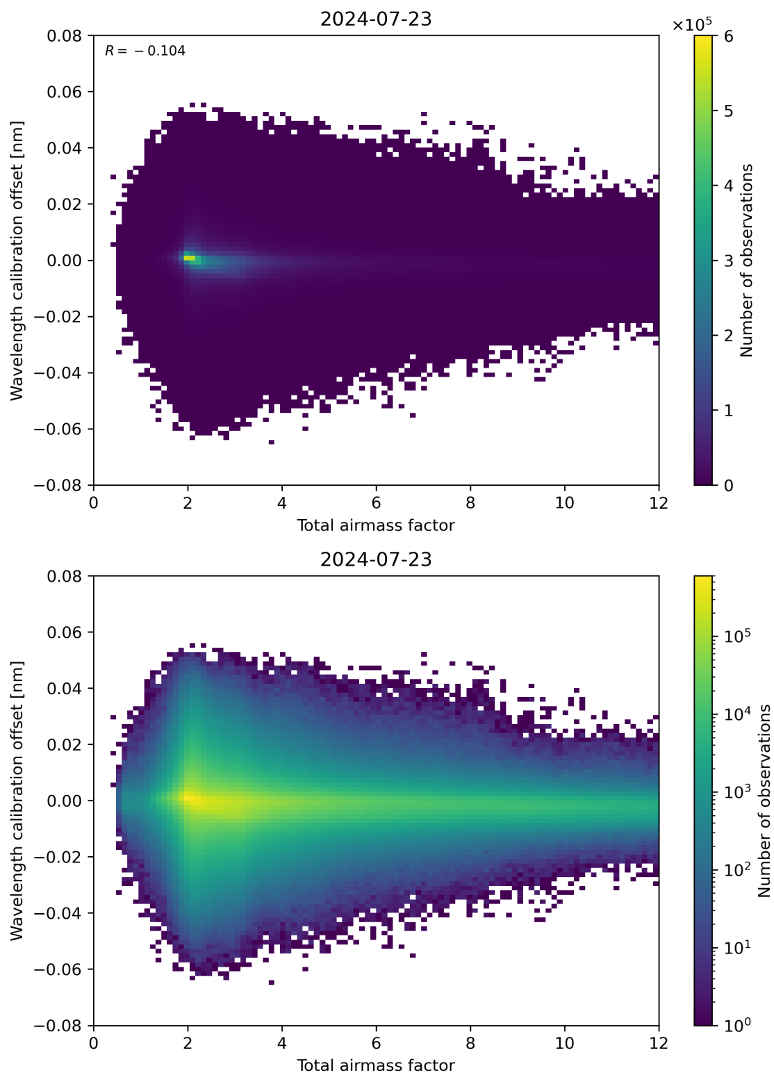
Figure 70: Scatter density plot of “Total airmass factor” against “Wavelength calibration offset” for 2024-07-22 to 2024-07-24.
