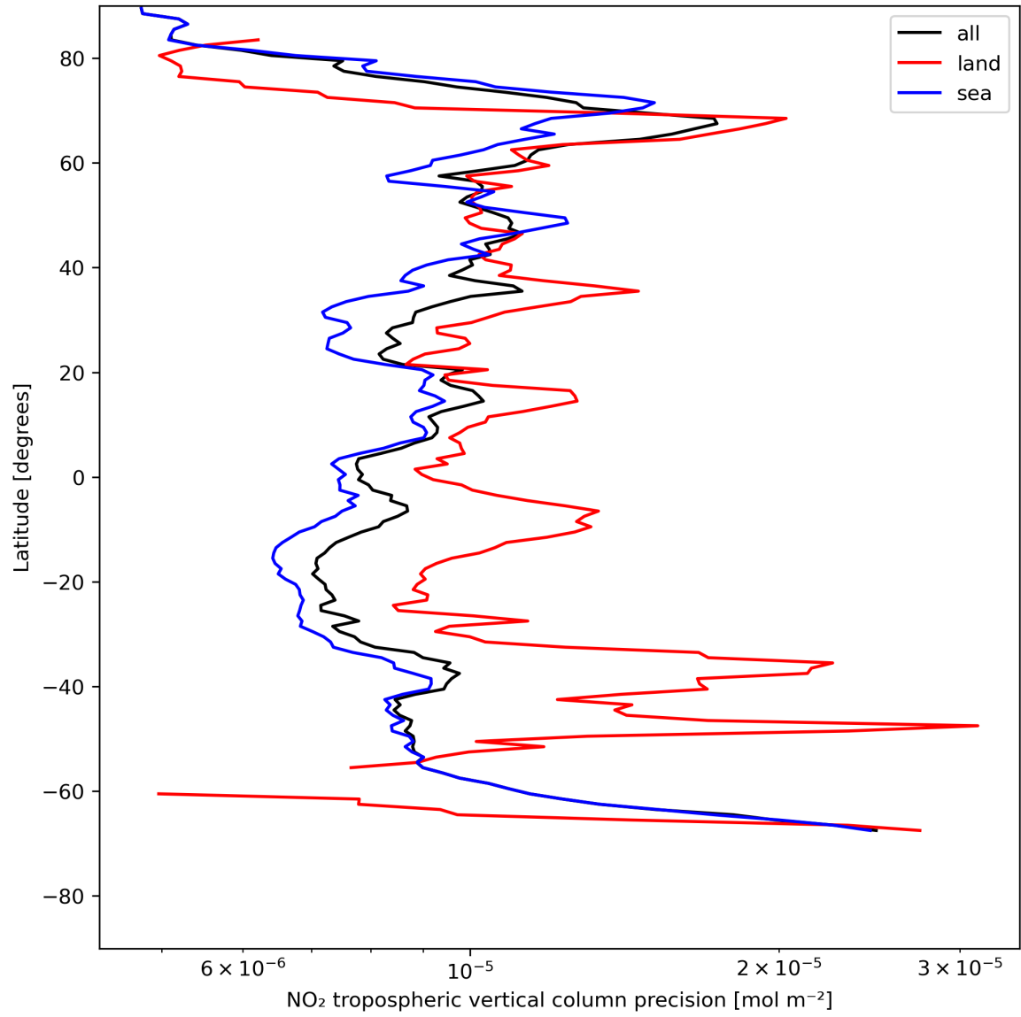
Figure 13: Zonal average of “NO 2 tropospheric vertical column precision” for 2024-07-22 to 2024-07-24.
