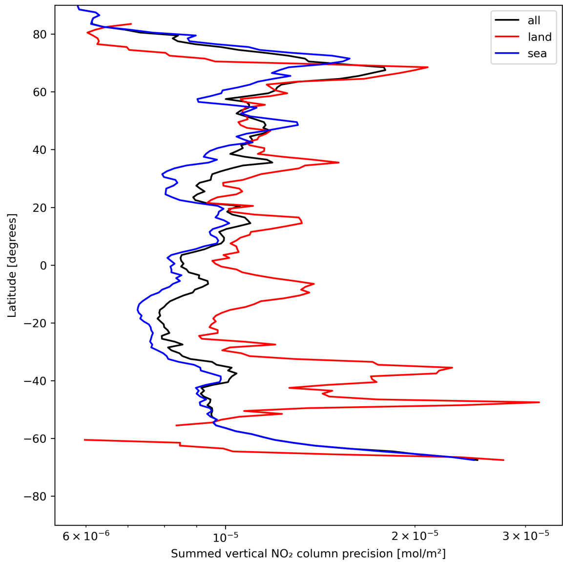
Figure 24: Zonal average of “Summed vertical NO 2 column precision” for 2024-07-22 to 2024-07-24.
