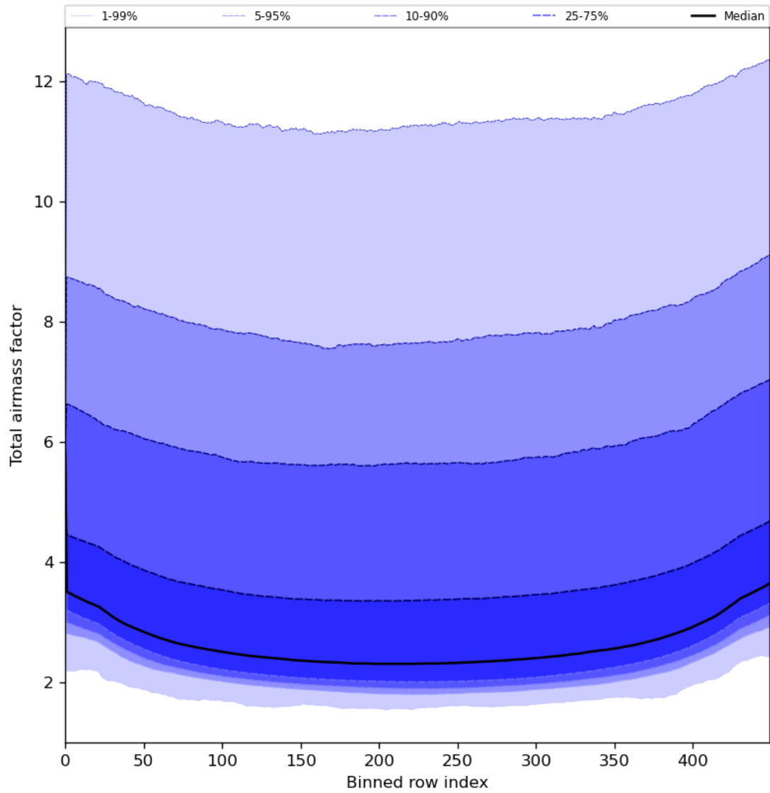
Figure 49: Along track statistics of “Total airmass factor” for 2024-07-22 to 2024-07-24
