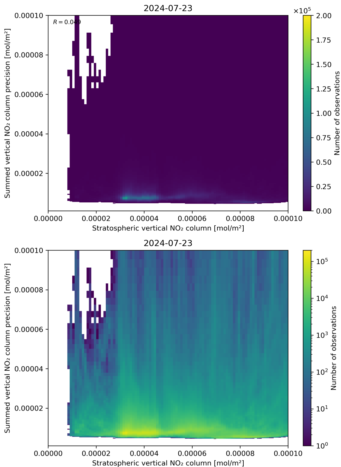
Figure 99: Scatter density plot of “Stratospheric vertical NO 2 column” against “Summed vertical NO 2 column precision” for 2024-07-22 to 2024-07-24.
