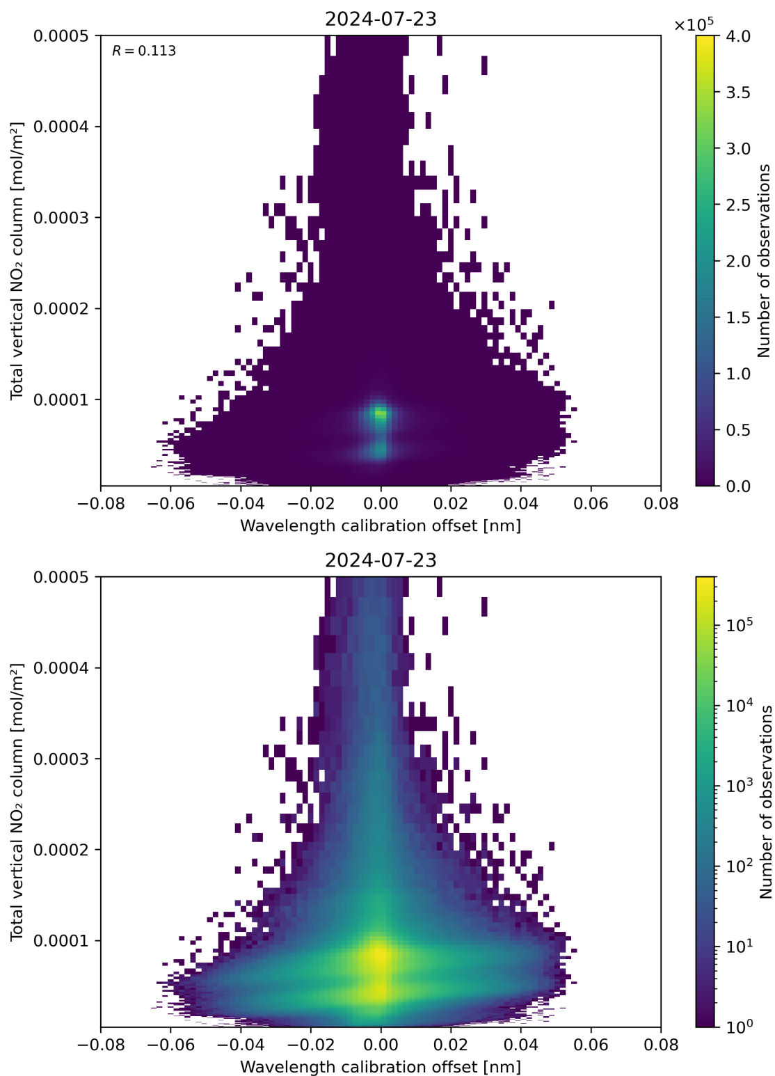
Figure 179: Scatter density plot of “Wavelength calibration offset” against “Total vertical NO 2 column” for 2024-07-22 to 2024-07-24.
