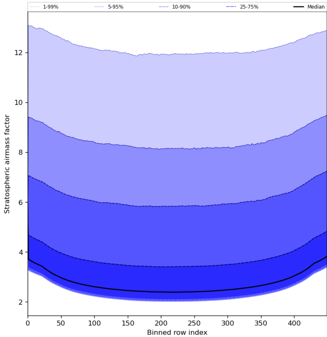
Figure 61: Along track statistics of “Stratospheric airmass factor” for 2024-07-22 to 2024-07-24
