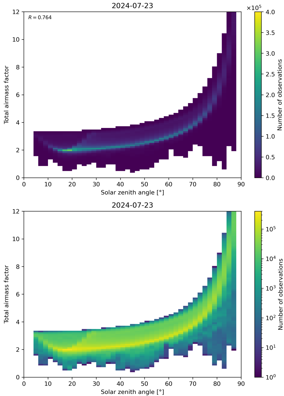
Figure 146: Scatter density plot of “Solar zenith angle” against “Total air mass factor” for 2024-07-22 to 2024-07-24.
