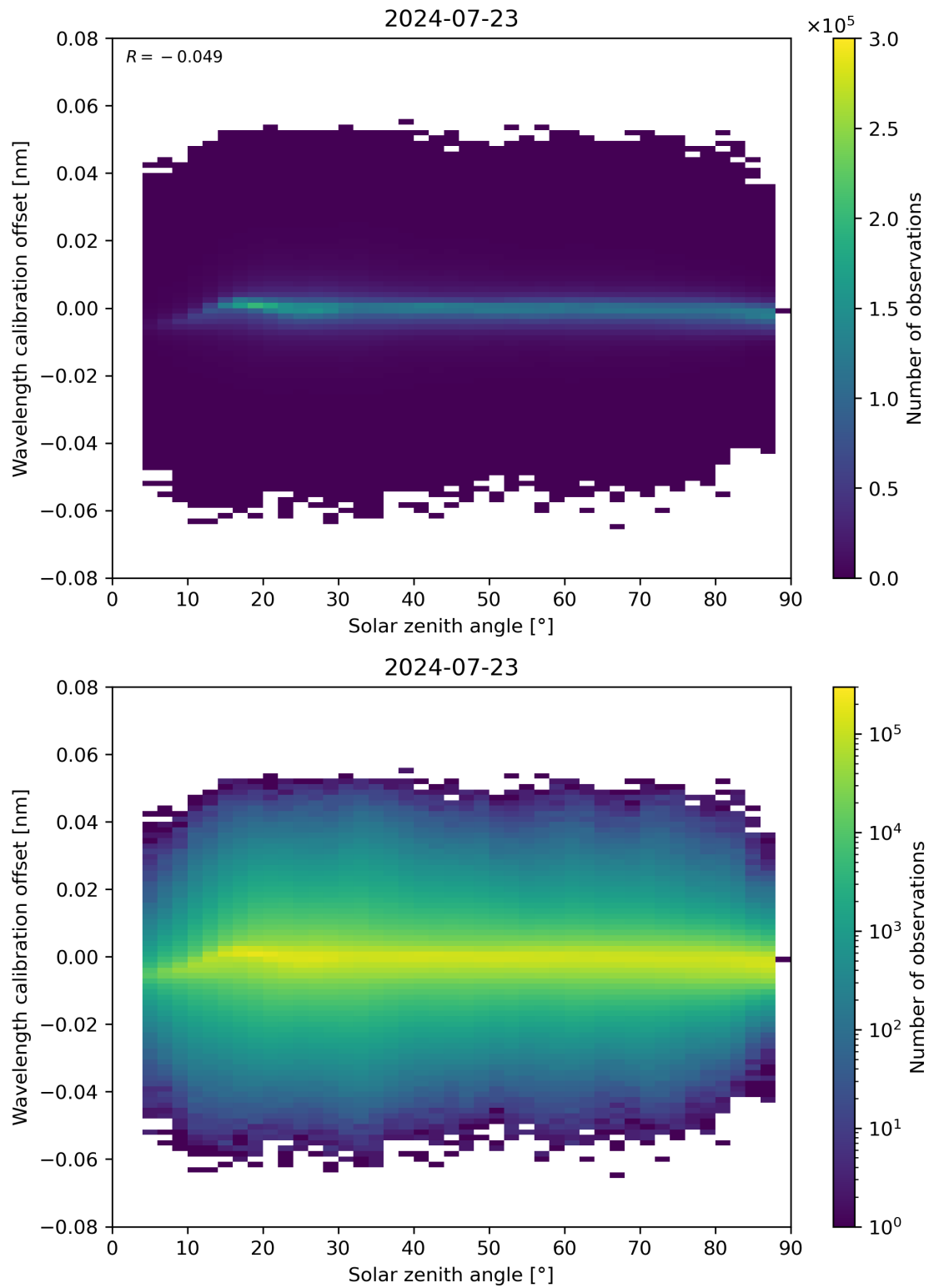
Figure 158: Scatter density plot of “Solar zenith angle” against “Wavelength calibration offset” for 2024-07-22 to 2024-07-24.
