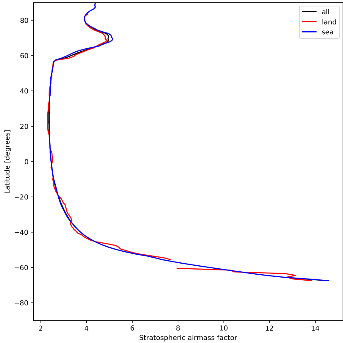
Figure 27: Zonal average of “Stratospheric air mass factor” for 2024-07-22 to 2024-07-24.
