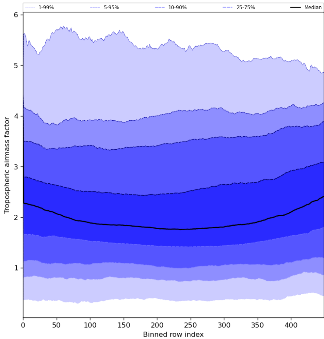
Figure 48: Along track statistics of “Tropospheric airmass factor” for 2024-07-22 to 2024-07-24
