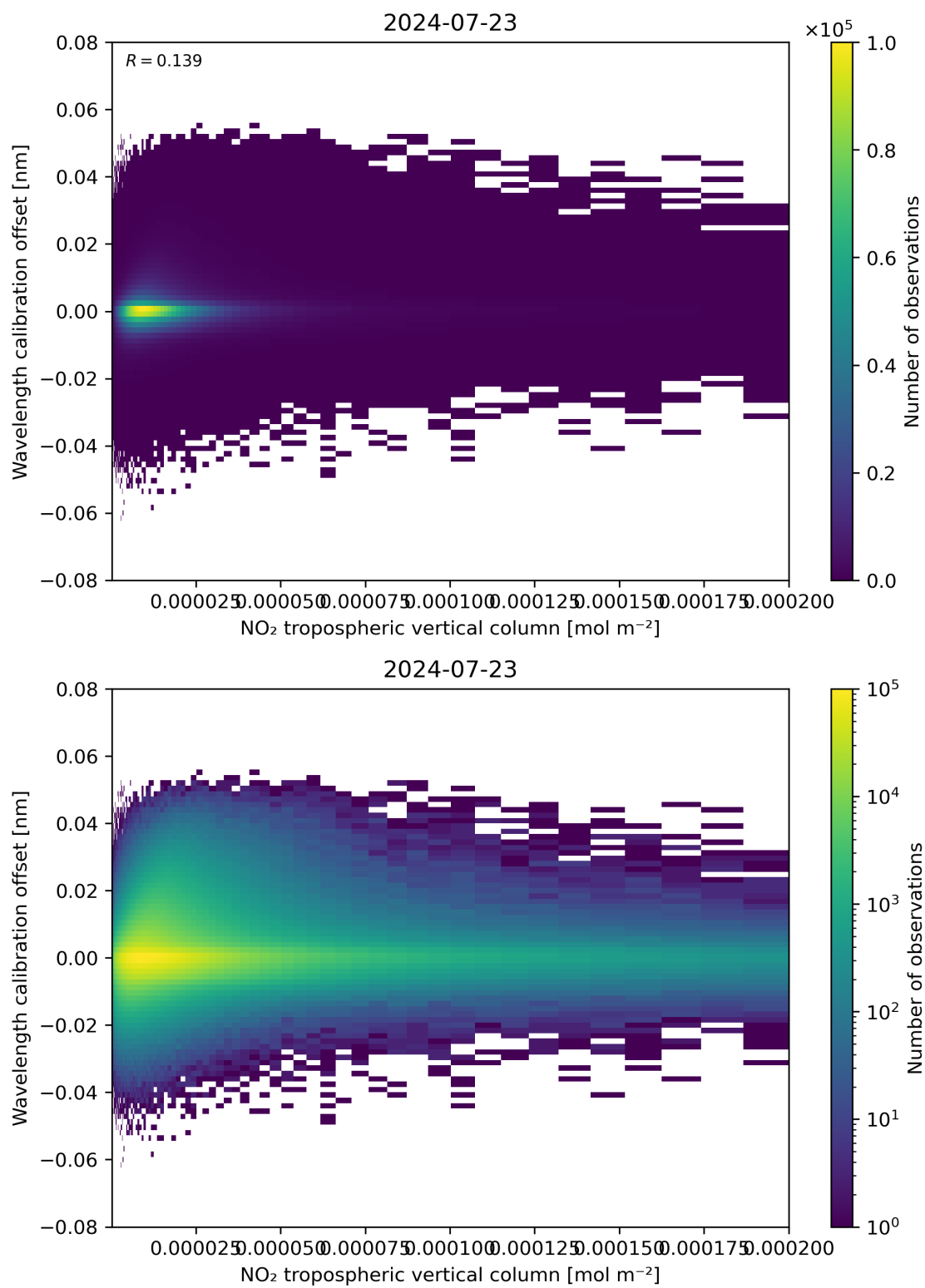
Figure 143: Scatter density plot of “NO 2 tropospheric vertical column” against “Wavelength calibration offset” for 2024-07-22 to 2024-07-24.
