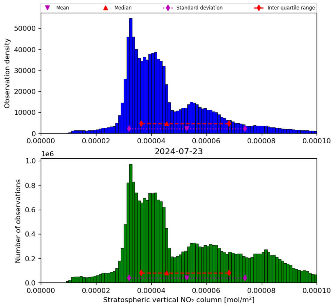
Figure 36: Histogram of “Stratospheric vertical NO 2 column” for 2024-07-22 to 2024-07-24
