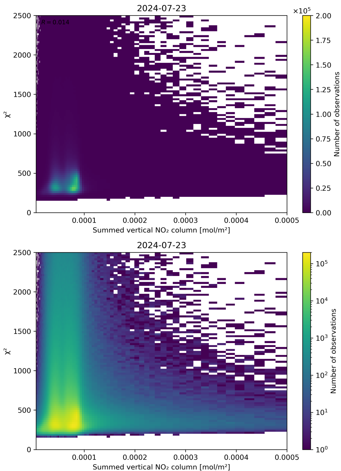
Figure 104: Scatter density plot of “Summed vertical NO 2 column” against “ \chi^2 ” for 2024-07-22 to 2024-07-24.
