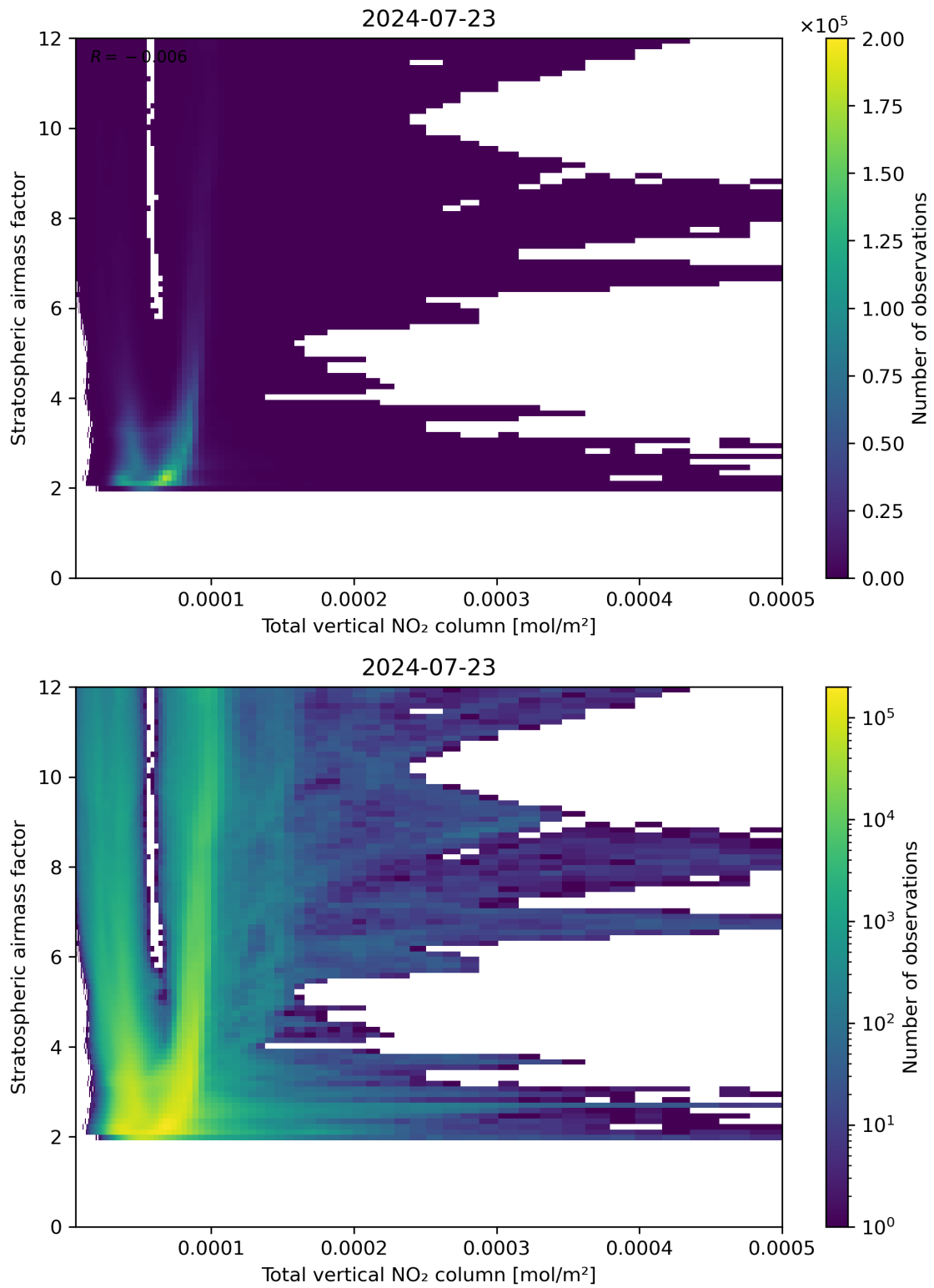
Figure 110: Scatter density plot of “Total vertical NO 2 column” against “Stratospheric airmass factor” for 2024-07-22 to 2024-07-24.
