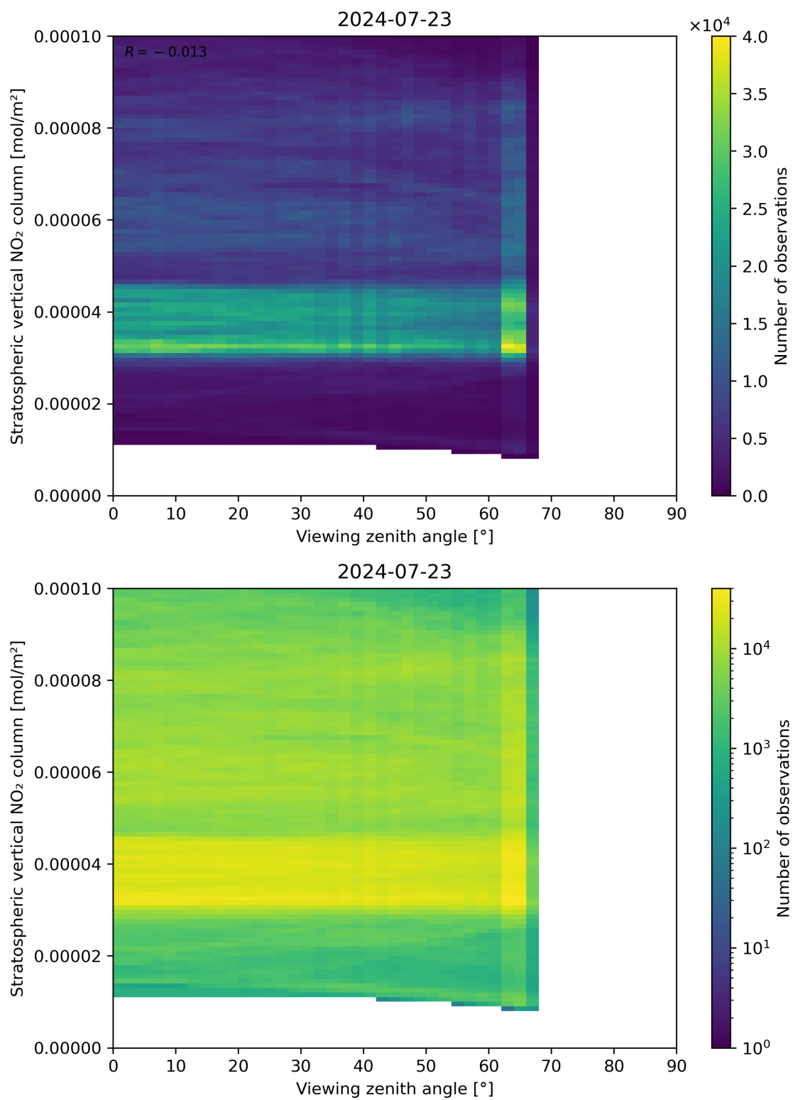
Figure 164: Scatter density plot of “Viewing zenith angle” against “Stratospheric vertical NO 2 column” for 2024-07-22 to 2024-07-24.
