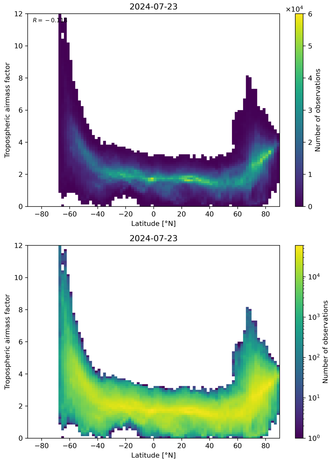
Figure 85: Scatter density plot of “Latitude” against “Tropospheric airmass factor” for 2024-07-22 to 2024-07-24.
