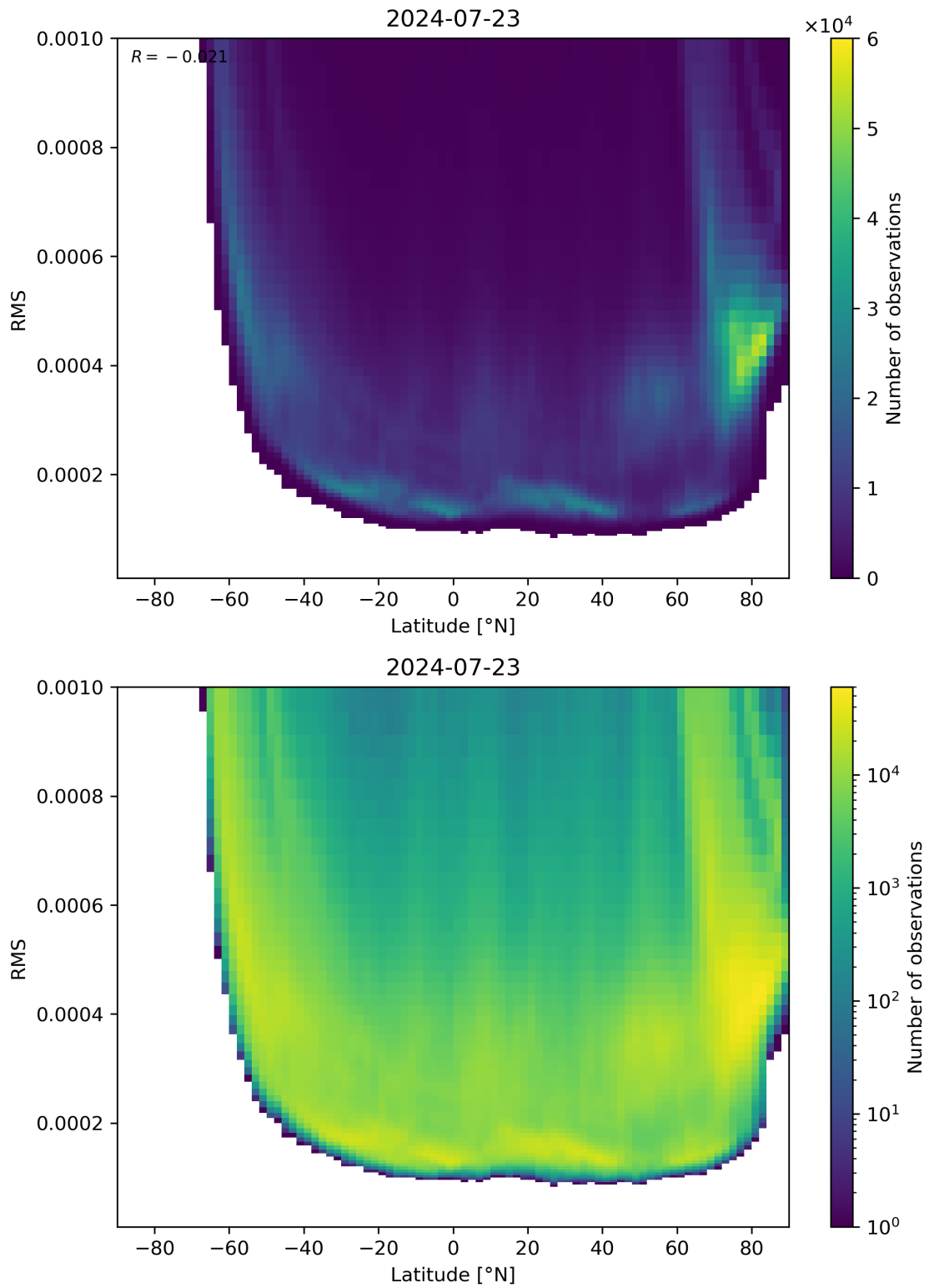
Figure 94: Scatter density plot of “Latitude” against “RMS” for 2024-07-22 to 2024-07-24.
