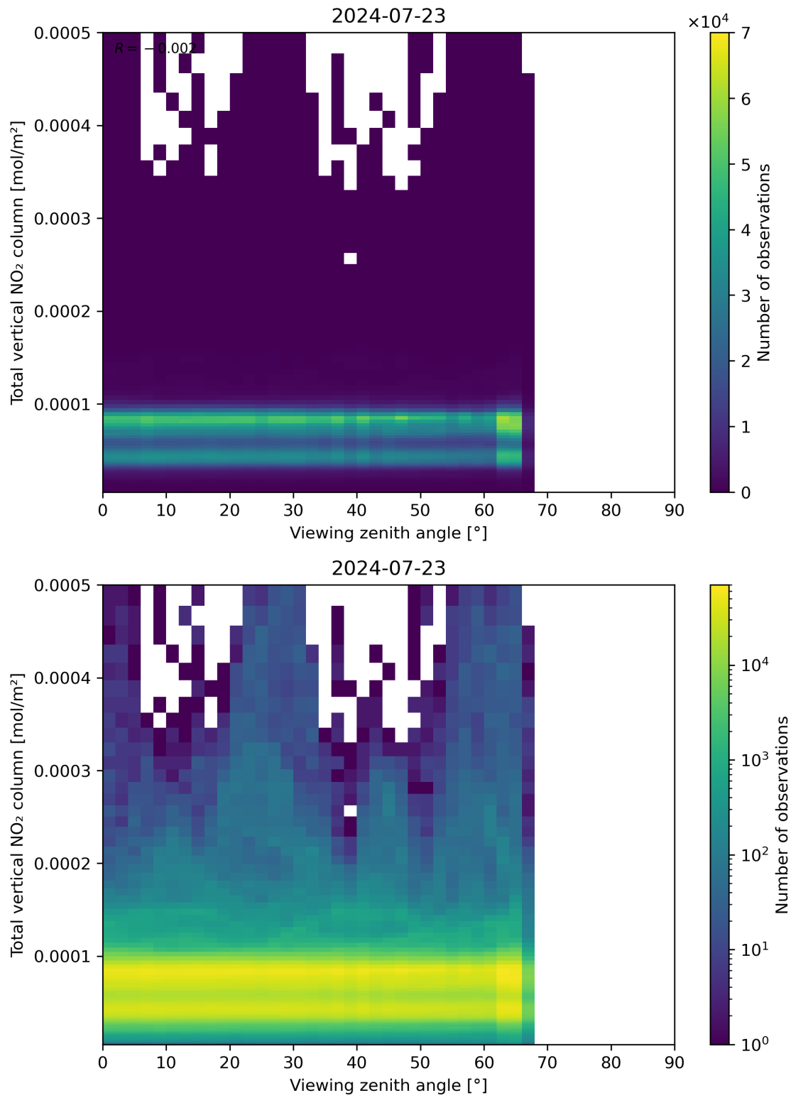
Figure 167: Scatter density plot of “Viewing zenith angle” against “Total vertical NO 2 column” for 2024-07-22 to 2024-07-24.
