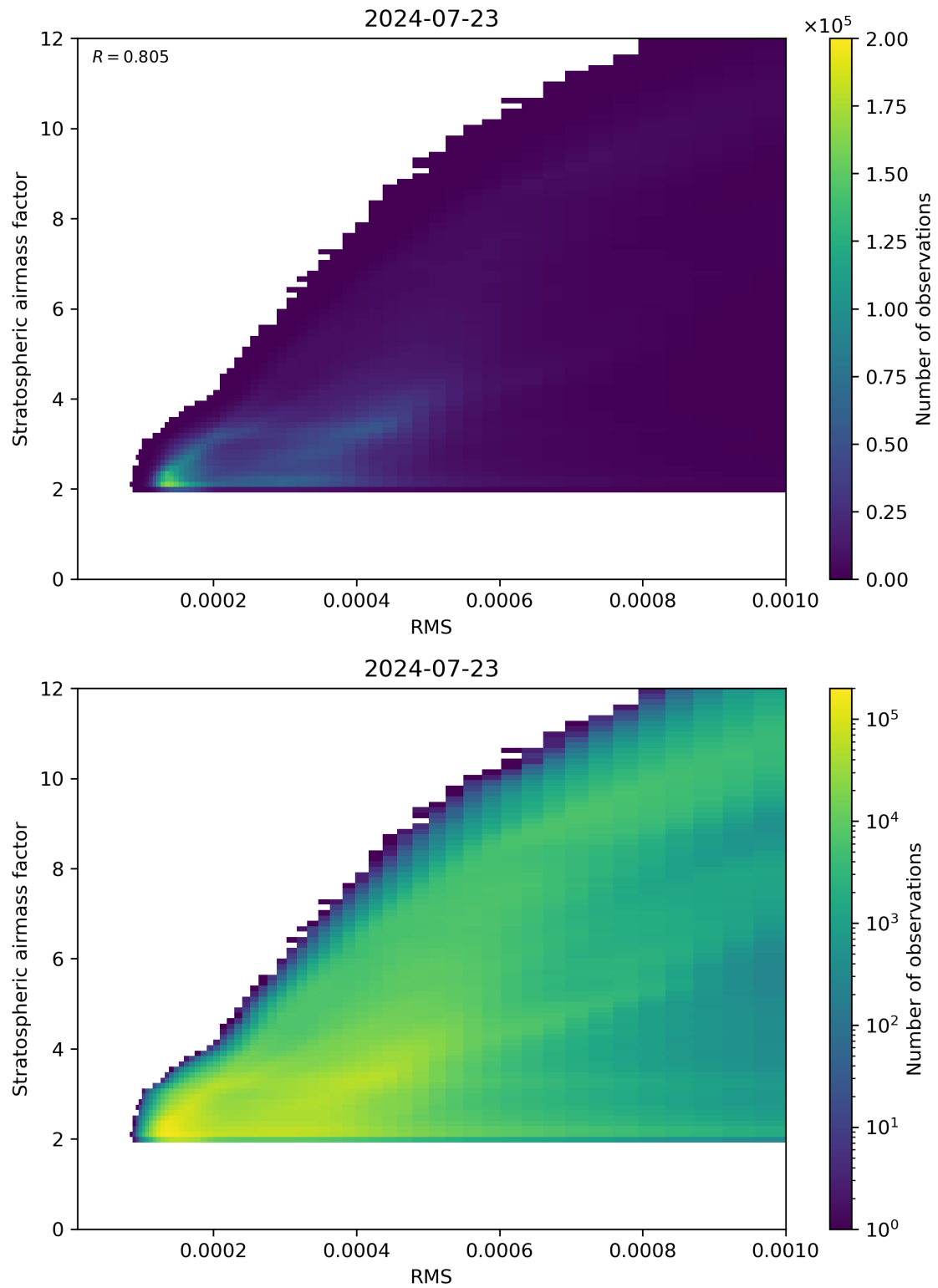
Figure 144: Scatter density plot of “RMS” against “Stratospheric airmass factor” for 2024-07-22 to 2024-07-24.
