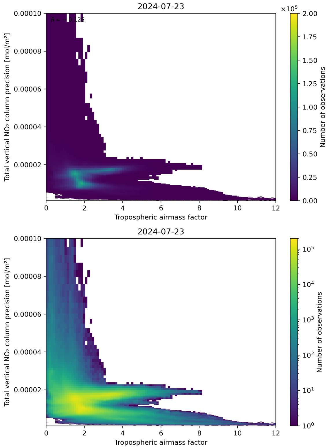
Figure 78: Scatter density plot of “Tropospheric air mass factor” against “Total vertical NO 2 column precision” for 2024-07-22 to 2024-07-24.
