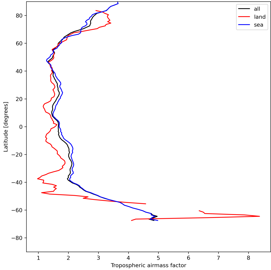
Figure 14: Zonal average of “Tropospheric airmass factor” for 2024-07-22 to 2024-07-24.
