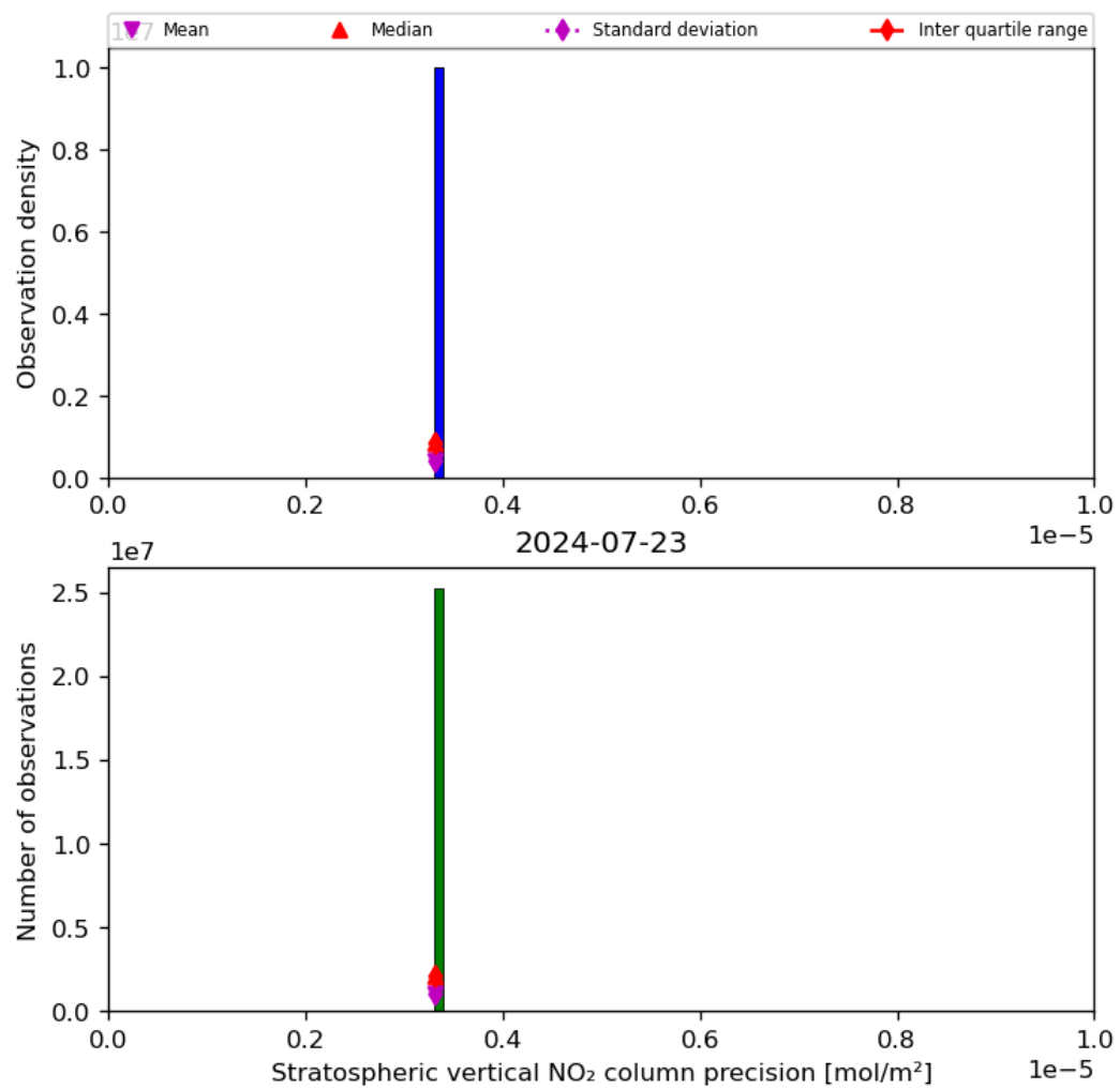
Figure 37: Histogram of “Stratospheric vertical NO 2 column precision” for 2024-07-22 to 2024-07-24
