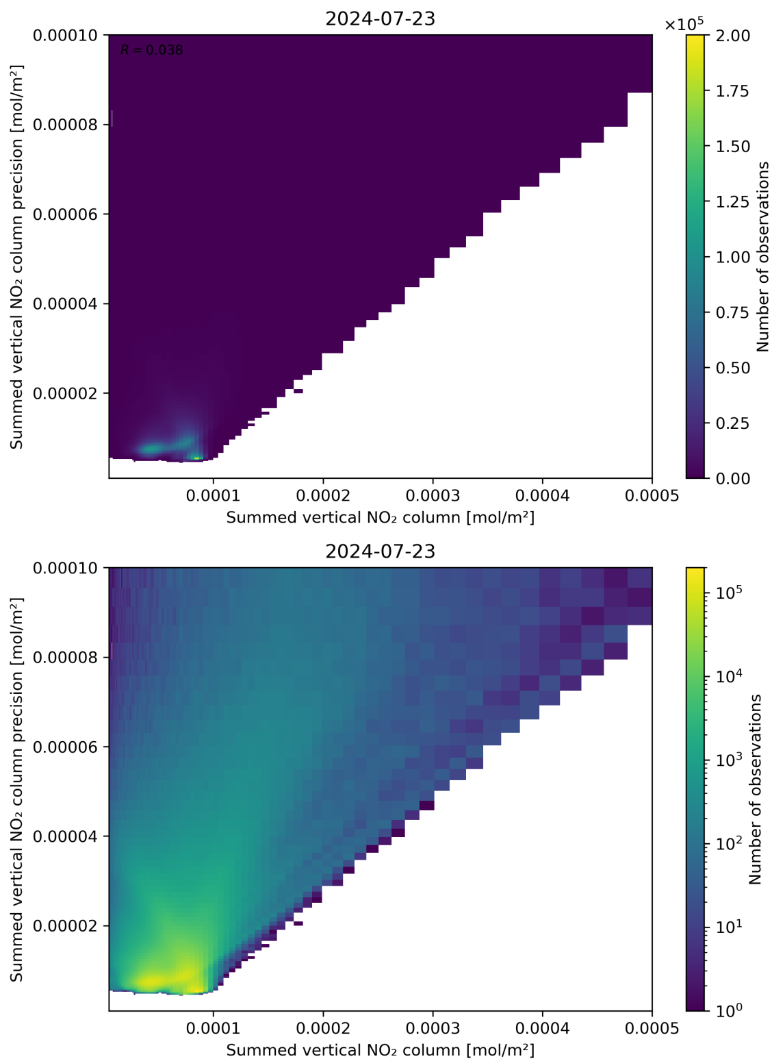
Figure 105: Scatter density plot of “Summed vertical NO 2 column” against “Summed vertical NO 2 column precision” for 2024-07-22 to 2024-07-24.
