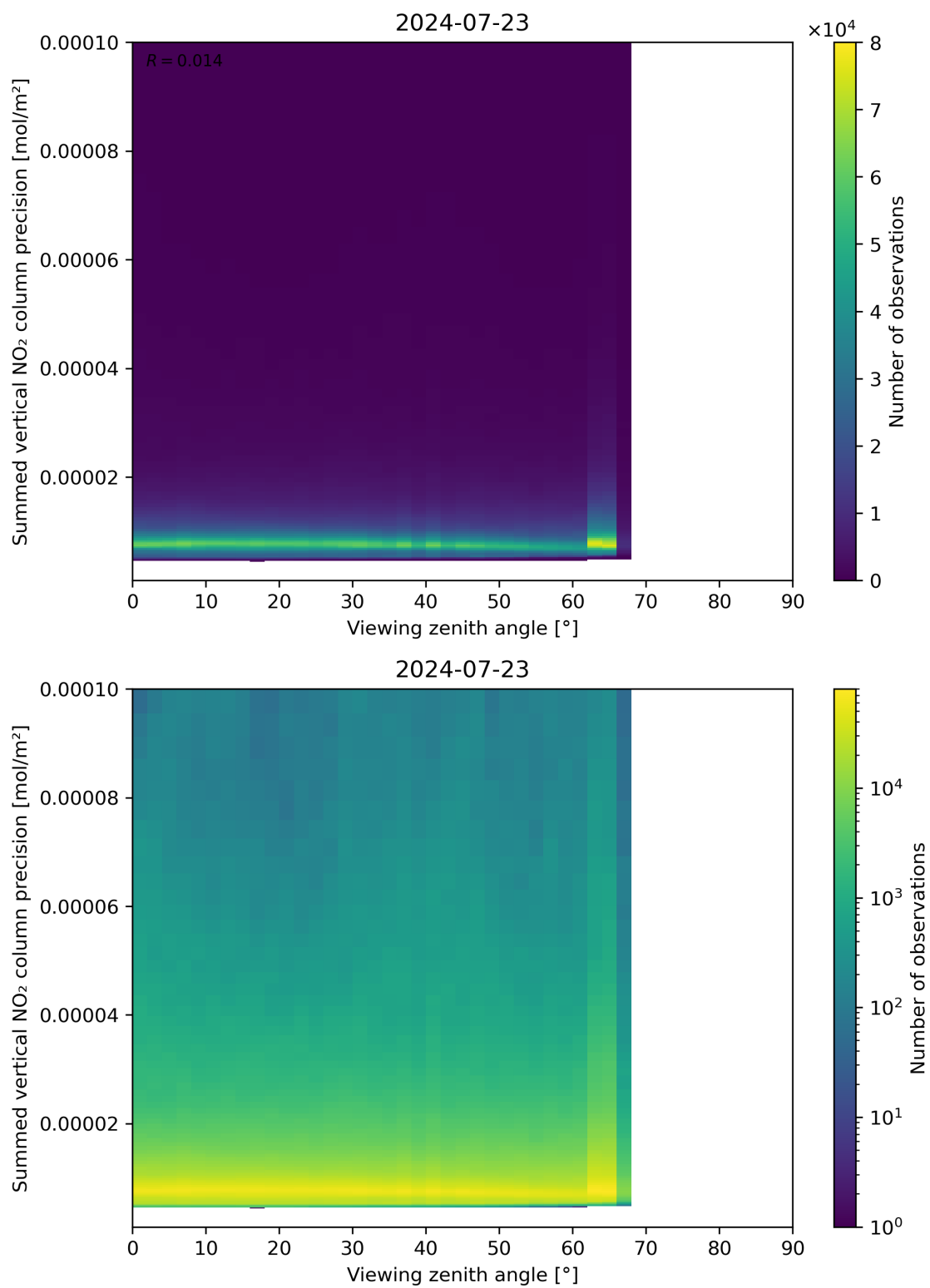
Figure 166: Scatter density plot of “Viewing zenith angle” against “Summed vertical NO 2 column precision” for 2024-07-22 to 2024-07-24.
