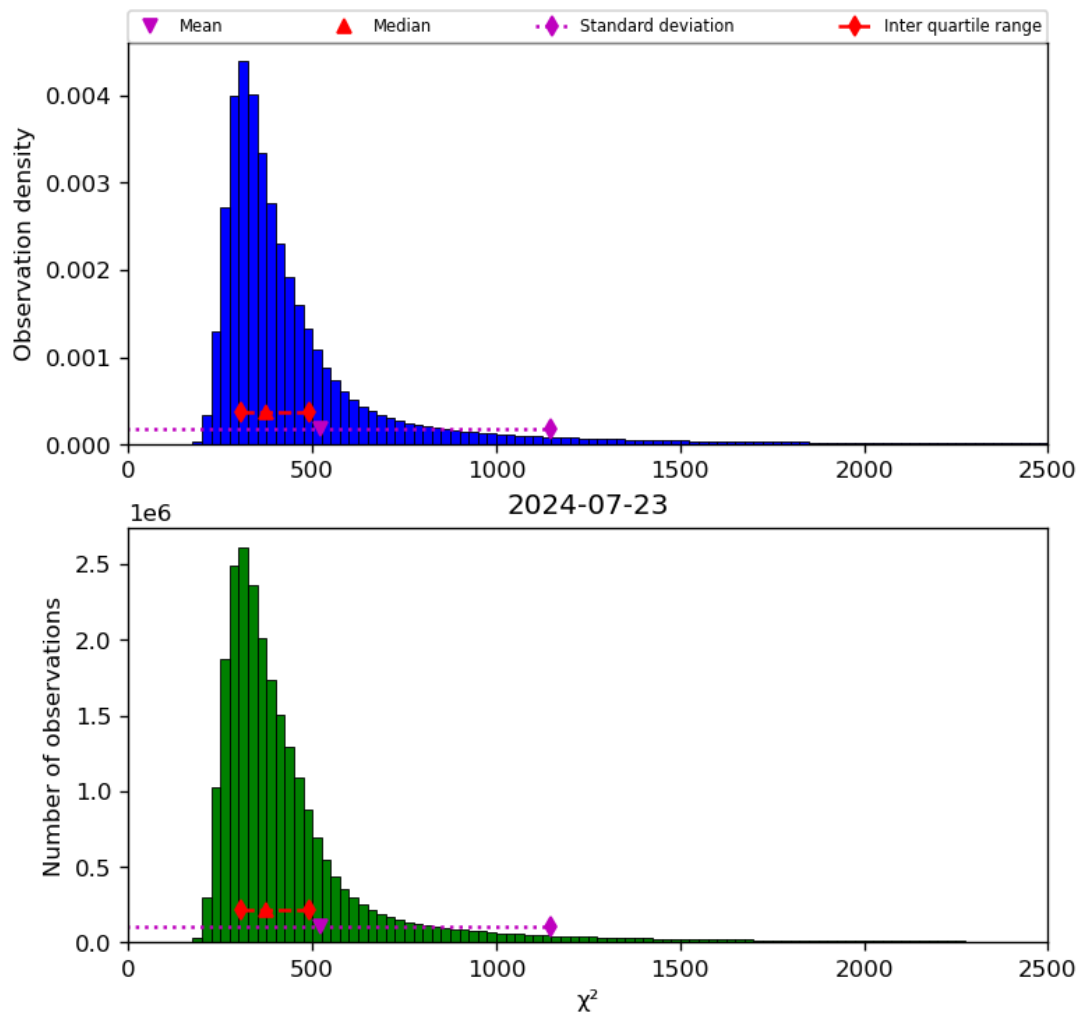
Figure 42: Histogram of “ \chi^2 ” for 2024-07-22 to 2024-07-24
