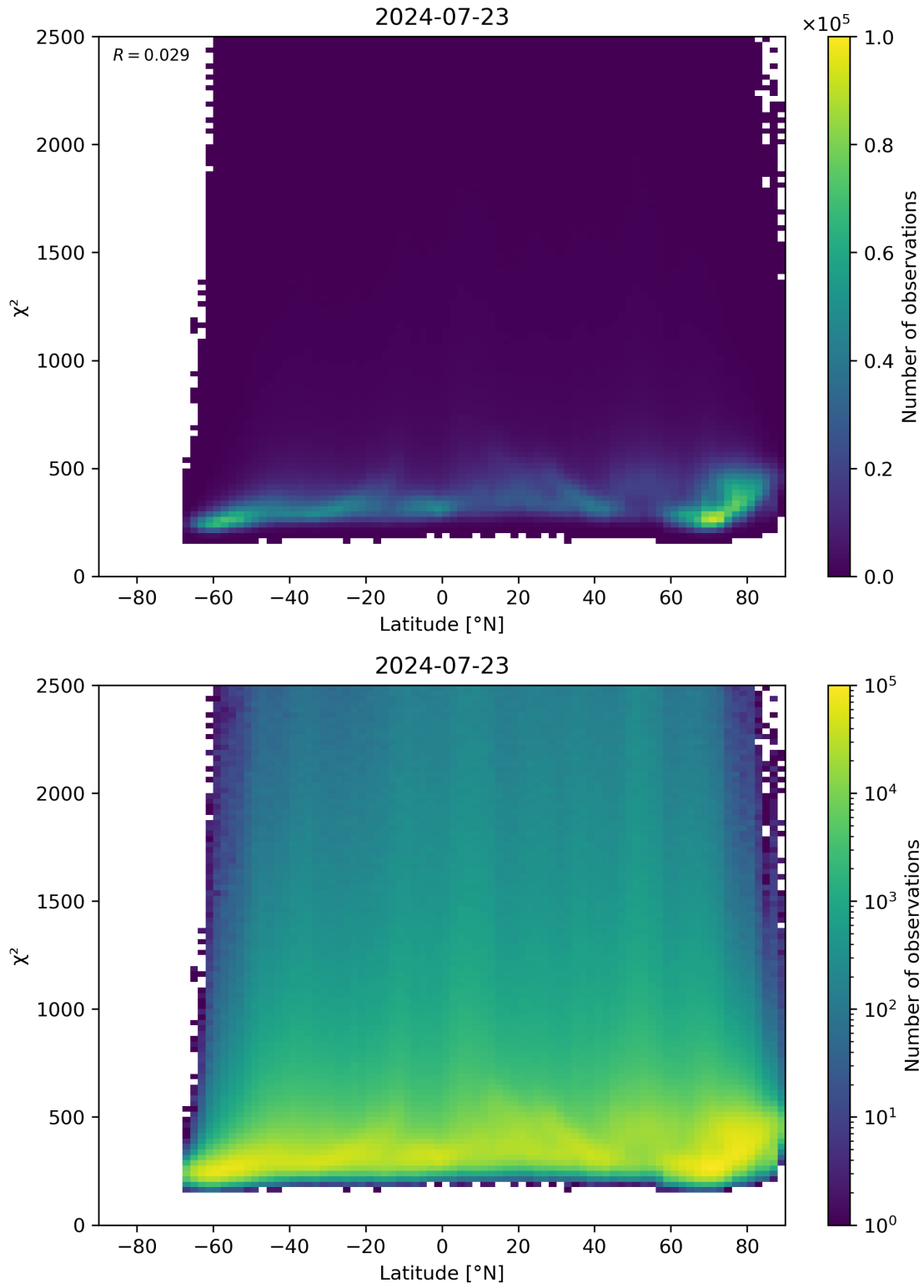
Figure 86: Scatter density plot of “Latitude” against “ \chi^2 ” for 2024-07-22 to 2024-07-24.
