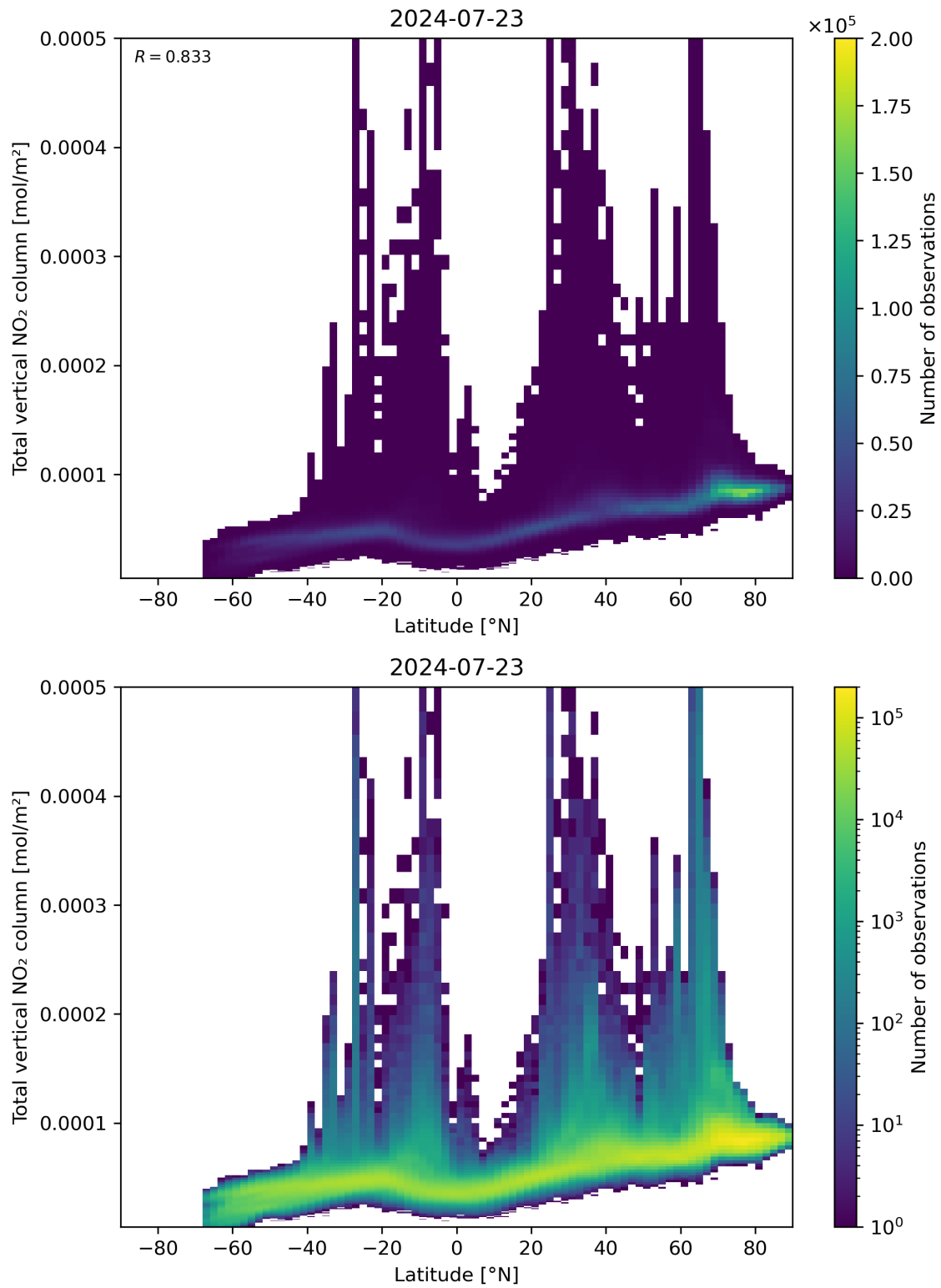
Figure 90: Scatter density plot of “Latitude” against “Total vertical NO 2 column” for 2024-07-22 to 2024-07-24.
