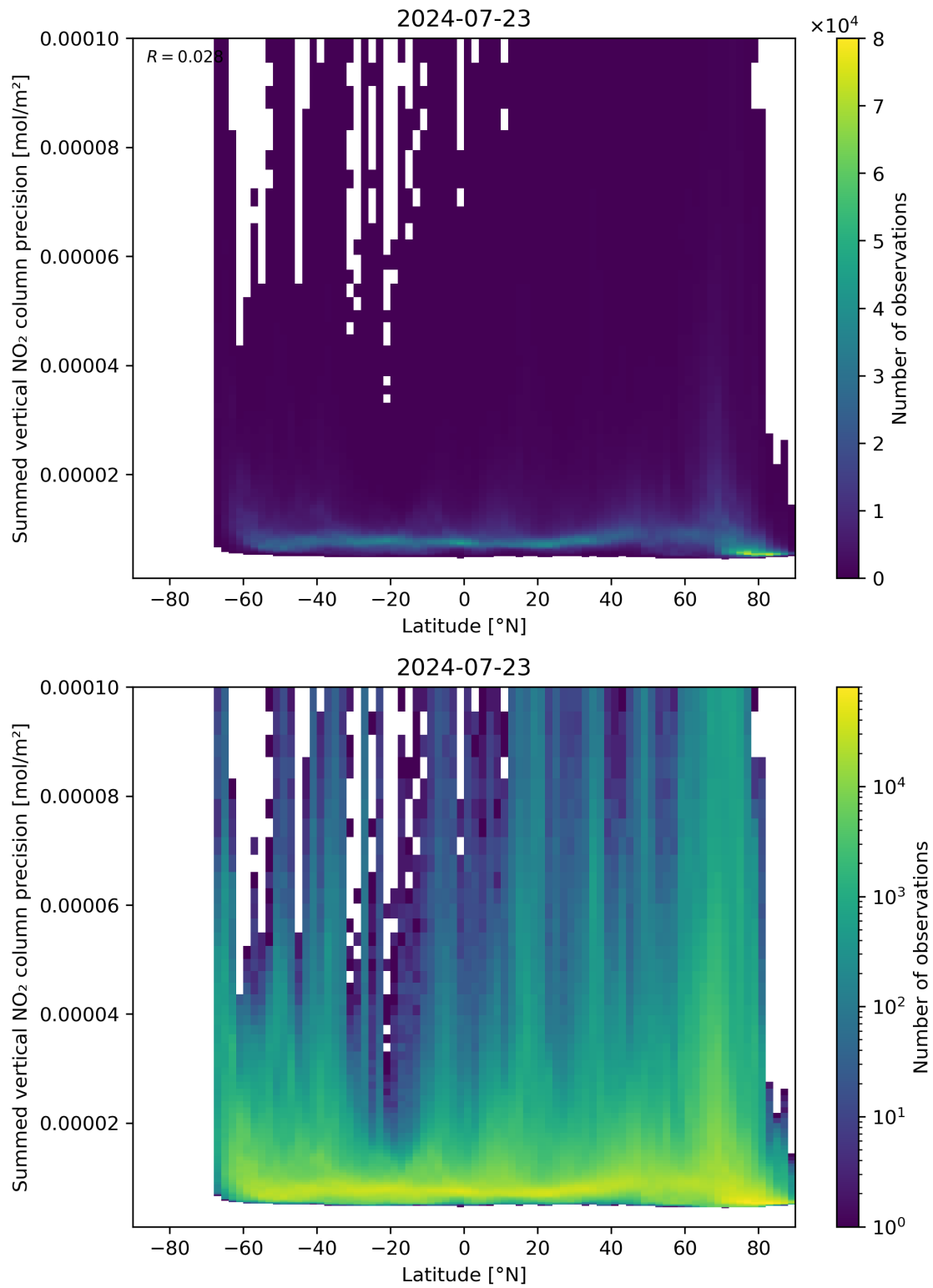
Figure 89: Scatter density plot of “Latitude” against “Summed vertical NO 2 column precision” for 2024-07-22 to 2024-07-24.
