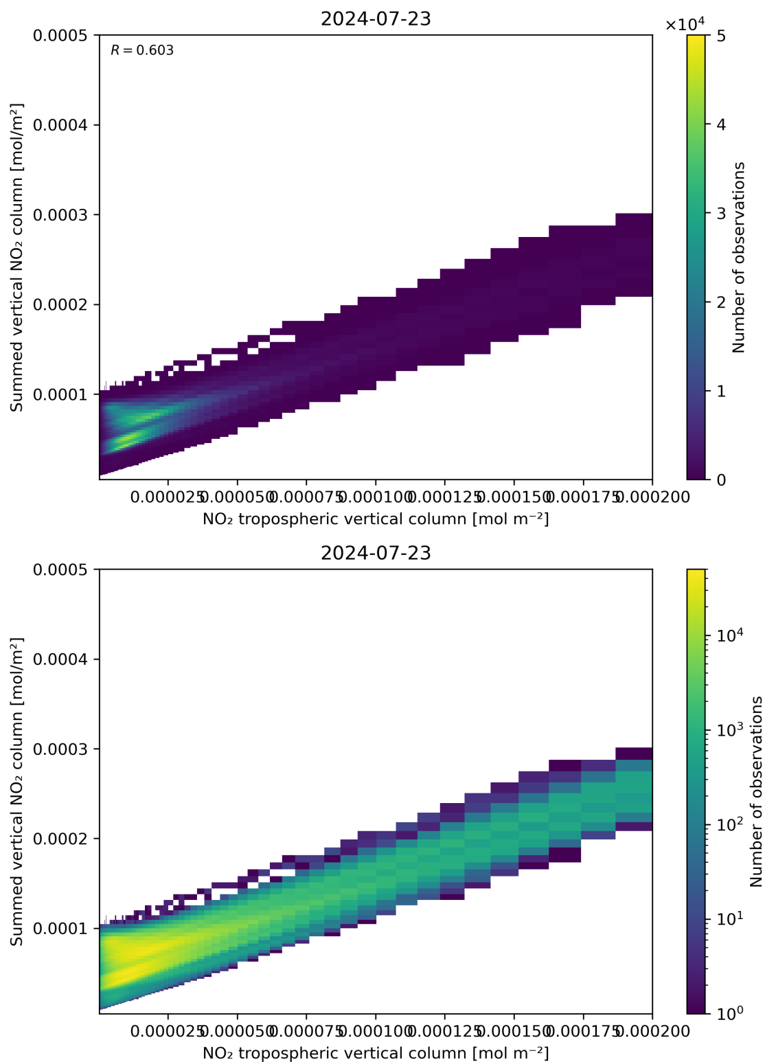
Figure 126: Scatter density plot of “NO 2 tropospheric vertical column” against “Summed vertical NO 2 column” for 2024-07-22 to 2024-07-24.
