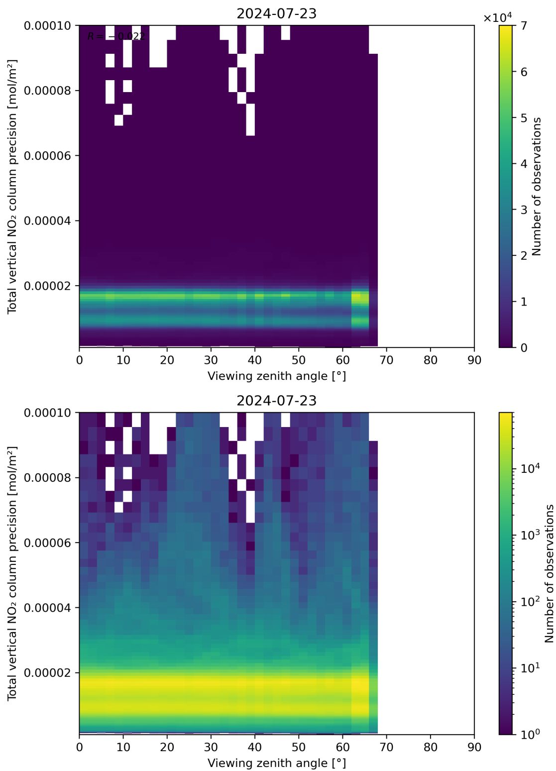
Figure 168: Scatter density plot of “Viewing zenith angle” against “Total vertical NO 2 column precision” for 2024-07-22 to 2024-07-24.
