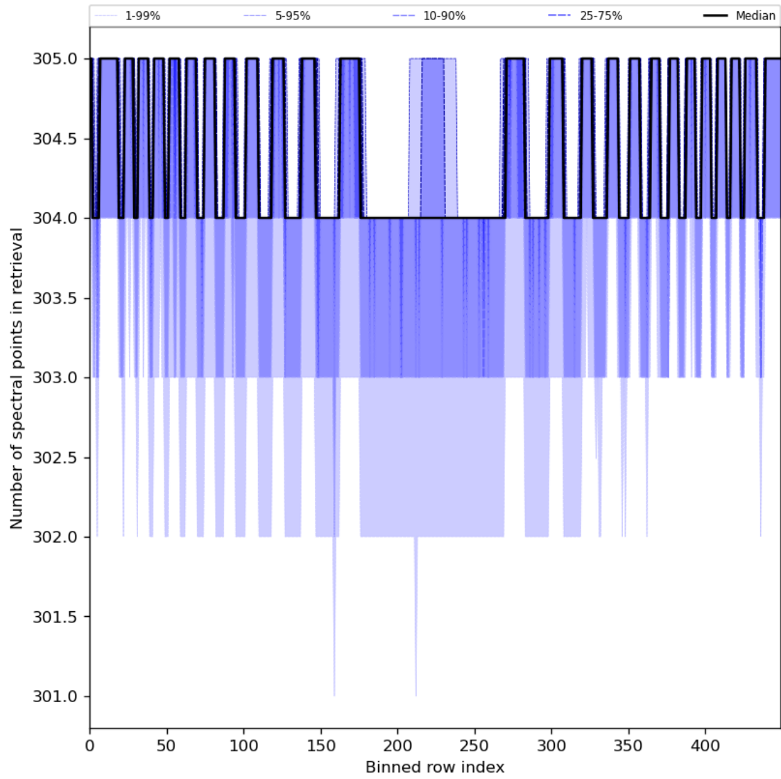
Figure 50: Along track statistics of “Number of spectral points in retrieval” for 2024-07-22 to 2024-07-24
