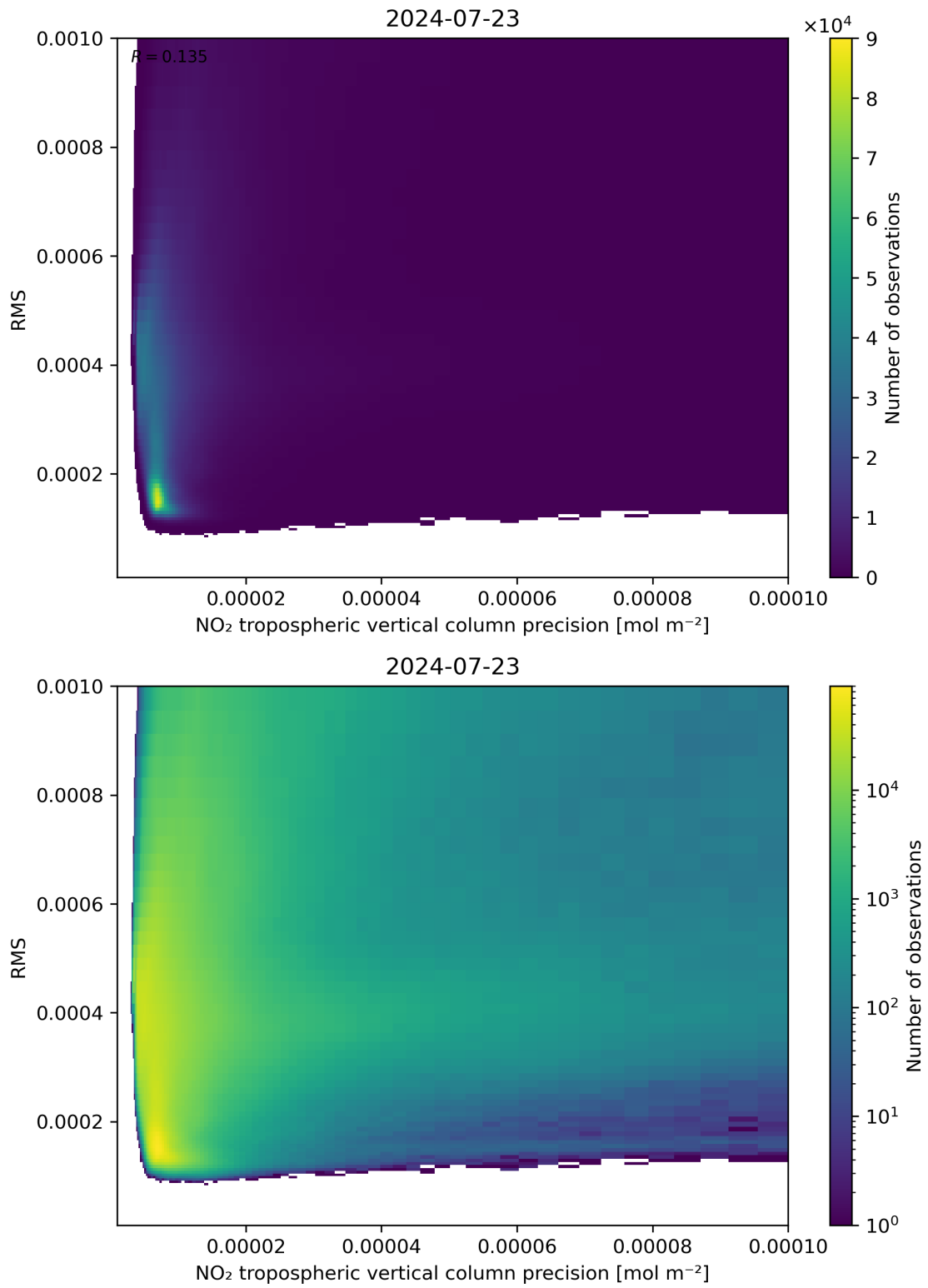
Figure 140: Scatter density plot of “NO 2 tropospheric vertical column precision” against “RMS” for 2024-07-22 to 2024-07-24.
