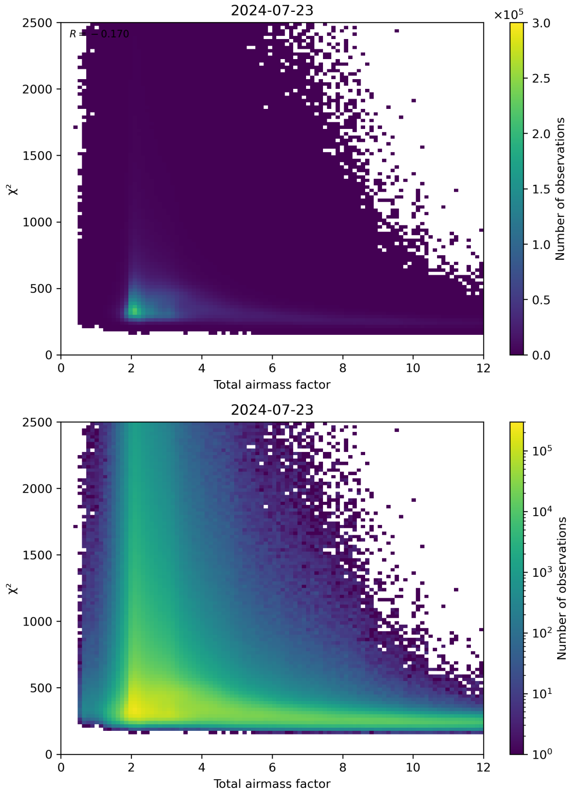
Figure 63: Scatter density plot of “Total airmass factor” against “ \chi^2 ” for 2024-07-22 to 2024-07-24.
