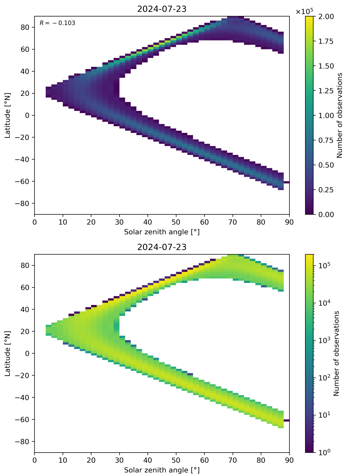
Figure 149: Scatter density plot of “Solar zenith angle” against “Latitude” for 2024-07-22 to 2024-07-24.
