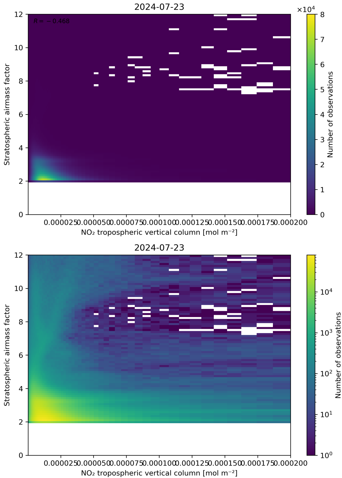
Figure 121: Scatter density plot of “NO 2 tropospheric vertical column” against “Stratospheric air mass factor” for 2024-07-22 to 2024-07-24.
