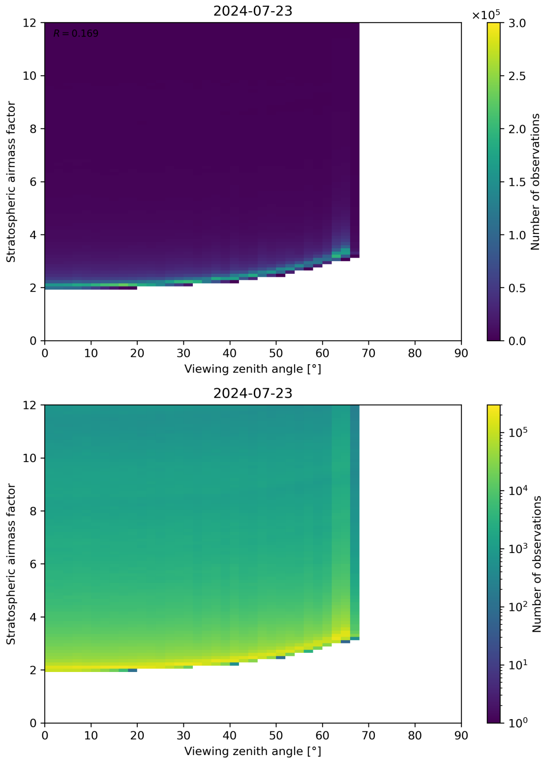
Figure 159: Scatter density plot of “Viewing zenith angle” against “Stratospheric airmass factor” for 2024-07-22 to 2024-07-24.
