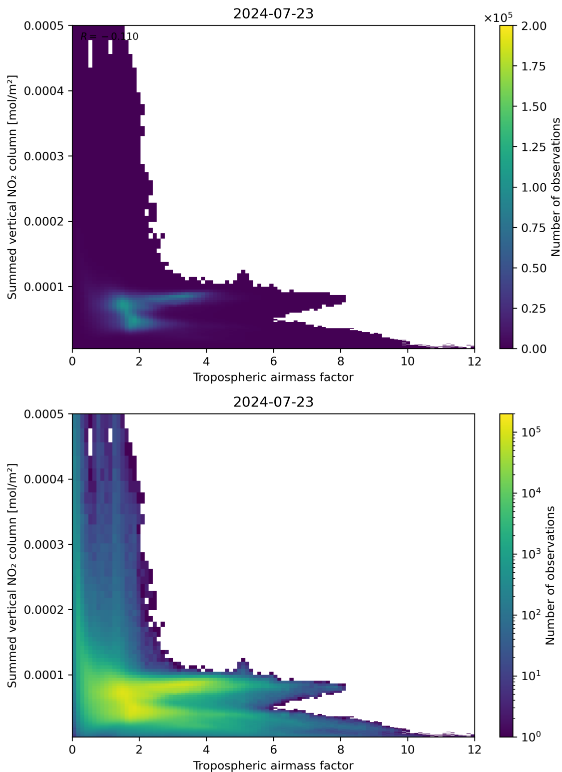
Figure 75: Scatter density plot of “Tropospheric airmass factor” against “Summed vertical NO 2 column” for 2024-07-22 to 2024-07-24.
