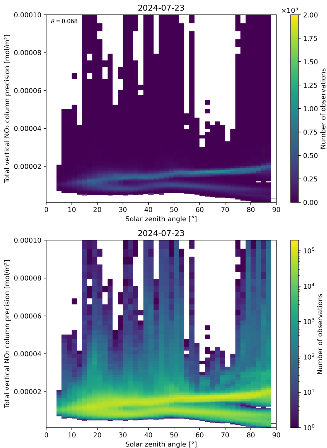
Figure 154: Scatter density plot of “Solar zenith angle” against “Total vertical NO 2 column precision” for 2024-07-22 to 2024-07-24.
