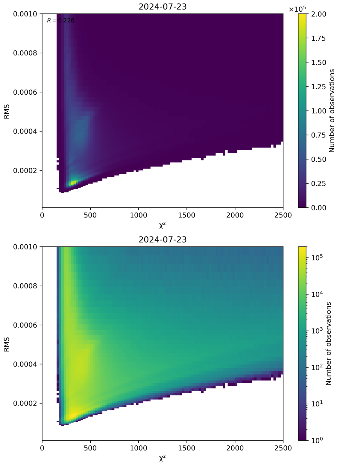
Figure 82: Scatter density plot of " \chi^2 " against "RMS" for 2024-07-22 to 2024-07-24.
