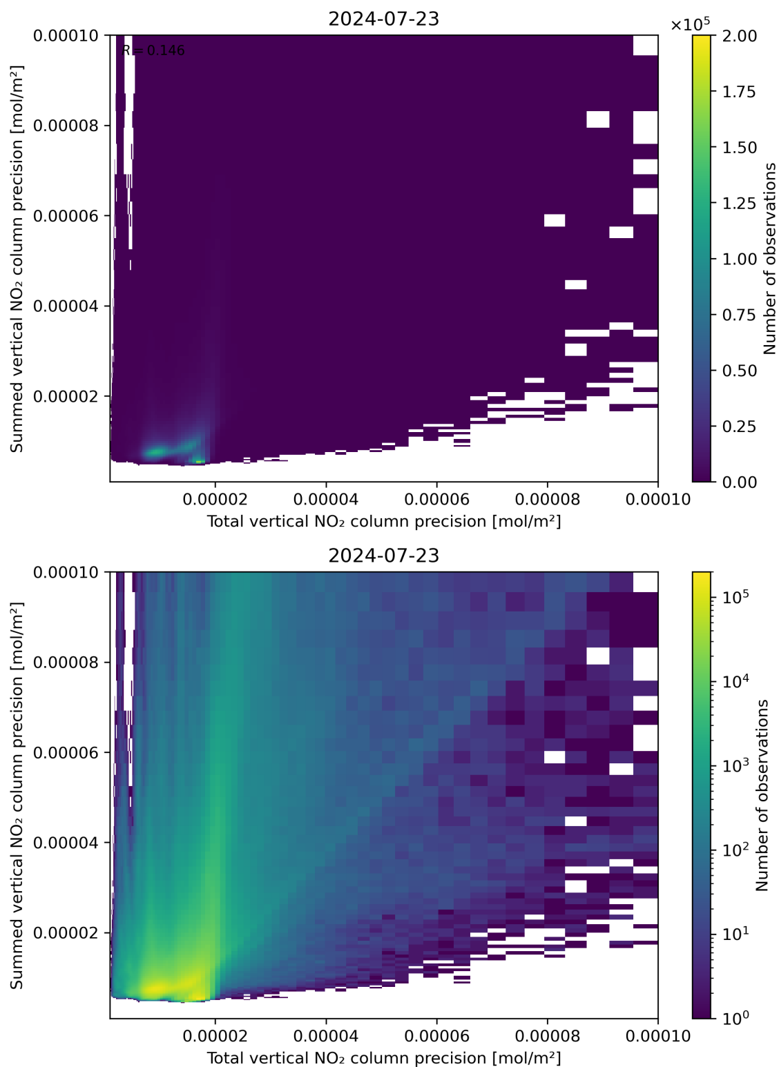
Figure 118: Scatter density plot of “Total vertical NO 2 column precision” against “Summed vertical NO 2 column precision” for 2024-07-22 to 2024-07-24.
