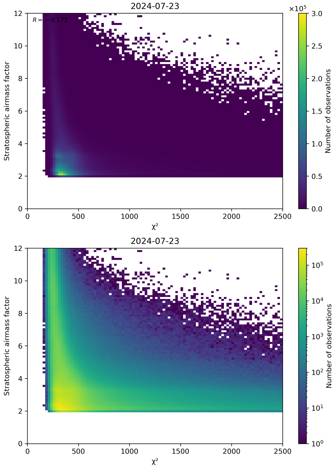
Figure 81: Scatter density plot of “ \chi^2 ” against “Stratospheric airmass factor” for 2024-07-22 to 2024-07-24.
