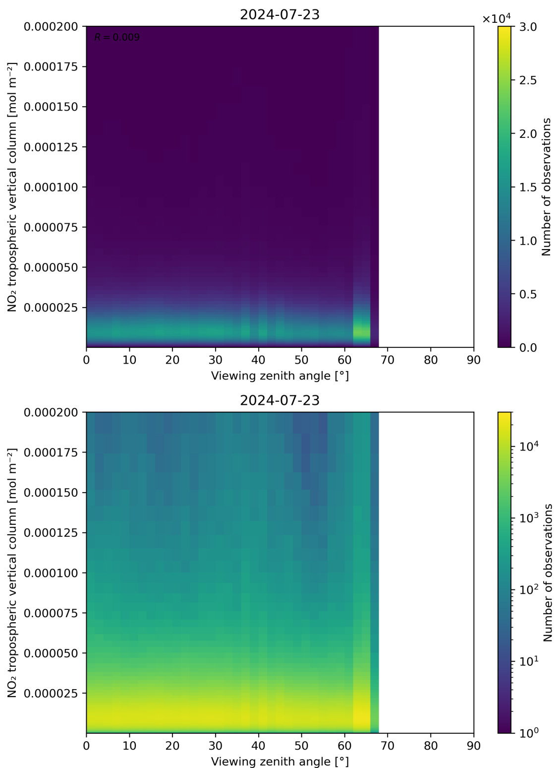
Figure 169: Scatter density plot of “Viewing zenith angle” against “NO 2 tropospheric vertical column” for 2024-07-22 to 2024-07-24.
