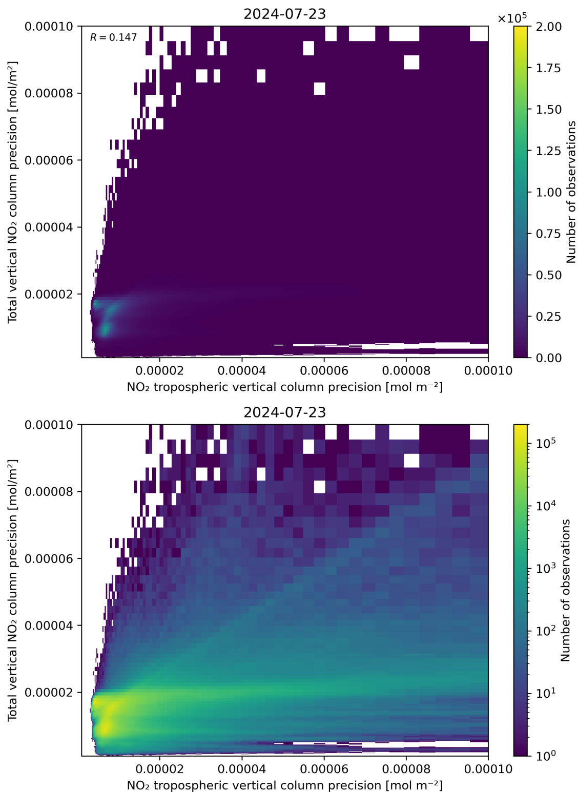
Figure 139: Scatter density plot of “NO 2 tropospheric vertical column precision” against “Total vertical NO 2 column precision” for 2024-07-22 to 2024-07-24.
