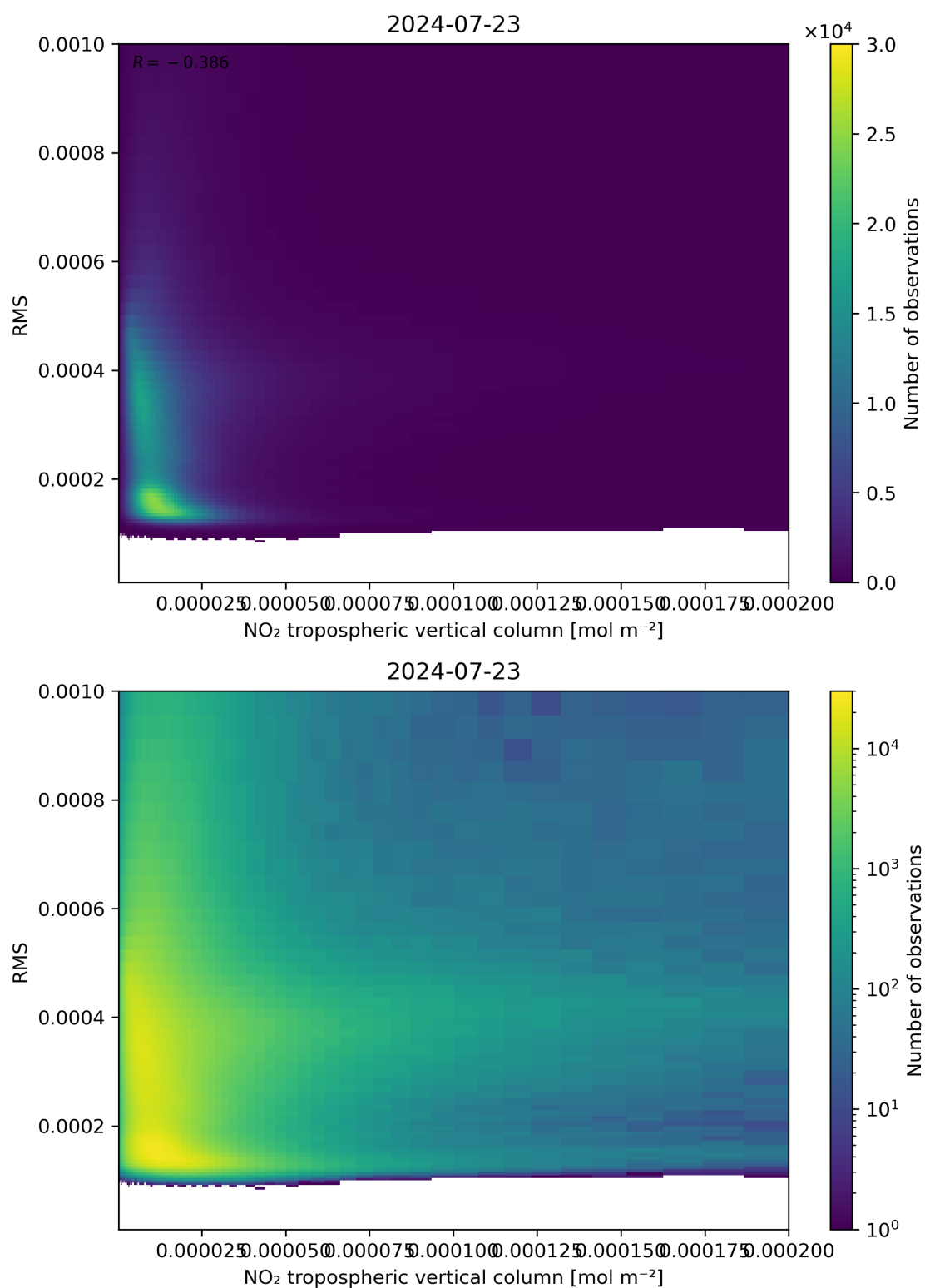
Figure 142: Scatter density plot of “NO 2 tropospheric vertical column” against “RMS” for 2024-07-22 to 2024-07-24.
