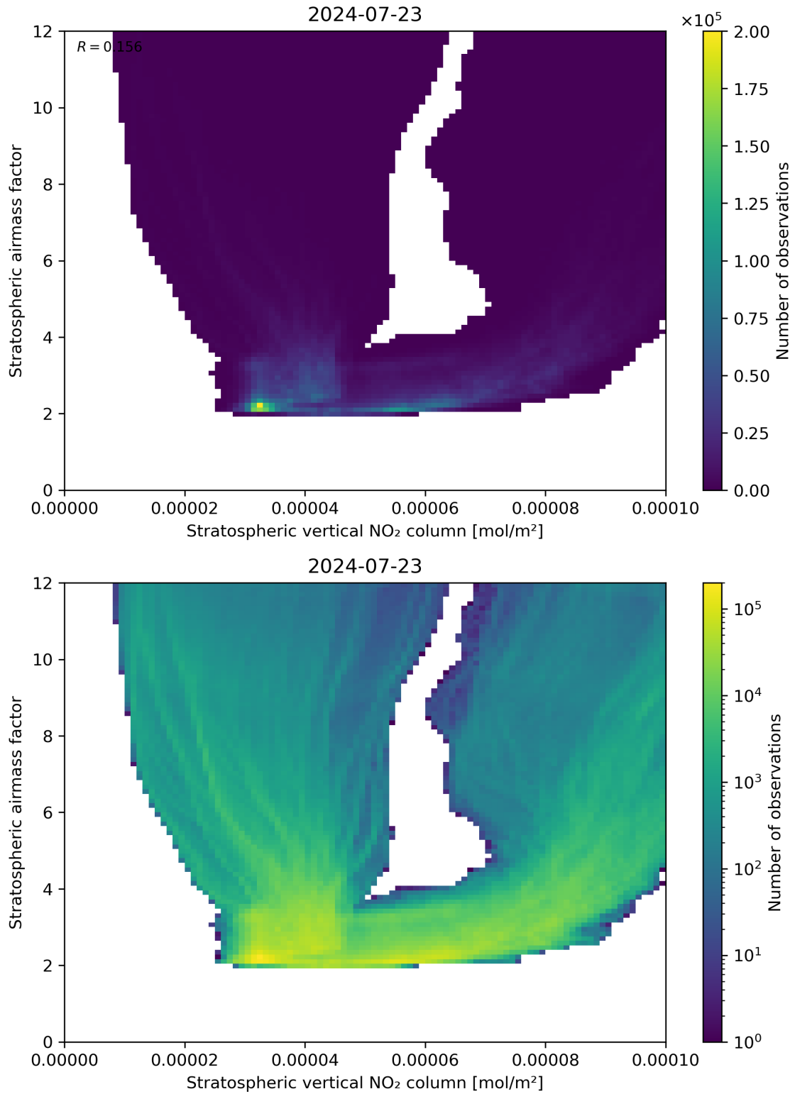
Figure 96: Scatter density plot of “Stratospheric vertical NO 2 column” against “Stratospheric airmass factor” for 2024-07-22 to 2024-07-24.
