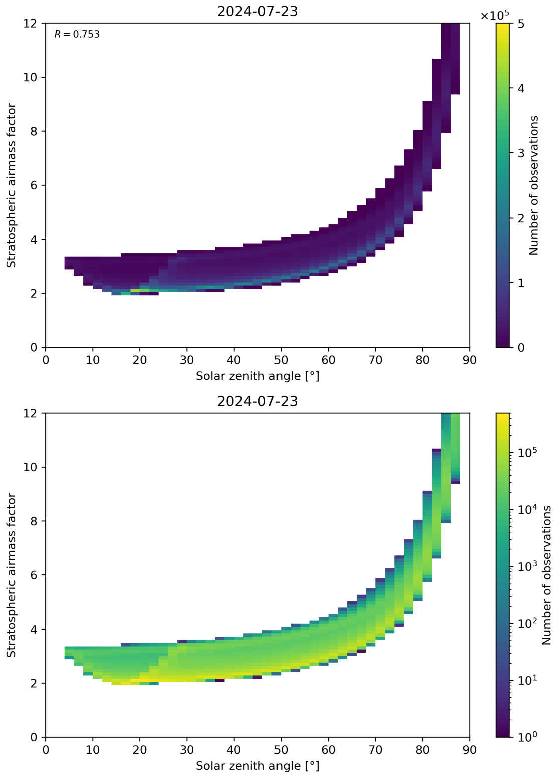
Figure 145: Scatter density plot of “Solar zenith angle” against “Stratospheric airmass factor” for 2024-07-22 to 2024-07-24.
