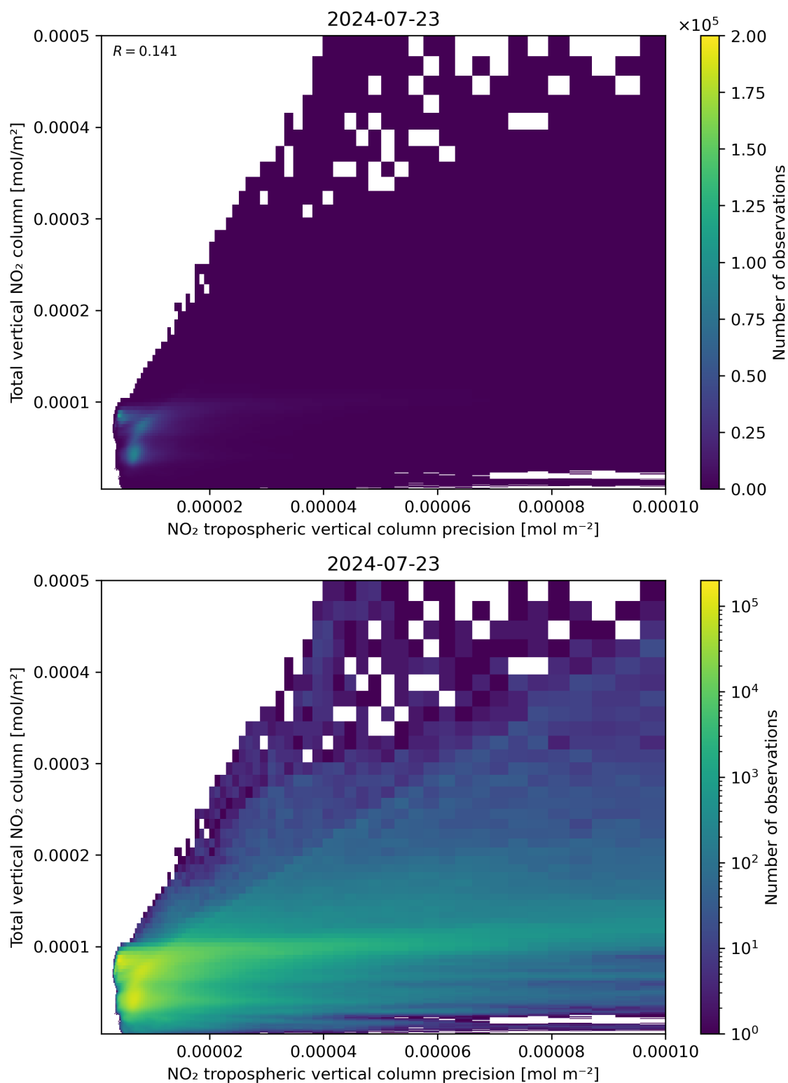
Figure 138: Scatter density plot of “NO 2 tropospheric vertical column precision” against “Total vertical NO 2 column” for 2024-07-22 to 2024-07-24.
