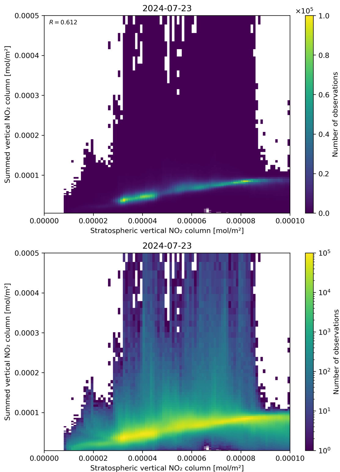
Figure 98: Scatter density plot of “Stratospheric vertical NO 2 column” against “Summed vertical NO 2 column” for 2024-07-22 to 2024-07-24.
