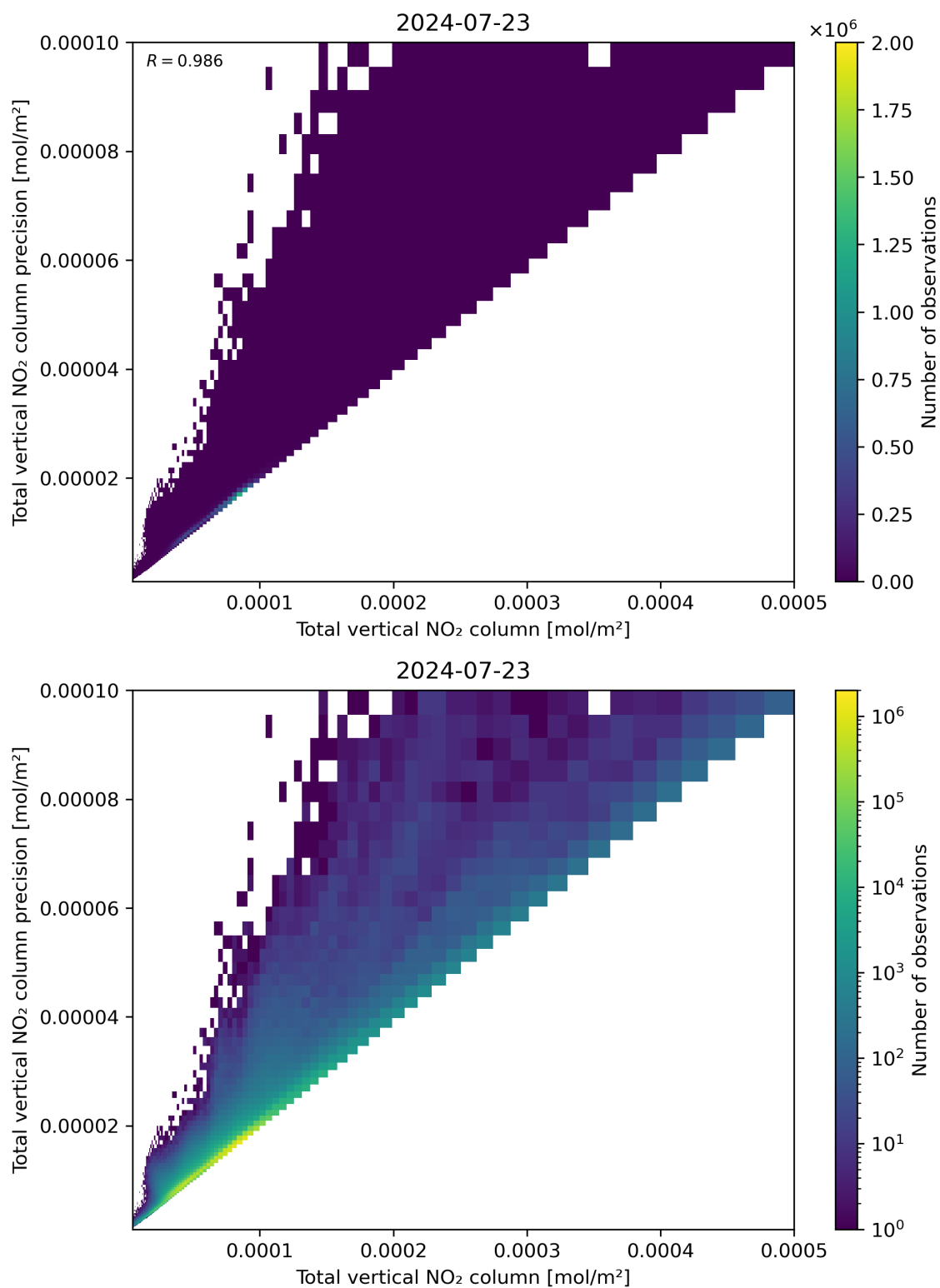
Figure 114: Scatter density plot of “Total vertical NO 2 column” against “Total vertical NO 2 column precision” for 2024-07-22 to 2024-07-24.
