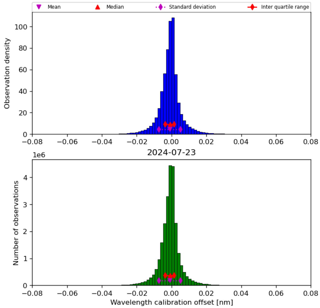
Figure 35: Histogram of “Wavelength calibration offset” for 2024-07-22 to 2024-07-24
