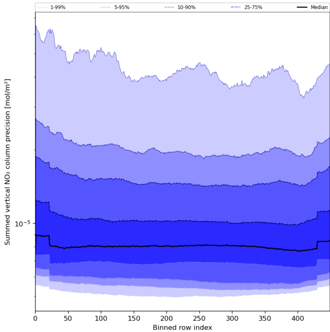
Figure 58: Along track statistics of “Summed vertical NO 2 column precision” for 2024-07-22 to 2024-07-24
