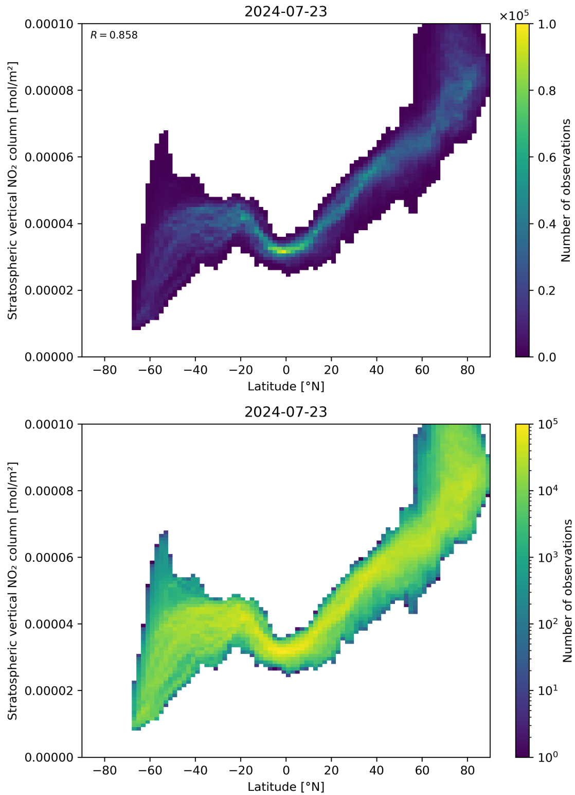
Figure 87: Scatter density plot of “Latitude” against “Stratospheric vertical NO 2 column” for 2024-07-22 to 2024-07-24.
