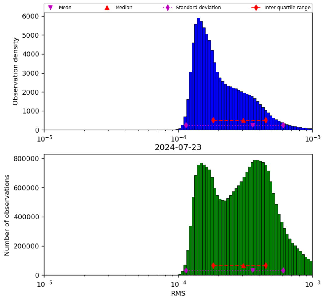
Figure 43: Histogram of “RMS” for 2024-07-22 to 2024-07-24
