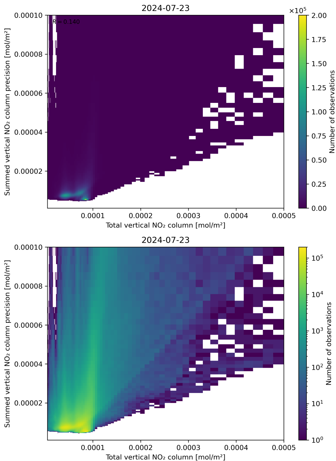
Figure 113: Scatter density plot of “Total vertical NO 2 column” against “Summed vertical NO 2 column precision” for 2024-07-22 to 2024-07-24.
