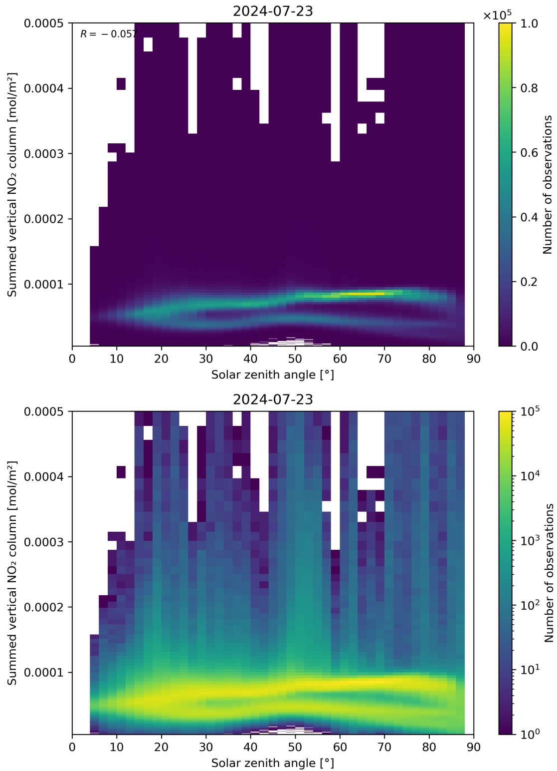
Figure 151: Scatter density plot of “Solar zenith angle” against “Summed vertical NO 2 column” for 2024-07-22 to 2024-07-24.
