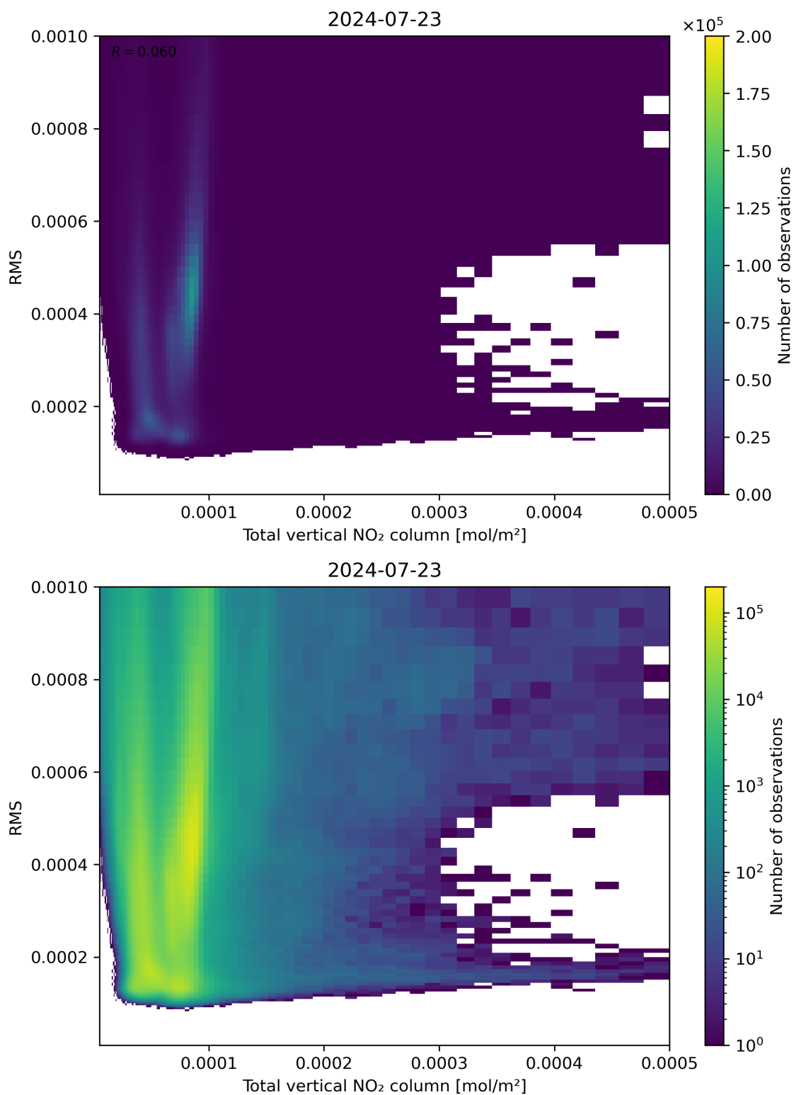
Figure 120: Scatter density plot of “Total vertical NO 2 column” against “RMS” for 2024-07-22 to 2024-07-24.
