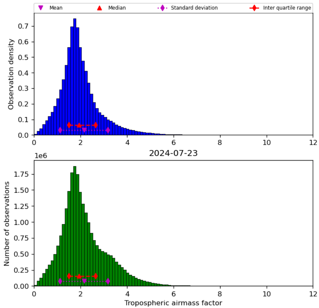
Figure 31: Histogram of “Tropospheric airmass factor” for 2024-07-22 to 2024-07-24
