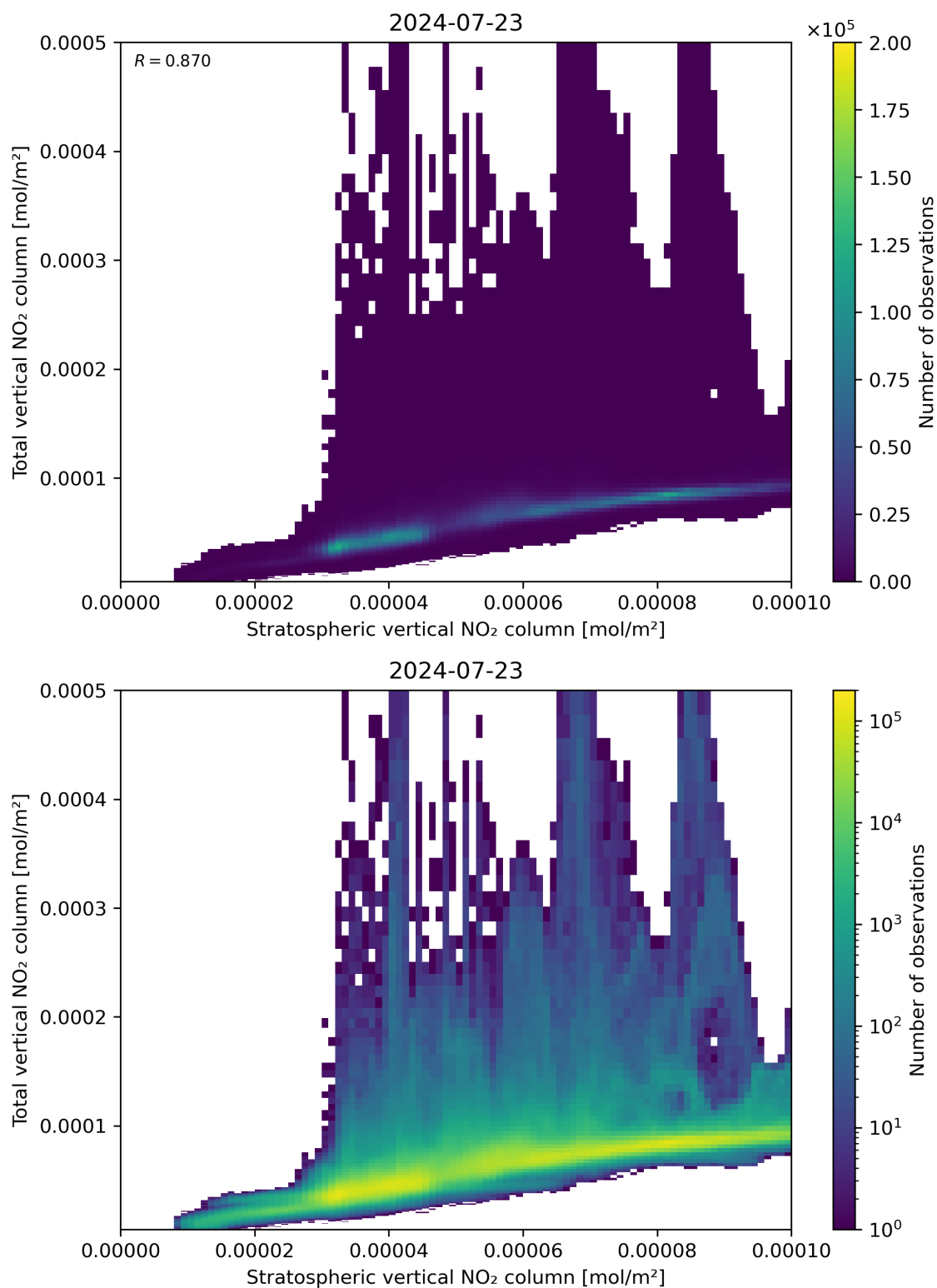
Figure 100: Scatter density plot of “Stratospheric vertical NO 2 column” against “Total vertical NO 2 column” for 2024-07-22 to 2024-07-24.
