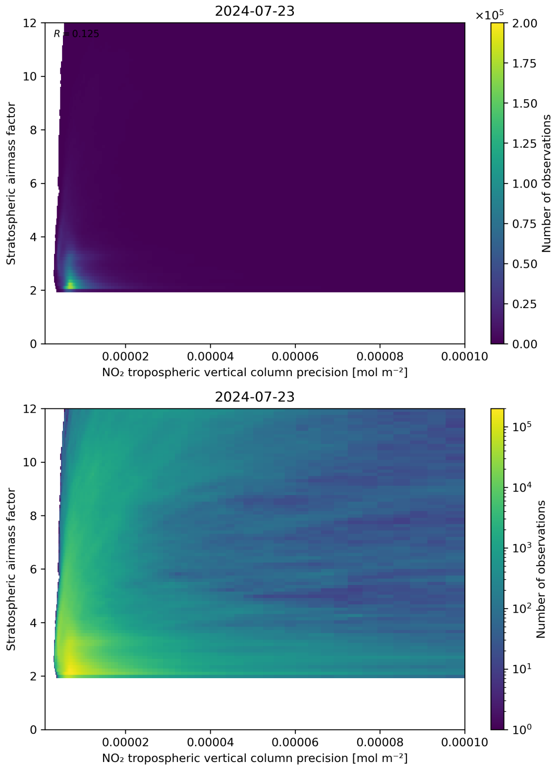
Figure 131: Scatter density plot of “NO 2 tropospheric vertical column precision” against “Stratospheric airmass factor” for 2024-07-22 to 2024-07-24.
