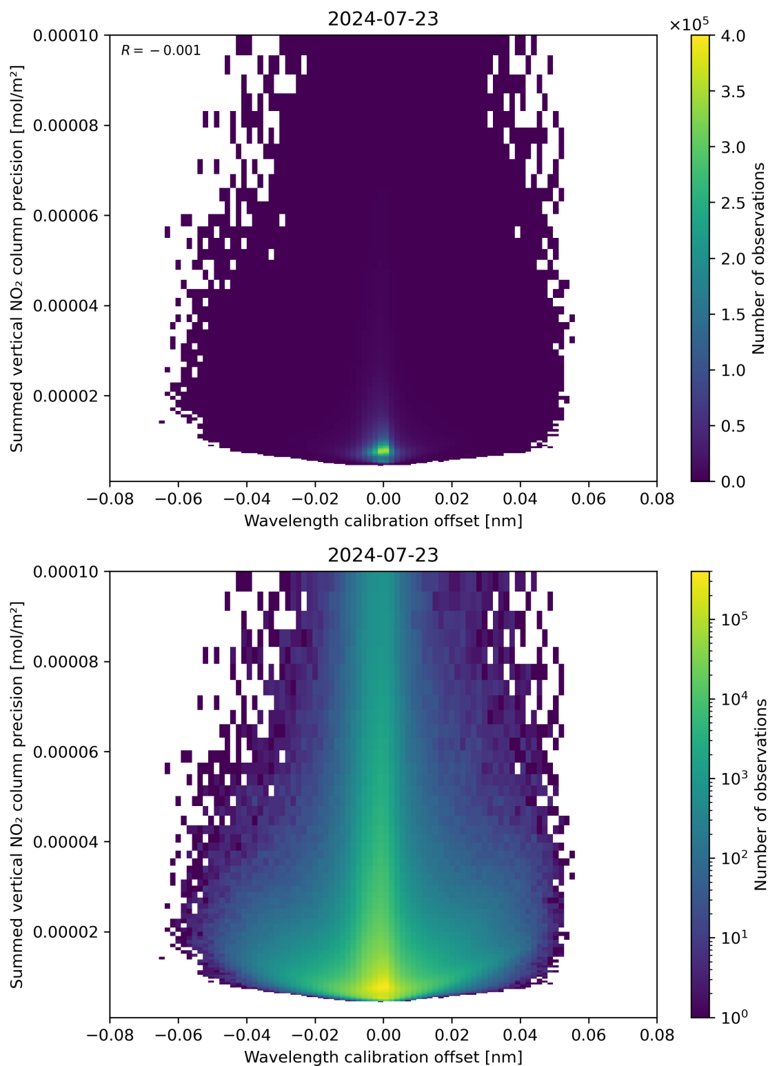
Figure 178: Scatter density plot of “Wavelength calibration offset” against “Summed vertical NO 2 column precision” for 2024-07-22 to 2024-07-24.
