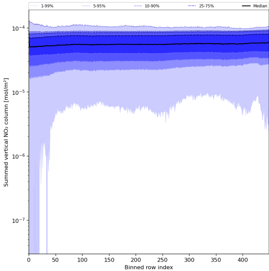
Figure 57: Along track statistics of “Summed vertical NO 2 column” for 2024-07-22 to 2024-07-24
