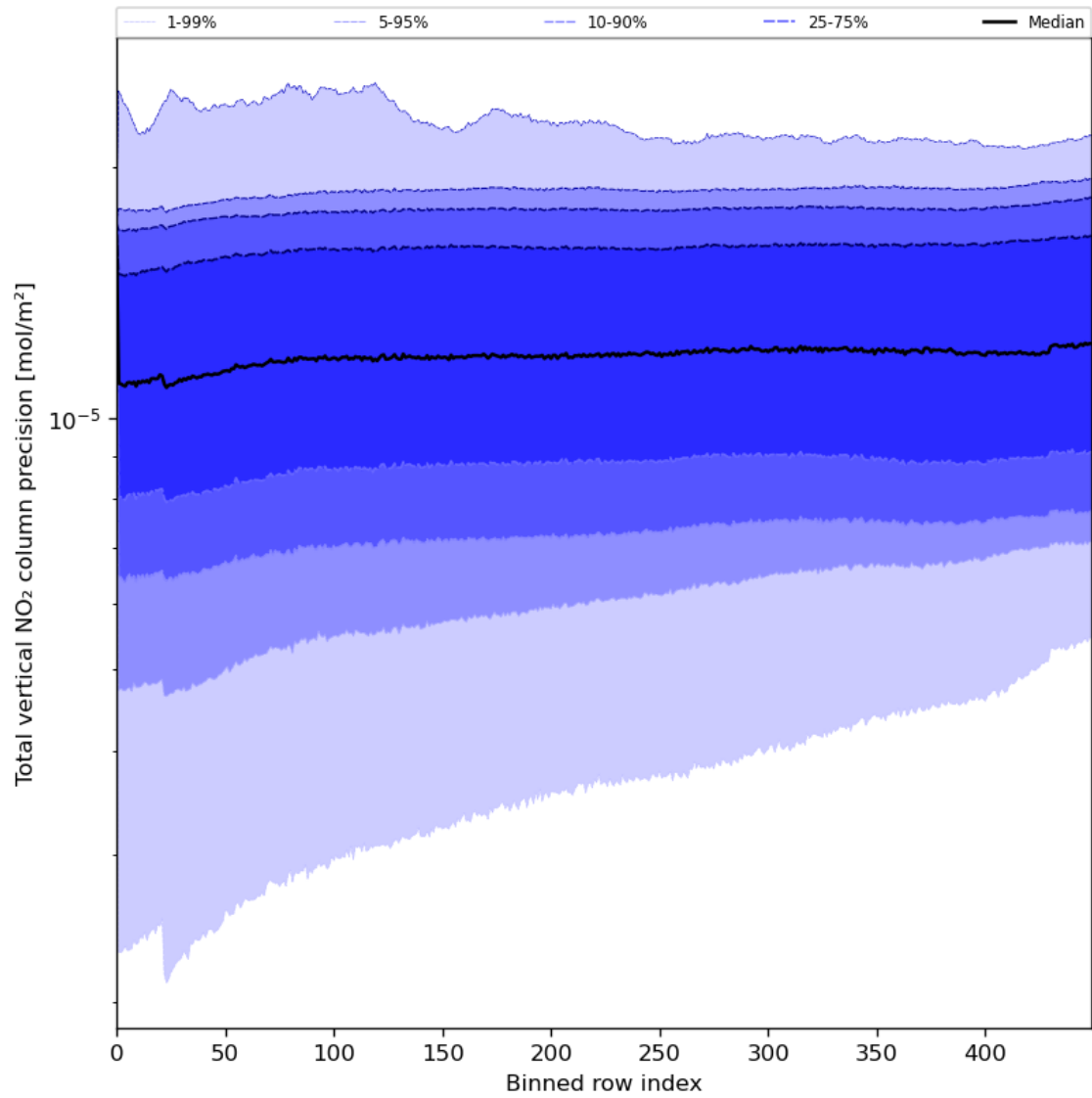
Figure 56: Along track statistics of “Total vertical NO 2 column precision” for 2024-07-22 to 2024-07-24
