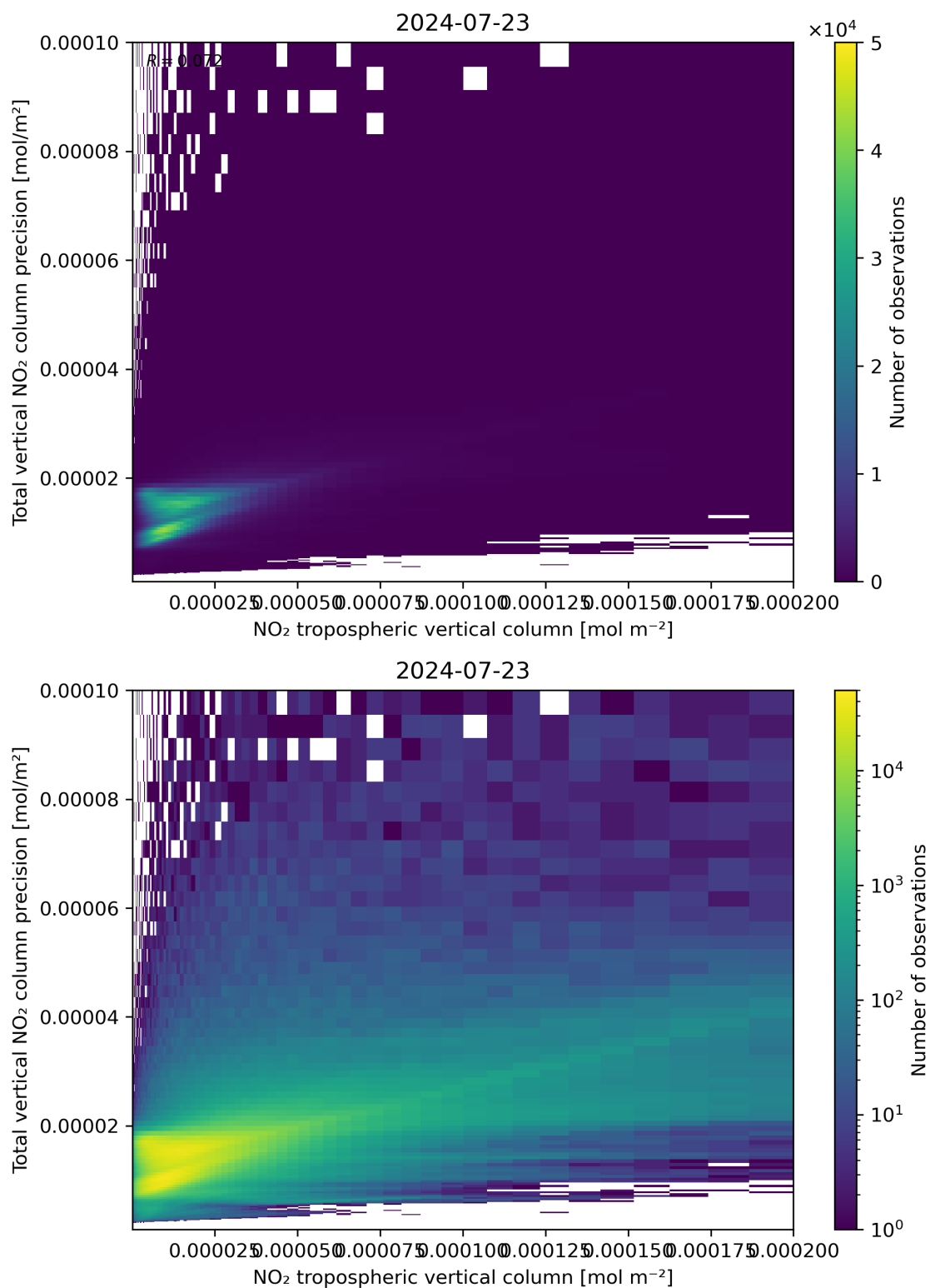
Figure 129: Scatter density plot of “NO 2 tropospheric vertical column” against “Total vertical NO 2 column precision” for 2024-07-22 to 2024-07-24.
