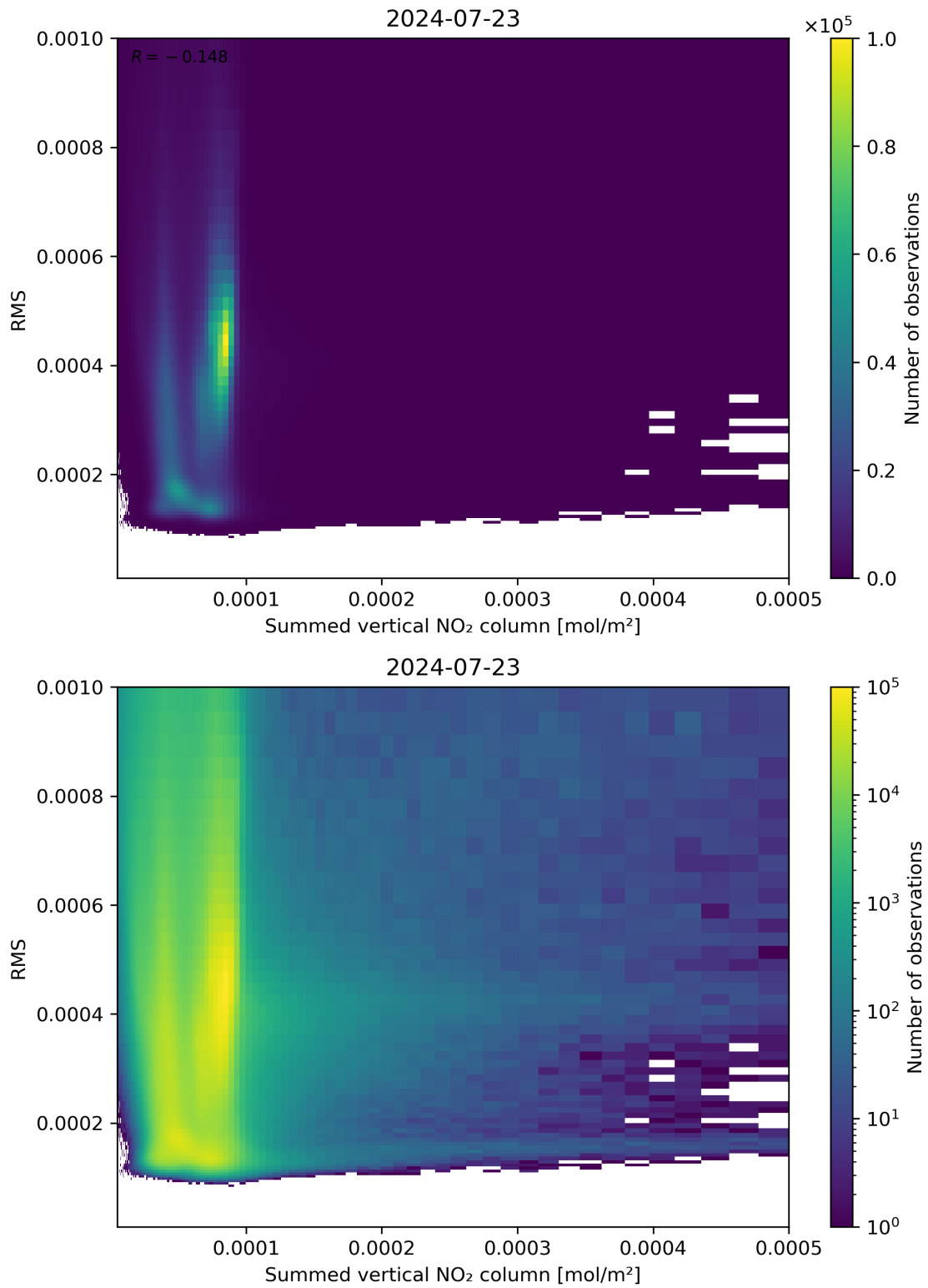
Figure 109: Scatter density plot of “Summed vertical NO 2 column” against “RMS” for 2024-07-22 to 2024-07-24.
