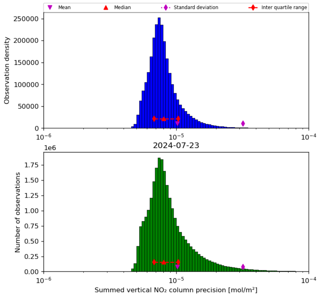
Figure 41: Histogram of "Summed vertical NO 2 column precision" for 2024-07-22 to 2024-07-24
