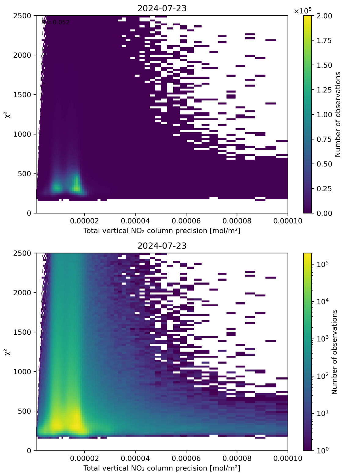
Figure 116: Scatter density plot of “Total vertical NO 2 column precision” against “ \chi^2 ” for 2024-07-22 to 2024-07-24.
