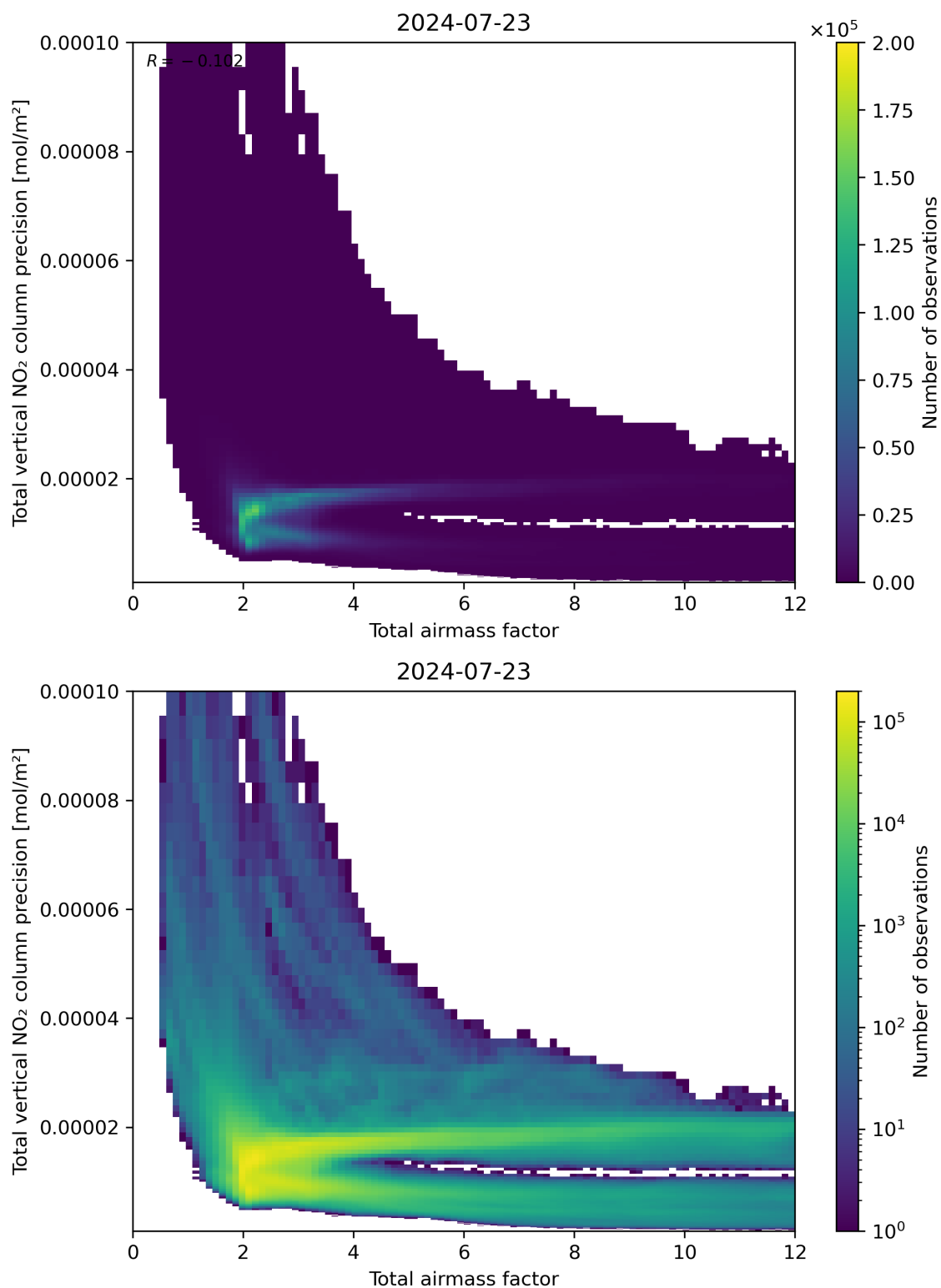
Figure 68: Scatter density plot of “Total airmass factor” against “Total vertical NO 2 column precision” for 2024-07-22 to 2024-07-24.
