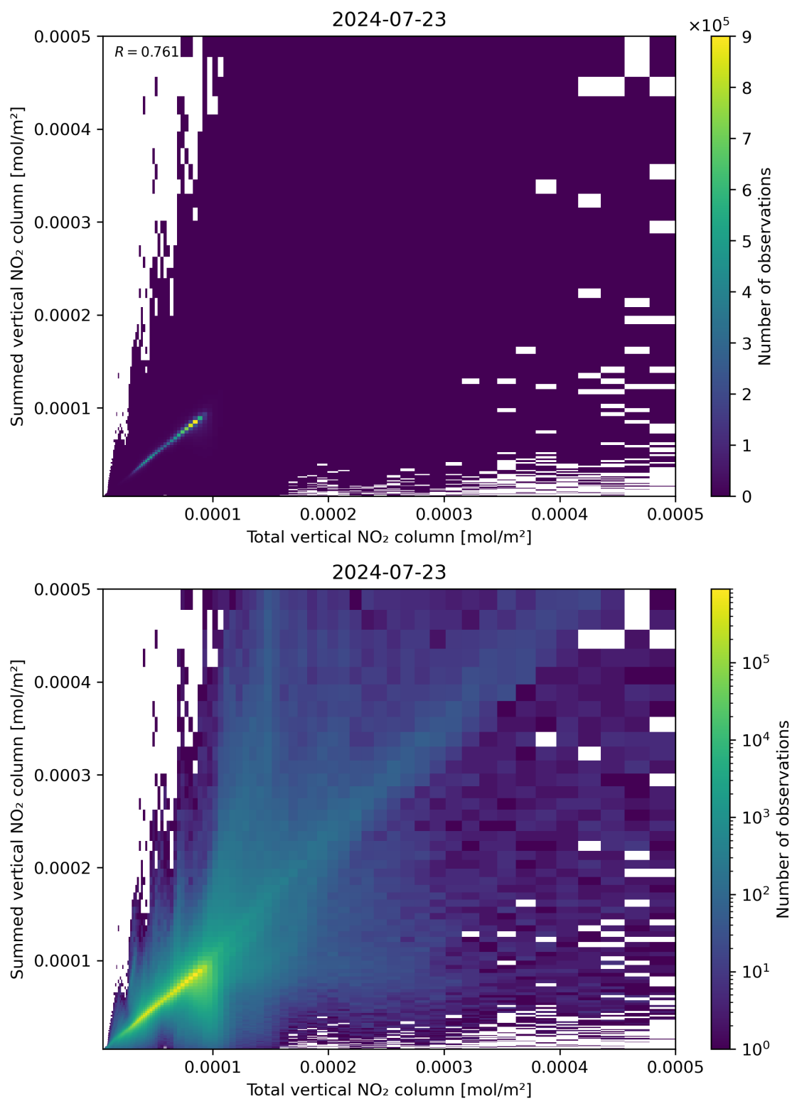
Figure 112: Scatter density plot of “Total vertical NO 2 column” against “Summed vertical NO 2 column” for 2024-07-22 to 2024-07-24.
