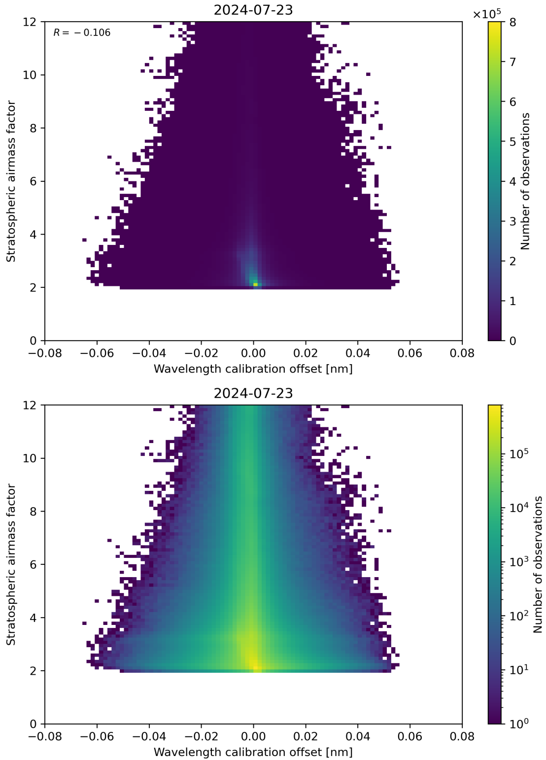
Figure 174: Scatter density plot of “Wavelength calibration offset” against “Stratospheric air mass factor” for 2024-07-22 to 2024-07-24.
