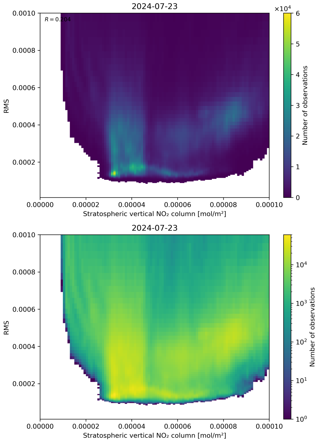
Figure 102: Scatter density plot of “Stratospheric vertical NO 2 column” against “RMS” for 2024-07-22 to 2024-07-24.
