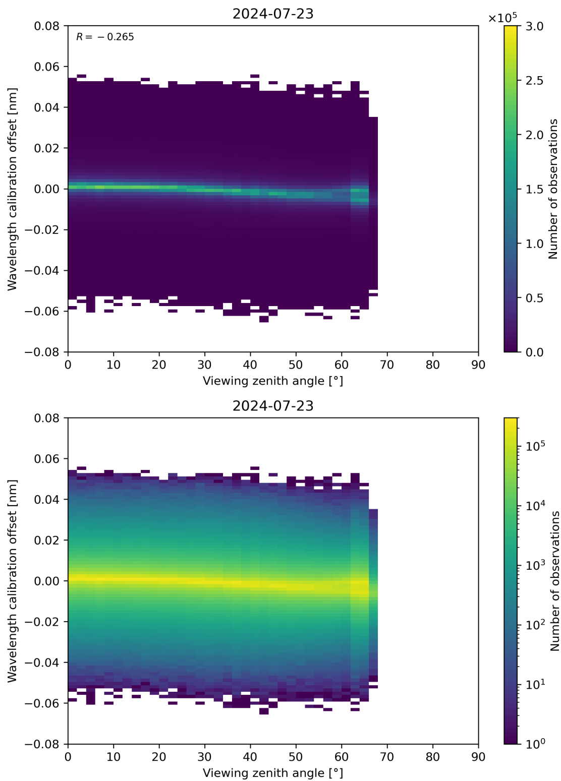
Figure 173: Scatter density plot of “Viewing zenith angle” against “Wavelength calibration offset” for 2024-07-22 to 2024-07-24.
