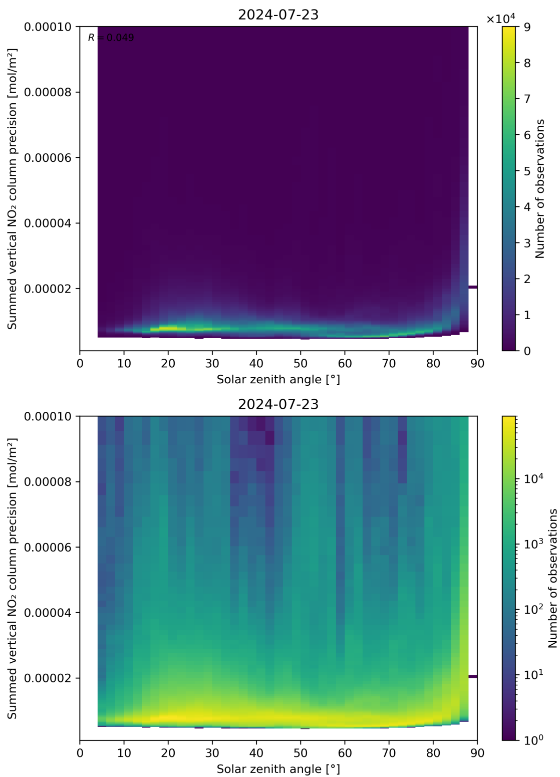
Figure 152: Scatter density plot of “Solar zenith angle” against “Summed vertical NO 2 column precision” for 2024-07-22 to 2024-07-24.
