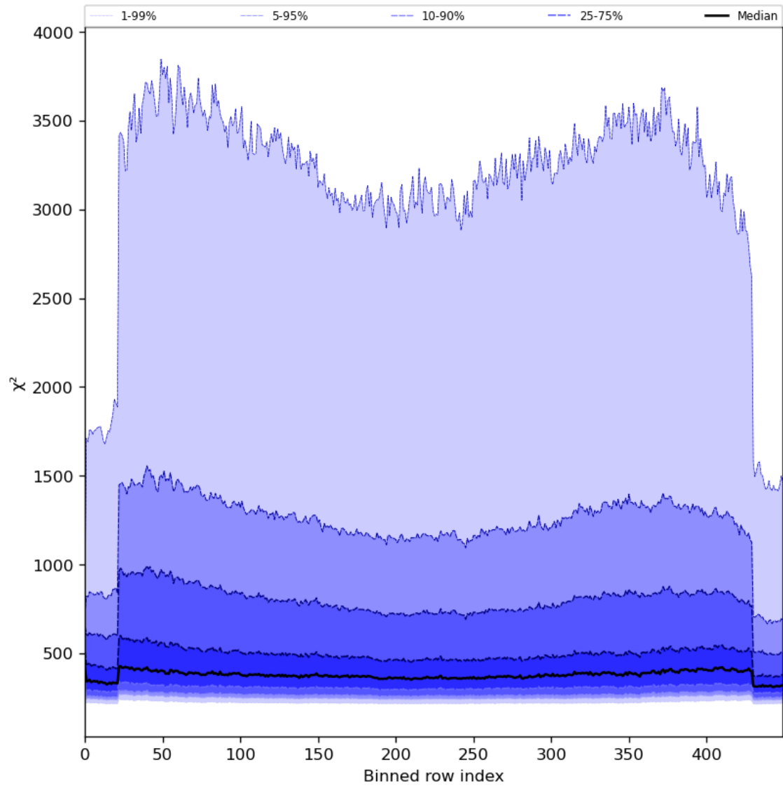
Figure 59: Along track statistics of “ \chi^2 ” for 2024-07-22 to 2024-07-24
