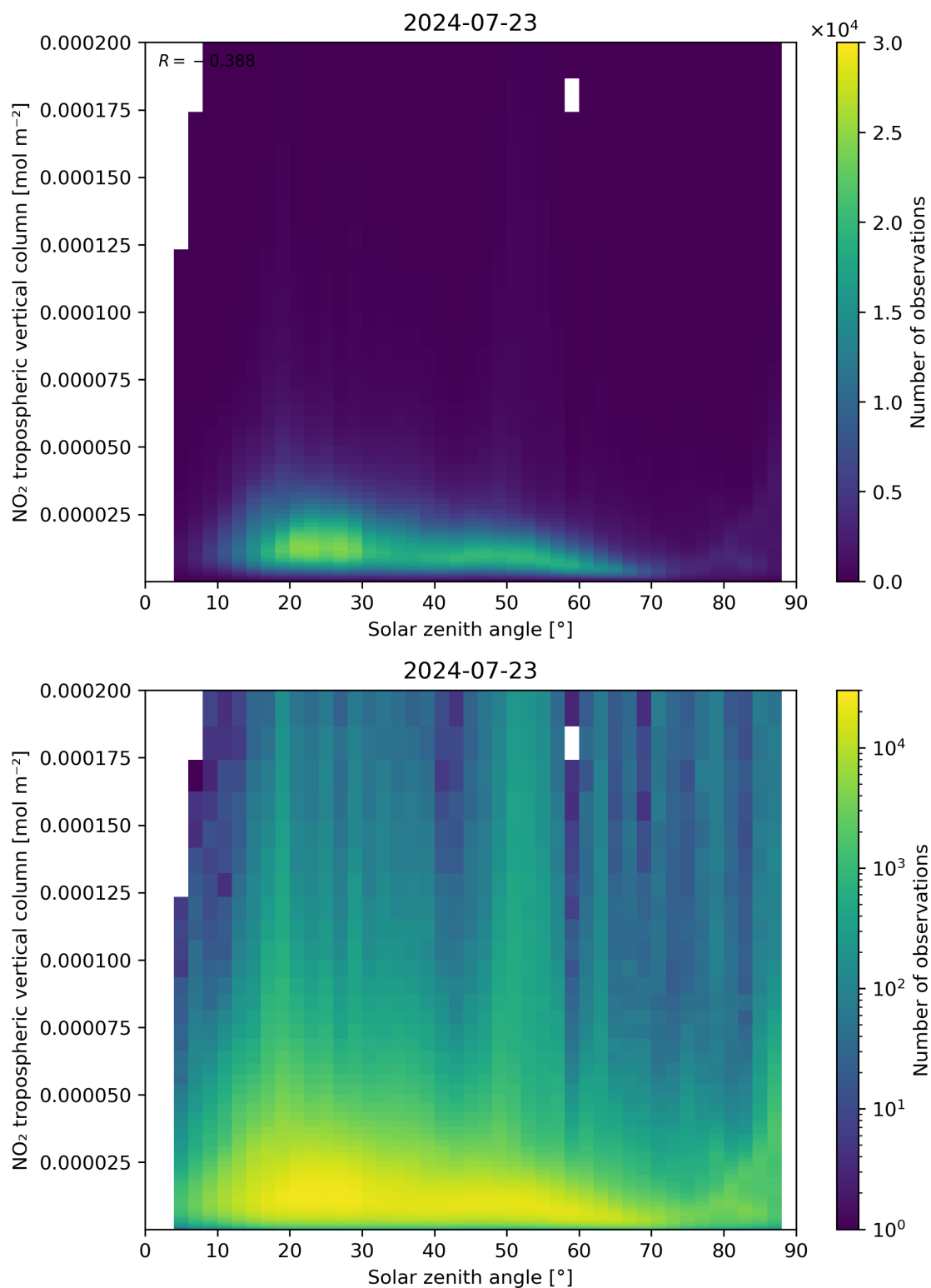
Figure 155: Scatter density plot of “Solar zenith angle” against “NO 2 tropospheric vertical column” for 2024-07-22 to 2024-07-24.
