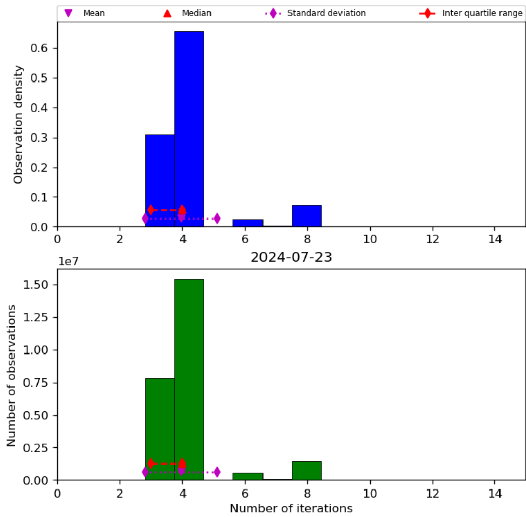
Figure 34: Histogram of “Number of iterations” for 2024-07-22 to 2024-07-24
