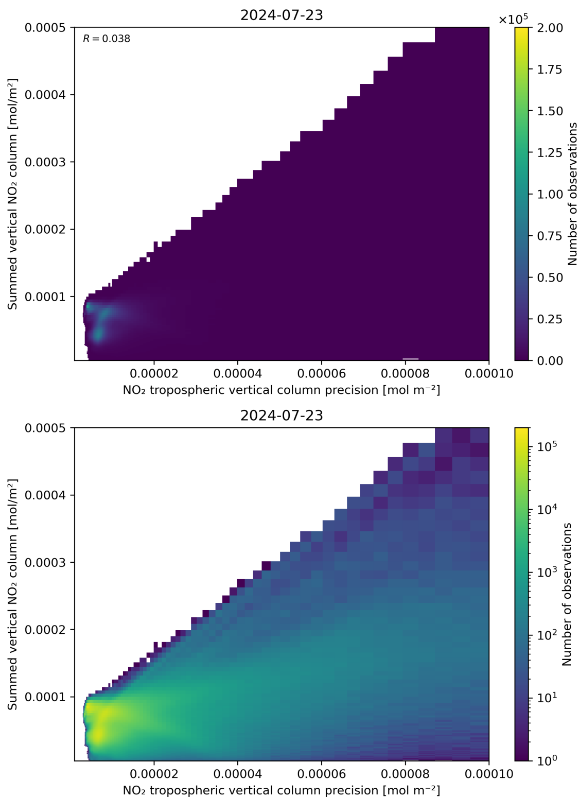
Figure 136: Scatter density plot of “NO 2 tropospheric vertical column precision” against “Summed vertical NO 2 column” for 2024-07-22 to 2024-07-24.
