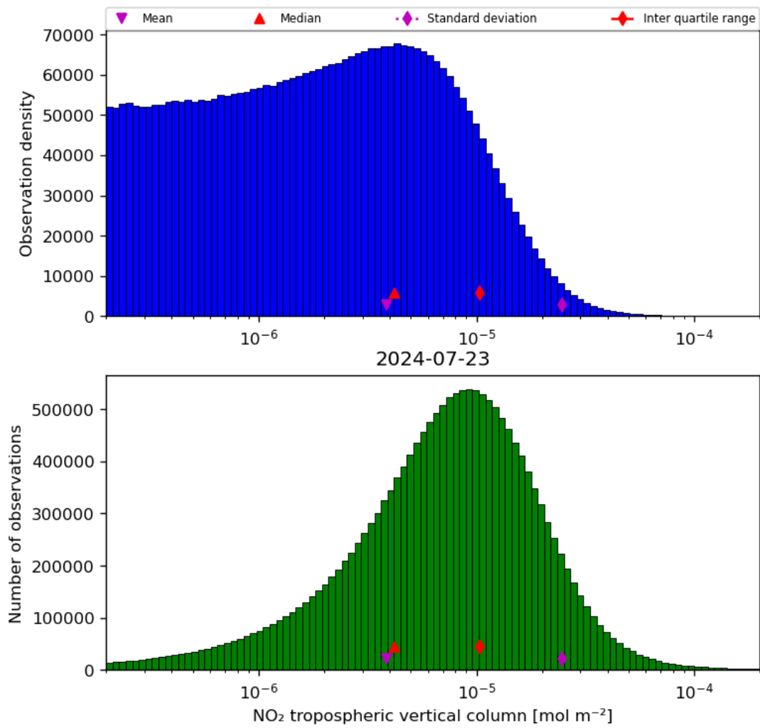
Figure 29: Histogram of “NO 2 tropospheric vertical column” for 2024-07-22 to 2024-07-24
