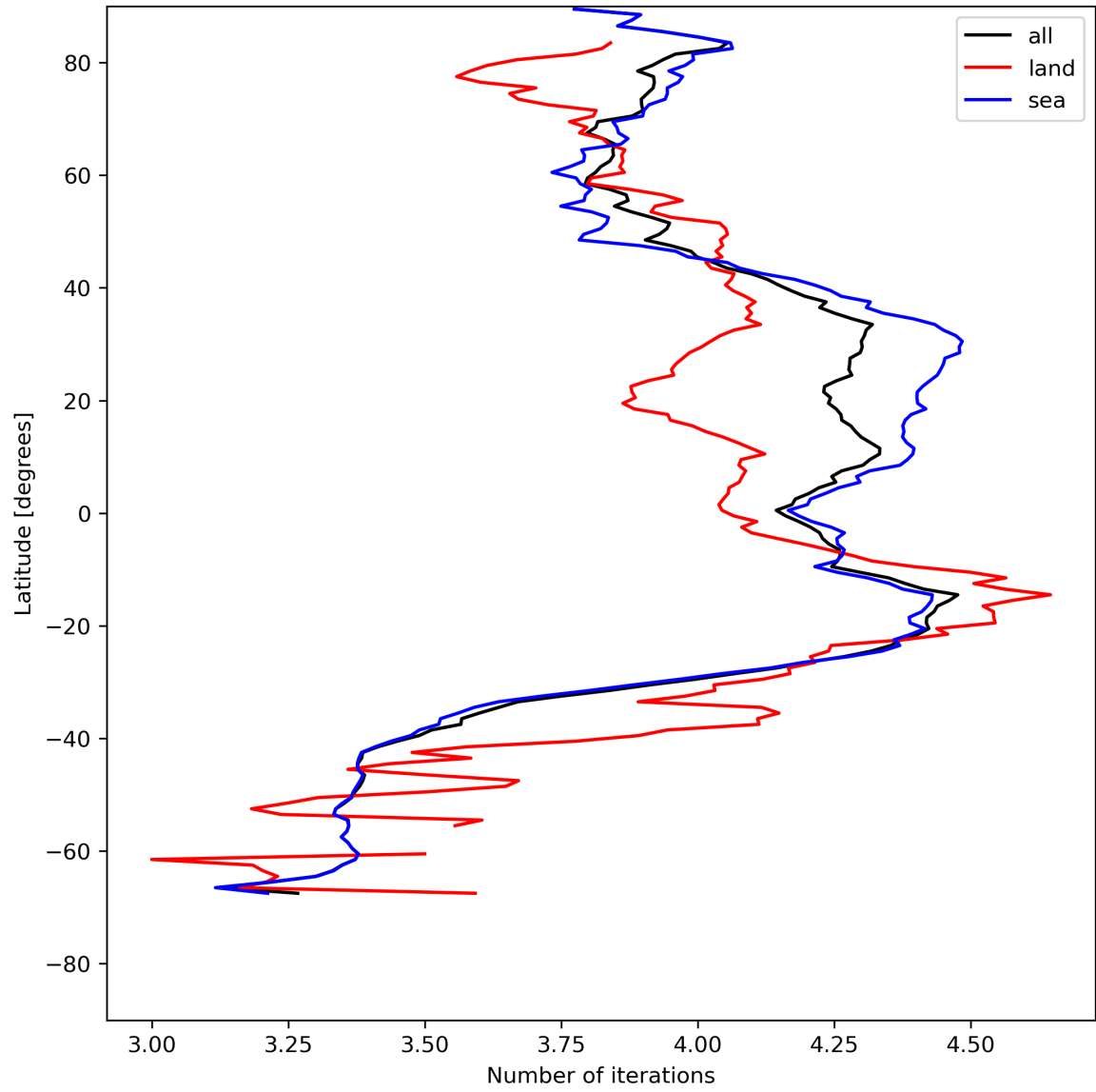
Figure 17: Zonal average of “Number of iterations” for 2024-07-22 to 2024-07-24.
