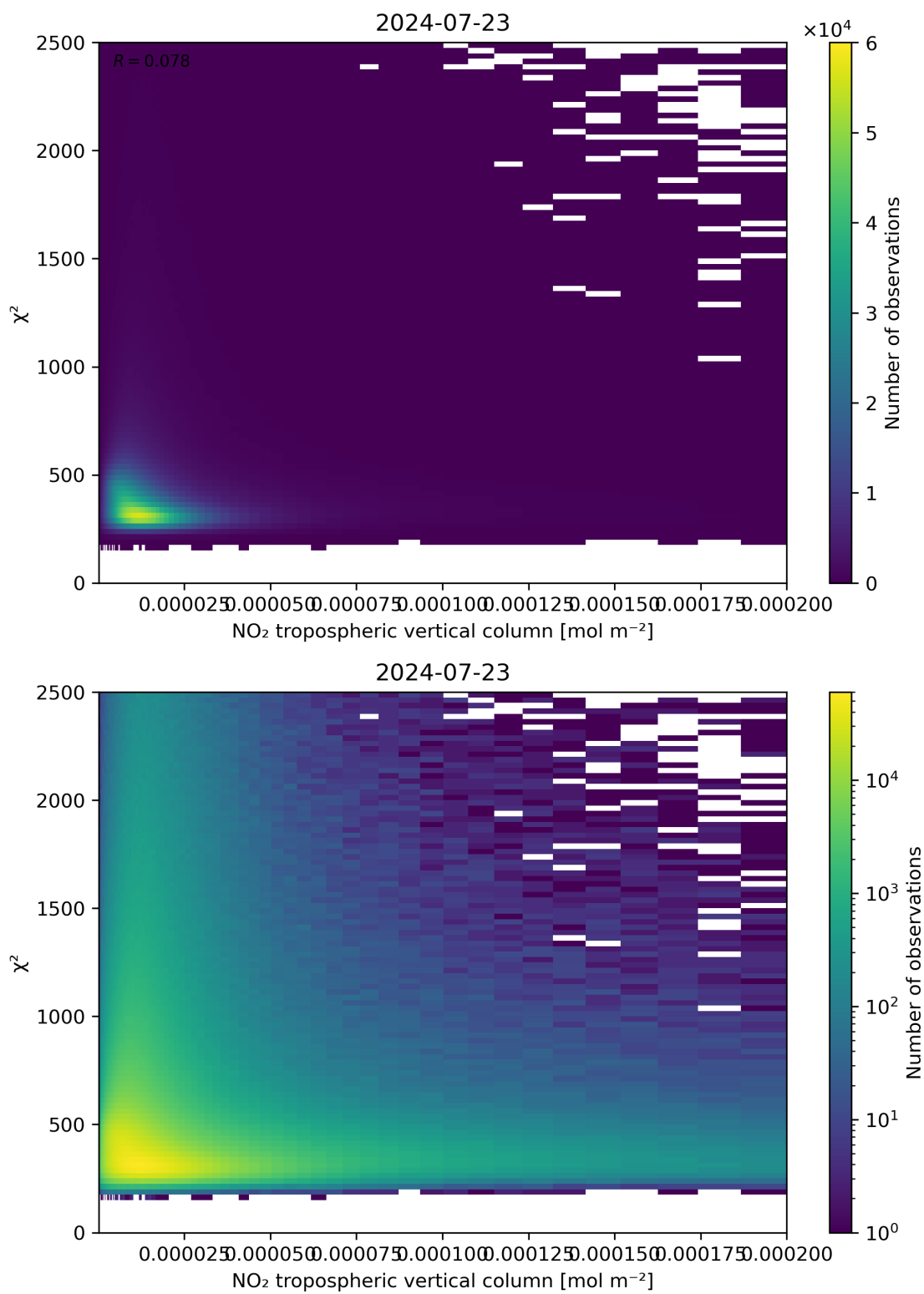
Figure 124: Scatter density plot of “NO 2 tropospheric vertical column” against “ \chi^2 ” for 2024-07-22 to 2024-07-24.
