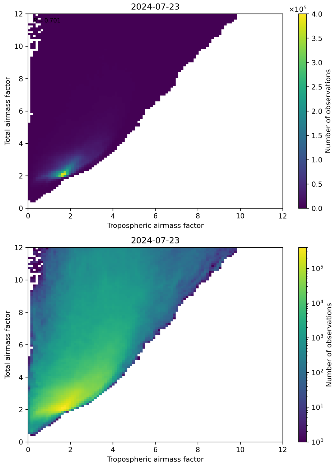
Figure 72: Scatter density plot of “Tropospheric airmass factor” against “Total airmass factor” for 2024-07-22 to 2024-07-24.
