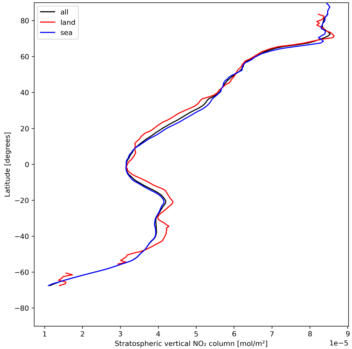
Figure 19: Zonal average of “Stratospheric vertical NO 2 column” for 2024-07-22 to 2024-07-24.
