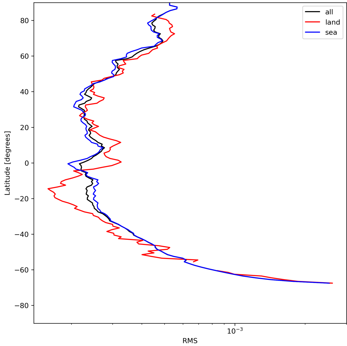
Figure 26: Zonal average of “RMS” for 2024-07-22 to 2024-07-24.
