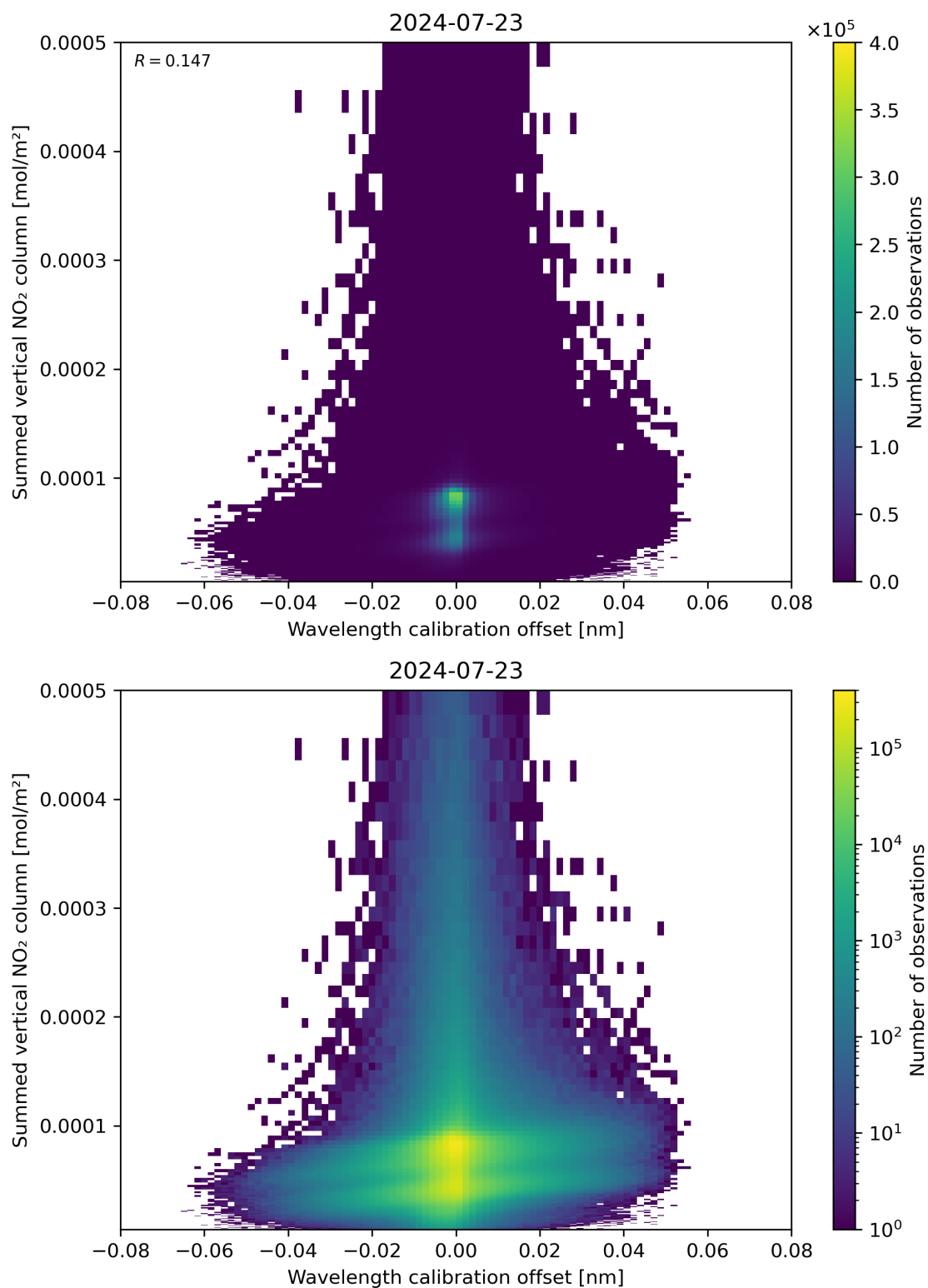
Figure 177: Scatter density plot of “Wavelength calibration offset” against “Summed vertical NO 2 column” for 2024-07-22 to 2024-07-24.
