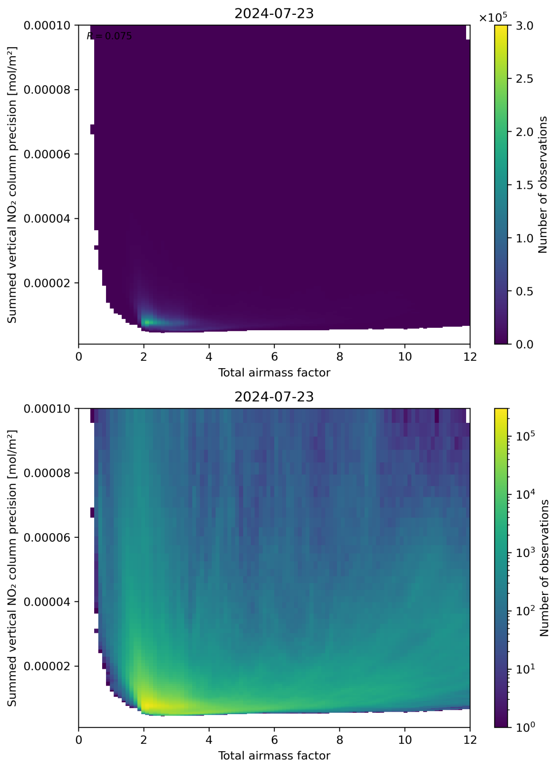
Figure 66: Scatter density plot of “Total airmass factor” against “Summed vertical NO 2 column precision” for 2024-07-22 to 2024-07-24.
