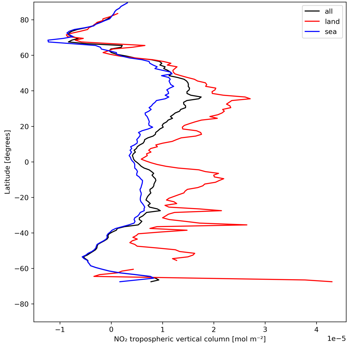
Figure 12: Zonal average of “NO 2 tropospheric vertical column” for 2024-07-22 to 2024-07-24.
