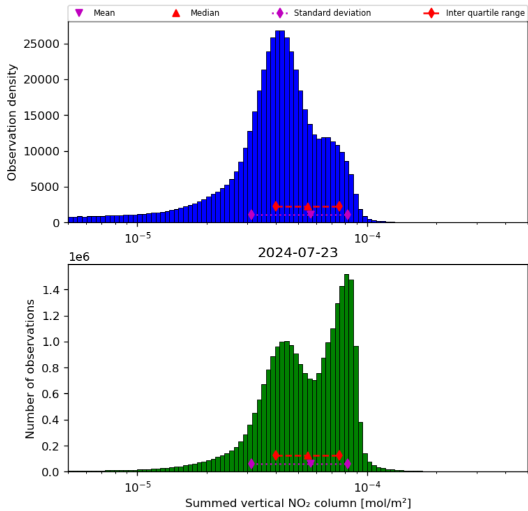
Figure 40: Histogram of “Summed vertical NO 2 column” for 2024-07-22 to 2024-07-24
