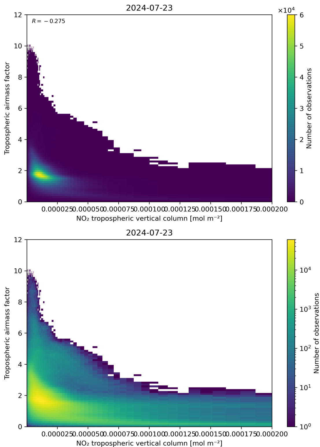
Figure 123: Scatter density plot of “NO 2 tropospheric vertical column” against “Tropospheric air mass factor” for 2024-07-22 to 2024-07-24.
