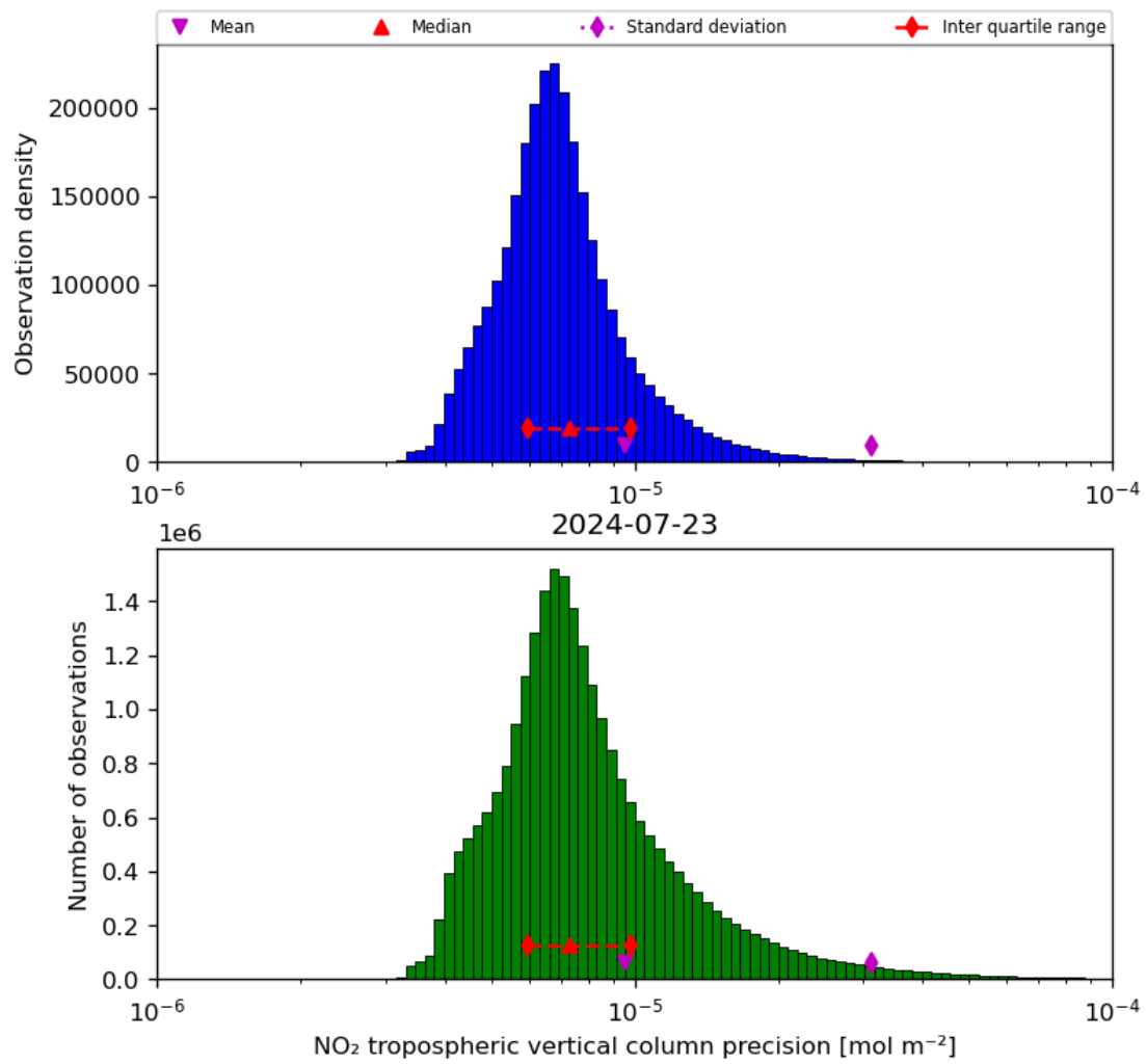
Figure 30: Histogram of “NO 2 tropospheric vertical column precision” for 2024-07-22 to 2024-07-24
