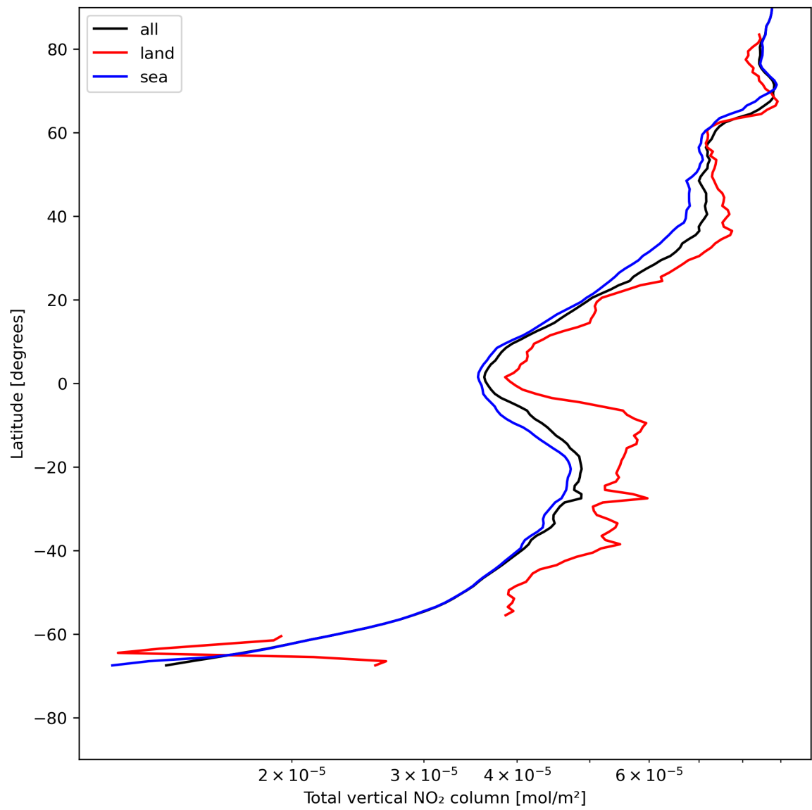
Figure 21: Zonal average of “Total vertical NO 2 column” for 2024-07-22 to 2024-07-24.
