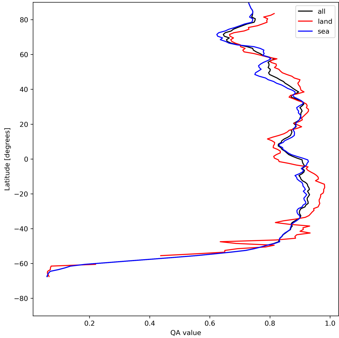
Figure 11: Zonal average of “QA value” for 2024-07-22 to 2024-07-24.
