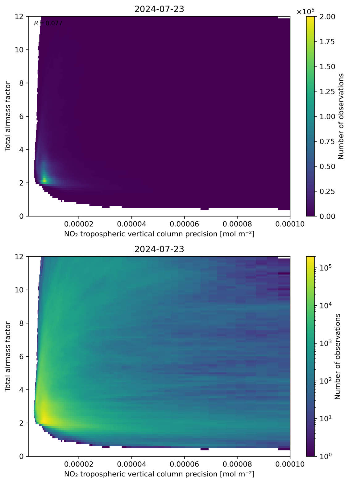
Figure 132: Scatter density plot of “NO 2 tropospheric vertical column precision” against “Total airmass factor” for 2024-07-22 to 2024-07-24.
