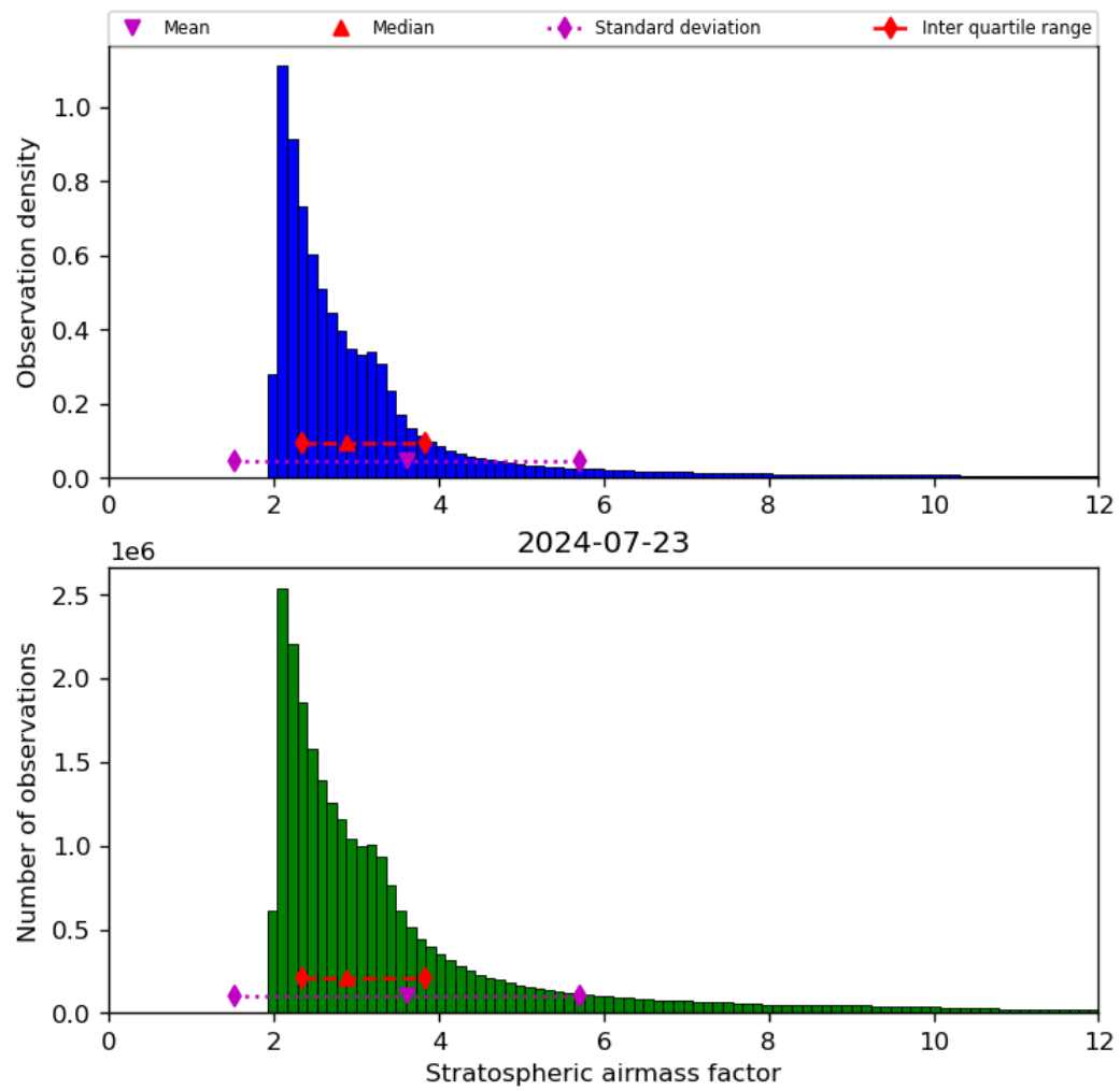
Figure 44: Histogram of “Stratospheric airmass factor” for 2024-07-22 to 2024-07-24
