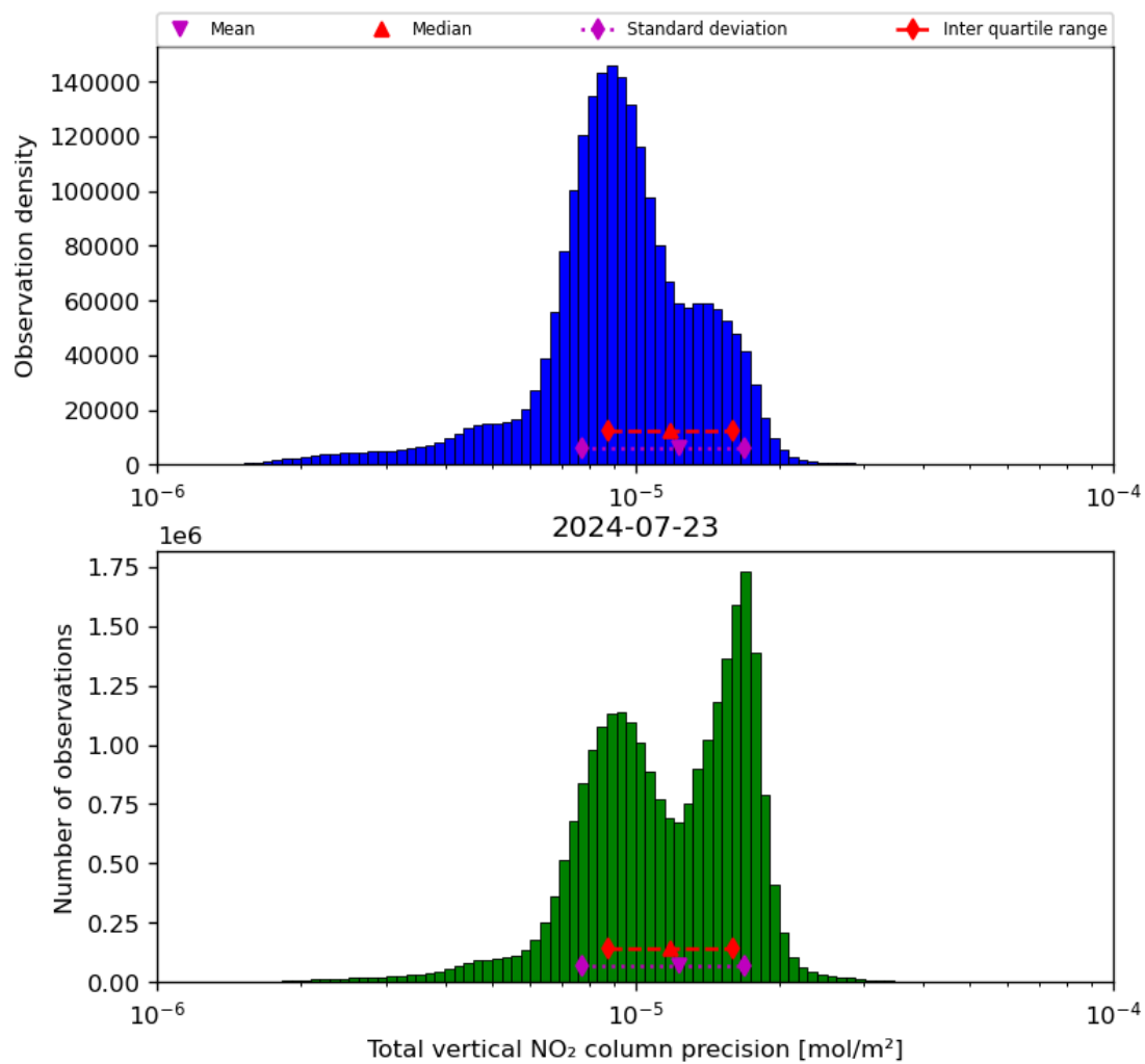
Figure 39: Histogram of “Total vertical NO 2 column precision” for 2024-07-22 to 2024-07-24
