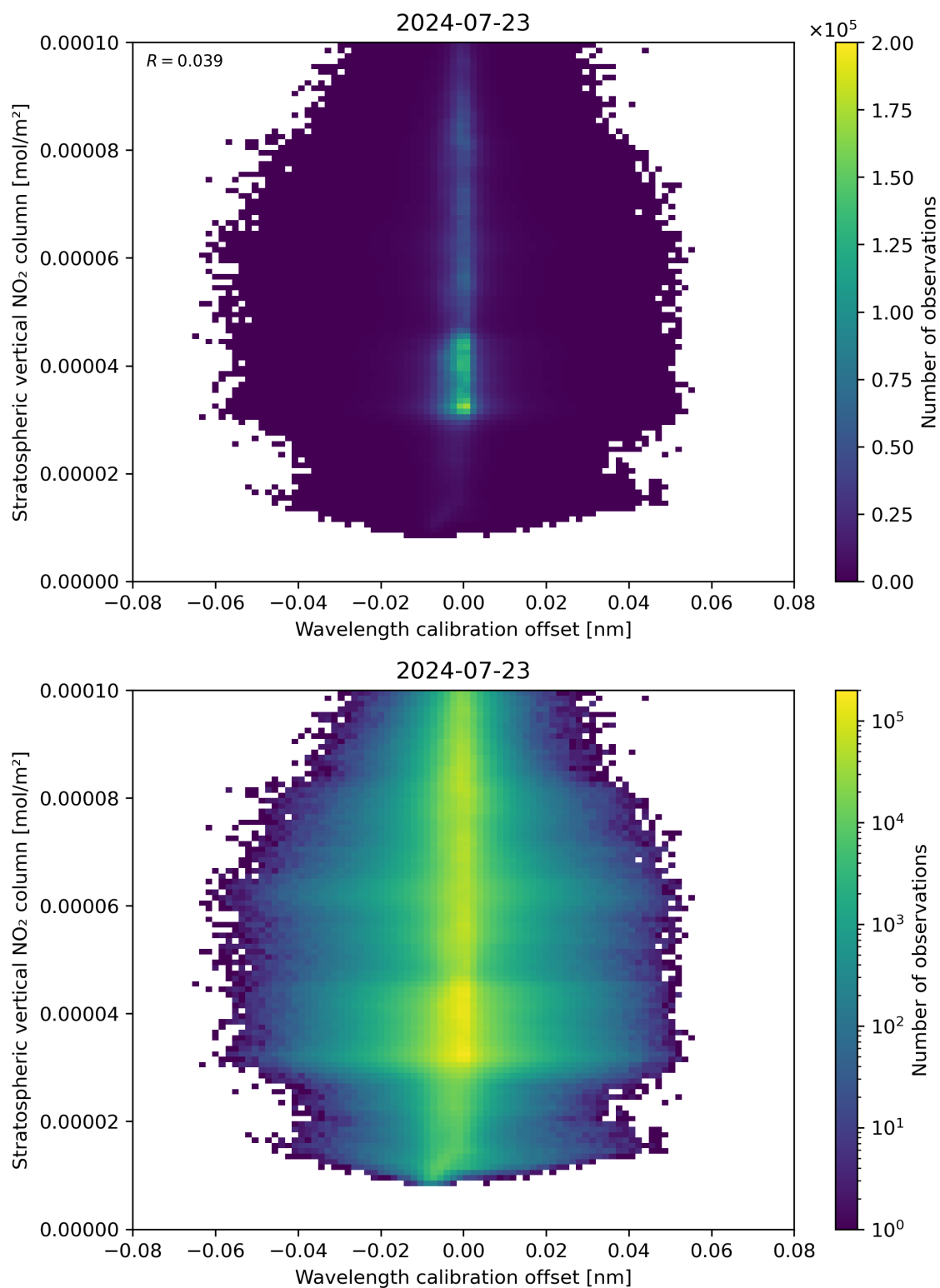
Figure 176: Scatter density plot of “Wavelength calibration offset” against “Stratospheric vertical NO 2 column” for 2024-07-22 to 2024-07-24.
