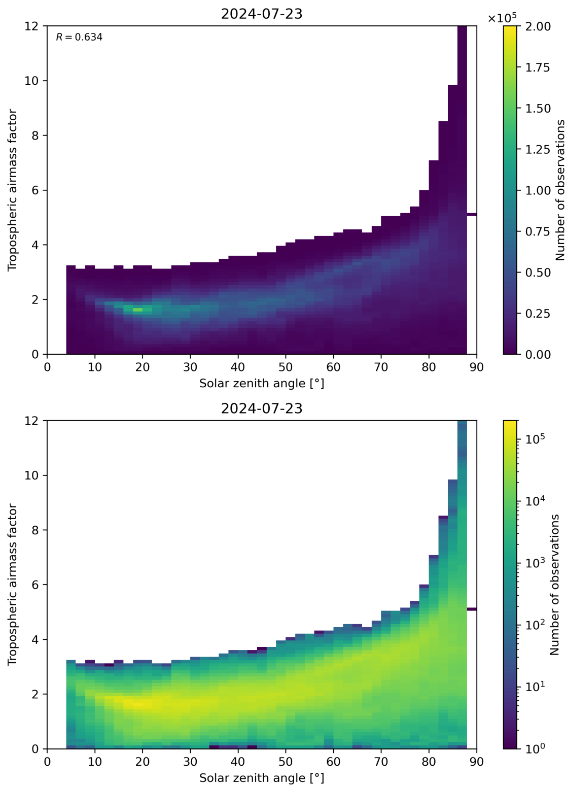
Figure 147: Scatter density plot of “Solar zenith angle” against “Tropospheric airmass factor” for 2024-07-22 to 2024-07-24.
