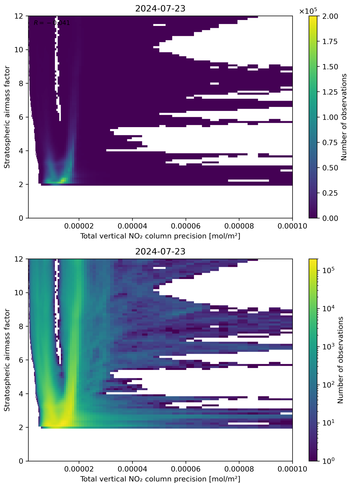
Figure 115: Scatter density plot of “Total vertical NO 2 column precision” against “Stratospheric air mass factor” for 2024-07-22 to 2024-07-24.
