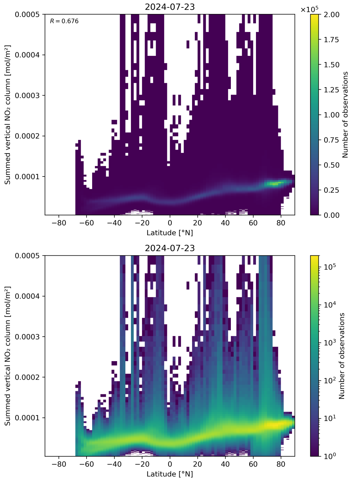
Figure 88: Scatter density plot of “Latitude” against “Summed vertical NO 2 column” for 2024-07-22 to 2024-07-24.
