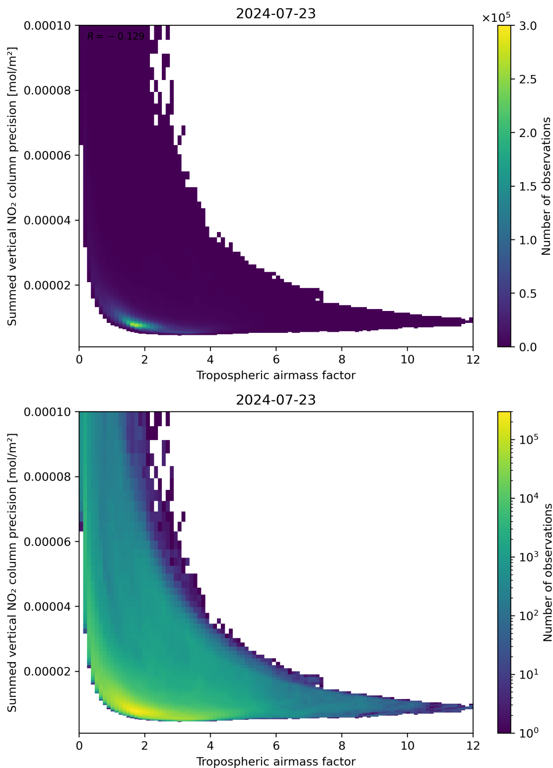
Figure 76: Scatter density plot of “Tropospheric air mass factor” against “Summed vertical NO 2 column precision” for 2024-07-22 to 2024-07-24.
