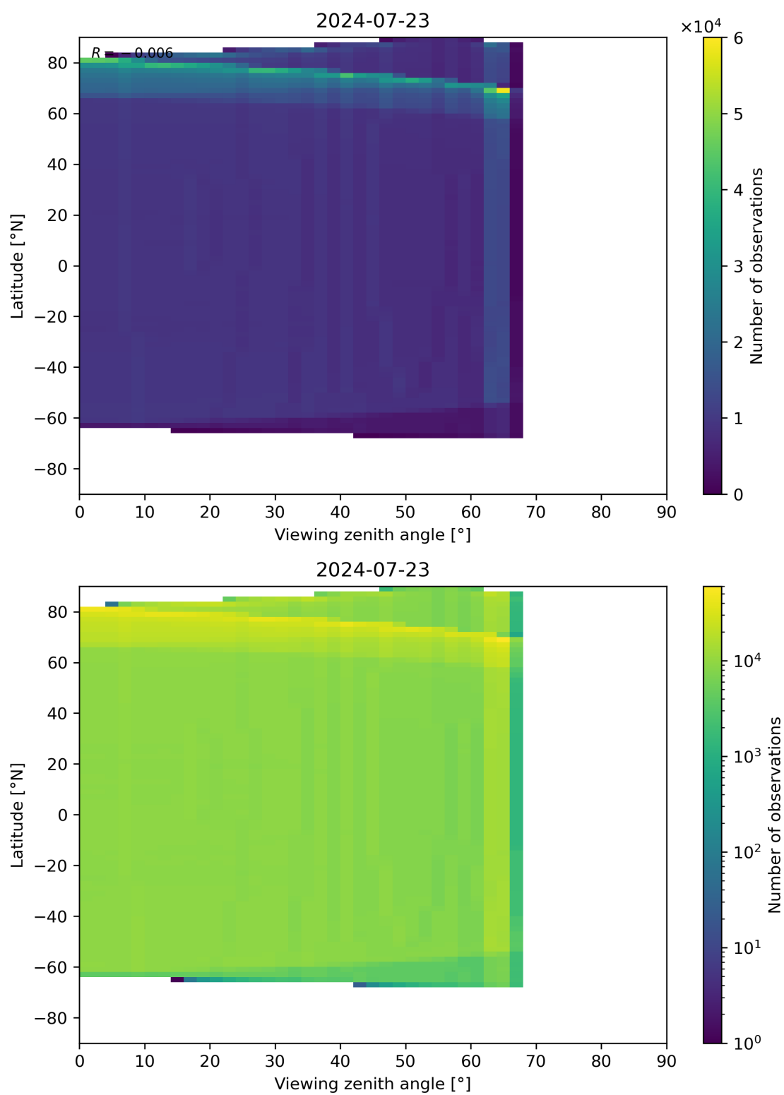
Figure 163: Scatter density plot of “Viewing zenith angle” against “Latitude” for 2024-07-22 to 2024-07-24.
