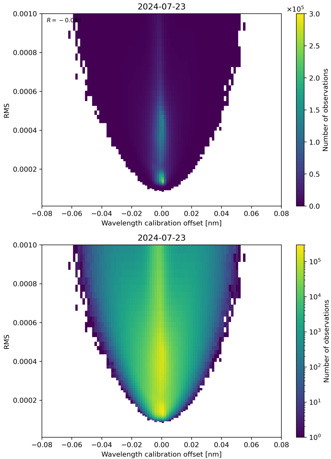
Figure 181: Scatter density plot of “Wavelength calibration offset” against “RMS” for 2024-07-22 to 2024-07-24.
