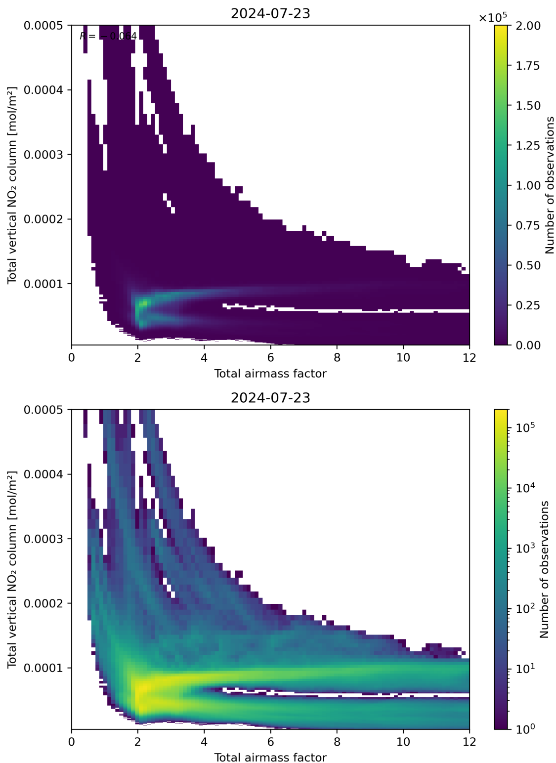
Figure 67: Scatter density plot of “Total airmass factor” against “Total vertical NO 2 column” for 2024-07-22 to 2024-07-24.
