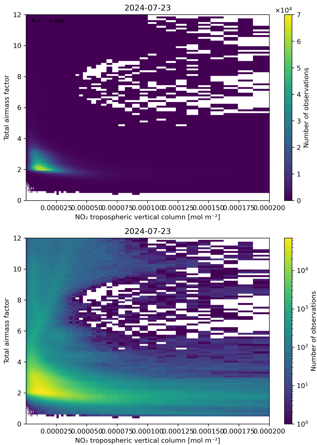
Figure 122: Scatter density plot of “NO 2 tropospheric vertical column” against “Total air mass factor” for 2024-07-22 to 2024-07-24.
