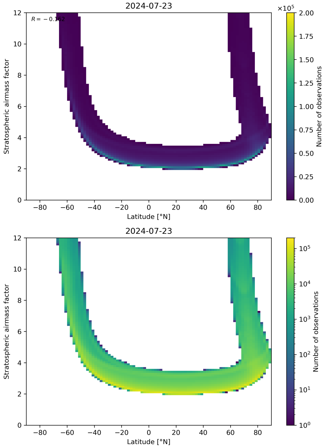
Figure 83: Scatter density plot of “Latitude” against “Stratospheric air mass factor” for 2024-07-22 to 2024-07-24.
