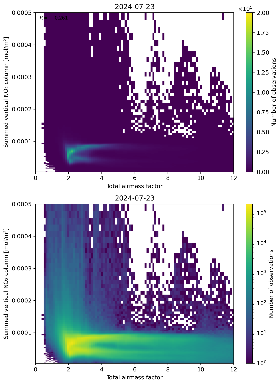
Figure 65: Scatter density plot of “Total airmass factor” against “Summed vertical NO 2 column” for 2024-07-22 to 2024-07-24.
