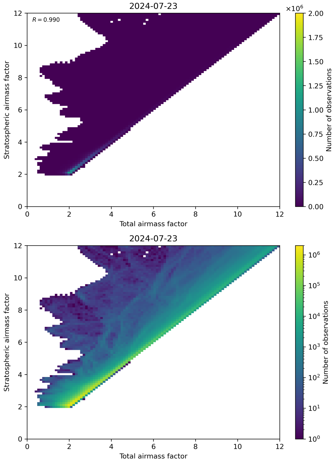
Figure 62: Scatter density plot of “Total airmass factor” against “Stratospheric airmass factor” for 2024-07-22 to 2024-07-24.
