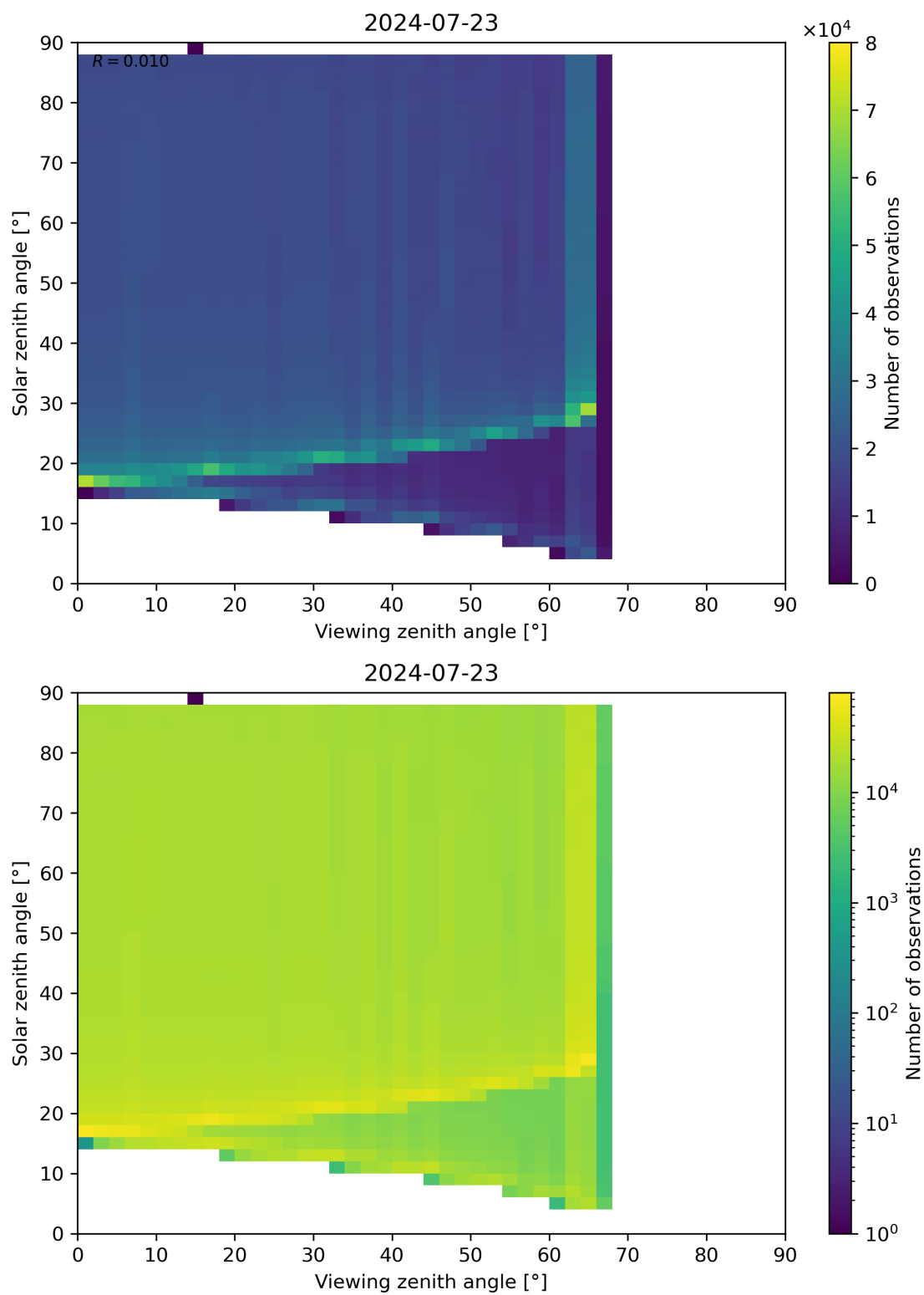
Figure 172: Scatter density plot of “Viewing zenith angle” against “Solar zenith angle” for 2024-07-22 to 2024-07-24.
