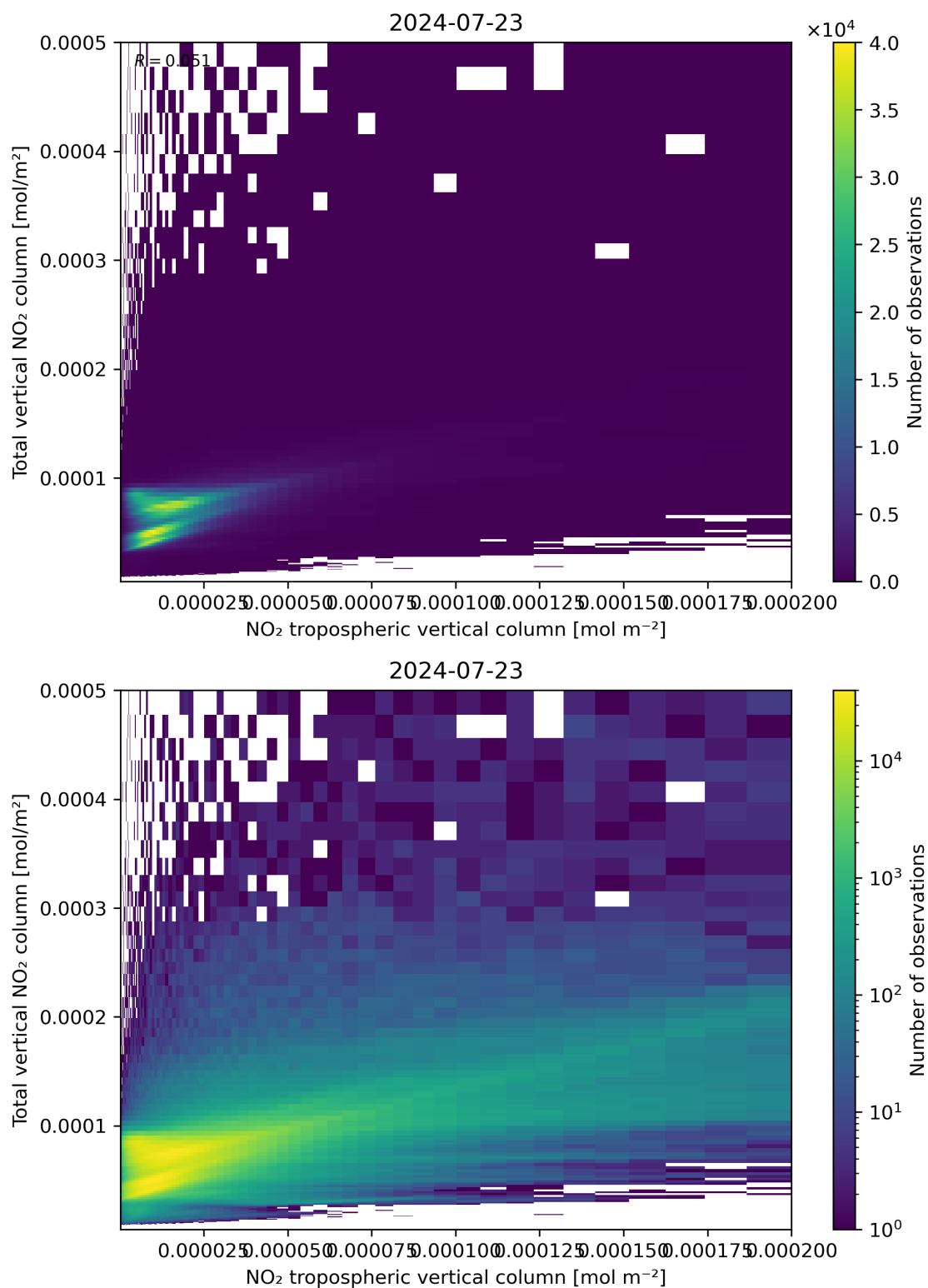
Figure 128: Scatter density plot of “NO 2 tropospheric vertical column” against “Total vertical NO 2 column” for 2024-07-22 to 2024-07-24.
