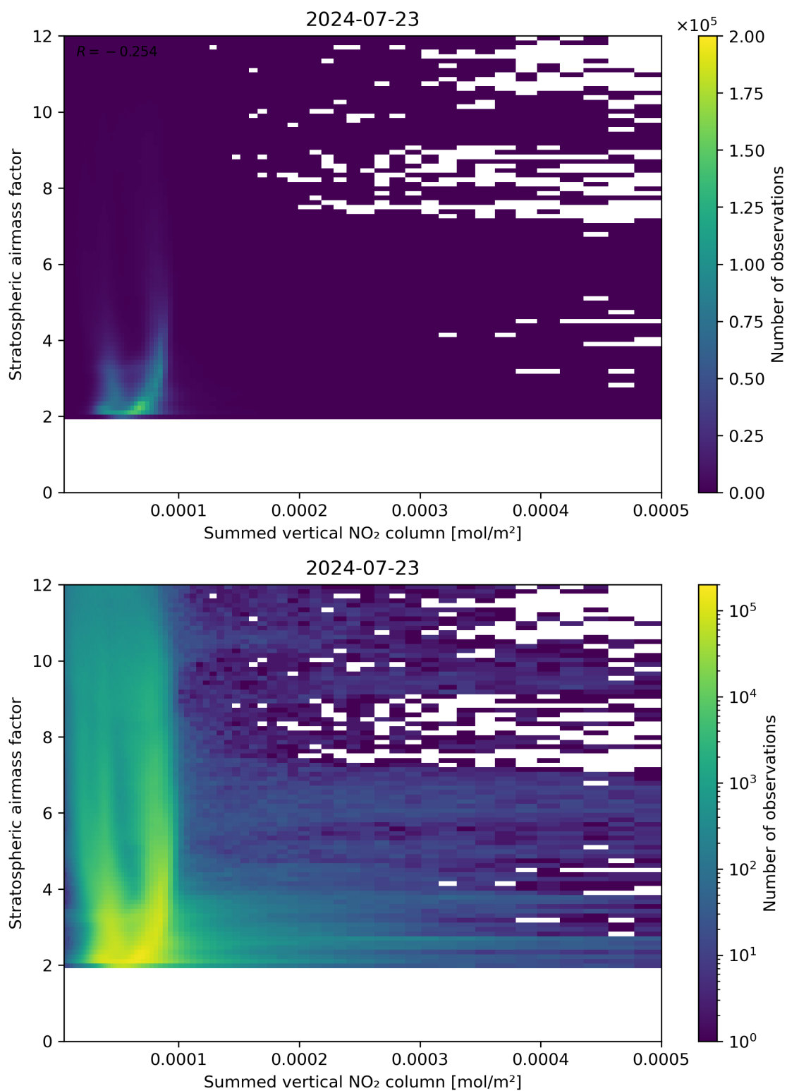
Figure 103: Scatter density plot of “Summed vertical NO 2 column” against “Stratospheric air mass factor” for 2024-07-22 to 2024-07-24.
