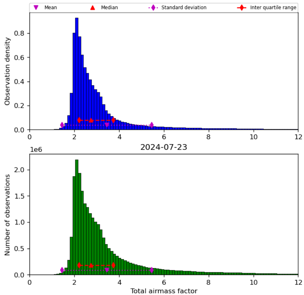
Figure 32: Histogram of “Total airmass factor” for 2024-07-22 to 2024-07-24
