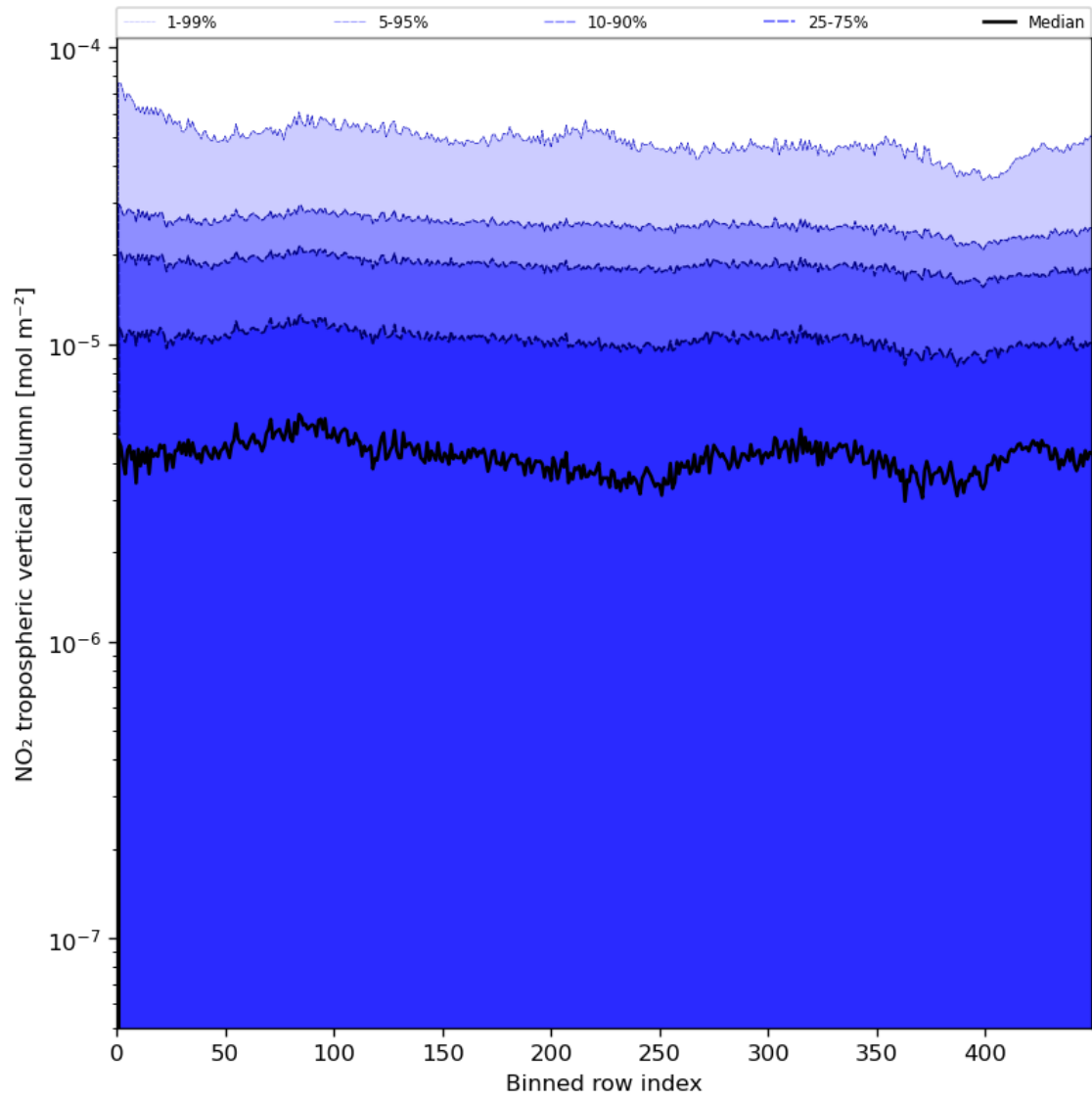
Figure 46: Along track statistics of “NO 2 tropospheric vertical column” for 2024-07-22 to 2024-07-24
