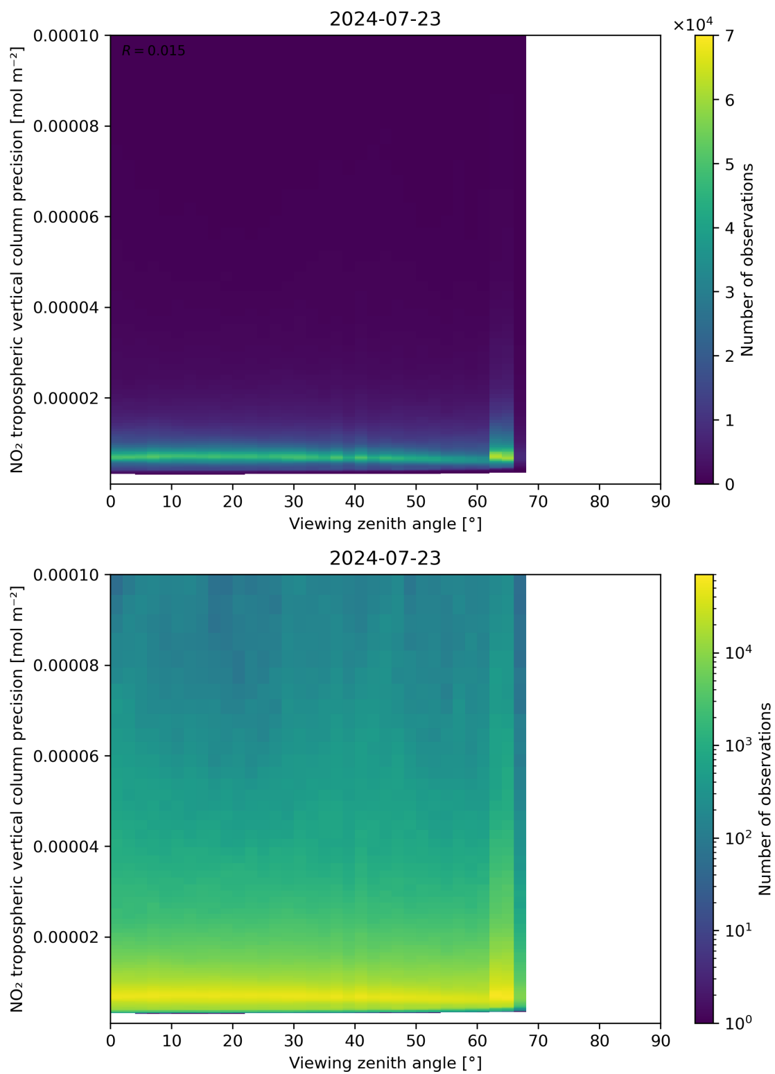
Figure 170: Scatter density plot of “Viewing zenith angle” against “NO 2 tropospheric vertical column precision” for 2024-07-22 to 2024-07-24.
