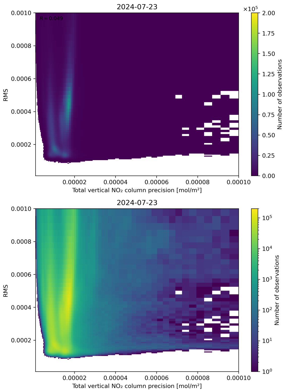
Figure 119: Scatter density plot of “Total vertical NO 2 column precision” against “RMS” for 2024-07-22 to 2024-07-24.
