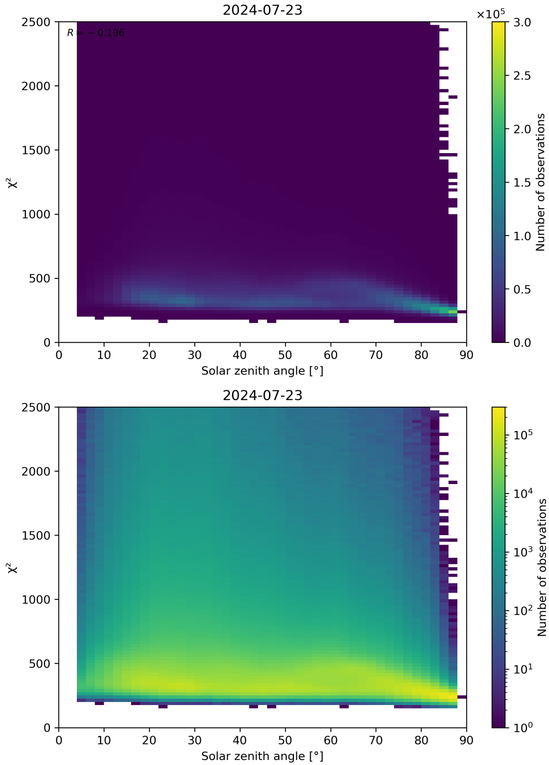
Figure 148: Scatter density plot of “Solar zenith angle” against “ \chi^2 ” for 2024-07-22 to 2024-07-24.
