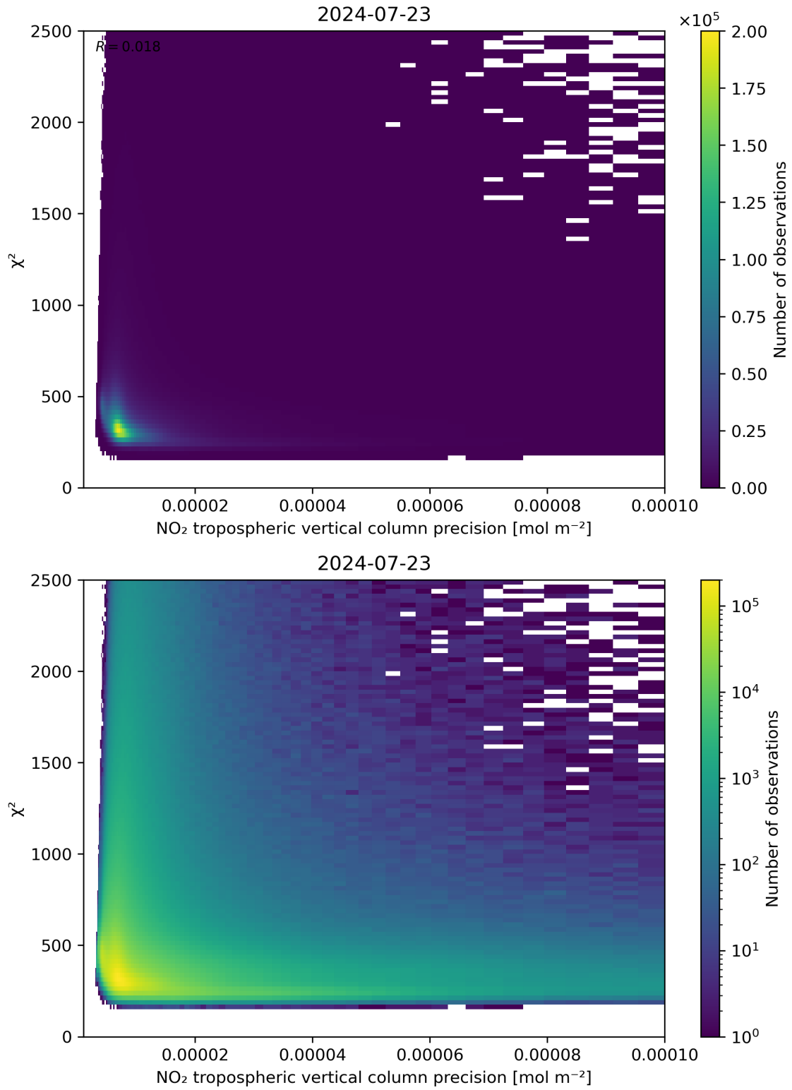
Figure 134: Scatter density plot of “NO 2 tropospheric vertical column precision” against “ \chi^2 ” for 2024-07-22 to 2024-07-24.
