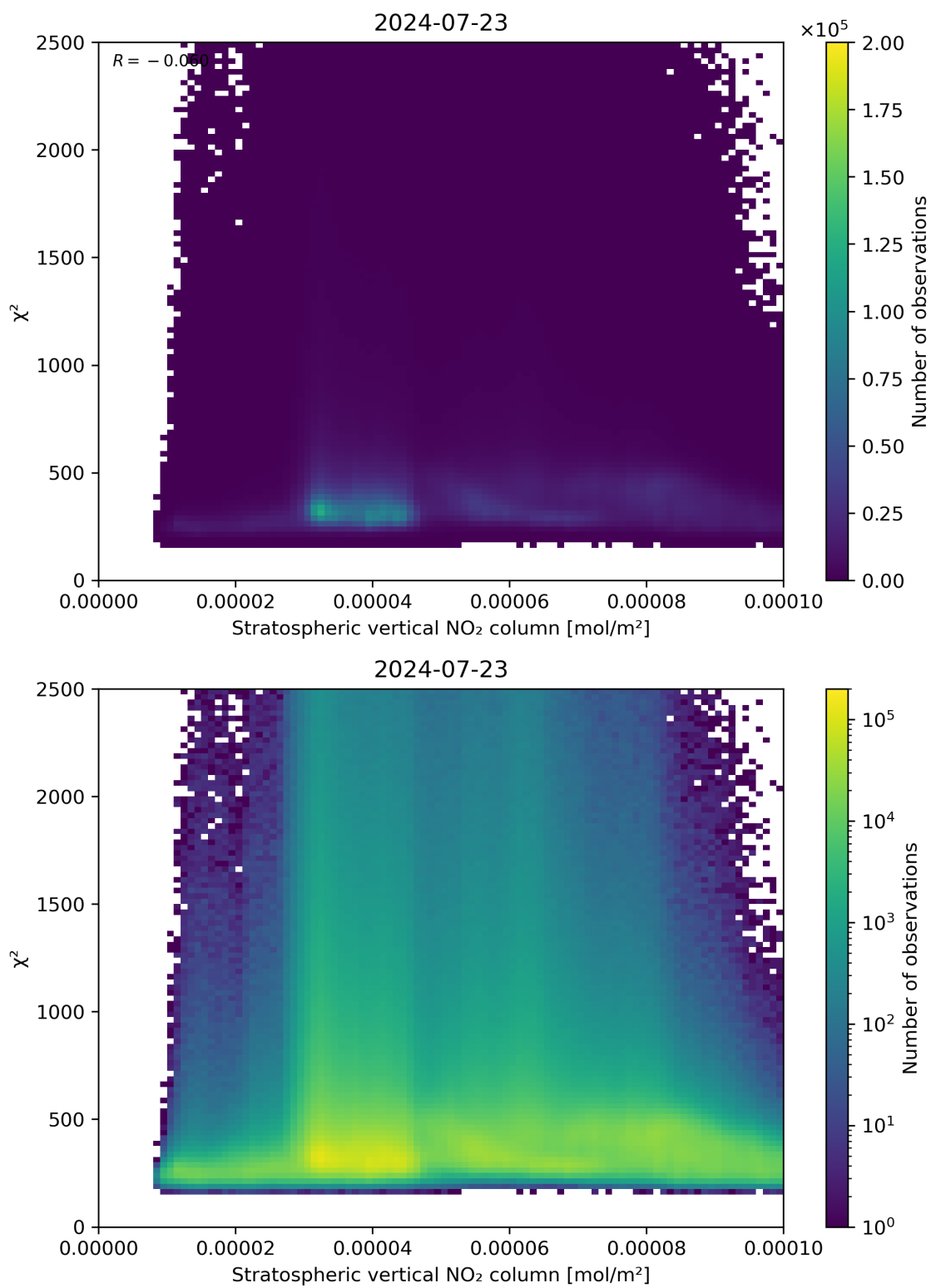
Figure 97: Scatter density plot of “Stratospheric vertical NO 2 column” against “ \chi^2 ” for 2024-07-22 to 2024-07-24.
