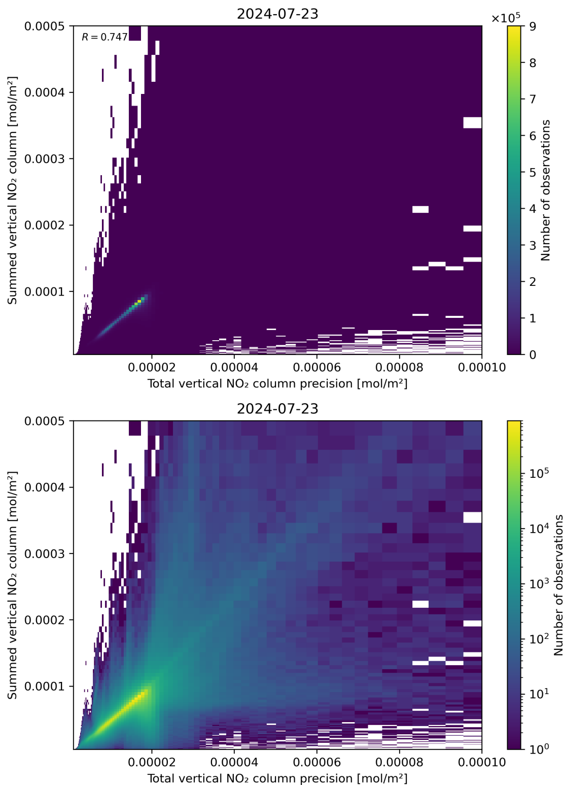
Figure 117: Scatter density plot of “Total vertical NO 2 column precision” against “Summed vertical NO 2 column” for 2024-07-22 to 2024-07-24.
