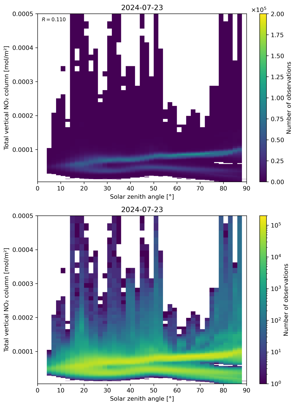
Figure 153: Scatter density plot of “Solar zenith angle” against “Total vertical NO 2 column” for 2024-07-22 to 2024-07-24.
