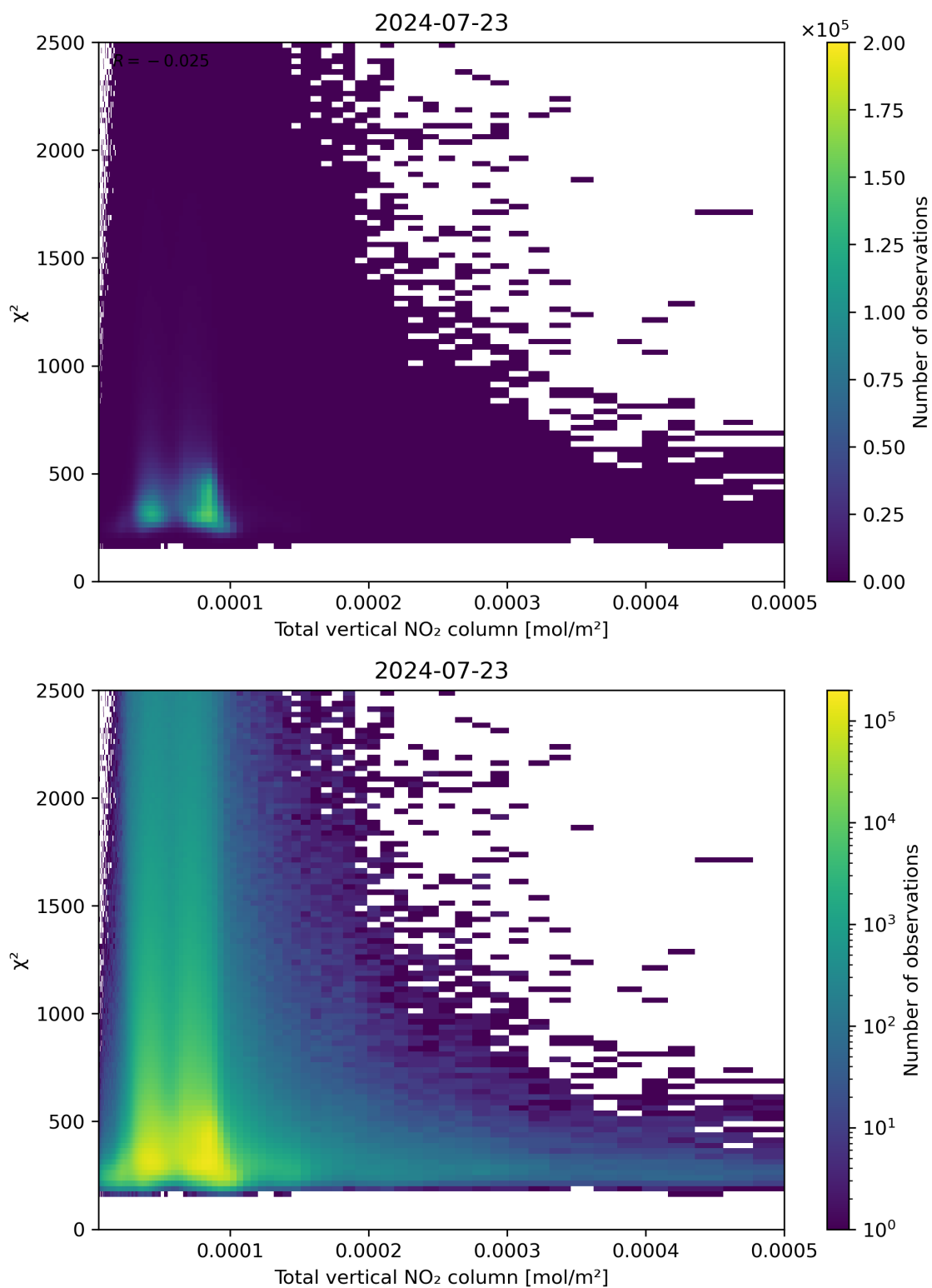
Figure 111: Scatter density plot of “Total vertical NO 2 column” against “ \chi^2 ” for 2024-07-22 to 2024-07-24.
