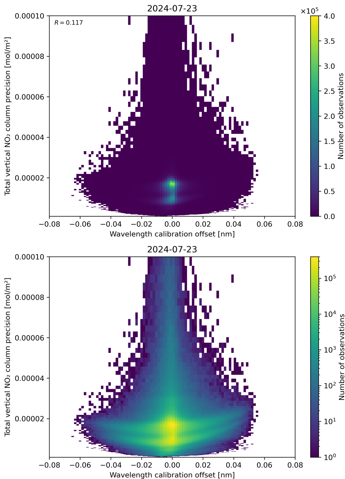
Figure 180: Scatter density plot of “Wavelength calibration offset” against “Total vertical NO 2 column precision” for 2024-07-22 to 2024-07-24.
