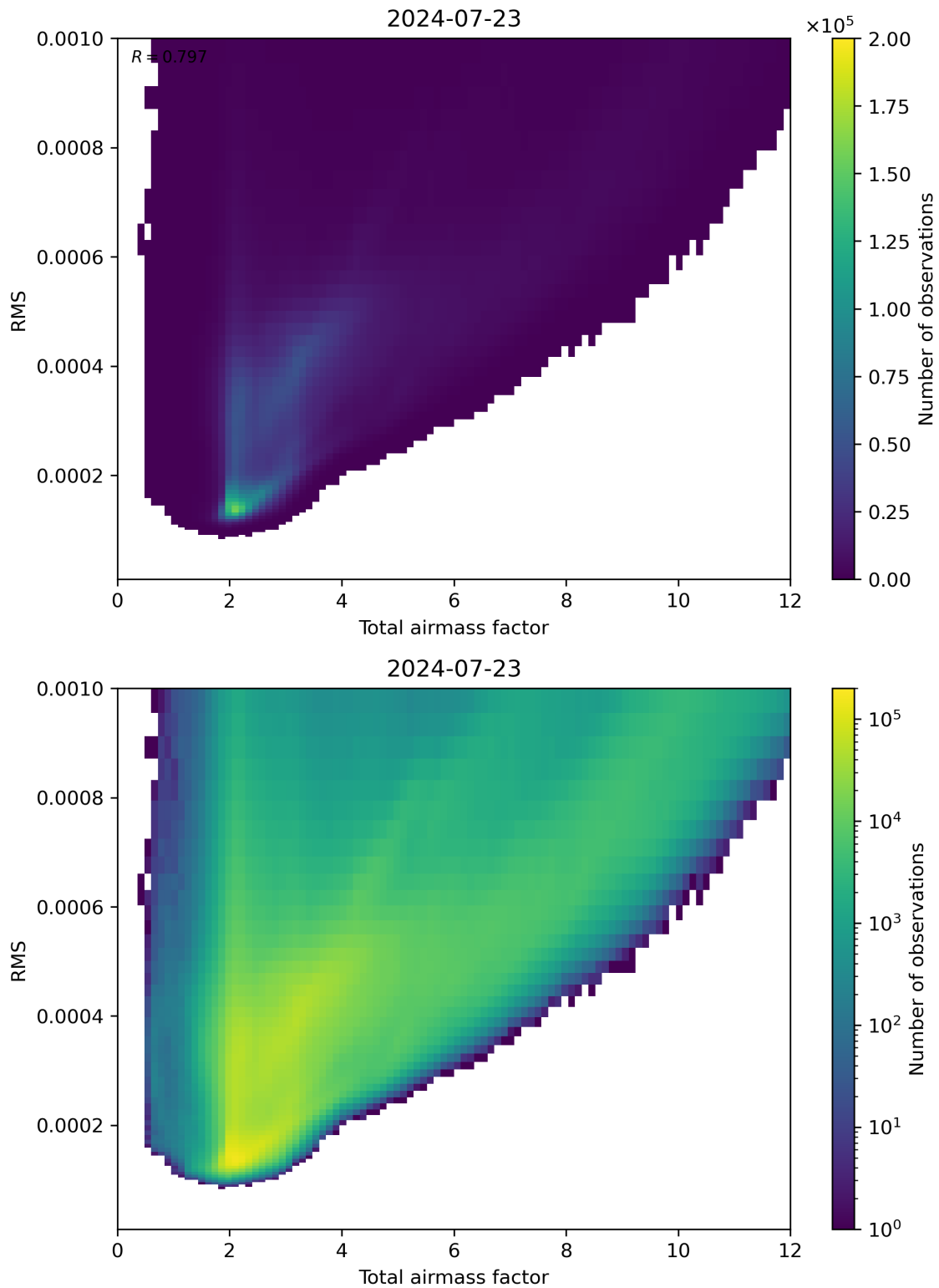
Figure 69: Scatter density plot of “Total airmass factor” against “RMS” for 2024-07-22 to 2024-07-24.
