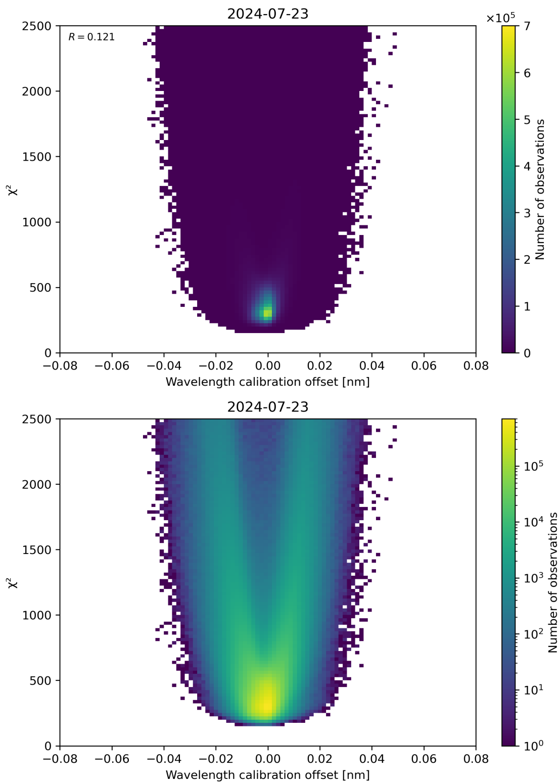
Figure 175: Scatter density plot of “Wavelength calibration offset” against “ \chi^2 ” for 2024-07-22 to 2024-07-24.
