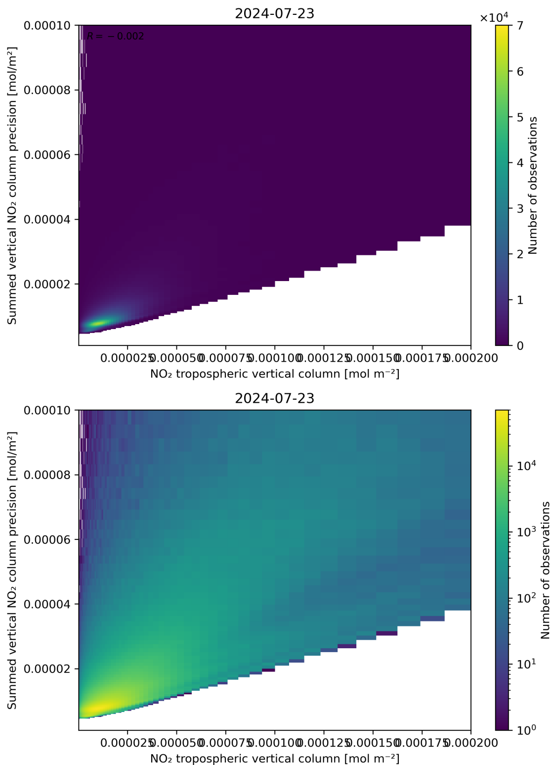
Figure 127: Scatter density plot of “NO 2 tropospheric vertical column” against “Summed vertical NO 2 column precision” for 2024-07-22 to 2024-07-24.
