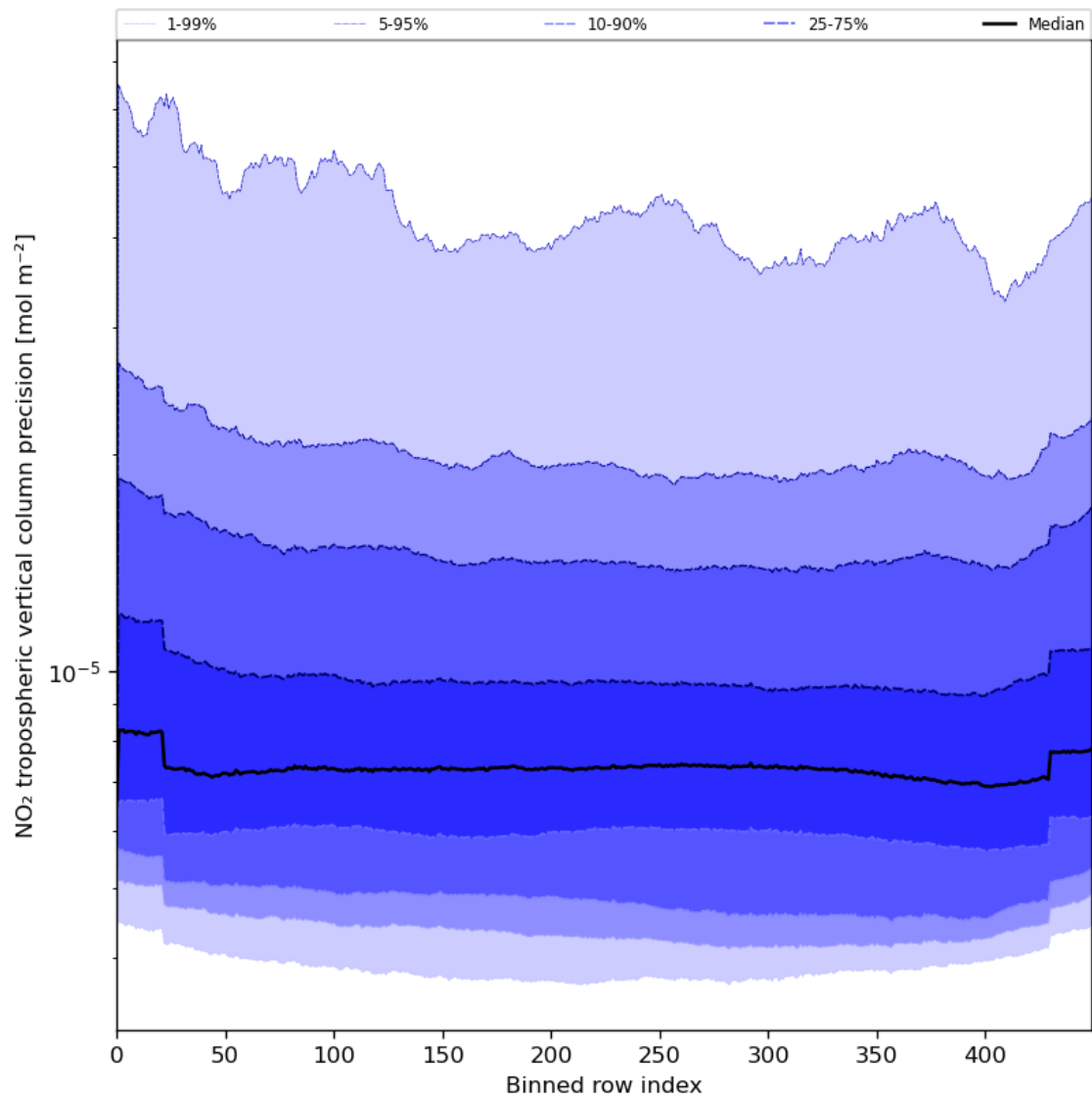
Figure 47: Along track statistics of “NO 2 tropospheric vertical column precision” for 2024-07-22 to 2024-07-24
