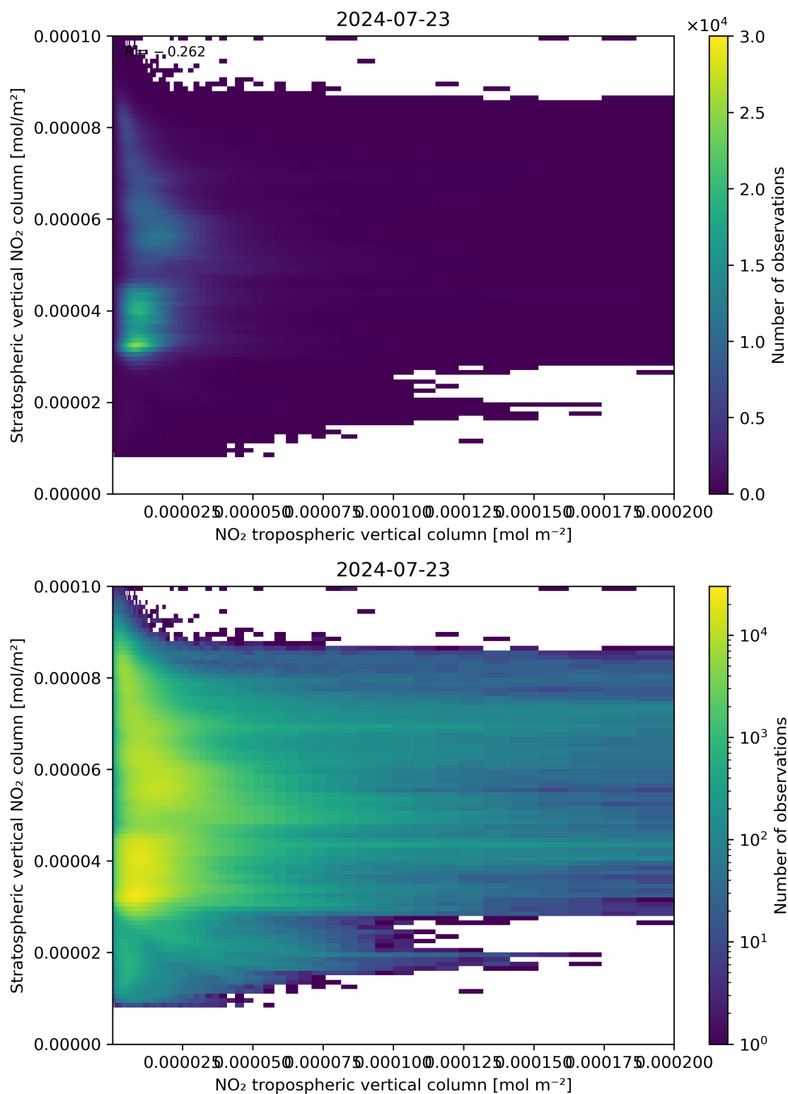
Figure 125: Scatter density plot of “NO 2 tropospheric vertical column” against “Stratospheric vertical NO 2 column” for 2024-07-22 to 2024-07-24.
