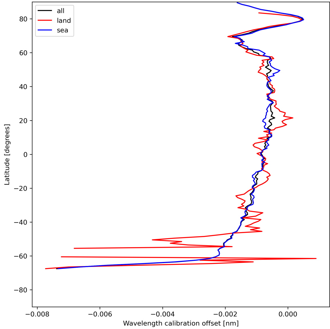
Figure 18: Zonal average of “Wavelength calibration offset” for 2024-07-22 to 2024-07-24.
