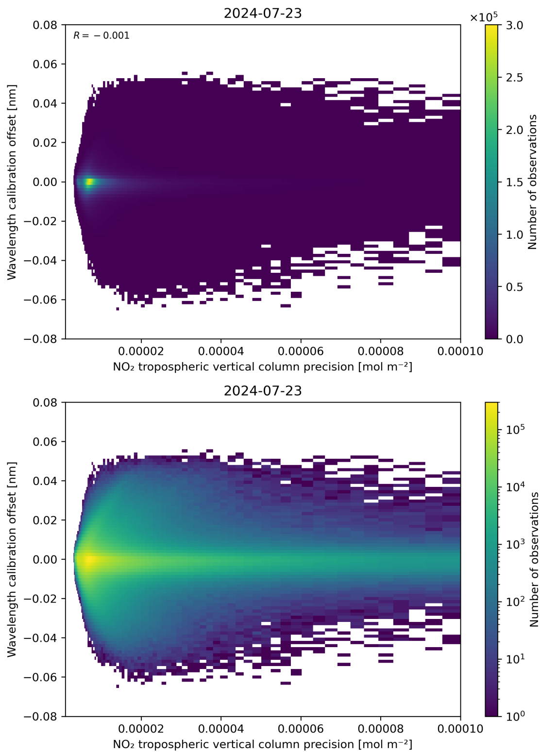
Figure 141: Scatter density plot of “NO 2 tropospheric vertical column precision” against “Wavelength calibration offset” for 2024-07-22 to 2024-07-24.
