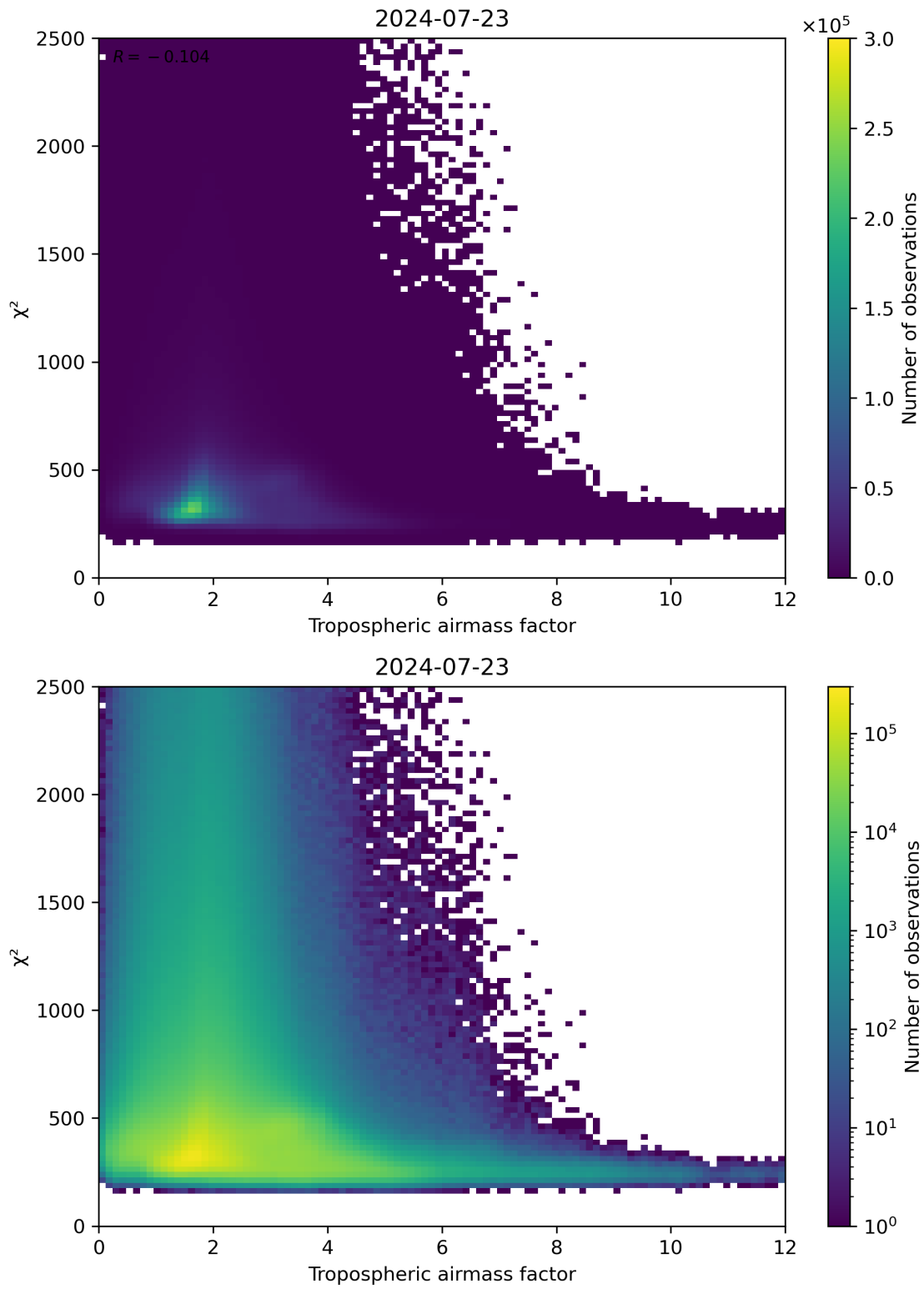
Figure 73: Scatter density plot of “Tropospheric airmass factor” against “ \chi^2 ” for 2024-07-22 to 2024-07-24.
