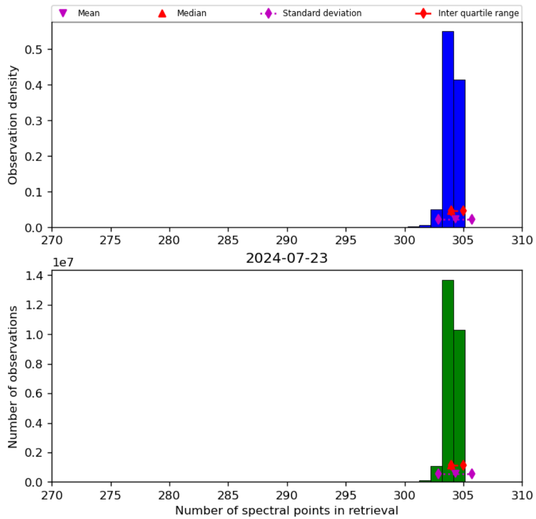
Figure 33: Histogram of “Number of spectral points in retrieval” for 2024-07-22 to 2024-07-24
