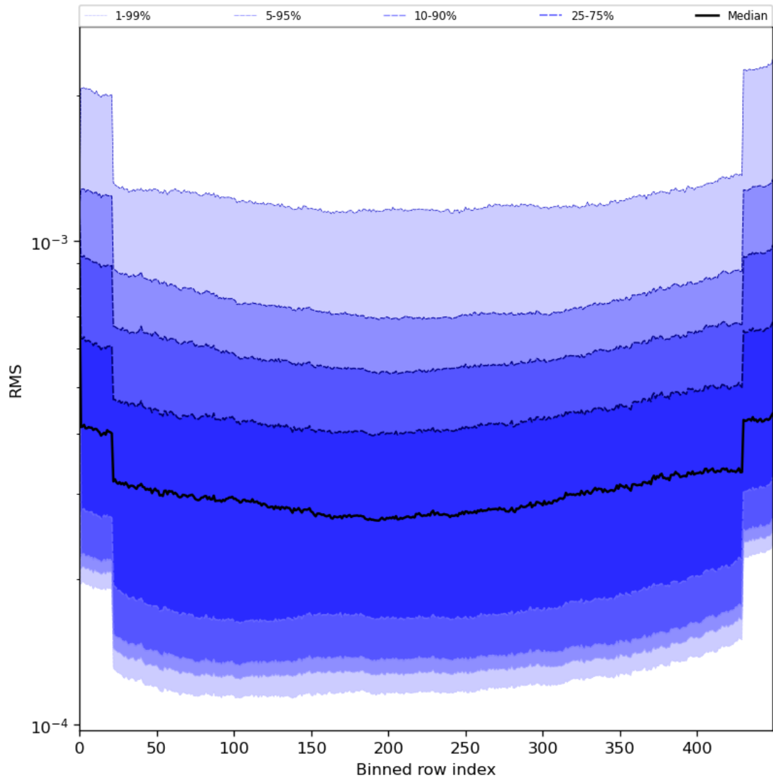
Figure 60: Along track statistics of “RMS” for 2024-07-22 to 2024-07-24
