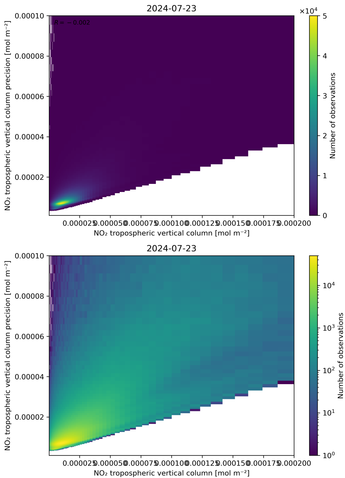
Figure 130: Scatter density plot of “NO 2 tropospheric vertical column” against “NO 2 tropospheric vertical column precision” for 2024-07-22 to 2024-07-24.
