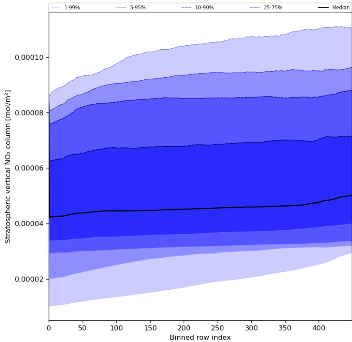
Figure 53: Along track statistics of “Stratospheric vertical NO 2 column” for 2024-07-22 to 2024-07-24
