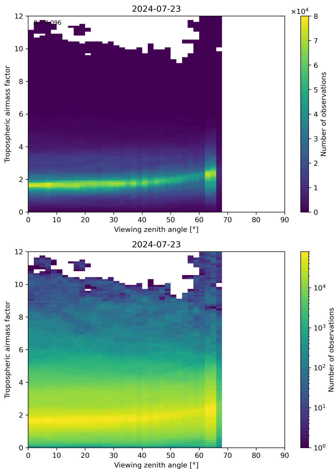
Figure 161: Scatter density plot of “Viewing zenith angle” against “Tropospheric airmass factor” for 2024-07-22 to 2024-07-24.
