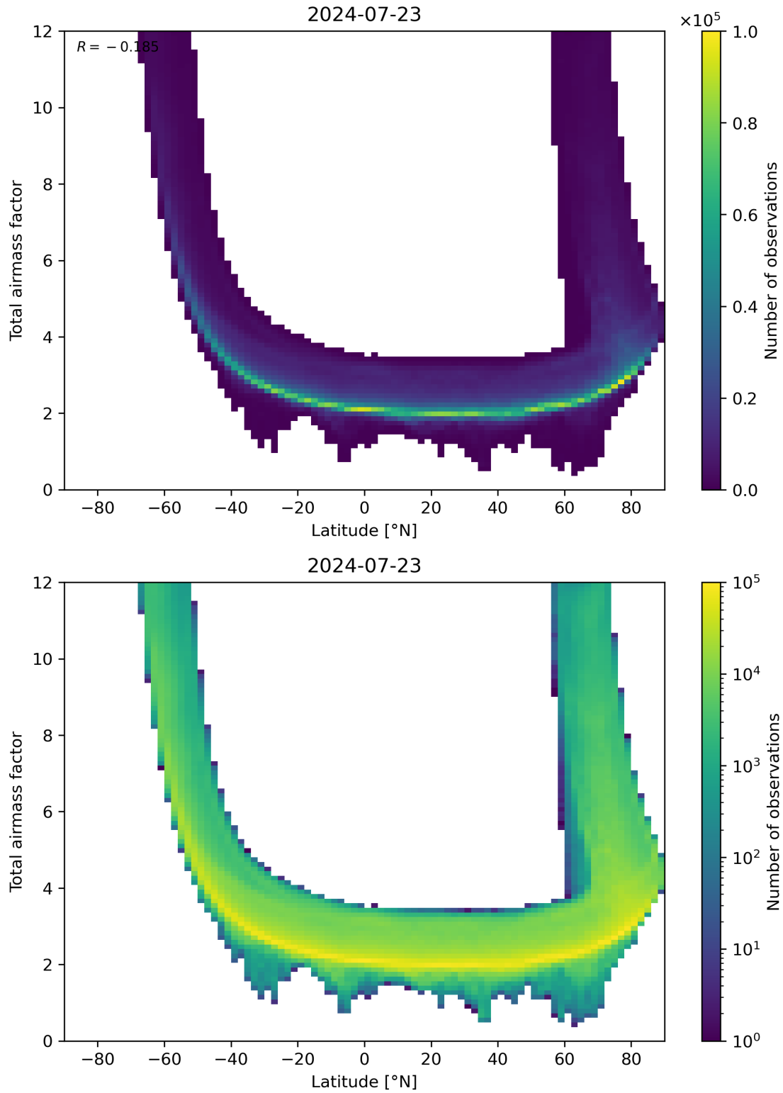
Figure 84: Scatter density plot of “Latitude” against “Total airmass factor” for 2024-07-22 to 2024-07-24.
