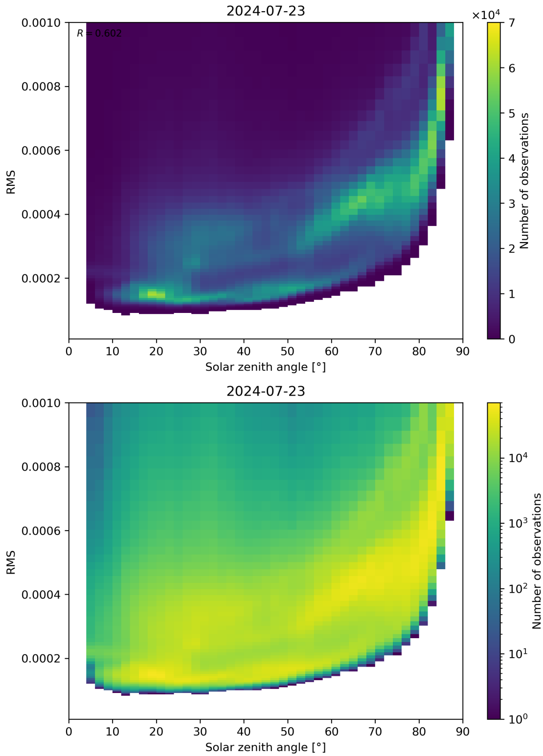
Figure 157: Scatter density plot of “Solar zenith angle” against “RMS” for 2024-07-22 to 2024-07-24.
