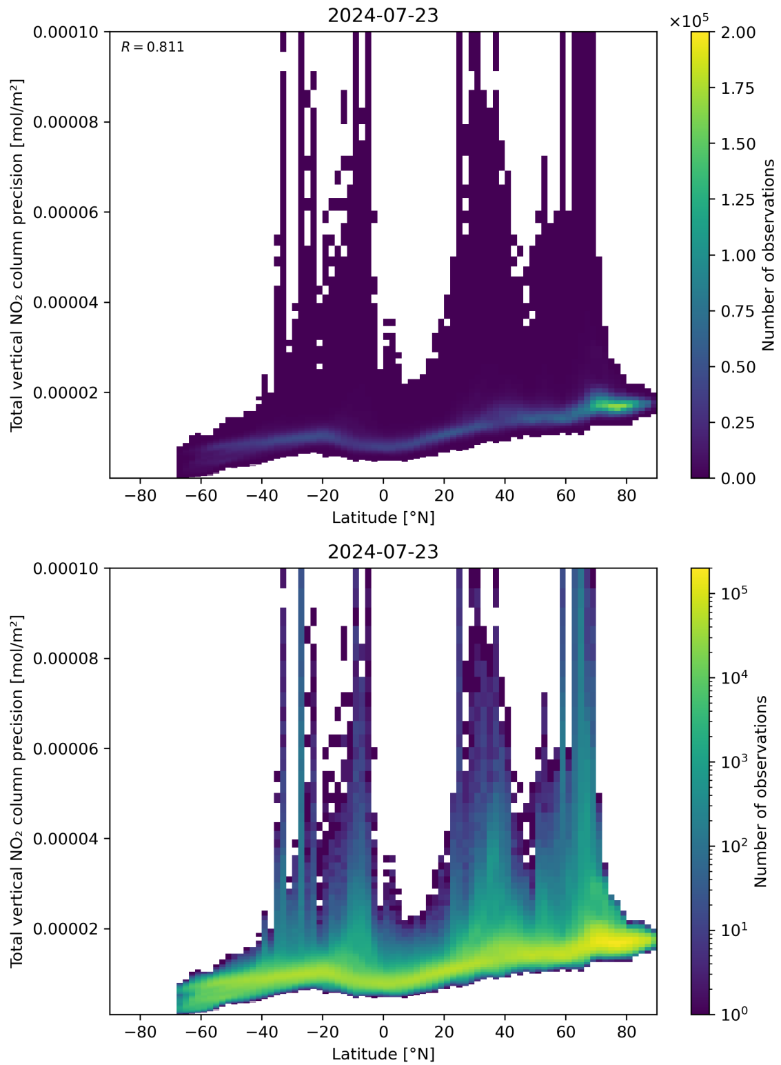
Figure 91: Scatter density plot of “Latitude” against “Total vertical NO 2 column precision” for 2024-07-22 to 2024-07-24.
