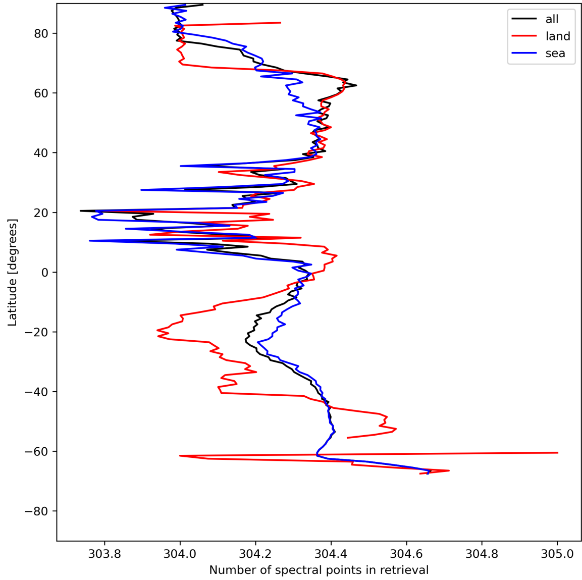
Figure 16: Zonal average of “Number of spectral points in retrieval” for 2024-07-22 to 2024-07-24.
