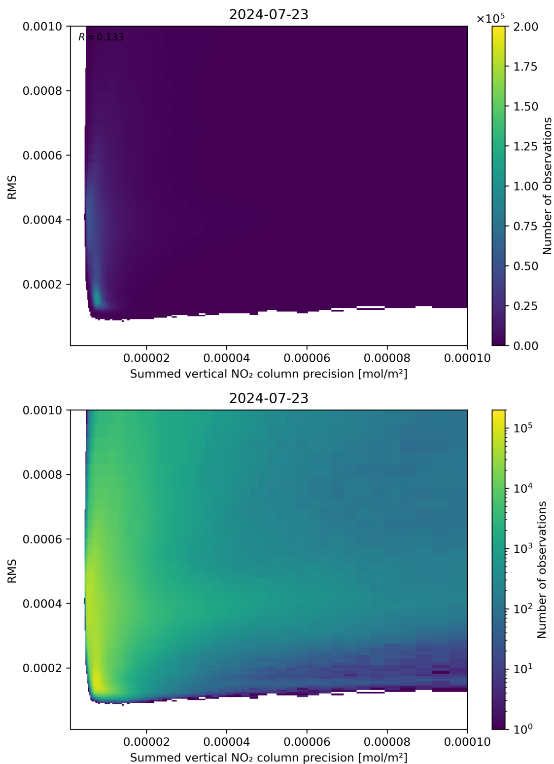
Figure 108: Scatter density plot of “Summed vertical NO 2 column precision” against “RMS” for 2024-07-22 to 2024-07-24.
