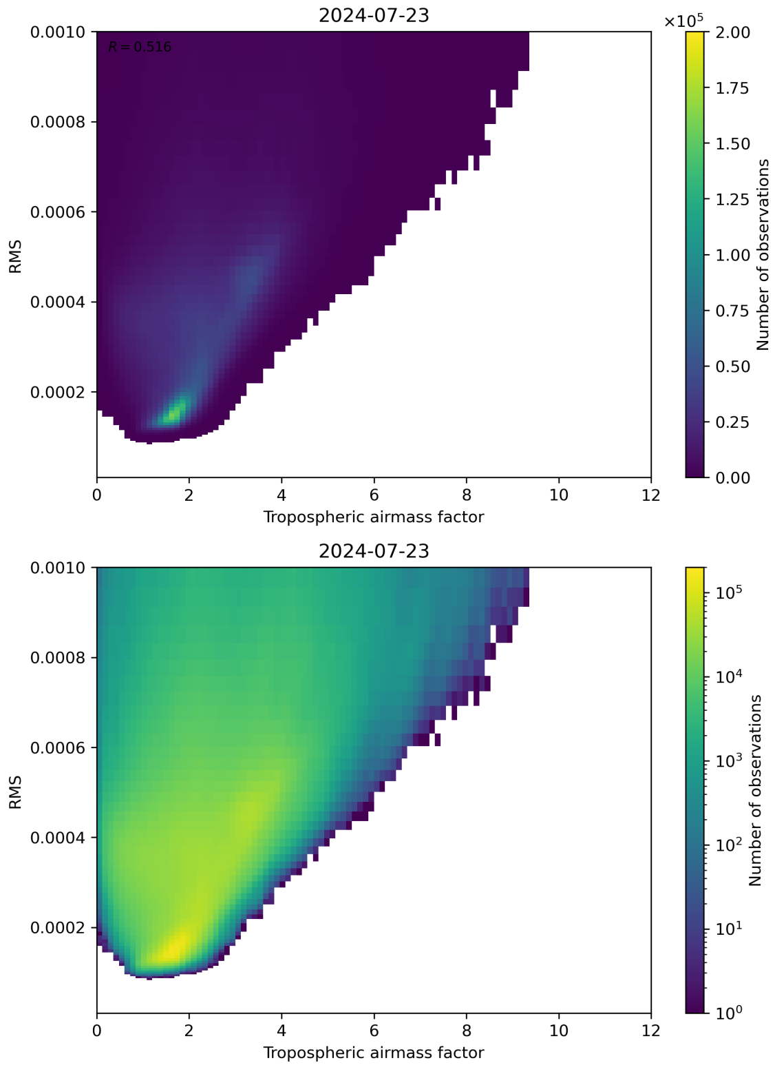
Figure 79: Scatter density plot of “Tropospheric airmass factor” against “RMS” for 2024-07-22 to 2024-07-24.
