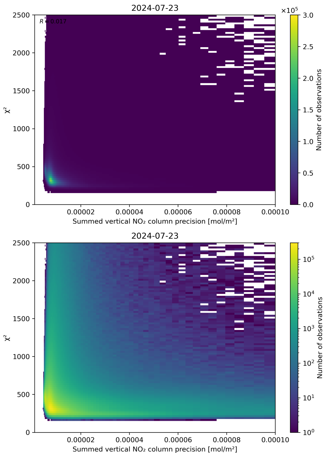
Figure 107: Scatter density plot of “Summed vertical NO 2 column precision” against “ \chi^2 ” for 2024-07-22 to 2024-07-24.
