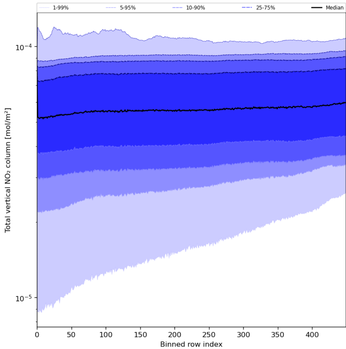
Figure 55: Along track statistics of “Total vertical NO 2 column” for 2024-07-22 to 2024-07-24
