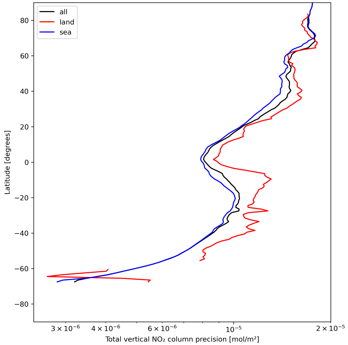
Figure 22: Zonal average of “Total vertical NO 2 column precision” for 2024-07-22 to 2024-07-24.
