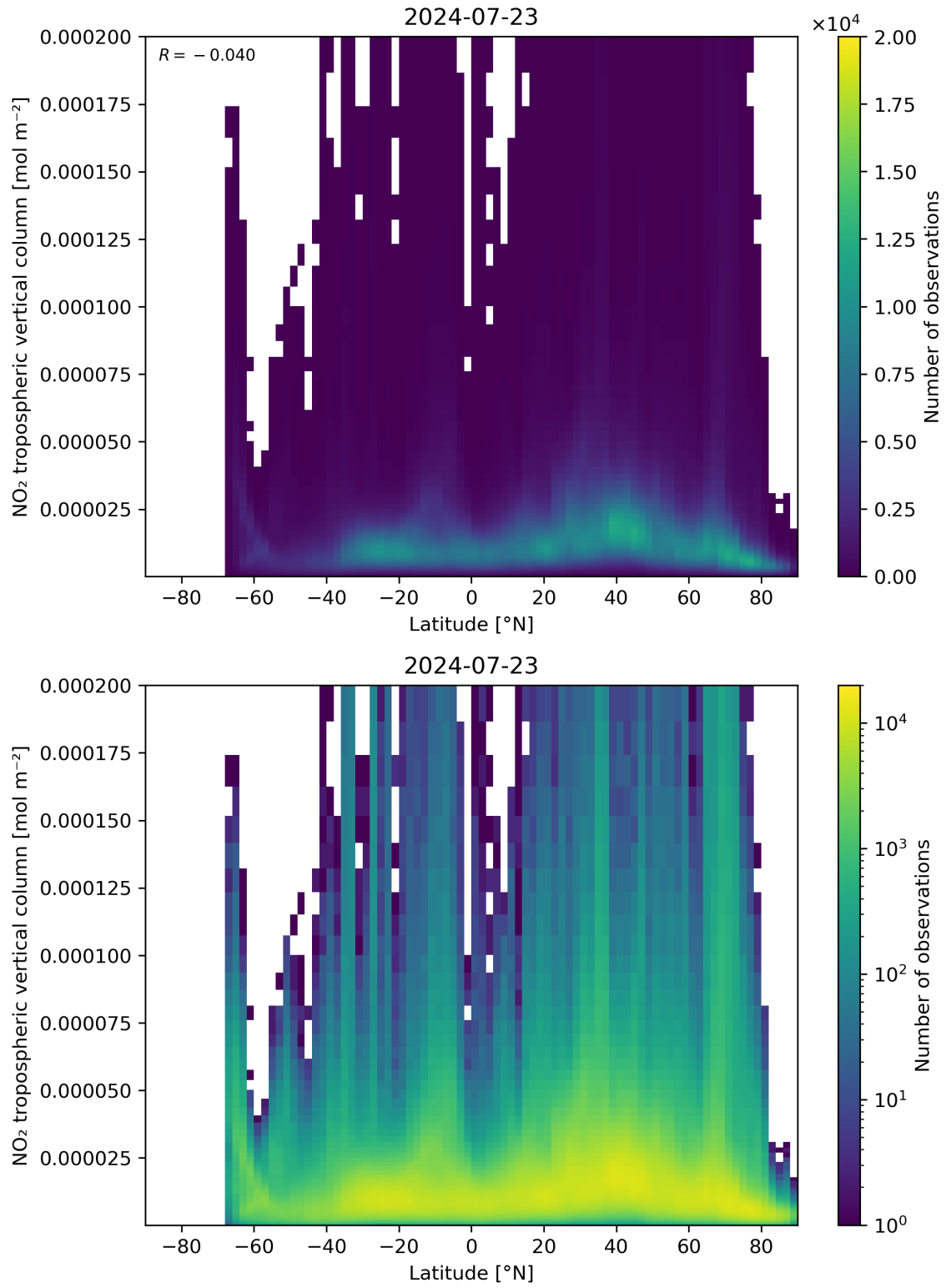
Figure 92: Scatter density plot of “Latitude” against “NO 2 tropospheric vertical column” for 2024-07-22 to 2024-07-24.
