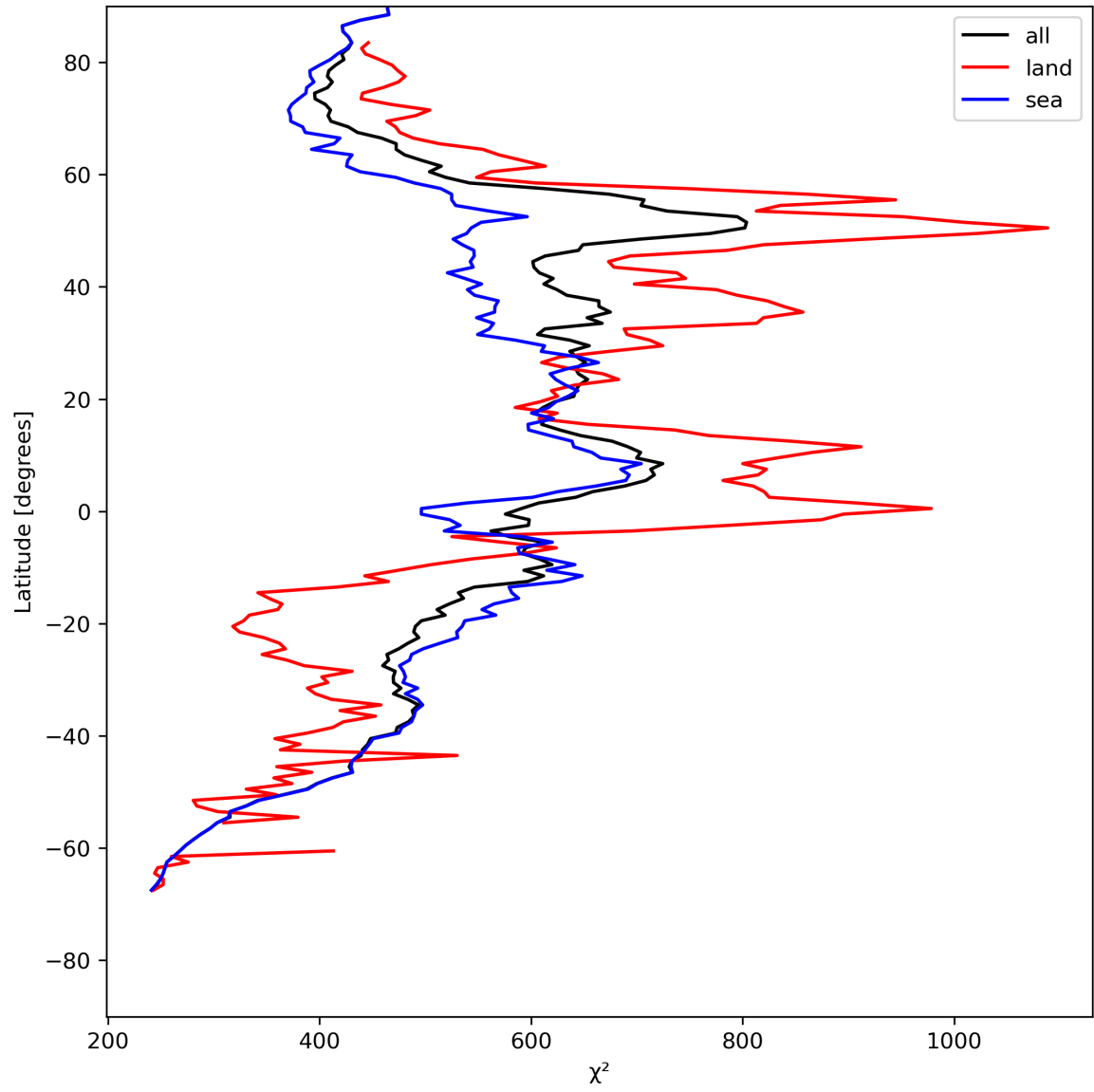
Figure 25: Zonal average of “ \chi^2 ” for 2024-07-22 to 2024-07-24.
