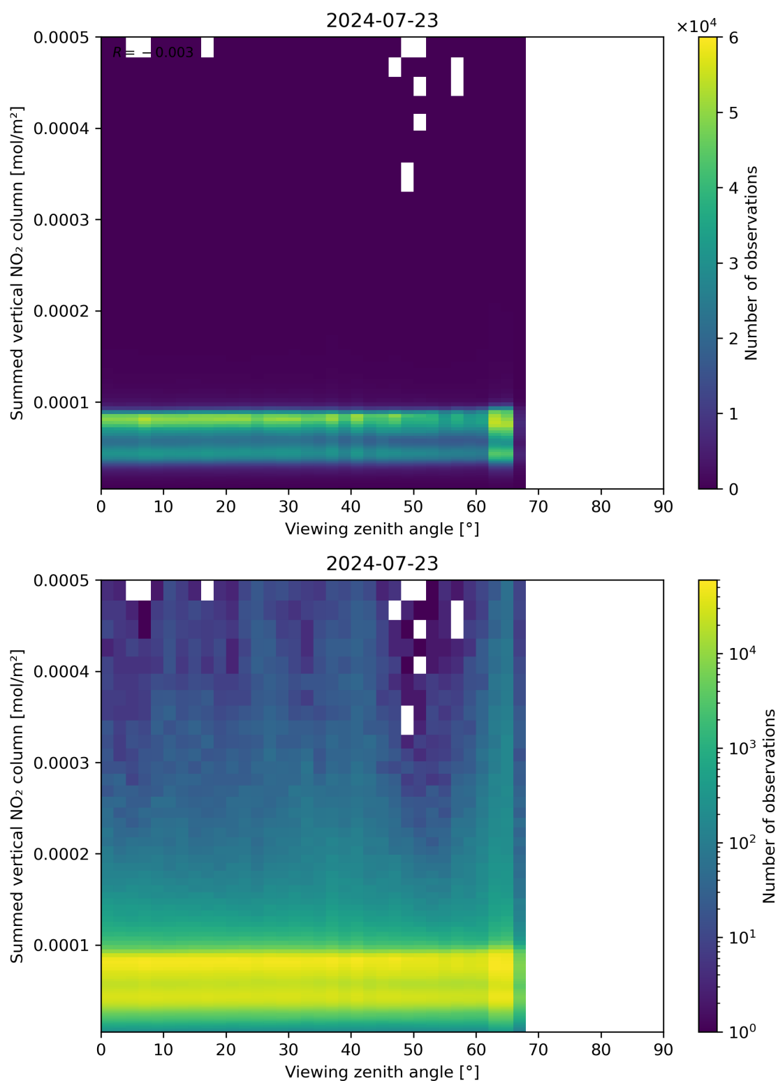
Figure 165: Scatter density plot of “Viewing zenith angle” against “Summed vertical NO 2 column” for 2024-07-22 to 2024-07-24.
