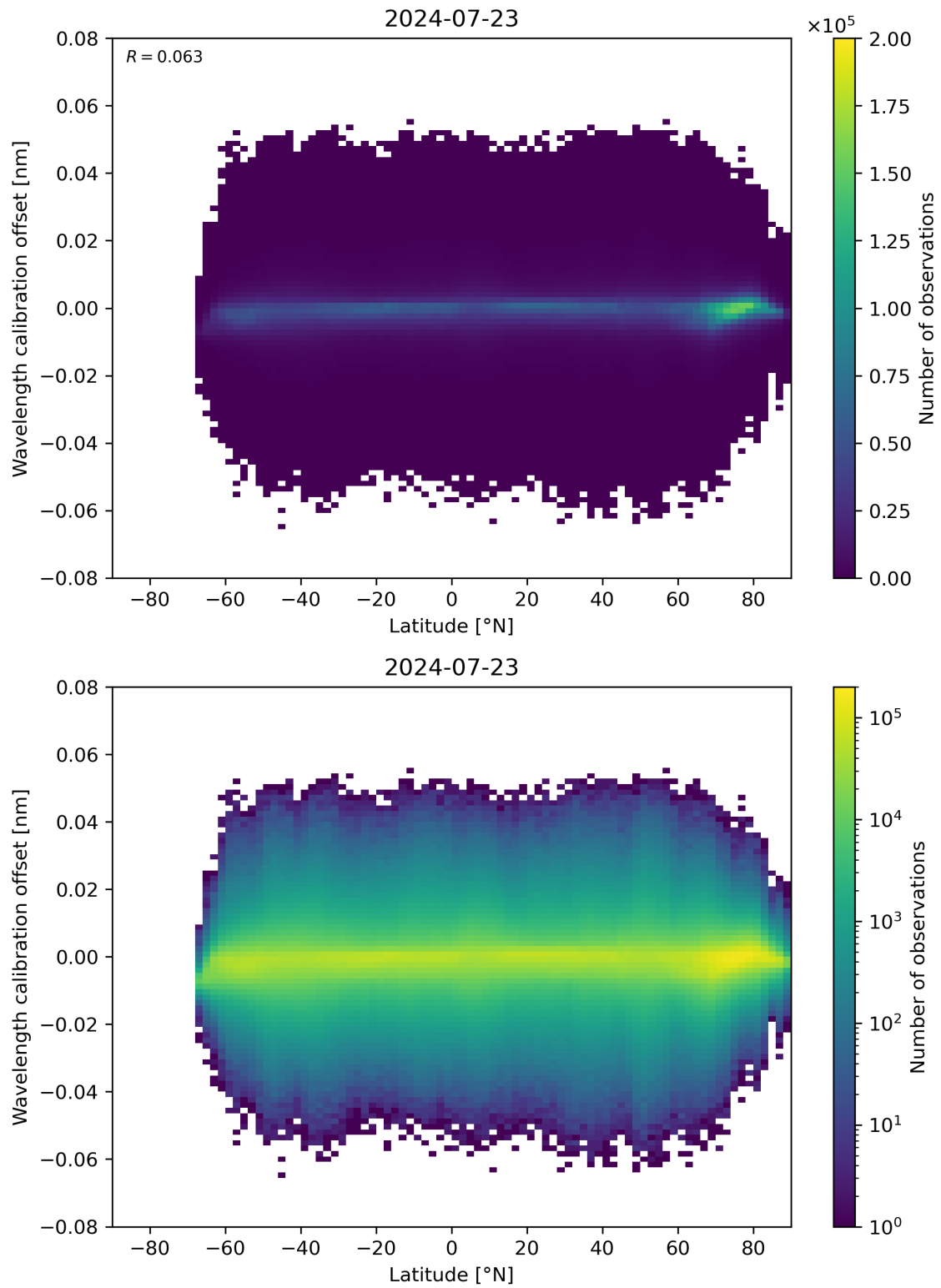
Figure 95: Scatter density plot of “Latitude” against “Wavelength calibration offset” for 2024-07-22 to 2024-07-24.
