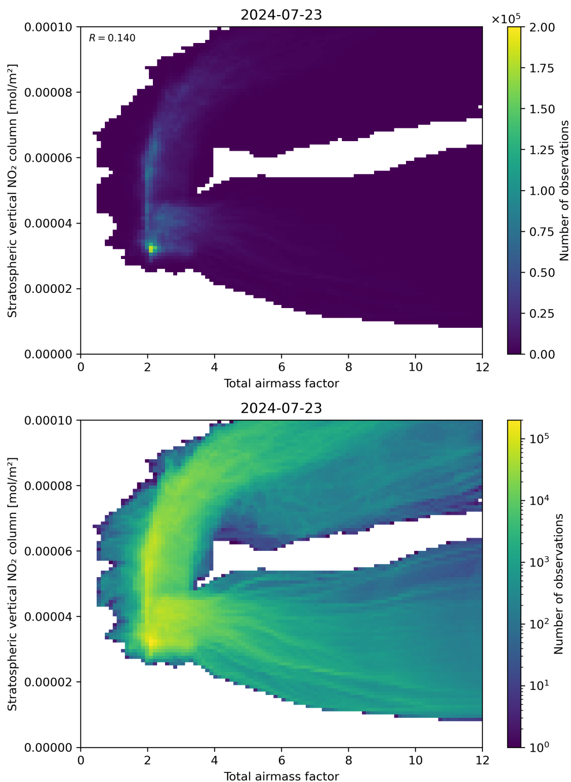
Figure 64: Scatter density plot of “Total airmass factor” against “Stratospheric vertical NO 2 column” for 2024-07-22 to 2024-07-24.
