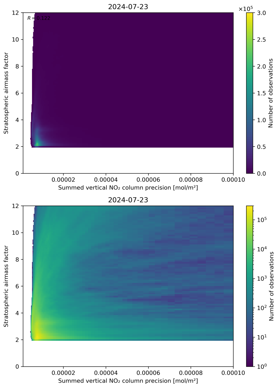
Figure 106: Scatter density plot of “Summed vertical NO 2 column precision” against “Stratospheric airmass factor” for 2024-07-22 to 2024-07-24.
