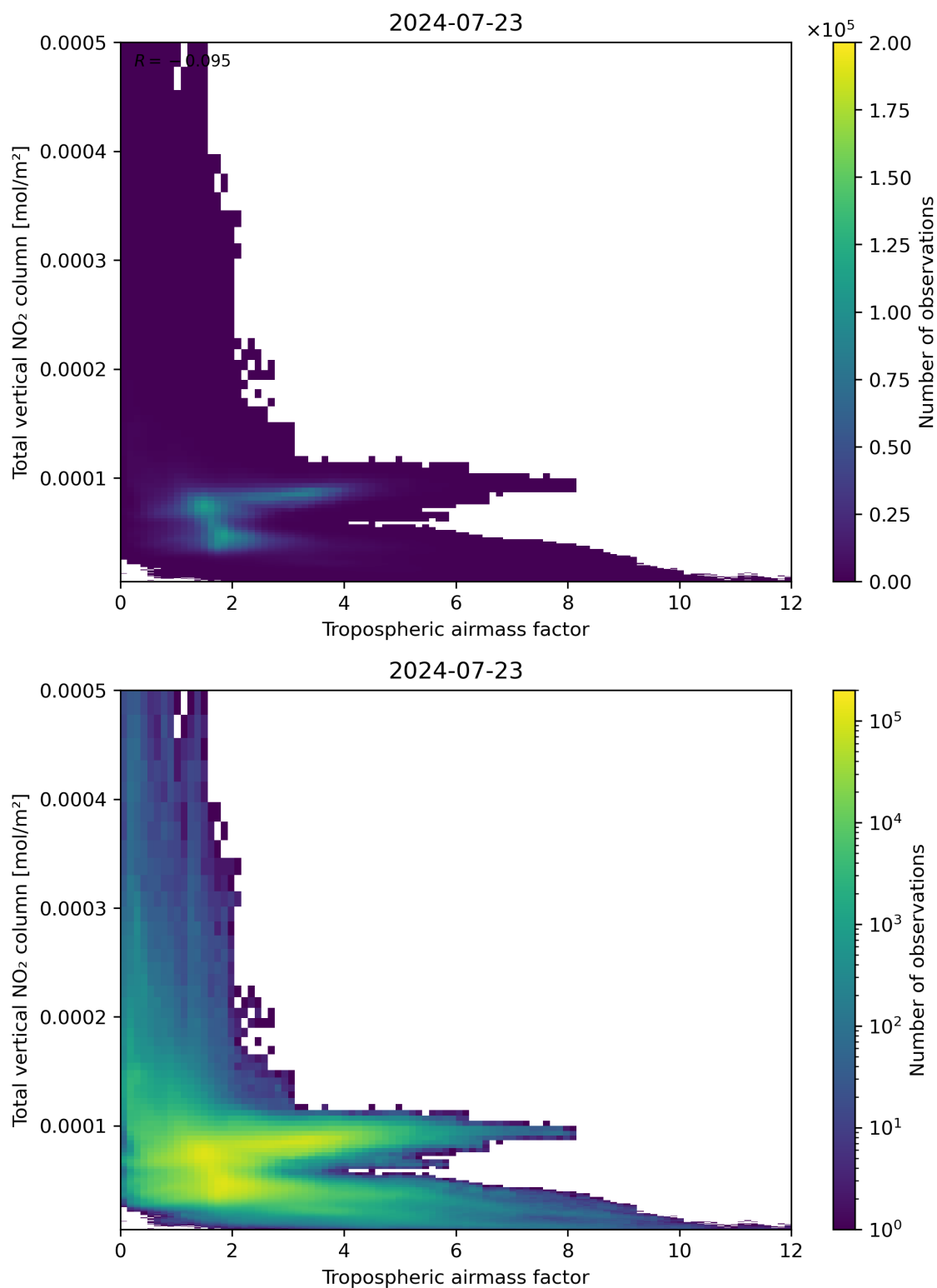
Figure 77: Scatter density plot of “Tropospheric airmass factor” against “Total vertical NO 2 column” for 2024-07-22 to 2024-07-24.
