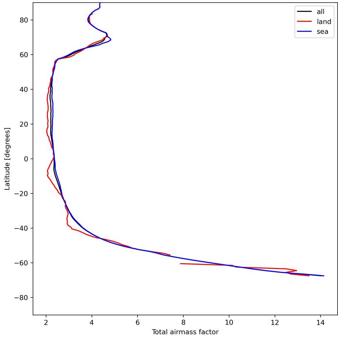
Figure 15: Zonal average of “Total airmass factor” for 2024-07-22 to 2024-07-24.
