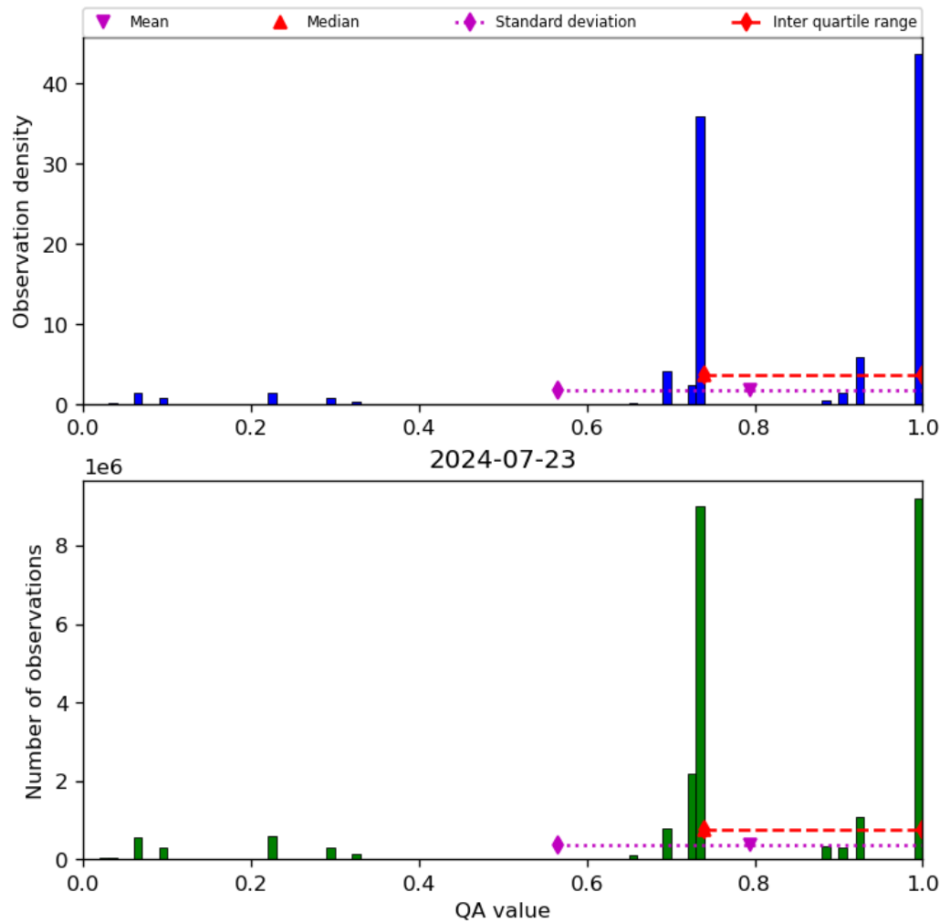
Figure 28: Histogram of “QA value” for 2024-07-22 to 2024-07-24
