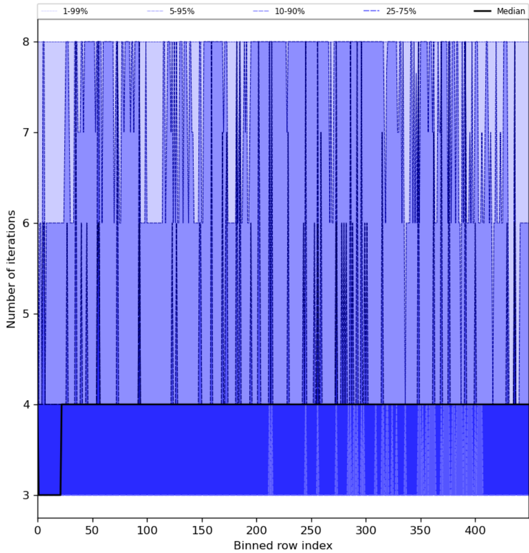
Figure 51: Along track statistics of “Number of iterations” for 2024-07-22 to 2024-07-24
