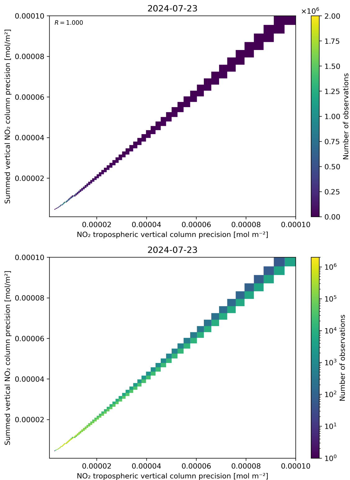
Figure 137: Scatter density plot of “NO 2 tropospheric vertical column precision” against “Summed vertical NO 2 column precision” for 2024-07-22 to 2024-07-24.
