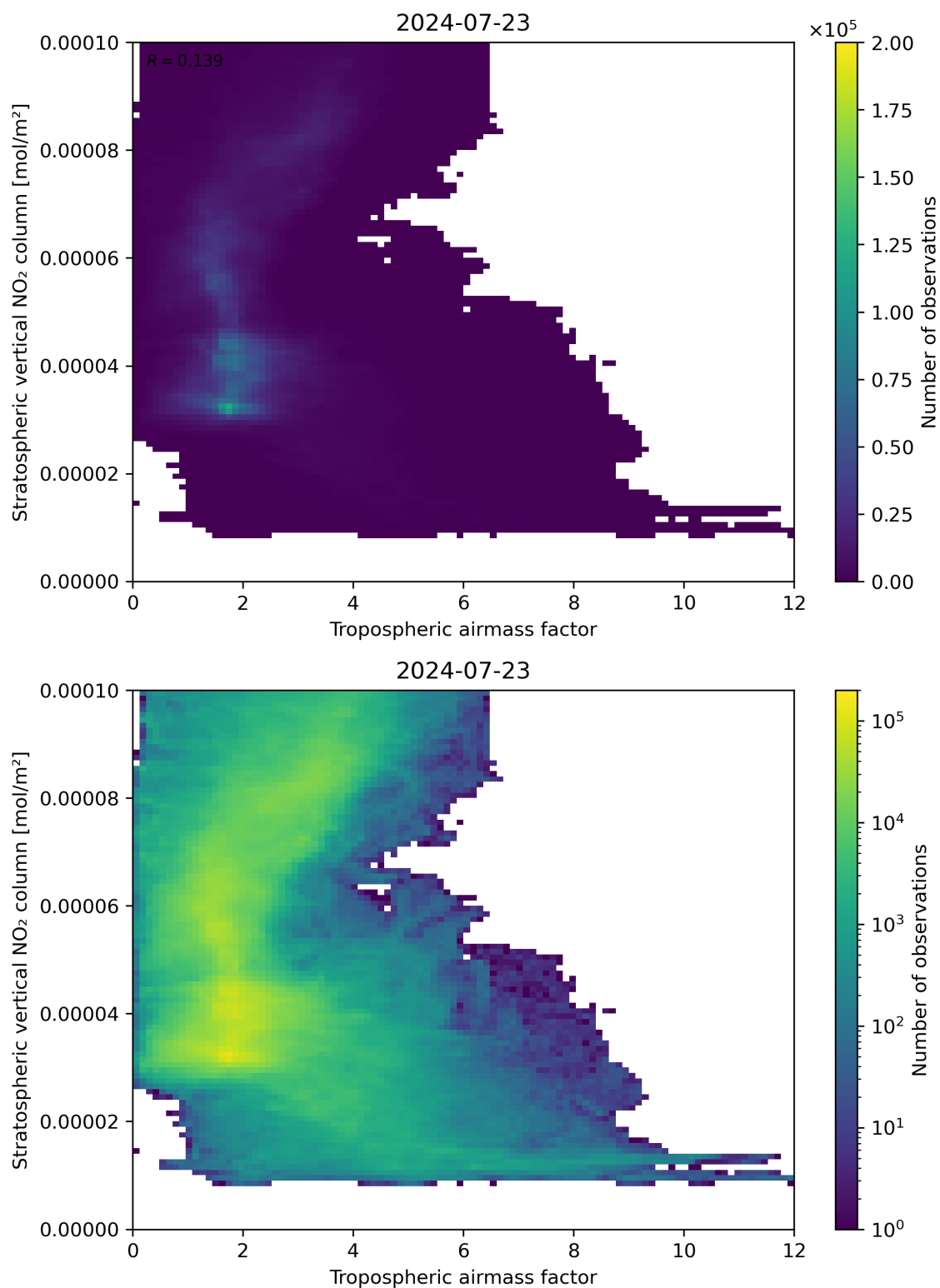
Figure 74: Scatter density plot of “Tropospheric air mass factor” against “Stratospheric vertical NO 2 column” for 2024-07-22 to 2024-07-24.
