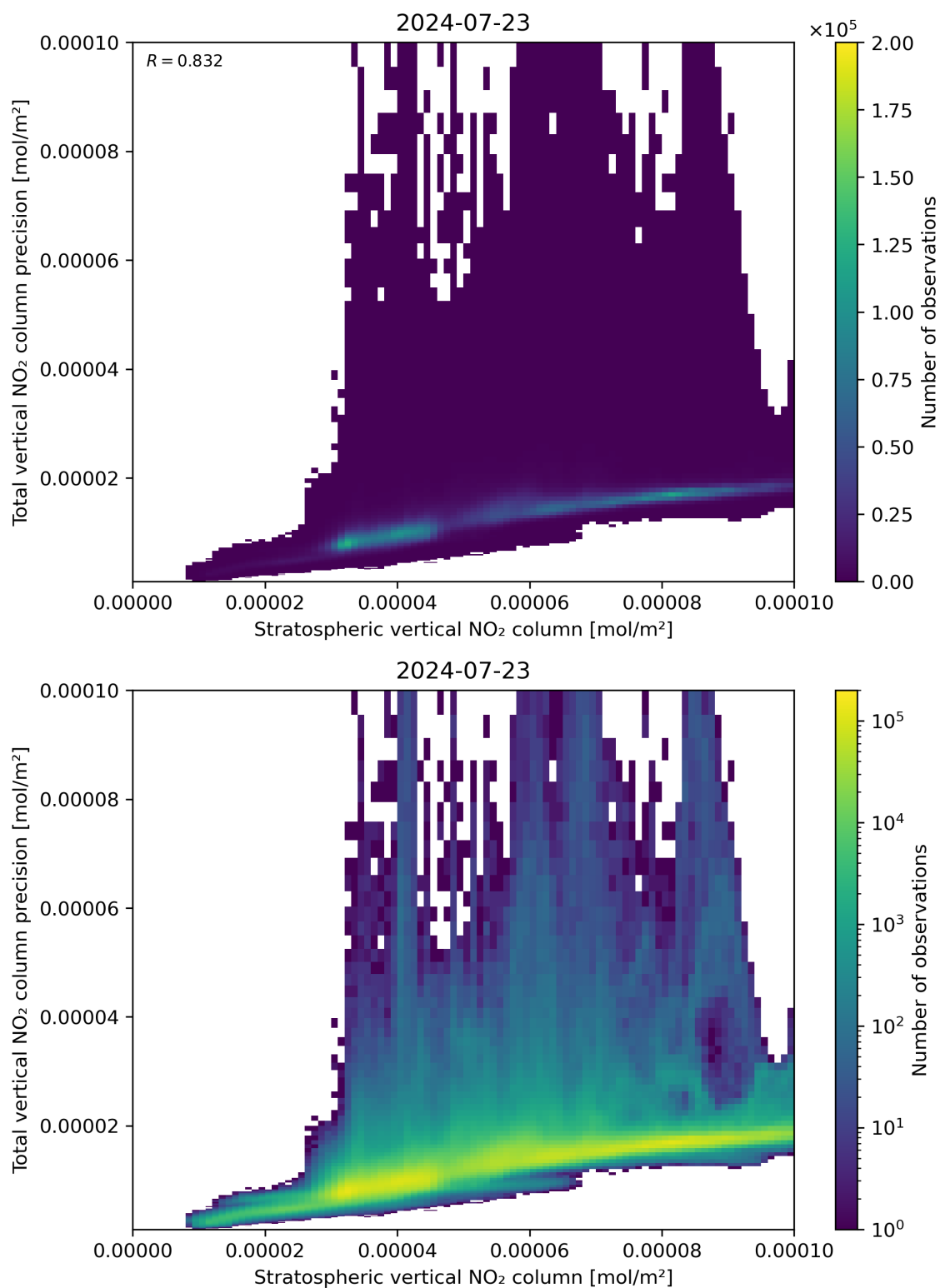
Figure 101: Scatter density plot of “Stratospheric vertical NO 2 column” against “Total vertical NO 2 column precision” for 2024-07-22 to 2024-07-24.
