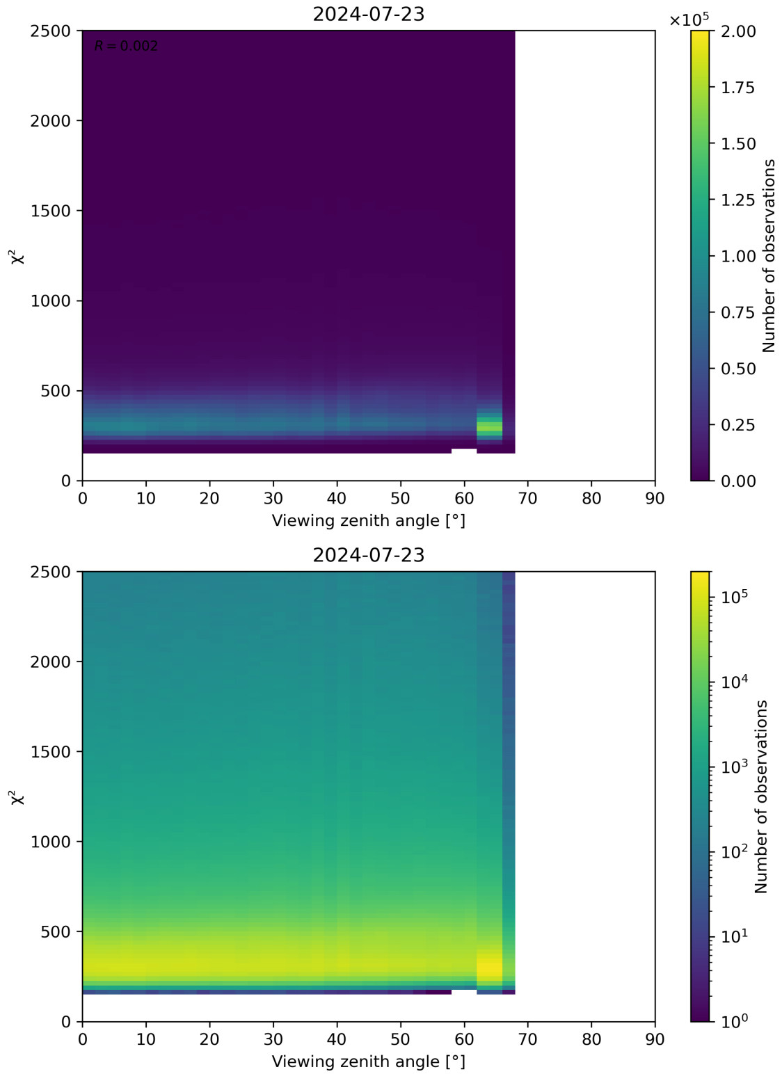
Figure 162: Scatter density plot of “Viewing zenith angle” against “ \chi^2 ” for 2024-07-22 to 2024-07-24.
