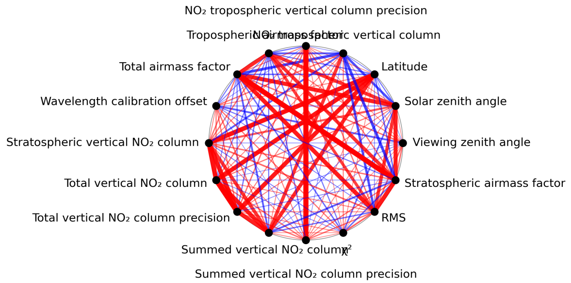
Figure 1: Map of correlation graph for 2024-07-22 to 2024-07-24.
