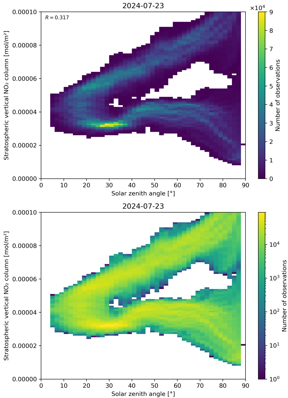
Figure 150: Scatter density plot of “Solar zenith angle” against “Stratospheric vertical NO 2 column” for 2024-07-22 to 2024-07-24.
