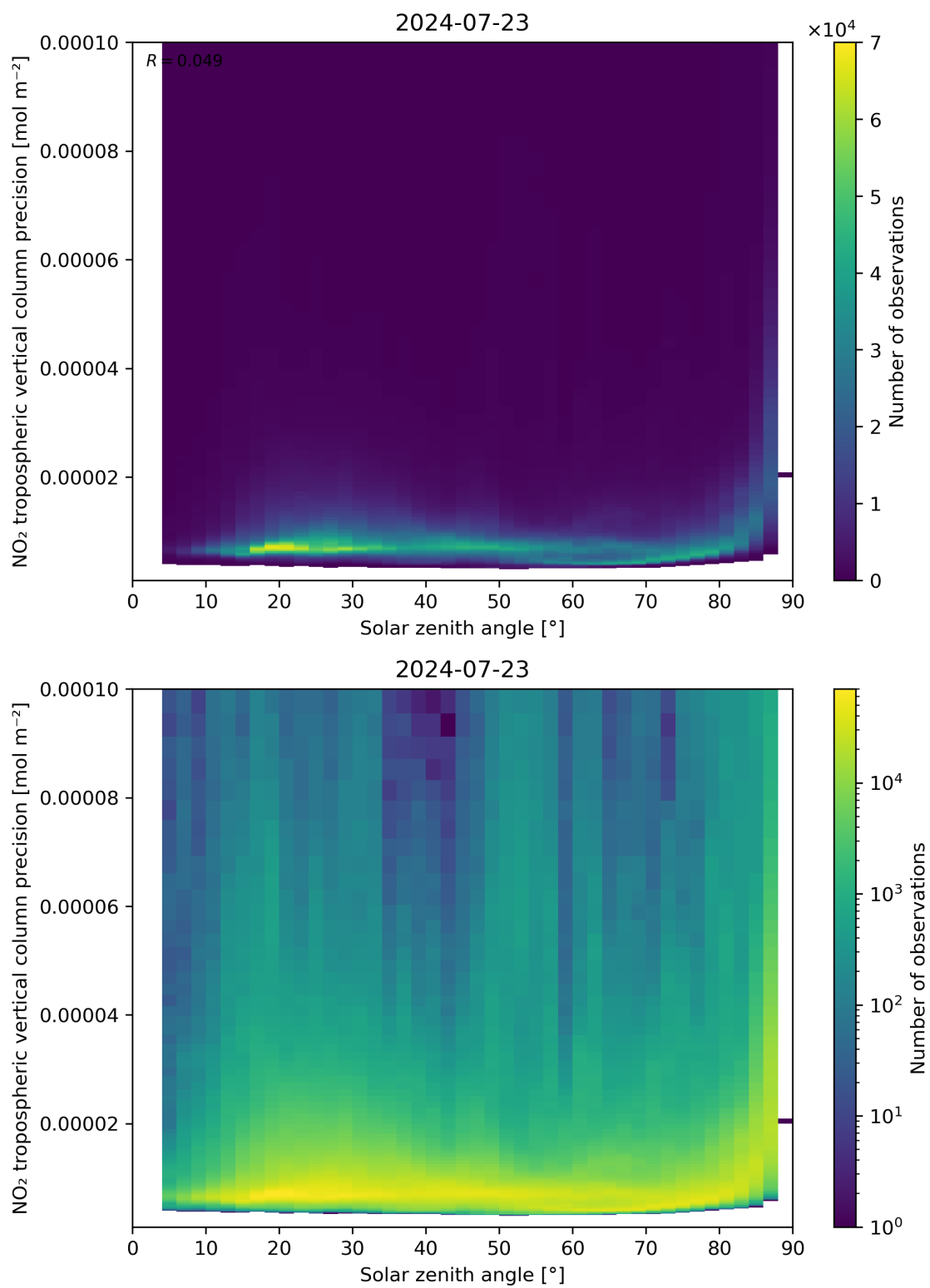
Figure 156: Scatter density plot of “Solar zenith angle” against “NO 2 tropospheric vertical column precision” for 2024-07-22 to 2024-07-24.
