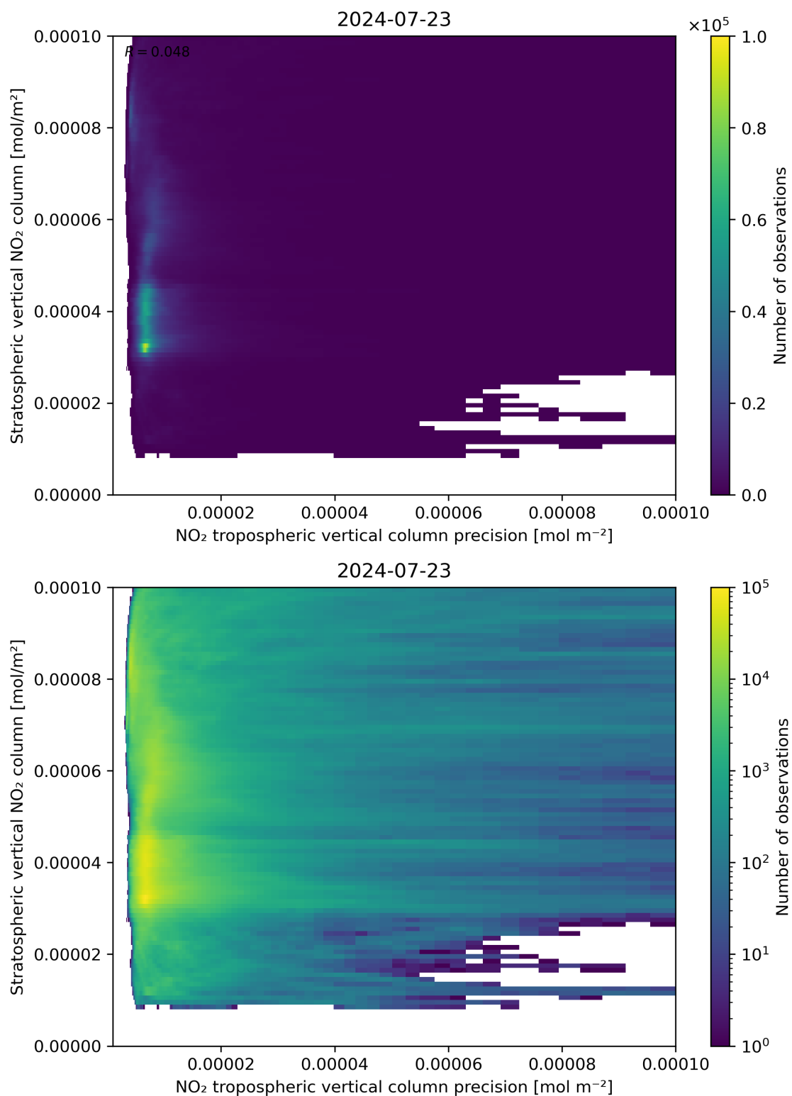
Figure 135: Scatter density plot of “NO 2 tropospheric vertical column precision” against “Stratospheric vertical NO 2 column” for 2024-07-22 to 2024-07-24.
