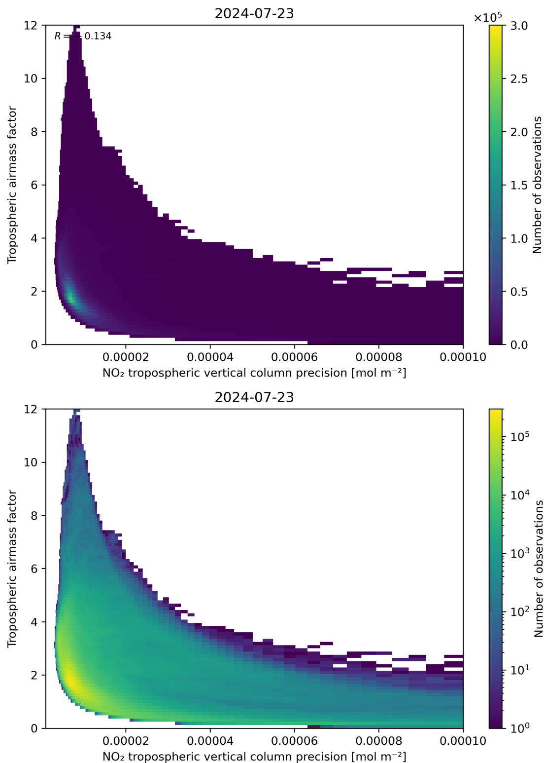
Figure 133: Scatter density plot of “NO 2 tropospheric vertical column precision” against “Tropospheric airmass factor” for 2024-07-22 to 2024-07-24.
