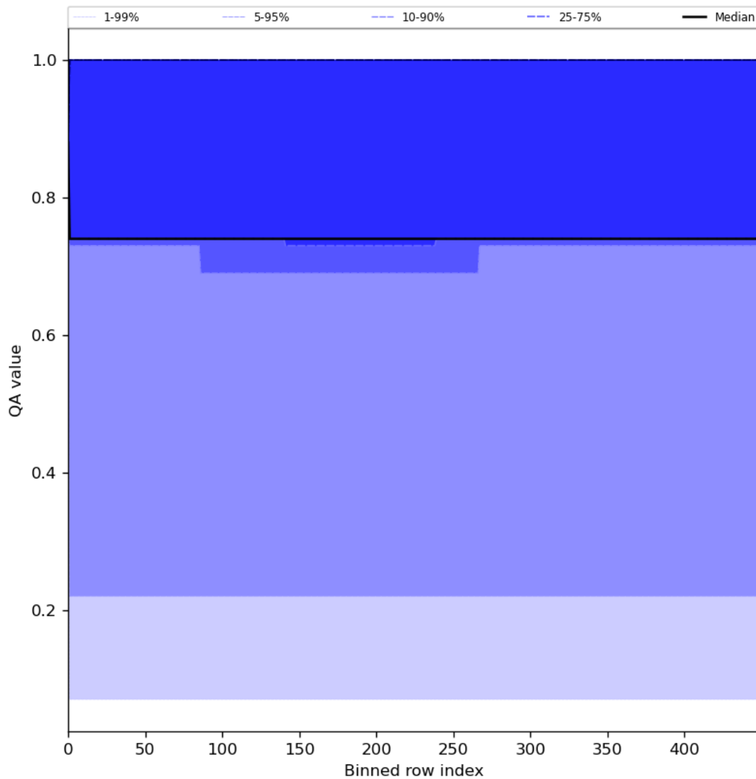
Figure 45: Along track statistics of “QA value” for 2024-07-22 to 2024-07-24
