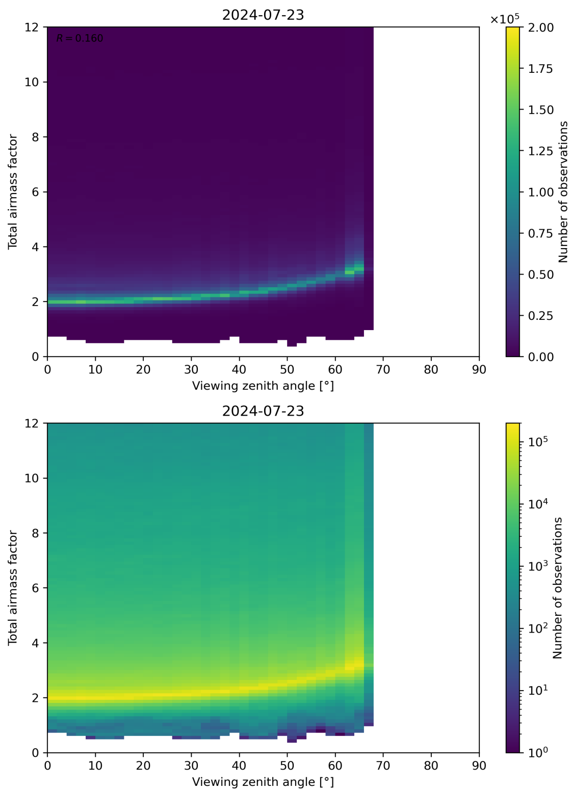
Figure 160: Scatter density plot of “Viewing zenith angle” against “Total airmass factor” for 2024-07-22 to 2024-07-24.
