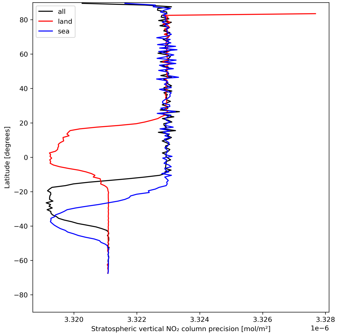
Figure 20: Zonal average of “Stratospheric vertical NO 2 column precision” for 2024-07-22 to 2024-07-24.
