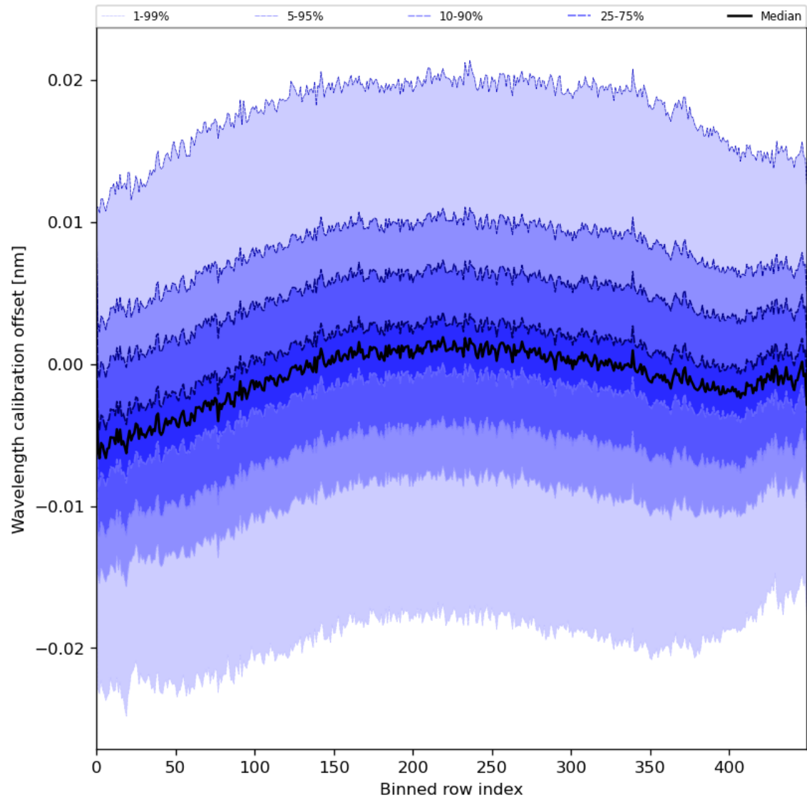
Figure 52: Along track statistics of “Wavelength calibration offset” for 2024-07-22 to 2024-07-24
