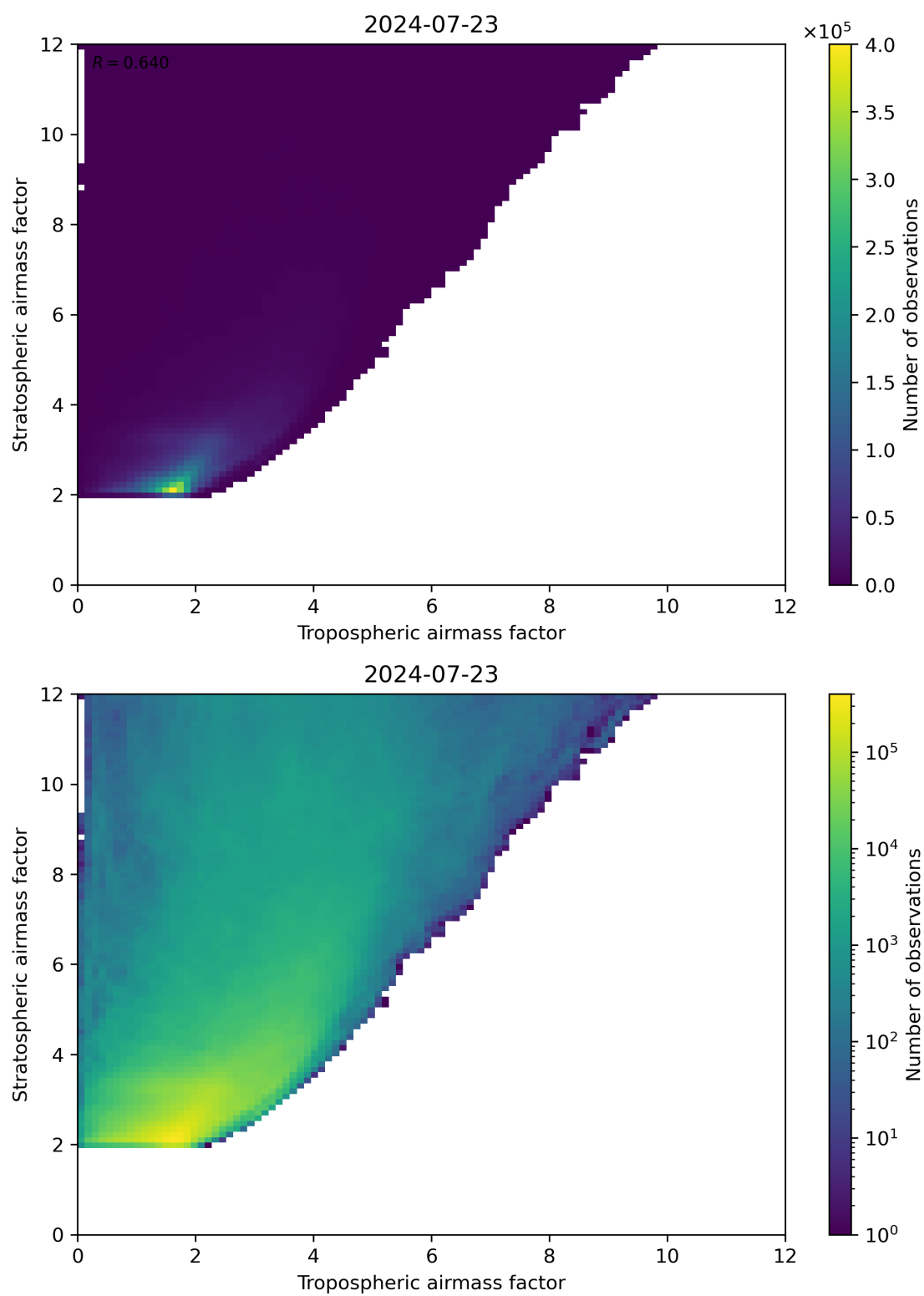
Figure 71: Scatter density plot of “Tropospheric airmass factor” against “Stratospheric airmass factor” for 2024-07-22 to 2024-07-24.
