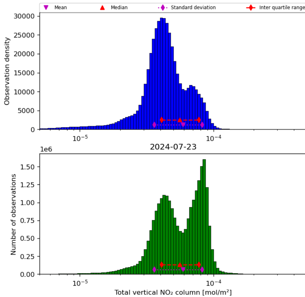
Figure 38: Histogram of “Total vertical NO 2 column” for 2024-07-22 to 2024-07-24
