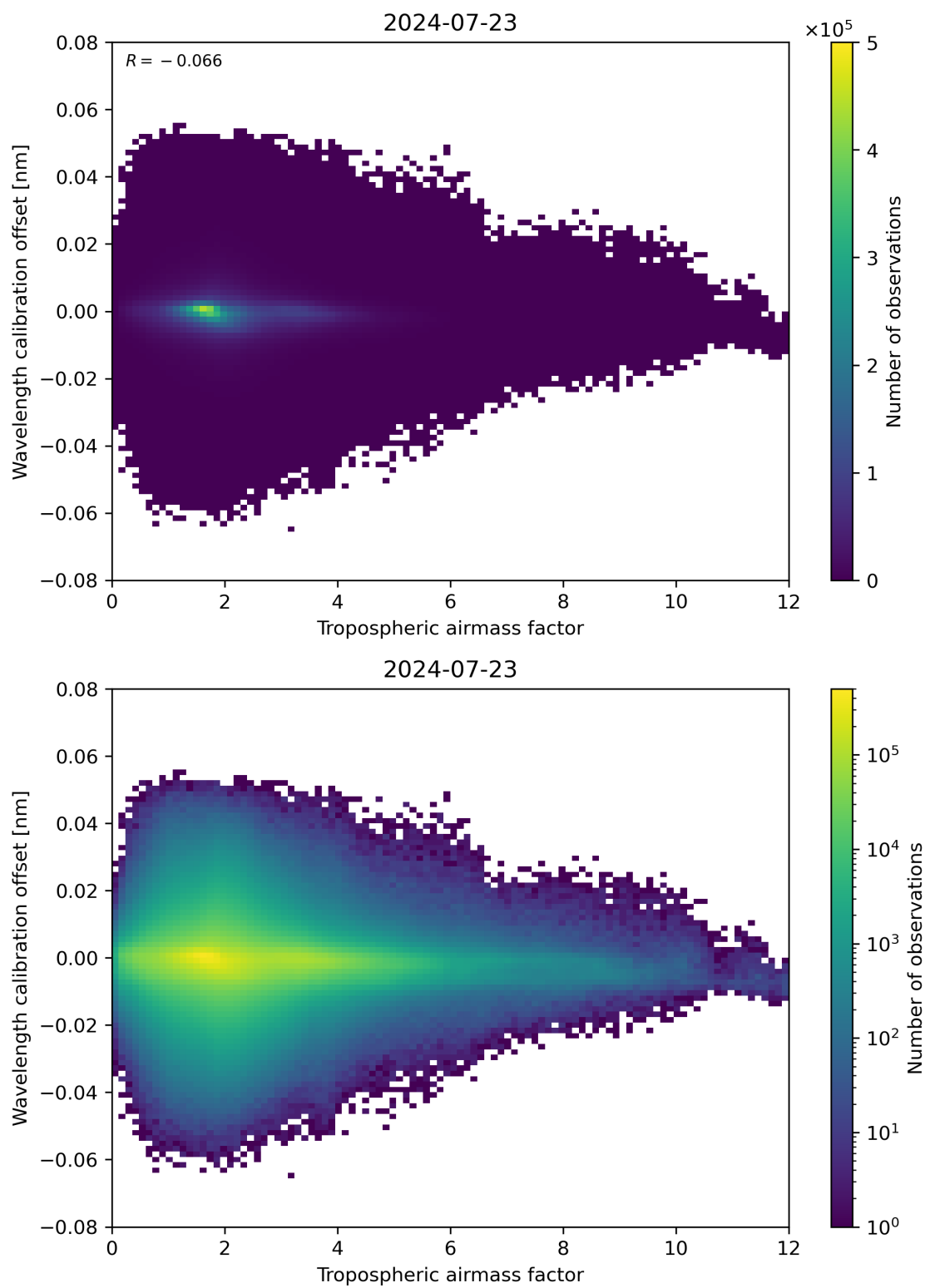
Figure 80: Scatter density plot of “Tropospheric airmass factor” against “Wavelength calibration offset” for 2024-07-22 to 2024-07-24.
