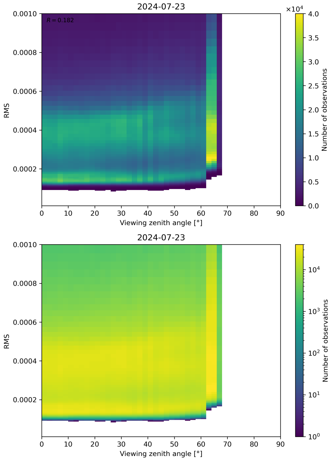
Figure 171: Scatter density plot of “Viewing zenith angle” against “RMS” for 2024-07-22 to 2024-07-24.
