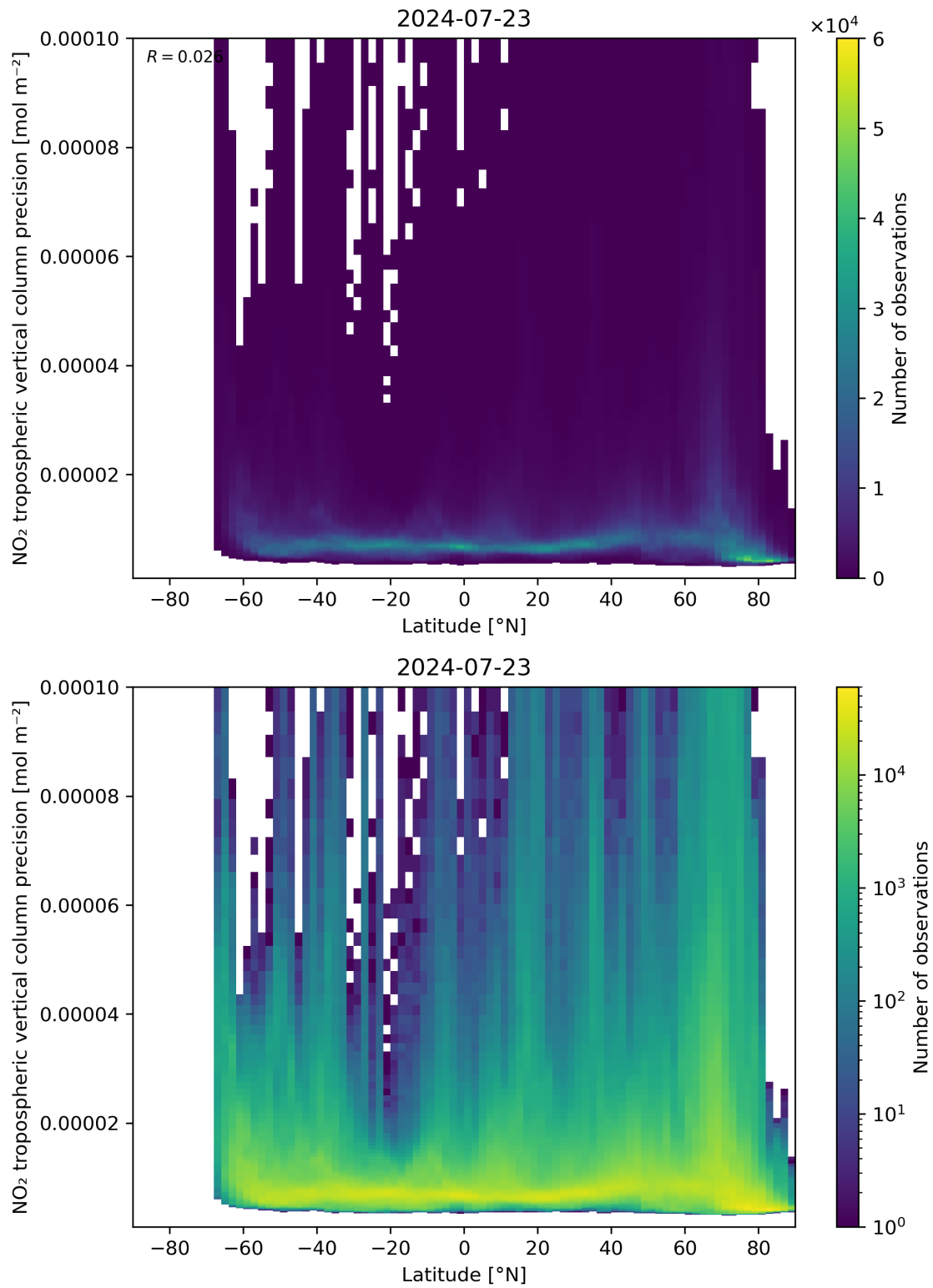
Figure 93: Scatter density plot of “Latitude” against “NO 2 tropospheric vertical column precision” for 2024-07-22 to 2024-07-24.
