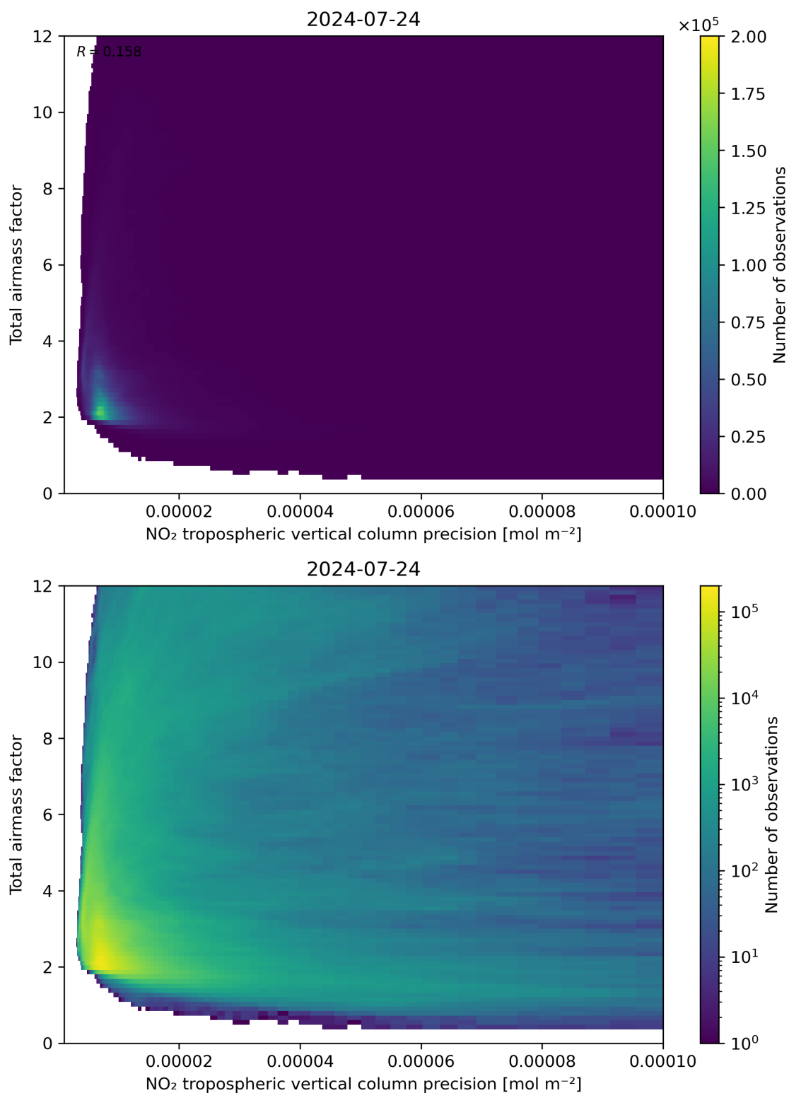
Figure 132: Scatter density plot of “NO 2 tropospheric vertical column precision” against “Total air mass factor” for 2024-07-23 to 2024-07-24.
