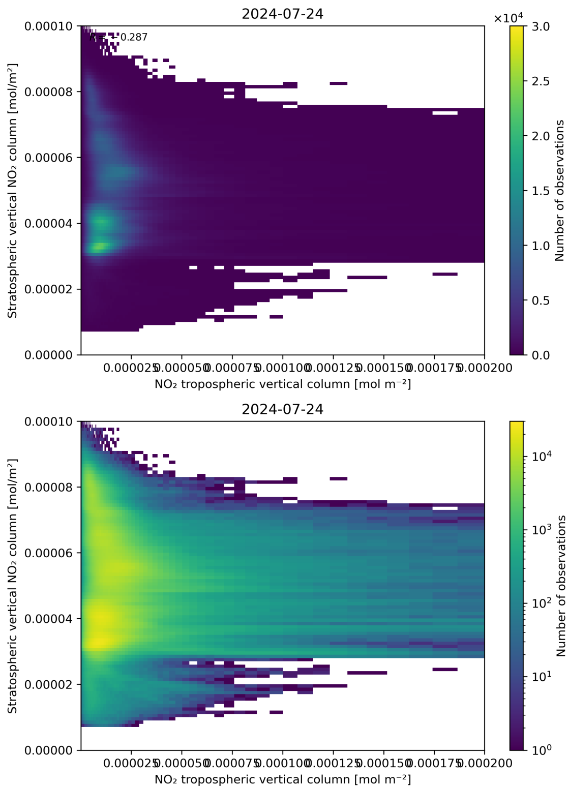
Figure 125: Scatter density plot of “NO 2 tropospheric vertical column” against “Stratospheric vertical NO 2 column” for 2024-07-23 to 2024-07-24.
