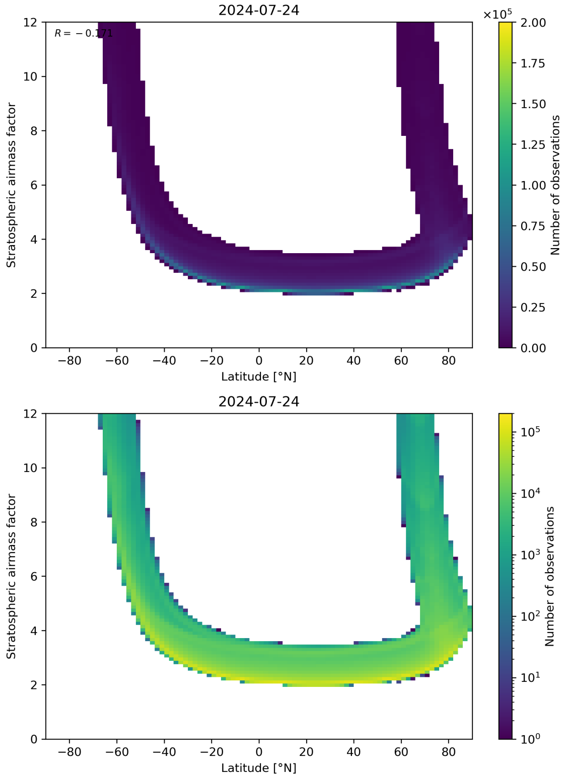
Figure 83: Scatter density plot of “Latitude” against “Stratospheric air mass factor” for 2024-07-23 to 2024-07-24.
