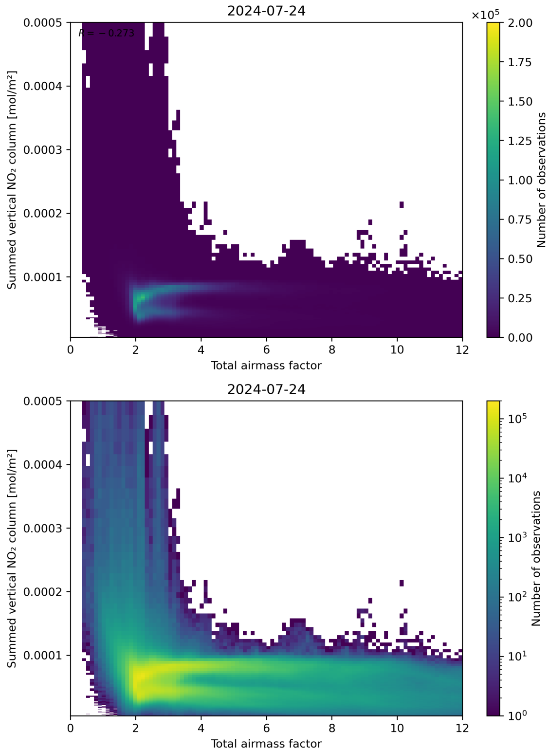
Figure 65: Scatter density plot of “Total airmass factor” against “Summed vertical NO 2 column” for 2024-07-23 to 2024-07-24.
