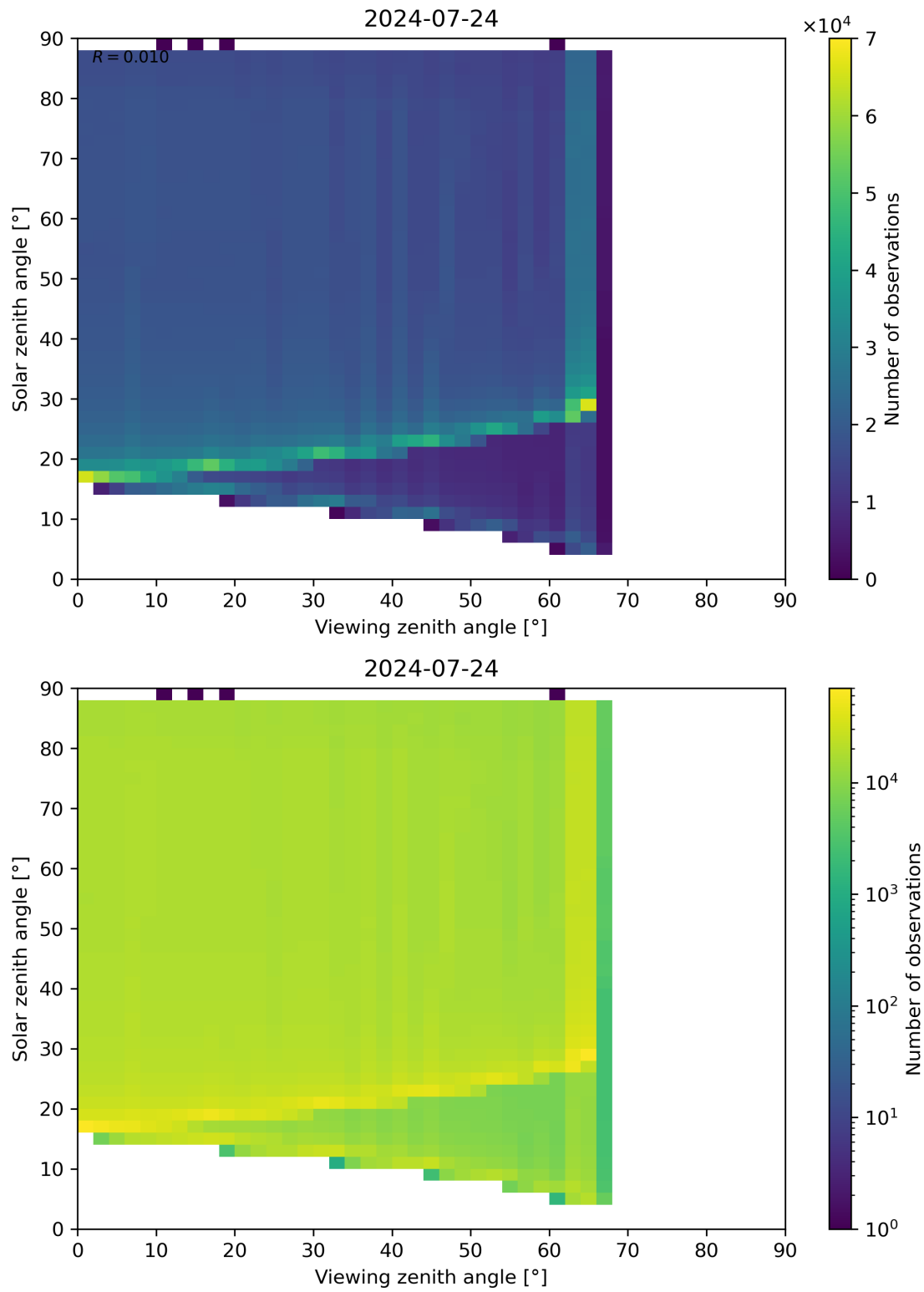
Figure 172: Scatter density plot of “Viewing zenith angle” against “Solar zenith angle” for 2024-07-23 to 2024-07-24.
