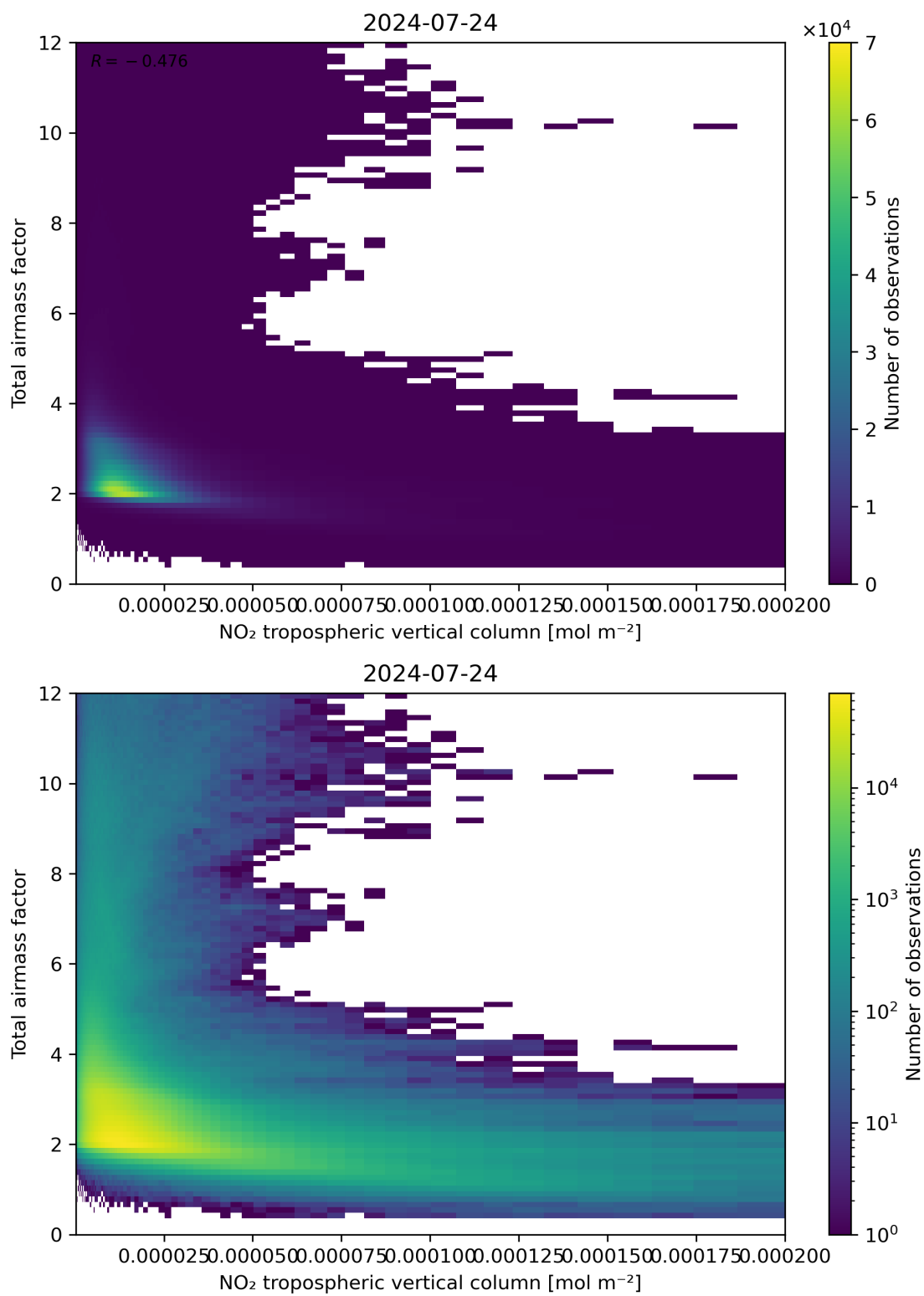
Figure 122: Scatter density plot of “NO 2 tropospheric vertical column” against “Total airmass factor” for 2024-07-23 to 2024-07-24.
