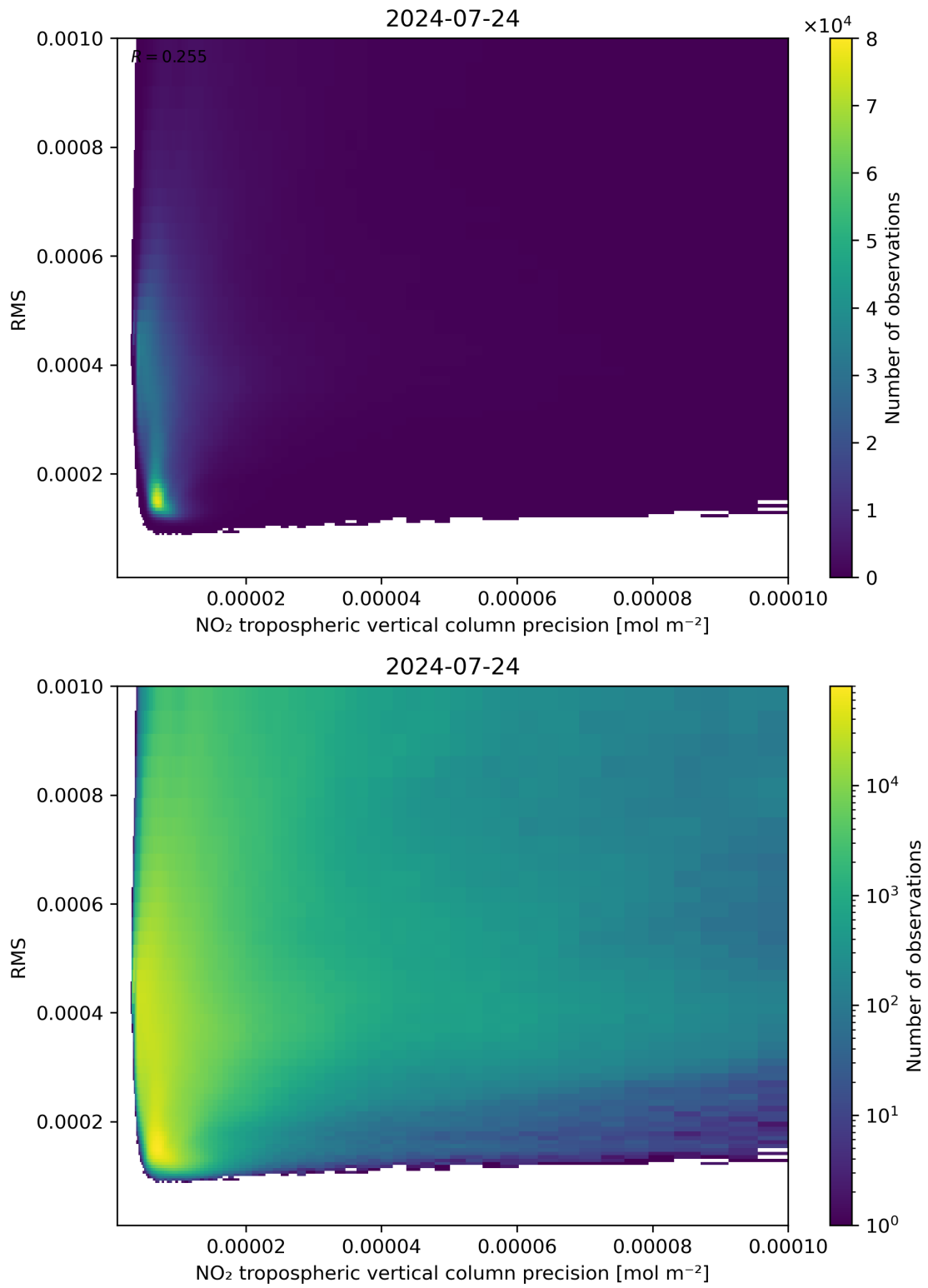
Figure 140: Scatter density plot of “NO 2 tropospheric vertical column precision” against “RMS” for 2024-07-23 to 2024-07-24.
