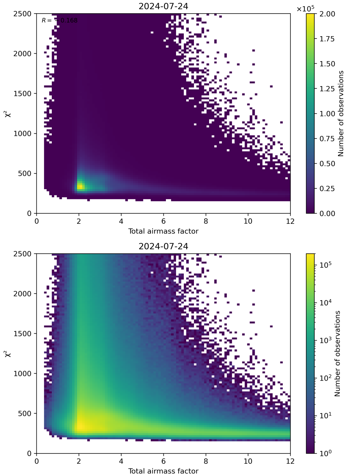
Figure 63: Scatter density plot of “Total airmass factor” against “ \chi^2 ” for 2024-07-23 to 2024-07-24.
