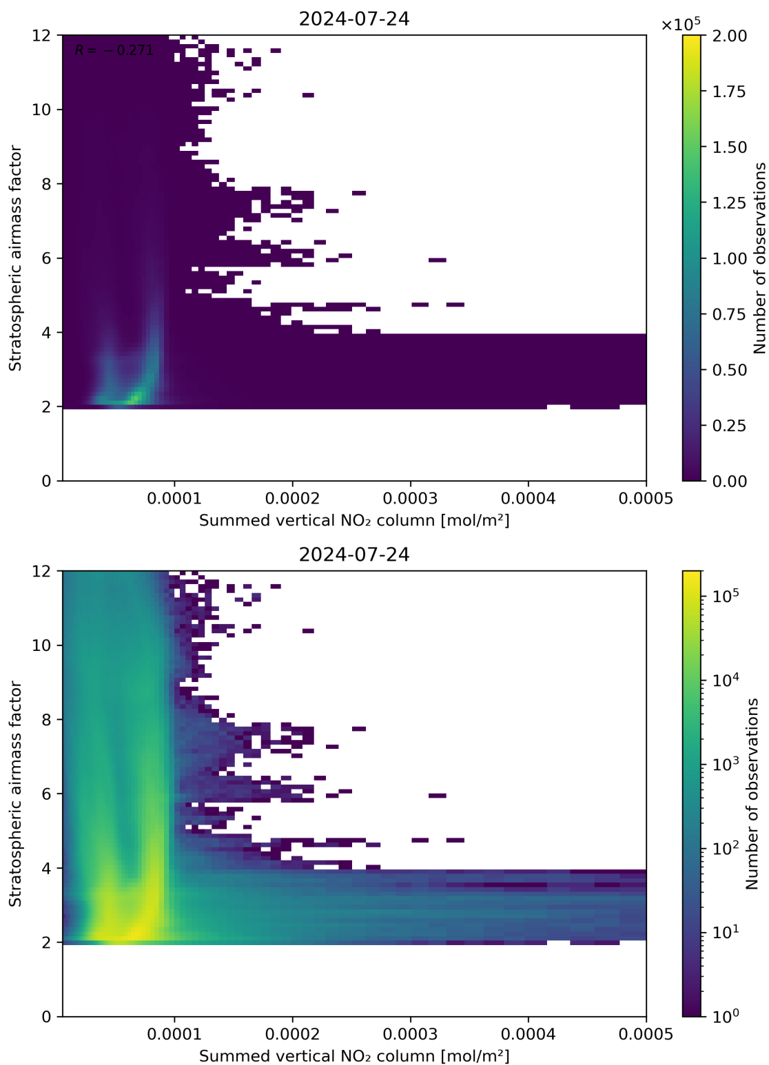
Figure 103: Scatter density plot of “Summed vertical NO 2 column” against “Stratospheric air mass factor” for 2024-07-23 to 2024-07-24.
