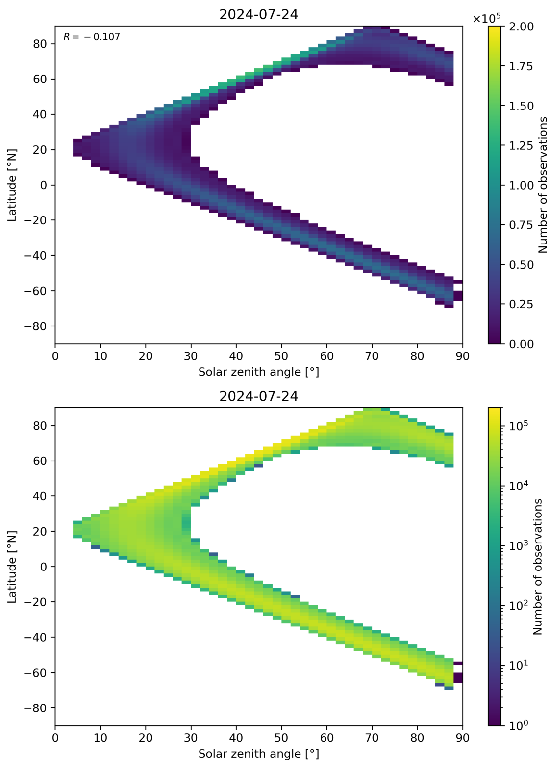
Figure 149: Scatter density plot of “Solar zenith angle” against “Latitude” for 2024-07-23 to 2024-07-24.
