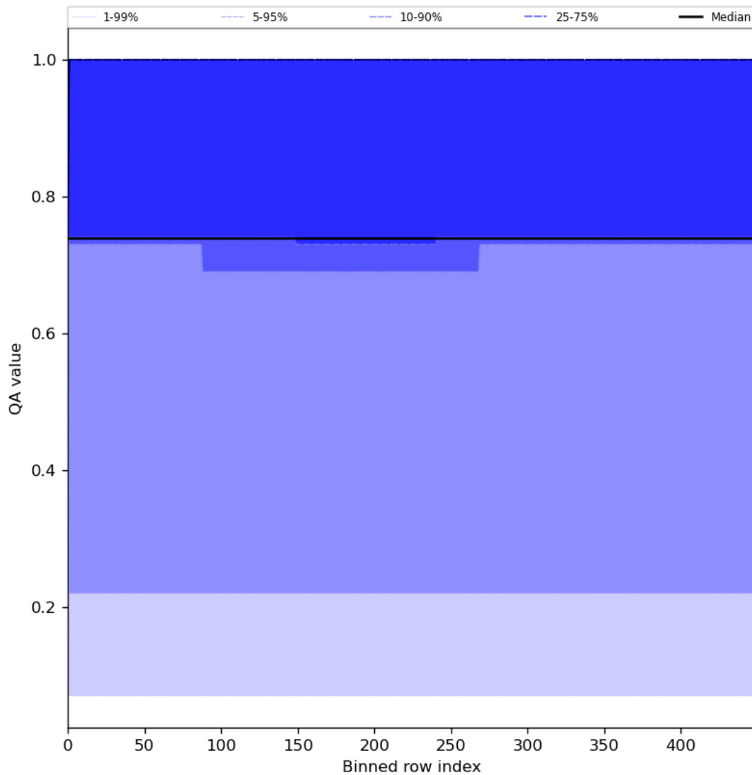
Figure 45: Along track statistics of “QA value” for 2024-07-23 to 2024-07-24
