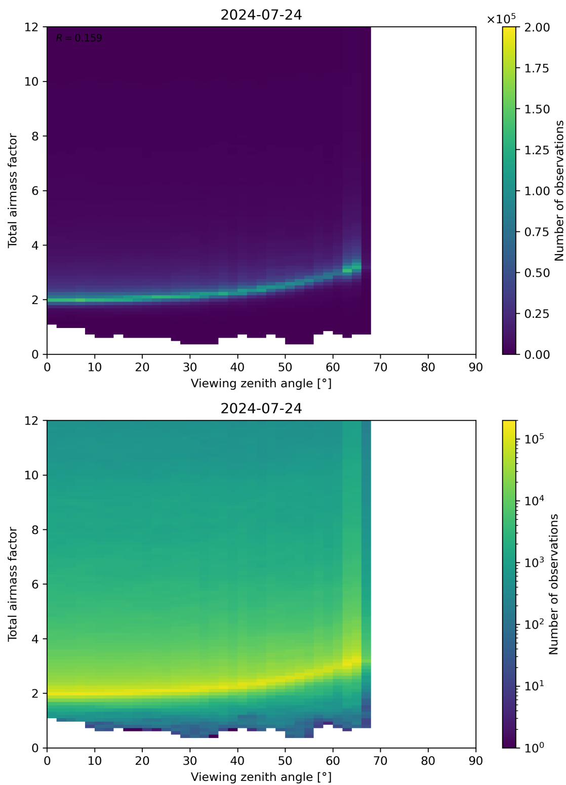
Figure 160: Scatter density plot of “Viewing zenith angle” against “Total airmass factor” for 2024-07-23 to 2024-07-24.
