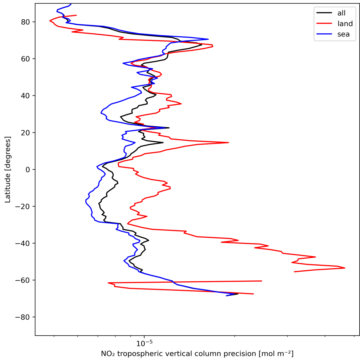
Figure 13: Zonal average of “NO 2 tropospheric vertical column precision” for 2024-07-23 to 2024-07-24.
