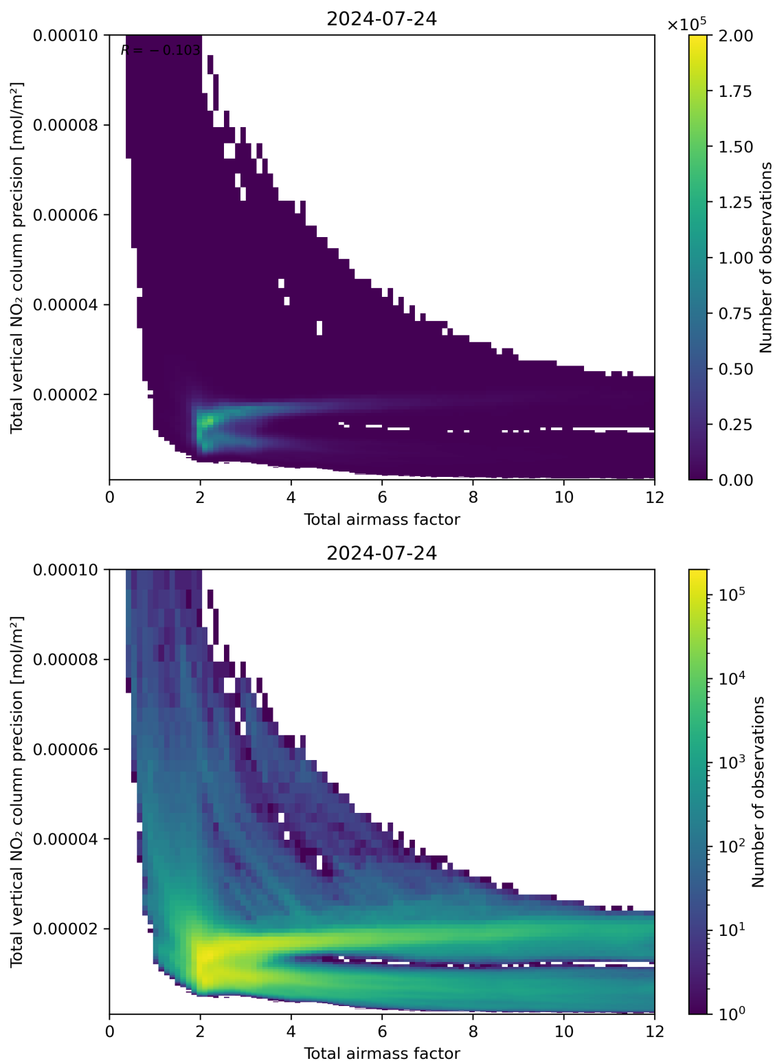
Figure 68: Scatter density plot of “Total airmass factor” against “Total vertical NO 2 column precision” for 2024-07-23 to 2024-07-24.
