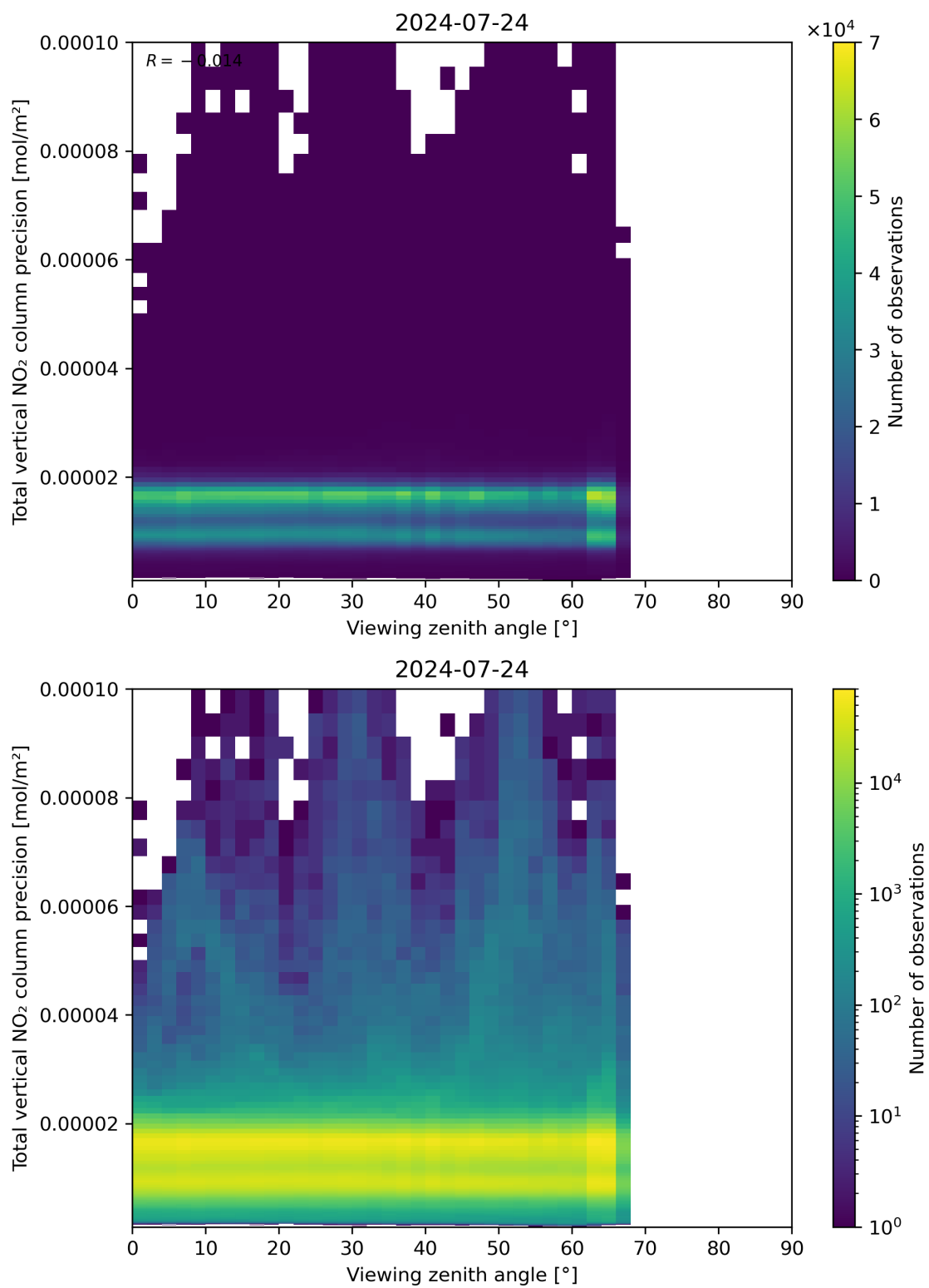
Figure 168: Scatter density plot of “Viewing zenith angle” against “Total vertical NO 2 column precision” for 2024-07-23 to 2024-07-24.
