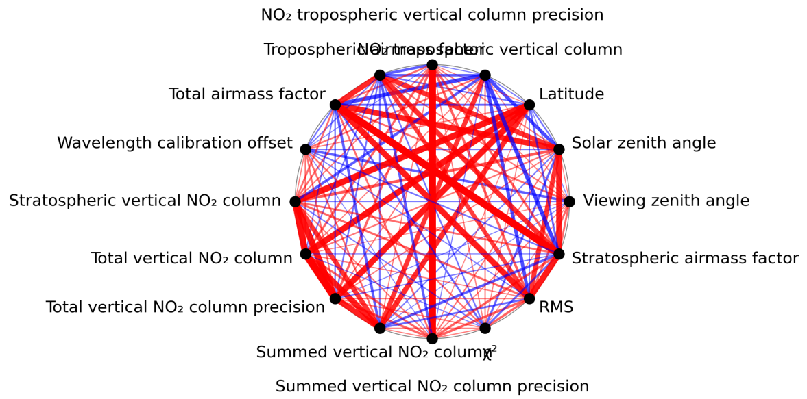
Figure 1: Map of correlation graph for 2024-07-23 to 2024-07-24.
