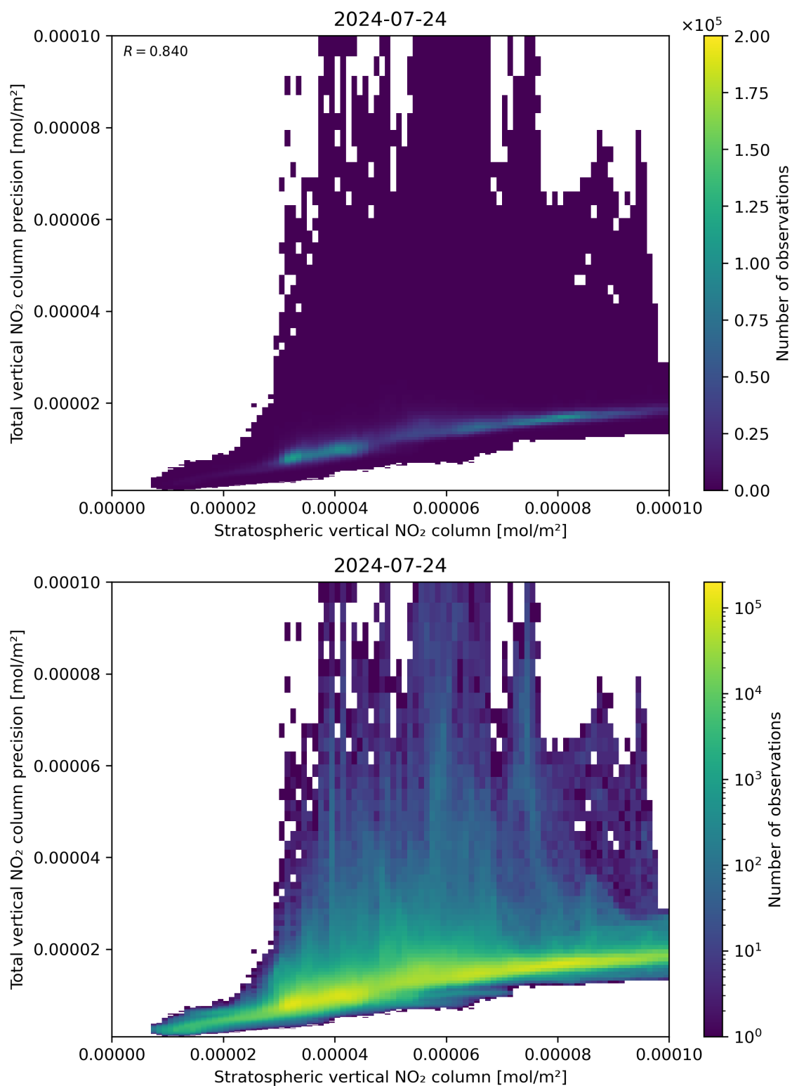
Figure 101: Scatter density plot of “Stratospheric vertical NO 2 column” against “Total vertical NO 2 column precision” for 2024-07-23 to 2024-07-24.
