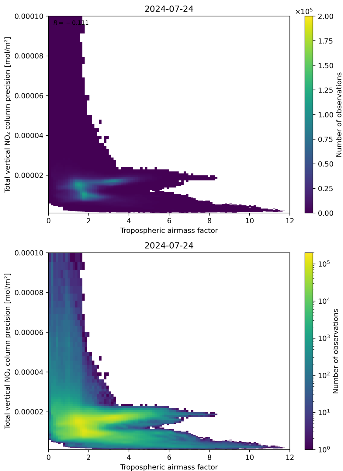
Figure 78: Scatter density plot of “Tropospheric air mass factor” against “Total vertical NO 2 column precision” for 2024-07-23 to 2024-07-24.
