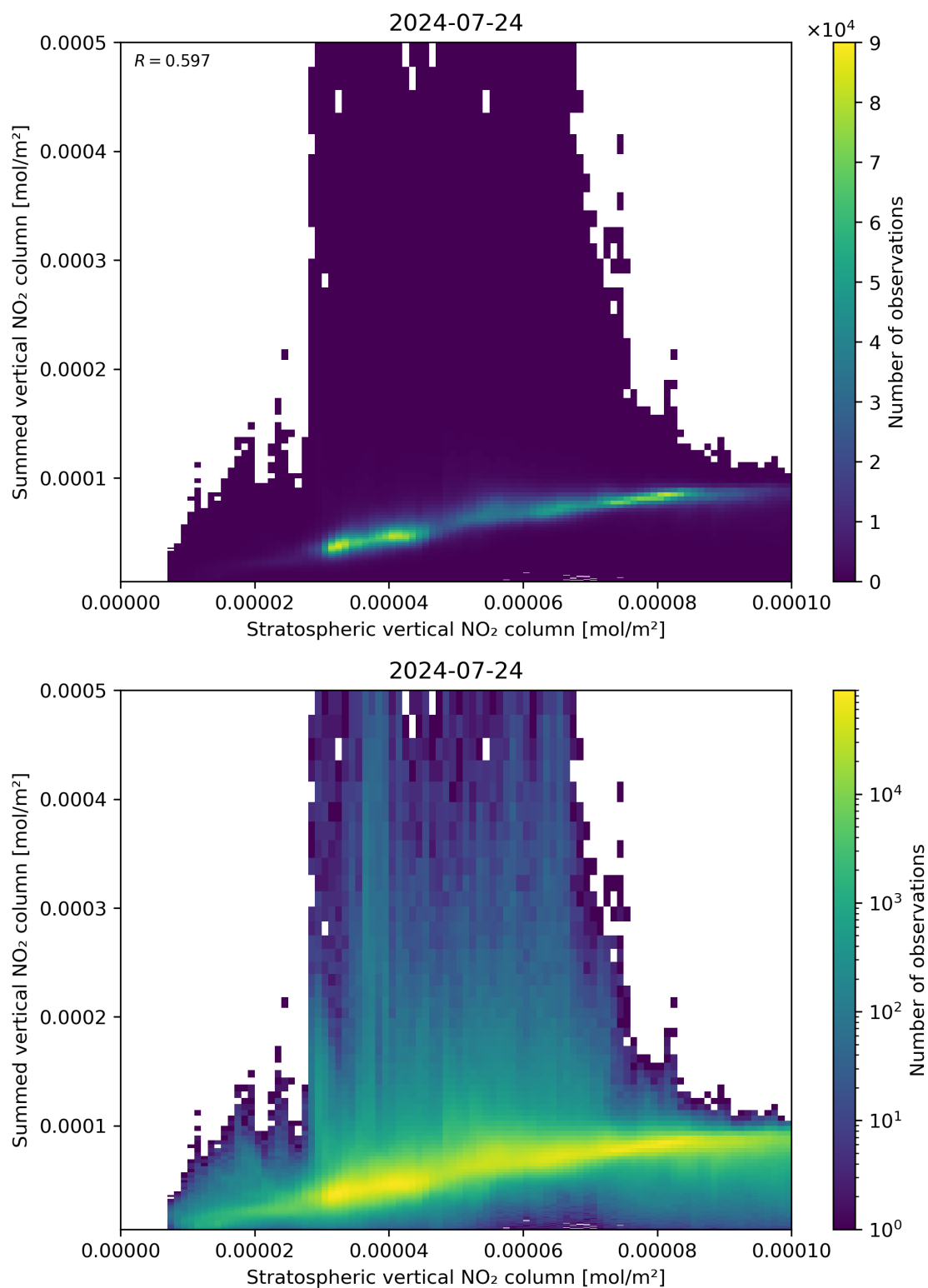
Figure 98: Scatter density plot of “Stratospheric vertical NO 2 column” against “Summed vertical NO 2 column” for 2024-07-23 to 2024-07-24.
