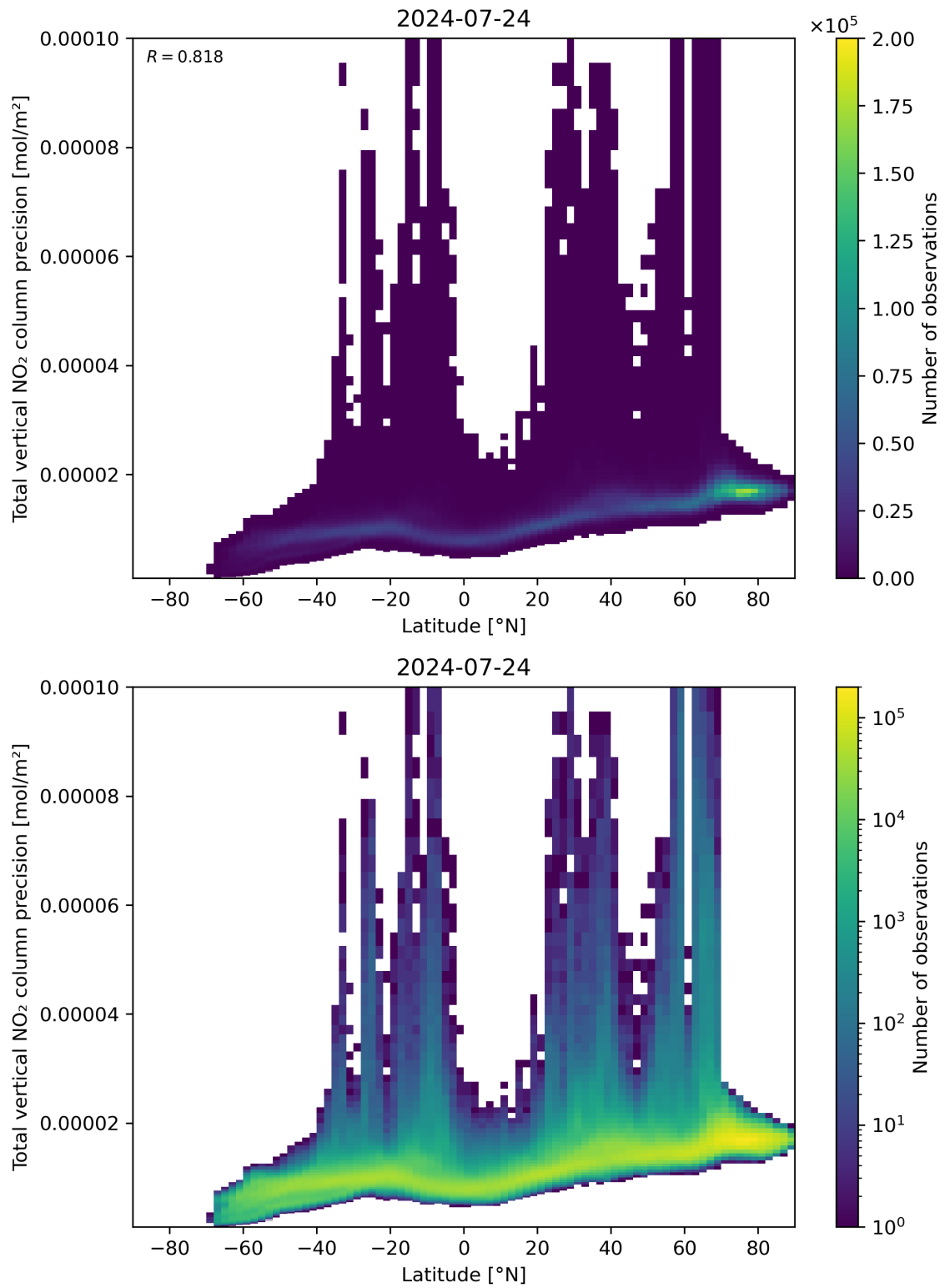
Figure 91: Scatter density plot of “Latitude” against “Total vertical NO 2 column precision” for 2024-07-23 to 2024-07-24.
