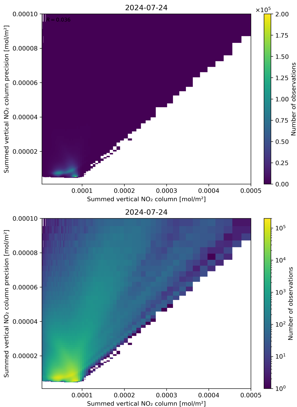
Figure 105: Scatter density plot of “Summed vertical NO 2 column” against “Summed vertical NO 2 column precision” for 2024-07-23 to 2024-07-24.
