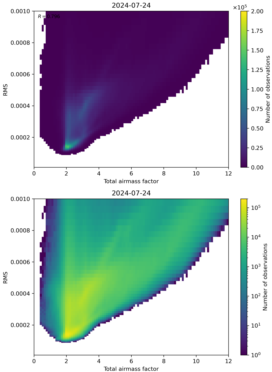
Figure 69: Scatter density plot of “Total airmass factor” against “RMS” for 2024-07-23 to 2024-07-24.
