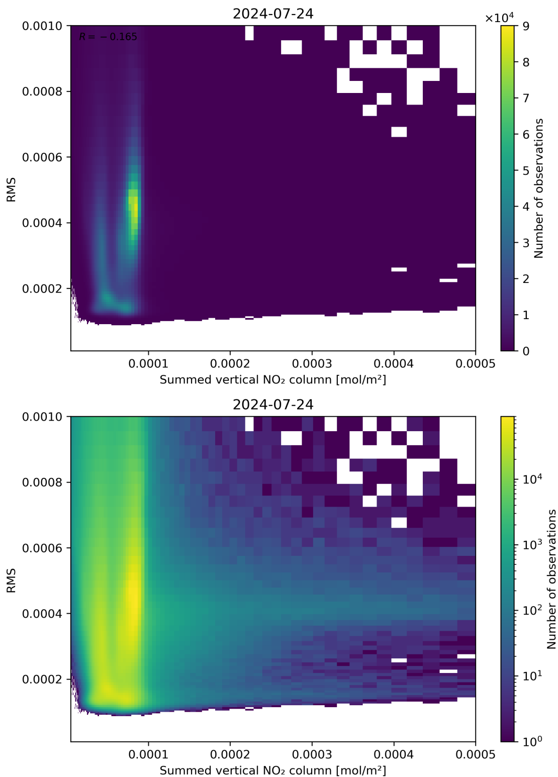
Figure 109: Scatter density plot of “Summed vertical NO 2 column” against “RMS” for 2024-07-23 to 2024-07-24.
