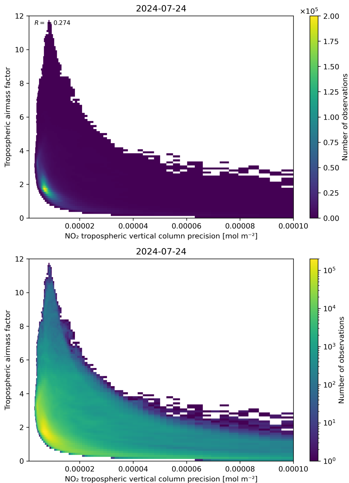
Figure 133: Scatter density plot of “NO 2 tropospheric vertical column precision” against “Tropospheric airmass factor” for 2024-07-23 to 2024-07-24.
