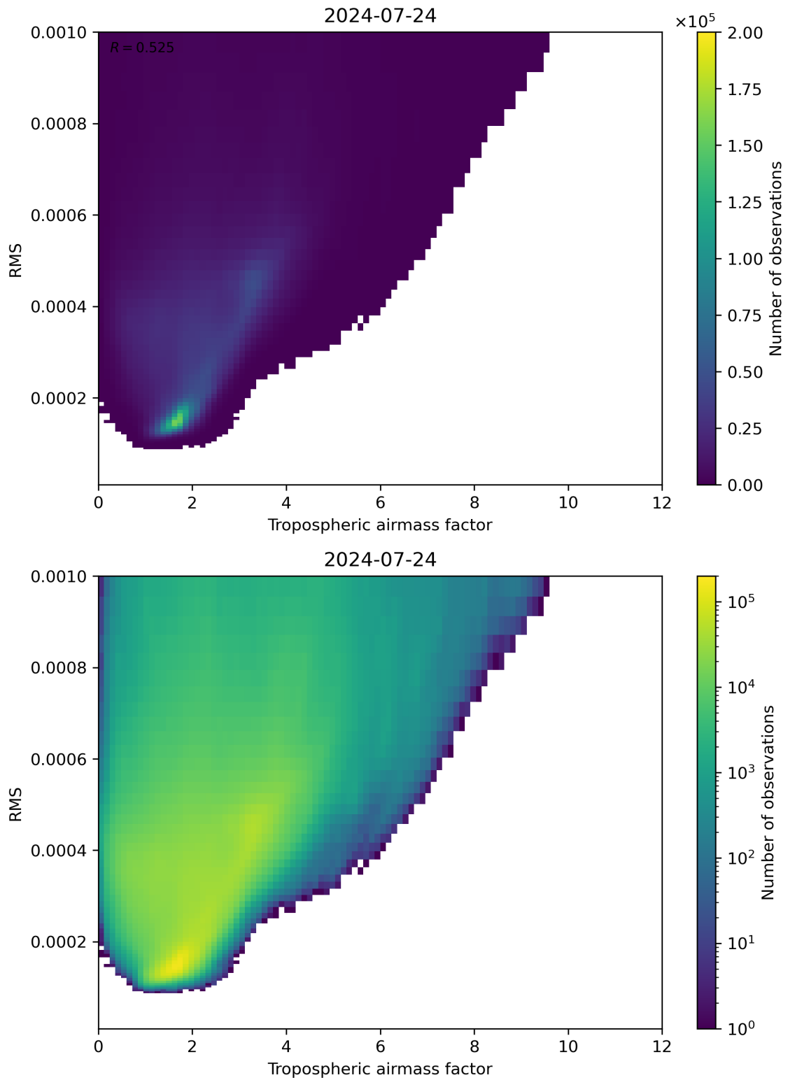
Figure 79: Scatter density plot of “Tropospheric airmass factor” against “RMS” for 2024-07-23 to 2024-07-24.
