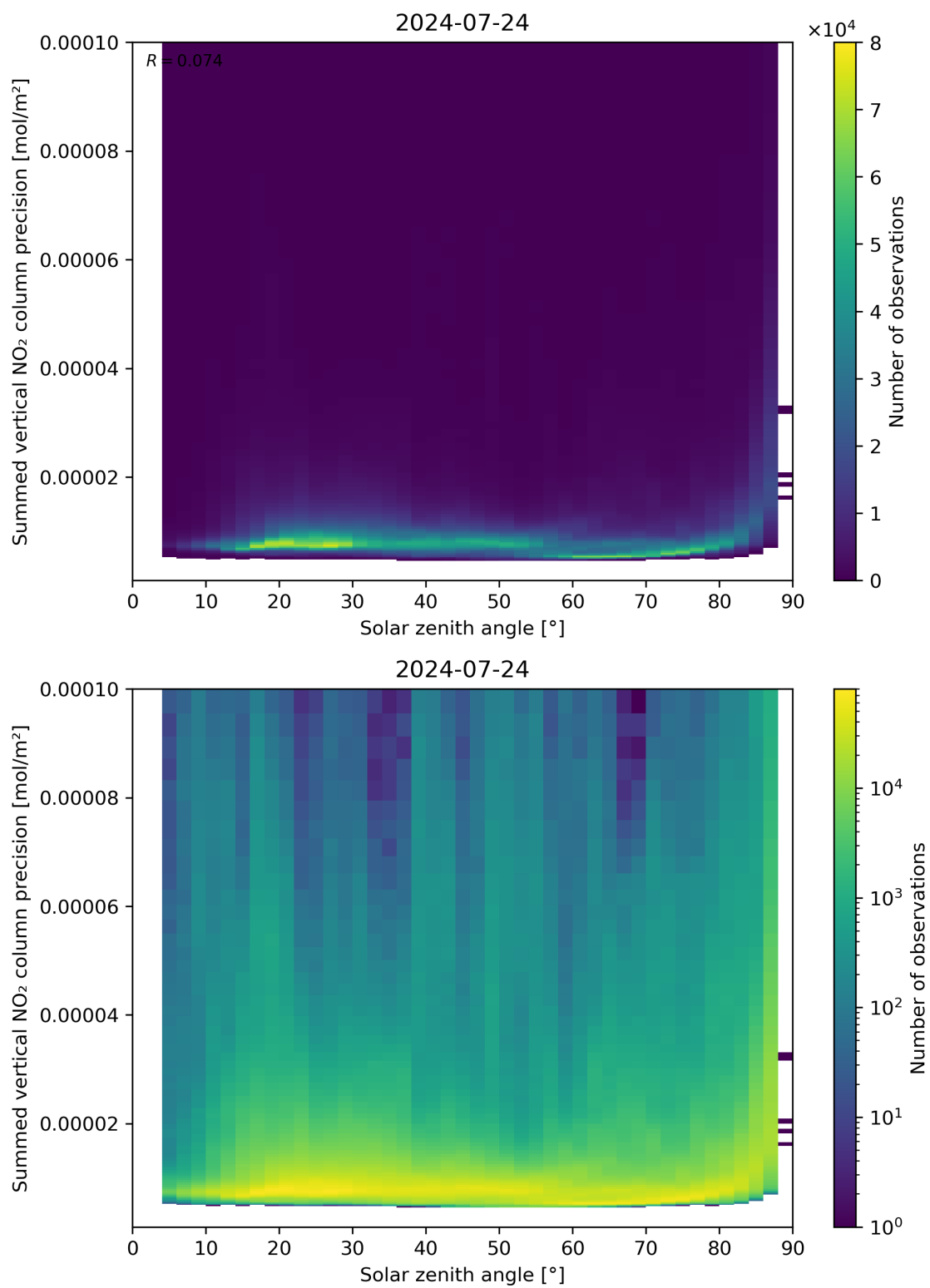
Figure 152: Scatter density plot of “Solar zenith angle” against “Summed vertical NO 2 column precision” for 2024-07-23 to 2024-07-24.
