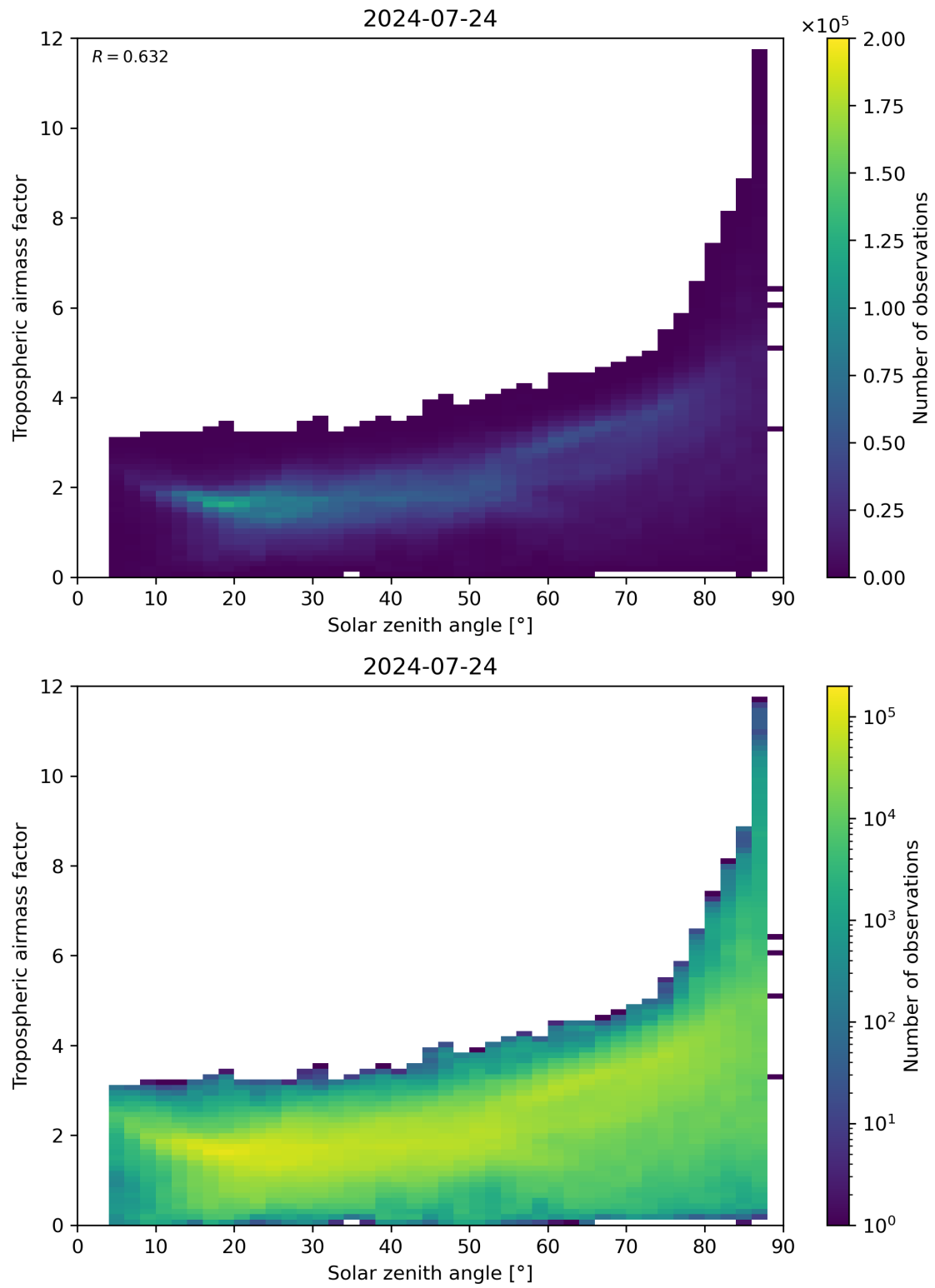
Figure 147: Scatter density plot of “Solar zenith angle” against “Tropospheric airmass factor” for 2024-07-23 to 2024-07-24.
