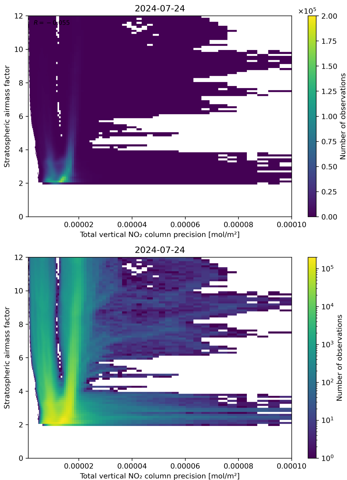
Figure 115: Scatter density plot of “Total vertical NO 2 column precision” against “Stratospheric air mass factor” for 2024-07-23 to 2024-07-24.
