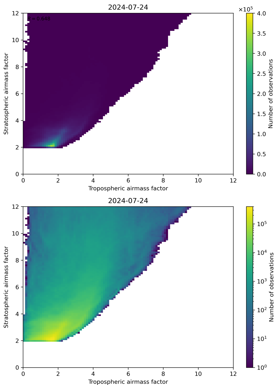
Figure 71: Scatter density plot of “Tropospheric airmass factor” against “Stratospheric airmass factor” for 2024-07-23 to 2024-07-24.
