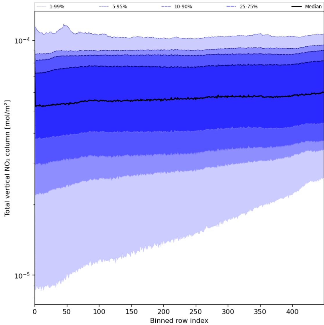
Figure 55: Along track statistics of “Total vertical NO 2 column” for 2024-07-23 to 2024-07-24
