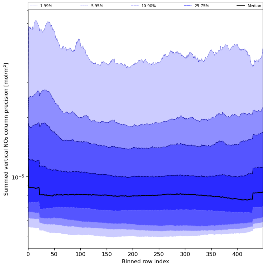
Figure 58: Along track statistics of “Summed vertical NO 2 column precision” for 2024-07-23 to 2024-07-24
