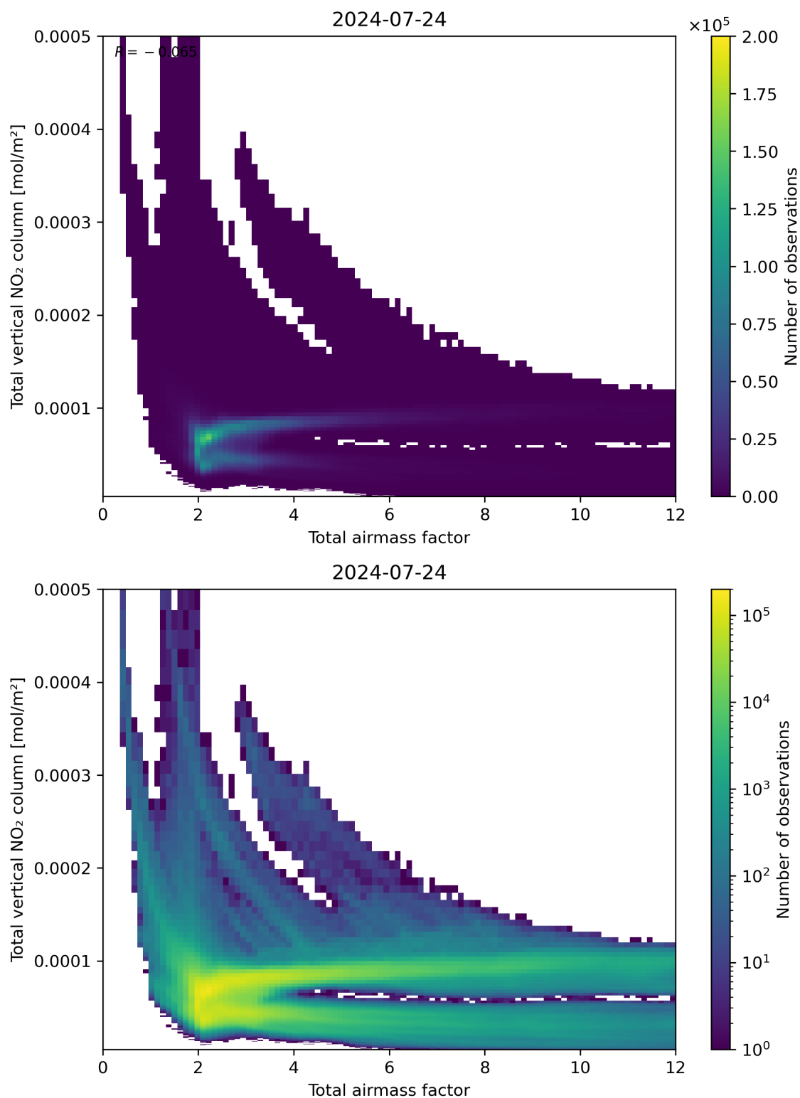
Figure 67: Scatter density plot of “Total airmass factor” against “Total vertical NO 2 column” for 2024-07-23 to 2024-07-24.
