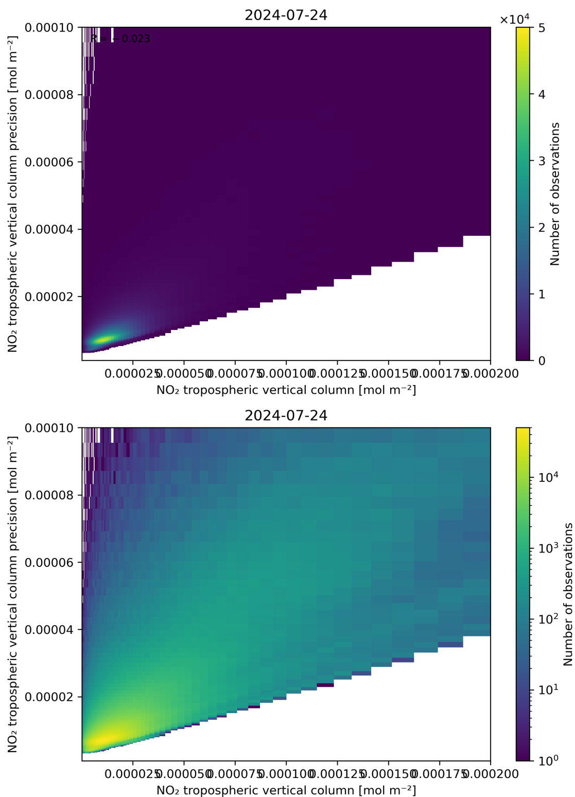
Figure 130: Scatter density plot of “NO 2 tropospheric vertical column” against “NO 2 tropospheric vertical column precision” for 2024-07-23 to 2024-07-24.
