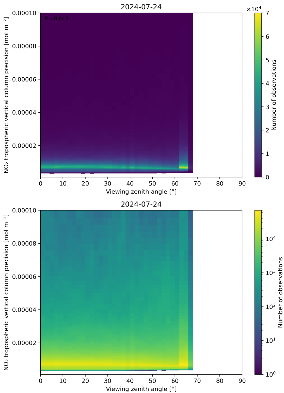
Figure 170: Scatter density plot of “Viewing zenith angle” against “NO 2 tropospheric vertical column precision” for 2024-07-23 to 2024-07-24.
