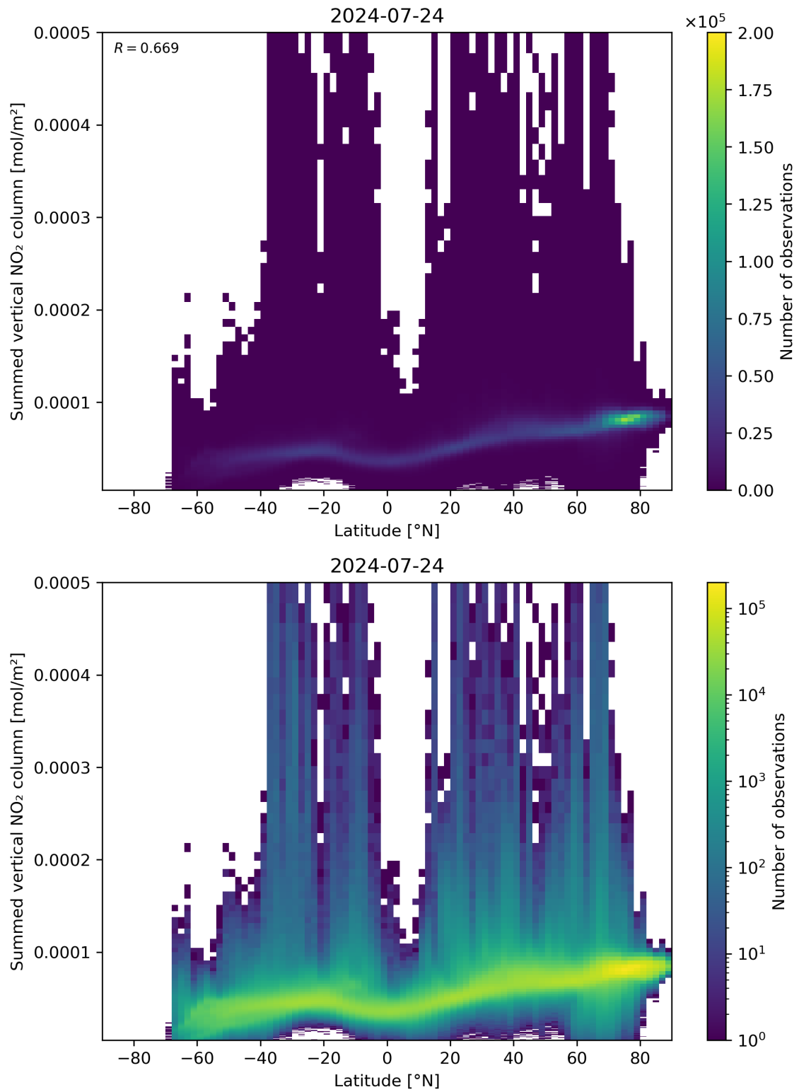
Figure 88: Scatter density plot of “Latitude” against “Summed vertical NO 2 column” for 2024-07-23 to 2024-07-24.
