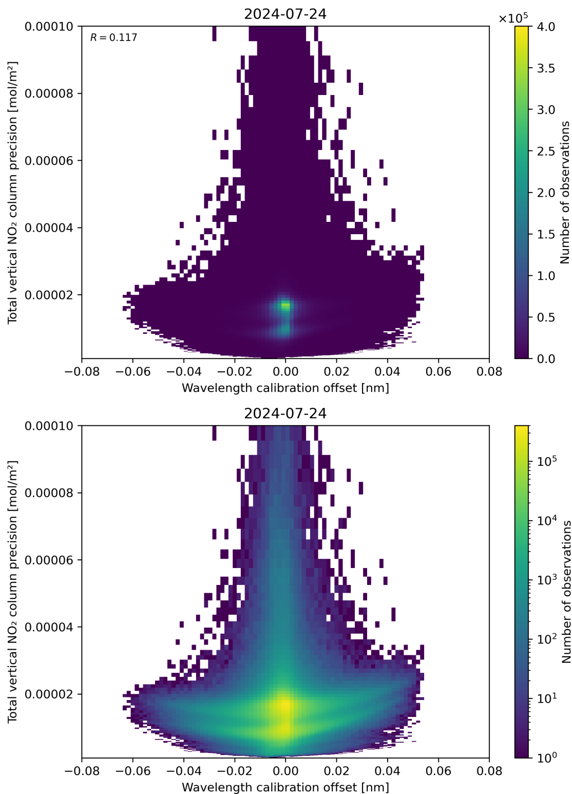
Figure 180: Scatter density plot of “Wavelength calibration offset” against “Total vertical NO 2 column precision” for 2024-07-23 to 2024-07-24.
