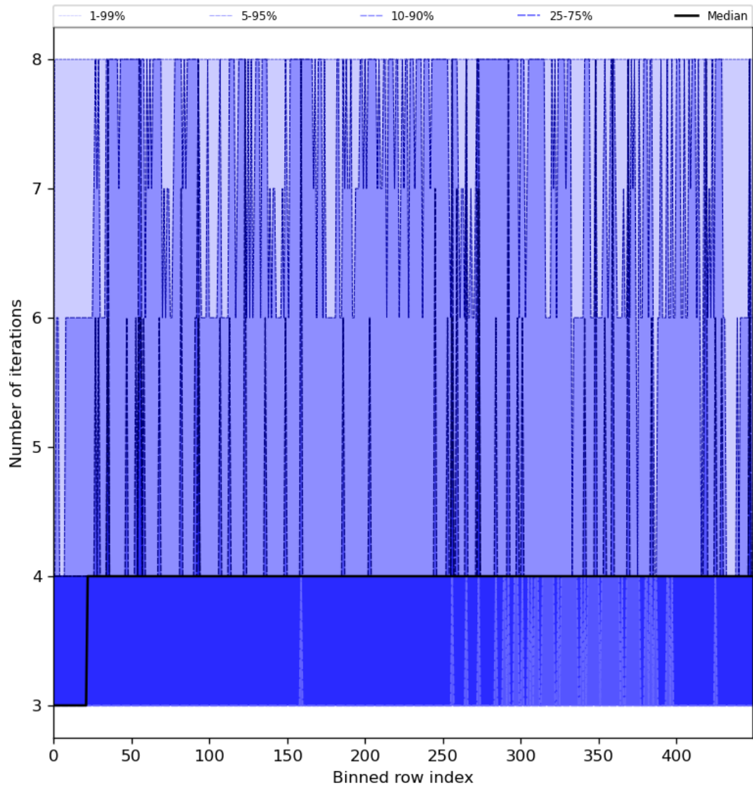
Figure 51: Along track statistics of “Number of iterations” for 2024-07-23 to 2024-07-24
