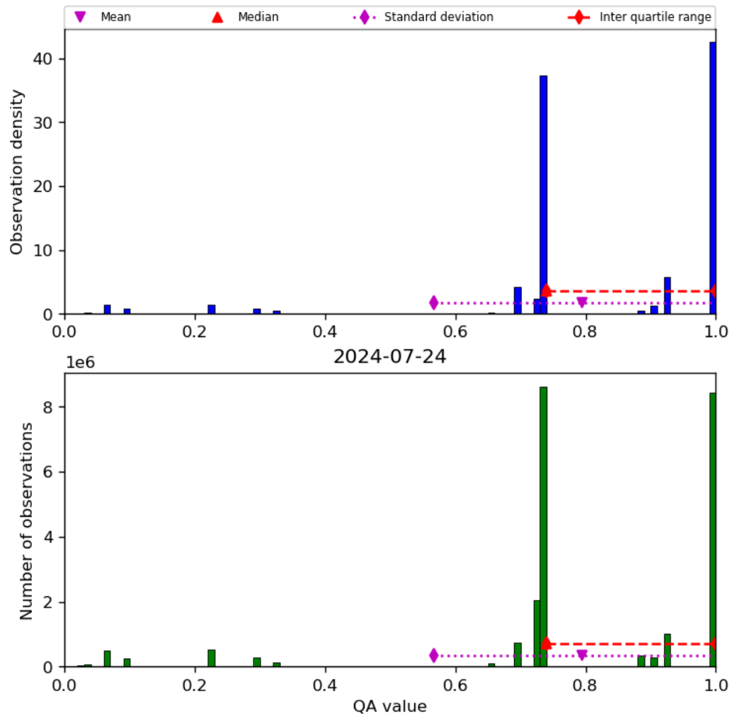
Figure 28: Histogram of “QA value” for 2024-07-23 to 2024-07-24
