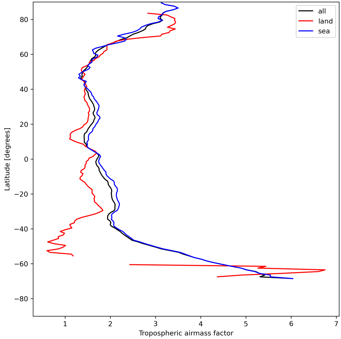
Figure 14: Zonal average of “Tropospheric airmass factor” for 2024-07-23 to 2024-07-24.
