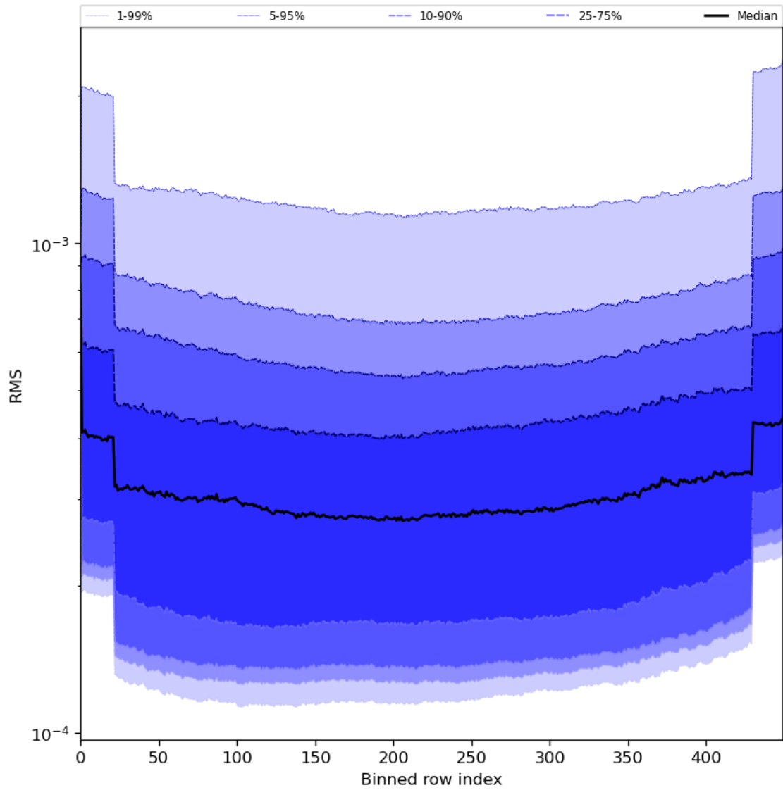
Figure 60: Along track statistics of “RMS” for 2024-07-23 to 2024-07-24
