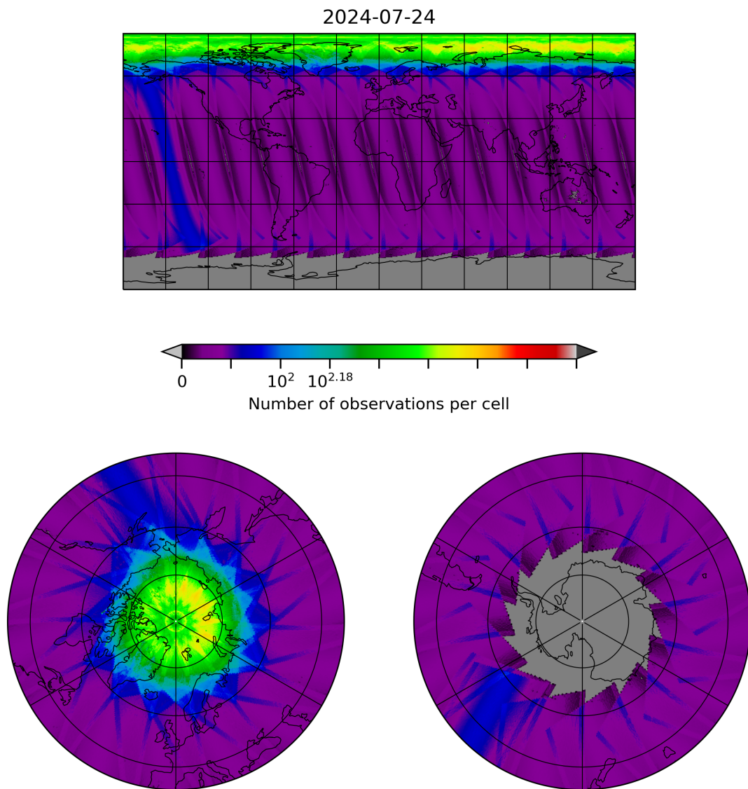
Figure 10: Map of the number of observations for 2024-07-23 to 2024-07-24
