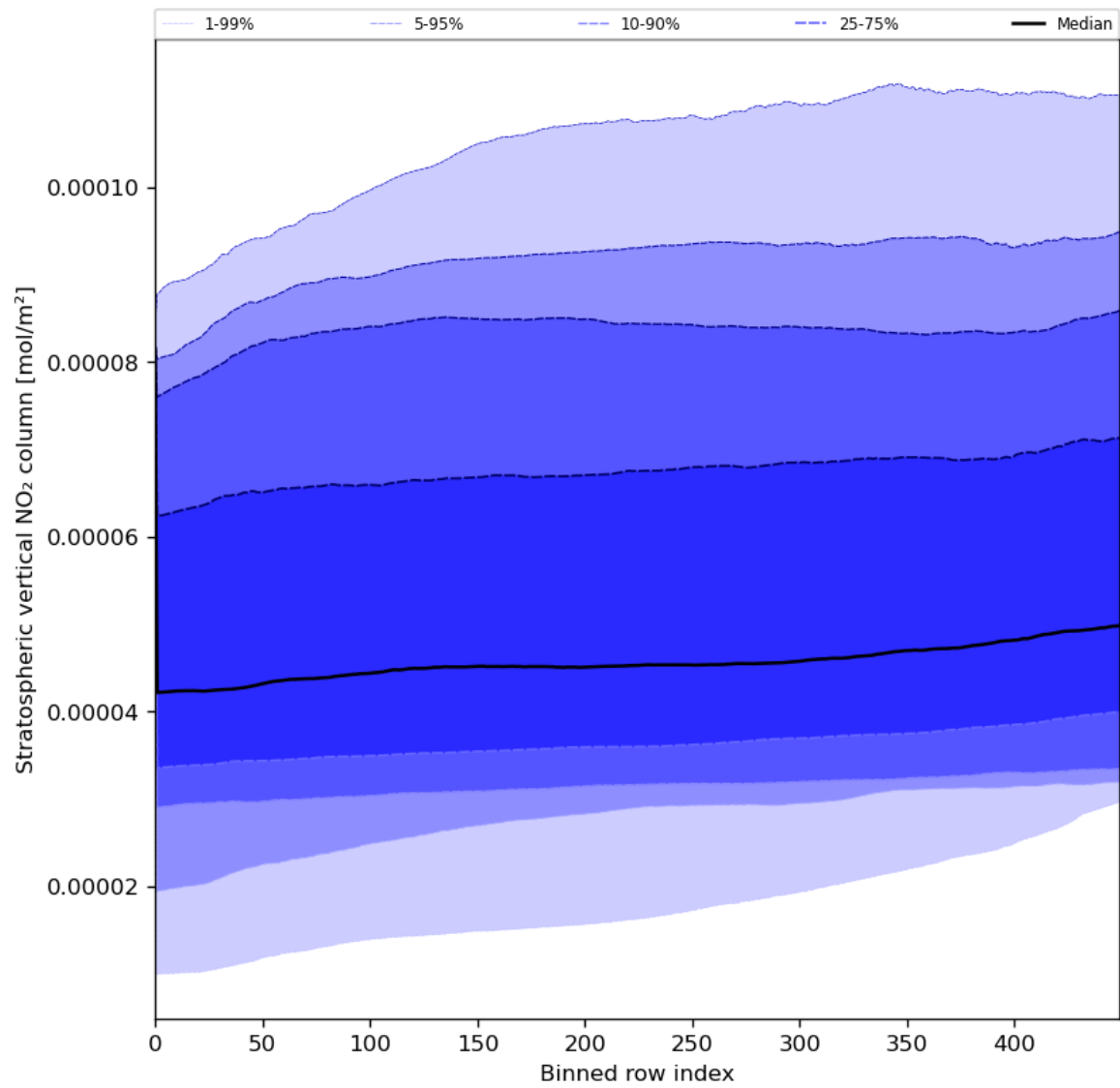
Figure 53: Along track statistics of “Stratospheric vertical NO 2 column” for 2024-07-23 to 2024-07-24
