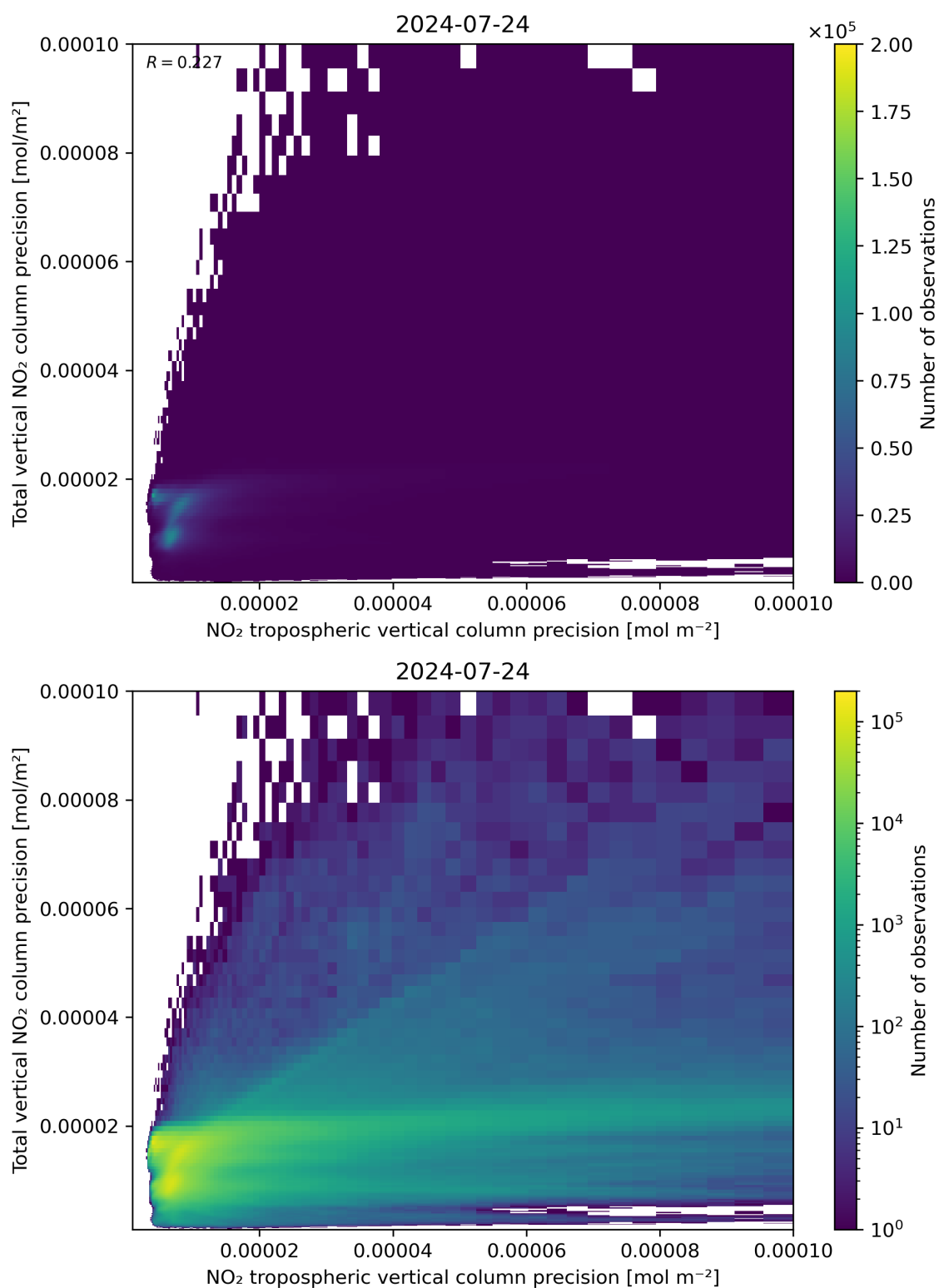
Figure 139: Scatter density plot of “NO 2 tropospheric vertical column precision” against “Total vertical NO 2 column precision” for 2024-07-23 to 2024-07-24.
