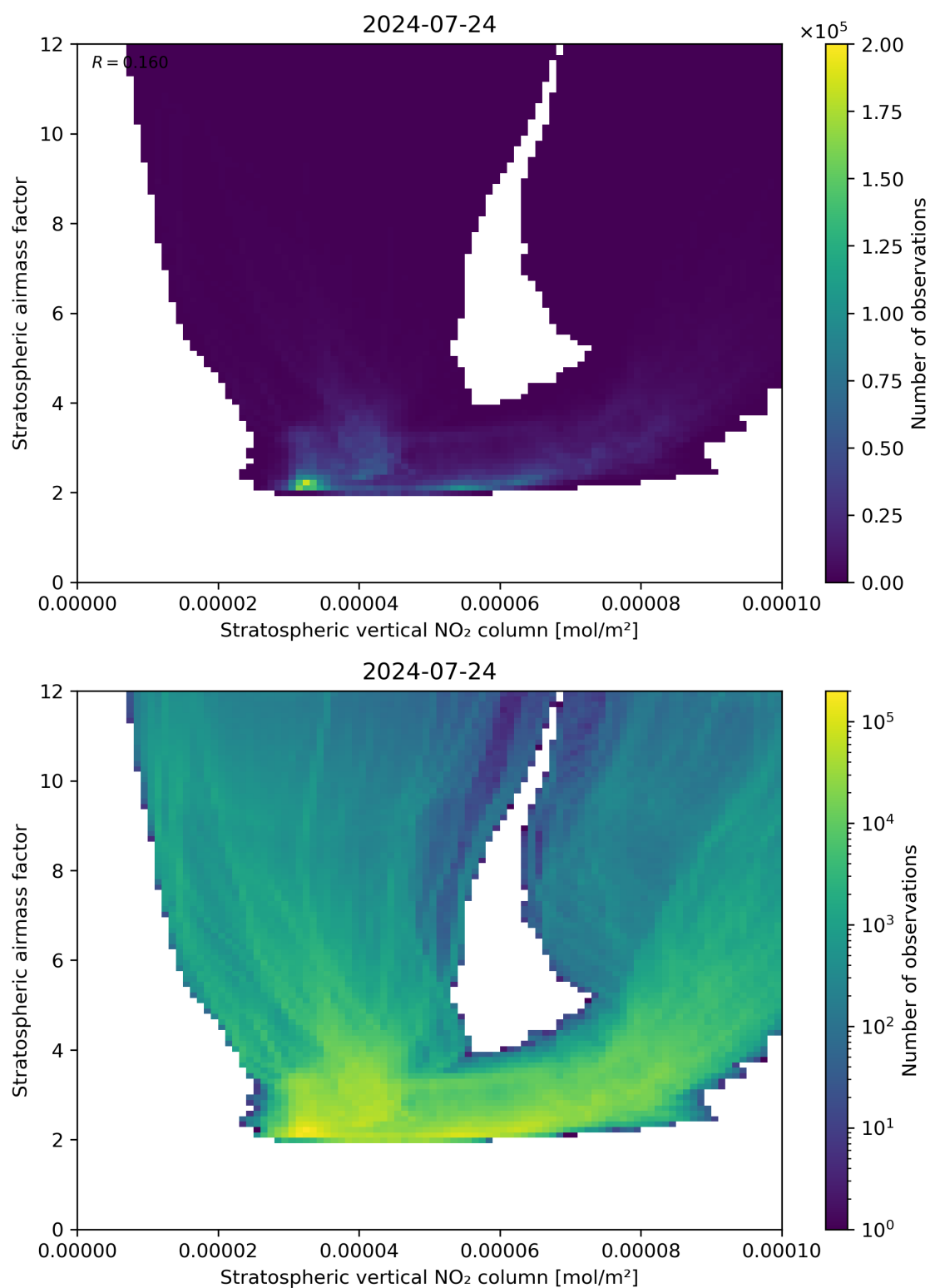
Figure 96: Scatter density plot of “Stratospheric vertical NO 2 column” against “Stratospheric airmass factor” for 2024-07-23 to 2024-07-24.
