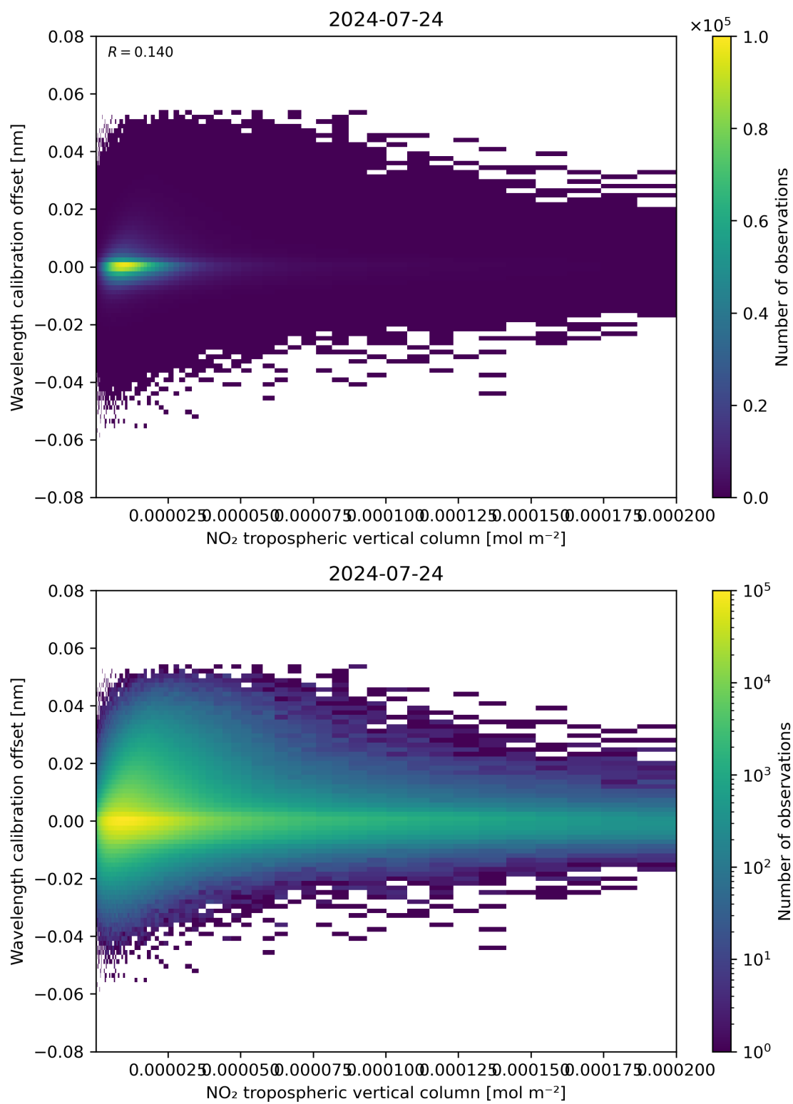
Figure 143: Scatter density plot of “NO 2 tropospheric vertical column” against “Wavelength calibration offset” for 2024-07-23 to 2024-07-24.
