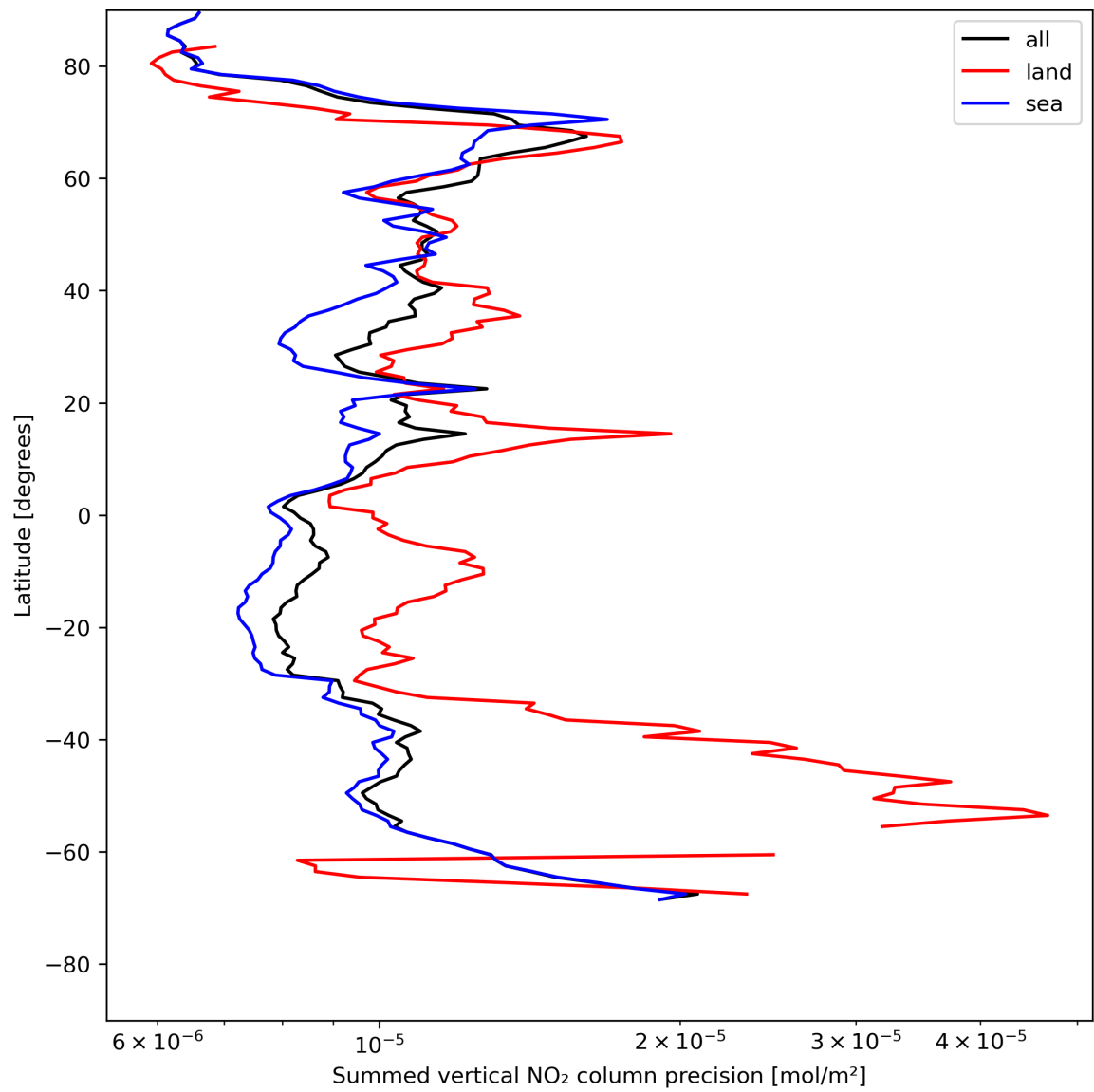
Figure 24: Zonal average of “Summed vertical NO 2 column precision” for 2024-07-23 to 2024-07-24.
