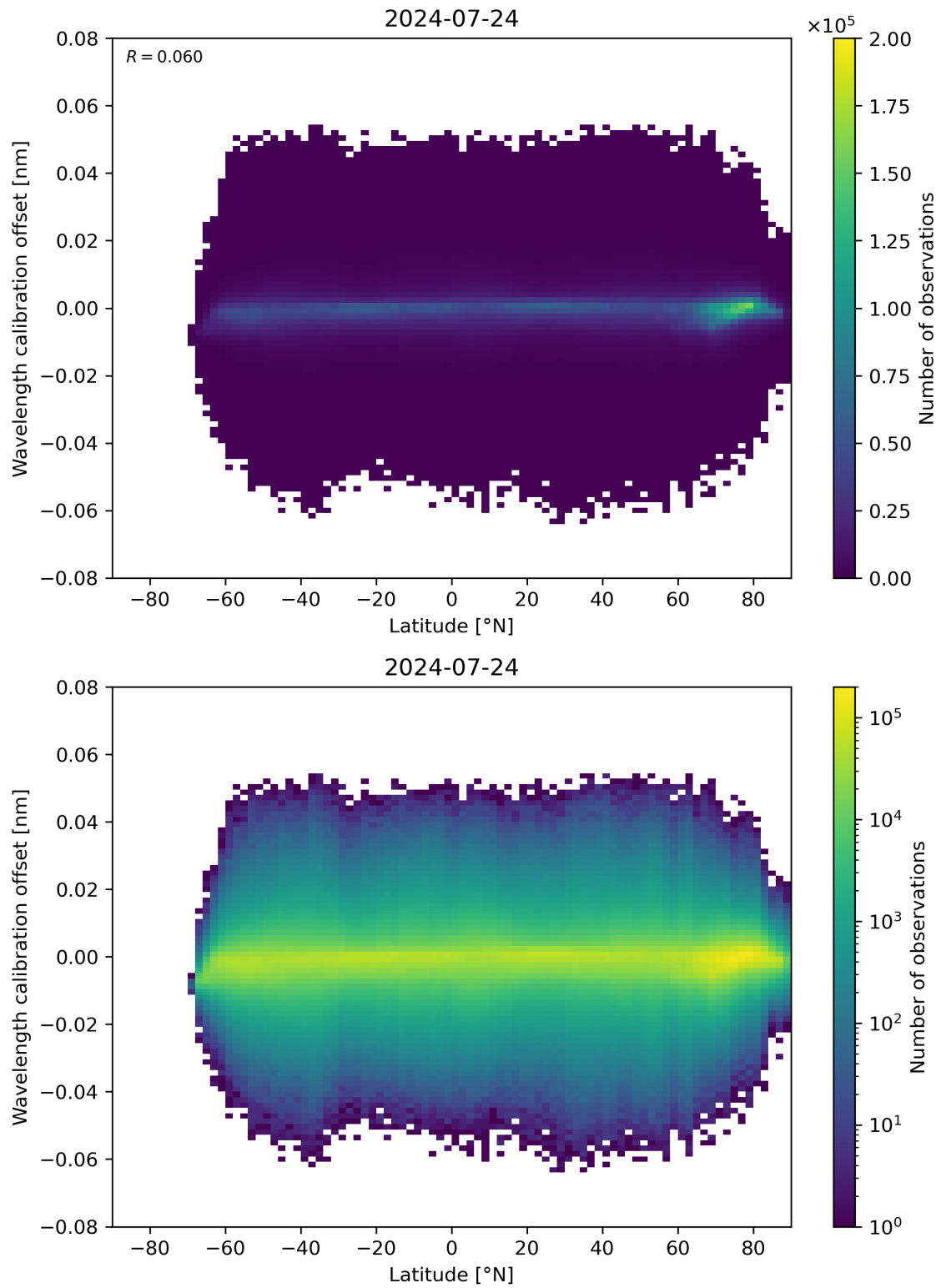
Figure 95: Scatter density plot of “Latitude” against “Wavelength calibration offset” for 2024-07-23 to 2024-07-24.
