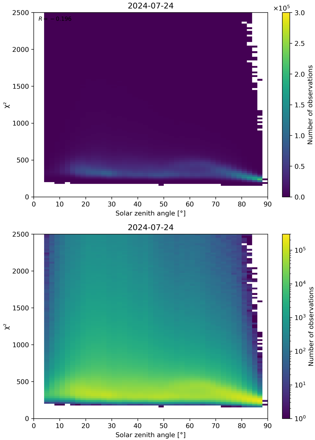
Figure 148: Scatter density plot of “Solar zenith angle” against “ \chi^2 ” for 2024-07-23 to 2024-07-24.
