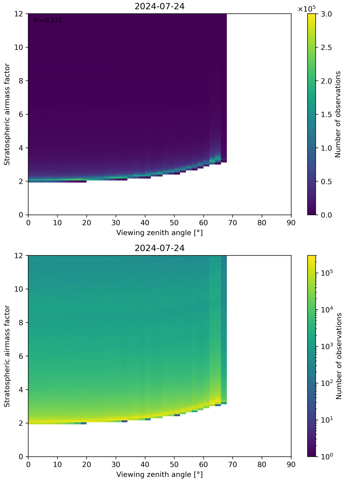
Figure 159: Scatter density plot of “Viewing zenith angle” against “Stratospheric airmass factor” for 2024-07-23 to 2024-07-24.
