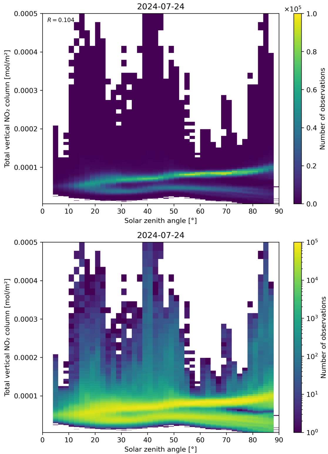
Figure 153: Scatter density plot of “Solar zenith angle” against “Total vertical NO 2 column” for 2024-07-23 to 2024-07-24.
