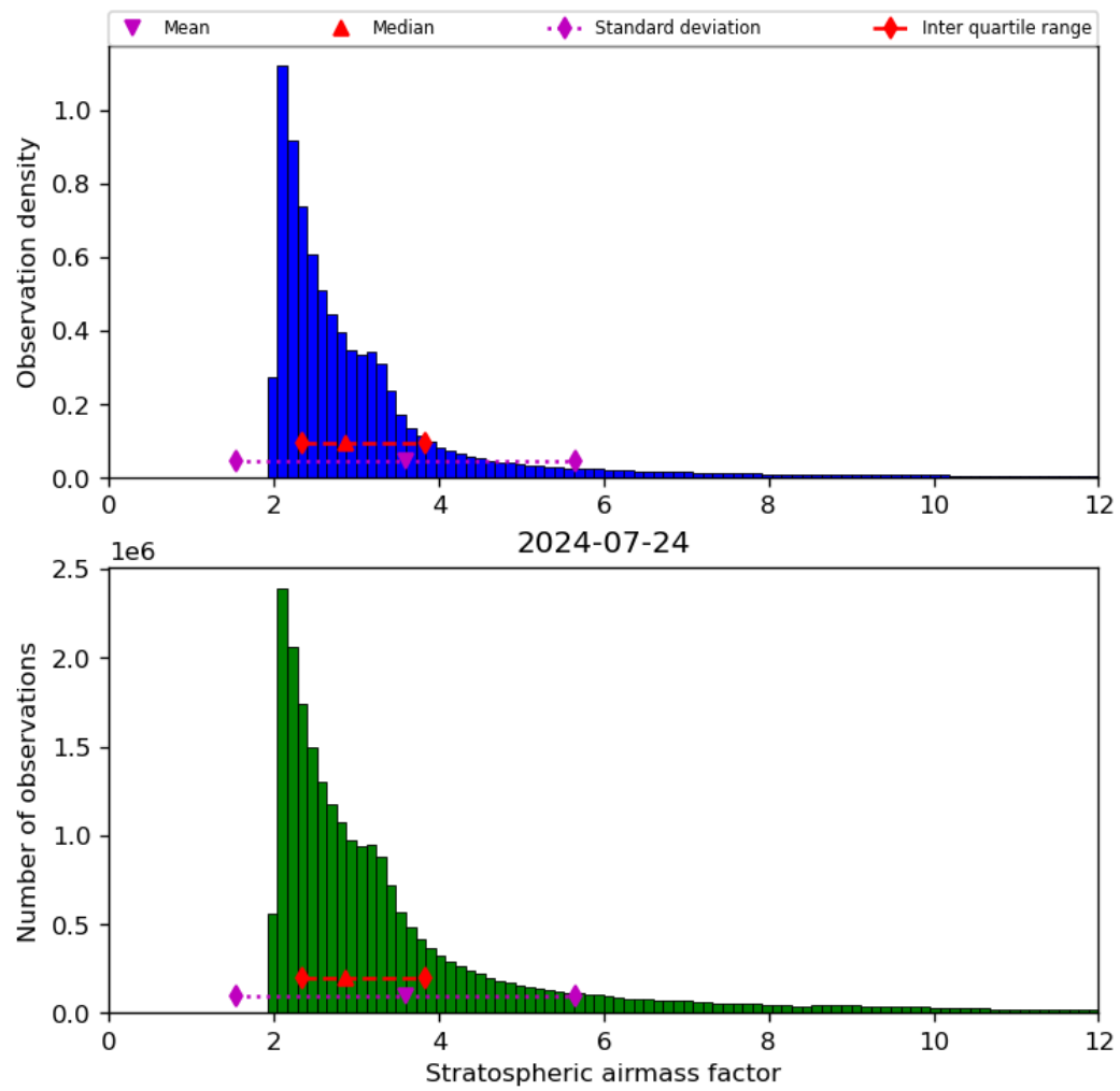
Figure 44: Histogram of “Stratospheric airmass factor” for 2024-07-23 to 2024-07-24
