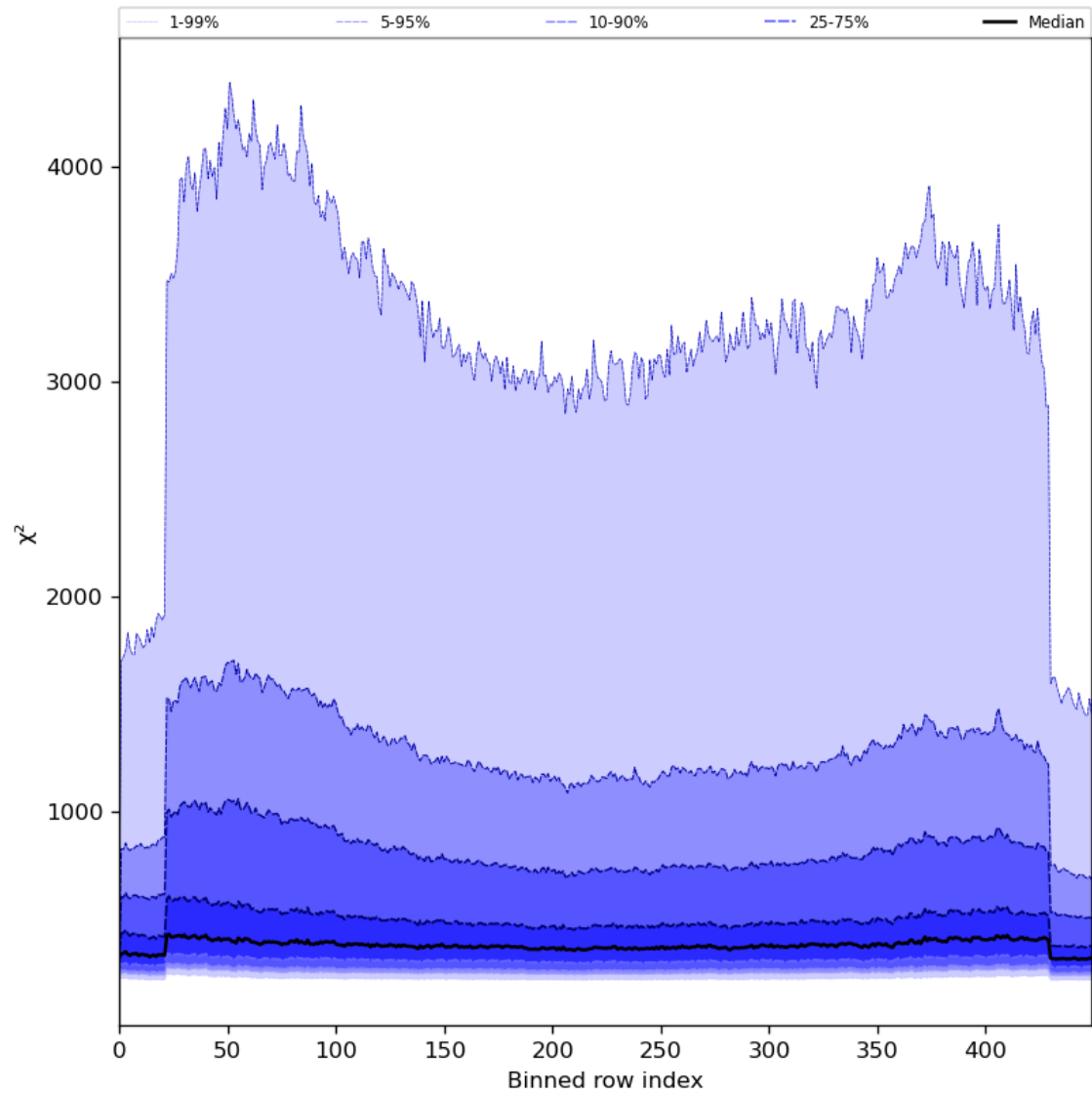
Figure 59: Along track statistics of “ \chi^2 ” for 2024-07-23 to 2024-07-24
