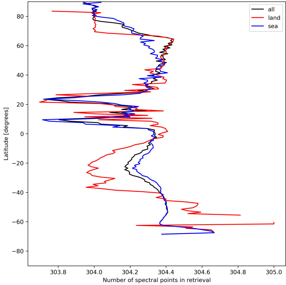
Figure 16: Zonal average of “Number of spectral points in retrieval” for 2024-07-23 to 2024-07-24.
