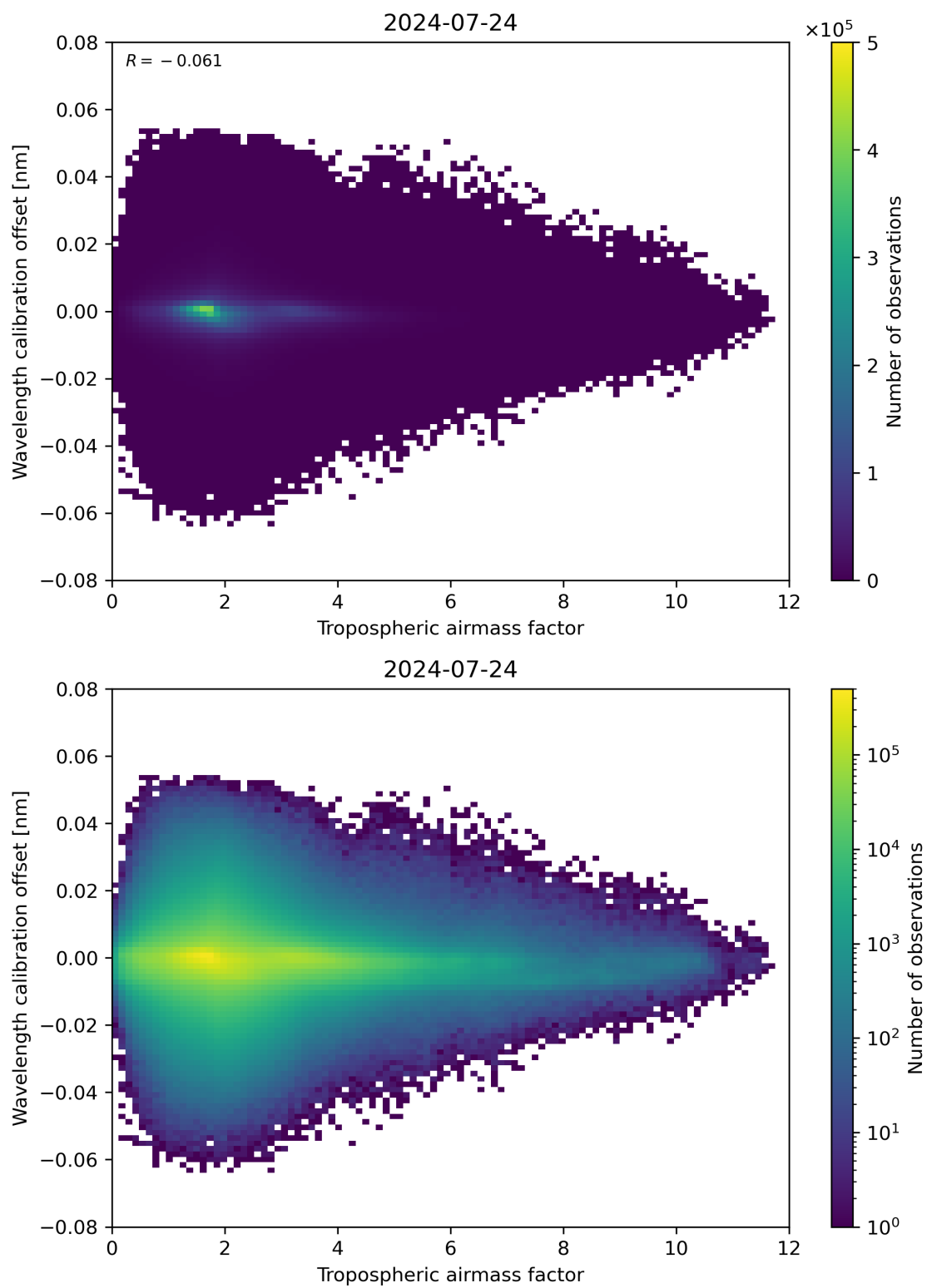
Figure 80: Scatter density plot of “Tropospheric air mass factor” against “Wavelength calibration offset” for 2024-07-23 to 2024-07-24.
