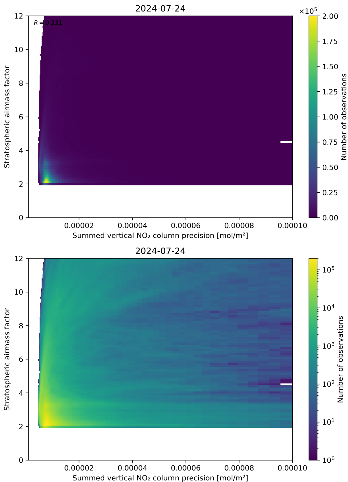
Figure 106: Scatter density plot of “Summed vertical NO 2 column precision” against “Stratospheric airmass factor” for 2024-07-23 to 2024-07-24.
