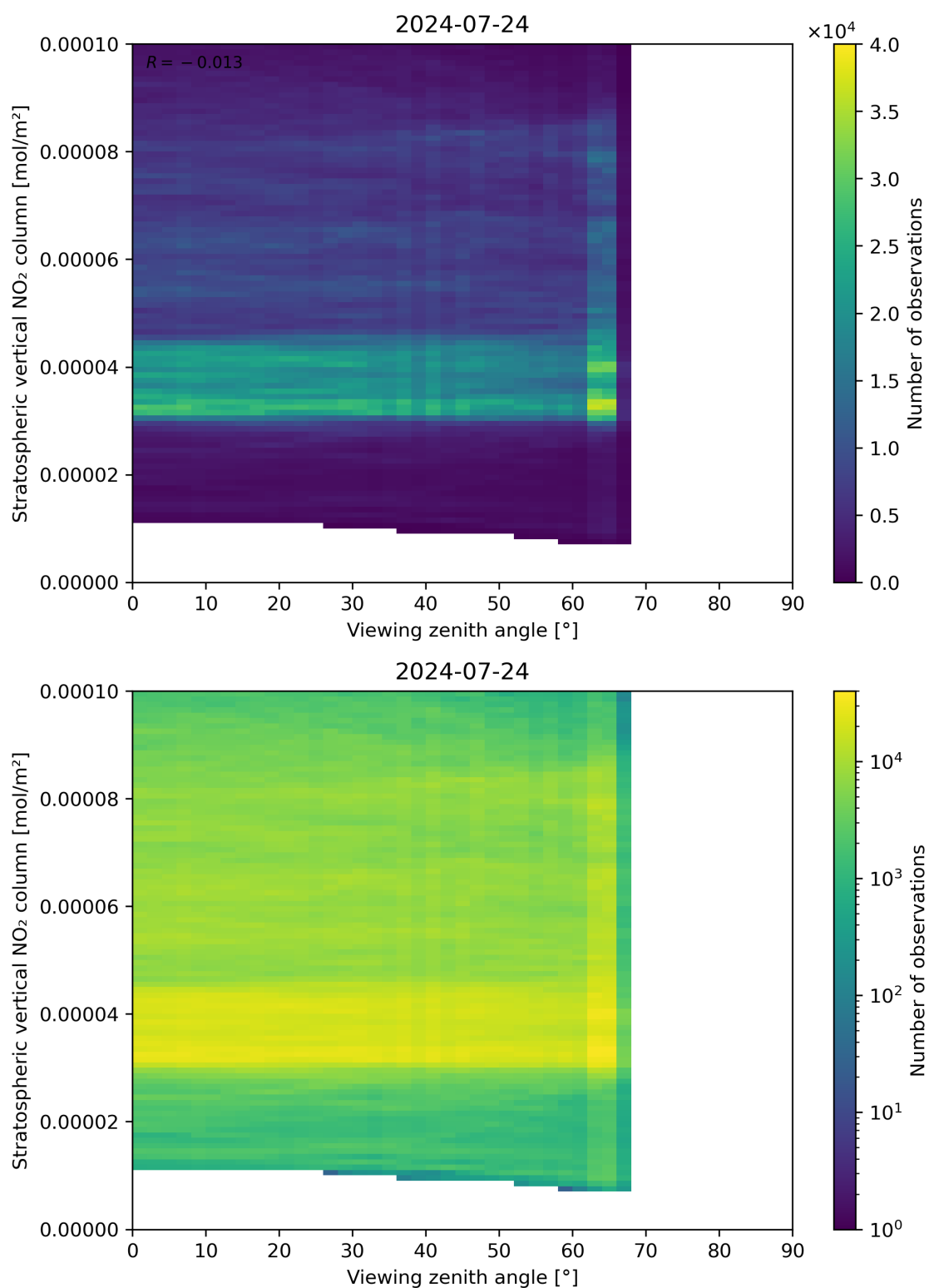
Figure 164: Scatter density plot of “Viewing zenith angle” against “Stratospheric vertical NO 2 column” for 2024-07-23 to 2024-07-24.
