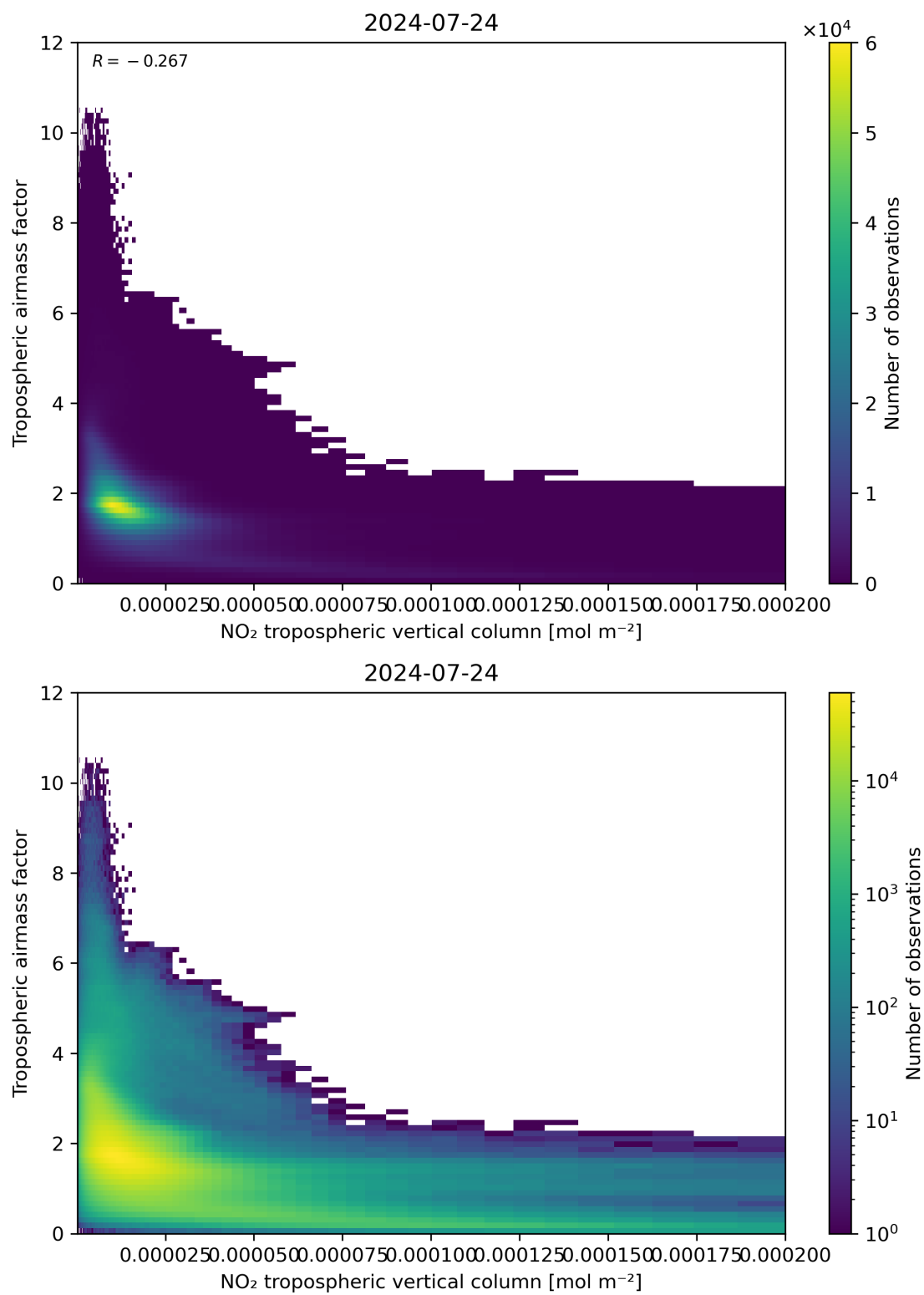
Figure 123: Scatter density plot of “NO 2 tropospheric vertical column” against “Tropospheric airmass factor” for 2024-07-23 to 2024-07-24.
