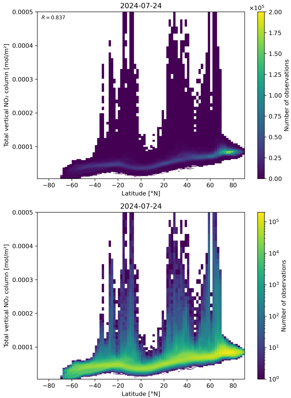
Figure 90: Scatter density plot of “Latitude” against “Total vertical NO 2 column” for 2024-07-23 to 2024-07-24.
