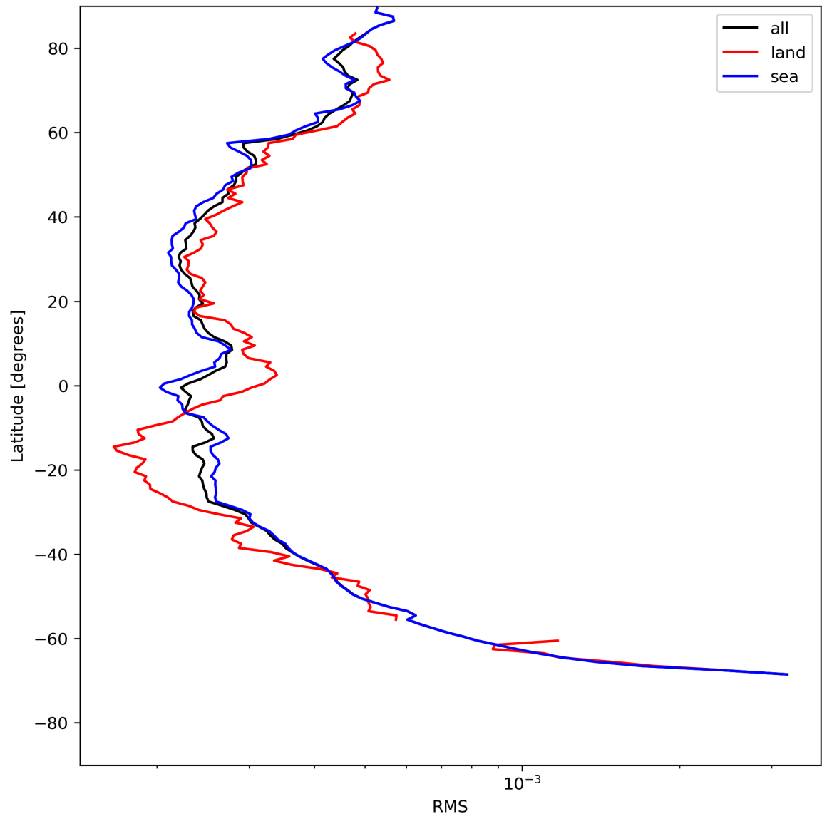
Figure 26: Zonal average of “RMS” for 2024-07-23 to 2024-07-24.
