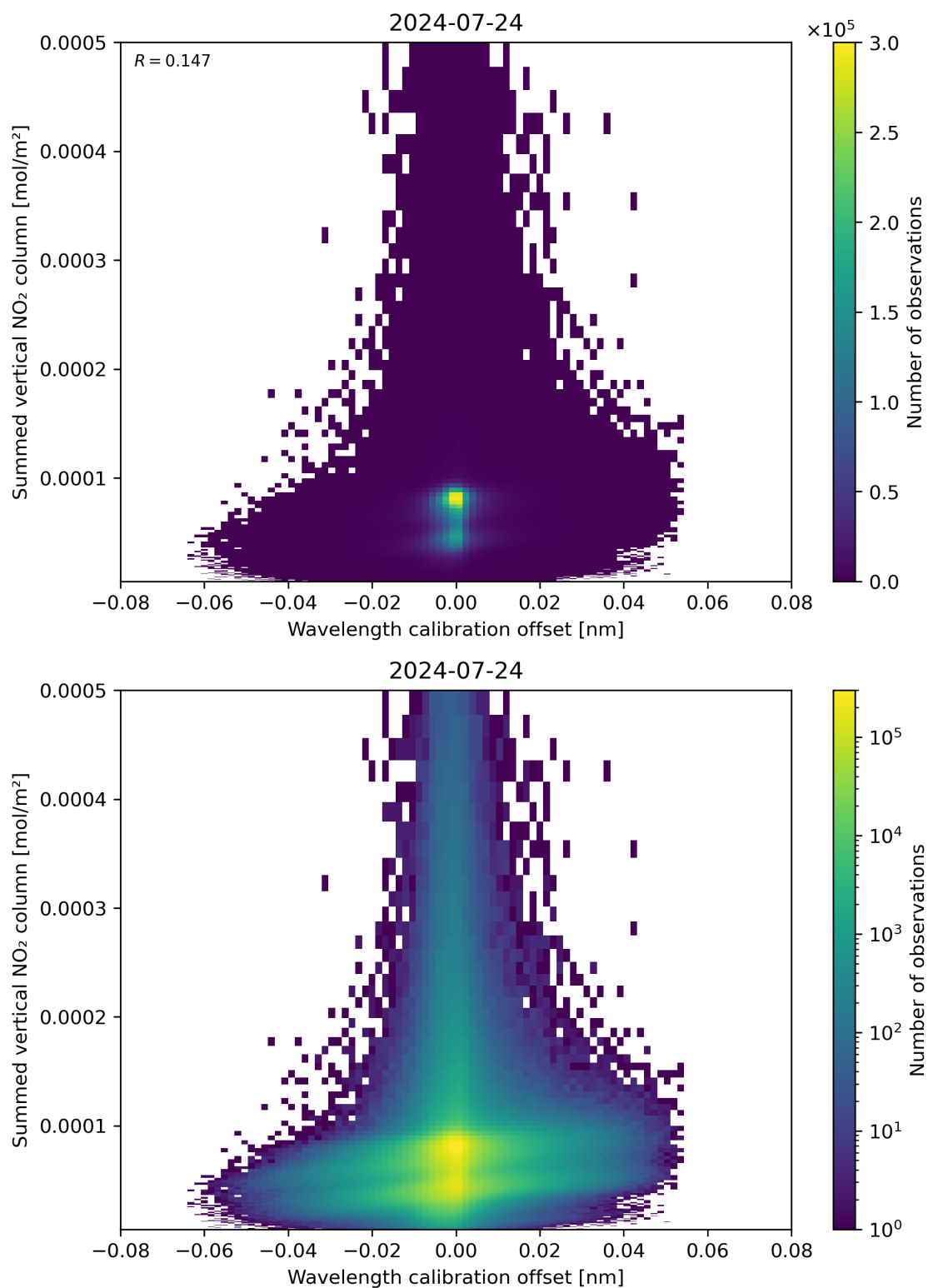
Figure 177: Scatter density plot of “Wavelength calibration offset” against “Summed vertical NO 2 column” for 2024-07-23 to 2024-07-24.
