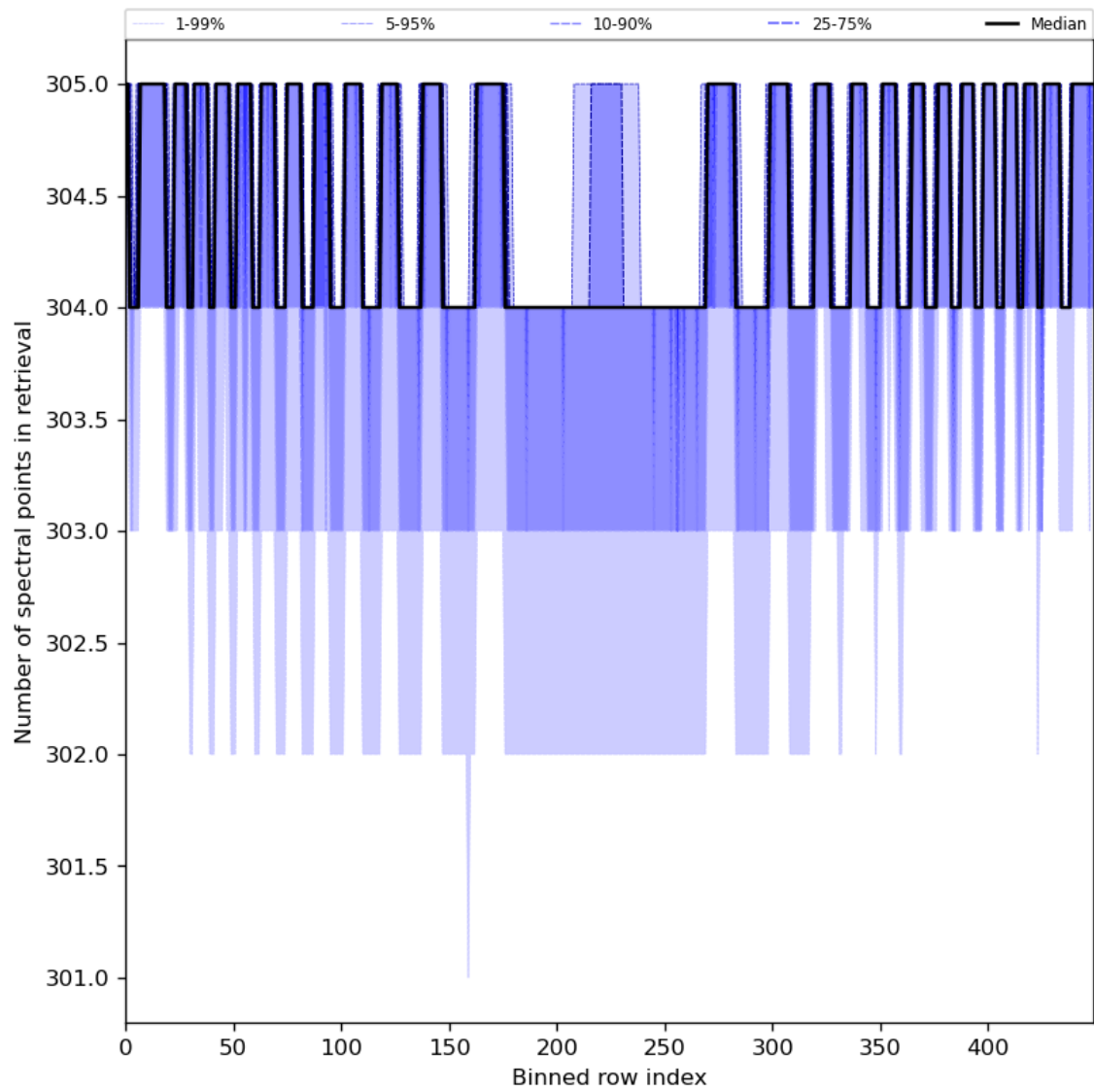
Figure 50: Along track statistics of “Number of spectral points in retrieval” for 2024-07-23 to 2024-07-24
