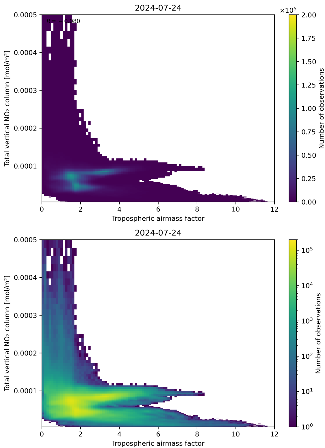
Figure 77: Scatter density plot of “Tropospheric airmass factor” against “Total vertical NO 2 column” for 2024-07-23 to 2024-07-24.
