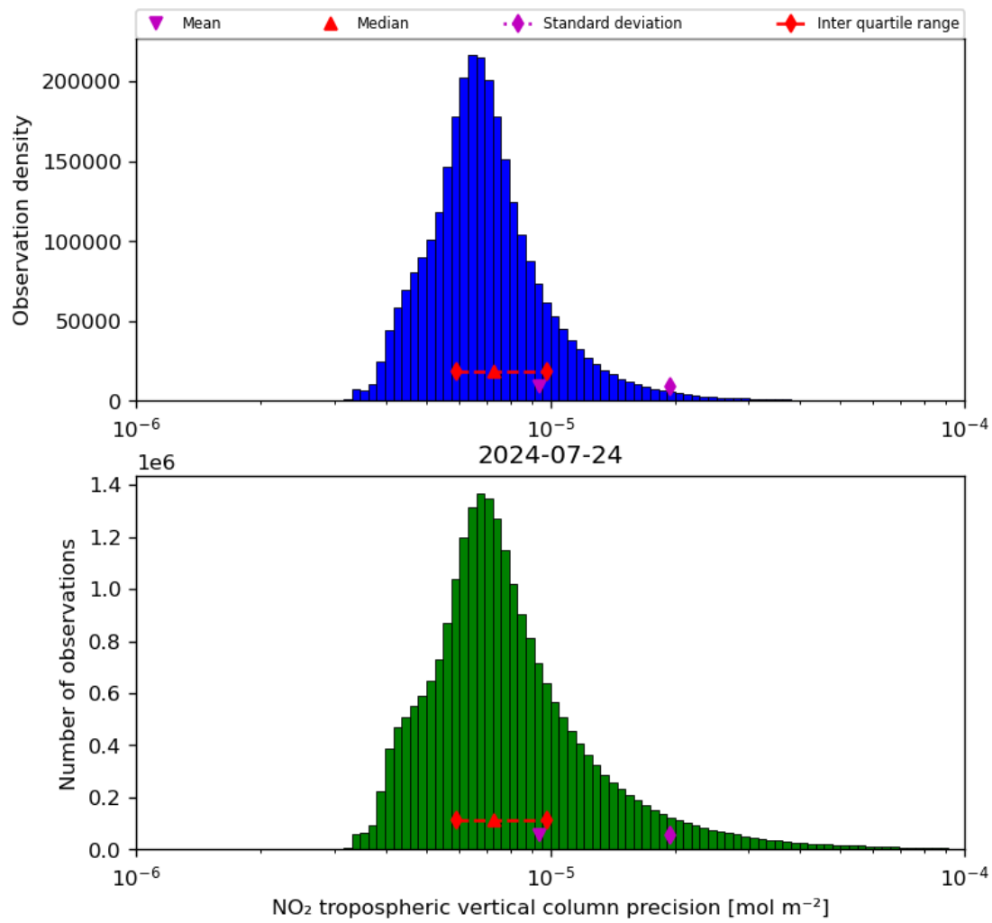
Figure 30: Histogram of “NO 2 tropospheric vertical column precision” for 2024-07-23 to 2024-07-24
