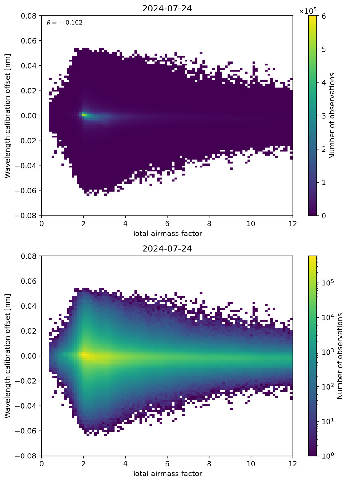
Figure 70: Scatter density plot of “Total airmass factor” against “Wavelength calibration offset” for 2024-07-23 to 2024-07-24.
