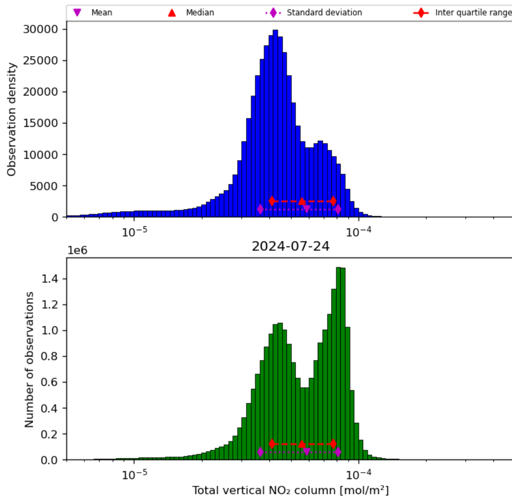
Figure 38: Histogram of “Total vertical NO 2 column” for 2024-07-23 to 2024-07-24
