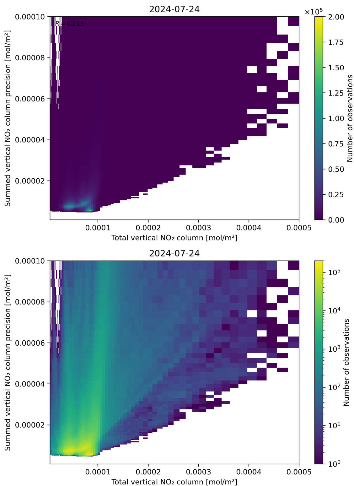
Figure 113: Scatter density plot of “Total vertical NO 2 column” against “Summed vertical NO 2 column precision” for 2024-07-23 to 2024-07-24.
