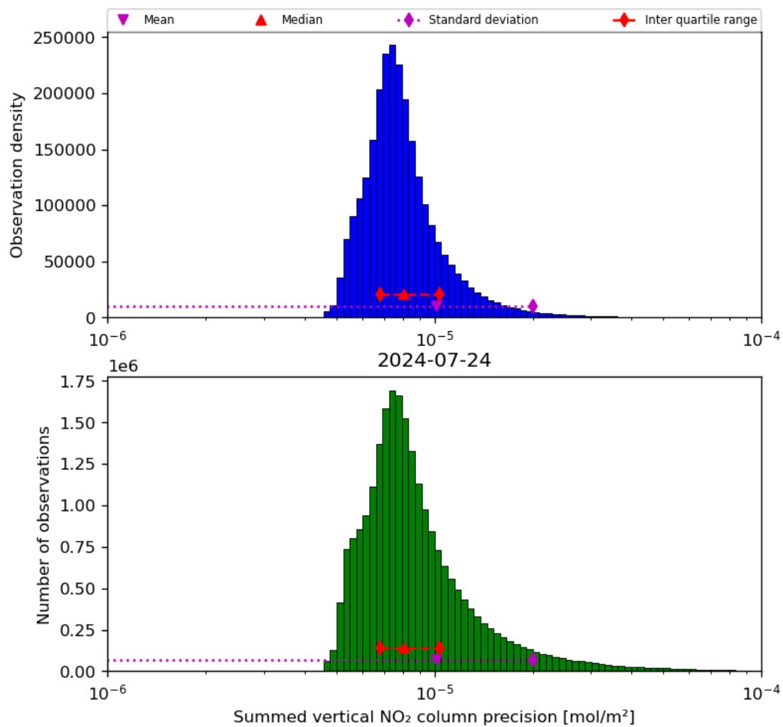
Figure 41: Histogram of “Summed vertical NO 2 column precision” for 2024-07-23 to 2024-07-24
