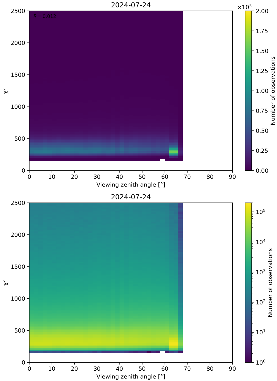
Figure 162: Scatter density plot of “Viewing zenith angle” against “ \chi^2 ” for 2024-07-23 to 2024-07-24.
