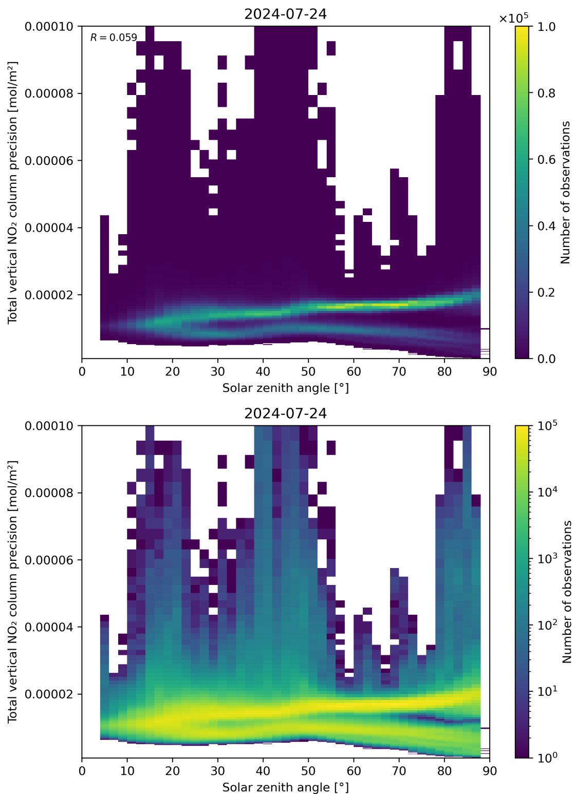
Figure 154: Scatter density plot of “Solar zenith angle” against “Total vertical NO 2 column precision” for 2024-07-23 to 2024-07-24.
