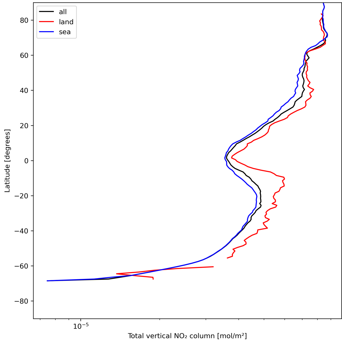
Figure 21: Zonal average of “Total vertical NO 2 column” for 2024-07-23 to 2024-07-24.
