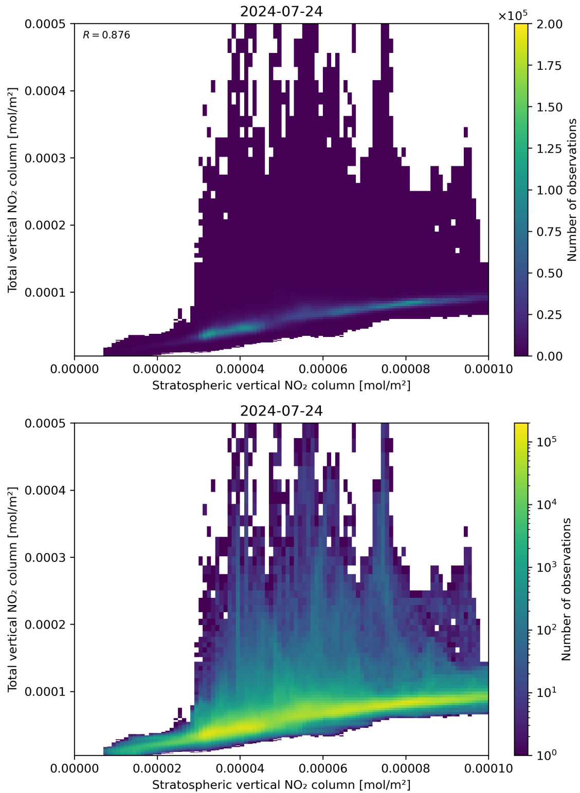
Figure 100: Scatter density plot of “Stratospheric vertical NO 2 column” against “Total vertical NO 2 column” for 2024-07-23 to 2024-07-24.
