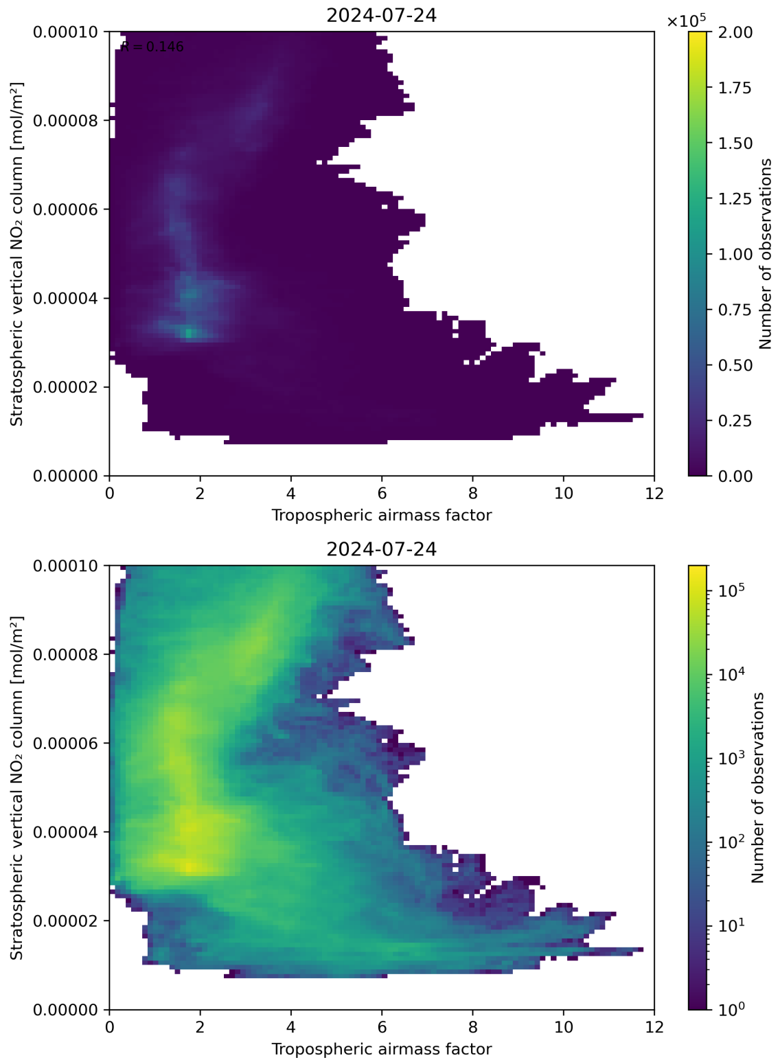
Figure 74: Scatter density plot of “Tropospheric air mass factor” against “Stratospheric vertical NO 2 column” for 2024-07-23 to 2024-07-24.
