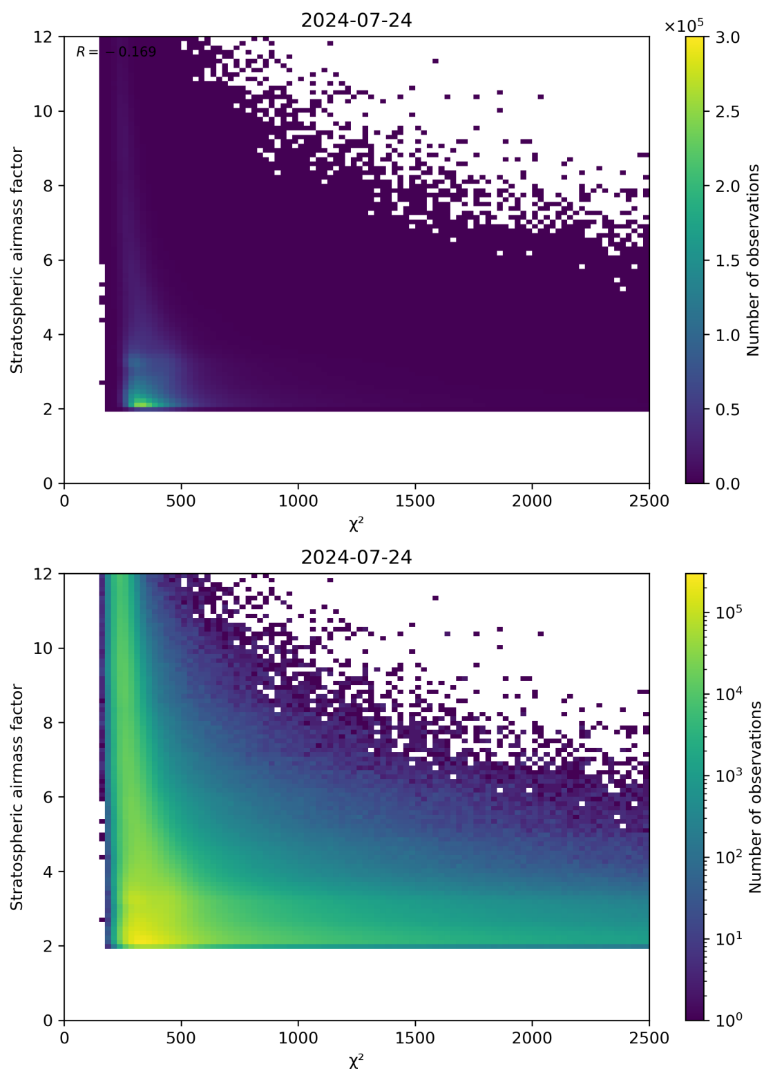
Figure 81: Scatter density plot of “ \chi^2 ” against “Stratospheric airmass factor” for 2024-07-23 to 2024-07-24.
