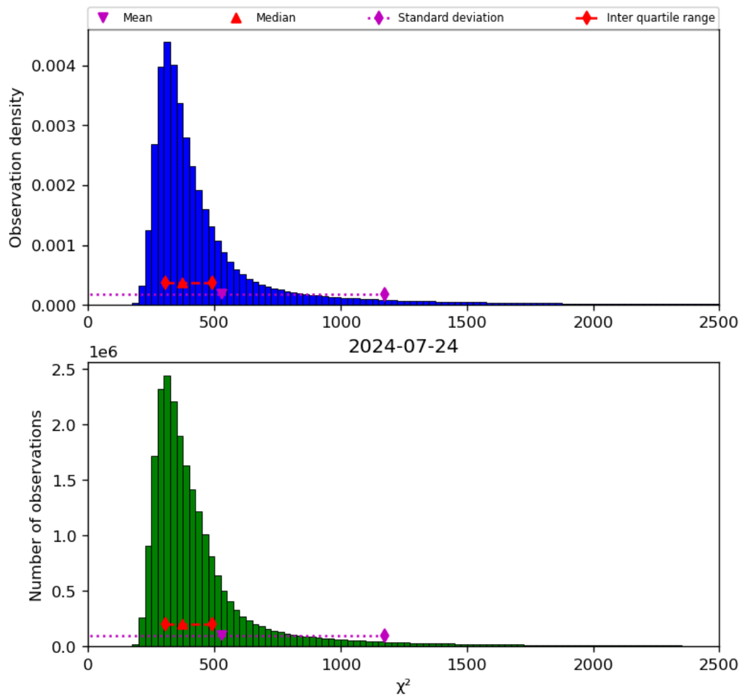
Figure 42: Histogram of “ \chi^2 ” for 2024-07-23 to 2024-07-24
