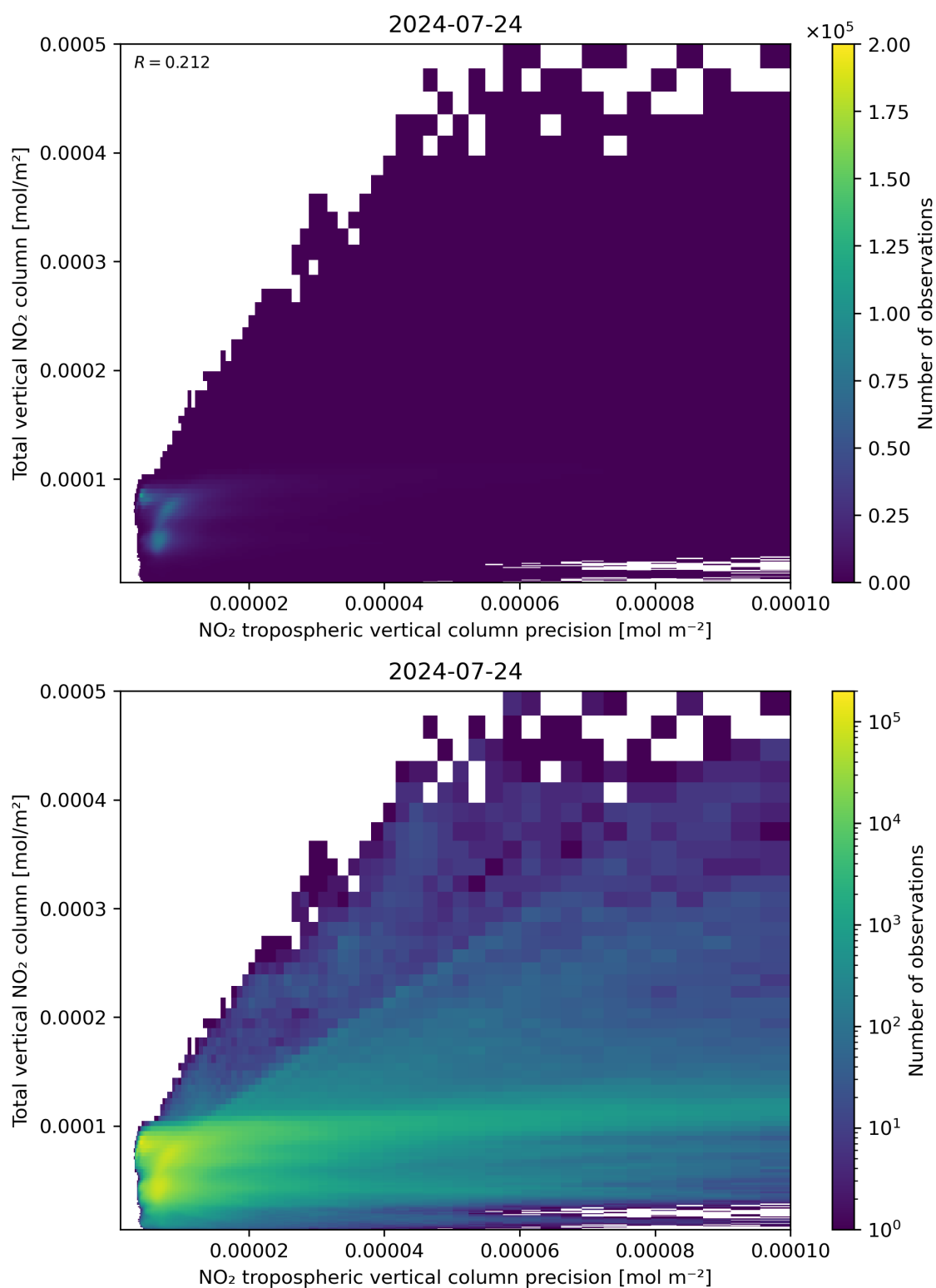
Figure 138: Scatter density plot of “NO 2 tropospheric vertical column precision” against “Total vertical NO 2 column” for 2024-07-23 to 2024-07-24.
