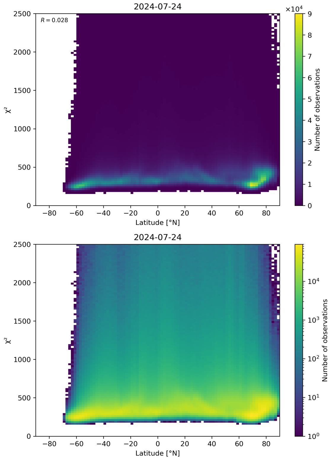
Figure 86: Scatter density plot of “Latitude” against “ \chi^2 ” for 2024-07-23 to 2024-07-24.
