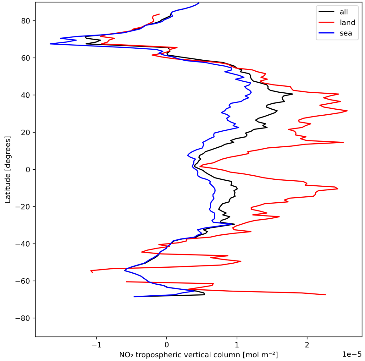
Figure 12: Zonal average of “NO 2 tropospheric vertical column” for 2024-07-23 to 2024-07-24.
