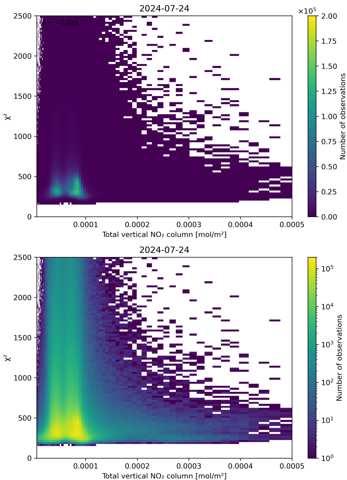
Figure 111: Scatter density plot of “Total vertical NO 2 column” against “ \chi^2 ” for 2024-07-23 to 2024-07-24.
