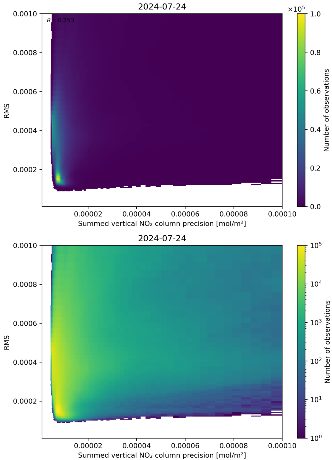
Figure 108: Scatter density plot of “Summed vertical NO 2 column precision” against “RMS” for 2024-07-23 to 2024-07-24.
