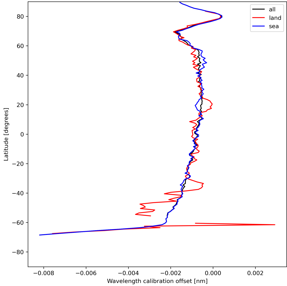
Figure 18: Zonal average of “Wavelength calibration offset” for 2024-07-23 to 2024-07-24.
