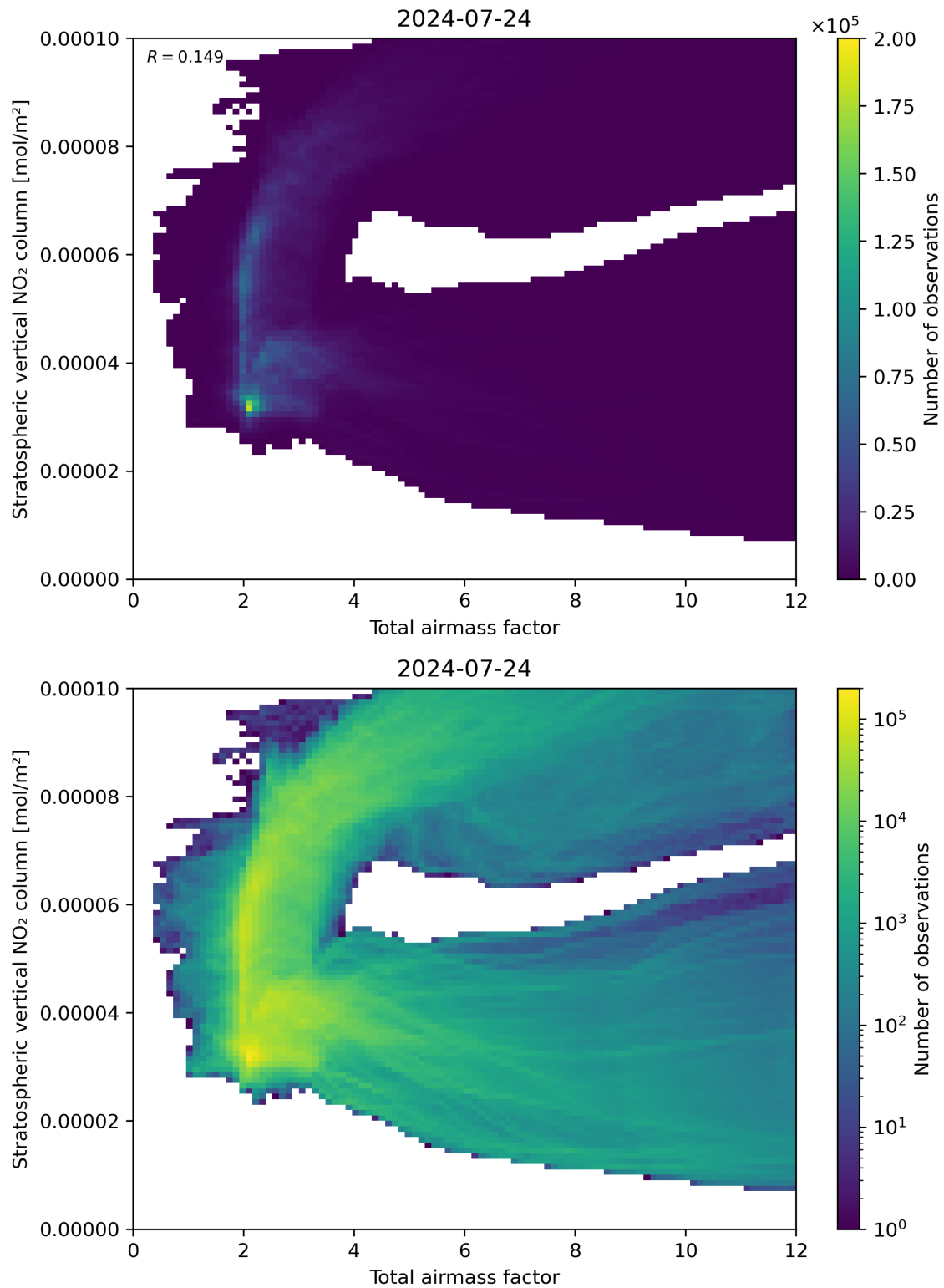
Figure 64: Scatter density plot of “Total airmass factor” against “Stratospheric vertical NO 2 column” for 2024-07-23 to 2024-07-24.
