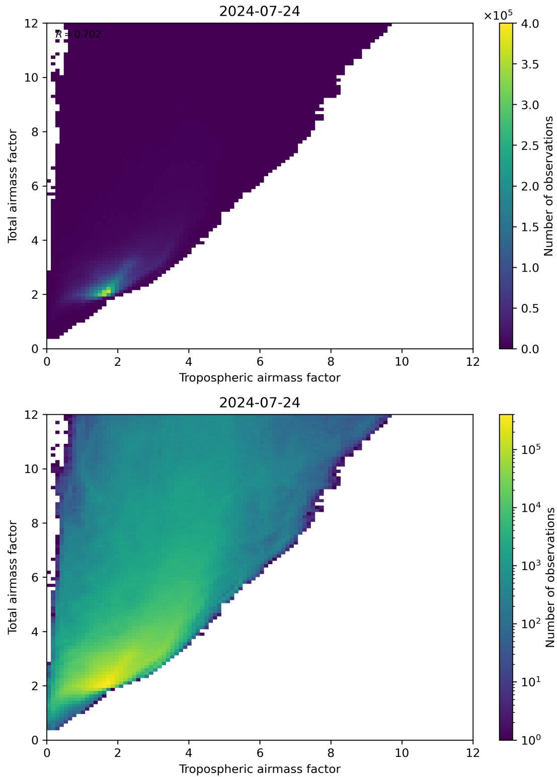
Figure 72: Scatter density plot of “Tropospheric airmass factor” against “Total airmass factor” for 2024-07-23 to 2024-07-24.
