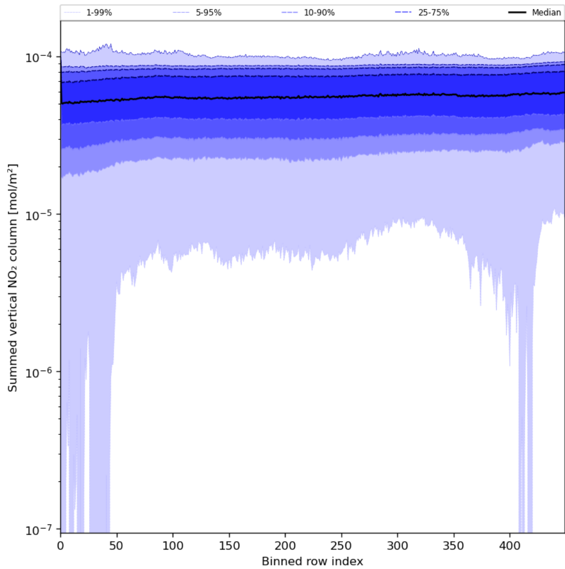
Figure 57: Along track statistics of “Summed vertical NO 2 column” for 2024-07-23 to 2024-07-24
