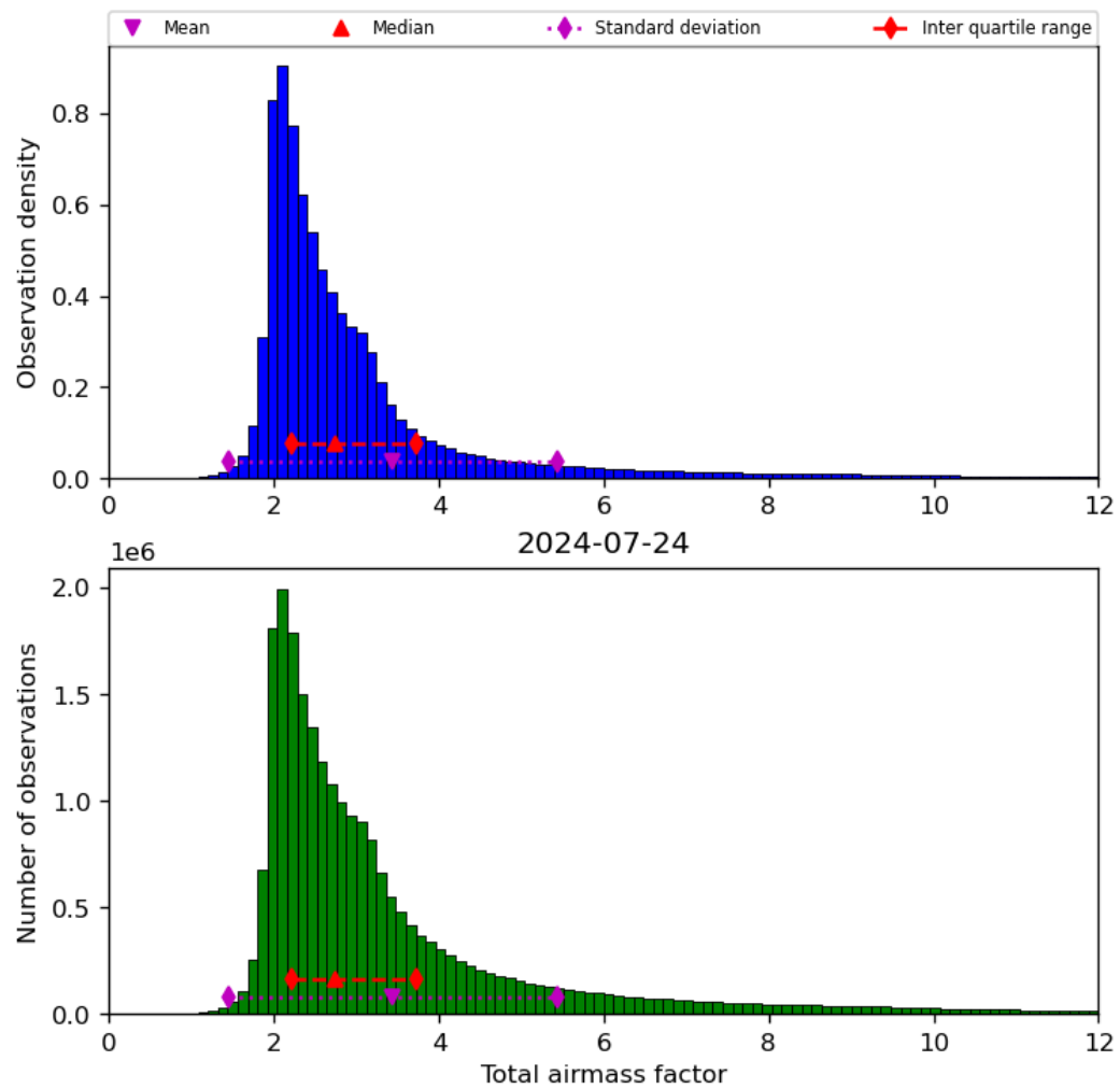
Figure 32: Histogram of “Total airmass factor” for 2024-07-23 to 2024-07-24
