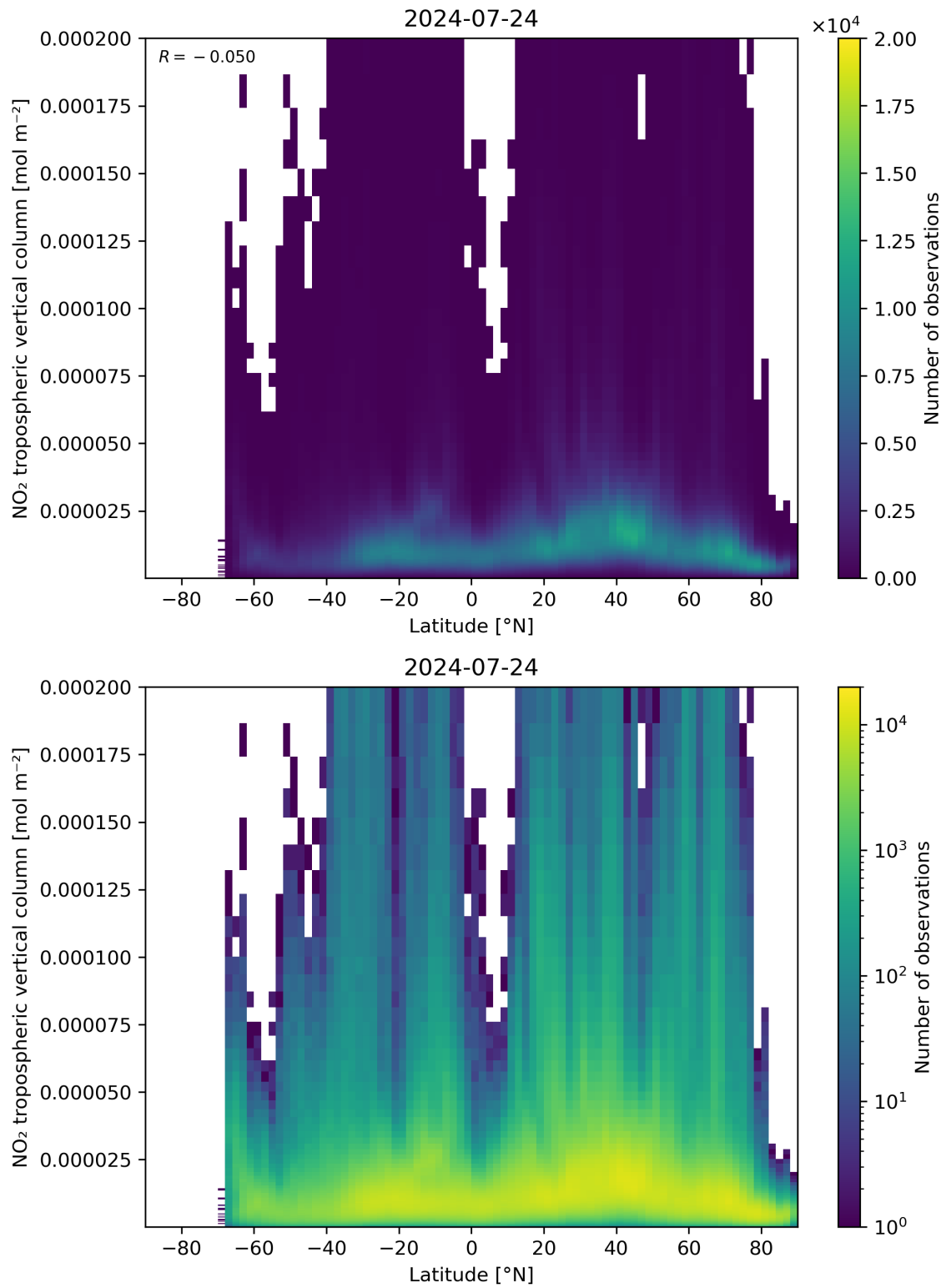
Figure 92: Scatter density plot of “Latitude” against “NO 2 tropospheric vertical column” for 2024-07-23 to 2024-07-24.
