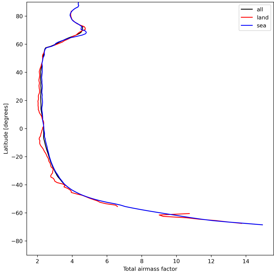
Figure 15: Zonal average of “Total airmass factor” for 2024-07-23 to 2024-07-24.
