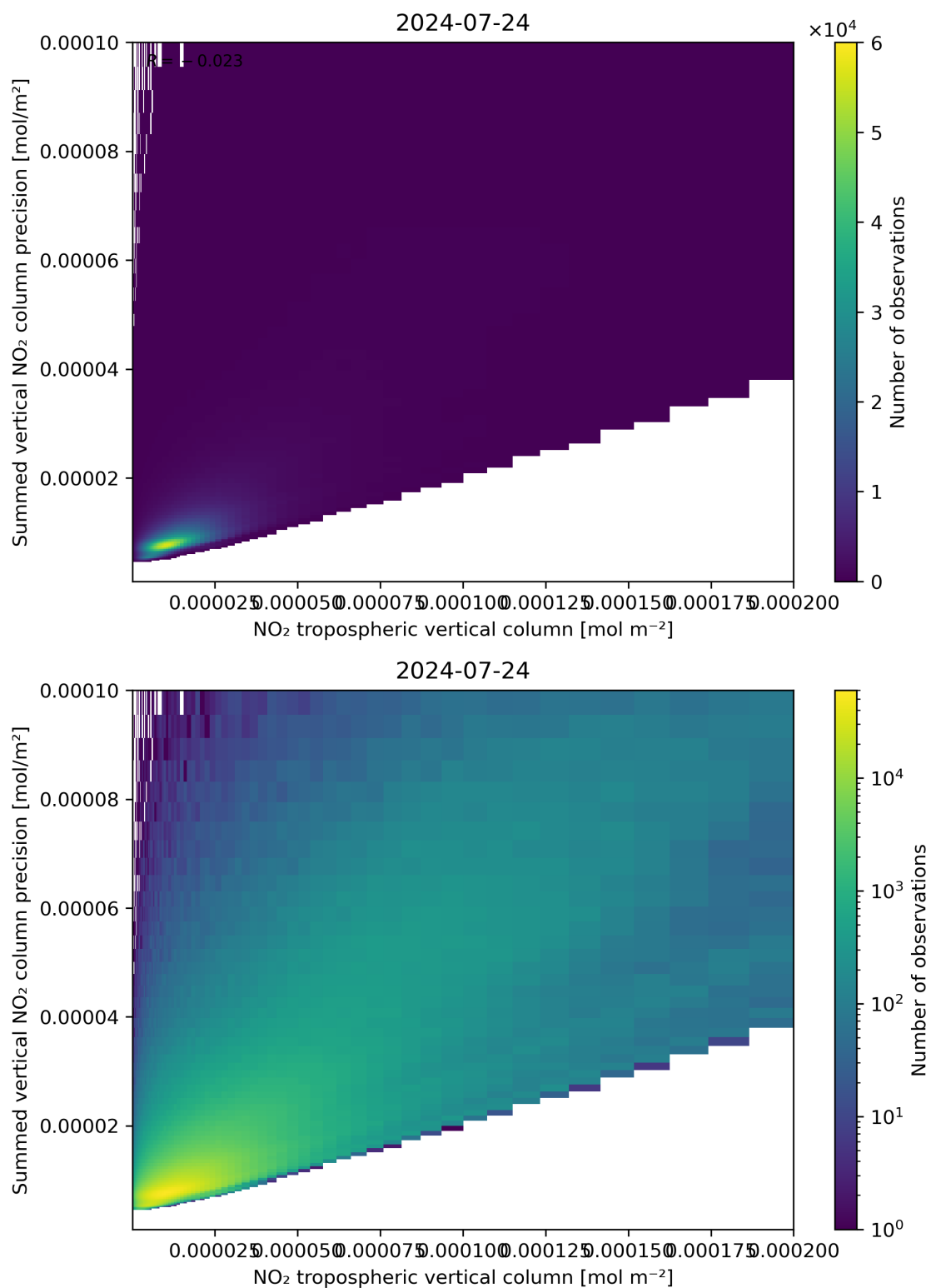
Figure 127: Scatter density plot of “NO 2 tropospheric vertical column” against “Summed vertical NO 2 column precision” for 2024-07-23 to 2024-07-24.
