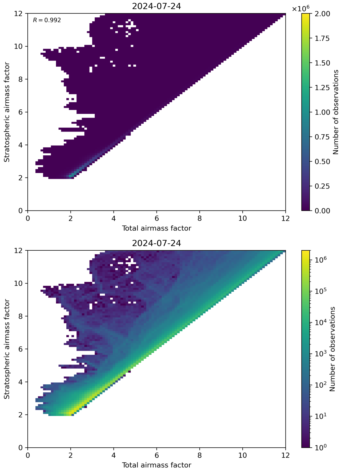
Figure 62: Scatter density plot of “Total airmass factor” against “Stratospheric airmass factor” for 2024-07-23 to 2024-07-24.
