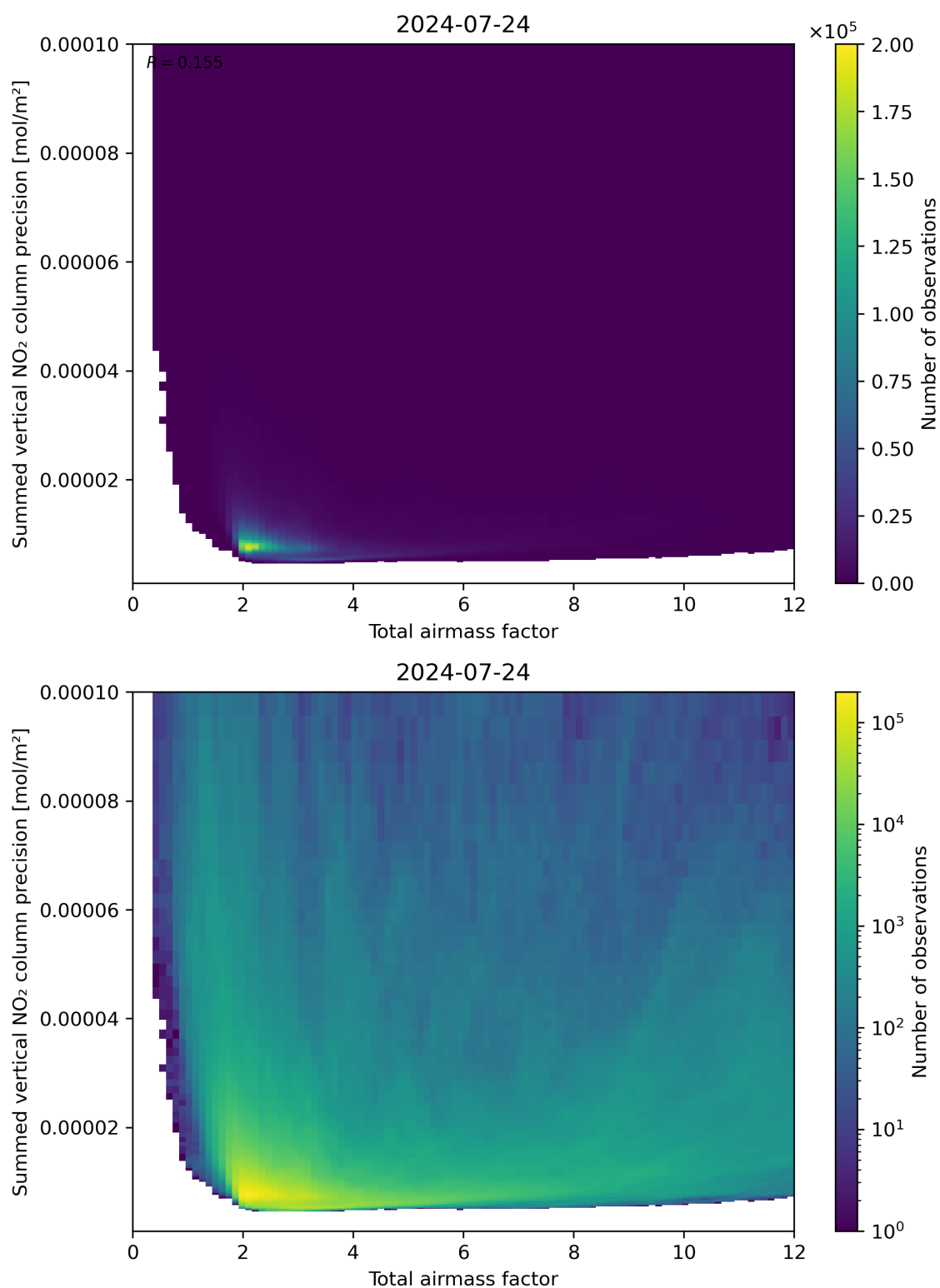
Figure 66: Scatter density plot of “Total airmass factor” against “Summed vertical NO 2 column precision” for 2024-07-23 to 2024-07-24.
