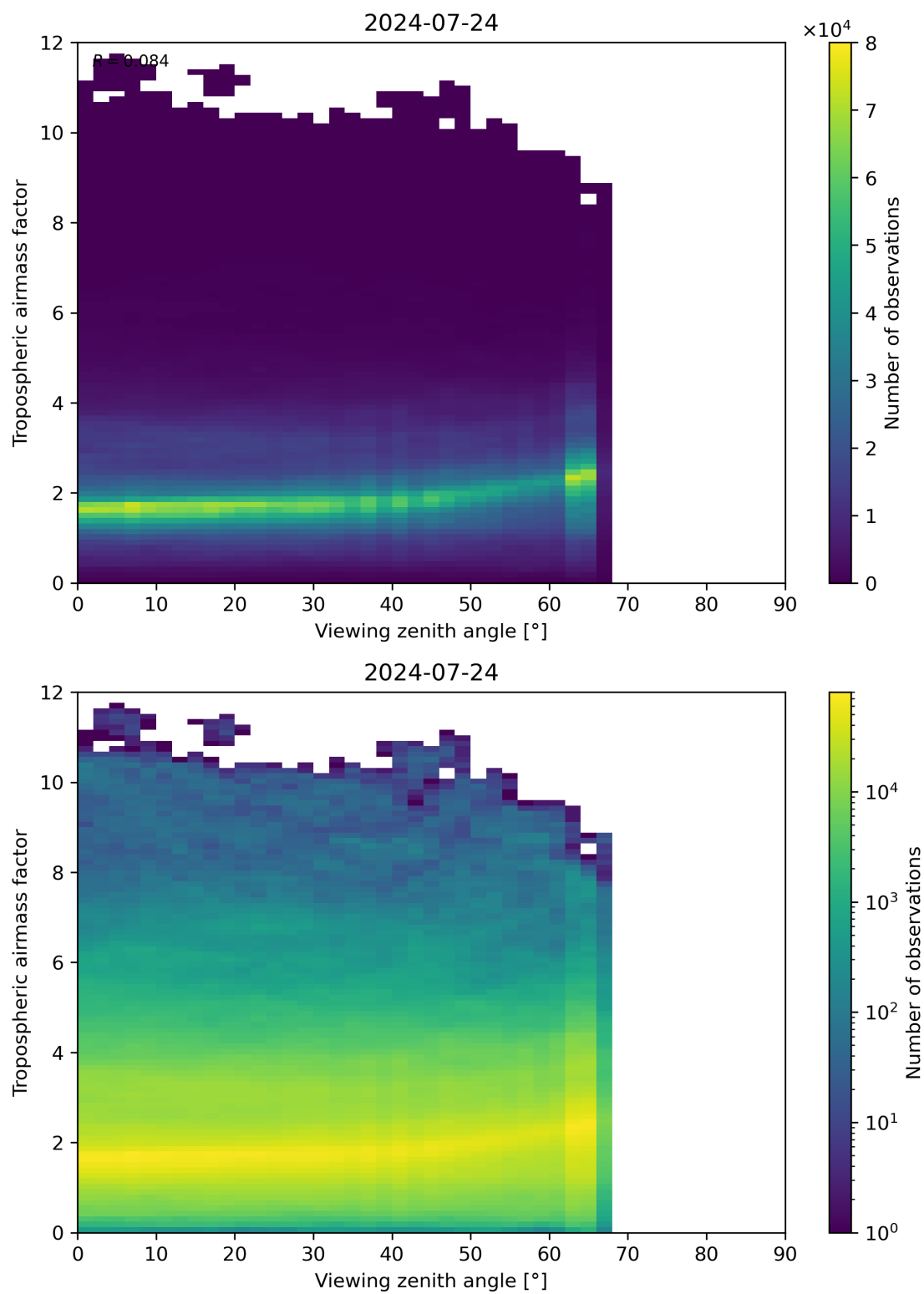
Figure 161: Scatter density plot of “Viewing zenith angle” against “Tropospheric airmass factor” for 2024-07-23 to 2024-07-24.
