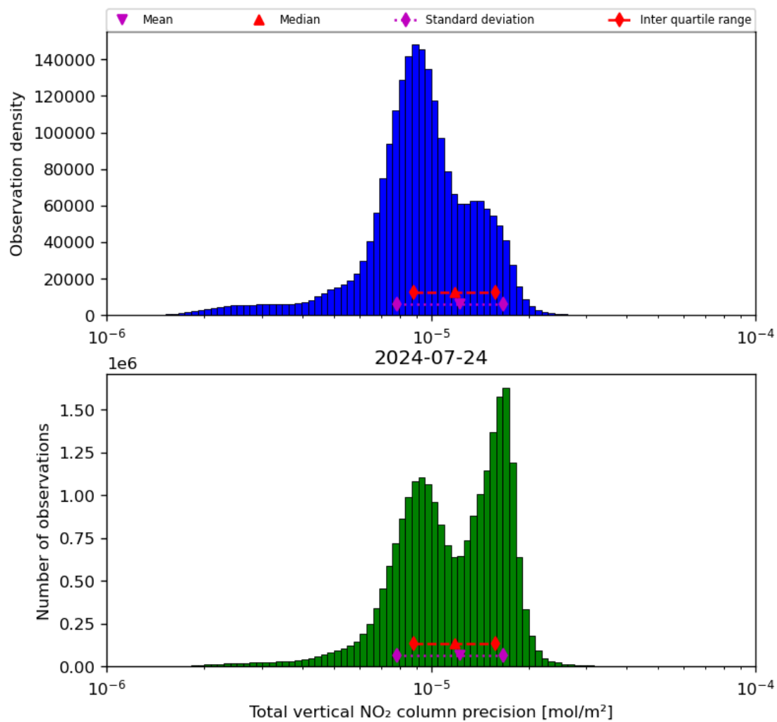
Figure 39: Histogram of “Total vertical NO 2 column precision” for 2024-07-23 to 2024-07-24
