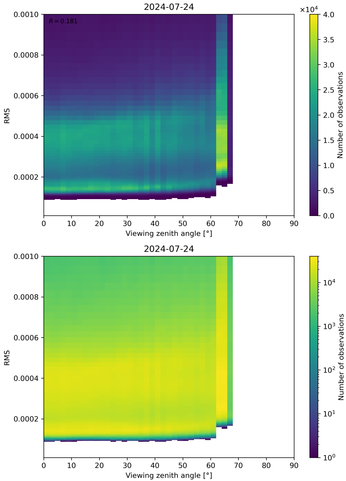
Figure 171: Scatter density plot of “Viewing zenith angle” against “RMS” for 2024-07-23 to 2024-07-24.
