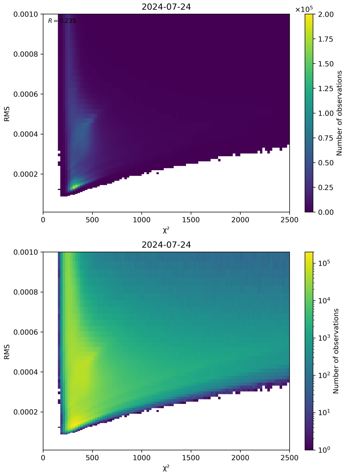
Figure 82: Scatter density plot of “ \chi^2 ” against “RMS” for 2024-07-23 to 2024-07-24.
