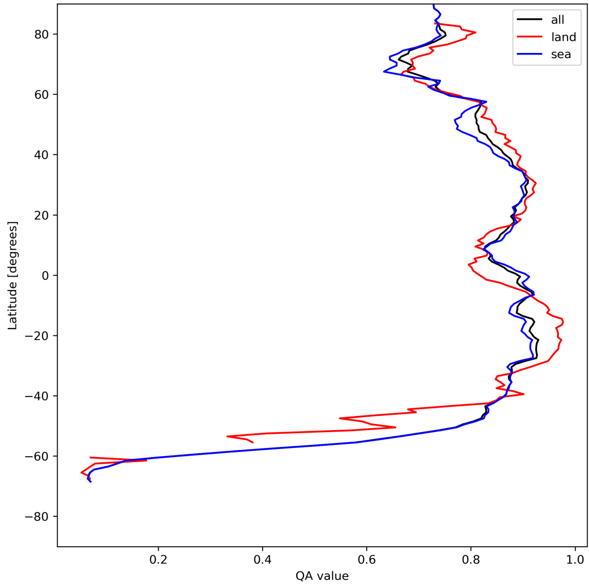
Figure 11: Zonal average of “QA value” for 2024-07-23 to 2024-07-24.
