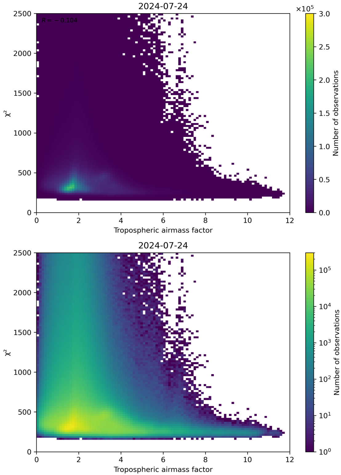
Figure 73: Scatter density plot of “Tropospheric airmass factor” against “ \chi^2 ” for 2024-07-23 to 2024-07-24.
