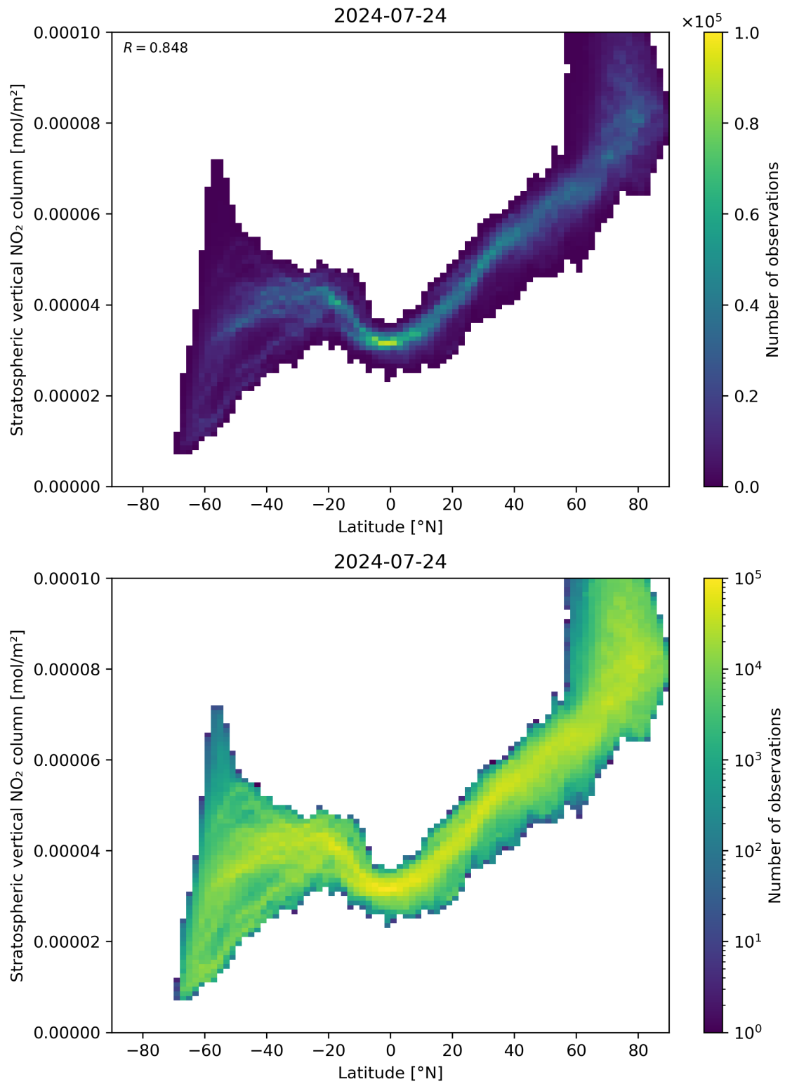
Figure 87: Scatter density plot of “Latitude” against “Stratospheric vertical NO 2 column” for 2024-07-23 to 2024-07-24.
