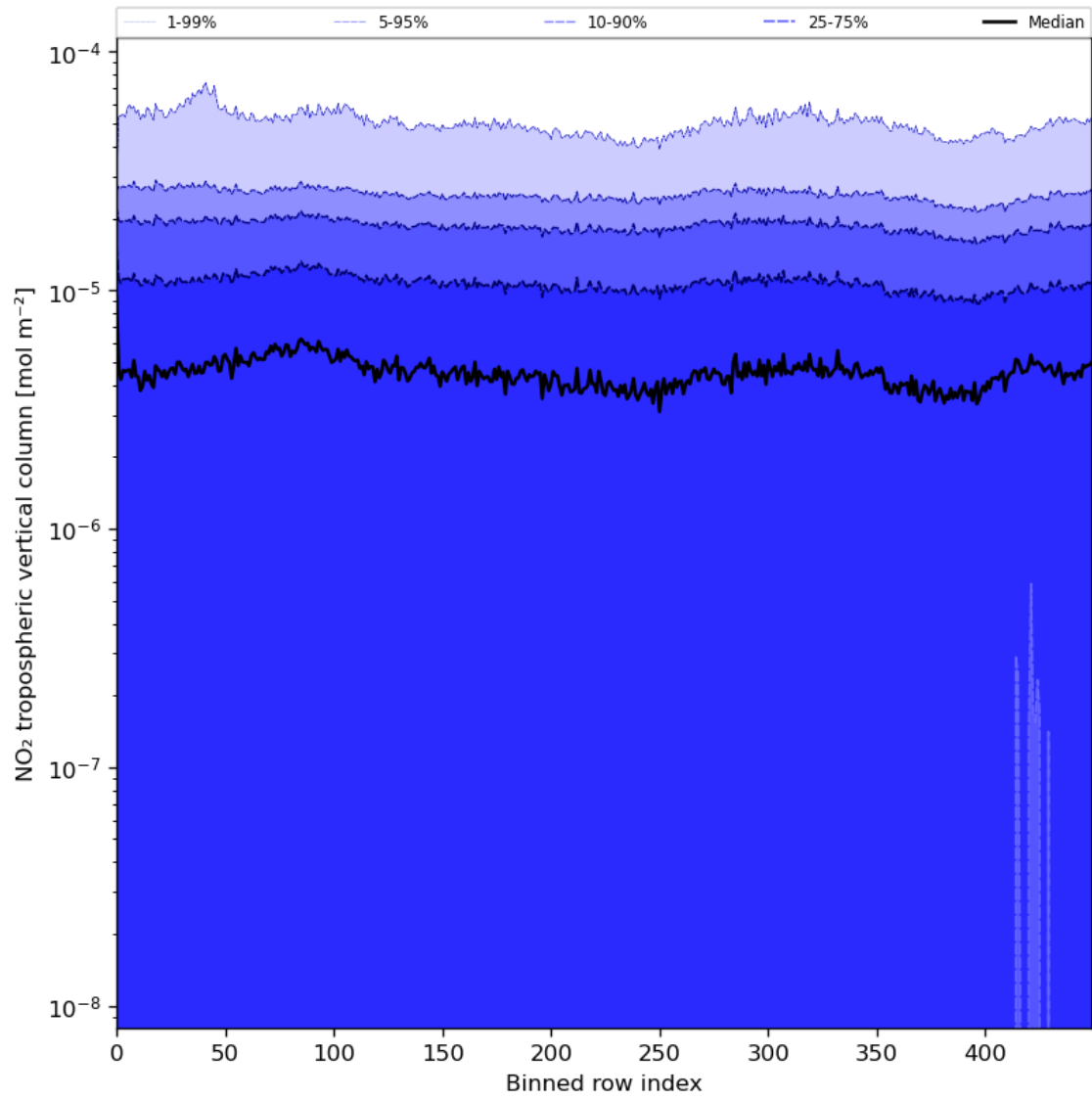
Figure 46: Along track statistics of “NO 2 tropospheric vertical column” for 2024-07-23 to 2024-07-24
