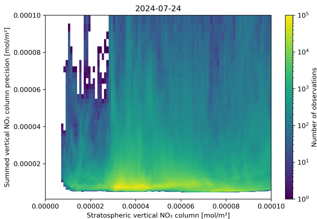
Figure 99: Scatter density plot of “Stratospheric vertical NO 2 column” against “Summed vertical NO 2 column precision” for 2024-07-23 to 2024-07-24.
