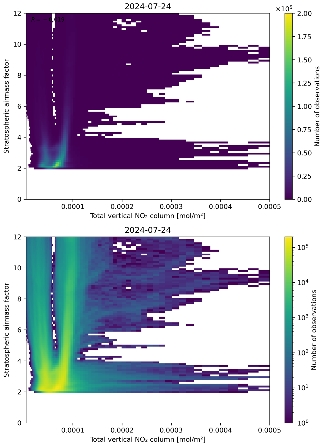
Figure 110: Scatter density plot of “Total vertical NO 2 column” against “Stratospheric air mass factor” for 2024-07-23 to 2024-07-24.
