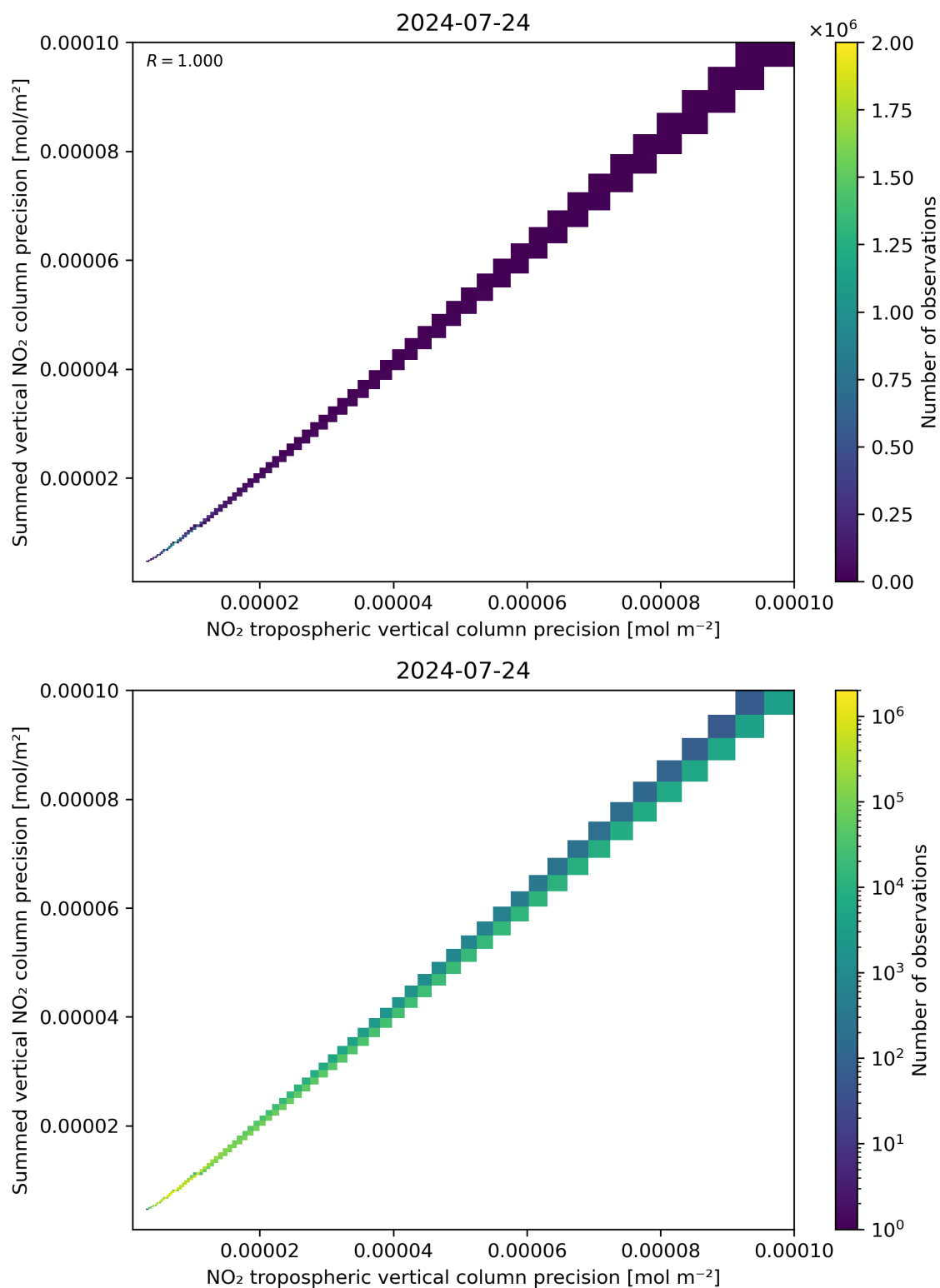
Figure 137: Scatter density plot of “NO 2 tropospheric vertical column precision” against “Summed vertical NO 2 column precision” for 2024-07-23 to 2024-07-24.
