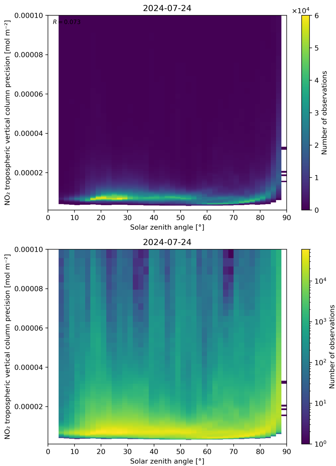
Figure 156: Scatter density plot of “Solar zenith angle” against “NO 2 tropospheric vertical column precision” for 2024-07-23 to 2024-07-24.
