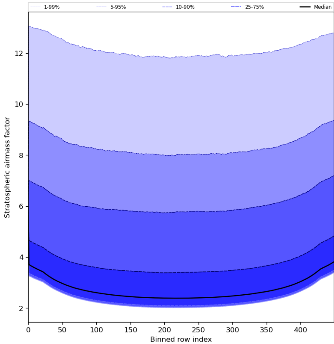
Figure 61: Along track statistics of “Stratospheric airmass factor” for 2024-07-23 to 2024-07-24
