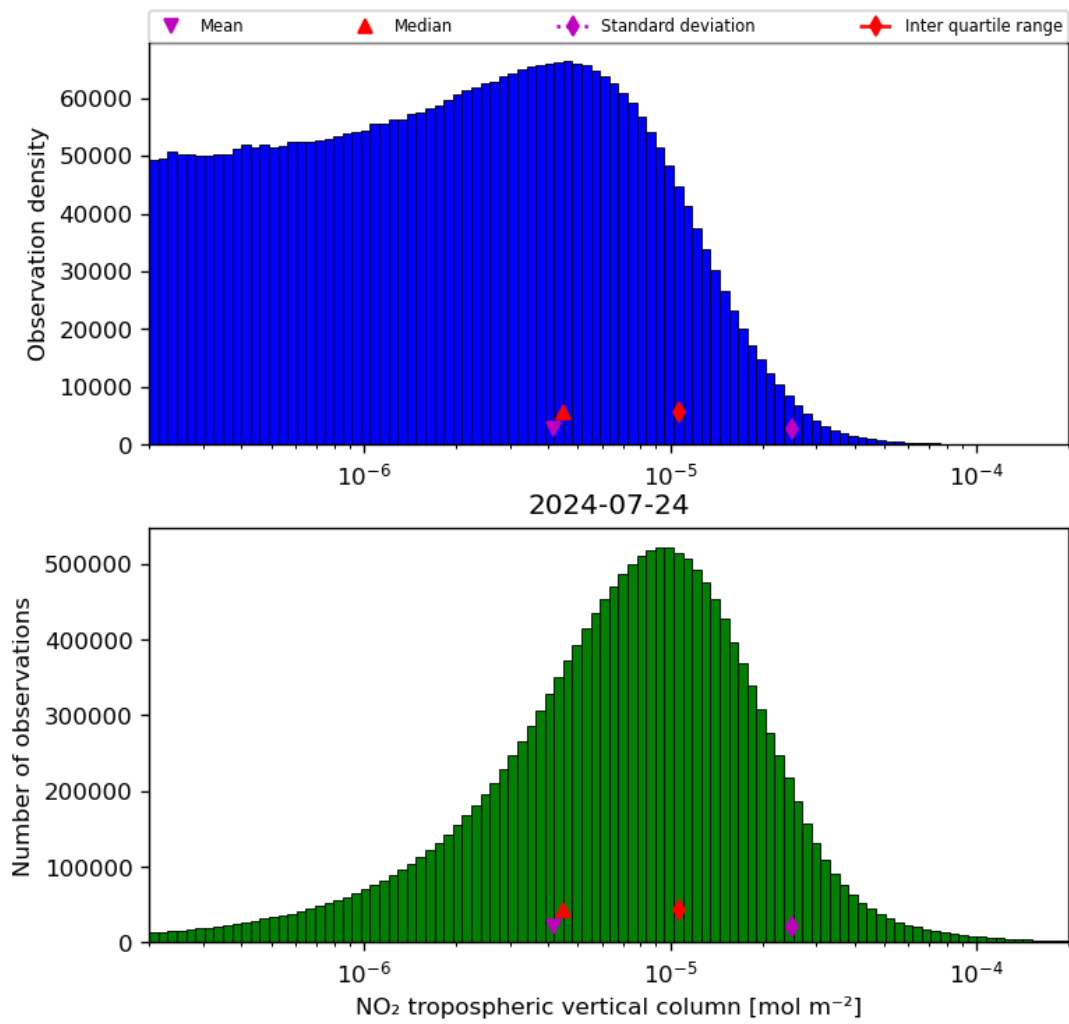
Figure 29: Histogram of “NO 2 tropospheric vertical column” for 2024-07-23 to 2024-07-24
