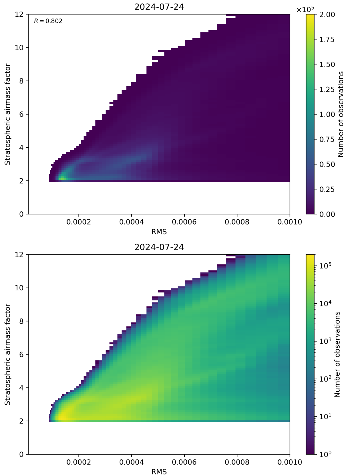
Figure 144: Scatter density plot of “RMS” against “Stratospheric airmass factor” for 2024-07-23 to 2024-07-24.
