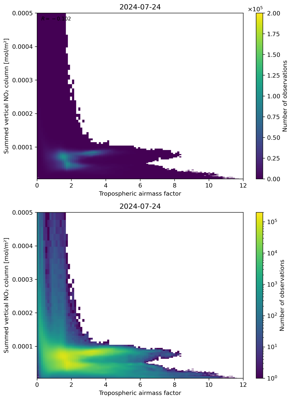
Figure 75: Scatter density plot of “Tropospheric air mass factor” against “Summed vertical NO 2 column” for 2024-07-23 to 2024-07-24.
