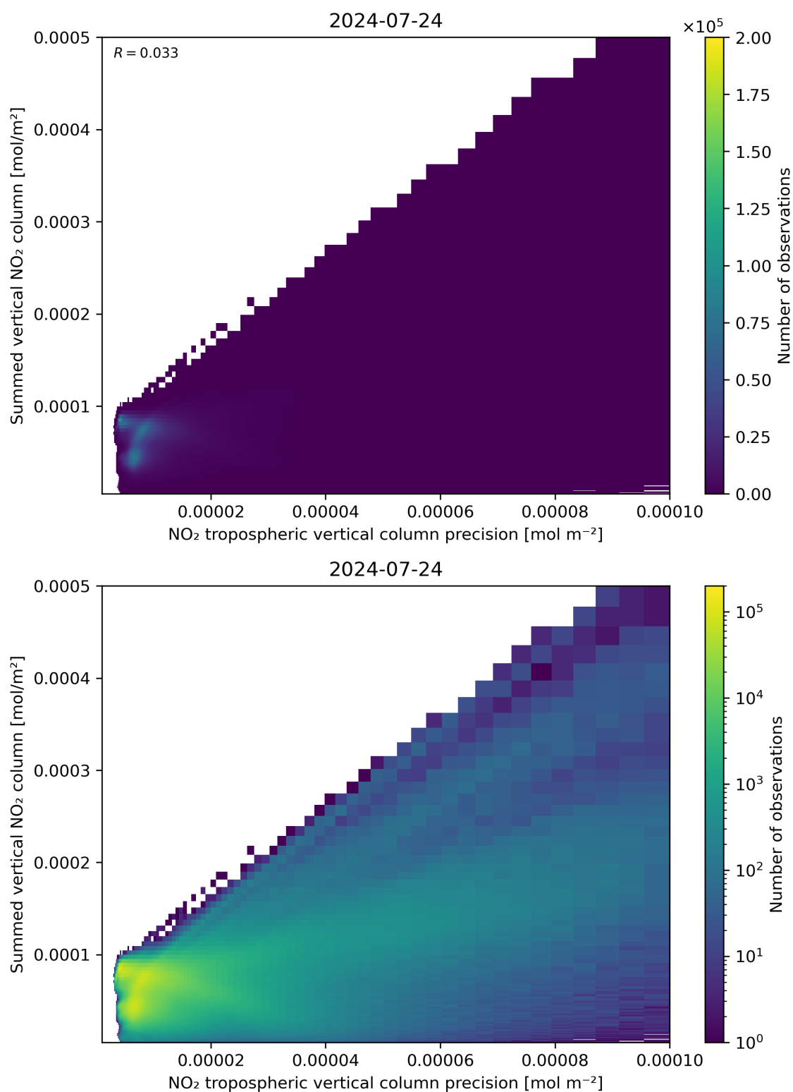
Figure 136: Scatter density plot of “NO 2 tropospheric vertical column precision” against “Summed vertical NO 2 column” for 2024-07-23 to 2024-07-24.
