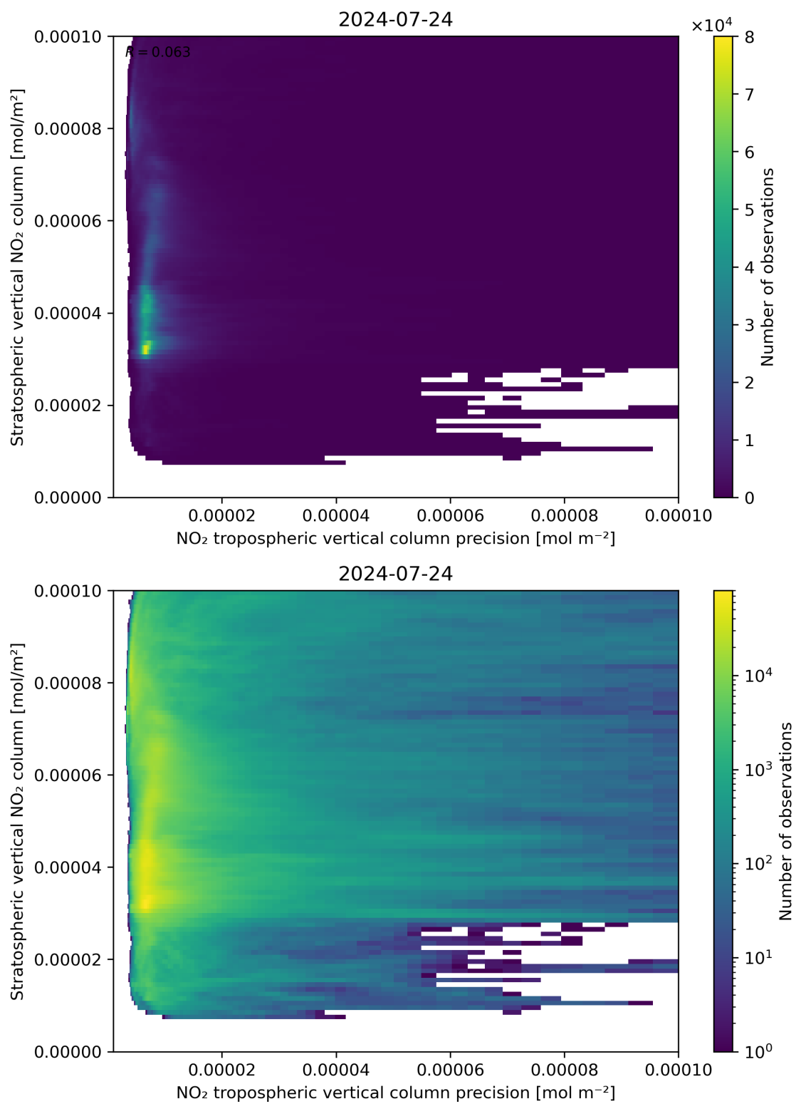
Figure 135: Scatter density plot of “NO 2 tropospheric vertical column precision” against “Stratospheric vertical NO 2 column” for 2024-07-23 to 2024-07-24.
