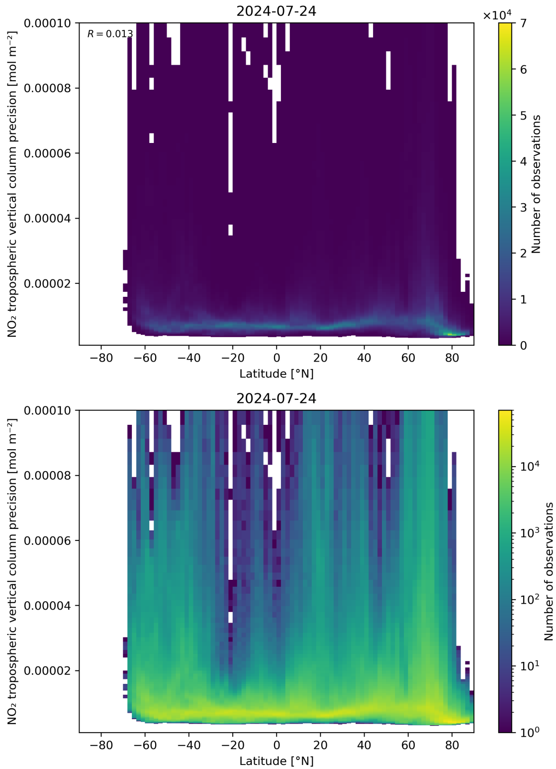
Figure 93: Scatter density plot of “Latitude” against “NO 2 tropospheric vertical column precision” for 2024-07-23 to 2024-07-24.
