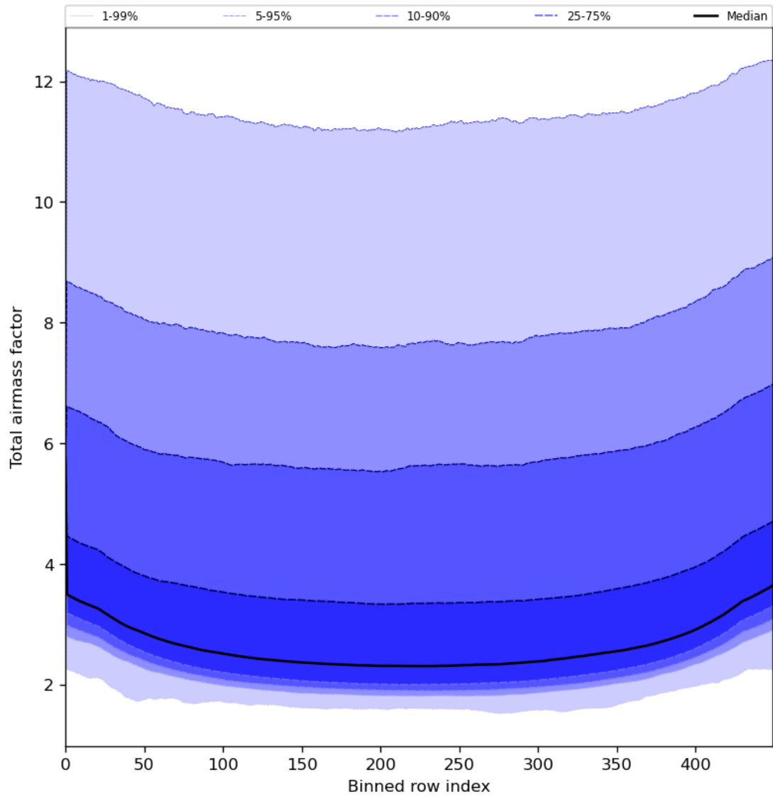
Figure 49: Along track statistics of “Total airmass factor” for 2024-07-23 to 2024-07-24
