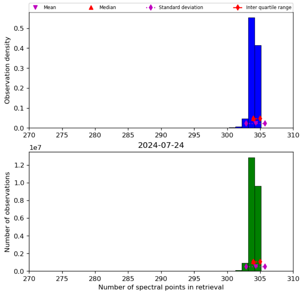
Figure 33: Histogram of “Number of spectral points in retrieval” for 2024-07-23 to 2024-07-24
