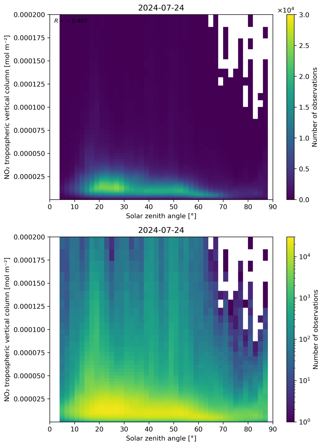
Figure 155: Scatter density plot of “Solar zenith angle” against “NO 2 tropospheric vertical column” for 2024-07-23 to 2024-07-24.
