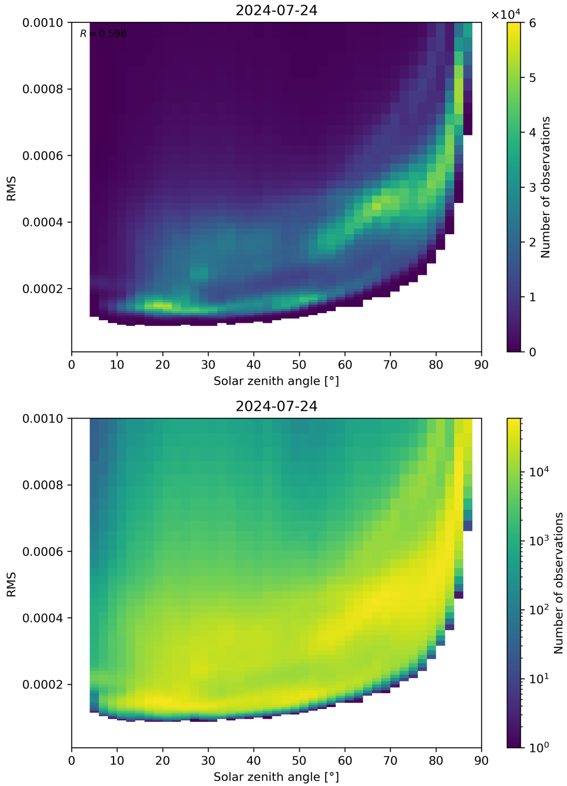
Figure 157: Scatter density plot of “Solar zenith angle” against “RMS” for 2024-07-23 to 2024-07-24.
