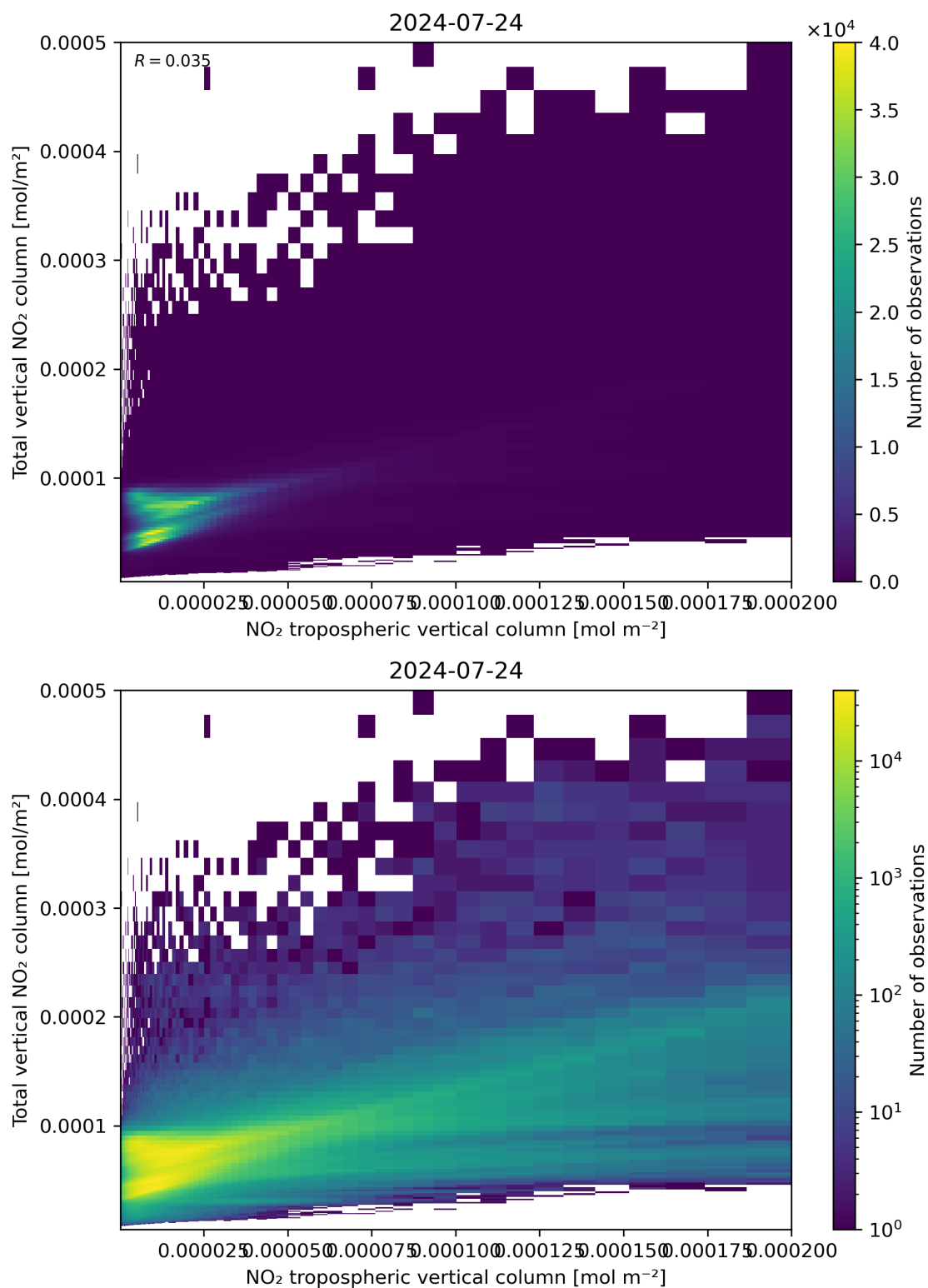
Figure 128: Scatter density plot of “NO 2 tropospheric vertical column” against “Total vertical NO 2 column” for 2024-07-23 to 2024-07-24.
