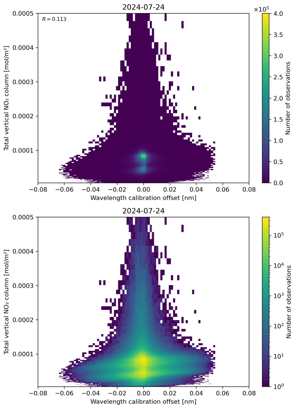
Figure 179: Scatter density plot of “Wavelength calibration offset” against “Total vertical NO 2 column” for 2024-07-23 to 2024-07-24.
