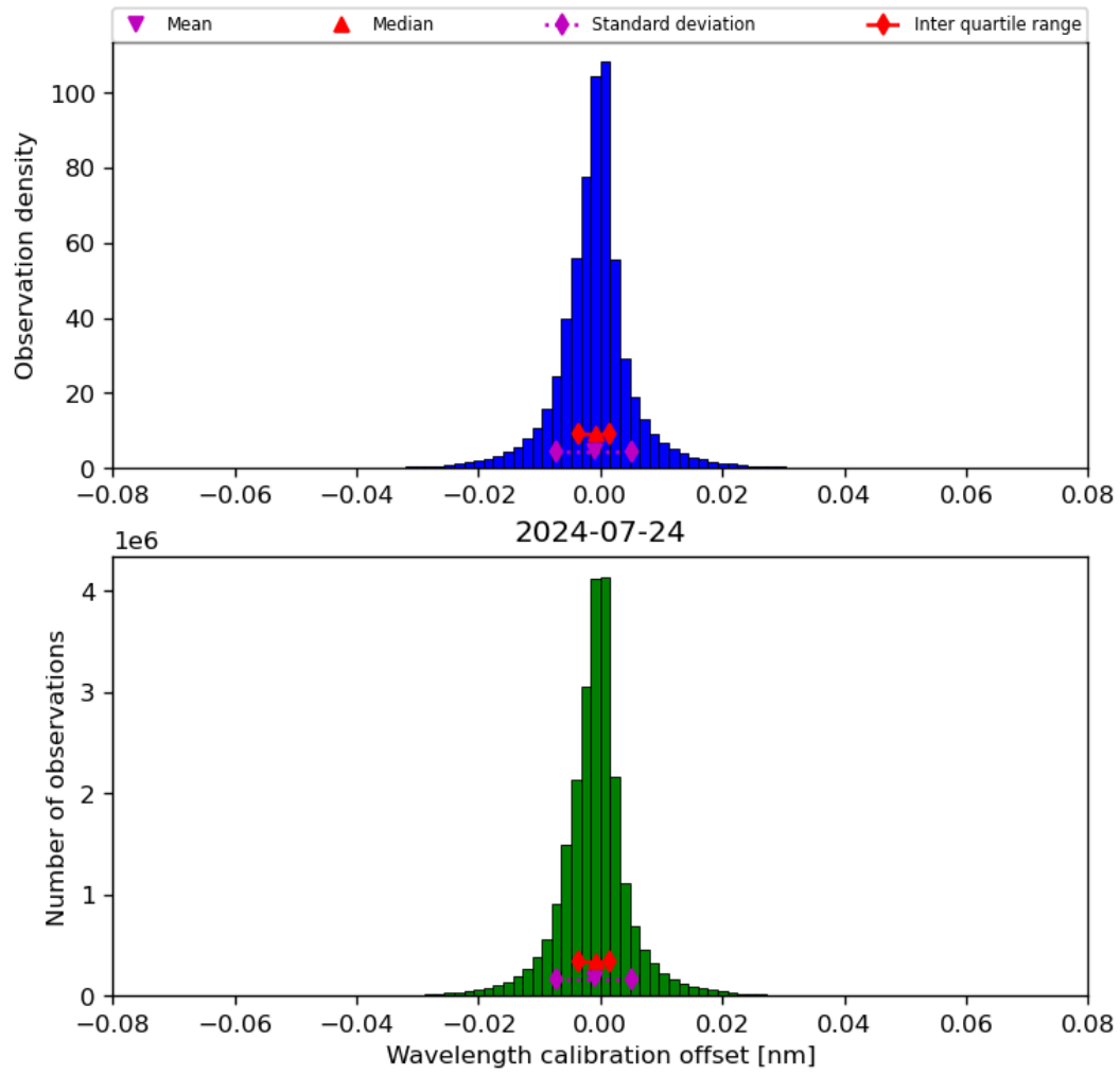
Figure 35: Histogram of “Wavelength calibration offset” for 2024-07-23 to 2024-07-24
