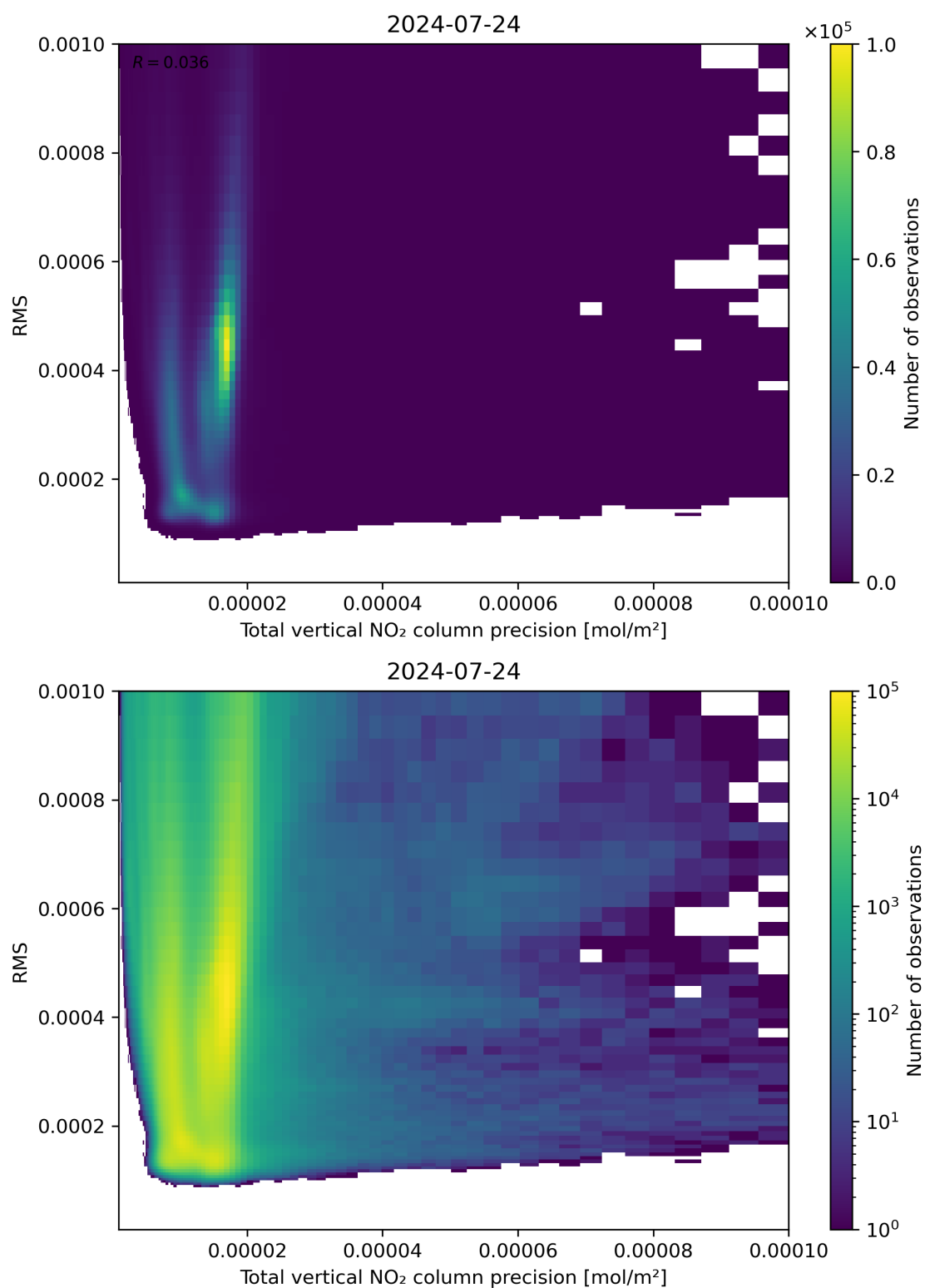
Figure 119: Scatter density plot of “Total vertical NO 2 column precision” against “RMS” for 2024-07-23 to 2024-07-24.
