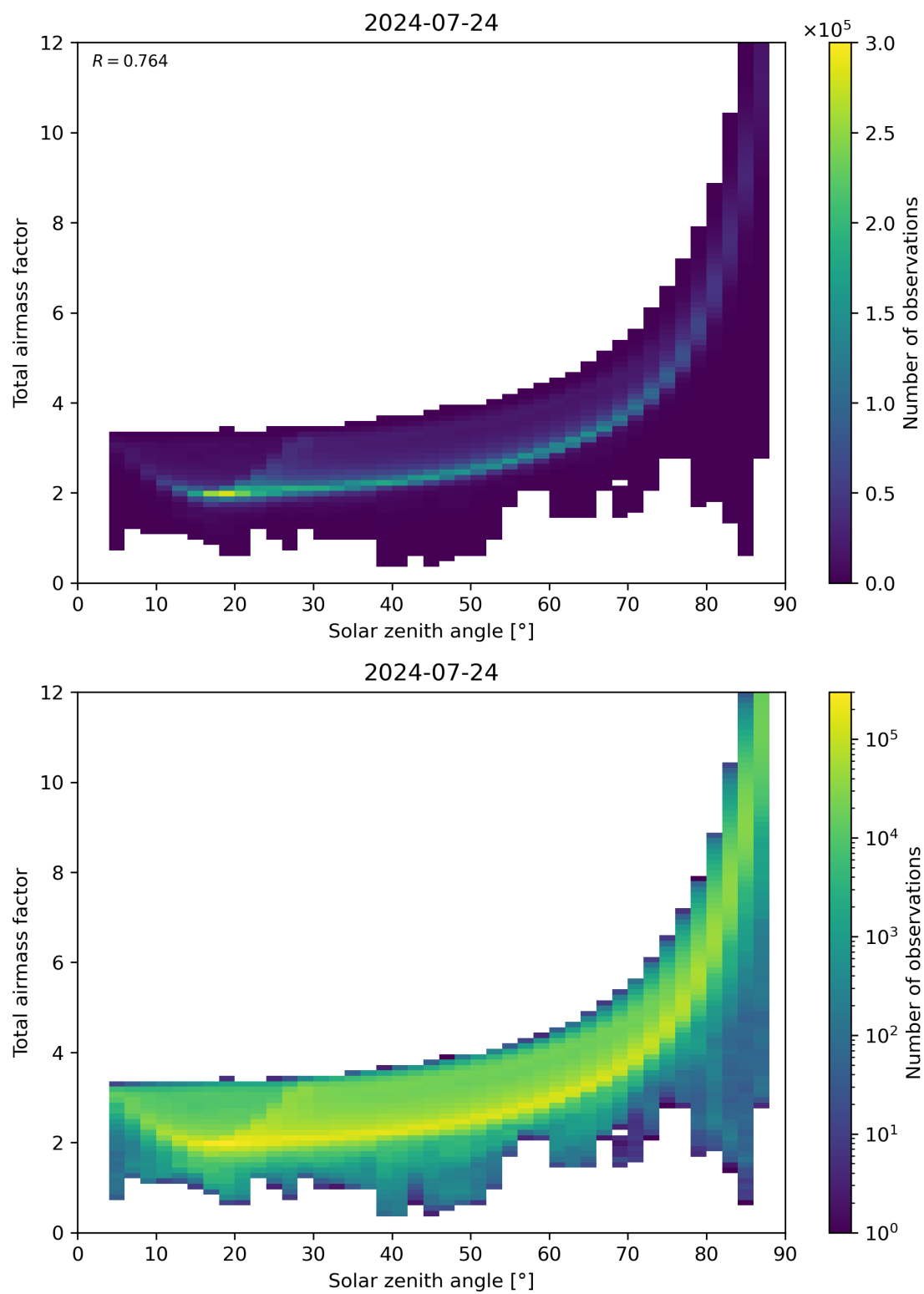
Figure 146: Scatter density plot of “Solar zenith angle” against “Total air mass factor” for 2024-07-23 to 2024-07-24.
