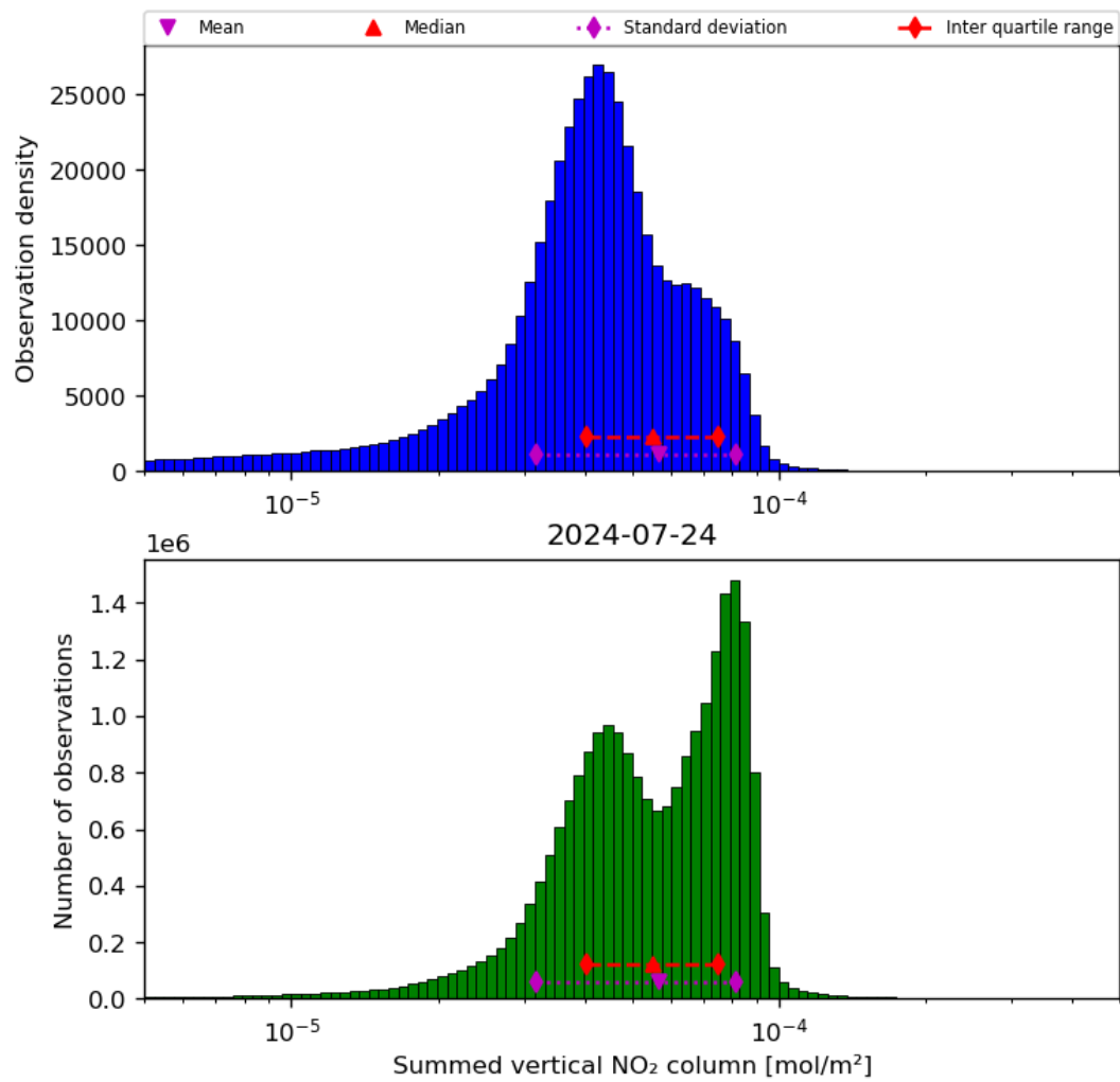
Figure 40: Histogram of “Summed vertical NO 2 column” for 2024-07-23 to 2024-07-24
