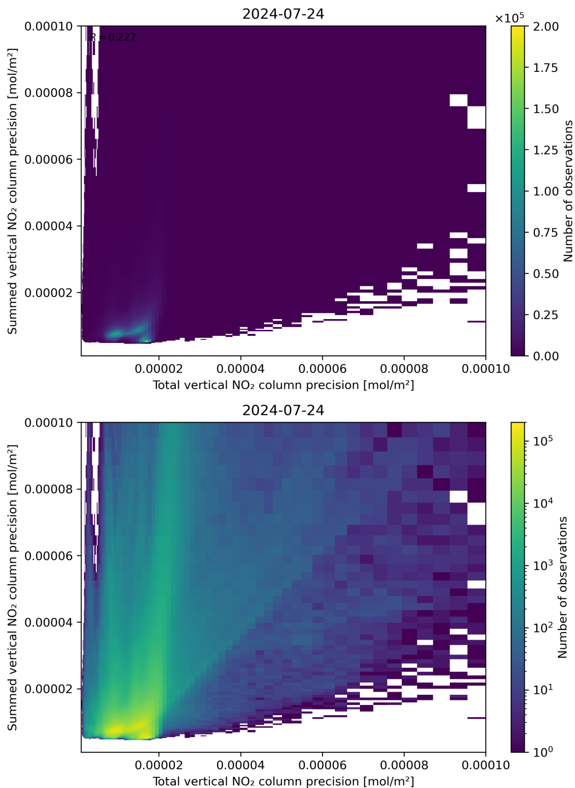
Figure 118: Scatter density plot of “Total vertical NO 2 column precision” against “Summed vertical NO 2 column precision” for 2024-07-23 to 2024-07-24.
