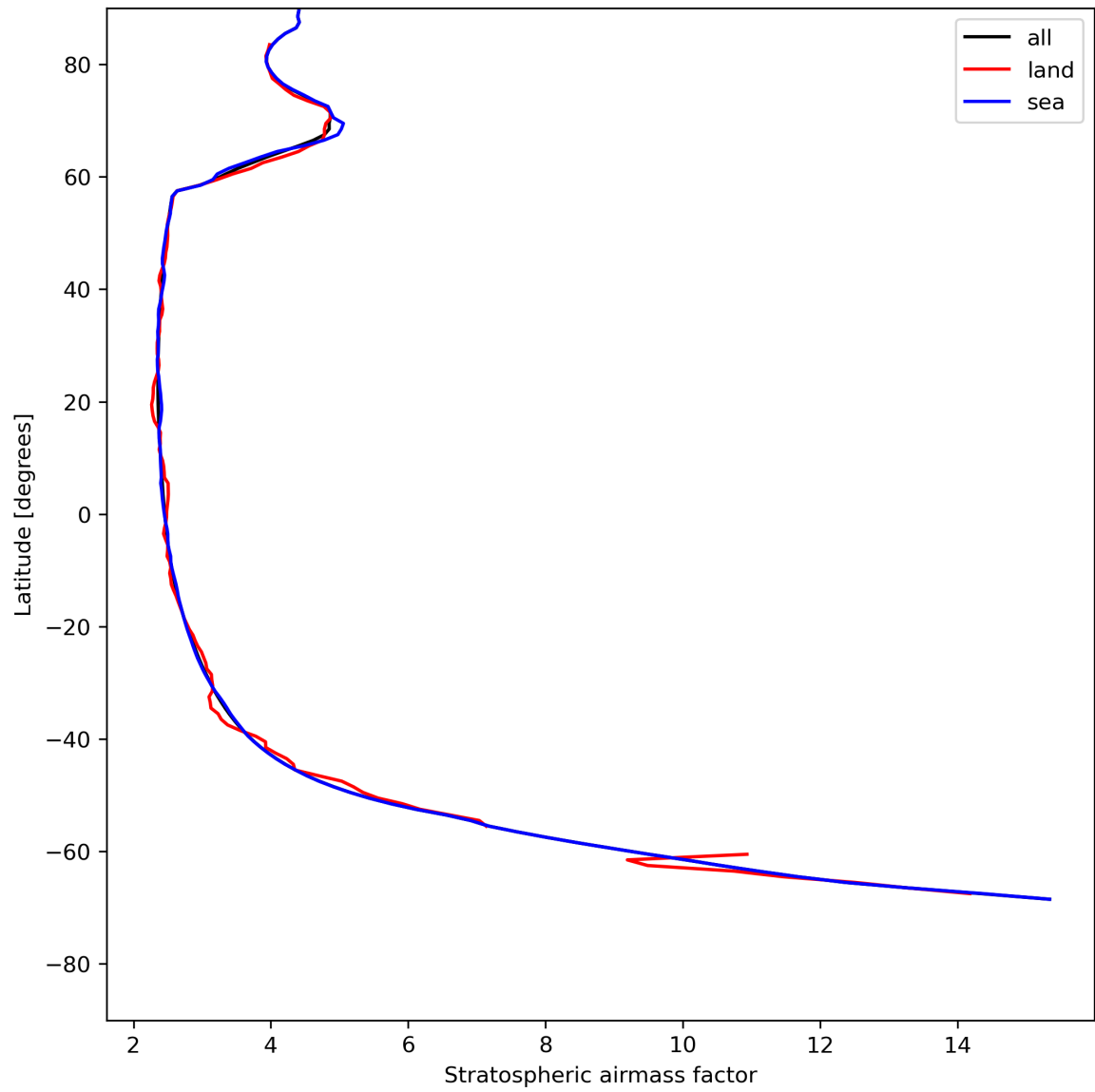
Figure 27: Zonal average of “Stratospheric airmass factor” for 2024-07-23 to 2024-07-24.
