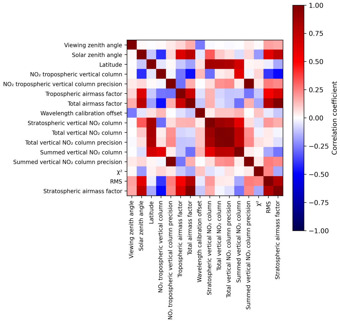
Figure 2: Map of correlation matrix for 2024-07-23 to 2024-07-24.
