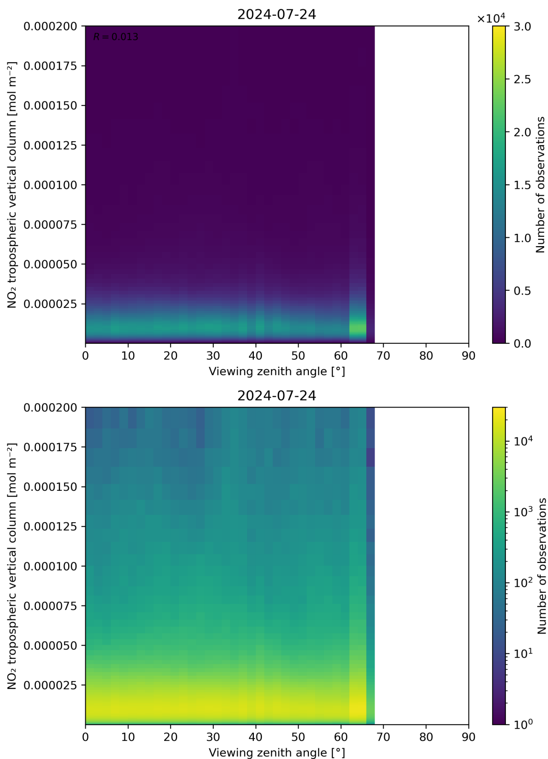
Figure 169: Scatter density plot of “Viewing zenith angle” against “NO 2 tropospheric vertical column” for 2024-07-23 to 2024-07-24.
