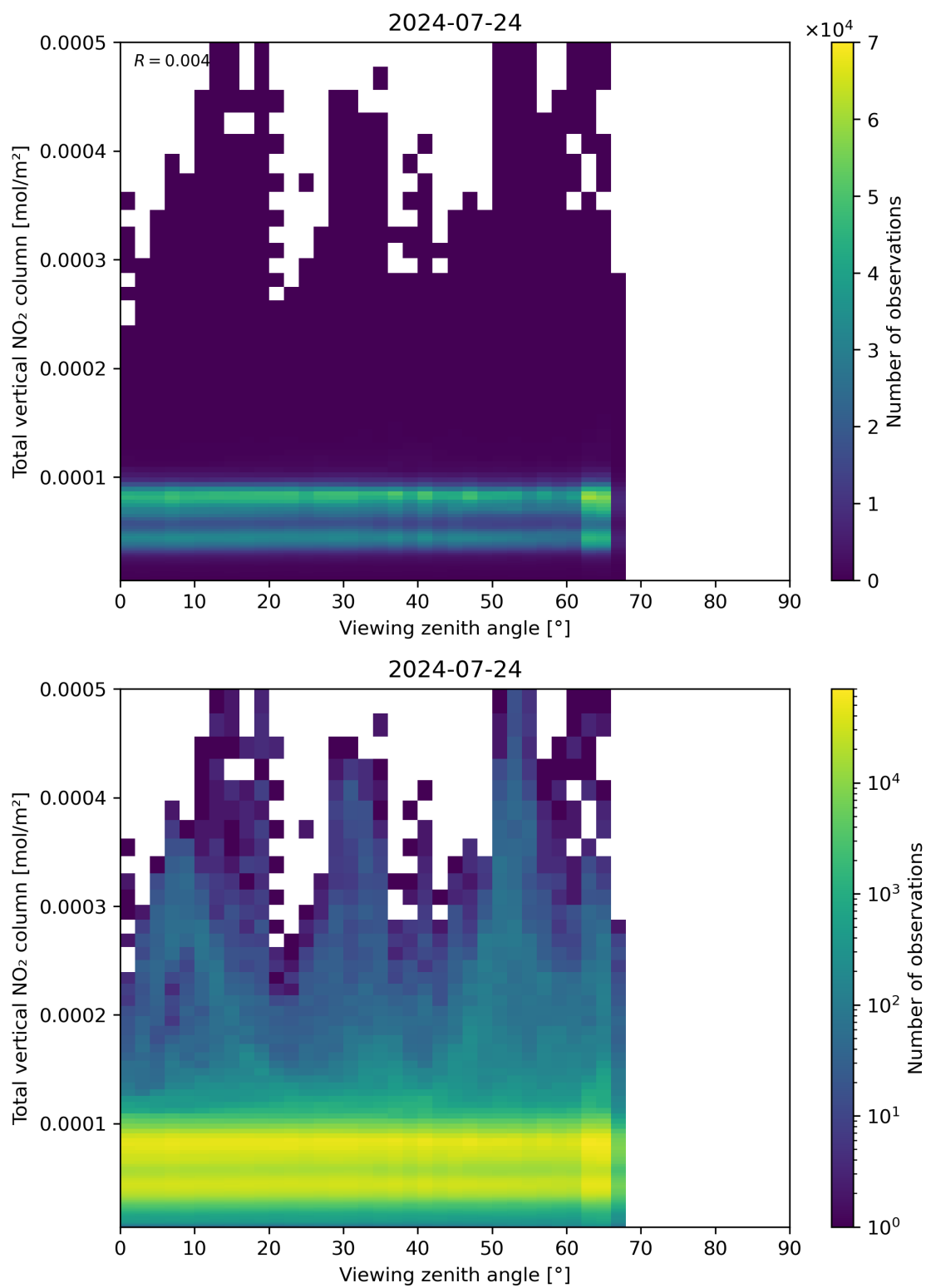
Figure 167: Scatter density plot of “Viewing zenith angle” against “Total vertical NO 2 column” for 2024-07-23 to 2024-07-24.
