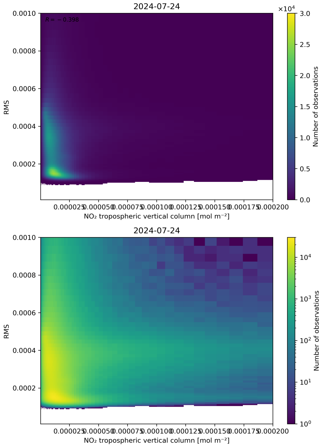
Figure 142: Scatter density plot of “NO 2 tropospheric vertical column” against “RMS” for 2024-07-23 to 2024-07-24.
