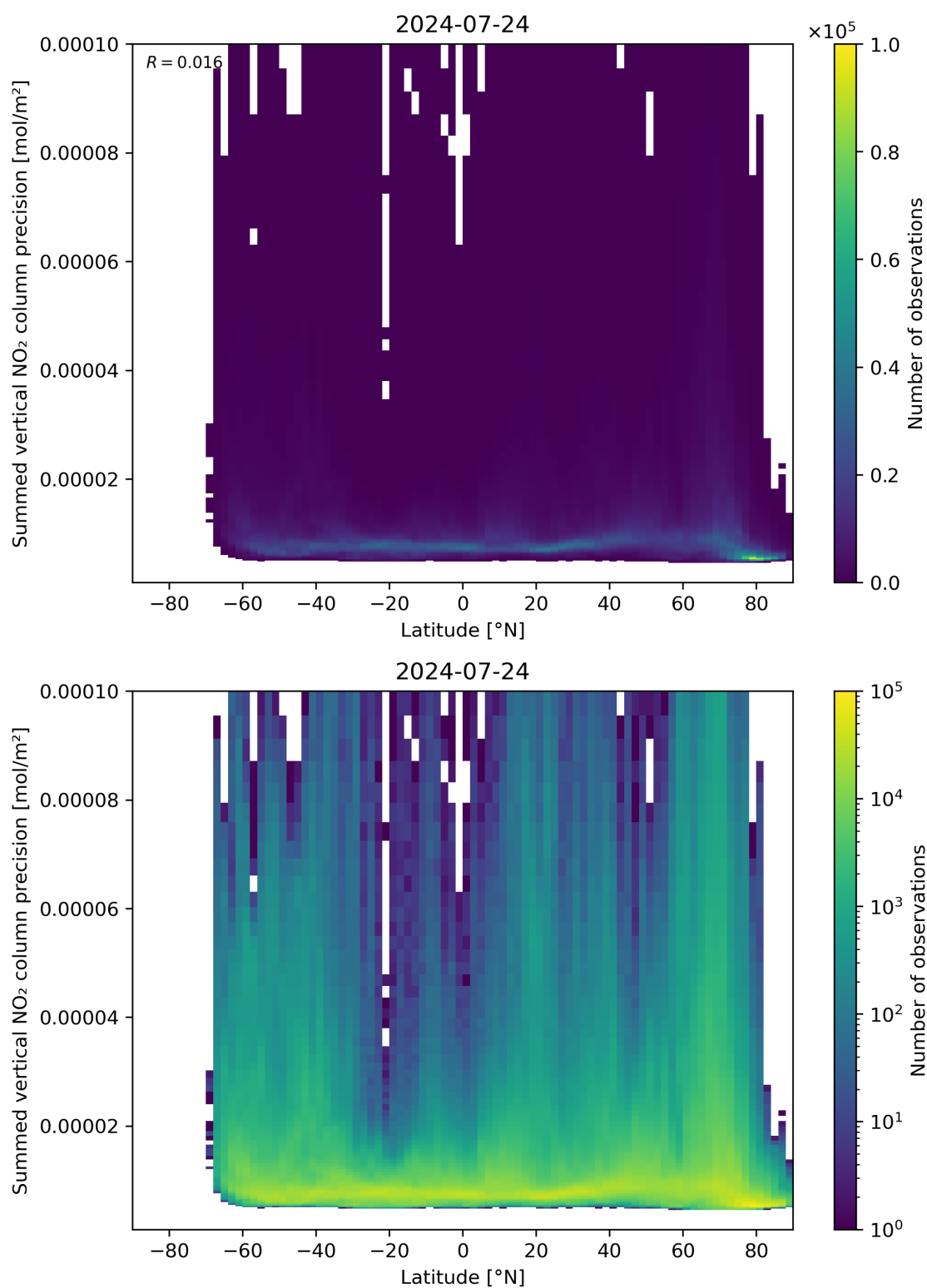
Figure 89: Scatter density plot of “Latitude” against “Summed vertical NO 2 column precision” for 2024-07-23 to 2024-07-24.
