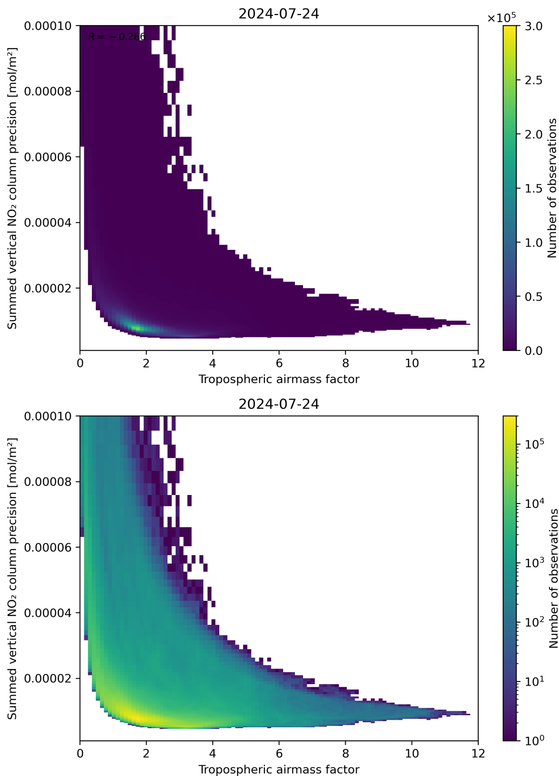
Figure 76: Scatter density plot of “Tropospheric air mass factor” against “Summed vertical NO 2 column precision” for 2024-07-23 to 2024-07-24.
