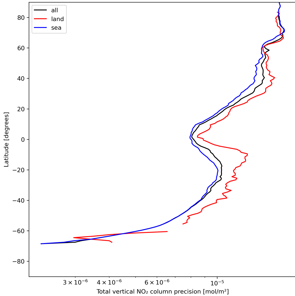
Figure 22: Zonal average of “Total vertical NO 2 column precision” for 2024-07-23 to 2024-07-24.
