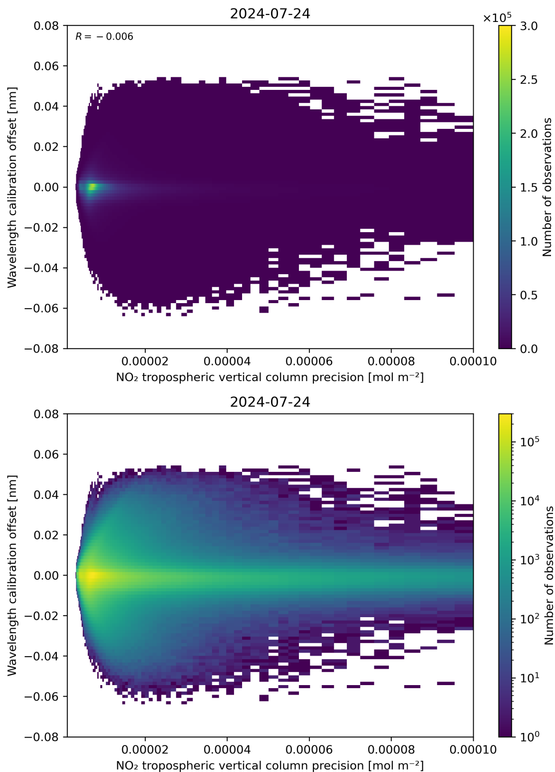
Figure 141: Scatter density plot of “NO 2 tropospheric vertical column precision” against “Wavelength calibration offset” for 2024-07-23 to 2024-07-24.
