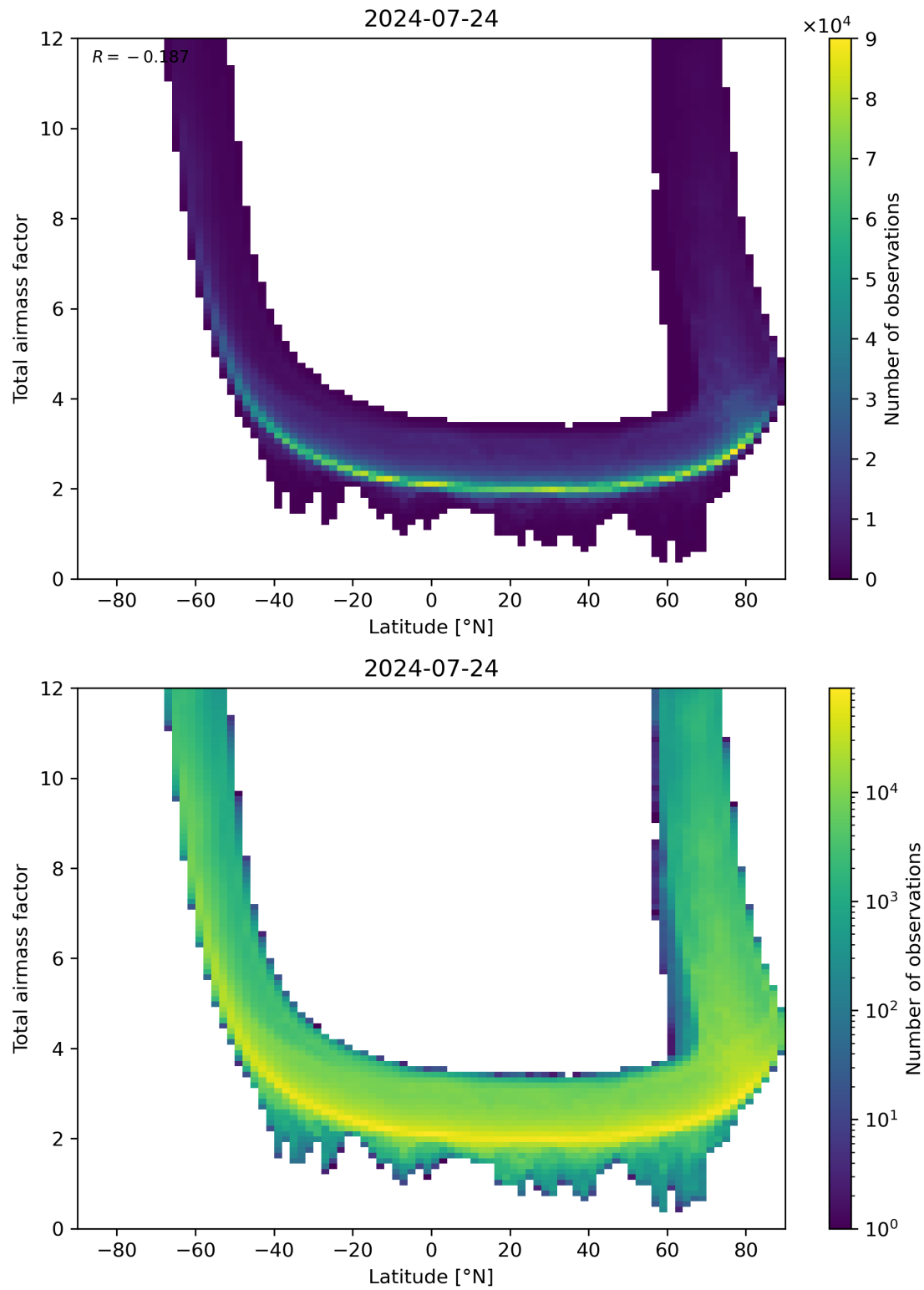
Figure 84: Scatter density plot of “Latitude” against “Total airmass factor” for 2024-07-23 to 2024-07-24.
