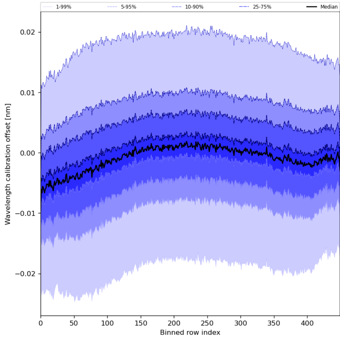
Figure 52: Along track statistics of “Wavelength calibration offset” for 2024-07-23 to 2024-07-24
