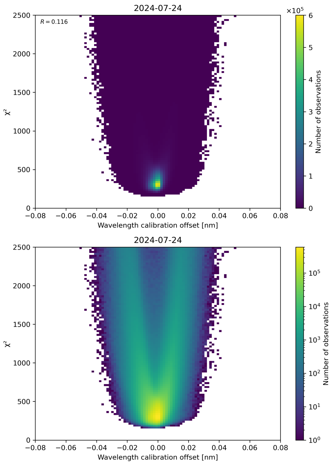
Figure 175: Scatter density plot of “Wavelength calibration offset” against “ \chi^2 ” for 2024-07-23 to 2024-07-24.
