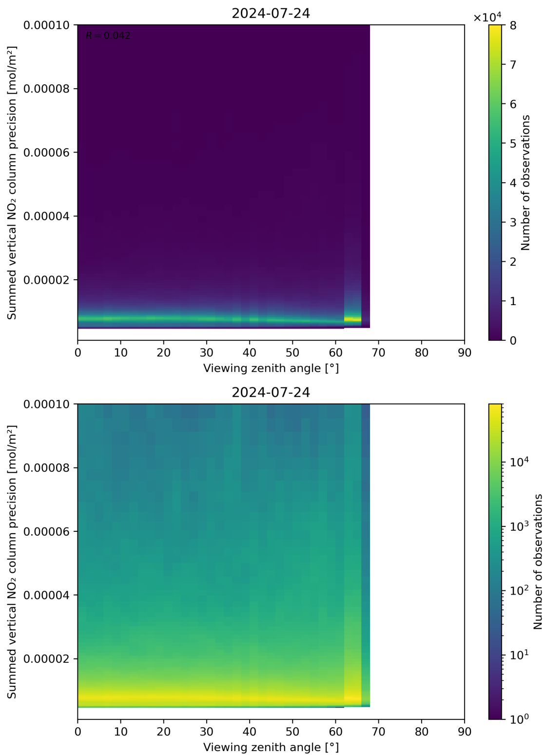
Figure 166: Scatter density plot of “Viewing zenith angle” against “Summed vertical NO 2 column precision” for 2024-07-23 to 2024-07-24.
