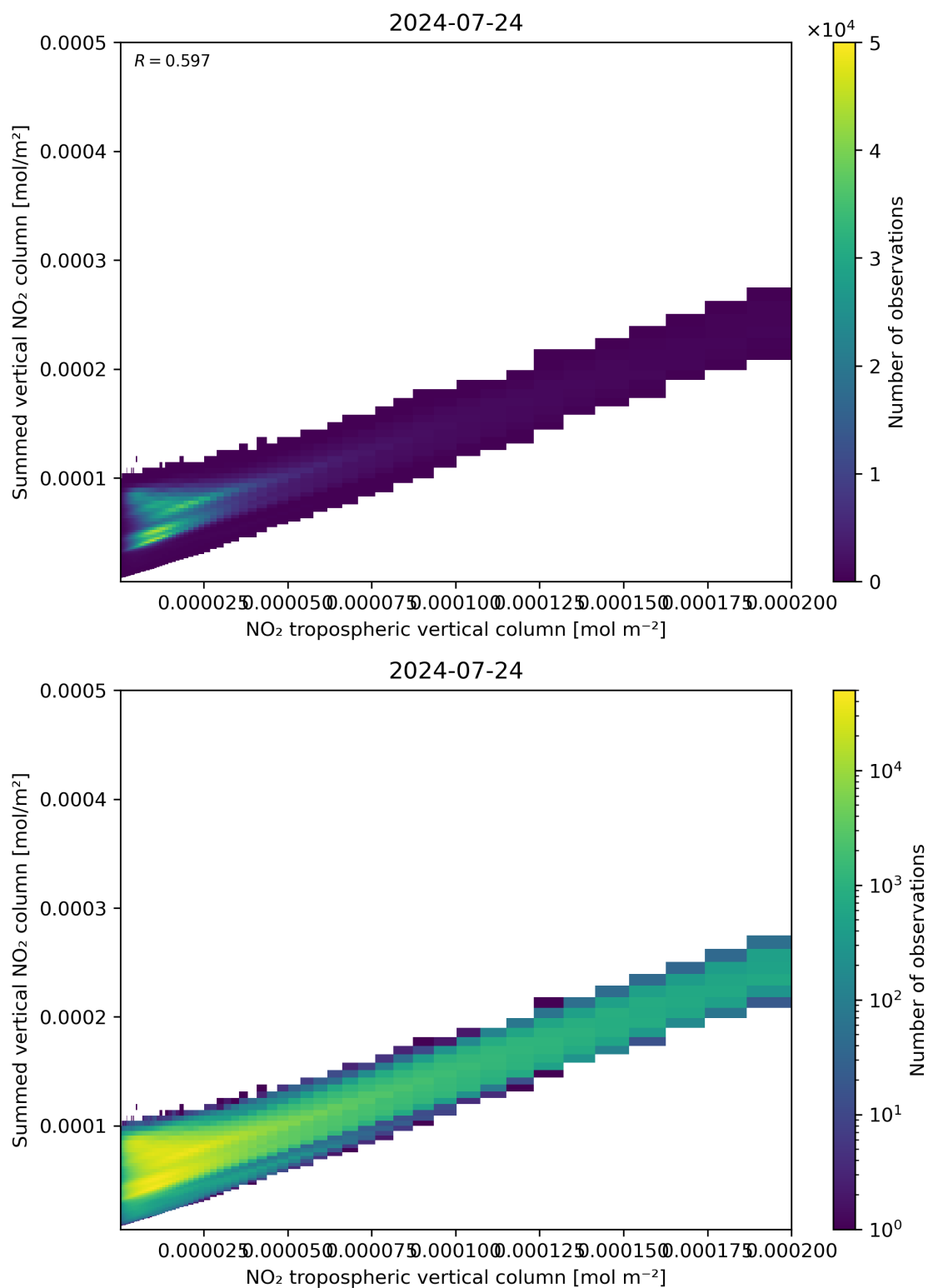
Figure 126: Scatter density plot of “NO 2 tropospheric vertical column” against “Summed vertical NO 2 column” for 2024-07-23 to 2024-07-24.
