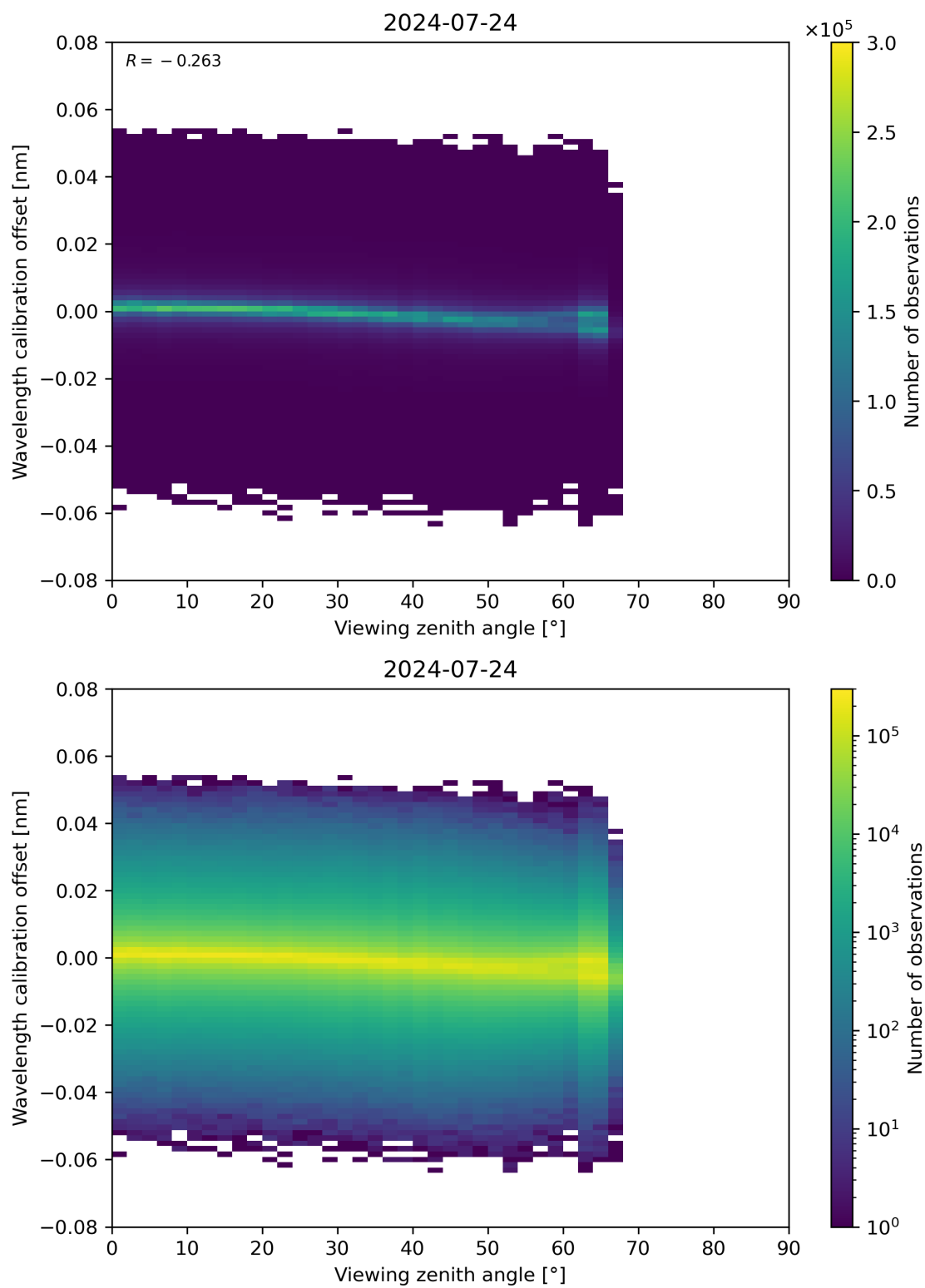
Figure 173: Scatter density plot of “Viewing zenith angle” against “Wavelength calibration offset” for 2024-07-23 to 2024-07-24.
