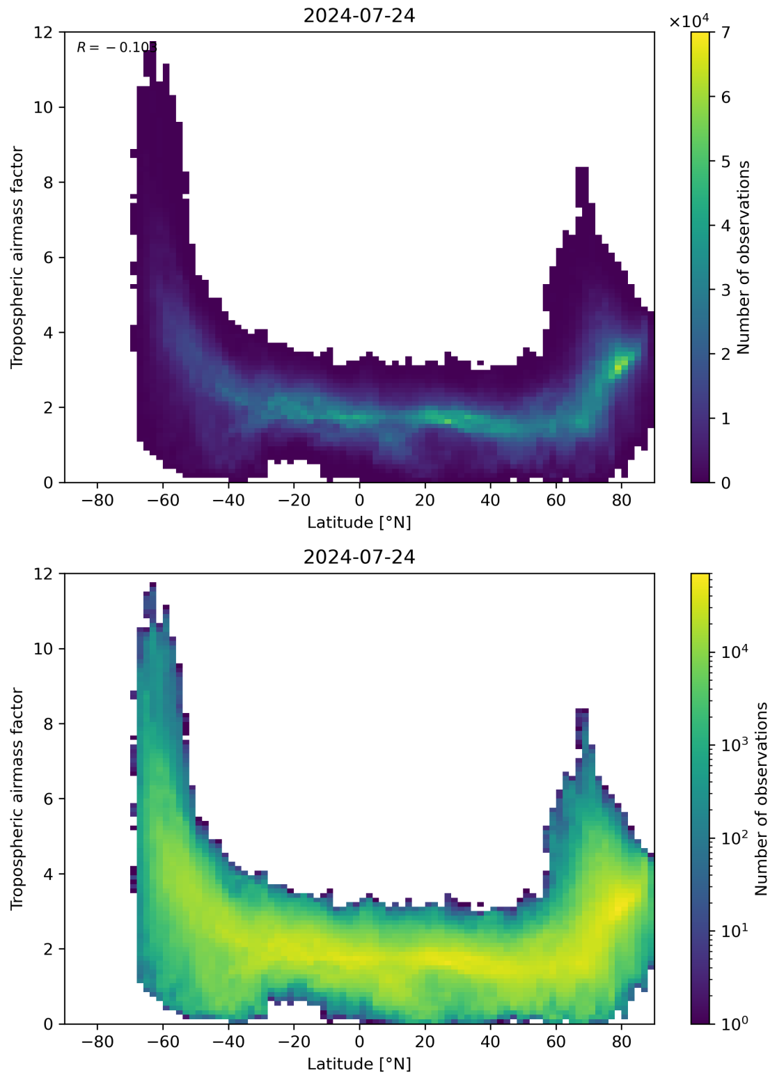
Figure 85: Scatter density plot of “Latitude” against “Tropospheric airmass factor” for 2024-07-23 to 2024-07-24.
