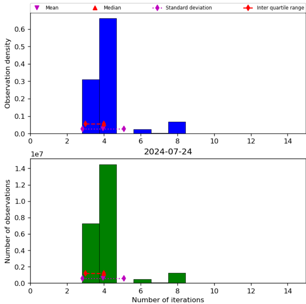
Figure 34: Histogram of “Number of iterations” for 2024-07-23 to 2024-07-24
