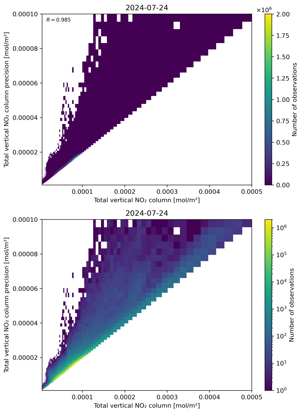
Figure 114: Scatter density plot of “Total vertical NO 2 column” against “Total vertical NO 2 column precision” for 2024-07-23 to 2024-07-24.
