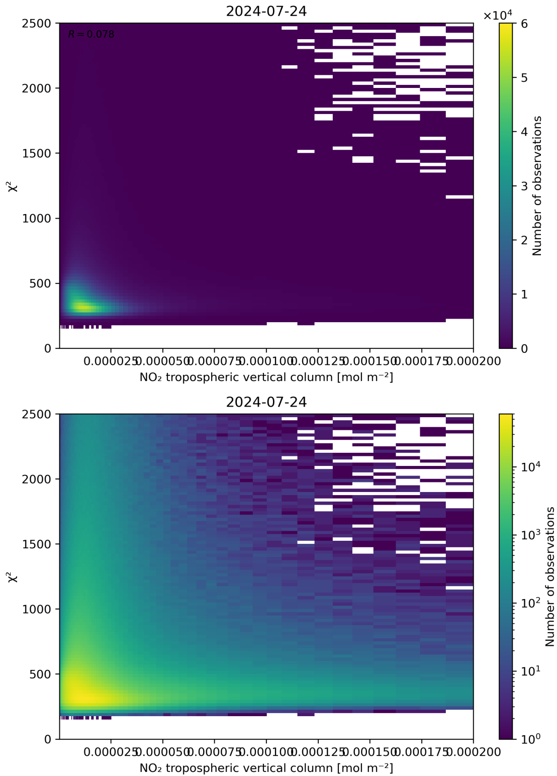
Figure 124: Scatter density plot of “NO 2 tropospheric vertical column” against “ \chi^2 ” for 2024-07-23 to 2024-07-24.
