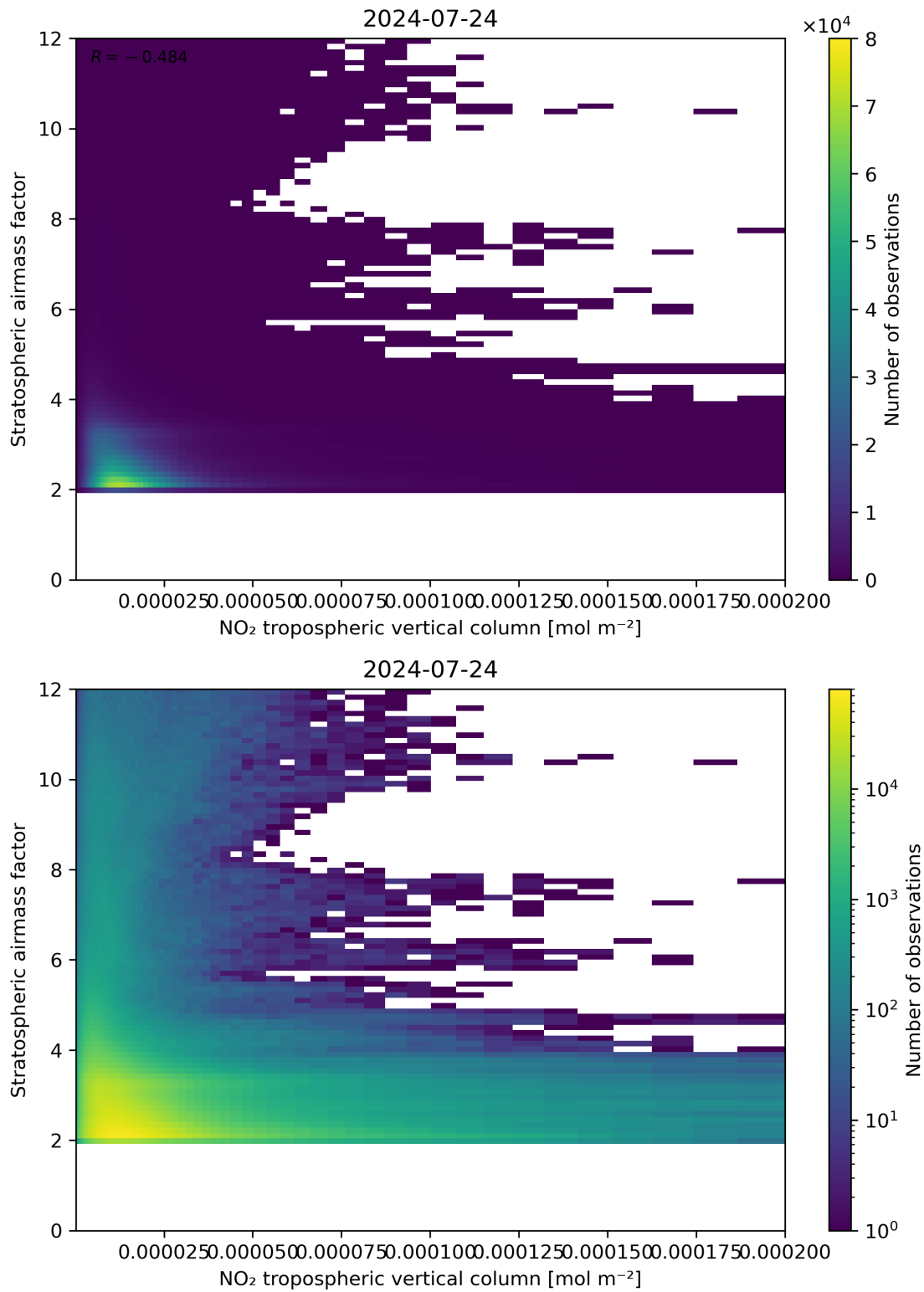
Figure 121: Scatter density plot of “NO 2 tropospheric vertical column” against “Stratospheric air mass factor” for 2024-07-23 to 2024-07-24.
