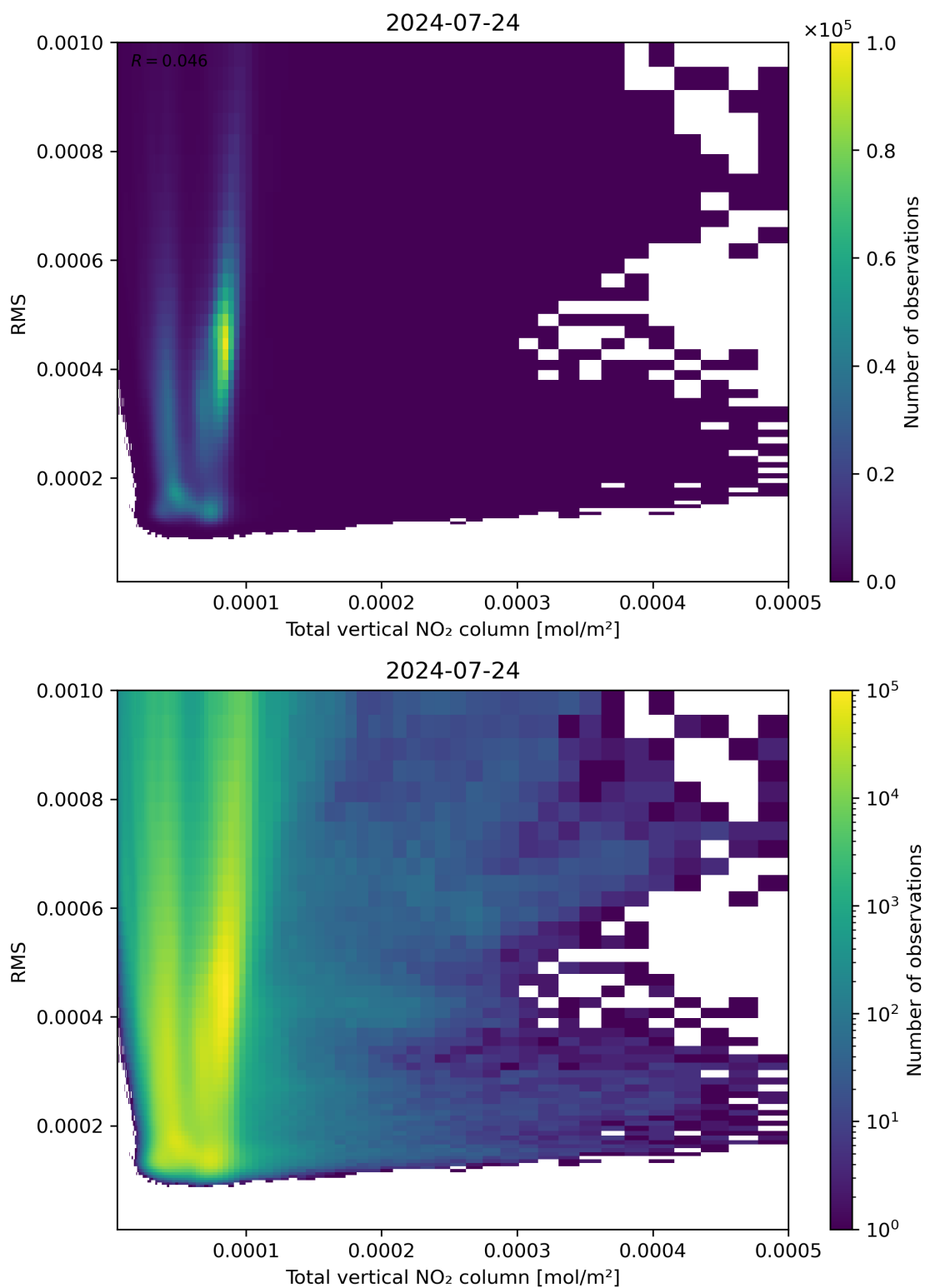
Figure 120: Scatter density plot of “Total vertical NO 2 column” against “RMS” for 2024-07-23 to 2024-07-24.
