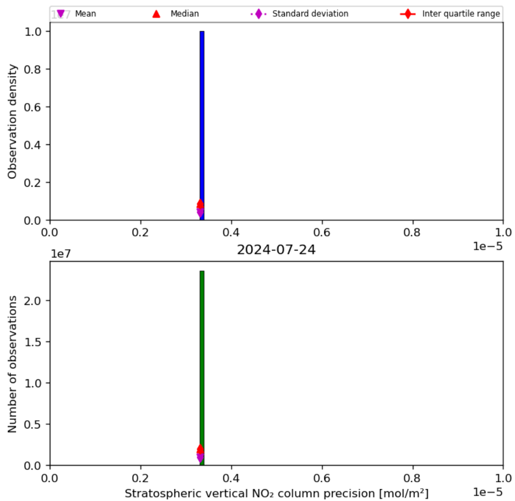
Figure 37: Histogram of “Stratospheric vertical NO 2 column precision” for 2024-07-23 to 2024-07-24
