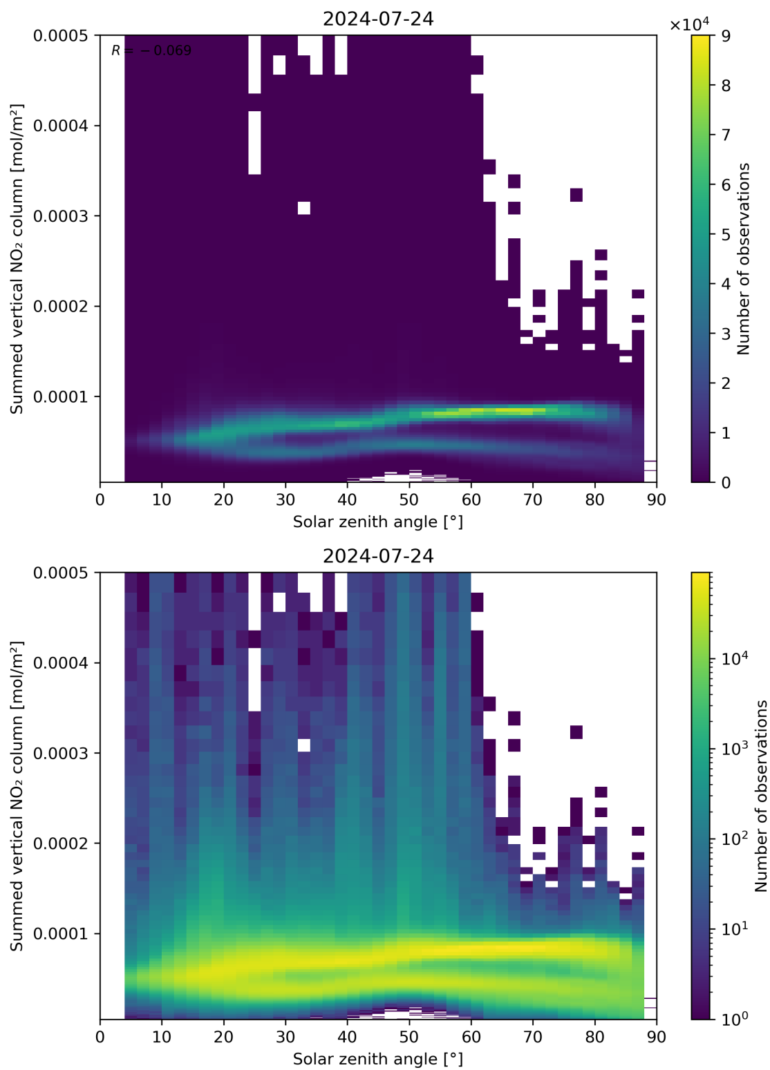
Figure 151: Scatter density plot of “Solar zenith angle” against “Summed vertical NO 2 column” for 2024-07-23 to 2024-07-24.
