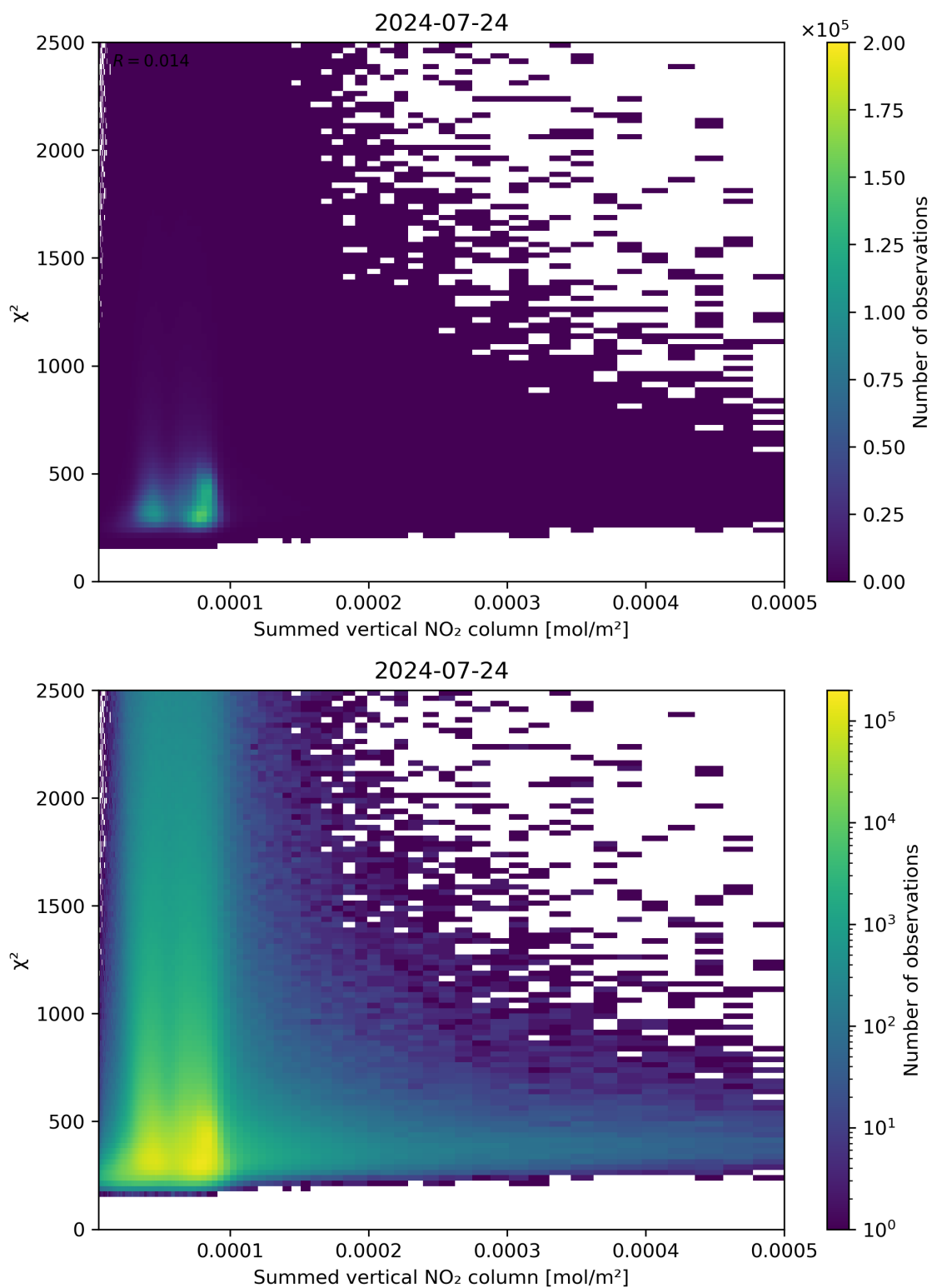
Figure 104: Scatter density plot of “Summed vertical NO 2 column” against “ \chi^2 ” for 2024-07-23 to 2024-07-24.
