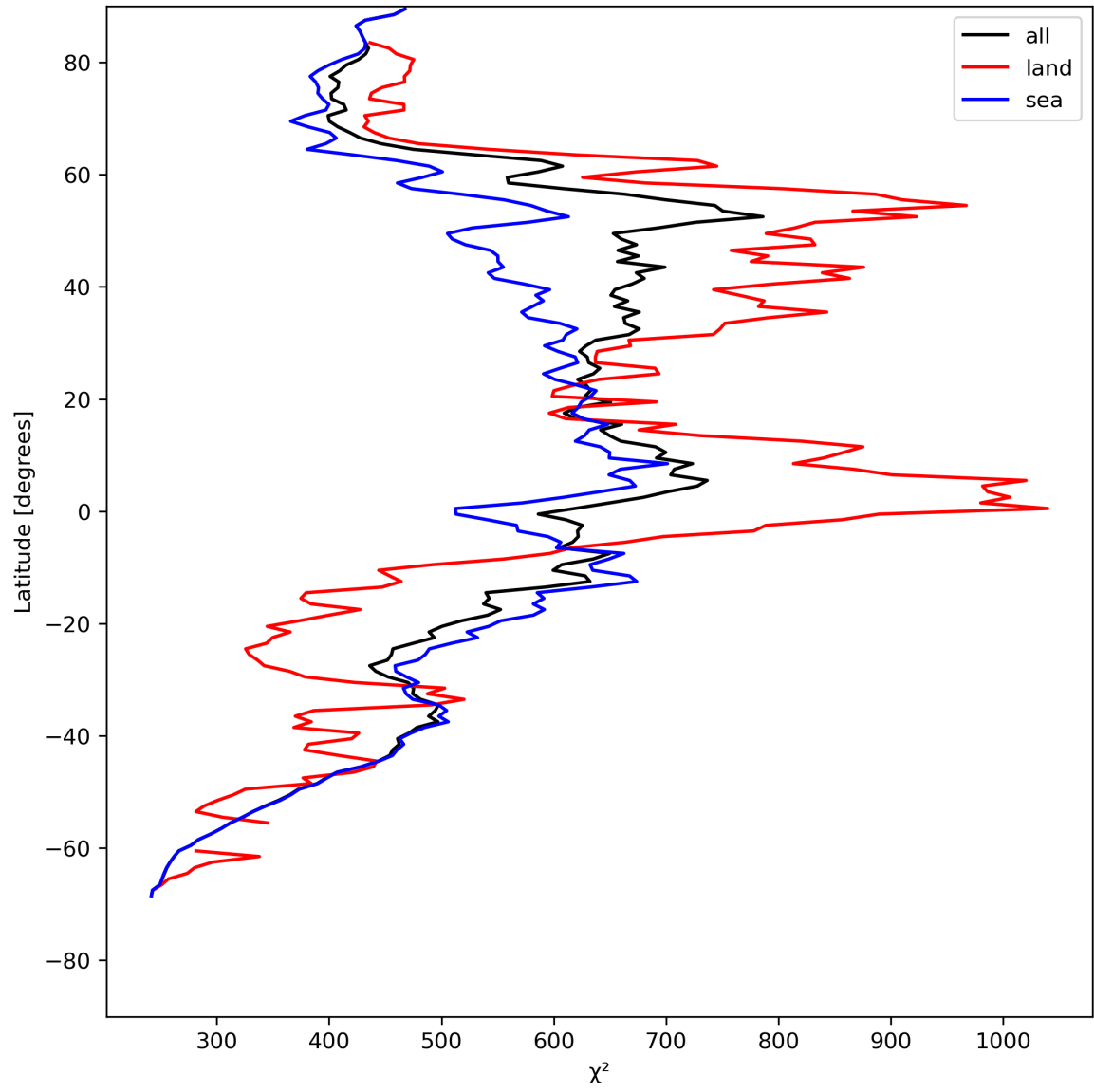
Figure 25: Zonal average of “ \chi^2 ” for 2024-07-23 to 2024-07-24.
