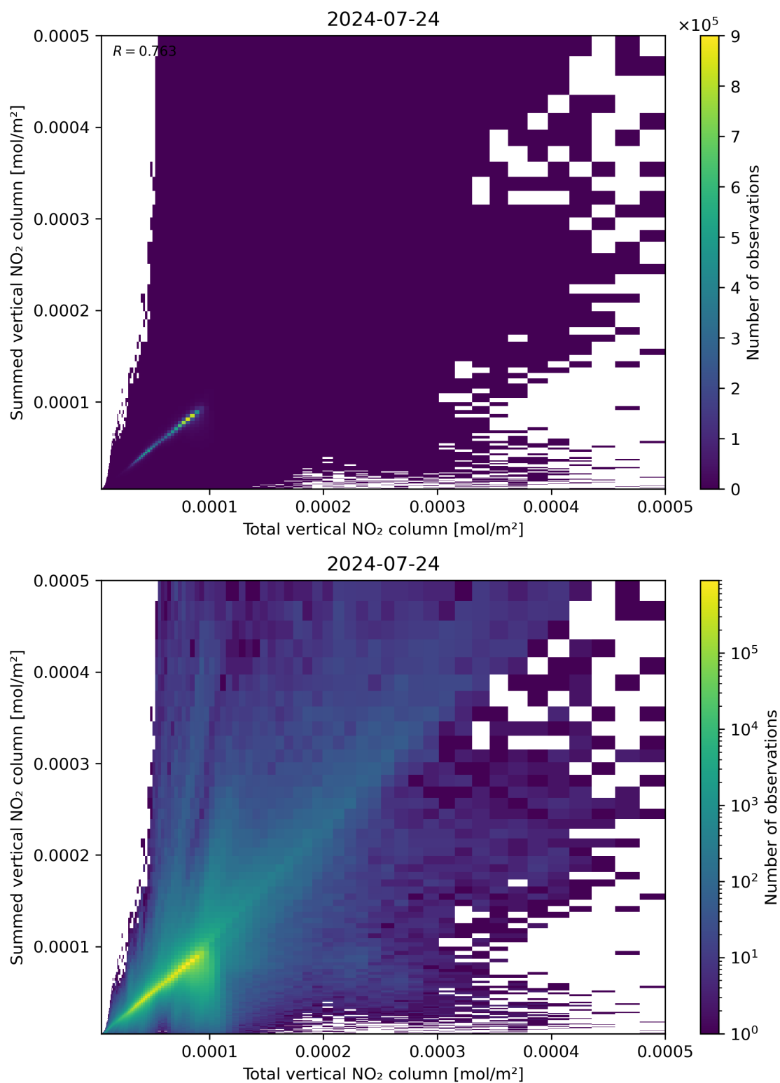
Figure 112: Scatter density plot of “Total vertical NO 2 column” against “Summed vertical NO 2 column” for 2024-07-23 to 2024-07-24.
