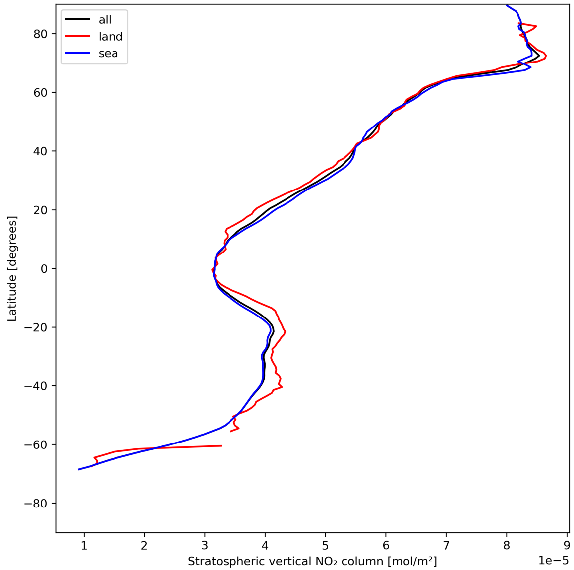
Figure 19: Zonal average of “Stratospheric vertical NO 2 column” for 2024-07-23 to 2024-07-24.
