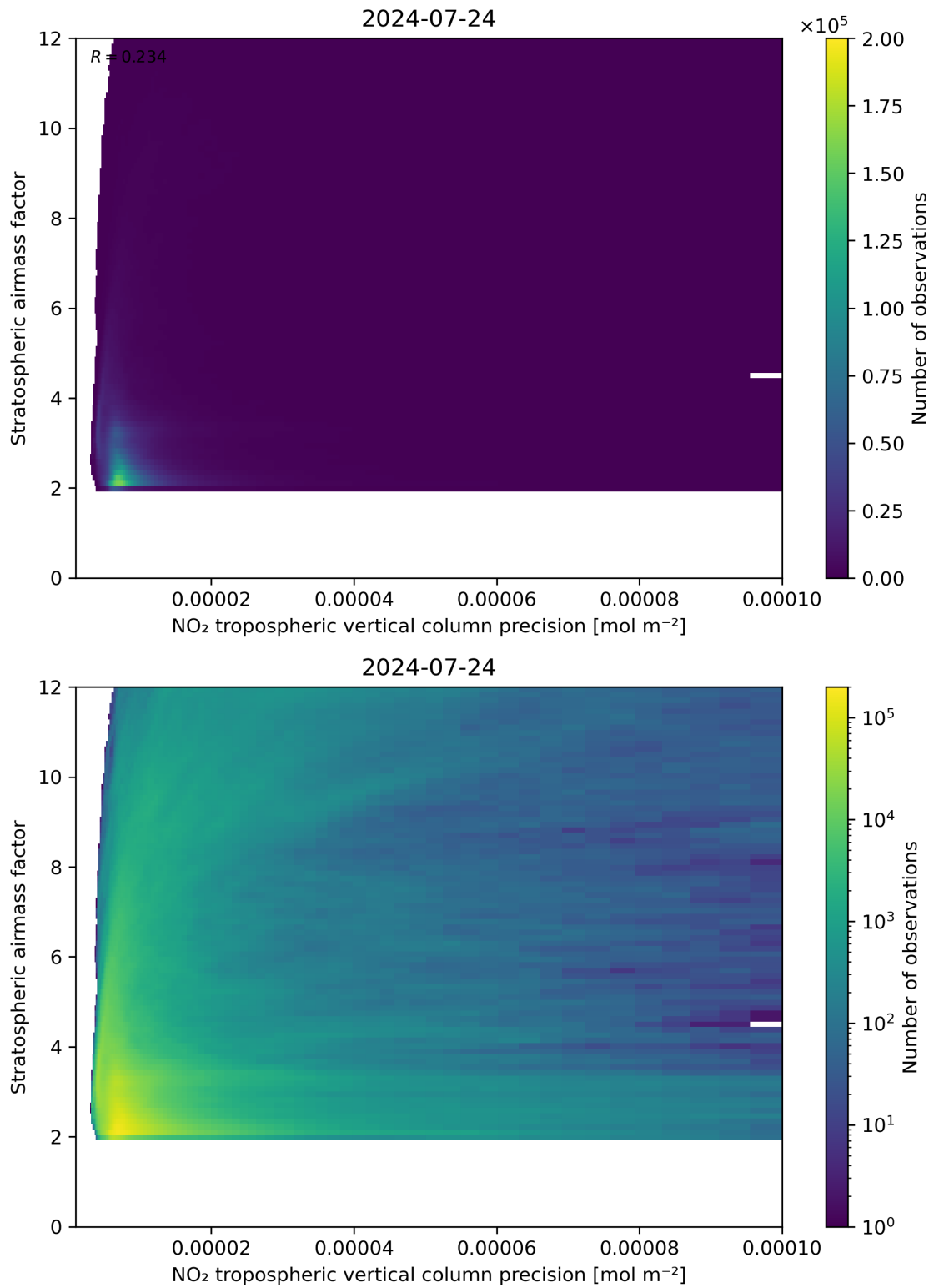
Figure 131: Scatter density plot of “NO 2 tropospheric vertical column precision” against “Stratospheric airmass factor” for 2024-07-23 to 2024-07-24.
