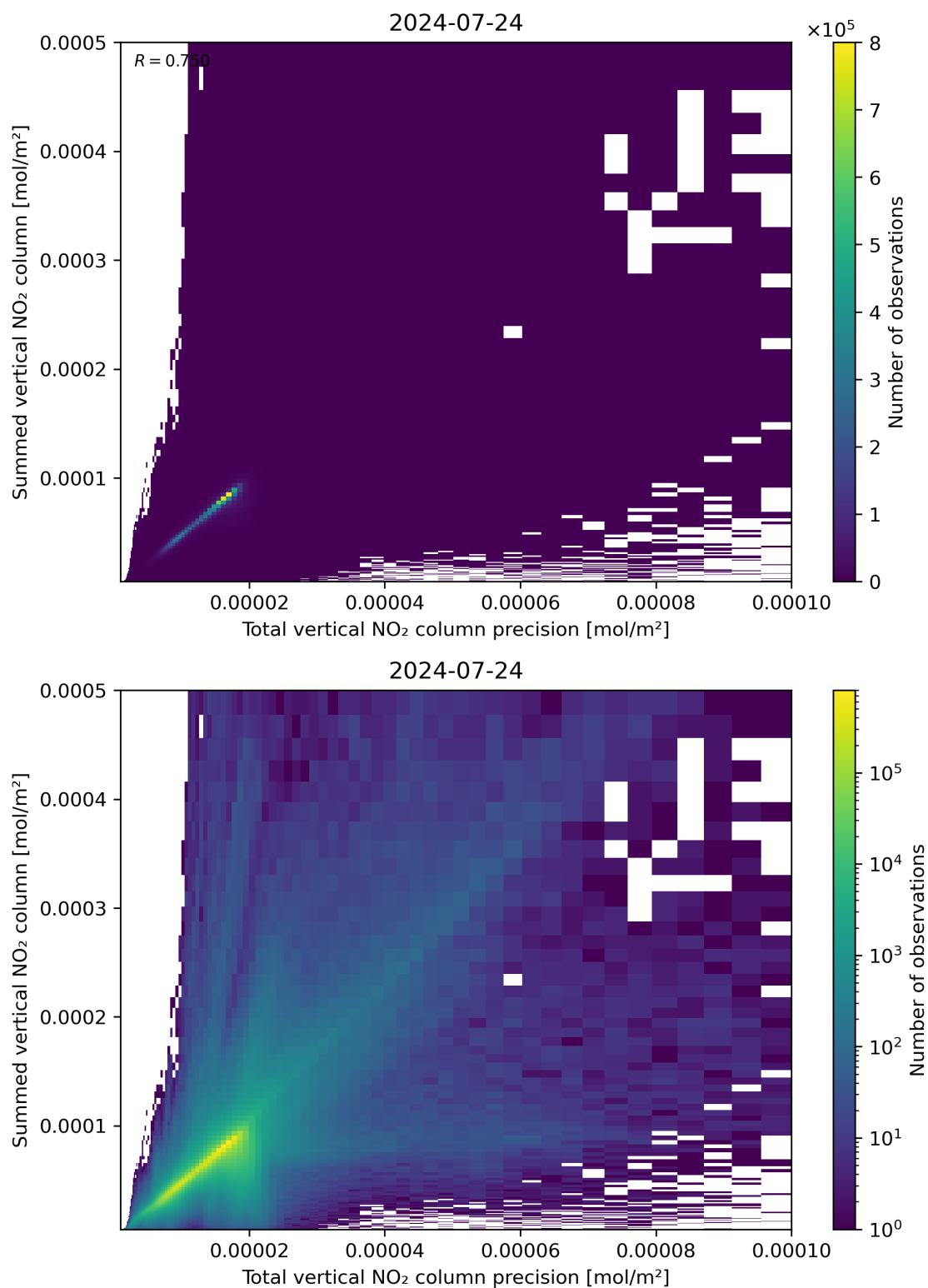
Figure 117: Scatter density plot of “Total vertical NO 2 column precision” against “Summed vertical NO 2 column” for 2024-07-23 to 2024-07-24.
