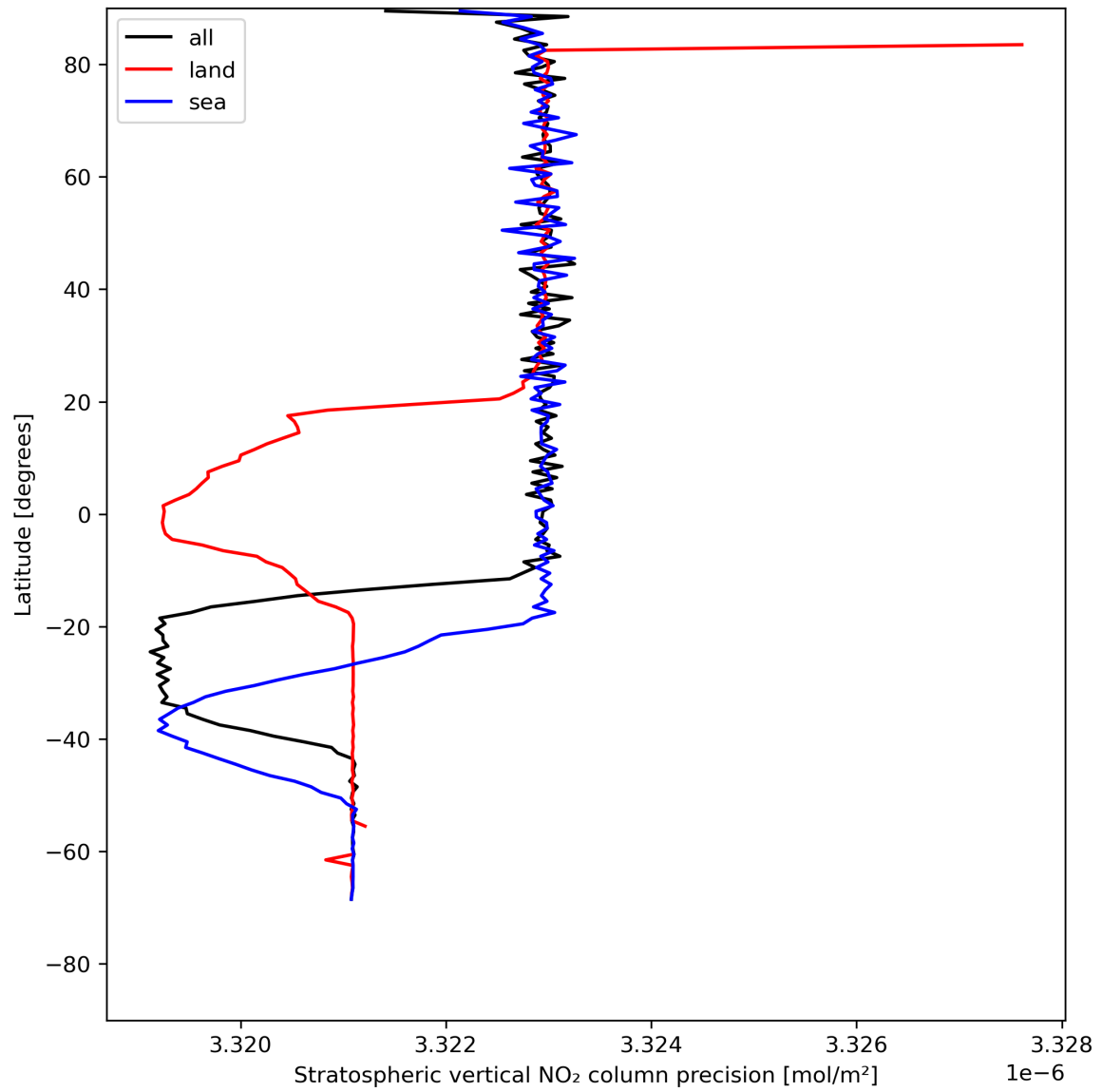
Figure 20: Zonal average of “Stratospheric vertical NO 2 column precision” for 2024-07-23 to 2024-07-24.
