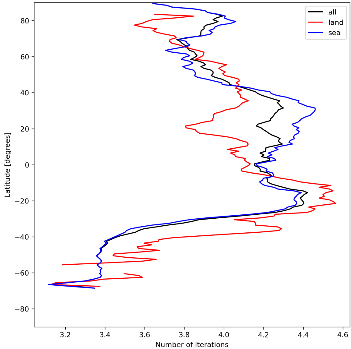
Figure 17: Zonal average of “Number of iterations” for 2024-07-23 to 2024-07-24.
