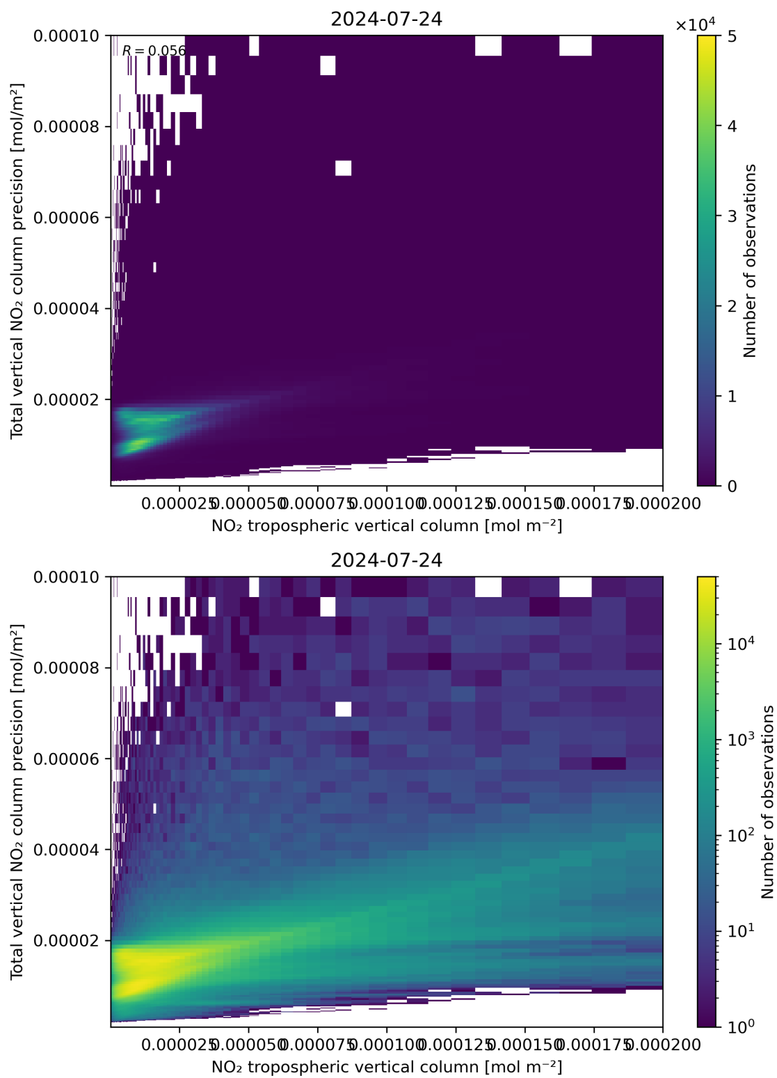
Figure 129: Scatter density plot of “NO 2 tropospheric vertical column” against “Total vertical NO 2 column precision” for 2024-07-23 to 2024-07-24.
