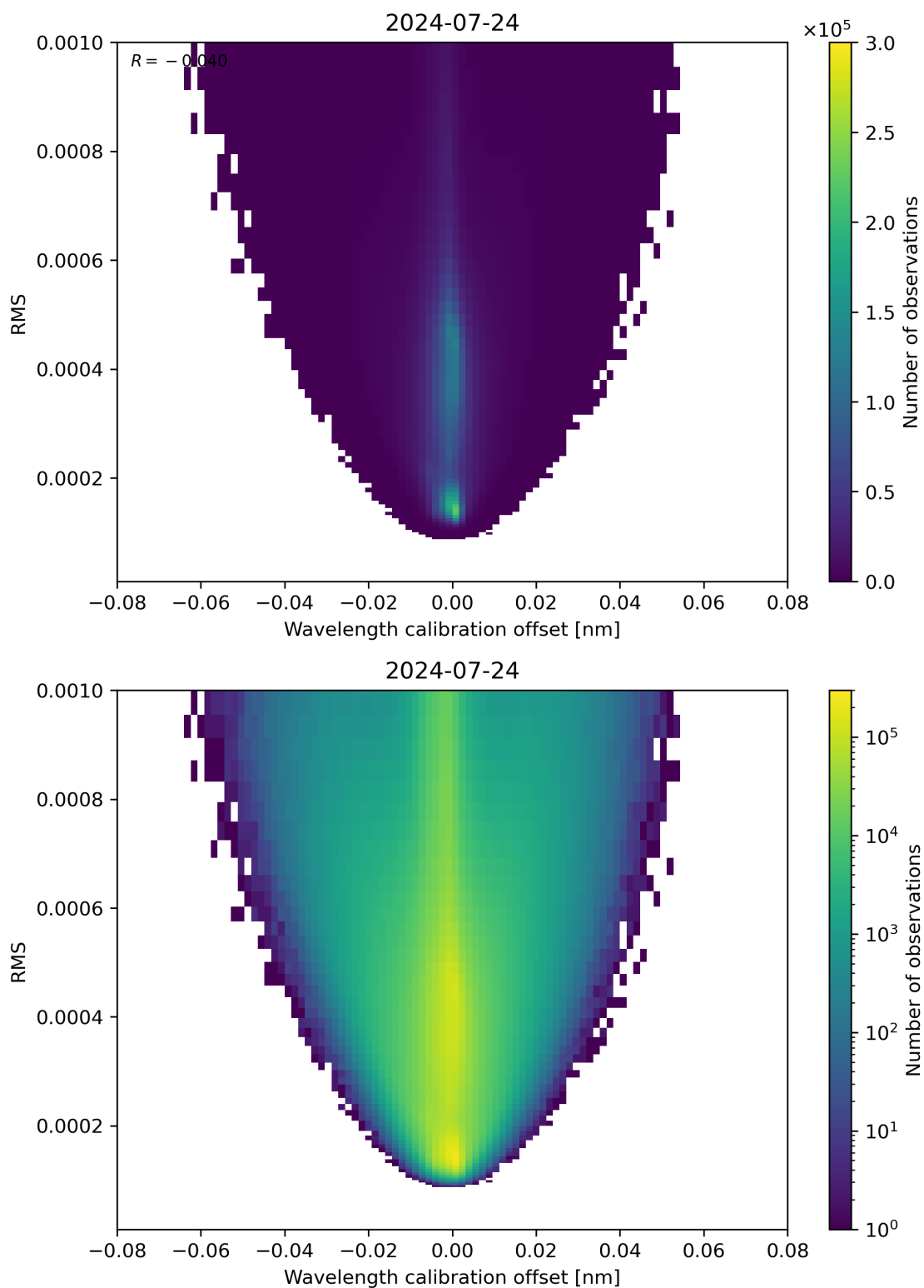
Figure 181: Scatter density plot of “Wavelength calibration offset” against “RMS” for 2024-07-23 to 2024-07-24.
