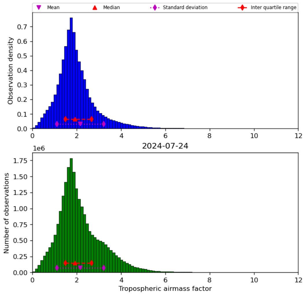
Figure 31: Histogram of “Tropospheric airmass factor” for 2024-07-23 to 2024-07-24
