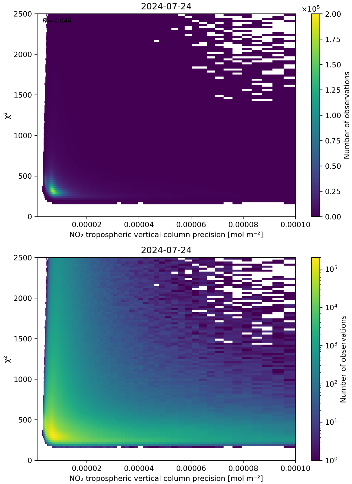
Figure 134: Scatter density plot of “NO 2 tropospheric vertical column precision” against “ \chi^2 ” for 2024-07-23 to 2024-07-24.
