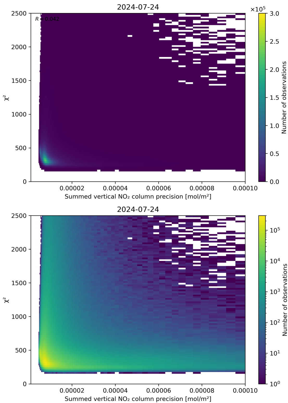
Figure 107: Scatter density plot of “Summed vertical NO 2 column precision” against “ \chi^2 ” for 2024-07-23 to 2024-07-24.
