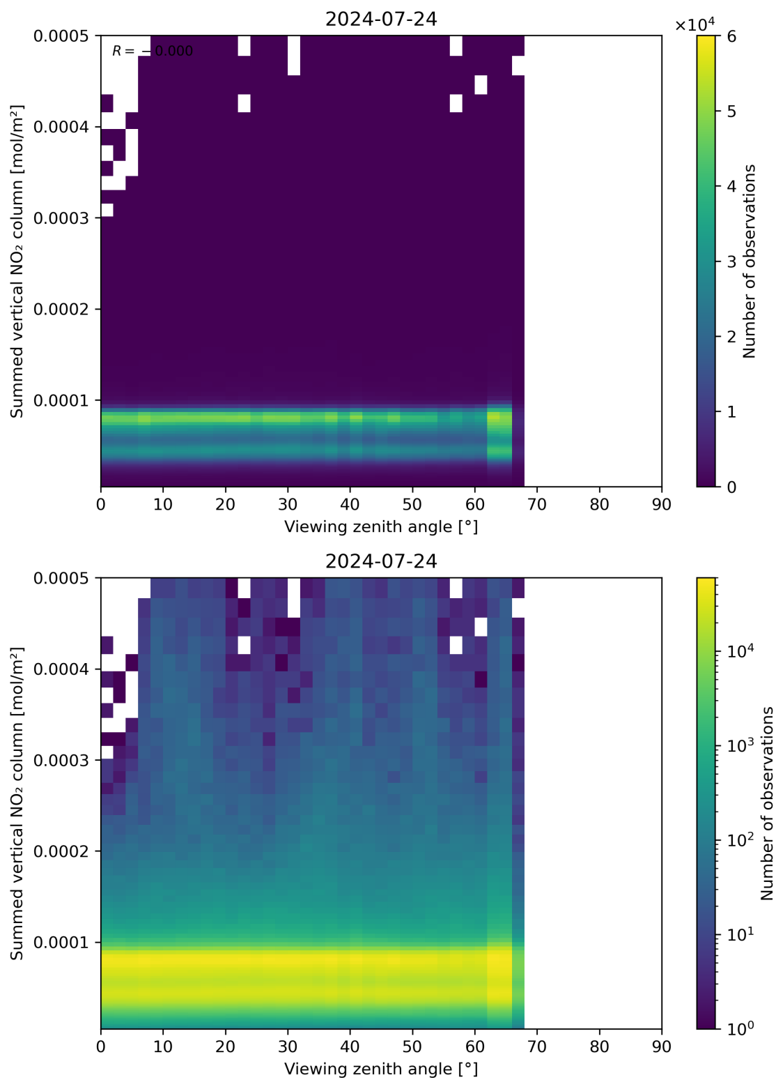
Figure 165: Scatter density plot of “Viewing zenith angle” against “Summed vertical NO 2 column” for 2024-07-23 to 2024-07-24.
