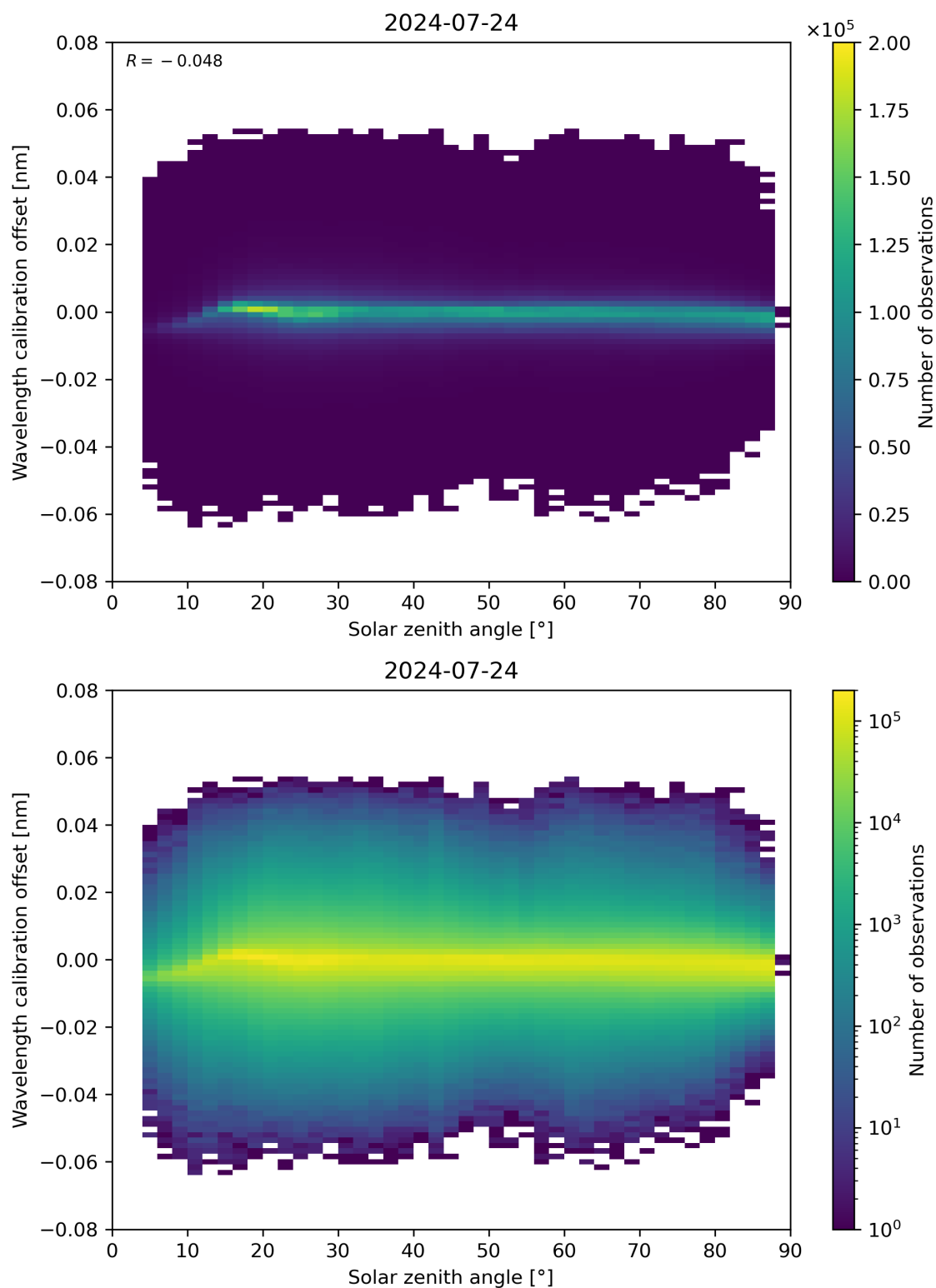
Figure 158: Scatter density plot of “Solar zenith angle” against “Wavelength calibration offset” for 2024-07-23 to 2024-07-24.
