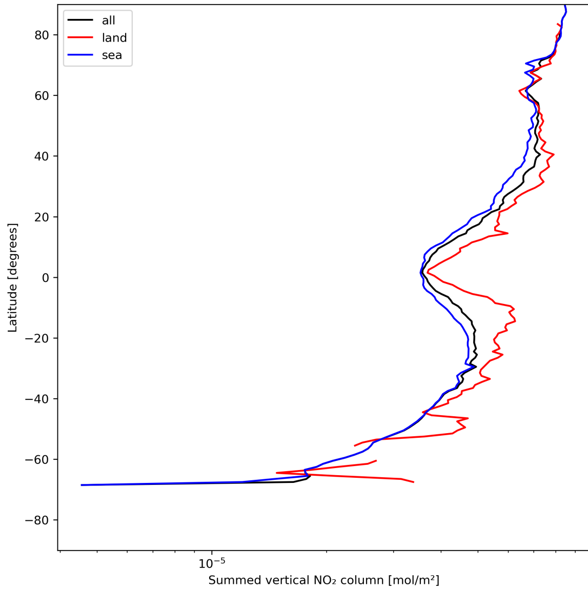
Figure 23: Zonal average of “Summed vertical NO 2 column” for 2024-07-23 to 2024-07-24.
