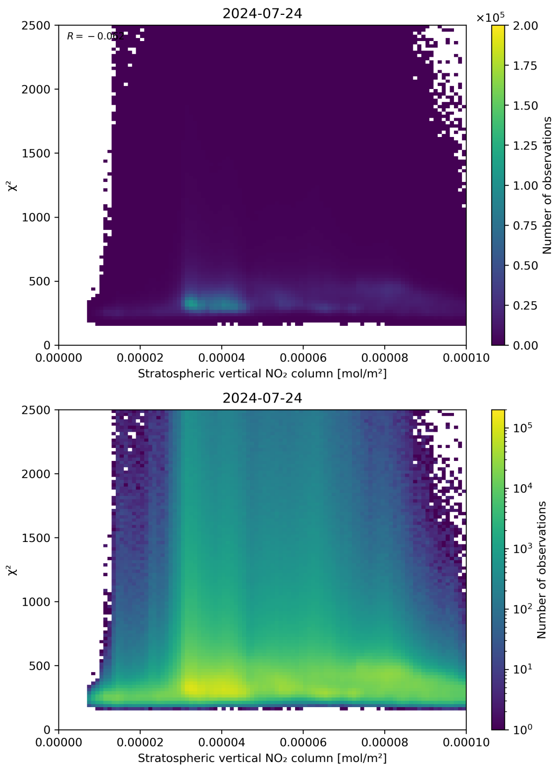
Figure 97: Scatter density plot of “Stratospheric vertical NO 2 column” against “ \chi^2 ” for 2024-07-23 to 2024-07-24.
