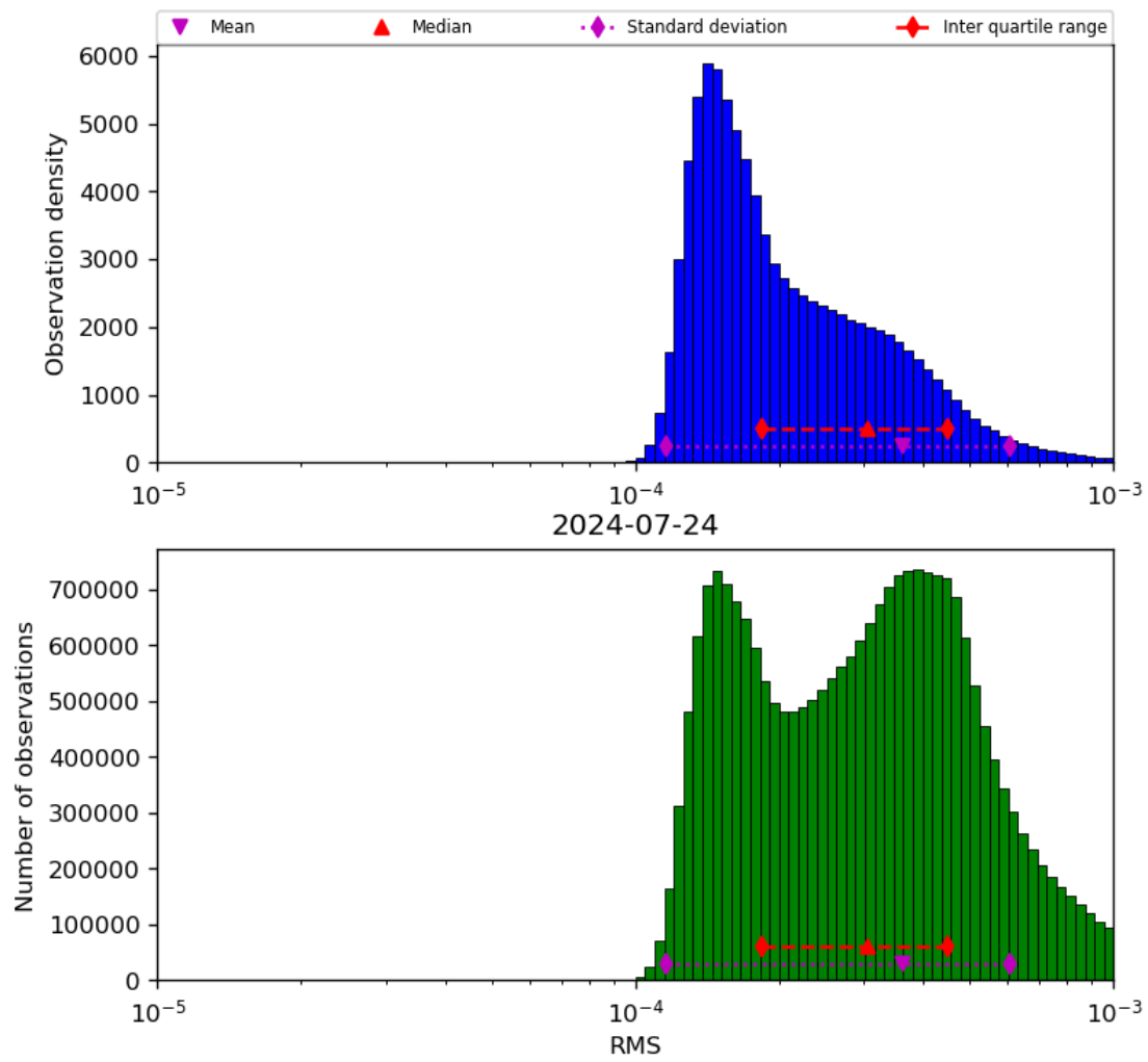
Figure 43: Histogram of “RMS” for 2024-07-23 to 2024-07-24
