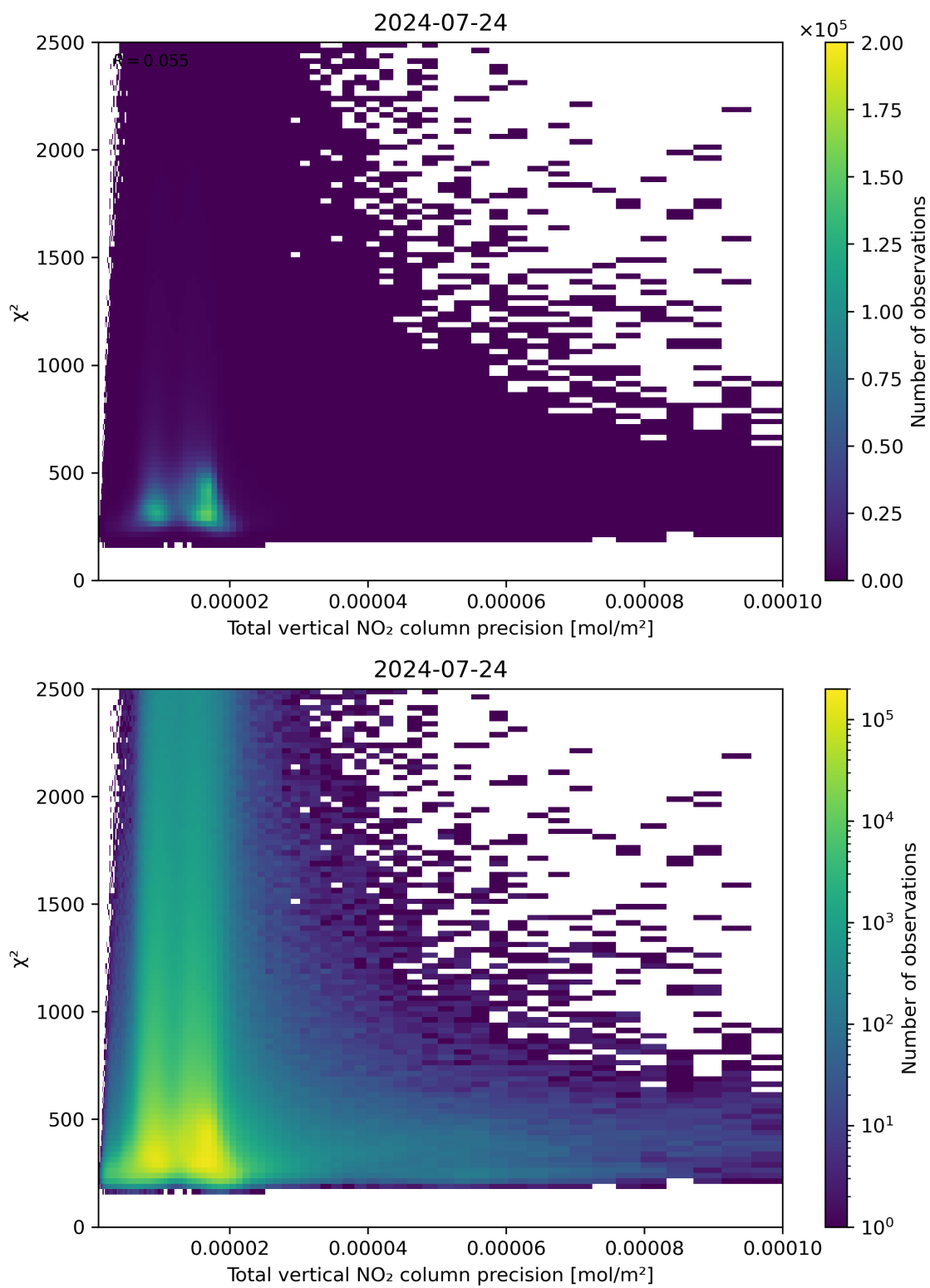
Figure 116: Scatter density plot of “Total vertical NO 2 column precision” against “ \chi^2 ” for 2024-07-23 to 2024-07-24.
