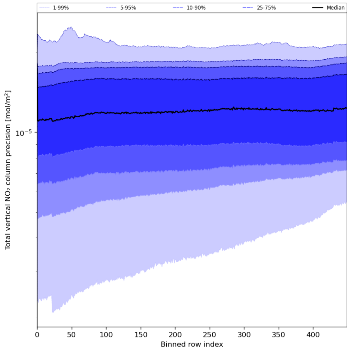
Figure 56: Along track statistics of “Total vertical NO 2 column precision” for 2024-07-23 to 2024-07-24
