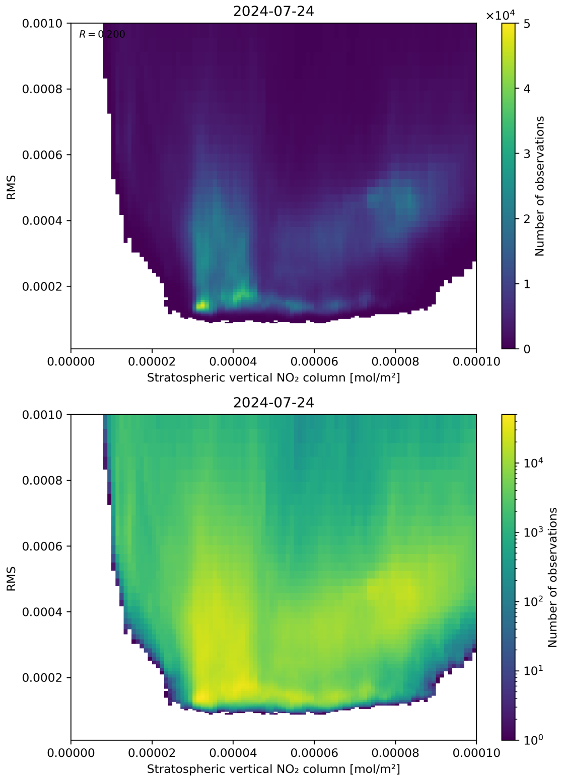
Figure 102: Scatter density plot of “Stratospheric vertical NO 2 column” against “RMS” for 2024-07-23 to 2024-07-24.
