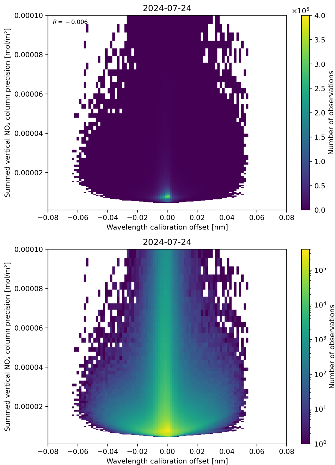
Figure 178: Scatter density plot of “Wavelength calibration offset” against “Summed vertical NO 2 column precision” for 2024-07-23 to 2024-07-24.
