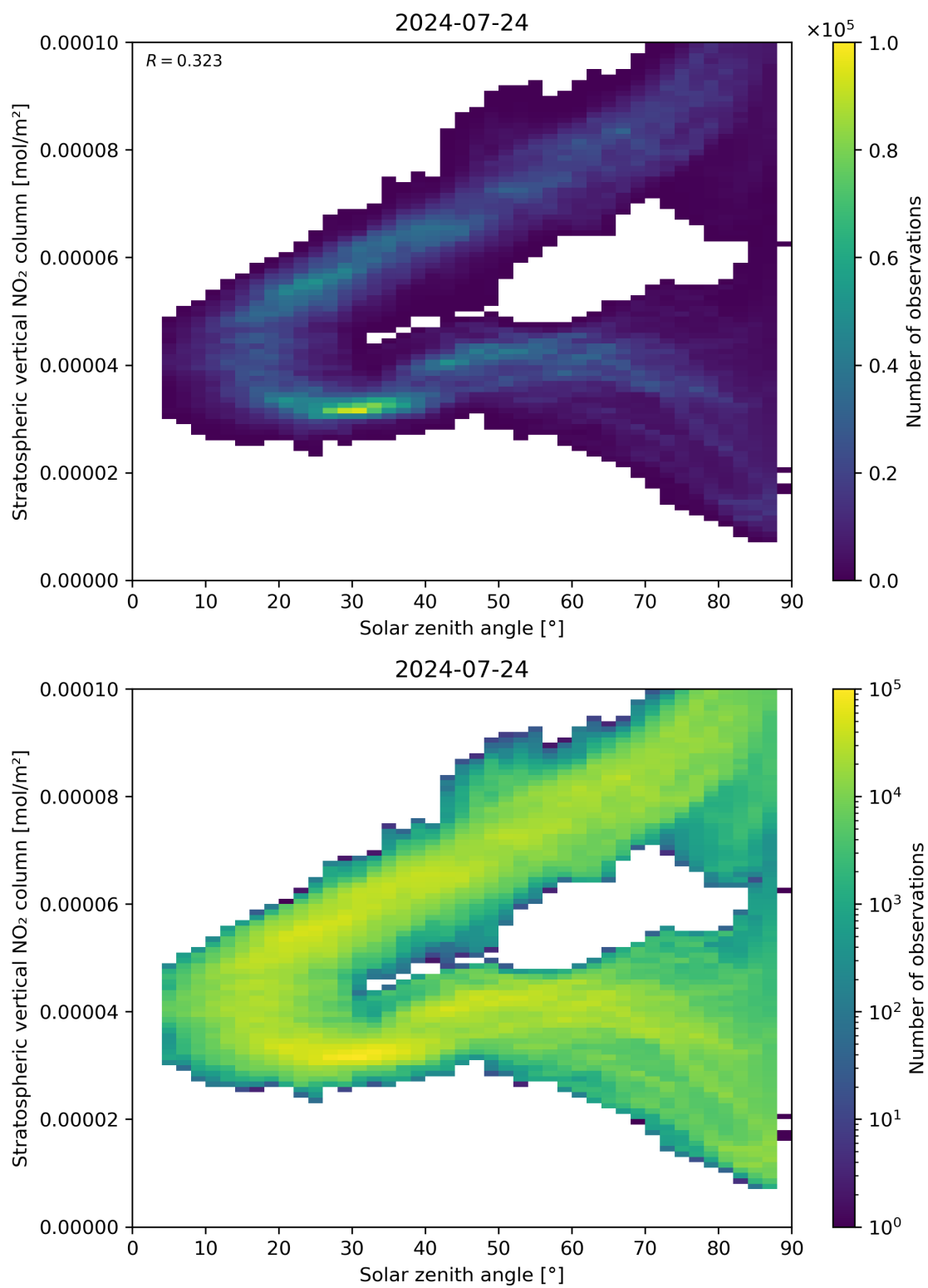
Figure 150: Scatter density plot of “Solar zenith angle” against “Stratospheric vertical NO 2 column” for 2024-07-23 to 2024-07-24.
