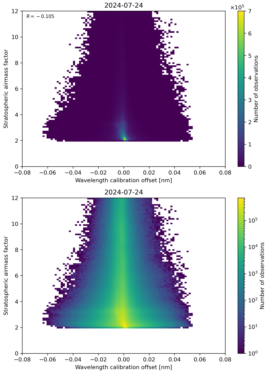
Figure 174: Scatter density plot of “Wavelength calibration offset” against “Stratospheric airmass factor” for 2024-07-23 to 2024-07-24.
