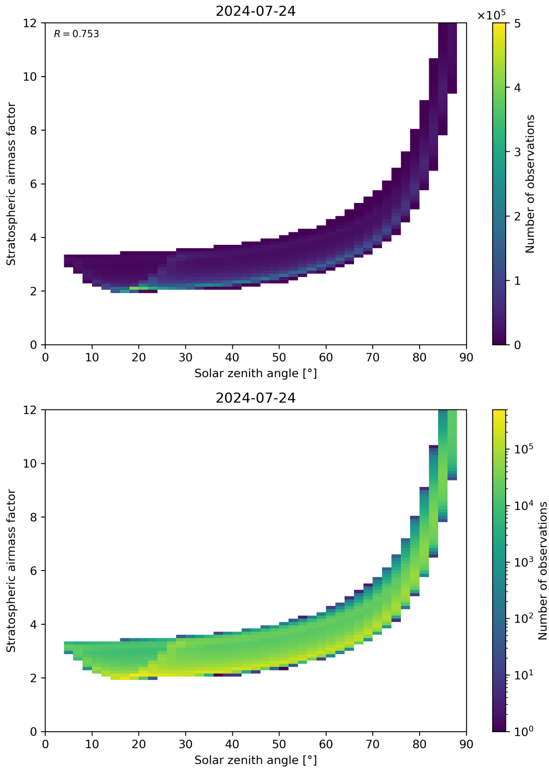
Figure 145: Scatter density plot of “Solar zenith angle” against “Stratospheric airmass factor” for 2024-07-23 to 2024-07-24.
