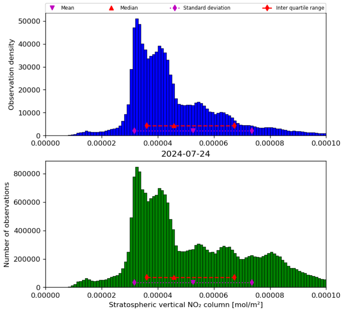
Figure 36: Histogram of “Stratospheric vertical NO 2 column” for 2024-07-23 to 2024-07-24
