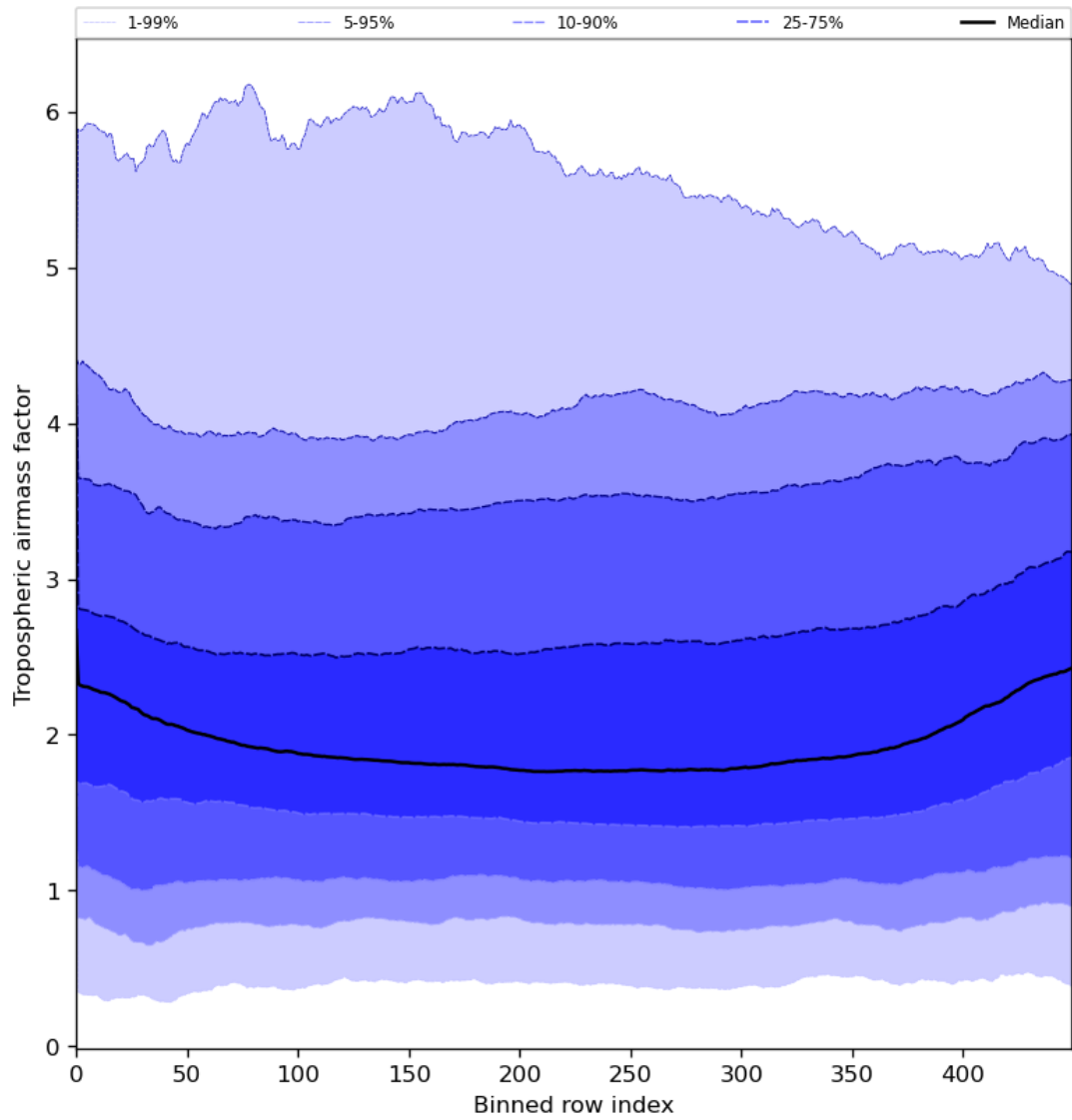
Figure 48: Along track statistics of “Tropospheric airmass factor” for 2024-07-23 to 2024-07-24
