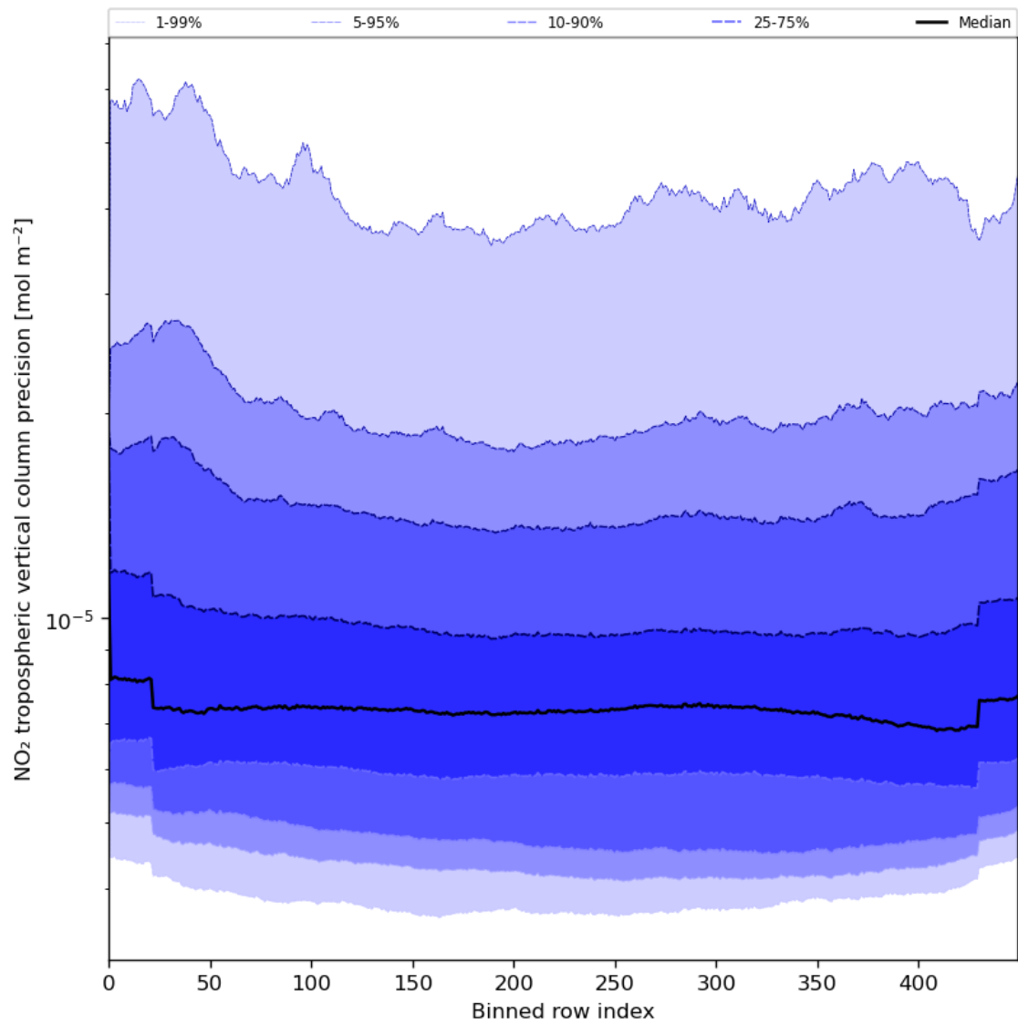
Figure 47: Along track statistics of “NO 2 tropospheric vertical column precision” for 2024-07-23 to 2024-07-24
