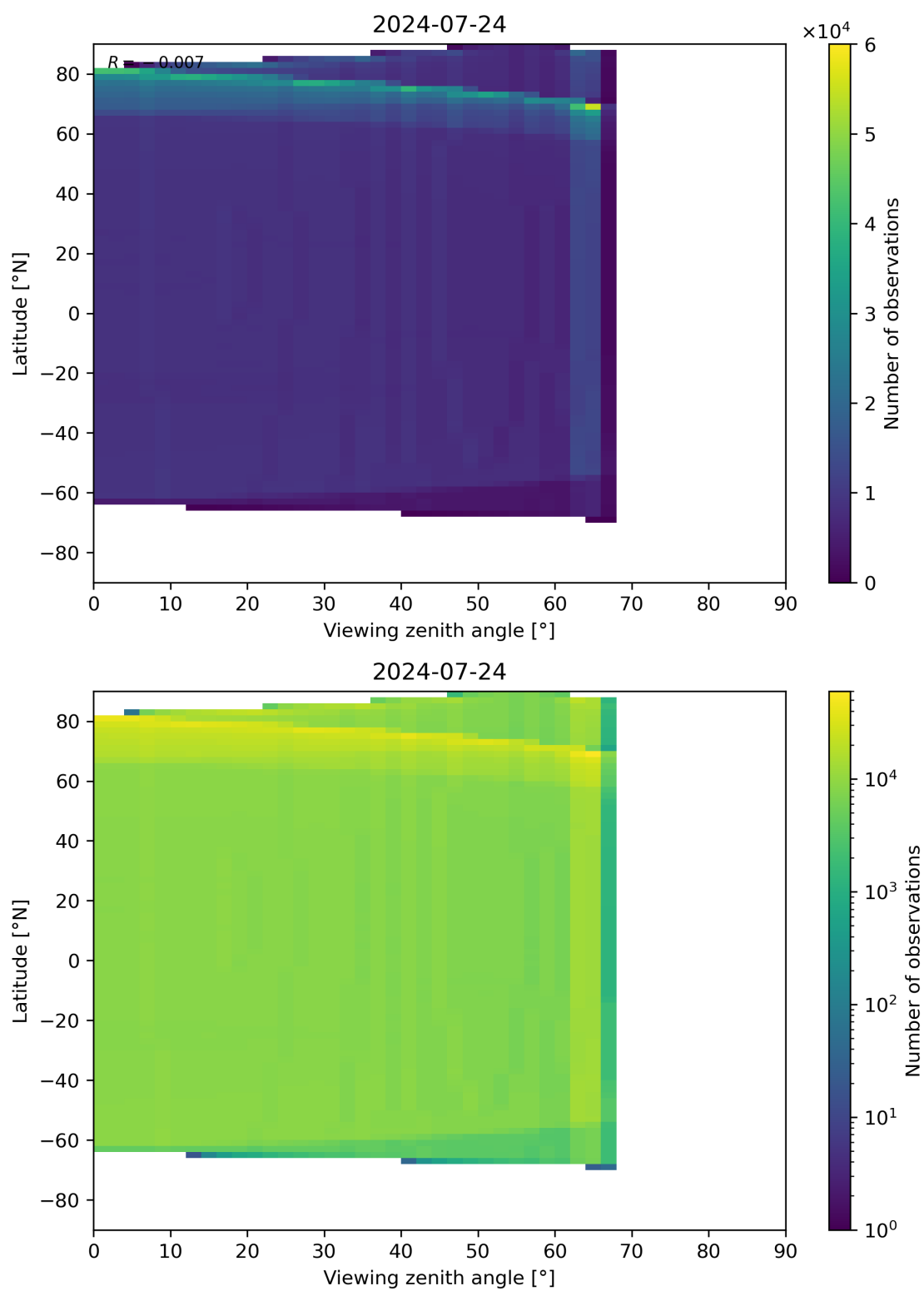
Figure 163: Scatter density plot of “Viewing zenith angle” against “Latitude” for 2024-07-23 to 2024-07-24.
