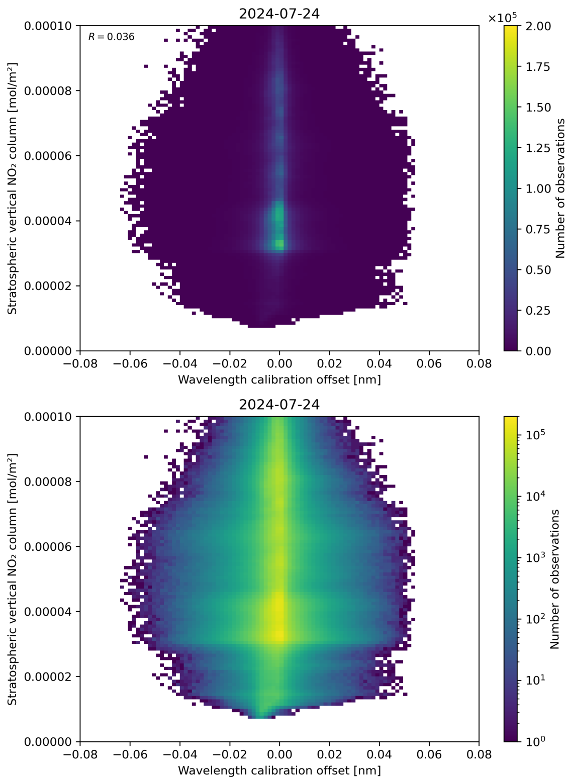
Figure 176: Scatter density plot of “Wavelength calibration offset” against “Stratospheric vertical NO 2 column” for 2024-07-23 to 2024-07-24.
