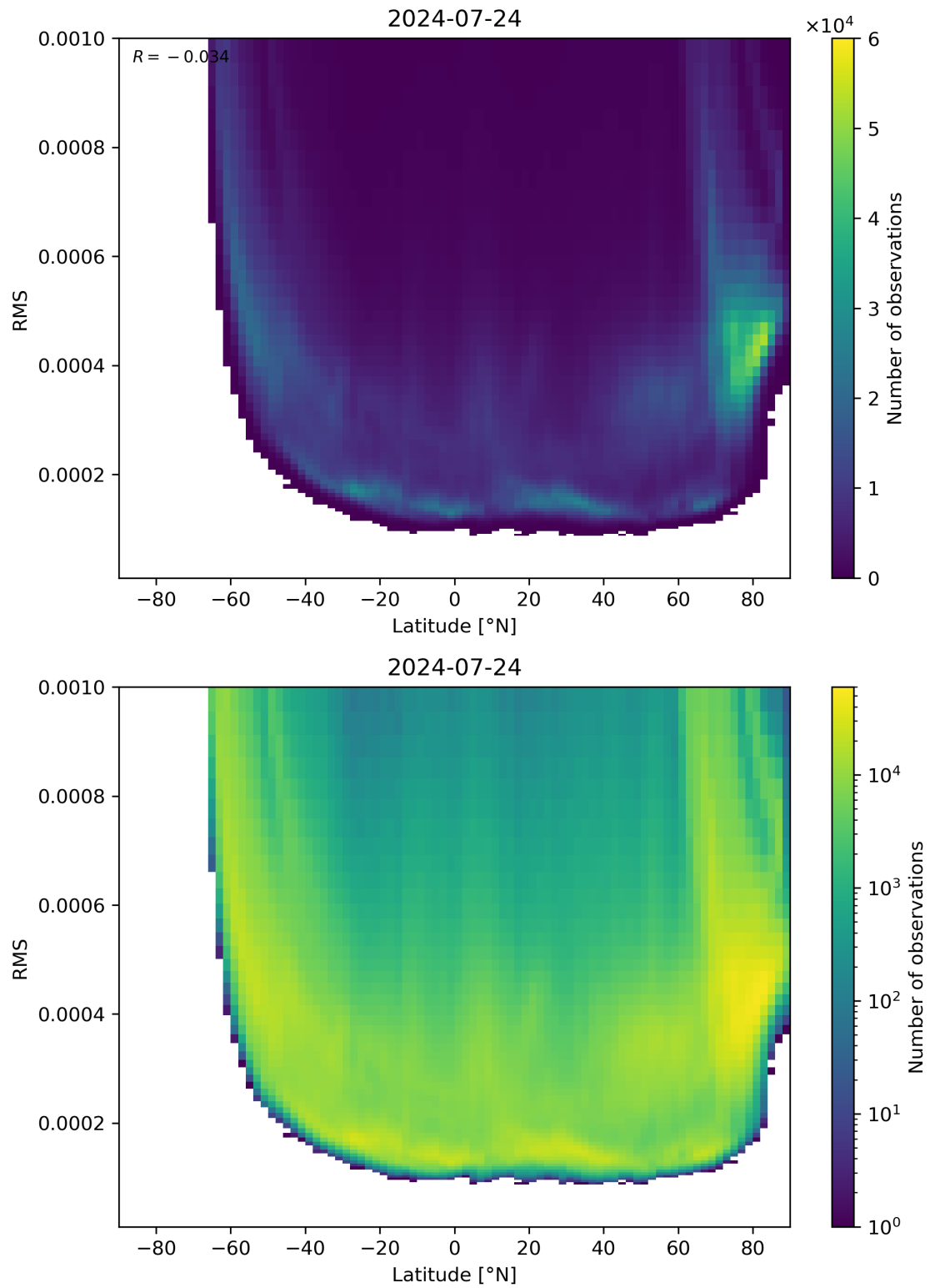
Figure 94: Scatter density plot of “Latitude” against “RMS” for 2024-07-23 to 2024-07-24.
