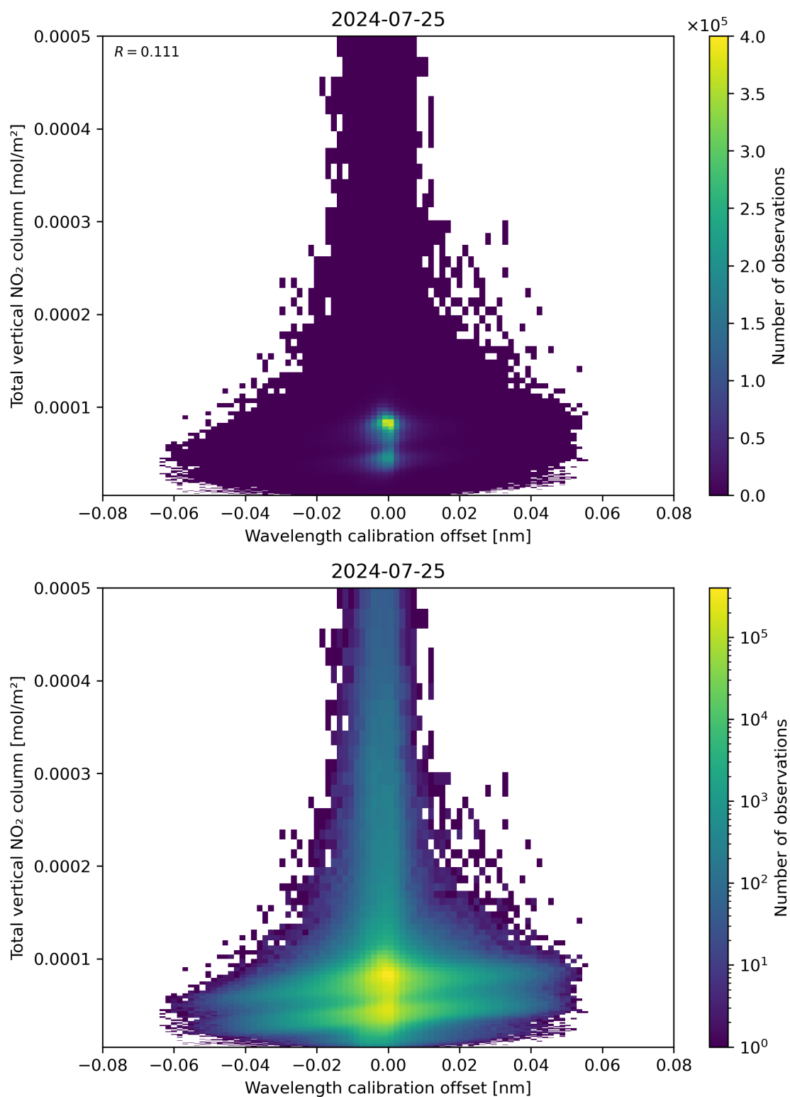
Figure 179: Scatter density plot of “Wavelength calibration offset” against “Total vertical NO 2 column” for 2024-07-24 to 2024-07-26.
