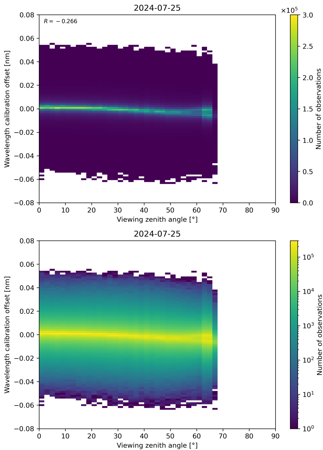
Figure 173: Scatter density plot of “Viewing zenith angle” against “Wavelength calibration offset” for 2024-07-24 to 2024-07-26.
