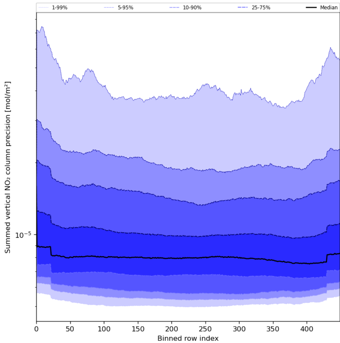
Figure 58: Along track statistics of “Summed vertical NO 2 column precision” for 2024-07-24 to 2024-07-26
