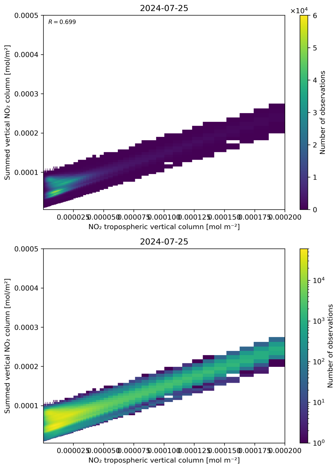
Figure 126: Scatter density plot of “NO 2 tropospheric vertical column” against “Summed vertical NO 2 column” for 2024-07-24 to 2024-07-26.
