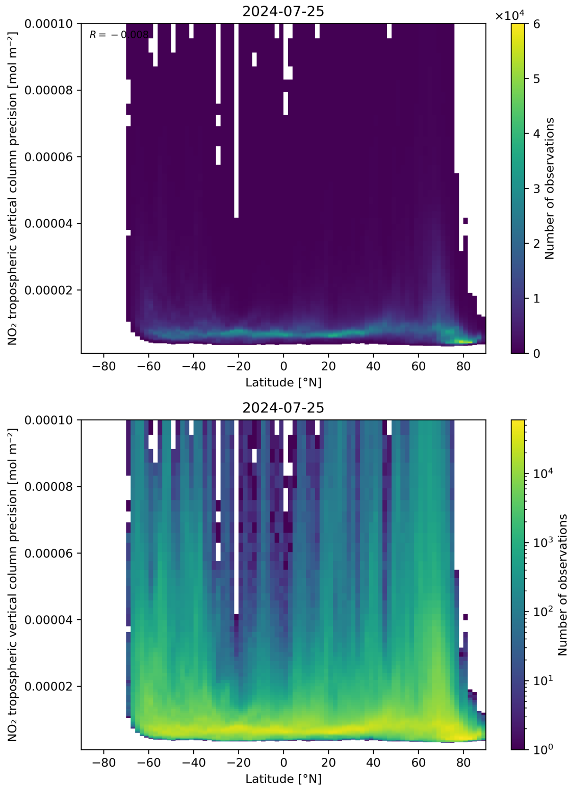
Figure 93: Scatter density plot of “Latitude” against “NO 2 tropospheric vertical column precision” for 2024-07-24 to 2024-07-26.
