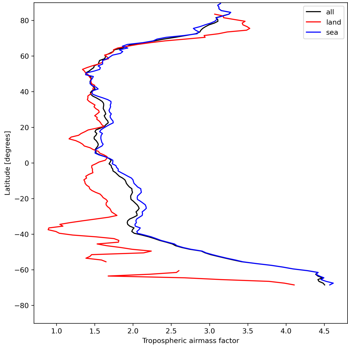
Figure 14: Zonal average of “Tropospheric air mass factor” for 2024-07-24 to 2024-07-26.
