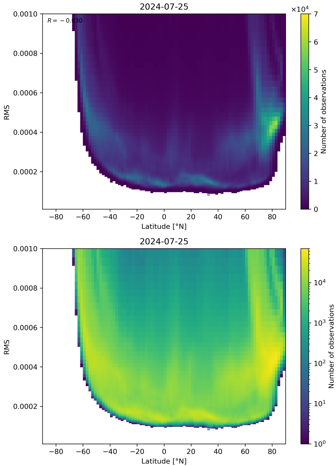
Figure 94: Scatter density plot of “Latitude” against “RMS” for 2024-07-24 to 2024-07-26.
