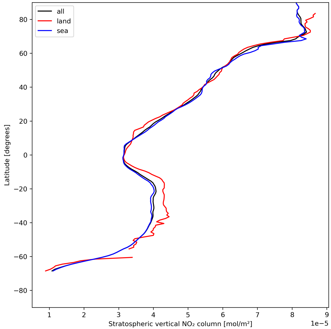
Figure 19: Zonal average of “Stratospheric vertical NO 2 column” for 2024-07-24 to 2024-07-26.
