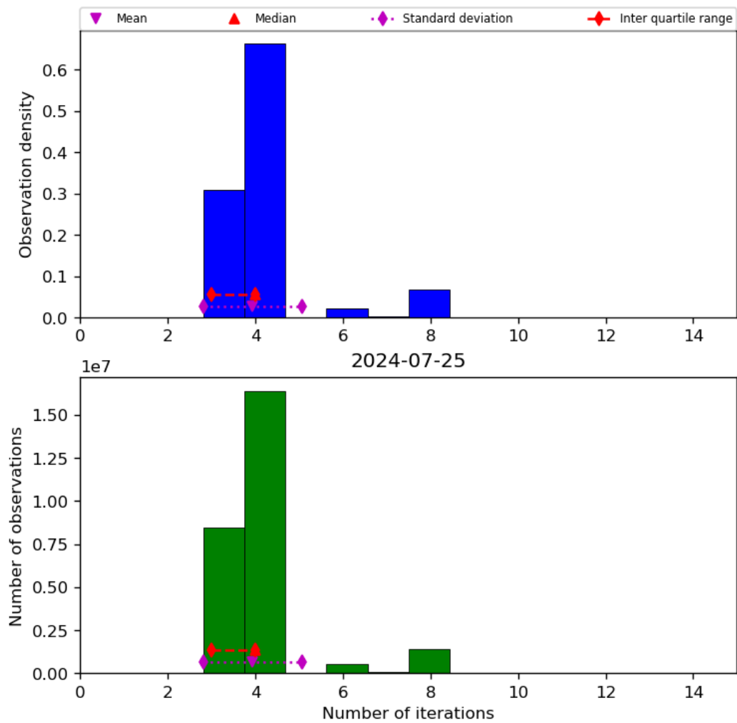
Figure 34: Histogram of “Number of iterations” for 2024-07-24 to 2024-07-26
