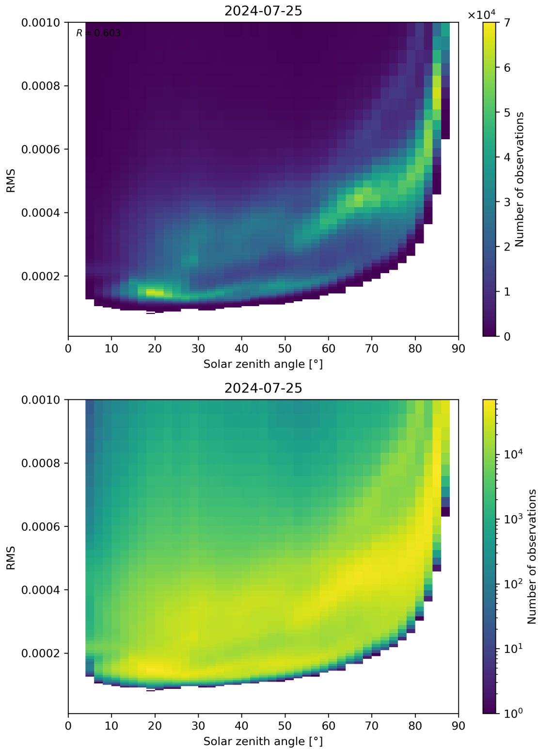
Figure 157: Scatter density plot of “Solar zenith angle” against “RMS” for 2024-07-24 to 2024-07-26.
