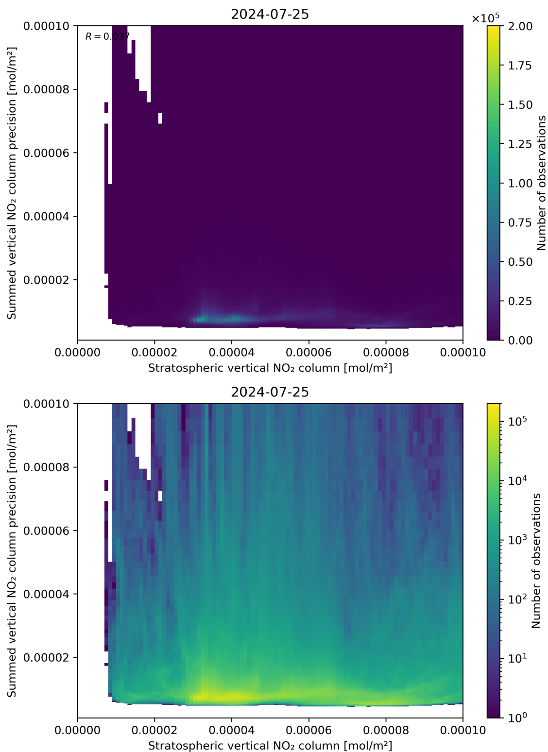
Figure 99: Scatter density plot of “Stratospheric vertical NO 2 column” against “Summed vertical NO 2 column precision” for 2024-07-24 to 2024-07-26.
