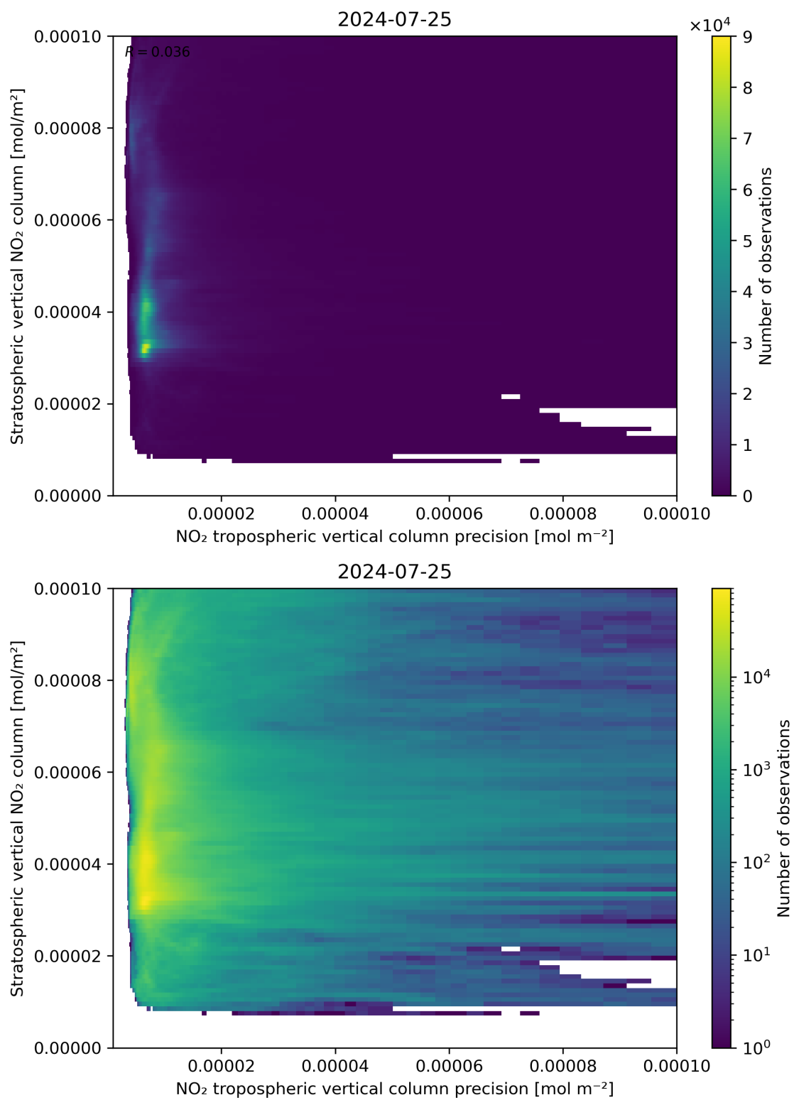
Figure 135: Scatter density plot of “NO 2 tropospheric vertical column precision” against “Stratospheric vertical NO 2 column” for 2024-07-24 to 2024-07-26.
