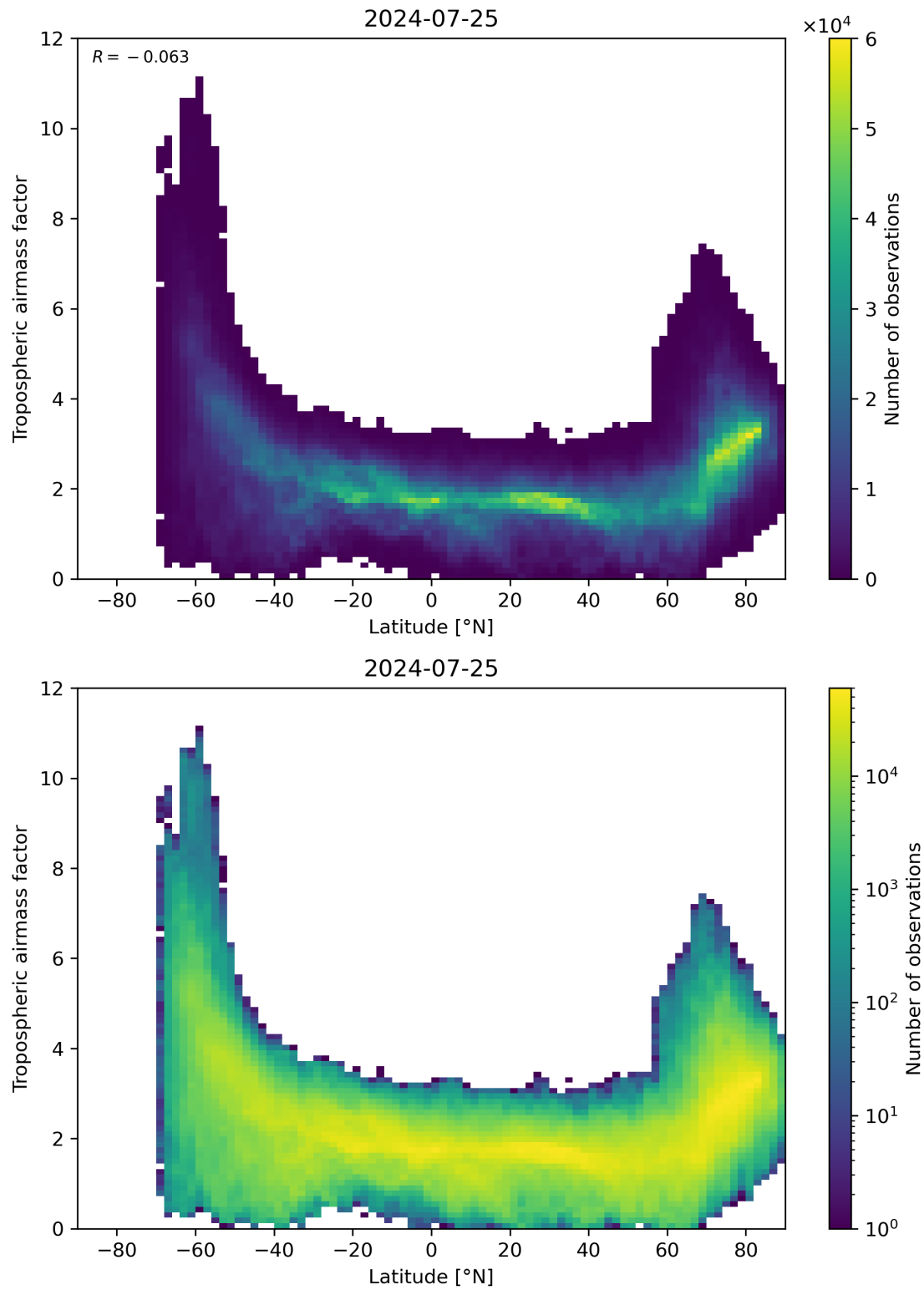
Figure 85: Scatter density plot of “Latitude” against “Tropospheric airmass factor” for 2024-07-24 to 2024-07-26.
