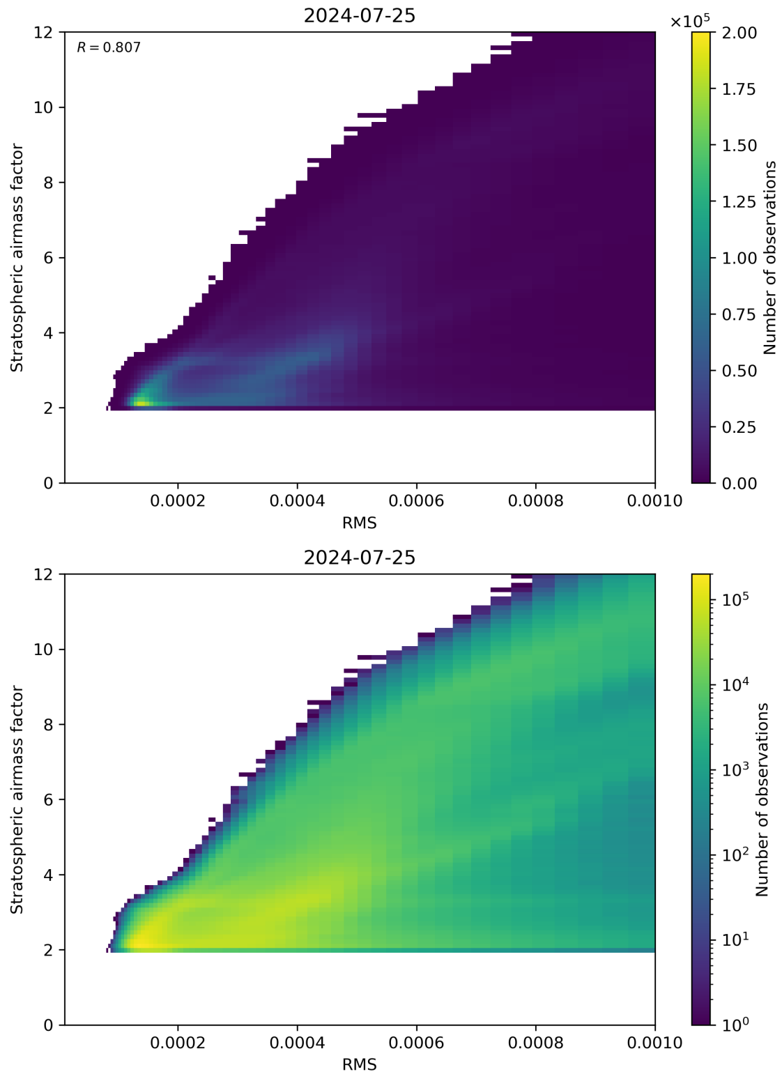
Figure 144: Scatter density plot of “RMS” against “Stratospheric airmass factor” for 2024-07-24 to 2024-07-26.
