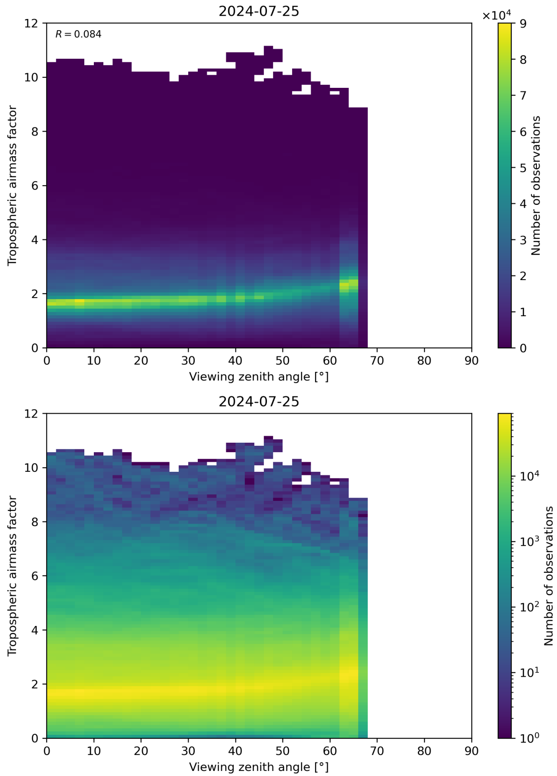
Figure 161: Scatter density plot of “Viewing zenith angle” against “Tropospheric airmass factor” for 2024-07-24 to 2024-07-26.
