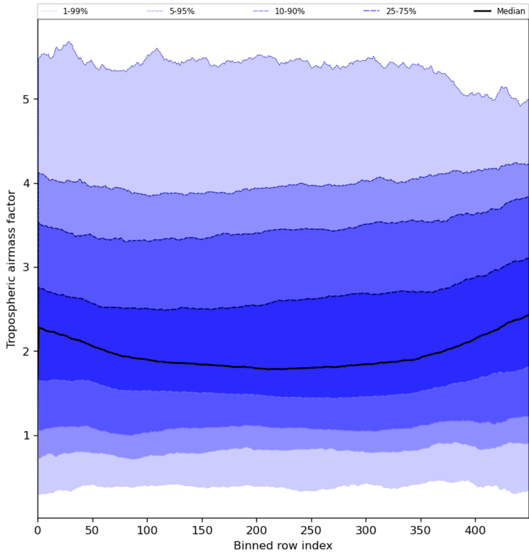
Figure 48: Along track statistics of “Tropospheric airmass factor” for 2024-07-24 to 2024-07-26
