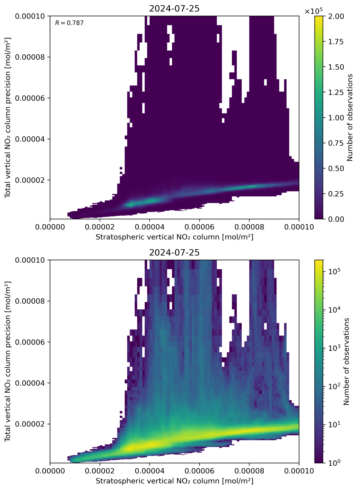
Figure 101: Scatter density plot of “Stratospheric vertical NO 2 column” against “Total vertical NO 2 column precision” for 2024-07-24 to 2024-07-26.
