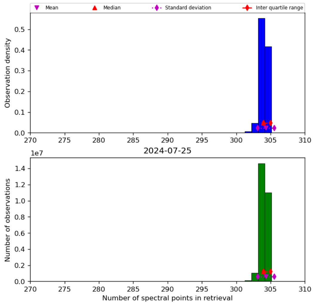
Figure 33: Histogram of “Number of spectral points in retrieval” for 2024-07-24 to 2024-07-26
