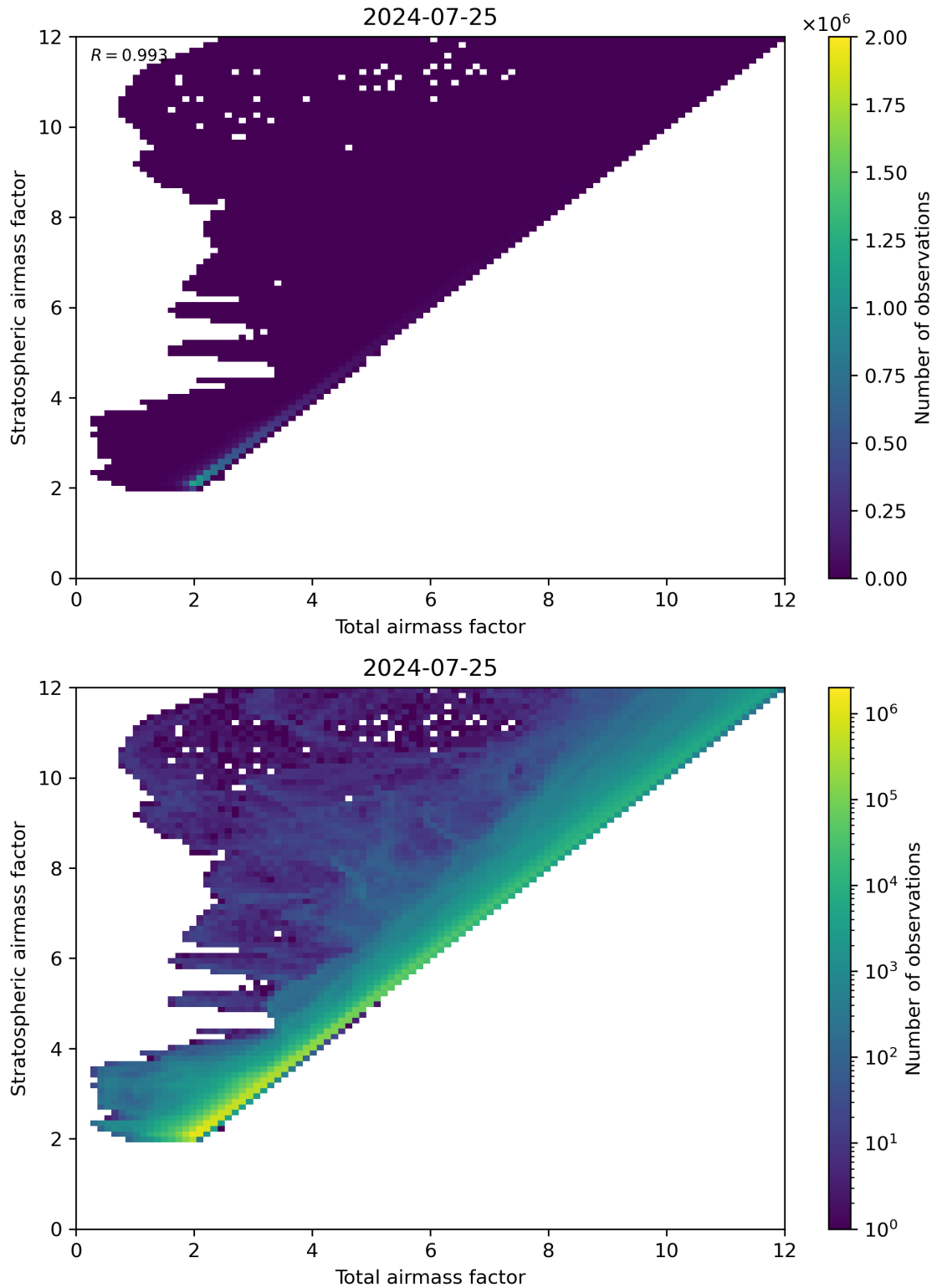
Figure 62: Scatter density plot of “Total airmass factor” against “Stratospheric airmass factor” for 2024-07-24 to 2024-07-26.
