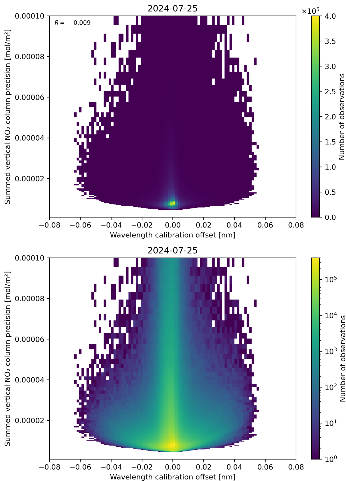
Figure 178: Scatter density plot of “Wavelength calibration offset” against “Summed vertical NO 2 column precision” for 2024-07-24 to 2024-07-26.
