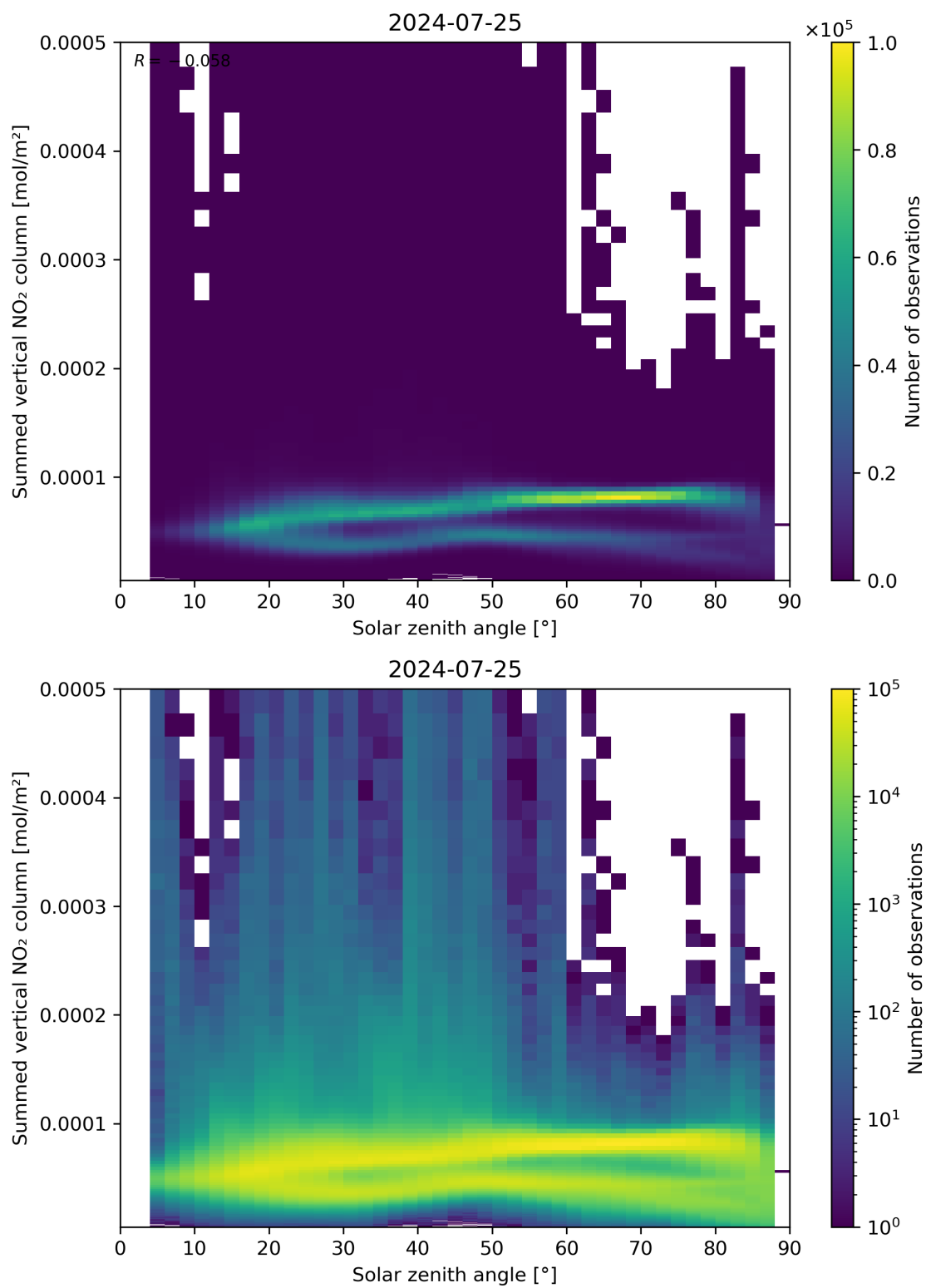
Figure 151: Scatter density plot of “Solar zenith angle” against “Summed vertical NO 2 column” for 2024-07-24 to 2024-07-26.
