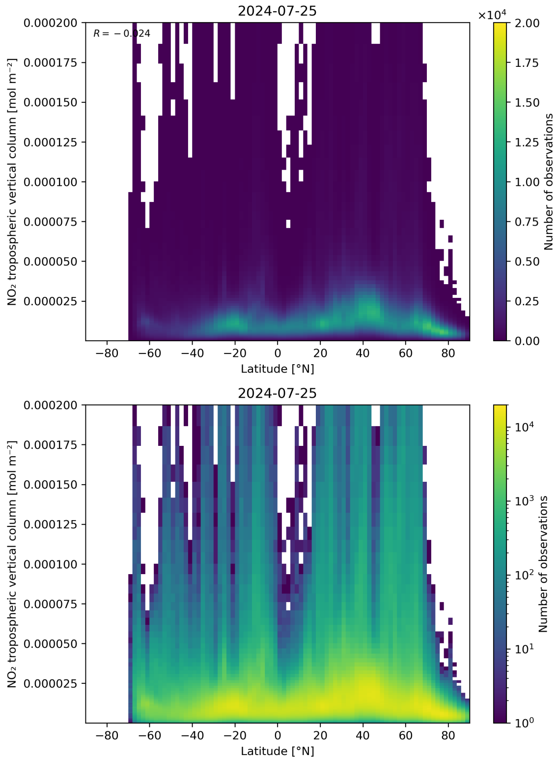
Figure 92: Scatter density plot of “Latitude” against “NO 2 tropospheric vertical column” for 2024-07-24 to 2024-07-26.
