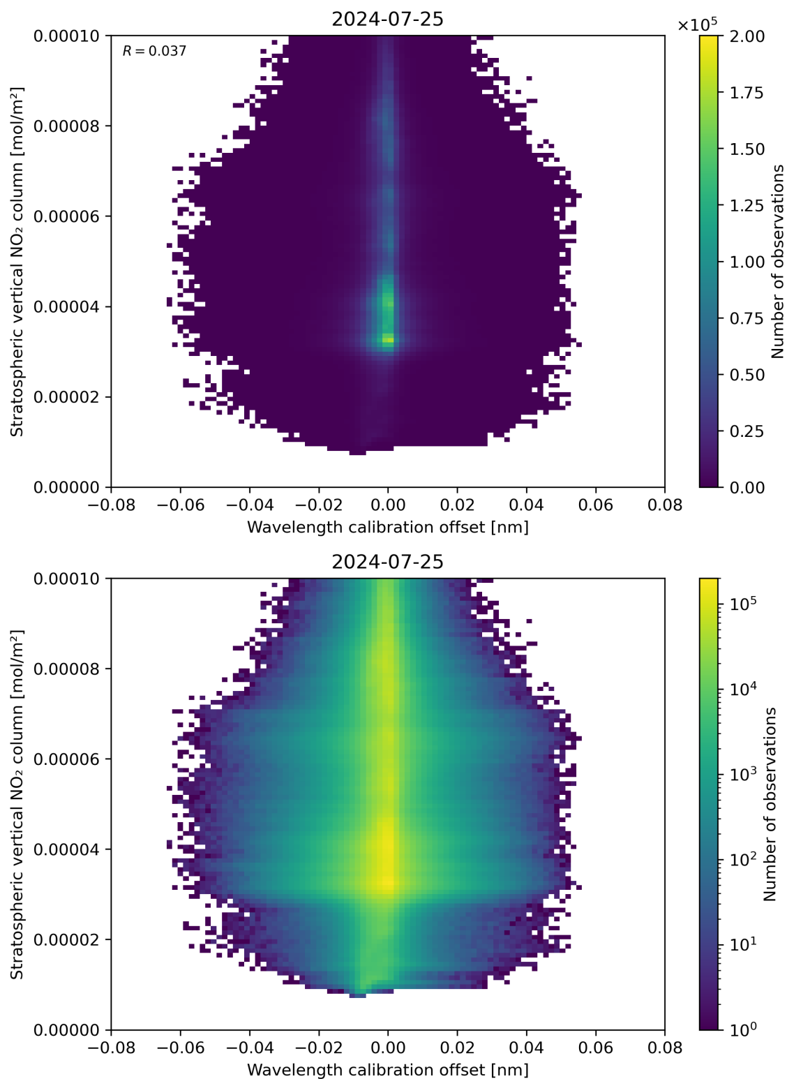
Figure 176: Scatter density plot of “Wavelength calibration offset” against “Stratospheric vertical NO 2 column” for 2024-07-24 to 2024-07-26.
