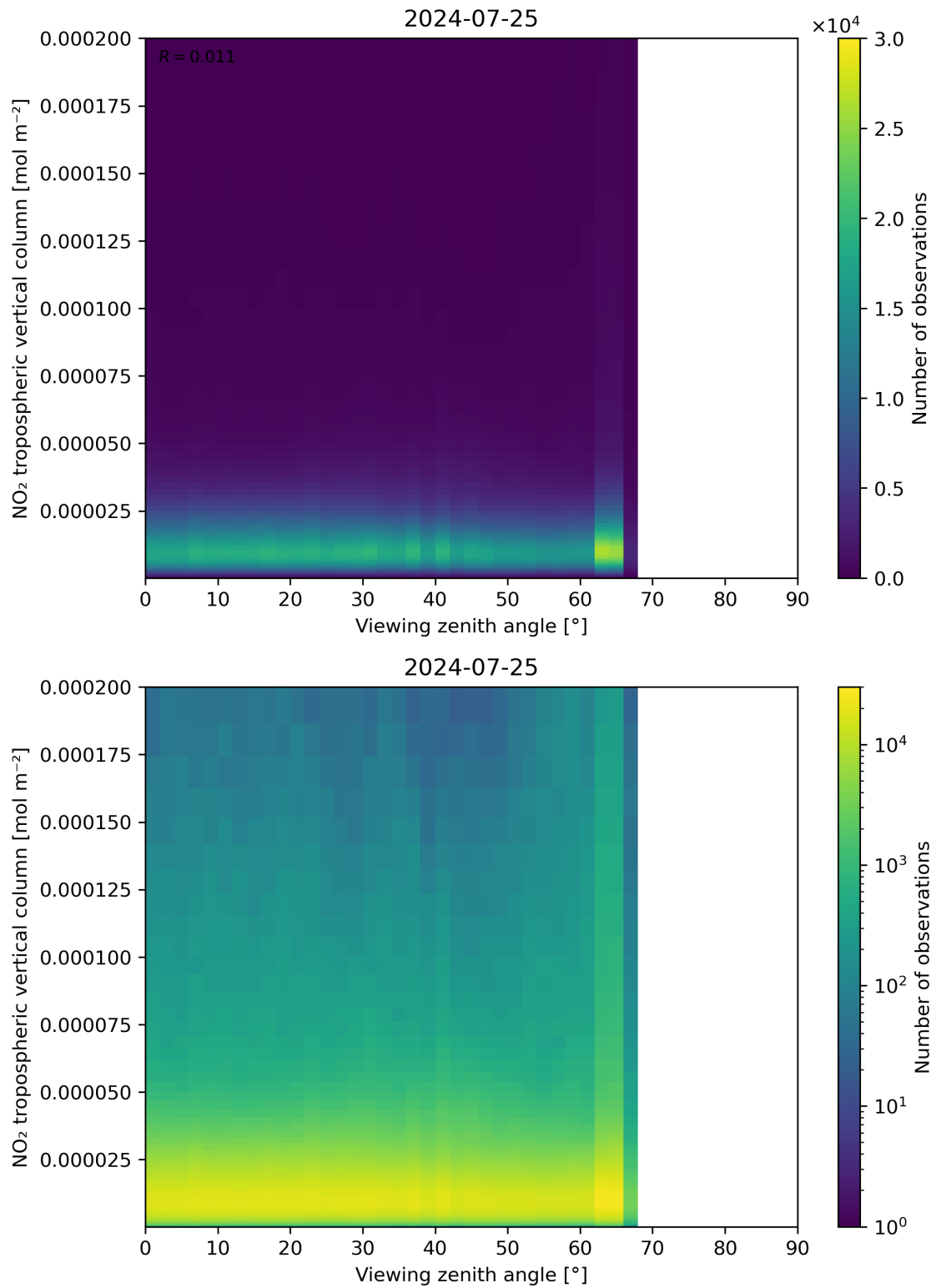
Figure 169: Scatter density plot of “Viewing zenith angle” against “NO 2 tropospheric vertical column” for 2024-07-24 to 2024-07-26.
