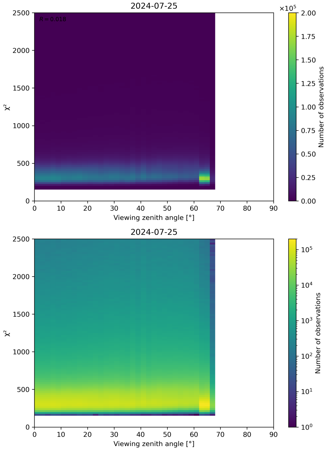
Figure 162: Scatter density plot of “Viewing zenith angle” against “ \chi^2 ” for 2024-07-24 to 2024-07-26.
