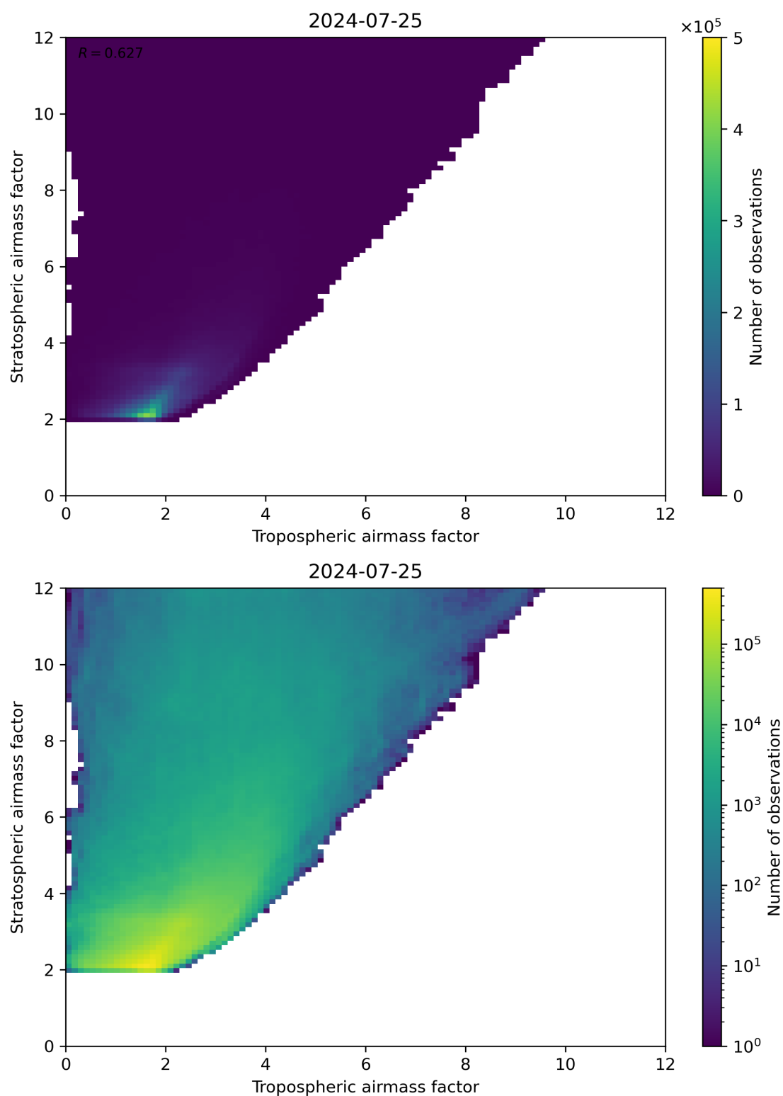
Figure 71: Scatter density plot of “Tropospheric airmass factor” against “Stratospheric airmass factor” for 2024-07-24 to 2024-07-26.
