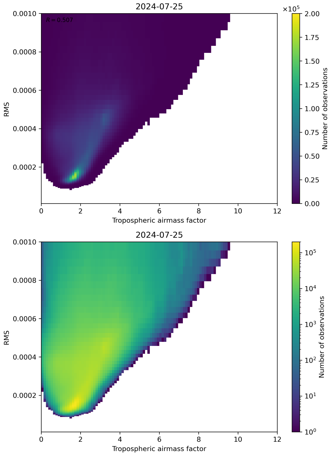
Figure 79: Scatter density plot of “Tropospheric airmass factor” against “RMS” for 2024-07-24 to 2024-07-26.
