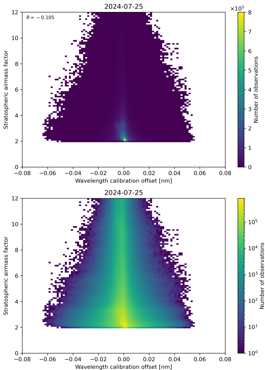
Figure 174: Scatter density plot of “Wavelength calibration offset” against “Stratospheric airmass factor” for 2024-07-24 to 2024-07-26.
