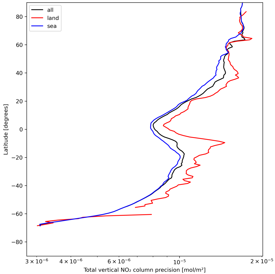
Figure 22: Zonal average of “Total vertical NO 2 column precision” for 2024-07-24 to 2024-07-26.
