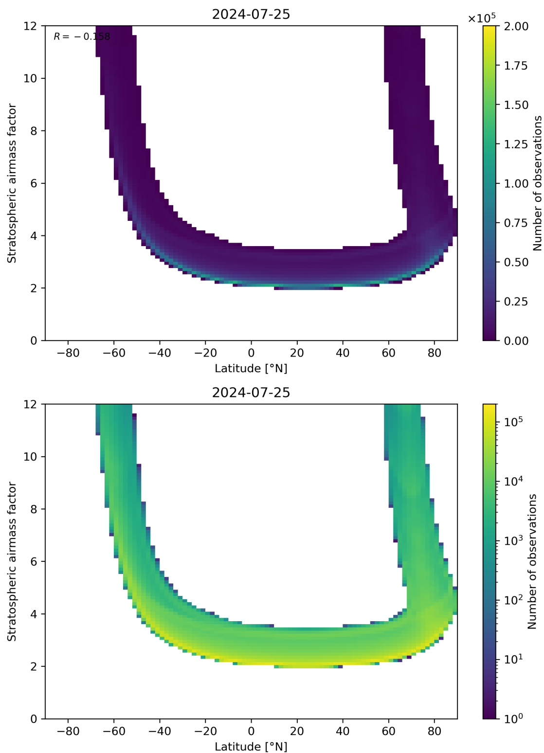
Figure 83: Scatter density plot of “Latitude” against “Stratospheric air mass factor” for 2024-07-24 to 2024-07-26.
