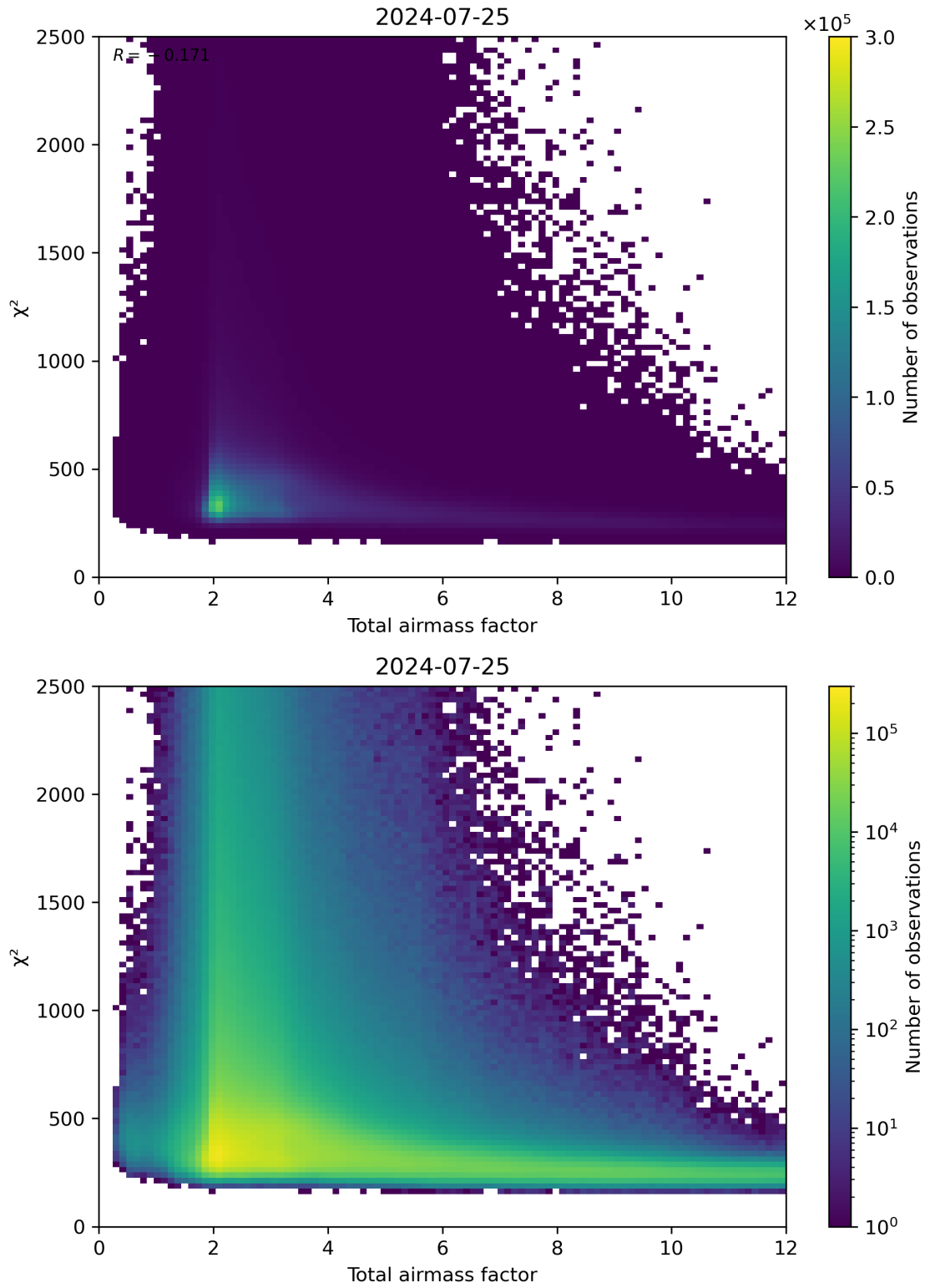
Figure 63: Scatter density plot of “Total airmass factor” against “ \chi^2 ” for 2024-07-24 to 2024-07-26.
