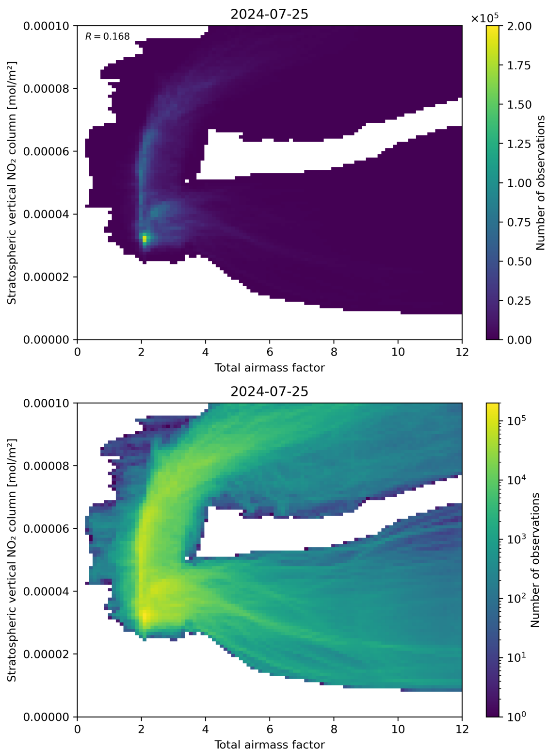
Figure 64: Scatter density plot of “Total airmass factor” against “Stratospheric vertical NO 2 column” for 2024-07-24 to 2024-07-26.
