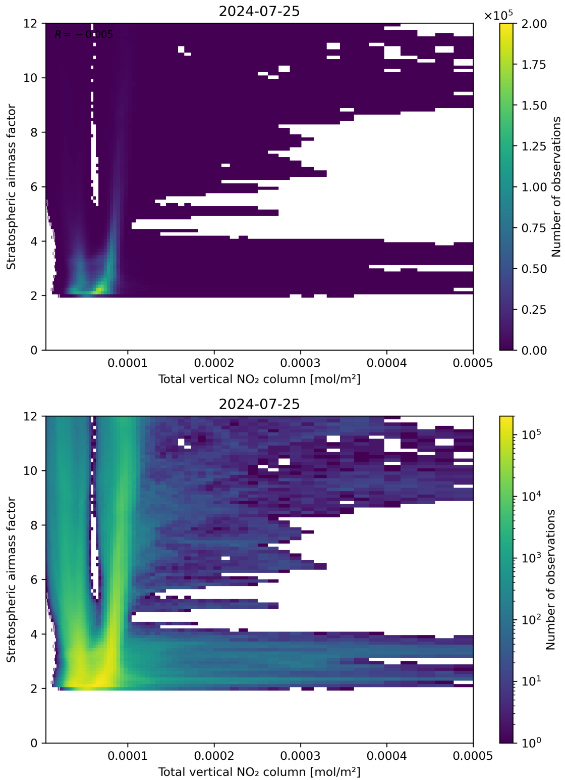
Figure 110: Scatter density plot of “Total vertical NO 2 column” against “Stratospheric airmass factor” for 2024-07-24 to 2024-07-26.
