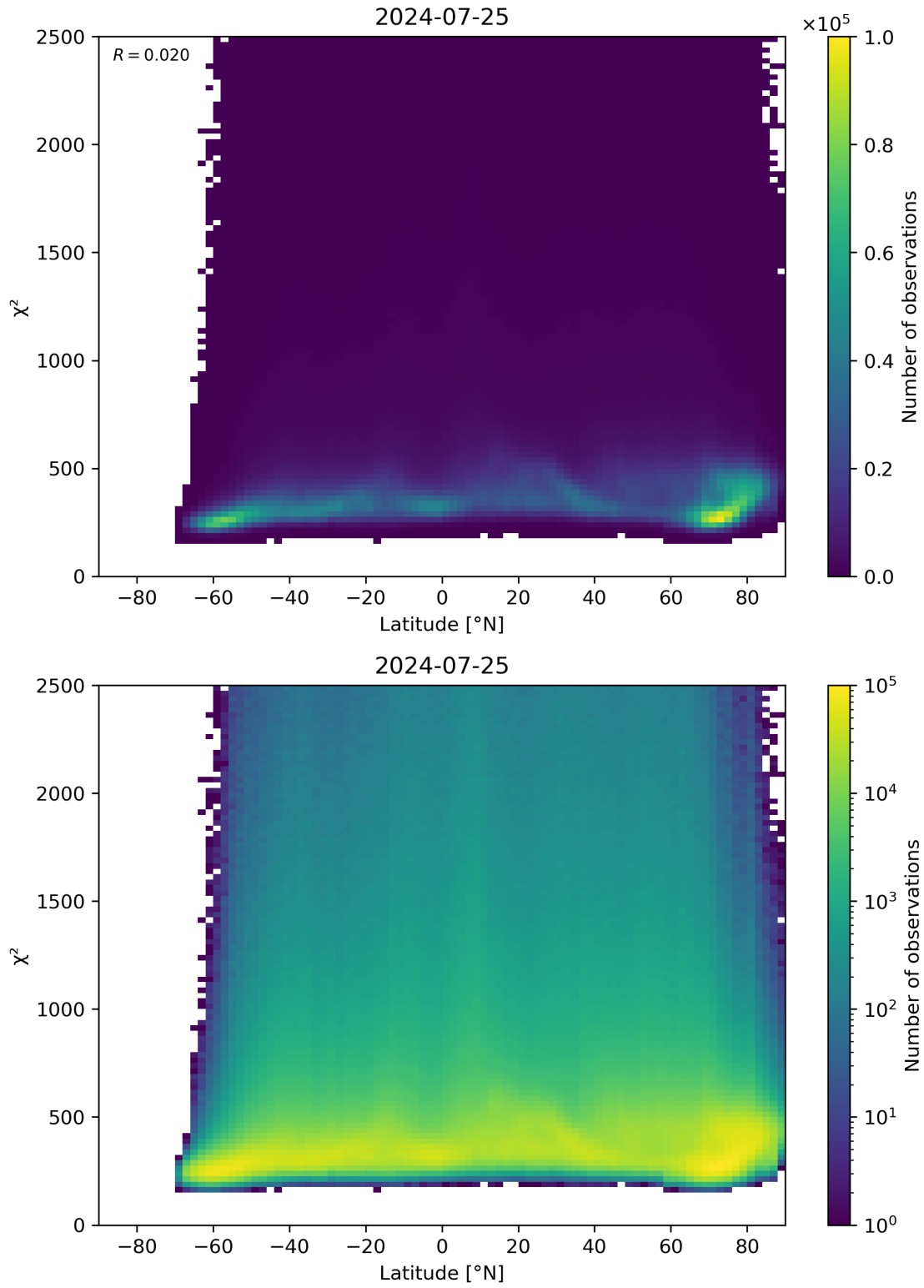
Figure 86: Scatter density plot of “Latitude” against “ \chi^2 ” for 2024-07-24 to 2024-07-26.
