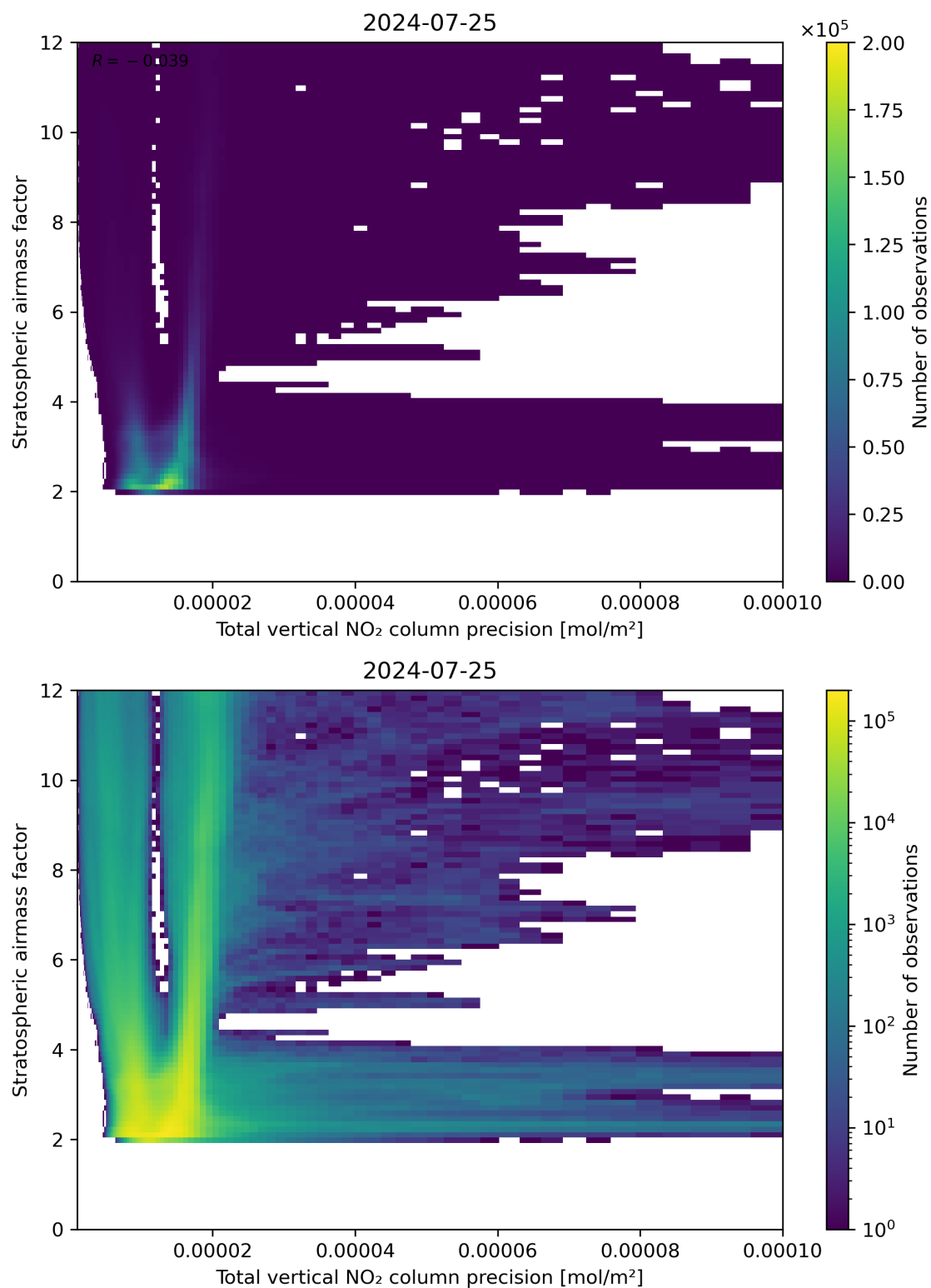
Figure 115: Scatter density plot of “Total vertical NO 2 column precision” against “Stratospheric air mass factor” for 2024-07-24 to 2024-07-26.
