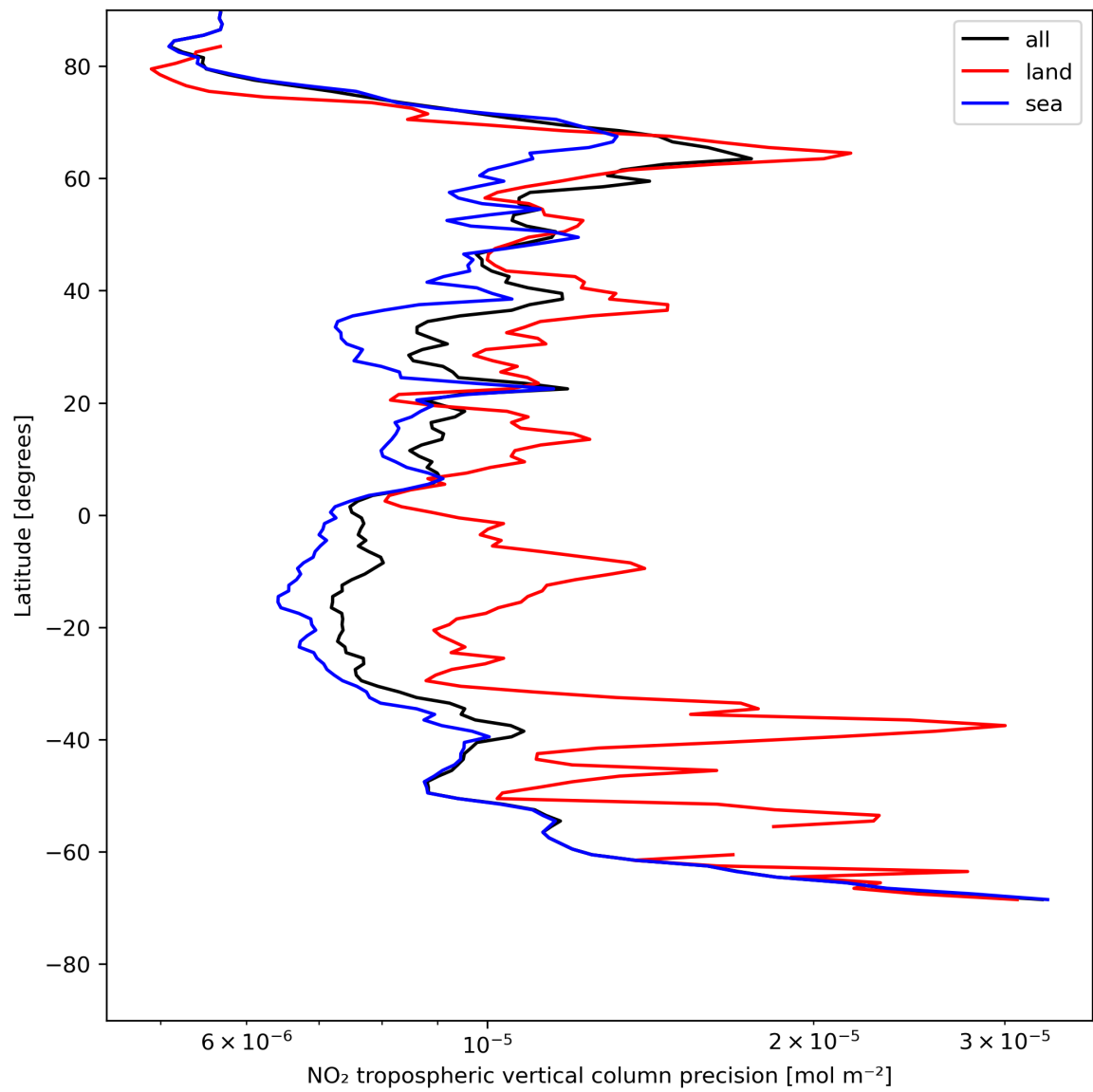
Figure 13: Zonal average of “NO 2 tropospheric vertical column precision” for 2024-07-24 to 2024-07-26.
