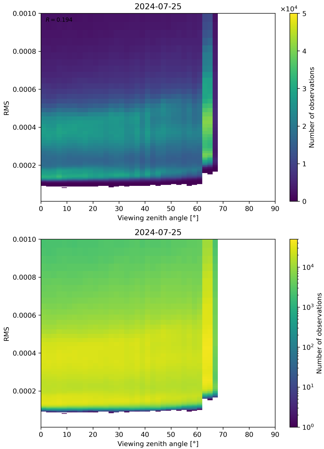
Figure 171: Scatter density plot of “Viewing zenith angle” against “RMS” for 2024-07-24 to 2024-07-26.
