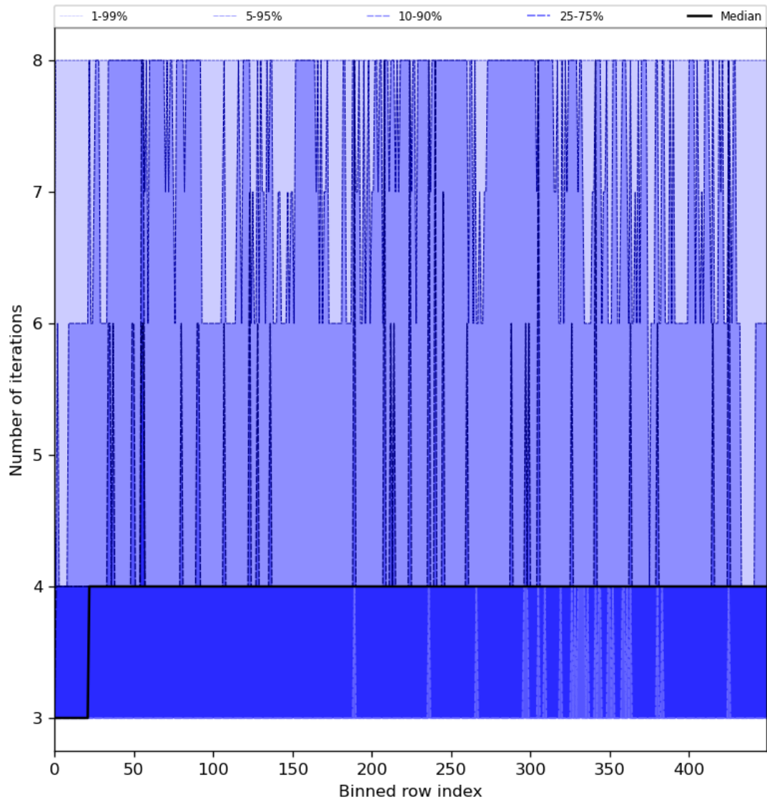
Figure 51: Along track statistics of “Number of iterations” for 2024-07-24 to 2024-07-26
