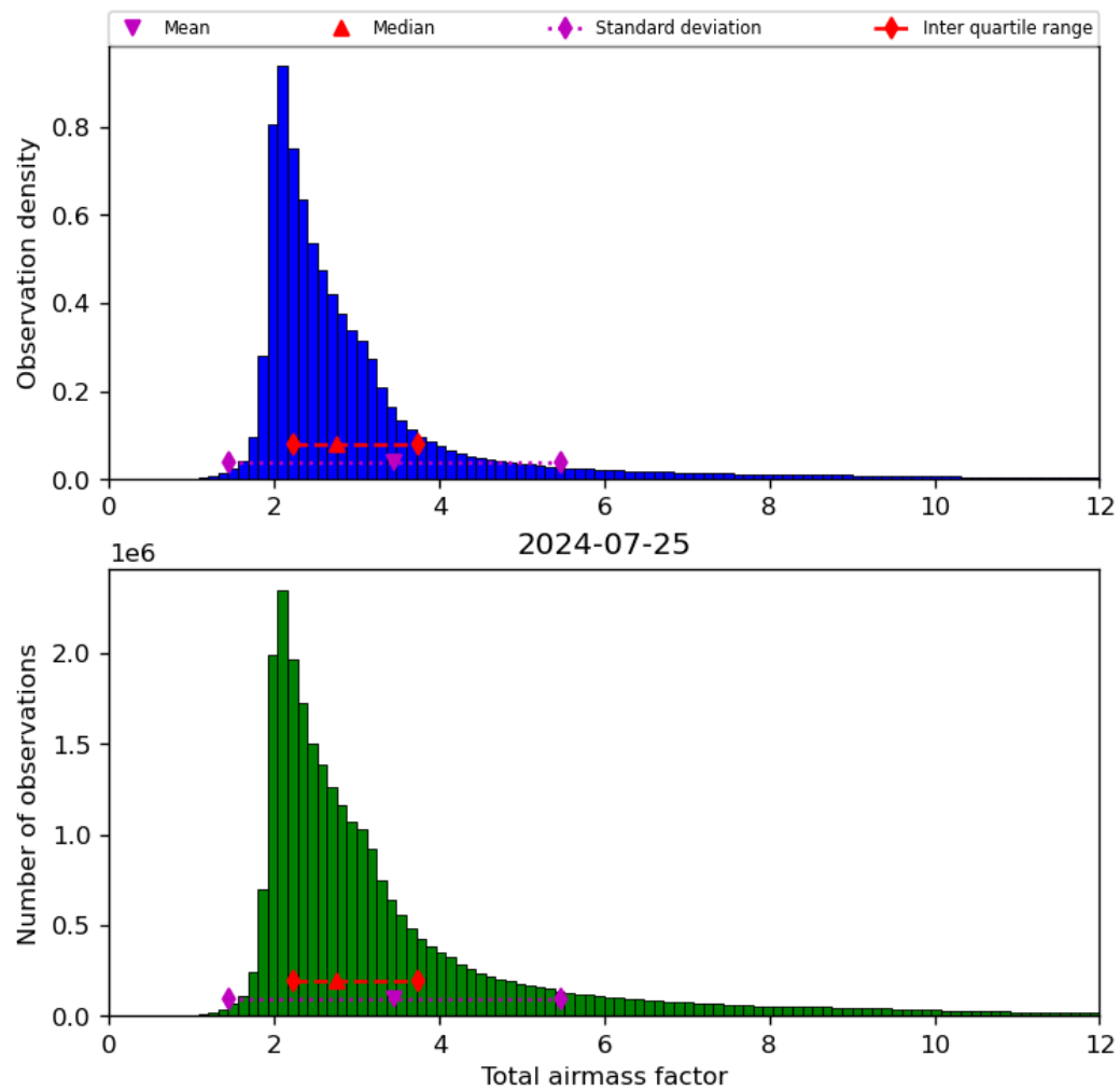
Figure 32: Histogram of “Total airmass factor” for 2024-07-24 to 2024-07-26
