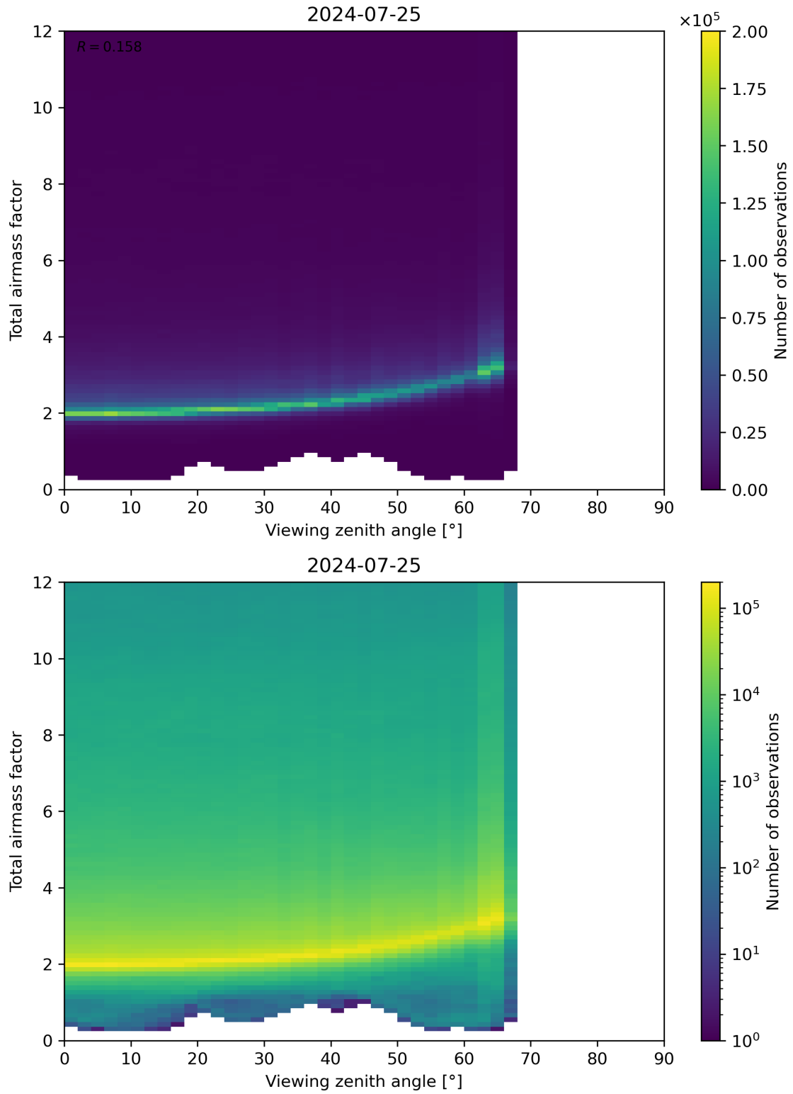
Figure 160: Scatter density plot of “Viewing zenith angle” against “Total airmass factor” for 2024-07-24 to 2024-07-26.
