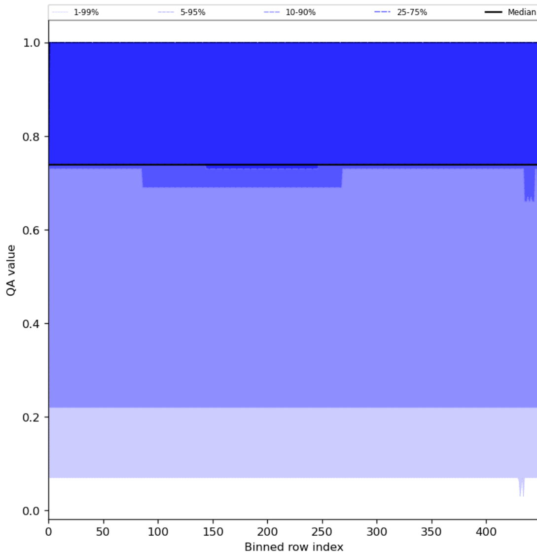
Figure 45: Along track statistics of “QA value” for 2024-07-24 to 2024-07-26
