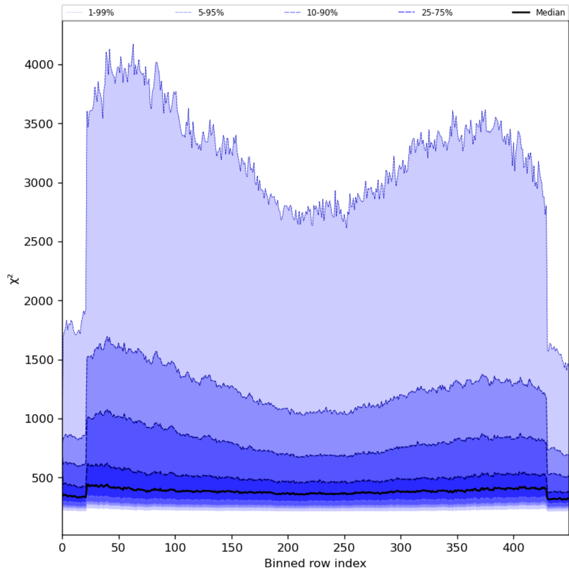
Figure 59: Along track statistics of “ \chi^2 ” for 2024-07-24 to 2024-07-26
