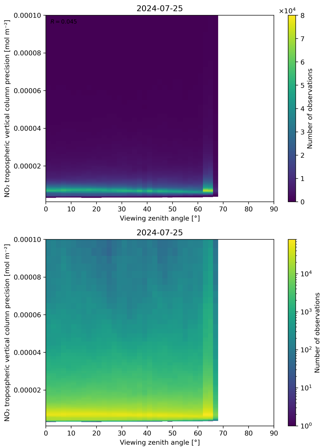
Figure 170: Scatter density plot of “Viewing zenith angle” against “NO 2 tropospheric vertical column precision” for 2024-07-24 to 2024-07-26.
