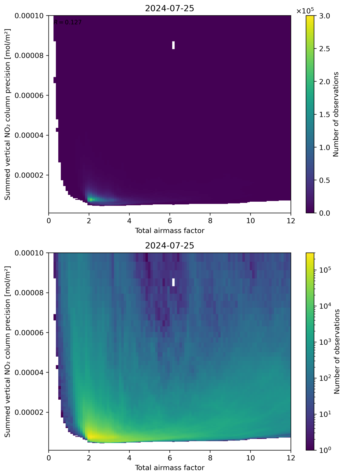
Figure 66: Scatter density plot of “Total airmass factor” against “Summed vertical NO 2 column precision” for 2024-07-24 to 2024-07-26.
