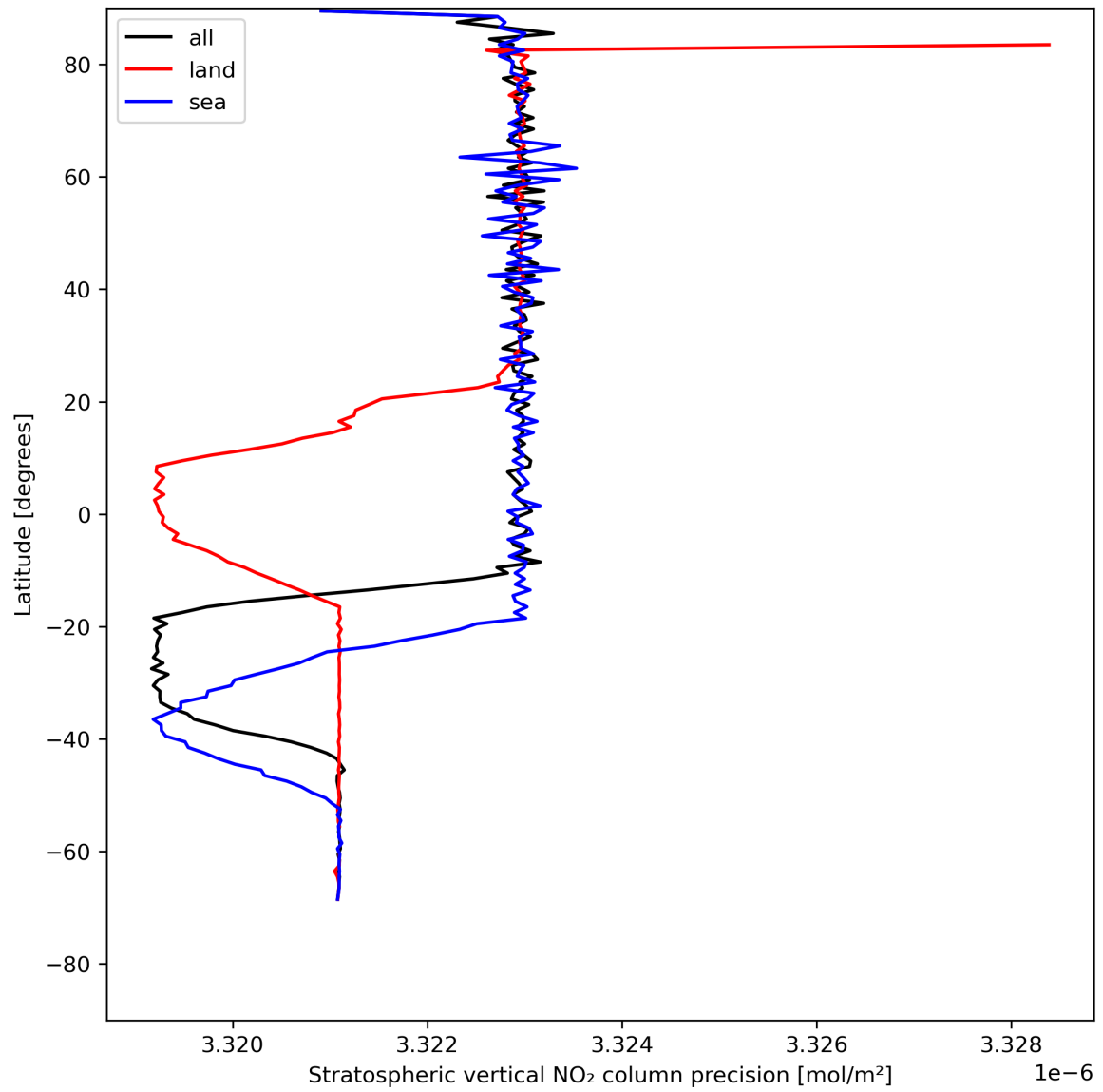
Figure 20: Zonal average of “Stratospheric vertical NO 2 column precision” for 2024-07-24 to 2024-07-26.
