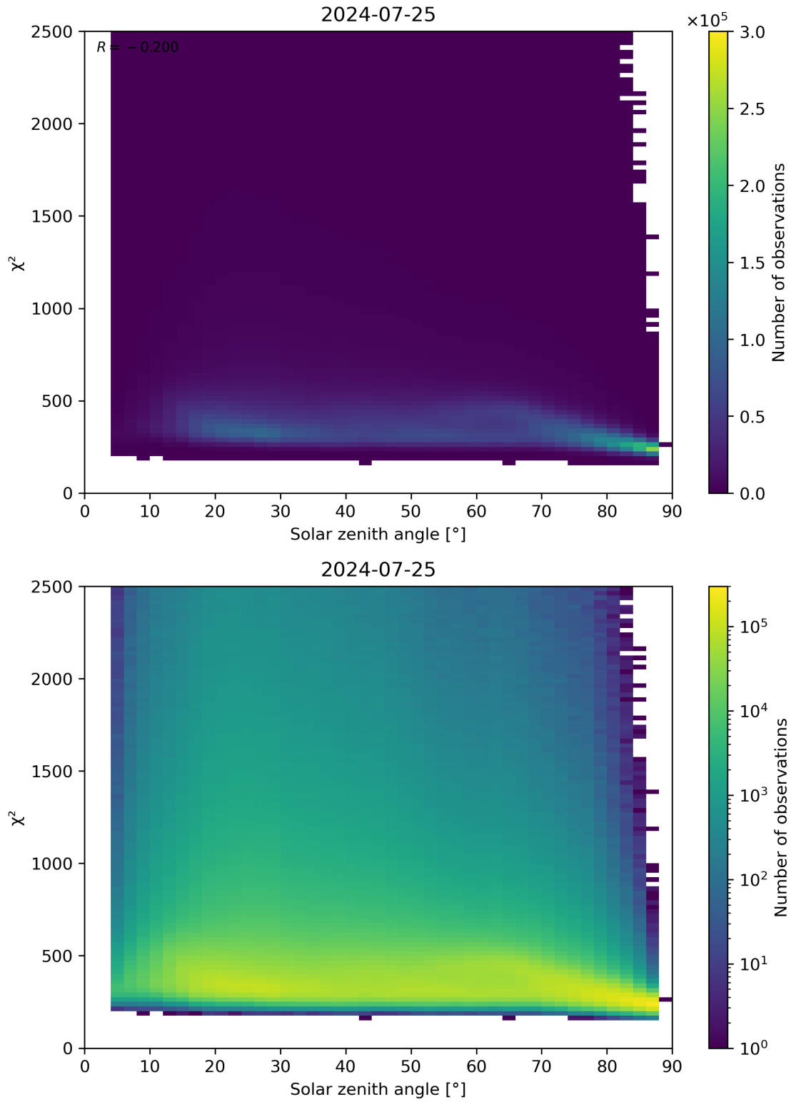
Figure 148: Scatter density plot of “Solar zenith angle” against “ \chi^2 ” for 2024-07-24 to 2024-07-26.
