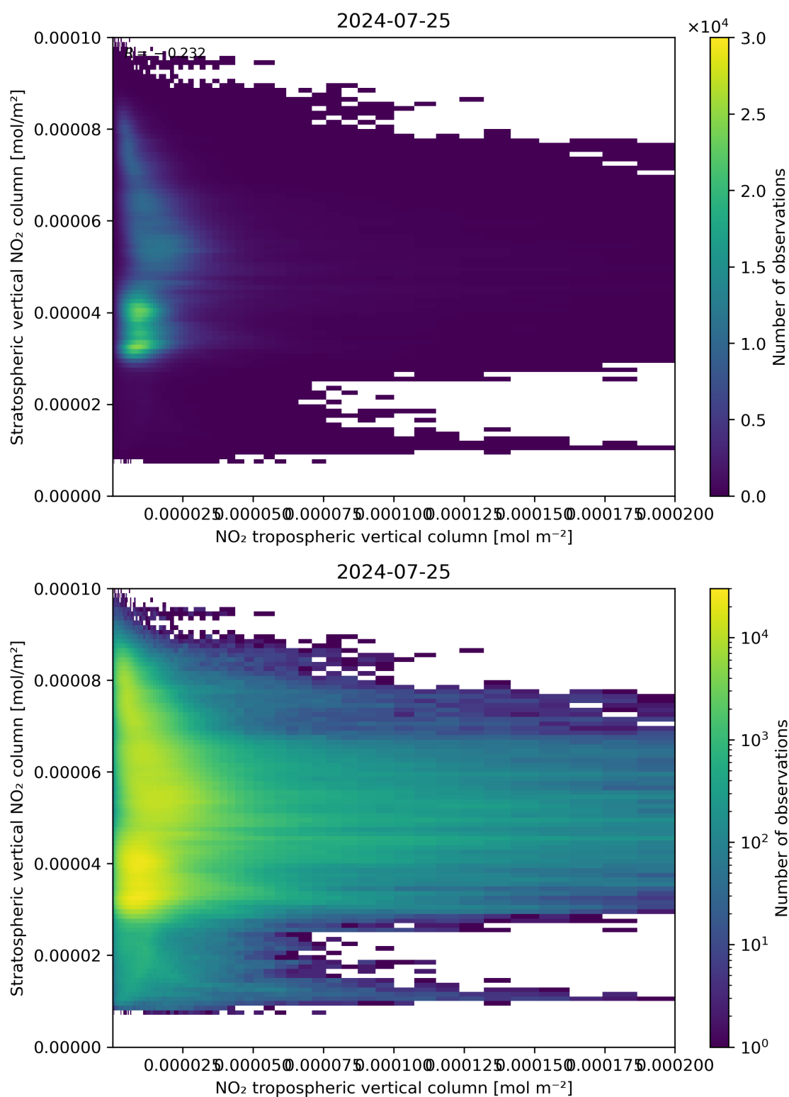
Figure 125: Scatter density plot of “NO 2 tropospheric vertical column” against “Stratospheric vertical NO 2 column” for 2024-07-24 to 2024-07-26.
