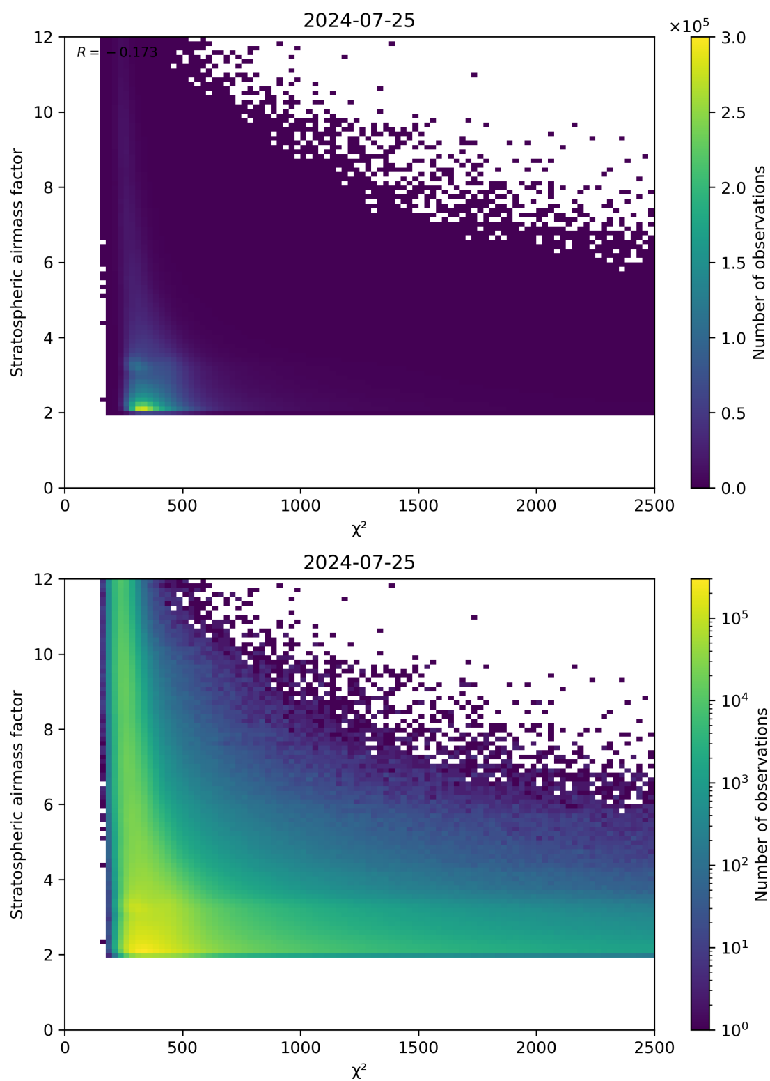
Figure 81: Scatter density plot of “ \chi^2 ” against “Stratospheric airmass factor” for 2024-07-24 to 2024-07-26.
