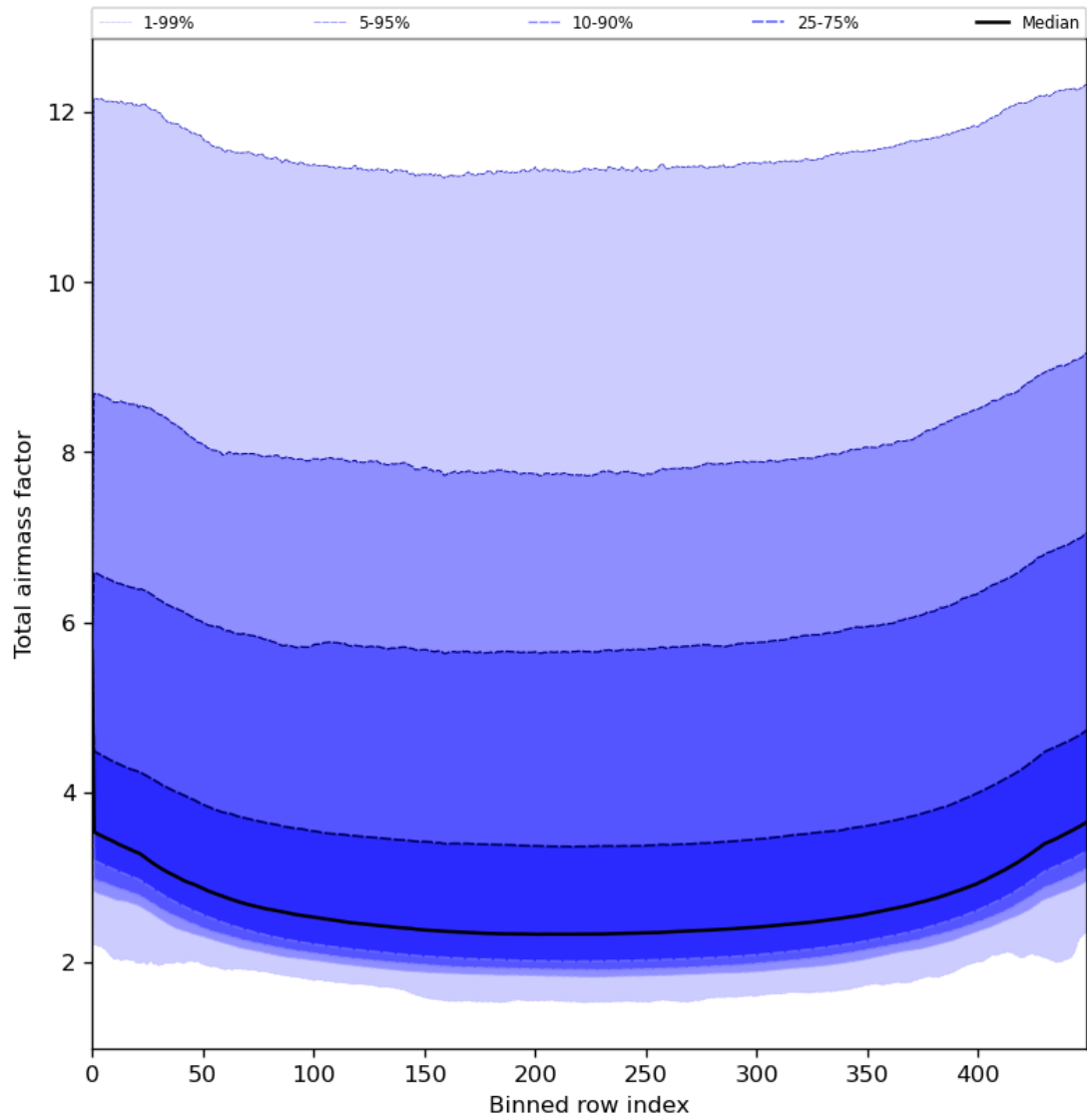
Figure 49: Along track statistics of “Total airmass factor” for 2024-07-24 to 2024-07-26
