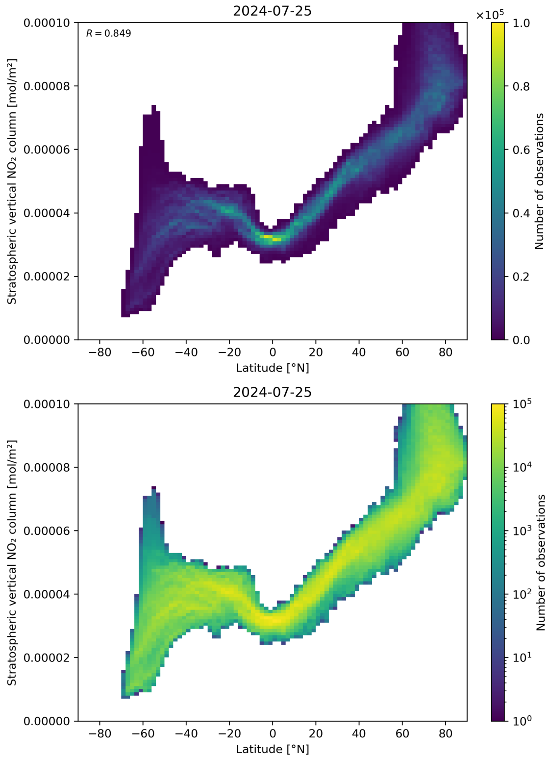
Figure 87: Scatter density plot of “Latitude” against “Stratospheric vertical NO 2 column” for 2024-07-24 to 2024-07-26.
