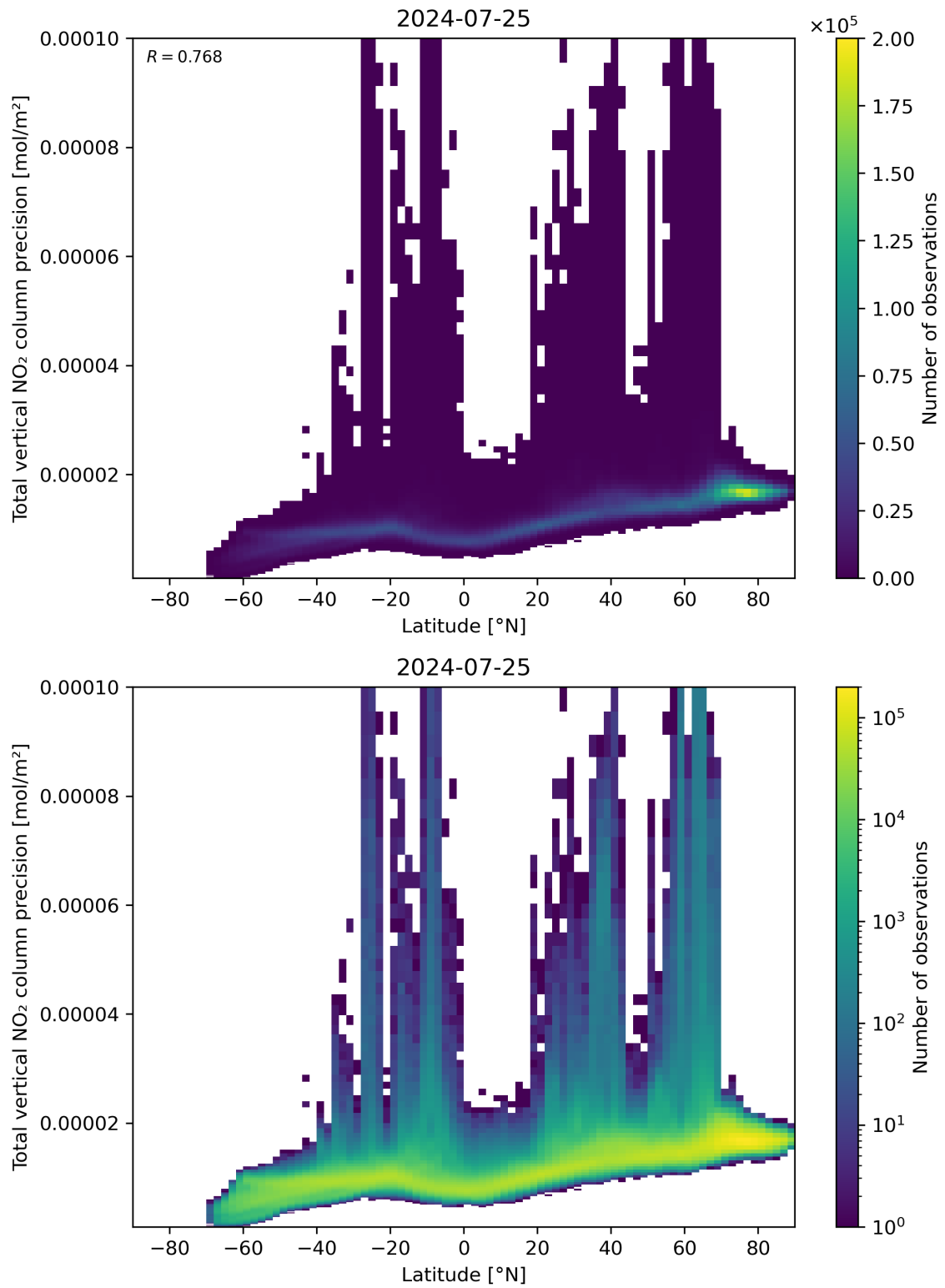
Figure 91: Scatter density plot of “Latitude” against “Total vertical NO 2 column precision” for 2024-07-24 to 2024-07-26.
