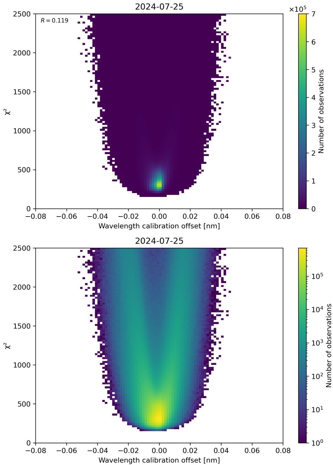
Figure 175: Scatter density plot of “Wavelength calibration offset” against “ \chi^2 ” for 2024-07-24 to 2024-07-26.
