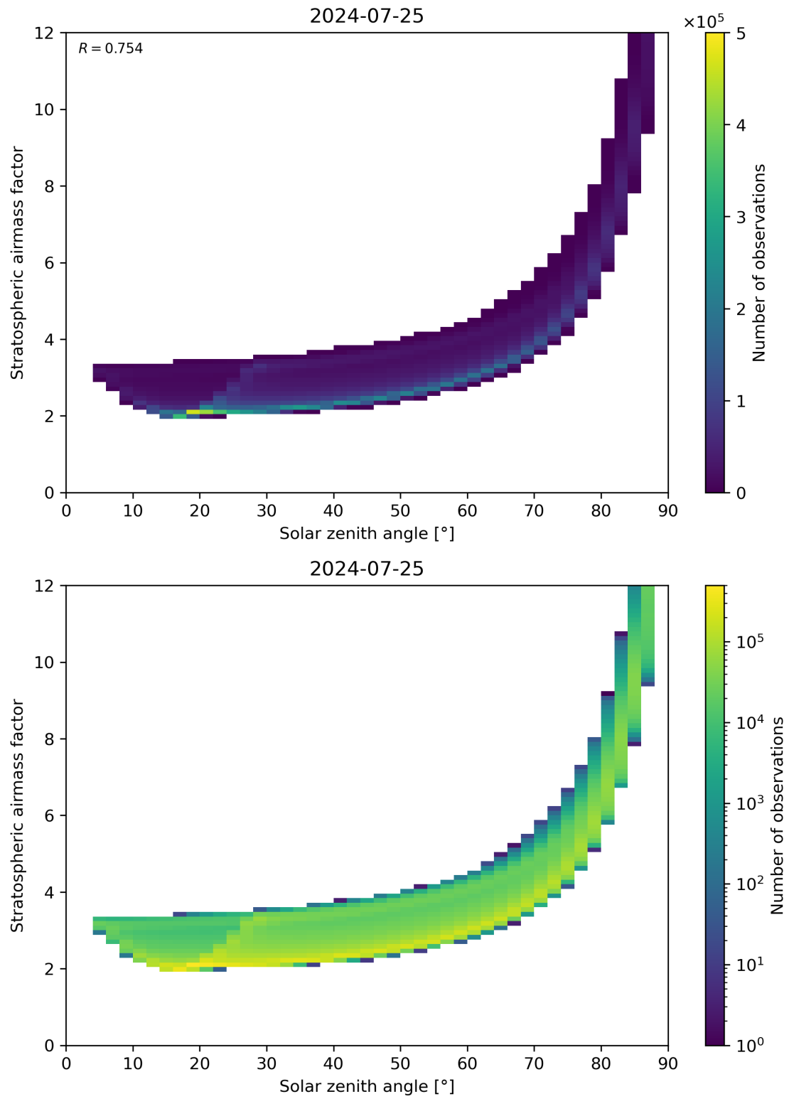
Figure 145: Scatter density plot of “Solar zenith angle” against “Stratospheric airmass factor” for 2024-07-24 to 2024-07-26.
