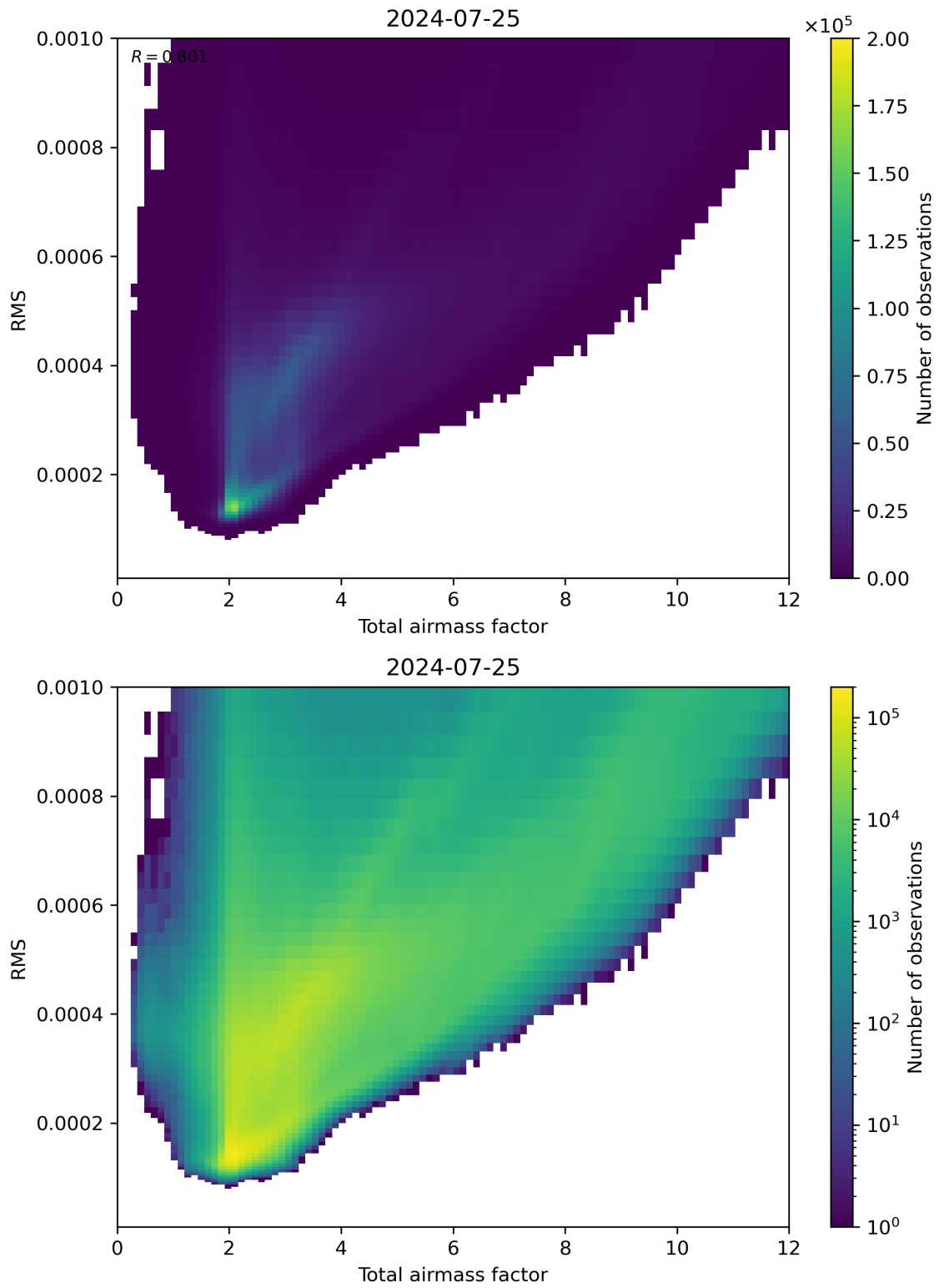
Figure 69: Scatter density plot of “Total airmass factor” against “RMS” for 2024-07-24 to 2024-07-26.
