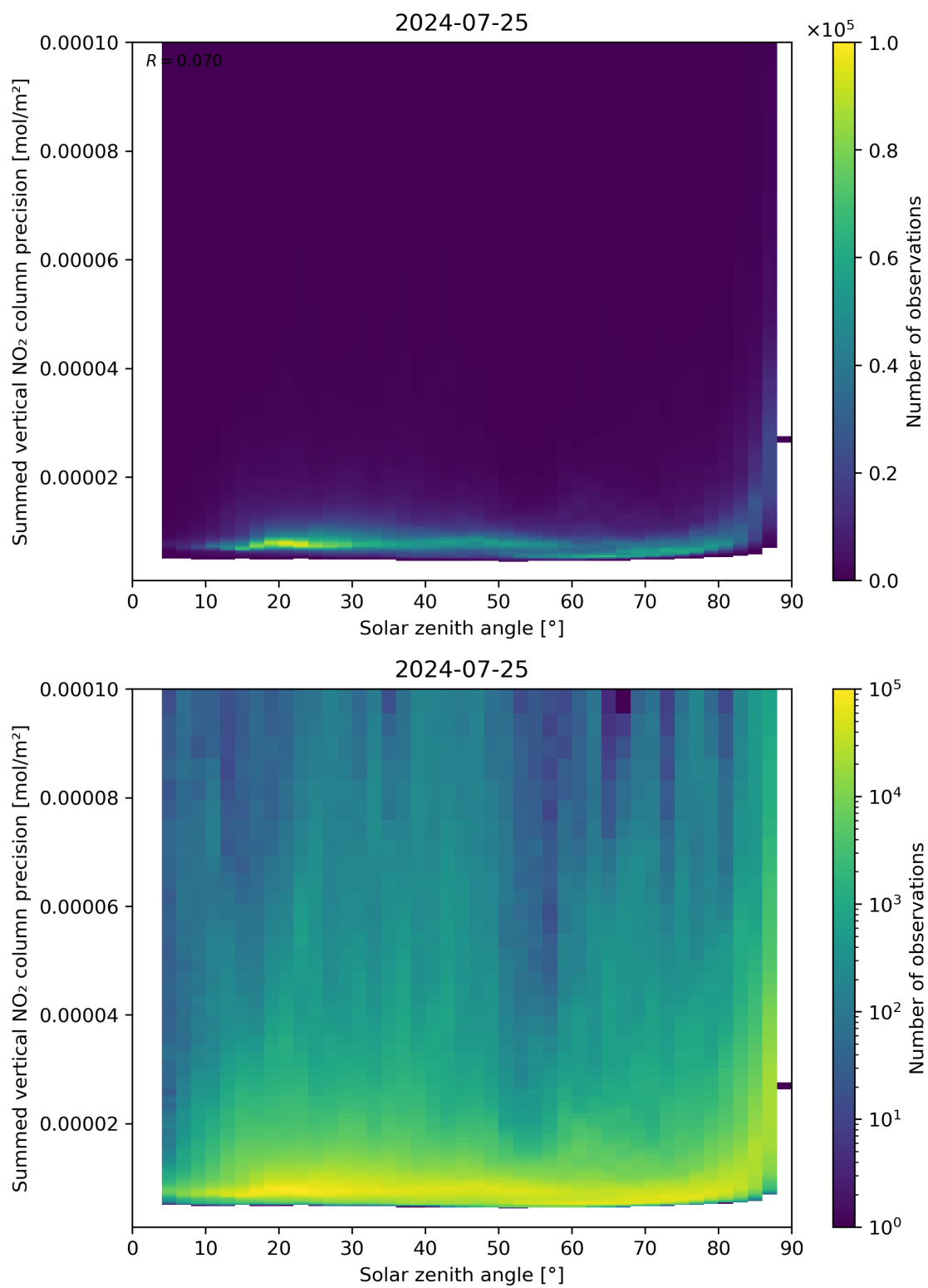
Figure 152: Scatter density plot of “Solar zenith angle” against “Summed vertical NO 2 column precision” for 2024-07-24 to 2024-07-26.
