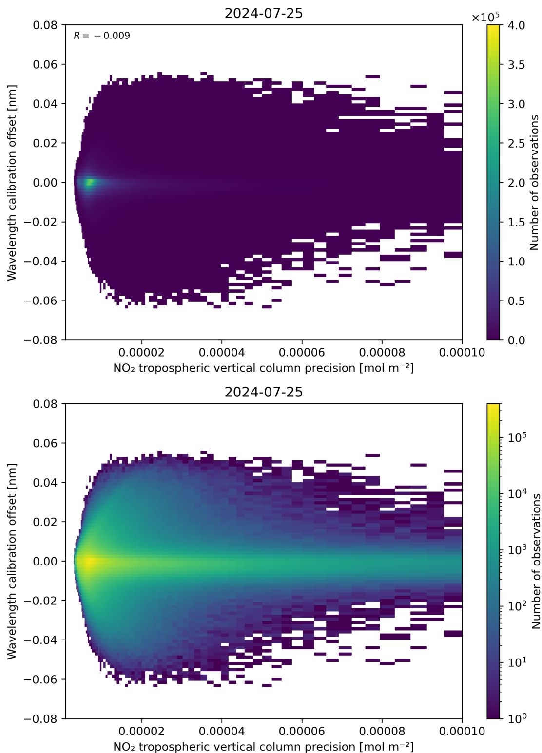
Figure 141: Scatter density plot of “NO 2 tropospheric vertical column precision” against “Wavelength calibration offset” for 2024-07-24 to 2024-07-26.
