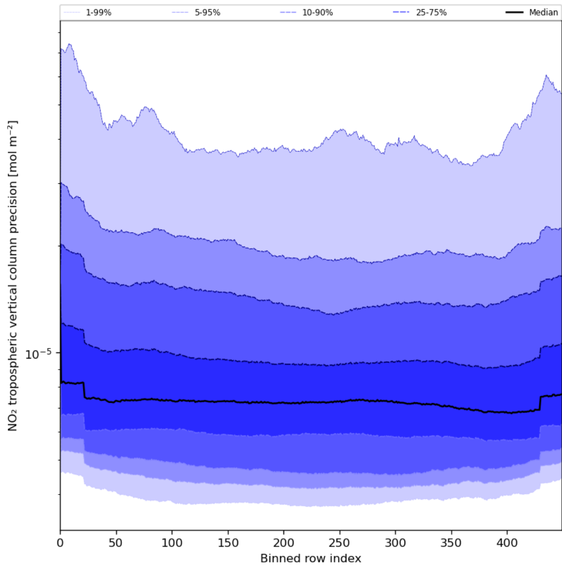
Figure 47: Along track statistics of “NO 2 tropospheric vertical column precision” for 2024-07-24 to 2024-07-26
