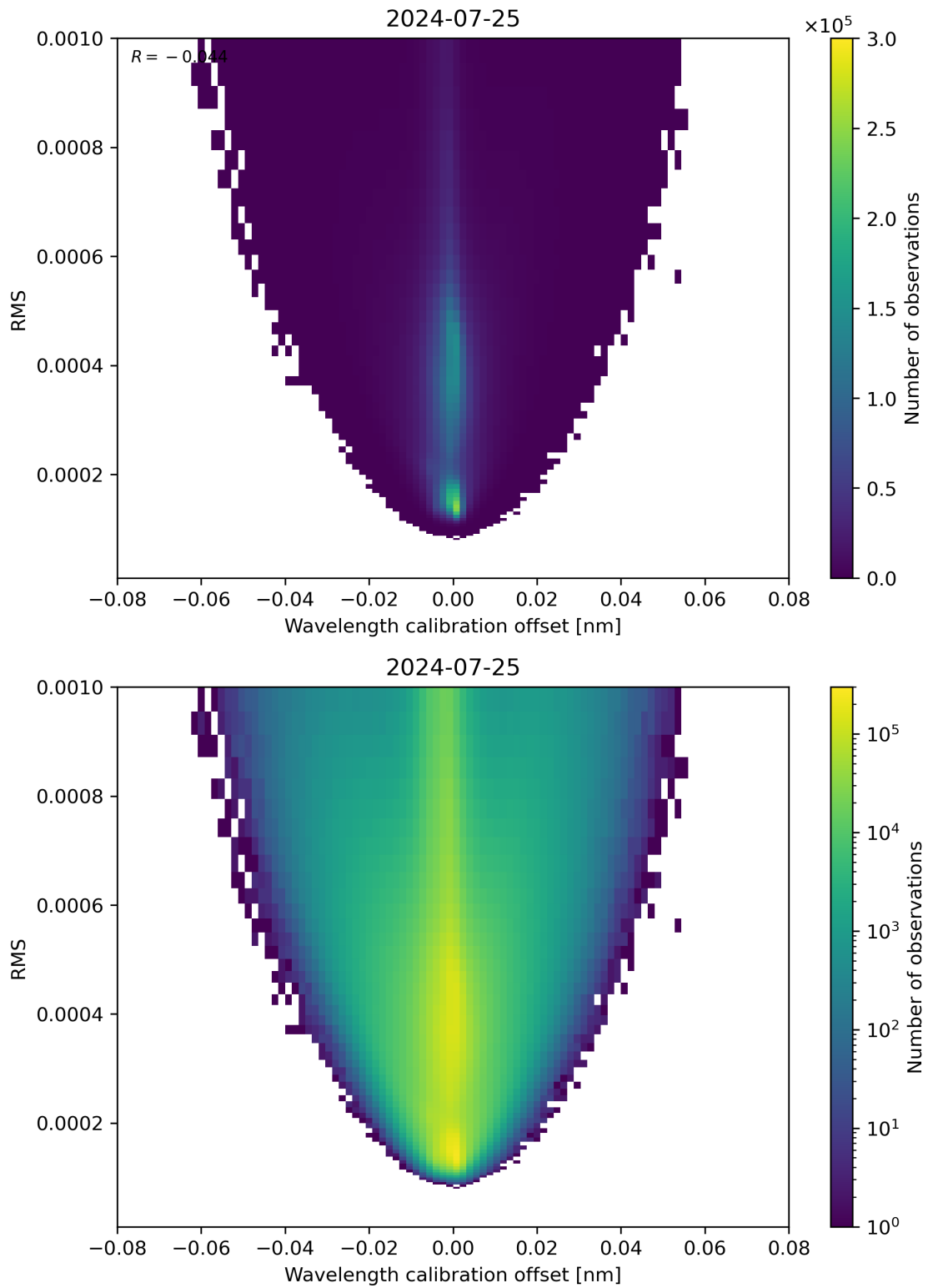
Figure 181: Scatter density plot of “Wavelength calibration offset” against “RMS” for 2024-07-24 to 2024-07-26.
