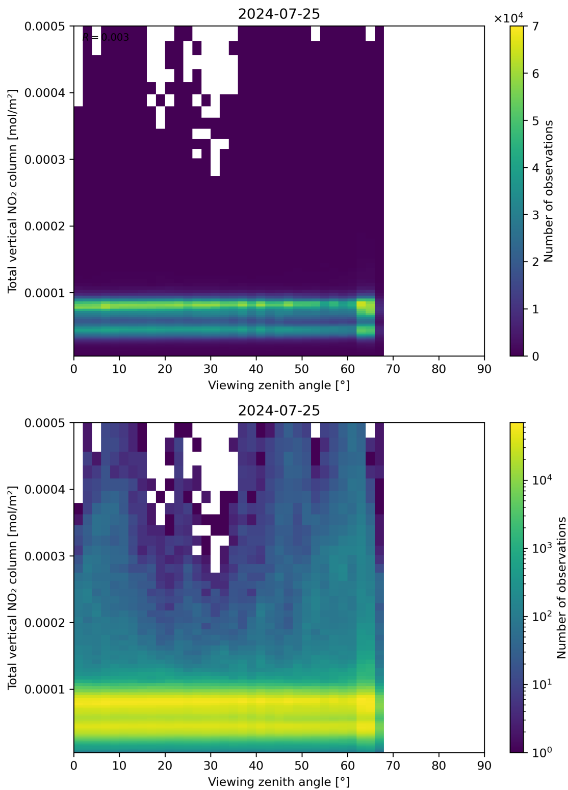
Figure 167: Scatter density plot of “Viewing zenith angle” against “Total vertical NO 2 column” for 2024-07-24 to 2024-07-26.
