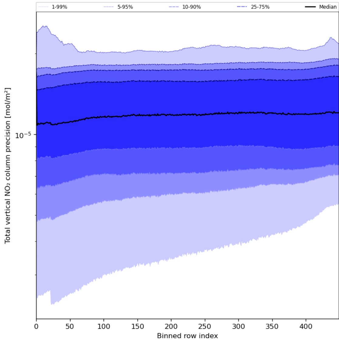
Figure 56: Along track statistics of “Total vertical NO 2 column precision” for 2024-07-24 to 2024-07-26
