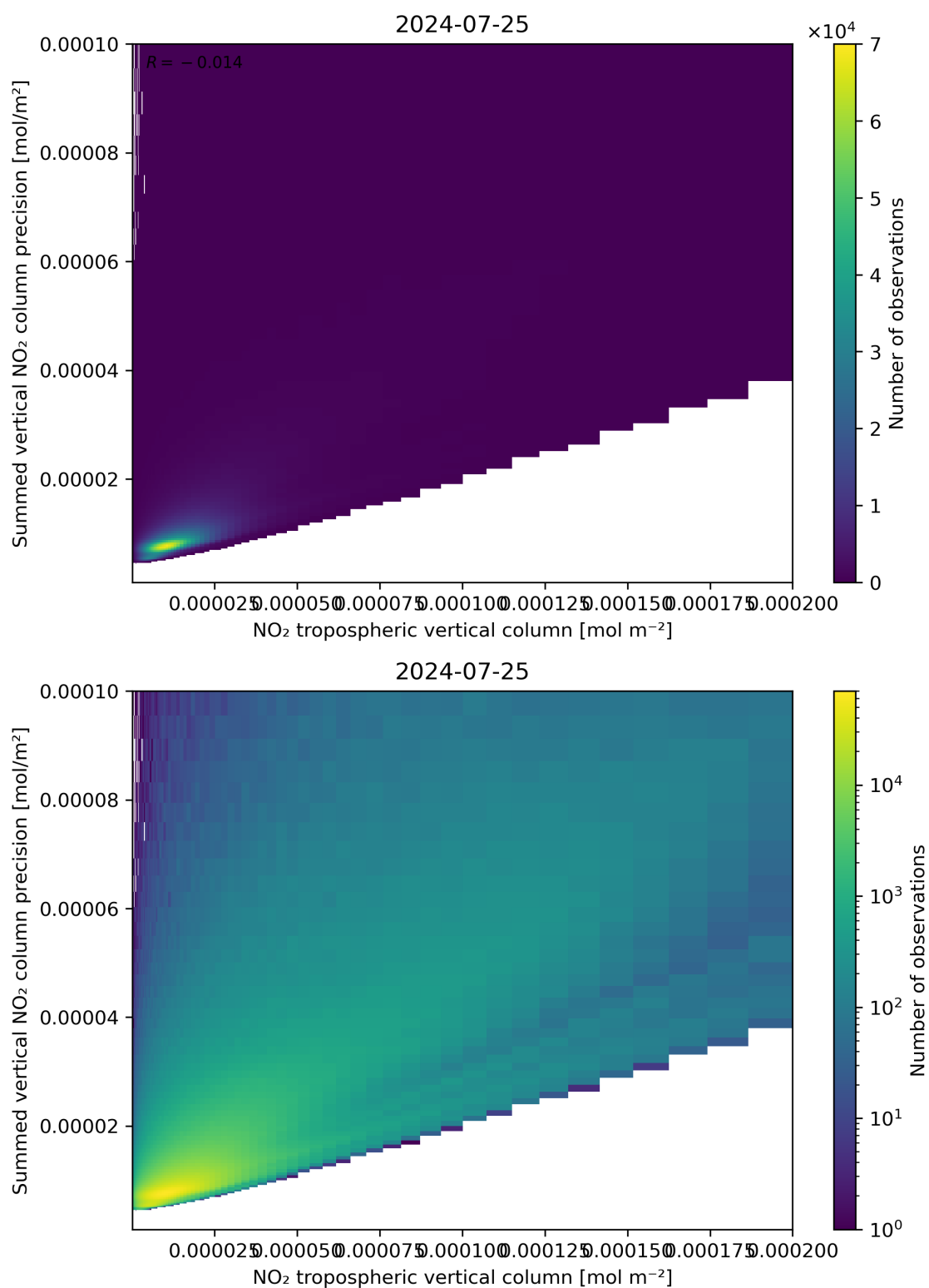
Figure 127: Scatter density plot of “NO 2 tropospheric vertical column” against “Summed vertical NO 2 column precision” for 2024-07-24 to 2024-07-26.
