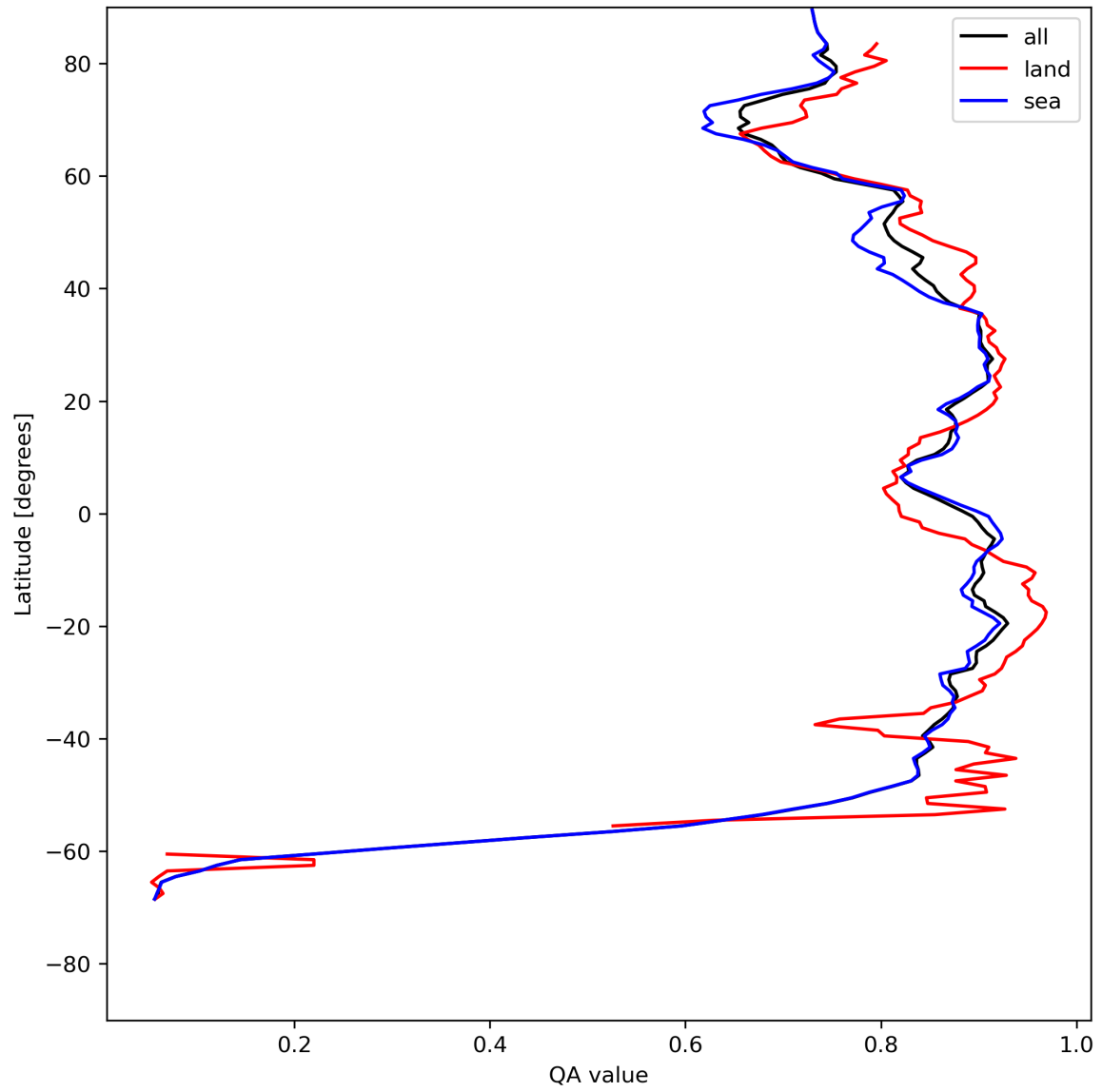
Figure 11: Zonal average of “QA value” for 2024-07-24 to 2024-07-26.
