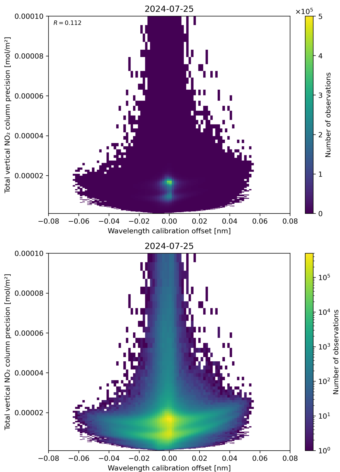
Figure 180: Scatter density plot of “Wavelength calibration offset” against “Total vertical NO 2 column precision” for 2024-07-24 to 2024-07-26.
