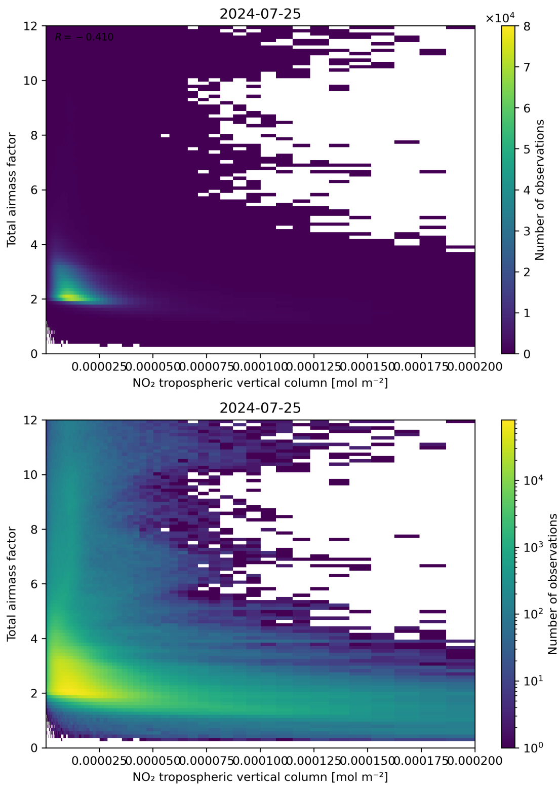
Figure 122: Scatter density plot of “NO 2 tropospheric vertical column” against “Total air mass factor” for 2024-07-24 to 2024-07-26.
