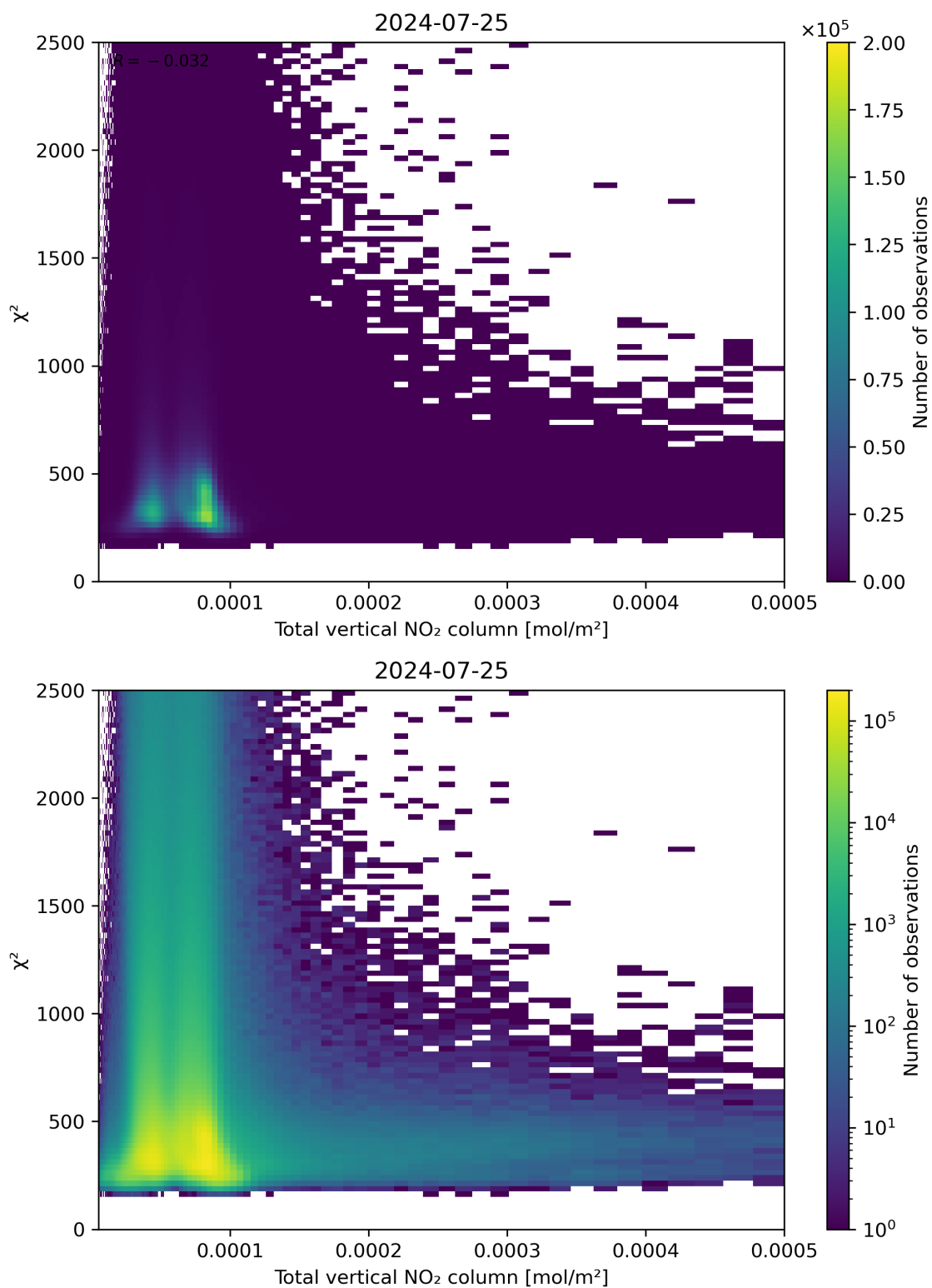
Figure 111: Scatter density plot of “Total vertical NO 2 column” against “ \chi^2 ” for 2024-07-24 to 2024-07-26.
