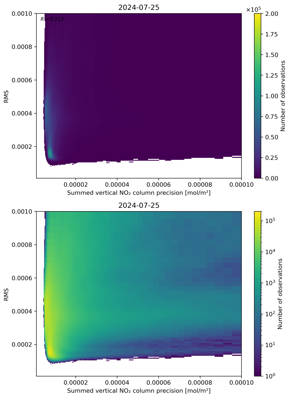
Figure 108: Scatter density plot of “Summed vertical NO 2 column precision” against “RMS” for 2024-07-24 to 2024-07-26.
