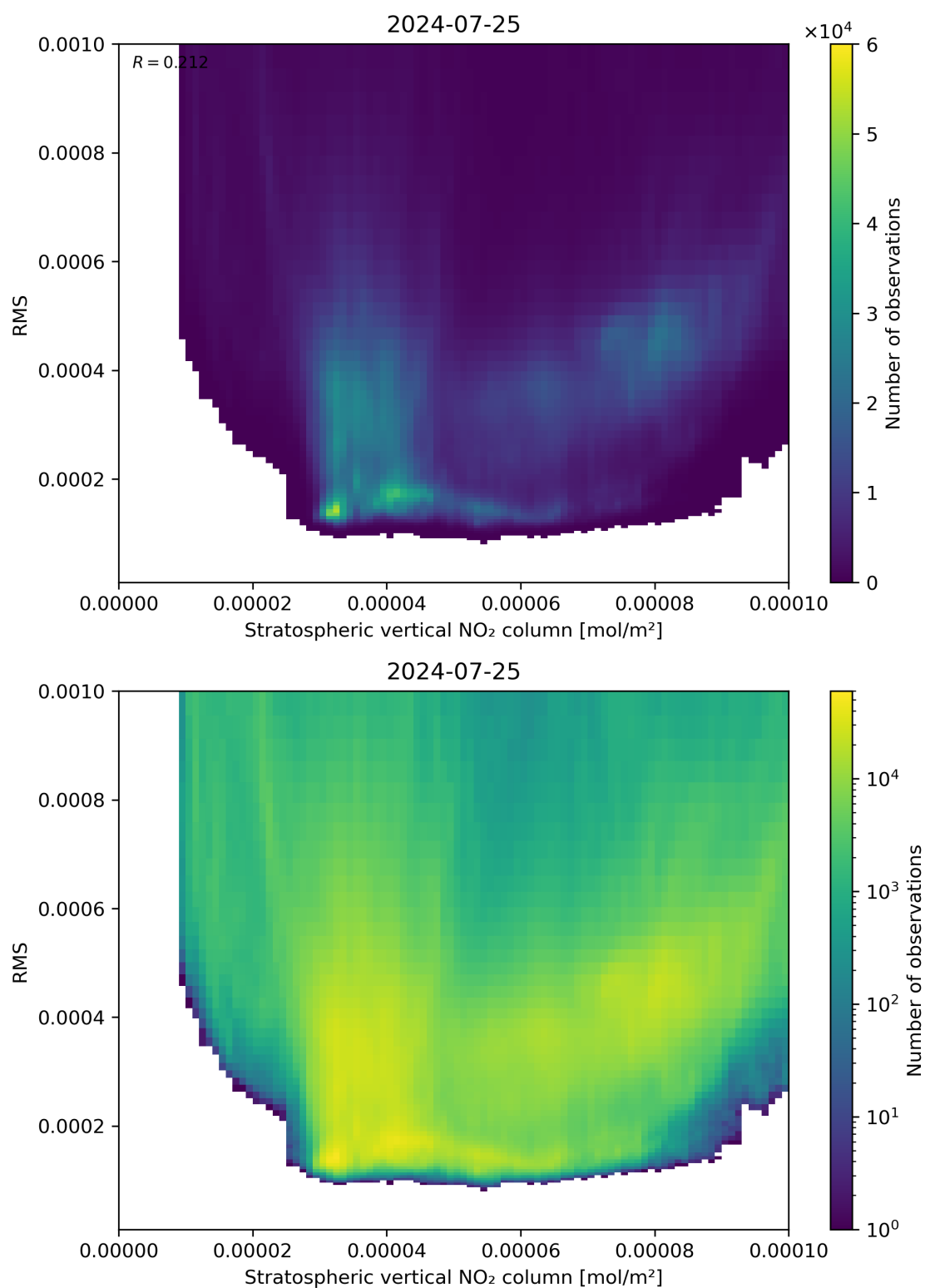
Figure 102: Scatter density plot of “Stratospheric vertical NO 2 column” against “RMS” for 2024-07-24 to 2024-07-26.
