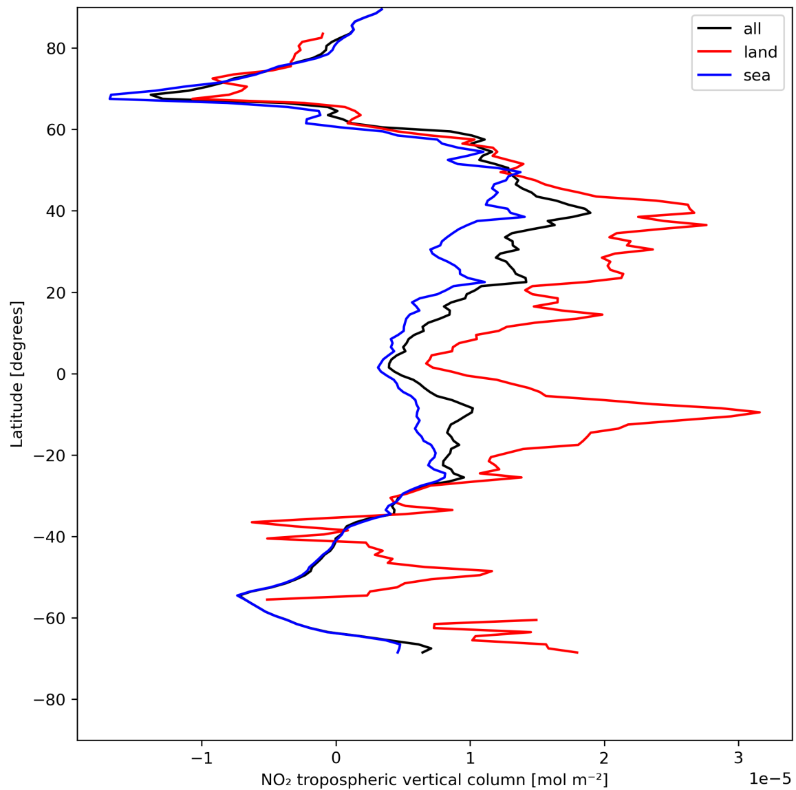
Figure 12: Zonal average of “NO 2 tropospheric vertical column” for 2024-07-24 to 2024-07-26.
