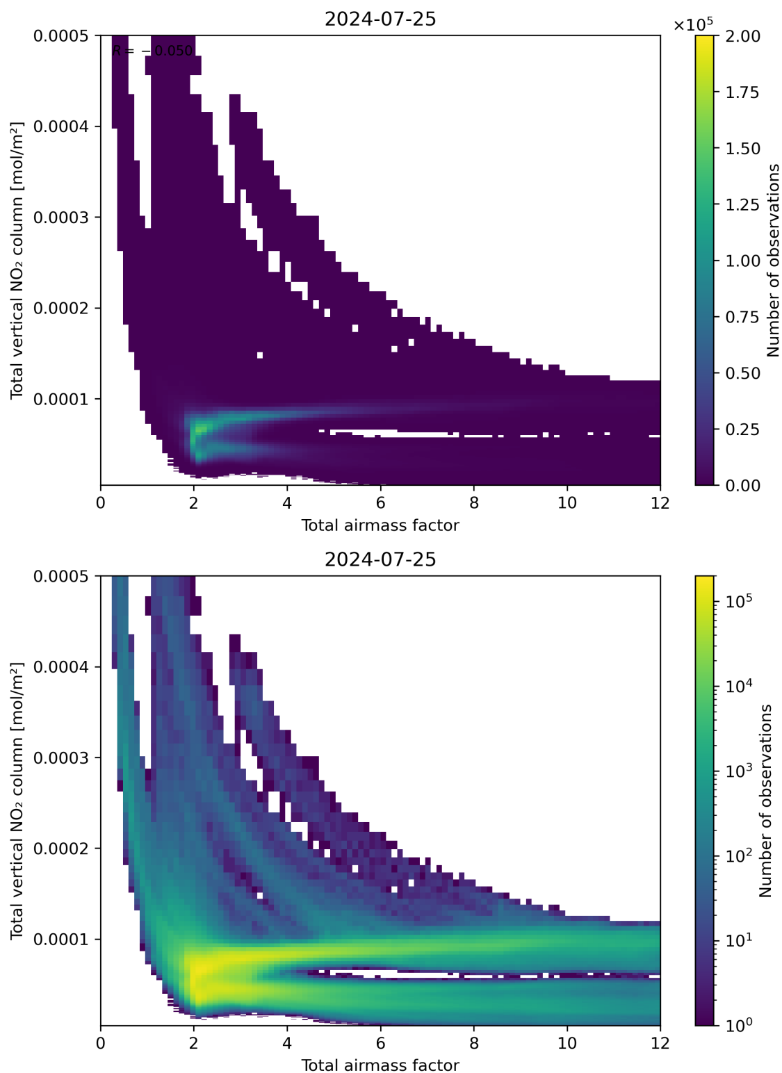
Figure 67: Scatter density plot of “Total airmass factor” against “Total vertical NO 2 column” for 2024-07-24 to 2024-07-26.
