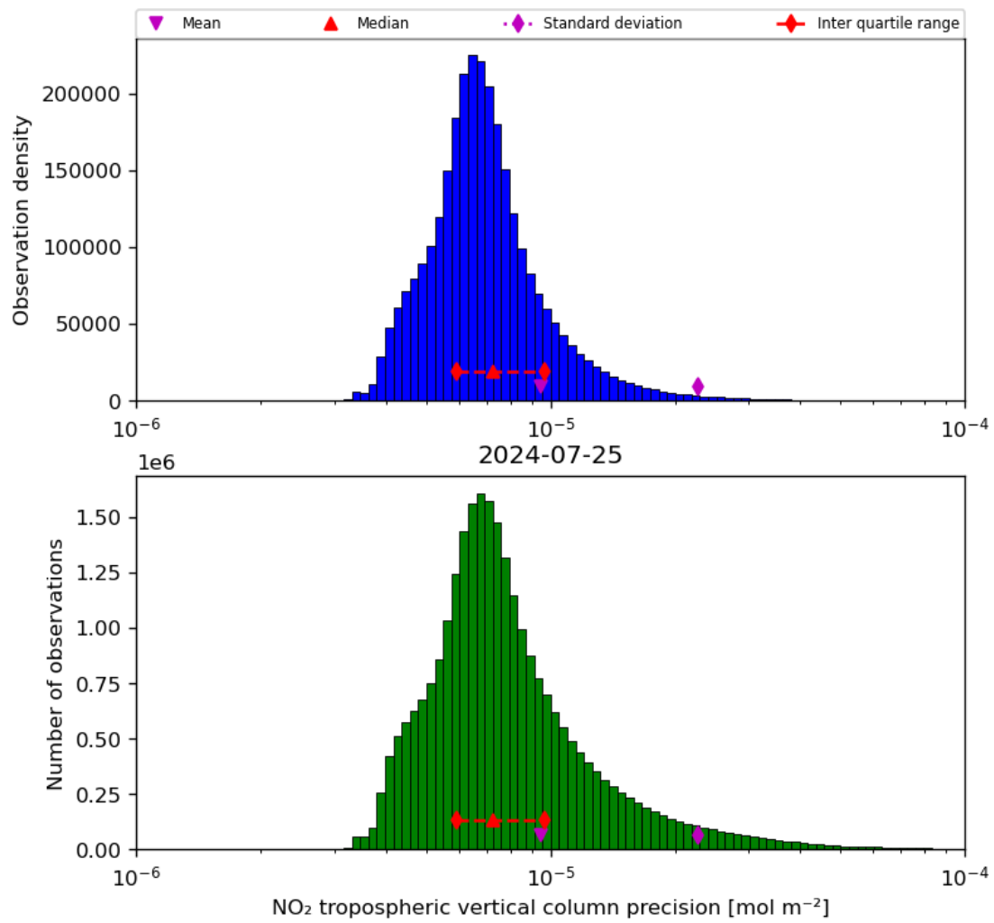
Figure 30: Histogram of “NO 2 tropospheric vertical column precision” for 2024-07-24 to 2024-07-26
