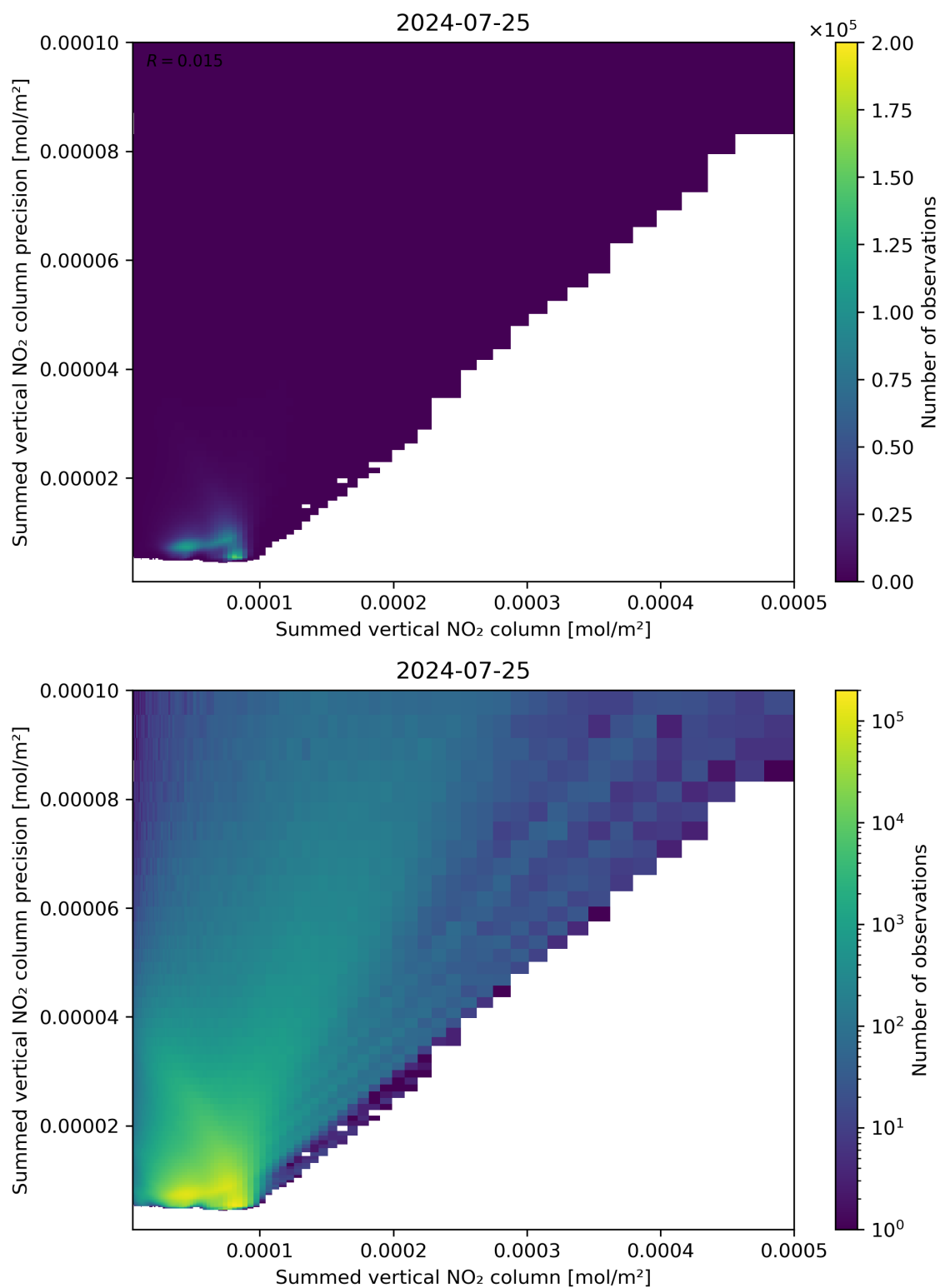
Figure 105: Scatter density plot of “Summed vertical NO 2 column” against “Summed vertical NO 2 column precision” for 2024-07-24 to 2024-07-26.
