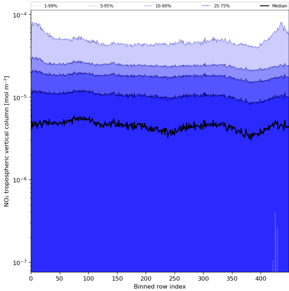
Figure 46: Along track statistics of “NO 2 tropospheric vertical column” for 2024-07-24 to 2024-07-26
