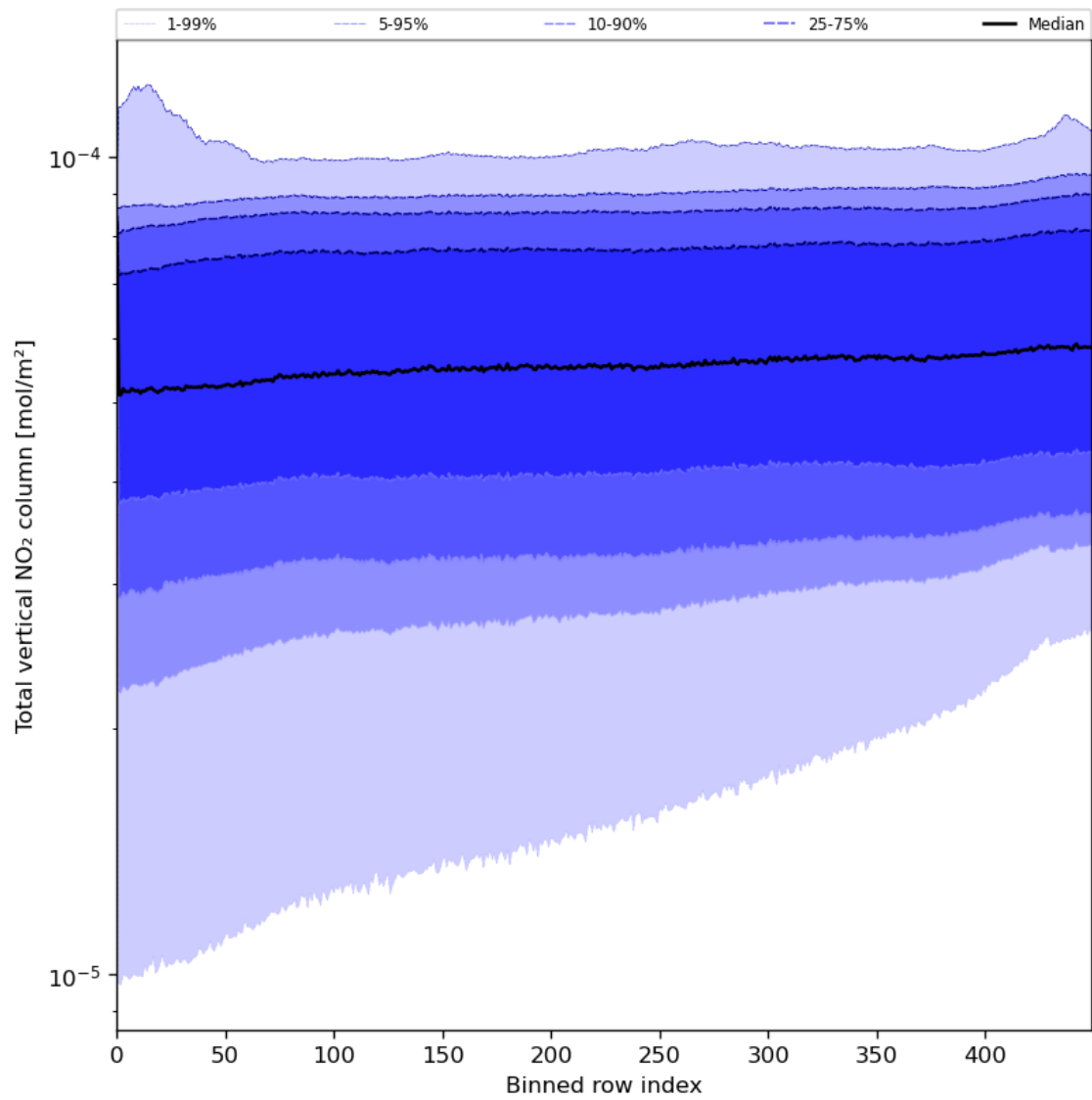
Figure 55: Along track statistics of “Total vertical NO 2 column” for 2024-07-24 to 2024-07-26
