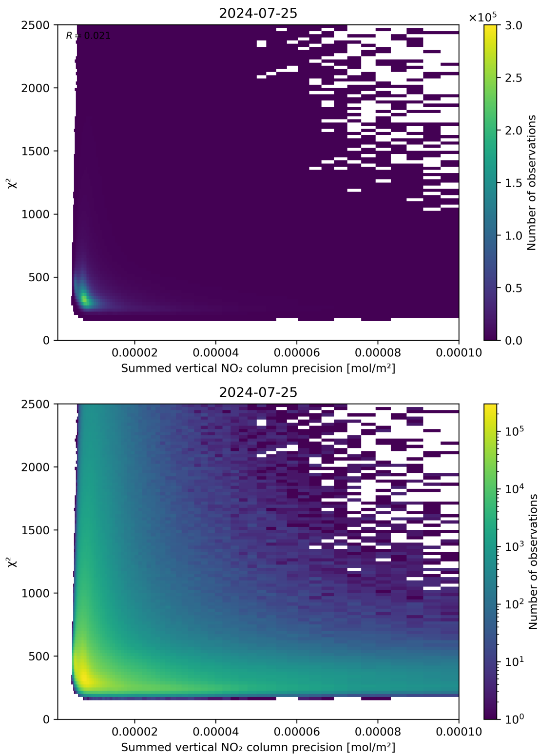
Figure 107: Scatter density plot of “Summed vertical NO 2 column precision” against “ \chi^2 ” for 2024-07-24 to 2024-07-26.
