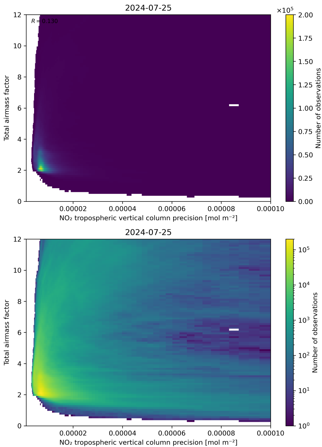
Figure 132: Scatter density plot of “NO 2 tropospheric vertical column precision” against “Total air mass factor” for 2024-07-24 to 2024-07-26.
