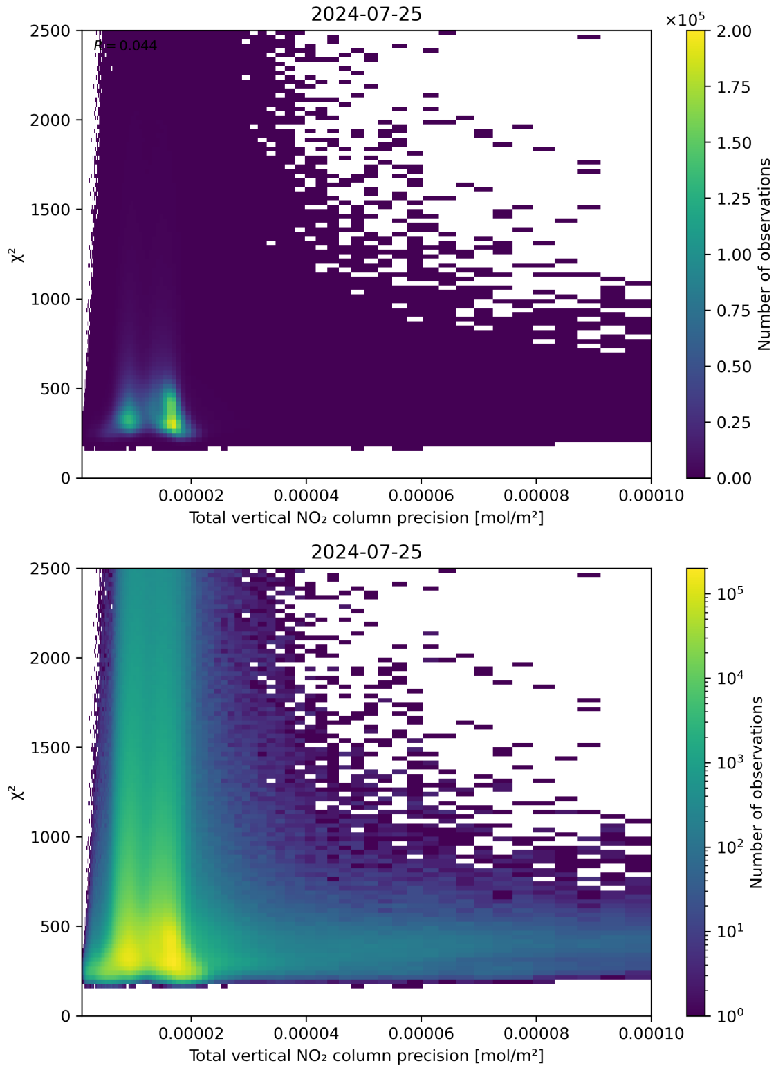
Figure 116: Scatter density plot of “Total vertical NO 2 column precision” against “ \chi^2 ” for 2024-07-24 to 2024-07-26.
