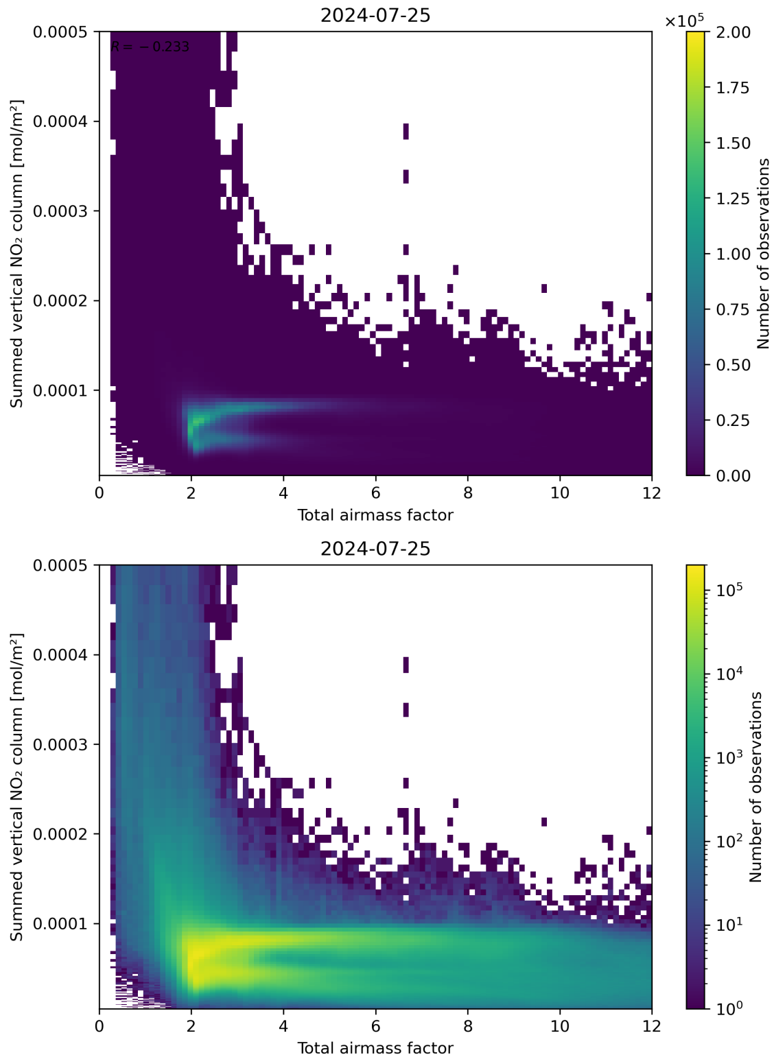
Figure 65: Scatter density plot of “Total airmass factor” against “Summed vertical NO 2 column” for 2024-07-24 to 2024-07-26.
