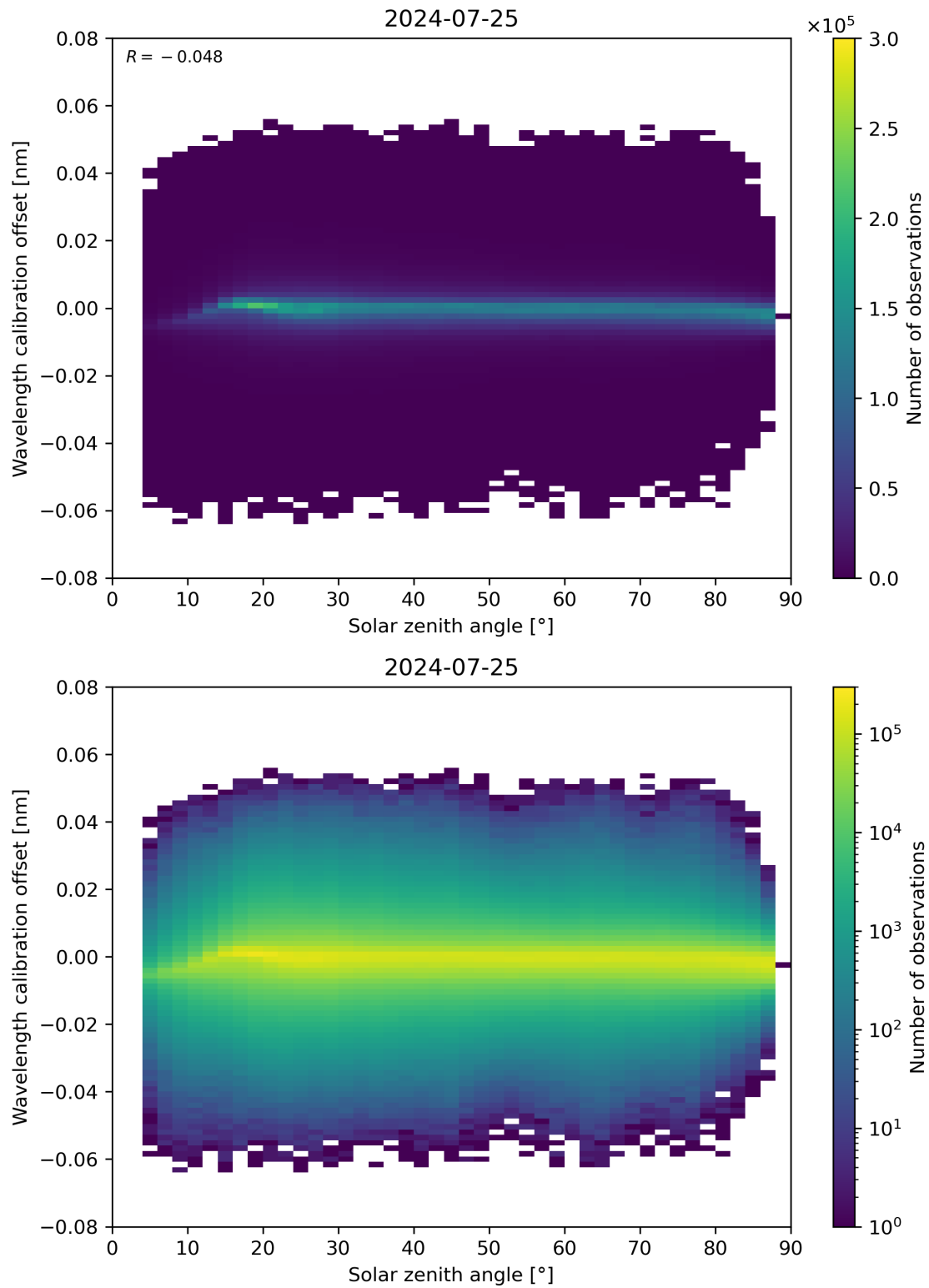
Figure 158: Scatter density plot of “Solar zenith angle” against “Wavelength calibration offset” for 2024-07-24 to 2024-07-26.
