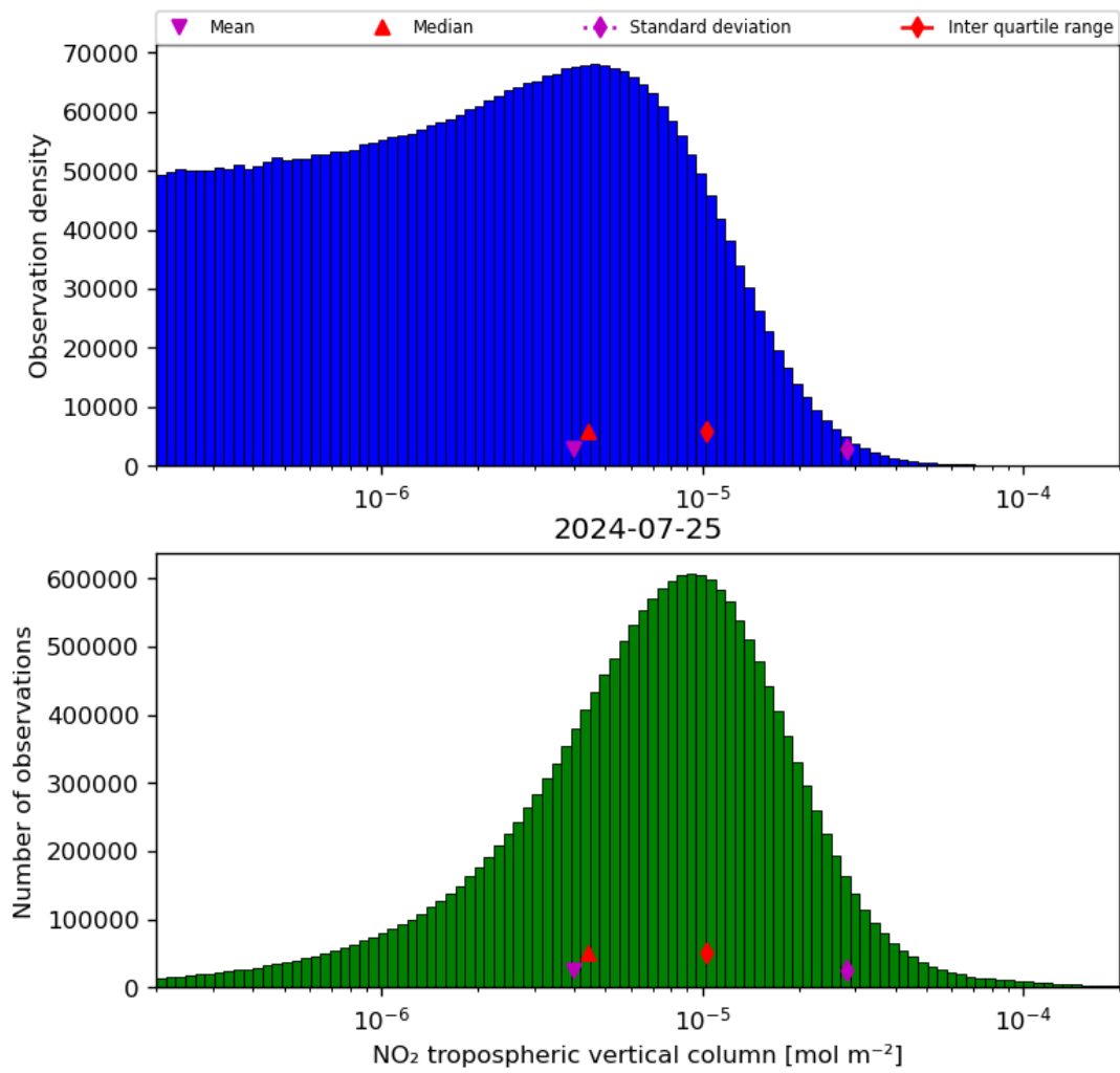
Figure 29: Histogram of “NO 2 tropospheric vertical column” for 2024-07-24 to 2024-07-26
