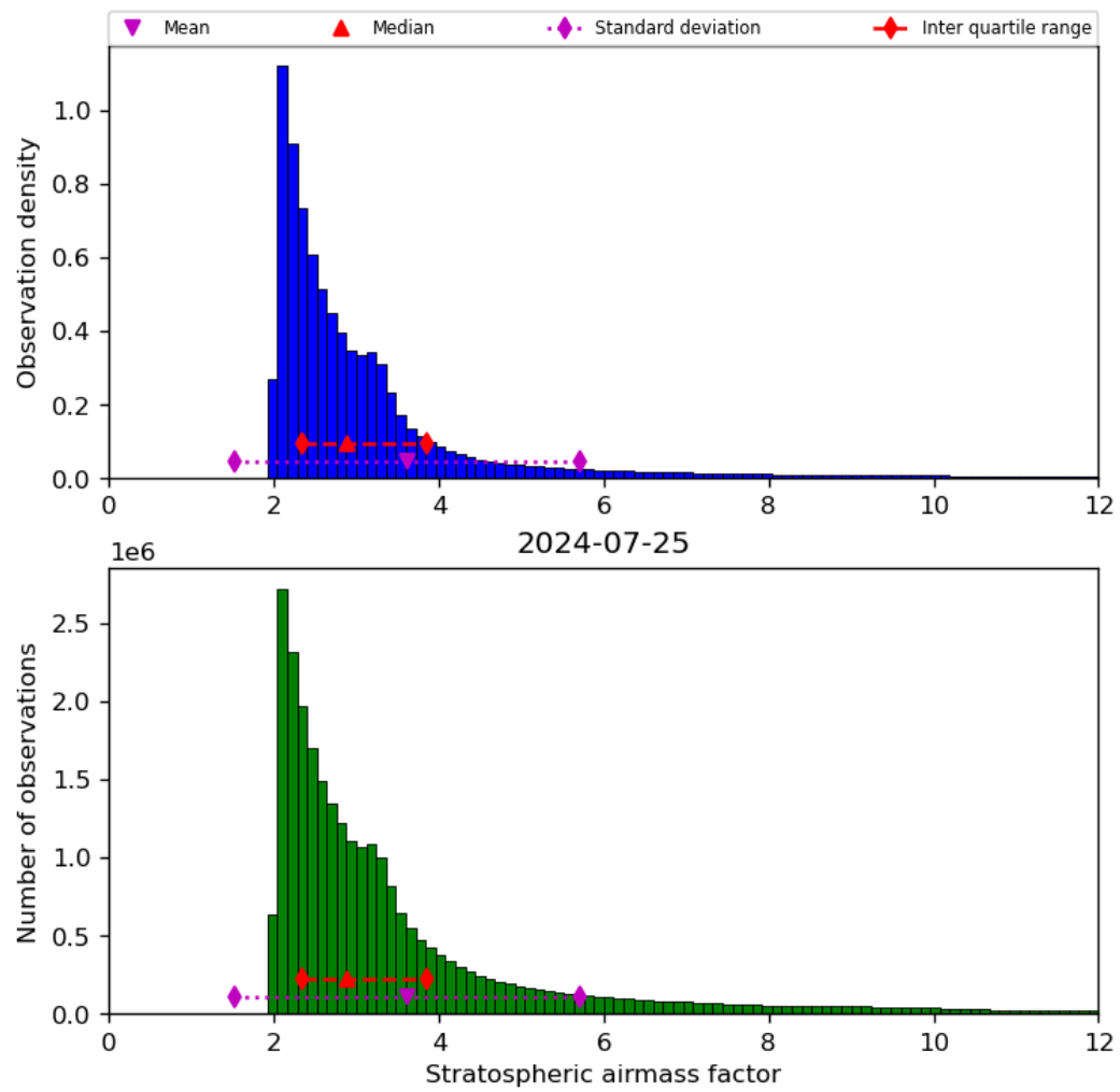
Figure 44: Histogram of “Stratospheric airmass factor” for 2024-07-24 to 2024-07-26
