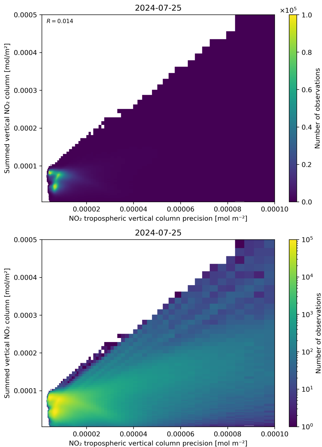
Figure 136: Scatter density plot of “NO 2 tropospheric vertical column precision” against “Summed vertical NO 2 column” for 2024-07-24 to 2024-07-26.
