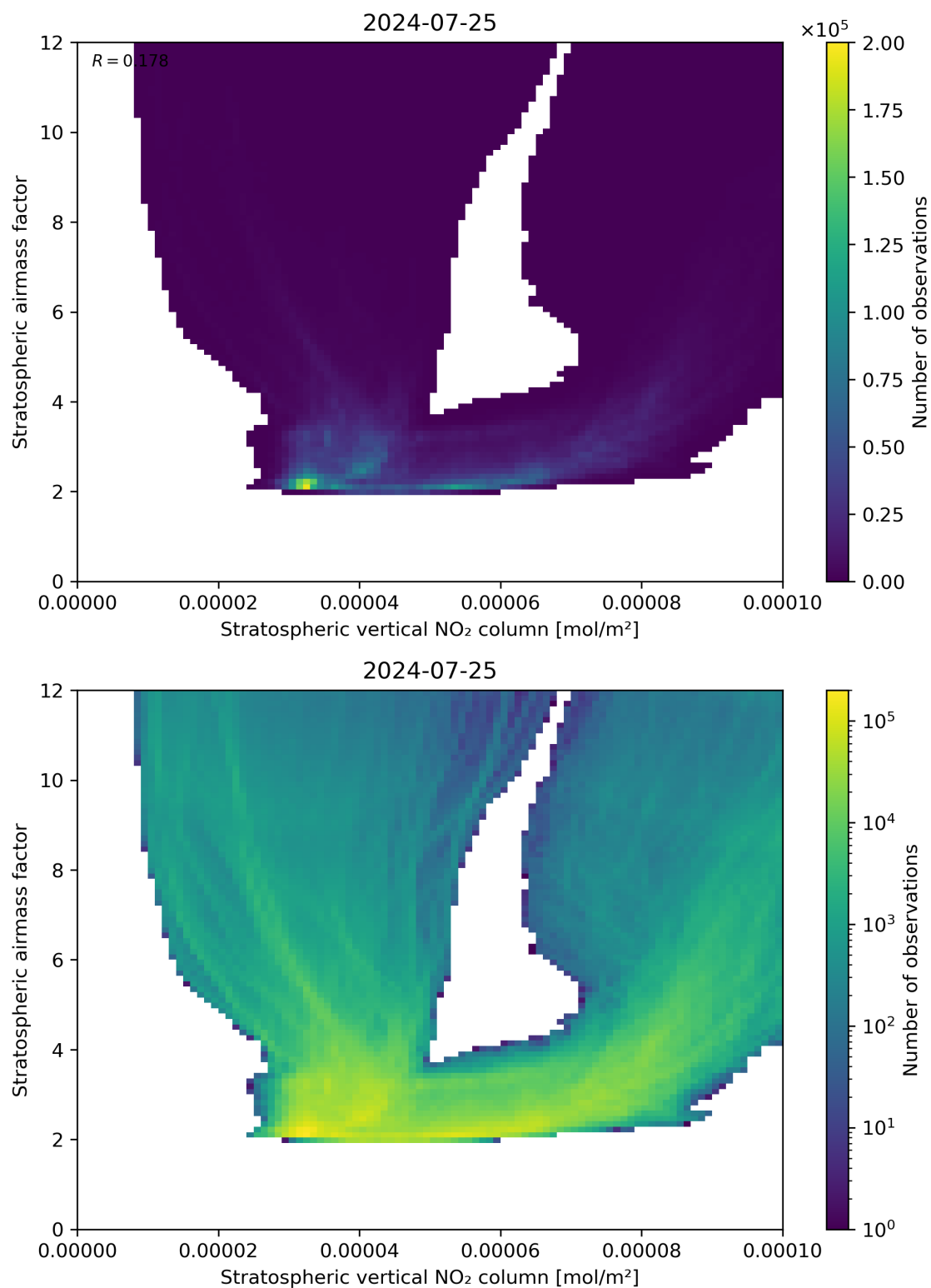
Figure 96: Scatter density plot of “Stratospheric vertical NO 2 column” against “Stratospheric airmass factor” for 2024-07-24 to 2024-07-26.
