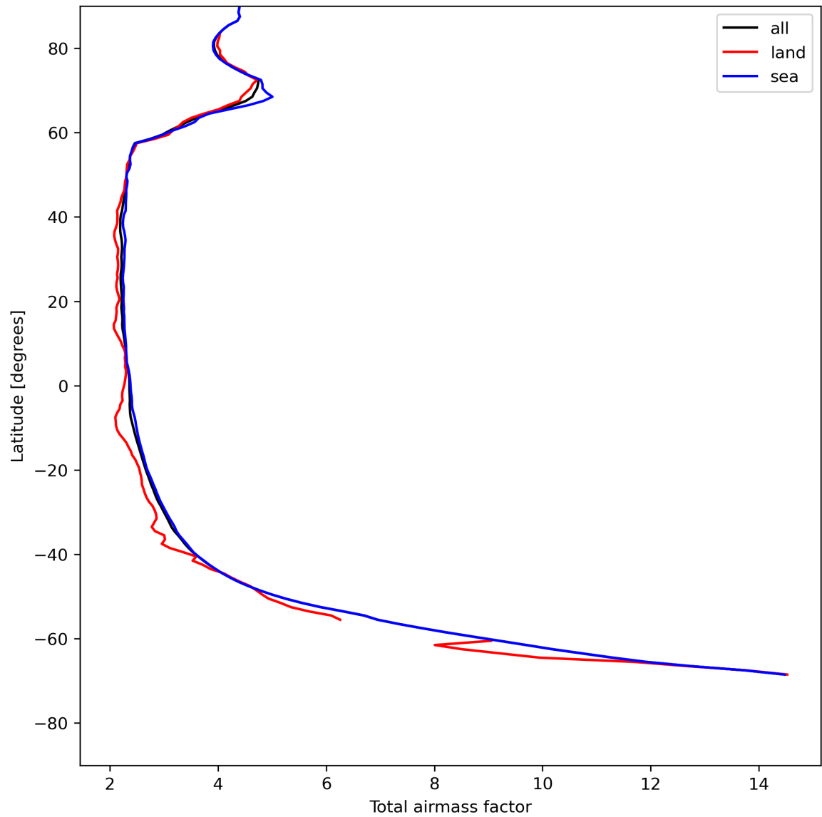
Figure 15: Zonal average of “Total airmass factor” for 2024-07-24 to 2024-07-26.
