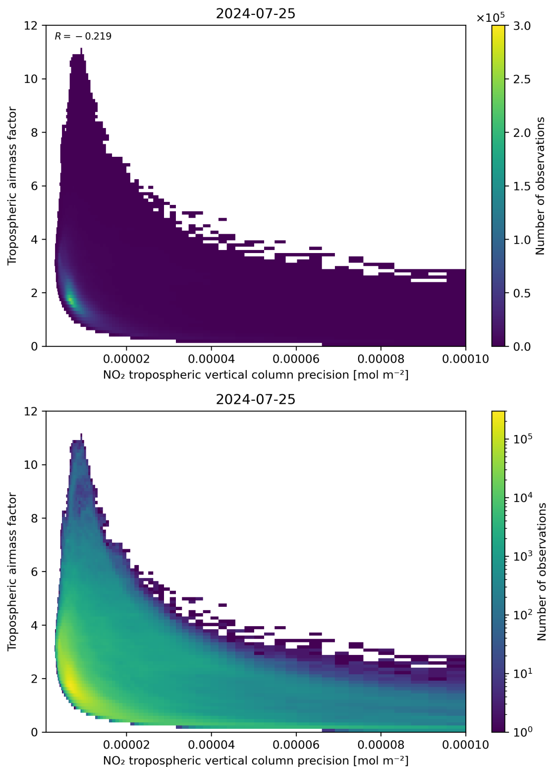
Figure 133: Scatter density plot of “NO 2 tropospheric vertical column precision” against “Tropospheric airmass factor” for 2024-07-24 to 2024-07-26.
