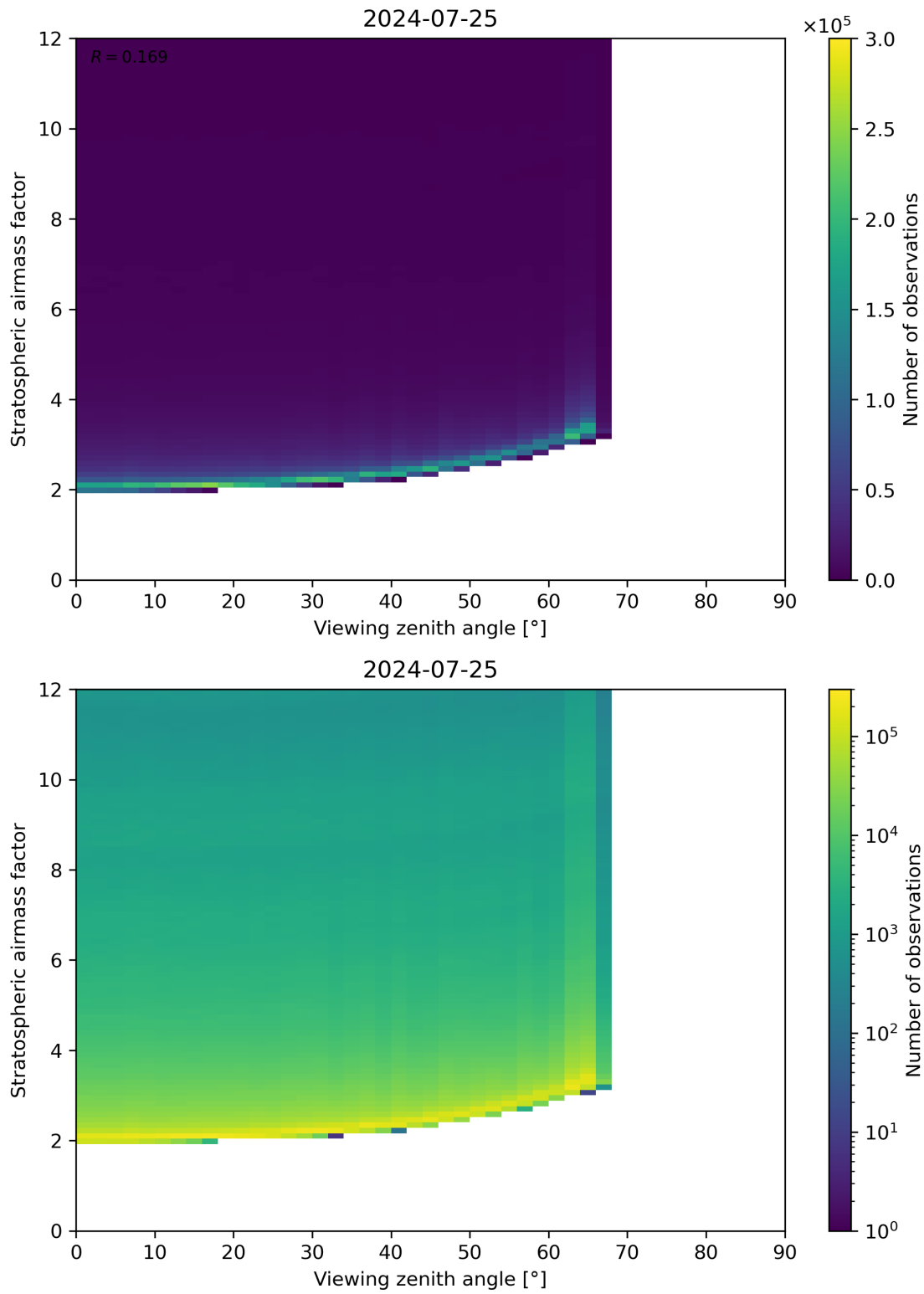
Figure 159: Scatter density plot of “Viewing zenith angle” against “Stratospheric airmass factor” for 2024-07-24 to 2024-07-26.
