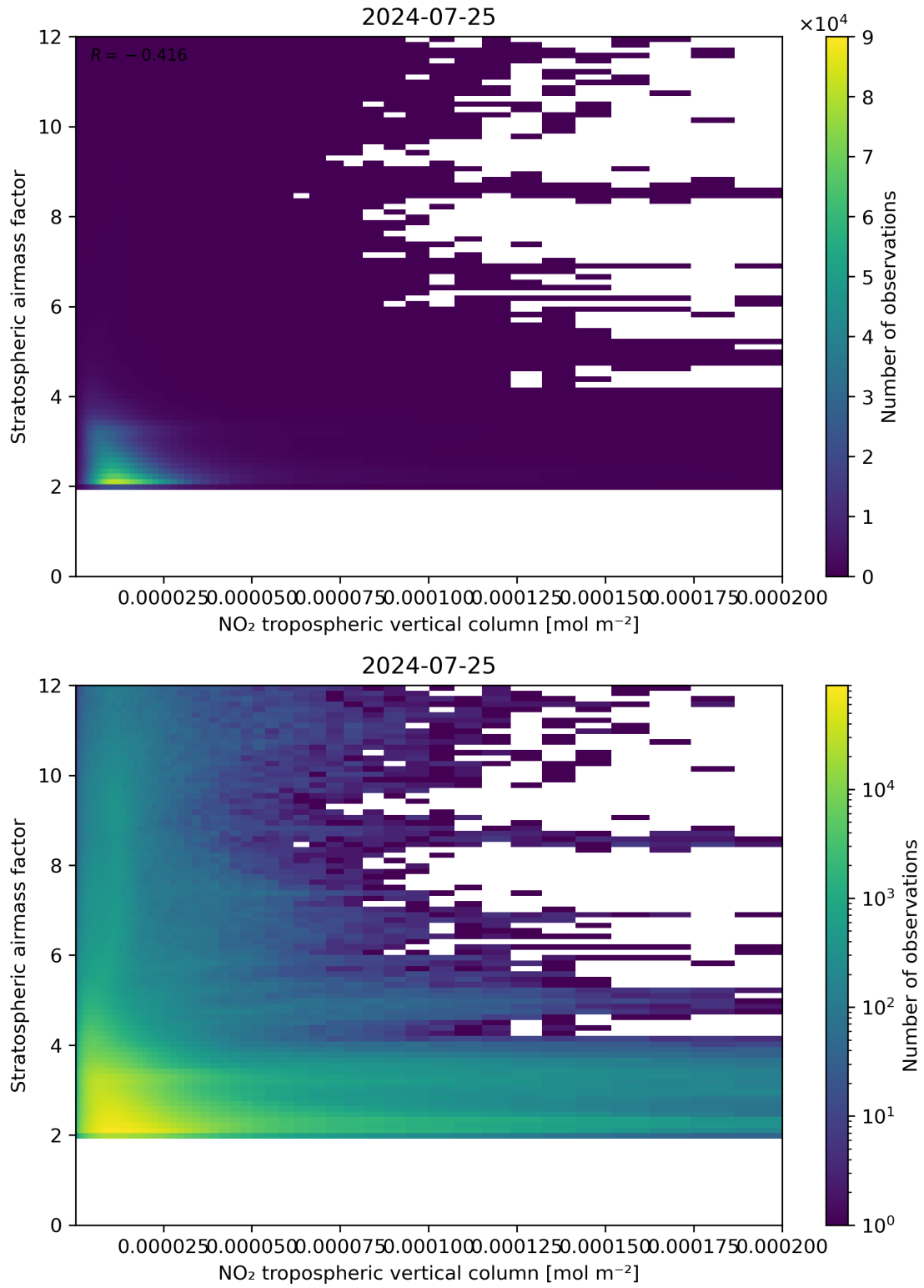
Figure 121: Scatter density plot of “NO 2 tropospheric vertical column” against “Stratospheric airmass factor” for 2024-07-24 to 2024-07-26.
