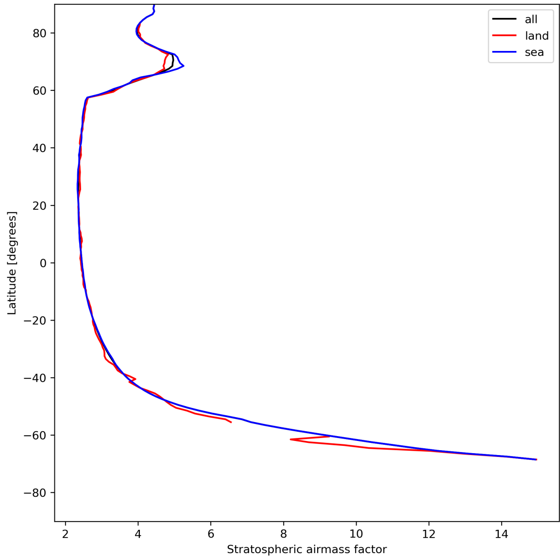
Figure 27: Zonal average of “Stratospheric air mass factor” for 2024-07-24 to 2024-07-26.
