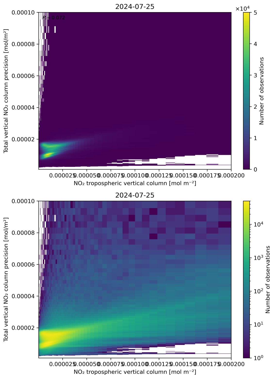
Figure 129: Scatter density plot of “NO 2 tropospheric vertical column” against “Total vertical NO 2 column precision” for 2024-07-24 to 2024-07-26.
