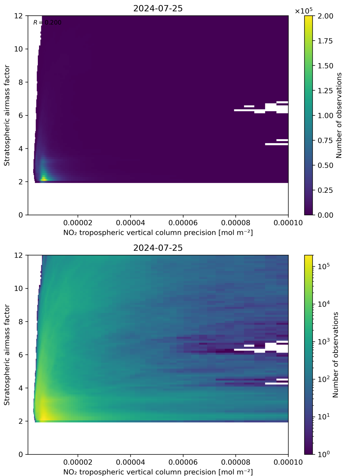
Figure 131: Scatter density plot of “NO 2 tropospheric vertical column precision” against “Stratospheric airmass factor” for 2024-07-24 to 2024-07-26.
