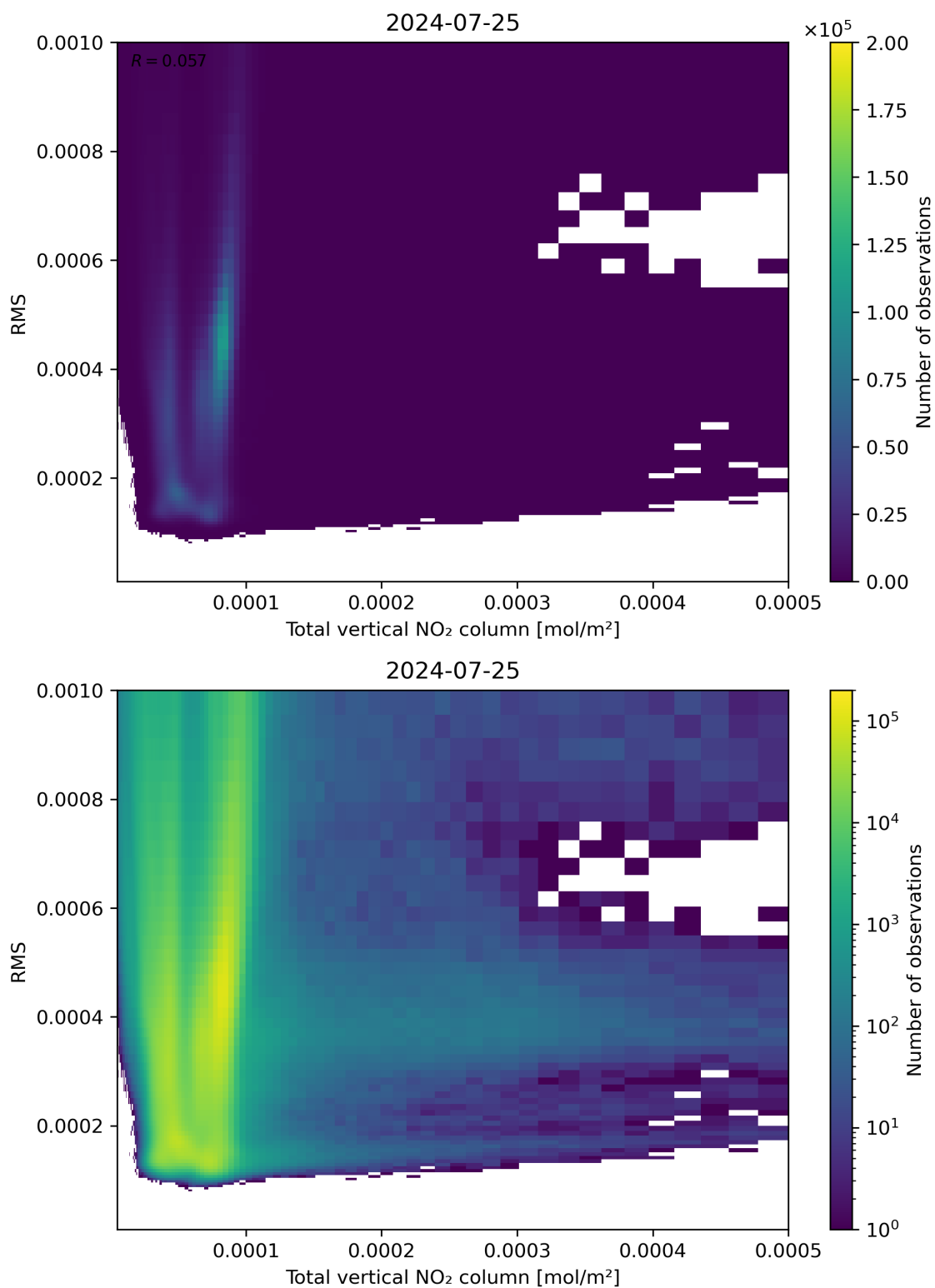
Figure 120: Scatter density plot of “Total vertical NO 2 column” against “RMS” for 2024-07-24 to 2024-07-26.
