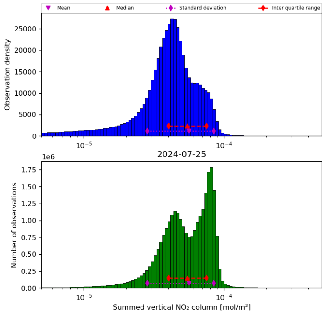
Figure 40: Histogram of “Summed vertical NO 2 column” for 2024-07-24 to 2024-07-26
