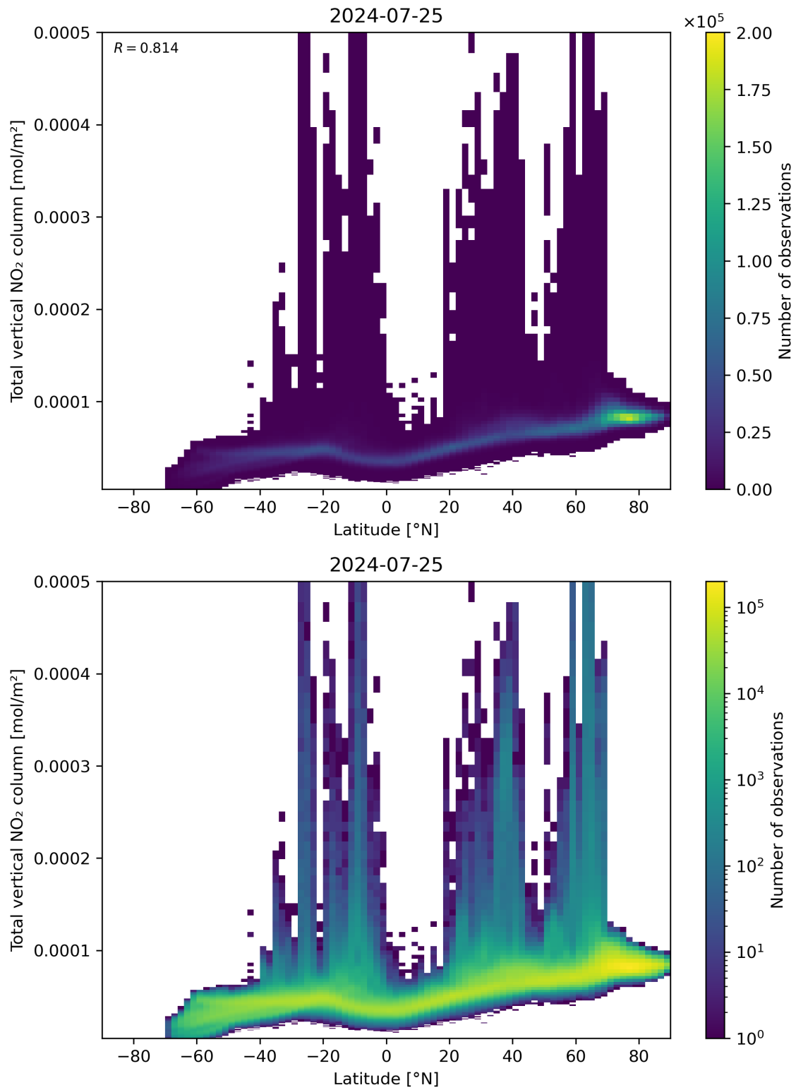
Figure 90: Scatter density plot of “Latitude” against “Total vertical NO 2 column” for 2024-07-24 to 2024-07-26.
