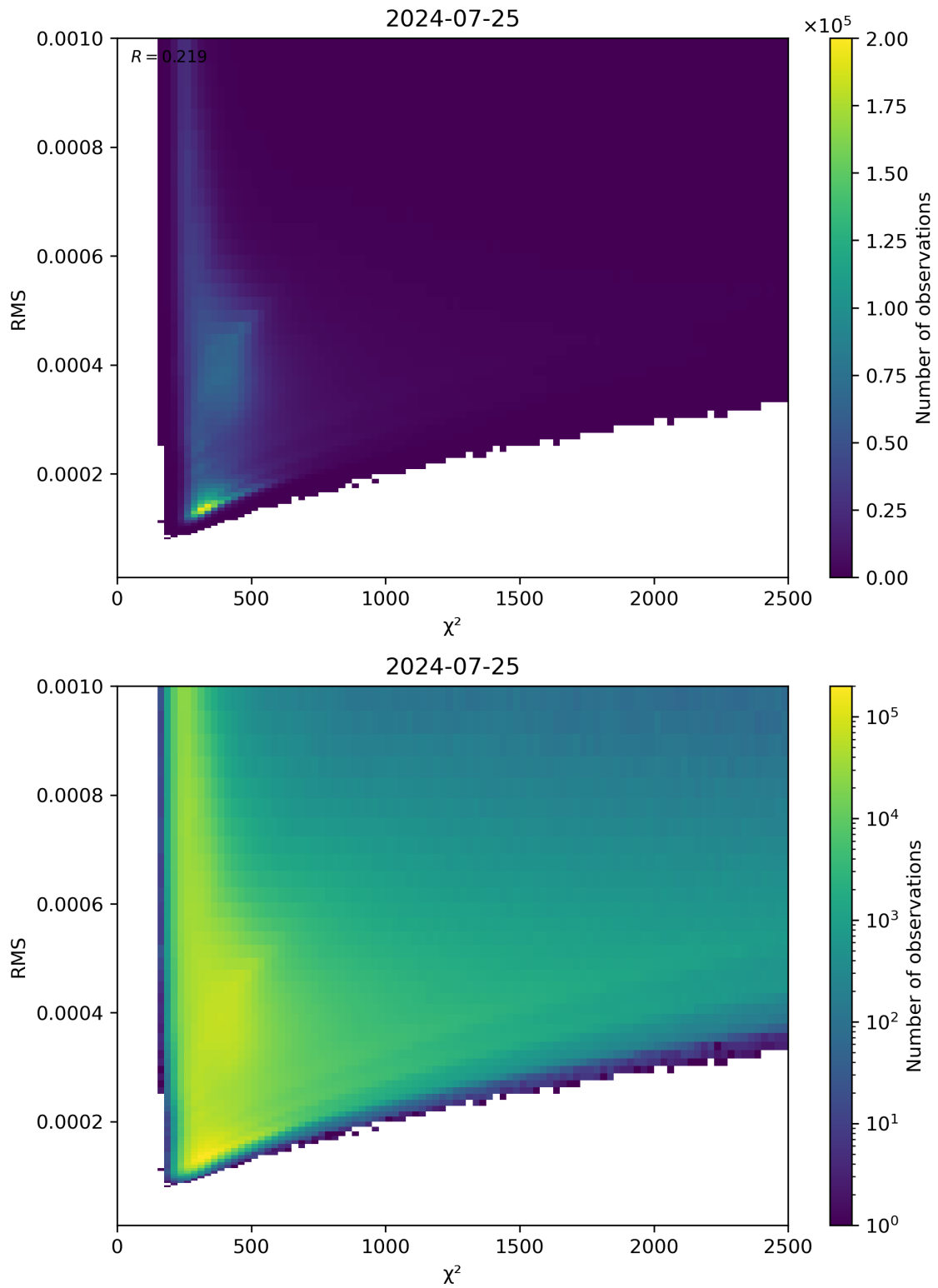
Figure 82: Scatter density plot of “ \chi^2 ” against “RMS” for 2024-07-24 to 2024-07-26.
