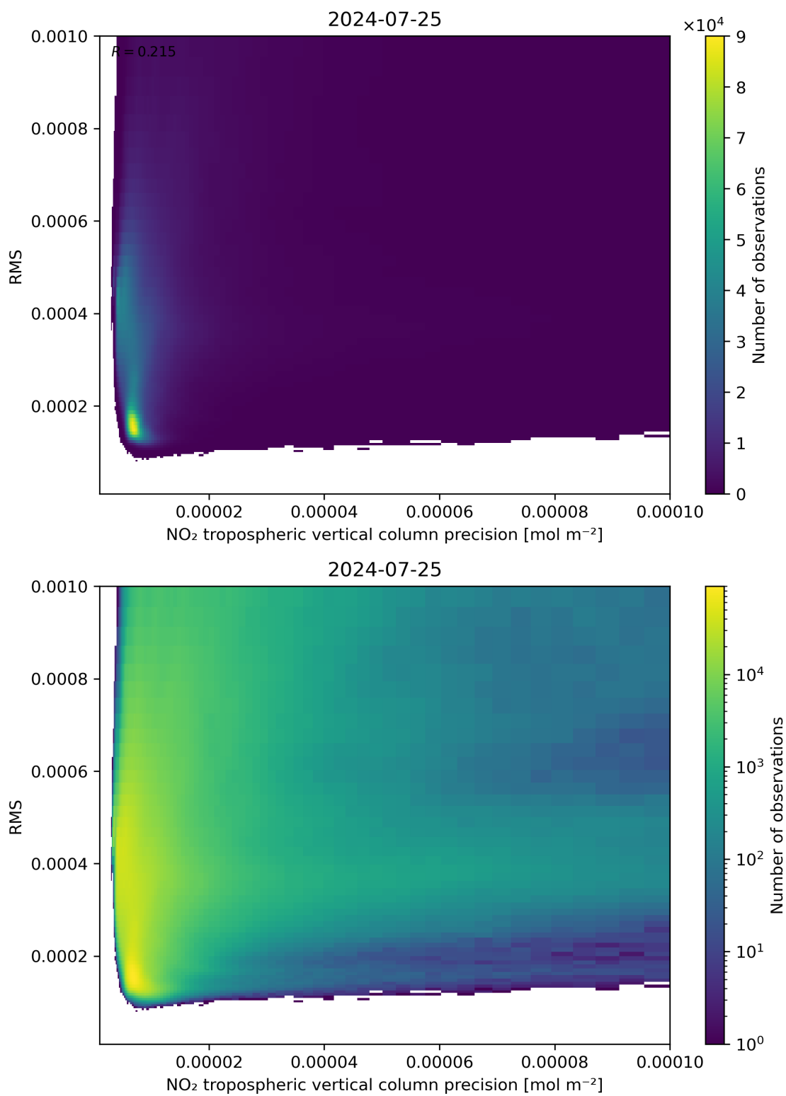
Figure 140: Scatter density plot of “NO 2 tropospheric vertical column precision” against “RMS” for 2024-07-24 to 2024-07-26.
