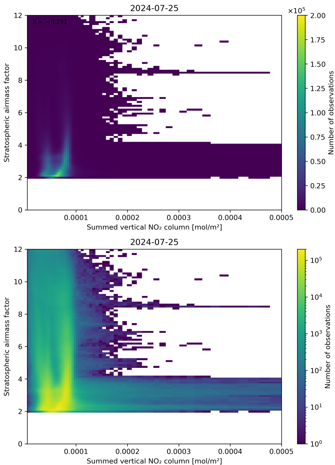
Figure 103: Scatter density plot of “Summed vertical NO 2 column” against “Stratospheric airmass factor” for 2024-07-24 to 2024-07-26.
