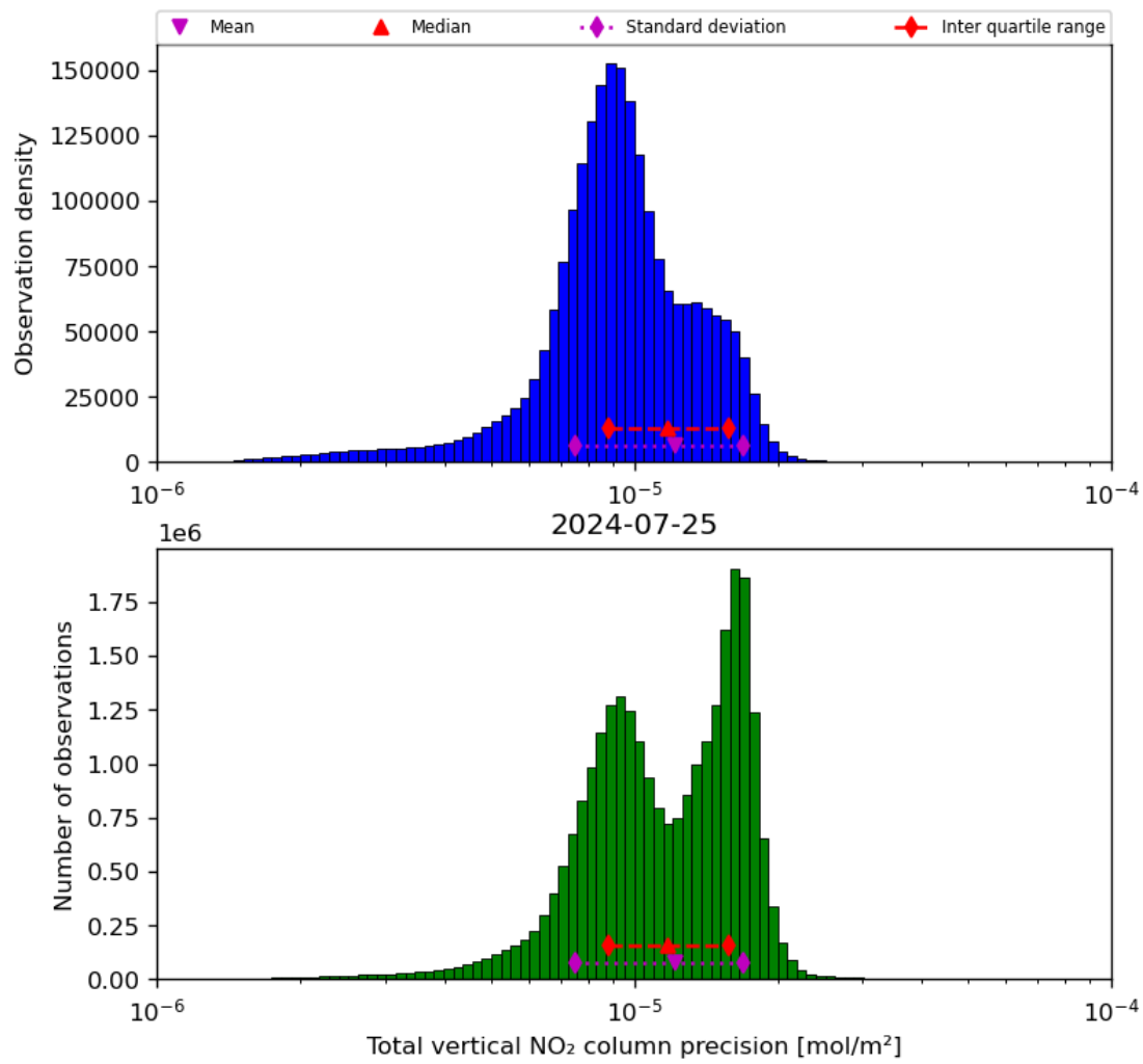
Figure 39: Histogram of “Total vertical NO 2 column precision” for 2024-07-24 to 2024-07-26
