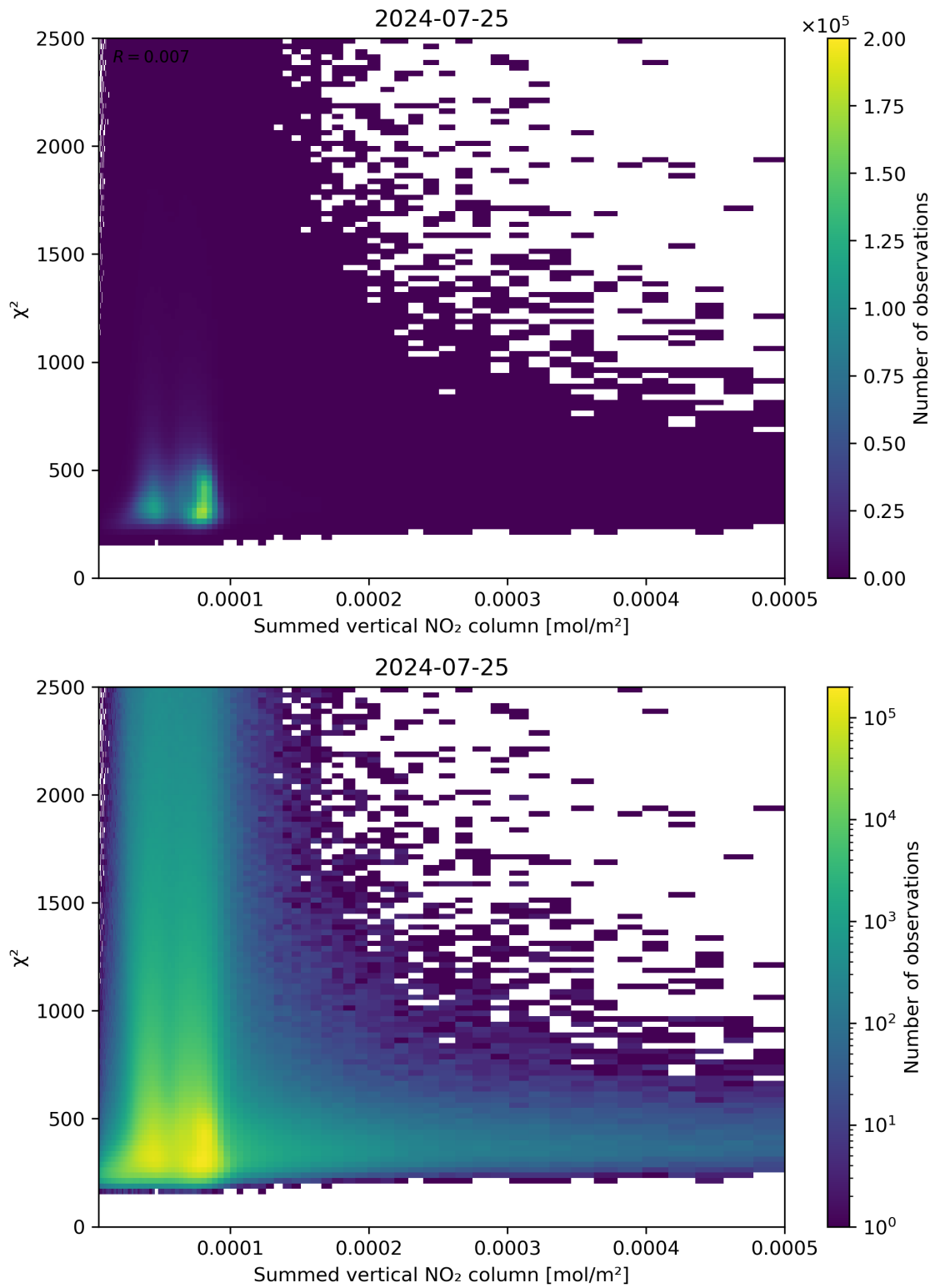
Figure 104: Scatter density plot of “Summed vertical NO 2 column” against “ \chi^2 ” for 2024-07-24 to 2024-07-26.
