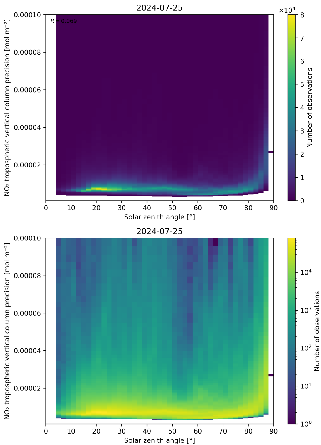
Figure 156: Scatter density plot of “Solar zenith angle” against “NO 2 tropospheric vertical column precision” for 2024-07-24 to 2024-07-26.
