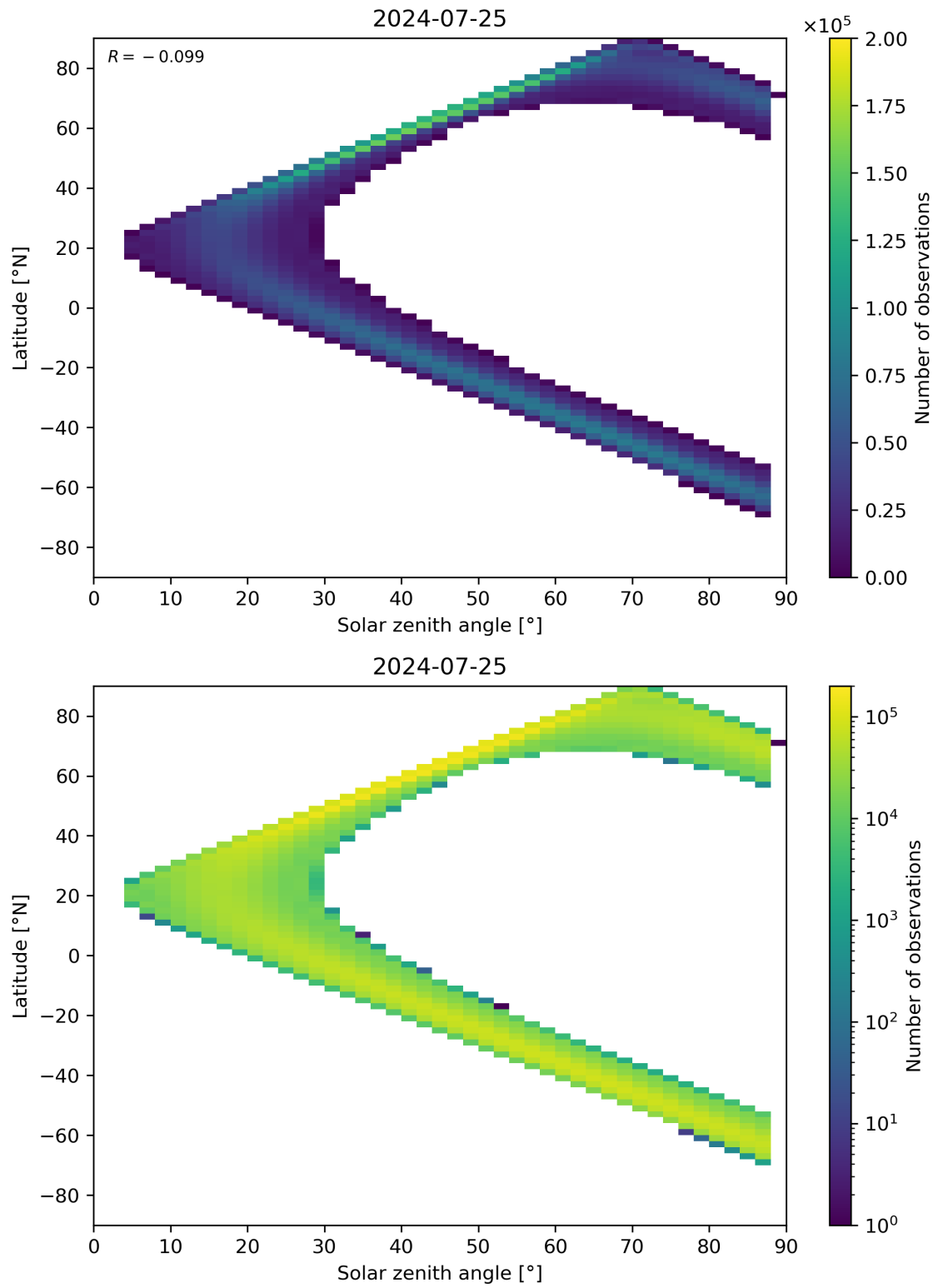
Figure 149: Scatter density plot of “Solar zenith angle” against “Latitude” for 2024-07-24 to 2024-07-26.
