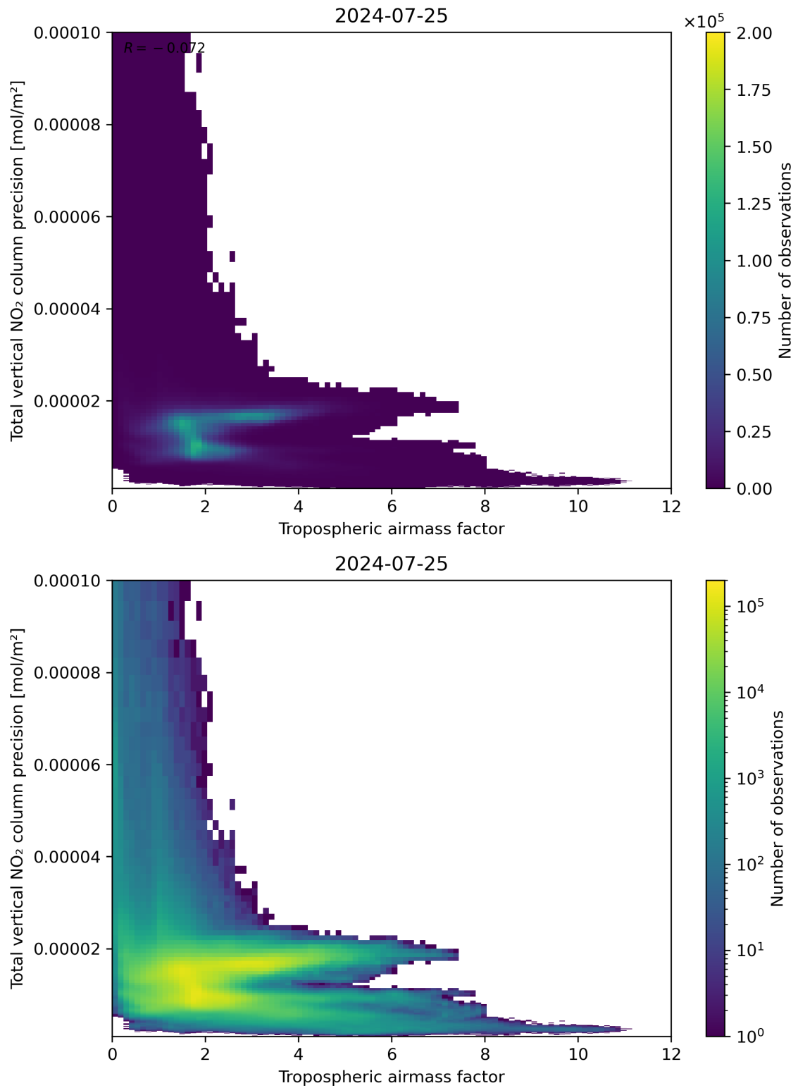
Figure 78: Scatter density plot of “Tropospheric air mass factor” against “Total vertical NO 2 column precision” for 2024-07-24 to 2024-07-26.
