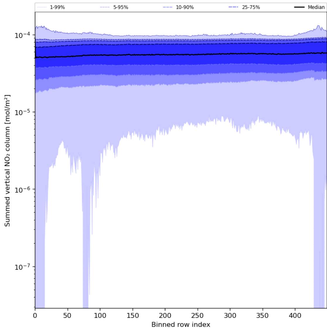
Figure 57: Along track statistics of “Summed vertical NO 2 column” for 2024-07-24 to 2024-07-26
