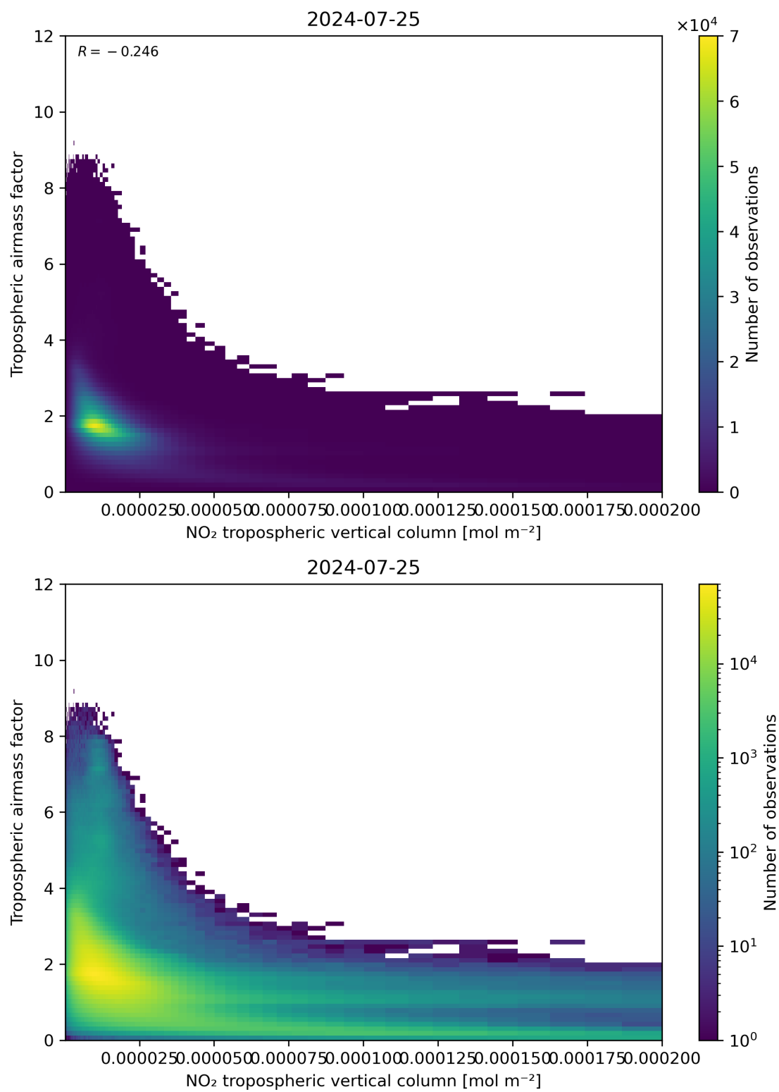
Figure 123: Scatter density plot of “NO 2 tropospheric vertical column” against “Tropospheric air mass factor” for 2024-07-24 to 2024-07-26.
