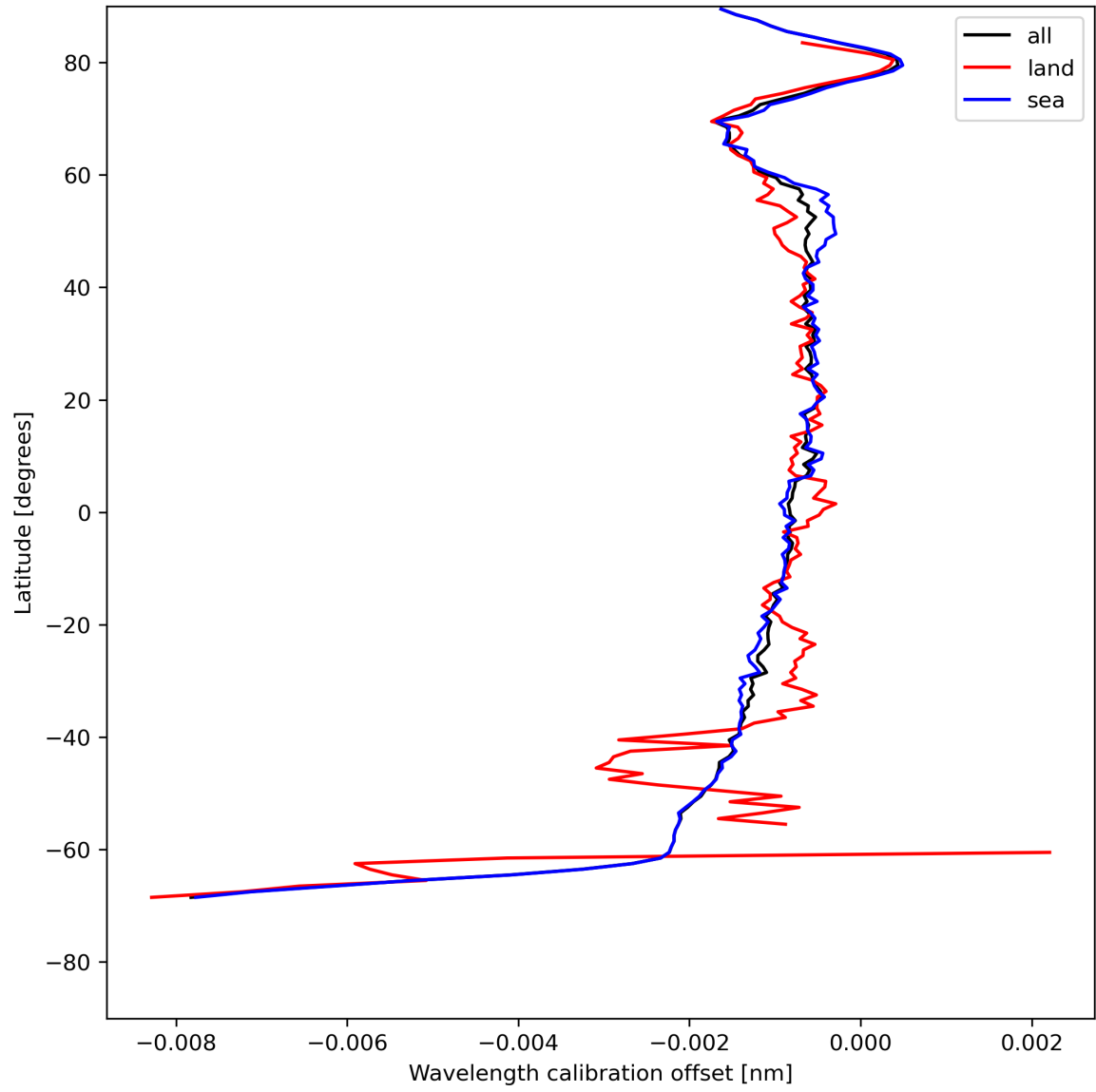
Figure 18: Zonal average of “Wavelength calibration offset” for 2024-07-24 to 2024-07-26.
