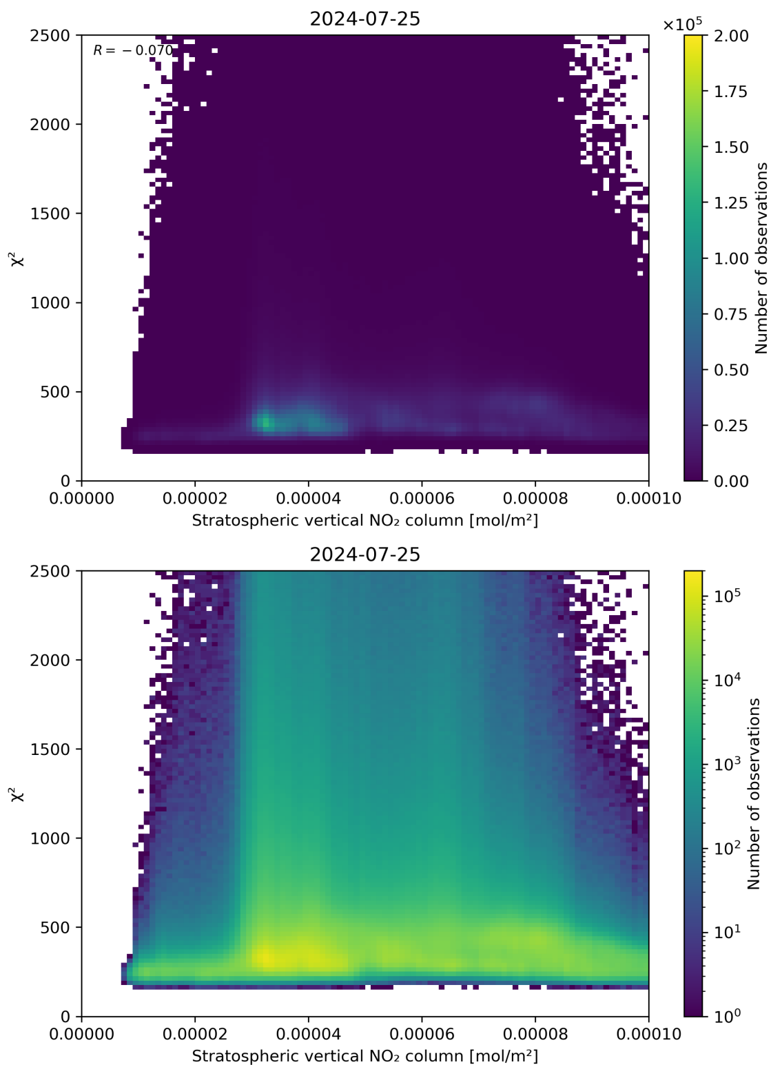
Figure 97: Scatter density plot of “Stratospheric vertical NO 2 column” against “ \chi^2 ” for 2024-07-24 to 2024-07-26.
