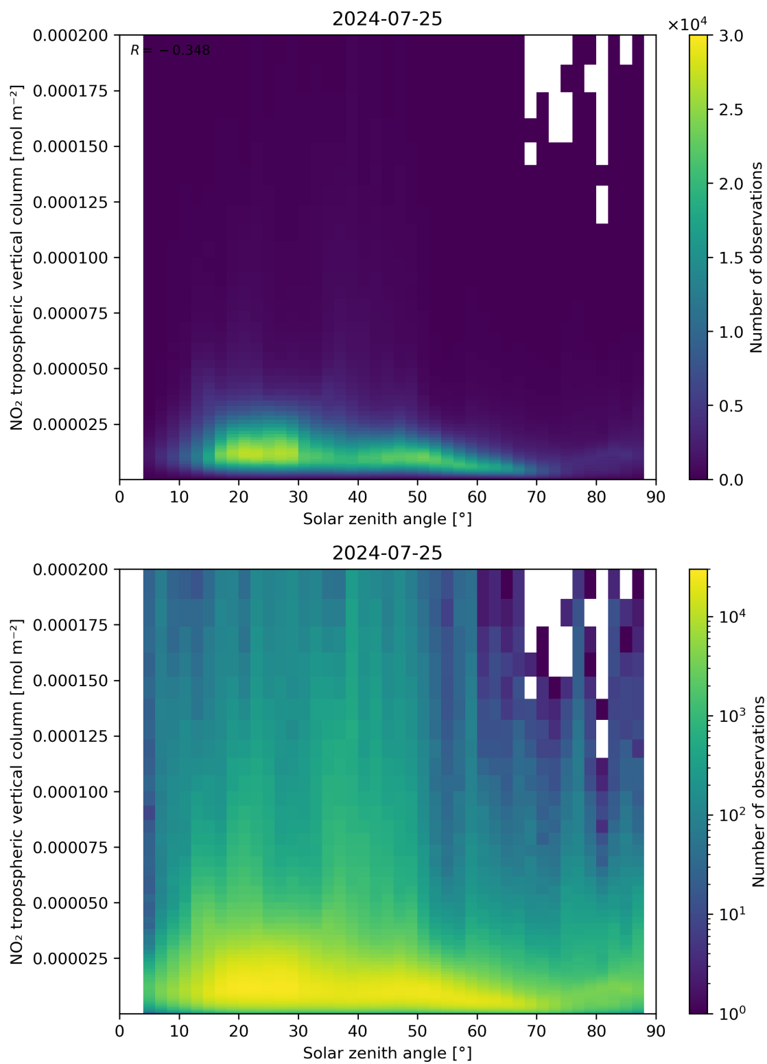
Figure 155: Scatter density plot of “Solar zenith angle” against “NO 2 tropospheric vertical column” for 2024-07-24 to 2024-07-26.
