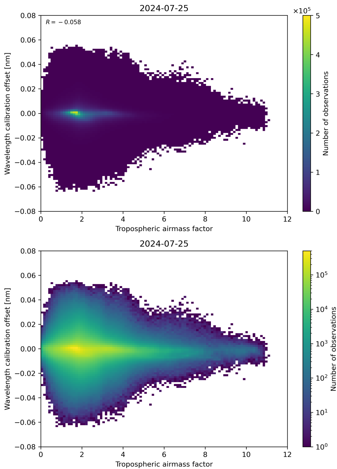
Figure 80: Scatter density plot of “Tropospheric air mass factor” against “Wavelength calibration offset” for 2024-07-24 to 2024-07-26.
