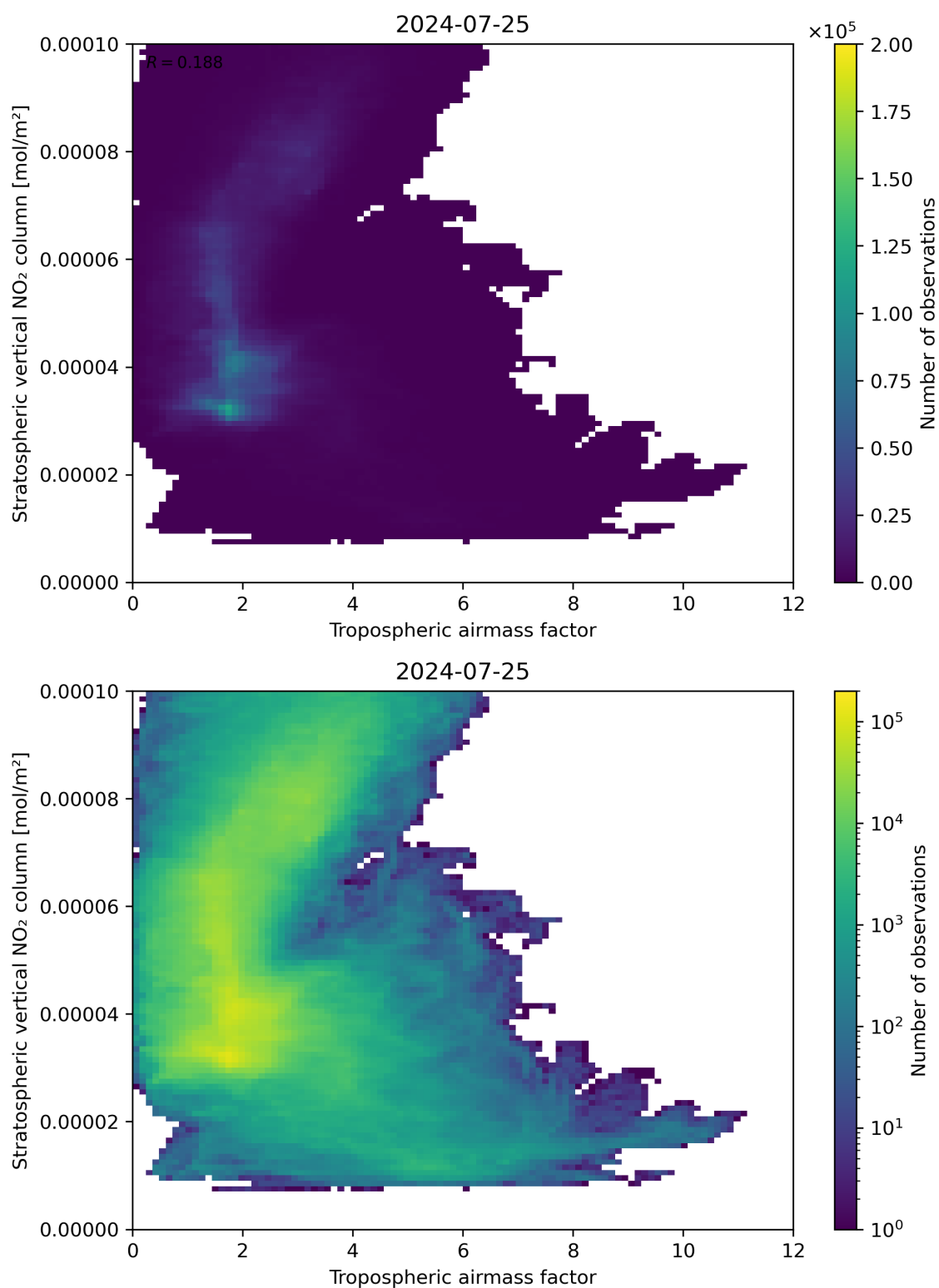
Figure 74: Scatter density plot of “Tropospheric air mass factor” against “Stratospheric vertical NO 2 column” for 2024-07-24 to 2024-07-26.
