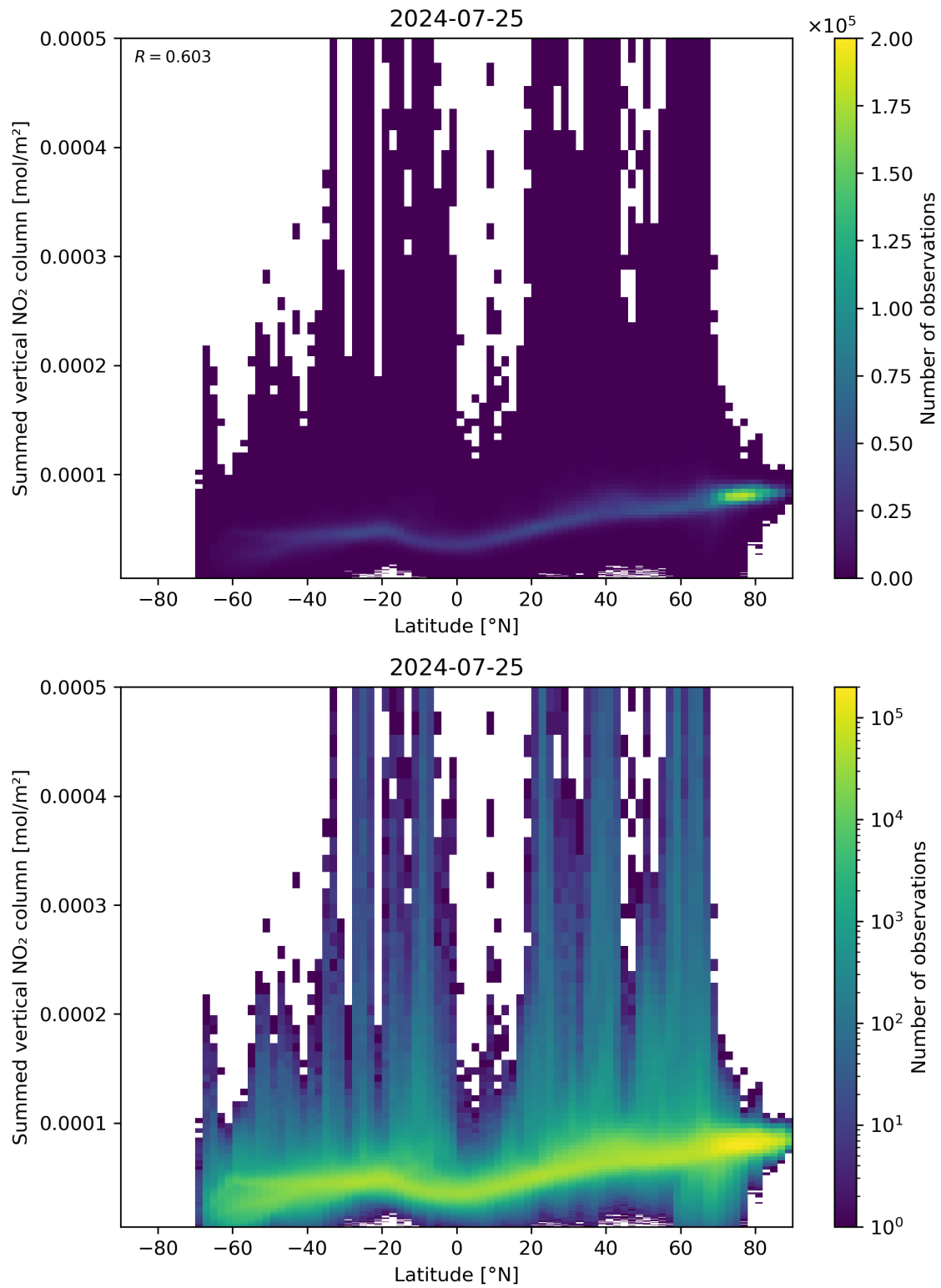
Figure 88: Scatter density plot of “Latitude” against “Summed vertical NO 2 column” for 2024-07-24 to 2024-07-26.
