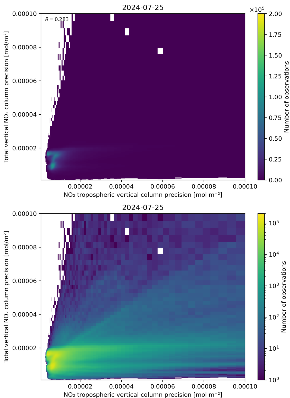
Figure 139: Scatter density plot of “NO 2 tropospheric vertical column precision” against “Total vertical NO 2 column precision” for 2024-07-24 to 2024-07-26.
