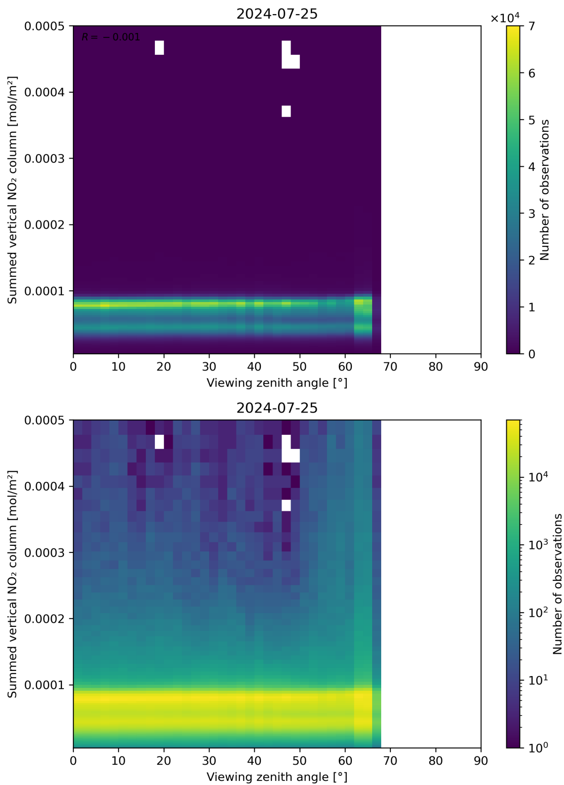
Figure 165: Scatter density plot of “Viewing zenith angle” against “Summed vertical NO 2 column” for 2024-07-24 to 2024-07-26.
