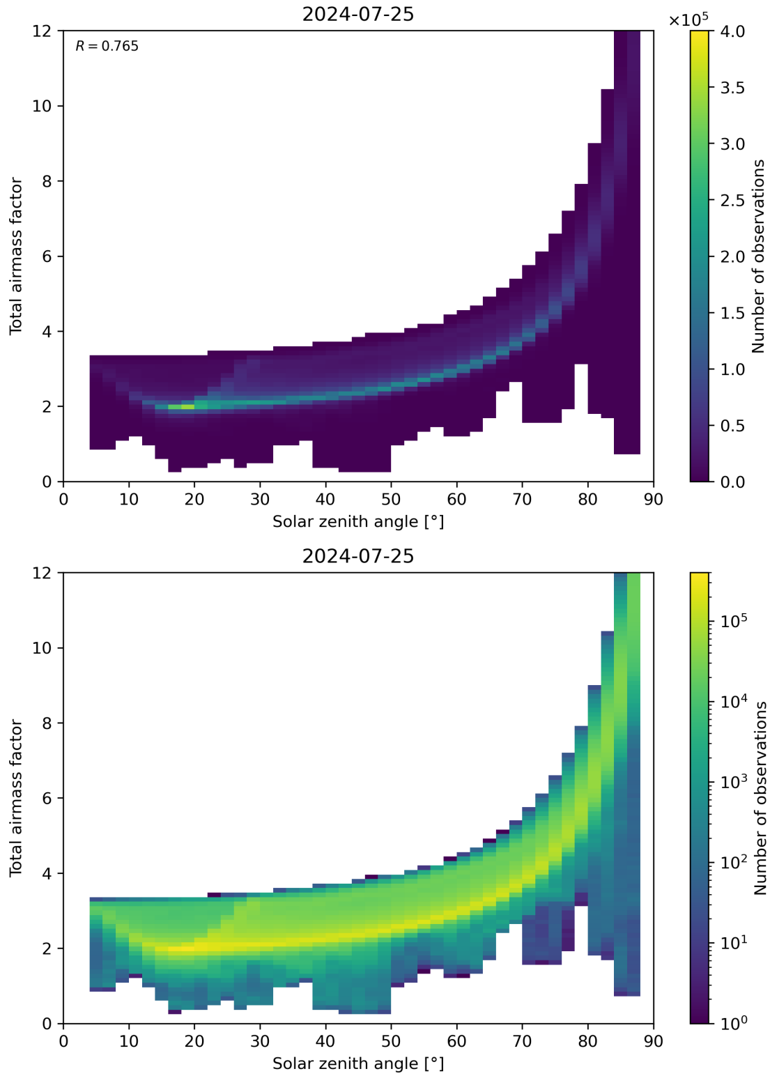
Figure 146: Scatter density plot of “Solar zenith angle” against “Total air mass factor” for 2024-07-24 to 2024-07-26.
