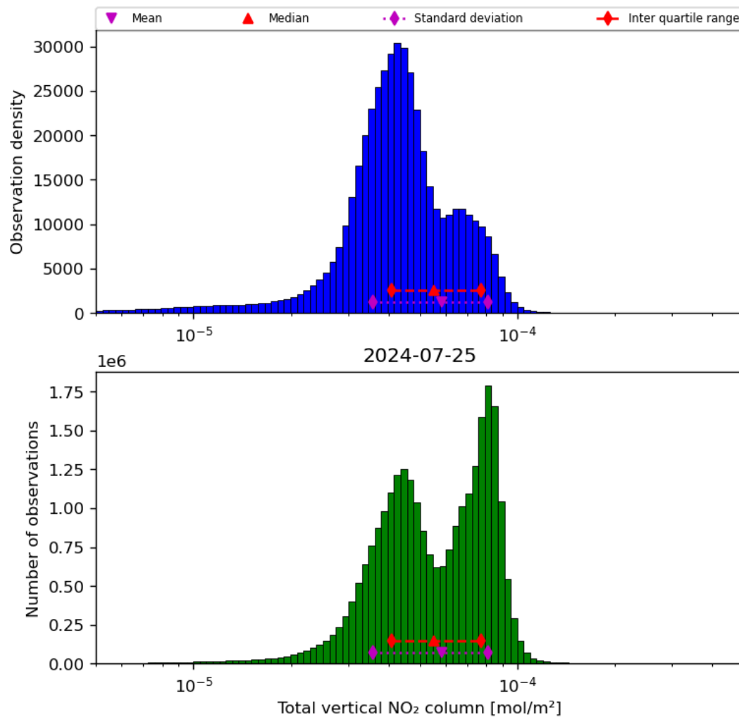
Figure 38: Histogram of “Total vertical NO 2 column” for 2024-07-24 to 2024-07-26
