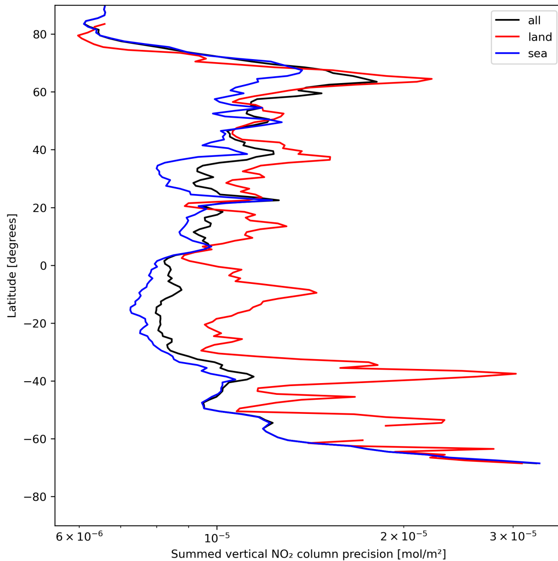
Figure 24: Zonal average of “Summed vertical NO 2 column precision” for 2024-07-24 to 2024-07-26.
