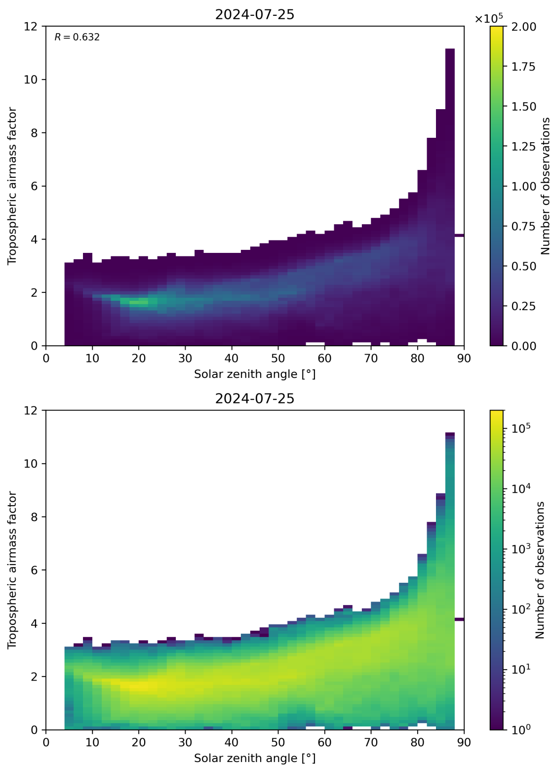
Figure 147: Scatter density plot of “Solar zenith angle” against “Tropospheric airmass factor” for 2024-07-24 to 2024-07-26.
