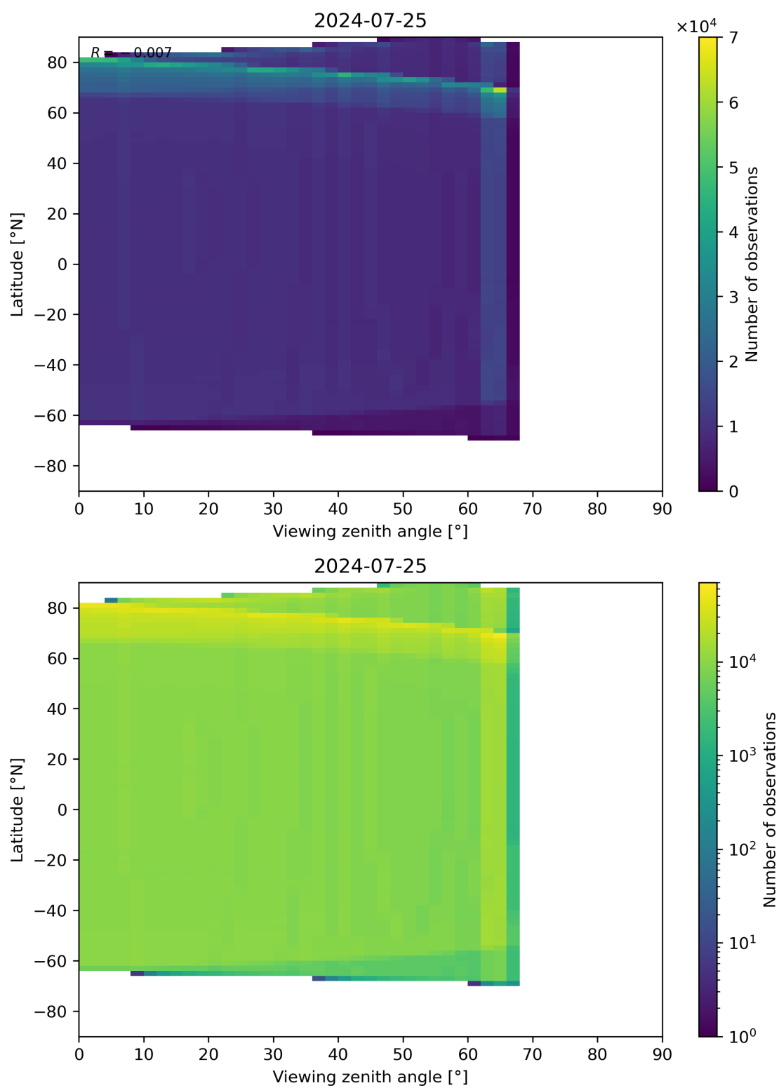
Figure 163: Scatter density plot of “Viewing zenith angle” against “Latitude” for 2024-07-24 to 2024-07-26.
