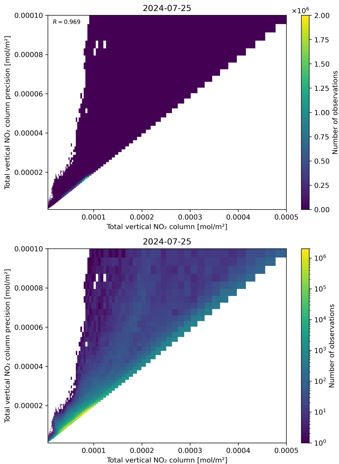
Figure 114: Scatter density plot of “Total vertical NO 2 column” against “Total vertical NO 2 column precision” for 2024-07-24 to 2024-07-26.
