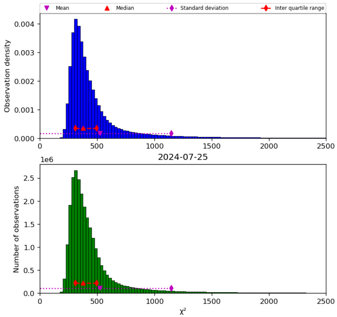
Figure 42: Histogram of “ \chi^2 ” for 2024-07-24 to 2024-07-26
