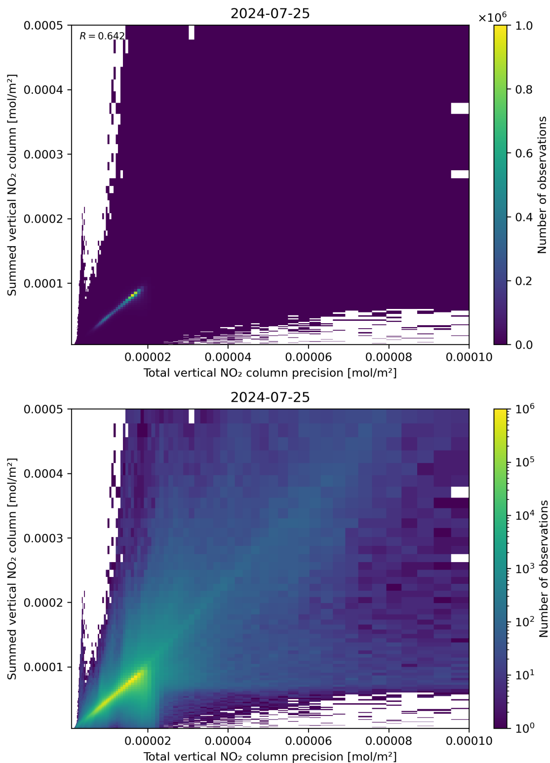
Figure 117: Scatter density plot of “Total vertical NO 2 column precision” against “Summed vertical NO 2 column” for 2024-07-24 to 2024-07-26.
