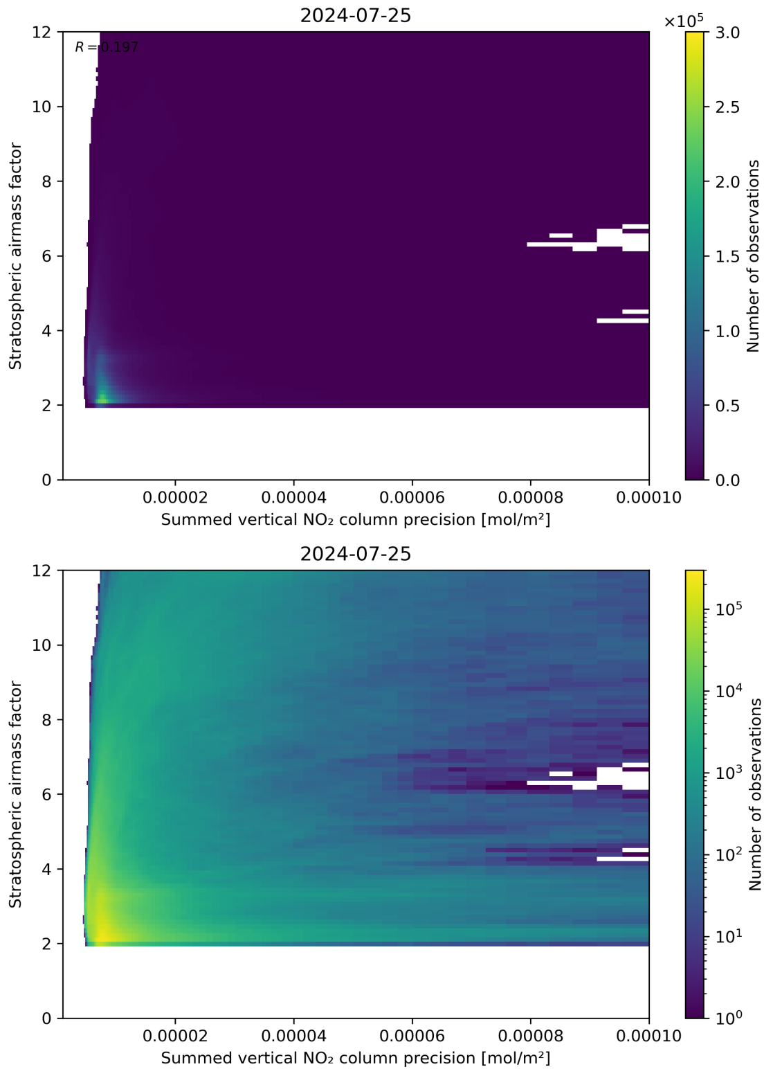
Figure 106: Scatter density plot of “Summed vertical NO 2 column precision” against “Stratospheric airmass factor” for 2024-07-24 to 2024-07-26.
