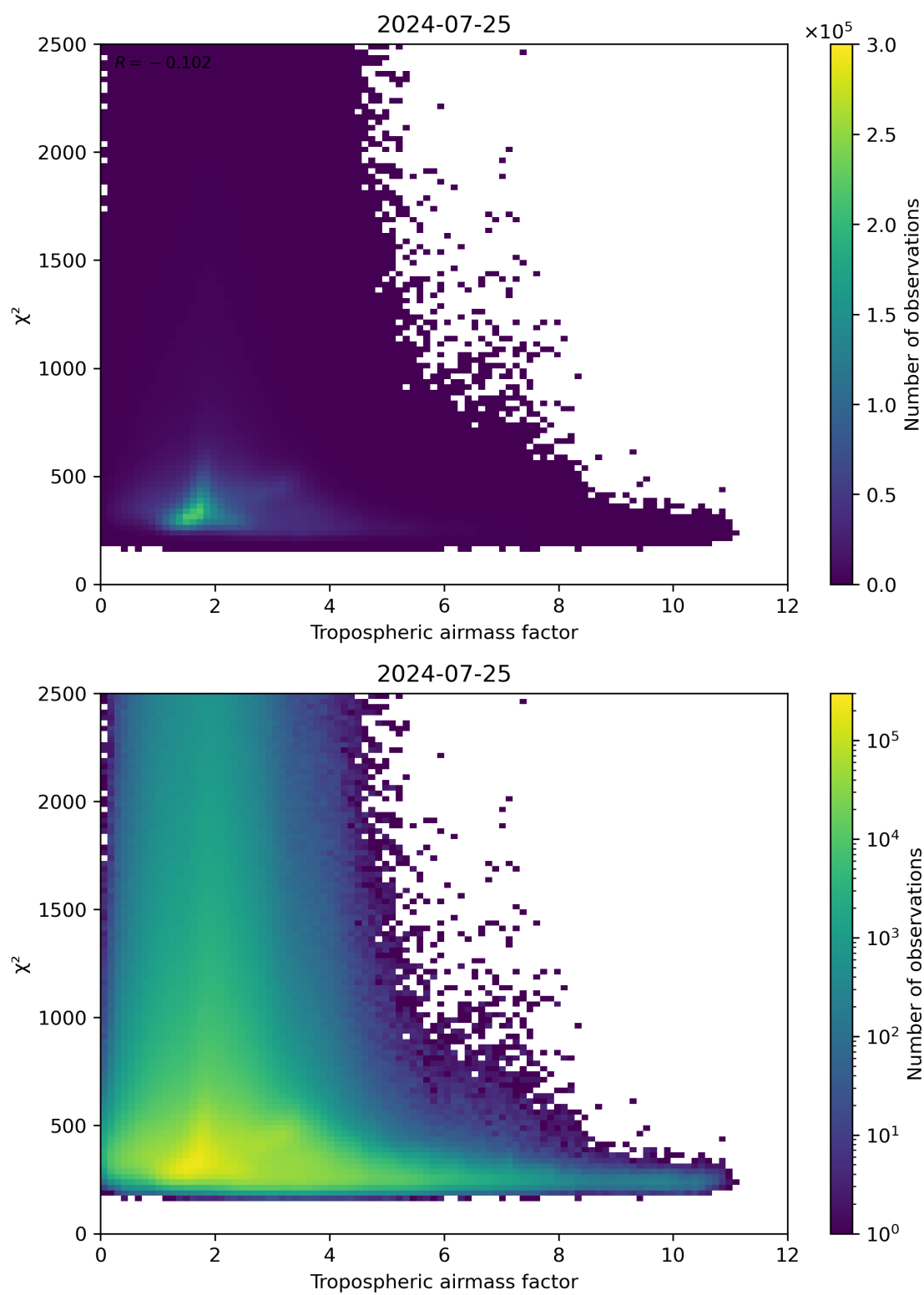
Figure 73: Scatter density plot of “Tropospheric airmass factor” against “ \chi^2 ” for 2024-07-24 to 2024-07-26.
