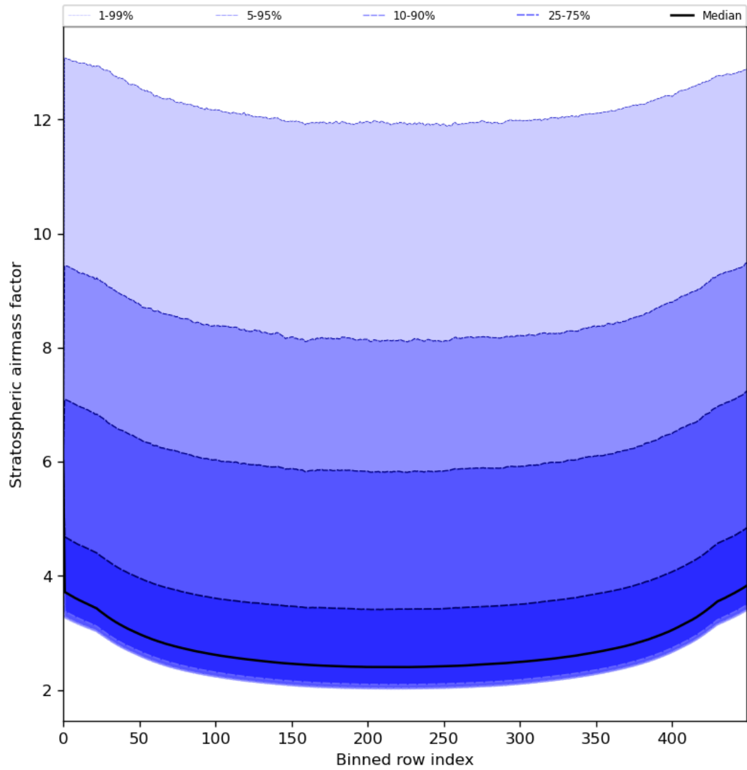
Figure 61: Along track statistics of “Stratospheric airmass factor” for 2024-07-24 to 2024-07-26
