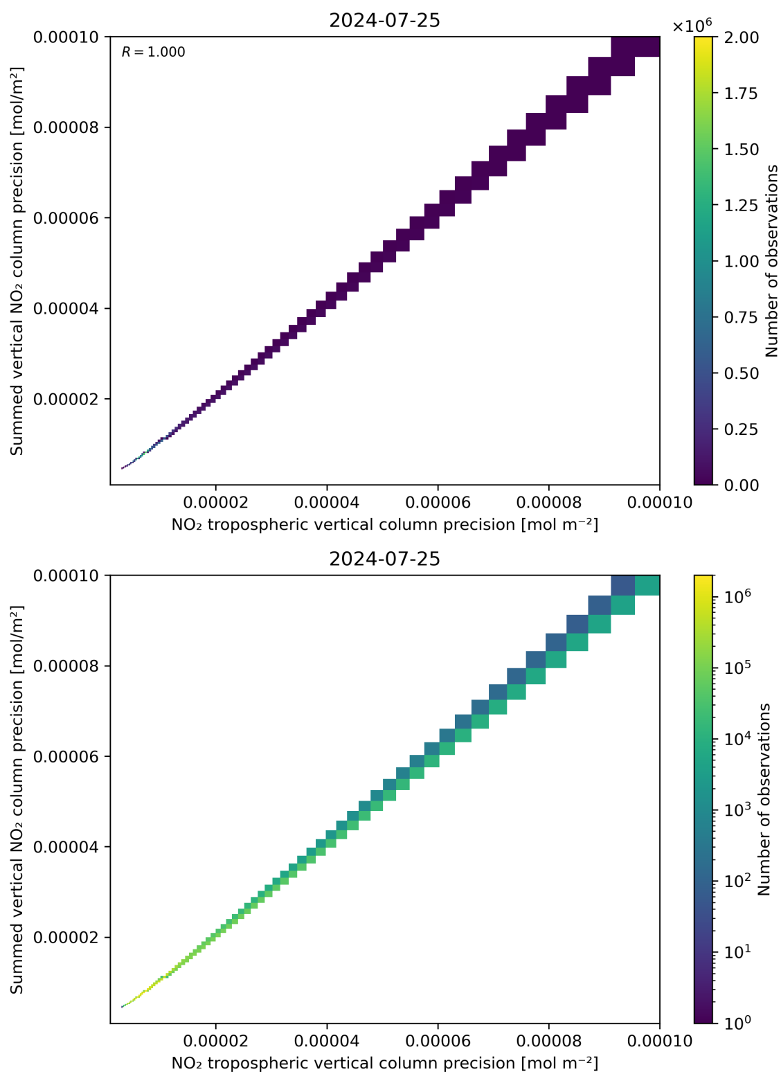
Figure 137: Scatter density plot of “NO 2 tropospheric vertical column precision” against “Summed vertical NO 2 column precision” for 2024-07-24 to 2024-07-26.
