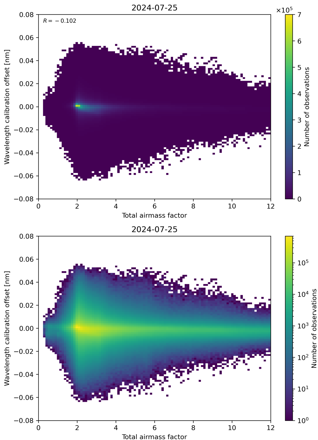
Figure 70: Scatter density plot of “Total airmass factor” against “Wavelength calibration offset” for 2024-07-24 to 2024-07-26.
