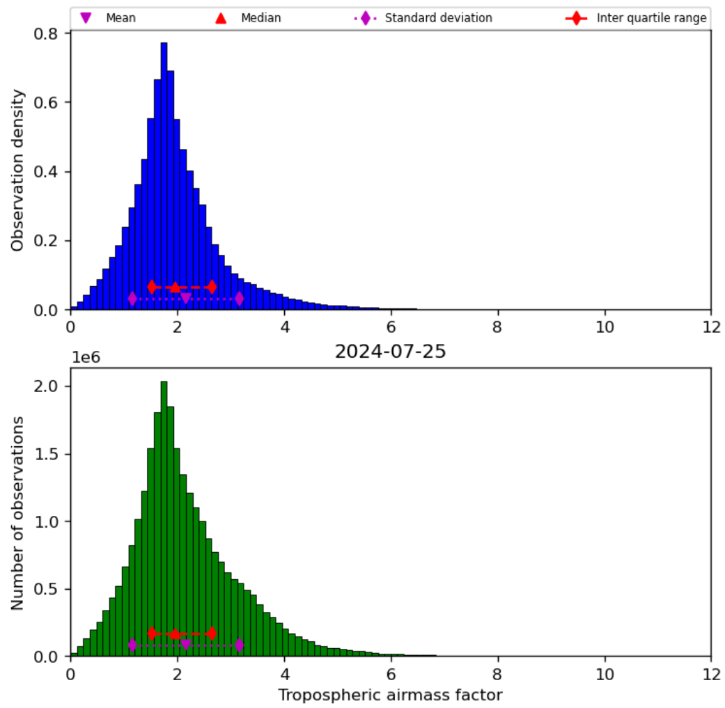
Figure 31: Histogram of “Tropospheric airmass factor” for 2024-07-24 to 2024-07-26
