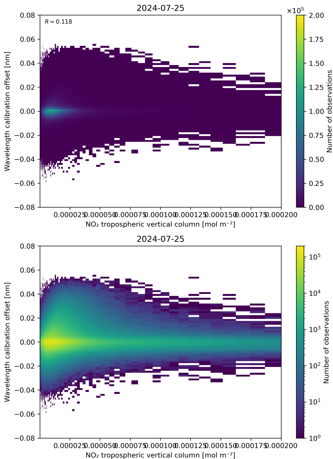
Figure 143: Scatter density plot of “NO 2 tropospheric vertical column” against “Wavelength calibration offset” for 2024-07-24 to 2024-07-26.
