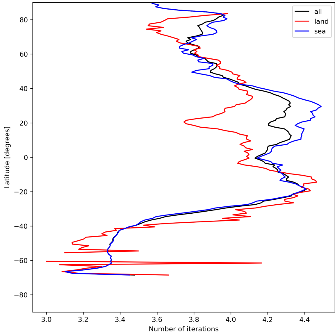
Figure 17: Zonal average of “Number of iterations” for 2024-07-24 to 2024-07-26.
