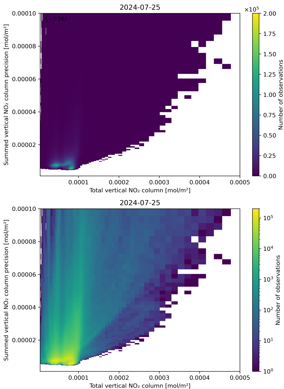
Figure 113: Scatter density plot of “Total vertical NO 2 column” against “Summed vertical NO 2 column precision” for 2024-07-24 to 2024-07-26.
