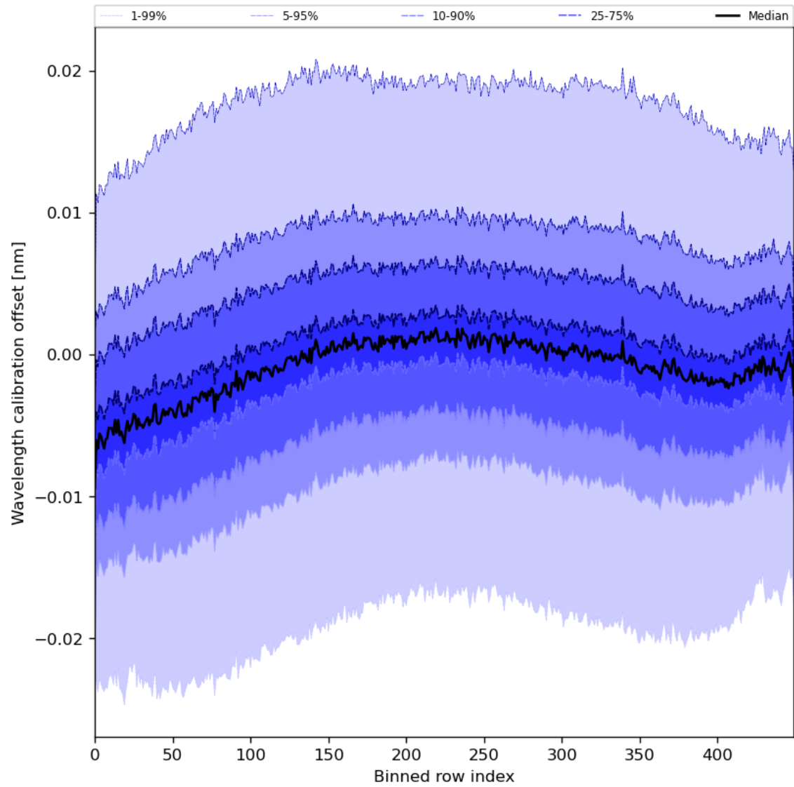
Figure 52: Along track statistics of “Wavelength calibration offset” for 2024-07-24 to 2024-07-26
