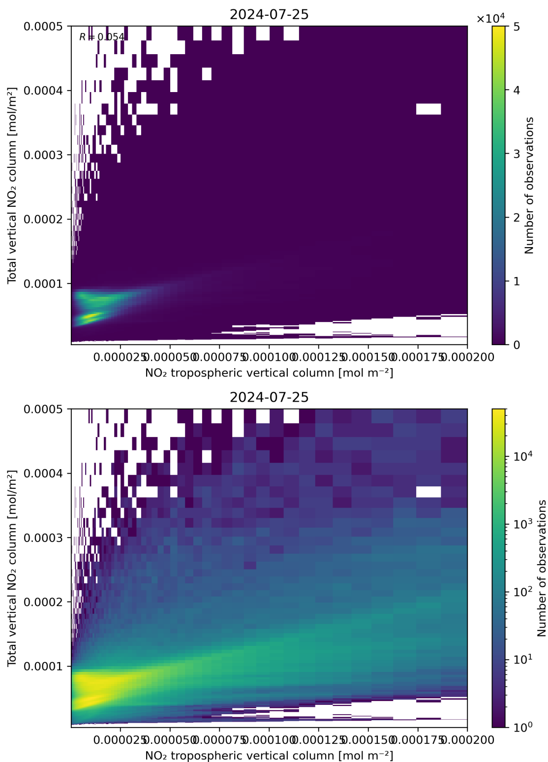
Figure 128: Scatter density plot of “NO 2 tropospheric vertical column” against “Total vertical NO 2 column” for 2024-07-24 to 2024-07-26.
