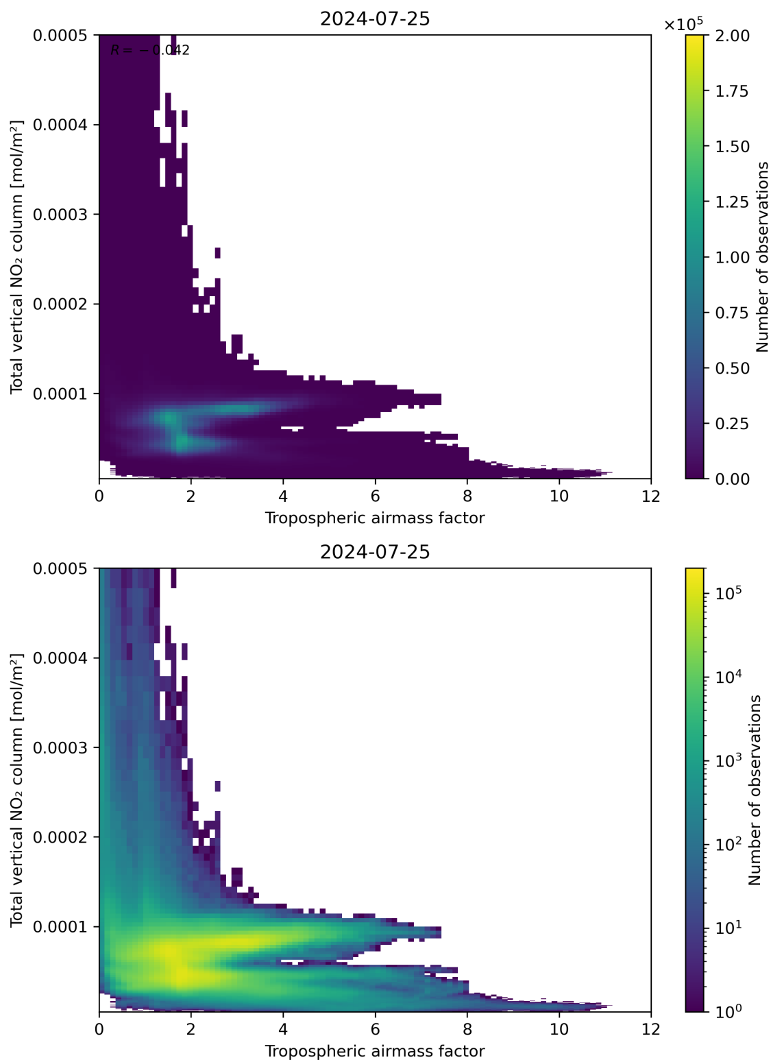
Figure 77: Scatter density plot of “Tropospheric airmass factor” against “Total vertical NO 2 column” for 2024-07-24 to 2024-07-26.
