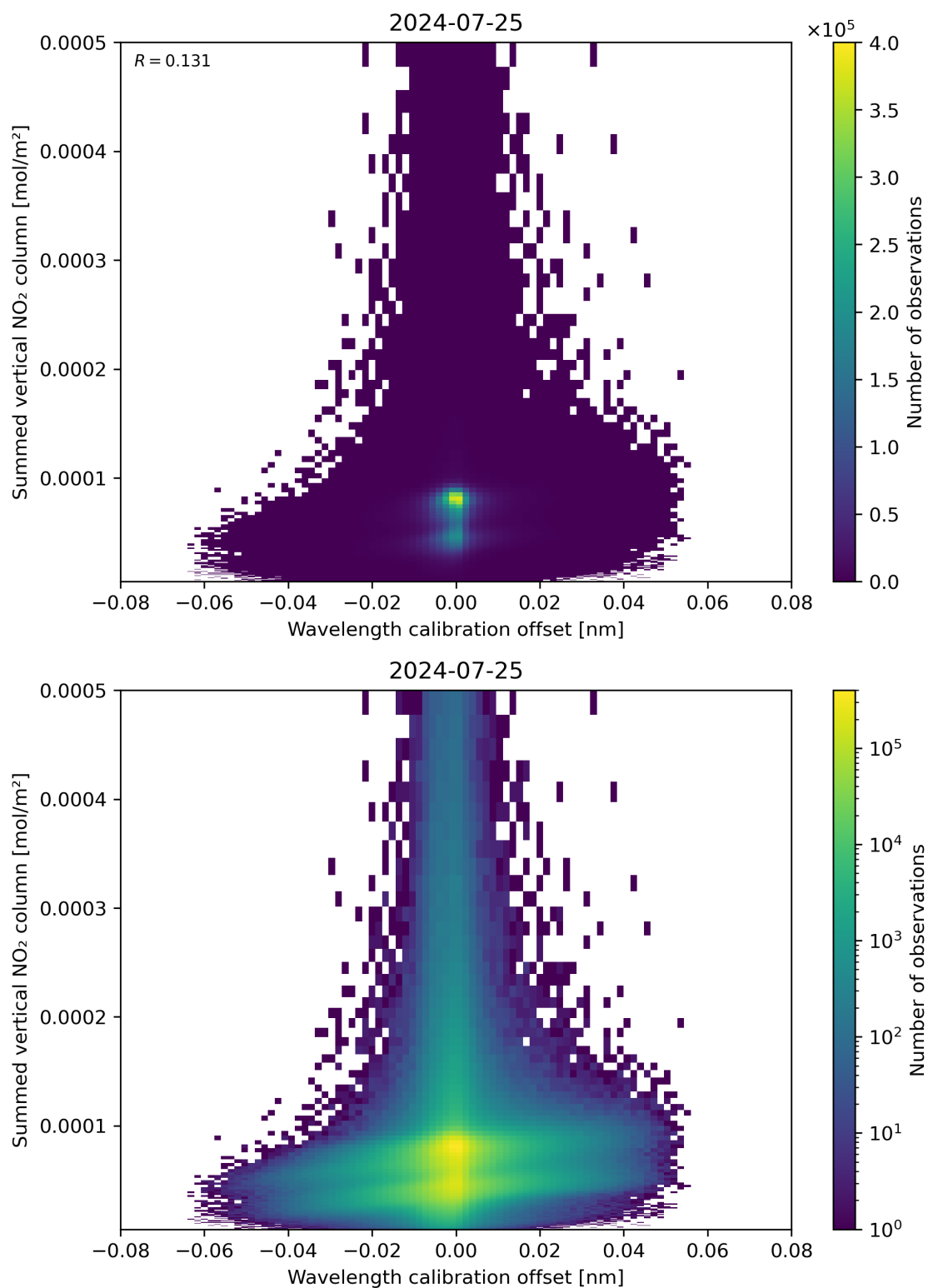
Figure 177: Scatter density plot of “Wavelength calibration offset” against “Summed vertical NO 2 column” for 2024-07-24 to 2024-07-26.
