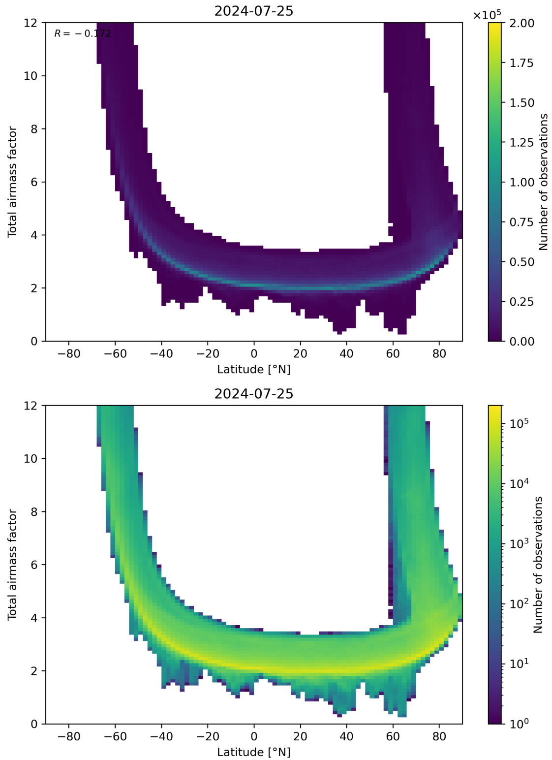
Figure 84: Scatter density plot of “Latitude” against “Total airmass factor” for 2024-07-24 to 2024-07-26.
