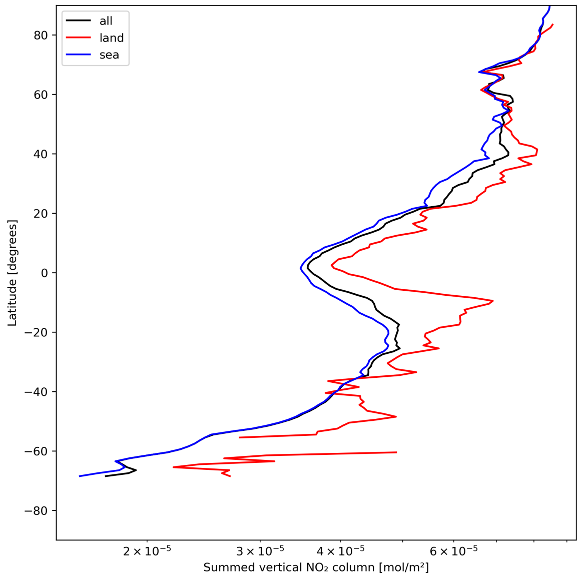
Figure 23: Zonal average of “Summed vertical NO 2 column” for 2024-07-24 to 2024-07-26.
