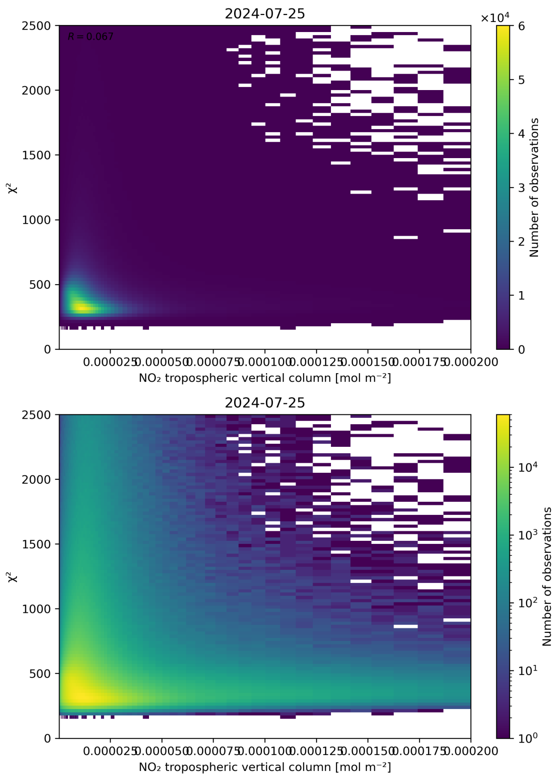
Figure 124: Scatter density plot of “NO 2 tropospheric vertical column” against “ \chi^2 ” for 2024-07-24 to 2024-07-26.
