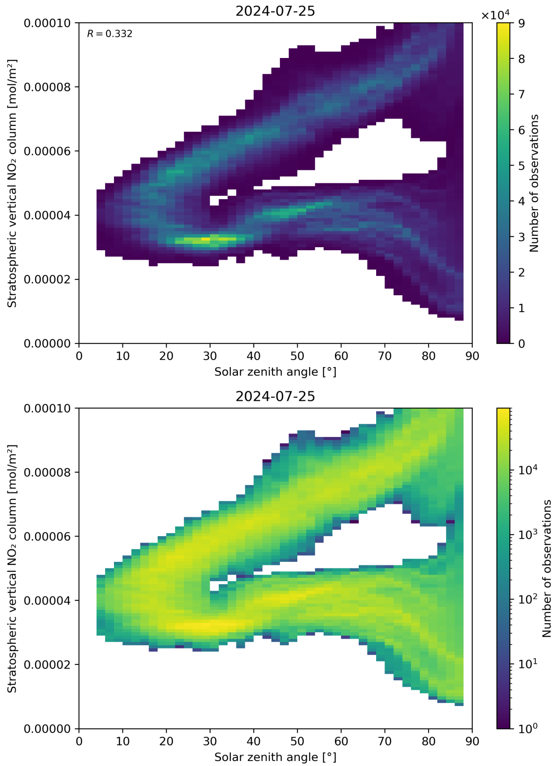
Figure 150: Scatter density plot of “Solar zenith angle” against “Stratospheric vertical NO 2 column” for 2024-07-24 to 2024-07-26.
