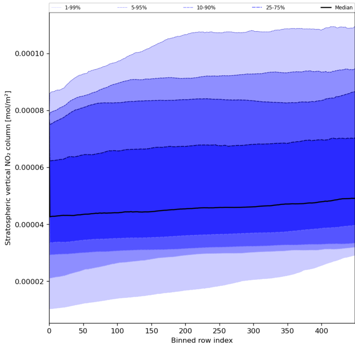
Figure 53: Along track statistics of “Stratospheric vertical NO 2 column” for 2024-07-24 to 2024-07-26
