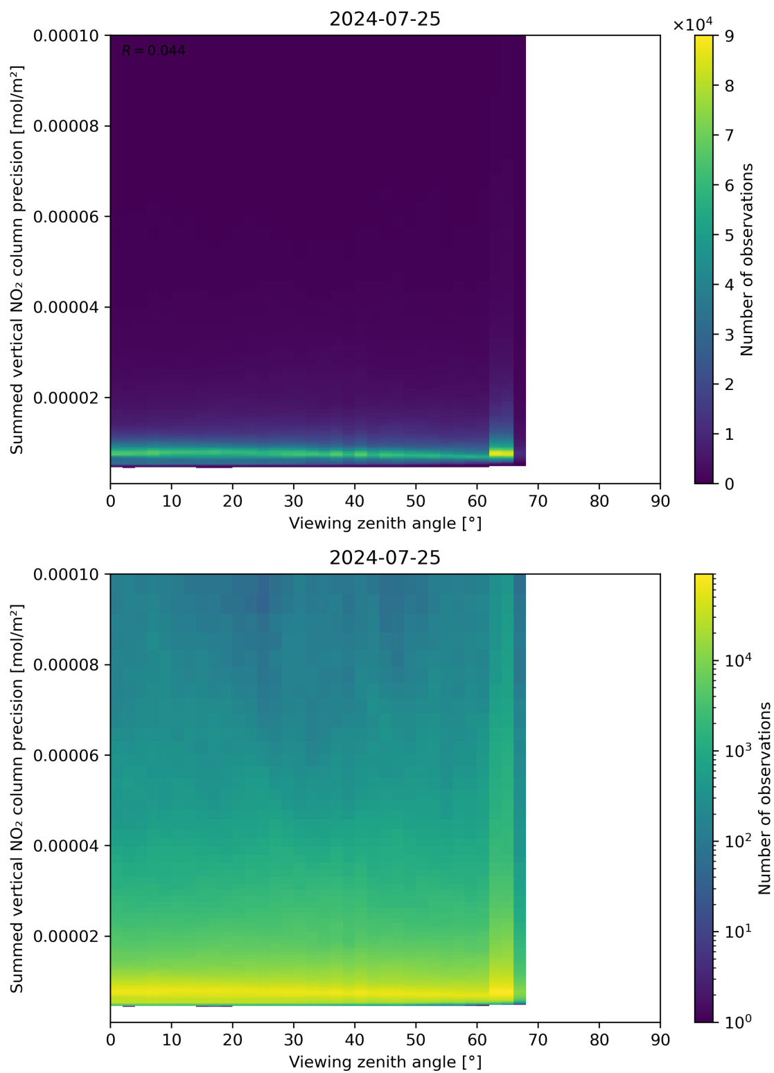
Figure 166: Scatter density plot of “Viewing zenith angle” against “Summed vertical NO 2 column precision” for 2024-07-24 to 2024-07-26.
