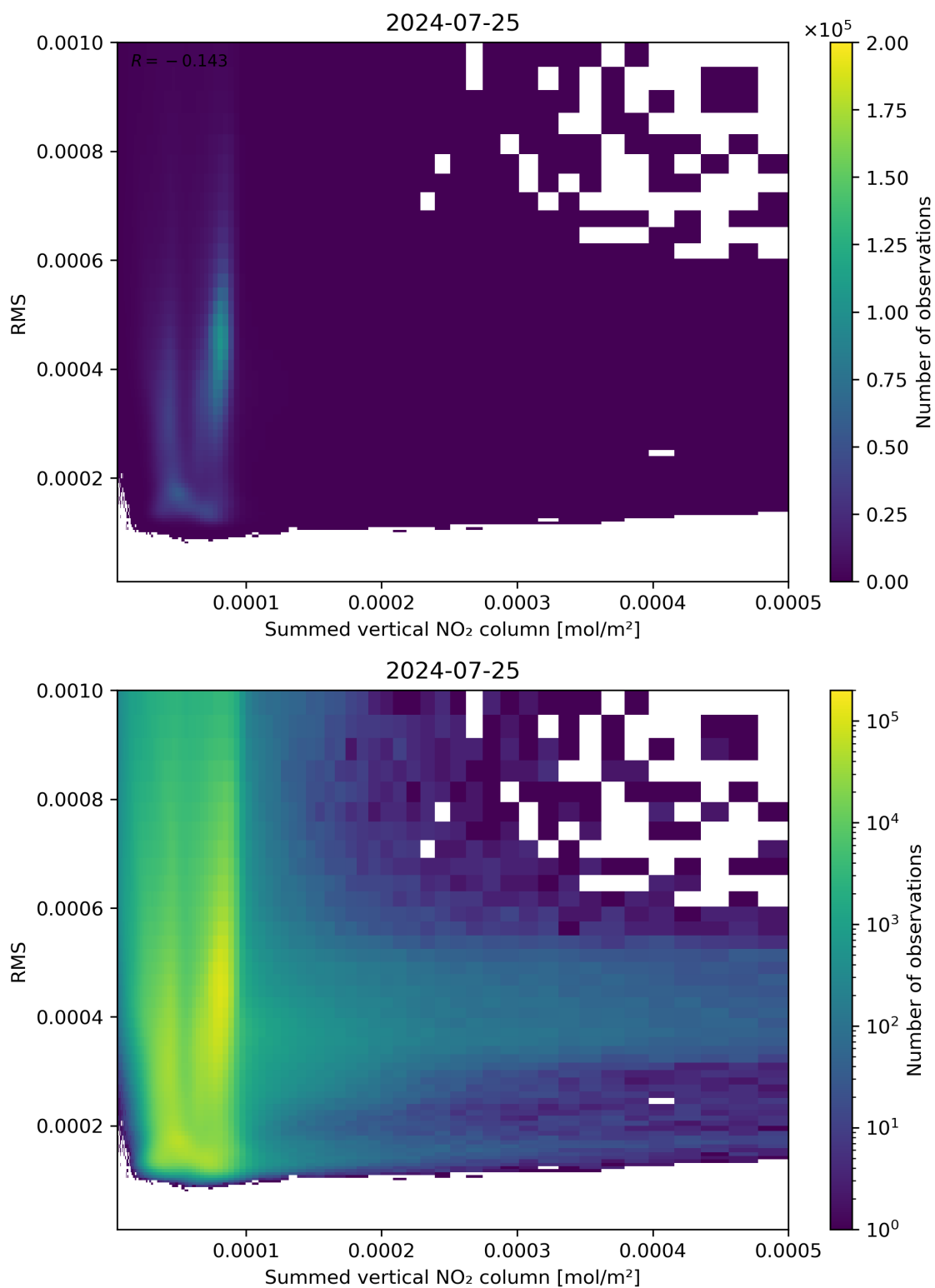
Figure 109: Scatter density plot of “Summed vertical NO 2 column” against “RMS” for 2024-07-24 to 2024-07-26.
