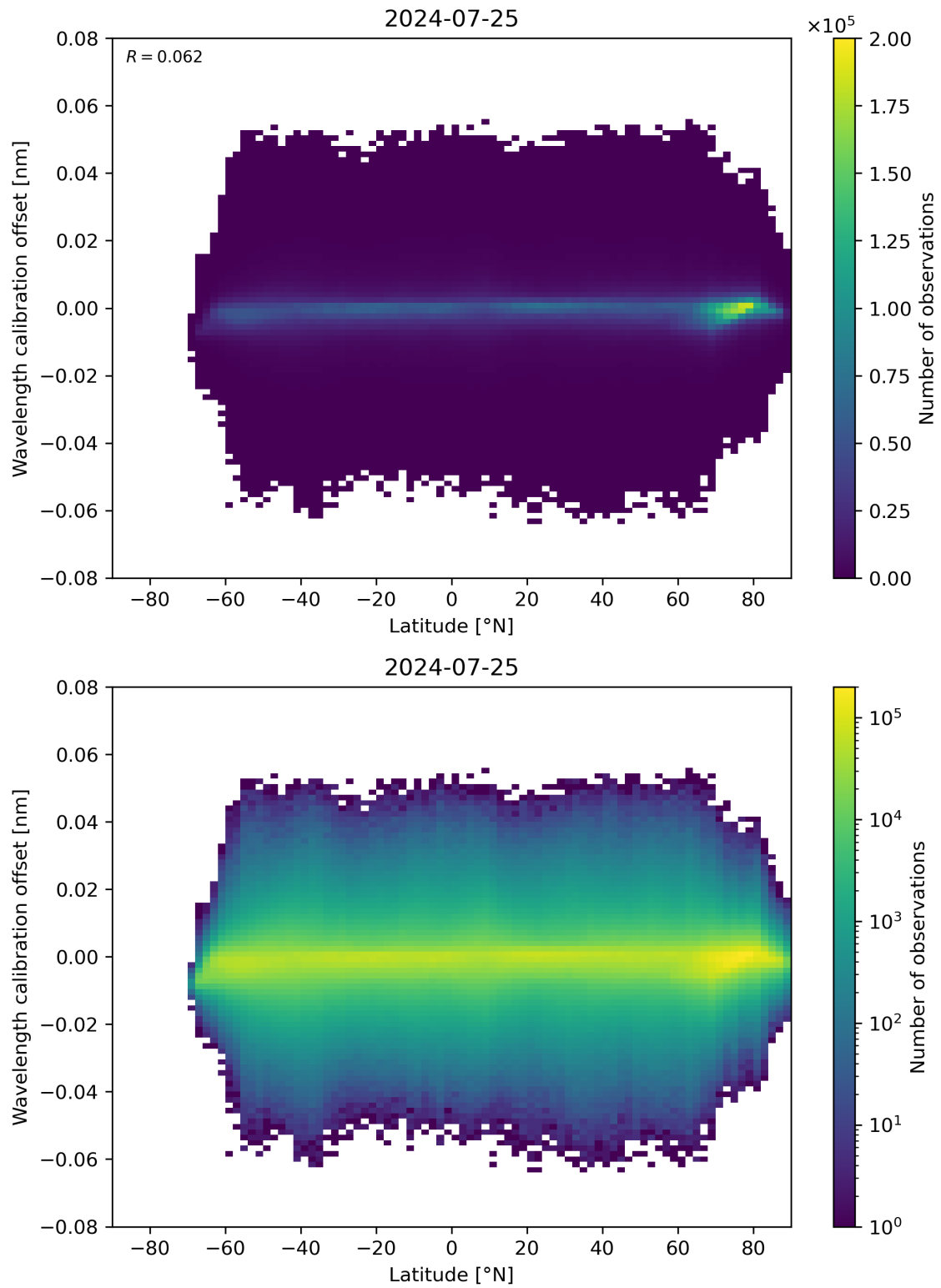
Figure 95: Scatter density plot of “Latitude” against “Wavelength calibration offset” for 2024-07-24 to 2024-07-26.
