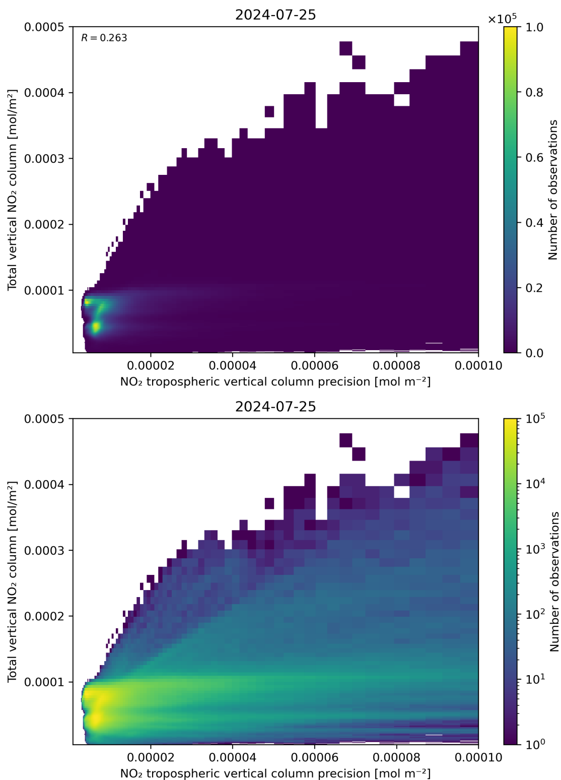
Figure 138: Scatter density plot of “NO 2 tropospheric vertical column precision” against “Total vertical NO 2 column” for 2024-07-24 to 2024-07-26.
