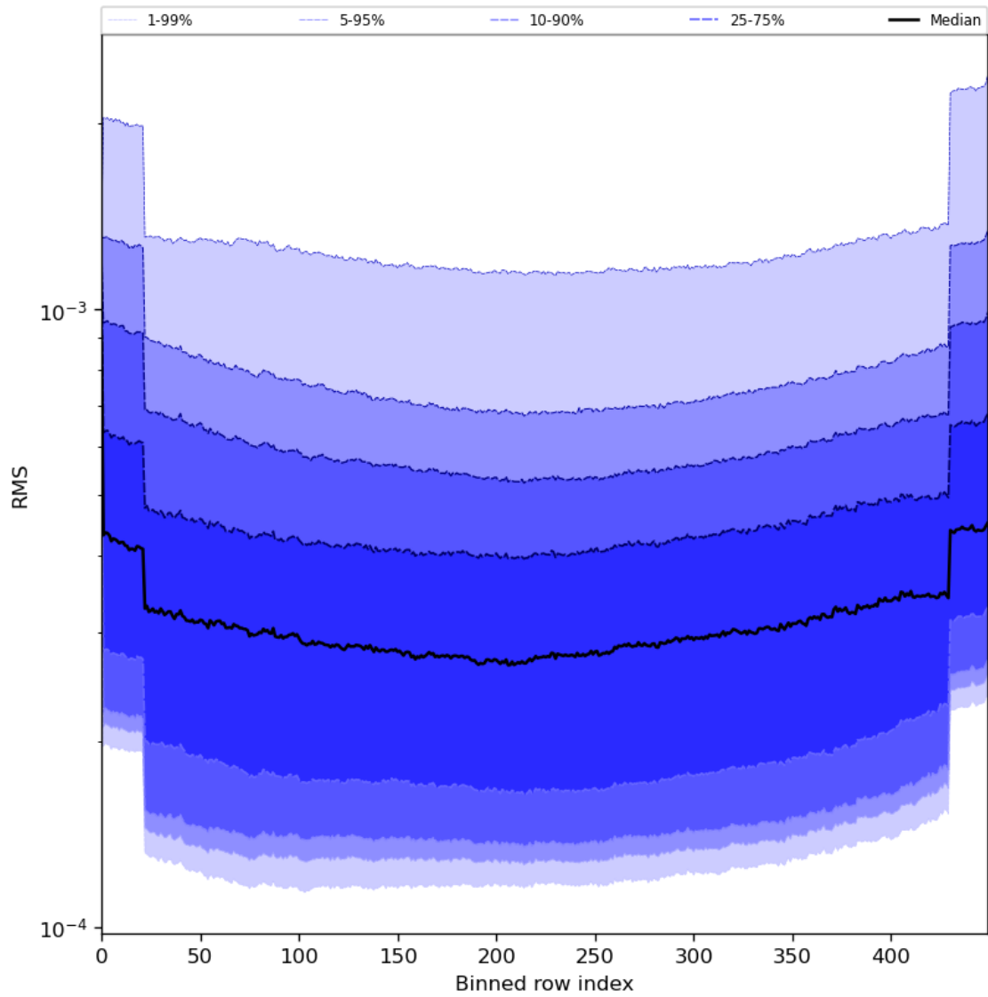
Figure 60: Along track statistics of “RMS” for 2024-07-24 to 2024-07-26
