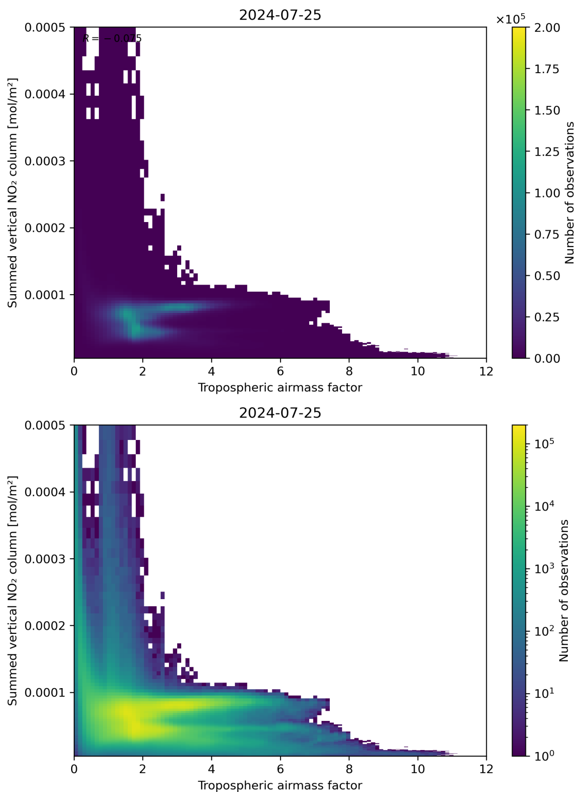
Figure 75: Scatter density plot of “Tropospheric air mass factor” against “Summed vertical NO 2 column” for 2024-07-24 to 2024-07-26.
