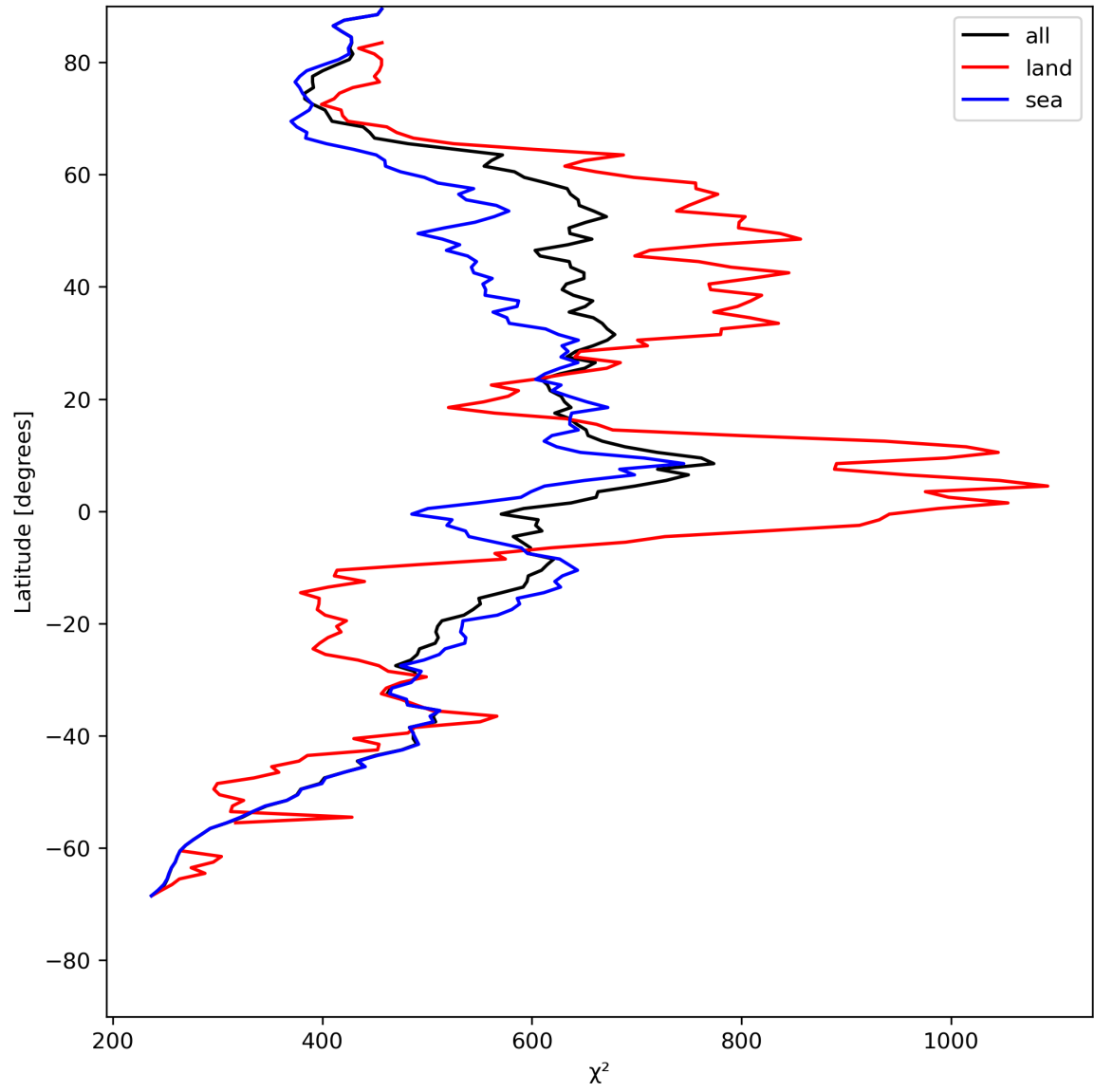
Figure 25: Zonal average of “ \chi^2 ” for 2024-07-24 to 2024-07-26.
