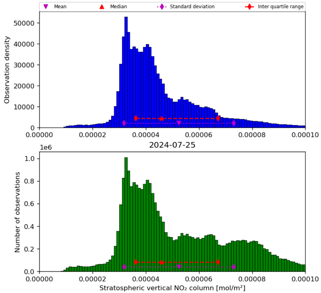
Figure 36: Histogram of “Stratospheric vertical NO 2 column” for 2024-07-24 to 2024-07-26
