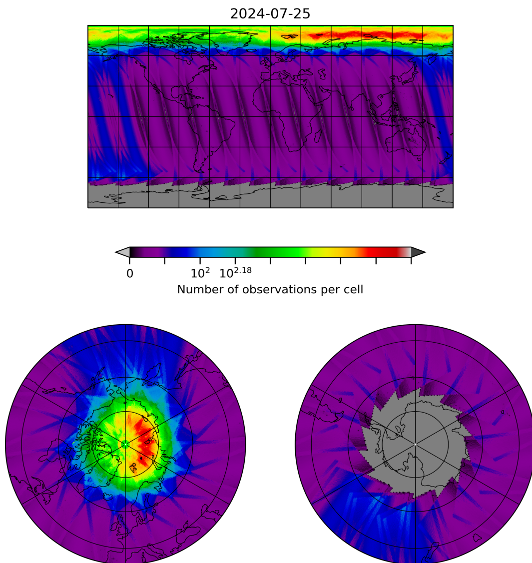
Figure 10: Map of the number of observations for 2024-07-24 to 2024-07-26
