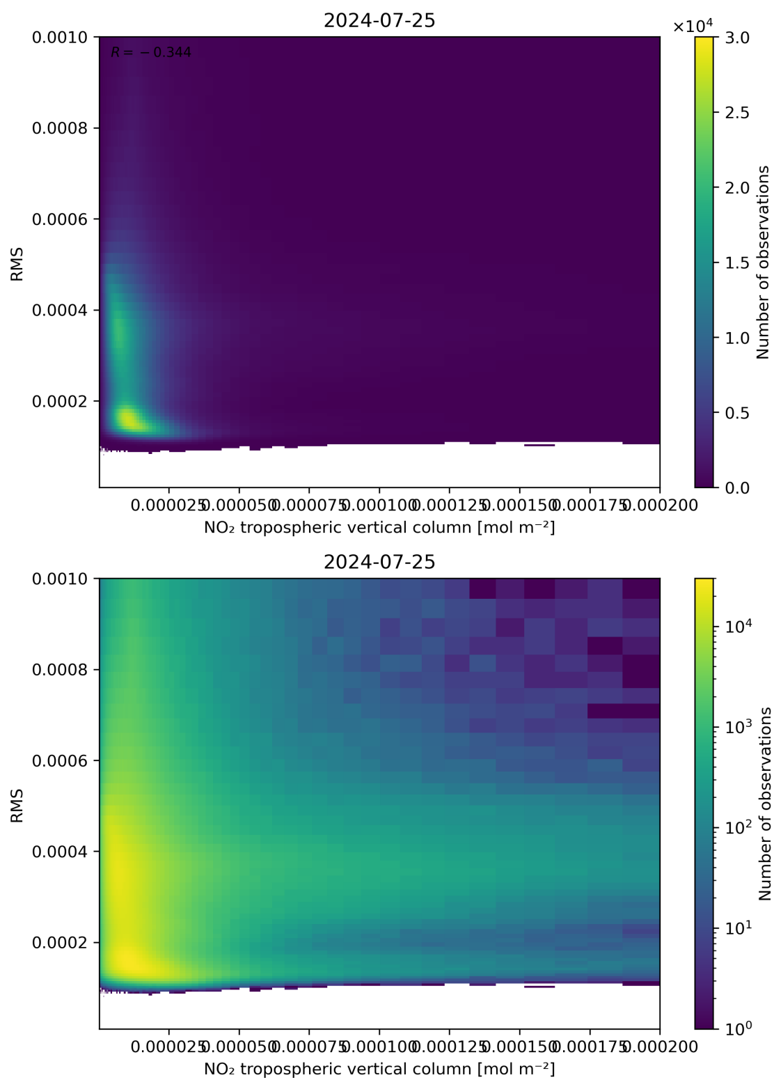
Figure 142: Scatter density plot of “NO 2 tropospheric vertical column” against “RMS” for 2024-07-24 to 2024-07-26.
