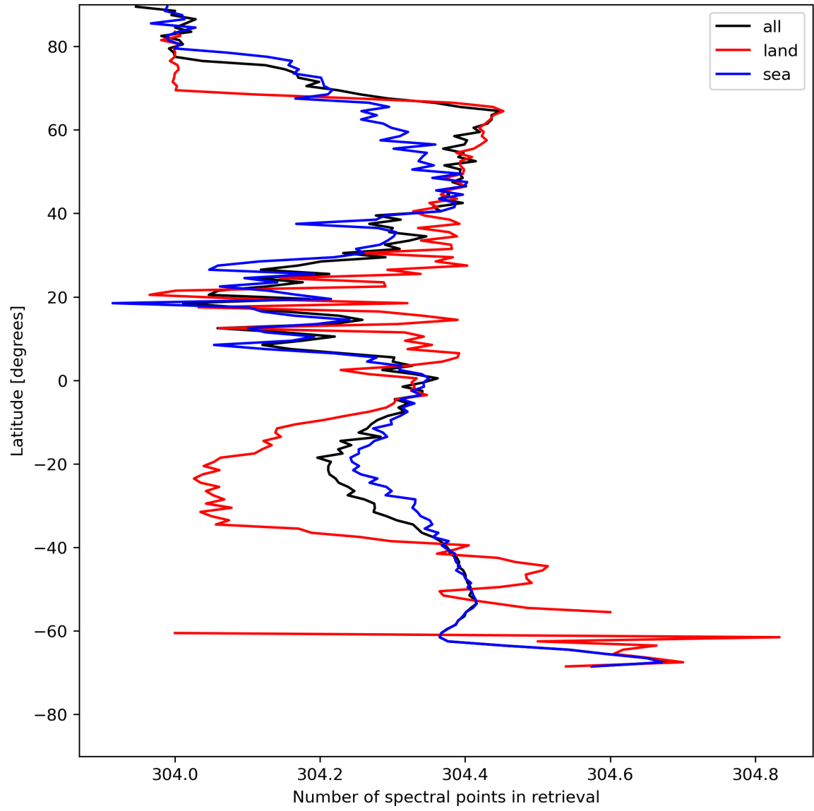
Figure 16: Zonal average of “Number of spectral points in retrieval” for 2024-07-24 to 2024-07-26.
