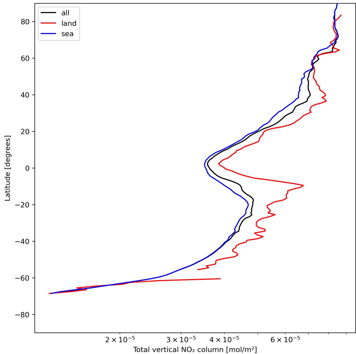
Figure 21: Zonal average of “Total vertical NO 2 column” for 2024-07-24 to 2024-07-26.
