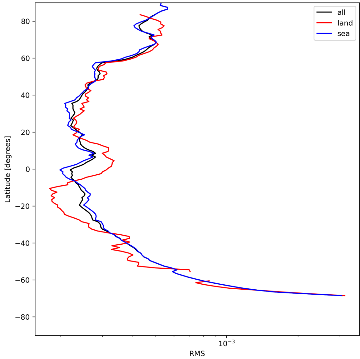
Figure 26: Zonal average of “RMS” for 2024-07-24 to 2024-07-26.
