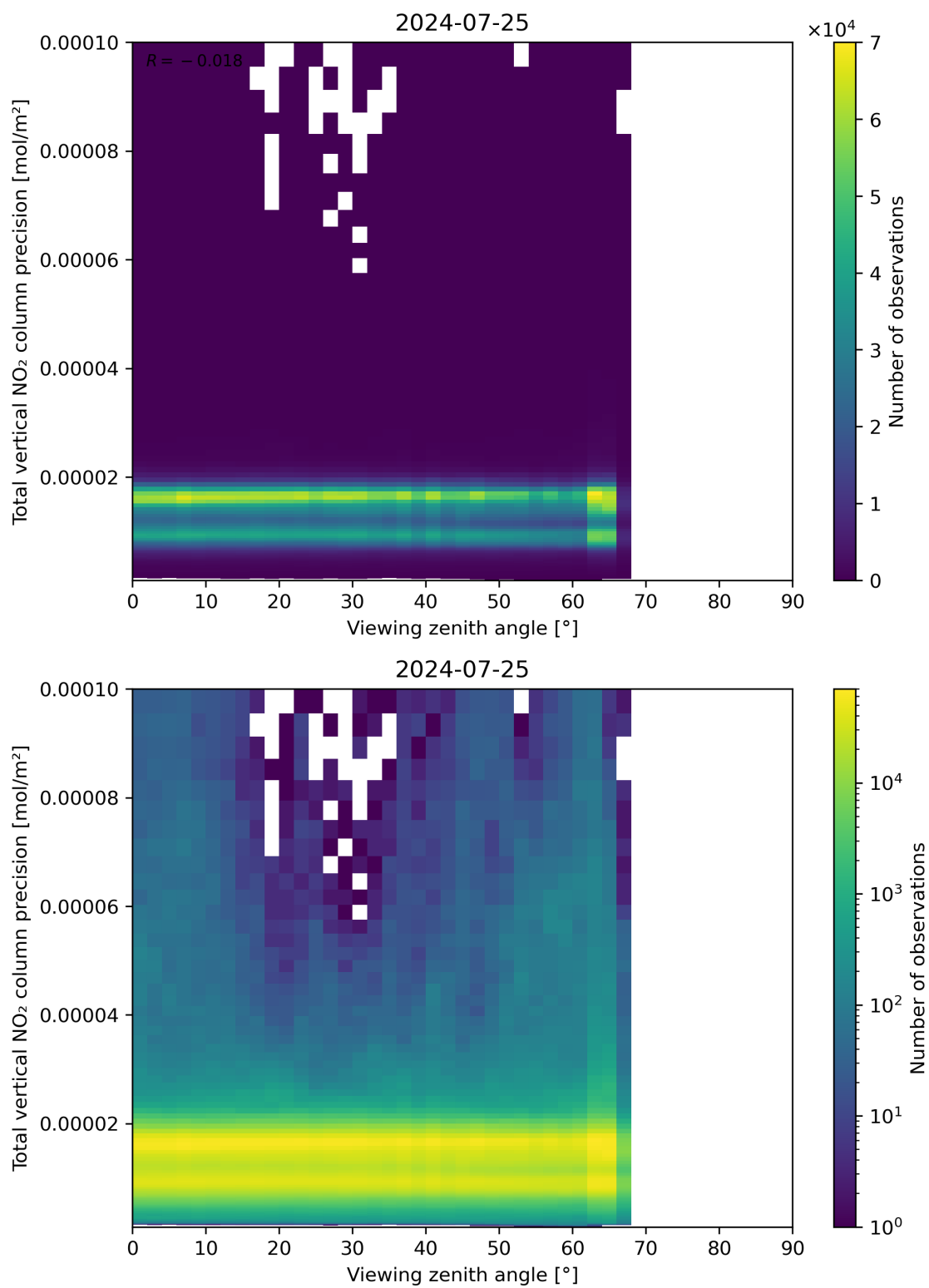
Figure 168: Scatter density plot of “Viewing zenith angle” against “Total vertical NO 2 column precision” for 2024-07-24 to 2024-07-26.
