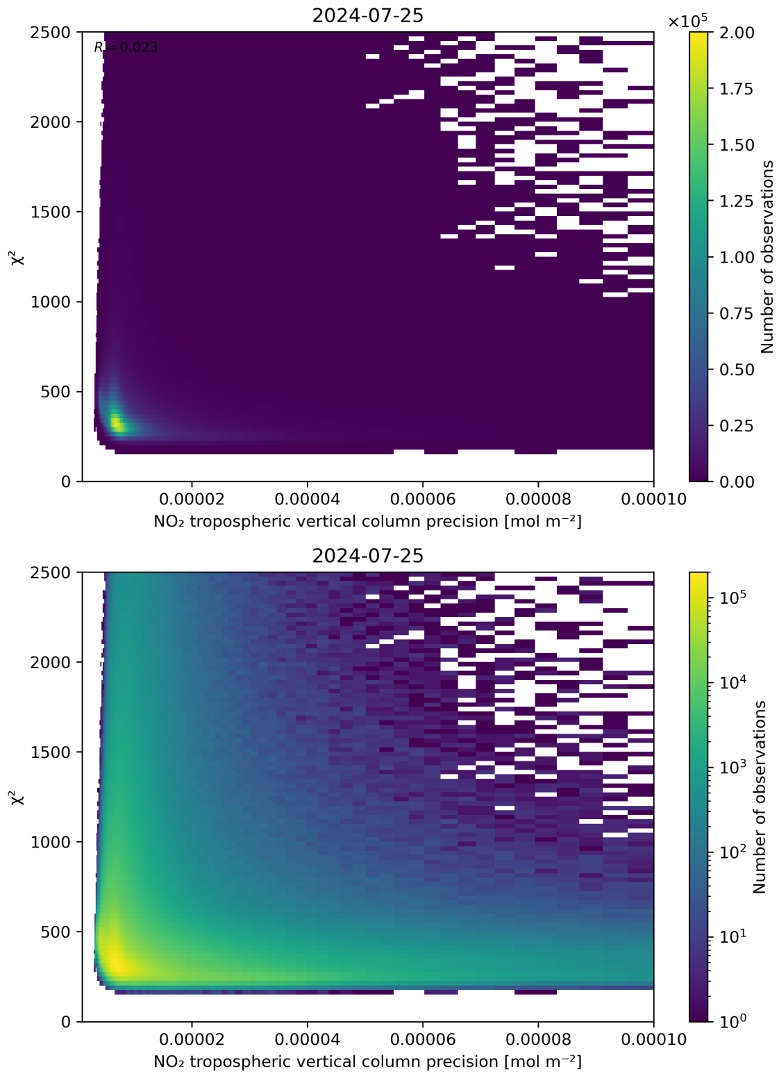
Figure 134: Scatter density plot of “NO 2 tropospheric vertical column precision” against “ \chi^2 ” for 2024-07-24 to 2024-07-26.
