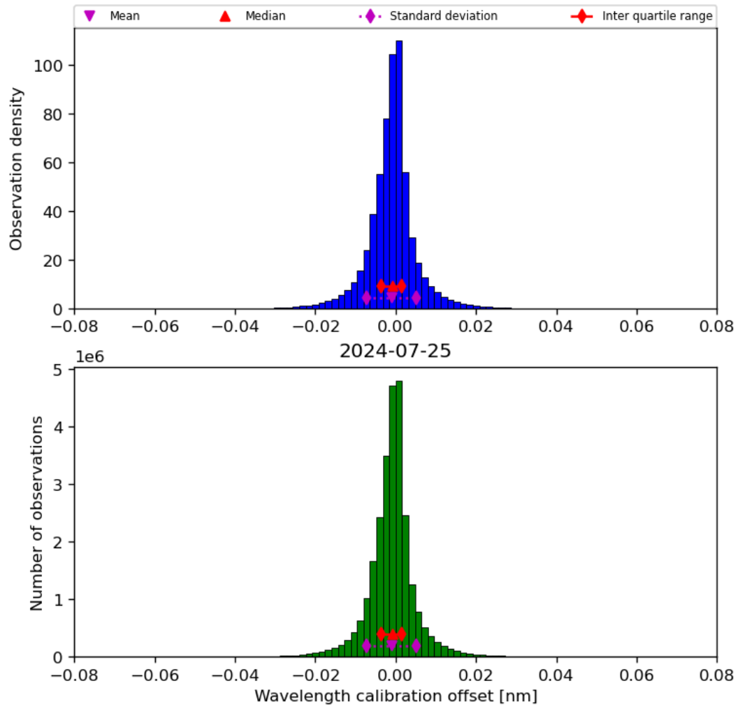
Figure 35: Histogram of “Wavelength calibration offset” for 2024-07-24 to 2024-07-26
