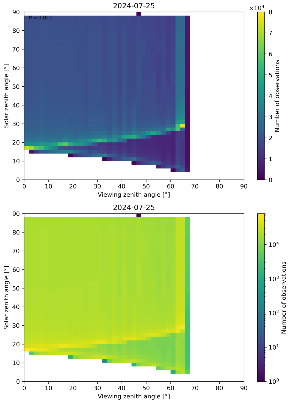
Figure 172: Scatter density plot of “Viewing zenith angle” against “Solar zenith angle” for 2024-07-24 to 2024-07-26.
