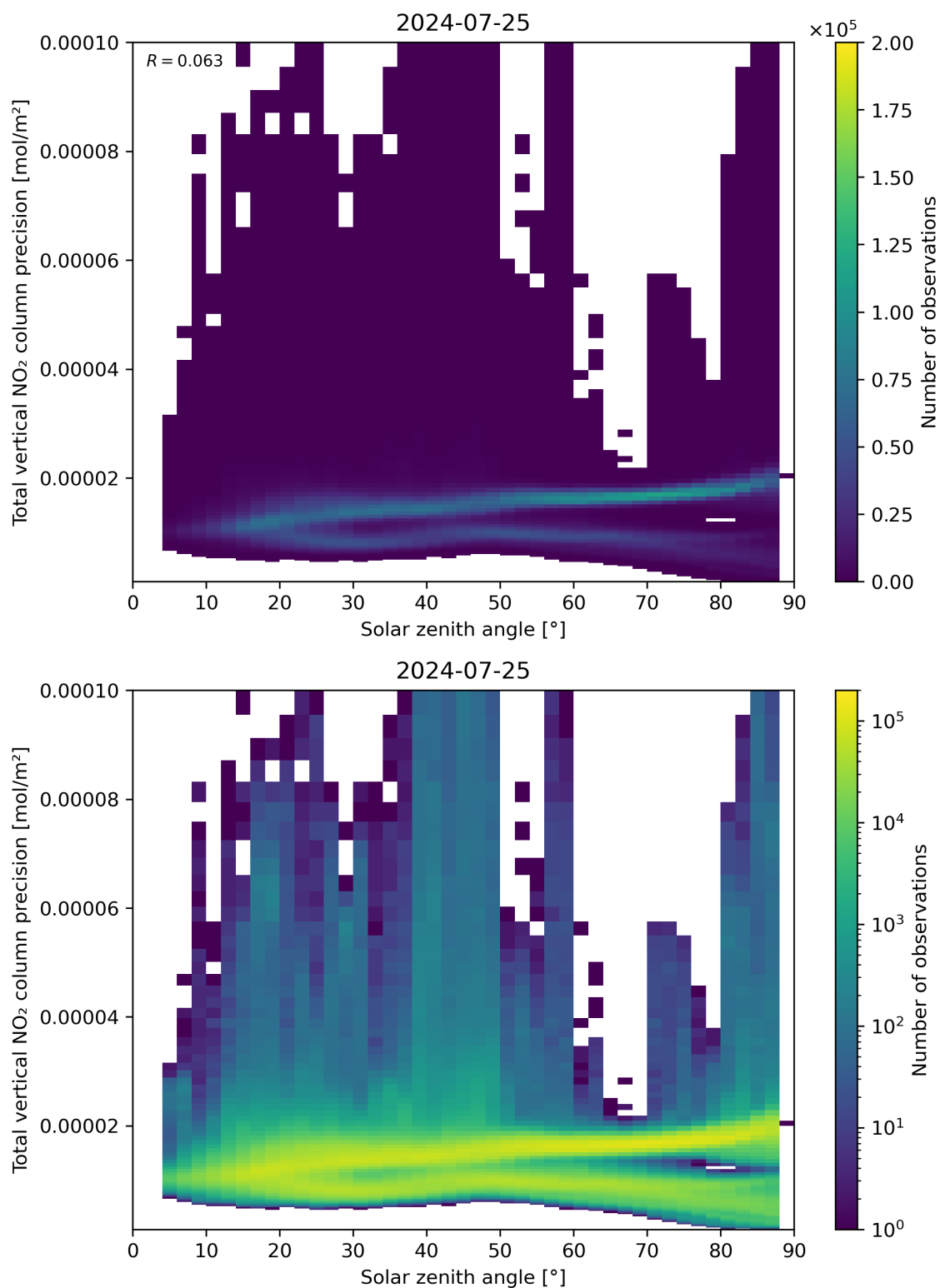
Figure 154: Scatter density plot of “Solar zenith angle” against “Total vertical NO 2 column precision” for 2024-07-24 to 2024-07-26.
