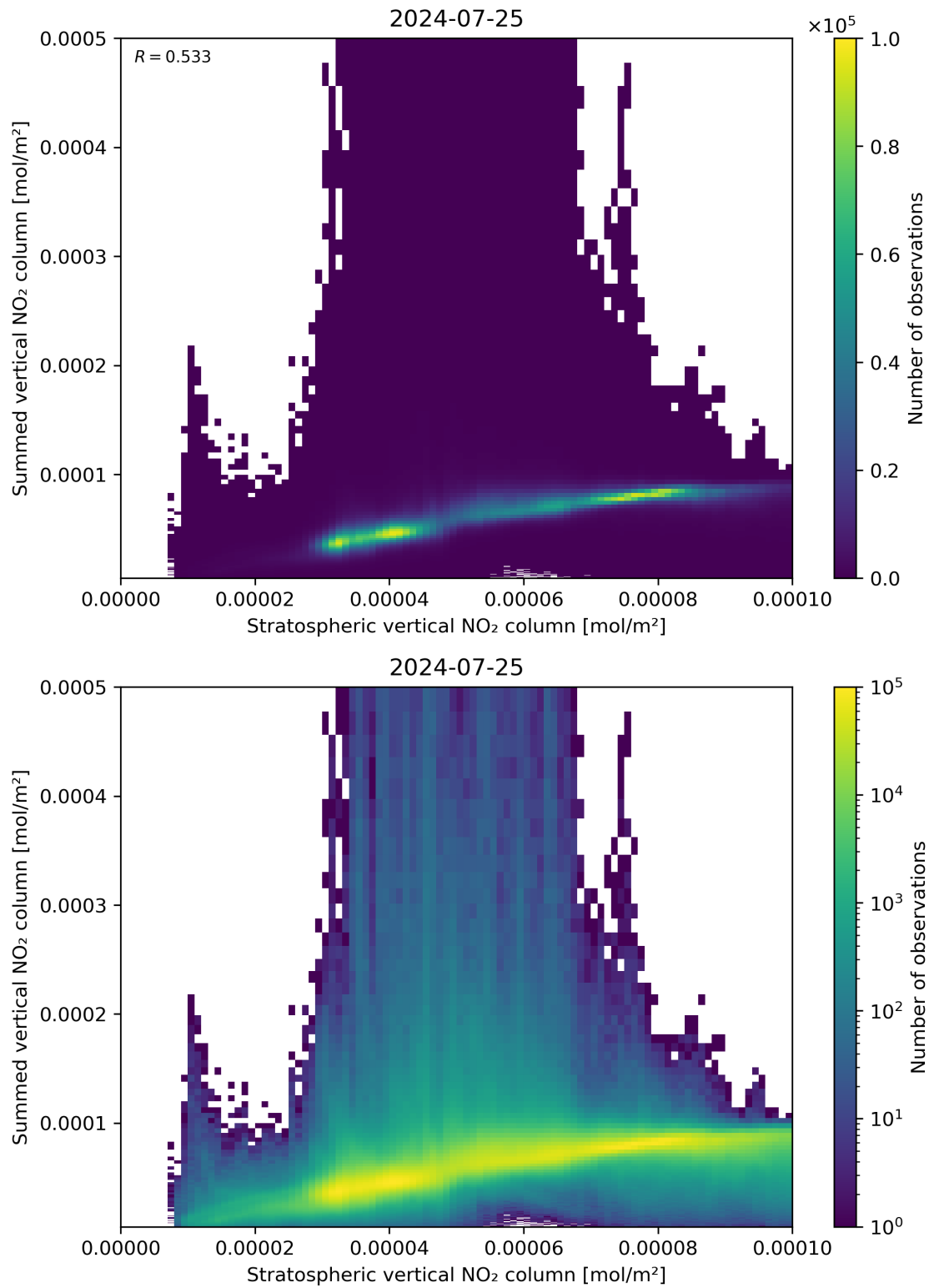
Figure 98: Scatter density plot of “Stratospheric vertical NO 2 column” against “Summed vertical NO 2 column” for 2024-07-24 to 2024-07-26.
