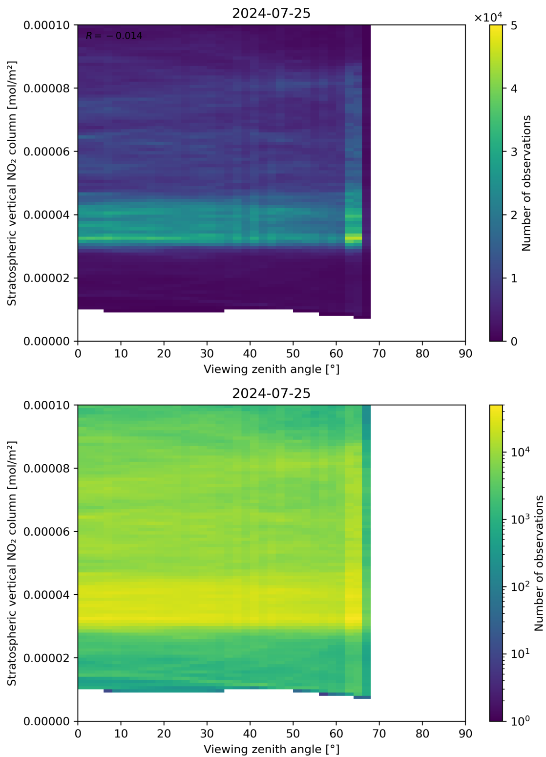
Figure 164: Scatter density plot of “Viewing zenith angle” against “Stratospheric vertical NO 2 column” for 2024-07-24 to 2024-07-26.
