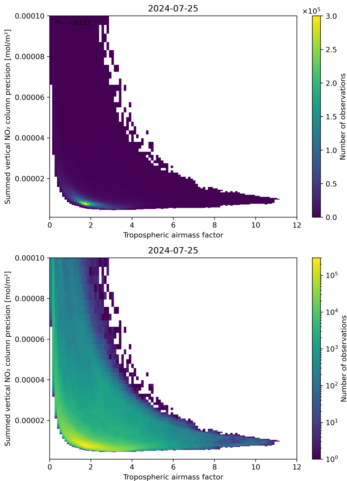
Figure 76: Scatter density plot of “Tropospheric air mass factor” against “Summed vertical NO 2 column precision” for 2024-07-24 to 2024-07-26.
