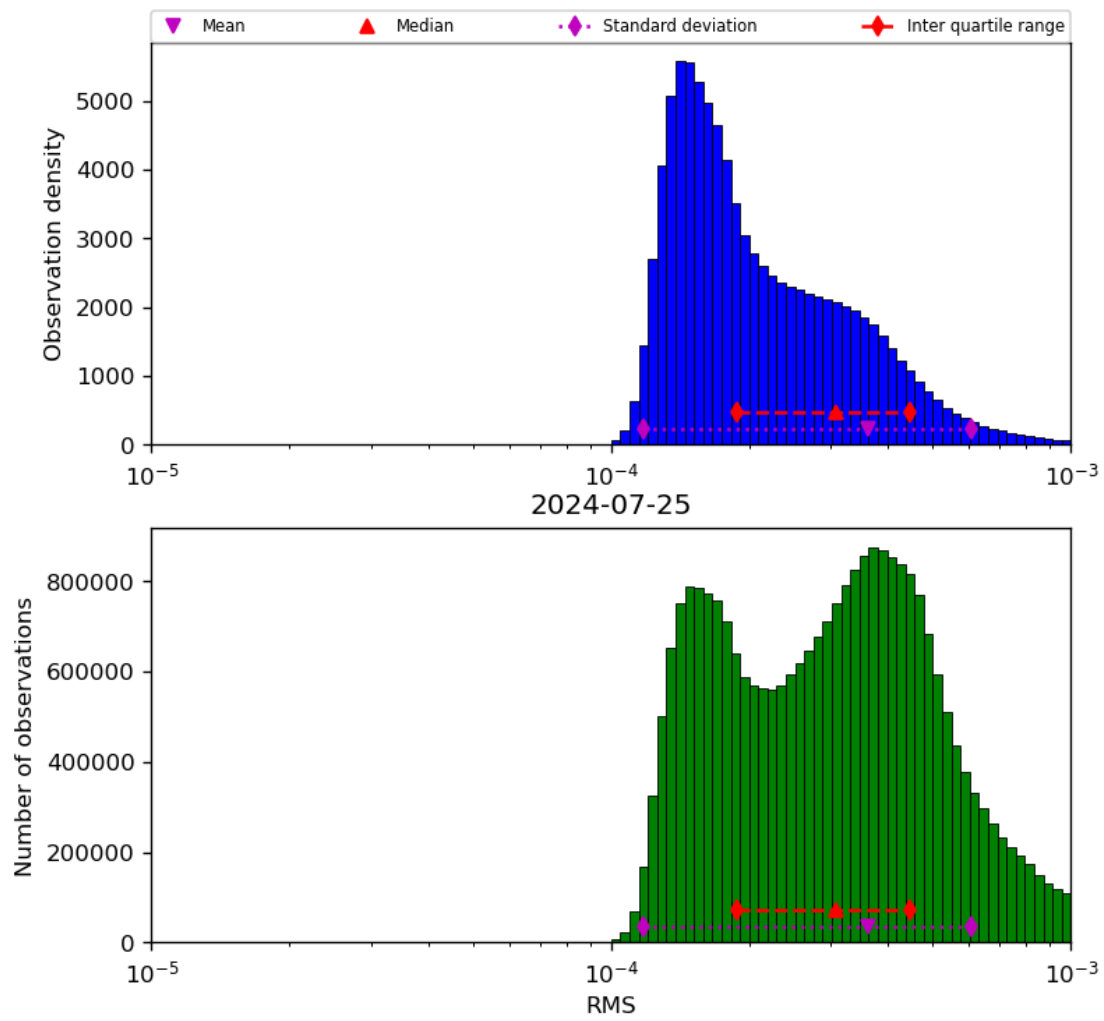
Figure 43: Histogram of “RMS” for 2024-07-24 to 2024-07-26
