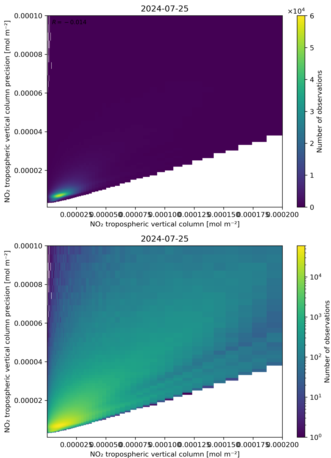
Figure 130: Scatter density plot of “NO 2 tropospheric vertical column” against “NO 2 tropospheric vertical column precision” for 2024-07-24 to 2024-07-26.
