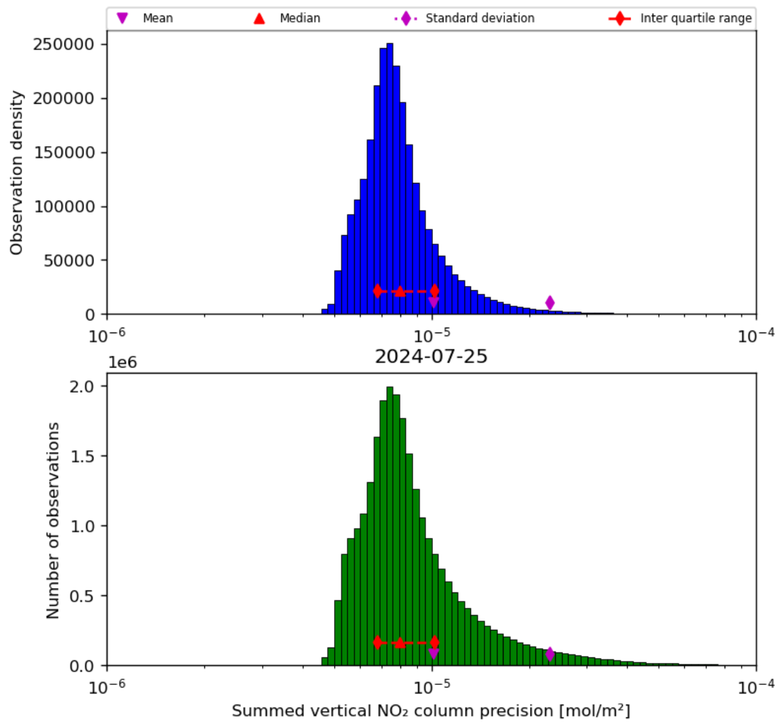
Figure 41: Histogram of "Summed vertical NO 2 column precision" for 2024-07-24 to 2024-07-26
