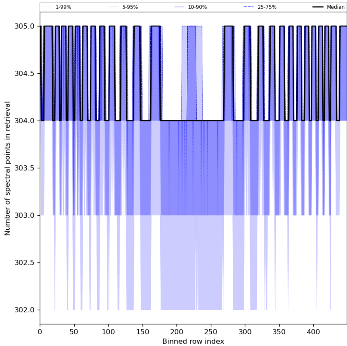
Figure 50: Along track statistics of “Number of spectral points in retrieval” for 2024-07-24 to 2024-07-26
