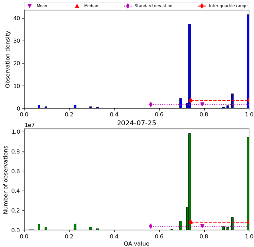
Figure 28: Histogram of “QA value” for 2024-07-24 to 2024-07-26
