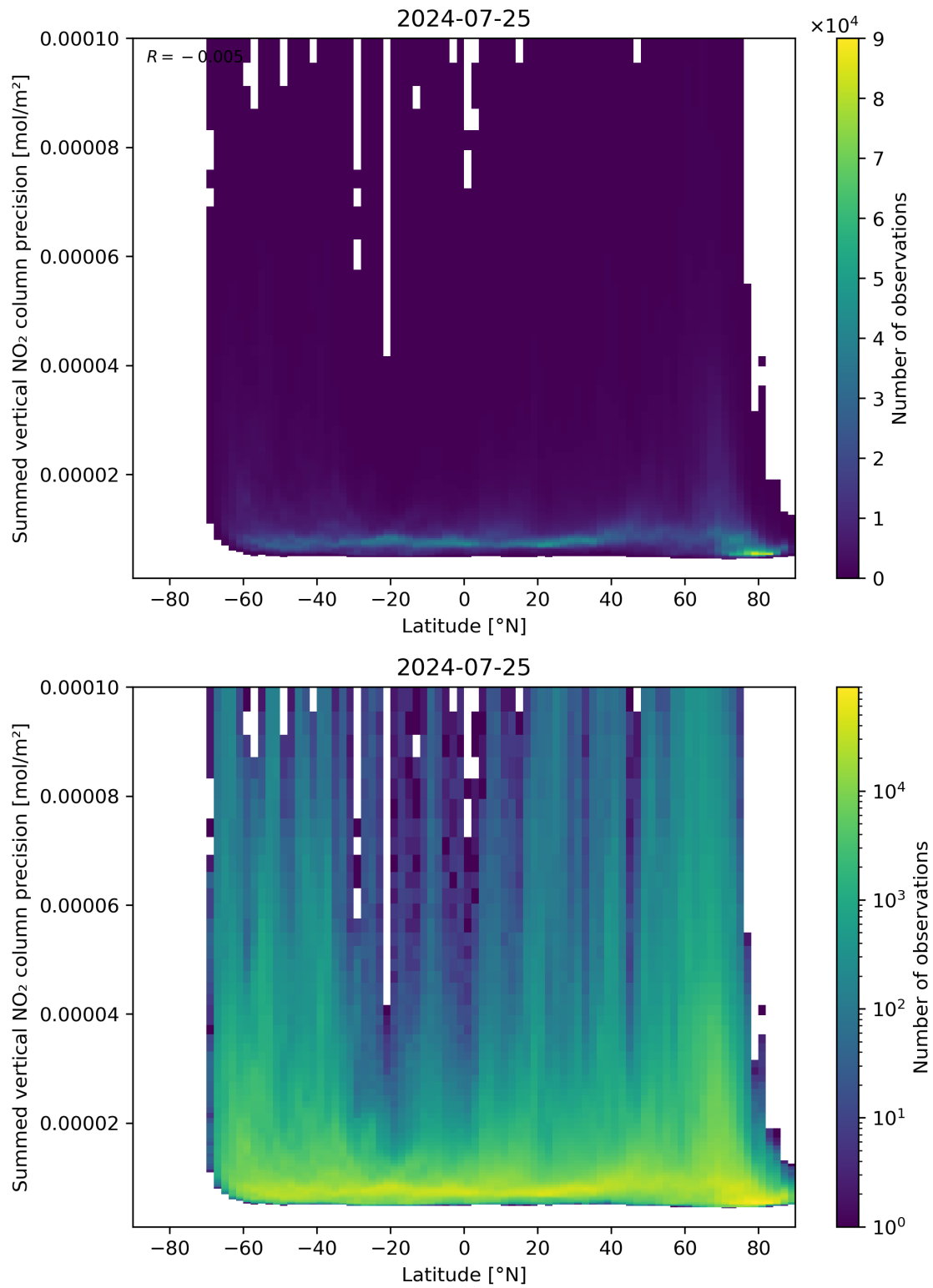
Figure 89: Scatter density plot of “Latitude” against “Summed vertical NO 2 column precision” for 2024-07-24 to 2024-07-26.
