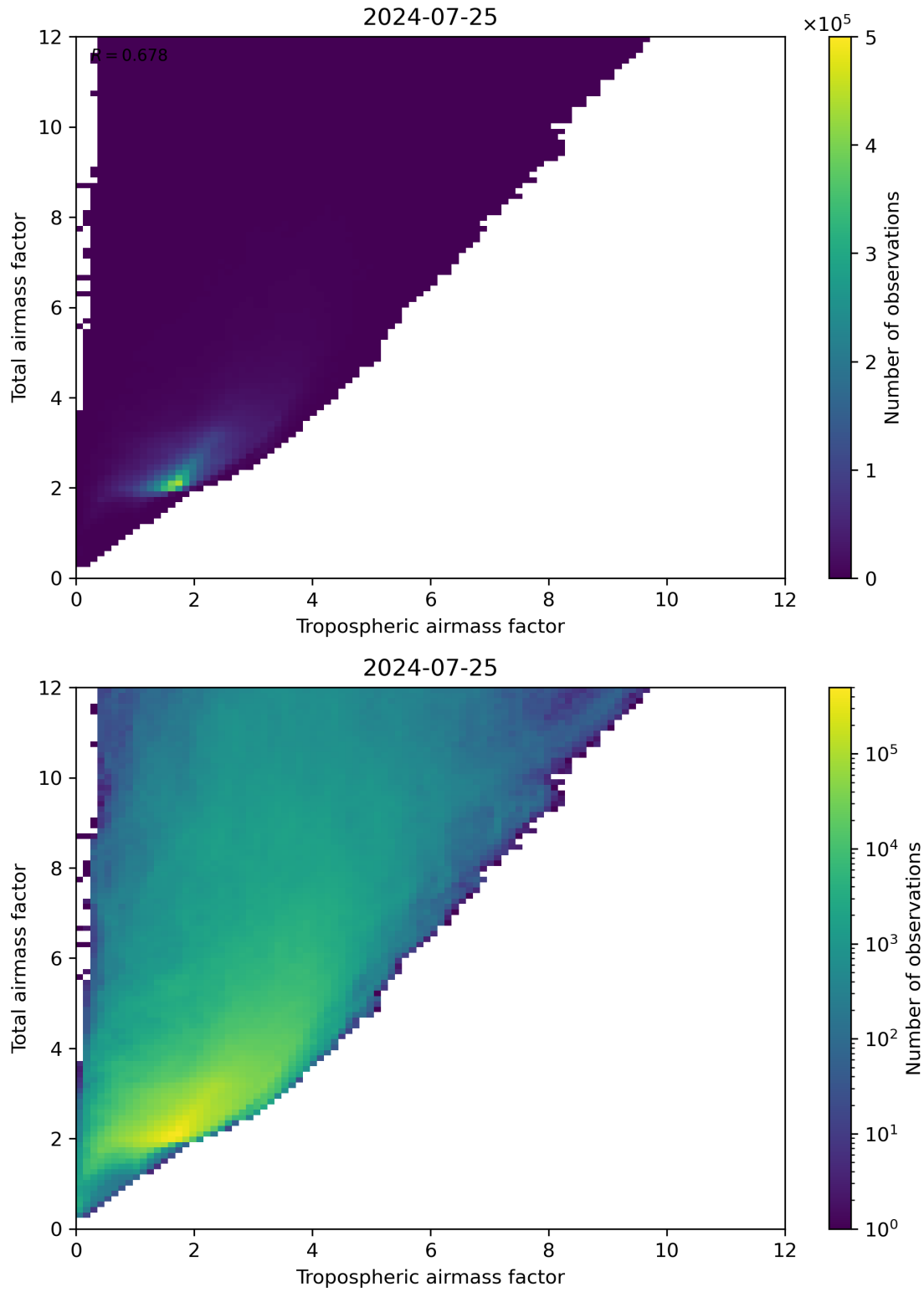
Figure 72: Scatter density plot of “Tropospheric airmass factor” against “Total airmass factor” for 2024-07-24 to 2024-07-26.
