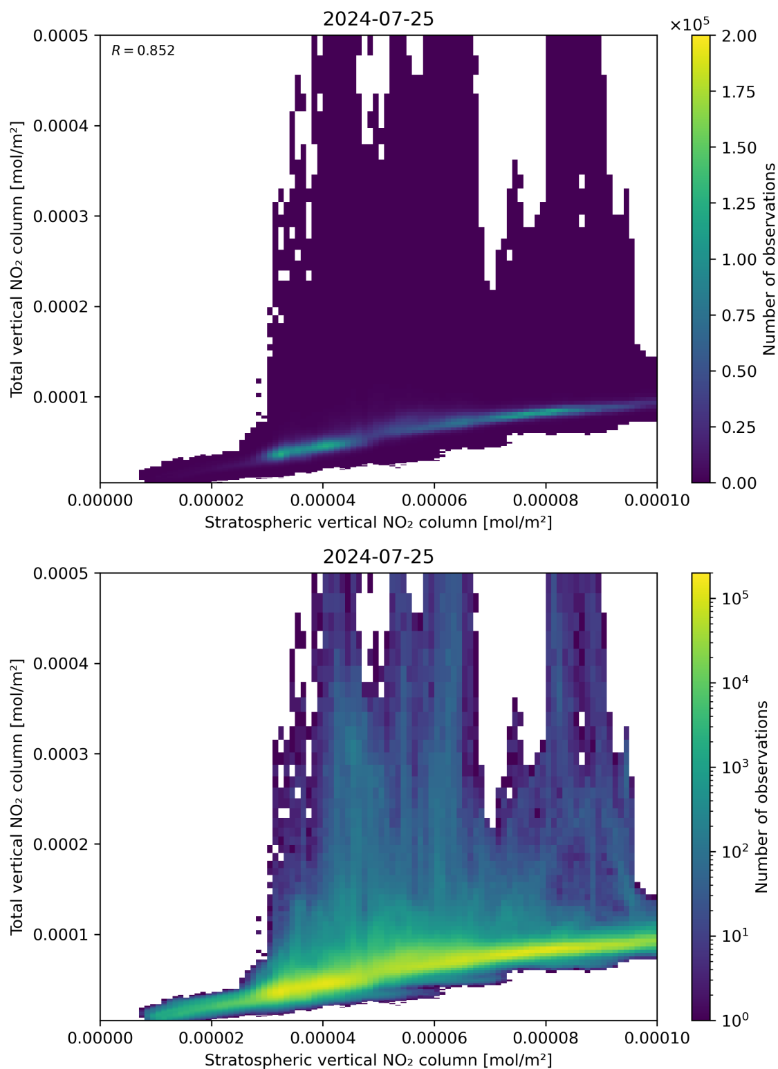
Figure 100: Scatter density plot of “Stratospheric vertical NO 2 column” against “Total vertical NO 2 column” for 2024-07-24 to 2024-07-26.
