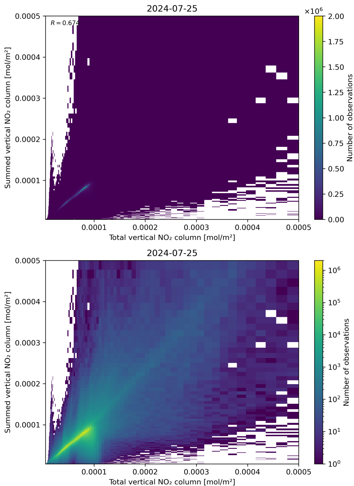
Figure 112: Scatter density plot of “Total vertical NO 2 column” against “Summed vertical NO 2 column” for 2024-07-24 to 2024-07-26.
