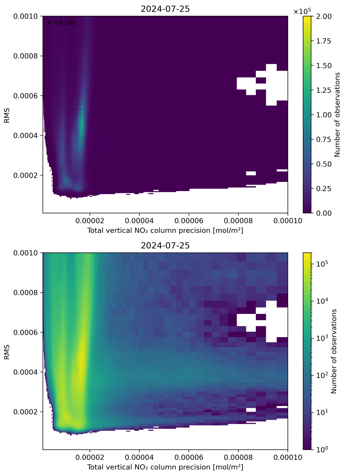
Figure 119: Scatter density plot of “Total vertical NO 2 column precision” against “RMS” for 2024-07-24 to 2024-07-26.
