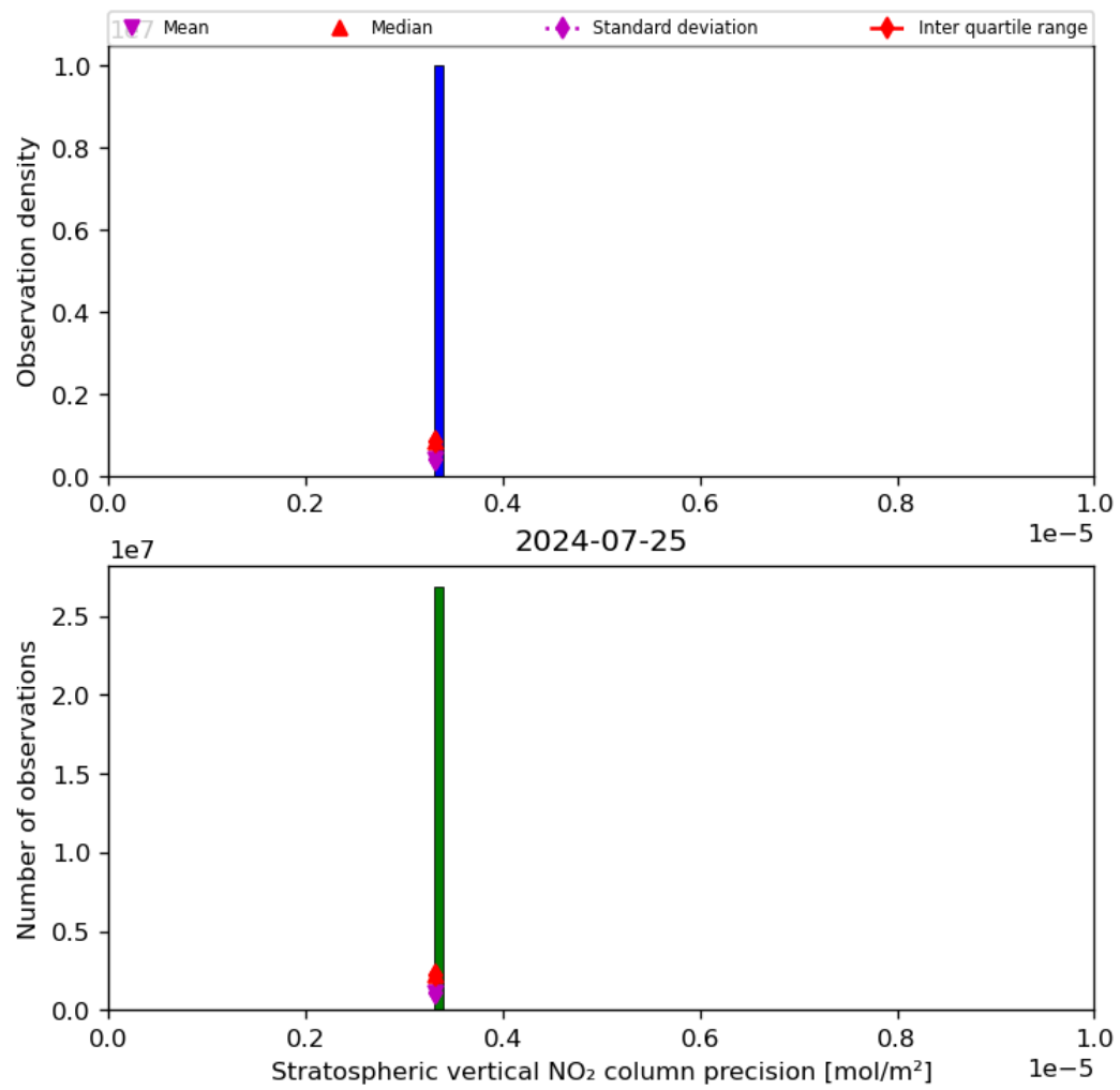
Figure 37: Histogram of “Stratospheric vertical NO 2 column precision” for 2024-07-24 to 2024-07-26
