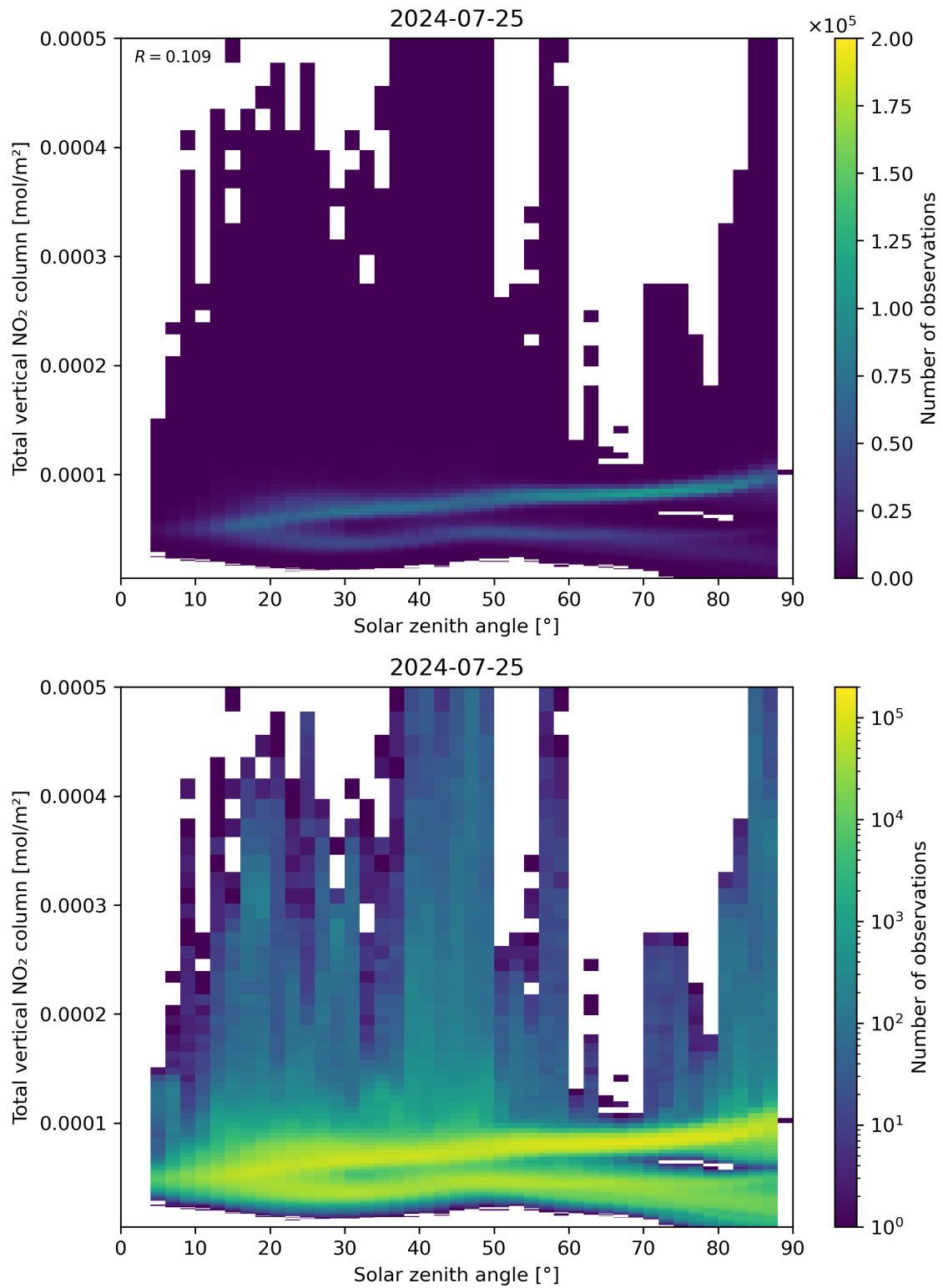
Figure 153: Scatter density plot of “Solar zenith angle” against “Total vertical \text{NO}_2 column” for 2024-07-24 to 2024-07-26.
