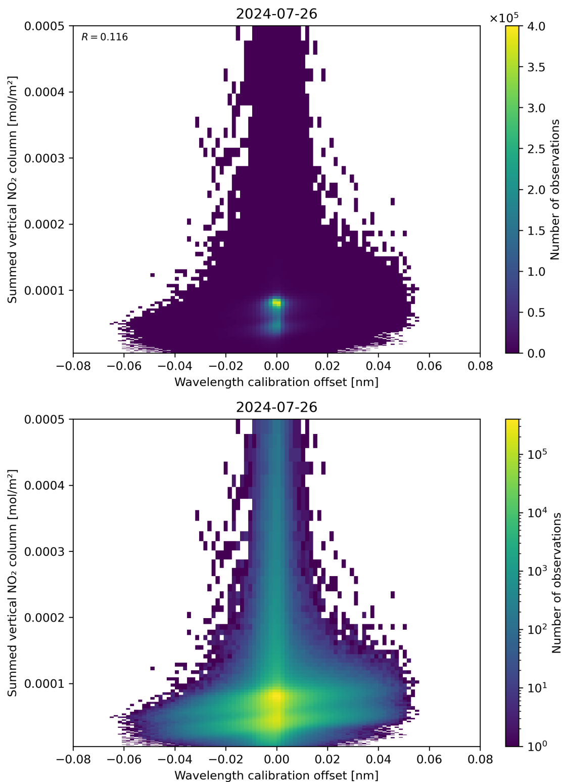
Figure 177: Scatter density plot of “Wavelength calibration offset” against “Summed vertical NO 2 column” for 2024-07-26 to 2024-07-27.
