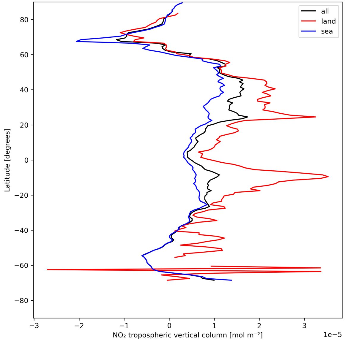
Figure 12: Zonal average of “NO 2 tropospheric vertical column” for 2024-07-26 to 2024-07-27.
