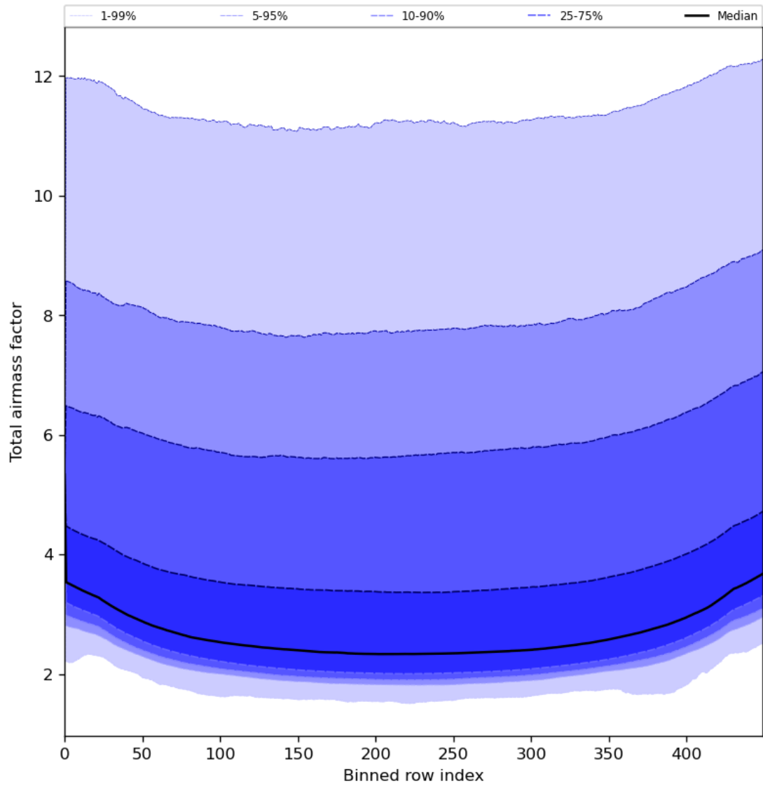
Figure 49: Along track statistics of “Total airmass factor” for 2024-07-26 to 2024-07-27
