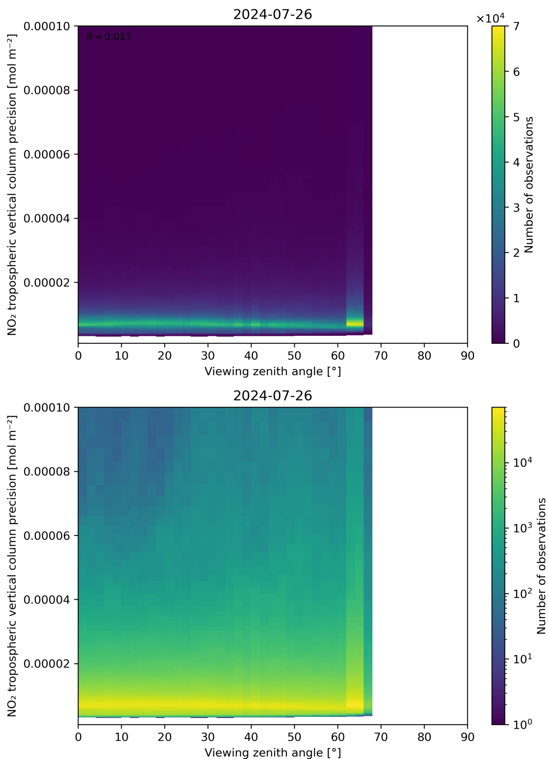
Figure 170: Scatter density plot of “Viewing zenith angle” against “NO 2 tropospheric vertical column precision” for 2024-07-26 to 2024-07-27.
