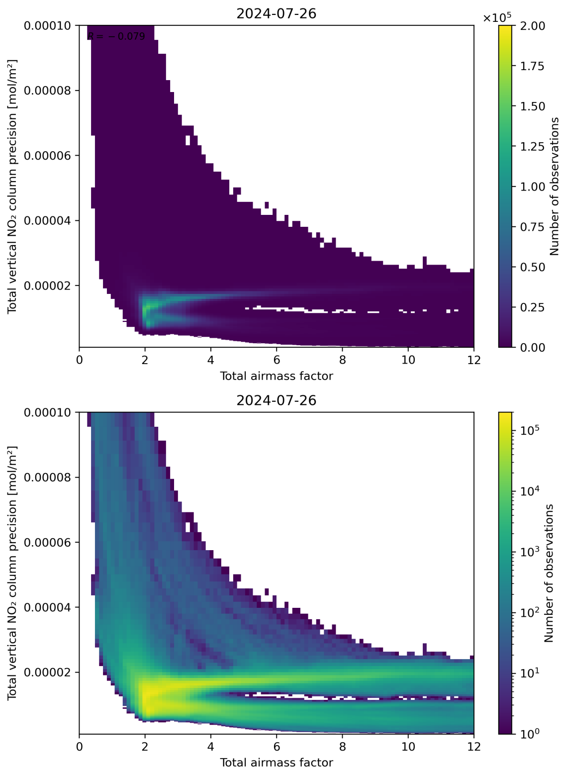
Figure 68: Scatter density plot of “Total airmass factor” against “Total vertical NO 2 column precision” for 2024-07-26 to 2024-07-27.
