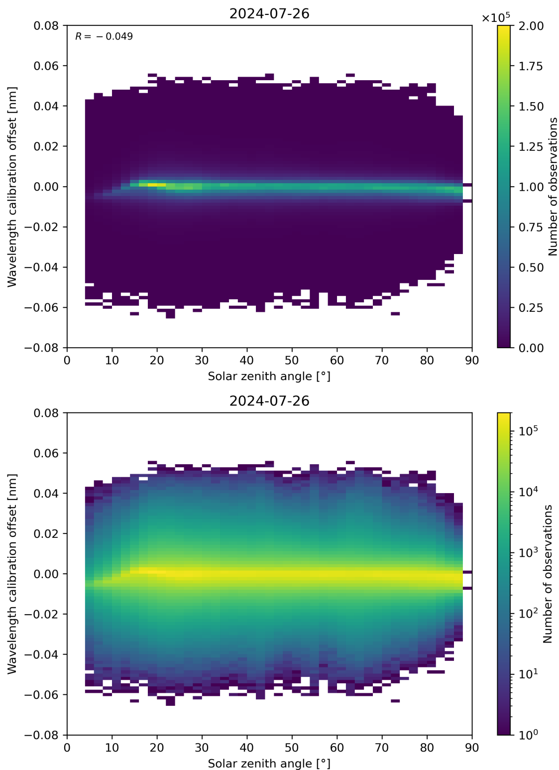
Figure 158: Scatter density plot of “Solar zenith angle” against “Wavelength calibration offset” for 2024-07-26 to 2024-07-27.
