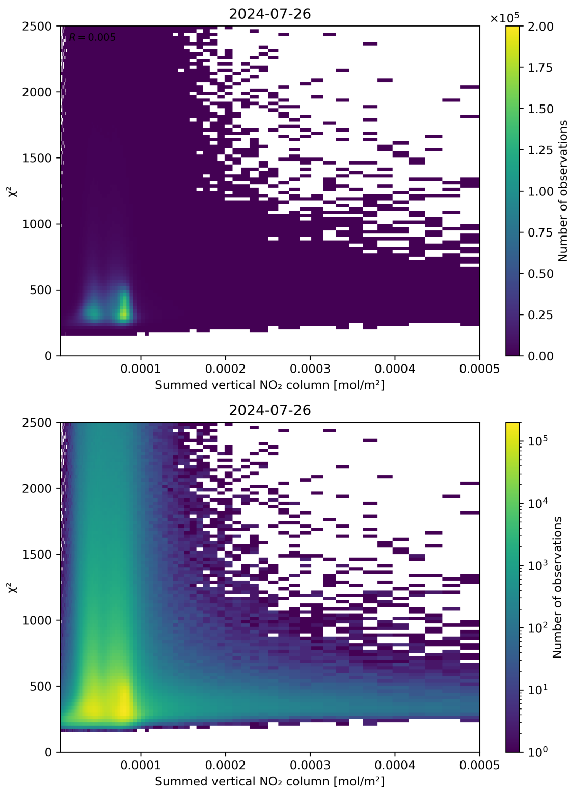
Figure 104: Scatter density plot of “Summed vertical NO 2 column” against “ \chi^2 ” for 2024-07-26 to 2024-07-27.
