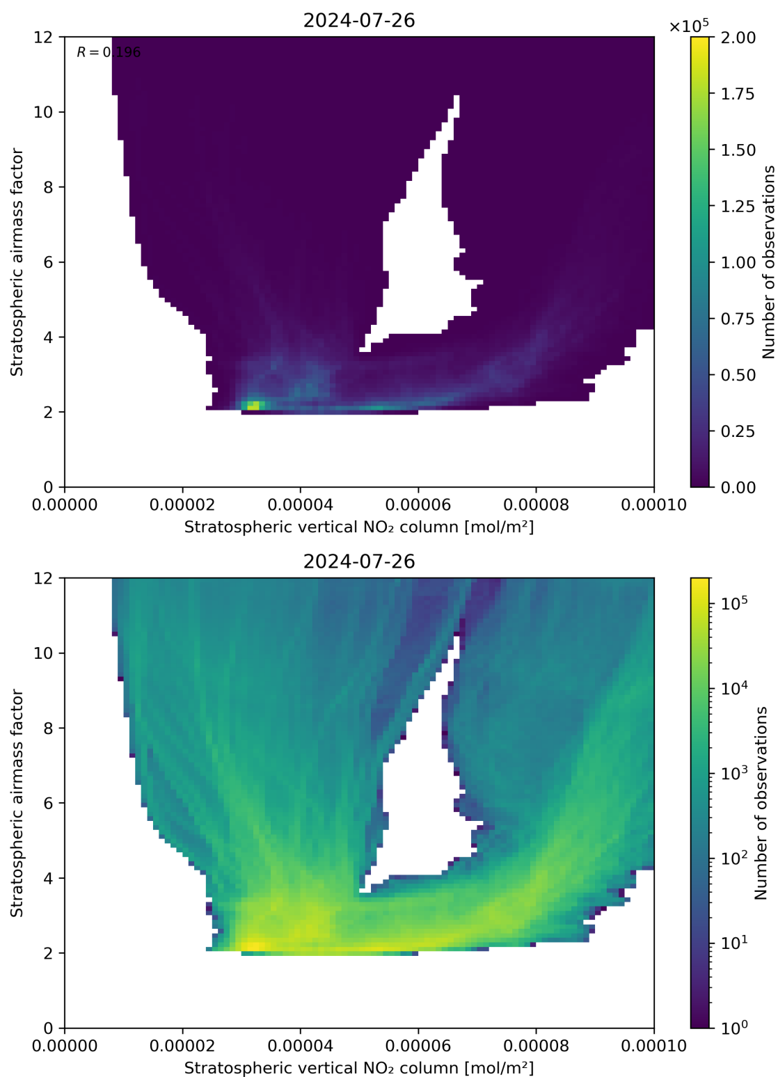
Figure 96: Scatter density plot of “Stratospheric vertical NO 2 column” against “Stratospheric airmass factor” for 2024-07-26 to 2024-07-27.
