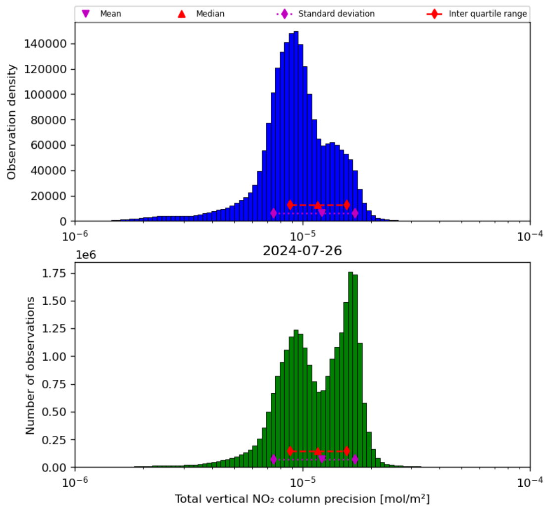
Figure 39: Histogram of “Total vertical NO 2 column precision” for 2024-07-26 to 2024-07-27
