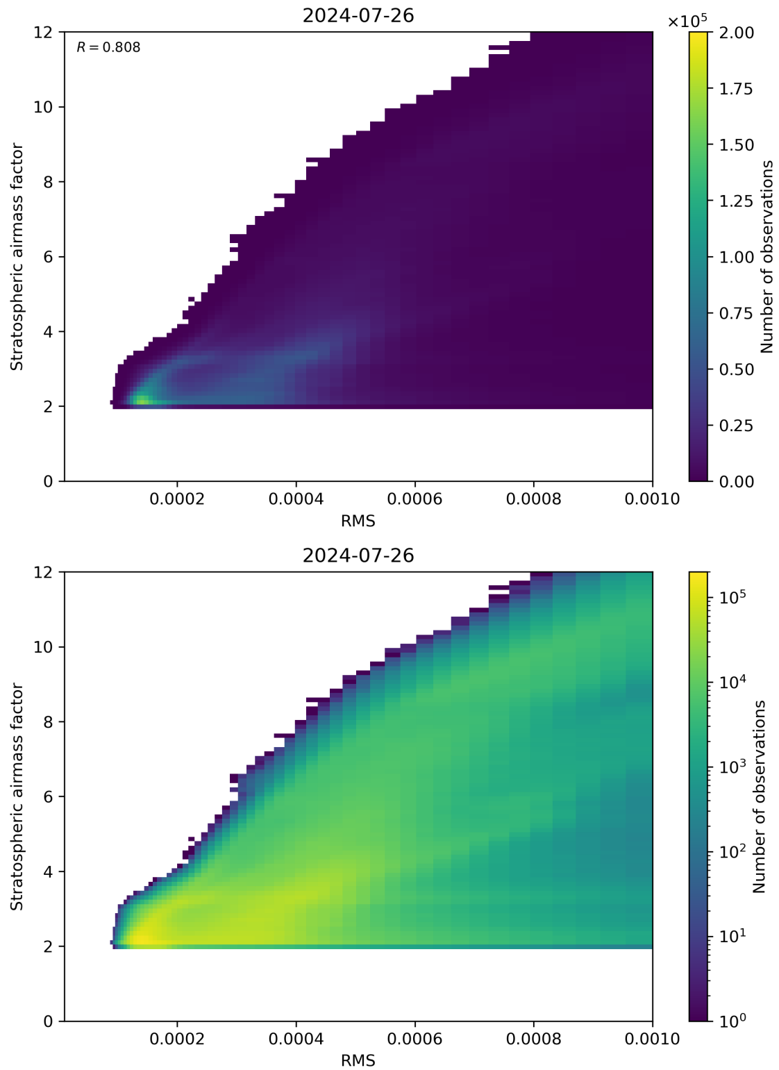
Figure 144: Scatter density plot of “RMS” against “Stratospheric airmass factor” for 2024-07-26 to 2024-07-27.
