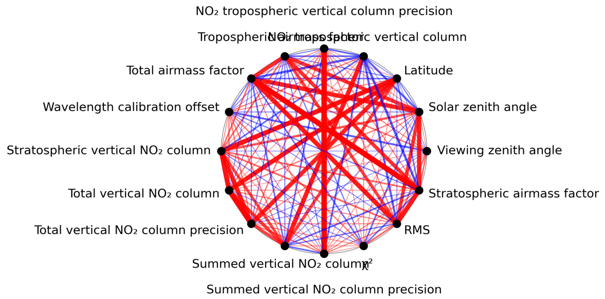
Figure 1: Map of correlation graph for 2024-07-26 to 2024-07-27.
