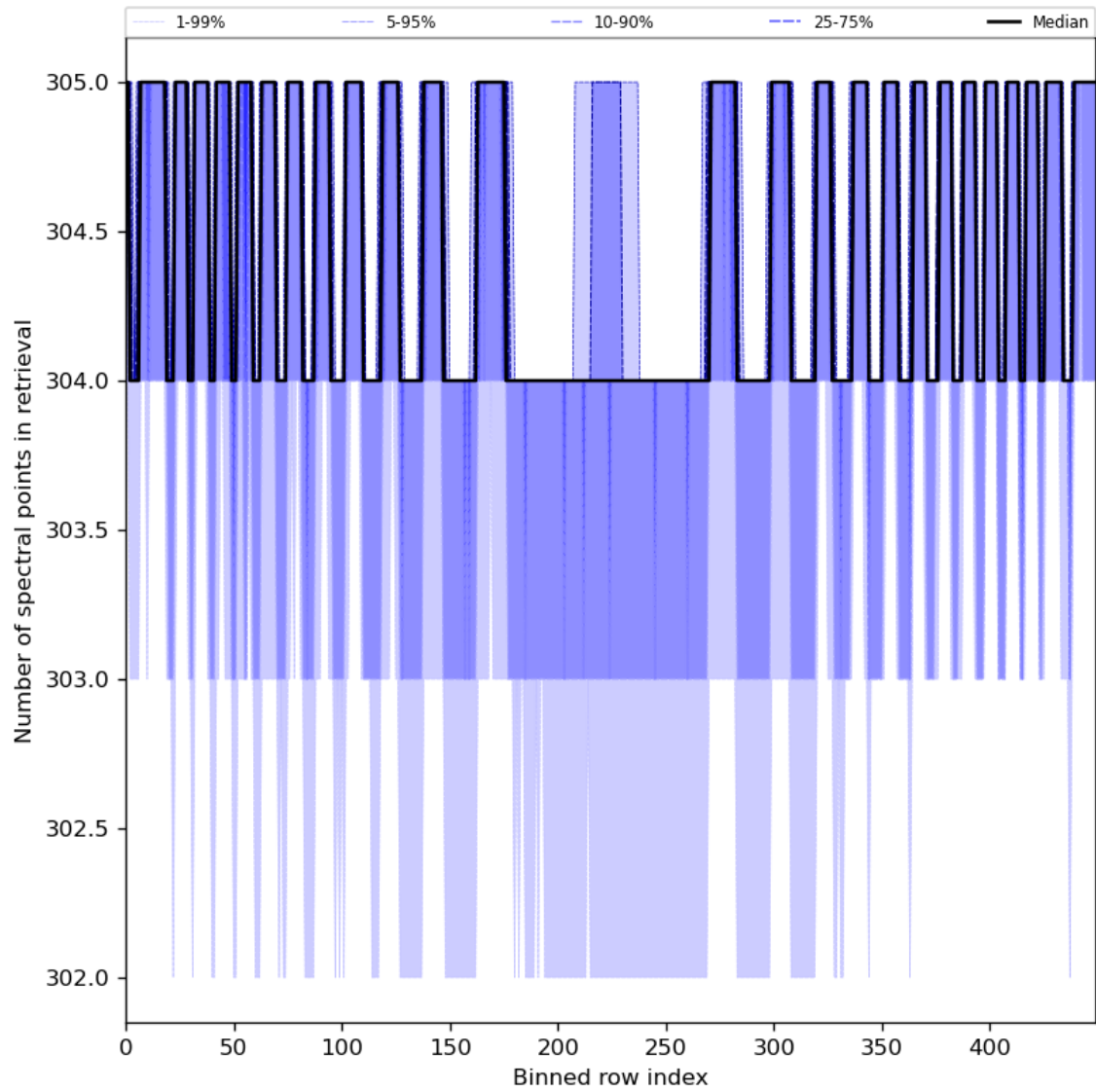
Figure 50: Along track statistics of “Number of spectral points in retrieval” for 2024-07-26 to 2024-07-27
