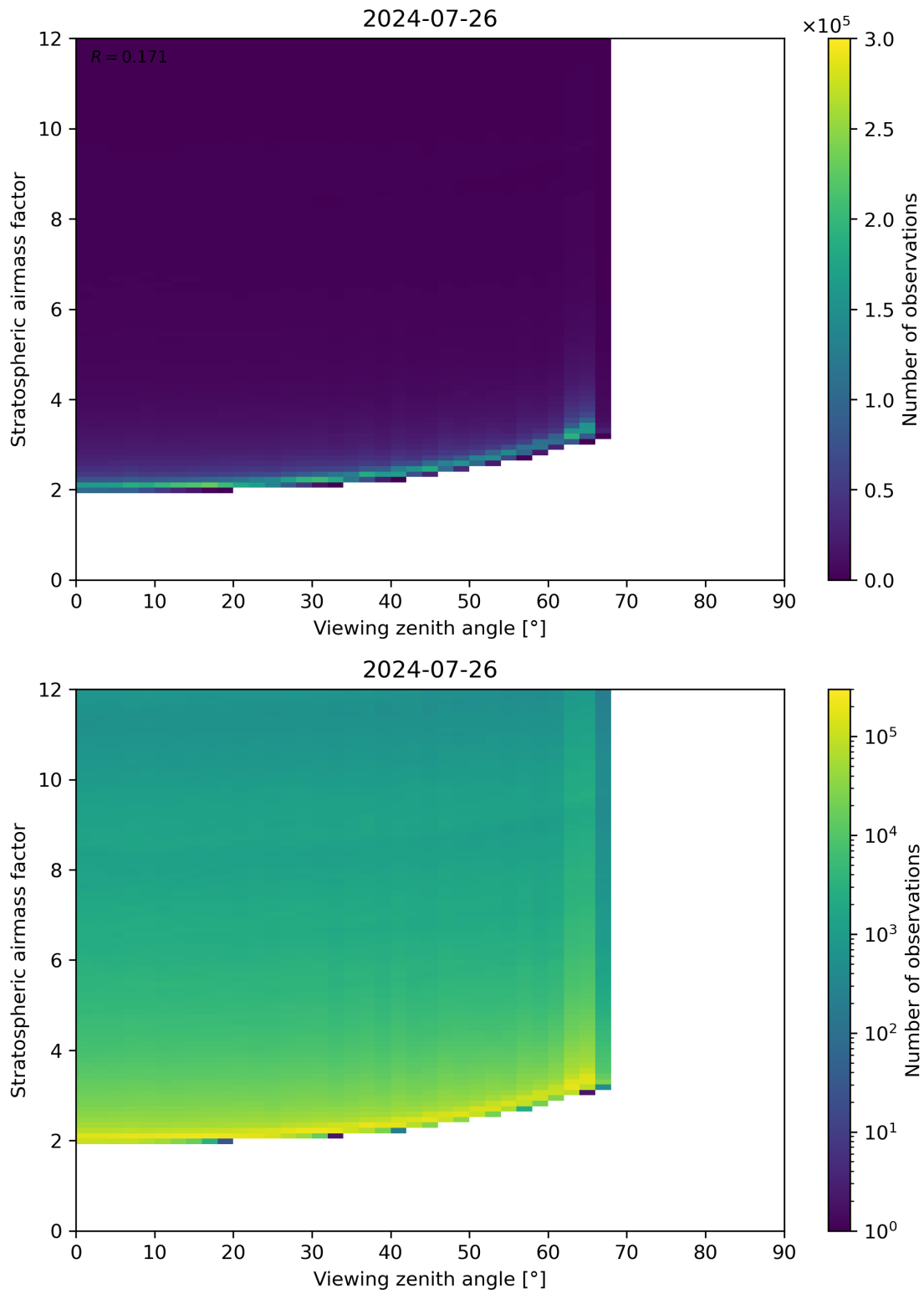
Figure 159: Scatter density plot of “Viewing zenith angle” against “Stratospheric airmass factor” for 2024-07-26 to 2024-07-27.
