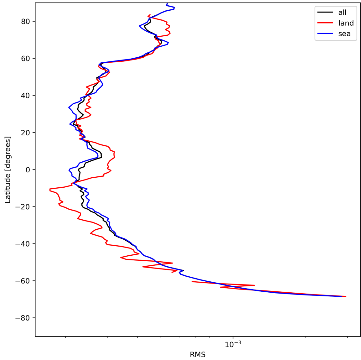
Figure 26: Zonal average of “RMS” for 2024-07-26 to 2024-07-27.
