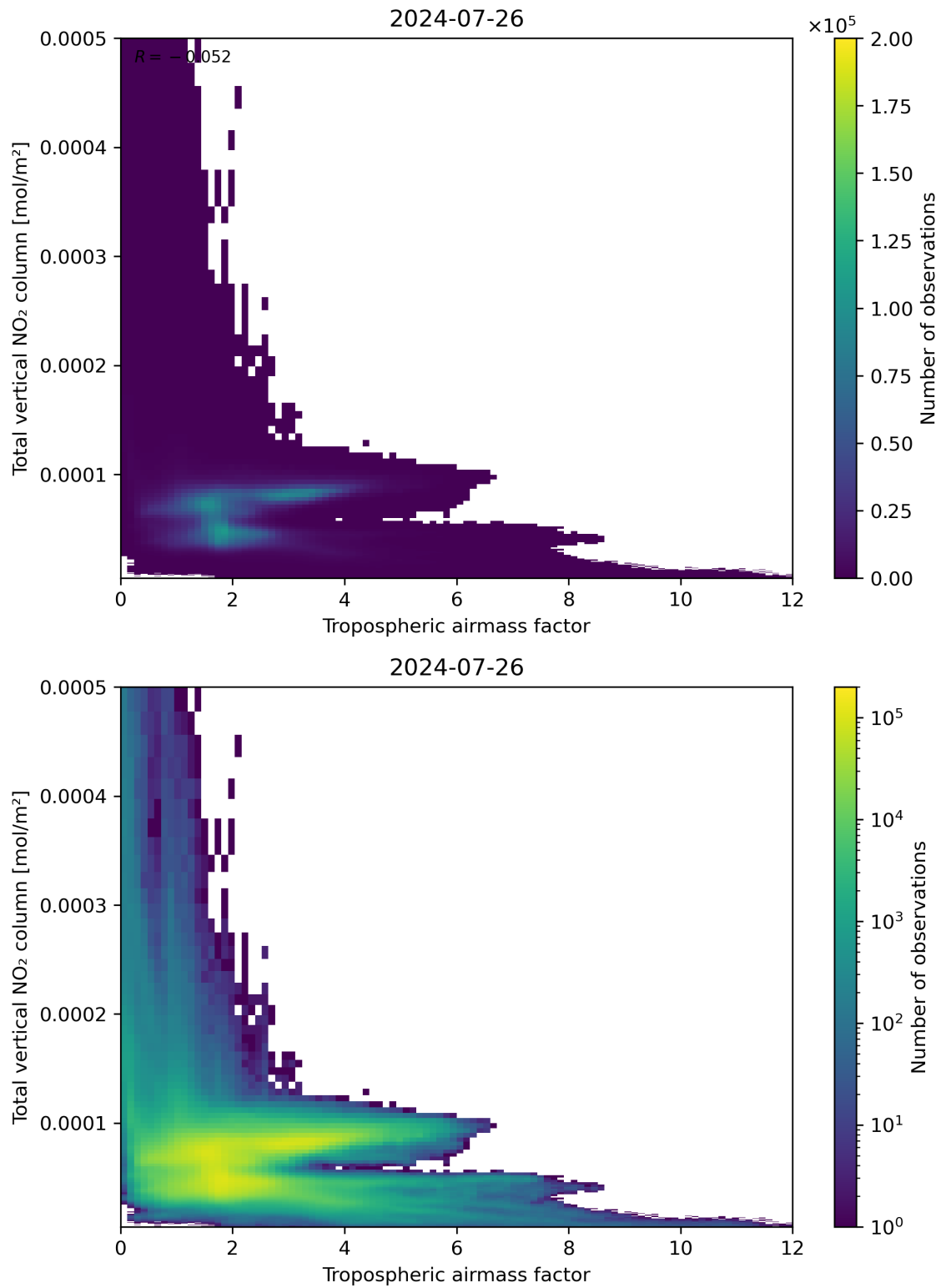
Figure 77: Scatter density plot of “Tropospheric airmass factor” against “Total vertical NO 2 column” for 2024-07-26 to 2024-07-27.
