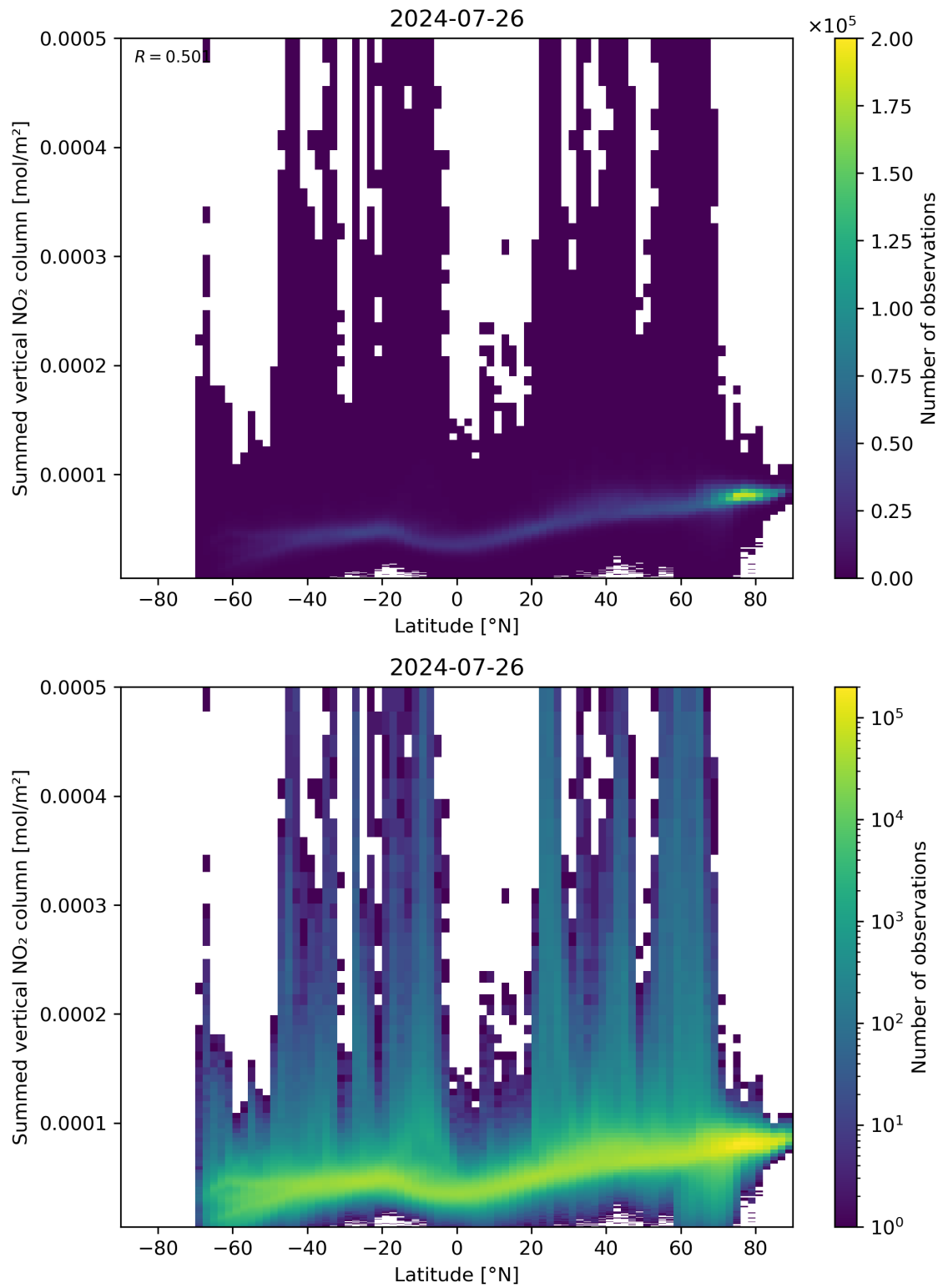
Figure 88: Scatter density plot of “Latitude” against “Summed vertical NO 2 column” for 2024-07-26 to 2024-07-27.
