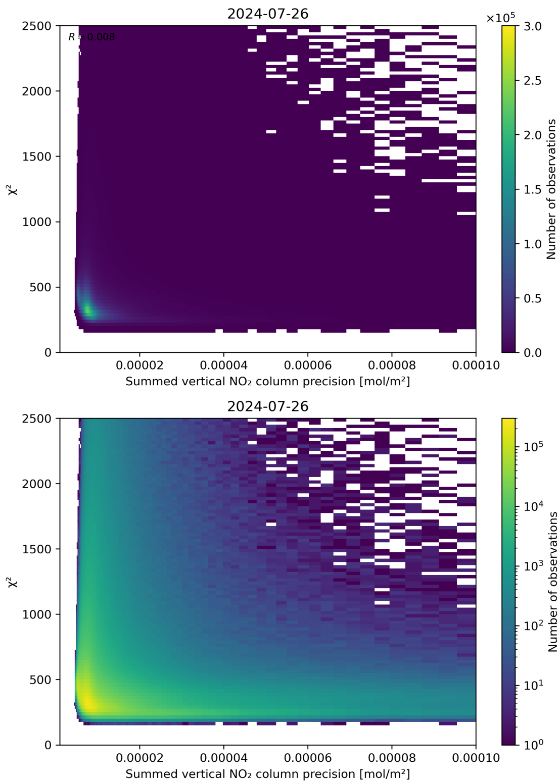
Figure 107: Scatter density plot of “Summed vertical NO 2 column precision” against “ \chi^2 ” for 2024-07-26 to 2024-07-27.
