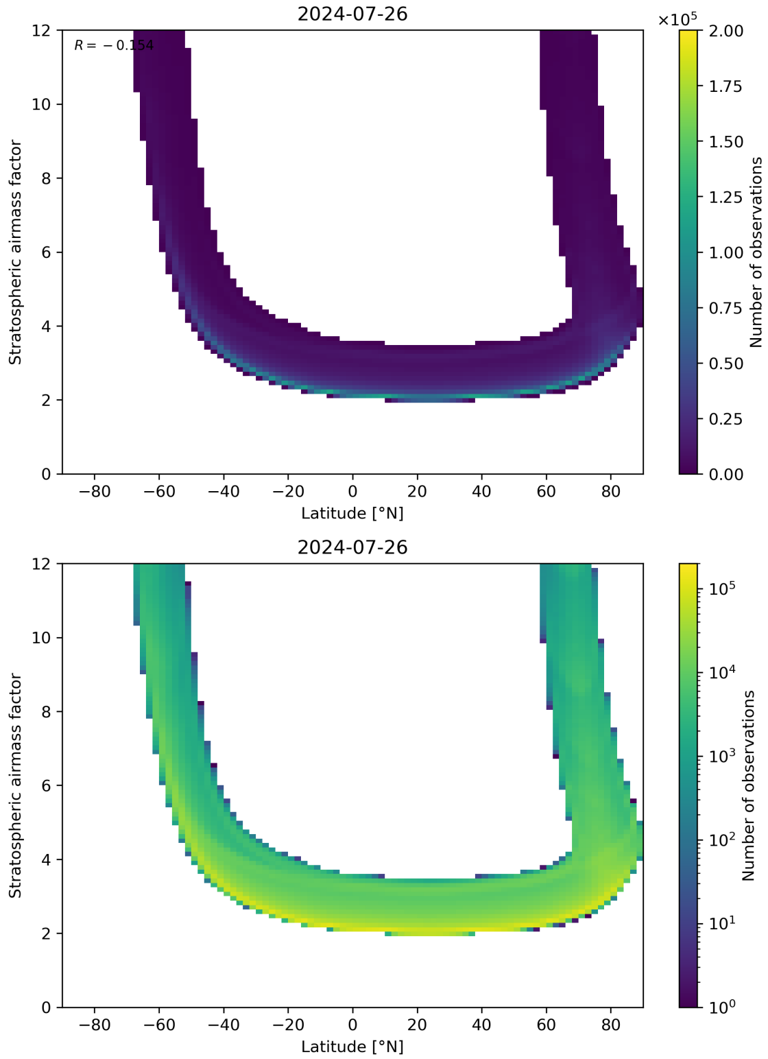
Figure 83: Scatter density plot of “Latitude” against “Stratospheric air mass factor” for 2024-07-26 to 2024-07-27.
