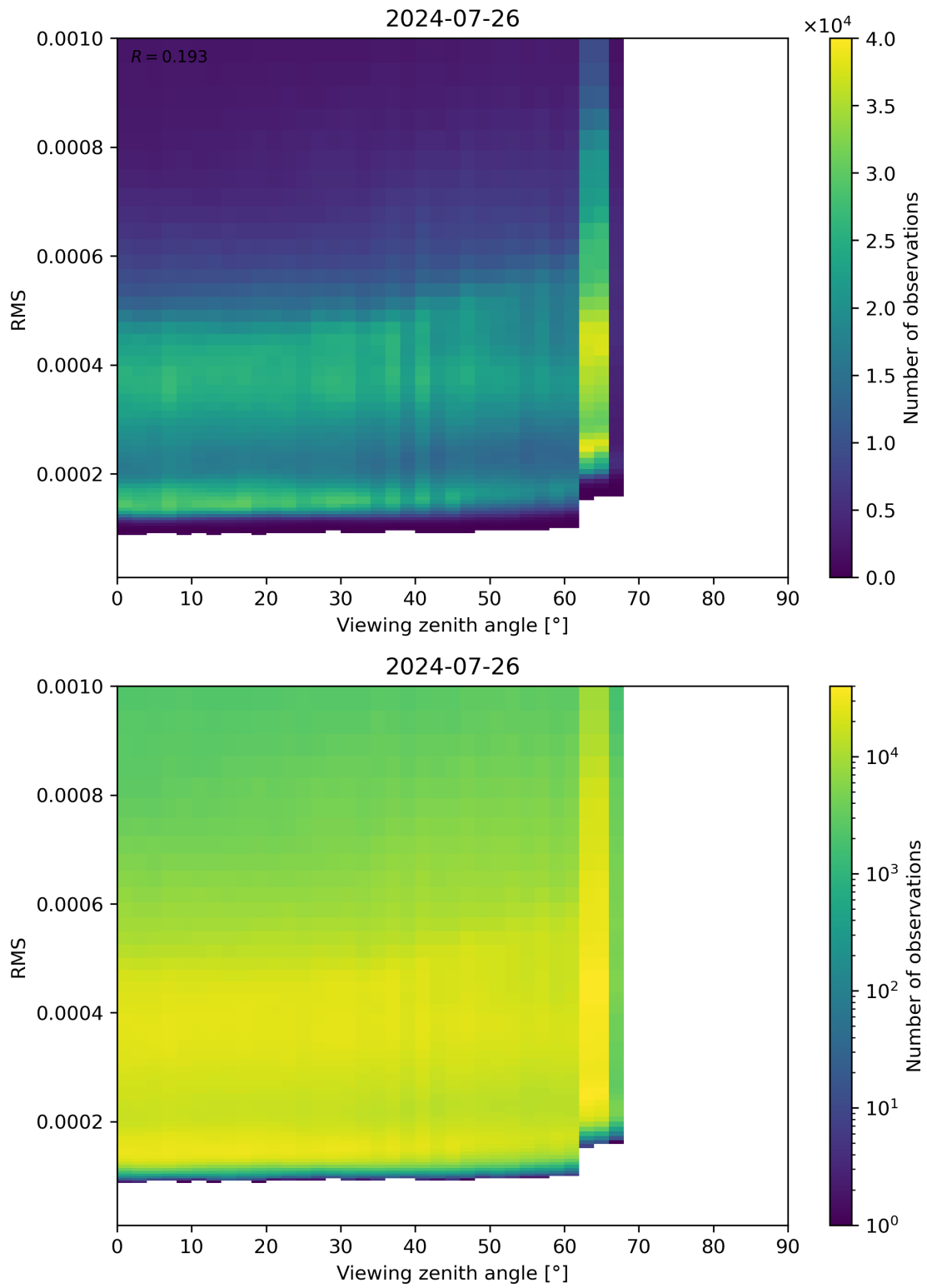
Figure 171: Scatter density plot of “Viewing zenith angle” against “RMS” for 2024-07-26 to 2024-07-27.
