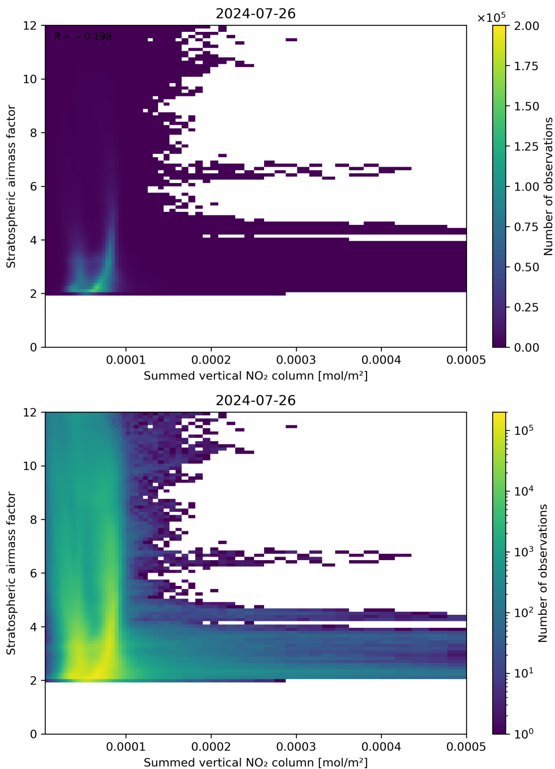
Figure 103: Scatter density plot of “Summed vertical NO 2 column” against “Stratospheric air mass factor” for 2024-07-26 to 2024-07-27.
