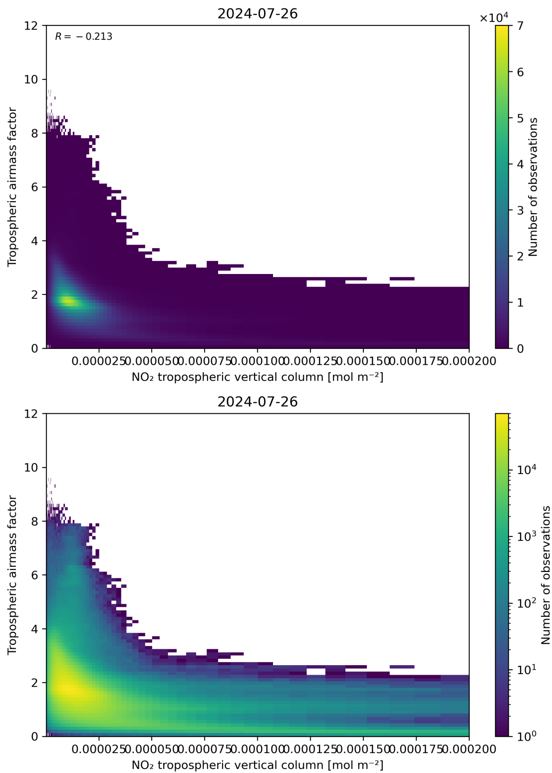
Figure 123: Scatter density plot of “NO 2 tropospheric vertical column” against “Tropospheric air mass factor” for 2024-07-26 to 2024-07-27.
