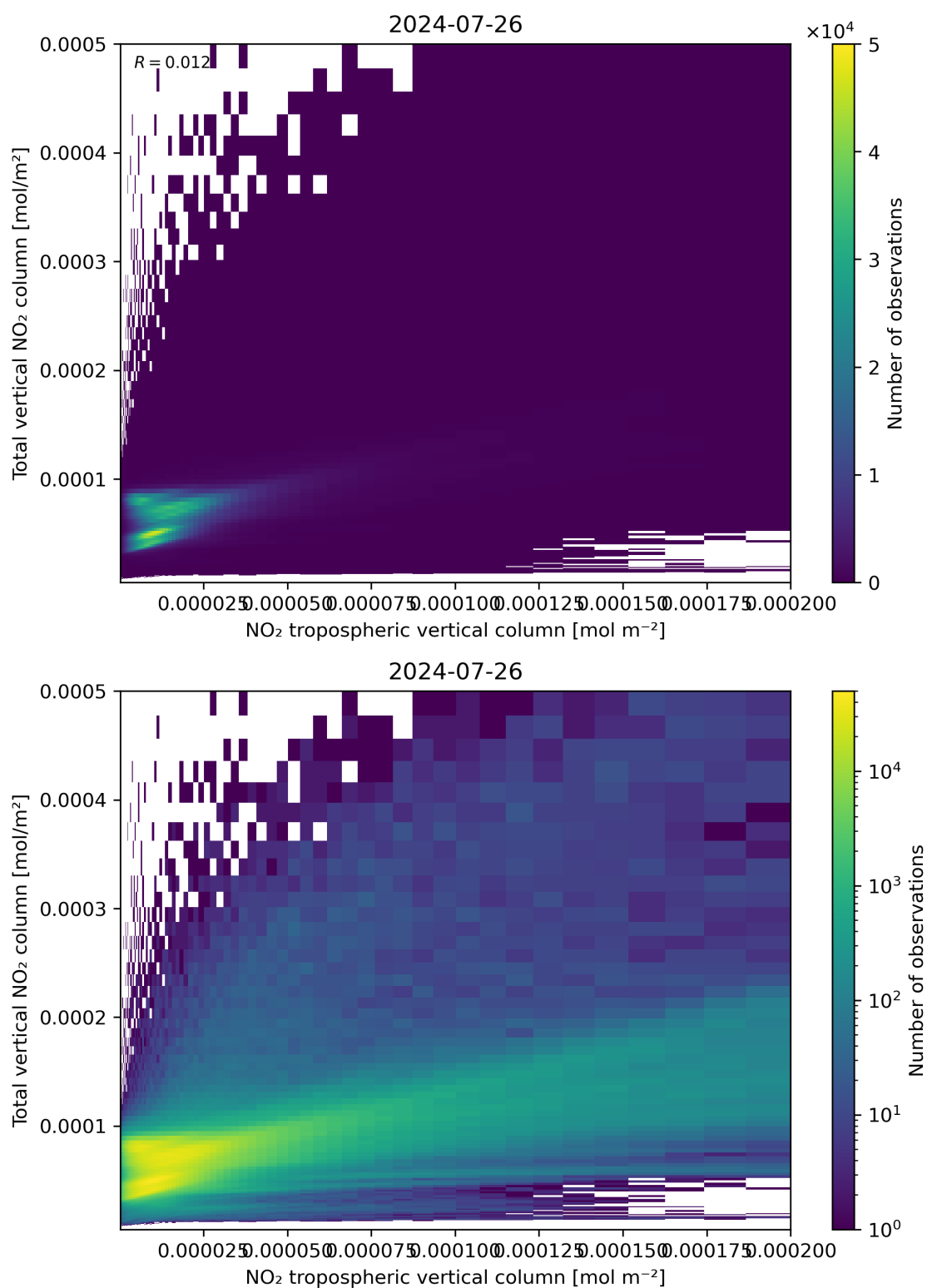
Figure 128: Scatter density plot of “NO 2 tropospheric vertical column” against “Total vertical NO 2 column” for 2024-07-26 to 2024-07-27.
