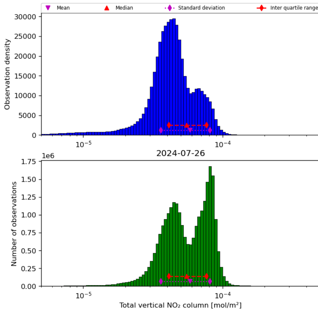
Figure 38: Histogram of “Total vertical NO 2 column” for 2024-07-26 to 2024-07-27
