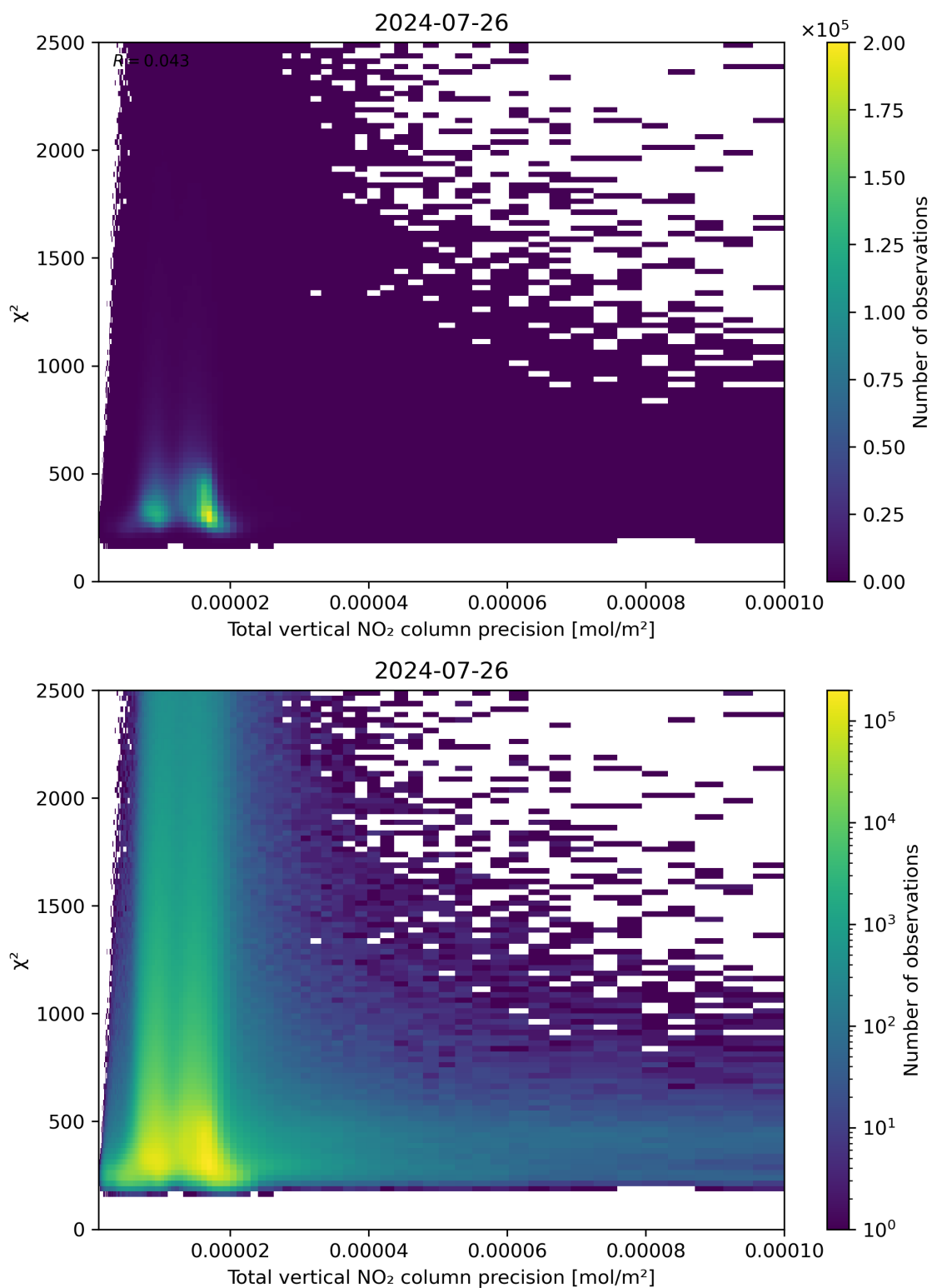
Figure 116: Scatter density plot of “Total vertical NO 2 column precision” against “ \chi^2 ” for 2024-07-26 to 2024-07-27.
