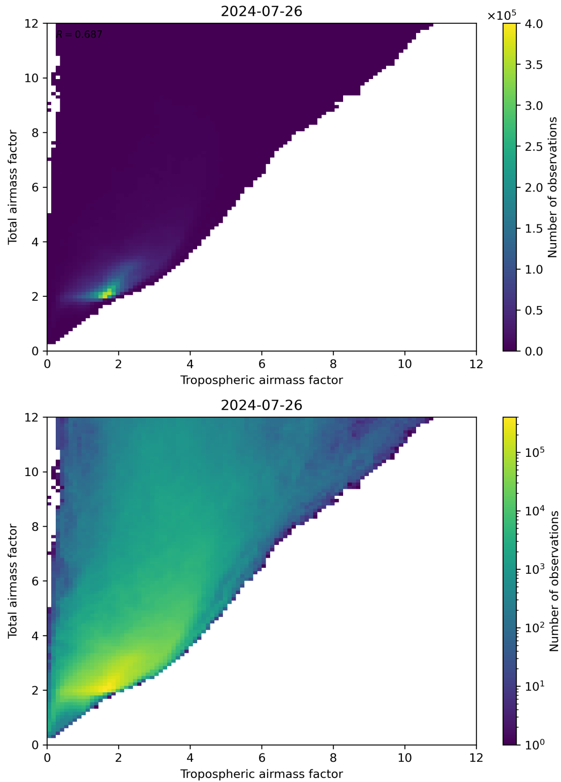
Figure 72: Scatter density plot of “Tropospheric airmass factor” against “Total airmass factor” for 2024-07-26 to 2024-07-27.
