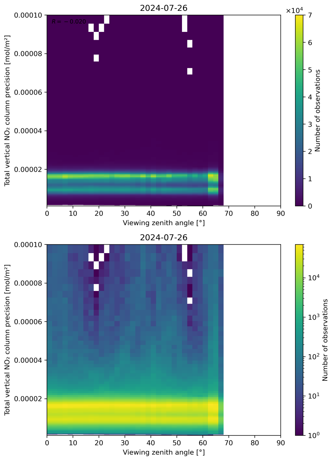
Figure 168: Scatter density plot of “Viewing zenith angle” against “Total vertical NO 2 column precision” for 2024-07-26 to 2024-07-27.
