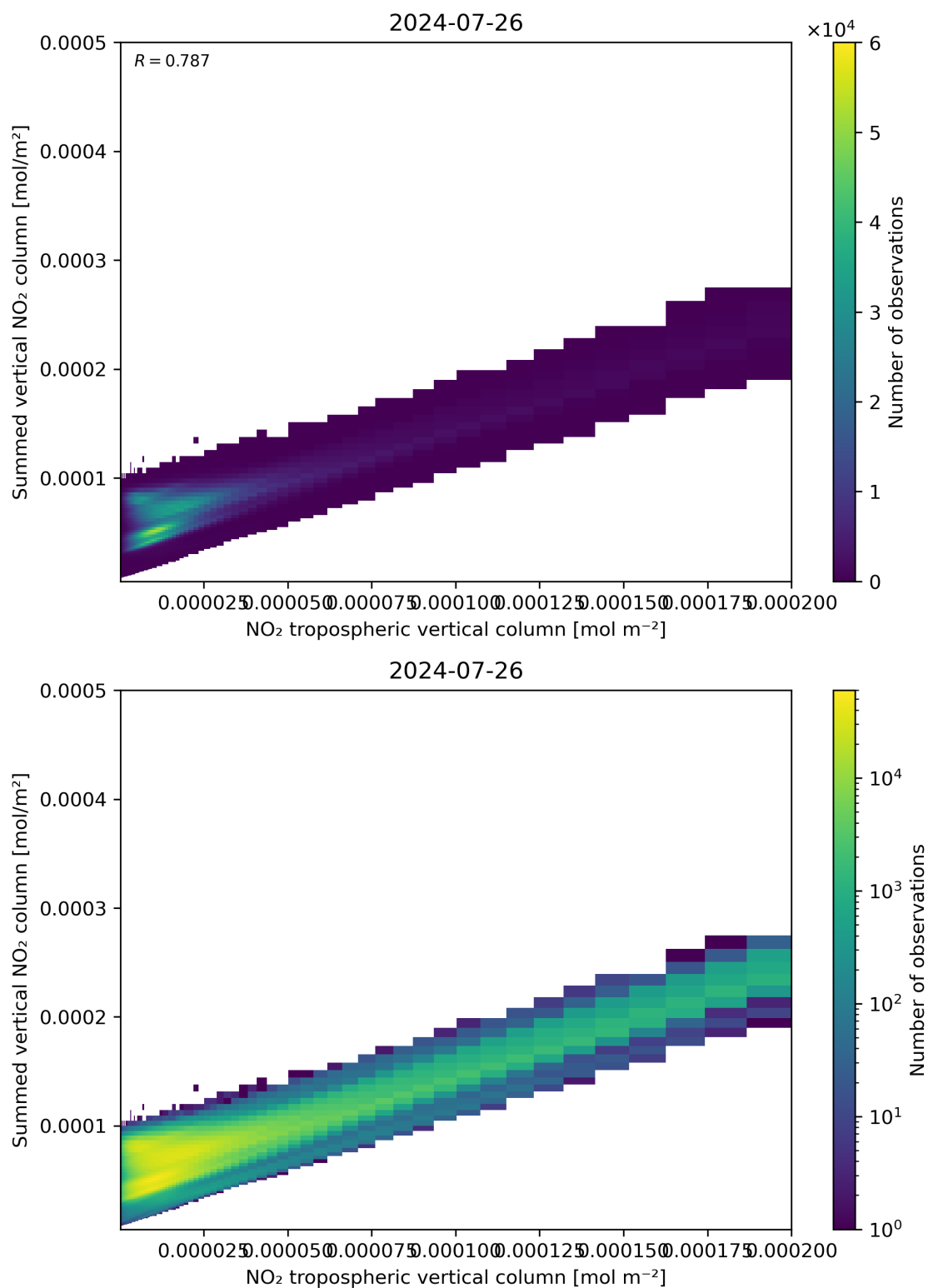
Figure 126: Scatter density plot of “NO 2 tropospheric vertical column” against “Summed vertical NO 2 column” for 2024-07-26 to 2024-07-27.
