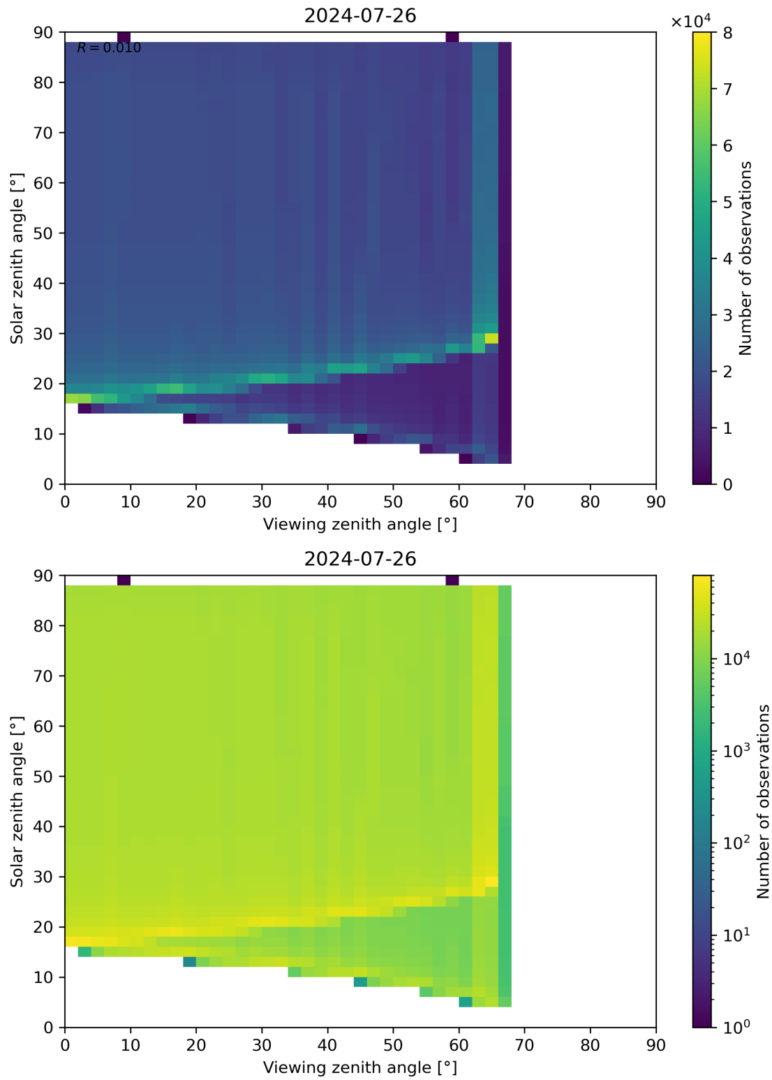
Figure 172: Scatter density plot of “Viewing zenith angle” against “Solar zenith angle” for 2024-07-26 to 2024-07-27.
