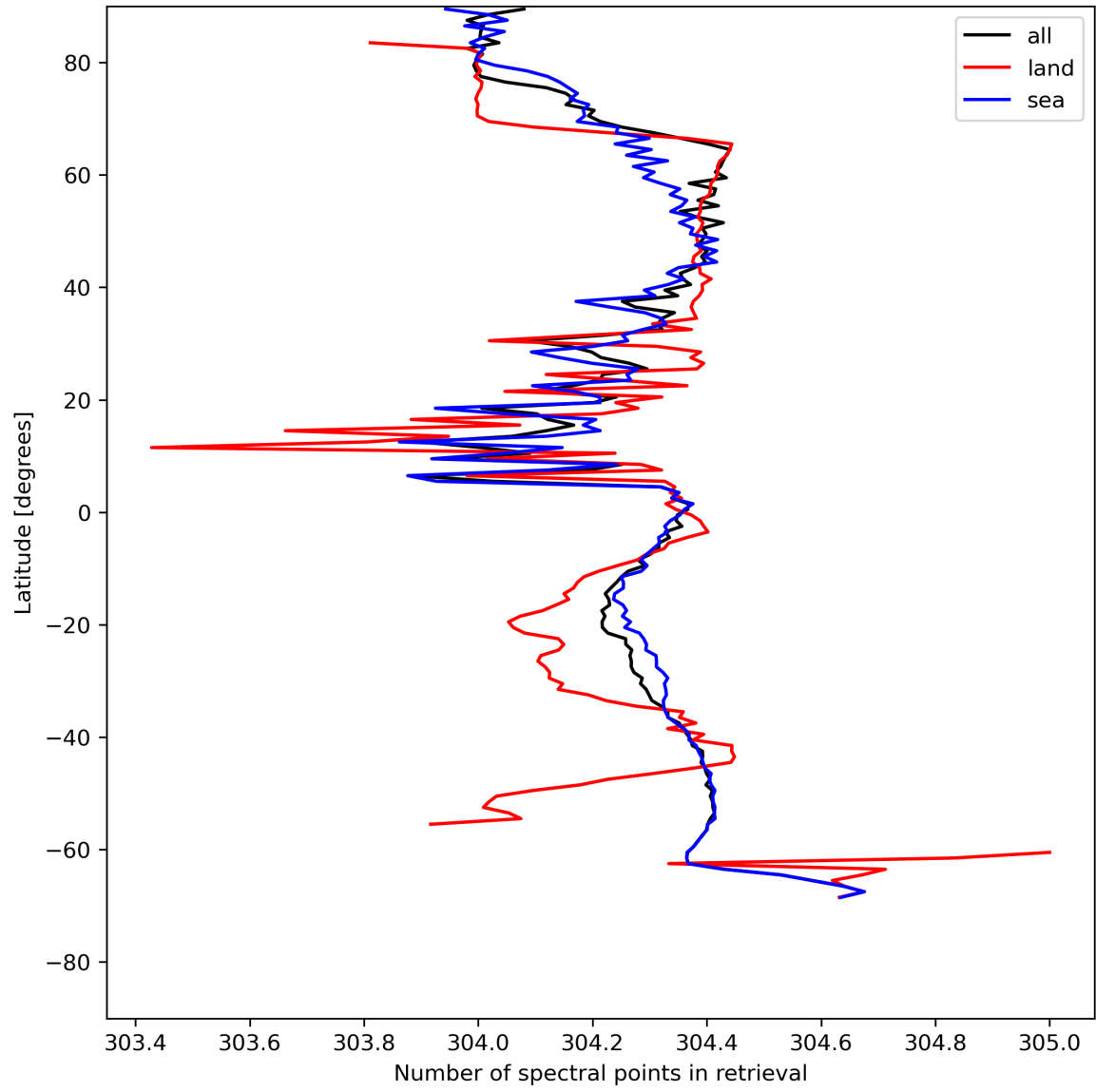
Figure 16: Zonal average of “Number of spectral points in retrieval” for 2024-07-26 to 2024-07-27.
