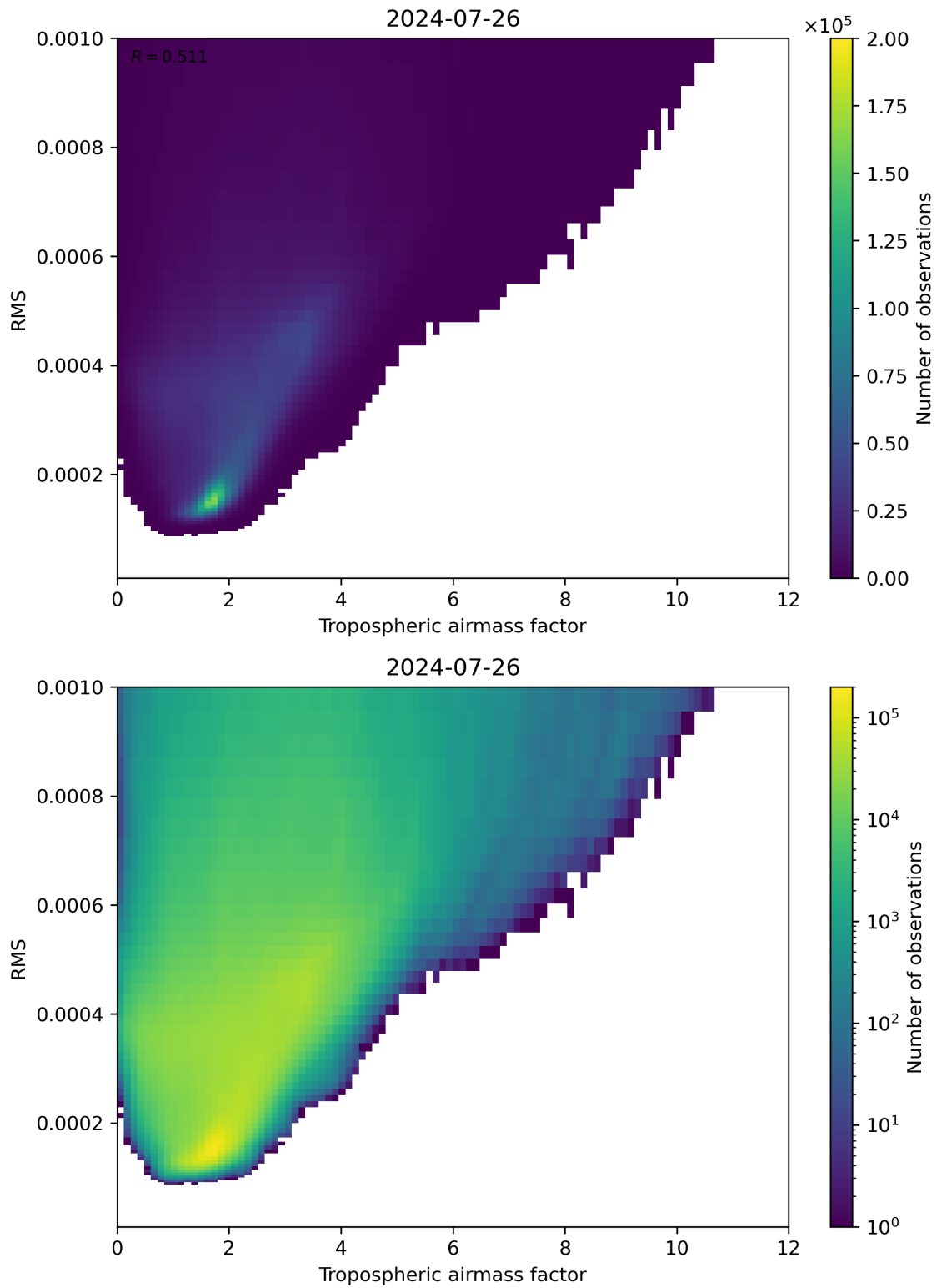
Figure 79: Scatter density plot of “Tropospheric airmass factor” against “RMS” for 2024-07-26 to 2024-07-27.
