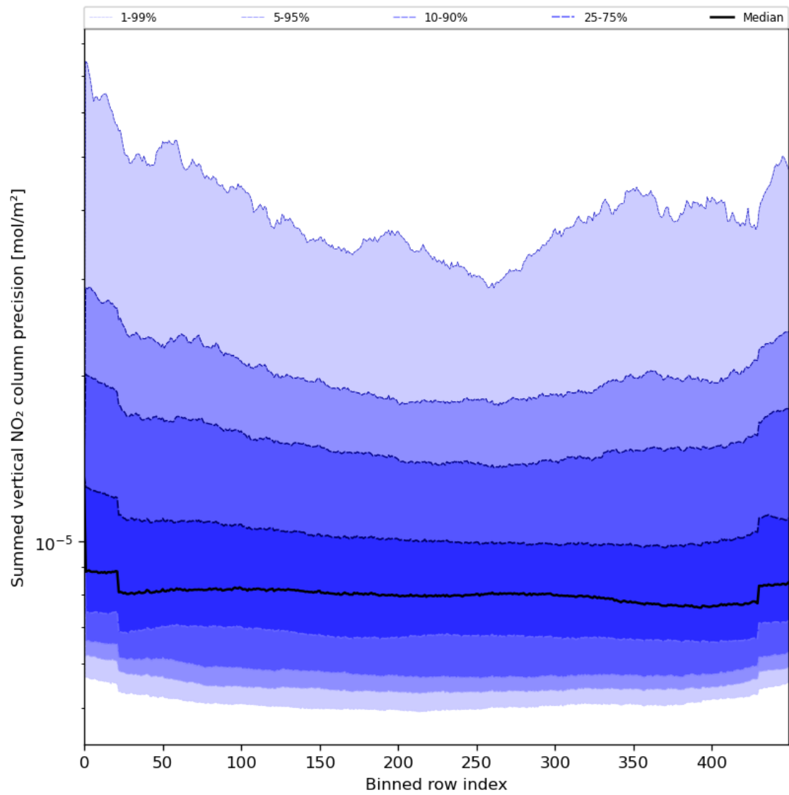
Figure 58: Along track statistics of “Summed vertical NO 2 column precision” for 2024-07-26 to 2024-07-27
