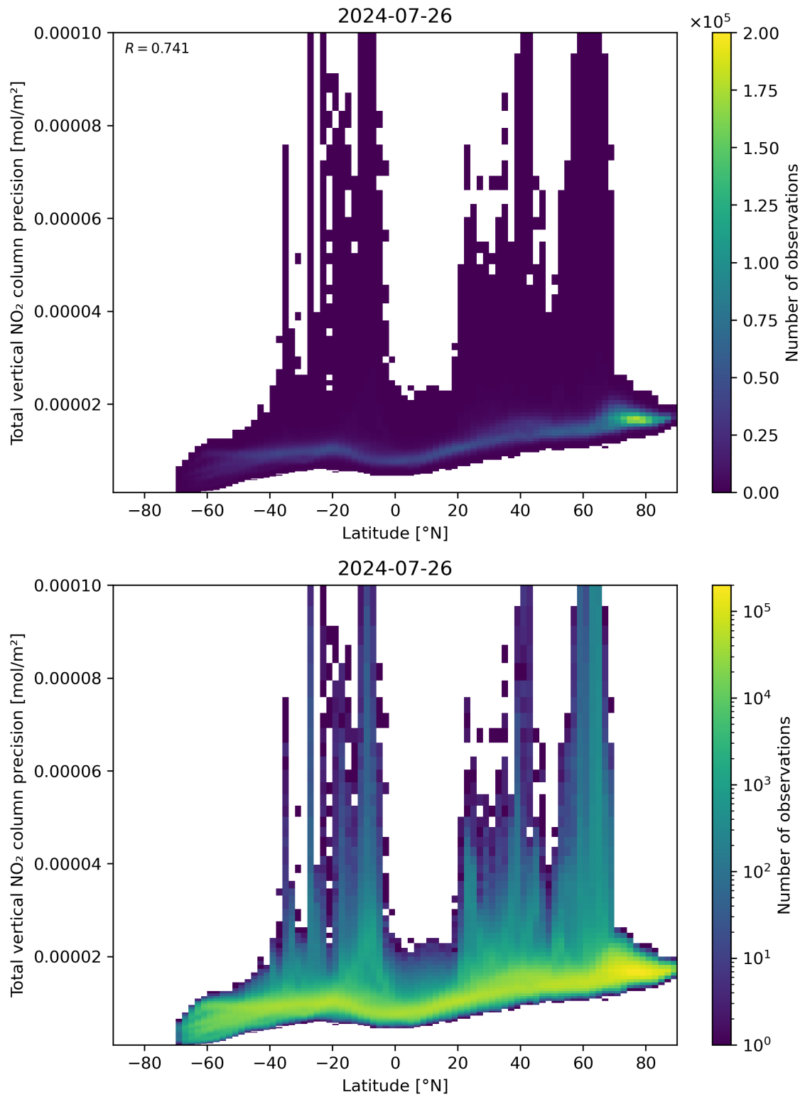
Figure 91: Scatter density plot of “Latitude” against “Total vertical NO 2 column precision” for 2024-07-26 to 2024-07-27.
