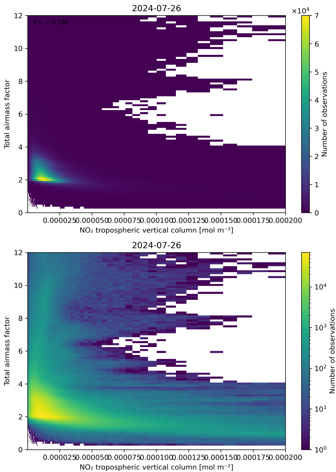
Figure 122: Scatter density plot of “NO 2 tropospheric vertical column” against “Total air mass factor” for 2024-07-26 to 2024-07-27.
