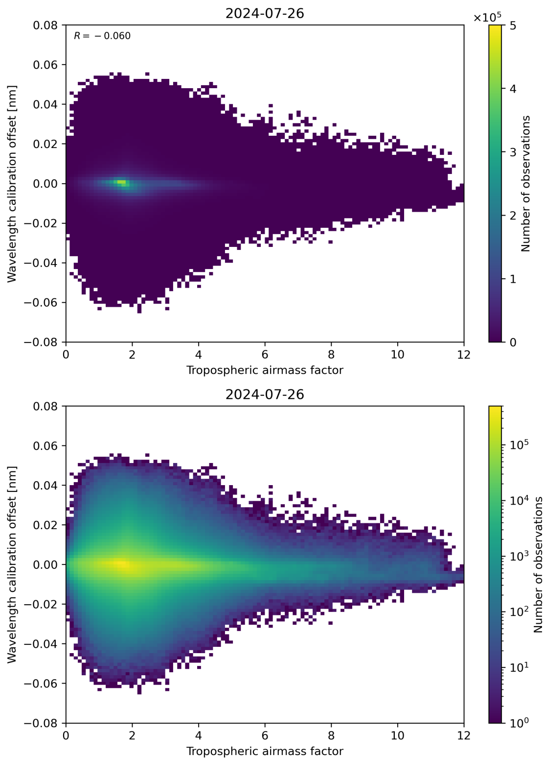
Figure 80: Scatter density plot of “Tropospheric air mass factor” against “Wavelength calibration offset” for 2024-07-26 to 2024-07-27.
