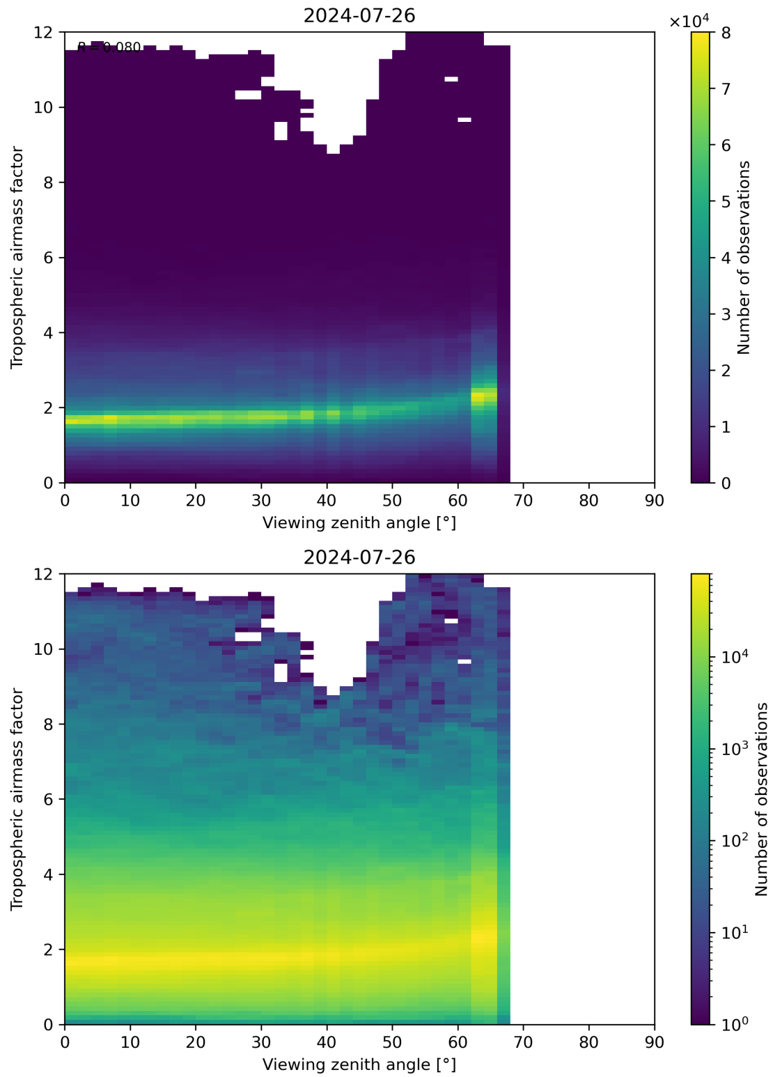
Figure 161: Scatter density plot of “Viewing zenith angle” against “Tropospheric airmass factor” for 2024-07-26 to 2024-07-27.
