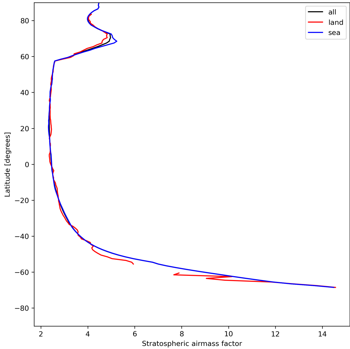
Figure 27: Zonal average of “Stratospheric air mass factor” for 2024-07-26 to 2024-07-27.
