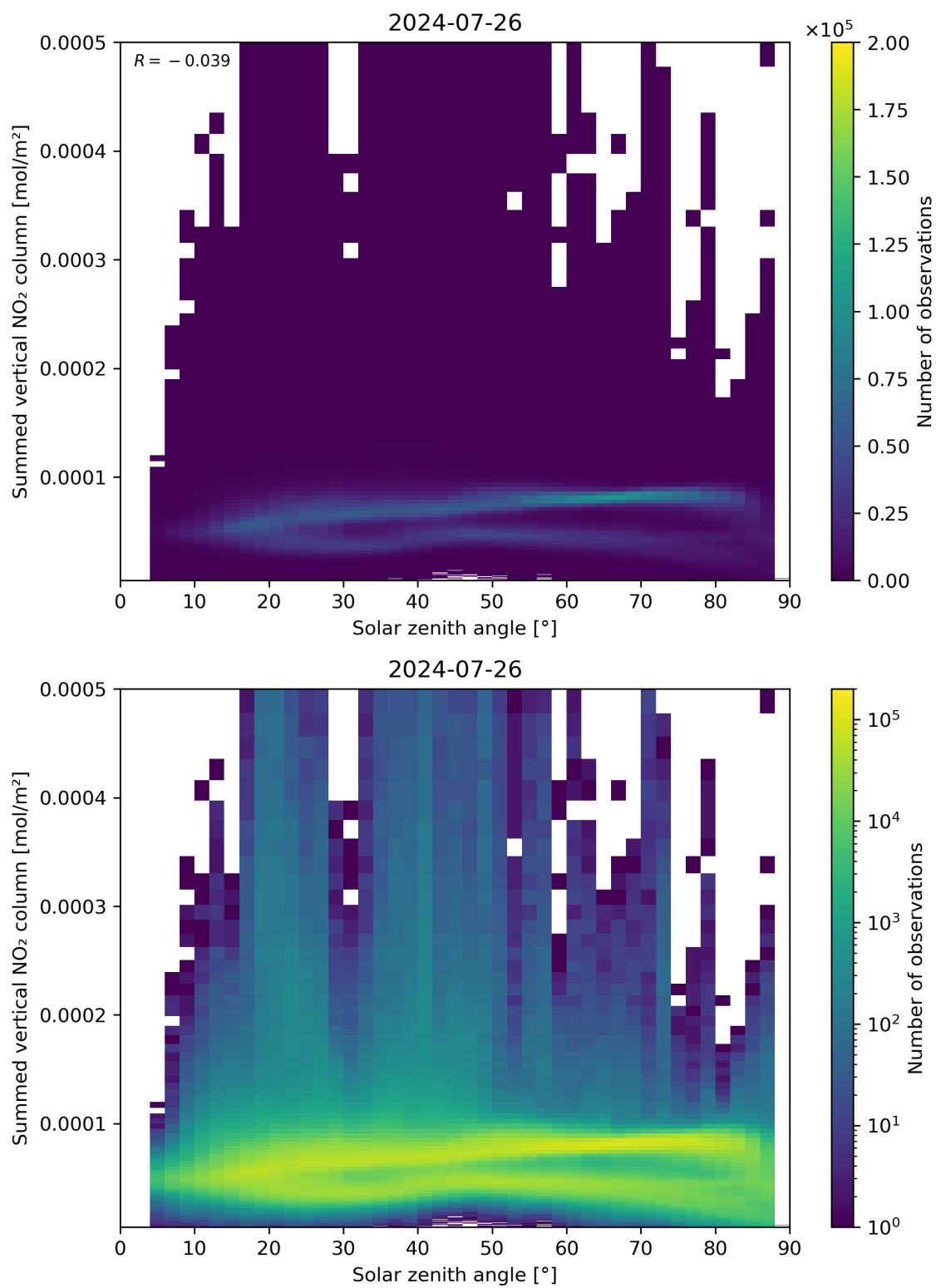
Figure 151: Scatter density plot of “Solar zenith angle” against “Summed vertical NO 2 column” for 2024-07-26 to 2024-07-27.
