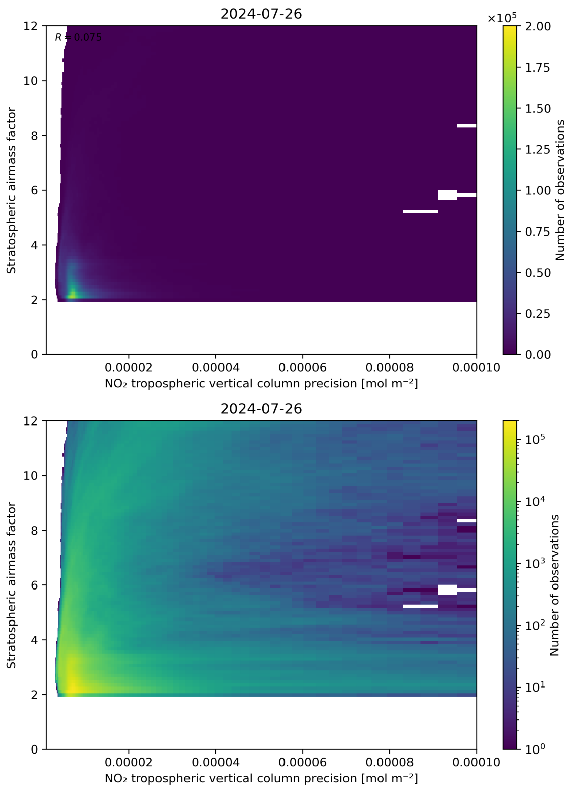
Figure 131: Scatter density plot of “NO 2 tropospheric vertical column precision” against “Stratospheric airmass factor” for 2024-07-26 to 2024-07-27.
