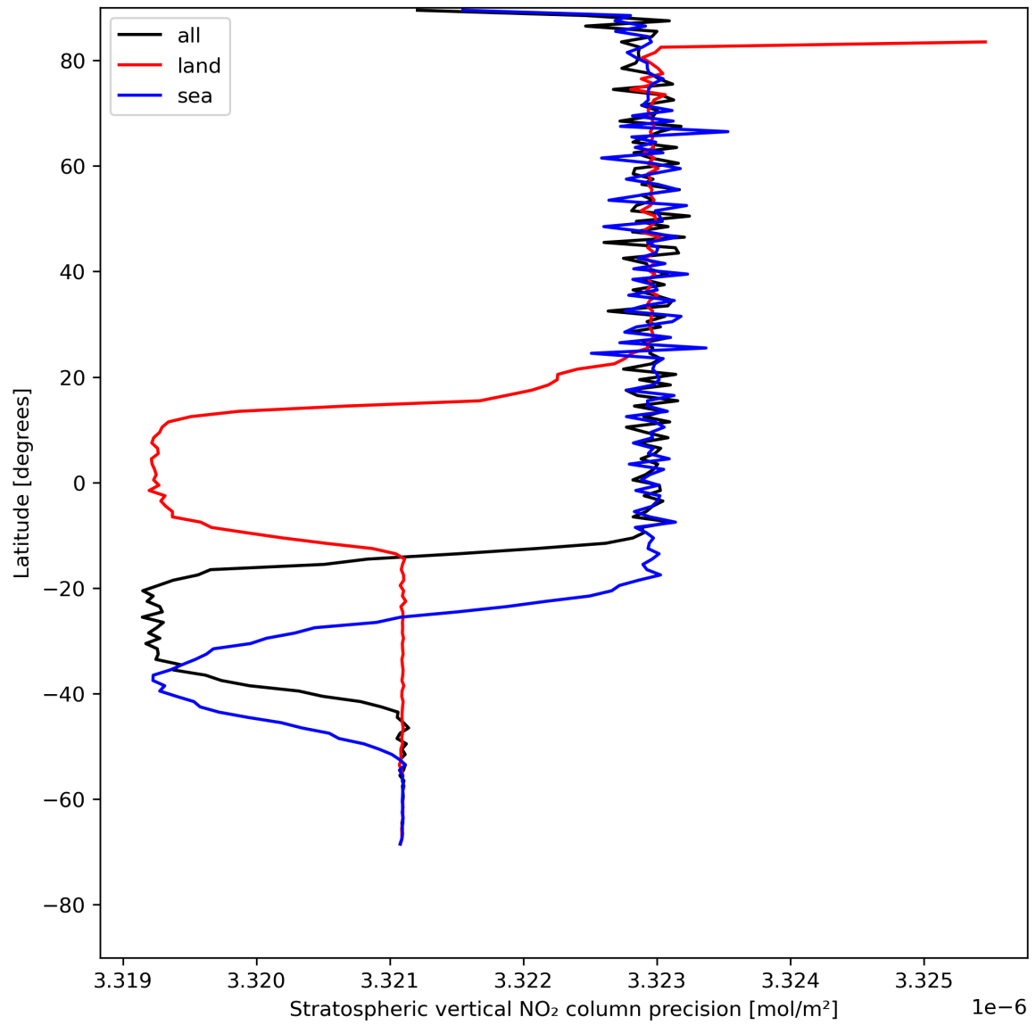
Figure 20: Zonal average of “Stratospheric vertical NO 2 column precision” for 2024-07-26 to 2024-07-27.
