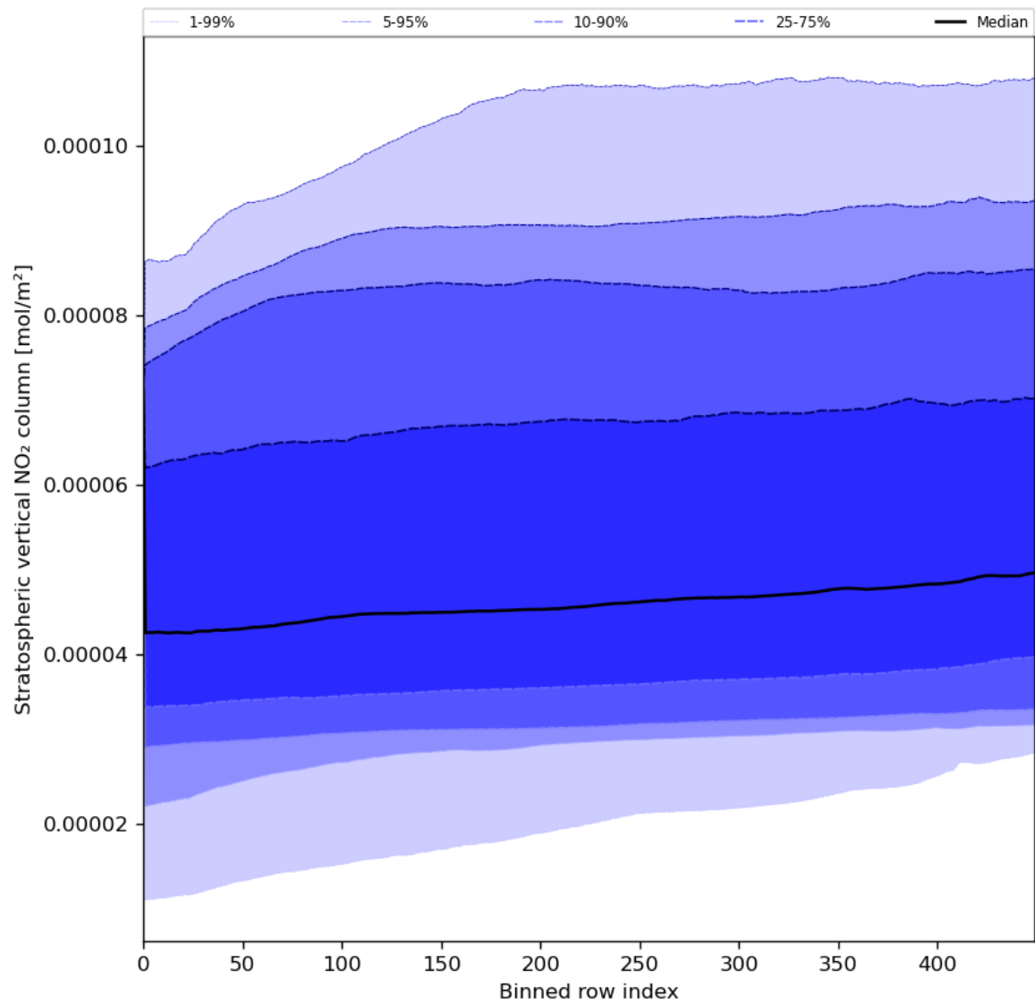
Figure 53: Along track statistics of “Stratospheric vertical NO 2 column” for 2024-07-26 to 2024-07-27
