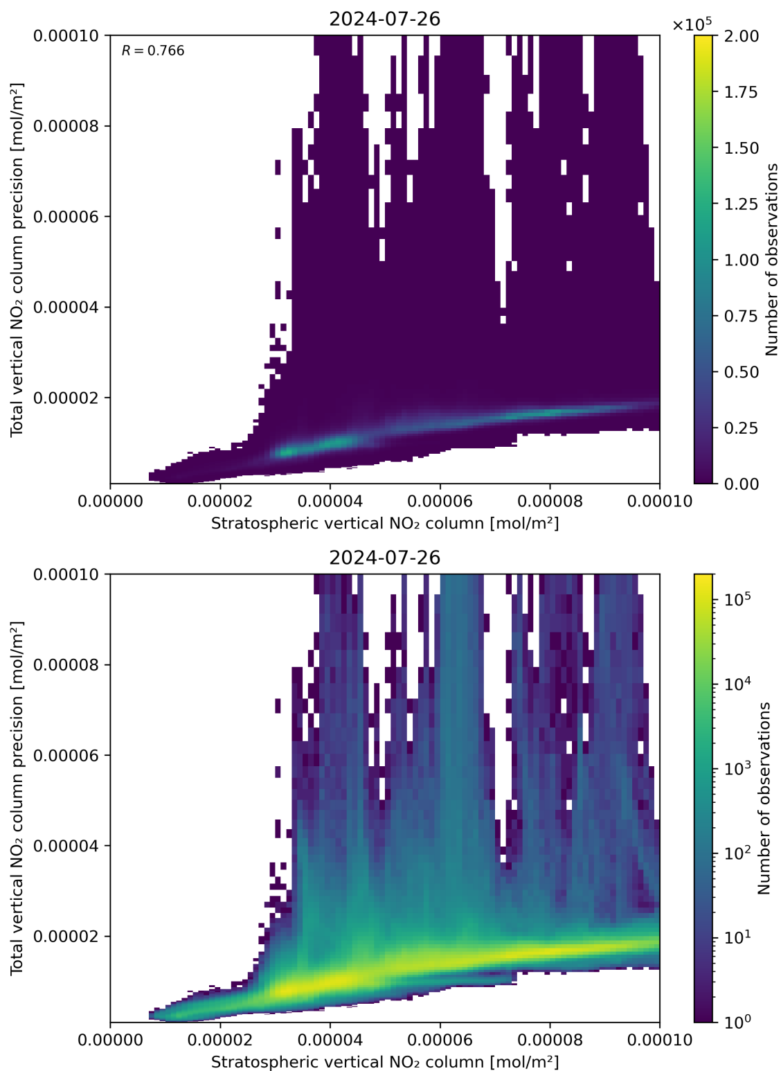
Figure 101: Scatter density plot of “Stratospheric vertical NO 2 column” against “Total vertical NO 2 column precision” for 2024-07-26 to 2024-07-27.
