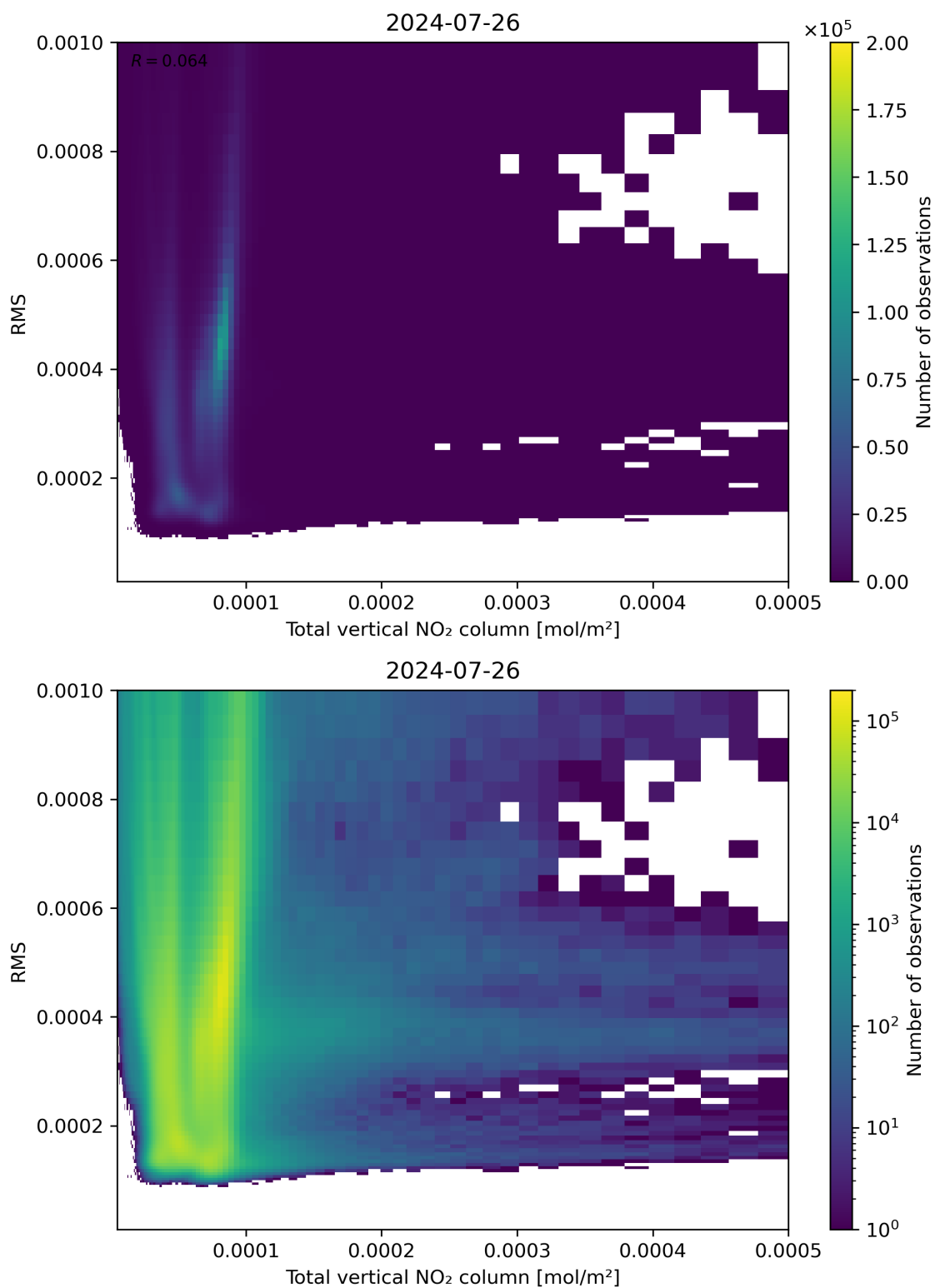
Figure 120: Scatter density plot of “Total vertical NO 2 column” against “RMS” for 2024-07-26 to 2024-07-27.
