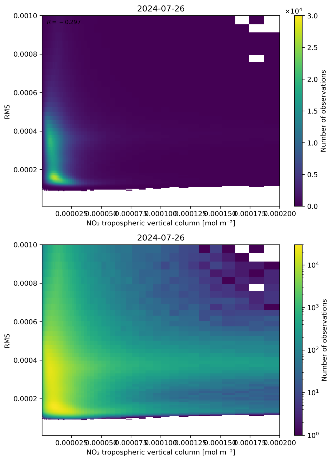
Figure 142: Scatter density plot of “NO 2 tropospheric vertical column” against “RMS” for 2024-07-26 to 2024-07-27.
