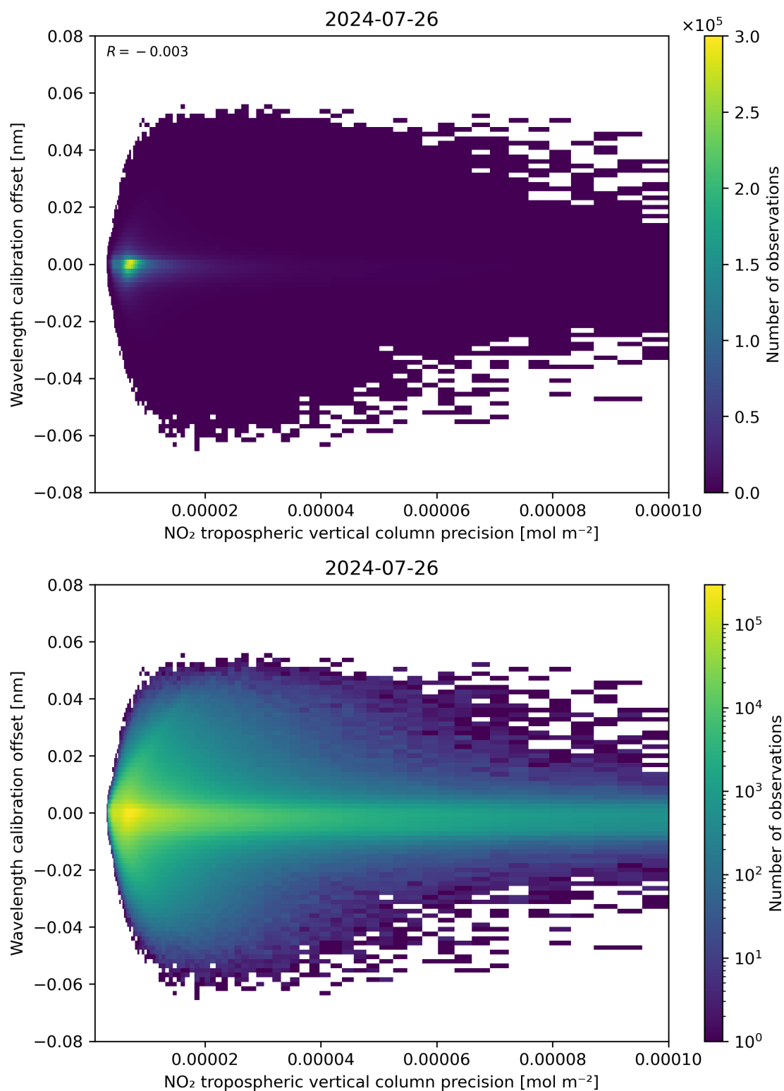
Figure 141: Scatter density plot of “NO 2 tropospheric vertical column precision” against “Wavelength calibration offset” for 2024-07-26 to 2024-07-27.
