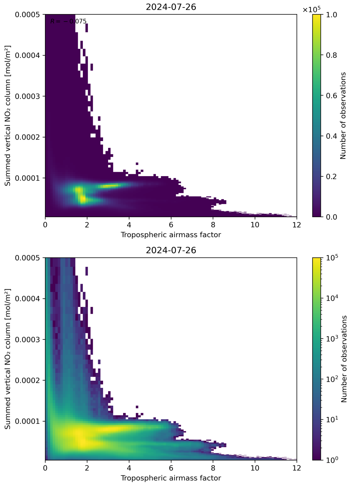
Figure 75: Scatter density plot of “Tropospheric airmass factor” against “Summed vertical NO 2 column” for 2024-07-26 to 2024-07-27.
