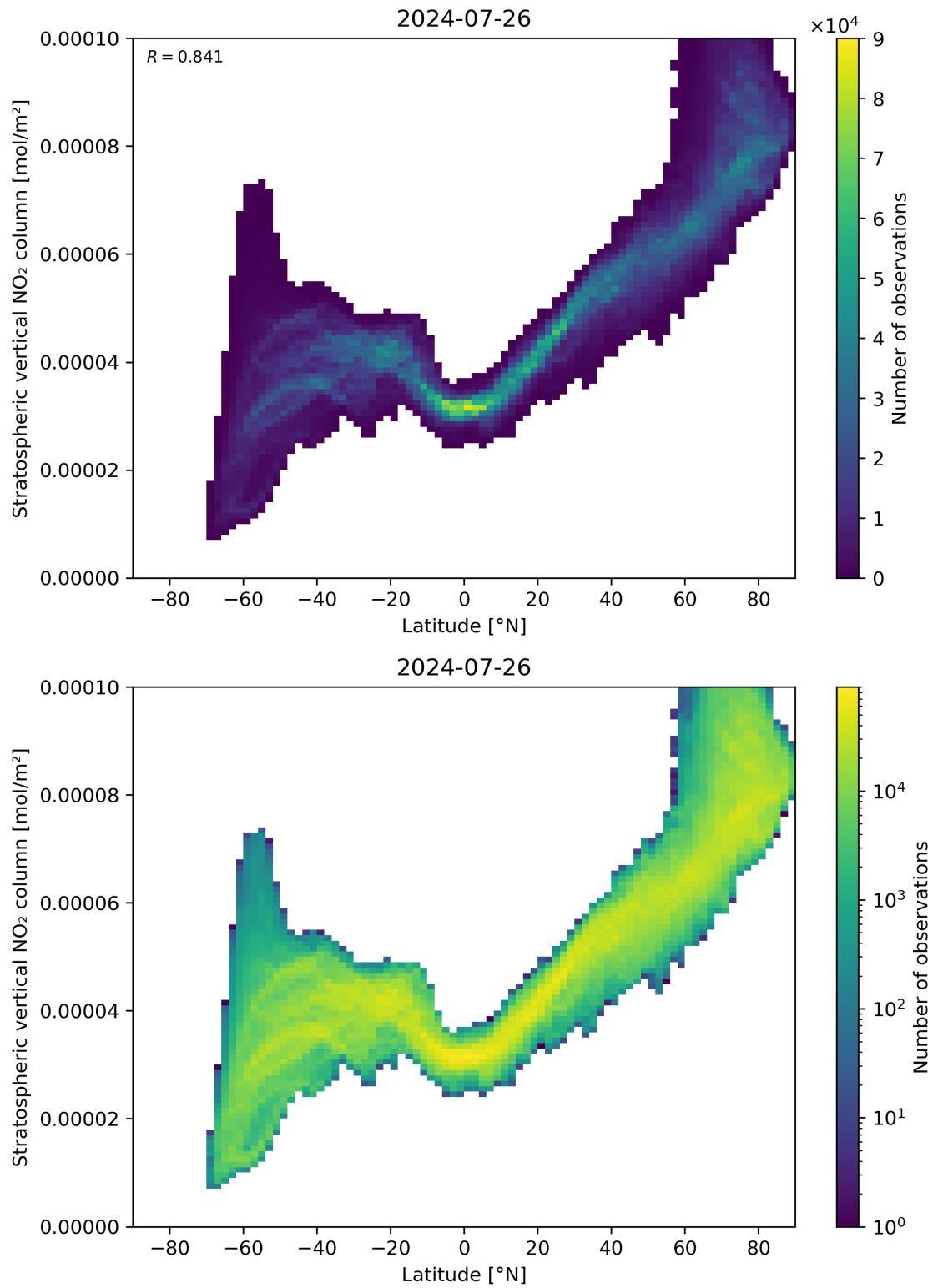
Figure 87: Scatter density plot of “Latitude” against “Stratospheric vertical NO 2 column” for 2024-07-26 to 2024-07-27.
