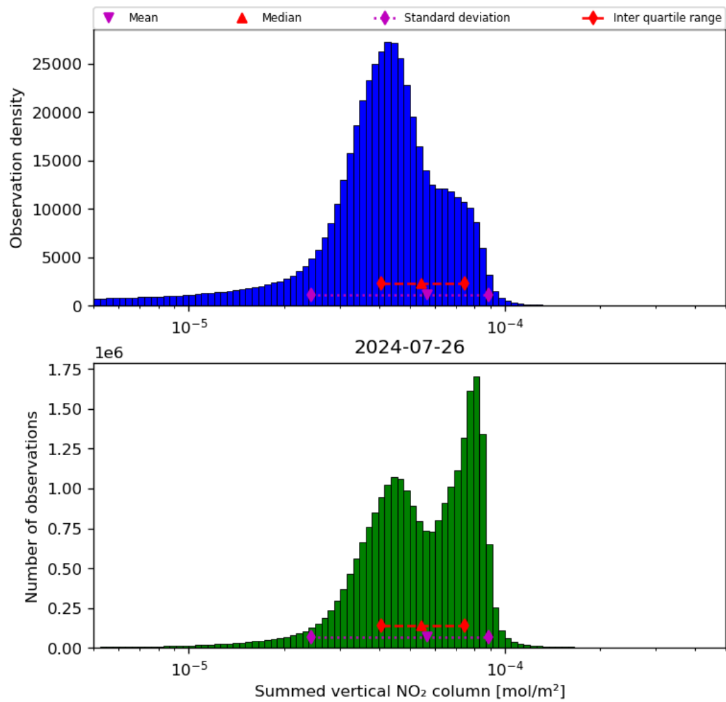
Figure 40: Histogram of “Summed vertical NO 2 column” for 2024-07-26 to 2024-07-27
