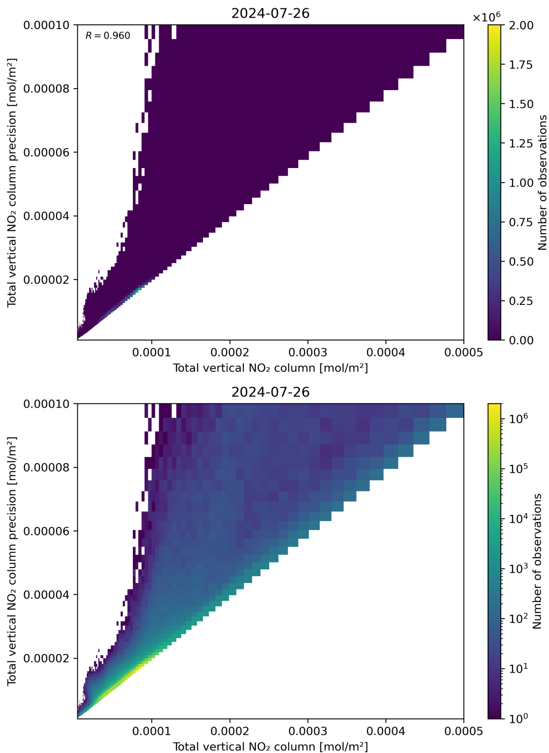
Figure 114: Scatter density plot of “Total vertical NO 2 column” against “Total vertical NO 2 column precision” for 2024-07-26 to 2024-07-27.
