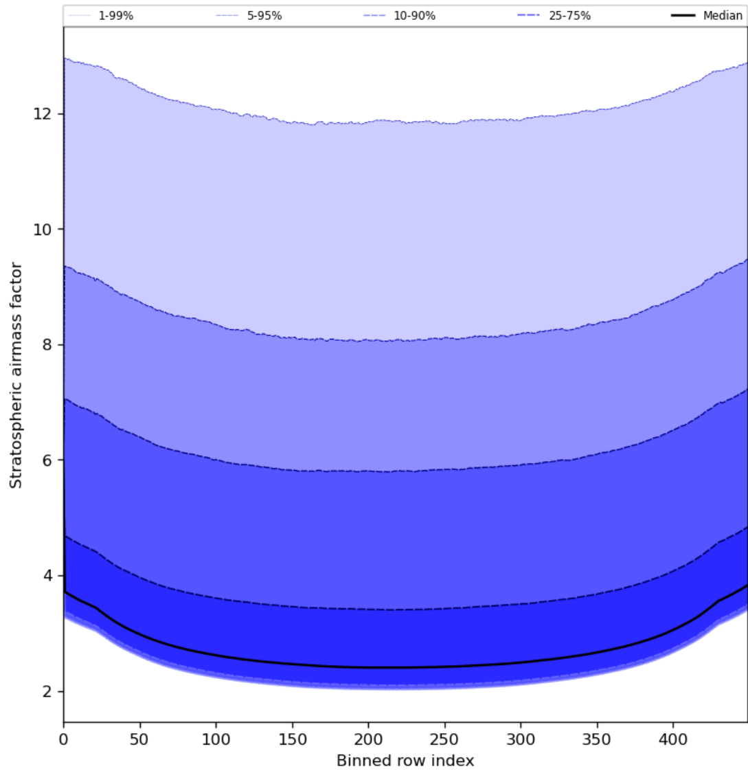
Figure 61: Along track statistics of “Stratospheric air mass factor” for 2024-07-26 to 2024-07-27
