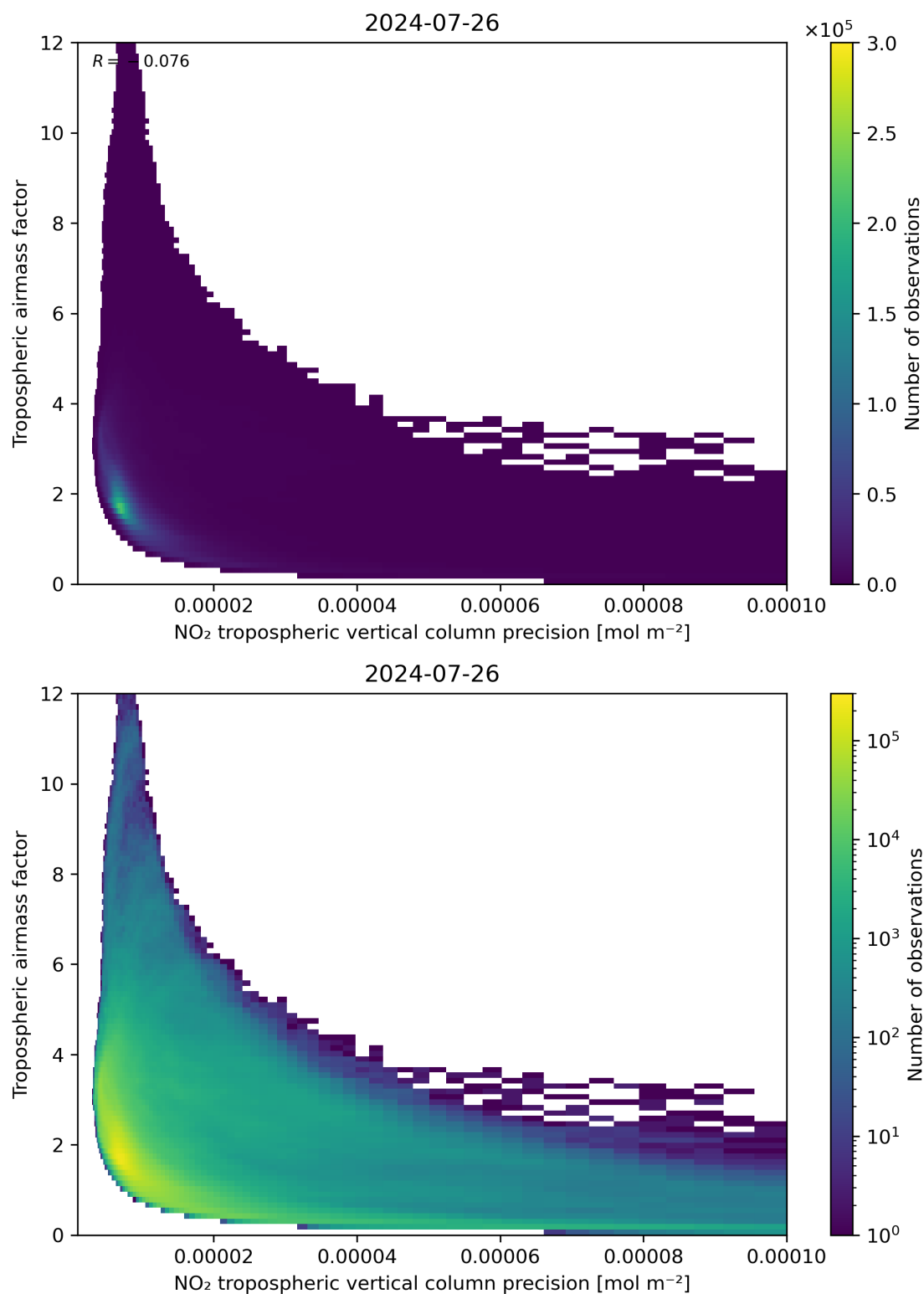
Figure 133: Scatter density plot of “NO 2 tropospheric vertical column precision” against “Tropospheric air mass factor” for 2024-07-26 to 2024-07-27.
