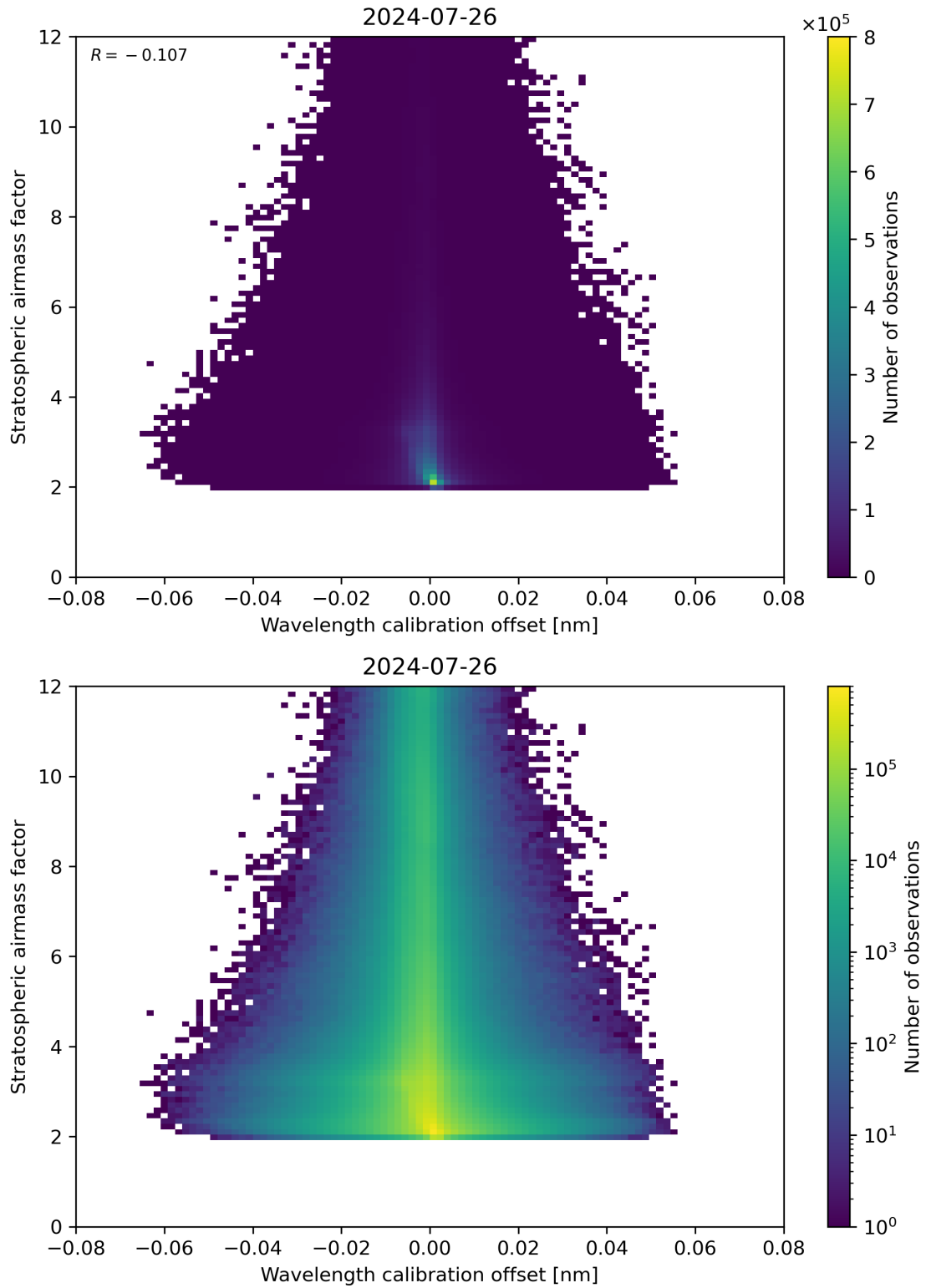
Figure 174: Scatter density plot of “Wavelength calibration offset” against “Stratospheric airmass factor” for 2024-07-26 to 2024-07-27.
