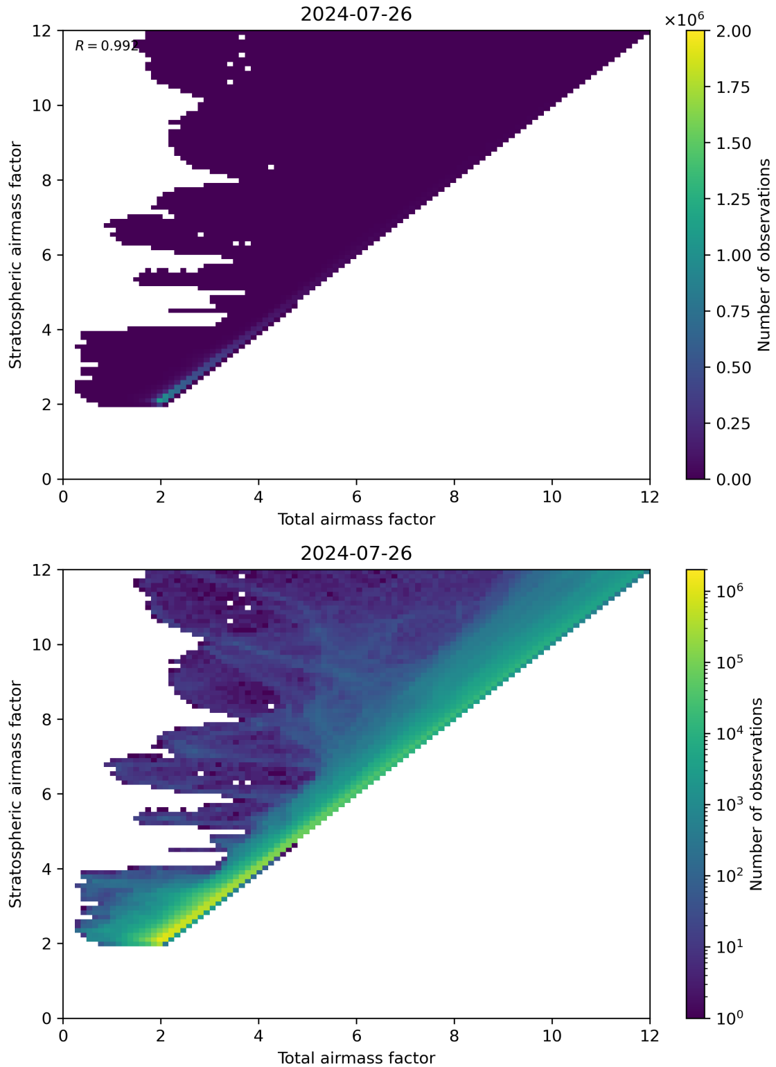
Figure 62: Scatter density plot of “Total air mass factor” against “Stratospheric air mass factor” for 2024-07-26 to 2024-07-27.
