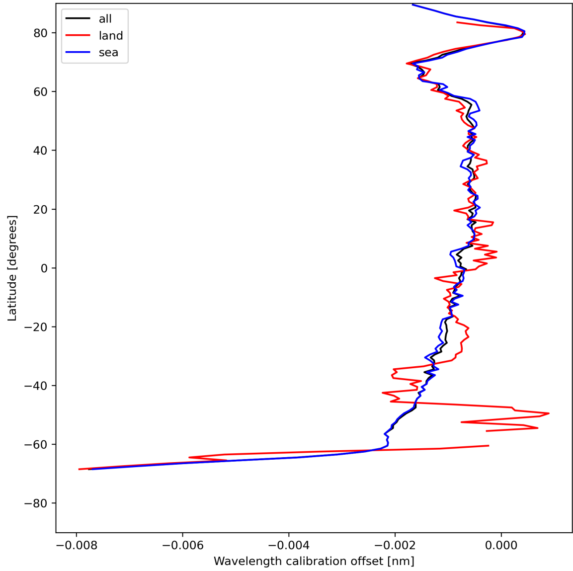
Figure 18: Zonal average of “Wavelength calibration offset” for 2024-07-26 to 2024-07-27.
