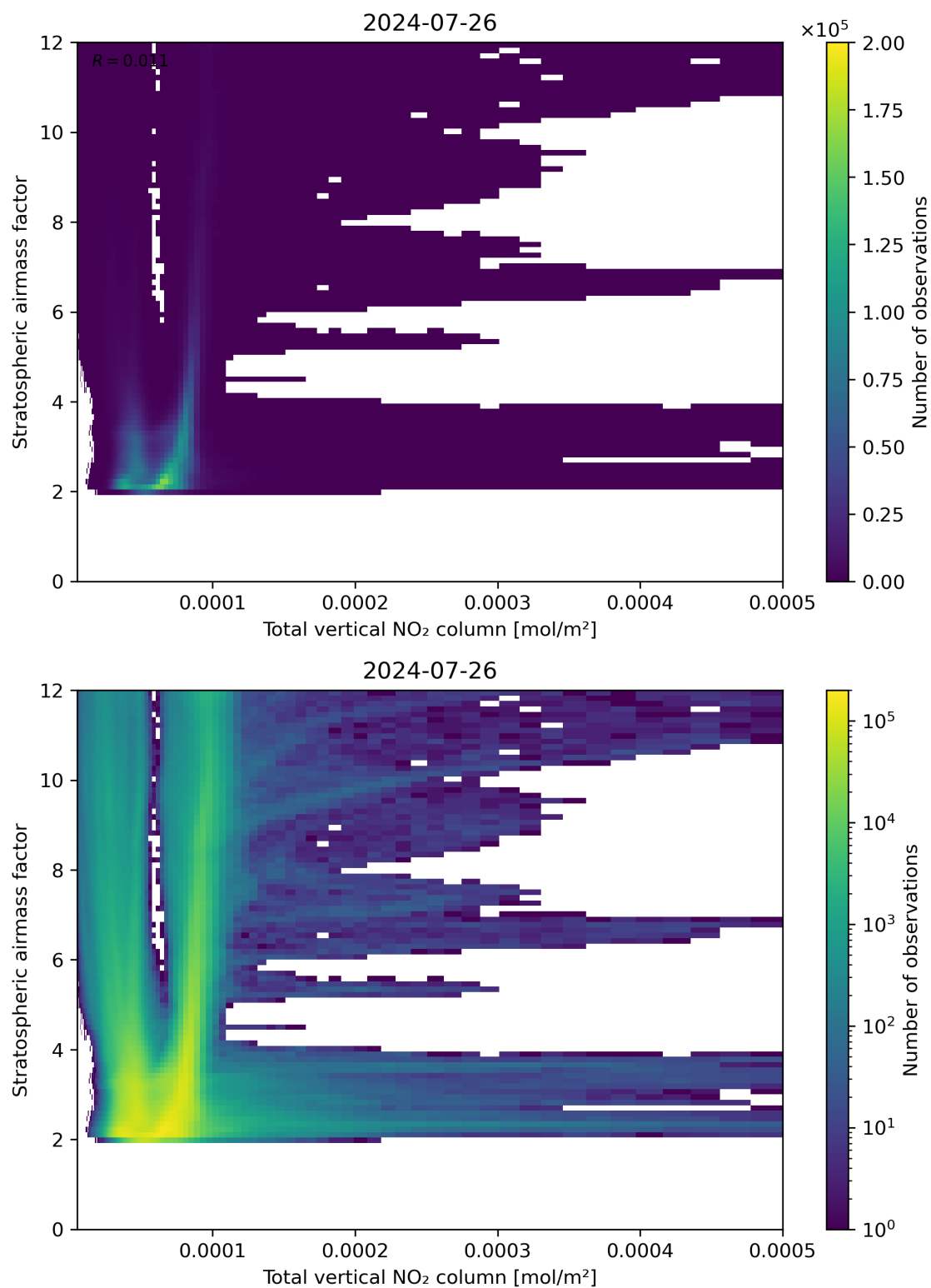
Figure 110: Scatter density plot of “Total vertical NO 2 column” against “Stratospheric air mass factor” for 2024-07-26 to 2024-07-27.
