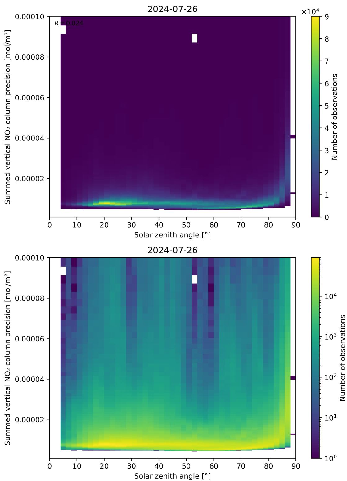
Figure 152: Scatter density plot of “Solar zenith angle” against “Summed vertical NO 2 column precision” for 2024-07-26 to 2024-07-27.
