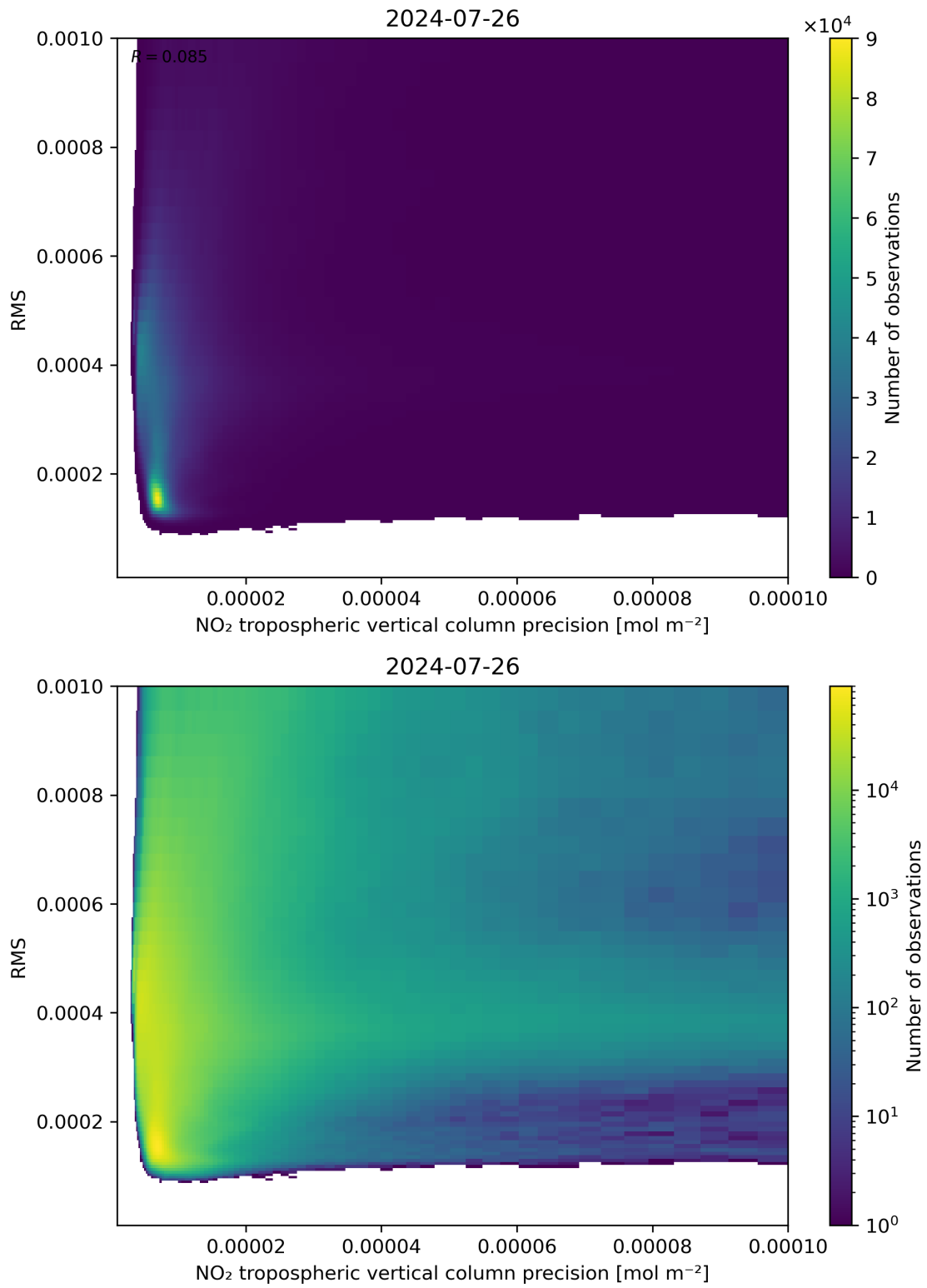
Figure 140: Scatter density plot of “NO 2 tropospheric vertical column precision” against “RMS” for 2024-07-26 to 2024-07-27.
