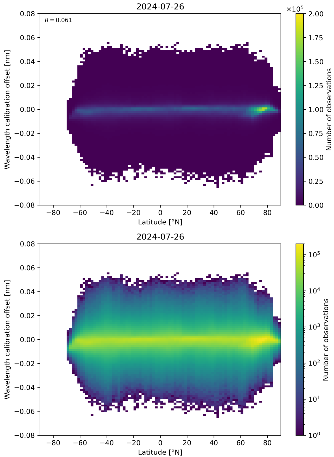
Figure 95: Scatter density plot of “Latitude” against “Wavelength calibration offset” for 2024-07-26 to 2024-07-27.
