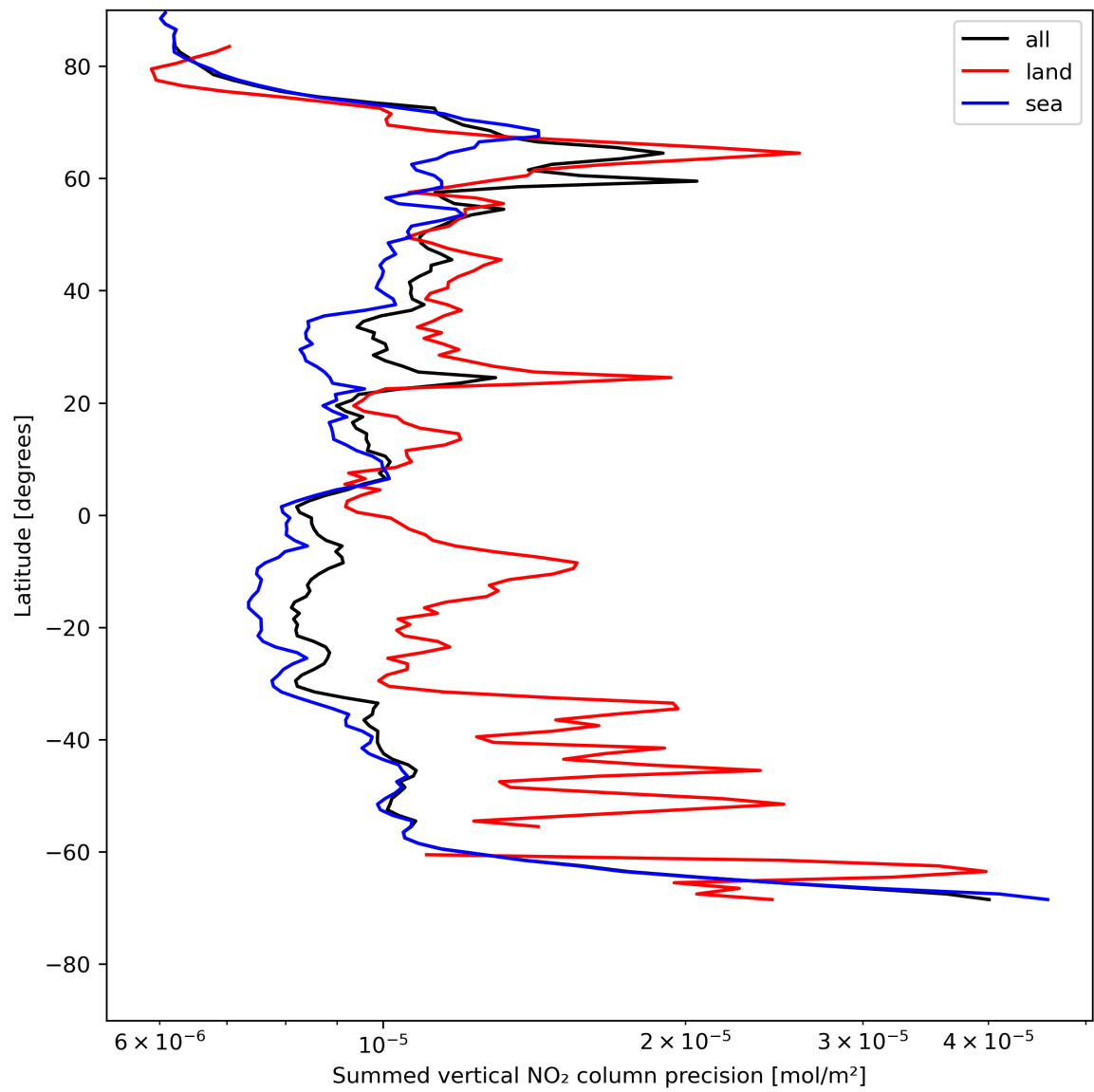
Figure 24: Zonal average of “Summed vertical NO 2 column precision” for 2024-07-26 to 2024-07-27.
