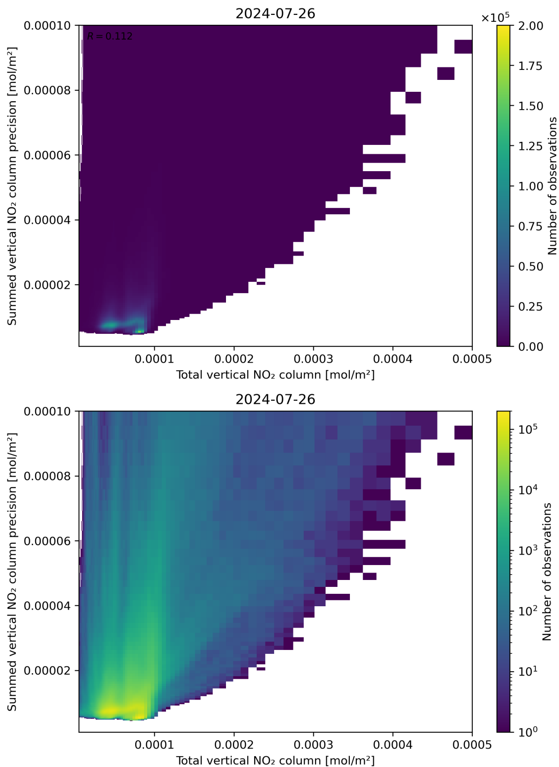
Figure 113: Scatter density plot of “Total vertical NO 2 column” against “Summed vertical NO 2 column precision” for 2024-07-26 to 2024-07-27.
