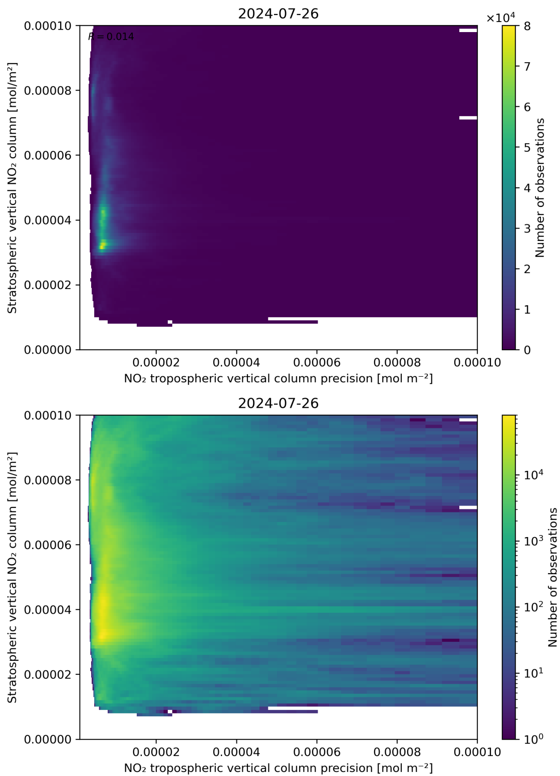
Figure 135: Scatter density plot of “NO 2 tropospheric vertical column precision” against “Stratospheric vertical NO 2 column” for 2024-07-26 to 2024-07-27.
