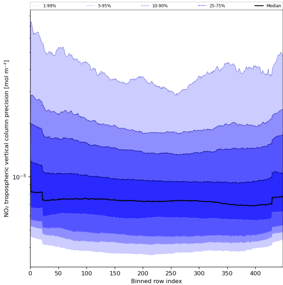
Figure 47: Along track statistics of “NO 2 tropospheric vertical column precision” for 2024-07-26 to 2024-07-27
