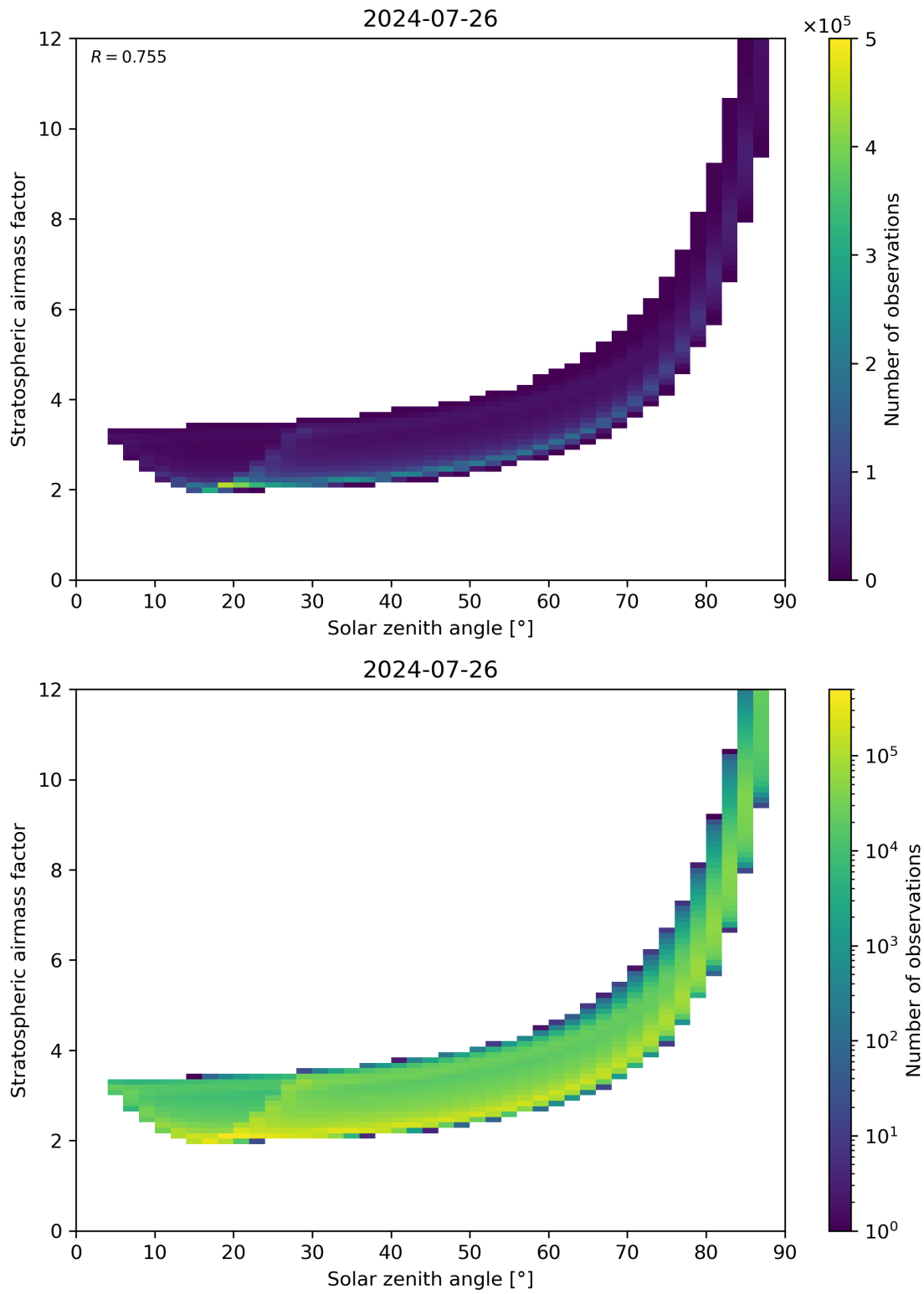
Figure 145: Scatter density plot of “Solar zenith angle” against “Stratospheric airmass factor” for 2024-07-26 to 2024-07-27.
