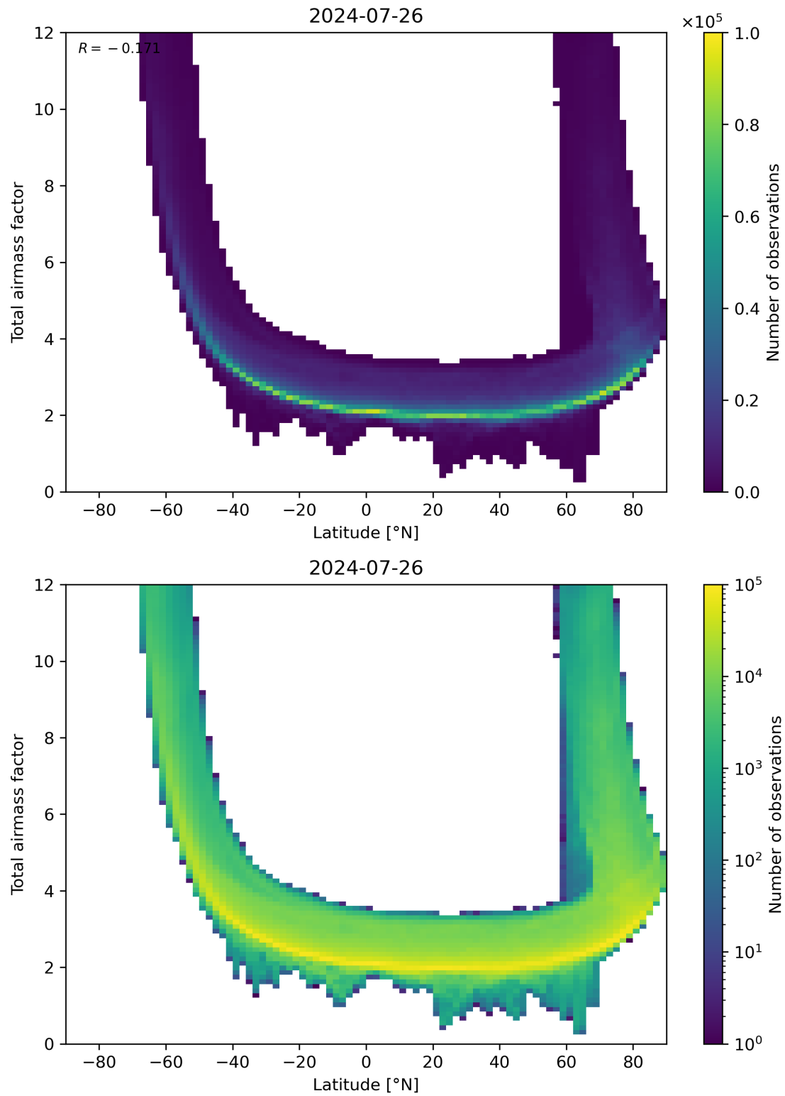
Figure 84: Scatter density plot of “Latitude” against “Total airmass factor” for 2024-07-26 to 2024-07-27.
