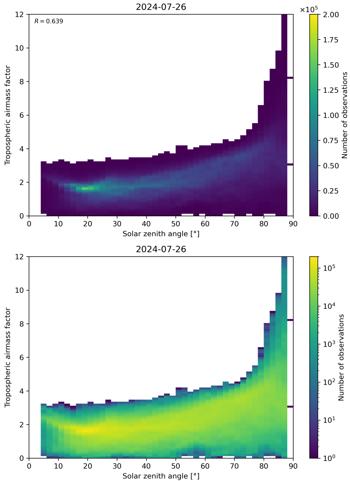
Figure 147: Scatter density plot of “Solar zenith angle” against “Tropospheric airmass factor” for 2024-07-26 to 2024-07-27.
