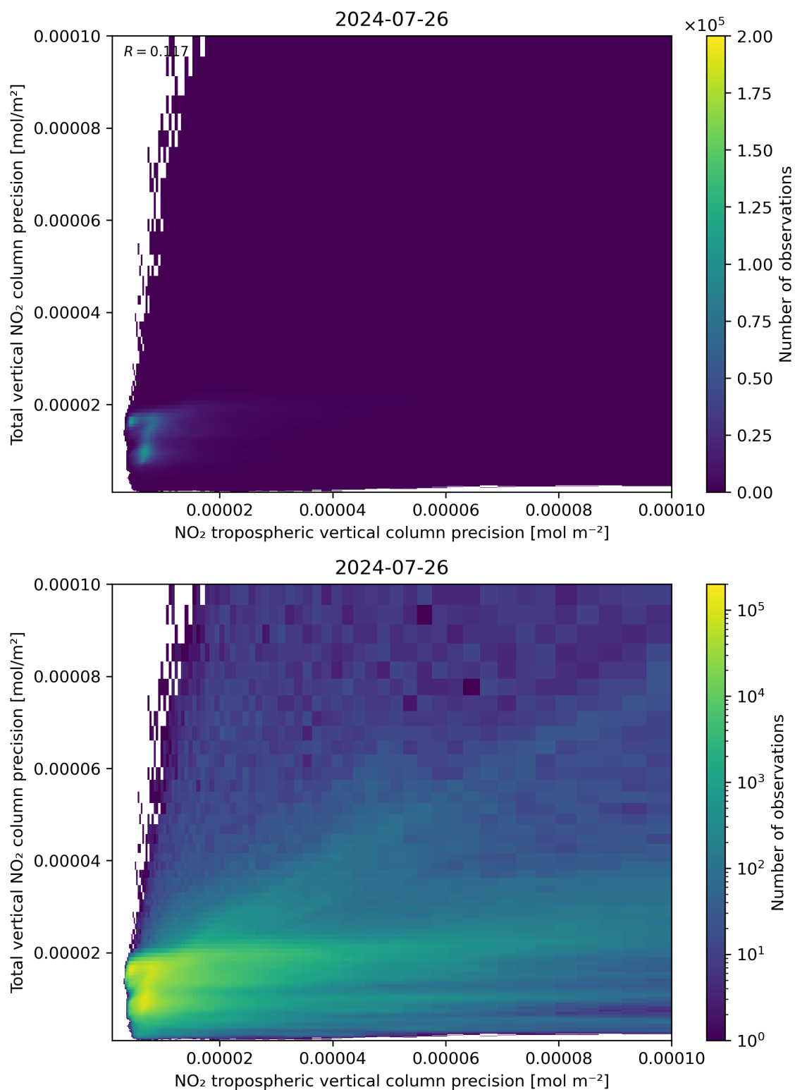
Figure 139: Scatter density plot of “NO 2 tropospheric vertical column precision” against “Total vertical NO 2 column precision” for 2024-07-26 to 2024-07-27.
