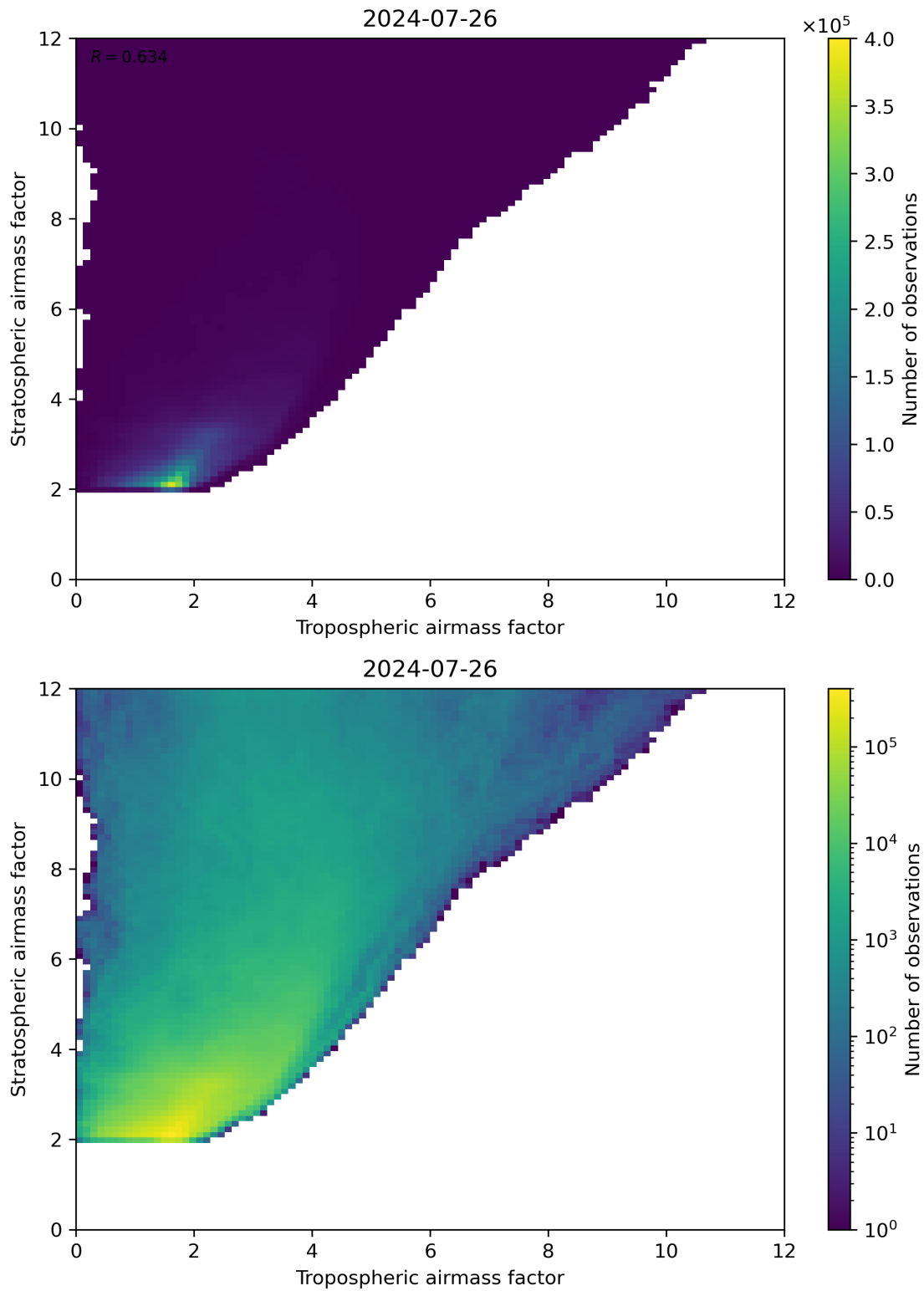
Figure 71: Scatter density plot of “Tropospheric airmass factor” against “Stratospheric airmass factor” for 2024-07-26 to 2024-07-27.
