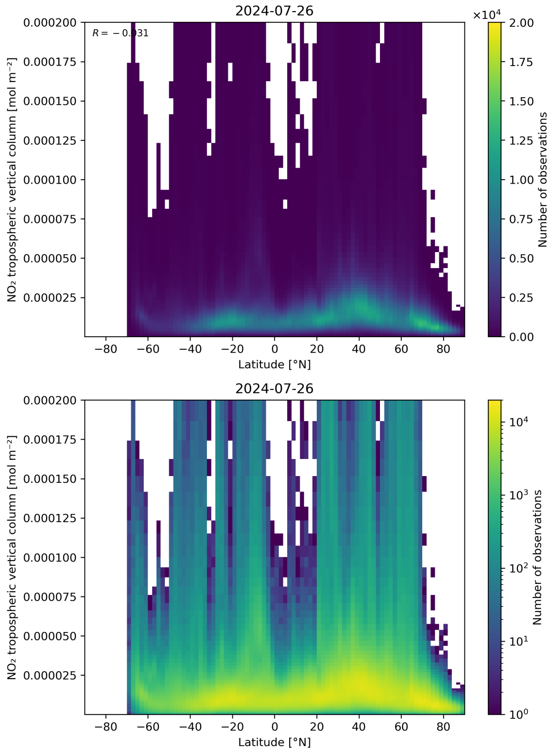
Figure 92: Scatter density plot of “Latitude” against “NO 2 tropospheric vertical column” for 2024-07-26 to 2024-07-27.
