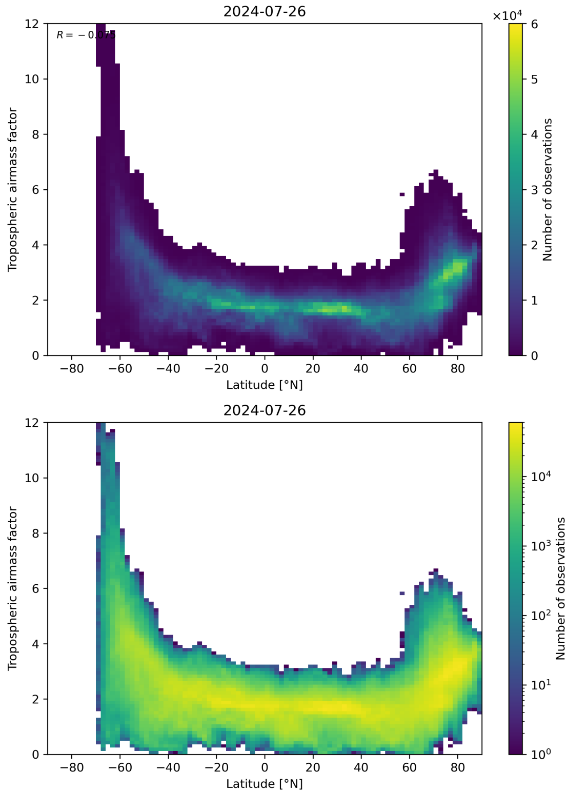
Figure 85: Scatter density plot of “Latitude” against “Tropospheric air mass factor” for 2024-07-26 to 2024-07-27.
