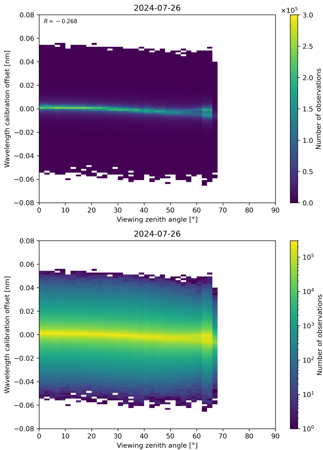
Figure 173: Scatter density plot of “Viewing zenith angle” against “Wavelength calibration offset” for 2024-07-26 to 2024-07-27.
