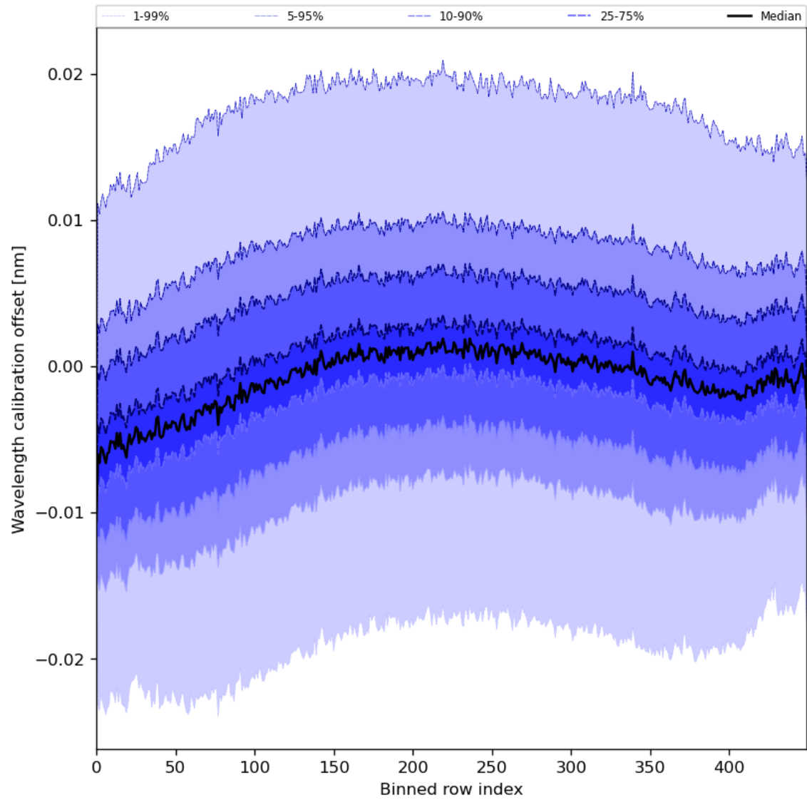
Figure 52: Along track statistics of “Wavelength calibration offset” for 2024-07-26 to 2024-07-27
