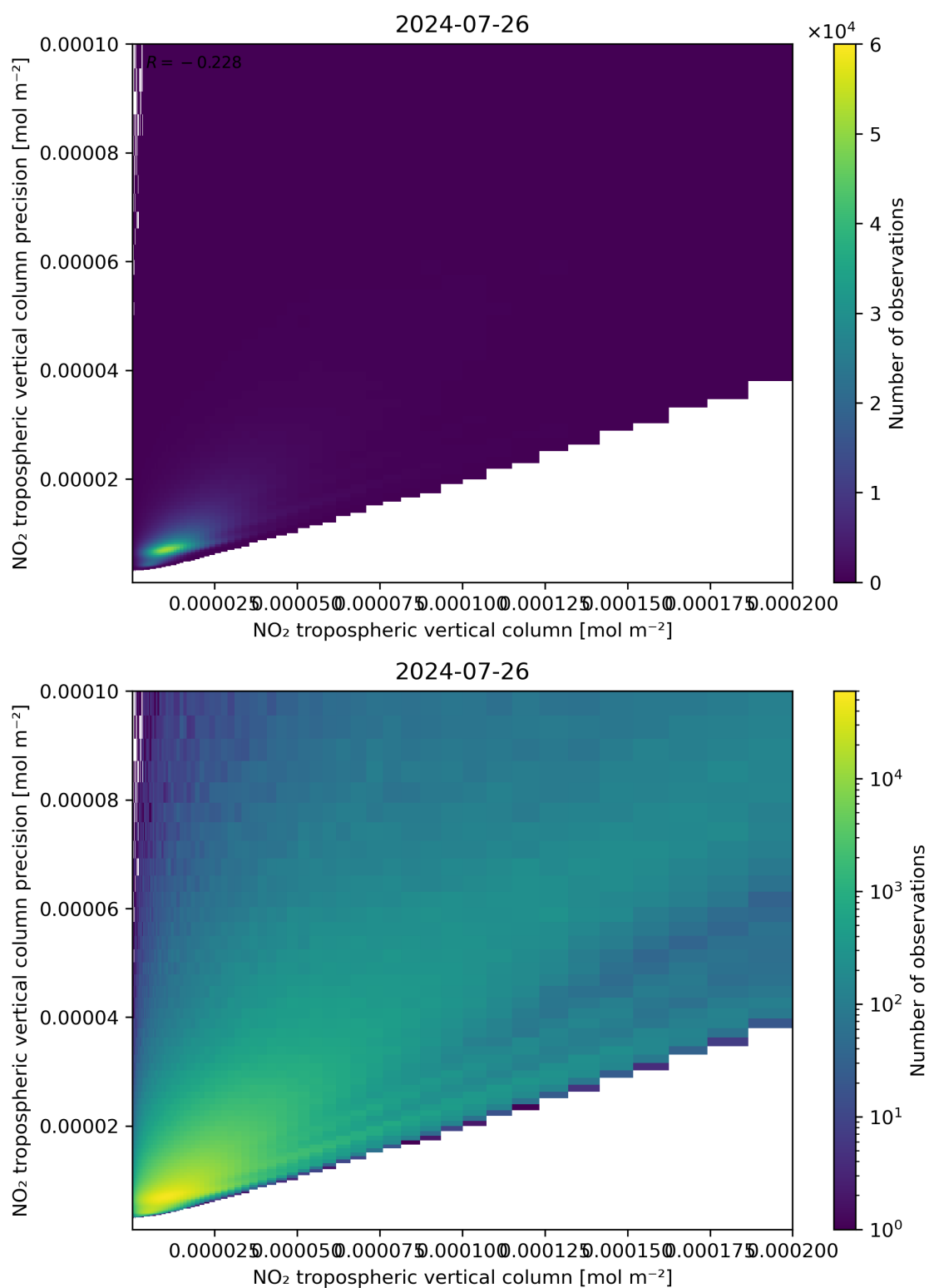
Figure 130: Scatter density plot of “NO 2 tropospheric vertical column” against “NO 2 tropospheric vertical column precision” for 2024-07-26 to 2024-07-27.
