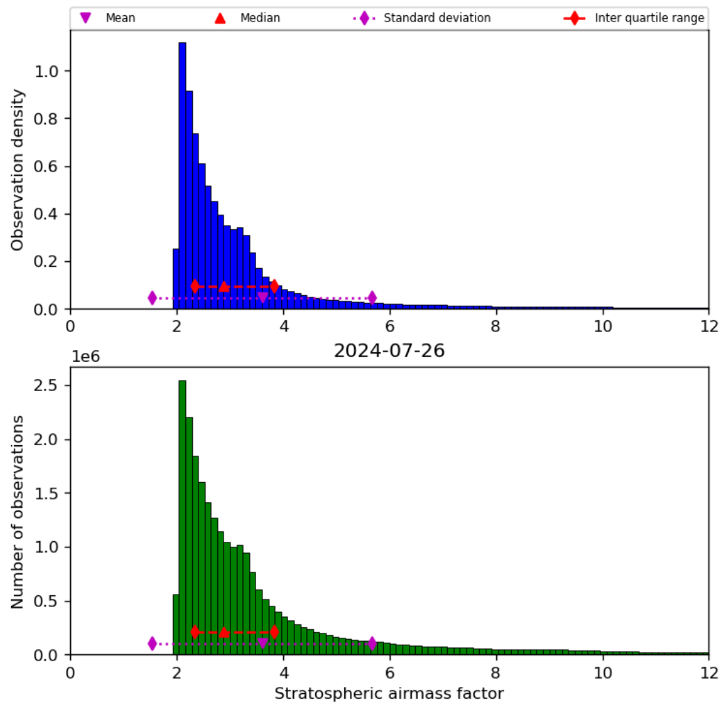
Figure 44: Histogram of “Stratospheric airmass factor” for 2024-07-26 to 2024-07-27
