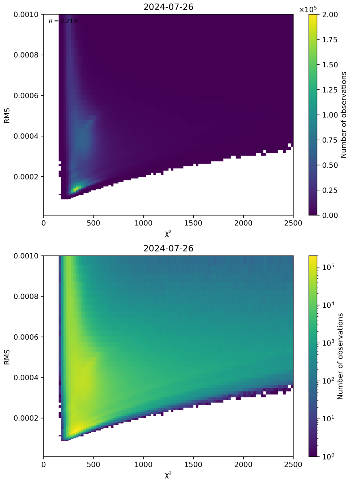
Figure 82: Scatter density plot of “ \chi^2 ” against “RMS” for 2024-07-26 to 2024-07-27.
