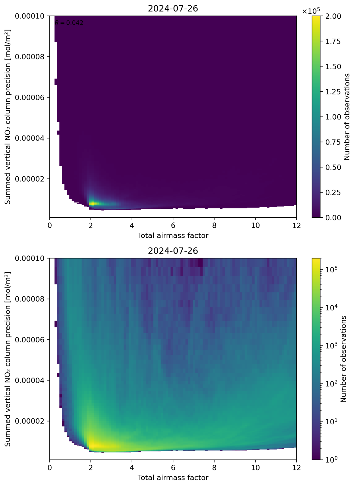
Figure 66: Scatter density plot of “Total airmass factor” against “Summed vertical NO 2 column precision” for 2024-07-26 to 2024-07-27.
