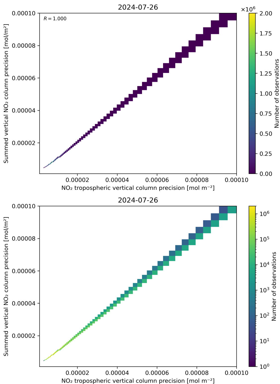
Figure 137: Scatter density plot of “NO 2 tropospheric vertical column precision” against “Summed vertical NO 2 column precision” for 2024-07-26 to 2024-07-27.
