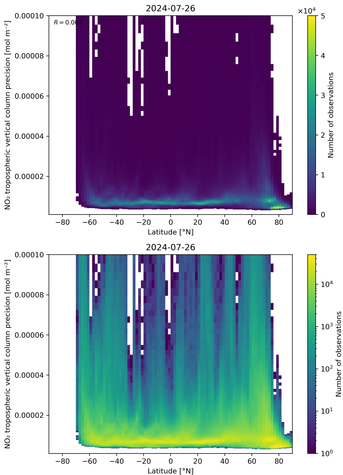
Figure 93: Scatter density plot of “Latitude” against “NO 2 tropospheric vertical column precision” for 2024-07-26 to 2024-07-27.
