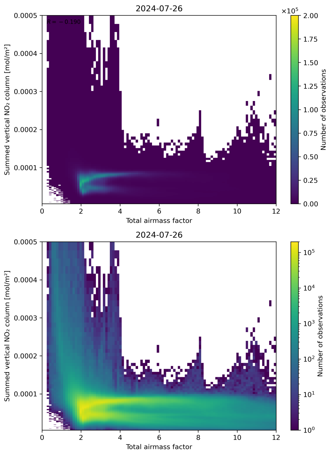
Figure 65: Scatter density plot of “Total airmass factor” against “Summed vertical NO 2 column” for 2024-07-26 to 2024-07-27.
