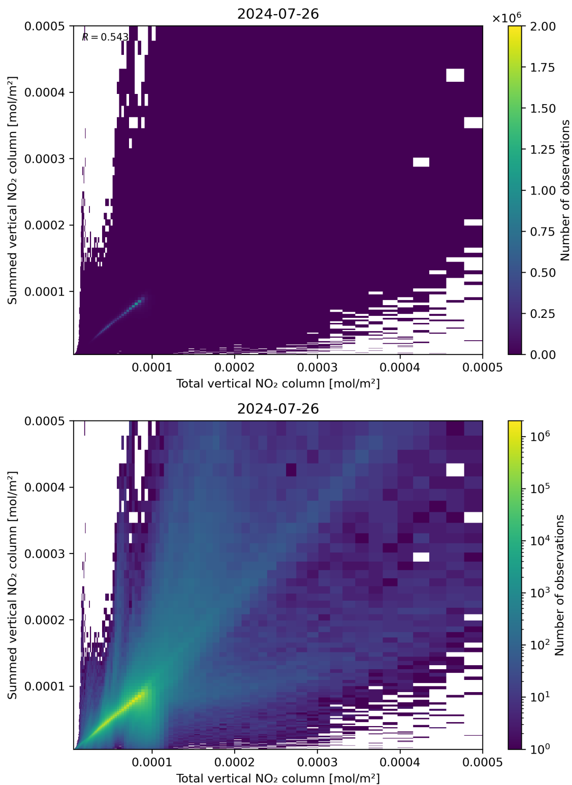
Figure 112: Scatter density plot of “Total vertical NO 2 column” against “Summed vertical NO 2 column” for 2024-07-26 to 2024-07-27.
