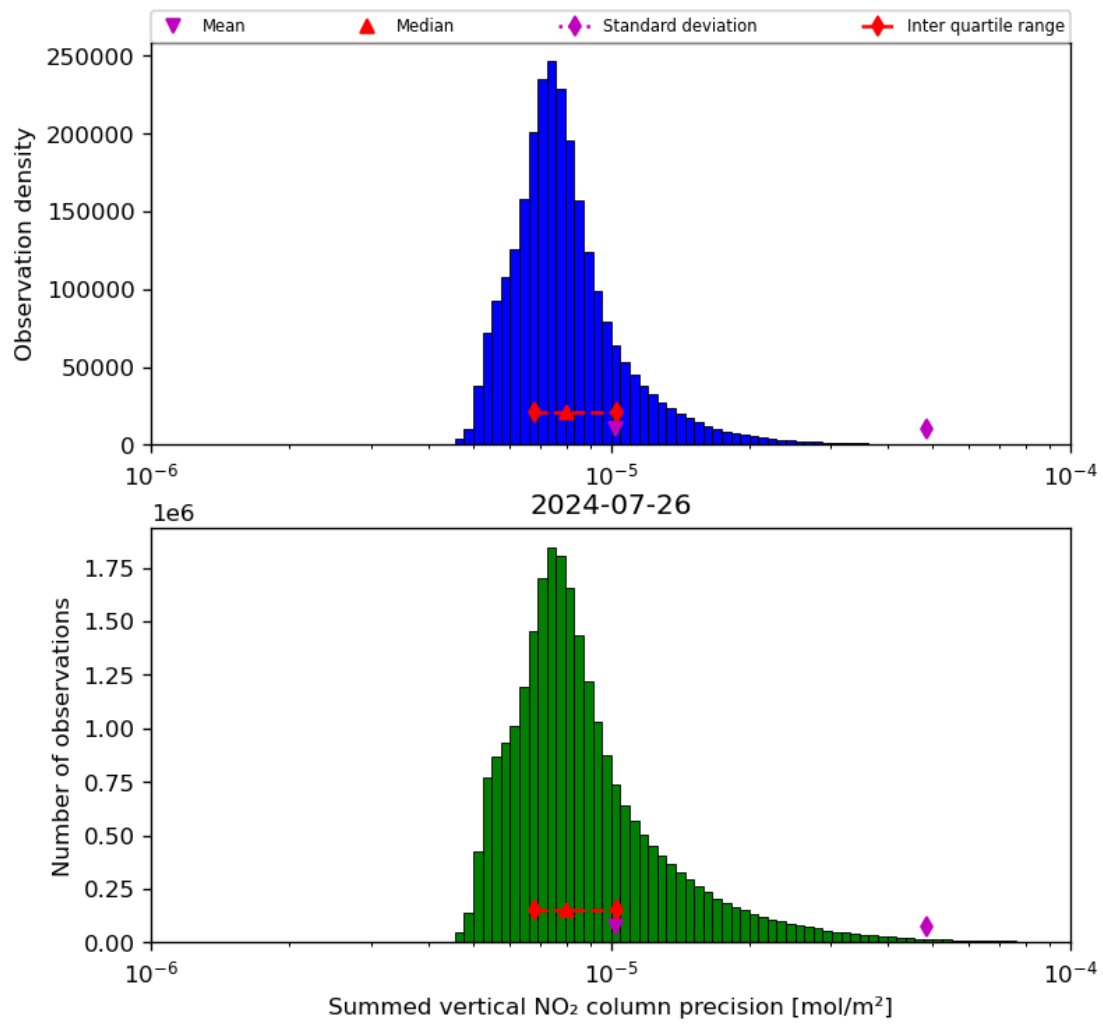
Figure 41: Histogram of “Summed vertical NO 2 column precision” for 2024-07-26 to 2024-07-27
