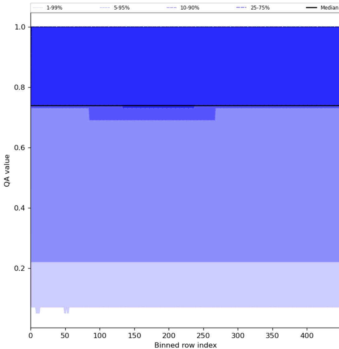
Figure 45: Along track statistics of “QA value” for 2024-07-26 to 2024-07-27
