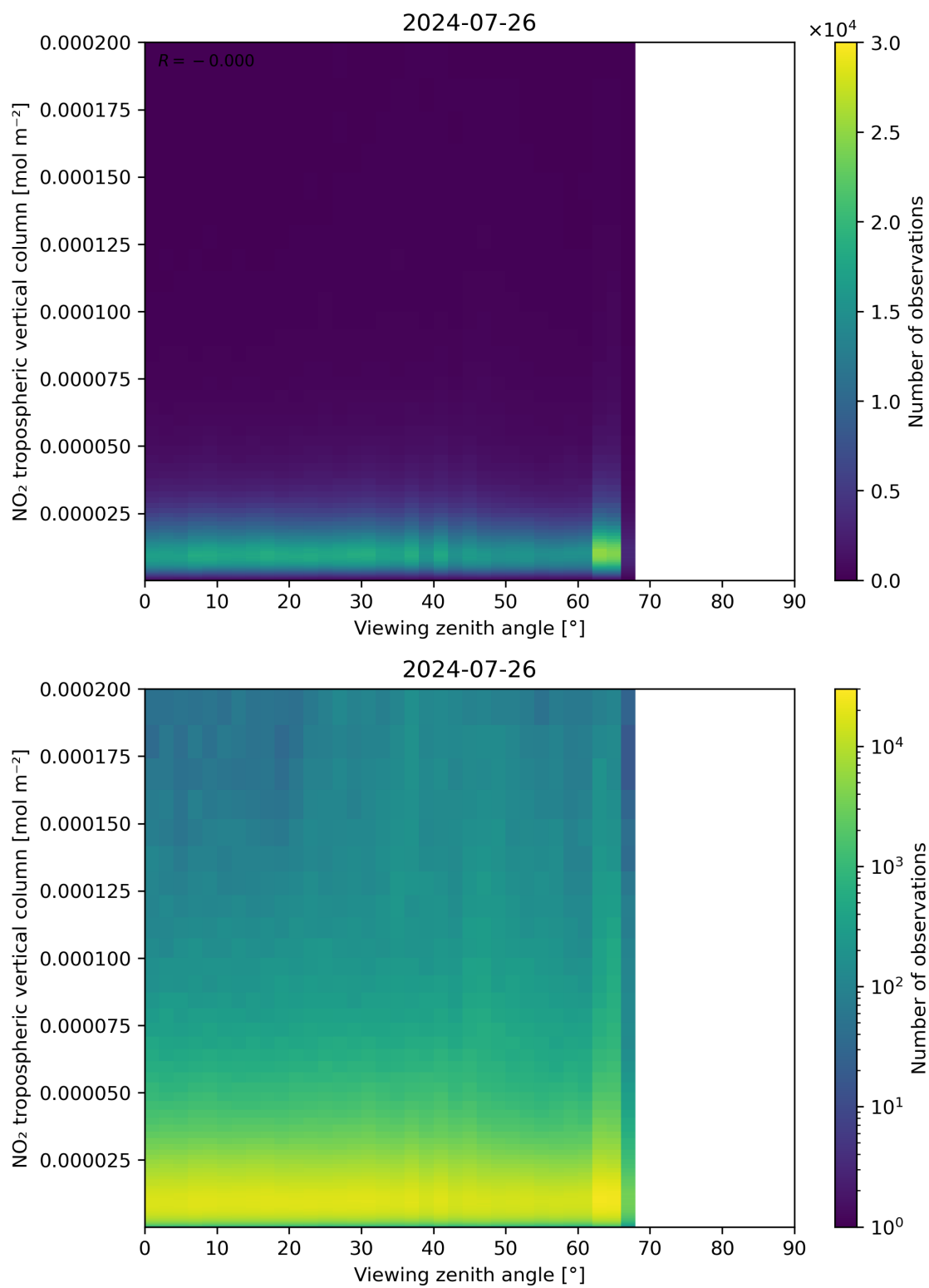
Figure 169: Scatter density plot of “Viewing zenith angle” against “NO 2 tropospheric vertical column” for 2024-07-26 to 2024-07-27.
