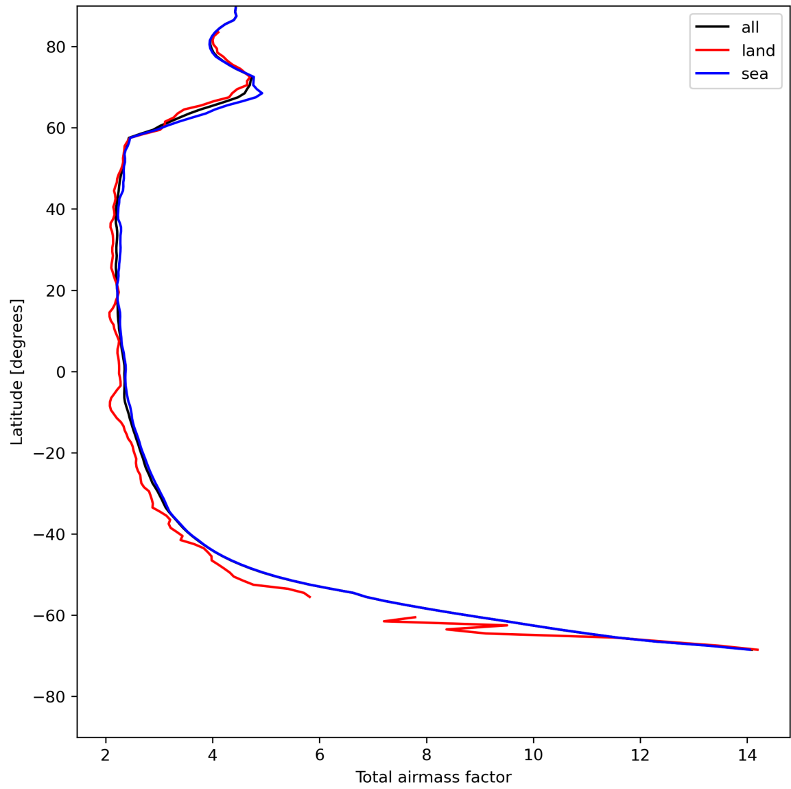
Figure 15: Zonal average of “Total airmass factor” for 2024-07-26 to 2024-07-27.
