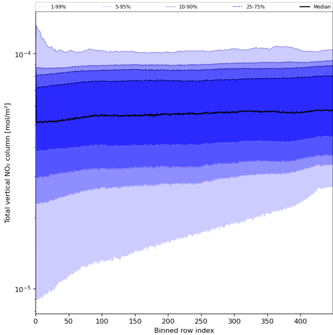
Figure 55: Along track statistics of "Total vertical NO 2 column" for 2024-07-26 to 2024-07-27
