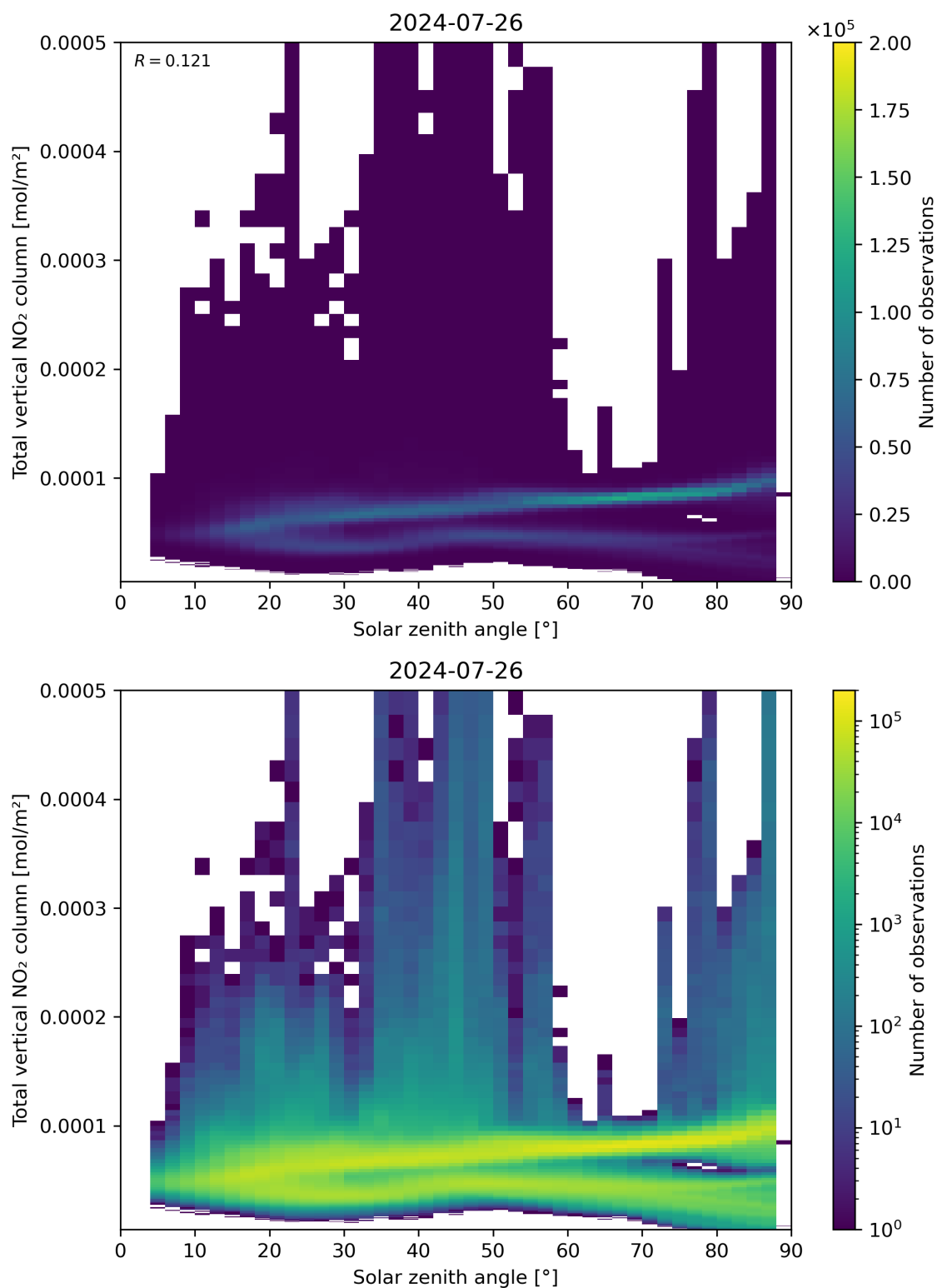
Figure 153: Scatter density plot of “Solar zenith angle” against “Total vertical NO 2 column” for 2024-07-26 to 2024-07-27.
