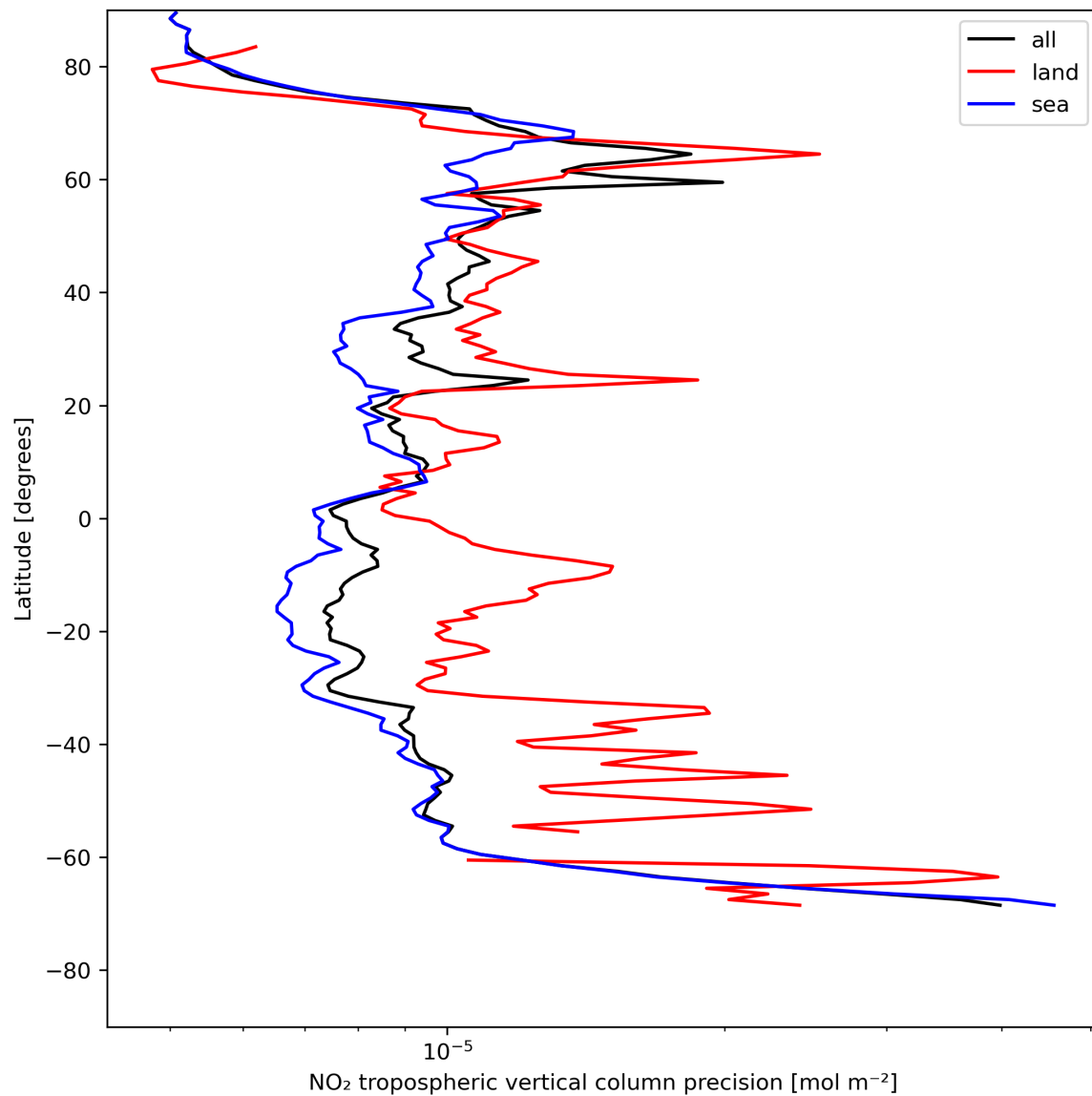
Figure 13: Zonal average of “NO 2 tropospheric vertical column precision” for 2024-07-26 to 2024-07-27.
