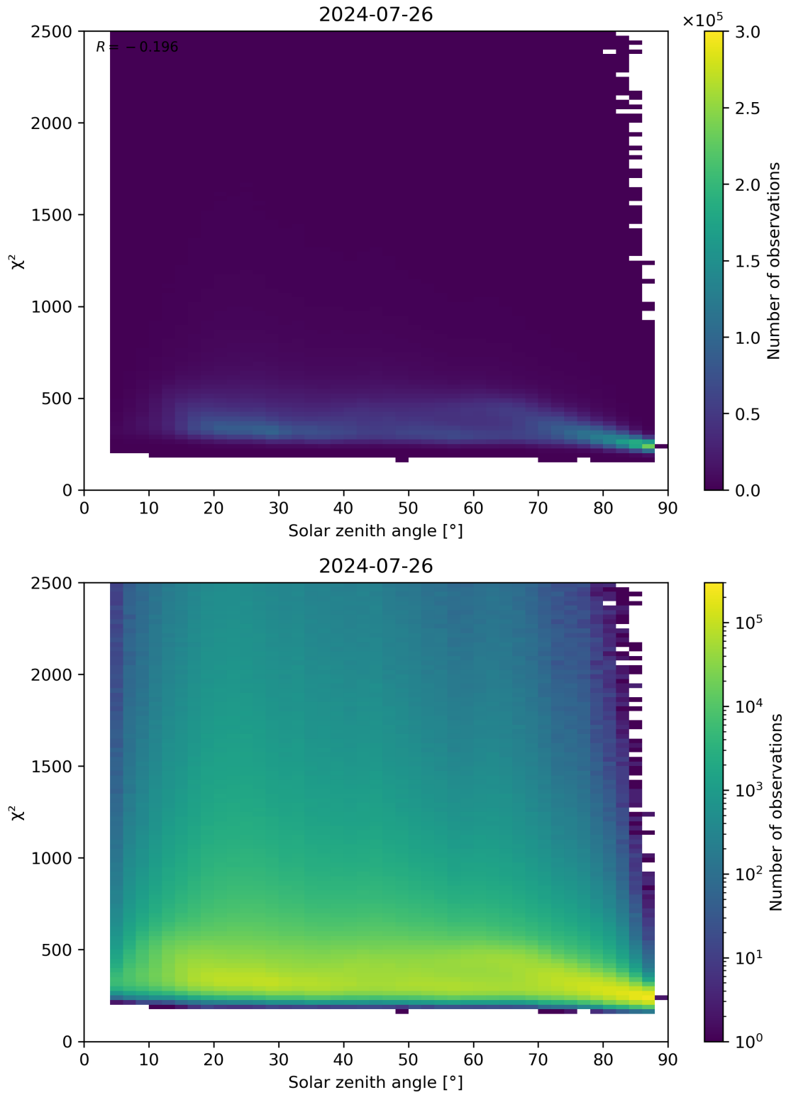
Figure 148: Scatter density plot of “Solar zenith angle” against “ \chi^2 ” for 2024-07-26 to 2024-07-27.
