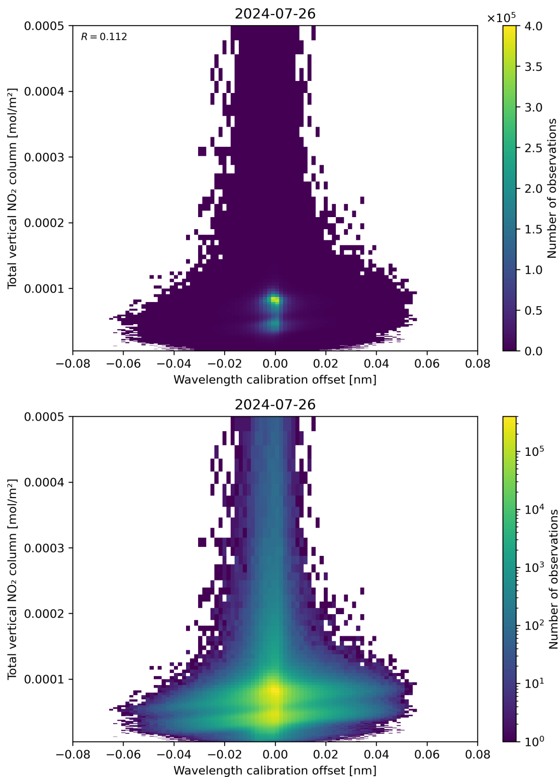
Figure 179: Scatter density plot of “Wavelength calibration offset” against “Total vertical NO 2 column” for 2024-07-26 to 2024-07-27.
