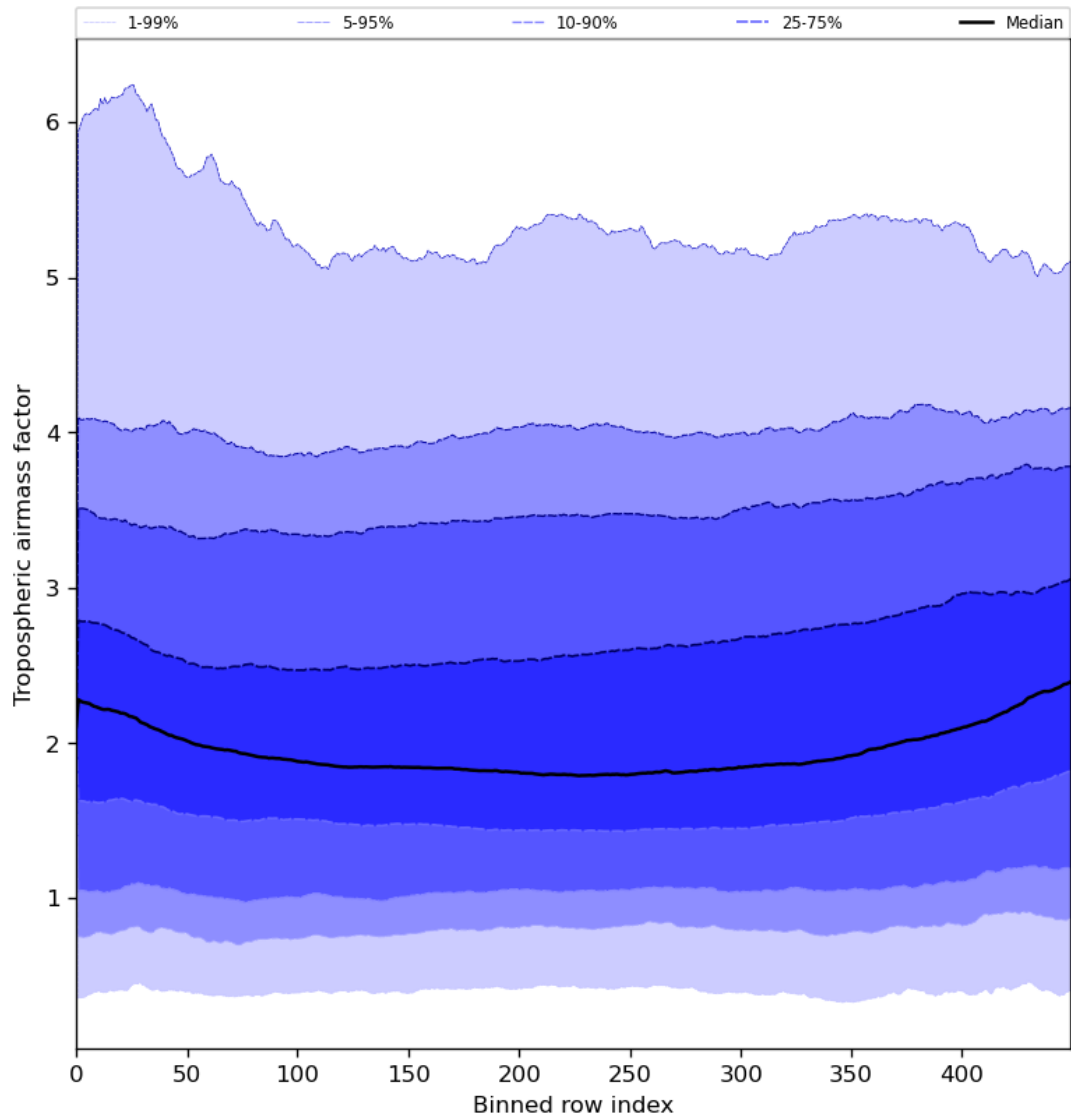
Figure 48: Along track statistics of “Tropospheric airmass factor” for 2024-07-26 to 2024-07-27
