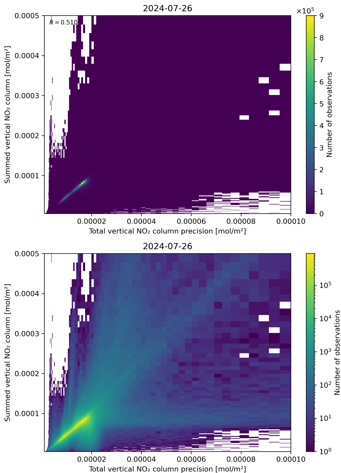
Figure 117: Scatter density plot of “Total vertical NO 2 column precision” against “Summed vertical NO 2 column” for 2024-07-26 to 2024-07-27.
