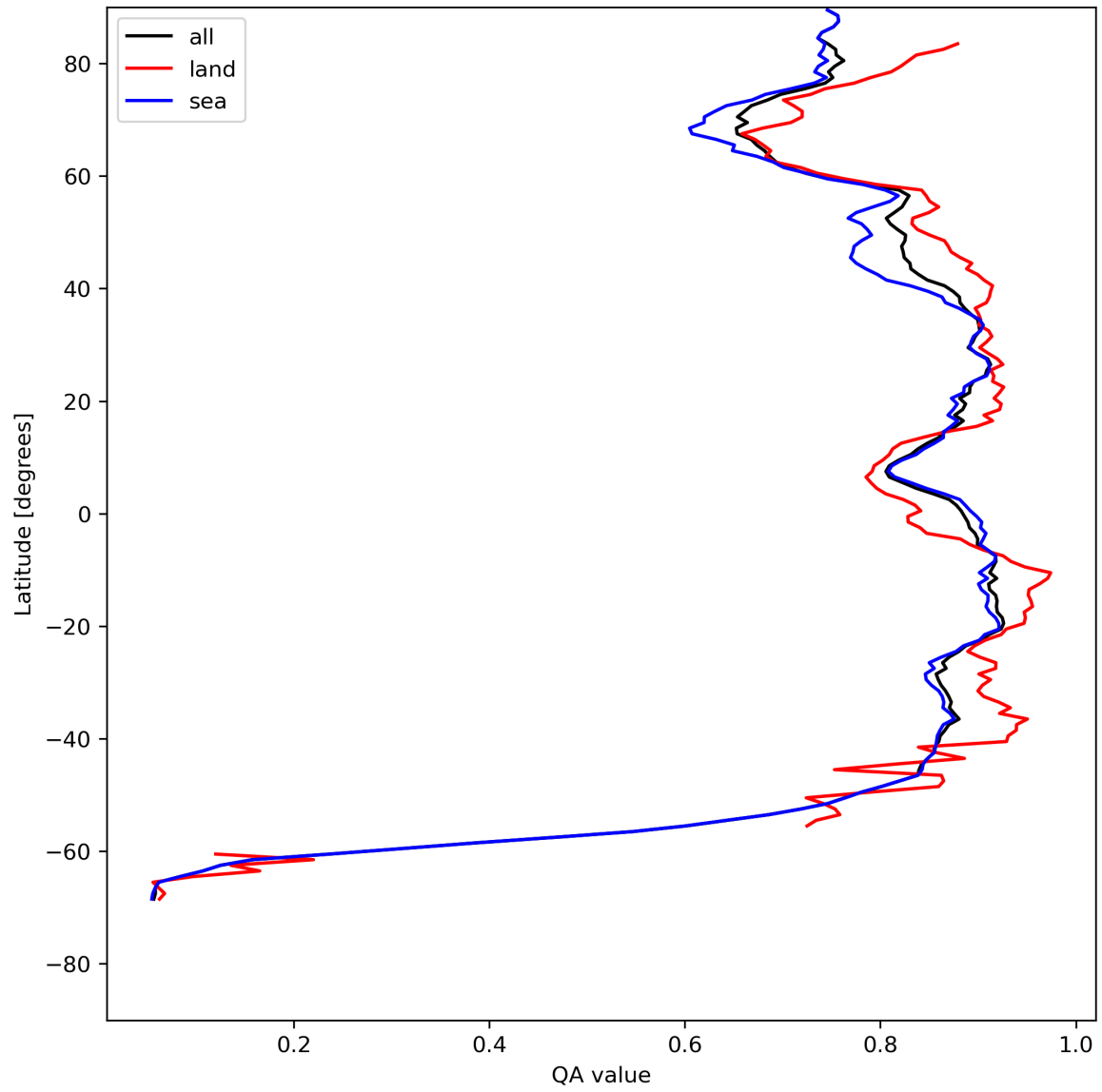
Figure 11: Zonal average of “QA value” for 2024-07-26 to 2024-07-27.
