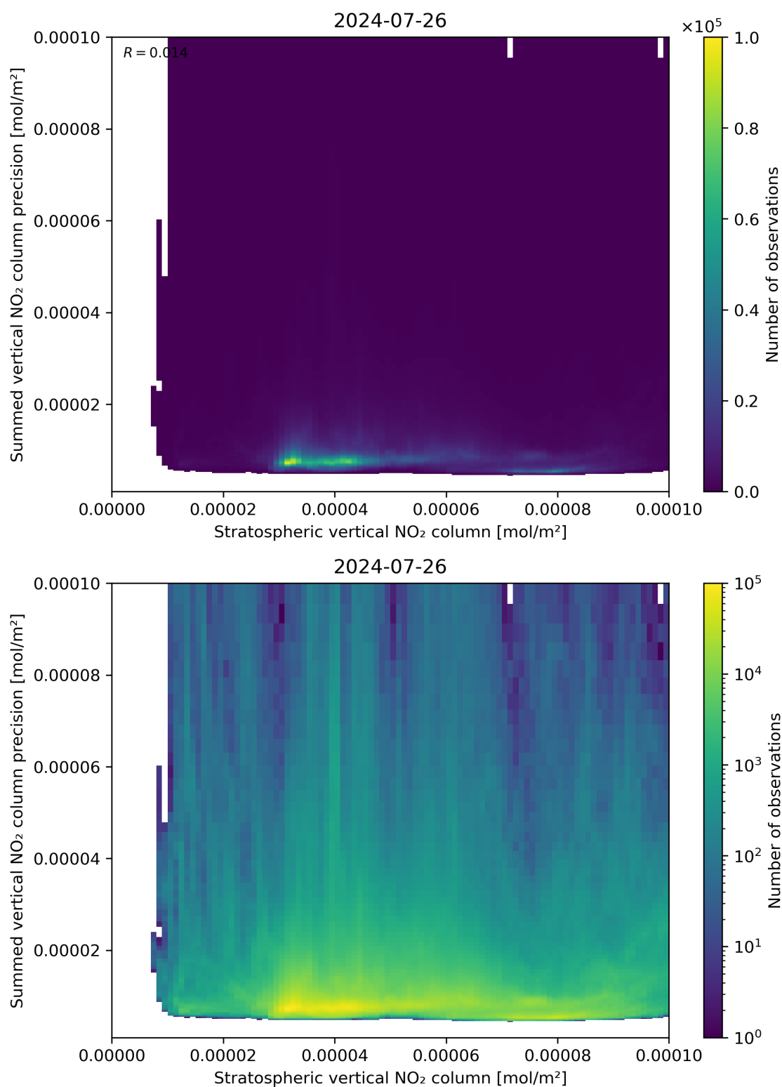
Figure 99: Scatter density plot of “Stratospheric vertical NO 2 column” against “Summed vertical NO 2 column precision” for 2024-07-26 to 2024-07-27.
