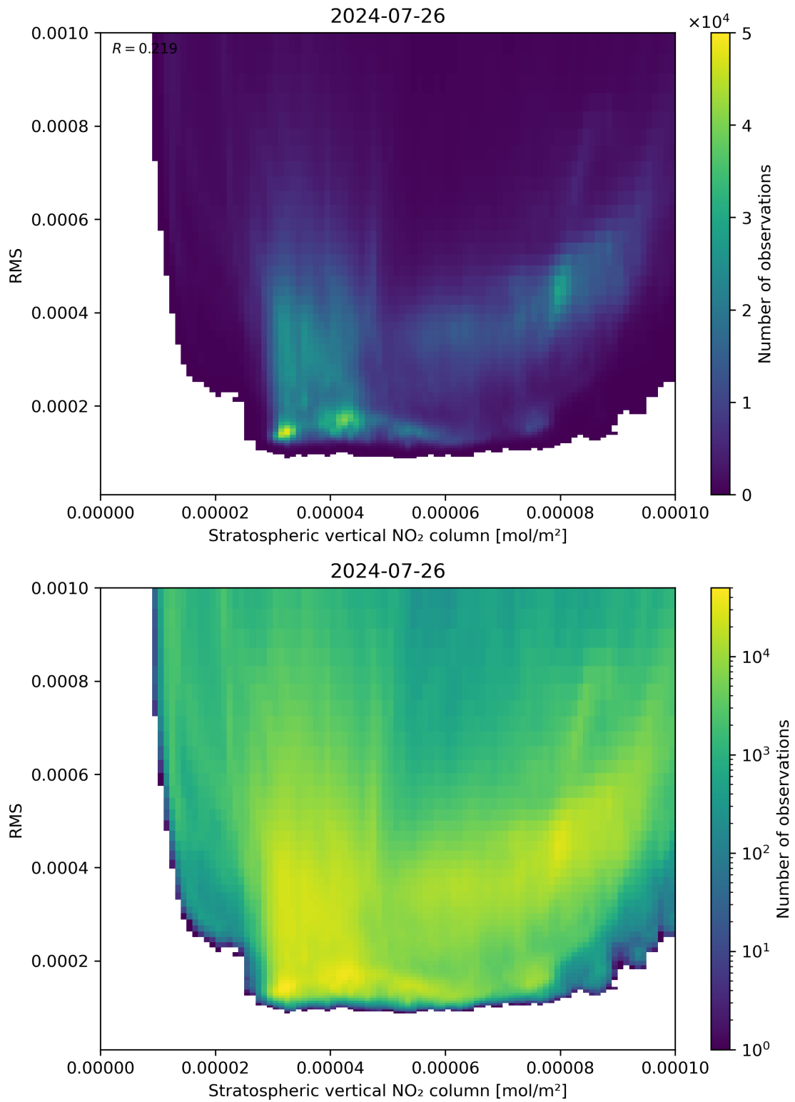
Figure 102: Scatter density plot of “Stratospheric vertical NO 2 column” against “RMS” for 2024-07-26 to 2024-07-27.
