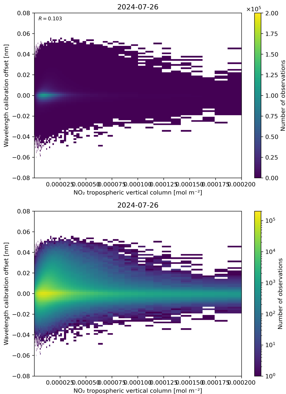
Figure 143: Scatter density plot of “NO 2 tropospheric vertical column” against “Wavelength calibration offset” for 2024-07-26 to 2024-07-27.
