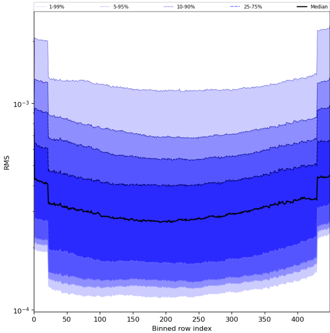
Figure 60: Along track statistics of “RMS” for 2024-07-26 to 2024-07-27
