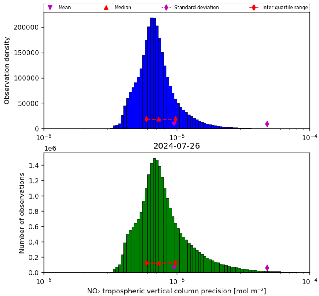
Figure 30: Histogram of “NO 2 tropospheric vertical column precision” for 2024-07-26 to 2024-07-27
