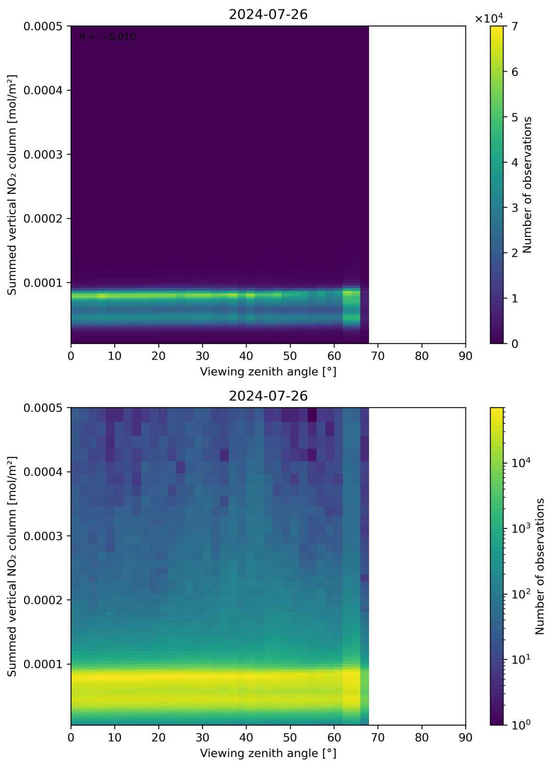
Figure 165: Scatter density plot of “Viewing zenith angle” against “Summed vertical NO 2 column” for 2024-07-26 to 2024-07-27.
