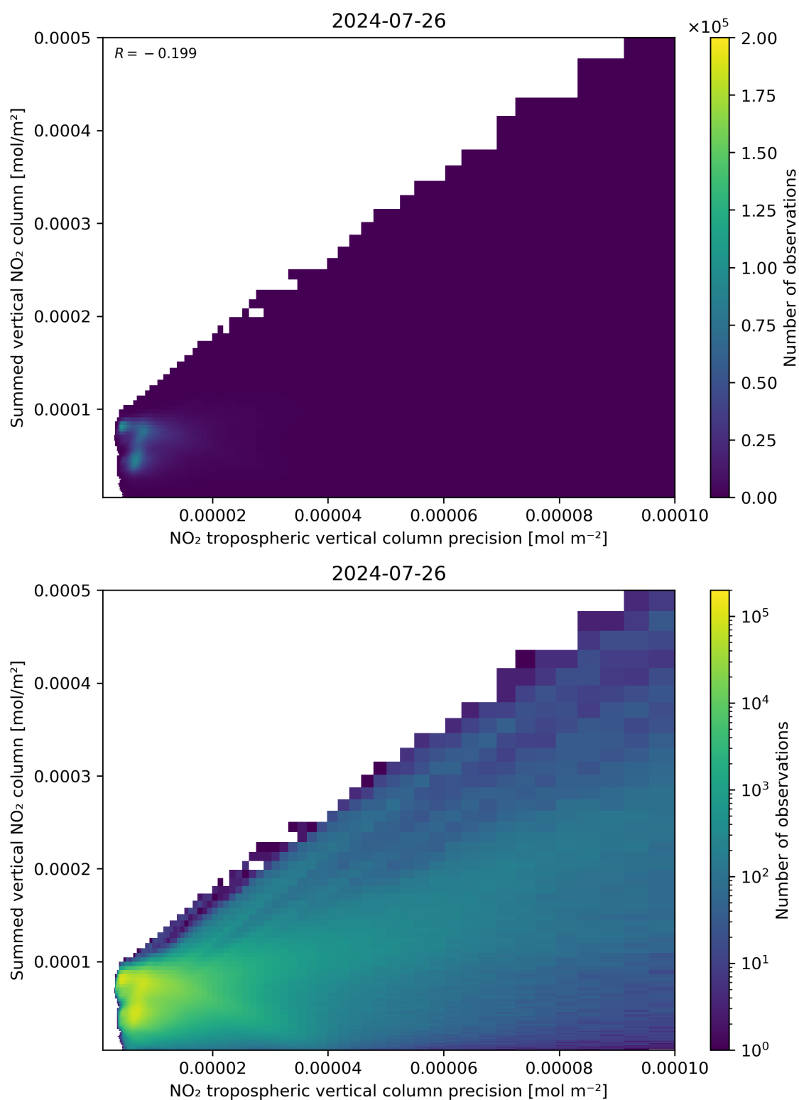
Figure 136: Scatter density plot of “NO 2 tropospheric vertical column precision” against “Summed vertical NO 2 column” for 2024-07-26 to 2024-07-27.
