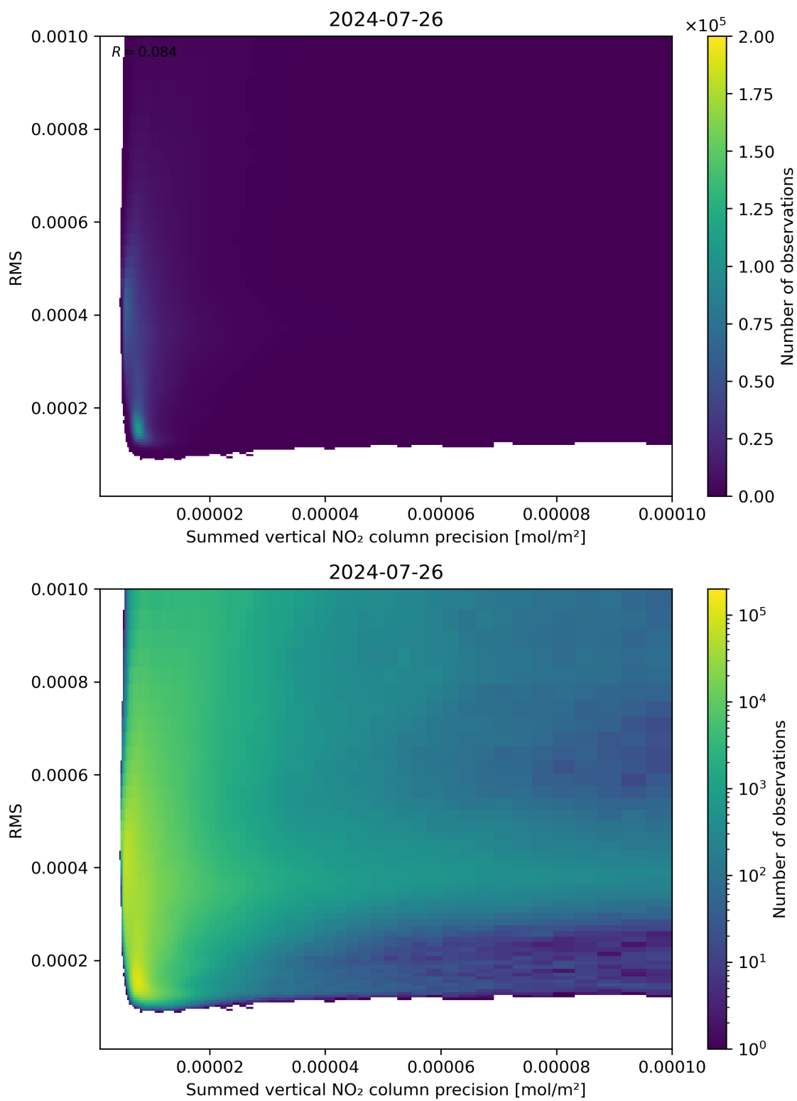
Figure 108: Scatter density plot of “Summed vertical NO 2 column precision” against “RMS” for 2024-07-26 to 2024-07-27.
