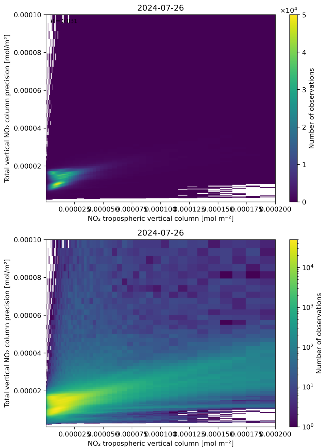
Figure 129: Scatter density plot of “NO 2 tropospheric vertical column” against “Total vertical NO 2 column precision” for 2024-07-26 to 2024-07-27.
