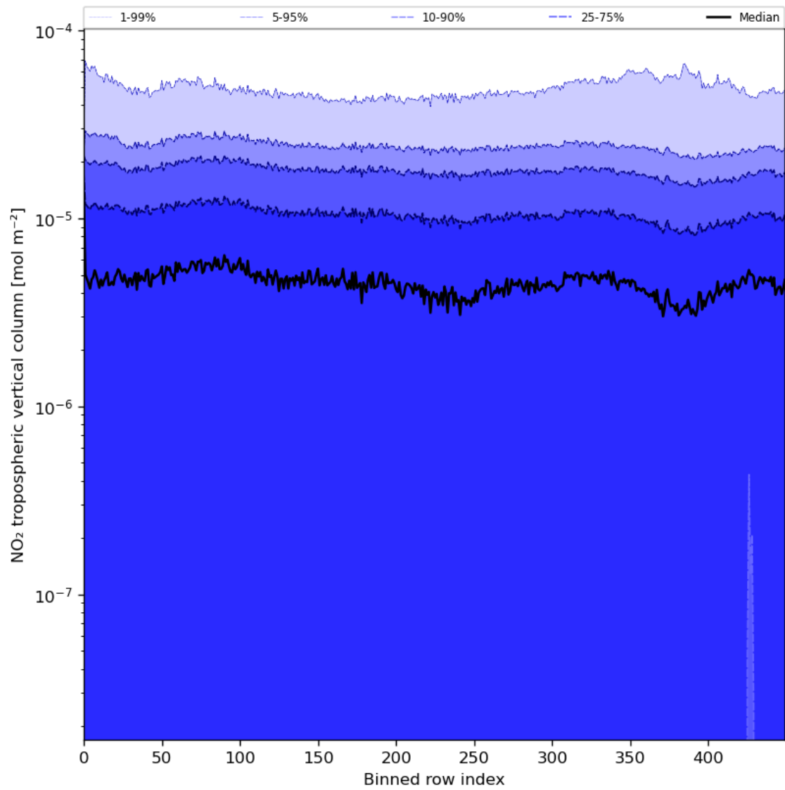
Figure 46: Along track statistics of “NO 2 tropospheric vertical column” for 2024-07-26 to 2024-07-27
