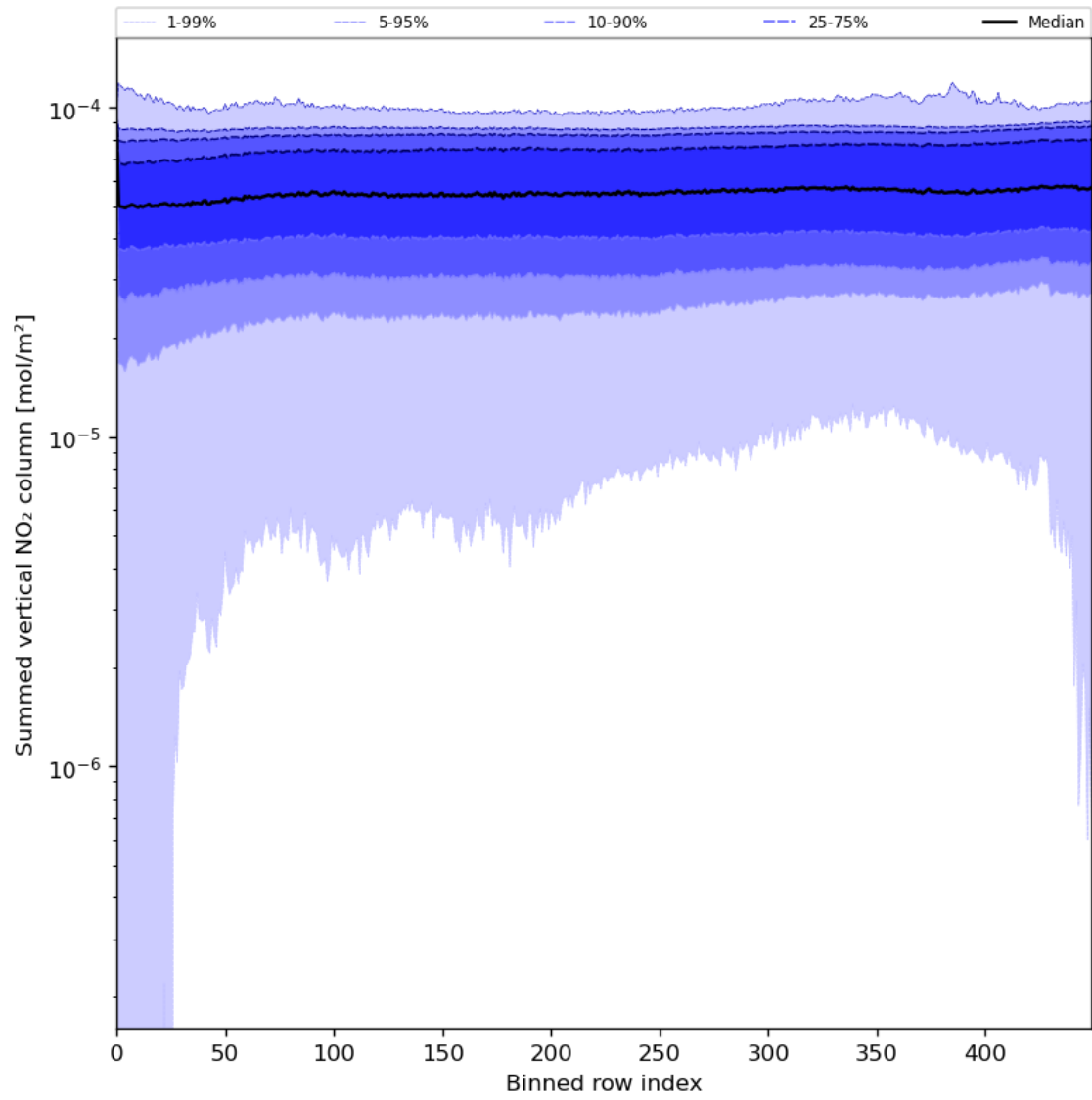
Figure 57: Along track statistics of “Summed vertical NO 2 column” for 2024-07-26 to 2024-07-27
