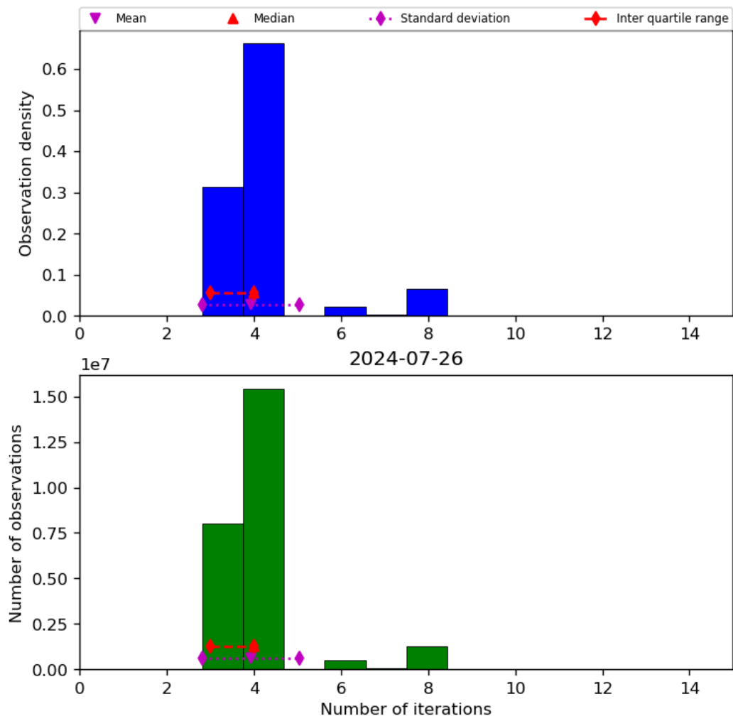
Figure 34: Histogram of “Number of iterations” for 2024-07-26 to 2024-07-27
