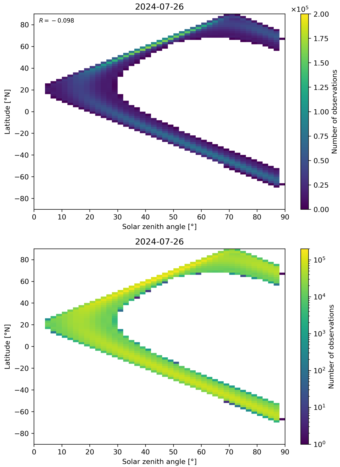
Figure 149: Scatter density plot of “Solar zenith angle” against “Latitude” for 2024-07-26 to 2024-07-27.
