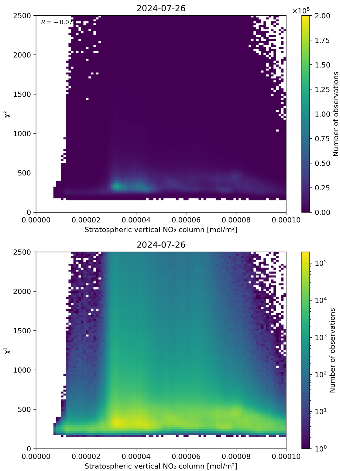
Figure 97: Scatter density plot of “Stratospheric vertical NO 2 column” against “ \chi^2 ” for 2024-07-26 to 2024-07-27.
