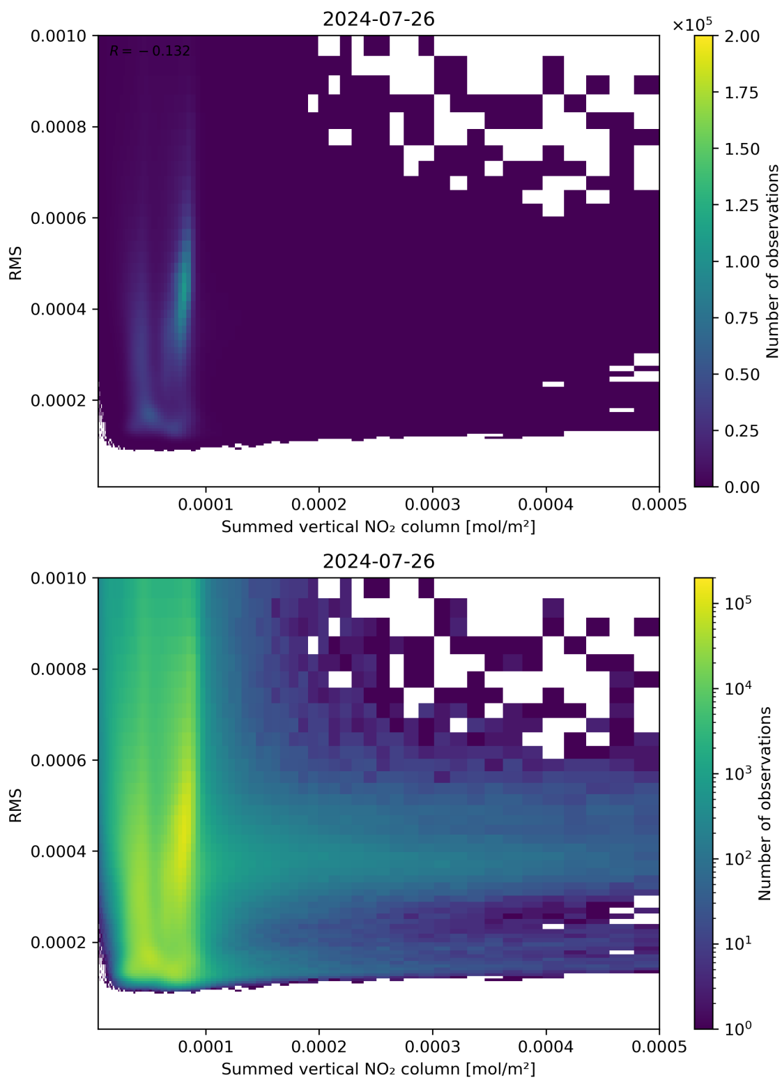
Figure 109: Scatter density plot of “Summed vertical NO 2 column” against “RMS” for 2024-07-26 to 2024-07-27.
