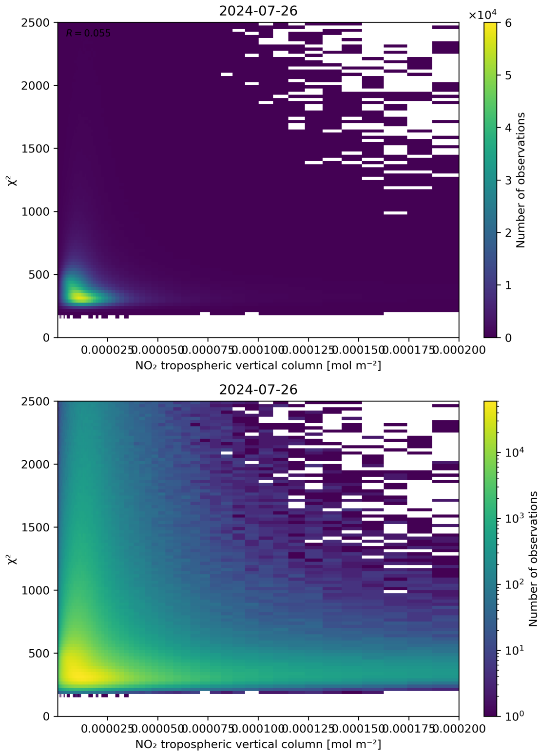
Figure 124: Scatter density plot of “NO 2 tropospheric vertical column” against “ \chi^2 ” for 2024-07-26 to 2024-07-27.
