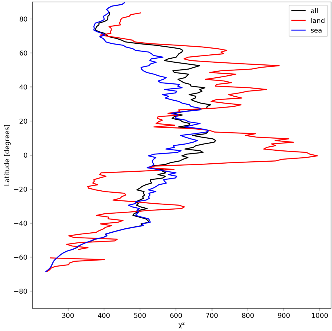
Figure 25: Zonal average of “ \chi^2 ” for 2024-07-26 to 2024-07-27.
