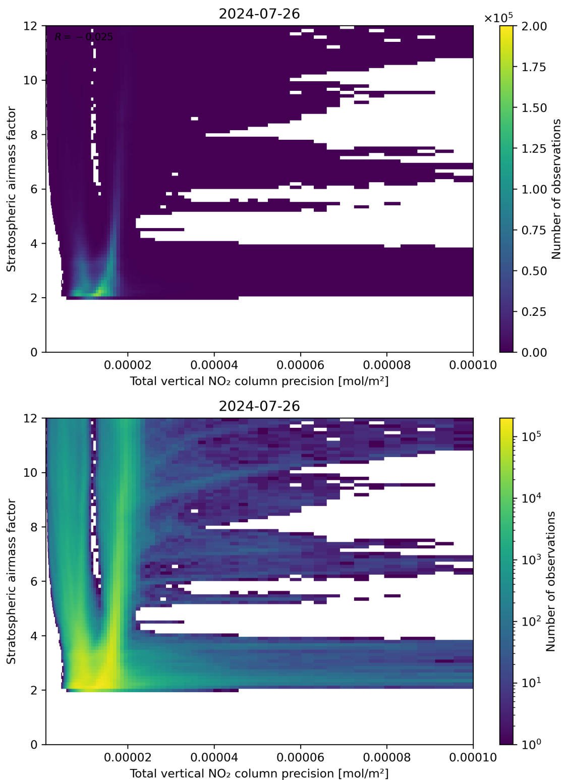
Figure 115: Scatter density plot of “Total vertical NO 2 column precision” against “Stratospheric air mass factor” for 2024-07-26 to 2024-07-27.
