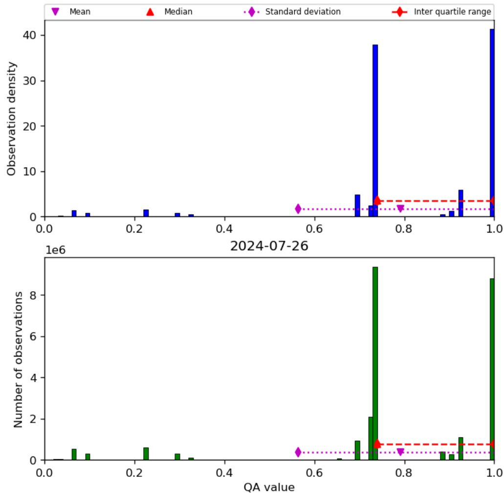
Figure 28: Histogram of “QA value” for 2024-07-26 to 2024-07-27
