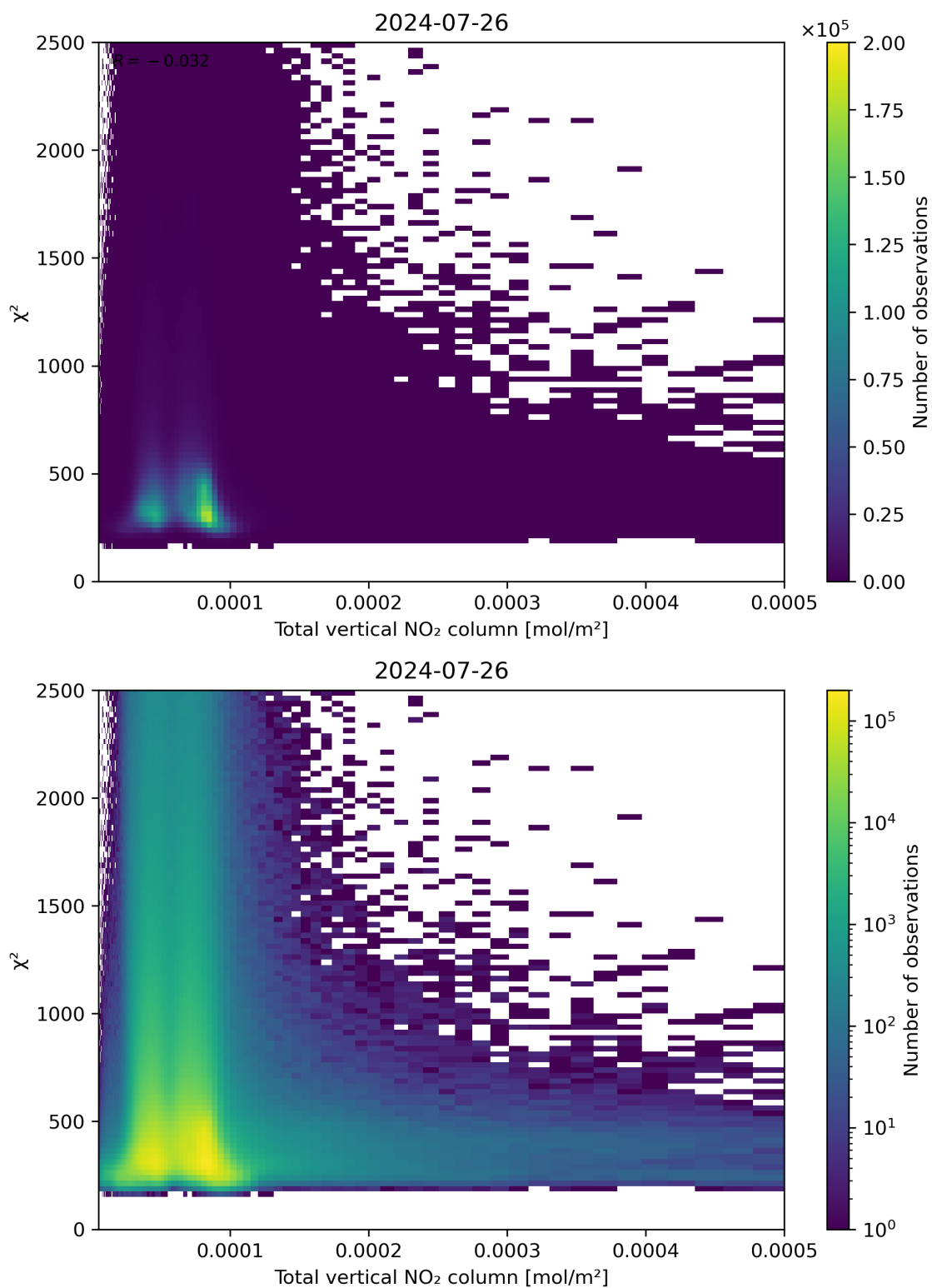
Figure 111: Scatter density plot of “Total vertical NO 2 column” against “ \chi^2 ” for 2024-07-26 to 2024-07-27.
