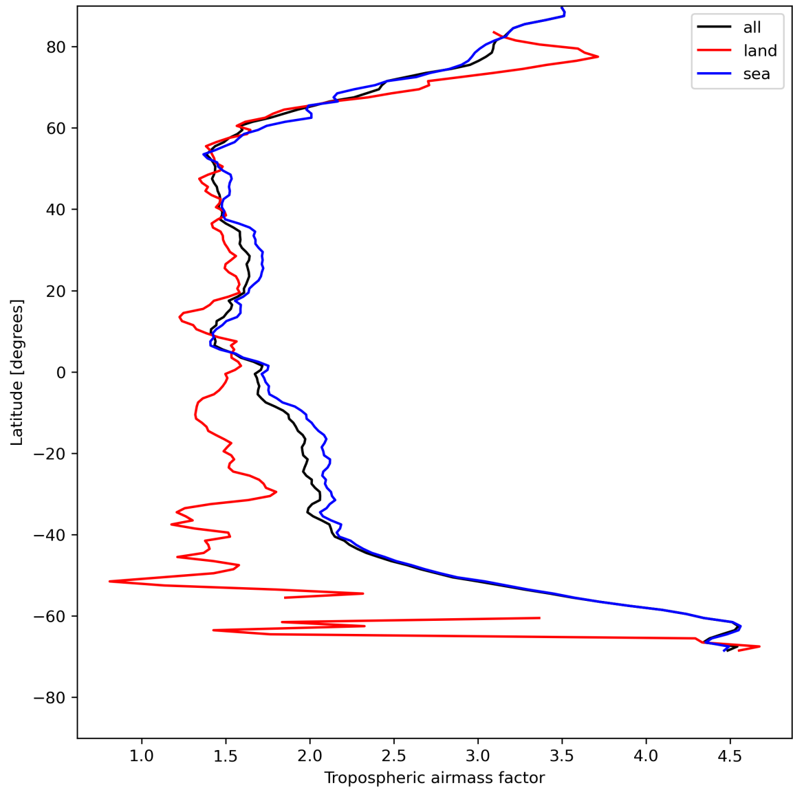
Figure 14: Zonal average of “Tropospheric airmass factor” for 2024-07-26 to 2024-07-27.
