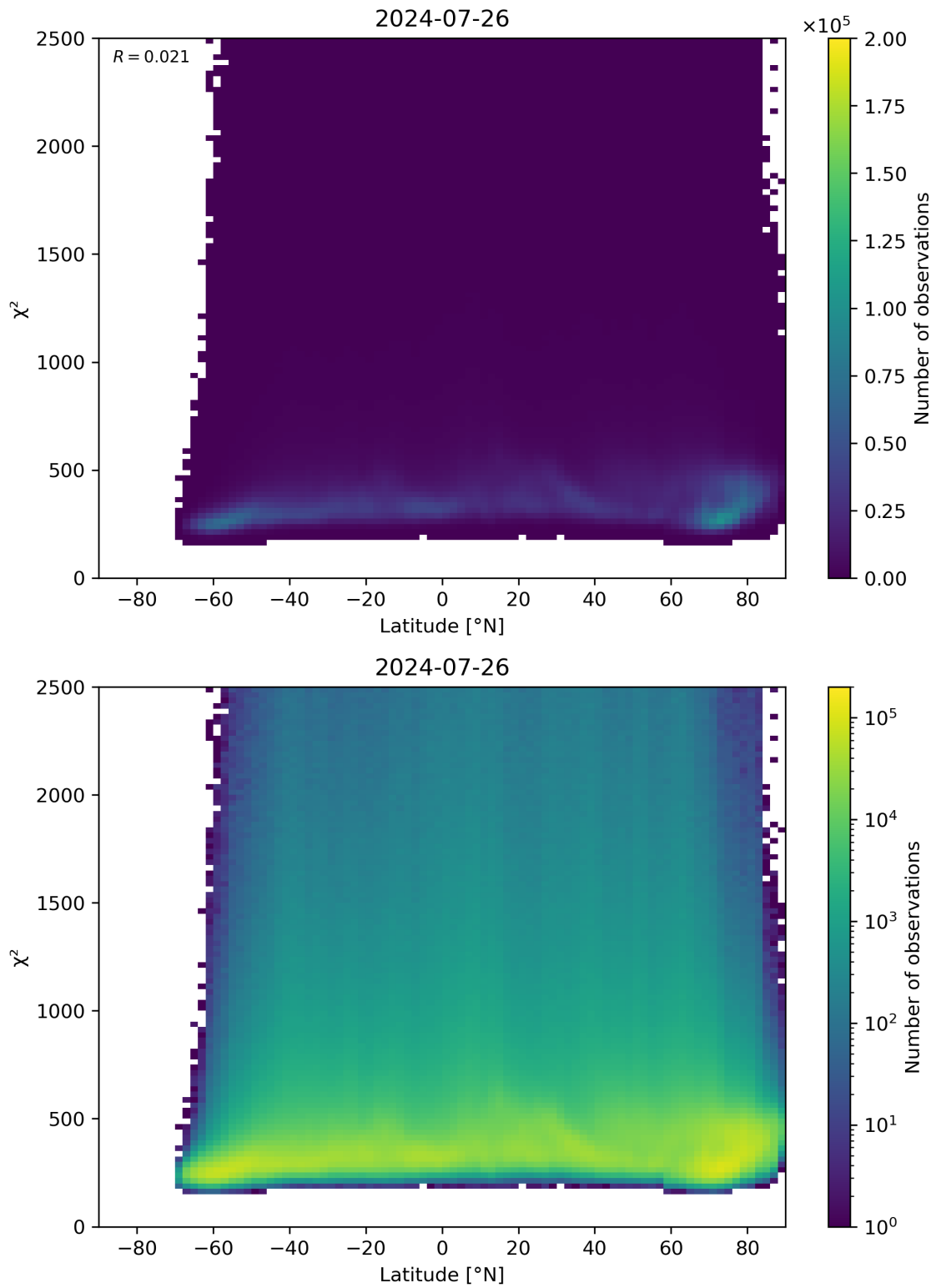
Figure 86: Scatter density plot of “Latitude” against “ \chi^2 ” for 2024-07-26 to 2024-07-27.
