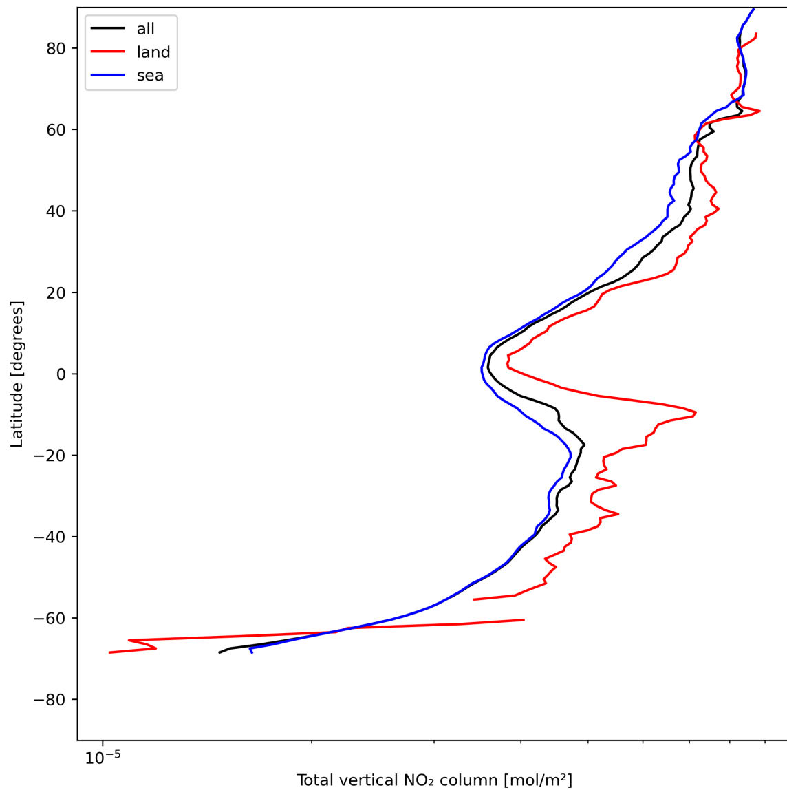
Figure 21: Zonal average of “Total vertical NO 2 column” for 2024-07-26 to 2024-07-27.
