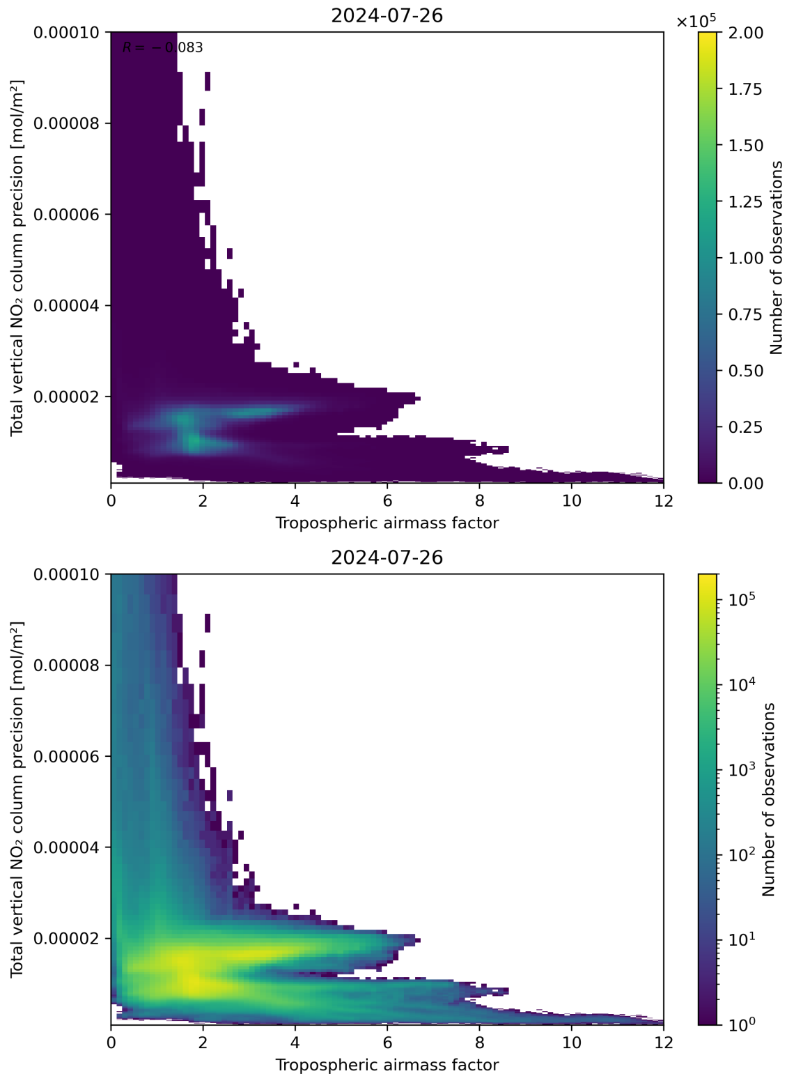
Figure 78: Scatter density plot of “Tropospheric air mass factor” against “Total vertical NO 2 column precision” for 2024-07-26 to 2024-07-27.
