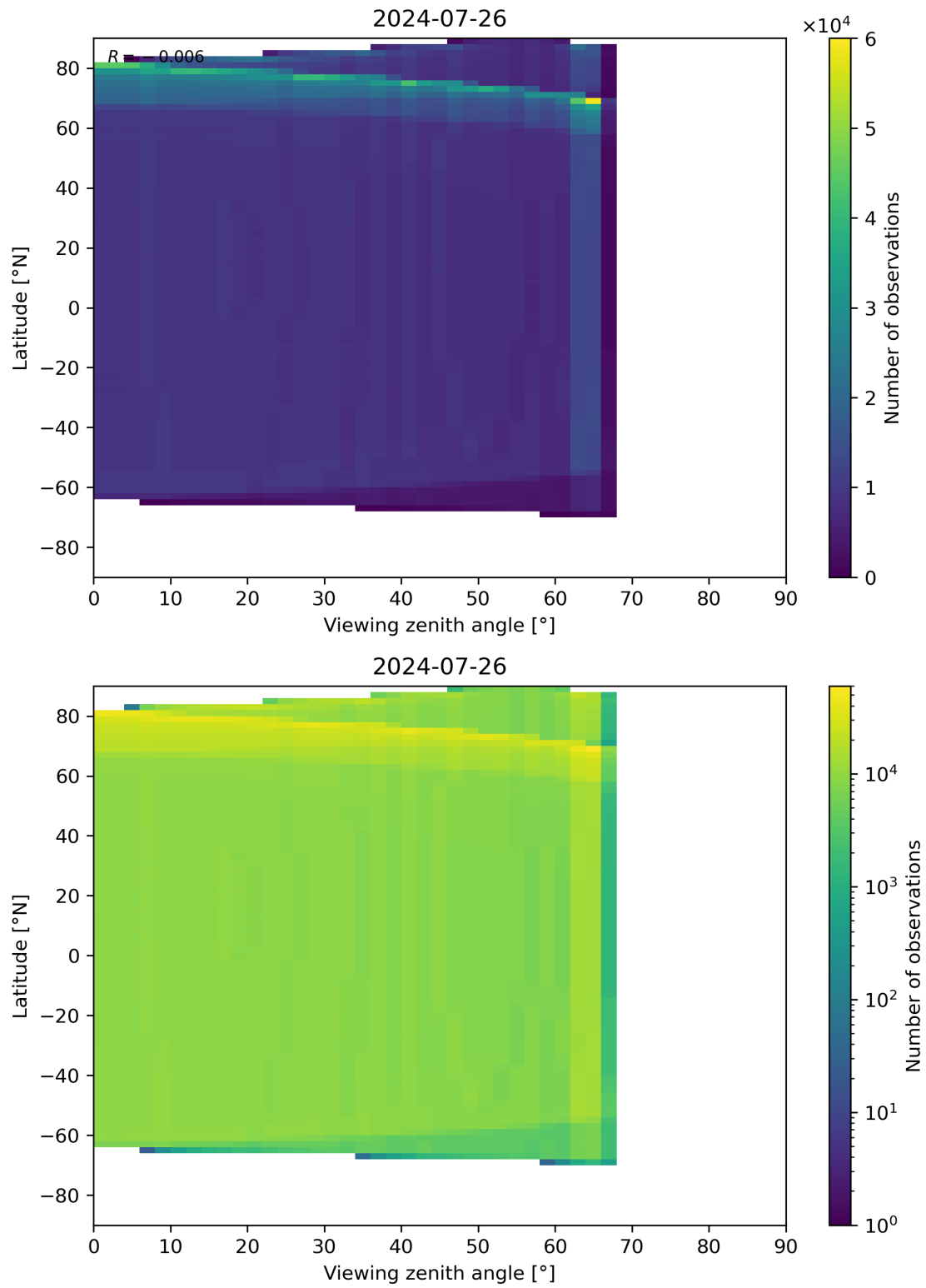
Figure 163: Scatter density plot of “Viewing zenith angle” against “Latitude” for 2024-07-26 to 2024-07-27.
