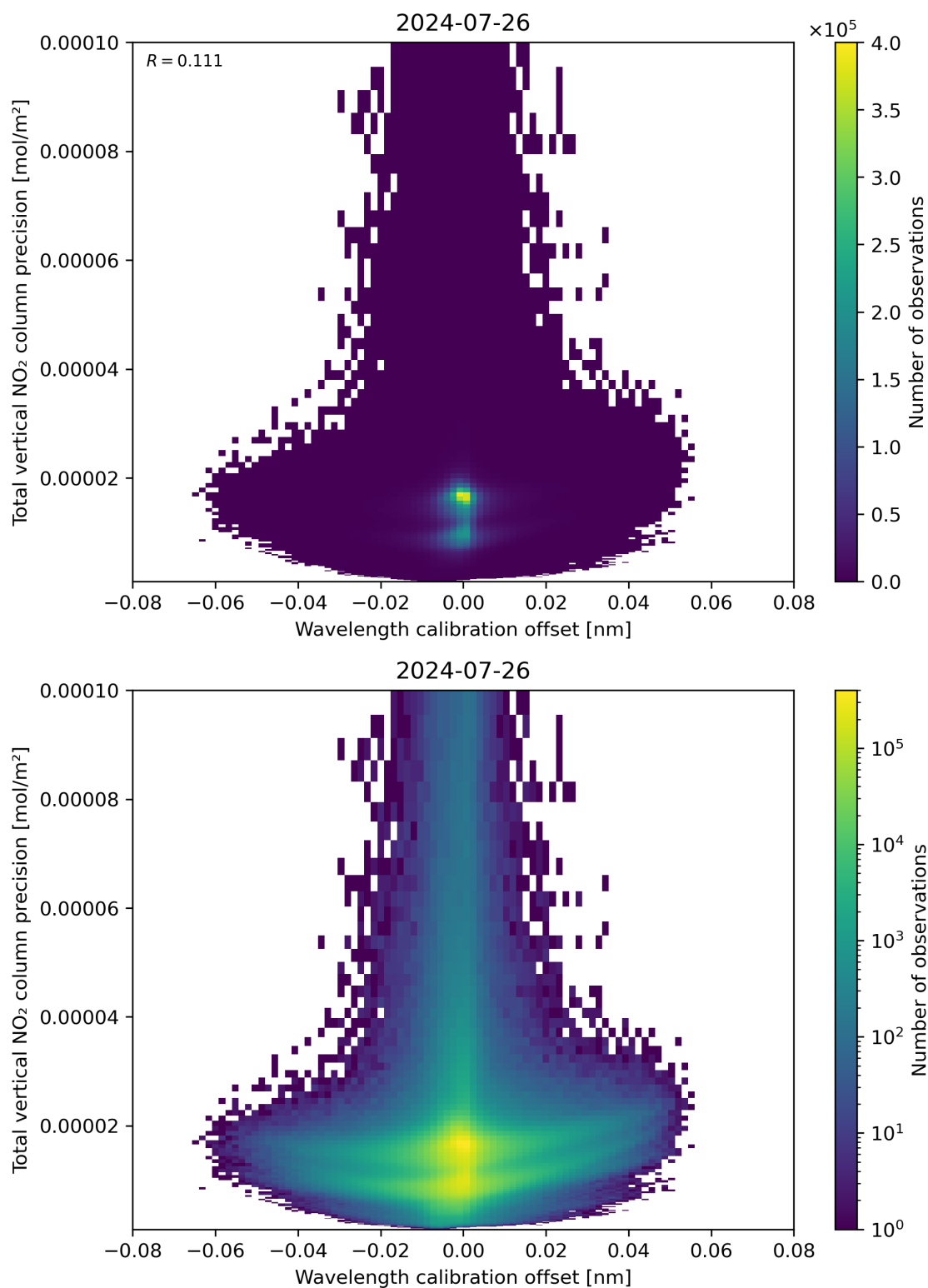
Figure 180: Scatter density plot of “Wavelength calibration offset” against “Total vertical NO 2 column precision” for 2024-07-26 to 2024-07-27.
