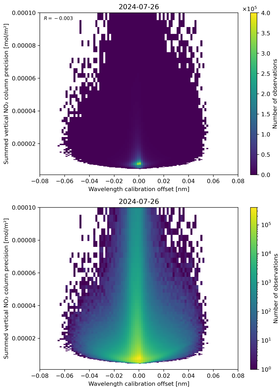
Figure 178: Scatter density plot of “Wavelength calibration offset” against “Summed vertical NO 2 column precision” for 2024-07-26 to 2024-07-27.
