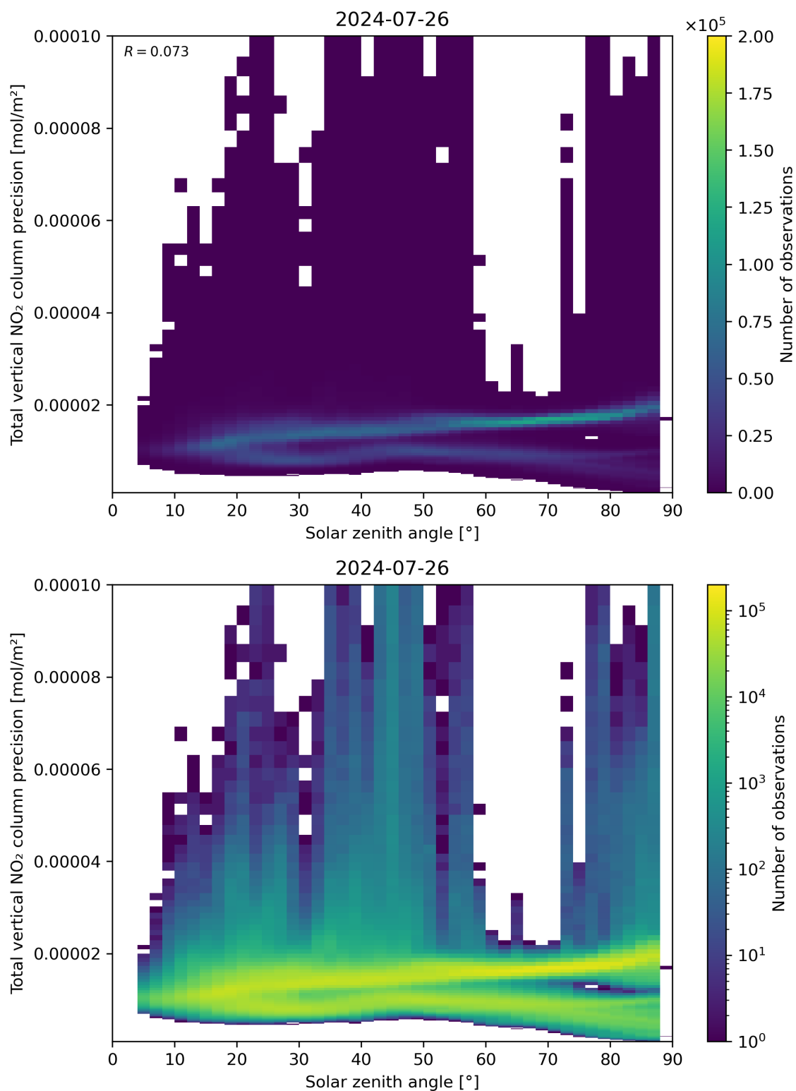
Figure 154: Scatter density plot of “Solar zenith angle” against “Total vertical NO 2 column precision” for 2024-07-26 to 2024-07-27.
