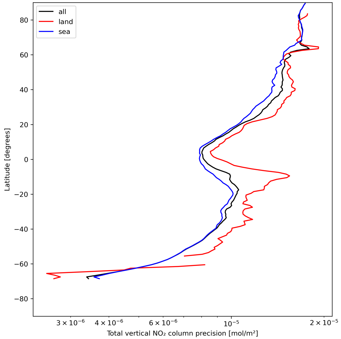
Figure 22: Zonal average of “Total vertical NO 2 column precision” for 2024-07-26 to 2024-07-27.
