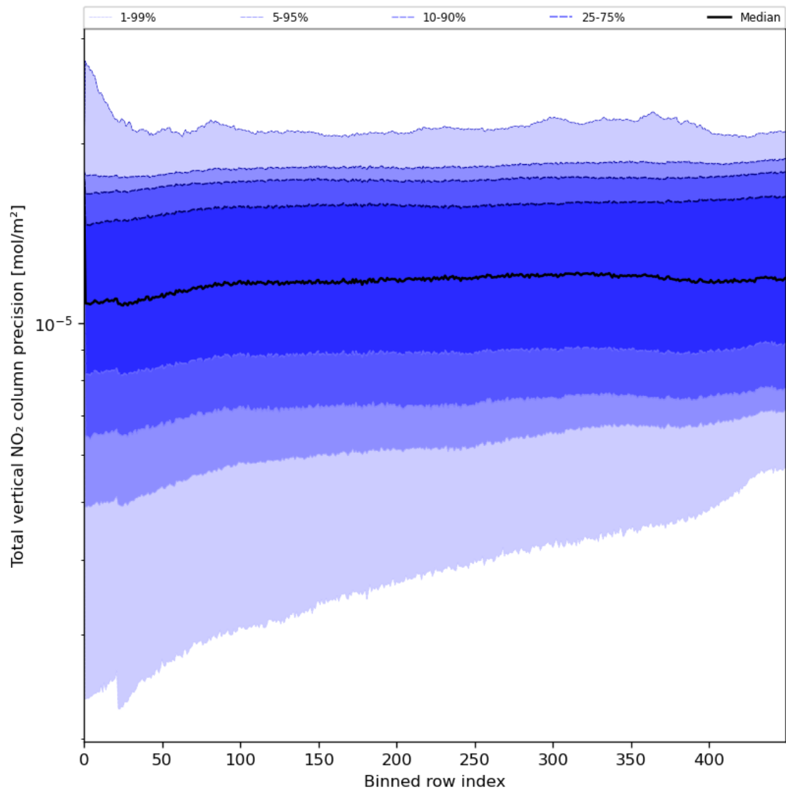
Figure 56: Along track statistics of “Total vertical NO 2 column precision” for 2024-07-26 to 2024-07-27
