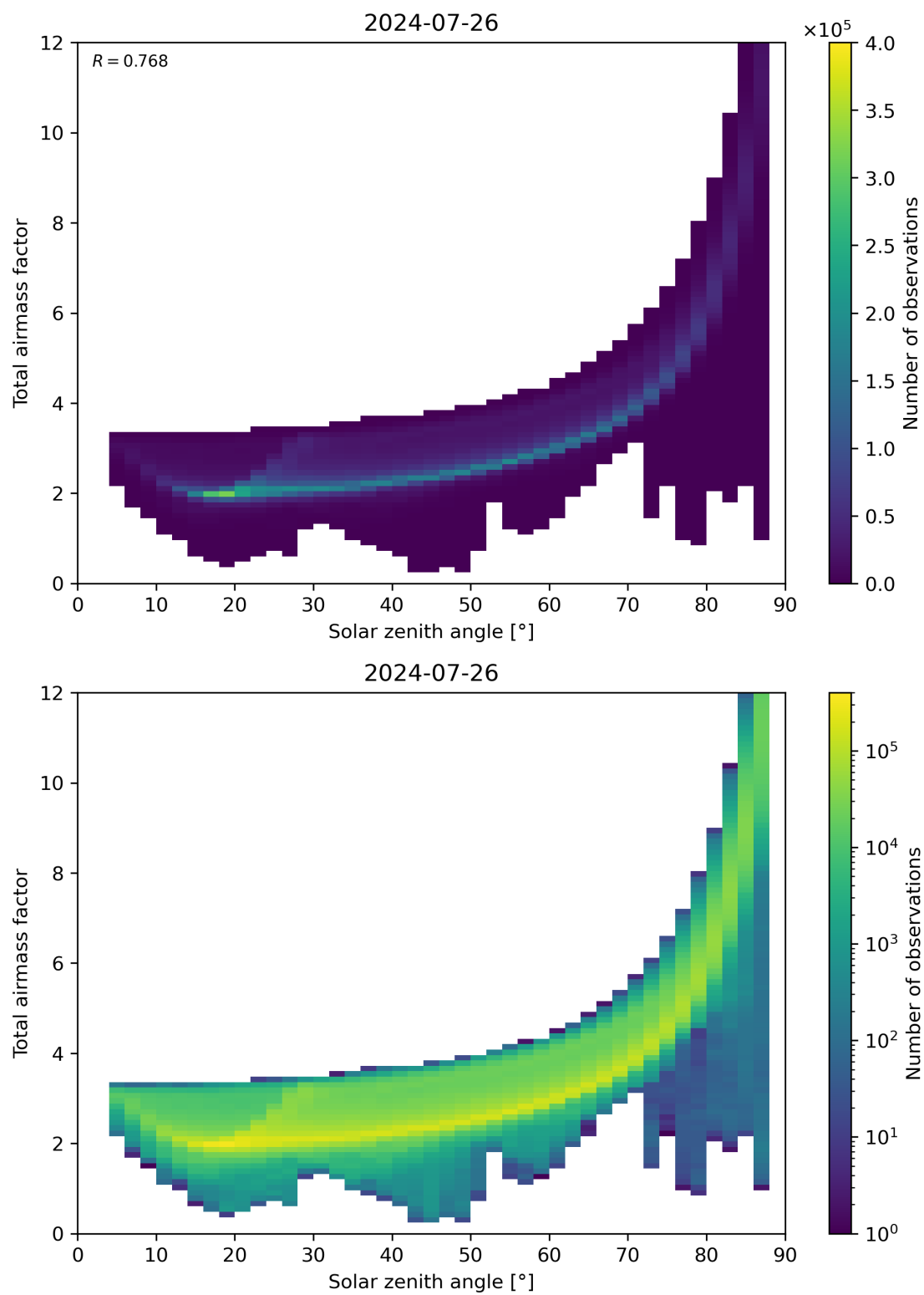
Figure 146: Scatter density plot of “Solar zenith angle” against “Total air mass factor” for 2024-07-26 to 2024-07-27.
