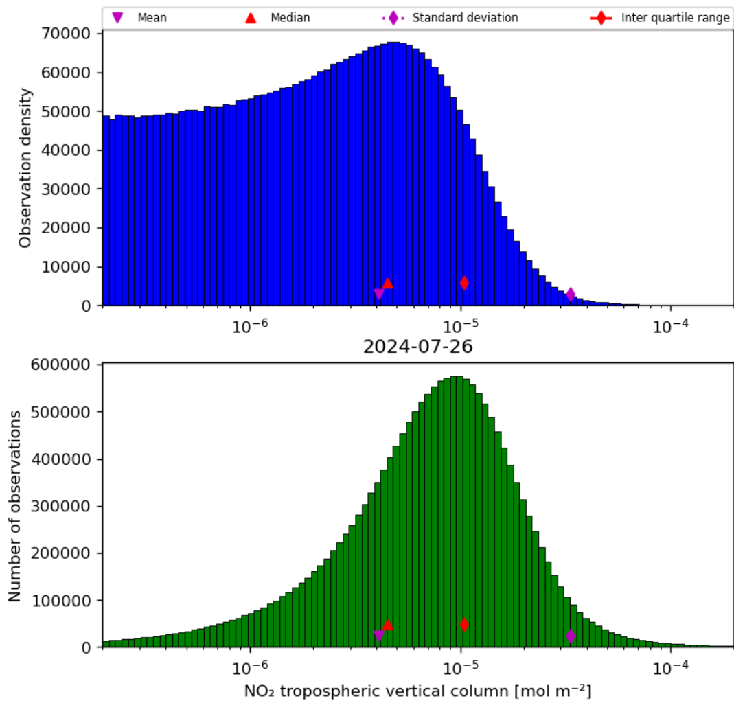
Figure 29: Histogram of “NO 2 tropospheric vertical column” for 2024-07-26 to 2024-07-27
