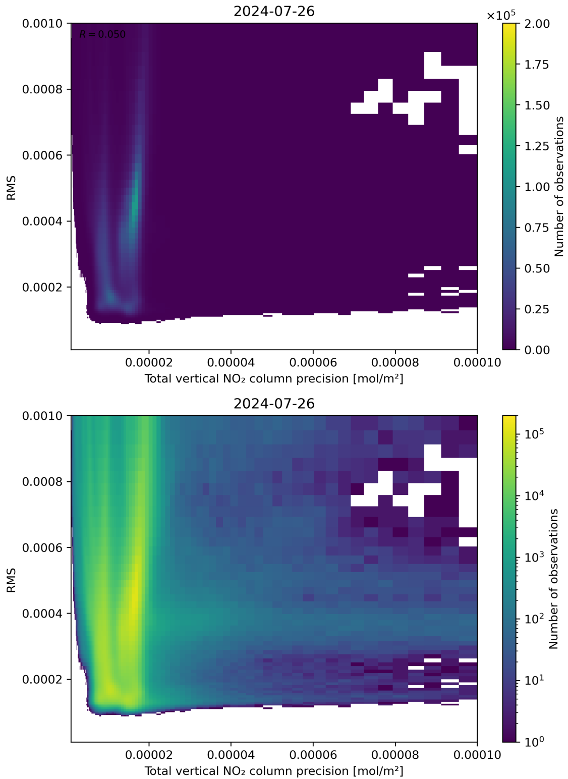
Figure 119: Scatter density plot of “Total vertical NO 2 column precision” against “RMS” for 2024-07-26 to 2024-07-27.
