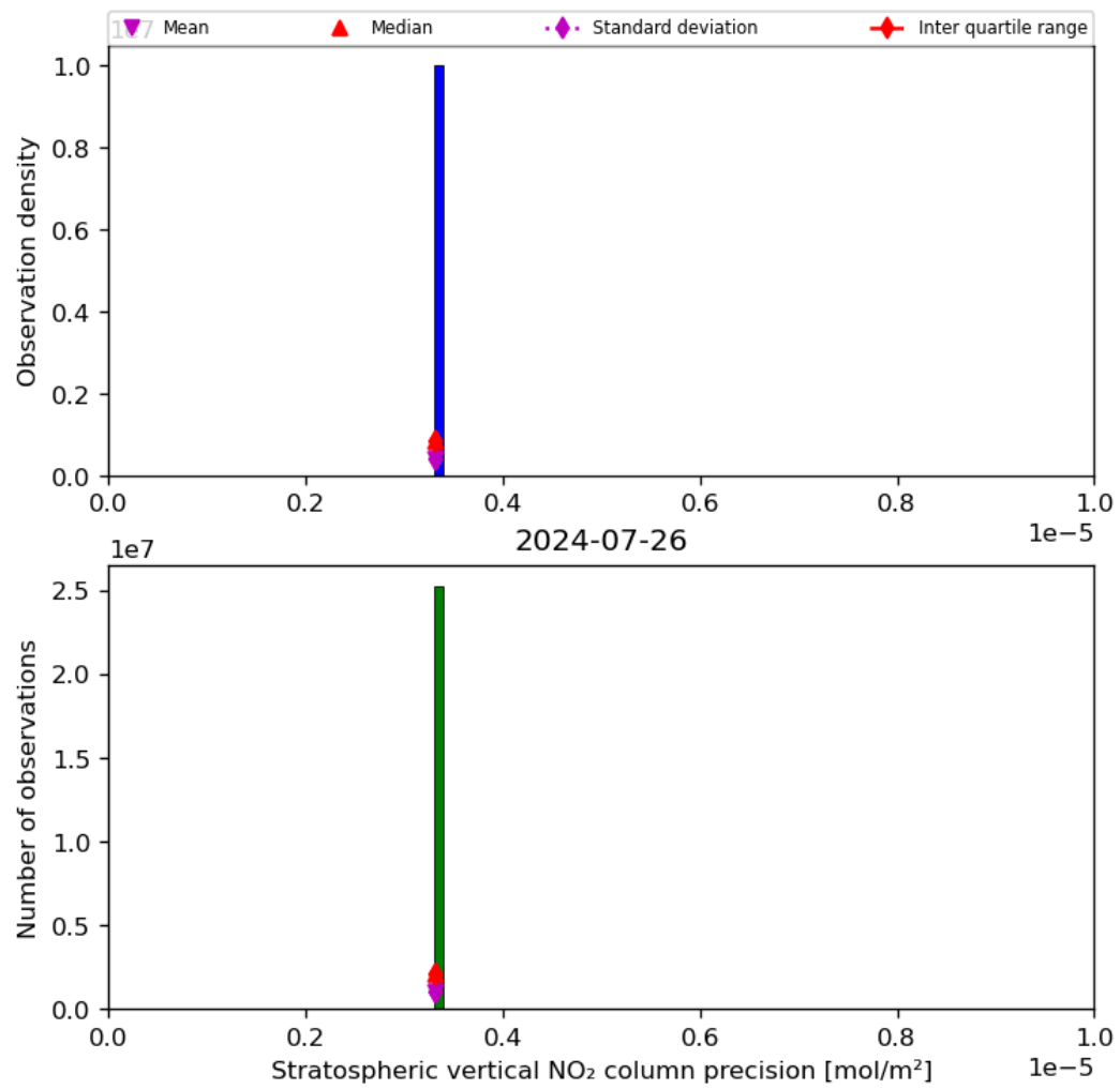
Figure 37: Histogram of “Stratospheric vertical NO 2 column precision” for 2024-07-26 to 2024-07-27
