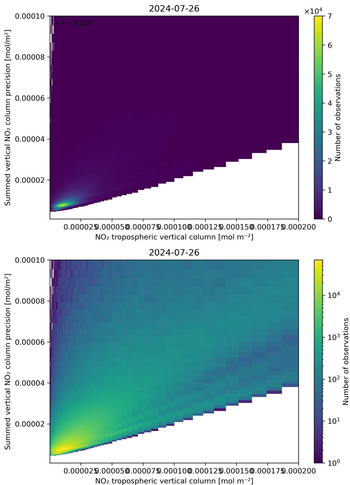
Figure 127: Scatter density plot of “NO 2 tropospheric vertical column” against “Summed vertical NO 2 column precision” for 2024-07-26 to 2024-07-27.
