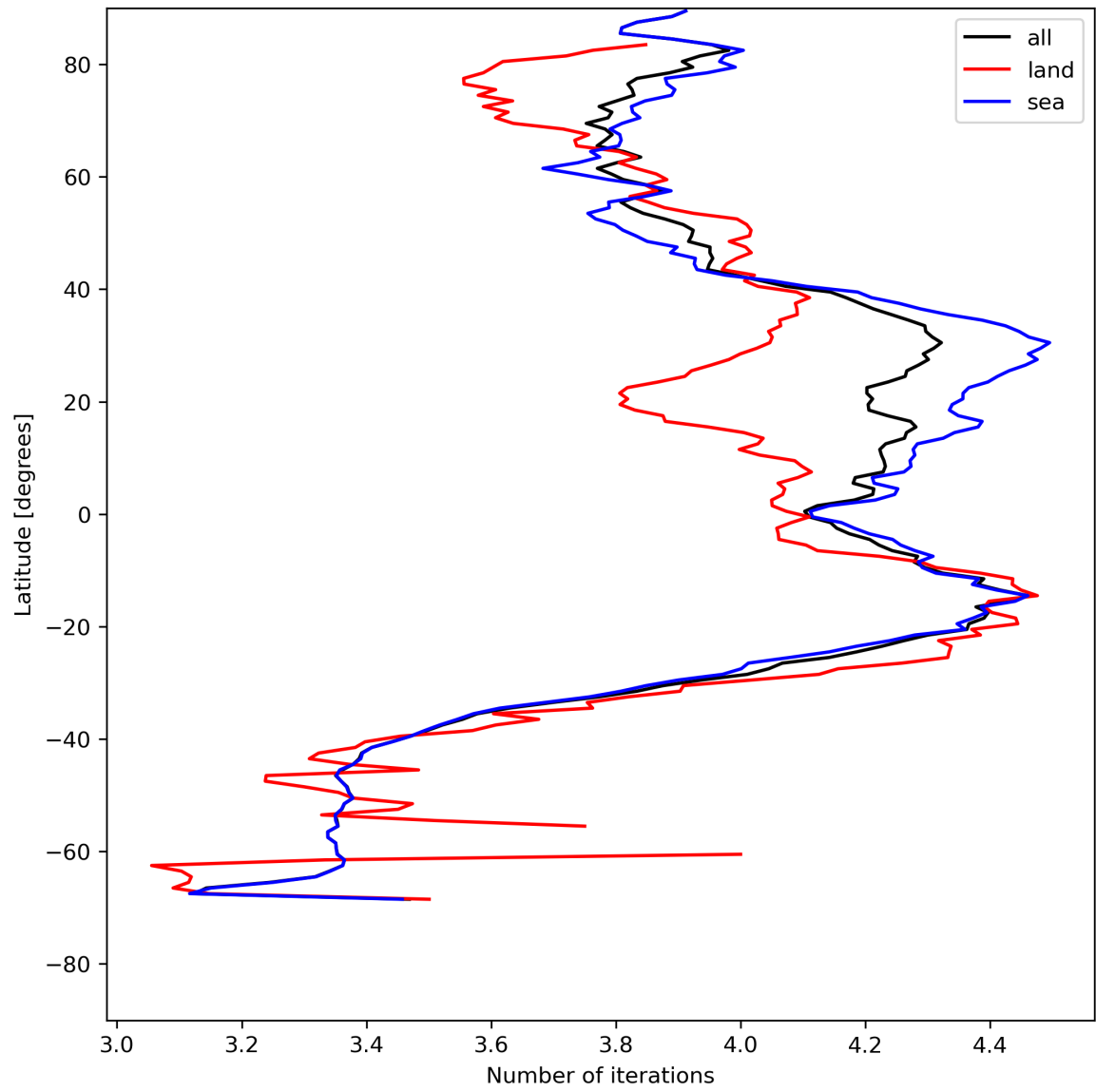
Figure 17: Zonal average of “Number of iterations” for 2024-07-26 to 2024-07-27.
