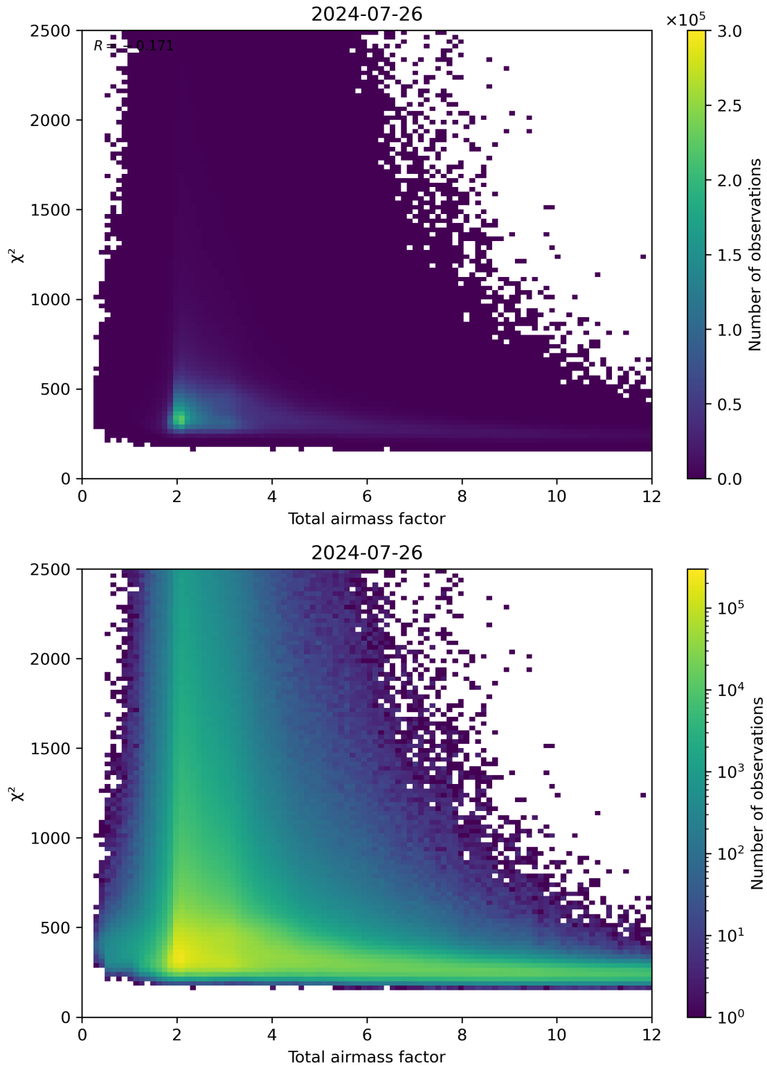
Figure 63: Scatter density plot of “Total airmass factor” against “ \chi^2 ” for 2024-07-26 to 2024-07-27.
