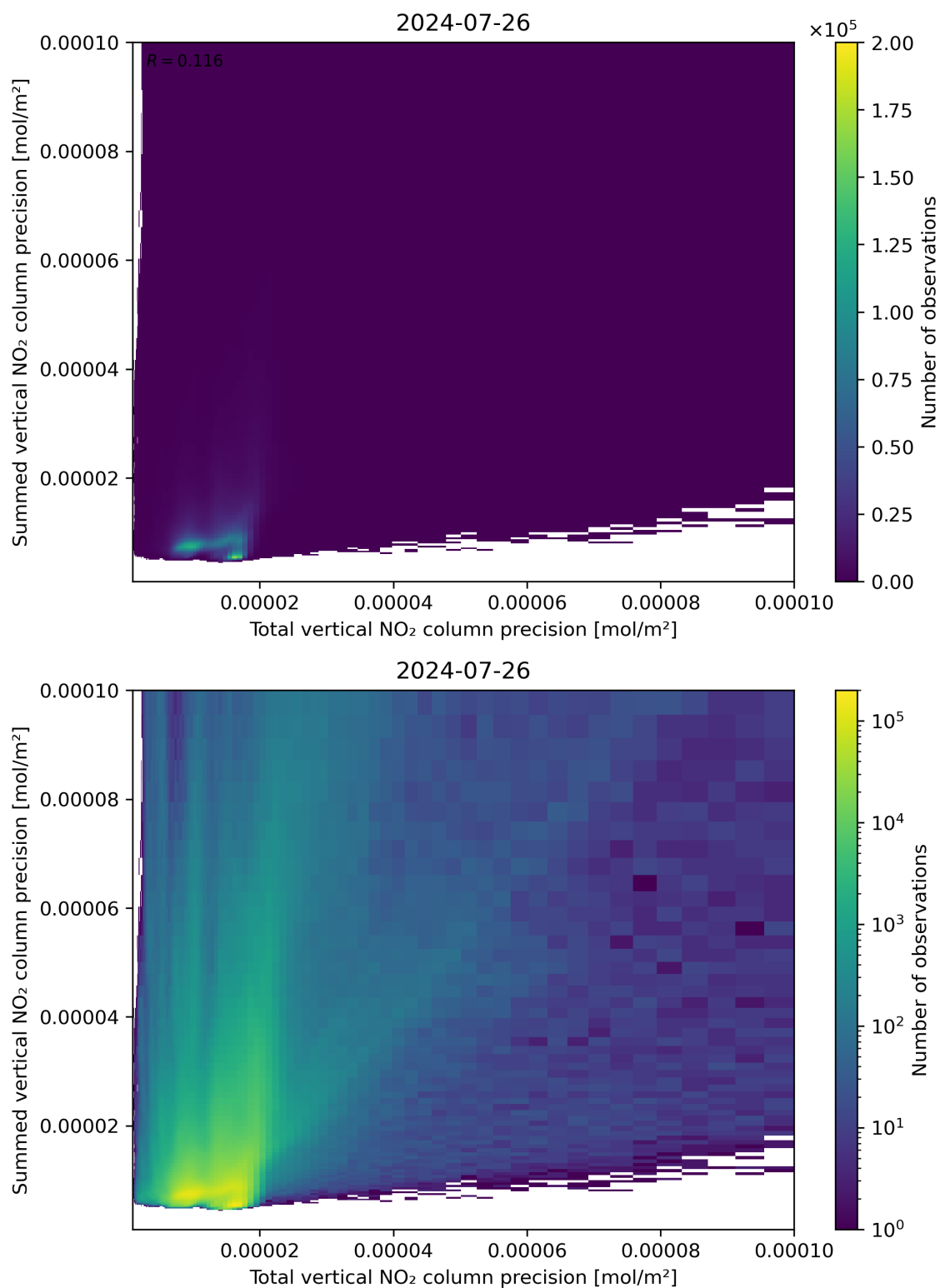
Figure 118: Scatter density plot of “Total vertical NO 2 column precision” against “Summed vertical NO 2 column precision” for 2024-07-26 to 2024-07-27.
