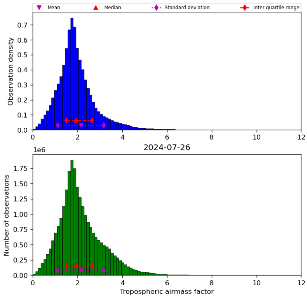
Figure 31: Histogram of “Tropospheric airmass factor” for 2024-07-26 to 2024-07-27
