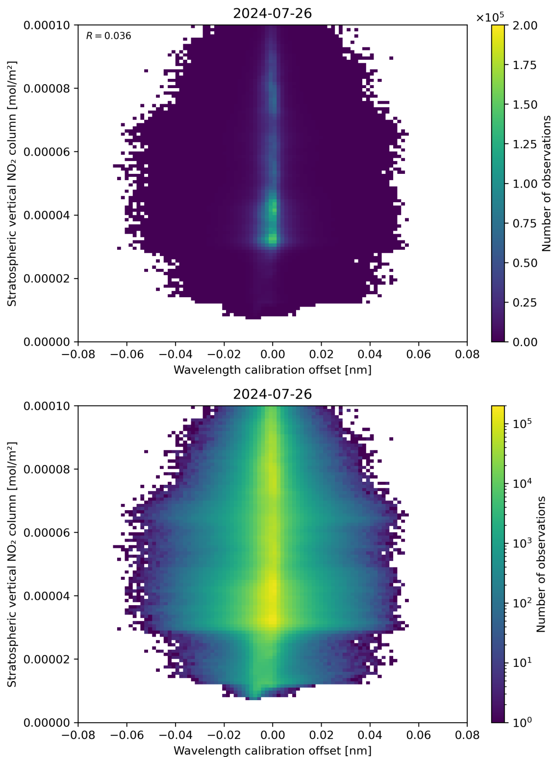
Figure 176: Scatter density plot of “Wavelength calibration offset” against “Stratospheric vertical NO 2 column” for 2024-07-26 to 2024-07-27.
