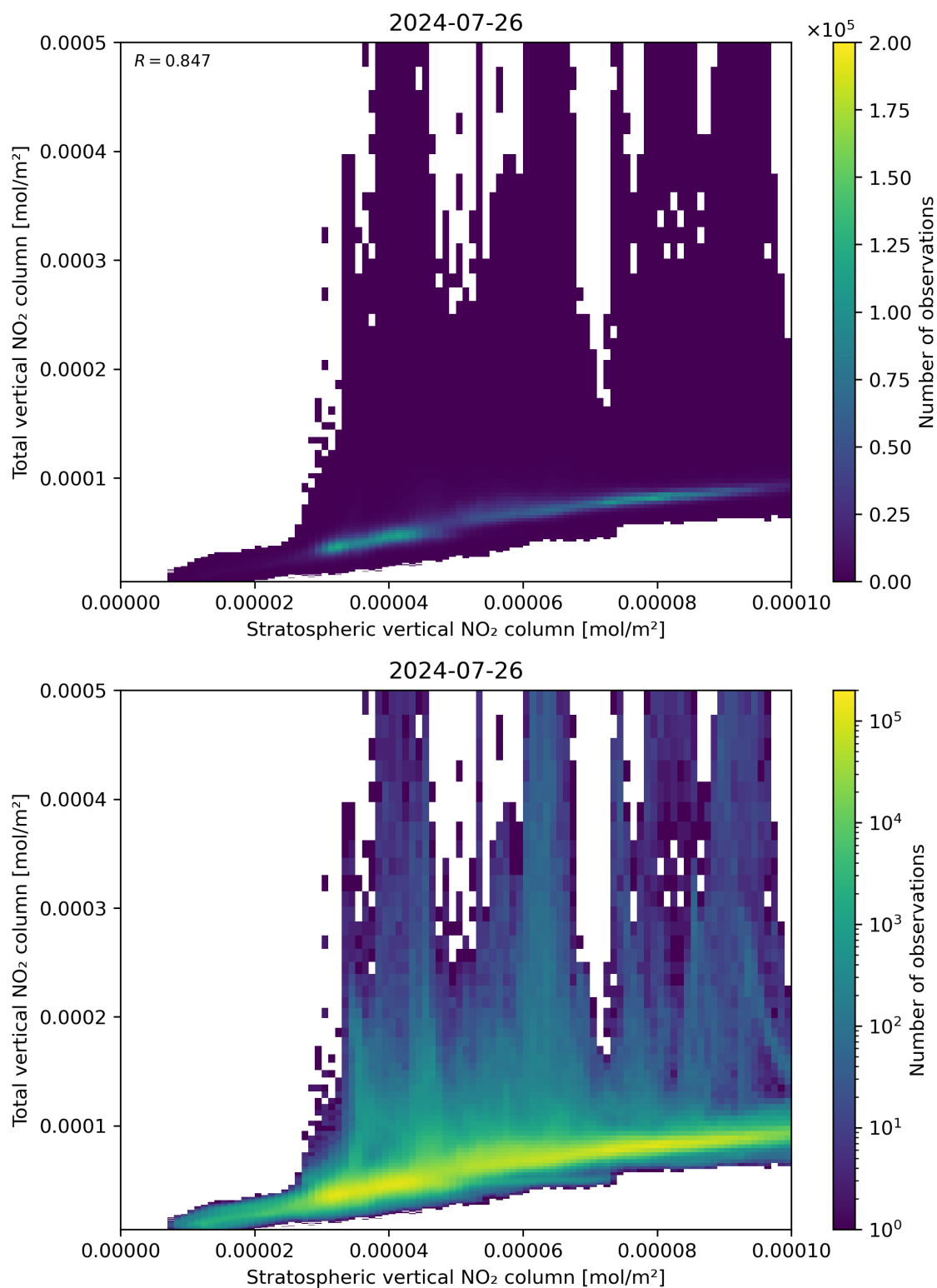
Figure 100: Scatter density plot of “Stratospheric vertical NO 2 column” against “Total vertical NO 2 column” for 2024-07-26 to 2024-07-27.
