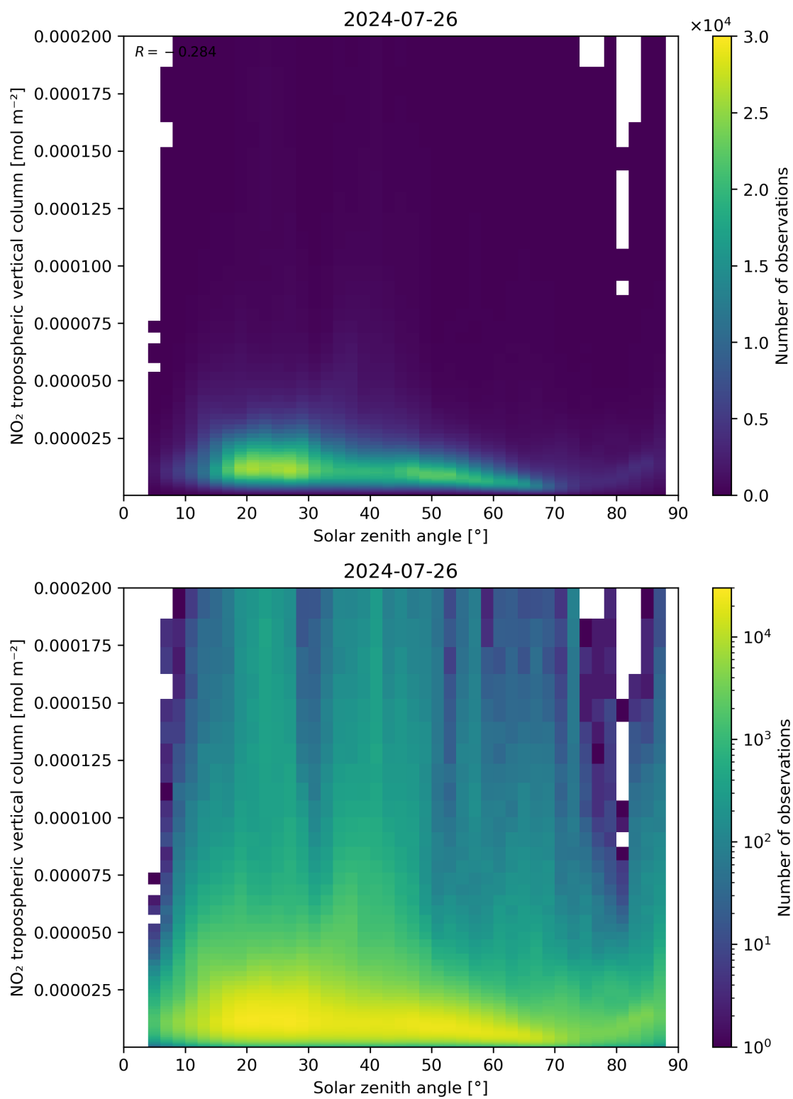
Figure 155: Scatter density plot of “Solar zenith angle” against “NO 2 tropospheric vertical column” for 2024-07-26 to 2024-07-27.
