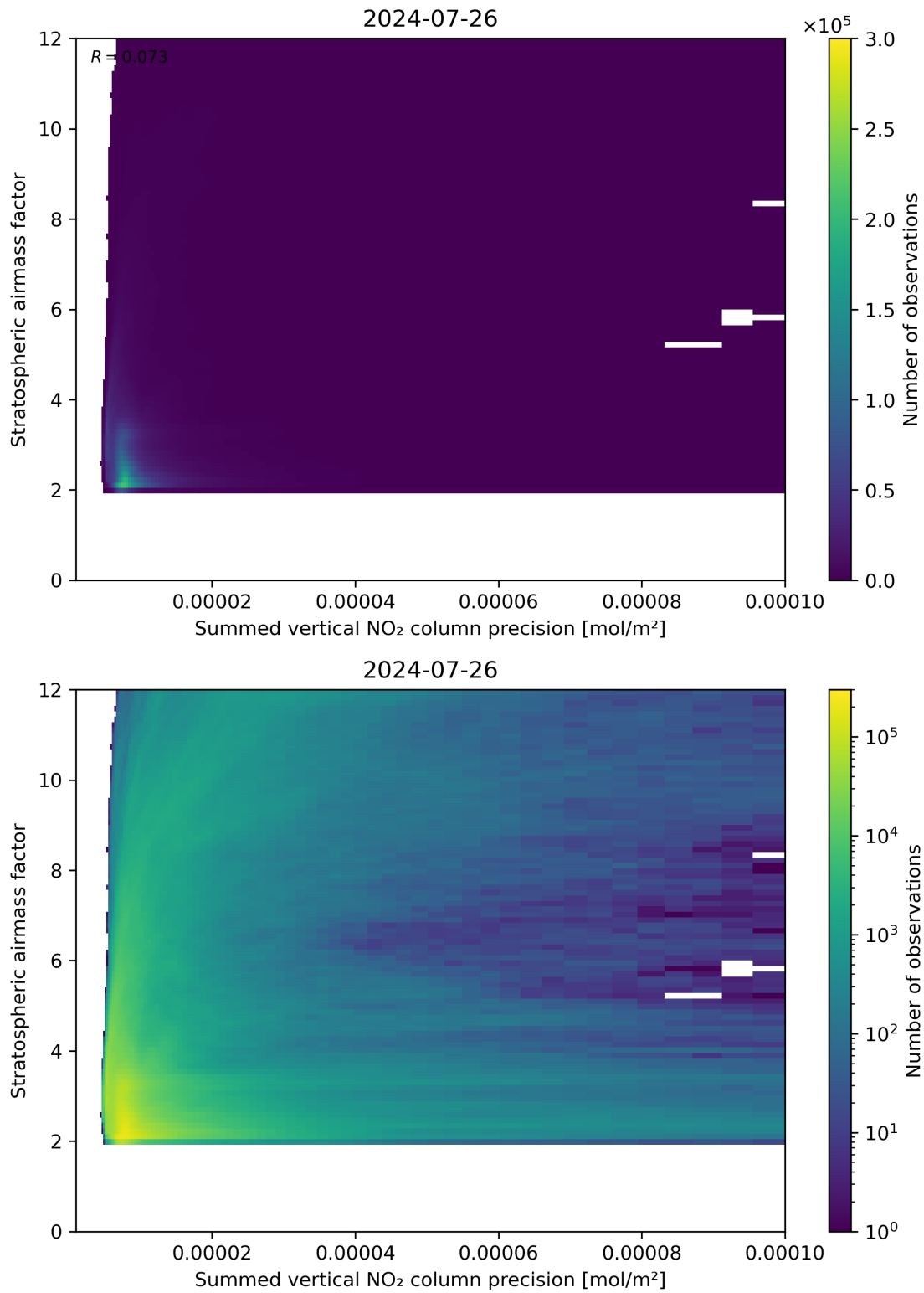
Figure 106: Scatter density plot of “Summed vertical NO 2 column precision” against “Stratospheric airmass factor” for 2024-07-26 to 2024-07-27.
