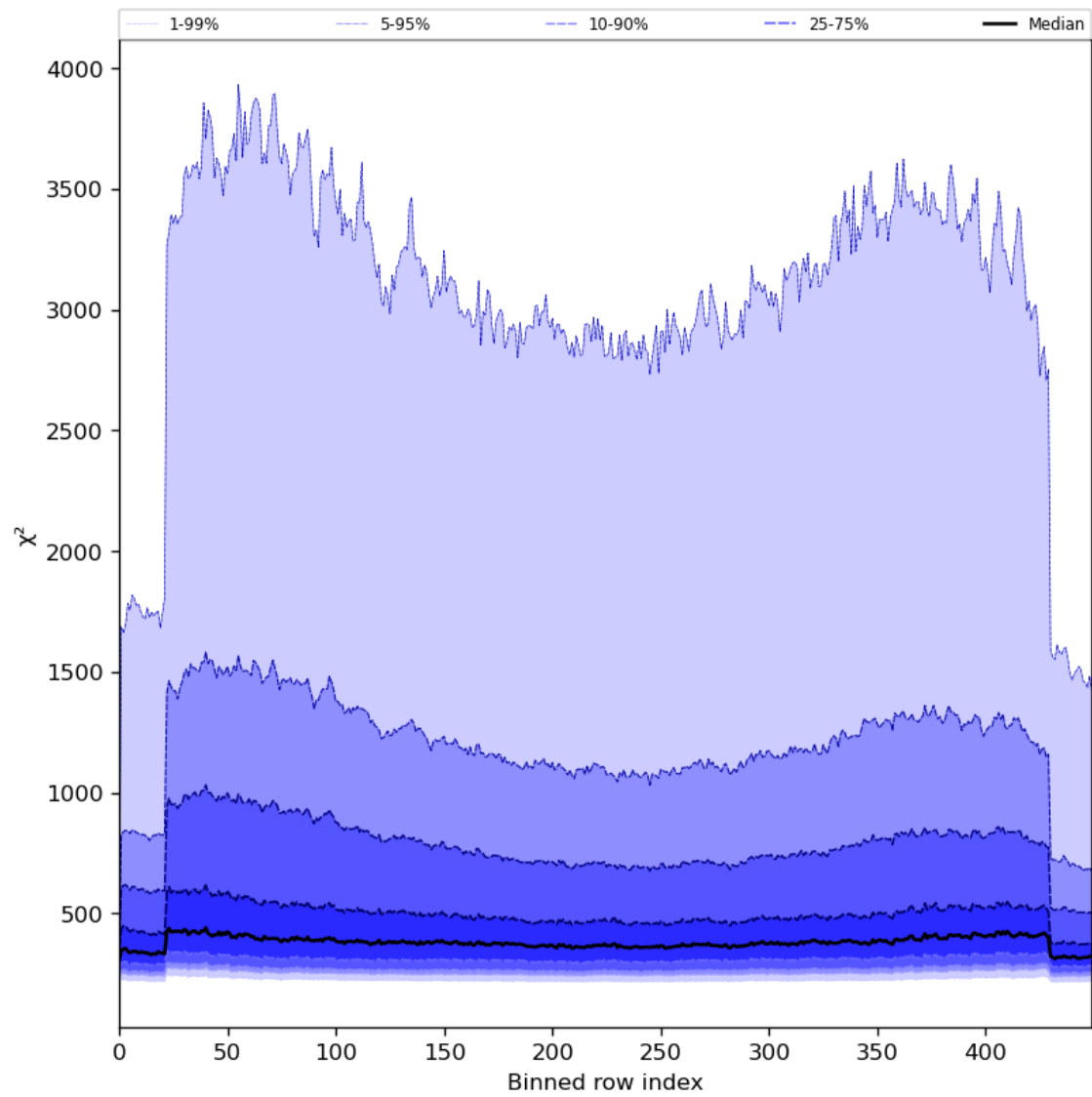
Figure 59: Along track statistics of “ \chi^2 ” for 2024-07-26 to 2024-07-27
