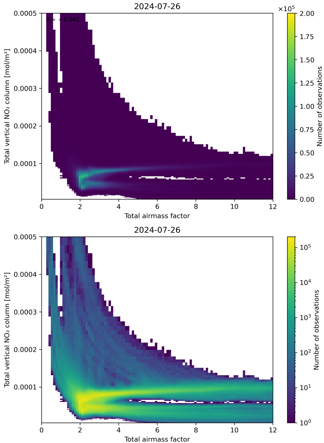
Figure 67: Scatter density plot of “Total airmass factor” against “Total vertical NO 2 column” for 2024-07-26 to 2024-07-27.
