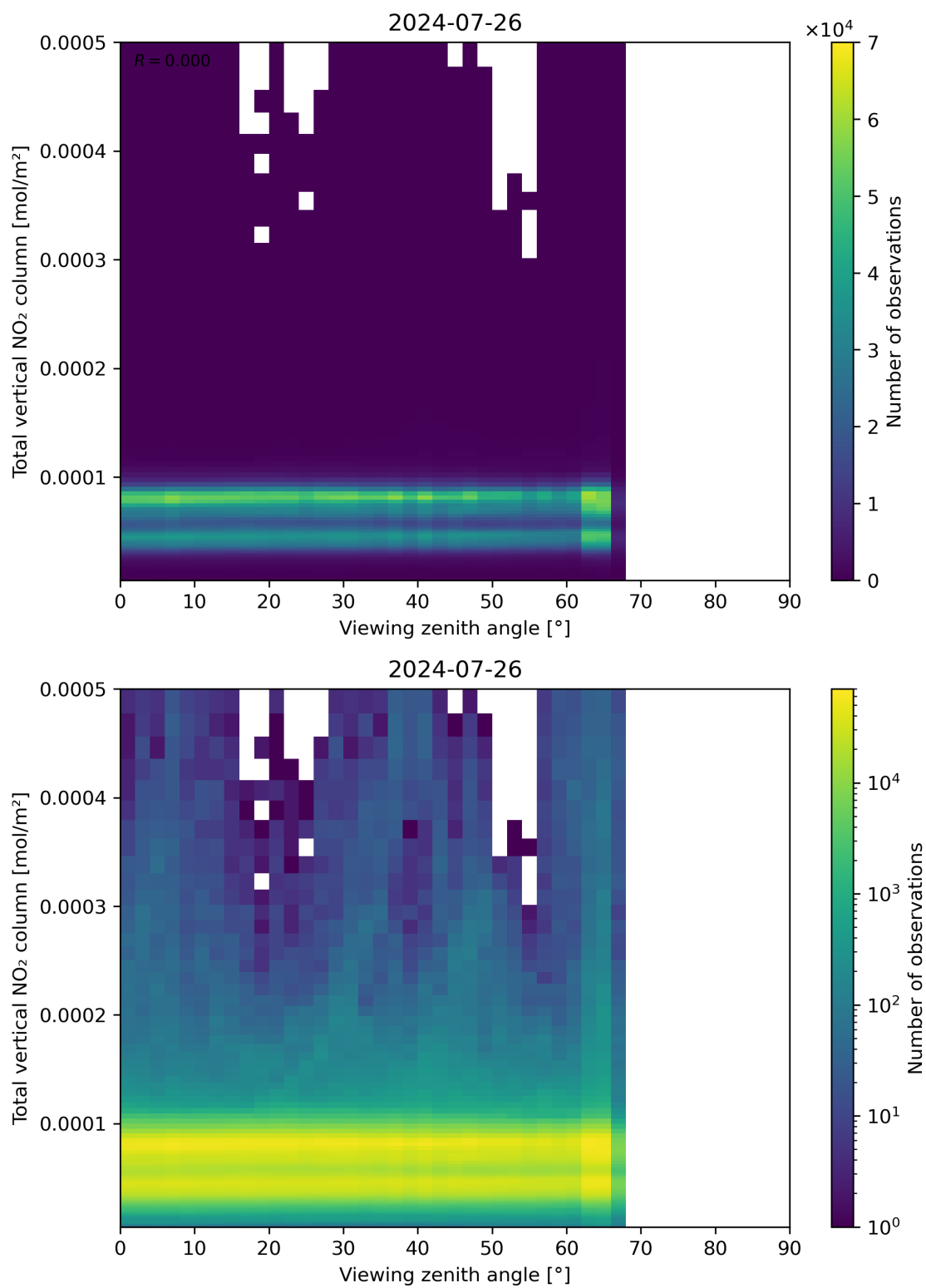
Figure 167: Scatter density plot of “Viewing zenith angle” against “Total vertical NO 2 column” for 2024-07-26 to 2024-07-27.
