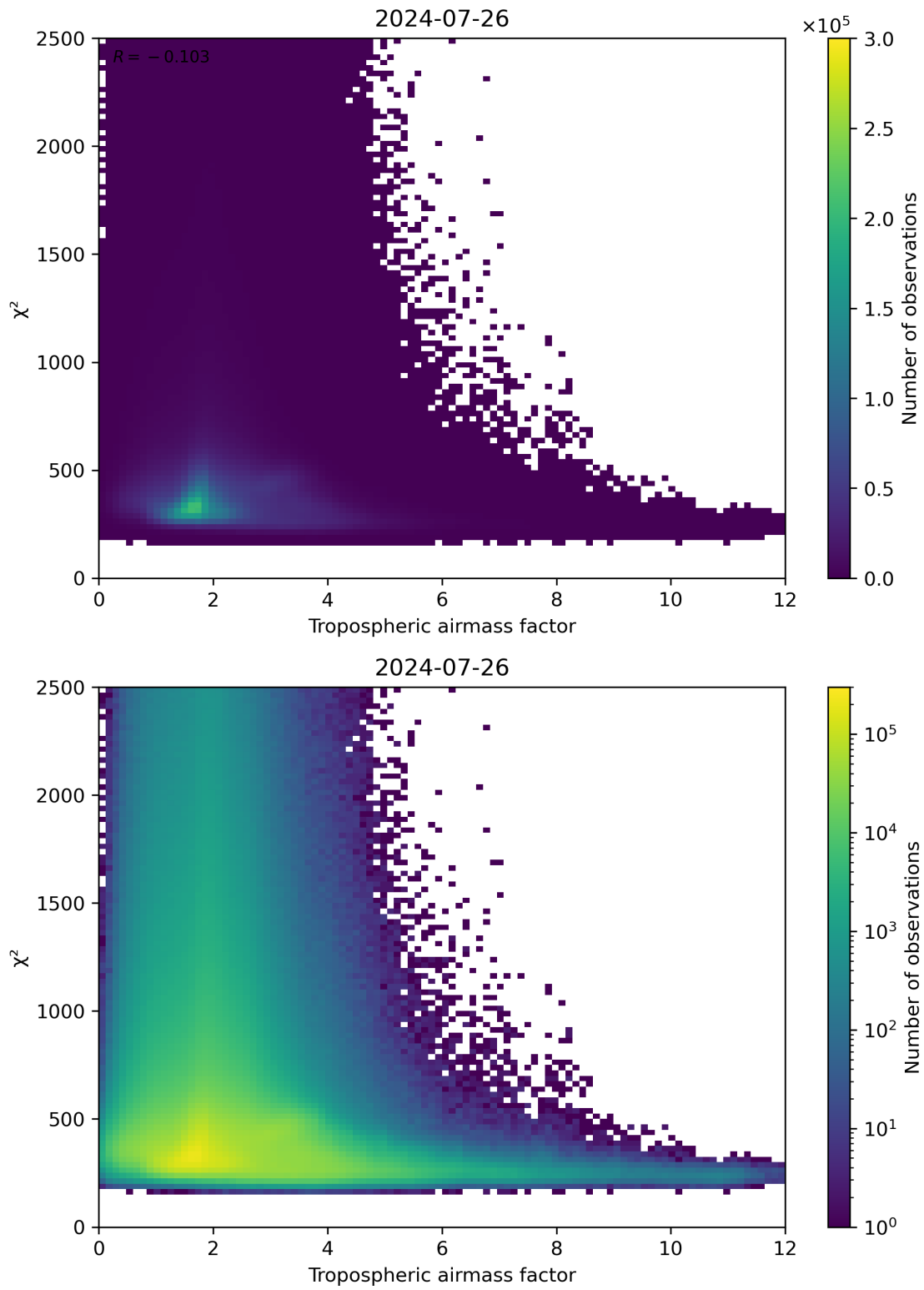
Figure 73: Scatter density plot of “Tropospheric airmass factor” against “ \chi^2 ” for 2024-07-26 to 2024-07-27.
