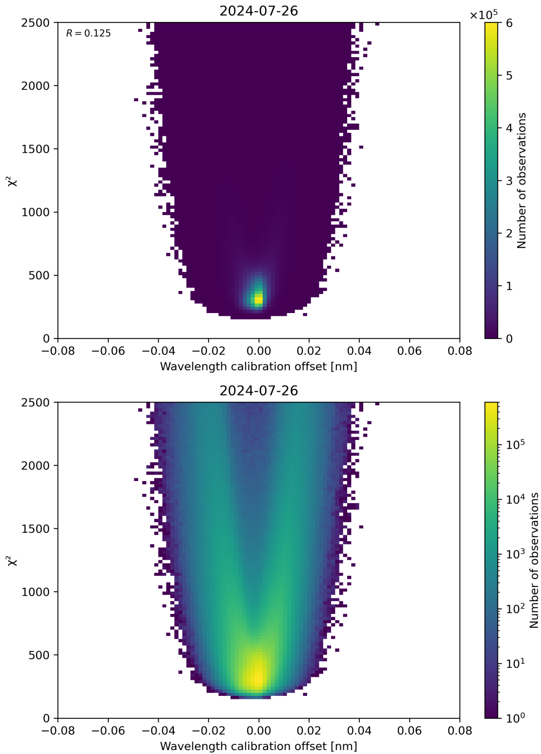
Figure 175: Scatter density plot of “Wavelength calibration offset” against “ \chi^2 ” for 2024-07-26 to 2024-07-27.
