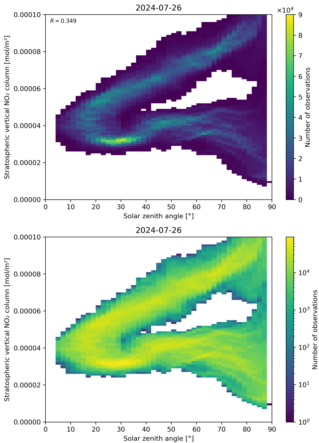
Figure 150: Scatter density plot of “Solar zenith angle” against “Stratospheric vertical NO 2 column” for 2024-07-26 to 2024-07-27.
