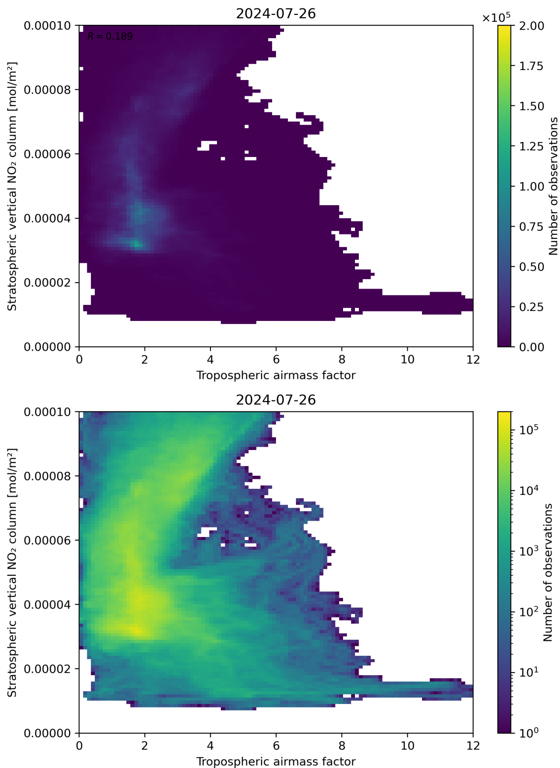
Figure 74: Scatter density plot of “Tropospheric air mass factor” against “Stratospheric vertical NO 2 column” for 2024-07-26 to 2024-07-27.
