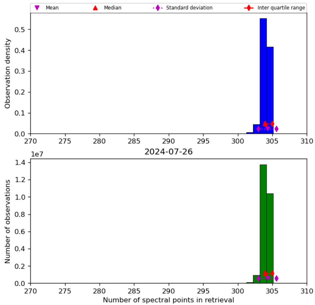
Figure 33: Histogram of “Number of spectral points in retrieval” for 2024-07-26 to 2024-07-27
