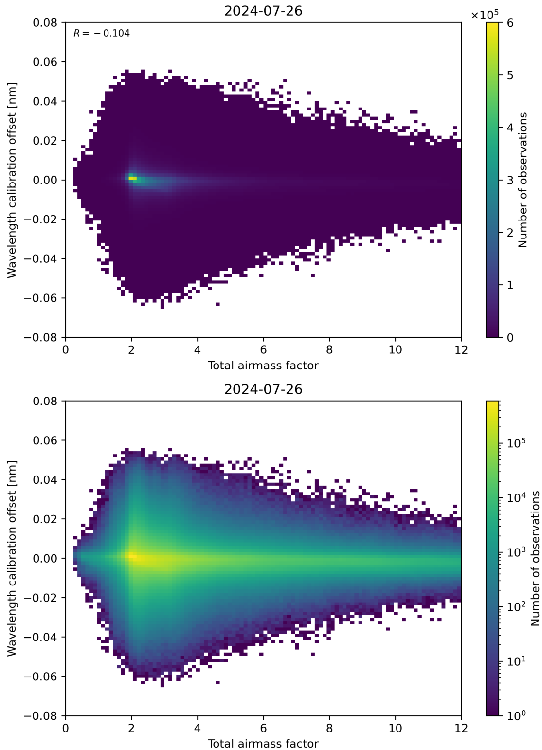
Figure 70: Scatter density plot of “Total airmass factor” against “Wavelength calibration offset” for 2024-07-26 to 2024-07-27.
