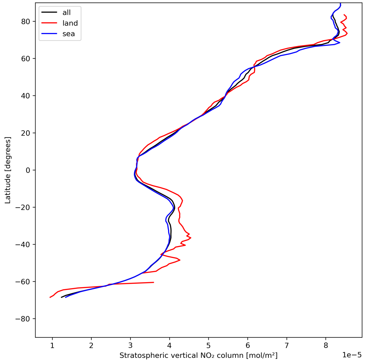
Figure 19: Zonal average of “Stratospheric vertical NO 2 column” for 2024-07-26 to 2024-07-27.
