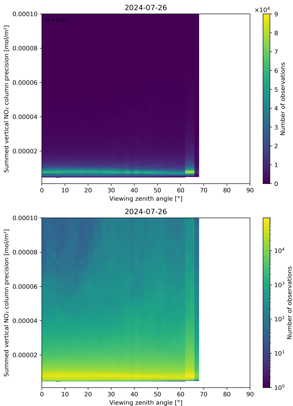
Figure 166: Scatter density plot of “Viewing zenith angle” against “Summed vertical NO 2 column precision” for 2024-07-26 to 2024-07-27.
