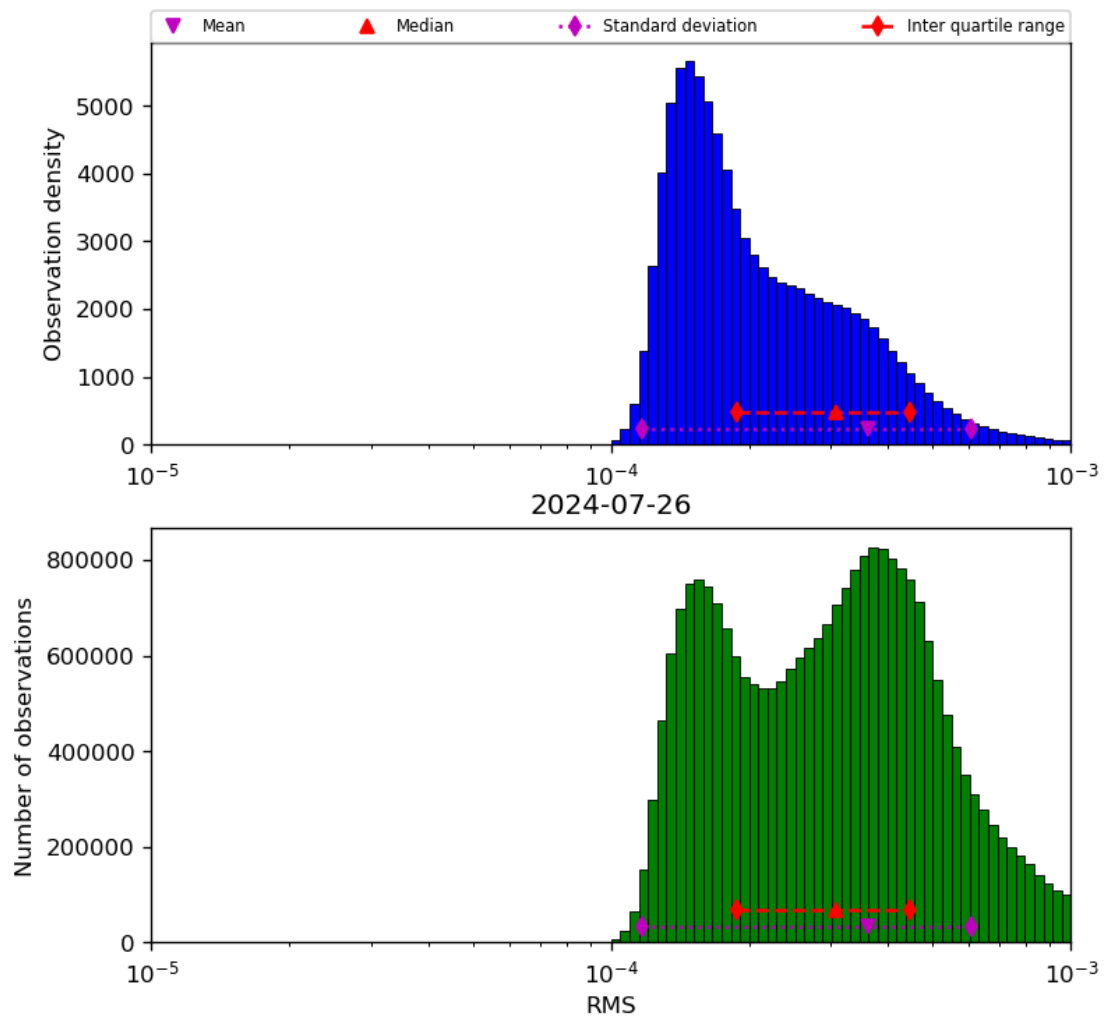
Figure 43: Histogram of “RMS” for 2024-07-26 to 2024-07-27
