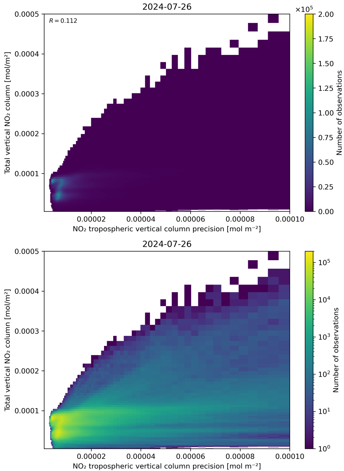
Figure 138: Scatter density plot of “NO 2 tropospheric vertical column precision” against “Total vertical NO 2 column” for 2024-07-26 to 2024-07-27.
