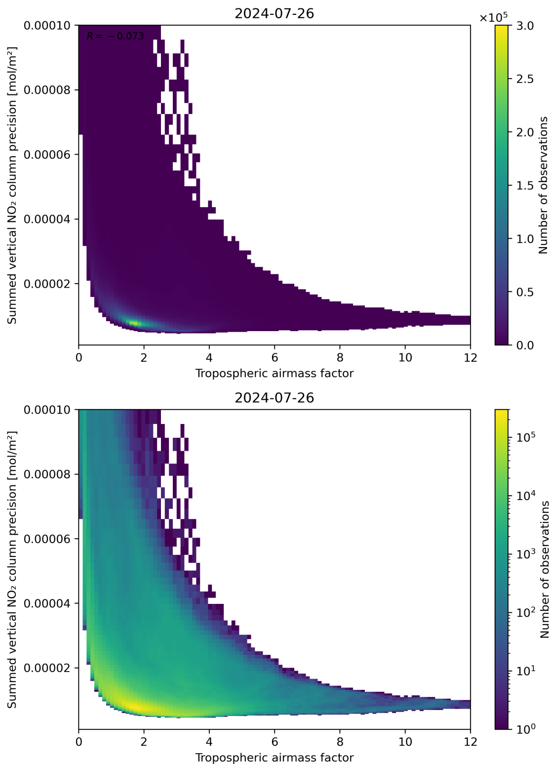
Figure 76: Scatter density plot of “Tropospheric air mass factor” against “Summed vertical NO 2 column precision” for 2024-07-26 to 2024-07-27.
