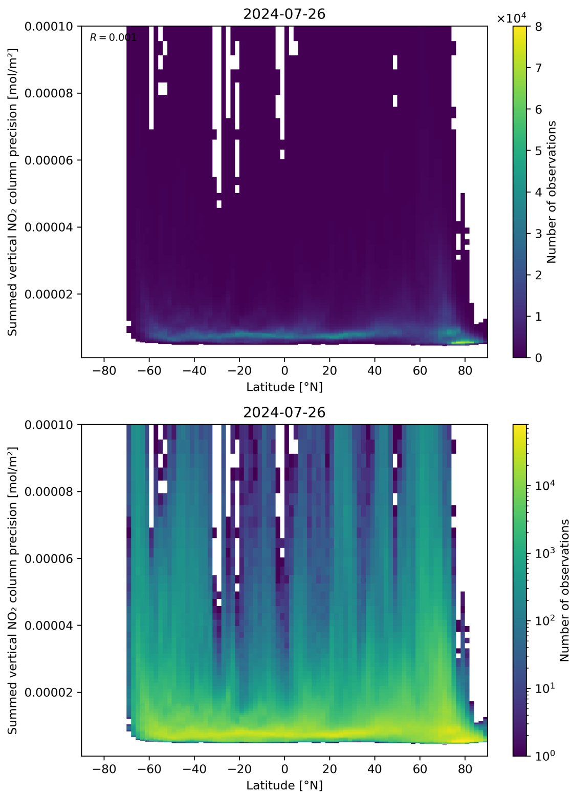
Figure 89: Scatter density plot of “Latitude” against “Summed vertical NO 2 column precision” for 2024-07-26 to 2024-07-27.
