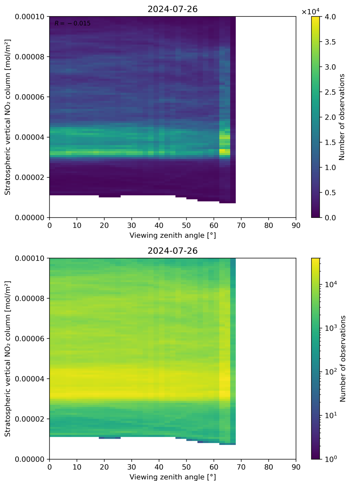
Figure 164: Scatter density plot of “Viewing zenith angle” against “Stratospheric vertical NO 2 column” for 2024-07-26 to 2024-07-27.
