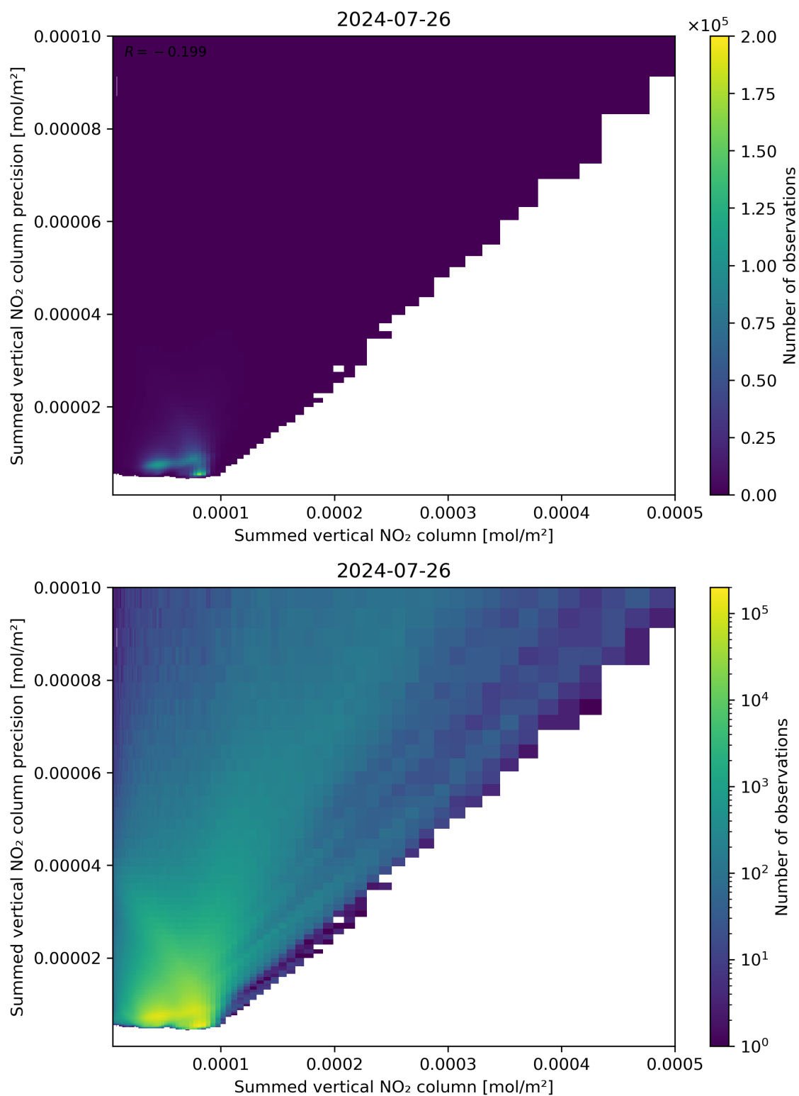
Figure 105: Scatter density plot of “Summed vertical NO 2 column” against “Summed vertical NO 2 column precision” for 2024-07-26 to 2024-07-27.
