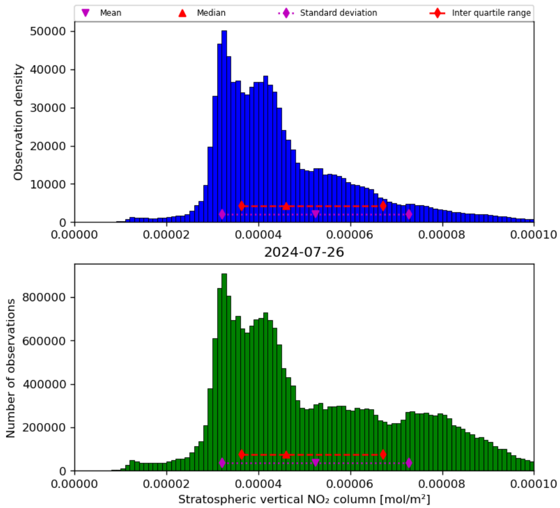
Figure 36: Histogram of “Stratospheric vertical NO 2 column” for 2024-07-26 to 2024-07-27
