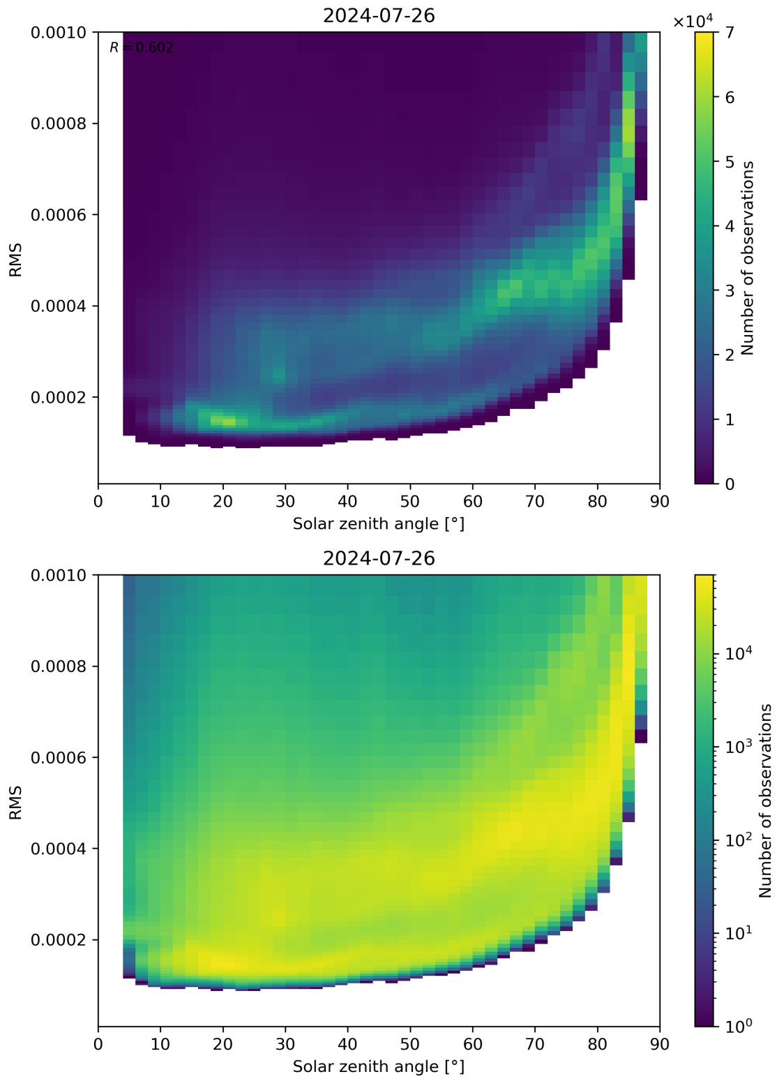
Figure 157: Scatter density plot of “Solar zenith angle” against “RMS” for 2024-07-26 to 2024-07-27.
