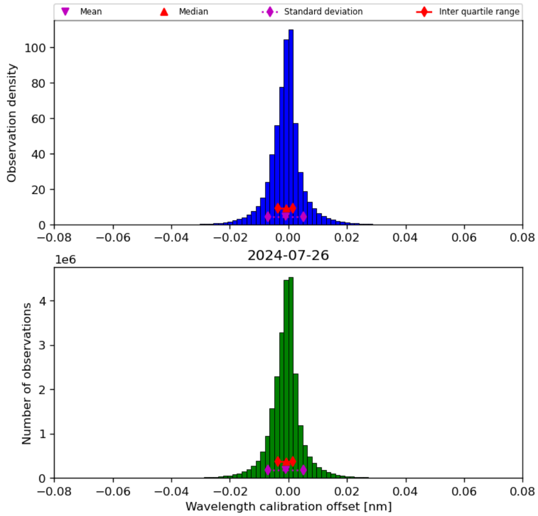
Figure 35: Histogram of “Wavelength calibration offset” for 2024-07-26 to 2024-07-27
