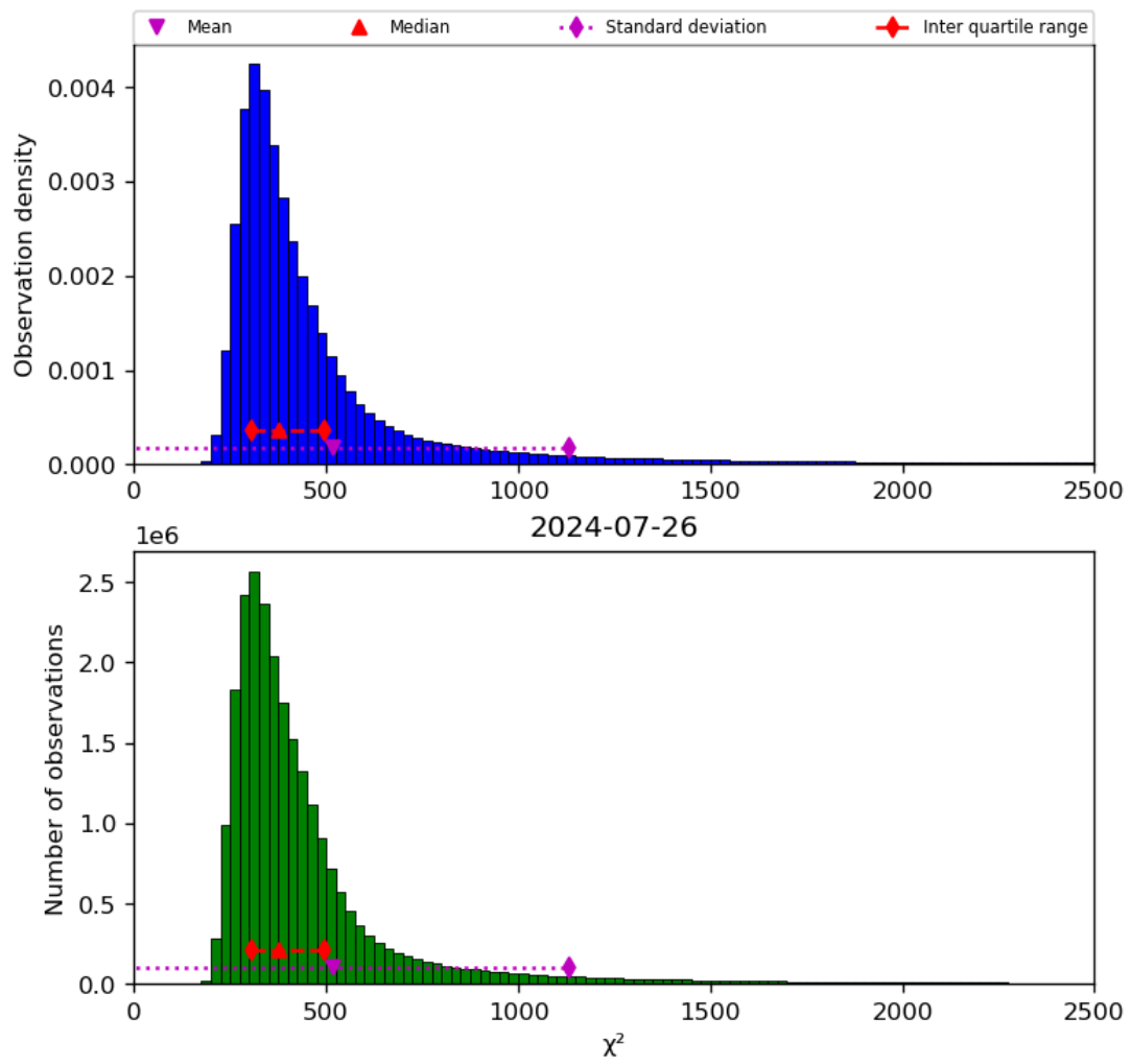
Figure 42: Histogram of “ \chi^2 ” for 2024-07-26 to 2024-07-27
