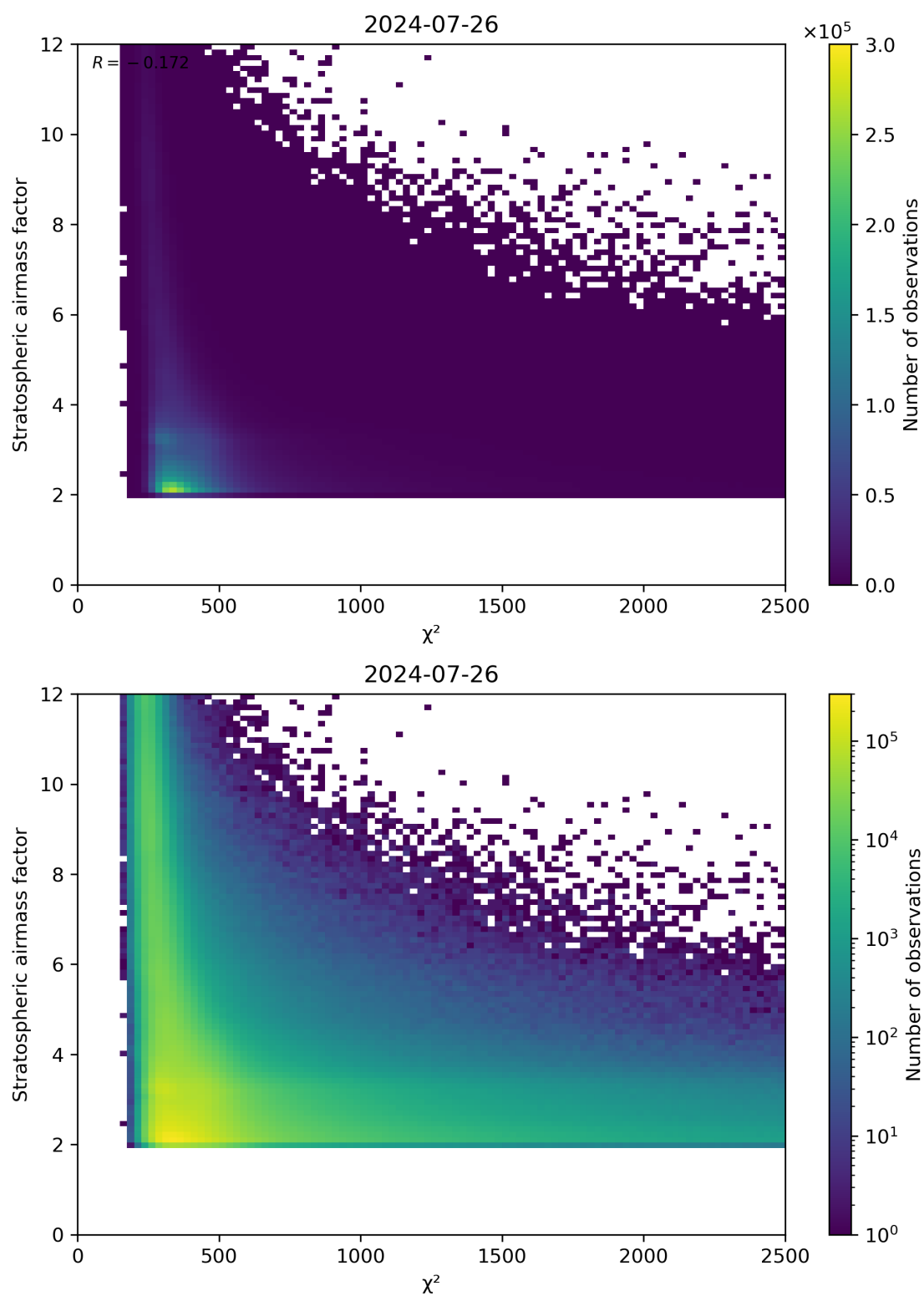
Figure 81: Scatter density plot of “ \chi^2 ” against “Stratospheric air mass factor” for 2024-07-26 to 2024-07-27.
