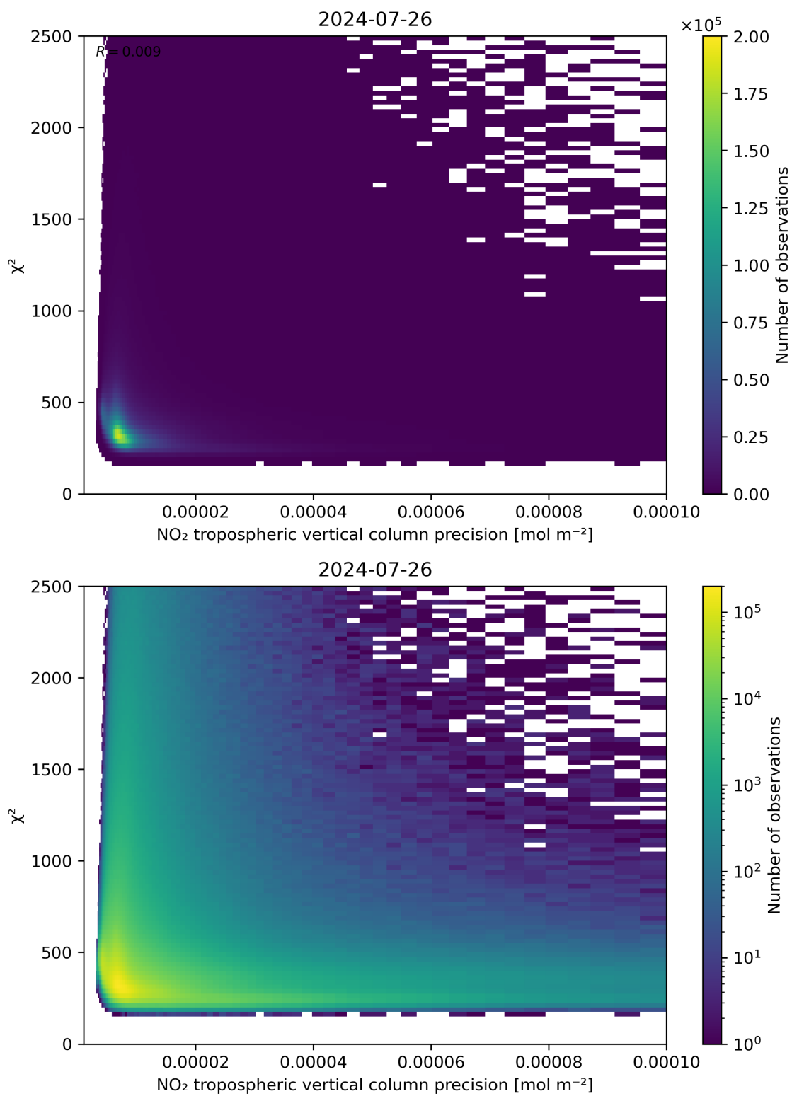
Figure 134: Scatter density plot of “NO 2 tropospheric vertical column precision” against “ \chi^2 ” for 2024-07-26 to 2024-07-27.
