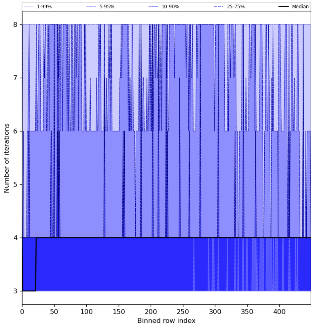
Figure 51: Along track statistics of “Number of iterations” for 2024-07-26 to 2024-07-27
