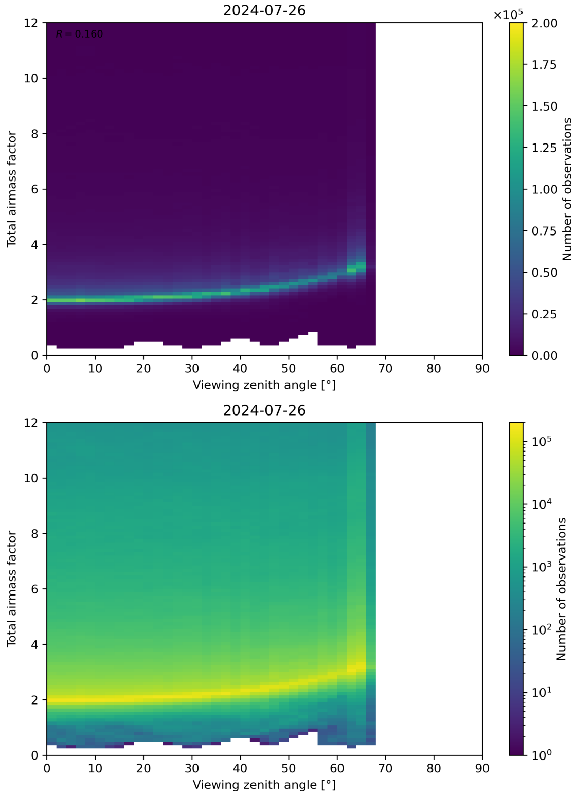
Figure 160: Scatter density plot of “Viewing zenith angle” against “Total airmass factor” for 2024-07-26 to 2024-07-27.
