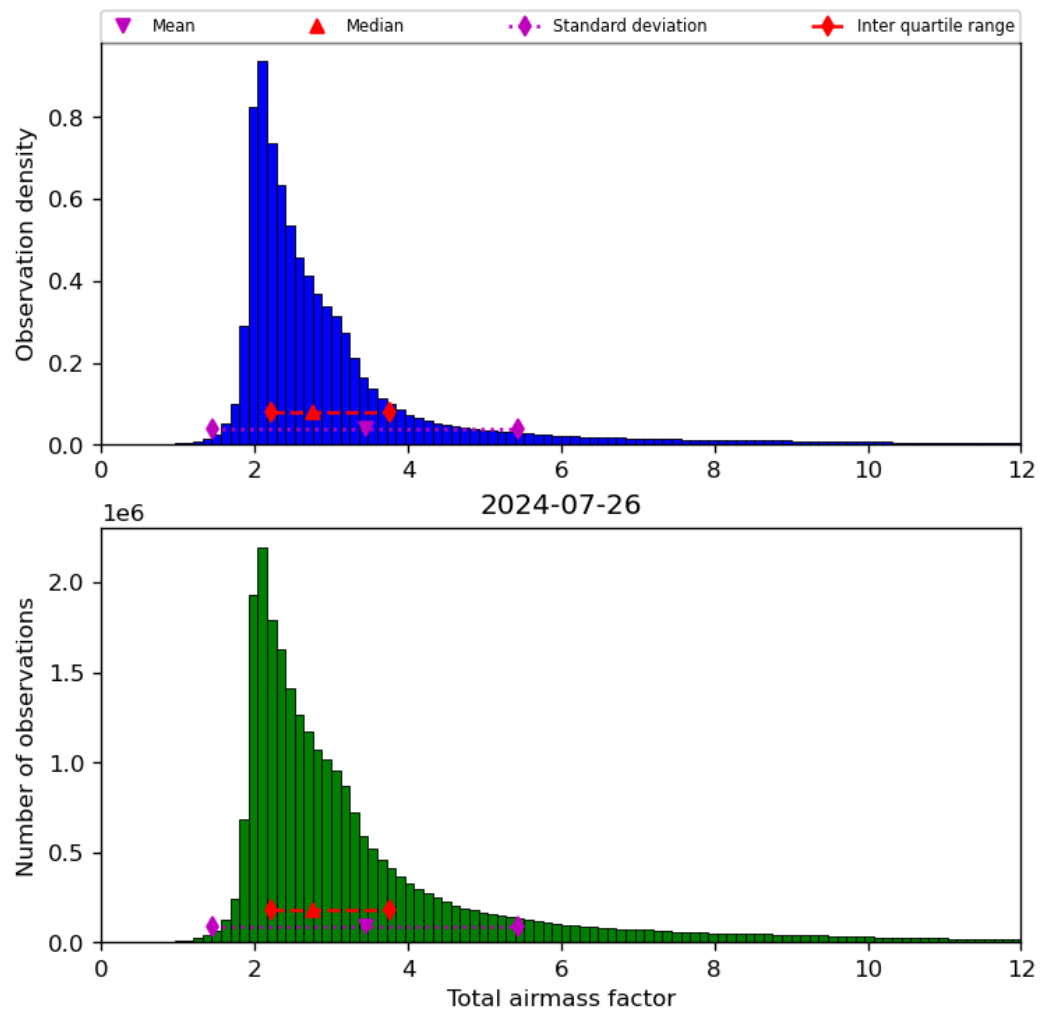
Figure 32: Histogram of “Total airmass factor” for 2024-07-26 to 2024-07-27
