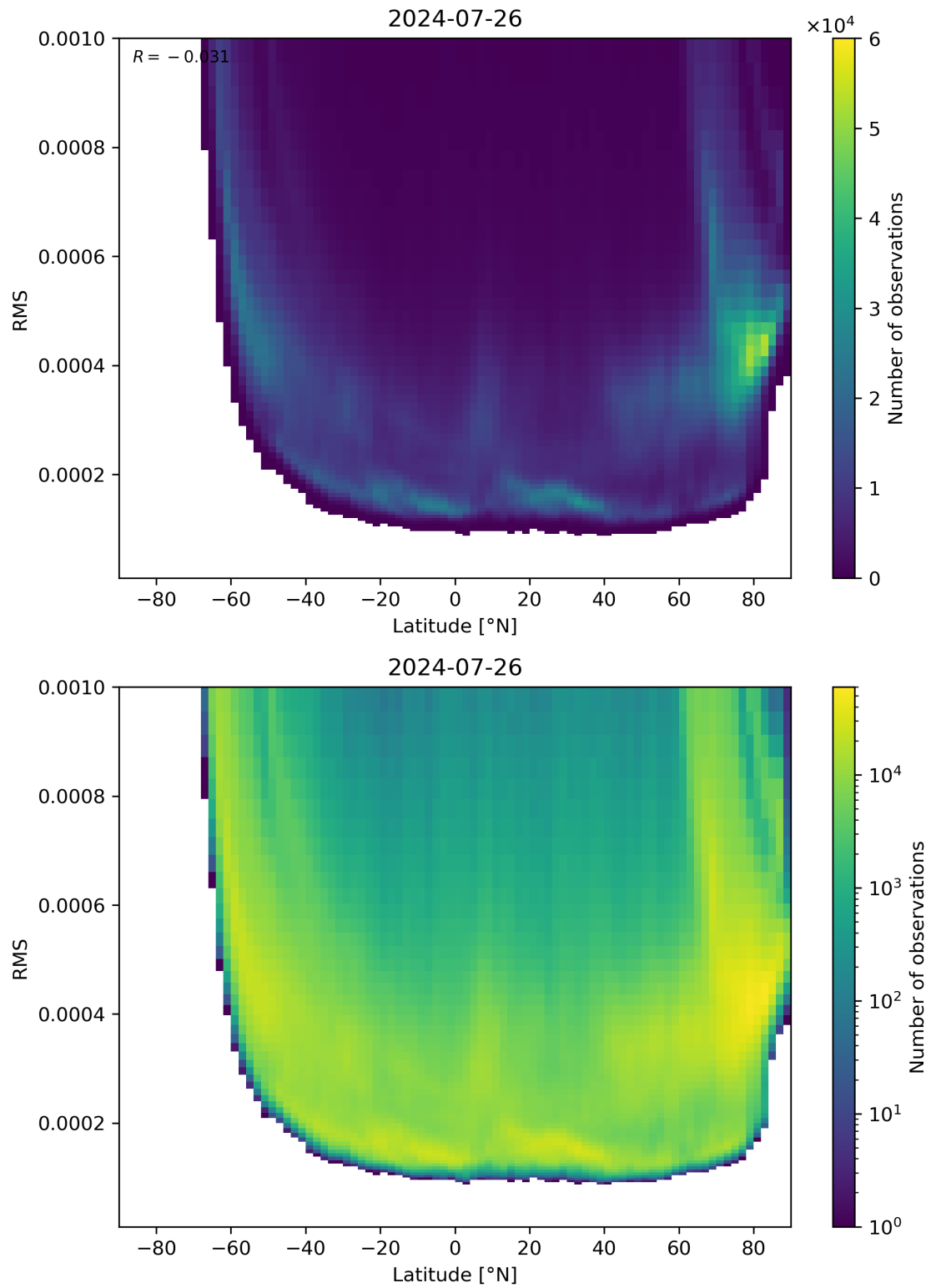
Figure 94: Scatter density plot of “Latitude” against “RMS” for 2024-07-26 to 2024-07-27.
