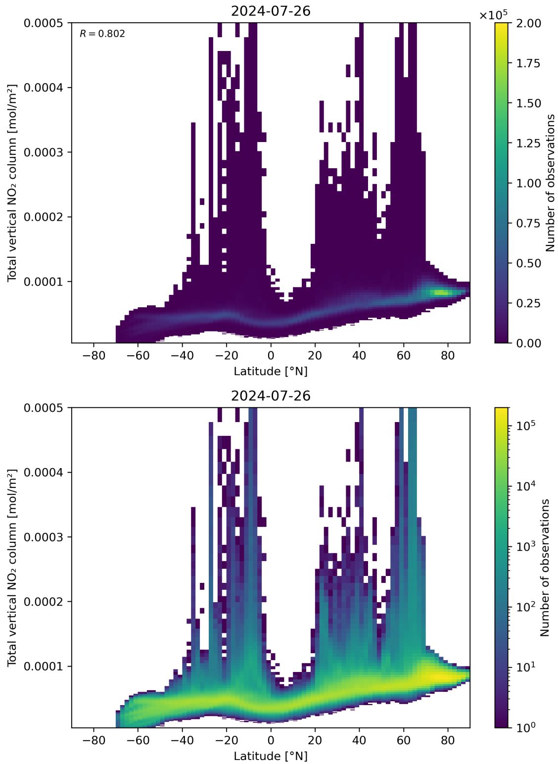
Figure 90: Scatter density plot of “Latitude” against “Total vertical NO 2 column” for 2024-07-26 to 2024-07-27.
