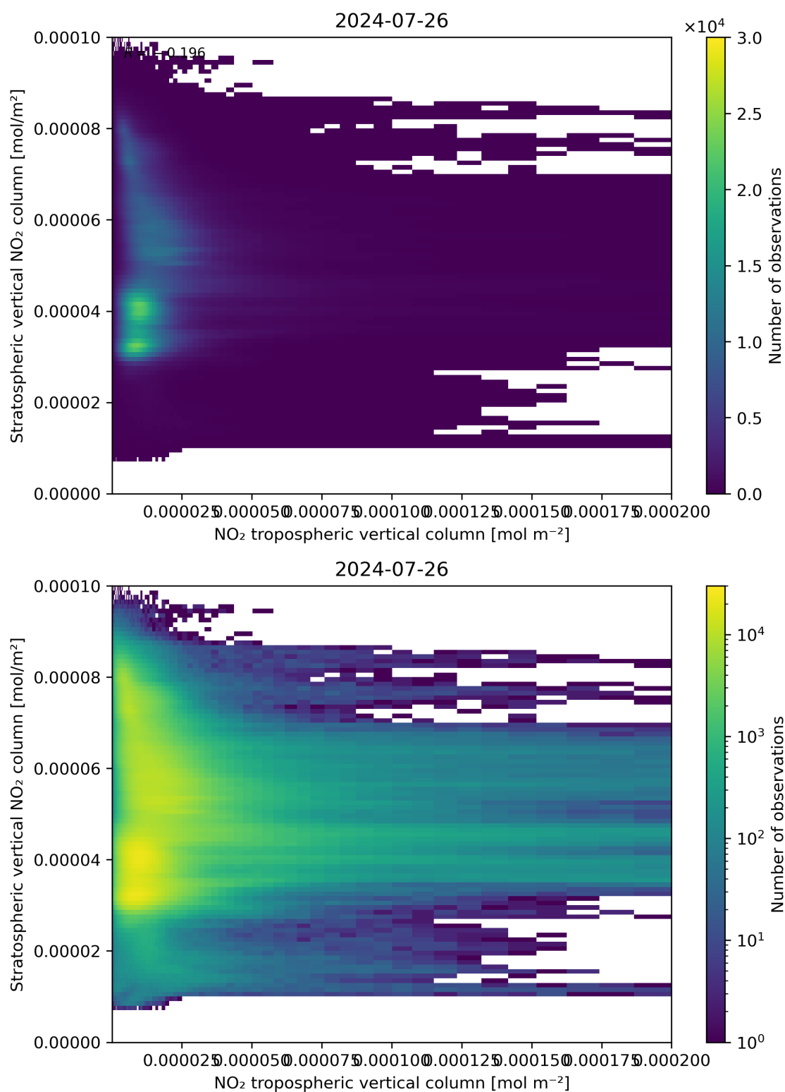
Figure 125: Scatter density plot of “NO 2 tropospheric vertical column” against “Stratospheric vertical NO 2 column” for 2024-07-26 to 2024-07-27.
