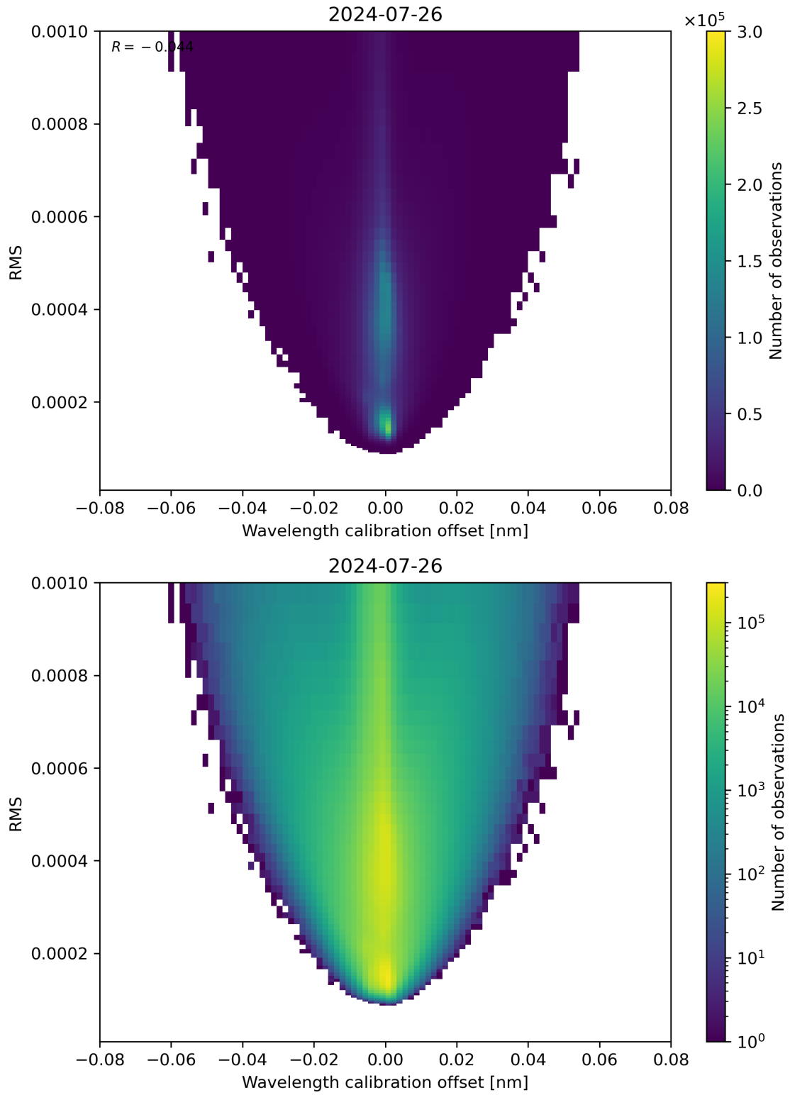
Figure 181: Scatter density plot of “Wavelength calibration offset” against “RMS” for 2024-07-26 to 2024-07-27.
