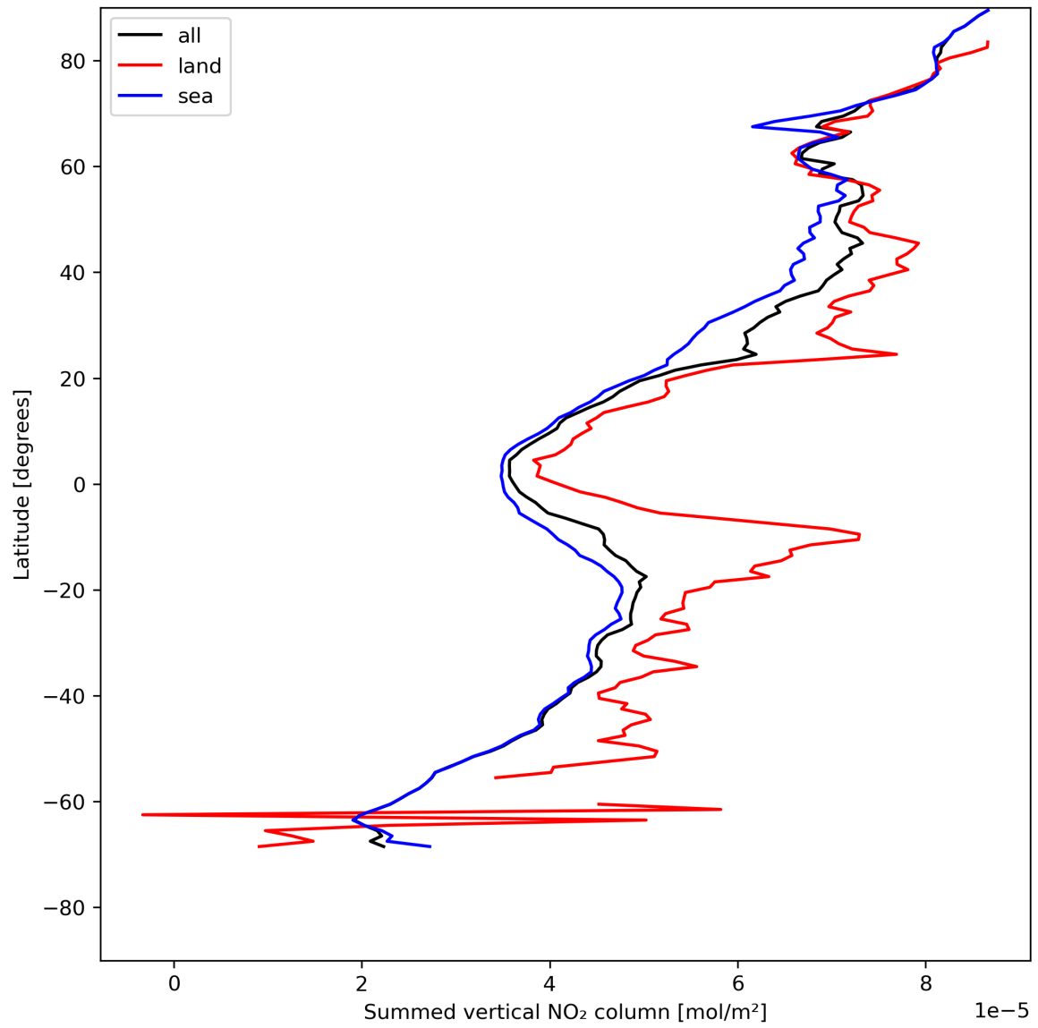
Figure 23: Zonal average of “Summed vertical NO 2 column” for 2024-07-26 to 2024-07-27.
