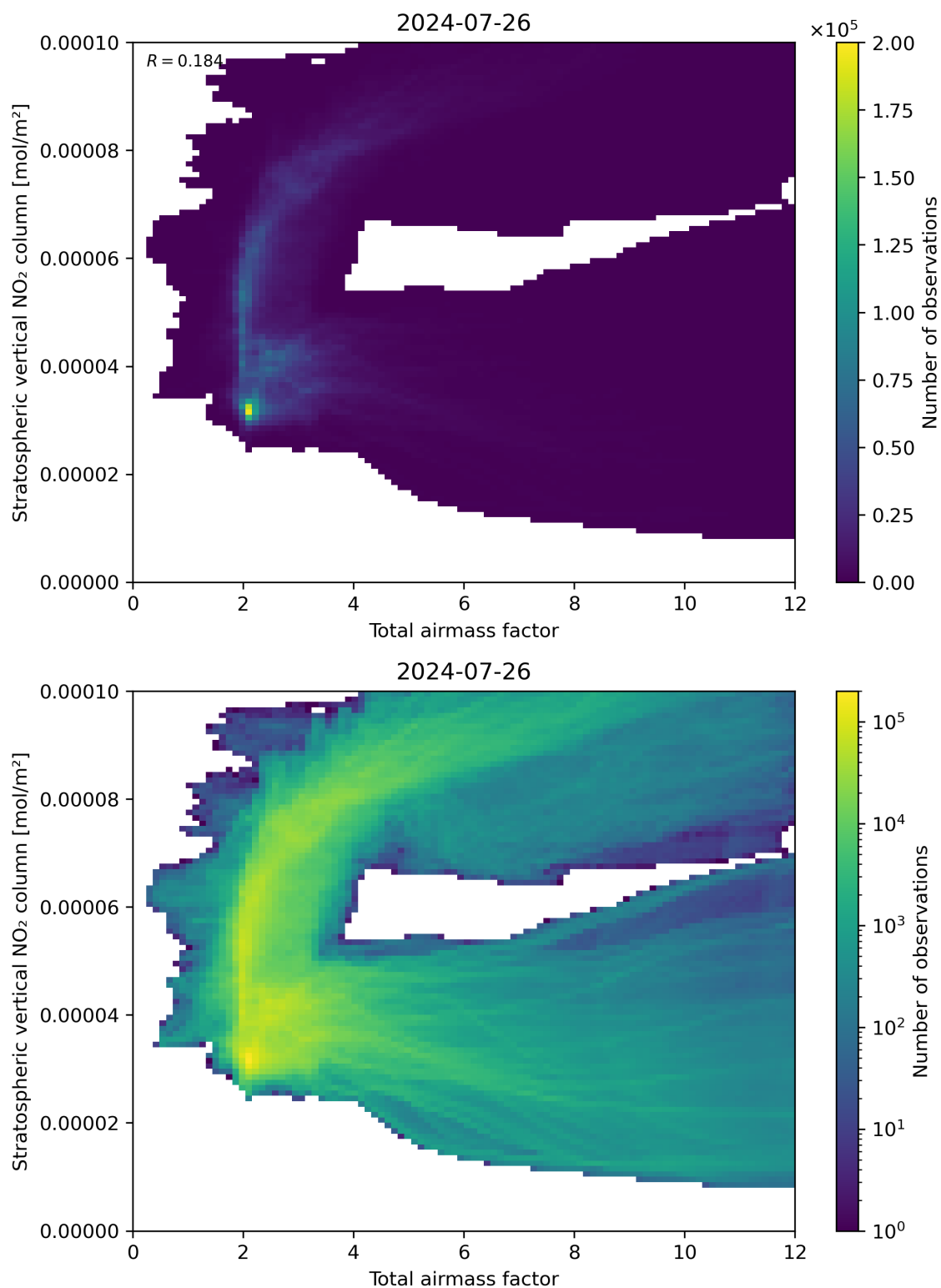
Figure 64: Scatter density plot of “Total airmass factor” against “Stratospheric vertical NO 2 column” for 2024-07-26 to 2024-07-27.
