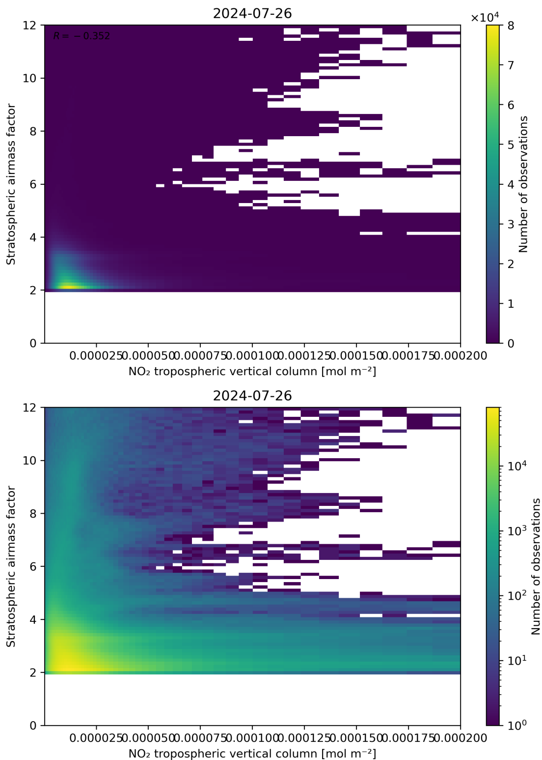
Figure 121: Scatter density plot of “NO 2 tropospheric vertical column” against “Stratospheric air mass factor” for 2024-07-26 to 2024-07-27.
