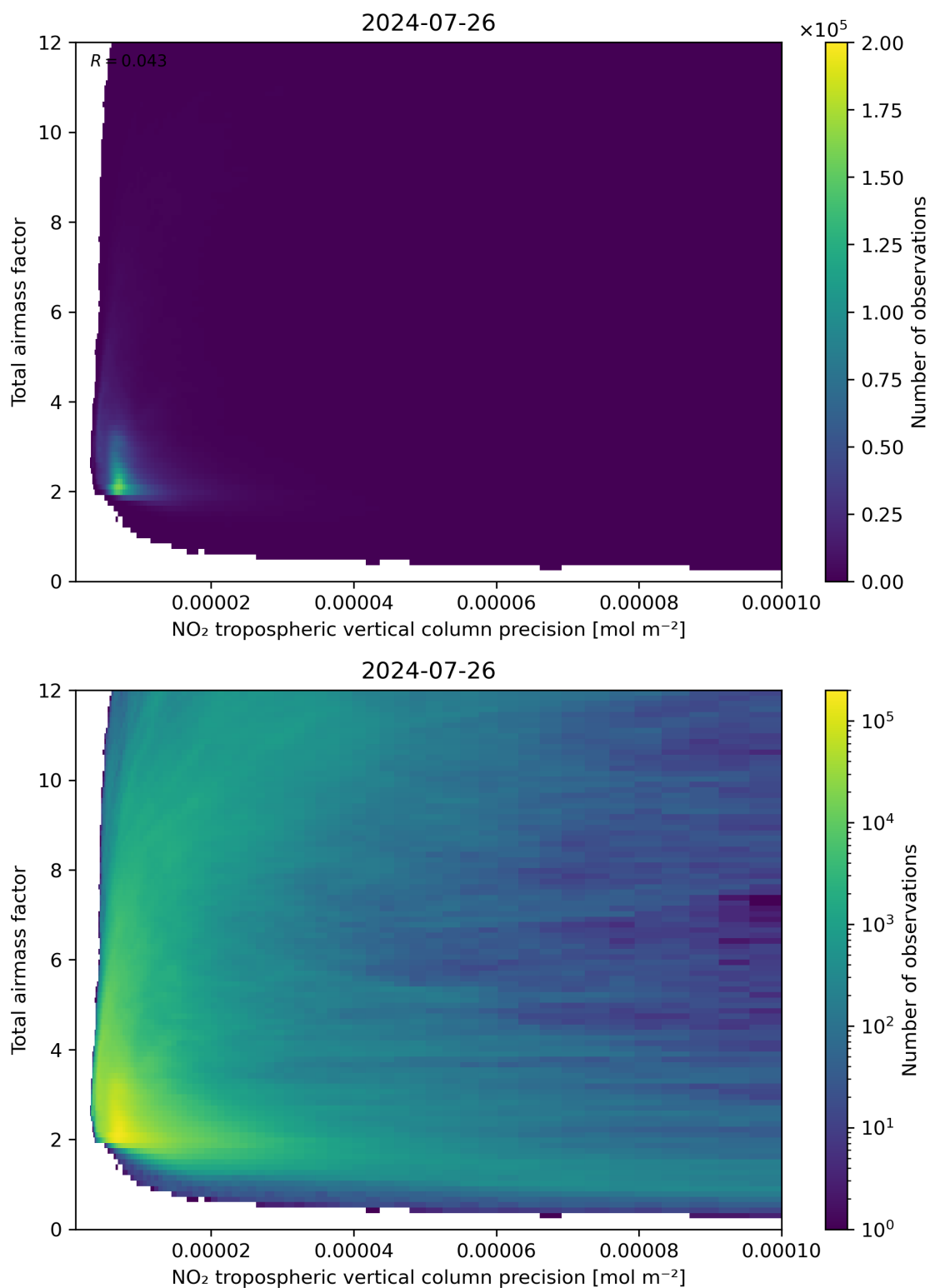
Figure 132: Scatter density plot of “NO 2 tropospheric vertical column precision” against “Total air mass factor” for 2024-07-26 to 2024-07-27.
