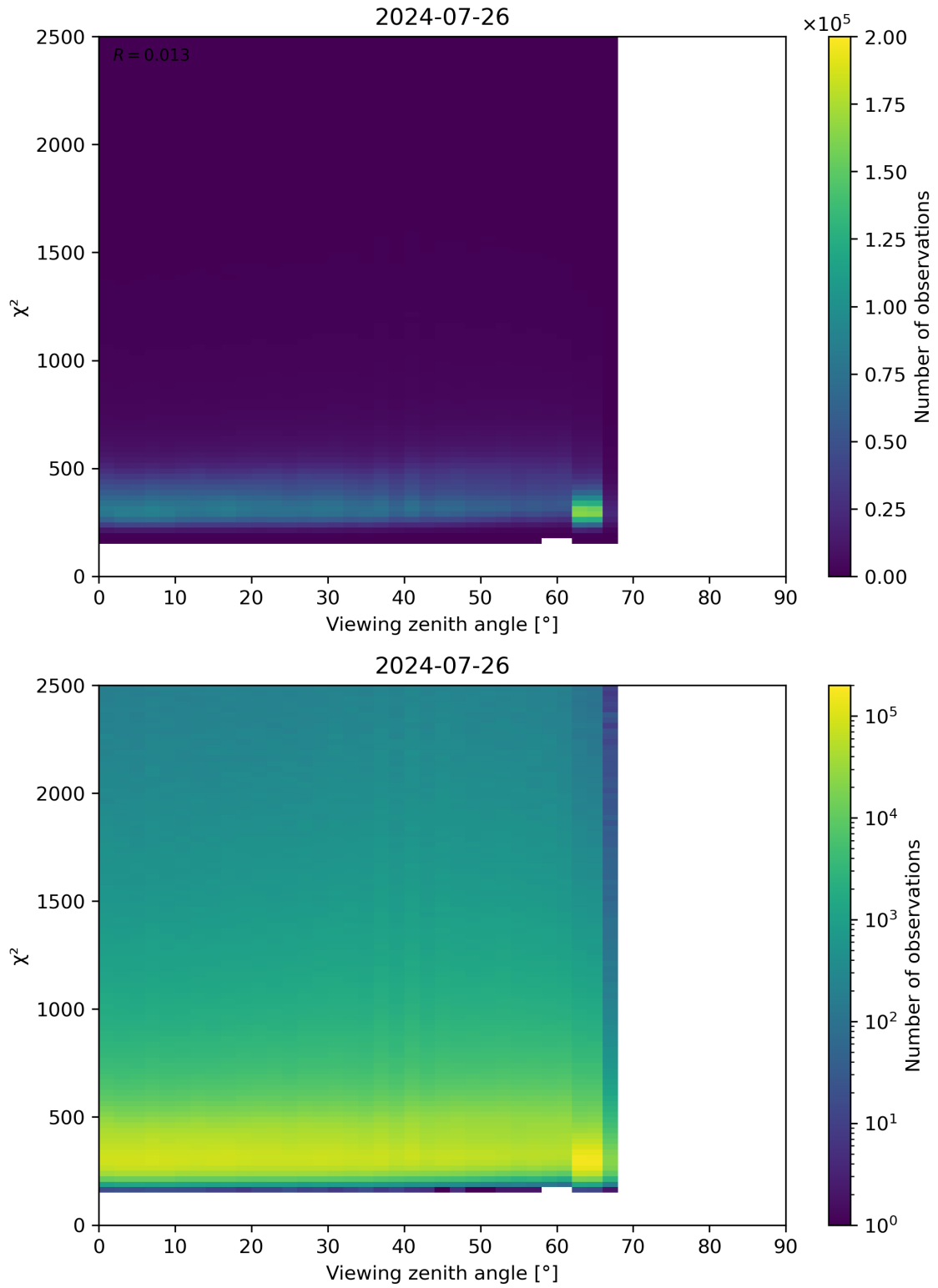
Figure 162: Scatter density plot of “Viewing zenith angle” against “ \chi^2 ” for 2024-07-26 to 2024-07-27.
