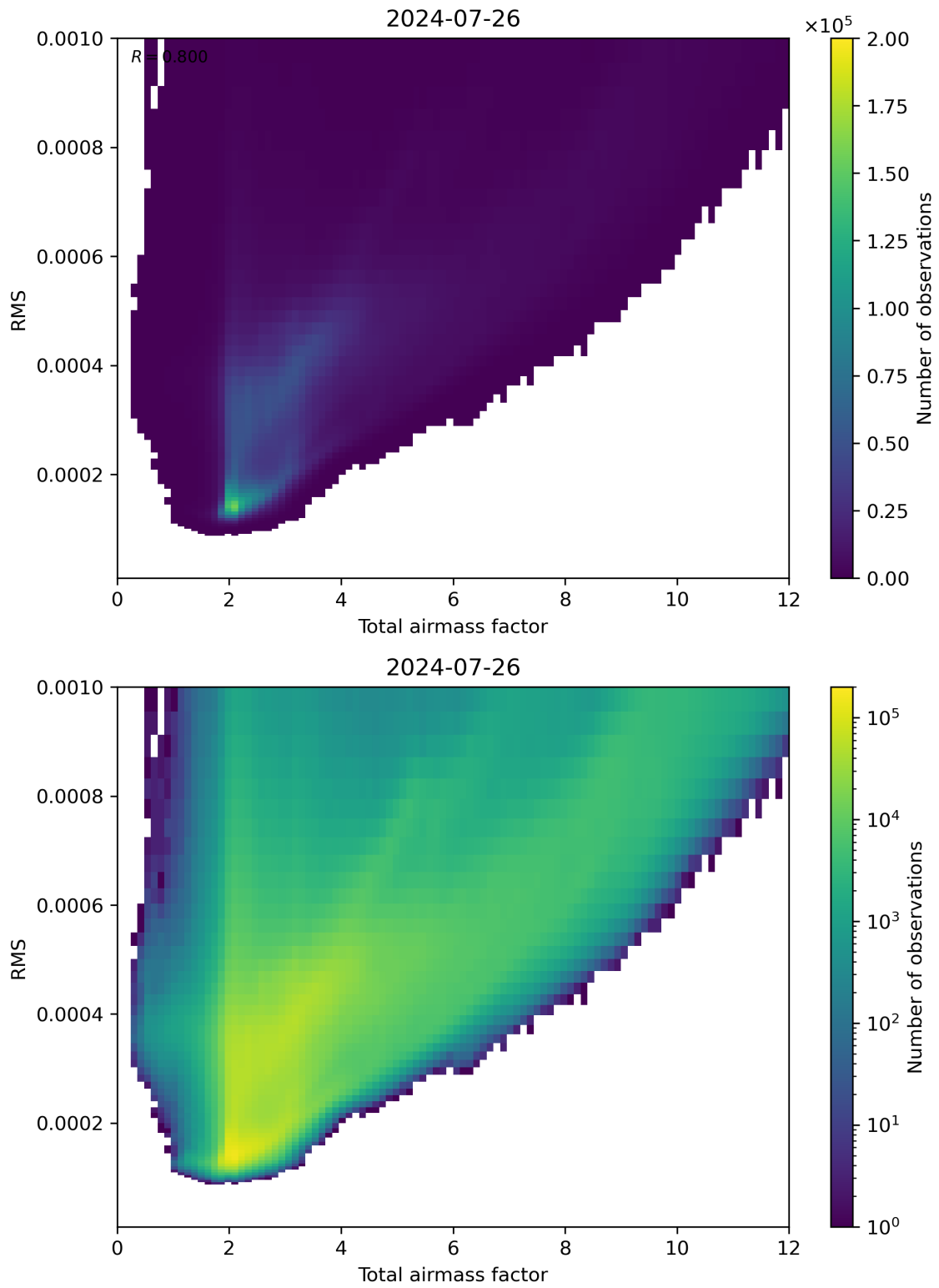
Figure 69: Scatter density plot of “Total airmass factor” against “RMS” for 2024-07-26 to 2024-07-27.
