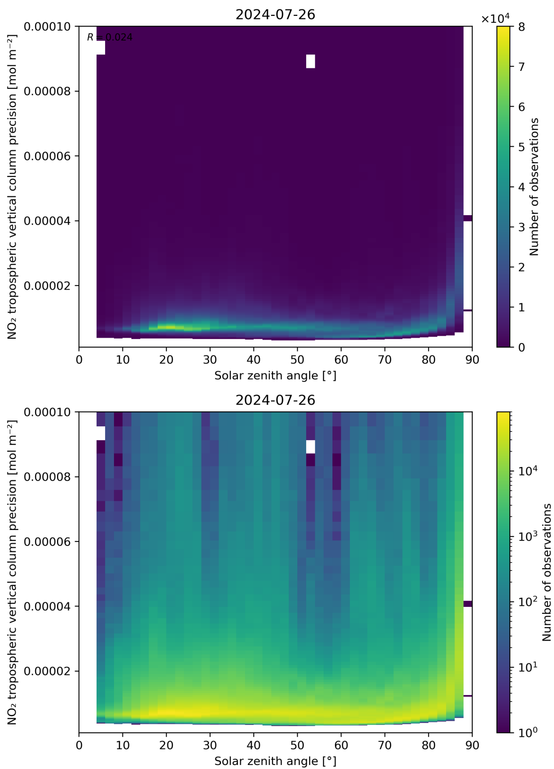
Figure 156: Scatter density plot of “Solar zenith angle” against “NO 2 tropospheric vertical column precision” for 2024-07-26 to 2024-07-27.
