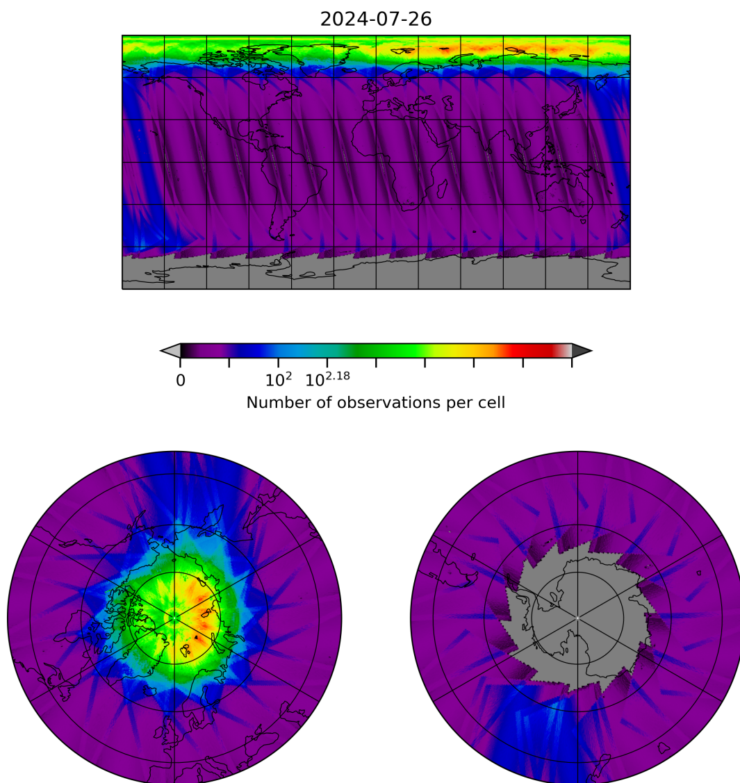
Figure 10: Map of the number of observations for 2024-07-26 to 2024-07-27
