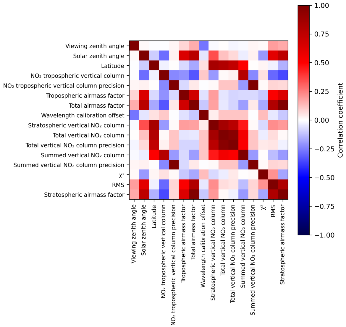
Figure 2: Map of correlation matrix for 2024-07-26 to 2024-07-27.
