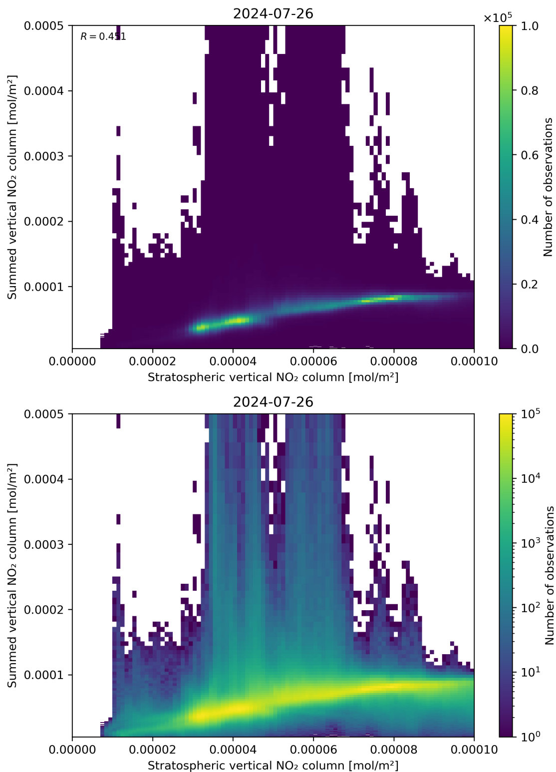
Figure 98: Scatter density plot of “Stratospheric vertical NO 2 column” against “Summed vertical NO 2 column” for 2024-07-26 to 2024-07-27.
