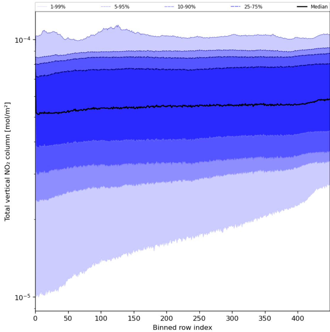
Figure 55: Along track statistics of “Total vertical NO 2 column” for 2024-07-26 to 2024-07-28
