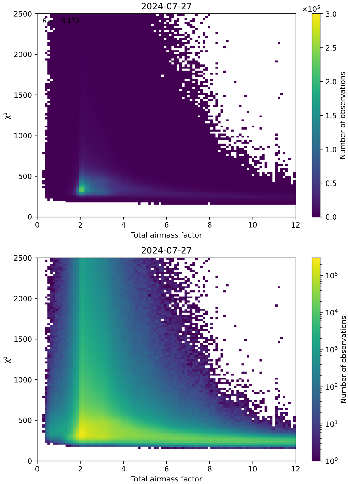
Figure 63: Scatter density plot of “Total airmass factor” against “ \chi^2 ” for 2024-07-26 to 2024-07-28.
