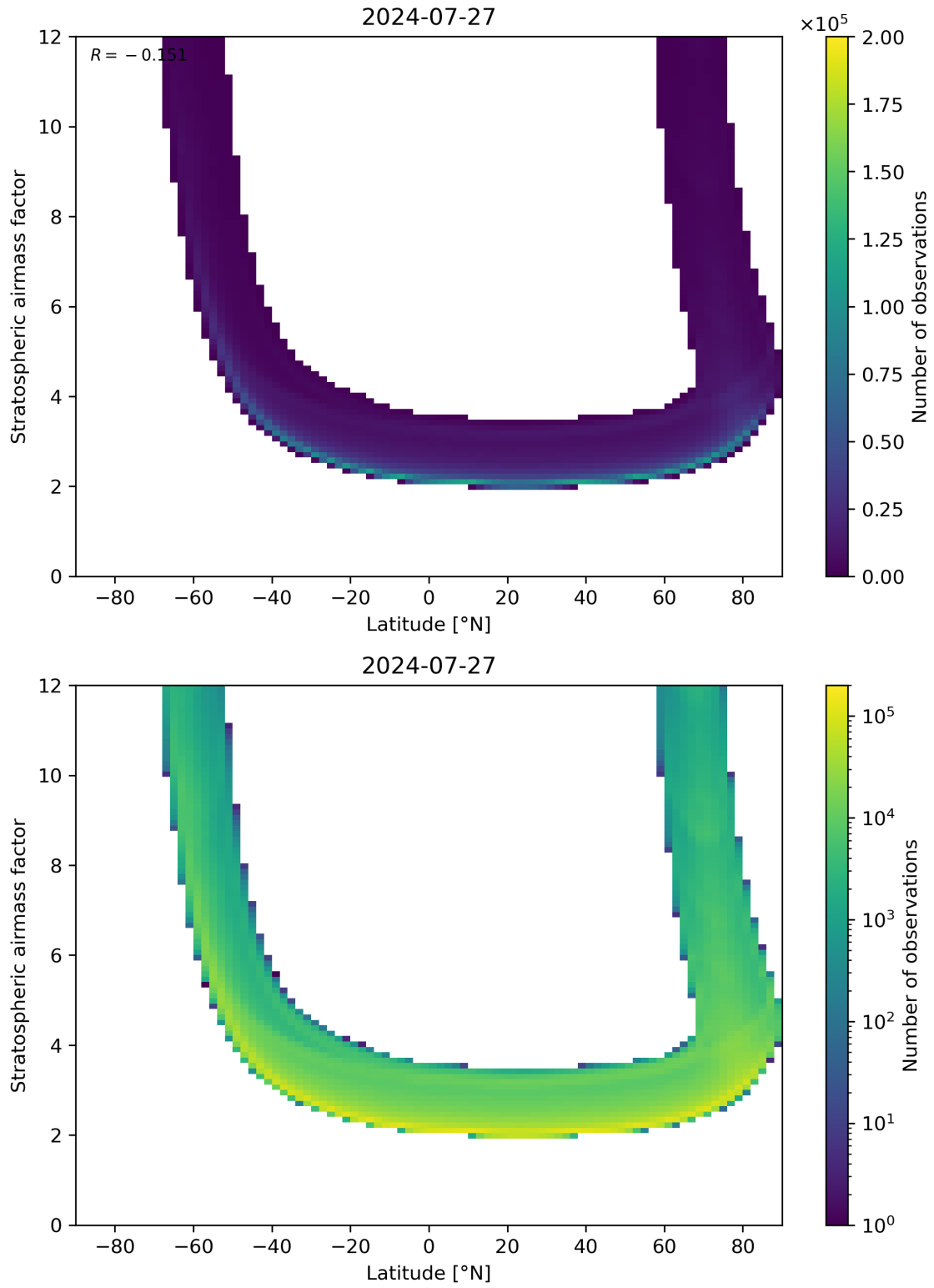
Figure 83: Scatter density plot of “Latitude” against “Stratospheric air mass factor” for 2024-07-26 to 2024-07-28.
