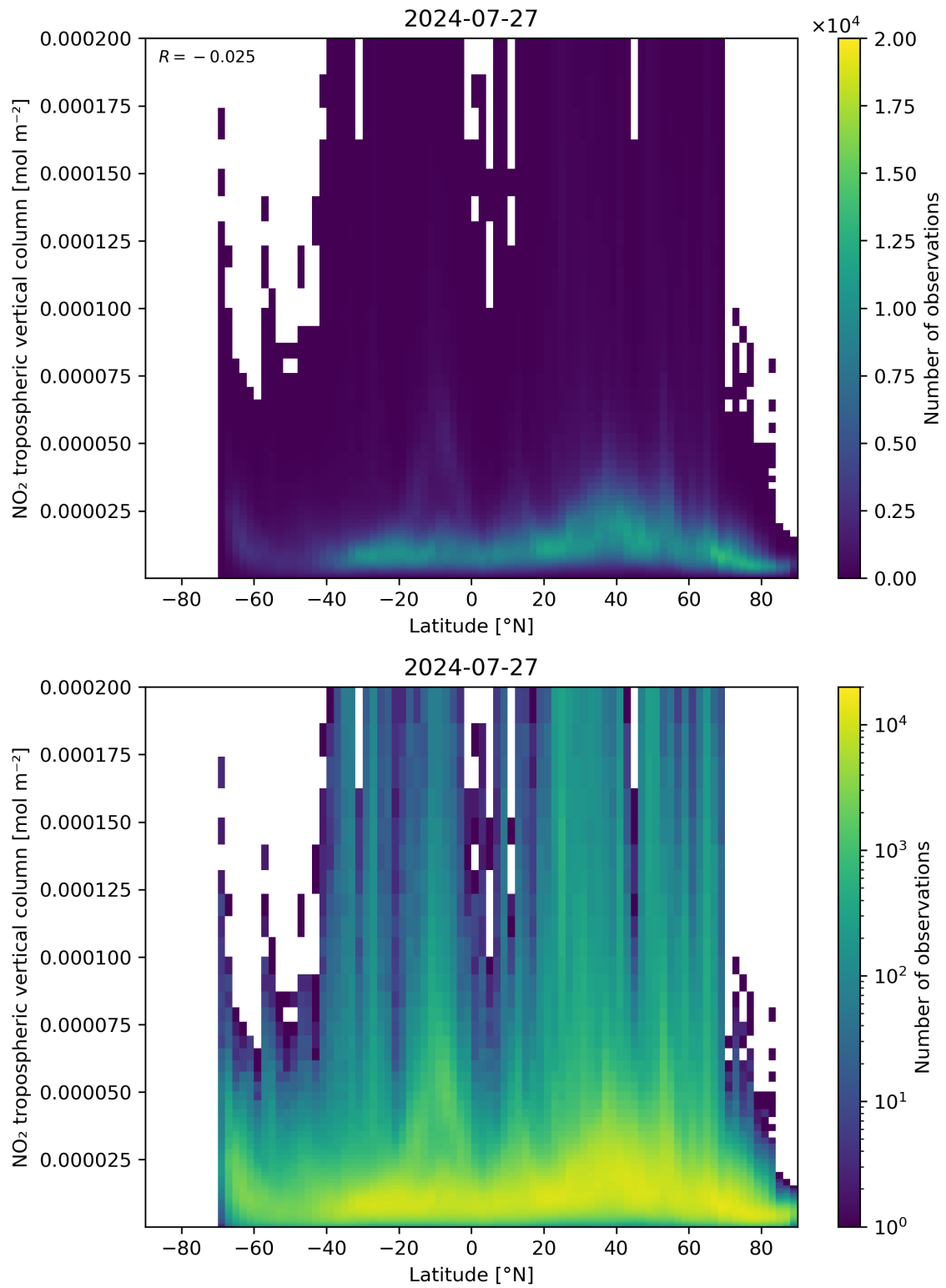
Figure 92: Scatter density plot of “Latitude” against “NO 2 tropospheric vertical column” for 2024-07-26 to 2024-07-28.
