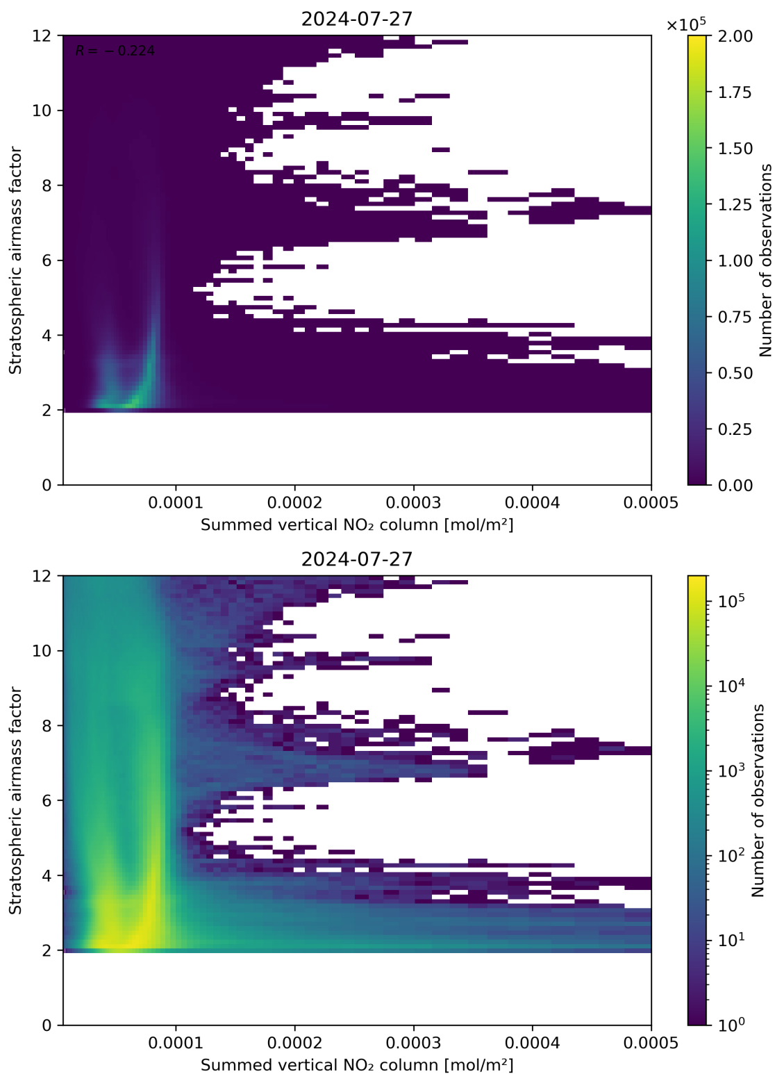
Figure 103: Scatter density plot of “Summed vertical NO 2 column” against “Stratospheric air mass factor” for 2024-07-26 to 2024-07-28.
