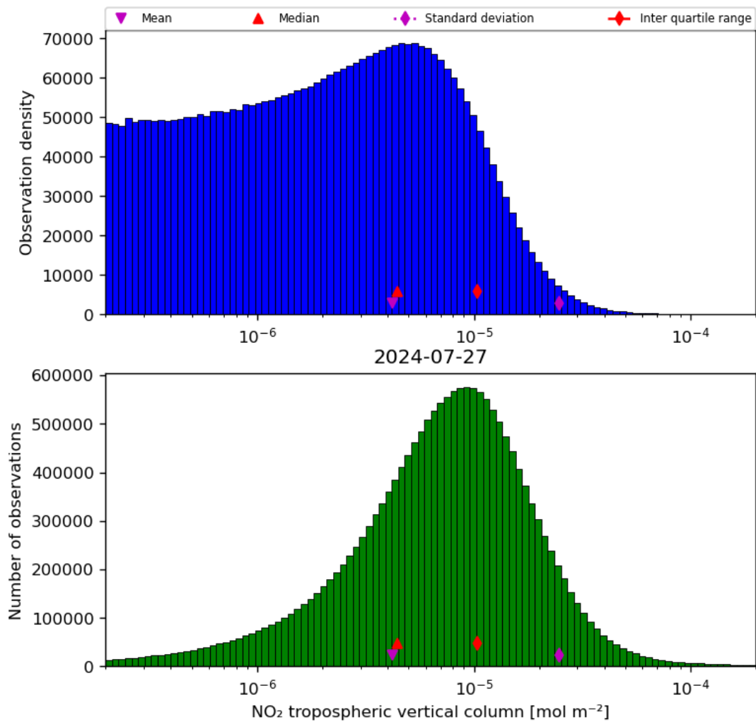
Figure 29: Histogram of “NO 2 tropospheric vertical column” for 2024-07-26 to 2024-07-28
