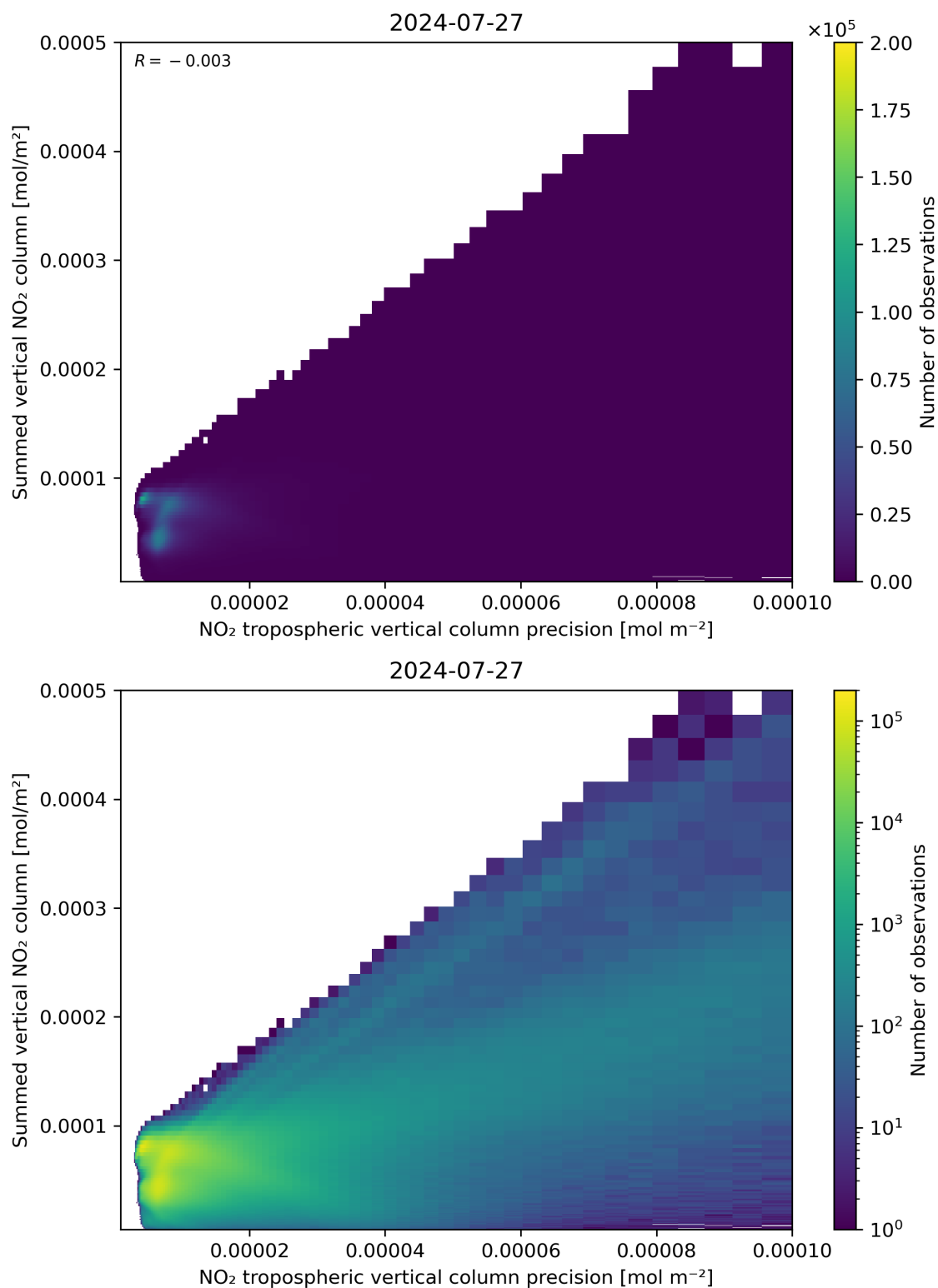
Figure 136: Scatter density plot of “NO 2 tropospheric vertical column precision” against “Summed vertical NO 2 column” for 2024-07-26 to 2024-07-28.
