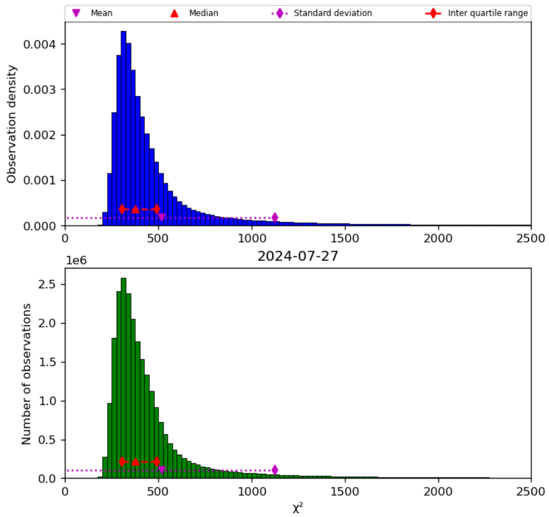
Figure 42: Histogram of “ \chi^2 ” for 2024-07-26 to 2024-07-28
