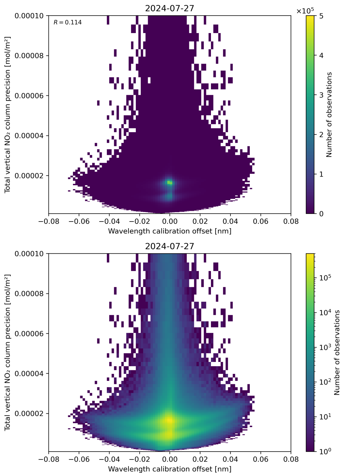
Figure 180: Scatter density plot of “Wavelength calibration offset” against “Total vertical NO 2 column precision” for 2024-07-26 to 2024-07-28.
