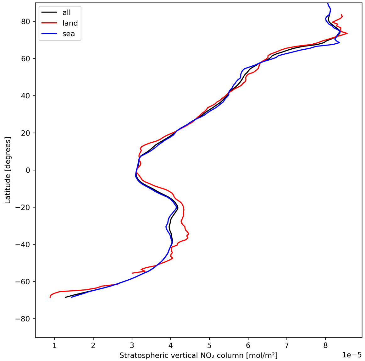
Figure 19: Zonal average of “Stratospheric vertical NO 2 column” for 2024-07-26 to 2024-07-28.
