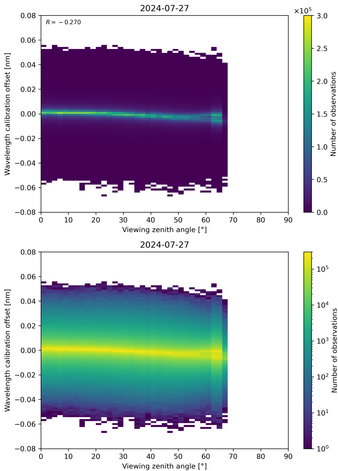
Figure 173: Scatter density plot of “Viewing zenith angle” against “Wavelength calibration offset” for 2024-07-26 to 2024-07-28.
