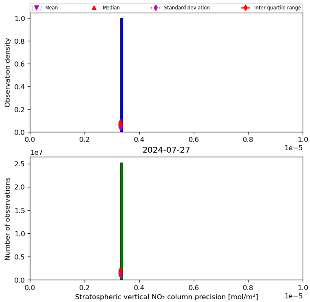
Figure 37: Histogram of “Stratospheric vertical NO 2 column precision” for 2024-07-26 to 2024-07-28
