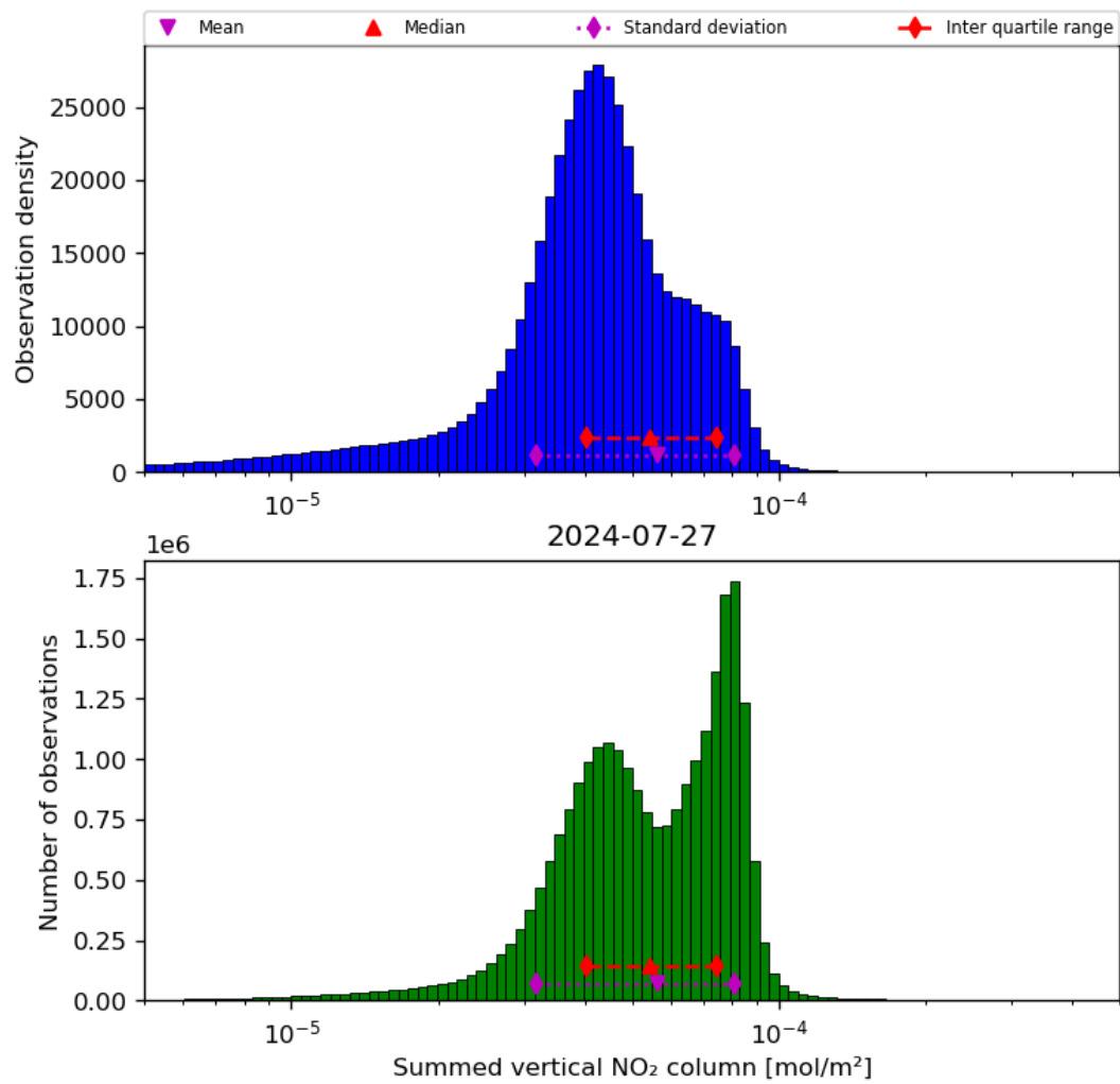
Figure 40: Histogram of “Summed vertical NO 2 column” for 2024-07-26 to 2024-07-28
