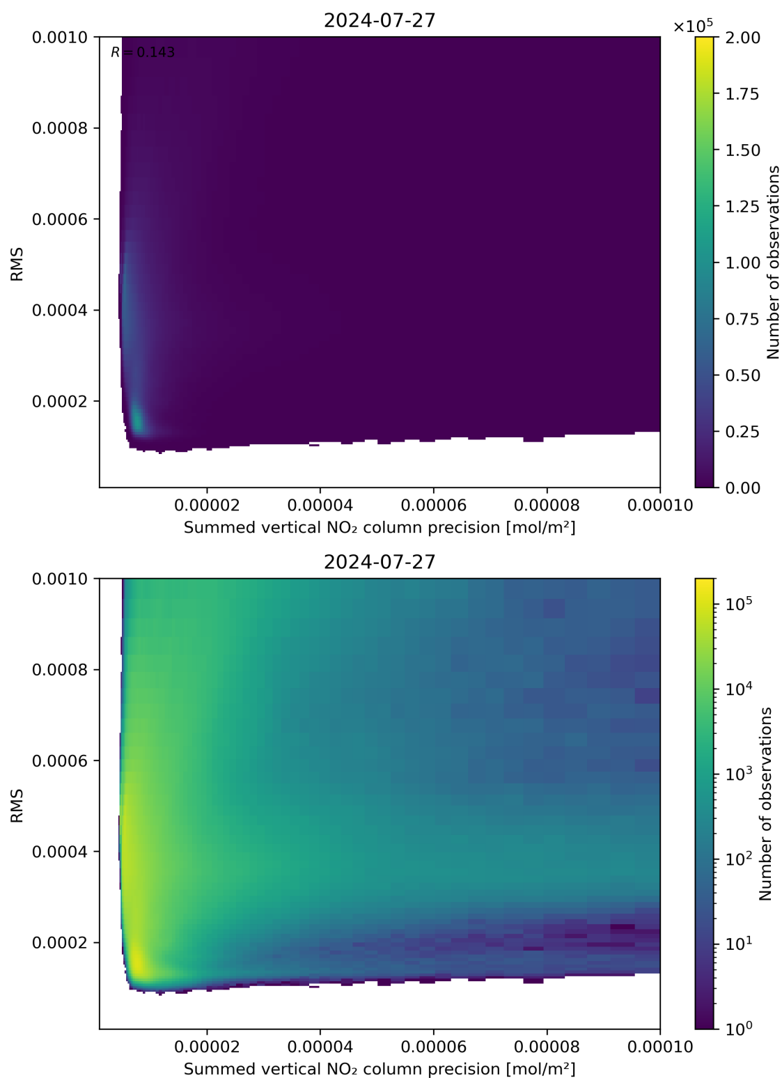
Figure 108: Scatter density plot of “Summed vertical NO 2 column precision” against “RMS” for 2024-07-26 to 2024-07-28.
