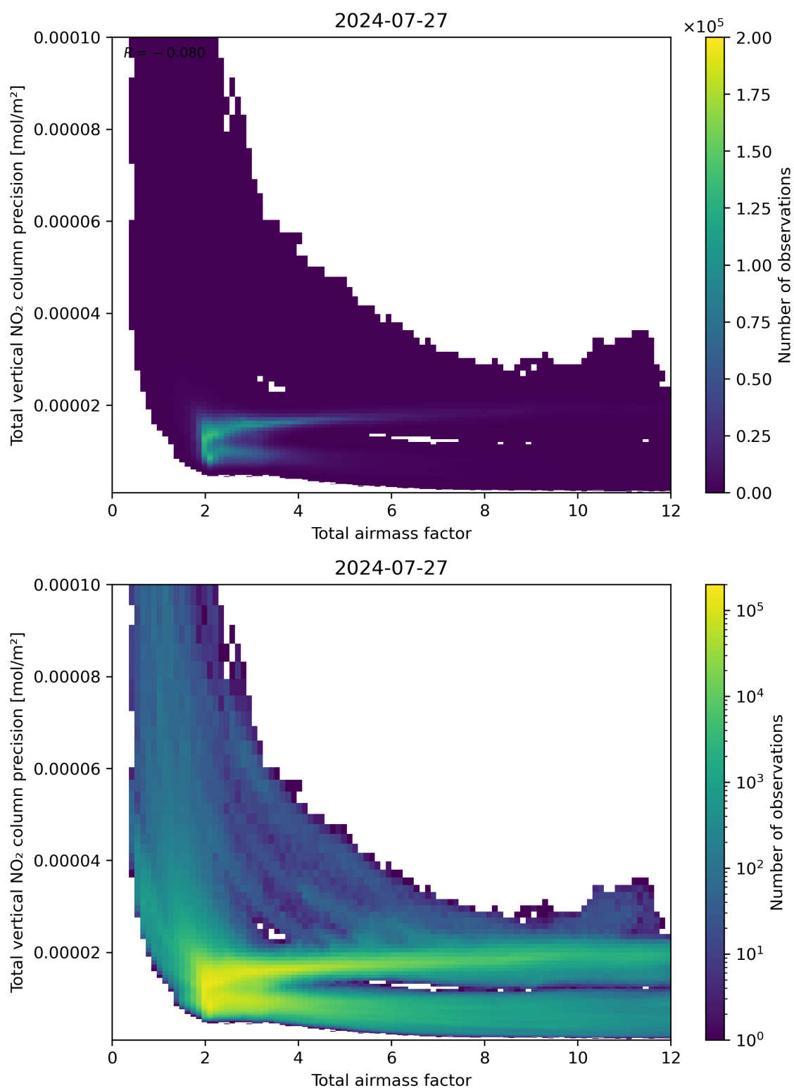
Figure 68: Scatter density plot of “Total airmass factor” against “Total vertical NO 2 column precision” for 2024-07-26 to 2024-07-28.
