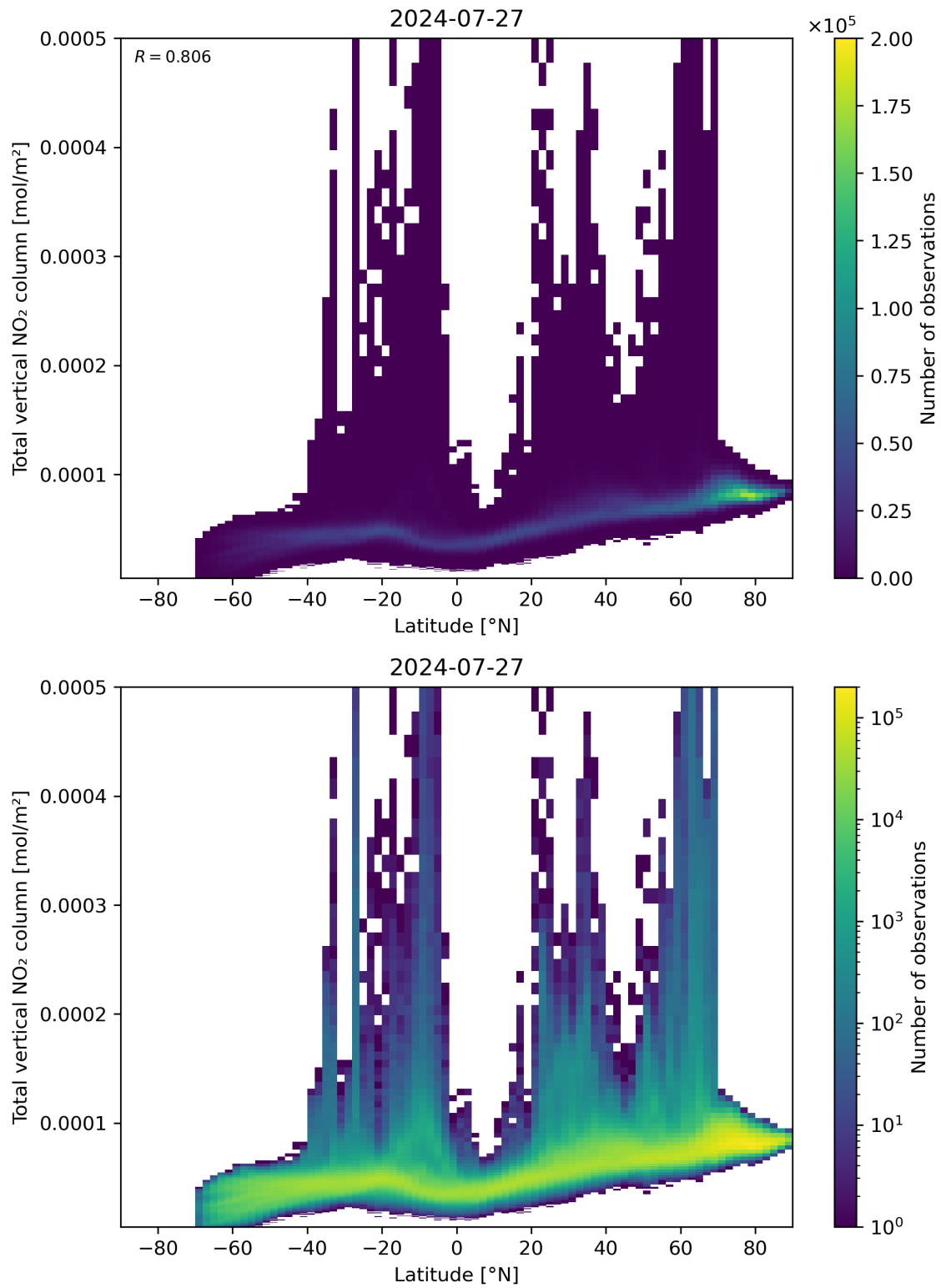
Figure 90: Scatter density plot of “Latitude” against “Total vertical NO 2 column” for 2024-07-26 to 2024-07-28.
