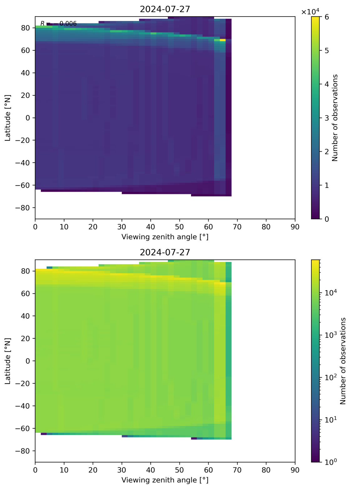
Figure 163: Scatter density plot of “Viewing zenith angle” against “Latitude” for 2024-07-26 to 2024-07-28.
