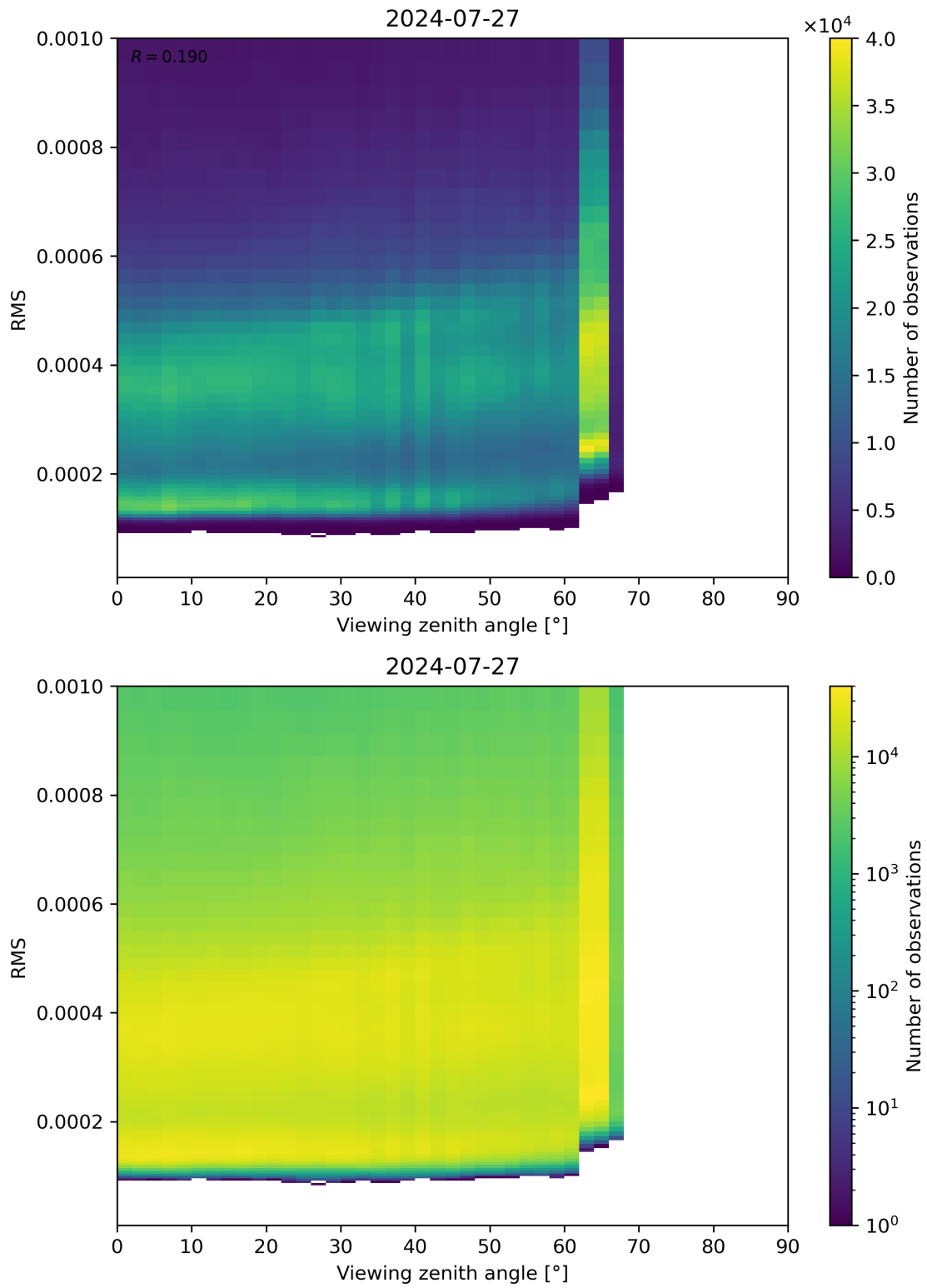
Figure 171: Scatter density plot of “Viewing zenith angle” against “RMS” for 2024-07-26 to 2024-07-28.
