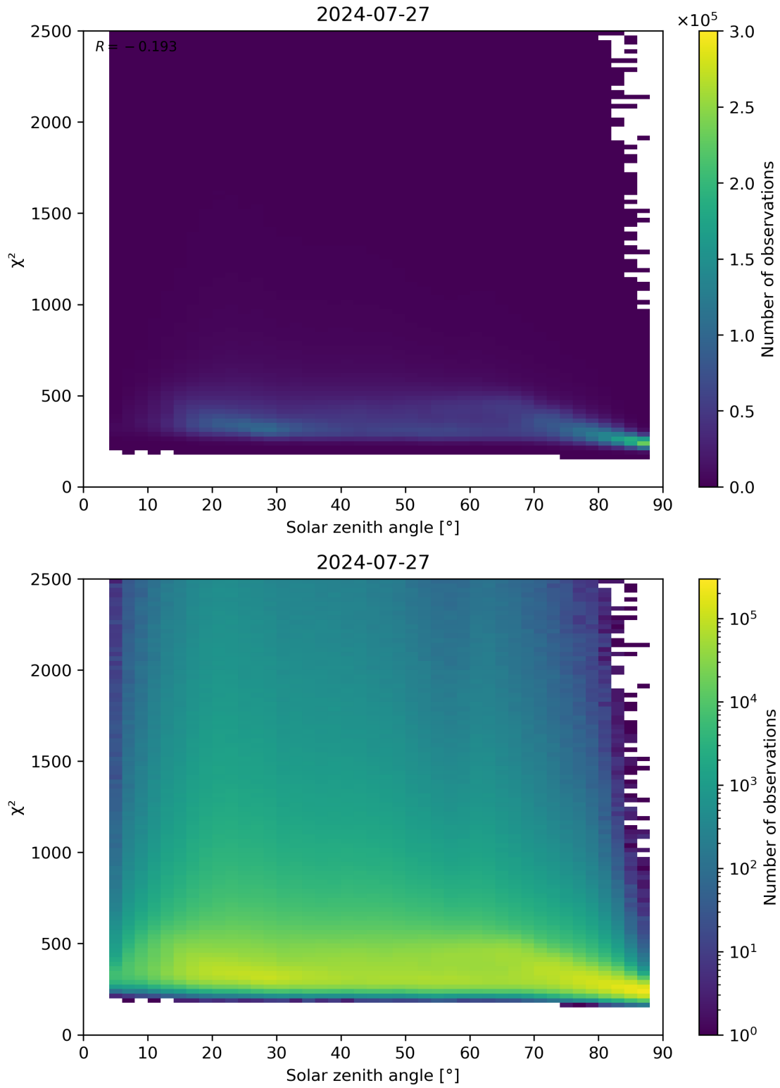
Figure 148: Scatter density plot of “Solar zenith angle” against “ \chi^2 ” for 2024-07-26 to 2024-07-28.
