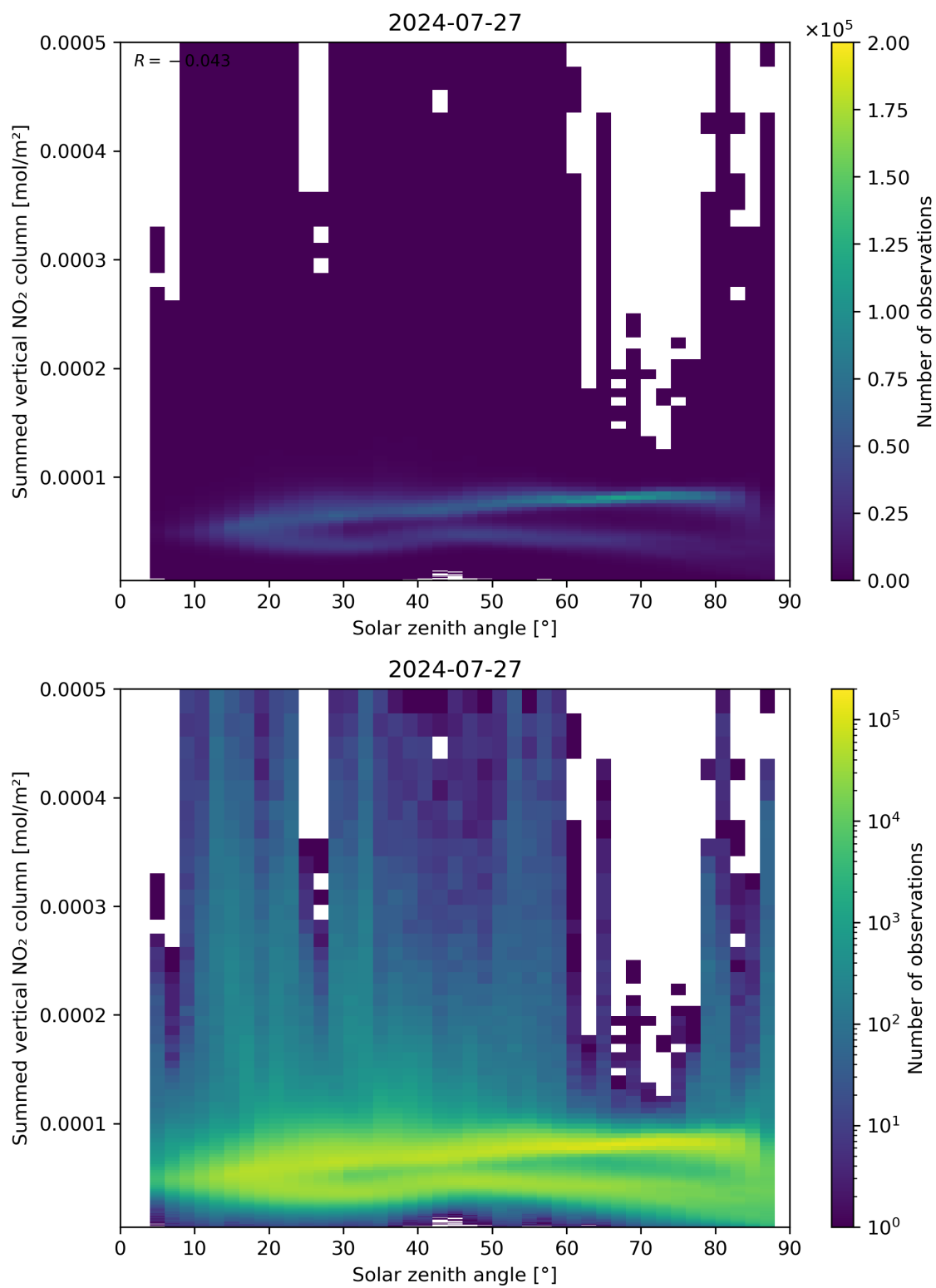
Figure 151: Scatter density plot of “Solar zenith angle” against “Summed vertical NO 2 column” for 2024-07-26 to 2024-07-28.
