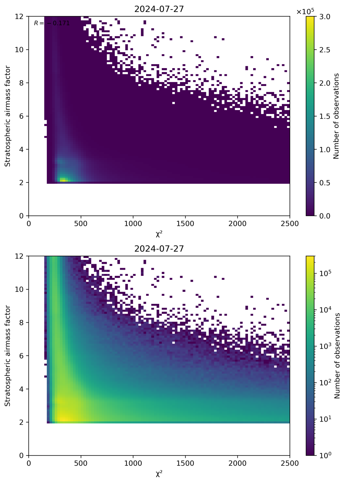
Figure 81: Scatter density plot of “ \chi^2 ” against “Stratospheric airmass factor” for 2024-07-26 to 2024-07-28.
