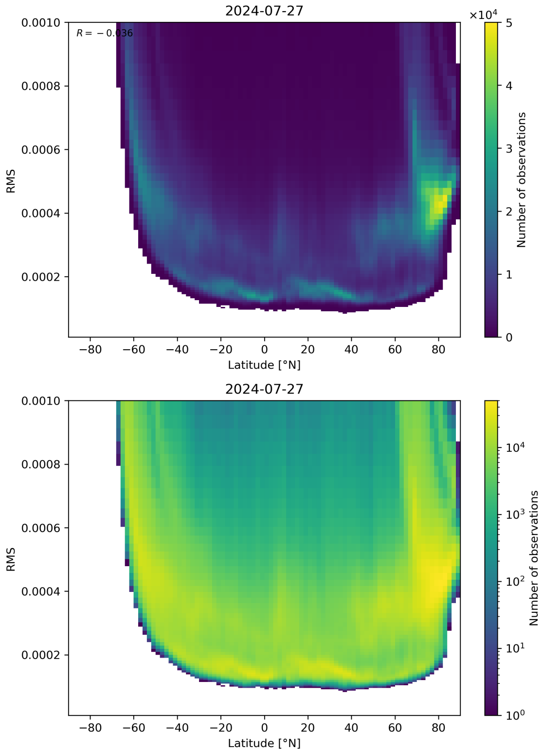
Figure 94: Scatter density plot of “Latitude” against “RMS” for 2024-07-26 to 2024-07-28.
