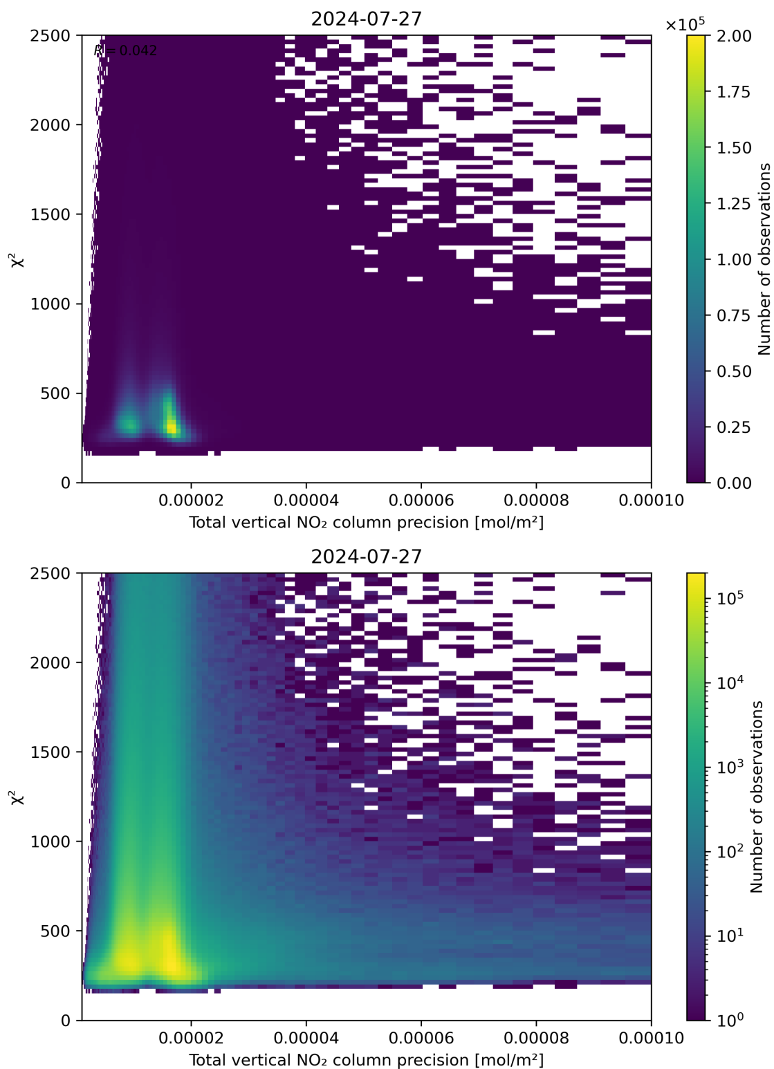
Figure 116: Scatter density plot of “Total vertical NO 2 column precision” against “ \chi^2 ” for 2024-07-26 to 2024-07-28.
