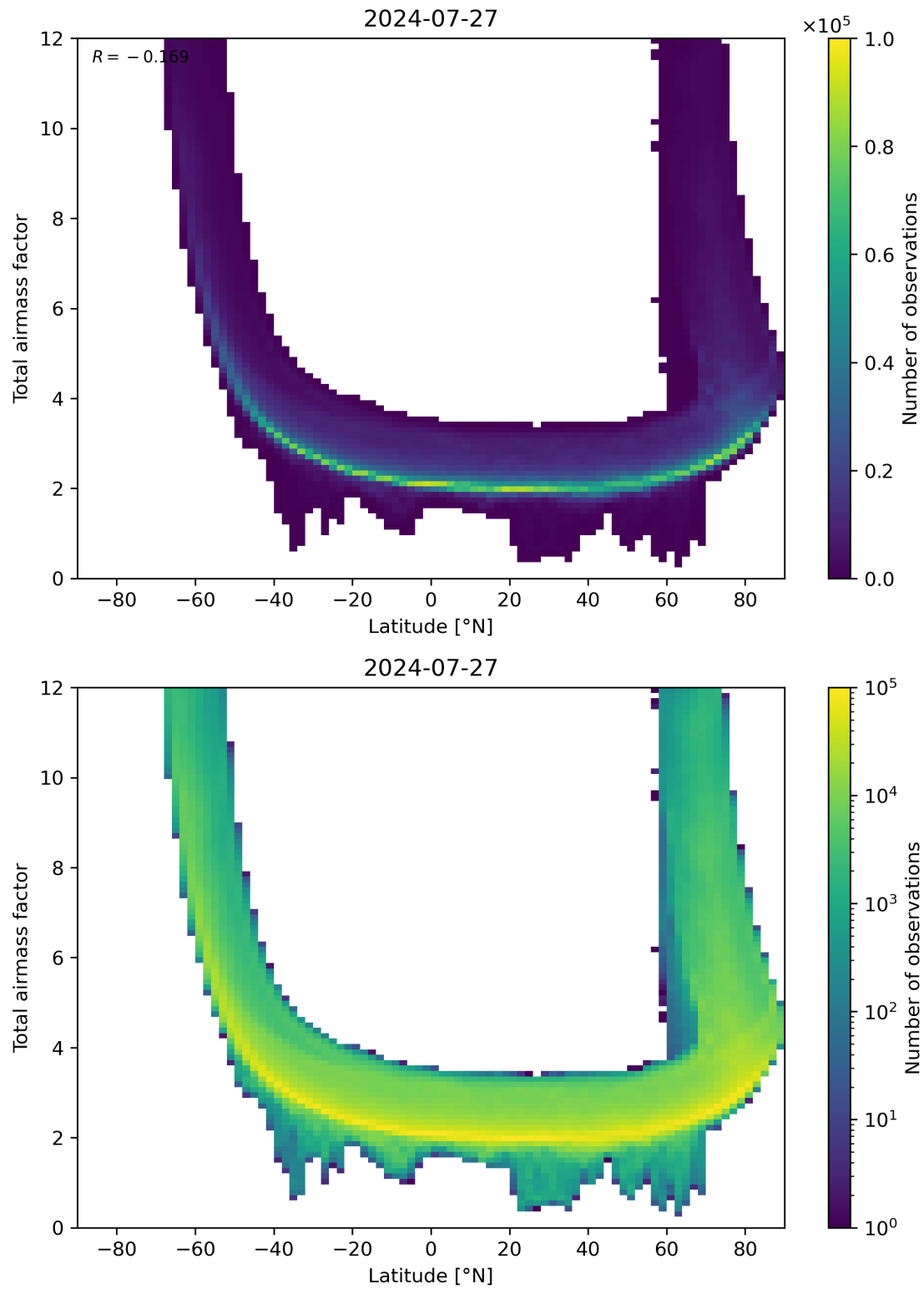
Figure 84: Scatter density plot of “Latitude” against “Total airmass factor” for 2024-07-26 to 2024-07-28.
