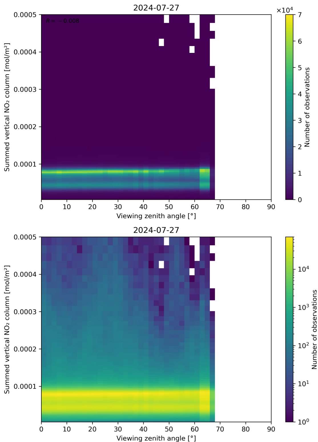
Figure 165: Scatter density plot of “Viewing zenith angle” against “Summed vertical NO 2 column” for 2024-07-26 to 2024-07-28.
