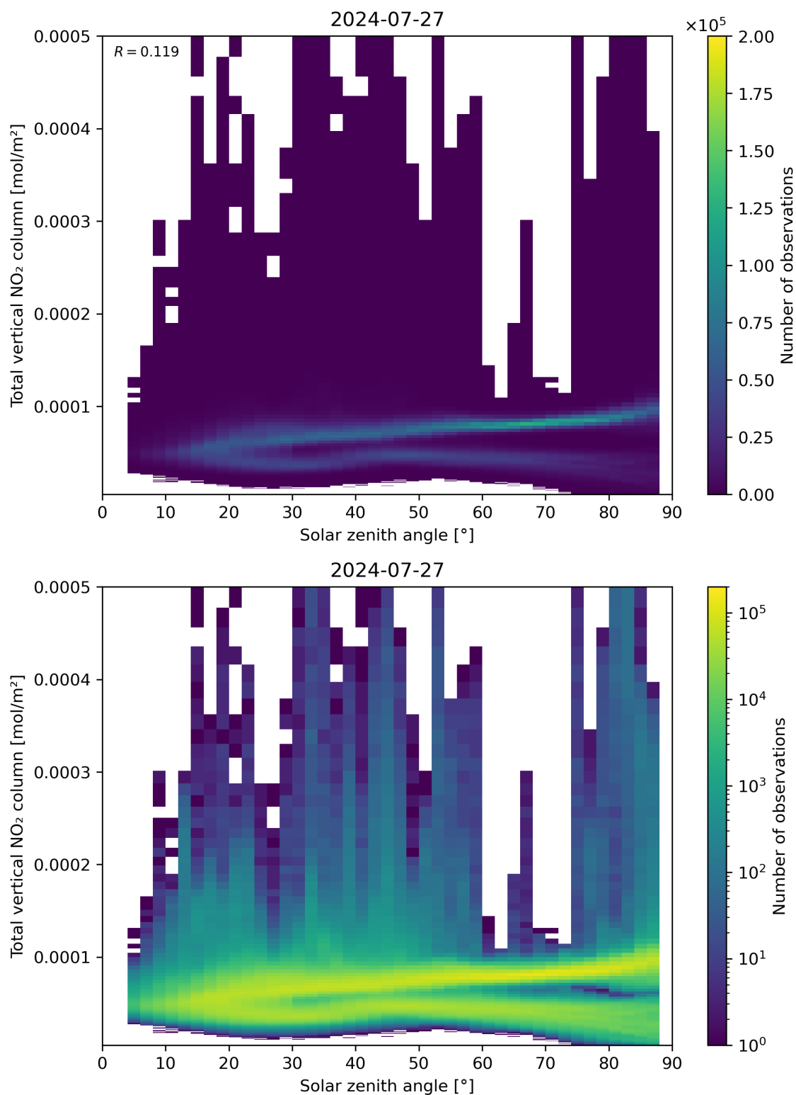
Figure 153: Scatter density plot of “Solar zenith angle” against “Total vertical NO 2 column” for 2024-07-26 to 2024-07-28.
