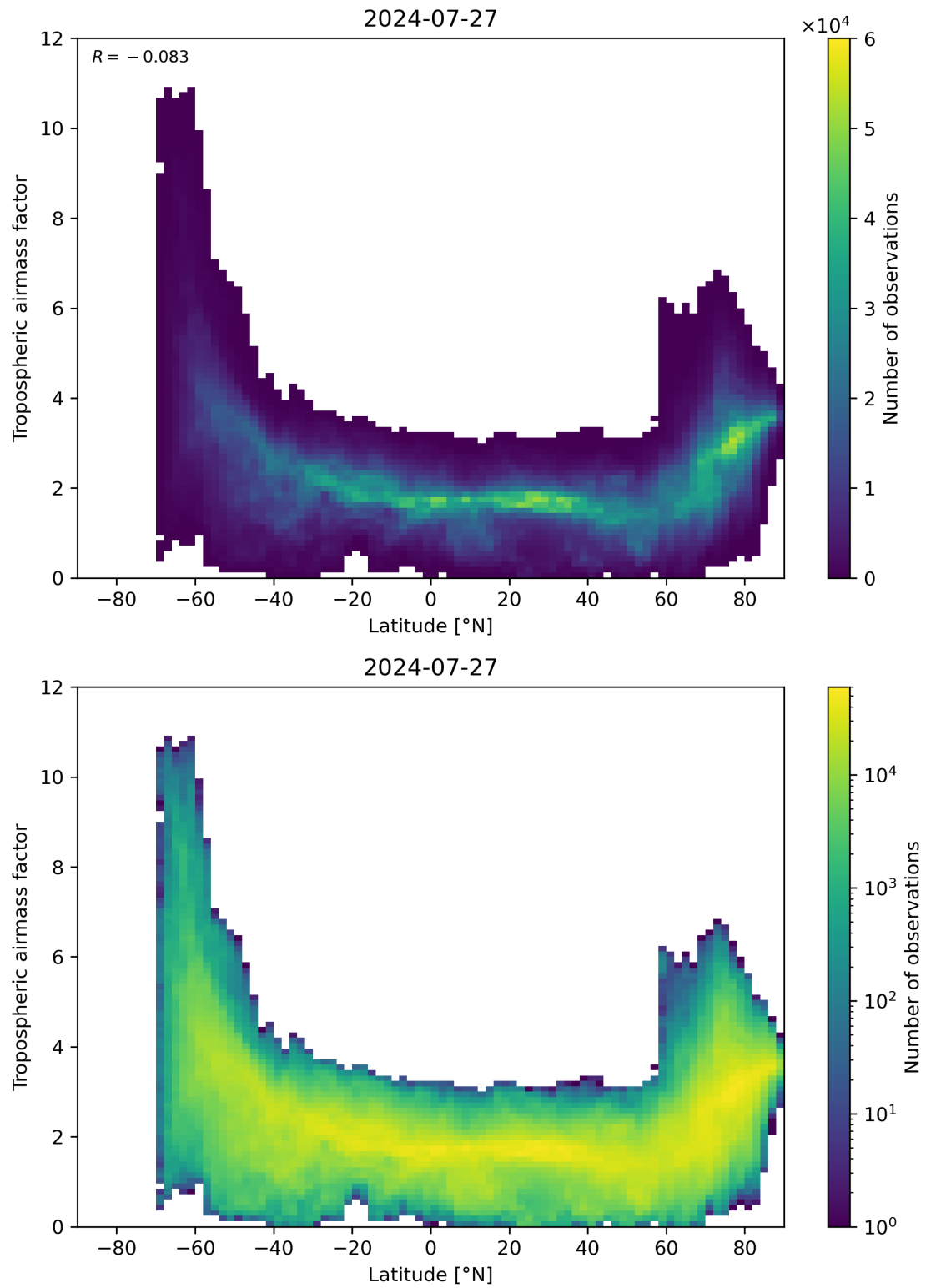
Figure 85: Scatter density plot of “Latitude” against “Tropospheric airmass factor” for 2024-07-26 to 2024-07-28.
