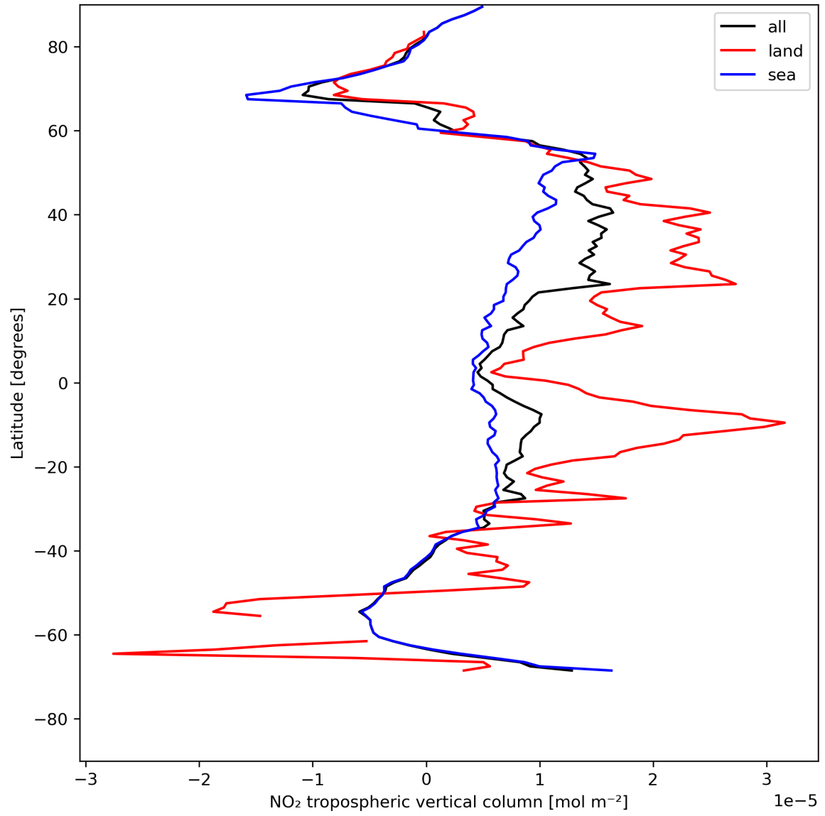
Figure 12: Zonal average of “NO 2 tropospheric vertical column” for 2024-07-26 to 2024-07-28.
