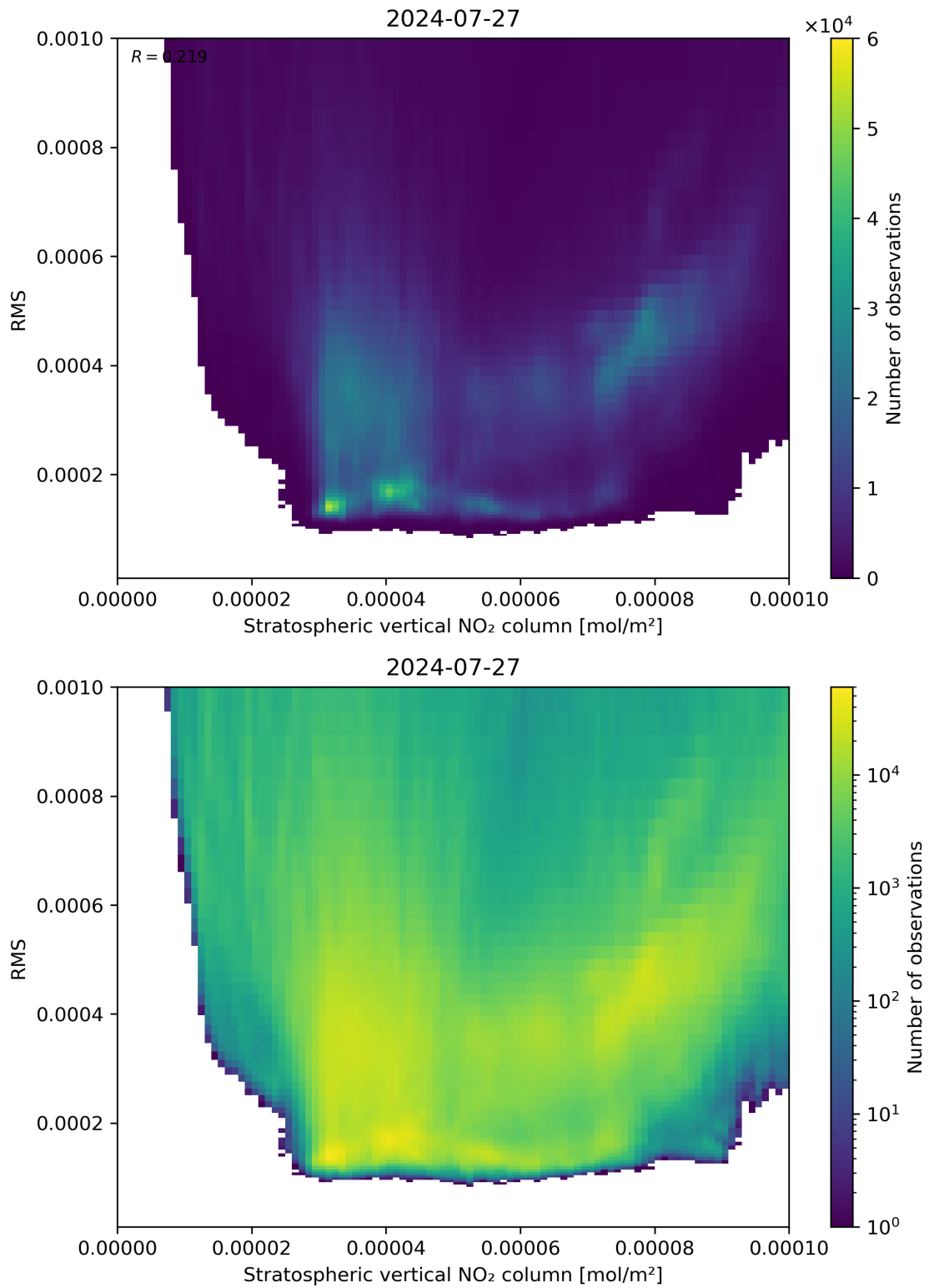
Figure 102: Scatter density plot of “Stratospheric vertical NO 2 column” against “RMS” for 2024-07-26 to 2024-07-28.
