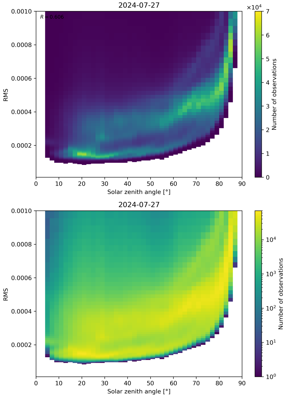
Figure 157: Scatter density plot of “Solar zenith angle” against “RMS” for 2024-07-26 to 2024-07-28.
