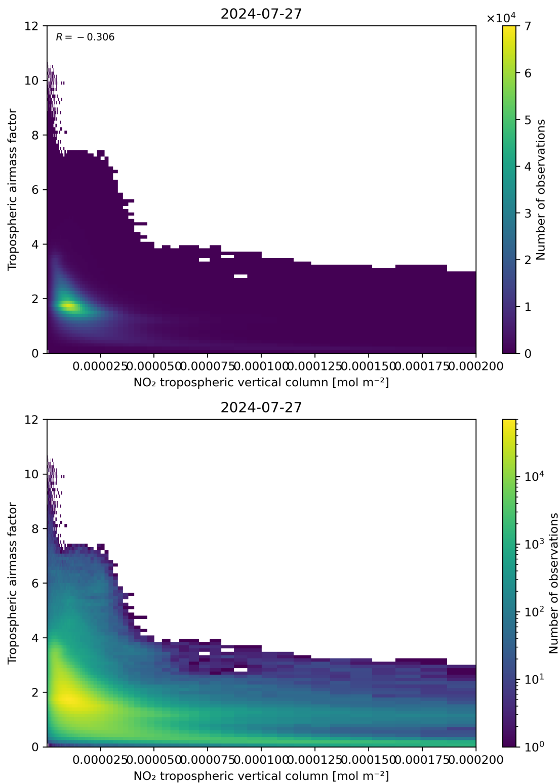
Figure 123: Scatter density plot of “NO 2 tropospheric vertical column” against “Tropospheric air mass factor” for 2024-07-26 to 2024-07-28.
