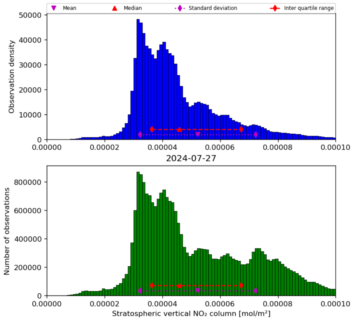
Figure 36: Histogram of “Stratospheric vertical NO 2 column” for 2024-07-26 to 2024-07-28
