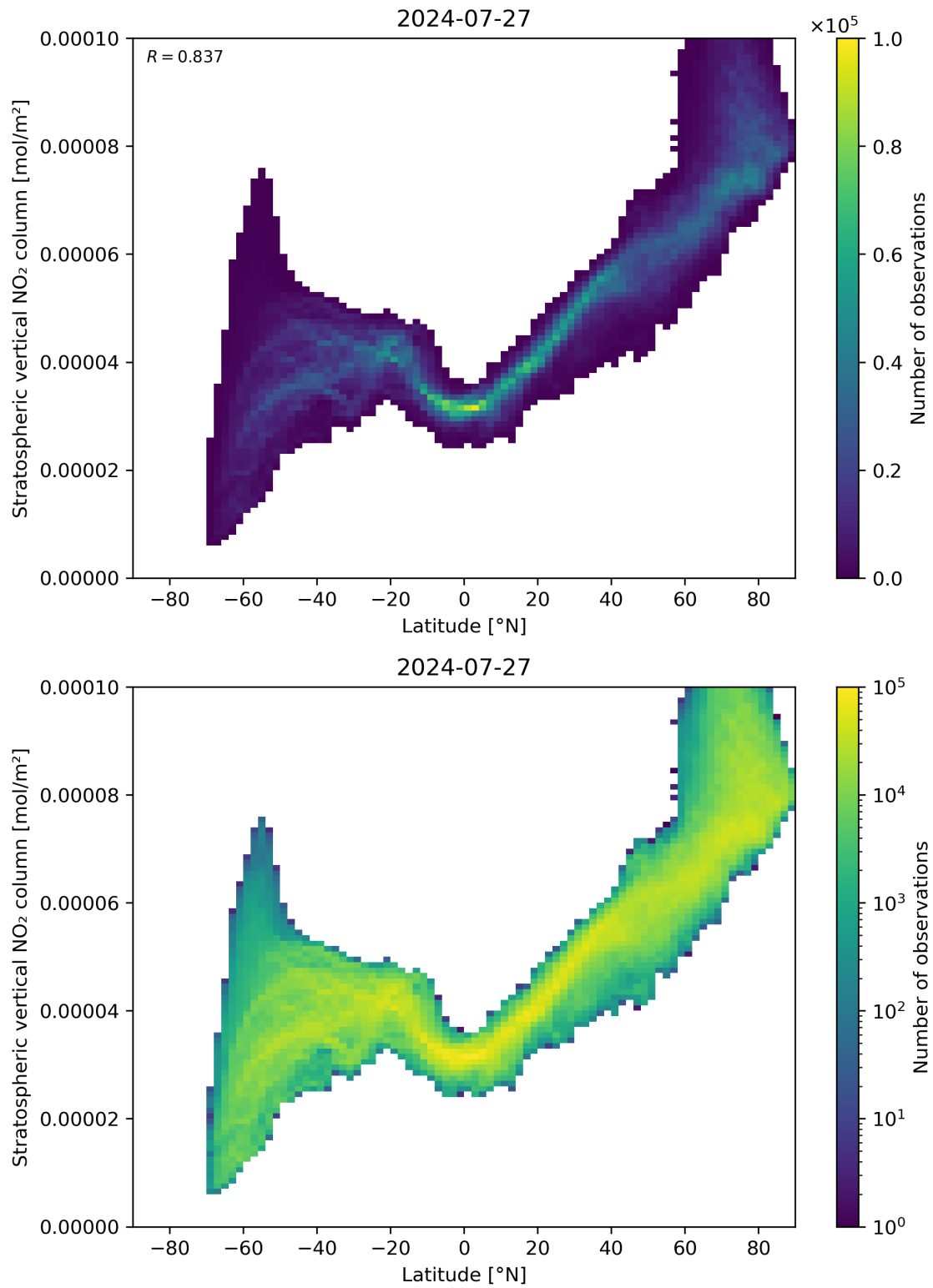
Figure 87: Scatter density plot of “Latitude” against “Stratospheric vertical NO 2 column” for 2024-07-26 to 2024-07-28.
