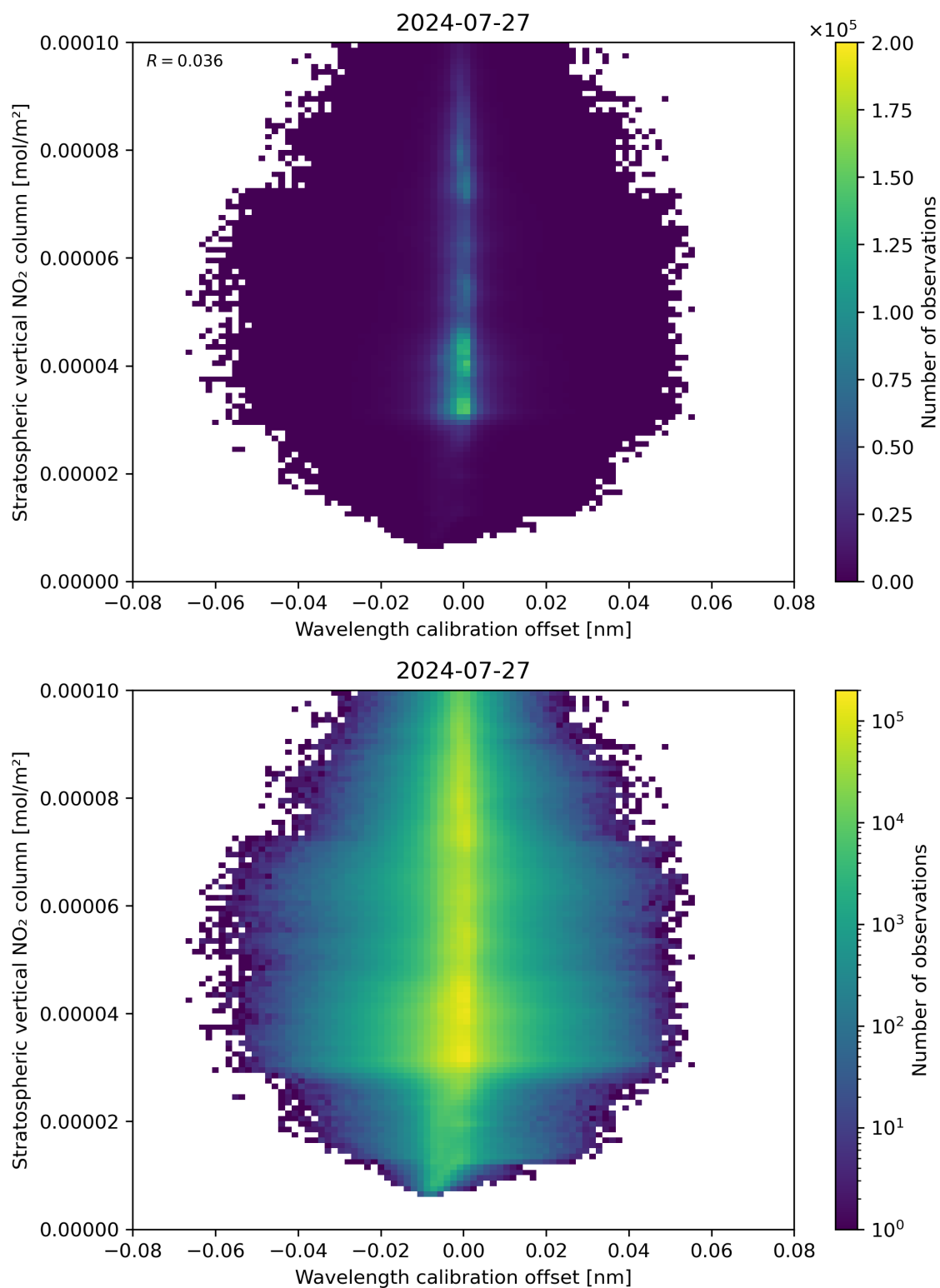
Figure 176: Scatter density plot of “Wavelength calibration offset” against “Stratospheric vertical NO 2 column” for 2024-07-26 to 2024-07-28.
