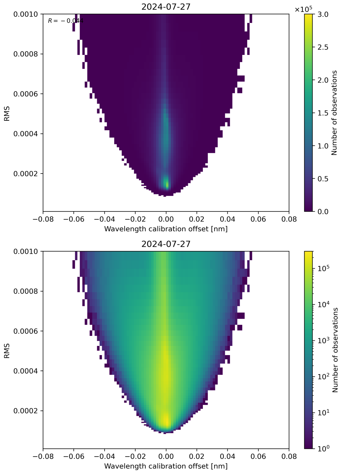
Figure 181: Scatter density plot of “Wavelength calibration offset” against “RMS” for 2024-07-26 to 2024-07-28.
