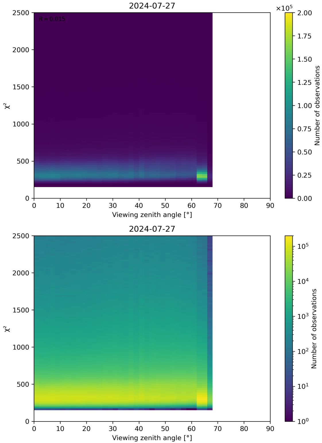
Figure 162: Scatter density plot of “Viewing zenith angle” against “ \chi^2 ” for 2024-07-26 to 2024-07-28.
