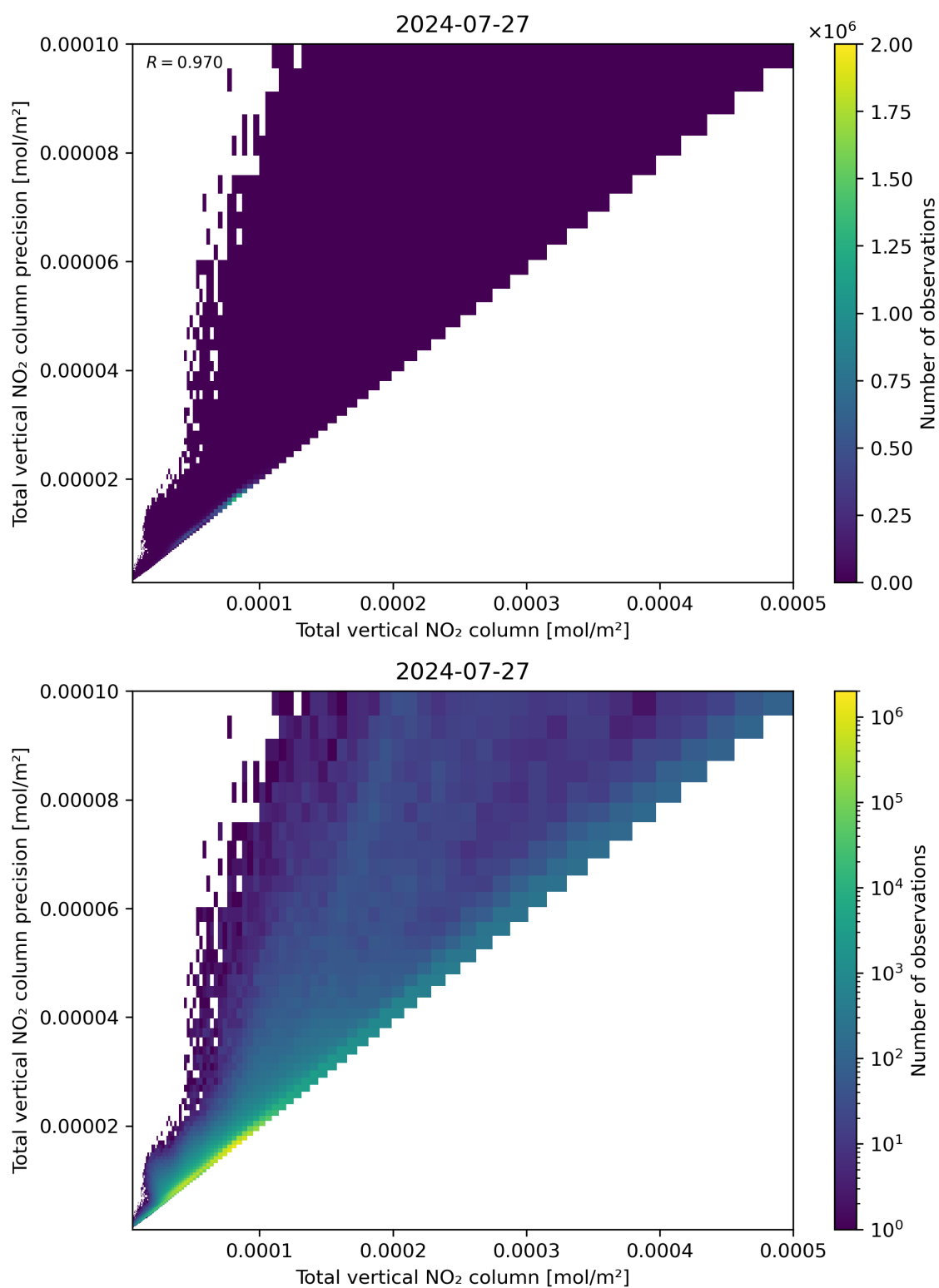
Figure 114: Scatter density plot of “Total vertical NO 2 column” against “Total vertical NO 2 column precision” for 2024-07-26 to 2024-07-28.
