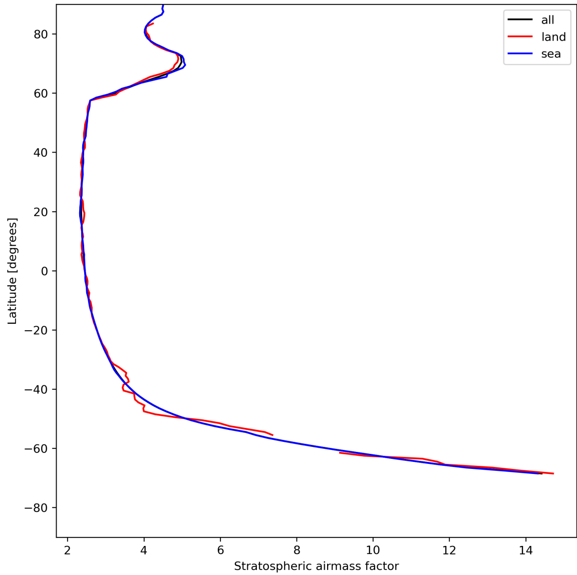
Figure 27: Zonal average of “Stratospheric airmass factor” for 2024-07-26 to 2024-07-28.
