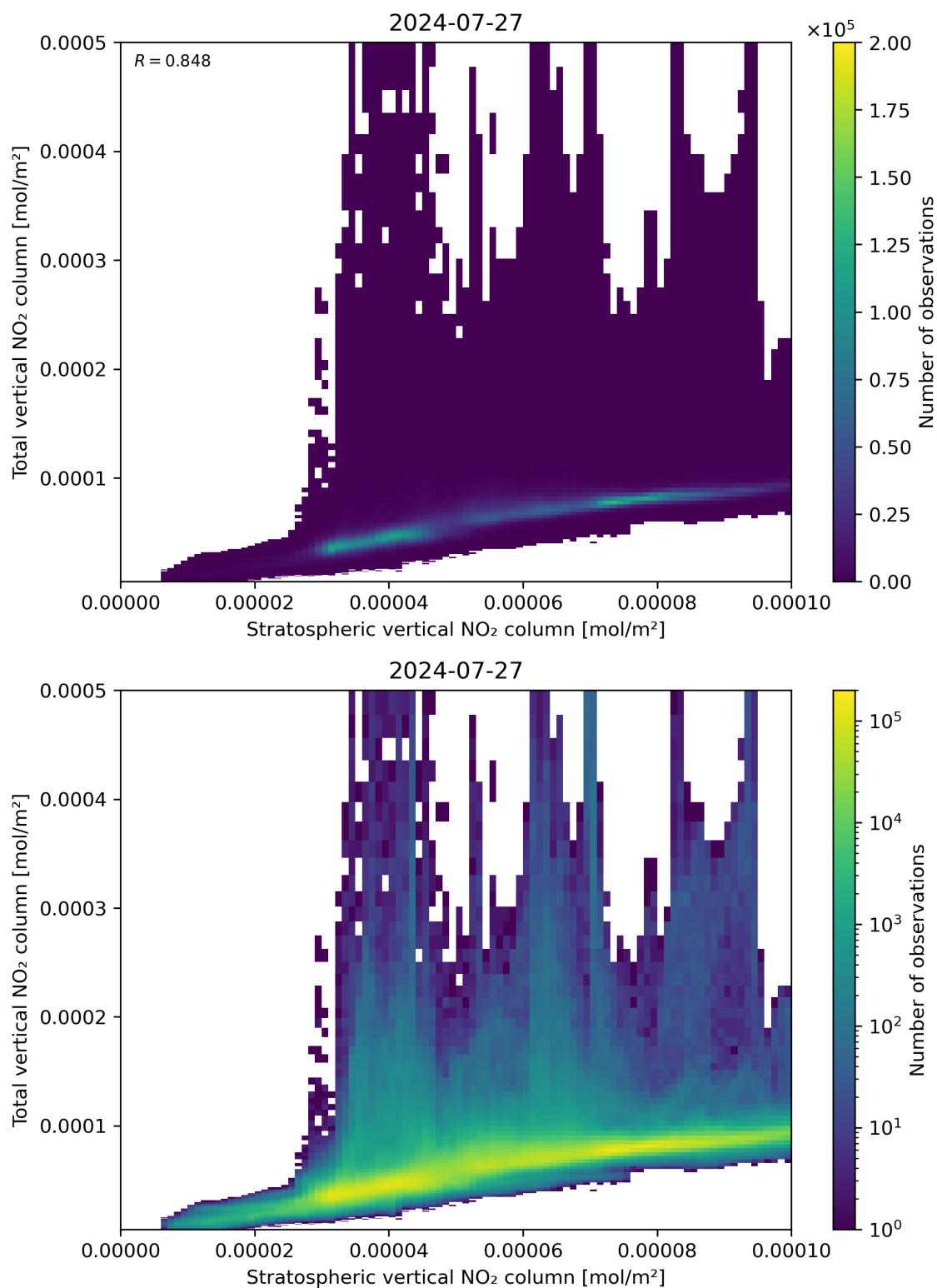
Figure 100: Scatter density plot of “Stratospheric vertical NO 2 column” against “Total vertical NO 2 column” for 2024-07-26 to 2024-07-28.
