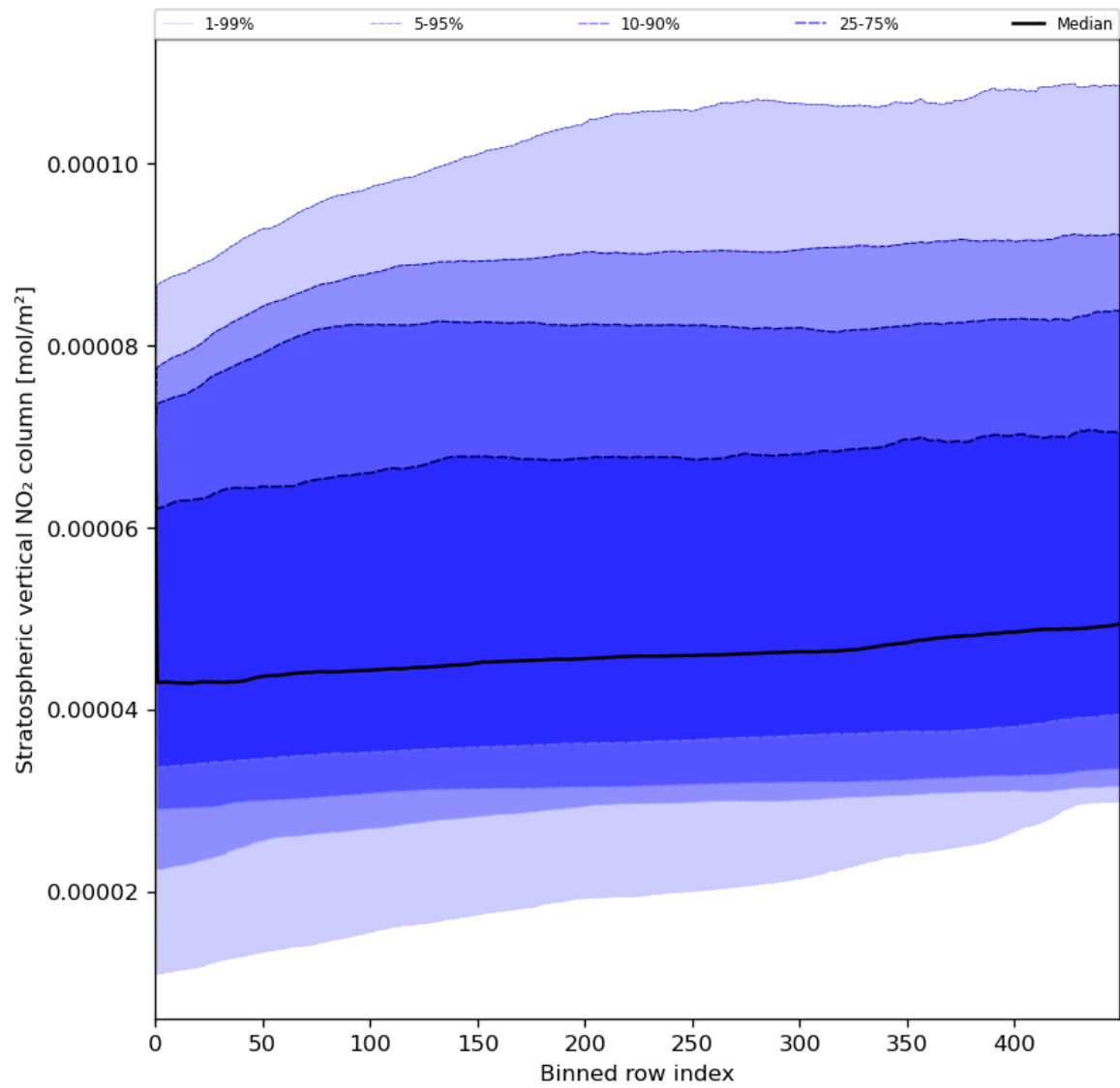
Figure 53: Along track statistics of “Stratospheric vertical NO 2 column” for 2024-07-26 to 2024-07-28
