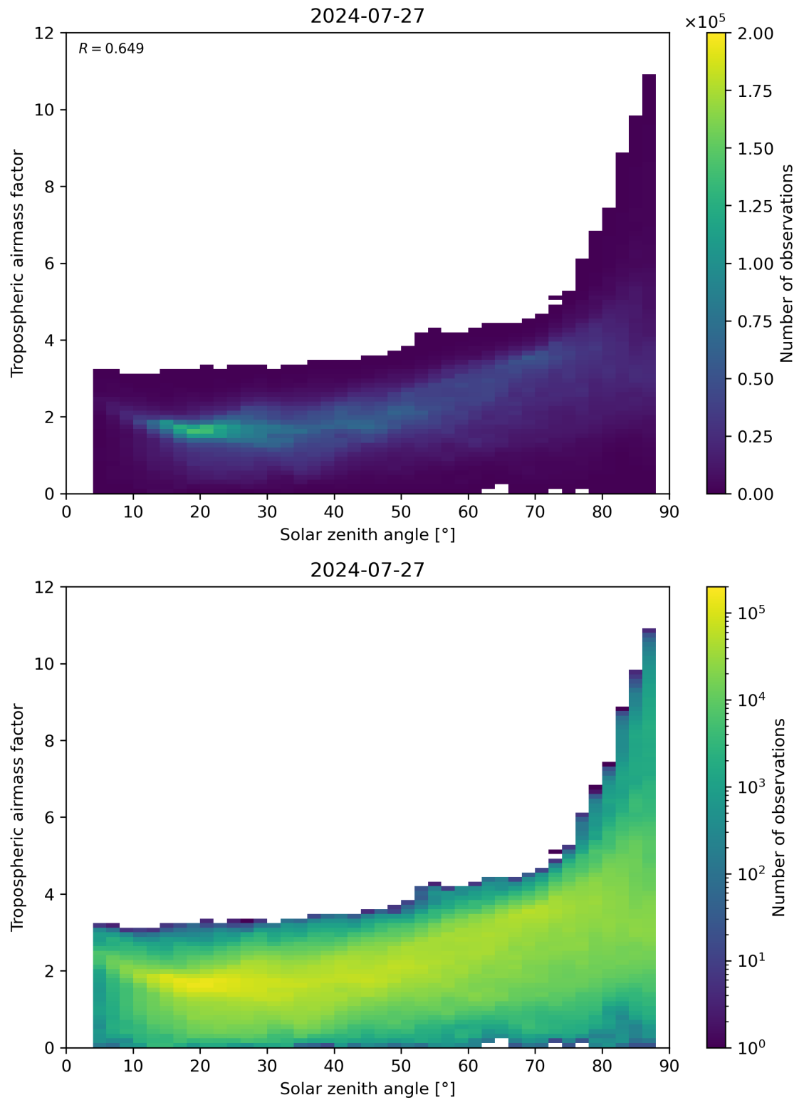
Figure 147: Scatter density plot of “Solar zenith angle” against “Tropospheric airmass factor” for 2024-07-26 to 2024-07-28.
