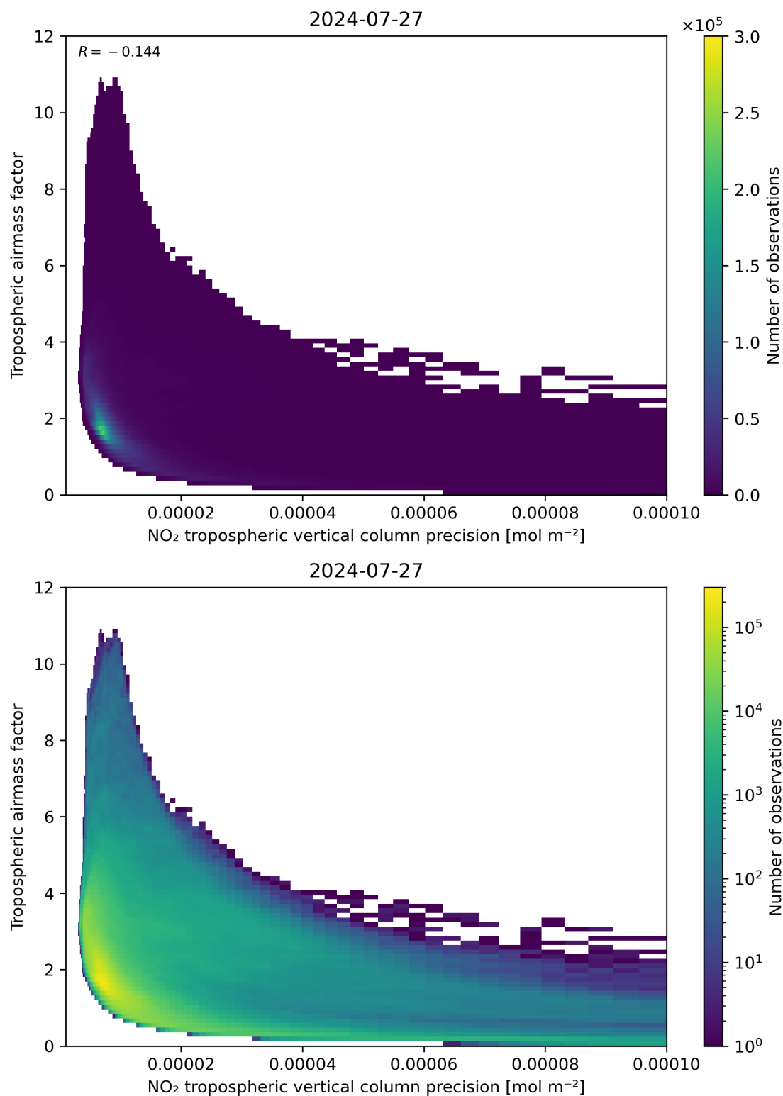
Figure 133: Scatter density plot of “NO 2 tropospheric vertical column precision” against “Tropospheric airmass factor” for 2024-07-26 to 2024-07-28.
