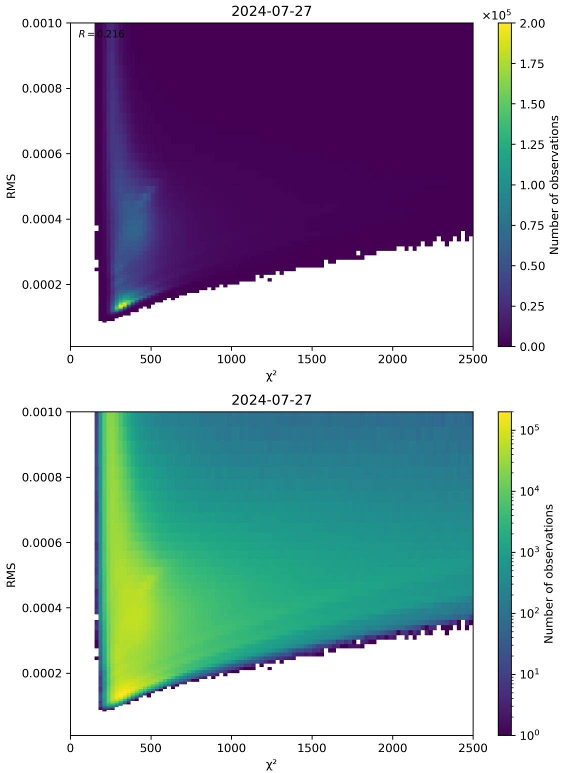
Figure 82: Scatter density plot of “ \chi^2 ” against “RMS” for 2024-07-26 to 2024-07-28.
