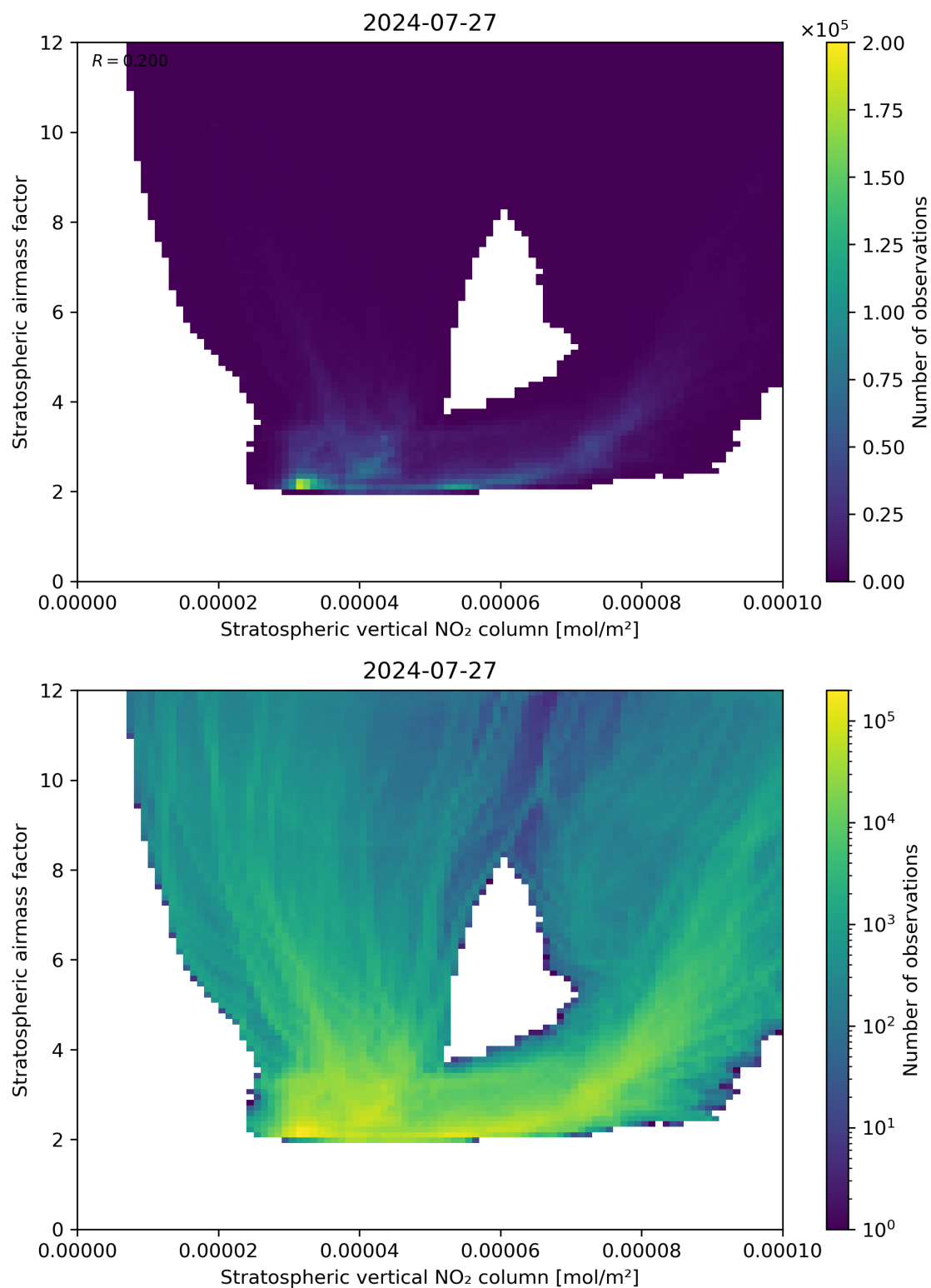
Figure 96: Scatter density plot of “Stratospheric vertical NO 2 column” against “Stratospheric airmass factor” for 2024-07-26 to 2024-07-28.
