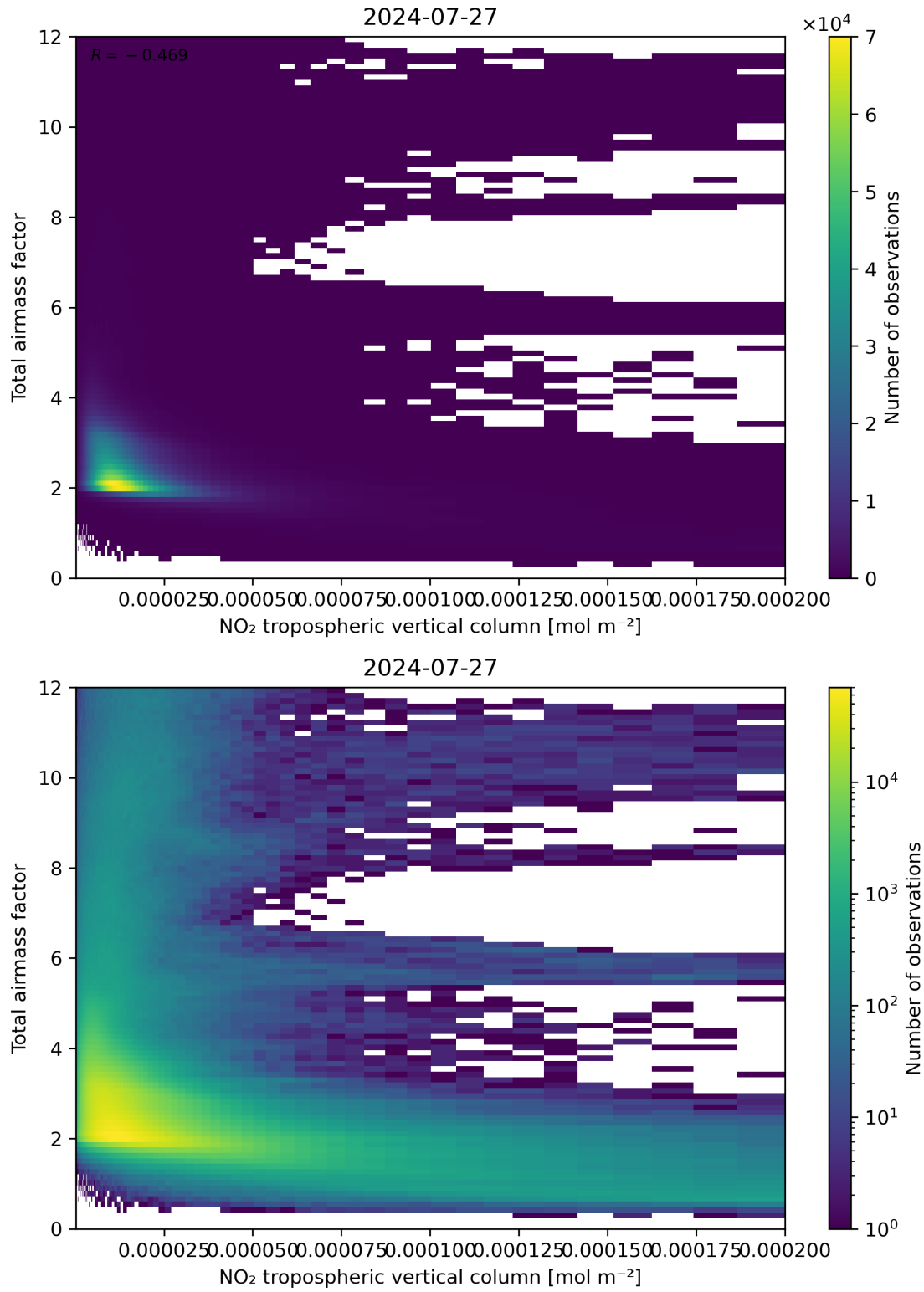
Figure 122: Scatter density plot of “NO 2 tropospheric vertical column” against “Total air mass factor” for 2024-07-26 to 2024-07-28.
