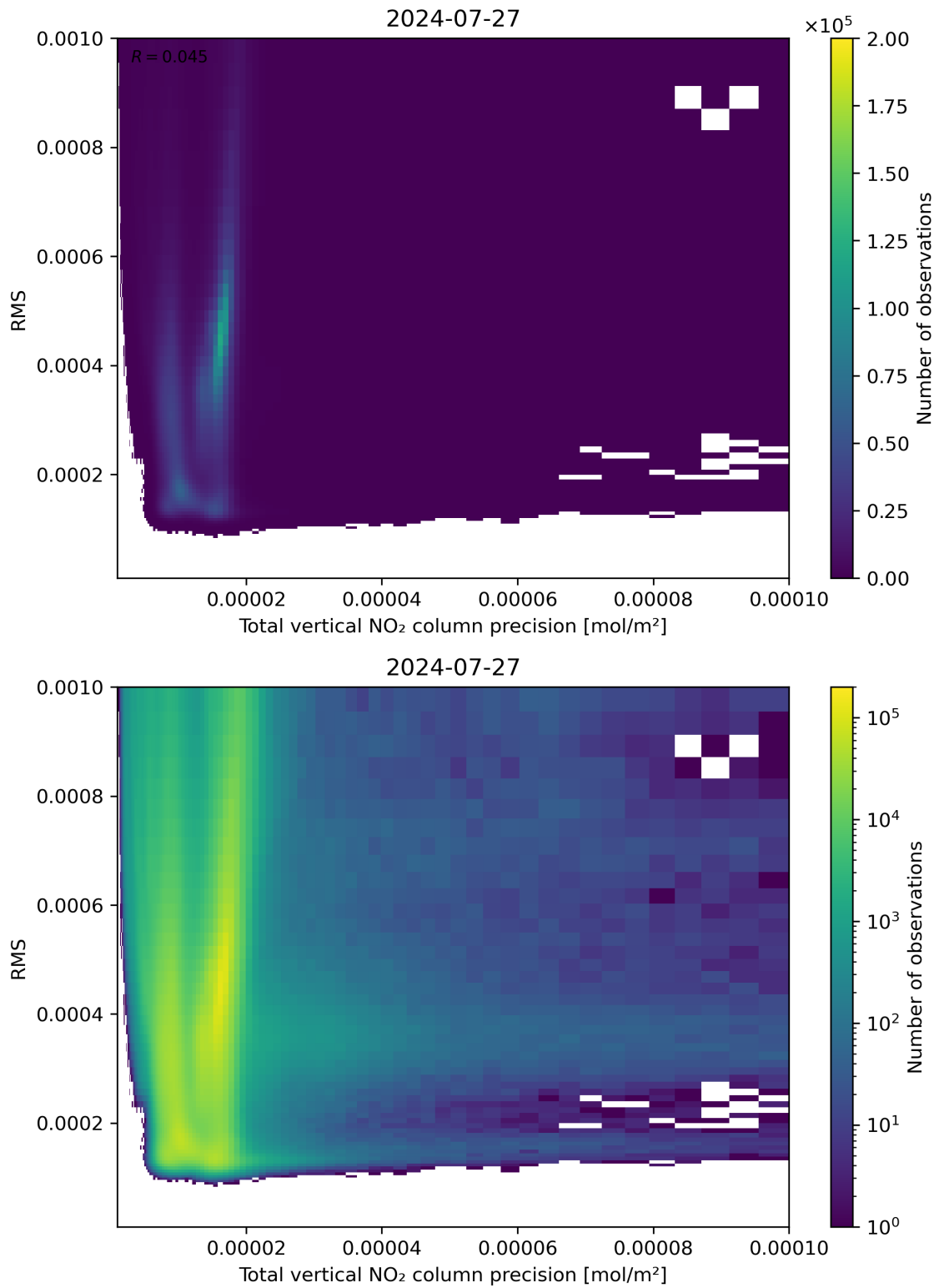
Figure 119: Scatter density plot of “Total vertical NO 2 column precision” against “RMS” for 2024-07-26 to 2024-07-28.
