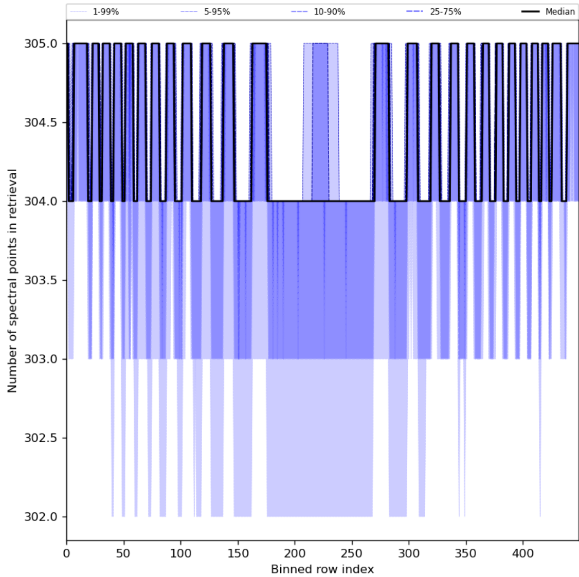
Figure 50: Along track statistics of “Number of spectral points in retrieval” for 2024-07-26 to 2024-07-28
