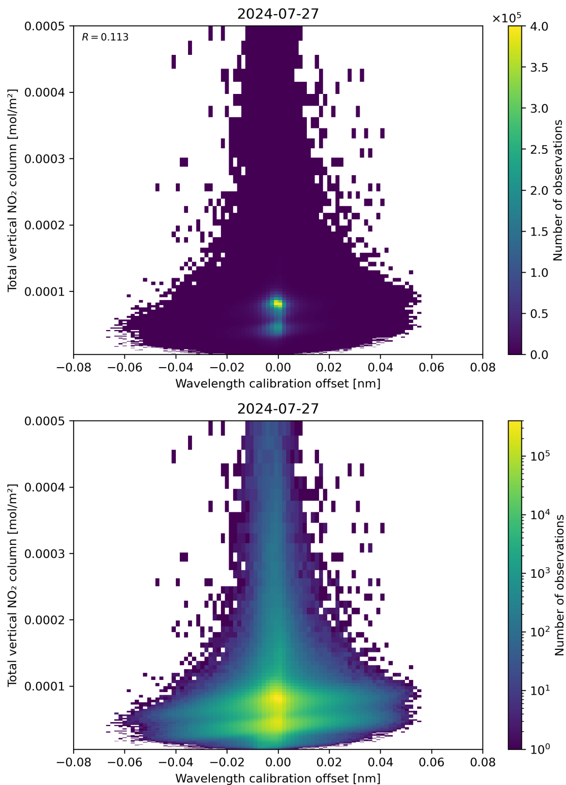
Figure 179: Scatter density plot of “Wavelength calibration offset” against “Total vertical NO 2 column” for 2024-07-26 to 2024-07-28.
