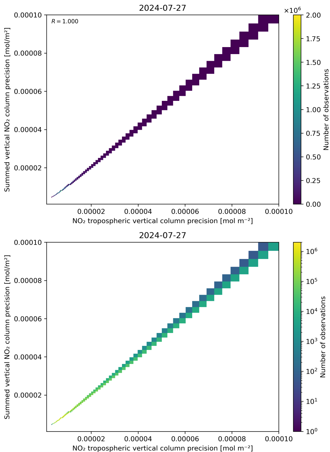
Figure 137: Scatter density plot of “NO 2 tropospheric vertical column precision” against “Summed vertical NO 2 column precision” for 2024-07-26 to 2024-07-28.
