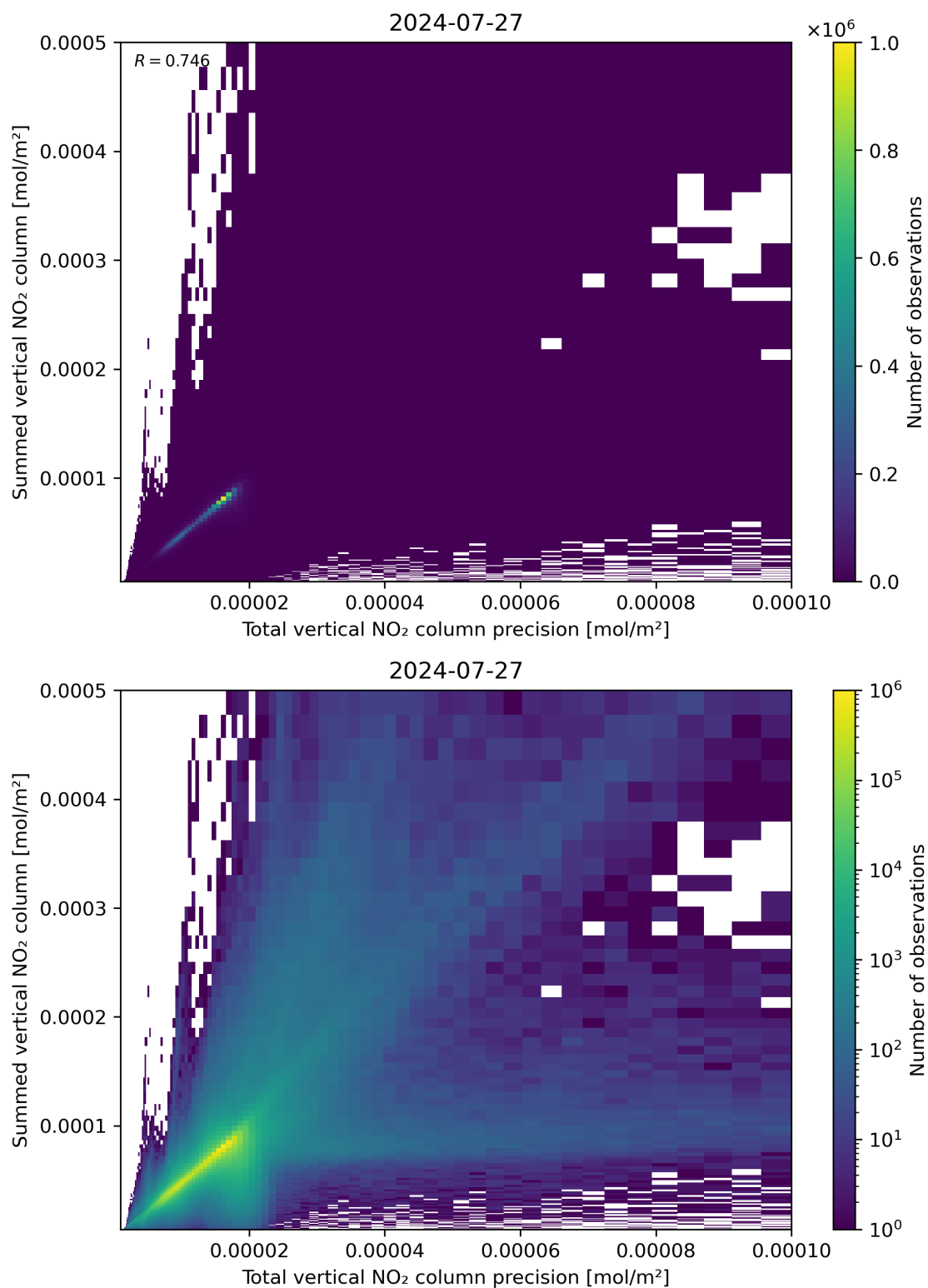
Figure 117: Scatter density plot of “Total vertical NO 2 column precision” against “Summed vertical NO 2 column” for 2024-07-26 to 2024-07-28.
