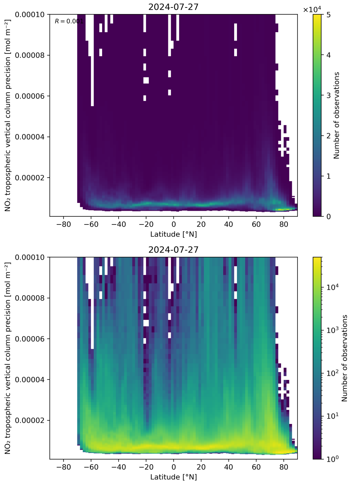
Figure 93: Scatter density plot of “Latitude” against “NO 2 tropospheric vertical column precision” for 2024-07-26 to 2024-07-28.
