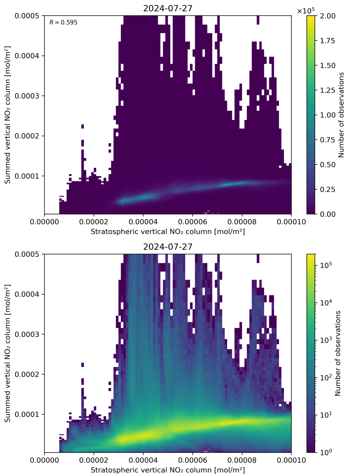
Figure 98: Scatter density plot of “Stratospheric vertical NO 2 column” against “Summed vertical NO 2 column” for 2024-07-26 to 2024-07-28.
