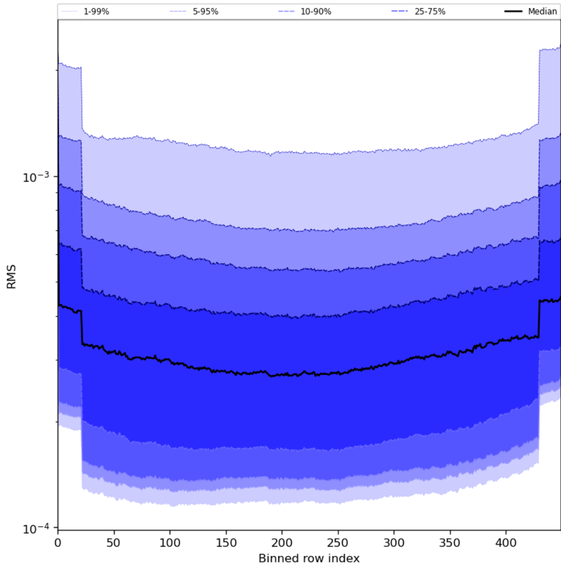
Figure 60: Along track statistics of “RMS” for 2024-07-26 to 2024-07-28
