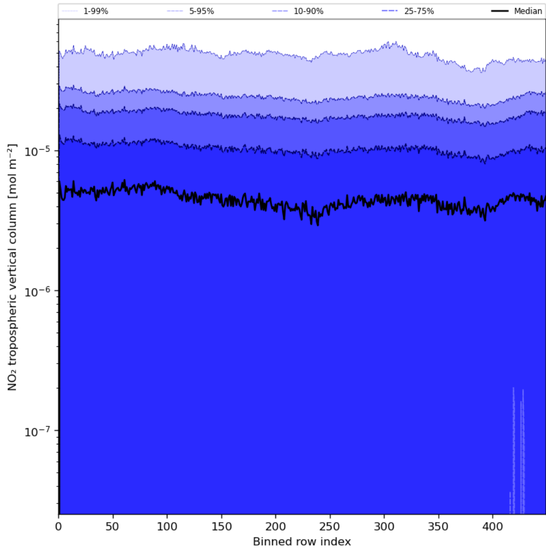
Figure 46: Along track statistics of “NO 2 tropospheric vertical column” for 2024-07-26 to 2024-07-28
