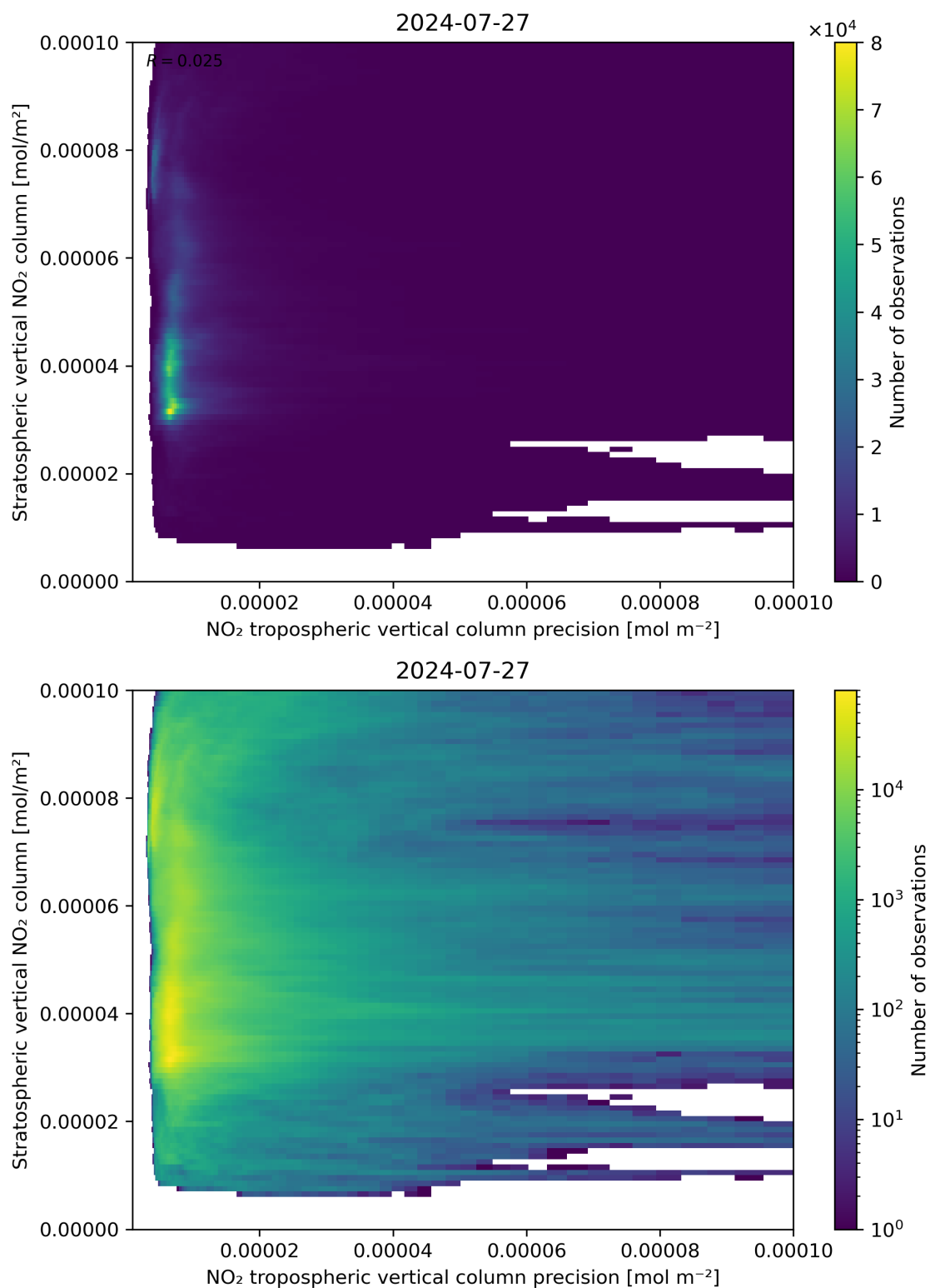
Figure 135: Scatter density plot of “NO 2 tropospheric vertical column precision” against “Stratospheric vertical NO 2 column” for 2024-07-26 to 2024-07-28.
