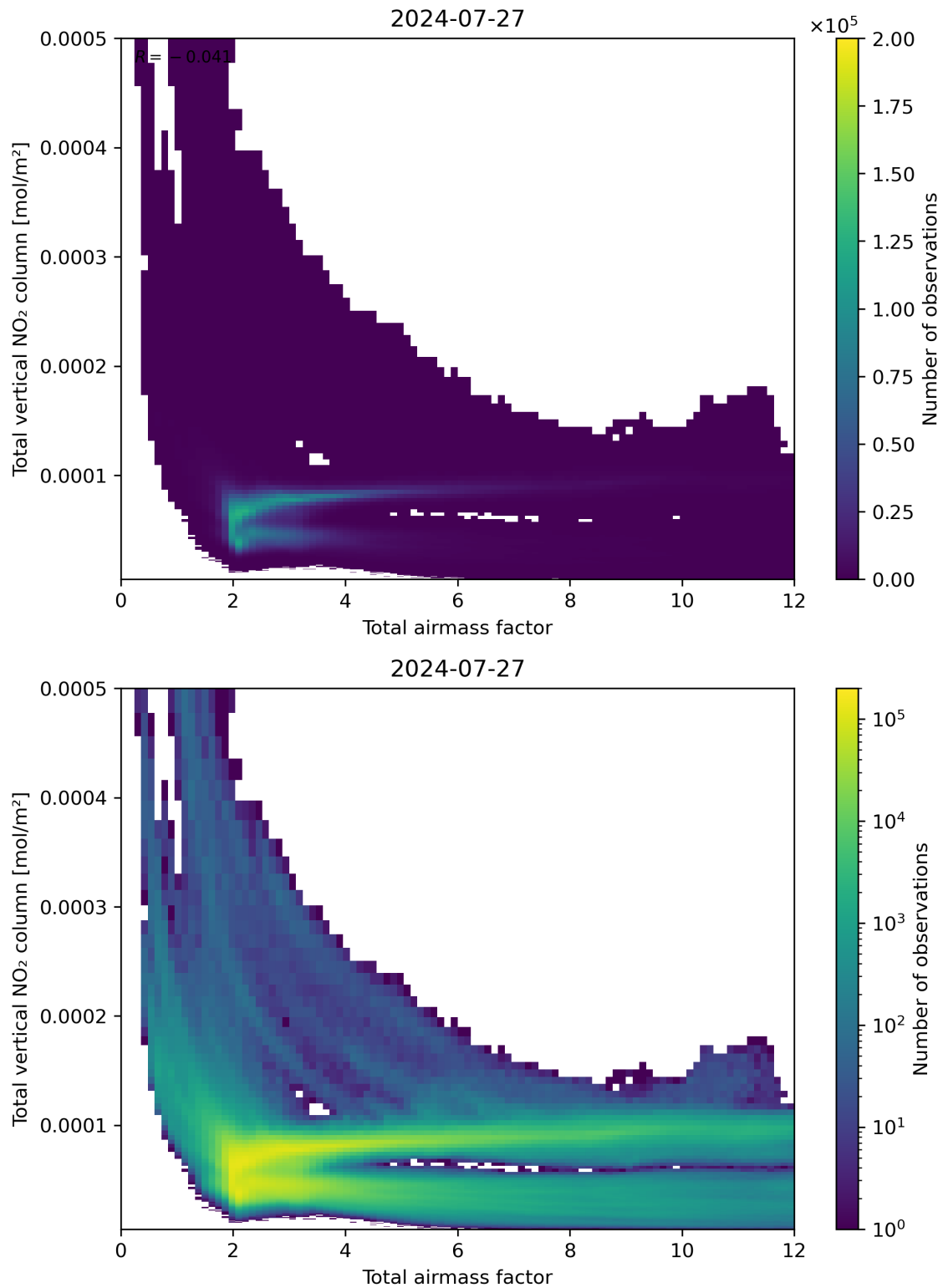
Figure 67: Scatter density plot of “Total airmass factor” against “Total vertical NO 2 column” for 2024-07-26 to 2024-07-28.
