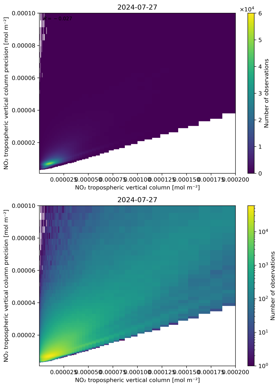
Figure 130: Scatter density plot of “NO 2 tropospheric vertical column” against “NO 2 tropospheric vertical column precision” for 2024-07-26 to 2024-07-28.
