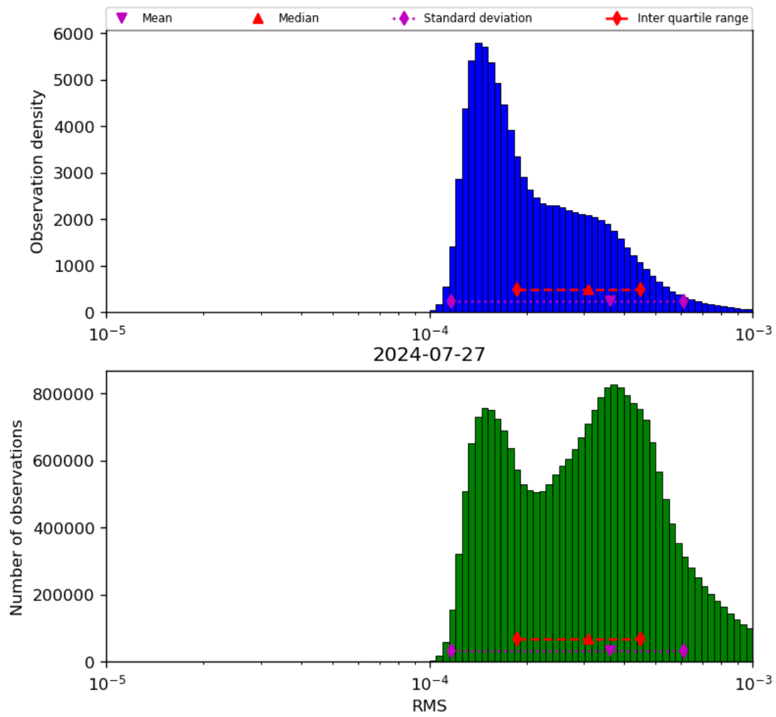
Figure 43: Histogram of “RMS” for 2024-07-26 to 2024-07-28
