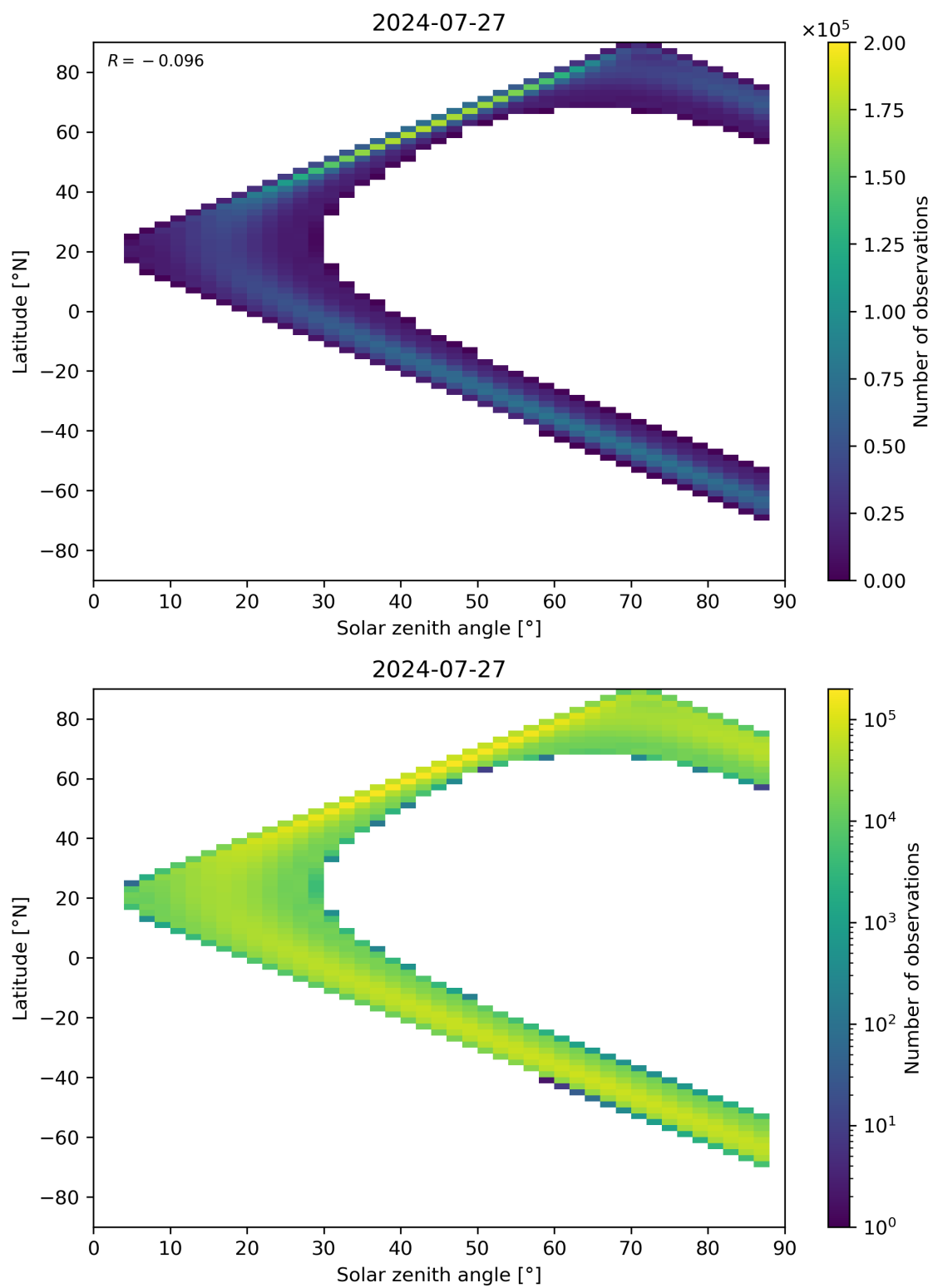
Figure 149: Scatter density plot of “Solar zenith angle” against “Latitude” for 2024-07-26 to 2024-07-28.
