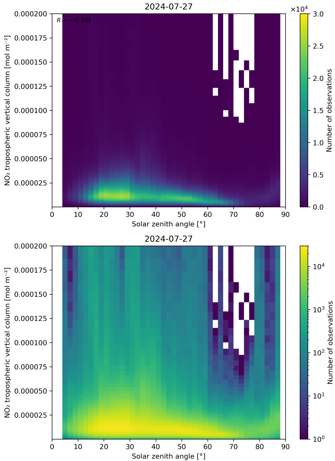
Figure 155: Scatter density plot of “Solar zenith angle” against “NO 2 tropospheric vertical column” for 2024-07-26 to 2024-07-28.
