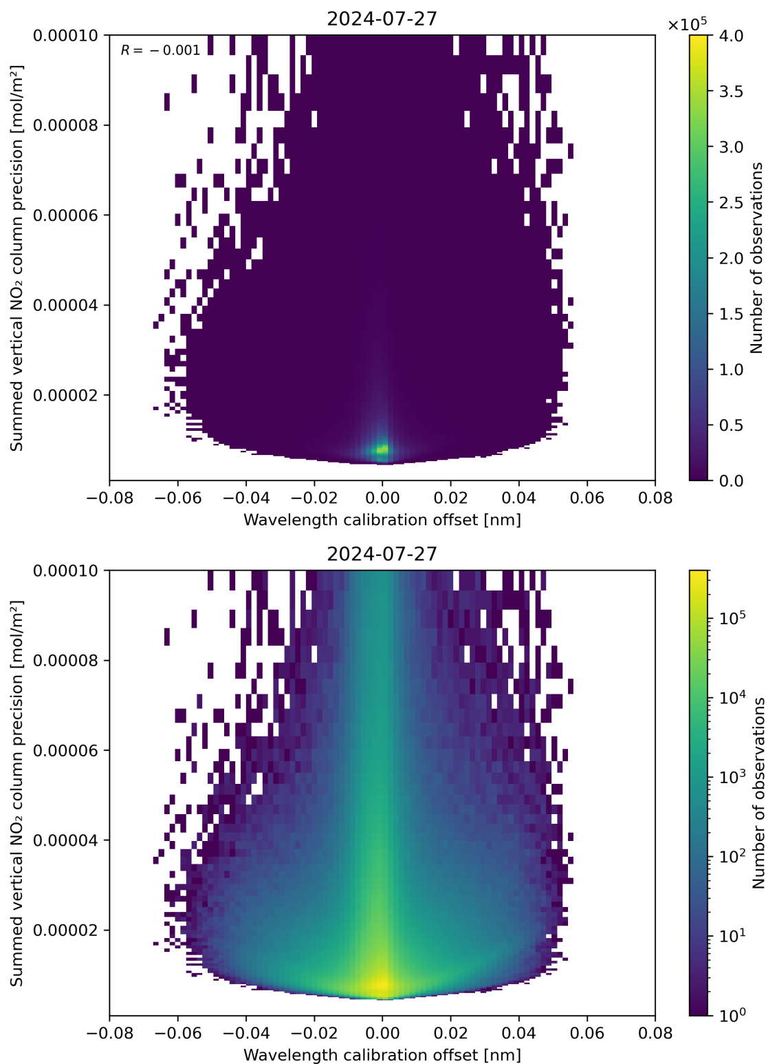
Figure 178: Scatter density plot of “Wavelength calibration offset” against “Summed vertical NO 2 column precision” for 2024-07-26 to 2024-07-28.
