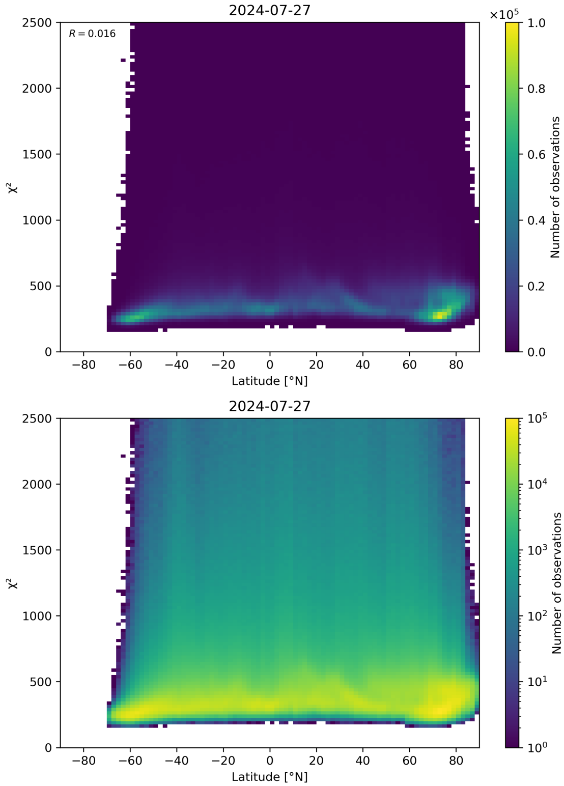
Figure 86: Scatter density plot of “Latitude” against “ \chi^2 ” for 2024-07-26 to 2024-07-28.
