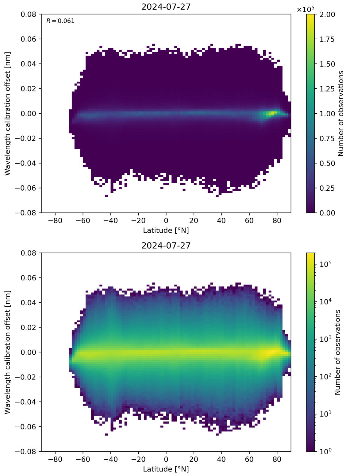
Figure 95: Scatter density plot of “Latitude” against “Wavelength calibration offset” for 2024-07-26 to 2024-07-28.
