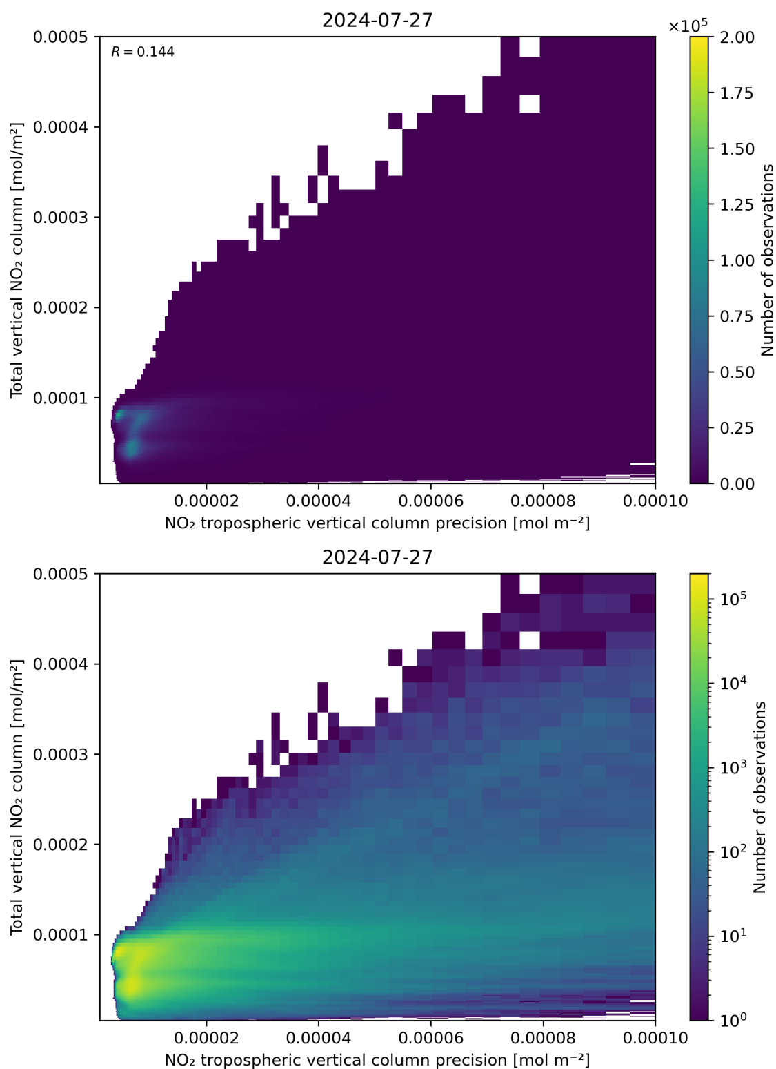
Figure 138: Scatter density plot of “NO 2 tropospheric vertical column precision” against “Total vertical NO 2 column” for 2024-07-26 to 2024-07-28.
