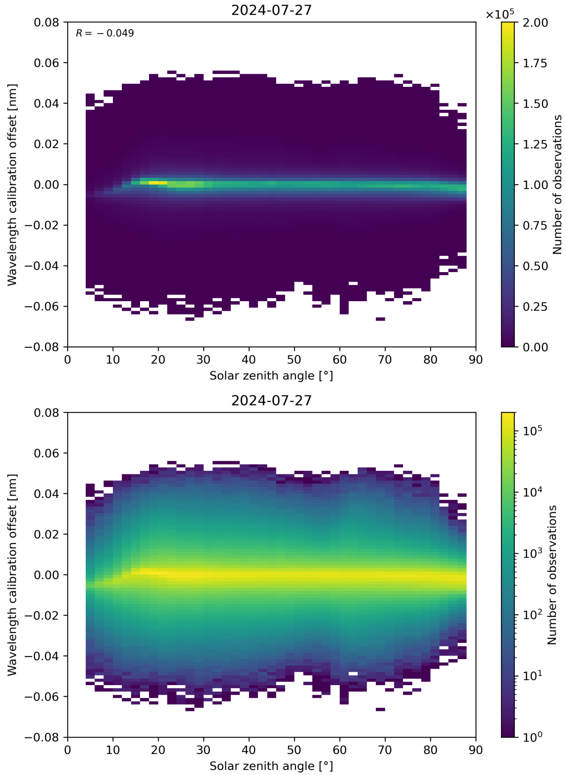
Figure 158: Scatter density plot of “Solar zenith angle” against “Wavelength calibration offset” for 2024-07-26 to 2024-07-28.
