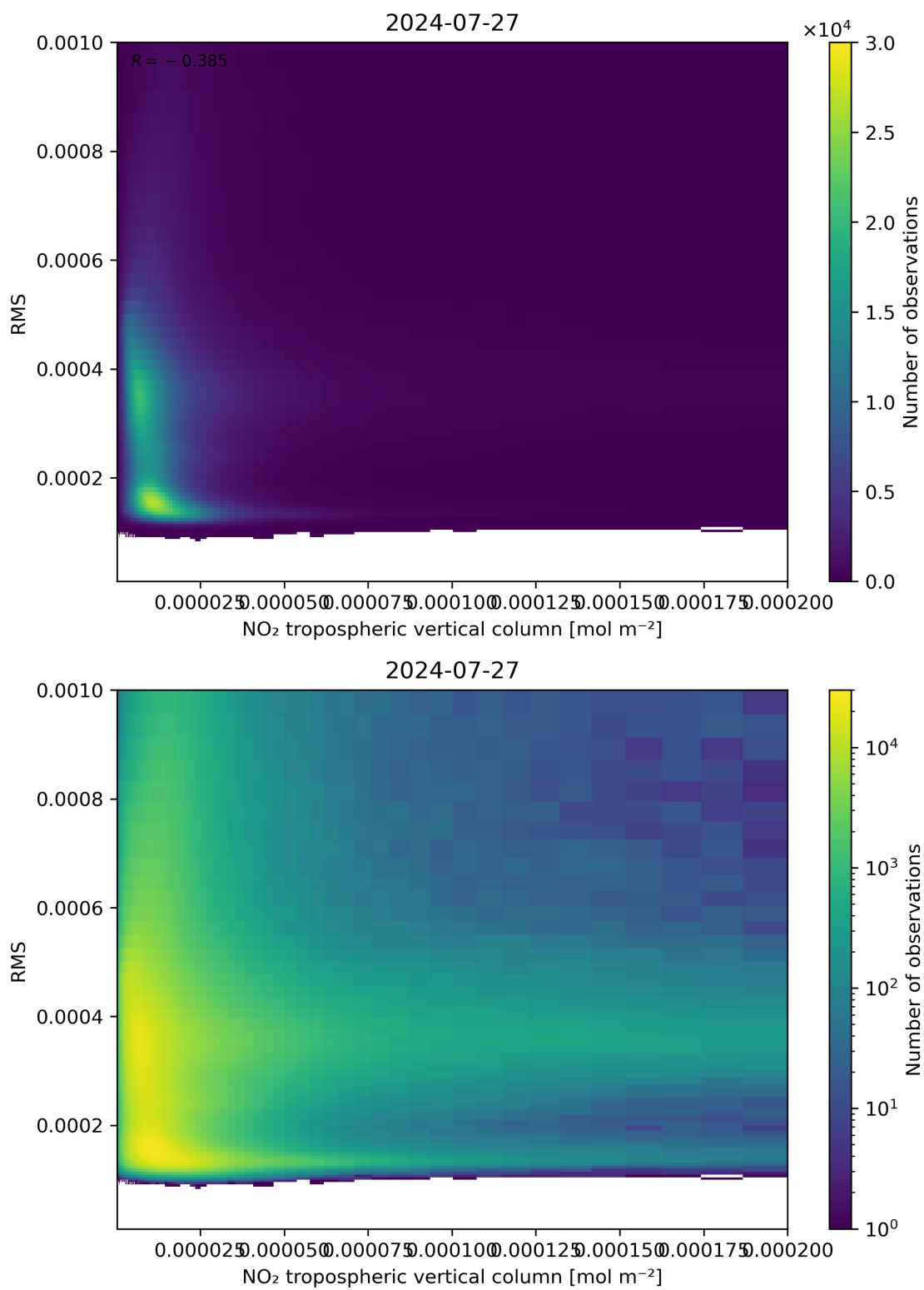
Figure 142: Scatter density plot of “NO 2 tropospheric vertical column” against “RMS” for 2024-07-26 to 2024-07-28.
