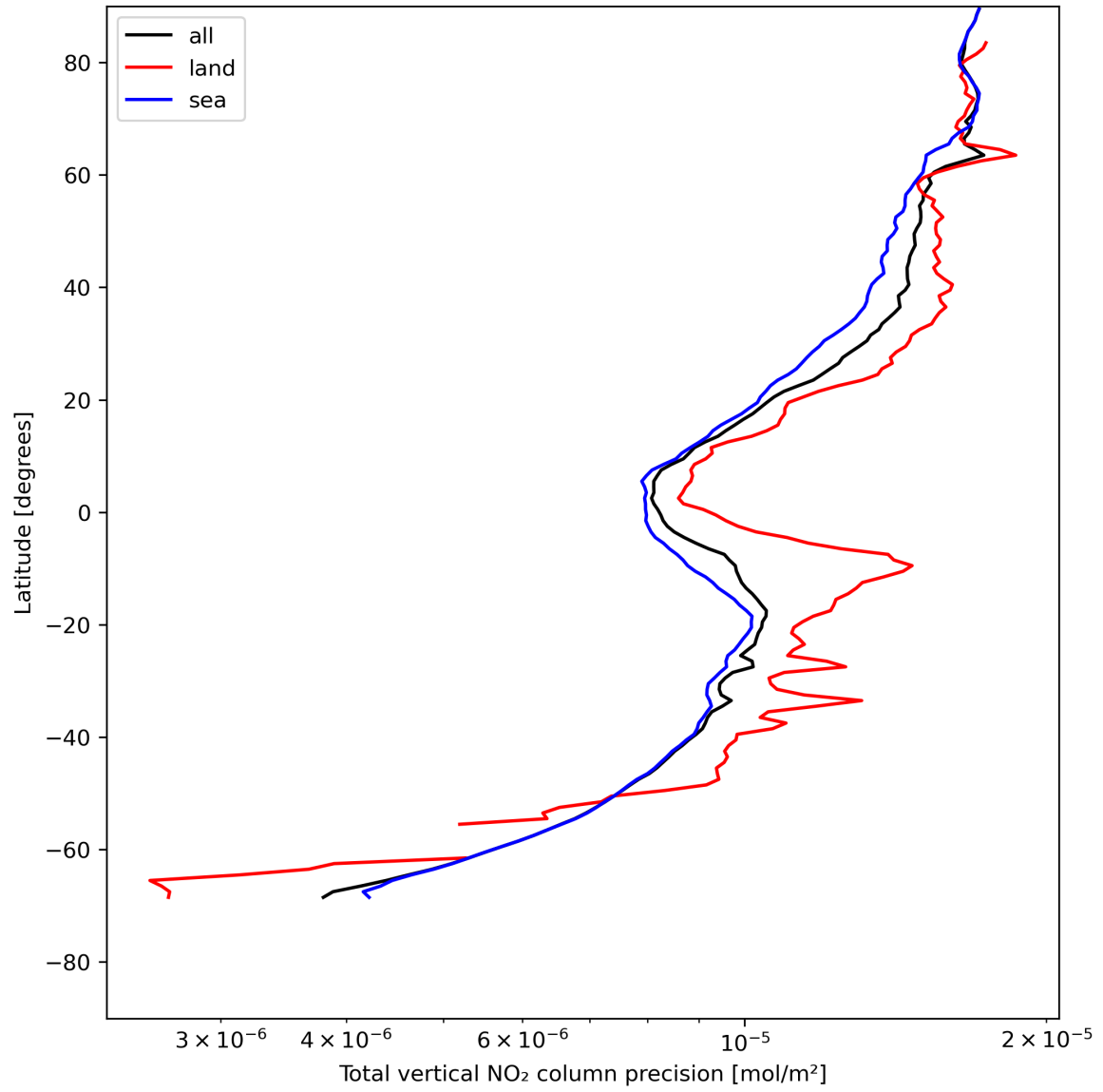
Figure 22: Zonal average of “Total vertical NO 2 column precision” for 2024-07-26 to 2024-07-28.
