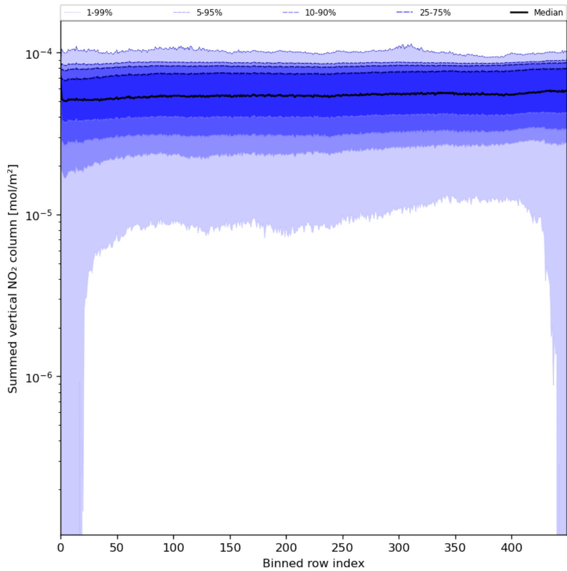
Figure 57: Along track statistics of “Summed vertical NO 2 column” for 2024-07-26 to 2024-07-28
