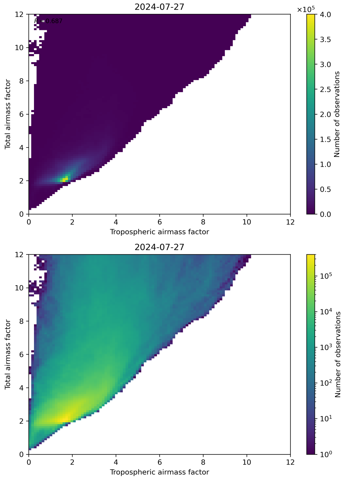
Figure 72: Scatter density plot of “Tropospheric airmass factor” against “Total airmass factor” for 2024-07-26 to 2024-07-28.
