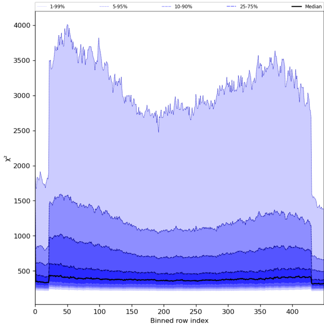
Figure 59: Along track statistics of “ \chi^2 ” for 2024-07-26 to 2024-07-28
