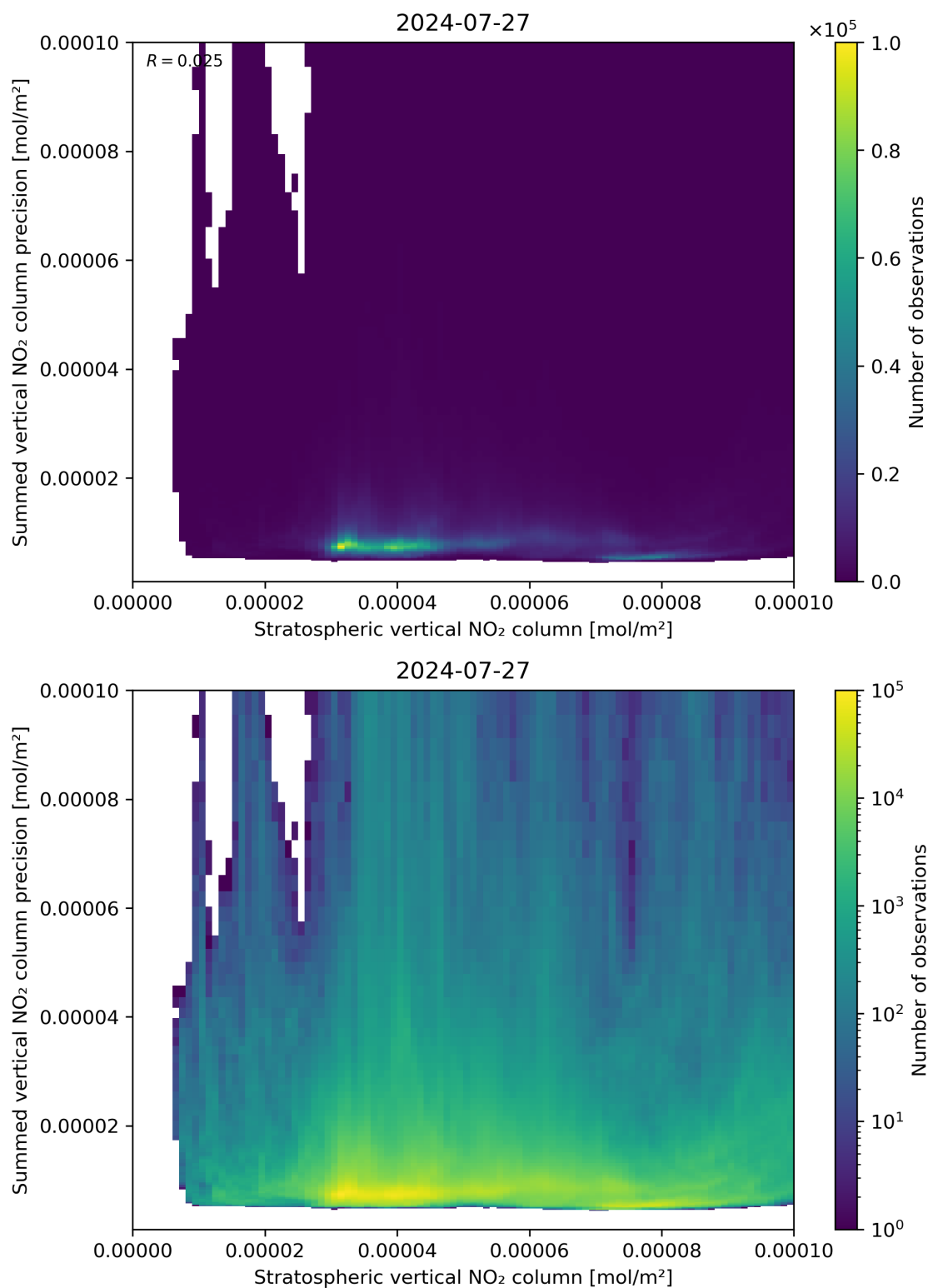
Figure 99: Scatter density plot of “Stratospheric vertical NO 2 column” against “Summed vertical NO 2 column precision” for 2024-07-26 to 2024-07-28.
