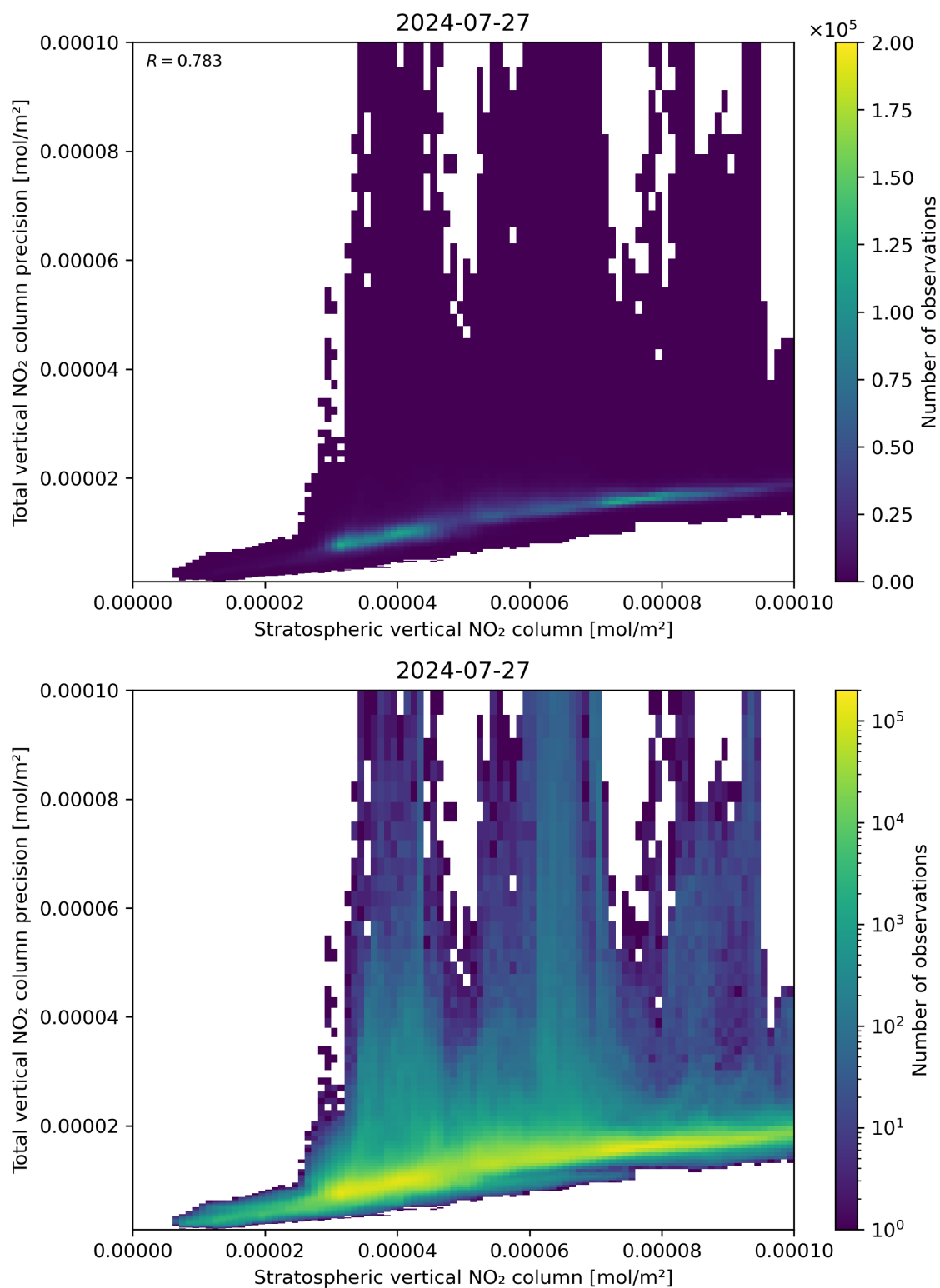
Figure 101: Scatter density plot of “Stratospheric vertical NO 2 column” against “Total vertical NO 2 column precision” for 2024-07-26 to 2024-07-28.
