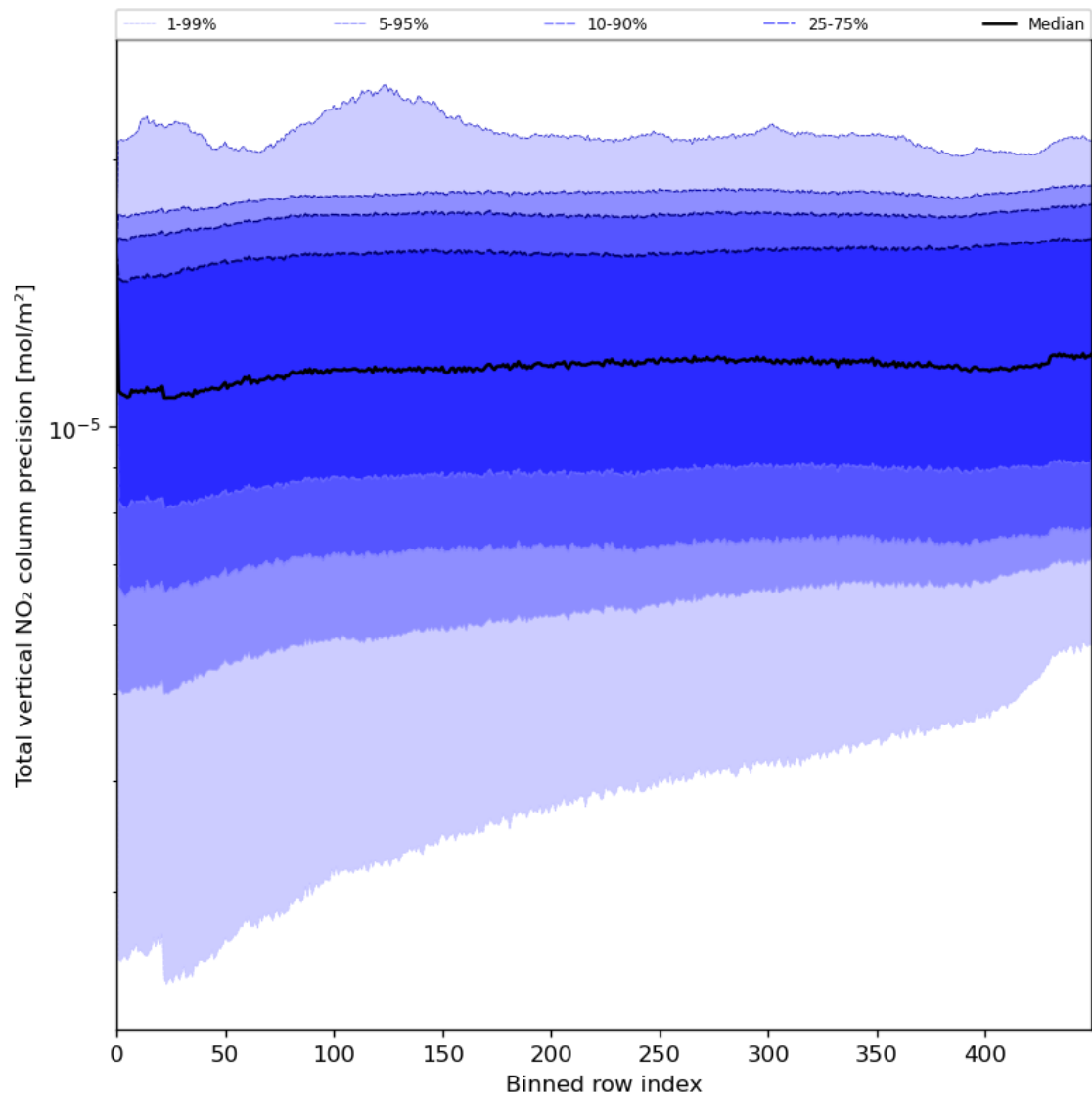
Figure 56: Along track statistics of “Total vertical NO 2 column precision” for 2024-07-26 to 2024-07-28
