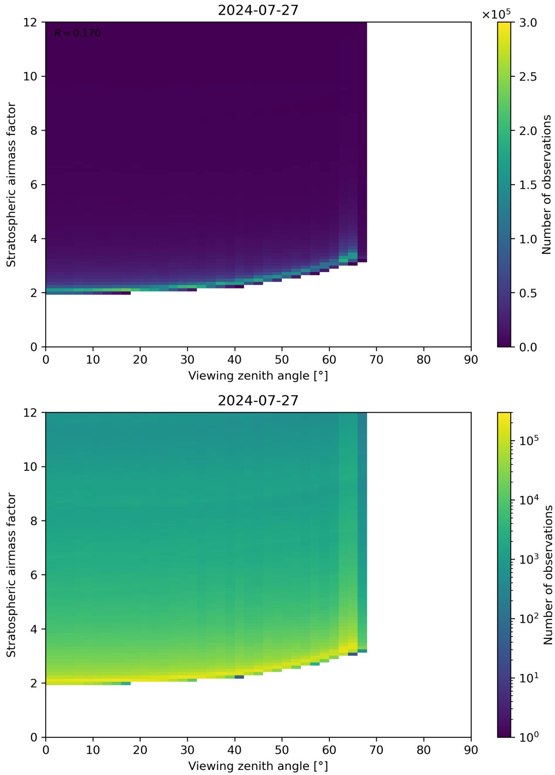
Figure 159: Scatter density plot of “Viewing zenith angle” against “Stratospheric airmass factor” for 2024-07-26 to 2024-07-28.
