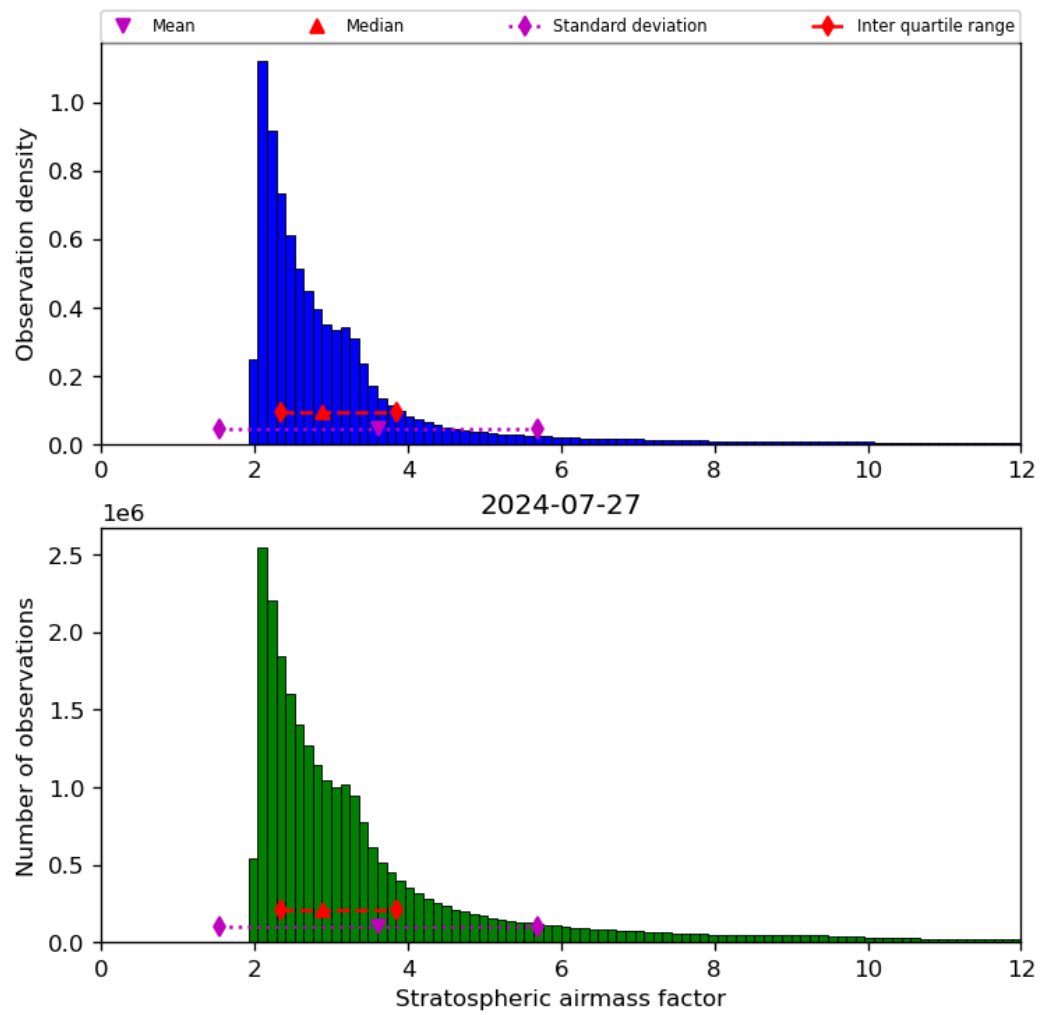
Figure 44: Histogram of “Stratospheric airmass factor” for 2024-07-26 to 2024-07-28
