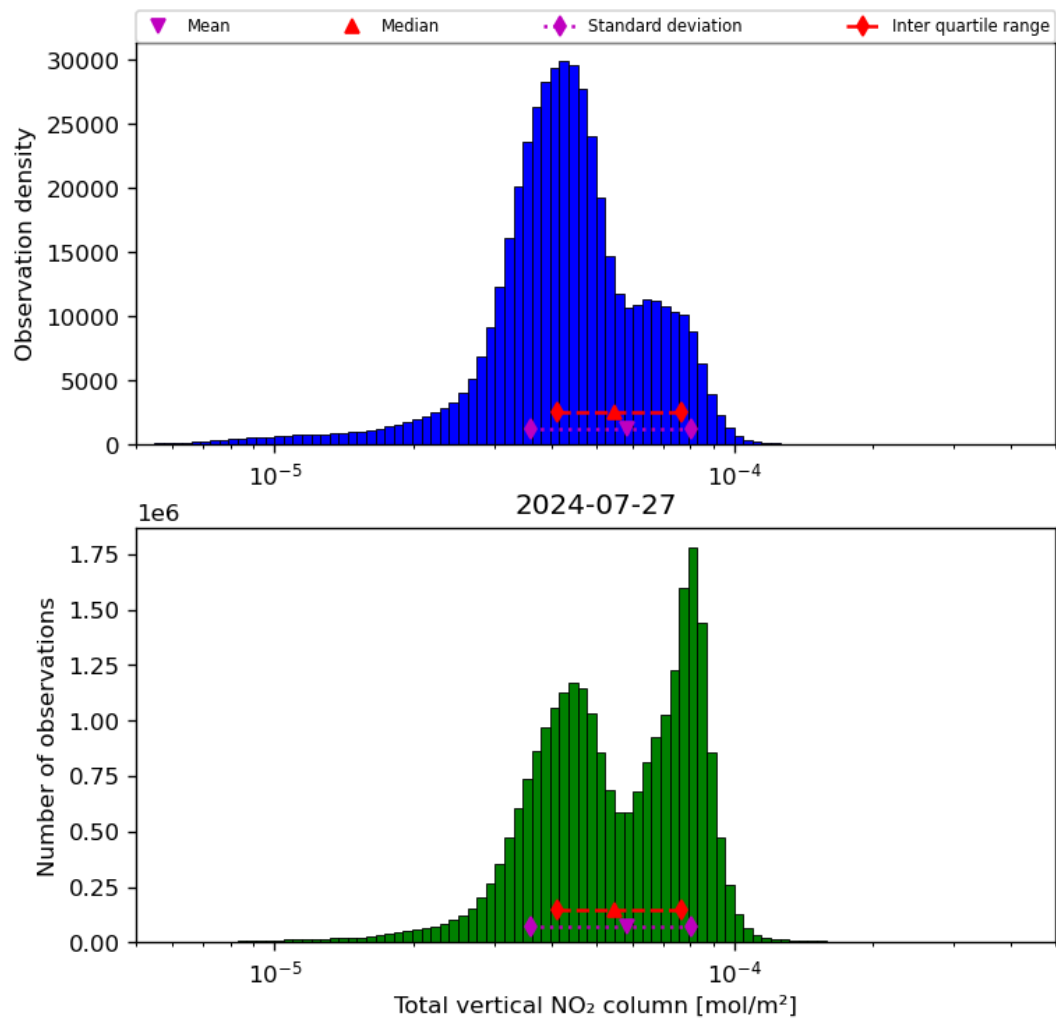
Figure 38: Histogram of “Total vertical NO 2 column” for 2024-07-26 to 2024-07-28
