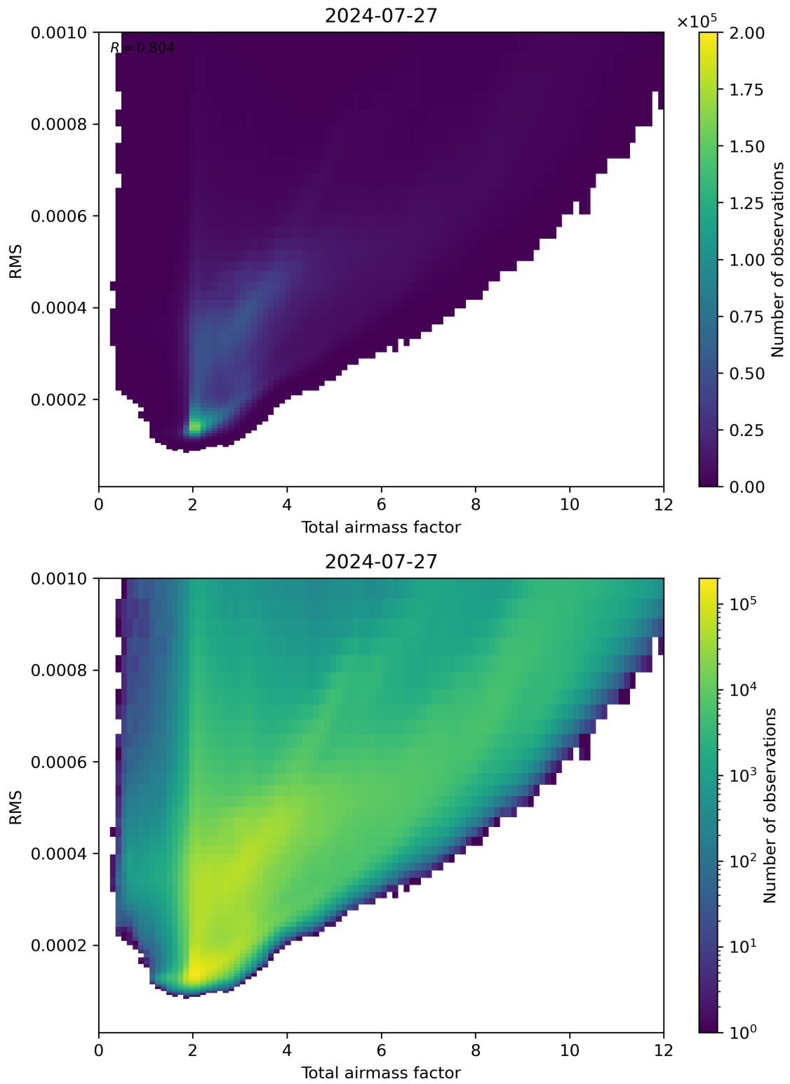
Figure 69: Scatter density plot of “Total airmass factor” against “RMS” for 2024-07-26 to 2024-07-28.
