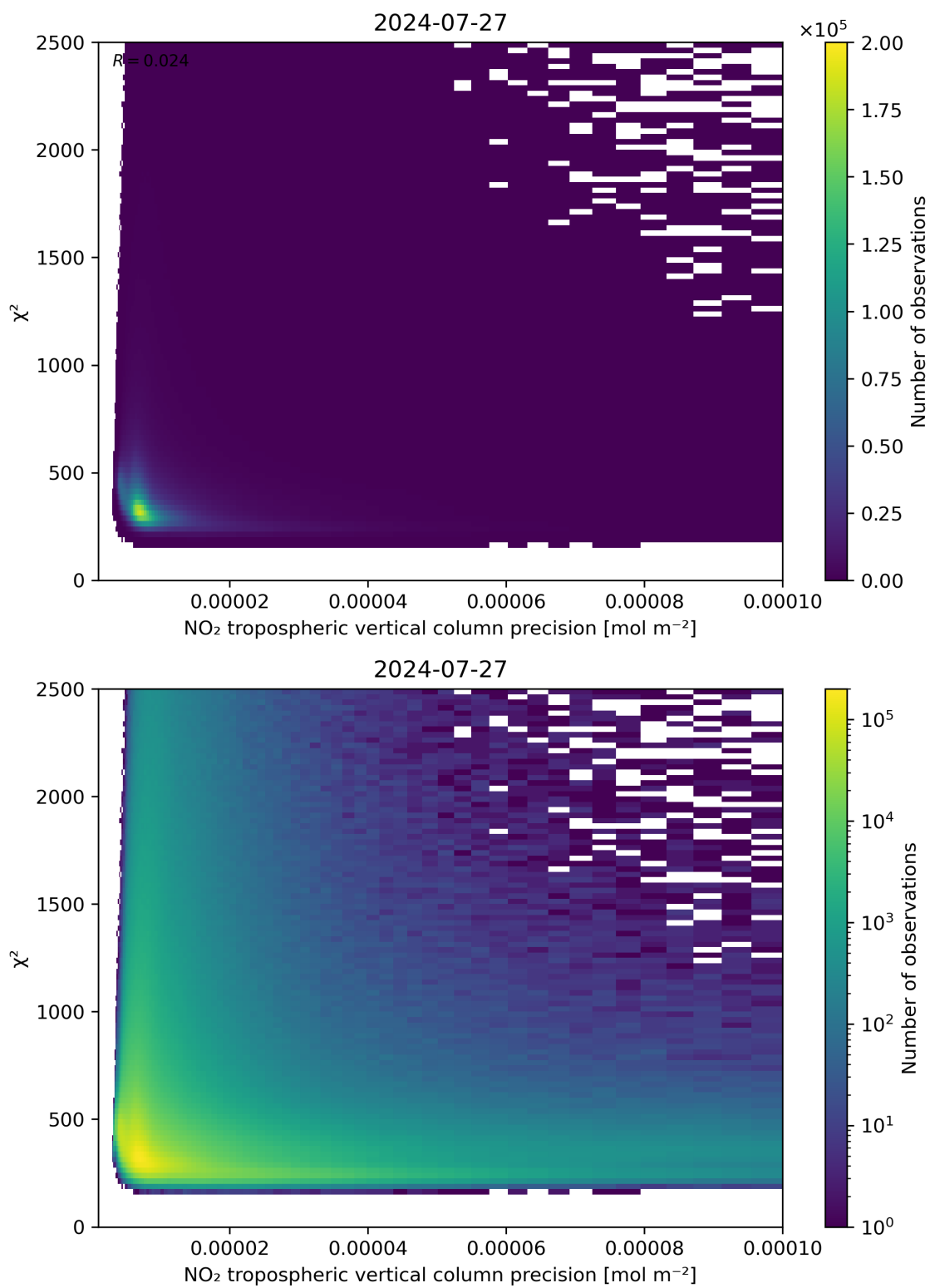
Figure 134: Scatter density plot of “NO 2 tropospheric vertical column precision” against “ \chi^2 ” for 2024-07-26 to 2024-07-28.
