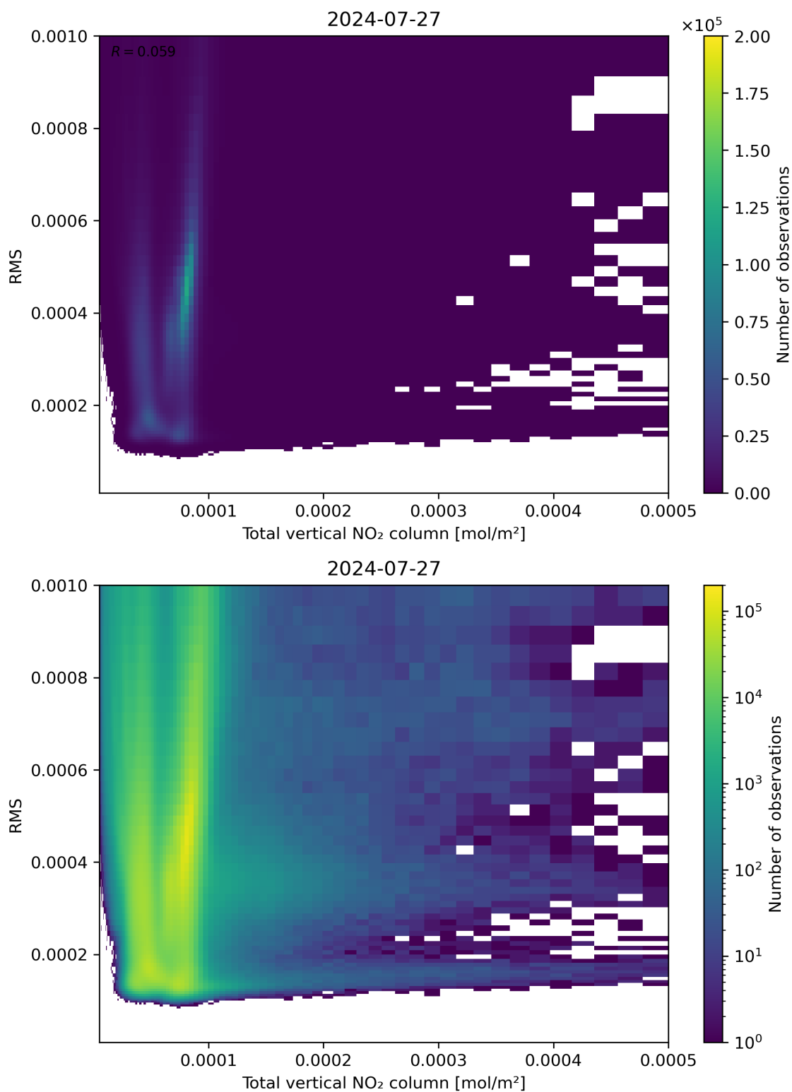
Figure 120: Scatter density plot of “Total vertical NO 2 column” against “RMS” for 2024-07-26 to 2024-07-28.
