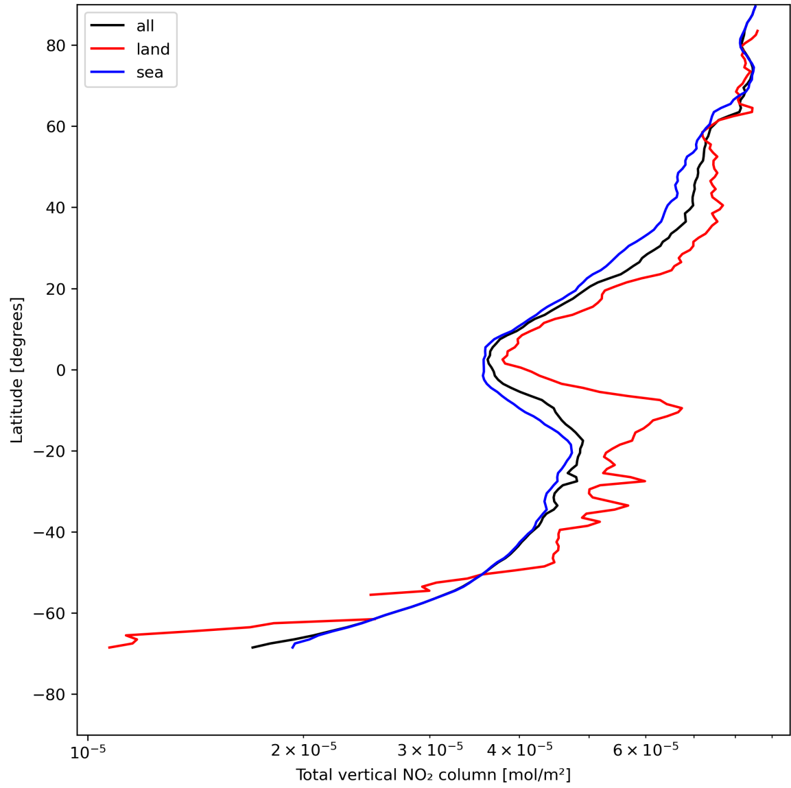
Figure 21: Zonal average of “Total vertical NO 2 column” for 2024-07-26 to 2024-07-28.
