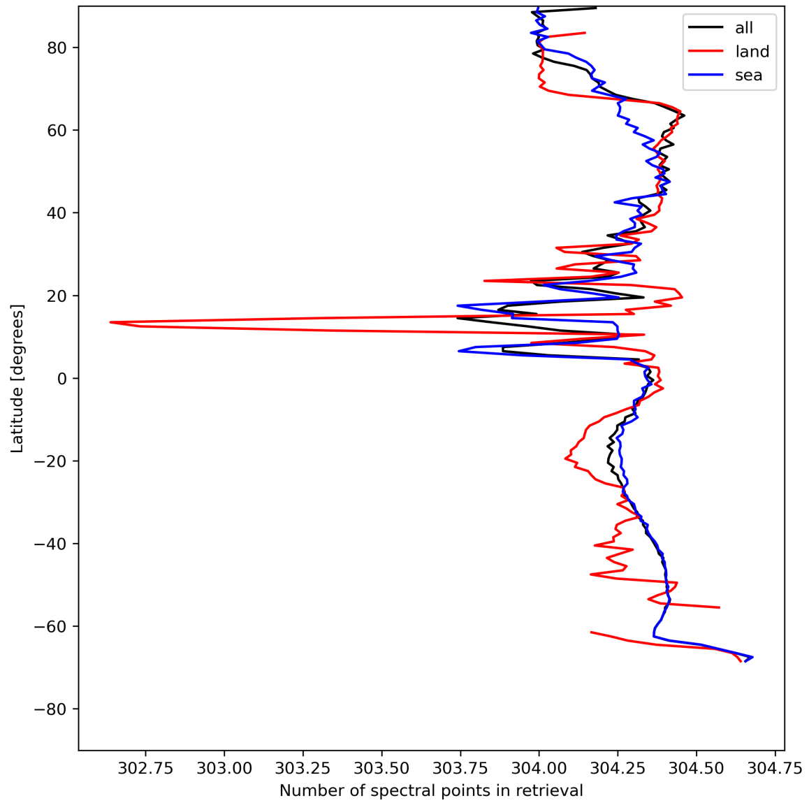
Figure 16: Zonal average of “Number of spectral points in retrieval” for 2024-07-26 to 2024-07-28.
