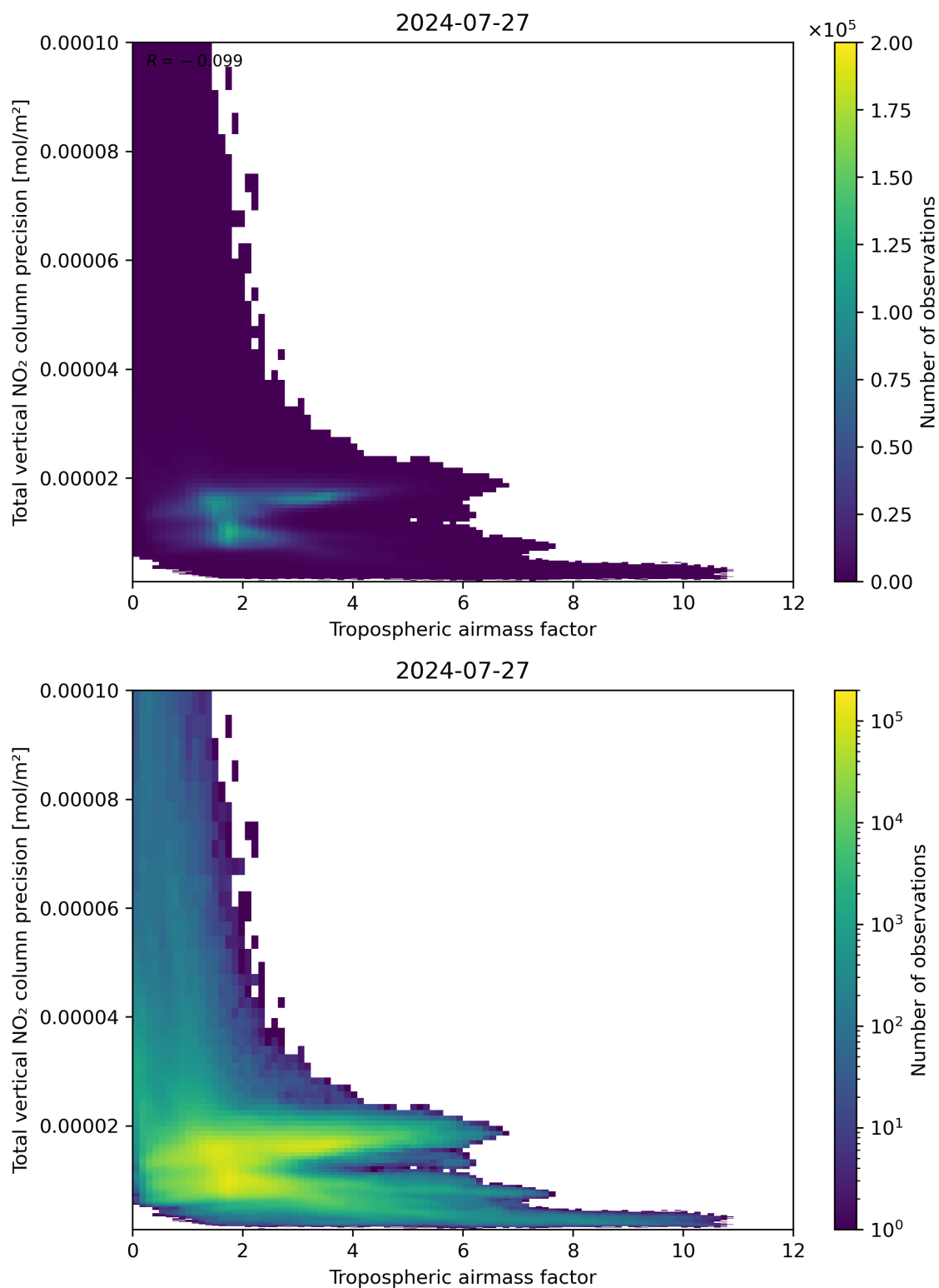
Figure 78: Scatter density plot of “Tropospheric air mass factor” against “Total vertical NO 2 column precision” for 2024-07-26 to 2024-07-28.
