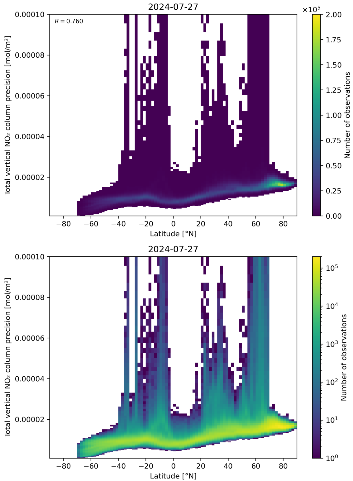
Figure 91: Scatter density plot of “Latitude” against “Total vertical NO 2 column precision” for 2024-07-26 to 2024-07-28.
