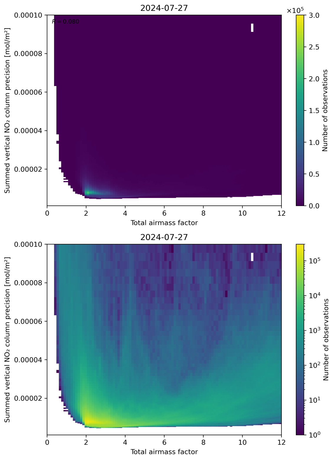
Figure 66: Scatter density plot of “Total airmass factor” against “Summed vertical NO 2 column precision” for 2024-07-26 to 2024-07-28.
