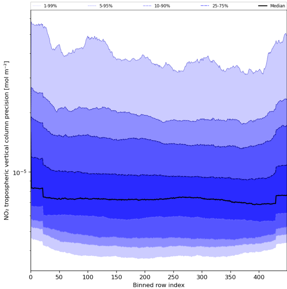
Figure 47: Along track statistics of “NO 2 tropospheric vertical column precision” for 2024-07-26 to 2024-07-28
