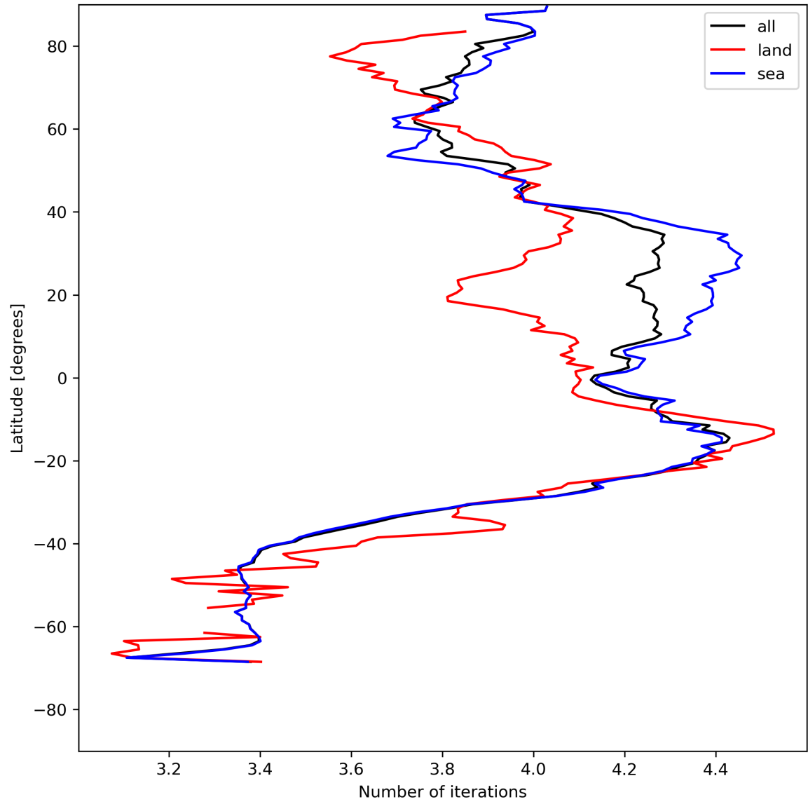
Figure 17: Zonal average of “Number of iterations” for 2024-07-26 to 2024-07-28.
