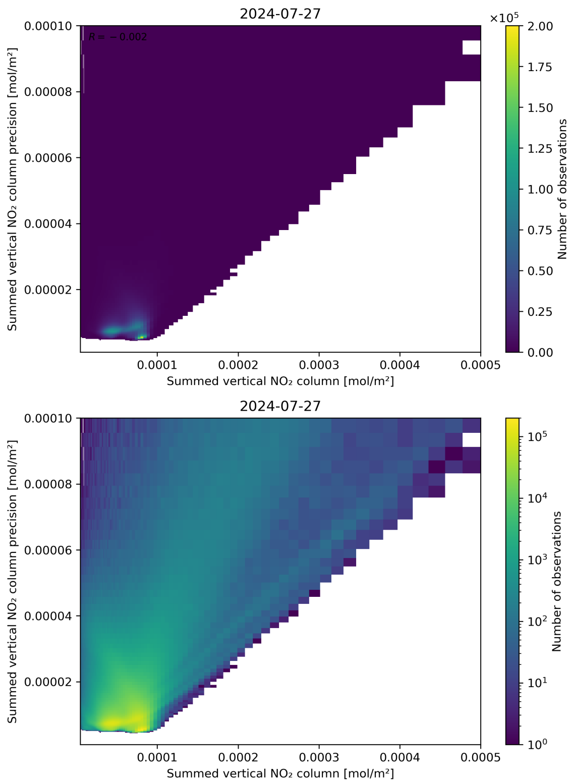
Figure 105: Scatter density plot of “Summed vertical NO 2 column” against “Summed vertical NO 2 column precision” for 2024-07-26 to 2024-07-28.
