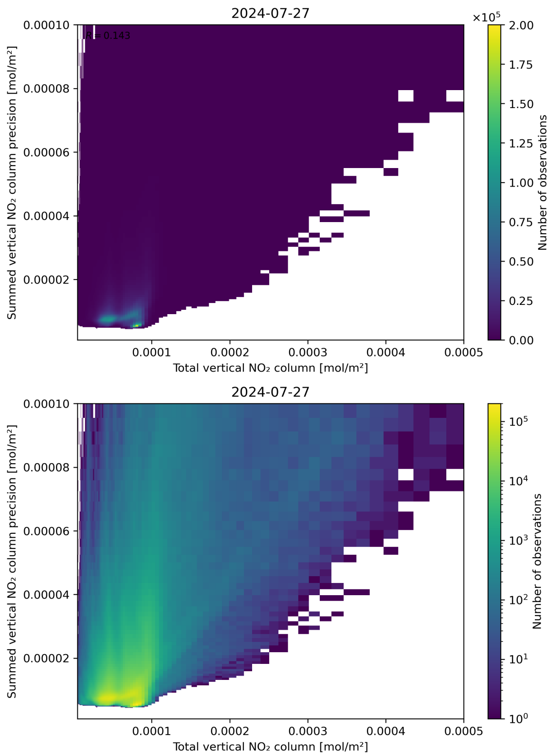
Figure 113: Scatter density plot of “Total vertical NO 2 column” against “Summed vertical NO 2 column precision” for 2024-07-26 to 2024-07-28.
