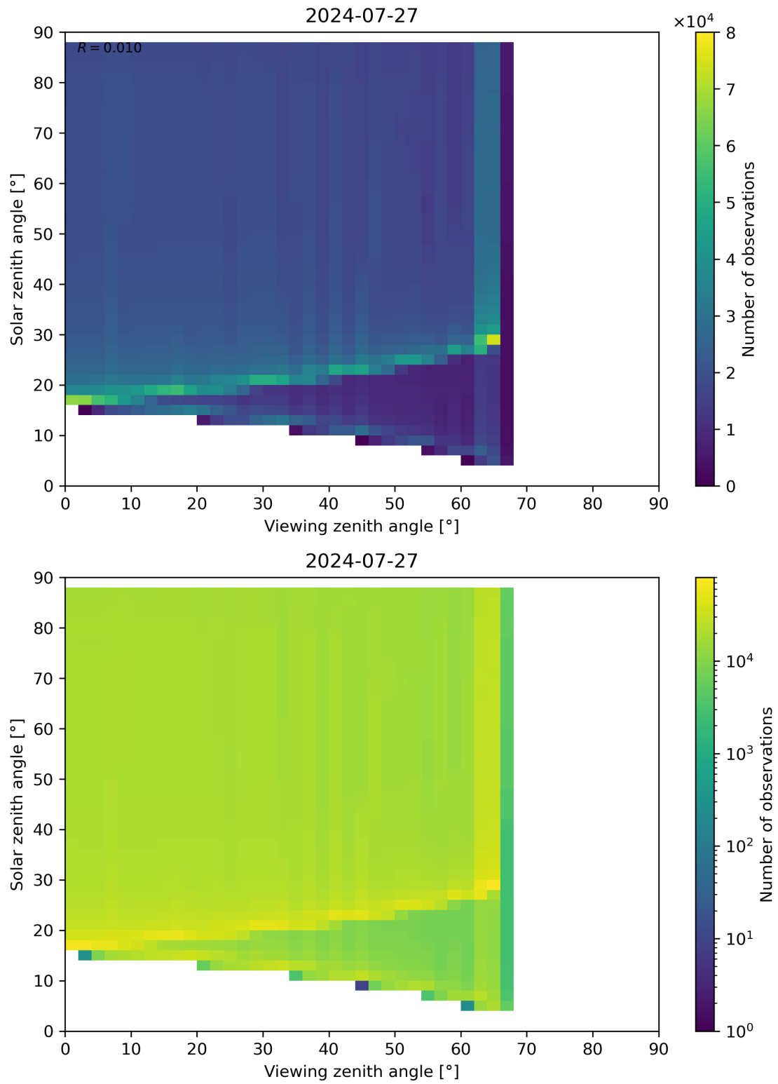
Figure 172: Scatter density plot of “Viewing zenith angle” against “Solar zenith angle” for 2024-07-26 to 2024-07-28.
