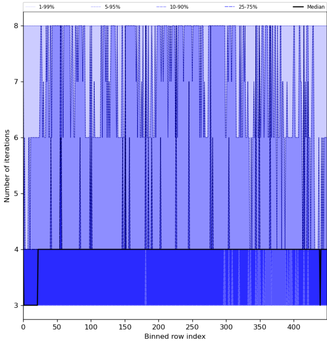
Figure 51: Along track statistics of “Number of iterations” for 2024-07-26 to 2024-07-28
