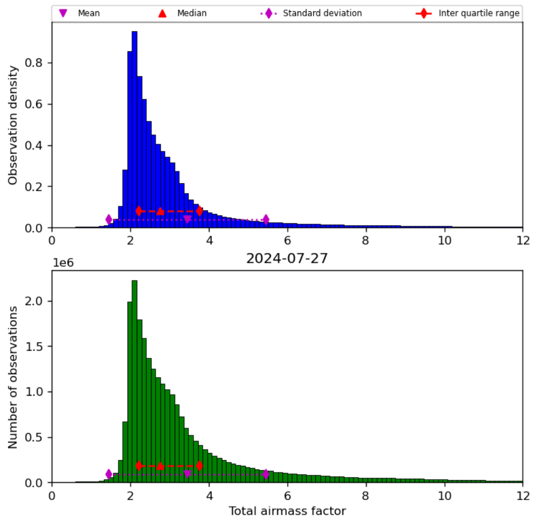
Figure 32: Histogram of “Total airmass factor” for 2024-07-26 to 2024-07-28
