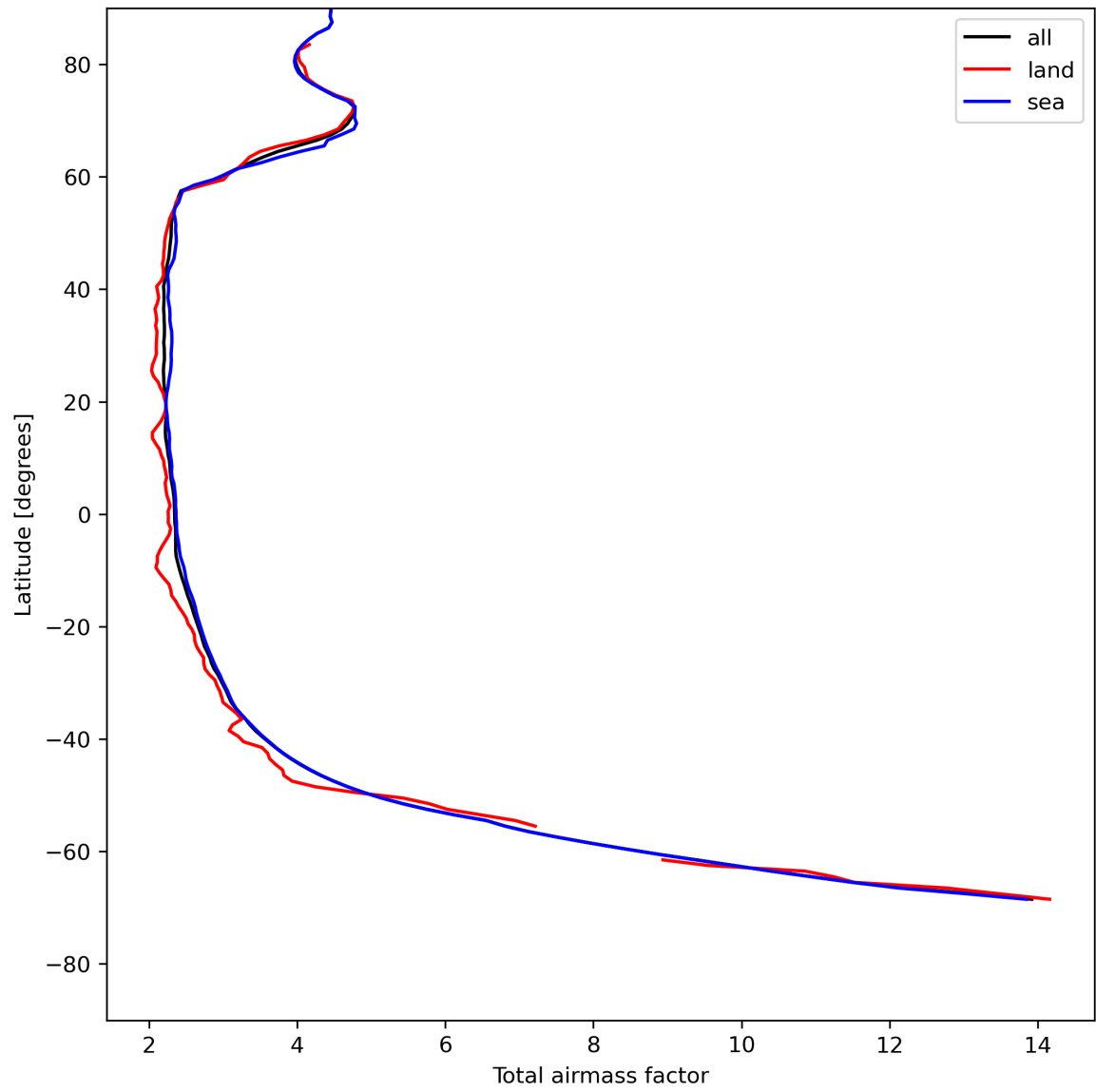
Figure 15: Zonal average of “Total airmass factor” for 2024-07-26 to 2024-07-28.
