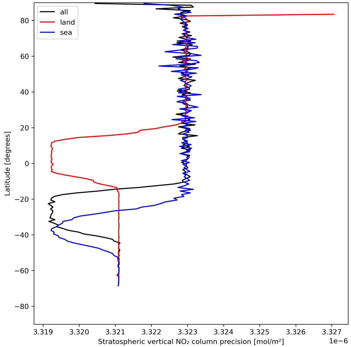
Figure 20: Zonal average of “Stratospheric vertical NO 2 column precision” for 2024-07-26 to 2024-07-28.
