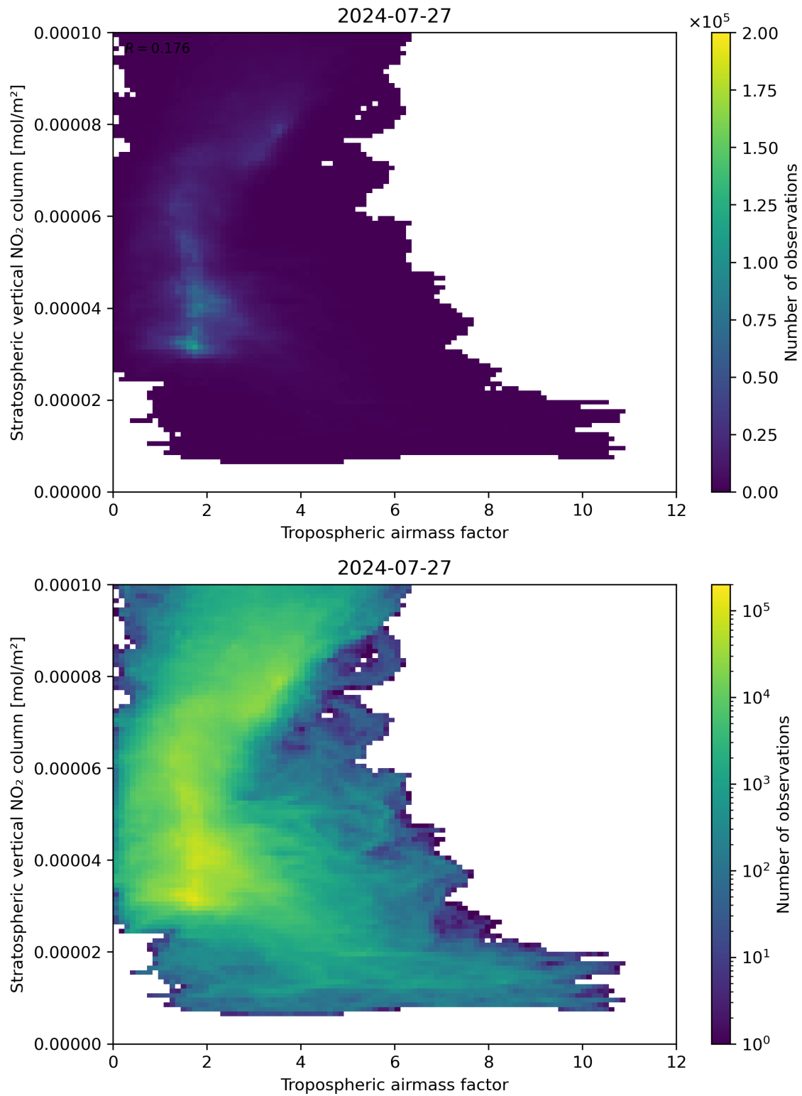
Figure 74: Scatter density plot of “Tropospheric air mass factor” against “Stratospheric vertical NO 2 column” for 2024-07-26 to 2024-07-28.
