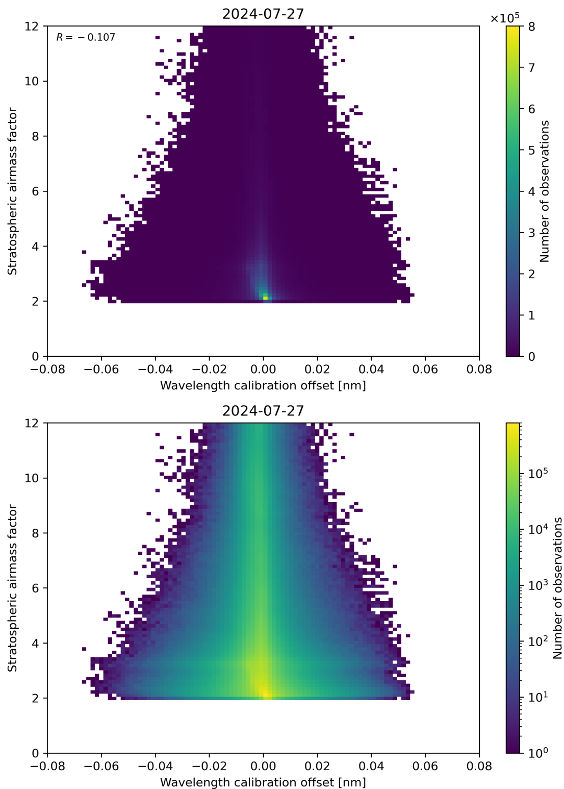
Figure 174: Scatter density plot of “Wavelength calibration offset” against “Stratospheric air mass factor” for 2024-07-26 to 2024-07-28.
