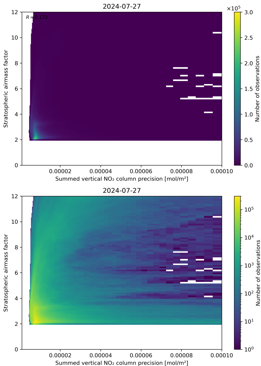
Figure 106: Scatter density plot of “Summed vertical NO 2 column precision” against “Stratospheric airmass factor” for 2024-07-26 to 2024-07-28.
