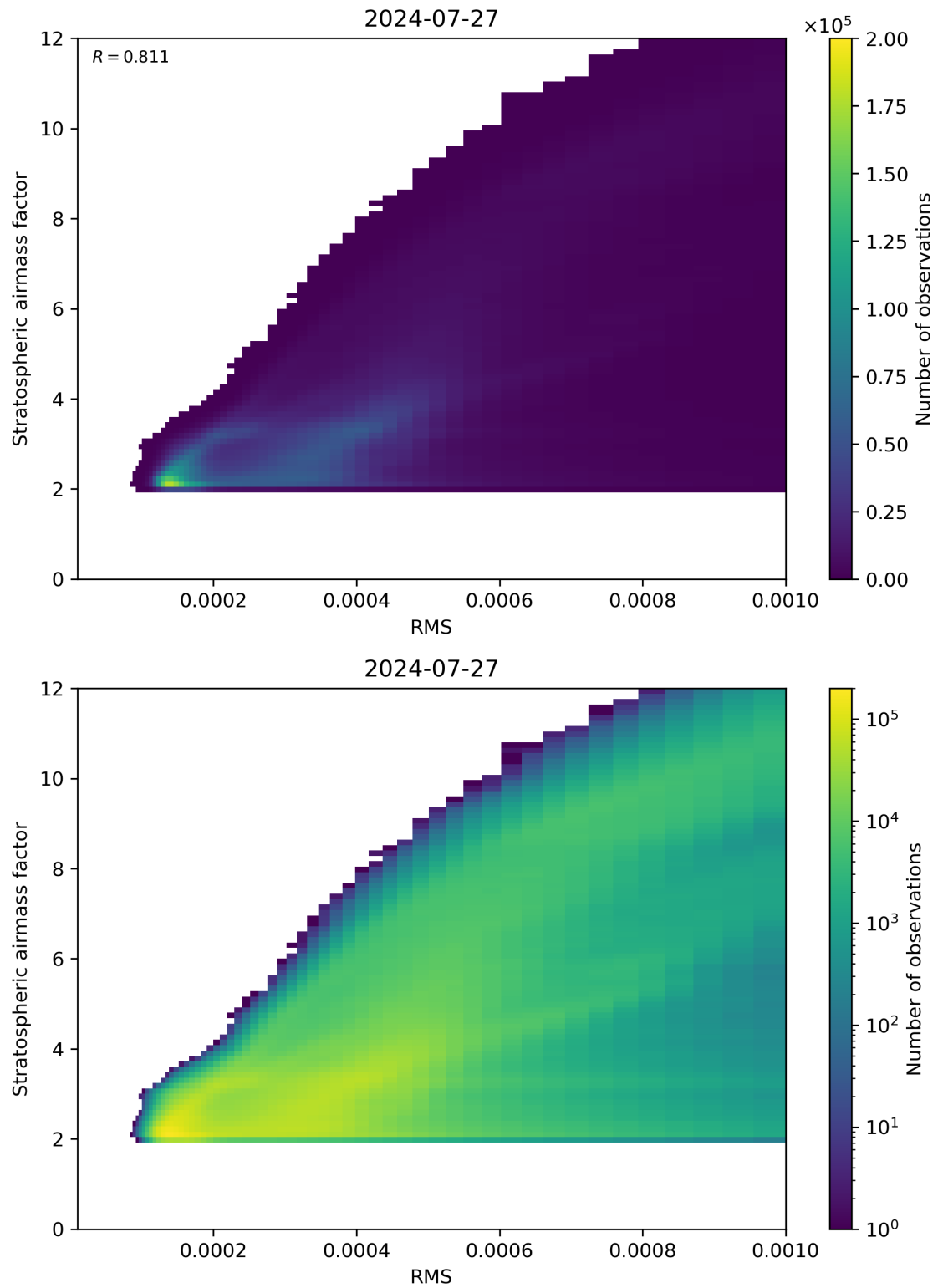
Figure 144: Scatter density plot of “RMS” against “Stratospheric airmass factor” for 2024-07-26 to 2024-07-28.
