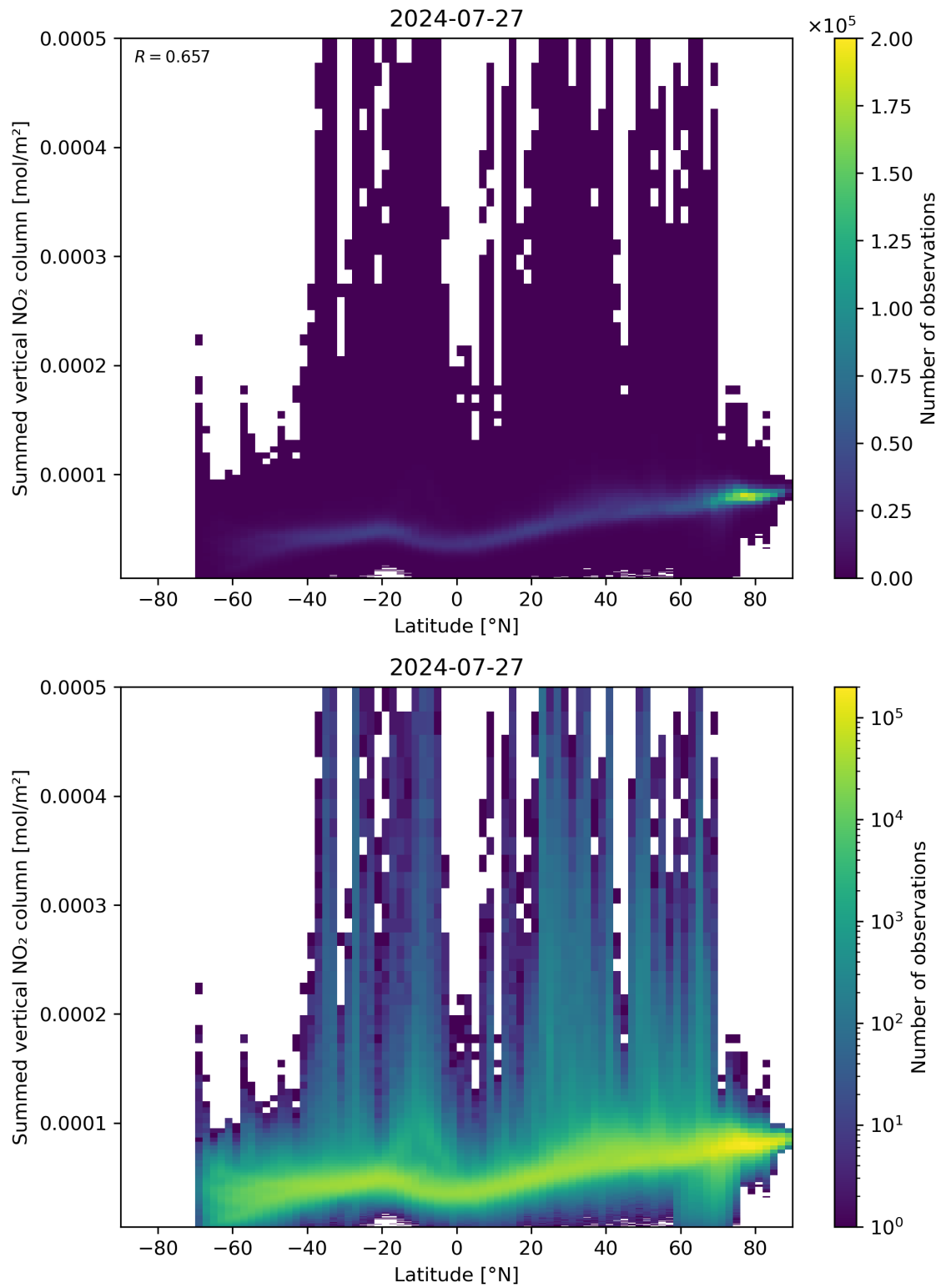
Figure 88: Scatter density plot of “Latitude” against “Summed vertical NO 2 column” for 2024-07-26 to 2024-07-28.
