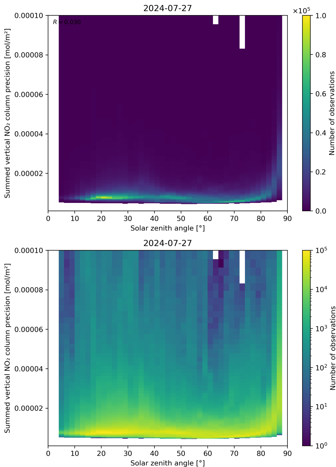
Figure 152: Scatter density plot of “Solar zenith angle” against “Summed vertical NO 2 column precision” for 2024-07-26 to 2024-07-28.
