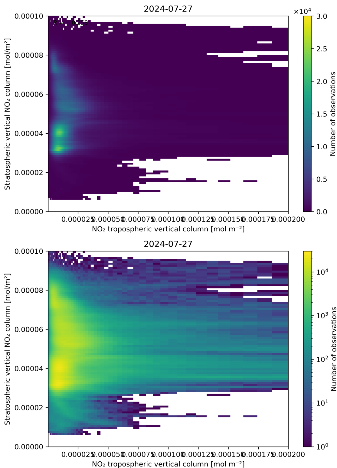
Figure 125: Scatter density plot of “NO 2 tropospheric vertical column” against “Stratospheric vertical NO 2 column” for 2024-07-26 to 2024-07-28.
