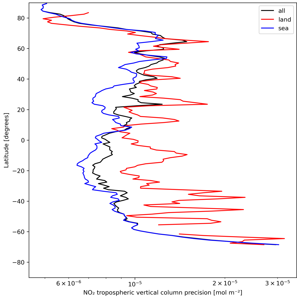
Figure 13: Zonal average of “NO 2 tropospheric vertical column precision” for 2024-07-26 to 2024-07-28.
