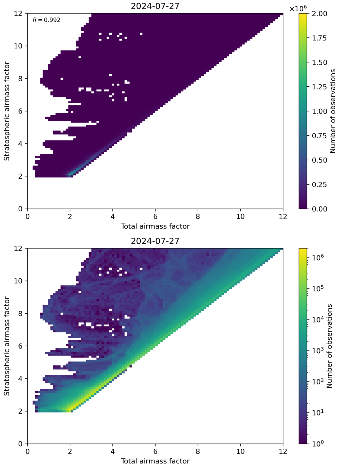
Figure 62: Scatter density plot of “Total airmass factor” against “Stratospheric airmass factor” for 2024-07-26 to 2024-07-28.
