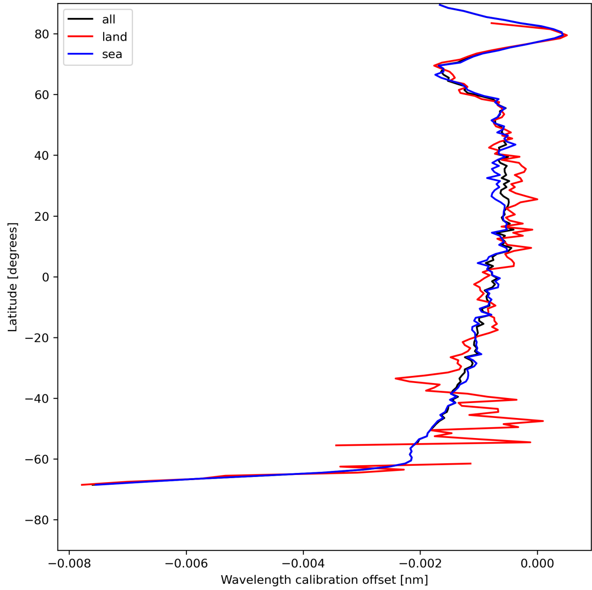
Figure 18: Zonal average of “Wavelength calibration offset” for 2024-07-26 to 2024-07-28.
