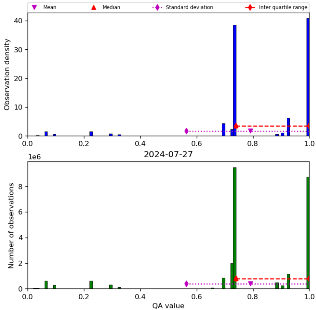
Figure 28: Histogram of “QA value” for 2024-07-26 to 2024-07-28
