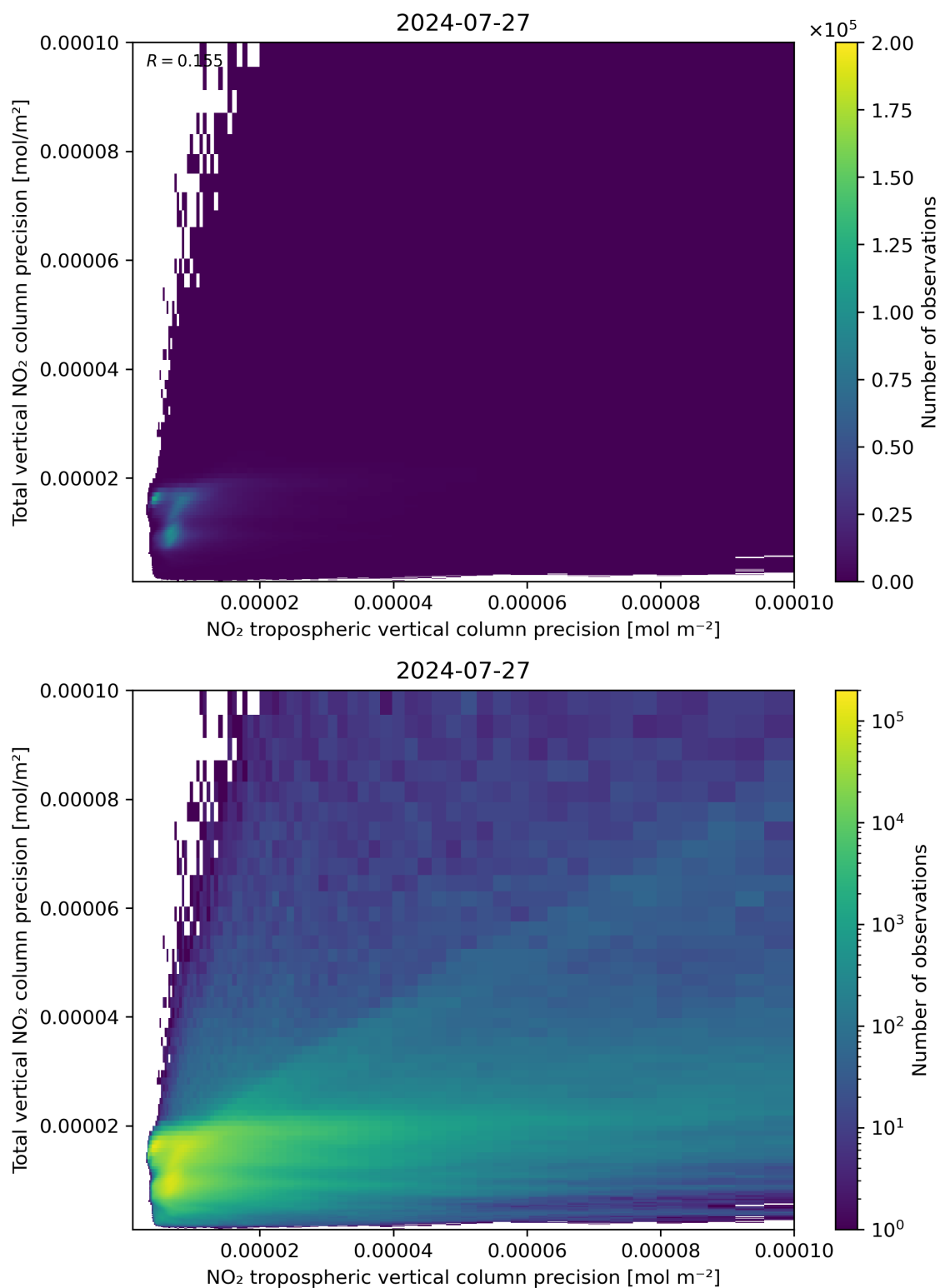
Figure 139: Scatter density plot of “NO 2 tropospheric vertical column precision” against “Total vertical NO 2 column precision” for 2024-07-26 to 2024-07-28.
