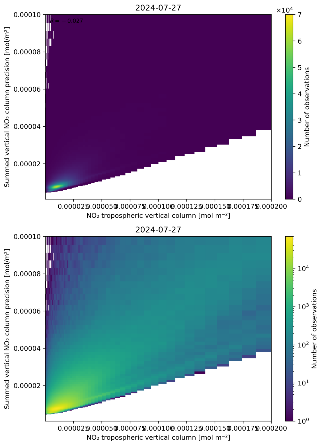
Figure 127: Scatter density plot of “NO 2 tropospheric vertical column” against “Summed vertical NO 2 column precision” for 2024-07-26 to 2024-07-28.
