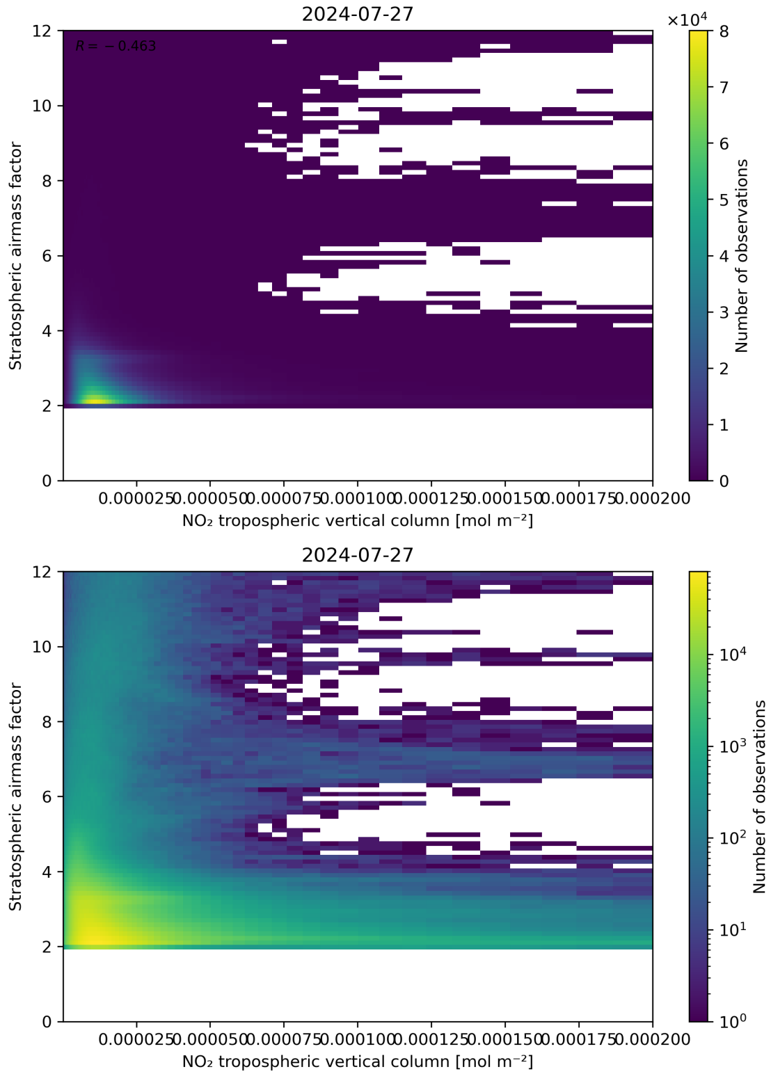
Figure 121: Scatter density plot of “NO 2 tropospheric vertical column” against “Stratospheric air mass factor” for 2024-07-26 to 2024-07-28.
