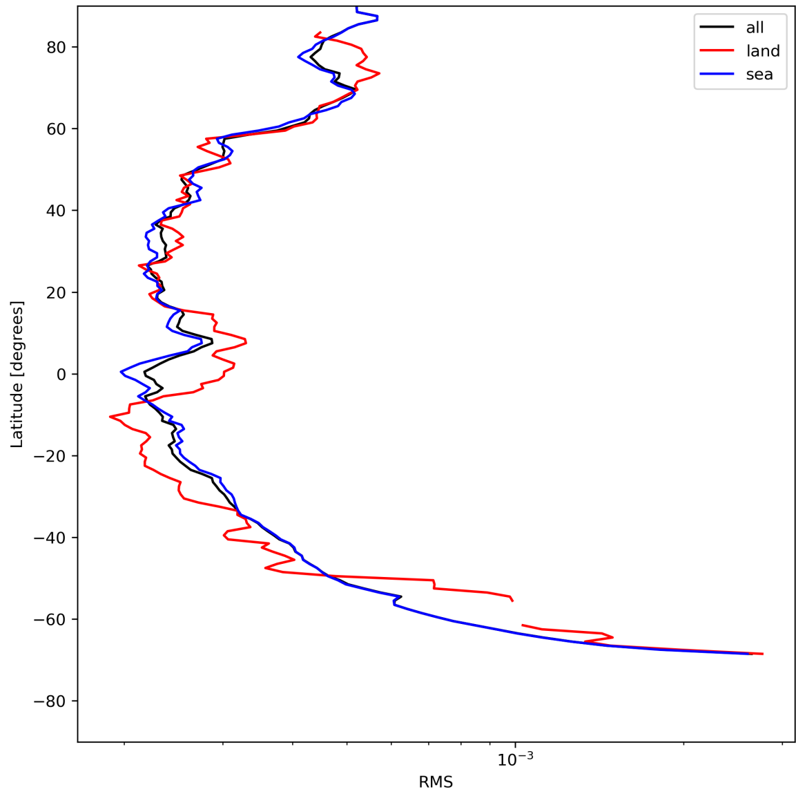
Figure 26: Zonal average of “RMS” for 2024-07-26 to 2024-07-28.
