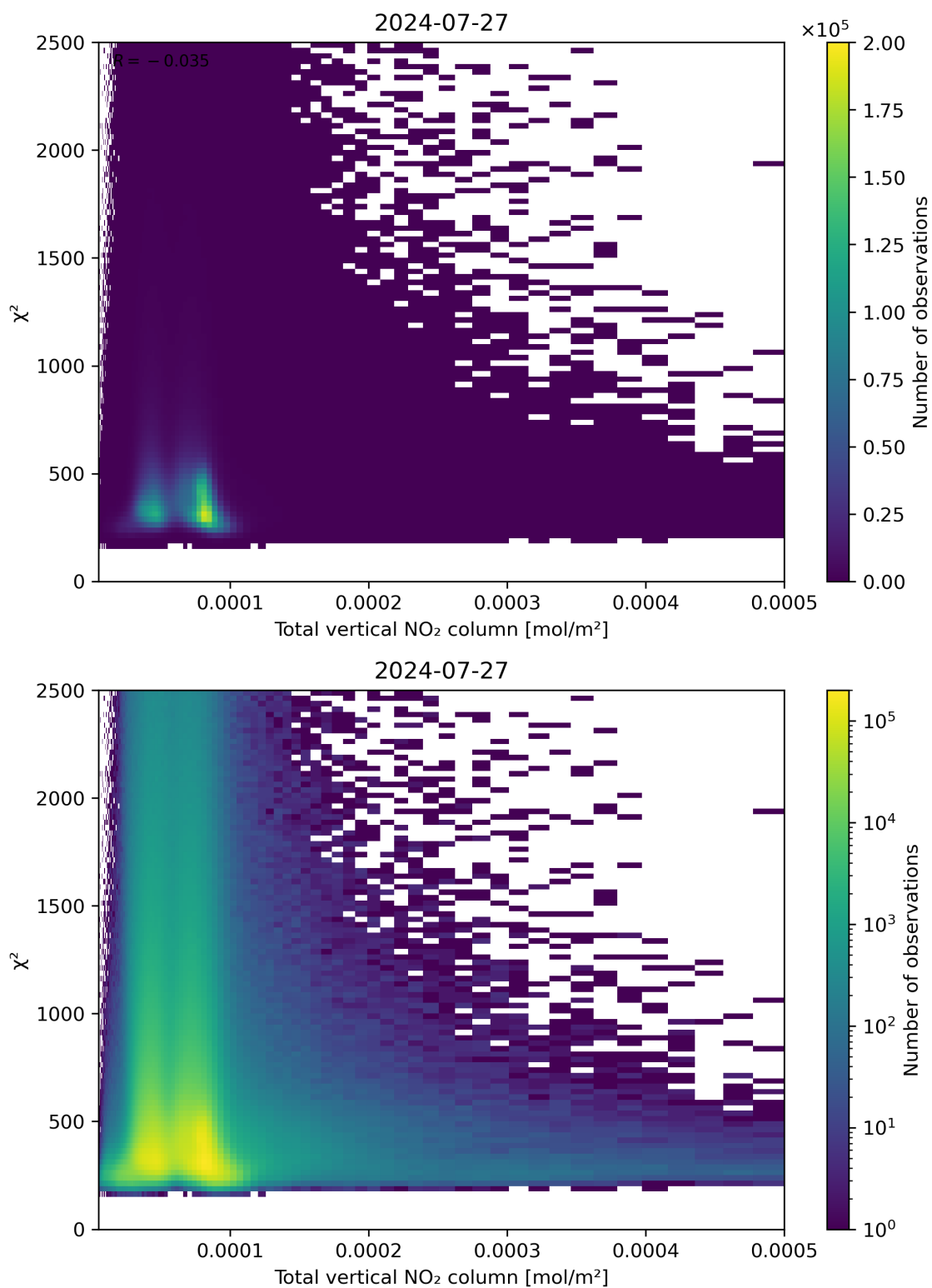
Figure 111: Scatter density plot of “Total vertical NO 2 column” against “ \chi^2 ” for 2024-07-26 to 2024-07-28.
