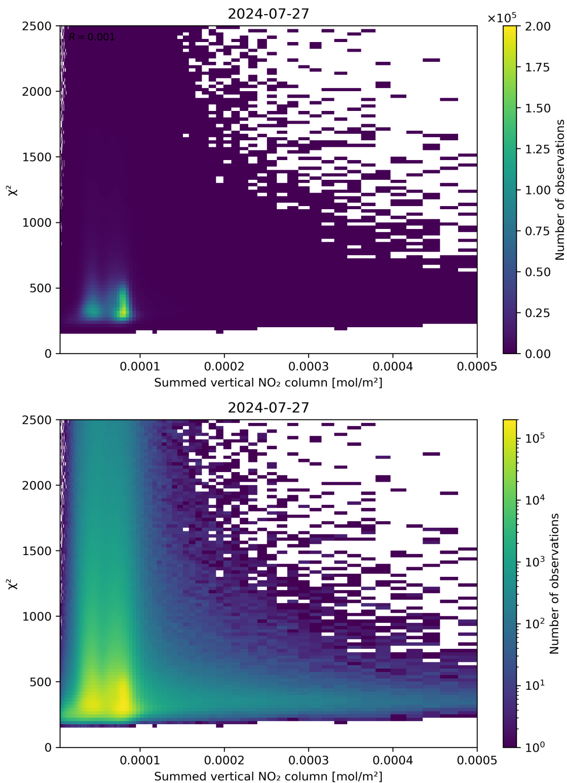
Figure 104: Scatter density plot of “Summed vertical NO 2 column” against “ \chi^2 ” for 2024-07-26 to 2024-07-28.
