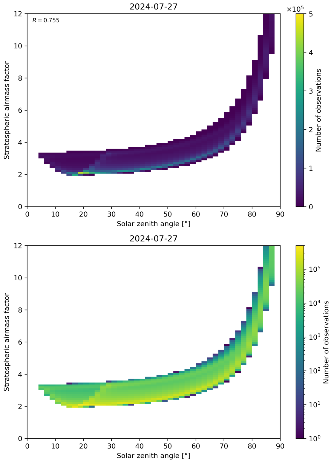
Figure 145: Scatter density plot of “Solar zenith angle” against “Stratospheric airmass factor” for 2024-07-26 to 2024-07-28.
