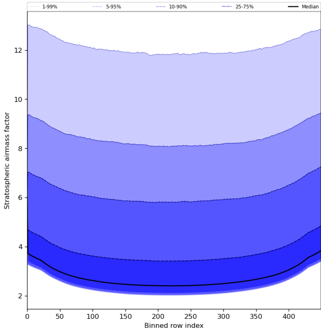
Figure 61: Along track statistics of “Stratospheric air mass factor” for 2024-07-26 to 2024-07-28
