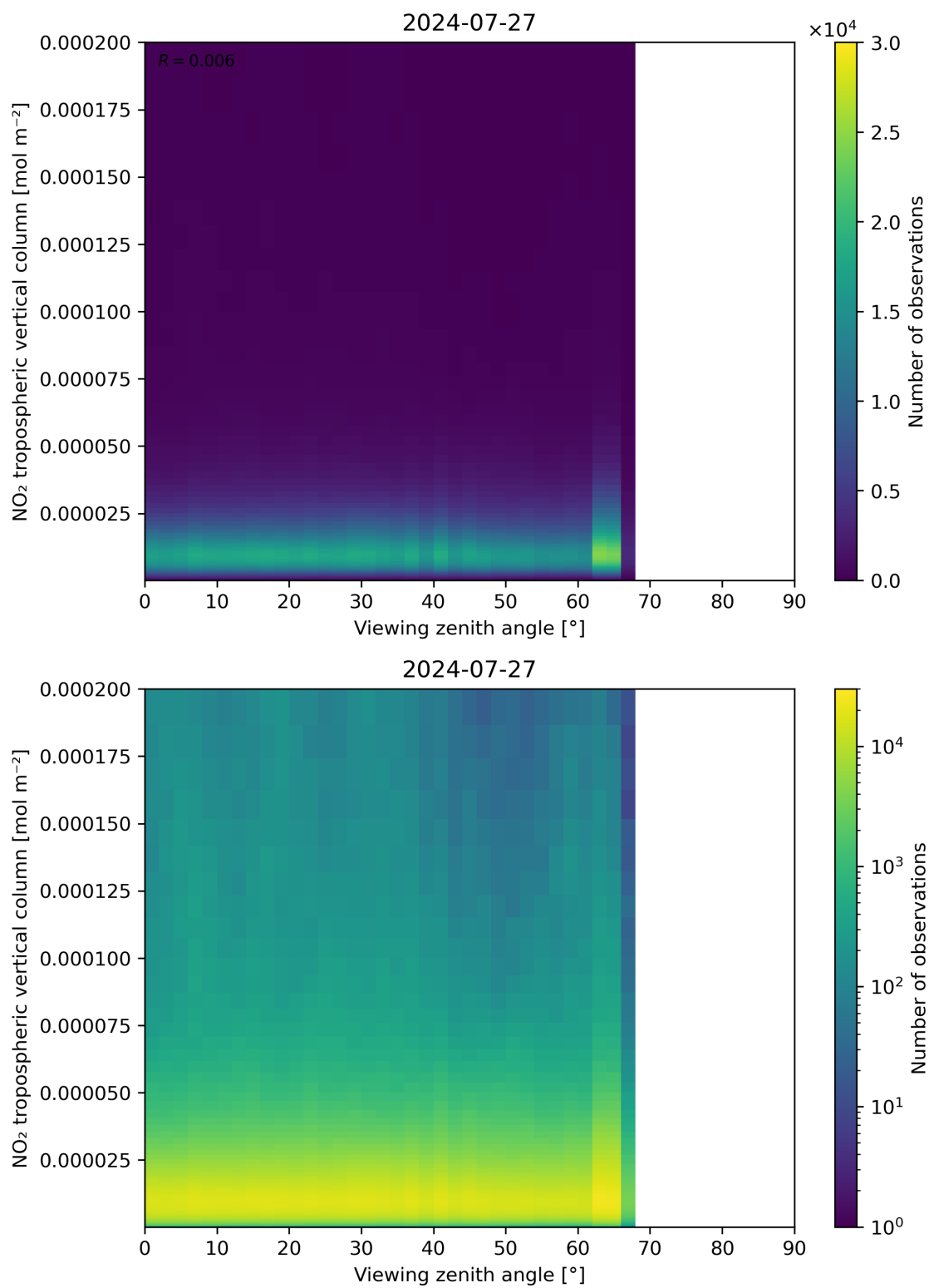
Figure 169: Scatter density plot of “Viewing zenith angle” against “NO 2 tropospheric vertical column” for 2024-07-26 to 2024-07-28.
