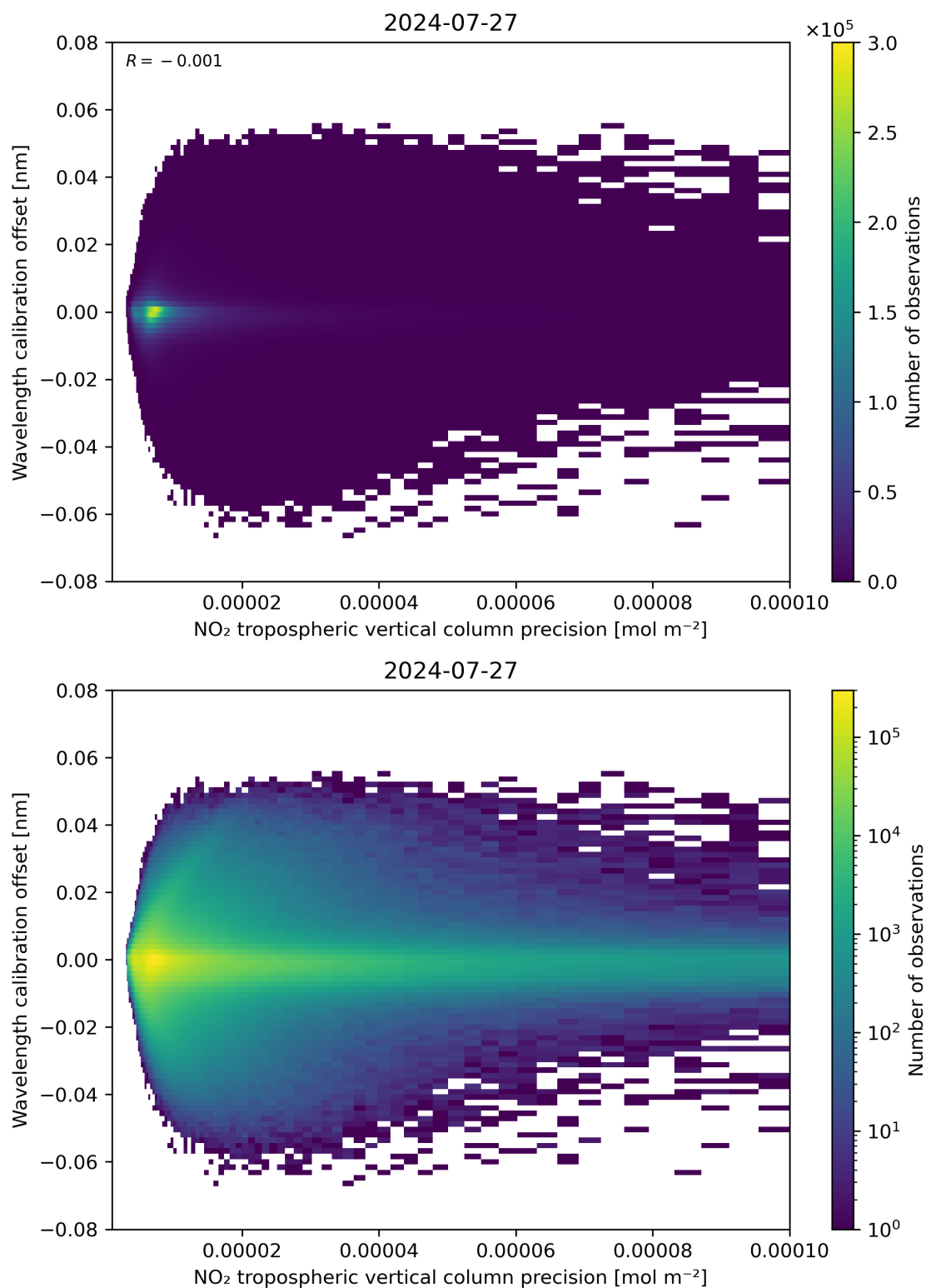
Figure 141: Scatter density plot of “NO 2 tropospheric vertical column precision” against “Wavelength calibration offset” for 2024-07-26 to 2024-07-28.
