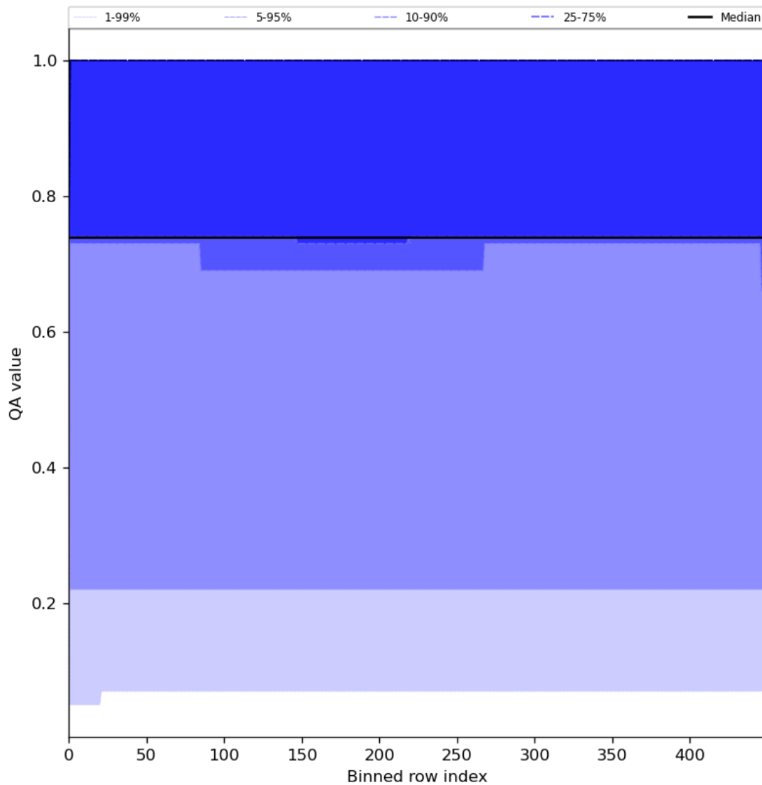
Figure 45: Along track statistics of “QA value” for 2024-07-26 to 2024-07-28
