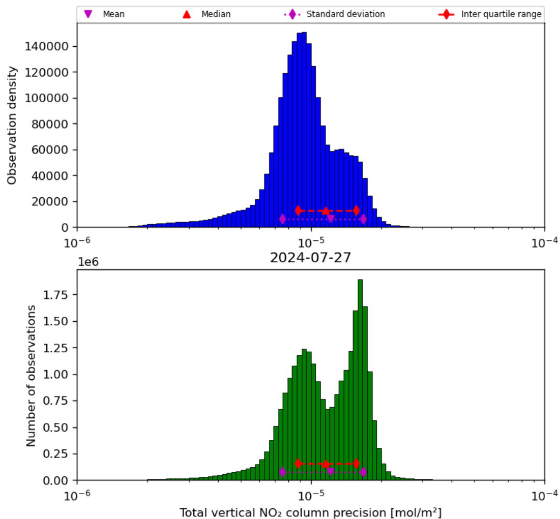
Figure 39: Histogram of “Total vertical NO 2 column precision” for 2024-07-26 to 2024-07-28
