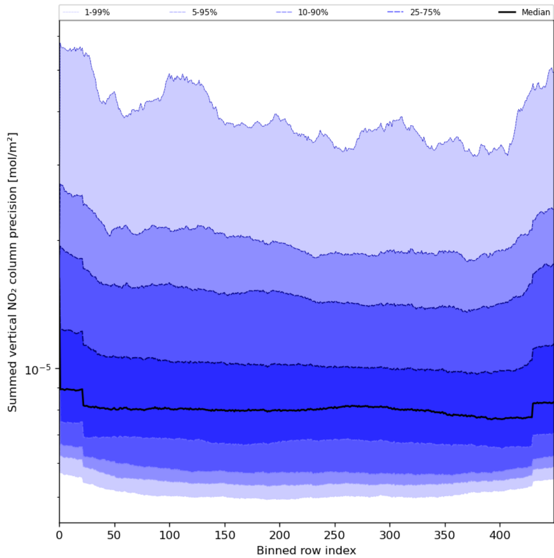
Figure 58: Along track statistics of “Summed vertical NO 2 column precision” for 2024-07-26 to 2024-07-28
