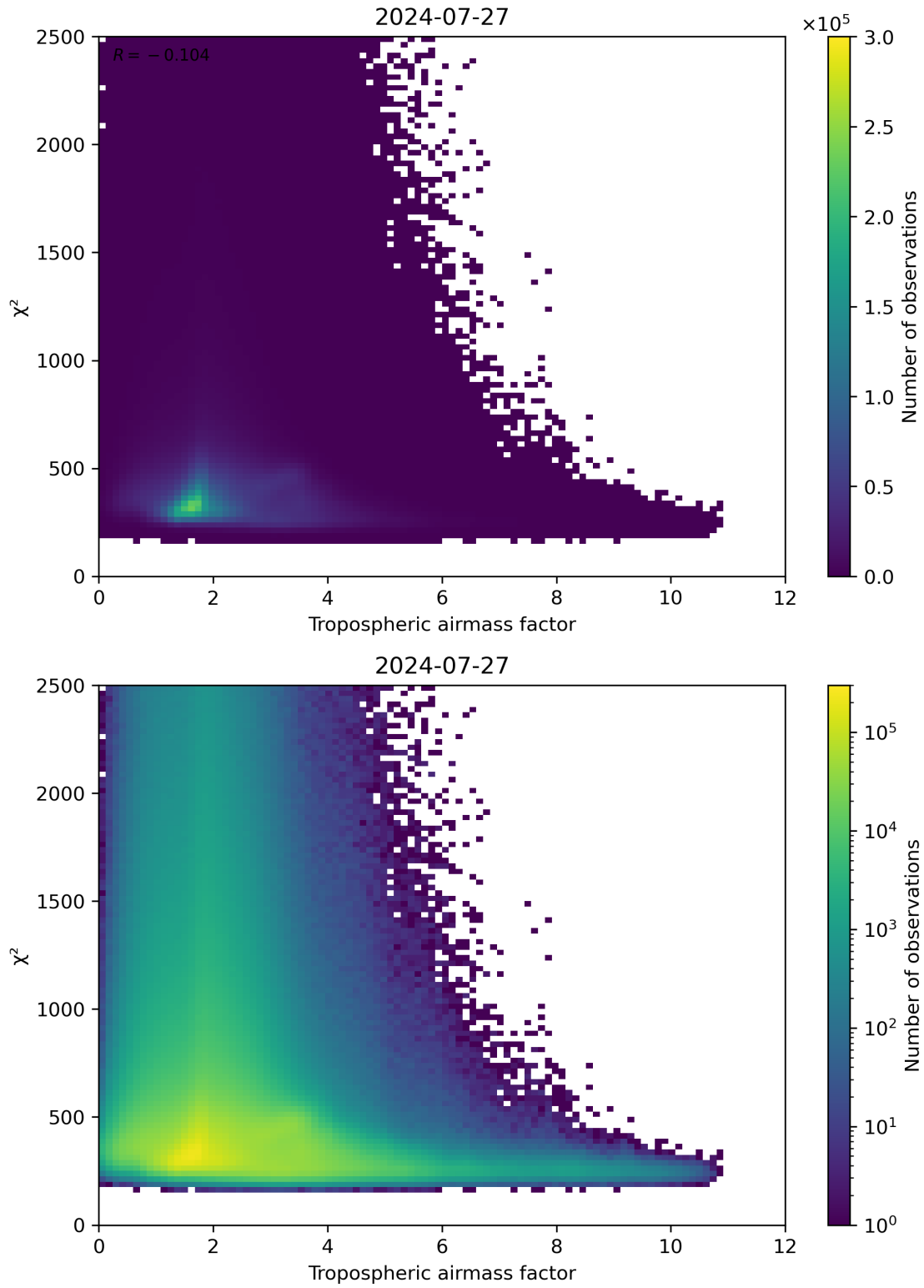
Figure 73: Scatter density plot of “Tropospheric airmass factor” against “ \chi^2 ” for 2024-07-26 to 2024-07-28.
