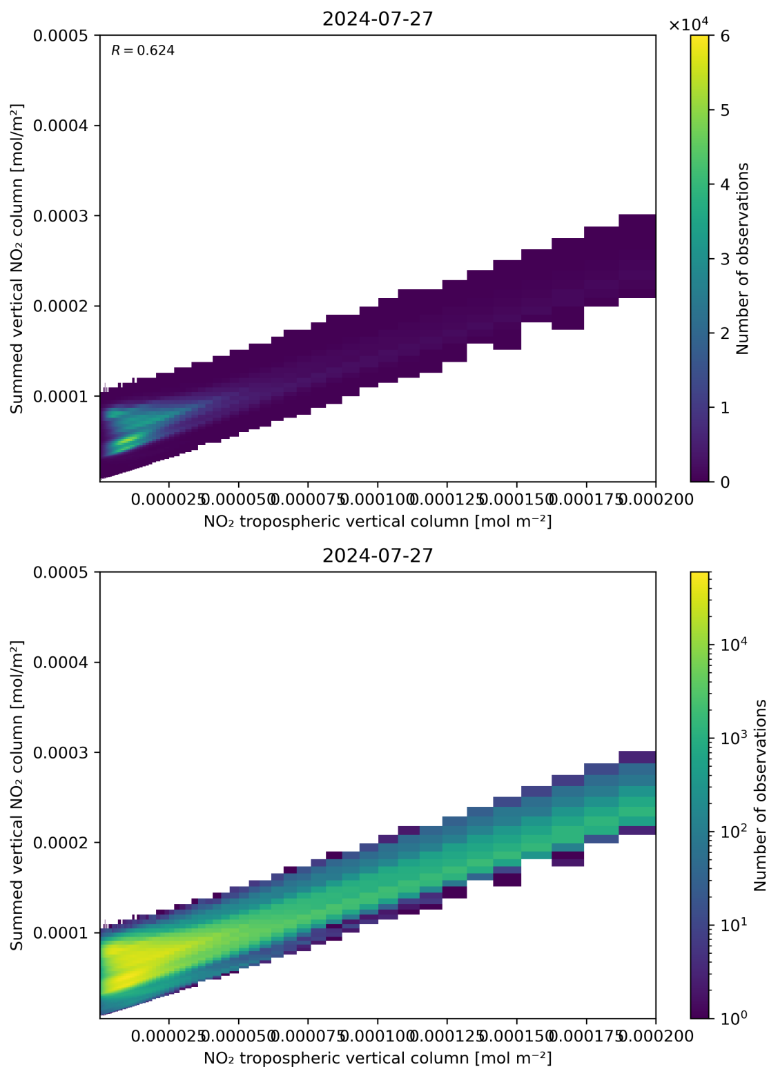
Figure 126: Scatter density plot of “NO 2 tropospheric vertical column” against “Summed vertical NO 2 column” for 2024-07-26 to 2024-07-28.
