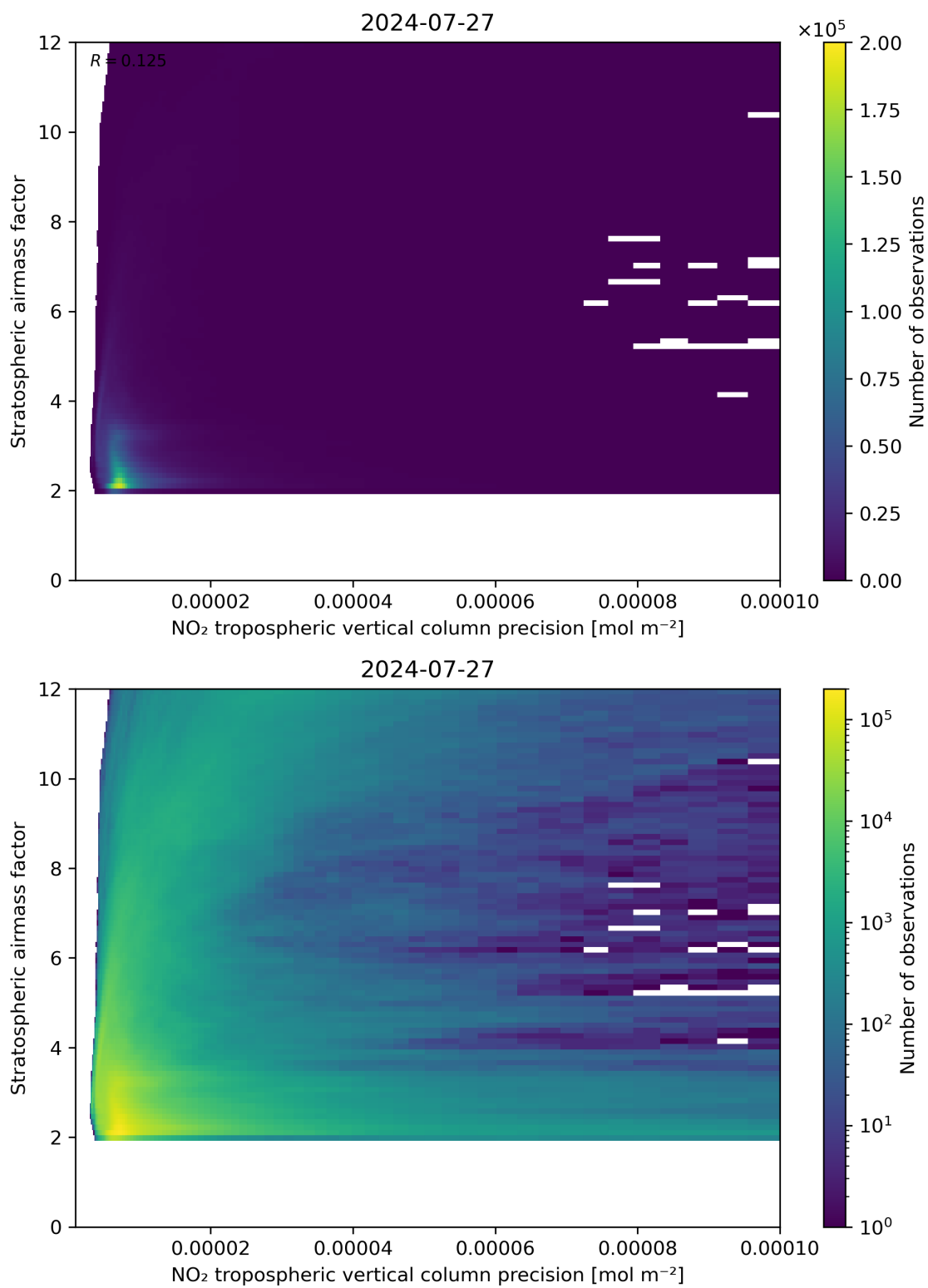
Figure 131: Scatter density plot of “NO 2 tropospheric vertical column precision” against “Stratospheric airmass factor” for 2024-07-26 to 2024-07-28.
