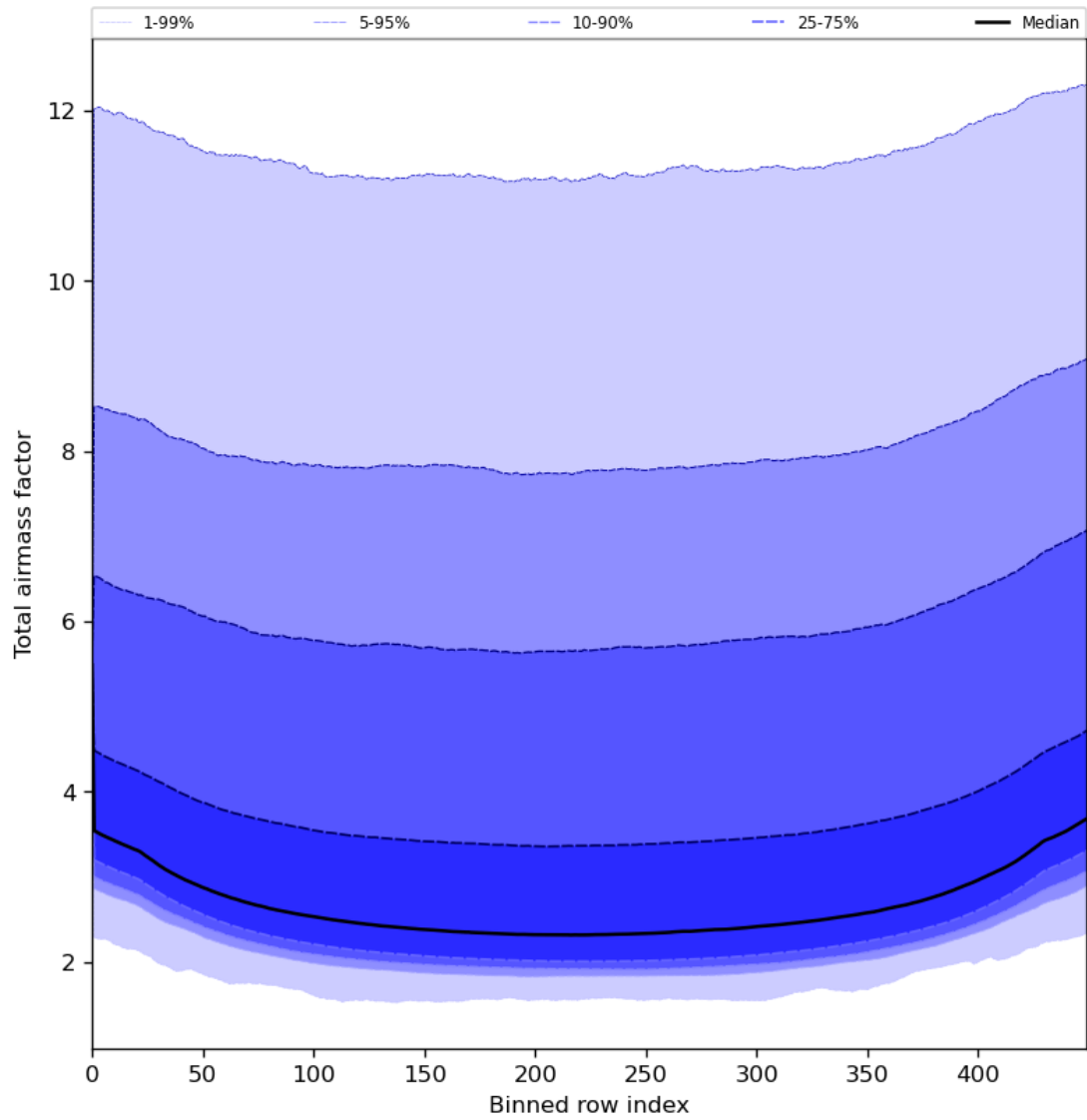
Figure 49: Along track statistics of “Total airmass factor” for 2024-07-26 to 2024-07-28
