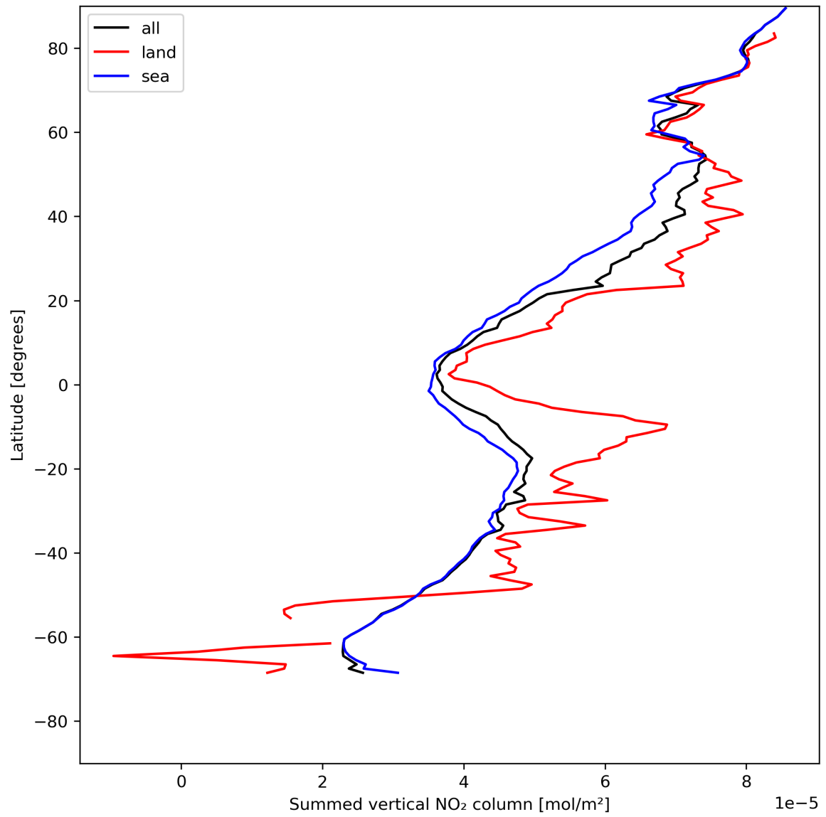
Figure 23: Zonal average of “Summed vertical NO 2 column” for 2024-07-26 to 2024-07-28.
