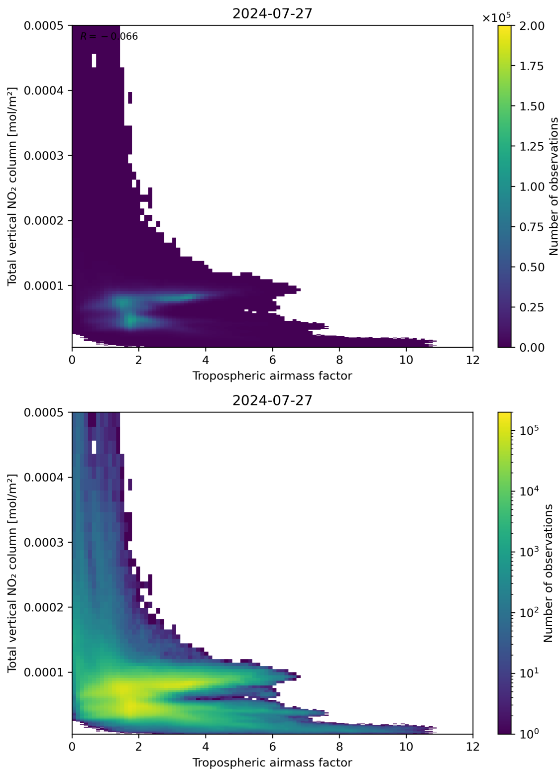
Figure 77: Scatter density plot of “Tropospheric airmass factor” against “Total vertical NO 2 column” for 2024-07-26 to 2024-07-28.
