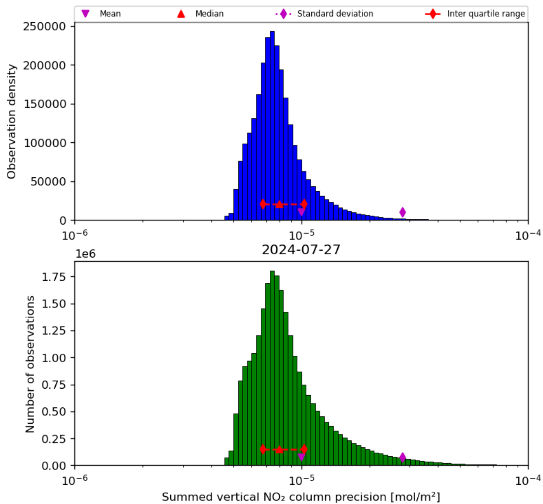
Figure 41: Histogram of “Summed vertical NO 2 column precision” for 2024-07-26 to 2024-07-28
