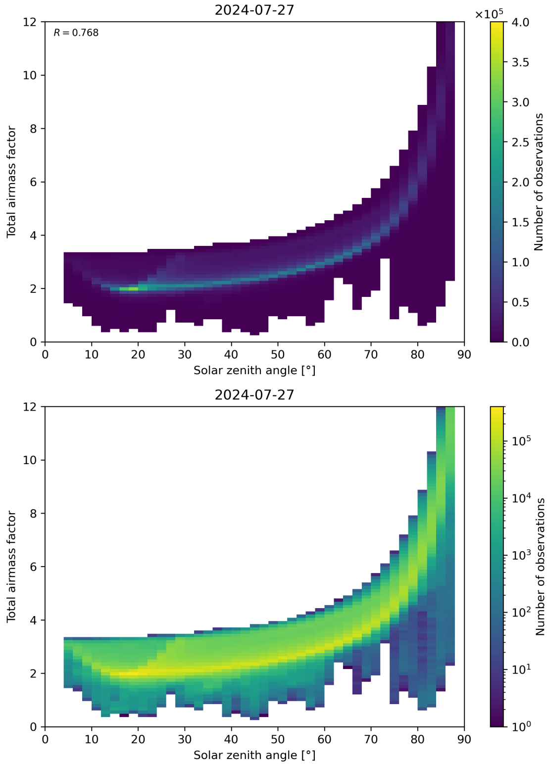
Figure 146: Scatter density plot of “Solar zenith angle” against “Total air mass factor” for 2024-07-26 to 2024-07-28.
