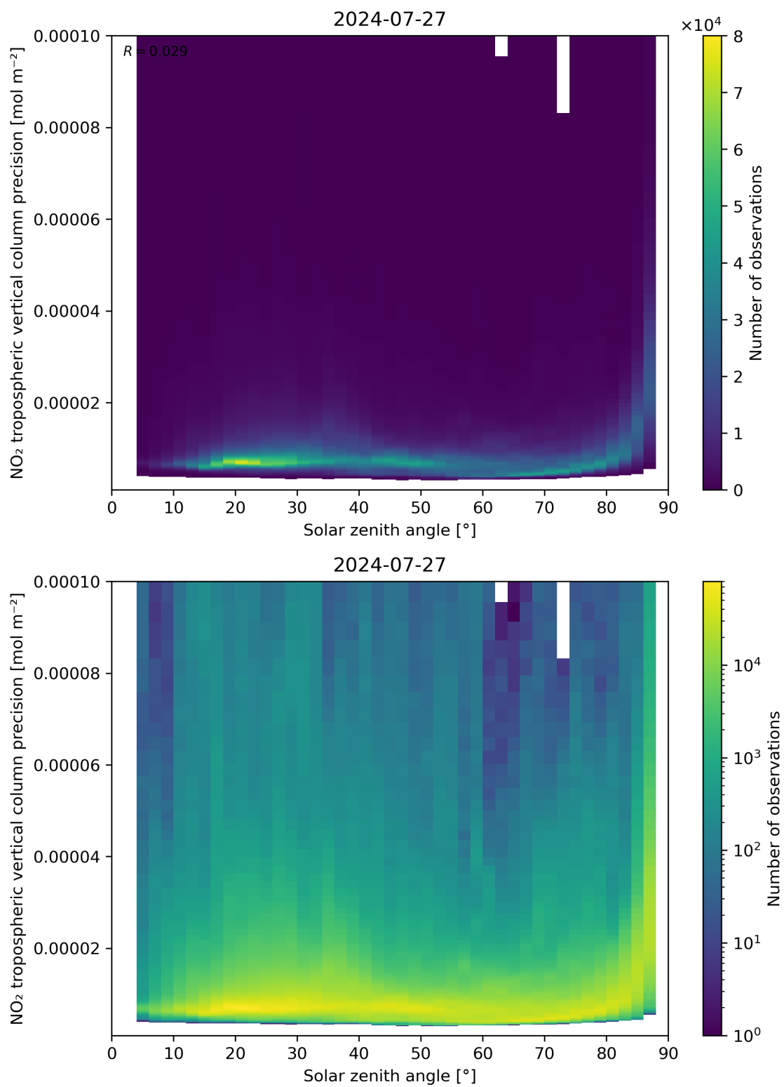
Figure 156: Scatter density plot of “Solar zenith angle” against “NO 2 tropospheric vertical column precision” for 2024-07-26 to 2024-07-28.
