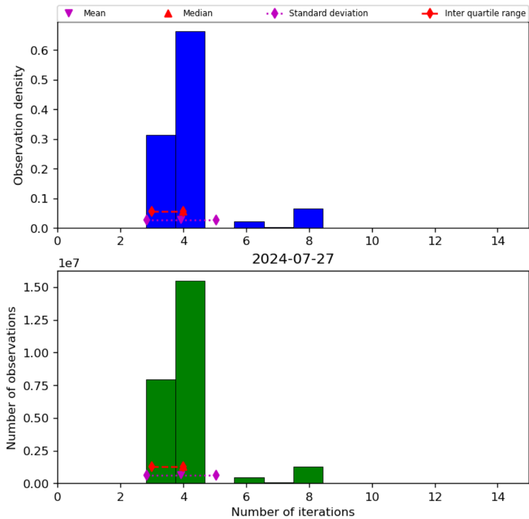
Figure 34: Histogram of “Number of iterations” for 2024-07-26 to 2024-07-28
