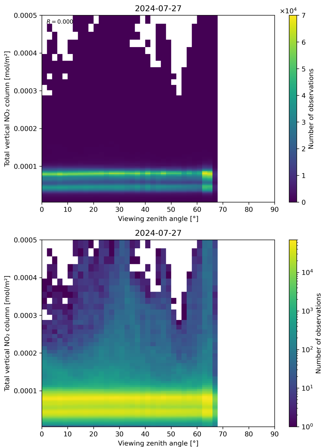
Figure 167: Scatter density plot of “Viewing zenith angle” against “Total vertical NO 2 column” for 2024-07-26 to 2024-07-28.
