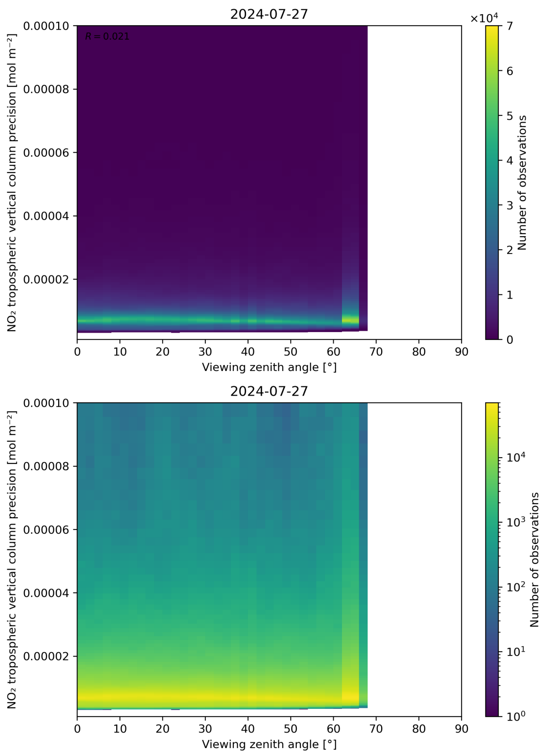
Figure 170: Scatter density plot of “Viewing zenith angle” against “NO 2 tropospheric vertical column precision” for 2024-07-26 to 2024-07-28.
