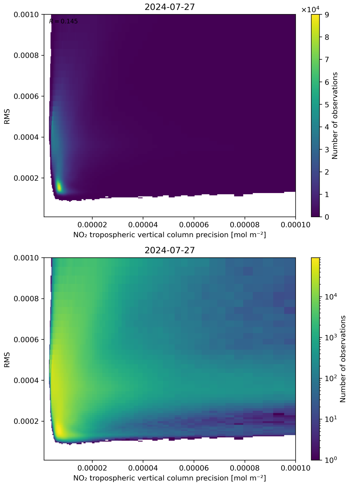
Figure 140: Scatter density plot of “NO 2 tropospheric vertical column precision” against “RMS” for 2024-07-26 to 2024-07-28.
