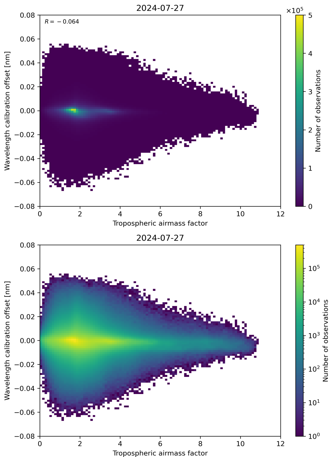
Figure 80: Scatter density plot of “Tropospheric airmass factor” against “Wavelength calibration offset” for 2024-07-26 to 2024-07-28.
