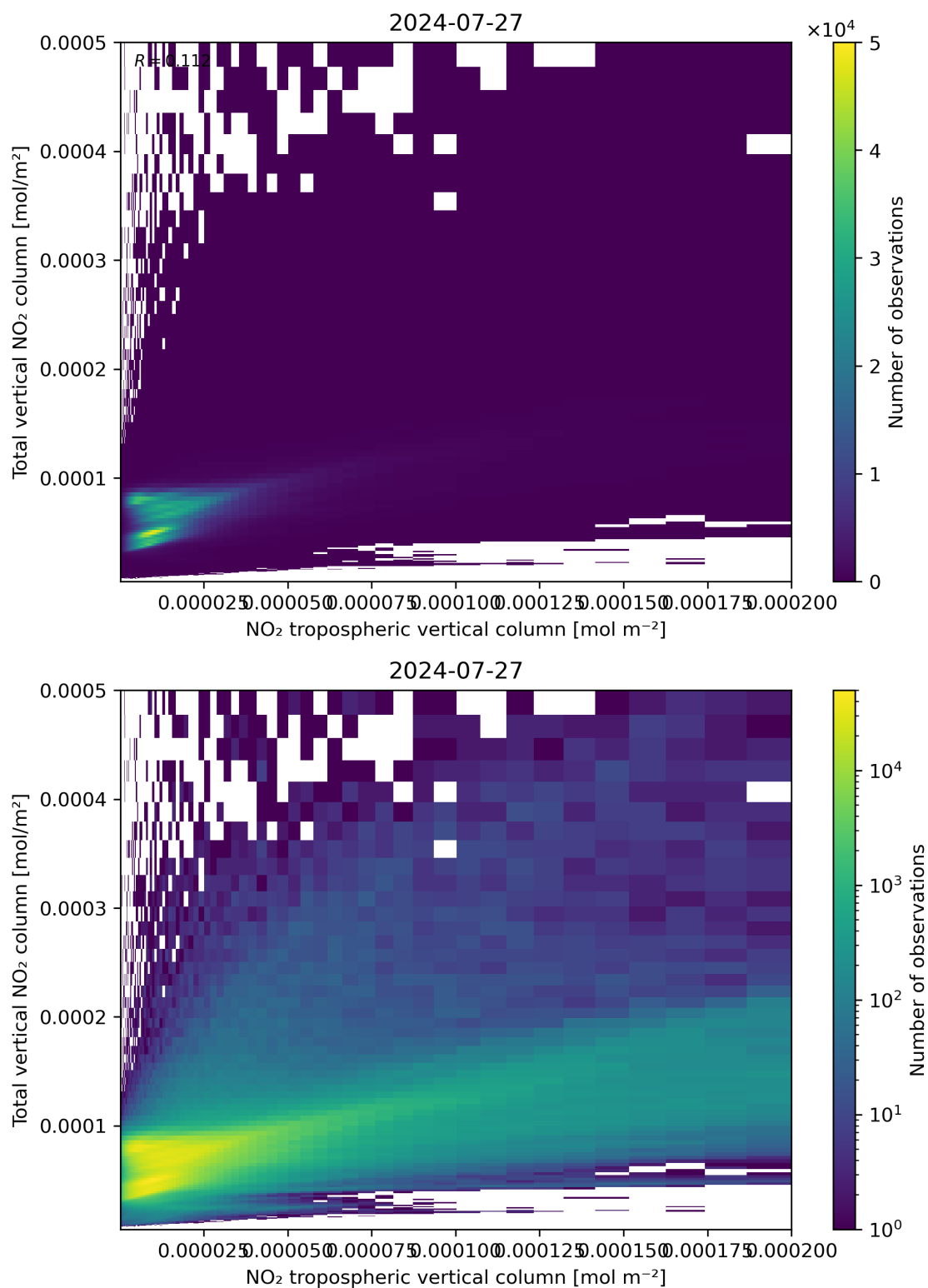
Figure 128: Scatter density plot of “NO 2 tropospheric vertical column” against “Total vertical NO 2 column” for 2024-07-26 to 2024-07-28.
