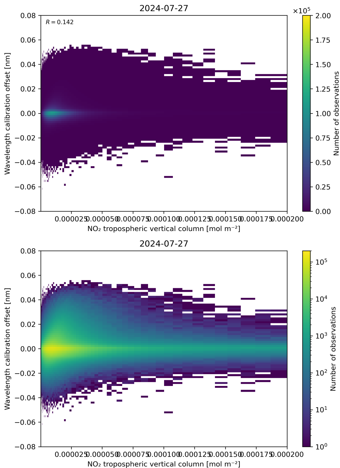
Figure 143: Scatter density plot of “NO 2 tropospheric vertical column” against “Wavelength calibration offset” for 2024-07-26 to 2024-07-28.
