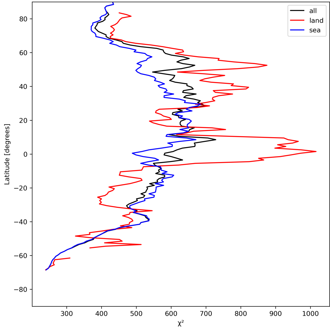
Figure 25: Zonal average of “ \chi^2 ” for 2024-07-26 to 2024-07-28.
