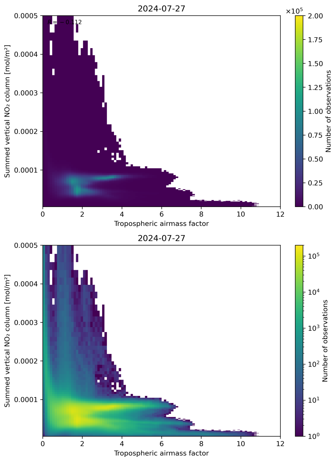
Figure 75: Scatter density plot of “Tropospheric airmass factor” against “Summed vertical NO 2 column” for 2024-07-26 to 2024-07-28.
