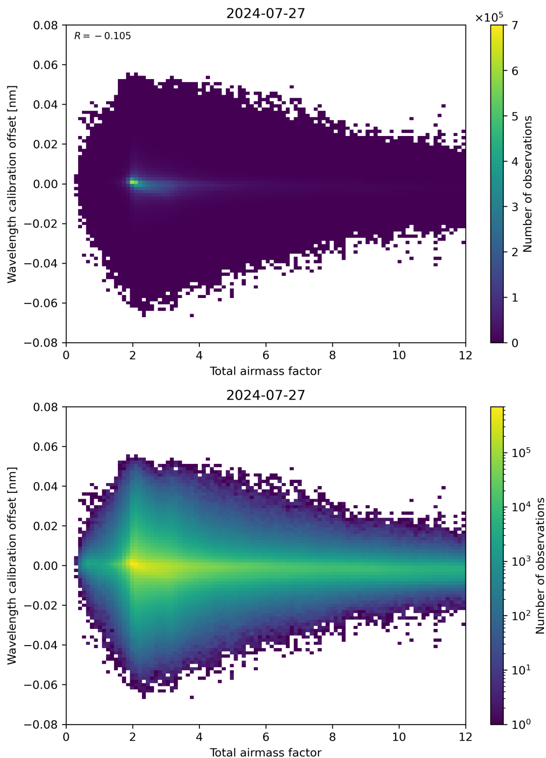
Figure 70: Scatter density plot of “Total airmass factor” against “Wavelength calibration offset” for 2024-07-26 to 2024-07-28.
