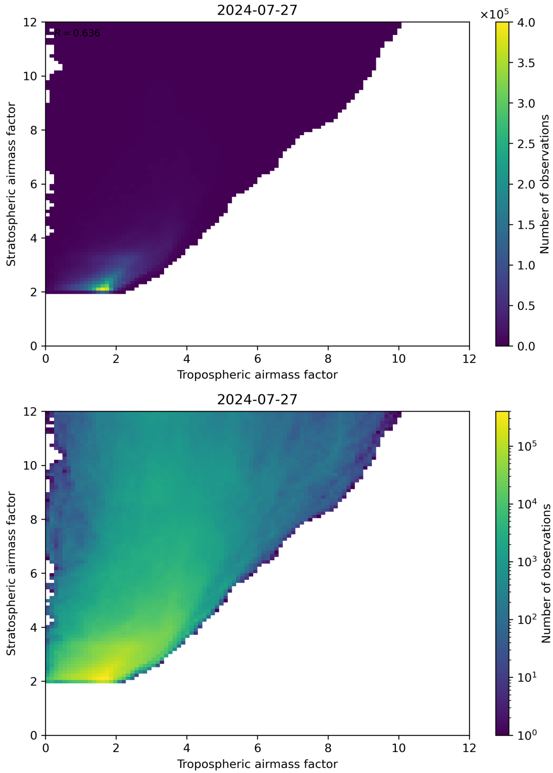
Figure 71: Scatter density plot of “Tropospheric airmass factor” against “Stratospheric airmass factor” for 2024-07-26 to 2024-07-28.
