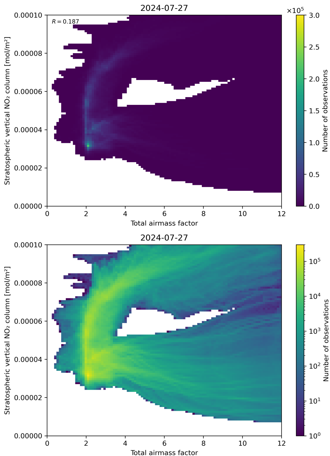
Figure 64: Scatter density plot of “Total airmass factor” against “Stratospheric vertical \text{NO}_2 column” for 2024-07-26 to 2024-07-28.
