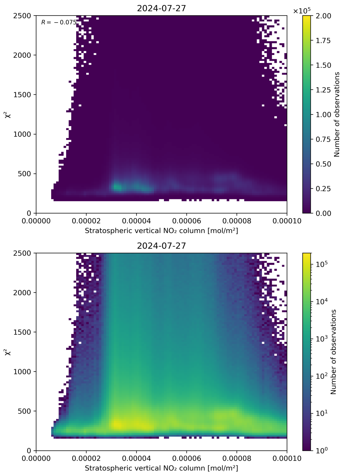
Figure 97: Scatter density plot of “Stratospheric vertical NO 2 column” against “ \chi^2 ” for 2024-07-26 to 2024-07-28.
