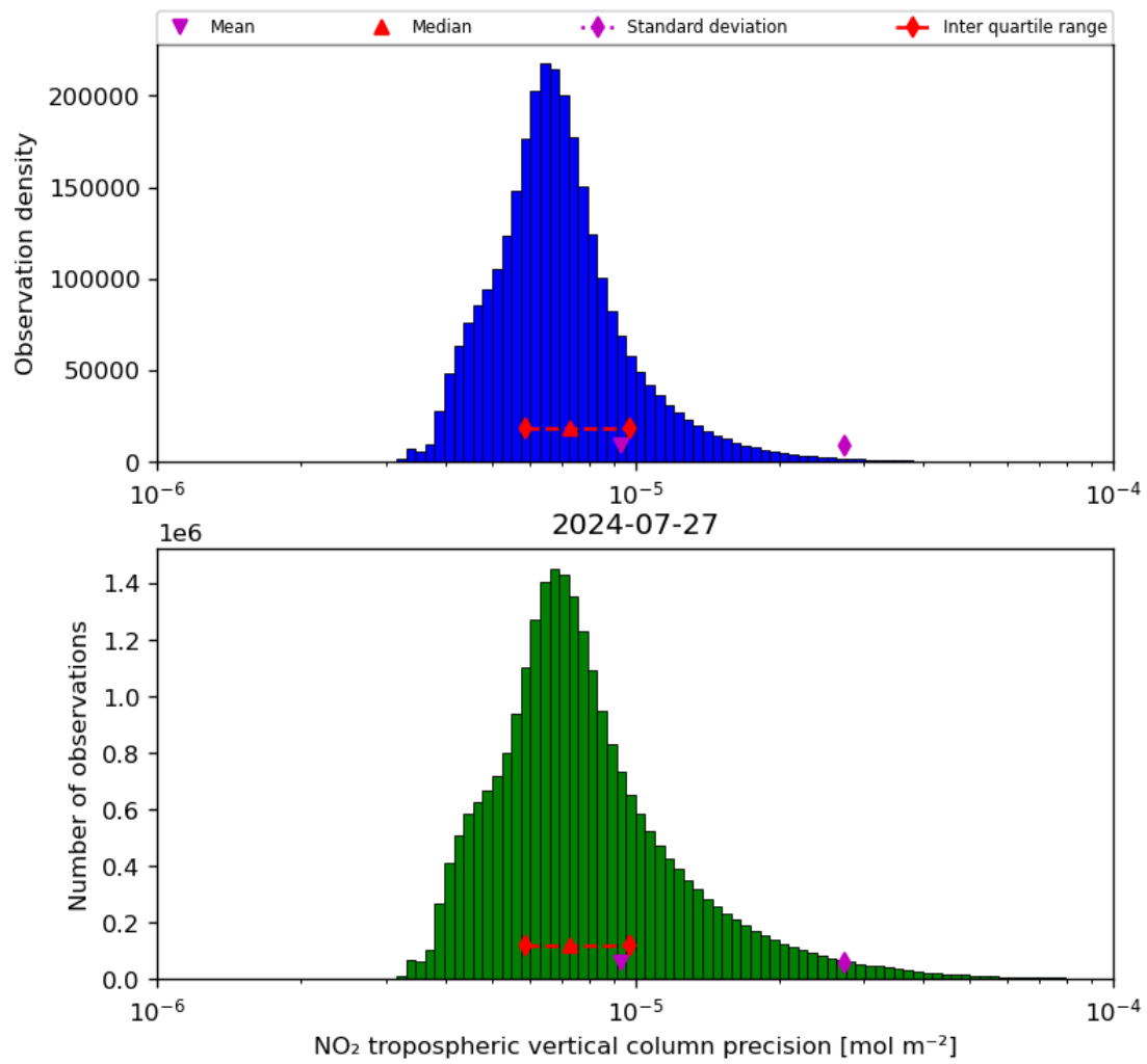
Figure 30: Histogram of “NO 2 tropospheric vertical column precision” for 2024-07-26 to 2024-07-28
