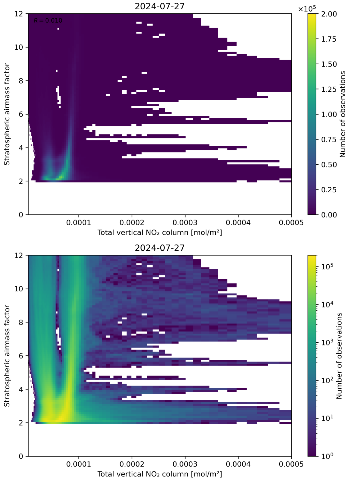
Figure 110: Scatter density plot of “Total vertical NO 2 column” against “Stratospheric airmass factor” for 2024-07-26 to 2024-07-28.
