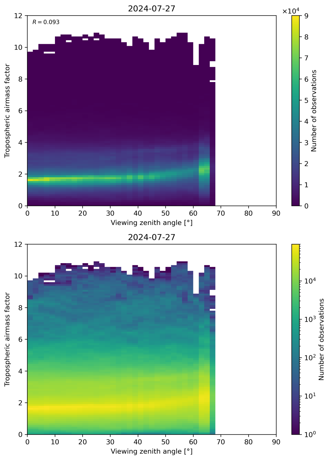
Figure 161: Scatter density plot of “Viewing zenith angle” against “Tropospheric airmass factor” for 2024-07-26 to 2024-07-28.
