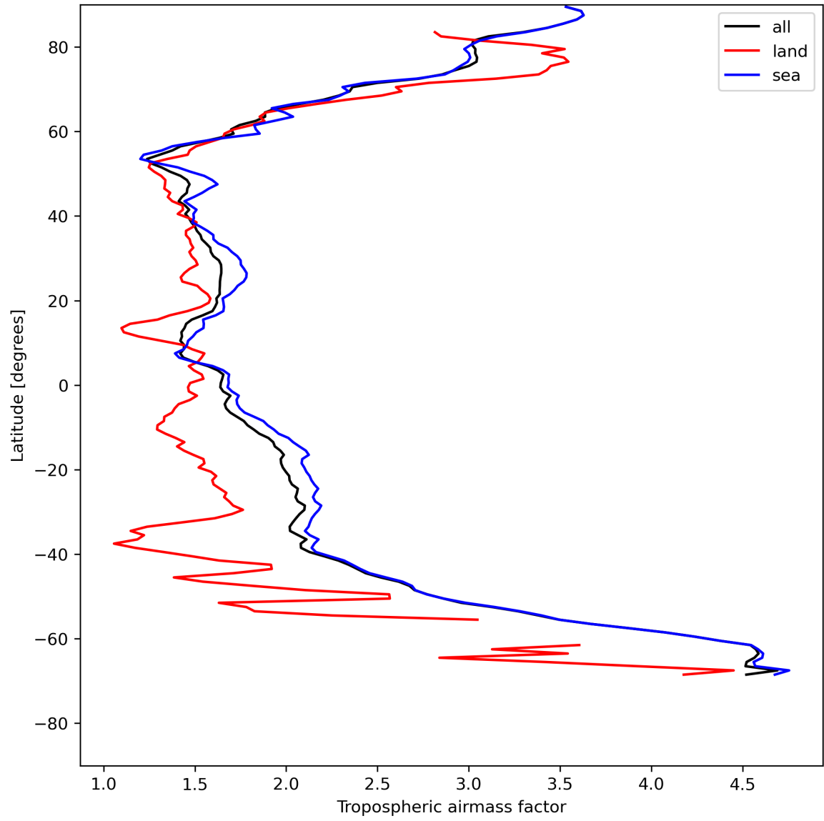
Figure 14: Zonal average of “Tropospheric airmass factor” for 2024-07-26 to 2024-07-28.
