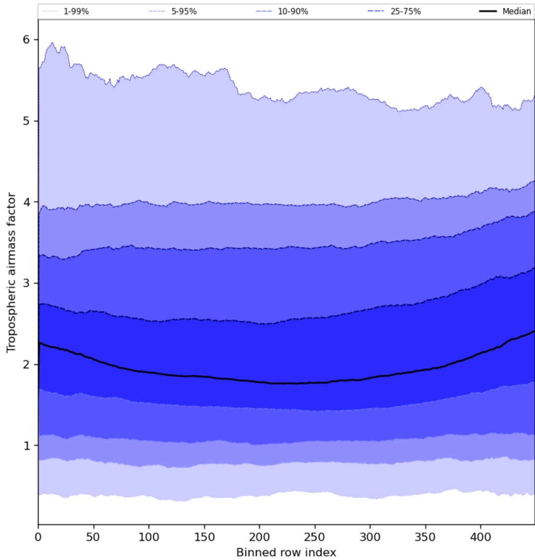
Figure 48: Along track statistics of “Tropospheric airmass factor” for 2024-07-26 to 2024-07-28
