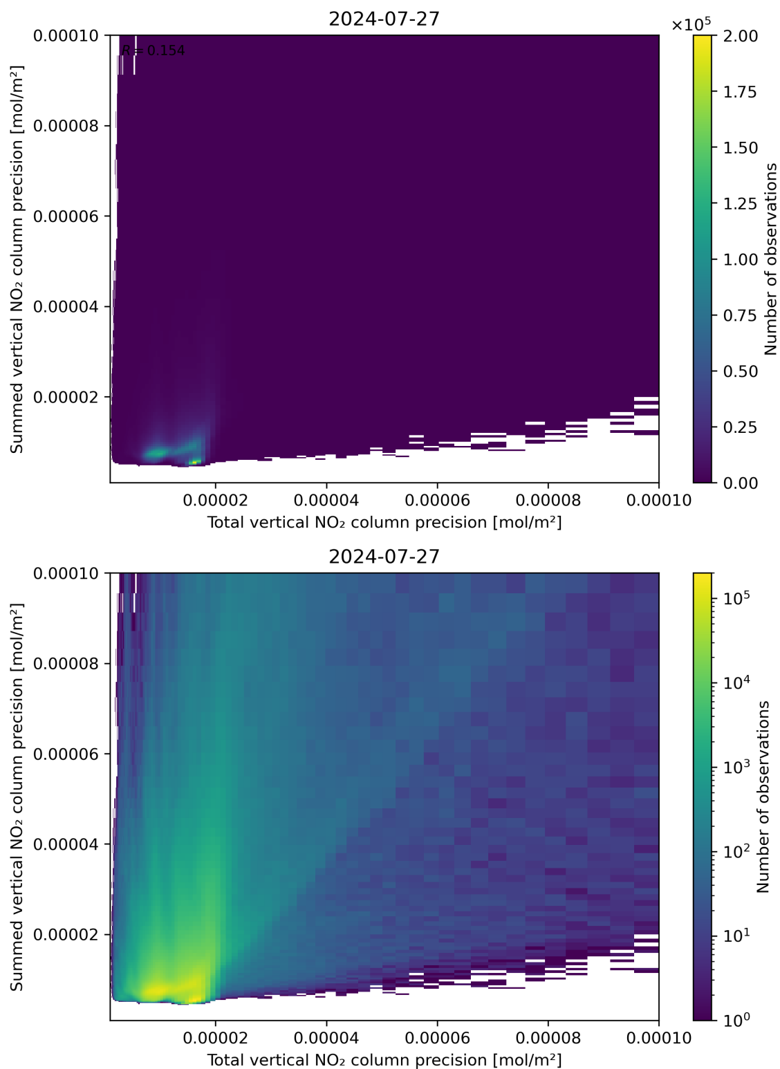
Figure 118: Scatter density plot of “Total vertical NO 2 column precision” against “Summed vertical NO 2 column precision” for 2024-07-26 to 2024-07-28.
