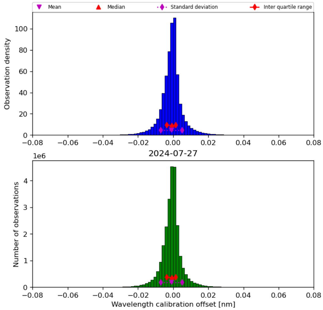
Figure 35: Histogram of “Wavelength calibration offset” for 2024-07-26 to 2024-07-28
