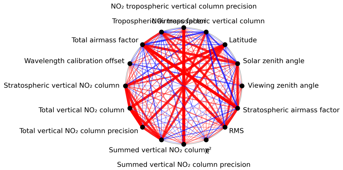
Figure 1: Map of correlation graph for 2024-07-26 to 2024-07-28.
