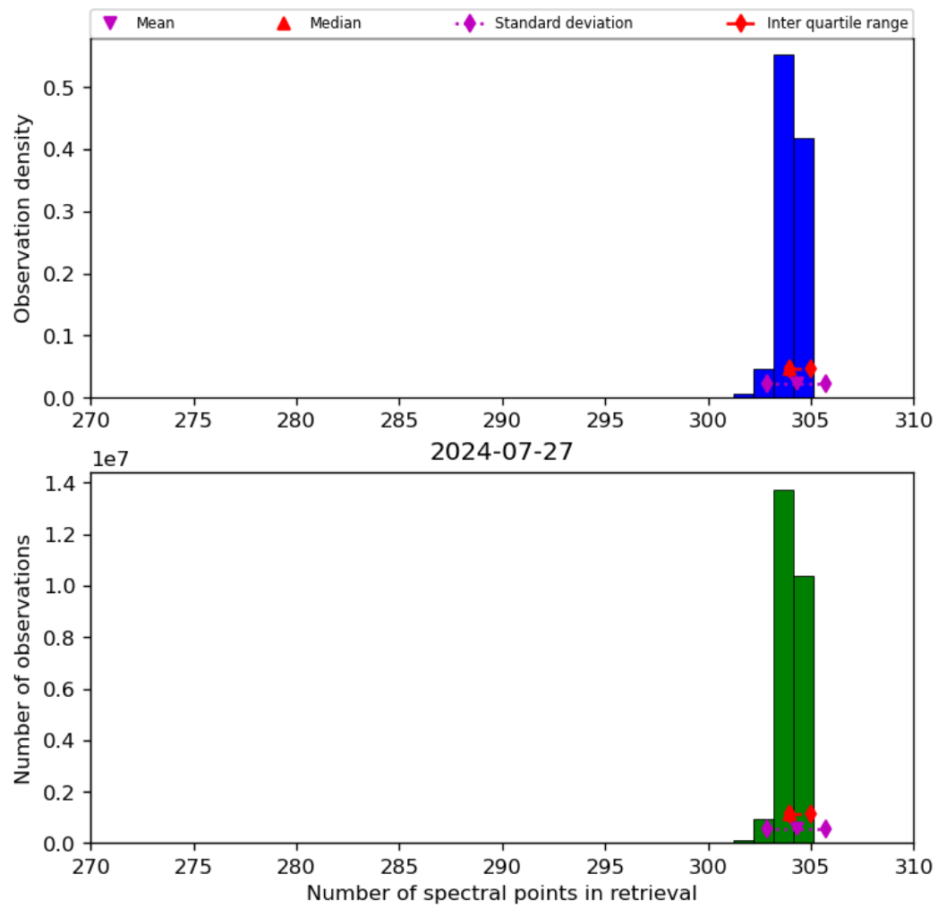
Figure 33: Histogram of “Number of spectral points in retrieval” for 2024-07-26 to 2024-07-28
