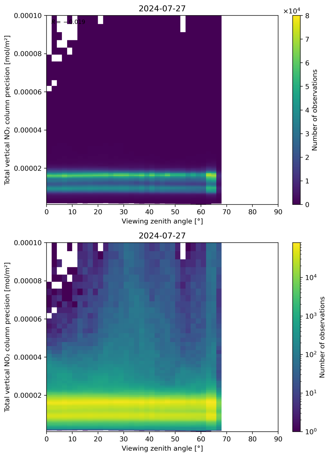
Figure 168: Scatter density plot of “Viewing zenith angle” against “Total vertical NO 2 column precision” for 2024-07-26 to 2024-07-28.
