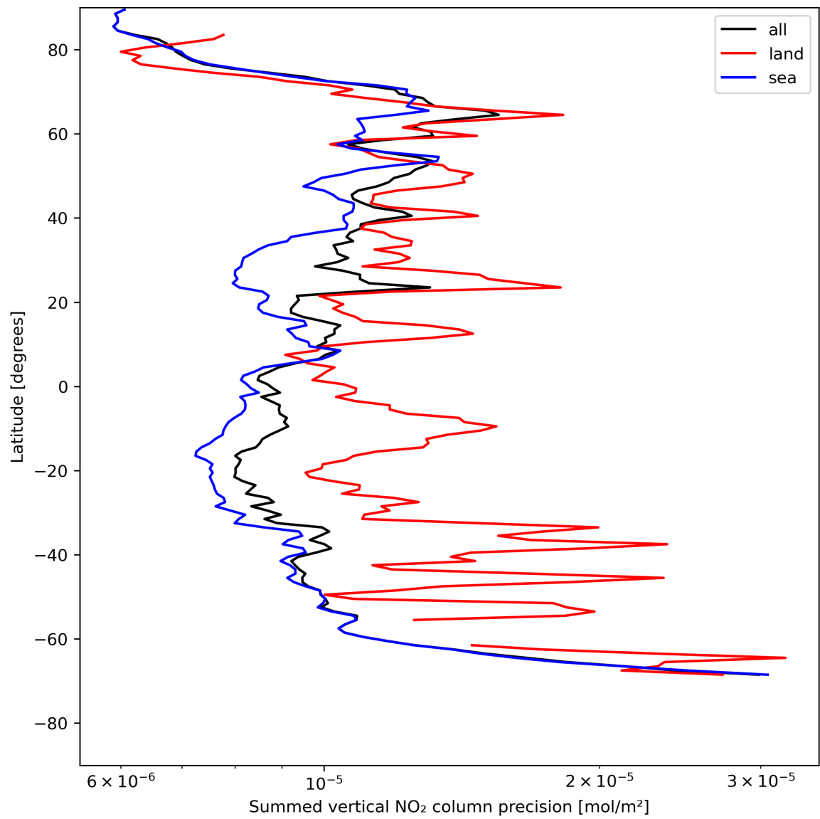
Figure 24: Zonal average of “Summed vertical NO 2 column precision” for 2024-07-26 to 2024-07-28.
