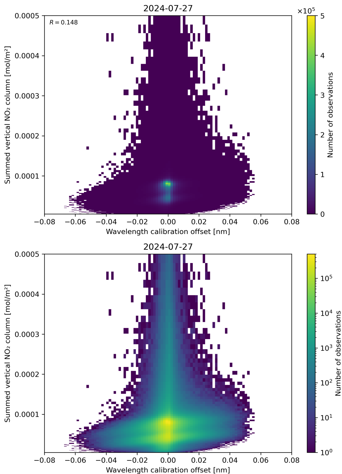
Figure 177: Scatter density plot of “Wavelength calibration offset” against “Summed vertical NO 2 column” for 2024-07-26 to 2024-07-28.
