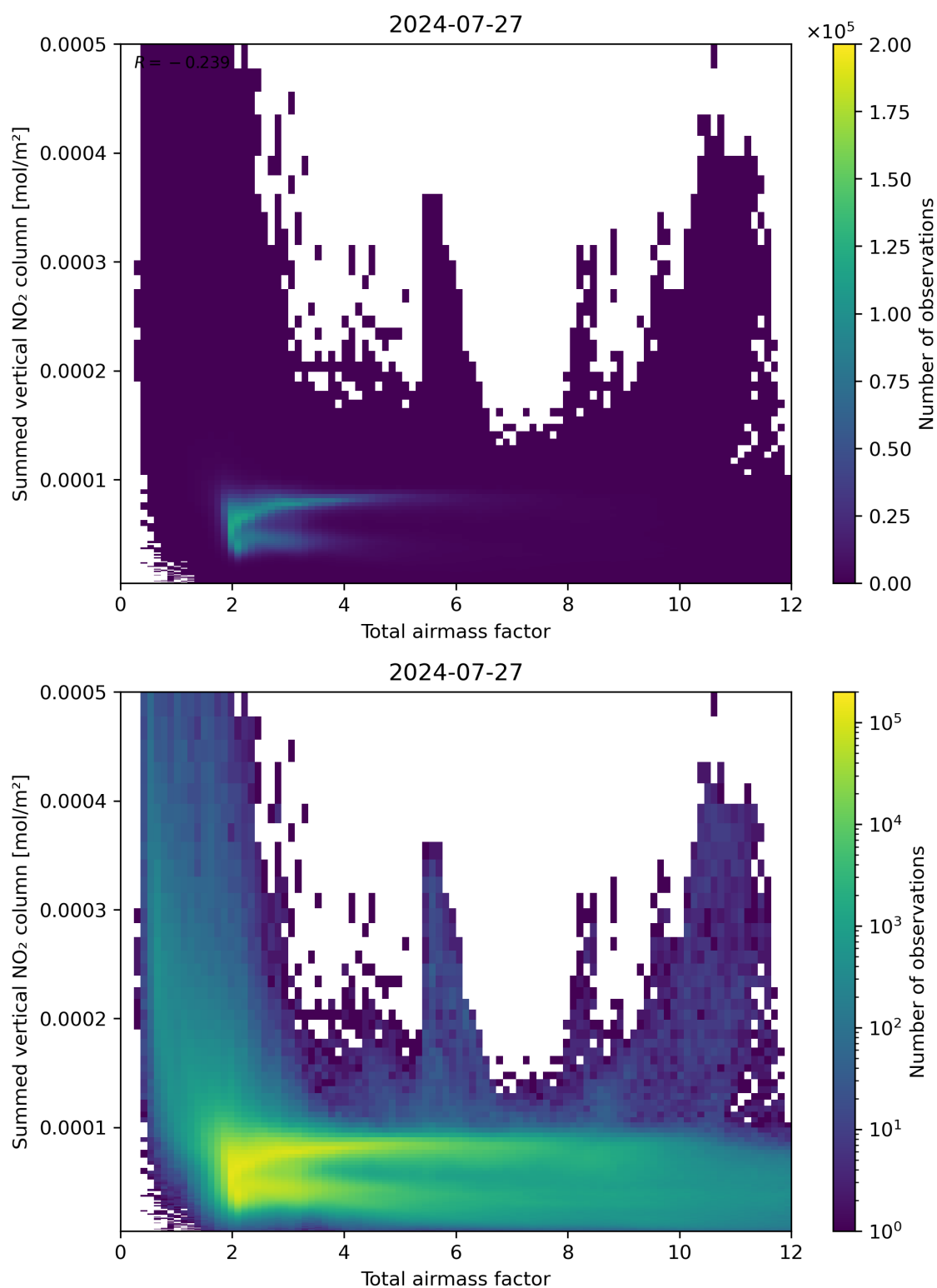
Figure 65: Scatter density plot of “Total airmass factor” against “Summed vertical NO 2 column” for 2024-07-26 to 2024-07-28.
