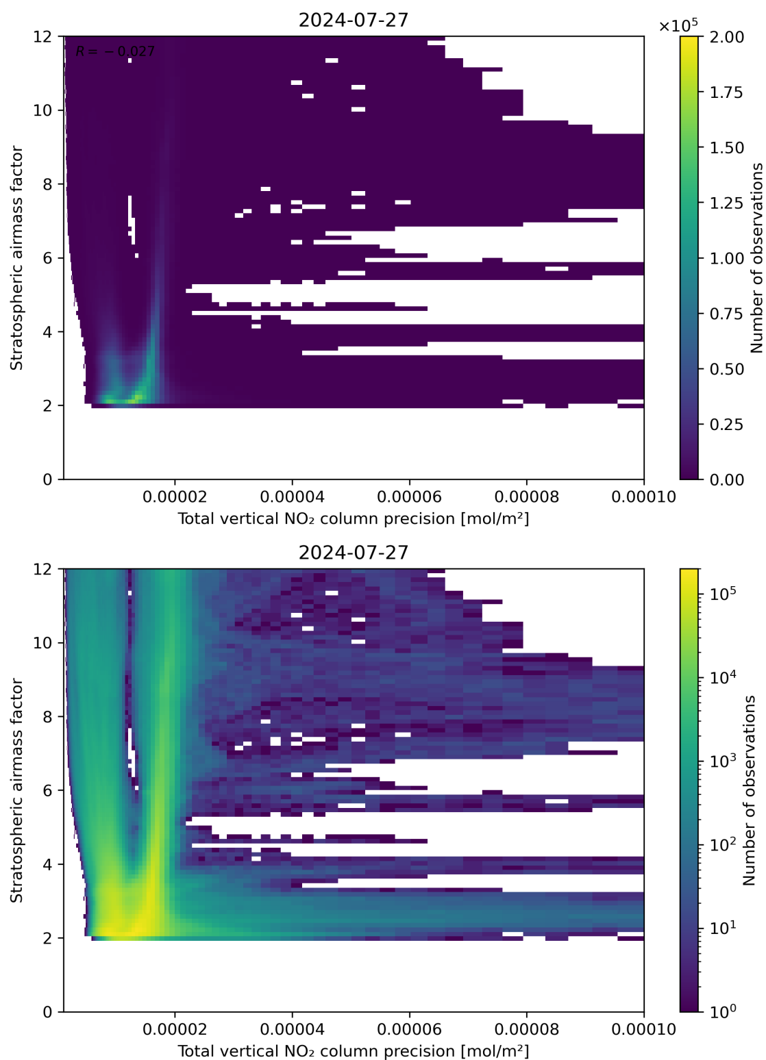
Figure 115: Scatter density plot of “Total vertical NO 2 column precision” against “Stratospheric air mass factor” for 2024-07-26 to 2024-07-28.
