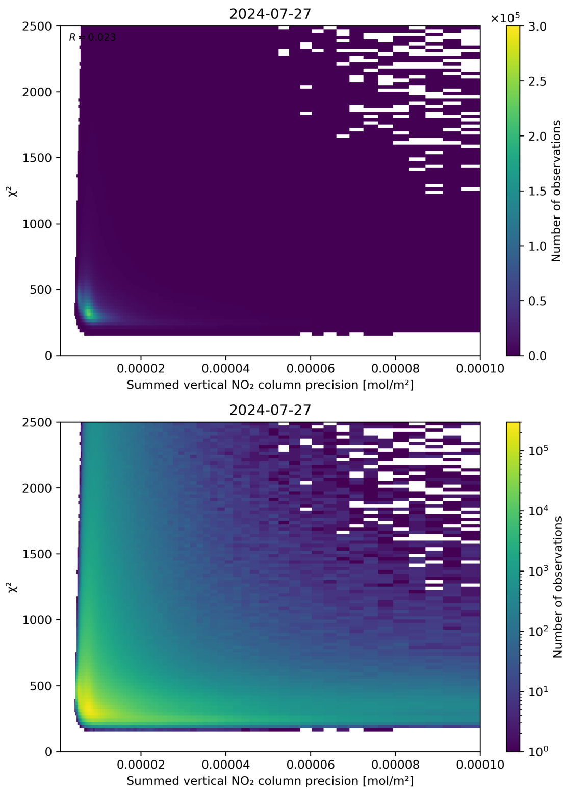
Figure 107: Scatter density plot of “Summed vertical NO 2 column precision” against “ \chi^2 ” for 2024-07-26 to 2024-07-28.
