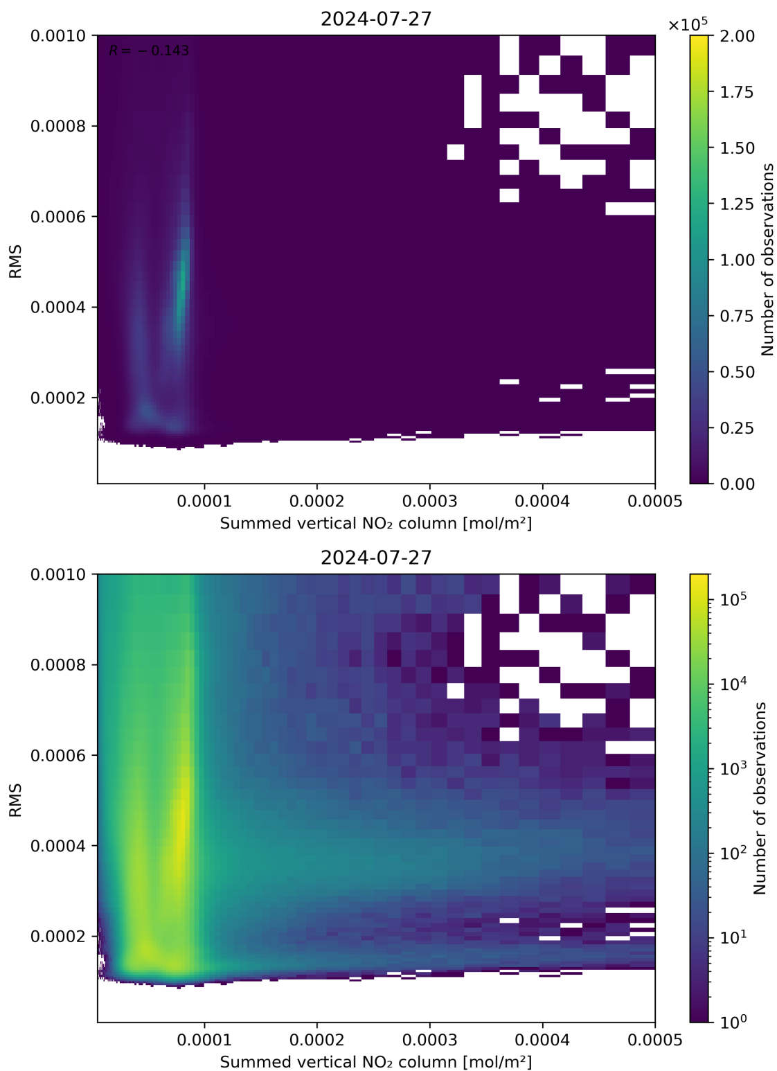
Figure 109: Scatter density plot of “Summed vertical NO 2 column” against “RMS” for 2024-07-26 to 2024-07-28.
