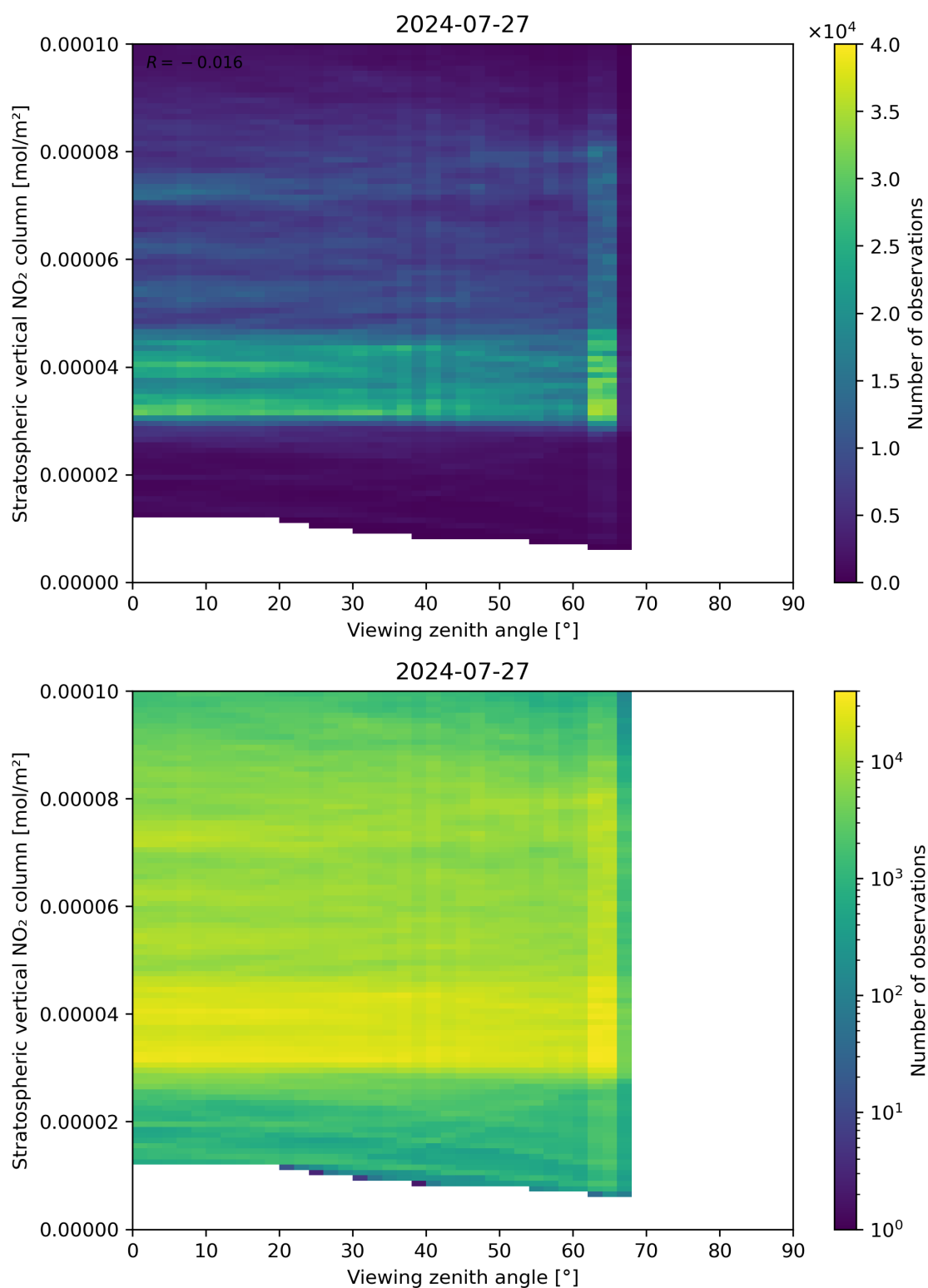
Figure 164: Scatter density plot of “Viewing zenith angle” against “Stratospheric vertical NO 2 column” for 2024-07-26 to 2024-07-28.
