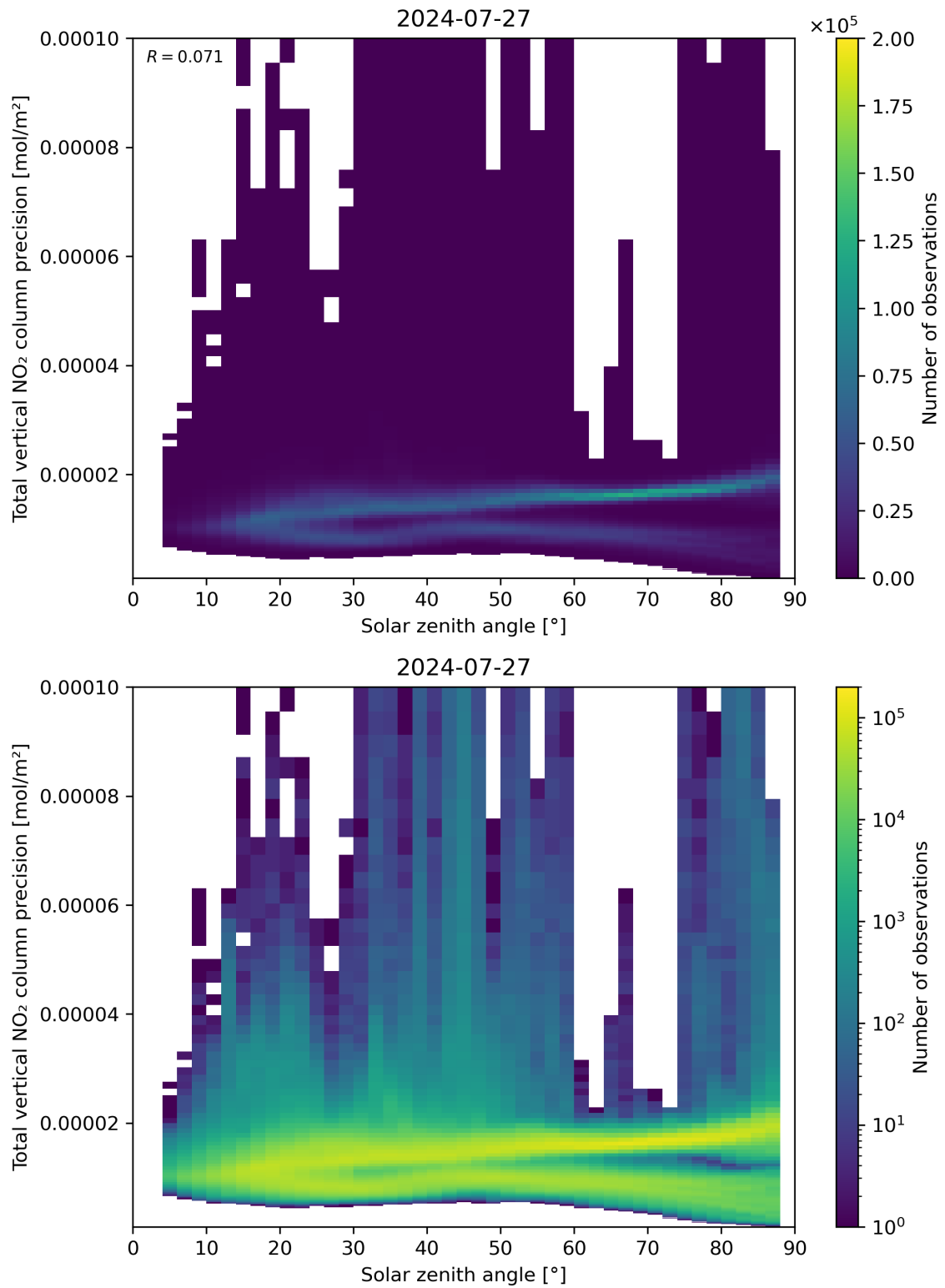
Figure 154: Scatter density plot of “Solar zenith angle” against “Total vertical NO 2 column precision” for 2024-07-26 to 2024-07-28.
