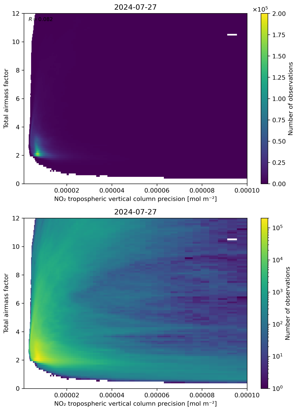
Figure 132: Scatter density plot of “NO 2 tropospheric vertical column precision” against “Total air mass factor” for 2024-07-26 to 2024-07-28.
