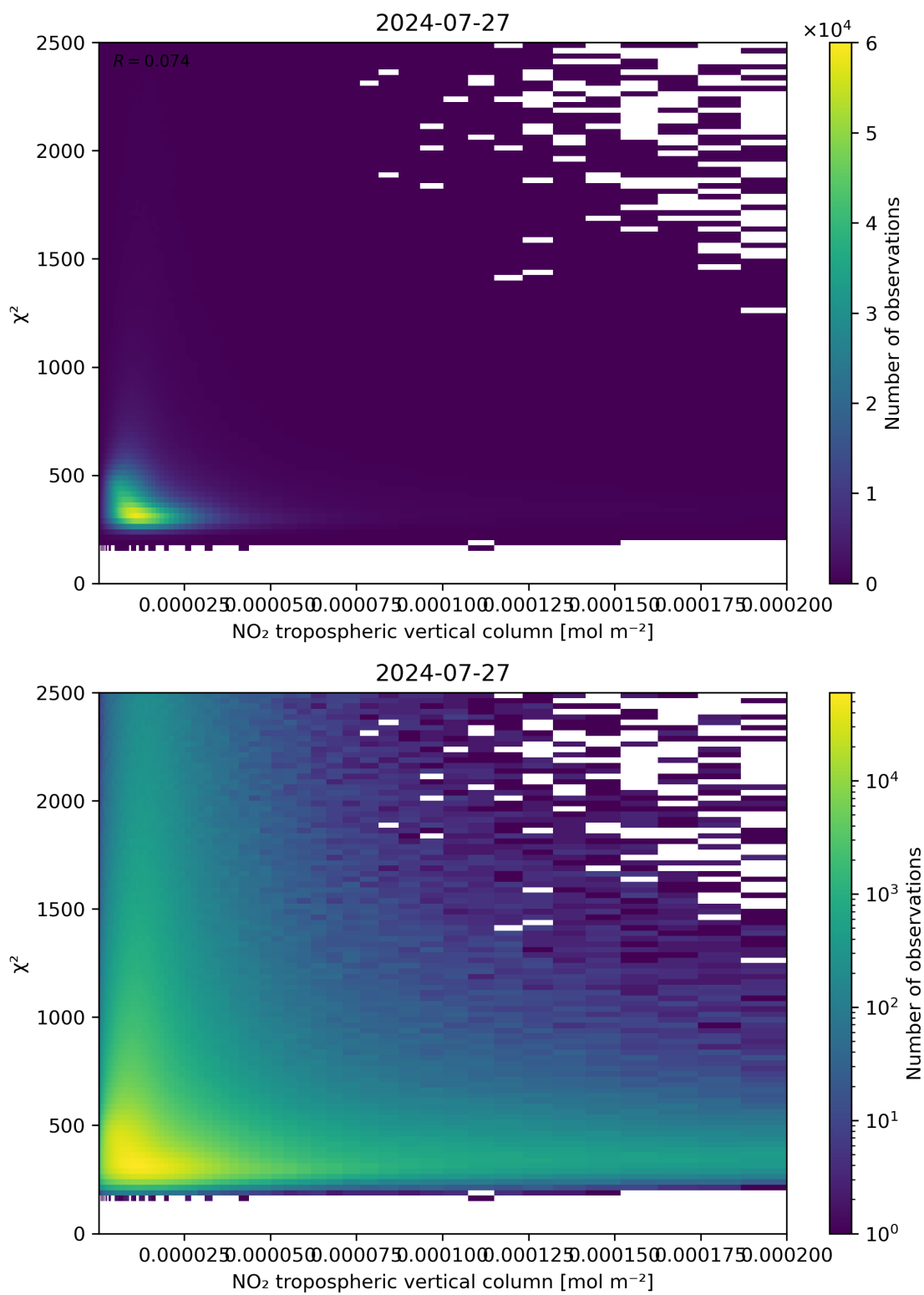
Figure 124: Scatter density plot of “NO 2 tropospheric vertical column” against “ \chi^2 ” for 2024-07-26 to 2024-07-28.
