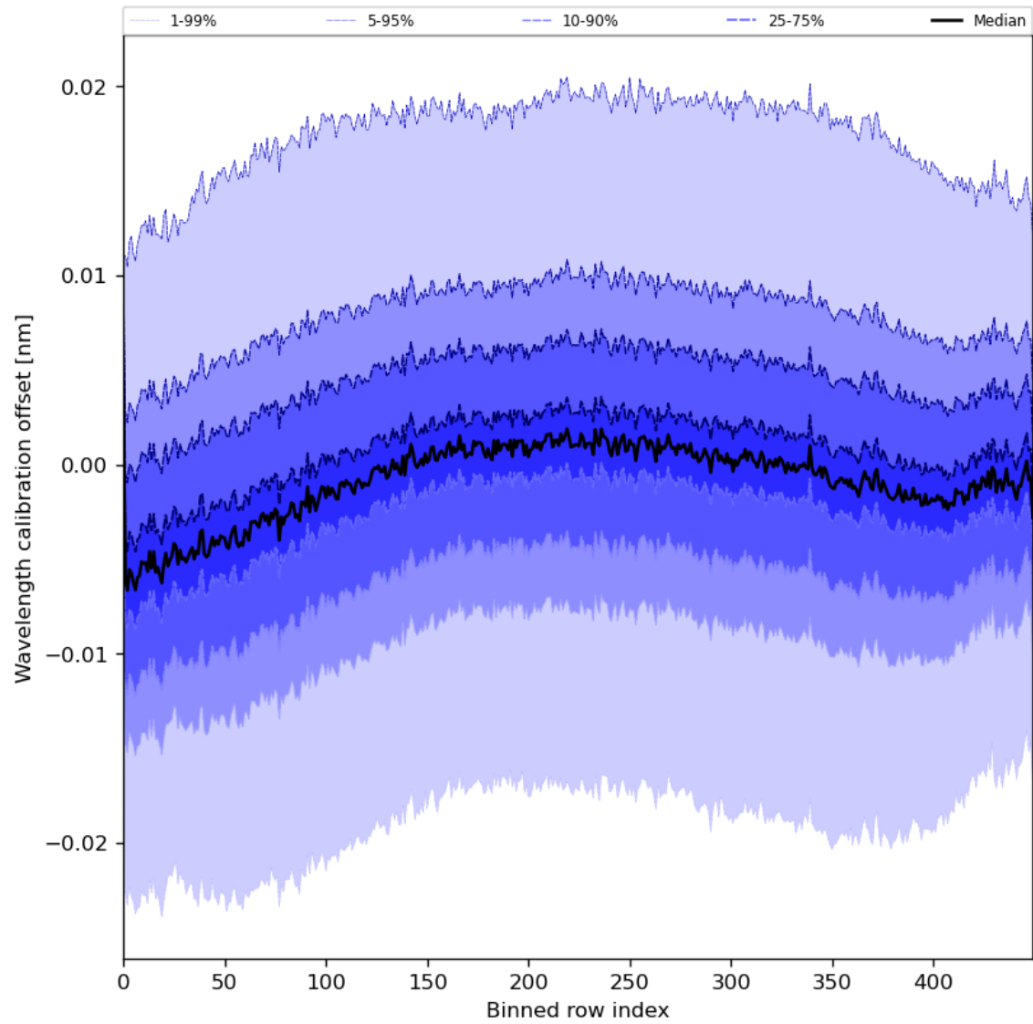
Figure 52: Along track statistics of “Wavelength calibration offset” for 2024-07-26 to 2024-07-28
