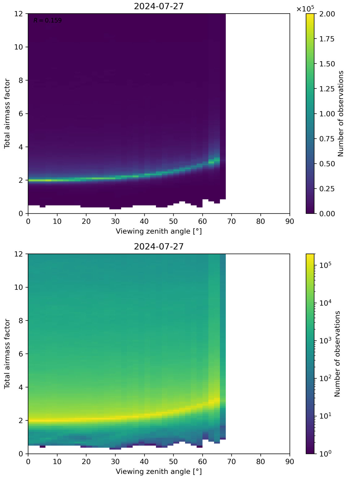
Figure 160: Scatter density plot of “Viewing zenith angle” against “Total airmass factor” for 2024-07-26 to 2024-07-28.
