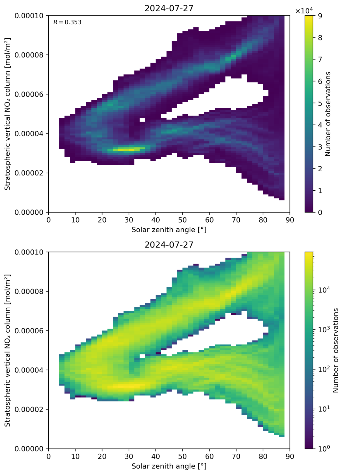
Figure 150: Scatter density plot of “Solar zenith angle” against “Stratospheric vertical NO 2 column” for 2024-07-26 to 2024-07-28.
