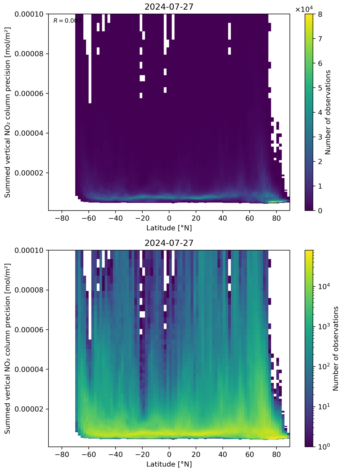
Figure 89: Scatter density plot of “Latitude” against “Summed vertical NO 2 column precision” for 2024-07-26 to 2024-07-28.
