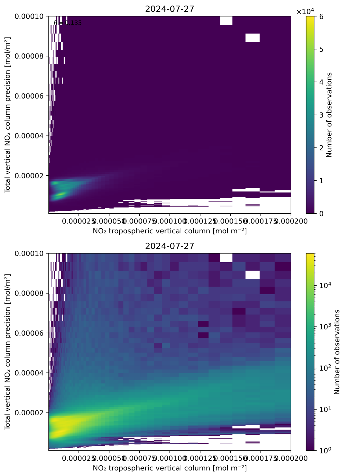
Figure 129: Scatter density plot of “NO 2 tropospheric vertical column” against “Total vertical NO 2 column precision” for 2024-07-26 to 2024-07-28.
