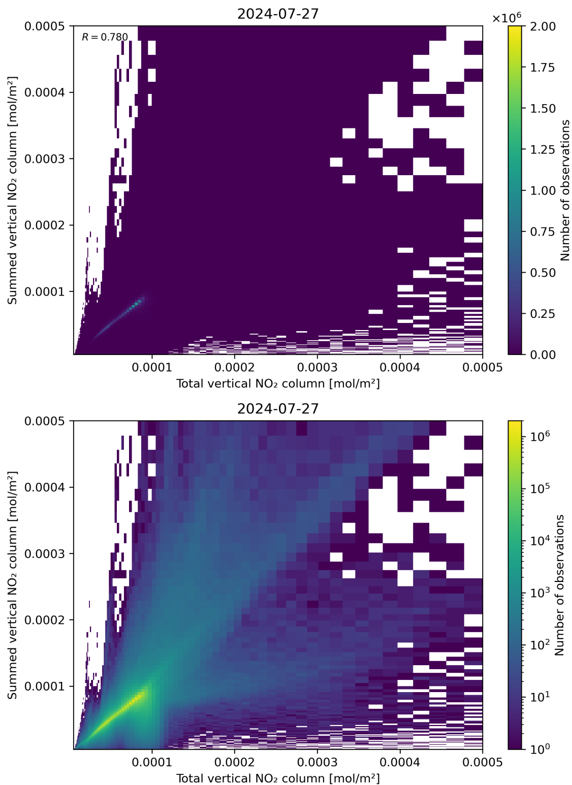
Figure 112: Scatter density plot of “Total vertical NO 2 column” against “Summed vertical NO 2 column” for 2024-07-26 to 2024-07-28.
