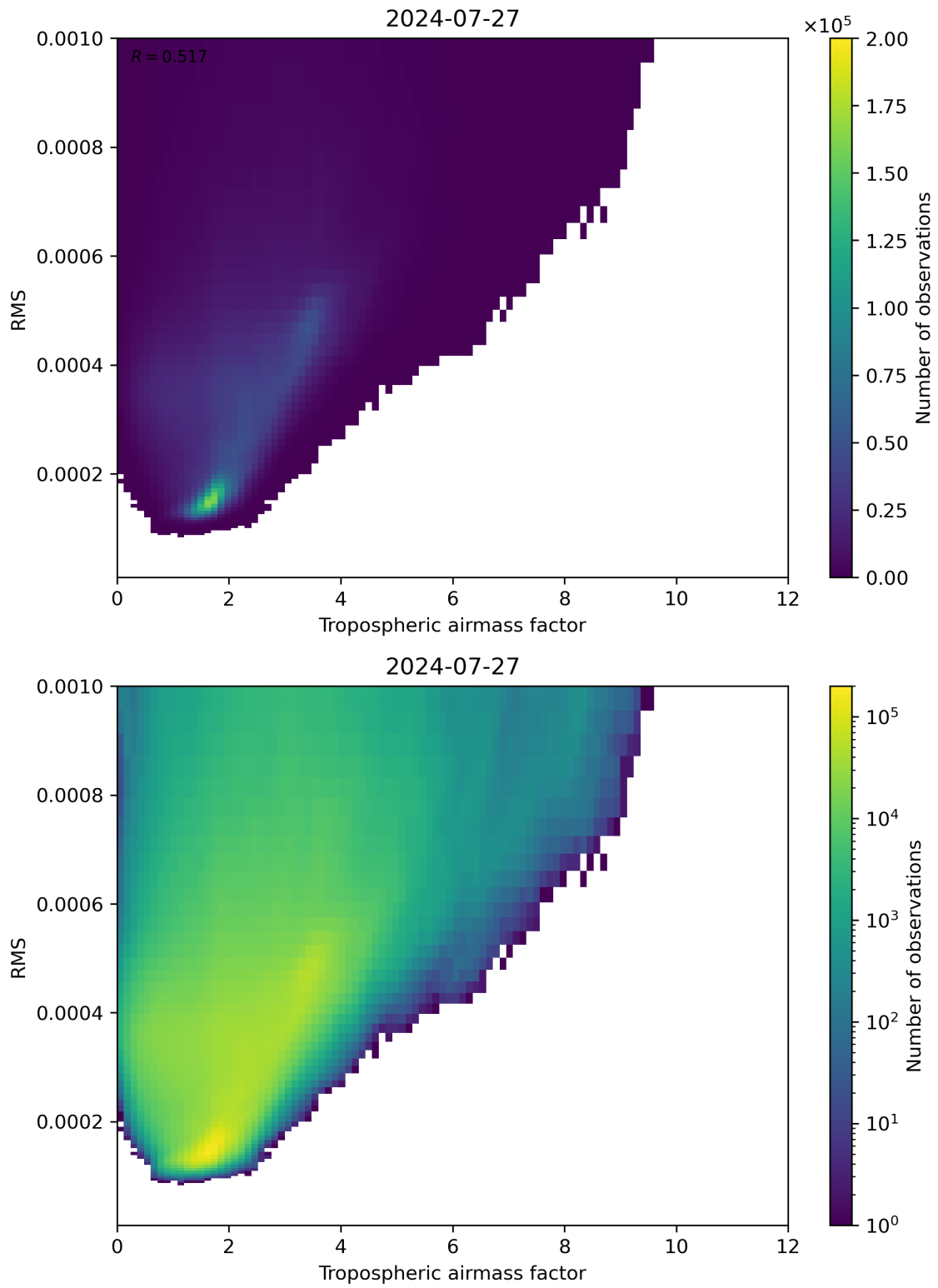
Figure 79: Scatter density plot of “Tropospheric airmass factor” against “RMS” for 2024-07-26 to 2024-07-28.
