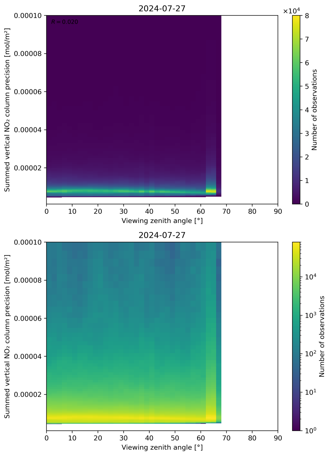
Figure 166: Scatter density plot of “Viewing zenith angle” against “Summed vertical NO 2 column precision” for 2024-07-26 to 2024-07-28.
