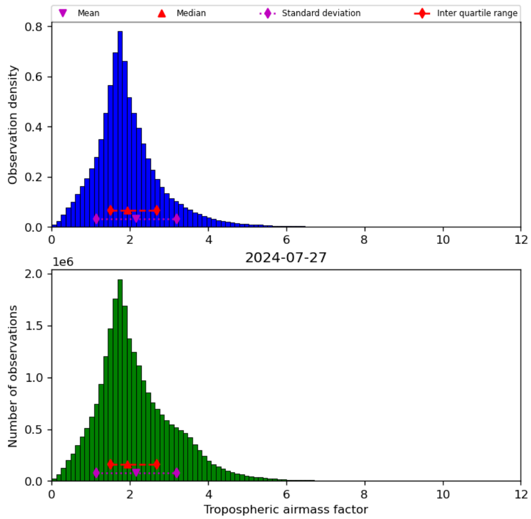
Figure 31: Histogram of “Tropospheric airmass factor” for 2024-07-26 to 2024-07-28
