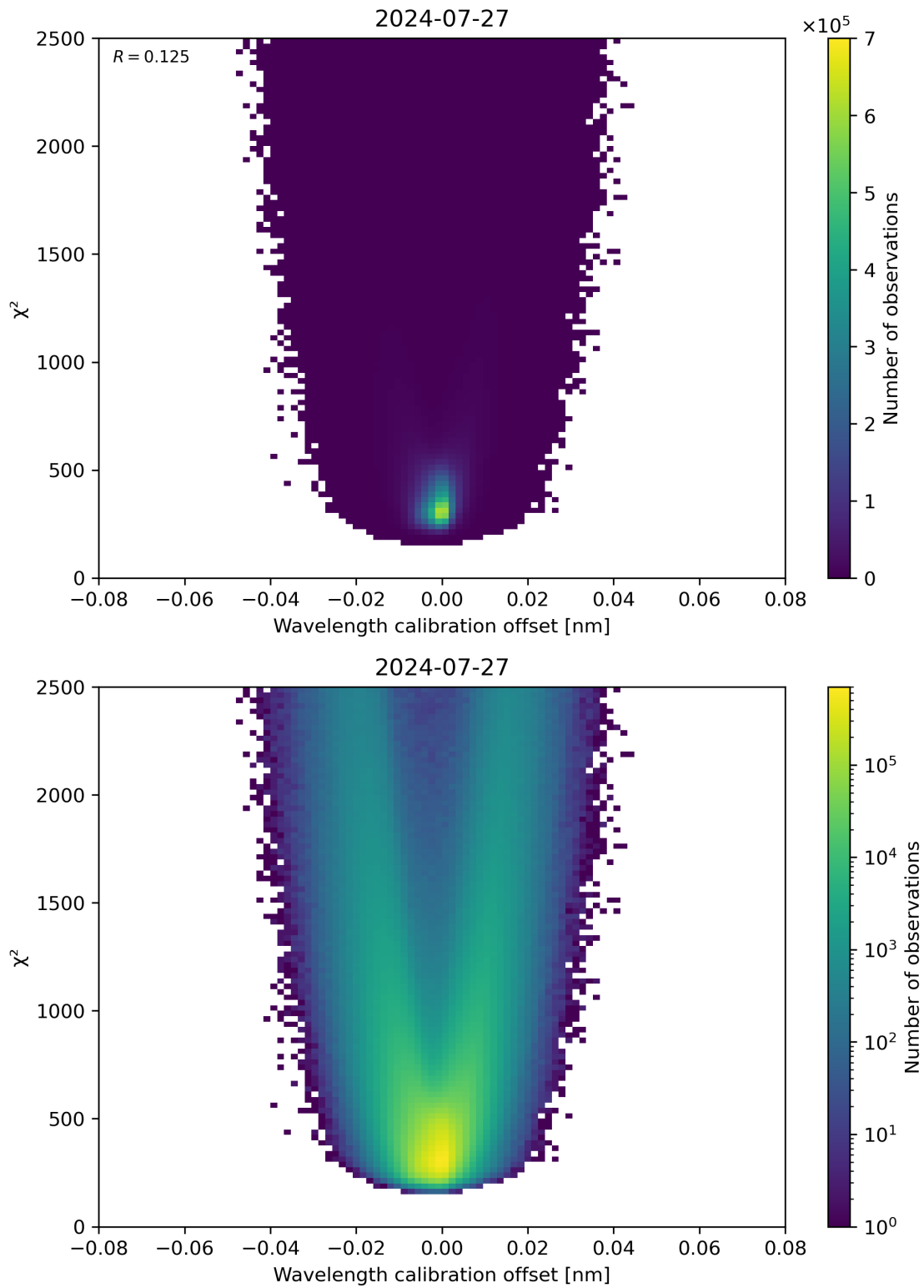
Figure 175: Scatter density plot of “Wavelength calibration offset” against “ \chi^2 ” for 2024-07-26 to 2024-07-28.
