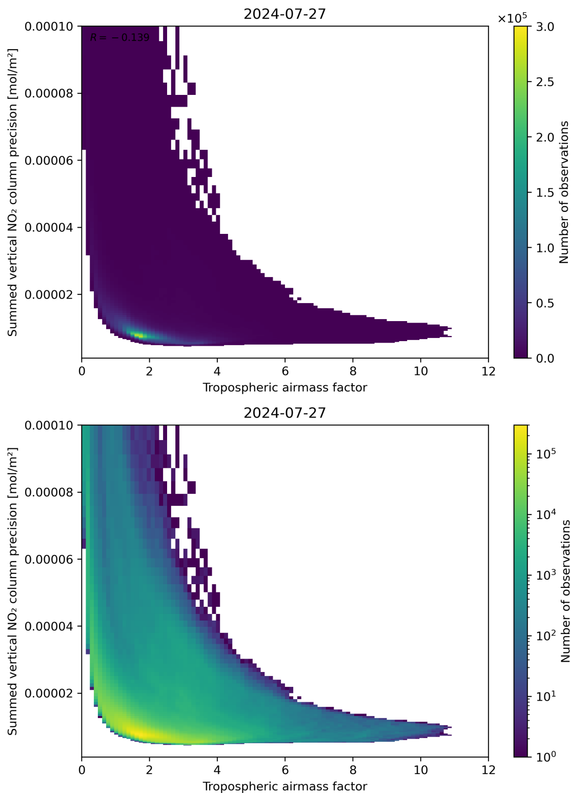
Figure 76: Scatter density plot of “Tropospheric air mass factor” against “Summed vertical NO 2 column precision” for 2024-07-26 to 2024-07-28.
