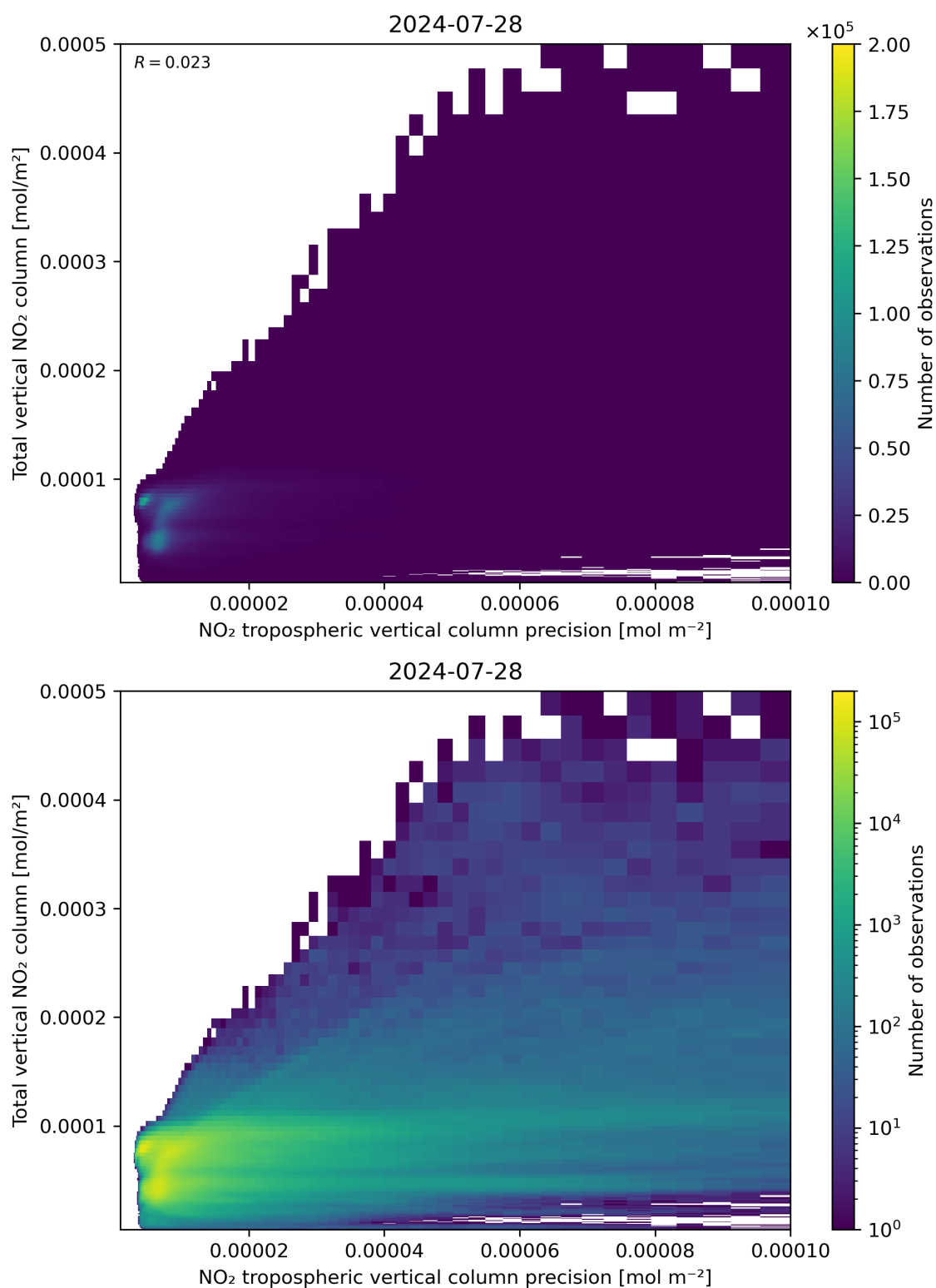
Figure 138: Scatter density plot of “NO 2 tropospheric vertical column precision” against “Total vertical NO 2 column” for 2024-07-27 to 2024-07-29.
