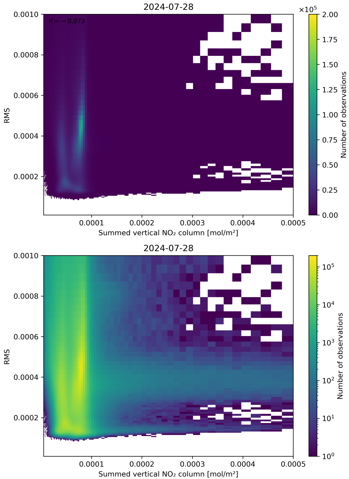
Figure 109: Scatter density plot of “Summed vertical NO 2 column” against “RMS” for 2024-07-27 to 2024-07-29.
