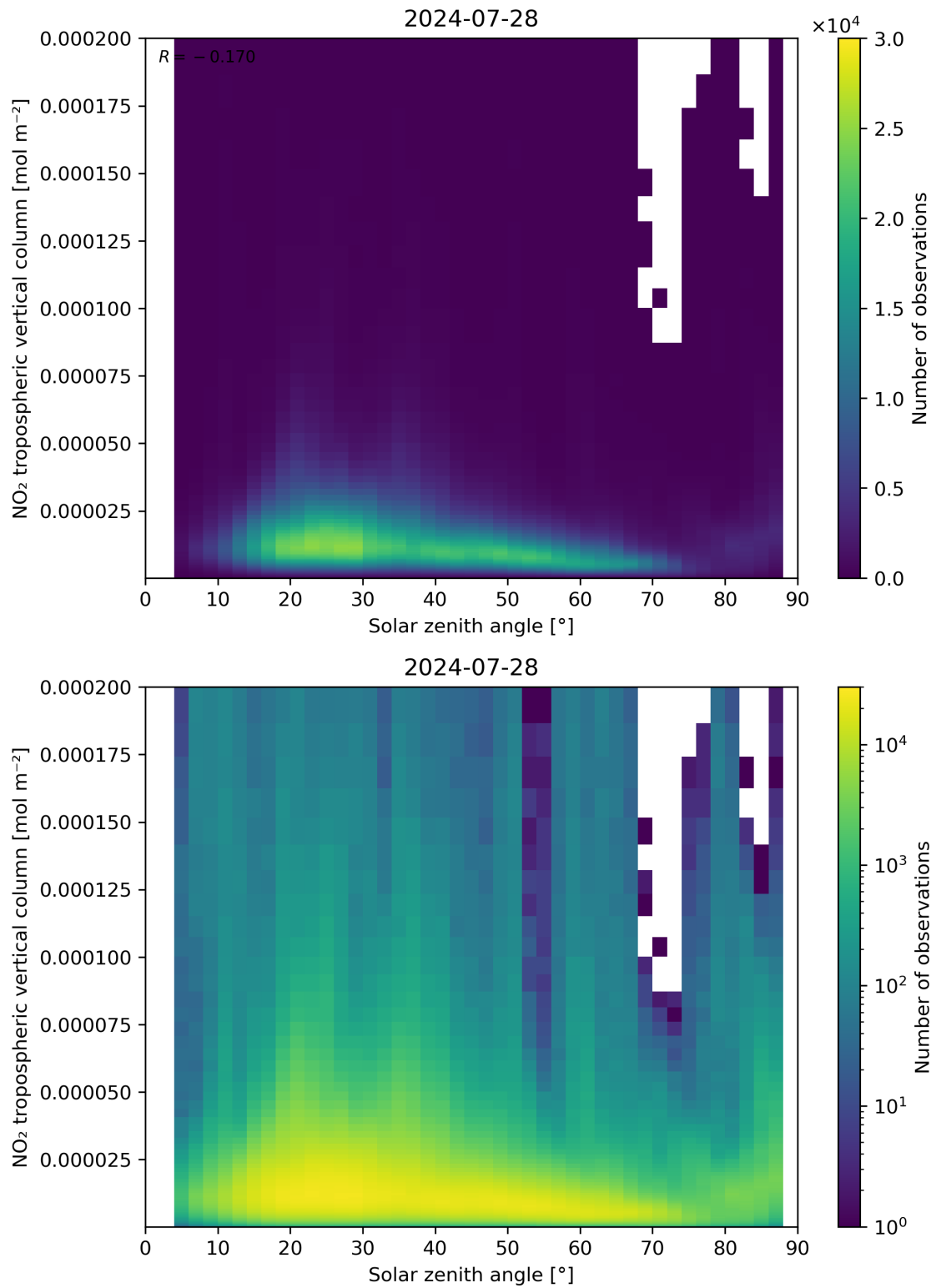
Figure 155: Scatter density plot of “Solar zenith angle” against “NO 2 tropospheric vertical column” for 2024-07-27 to 2024-07-29.
