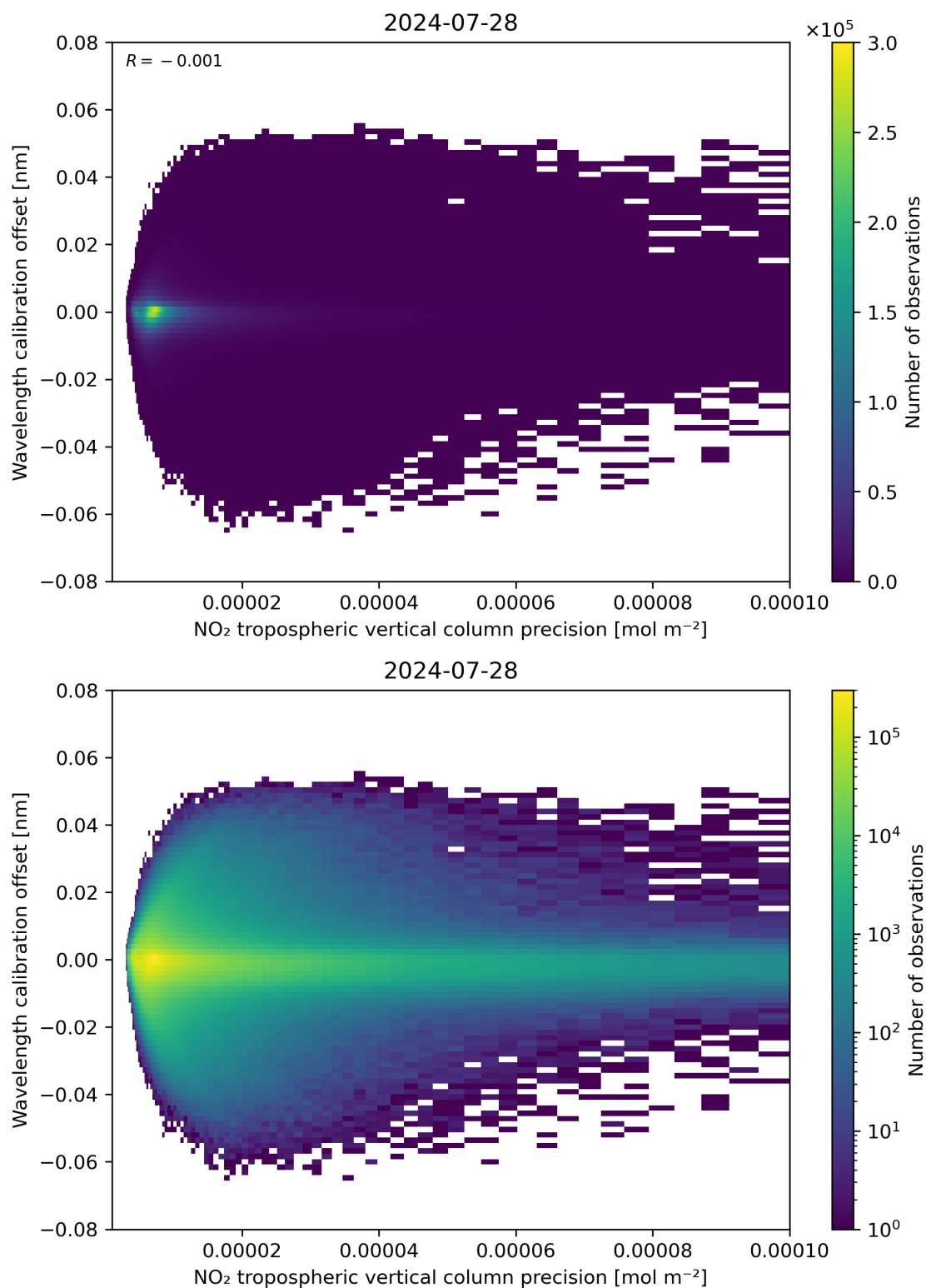
Figure 141: Scatter density plot of “NO 2 tropospheric vertical column precision” against “Wavelength calibration offset” for 2024-07-27 to 2024-07-29.
