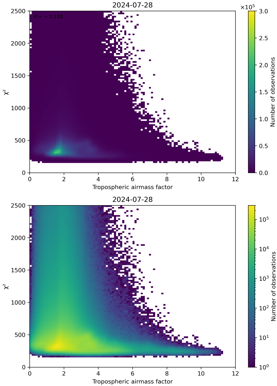
Figure 73: Scatter density plot of “Tropospheric airmass factor” against “ \chi^2 ” for 2024-07-27 to 2024-07-29.
