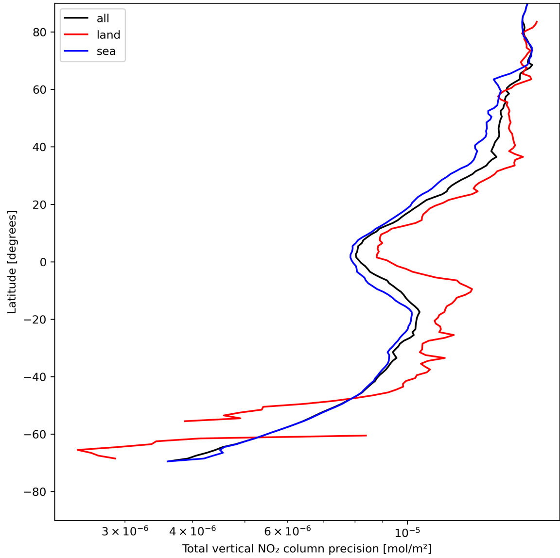
Figure 22: Zonal average of “Total vertical NO 2 column precision” for 2024-07-27 to 2024-07-29.
