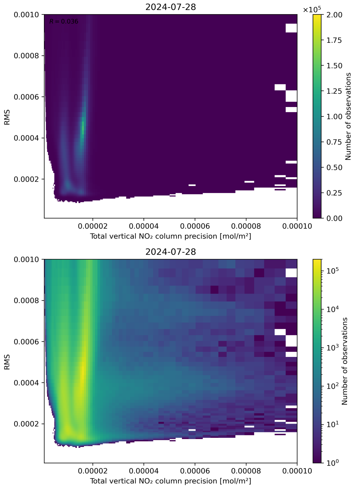
Figure 119: Scatter density plot of “Total vertical NO 2 column precision” against “RMS” for 2024-07-27 to 2024-07-29.
