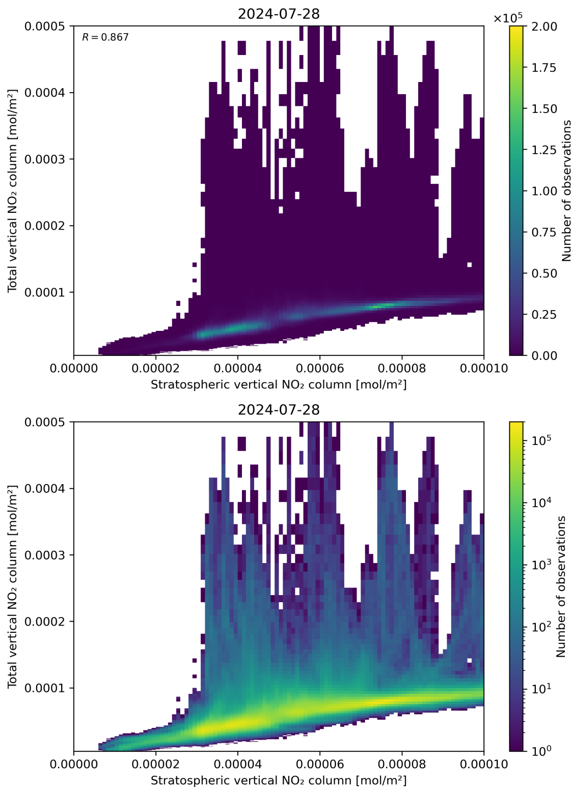
Figure 100: Scatter density plot of “Stratospheric vertical NO 2 column” against “Total vertical NO 2 column” for 2024-07-27 to 2024-07-29.
