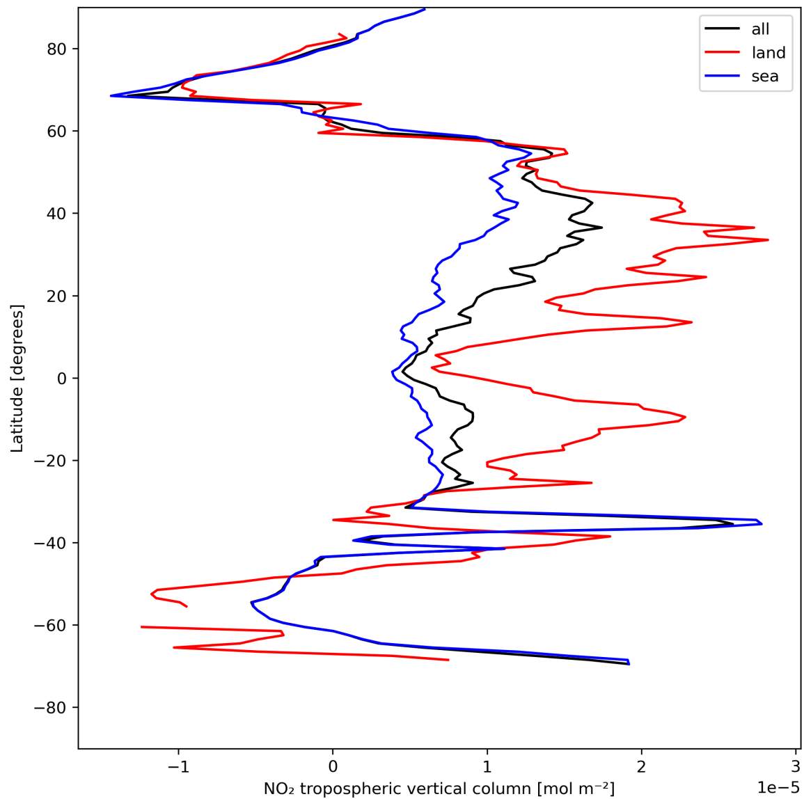
Figure 12: Zonal average of “NO 2 tropospheric vertical column” for 2024-07-27 to 2024-07-29.
