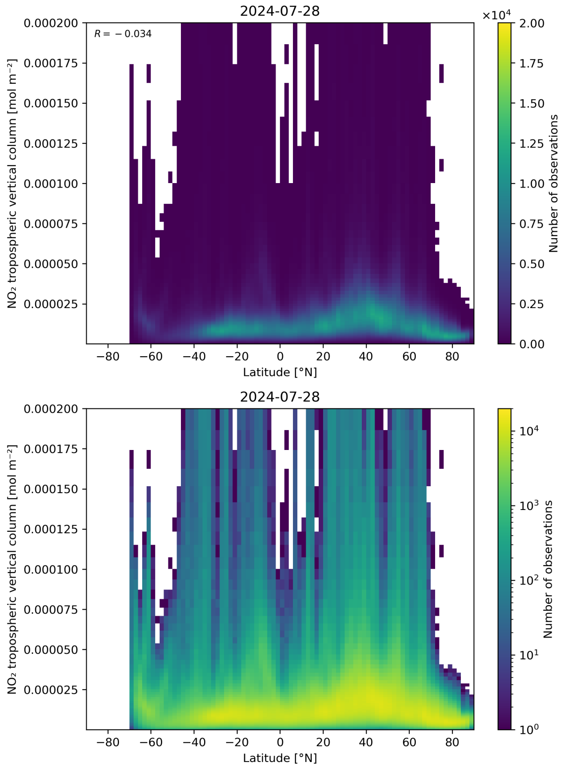
Figure 92: Scatter density plot of “Latitude” against “NO 2 tropospheric vertical column” for 2024-07-27 to 2024-07-29.
