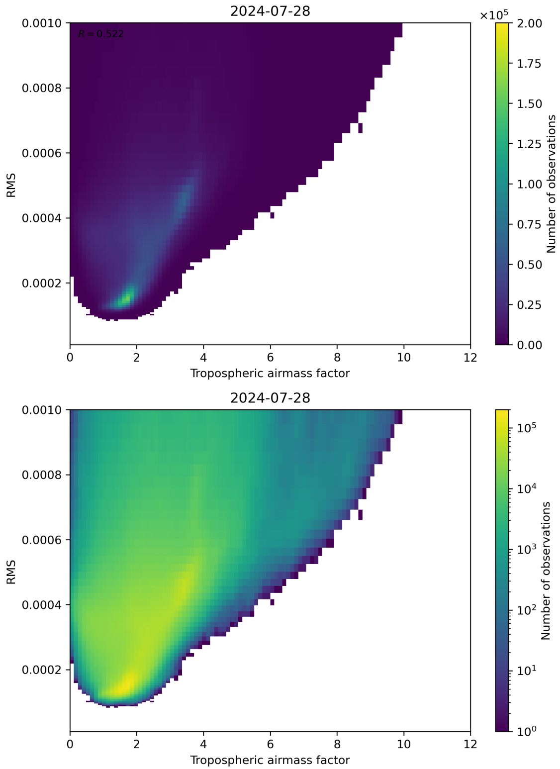
Figure 79: Scatter density plot of “Tropospheric airmass factor” against “RMS” for 2024-07-27 to 2024-07-29.
