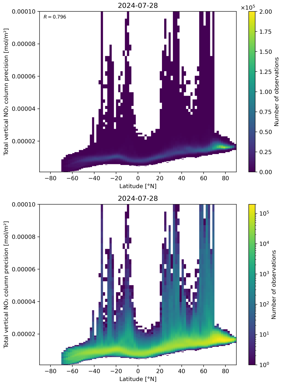
Figure 91: Scatter density plot of “Latitude” against “Total vertical NO 2 column precision” for 2024-07-27 to 2024-07-29.
