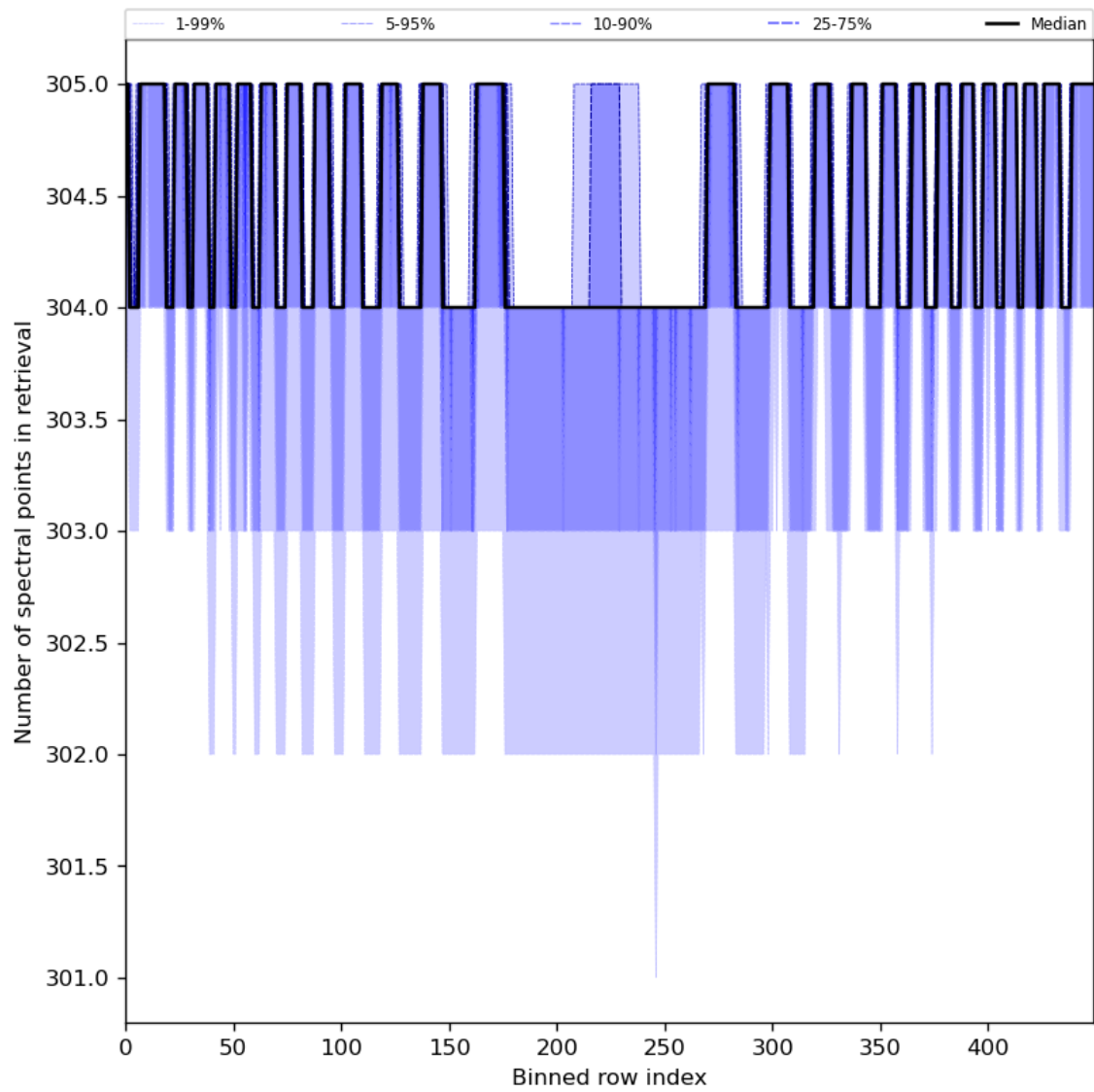
Figure 50: Along track statistics of “Number of spectral points in retrieval” for 2024-07-27 to 2024-07-29
