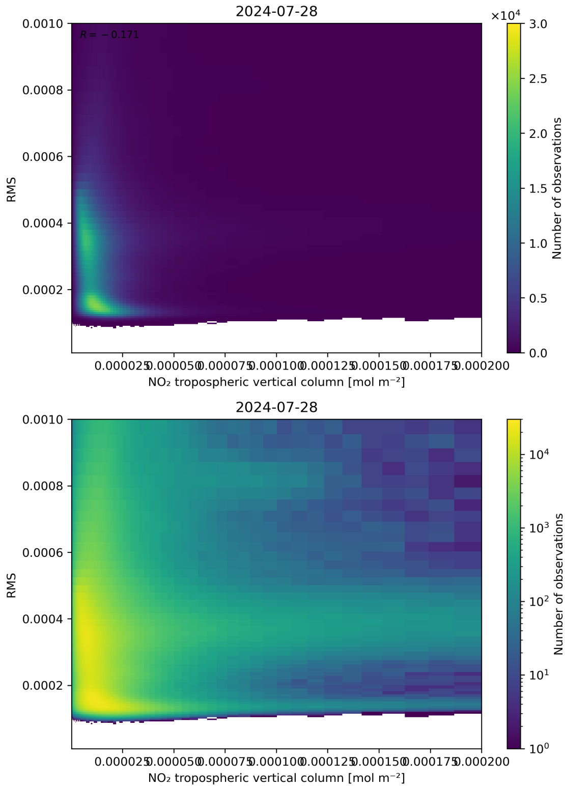
Figure 142: Scatter density plot of “NO 2 tropospheric vertical column” against “RMS” for 2024-07-27 to 2024-07-29.
