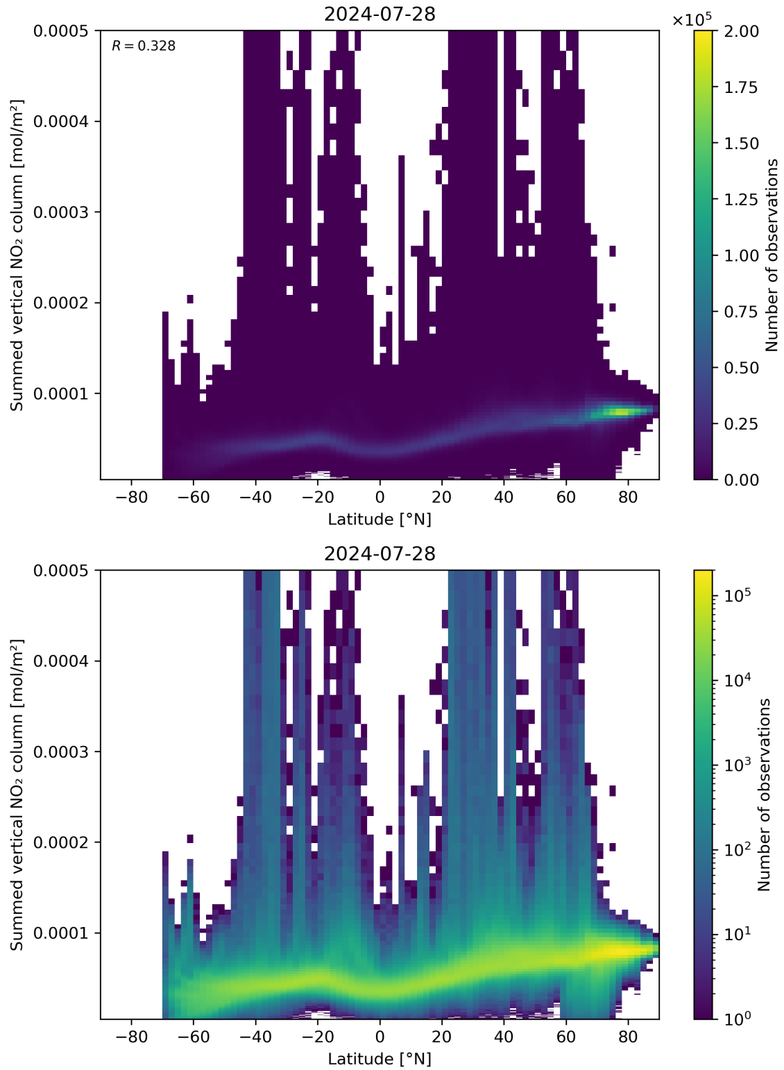
Figure 88: Scatter density plot of “Latitude” against “Summed vertical NO 2 column” for 2024-07-27 to 2024-07-29.
