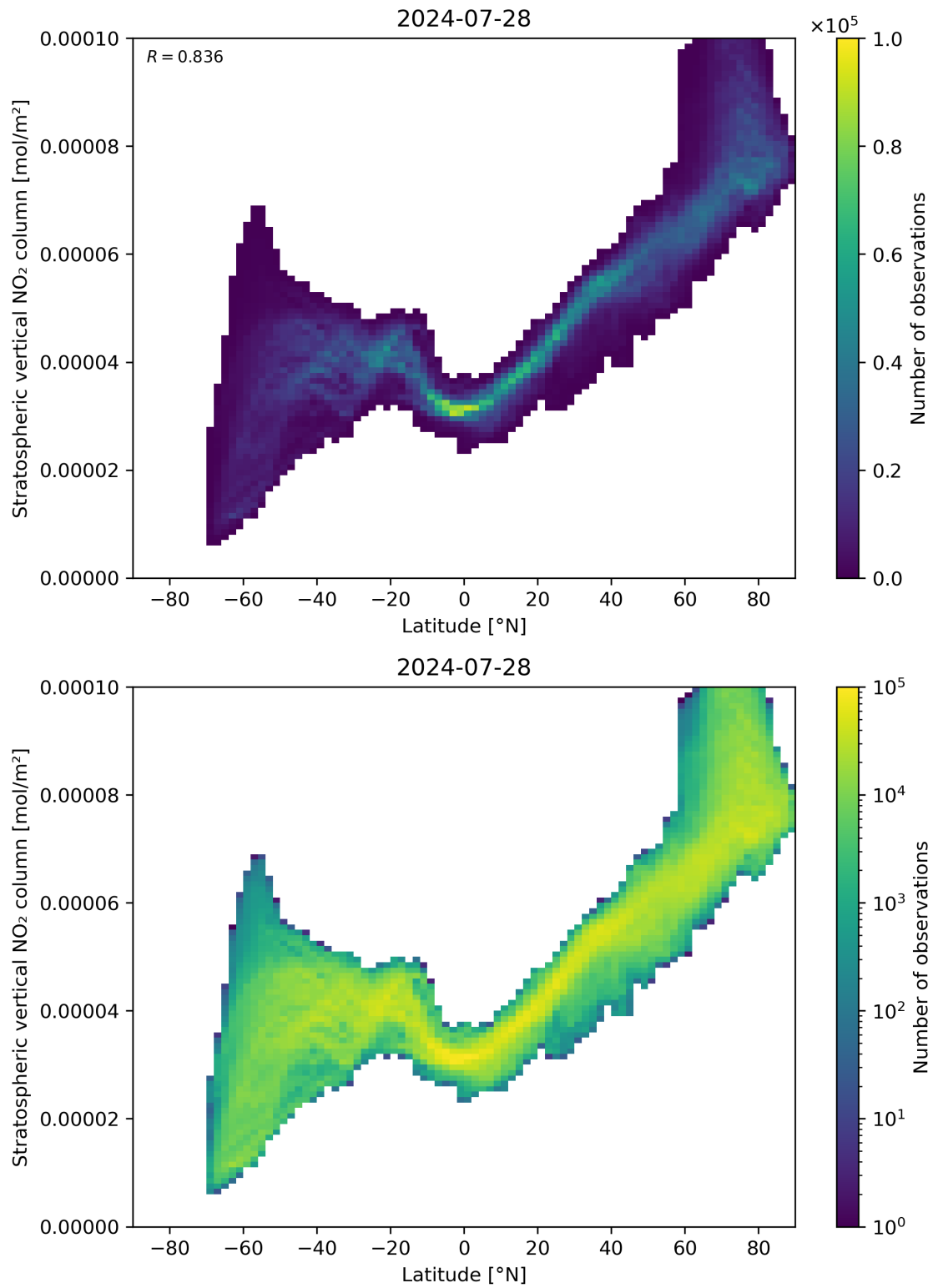
Figure 87: Scatter density plot of “Latitude” against “Stratospheric vertical NO 2 column” for 2024-07-27 to 2024-07-29.
