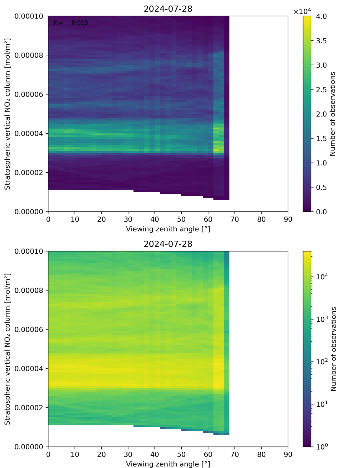
Figure 164: Scatter density plot of “Viewing zenith angle” against “Stratospheric vertical NO 2 column” for 2024-07-27 to 2024-07-29.
