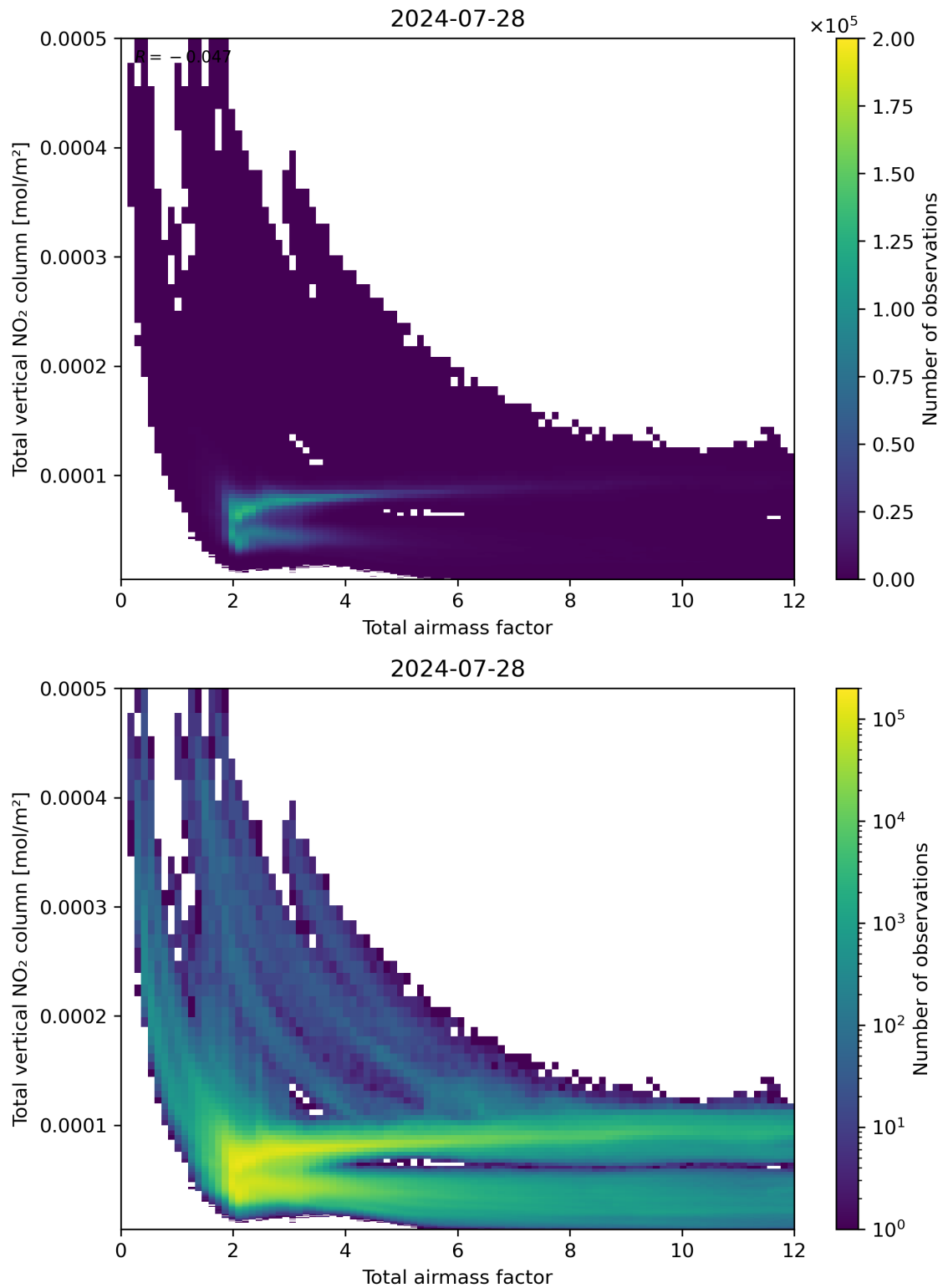
Figure 67: Scatter density plot of “Total airmass factor” against “Total vertical NO 2 column” for 2024-07-27 to 2024-07-29.
