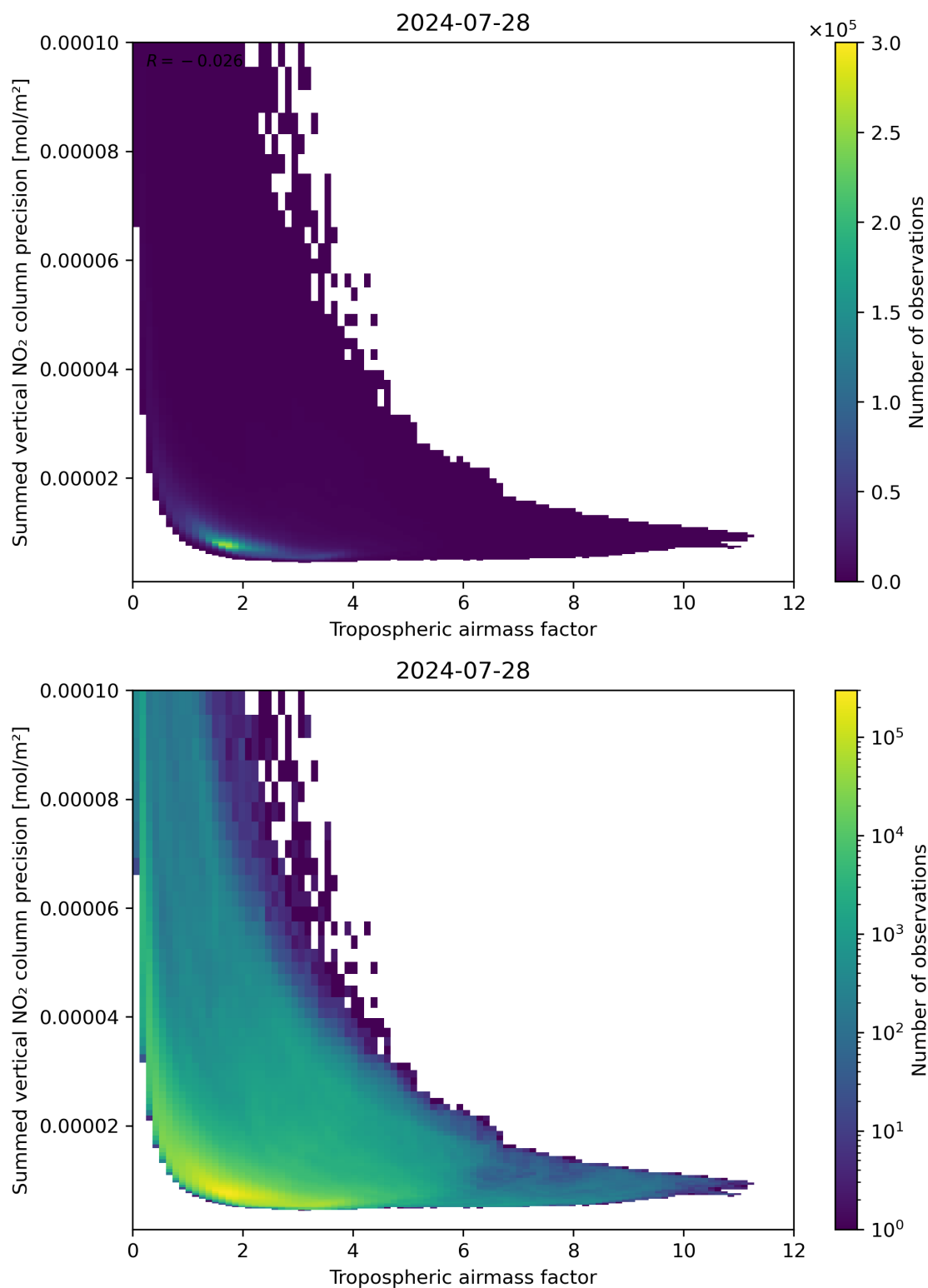
Figure 76: Scatter density plot of “Tropospheric air mass factor” against “Summed vertical NO 2 column precision” for 2024-07-27 to 2024-07-29.
