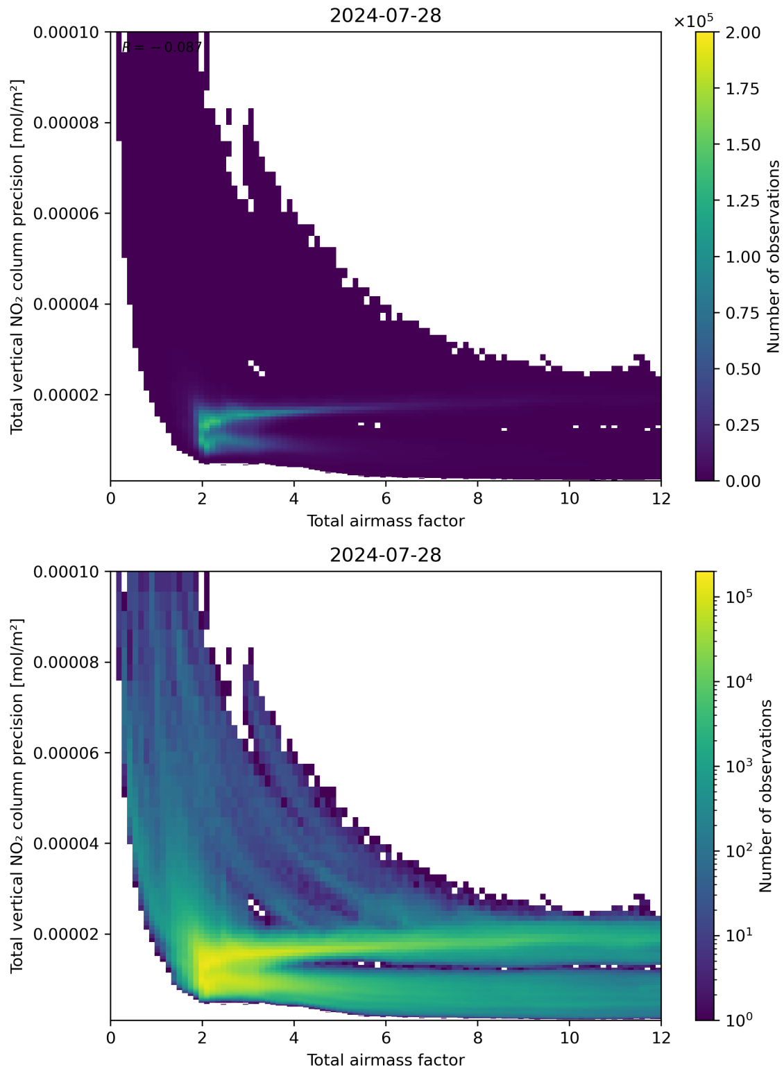
Figure 68: Scatter density plot of “Total airmass factor” against “Total vertical NO 2 column precision” for 2024-07-27 to 2024-07-29.
