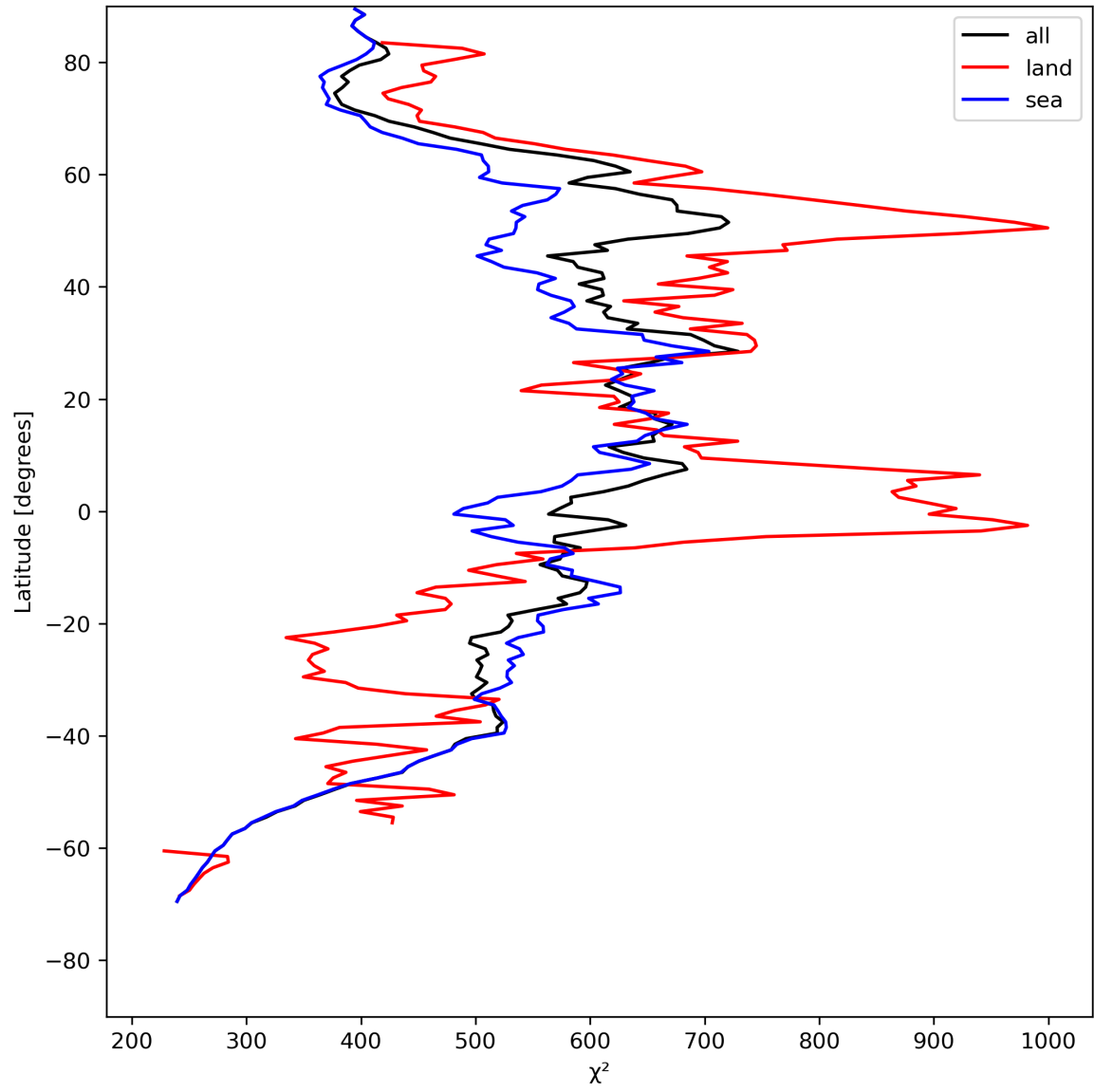
Figure 25: Zonal average of “ \chi^2 ” for 2024-07-27 to 2024-07-29.
