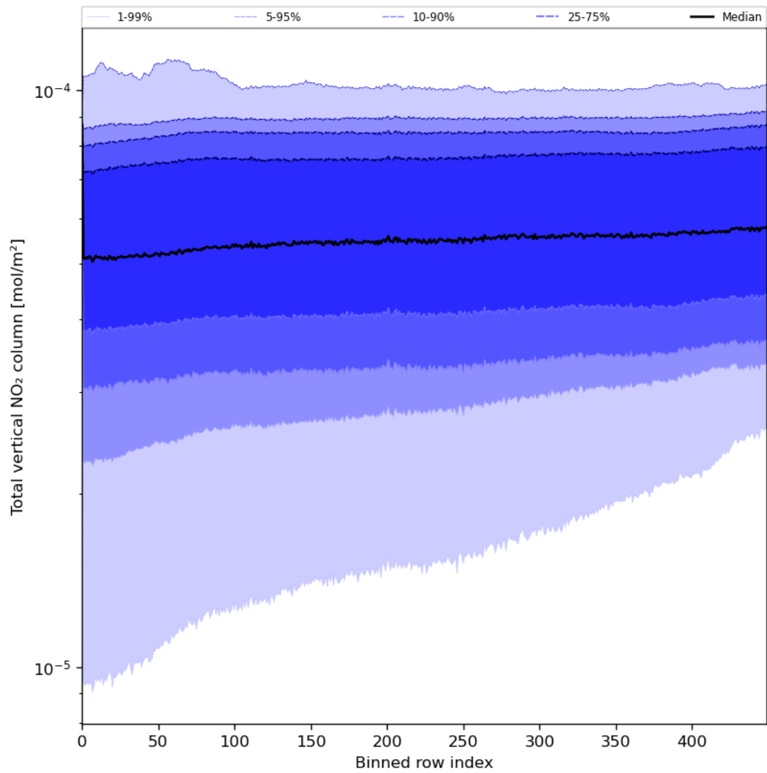
Figure 55: Along track statistics of “Total vertical NO 2 column” for 2024-07-27 to 2024-07-29
