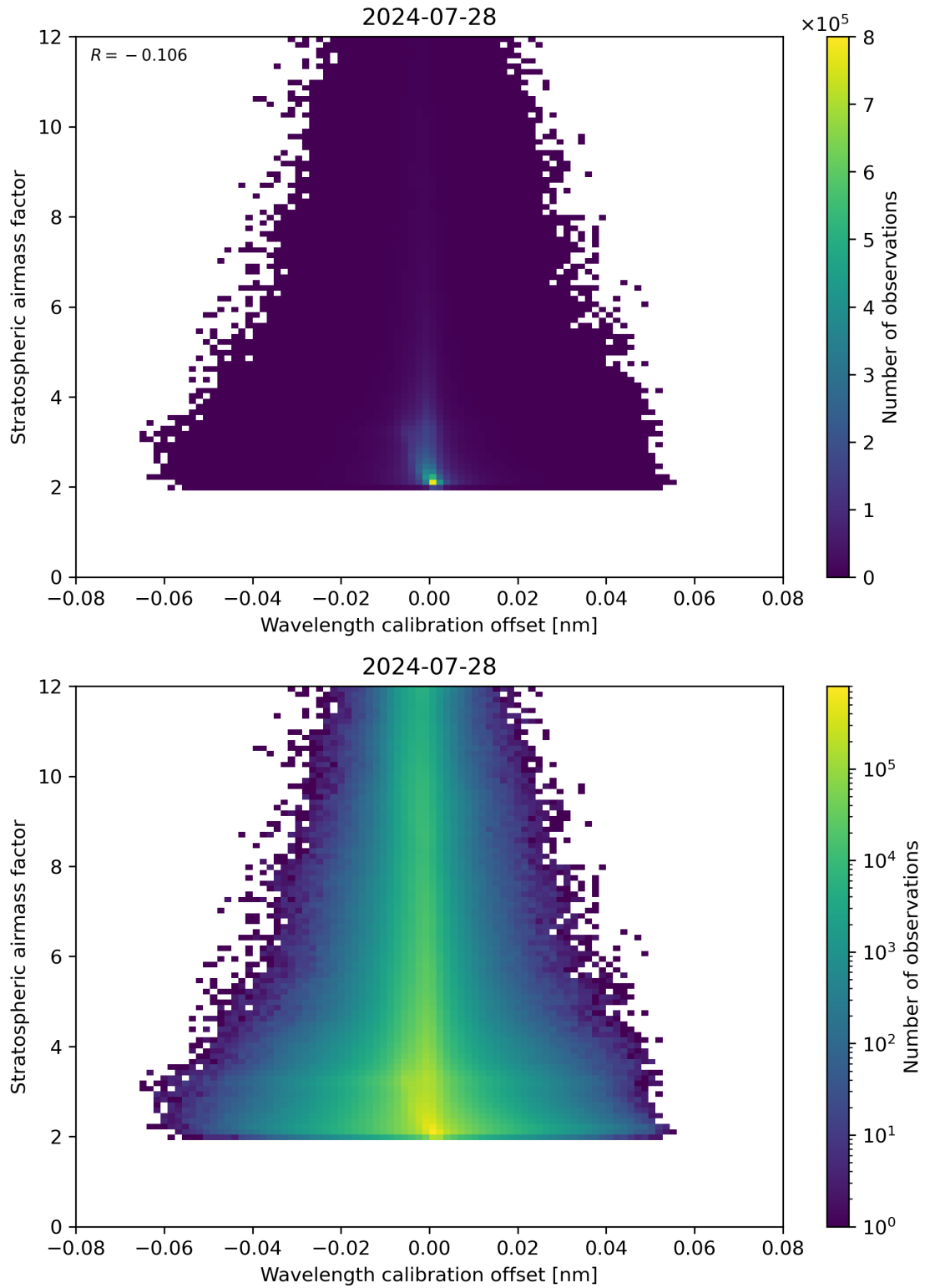
Figure 174: Scatter density plot of “Wavelength calibration offset” against “Stratospheric air mass factor” for 2024-07-27 to 2024-07-29.
