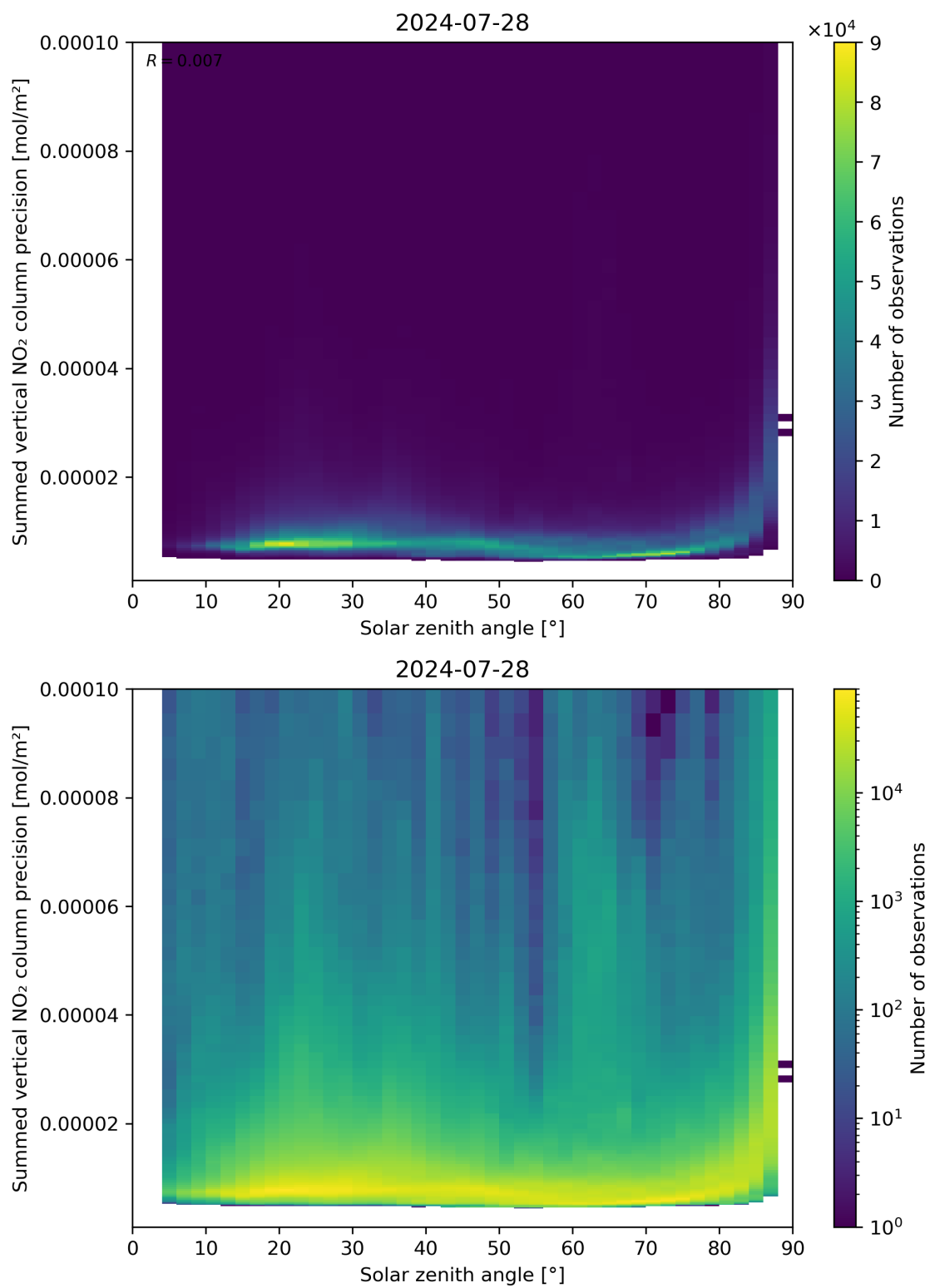
Figure 152: Scatter density plot of “Solar zenith angle” against “Summed vertical NO 2 column precision” for 2024-07-27 to 2024-07-29.
