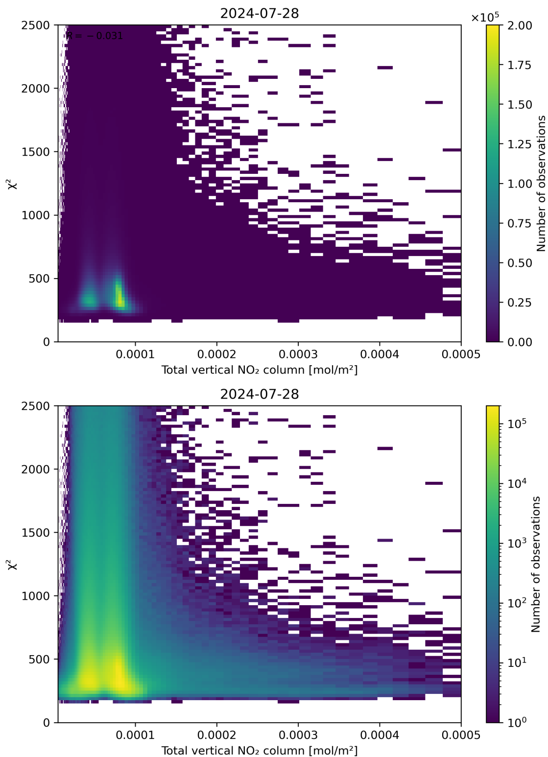
Figure 111: Scatter density plot of “Total vertical NO 2 column” against “ \chi^2 ” for 2024-07-27 to 2024-07-29.
