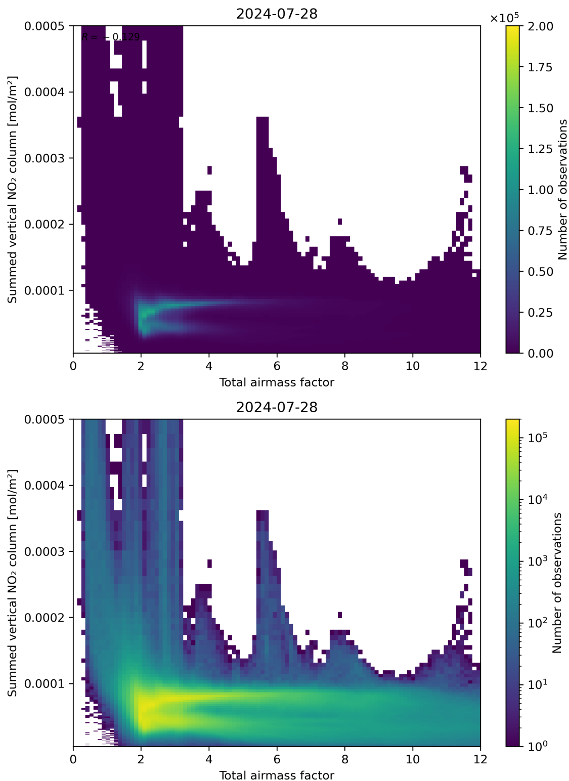
Figure 65: Scatter density plot of “Total airmass factor” against “Summed vertical NO 2 column” for 2024-07-27 to 2024-07-29.
