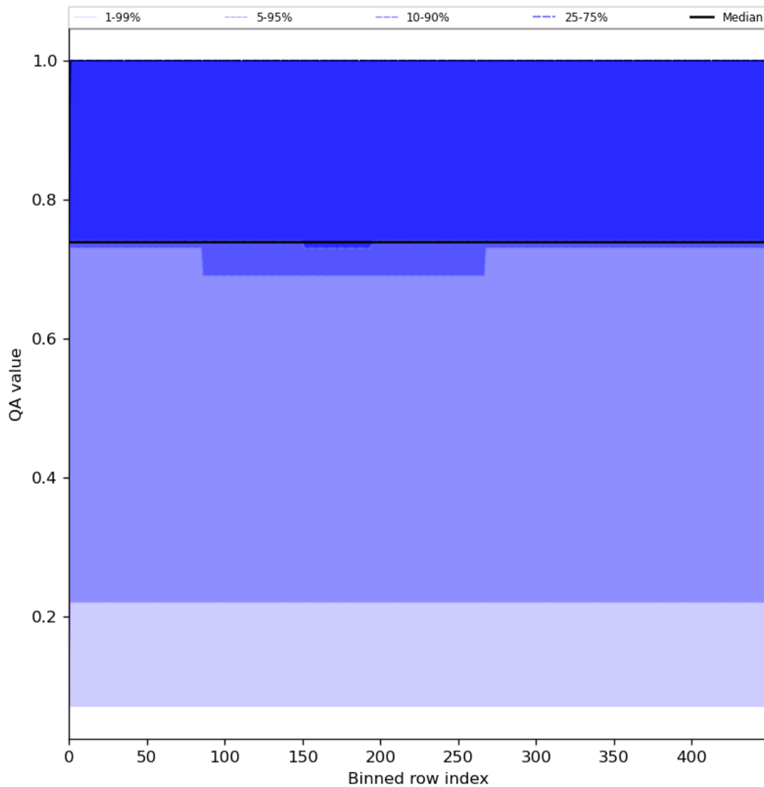
Figure 45: Along track statistics of “QA value” for 2024-07-27 to 2024-07-29
