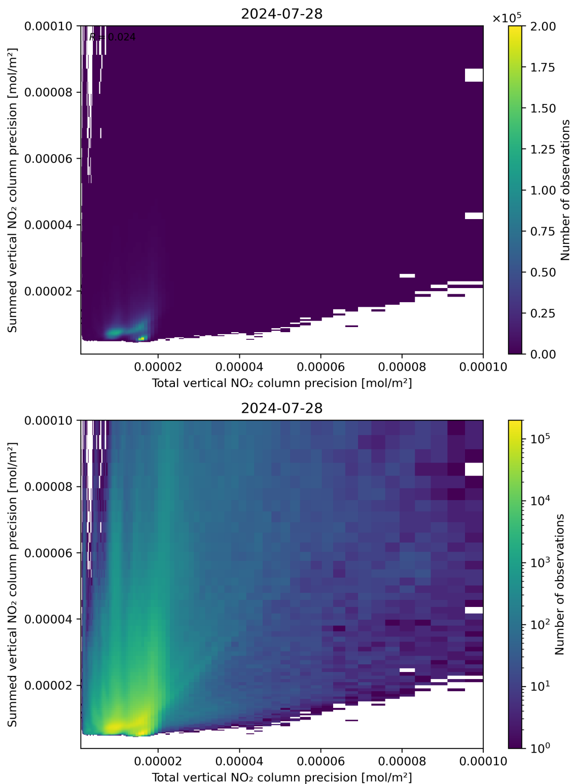
Figure 118: Scatter density plot of “Total vertical NO 2 column precision” against “Summed vertical NO 2 column precision” for 2024-07-27 to 2024-07-29.
