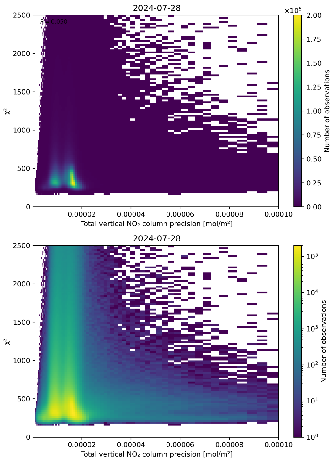
Figure 116: Scatter density plot of “Total vertical NO 2 column precision” against “ \chi^2 ” for 2024-07-27 to 2024-07-29.
