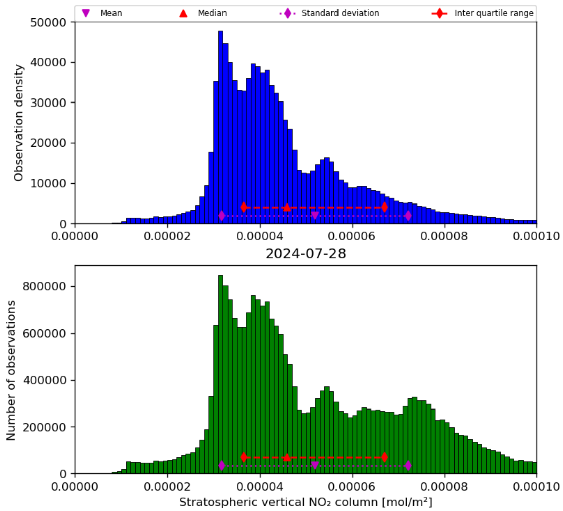
Figure 36: Histogram of “Stratospheric vertical NO 2 column” for 2024-07-27 to 2024-07-29
