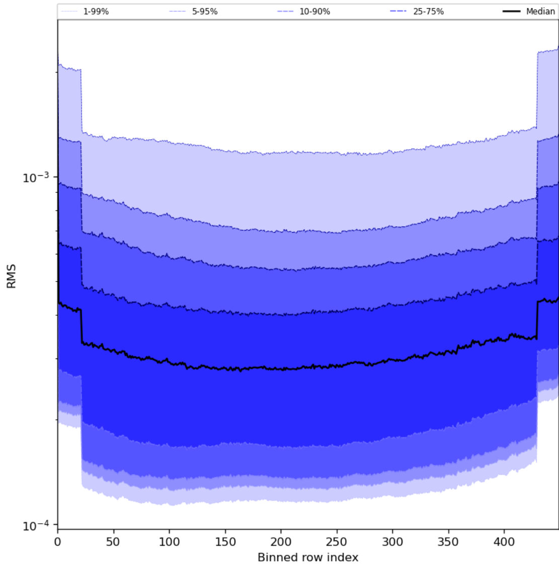
Figure 60: Along track statistics of “RMS” for 2024-07-27 to 2024-07-29
