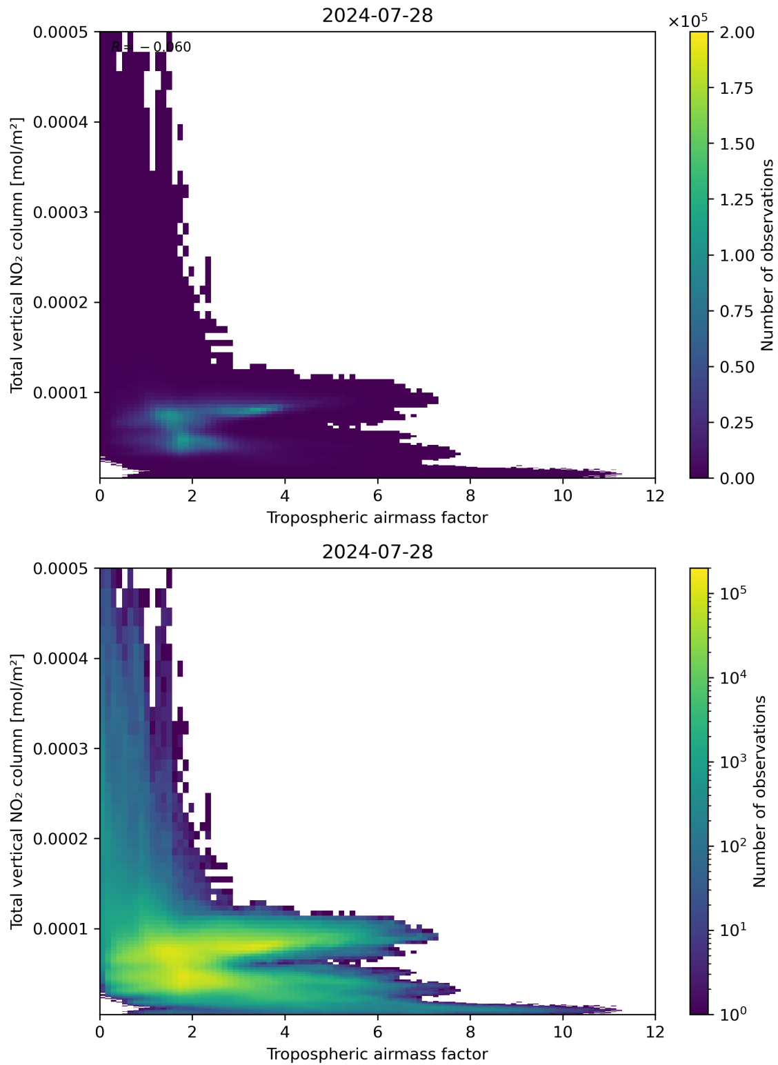
Figure 77: Scatter density plot of “Tropospheric airmass factor” against “Total vertical NO 2 column” for 2024-07-27 to 2024-07-29.
