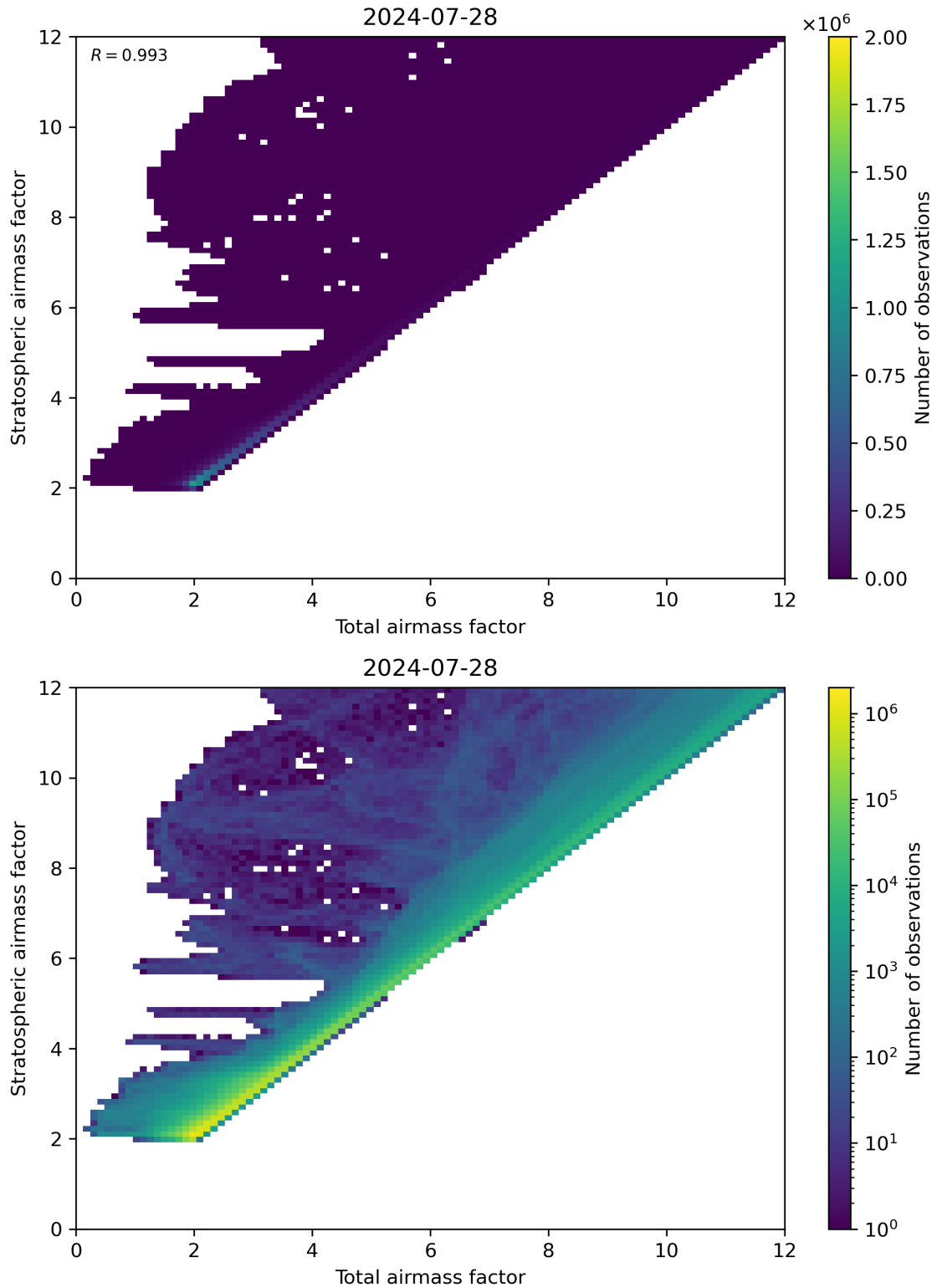
Figure 62: Scatter density plot of “Total airmass factor” against “Stratospheric airmass factor” for 2024-07-27 to 2024-07-29.
