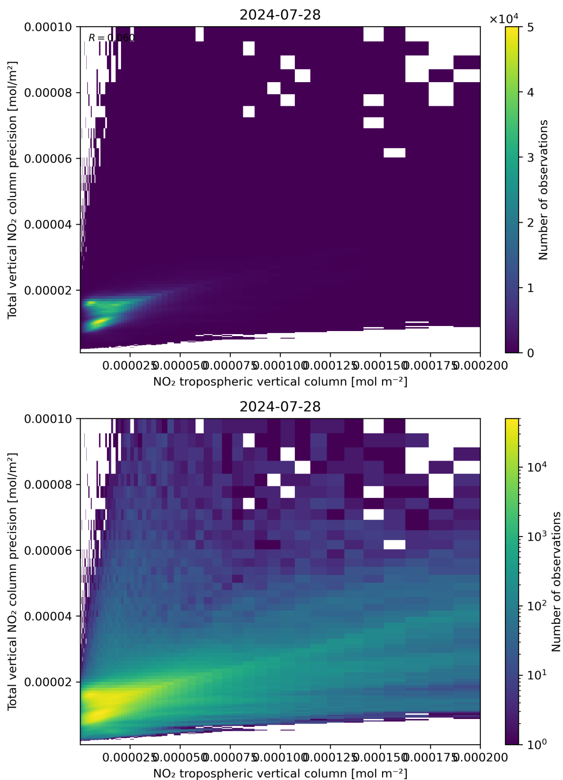
Figure 129: Scatter density plot of “NO 2 tropospheric vertical column” against “Total vertical NO 2 column precision” for 2024-07-27 to 2024-07-29.
