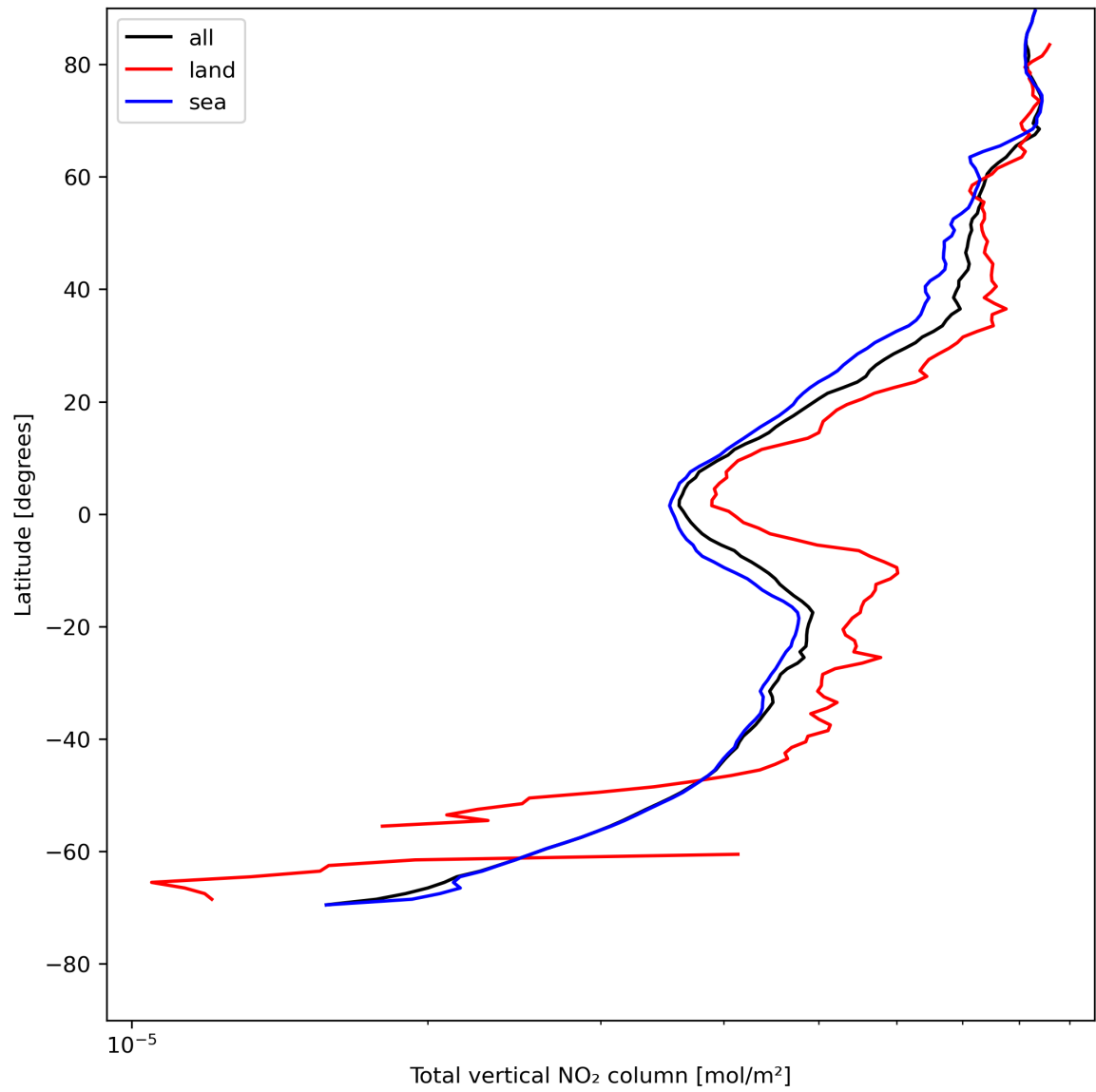
Figure 21: Zonal average of “Total vertical NO 2 column” for 2024-07-27 to 2024-07-29.
