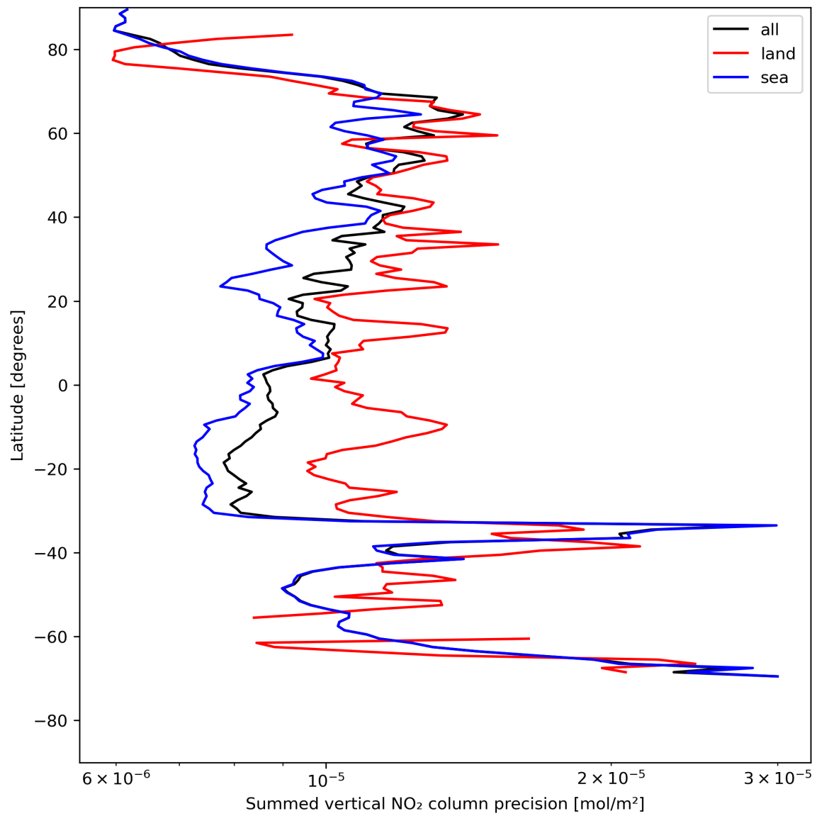
Figure 24: Zonal average of “Summed vertical NO 2 column precision” for 2024-07-27 to 2024-07-29.
