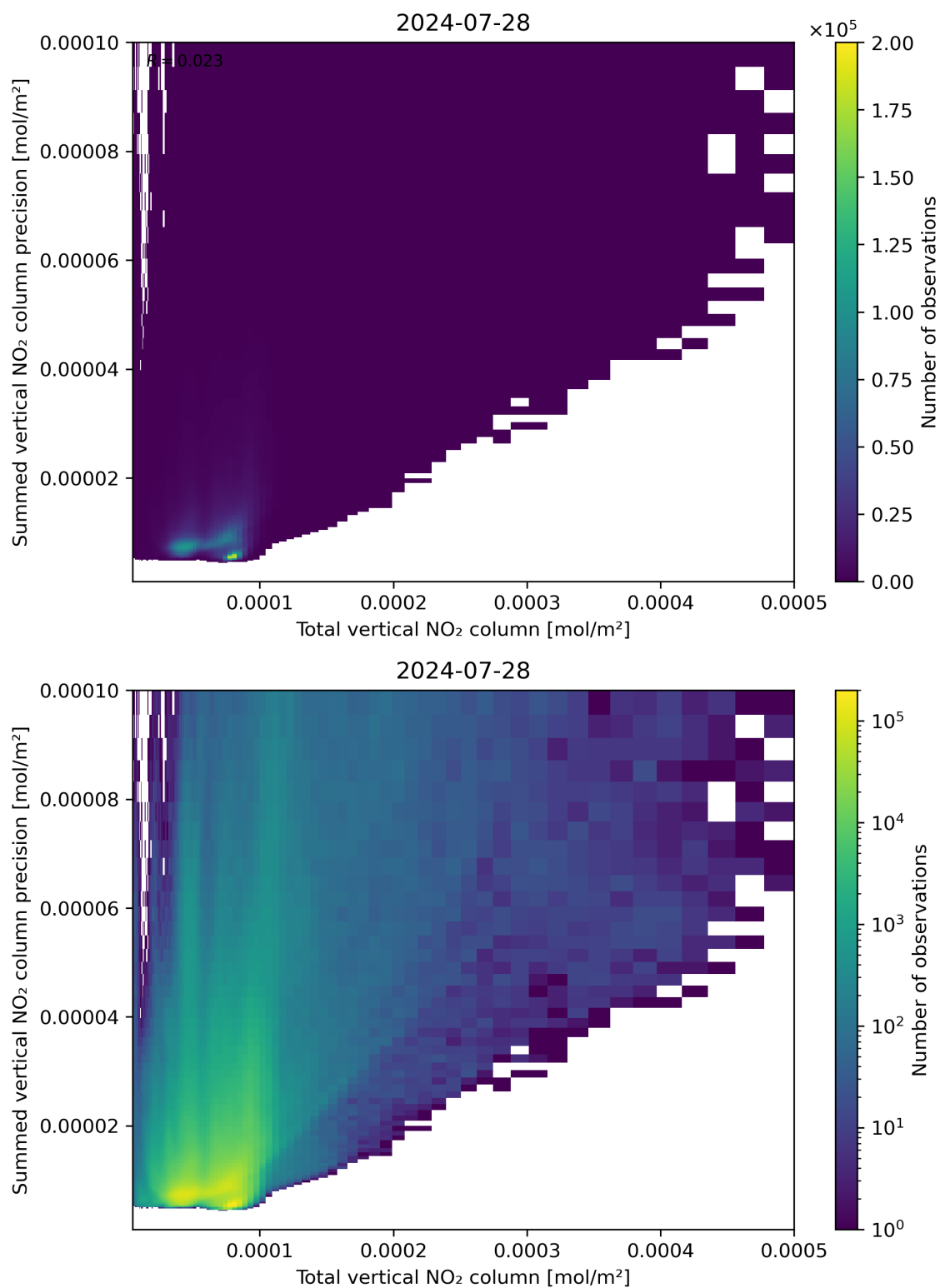
Figure 113: Scatter density plot of “Total vertical NO 2 column” against “Summed vertical NO 2 column precision” for 2024-07-27 to 2024-07-29.
