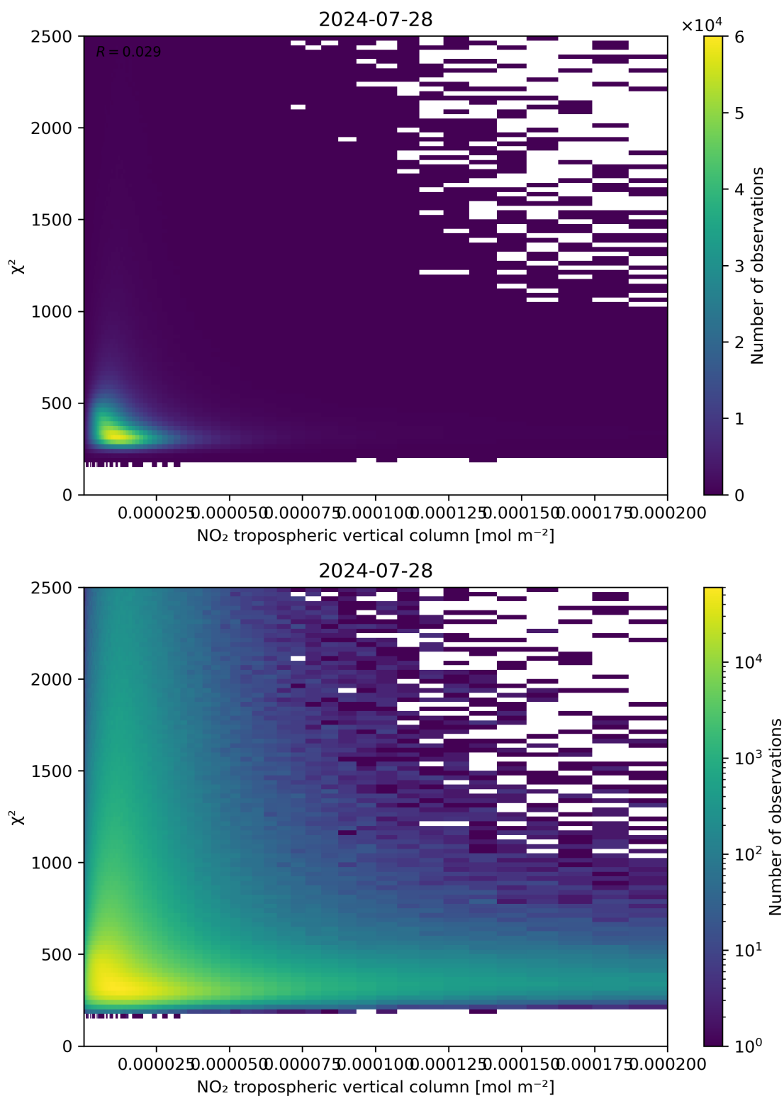
Figure 124: Scatter density plot of “NO 2 tropospheric vertical column” against “ \chi^2 ” for 2024-07-27 to 2024-07-29.
