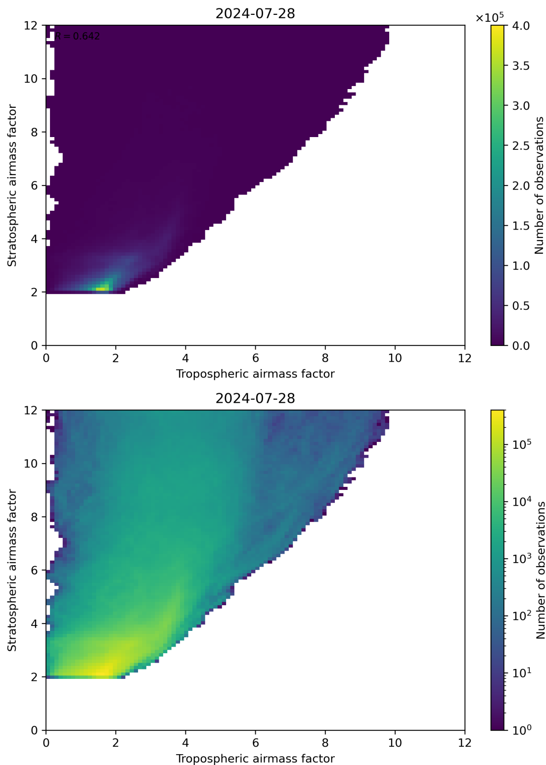
Figure 71: Scatter density plot of “Tropospheric airmass factor” against “Stratospheric airmass factor” for 2024-07-27 to 2024-07-29.
