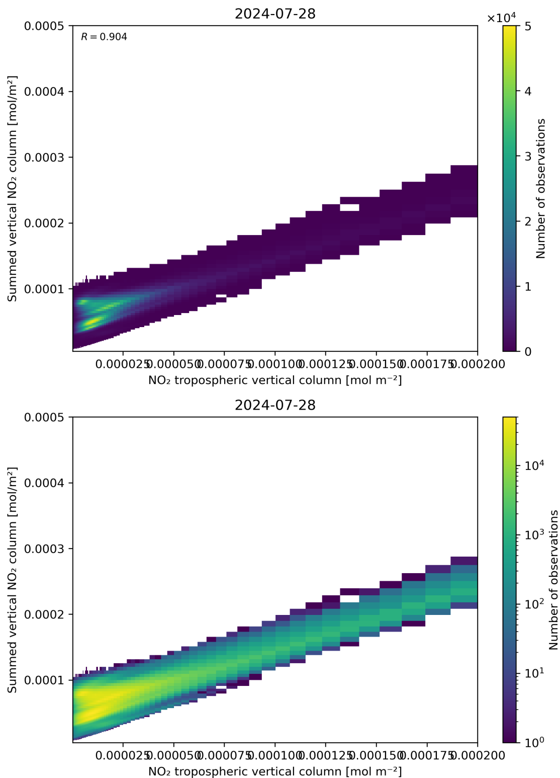
Figure 126: Scatter density plot of “NO 2 tropospheric vertical column” against “Summed vertical NO 2 column” for 2024-07-27 to 2024-07-29.
