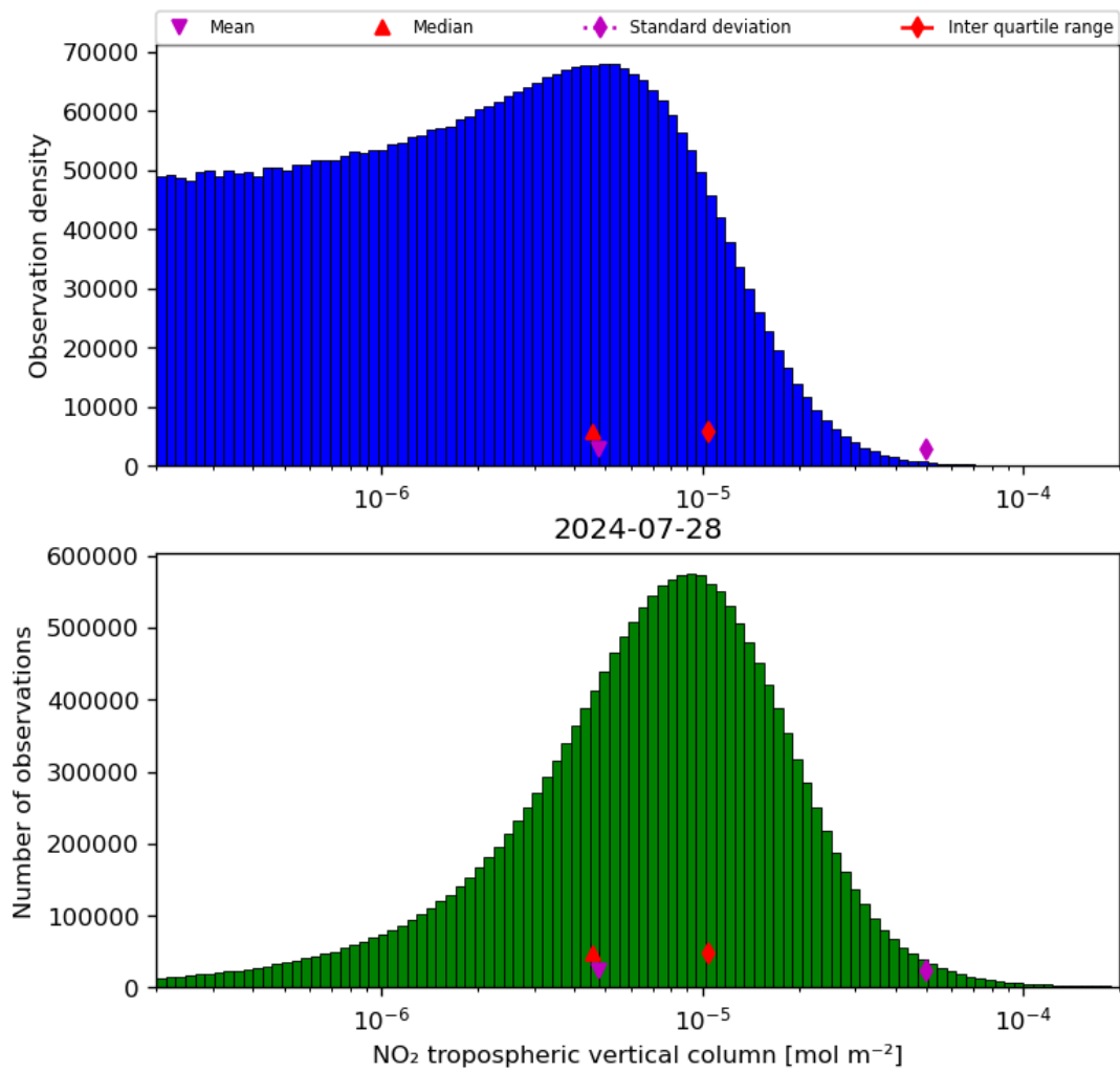
Figure 29: Histogram of “NO 2 tropospheric vertical column” for 2024-07-27 to 2024-07-29
