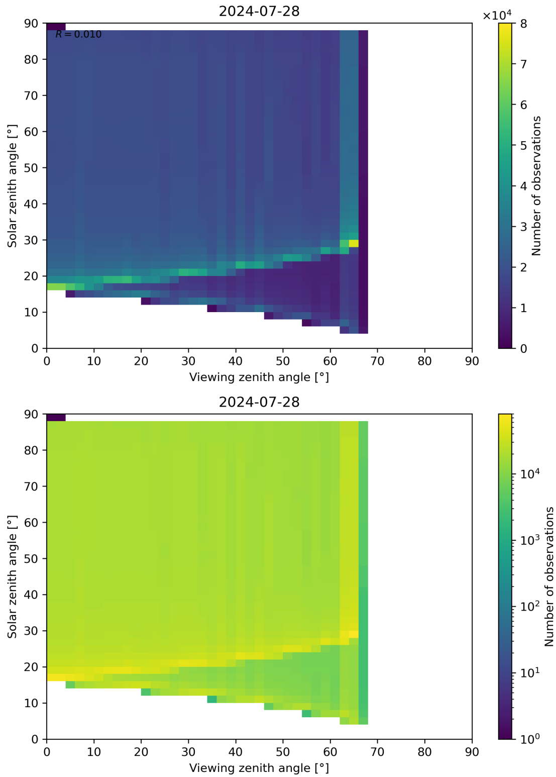
Figure 172: Scatter density plot of “Viewing zenith angle” against “Solar zenith angle” for 2024-07-27 to 2024-07-29.
