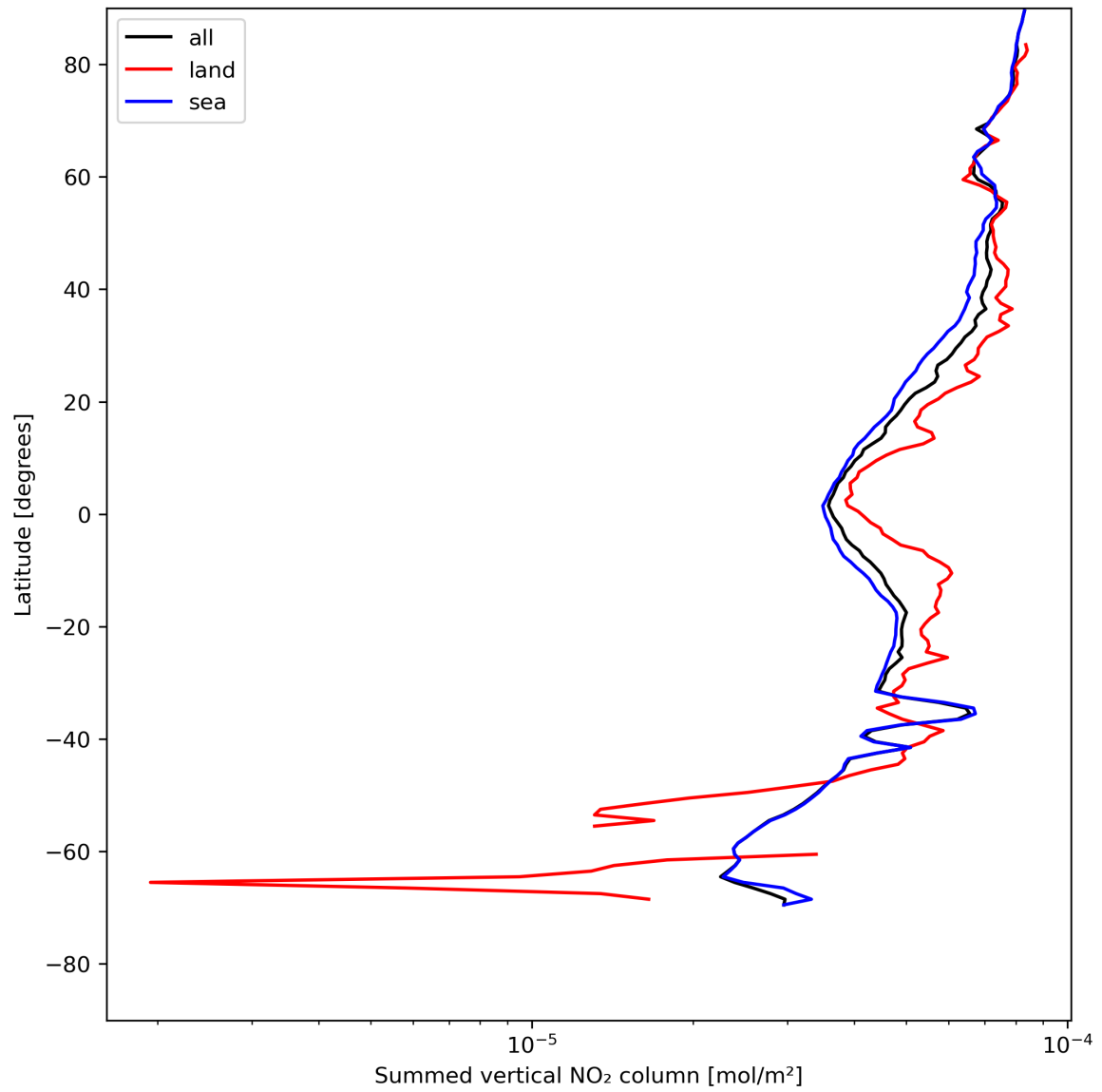
Figure 23: Zonal average of “Summed vertical NO 2 column” for 2024-07-27 to 2024-07-29.
