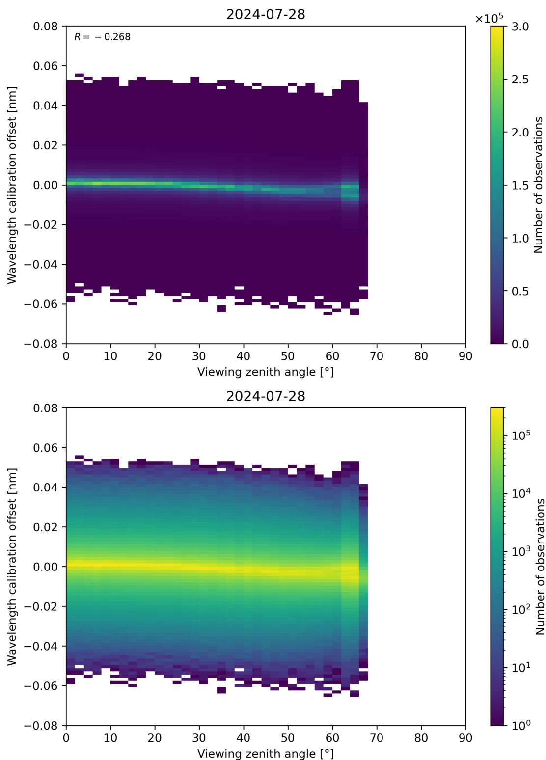
Figure 173: Scatter density plot of “Viewing zenith angle” against “Wavelength calibration offset” for 2024-07-27 to 2024-07-29.
