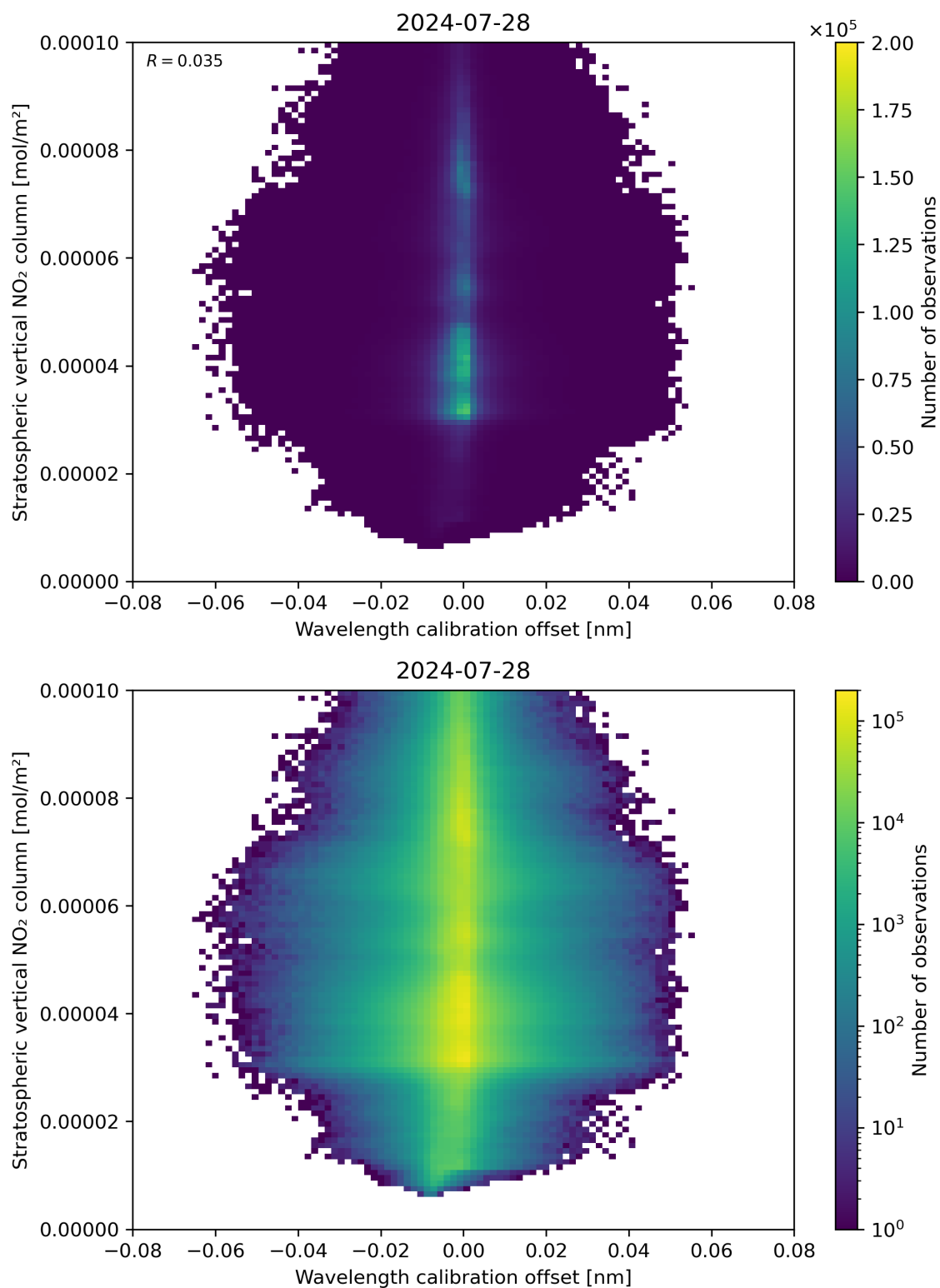
Figure 176: Scatter density plot of “Wavelength calibration offset” against “Stratospheric vertical NO 2 column” for 2024-07-27 to 2024-07-29.
