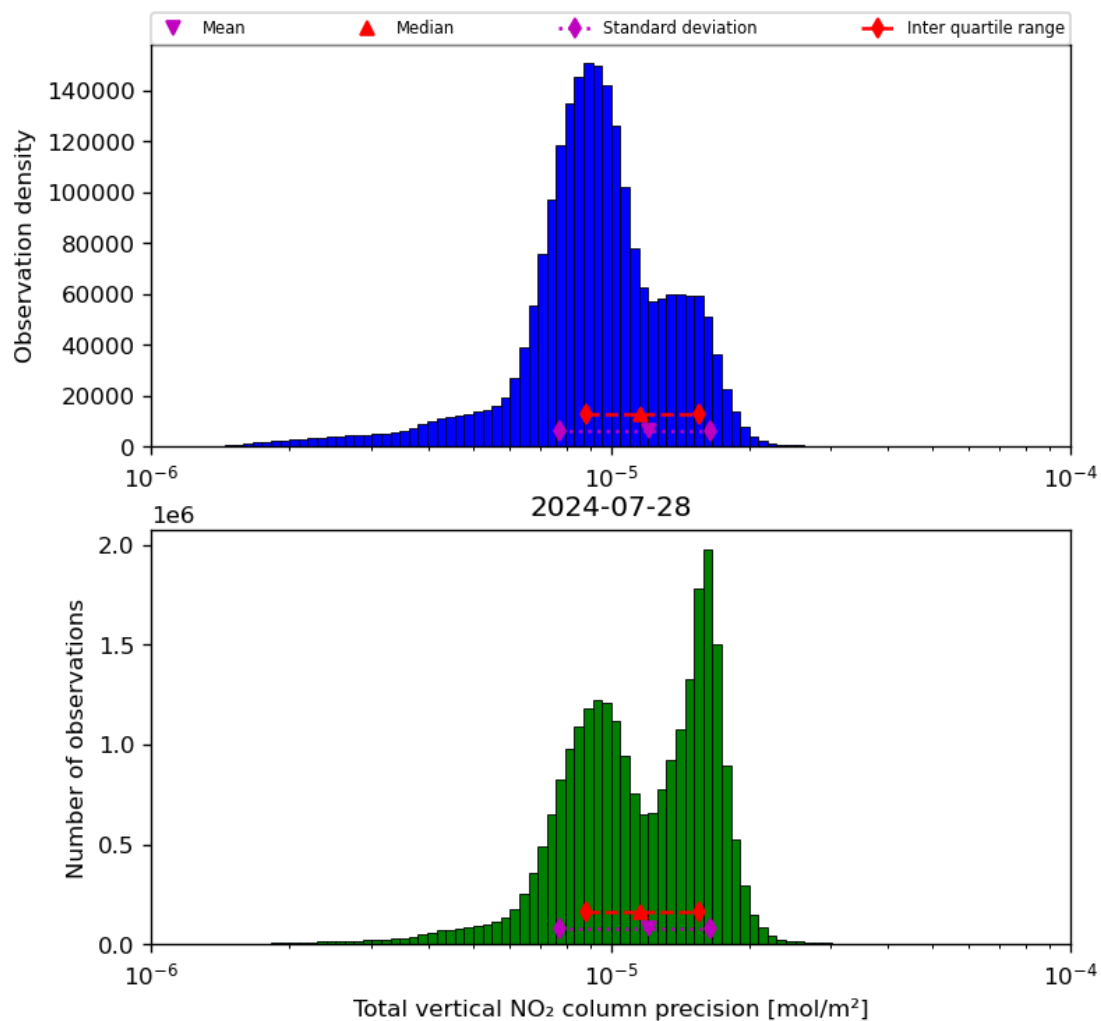
Figure 39: Histogram of “Total vertical NO 2 column precision” for 2024-07-27 to 2024-07-29
