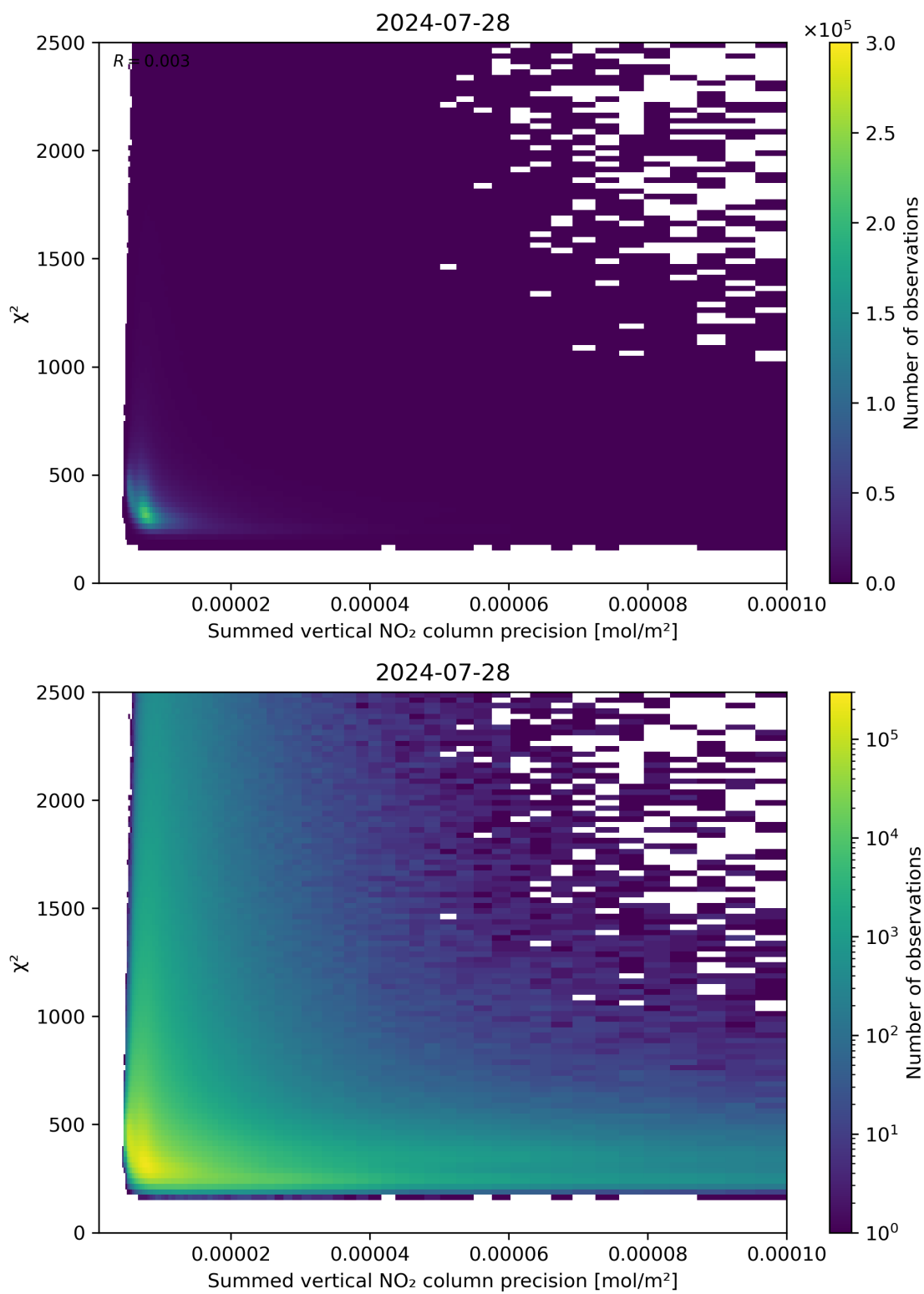
Figure 107: Scatter density plot of “Summed vertical NO 2 column precision” against “ \chi^2 ” for 2024-07-27 to 2024-07-29.
