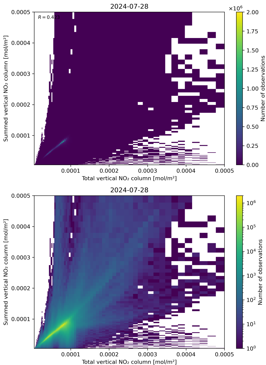
Figure 112: Scatter density plot of “Total vertical NO 2 column” against “Summed vertical NO 2 column” for 2024-07-27 to 2024-07-29.
