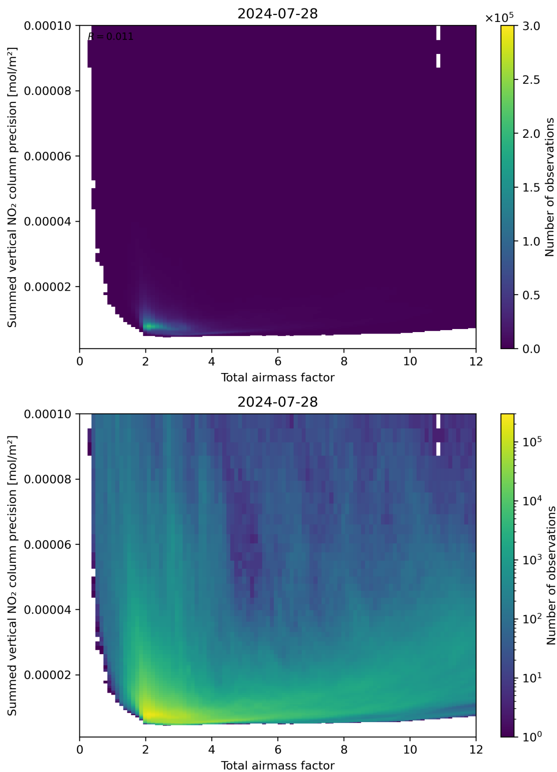
Figure 66: Scatter density plot of “Total airmass factor” against “Summed vertical NO 2 column precision” for 2024-07-27 to 2024-07-29.
