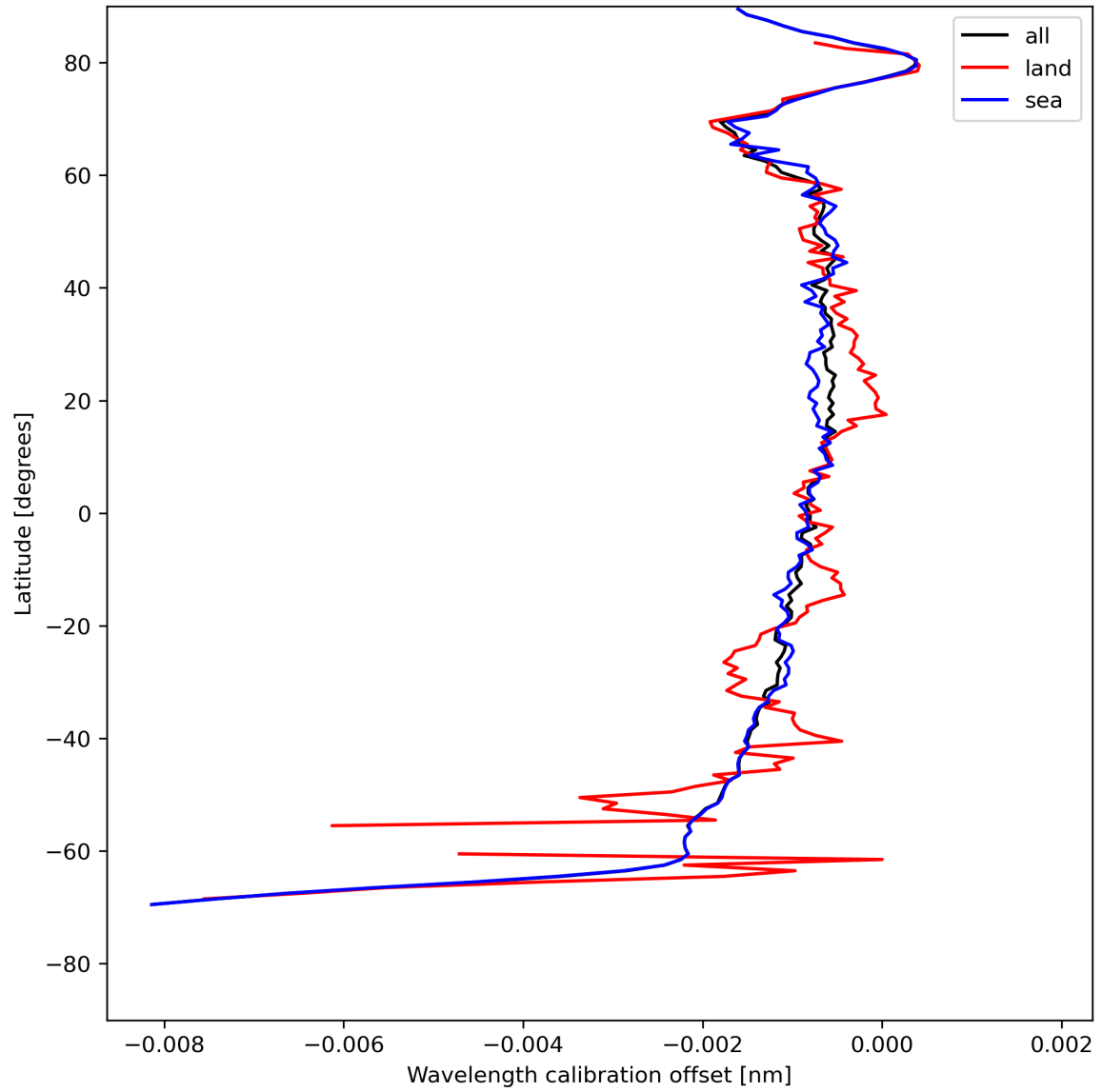
Figure 18: Zonal average of “Wavelength calibration offset” for 2024-07-27 to 2024-07-29.
