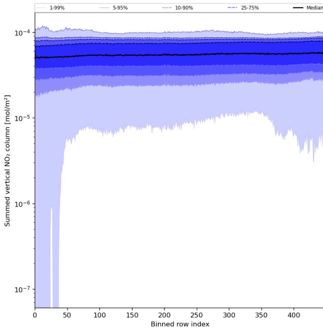
Figure 57: Along track statistics of “Summed vertical NO 2 column” for 2024-07-27 to 2024-07-29
