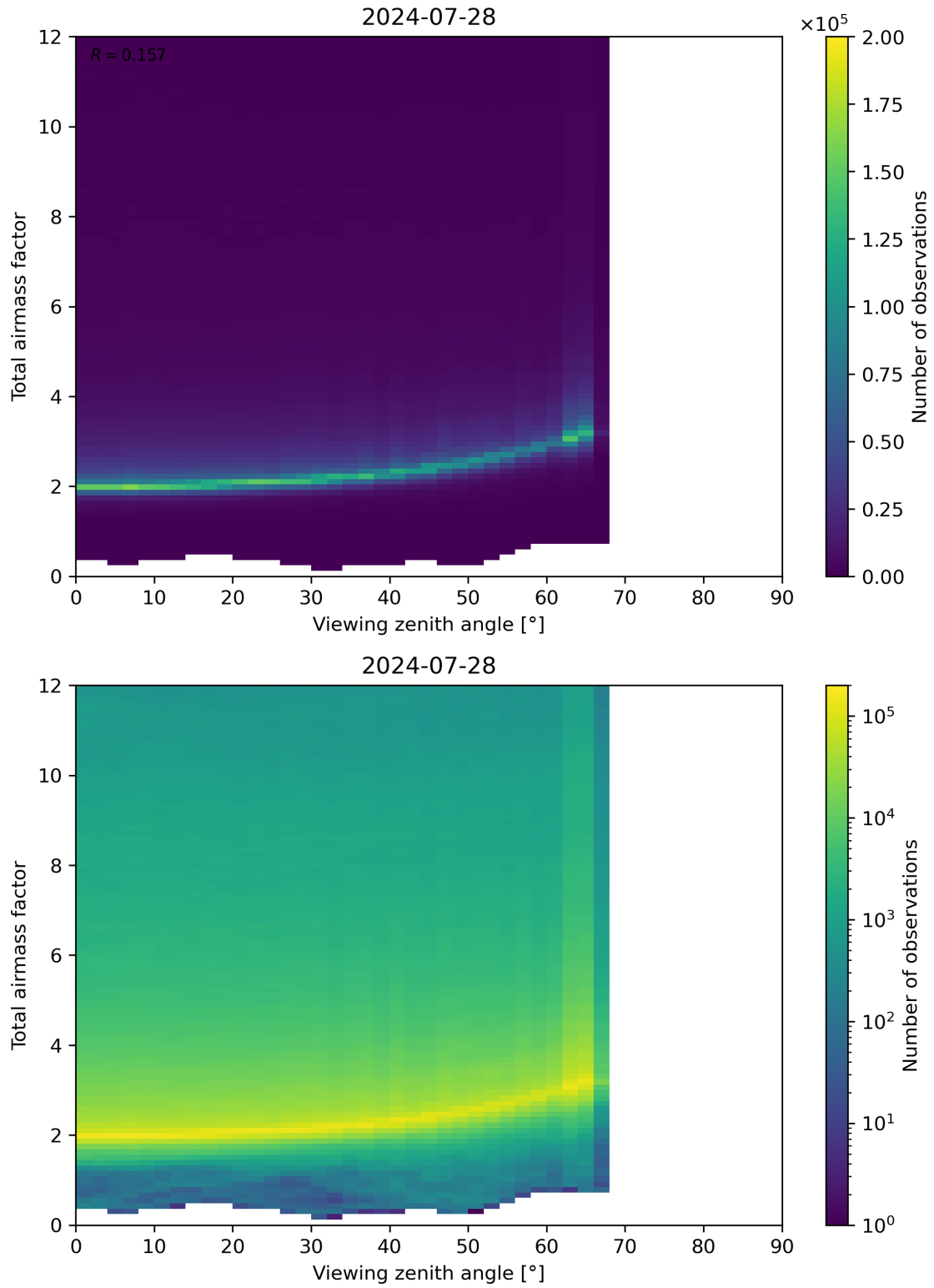
Figure 160: Scatter density plot of “Viewing zenith angle” against “Total airmass factor” for 2024-07-27 to 2024-07-29.
