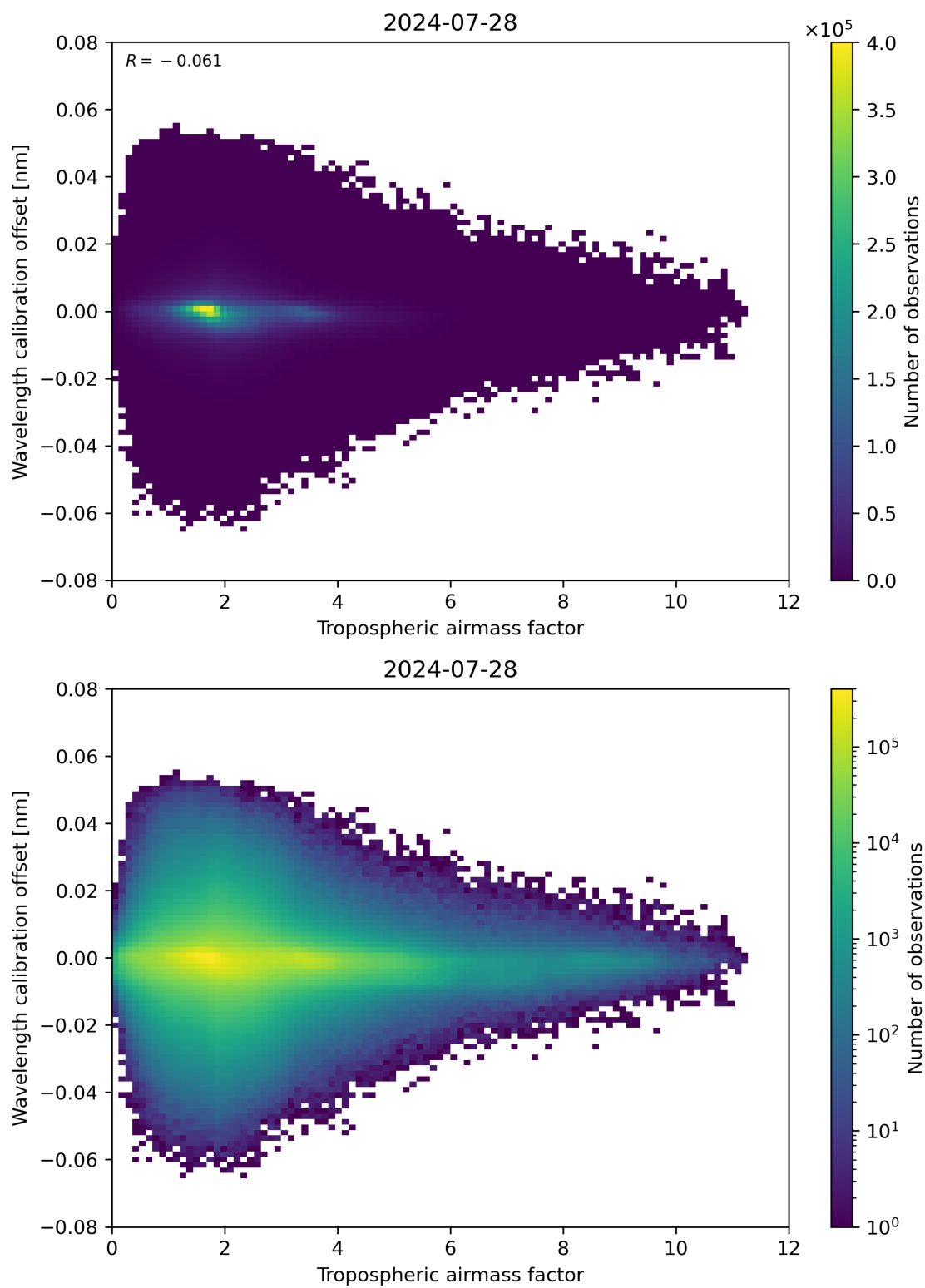
Figure 80: Scatter density plot of “Tropospheric airmass factor” against “Wavelength calibration offset” for 2024-07-27 to 2024-07-29.
