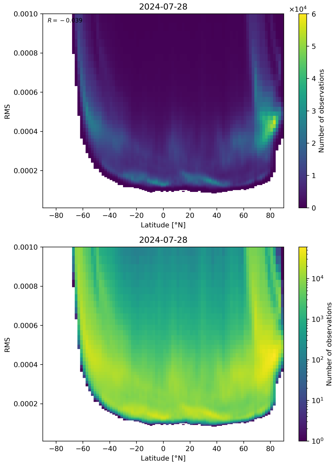
Figure 94: Scatter density plot of “Latitude” against “RMS” for 2024-07-27 to 2024-07-29.
