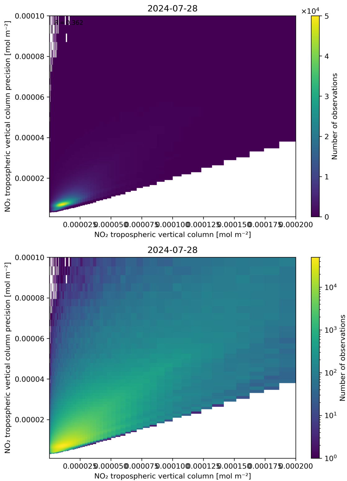
Figure 130: Scatter density plot of “NO 2 tropospheric vertical column” against “NO 2 tropospheric vertical column precision” for 2024-07-27 to 2024-07-29.
