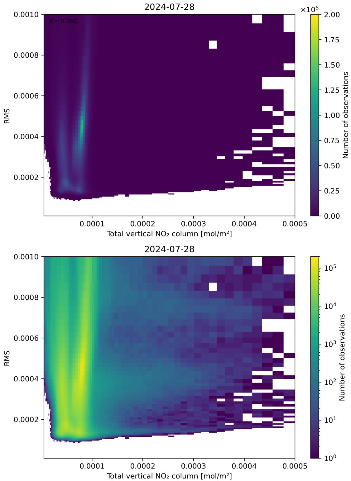
Figure 120: Scatter density plot of “Total vertical NO 2 column” against “RMS” for 2024-07-27 to 2024-07-29.
