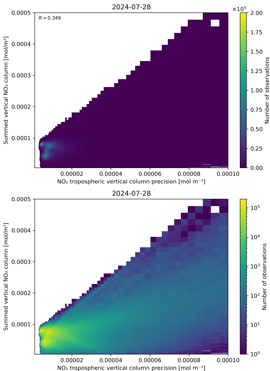
Figure 136: Scatter density plot of “NO 2 tropospheric vertical column precision” against “Summed vertical NO 2 column” for 2024-07-27 to 2024-07-29.
