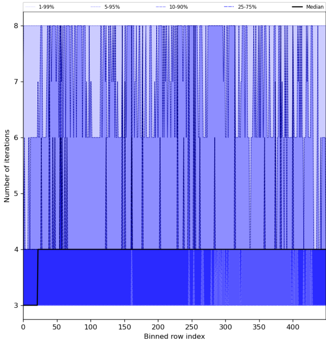
Figure 51: Along track statistics of “Number of iterations” for 2024-07-27 to 2024-07-29
