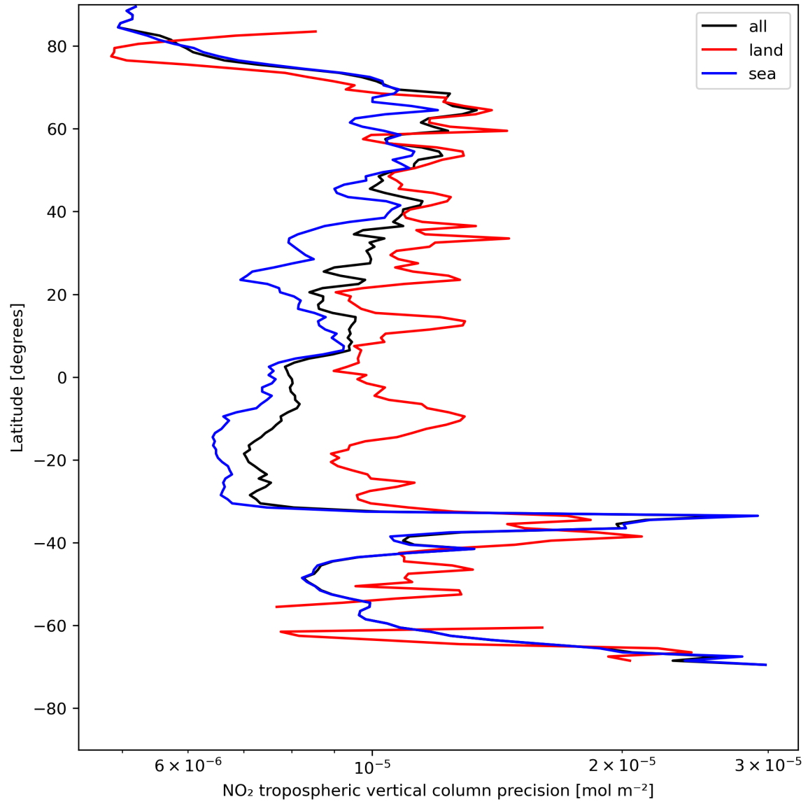
Figure 13: Zonal average of “NO 2 tropospheric vertical column precision” for 2024-07-27 to 2024-07-29.
