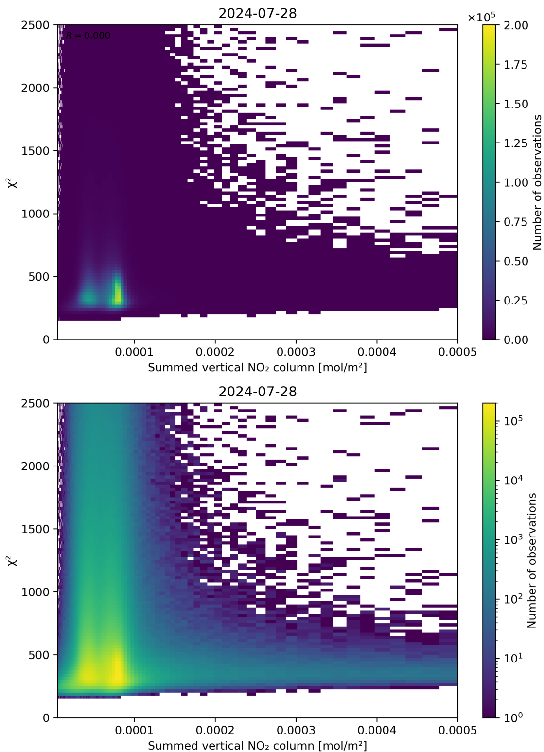
Figure 104: Scatter density plot of “Summed vertical NO 2 column” against “ \chi^2 ” for 2024-07-27 to 2024-07-29.
