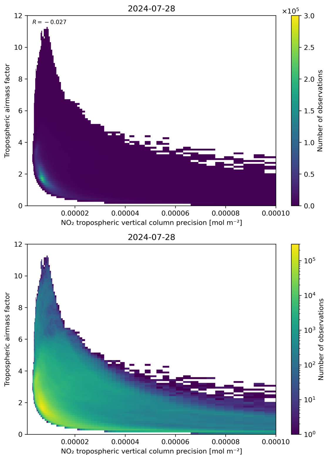
Figure 133: Scatter density plot of “NO 2 tropospheric vertical column precision” against “Tropospheric airmass factor” for 2024-07-27 to 2024-07-29.
