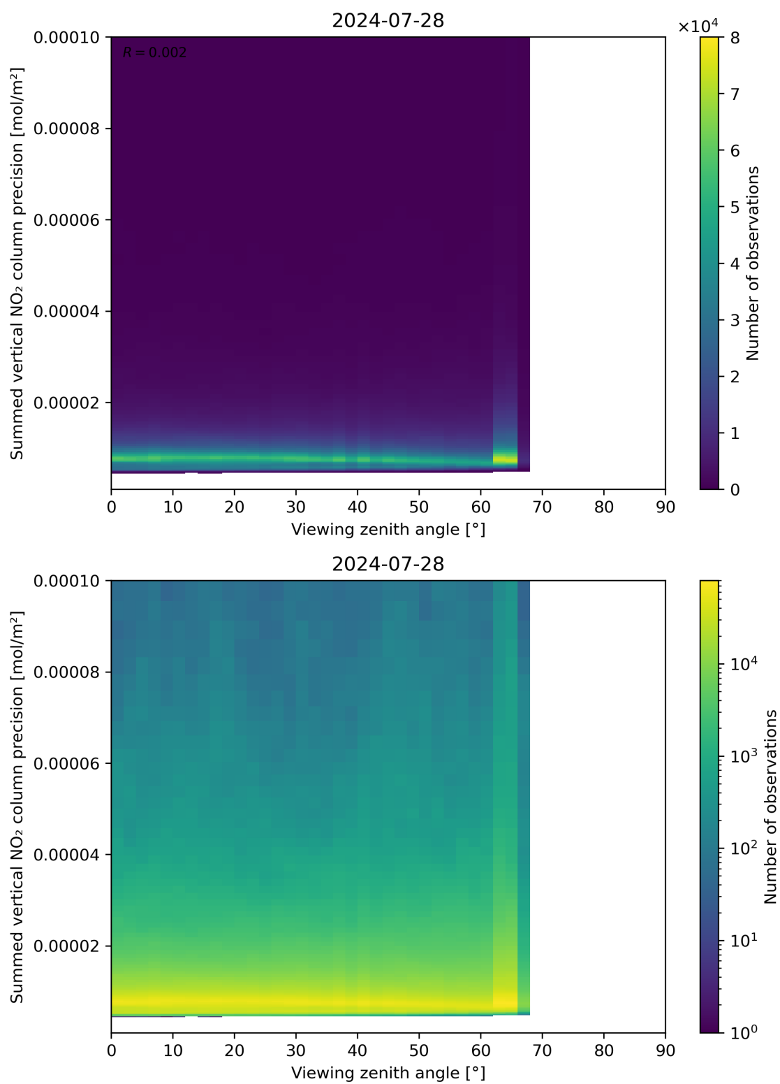
Figure 166: Scatter density plot of “Viewing zenith angle” against “Summed vertical NO 2 column precision” for 2024-07-27 to 2024-07-29.
