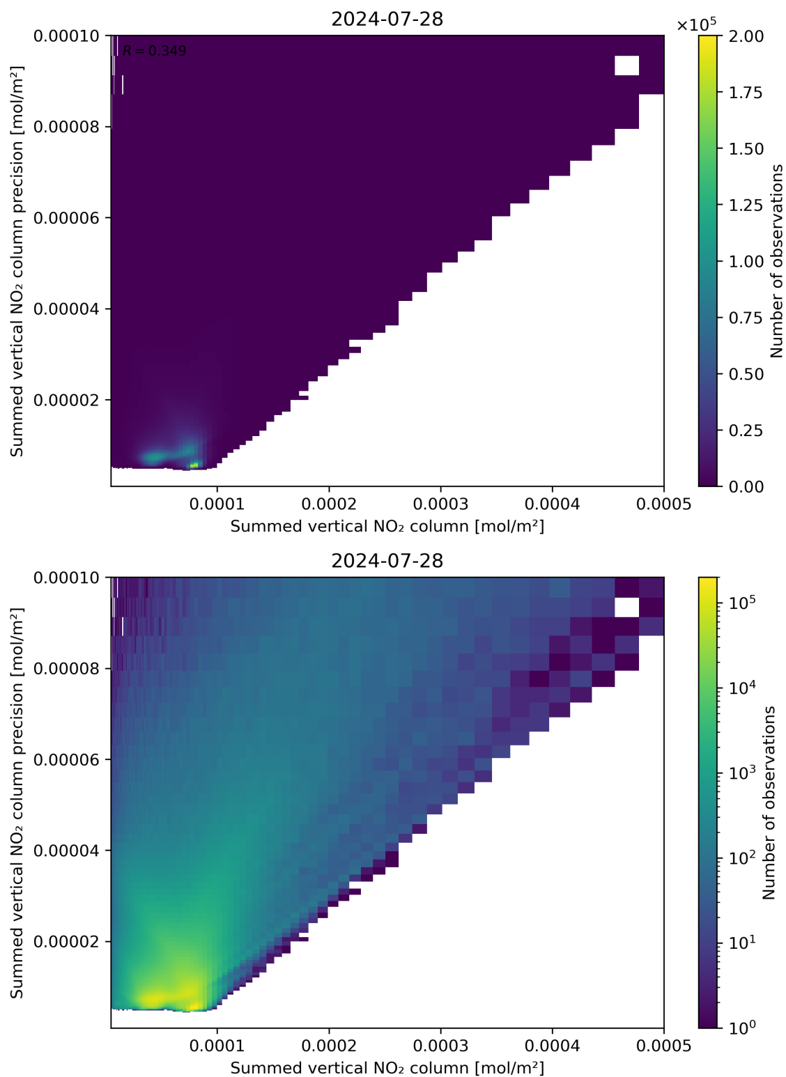
Figure 105: Scatter density plot of “Summed vertical NO 2 column” against “Summed vertical NO 2 column precision” for 2024-07-27 to 2024-07-29.
