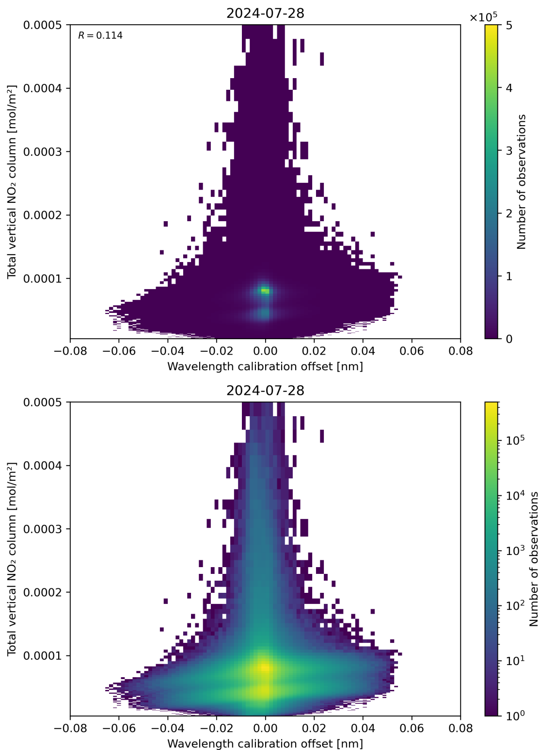
Figure 179: Scatter density plot of “Wavelength calibration offset” against “Total vertical NO 2 column” for 2024-07-27 to 2024-07-29.
