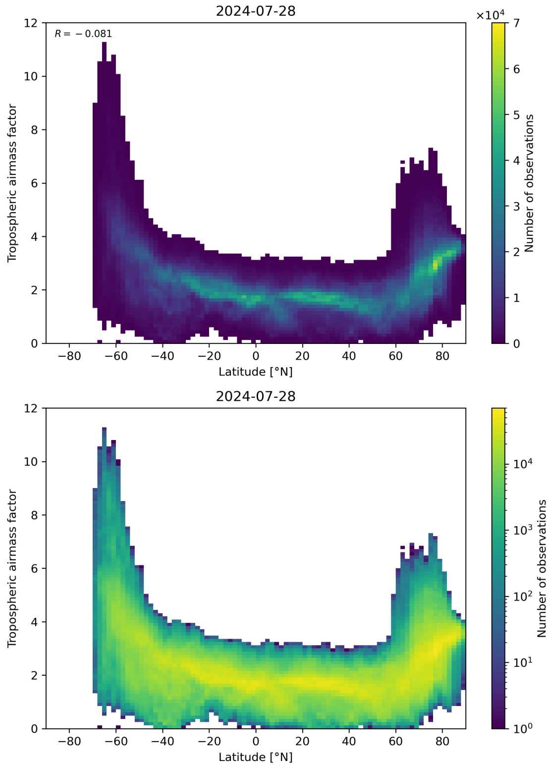
Figure 85: Scatter density plot of “Latitude” against “Tropospheric airmass factor” for 2024-07-27 to 2024-07-29.
