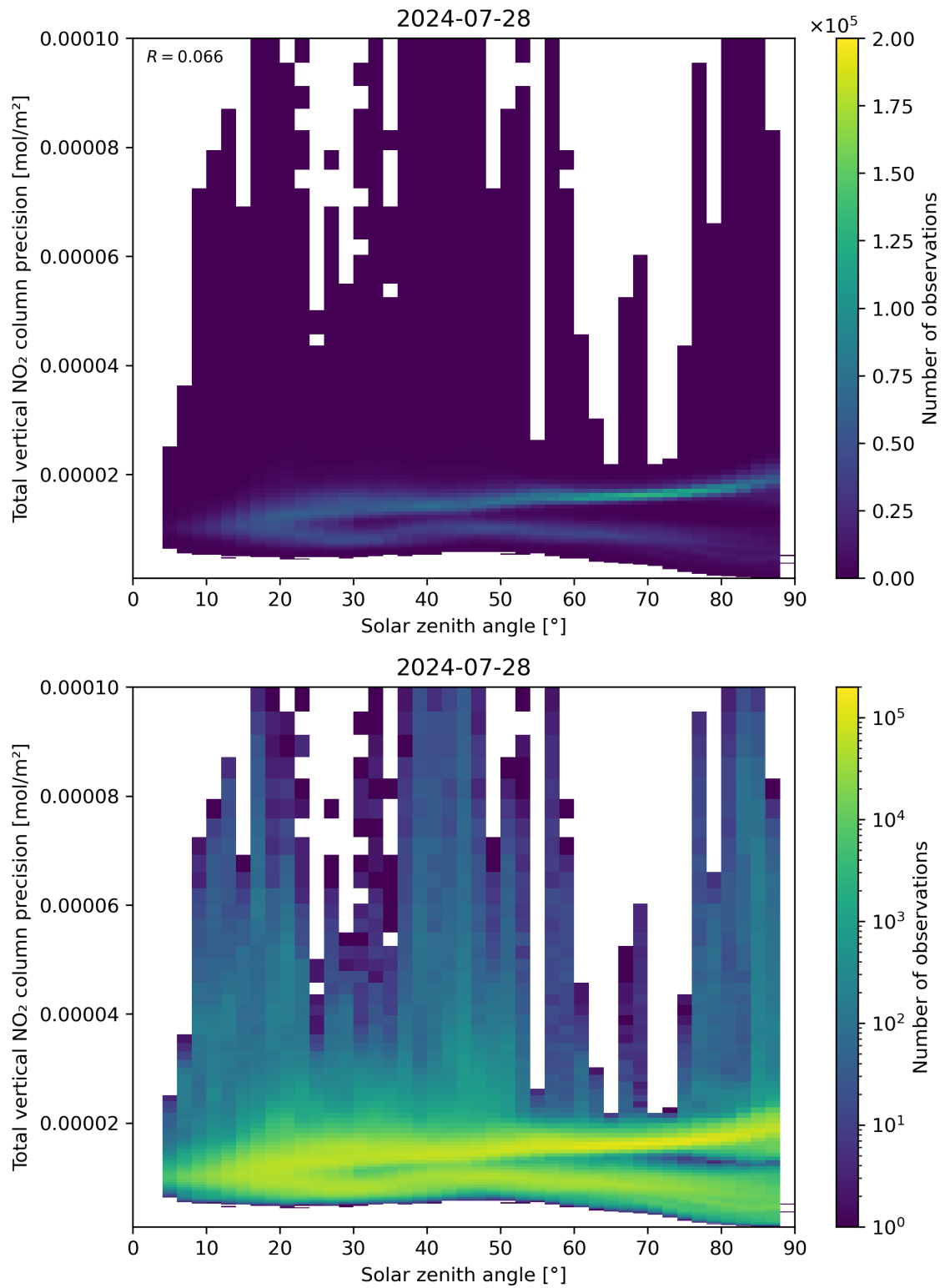
Figure 154: Scatter density plot of “Solar zenith angle” against “Total vertical NO 2 column precision” for 2024-07-27 to 2024-07-29.
