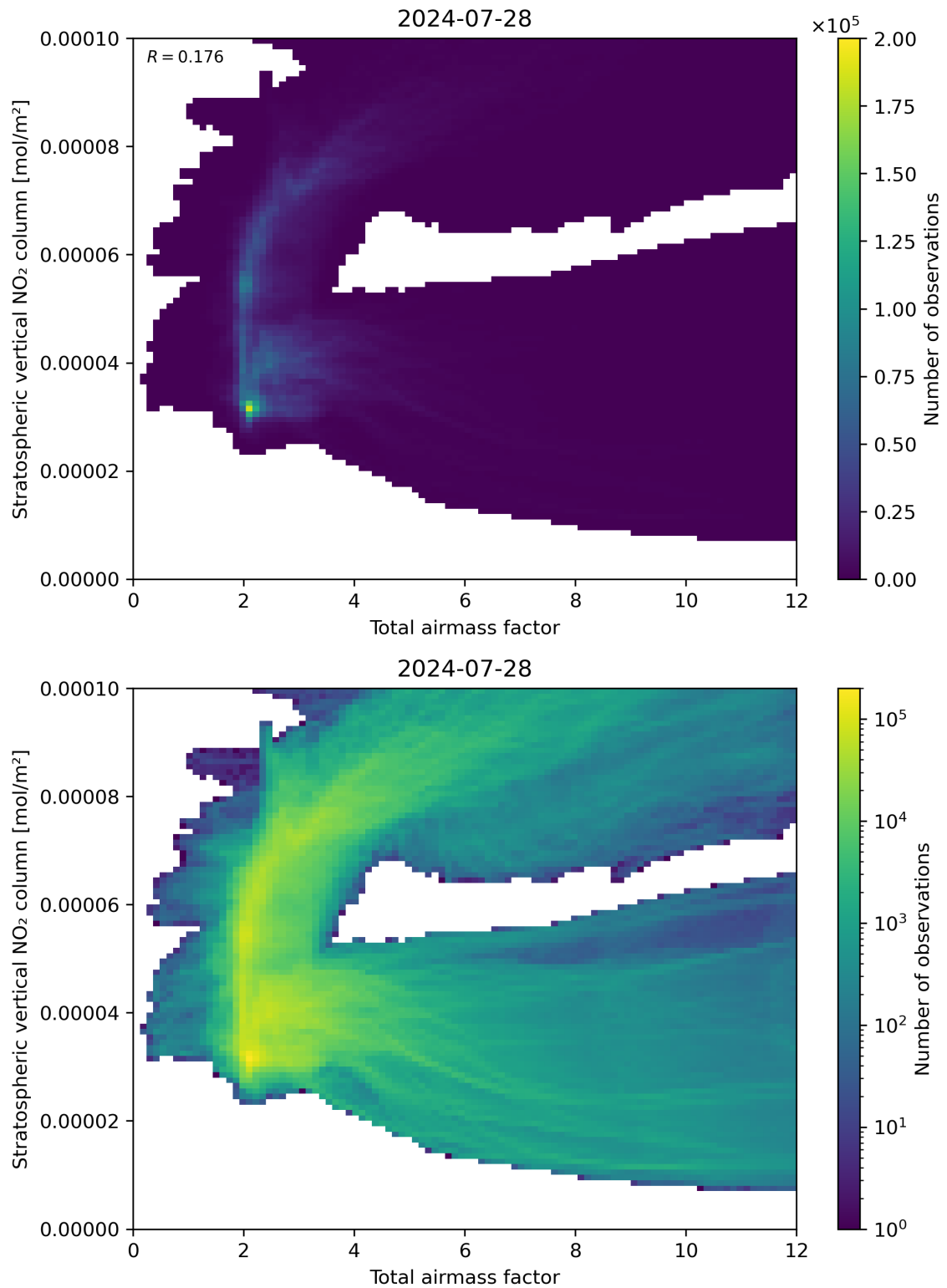
Figure 64: Scatter density plot of “Total airmass factor” against “Stratospheric vertical NO 2 column” for 2024-07-27 to 2024-07-29.
