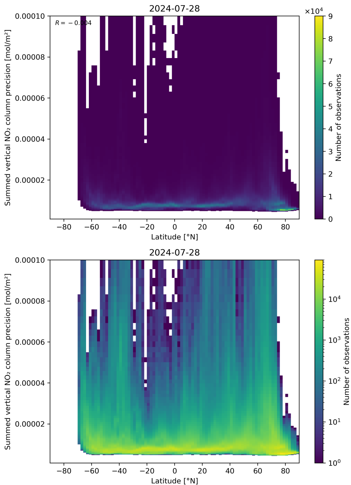
Figure 89: Scatter density plot of “Latitude” against “Summed vertical NO 2 column precision” for 2024-07-27 to 2024-07-29.
