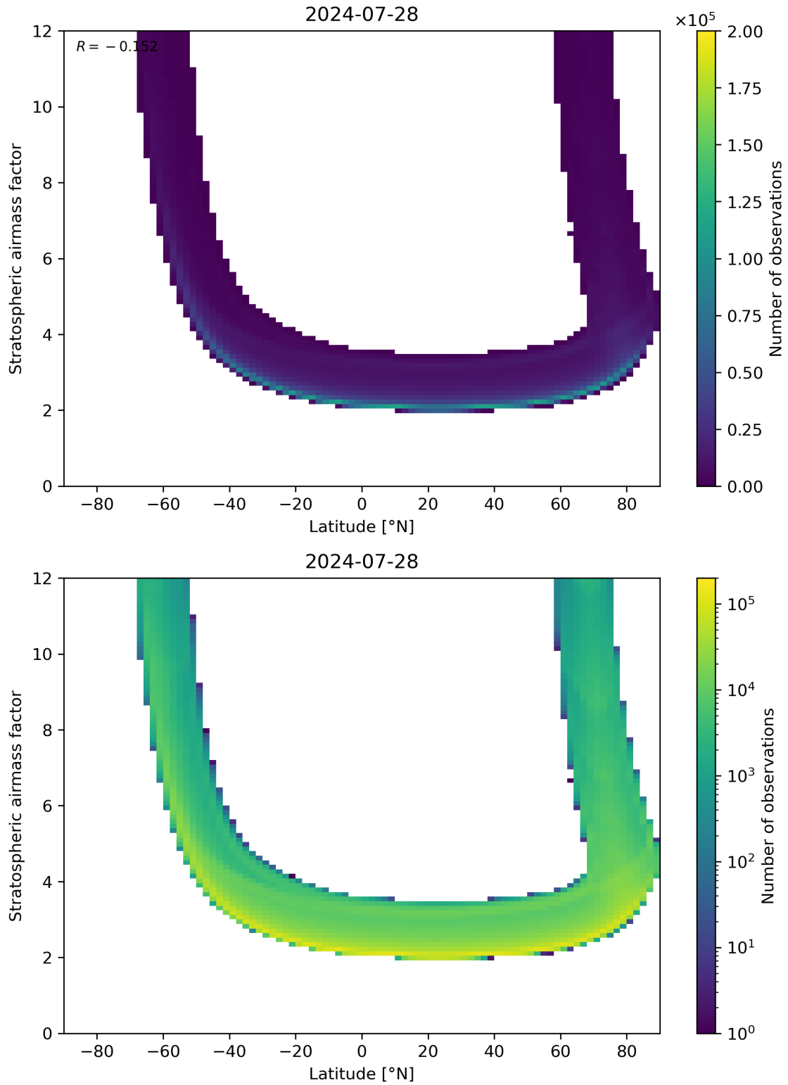
Figure 83: Scatter density plot of “Latitude” against “Stratospheric airmass factor” for 2024-07-27 to 2024-07-29.
