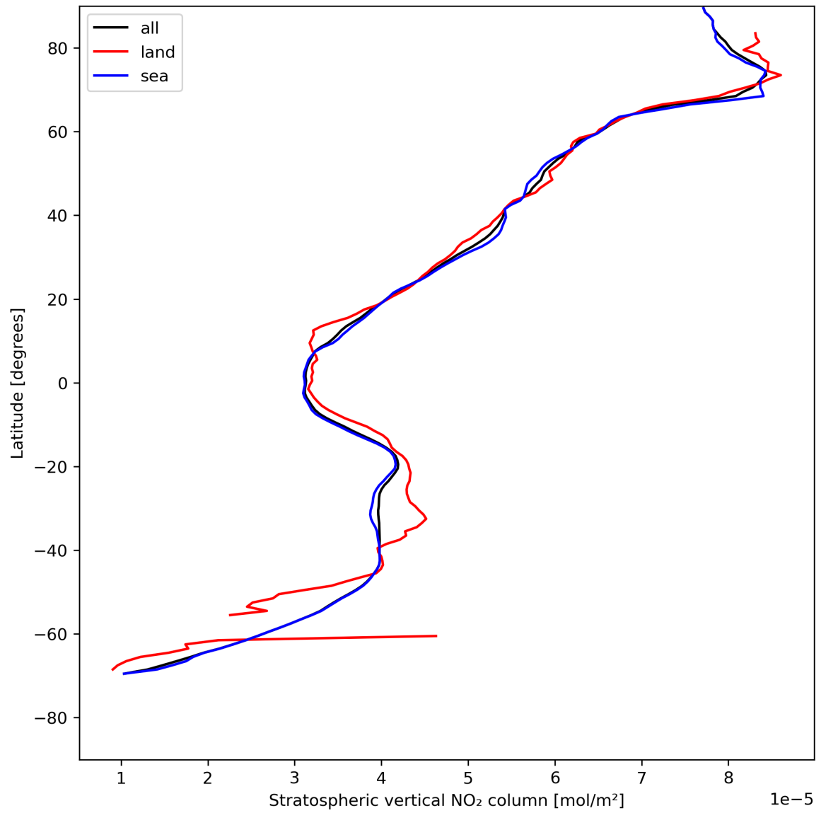
Figure 19: Zonal average of “Stratospheric vertical NO 2 column” for 2024-07-27 to 2024-07-29.
