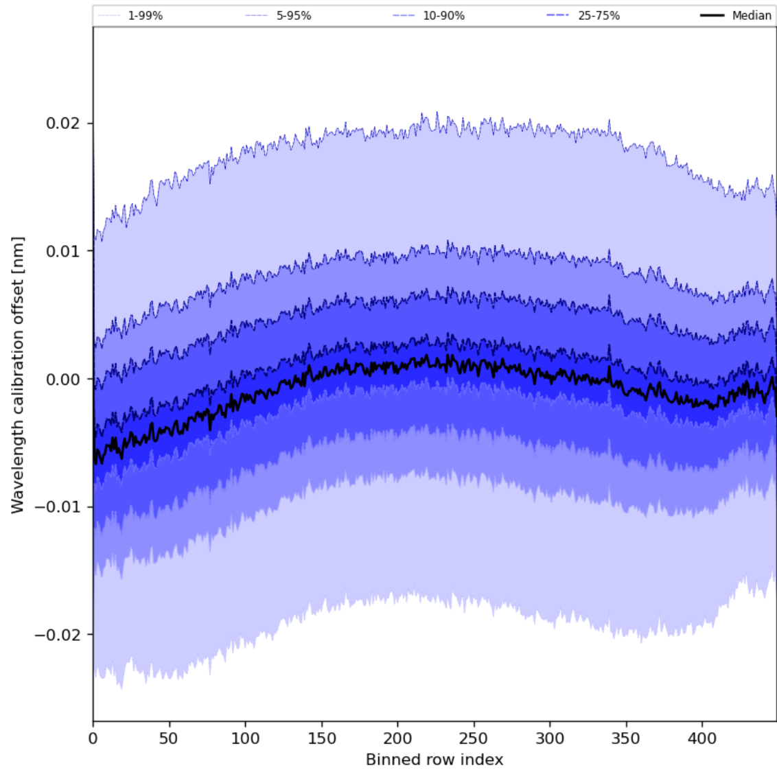
Figure 52: Along track statistics of “Wavelength calibration offset” for 2024-07-27 to 2024-07-29
