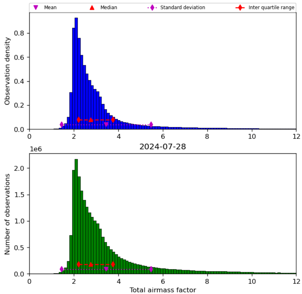
Figure 32: Histogram of “Total airmass factor” for 2024-07-27 to 2024-07-29
