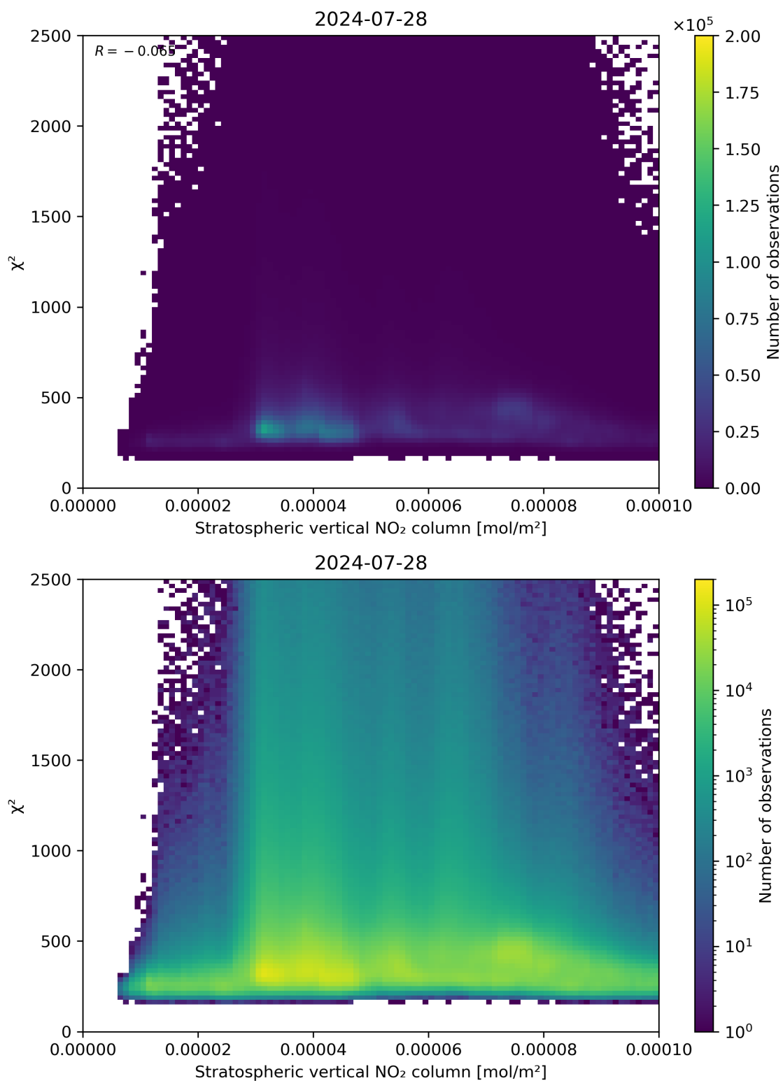
Figure 97: Scatter density plot of “Stratospheric vertical NO 2 column” against “ \chi^2 ” for 2024-07-27 to 2024-07-29.
