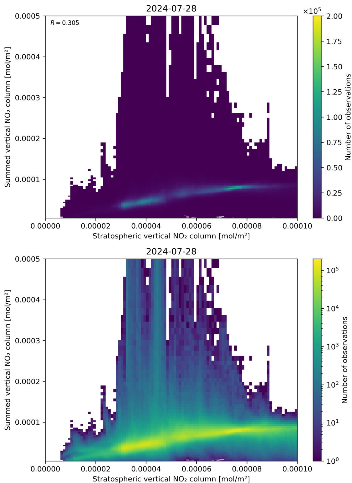
Figure 98: Scatter density plot of “Stratospheric vertical NO 2 column” against “Summed vertical NO 2 column” for 2024-07-27 to 2024-07-29.
