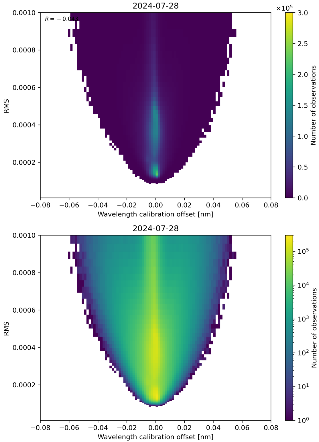
Figure 181: Scatter density plot of “Wavelength calibration offset” against “RMS” for 2024-07-27 to 2024-07-29.
