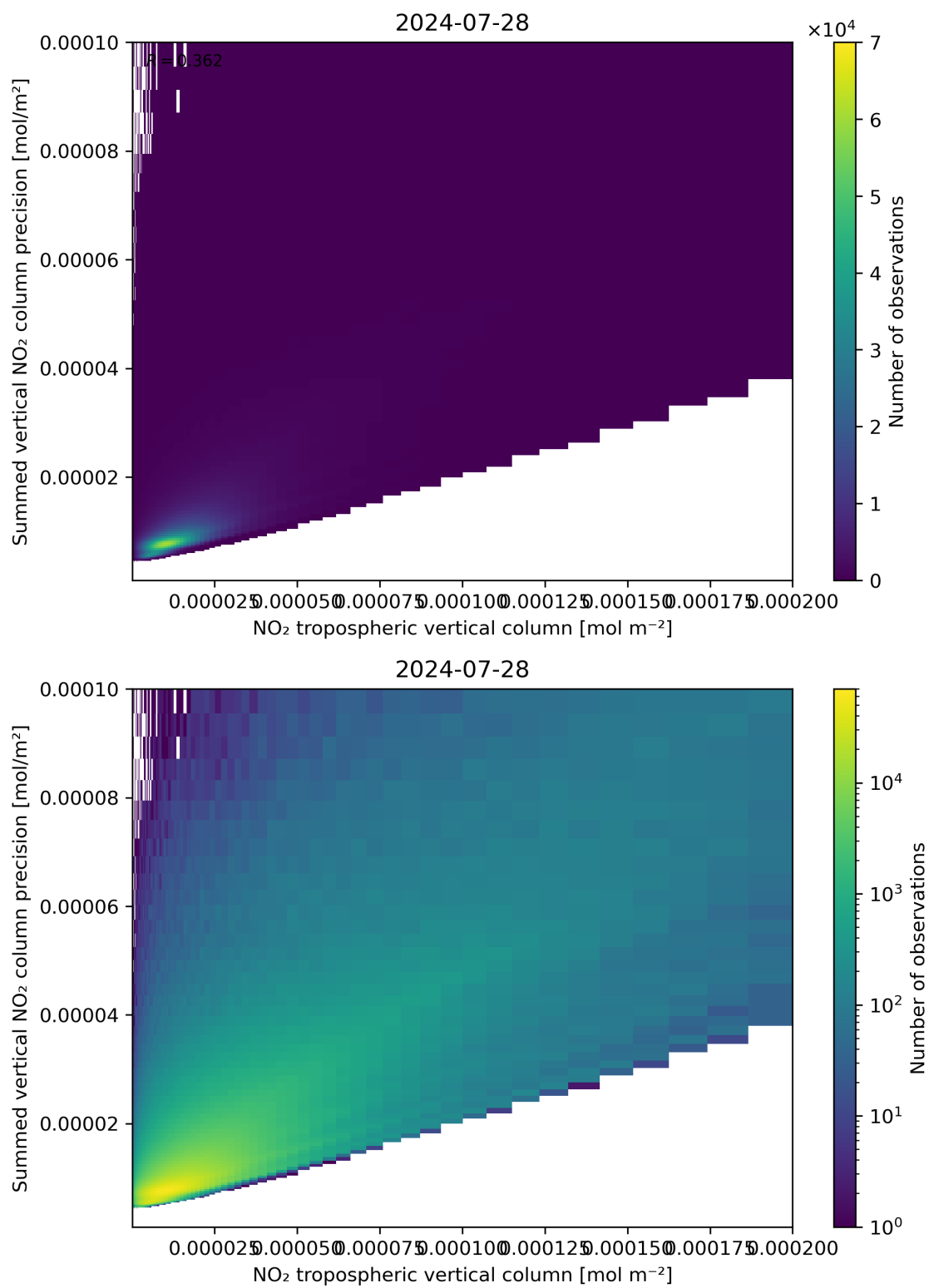
Figure 127: Scatter density plot of “NO 2 tropospheric vertical column” against “Summed vertical NO 2 column precision” for 2024-07-27 to 2024-07-29.
