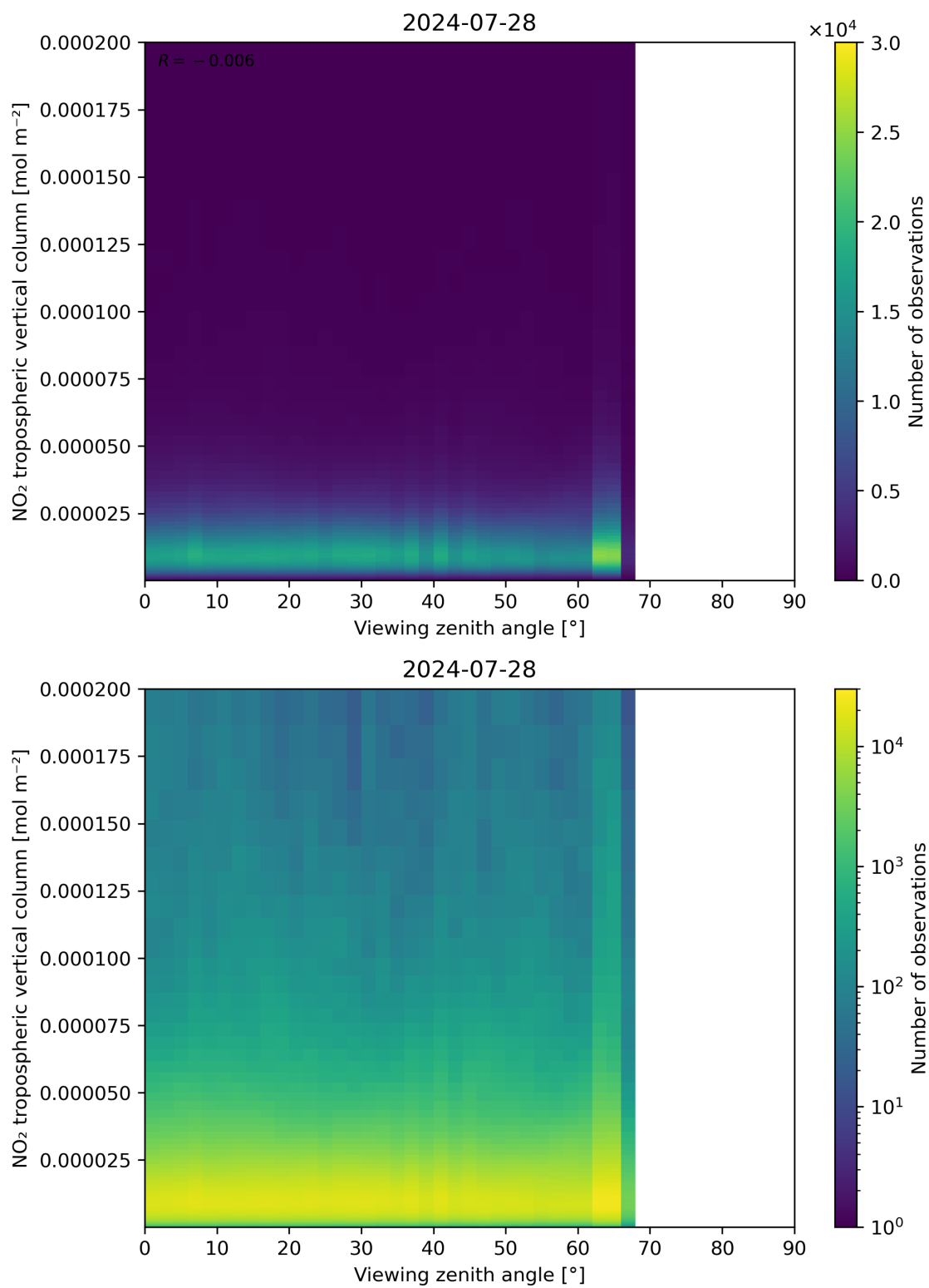
Figure 169: Scatter density plot of “Viewing zenith angle” against “NO 2 tropospheric vertical column” for 2024-07-27 to 2024-07-29.
