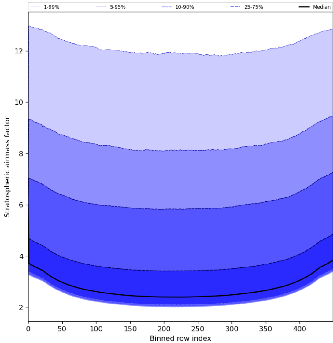
Figure 61: Along track statistics of “Stratospheric airmass factor” for 2024-07-27 to 2024-07-29
