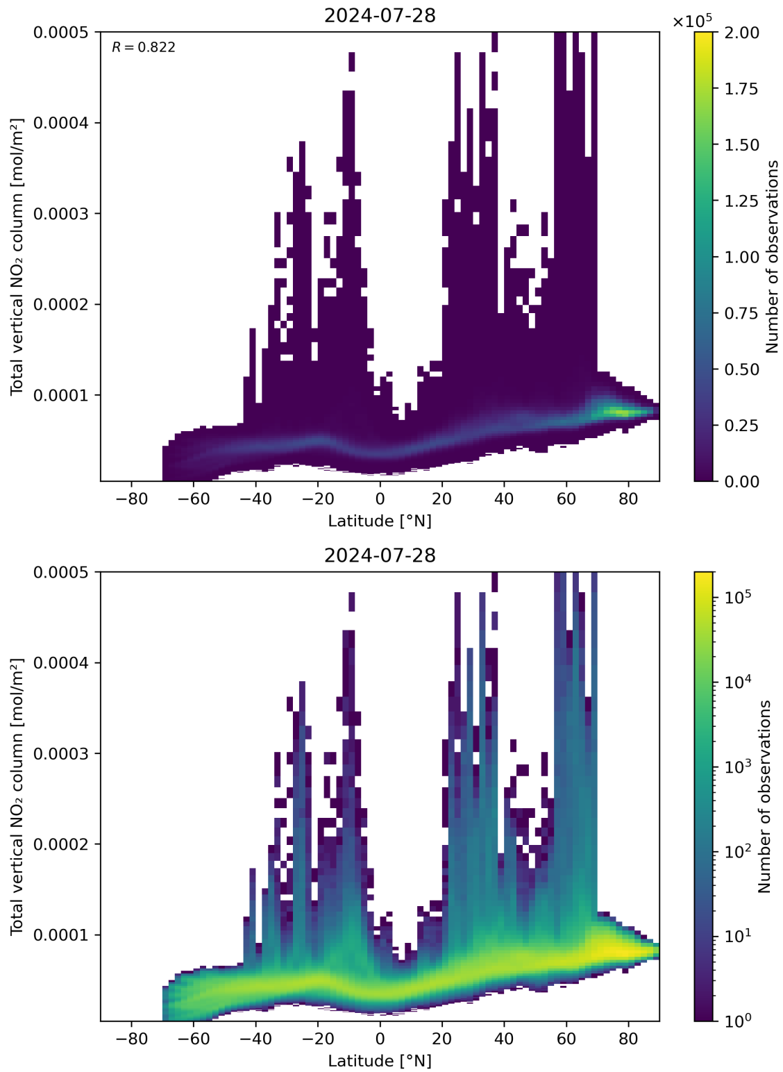
Figure 90: Scatter density plot of “Latitude” against “Total vertical NO 2 column” for 2024-07-27 to 2024-07-29.
