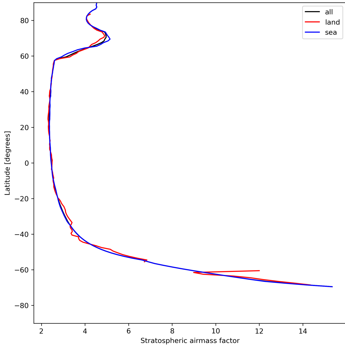
Figure 27: Zonal average of “Stratospheric air mass factor” for 2024-07-27 to 2024-07-29.
