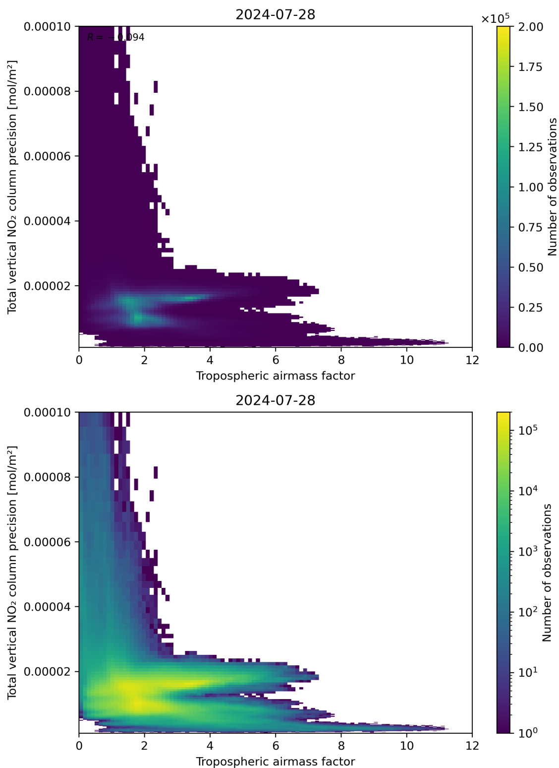
Figure 78: Scatter density plot of “Tropospheric air mass factor” against “Total vertical NO 2 column precision” for 2024-07-27 to 2024-07-29.
