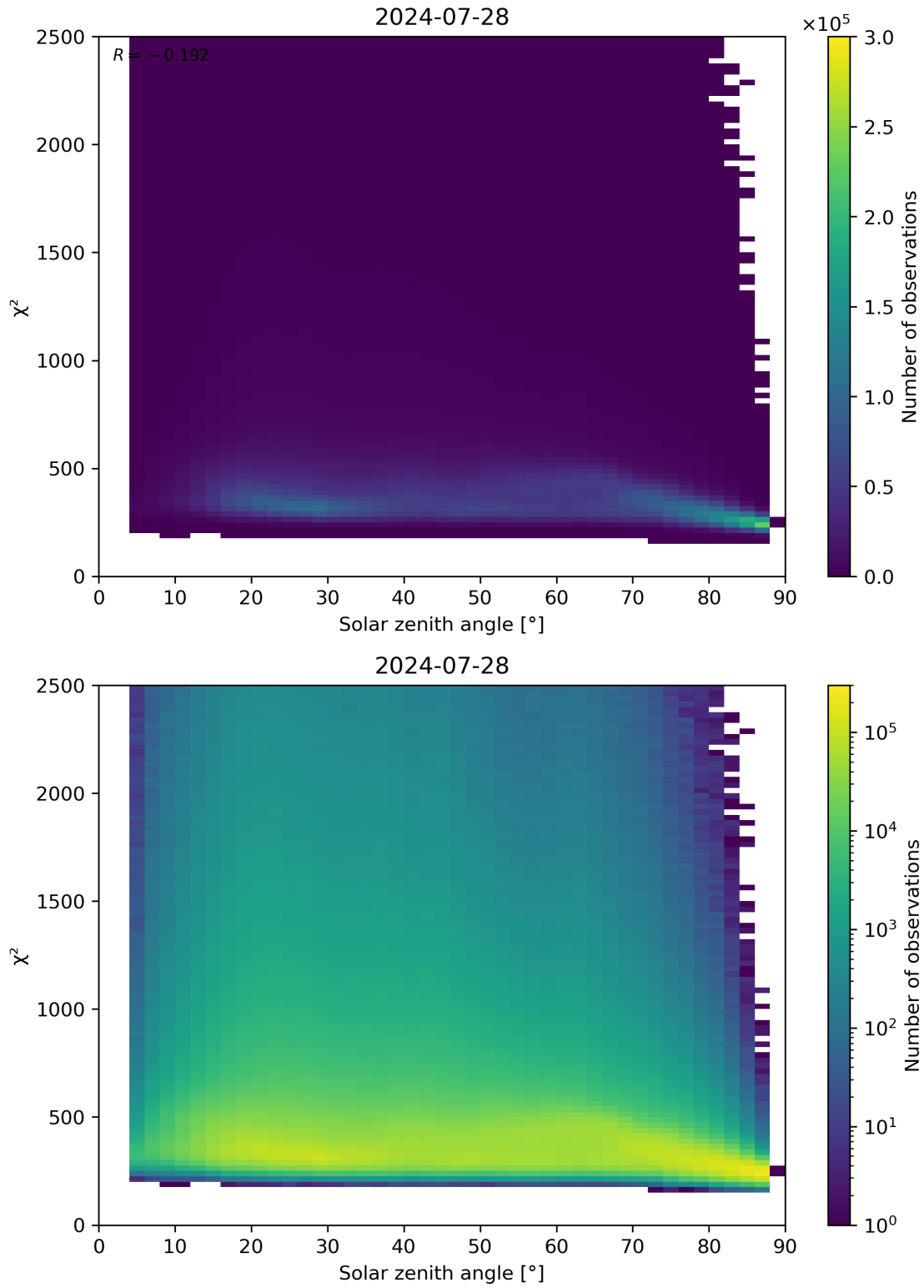
Figure 148: Scatter density plot of “Solar zenith angle” against “ \chi^2 ” for 2024-07-27 to 2024-07-29.
