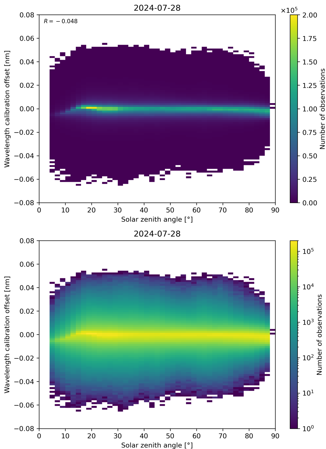
Figure 158: Scatter density plot of “Solar zenith angle” against “Wavelength calibration offset” for 2024-07-27 to 2024-07-29.
