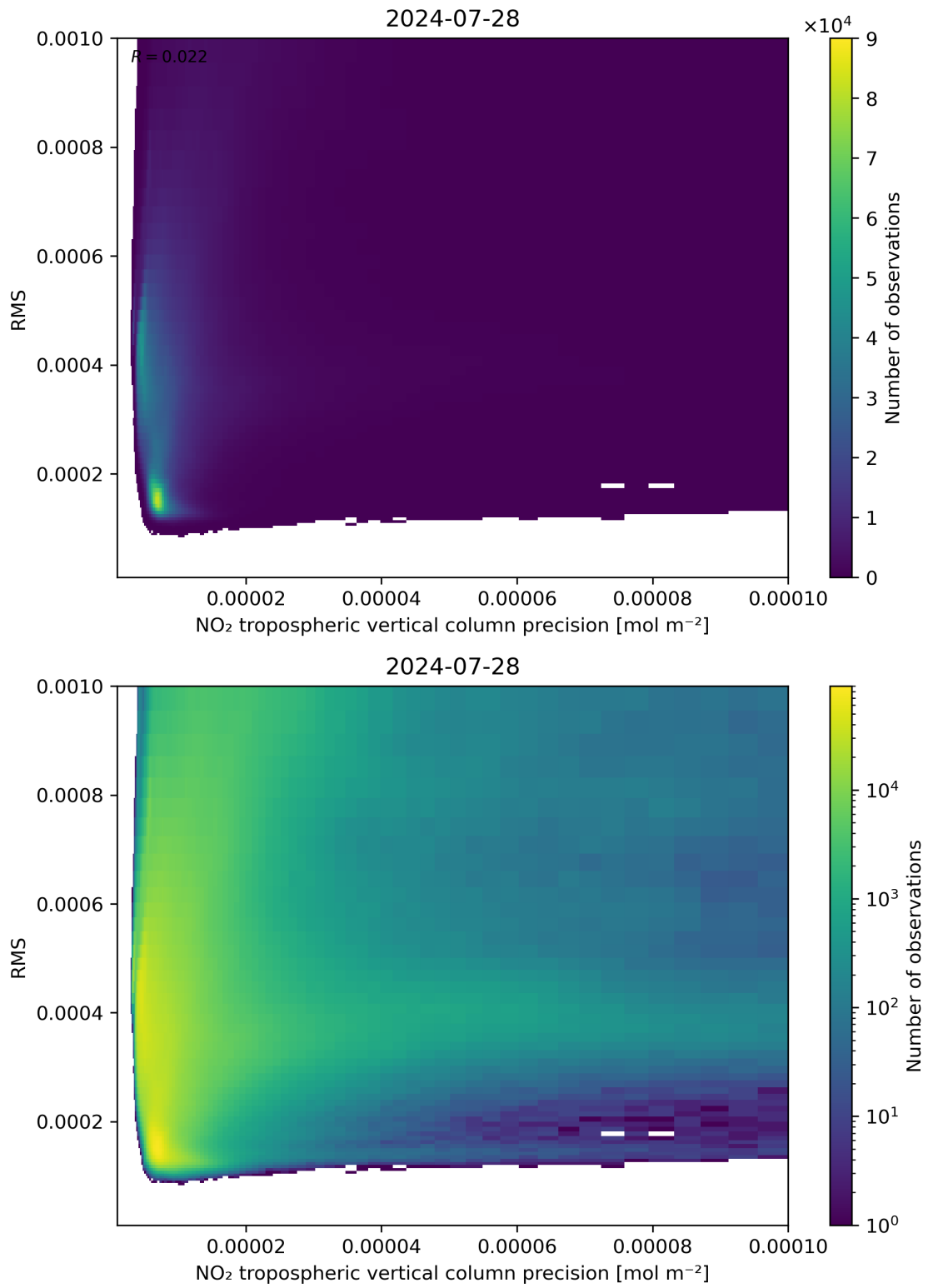
Figure 140: Scatter density plot of “NO 2 tropospheric vertical column precision” against “RMS” for 2024-07-27 to 2024-07-29.
