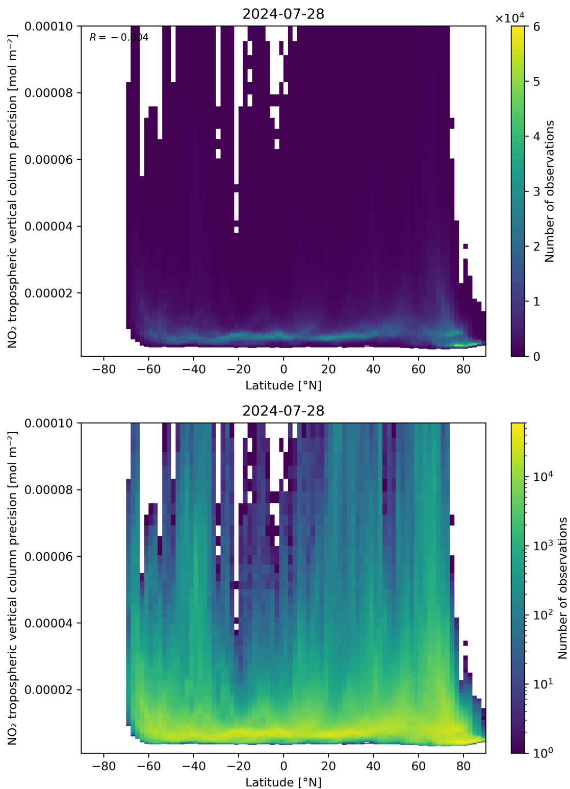
Figure 93: Scatter density plot of “Latitude” against “NO 2 tropospheric vertical column precision” for 2024-07-27 to 2024-07-29.
