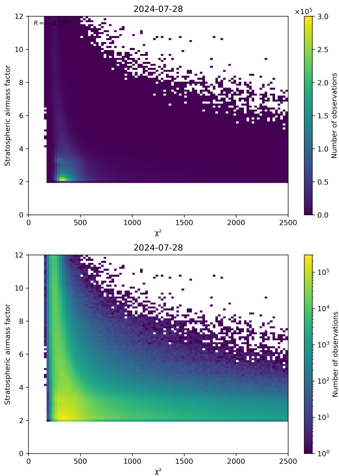
Figure 81: Scatter density plot of “ \chi^2 ” against “Stratospheric airmass factor” for 2024-07-27 to 2024-07-29.
