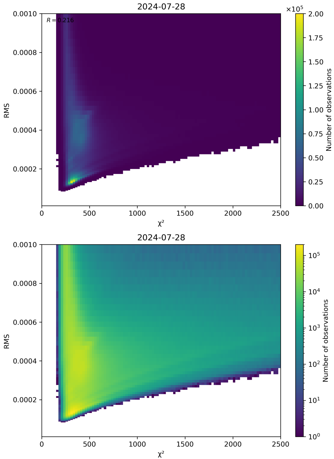
Figure 82: Scatter density plot of “ \chi^2 ” against “RMS” for 2024-07-27 to 2024-07-29.
