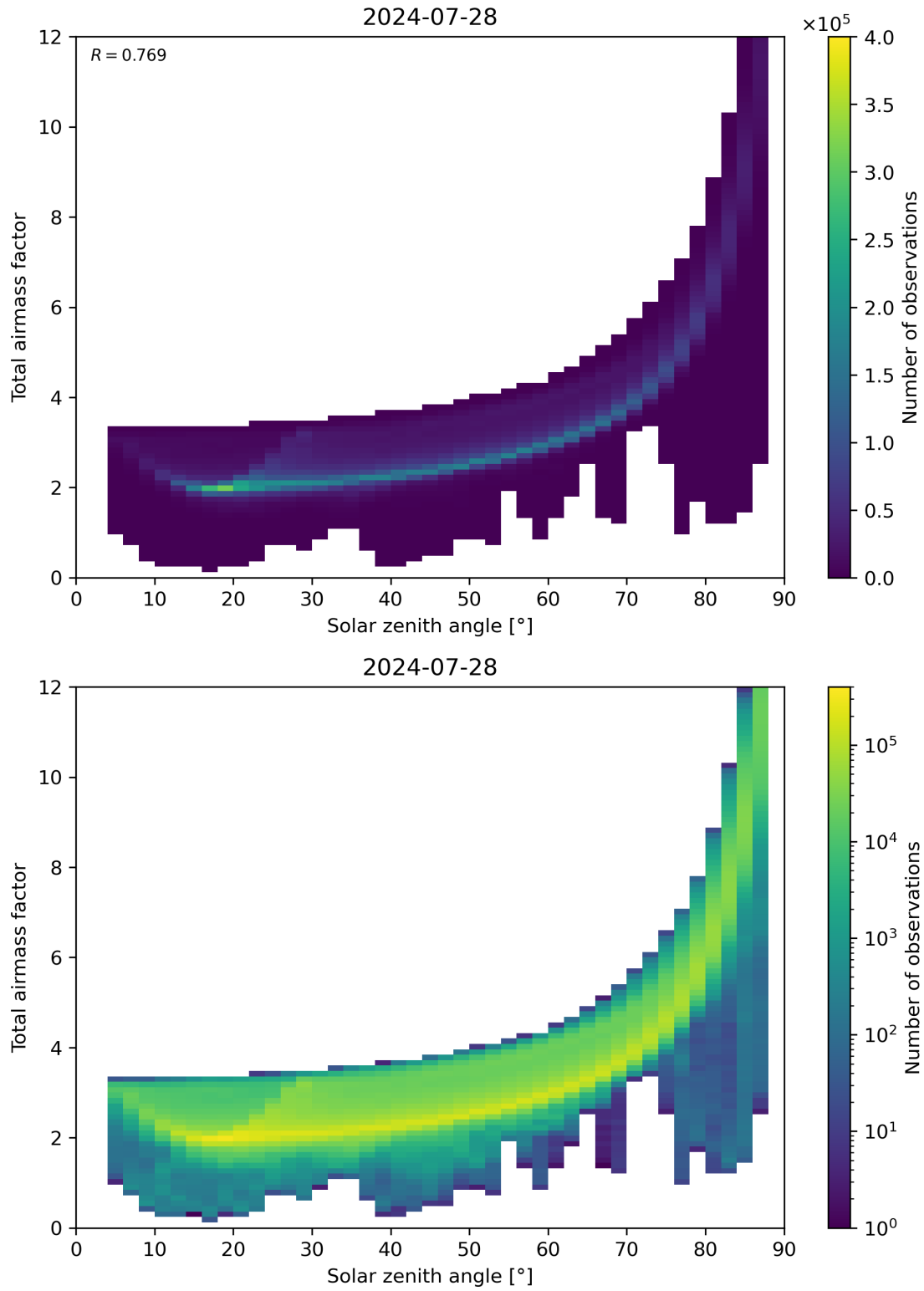
Figure 146: Scatter density plot of “Solar zenith angle” against “Total air mass factor” for 2024-07-27 to 2024-07-29.
