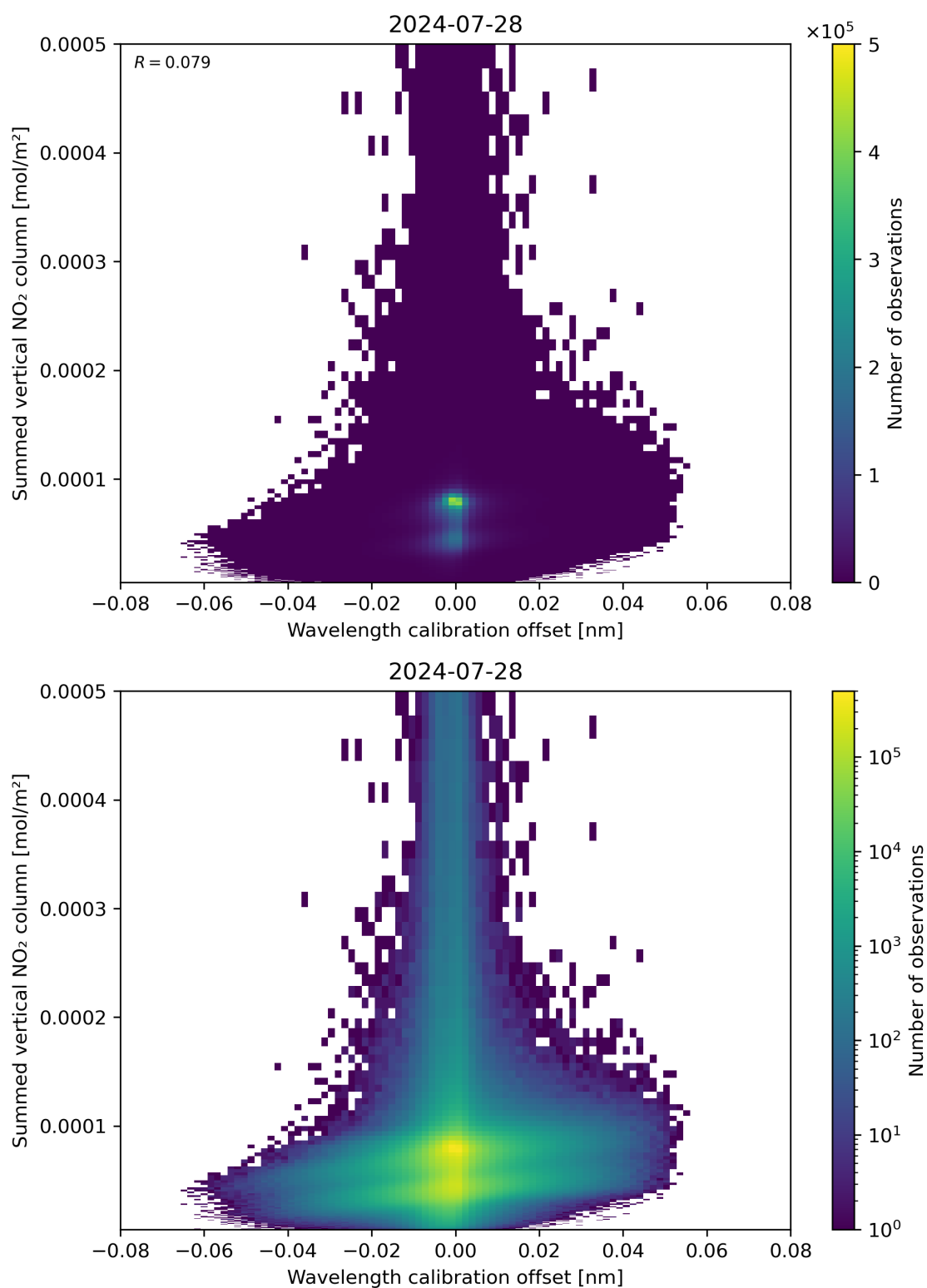
Figure 177: Scatter density plot of “Wavelength calibration offset” against “Summed vertical NO 2 column” for 2024-07-27 to 2024-07-29.
