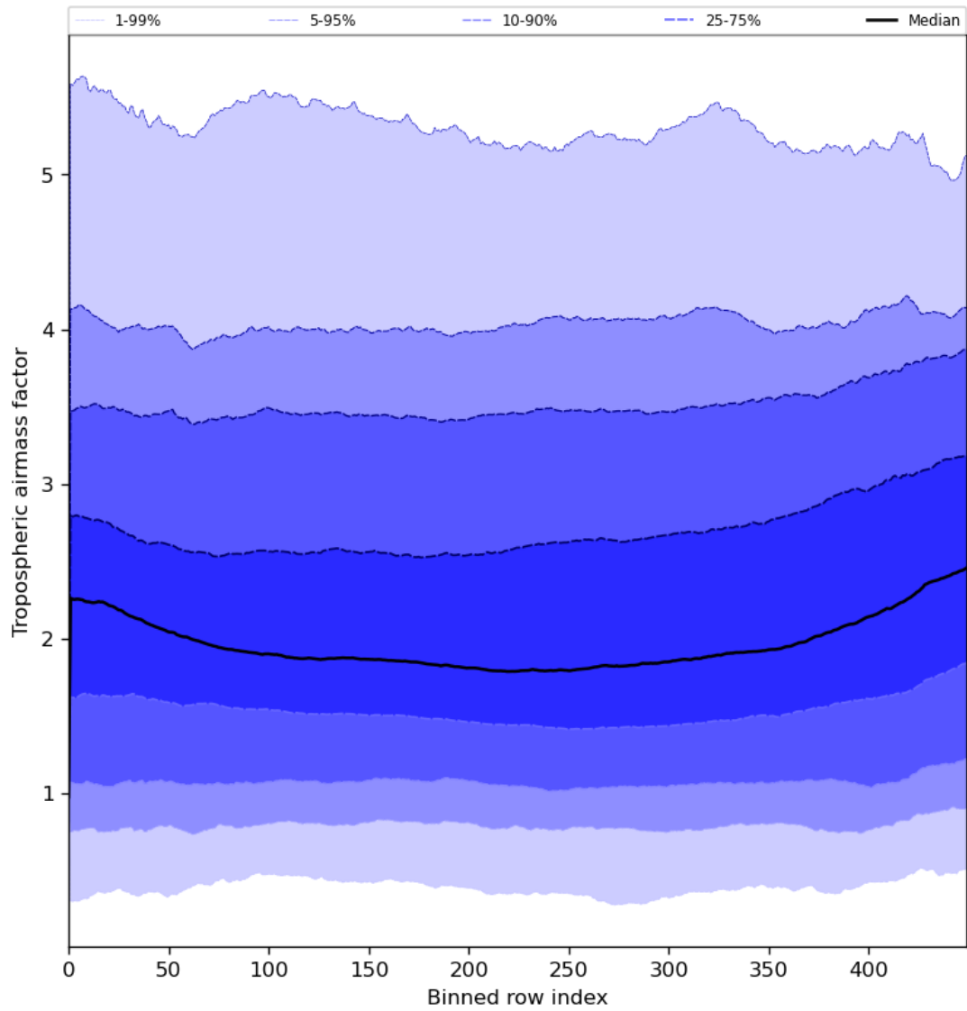
Figure 48: Along track statistics of “Tropospheric airmass factor” for 2024-07-27 to 2024-07-29
