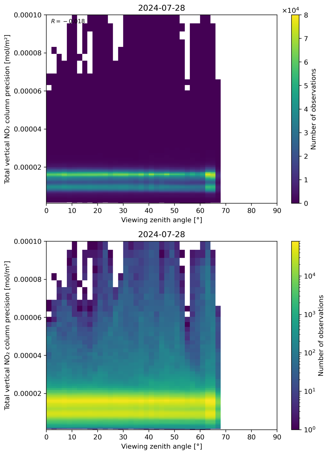
Figure 168: Scatter density plot of “Viewing zenith angle” against “Total vertical NO 2 column precision” for 2024-07-27 to 2024-07-29.
