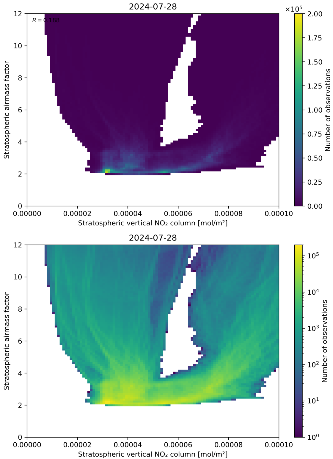
Figure 96: Scatter density plot of “Stratospheric vertical NO 2 column” against “Stratospheric airmass factor” for 2024-07-27 to 2024-07-29.
