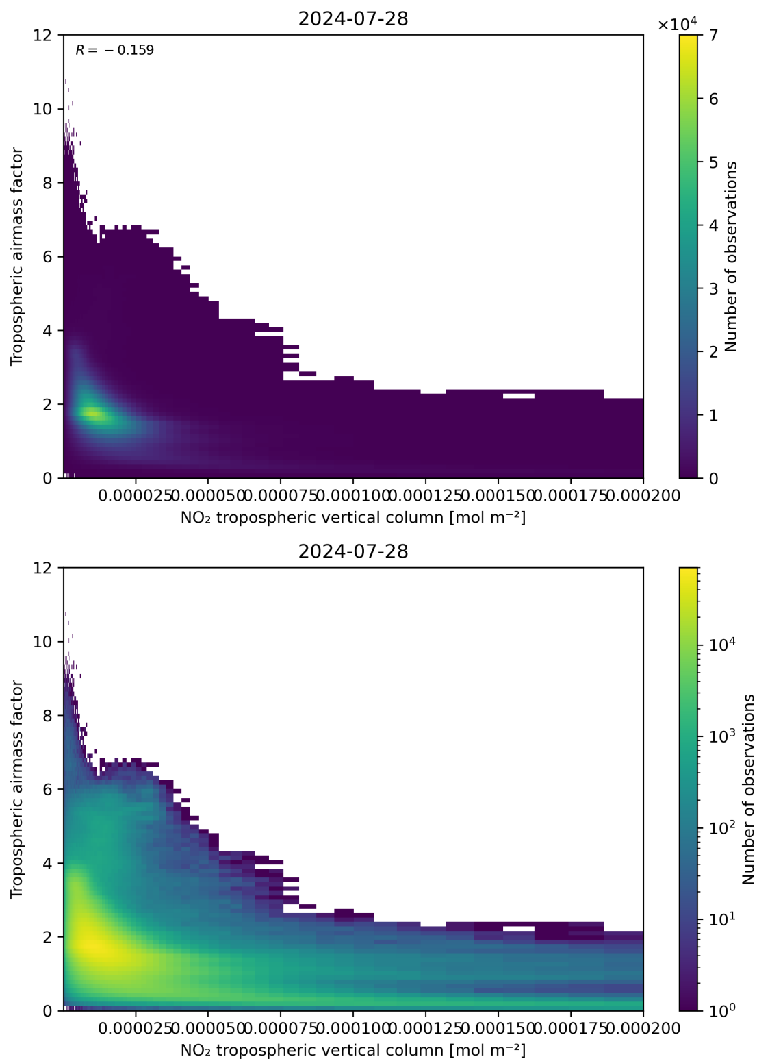
Figure 123: Scatter density plot of “NO 2 tropospheric vertical column” against “Tropospheric airmass factor” for 2024-07-27 to 2024-07-29.
