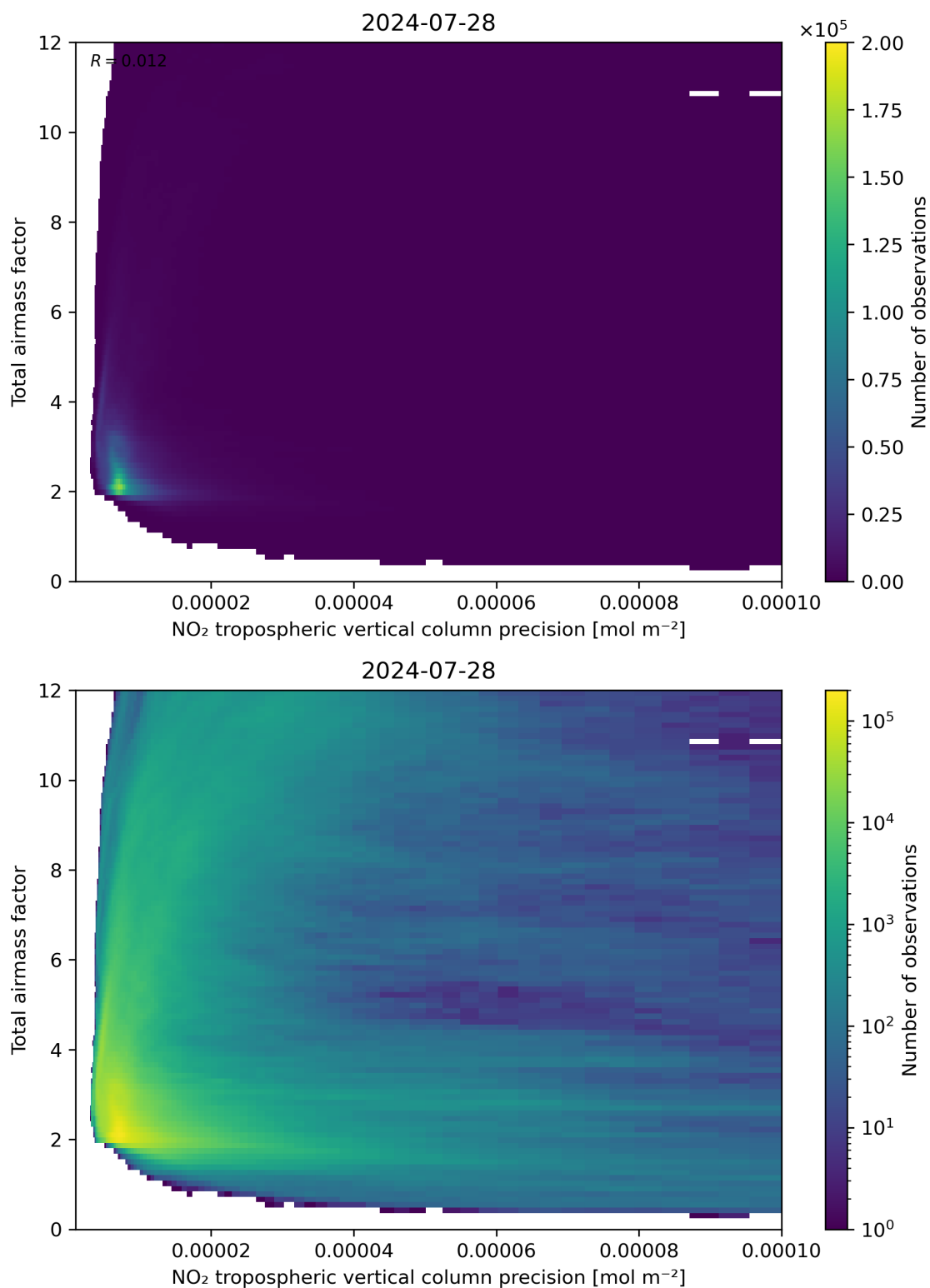
Figure 132: Scatter density plot of “NO 2 tropospheric vertical column precision” against “Total air mass factor” for 2024-07-27 to 2024-07-29.
