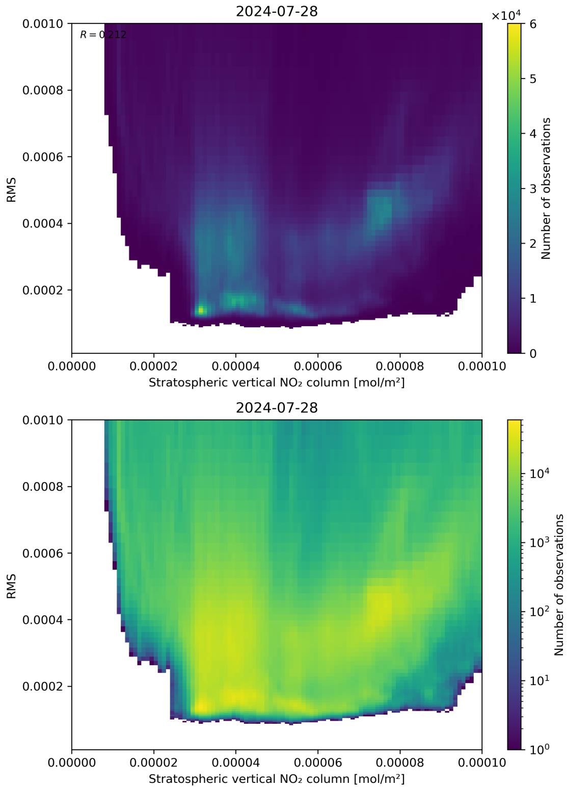
Figure 102: Scatter density plot of “Stratospheric vertical NO 2 column” against “RMS” for 2024-07-27 to 2024-07-29.
