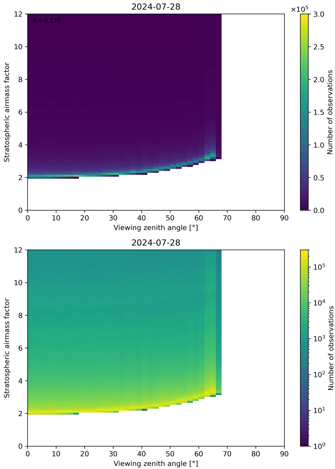
Figure 159: Scatter density plot of “Viewing zenith angle” against “Stratospheric airmass factor” for 2024-07-27 to 2024-07-29.
