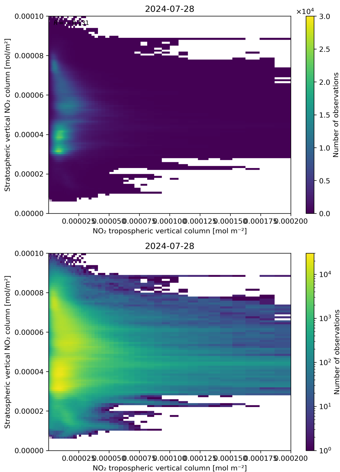
Figure 125: Scatter density plot of “NO 2 tropospheric vertical column” against “Stratospheric vertical NO 2 column” for 2024-07-27 to 2024-07-29.
