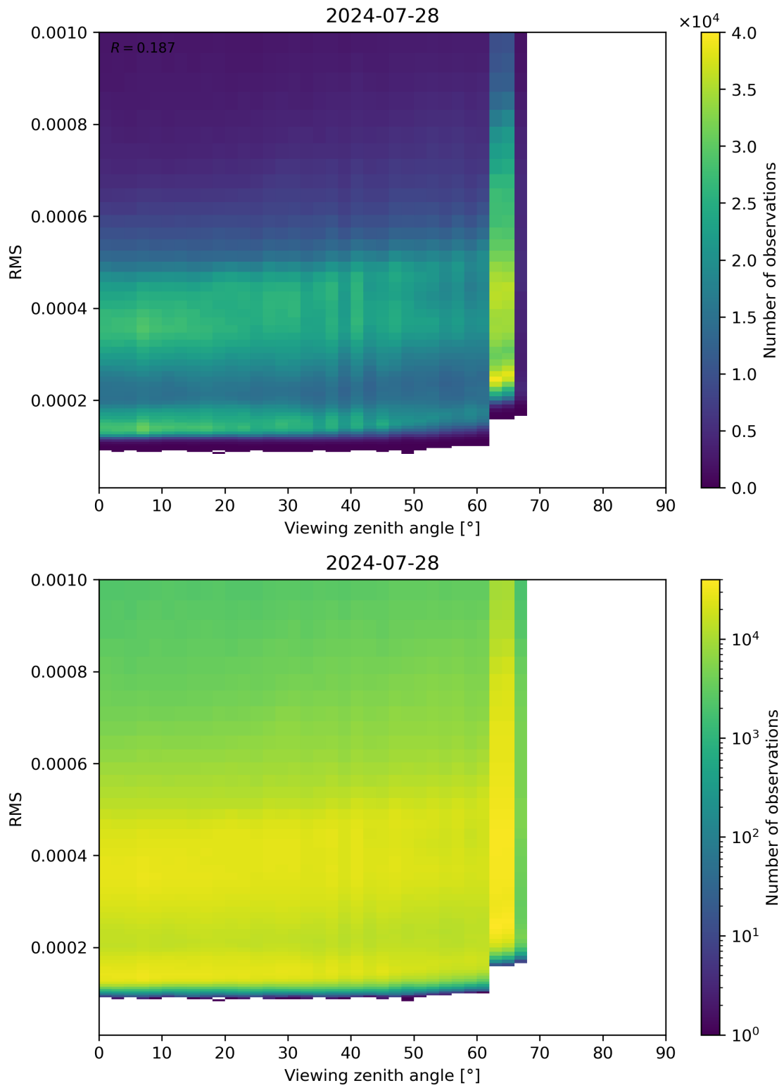
Figure 171: Scatter density plot of “Viewing zenith angle” against “RMS” for 2024-07-27 to 2024-07-29.
