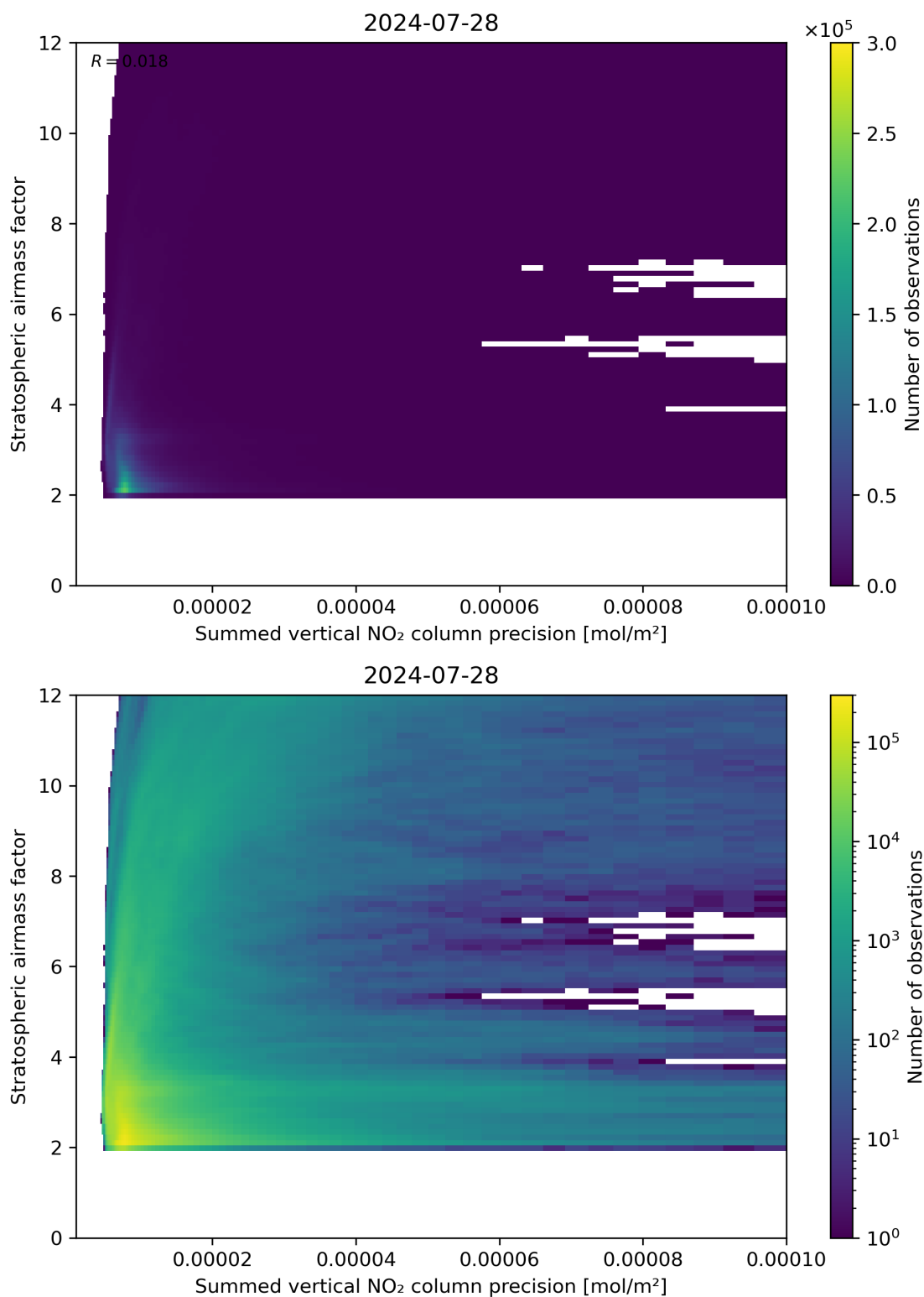
Figure 106: Scatter density plot of “Summed vertical NO 2 column precision” against “Stratospheric airmass factor” for 2024-07-27 to 2024-07-29.
