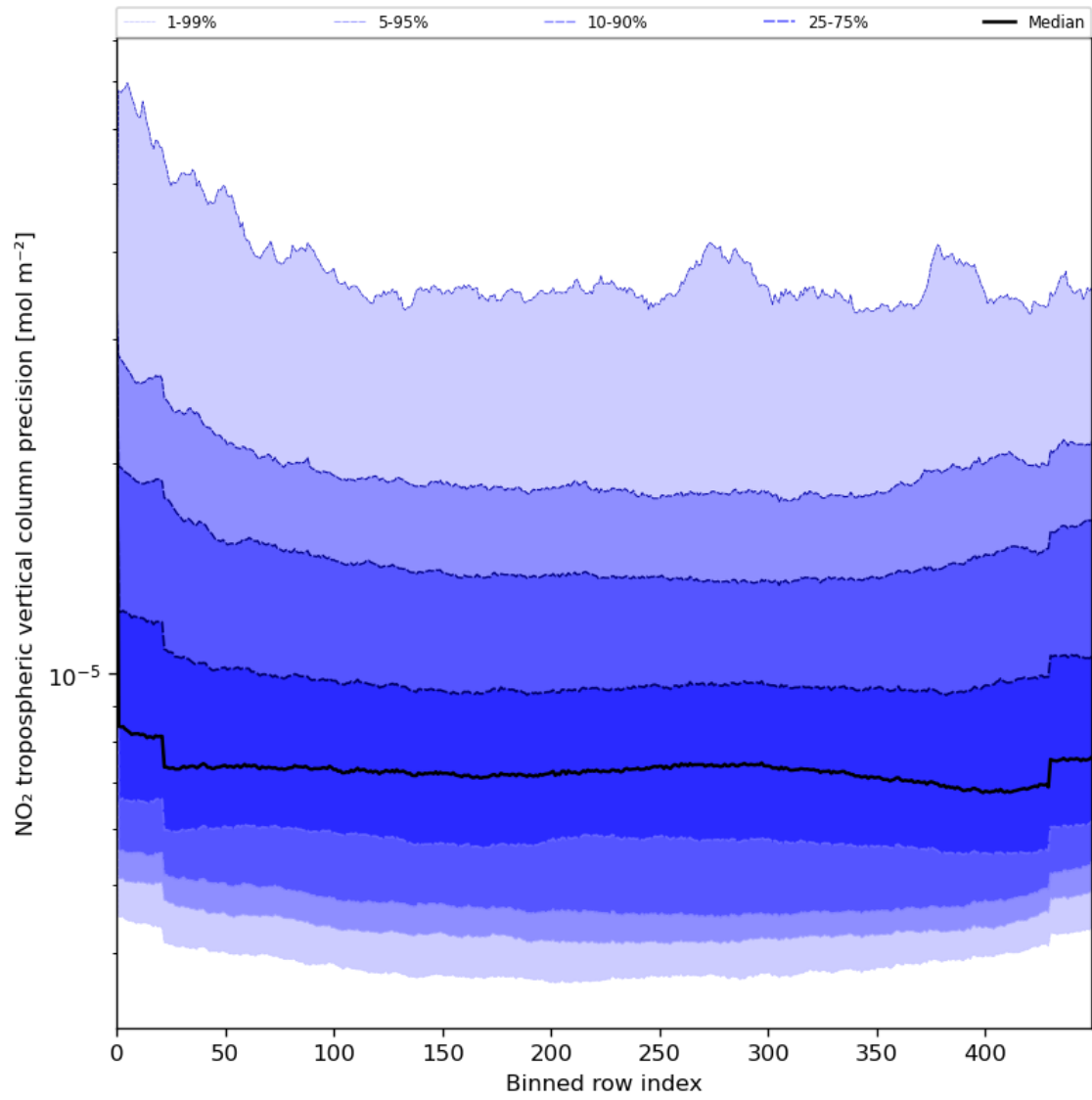
Figure 47: Along track statistics of “NO 2 tropospheric vertical column precision” for 2024-07-27 to 2024-07-29
