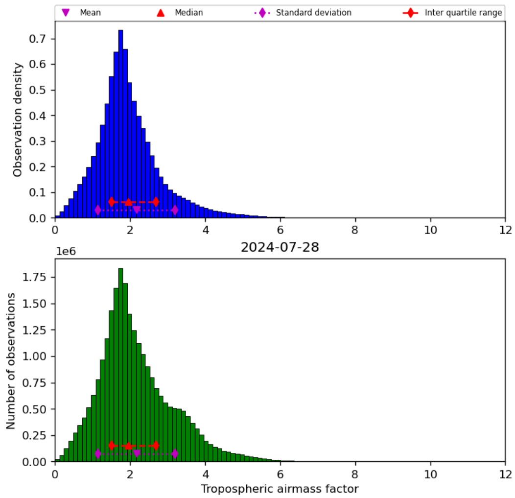
Figure 31: Histogram of “Tropospheric airmass factor” for 2024-07-27 to 2024-07-29
