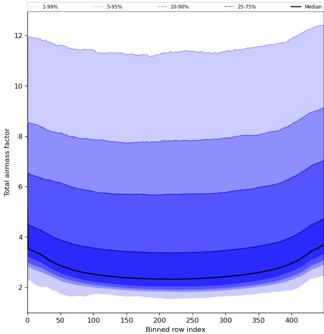
Figure 49: Along track statistics of “Total airmass factor” for 2024-07-27 to 2024-07-29
