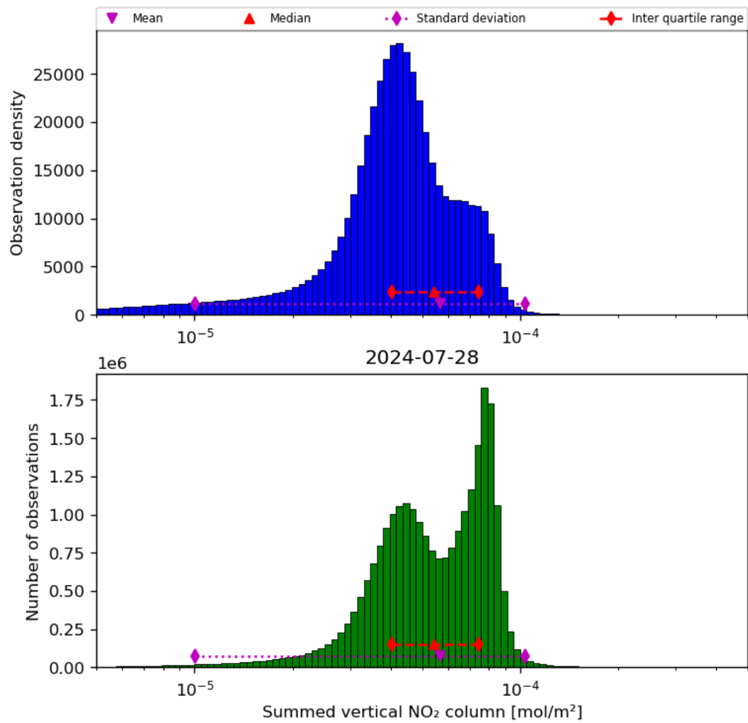
Figure 40: Histogram of “Summed vertical NO 2 column” for 2024-07-27 to 2024-07-29
