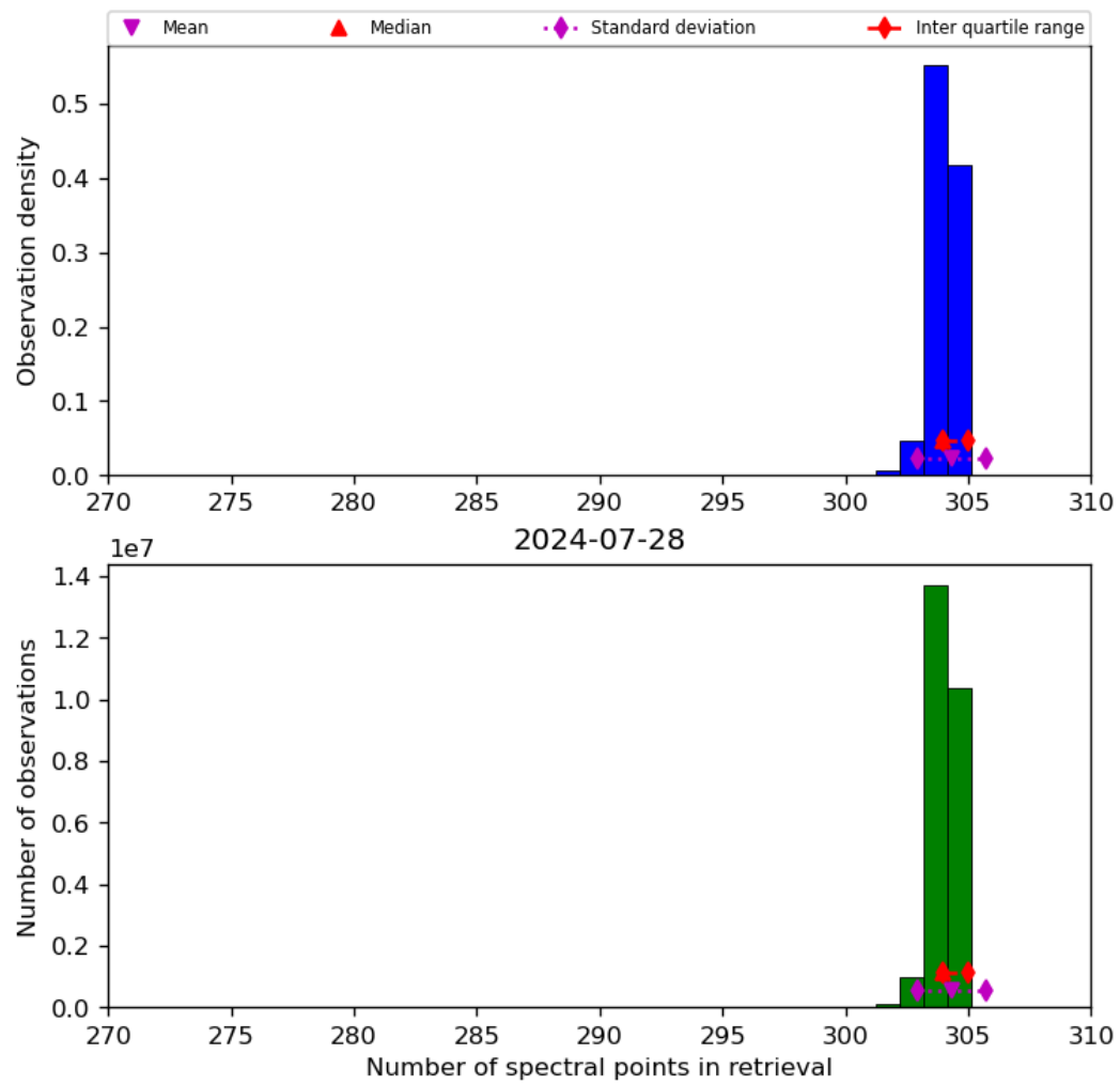
Figure 33: Histogram of “Number of spectral points in retrieval” for 2024-07-27 to 2024-07-29
