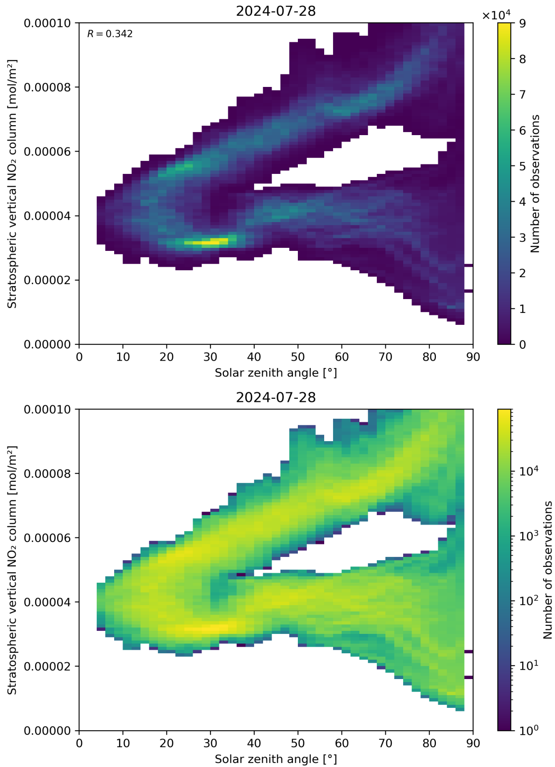
Figure 150: Scatter density plot of “Solar zenith angle” against “Stratospheric vertical NO 2 column” for 2024-07-27 to 2024-07-29.
