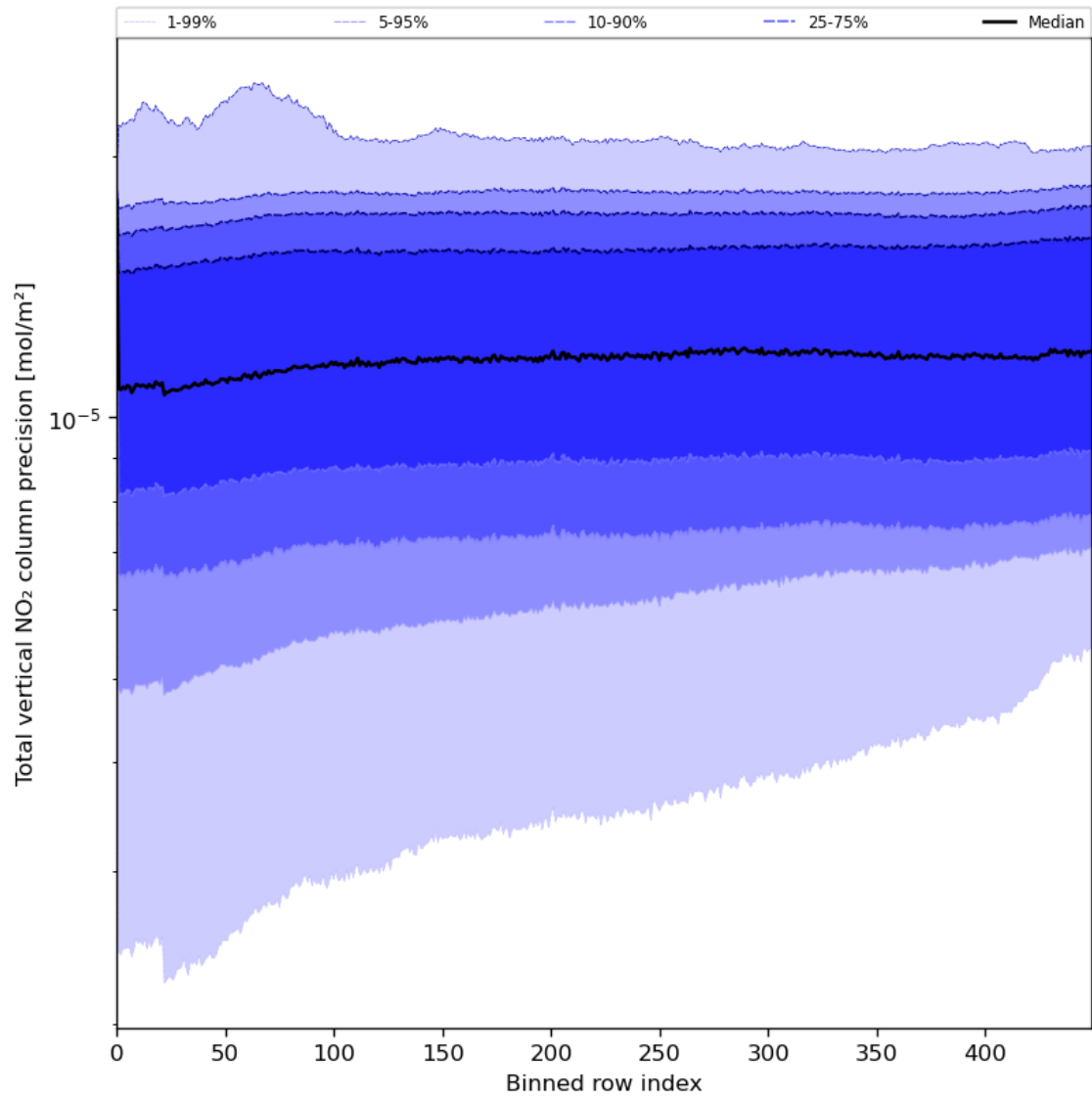
Figure 56: Along track statistics of “Total vertical NO 2 column precision” for 2024-07-27 to 2024-07-29
