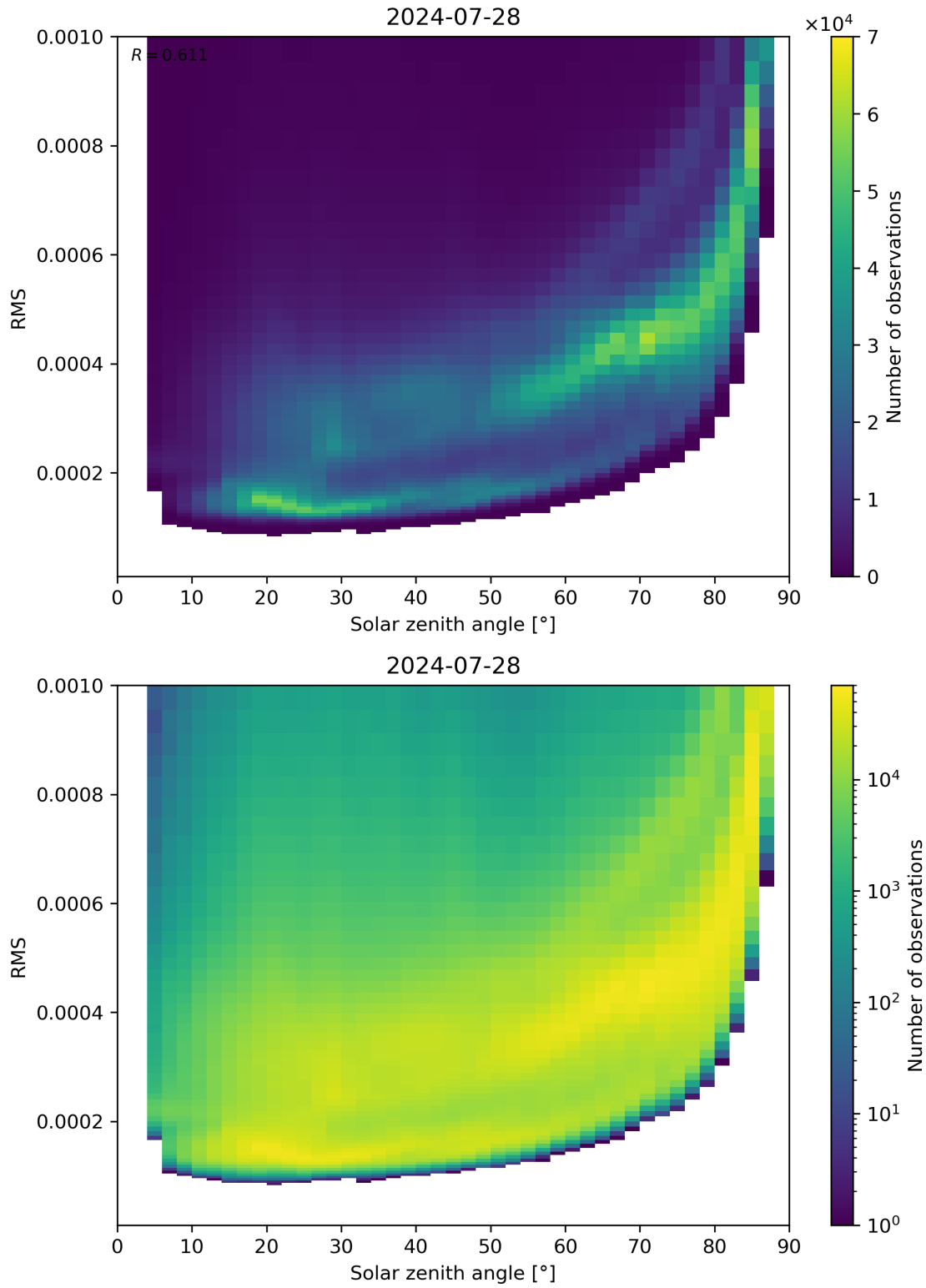
Figure 157: Scatter density plot of “Solar zenith angle” against “RMS” for 2024-07-27 to 2024-07-29.
