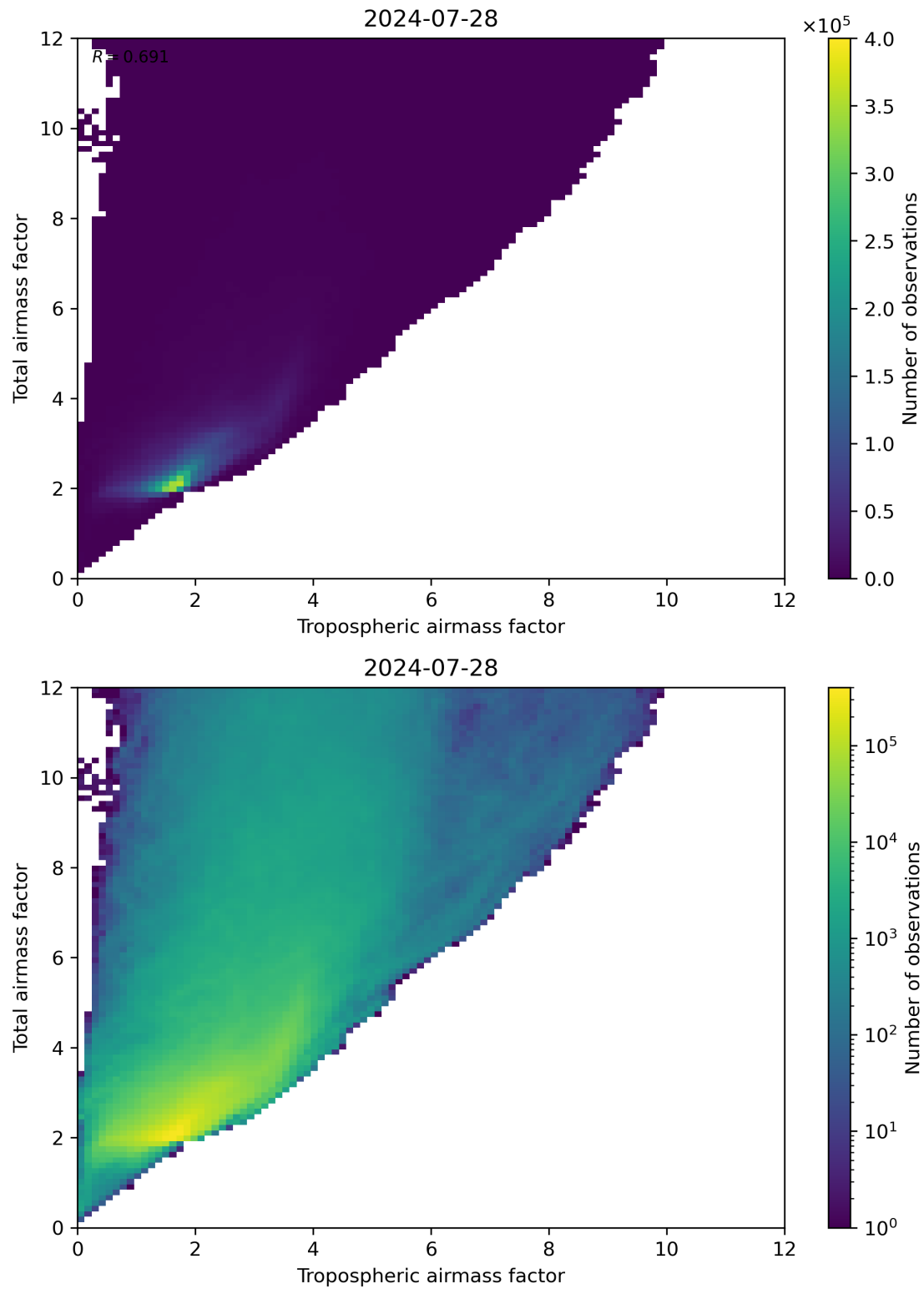
Figure 72: Scatter density plot of “Tropospheric airmass factor” against “Total airmass factor” for 2024-07-27 to 2024-07-29.
