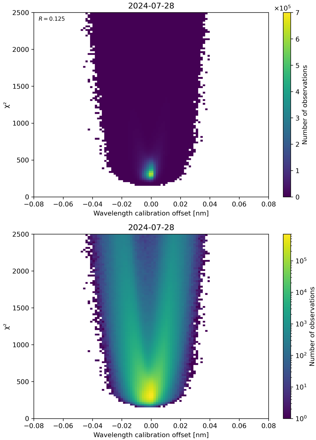
Figure 175: Scatter density plot of “Wavelength calibration offset” against “ \chi^2 ” for 2024-07-27 to 2024-07-29.
