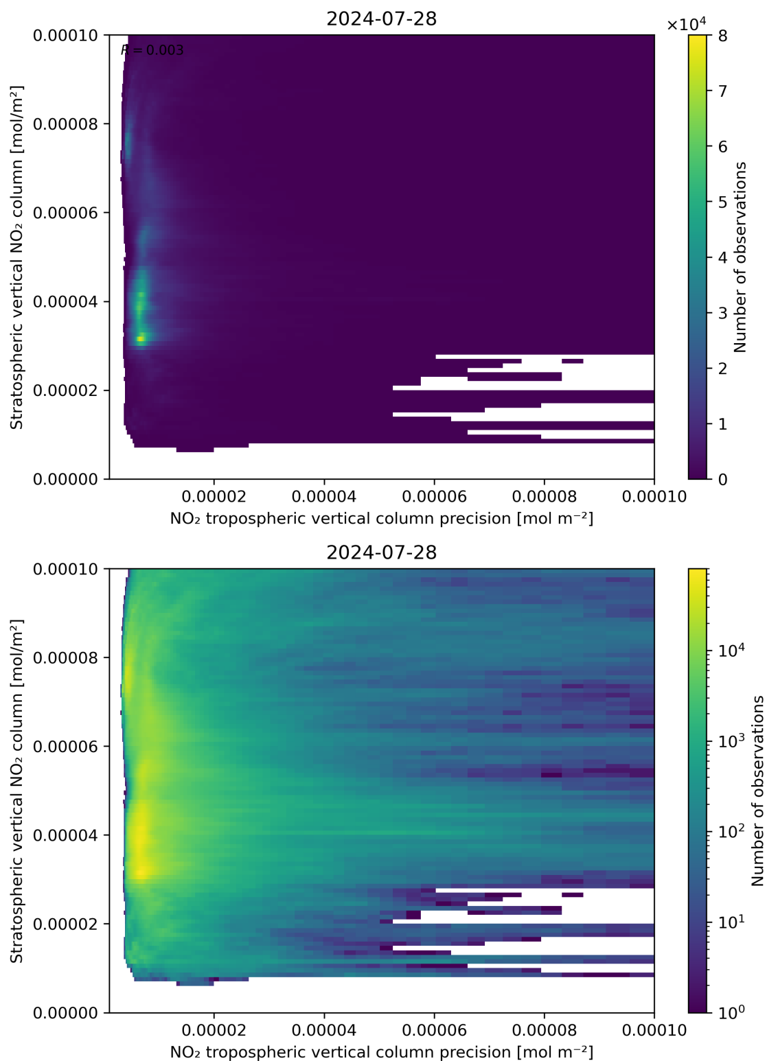
Figure 135: Scatter density plot of “NO 2 tropospheric vertical column precision” against “Stratospheric vertical NO 2 column” for 2024-07-27 to 2024-07-29.
