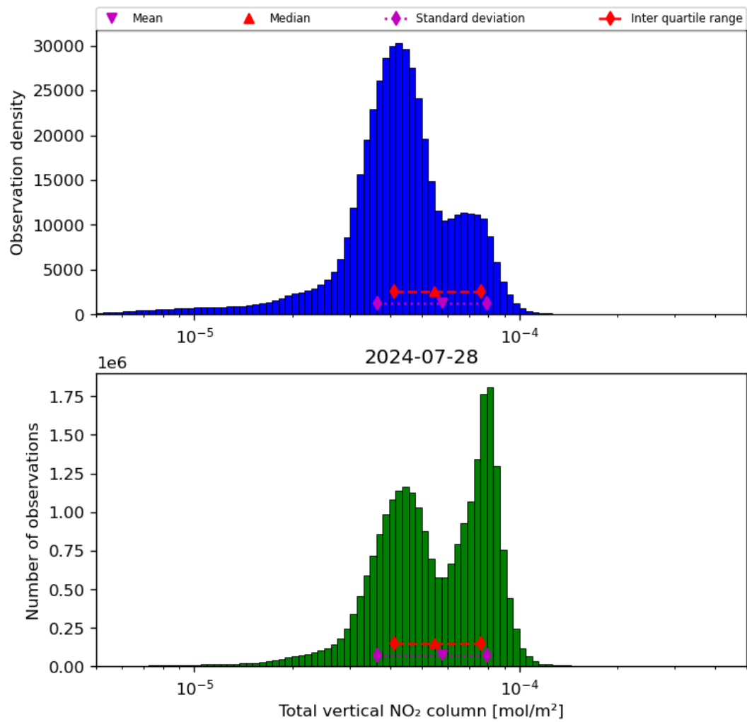
Figure 38: Histogram of “Total vertical NO 2 column” for 2024-07-27 to 2024-07-29
