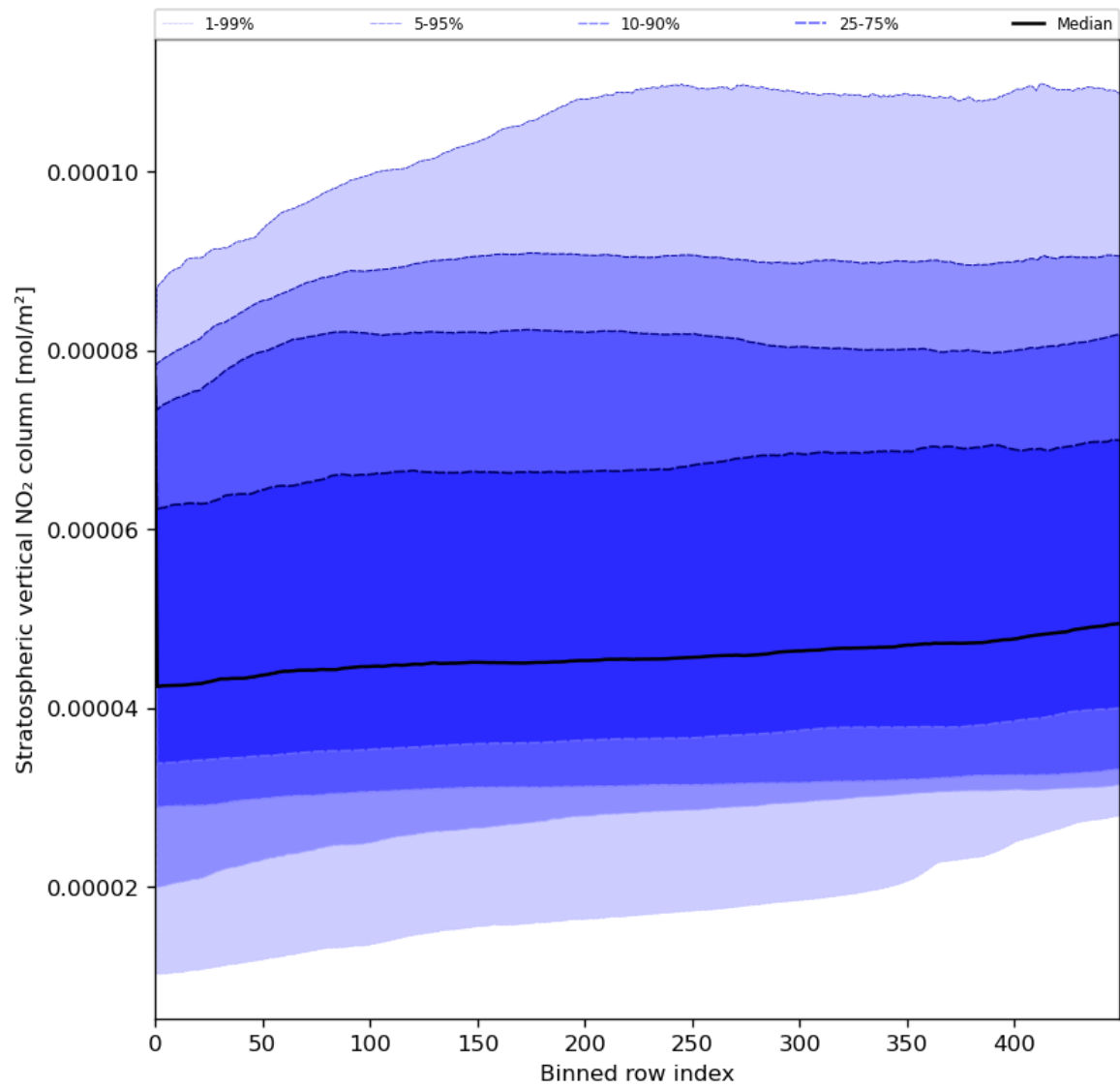
Figure 53: Along track statistics of “Stratospheric vertical NO 2 column” for 2024-07-27 to 2024-07-29
