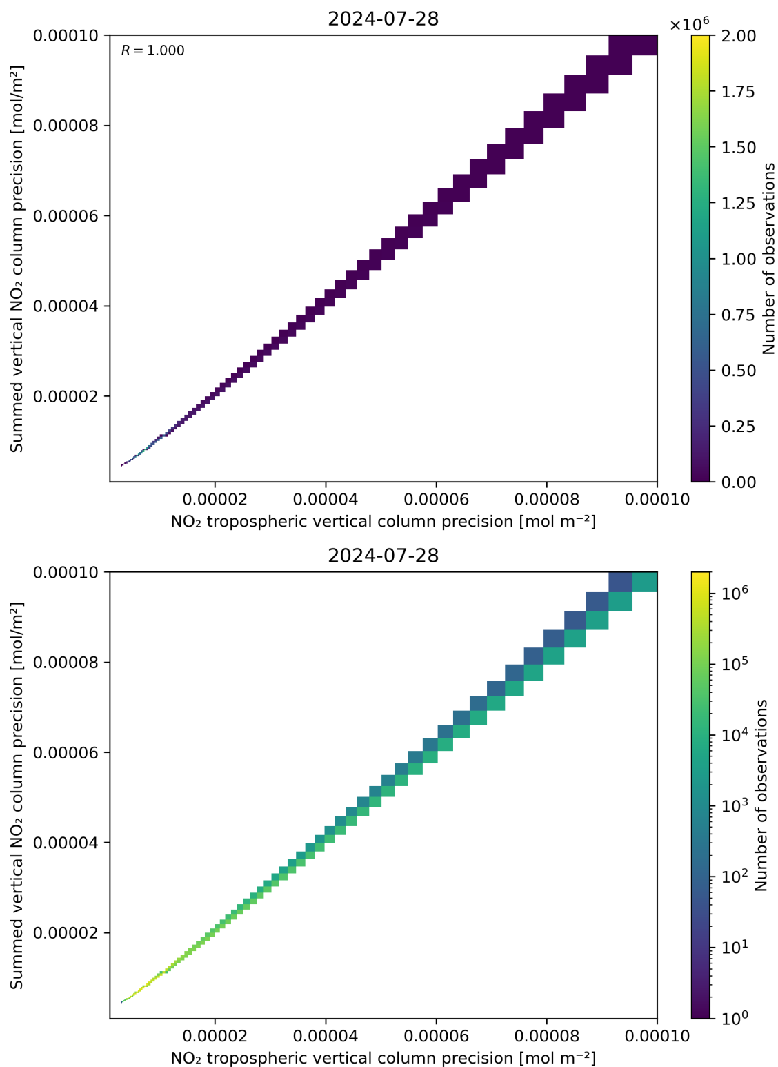
Figure 137: Scatter density plot of “NO 2 tropospheric vertical column precision” against “Summed vertical NO 2 column precision” for 2024-07-27 to 2024-07-29.
