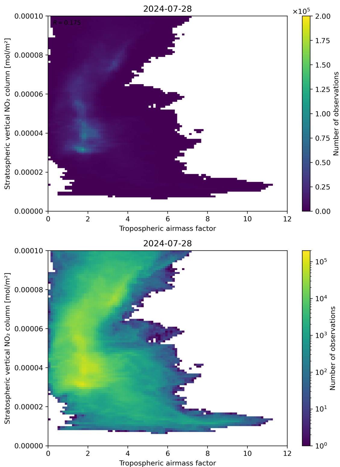
Figure 74: Scatter density plot of “Tropospheric air mass factor” against “Stratospheric vertical NO 2 column” for 2024-07-27 to 2024-07-29.
