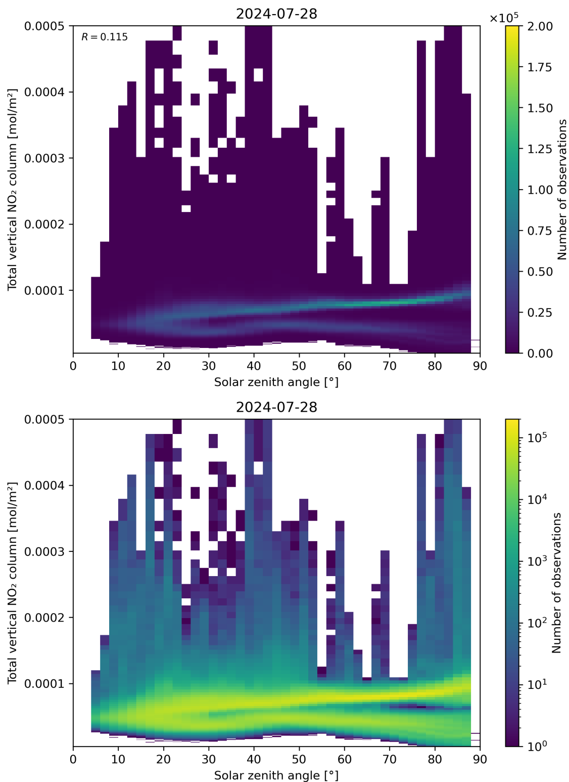
Figure 153: Scatter density plot of “Solar zenith angle” against “Total vertical NO 2 column” for 2024-07-27 to 2024-07-29.
