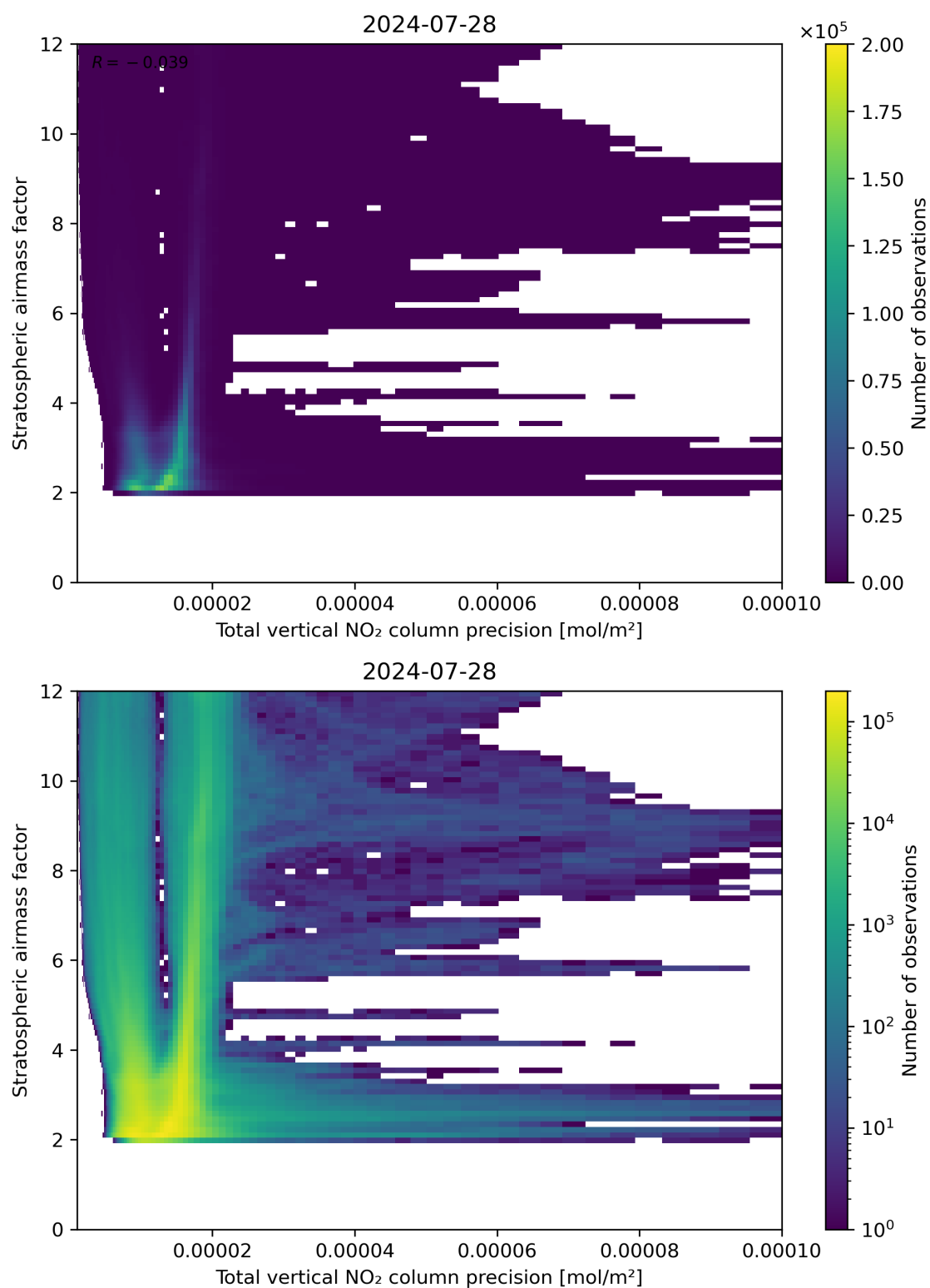
Figure 115: Scatter density plot of “Total vertical NO 2 column precision” against “Stratospheric air mass factor” for 2024-07-27 to 2024-07-29.
