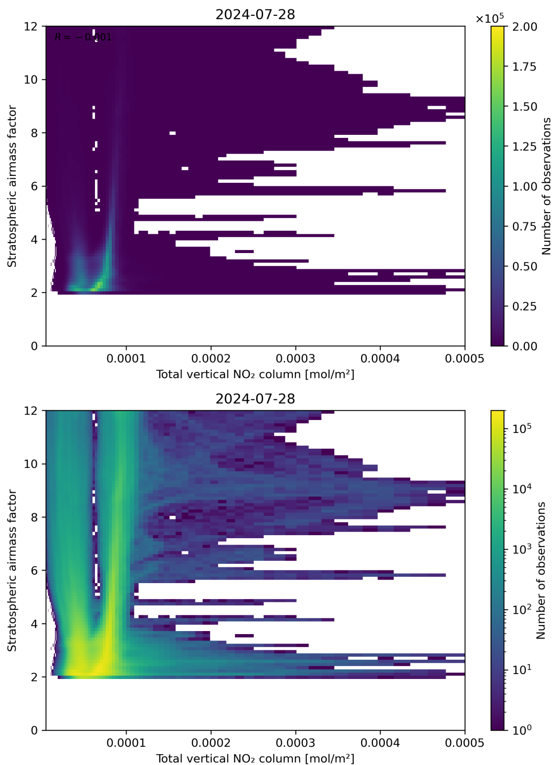
Figure 110: Scatter density plot of “Total vertical NO 2 column” against “Stratospheric air mass factor” for 2024-07-27 to 2024-07-29.
