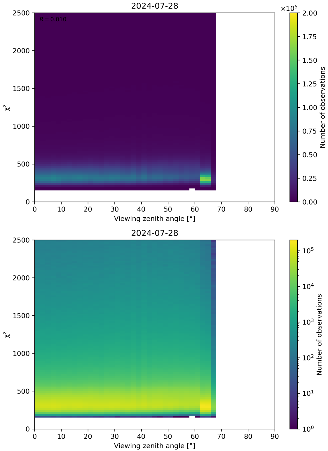
Figure 162: Scatter density plot of “Viewing zenith angle” against “ \chi^2 ” for 2024-07-27 to 2024-07-29.
