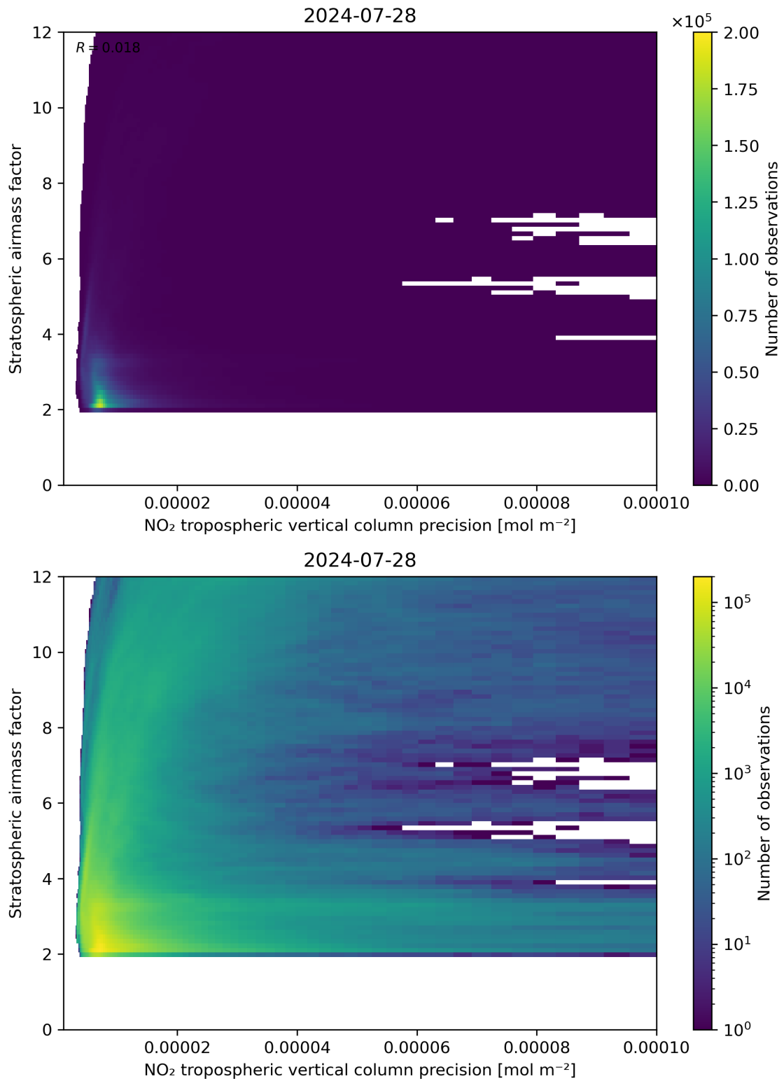
Figure 131: Scatter density plot of “NO 2 tropospheric vertical column precision” against “Stratospheric airmass factor” for 2024-07-27 to 2024-07-29.
