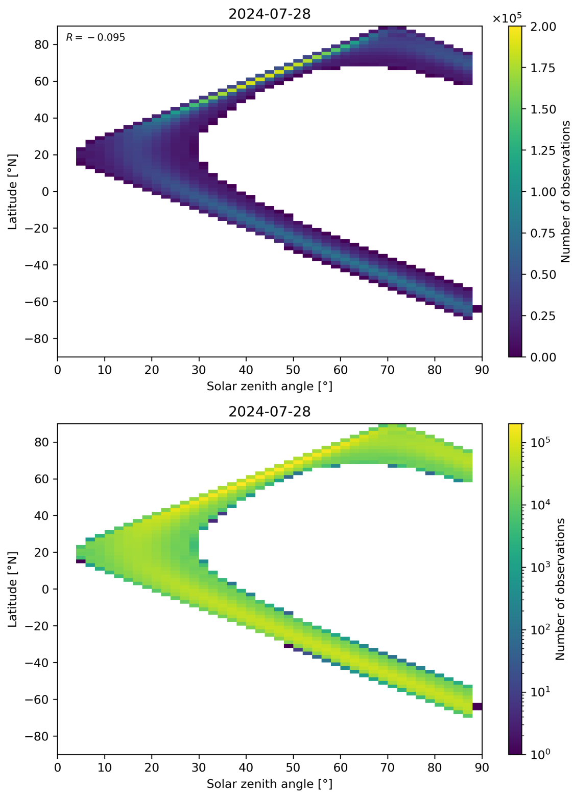
Figure 149: Scatter density plot of “Solar zenith angle” against “Latitude” for 2024-07-27 to 2024-07-29.
