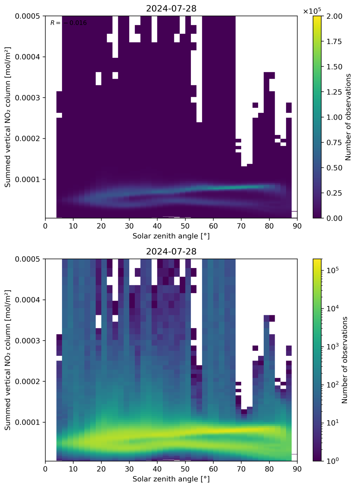
Figure 151: Scatter density plot of “Solar zenith angle” against “Summed vertical NO 2 column” for 2024-07-27 to 2024-07-29.
