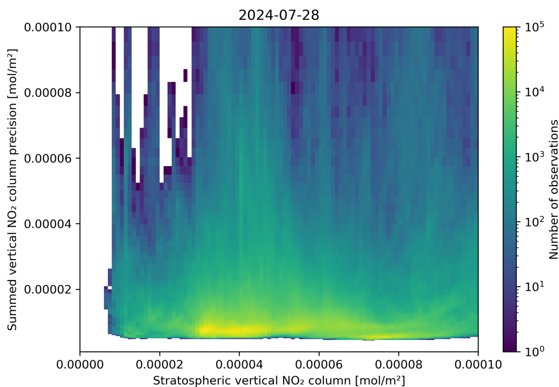
Figure 99: Scatter density plot of “Stratospheric vertical NO 2 column” against “Summed vertical NO 2 column precision” for 2024-07-27 to 2024-07-29.
