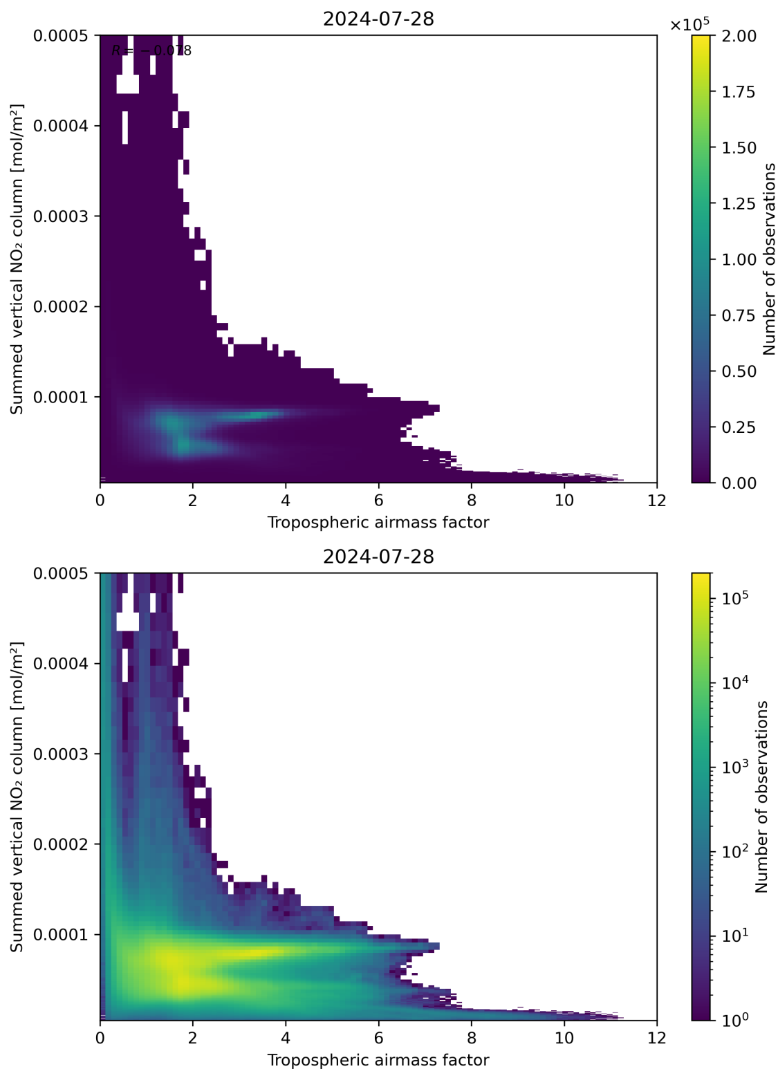
Figure 75: Scatter density plot of “Tropospheric airmass factor” against “Summed vertical NO 2 column” for 2024-07-27 to 2024-07-29.
