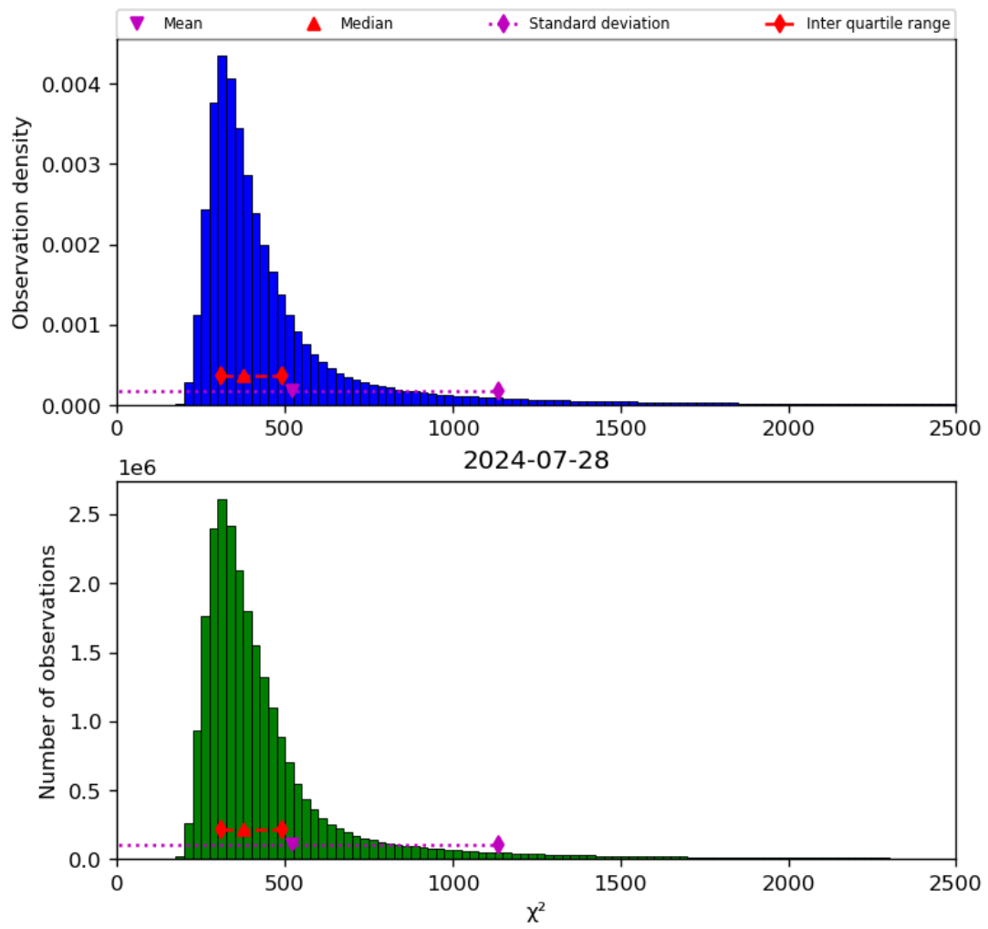
Figure 42: Histogram of “ \chi^2 ” for 2024-07-27 to 2024-07-29
