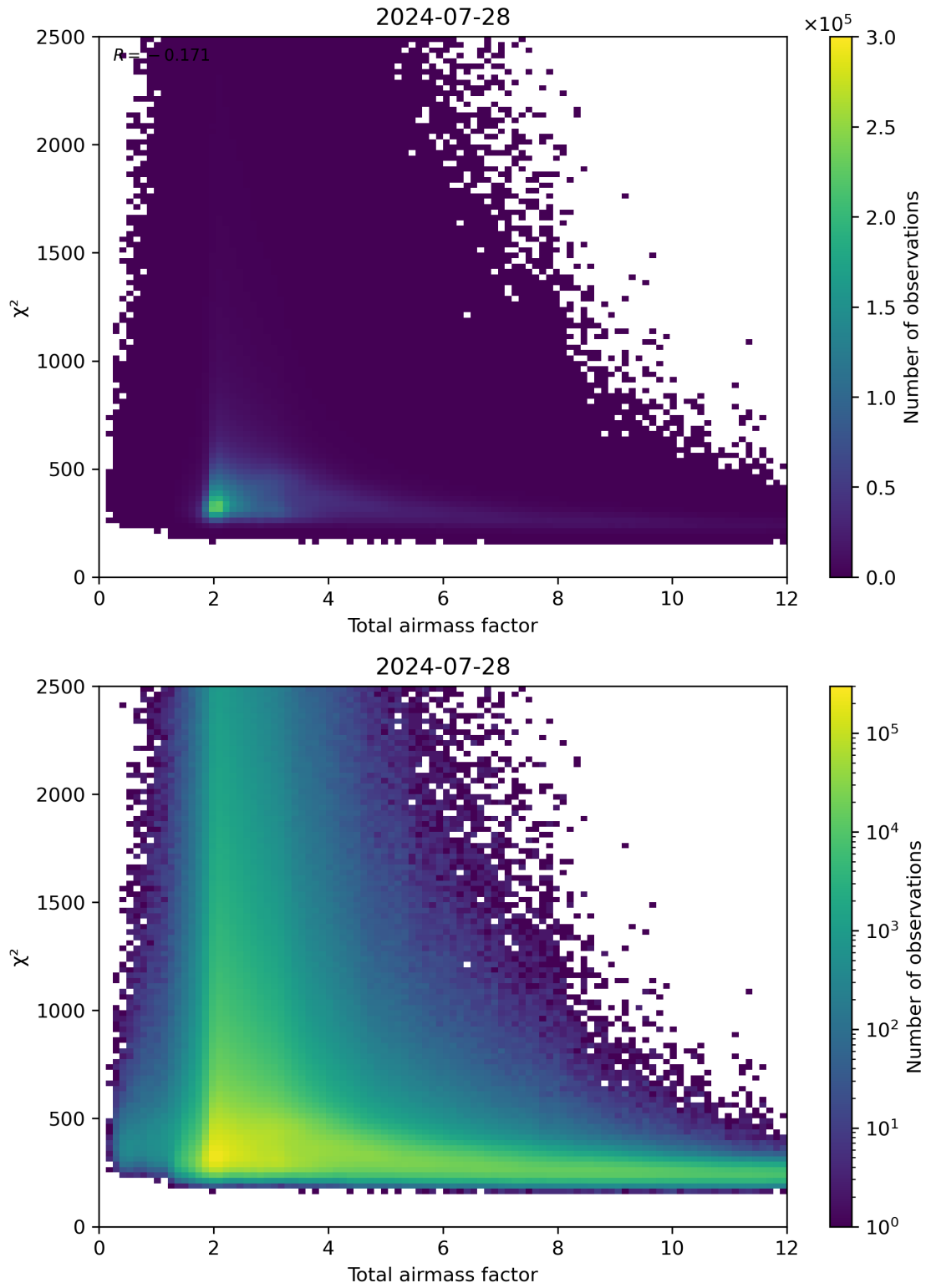
Figure 63: Scatter density plot of “Total airmass factor” against “ \chi^2 ” for 2024-07-27 to 2024-07-29.
