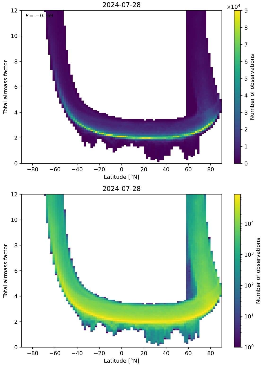
Figure 84: Scatter density plot of “Latitude” against “Total airmass factor” for 2024-07-27 to 2024-07-29.
