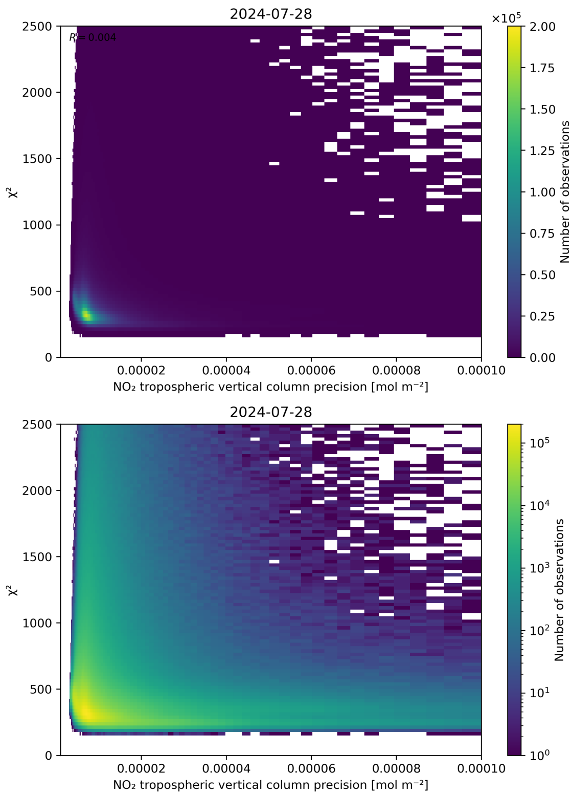
Figure 134: Scatter density plot of “NO 2 tropospheric vertical column precision” against “ \chi^2 ” for 2024-07-27 to 2024-07-29.
