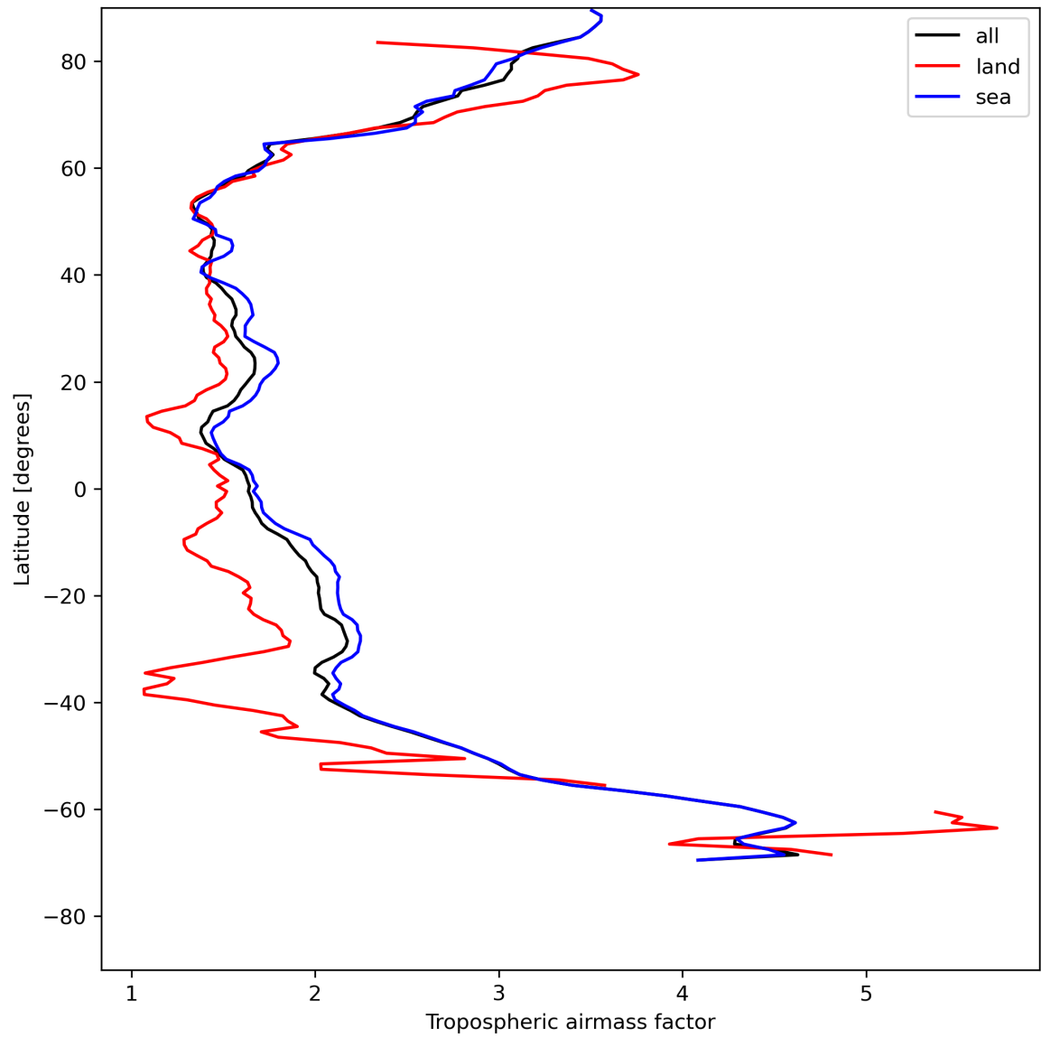
Figure 14: Zonal average of “Tropospheric airmass factor” for 2024-07-27 to 2024-07-29.
