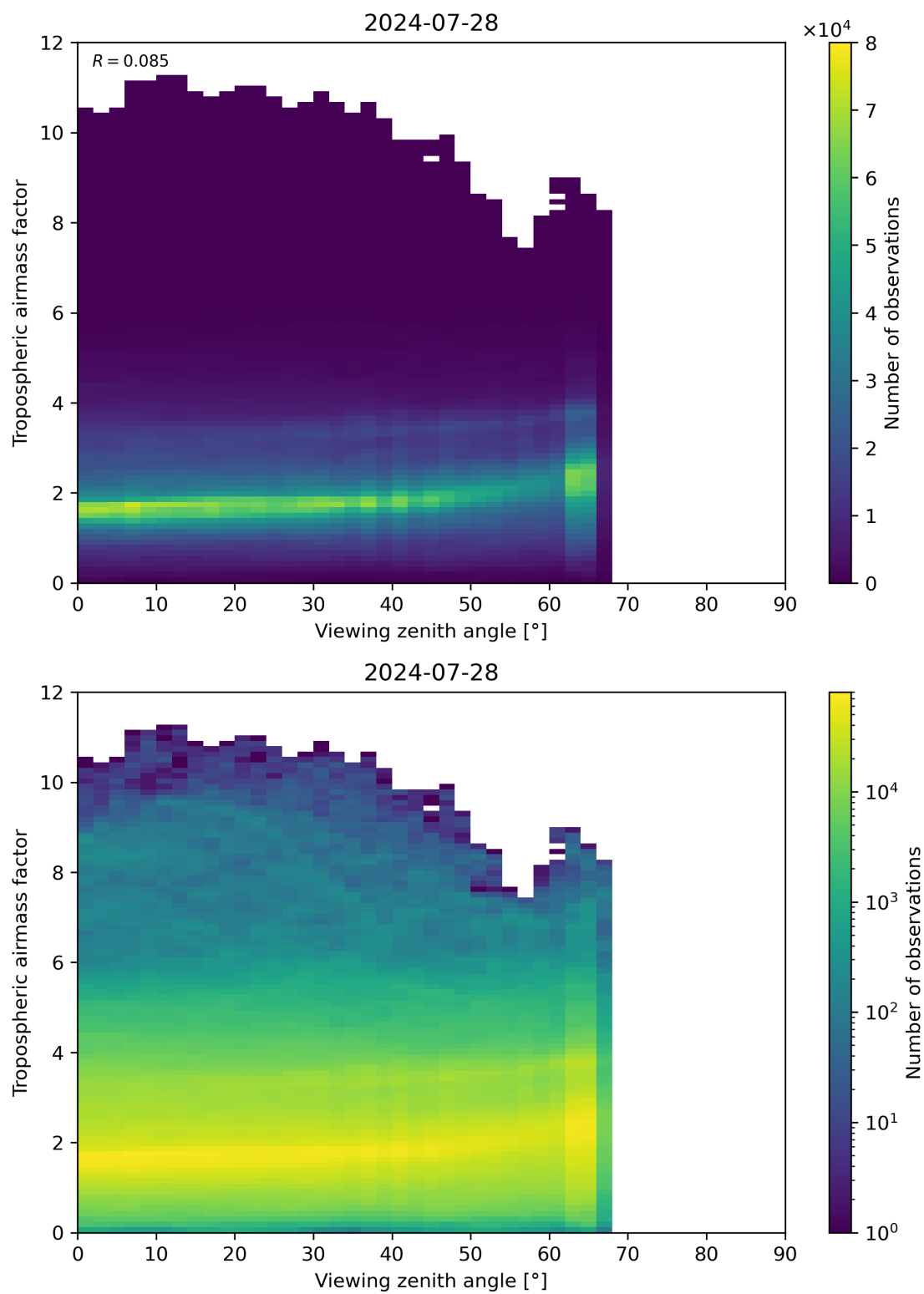
Figure 161: Scatter density plot of “Viewing zenith angle” against “Tropospheric airmass factor” for 2024-07-27 to 2024-07-29.
