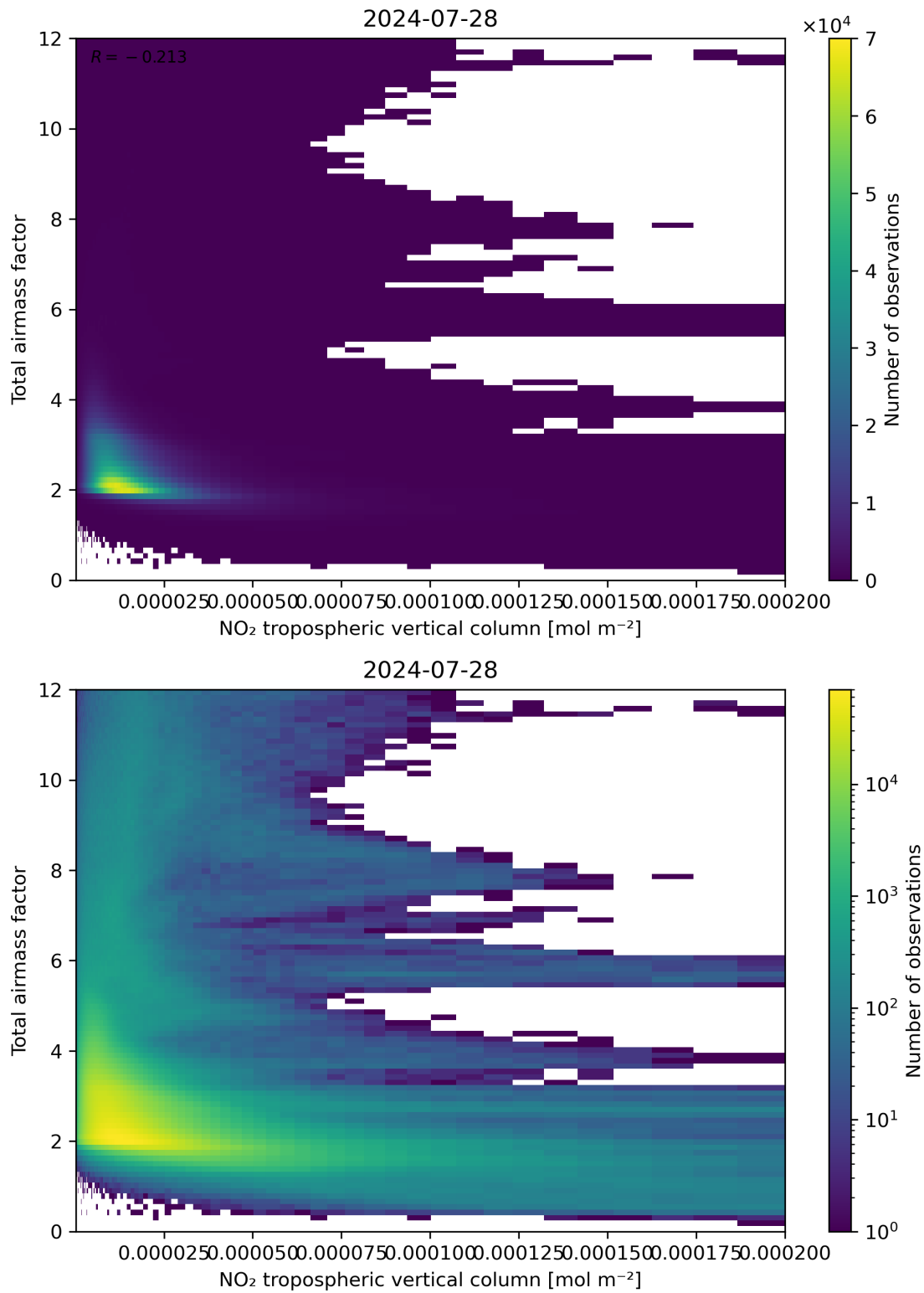
Figure 122: Scatter density plot of “NO 2 tropospheric vertical column” against “Total air mass factor” for 2024-07-27 to 2024-07-29.
