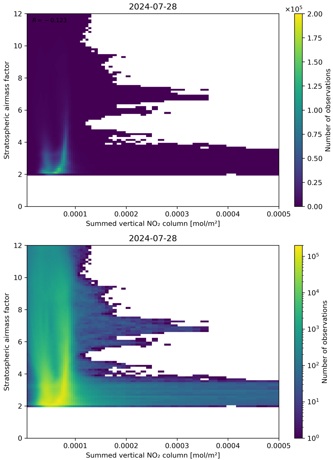
Figure 103: Scatter density plot of “Summed vertical NO 2 column” against “Stratospheric air mass factor” for 2024-07-27 to 2024-07-29.
