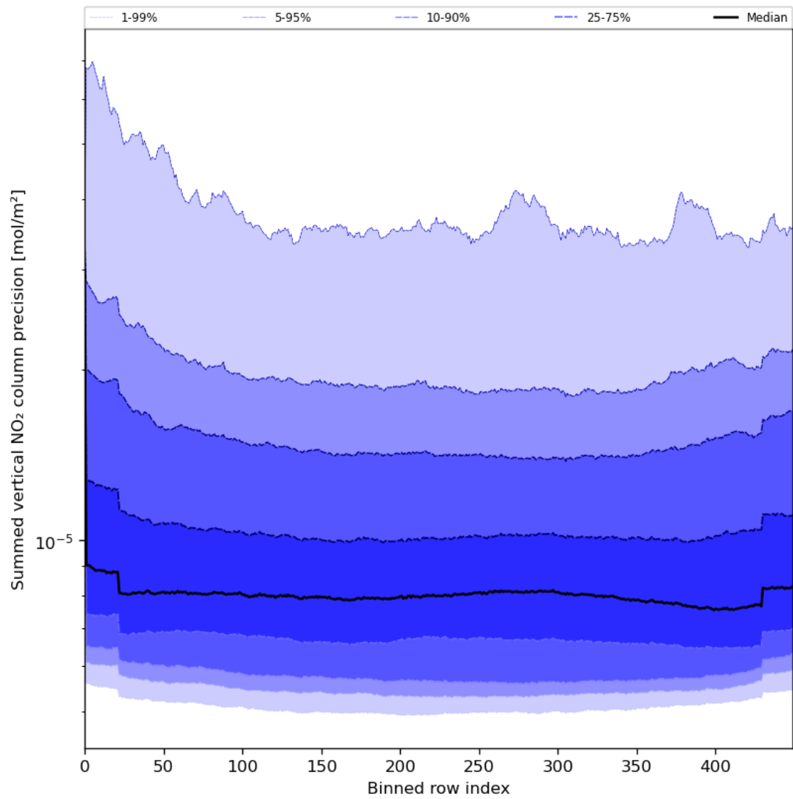
Figure 58: Along track statistics of “Summed vertical NO 2 column precision” for 2024-07-27 to 2024-07-29
