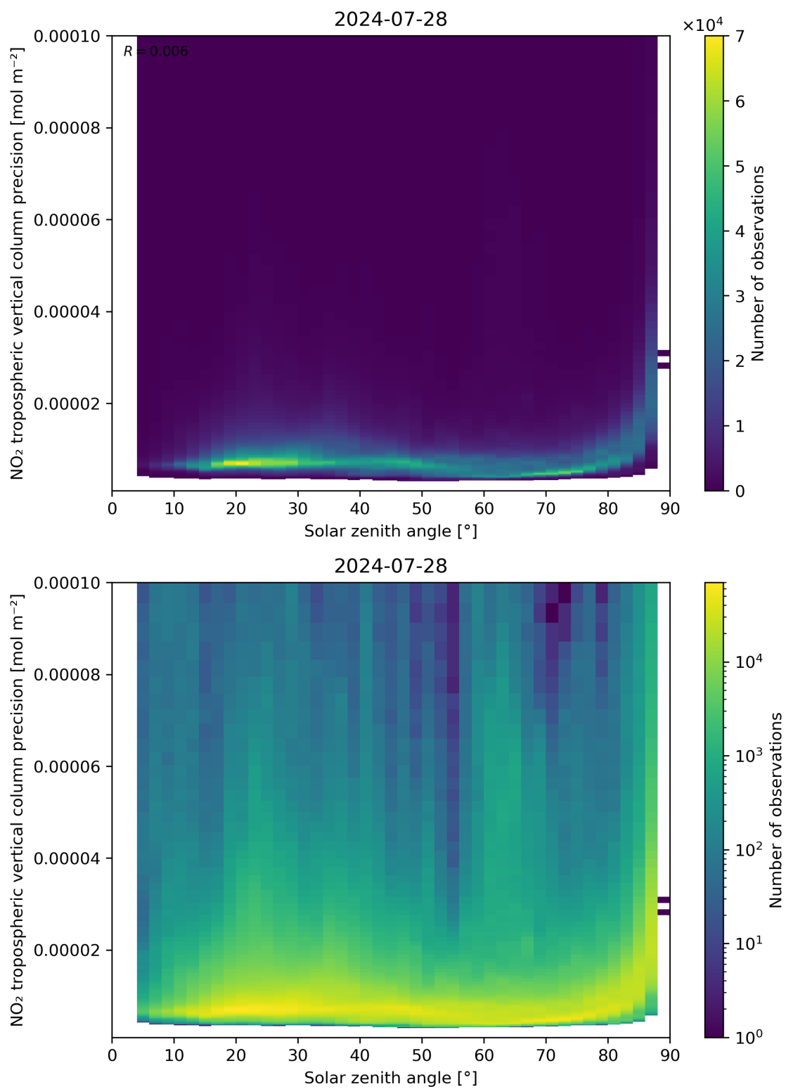
Figure 156: Scatter density plot of “Solar zenith angle” against “NO 2 tropospheric vertical column precision” for 2024-07-27 to 2024-07-29.
