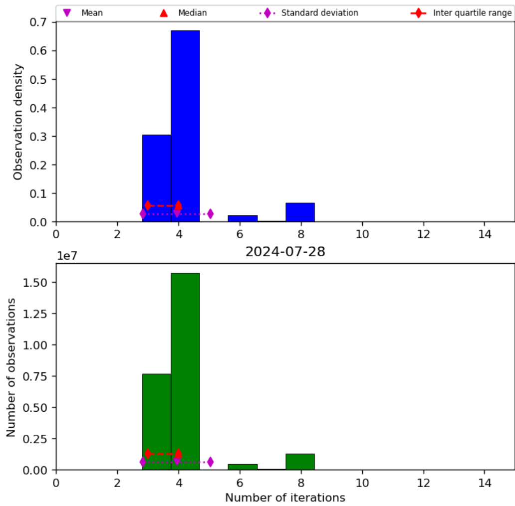
Figure 34: Histogram of “Number of iterations” for 2024-07-27 to 2024-07-29
