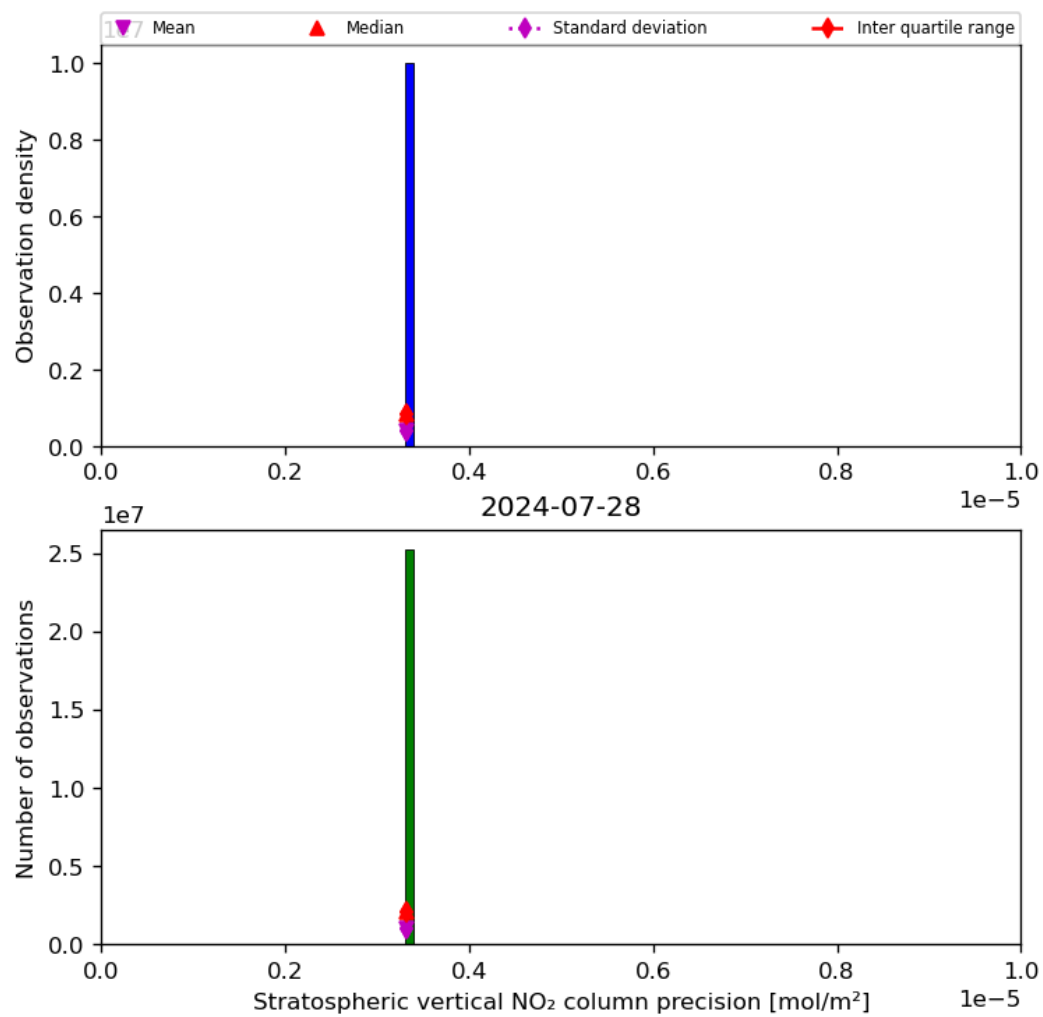
Figure 37: Histogram of “Stratospheric vertical NO 2 column precision” for 2024-07-27 to 2024-07-29
