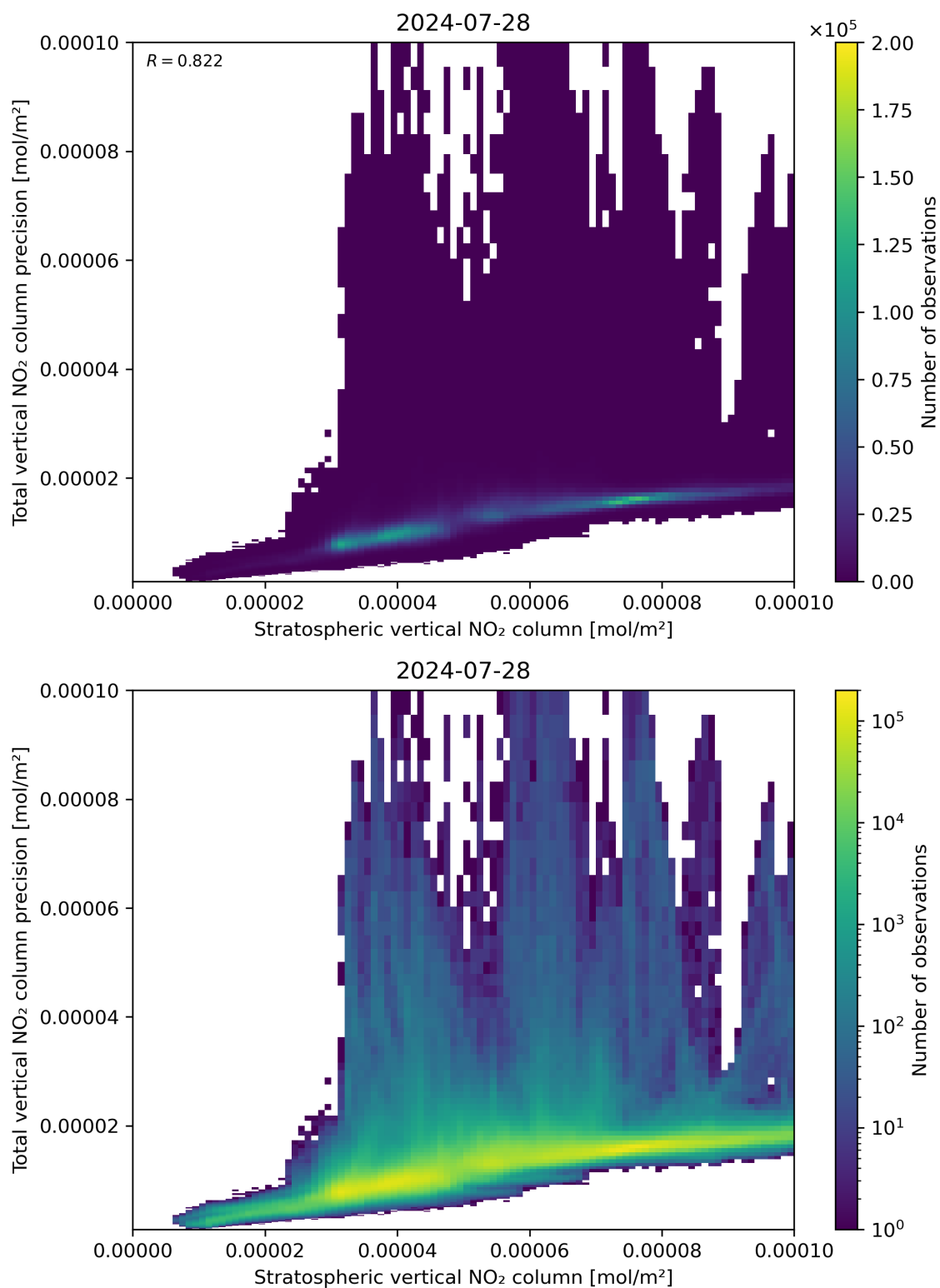
Figure 101: Scatter density plot of “Stratospheric vertical NO 2 column” against “Total vertical NO 2 column precision” for 2024-07-27 to 2024-07-29.
