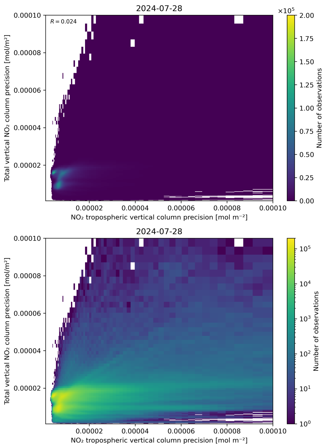
Figure 139: Scatter density plot of “NO 2 tropospheric vertical column precision” against “Total vertical NO 2 column precision” for 2024-07-27 to 2024-07-29.
