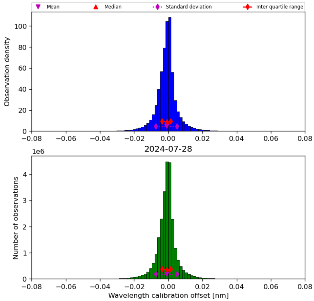
Figure 35: Histogram of “Wavelength calibration offset” for 2024-07-27 to 2024-07-29
