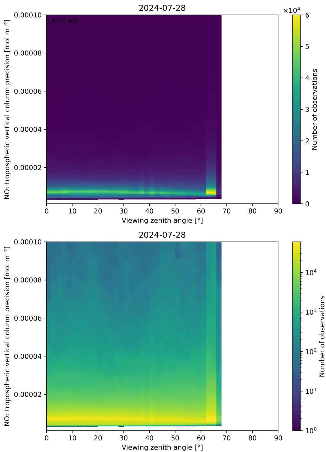
Figure 170: Scatter density plot of “Viewing zenith angle” against “NO 2 tropospheric vertical column precision” for 2024-07-27 to 2024-07-29.
