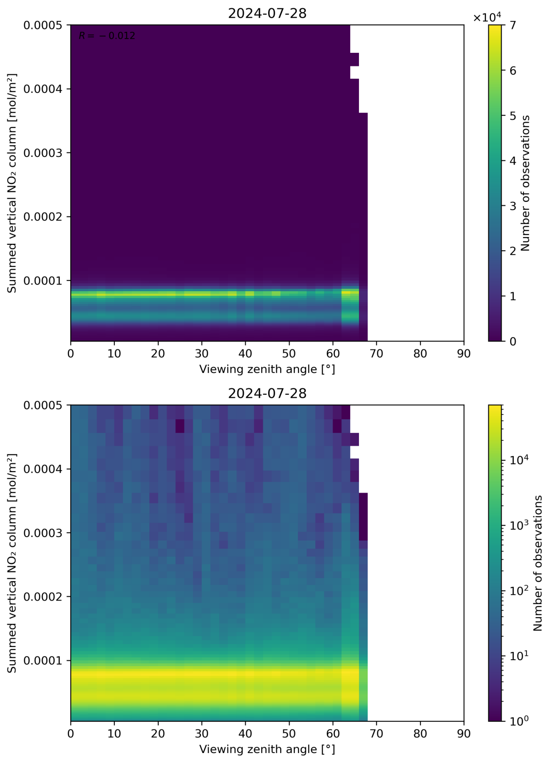
Figure 165: Scatter density plot of “Viewing zenith angle” against “Summed vertical NO 2 column” for 2024-07-27 to 2024-07-29.
