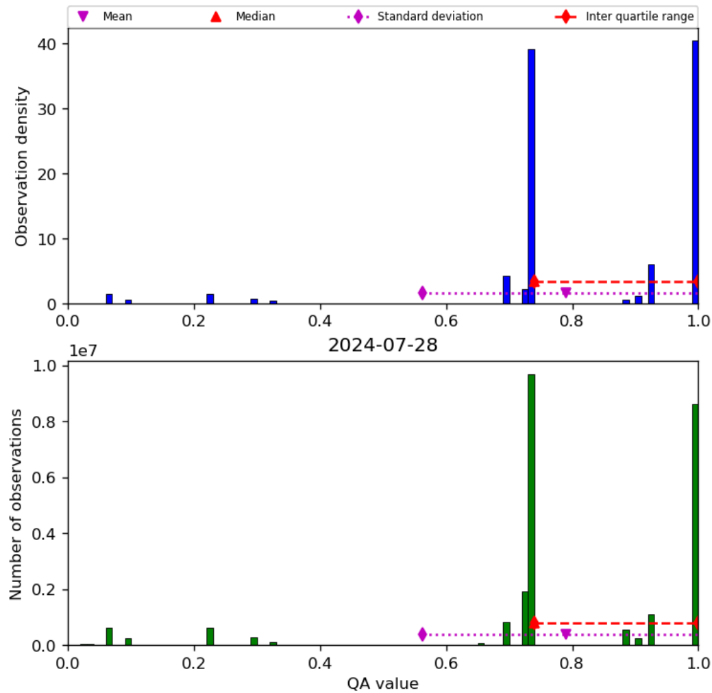
Figure 28: Histogram of “QA value” for 2024-07-27 to 2024-07-29
