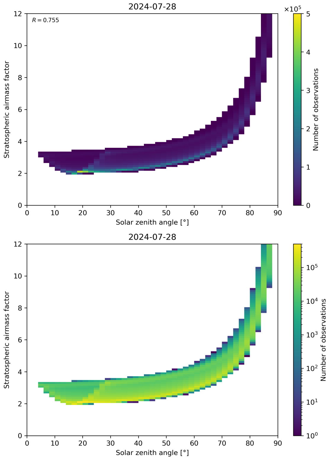
Figure 145: Scatter density plot of “Solar zenith angle” against “Stratospheric airmass factor” for 2024-07-27 to 2024-07-29.
