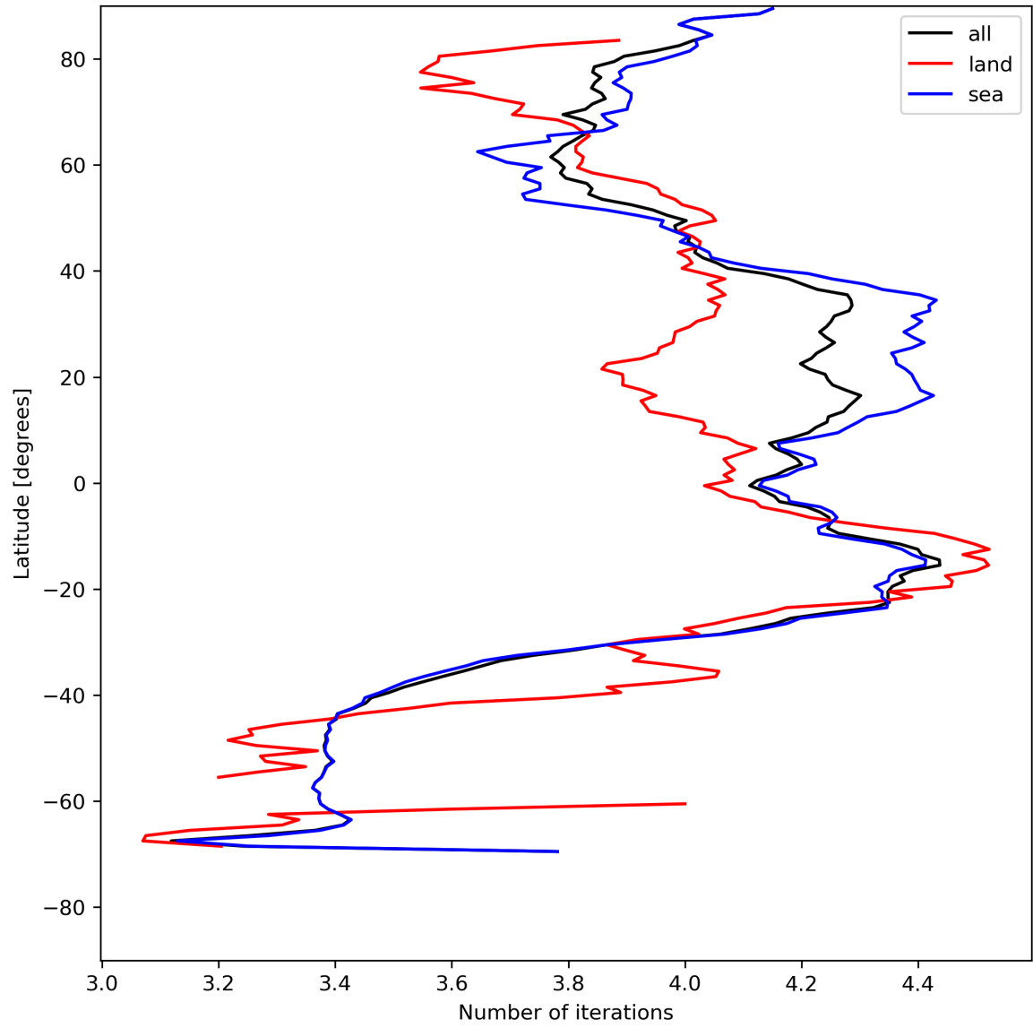
Figure 17: Zonal average of “Number of iterations” for 2024-07-27 to 2024-07-29.
