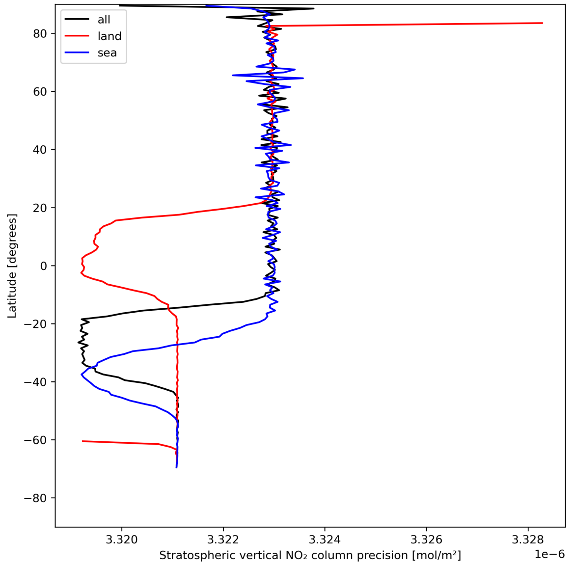
Figure 20: Zonal average of “Stratospheric vertical NO 2 column precision” for 2024-07-27 to 2024-07-29.
