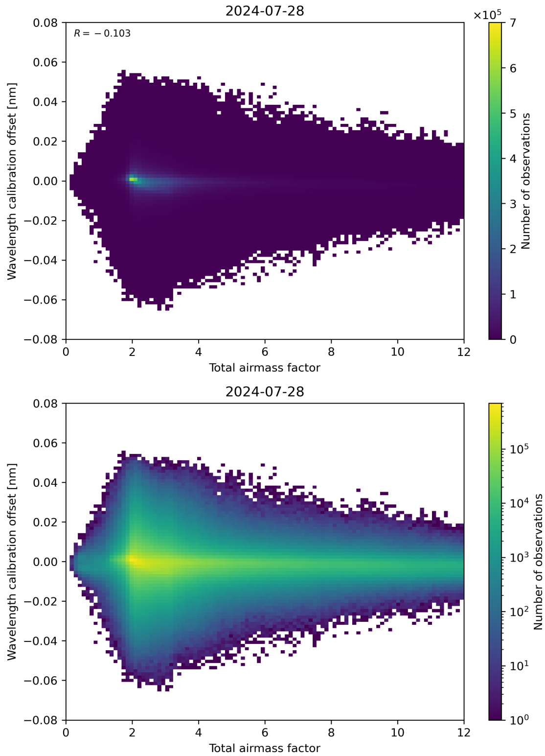
Figure 70: Scatter density plot of “Total airmass factor” against “Wavelength calibration offset” for 2024-07-27 to 2024-07-29.
