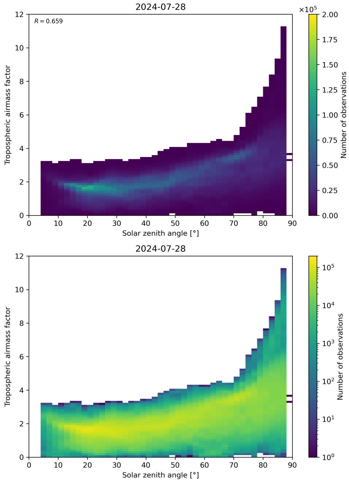
Figure 147: Scatter density plot of “Solar zenith angle” against “Tropospheric airmass factor” for 2024-07-27 to 2024-07-29.
