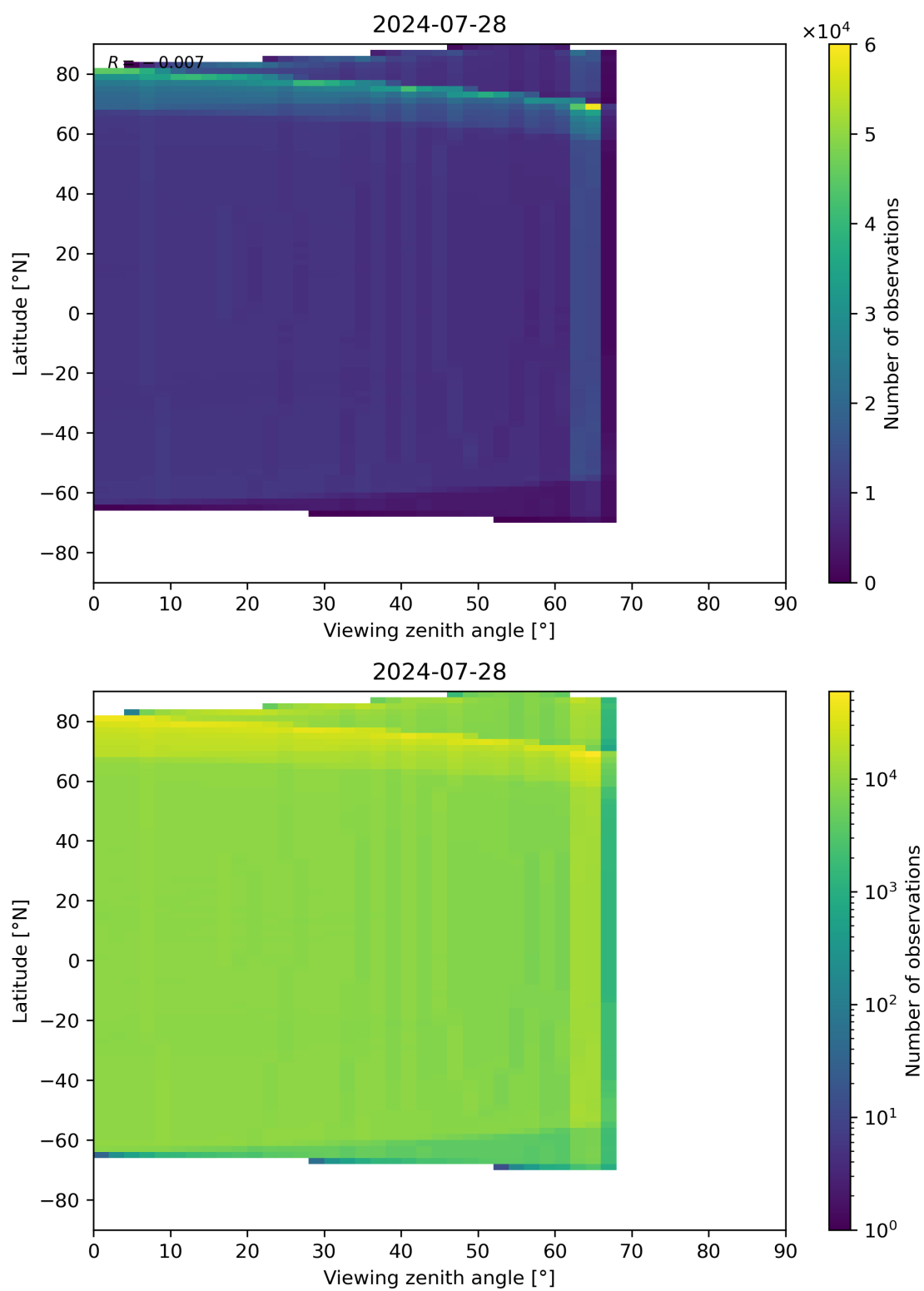
Figure 163: Scatter density plot of “Viewing zenith angle” against “Latitude” for 2024-07-27 to 2024-07-29.
