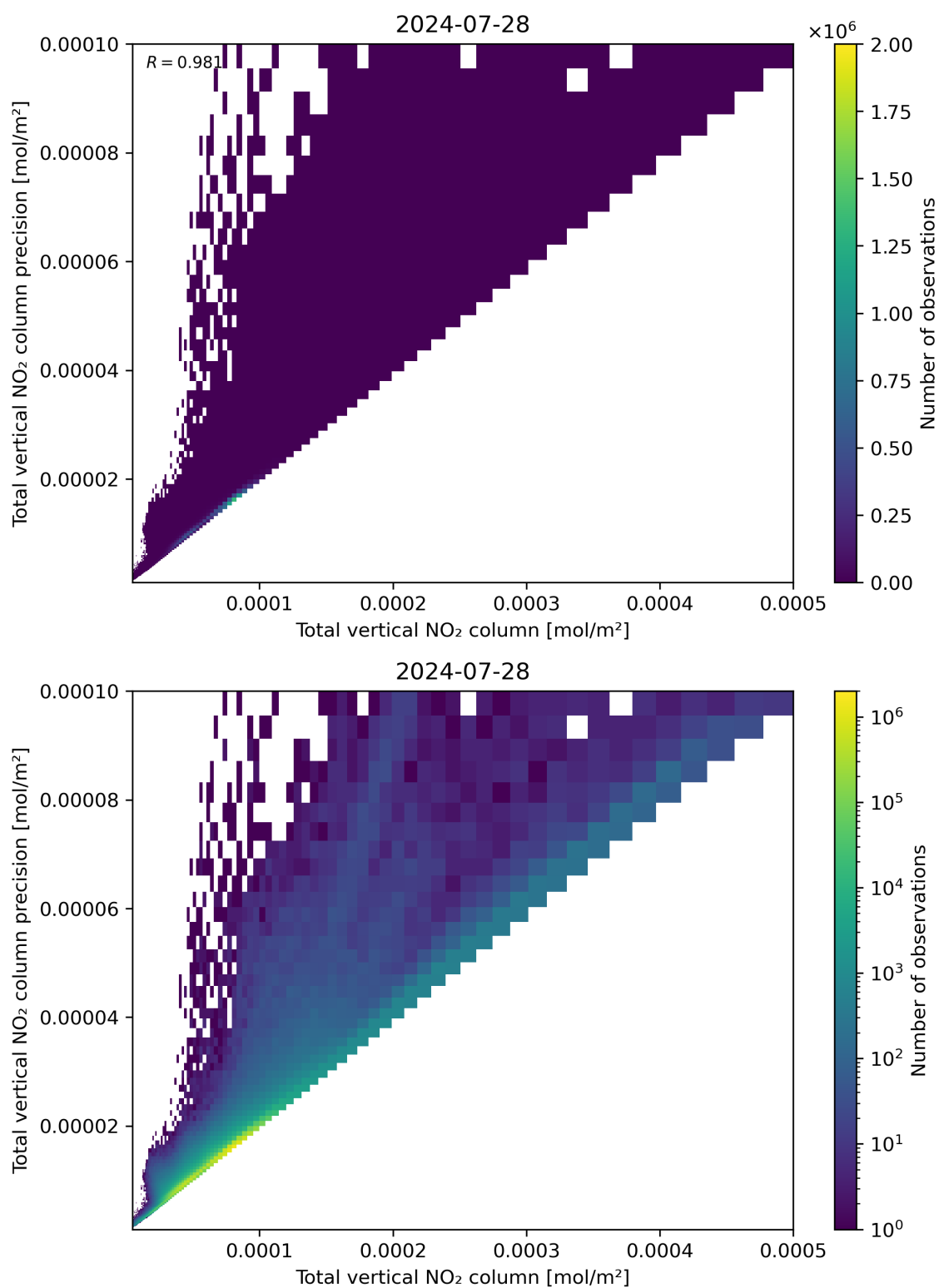
Figure 114: Scatter density plot of “Total vertical NO 2 column” against “Total vertical NO 2 column precision” for 2024-07-27 to 2024-07-29.
