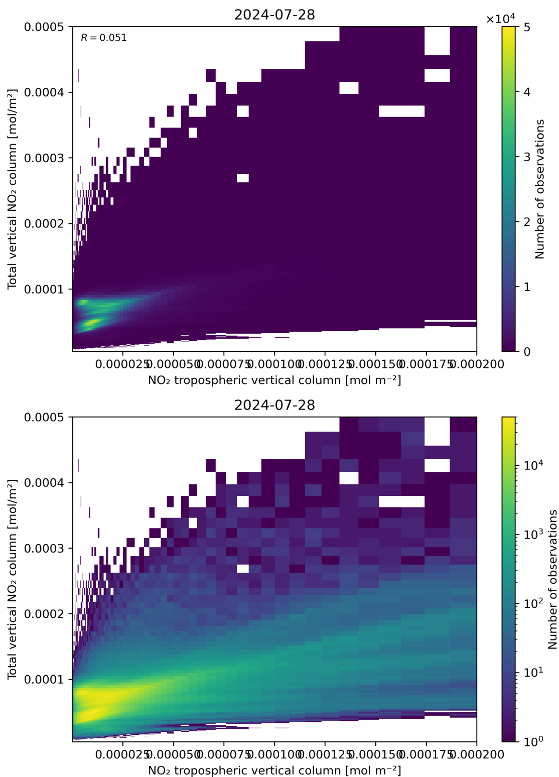
Figure 128: Scatter density plot of “NO 2 tropospheric vertical column” against “Total vertical NO 2 column” for 2024-07-27 to 2024-07-29.
