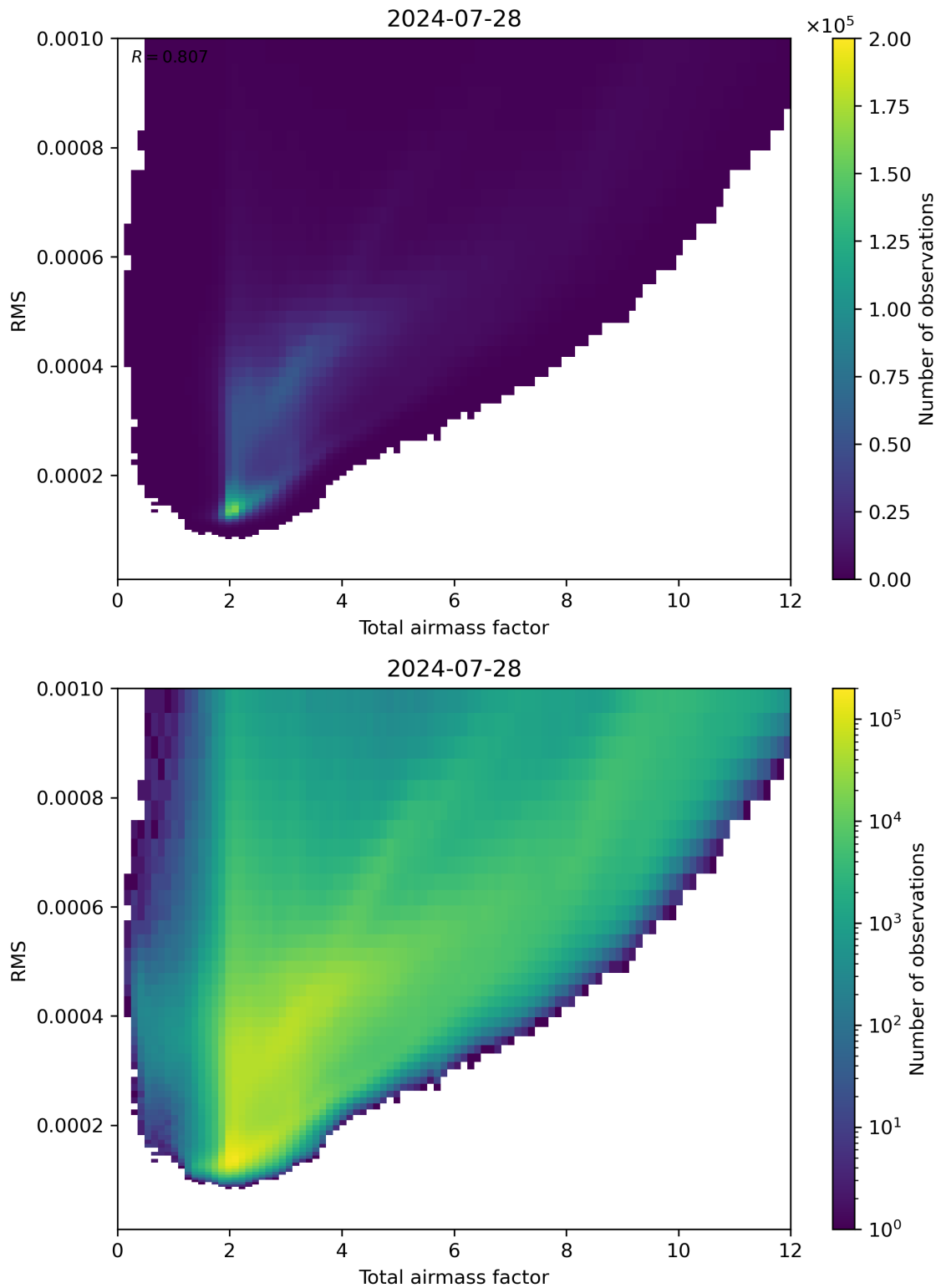
Figure 69: Scatter density plot of “Total airmass factor” against “RMS” for 2024-07-27 to 2024-07-29.
