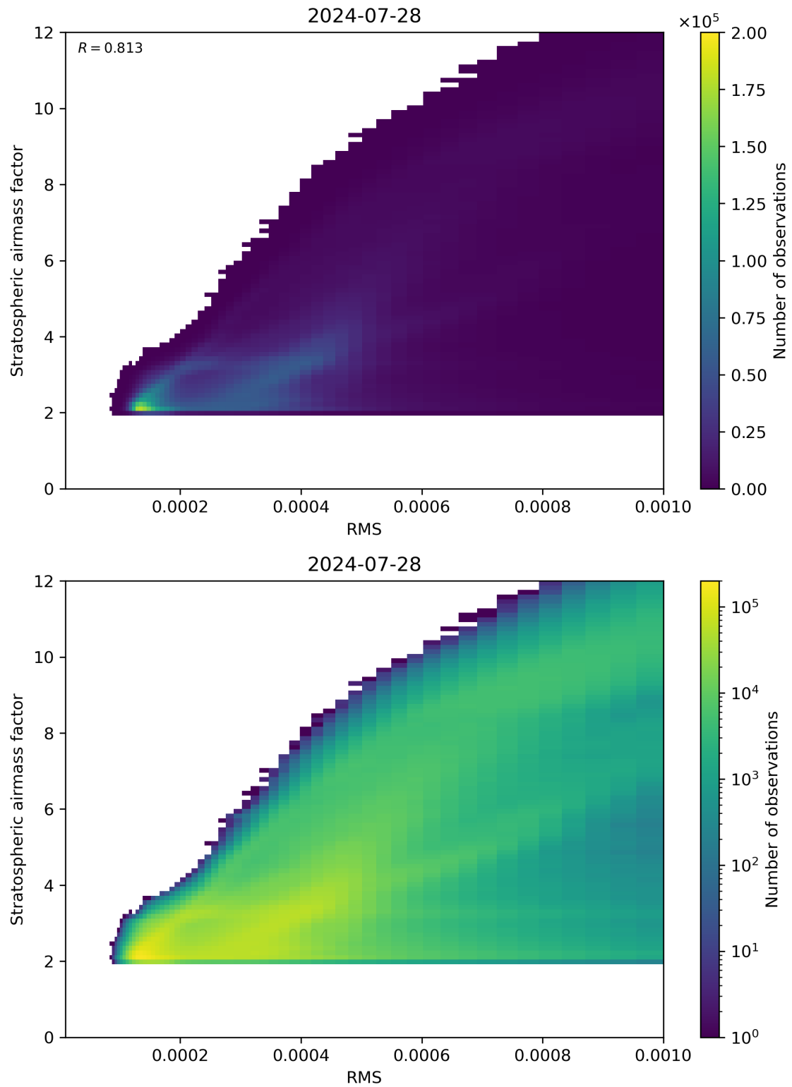
Figure 144: Scatter density plot of “RMS” against “Stratospheric airmass factor” for 2024-07-27 to 2024-07-29.
