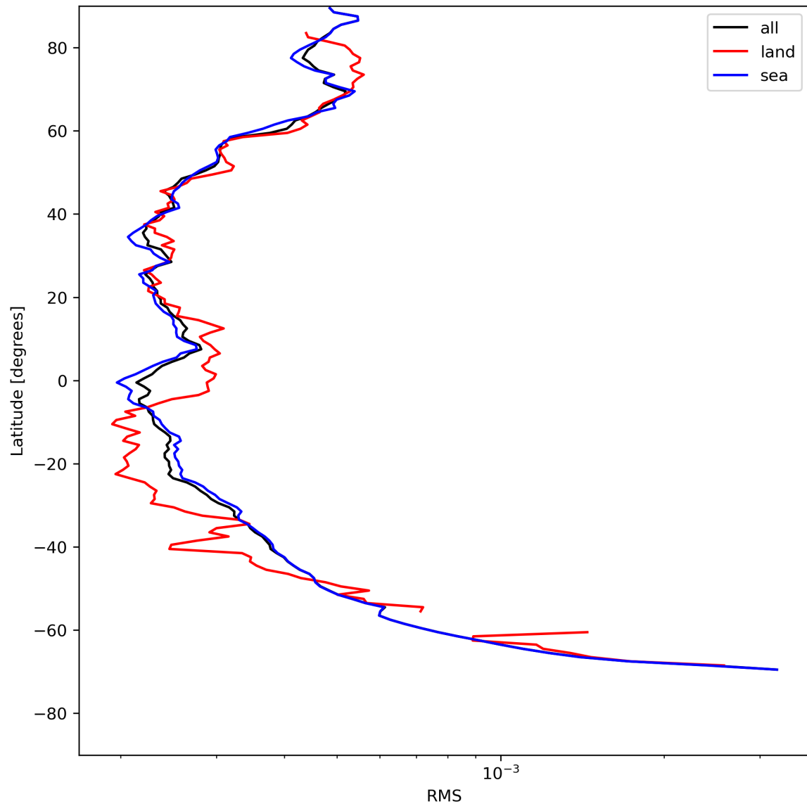
Figure 26: Zonal average of “RMS” for 2024-07-27 to 2024-07-29.
