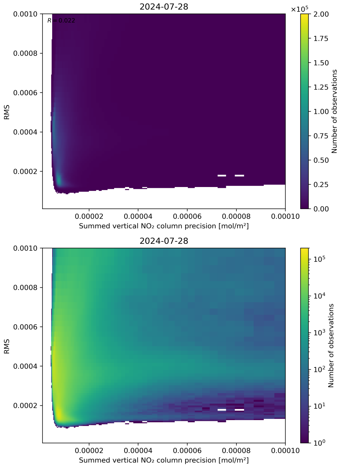
Figure 108: Scatter density plot of “Summed vertical NO 2 column precision” against “RMS” for 2024-07-27 to 2024-07-29.
