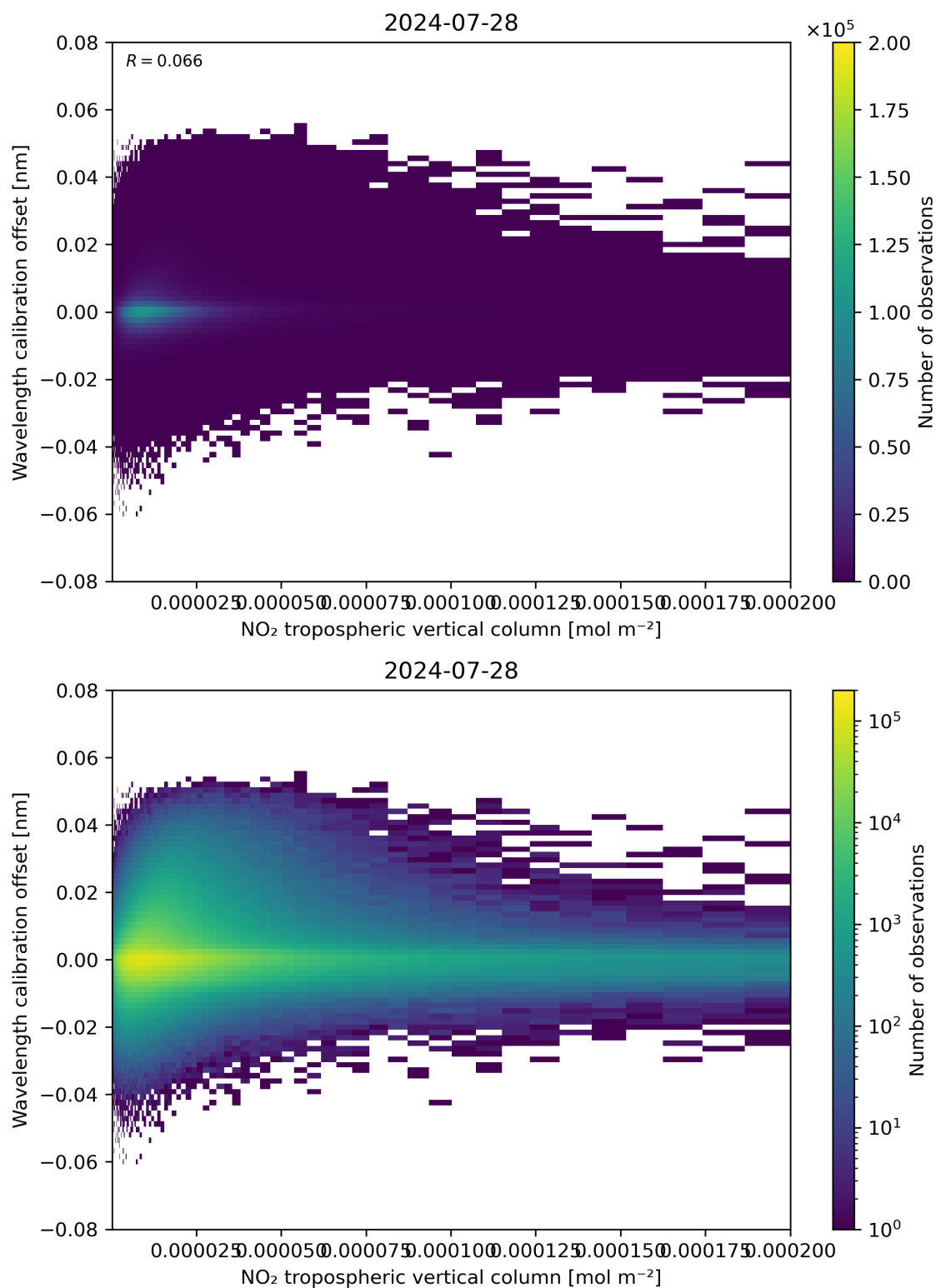
Figure 143: Scatter density plot of “NO 2 tropospheric vertical column” against “Wavelength calibration offset” for 2024-07-27 to 2024-07-29.
