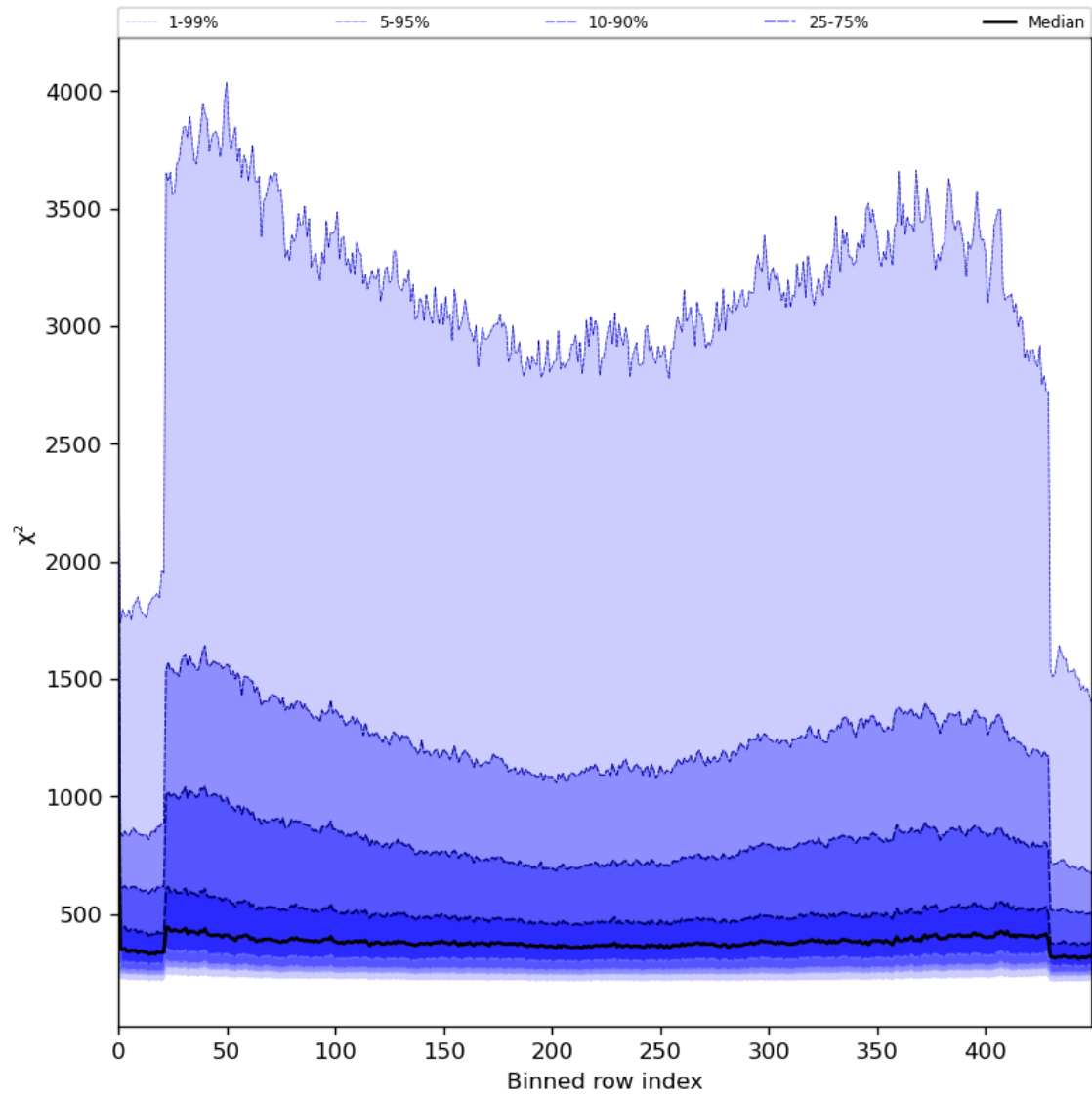
Figure 59: Along track statistics of “ \chi^2 ” for 2024-07-27 to 2024-07-29
