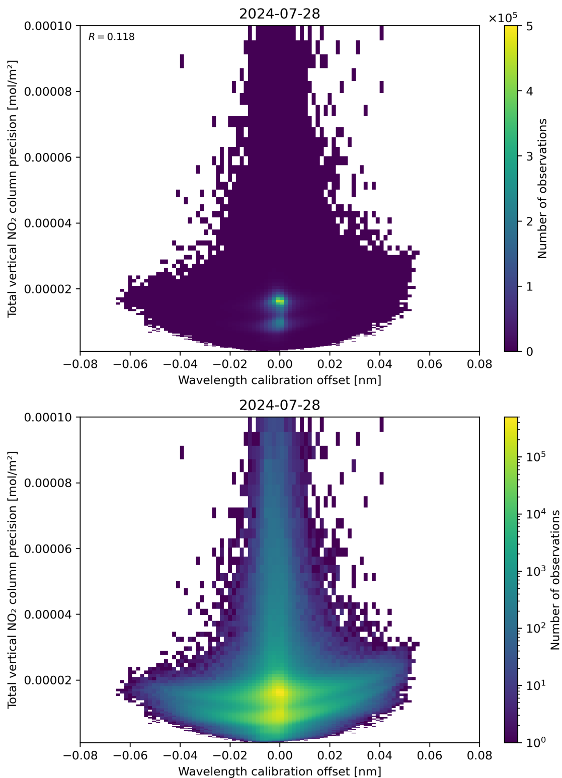
Figure 180: Scatter density plot of “Wavelength calibration offset” against “Total vertical NO 2 column precision” for 2024-07-27 to 2024-07-29.
