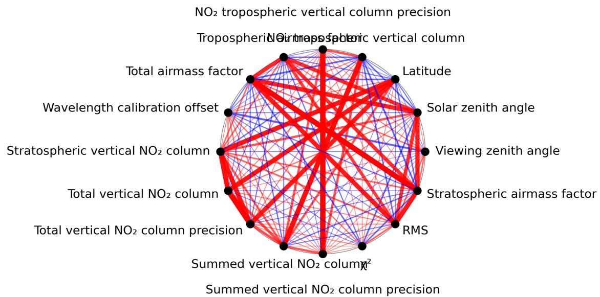
Figure 1: Map of correlation graph for 2024-07-27 to 2024-07-29.
