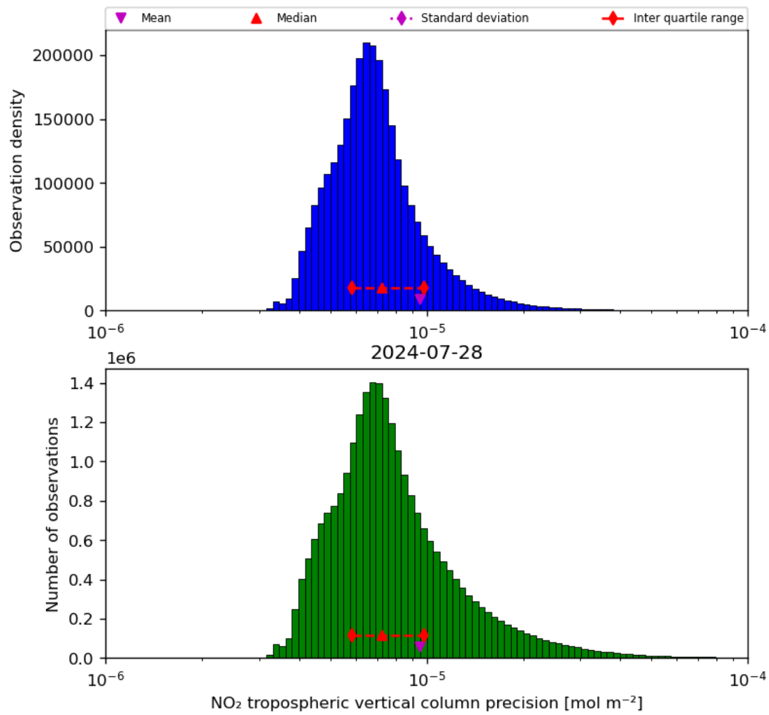
Figure 30: Histogram of “NO 2 tropospheric vertical column precision” for 2024-07-27 to 2024-07-29
