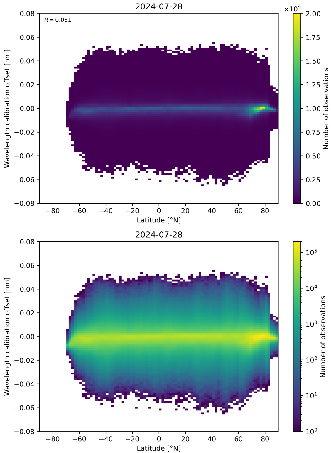
Figure 95: Scatter density plot of “Latitude” against “Wavelength calibration offset” for 2024-07-27 to 2024-07-29.
