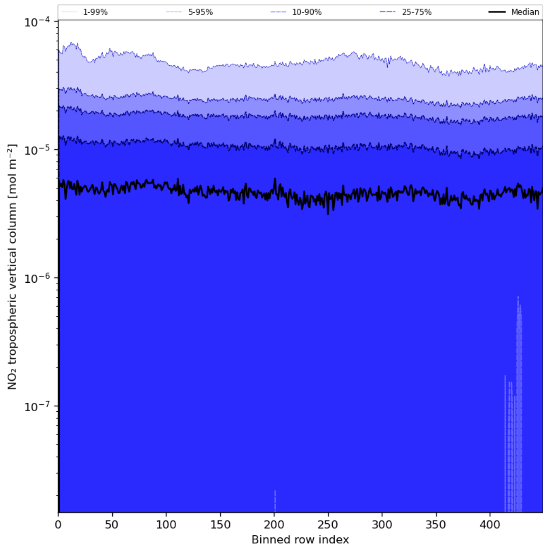
Figure 46: Along track statistics of “NO 2 tropospheric vertical column” for 2024-07-27 to 2024-07-29
