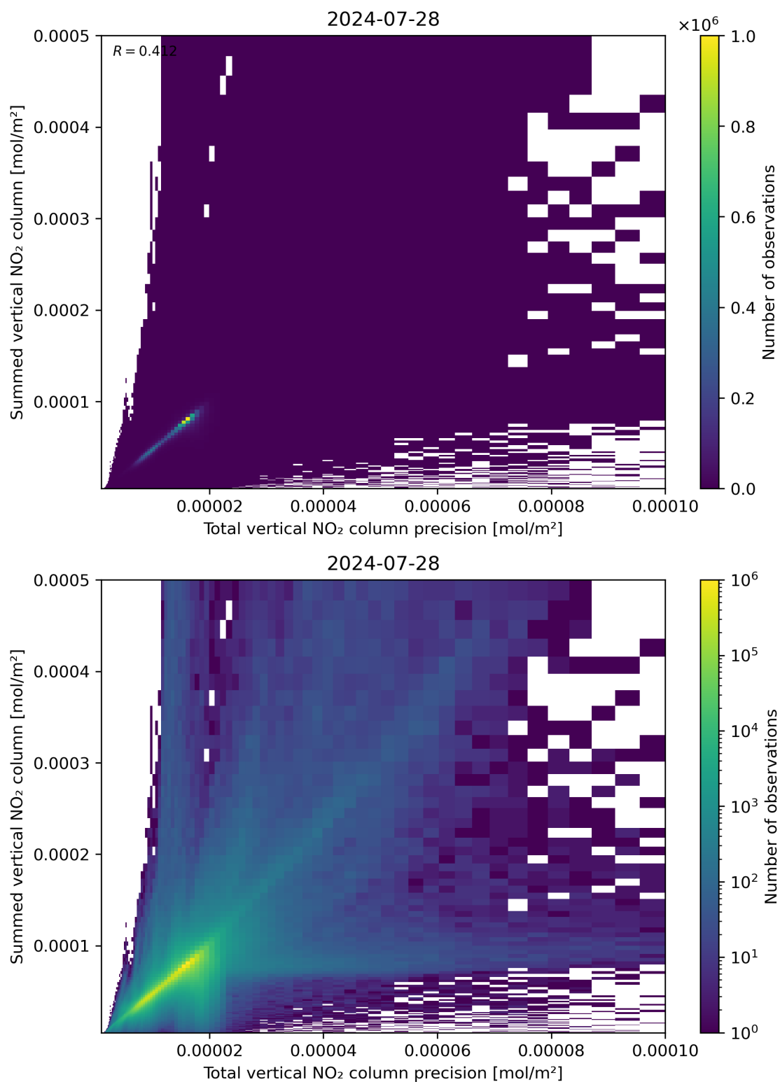
Figure 117: Scatter density plot of “Total vertical NO 2 column precision” against “Summed vertical NO 2 column” for 2024-07-27 to 2024-07-29.
