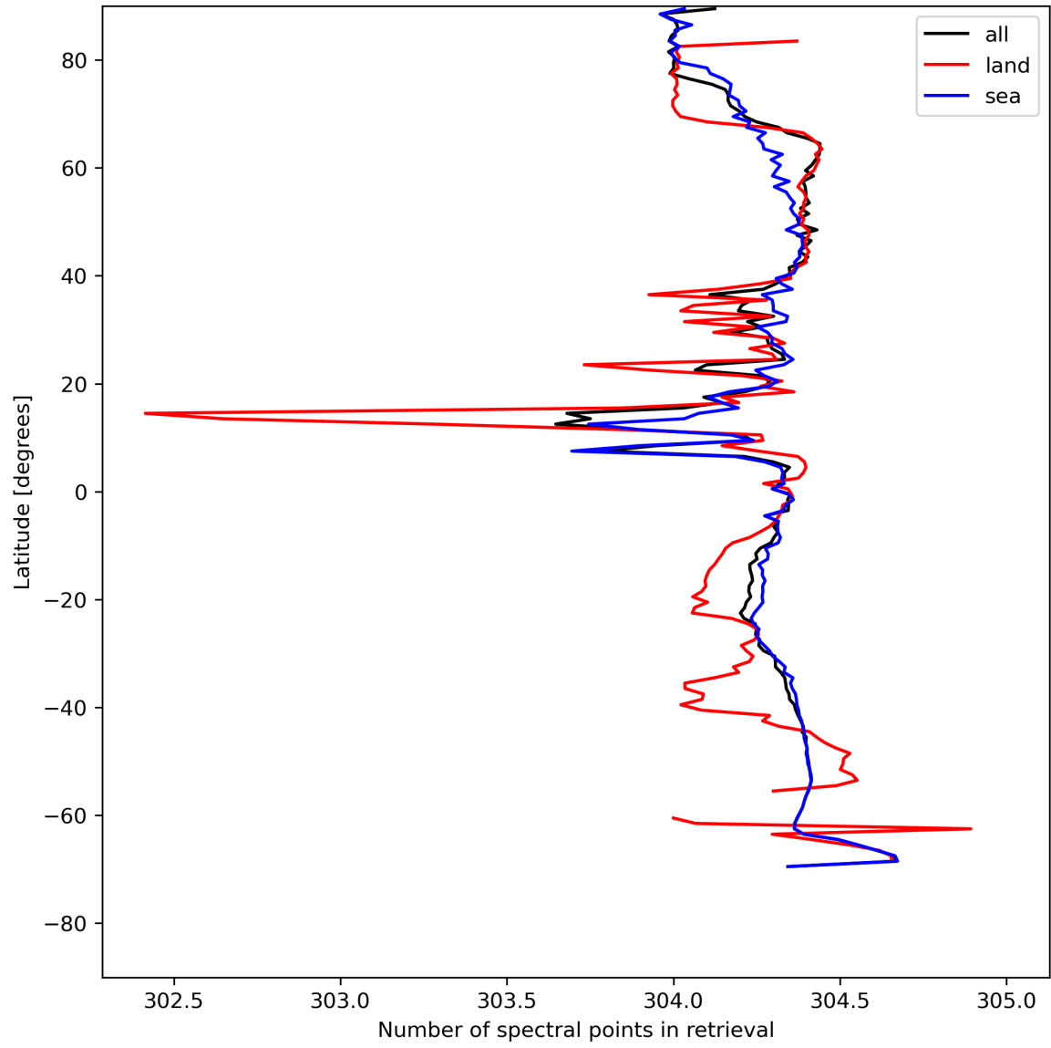
Figure 16: Zonal average of “Number of spectral points in retrieval” for 2024-07-27 to 2024-07-29.
