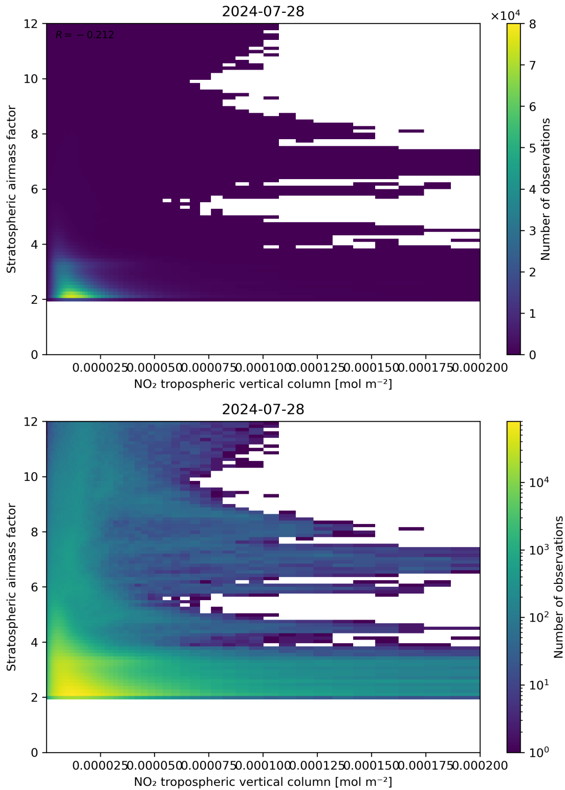
Figure 121: Scatter density plot of “NO 2 tropospheric vertical column” against “Stratospheric air mass factor” for 2024-07-27 to 2024-07-29.
