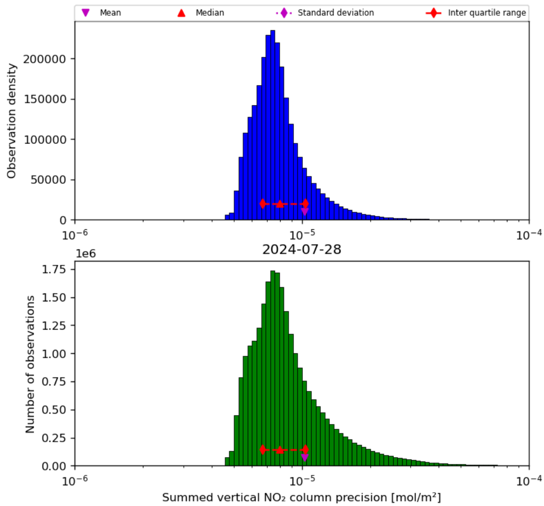
Figure 41: Histogram of "Summed vertical NO 2 column precision" for 2024-07-27 to 2024-07-29
