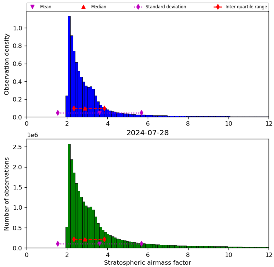
Figure 44: Histogram of “Stratospheric airmass factor” for 2024-07-27 to 2024-07-29
