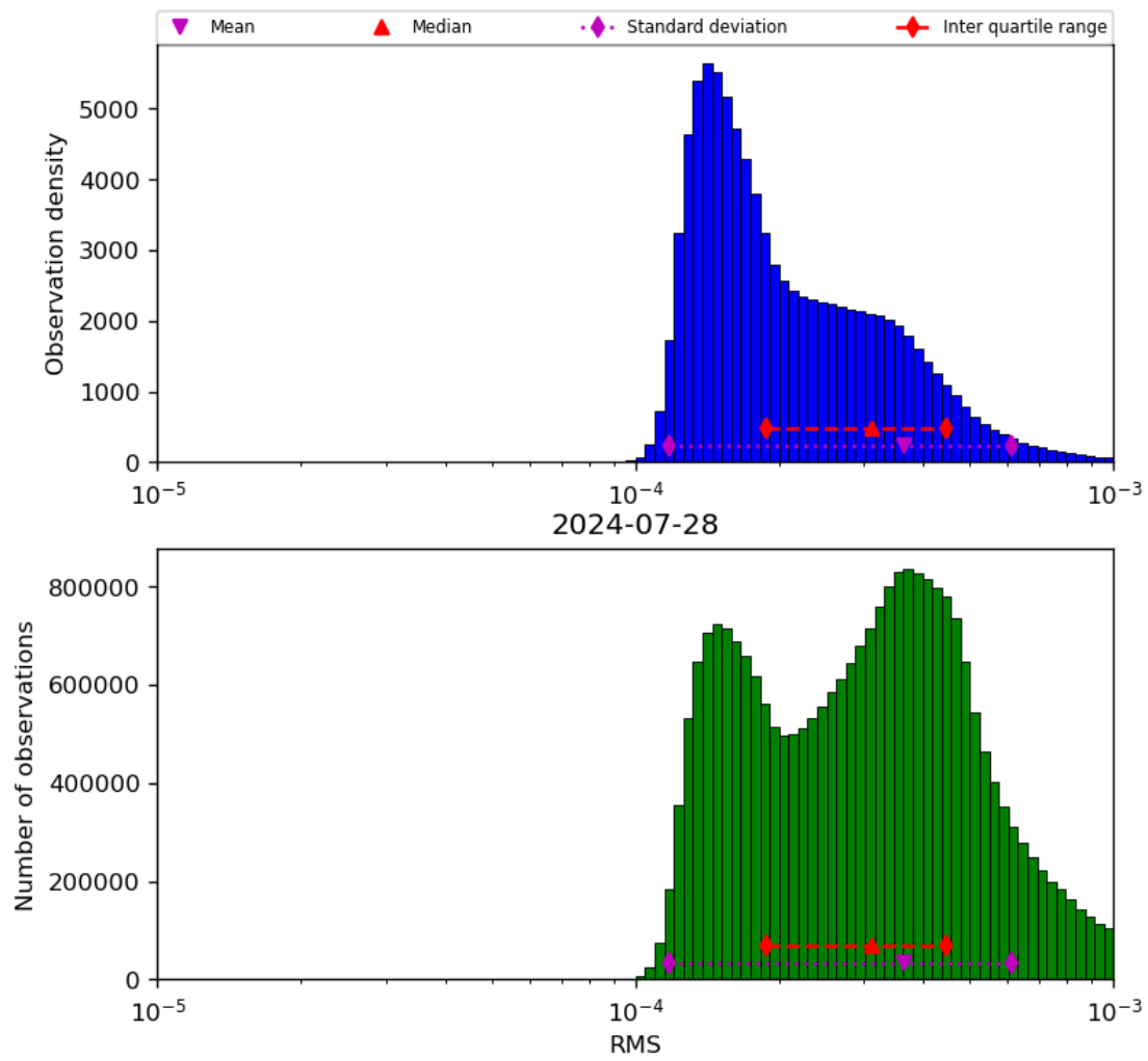
Figure 43: Histogram of “RMS” for 2024-07-27 to 2024-07-29
