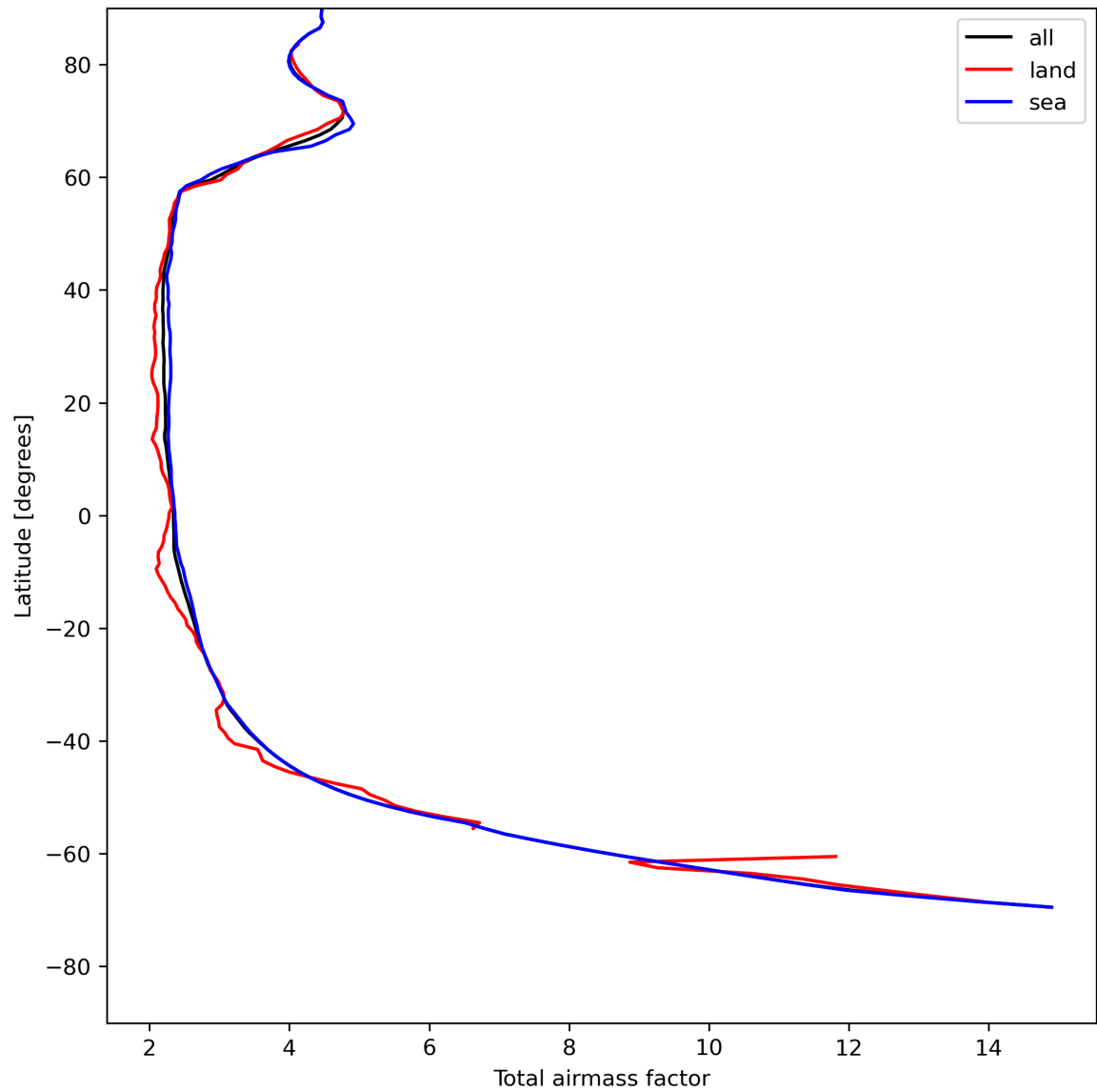
Figure 15: Zonal average of “Total airmass factor” for 2024-07-27 to 2024-07-29.
