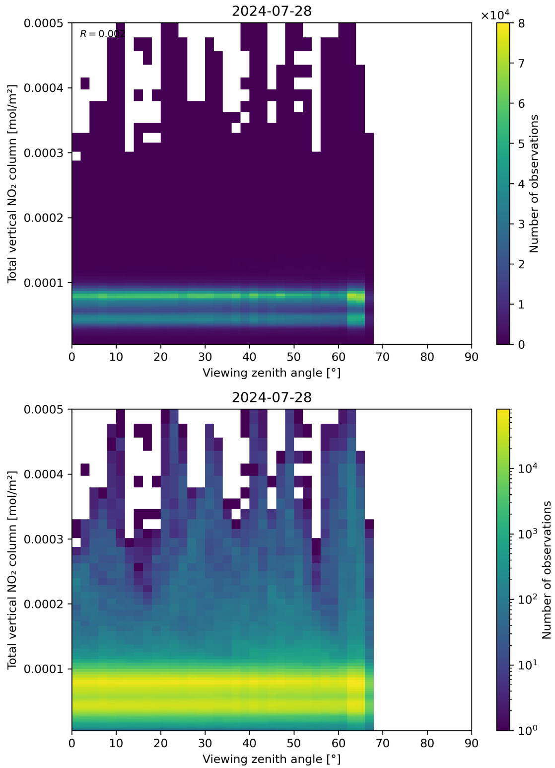
Figure 167: Scatter density plot of “Viewing zenith angle” against “Total vertical NO 2 column” for 2024-07-27 to 2024-07-29.
