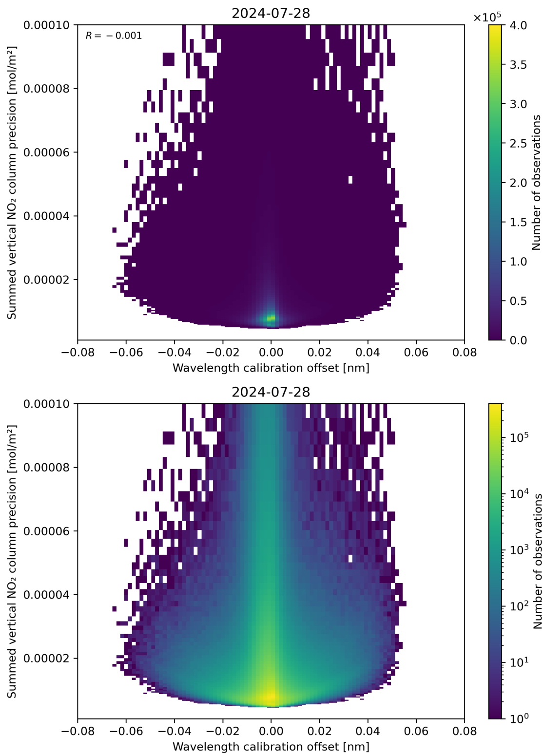
Figure 178: Scatter density plot of “Wavelength calibration offset” against “Summed vertical NO 2 column precision” for 2024-07-27 to 2024-07-29.
