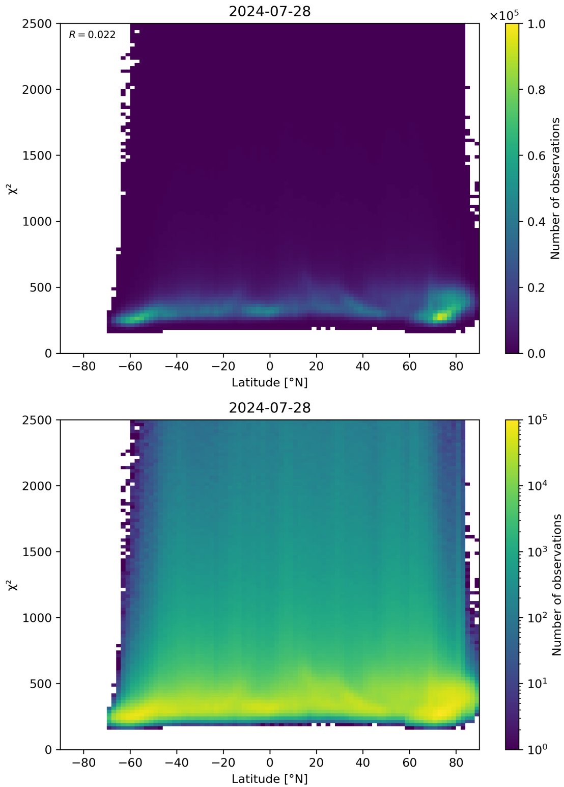
Figure 86: Scatter density plot of “Latitude” against “ \chi^2 ” for 2024-07-27 to 2024-07-29.
