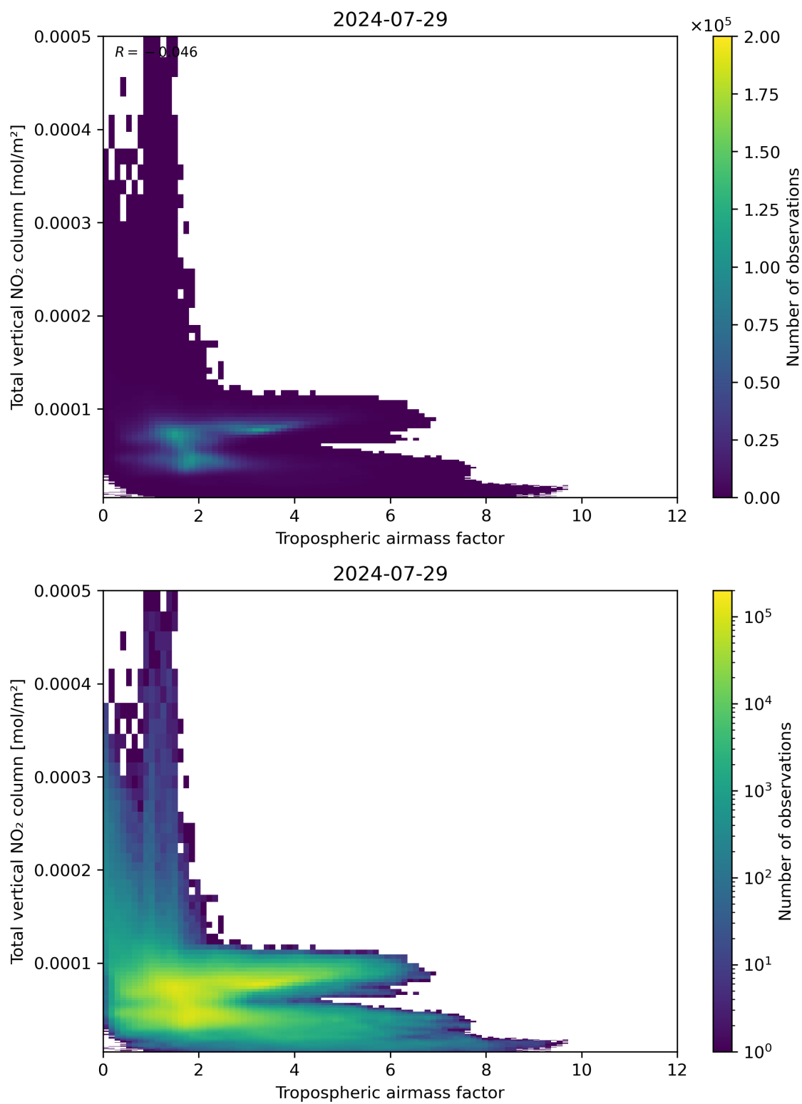
Figure 77: Scatter density plot of “Tropospheric airmass factor” against “Total vertical NO 2 column” for 2024-07-28 to 2024-07-30.
