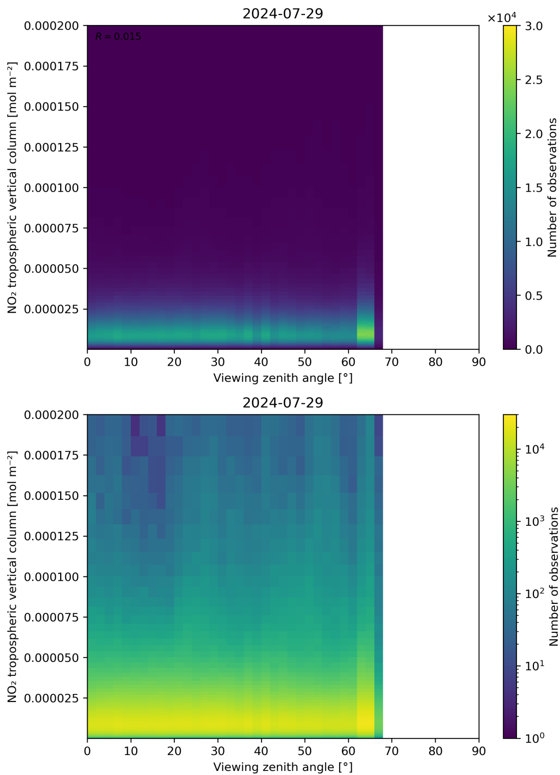
Figure 169: Scatter density plot of “Viewing zenith angle” against “NO 2 tropospheric vertical column” for 2024-07-28 to 2024-07-30.
