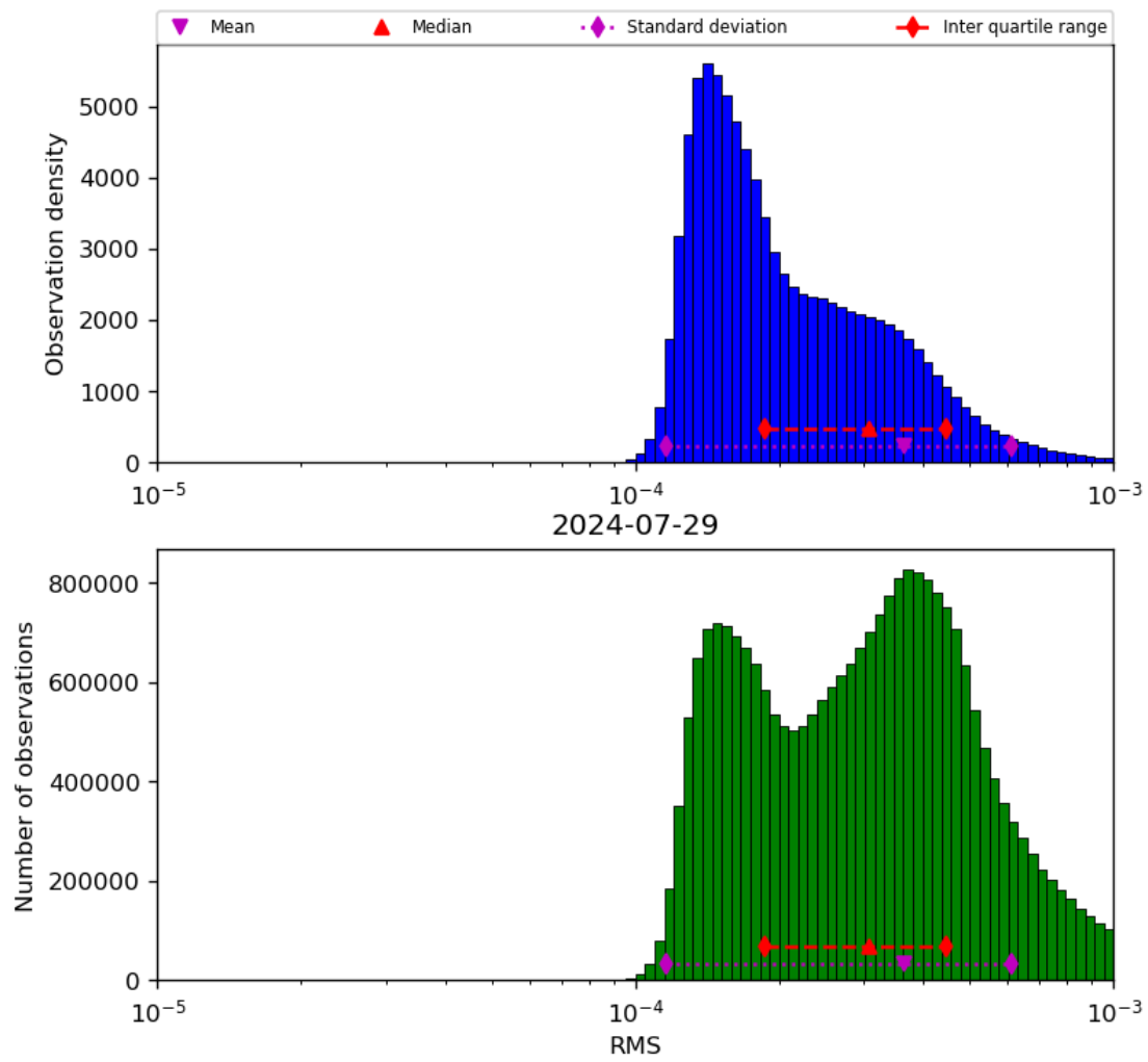
Figure 43: Histogram of “RMS” for 2024-07-28 to 2024-07-30
