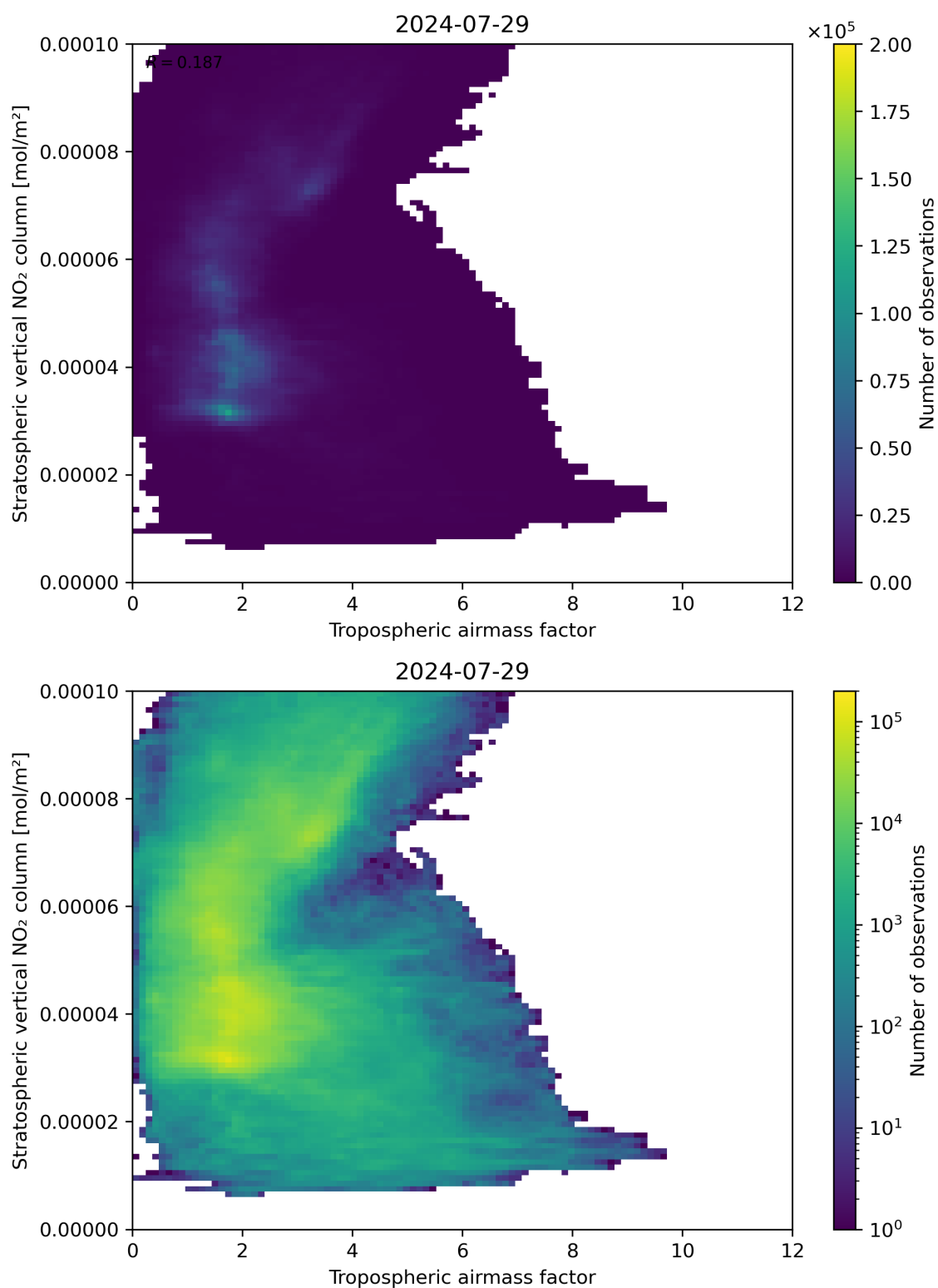
Figure 74: Scatter density plot of “Tropospheric air mass factor” against “Stratospheric vertical NO 2 column” for 2024-07-28 to 2024-07-30.
