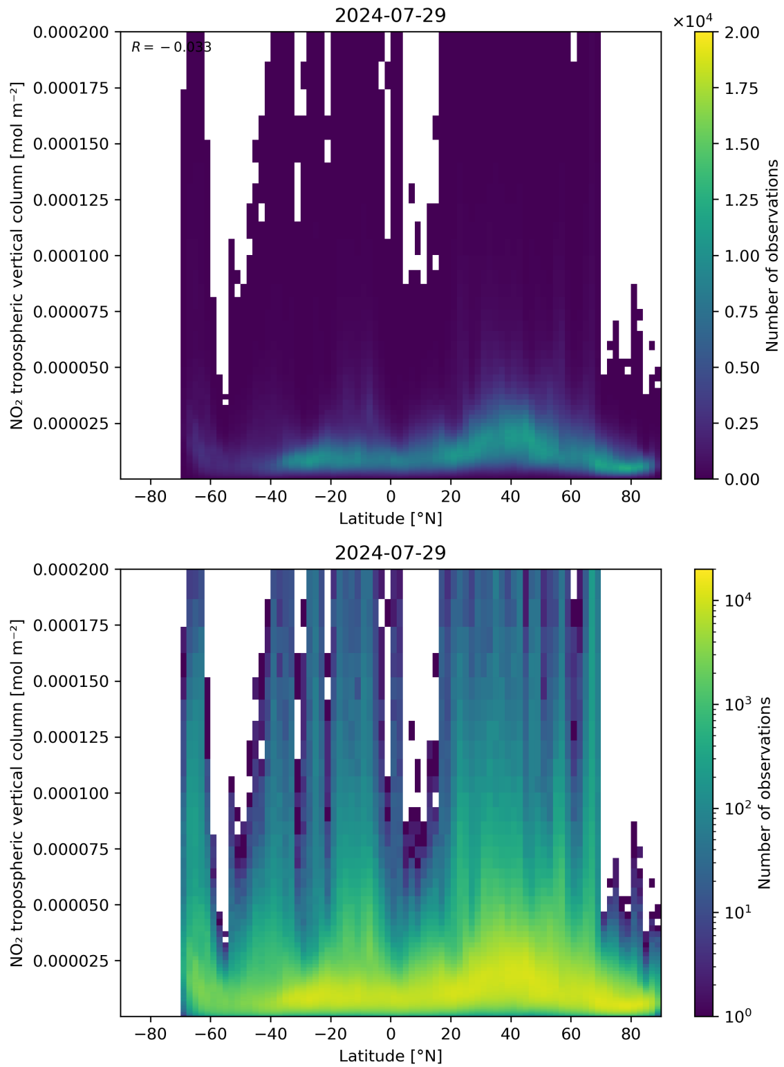
Figure 92: Scatter density plot of “Latitude” against “NO 2 tropospheric vertical column” for 2024-07-28 to 2024-07-30.
