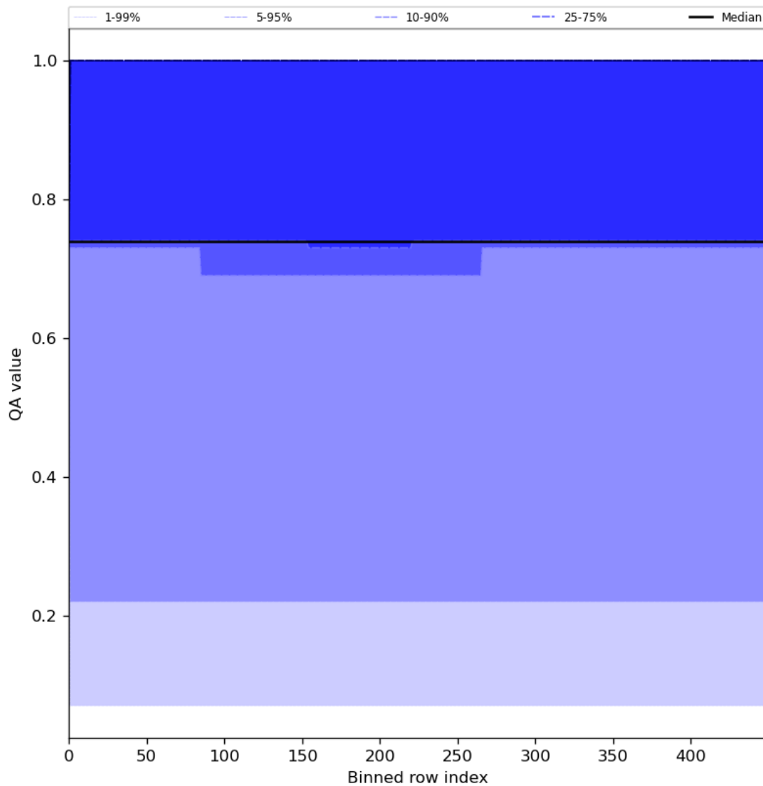
Figure 45: Along track statistics of “QA value” for 2024-07-28 to 2024-07-30
