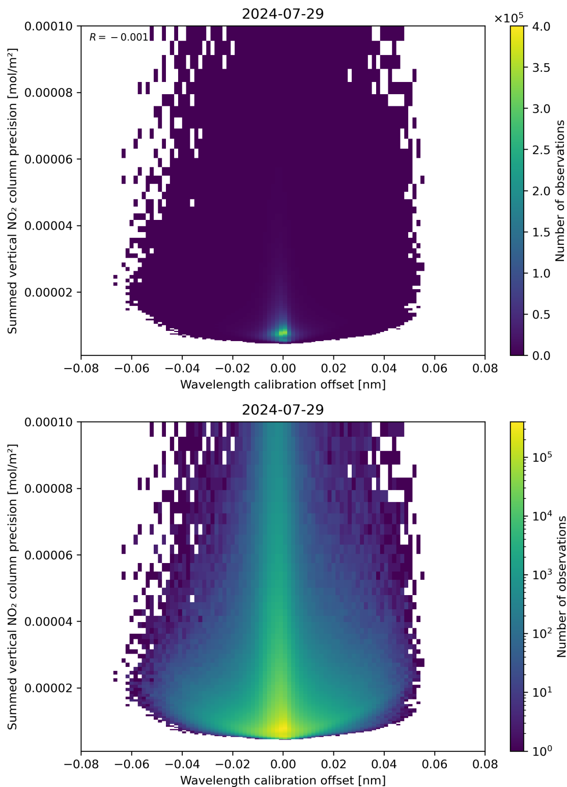
Figure 178: Scatter density plot of “Wavelength calibration offset” against “Summed vertical NO 2 column precision” for 2024-07-28 to 2024-07-30.
