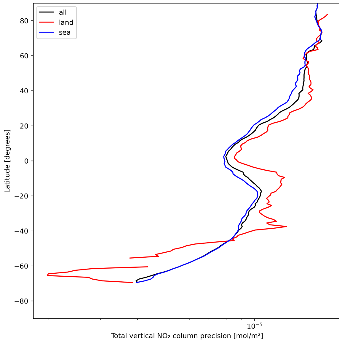
Figure 22: Zonal average of “Total vertical NO 2 column precision” for 2024-07-28 to 2024-07-30.
