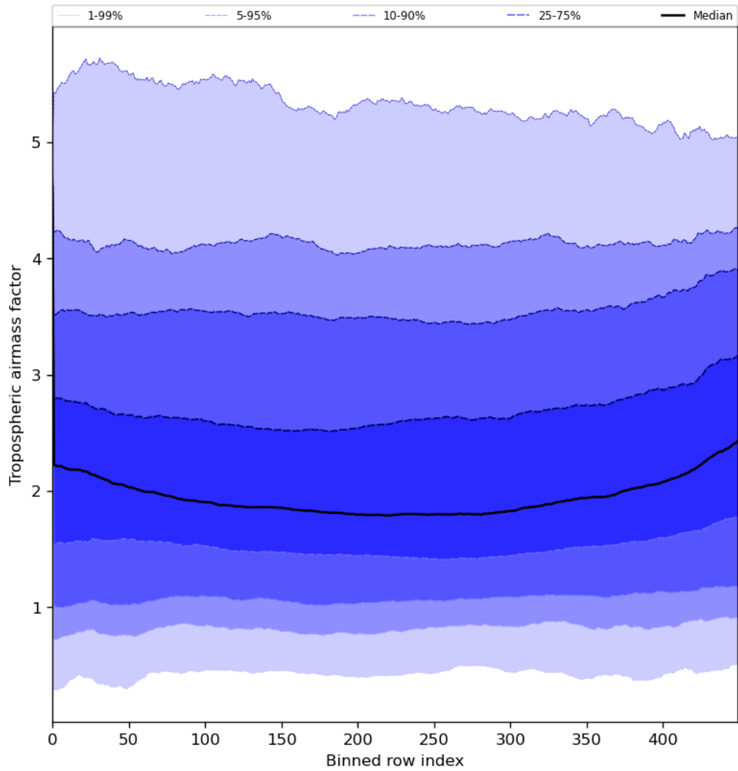
Figure 48: Along track statistics of “Tropospheric airmass factor” for 2024-07-28 to 2024-07-30
