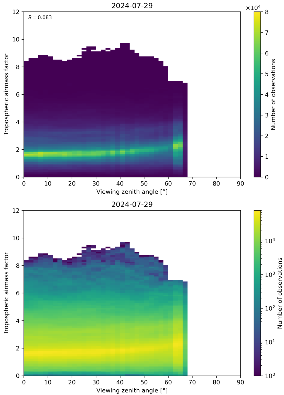
Figure 161: Scatter density plot of “Viewing zenith angle” against “Tropospheric airmass factor” for 2024-07-28 to 2024-07-30.
