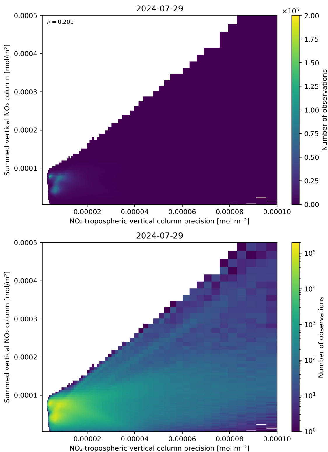
Figure 136: Scatter density plot of “NO 2 tropospheric vertical column precision” against “Summed vertical NO 2 column” for 2024-07-28 to 2024-07-30.
