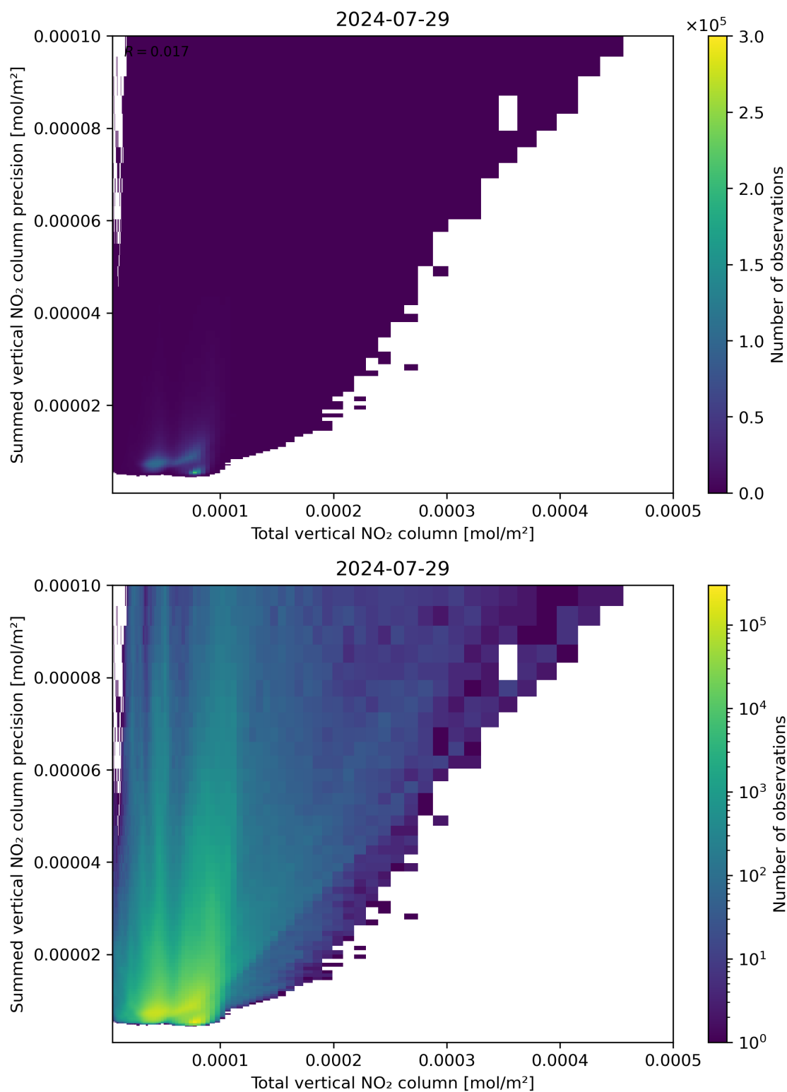
Figure 113: Scatter density plot of “Total vertical NO 2 column” against “Summed vertical NO 2 column precision” for 2024-07-28 to 2024-07-30.
