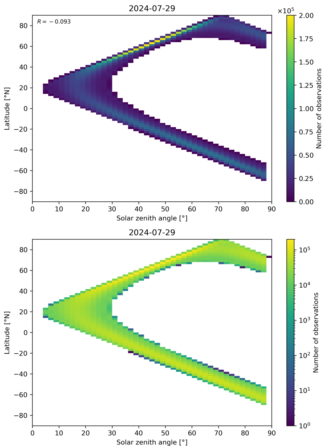
Figure 149: Scatter density plot of “Solar zenith angle” against “Latitude” for 2024-07-28 to 2024-07-30.
