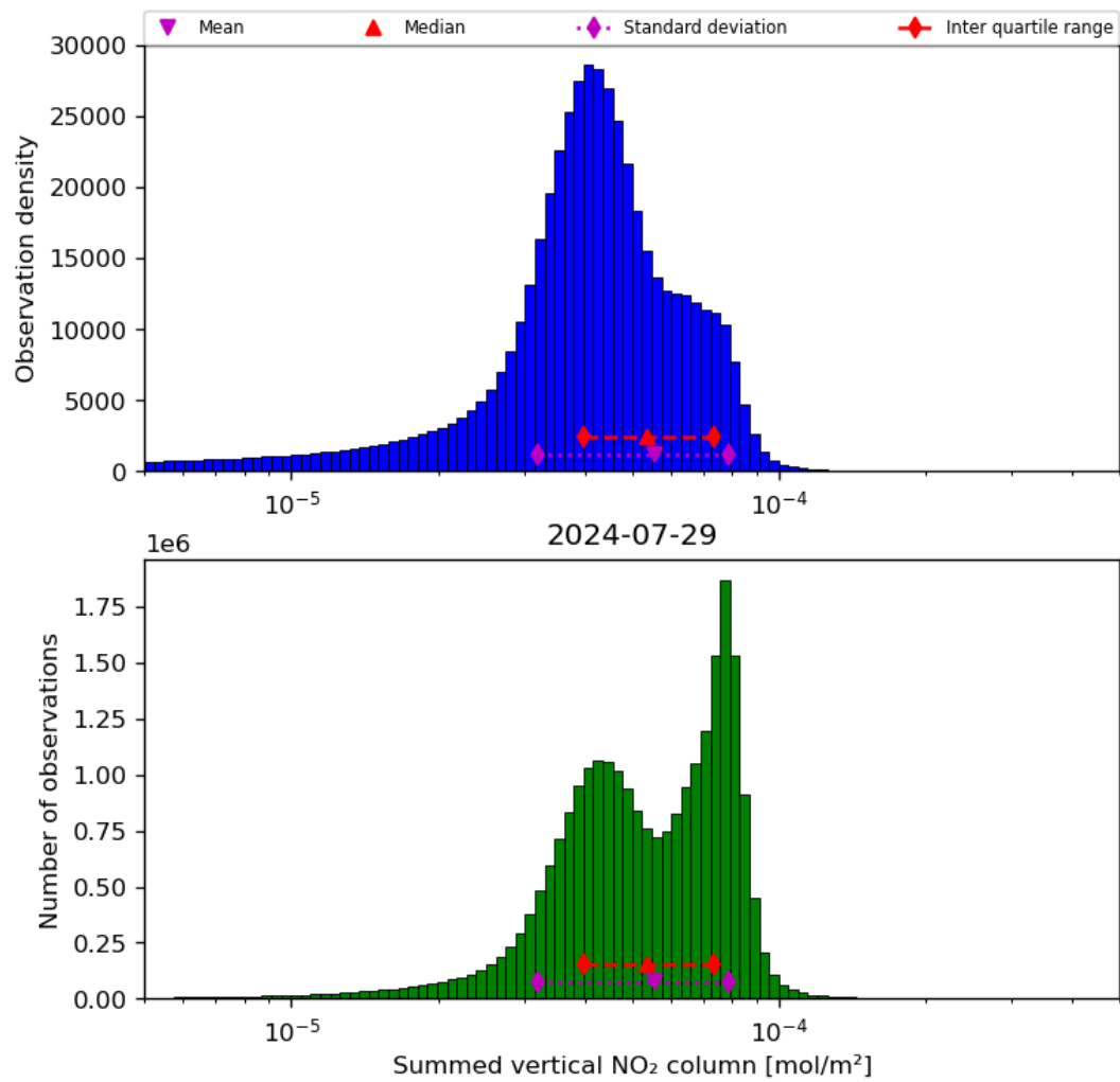
Figure 40: Histogram of “Summed vertical NO 2 column” for 2024-07-28 to 2024-07-30
