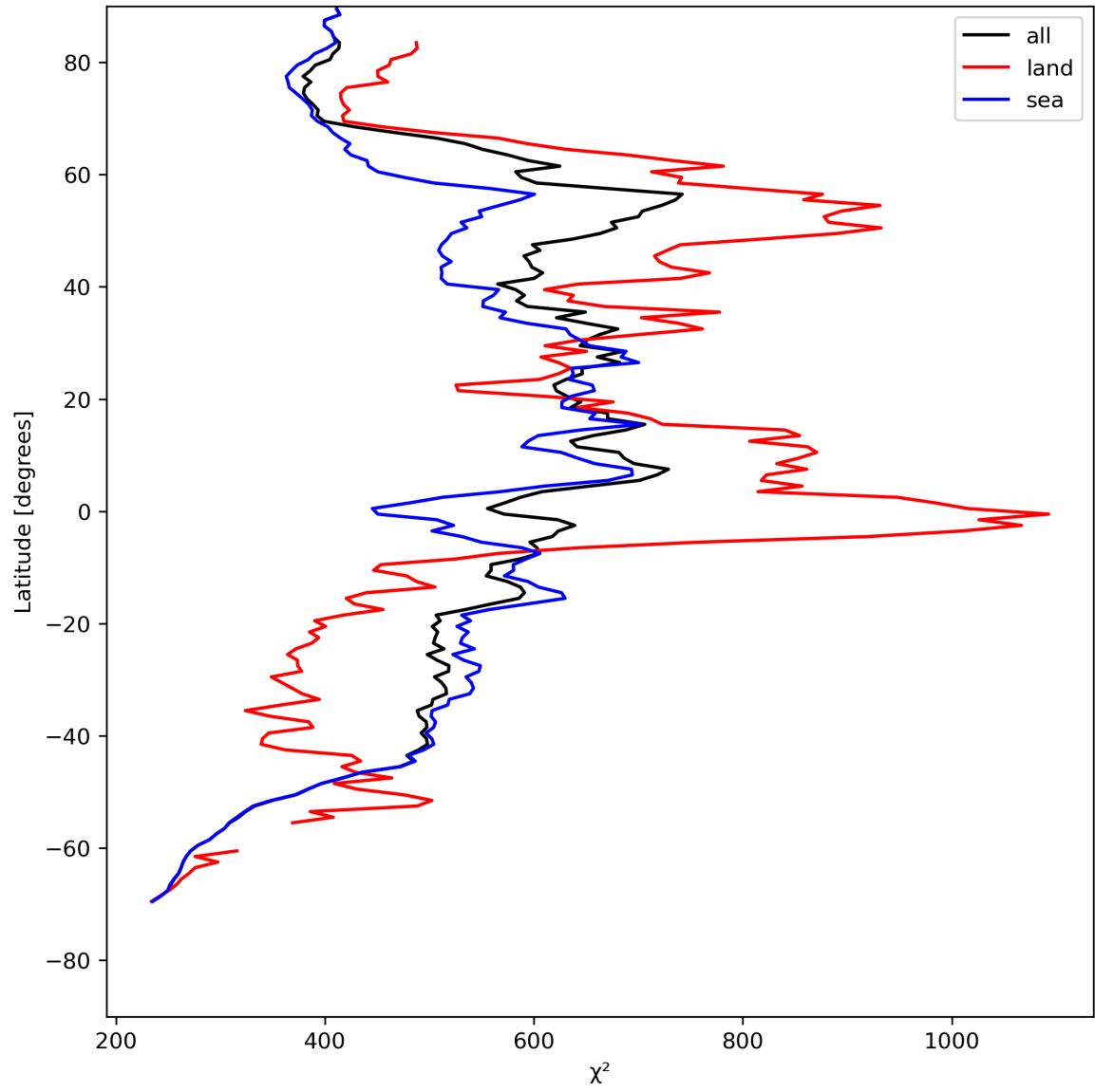
Figure 25: Zonal average of “ \chi^2 ” for 2024-07-28 to 2024-07-30.
