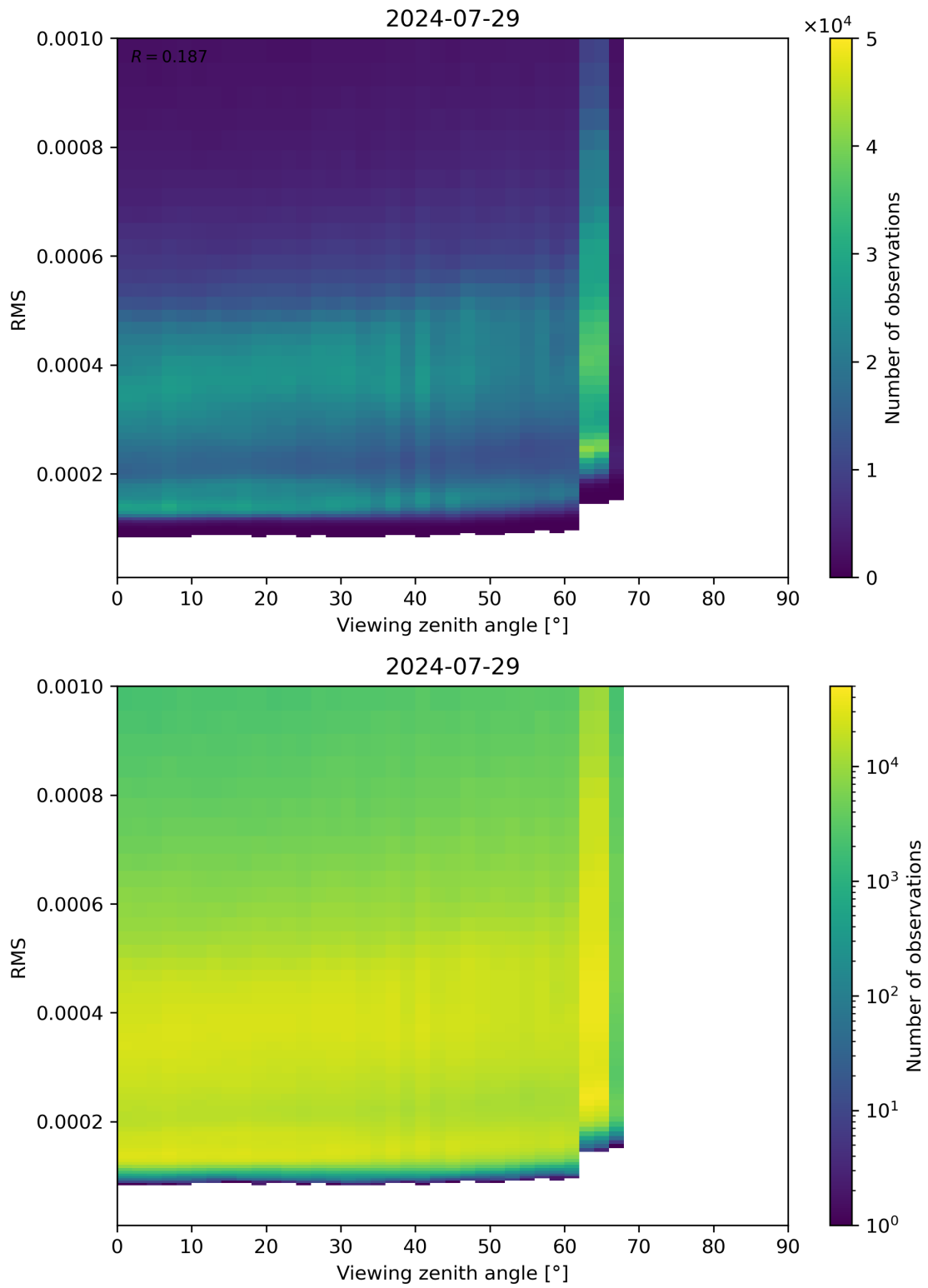
Figure 171: Scatter density plot of “Viewing zenith angle” against “RMS” for 2024-07-28 to 2024-07-30.
