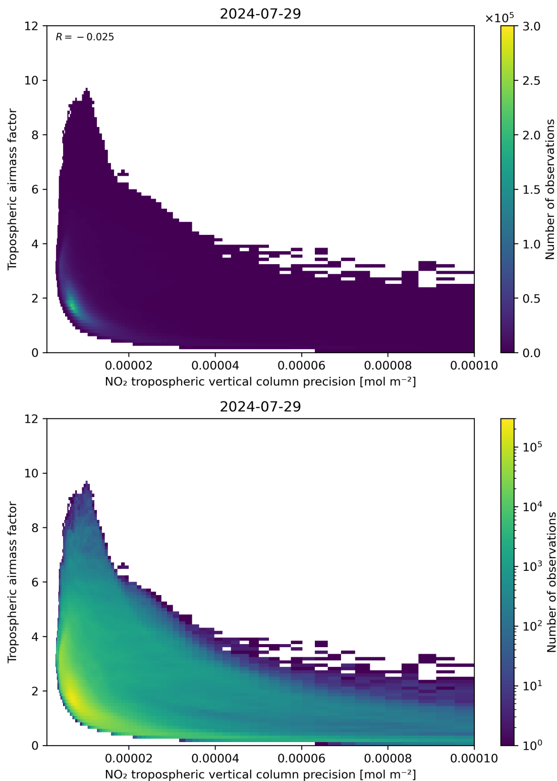
Figure 133: Scatter density plot of “NO 2 tropospheric vertical column precision” against “Tropospheric airmass factor” for 2024-07-28 to 2024-07-30.
