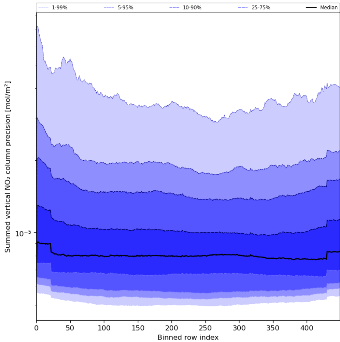
Figure 58: Along track statistics of “Summed vertical NO 2 column precision” for 2024-07-28 to 2024-07-30
