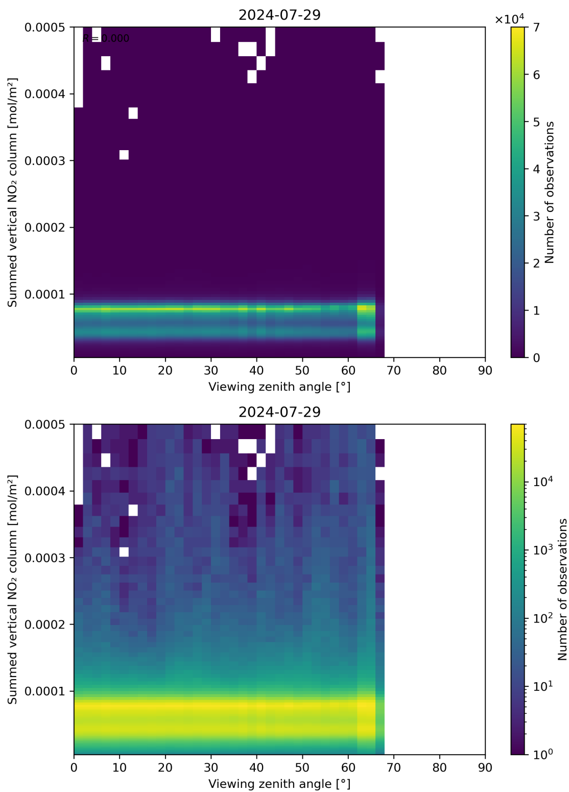
Figure 165: Scatter density plot of “Viewing zenith angle” against “Summed vertical NO 2 column” for 2024-07-28 to 2024-07-30.
