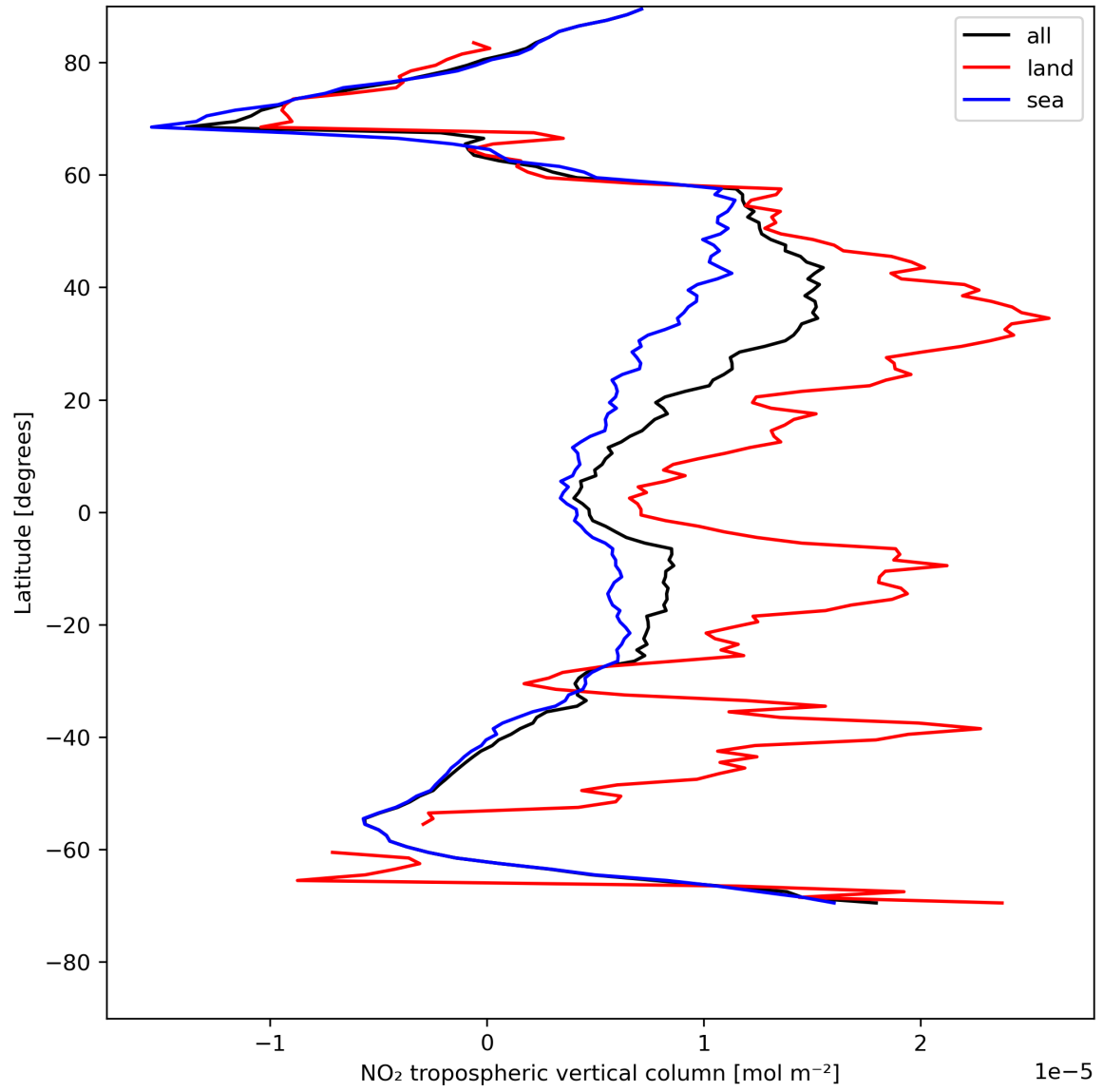
Figure 12: Zonal average of “NO 2 tropospheric vertical column” for 2024-07-28 to 2024-07-30.
