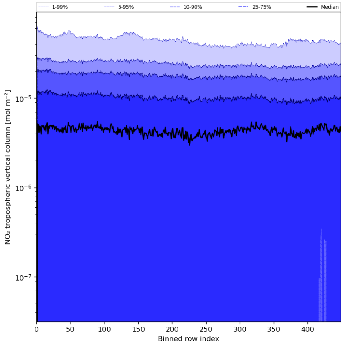
Figure 46: Along track statistics of “NO 2 tropospheric vertical column” for 2024-07-28 to 2024-07-30
