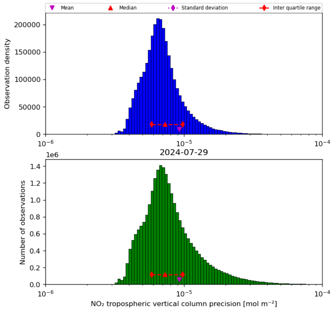
Figure 30: Histogram of “NO 2 tropospheric vertical column precision” for 2024-07-28 to 2024-07-30
