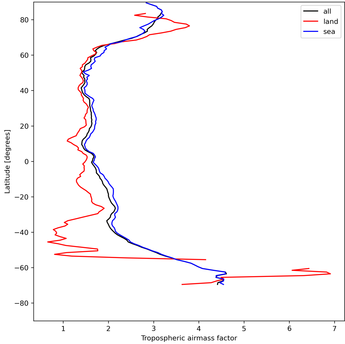
Figure 14: Zonal average of “Tropospheric air mass factor” for 2024-07-28 to 2024-07-30.
