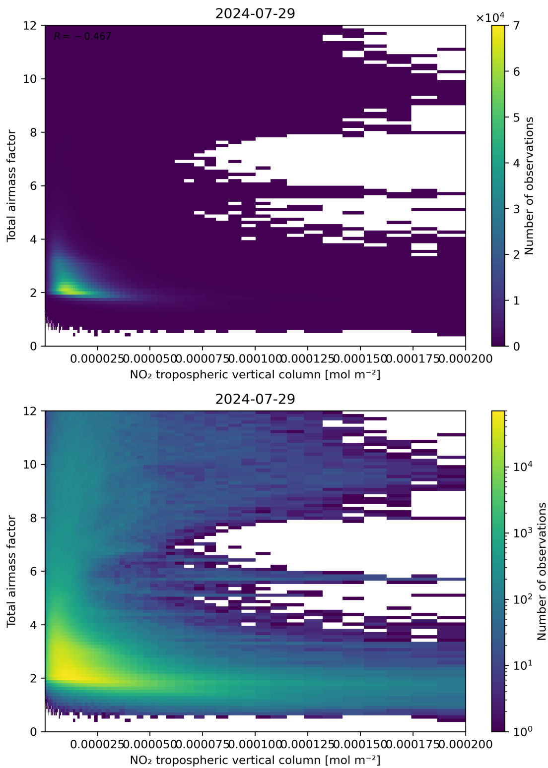
Figure 122: Scatter density plot of “NO 2 tropospheric vertical column” against “Total air mass factor” for 2024-07-28 to 2024-07-30.
