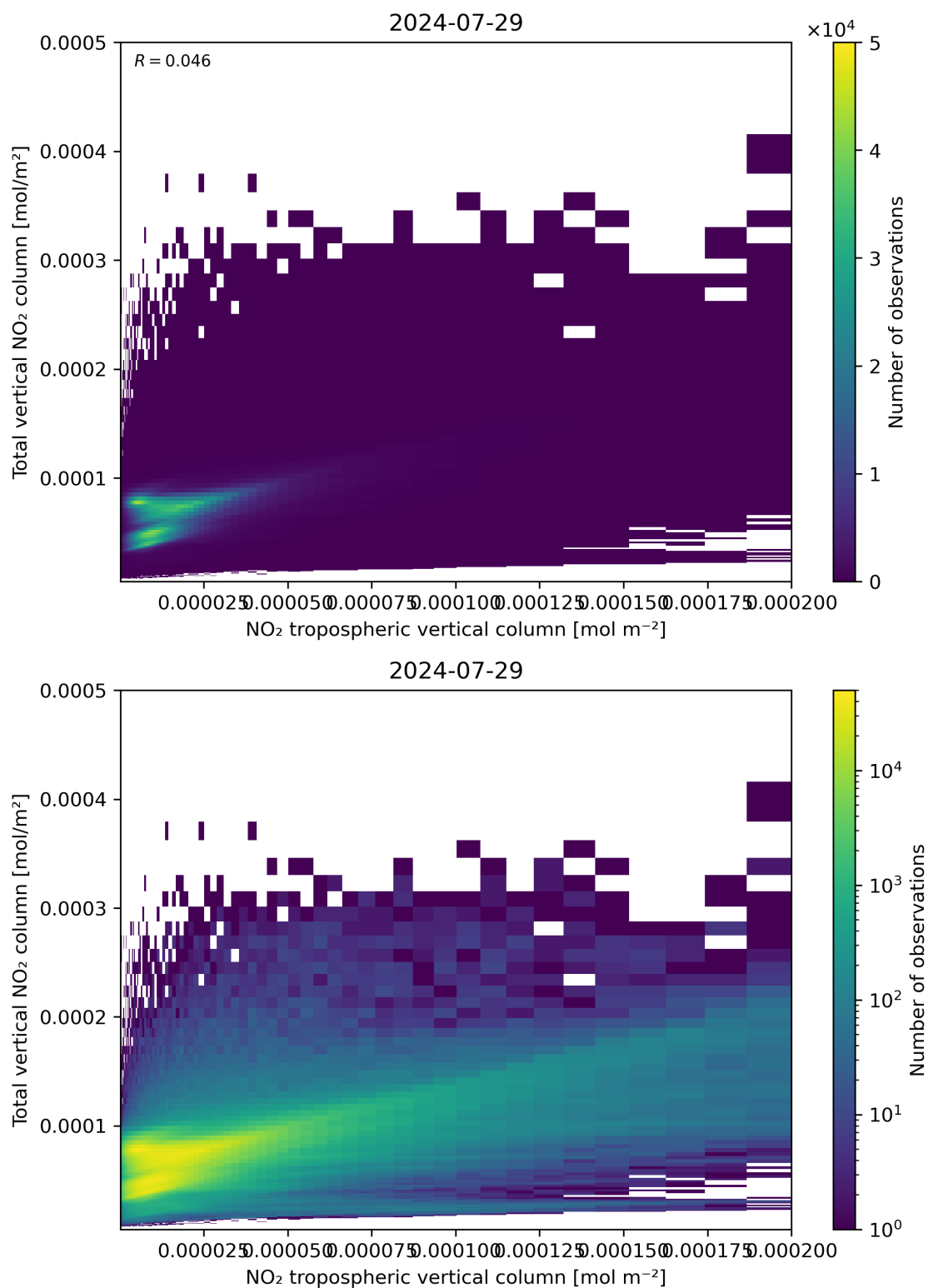
Figure 128: Scatter density plot of “NO 2 tropospheric vertical column” against “Total vertical NO 2 column” for 2024-07-28 to 2024-07-30.
