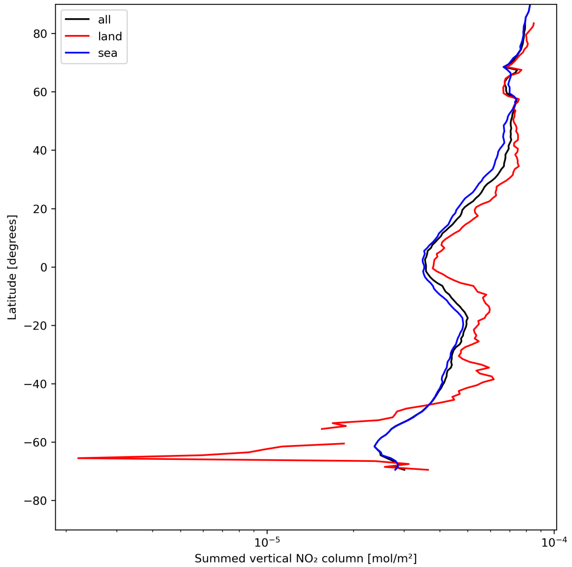
Figure 23: Zonal average of “Summed vertical NO 2 column” for 2024-07-28 to 2024-07-30.
