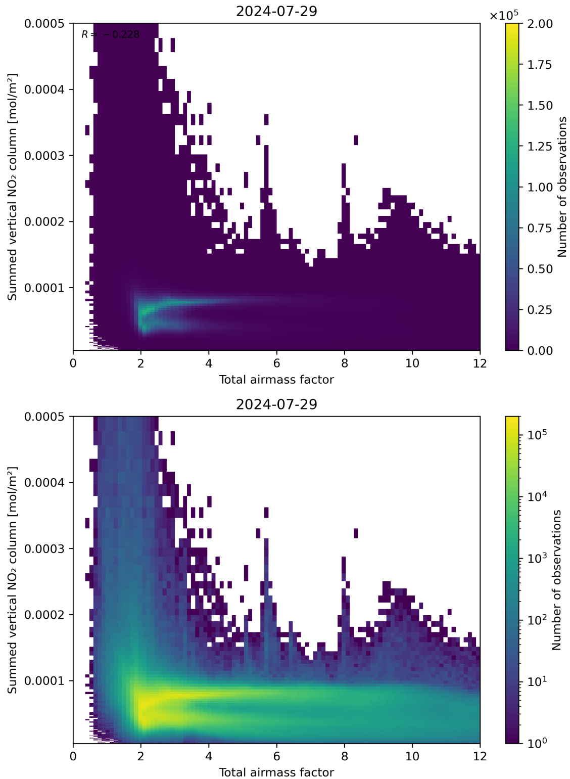
Figure 65: Scatter density plot of “Total airmass factor” against “Summed vertical NO 2 column” for 2024-07-28 to 2024-07-30.
