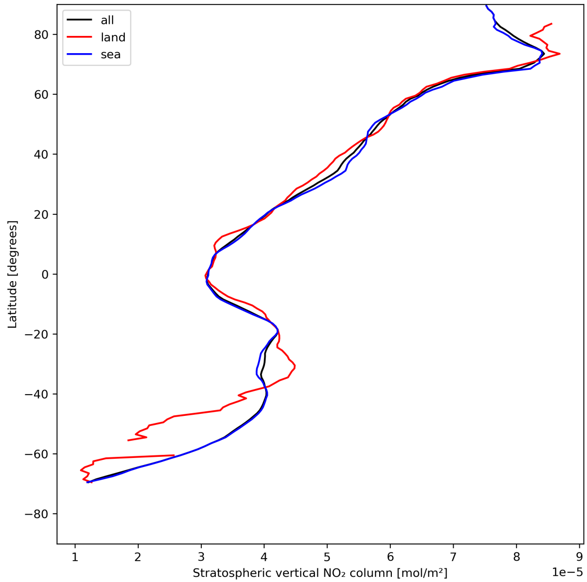
Figure 19: Zonal average of “Stratospheric vertical NO 2 column” for 2024-07-28 to 2024-07-30.
