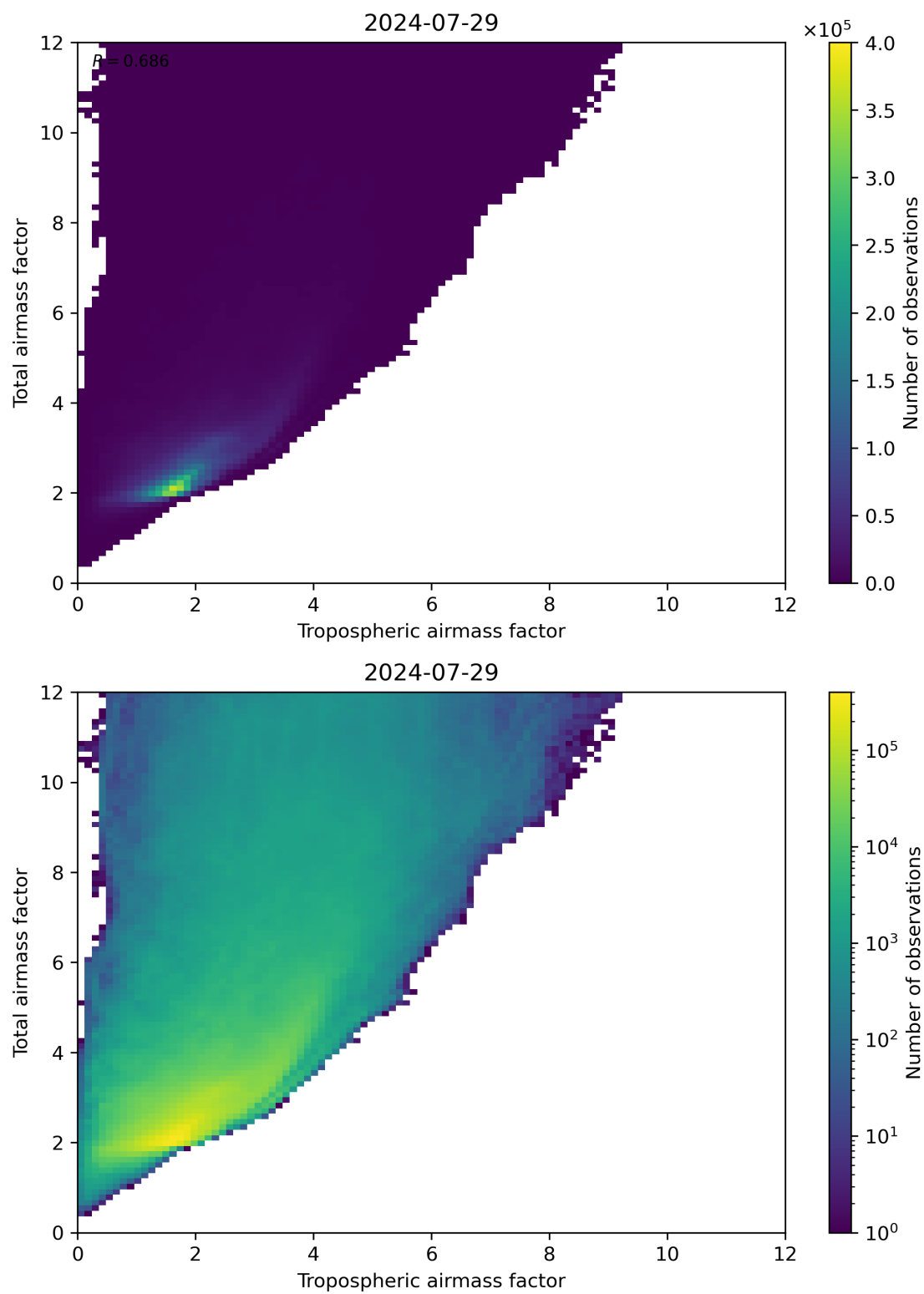
Figure 72: Scatter density plot of “Tropospheric airmass factor” against “Total airmass factor” for 2024-07-28 to 2024-07-30.
