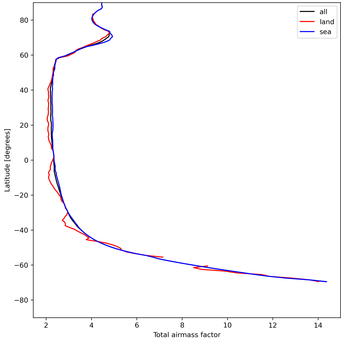
Figure 15: Zonal average of “Total airmass factor” for 2024-07-28 to 2024-07-30.
