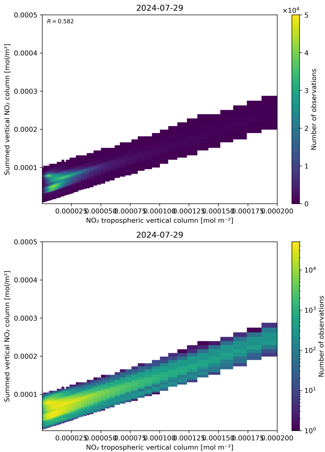
Figure 126: Scatter density plot of “NO 2 tropospheric vertical column” against “Summed vertical NO 2 column” for 2024-07-28 to 2024-07-30.
