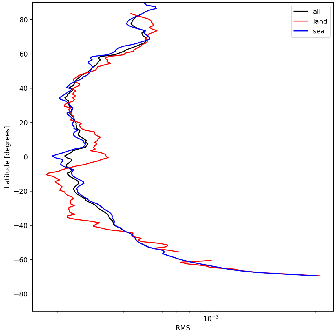
Figure 26: Zonal average of “RMS” for 2024-07-28 to 2024-07-30.
