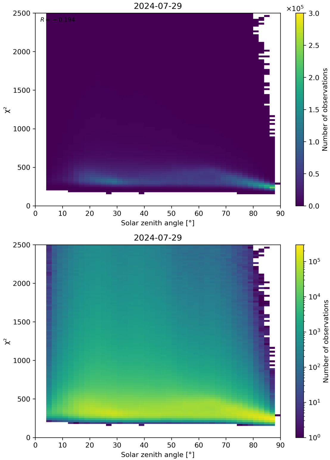
Figure 148: Scatter density plot of “Solar zenith angle” against “ \chi^2 ” for 2024-07-28 to 2024-07-30.
