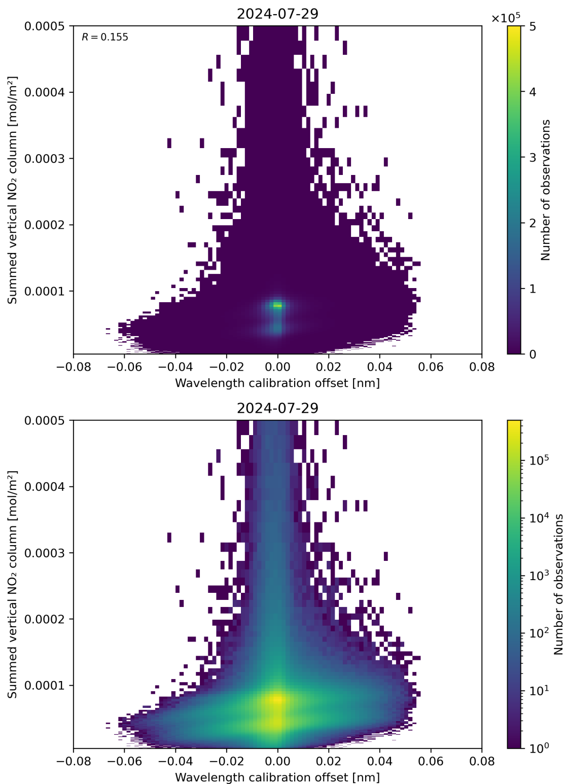
Figure 177: Scatter density plot of “Wavelength calibration offset” against “Summed vertical NO 2 column” for 2024-07-28 to 2024-07-30.
