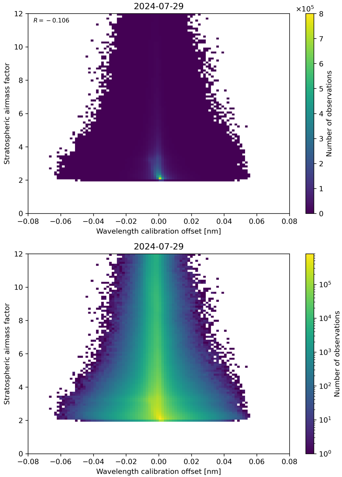
Figure 174: Scatter density plot of “Wavelength calibration offset” against “Stratospheric airmass factor” for 2024-07-28 to 2024-07-30.
