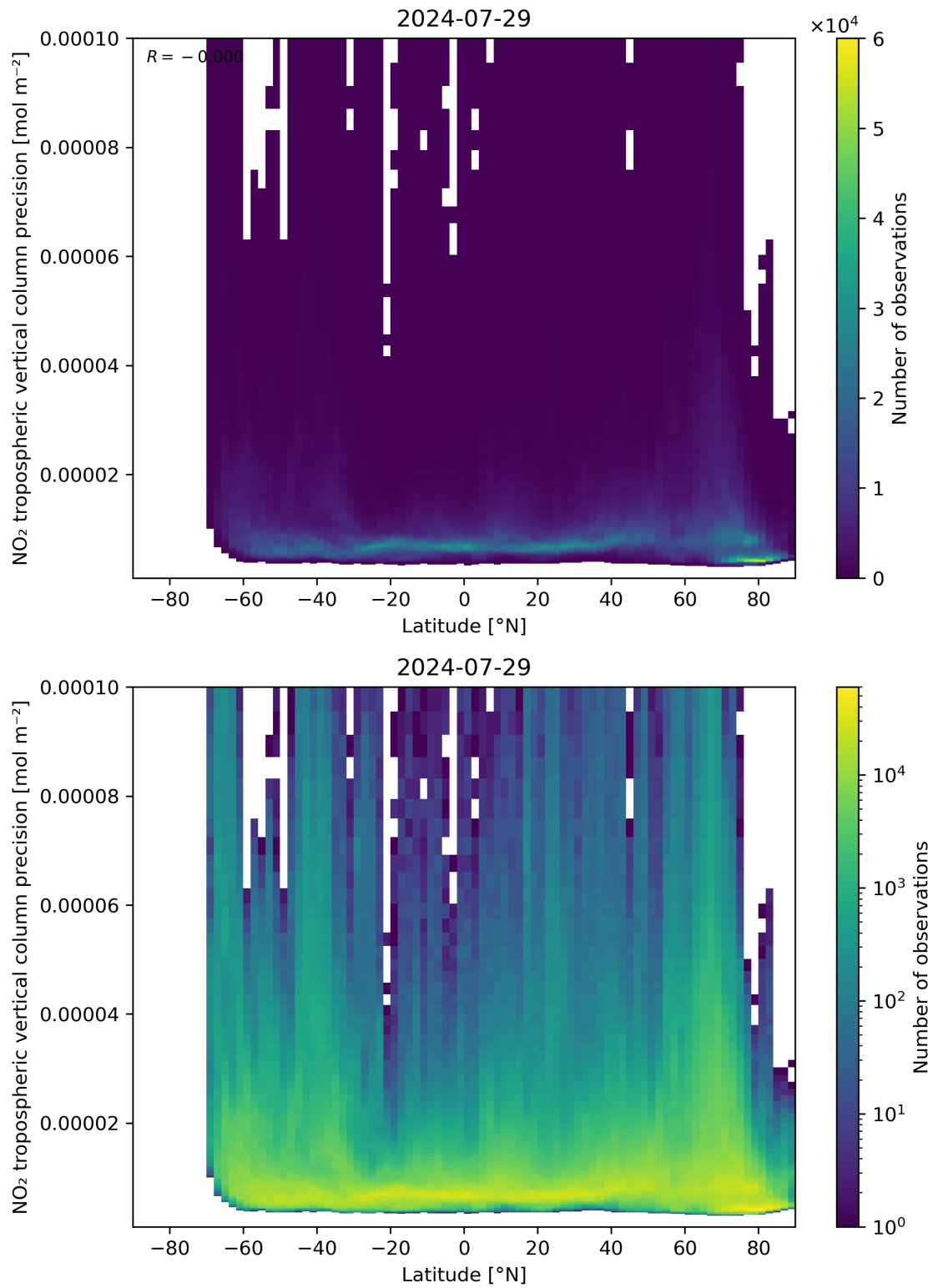
Figure 93: Scatter density plot of “Latitude” against “NO 2 tropospheric vertical column precision” for 2024-07-28 to 2024-07-30.
