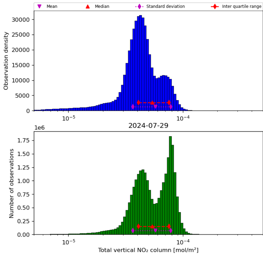
Figure 38: Histogram of “Total vertical NO 2 column” for 2024-07-28 to 2024-07-30
