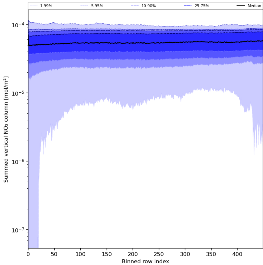
Figure 57: Along track statistics of “Summed vertical NO 2 column” for 2024-07-28 to 2024-07-30
