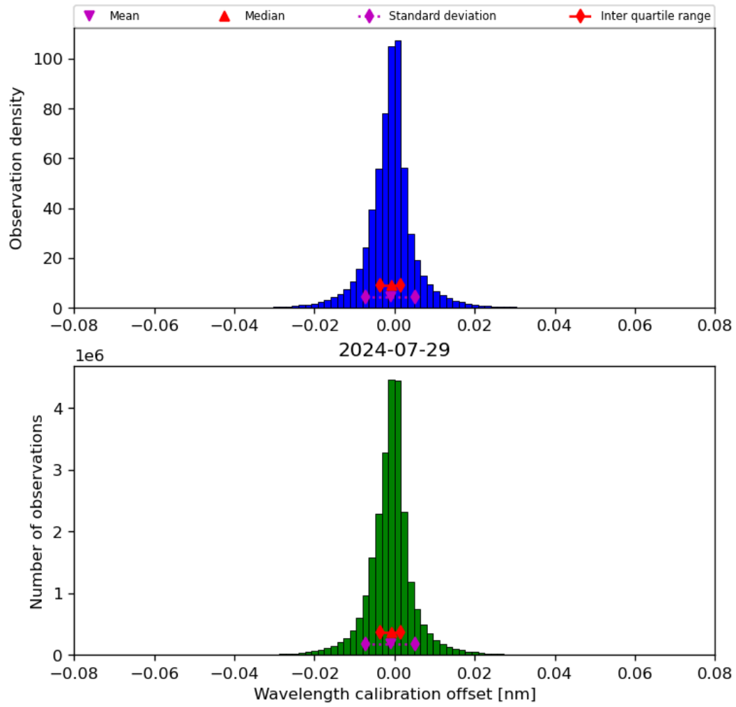
Figure 35: Histogram of “Wavelength calibration offset” for 2024-07-28 to 2024-07-30
