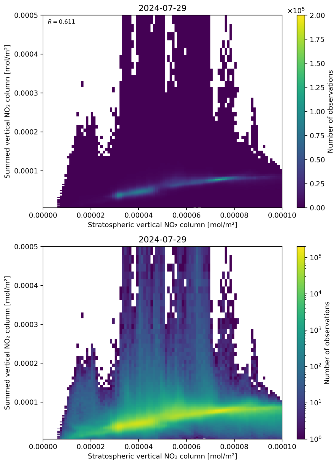
Figure 98: Scatter density plot of “Stratospheric vertical NO 2 column” against “Summed vertical NO 2 column” for 2024-07-28 to 2024-07-30.
