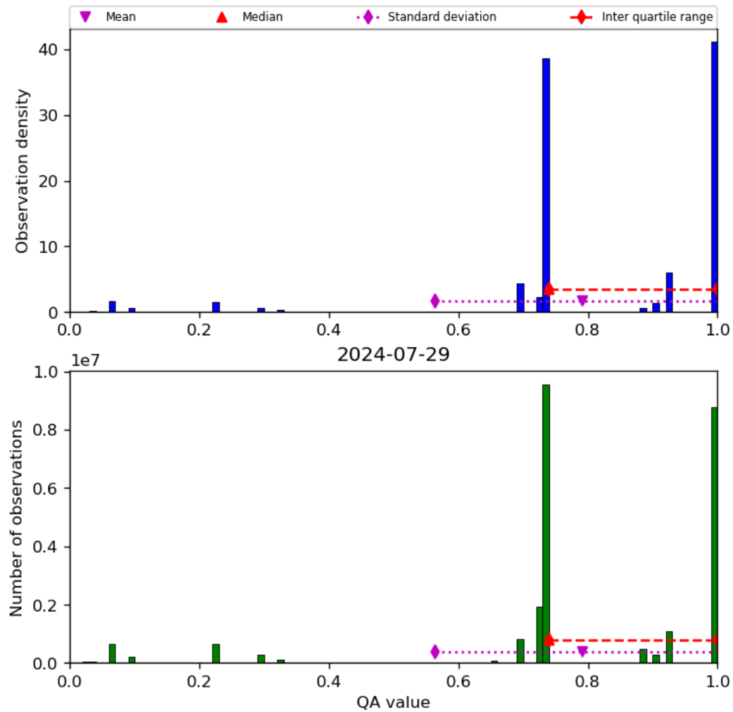
Figure 28: Histogram of “QA value” for 2024-07-28 to 2024-07-30
