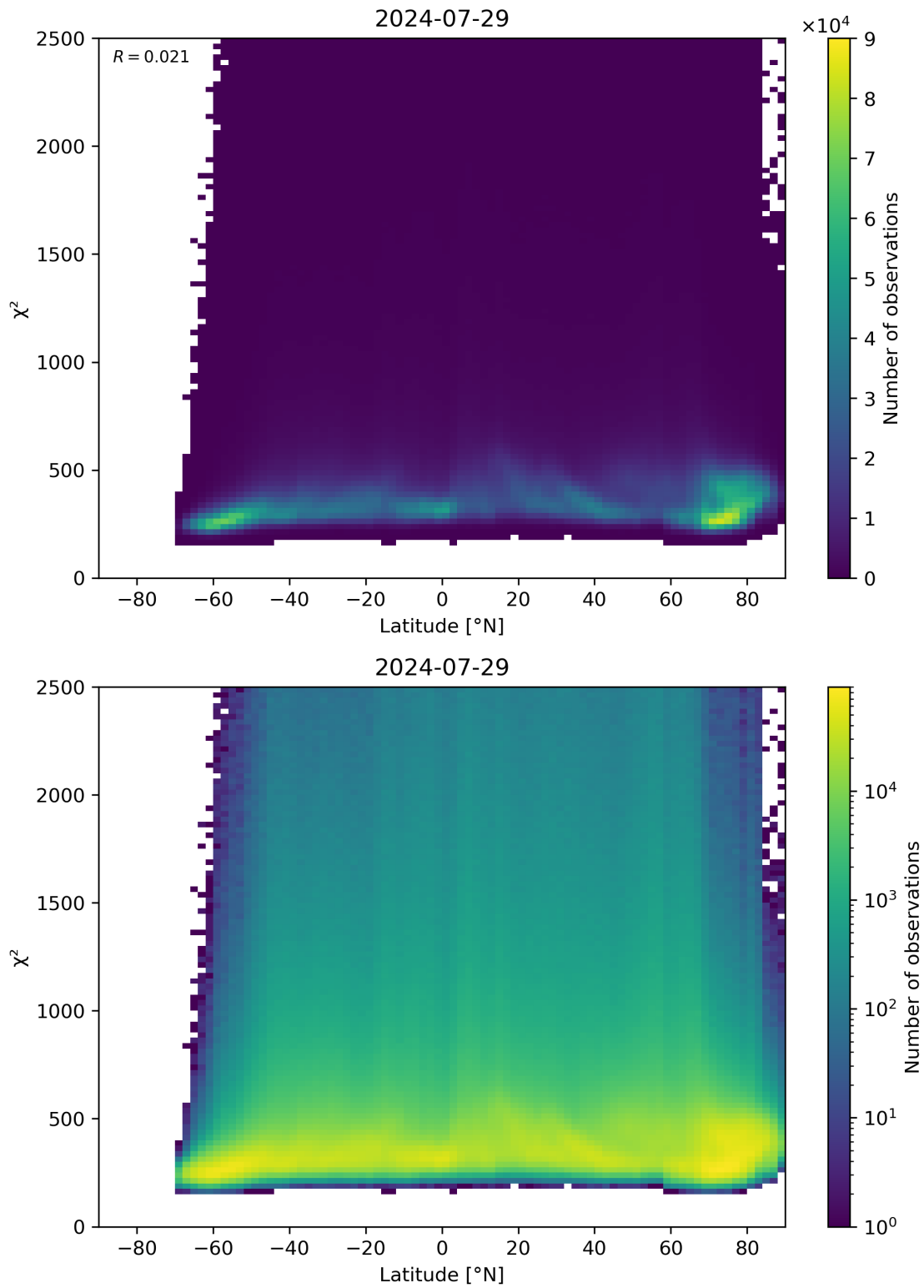
Figure 86: Scatter density plot of “Latitude” against “ \chi^2 ” for 2024-07-28 to 2024-07-30.
