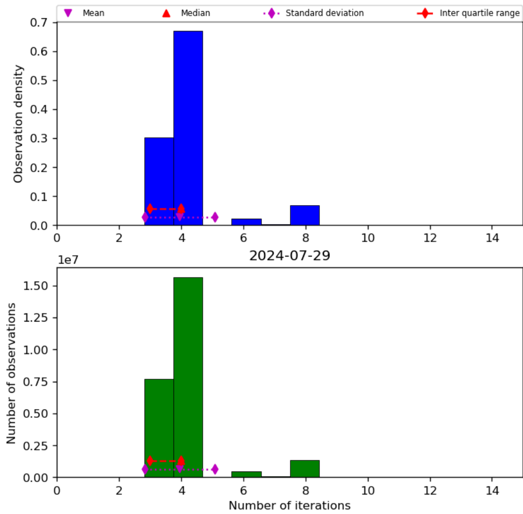
Figure 34: Histogram of “Number of iterations” for 2024-07-28 to 2024-07-30
