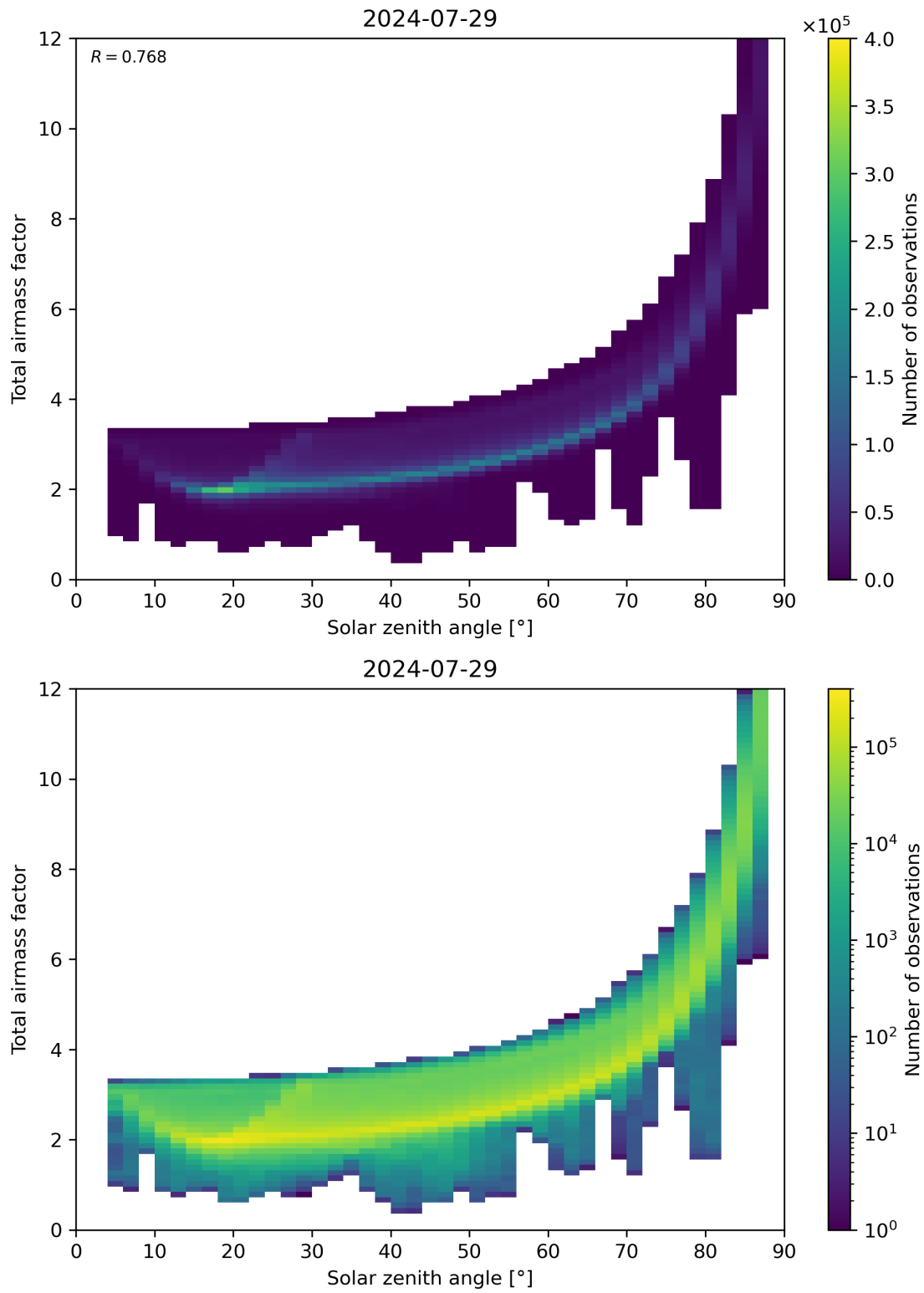
Figure 146: Scatter density plot of “Solar zenith angle” against “Total air mass factor” for 2024-07-28 to 2024-07-30.
