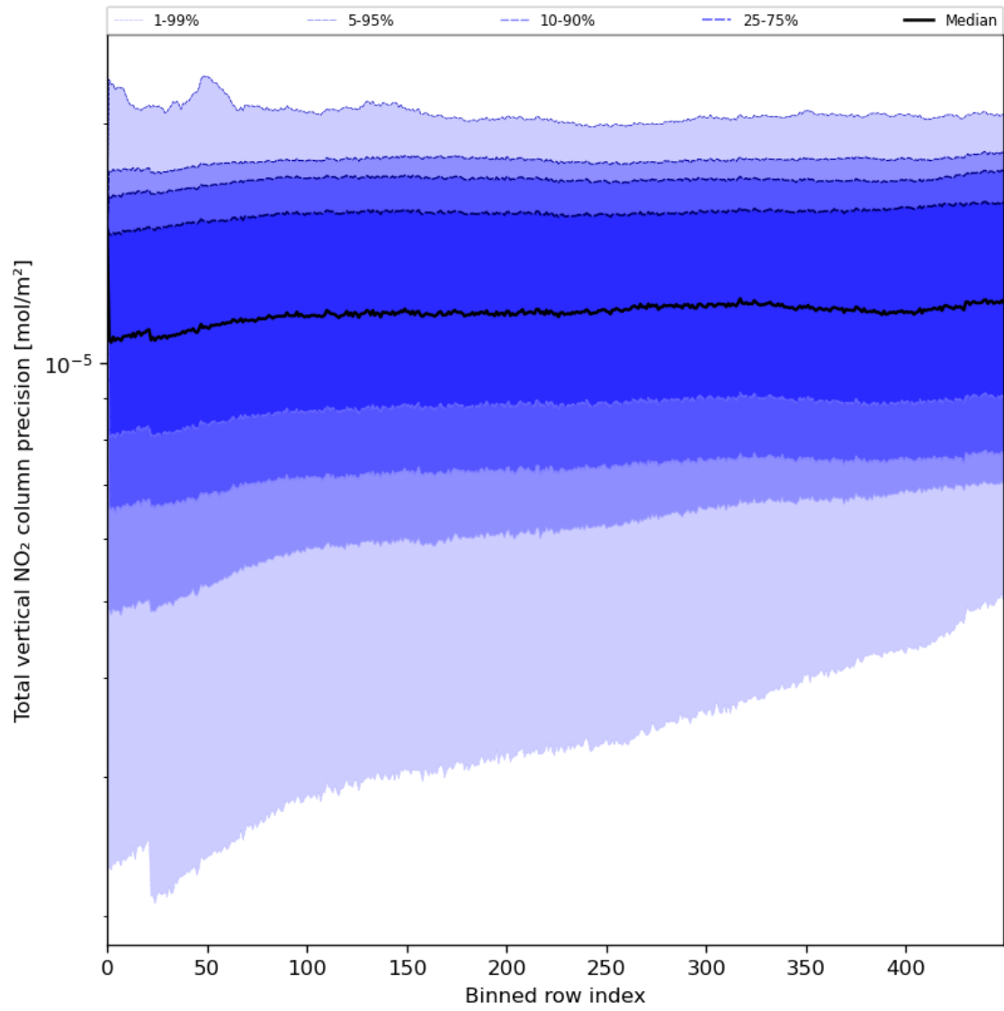
Figure 56: Along track statistics of “Total vertical NO 2 column precision” for 2024-07-28 to 2024-07-30
