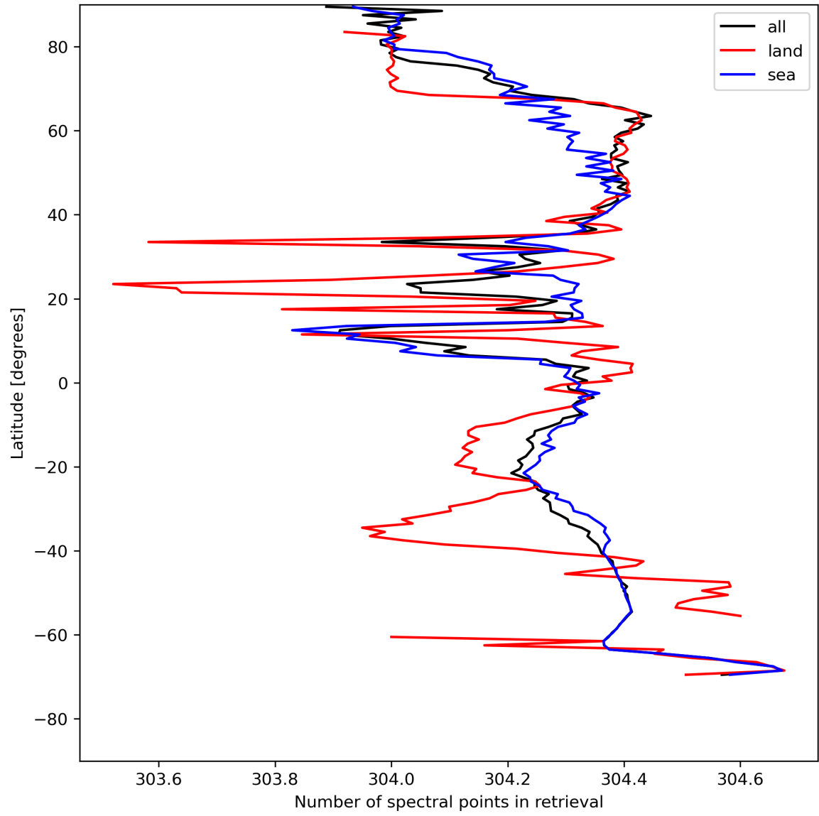
Figure 16: Zonal average of “Number of spectral points in retrieval” for 2024-07-28 to 2024-07-30.
