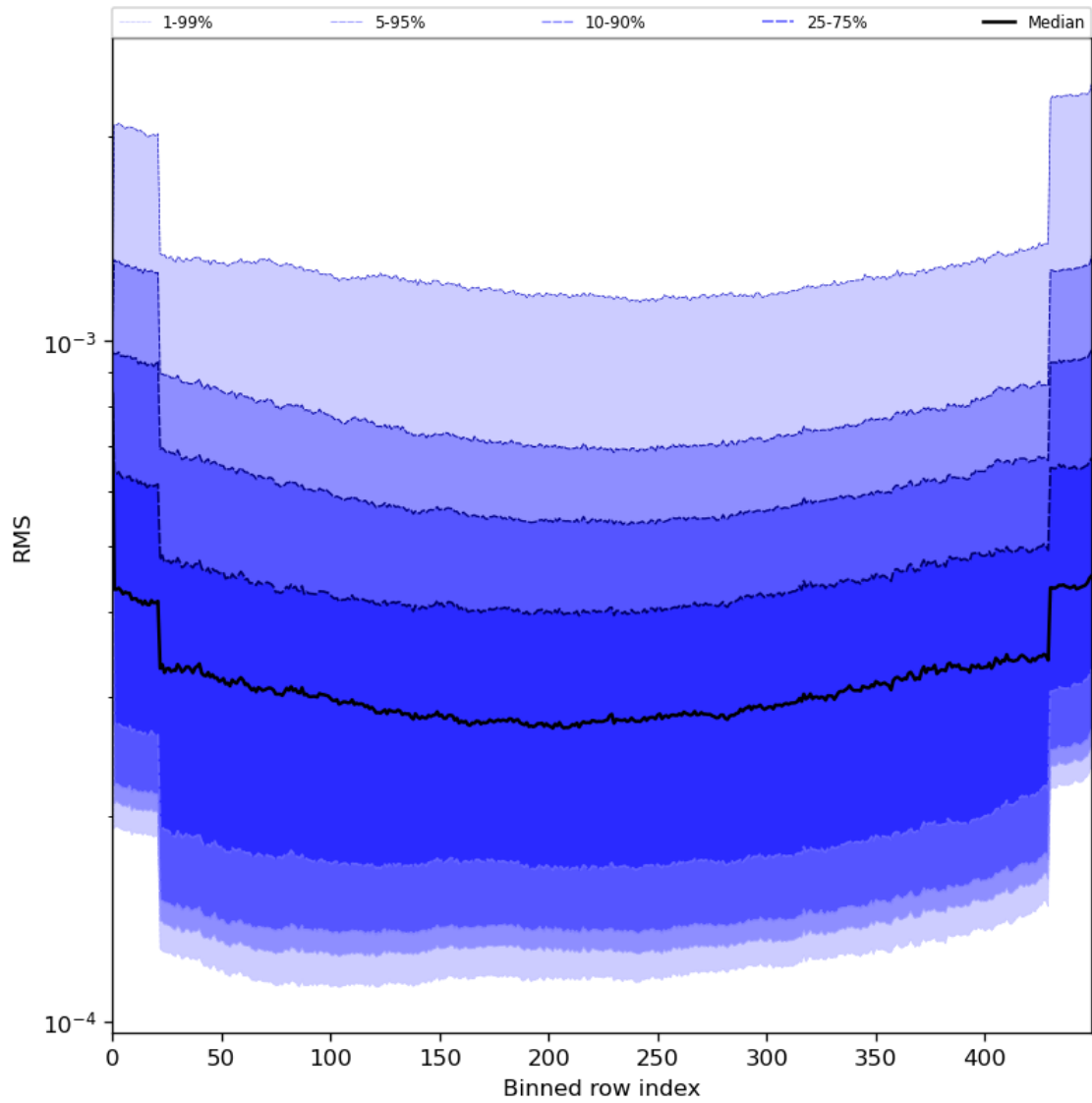
Figure 60: Along track statistics of “RMS” for 2024-07-28 to 2024-07-30
