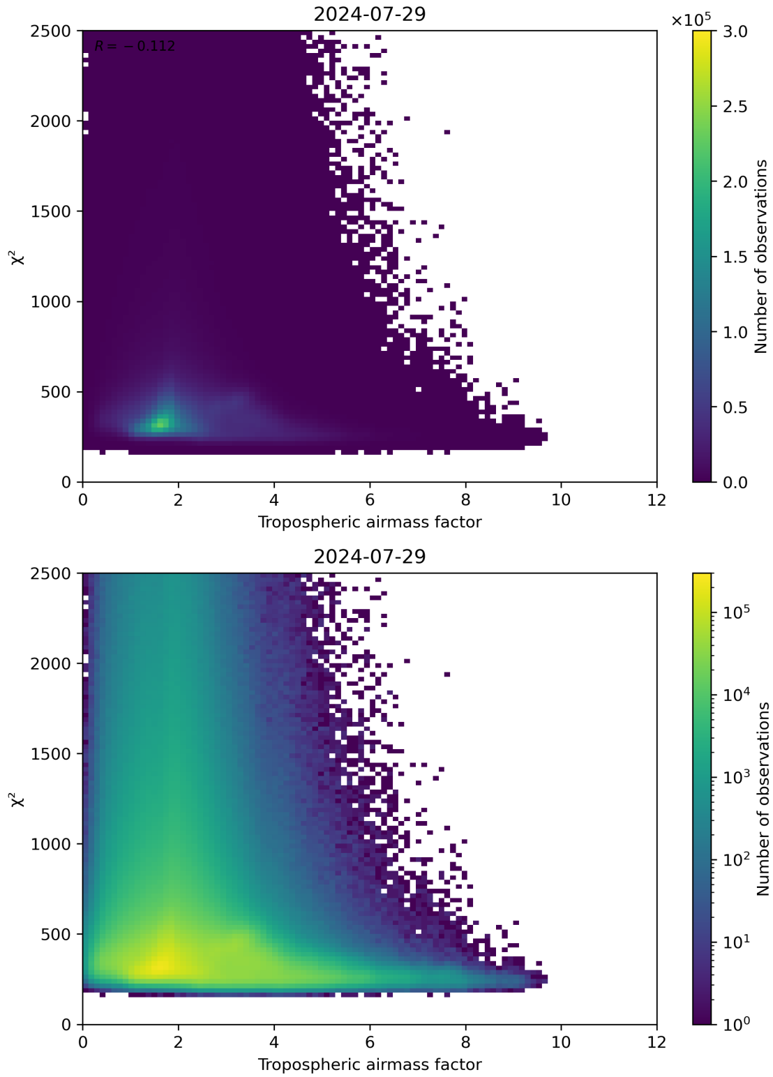
Figure 73: Scatter density plot of “Tropospheric airmass factor” against “ \chi^2 ” for 2024-07-28 to 2024-07-30.
