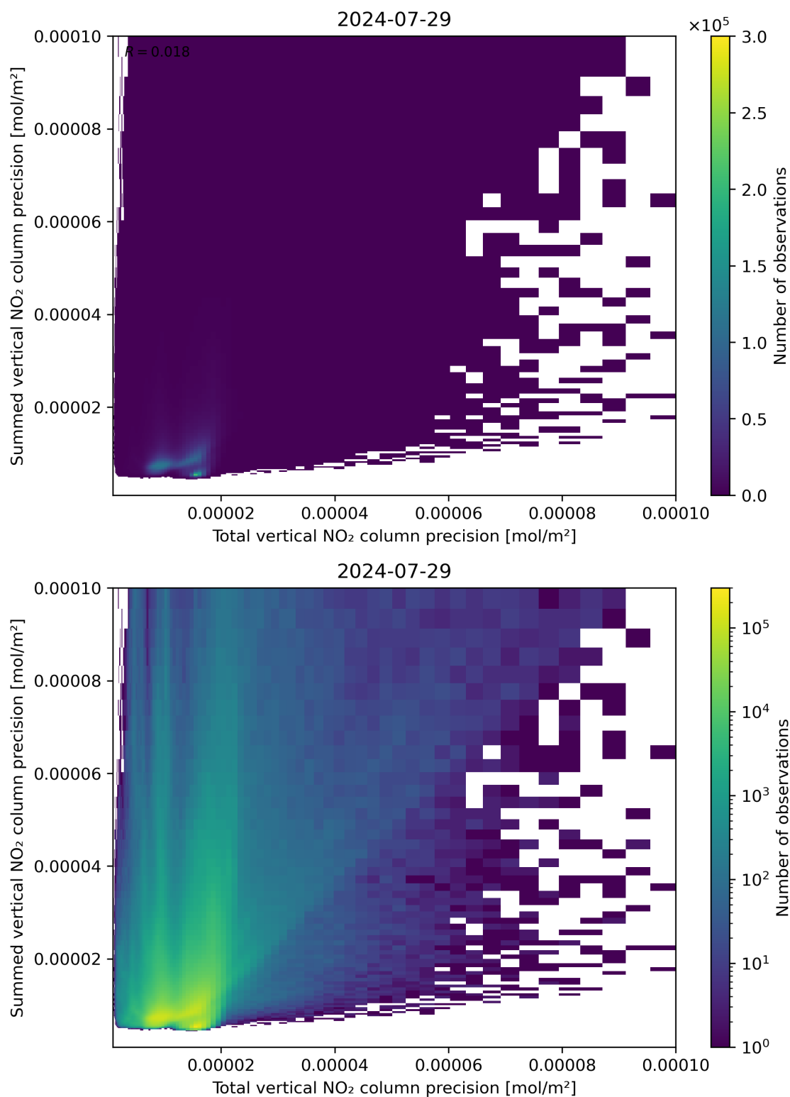
Figure 118: Scatter density plot of “Total vertical NO 2 column precision” against “Summed vertical NO 2 column precision” for 2024-07-28 to 2024-07-30.
