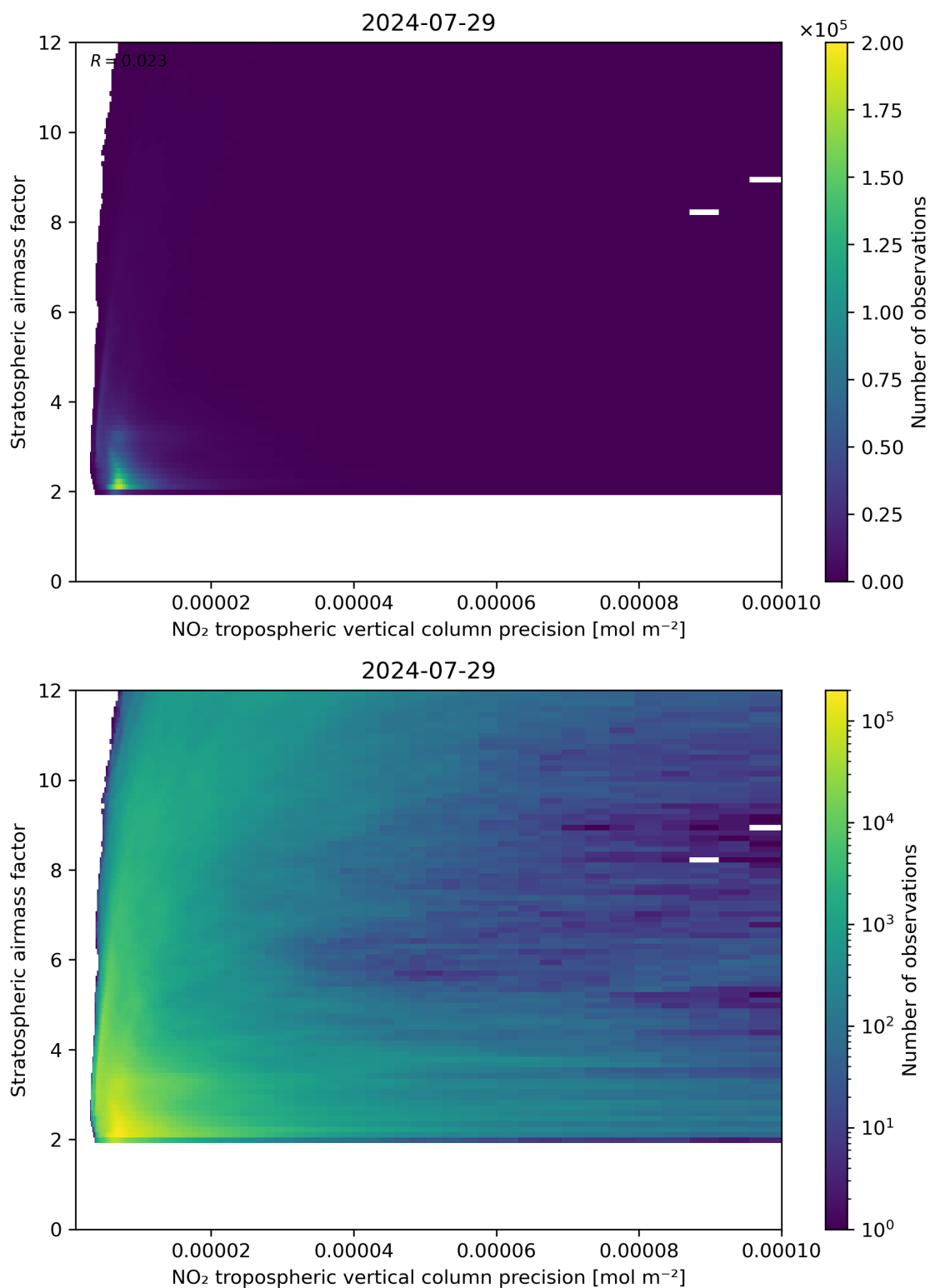
Figure 131: Scatter density plot of “NO 2 tropospheric vertical column precision” against “Stratospheric airmass factor” for 2024-07-28 to 2024-07-30.
