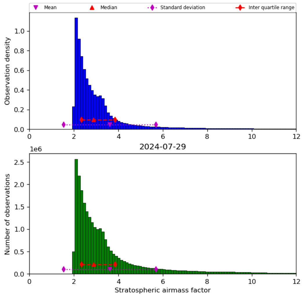
Figure 44: Histogram of “Stratospheric airmass factor” for 2024-07-28 to 2024-07-30
