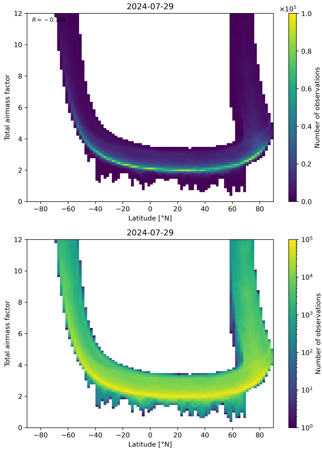
Figure 84: Scatter density plot of “Latitude” against “Total airmass factor” for 2024-07-28 to 2024-07-30.
