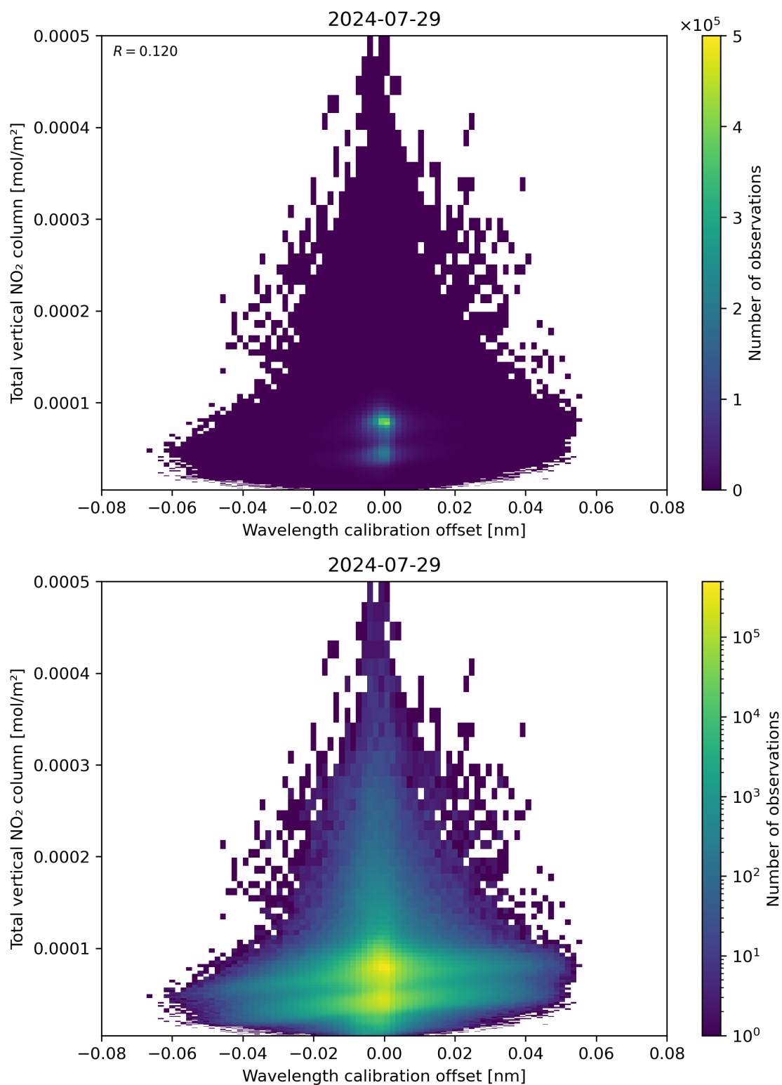
Figure 179: Scatter density plot of “Wavelength calibration offset” against “Total vertical NO 2 column” for 2024-07-28 to 2024-07-30.
