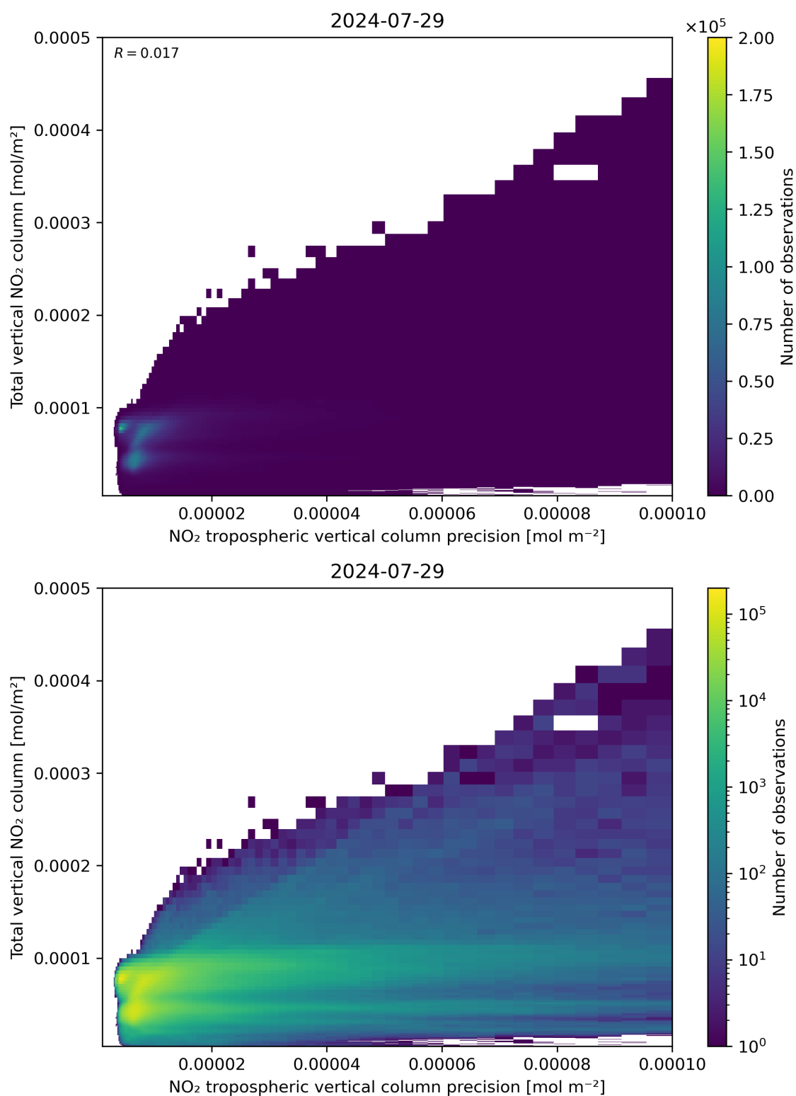
Figure 138: Scatter density plot of “NO 2 tropospheric vertical column precision” against “Total vertical NO 2 column” for 2024-07-28 to 2024-07-30.
