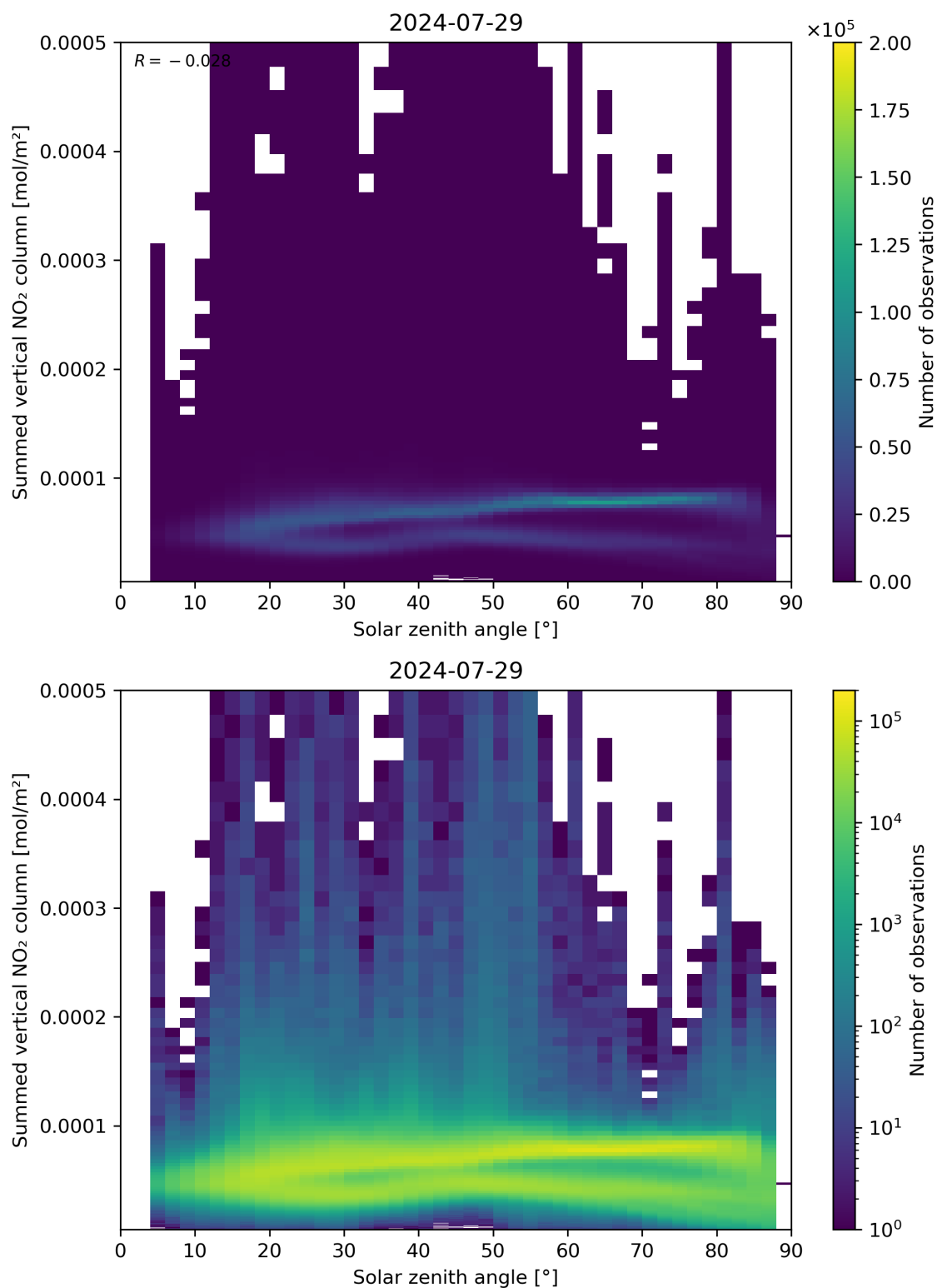
Figure 151: Scatter density plot of “Solar zenith angle” against “Summed vertical NO 2 column” for 2024-07-28 to 2024-07-30.
