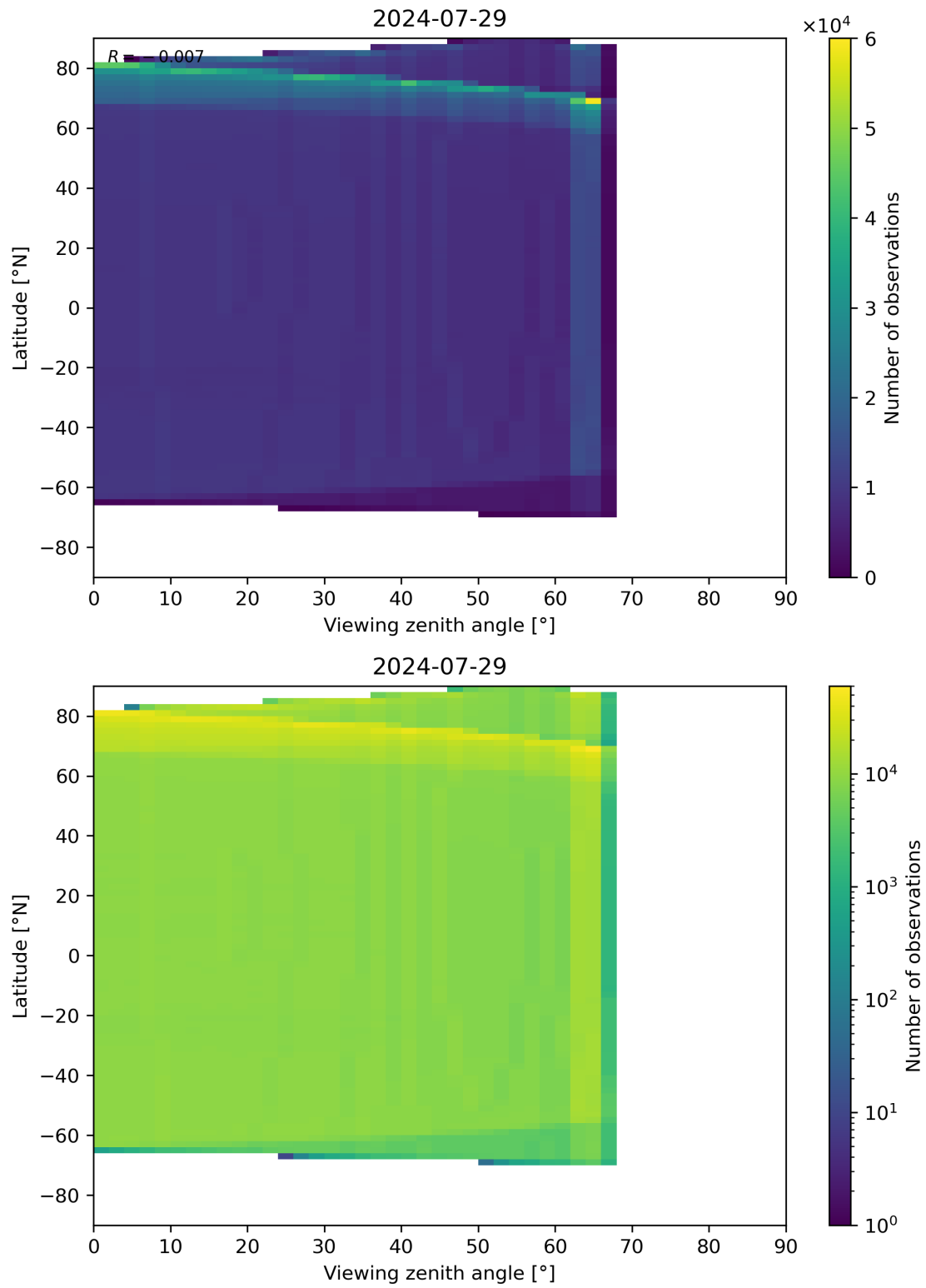
Figure 163: Scatter density plot of “Viewing zenith angle” against “Latitude” for 2024-07-28 to 2024-07-30.
