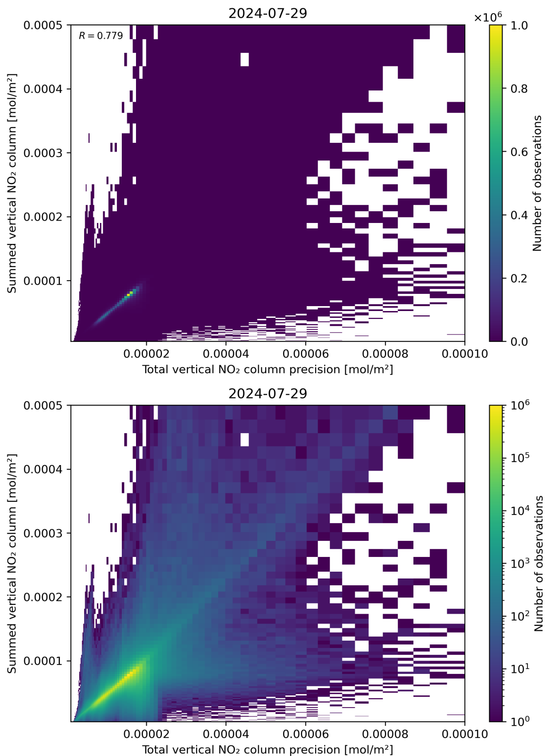
Figure 117: Scatter density plot of “Total vertical NO 2 column precision” against “Summed vertical NO 2 column” for 2024-07-28 to 2024-07-30.
