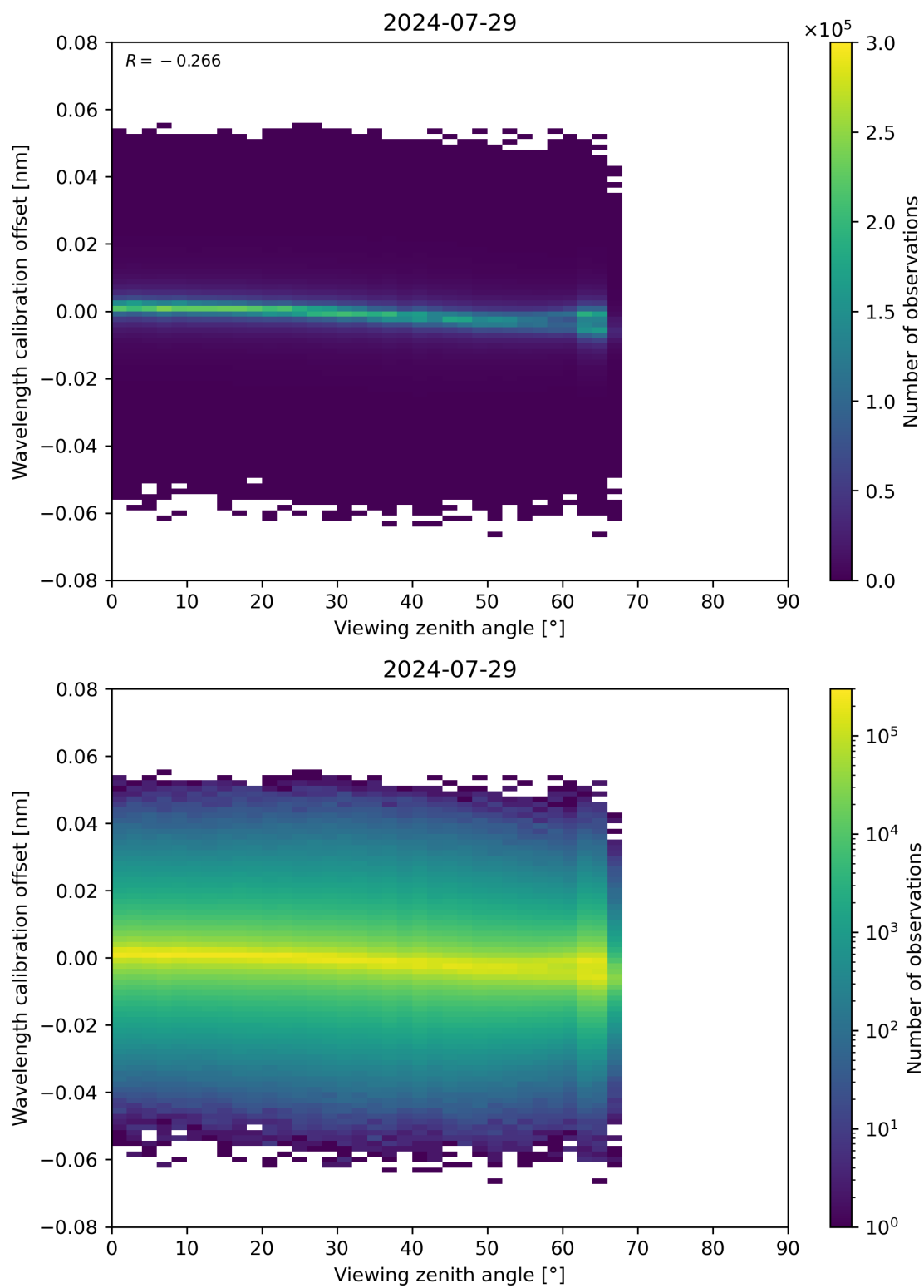
Figure 173: Scatter density plot of “Viewing zenith angle” against “Wavelength calibration offset” for 2024-07-28 to 2024-07-30.
