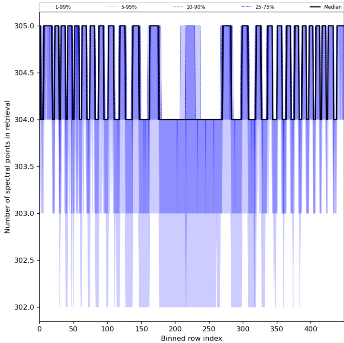
Figure 50: Along track statistics of “Number of spectral points in retrieval” for 2024-07-28 to 2024-07-30
