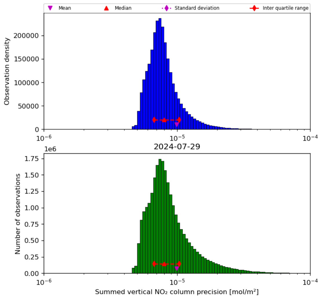
Figure 41: Histogram of "Summed vertical NO 2 column precision" for 2024-07-28 to 2024-07-30
