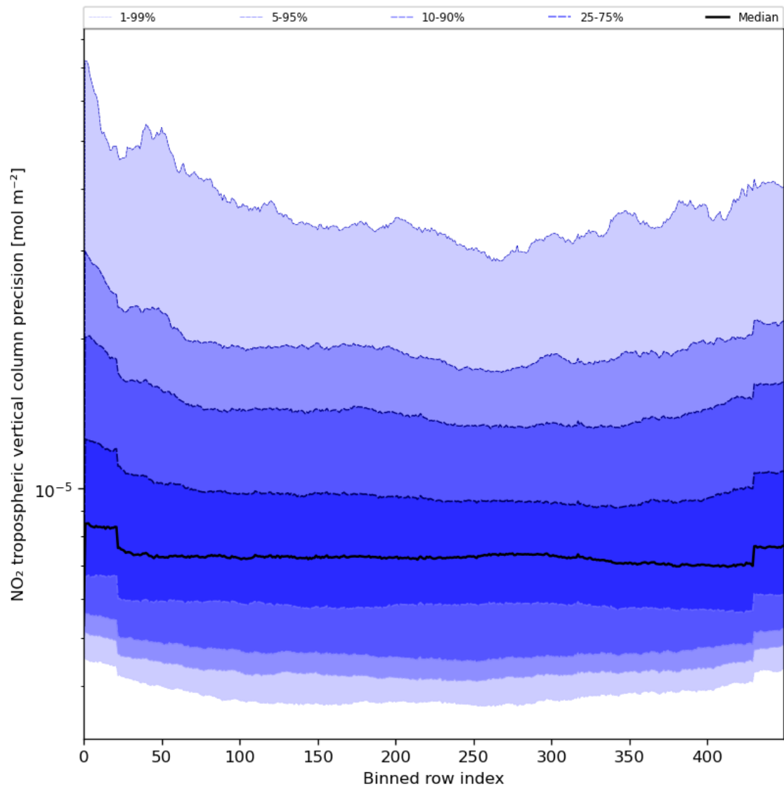
Figure 47: Along track statistics of “NO 2 tropospheric vertical column precision” for 2024-07-28 to 2024-07-30
