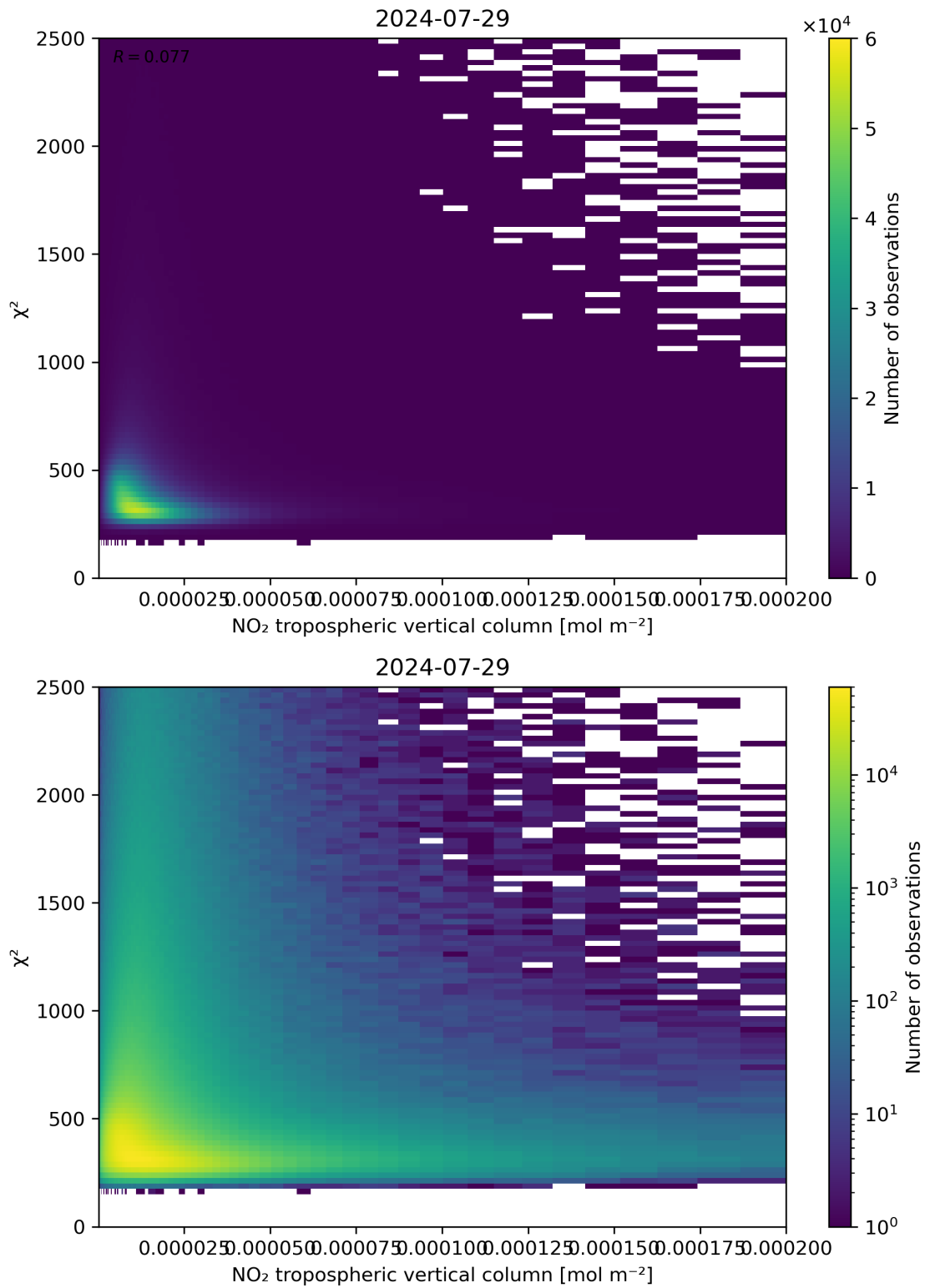
Figure 124: Scatter density plot of “NO 2 tropospheric vertical column” against “ \chi^2 ” for 2024-07-28 to 2024-07-30.
