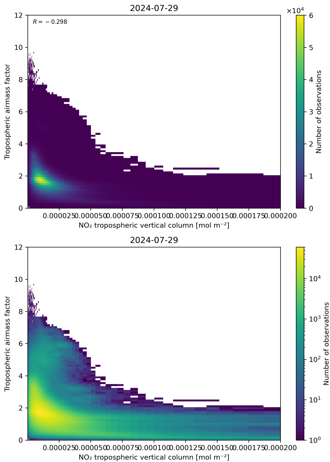
Figure 123: Scatter density plot of “NO 2 tropospheric vertical column” against “Tropospheric air mass factor” for 2024-07-28 to 2024-07-30.
