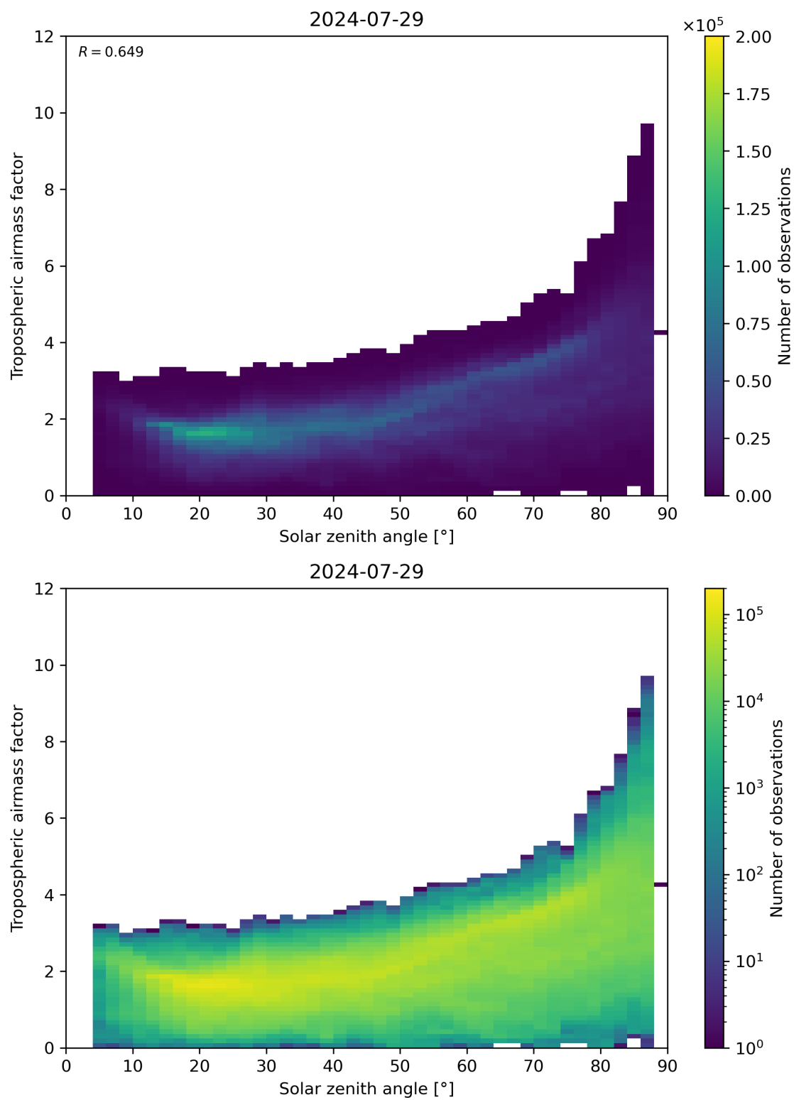
Figure 147: Scatter density plot of “Solar zenith angle” against “Tropospheric airmass factor” for 2024-07-28 to 2024-07-30.
