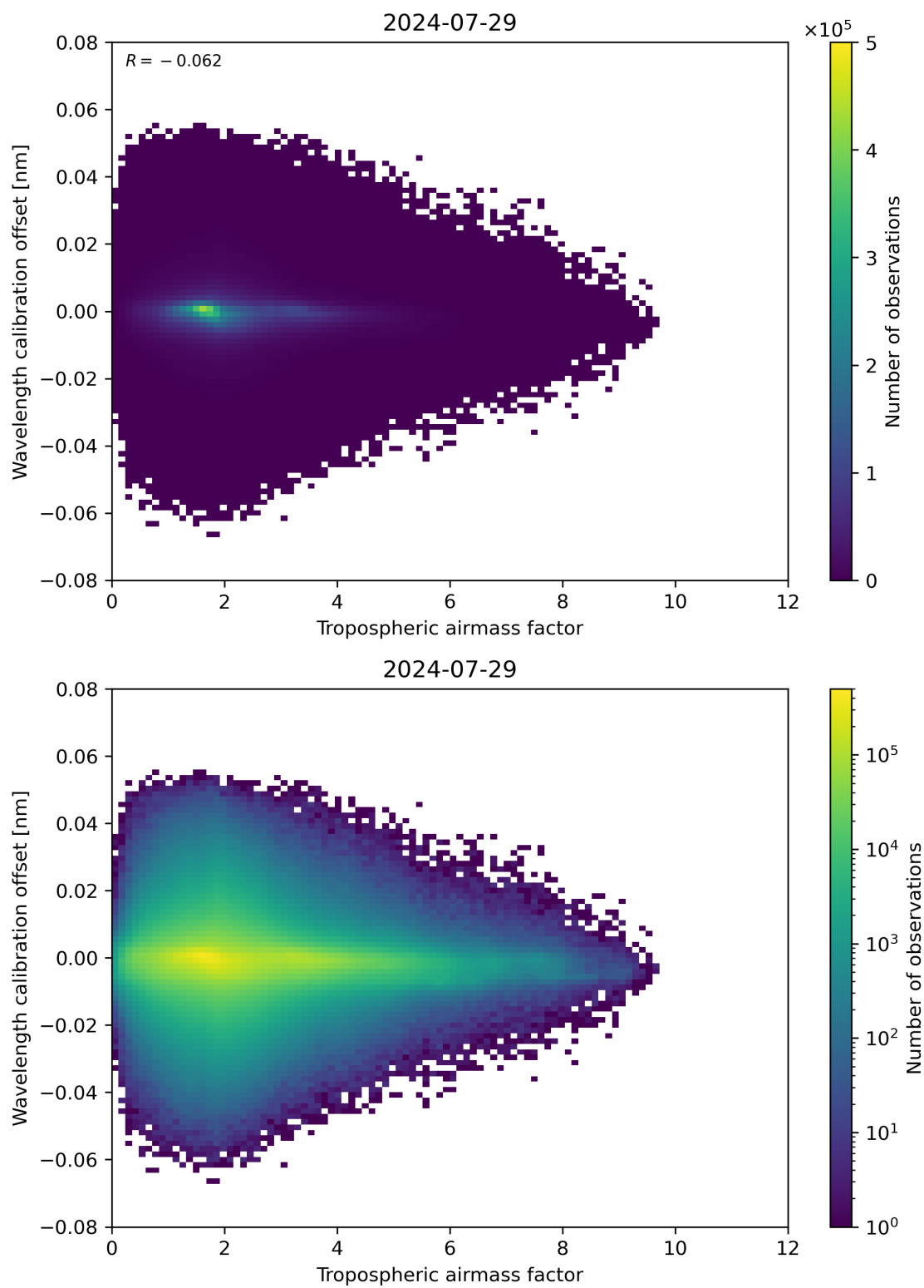
Figure 80: Scatter density plot of “Tropospheric airmass factor” against “Wavelength calibration offset” for 2024-07-28 to 2024-07-30.
