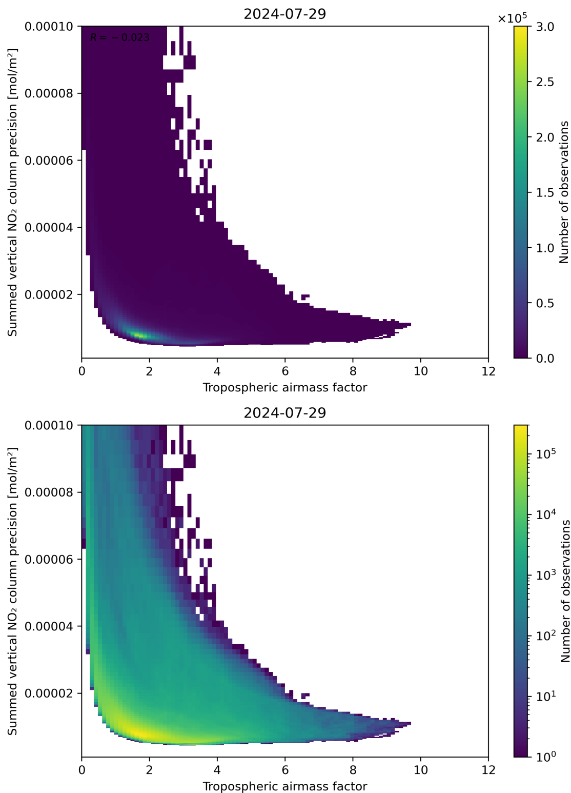
Figure 76: Scatter density plot of “Tropospheric air mass factor” against “Summed vertical NO 2 column precision” for 2024-07-28 to 2024-07-30.
