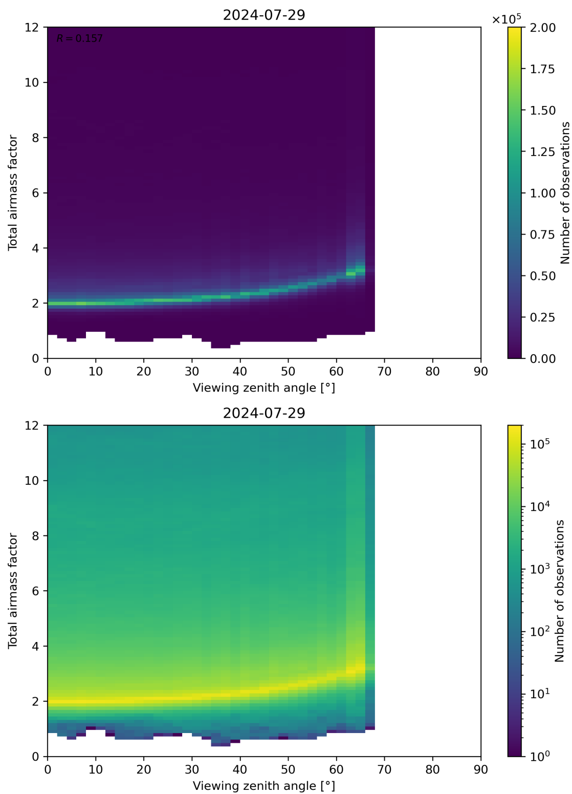
Figure 160: Scatter density plot of “Viewing zenith angle” against “Total airmass factor” for 2024-07-28 to 2024-07-30.
