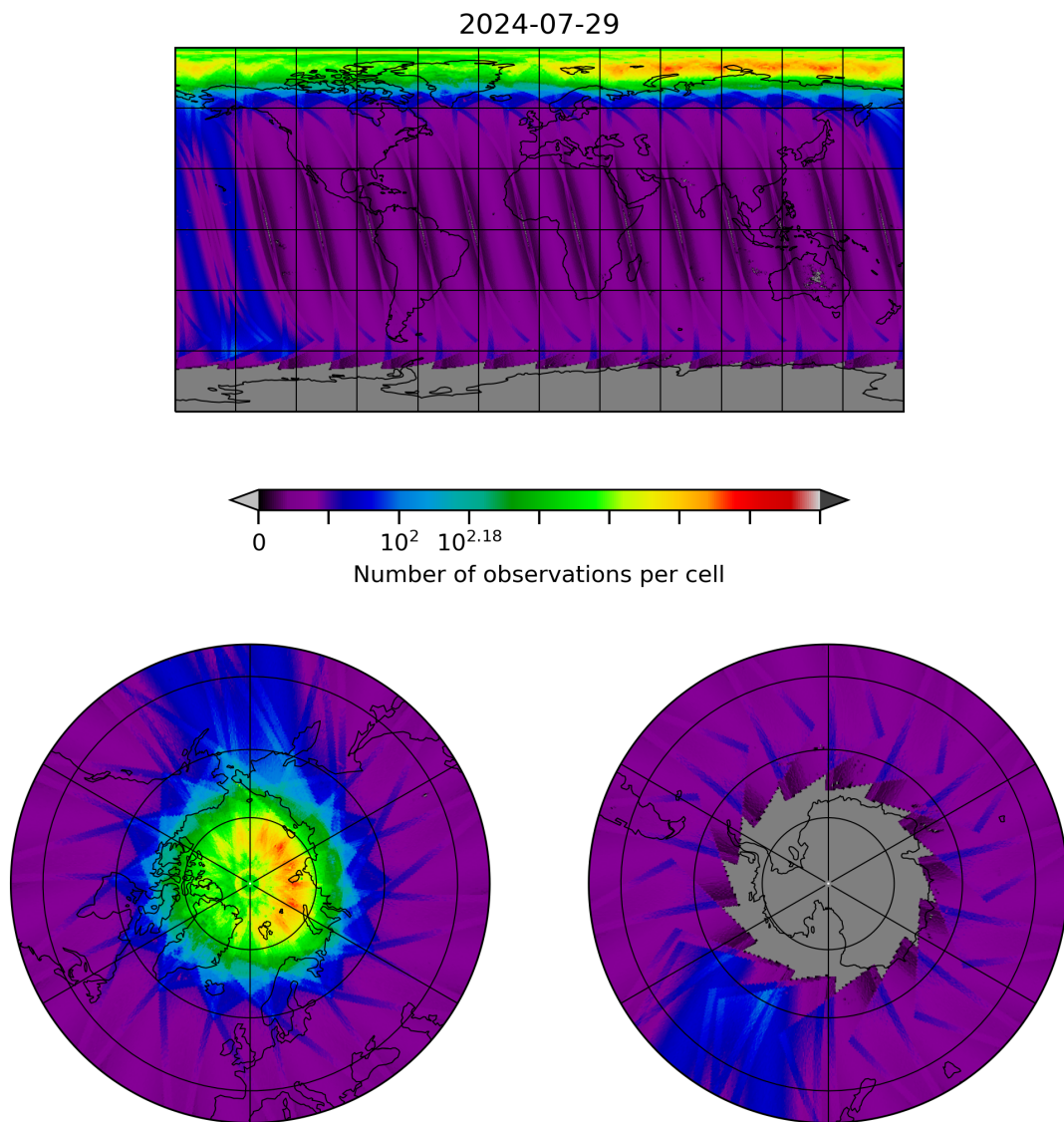
Figure 10: Map of the number of observations for 2024-07-28 to 2024-07-30
