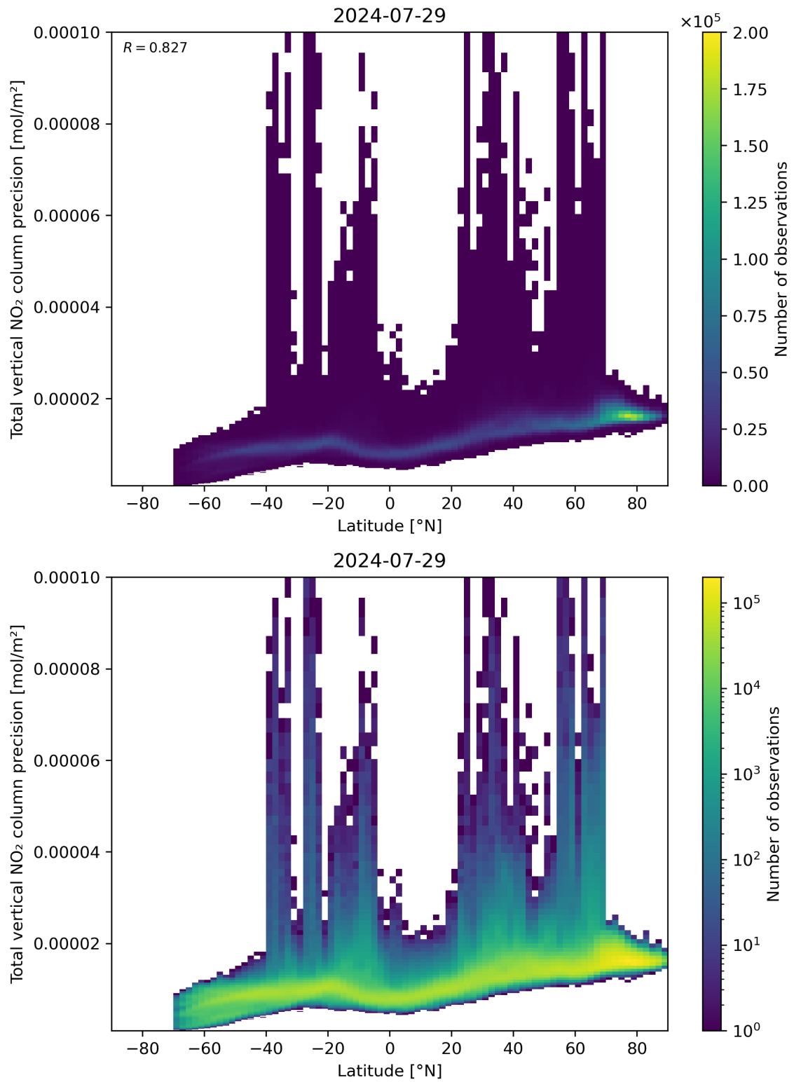
Figure 91: Scatter density plot of “Latitude” against “Total vertical NO 2 column precision” for 2024-07-28 to 2024-07-30.
