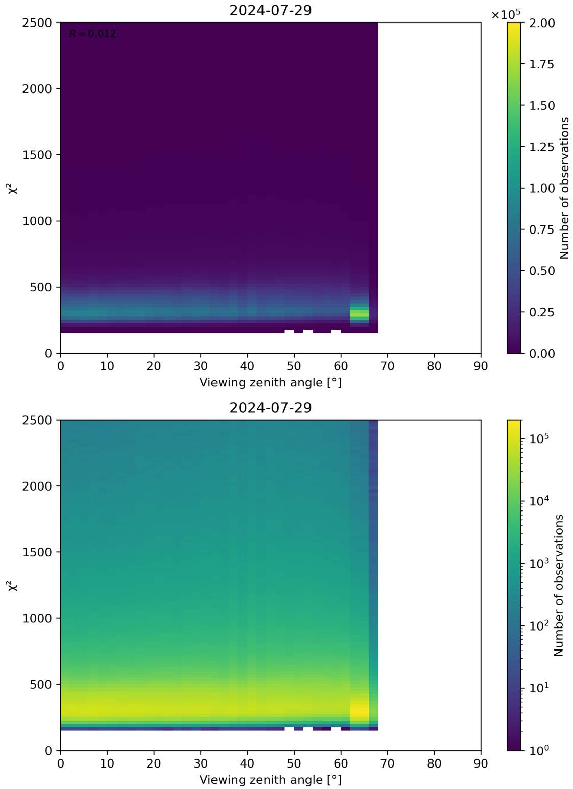
Figure 162: Scatter density plot of “Viewing zenith angle” against “ \chi^2 ” for 2024-07-28 to 2024-07-30.
