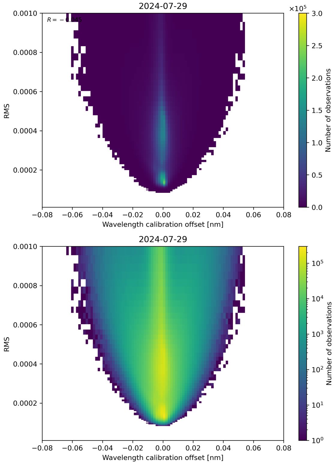
Figure 181: Scatter density plot of “Wavelength calibration offset” against “RMS” for 2024-07-28 to 2024-07-30.
