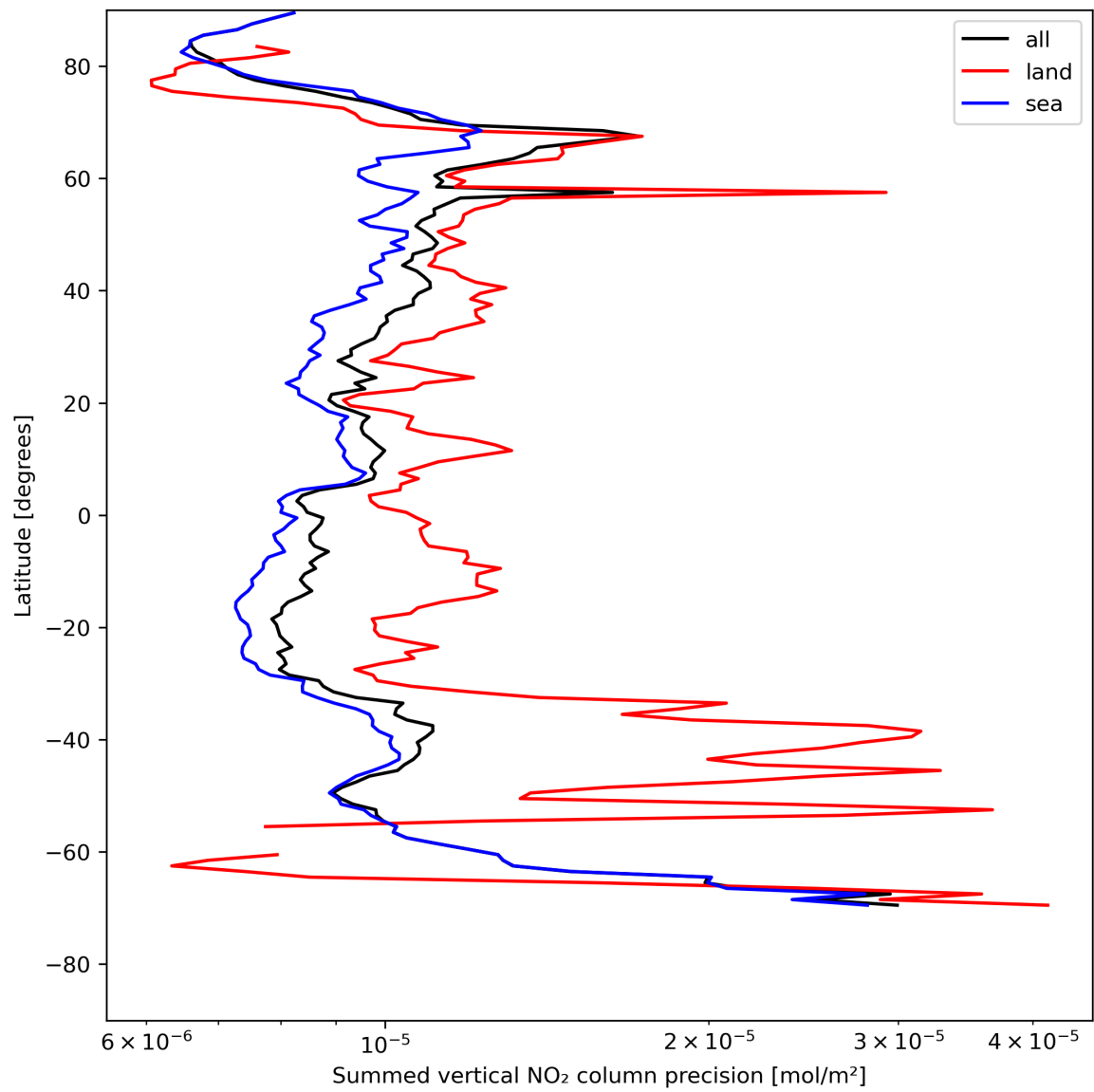
Figure 24: Zonal average of “Summed vertical NO 2 column precision” for 2024-07-28 to 2024-07-30.
