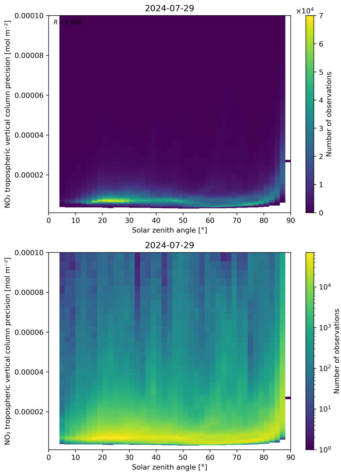
Figure 156: Scatter density plot of “Solar zenith angle” against “NO 2 tropospheric vertical column precision” for 2024-07-28 to 2024-07-30.
