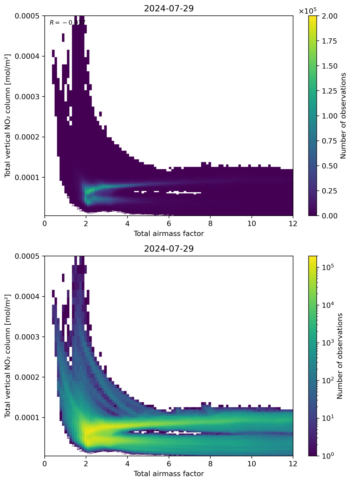
Figure 67: Scatter density plot of “Total airmass factor” against “Total vertical NO 2 column” for 2024-07-28 to 2024-07-30.
