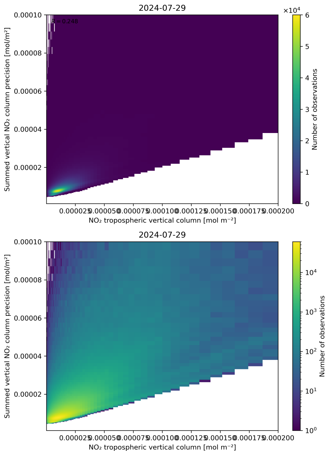
Figure 127: Scatter density plot of “NO 2 tropospheric vertical column” against “Summed vertical NO 2 column precision” for 2024-07-28 to 2024-07-30.
