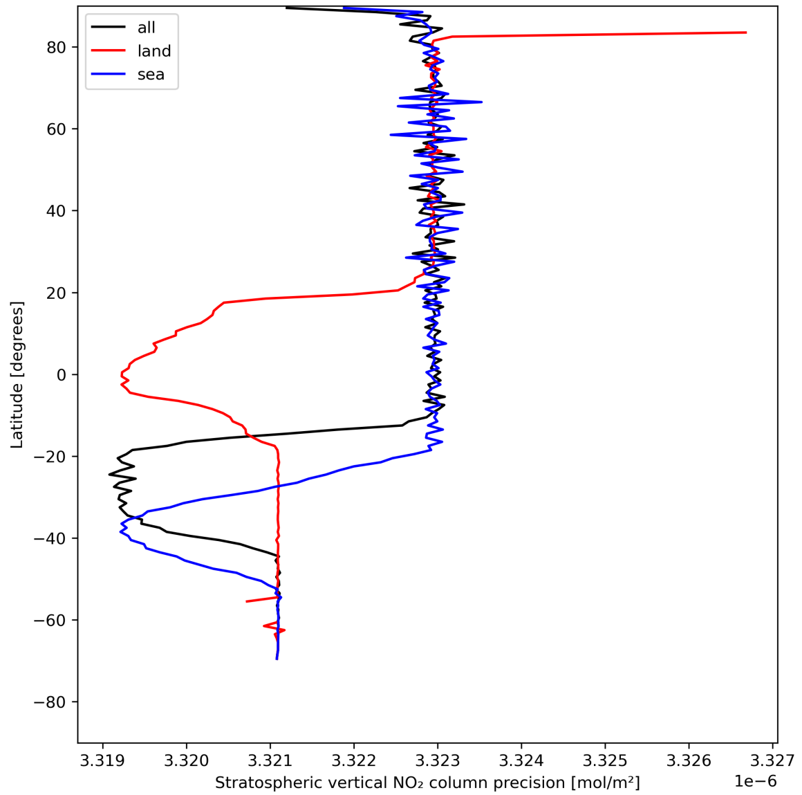
Figure 20: Zonal average of “Stratospheric vertical NO 2 column precision” for 2024-07-28 to 2024-07-30.
