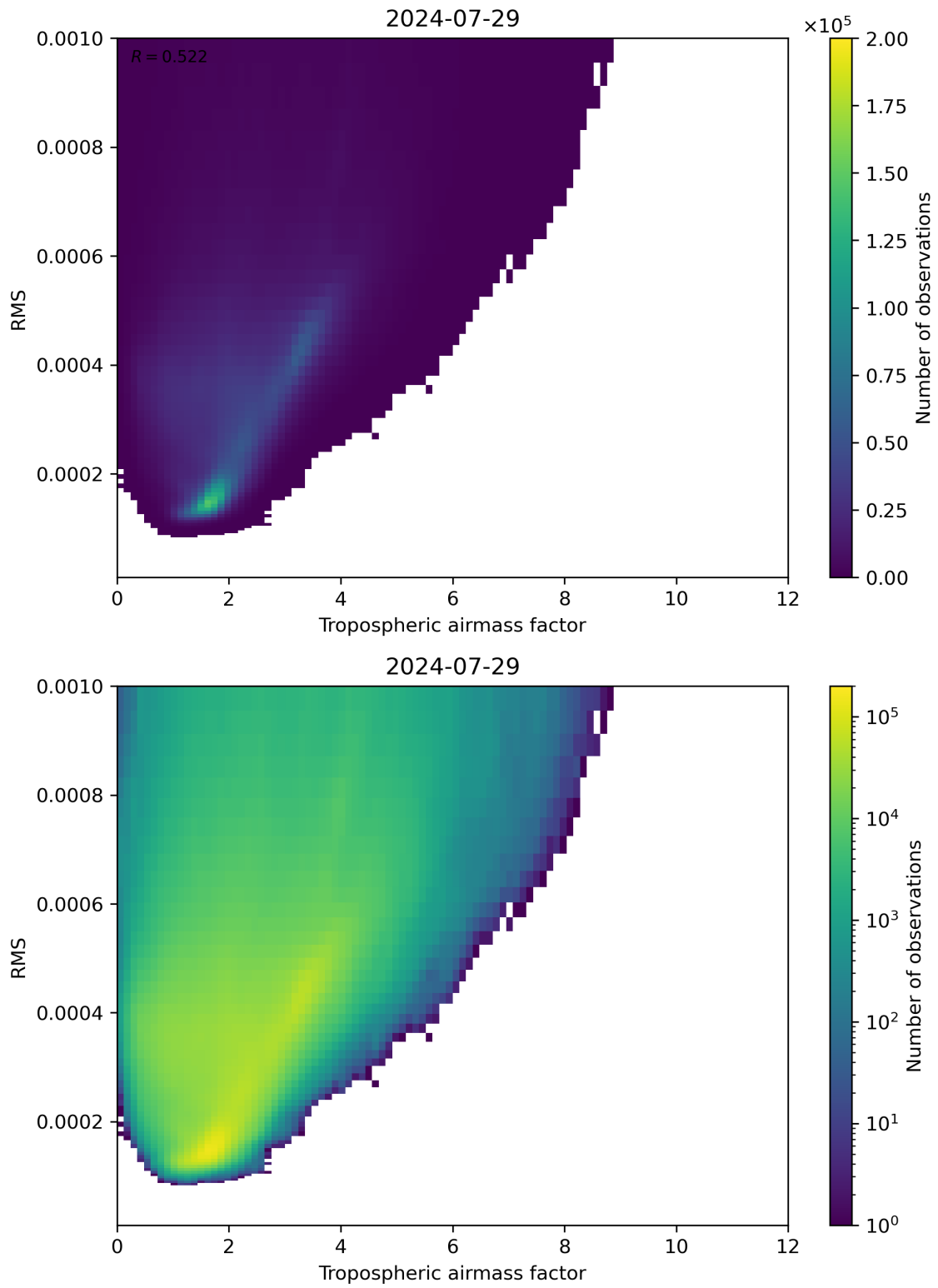
Figure 79: Scatter density plot of “Tropospheric airmass factor” against “RMS” for 2024-07-28 to 2024-07-30.
