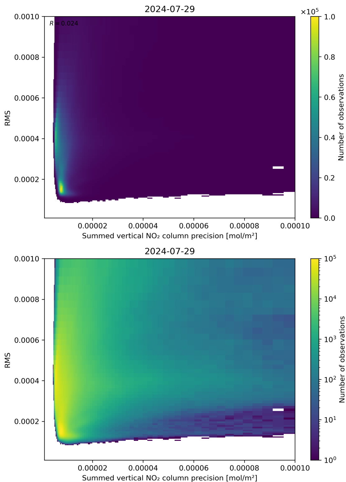
Figure 108: Scatter density plot of “Summed vertical NO 2 column precision” against “RMS” for 2024-07-28 to 2024-07-30.
