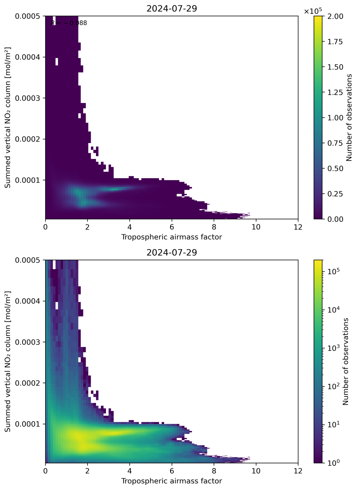
Figure 75: Scatter density plot of “Tropospheric air mass factor” against “Summed vertical NO 2 column” for 2024-07-28 to 2024-07-30.
