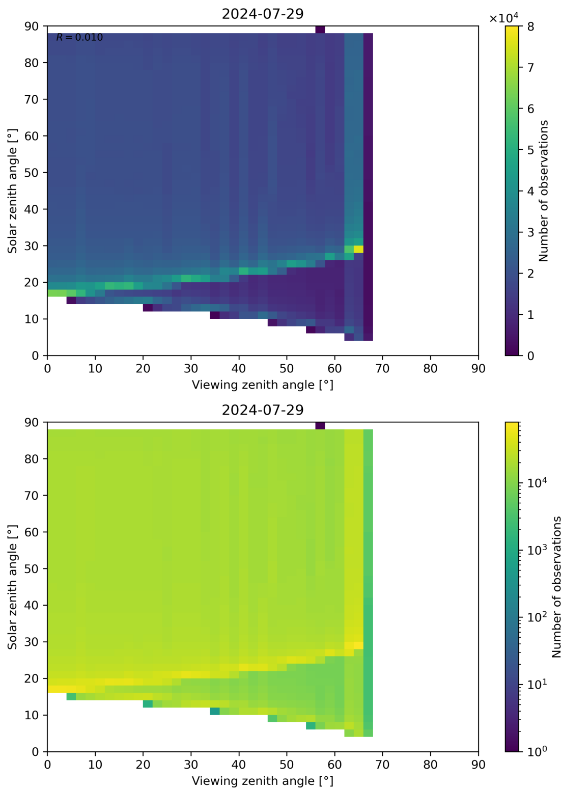
Figure 172: Scatter density plot of “Viewing zenith angle” against “Solar zenith angle” for 2024-07-28 to 2024-07-30.
