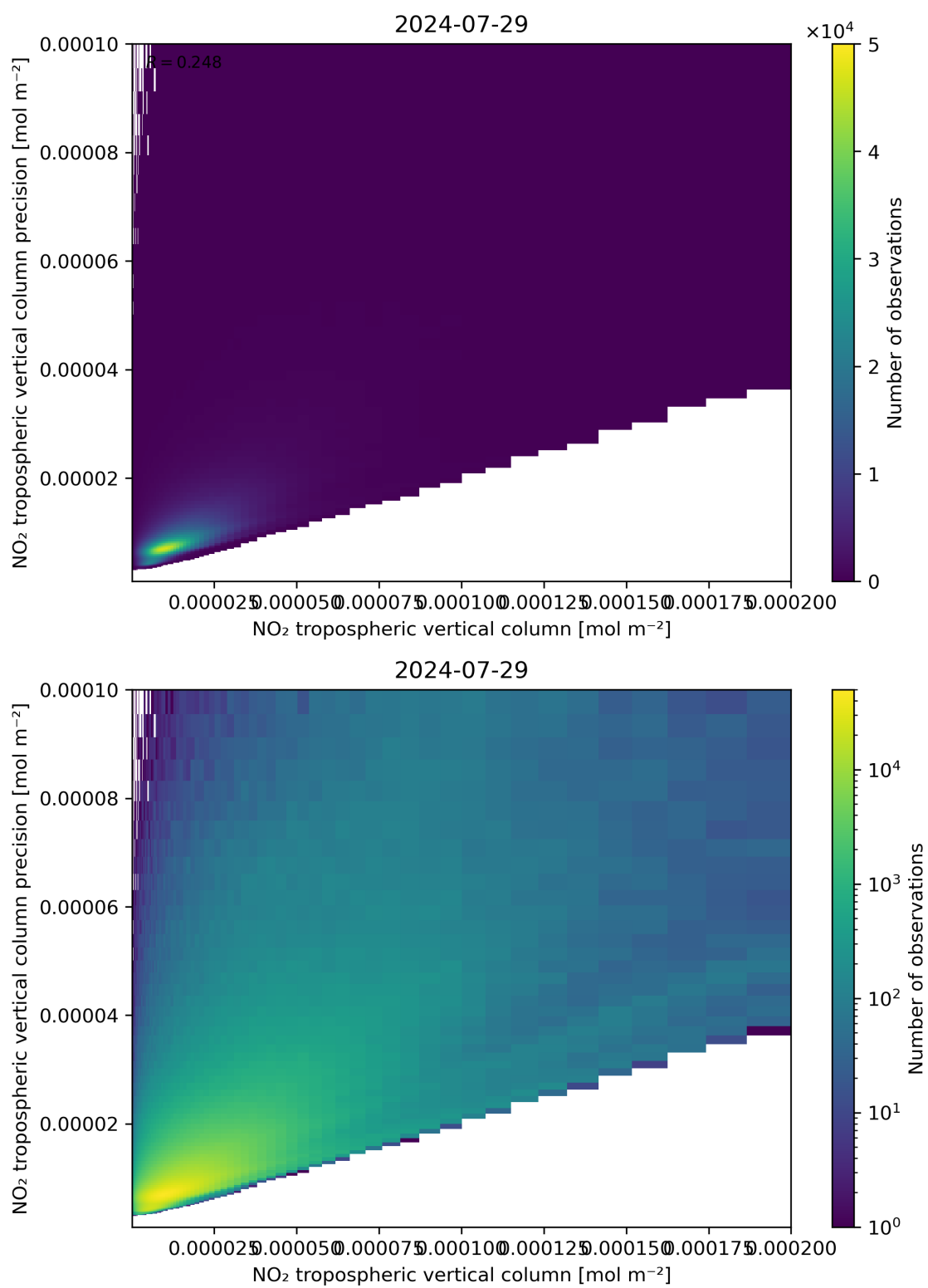
Figure 130: Scatter density plot of “NO 2 tropospheric vertical column” against “NO 2 tropospheric vertical column precision” for 2024-07-28 to 2024-07-30.
