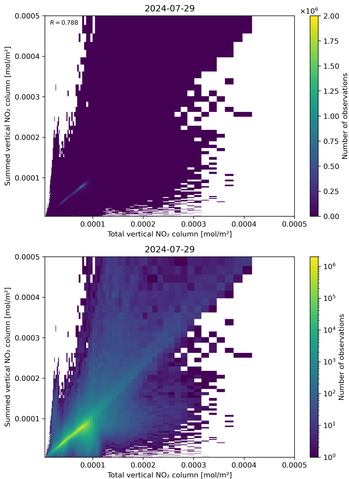
Figure 112: Scatter density plot of “Total vertical NO 2 column” against “Summed vertical NO 2 column” for 2024-07-28 to 2024-07-30.
