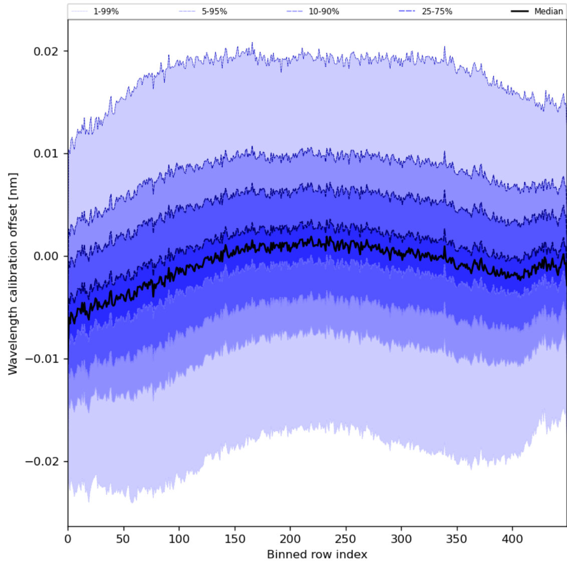
Figure 52: Along track statistics of “Wavelength calibration offset” for 2024-07-28 to 2024-07-30
