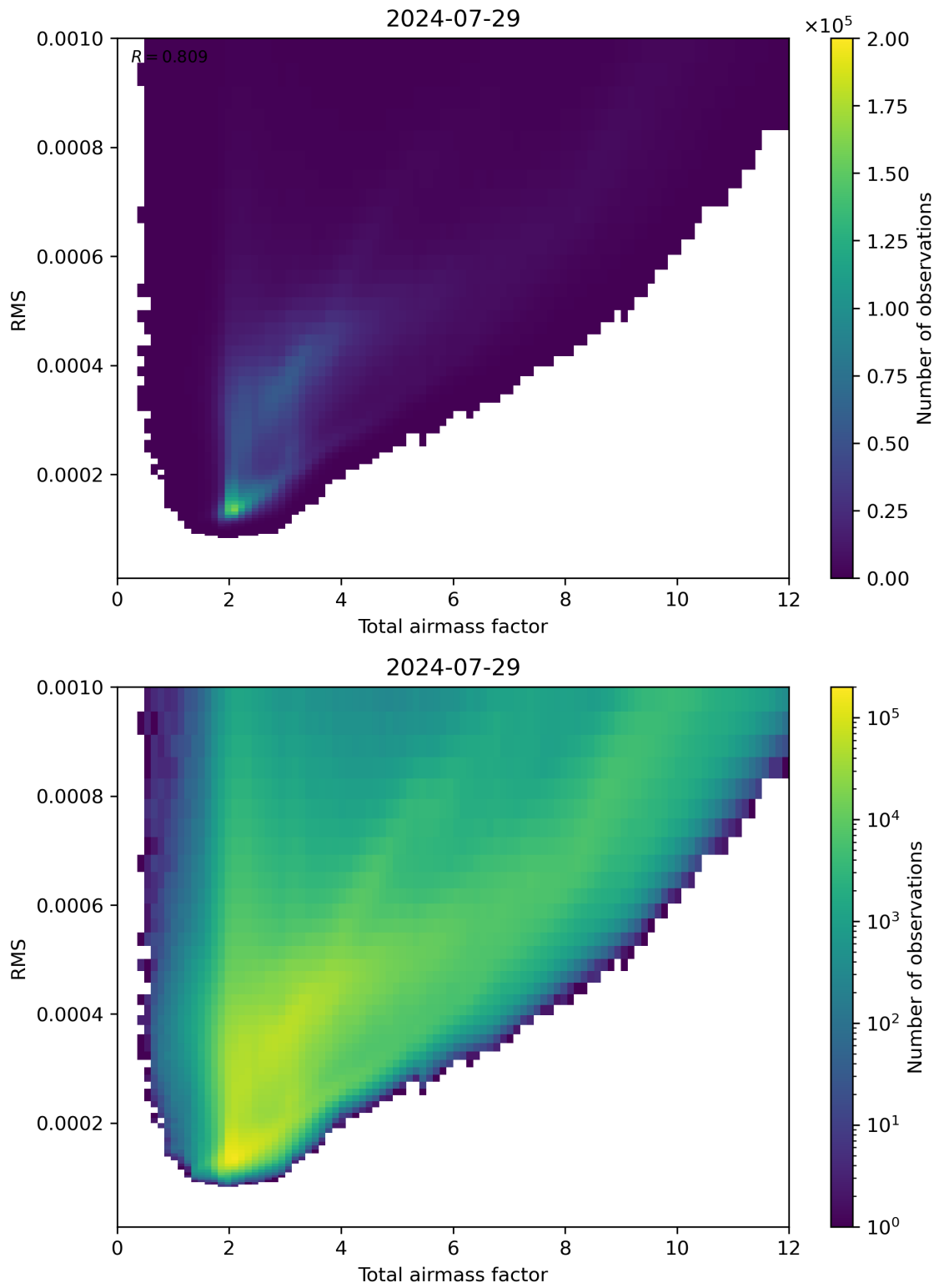
Figure 69: Scatter density plot of “Total airmass factor” against “RMS” for 2024-07-28 to 2024-07-30.
