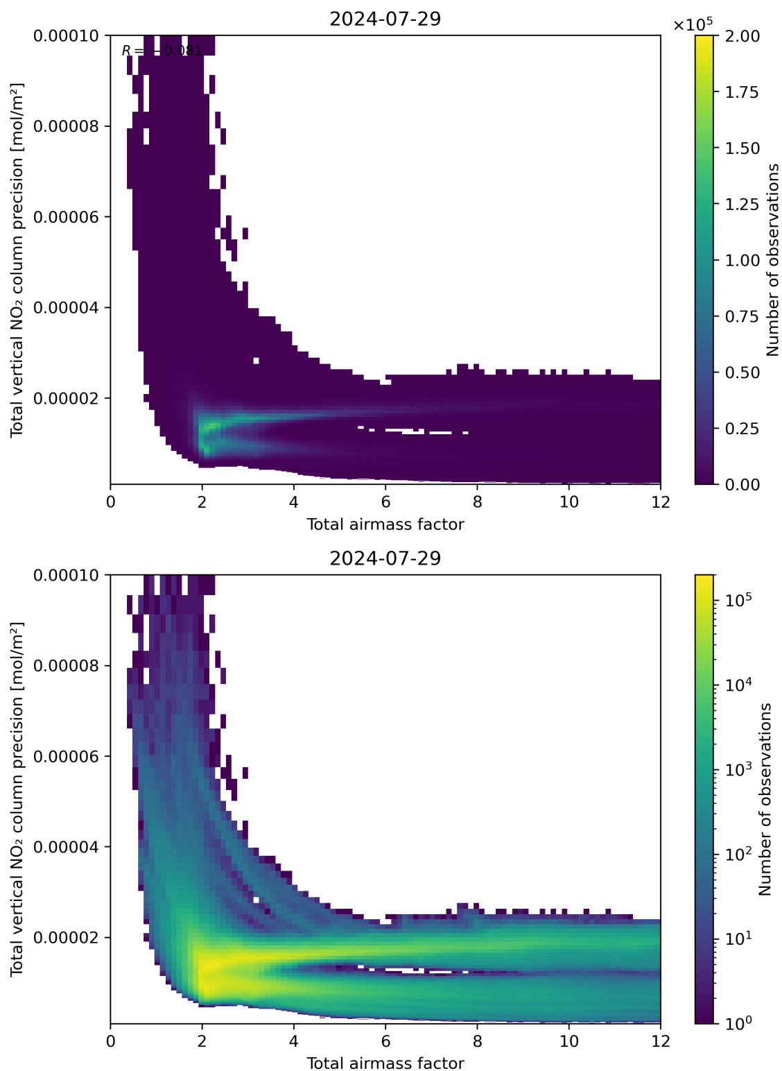
Figure 68: Scatter density plot of “Total airmass factor” against “Total vertical NO 2 column precision” for 2024-07-28 to 2024-07-30.
