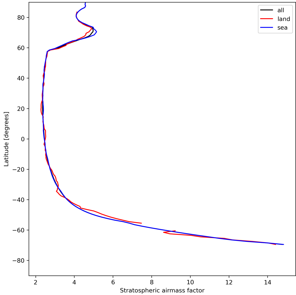
Figure 27: Zonal average of “Stratospheric air mass factor” for 2024-07-28 to 2024-07-30.
