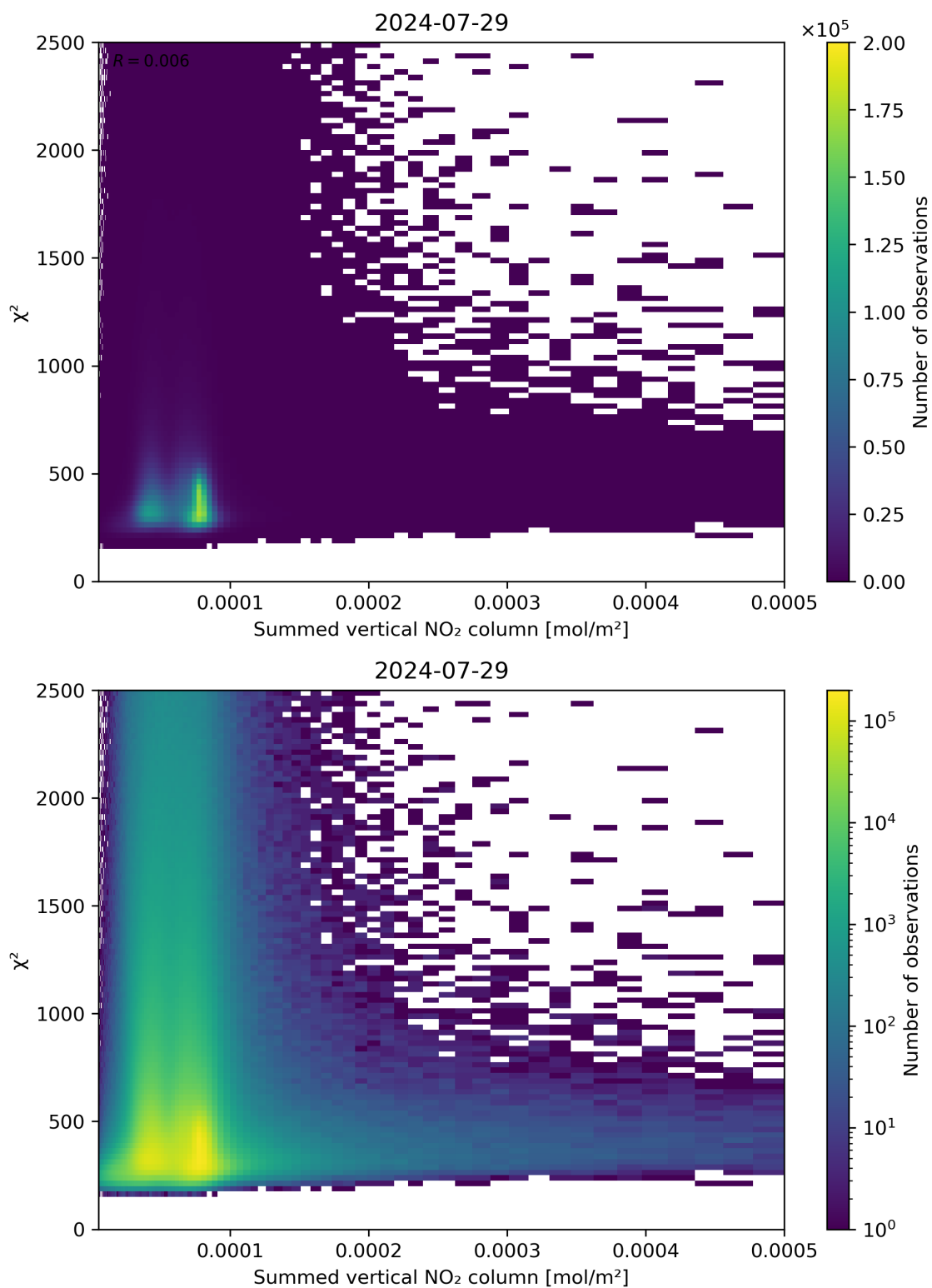
Figure 104: Scatter density plot of “Summed vertical NO 2 column” against “ \chi^2 ” for 2024-07-28 to 2024-07-30.
