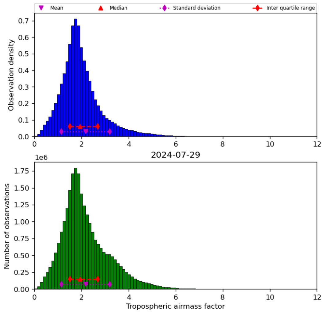
Figure 31: Histogram of “Tropospheric airmass factor” for 2024-07-28 to 2024-07-30
