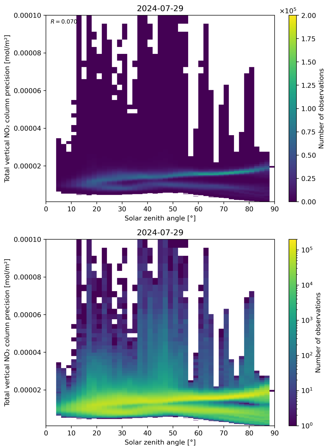
Figure 154: Scatter density plot of “Solar zenith angle” against “Total vertical NO 2 column precision” for 2024-07-28 to 2024-07-30.
