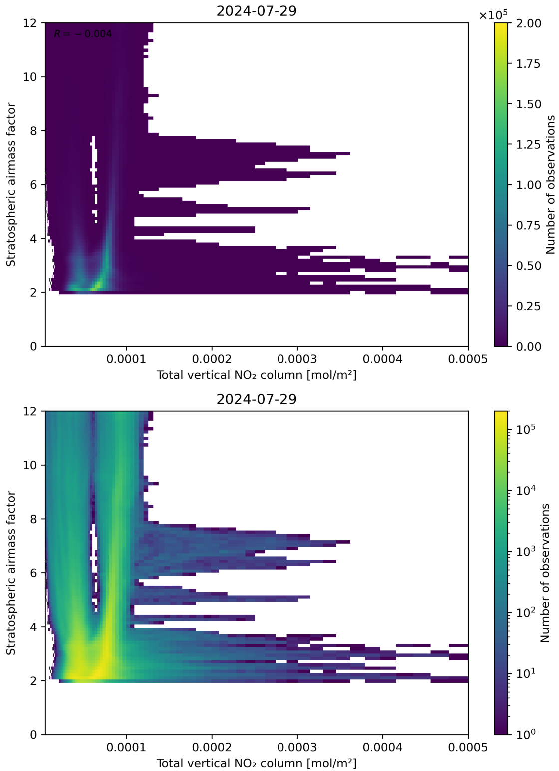
Figure 110: Scatter density plot of “Total vertical NO 2 column” against “Stratospheric airmass factor” for 2024-07-28 to 2024-07-30.
