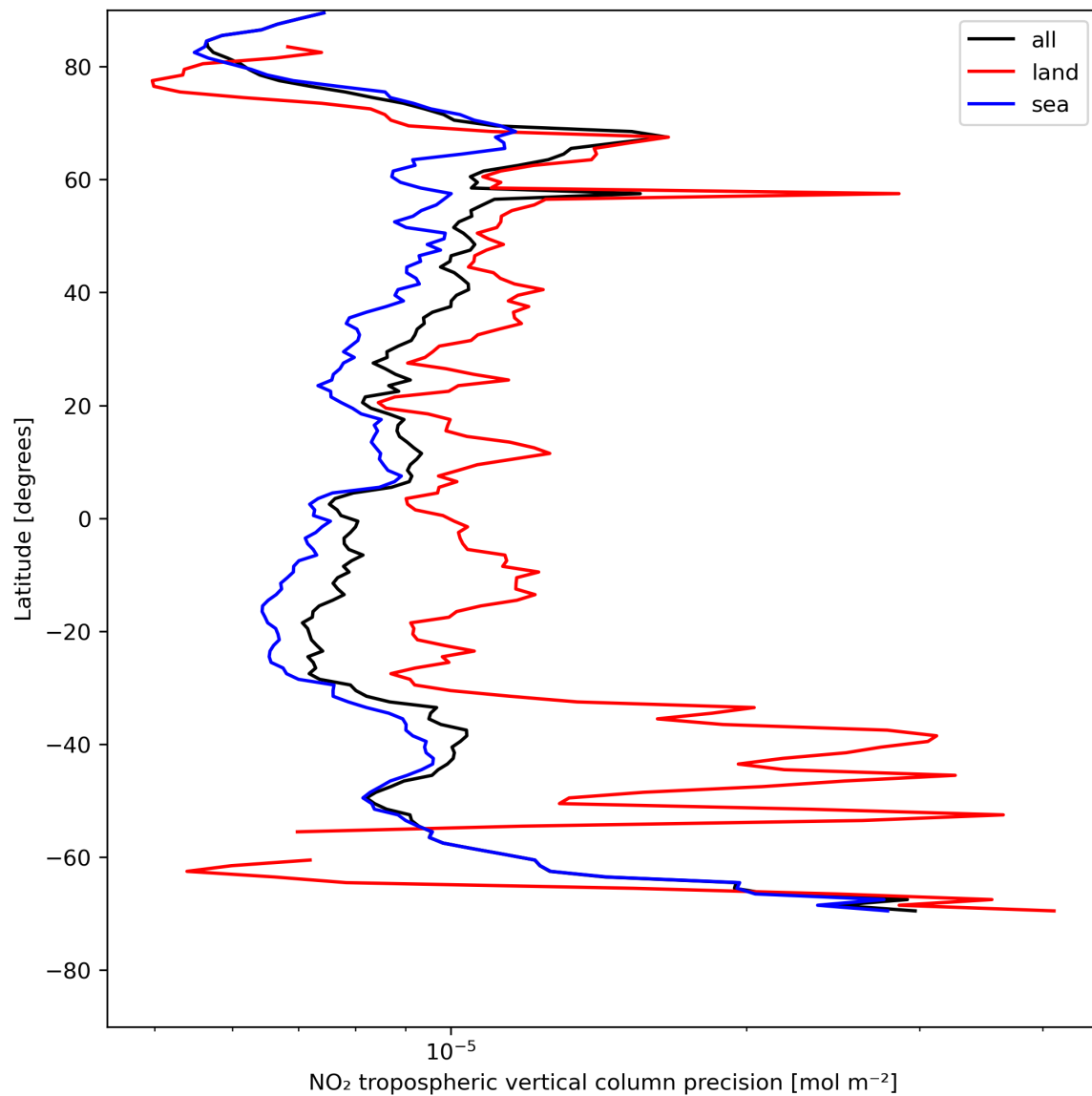
Figure 13: Zonal average of “NO 2 tropospheric vertical column precision” for 2024-07-28 to 2024-07-30.
