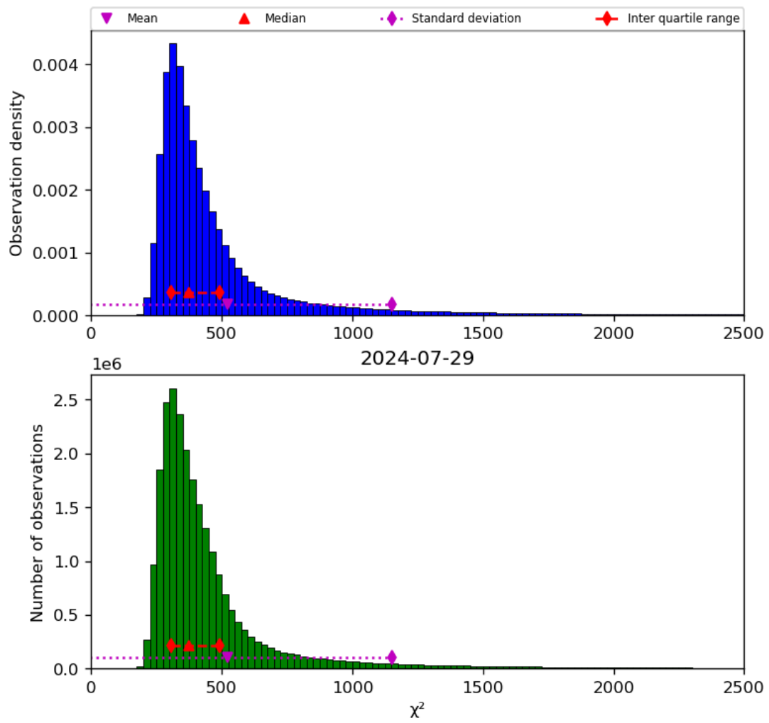
Figure 42: Histogram of " \chi^2 " for 2024-07-28 to 2024-07-30
