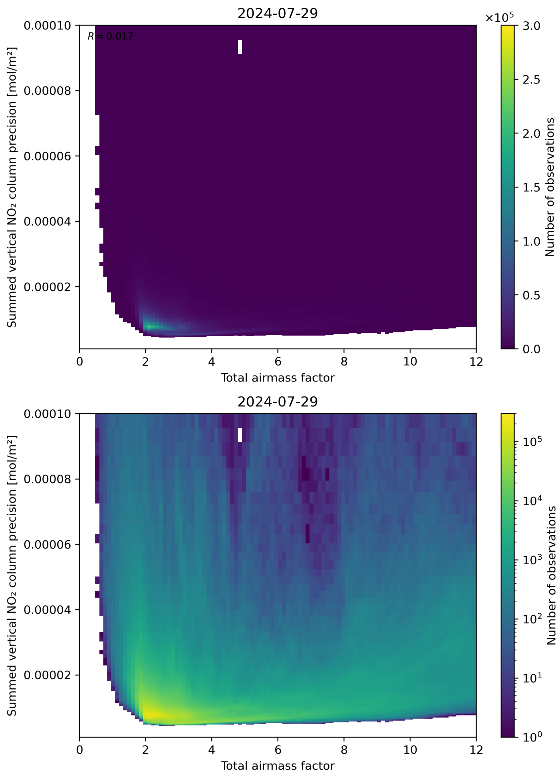
Figure 66: Scatter density plot of “Total airmass factor” against “Summed vertical NO 2 column precision” for 2024-07-28 to 2024-07-30.
