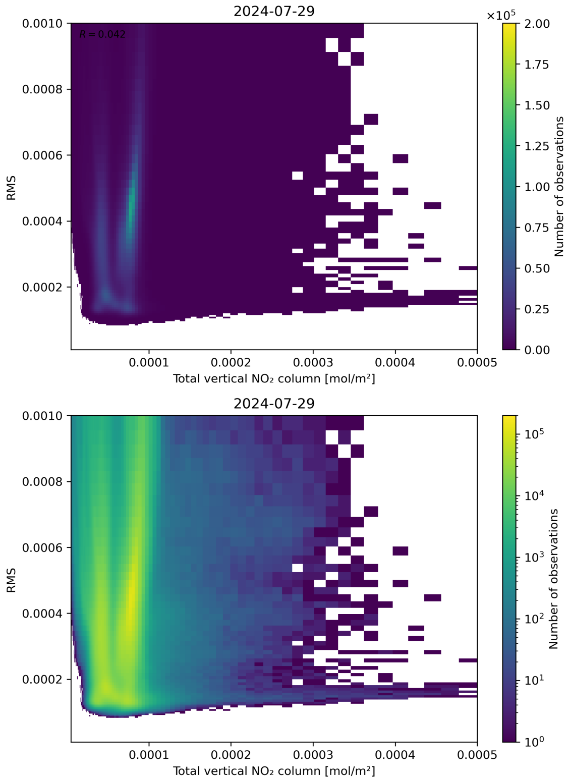
Figure 120: Scatter density plot of “Total vertical NO 2 column” against “RMS” for 2024-07-28 to 2024-07-30.
