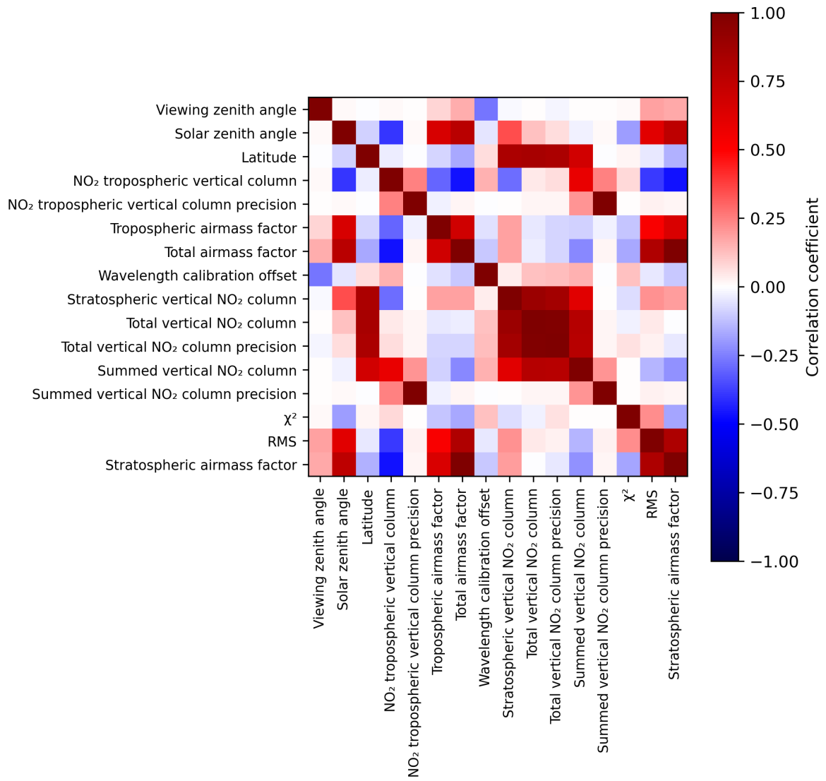
Figure 2: Map of correlation matrix for 2024-07-28 to 2024-07-30.
