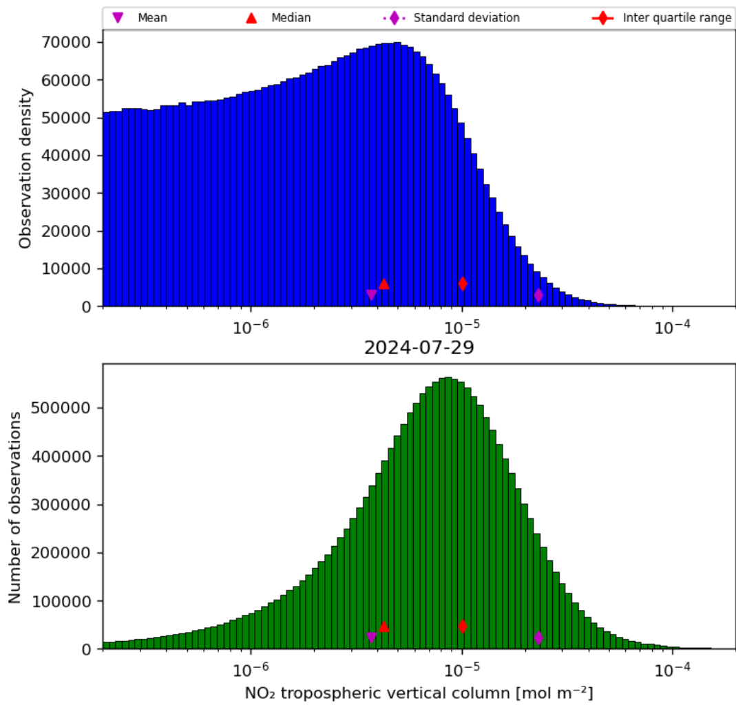
Figure 29: Histogram of “NO 2 tropospheric vertical column” for 2024-07-28 to 2024-07-30
