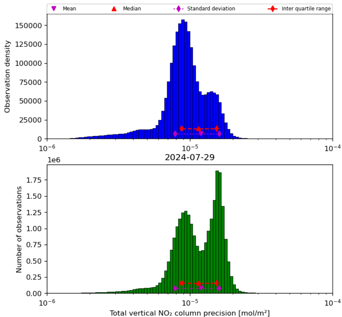
Figure 39: Histogram of “Total vertical NO 2 column precision” for 2024-07-28 to 2024-07-30
