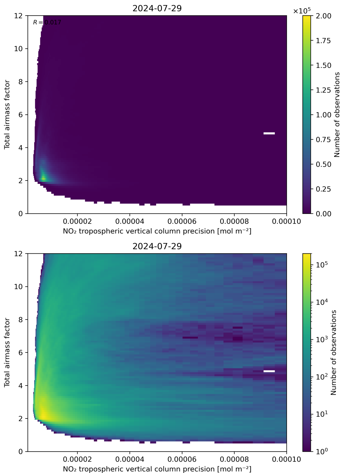
Figure 132: Scatter density plot of “NO 2 tropospheric vertical column precision” against “Total air mass factor” for 2024-07-28 to 2024-07-30.
