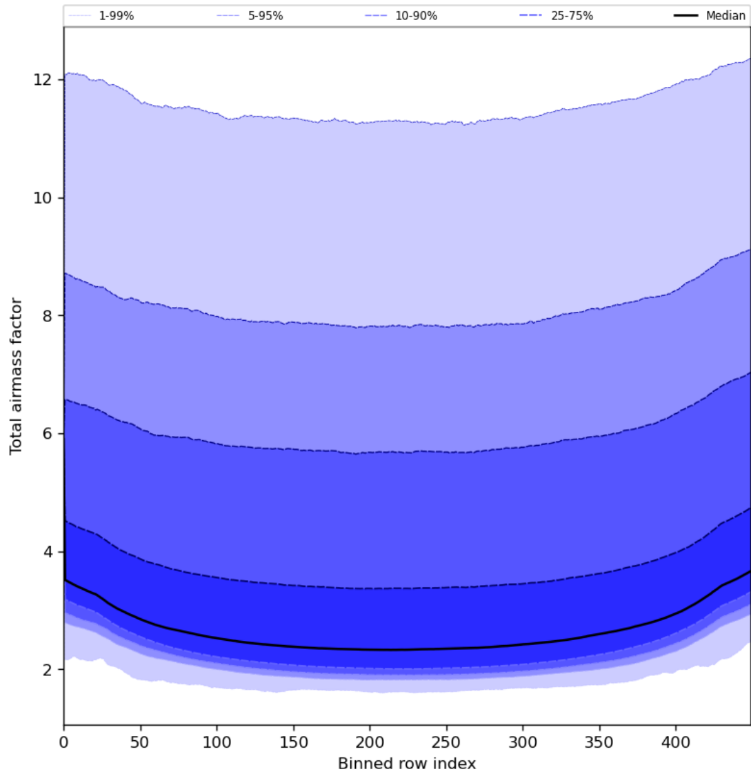
Figure 49: Along track statistics of “Total airmass factor” for 2024-07-28 to 2024-07-30
