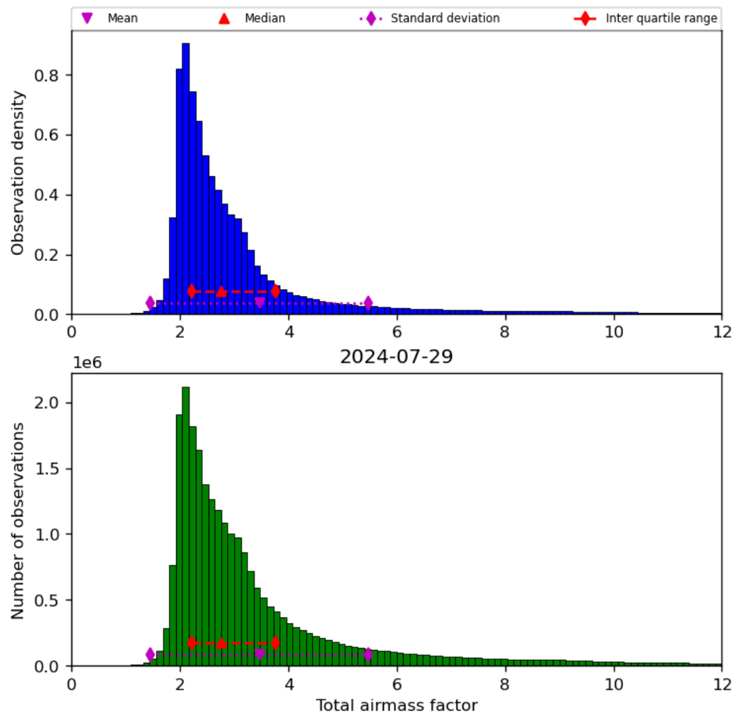
Figure 32: Histogram of “Total airmass factor” for 2024-07-28 to 2024-07-30
