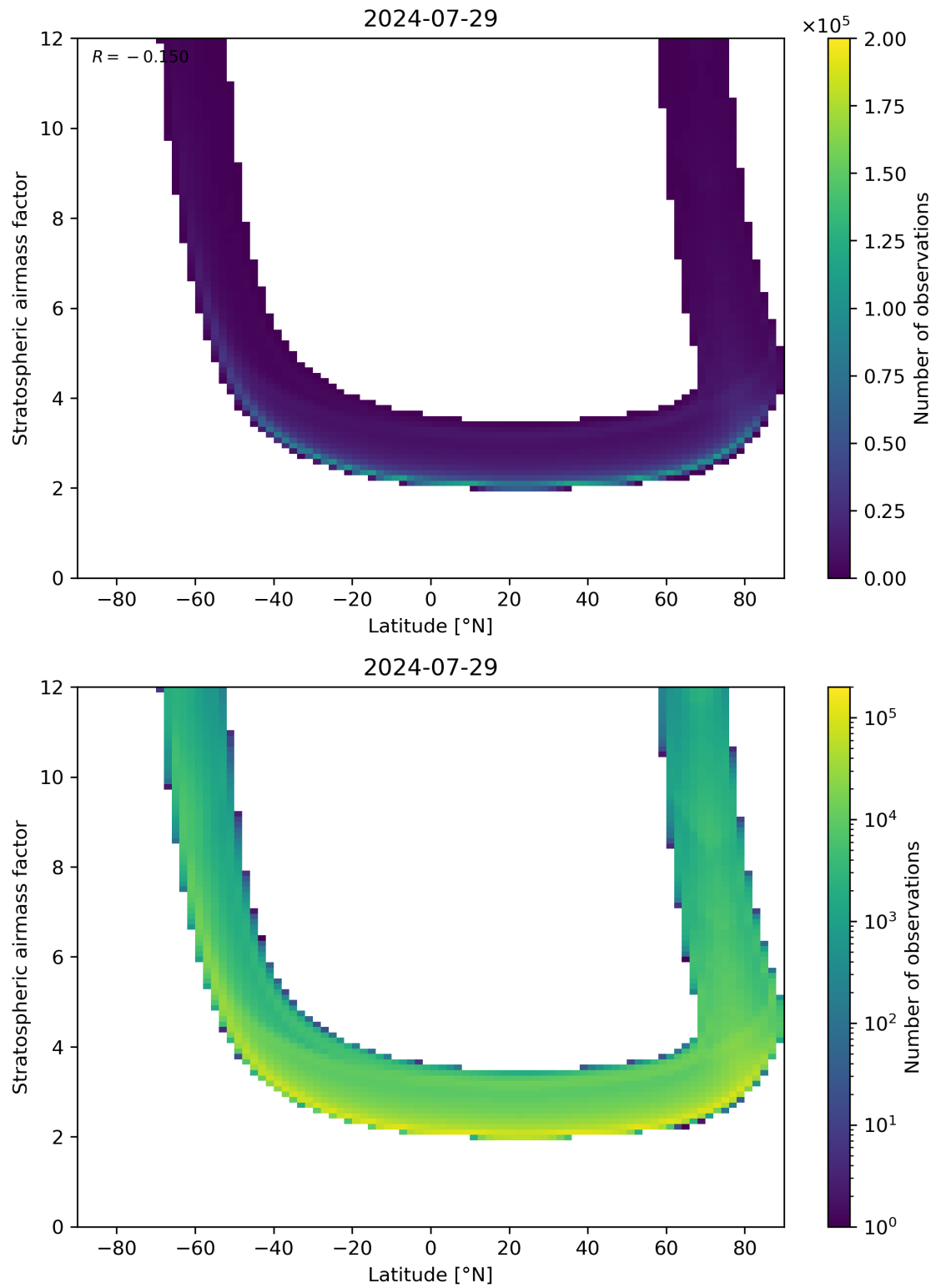
Figure 83: Scatter density plot of “Latitude” against “Stratospheric air mass factor” for 2024-07-28 to 2024-07-30.
