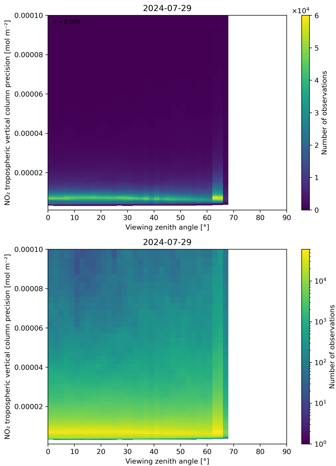
Figure 170: Scatter density plot of “Viewing zenith angle” against “NO 2 tropospheric vertical column precision” for 2024-07-28 to 2024-07-30.
