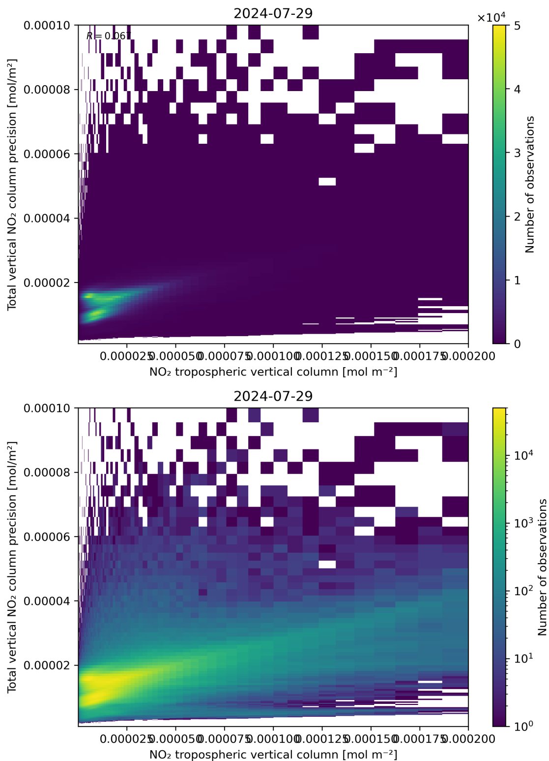
Figure 129: Scatter density plot of “NO 2 tropospheric vertical column” against “Total vertical NO 2 column precision” for 2024-07-28 to 2024-07-30.
