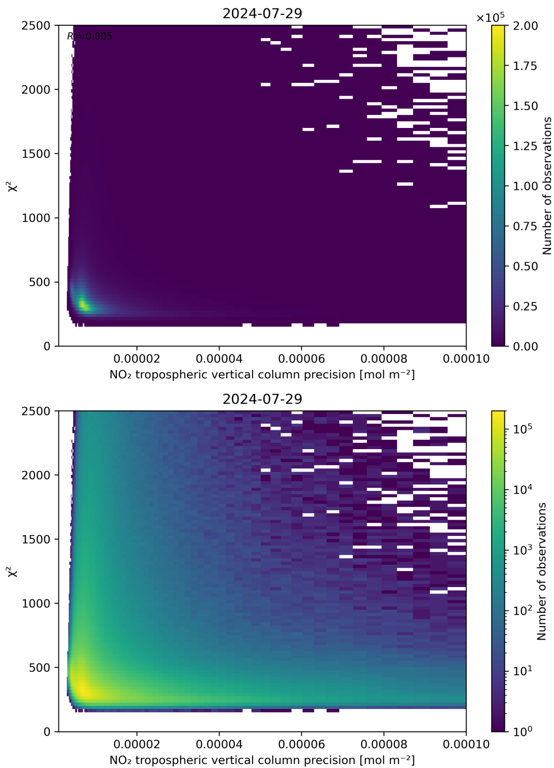
Figure 134: Scatter density plot of “NO 2 tropospheric vertical column precision” against “ \chi^2 ” for 2024-07-28 to 2024-07-30.
