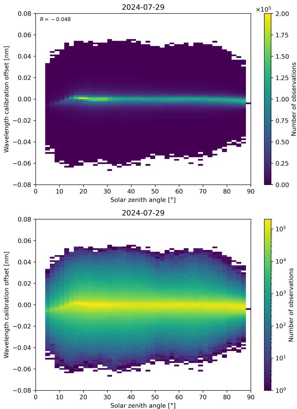
Figure 158: Scatter density plot of “Solar zenith angle” against “Wavelength calibration offset” for 2024-07-28 to 2024-07-30.
