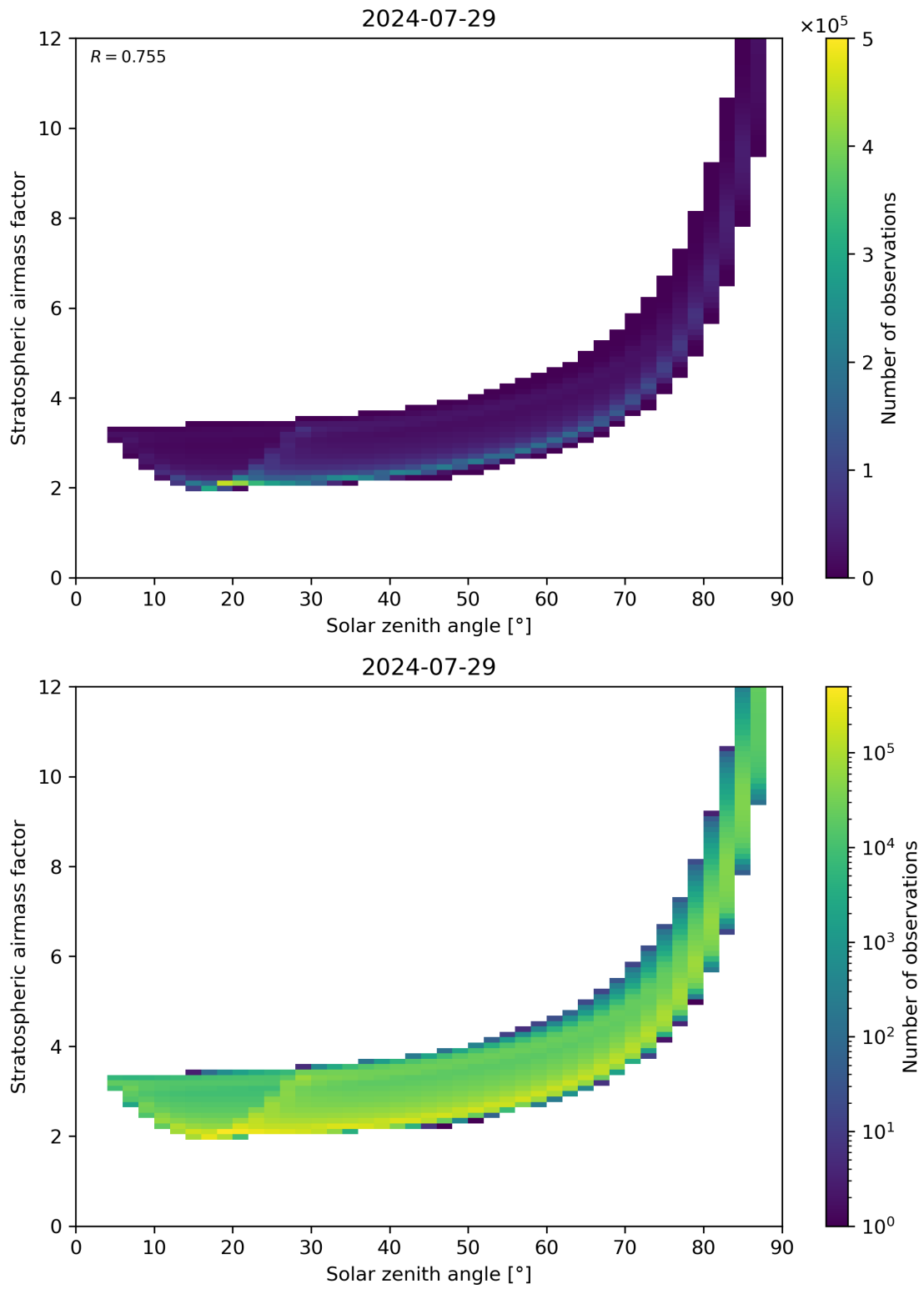
Figure 145: Scatter density plot of “Solar zenith angle” against “Stratospheric airmass factor” for 2024-07-28 to 2024-07-30.
