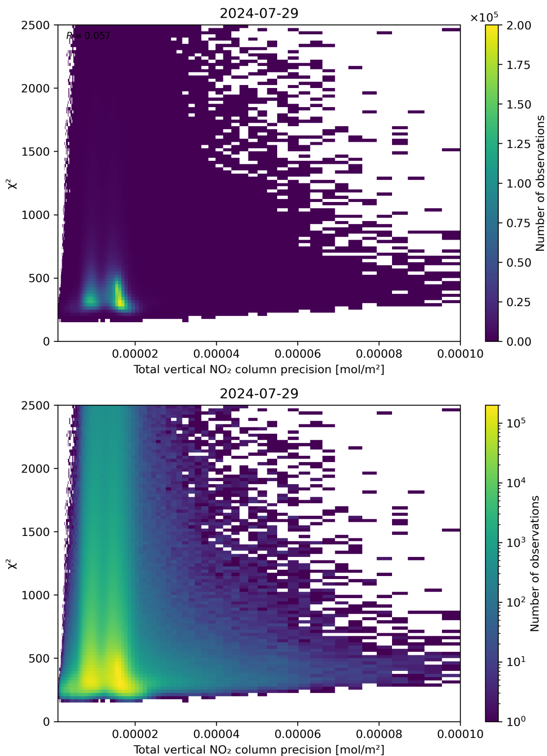
Figure 116: Scatter density plot of “Total vertical NO 2 column precision” against “ \chi^2 ” for 2024-07-28 to 2024-07-30.
