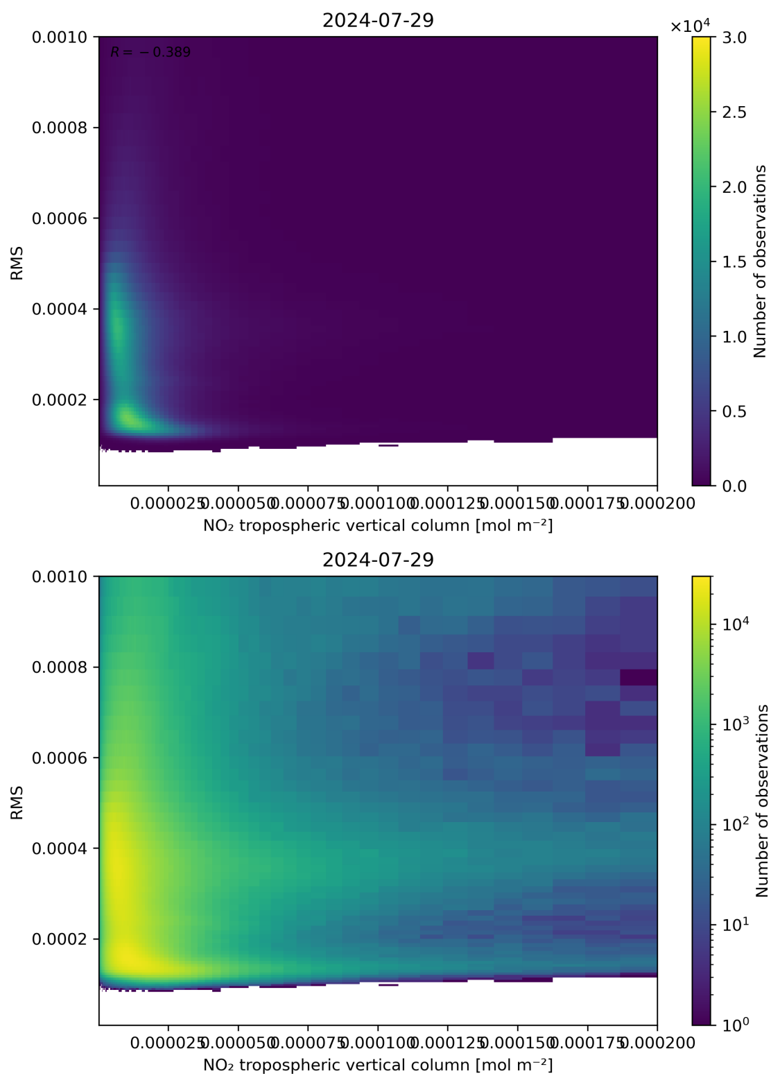
Figure 142: Scatter density plot of “NO 2 tropospheric vertical column” against “RMS” for 2024-07-28 to 2024-07-30.
