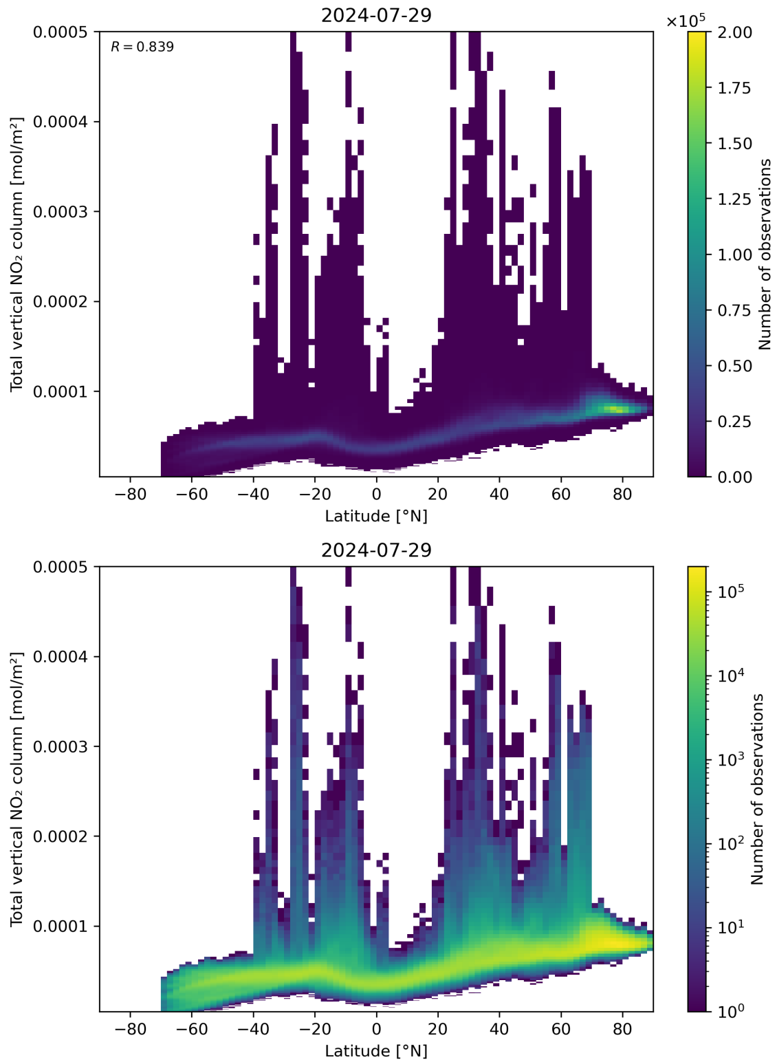
Figure 90: Scatter density plot of “Latitude” against “Total vertical NO 2 column” for 2024-07-28 to 2024-07-30.
