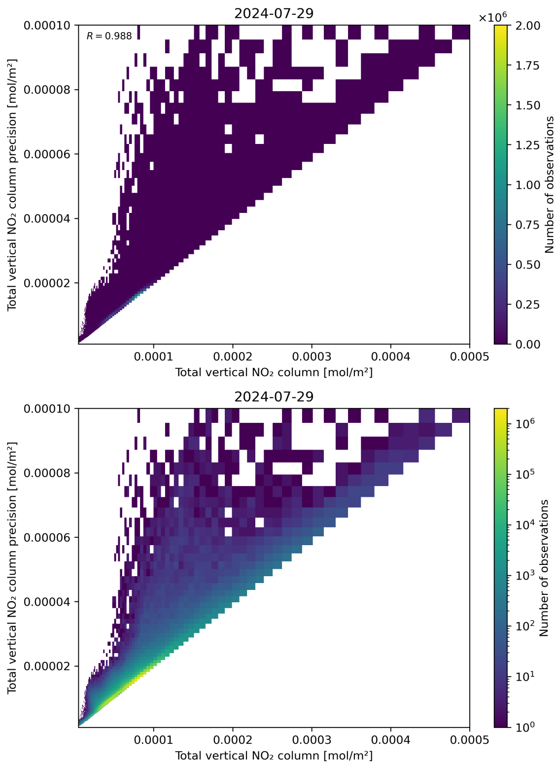
Figure 114: Scatter density plot of “Total vertical NO 2 column” against “Total vertical NO 2 column precision” for 2024-07-28 to 2024-07-30.
