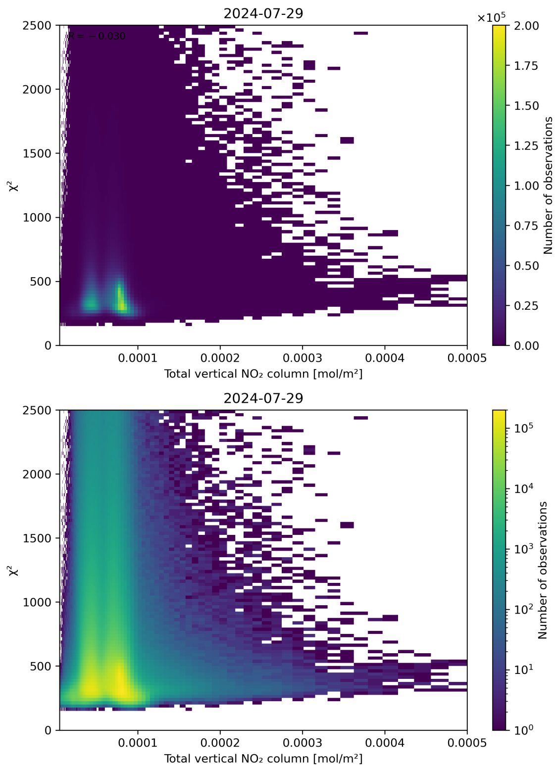
Figure 111: Scatter density plot of “Total vertical NO 2 column” against “ \chi^2 ” for 2024-07-28 to 2024-07-30.
