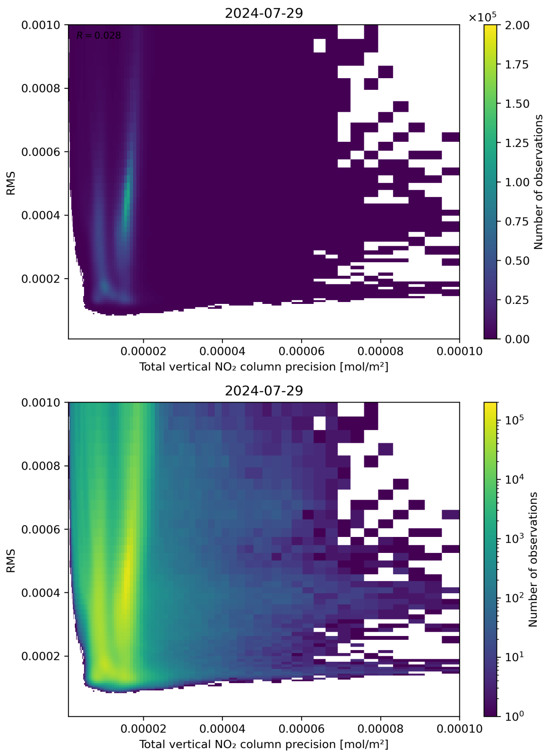
Figure 119: Scatter density plot of “Total vertical NO 2 column precision” against “RMS” for 2024-07-28 to 2024-07-30.
