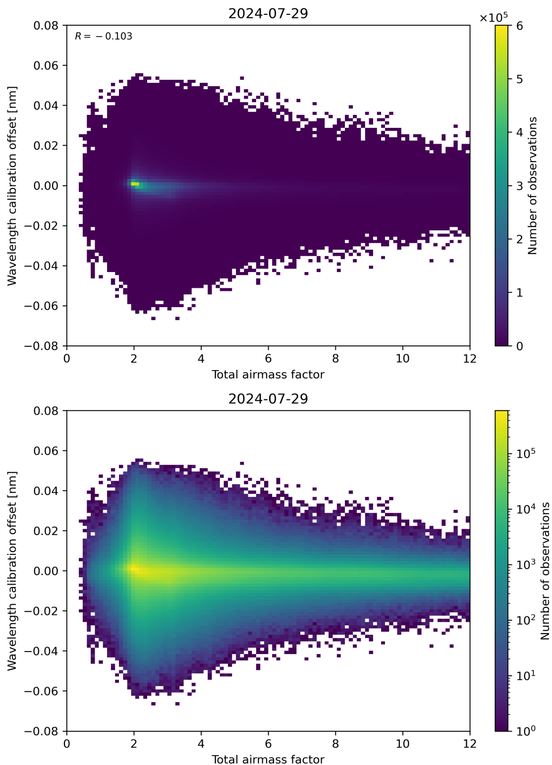
Figure 70: Scatter density plot of “Total airmass factor” against “Wavelength calibration offset” for 2024-07-28 to 2024-07-30.
