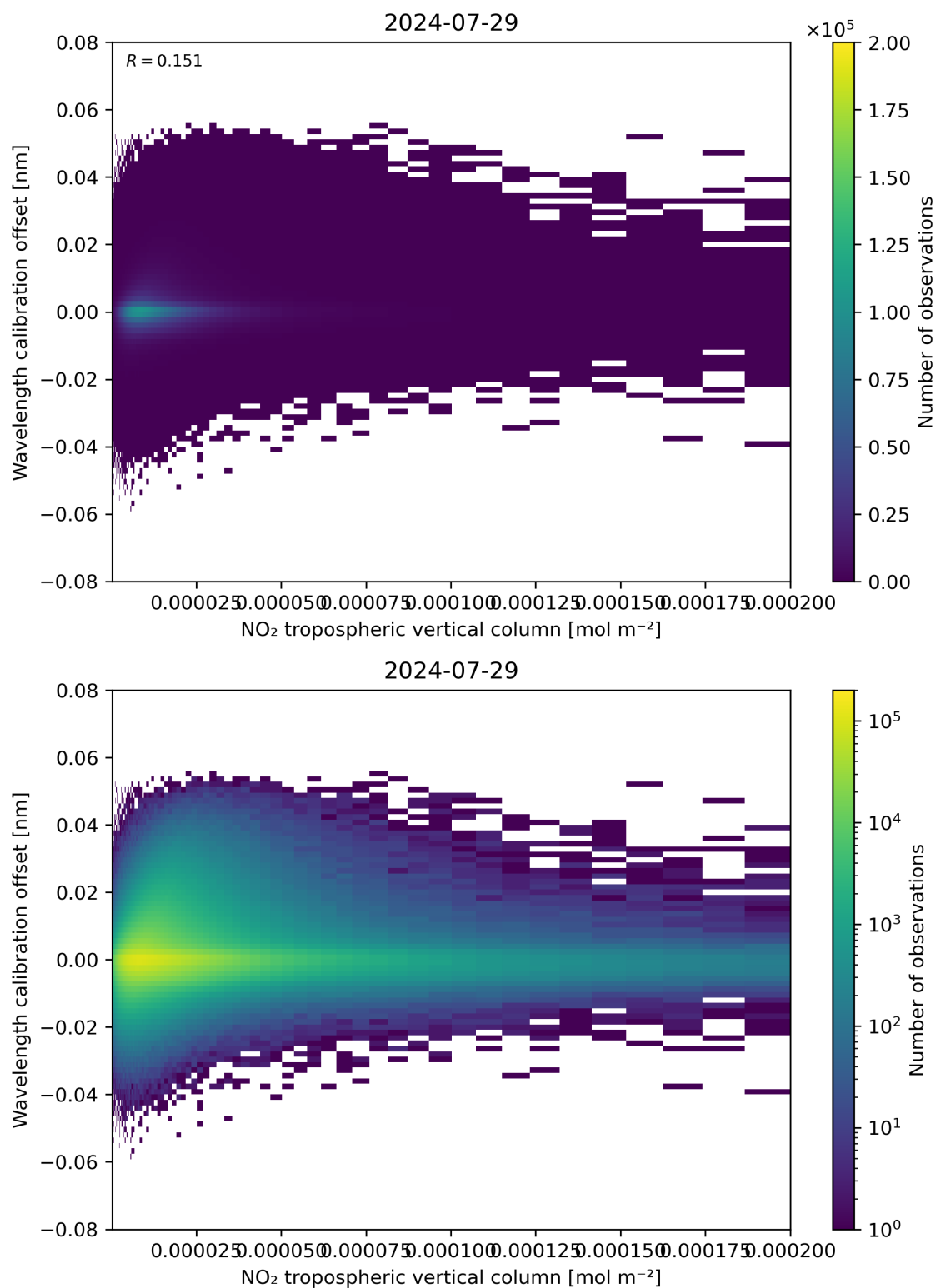
Figure 143: Scatter density plot of “NO 2 tropospheric vertical column” against “Wavelength calibration offset” for 2024-07-28 to 2024-07-30.
