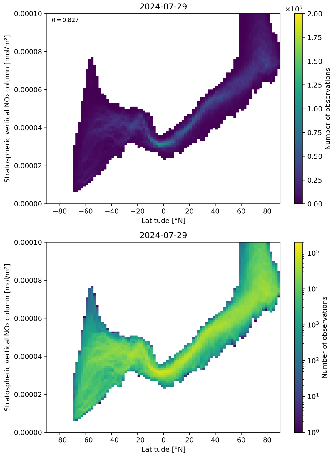
Figure 87: Scatter density plot of “Latitude” against “Stratospheric vertical \text{NO}_2 column” for 2024-07-28 to 2024-07-30.
