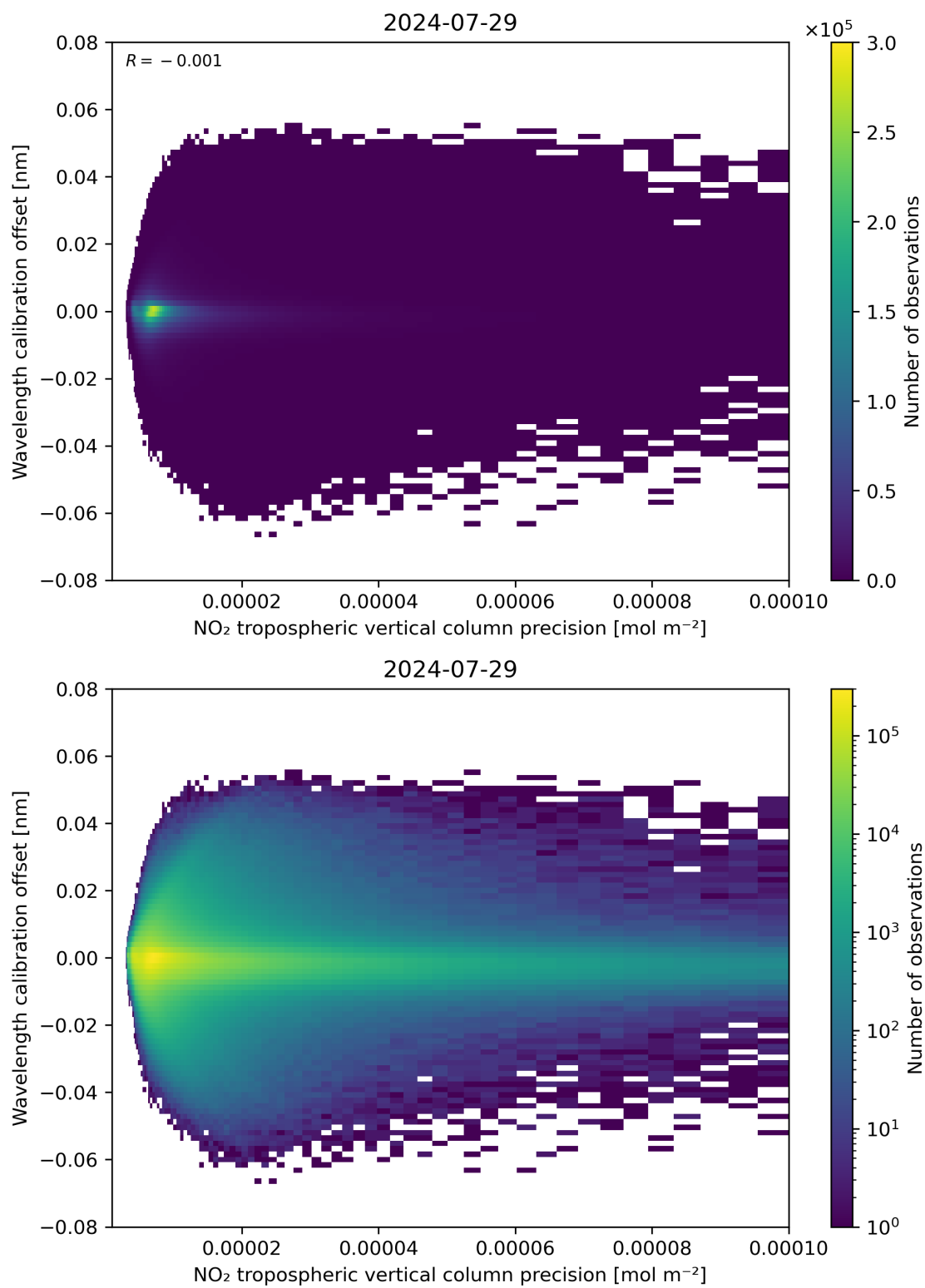
Figure 141: Scatter density plot of “NO 2 tropospheric vertical column precision” against “Wavelength calibration offset” for 2024-07-28 to 2024-07-30.
