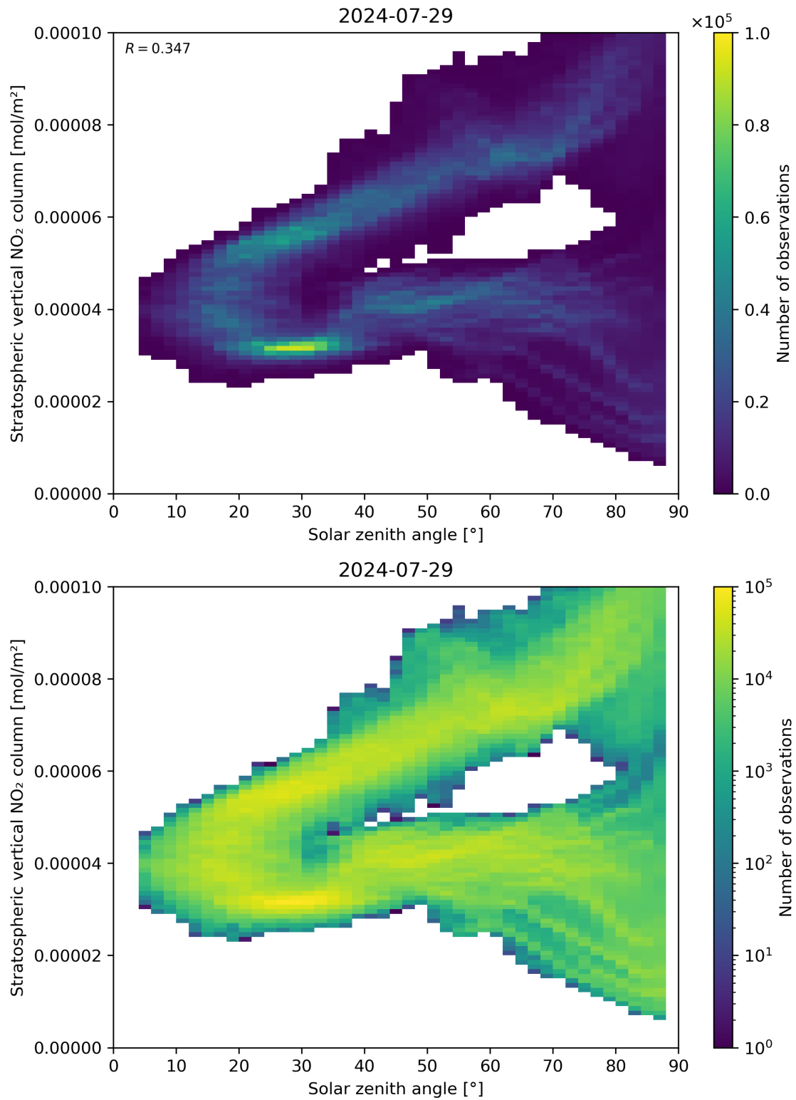
Figure 150: Scatter density plot of “Solar zenith angle” against “Stratospheric vertical NO 2 column” for 2024-07-28 to 2024-07-30.
