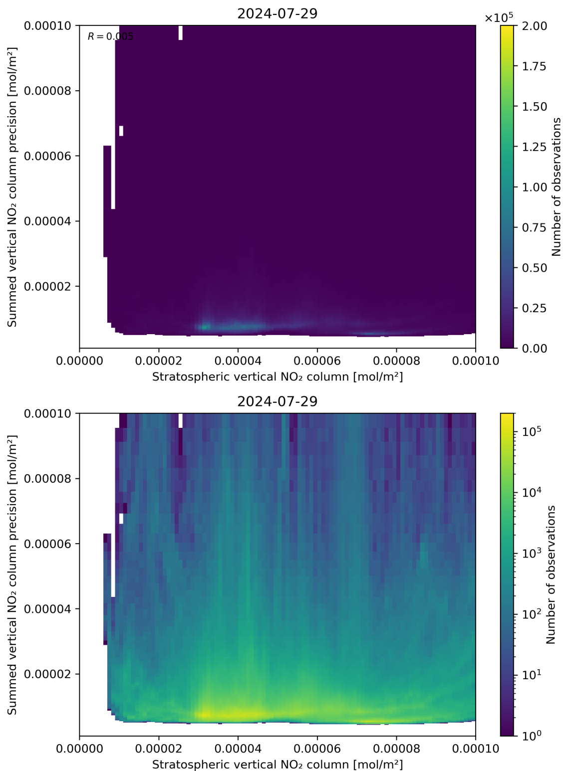
Figure 99: Scatter density plot of “Stratospheric vertical NO 2 column” against “Summed vertical NO 2 column precision” for 2024-07-28 to 2024-07-30.
