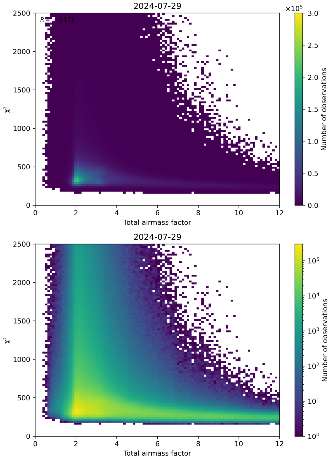
Figure 63: Scatter density plot of “Total airmass factor” against “ \chi^2 ” for 2024-07-28 to 2024-07-30.
