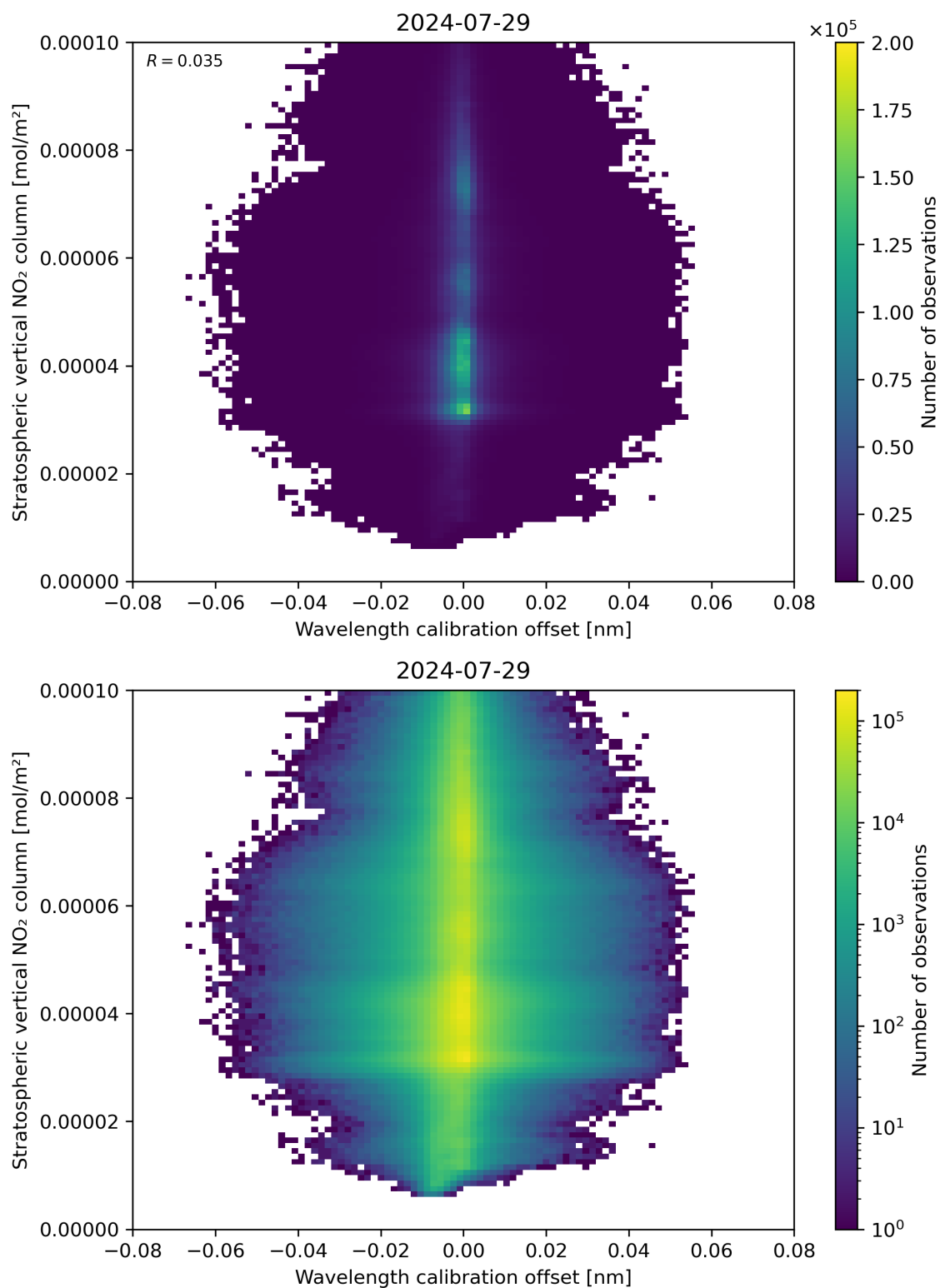
Figure 176: Scatter density plot of “Wavelength calibration offset” against “Stratospheric vertical NO 2 column” for 2024-07-28 to 2024-07-30.
