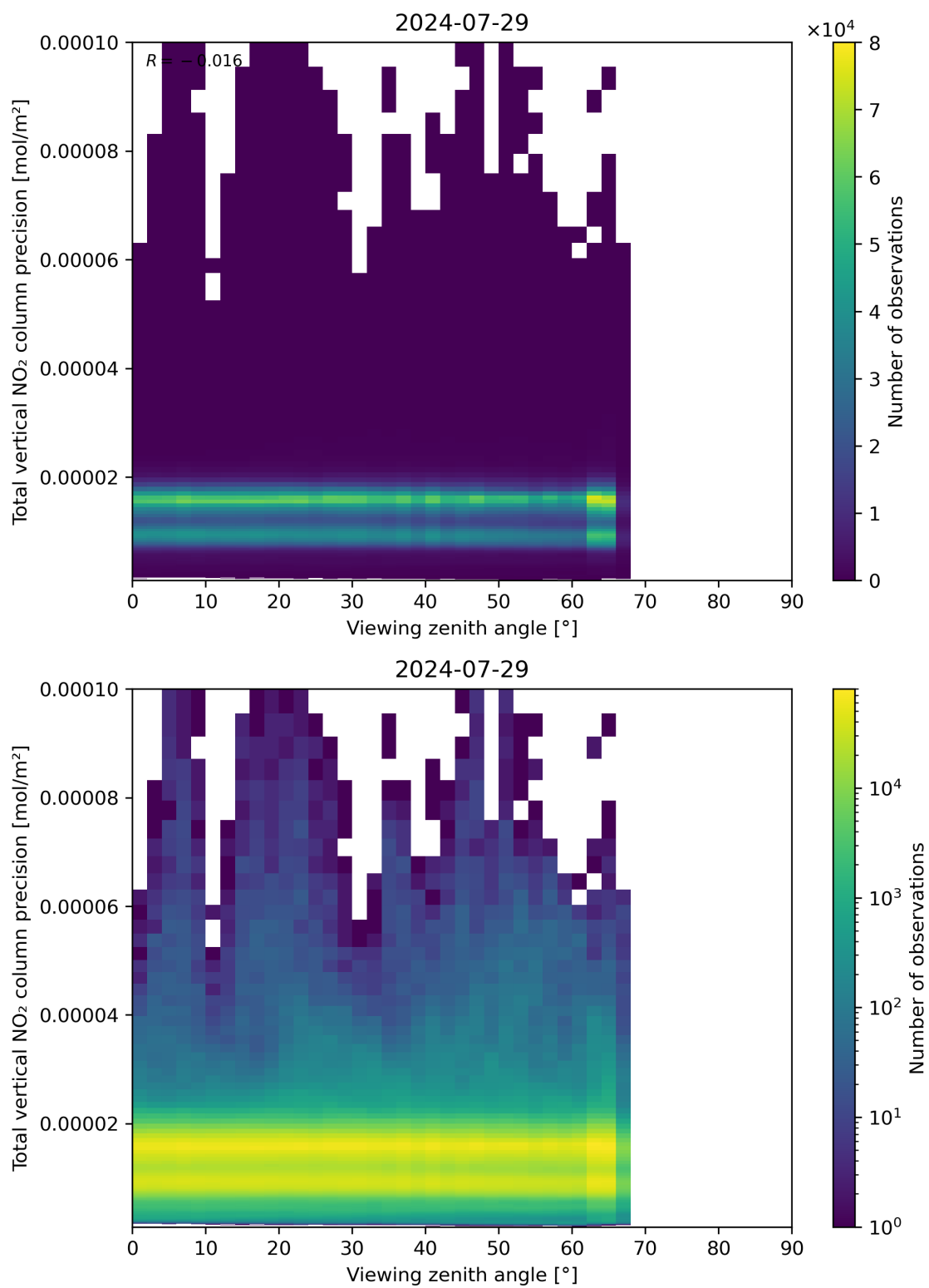
Figure 168: Scatter density plot of “Viewing zenith angle” against “Total vertical NO 2 column precision” for 2024-07-28 to 2024-07-30.
