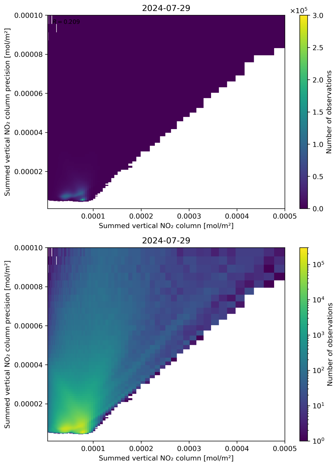
Figure 105: Scatter density plot of “Summed vertical NO 2 column” against “Summed vertical NO 2 column precision” for 2024-07-28 to 2024-07-30.
