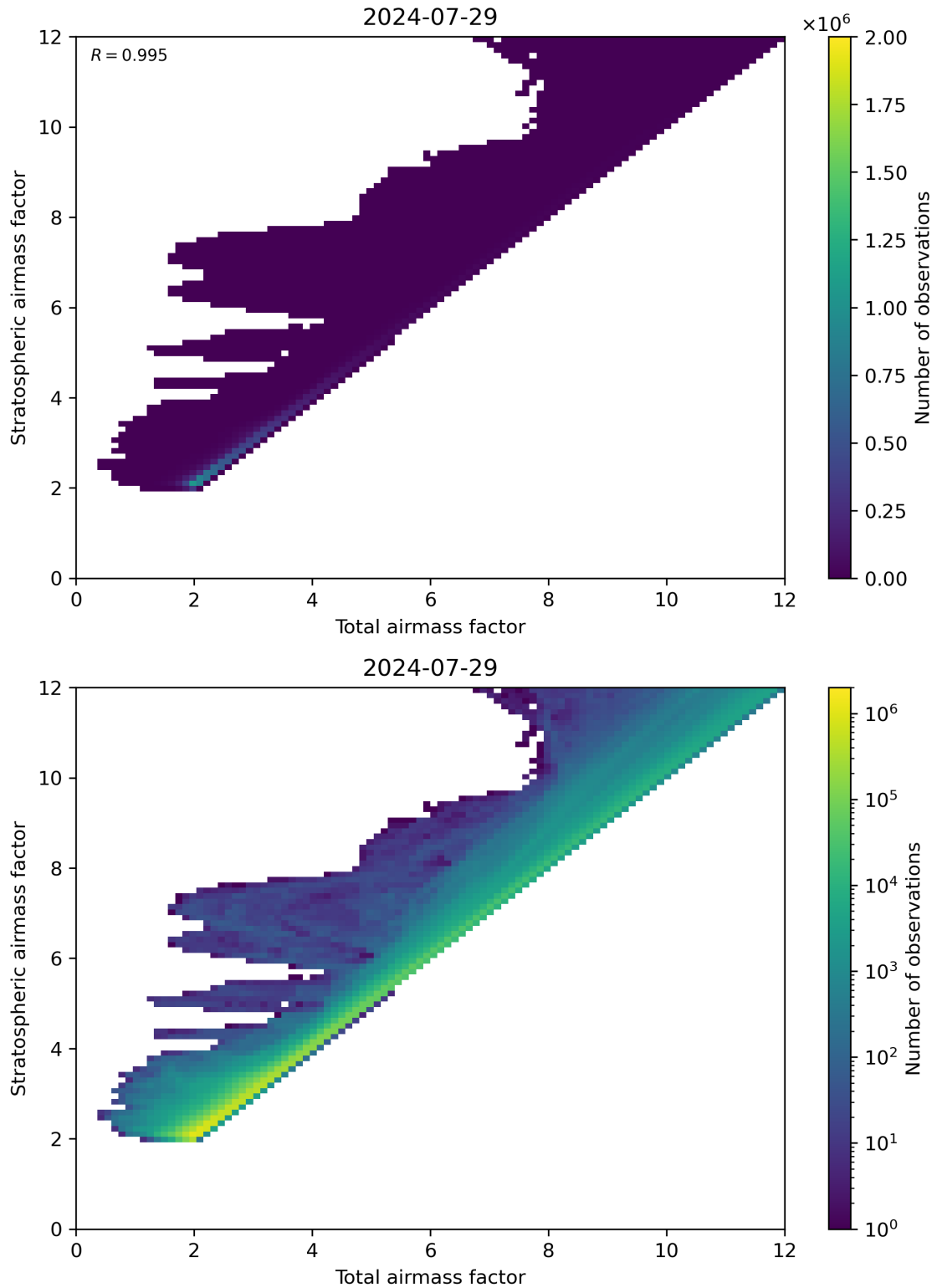
Figure 62: Scatter density plot of “Total airmass factor” against “Stratospheric airmass factor” for 2024-07-28 to 2024-07-30.
