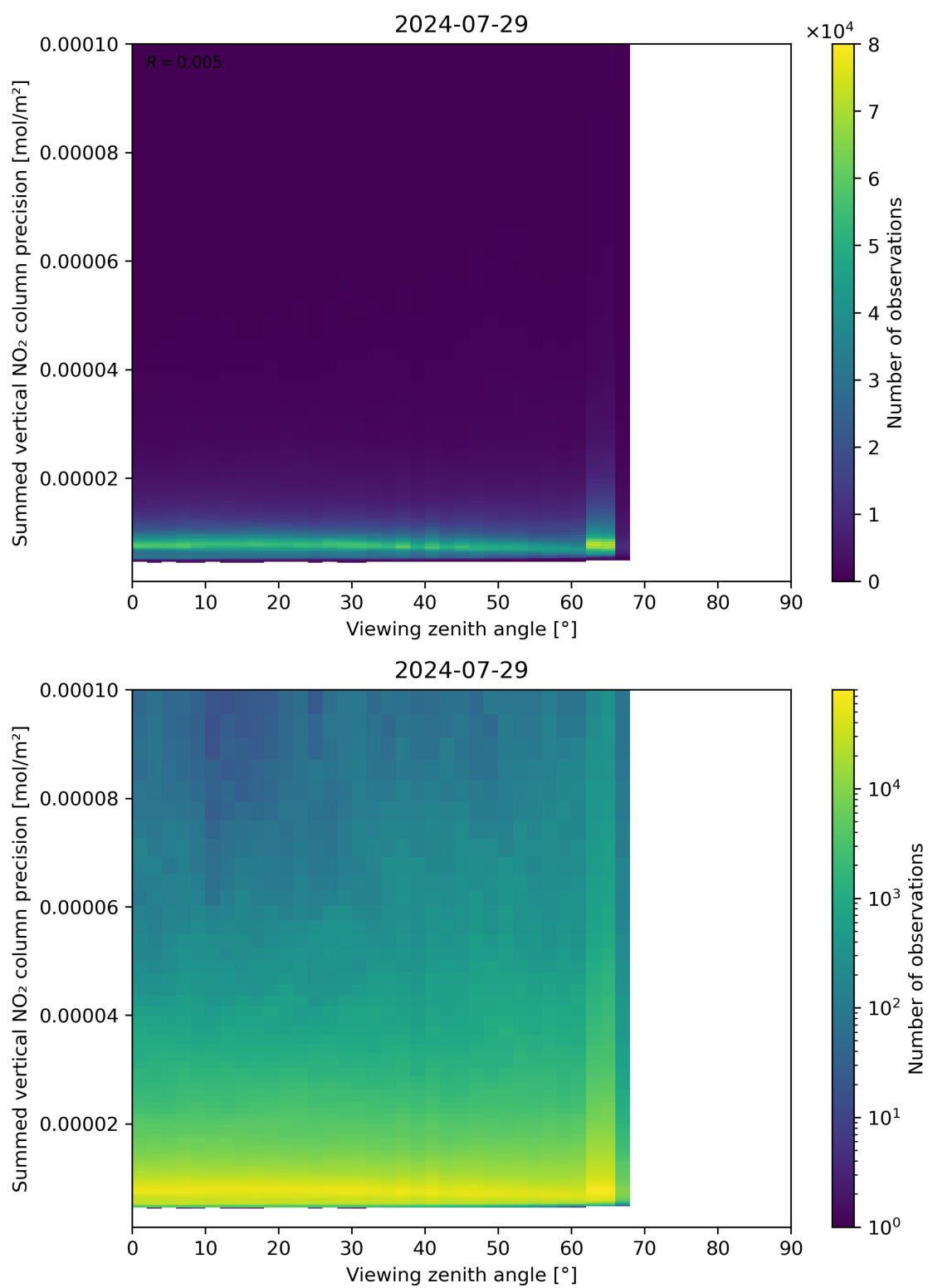
Figure 166: Scatter density plot of “Viewing zenith angle” against “Summed vertical NO 2 column precision” for 2024-07-28 to 2024-07-30.
