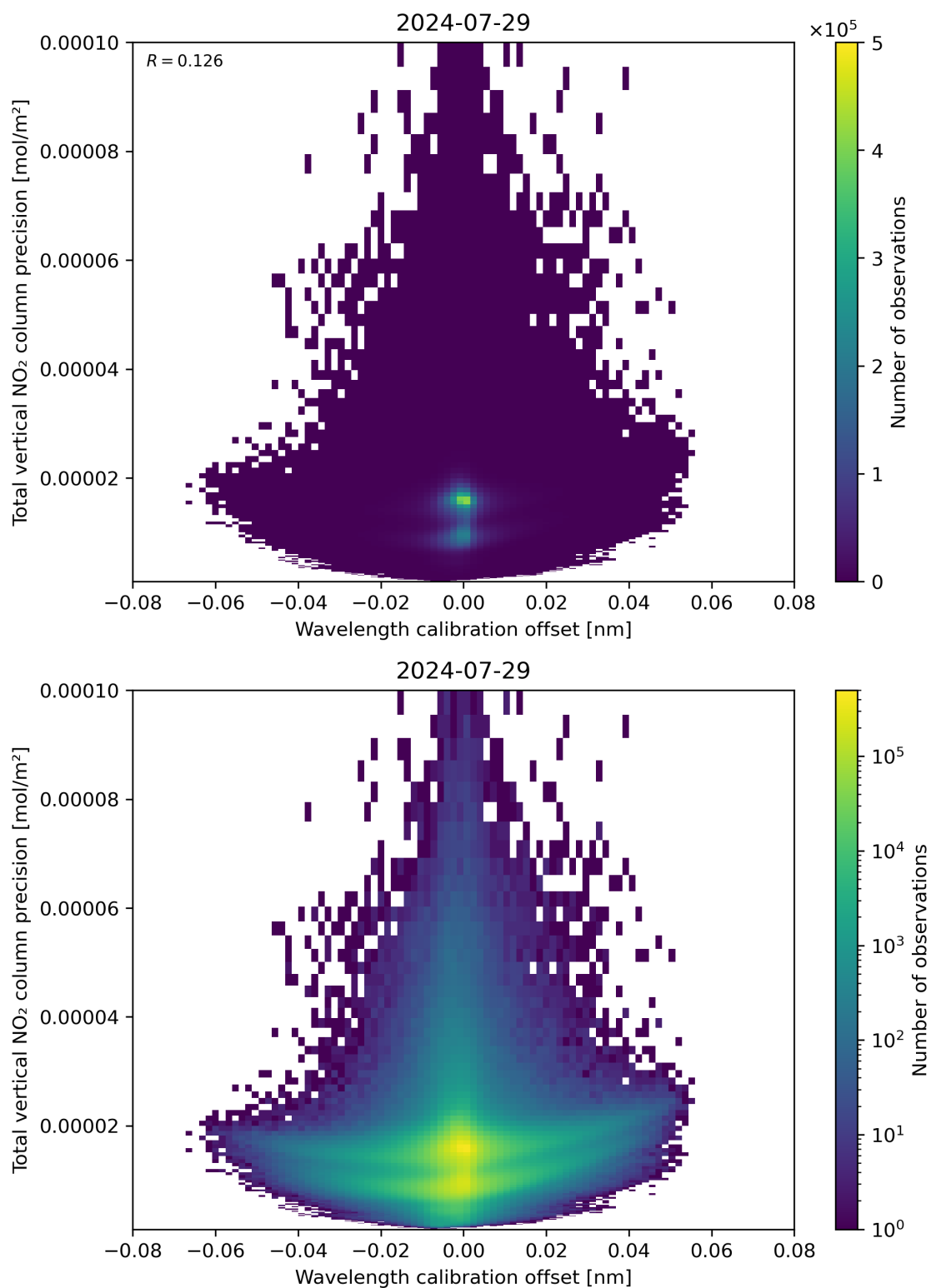
Figure 180: Scatter density plot of “Wavelength calibration offset” against “Total vertical NO 2 column precision” for 2024-07-28 to 2024-07-30.
