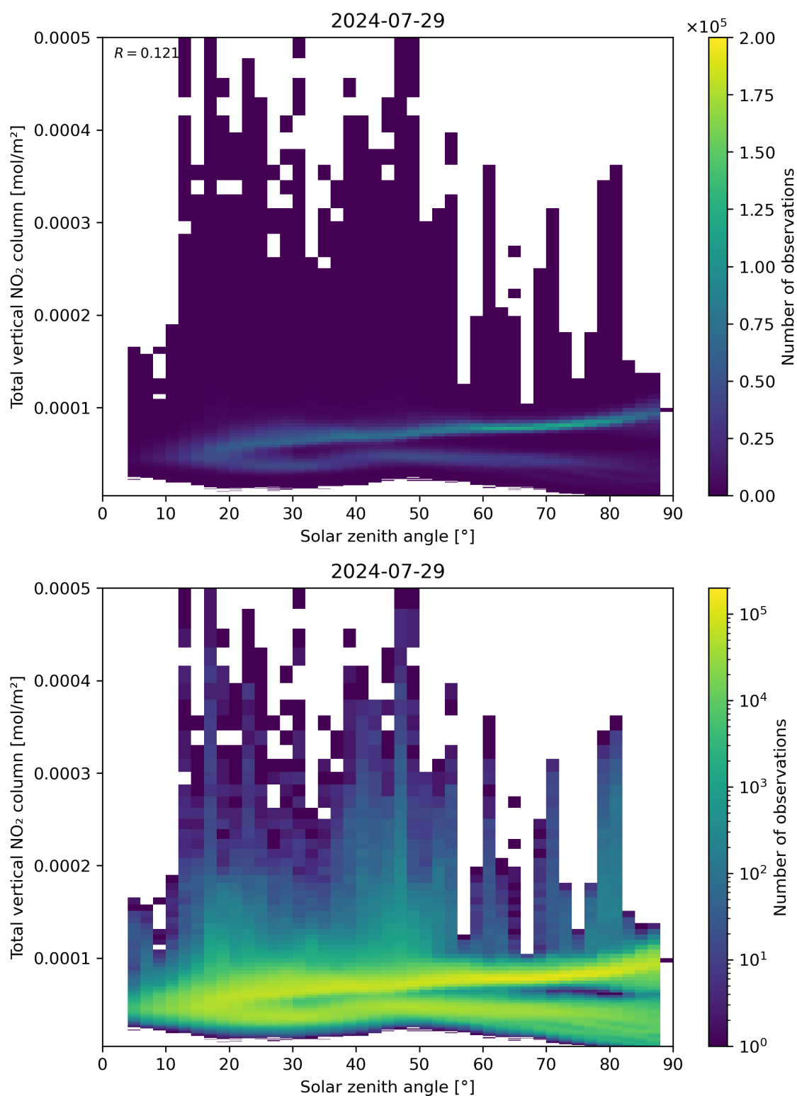
Figure 153: Scatter density plot of “Solar zenith angle” against “Total vertical NO 2 column” for 2024-07-28 to 2024-07-30.
