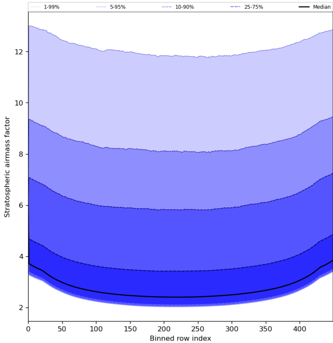
Figure 61: Along track statistics of “Stratospheric airmass factor” for 2024-07-28 to 2024-07-30
