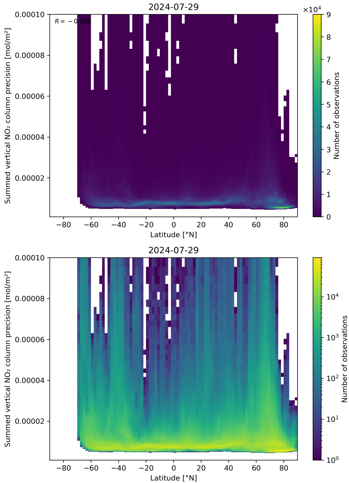
Figure 89: Scatter density plot of “Latitude” against “Summed vertical NO 2 column precision” for 2024-07-28 to 2024-07-30.
