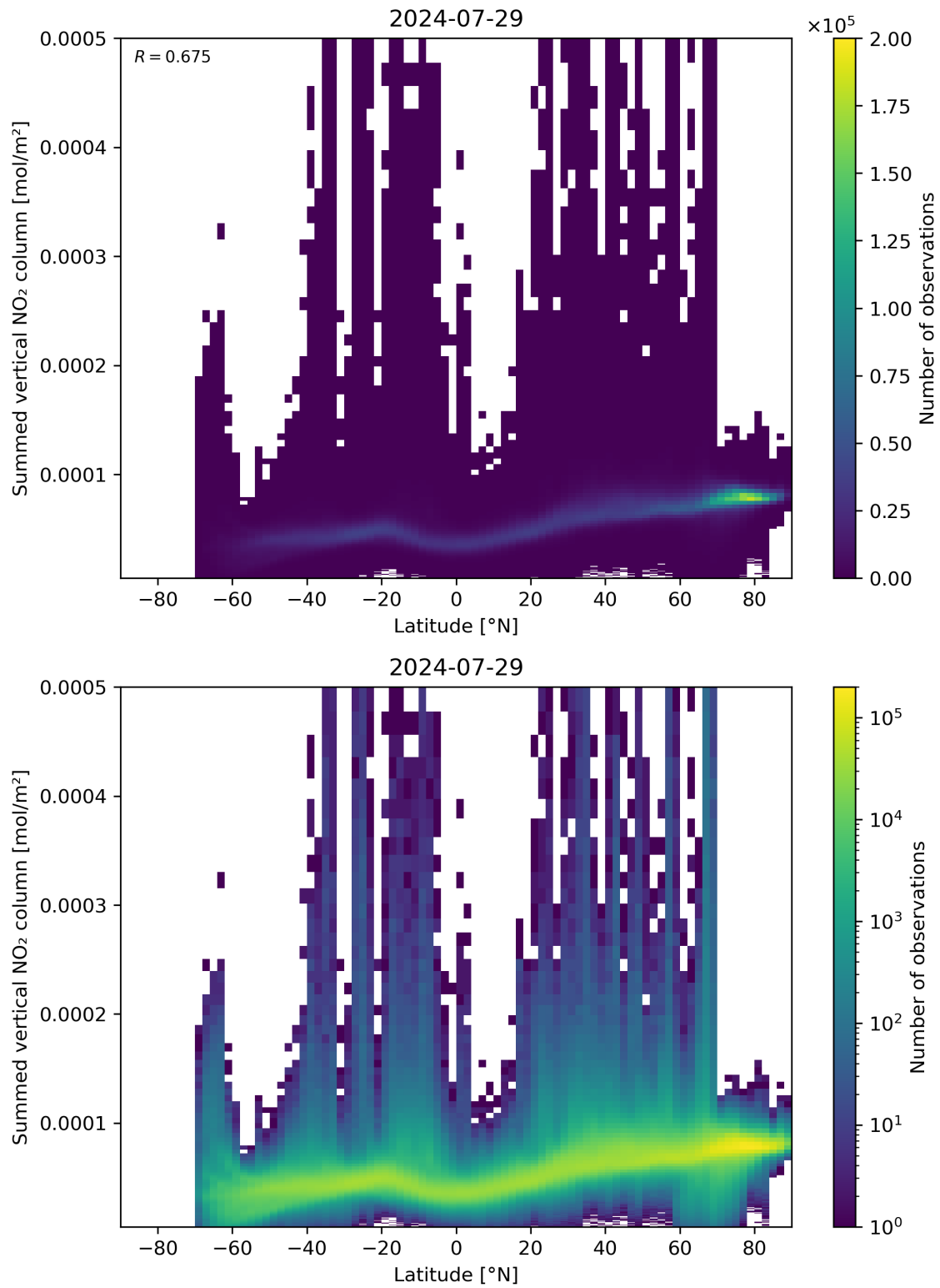
Figure 88: Scatter density plot of “Latitude” against “Summed vertical NO 2 column” for 2024-07-28 to 2024-07-30.
