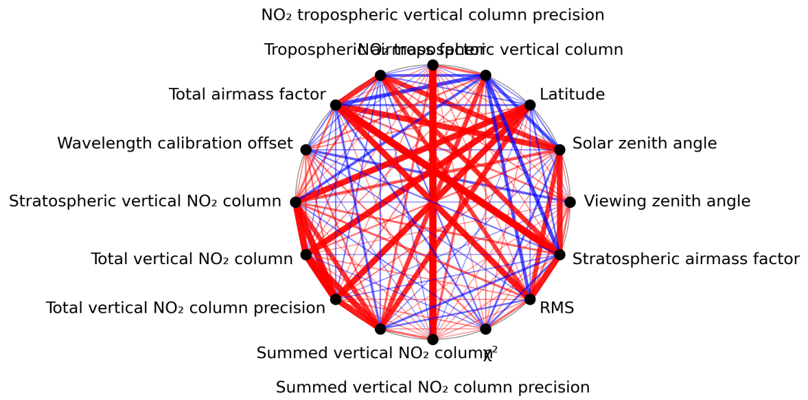
Figure 1: Map of correlation graph for 2024-07-28 to 2024-07-30.
