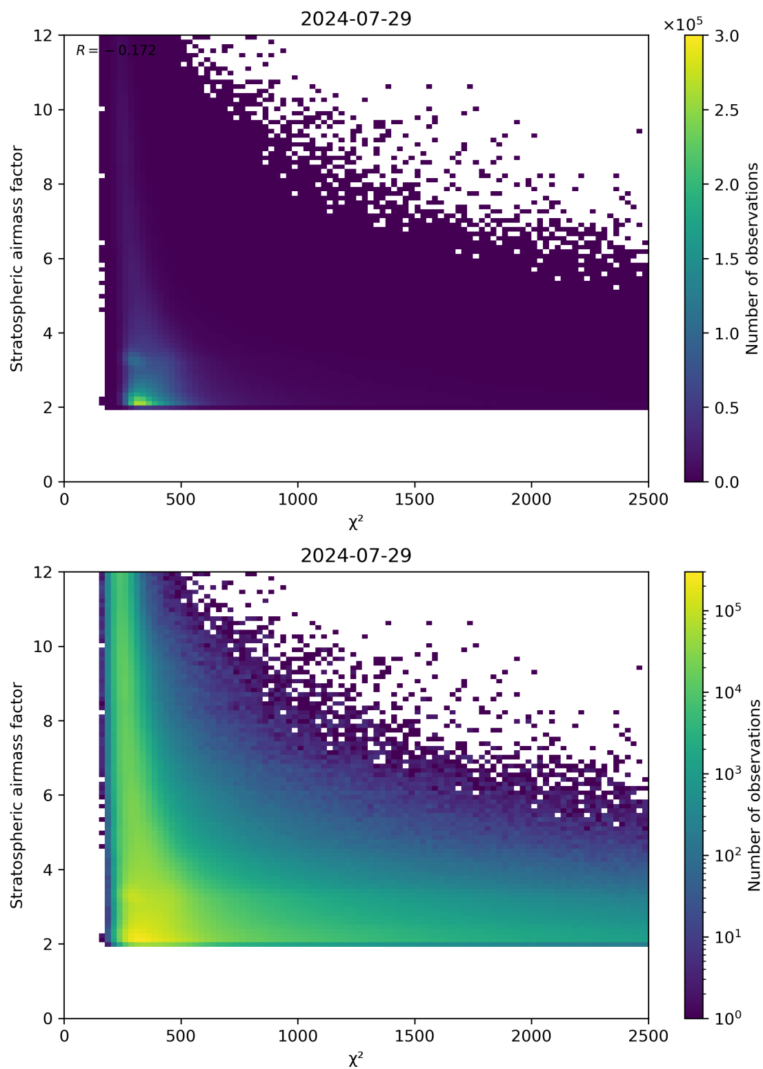
Figure 81: Scatter density plot of “ \chi^2 ” against “Stratospheric airmass factor” for 2024-07-28 to 2024-07-30.
