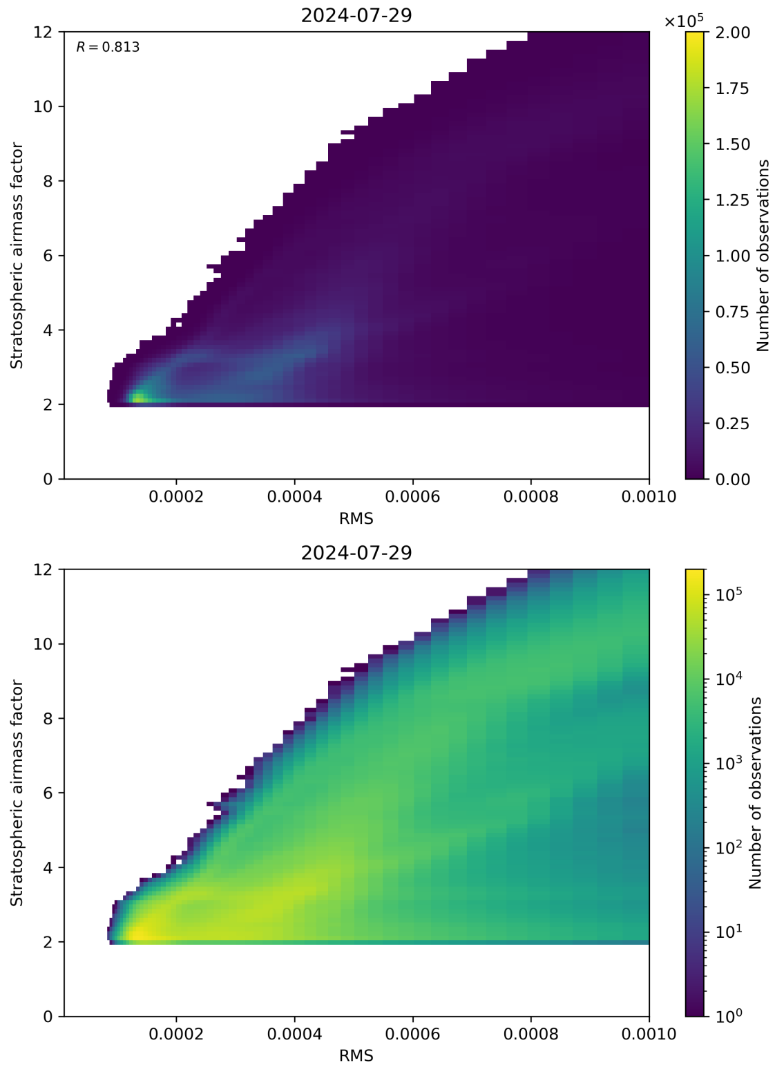
Figure 144: Scatter density plot of “RMS” against “Stratospheric airmass factor” for 2024-07-28 to 2024-07-30.
