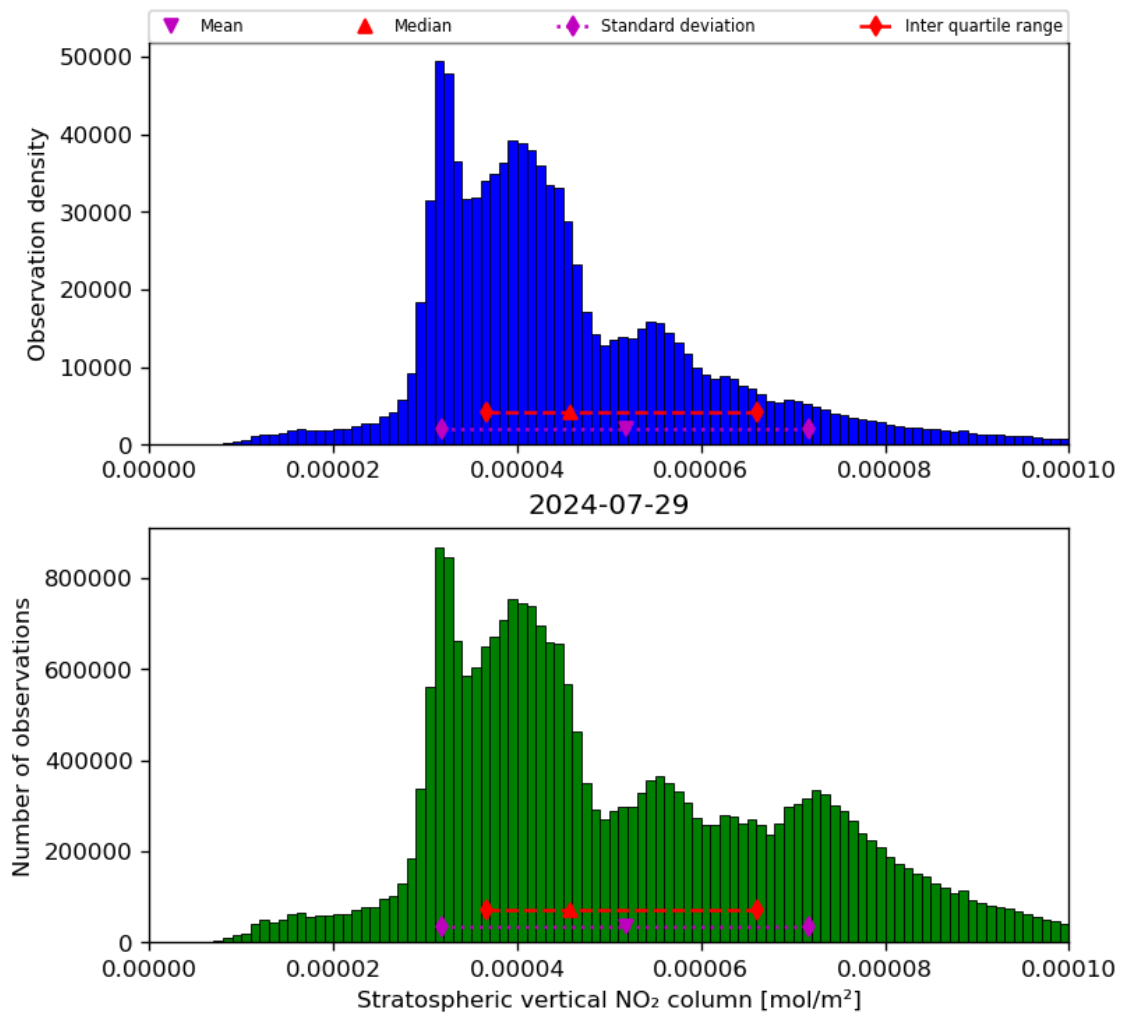
Figure 36: Histogram of “Stratospheric vertical NO 2 column” for 2024-07-28 to 2024-07-30
