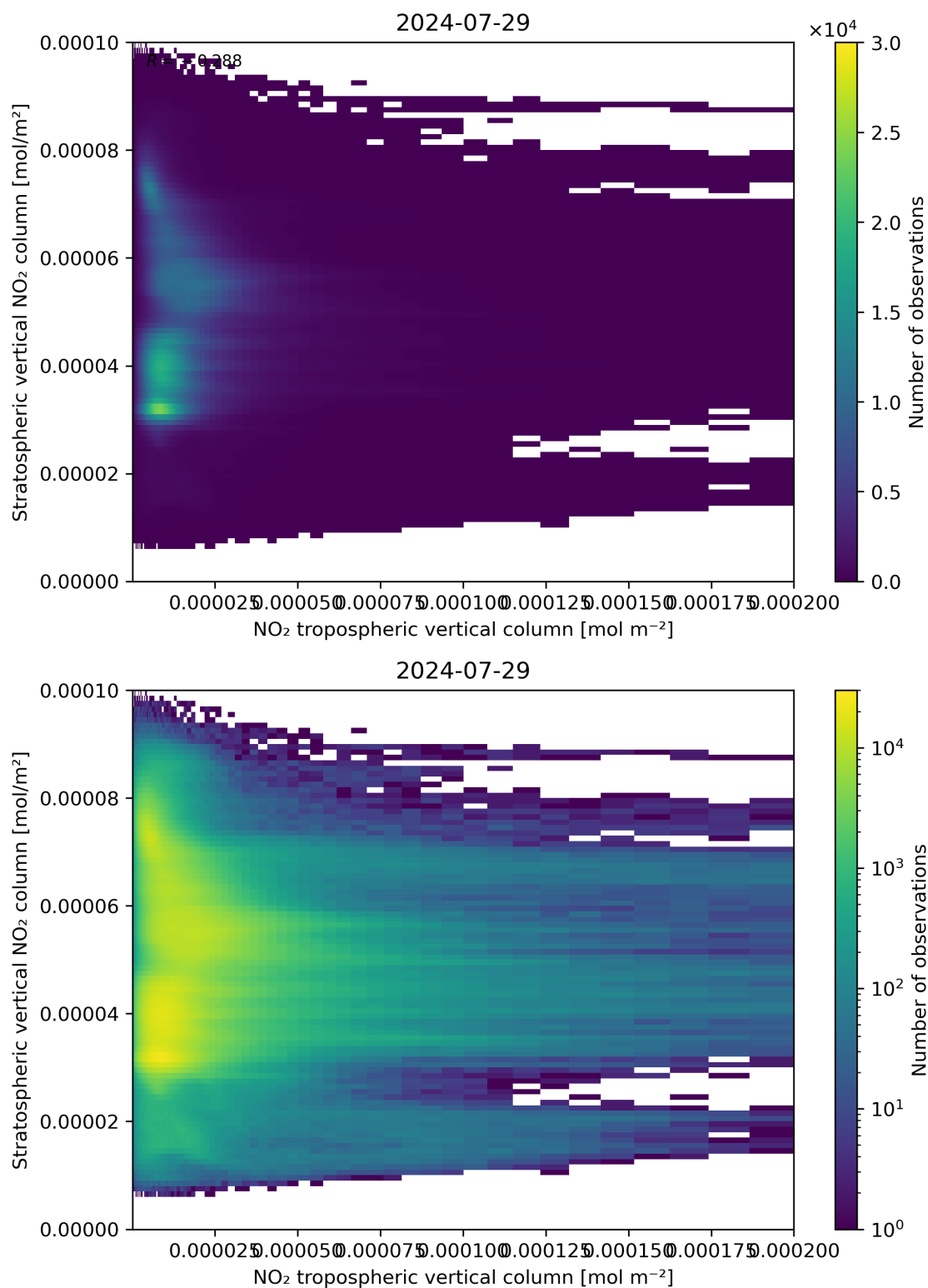
Figure 125: Scatter density plot of “NO 2 tropospheric vertical column” against “Stratospheric vertical NO 2 column” for 2024-07-28 to 2024-07-30.
