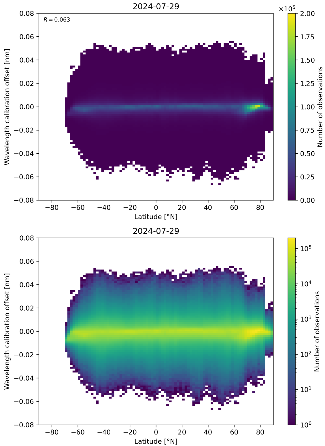
Figure 95: Scatter density plot of “Latitude” against “Wavelength calibration offset” for 2024-07-28 to 2024-07-30.
