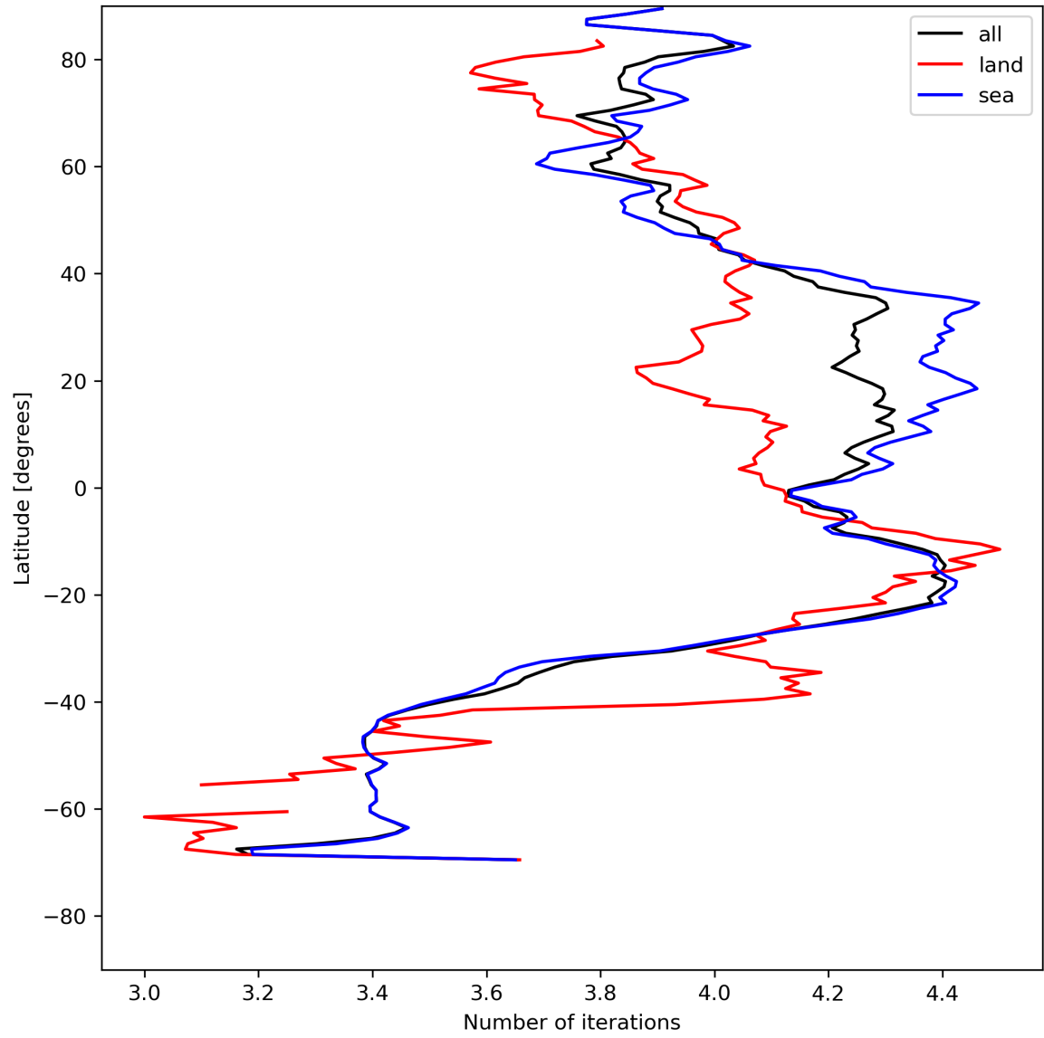
Figure 17: Zonal average of “Number of iterations” for 2024-07-28 to 2024-07-30.
