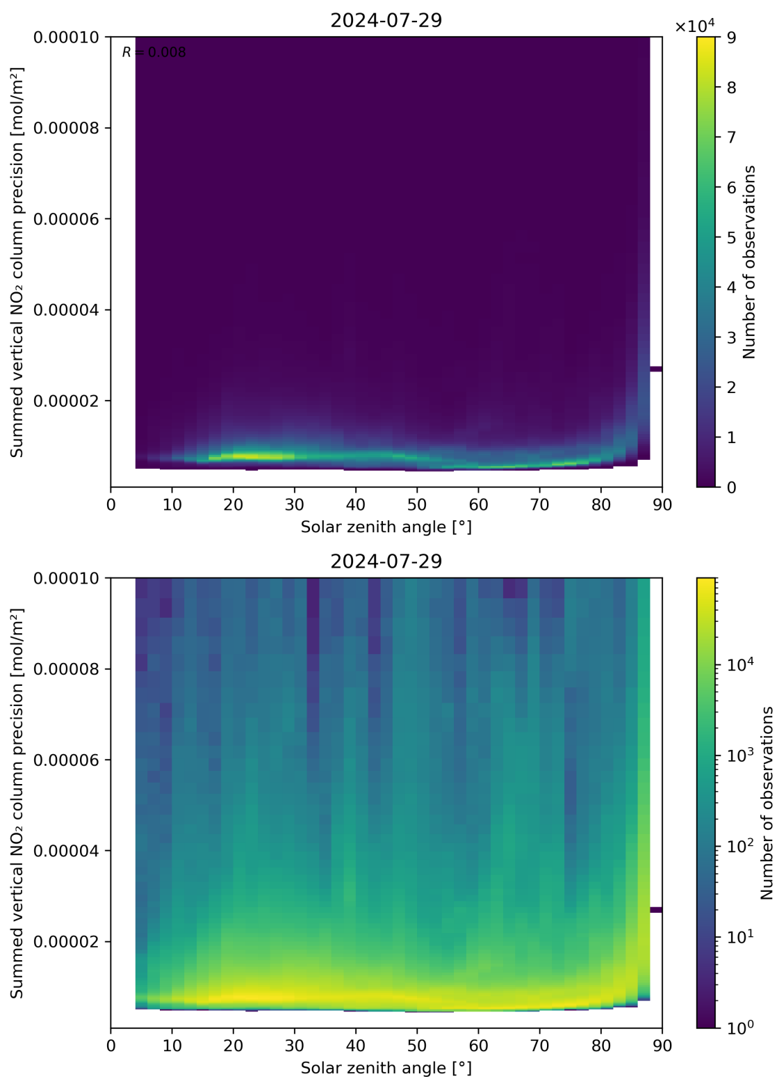
Figure 152: Scatter density plot of “Solar zenith angle” against “Summed vertical NO 2 column precision” for 2024-07-28 to 2024-07-30.
