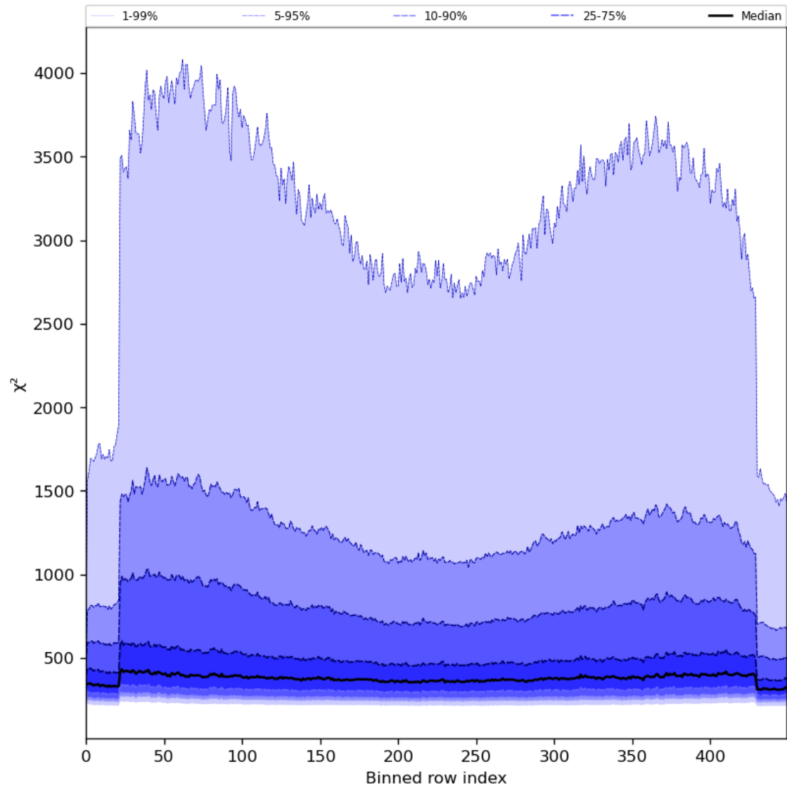
Figure 59: Along track statistics of “ \chi^2 ” for 2024-07-28 to 2024-07-30
