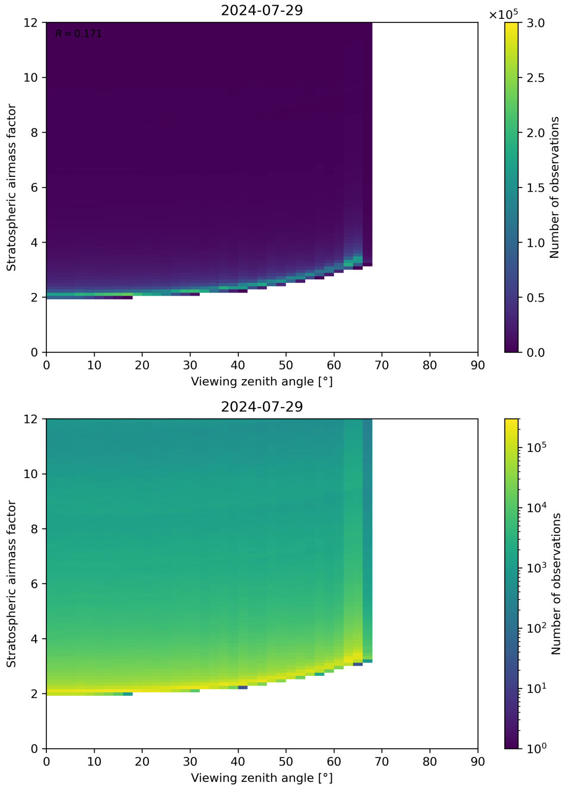
Figure 159: Scatter density plot of “Viewing zenith angle” against “Stratospheric airmass factor” for 2024-07-28 to 2024-07-30.
