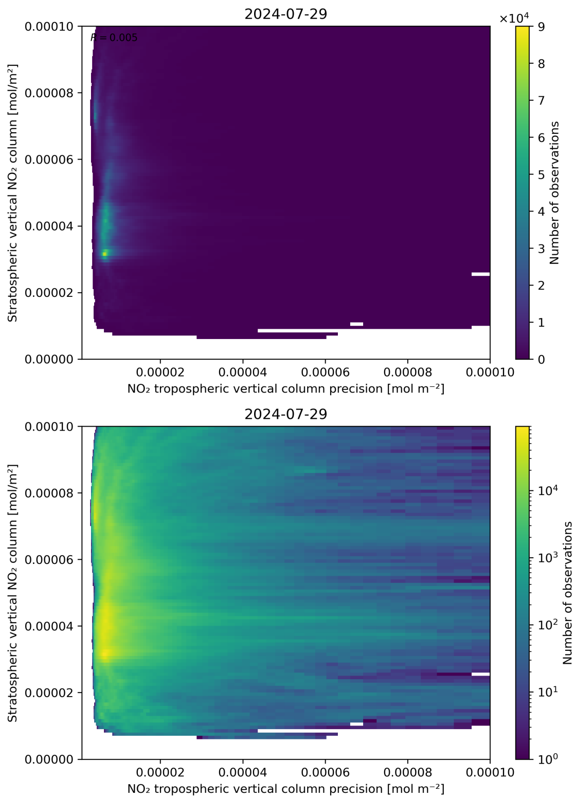
Figure 135: Scatter density plot of “NO 2 tropospheric vertical column precision” against “Stratospheric vertical NO 2 column” for 2024-07-28 to 2024-07-30.
