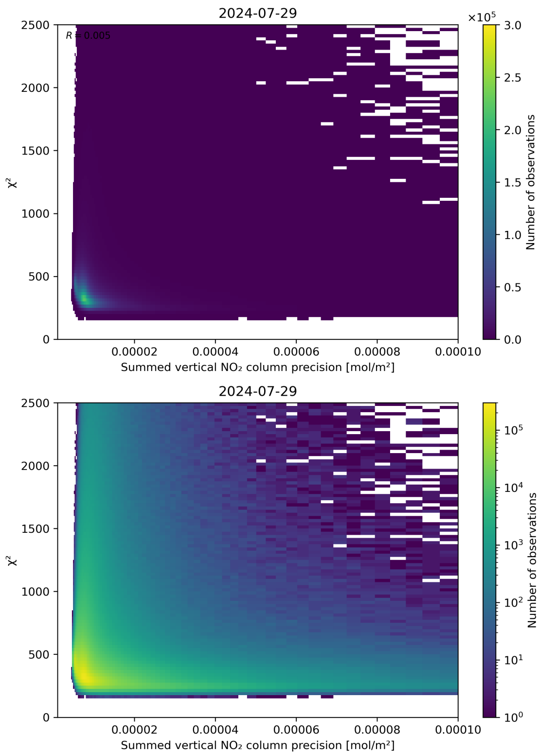
Figure 107: Scatter density plot of “Summed vertical NO 2 column precision” against “ \chi^2 ” for 2024-07-28 to 2024-07-30.
