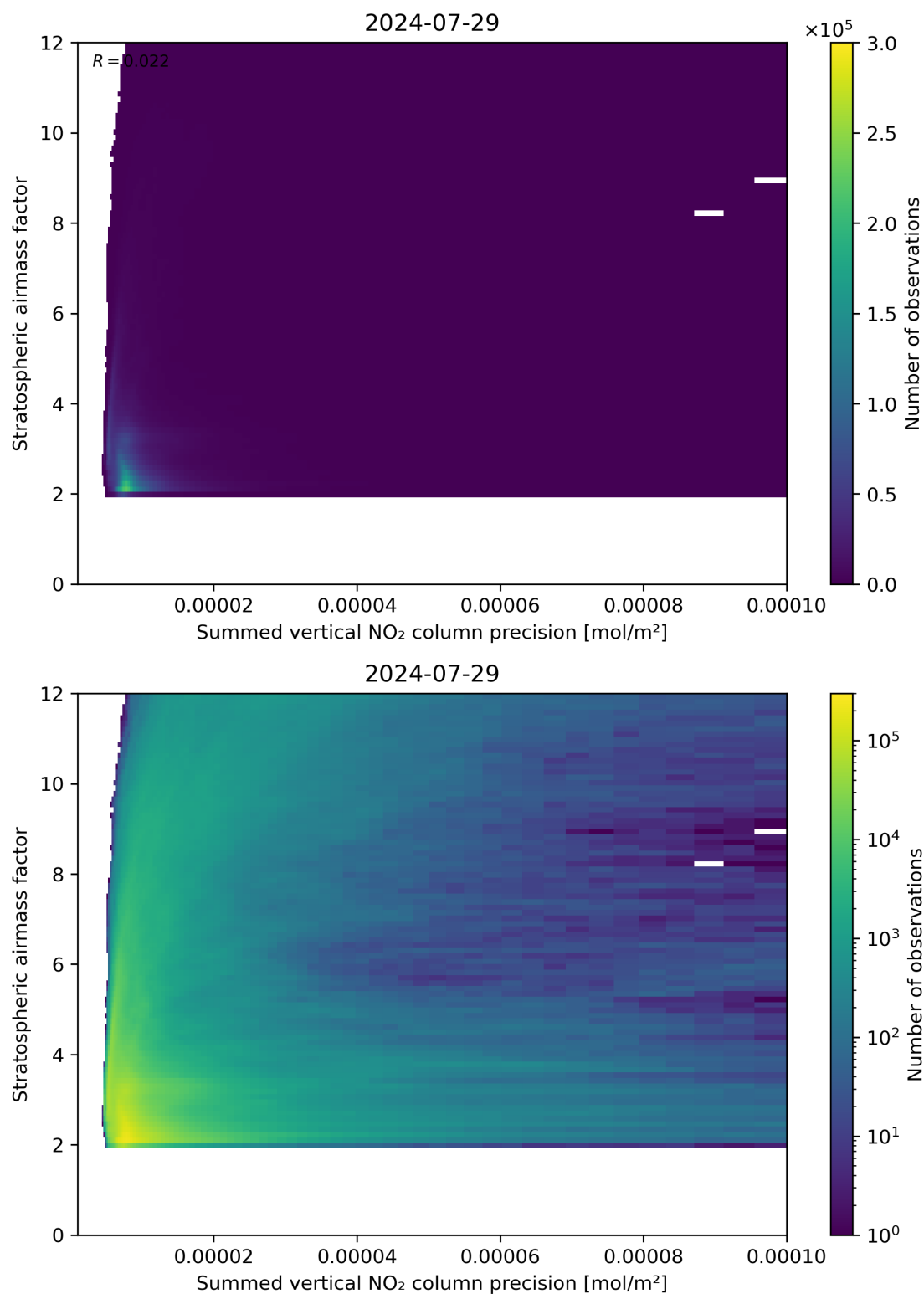
Figure 106: Scatter density plot of “Summed vertical NO 2 column precision” against “Stratospheric airmass factor” for 2024-07-28 to 2024-07-30.
