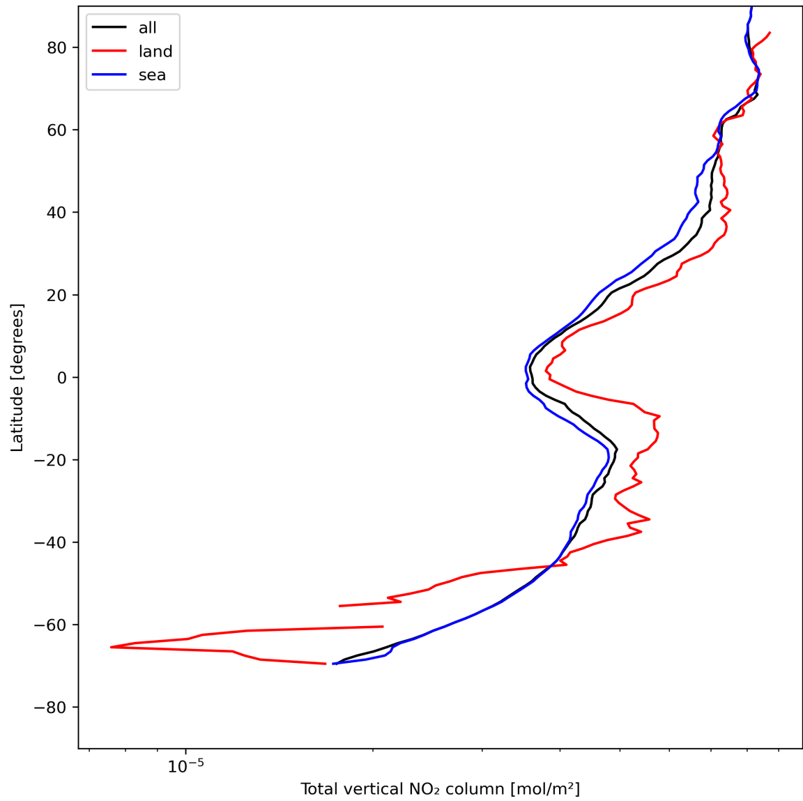
Figure 21: Zonal average of “Total vertical NO 2 column” for 2024-07-28 to 2024-07-30.
