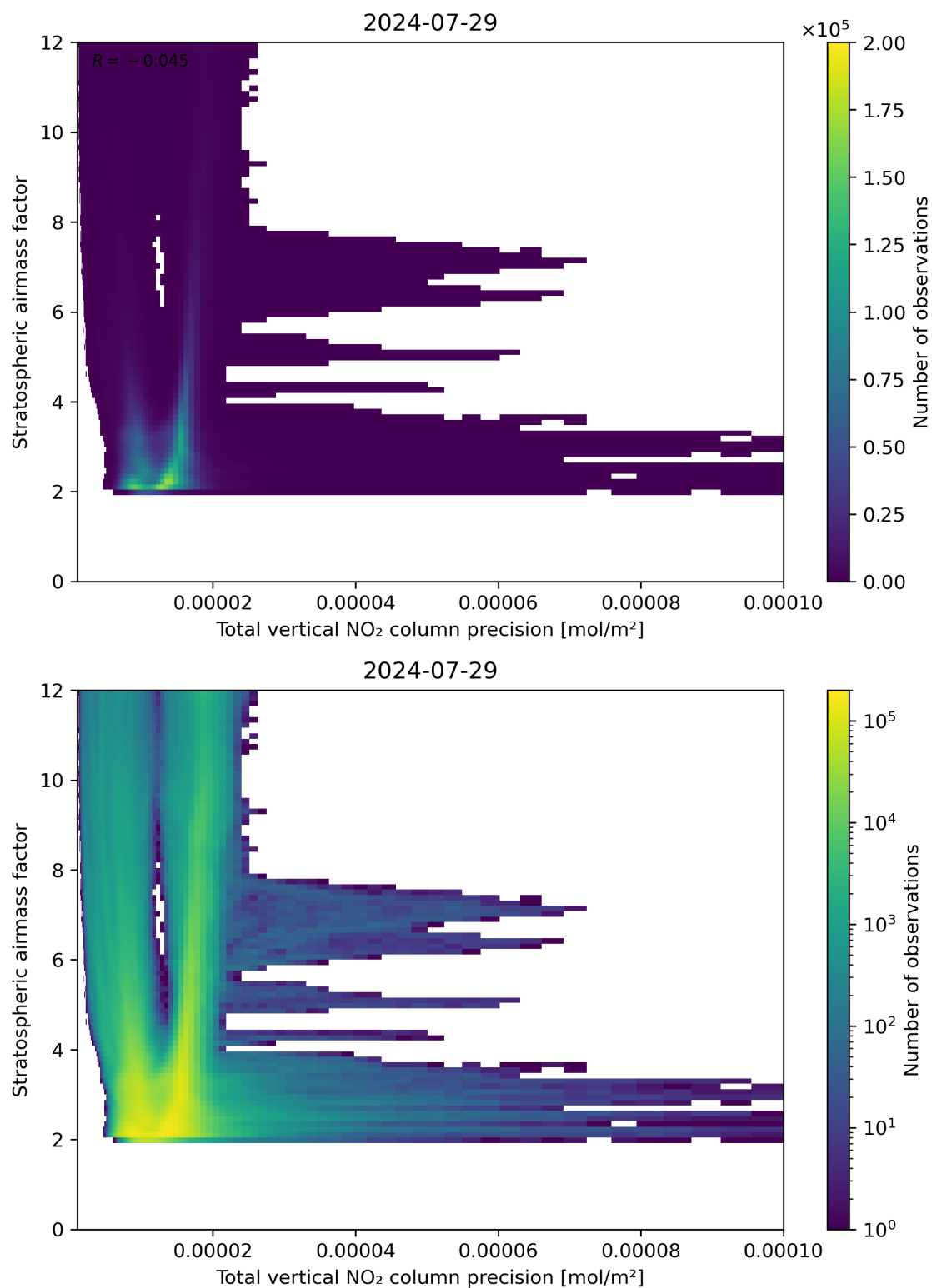
Figure 115: Scatter density plot of “Total vertical NO 2 column precision” against “Stratospheric air mass factor” for 2024-07-28 to 2024-07-30.
