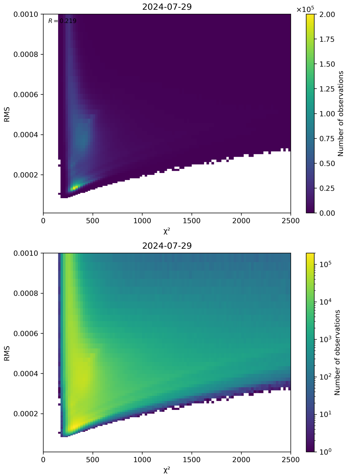
Figure 82: Scatter density plot of “ \chi^2 ” against “RMS” for 2024-07-28 to 2024-07-30.
