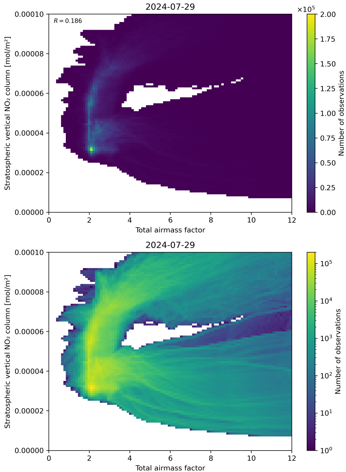
Figure 64: Scatter density plot of “Total airmass factor” against “Stratospheric vertical NO 2 column” for 2024-07-28 to 2024-07-30.
