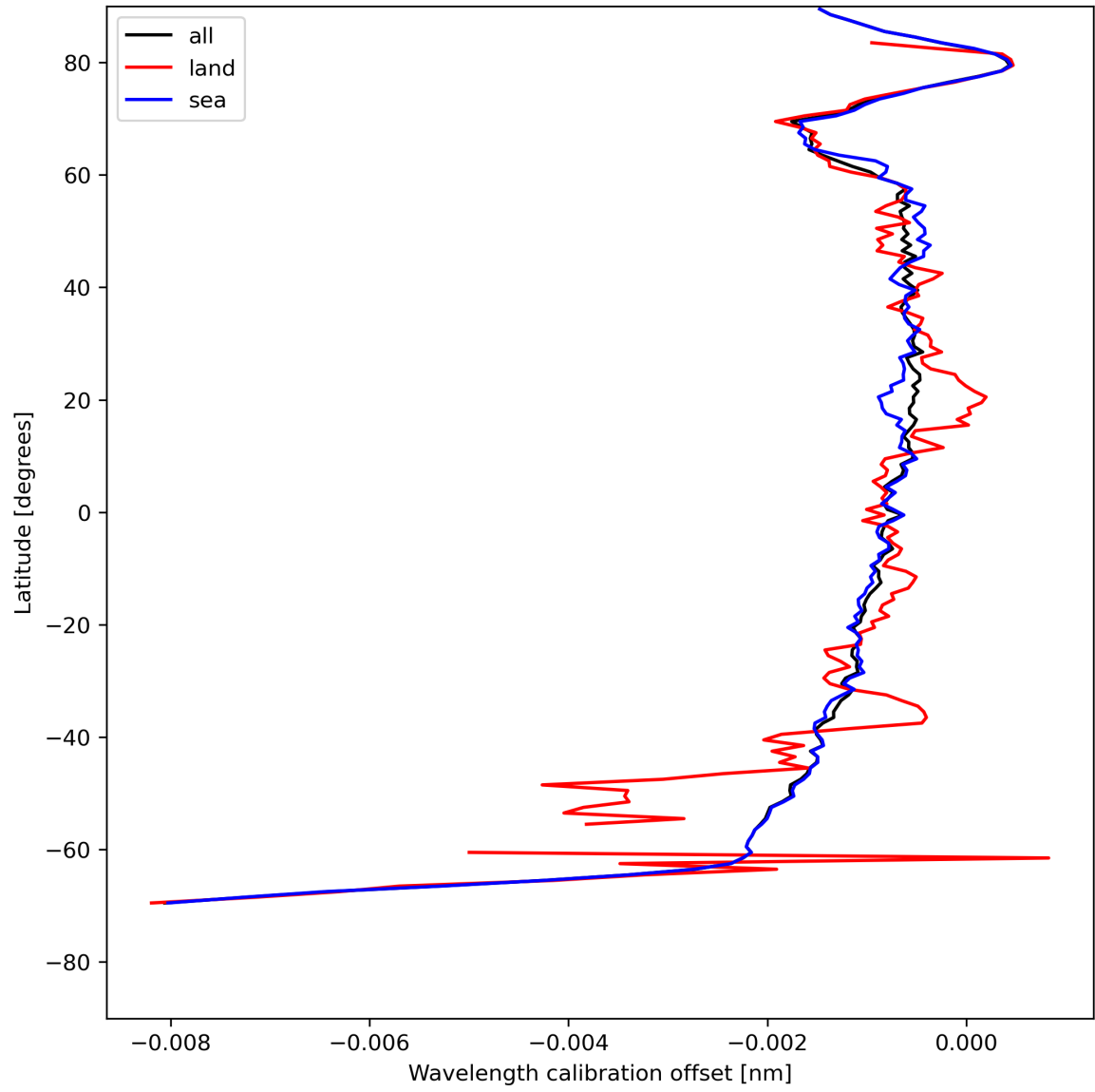
Figure 18: Zonal average of “Wavelength calibration offset” for 2024-07-28 to 2024-07-30.
