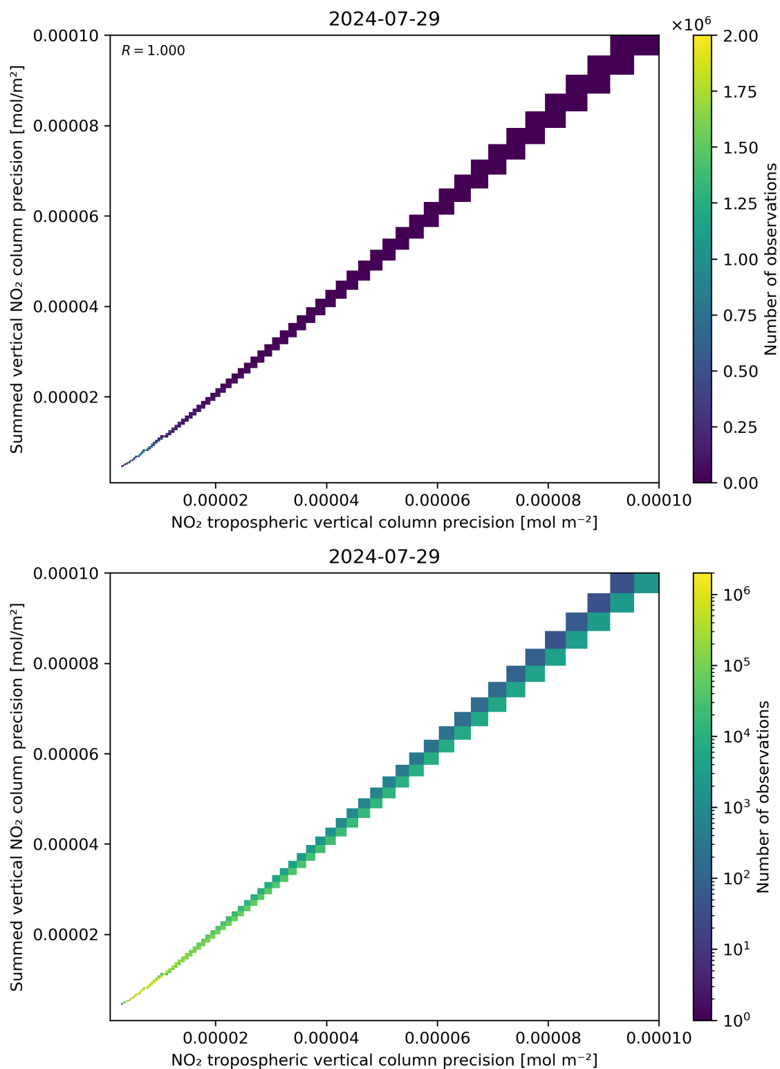
Figure 137: Scatter density plot of “NO 2 tropospheric vertical column precision” against “Summed vertical NO 2 column precision” for 2024-07-28 to 2024-07-30.
