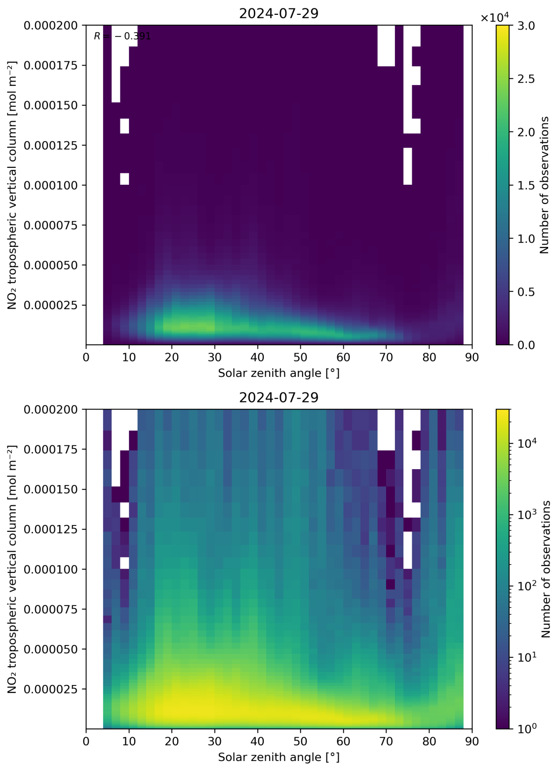
Figure 155: Scatter density plot of “Solar zenith angle” against “NO 2 tropospheric vertical column” for 2024-07-28 to 2024-07-30.
