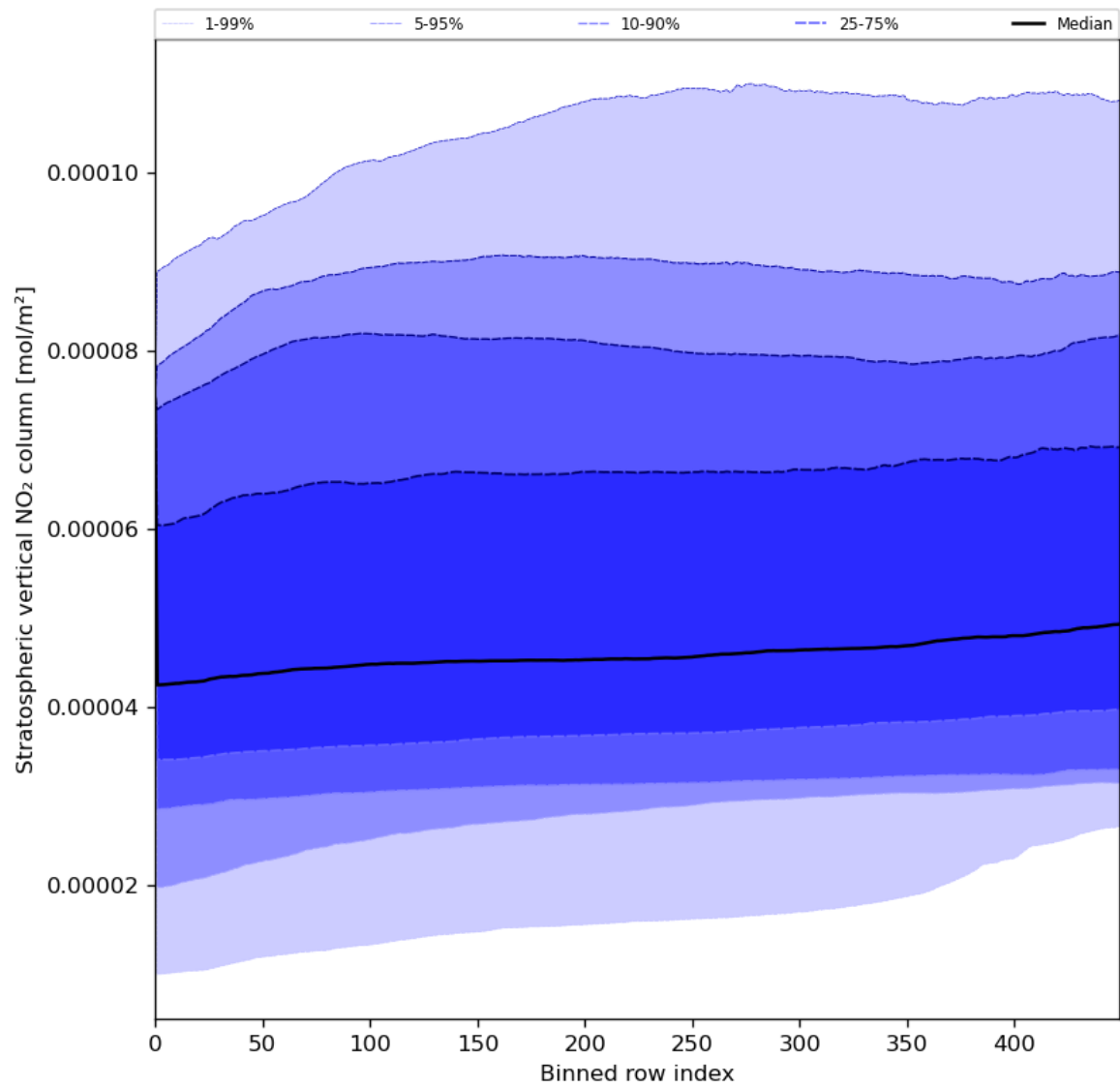
Figure 53: Along track statistics of “Stratospheric vertical NO 2 column” for 2024-07-28 to 2024-07-30
