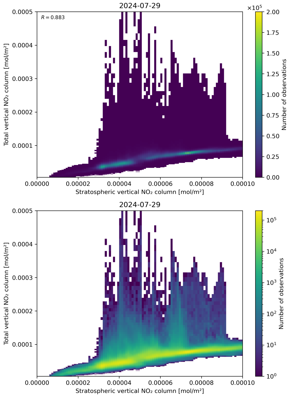
Figure 100: Scatter density plot of “Stratospheric vertical NO 2 column” against “Total vertical NO 2 column” for 2024-07-28 to 2024-07-30.
