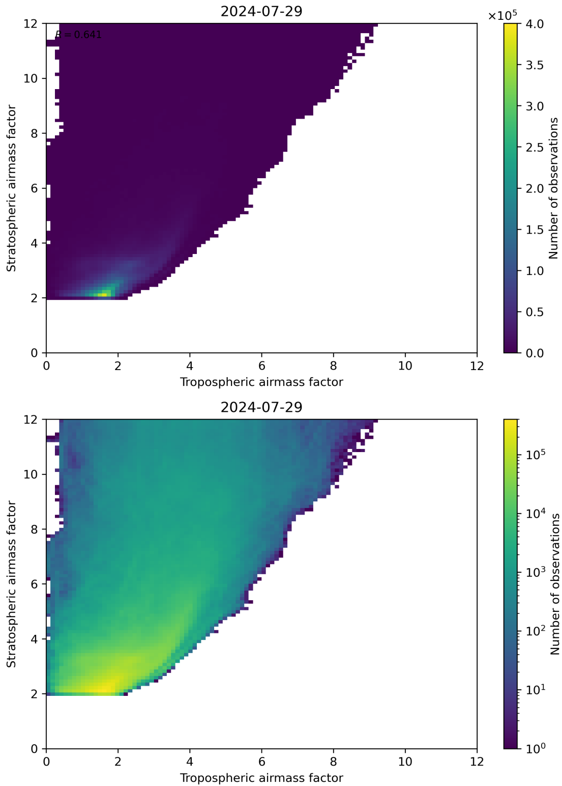
Figure 71: Scatter density plot of “Tropospheric airmass factor” against “Stratospheric airmass factor” for 2024-07-28 to 2024-07-30.
