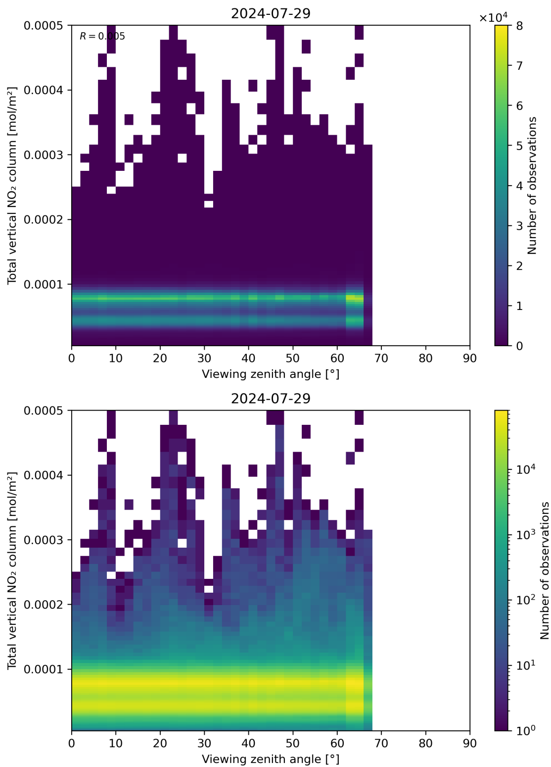
Figure 167: Scatter density plot of “Viewing zenith angle” against “Total vertical NO 2 column” for 2024-07-28 to 2024-07-30.
