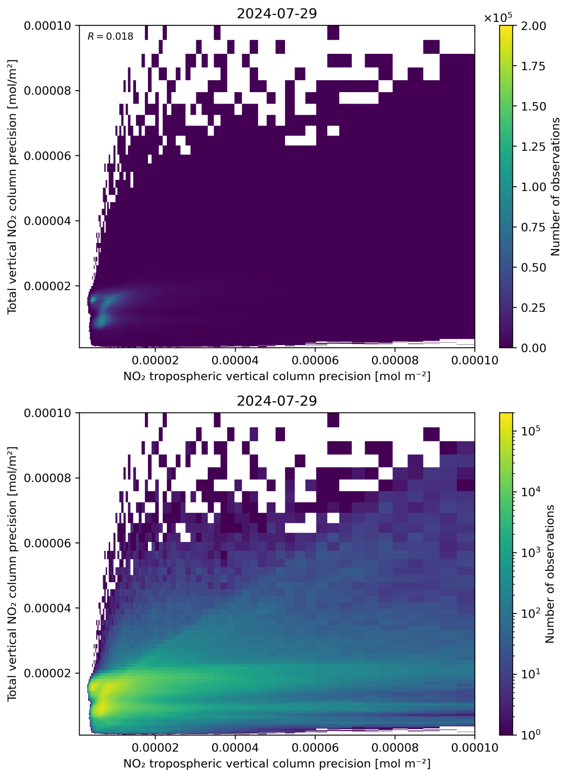
Figure 139: Scatter density plot of “NO 2 tropospheric vertical column precision” against “Total vertical NO 2 column precision” for 2024-07-28 to 2024-07-30.
