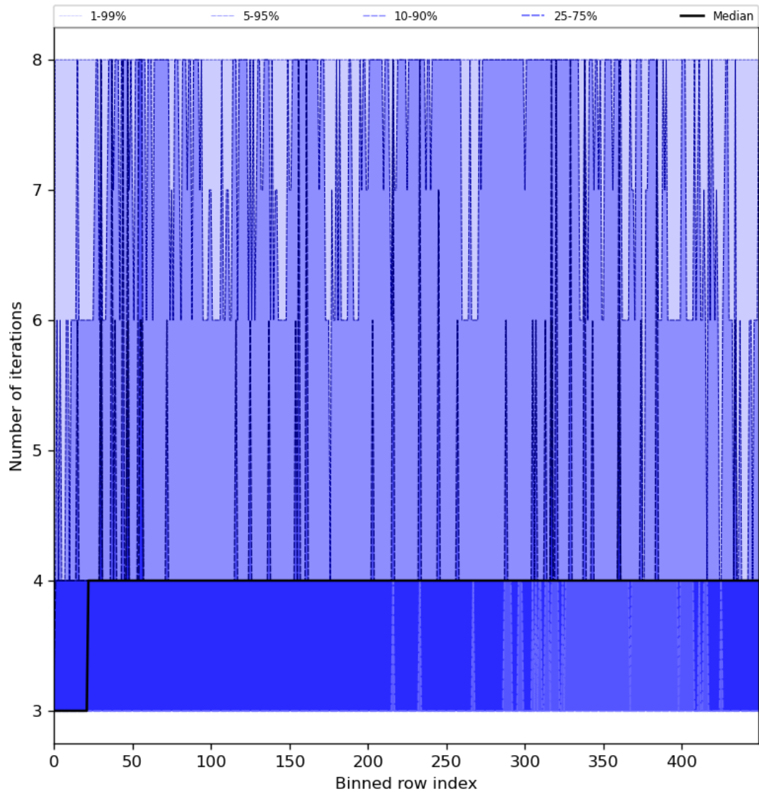
Figure 51: Along track statistics of “Number of iterations” for 2024-07-28 to 2024-07-30
