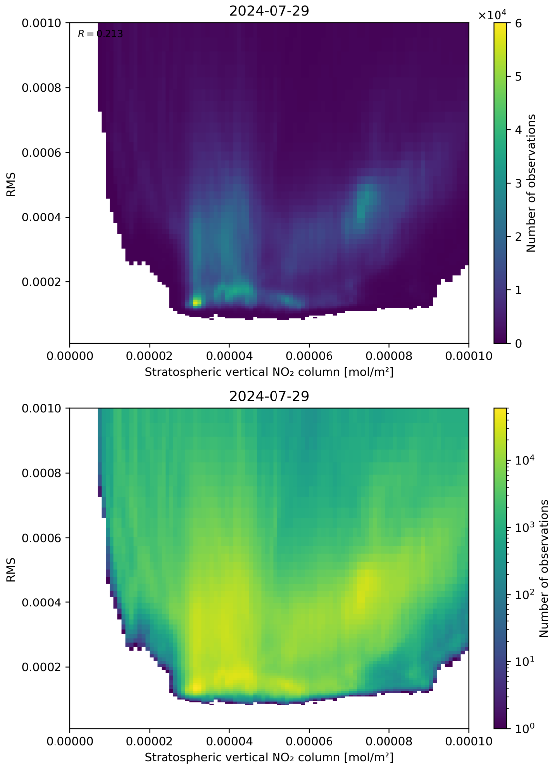
Figure 102: Scatter density plot of “Stratospheric vertical NO 2 column” against “RMS” for 2024-07-28 to 2024-07-30.
