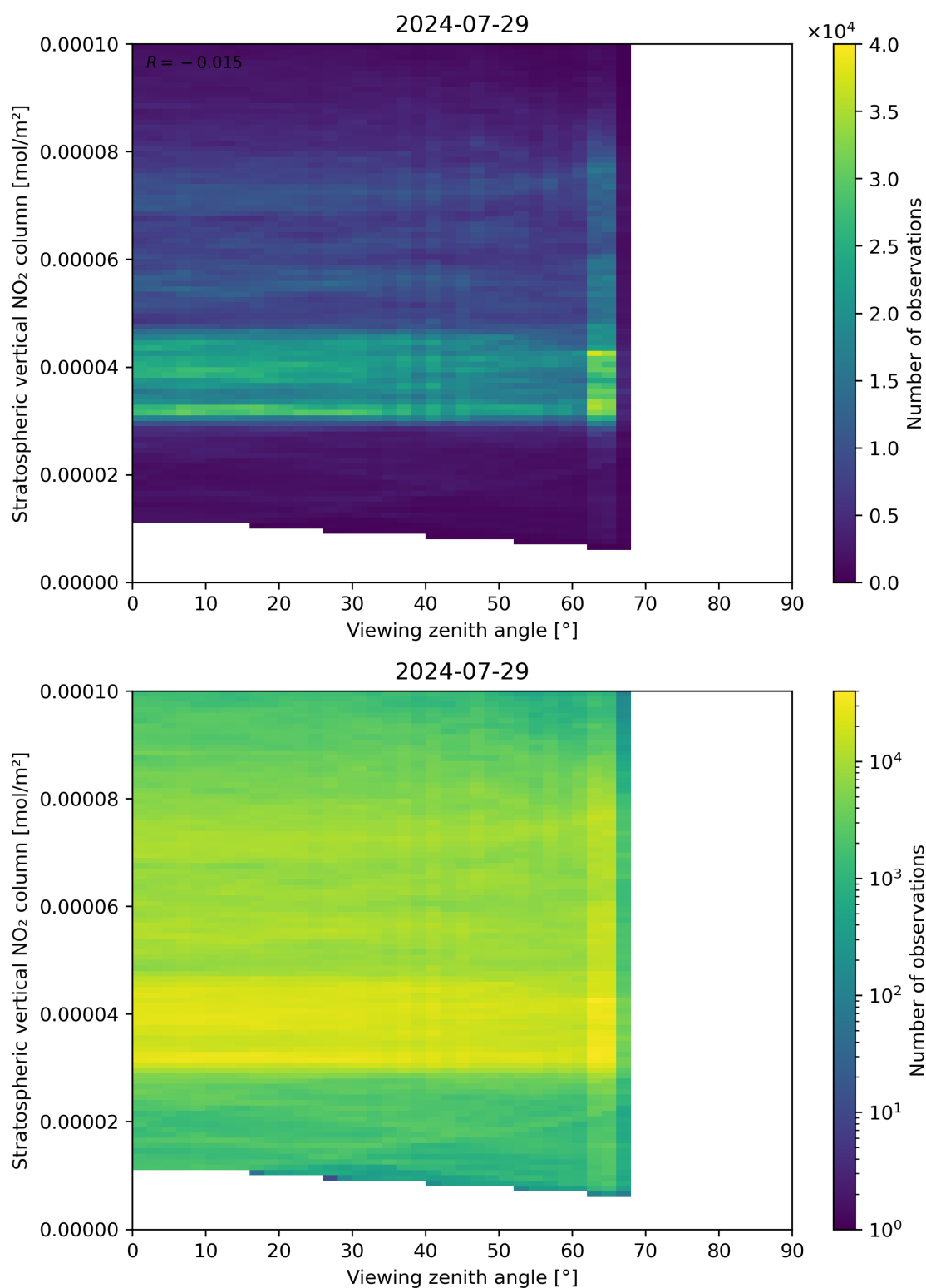
Figure 164: Scatter density plot of “Viewing zenith angle” against “Stratospheric vertical NO 2 column” for 2024-07-28 to 2024-07-30.
