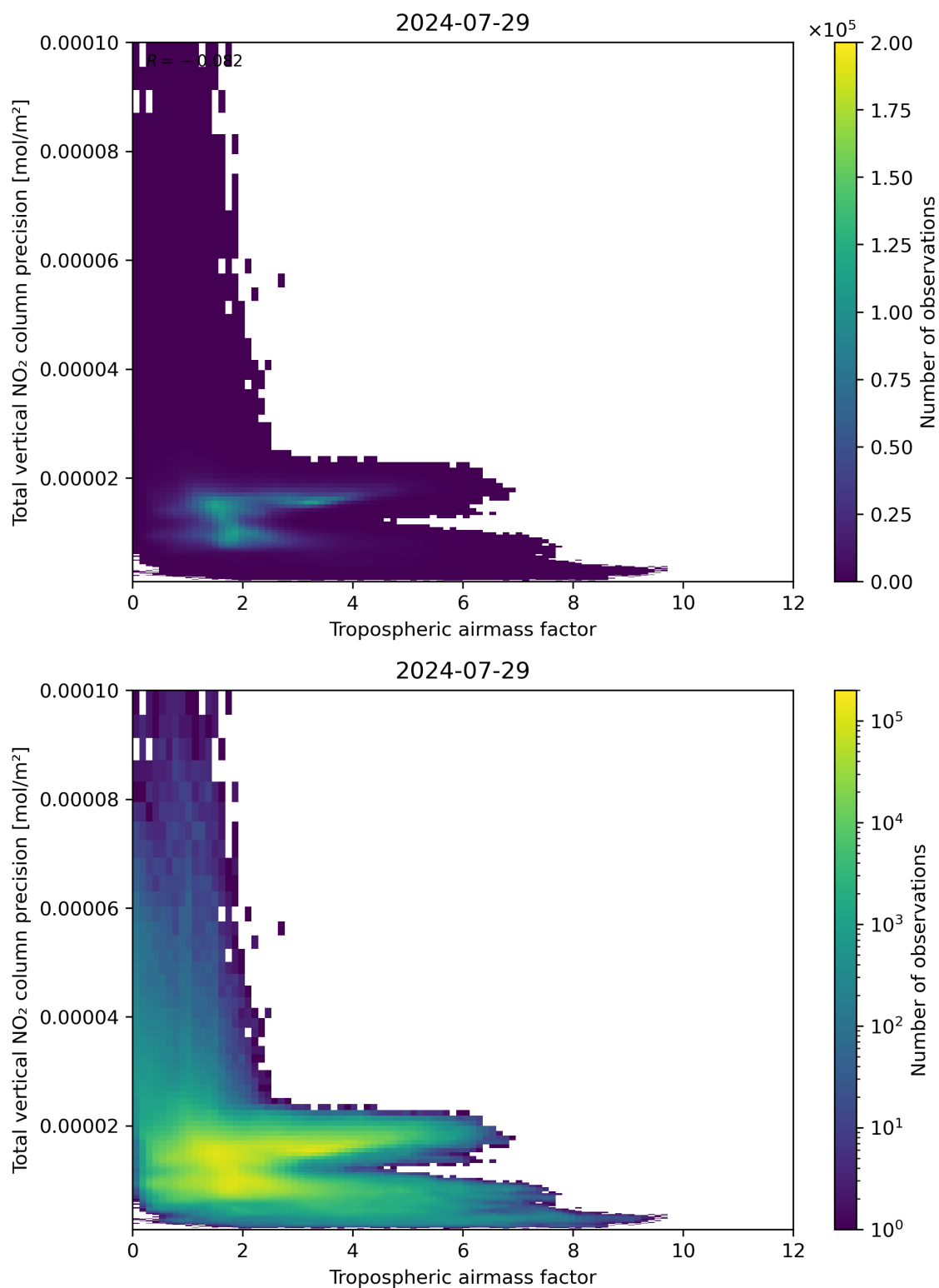
Figure 78: Scatter density plot of “Tropospheric air mass factor” against “Total vertical NO 2 column precision” for 2024-07-28 to 2024-07-30.
