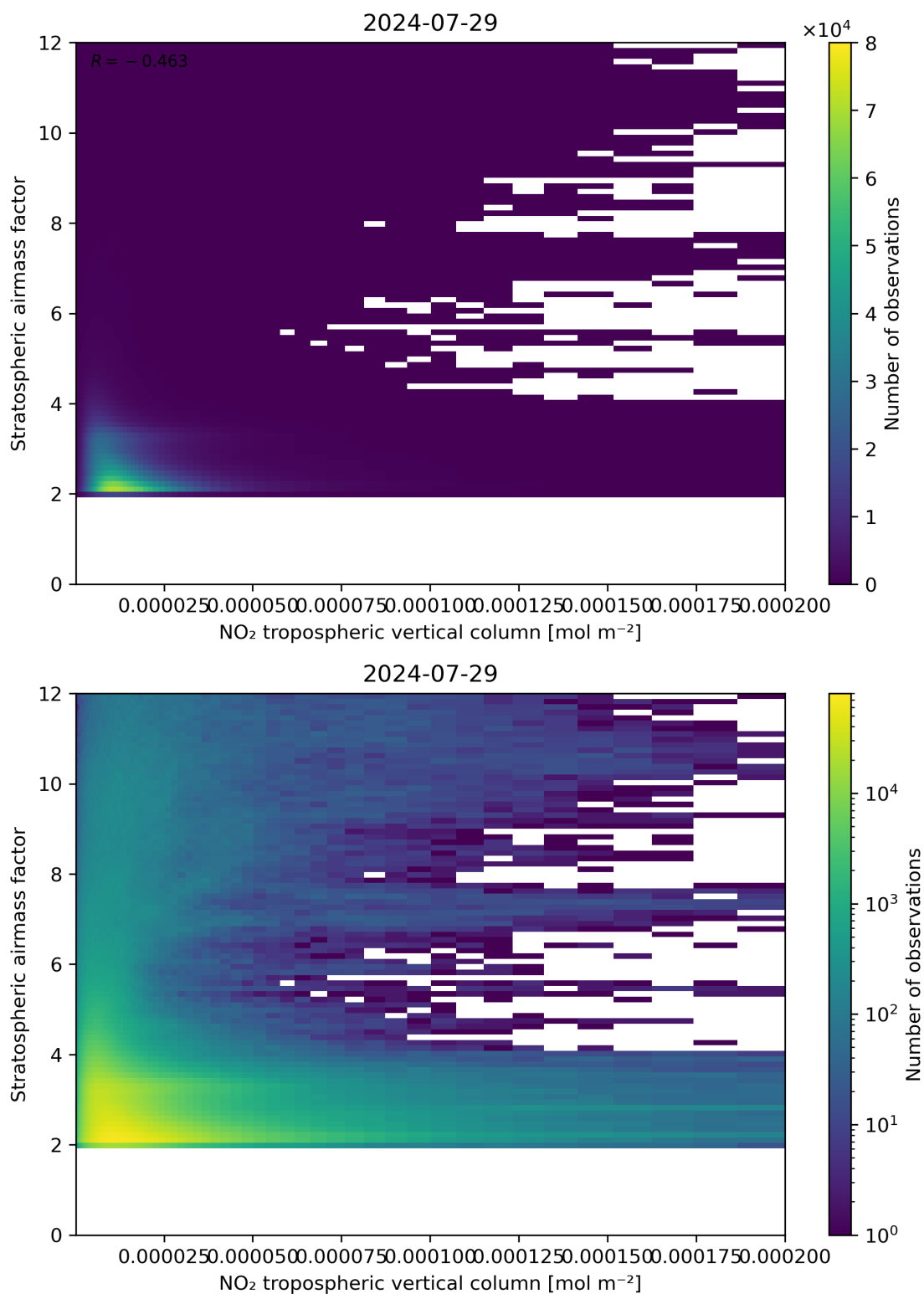
Figure 121: Scatter density plot of “NO 2 tropospheric vertical column” against “Stratospheric air mass factor” for 2024-07-28 to 2024-07-30.
