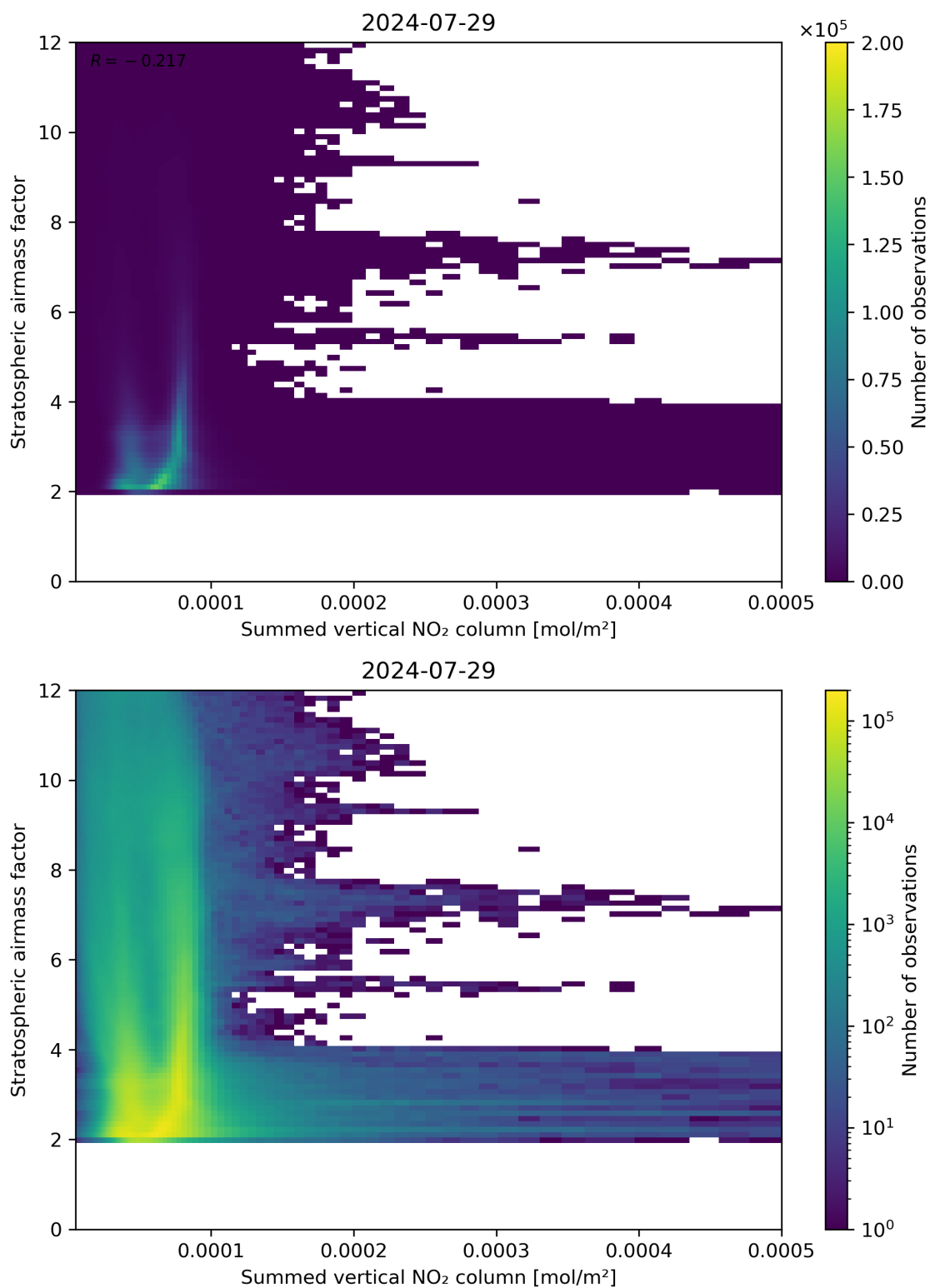
Figure 103: Scatter density plot of “Summed vertical NO 2 column” against “Stratospheric air mass factor” for 2024-07-28 to 2024-07-30.
