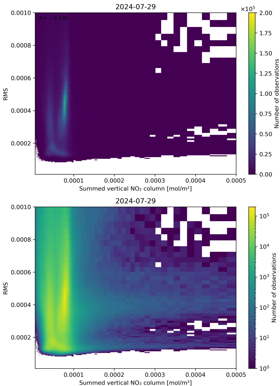
Figure 109: Scatter density plot of “Summed vertical NO 2 column” against “RMS” for 2024-07-28 to 2024-07-30.
