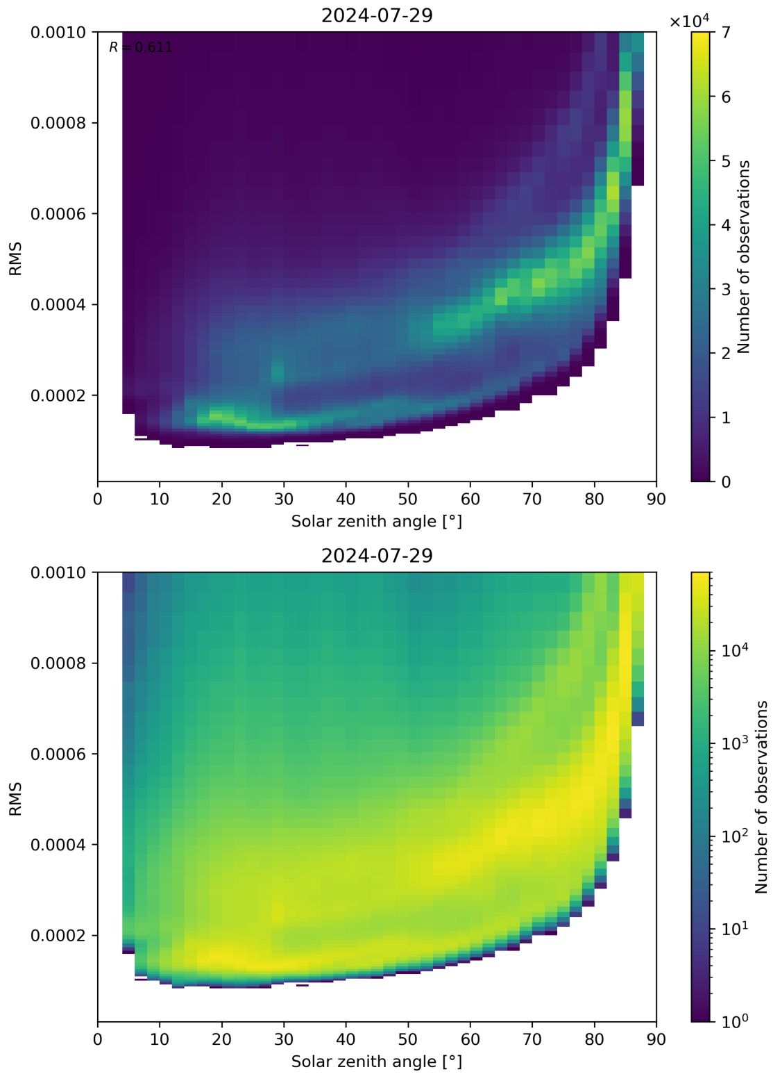
Figure 157: Scatter density plot of “Solar zenith angle” against “RMS” for 2024-07-28 to 2024-07-30.
