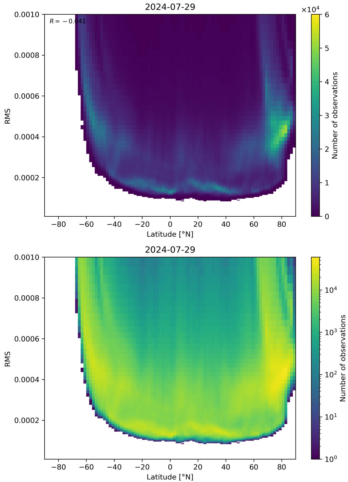
Figure 94: Scatter density plot of “Latitude” against “RMS” for 2024-07-28 to 2024-07-30.
