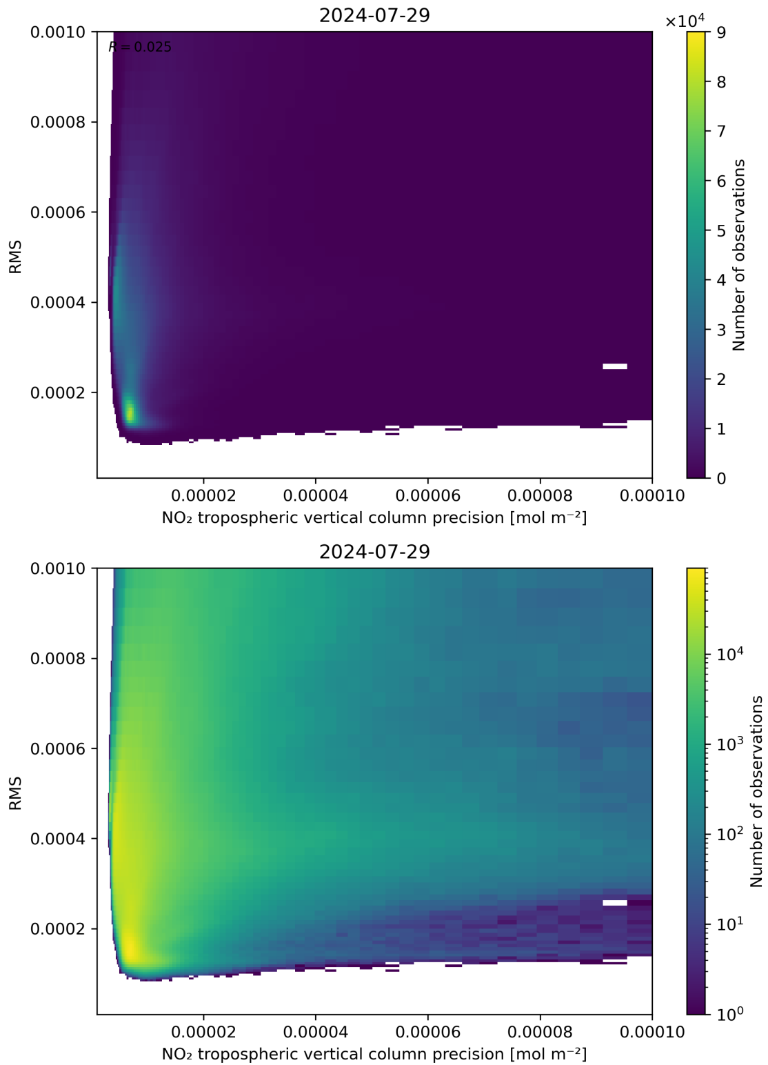
Figure 140: Scatter density plot of “NO 2 tropospheric vertical column precision” against “RMS” for 2024-07-28 to 2024-07-30.
