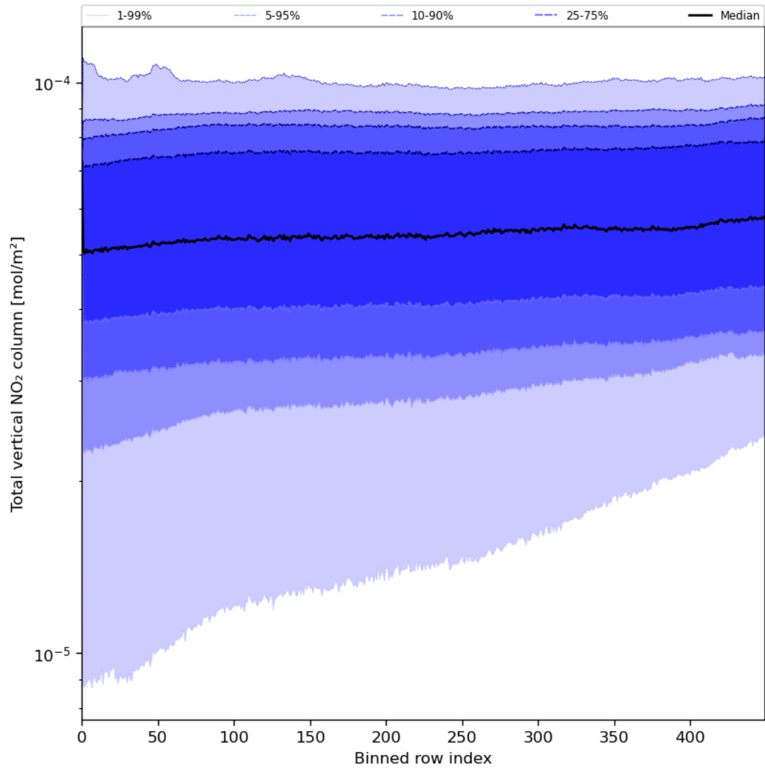
Figure 55: Along track statistics of “Total vertical NO 2 column” for 2024-07-28 to 2024-07-30
