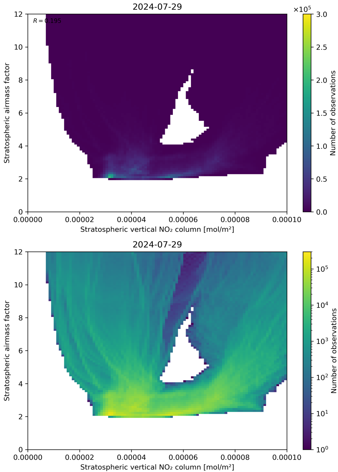
Figure 96: Scatter density plot of “Stratospheric vertical NO 2 column” against “Stratospheric airmass factor” for 2024-07-28 to 2024-07-30.
