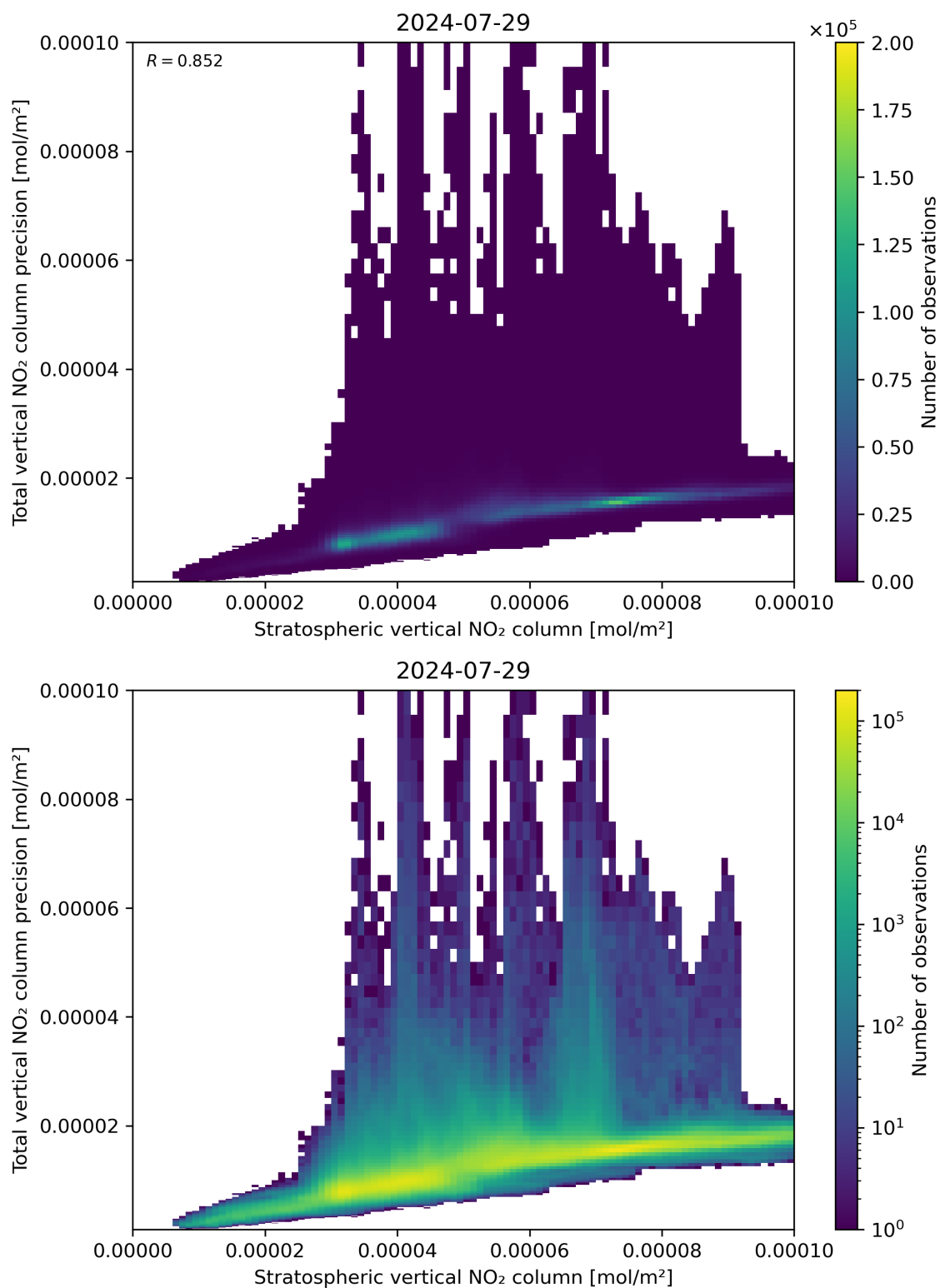
Figure 101: Scatter density plot of “Stratospheric vertical NO 2 column” against “Total vertical NO 2 column precision” for 2024-07-28 to 2024-07-30.
