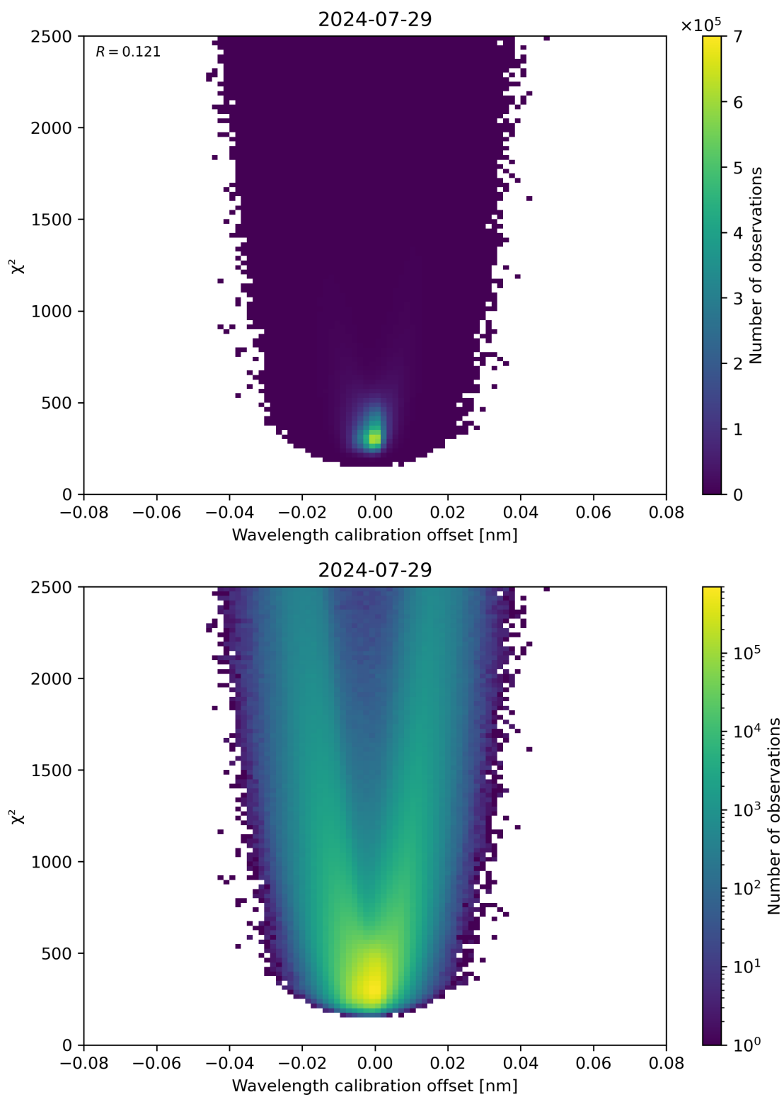
Figure 175: Scatter density plot of “Wavelength calibration offset” against “ \chi^2 ” for 2024-07-28 to 2024-07-30.
