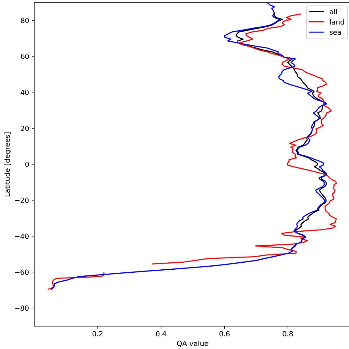
Figure 11: Zonal average of “QA value” for 2024-07-28 to 2024-07-30.
