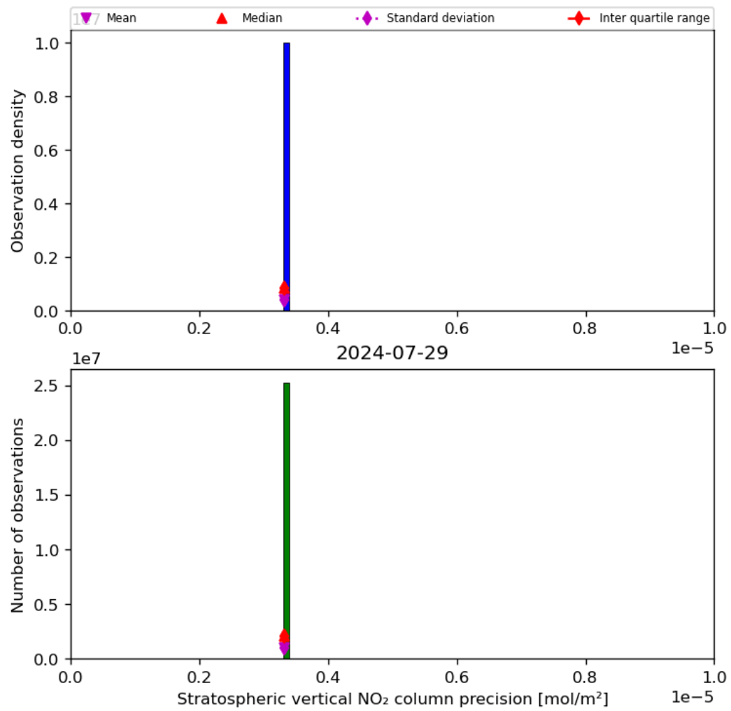
Figure 37: Histogram of “Stratospheric vertical NO 2 column precision” for 2024-07-28 to 2024-07-30
