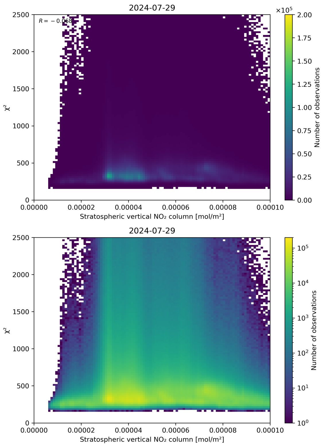
Figure 97: Scatter density plot of “Stratospheric vertical NO 2 column” against “ \chi^2 ” for 2024-07-28 to 2024-07-30.
