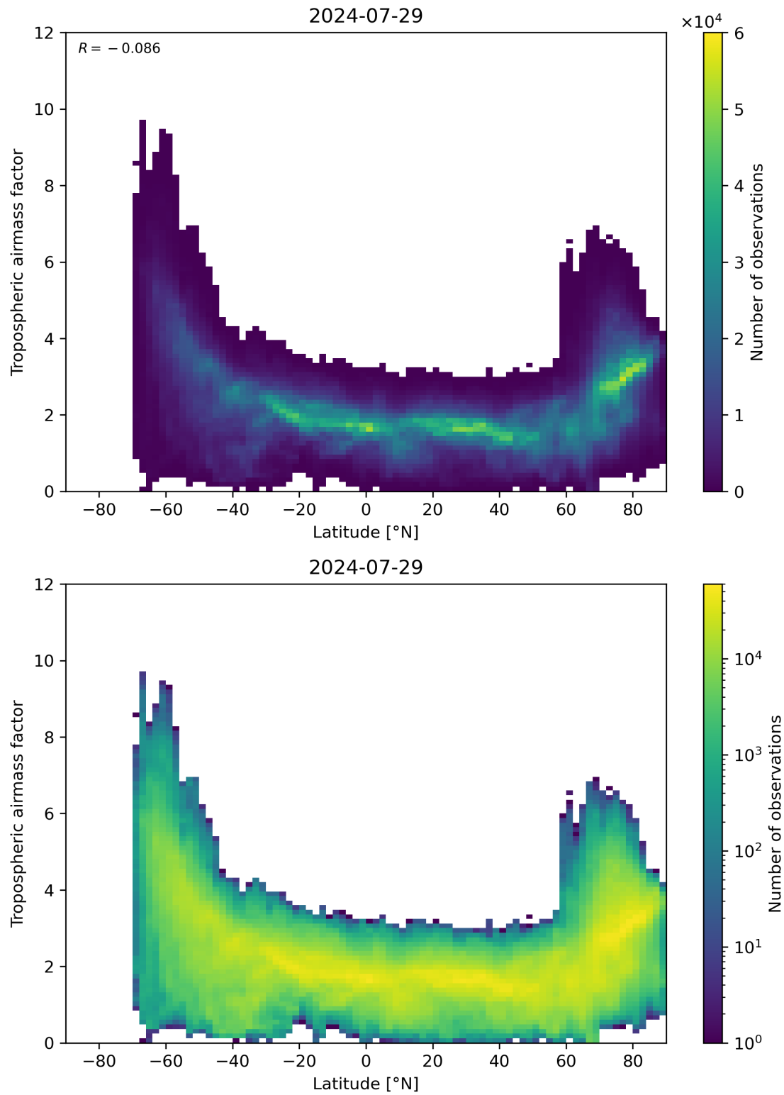
Figure 85: Scatter density plot of “Latitude” against “Tropospheric air mass factor” for 2024-07-28 to 2024-07-30.
