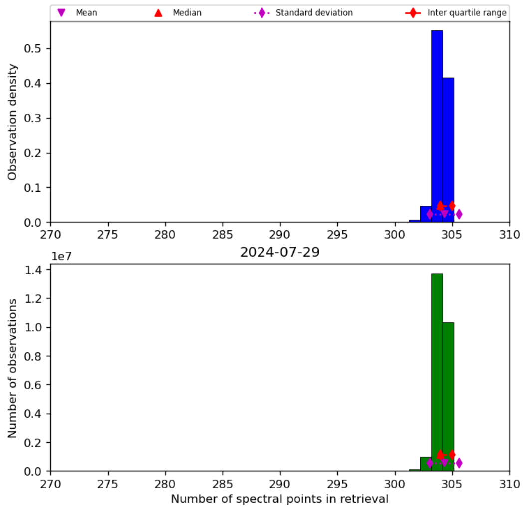
Figure 33: Histogram of “Number of spectral points in retrieval” for 2024-07-28 to 2024-07-30
