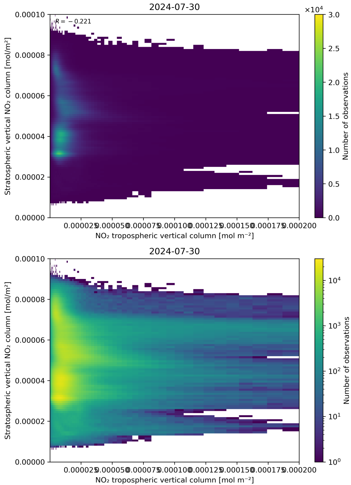
Figure 125: Scatter density plot of “NO 2 tropospheric vertical column” against “Stratospheric vertical NO 2 column” for 2024-07-29 to 2024-07-31.
