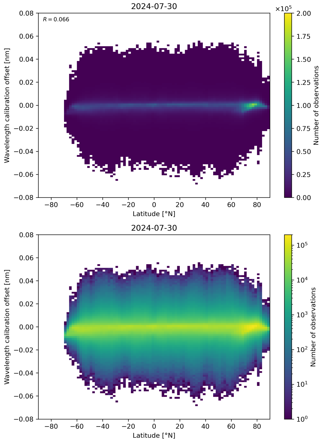
Figure 95: Scatter density plot of “Latitude” against “Wavelength calibration offset” for 2024-07-29 to 2024-07-31.
