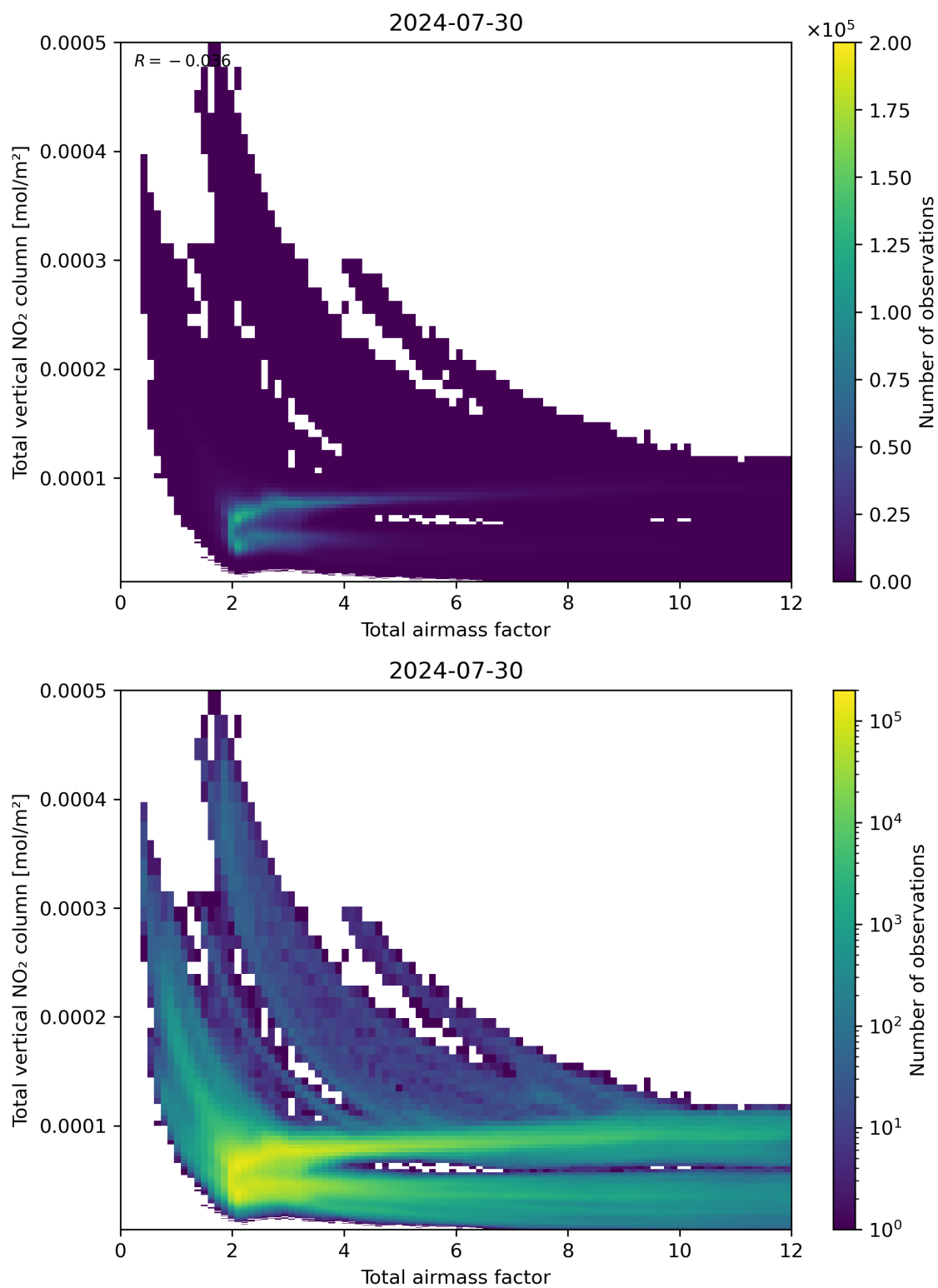
Figure 67: Scatter density plot of “Total air mass factor” against “Total vertical NO 2 column” for 2024-07-29 to 2024-07-31.
