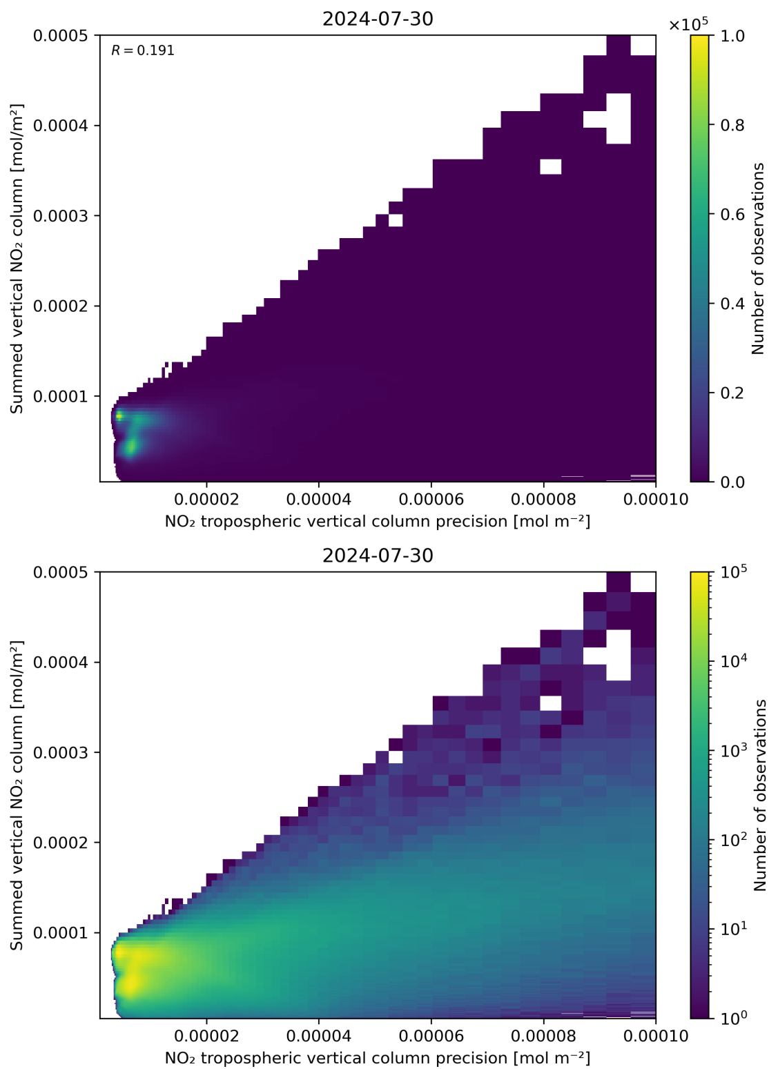
Figure 136: Scatter density plot of “NO 2 tropospheric vertical column precision” against “Summed vertical NO 2 column” for 2024-07-29 to 2024-07-31.
