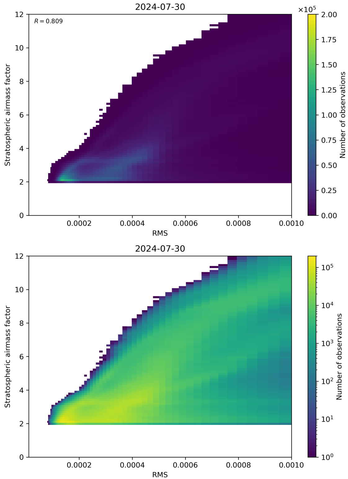
Figure 144: Scatter density plot of “RMS” against “Stratospheric airmass factor” for 2024-07-29 to 2024-07-31.
