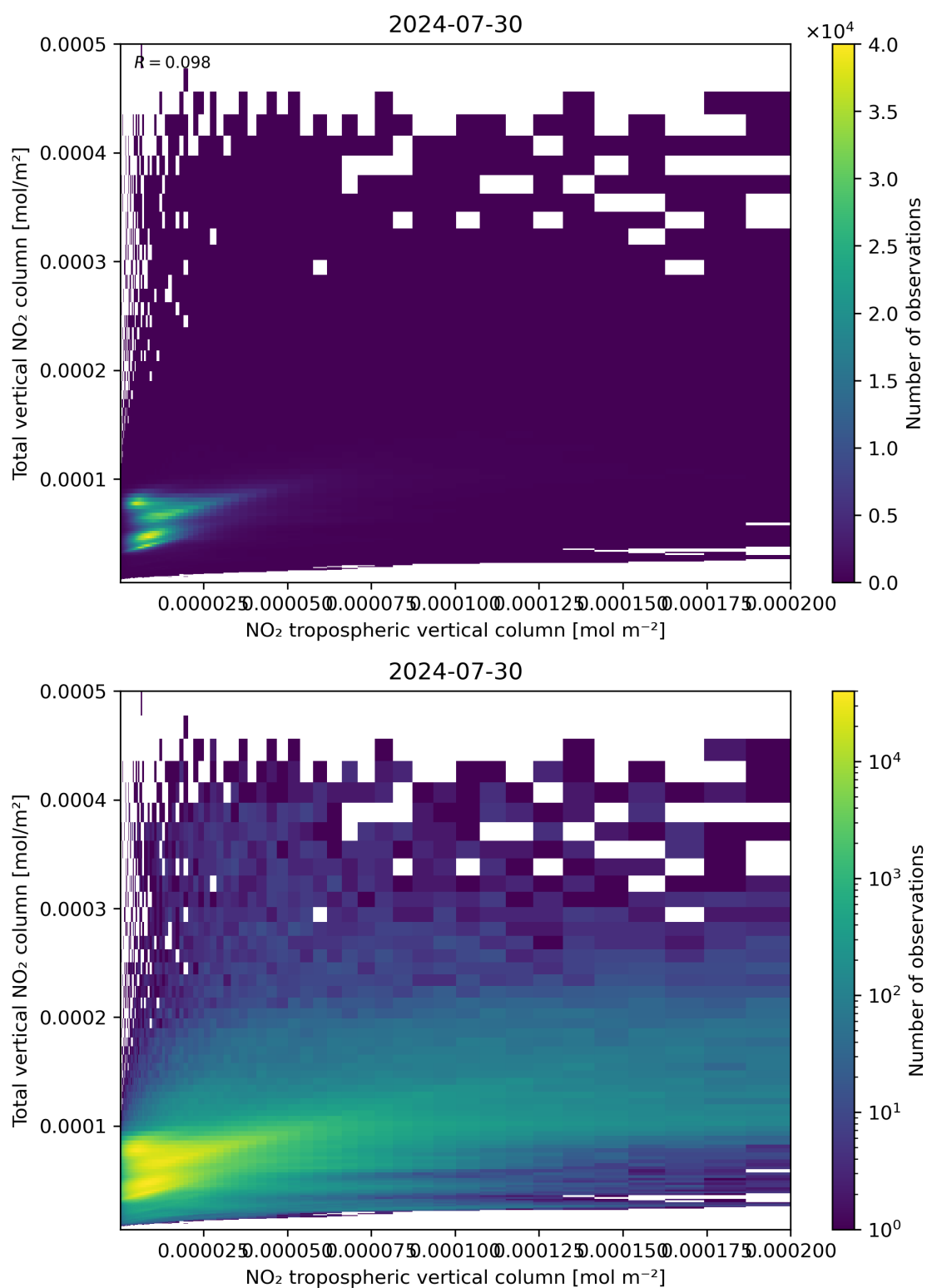
Figure 128: Scatter density plot of “NO 2 tropospheric vertical column” against “Total vertical NO 2 column” for 2024-07-29 to 2024-07-31.
