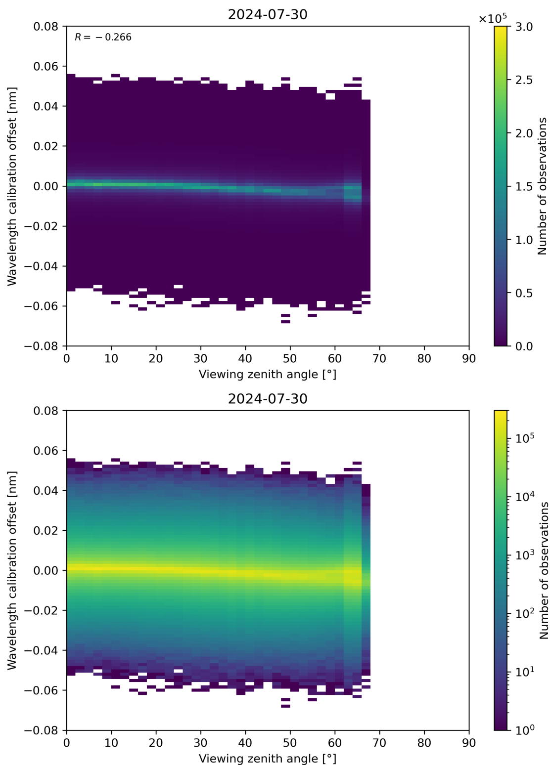
Figure 173: Scatter density plot of “Viewing zenith angle” against “Wavelength calibration offset” for 2024-07-29 to 2024-07-31.
