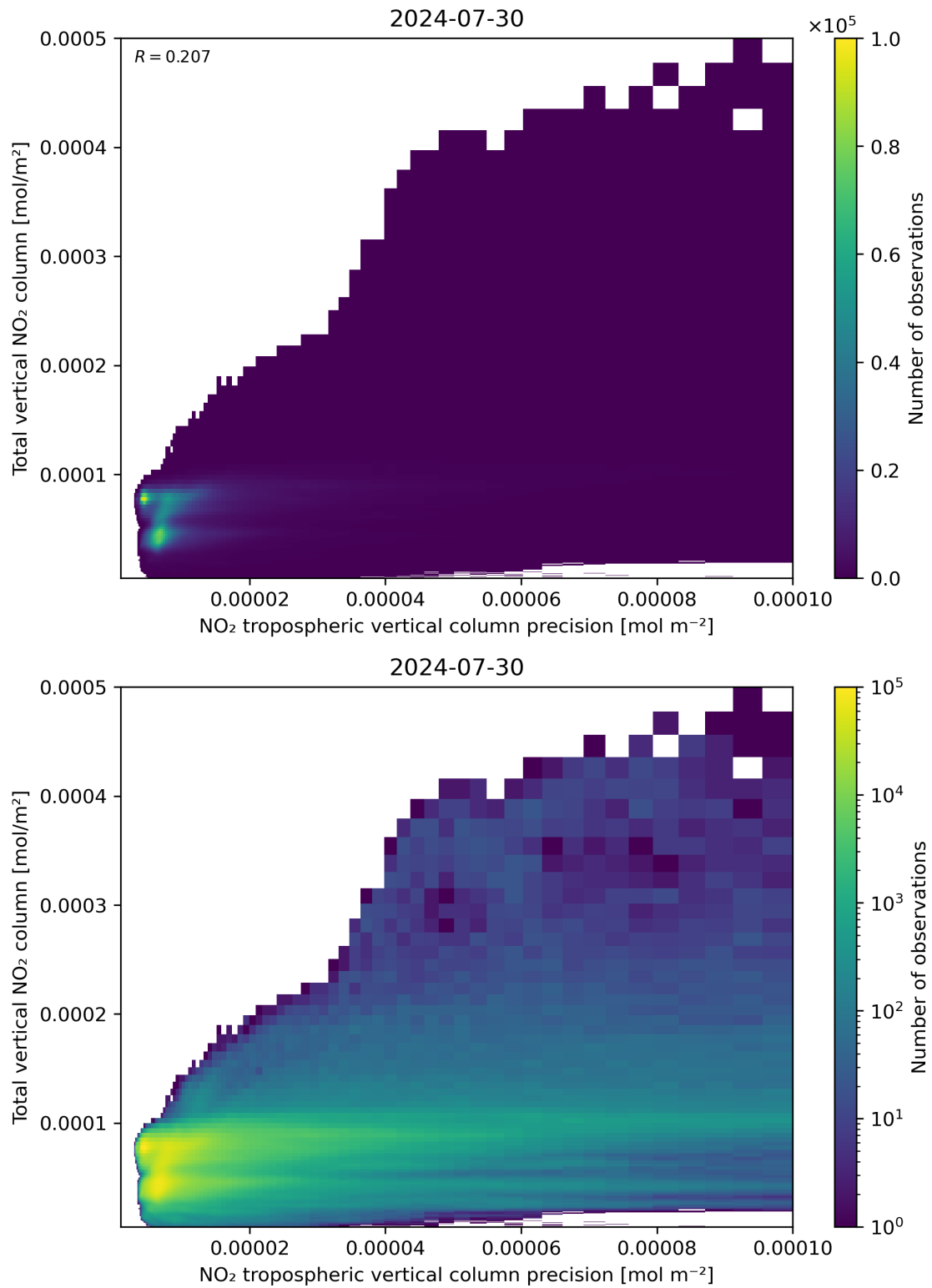
Figure 138: Scatter density plot of “NO 2 tropospheric vertical column precision” against “Total vertical NO 2 column” for 2024-07-29 to 2024-07-31.
