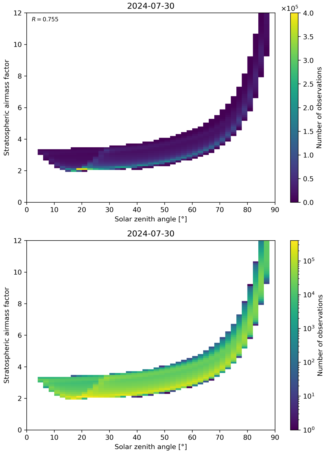
Figure 145: Scatter density plot of “Solar zenith angle” against “Stratospheric airmass factor” for 2024-07-29 to 2024-07-31.
