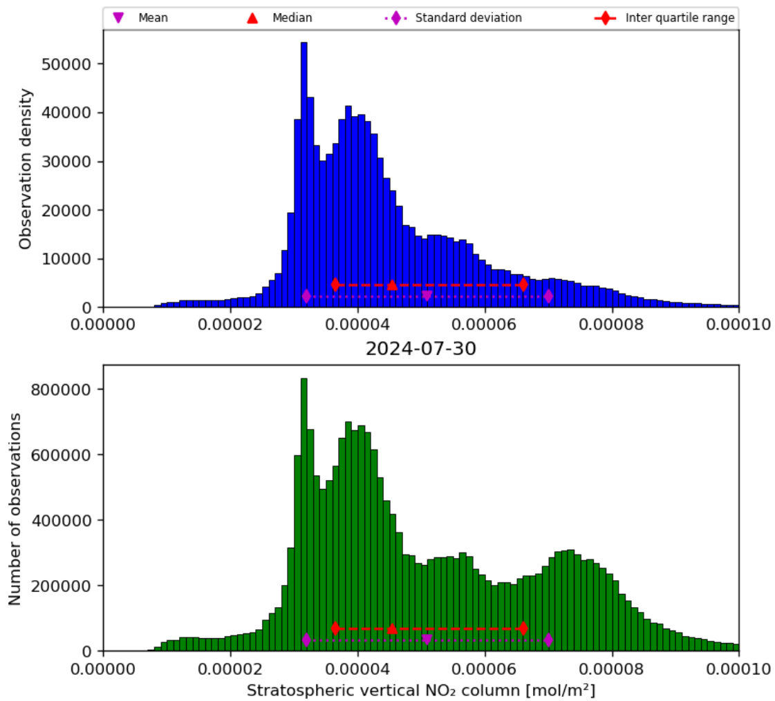
Figure 36: Histogram of “Stratospheric vertical NO 2 column” for 2024-07-29 to 2024-07-31
