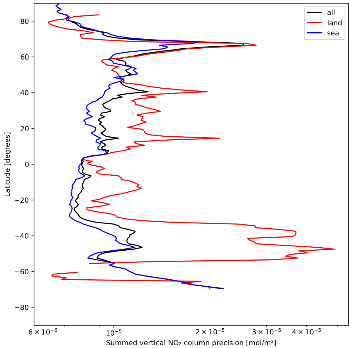
Figure 24: Zonal average of “Summed vertical NO 2 column precision” for 2024-07-29 to 2024-07-31.
