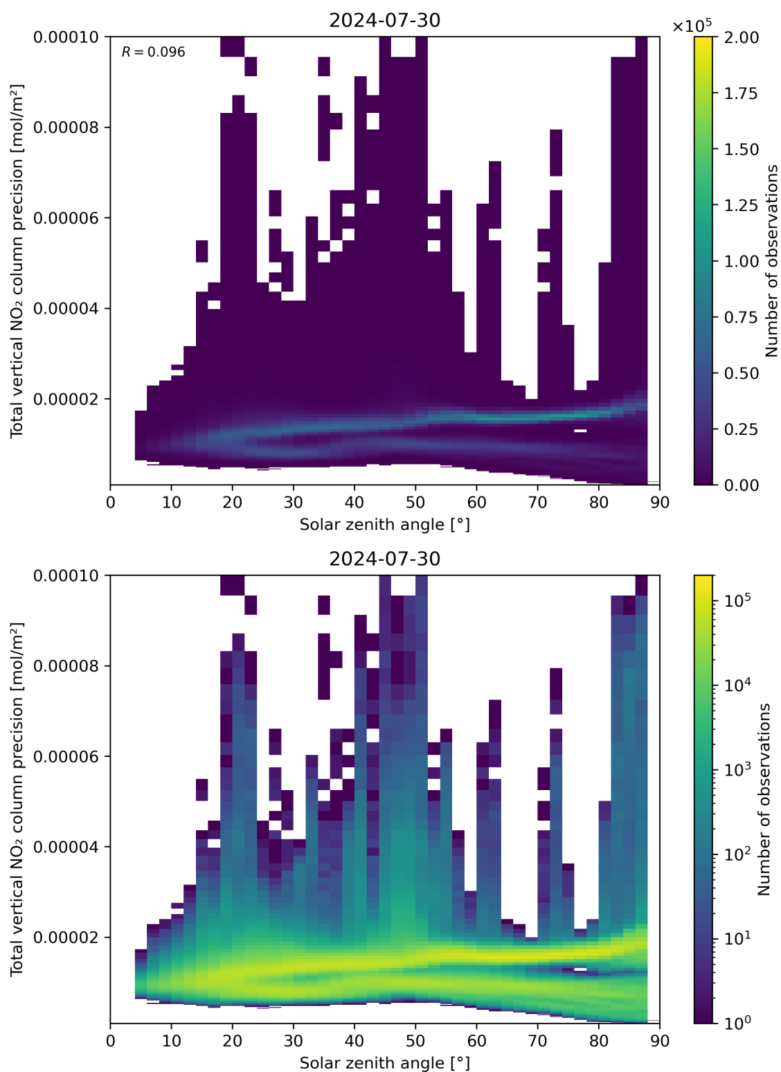
Figure 154: Scatter density plot of “Solar zenith angle” against “Total vertical NO 2 column precision” for 2024-07-29 to 2024-07-31.
