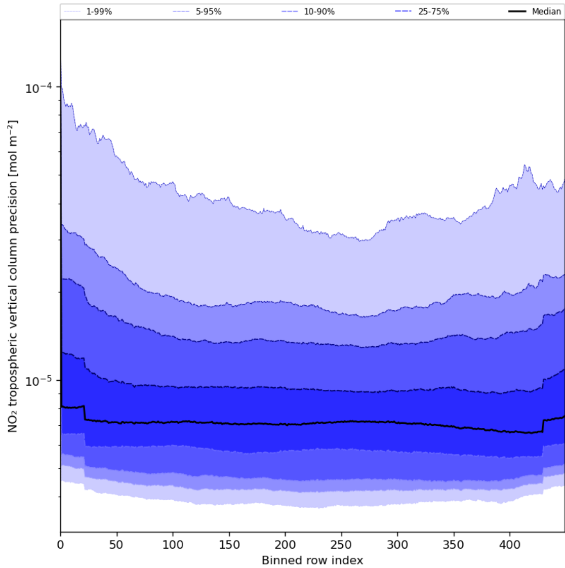
Figure 47: Along track statistics of “NO 2 tropospheric vertical column precision” for 2024-07-29 to 2024-07-31
