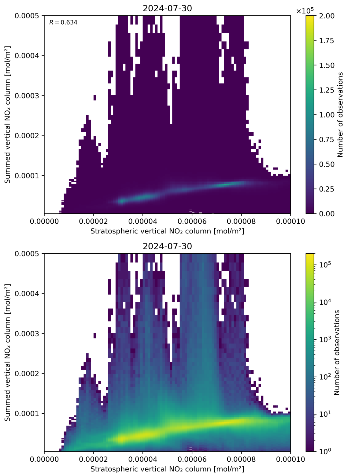
Figure 98: Scatter density plot of “Stratospheric vertical NO 2 column” against “Summed vertical NO 2 column” for 2024-07-29 to 2024-07-31.
