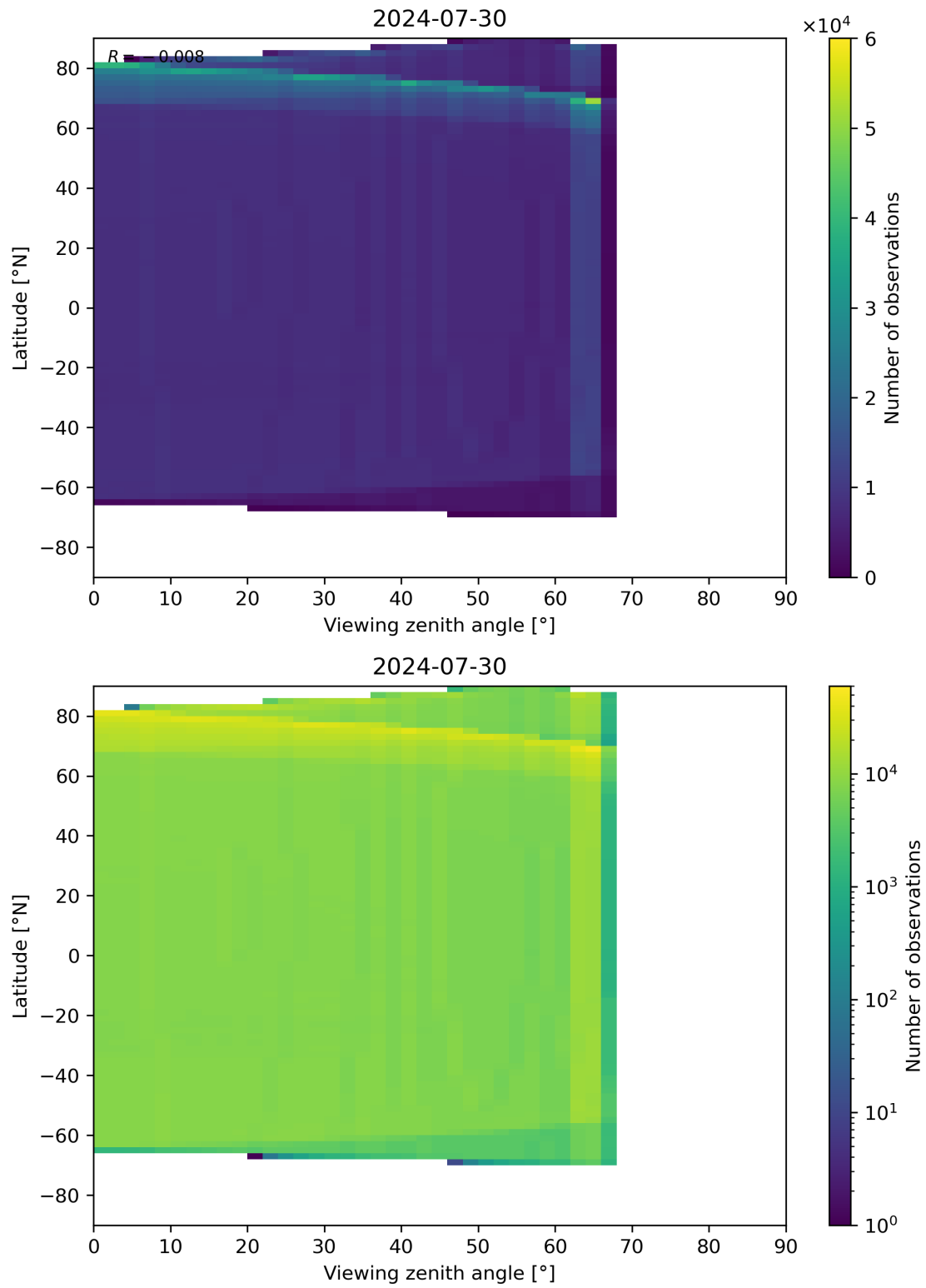
Figure 163: Scatter density plot of “Viewing zenith angle” against “Latitude” for 2024-07-29 to 2024-07-31.
