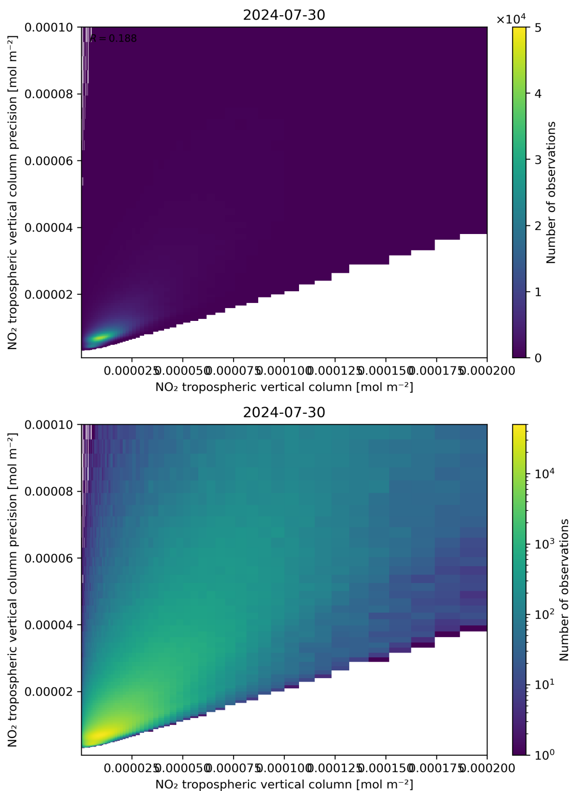
Figure 130: Scatter density plot of “NO 2 tropospheric vertical column” against “NO 2 tropospheric vertical column precision” for 2024-07-29 to 2024-07-31.
