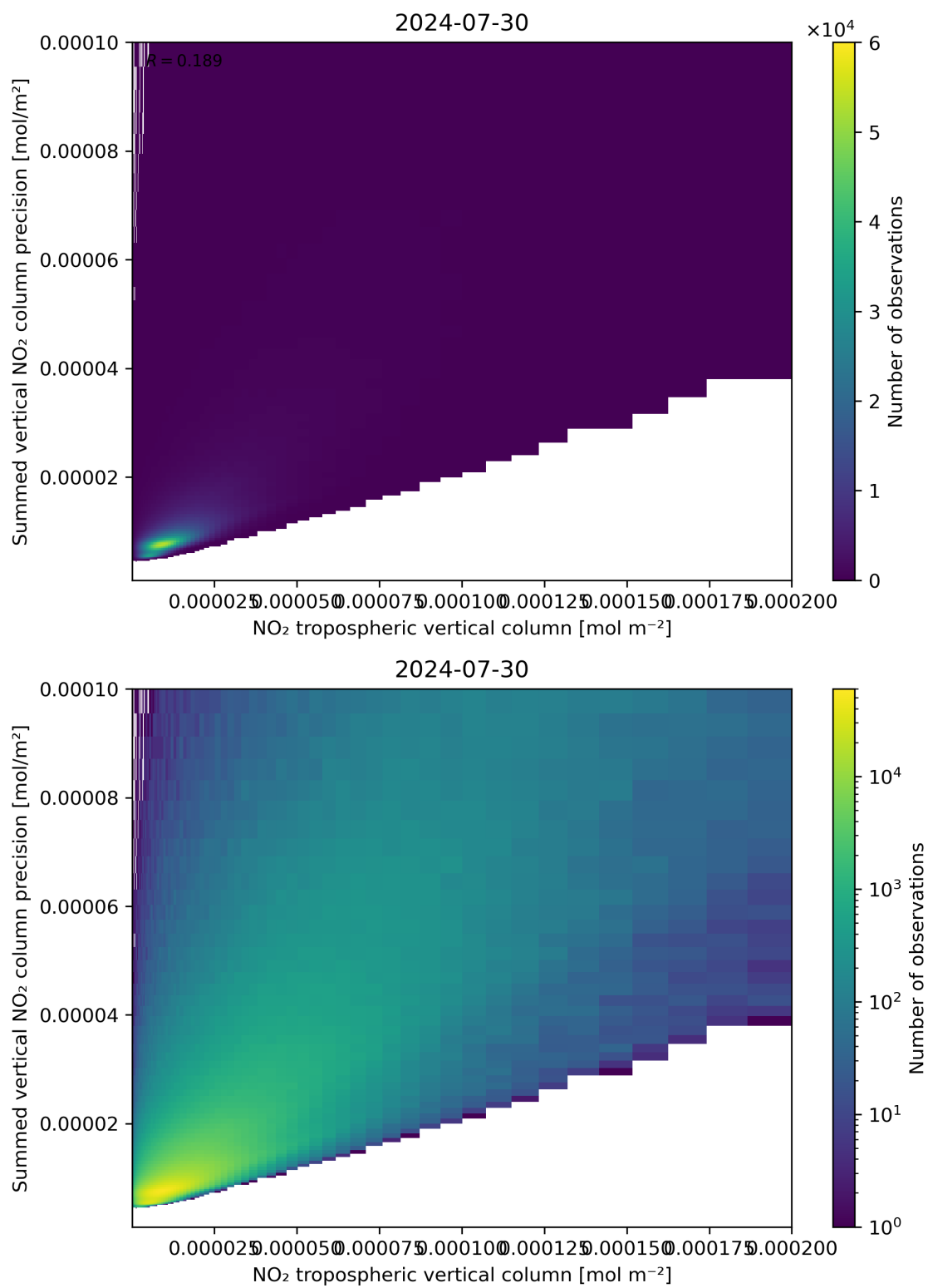
Figure 127: Scatter density plot of “NO 2 tropospheric vertical column” against “Summed vertical NO 2 column precision” for 2024-07-29 to 2024-07-31.
