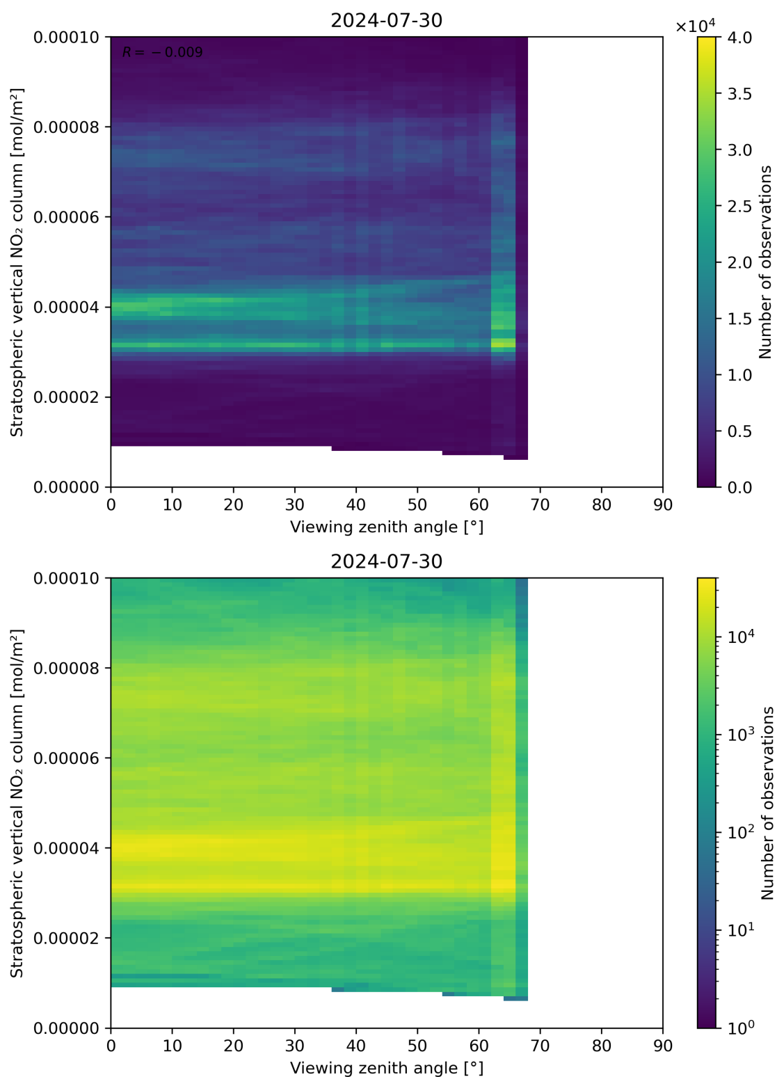
Figure 164: Scatter density plot of “Viewing zenith angle” against “Stratospheric vertical NO 2 column” for 2024-07-29 to 2024-07-31.
