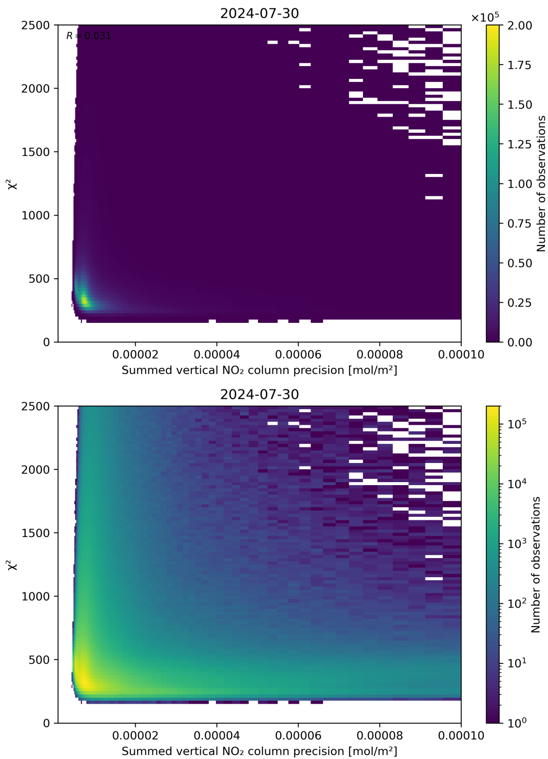
Figure 107: Scatter density plot of “Summed vertical NO 2 column precision” against “ \chi^2 ” for 2024-07-29 to 2024-07-31.
