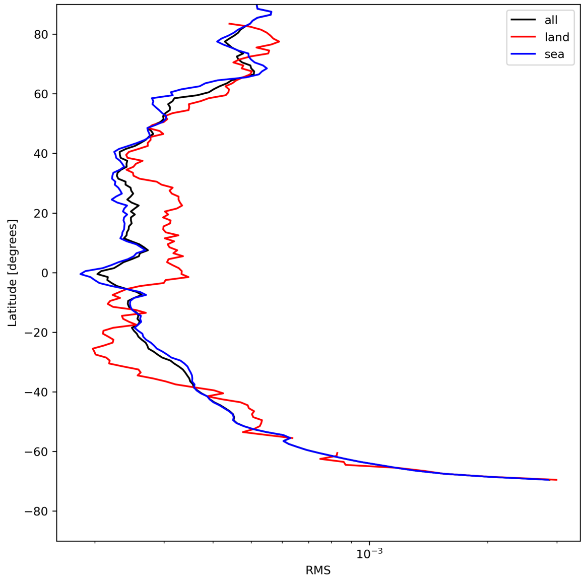
Figure 26: Zonal average of “RMS” for 2024-07-29 to 2024-07-31.
