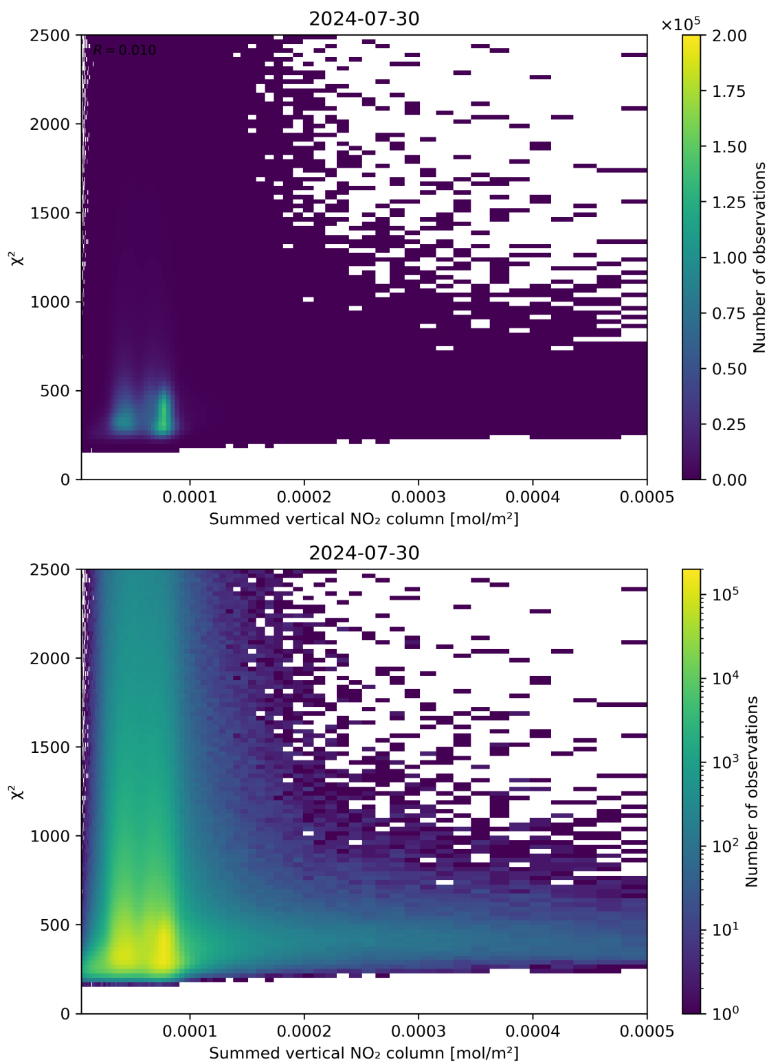
Figure 104: Scatter density plot of “Summed vertical NO 2 column” against “ \chi^2 ” for 2024-07-29 to 2024-07-31.
