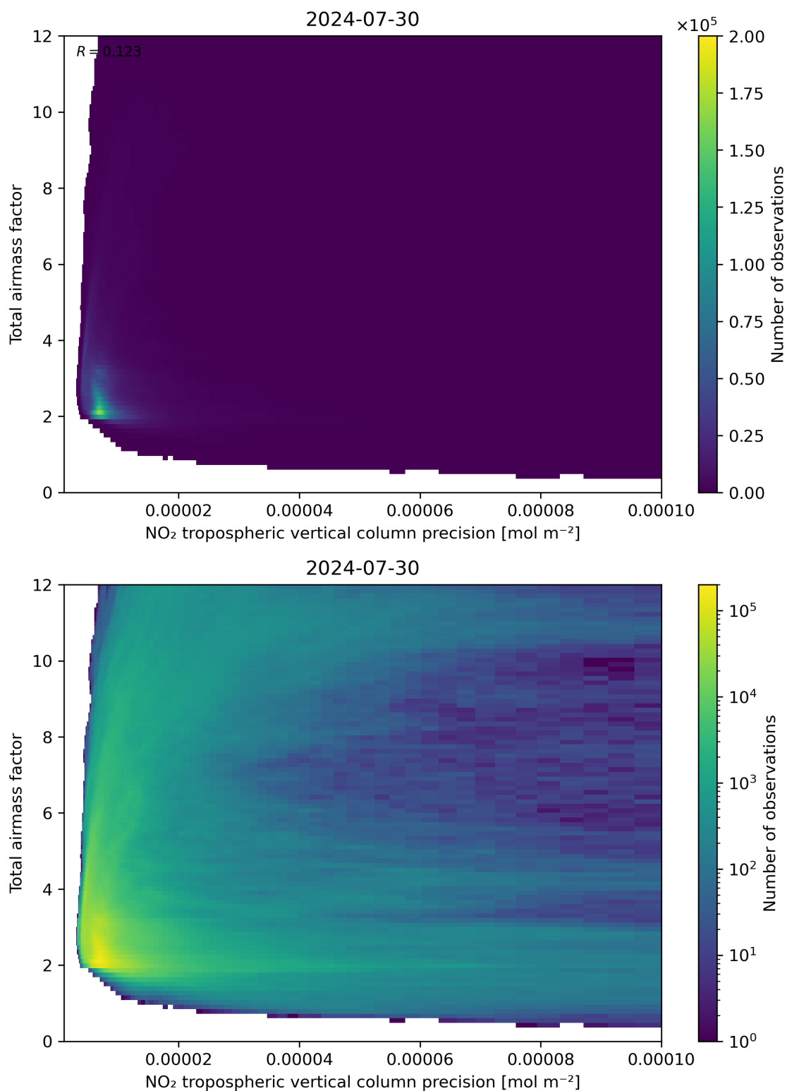
Figure 132: Scatter density plot of “NO 2 tropospheric vertical column precision” against “Total air mass factor” for 2024-07-29 to 2024-07-31.
