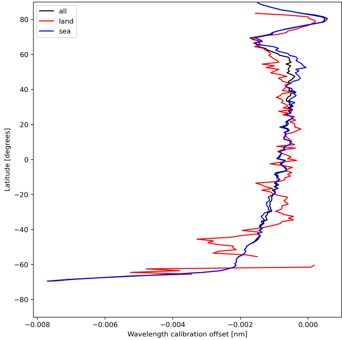
Figure 18: Zonal average of “Wavelength calibration offset” for 2024-07-29 to 2024-07-31.
