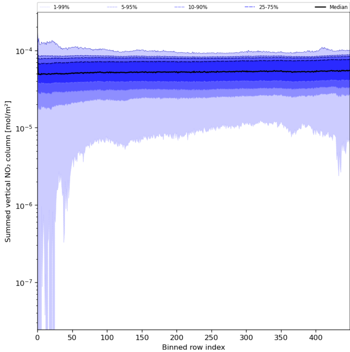
Figure 57: Along track statistics of “Summed vertical NO 2 column” for 2024-07-29 to 2024-07-31
