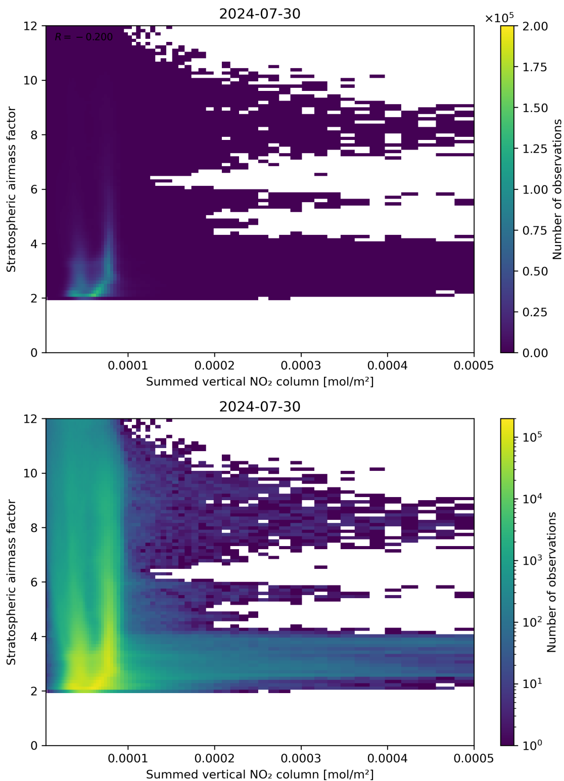
Figure 103: Scatter density plot of “Summed vertical NO 2 column” against “Stratospheric air mass factor” for 2024-07-29 to 2024-07-31.
