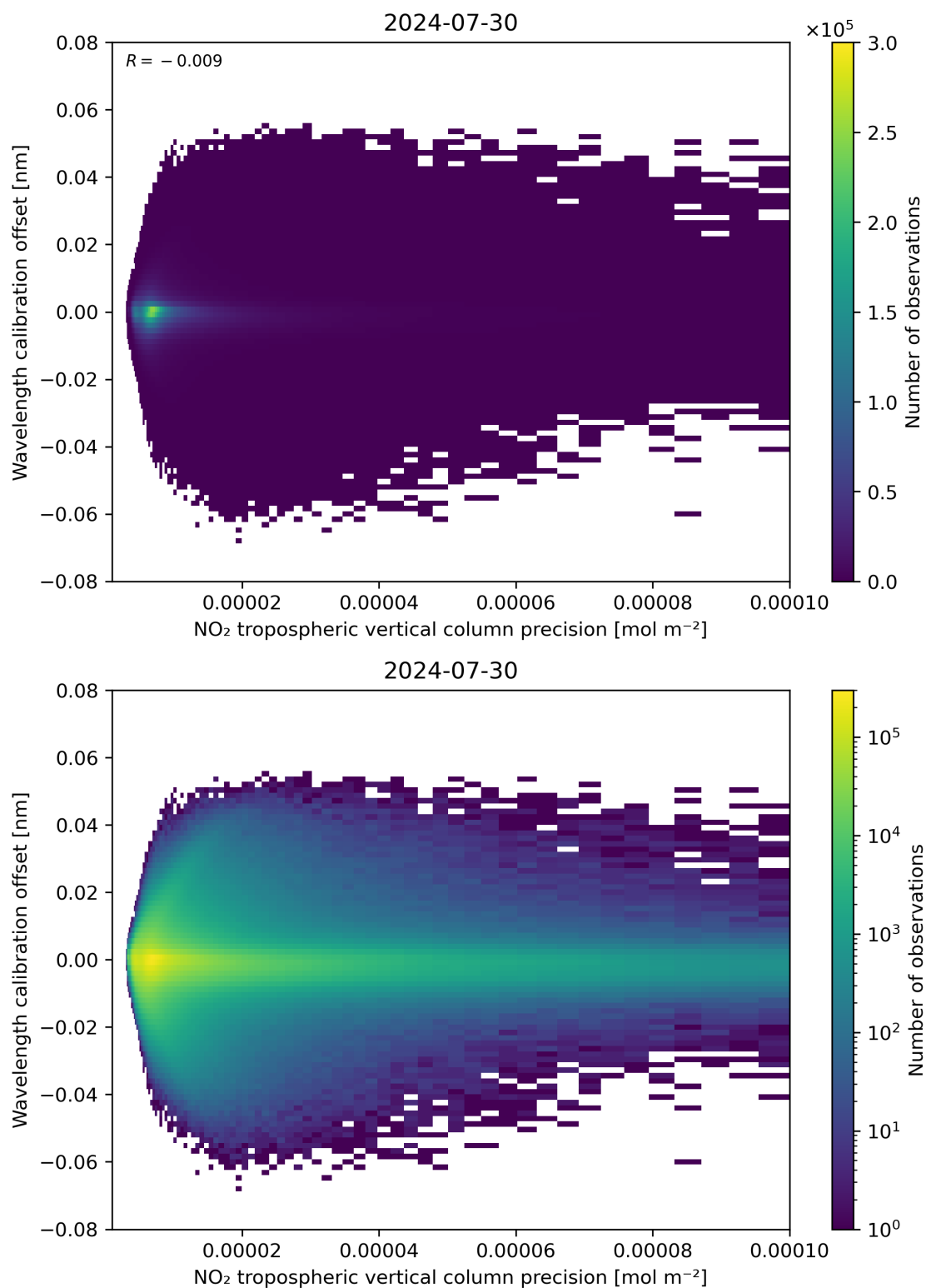
Figure 141: Scatter density plot of “NO 2 tropospheric vertical column precision” against “Wavelength calibration offset” for 2024-07-29 to 2024-07-31.
