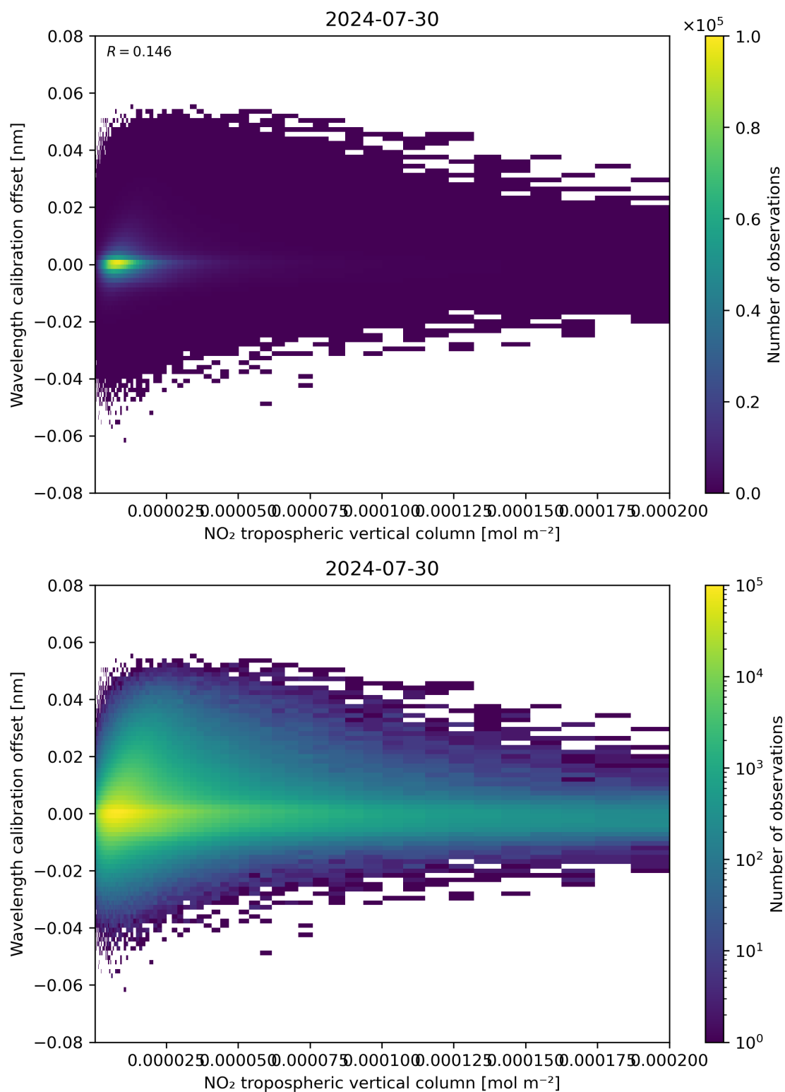
Figure 143: Scatter density plot of “NO 2 tropospheric vertical column” against “Wavelength calibration offset” for 2024-07-29 to 2024-07-31.
