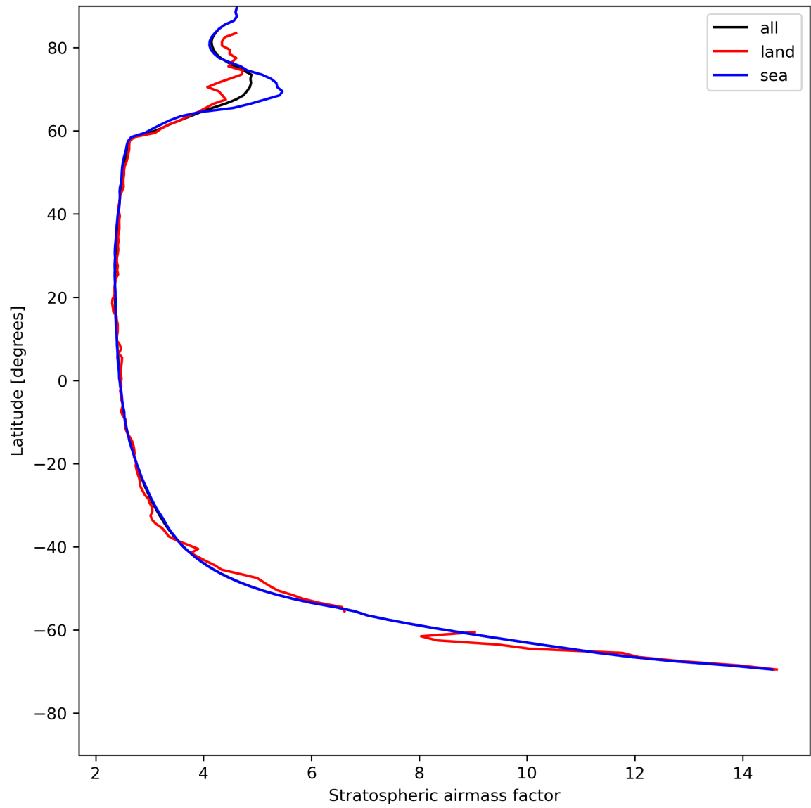
Figure 27: Zonal average of “Stratospheric air mass factor” for 2024-07-29 to 2024-07-31.
