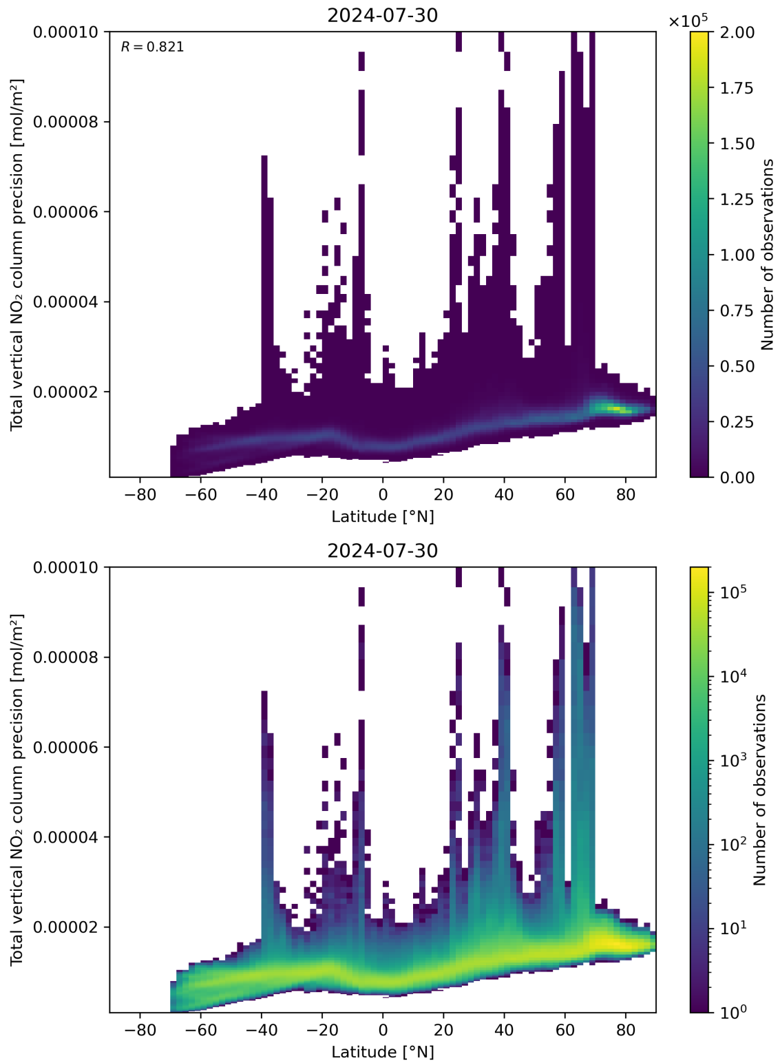
Figure 91: Scatter density plot of “Latitude” against “Total vertical NO 2 column precision” for 2024-07-29 to 2024-07-31.
