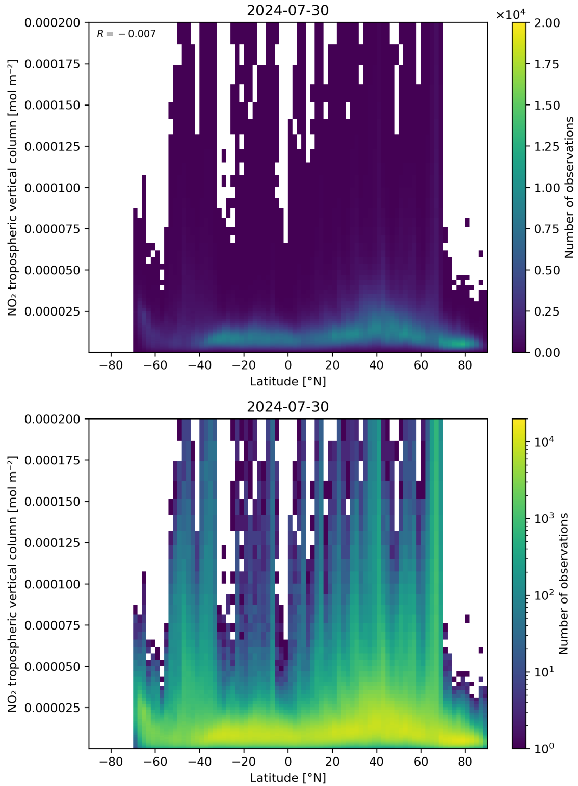
Figure 92: Scatter density plot of “Latitude” against “NO 2 tropospheric vertical column” for 2024-07-29 to 2024-07-31.
