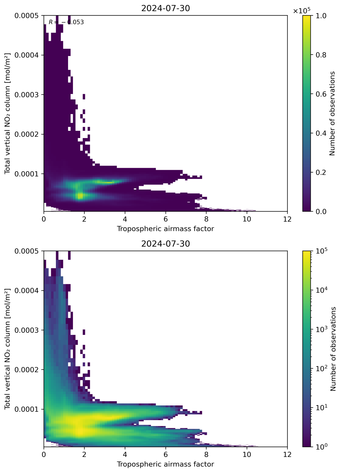
Figure 77: Scatter density plot of “Tropospheric airmass factor” against “Total vertical NO 2 column” for 2024-07-29 to 2024-07-31.
