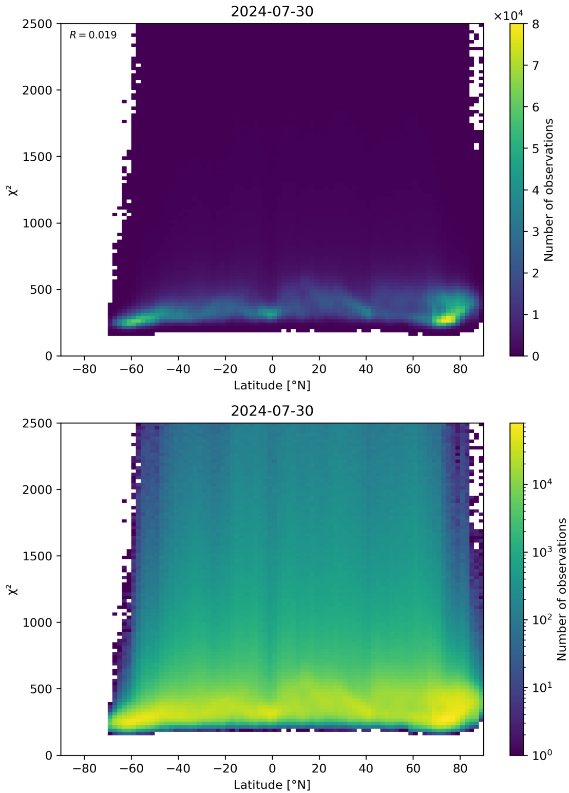
Figure 86: Scatter density plot of “Latitude” against “ \chi^2 ” for 2024-07-29 to 2024-07-31.
