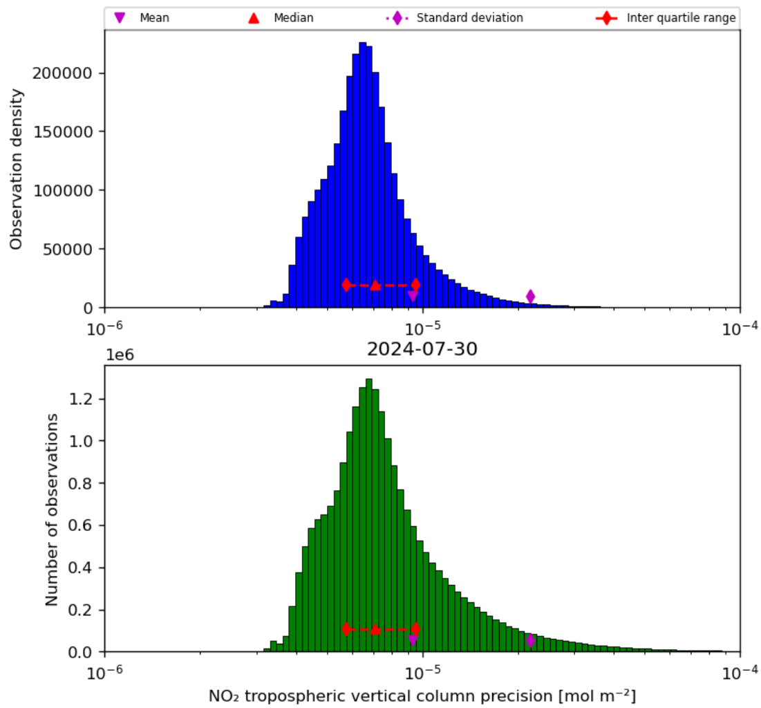
Figure 30: Histogram of “NO 2 tropospheric vertical column precision” for 2024-07-29 to 2024-07-31
