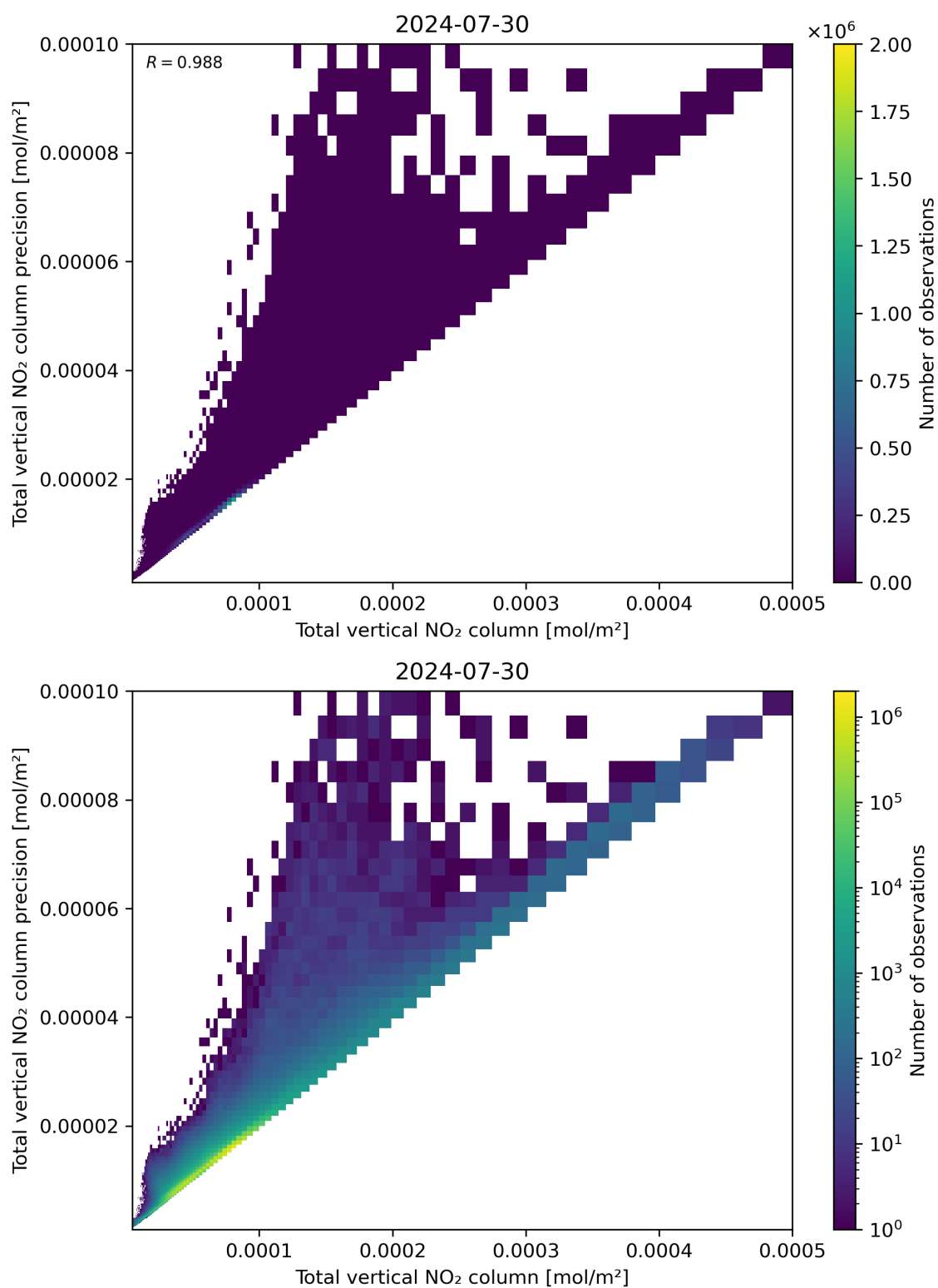
Figure 114: Scatter density plot of “Total vertical NO 2 column” against “Total vertical NO 2 column precision” for 2024-07-29 to 2024-07-31.
