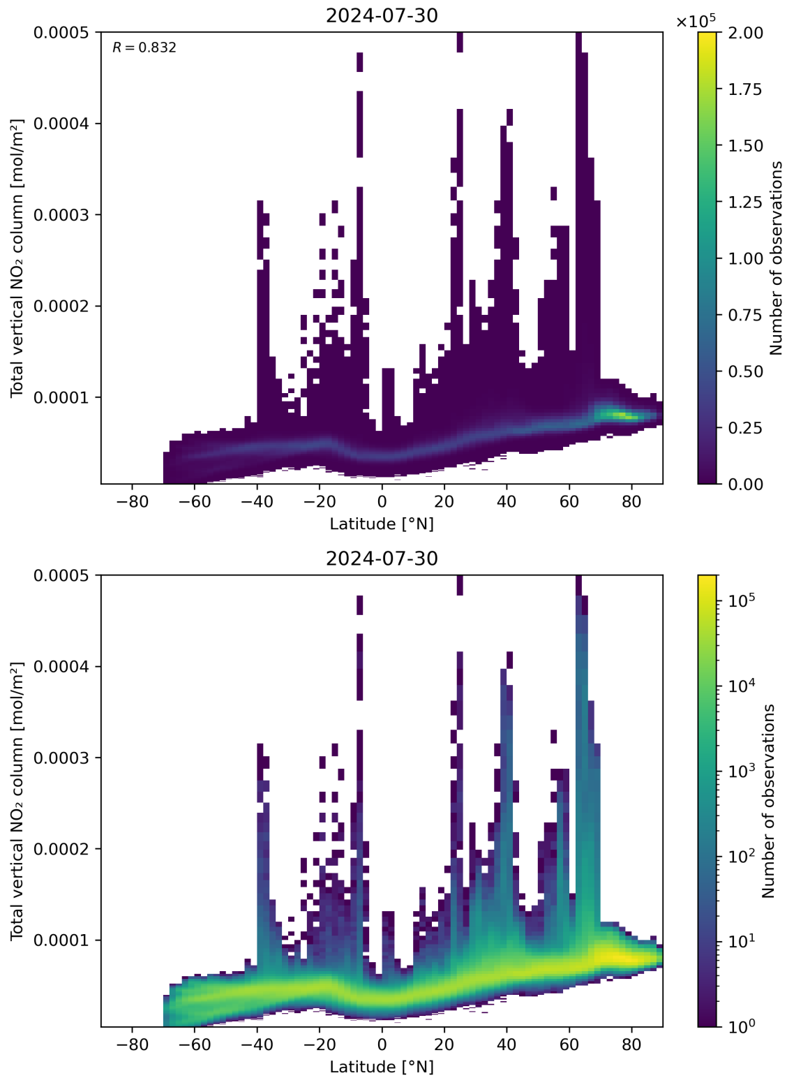
Figure 90: Scatter density plot of “Latitude” against “Total vertical NO 2 column” for 2024-07-29 to 2024-07-31.
