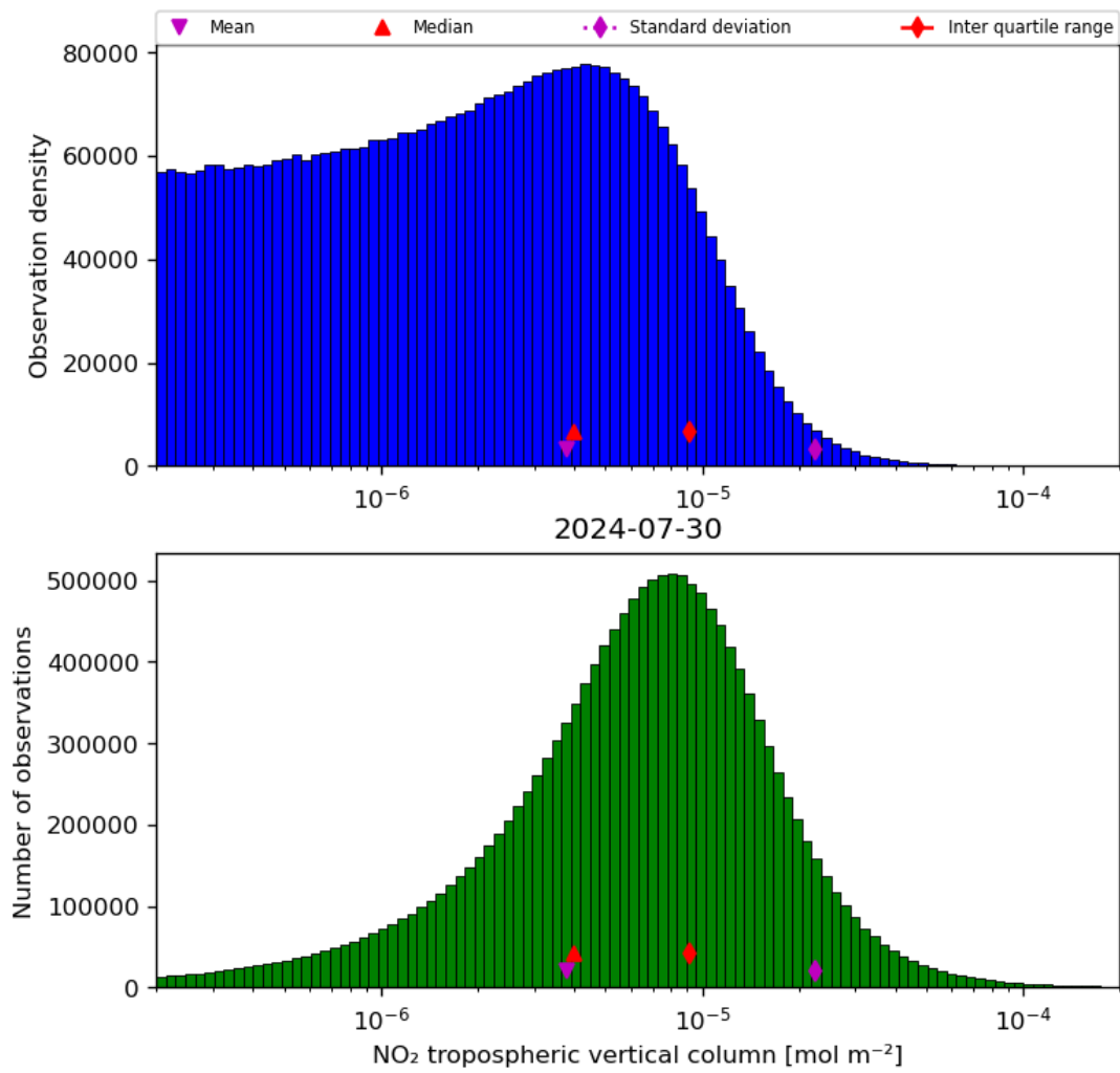
Figure 29: Histogram of “NO 2 tropospheric vertical column” for 2024-07-29 to 2024-07-31
