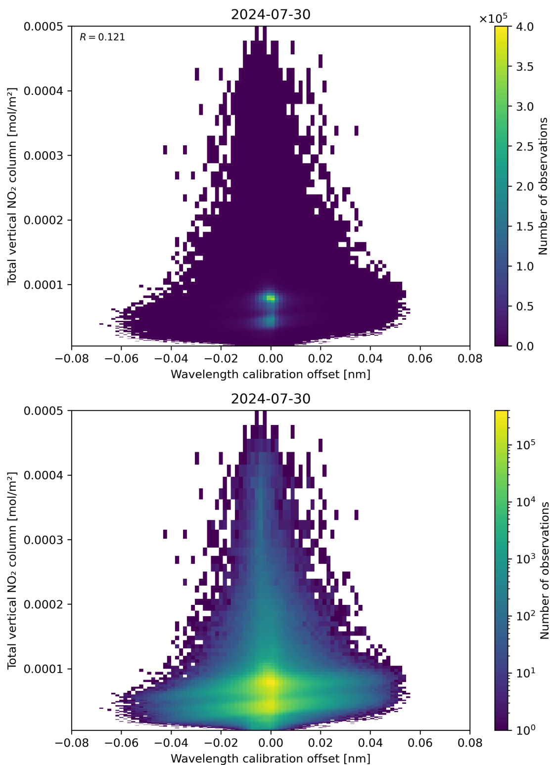
Figure 179: Scatter density plot of “Wavelength calibration offset” against “Total vertical NO 2 column” for 2024-07-29 to 2024-07-31.
