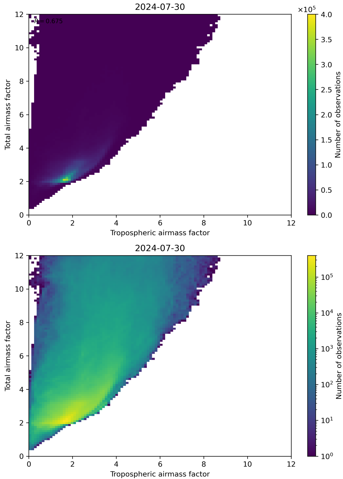
Figure 72: Scatter density plot of “Tropospheric airmass factor” against “Total airmass factor” for 2024-07-29 to 2024-07-31.
