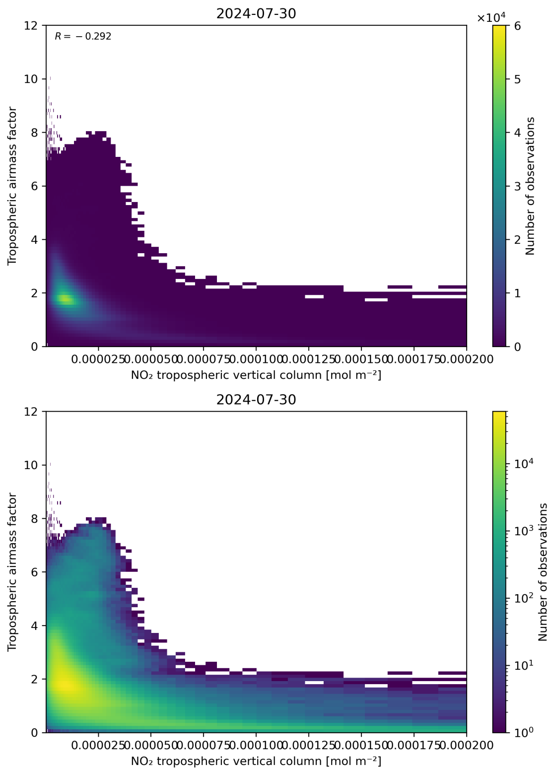
Figure 123: Scatter density plot of “NO 2 tropospheric vertical column” against “Tropospheric air mass factor” for 2024-07-29 to 2024-07-31.
