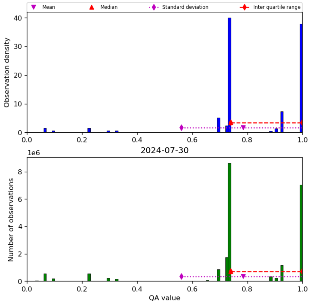
Figure 28: Histogram of “QA value” for 2024-07-29 to 2024-07-31
