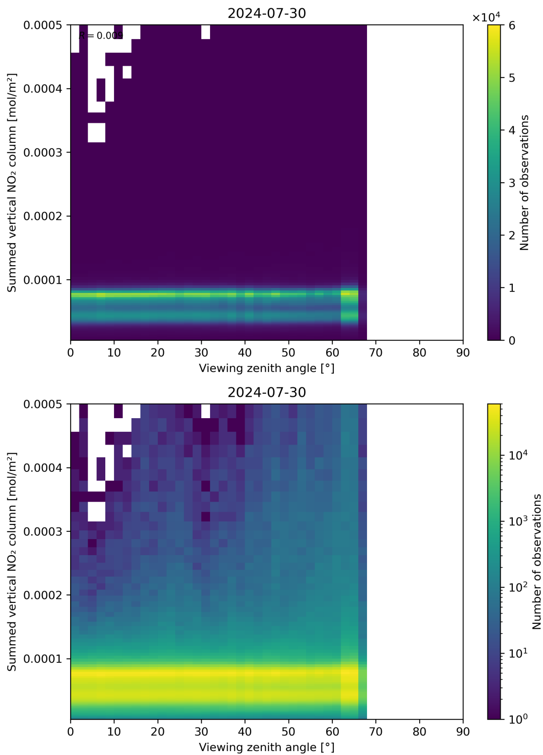
Figure 165: Scatter density plot of “Viewing zenith angle” against “Summed vertical NO 2 column” for 2024-07-29 to 2024-07-31.
