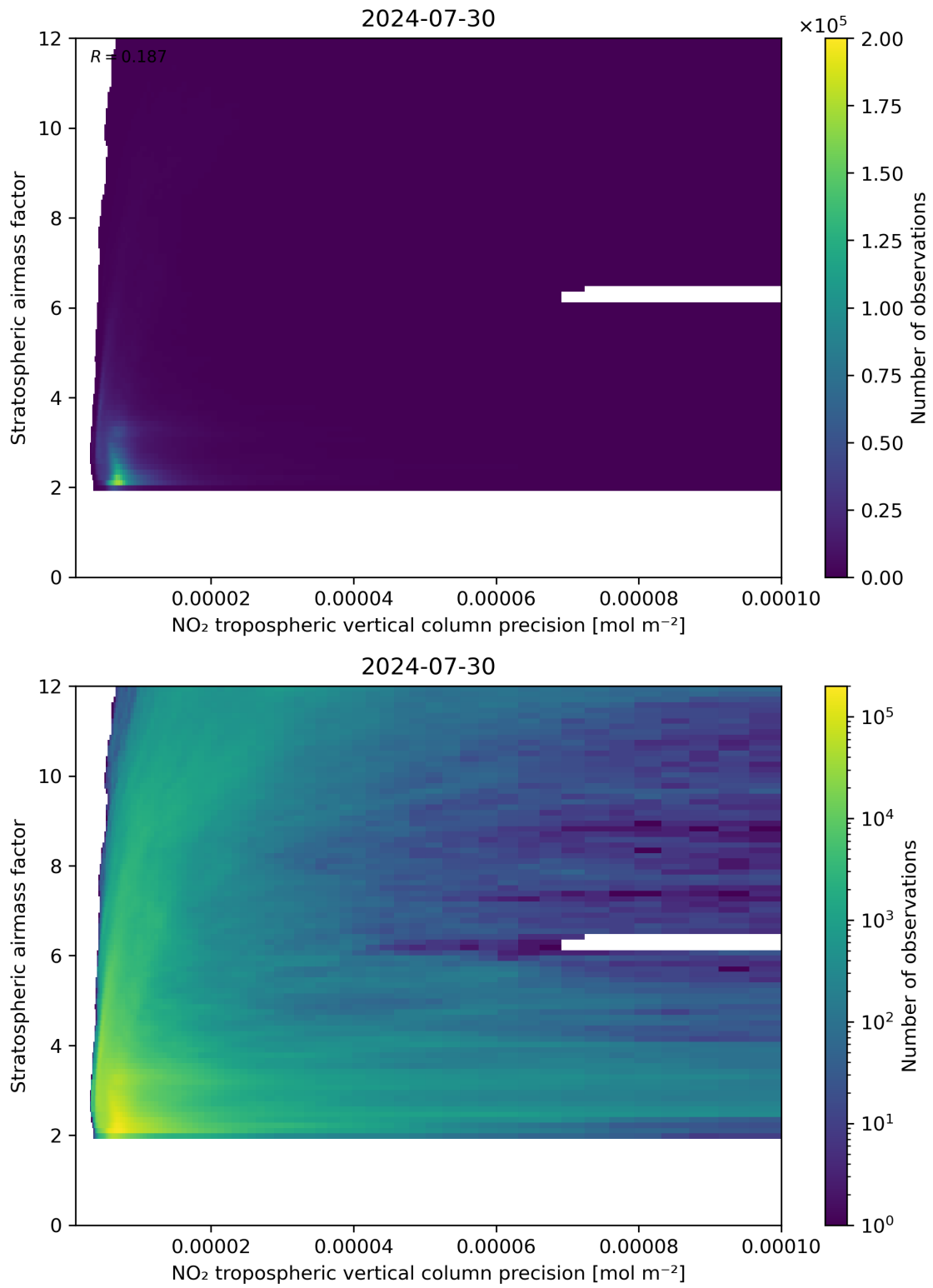
Figure 131: Scatter density plot of “NO 2 tropospheric vertical column precision” against “Stratospheric airmass factor” for 2024-07-29 to 2024-07-31.
