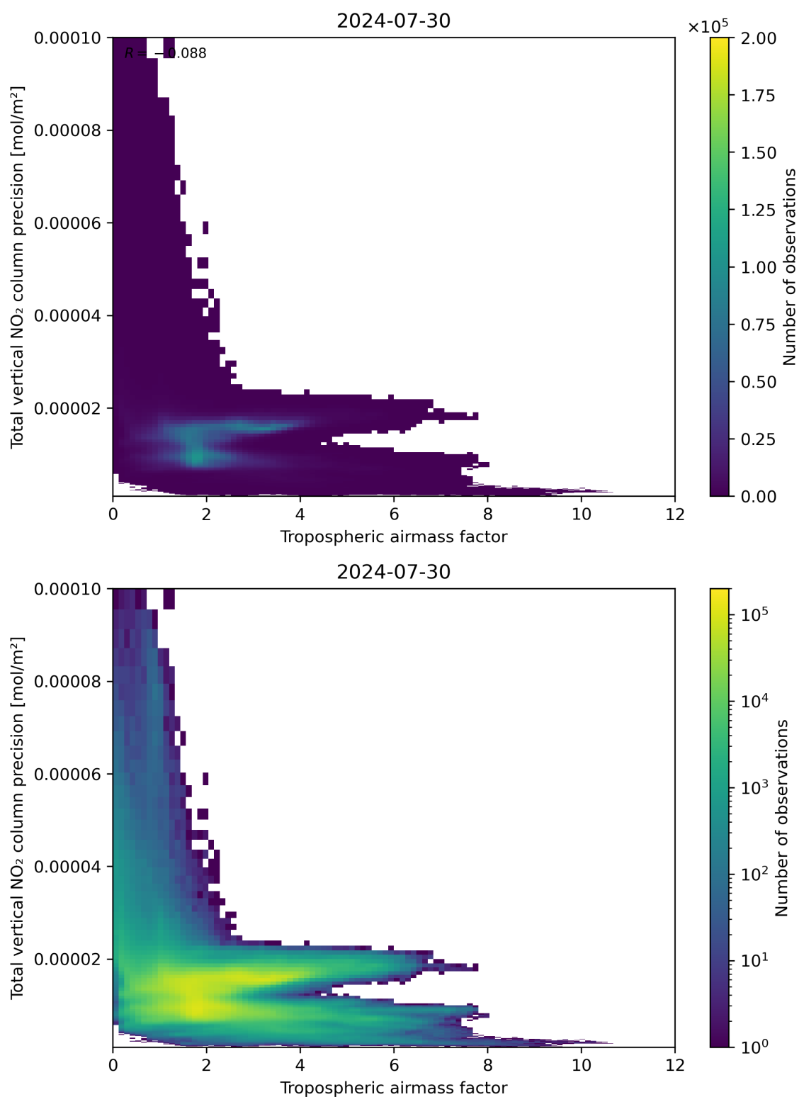
Figure 78: Scatter density plot of “Tropospheric air mass factor” against “Total vertical NO 2 column precision” for 2024-07-29 to 2024-07-31.
