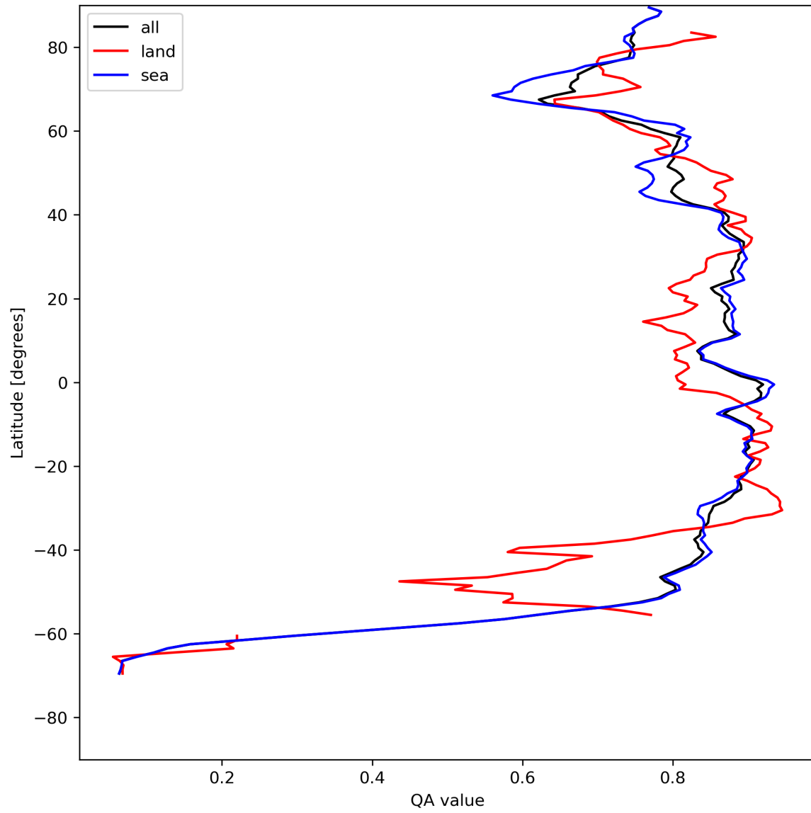
Figure 11: Zonal average of “QA value” for 2024-07-29 to 2024-07-31.
