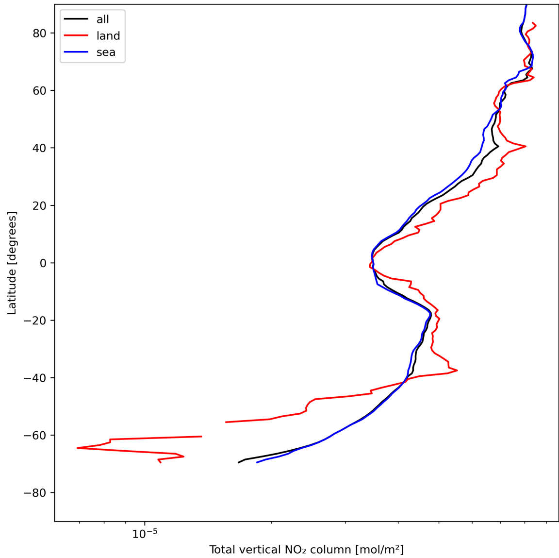
Figure 21: Zonal average of “Total vertical NO 2 column” for 2024-07-29 to 2024-07-31.
