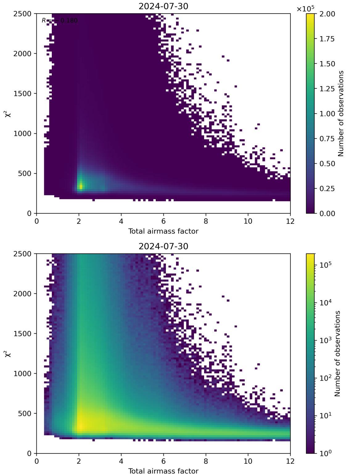
Figure 63: Scatter density plot of “Total airmass factor” against “ \chi^2 ” for 2024-07-29 to 2024-07-31.
