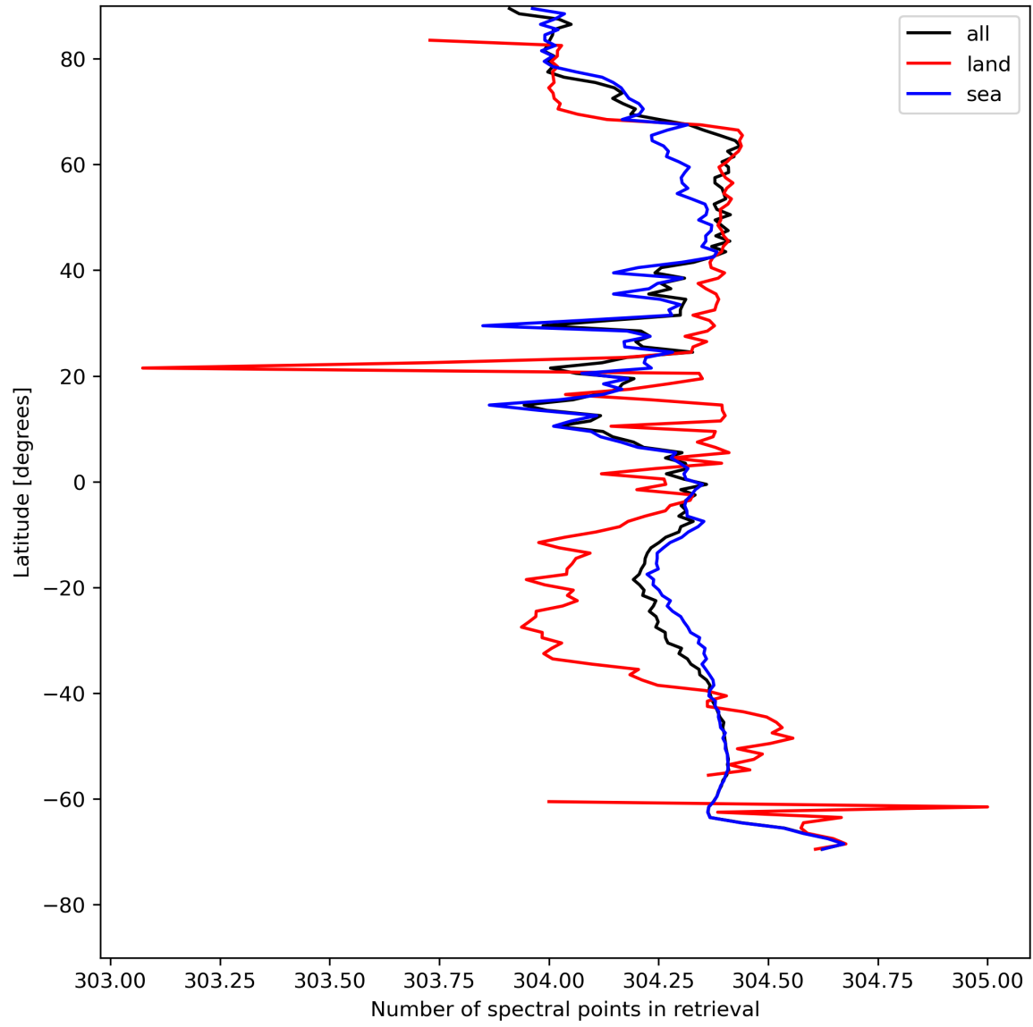
Figure 16: Zonal average of “Number of spectral points in retrieval” for 2024-07-29 to 2024-07-31.
