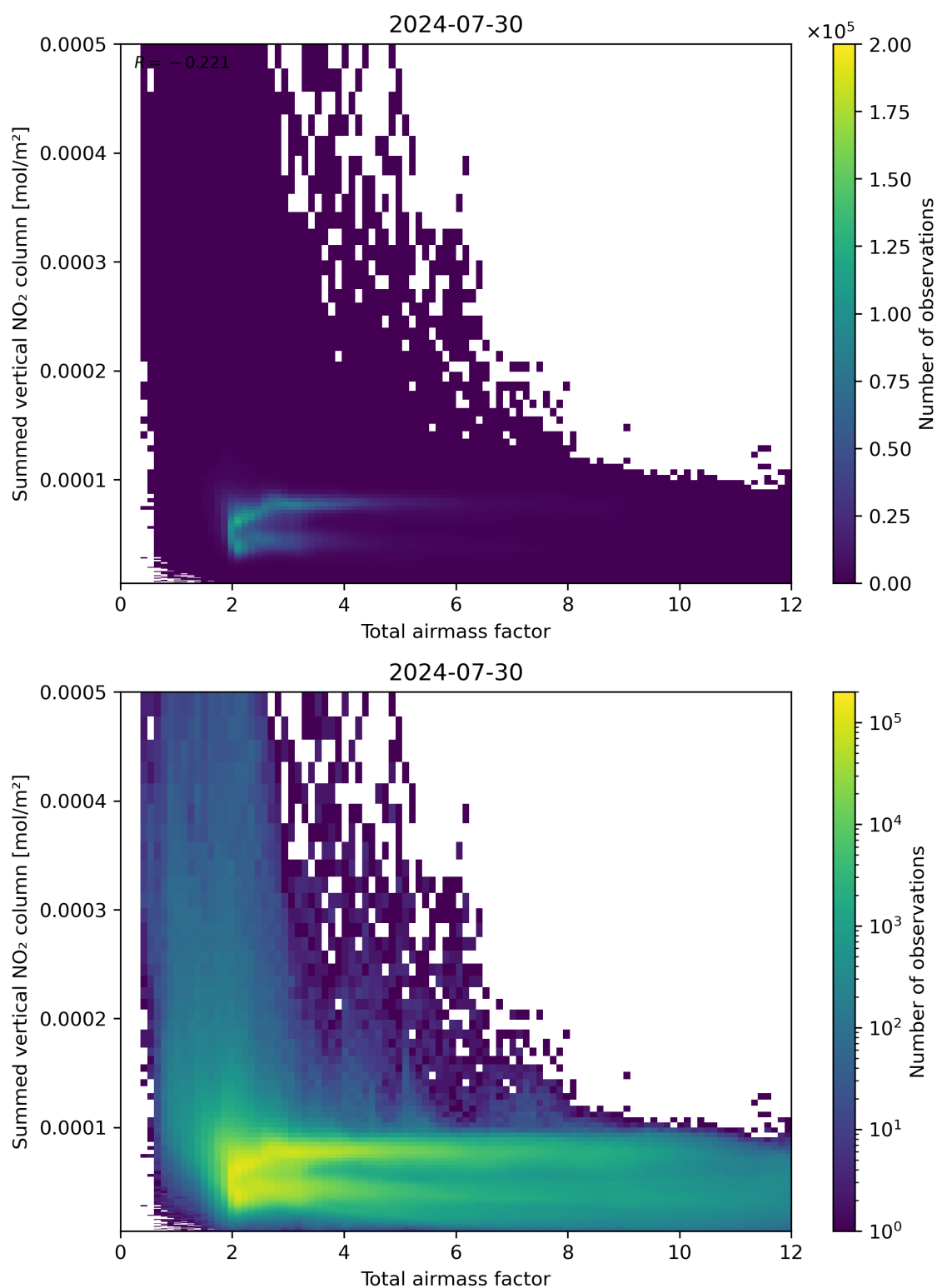
Figure 65: Scatter density plot of “Total airmass factor” against “Summed vertical NO 2 column” for 2024-07-29 to 2024-07-31.
