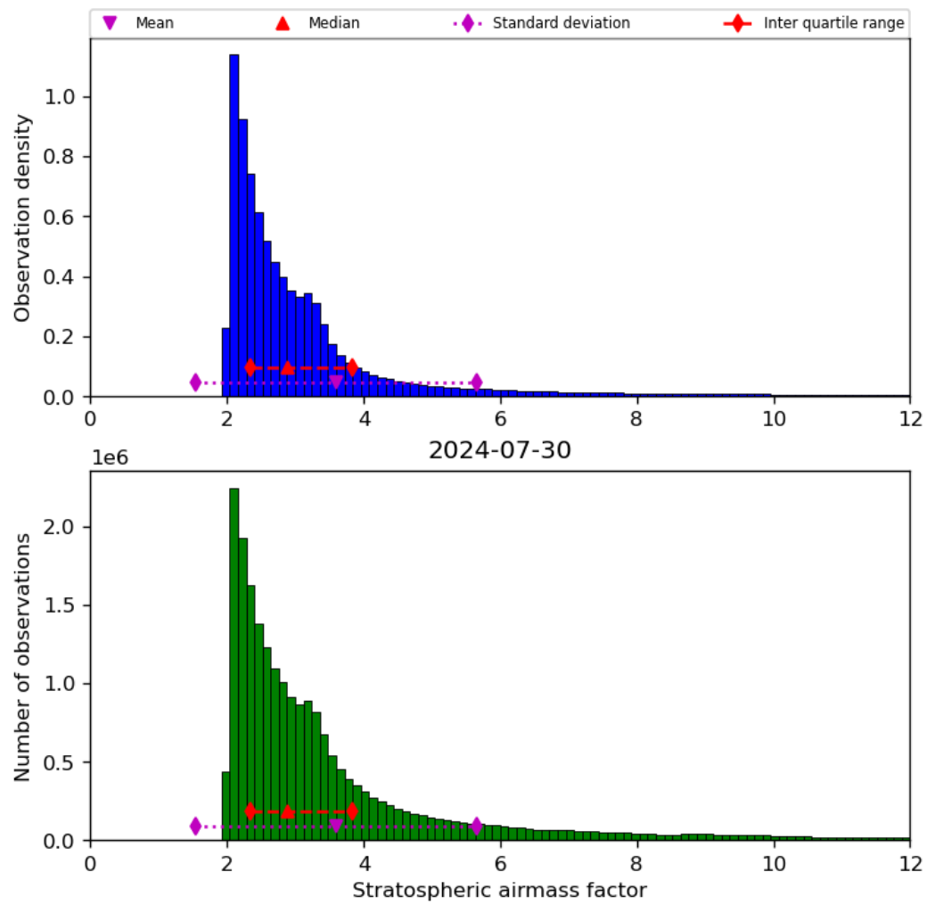
Figure 44: Histogram of “Stratospheric airmass factor” for 2024-07-29 to 2024-07-31
