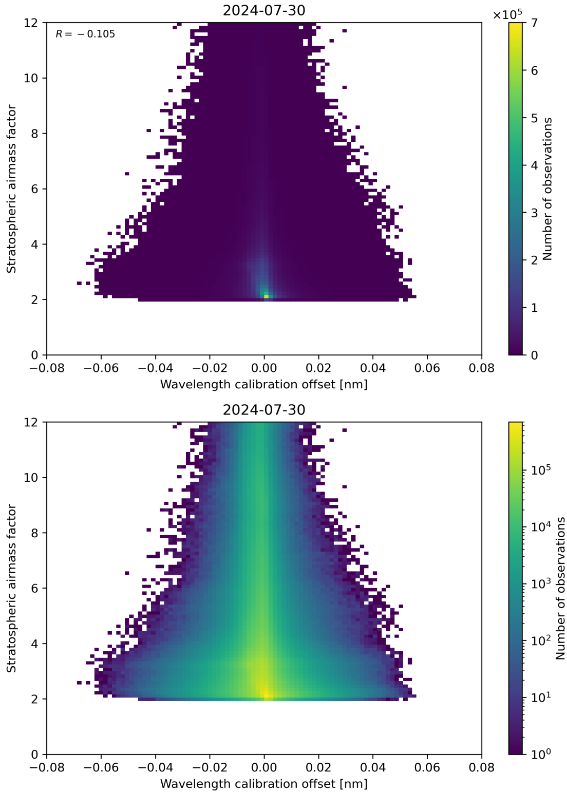
Figure 174: Scatter density plot of “Wavelength calibration offset” against “Stratospheric air mass factor” for 2024-07-29 to 2024-07-31.
