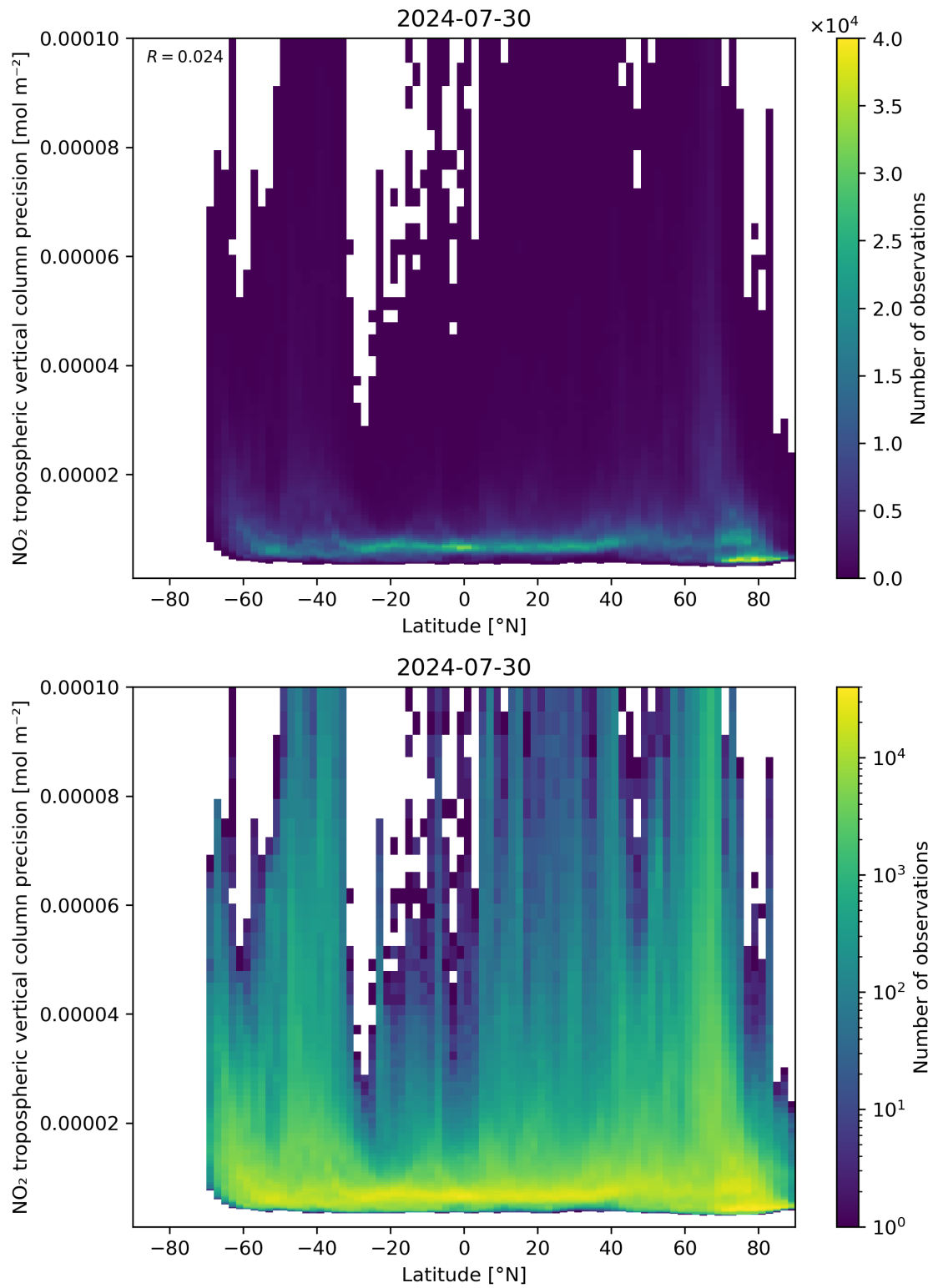
Figure 93: Scatter density plot of “Latitude” against “NO 2 tropospheric vertical column precision” for 2024-07-29 to 2024-07-31.
