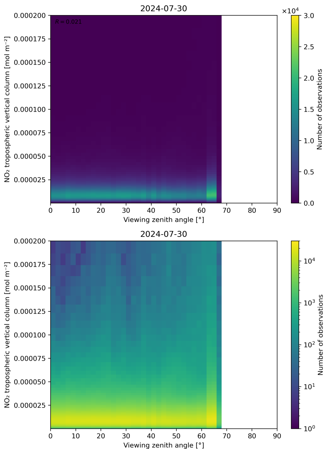
Figure 169: Scatter density plot of “Viewing zenith angle” against “NO 2 tropospheric vertical column” for 2024-07-29 to 2024-07-31.
