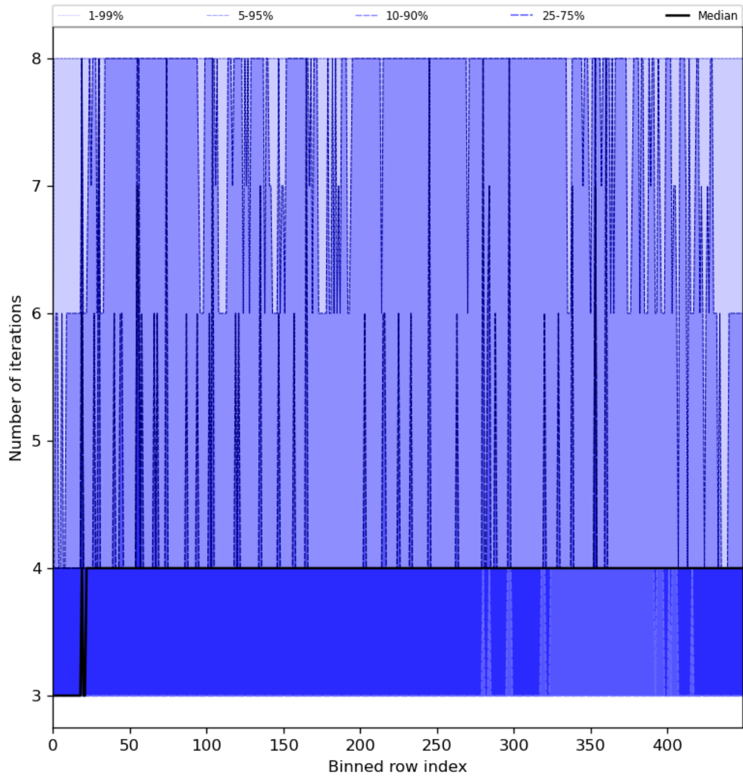
Figure 51: Along track statistics of “Number of iterations” for 2024-07-29 to 2024-07-31
