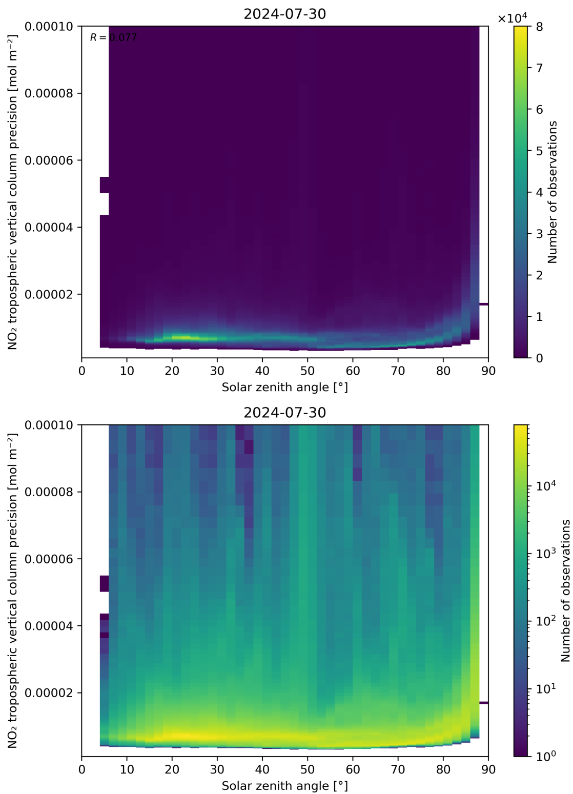
Figure 156: Scatter density plot of “Solar zenith angle” against “NO 2 tropospheric vertical column precision” for 2024-07-29 to 2024-07-31.
