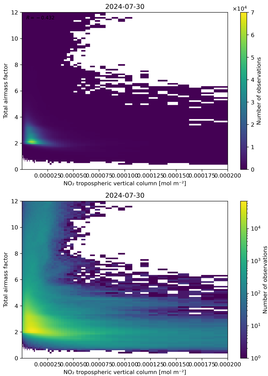
Figure 122: Scatter density plot of “NO 2 tropospheric vertical column” against “Total air mass factor” for 2024-07-29 to 2024-07-31.
