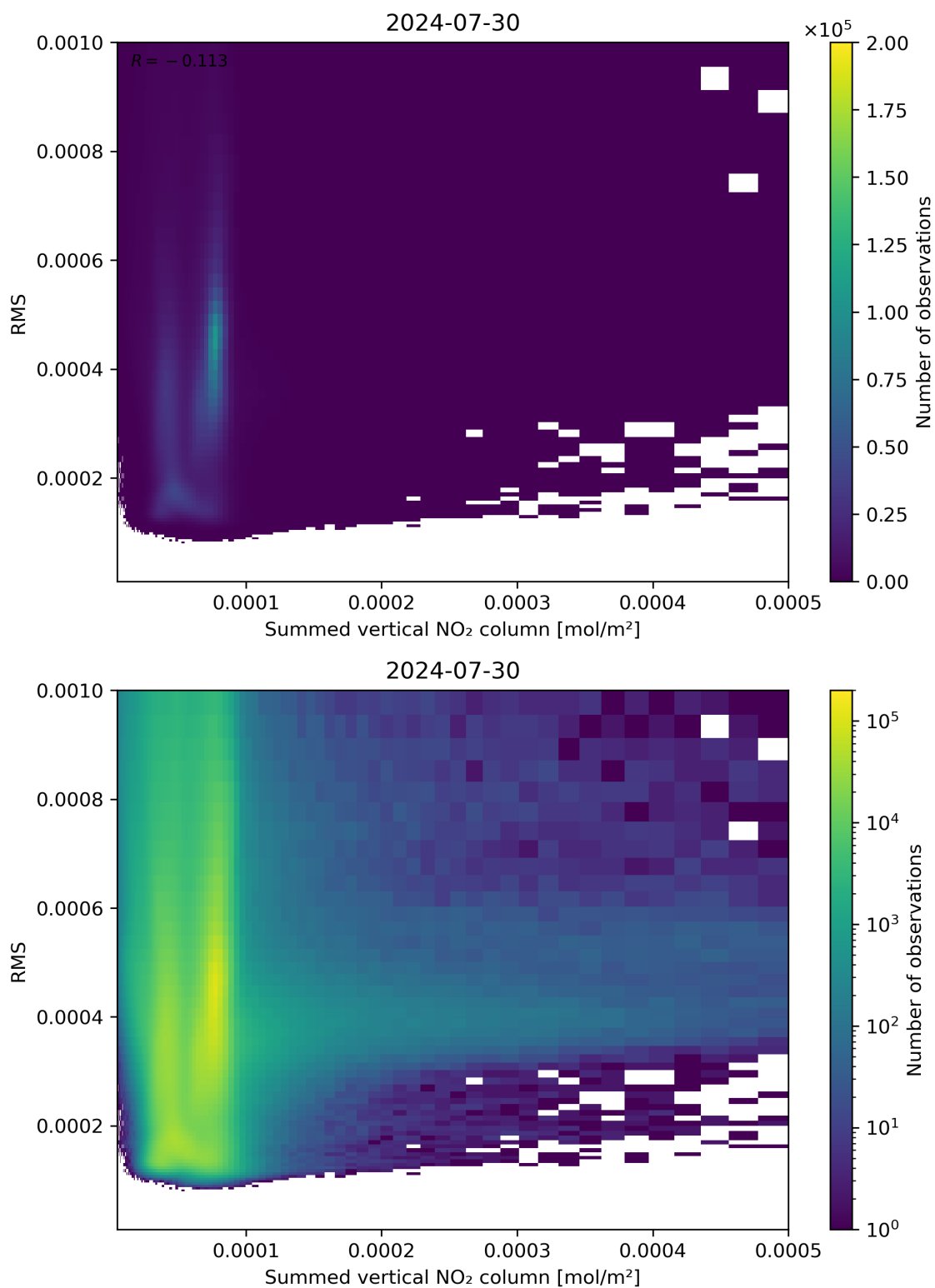
Figure 109: Scatter density plot of “Summed vertical NO 2 column” against “RMS” for 2024-07-29 to 2024-07-31.
