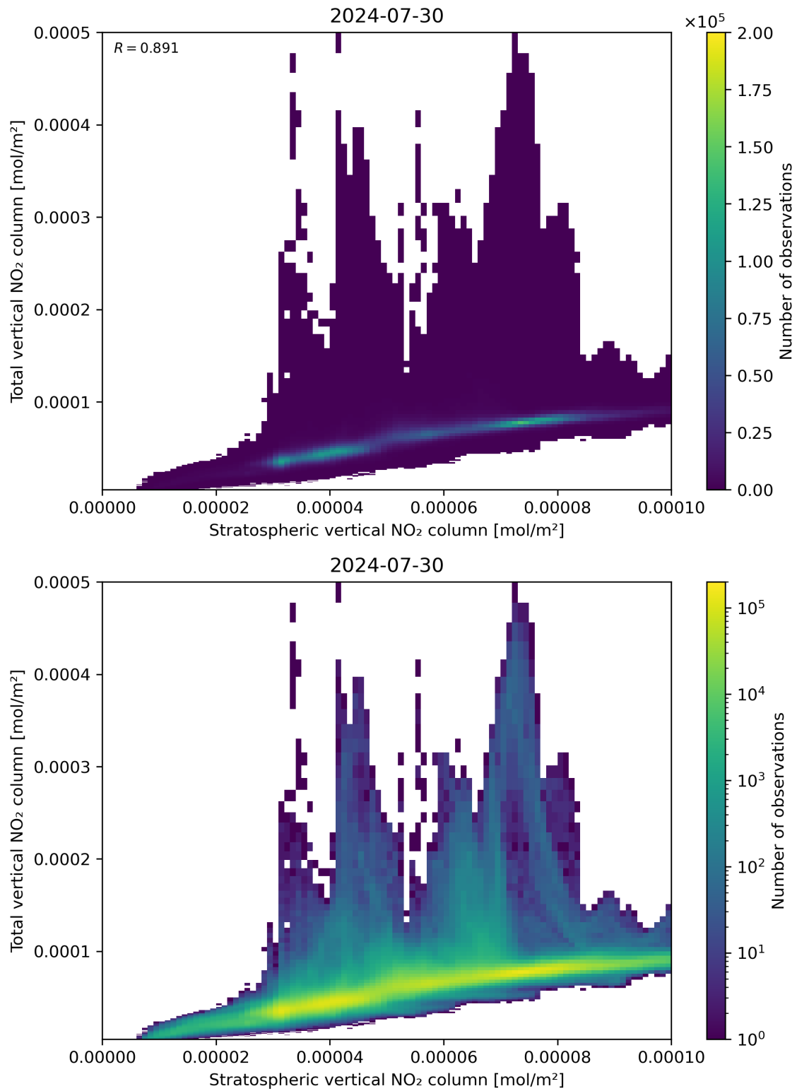
Figure 100: Scatter density plot of “Stratospheric vertical NO 2 column” against “Total vertical NO 2 column” for 2024-07-29 to 2024-07-31.
