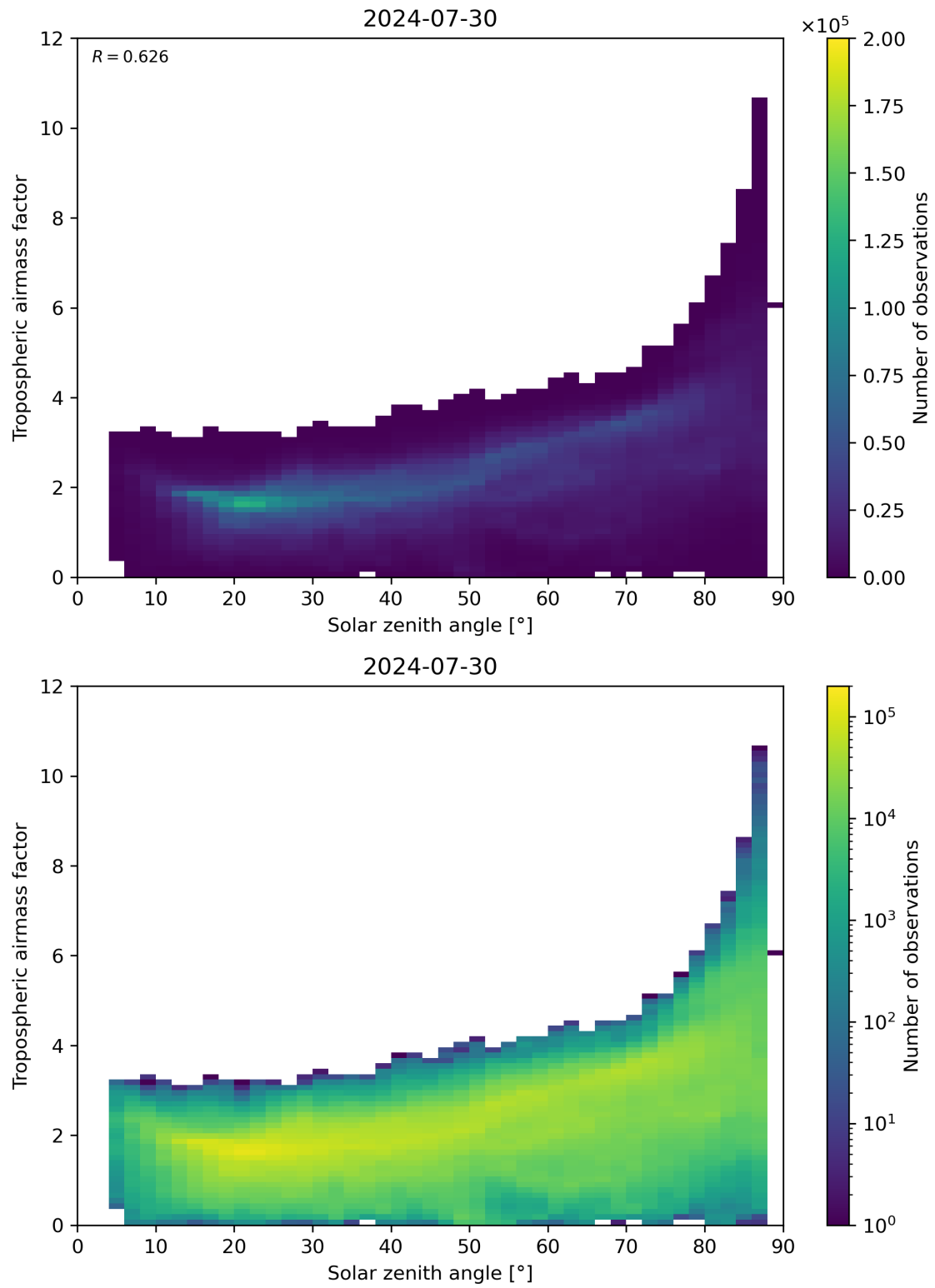
Figure 147: Scatter density plot of “Solar zenith angle” against “Tropospheric airmass factor” for 2024-07-29 to 2024-07-31.
