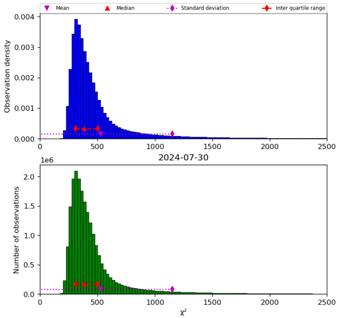
Figure 42: Histogram of “ \chi^2 ” for 2024-07-29 to 2024-07-31
