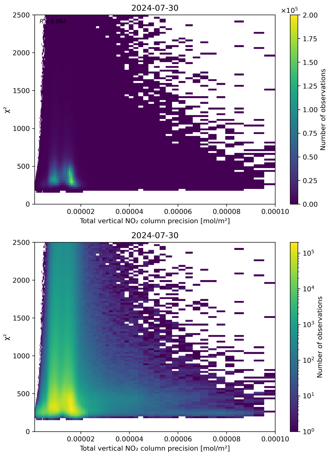
Figure 116: Scatter density plot of “Total vertical NO 2 column precision” against “ \chi^2 ” for 2024-07-29 to 2024-07-31.
