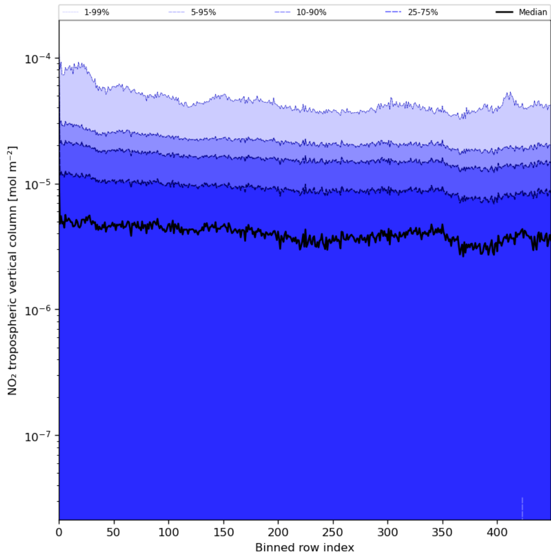
Figure 46: Along track statistics of “NO 2 tropospheric vertical column” for 2024-07-29 to 2024-07-31
