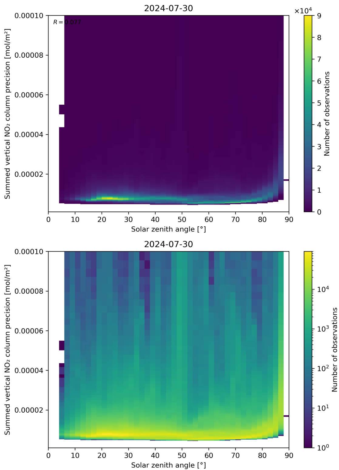
Figure 152: Scatter density plot of “Solar zenith angle” against “Summed vertical NO 2 column precision” for 2024-07-29 to 2024-07-31.
