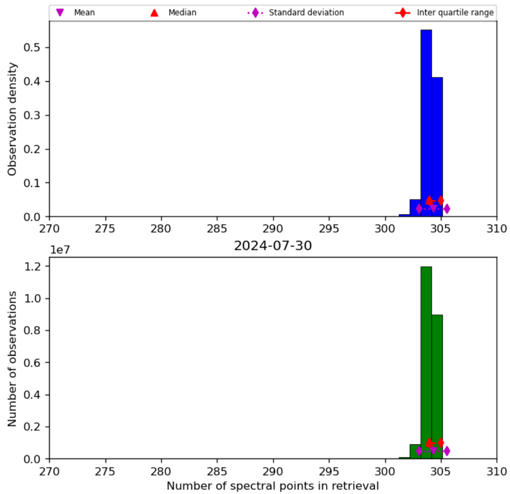
Figure 33: Histogram of “Number of spectral points in retrieval” for 2024-07-29 to 2024-07-31
