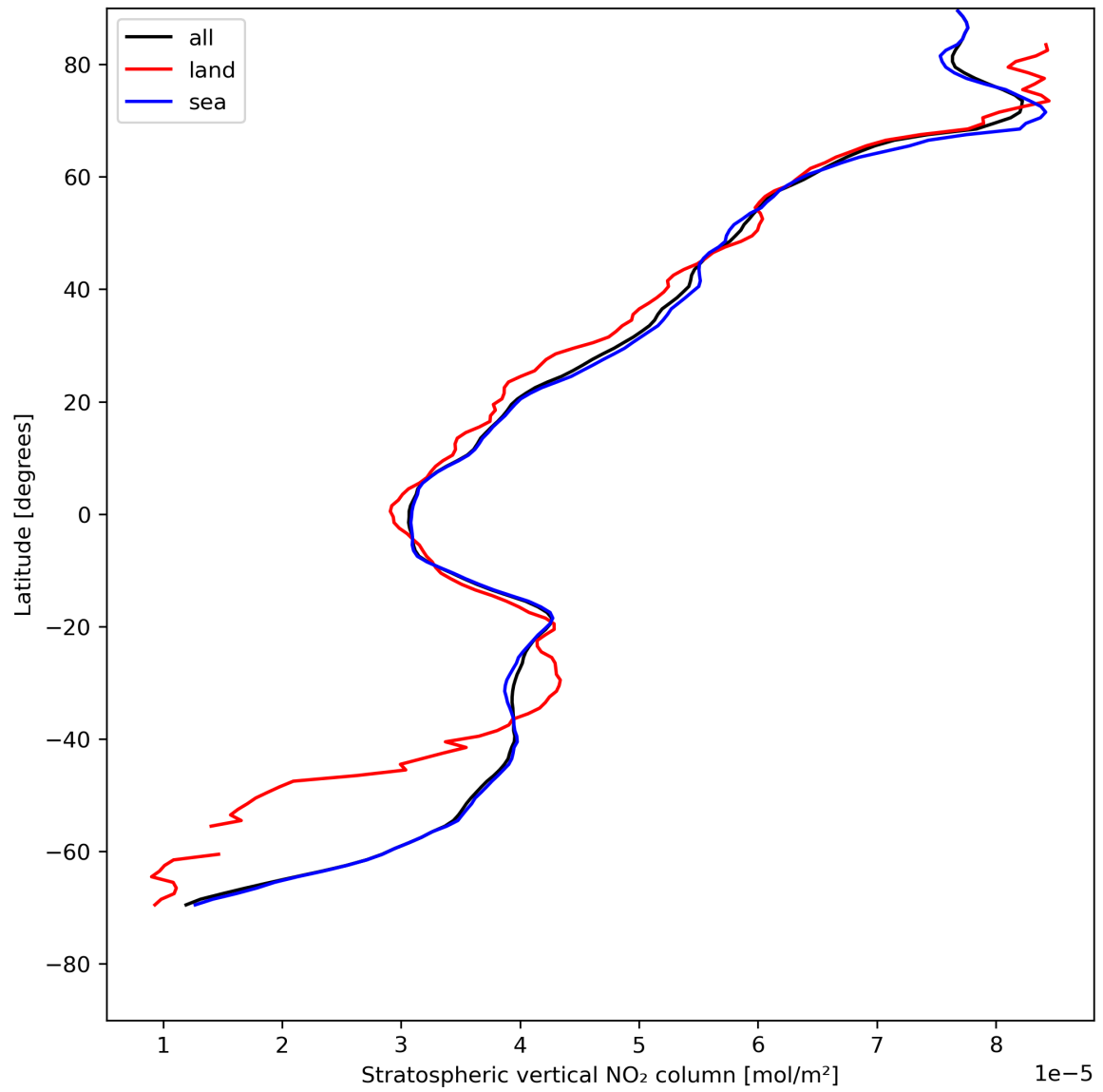
Figure 19: Zonal average of “Stratospheric vertical NO 2 column” for 2024-07-29 to 2024-07-31.
