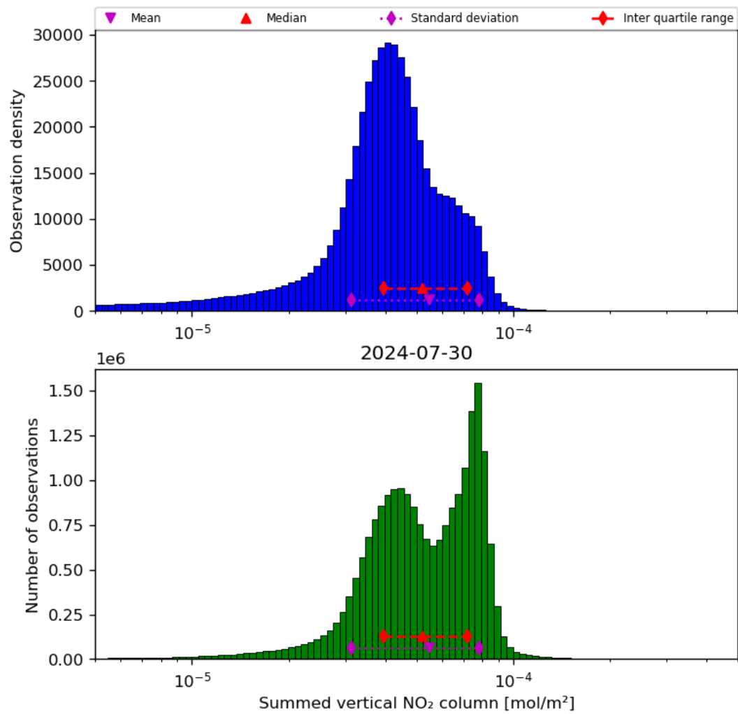
Figure 40: Histogram of “Summed vertical NO 2 column” for 2024-07-29 to 2024-07-31
