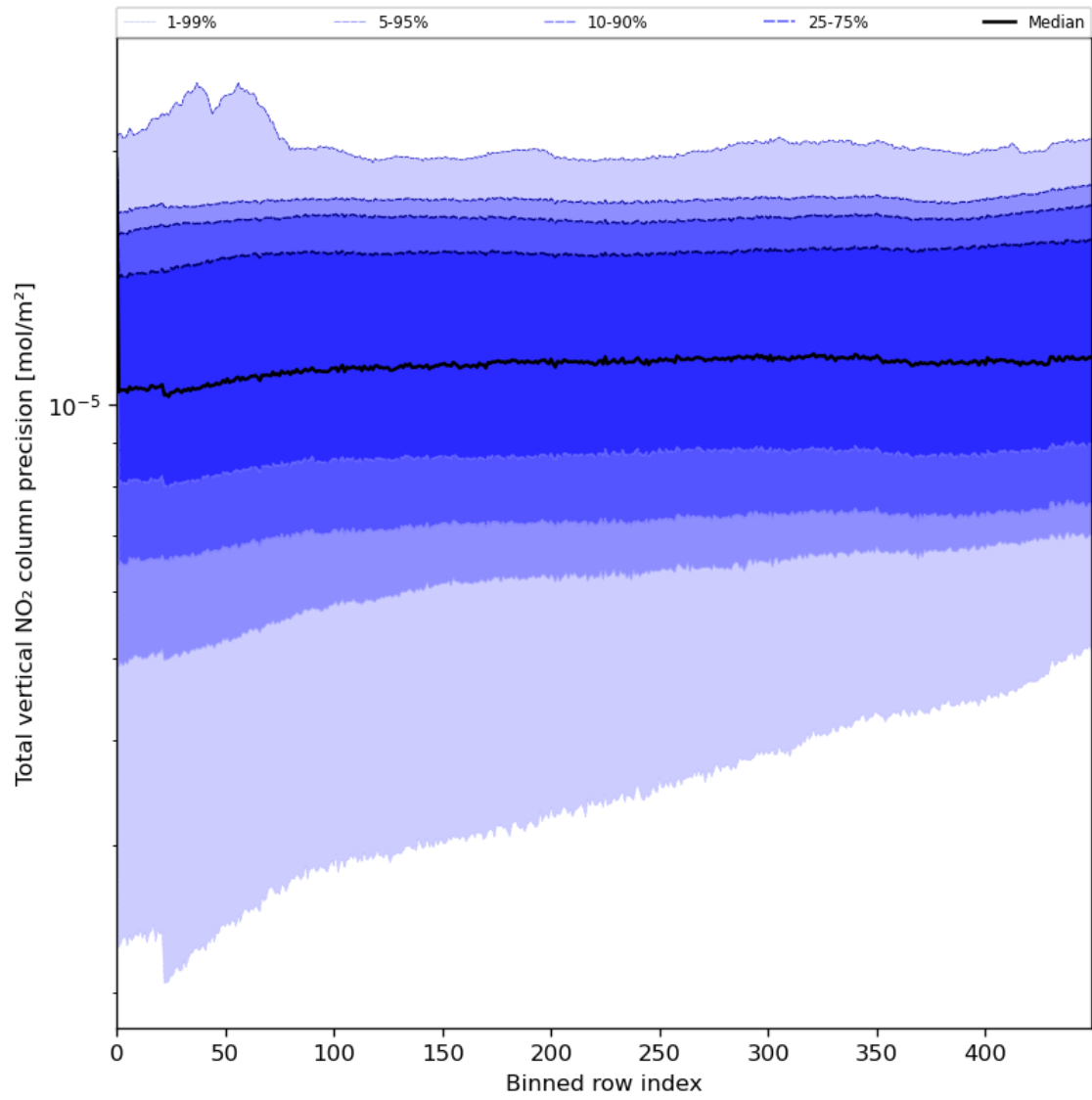
Figure 56: Along track statistics of “Total vertical NO 2 column precision” for 2024-07-29 to 2024-07-31
