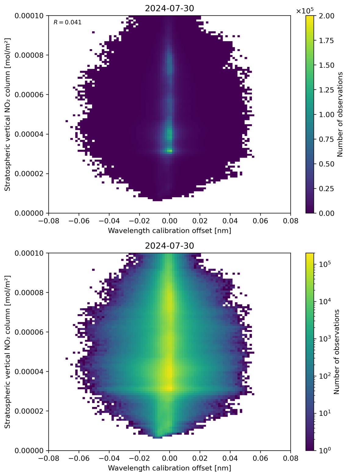
Figure 176: Scatter density plot of “Wavelength calibration offset” against “Stratospheric vertical NO 2 column” for 2024-07-29 to 2024-07-31.
