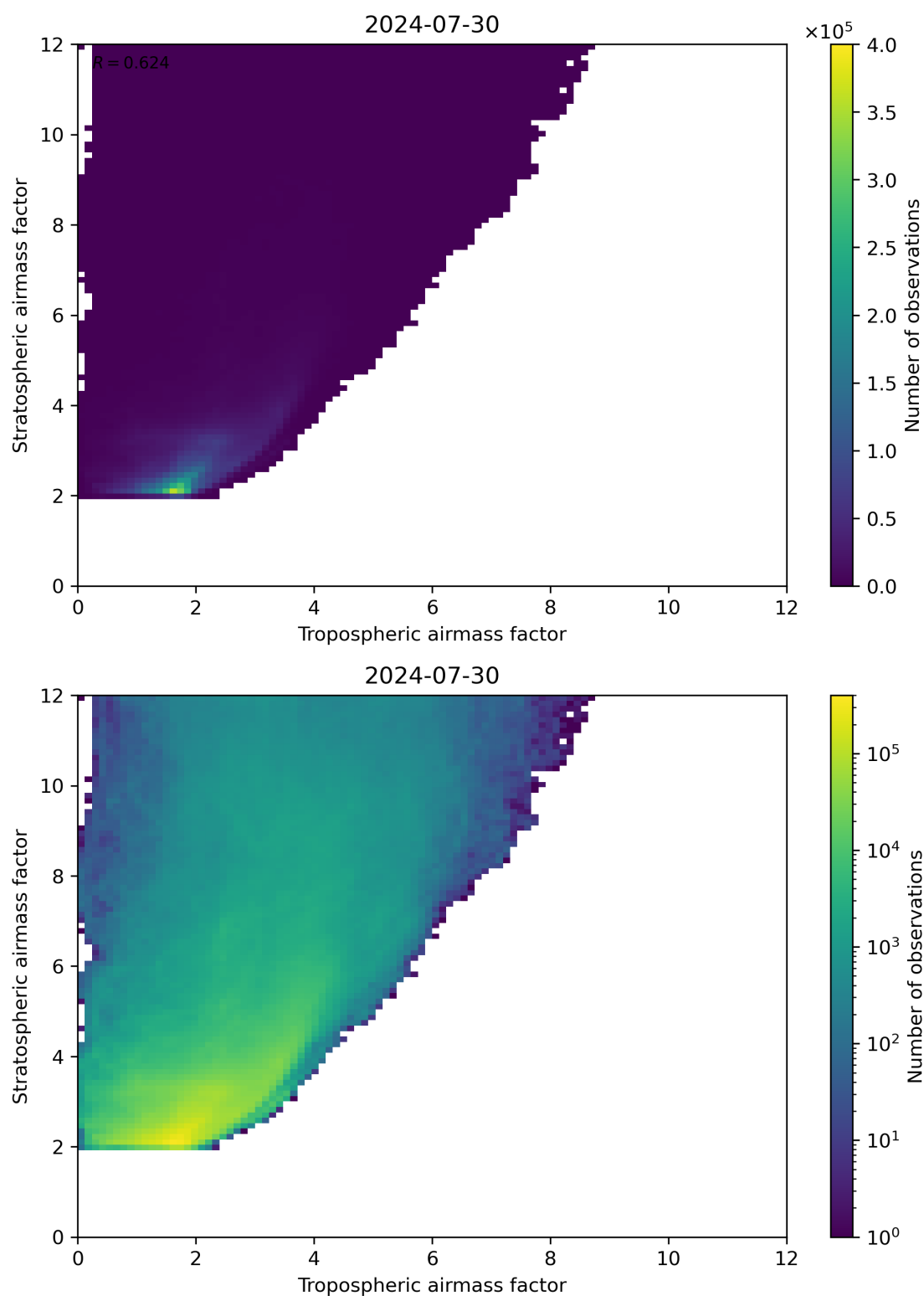
Figure 71: Scatter density plot of “Tropospheric airmass factor” against “Stratospheric airmass factor” for 2024-07-29 to 2024-07-31.
