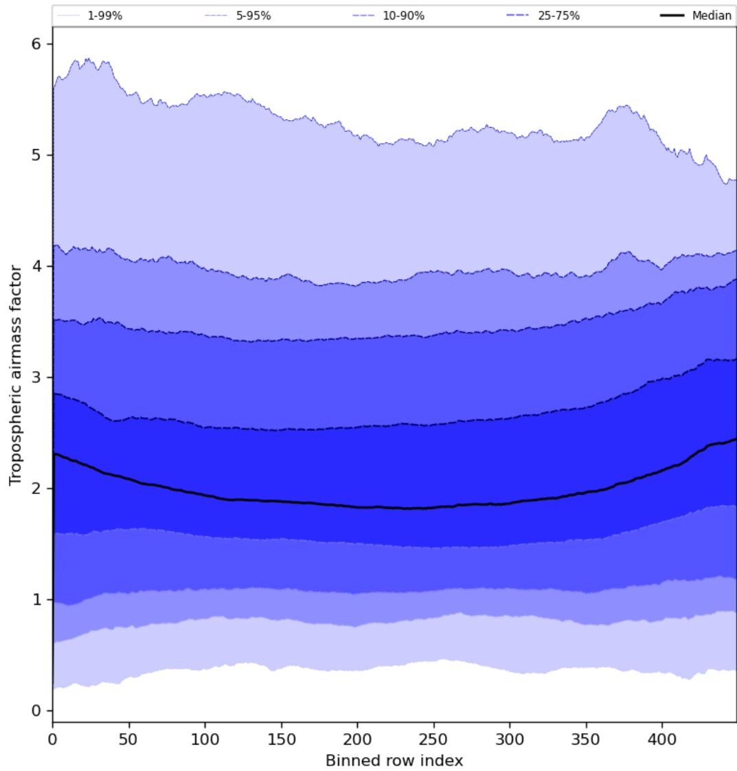
Figure 48: Along track statistics of “Tropospheric airmass factor” for 2024-07-29 to 2024-07-31
