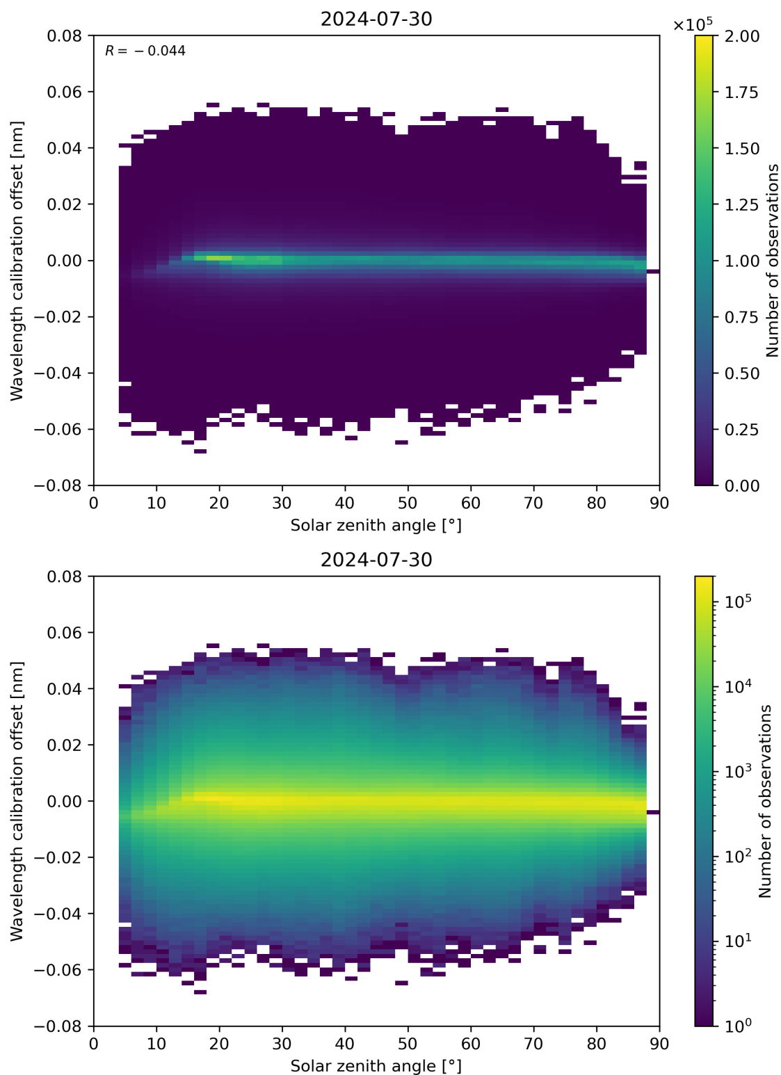
Figure 158: Scatter density plot of “Solar zenith angle” against “Wavelength calibration offset” for 2024-07-29 to 2024-07-31.
