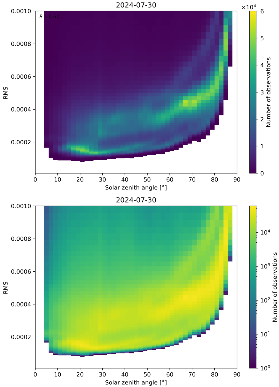
Figure 157: Scatter density plot of “Solar zenith angle” against “RMS” for 2024-07-29 to 2024-07-31.
