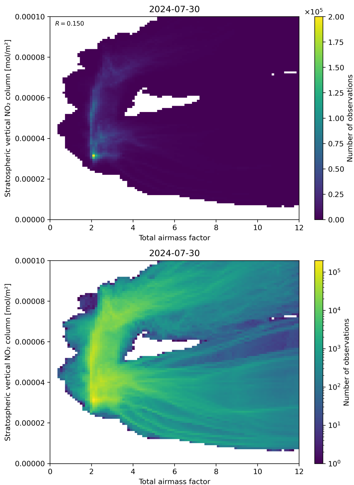
Figure 64: Scatter density plot of “Total airmass factor” against “Stratospheric vertical NO 2 column” for 2024-07-29 to 2024-07-31.
