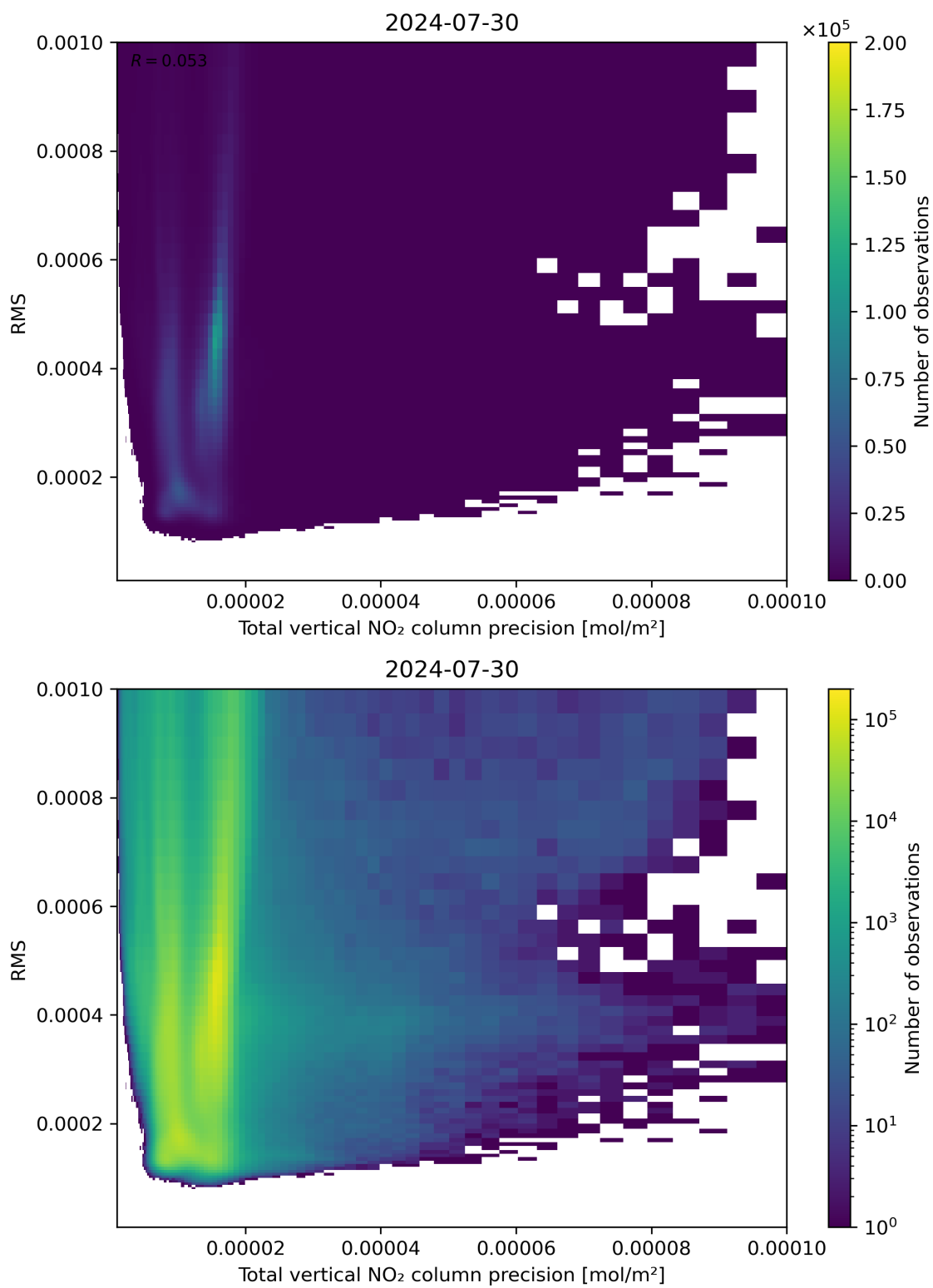
Figure 119: Scatter density plot of “Total vertical NO 2 column precision” against “RMS” for 2024-07-29 to 2024-07-31.
