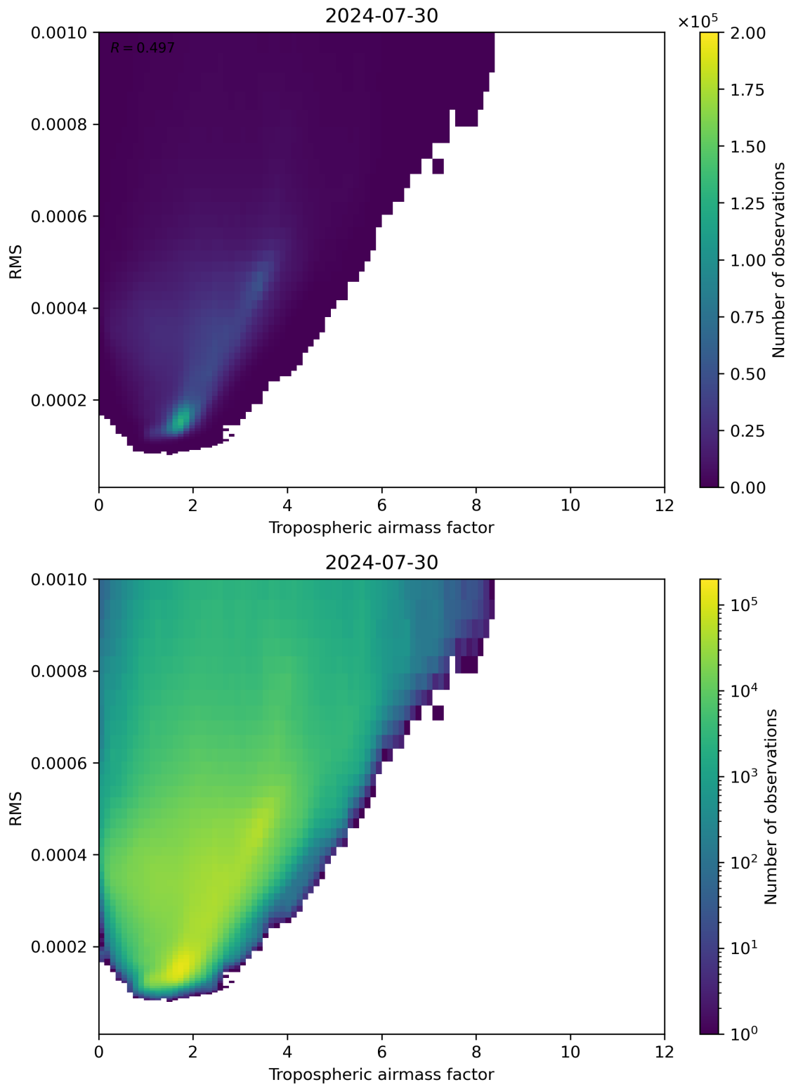
Figure 79: Scatter density plot of “Tropospheric airmass factor” against “RMS” for 2024-07-29 to 2024-07-31.
