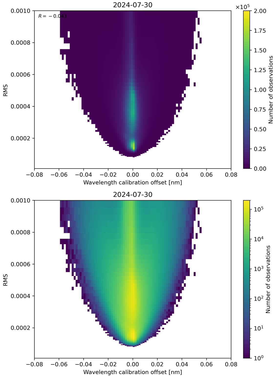
Figure 181: Scatter density plot of “Wavelength calibration offset” against “RMS” for 2024-07-29 to 2024-07-31.
