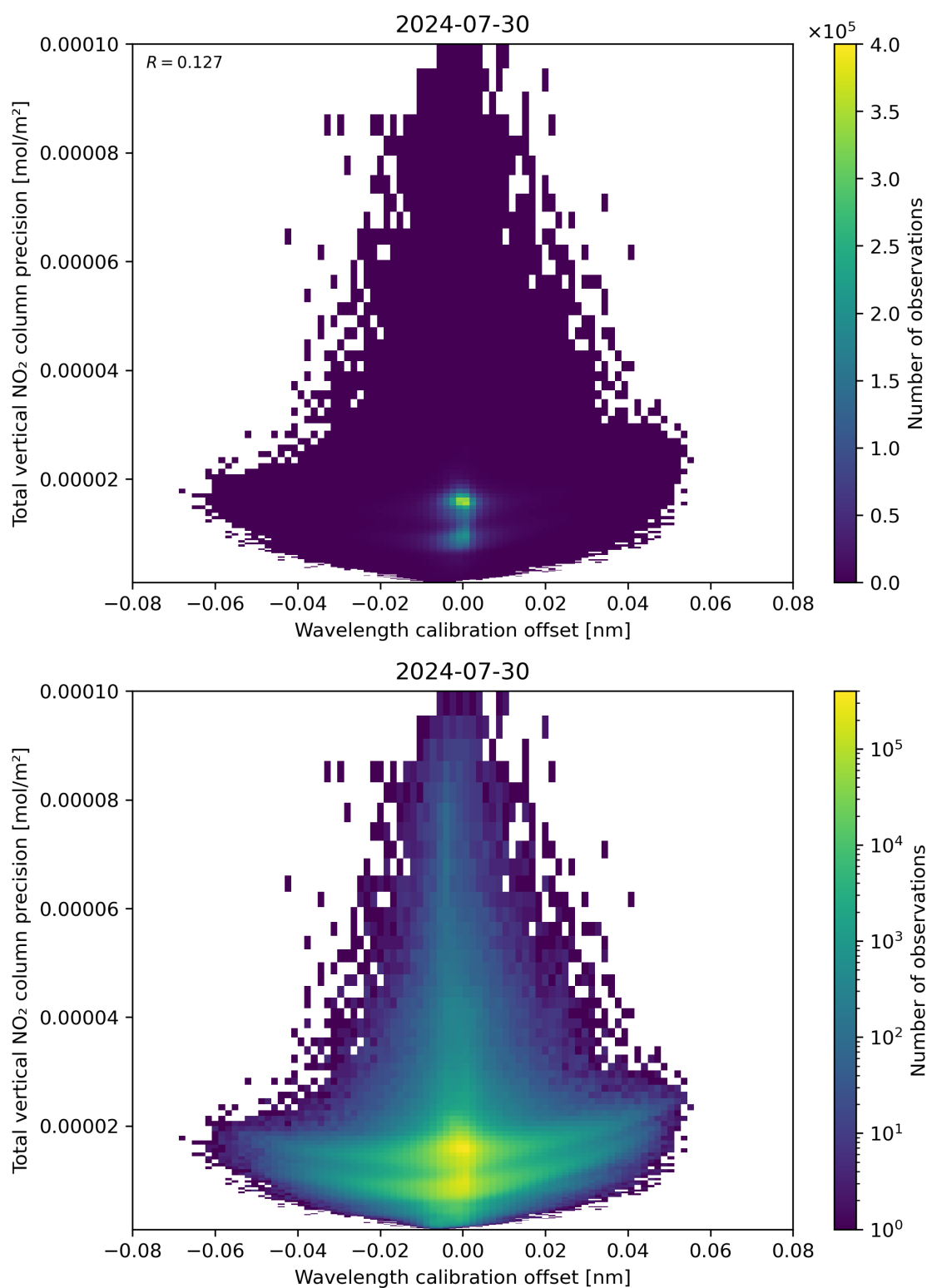
Figure 180: Scatter density plot of “Wavelength calibration offset” against “Total vertical NO 2 column precision” for 2024-07-29 to 2024-07-31.
