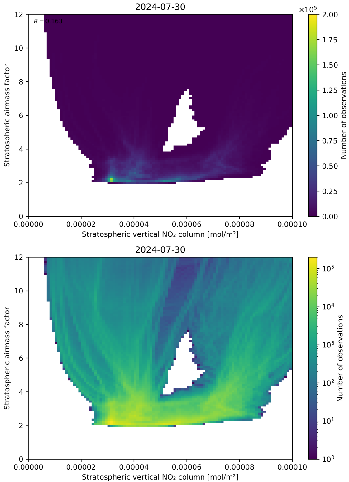
Figure 96: Scatter density plot of “Stratospheric vertical NO 2 column” against “Stratospheric airmass factor” for 2024-07-29 to 2024-07-31.
