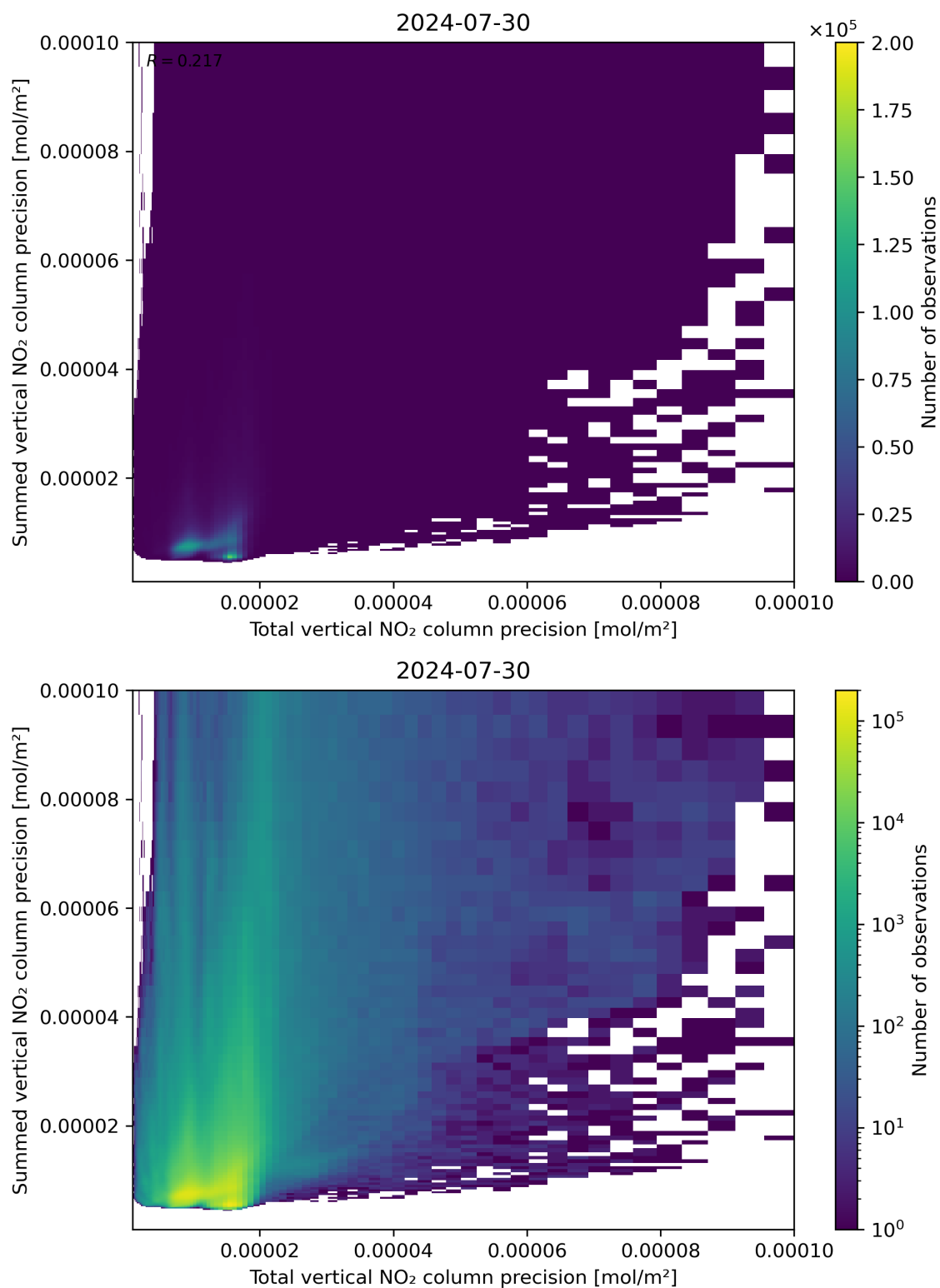
Figure 118: Scatter density plot of “Total vertical NO 2 column precision” against “Summed vertical NO 2 column precision” for 2024-07-29 to 2024-07-31.
