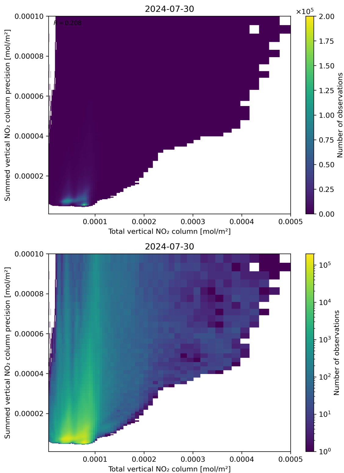
Figure 113: Scatter density plot of “Total vertical NO 2 column” against “Summed vertical NO 2 column precision” for 2024-07-29 to 2024-07-31.
