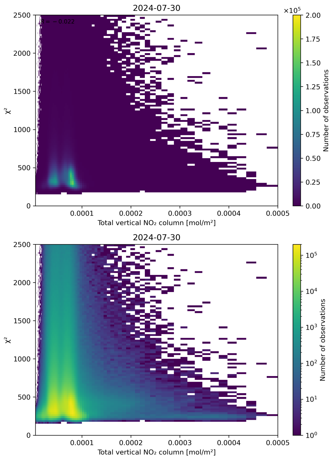
Figure 111: Scatter density plot of “Total vertical NO 2 column” against “ \chi^2 ” for 2024-07-29 to 2024-07-31.
