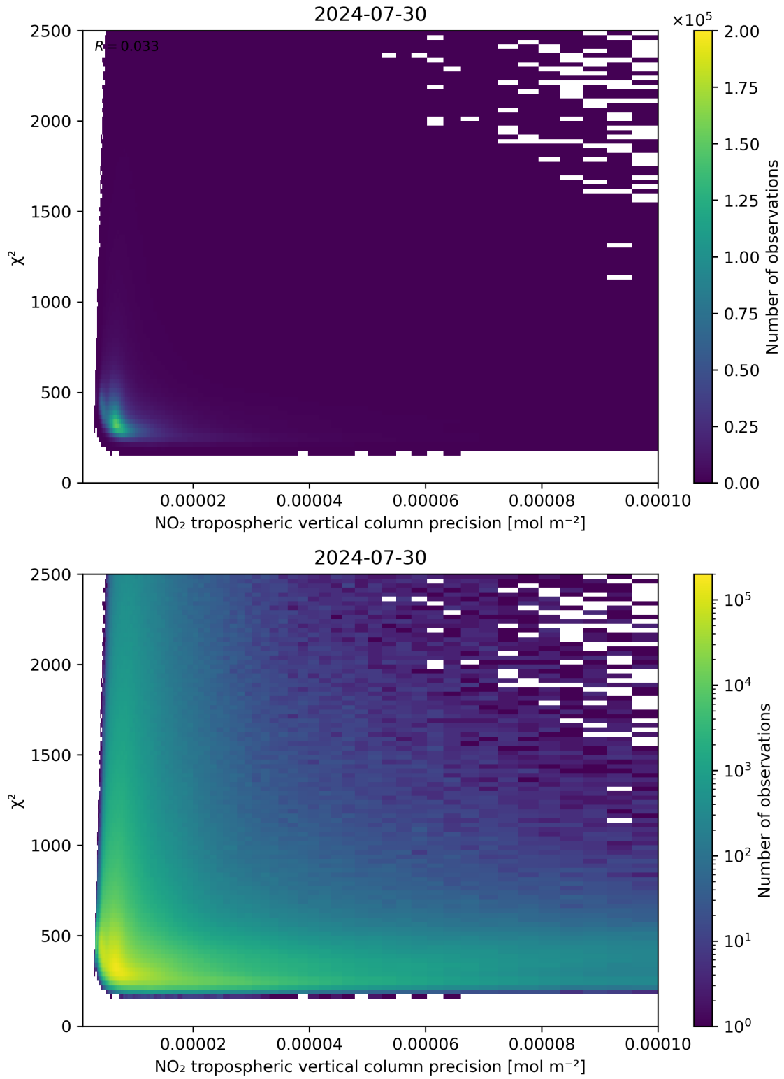
Figure 134: Scatter density plot of “NO 2 tropospheric vertical column precision” against “ \chi^2 ” for 2024-07-29 to 2024-07-31.
