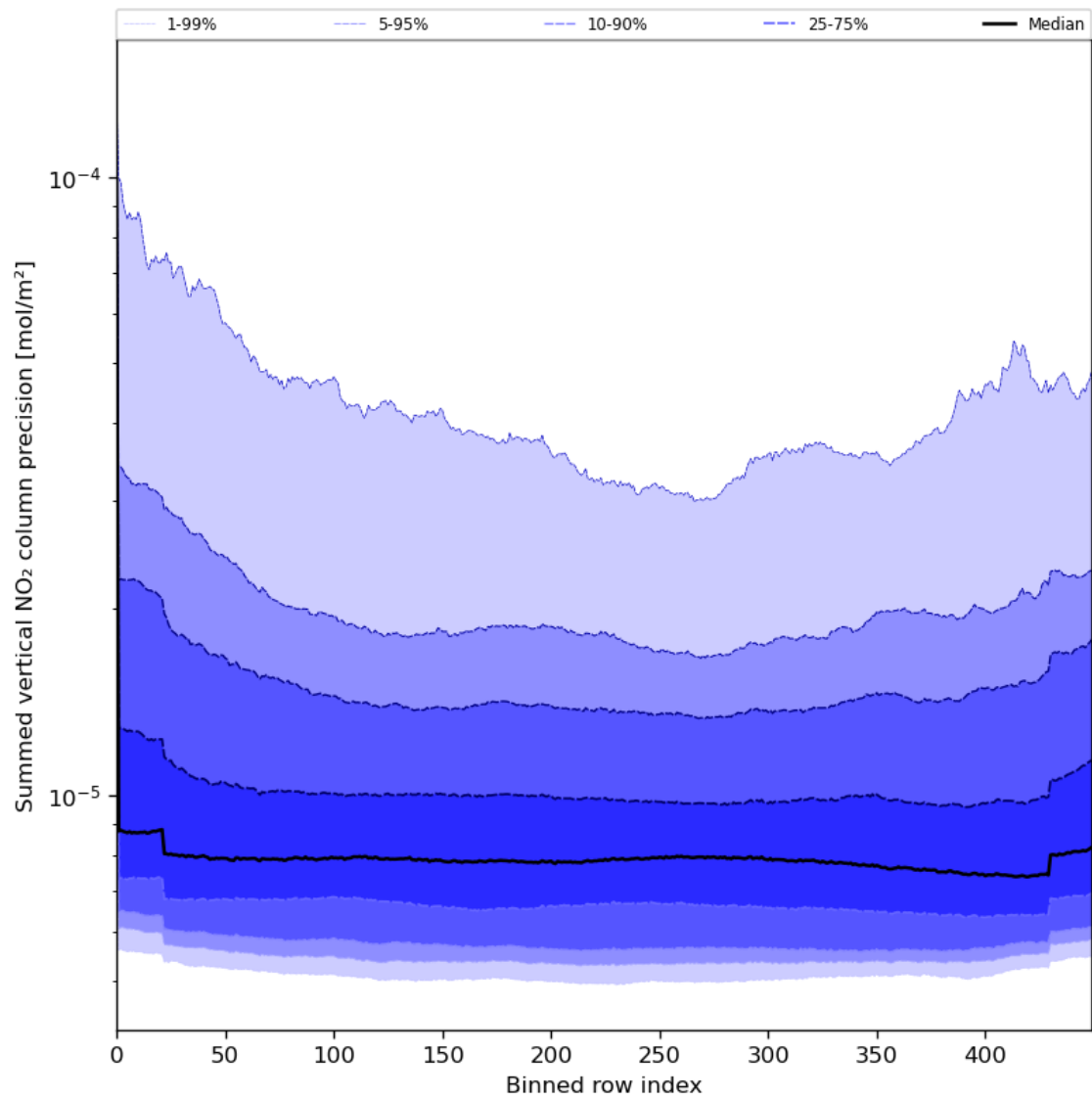
Figure 58: Along track statistics of “Summed vertical NO 2 column precision” for 2024-07-29 to 2024-07-31
