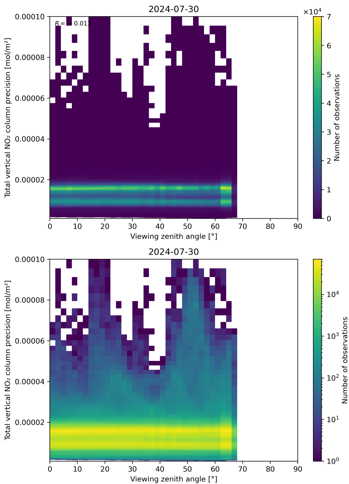
Figure 168: Scatter density plot of “Viewing zenith angle” against “Total vertical NO 2 column precision” for 2024-07-29 to 2024-07-31.
