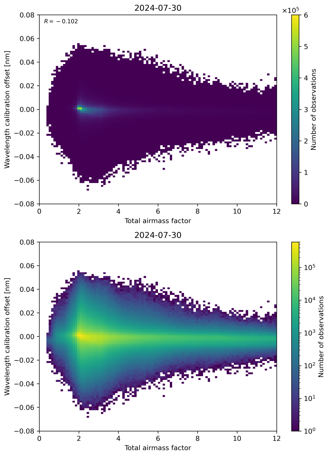
Figure 70: Scatter density plot of “Total airmass factor” against “Wavelength calibration offset” for 2024-07-29 to 2024-07-31.
