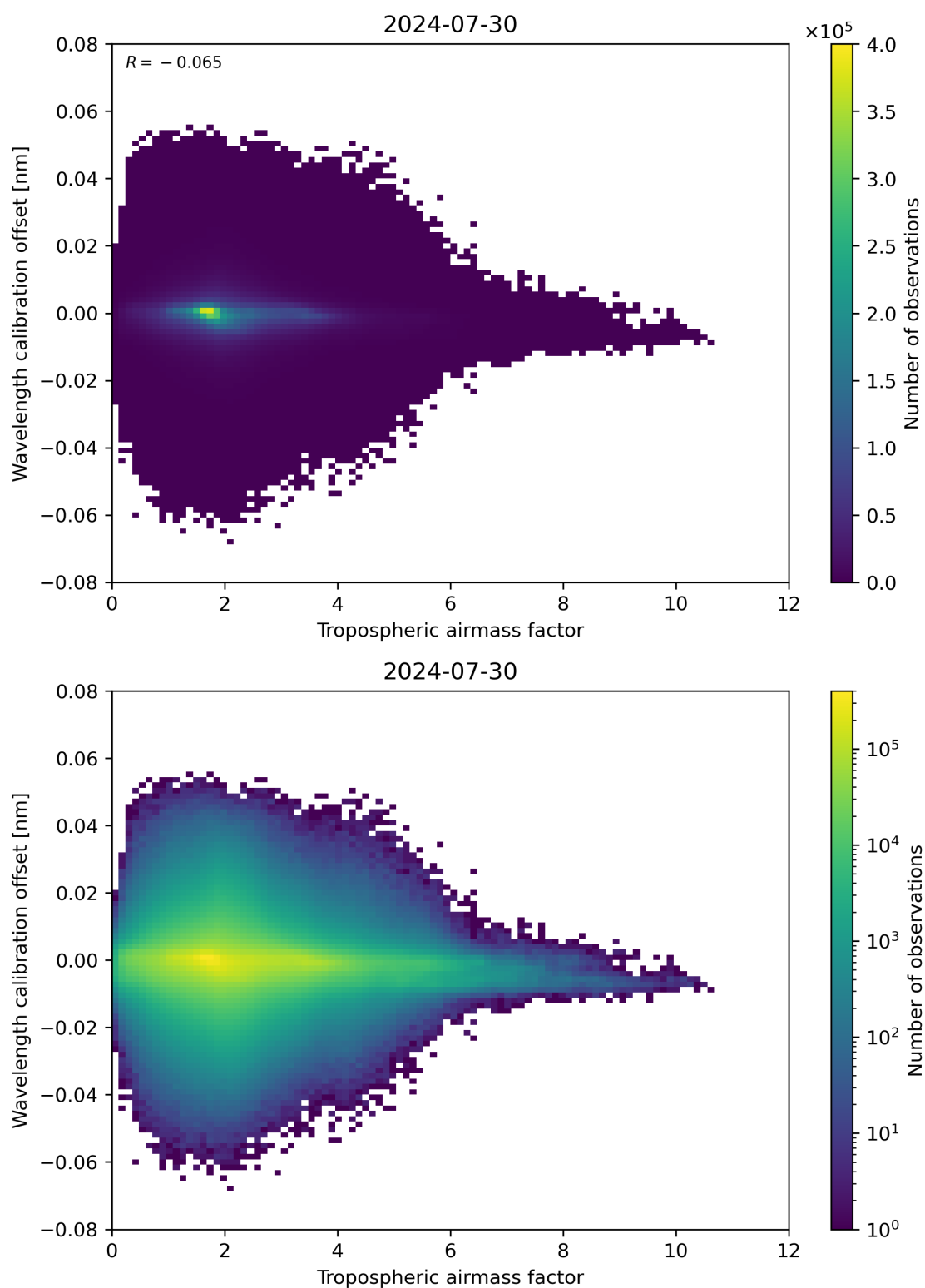
Figure 80: Scatter density plot of “Tropospheric airmass factor” against “Wavelength calibration offset” for 2024-07-29 to 2024-07-31.
