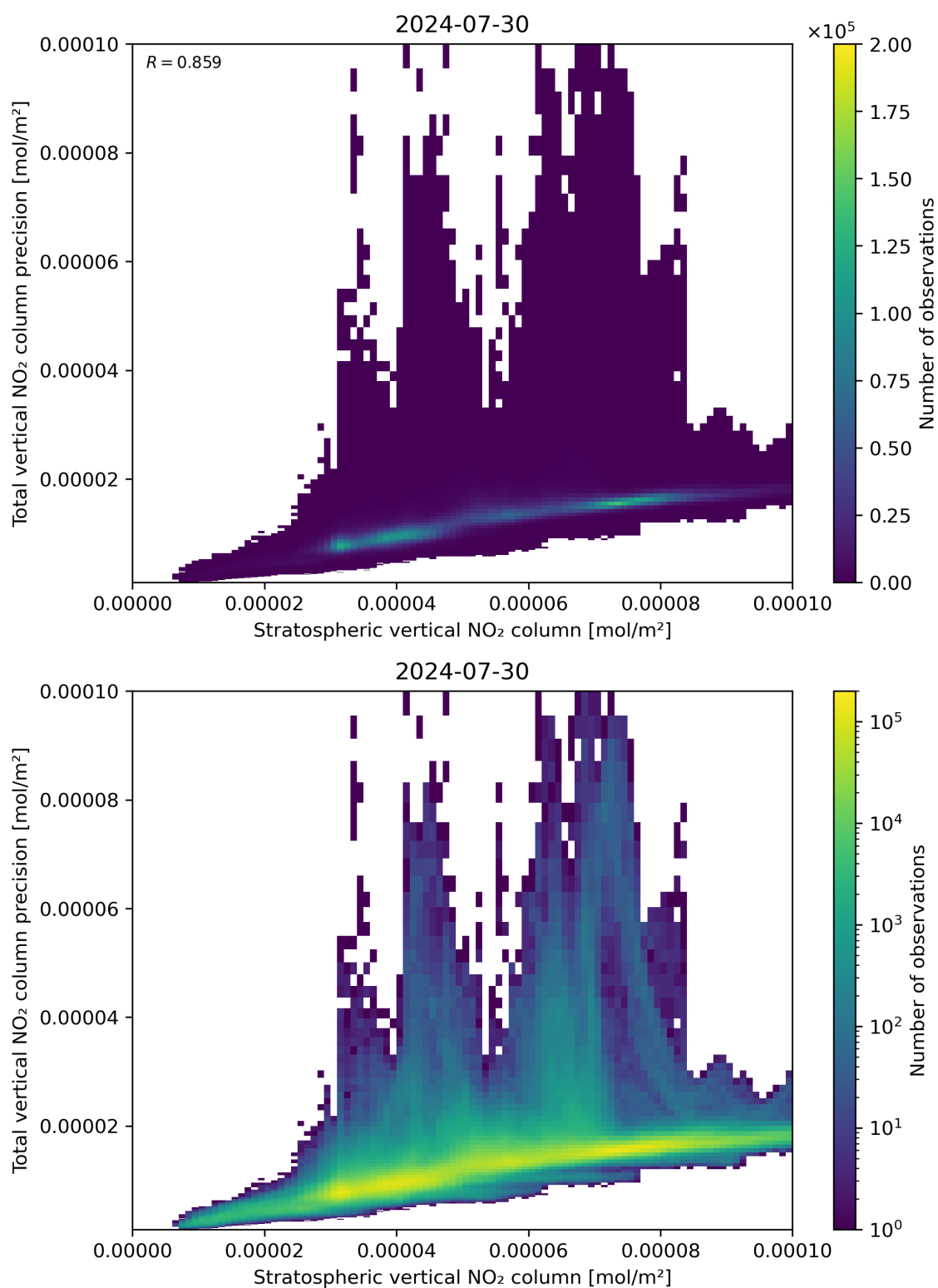
Figure 101: Scatter density plot of “Stratospheric vertical NO 2 column” against “Total vertical NO 2 column precision” for 2024-07-29 to 2024-07-31.
