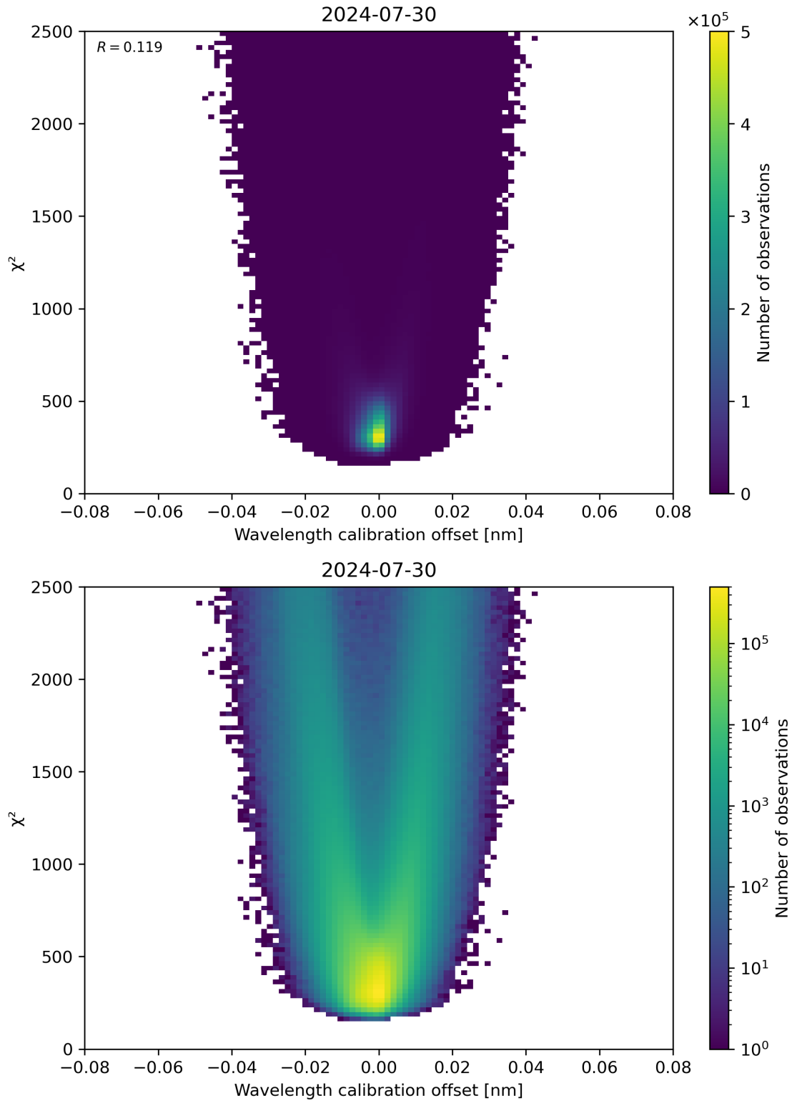
Figure 175: Scatter density plot of “Wavelength calibration offset” against “ \chi^2 ” for 2024-07-29 to 2024-07-31.
