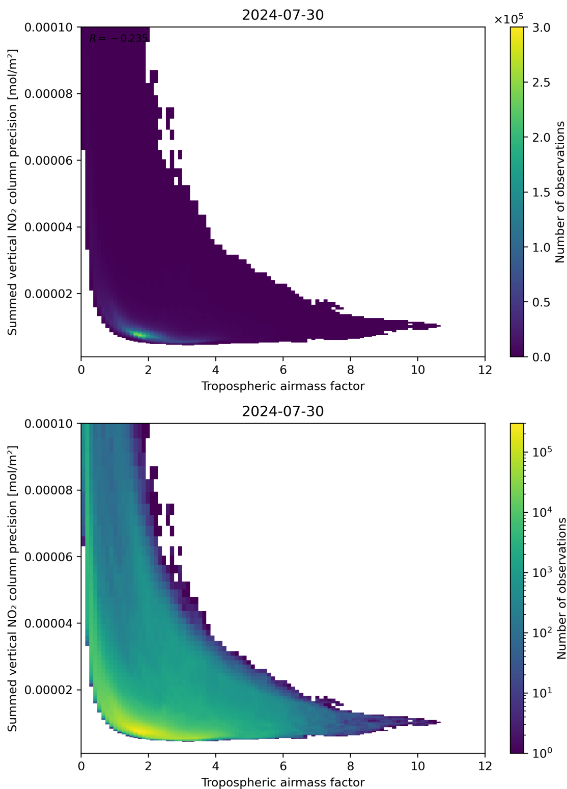
Figure 76: Scatter density plot of “Tropospheric air mass factor” against “Summed vertical NO 2 column precision” for 2024-07-29 to 2024-07-31.
