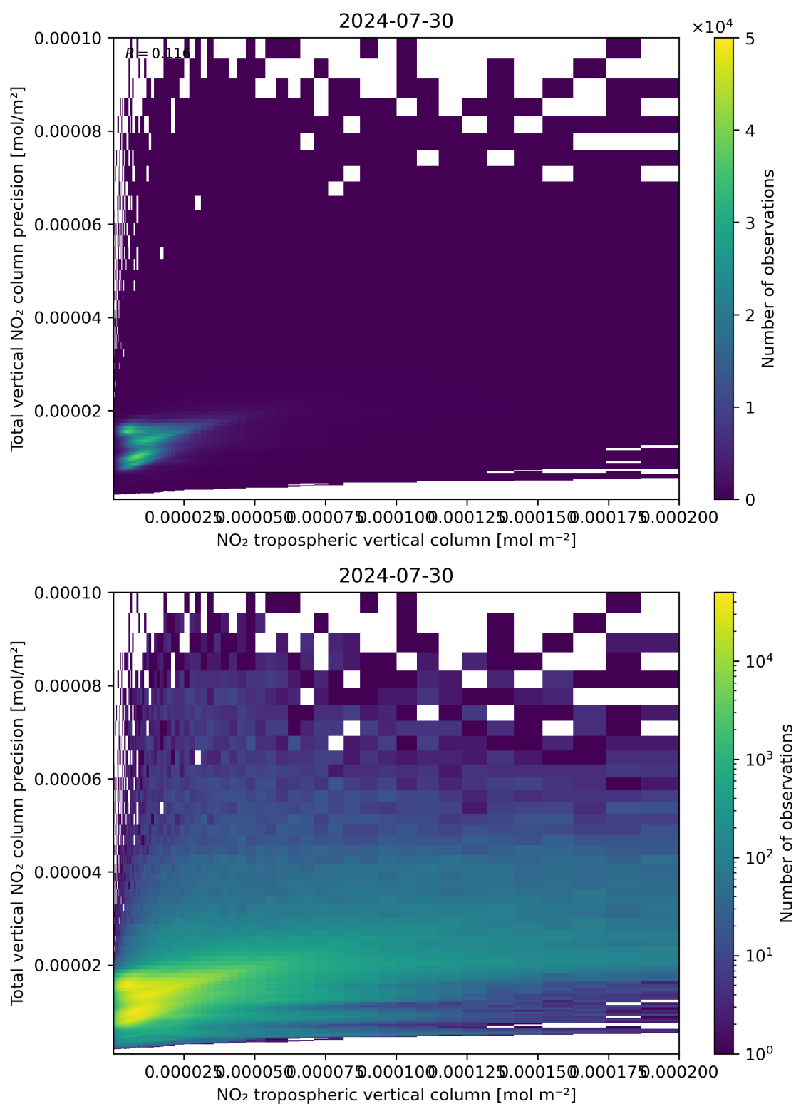
Figure 129: Scatter density plot of “NO 2 tropospheric vertical column” against “Total vertical NO 2 column precision” for 2024-07-29 to 2024-07-31.
