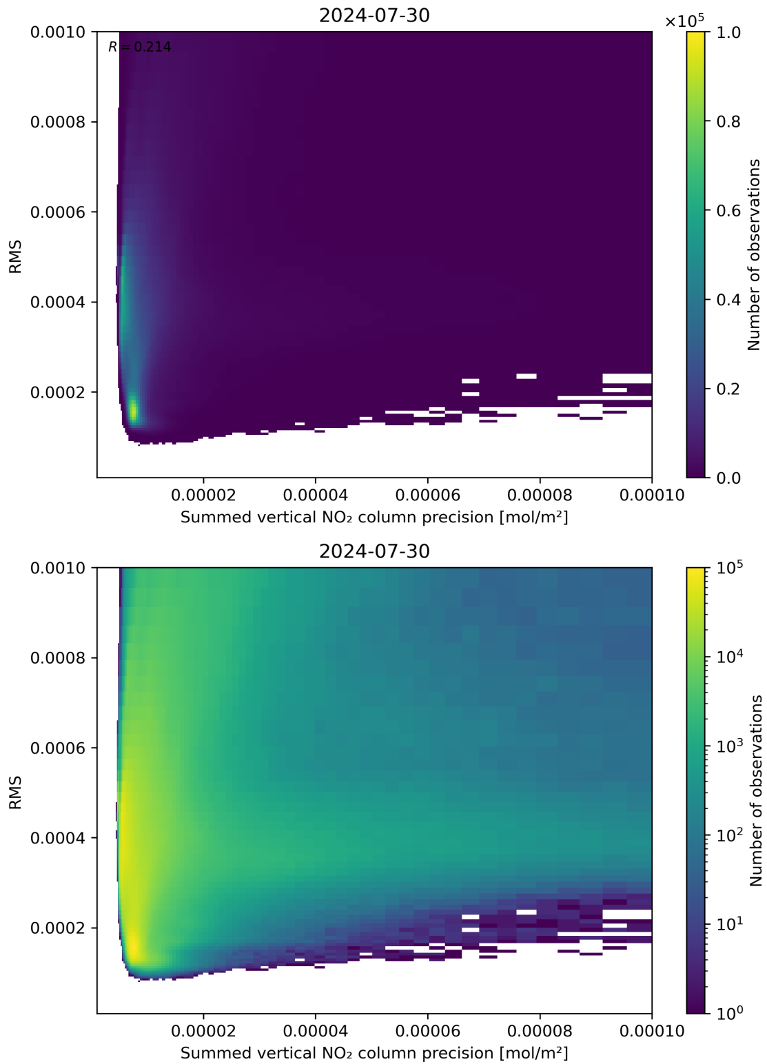
Figure 108: Scatter density plot of “Summed vertical NO 2 column precision” against “RMS” for 2024-07-29 to 2024-07-31.
