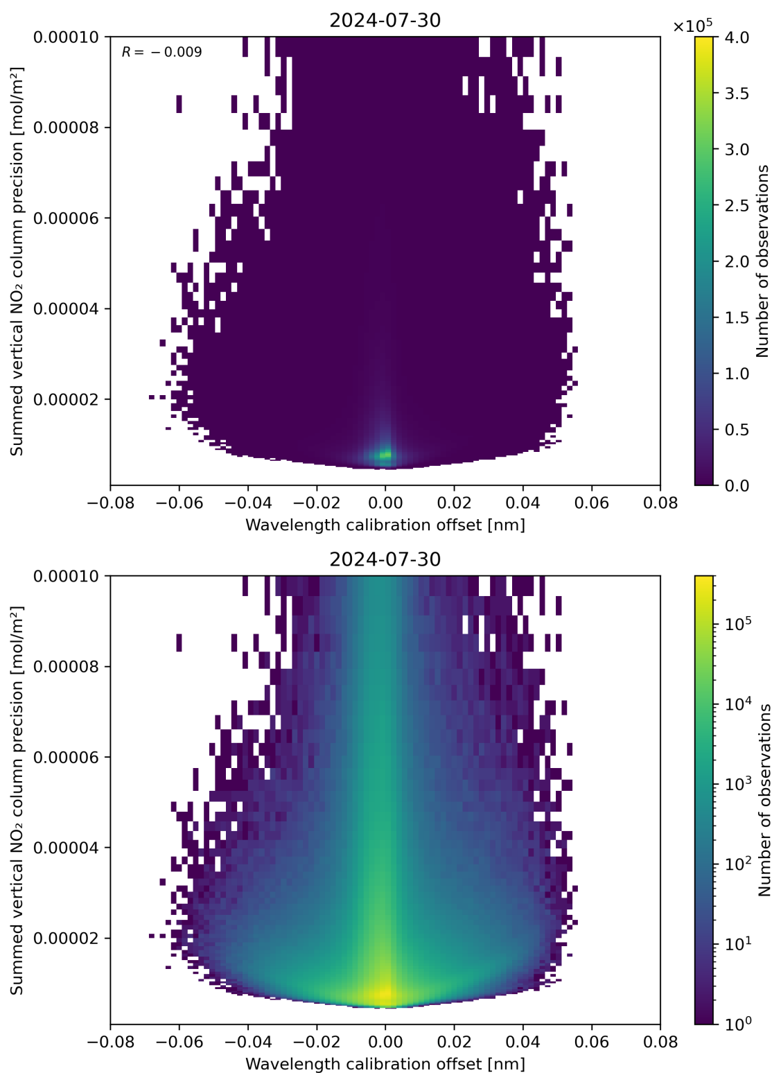
Figure 178: Scatter density plot of “Wavelength calibration offset” against “Summed vertical NO 2 column precision” for 2024-07-29 to 2024-07-31.
