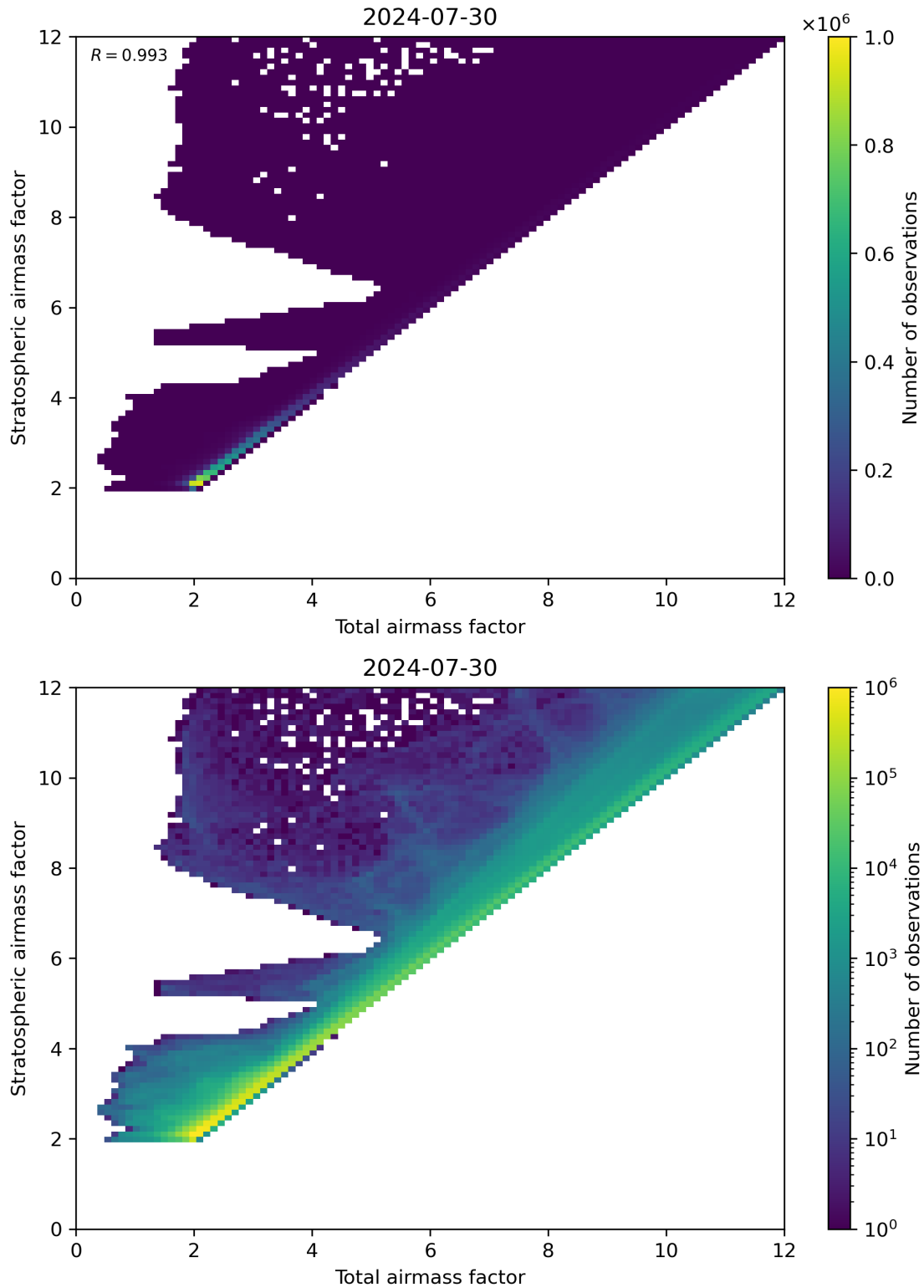
Figure 62: Scatter density plot of “Total airmass factor” against “Stratospheric airmass factor” for 2024-07-29 to 2024-07-31.
