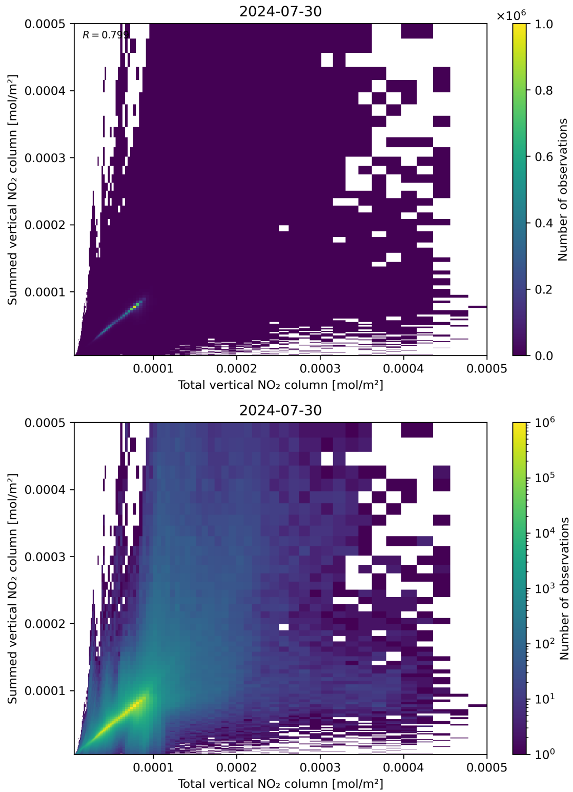
Figure 112: Scatter density plot of “Total vertical NO 2 column” against “Summed vertical NO 2 column” for 2024-07-29 to 2024-07-31.
