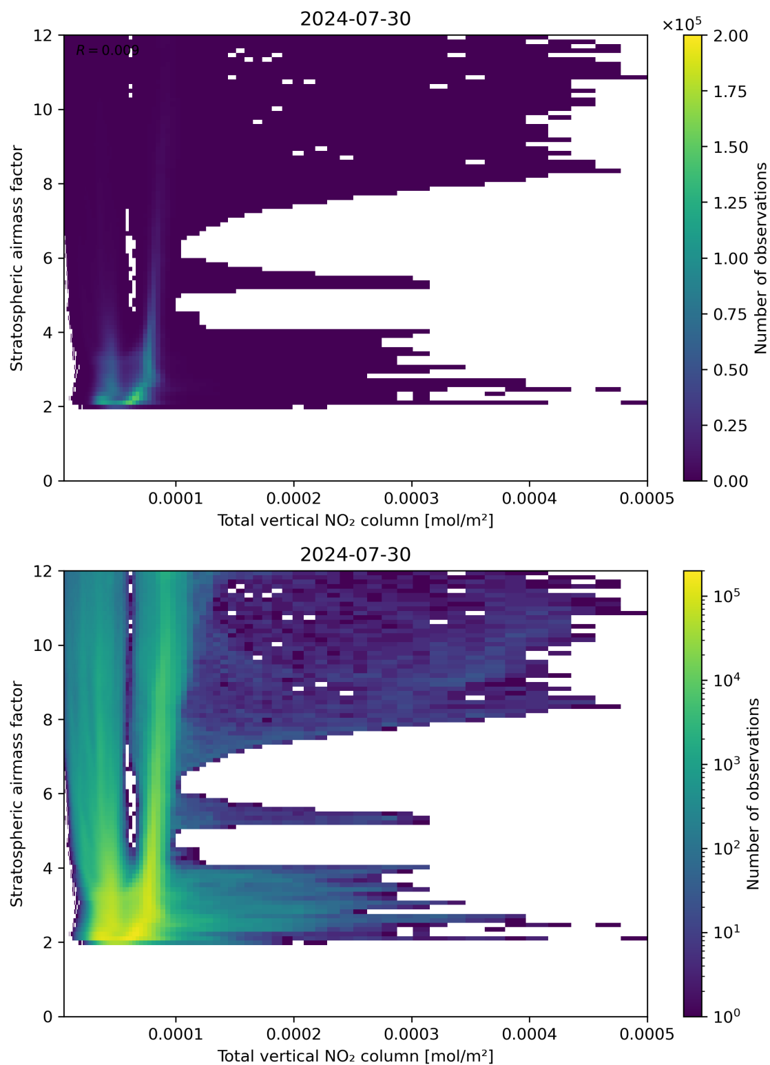
Figure 110: Scatter density plot of “Total vertical NO 2 column” against “Stratospheric airmass factor” for 2024-07-29 to 2024-07-31.
