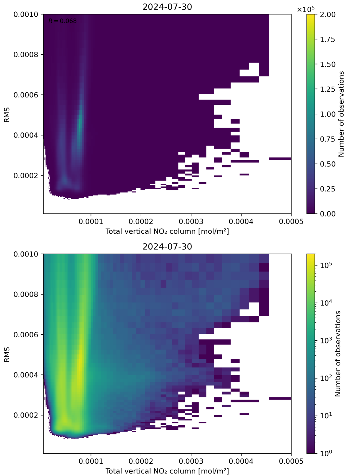
Figure 120: Scatter density plot of “Total vertical NO 2 column” against “RMS” for 2024-07-29 to 2024-07-31.
