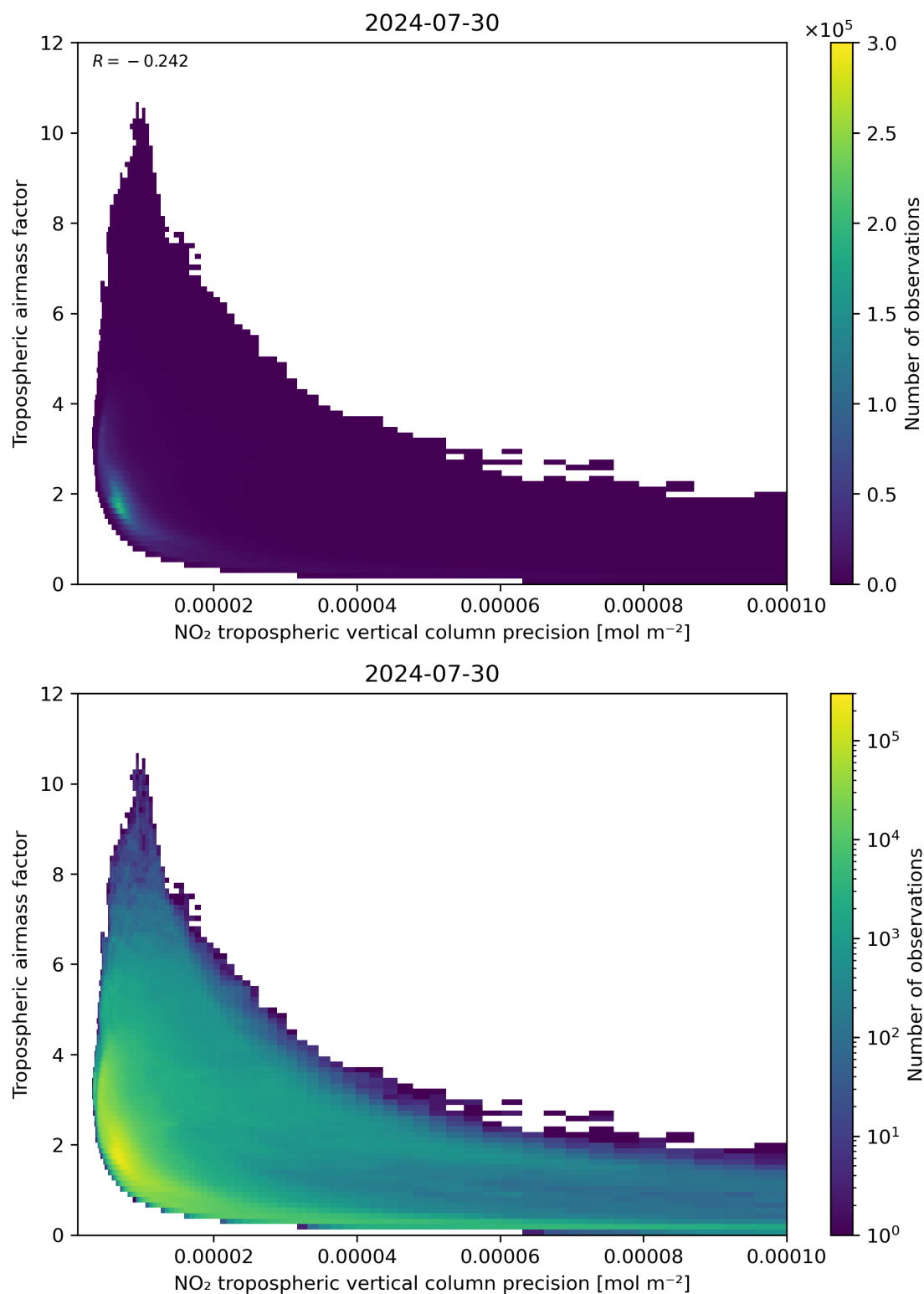
Figure 133: Scatter density plot of “NO 2 tropospheric vertical column precision” against “Tropospheric airmass factor” for 2024-07-29 to 2024-07-31.
