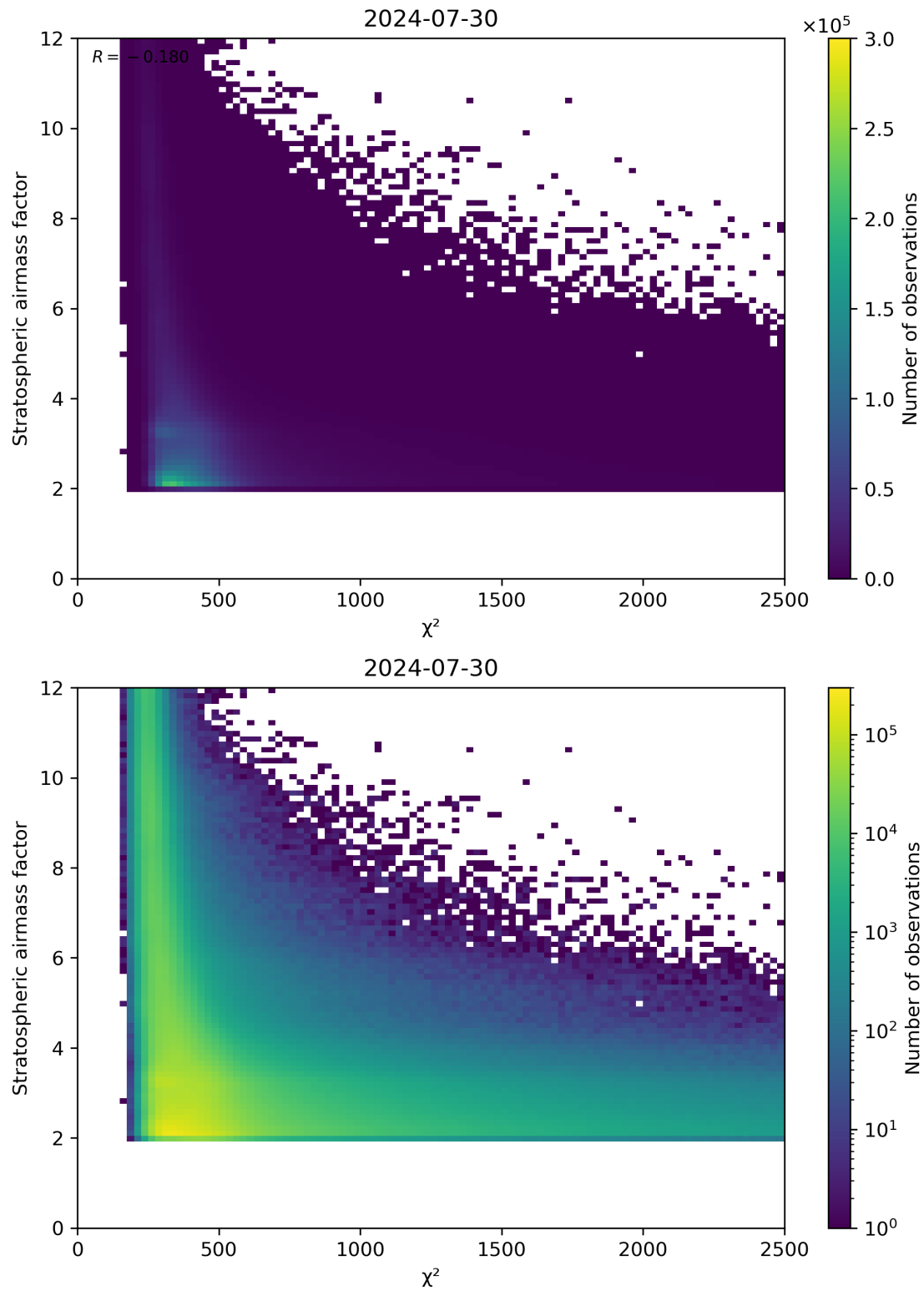
Figure 81: Scatter density plot of “ \chi^2 ” against “Stratospheric airmass factor” for 2024-07-29 to 2024-07-31.
