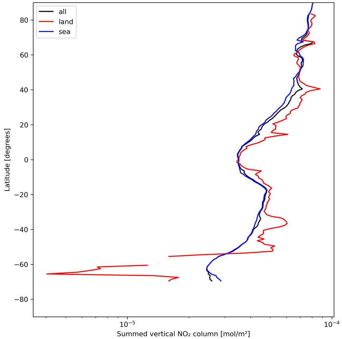
Figure 23: Zonal average of “Summed vertical NO 2 column” for 2024-07-29 to 2024-07-31.
