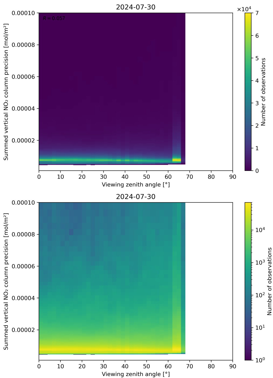
Figure 166: Scatter density plot of “Viewing zenith angle” against “Summed vertical NO 2 column precision” for 2024-07-29 to 2024-07-31.
