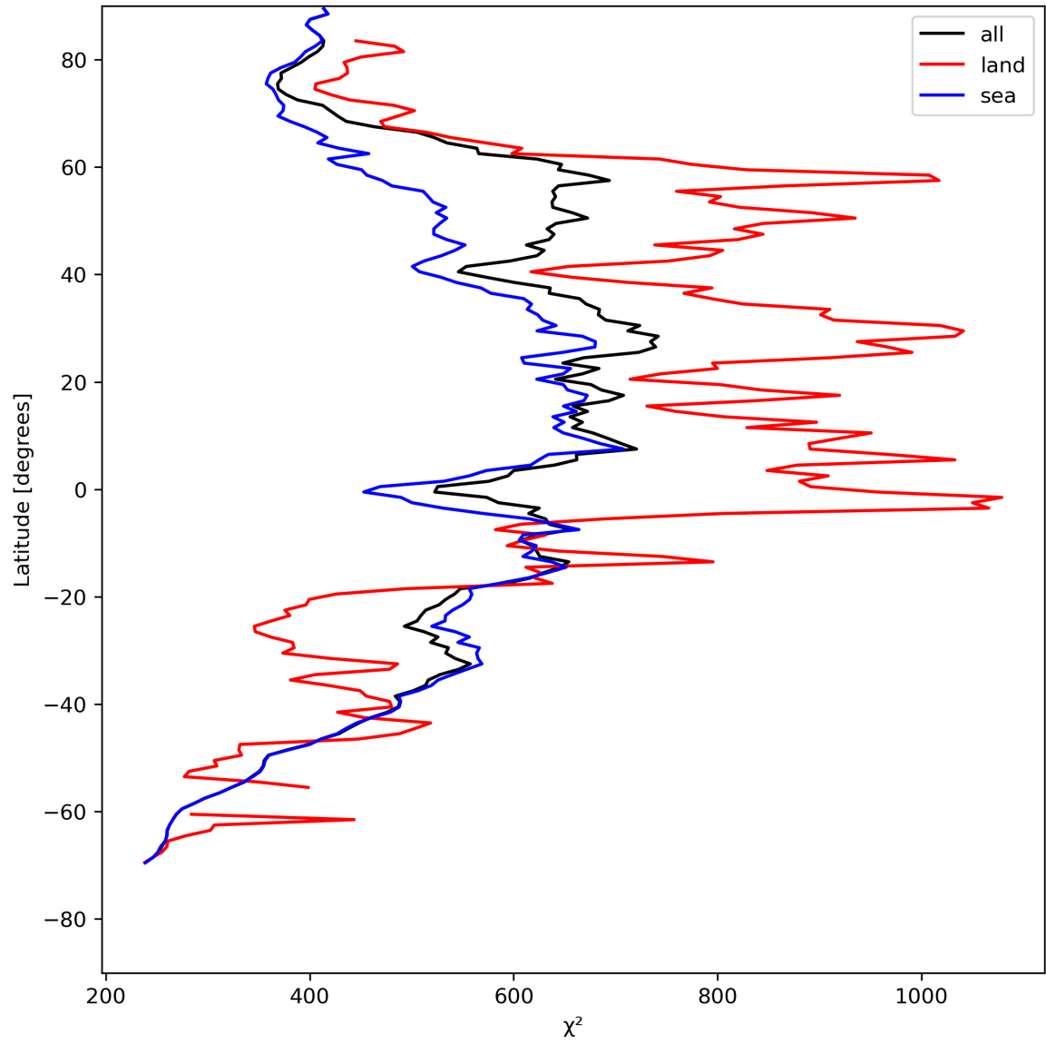
Figure 25: Zonal average of “ \chi^2 ” for 2024-07-29 to 2024-07-31.
