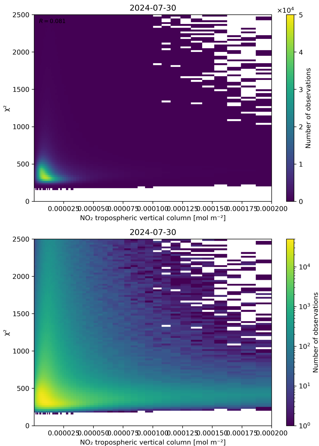
Figure 124: Scatter density plot of “NO 2 tropospheric vertical column” against “ \chi^2 ” for 2024-07-29 to 2024-07-31.
