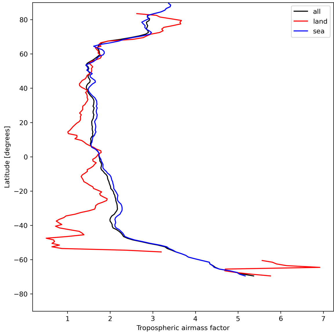
Figure 14: Zonal average of “Tropospheric airmass factor” for 2024-07-29 to 2024-07-31.
