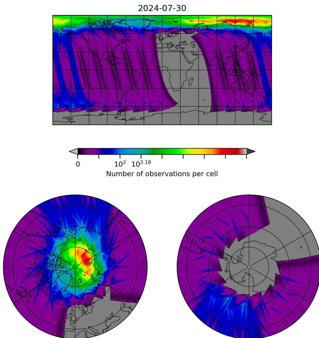
Figure 10: Map of the number of observations for 2024-07-29 to 2024-07-31
