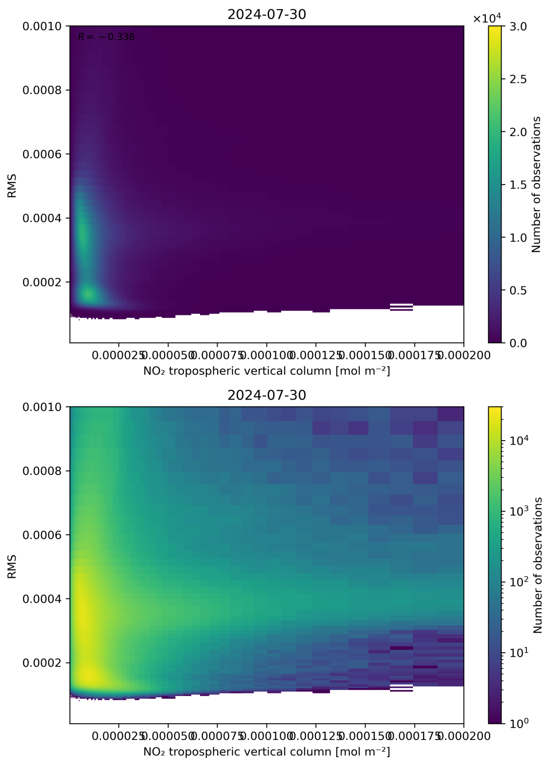
Figure 142: Scatter density plot of “NO 2 tropospheric vertical column” against “RMS” for 2024-07-29 to 2024-07-31.
