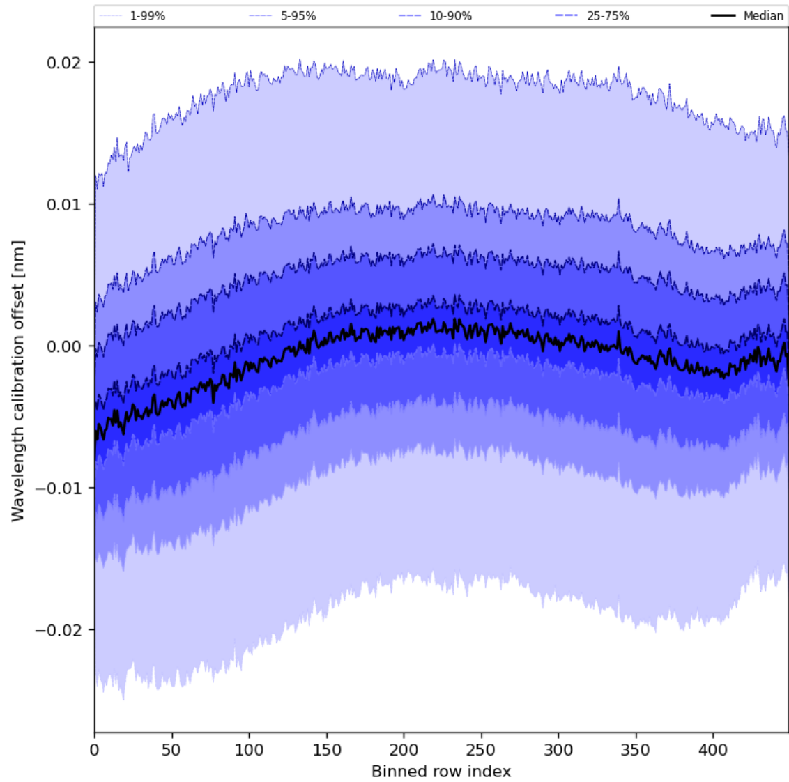
Figure 52: Along track statistics of “Wavelength calibration offset” for 2024-07-29 to 2024-07-31
