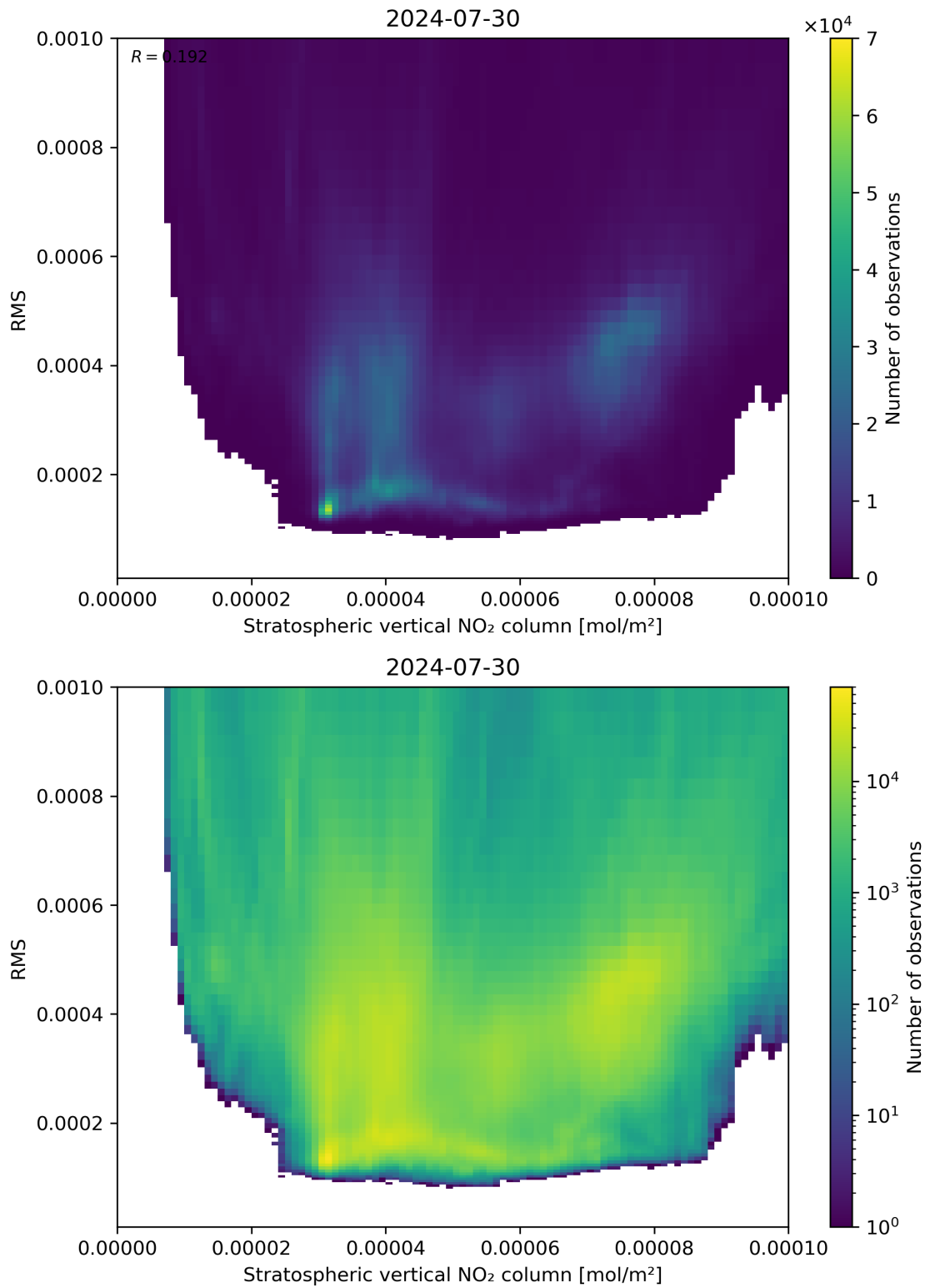
Figure 102: Scatter density plot of “Stratospheric vertical NO 2 column” against “RMS” for 2024-07-29 to 2024-07-31.
