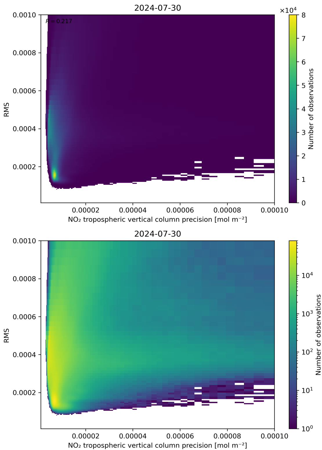
Figure 140: Scatter density plot of “NO 2 tropospheric vertical column precision” against “RMS” for 2024-07-29 to 2024-07-31.
