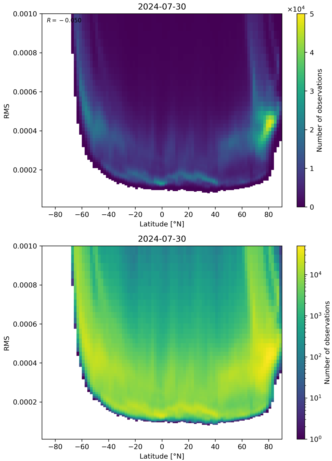
Figure 94: Scatter density plot of “Latitude” against “RMS” for 2024-07-29 to 2024-07-31.
