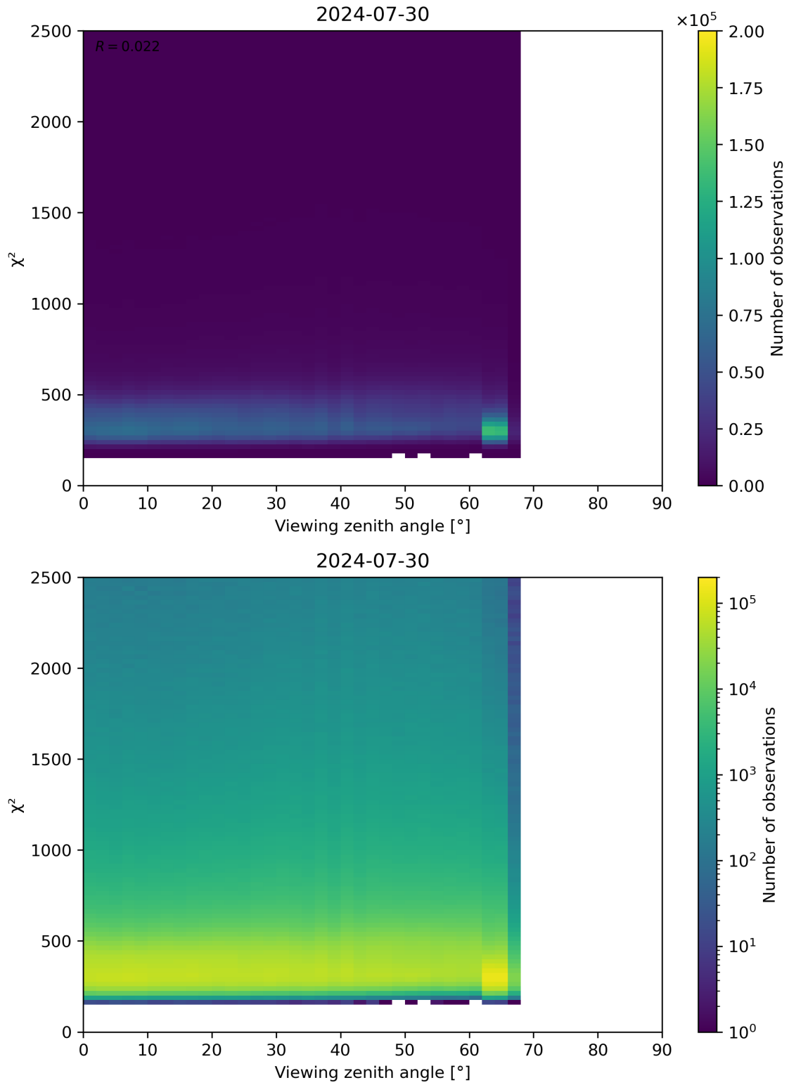
Figure 162: Scatter density plot of “Viewing zenith angle” against “ \chi^2 ” for 2024-07-29 to 2024-07-31.
