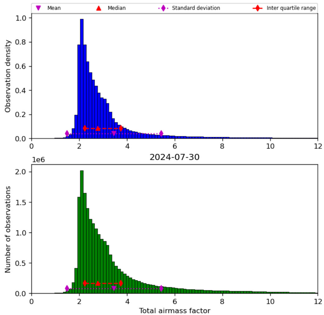
Figure 32: Histogram of “Total airmass factor” for 2024-07-29 to 2024-07-31
