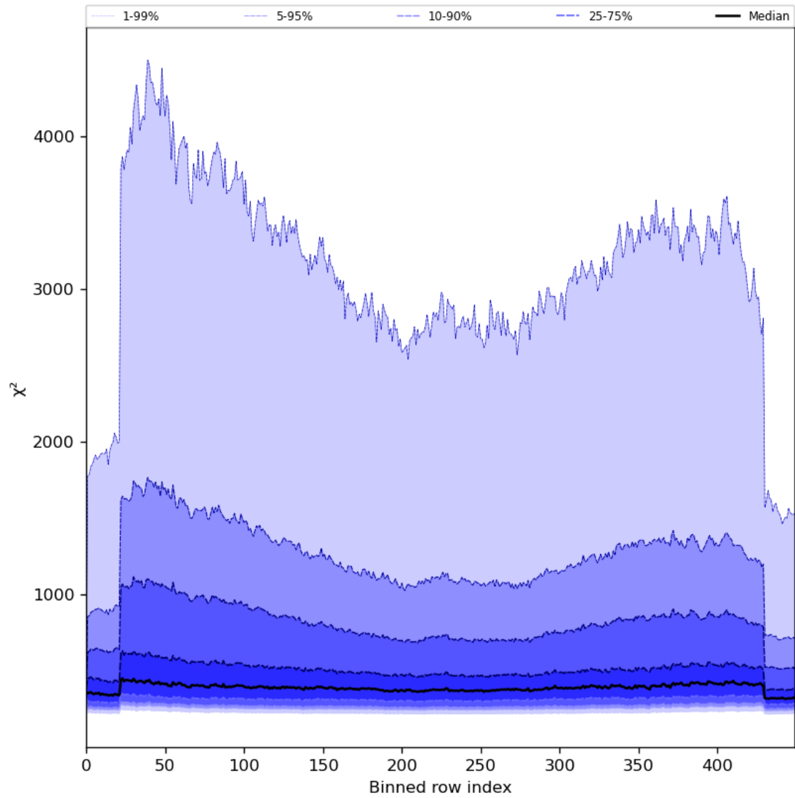
Figure 59: Along track statistics of “ \chi^2 ” for 2024-07-29 to 2024-07-31
