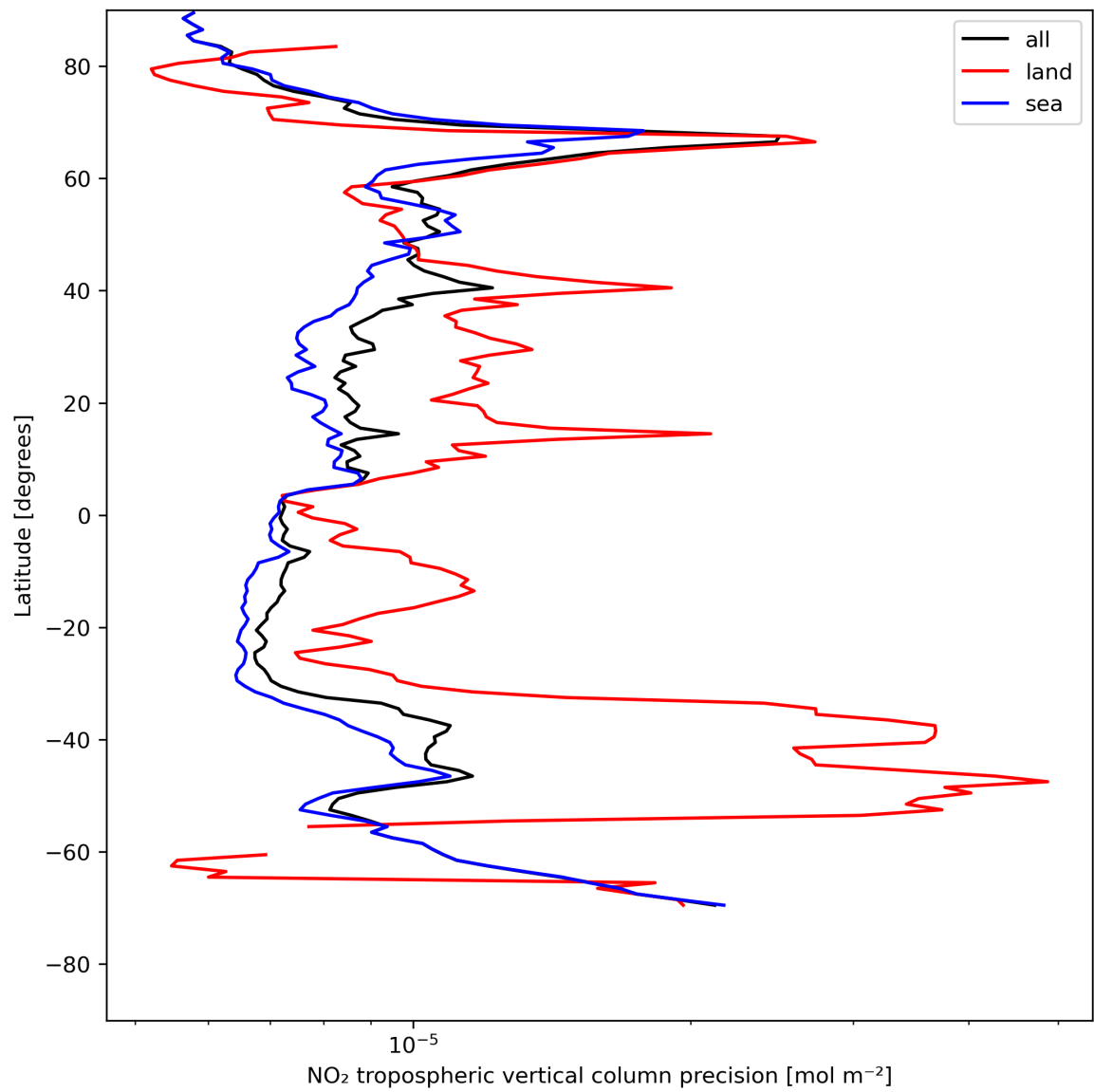
Figure 13: Zonal average of “NO 2 tropospheric vertical column precision” for 2024-07-29 to 2024-07-31.
