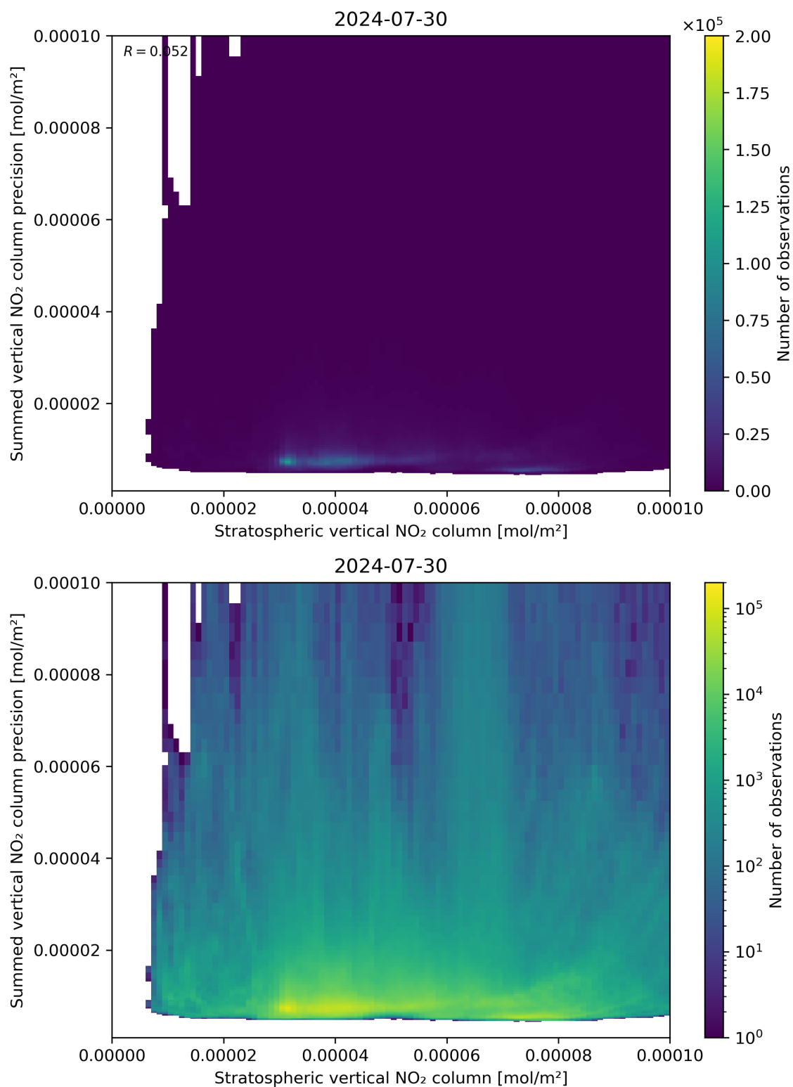
Figure 99: Scatter density plot of “Stratospheric vertical NO 2 column” against “Summed vertical NO 2 column precision” for 2024-07-29 to 2024-07-31.
