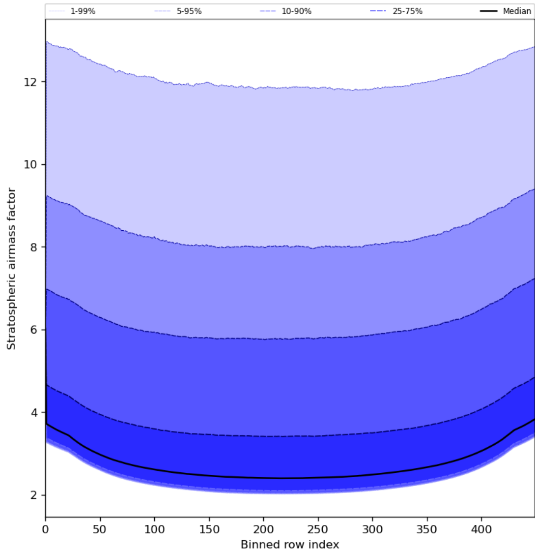
Figure 61: Along track statistics of “Stratospheric air mass factor” for 2024-07-29 to 2024-07-31
