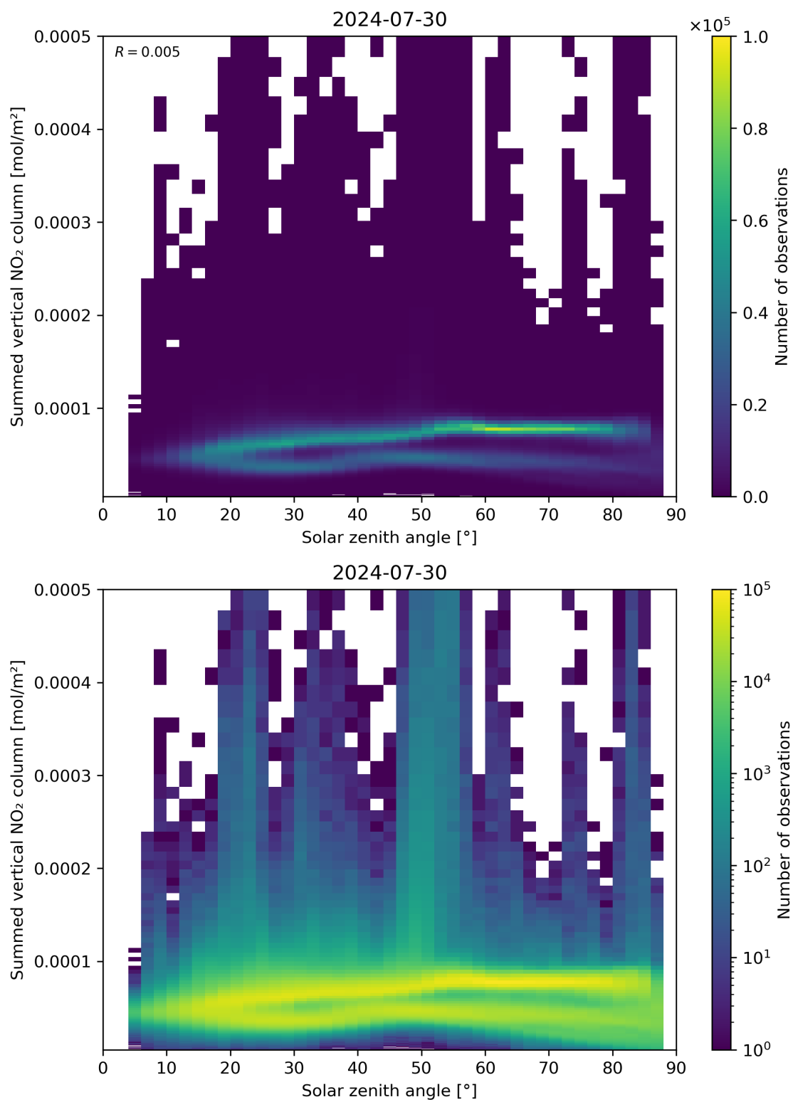
Figure 151: Scatter density plot of “Solar zenith angle” against “Summed vertical NO 2 column” for 2024-07-29 to 2024-07-31.
