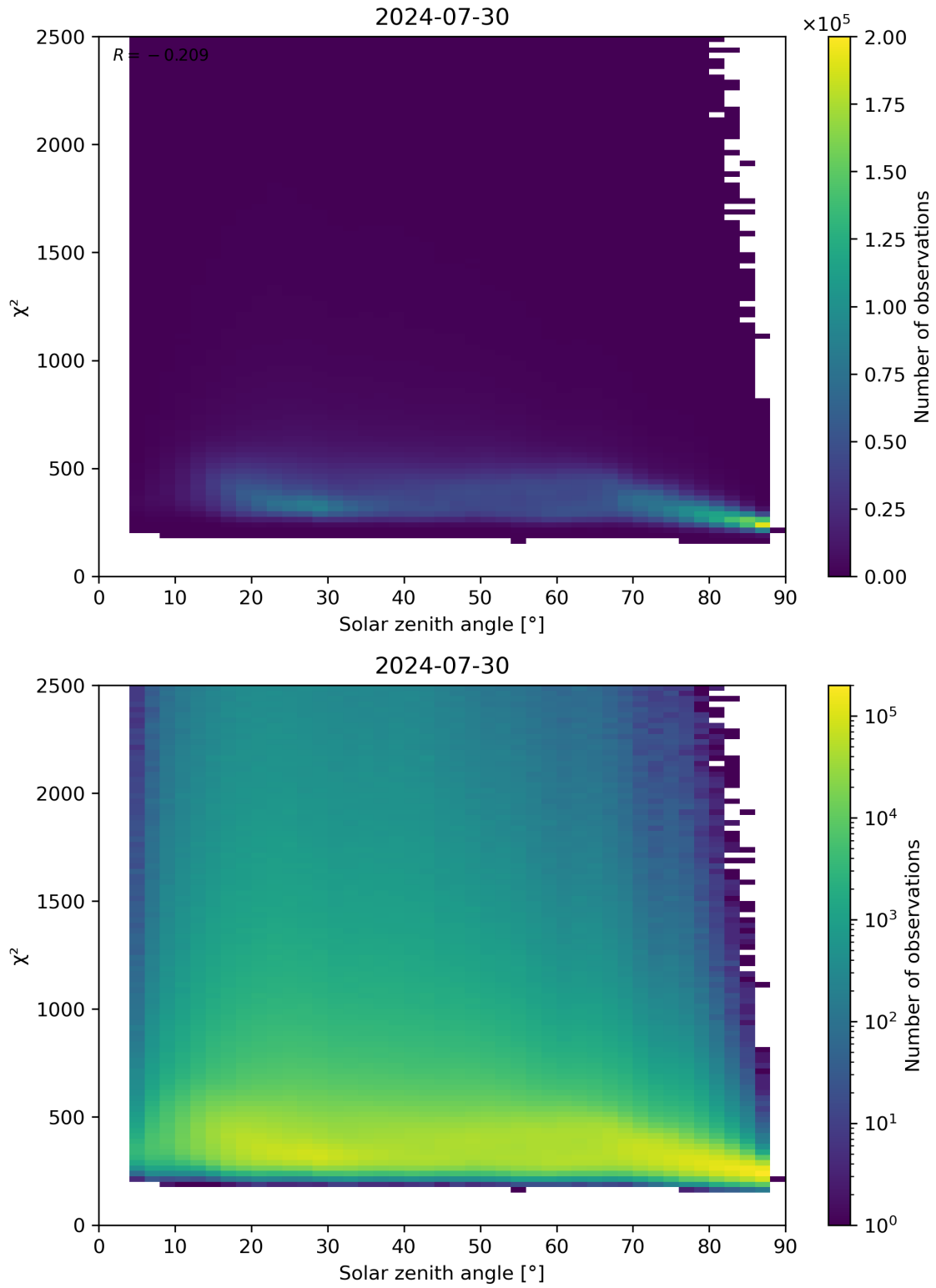
Figure 148: Scatter density plot of “Solar zenith angle” against “ \chi^2 ” for 2024-07-29 to 2024-07-31.
