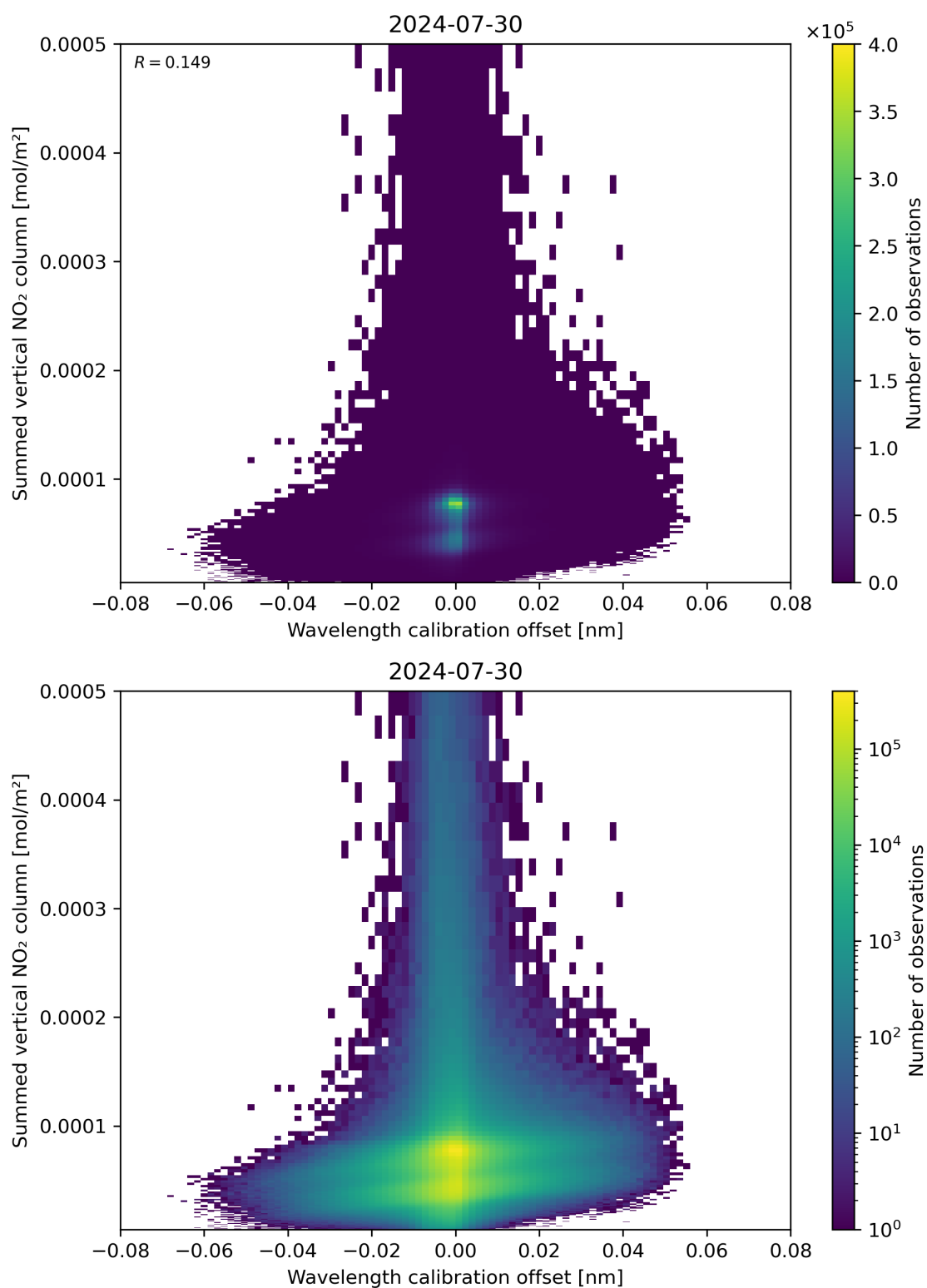
Figure 177: Scatter density plot of “Wavelength calibration offset” against “Summed vertical NO 2 column” for 2024-07-29 to 2024-07-31.
