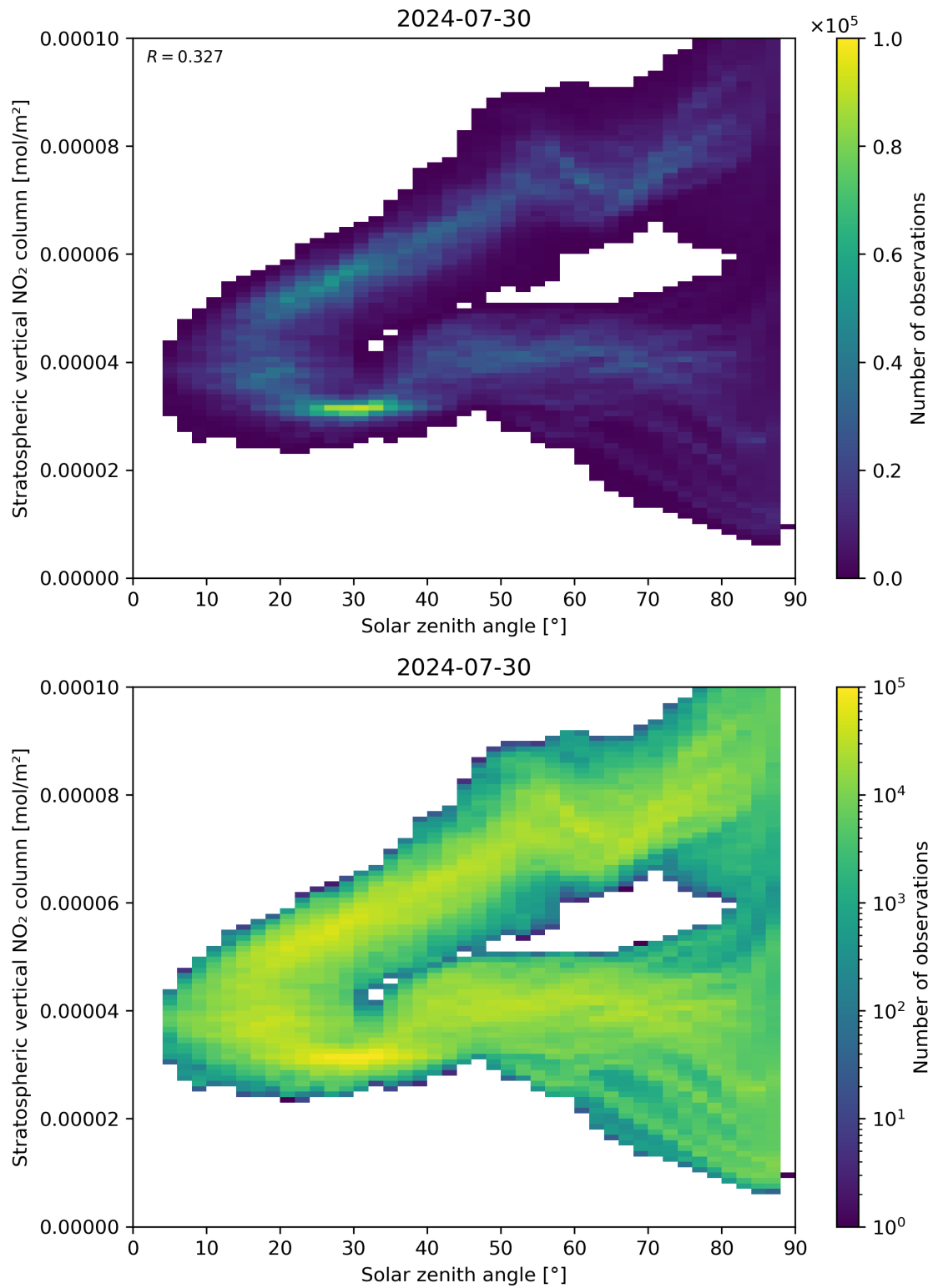
Figure 150: Scatter density plot of “Solar zenith angle” against “Stratospheric vertical NO 2 column” for 2024-07-29 to 2024-07-31.
