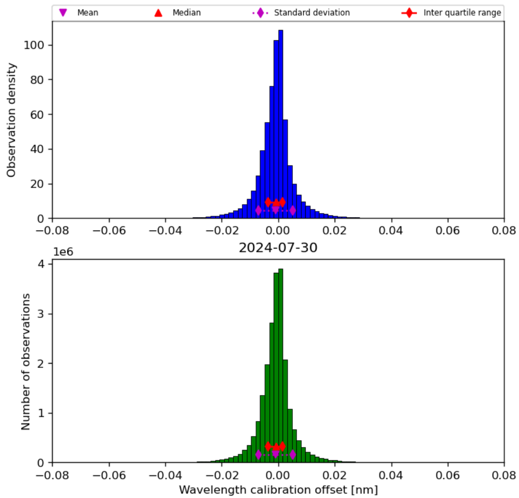
Figure 35: Histogram of “Wavelength calibration offset” for 2024-07-29 to 2024-07-31
