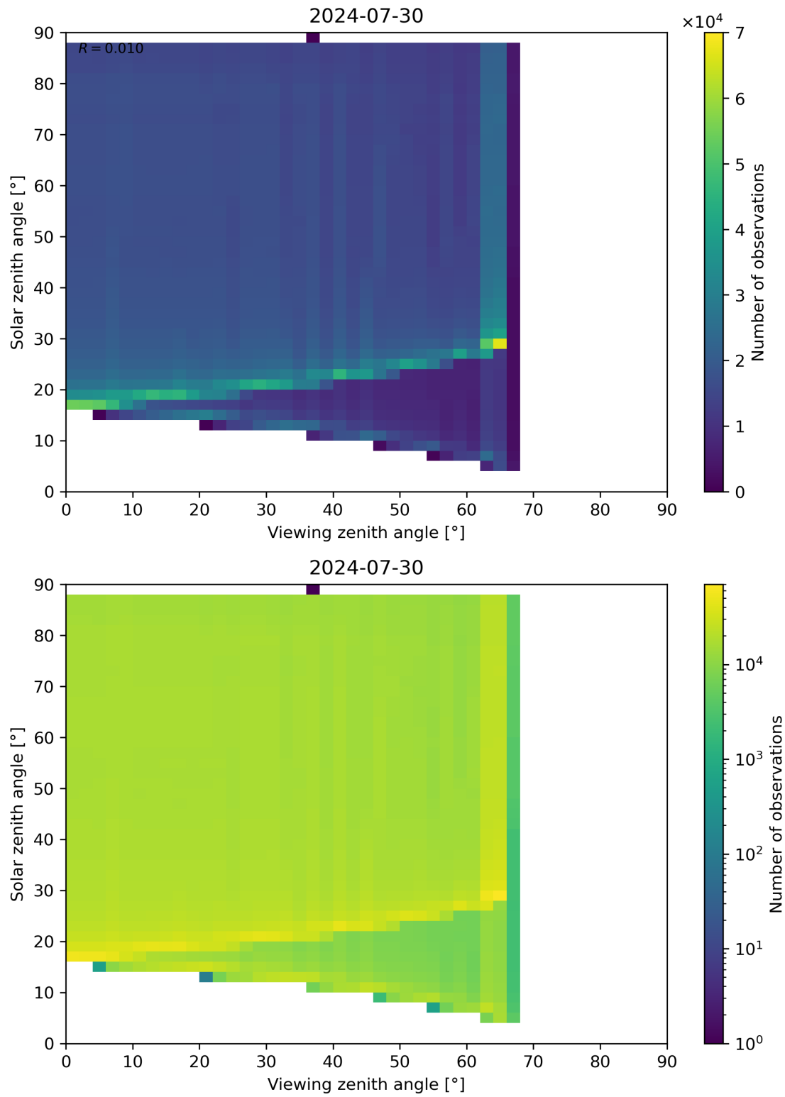
Figure 172: Scatter density plot of “Viewing zenith angle” against “Solar zenith angle” for 2024-07-29 to 2024-07-31.
