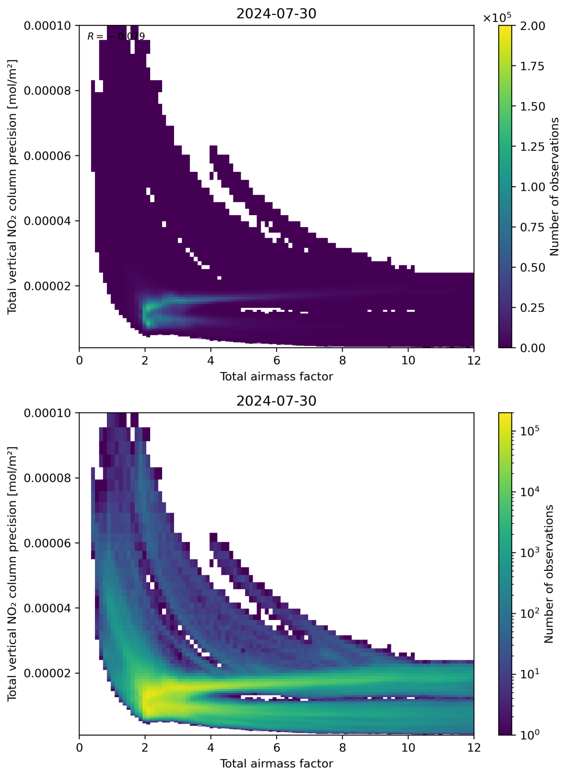
Figure 68: Scatter density plot of “Total airmass factor” against “Total vertical NO 2 column precision” for 2024-07-29 to 2024-07-31.
