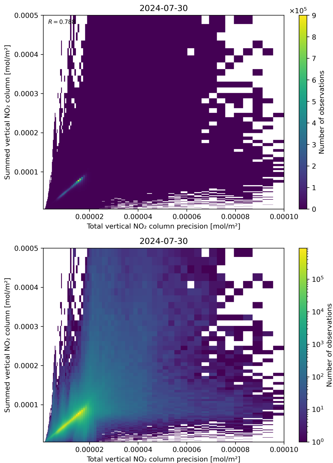
Figure 117: Scatter density plot of “Total vertical NO 2 column precision” against “Summed vertical NO 2 column” for 2024-07-29 to 2024-07-31.
