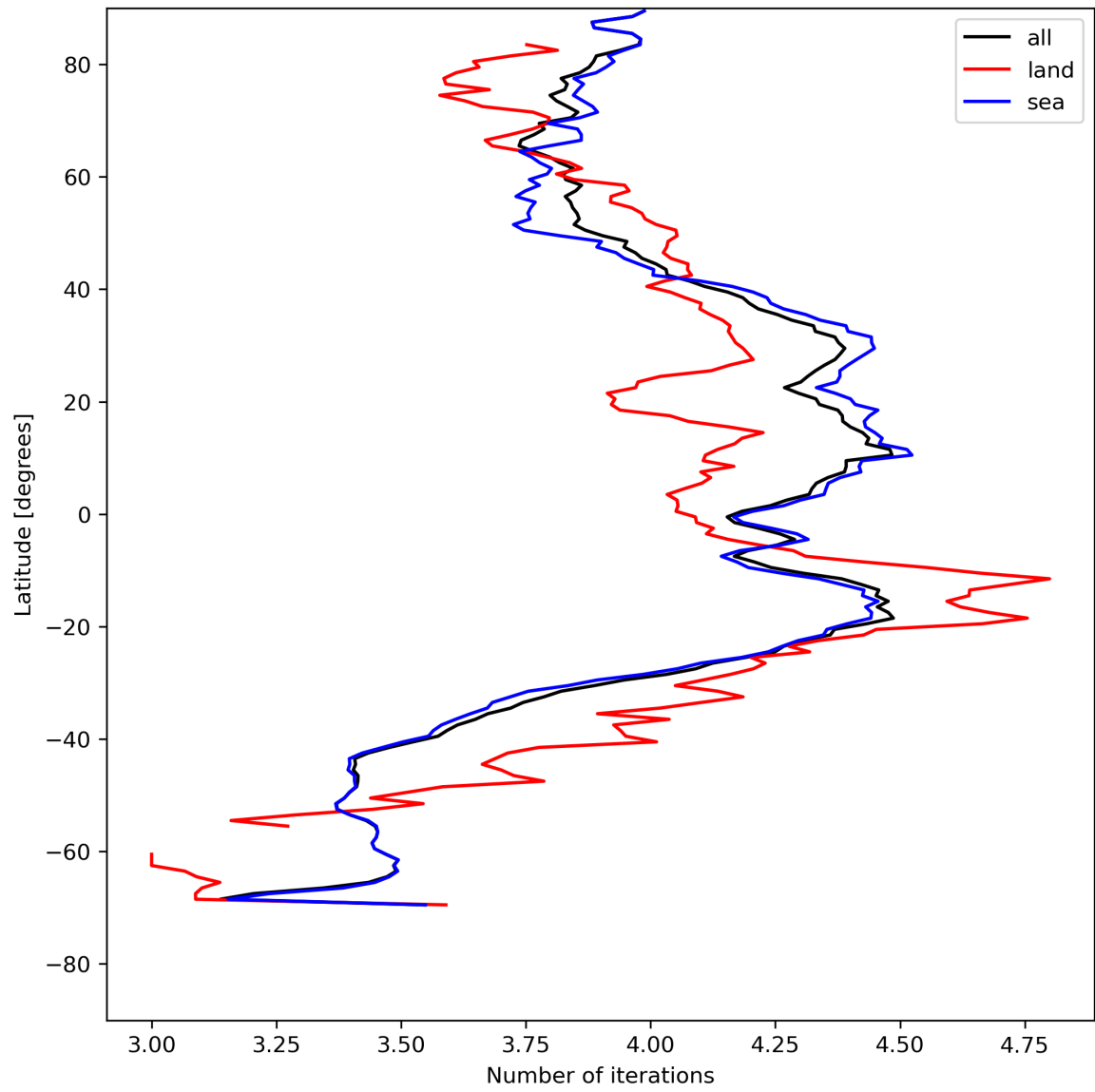
Figure 17: Zonal average of “Number of iterations” for 2024-07-29 to 2024-07-31.
