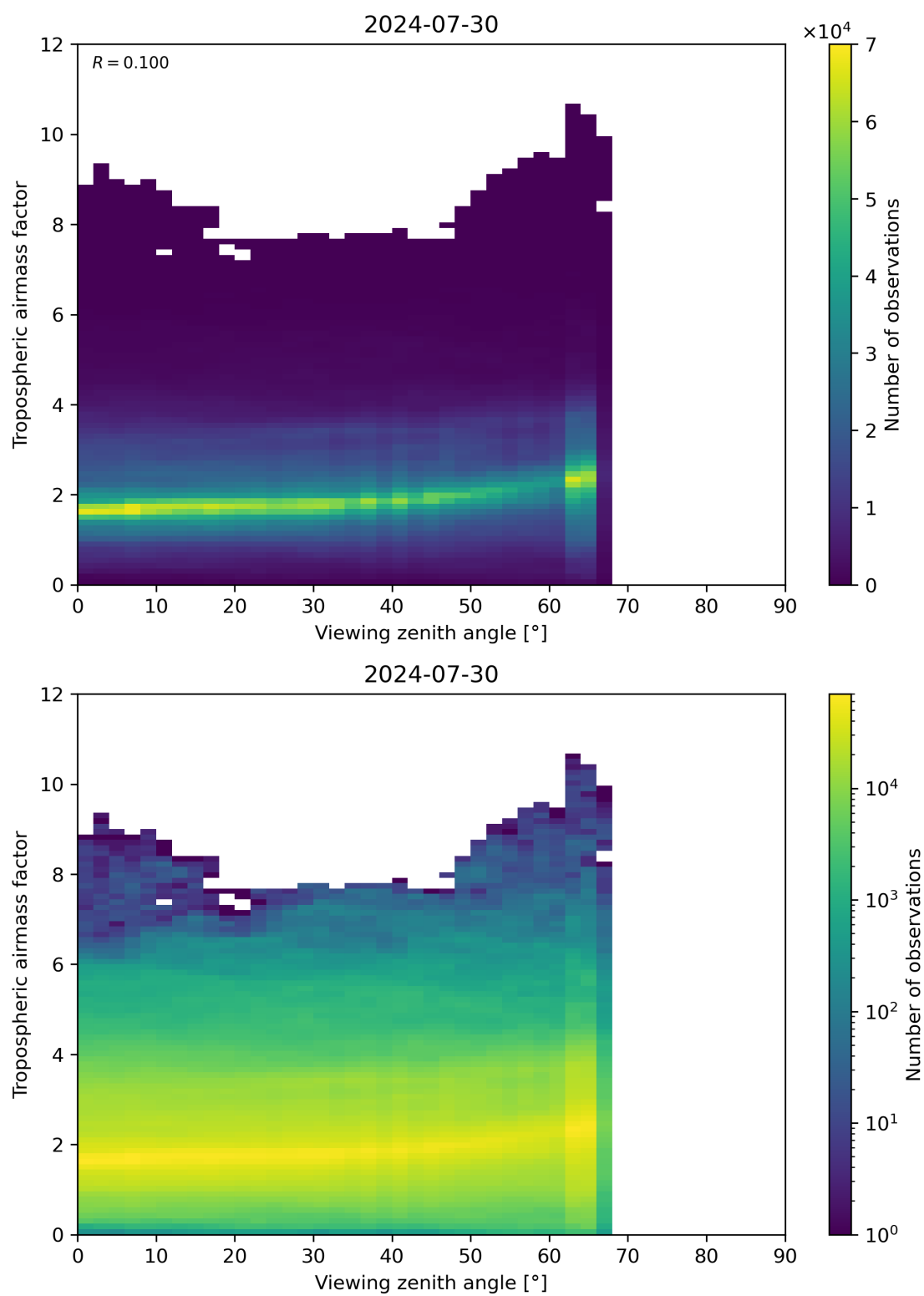
Figure 161: Scatter density plot of “Viewing zenith angle” against “Tropospheric airmass factor” for 2024-07-29 to 2024-07-31.
