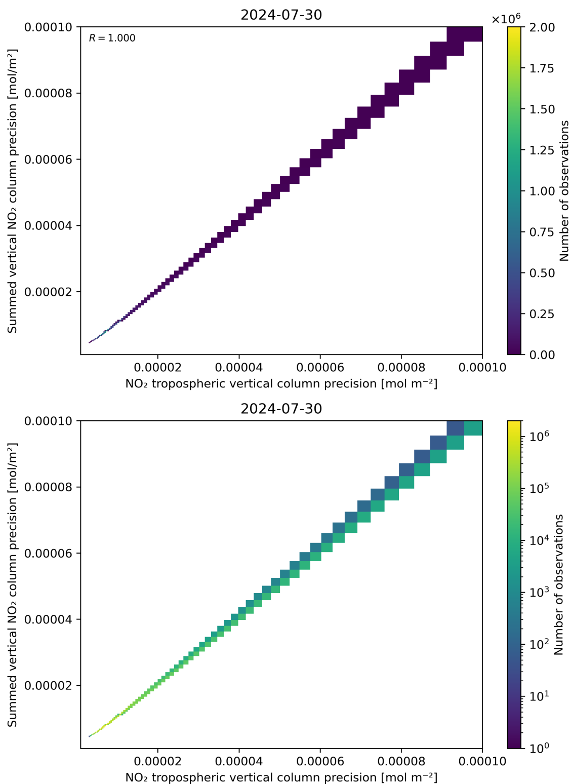
Figure 137: Scatter density plot of “NO 2 tropospheric vertical column precision” against “Summed vertical NO 2 column precision” for 2024-07-29 to 2024-07-31.
