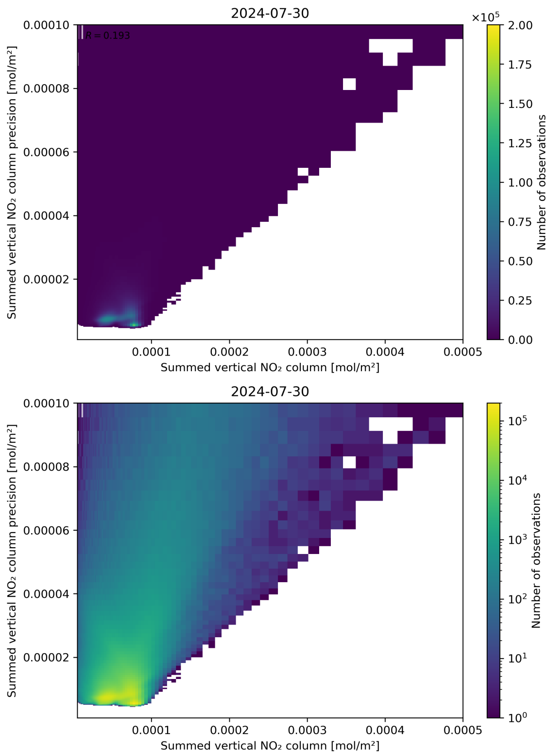
Figure 105: Scatter density plot of “Summed vertical NO 2 column” against “Summed vertical NO 2 column precision” for 2024-07-29 to 2024-07-31.
