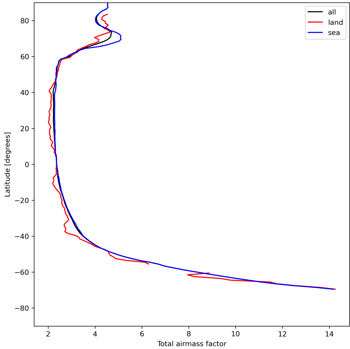
Figure 15: Zonal average of “Total airmass factor” for 2024-07-29 to 2024-07-31.
