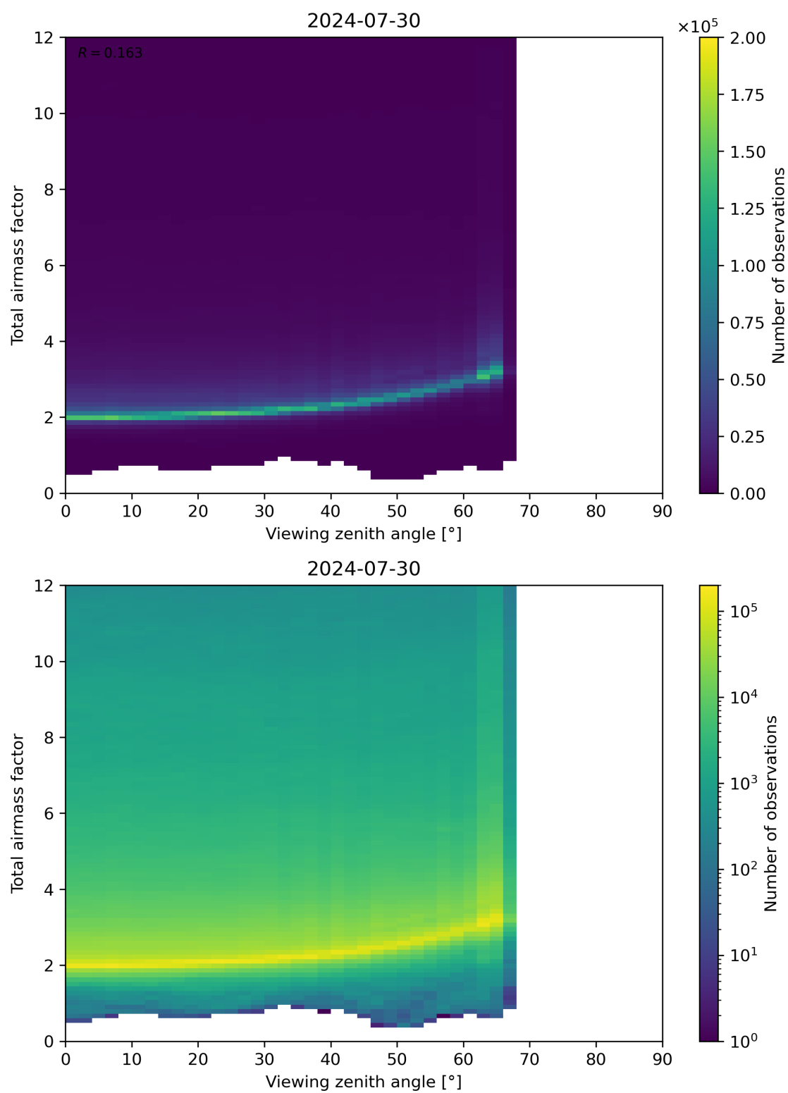
Figure 160: Scatter density plot of “Viewing zenith angle” against “Total airmass factor” for 2024-07-29 to 2024-07-31.
