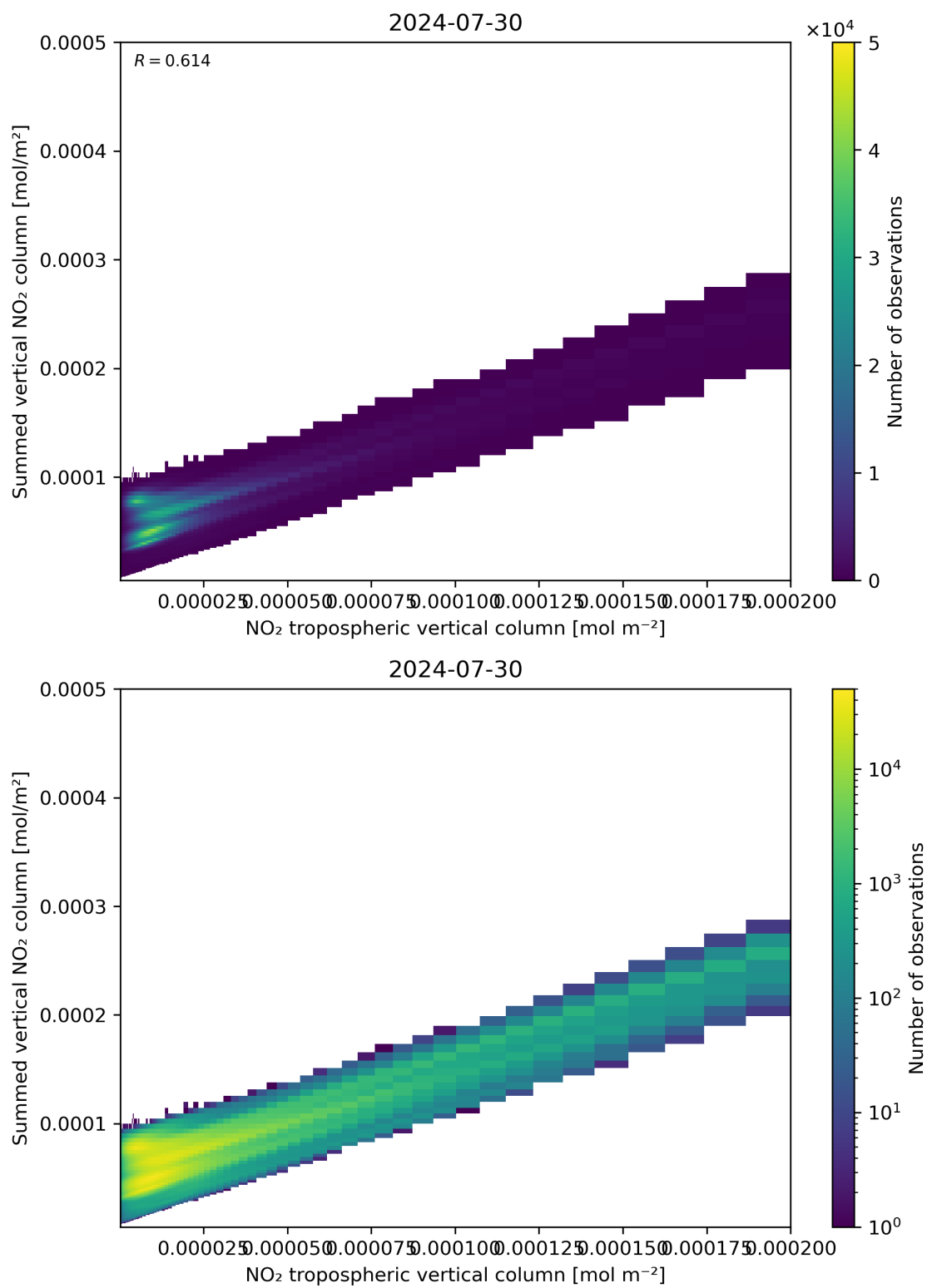
Figure 126: Scatter density plot of “NO 2 tropospheric vertical column” against “Summed vertical NO 2 column” for 2024-07-29 to 2024-07-31.
