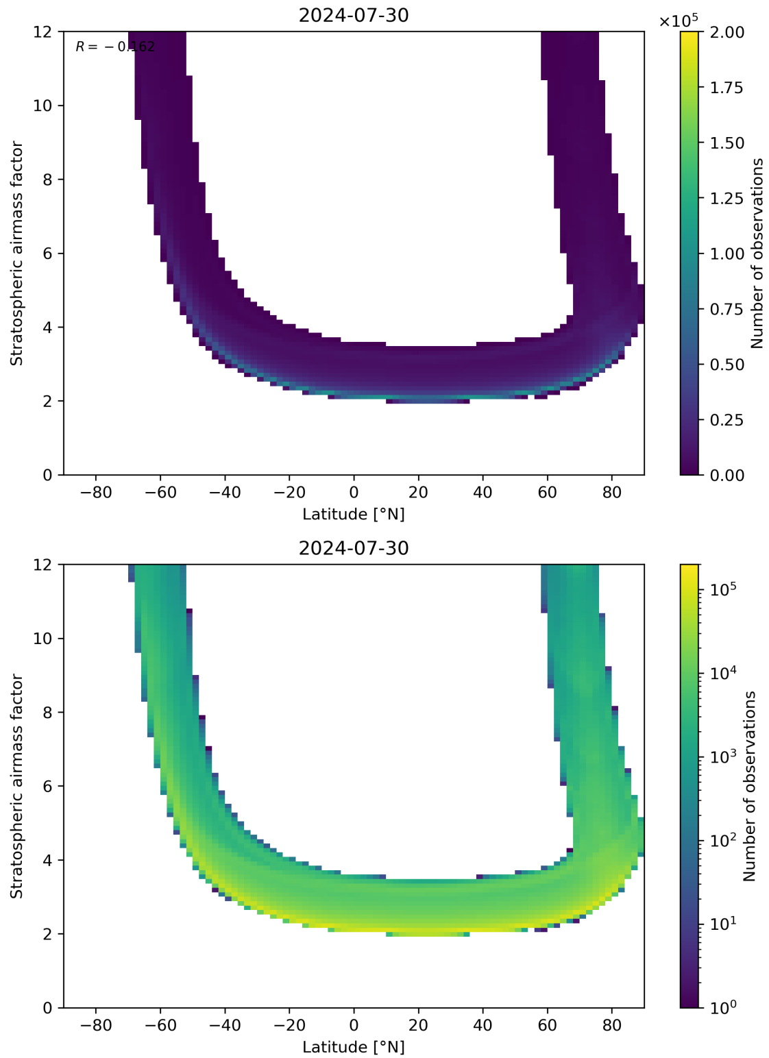
Figure 83: Scatter density plot of “Latitude” against “Stratospheric air mass factor” for 2024-07-29 to 2024-07-31.
