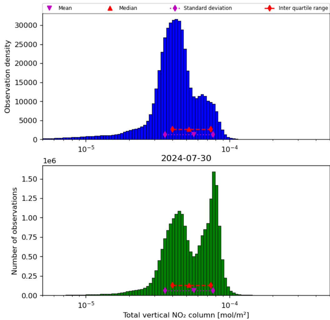
Figure 38: Histogram of “Total vertical NO 2 column” for 2024-07-29 to 2024-07-31
