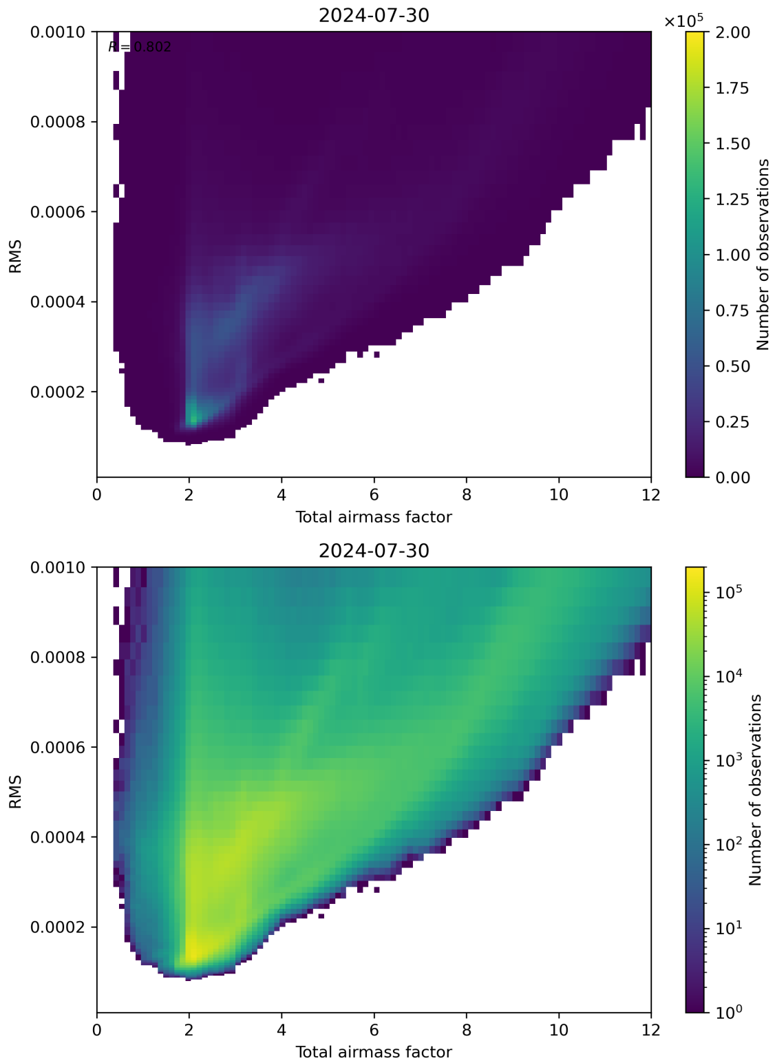
Figure 69: Scatter density plot of “Total airmass factor” against “RMS” for 2024-07-29 to 2024-07-31.
