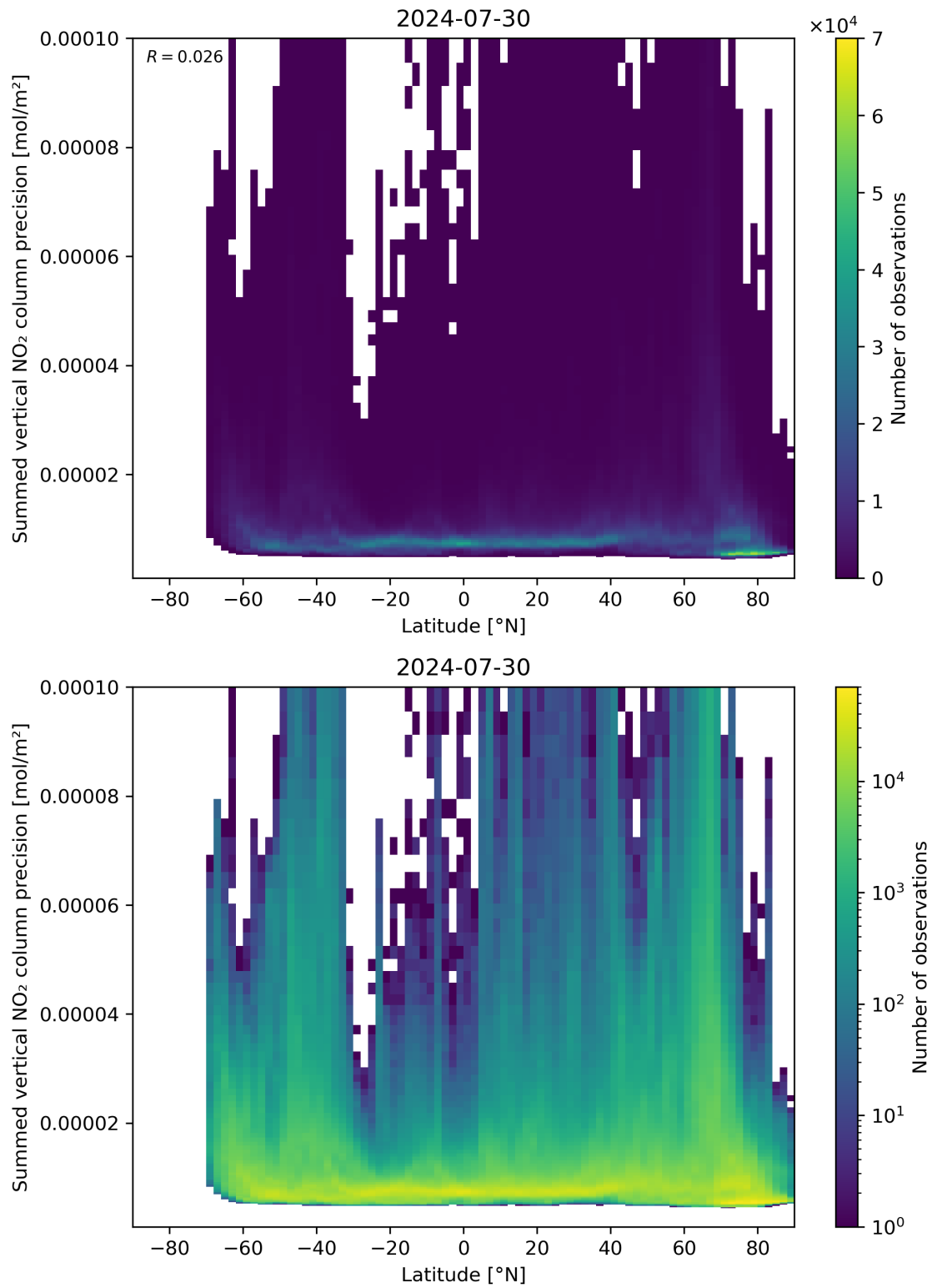
Figure 89: Scatter density plot of “Latitude” against “Summed vertical NO 2 column precision” for 2024-07-29 to 2024-07-31.
