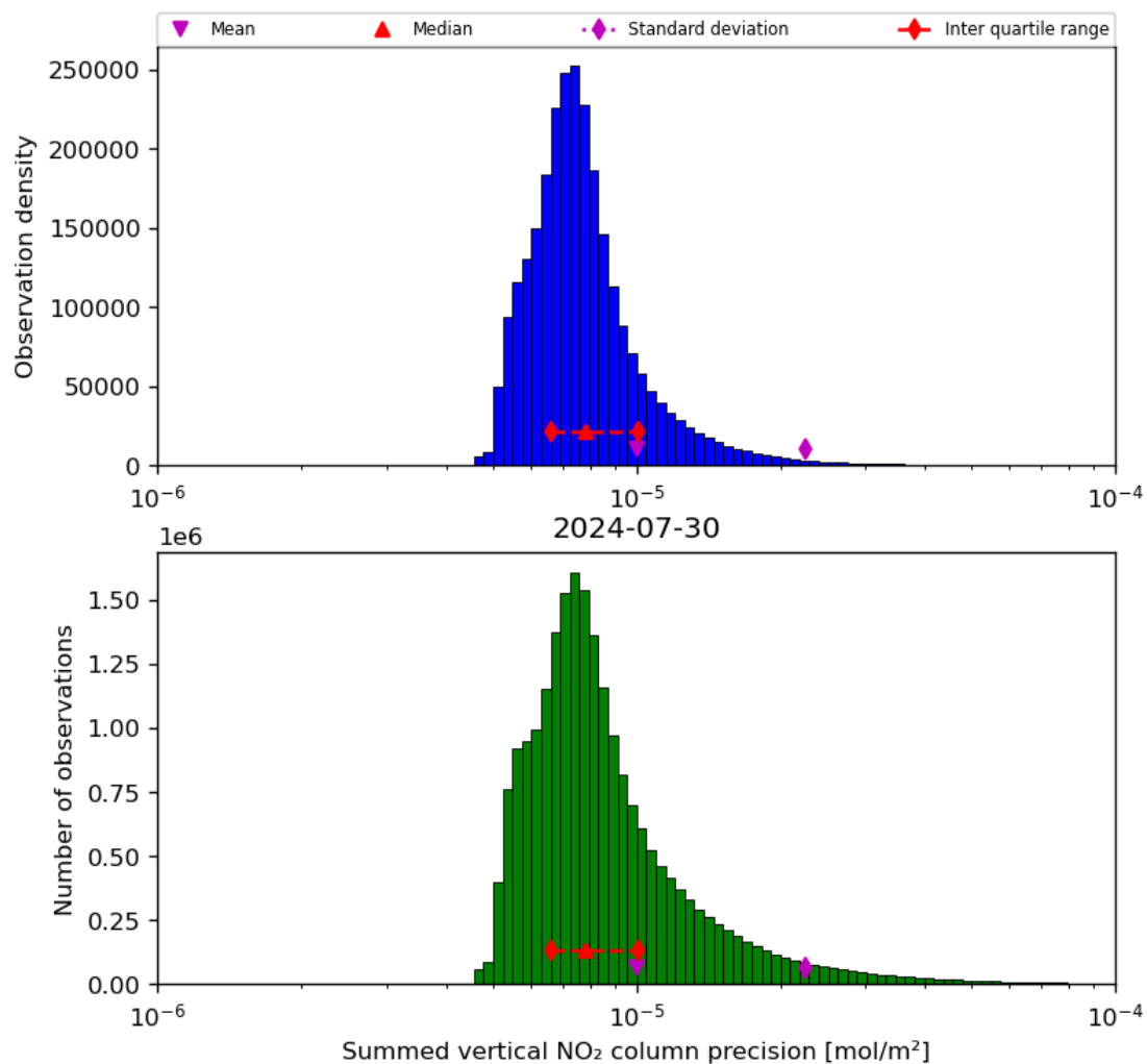
Figure 41: Histogram of “Summed vertical NO 2 column precision” for 2024-07-29 to 2024-07-31
