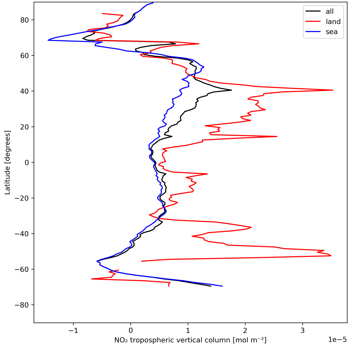
Figure 12: Zonal average of “NO 2 tropospheric vertical column” for 2024-07-29 to 2024-07-31.
