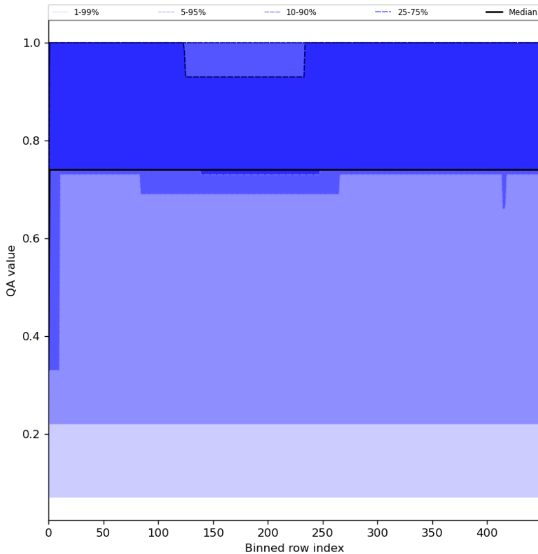
Figure 45: Along track statistics of “QA value” for 2024-07-29 to 2024-07-31
