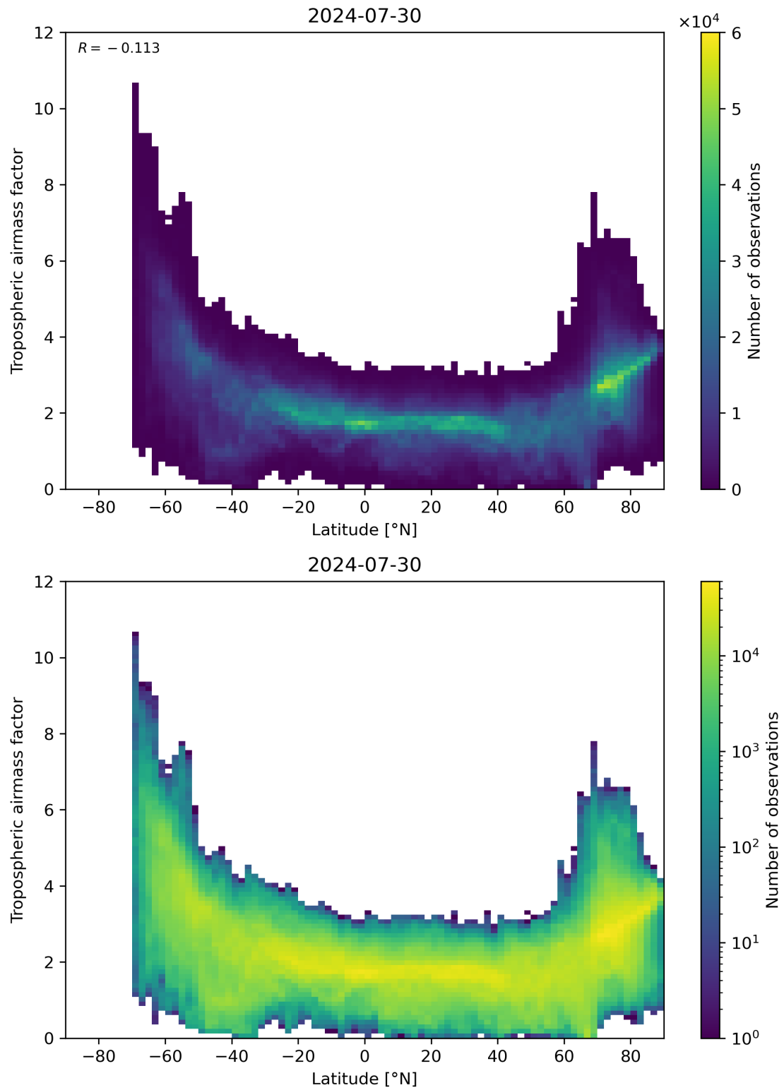
Figure 85: Scatter density plot of “Latitude” against “Tropospheric air mass factor” for 2024-07-29 to 2024-07-31.
