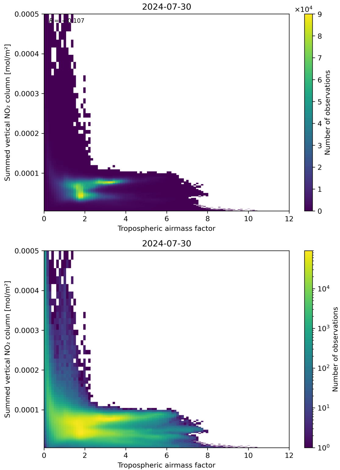
Figure 75: Scatter density plot of “Tropospheric air mass factor” against “Summed vertical NO 2 column” for 2024-07-29 to 2024-07-31.
