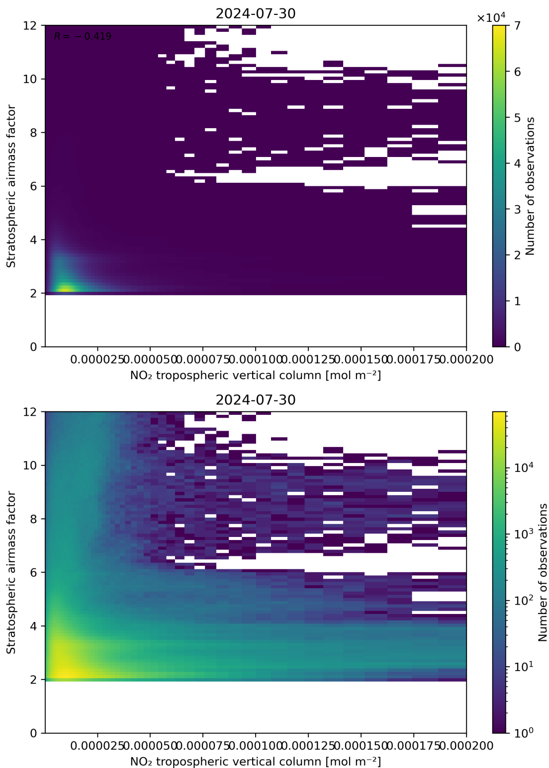
Figure 121: Scatter density plot of “NO 2 tropospheric vertical column” against “Stratospheric air mass factor” for 2024-07-29 to 2024-07-31.
