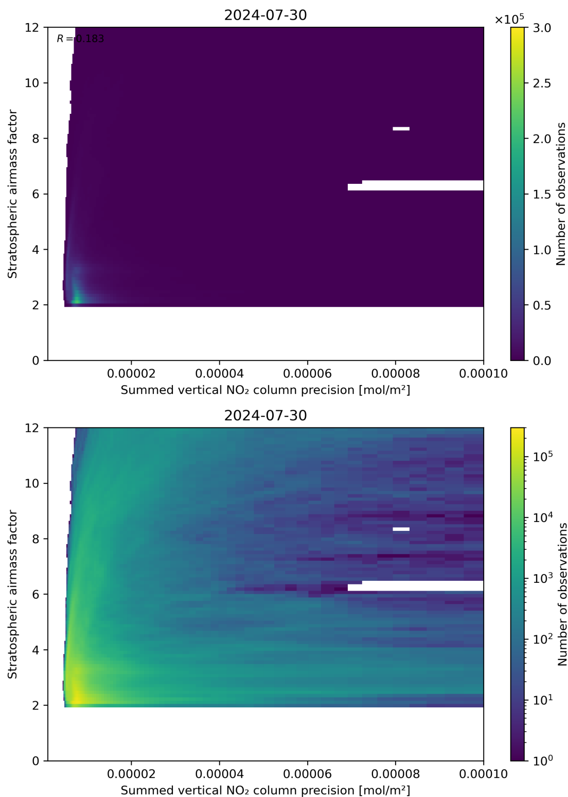
Figure 106: Scatter density plot of “Summed vertical NO 2 column precision” against “Stratospheric airmass factor” for 2024-07-29 to 2024-07-31.
