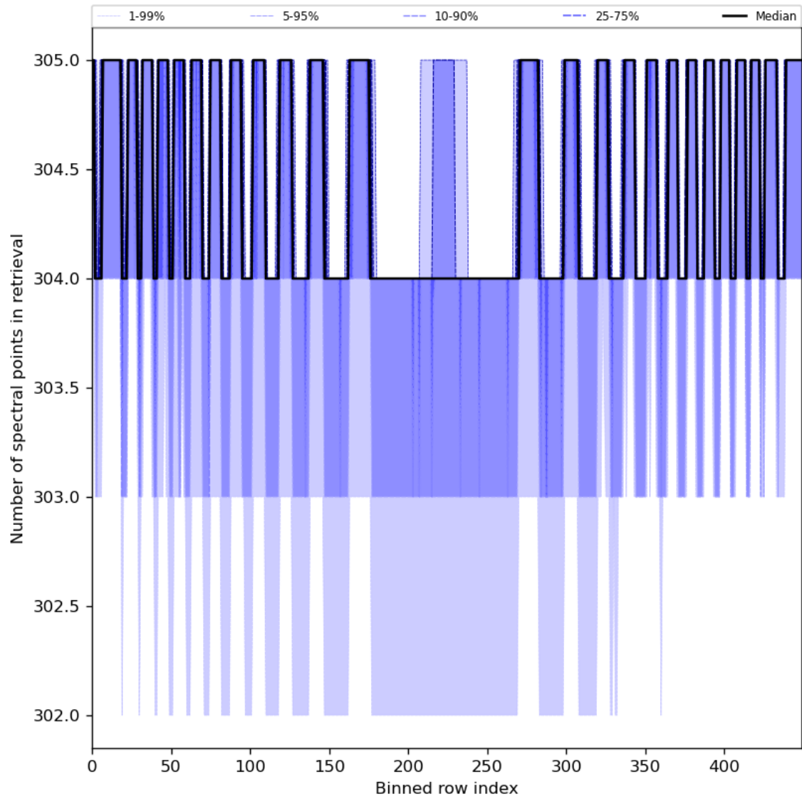
Figure 50: Along track statistics of “Number of spectral points in retrieval” for 2024-07-29 to 2024-07-31
