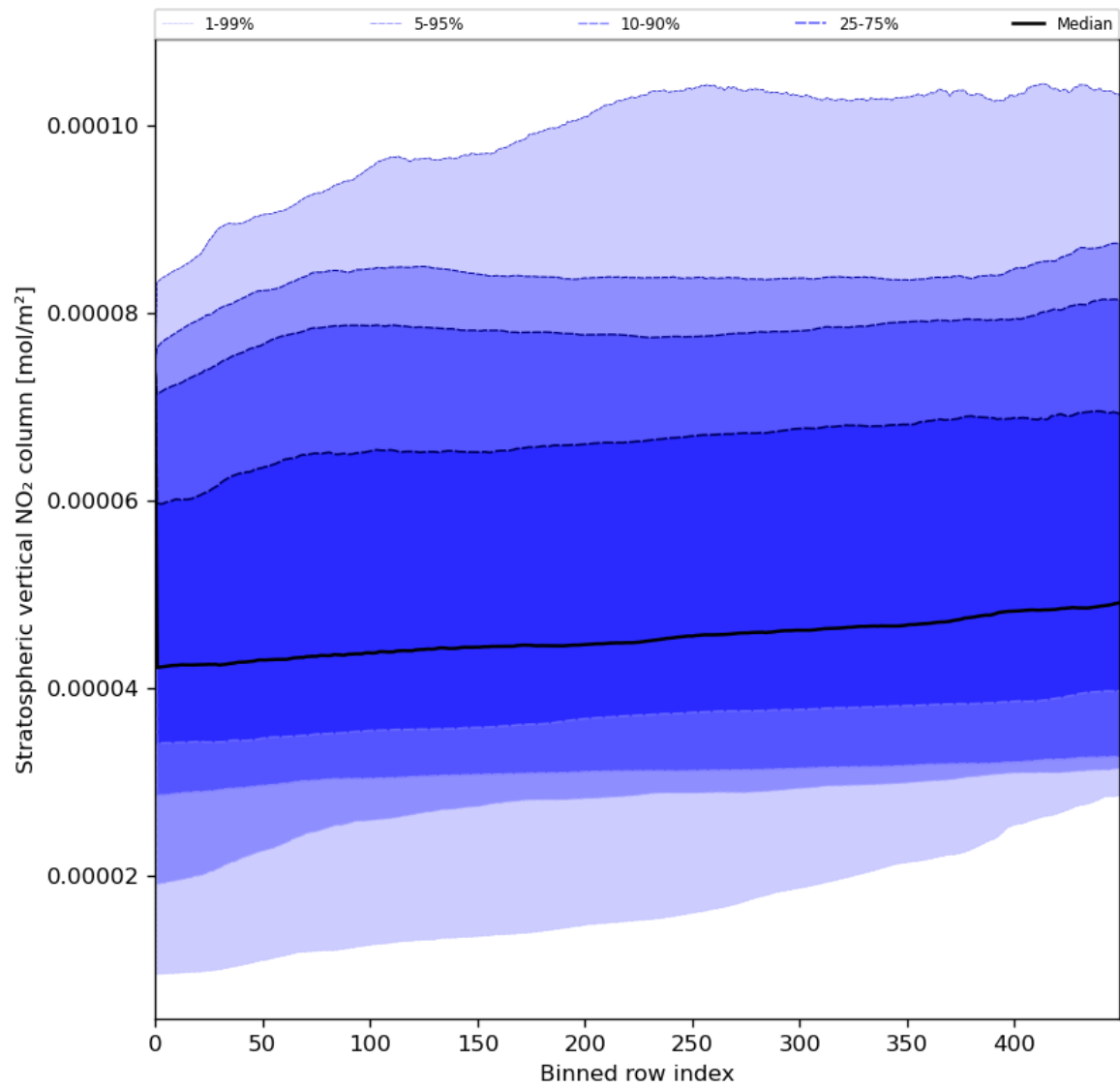
Figure 53: Along track statistics of "Stratospheric vertical NO 2 column" for 2024-07-29 to 2024-07-31
