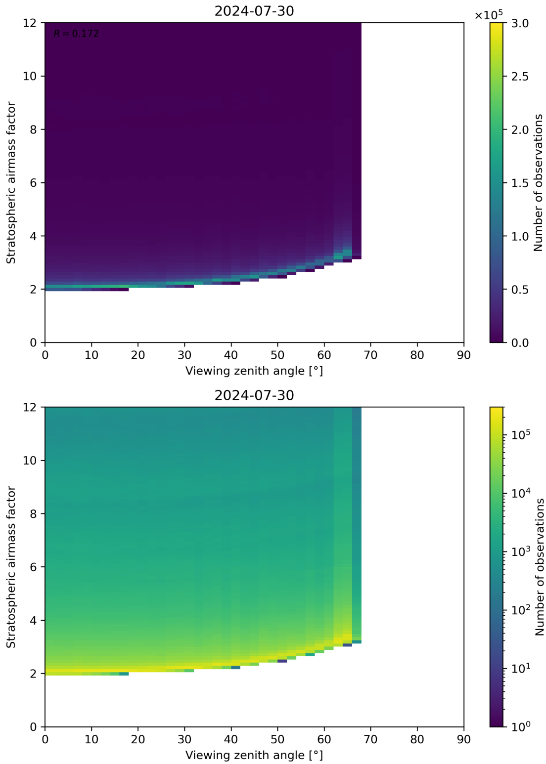
Figure 159: Scatter density plot of “Viewing zenith angle” against “Stratospheric airmass factor” for 2024-07-29 to 2024-07-31.
