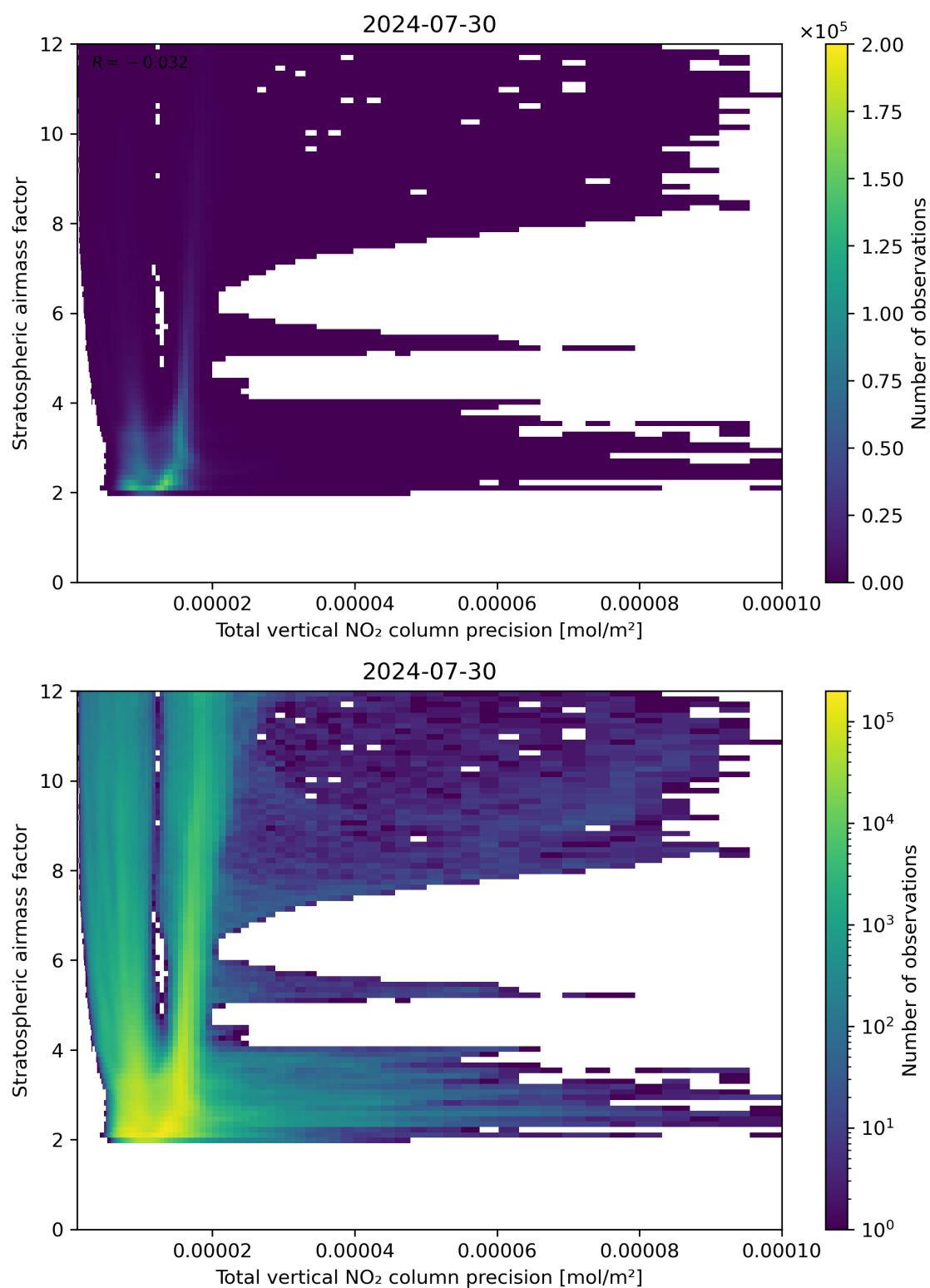
Figure 115: Scatter density plot of “Total vertical NO 2 column precision” against “Stratospheric airmass factor” for 2024-07-29 to 2024-07-31.
