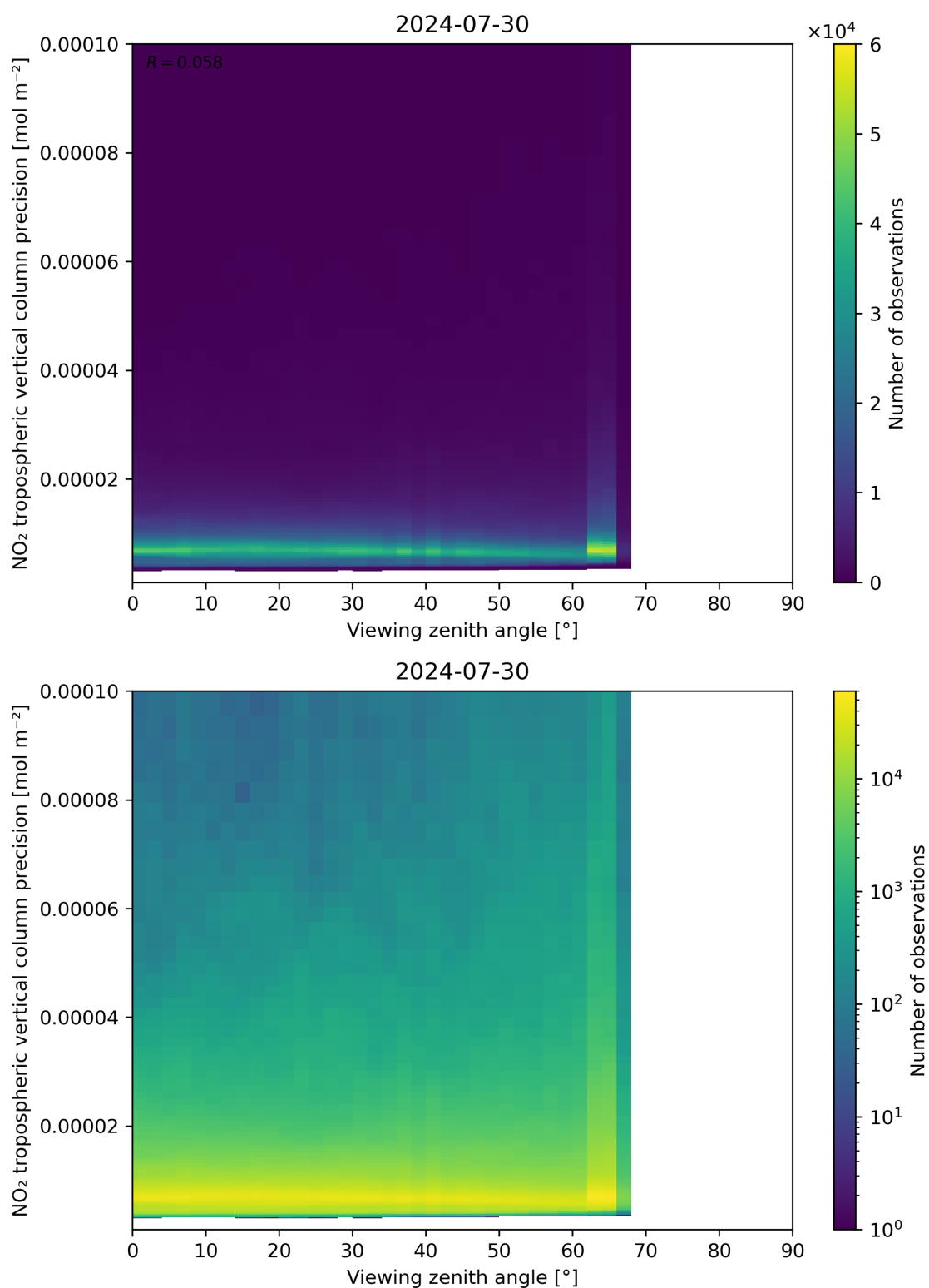
Figure 170: Scatter density plot of “Viewing zenith angle” against “NO 2 tropospheric vertical column precision” for 2024-07-29 to 2024-07-31.
