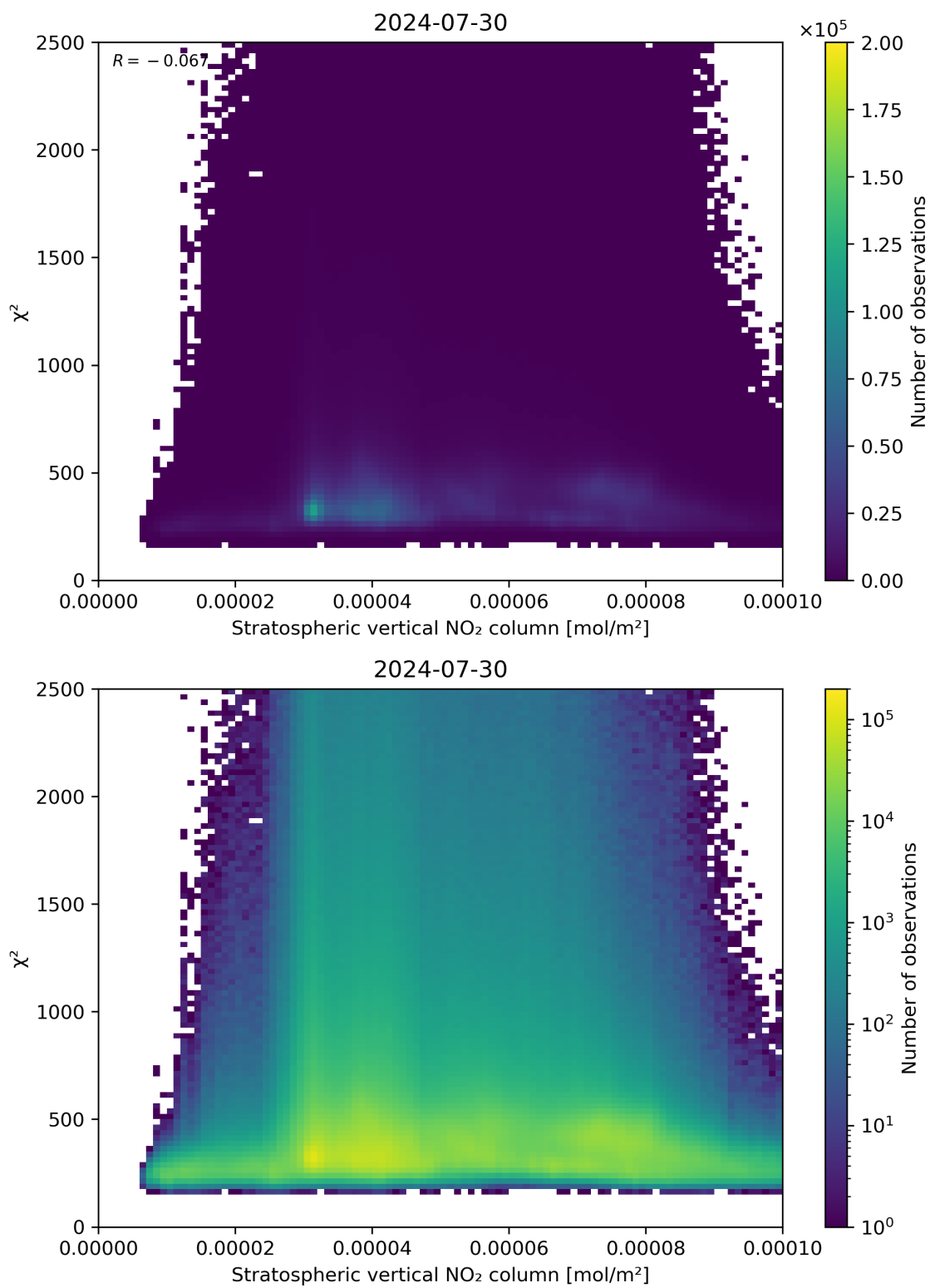
Figure 97: Scatter density plot of “Stratospheric vertical NO 2 column” against “ \chi^2 ” for 2024-07-29 to 2024-07-31.
