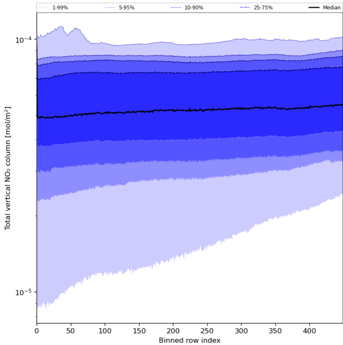
Figure 55: Along track statistics of “Total vertical NO 2 column” for 2024-07-29 to 2024-07-31
