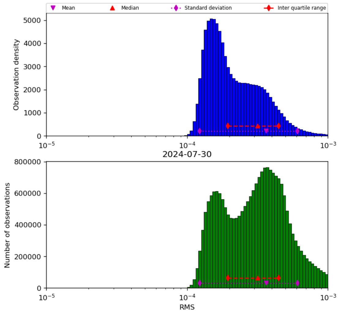
Figure 43: Histogram of “RMS” for 2024-07-29 to 2024-07-31
