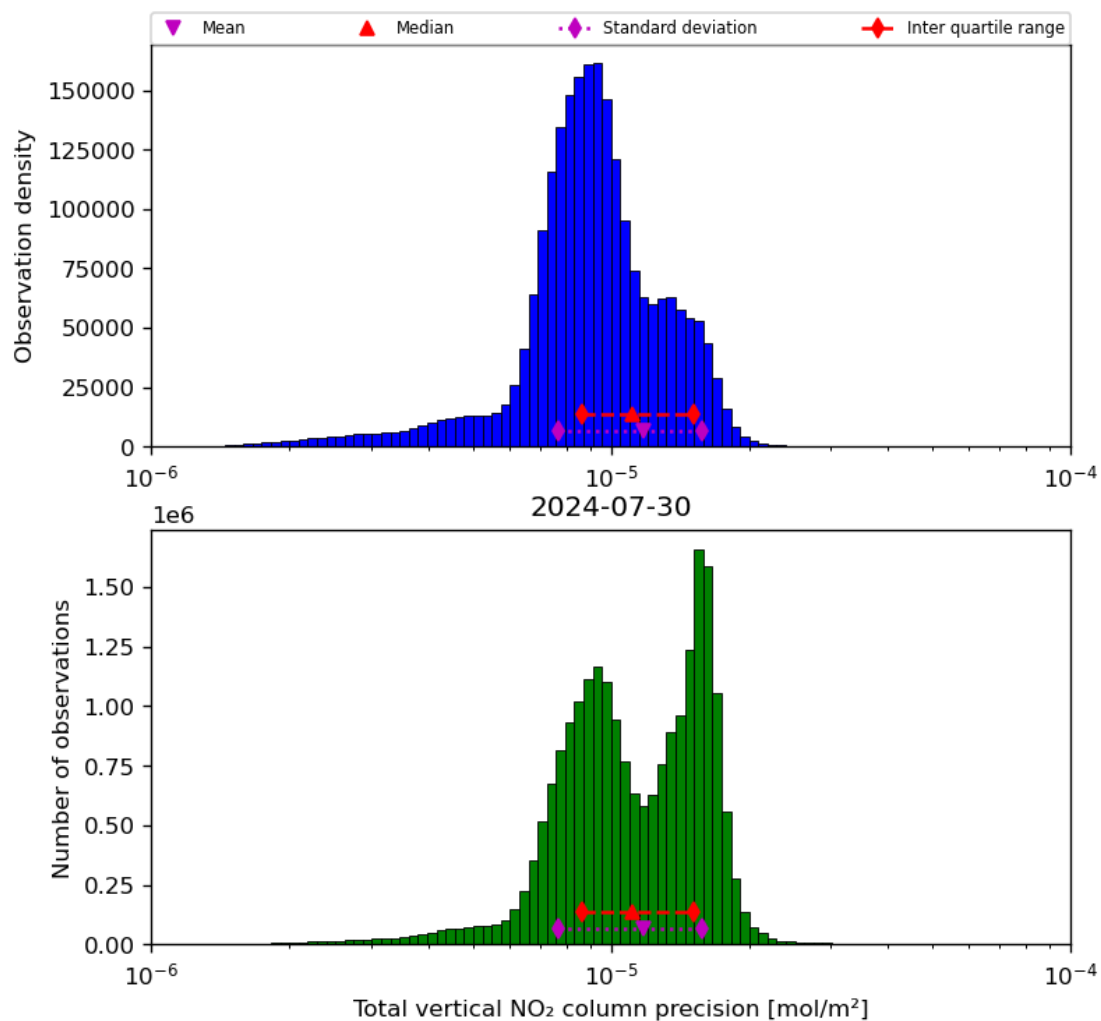
Figure 39: Histogram of “Total vertical NO 2 column precision” for 2024-07-29 to 2024-07-31
