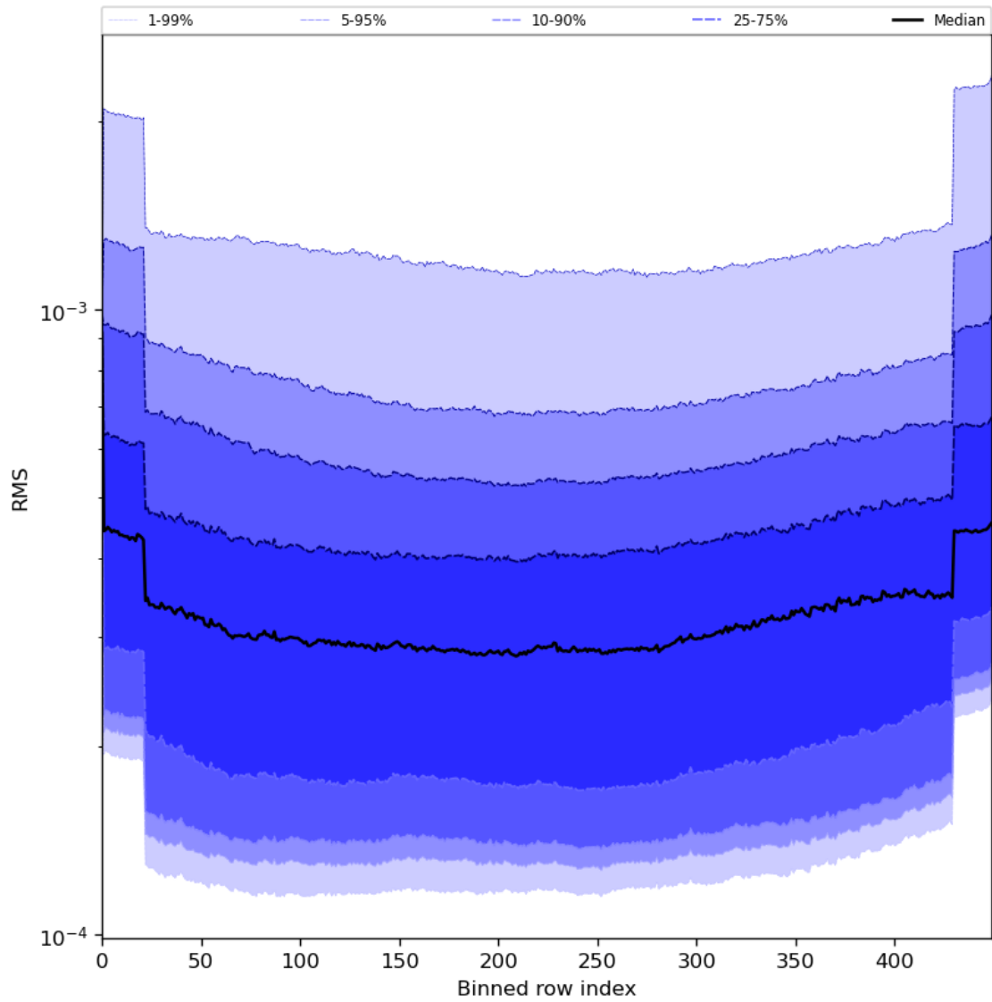
Figure 60: Along track statistics of “RMS” for 2024-07-29 to 2024-07-31
