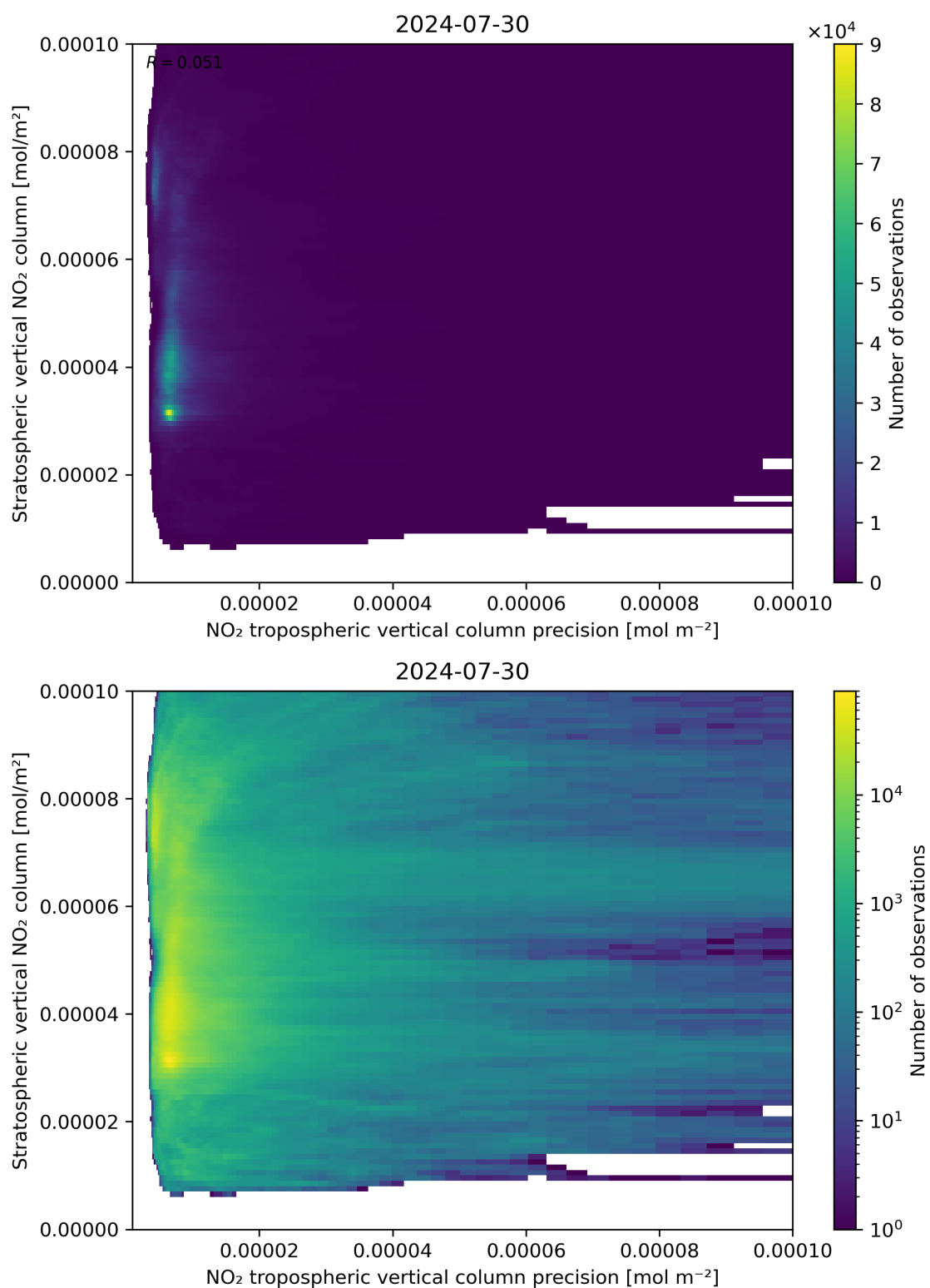
Figure 135: Scatter density plot of “NO 2 tropospheric vertical column precision” against “Stratospheric vertical NO 2 column” for 2024-07-29 to 2024-07-31.
