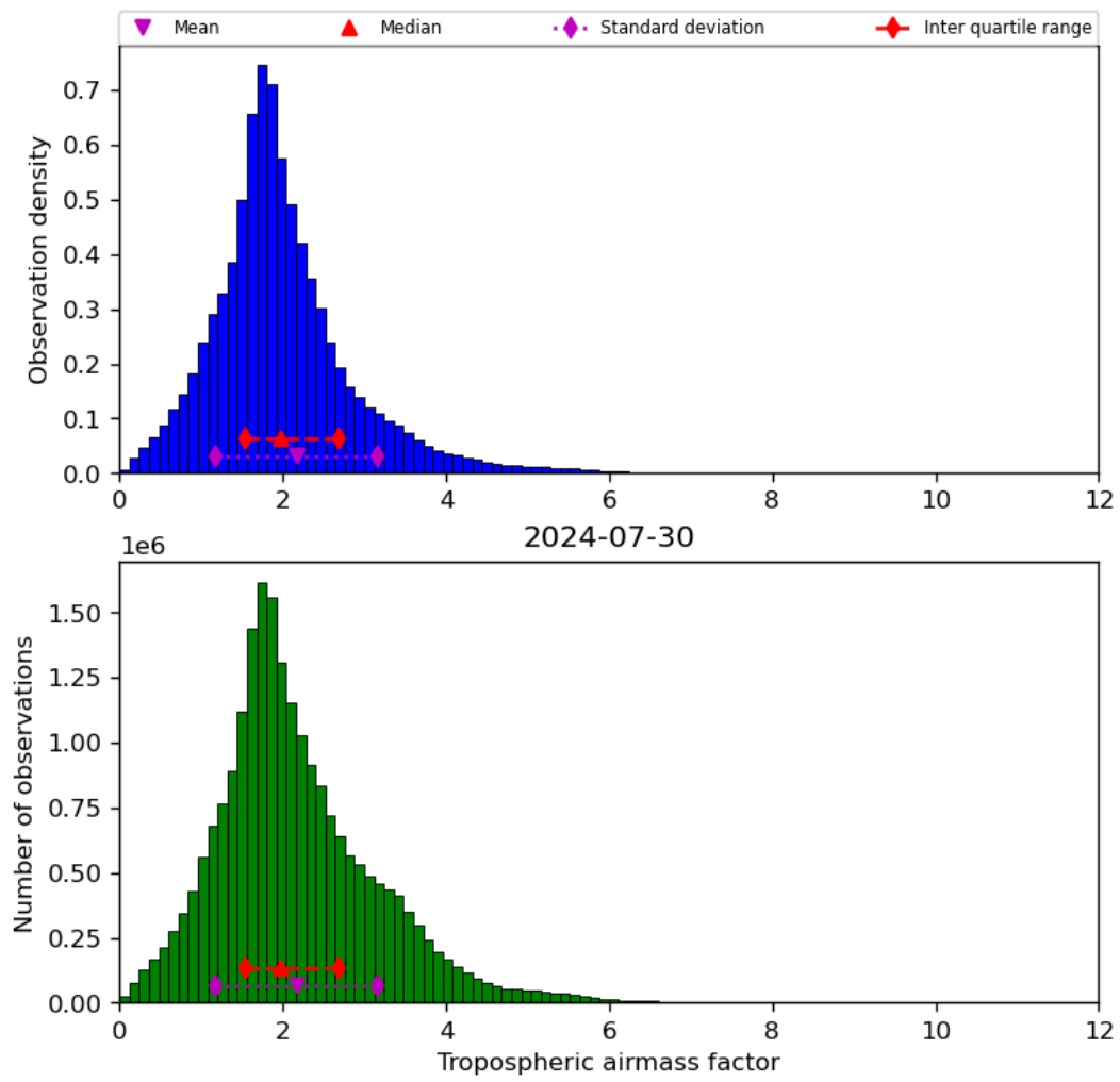
Figure 31: Histogram of “Tropospheric airmass factor” for 2024-07-29 to 2024-07-31
