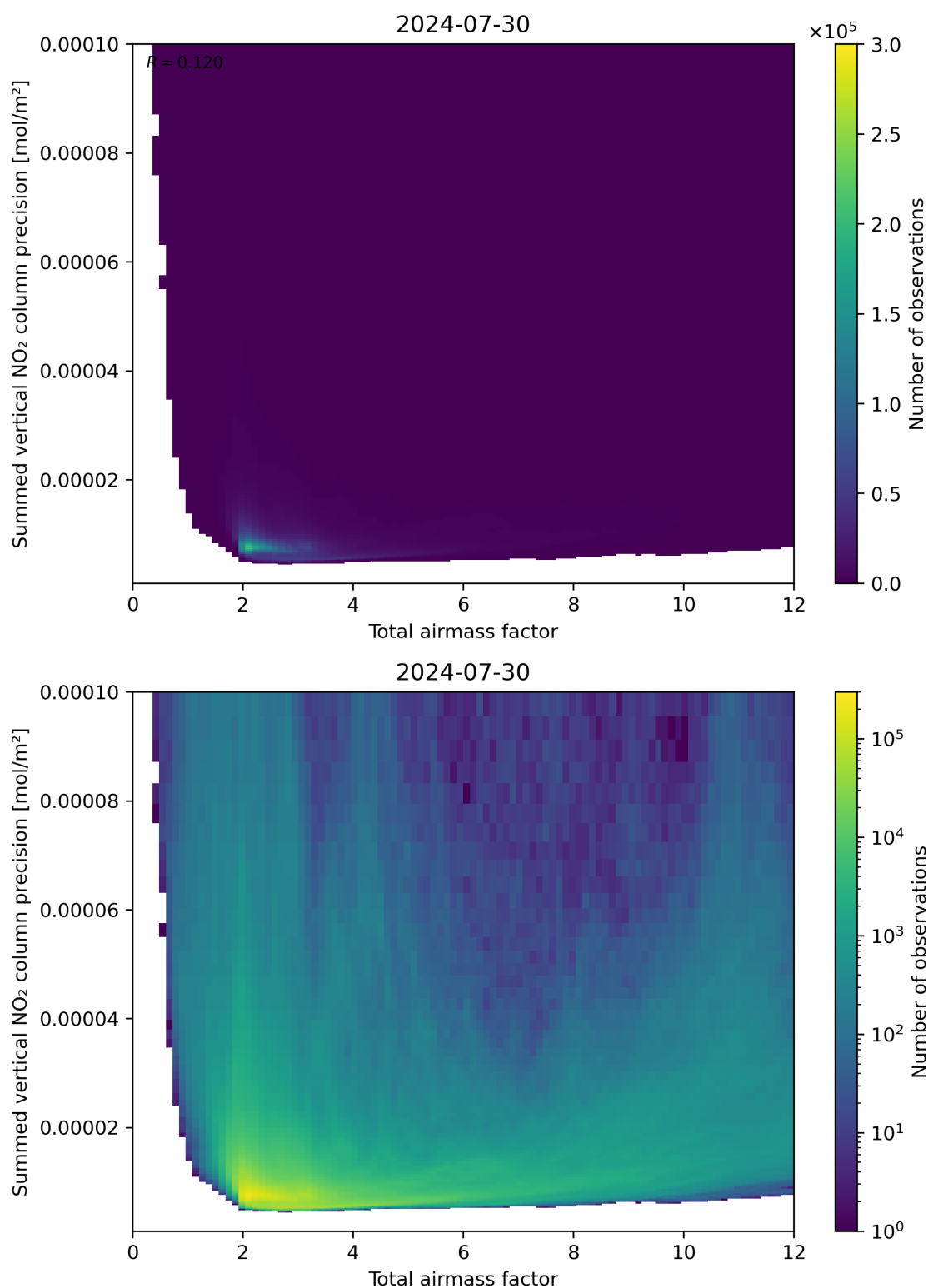
Figure 66: Scatter density plot of “Total airmass factor” against “Summed vertical NO 2 column precision” for 2024-07-29 to 2024-07-31.
