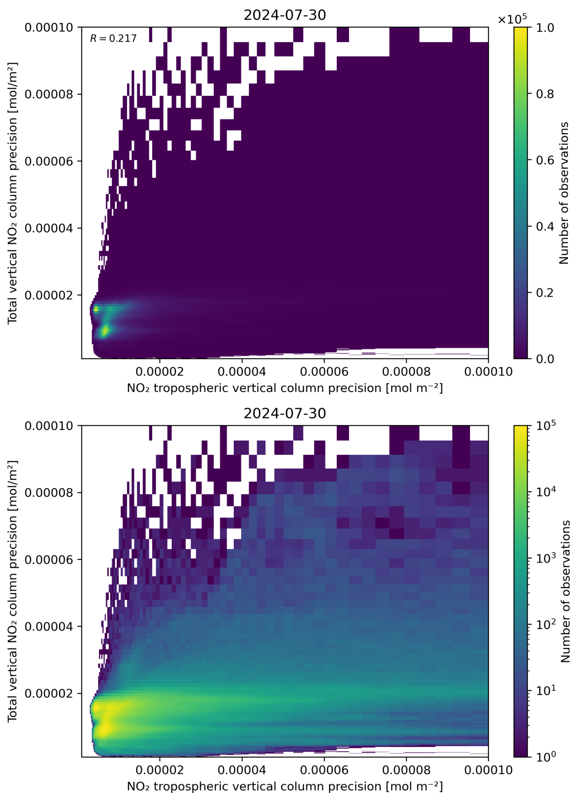
Figure 139: Scatter density plot of “NO 2 tropospheric vertical column precision” against “Total vertical NO 2 column precision” for 2024-07-29 to 2024-07-31.
