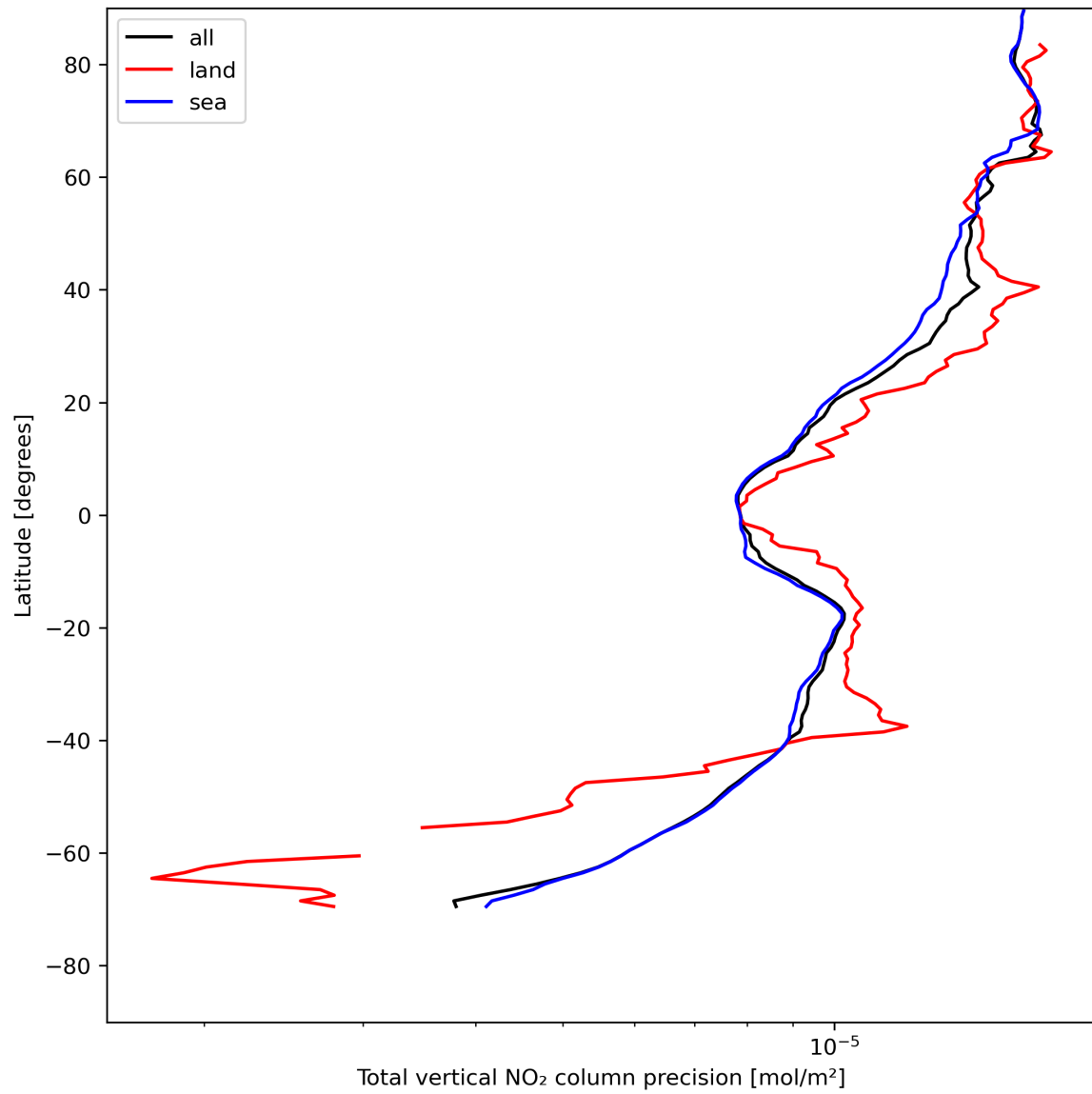
Figure 22: Zonal average of “Total vertical NO 2 column precision” for 2024-07-29 to 2024-07-31.
