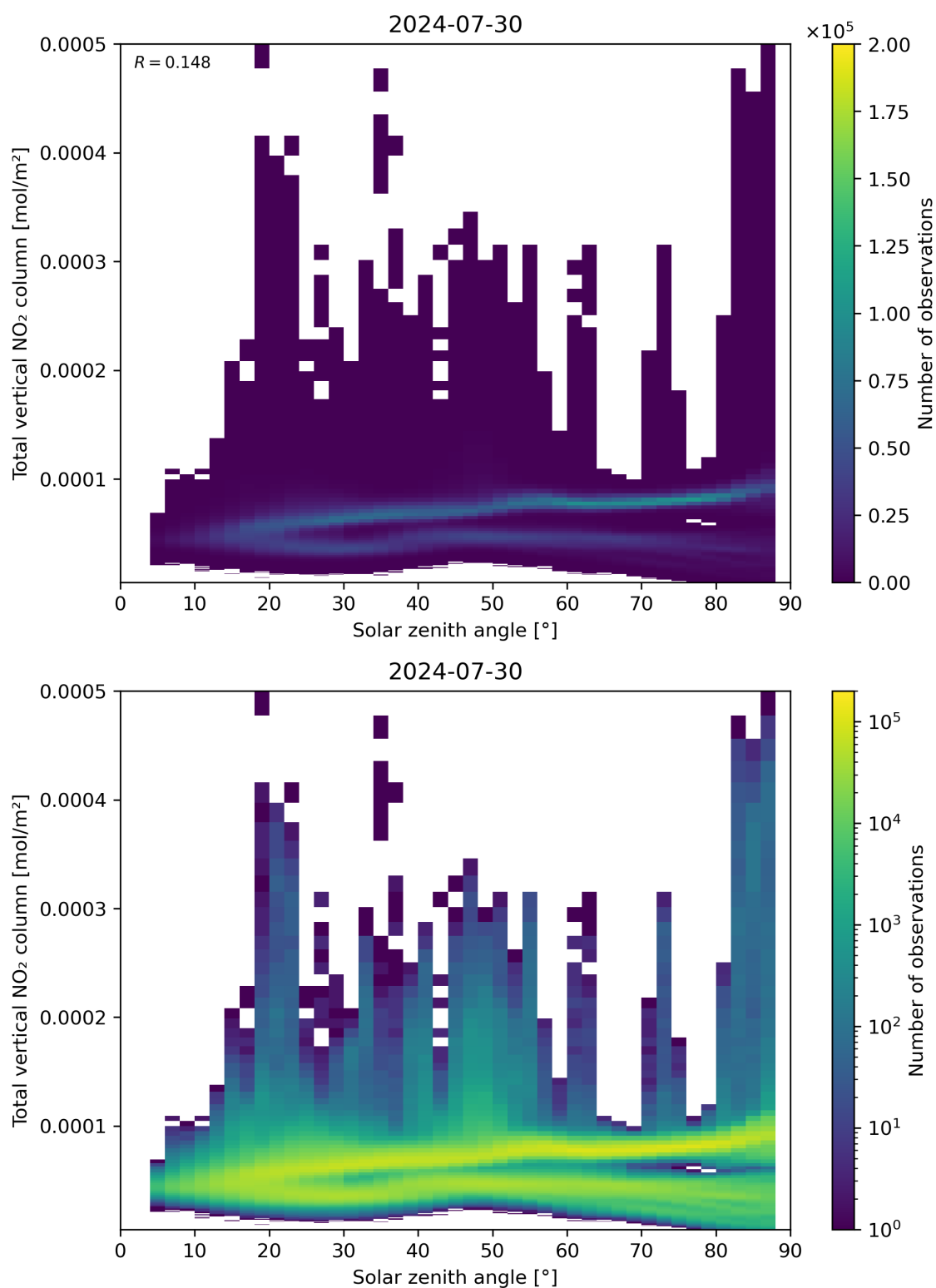
Figure 153: Scatter density plot of “Solar zenith angle” against “Total vertical NO 2 column” for 2024-07-29 to 2024-07-31.
