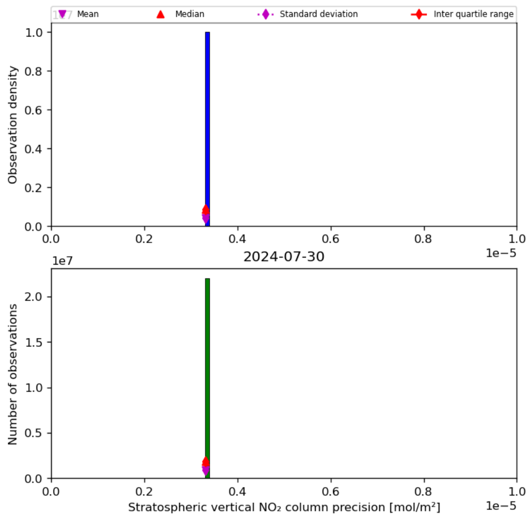
Figure 37: Histogram of “Stratospheric vertical NO 2 column precision” for 2024-07-29 to 2024-07-31
