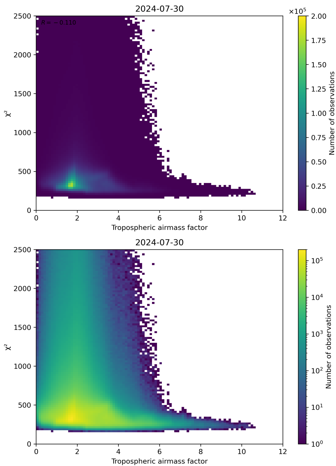
Figure 73: Scatter density plot of “Tropospheric airmass factor” against “ \chi^2 ” for 2024-07-29 to 2024-07-31.
