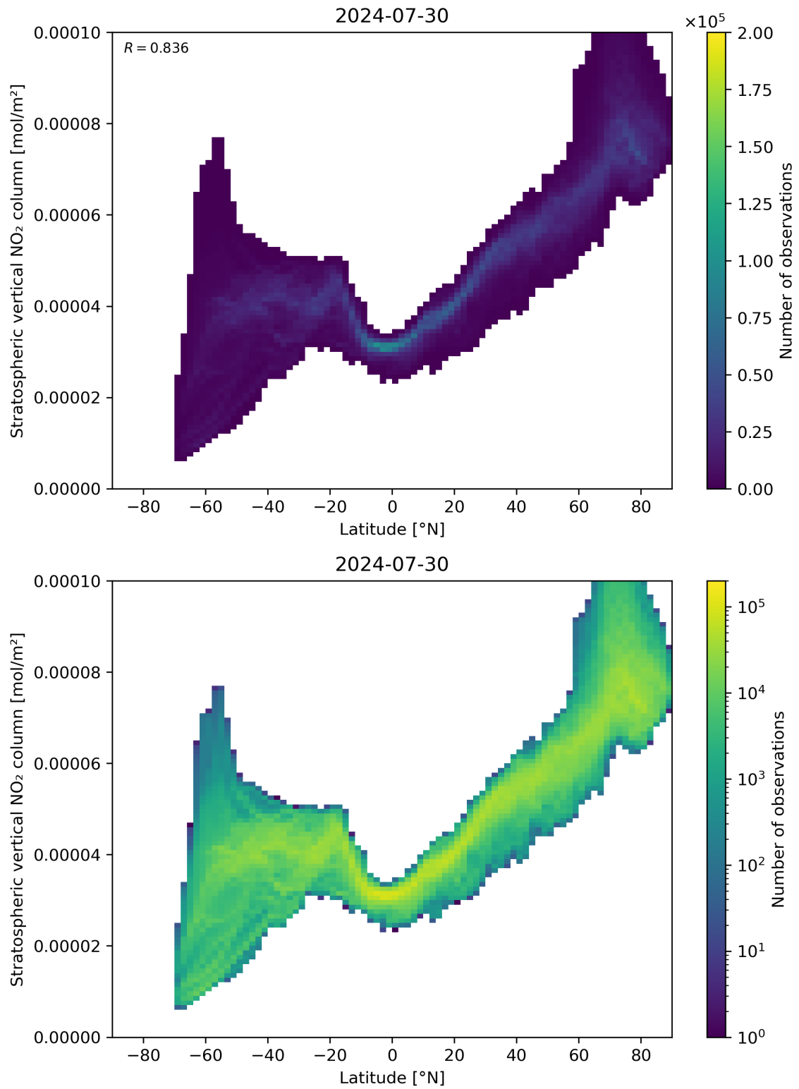
Figure 87: Scatter density plot of “Latitude” against “Stratospheric vertical NO 2 column” for 2024-07-29 to 2024-07-31.
