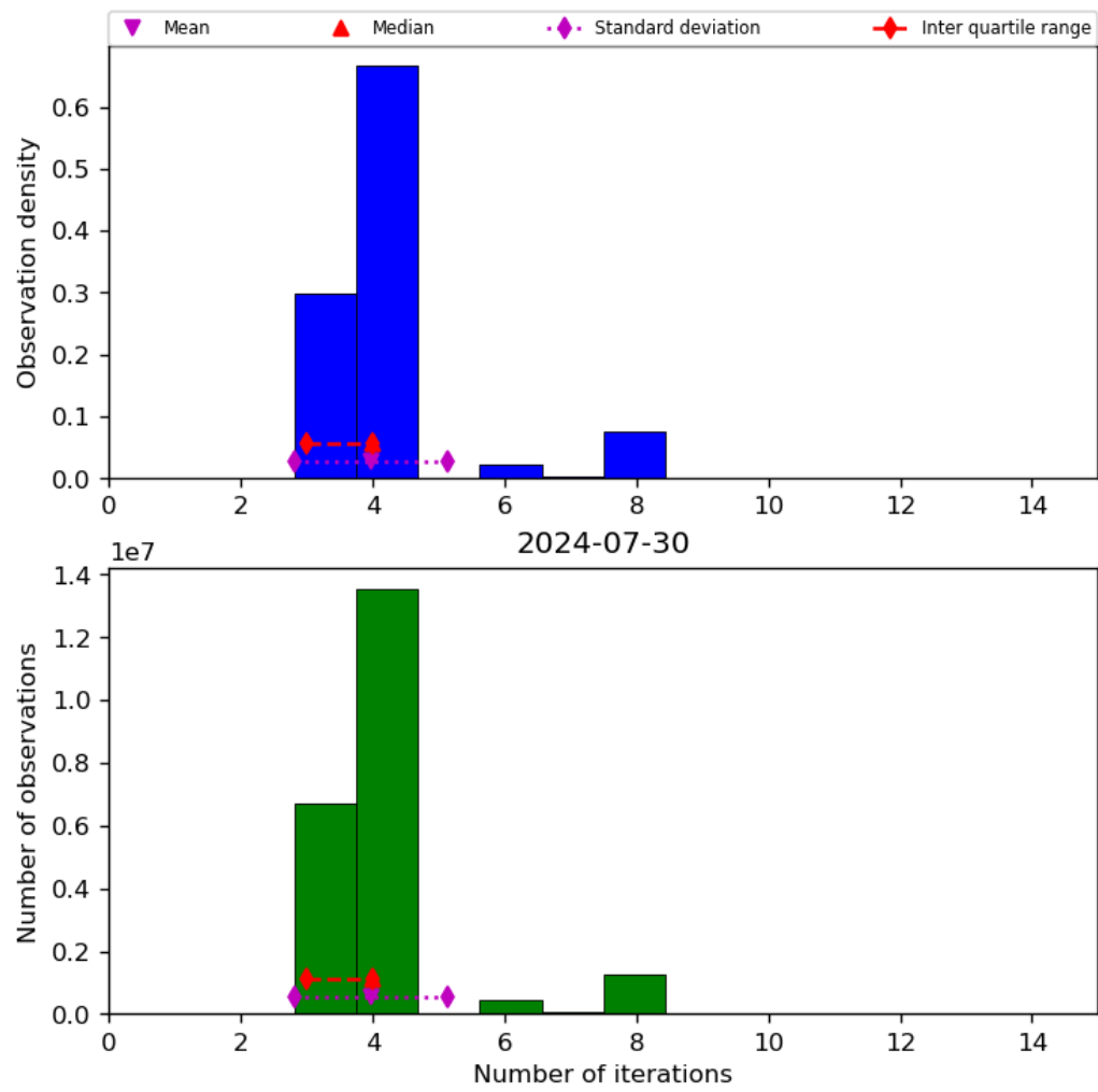
Figure 34: Histogram of “Number of iterations” for 2024-07-29 to 2024-07-31
