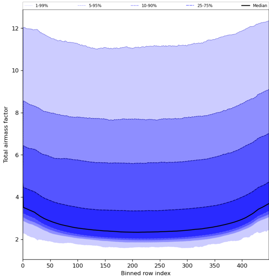
Figure 49: Along track statistics of “Total airmass factor” for 2024-07-29 to 2024-07-31
