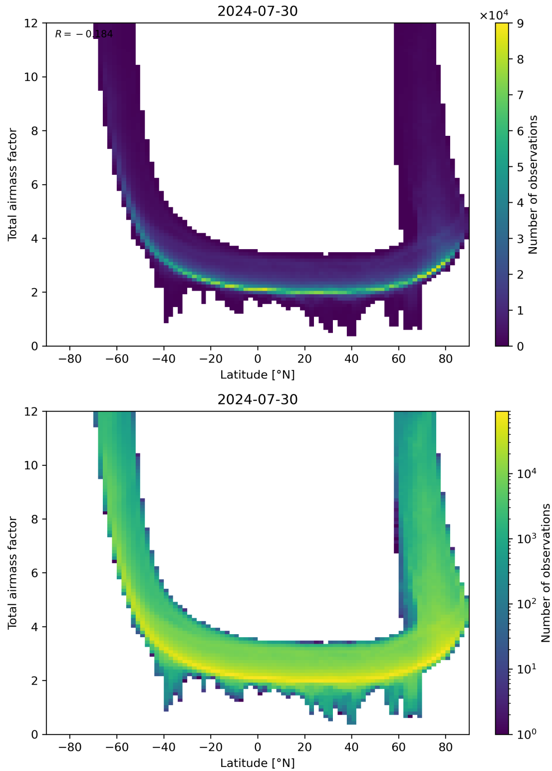
Figure 84: Scatter density plot of “Latitude” against “Total airmass factor” for 2024-07-29 to 2024-07-31.
