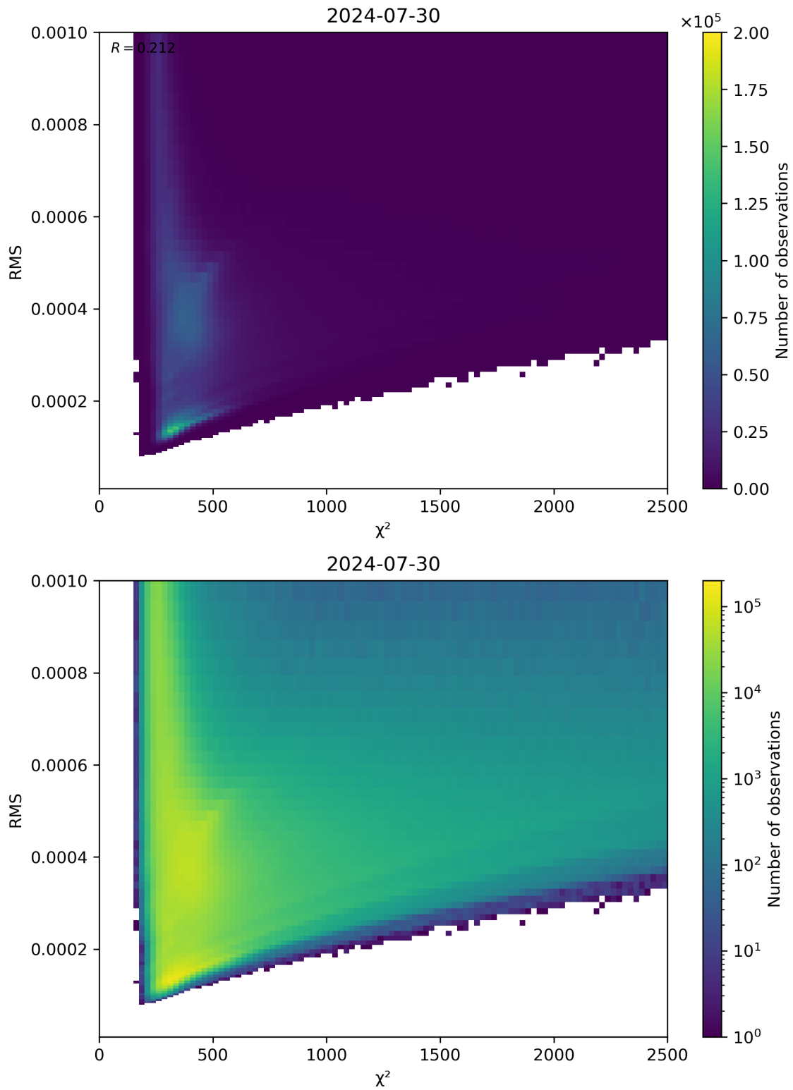
Figure 82: Scatter density plot of “ \chi^2 ” against “RMS” for 2024-07-29 to 2024-07-31.
