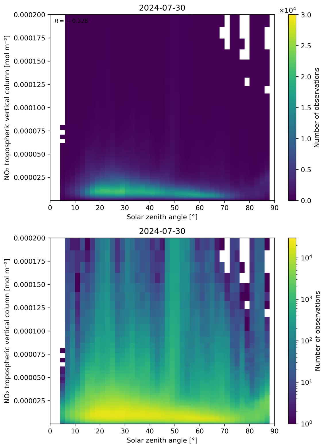
Figure 155: Scatter density plot of “Solar zenith angle” against “NO 2 tropospheric vertical column” for 2024-07-29 to 2024-07-31.
