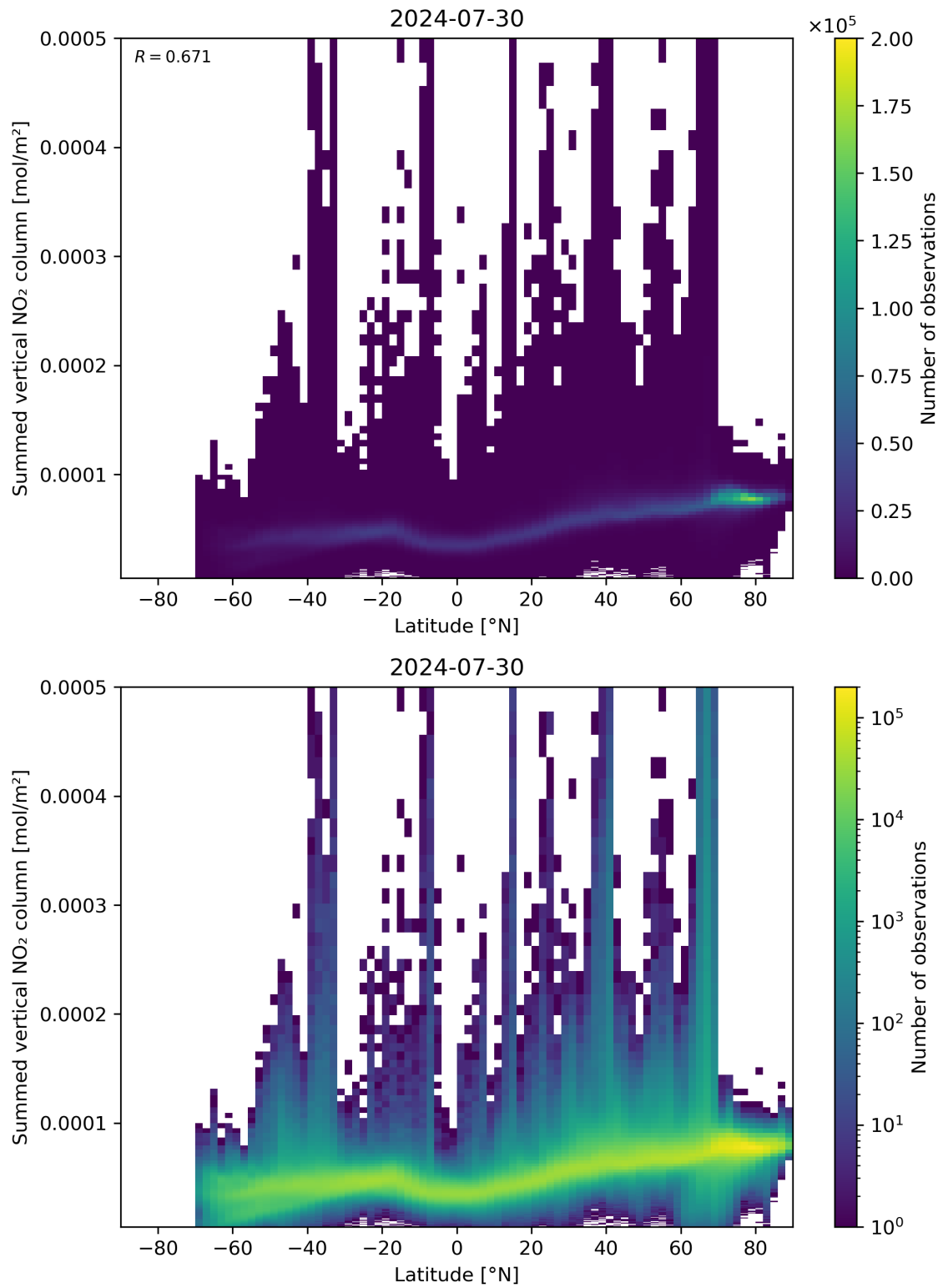
Figure 88: Scatter density plot of “Latitude” against “Summed vertical NO 2 column” for 2024-07-29 to 2024-07-31.
