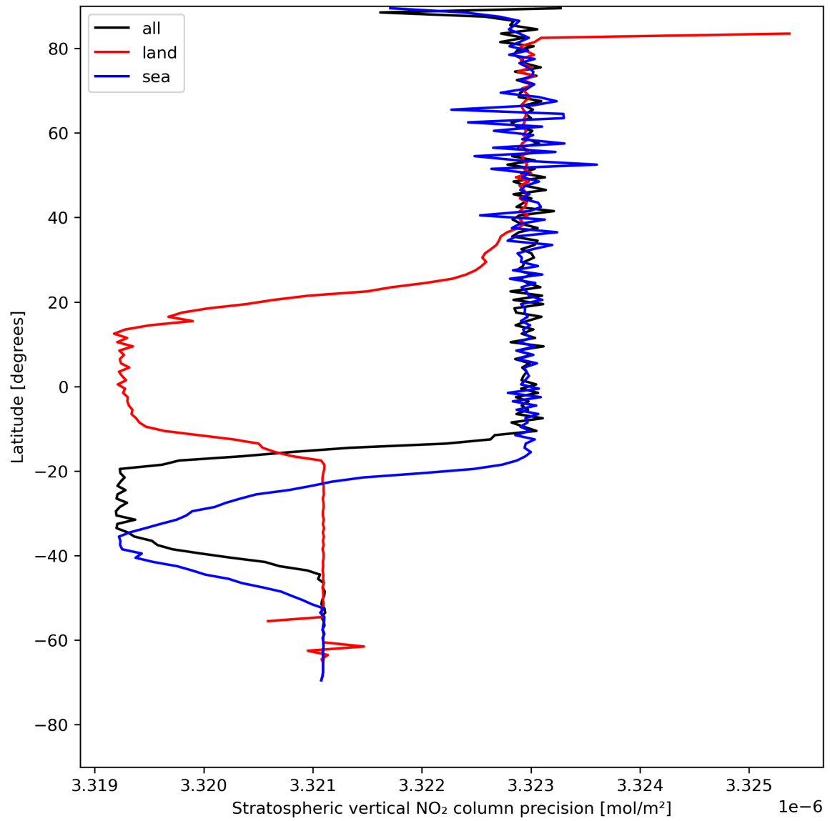
Figure 20: Zonal average of “Stratospheric vertical NO 2 column precision” for 2024-07-29 to 2024-07-31.
