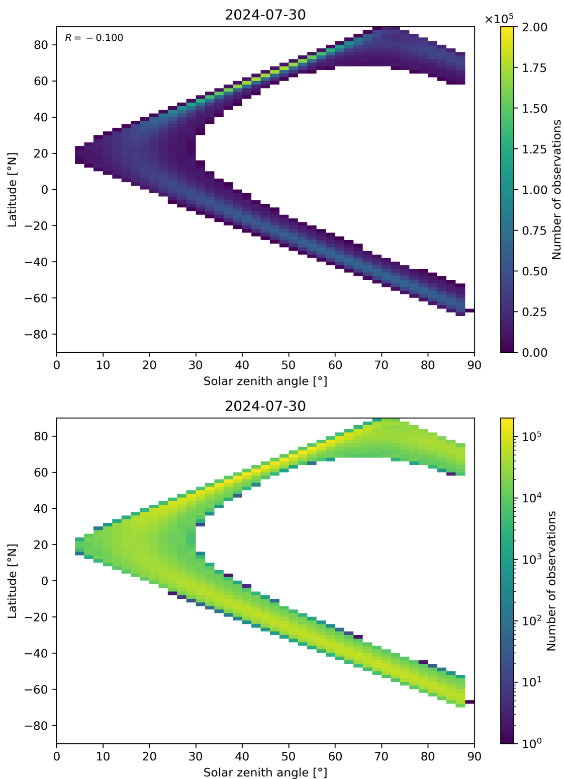
Figure 149: Scatter density plot of “Solar zenith angle” against “Latitude” for 2024-07-29 to 2024-07-31.
