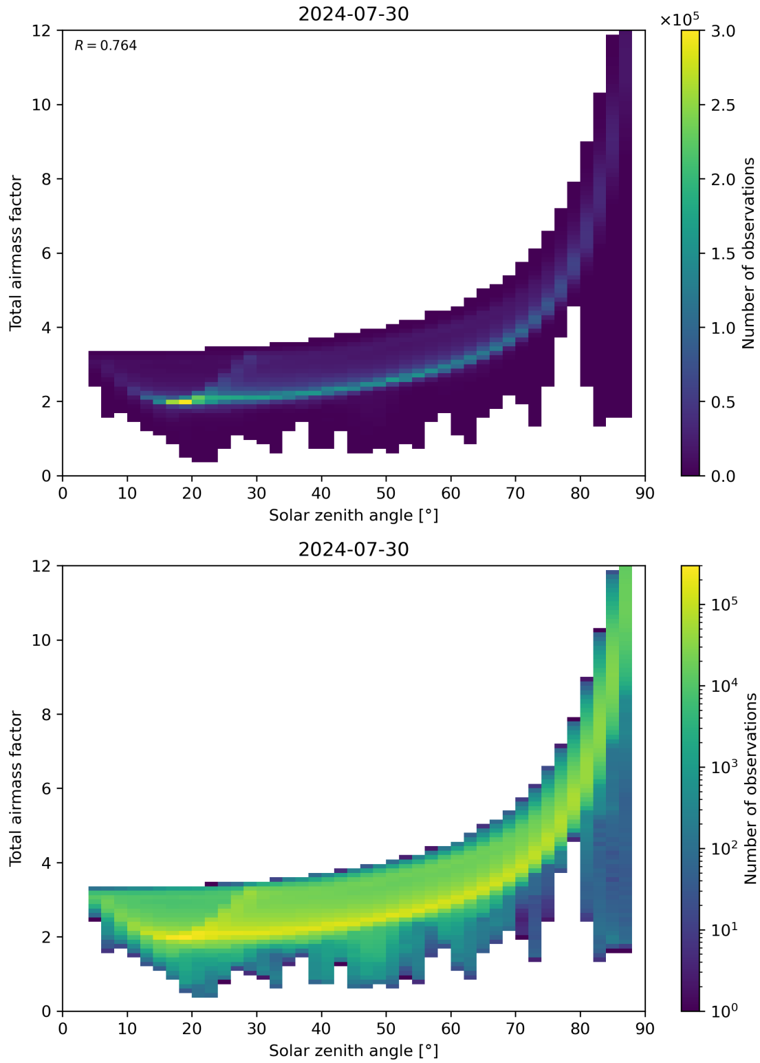
Figure 146: Scatter density plot of “Solar zenith angle” against “Total air mass factor” for 2024-07-29 to 2024-07-31.
