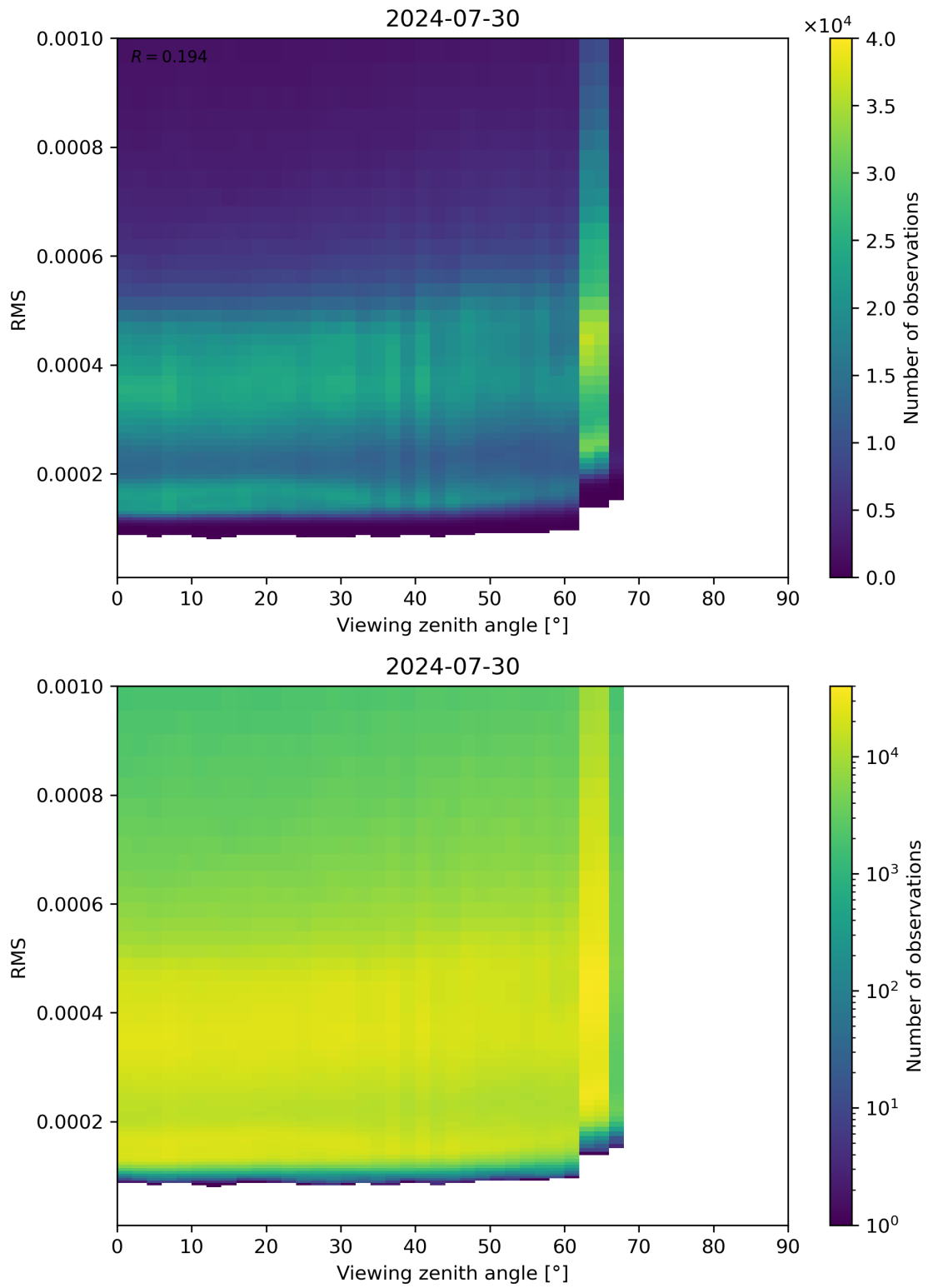
Figure 171: Scatter density plot of “Viewing zenith angle” against “RMS” for 2024-07-29 to 2024-07-31.
