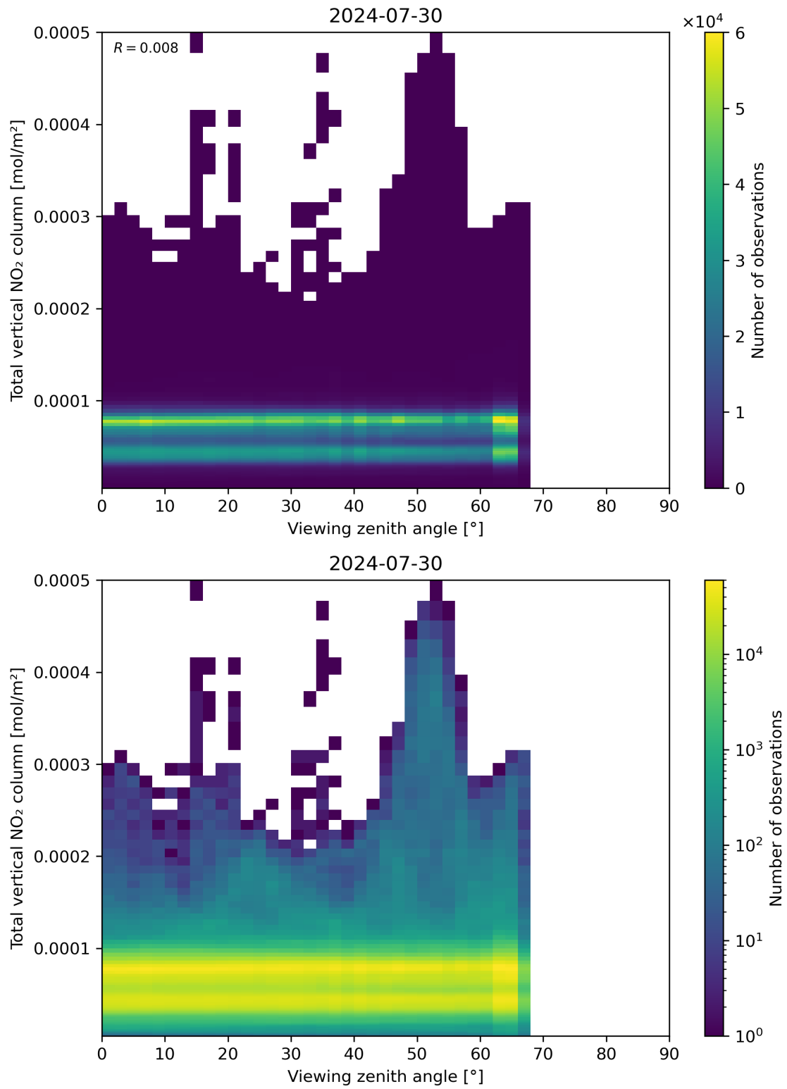
Figure 167: Scatter density plot of “Viewing zenith angle” against “Total vertical NO 2 column” for 2024-07-29 to 2024-07-31.
