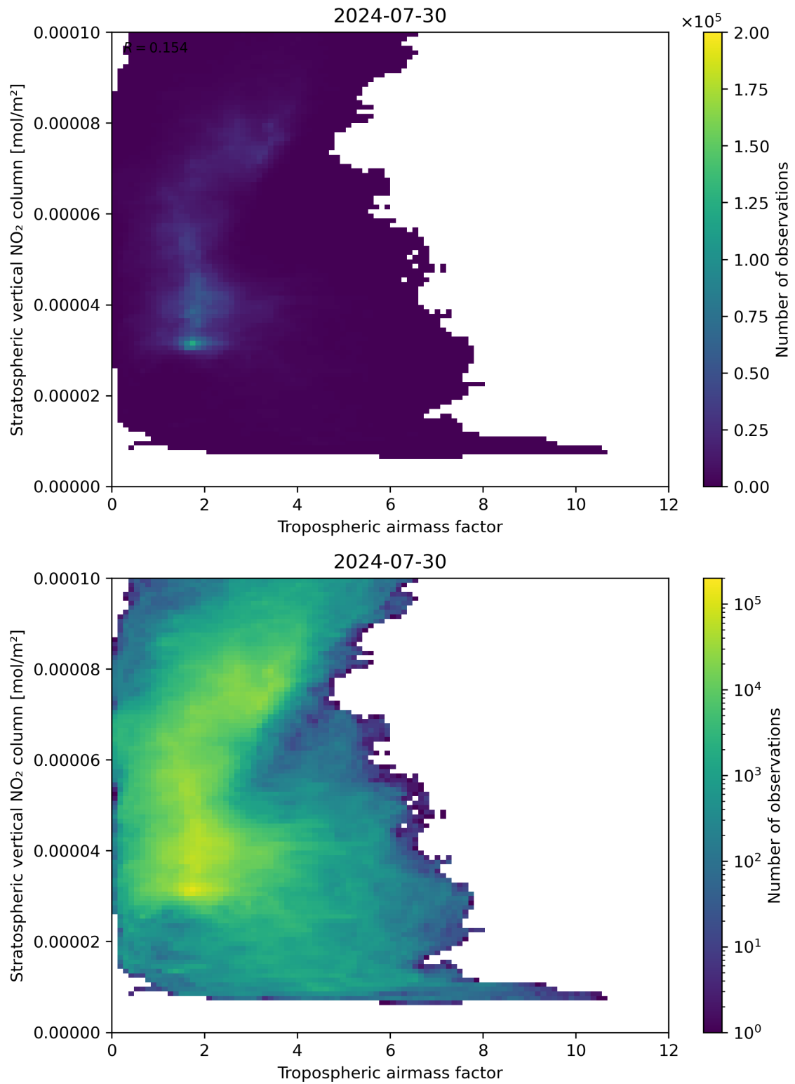
Figure 74: Scatter density plot of “Tropospheric air mass factor” against “Stratospheric vertical NO 2 column” for 2024-07-29 to 2024-07-31.
