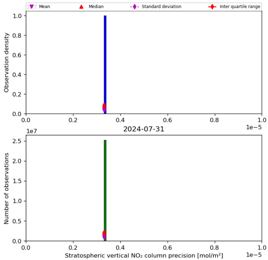
Figure 37: Histogram of “Stratospheric vertical NO 2 column precision” for 2024-07-31 to 2024-08-01
