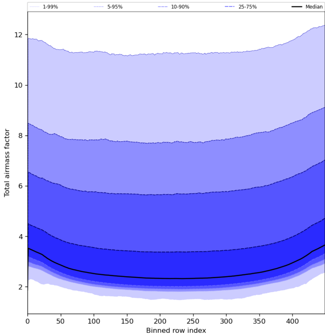
Figure 49: Along track statistics of “Total airmass factor” for 2024-07-31 to 2024-08-01
