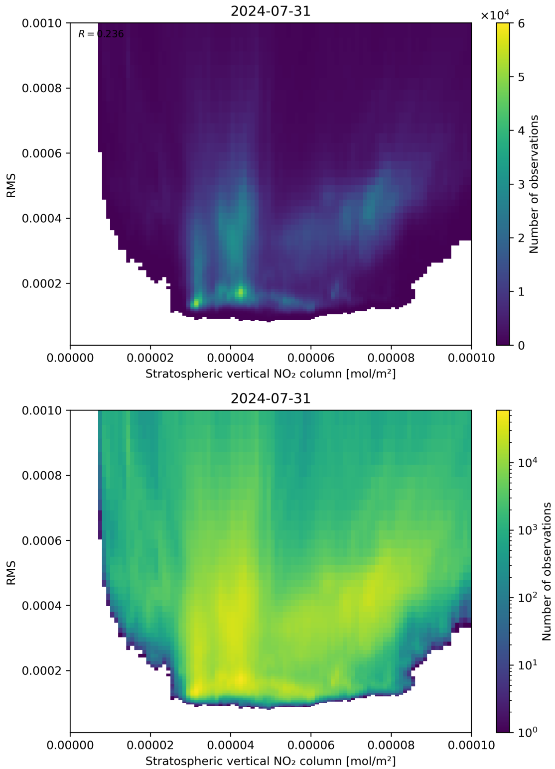
Figure 102: Scatter density plot of “Stratospheric vertical NO 2 column” against “RMS” for 2024-07-31 to 2024-08-01.
