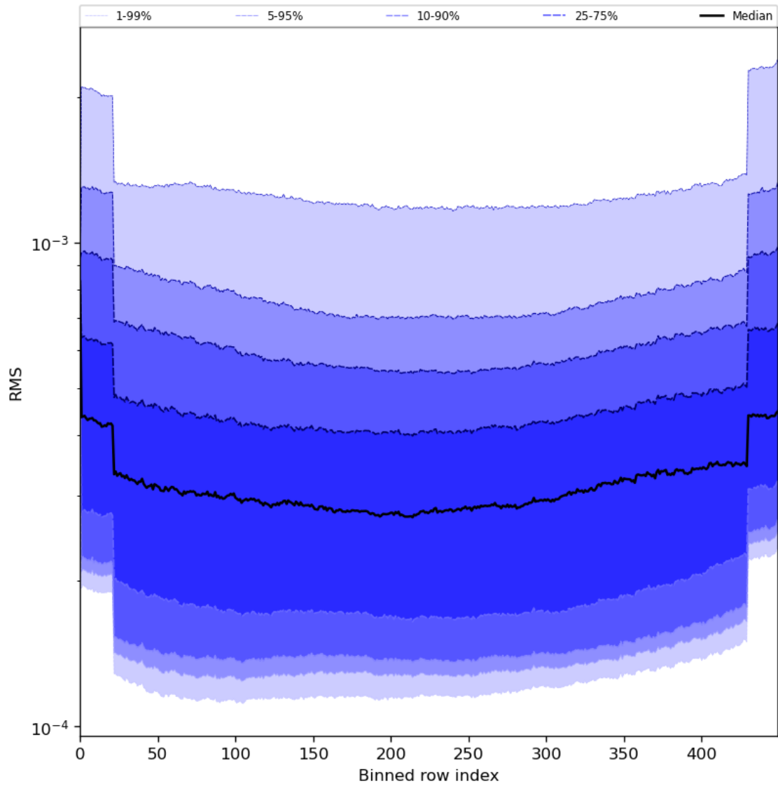
Figure 60: Along track statistics of “RMS” for 2024-07-31 to 2024-08-01
