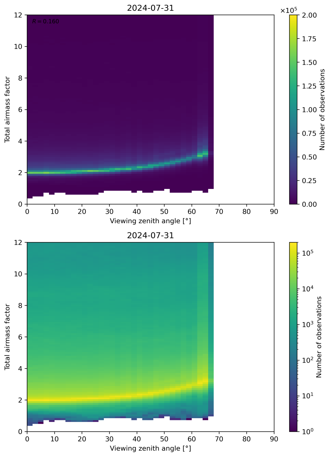
Figure 160: Scatter density plot of “Viewing zenith angle” against “Total airmass factor” for 2024-07-31 to 2024-08-01.
