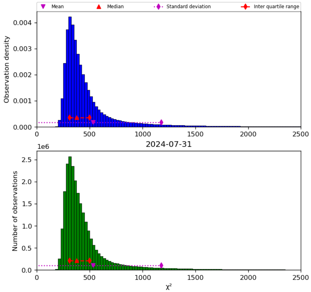
Figure 42: Histogram of “ \chi^2 ” for 2024-07-31 to 2024-08-01
