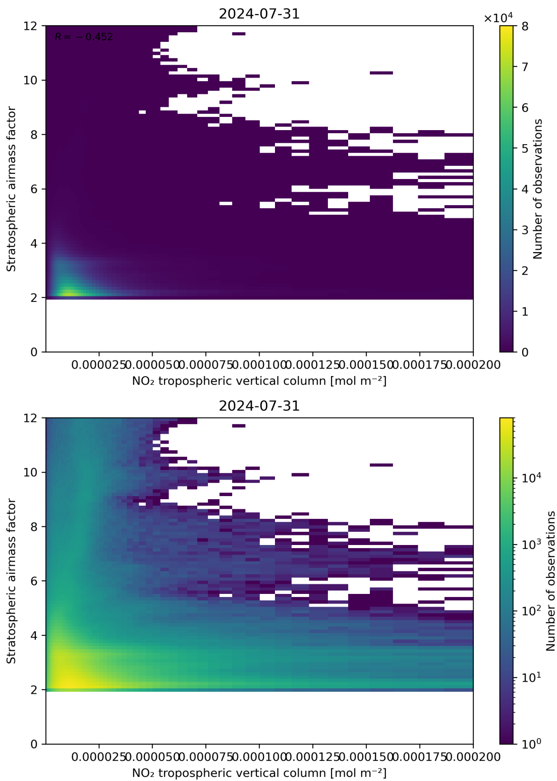
Figure 121: Scatter density plot of “NO 2 tropospheric vertical column” against “Stratospheric air mass factor” for 2024-07-31 to 2024-08-01.
