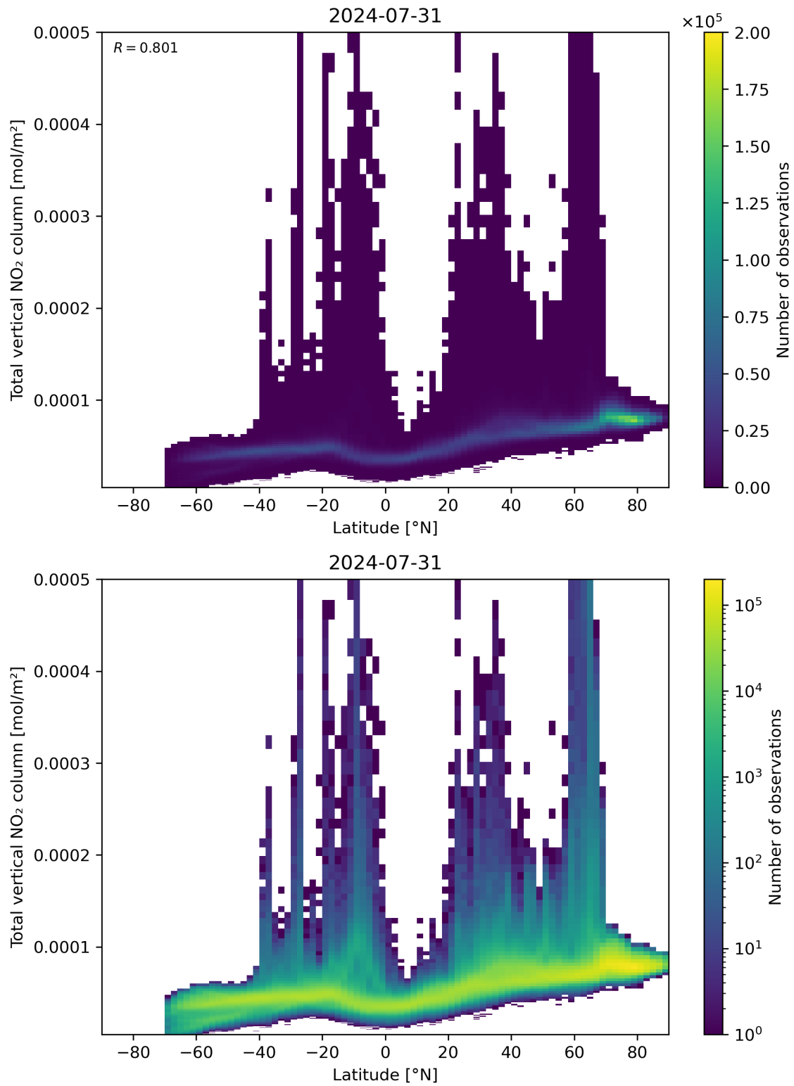
Figure 90: Scatter density plot of “Latitude” against “Total vertical NO 2 column” for 2024-07-31 to 2024-08-01.
