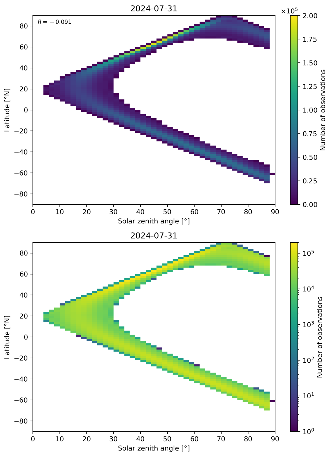
Figure 149: Scatter density plot of “Solar zenith angle” against “Latitude” for 2024-07-31 to 2024-08-01.
