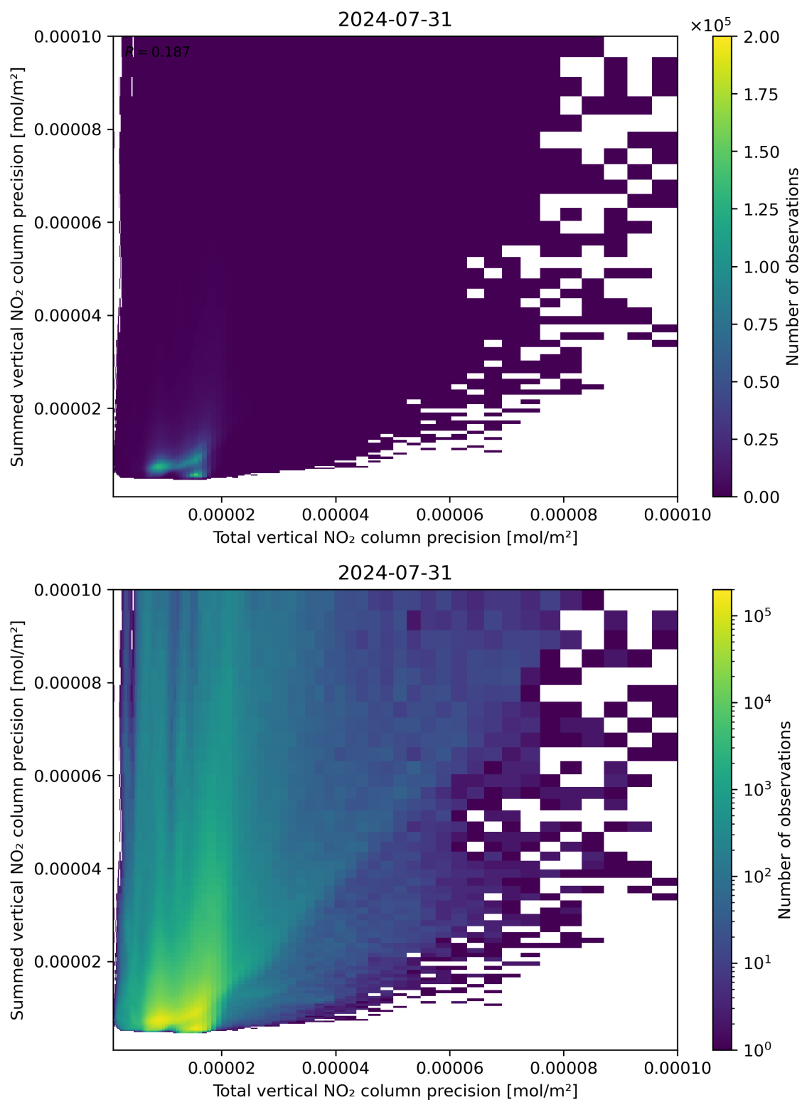
Figure 118: Scatter density plot of “Total vertical NO 2 column precision” against “Summed vertical NO 2 column precision” for 2024-07-31 to 2024-08-01.
