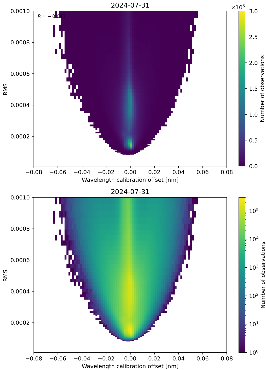
Figure 181: Scatter density plot of “Wavelength calibration offset” against “RMS” for 2024-07-31 to 2024-08-01.
