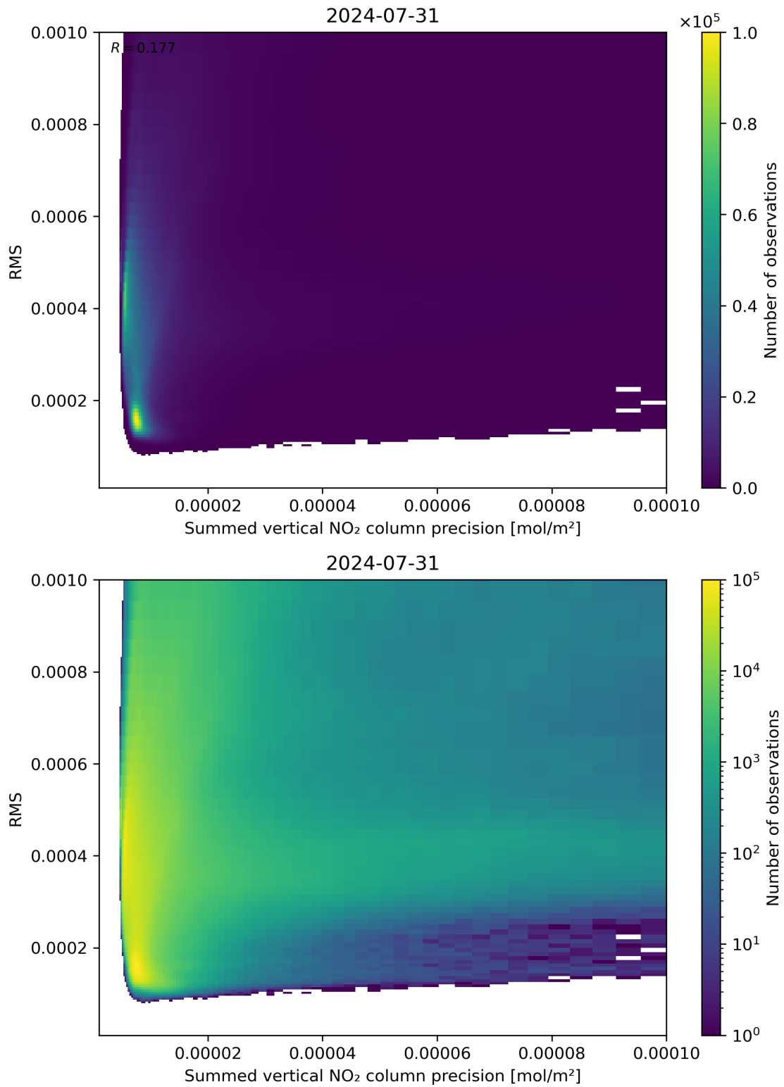
Figure 108: Scatter density plot of “Summed vertical NO 2 column precision” against “RMS” for 2024-07-31 to 2024-08-01.
