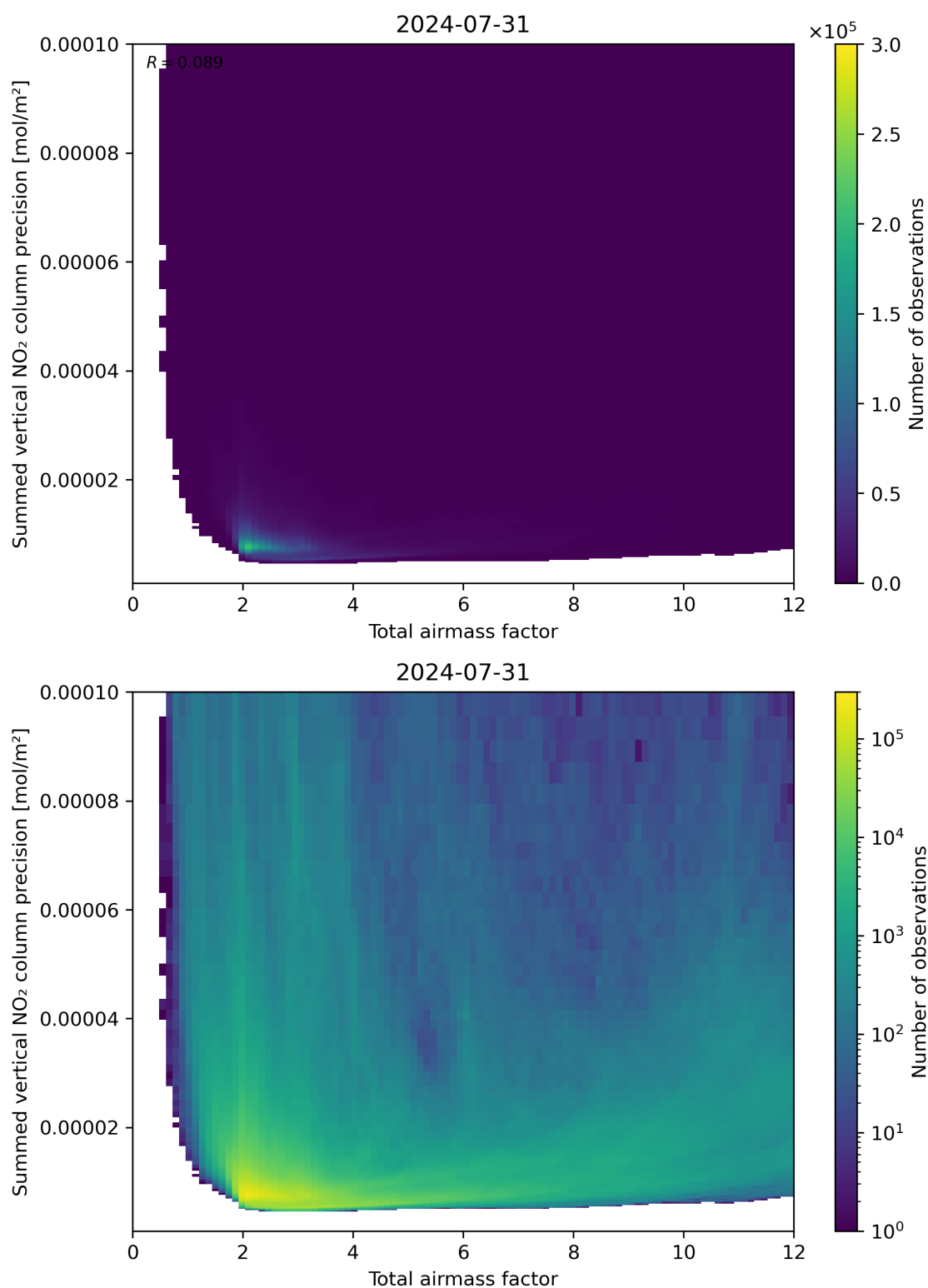
Figure 66: Scatter density plot of “Total airmass factor” against “Summed vertical NO 2 column precision” for 2024-07-31 to 2024-08-01.
