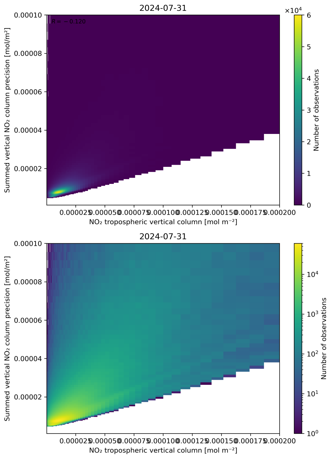
Figure 127: Scatter density plot of “NO 2 tropospheric vertical column” against “Summed vertical NO 2 column precision” for 2024-07-31 to 2024-08-01.
