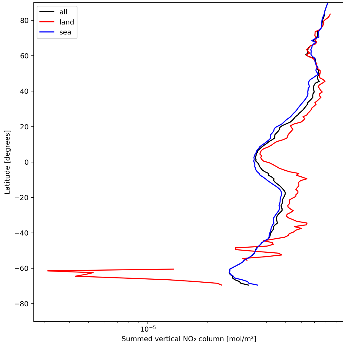
Figure 23: Zonal average of “Summed vertical NO 2 column” for 2024-07-31 to 2024-08-01.
