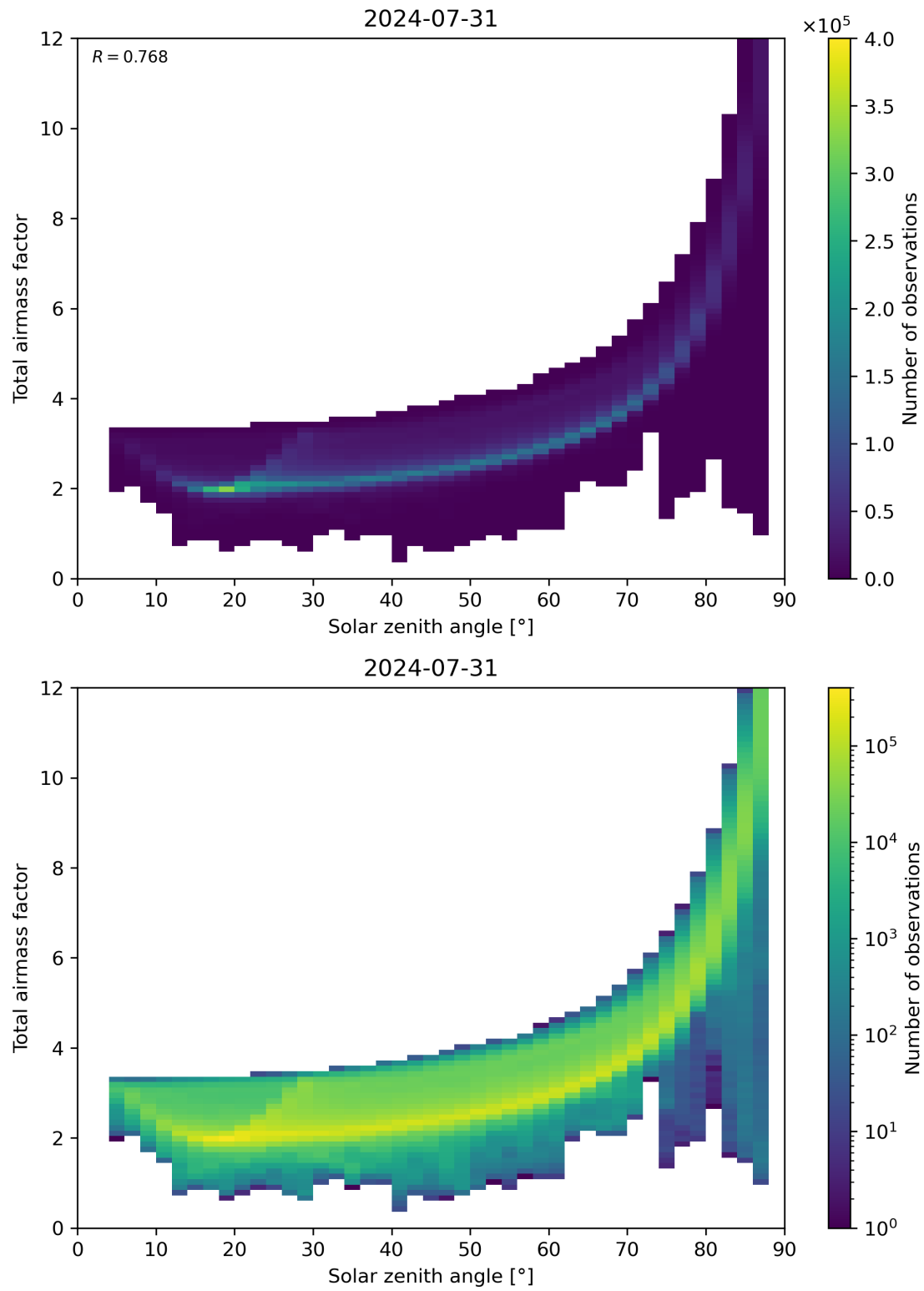
Figure 146: Scatter density plot of “Solar zenith angle” against “Total air mass factor” for 2024-07-31 to 2024-08-01.
