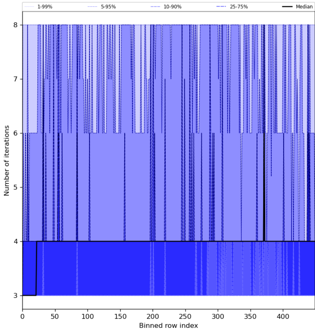
Figure 51: Along track statistics of “Number of iterations” for 2024-07-31 to 2024-08-01
