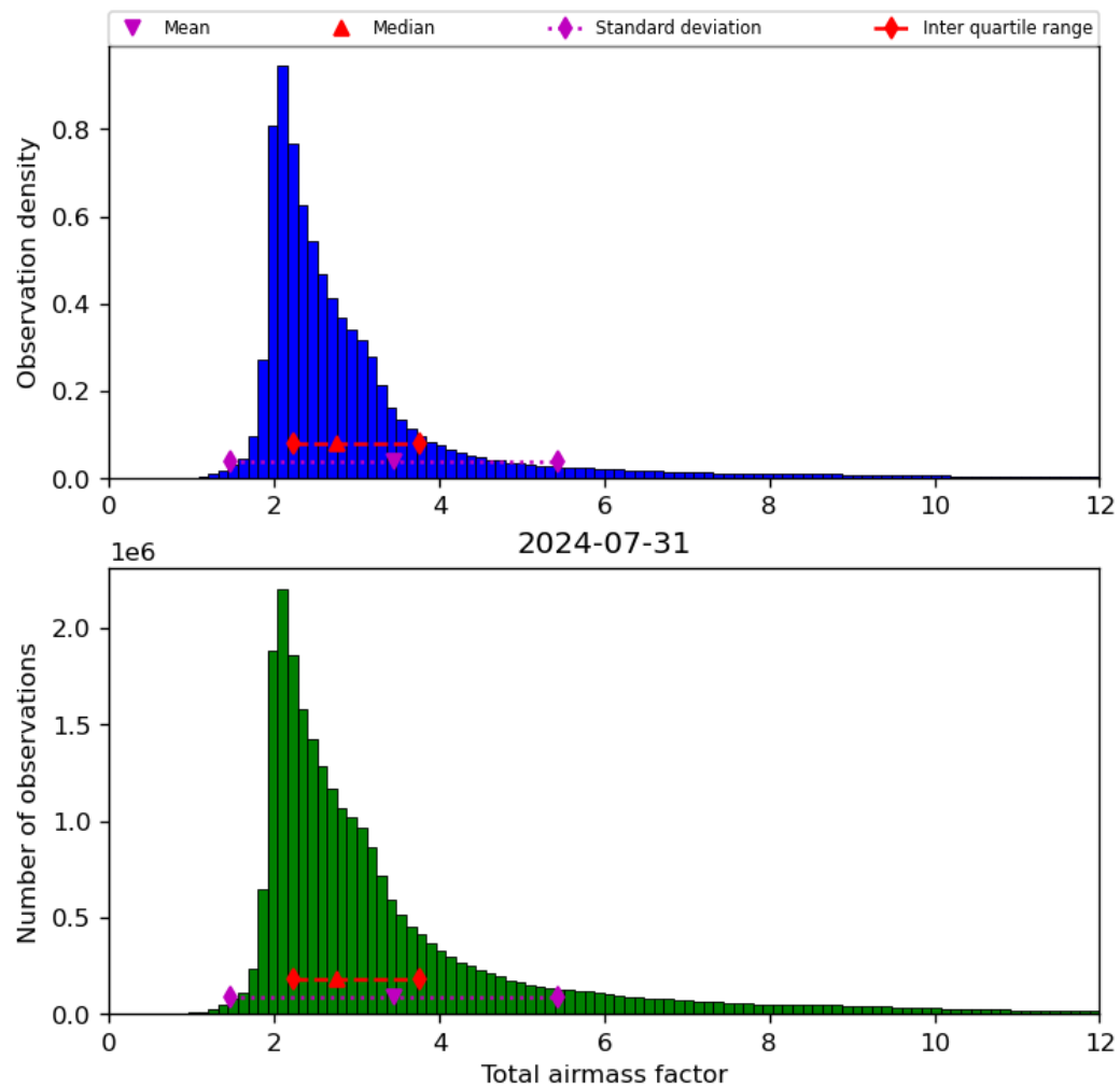
Figure 32: Histogram of “Total airmass factor” for 2024-07-31 to 2024-08-01
