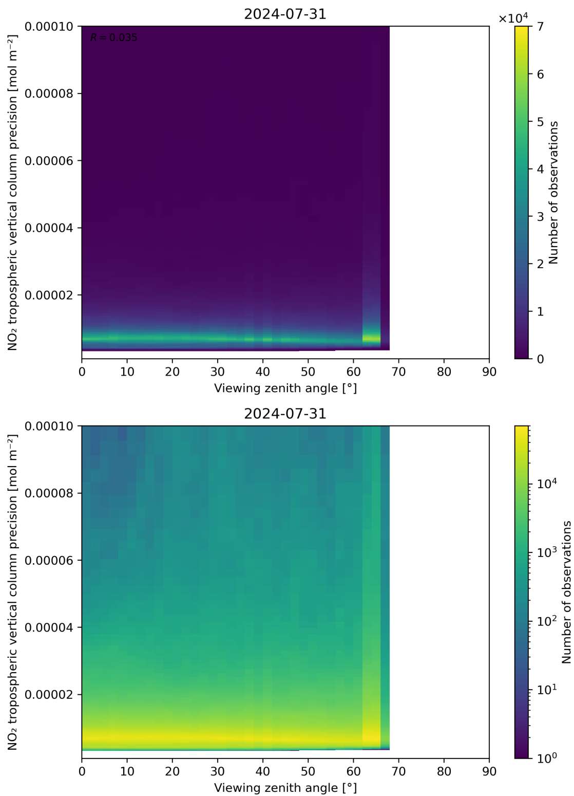
Figure 170: Scatter density plot of “Viewing zenith angle” against “NO 2 tropospheric vertical column precision” for 2024-07-31 to 2024-08-01.
