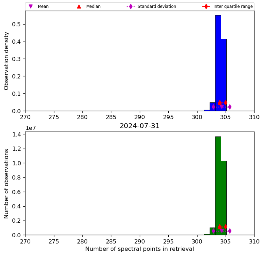
Figure 33: Histogram of “Number of spectral points in retrieval” for 2024-07-31 to 2024-08-01
