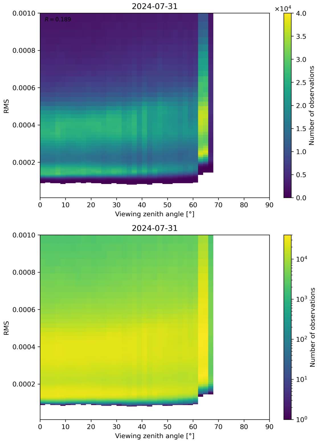
Figure 171: Scatter density plot of “Viewing zenith angle” against “RMS” for 2024-07-31 to 2024-08-01.
