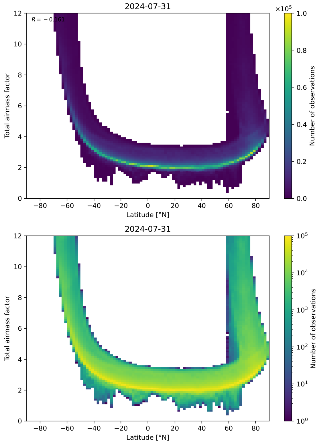
Figure 84: Scatter density plot of “Latitude” against “Total airmass factor” for 2024-07-31 to 2024-08-01.
