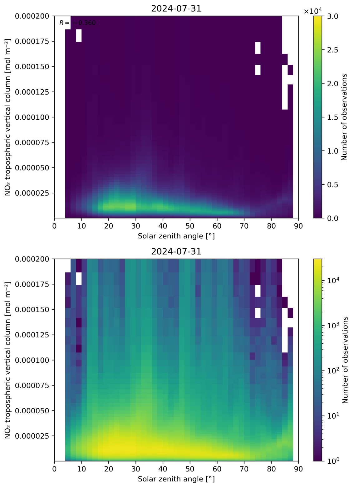
Figure 155: Scatter density plot of “Solar zenith angle” against “NO 2 tropospheric vertical column” for 2024-07-31 to 2024-08-01.
