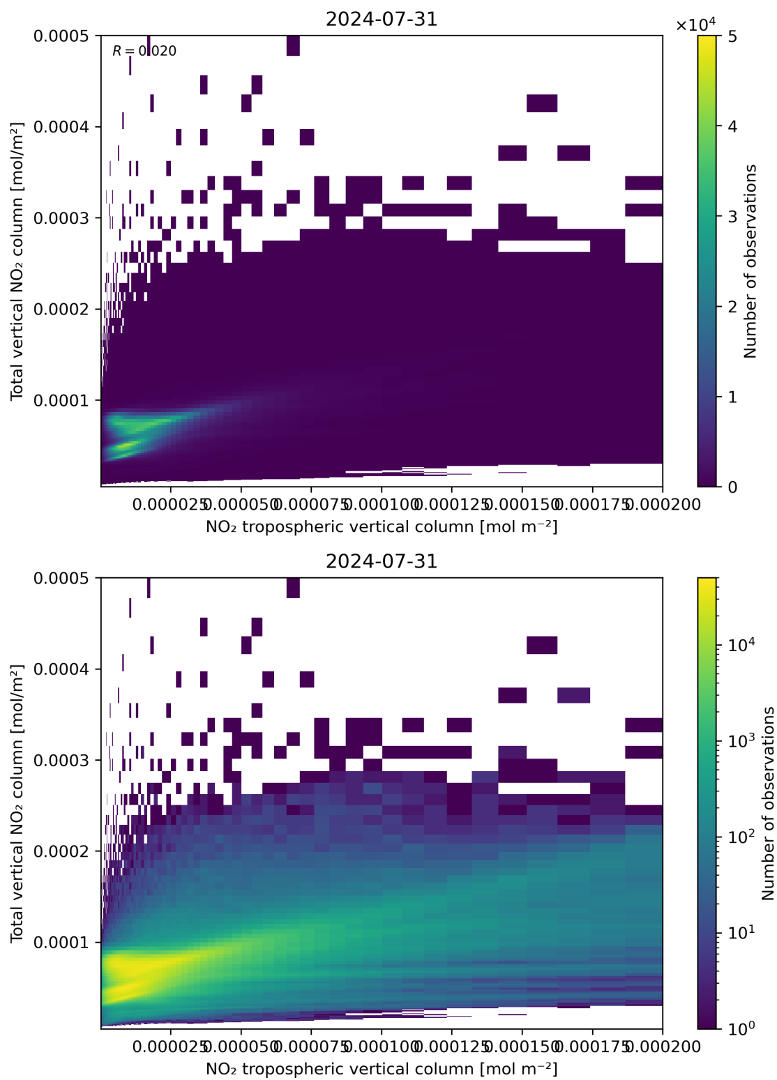
Figure 128: Scatter density plot of “NO 2 tropospheric vertical column” against “Total vertical NO 2 column” for 2024-07-31 to 2024-08-01.
