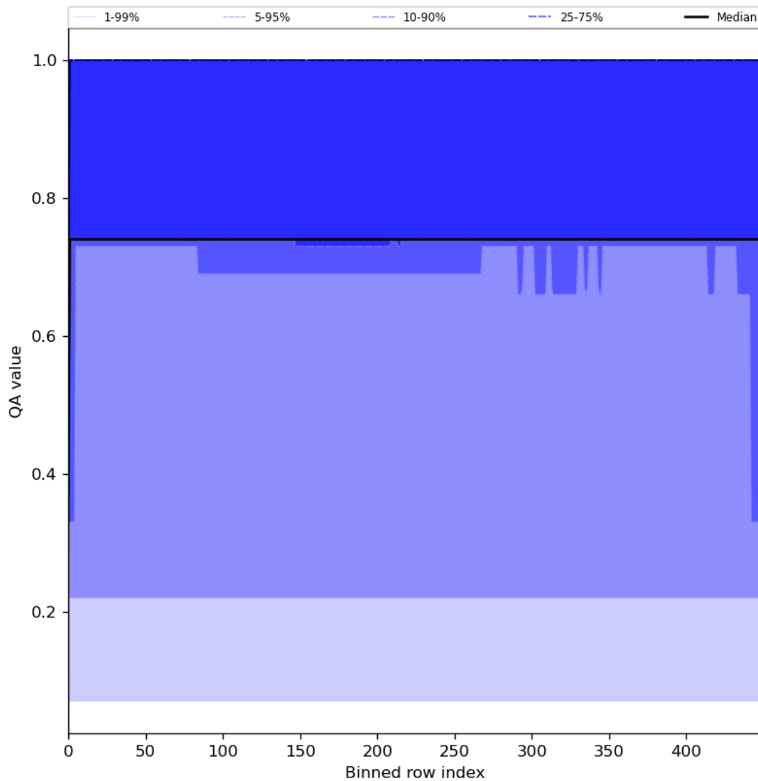
Figure 45: Along track statistics of “QA value” for 2024-07-31 to 2024-08-01
