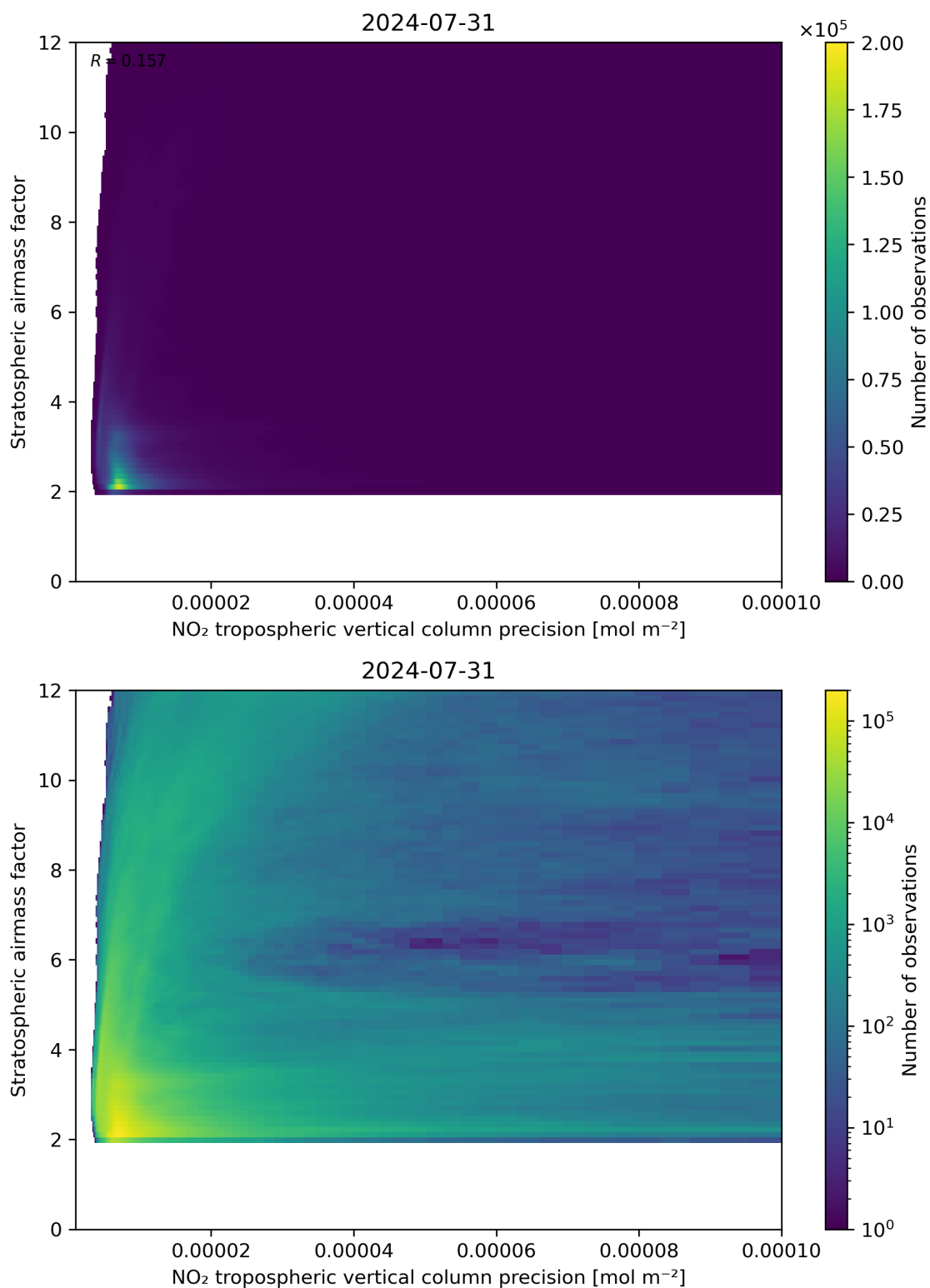
Figure 131: Scatter density plot of “NO 2 tropospheric vertical column precision” against “Stratospheric airmass factor” for 2024-07-31 to 2024-08-01.
