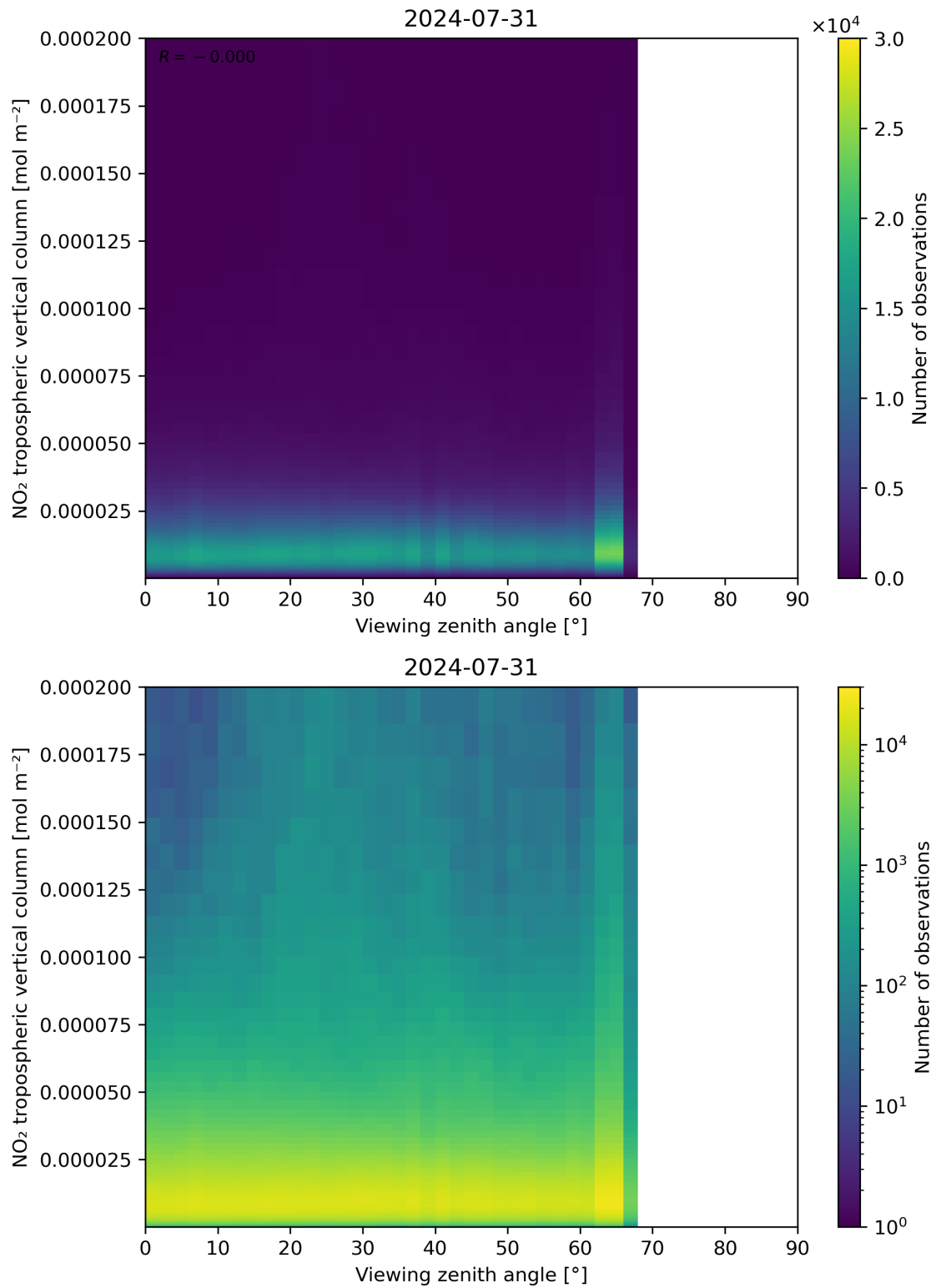
Figure 169: Scatter density plot of “Viewing zenith angle” against “NO 2 tropospheric vertical column” for 2024-07-31 to 2024-08-01.
