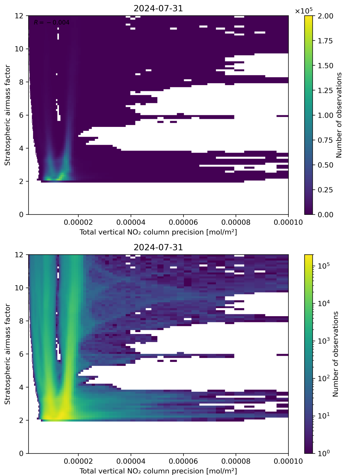
Figure 115: Scatter density plot of “Total vertical NO 2 column precision” against “Stratospheric air mass factor” for 2024-07-31 to 2024-08-01.
