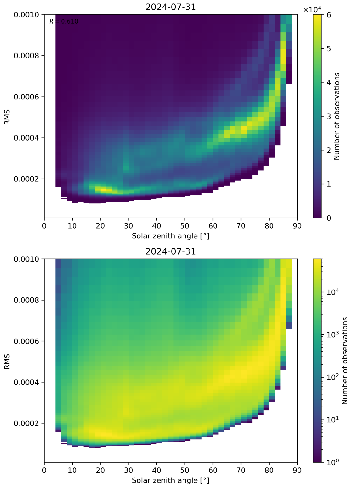
Figure 157: Scatter density plot of “Solar zenith angle” against “RMS” for 2024-07-31 to 2024-08-01.
