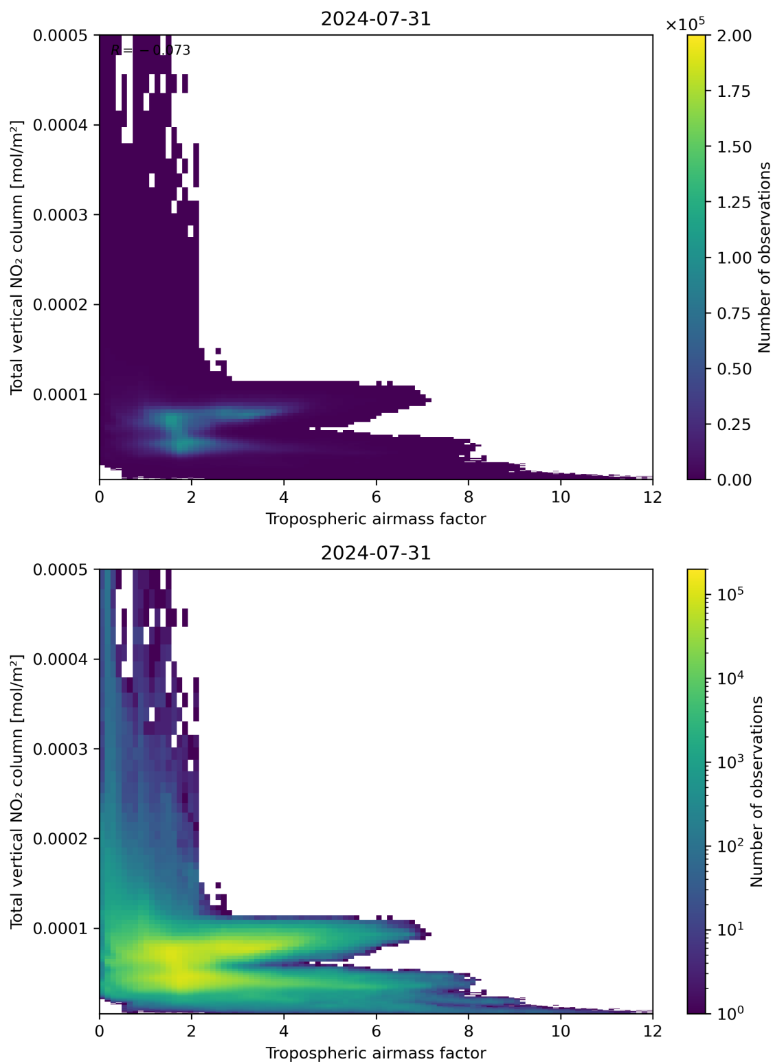
Figure 77: Scatter density plot of “Tropospheric airmass factor” against “Total vertical NO 2 column” for 2024-07-31 to 2024-08-01.
