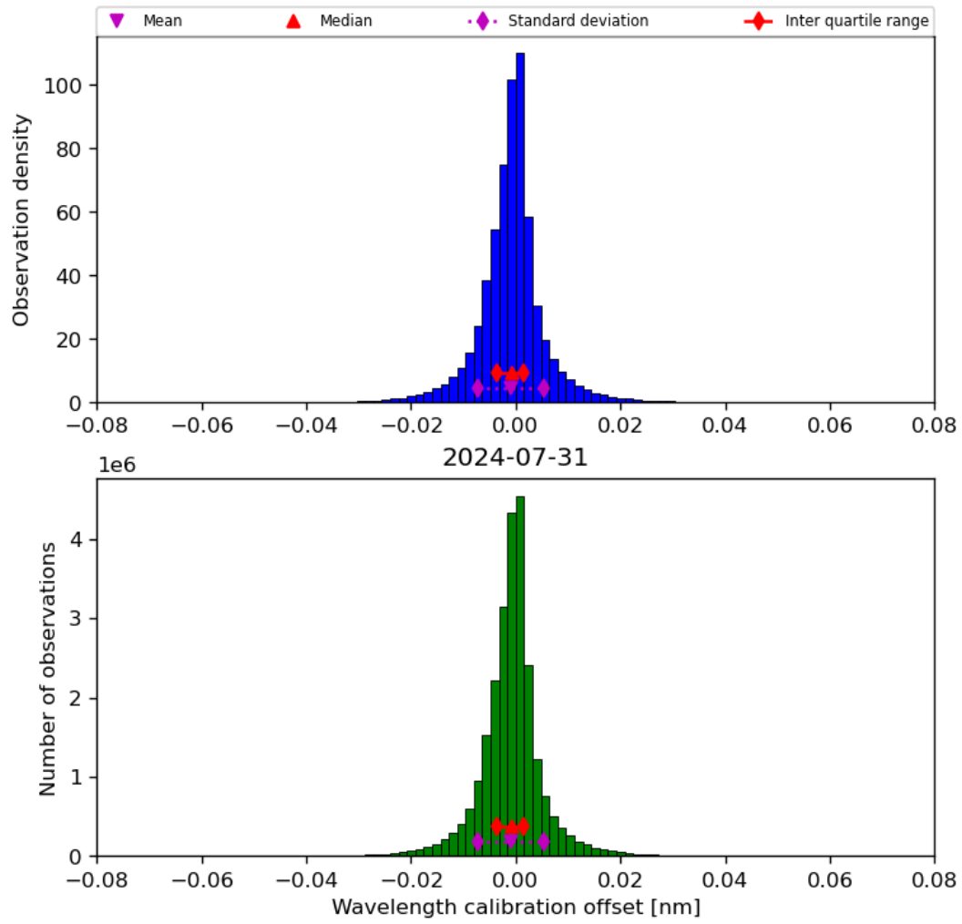
Figure 35: Histogram of “Wavelength calibration offset” for 2024-07-31 to 2024-08-01
