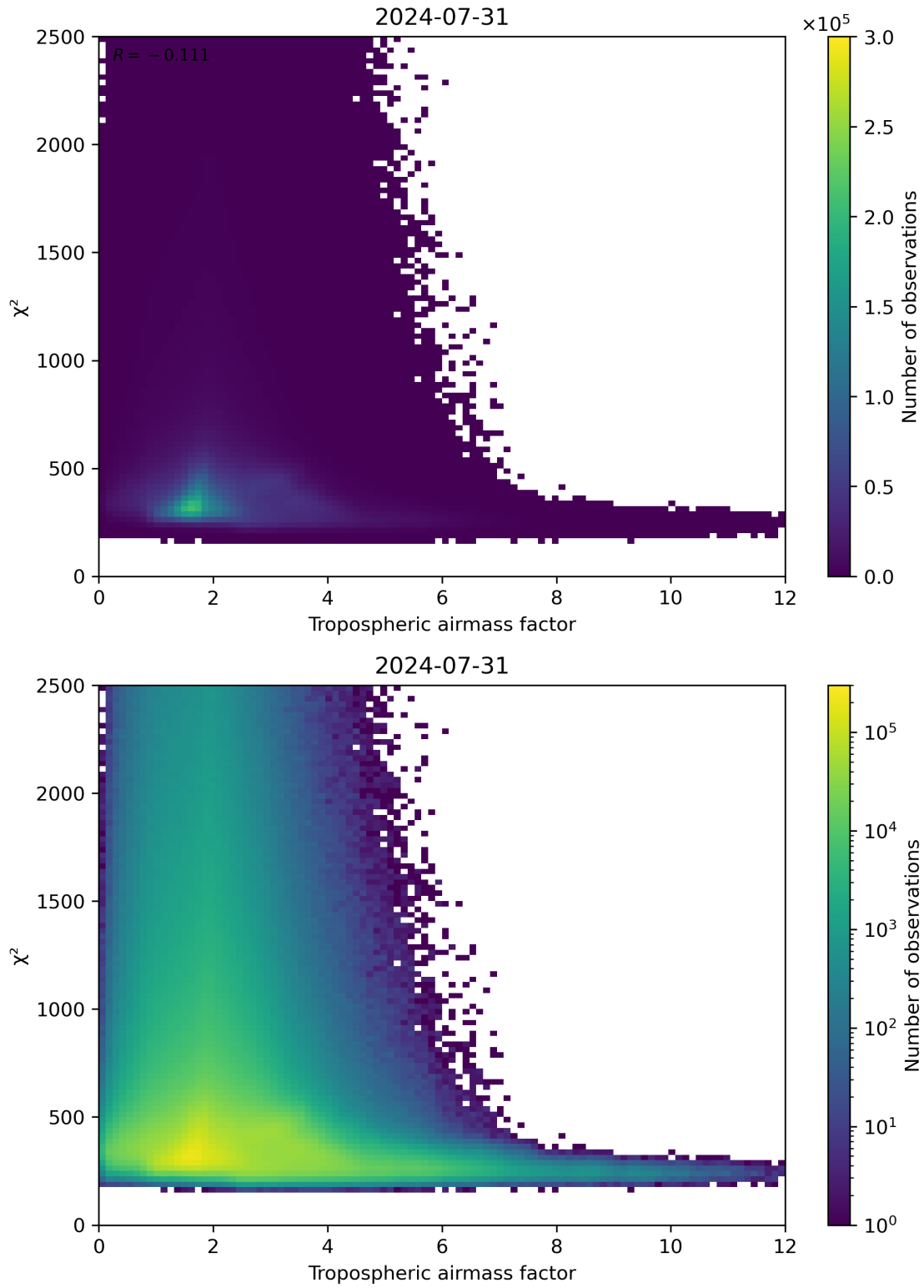
Figure 73: Scatter density plot of “Tropospheric airmass factor” against “ \chi^2 ” for 2024-07-31 to 2024-08-01.
