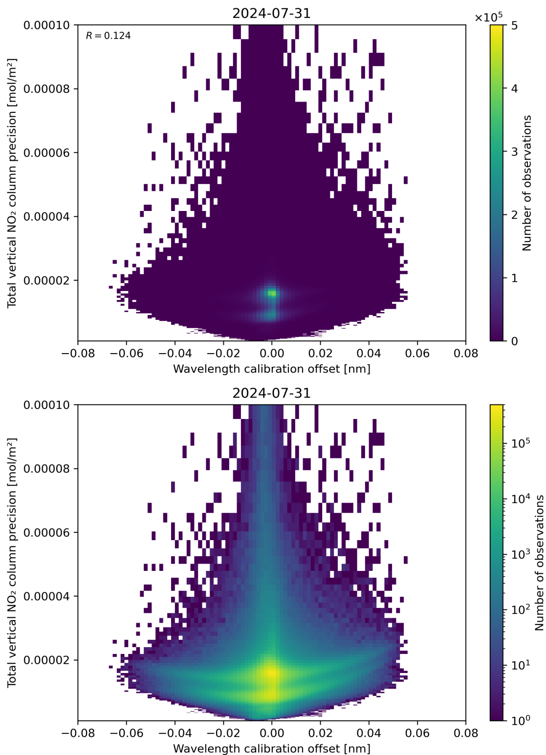
Figure 180: Scatter density plot of “Wavelength calibration offset” against “Total vertical NO 2 column precision” for 2024-07-31 to 2024-08-01.
