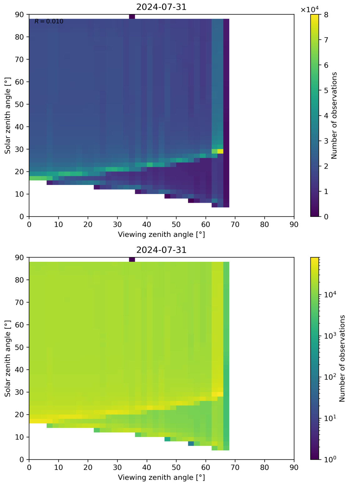
Figure 172: Scatter density plot of “Viewing zenith angle” against “Solar zenith angle” for 2024-07-31 to 2024-08-01.
