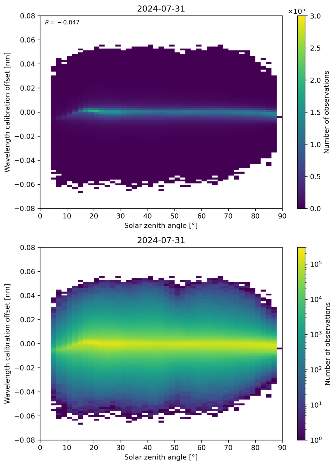
Figure 158: Scatter density plot of “Solar zenith angle” against “Wavelength calibration offset” for 2024-07-31 to 2024-08-01.
