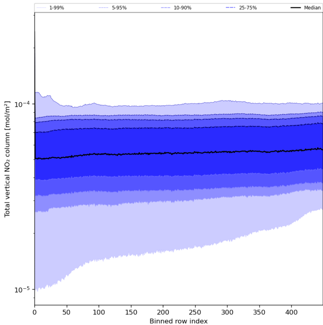
Figure 55: Along track statistics of “Total vertical NO 2 column” for 2024-07-31 to 2024-08-01
