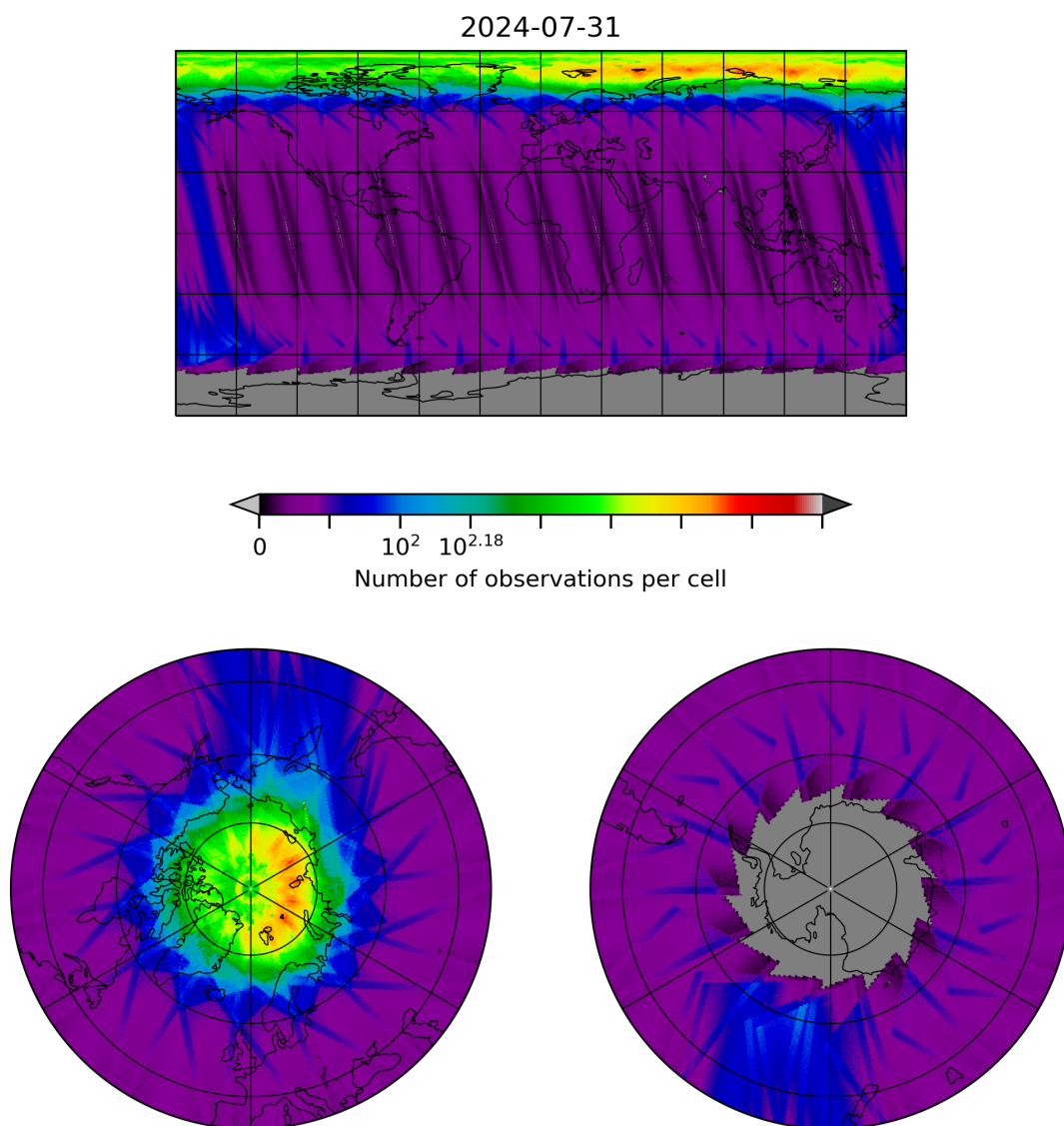
Figure 10: Map of the number of observations for 2024-07-31 to 2024-08-01
