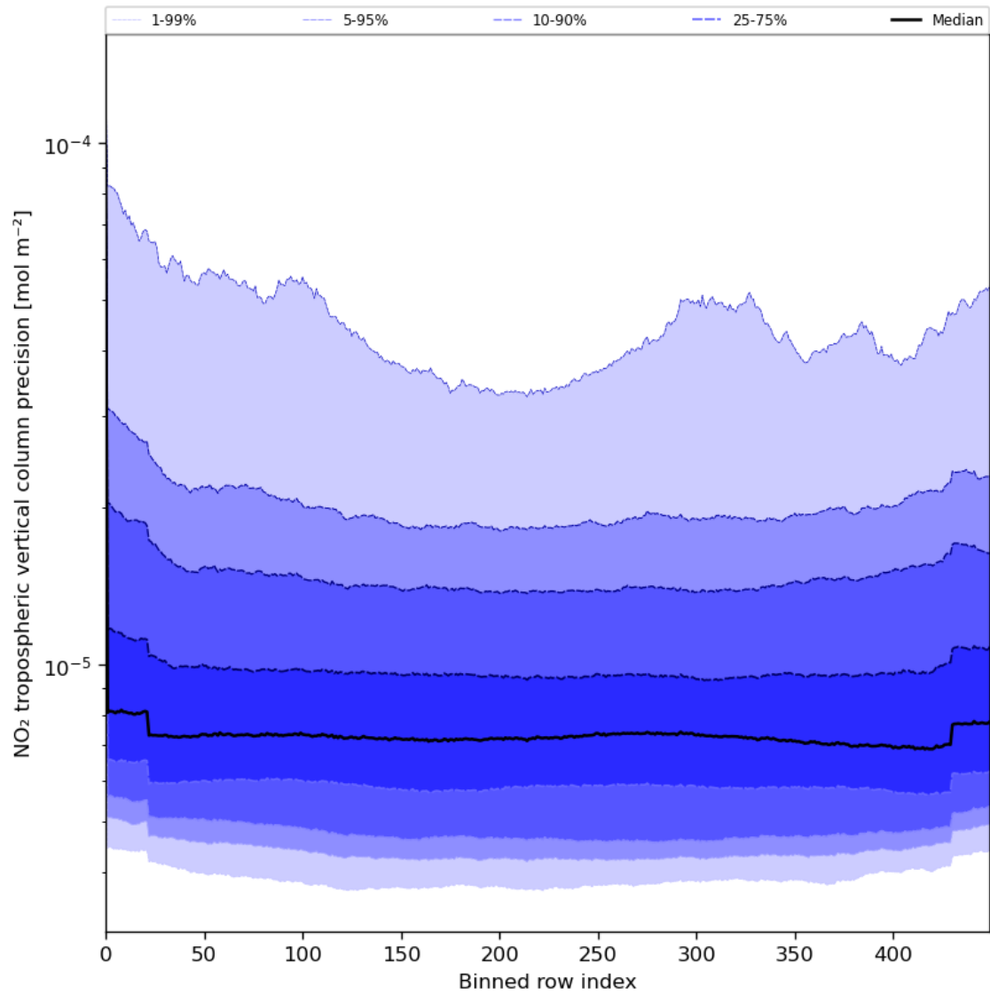
Figure 47: Along track statistics of “NO 2 tropospheric vertical column precision” for 2024-07-31 to 2024-08-01
