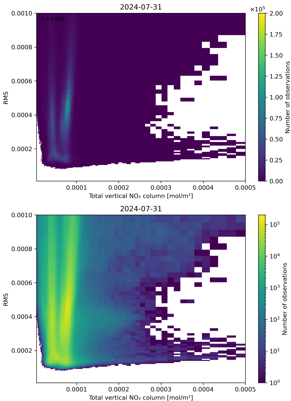
Figure 120: Scatter density plot of “Total vertical NO 2 column” against “RMS” for 2024-07-31 to 2024-08-01.
