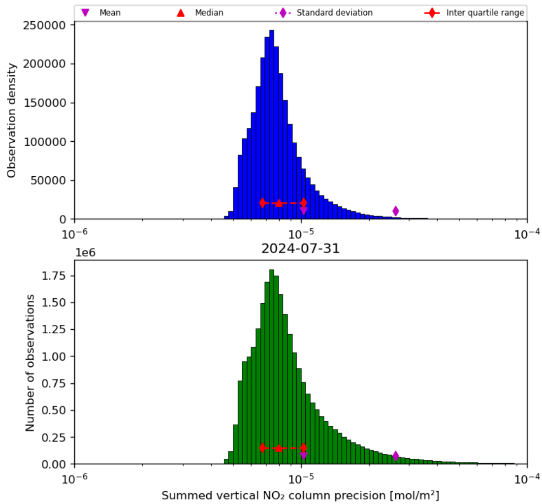
Figure 41: Histogram of "Summed vertical NO 2 column precision" for 2024-07-31 to 2024-08-01
