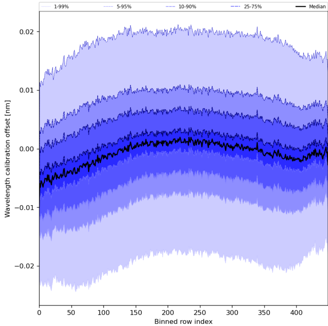
Figure 52: Along track statistics of “Wavelength calibration offset” for 2024-07-31 to 2024-08-01
