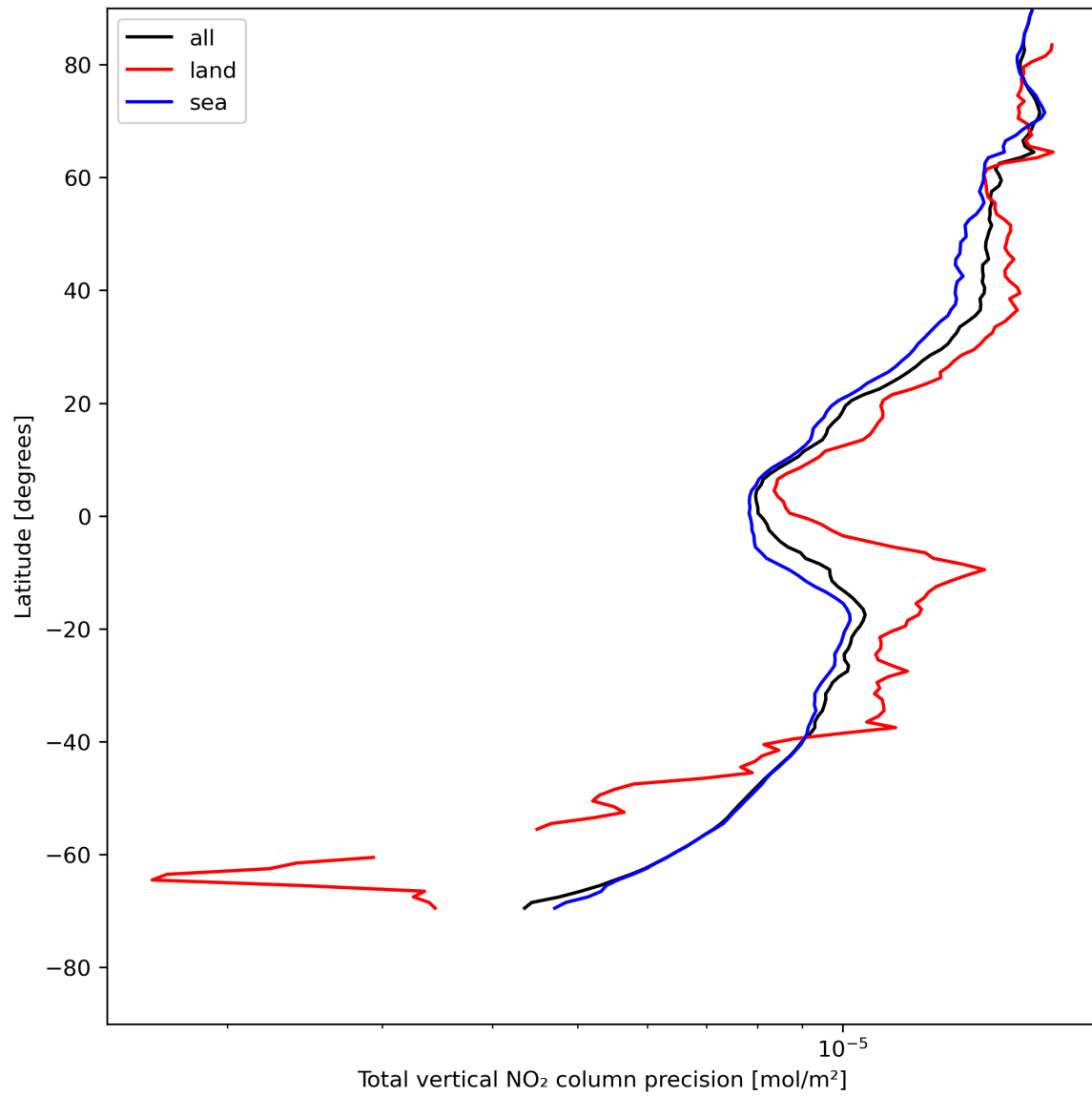
Figure 22: Zonal average of “Total vertical NO 2 column precision” for 2024-07-31 to 2024-08-01.
