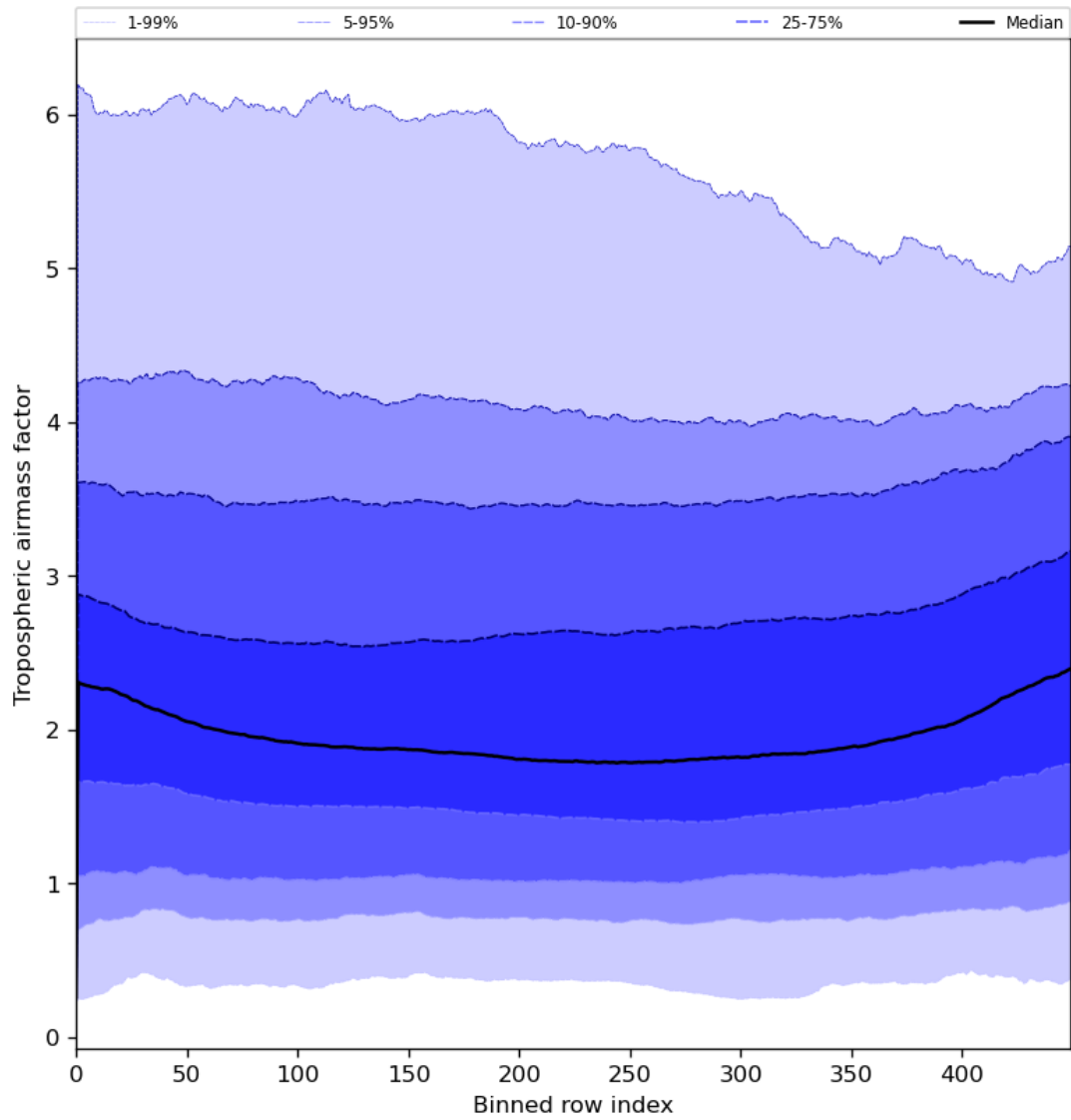
Figure 48: Along track statistics of “Tropospheric airmass factor” for 2024-07-31 to 2024-08-01
