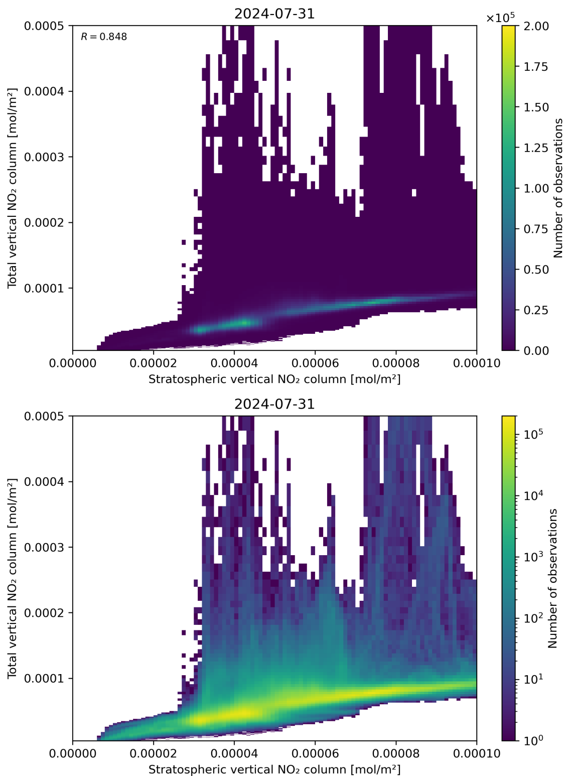
Figure 100: Scatter density plot of “Stratospheric vertical NO 2 column” against “Total vertical NO 2 column” for 2024-07-31 to 2024-08-01.
