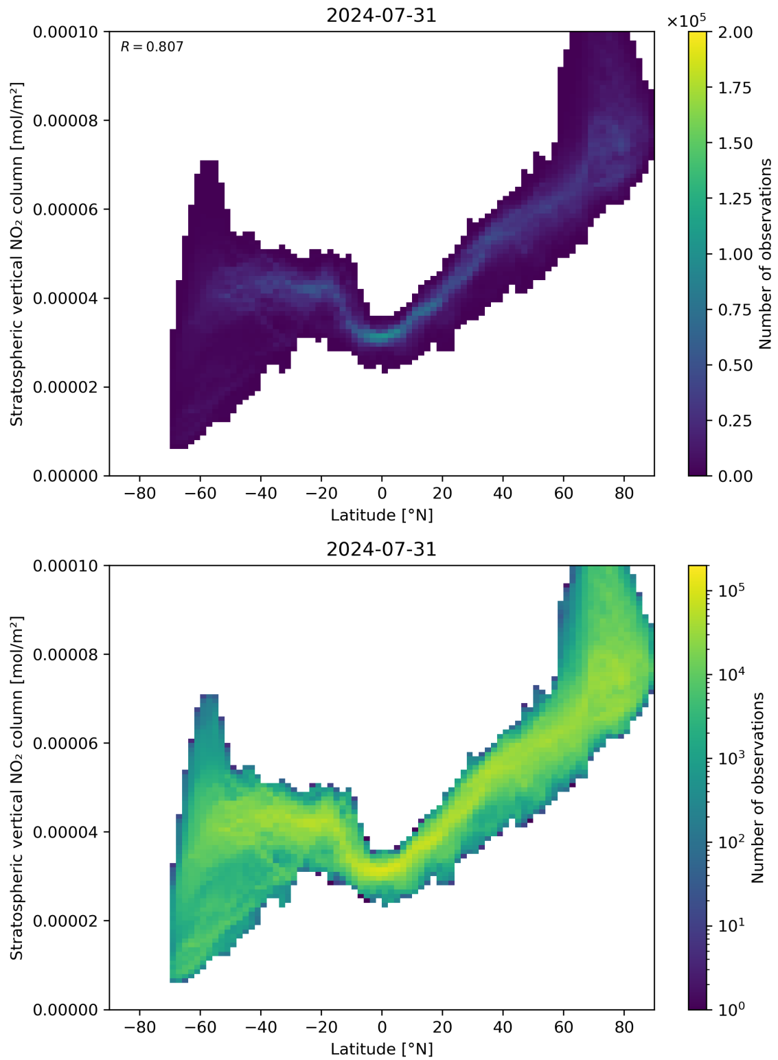
Figure 87: Scatter density plot of “Latitude” against “Stratospheric vertical NO 2 column” for 2024-07-31 to 2024-08-01.
