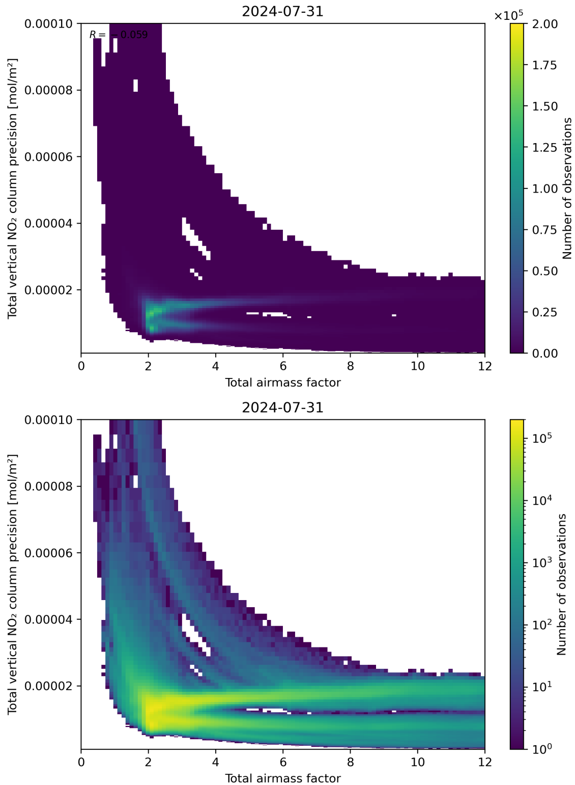
Figure 68: Scatter density plot of “Total airmass factor” against “Total vertical NO 2 column precision” for 2024-07-31 to 2024-08-01.
