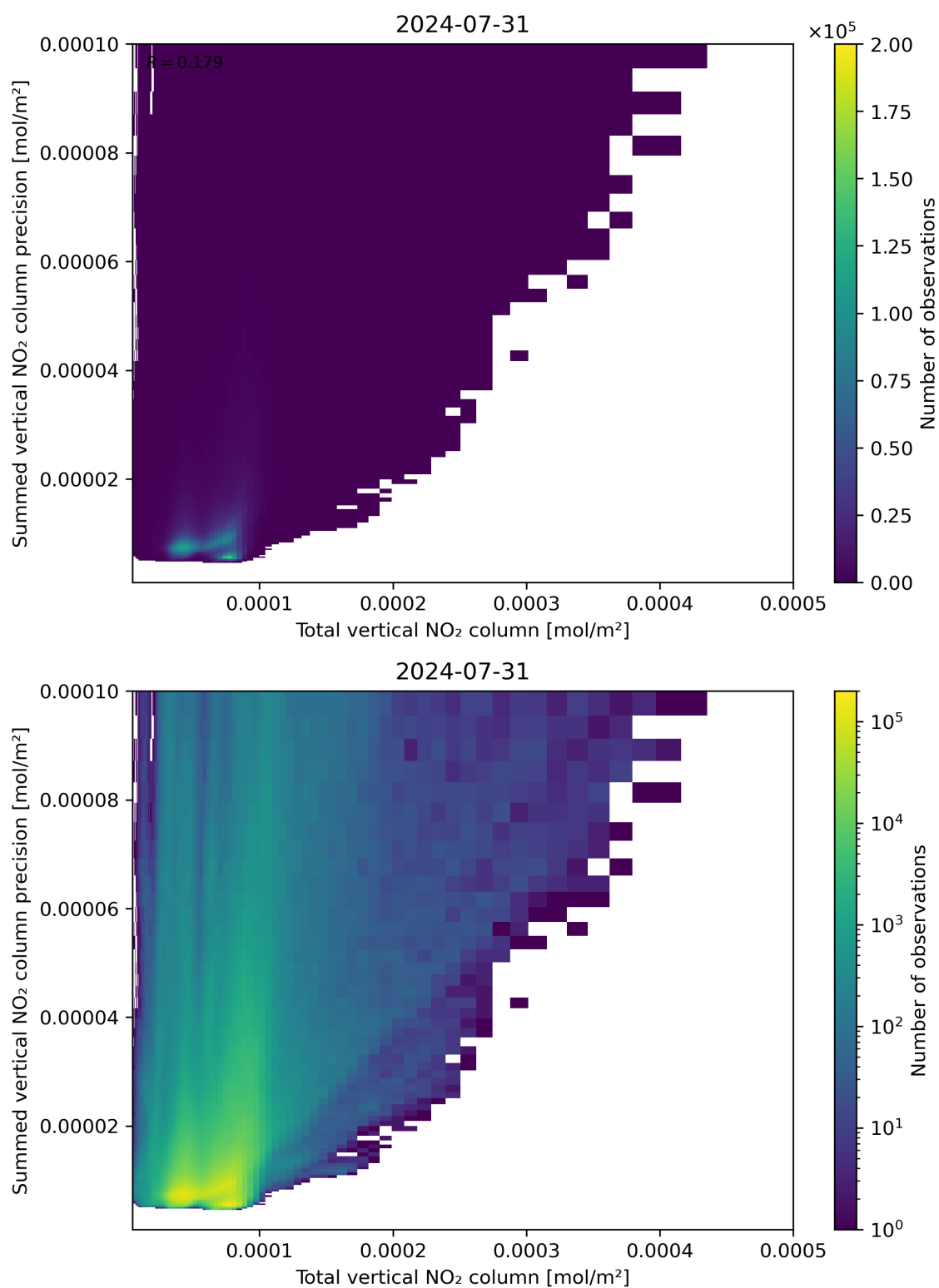
Figure 113: Scatter density plot of “Total vertical NO 2 column” against “Summed vertical NO 2 column precision” for 2024-07-31 to 2024-08-01.
