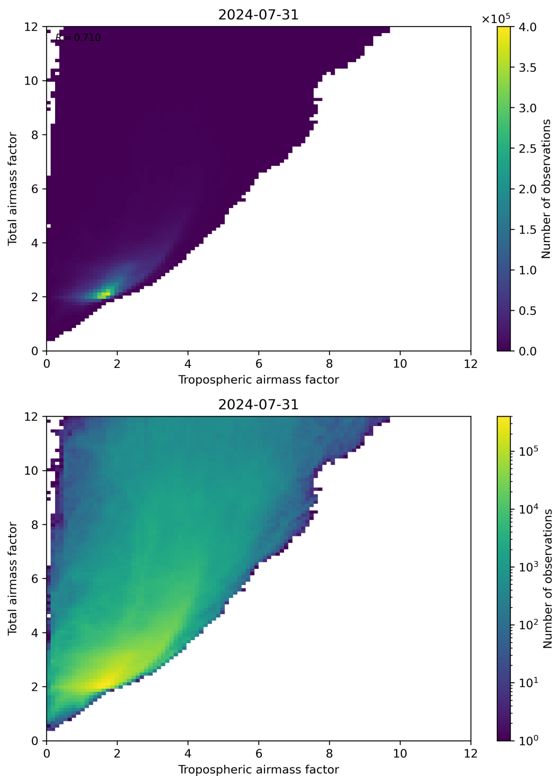
Figure 72: Scatter density plot of “Tropospheric airmass factor” against “Total airmass factor” for 2024-07-31 to 2024-08-01.
