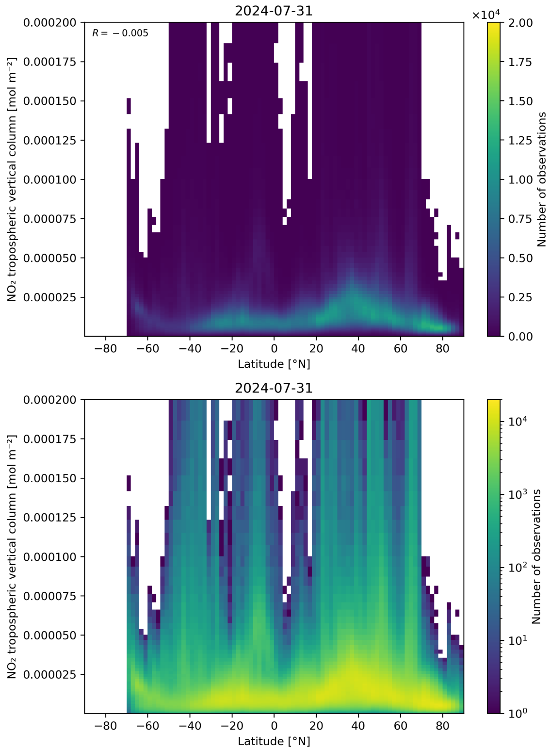
Figure 92: Scatter density plot of “Latitude” against “NO 2 tropospheric vertical column” for 2024-07-31 to 2024-08-01.
