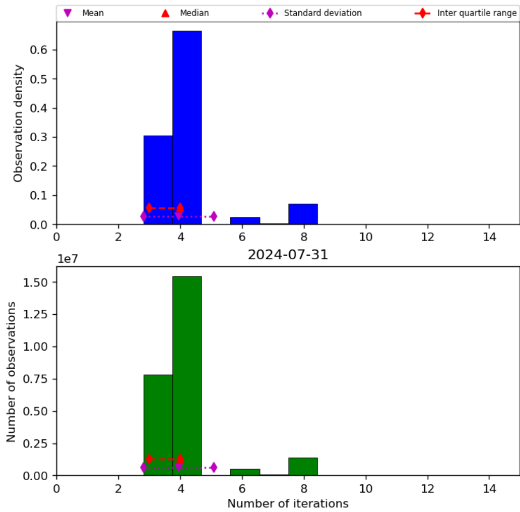
Figure 34: Histogram of “Number of iterations” for 2024-07-31 to 2024-08-01
