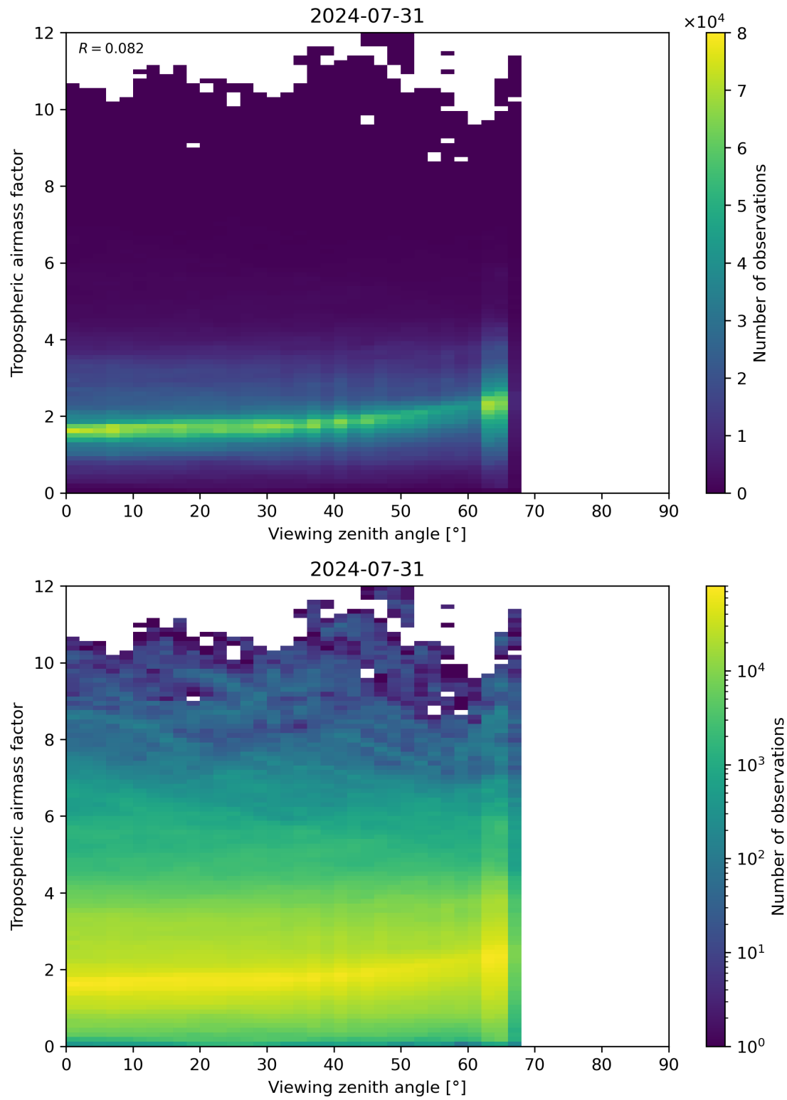
Figure 161: Scatter density plot of “Viewing zenith angle” against “Tropospheric airmass factor” for 2024-07-31 to 2024-08-01.
