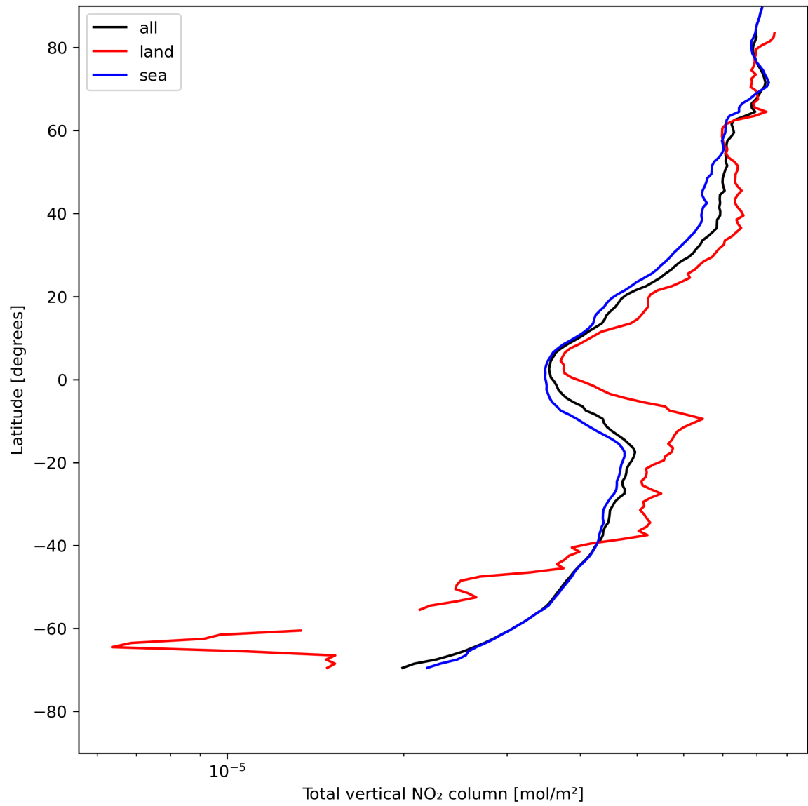
Figure 21: Zonal average of “Total vertical NO 2 column” for 2024-07-31 to 2024-08-01.
