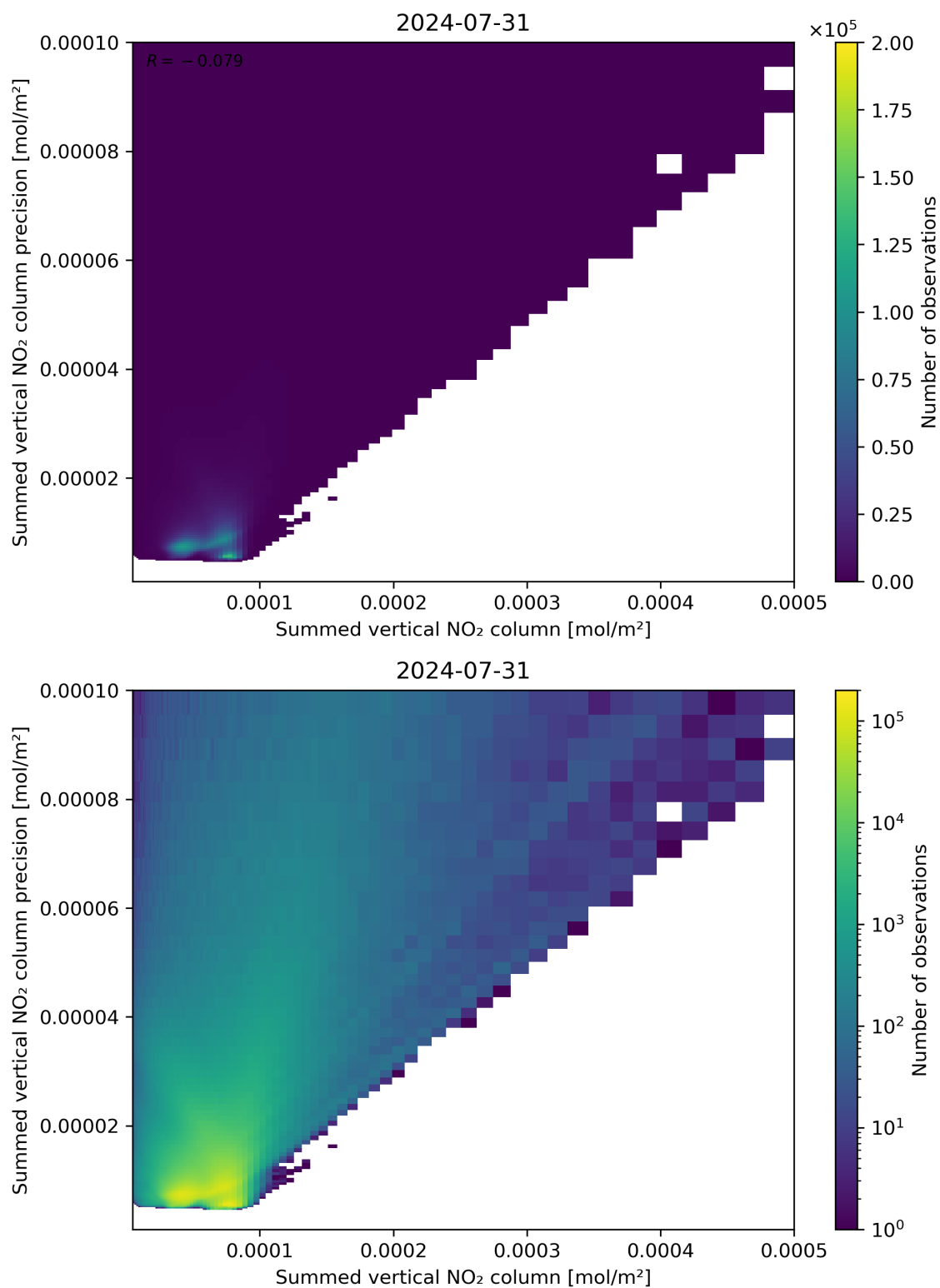
Figure 105: Scatter density plot of “Summed vertical NO 2 column” against “Summed vertical NO 2 column precision” for 2024-07-31 to 2024-08-01.
