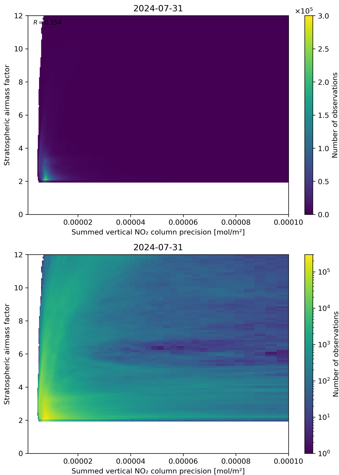
Figure 106: Scatter density plot of “Summed vertical NO 2 column precision” against “Stratospheric airmass factor” for 2024-07-31 to 2024-08-01.
