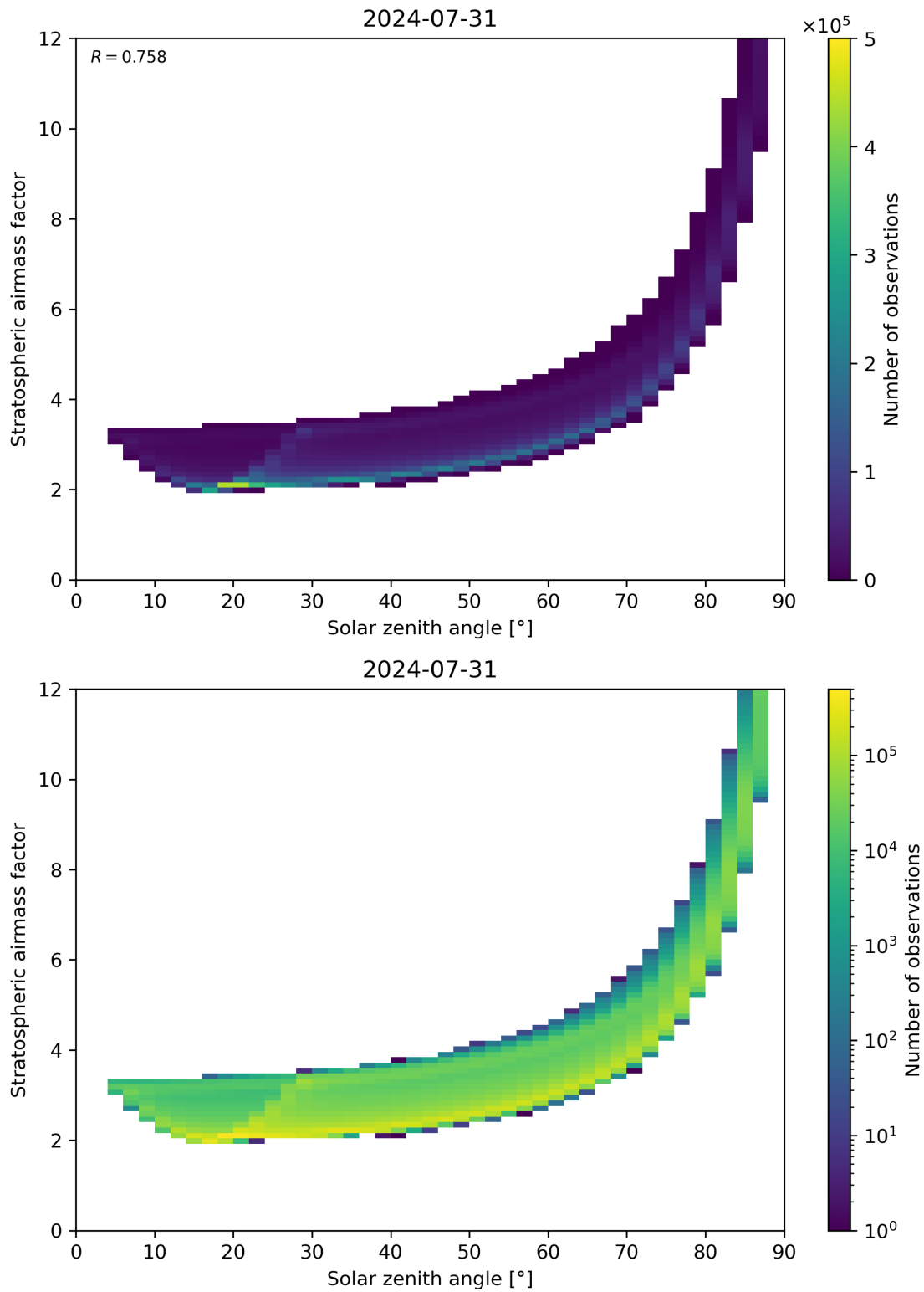
Figure 145: Scatter density plot of “Solar zenith angle” against “Stratospheric airmass factor” for 2024-07-31 to 2024-08-01.
