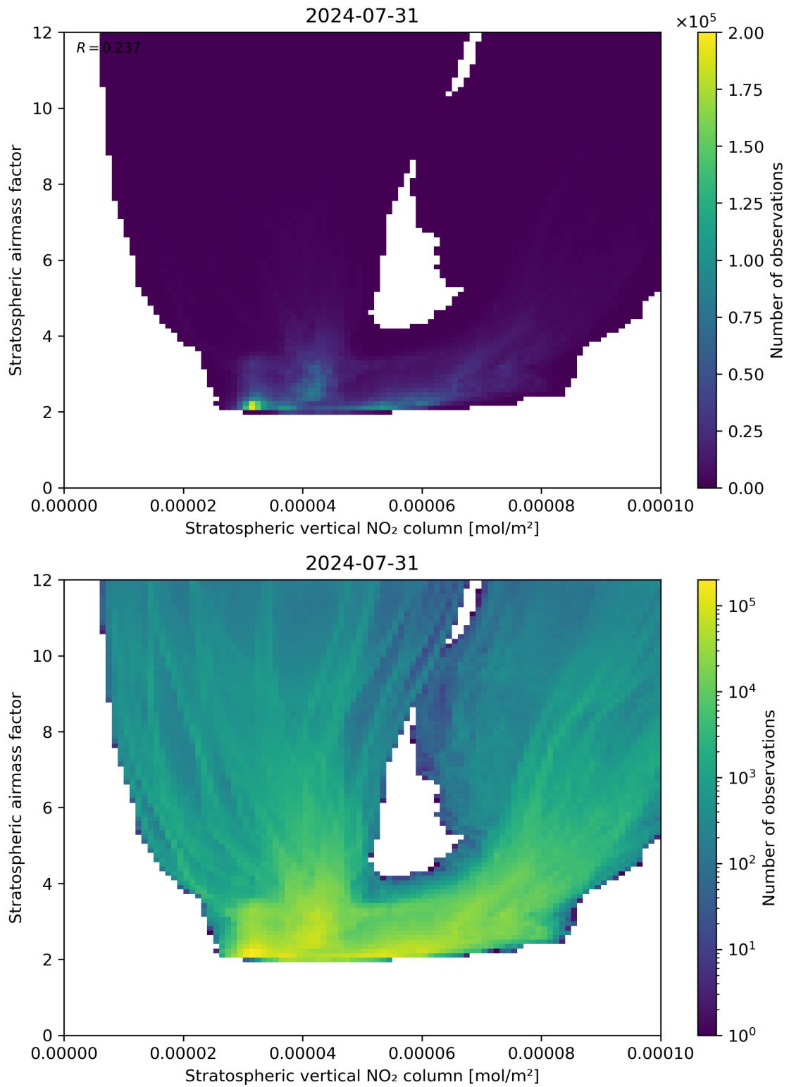
Figure 96: Scatter density plot of “Stratospheric vertical NO 2 column” against “Stratospheric airmass factor” for 2024-07-31 to 2024-08-01.
