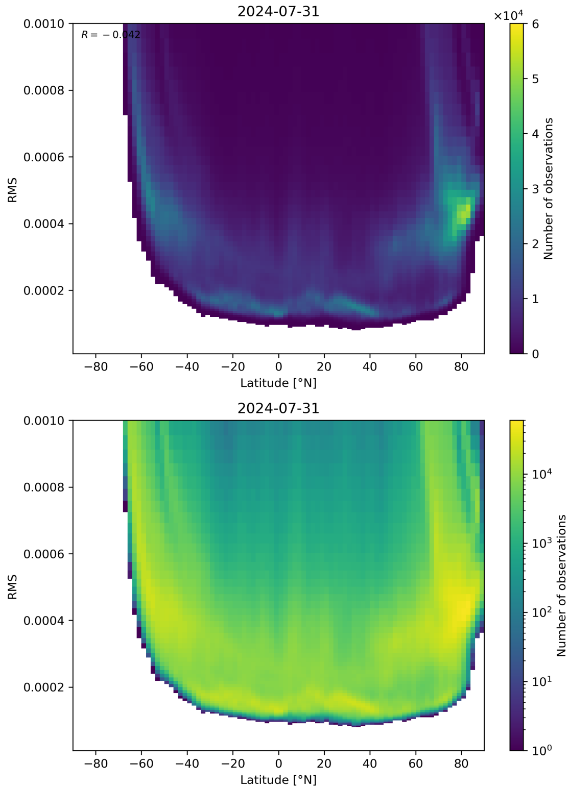
Figure 94: Scatter density plot of “Latitude” against “RMS” for 2024-07-31 to 2024-08-01.
