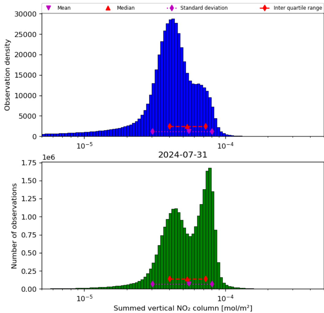
Figure 40: Histogram of “Summed vertical NO 2 column” for 2024-07-31 to 2024-08-01
