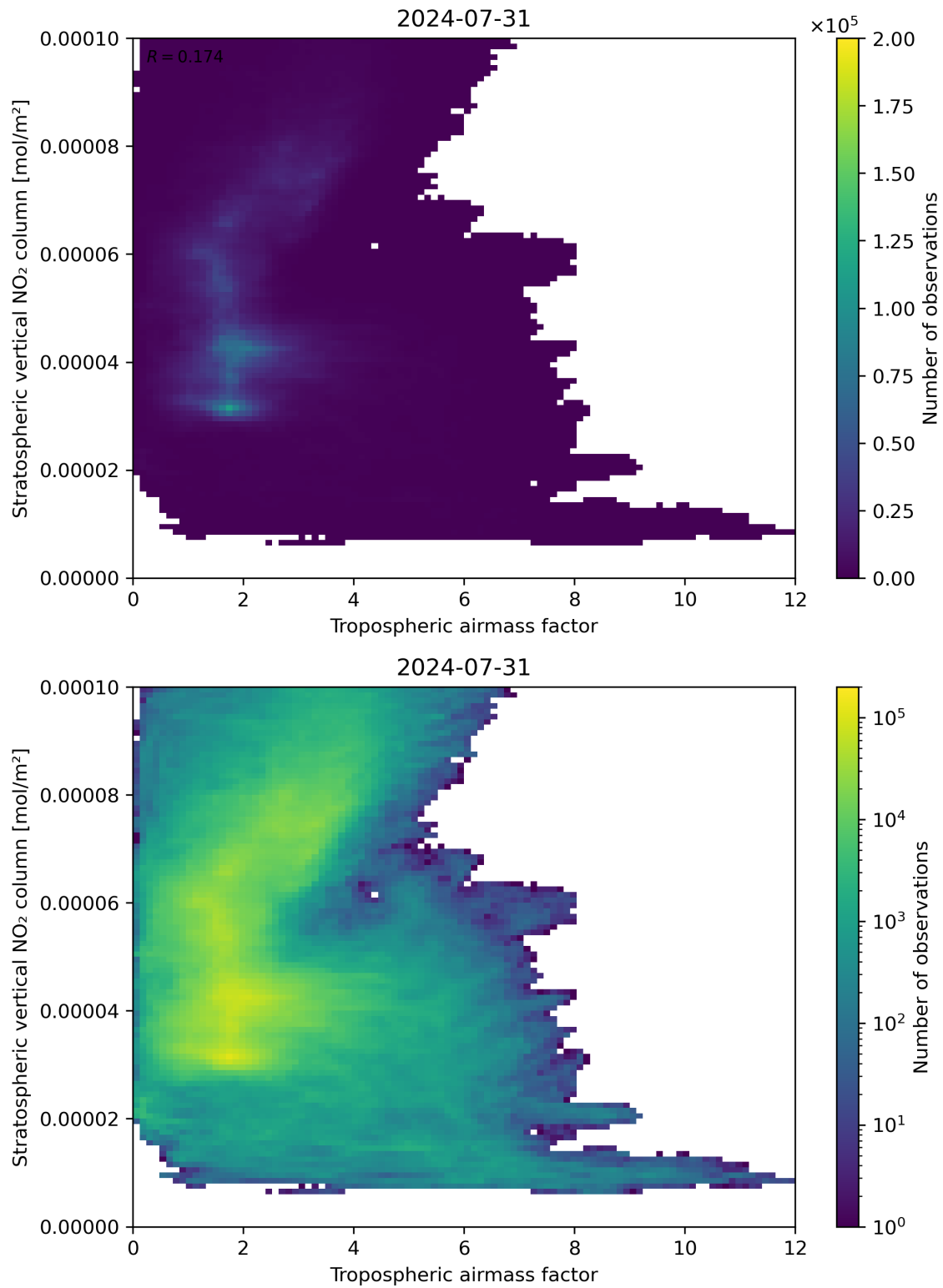
Figure 74: Scatter density plot of “Tropospheric airmass factor” against “Stratospheric vertical NO 2 column” for 2024-07-31 to 2024-08-01.
