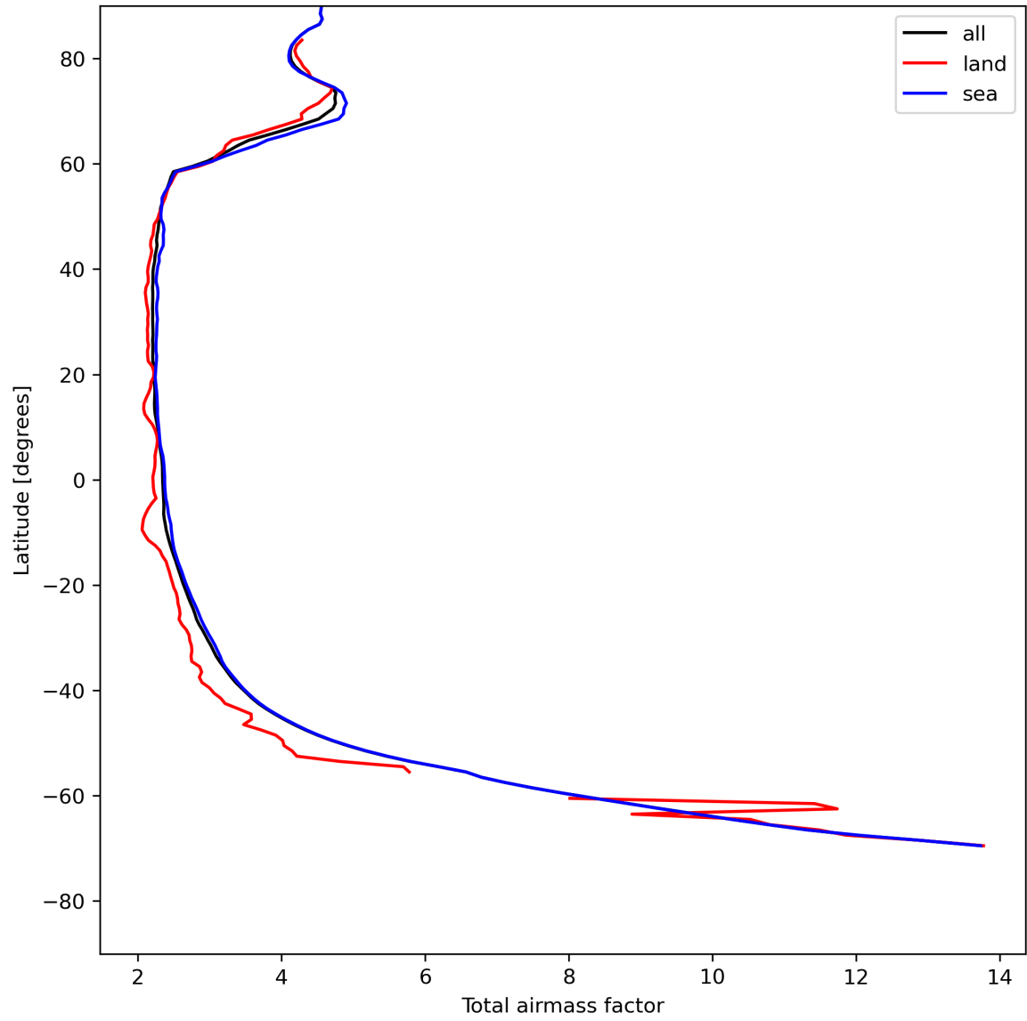
Figure 15: Zonal average of “Total airmass factor” for 2024-07-31 to 2024-08-01.
