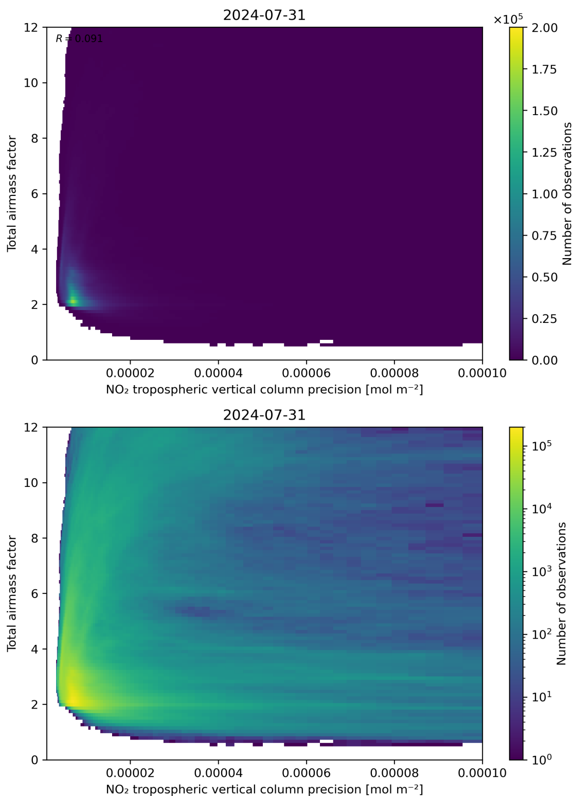
Figure 132: Scatter density plot of “NO 2 tropospheric vertical column precision” against “Total air mass factor” for 2024-07-31 to 2024-08-01.
