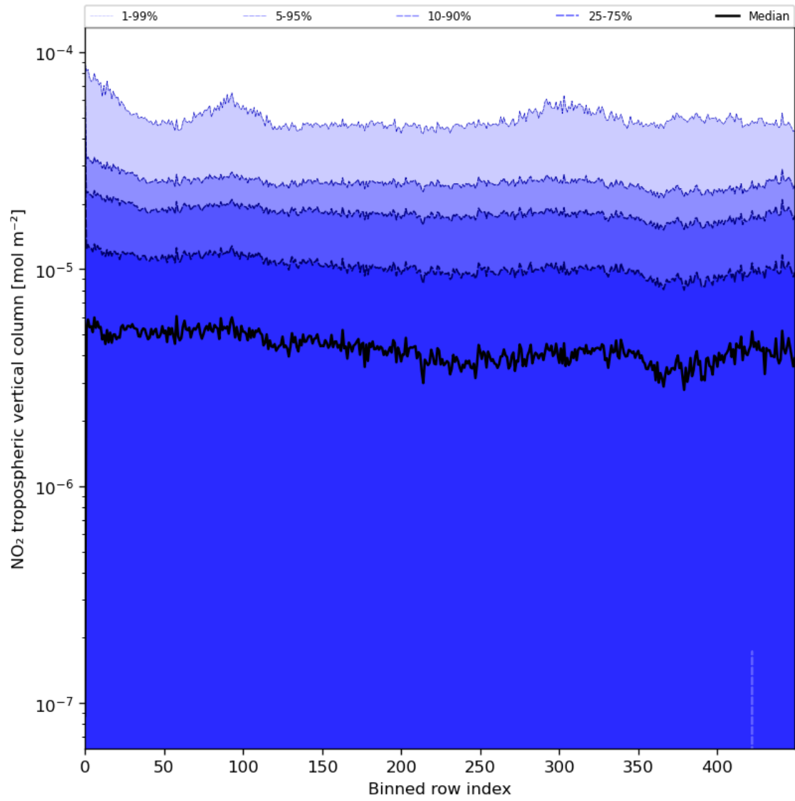
Figure 46: Along track statistics of “NO 2 tropospheric vertical column” for 2024-07-31 to 2024-08-01
