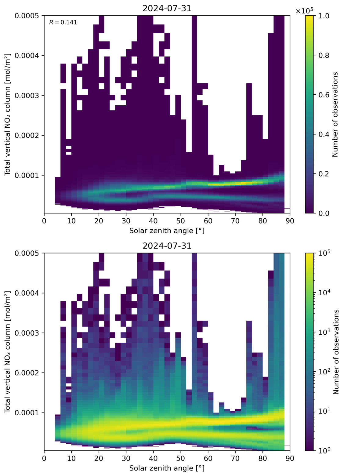
Figure 153: Scatter density plot of “Solar zenith angle” against “Total vertical NO 2 column” for 2024-07-31 to 2024-08-01.
