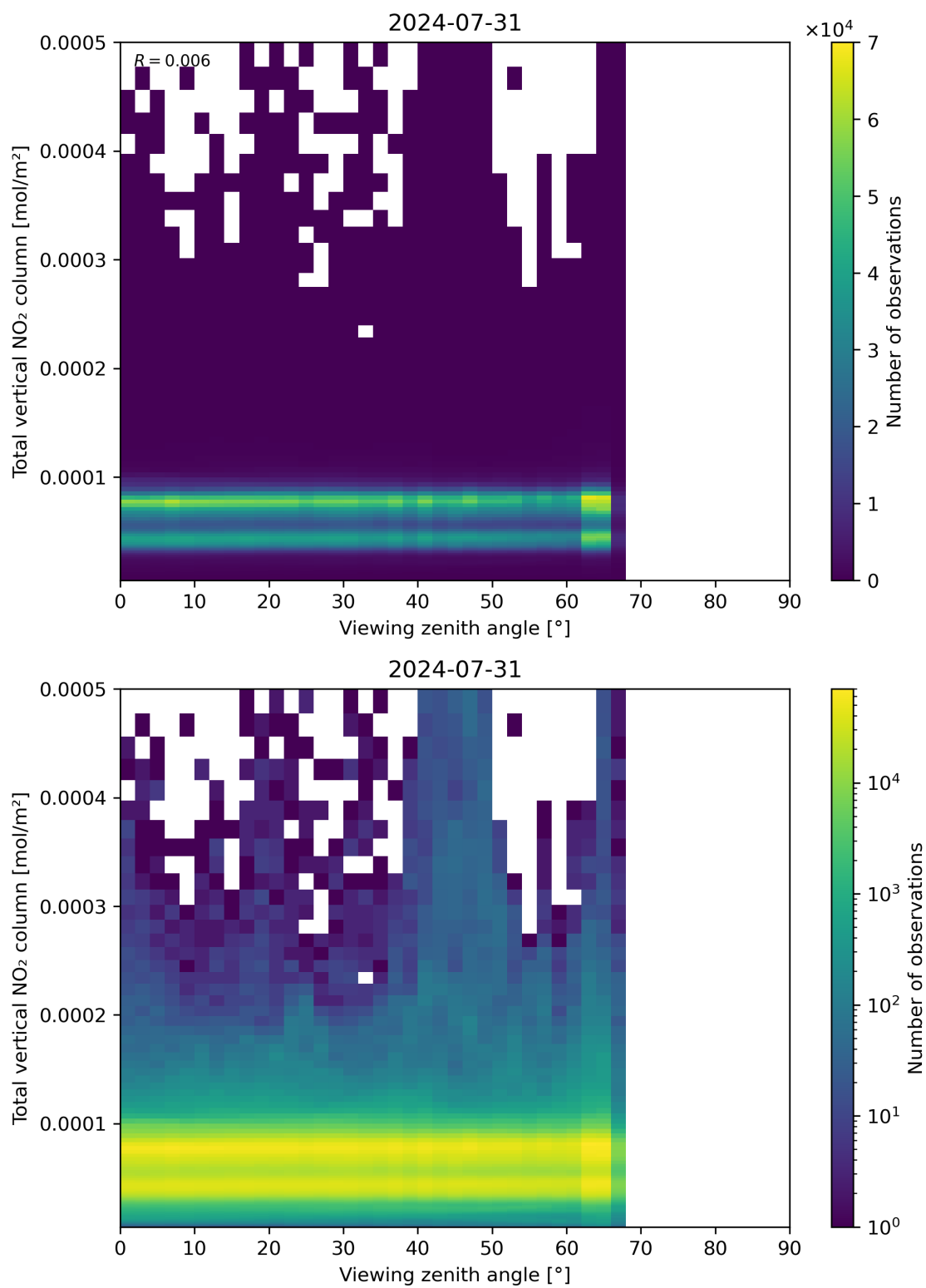
Figure 167: Scatter density plot of “Viewing zenith angle” against “Total vertical NO 2 column” for 2024-07-31 to 2024-08-01.
