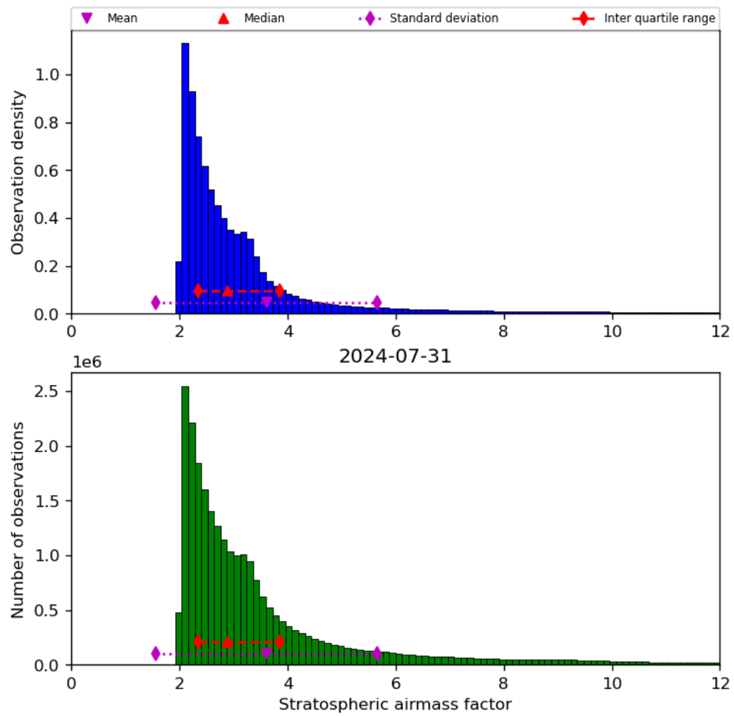
Figure 44: Histogram of “Stratospheric airmass factor” for 2024-07-31 to 2024-08-01
