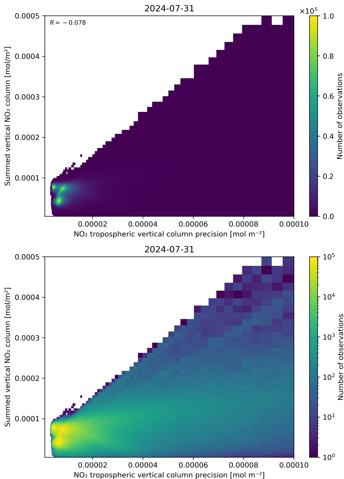
Figure 136: Scatter density plot of “NO 2 tropospheric vertical column precision” against “Summed vertical NO 2 column” for 2024-07-31 to 2024-08-01.
