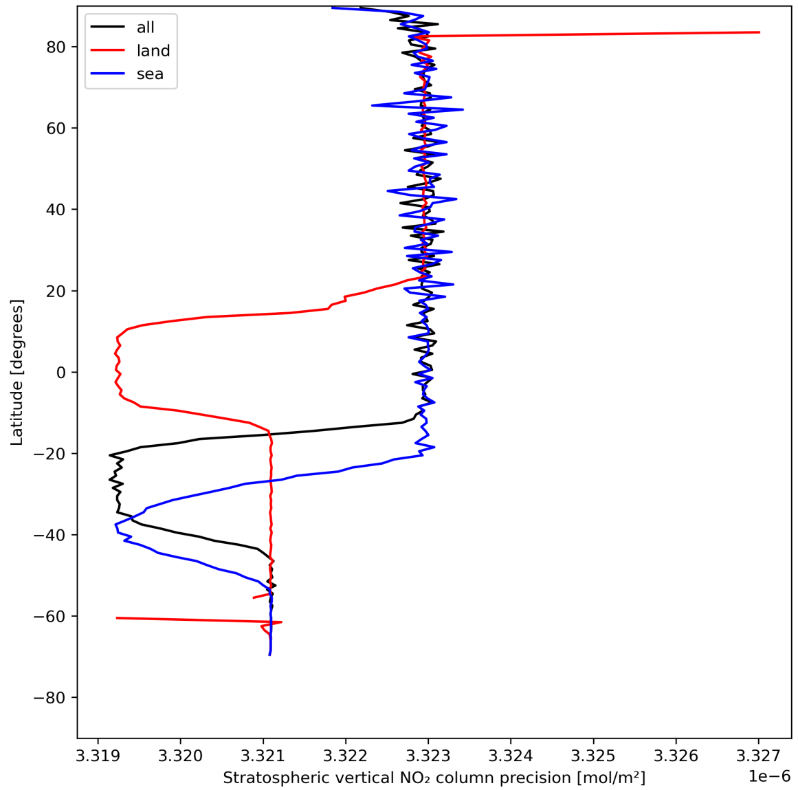
Figure 20: Zonal average of “Stratospheric vertical NO 2 column precision” for 2024-07-31 to 2024-08-01.
