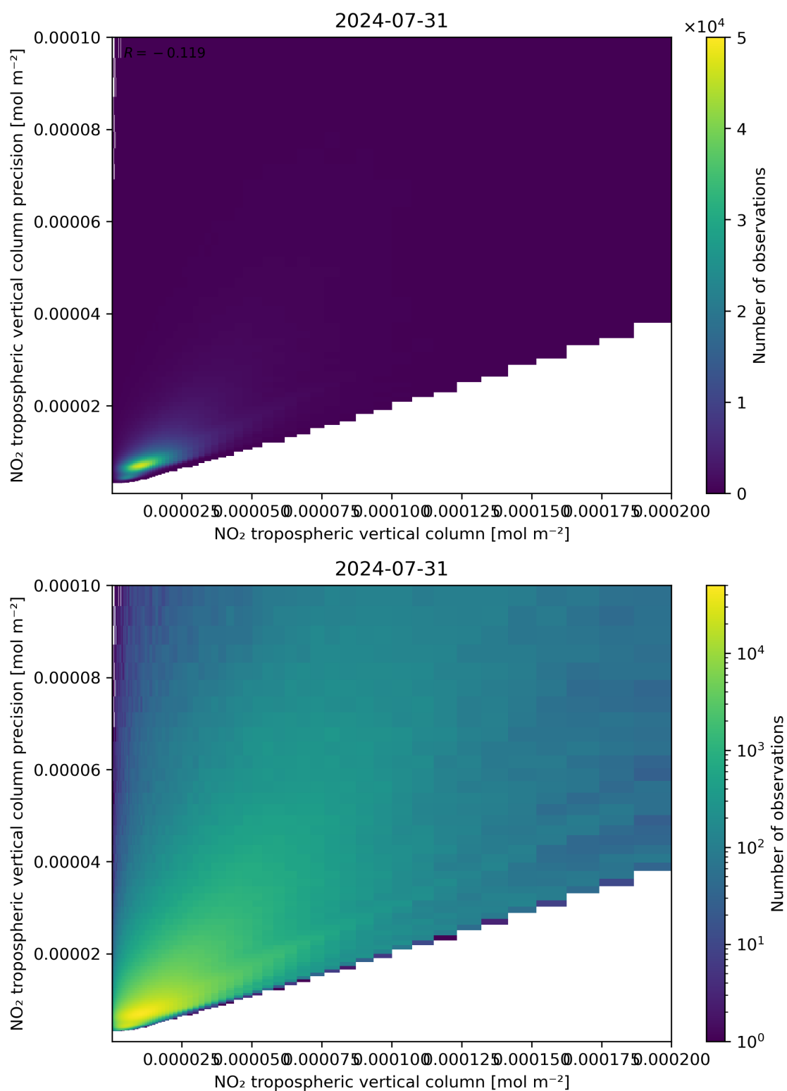
Figure 130: Scatter density plot of “NO 2 tropospheric vertical column” against “NO 2 tropospheric vertical column precision” for 2024-07-31 to 2024-08-01.
