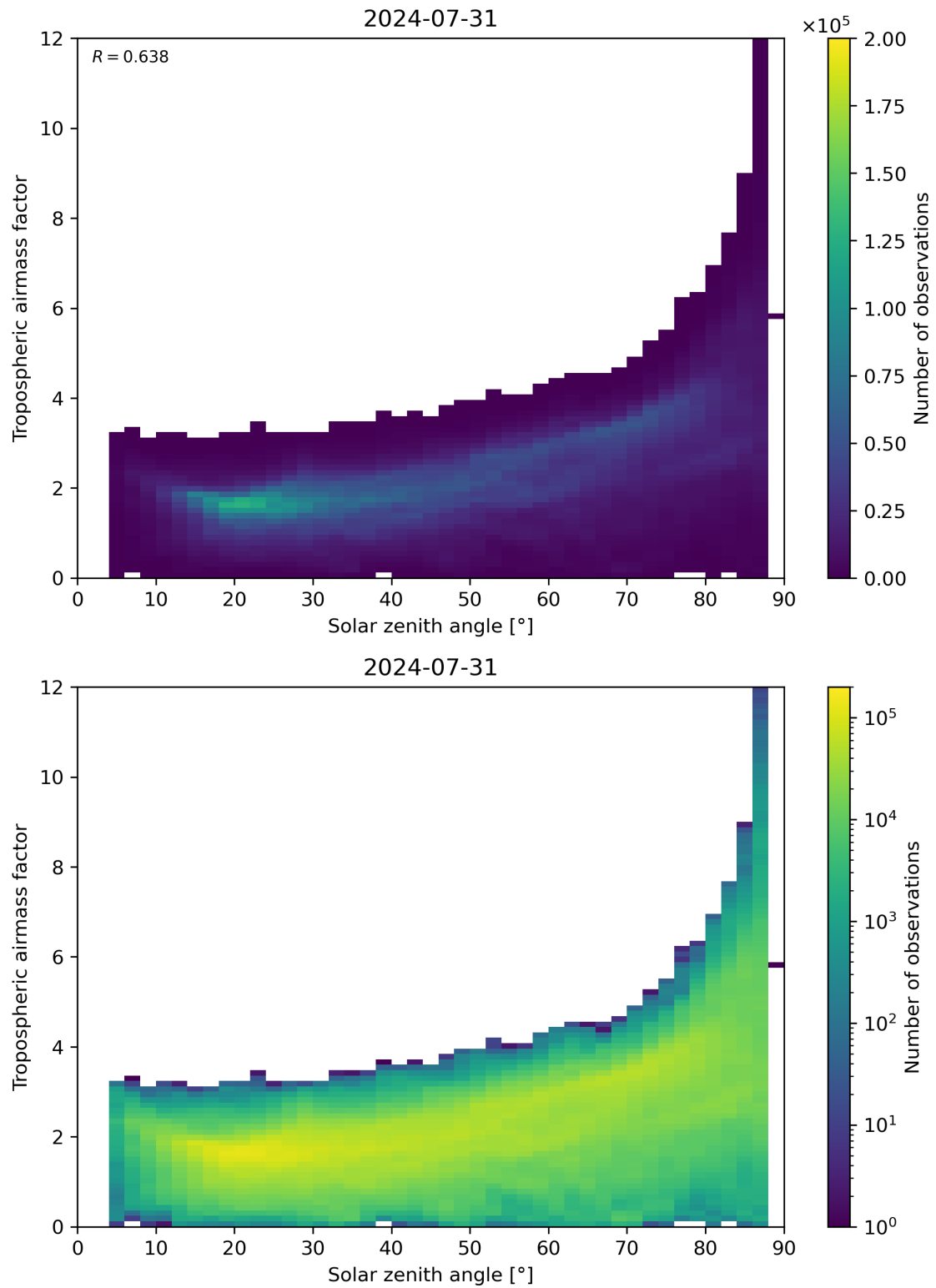
Figure 147: Scatter density plot of “Solar zenith angle” against “Tropospheric airmass factor” for 2024-07-31 to 2024-08-01.
