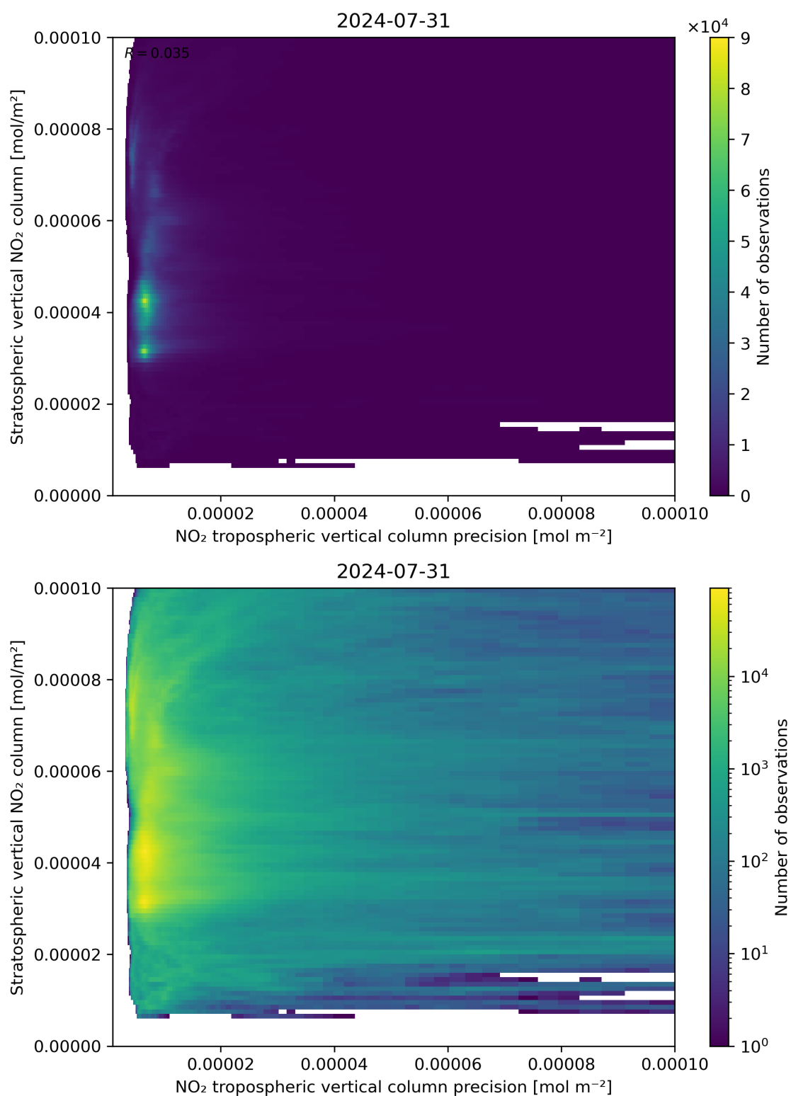
Figure 135: Scatter density plot of “NO 2 tropospheric vertical column precision” against “Stratospheric vertical NO 2 column” for 2024-07-31 to 2024-08-01.
