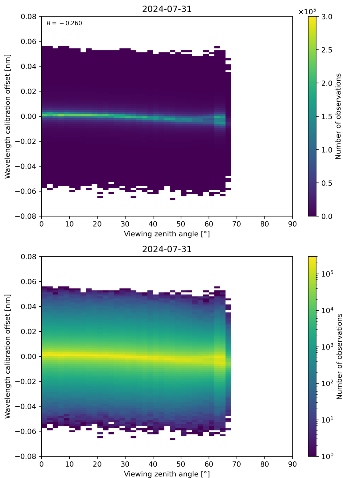
Figure 173: Scatter density plot of “Viewing zenith angle” against “Wavelength calibration offset” for 2024-07-31 to 2024-08-01.
