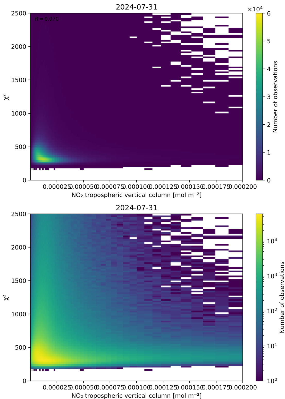
Figure 124: Scatter density plot of “NO 2 tropospheric vertical column” against “ \chi^2 ” for 2024-07-31 to 2024-08-01.
