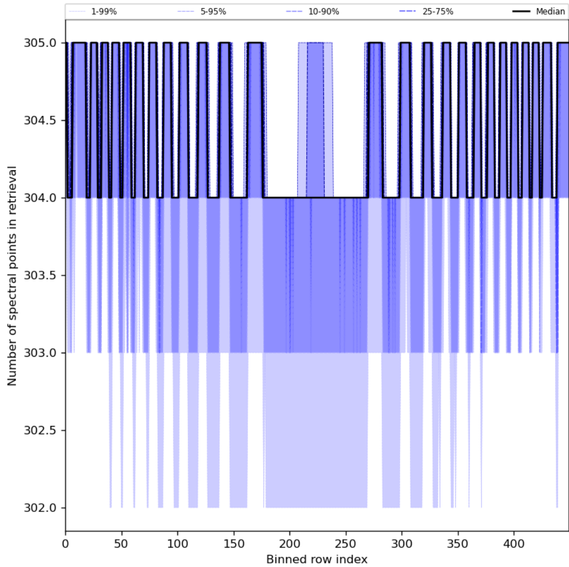
Figure 50: Along track statistics of “Number of spectral points in retrieval” for 2024-07-31 to 2024-08-01
