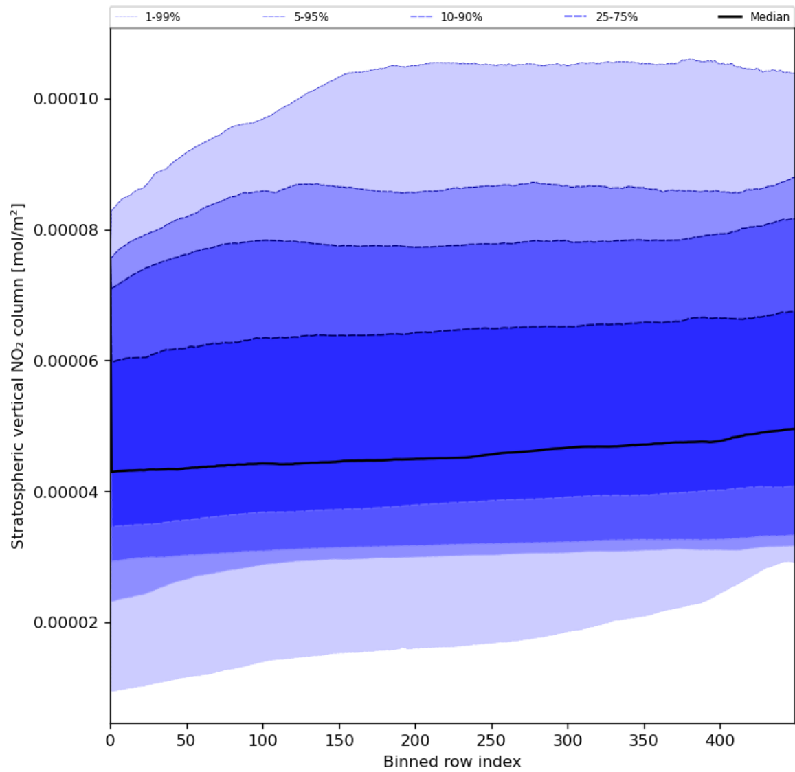
Figure 53: Along track statistics of “Stratospheric vertical NO 2 column” for 2024-07-31 to 2024-08-01
