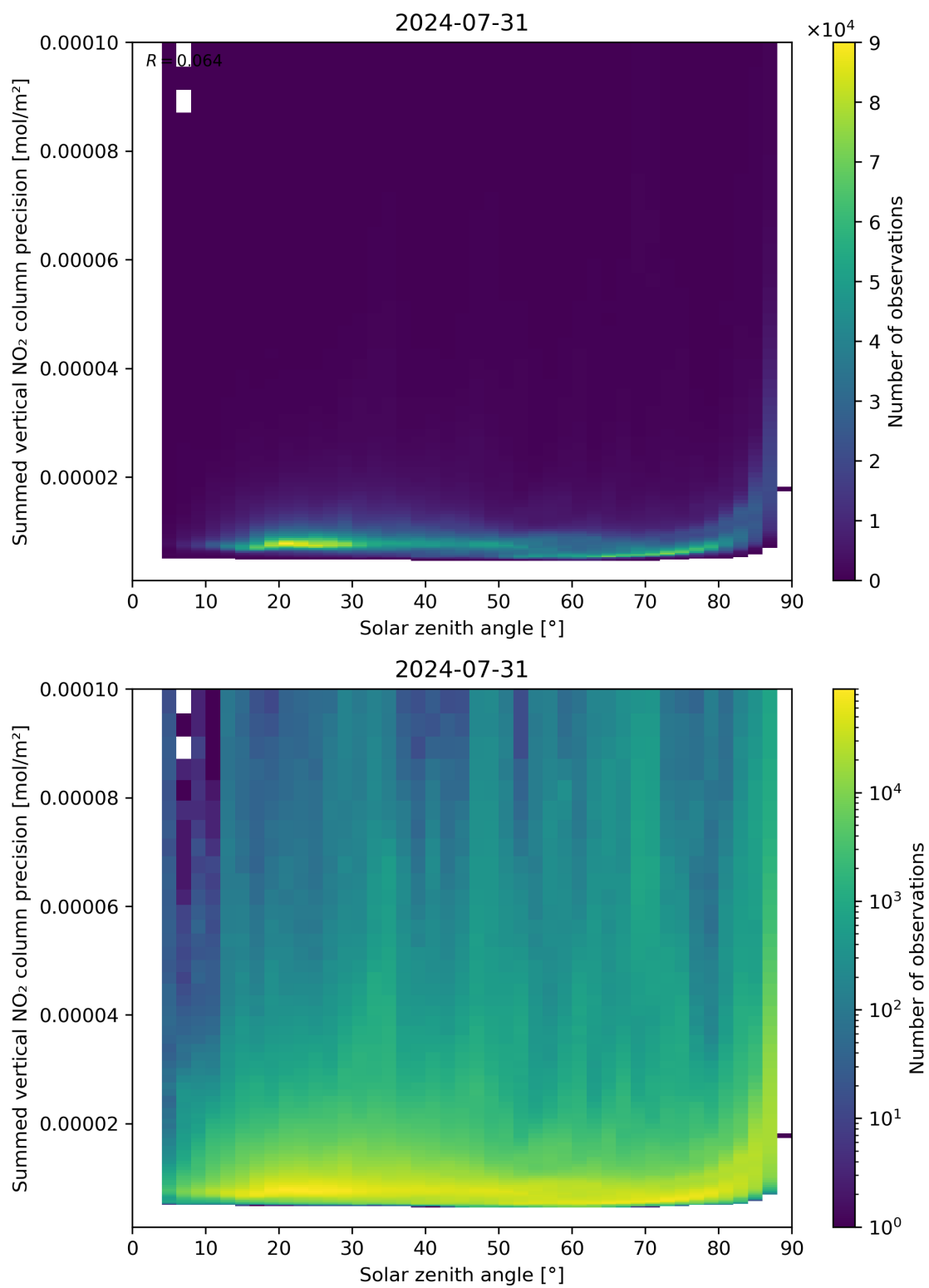
Figure 152: Scatter density plot of “Solar zenith angle” against “Summed vertical NO 2 column precision” for 2024-07-31 to 2024-08-01.
