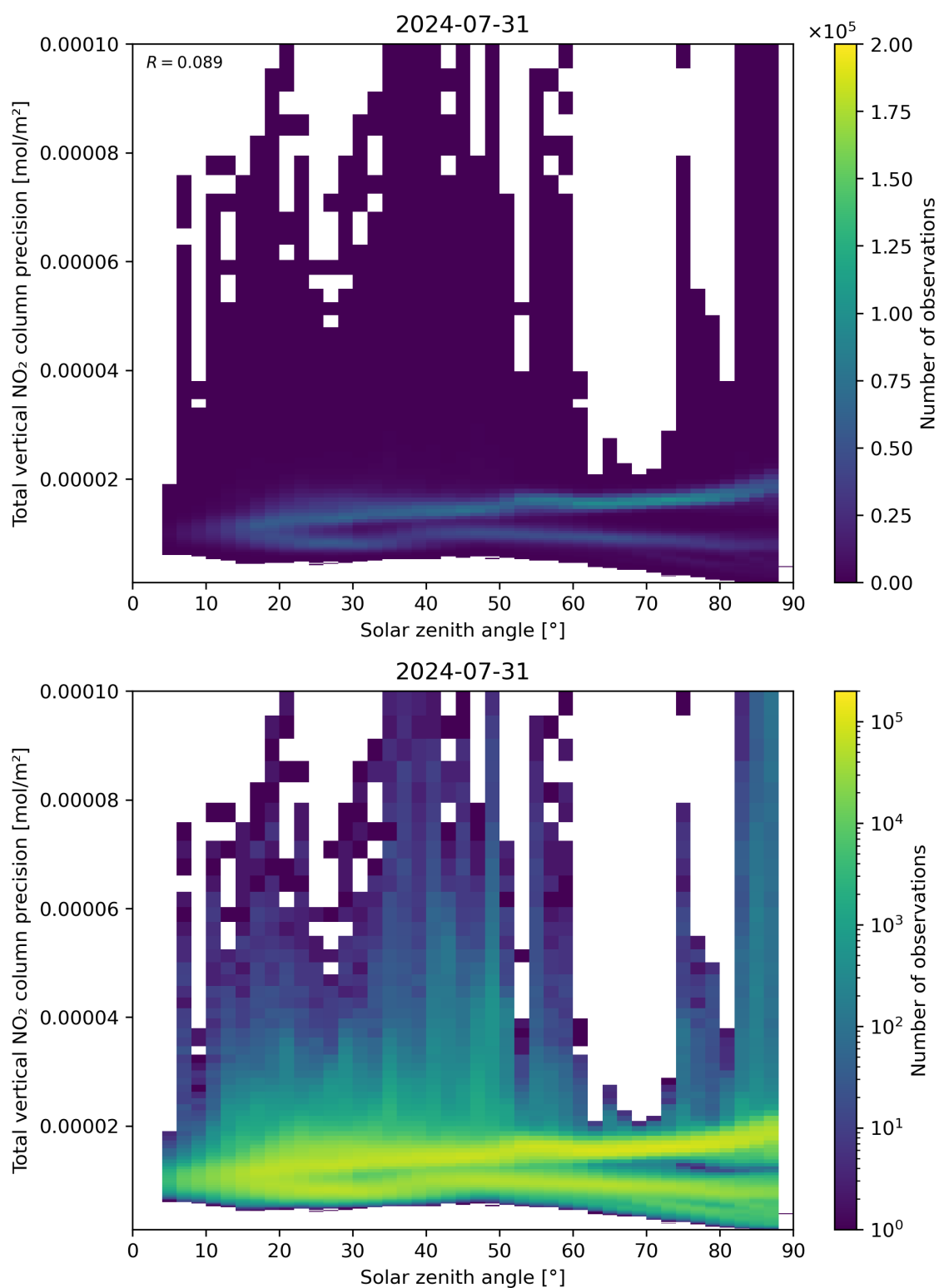
Figure 154: Scatter density plot of “Solar zenith angle” against “Total vertical NO 2 column precision” for 2024-07-31 to 2024-08-01.
