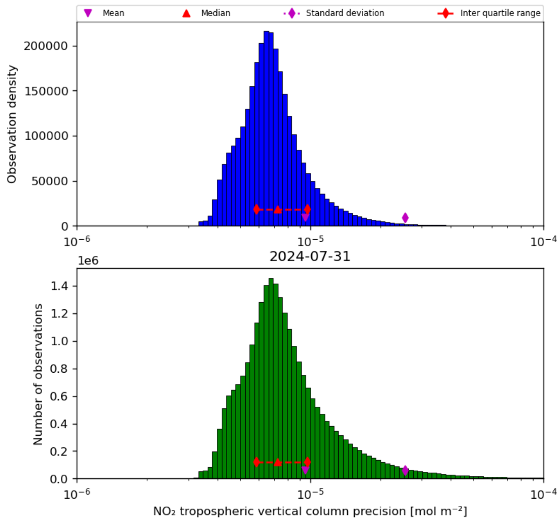
Figure 30: Histogram of “NO 2 tropospheric vertical column precision” for 2024-07-31 to 2024-08-01
