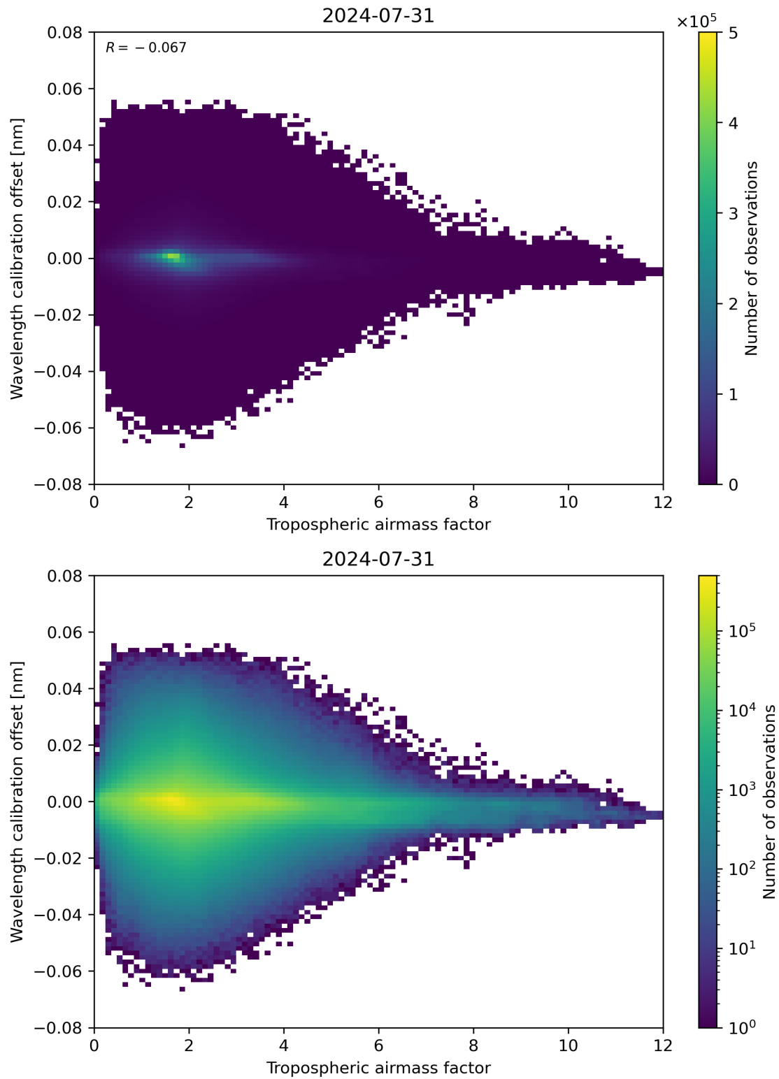
Figure 80: Scatter density plot of “Tropospheric air mass factor” against “Wavelength calibration offset” for 2024-07-31 to 2024-08-01.
