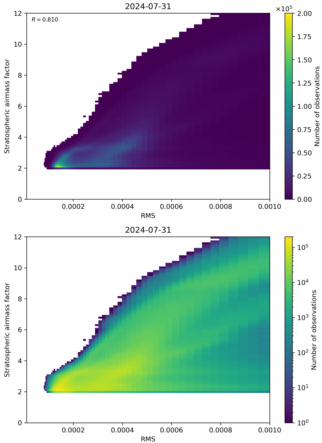
Figure 144: Scatter density plot of “RMS” against “Stratospheric airmass factor” for 2024-07-31 to 2024-08-01.
