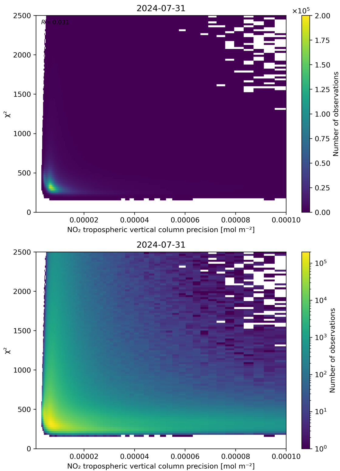
Figure 134: Scatter density plot of “NO 2 tropospheric vertical column precision” against “ \chi^2 ” for 2024-07-31 to 2024-08-01.
