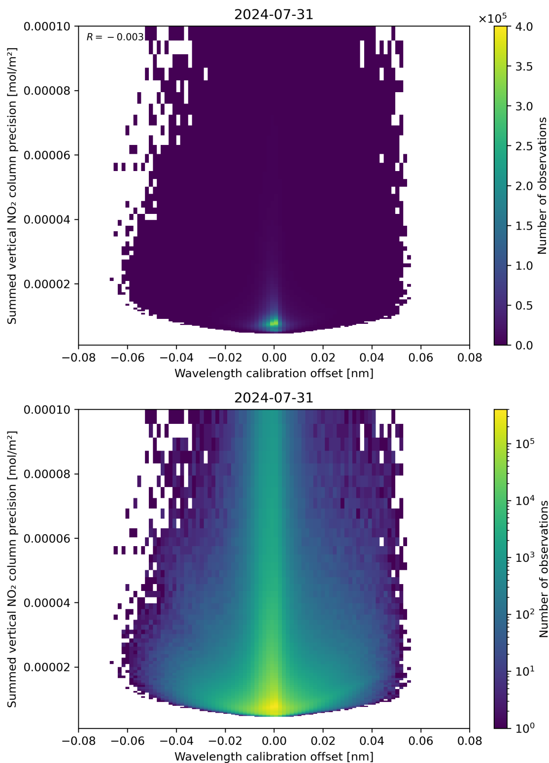
Figure 178: Scatter density plot of “Wavelength calibration offset” against “Summed vertical NO 2 column precision” for 2024-07-31 to 2024-08-01.
