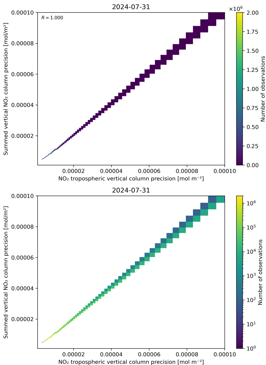
Figure 137: Scatter density plot of “NO 2 tropospheric vertical column precision” against “Summed vertical NO 2 column precision” for 2024-07-31 to 2024-08-01.
