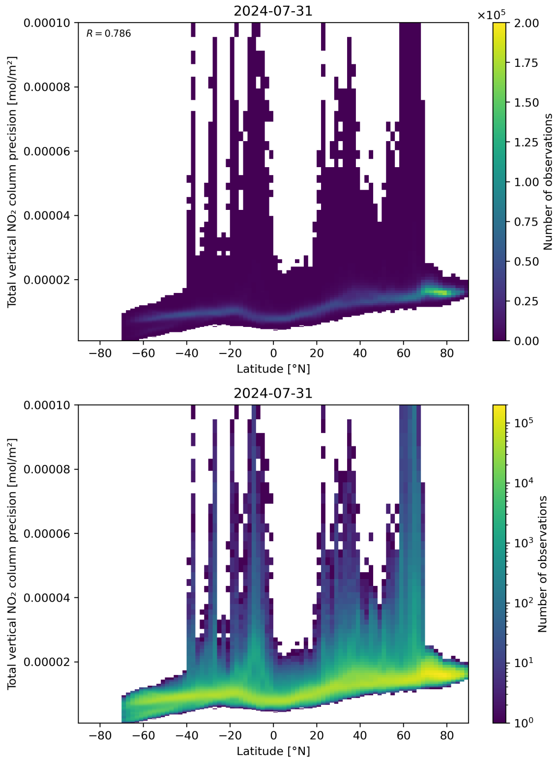
Figure 91: Scatter density plot of “Latitude” against “Total vertical NO 2 column precision” for 2024-07-31 to 2024-08-01.
