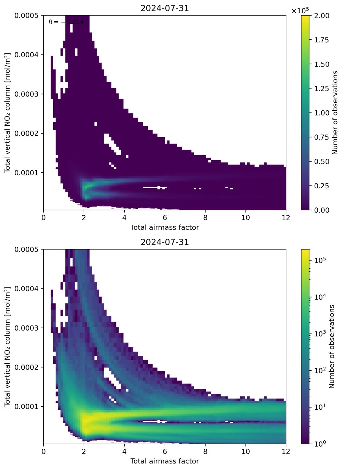
Figure 67: Scatter density plot of “Total airmass factor” against “Total vertical NO 2 column” for 2024-07-31 to 2024-08-01.
