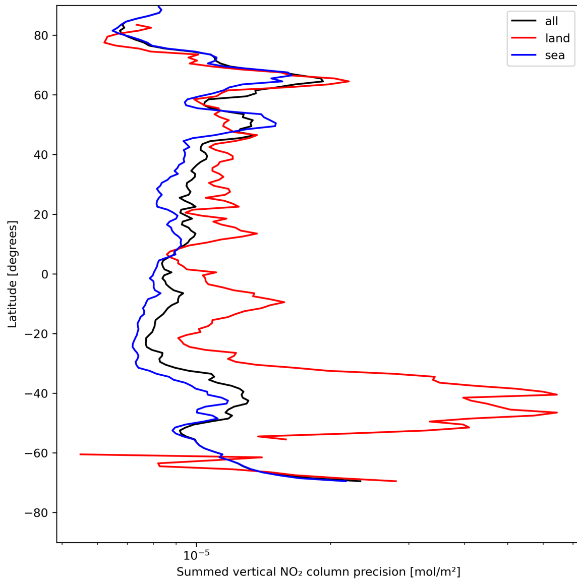
Figure 24: Zonal average of “Summed vertical NO 2 column precision” for 2024-07-31 to 2024-08-01.
