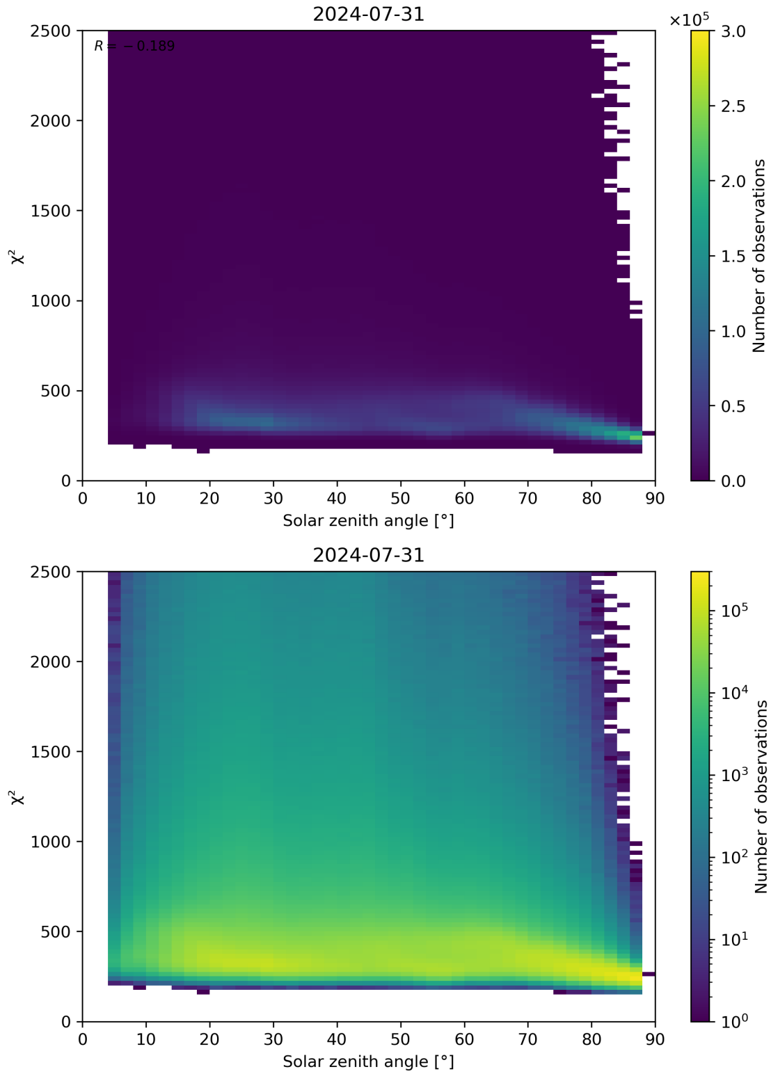
Figure 148: Scatter density plot of “Solar zenith angle” against “ \chi^2 ” for 2024-07-31 to 2024-08-01.
