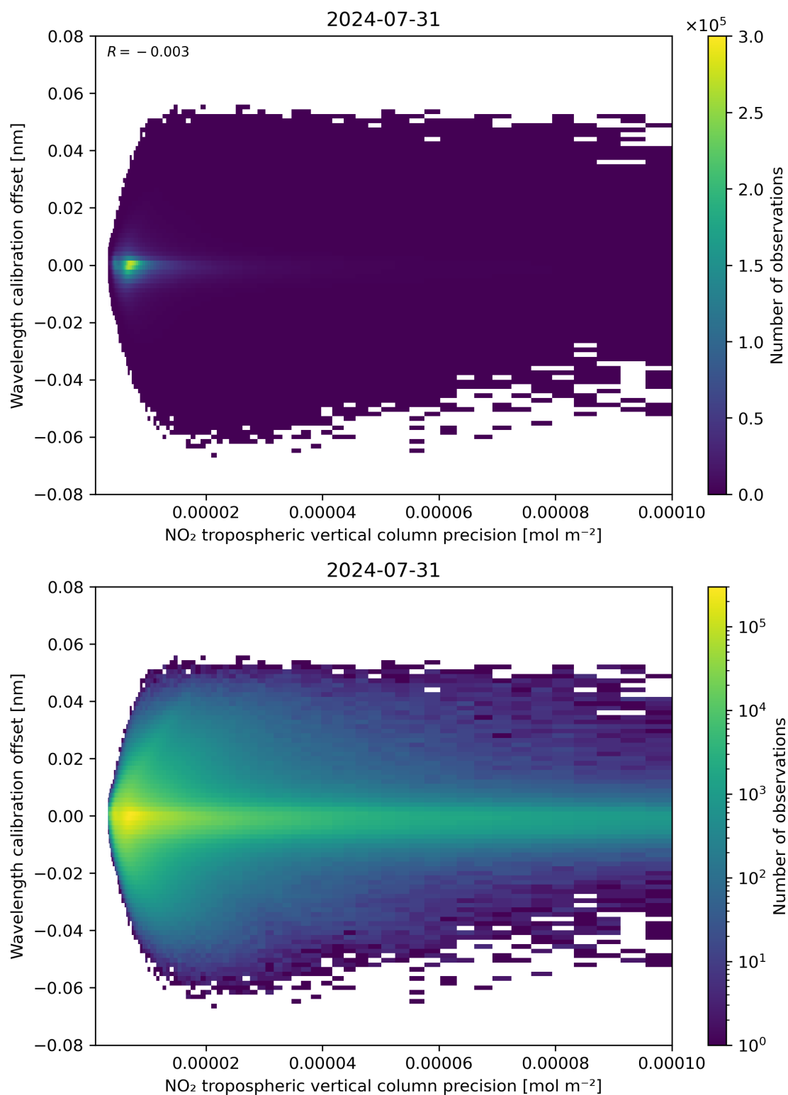
Figure 141: Scatter density plot of “NO 2 tropospheric vertical column precision” against “Wavelength calibration offset” for 2024-07-31 to 2024-08-01.
