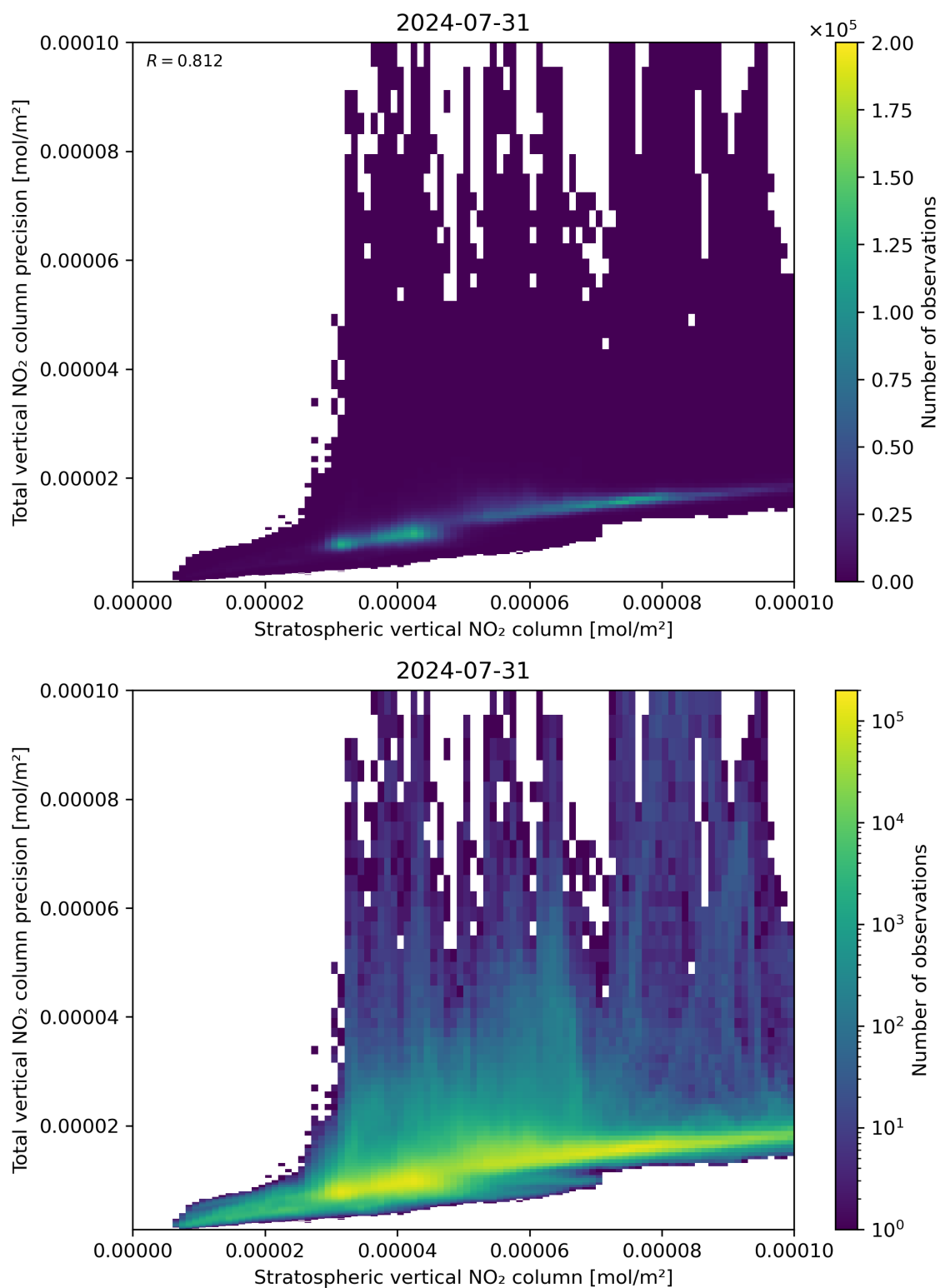
Figure 101: Scatter density plot of “Stratospheric vertical NO 2 column” against “Total vertical NO 2 column precision” for 2024-07-31 to 2024-08-01.
