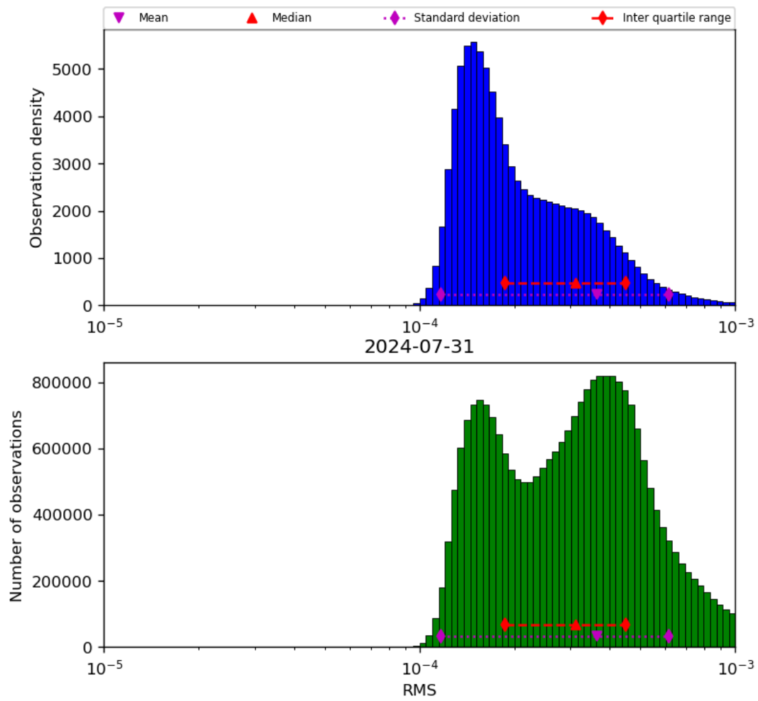
Figure 43: Histogram of “RMS” for 2024-07-31 to 2024-08-01
