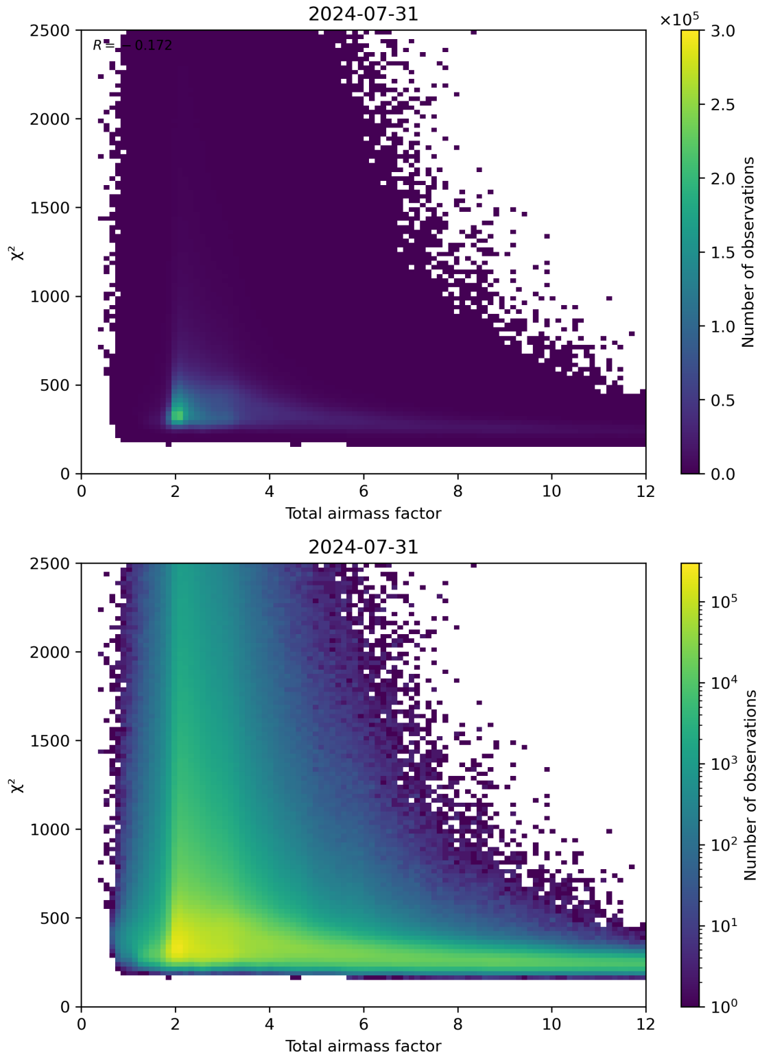
Figure 63: Scatter density plot of “Total airmass factor” against “ \chi^2 ” for 2024-07-31 to 2024-08-01.
