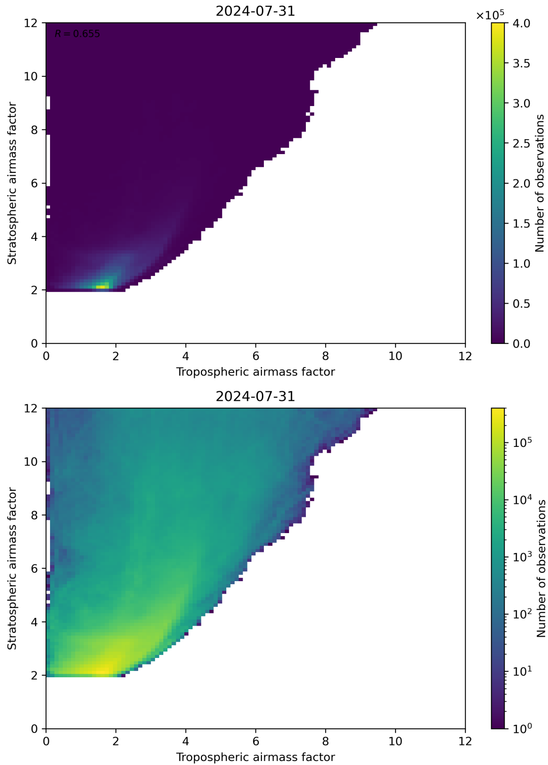
Figure 71: Scatter density plot of “Tropospheric airmass factor” against “Stratospheric airmass factor” for 2024-07-31 to 2024-08-01.
