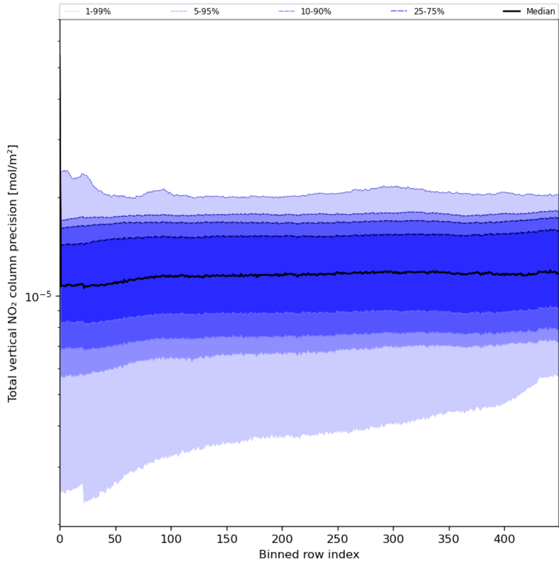
Figure 56: Along track statistics of “Total vertical NO 2 column precision” for 2024-07-31 to 2024-08-01
