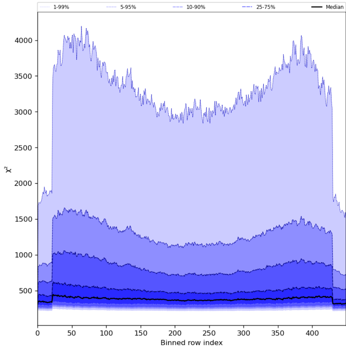
Figure 59: Along track statistics of “ \chi^2 ” for 2024-07-31 to 2024-08-01
