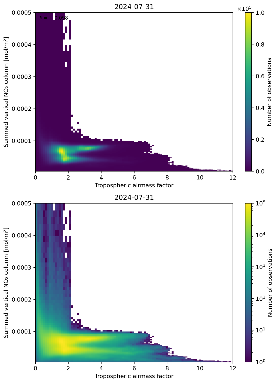
Figure 75: Scatter density plot of “Tropospheric airmass factor” against “Summed vertical NO 2 column” for 2024-07-31 to 2024-08-01.
