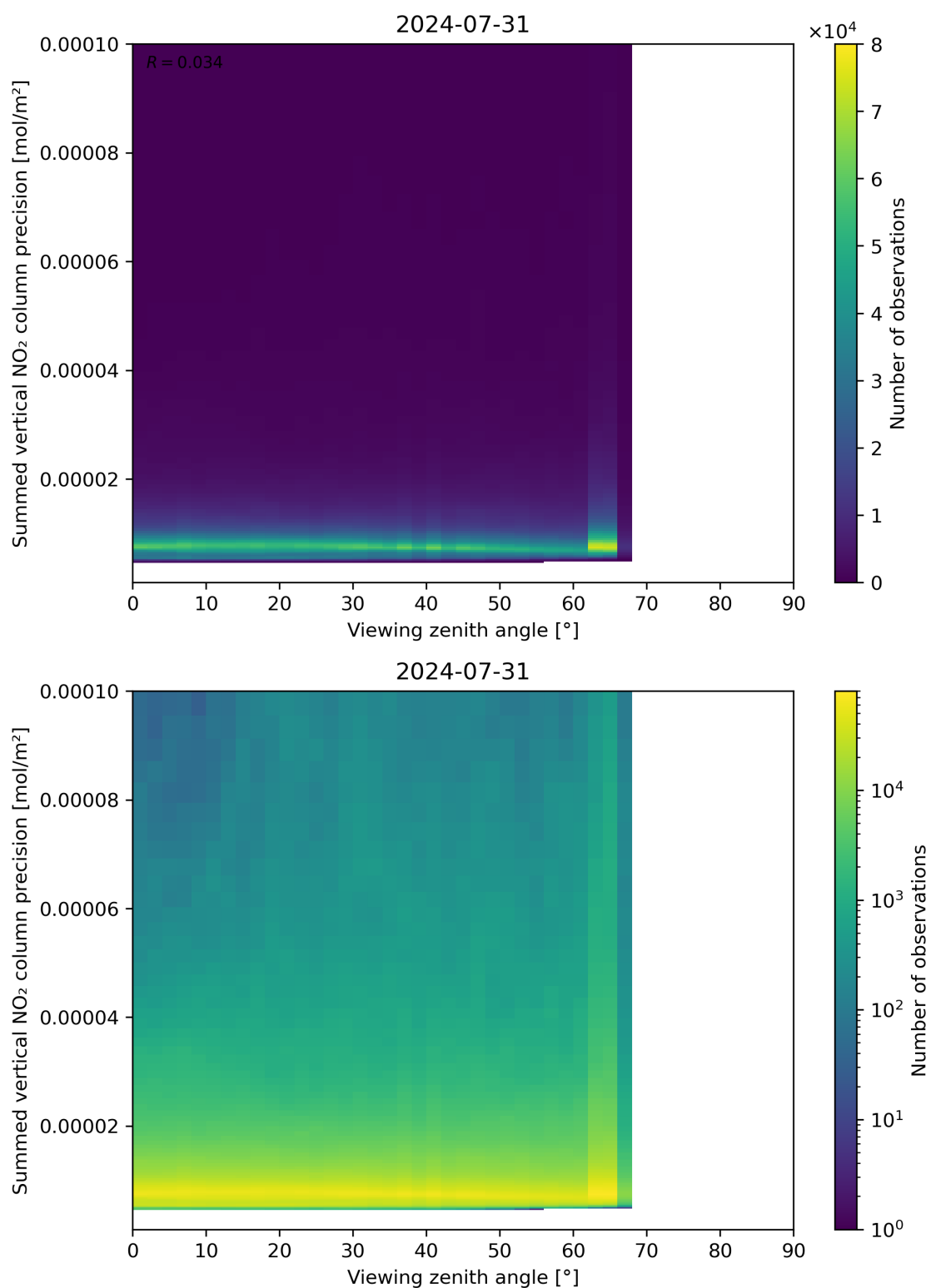
Figure 166: Scatter density plot of “Viewing zenith angle” against “Summed vertical NO 2 column precision” for 2024-07-31 to 2024-08-01.
