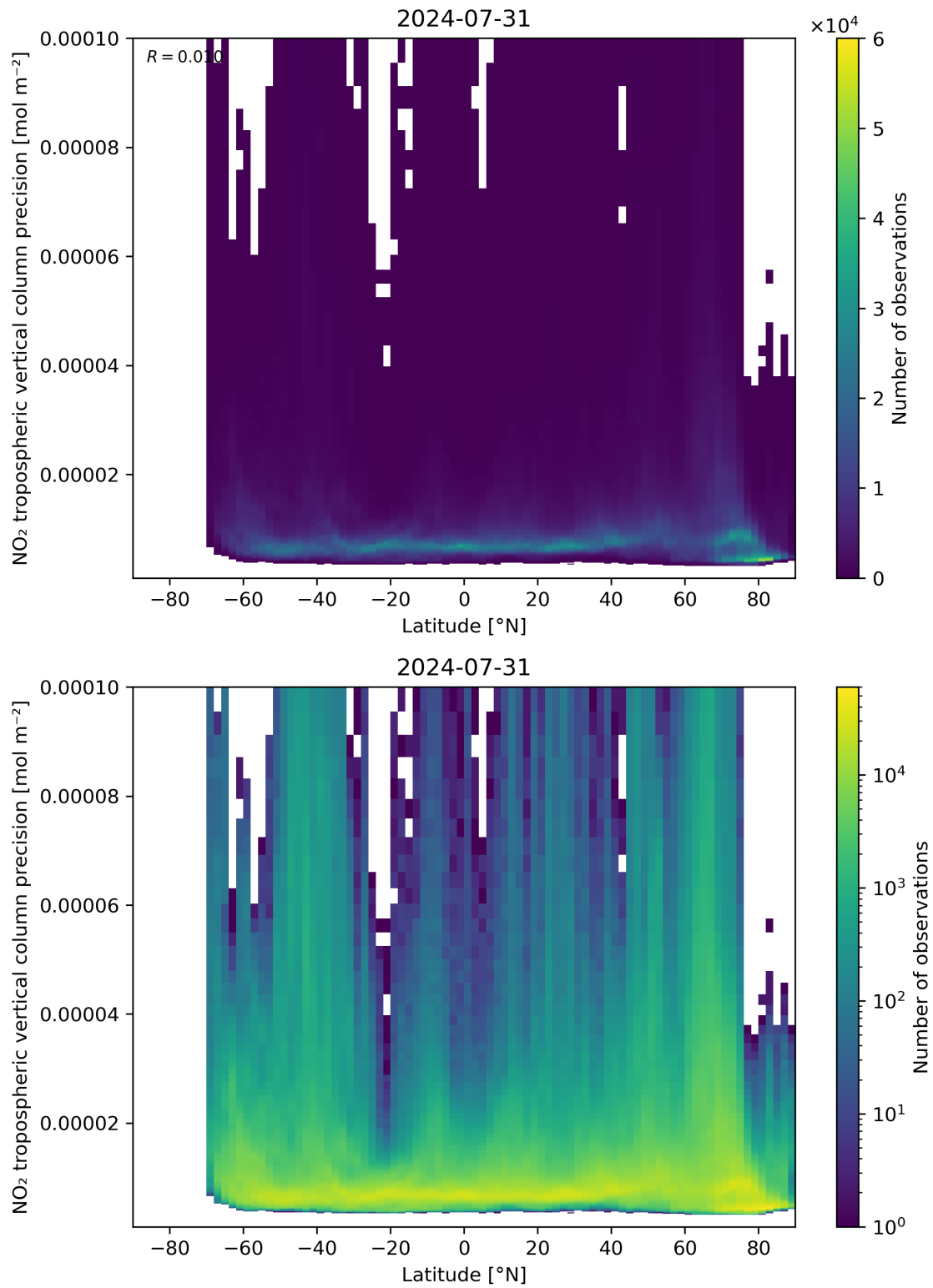
Figure 93: Scatter density plot of “Latitude” against “NO 2 tropospheric vertical column precision” for 2024-07-31 to 2024-08-01.
