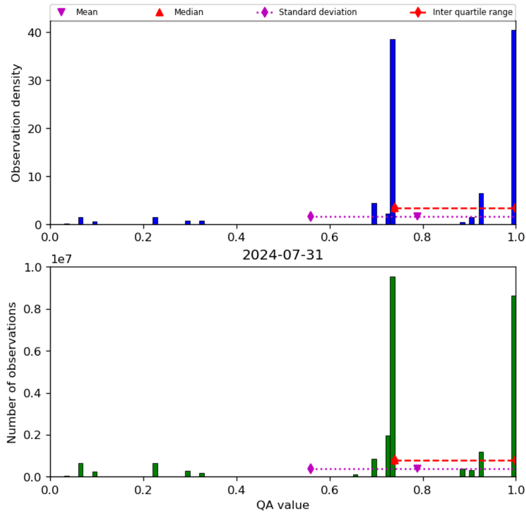
Figure 28: Histogram of “QA value” for 2024-07-31 to 2024-08-01
