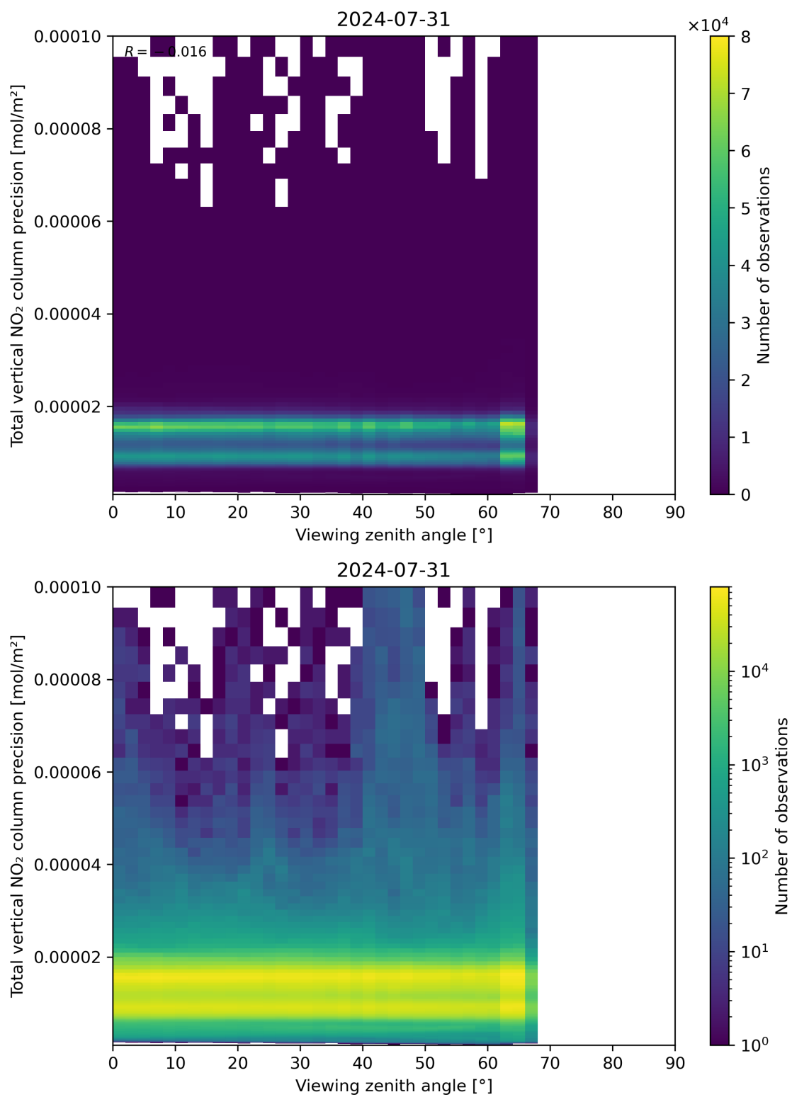
Figure 168: Scatter density plot of “Viewing zenith angle” against “Total vertical NO 2 column precision” for 2024-07-31 to 2024-08-01.
