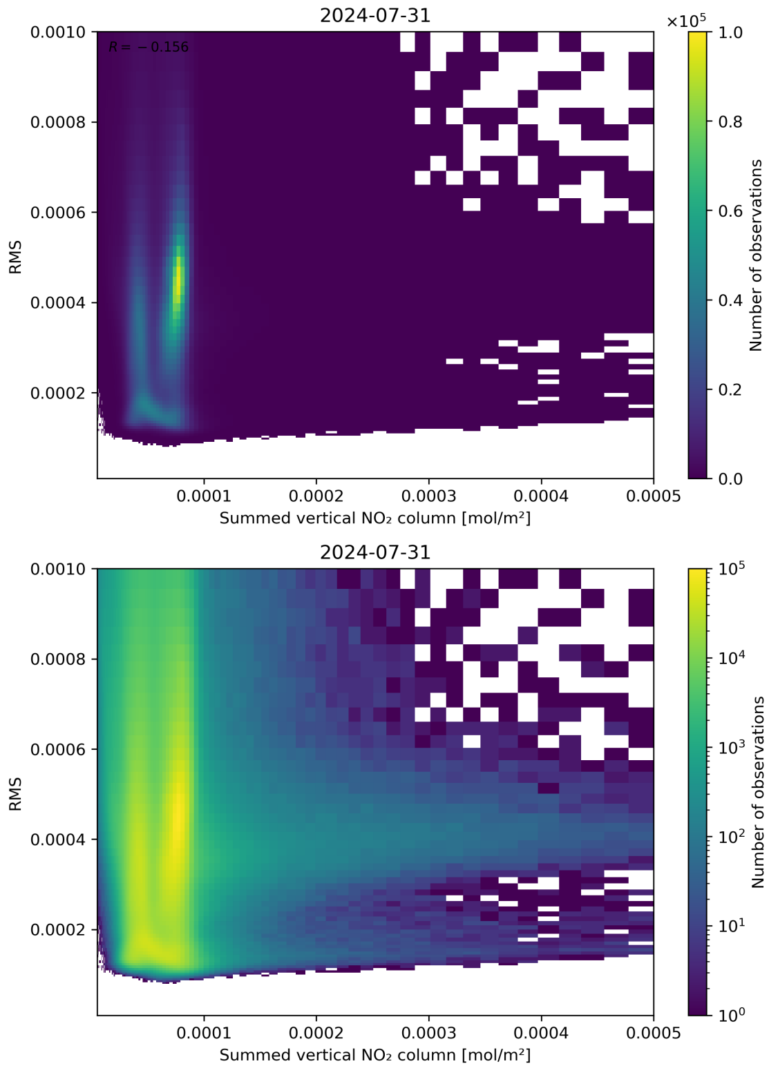
Figure 109: Scatter density plot of “Summed vertical NO 2 column” against “RMS” for 2024-07-31 to 2024-08-01.
