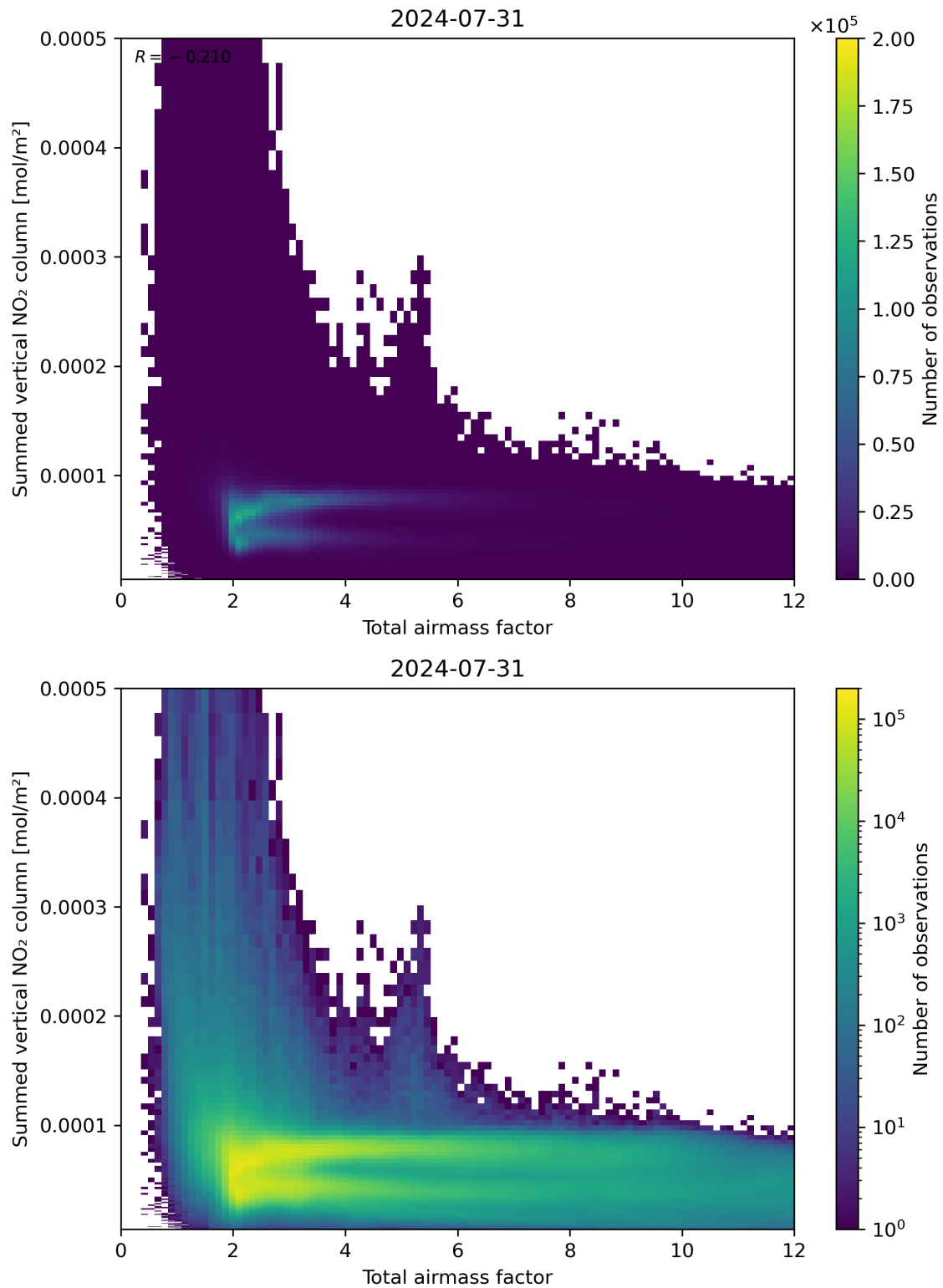
Figure 65: Scatter density plot of “Total airmass factor” against “Summed vertical NO 2 column” for 2024-07-31 to 2024-08-01.
