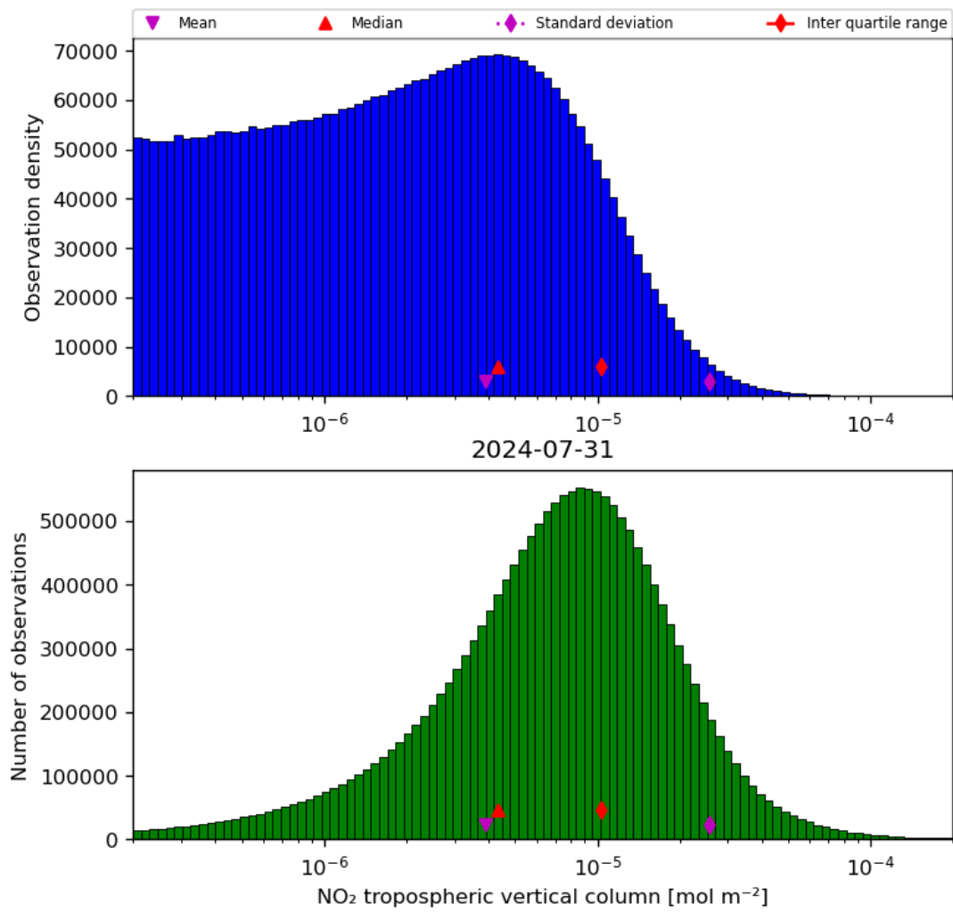
Figure 29: Histogram of “NO 2 tropospheric vertical column” for 2024-07-31 to 2024-08-01
