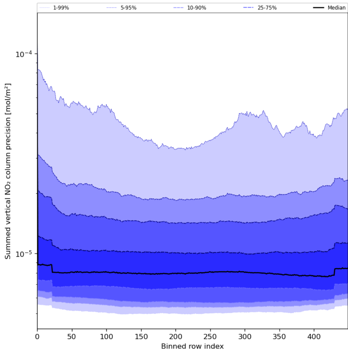
Figure 58: Along track statistics of “Summed vertical NO 2 column precision” for 2024-07-31 to 2024-08-01
