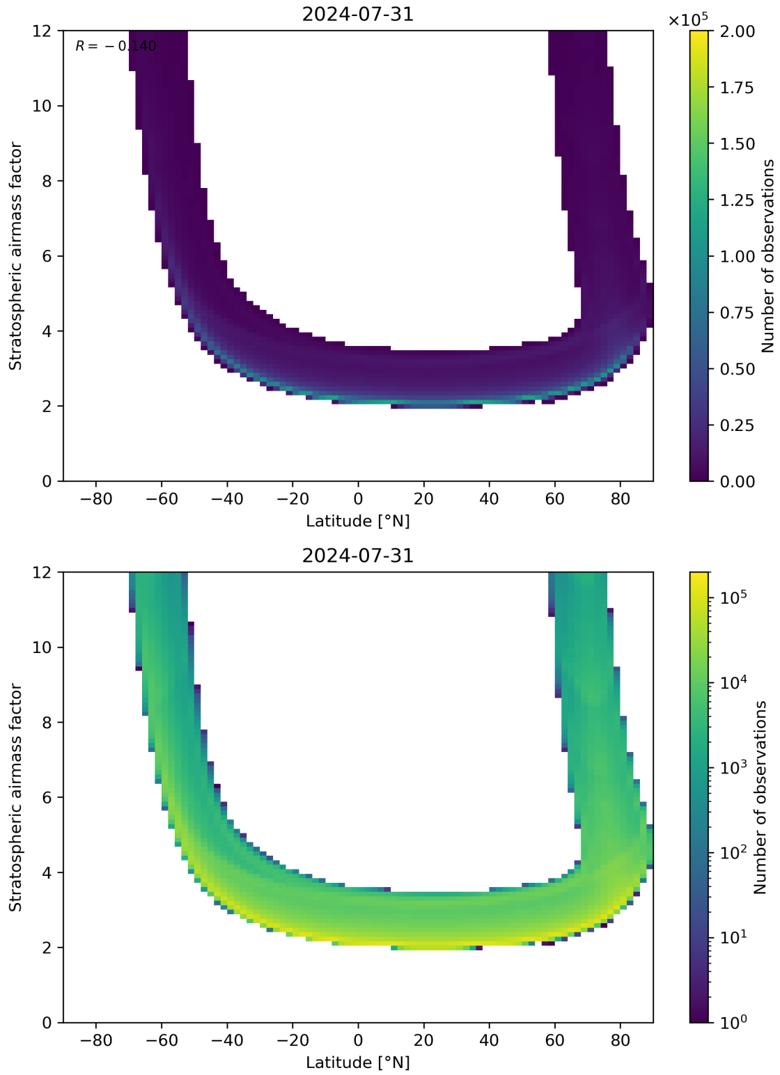
Figure 83: Scatter density plot of “Latitude” against “Stratospheric air mass factor” for 2024-07-31 to 2024-08-01.
