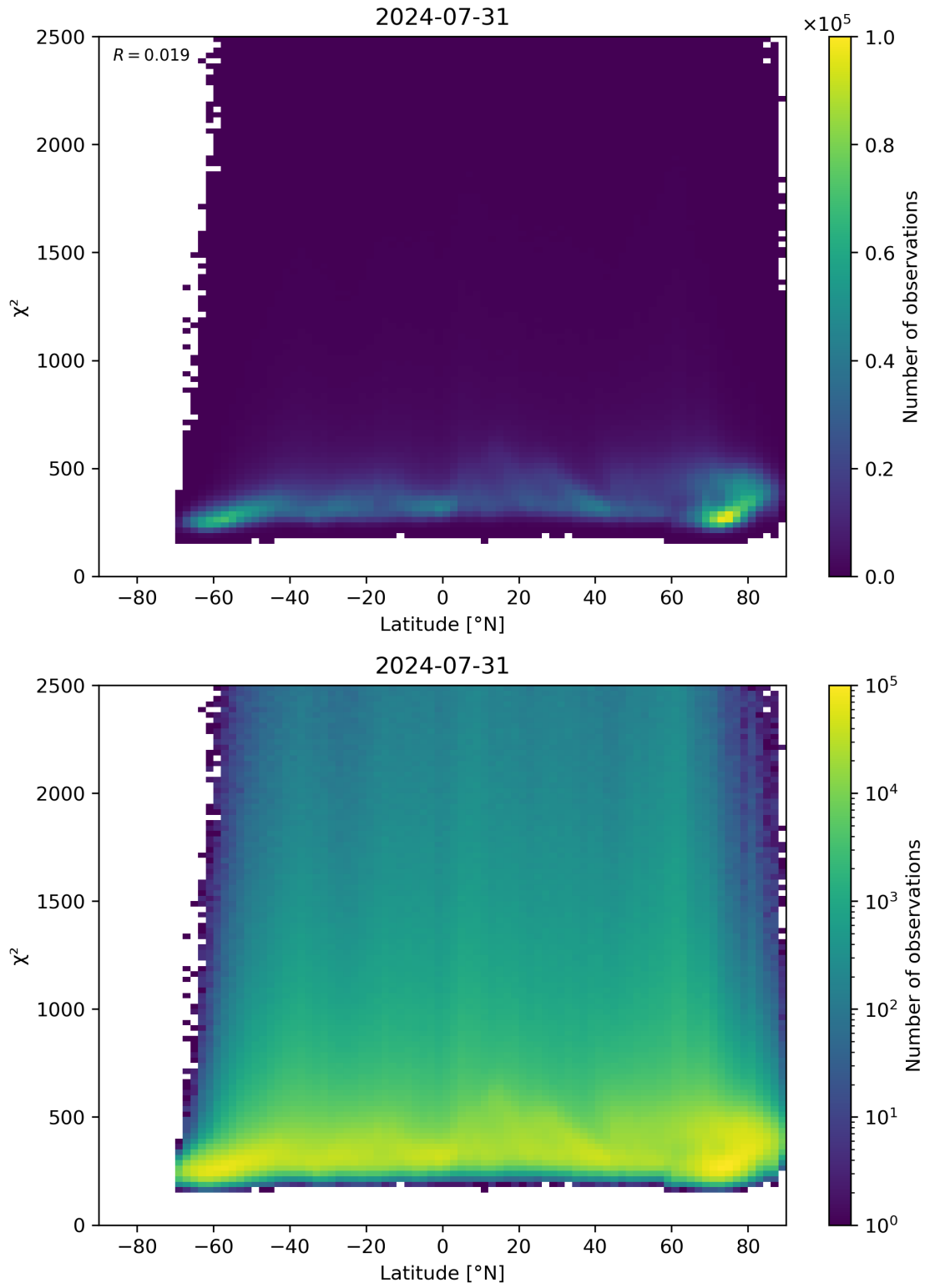
Figure 86: Scatter density plot of “Latitude” against “ \chi^2 ” for 2024-07-31 to 2024-08-01.
