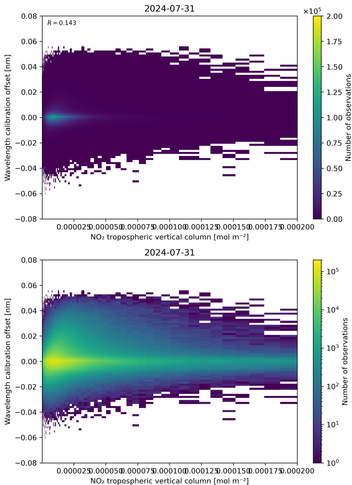
Figure 143: Scatter density plot of “NO 2 tropospheric vertical column” against “Wavelength calibration offset” for 2024-07-31 to 2024-08-01.
