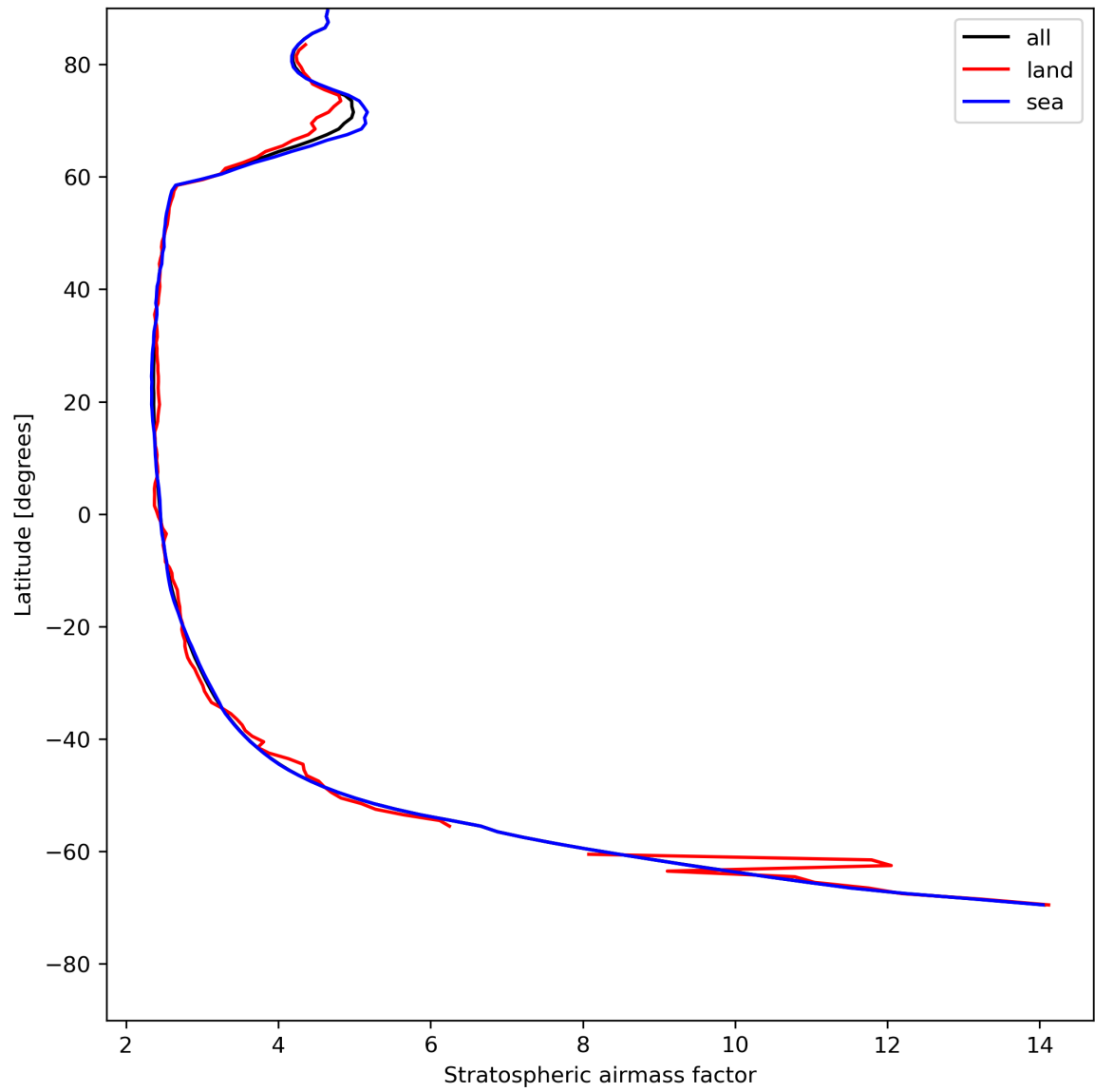
Figure 27: Zonal average of “Stratospheric airmass factor” for 2024-07-31 to 2024-08-01.
