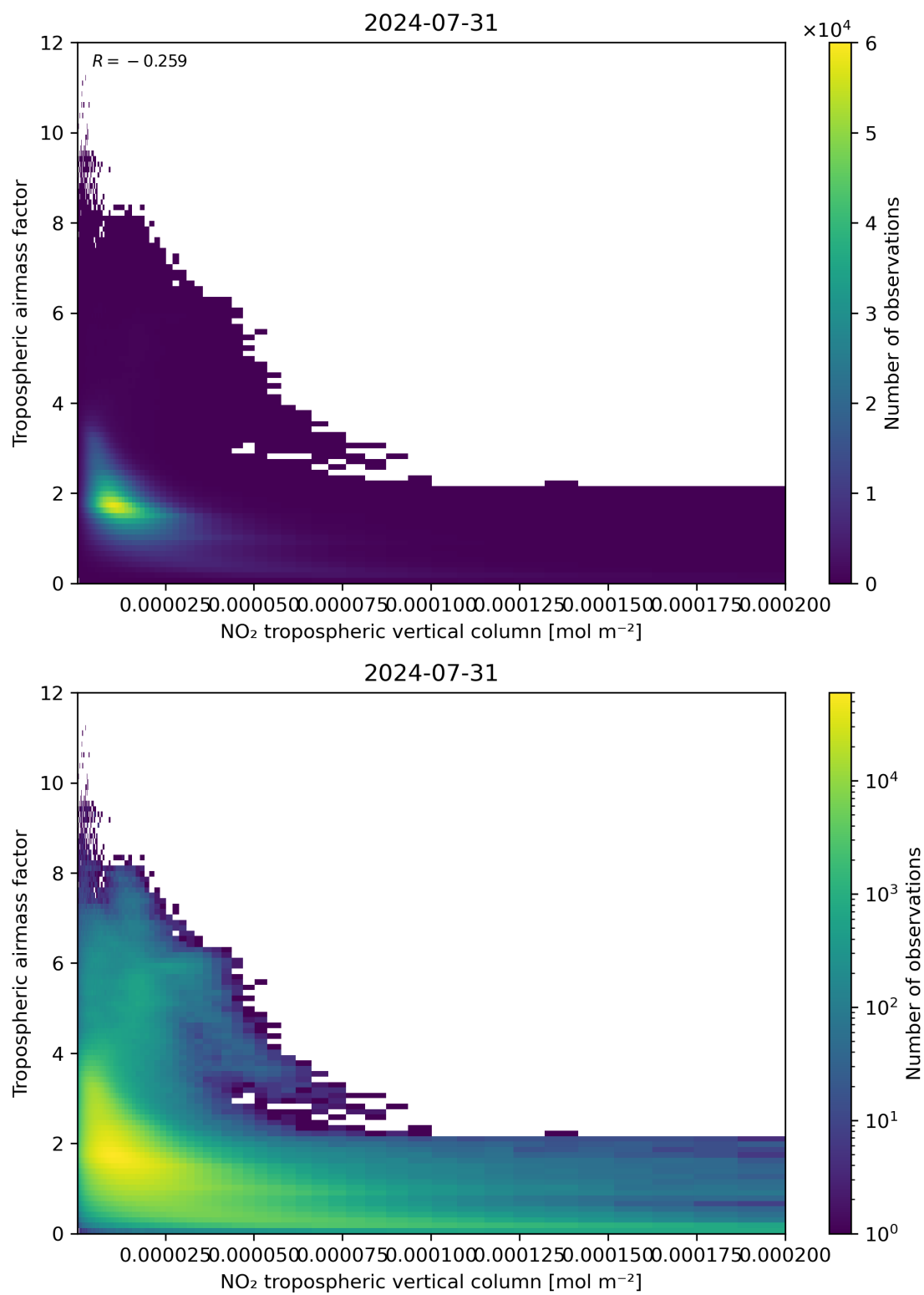
Figure 123: Scatter density plot of “NO 2 tropospheric vertical column” against “Tropospheric air mass factor” for 2024-07-31 to 2024-08-01.
