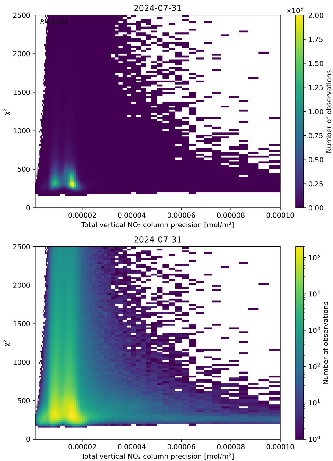
Figure 116: Scatter density plot of “Total vertical NO 2 column precision” against “ \chi^2 ” for 2024-07-31 to 2024-08-01.
