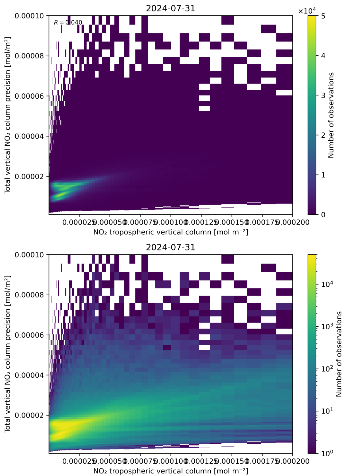
Figure 129: Scatter density plot of “NO 2 tropospheric vertical column” against “Total vertical NO 2 column precision” for 2024-07-31 to 2024-08-01.
