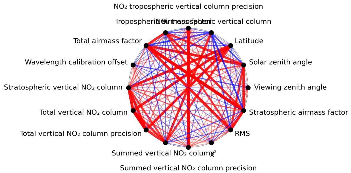
Figure 1: Map of correlation graph for 2024-07-31 to 2024-08-01.
