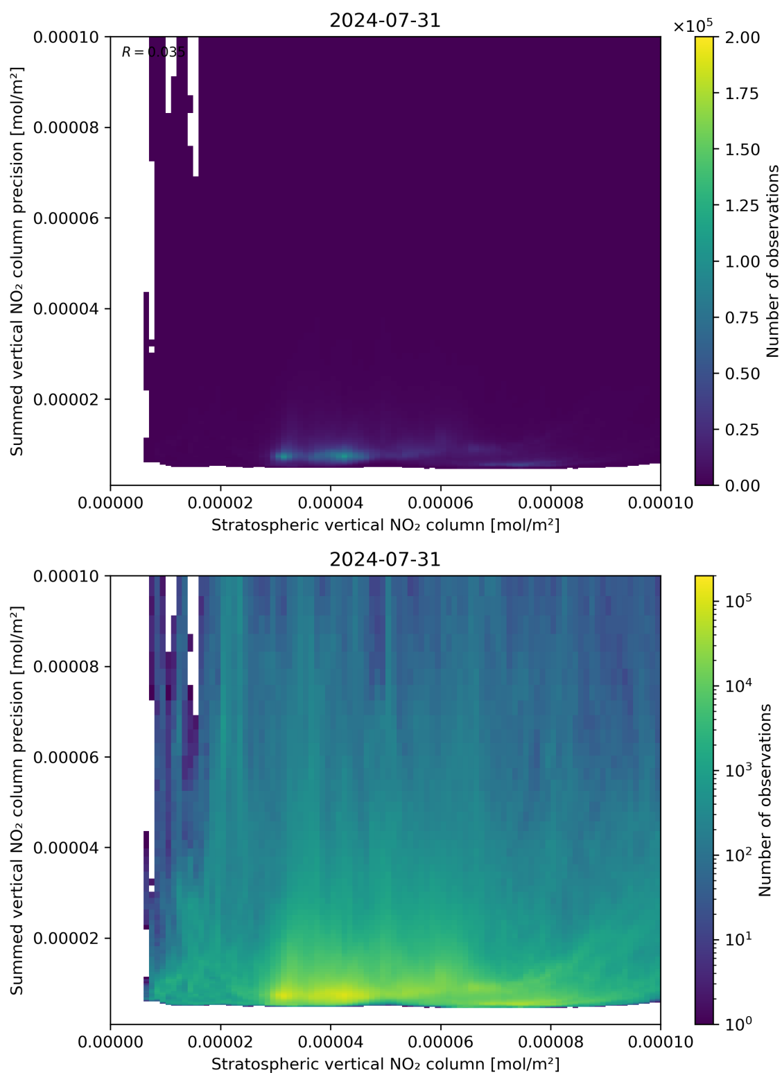
Figure 99: Scatter density plot of “Stratospheric vertical NO 2 column” against “Summed vertical NO 2 column precision” for 2024-07-31 to 2024-08-01.
