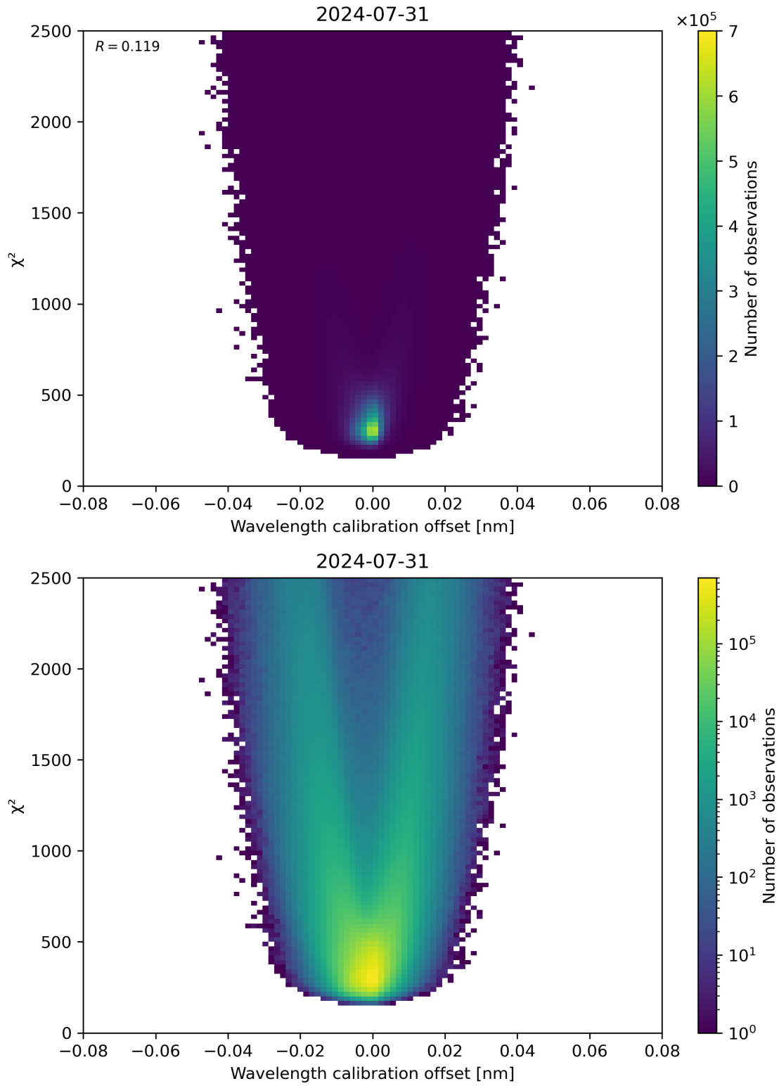
Figure 175: Scatter density plot of “Wavelength calibration offset” against “ \chi^2 ” for 2024-07-31 to 2024-08-01.
