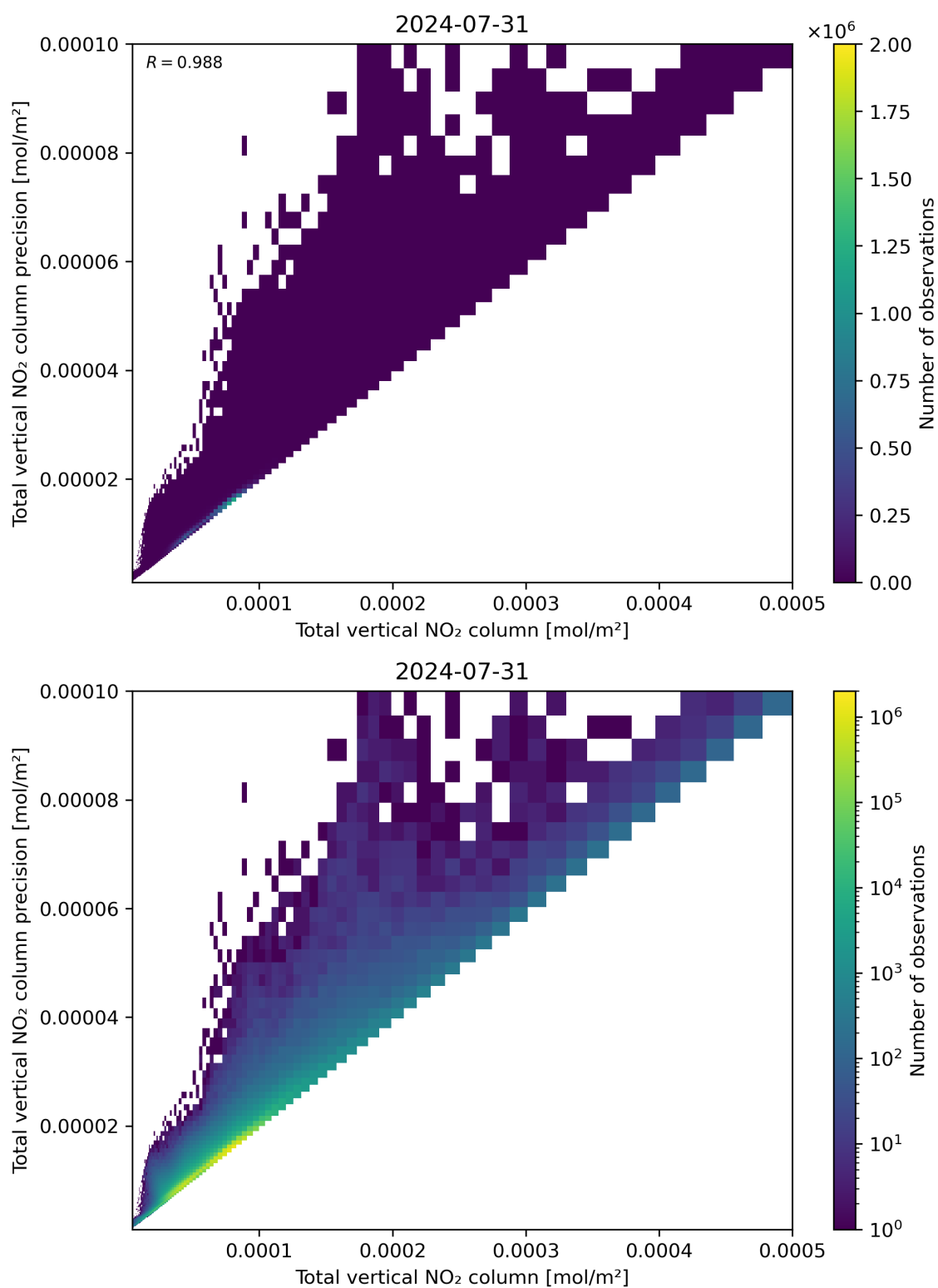
Figure 114: Scatter density plot of “Total vertical NO 2 column” against “Total vertical NO 2 column precision” for 2024-07-31 to 2024-08-01.
