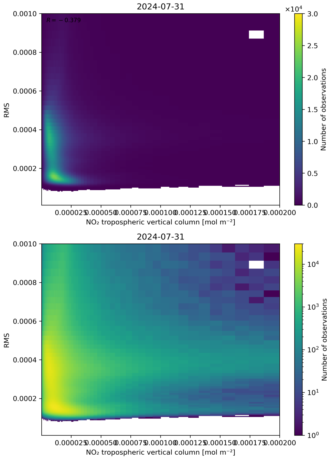
Figure 142: Scatter density plot of “NO 2 tropospheric vertical column” against “RMS” for 2024-07-31 to 2024-08-01.
