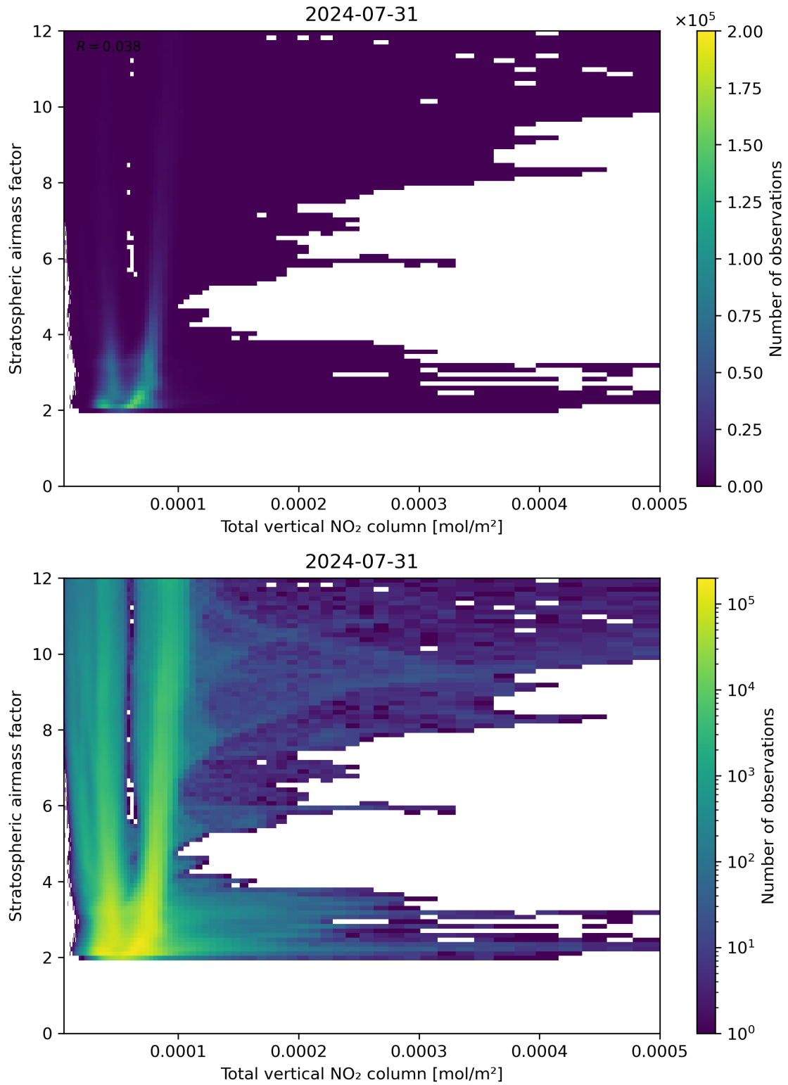
Figure 110: Scatter density plot of “Total vertical NO 2 column” against “Stratospheric airmass factor” for 2024-07-31 to 2024-08-01.
