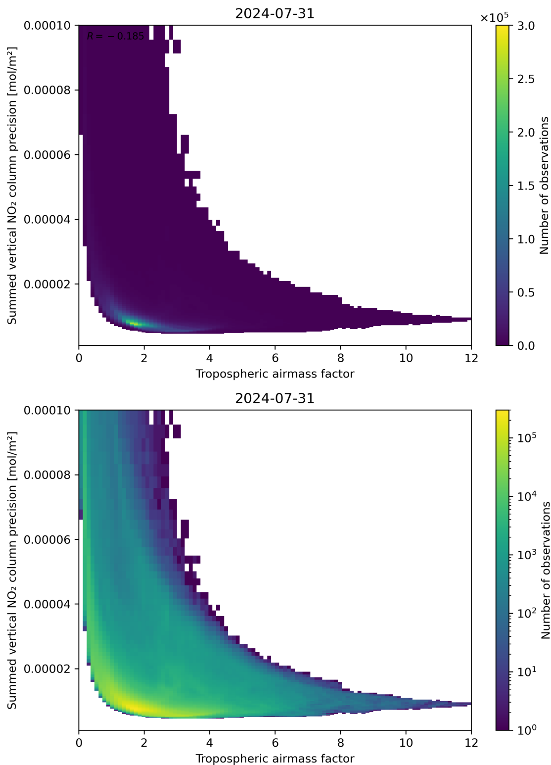
Figure 76: Scatter density plot of “Tropospheric air mass factor” against “Summed vertical NO 2 column precision” for 2024-07-31 to 2024-08-01.
