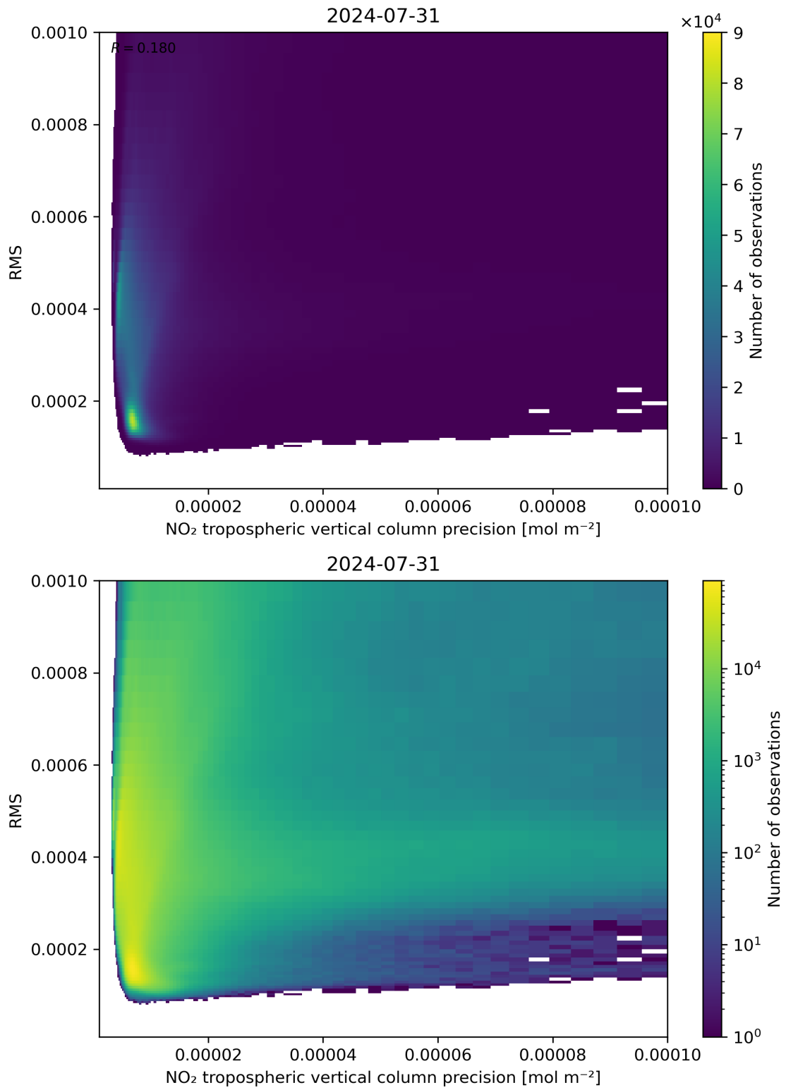
Figure 140: Scatter density plot of “NO 2 tropospheric vertical column precision” against “RMS” for 2024-07-31 to 2024-08-01.
