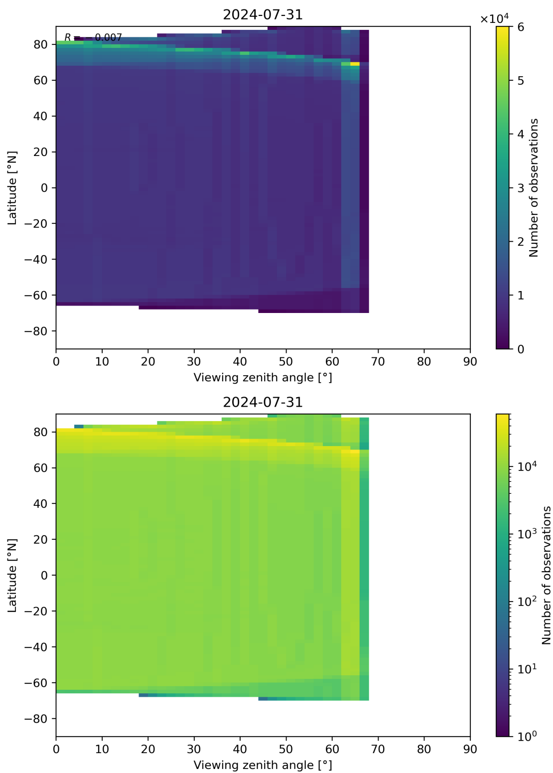
Figure 163: Scatter density plot of “Viewing zenith angle” against “Latitude” for 2024-07-31 to 2024-08-01.
