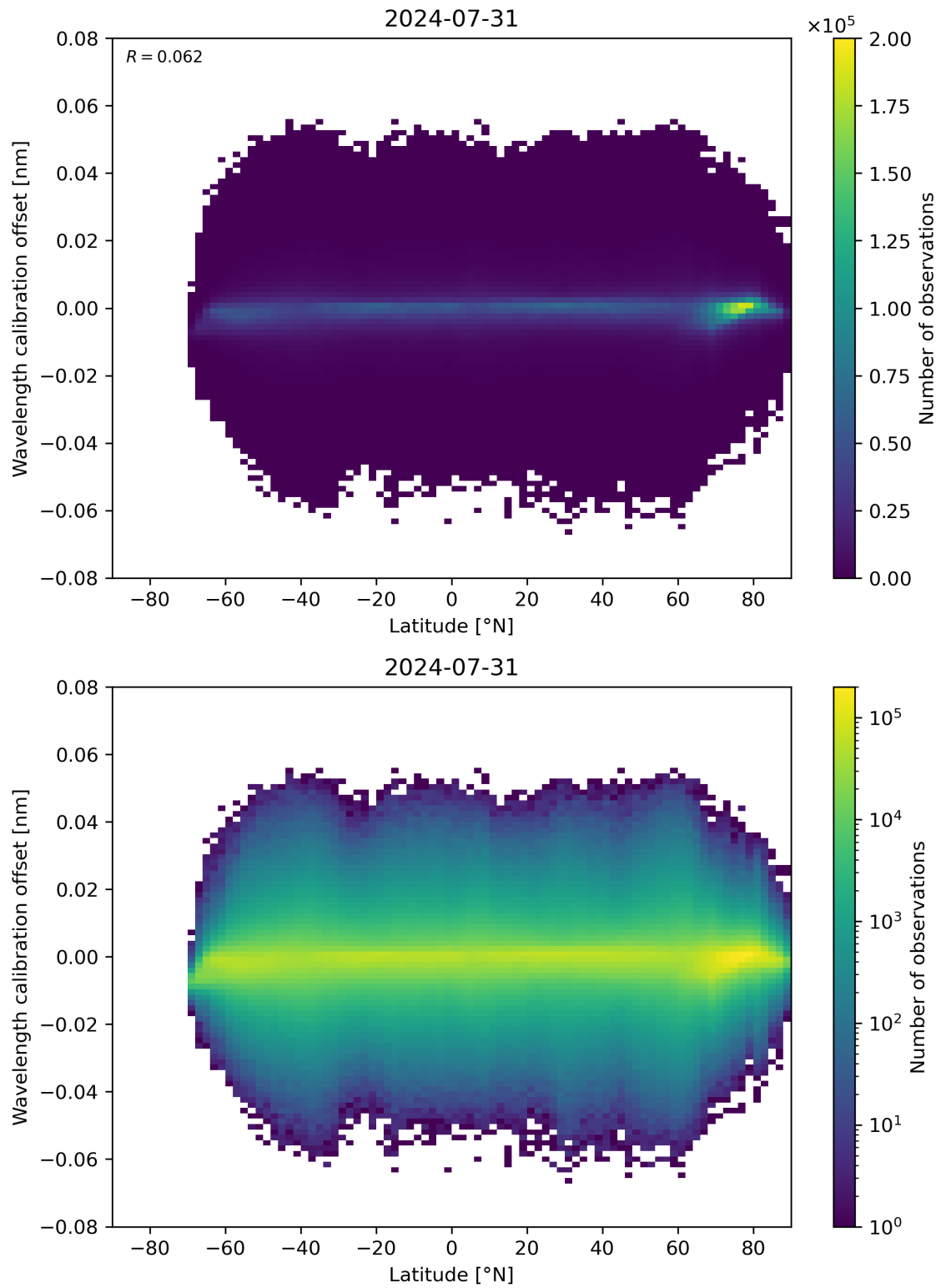
Figure 95: Scatter density plot of “Latitude” against “Wavelength calibration offset” for 2024-07-31 to 2024-08-01.
