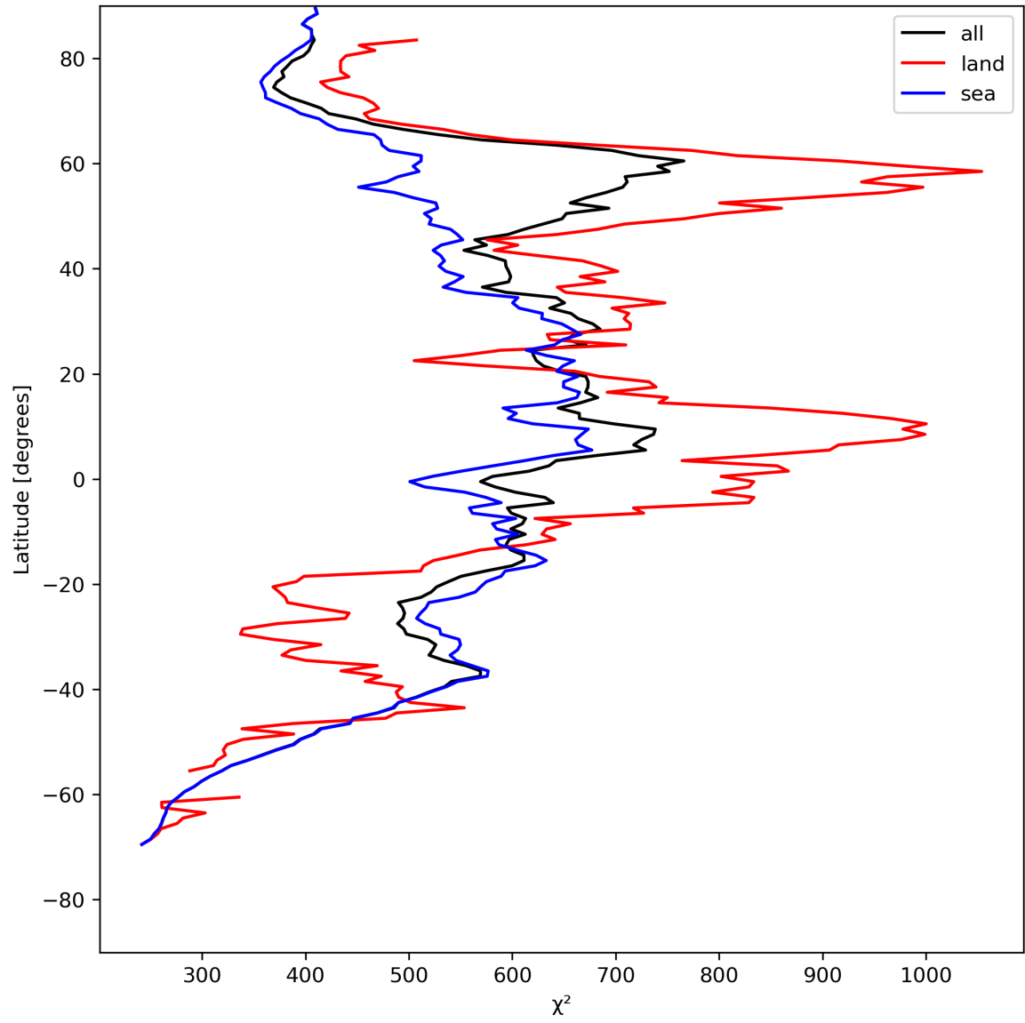
Figure 25: Zonal average of “ \chi^2 ” for 2024-07-31 to 2024-08-01.
