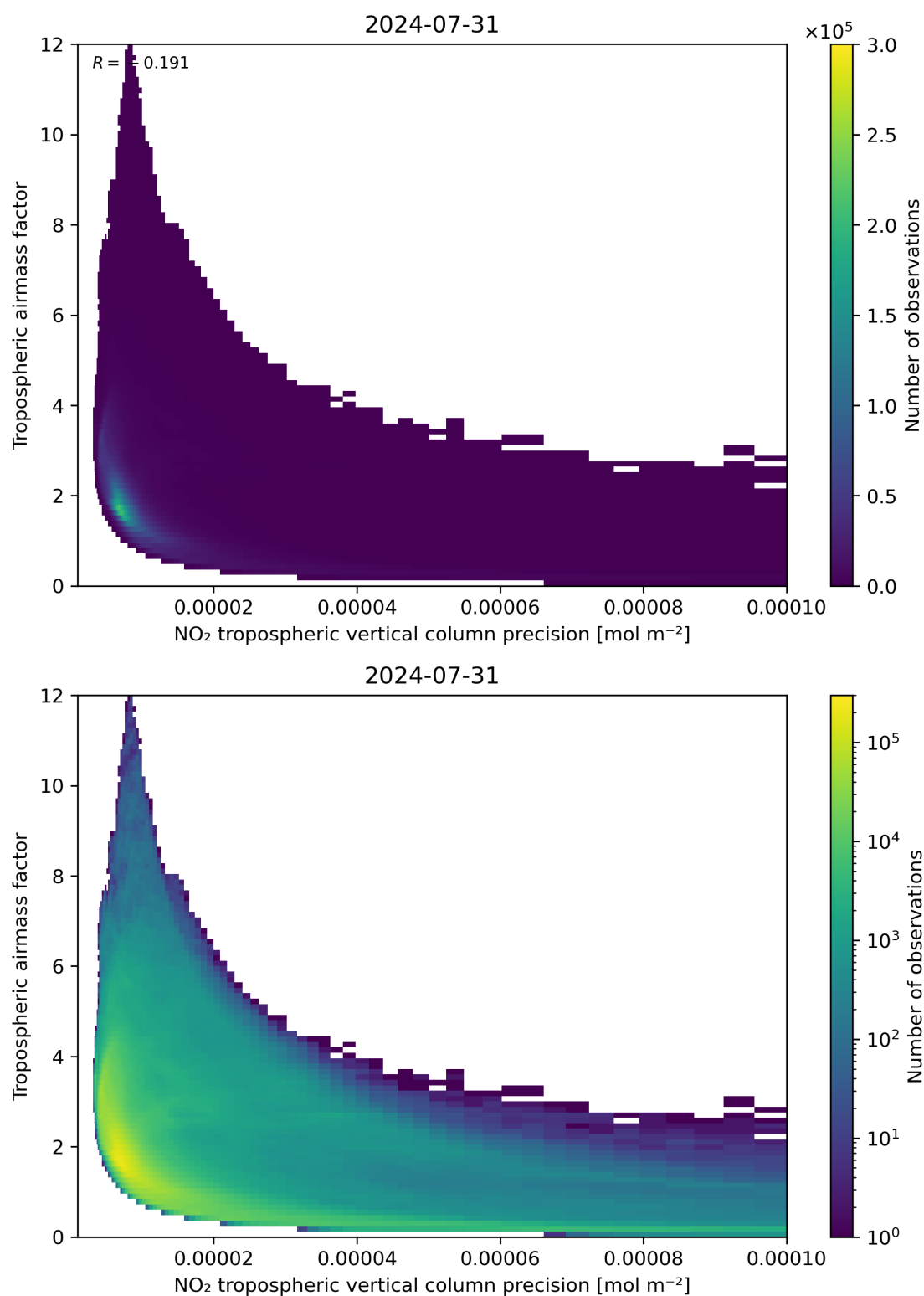
Figure 133: Scatter density plot of “NO 2 tropospheric vertical column precision” against “Tropospheric airmass factor” for 2024-07-31 to 2024-08-01.
