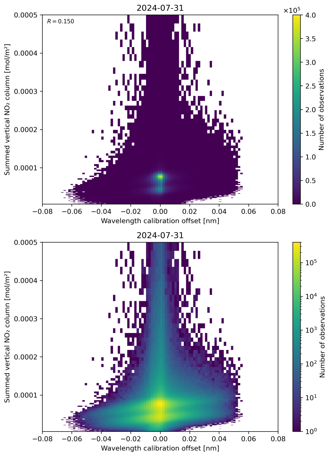
Figure 177: Scatter density plot of “Wavelength calibration offset” against “Summed vertical NO 2 column” for 2024-07-31 to 2024-08-01.
