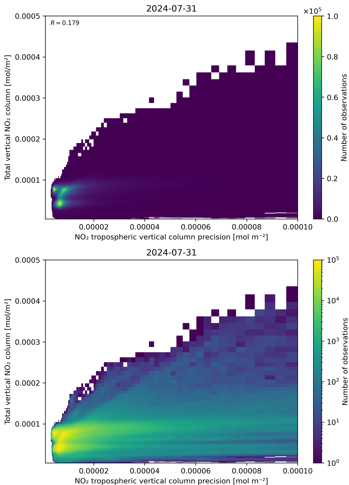
Figure 138: Scatter density plot of “NO 2 tropospheric vertical column precision” against “Total vertical NO 2 column” for 2024-07-31 to 2024-08-01.
