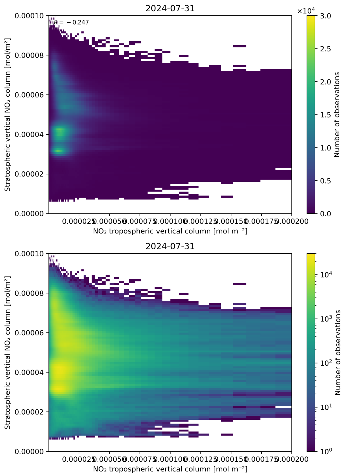
Figure 125: Scatter density plot of “NO 2 tropospheric vertical column” against “Stratospheric vertical NO 2 column” for 2024-07-31 to 2024-08-01.
