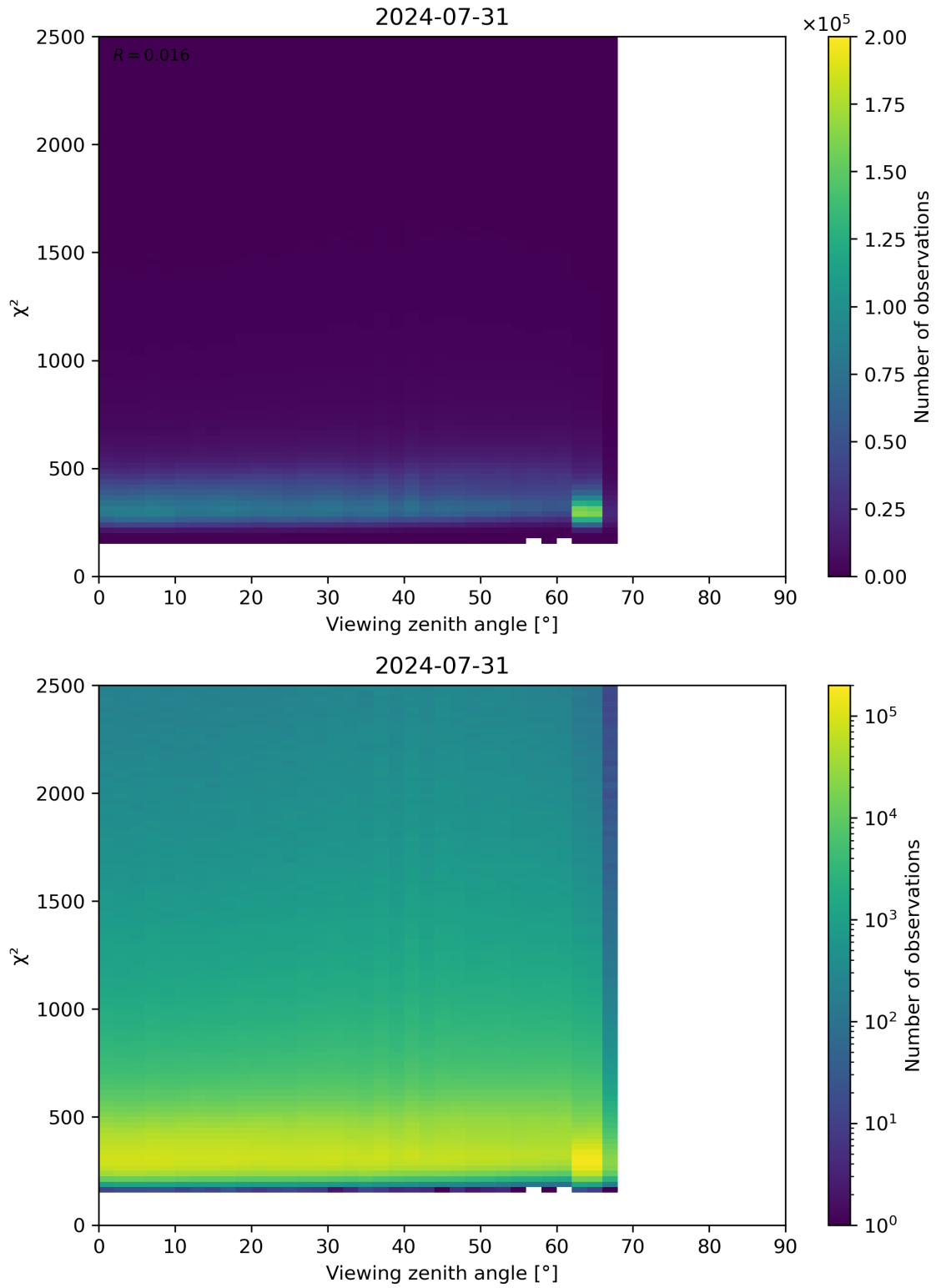
Figure 162: Scatter density plot of “Viewing zenith angle” against “ \chi^2 ” for 2024-07-31 to 2024-08-01.
