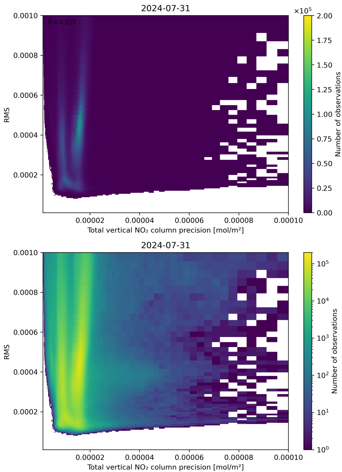
Figure 119: Scatter density plot of “Total vertical NO 2 column precision” against “RMS” for 2024-07-31 to 2024-08-01.
