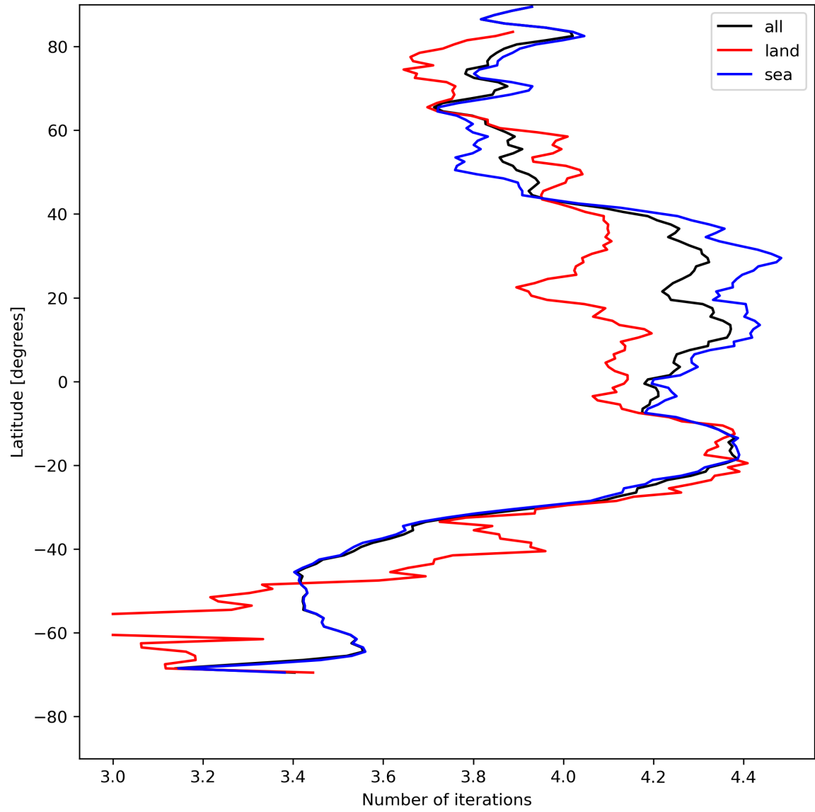
Figure 17: Zonal average of “Number of iterations” for 2024-07-31 to 2024-08-01.
