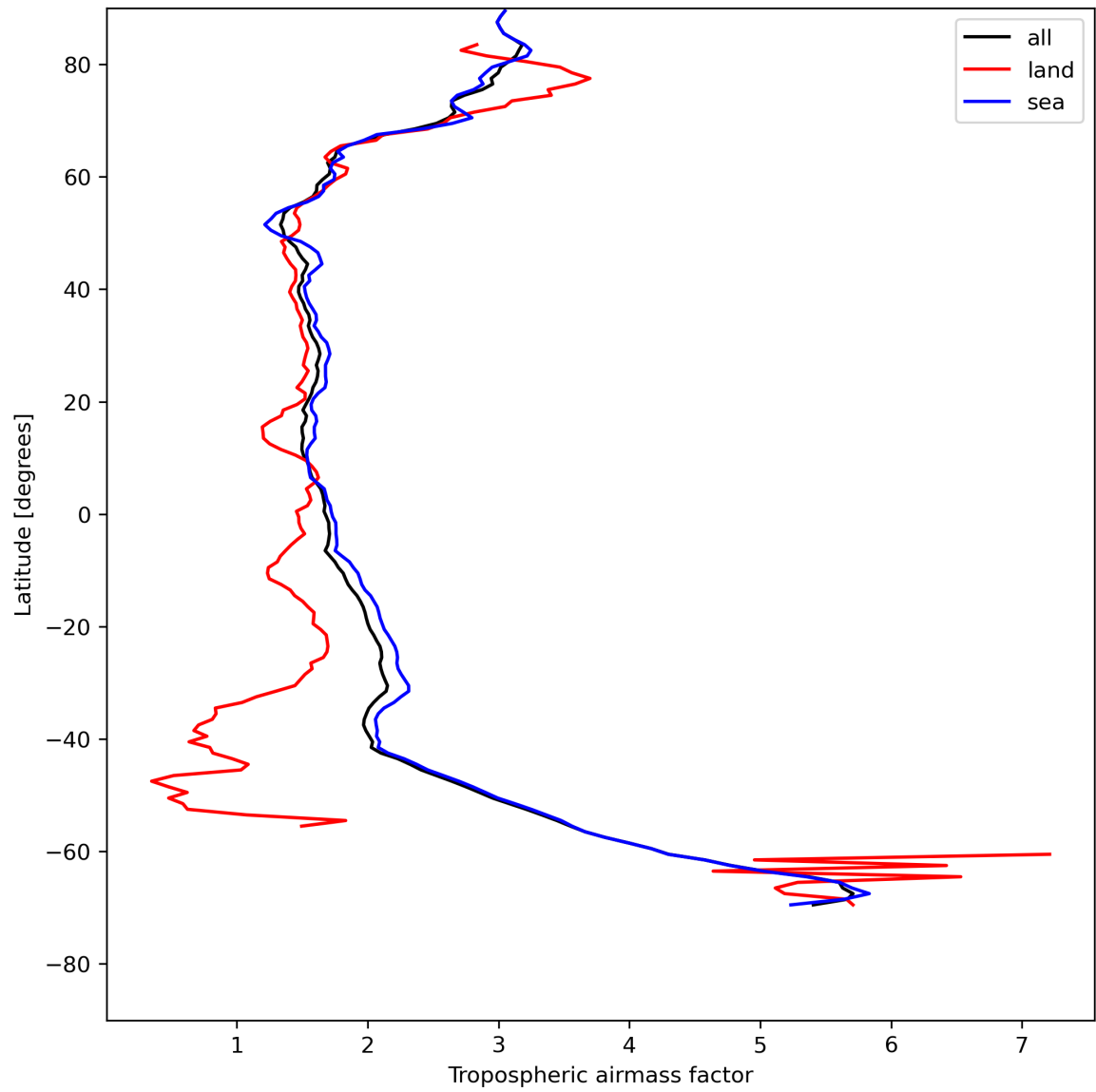
Figure 14: Zonal average of “Tropospheric airmass factor” for 2024-07-31 to 2024-08-01.
