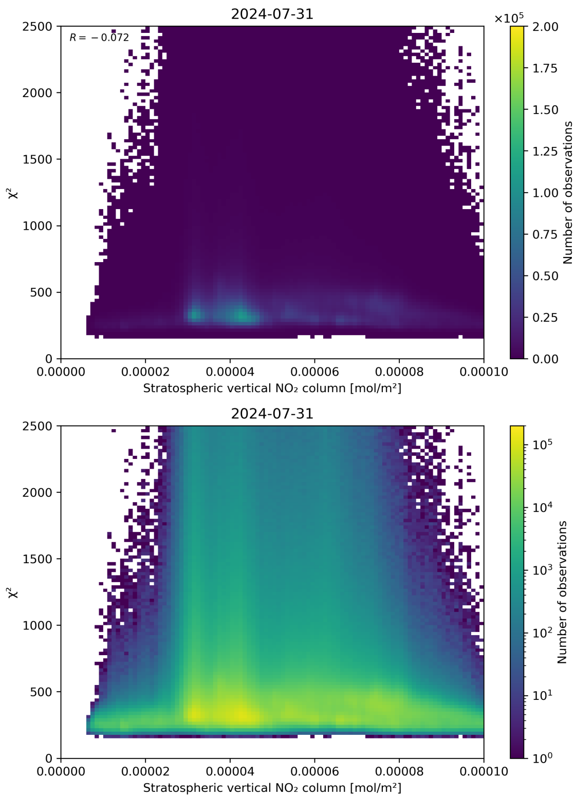
Figure 97: Scatter density plot of “Stratospheric vertical NO 2 column” against “ \chi^2 ” for 2024-07-31 to 2024-08-01.
