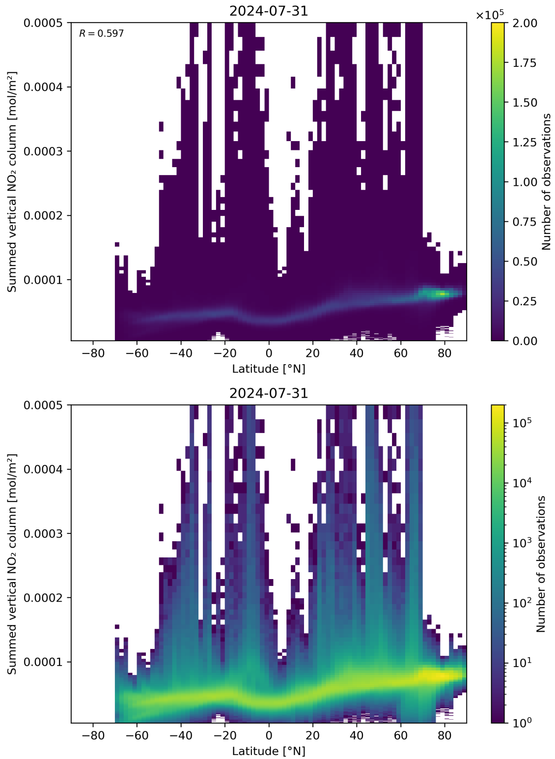
Figure 88: Scatter density plot of “Latitude” against “Summed vertical NO 2 column” for 2024-07-31 to 2024-08-01.
