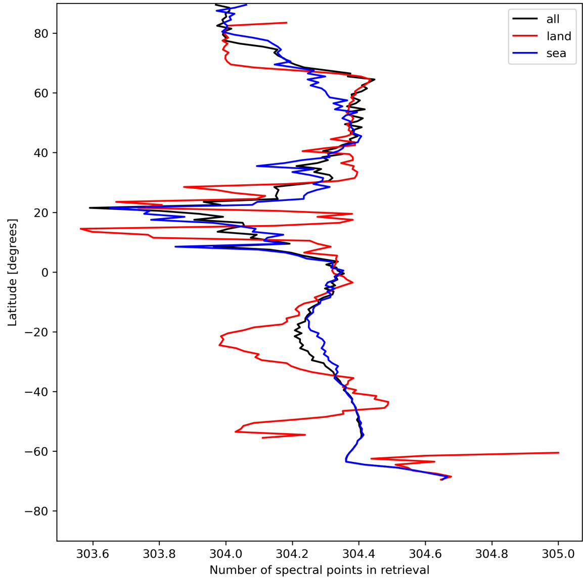
Figure 16: Zonal average of “Number of spectral points in retrieval” for 2024-07-31 to 2024-08-01.
