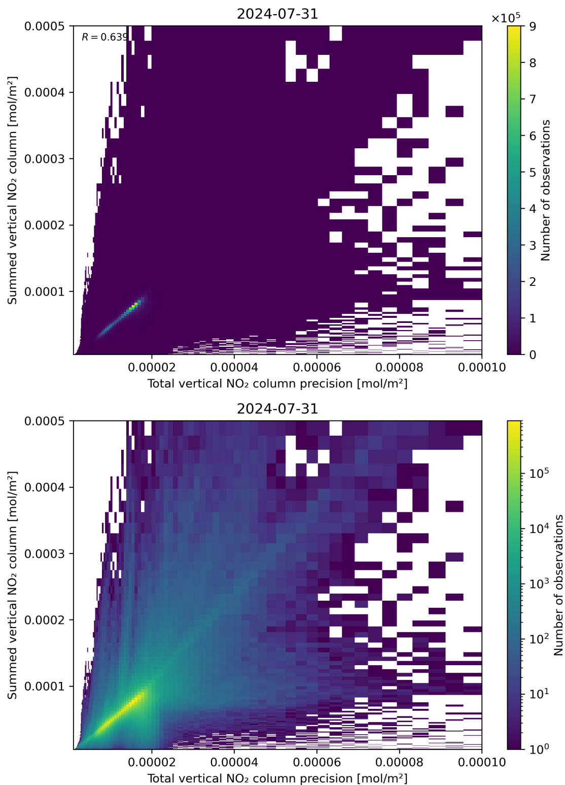
Figure 117: Scatter density plot of “Total vertical NO 2 column precision” against “Summed vertical NO 2 column” for 2024-07-31 to 2024-08-01.
