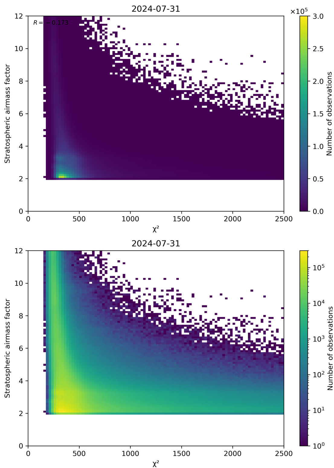
Figure 81: Scatter density plot of “ \chi^2 ” against “Stratospheric airmass factor” for 2024-07-31 to 2024-08-01.
