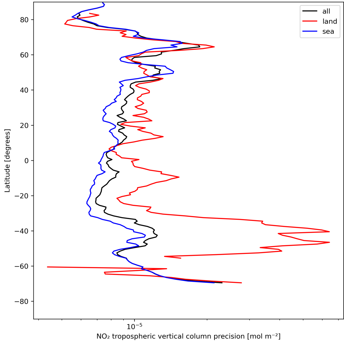
Figure 13: Zonal average of “NO 2 tropospheric vertical column precision” for 2024-07-31 to 2024-08-01.
