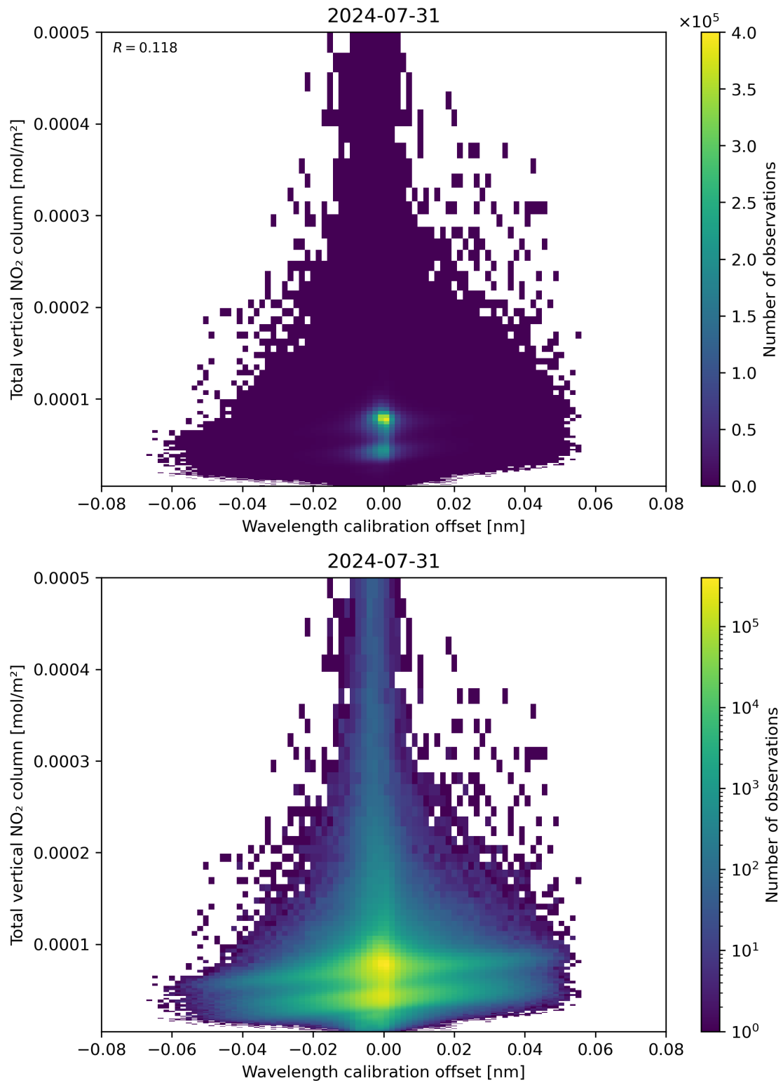
Figure 179: Scatter density plot of “Wavelength calibration offset” against “Total vertical NO 2 column” for 2024-07-31 to 2024-08-01.
