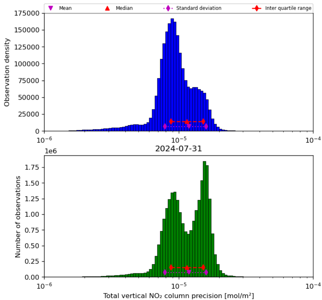
Figure 39: Histogram of “Total vertical NO 2 column precision” for 2024-07-31 to 2024-08-01
