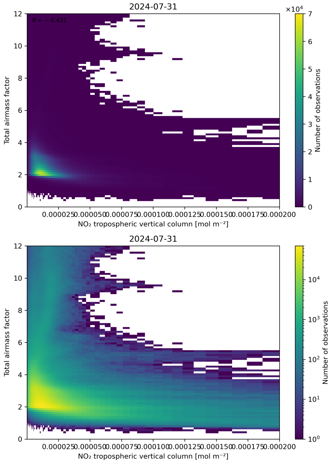
Figure 122: Scatter density plot of “NO 2 tropospheric vertical column” against “Total air mass factor” for 2024-07-31 to 2024-08-01.
