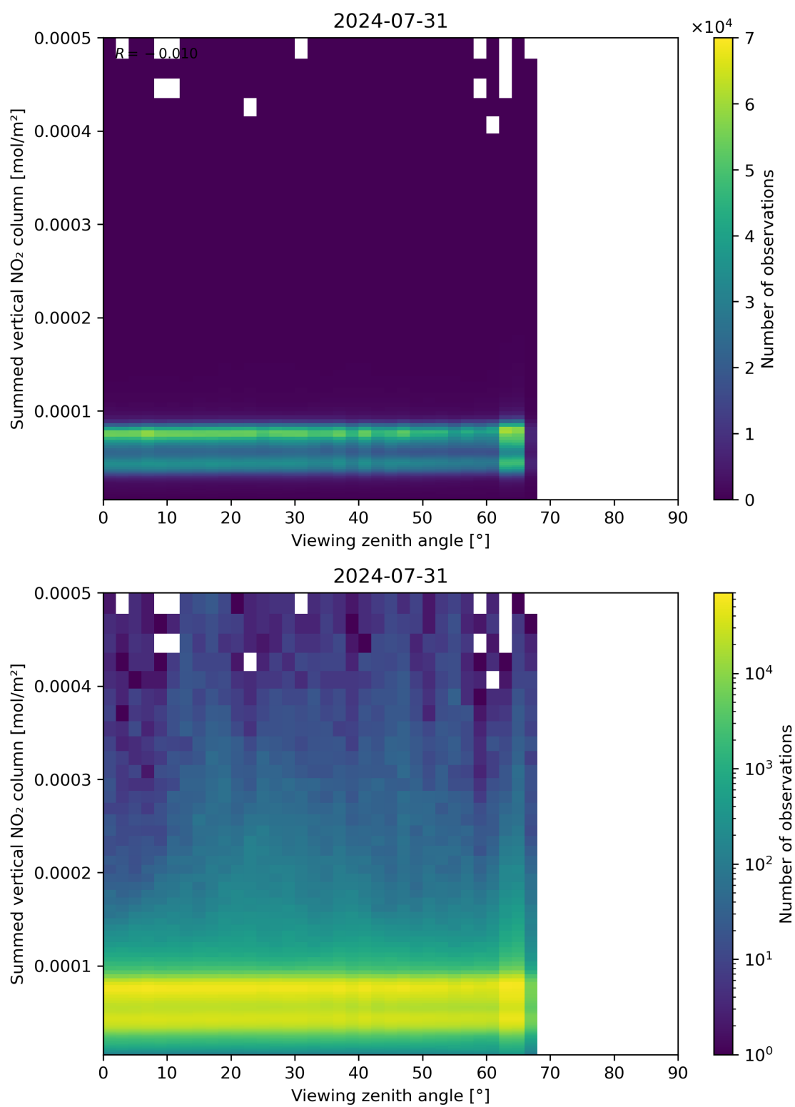
Figure 165: Scatter density plot of “Viewing zenith angle” against “Summed vertical NO 2 column” for 2024-07-31 to 2024-08-01.
