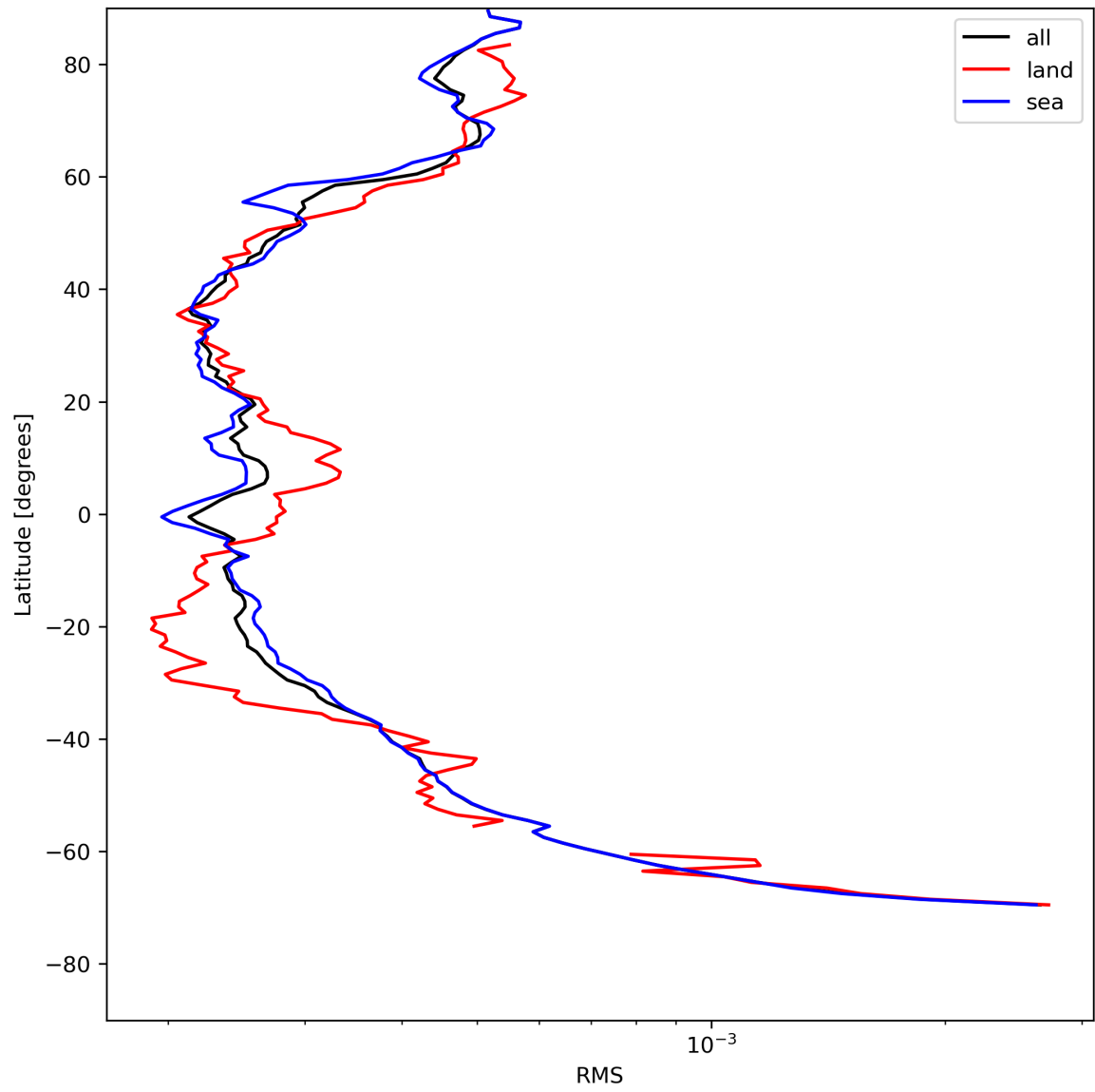
Figure 26: Zonal average of “RMS” for 2024-07-31 to 2024-08-01.
