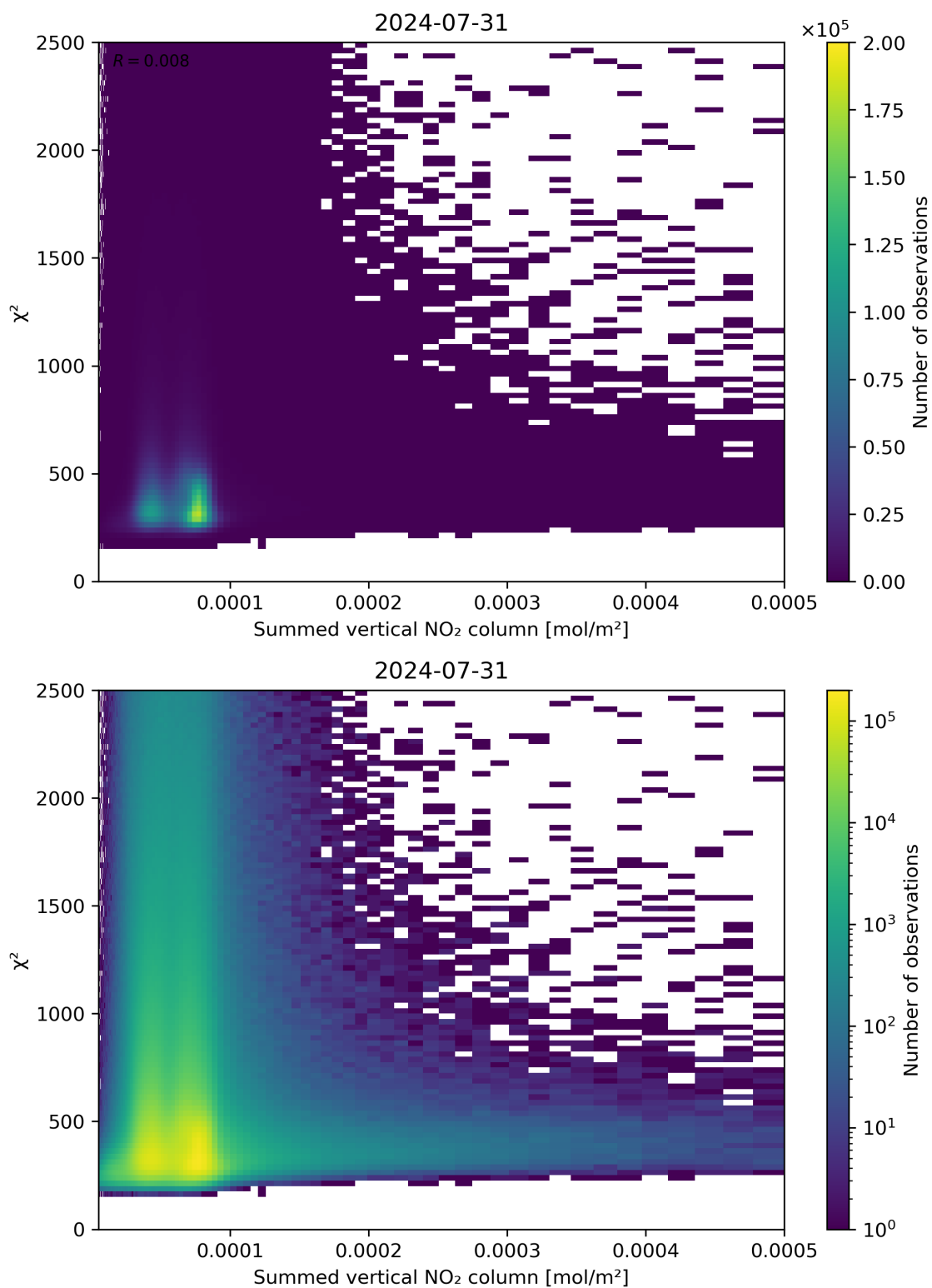
Figure 104: Scatter density plot of “Summed vertical NO 2 column” against “ \chi^2 ” for 2024-07-31 to 2024-08-01.
