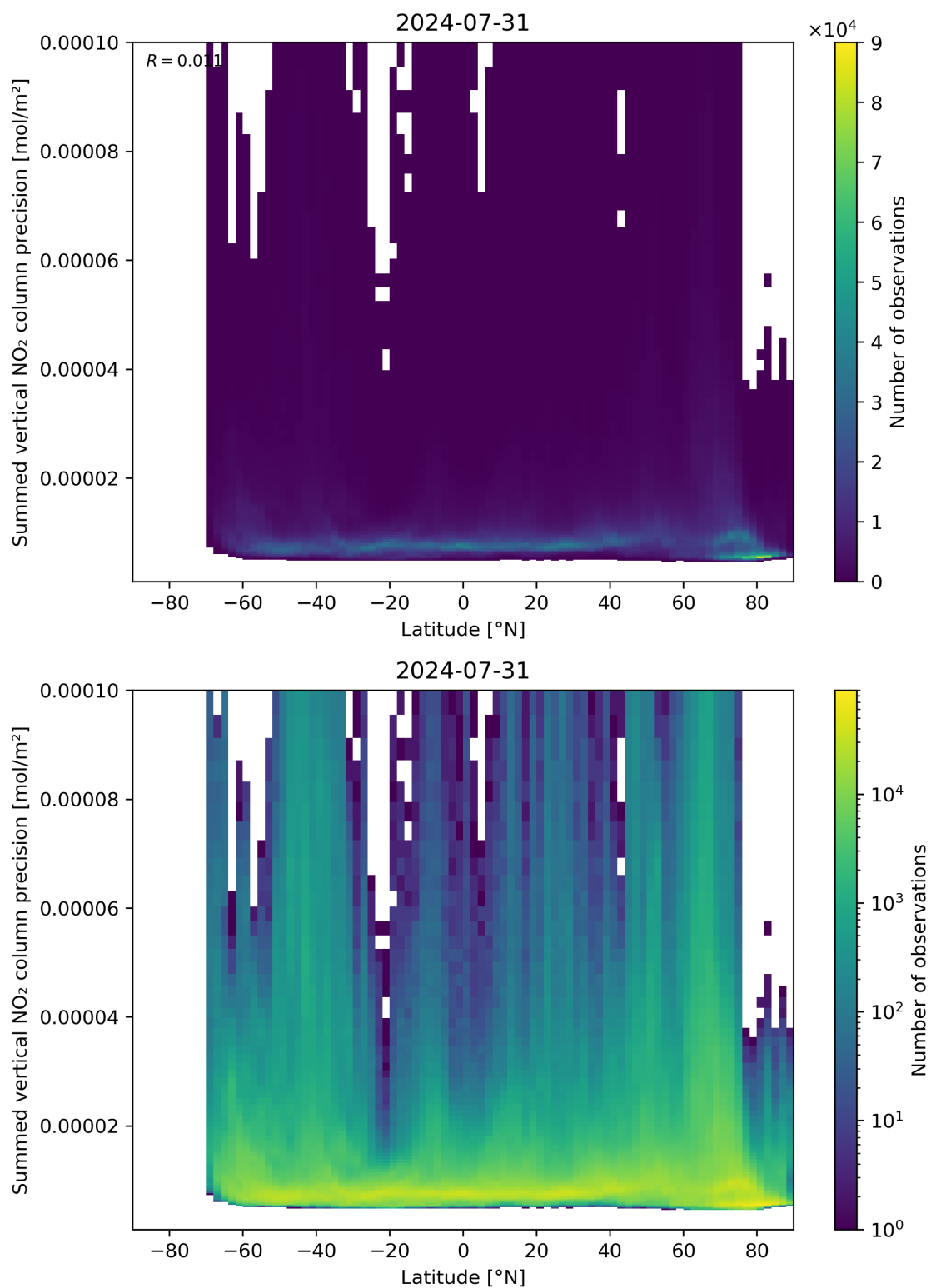
Figure 89: Scatter density plot of “Latitude” against “Summed vertical NO 2 column precision” for 2024-07-31 to 2024-08-01.
