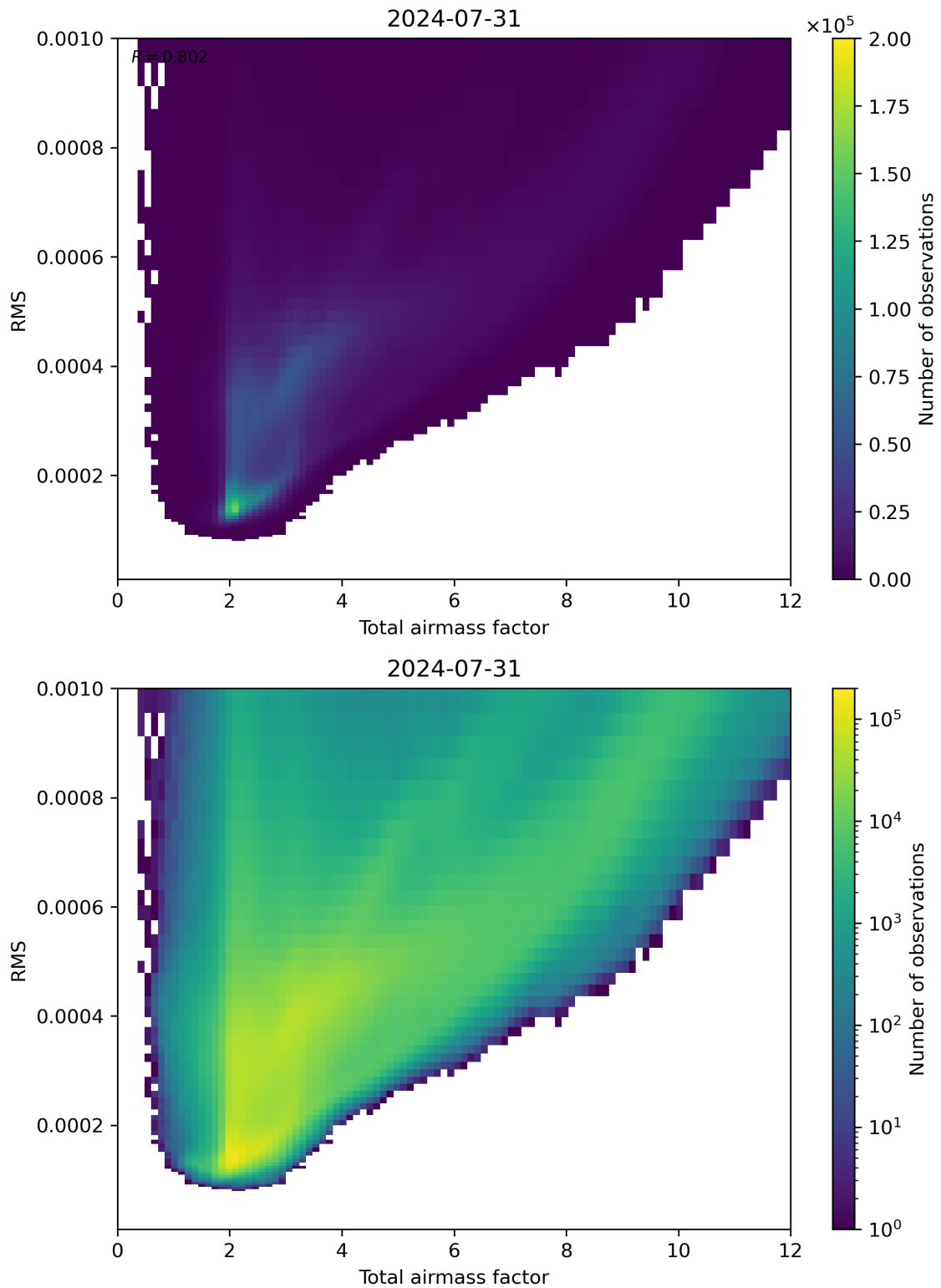
Figure 69: Scatter density plot of “Total airmass factor” against “RMS” for 2024-07-31 to 2024-08-01.
