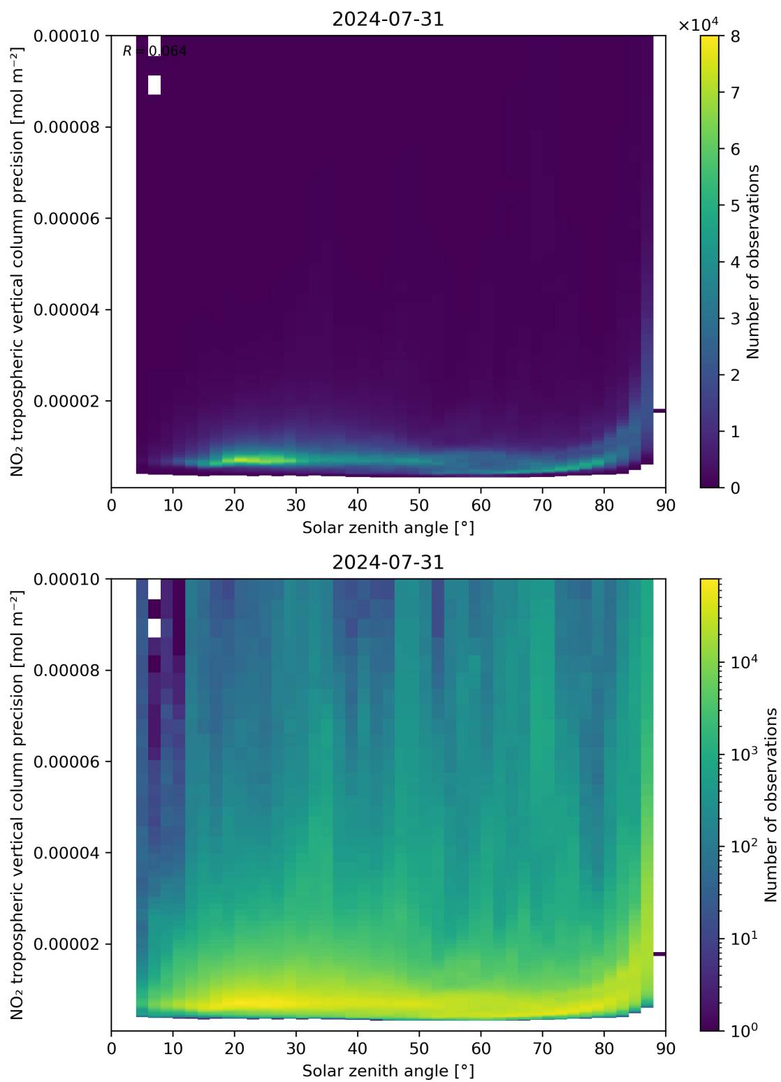
Figure 156: Scatter density plot of “Solar zenith angle” against “NO 2 tropospheric vertical column precision” for 2024-07-31 to 2024-08-01.
