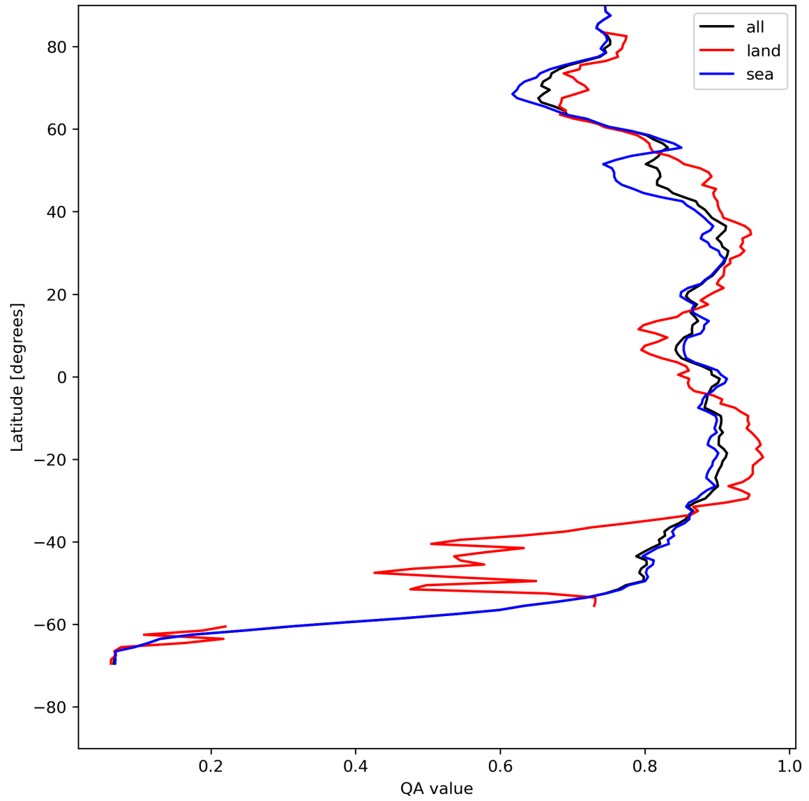
Figure 11: Zonal average of “QA value” for 2024-07-31 to 2024-08-01.
