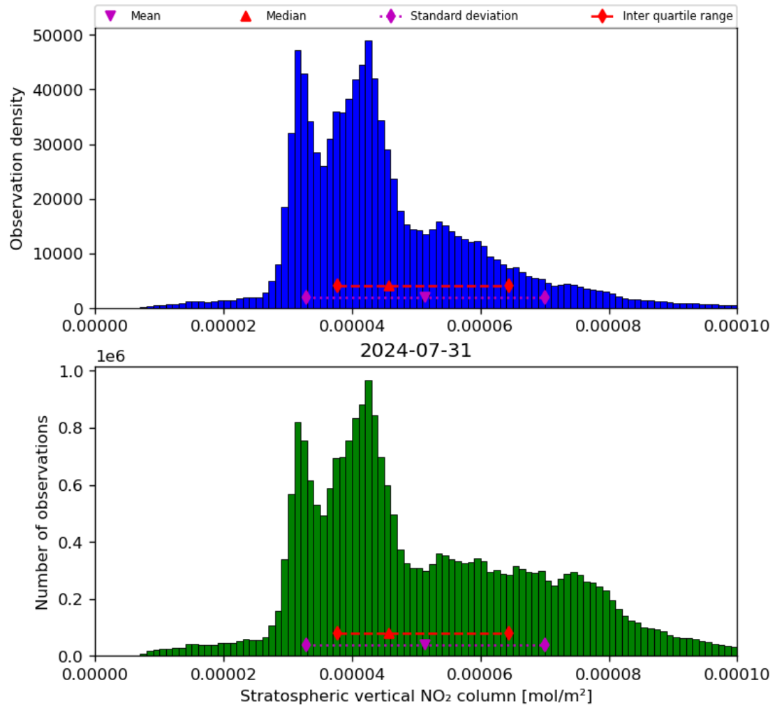
Figure 36: Histogram of “Stratospheric vertical NO 2 column” for 2024-07-31 to 2024-08-01
