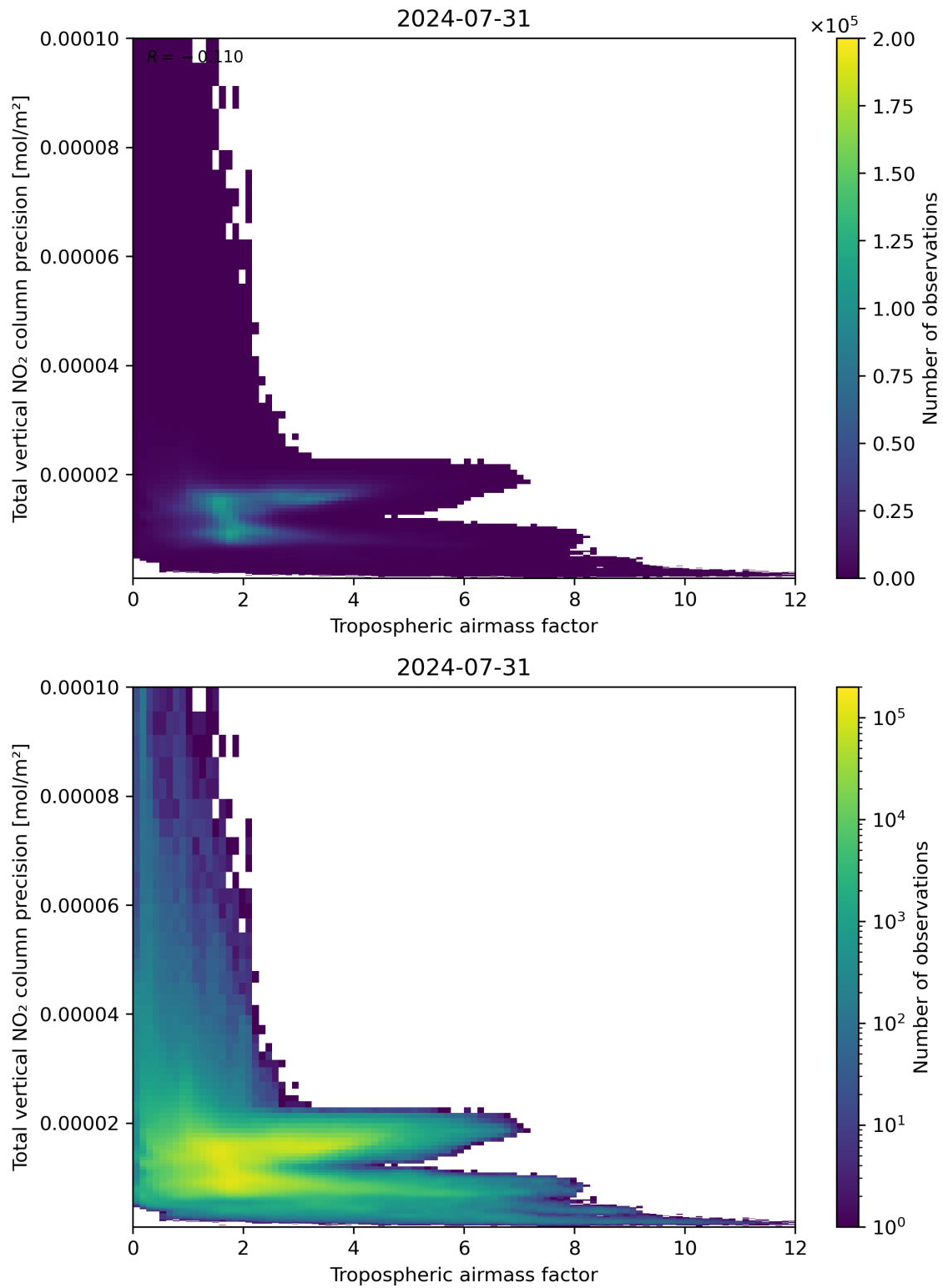
Figure 78: Scatter density plot of “Tropospheric air mass factor” against “Total vertical NO 2 column precision” for 2024-07-31 to 2024-08-01.
