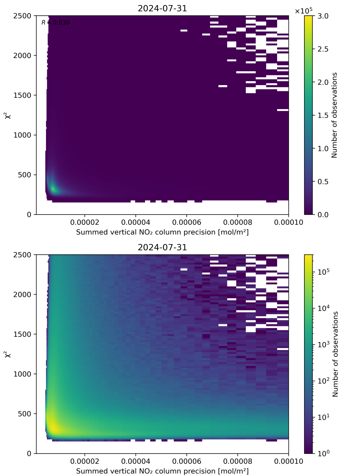
Figure 107: Scatter density plot of “Summed vertical NO 2 column precision” against “ \chi^2 ” for 2024-07-31 to 2024-08-01.
