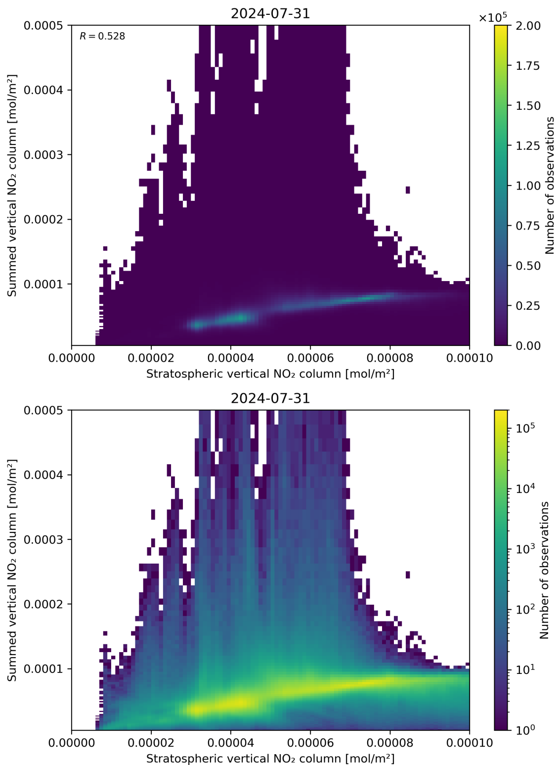
Figure 98: Scatter density plot of “Stratospheric vertical NO 2 column” against “Summed vertical NO 2 column” for 2024-07-31 to 2024-08-01.
