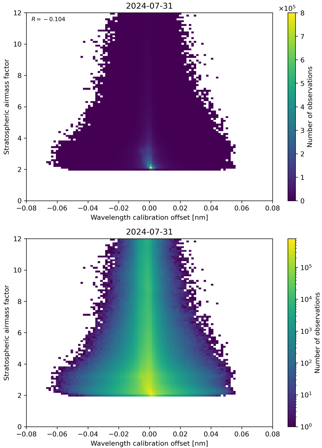
Figure 174: Scatter density plot of “Wavelength calibration offset” against “Stratospheric air mass factor” for 2024-07-31 to 2024-08-01.
