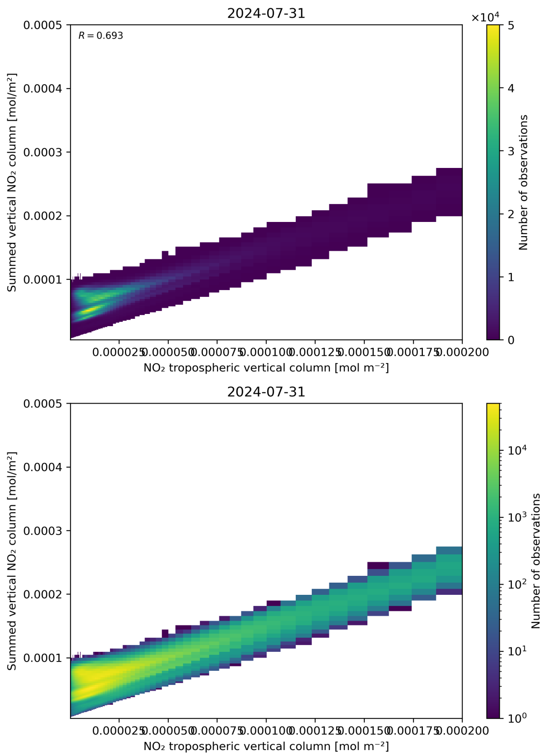
Figure 126: Scatter density plot of “NO 2 tropospheric vertical column” against “Summed vertical NO 2 column” for 2024-07-31 to 2024-08-01.
