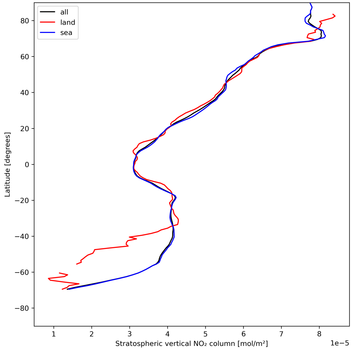
Figure 19: Zonal average of “Stratospheric vertical NO 2 column” for 2024-07-31 to 2024-08-01.
