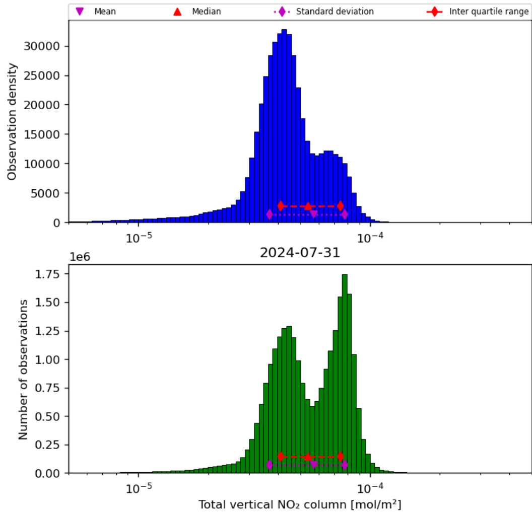
Figure 38: Histogram of "Total vertical NO 2 column" for 2024-07-31 to 2024-08-01
