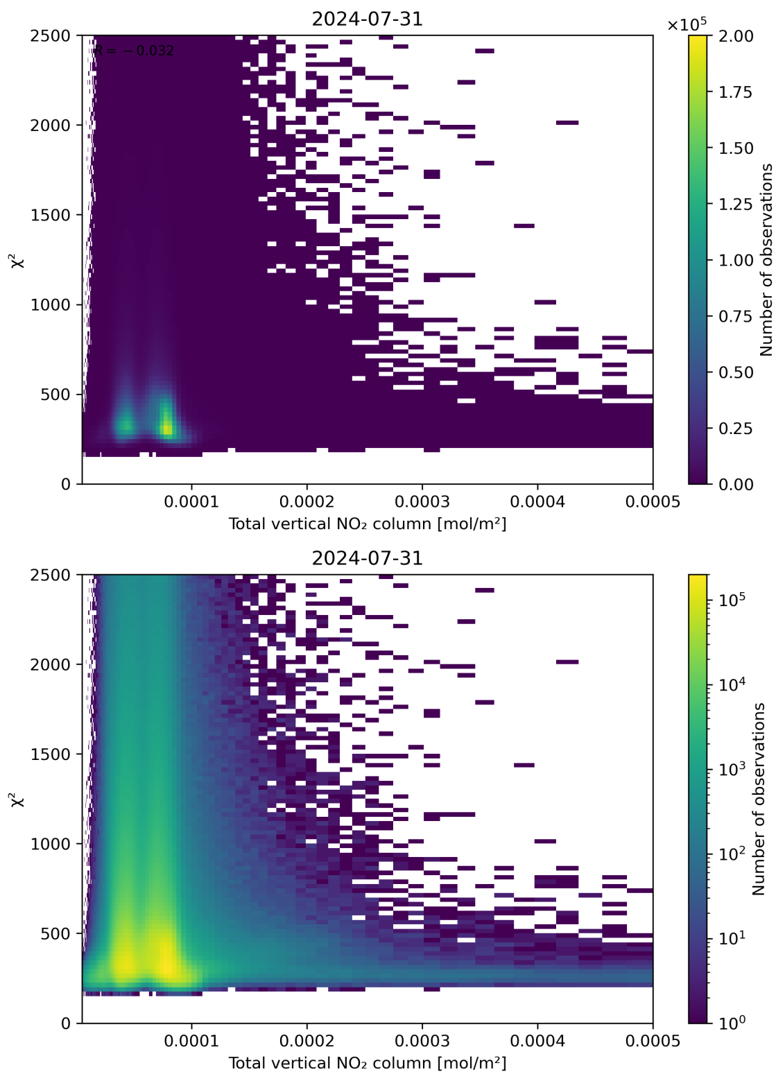
Figure 111: Scatter density plot of “Total vertical NO 2 column” against “ \chi^2 ” for 2024-07-31 to 2024-08-01.
