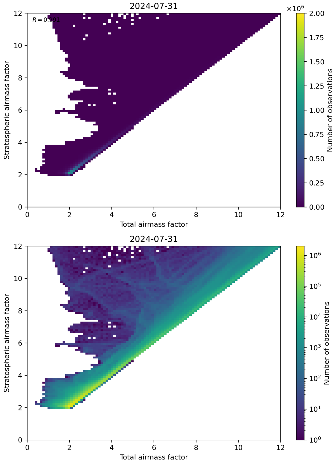
Figure 62: Scatter density plot of “Total airmass factor” against “Stratospheric airmass factor” for 2024-07-31 to 2024-08-01.
