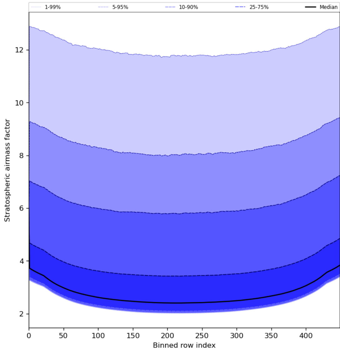
Figure 61: Along track statistics of “Stratospheric airmass factor” for 2024-07-31 to 2024-08-01
