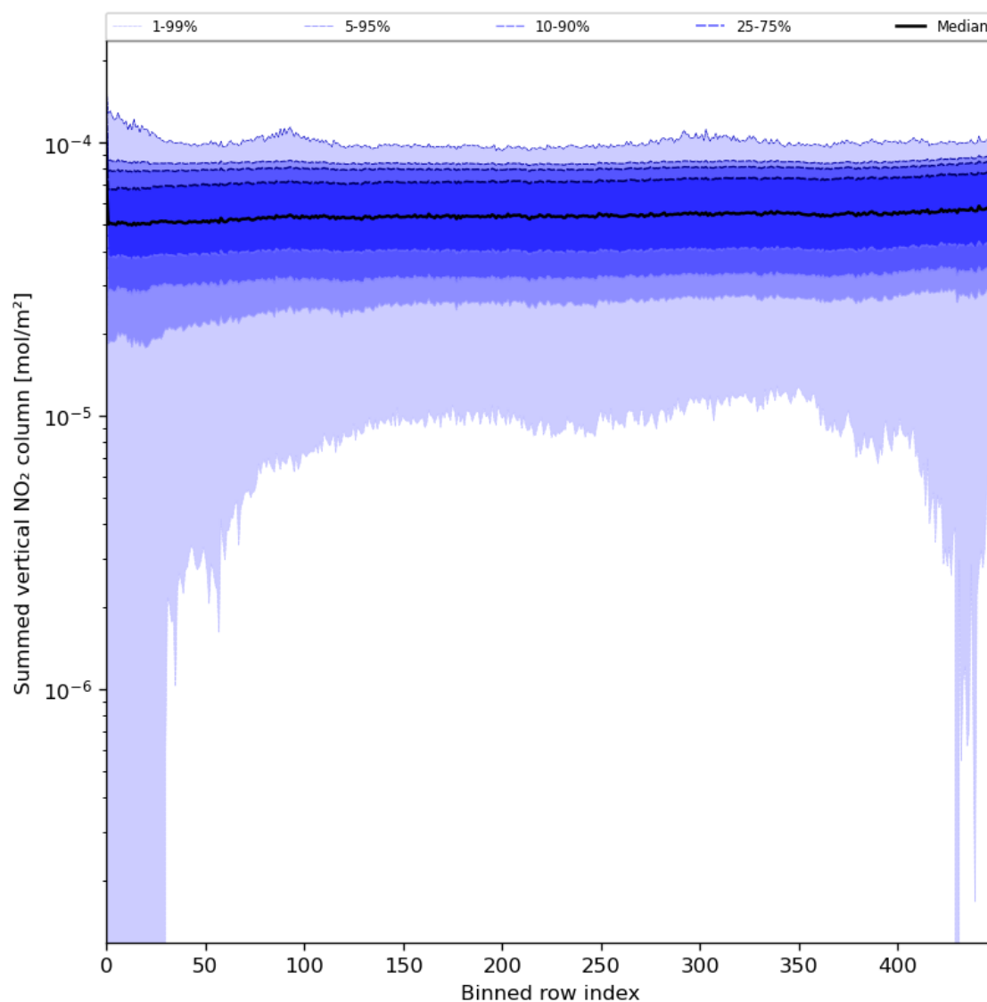
Figure 57: Along track statistics of “Summed vertical NO 2 column” for 2024-07-31 to 2024-08-01
