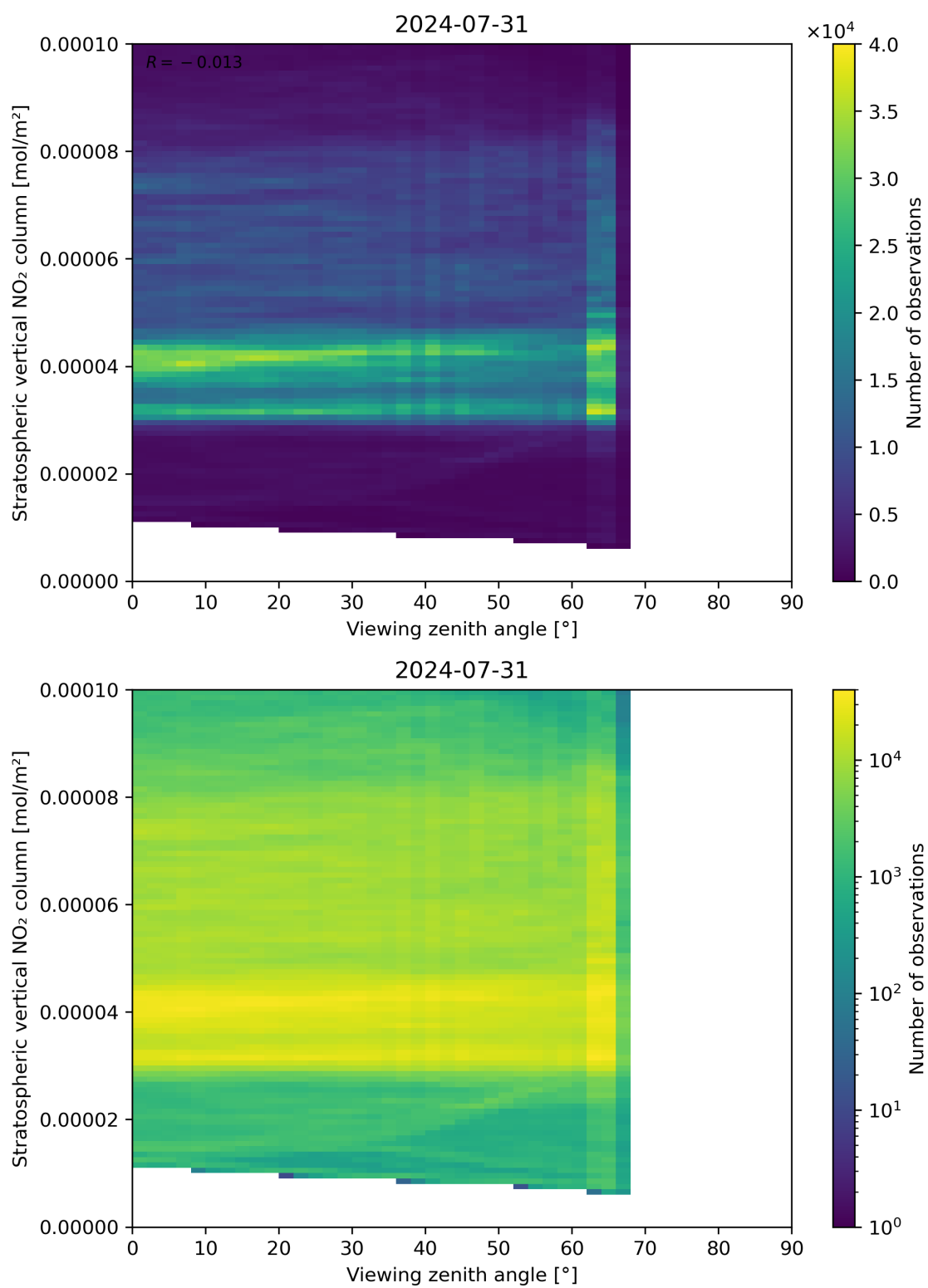
Figure 164: Scatter density plot of “Viewing zenith angle” against “Stratospheric vertical NO 2 column” for 2024-07-31 to 2024-08-01.
