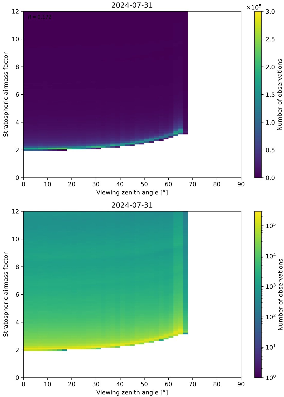
Figure 159: Scatter density plot of “Viewing zenith angle” against “Stratospheric airmass factor” for 2024-07-31 to 2024-08-01.
