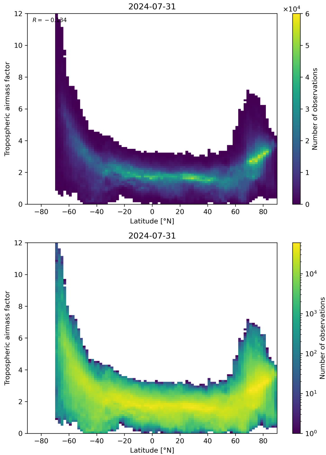
Figure 85: Scatter density plot of “Latitude” against “Tropospheric air mass factor” for 2024-07-31 to 2024-08-01.
