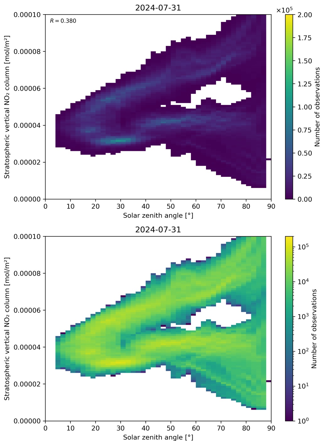
Figure 150: Scatter density plot of “Solar zenith angle” against “Stratospheric vertical NO 2 column” for 2024-07-31 to 2024-08-01.
