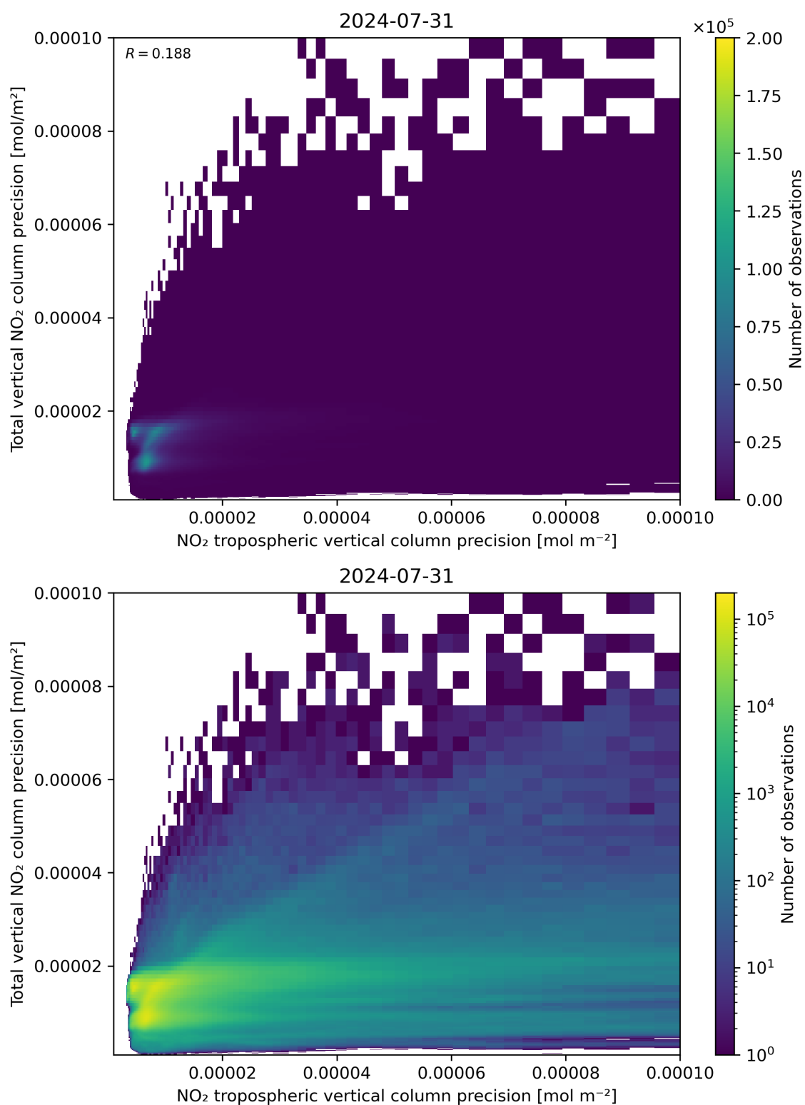
Figure 139: Scatter density plot of “NO 2 tropospheric vertical column precision” against “Total vertical NO 2 column precision” for 2024-07-31 to 2024-08-01.
