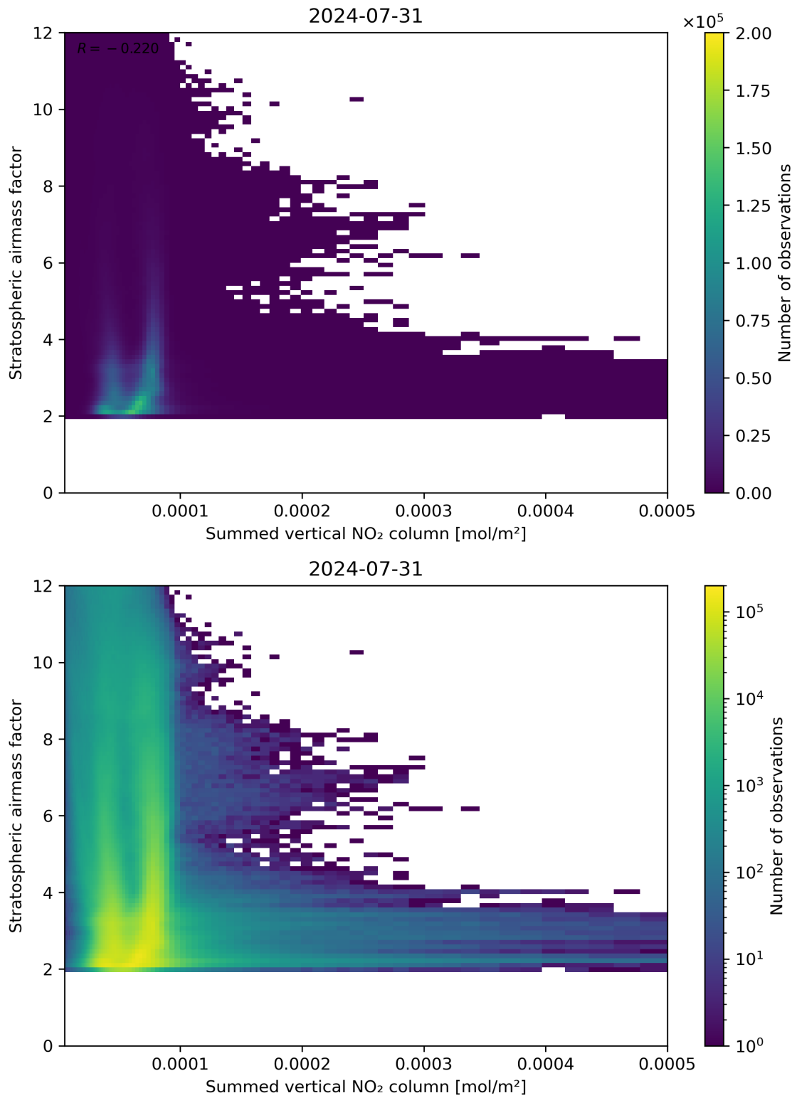
Figure 103: Scatter density plot of “Summed vertical NO 2 column” against “Stratospheric air mass factor” for 2024-07-31 to 2024-08-01.
