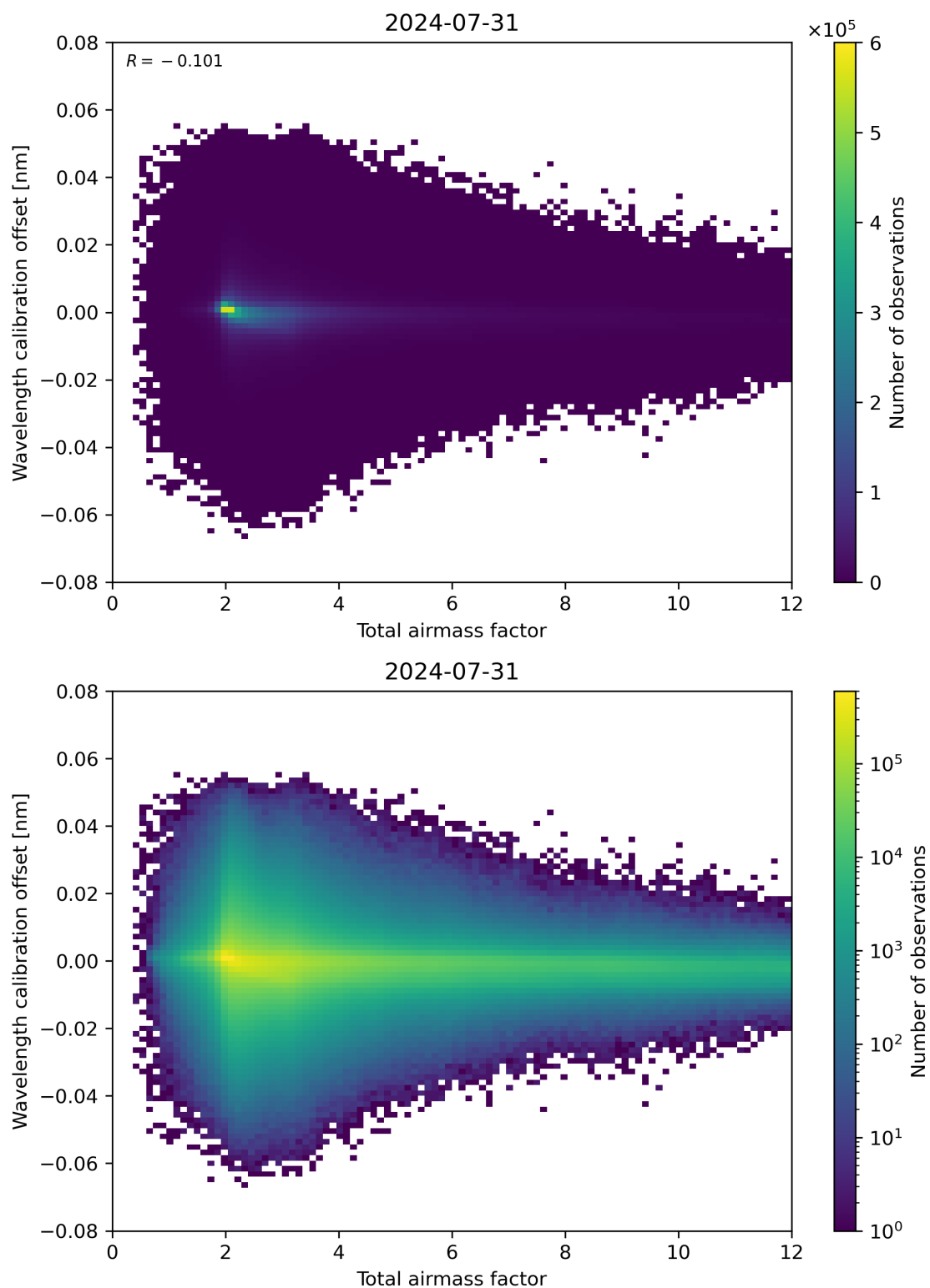
Figure 70: Scatter density plot of “Total airmass factor” against “Wavelength calibration offset” for 2024-07-31 to 2024-08-01.
