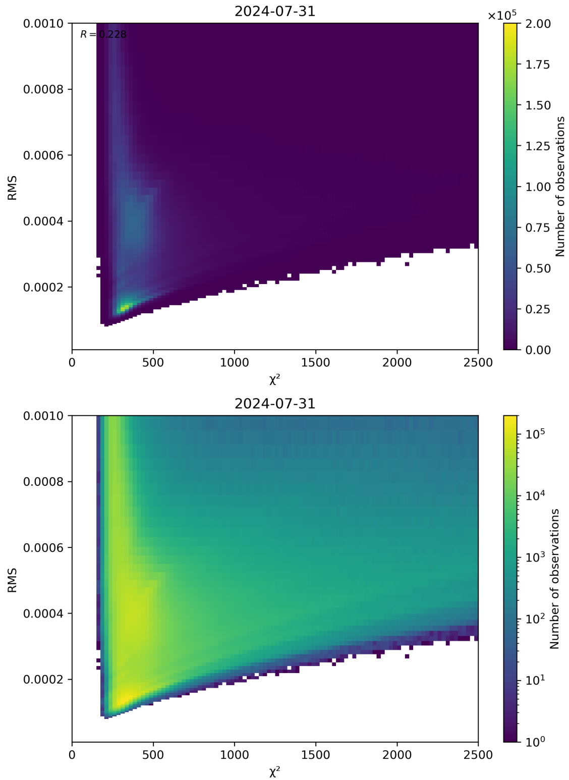
Figure 82: Scatter density plot of “ \chi^2 ” against “RMS” for 2024-07-31 to 2024-08-01.
