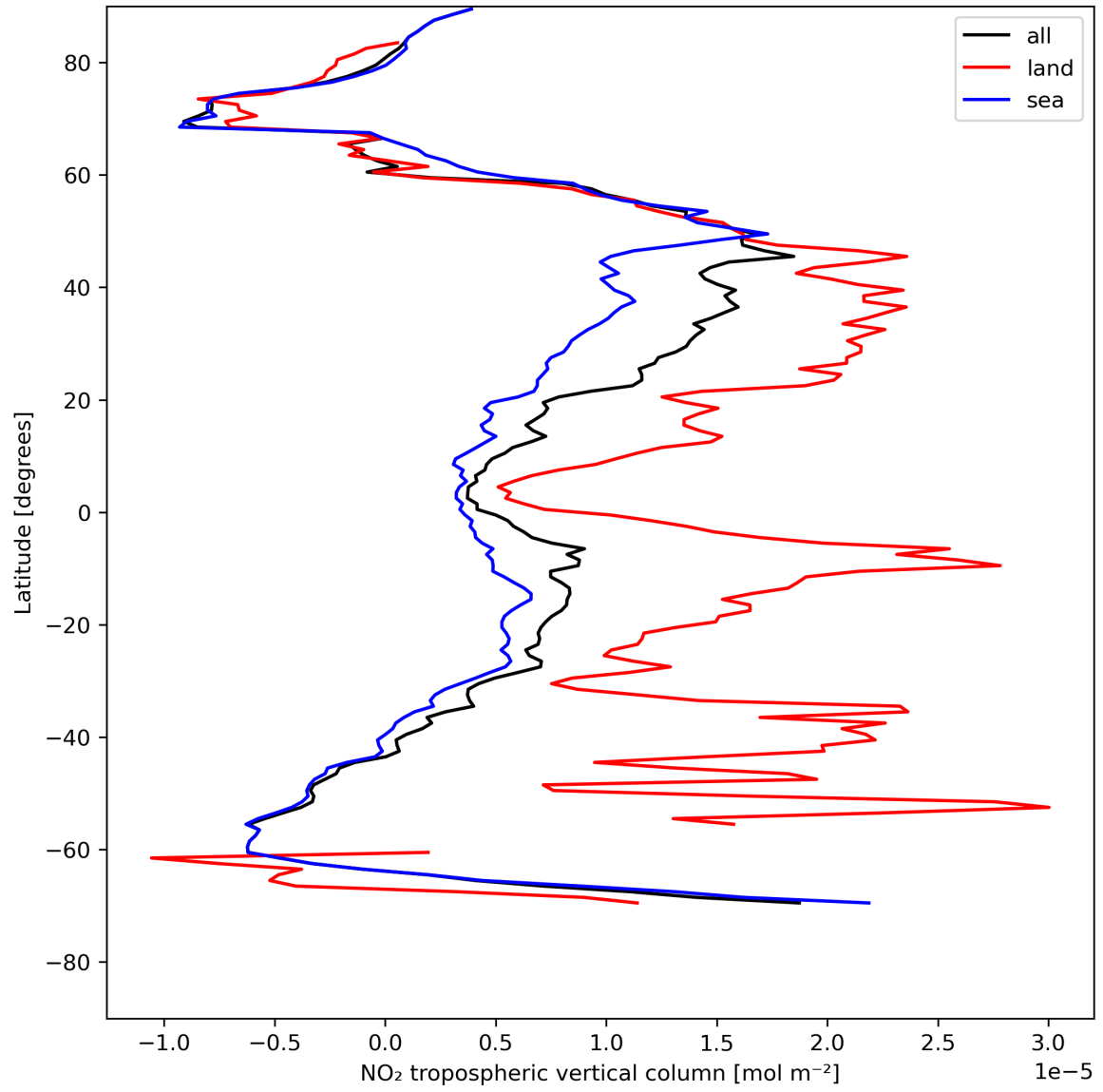
Figure 12: Zonal average of “NO 2 tropospheric vertical column” for 2024-07-31 to 2024-08-01.
