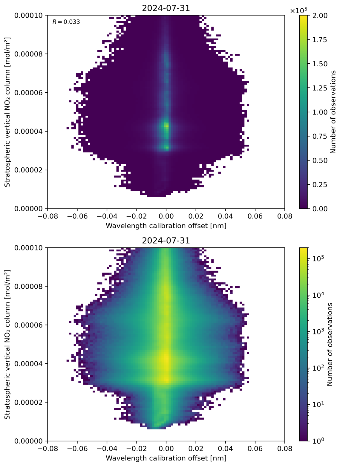
Figure 176: Scatter density plot of “Wavelength calibration offset” against “Stratospheric vertical NO 2 column” for 2024-07-31 to 2024-08-01.
