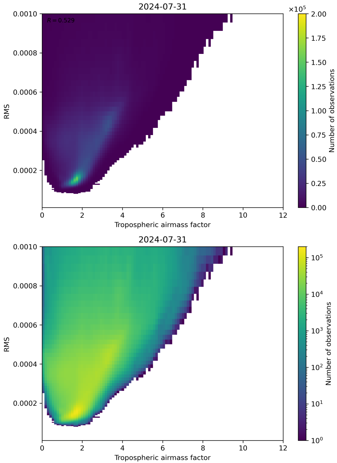
Figure 79: Scatter density plot of “Tropospheric airmass factor” against “RMS” for 2024-07-31 to 2024-08-01.
