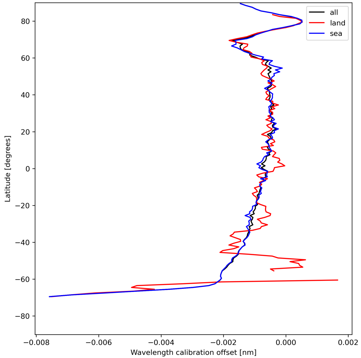
Figure 18: Zonal average of “Wavelength calibration offset” for 2024-07-31 to 2024-08-01.
