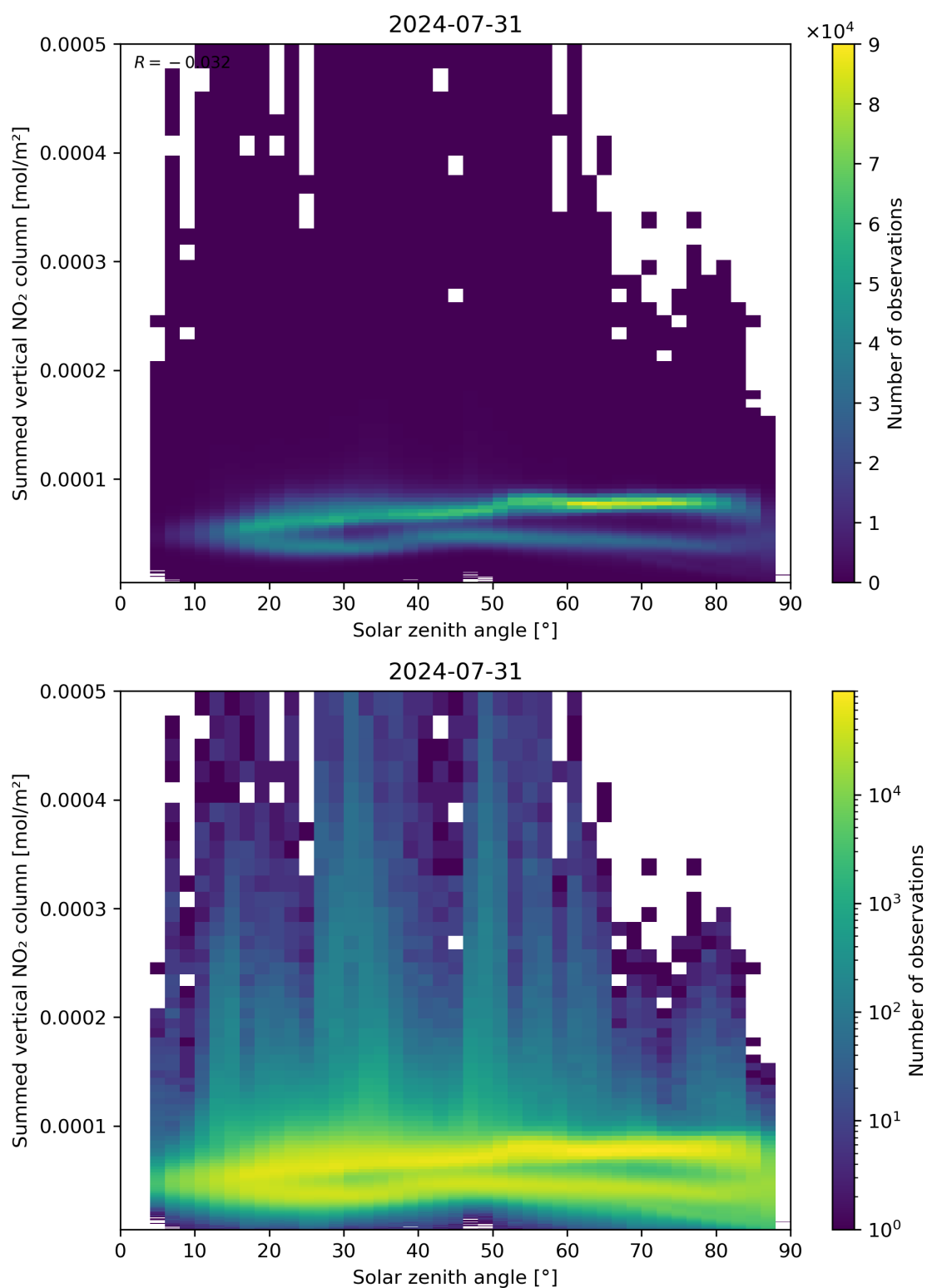
Figure 151: Scatter density plot of “Solar zenith angle” against “Summed vertical NO 2 column” for 2024-07-31 to 2024-08-01.
