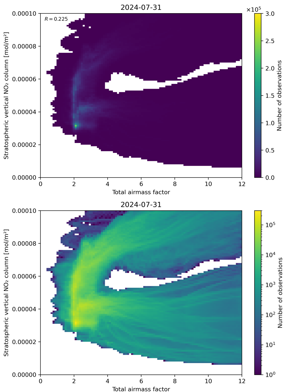
Figure 64: Scatter density plot of “Total airmass factor” against “Stratospheric vertical NO 2 column” for 2024-07-31 to 2024-08-01.
