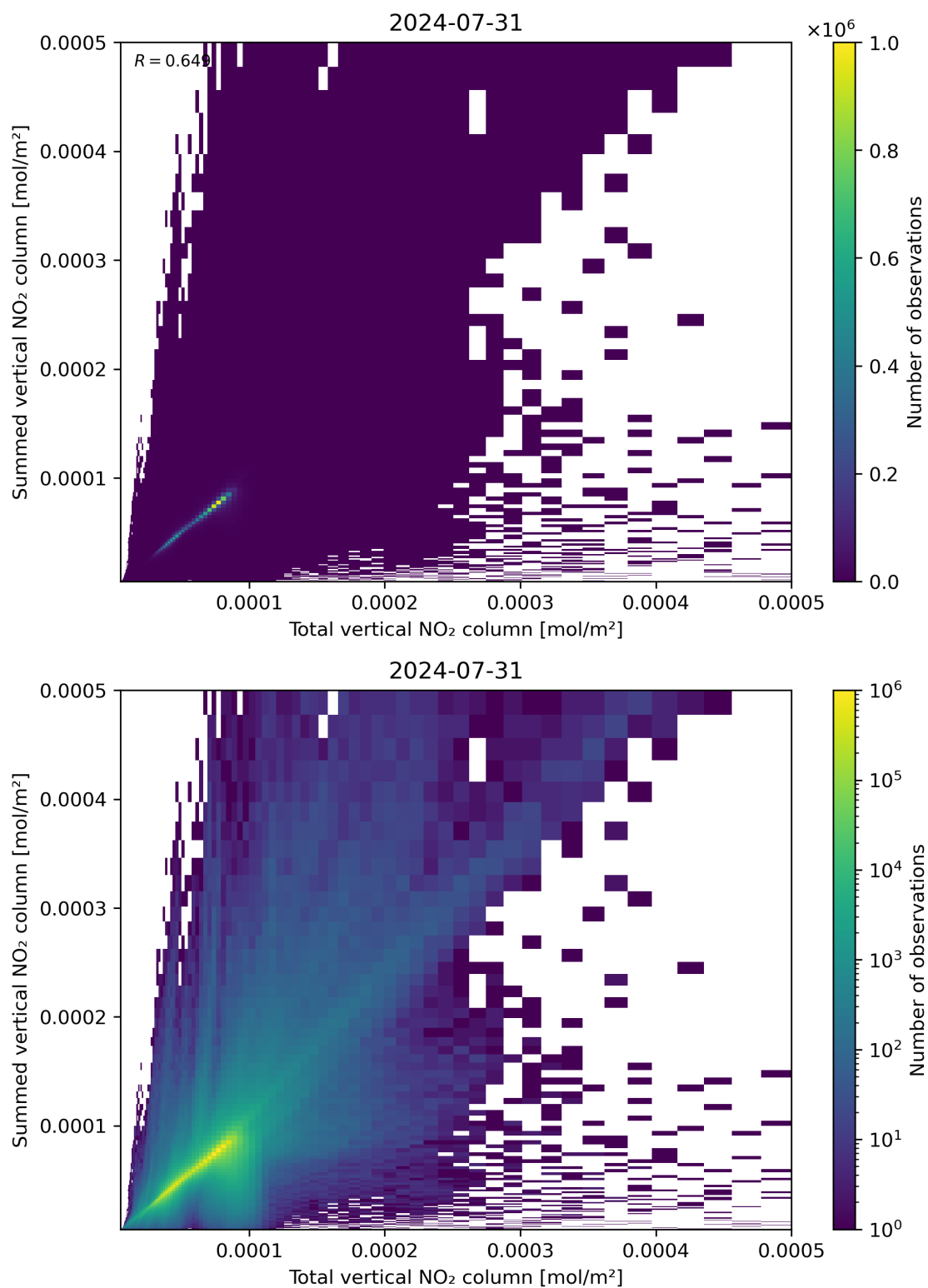
Figure 112: Scatter density plot of “Total vertical NO 2 column” against “Summed vertical NO 2 column” for 2024-07-31 to 2024-08-01.
