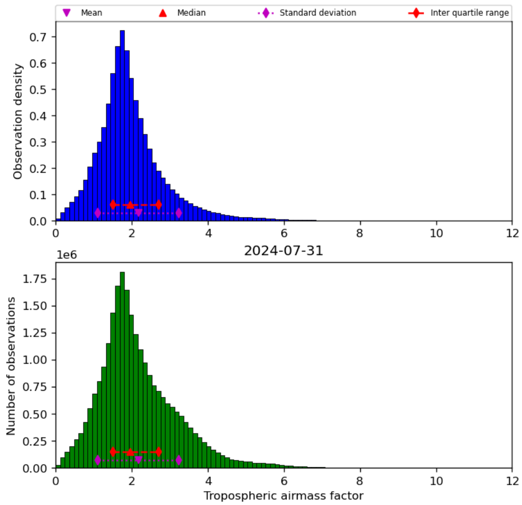
Figure 31: Histogram of “Tropospheric airmass factor” for 2024-07-31 to 2024-08-01
