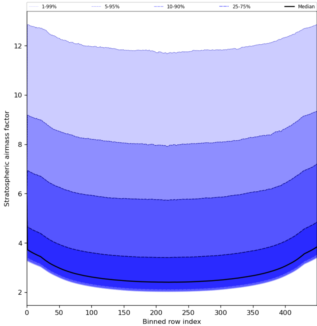
Figure 61: Along track statistics of “Stratospheric airmass factor” for 2024-07-31 to 2024-08-02
