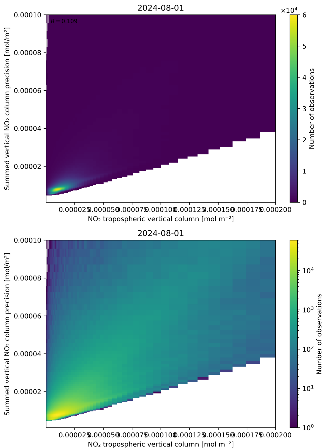
Figure 127: Scatter density plot of “NO 2 tropospheric vertical column” against “Summed vertical NO 2 column precision” for 2024-07-31 to 2024-08-02.
