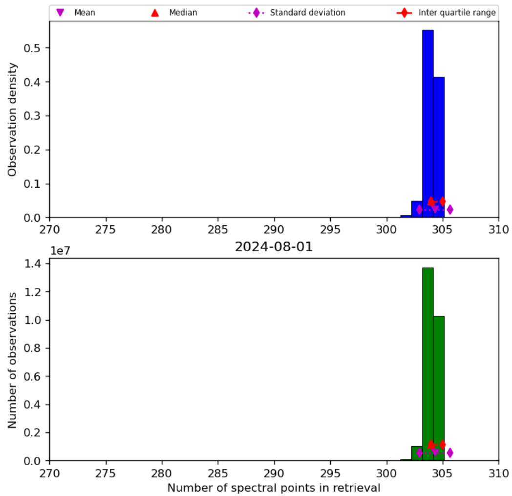
Figure 33: Histogram of “Number of spectral points in retrieval” for 2024-07-31 to 2024-08-02
