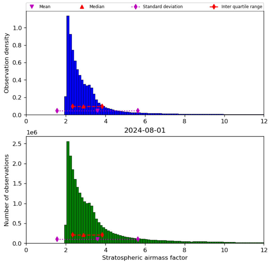
Figure 44: Histogram of “Stratospheric airmass factor” for 2024-07-31 to 2024-08-02
