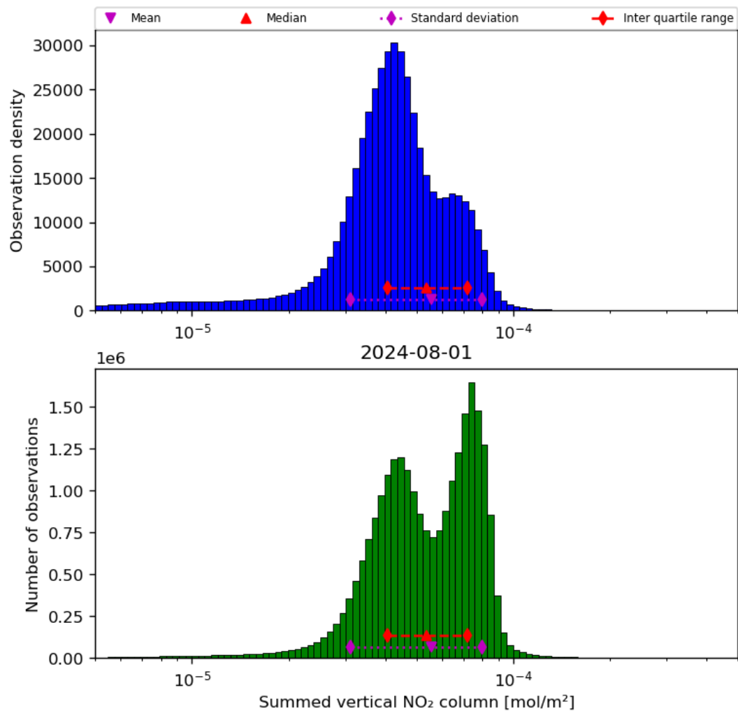
Figure 40: Histogram of “Summed vertical NO 2 column” for 2024-07-31 to 2024-08-02
