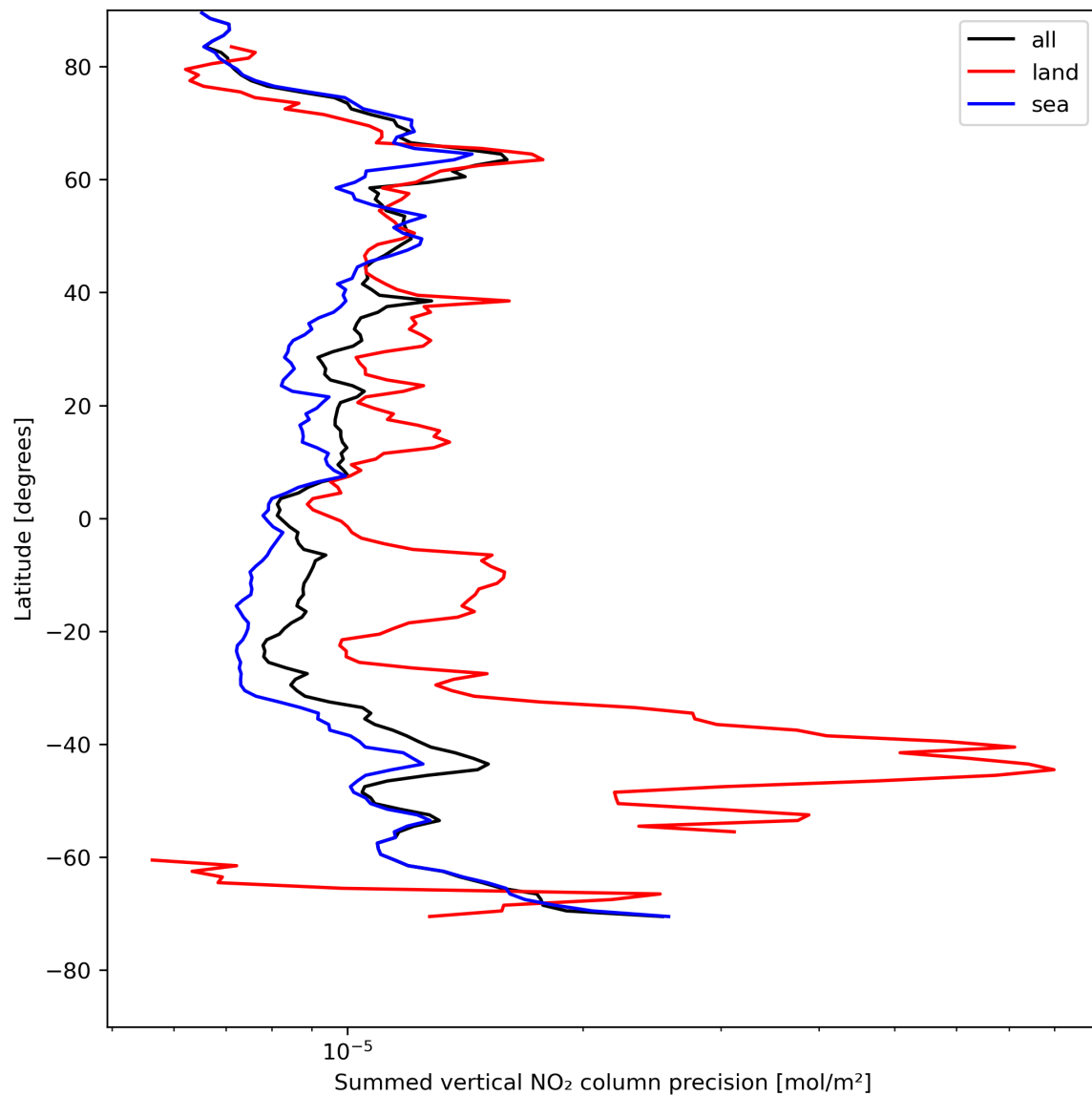
Figure 24: Zonal average of “Summed vertical NO 2 column precision” for 2024-07-31 to 2024-08-02.
