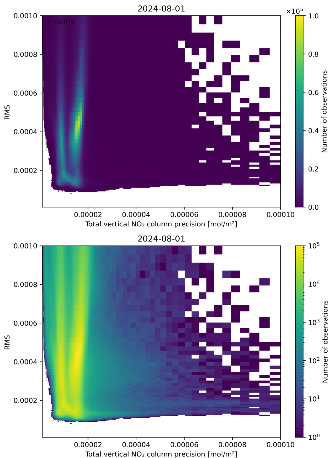
Figure 119: Scatter density plot of “Total vertical NO 2 column precision” against “RMS” for 2024-07-31 to 2024-08-02.
