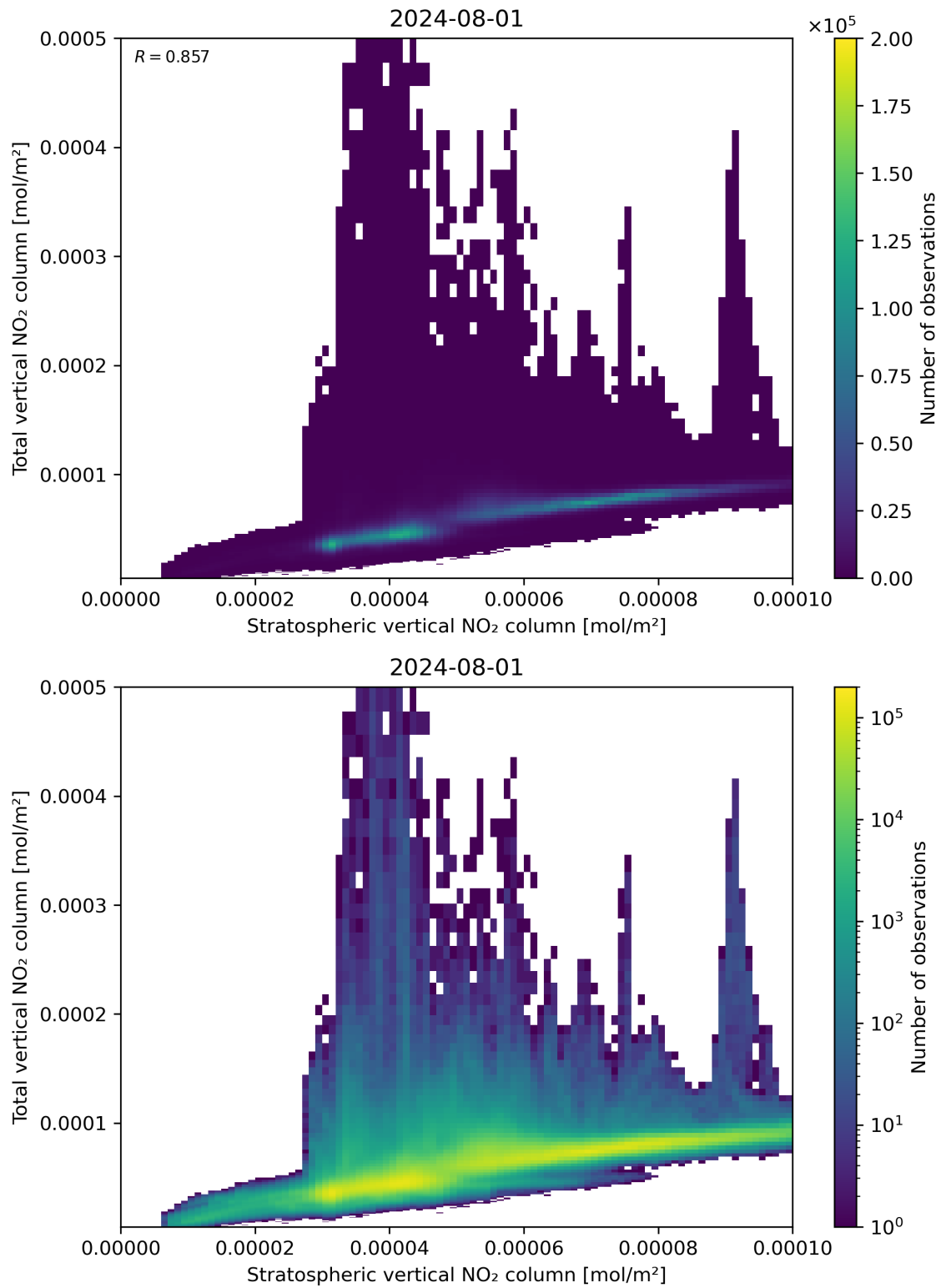
Figure 100: Scatter density plot of “Stratospheric vertical NO 2 column” against “Total vertical NO 2 column” for 2024-07-31 to 2024-08-02.
