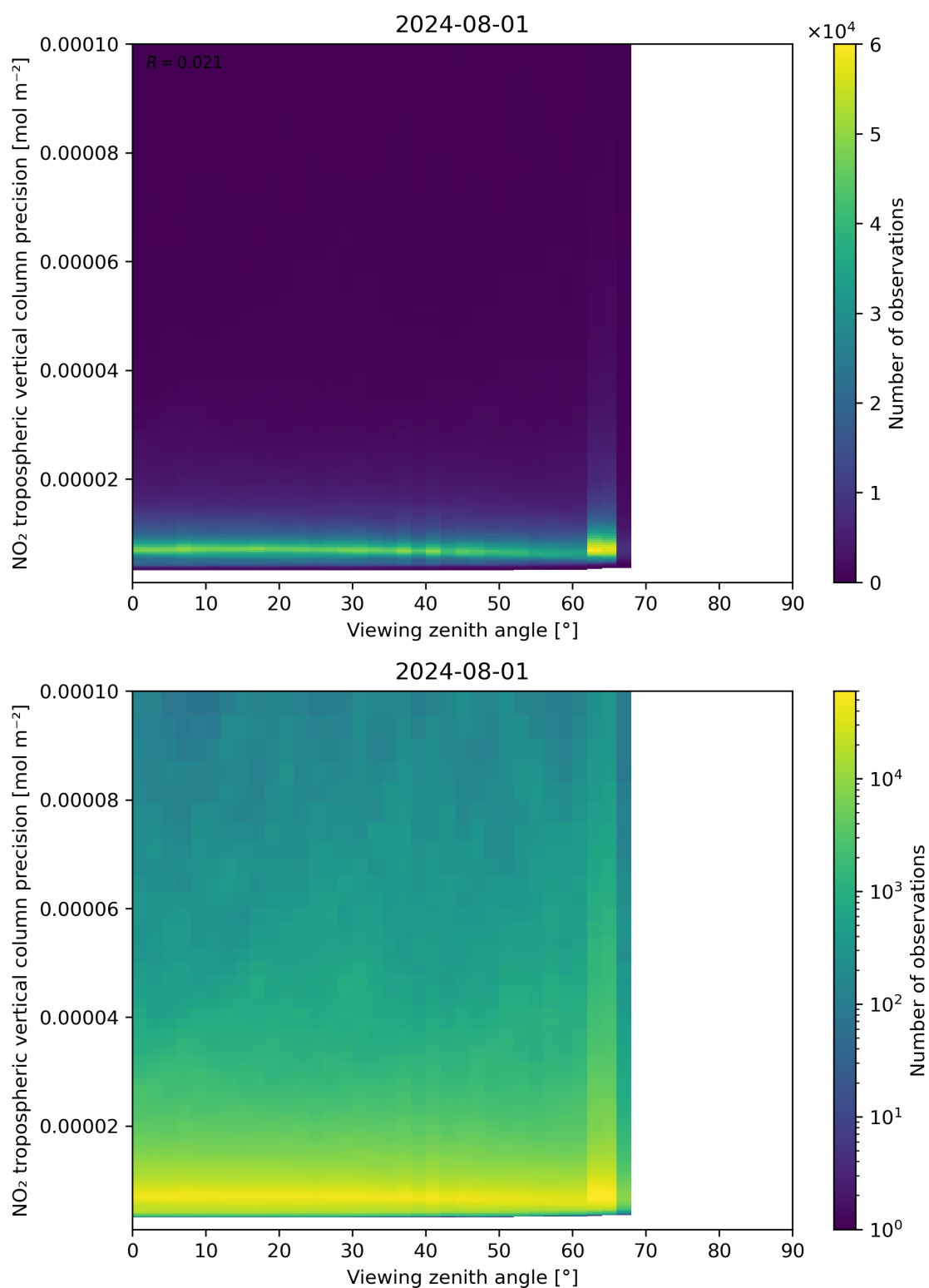
Figure 170: Scatter density plot of “Viewing zenith angle” against “NO 2 tropospheric vertical column precision” for 2024-07-31 to 2024-08-02.
