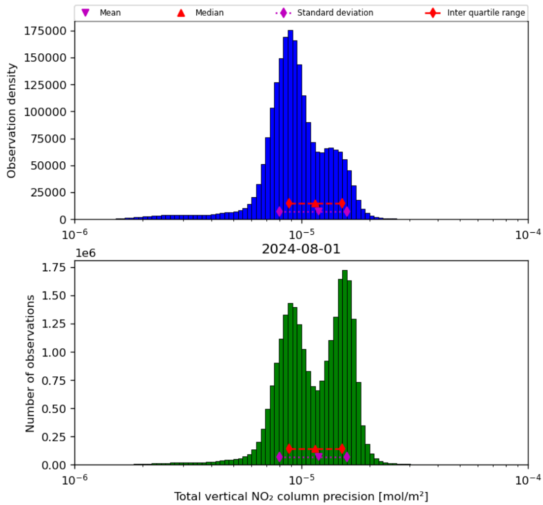
Figure 39: Histogram of “Total vertical NO 2 column precision” for 2024-07-31 to 2024-08-02
