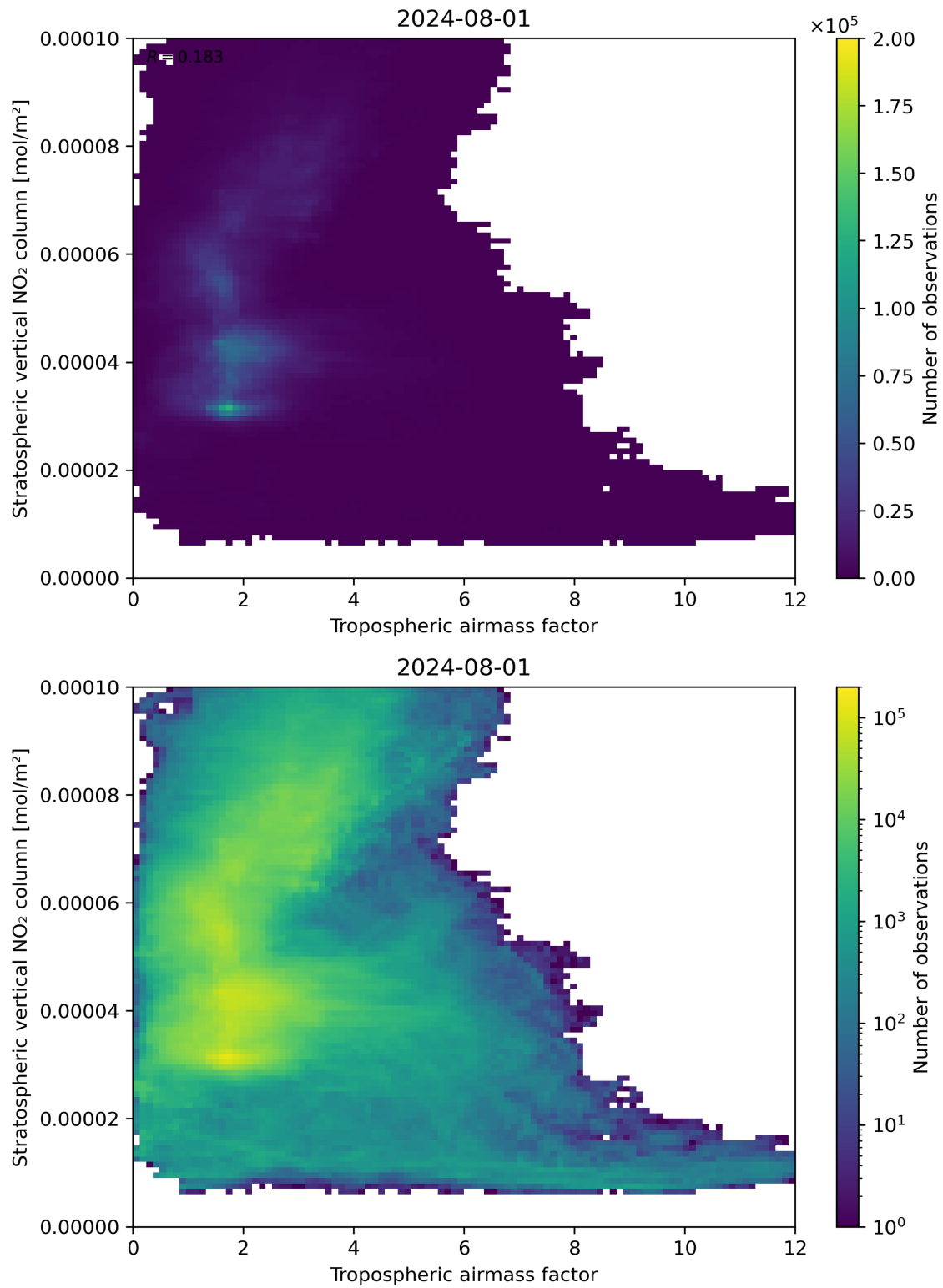
Figure 74: Scatter density plot of “Tropospheric air mass factor” against “Stratospheric vertical NO 2 column” for 2024-07-31 to 2024-08-02.
