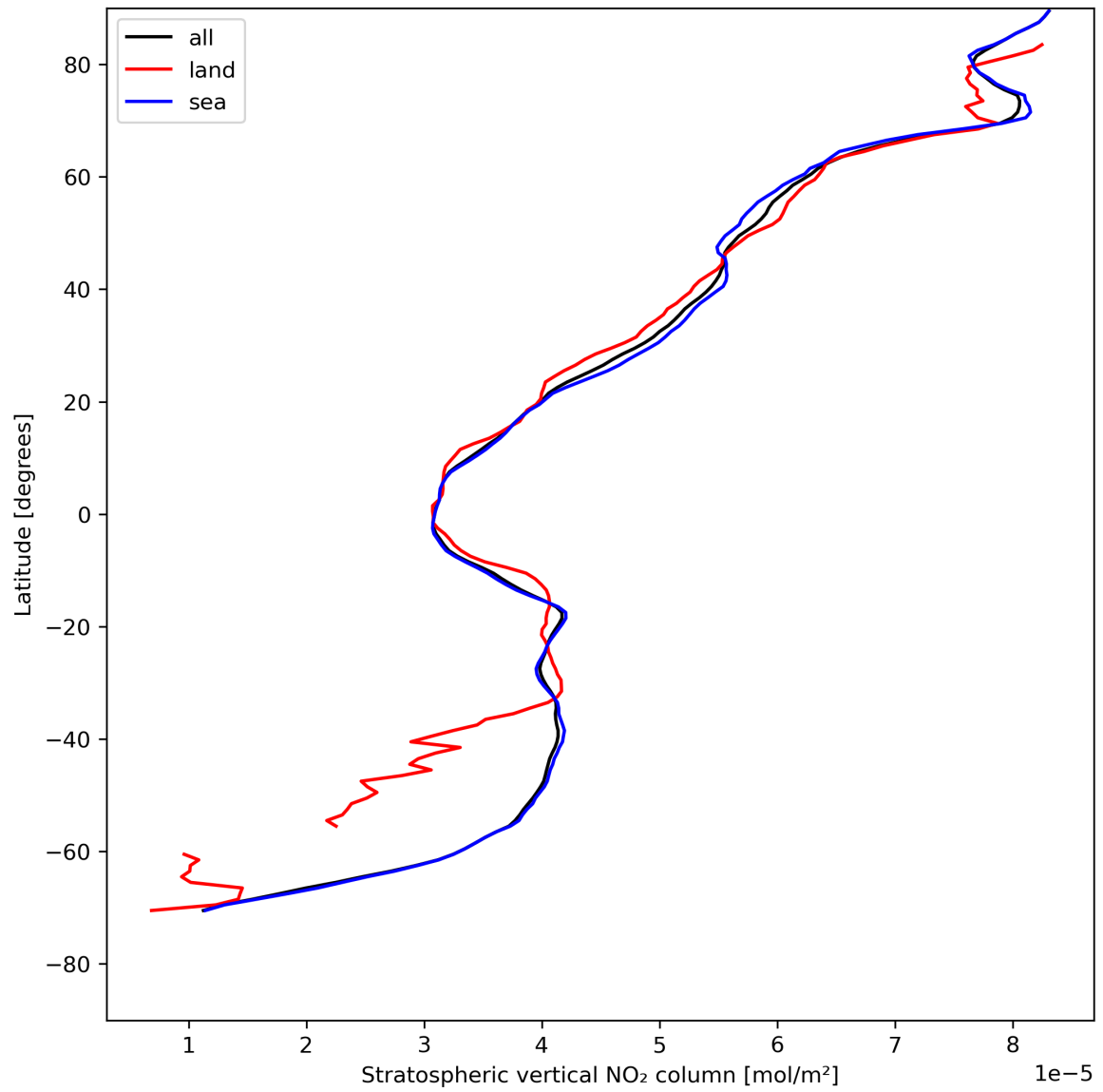
Figure 19: Zonal average of “Stratospheric vertical NO 2 column” for 2024-07-31 to 2024-08-02.
