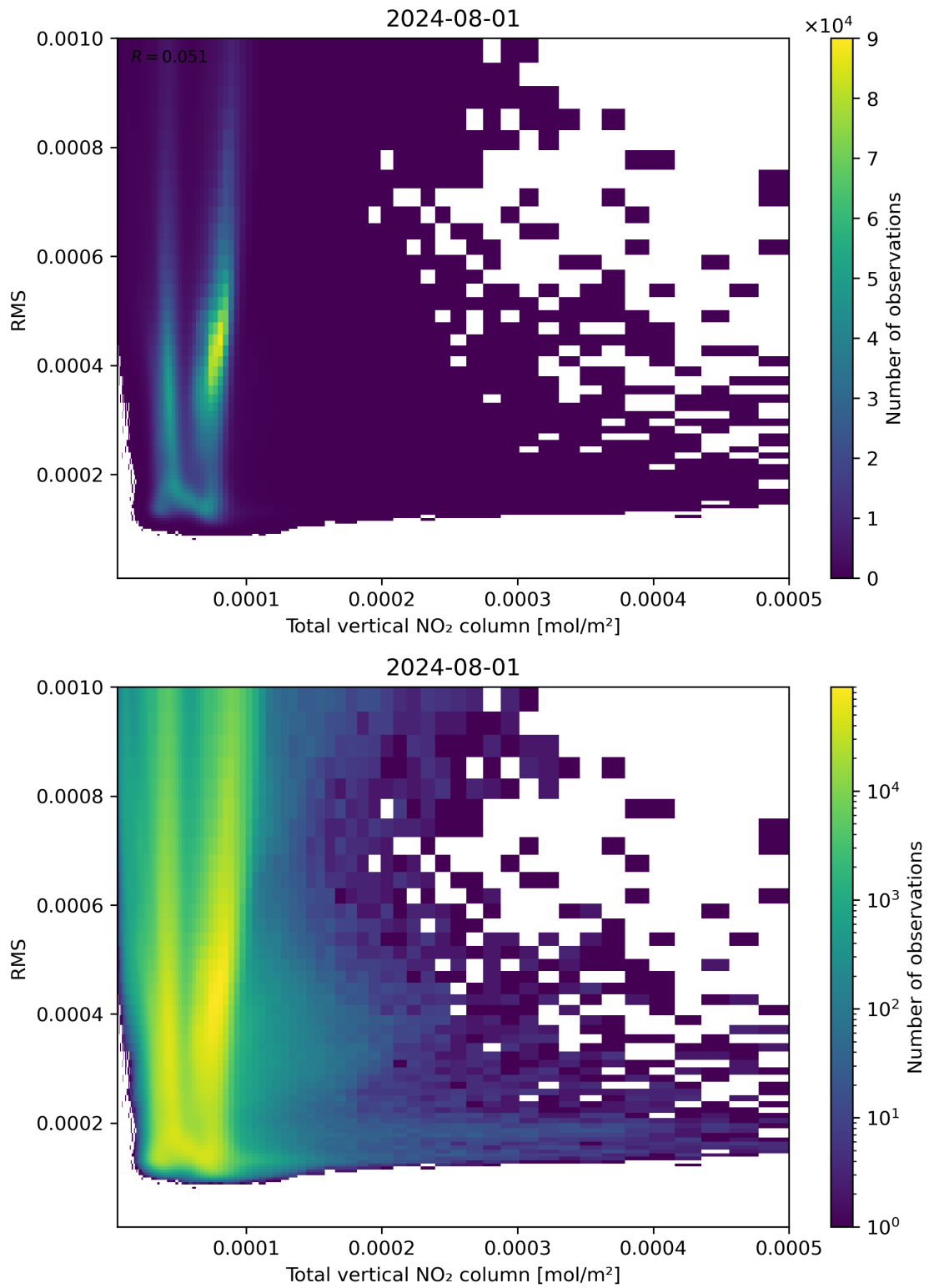
Figure 120: Scatter density plot of “Total vertical NO 2 column” against “RMS” for 2024-07-31 to 2024-08-02.
