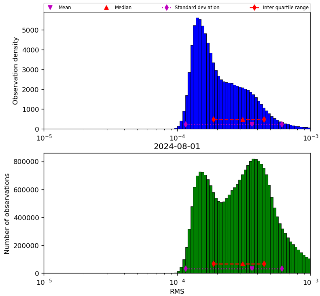
Figure 43: Histogram of “RMS” for 2024-07-31 to 2024-08-02
