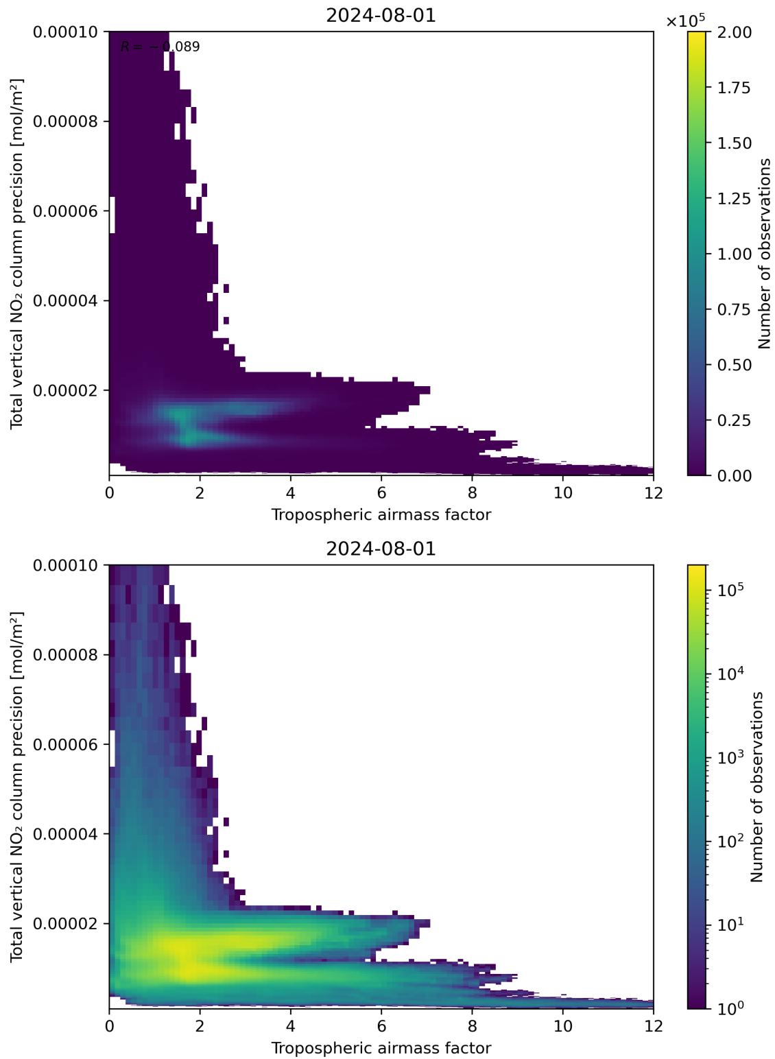
Figure 78: Scatter density plot of “Tropospheric air mass factor” against “Total vertical NO 2 column precision” for 2024-07-31 to 2024-08-02.
