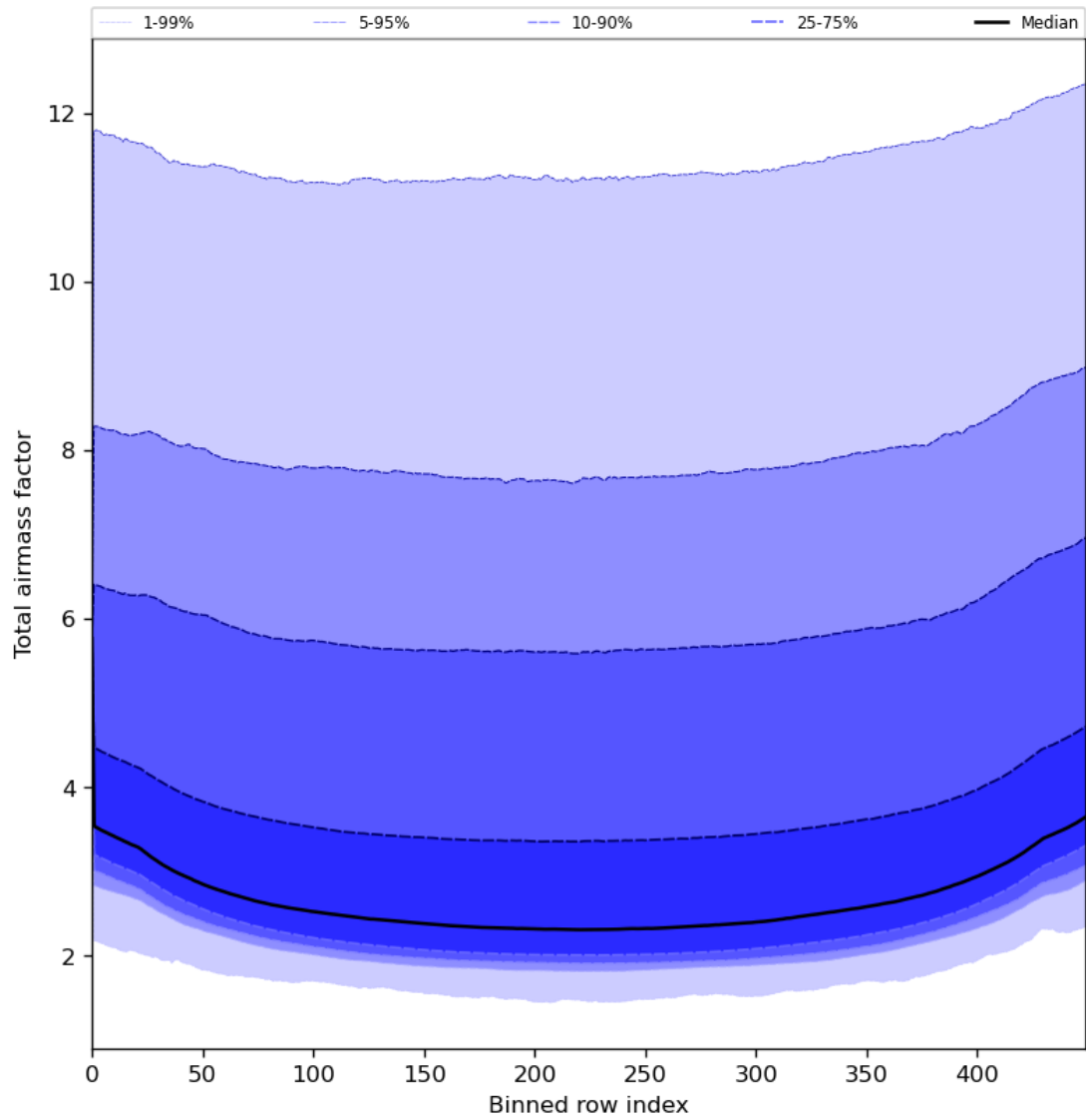
Figure 49: Along track statistics of “Total airmass factor” for 2024-07-31 to 2024-08-02
