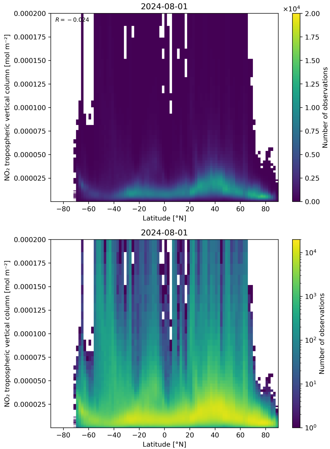
Figure 92: Scatter density plot of “Latitude” against “NO 2 tropospheric vertical column” for 2024-07-31 to 2024-08-02.
