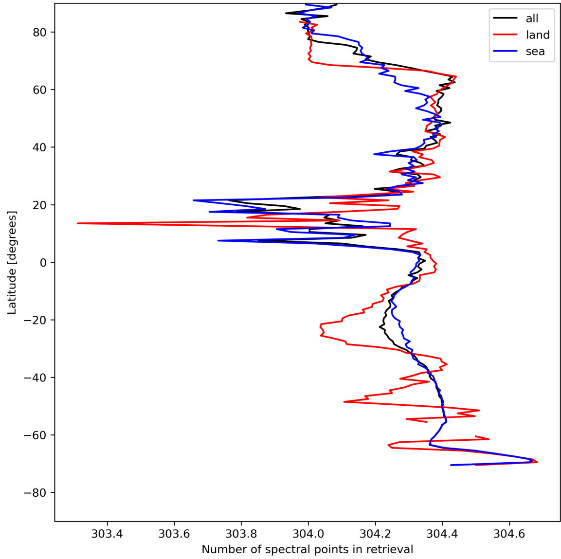
Figure 16: Zonal average of “Number of spectral points in retrieval” for 2024-07-31 to 2024-08-02.
