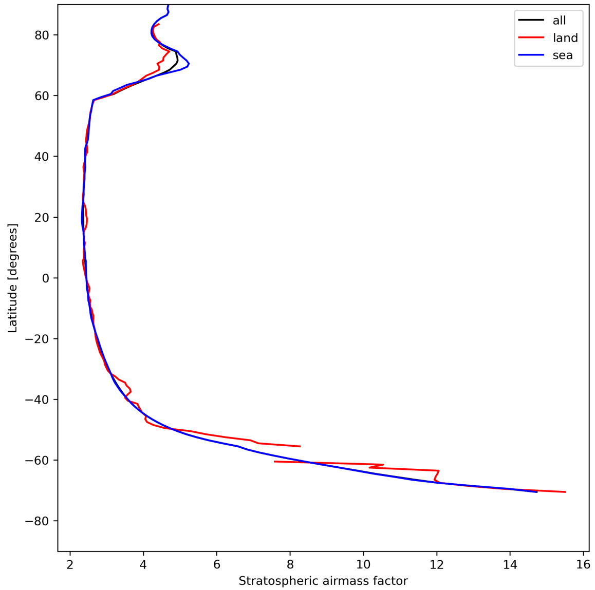
Figure 27: Zonal average of “Stratospheric airmass factor” for 2024-07-31 to 2024-08-02.
