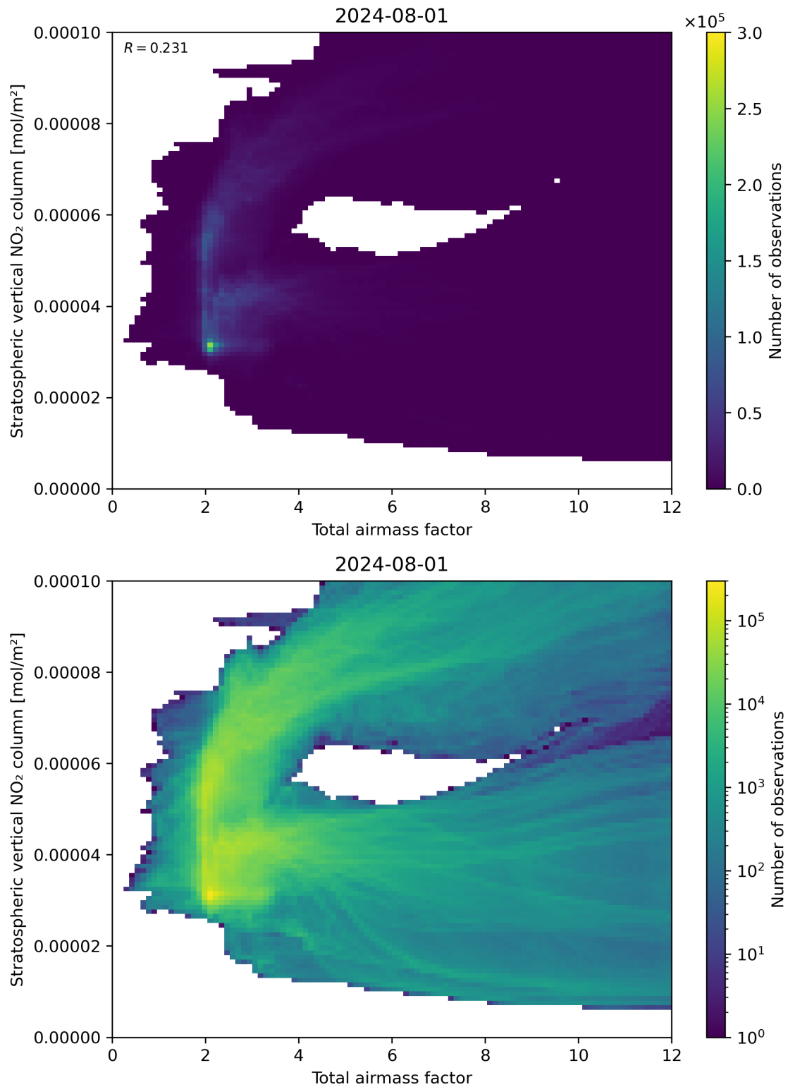
Figure 64: Scatter density plot of “Total airmass factor” against “Stratospheric vertical \text{NO}_2 column” for 2024-07-31 to 2024-08-02.
