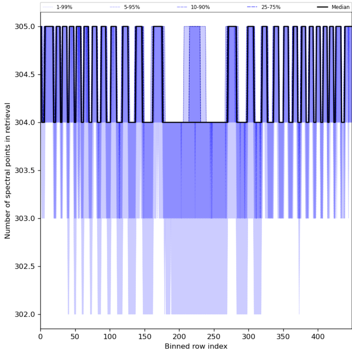
Figure 50: Along track statistics of “Number of spectral points in retrieval” for 2024-07-31 to 2024-08-02
