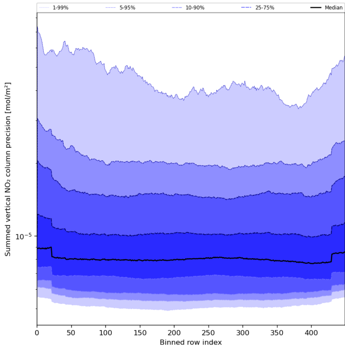
Figure 58: Along track statistics of “Summed vertical NO 2 column precision” for 2024-07-31 to 2024-08-02
