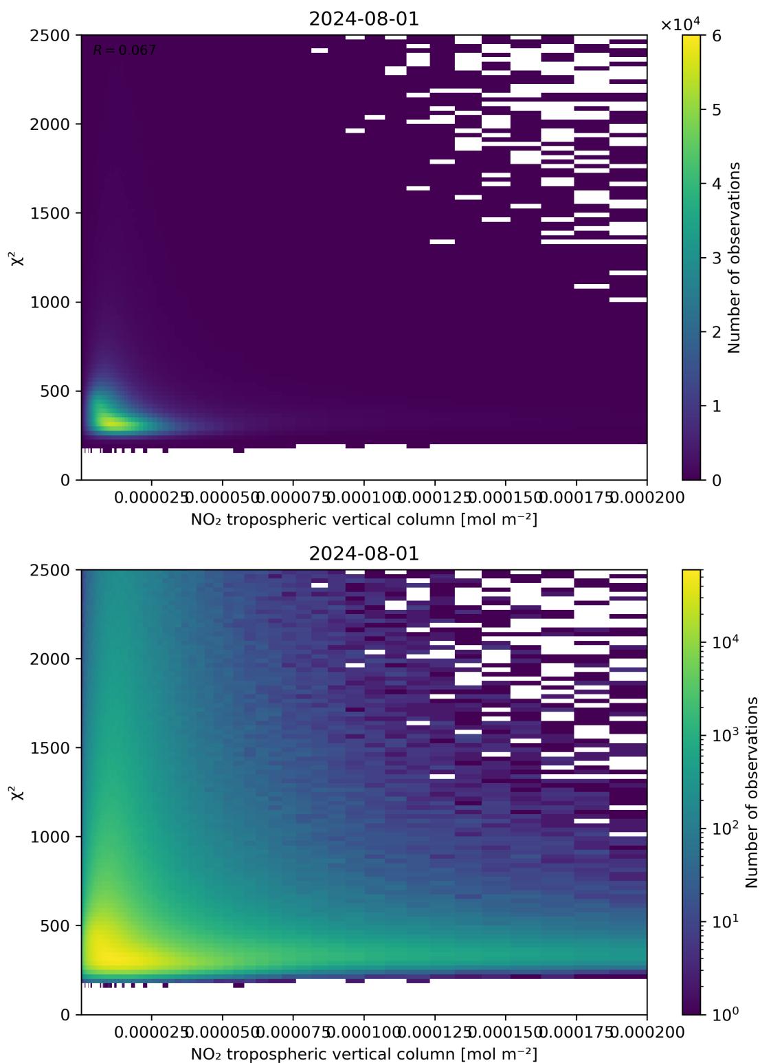
Figure 124: Scatter density plot of “NO 2 tropospheric vertical column” against “ \chi^2 ” for 2024-07-31 to 2024-08-02.
