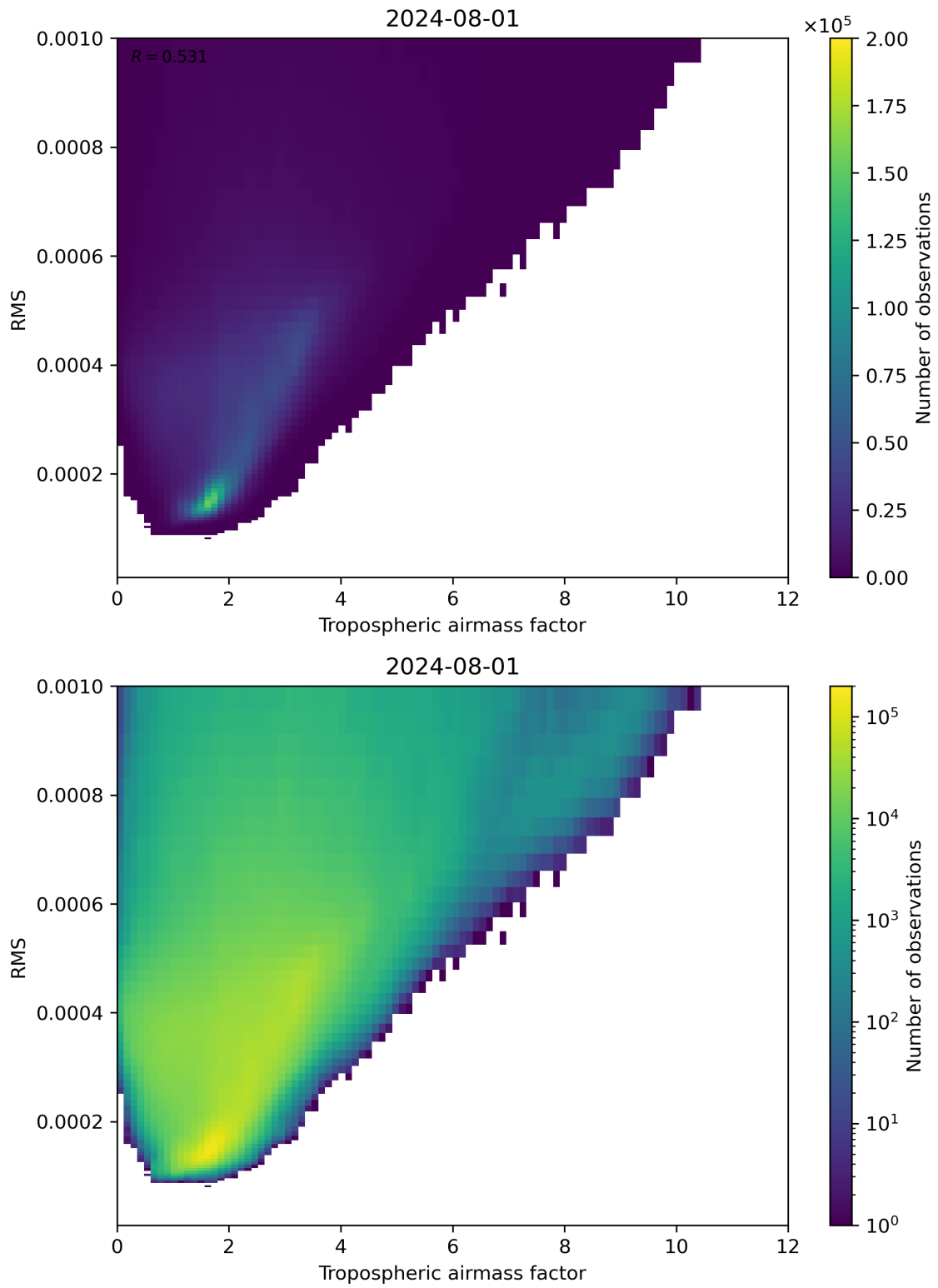
Figure 79: Scatter density plot of “Tropospheric airmass factor” against “RMS” for 2024-07-31 to 2024-08-02.
