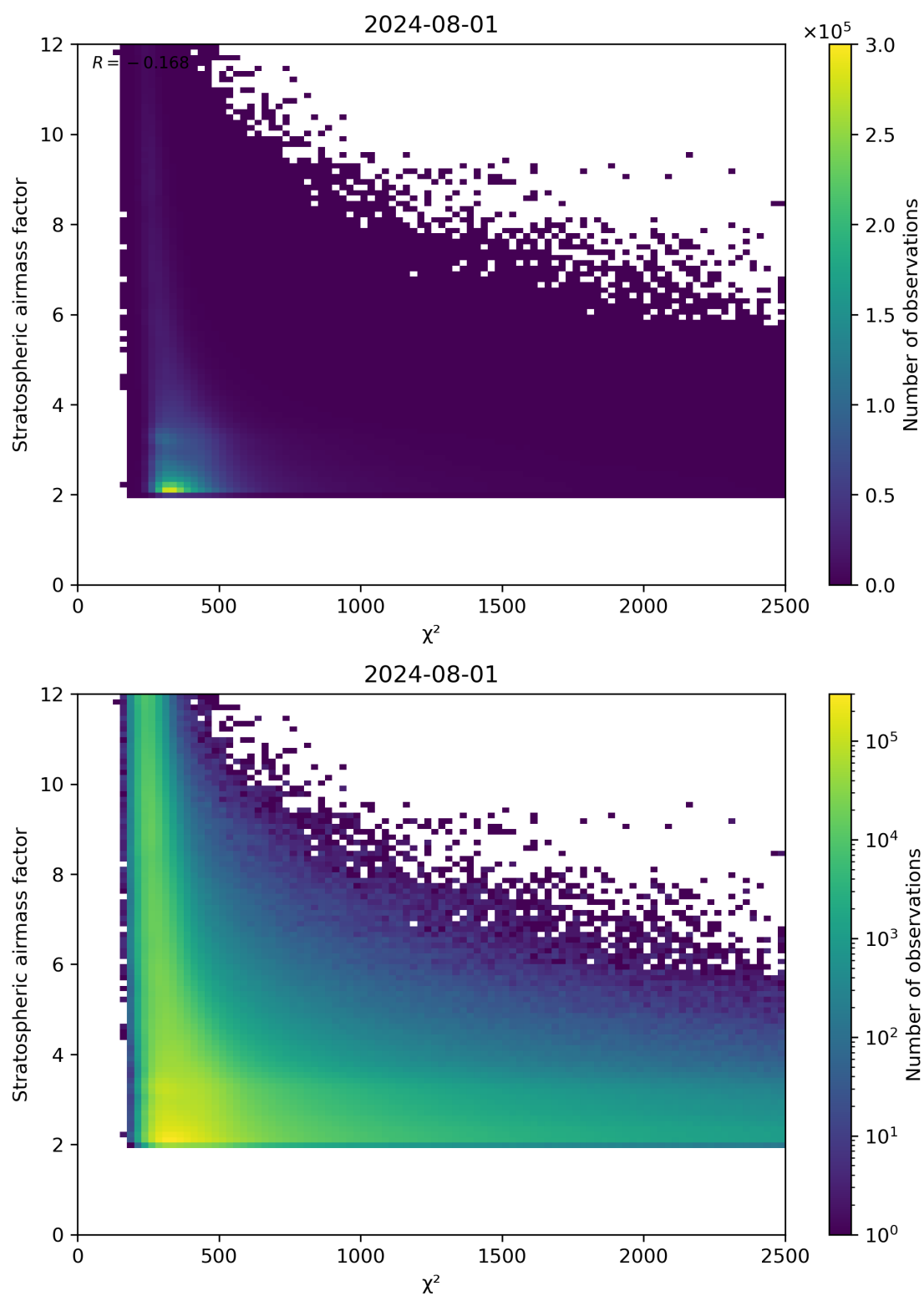
Figure 81: Scatter density plot of “ \chi^2 ” against “Stratospheric airmass factor” for 2024-07-31 to 2024-08-02.
