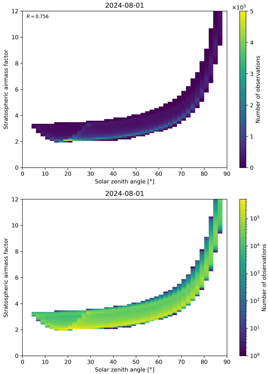
Figure 145: Scatter density plot of “Solar zenith angle” against “Stratospheric airmass factor” for 2024-07-31 to 2024-08-02.
