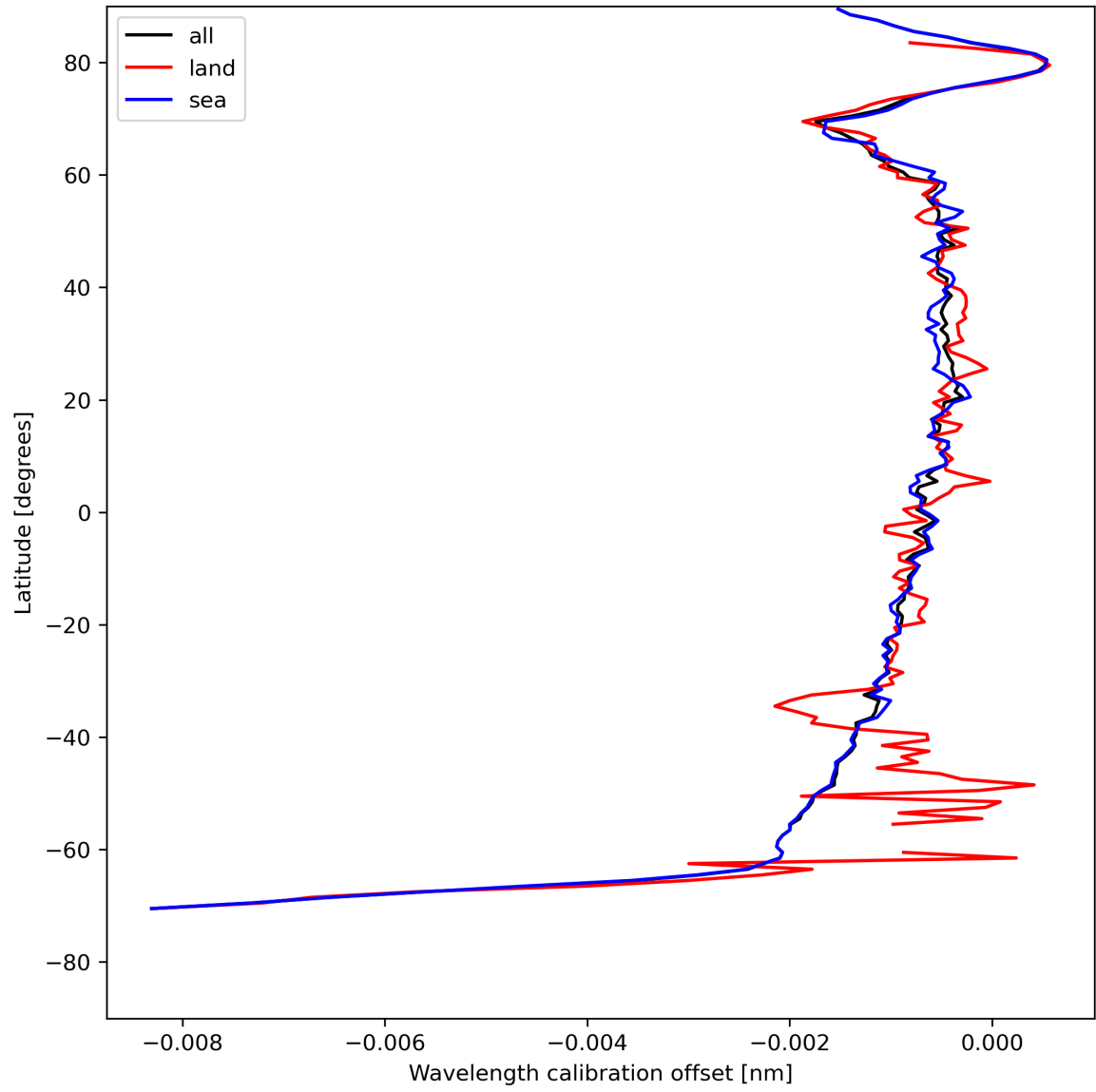
Figure 18: Zonal average of “Wavelength calibration offset” for 2024-07-31 to 2024-08-02.
