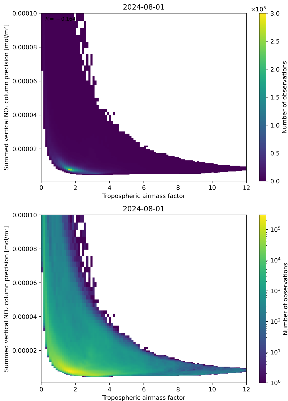
Figure 76: Scatter density plot of “Tropospheric air mass factor” against “Summed vertical NO 2 column precision” for 2024-07-31 to 2024-08-02.
