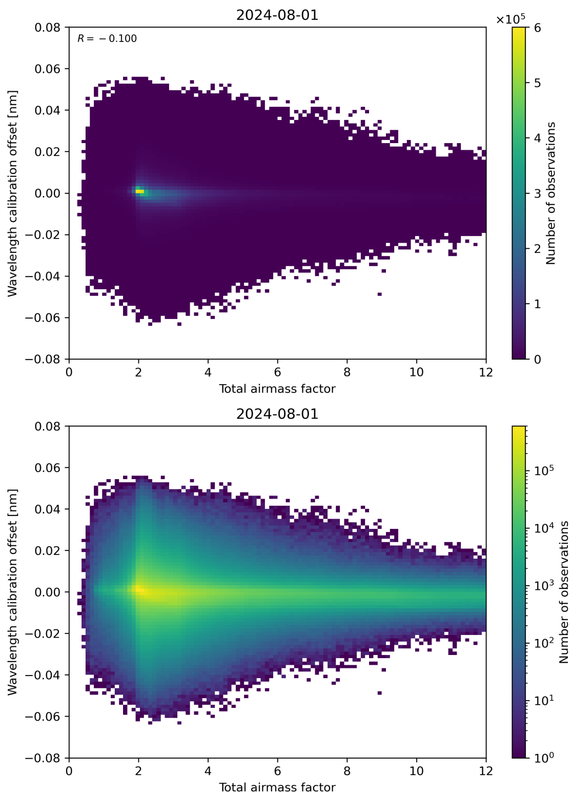
Figure 70: Scatter density plot of “Total airmass factor” against “Wavelength calibration offset” for 2024-07-31 to 2024-08-02.
