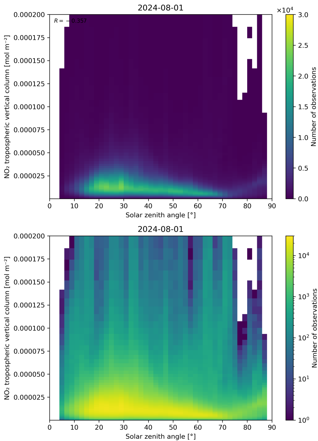
Figure 155: Scatter density plot of “Solar zenith angle” against “NO 2 tropospheric vertical column” for 2024-07-31 to 2024-08-02.
