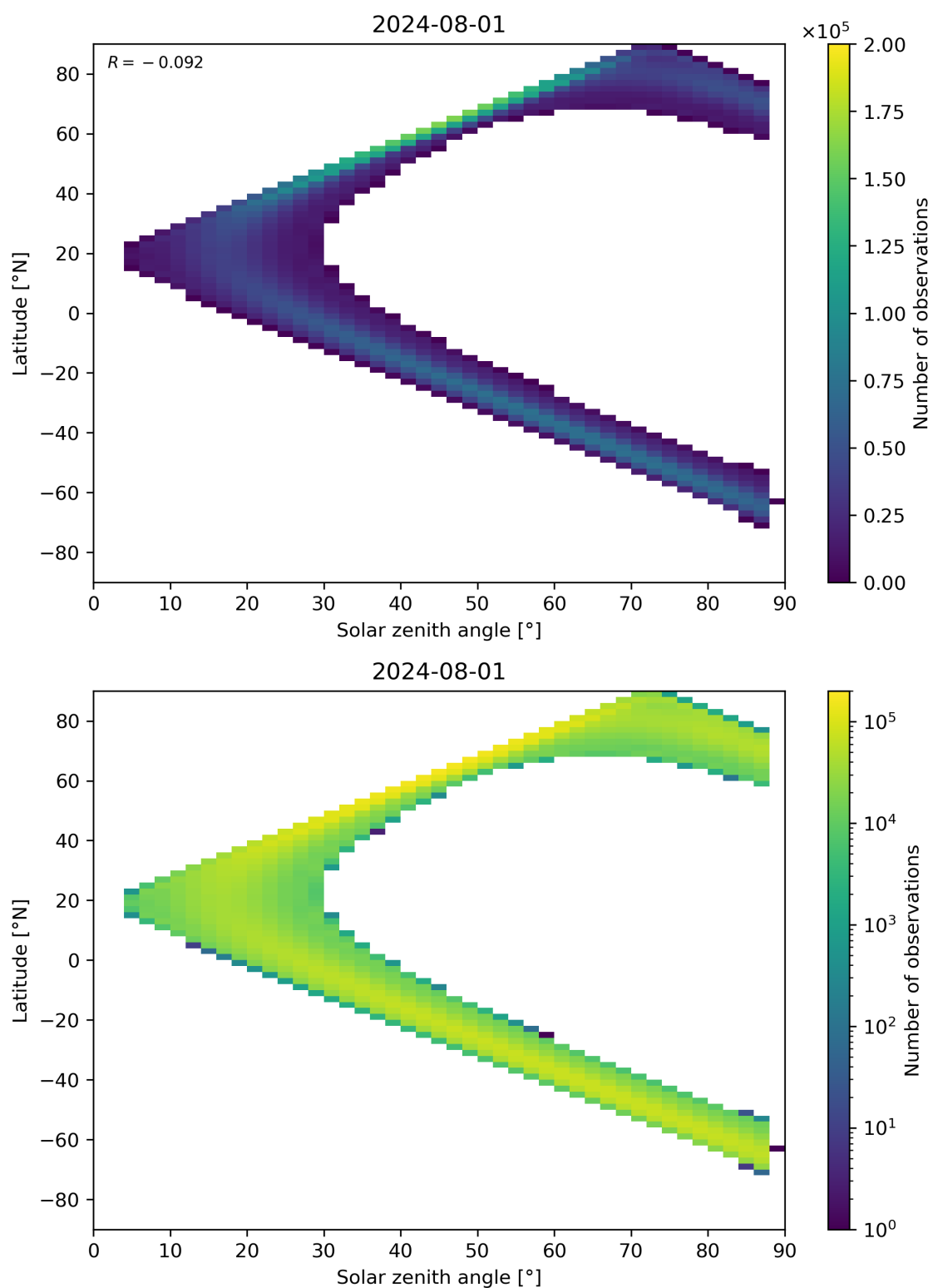
Figure 149: Scatter density plot of “Solar zenith angle” against “Latitude” for 2024-07-31 to 2024-08-02.
