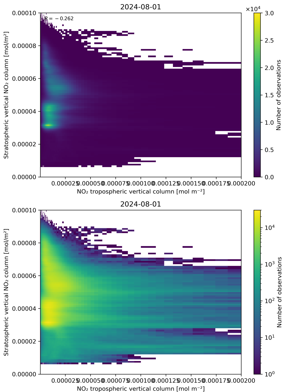
Figure 125: Scatter density plot of “NO 2 tropospheric vertical column” against “Stratospheric vertical NO 2 column” for 2024-07-31 to 2024-08-02.
