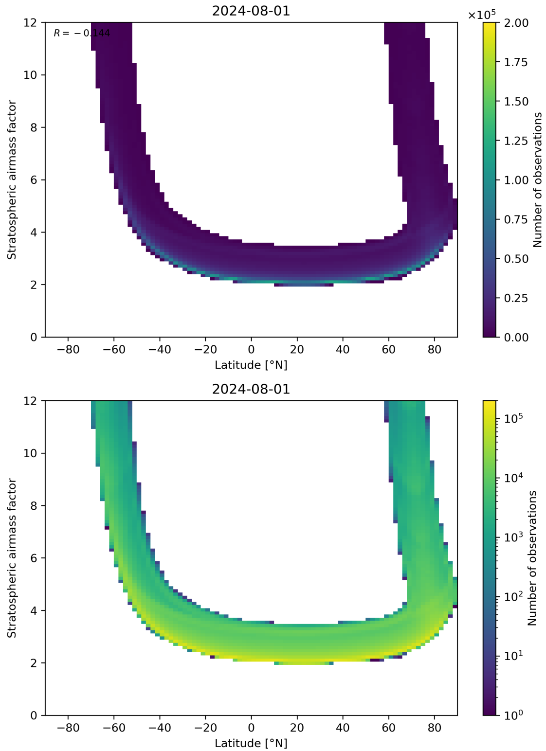
Figure 83: Scatter density plot of “Latitude” against “Stratospheric air mass factor” for 2024-07-31 to 2024-08-02.
