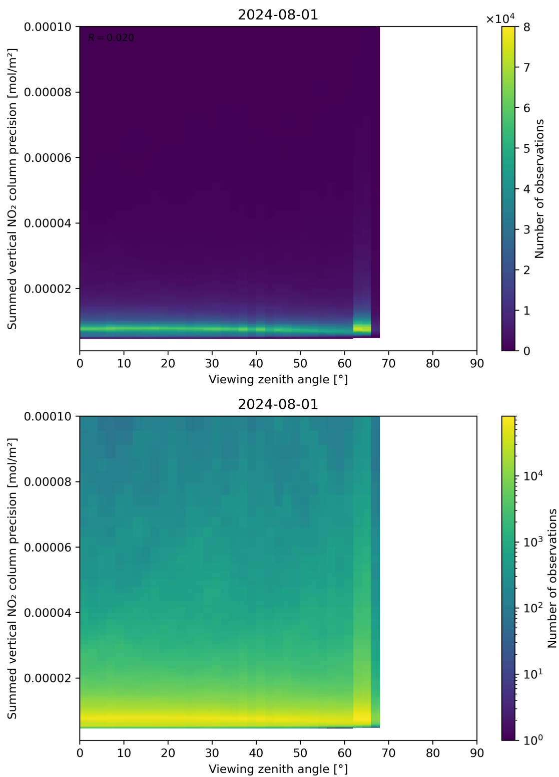
Figure 166: Scatter density plot of “Viewing zenith angle” against “Summed vertical NO 2 column precision” for 2024-07-31 to 2024-08-02.
