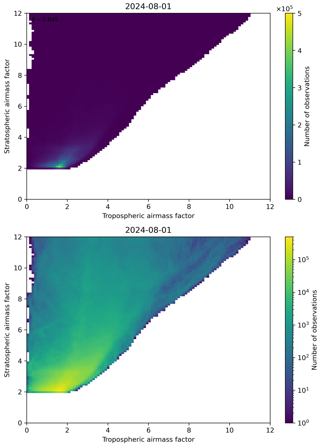
Figure 71: Scatter density plot of “Tropospheric airmass factor” against “Stratospheric airmass factor” for 2024-07-31 to 2024-08-02.
