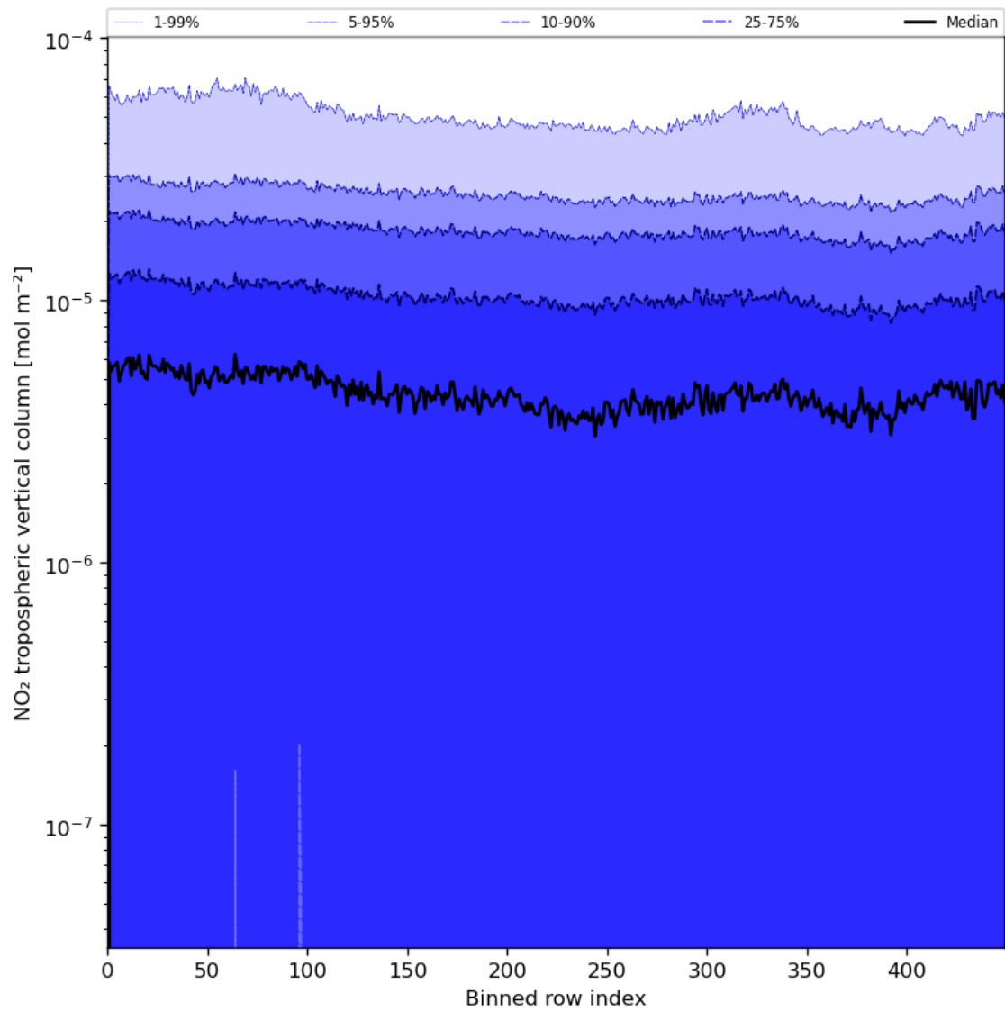
Figure 46: Along track statistics of "NO 2 tropospheric vertical column" for 2024-07-31 to 2024-08-02
