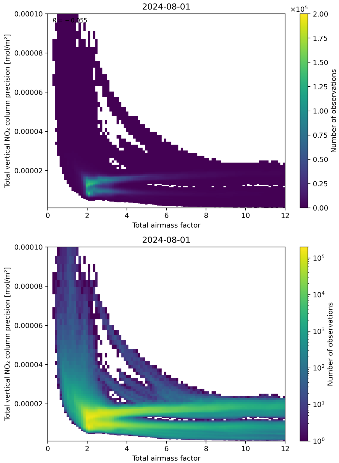
Figure 68: Scatter density plot of “Total airmass factor” against “Total vertical NO 2 column precision” for 2024-07-31 to 2024-08-02.
