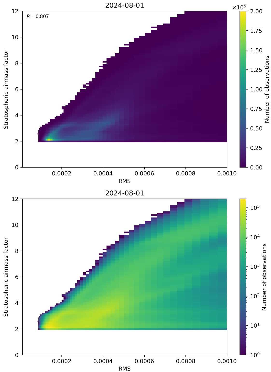
Figure 144: Scatter density plot of “RMS” against “Stratospheric airmass factor” for 2024-07-31 to 2024-08-02.
