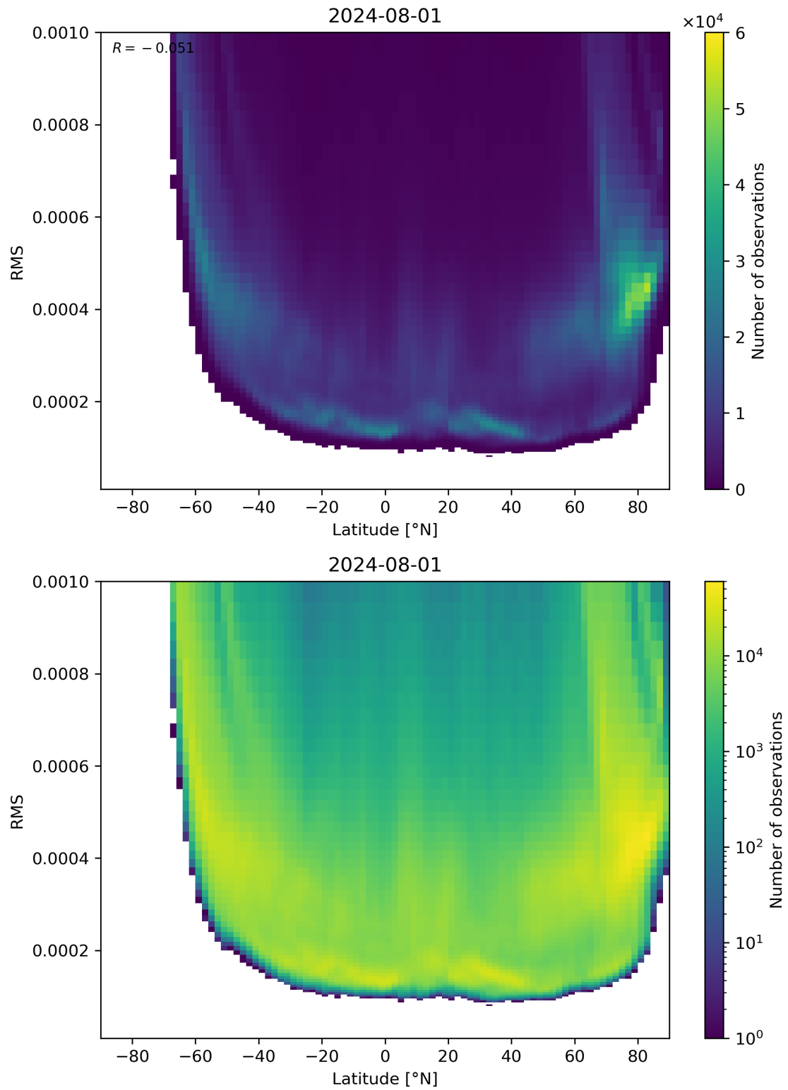
Figure 94: Scatter density plot of “Latitude” against “RMS” for 2024-07-31 to 2024-08-02.
