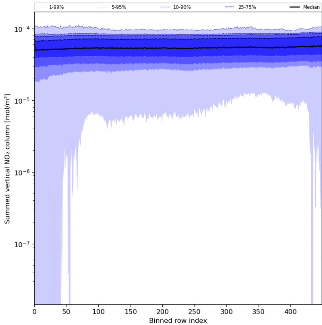
Figure 57: Along track statistics of “Summed vertical NO 2 column” for 2024-07-31 to 2024-08-02
