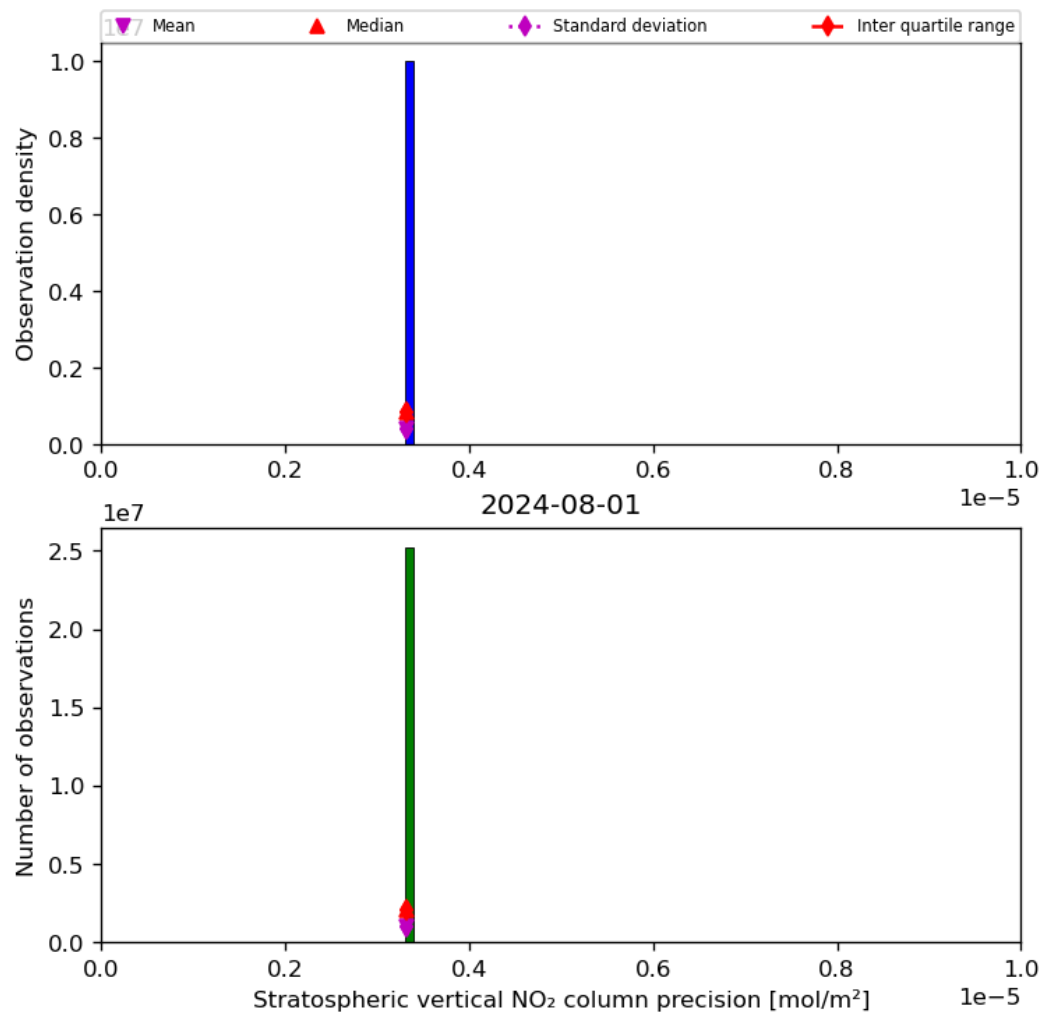
Figure 37: Histogram of “Stratospheric vertical NO 2 column precision” for 2024-07-31 to 2024-08-02
