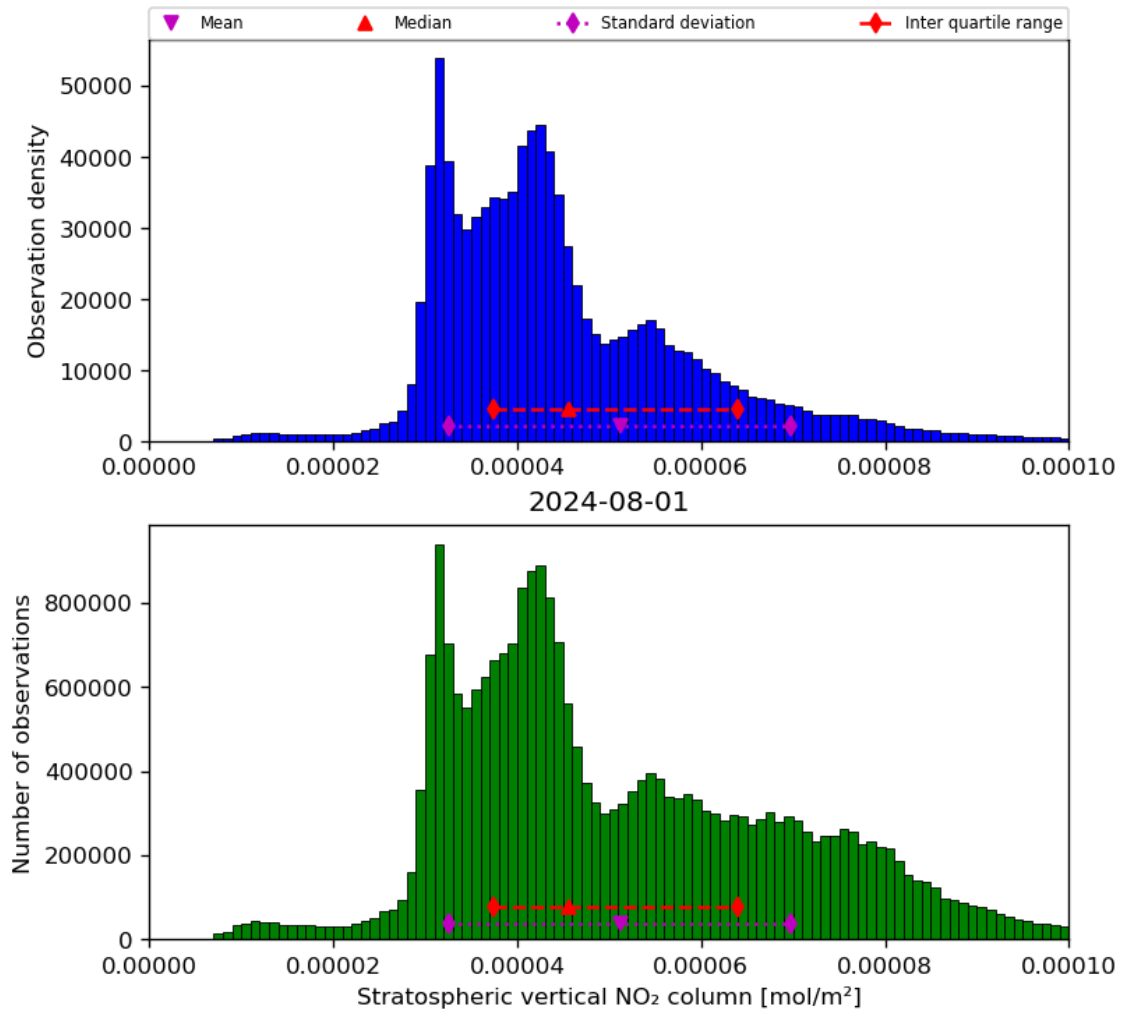
Figure 36: Histogram of “Stratospheric vertical NO 2 column” for 2024-07-31 to 2024-08-02
