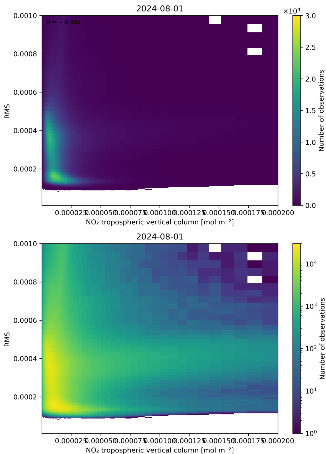
Figure 142: Scatter density plot of “NO 2 tropospheric vertical column” against “RMS” for 2024-07-31 to 2024-08-02.
