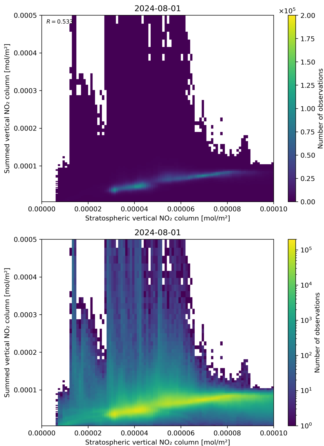
Figure 98: Scatter density plot of “Stratospheric vertical NO 2 column” against “Summed vertical NO 2 column” for 2024-07-31 to 2024-08-02.
