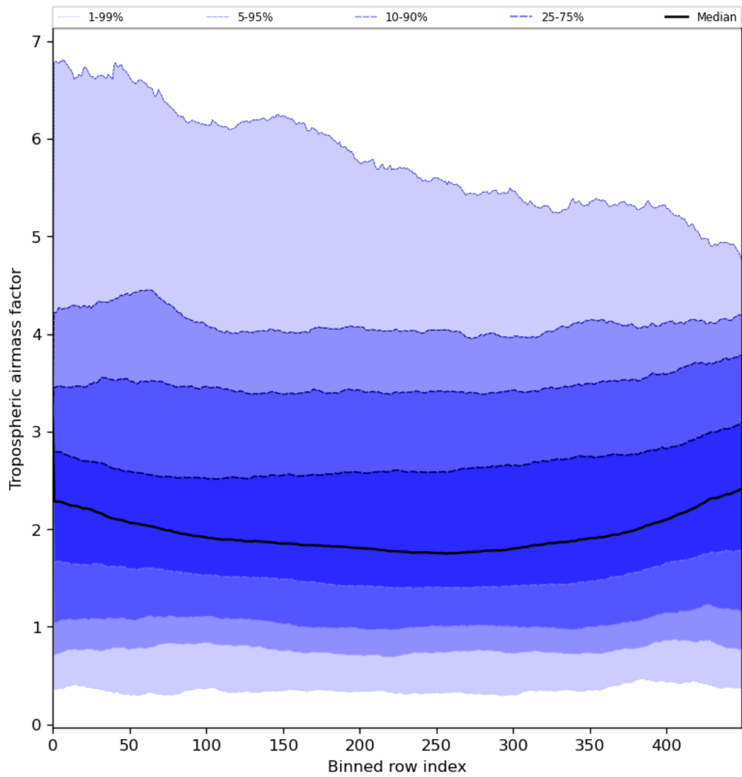
Figure 48: Along track statistics of “Tropospheric airmass factor” for 2024-07-31 to 2024-08-02
