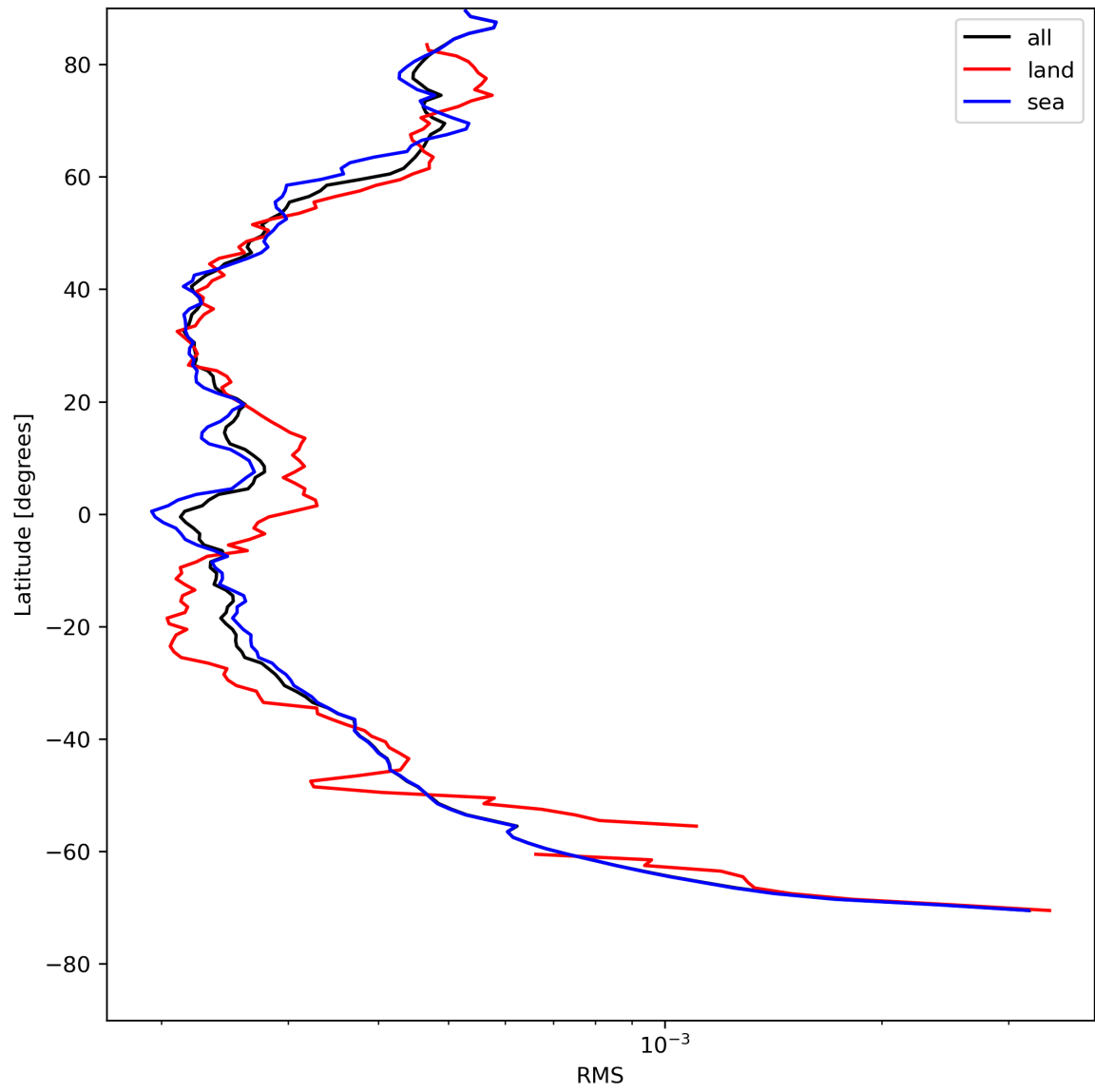
Figure 26: Zonal average of “RMS” for 2024-07-31 to 2024-08-02.
