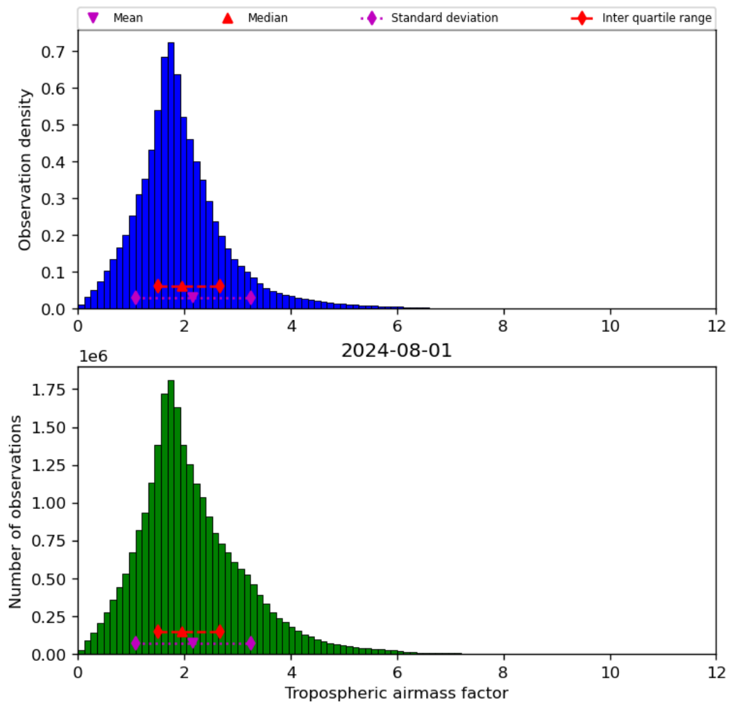
Figure 31: Histogram of “Tropospheric airmass factor” for 2024-07-31 to 2024-08-02
