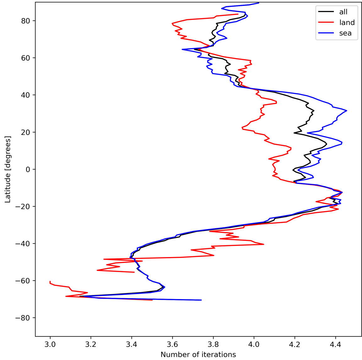
Figure 17: Zonal average of “Number of iterations” for 2024-07-31 to 2024-08-02.
