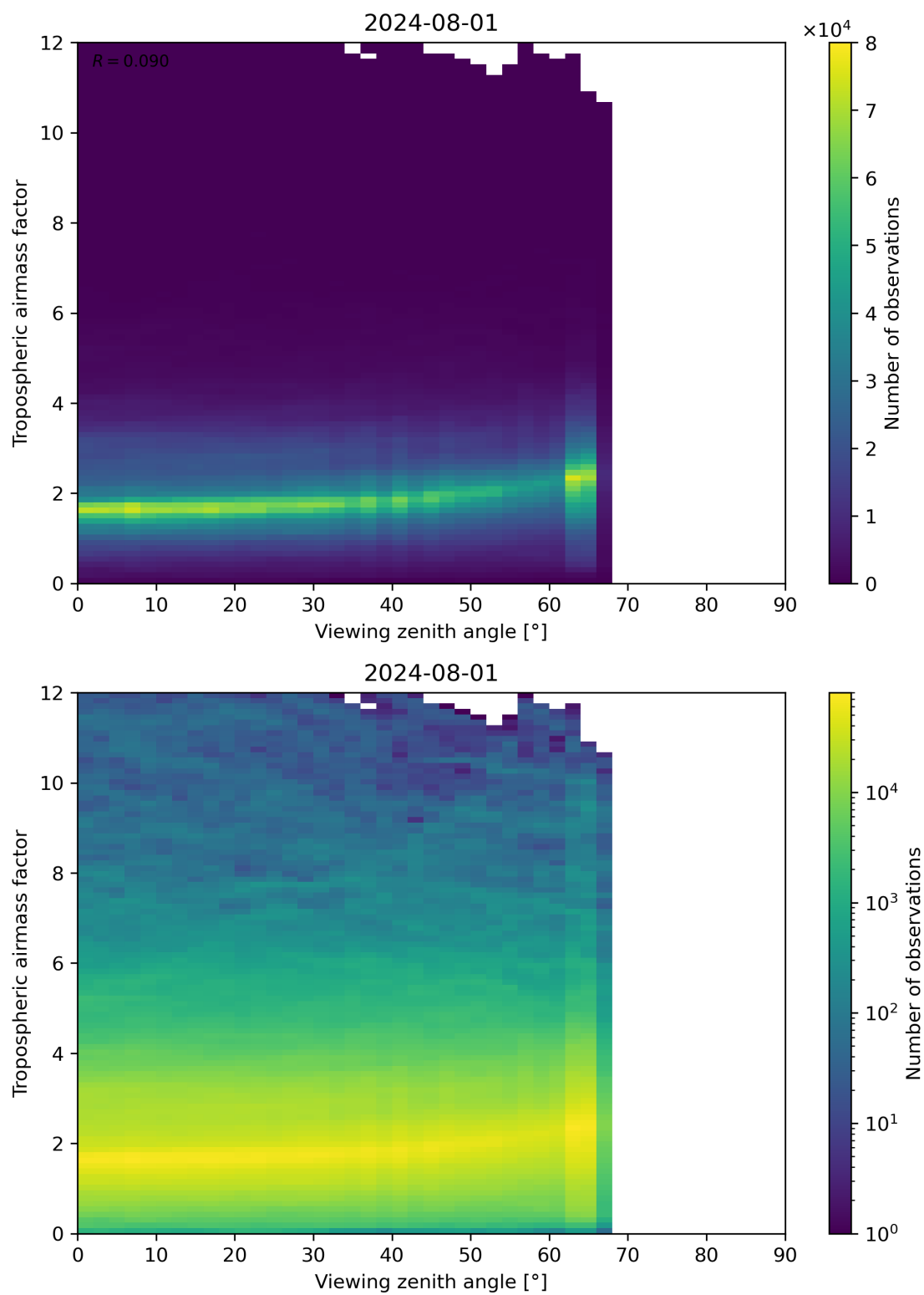
Figure 161: Scatter density plot of “Viewing zenith angle” against “Tropospheric airmass factor” for 2024-07-31 to 2024-08-02.
