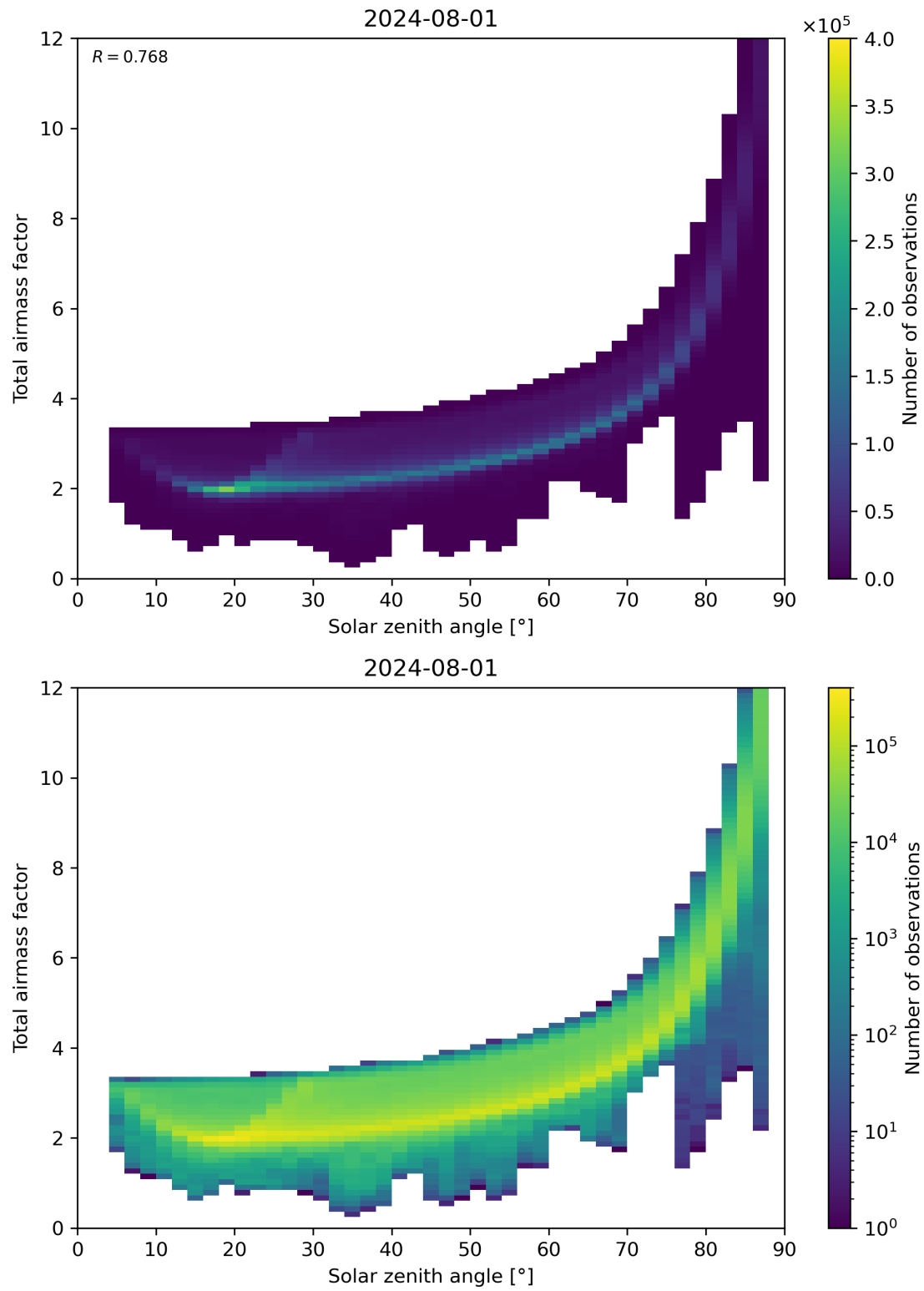
Figure 146: Scatter density plot of “Solar zenith angle” against “Total air mass factor” for 2024-07-31 to 2024-08-02.
