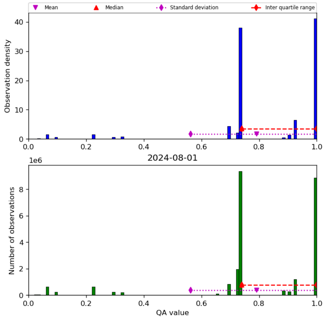
Figure 28: Histogram of “QA value” for 2024-07-31 to 2024-08-02
