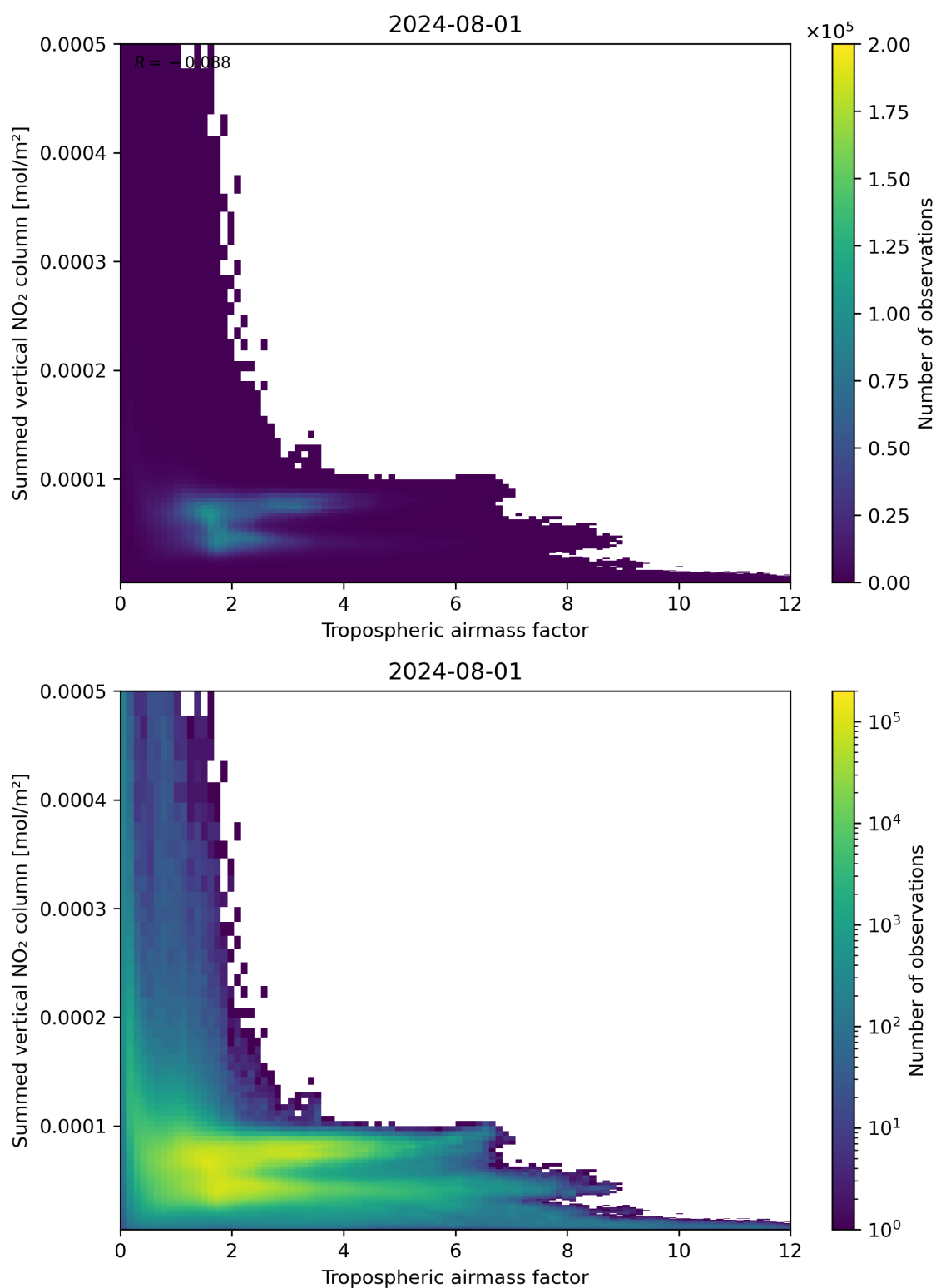
Figure 75: Scatter density plot of “Tropospheric airmass factor” against “Summed vertical NO 2 column” for 2024-07-31 to 2024-08-02.
