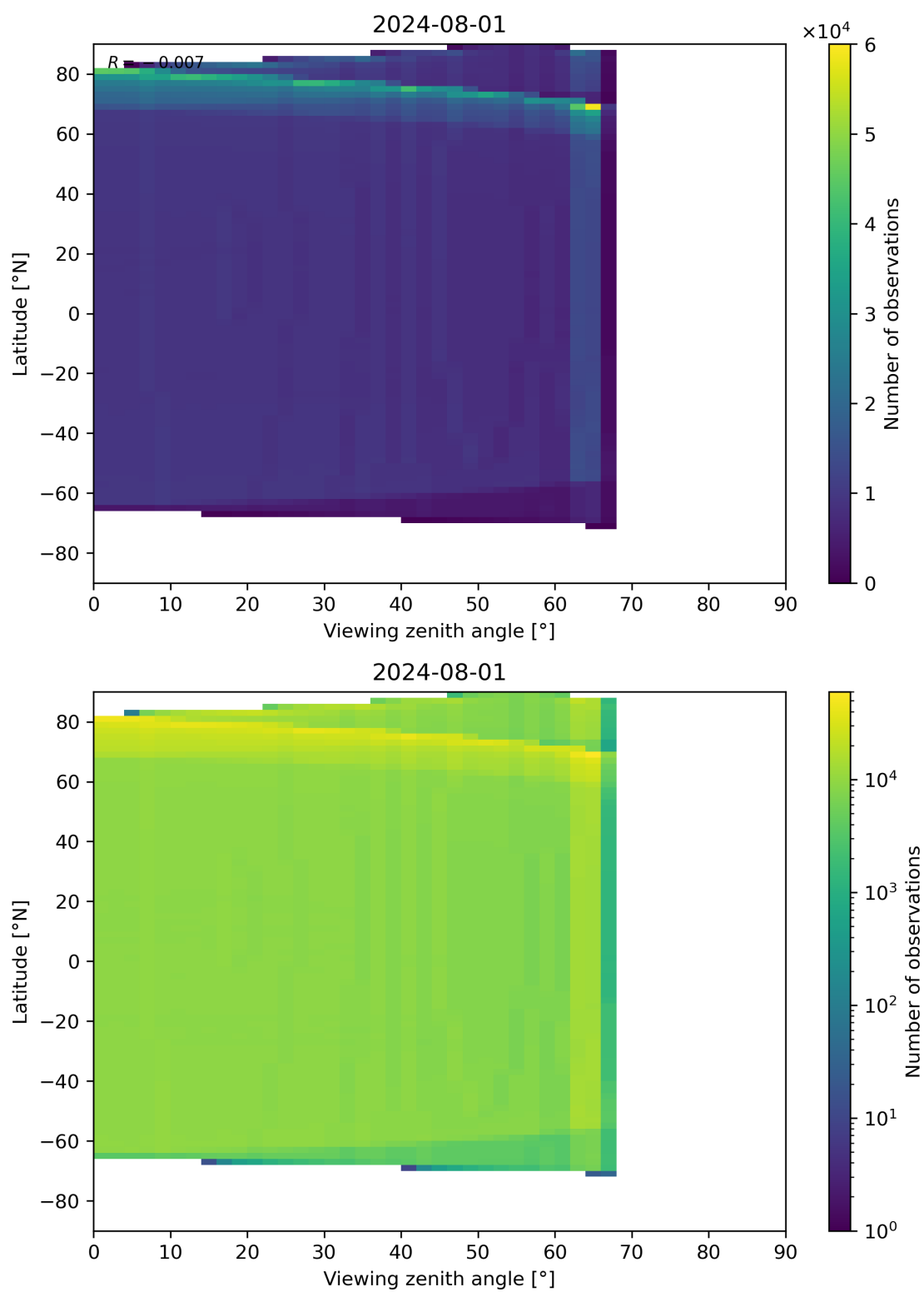
Figure 163: Scatter density plot of “Viewing zenith angle” against “Latitude” for 2024-07-31 to 2024-08-02.
