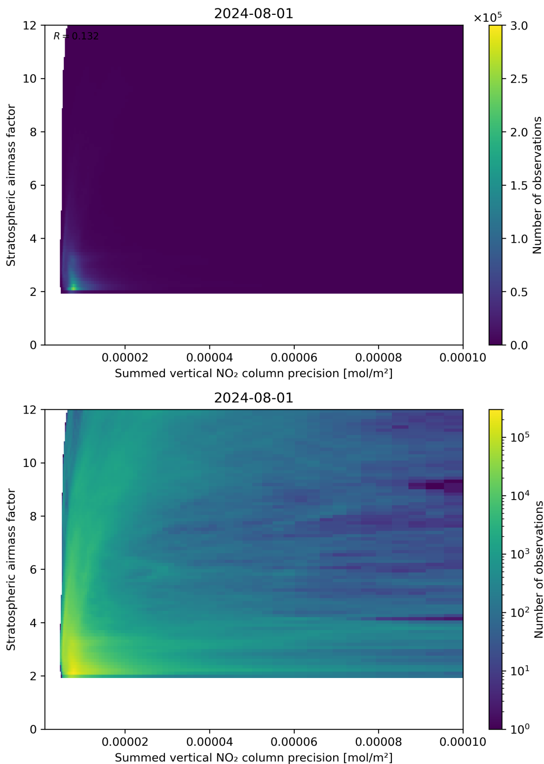
Figure 106: Scatter density plot of “Summed vertical NO 2 column precision” against “Stratospheric airmass factor” for 2024-07-31 to 2024-08-02.
