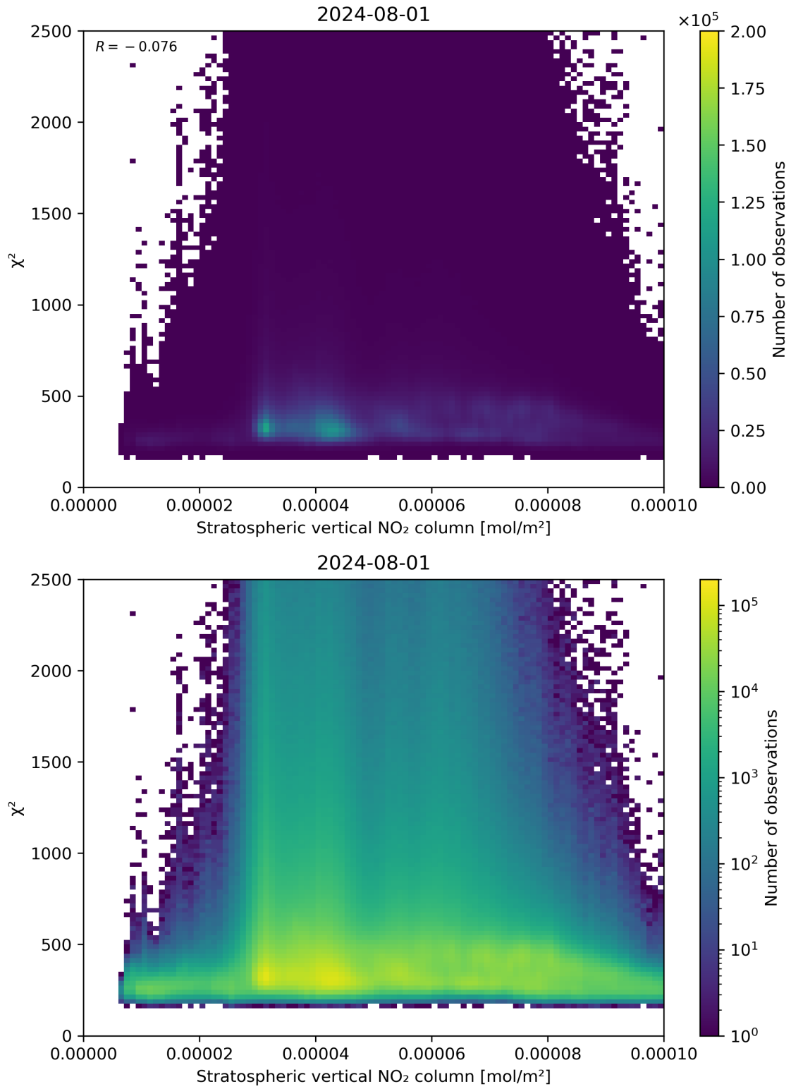
Figure 97: Scatter density plot of “Stratospheric vertical NO 2 column” against “ \chi^2 ” for 2024-07-31 to 2024-08-02.
