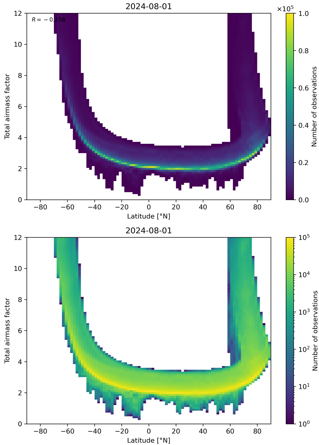
Figure 84: Scatter density plot of “Latitude” against “Total airmass factor” for 2024-07-31 to 2024-08-02.
