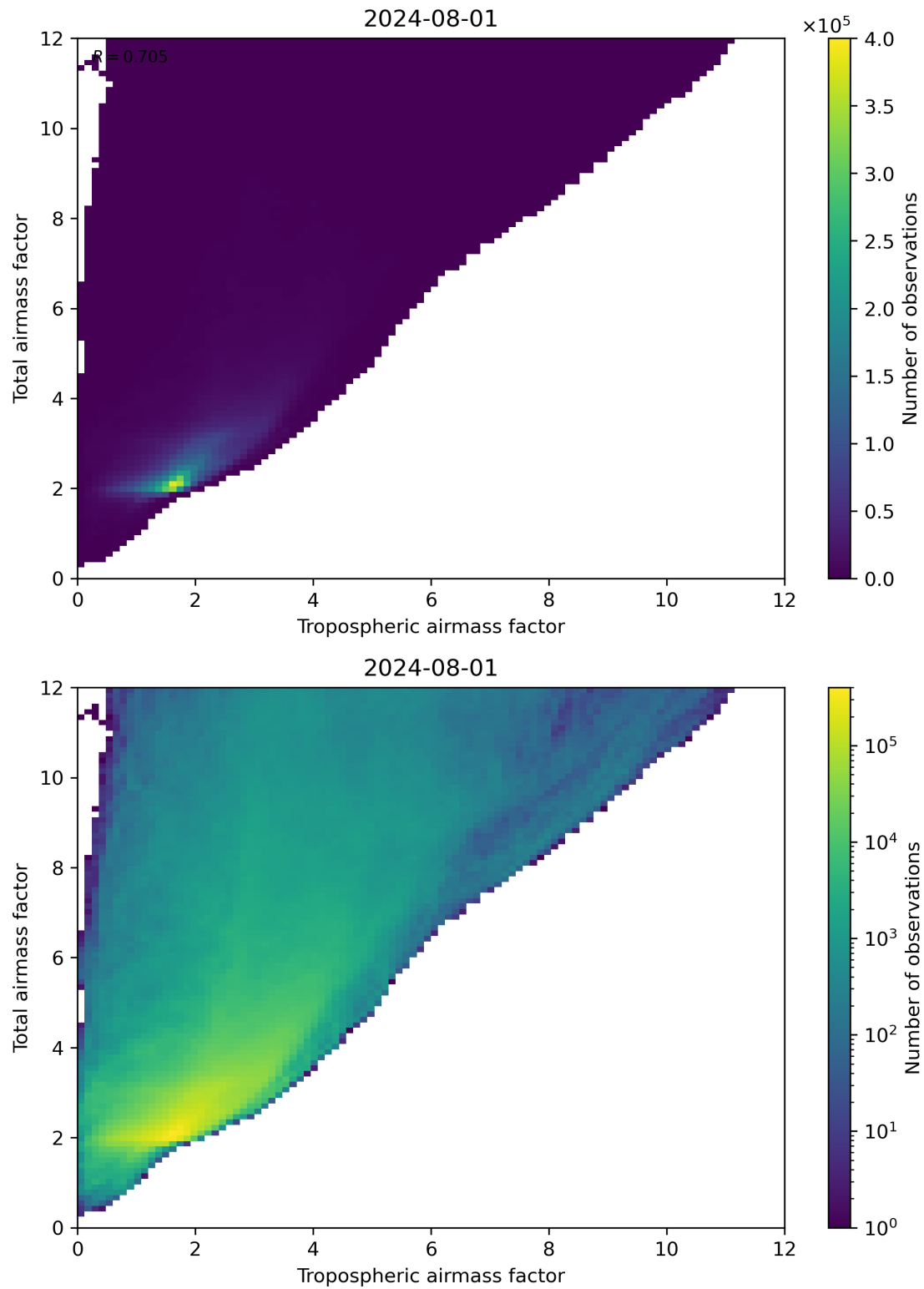
Figure 72: Scatter density plot of “Tropospheric airmass factor” against “Total airmass factor” for 2024-07-31 to 2024-08-02.
