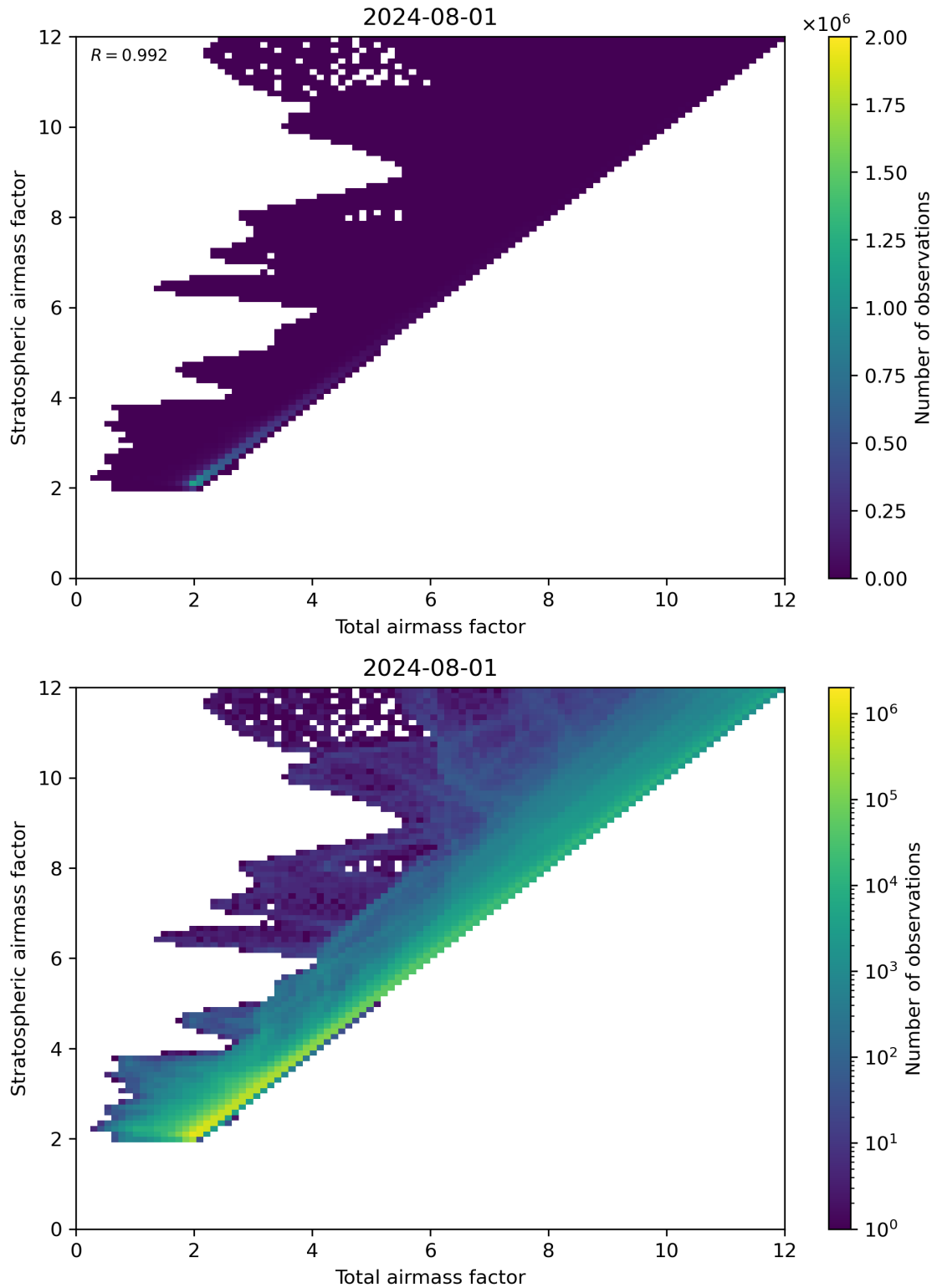
Figure 62: Scatter density plot of “Total airmass factor” against “Stratospheric airmass factor” for 2024-07-31 to 2024-08-02.
