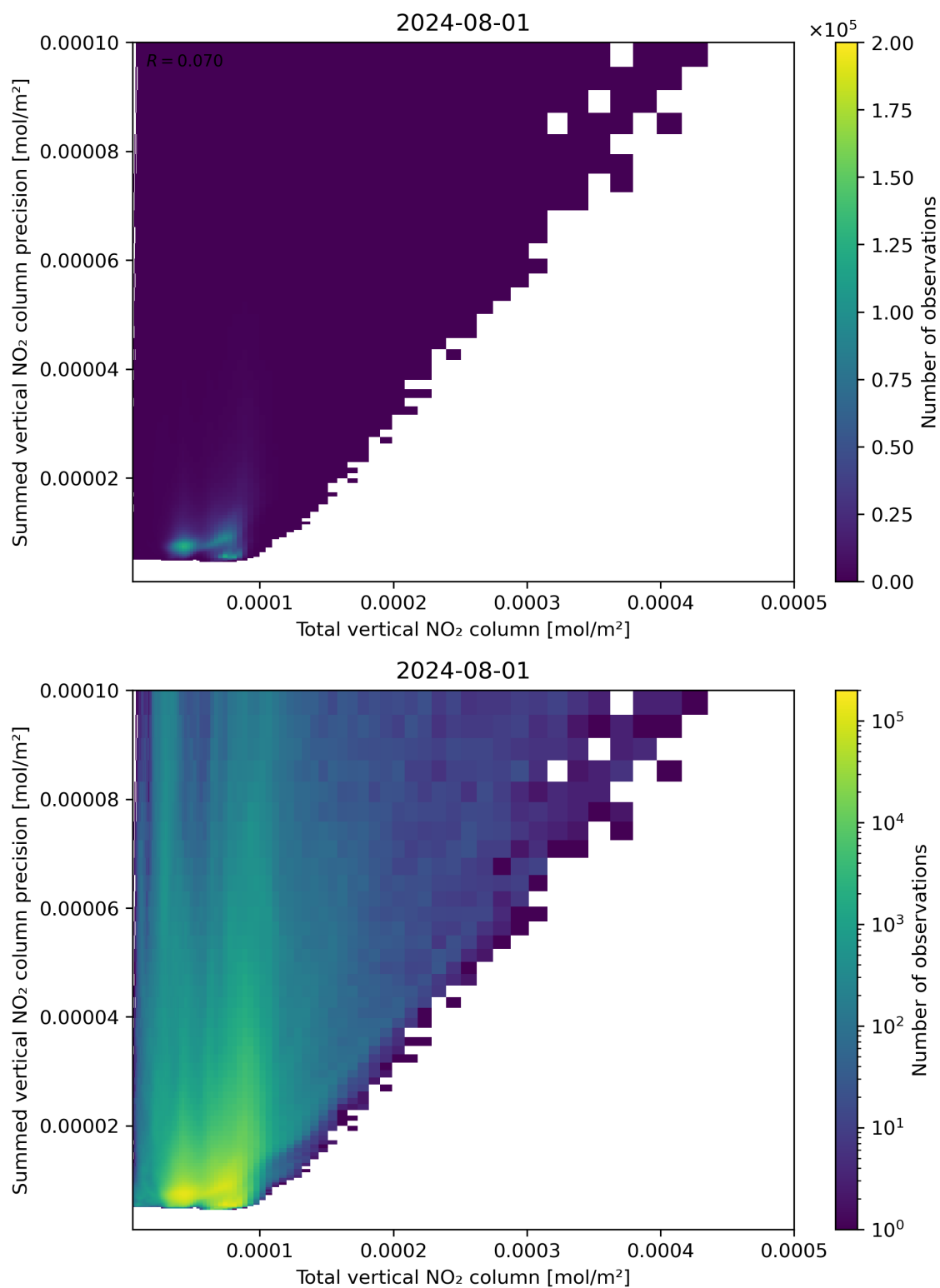
Figure 113: Scatter density plot of “Total vertical NO 2 column” against “Summed vertical NO 2 column precision” for 2024-07-31 to 2024-08-02.
