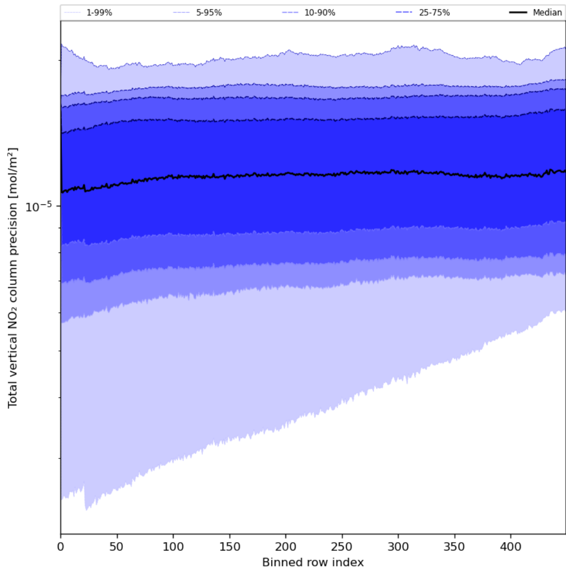
Figure 56: Along track statistics of “Total vertical NO 2 column precision” for 2024-07-31 to 2024-08-02
