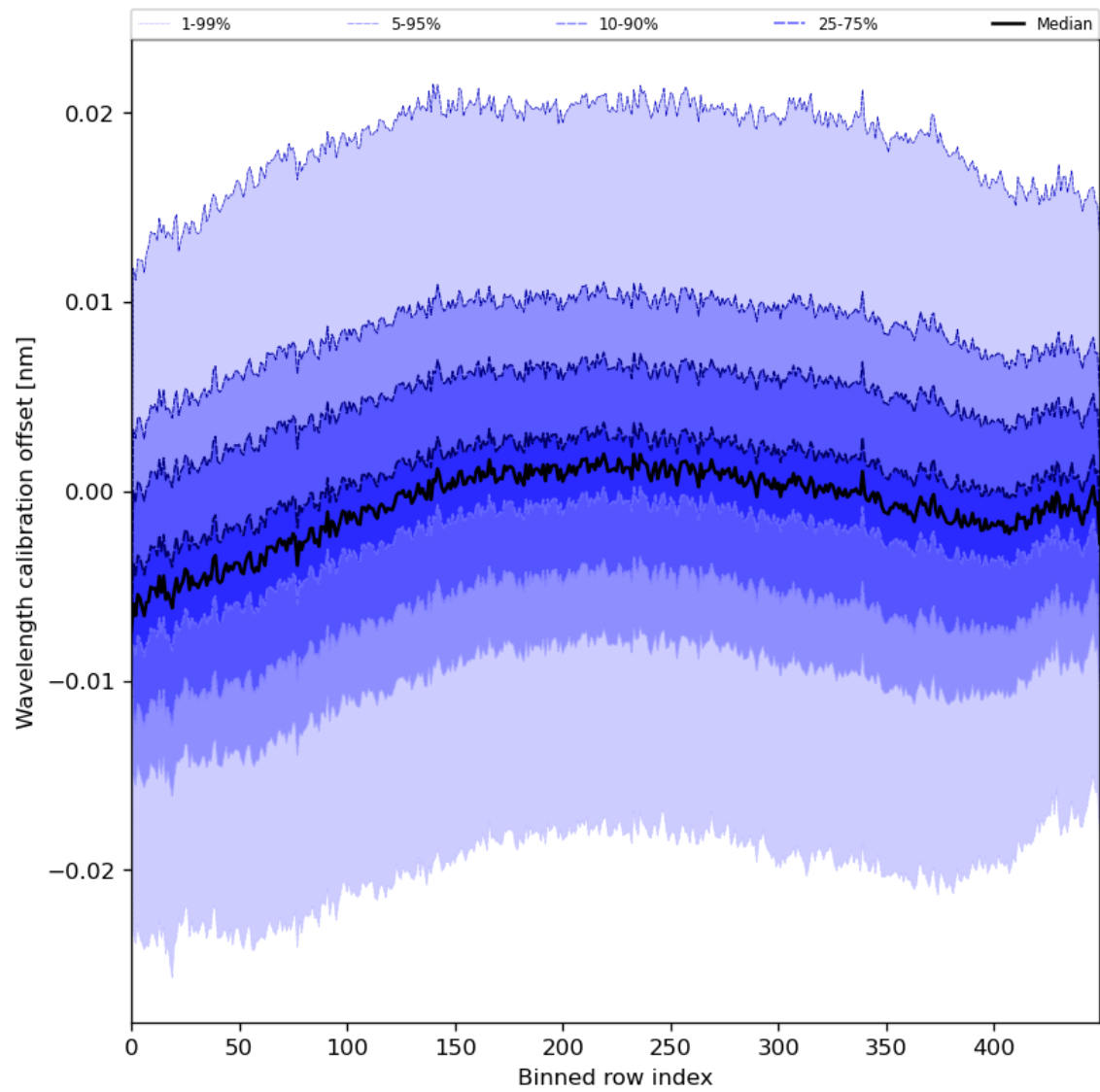
Figure 52: Along track statistics of “Wavelength calibration offset” for 2024-07-31 to 2024-08-02
