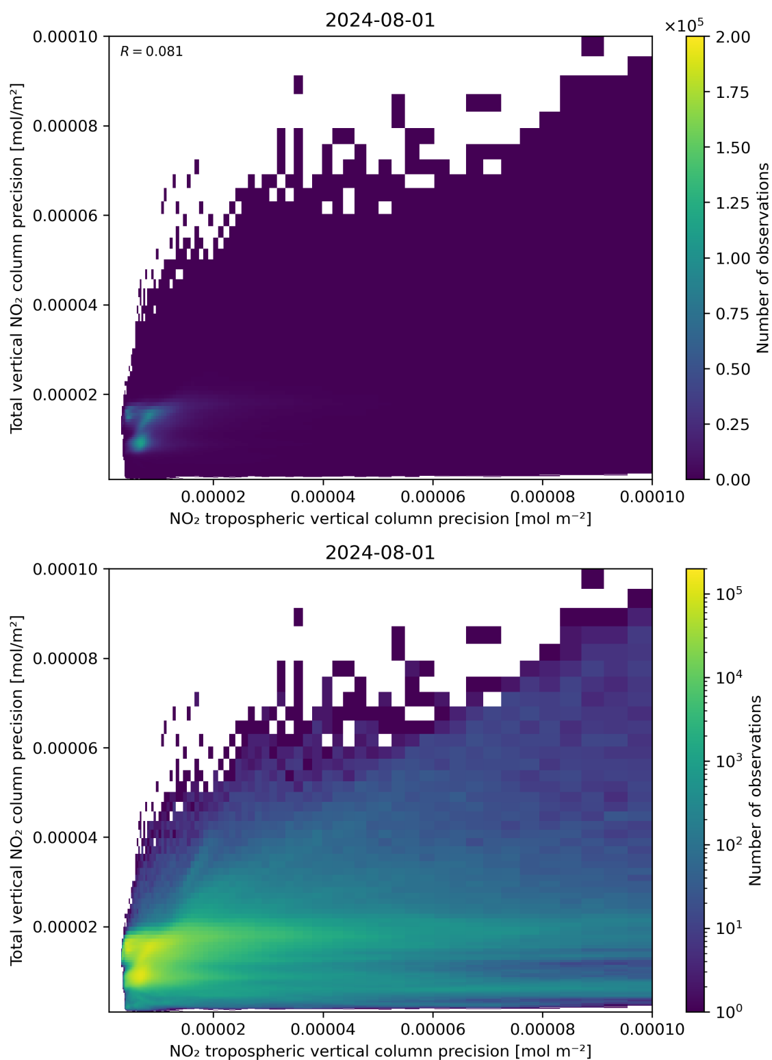
Figure 139: Scatter density plot of “NO 2 tropospheric vertical column precision” against “Total vertical NO 2 column precision” for 2024-07-31 to 2024-08-02.
