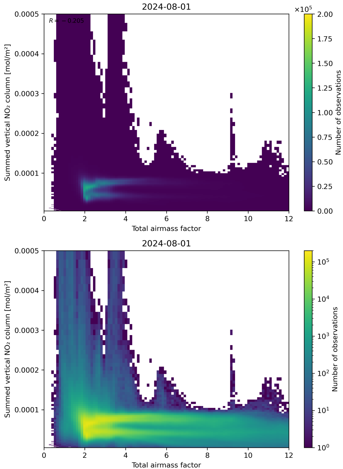
Figure 65: Scatter density plot of “Total airmass factor” against “Summed vertical NO 2 column” for 2024-07-31 to 2024-08-02.
