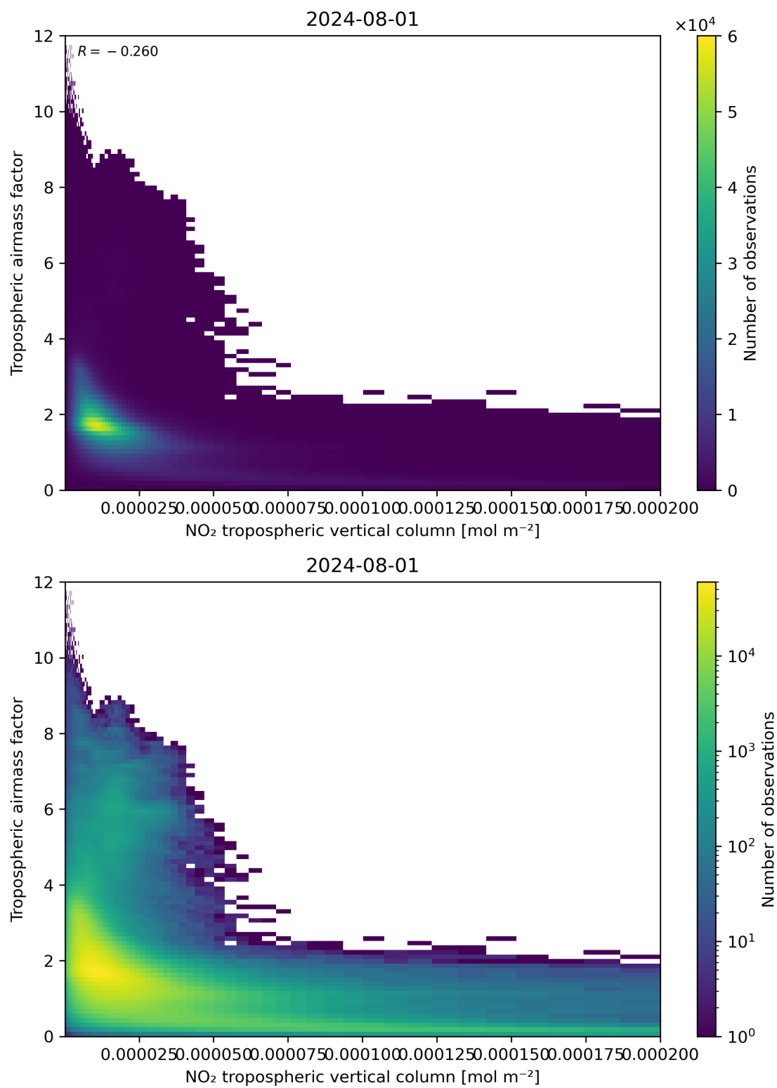
Figure 123: Scatter density plot of “NO 2 tropospheric vertical column” against “Tropospheric air mass factor” for 2024-07-31 to 2024-08-02.
