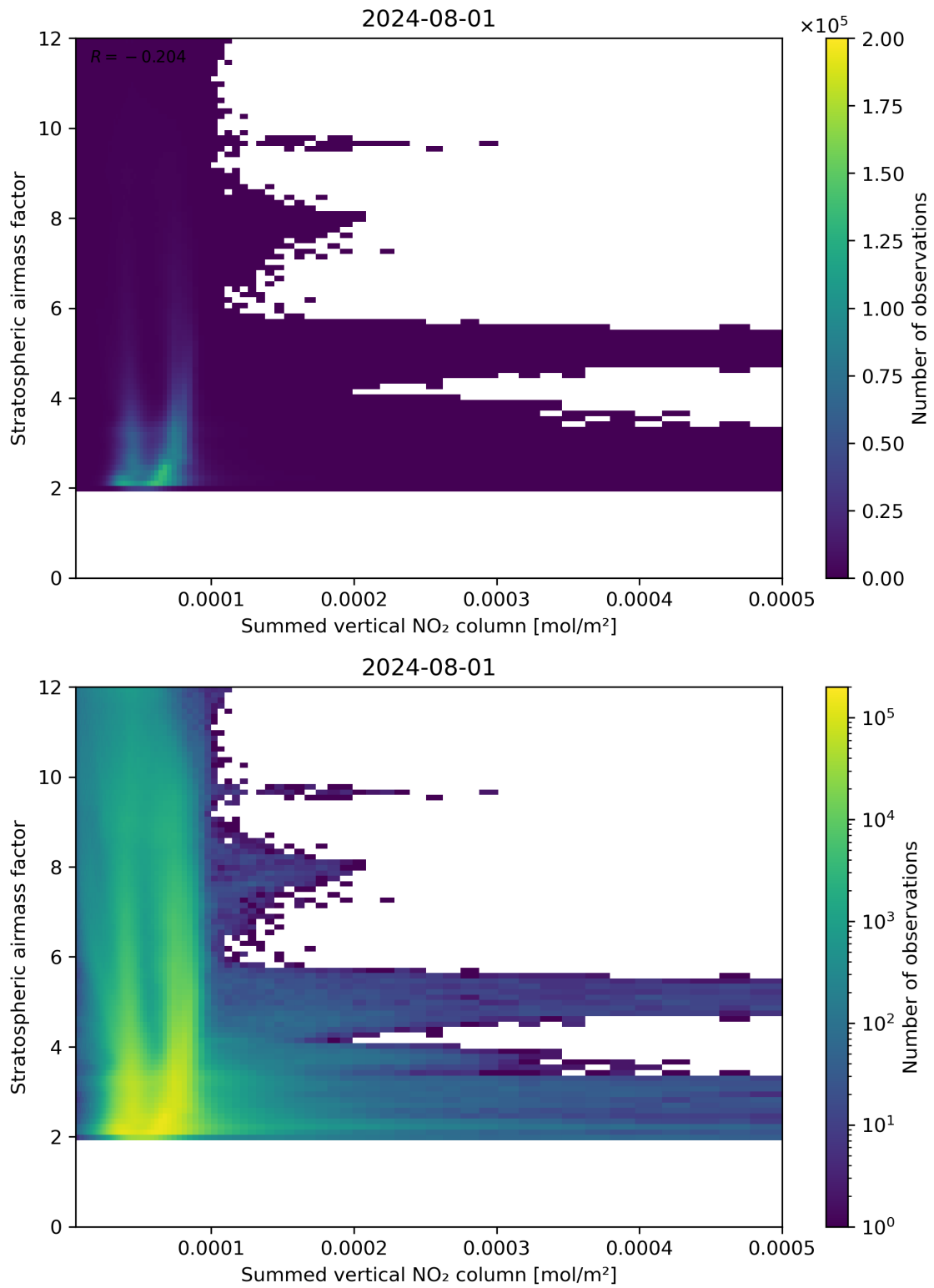
Figure 103: Scatter density plot of “Summed vertical NO 2 column” against “Stratospheric air mass factor” for 2024-07-31 to 2024-08-02.
