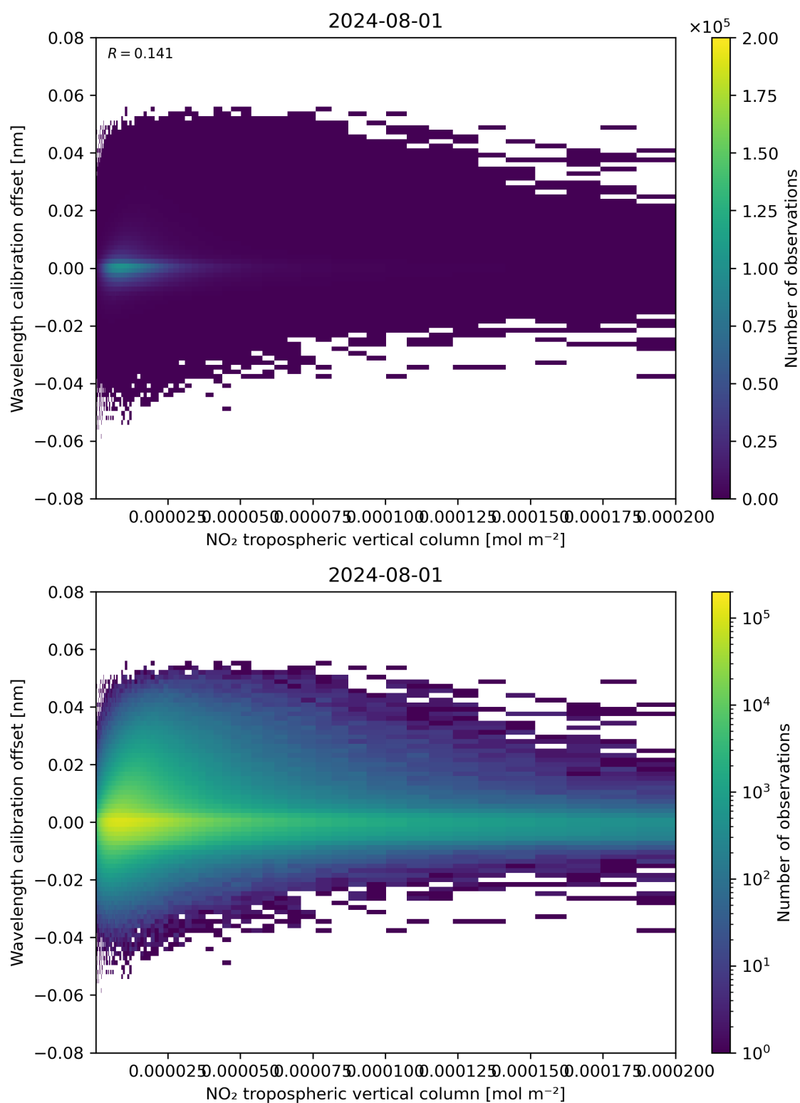
Figure 143: Scatter density plot of “NO 2 tropospheric vertical column” against “Wavelength calibration offset” for 2024-07-31 to 2024-08-02.
