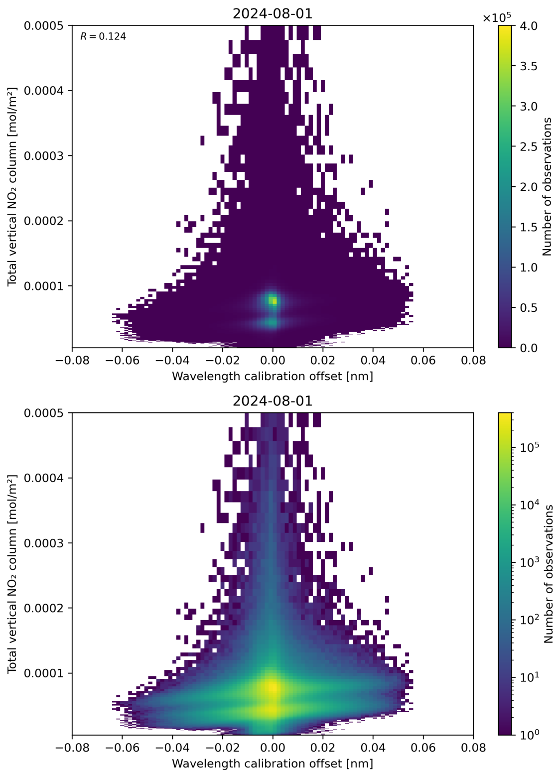
Figure 179: Scatter density plot of “Wavelength calibration offset” against “Total vertical NO 2 column” for 2024-07-31 to 2024-08-02.
