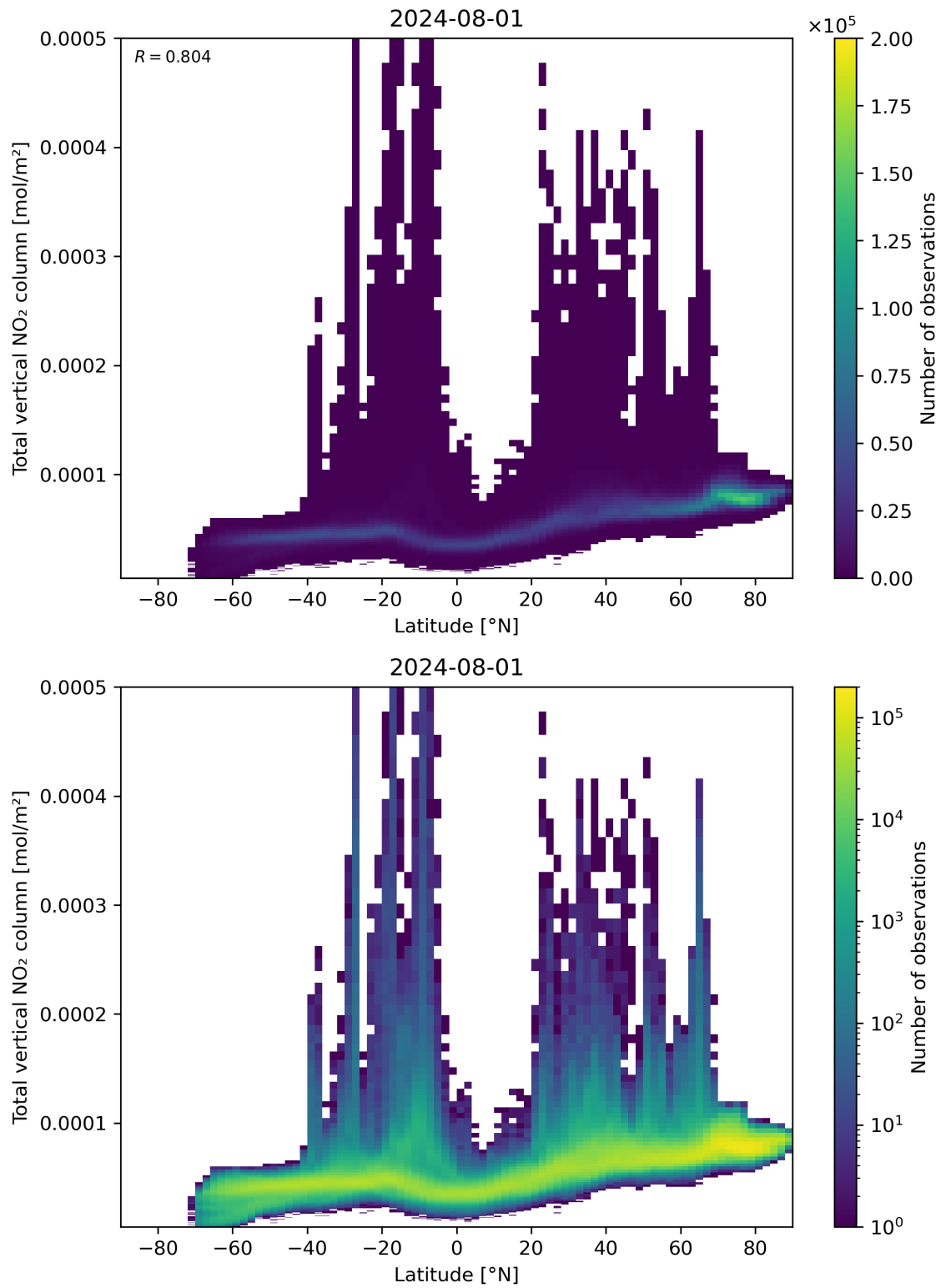
Figure 90: Scatter density plot of “Latitude” against “Total vertical NO 2 column” for 2024-07-31 to 2024-08-02.
