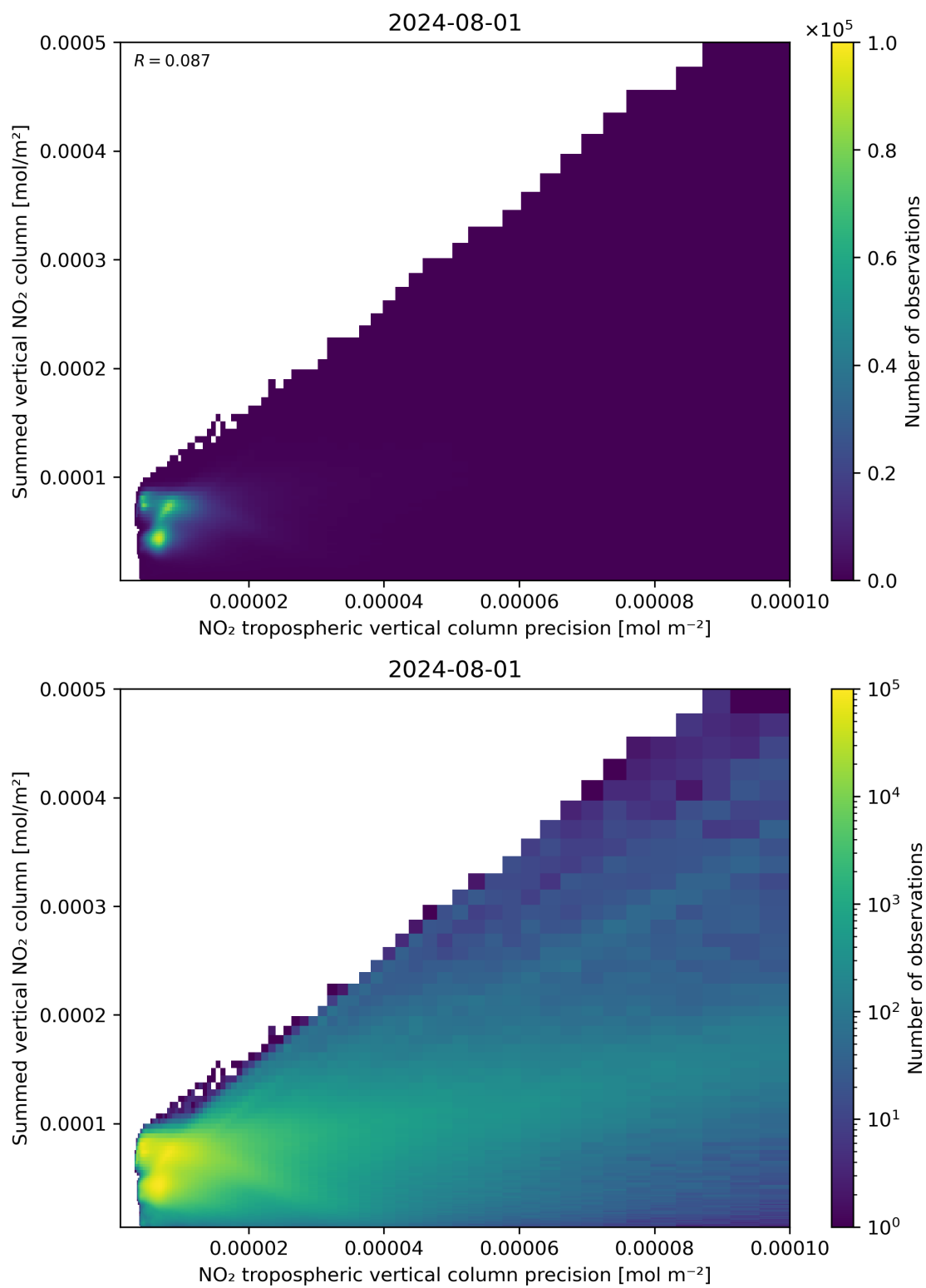
Figure 136: Scatter density plot of “NO 2 tropospheric vertical column precision” against “Summed vertical NO 2 column” for 2024-07-31 to 2024-08-02.
