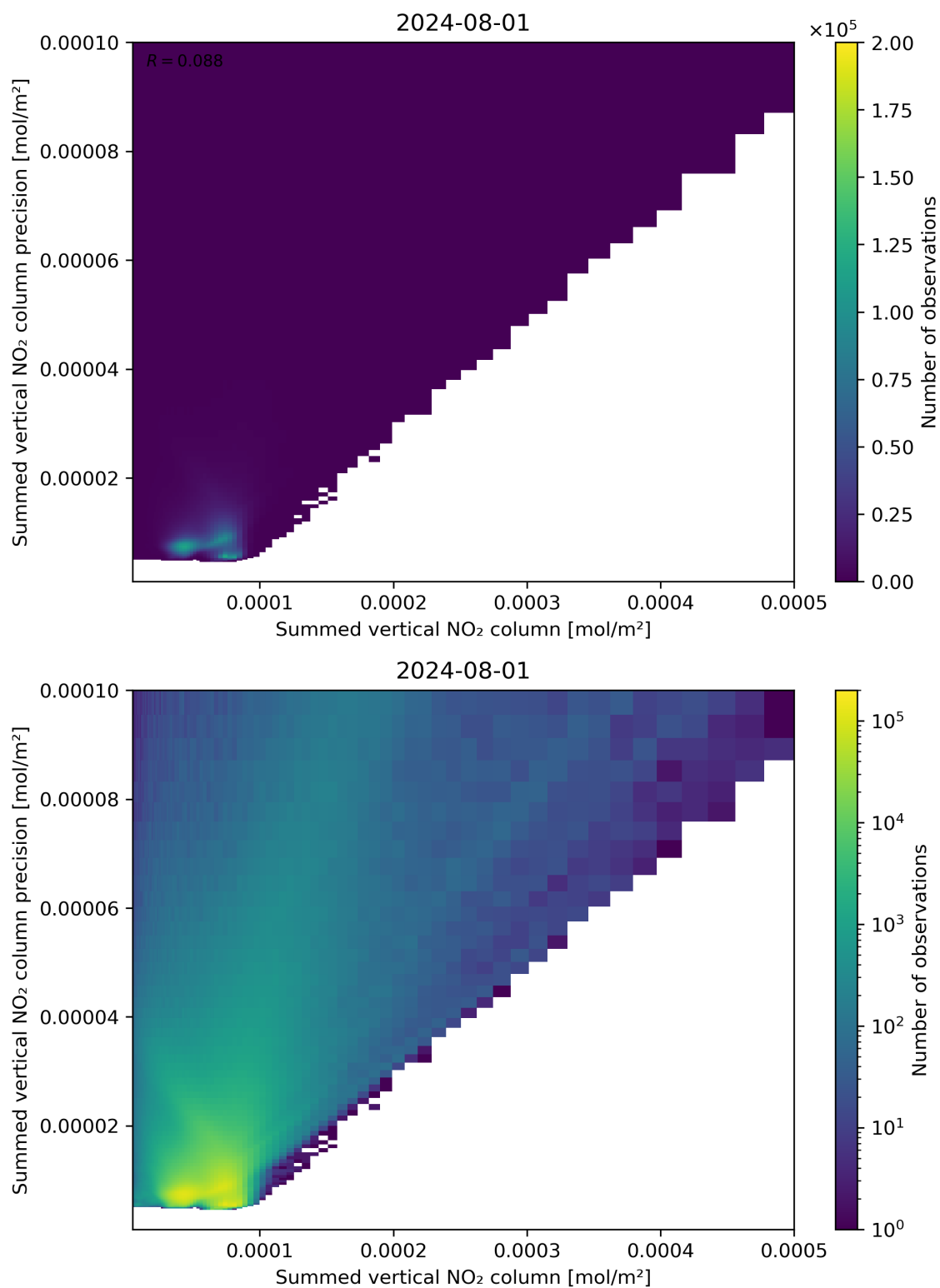
Figure 105: Scatter density plot of “Summed vertical NO 2 column” against “Summed vertical NO 2 column precision” for 2024-07-31 to 2024-08-02.
