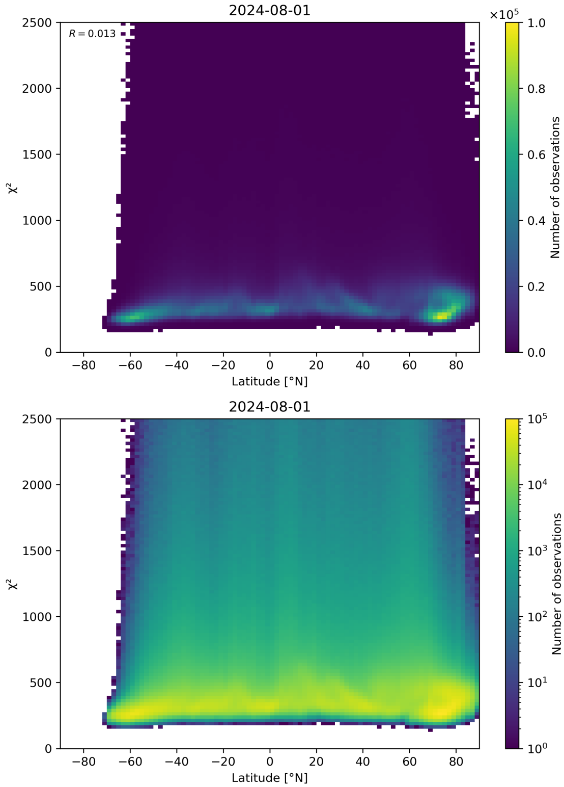
Figure 86: Scatter density plot of “Latitude” against “ \chi^2 ” for 2024-07-31 to 2024-08-02.
