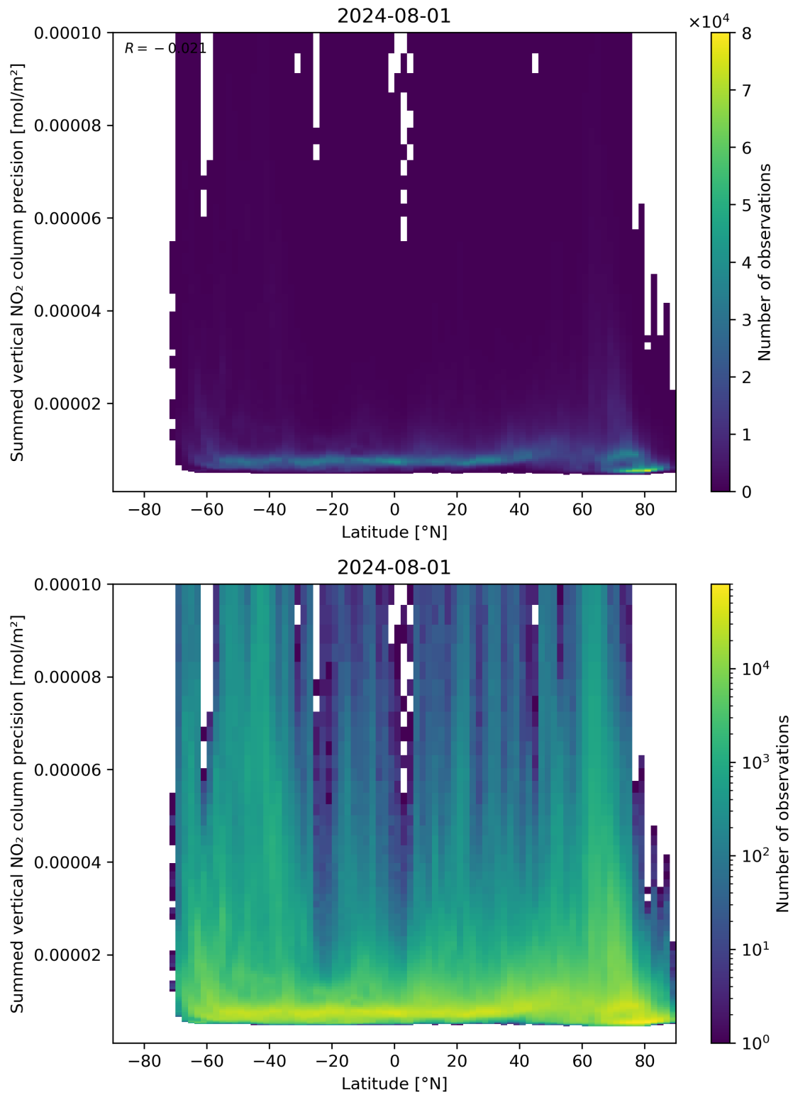
Figure 89: Scatter density plot of “Latitude” against “Summed vertical NO 2 column precision” for 2024-07-31 to 2024-08-02.
