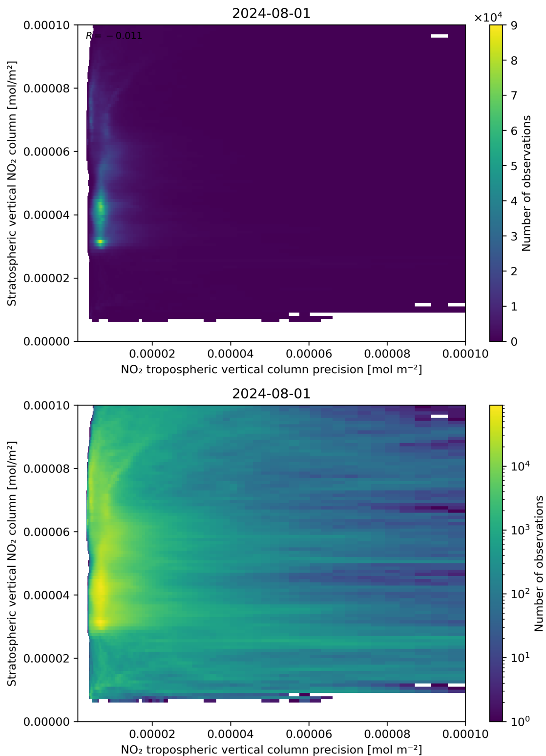
Figure 135: Scatter density plot of “NO 2 tropospheric vertical column precision” against “Stratospheric vertical NO 2 column” for 2024-07-31 to 2024-08-02.
