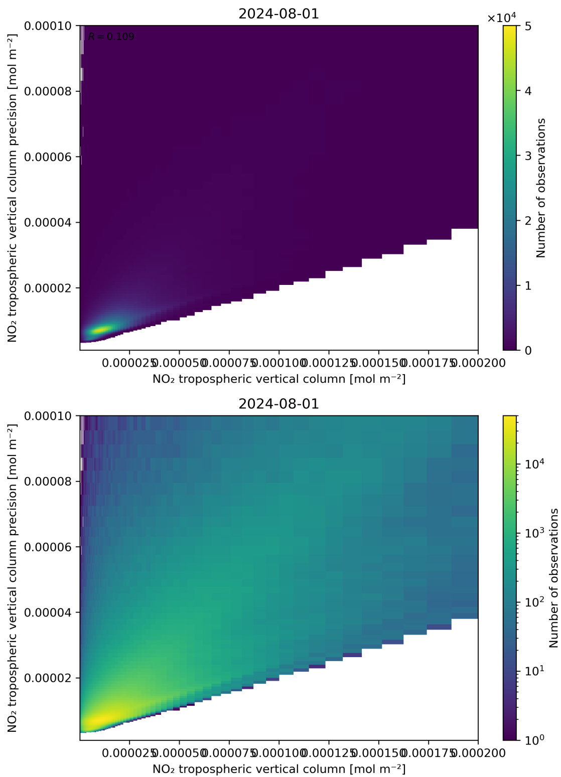
Figure 130: Scatter density plot of “NO 2 tropospheric vertical column” against “NO 2 tropospheric vertical column precision” for 2024-07-31 to 2024-08-02.
