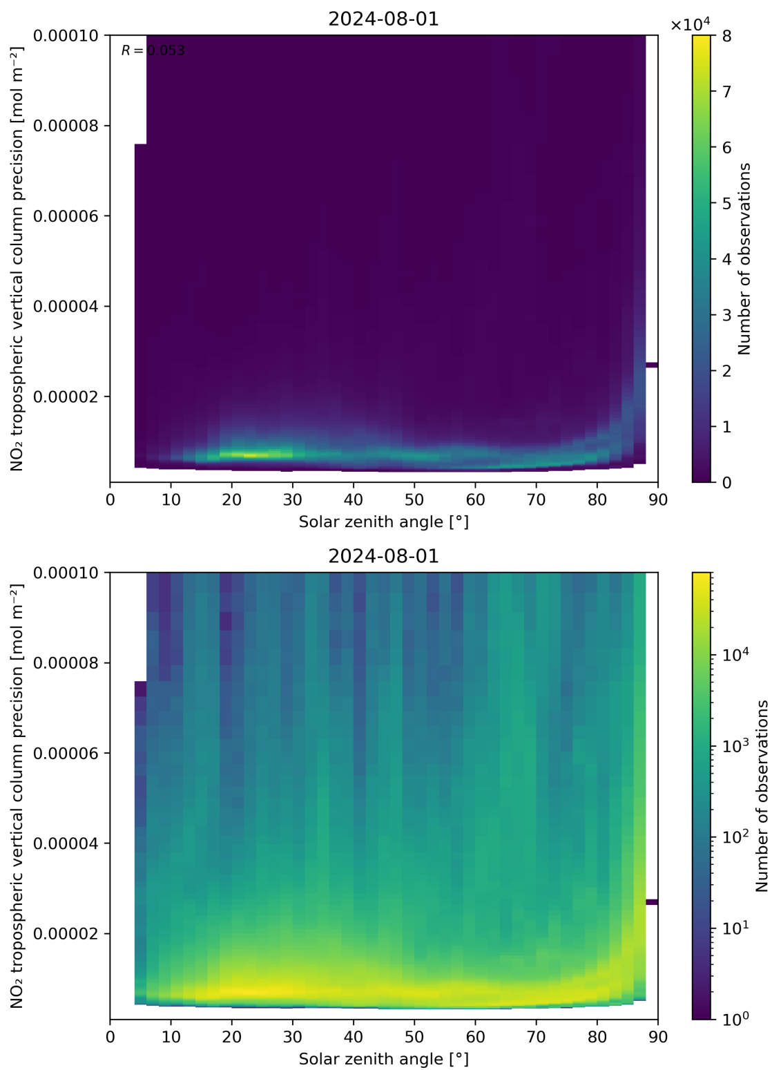
Figure 156: Scatter density plot of “Solar zenith angle” against “NO 2 tropospheric vertical column precision” for 2024-07-31 to 2024-08-02.
