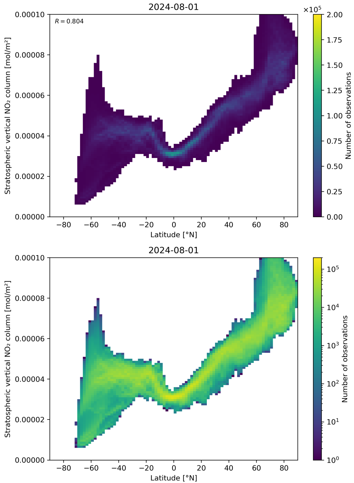
Figure 87: Scatter density plot of “Latitude” against “Stratospheric vertical NO 2 column” for 2024-07-31 to 2024-08-02.
