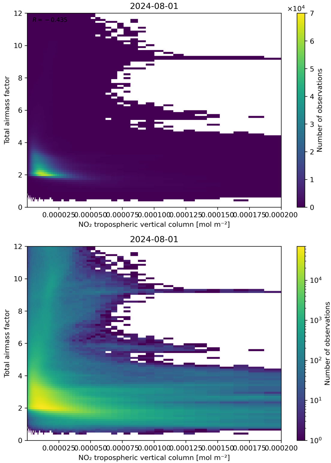
Figure 122: Scatter density plot of “NO 2 tropospheric vertical column” against “Total air mass factor” for 2024-07-31 to 2024-08-02.
