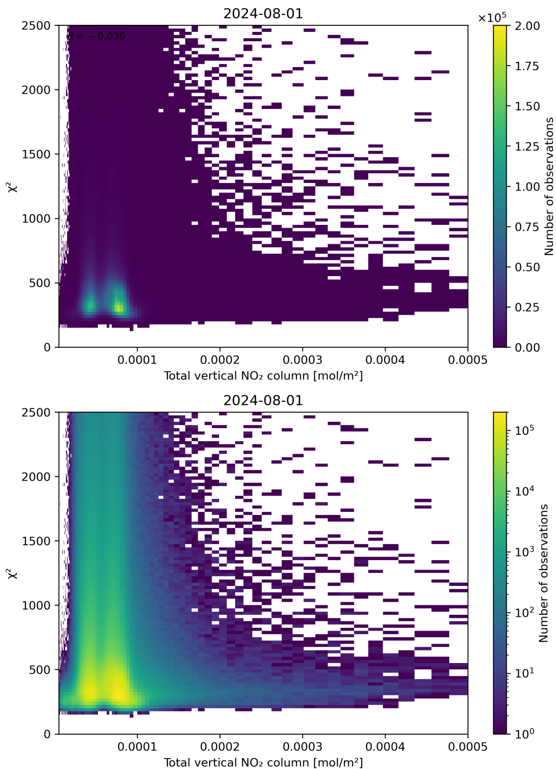
Figure 111: Scatter density plot of “Total vertical NO 2 column” against “ \chi^2 ” for 2024-07-31 to 2024-08-02.
