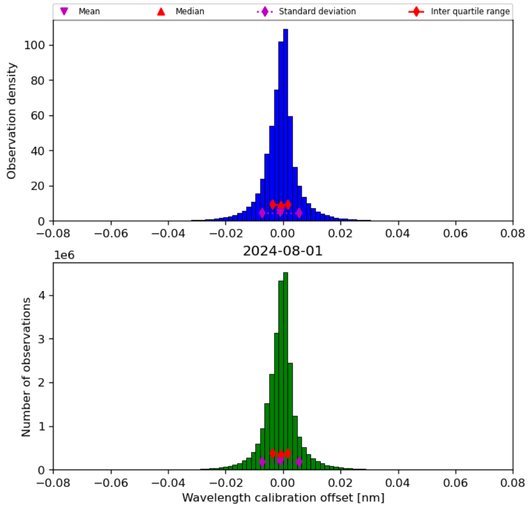
Figure 35: Histogram of “Wavelength calibration offset” for 2024-07-31 to 2024-08-02
