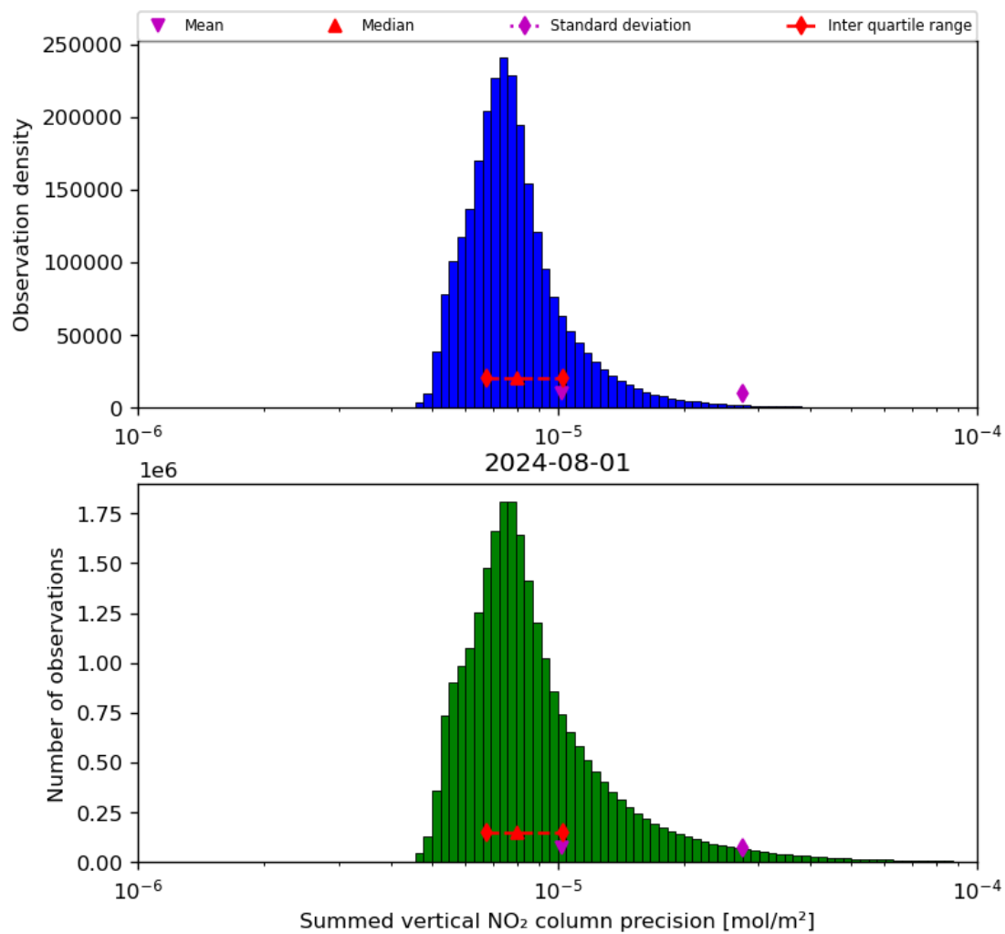
Figure 41: Histogram of “Summed vertical NO 2 column precision” for 2024-07-31 to 2024-08-02
