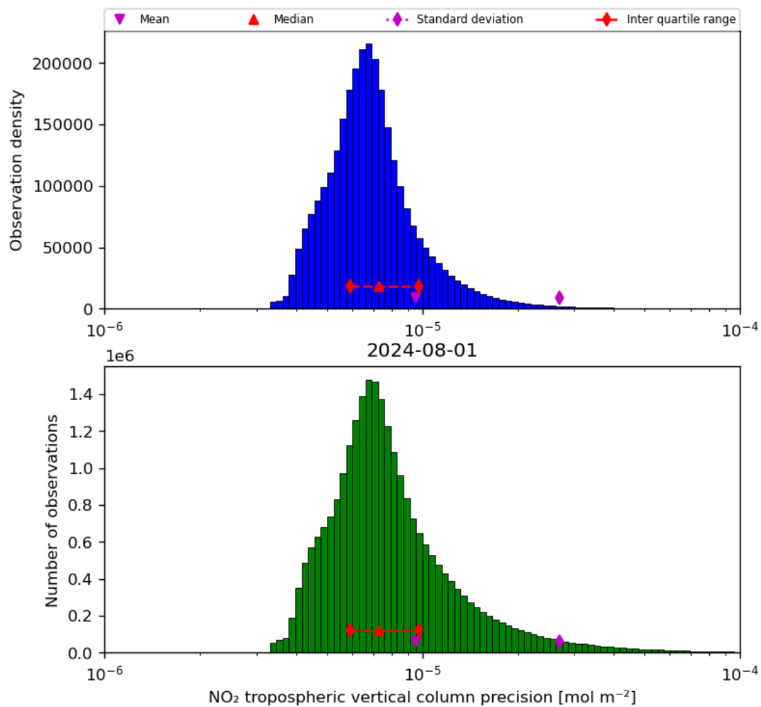
Figure 30: Histogram of “NO 2 tropospheric vertical column precision” for 2024-07-31 to 2024-08-02
