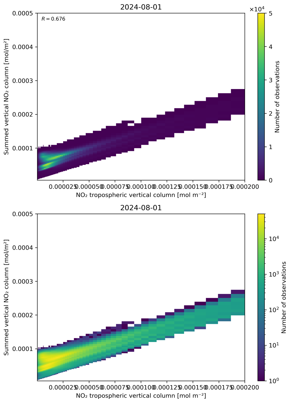
Figure 126: Scatter density plot of “NO 2 tropospheric vertical column” against “Summed vertical NO 2 column” for 2024-07-31 to 2024-08-02.
