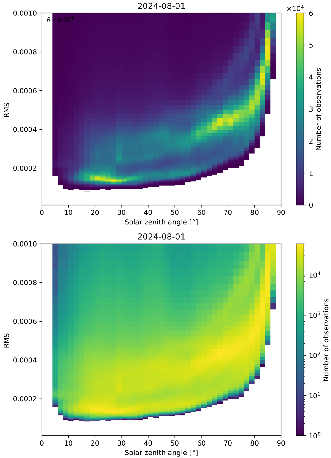
Figure 157: Scatter density plot of “Solar zenith angle” against “RMS” for 2024-07-31 to 2024-08-02.
