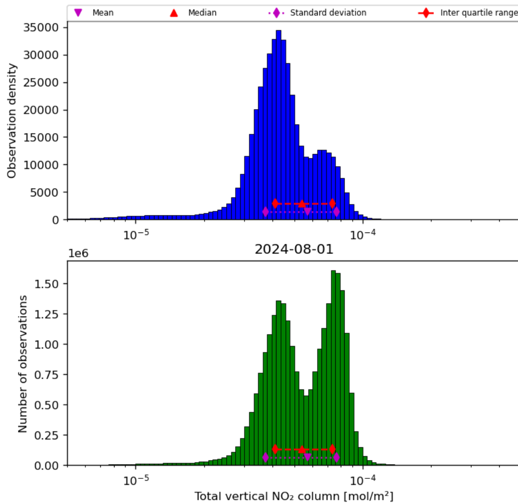
Figure 38: Histogram of “Total vertical NO 2 column” for 2024-07-31 to 2024-08-02
