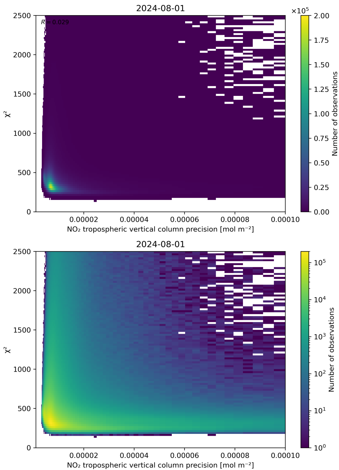
Figure 134: Scatter density plot of “NO 2 tropospheric vertical column precision” against “ \chi^2 ” for 2024-07-31 to 2024-08-02.
