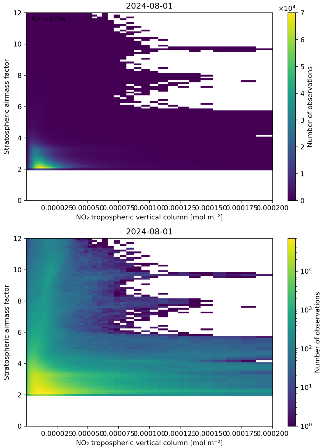
Figure 121: Scatter density plot of “NO 2 tropospheric vertical column” against “Stratospheric air mass factor” for 2024-07-31 to 2024-08-02.
