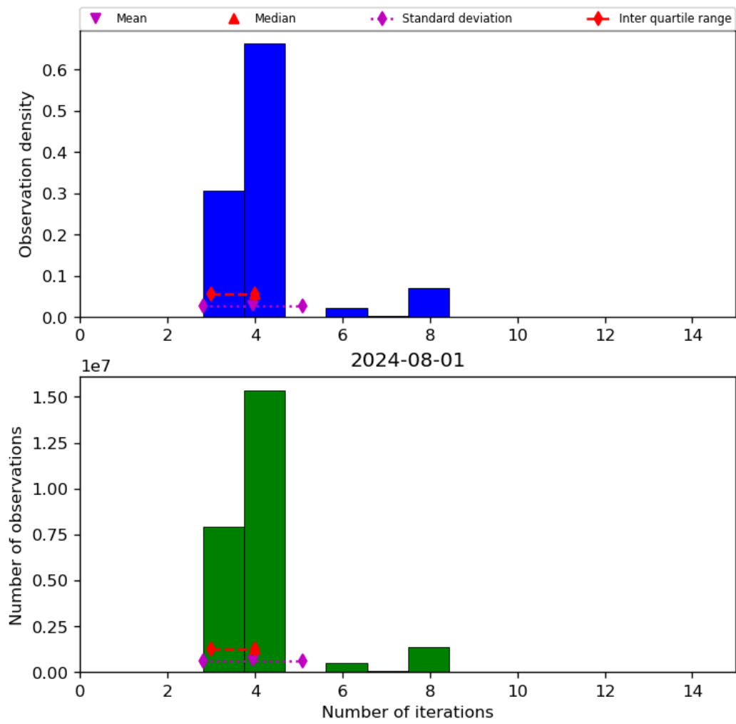
Figure 34: Histogram of “Number of iterations” for 2024-07-31 to 2024-08-02
