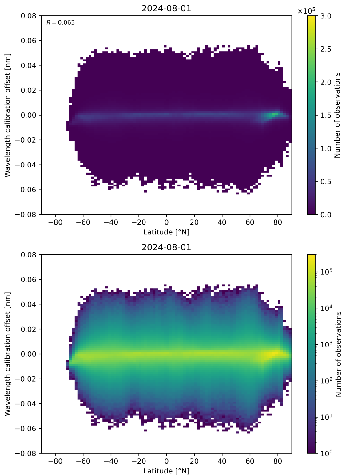
Figure 95: Scatter density plot of “Latitude” against “Wavelength calibration offset” for 2024-07-31 to 2024-08-02.
