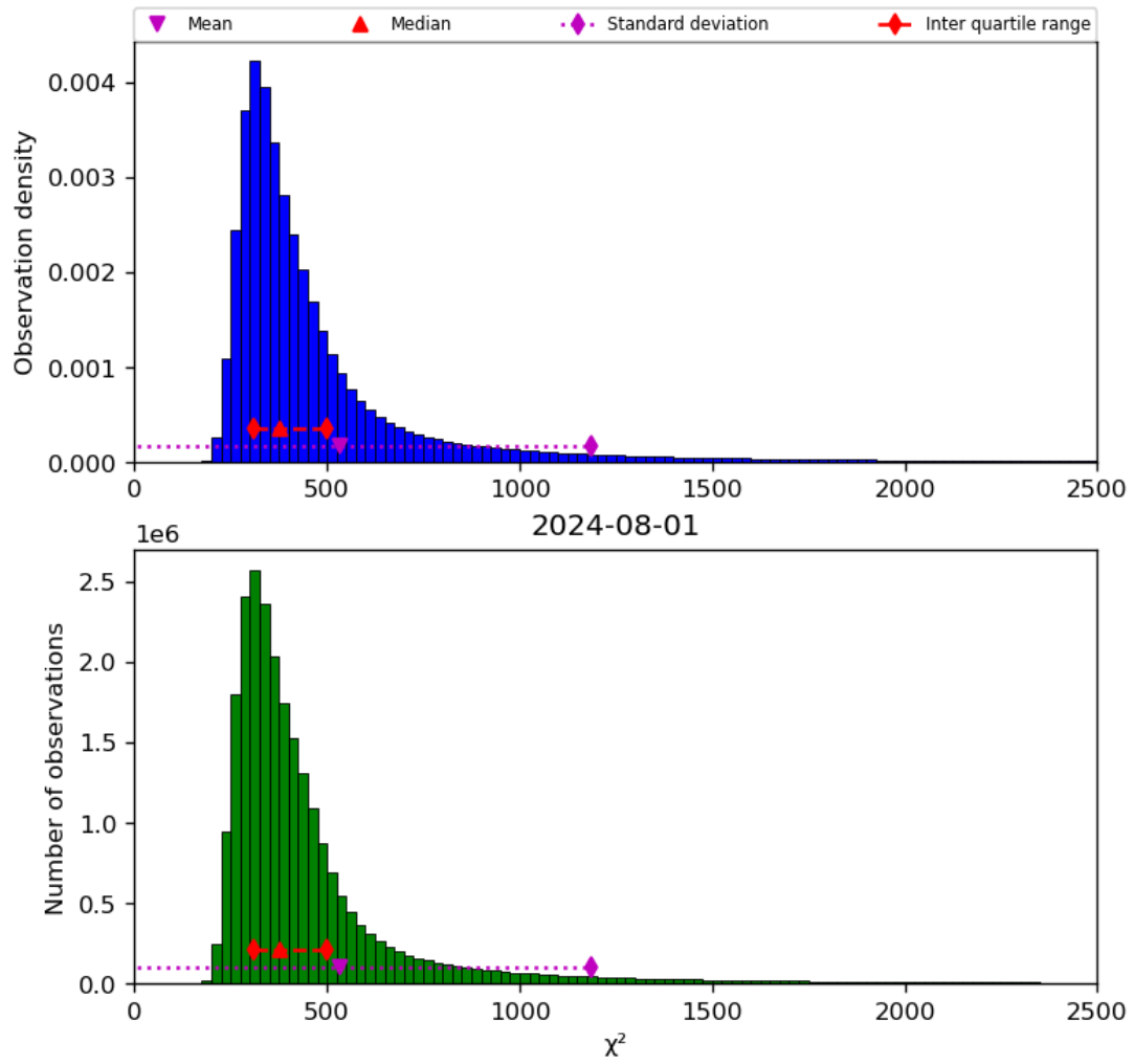
Figure 42: Histogram of “ \chi^2 ” for 2024-07-31 to 2024-08-02
