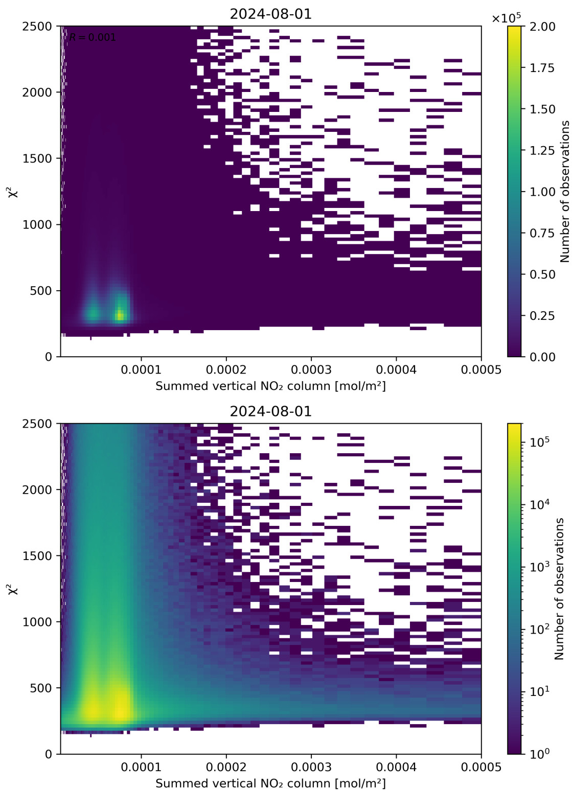
Figure 104: Scatter density plot of “Summed vertical NO 2 column” against “ \chi^2 ” for 2024-07-31 to 2024-08-02.
