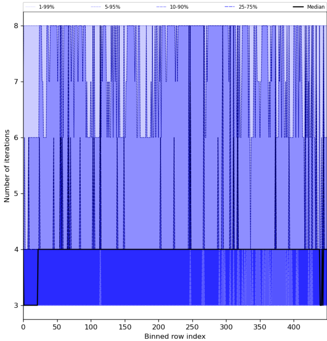
Figure 51: Along track statistics of “Number of iterations” for 2024-07-31 to 2024-08-02
