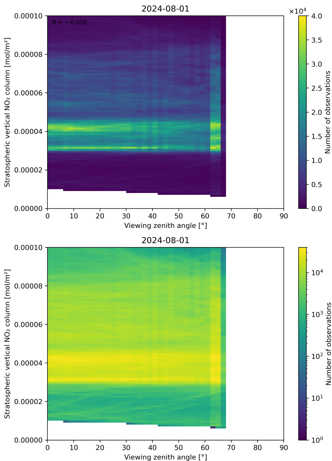
Figure 164: Scatter density plot of “Viewing zenith angle” against “Stratospheric vertical NO 2 column” for 2024-07-31 to 2024-08-02.
