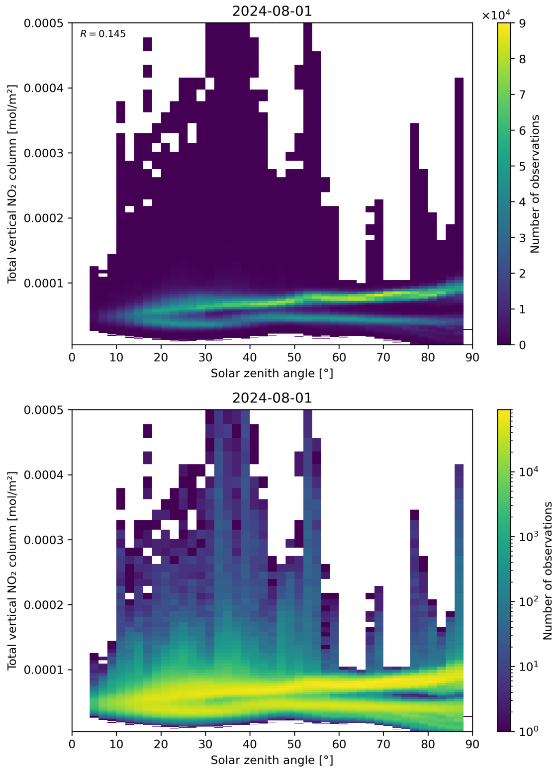
Figure 153: Scatter density plot of “Solar zenith angle” against “Total vertical NO 2 column” for 2024-07-31 to 2024-08-02.
