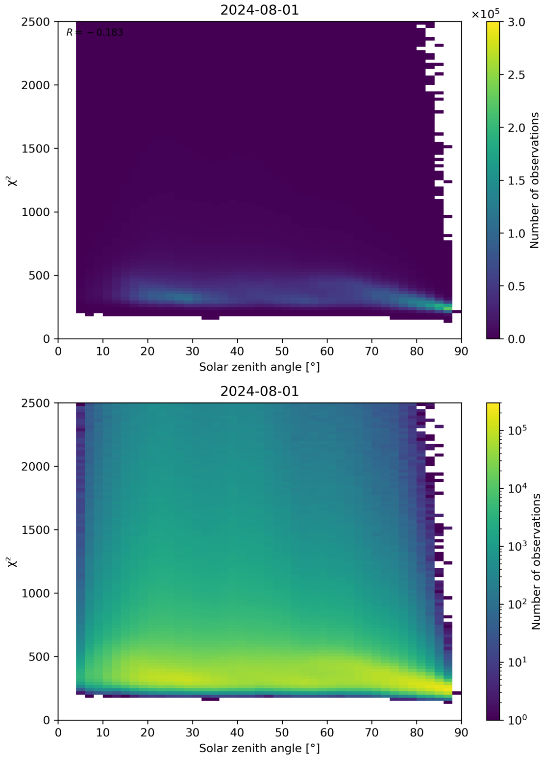
Figure 148: Scatter density plot of “Solar zenith angle” against “ \chi^2 ” for 2024-07-31 to 2024-08-02.
