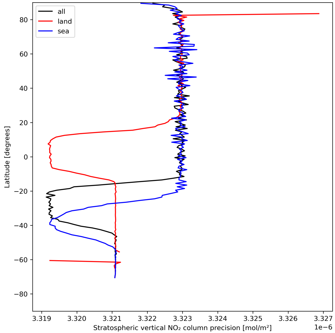
Figure 20: Zonal average of “Stratospheric vertical NO 2 column precision” for 2024-07-31 to 2024-08-02.
