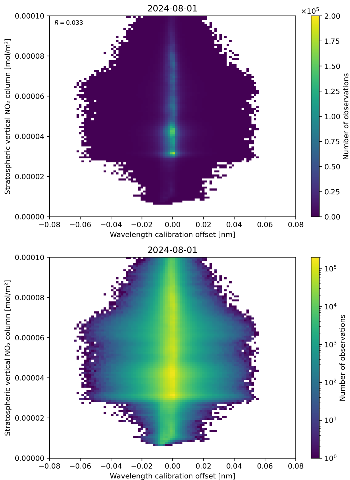
Figure 176: Scatter density plot of “Wavelength calibration offset” against “Stratospheric vertical NO 2 column” for 2024-07-31 to 2024-08-02.
