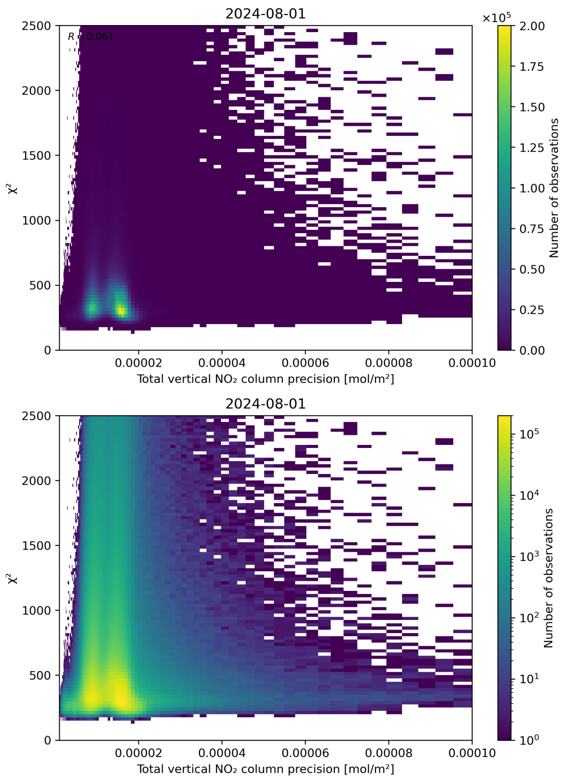
Figure 116: Scatter density plot of “Total vertical NO 2 column precision” against “ \chi^2 ” for 2024-07-31 to 2024-08-02.
