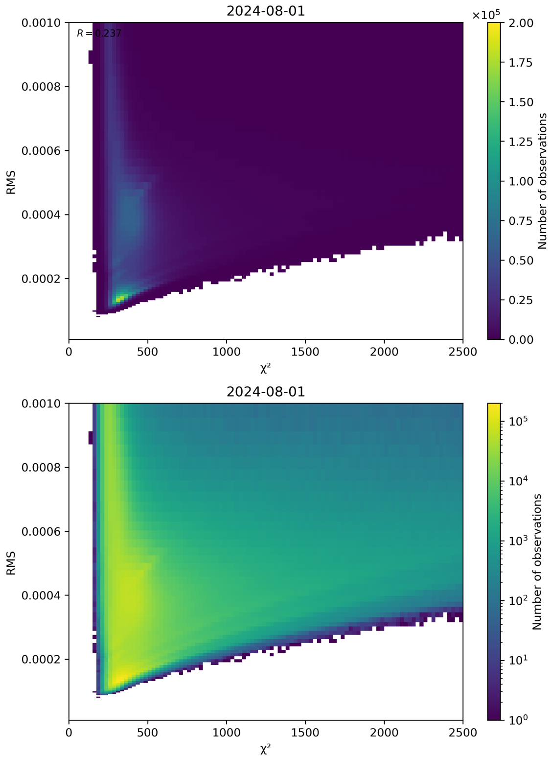
Figure 82: Scatter density plot of “ \chi^2 ” against “RMS” for 2024-07-31 to 2024-08-02.
