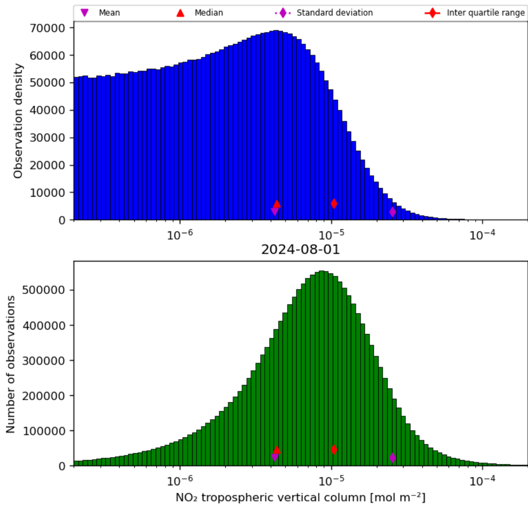
Figure 29: Histogram of “NO 2 tropospheric vertical column” for 2024-07-31 to 2024-08-02
