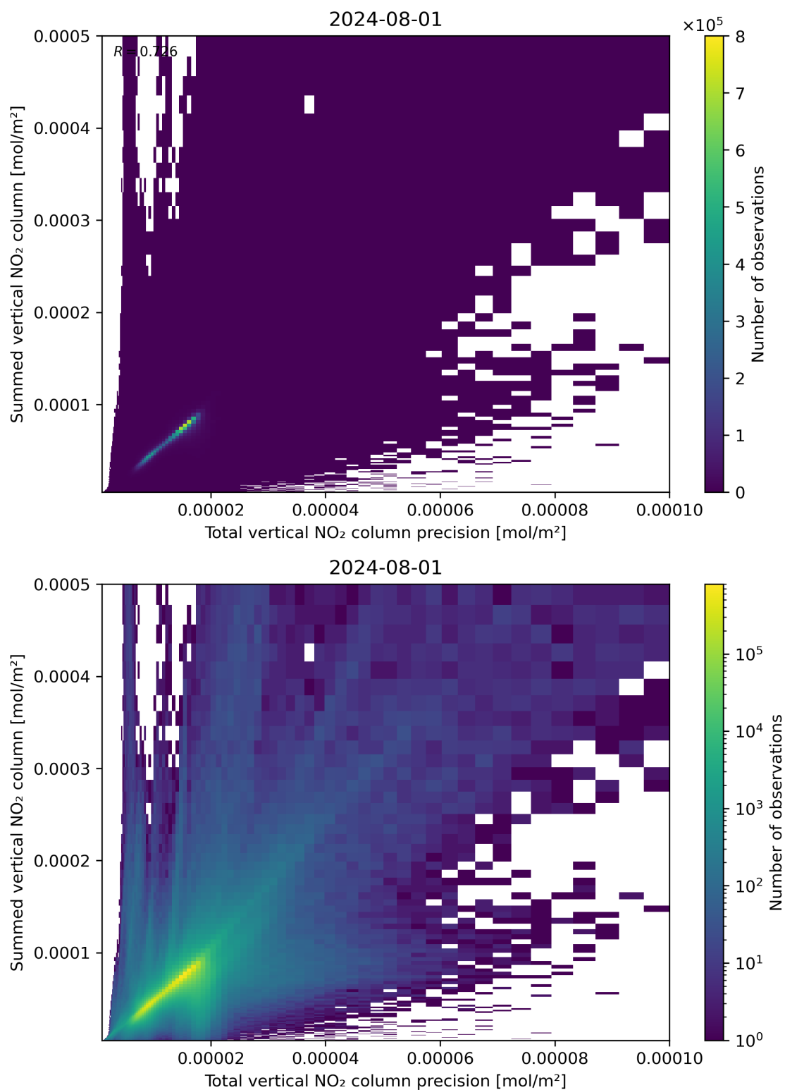
Figure 117: Scatter density plot of “Total vertical NO 2 column precision” against “Summed vertical NO 2 column” for 2024-07-31 to 2024-08-02.
