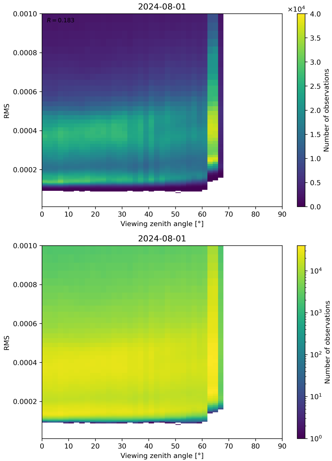
Figure 171: Scatter density plot of “Viewing zenith angle” against “RMS” for 2024-07-31 to 2024-08-02.
