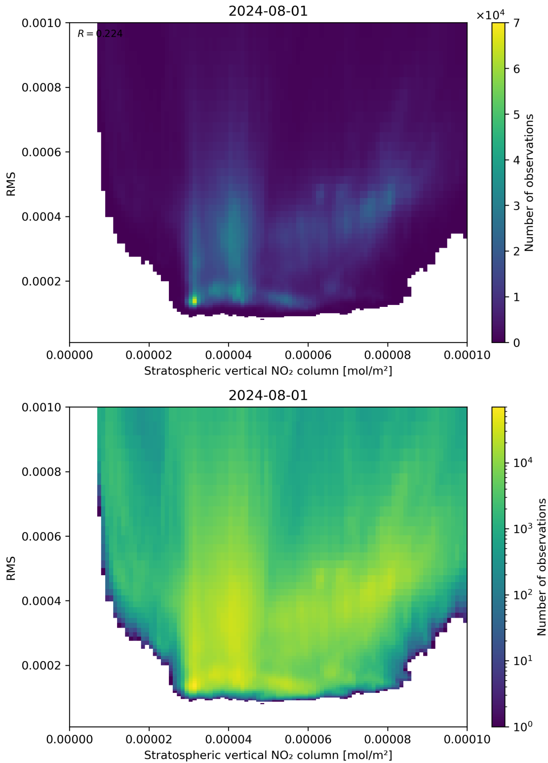
Figure 102: Scatter density plot of “Stratospheric vertical NO 2 column” against “RMS” for 2024-07-31 to 2024-08-02.
