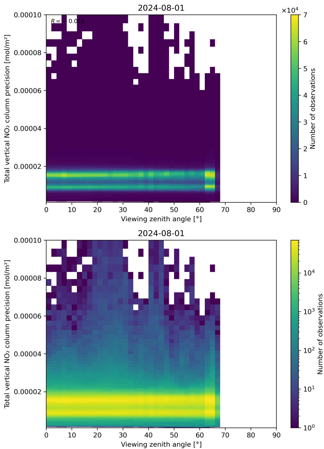
Figure 168: Scatter density plot of “Viewing zenith angle” against “Total vertical NO 2 column precision” for 2024-07-31 to 2024-08-02.
