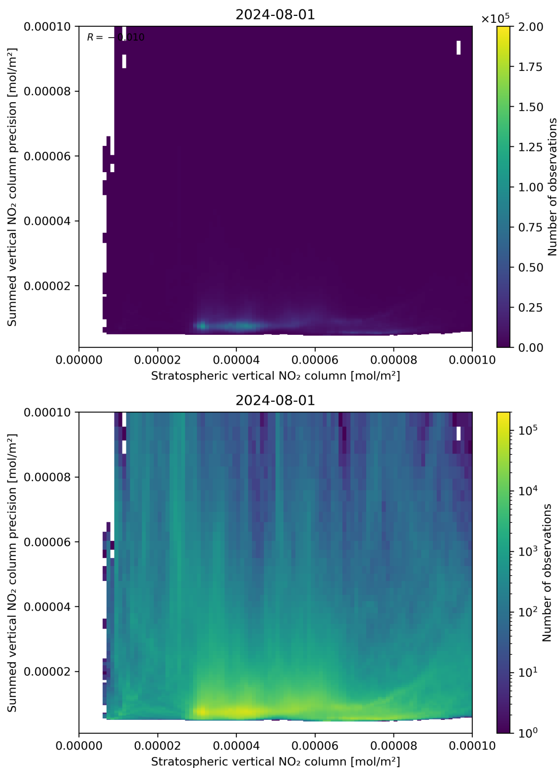
Figure 99: Scatter density plot of “Stratospheric vertical NO 2 column” against “Summed vertical NO 2 column precision” for 2024-07-31 to 2024-08-02.
