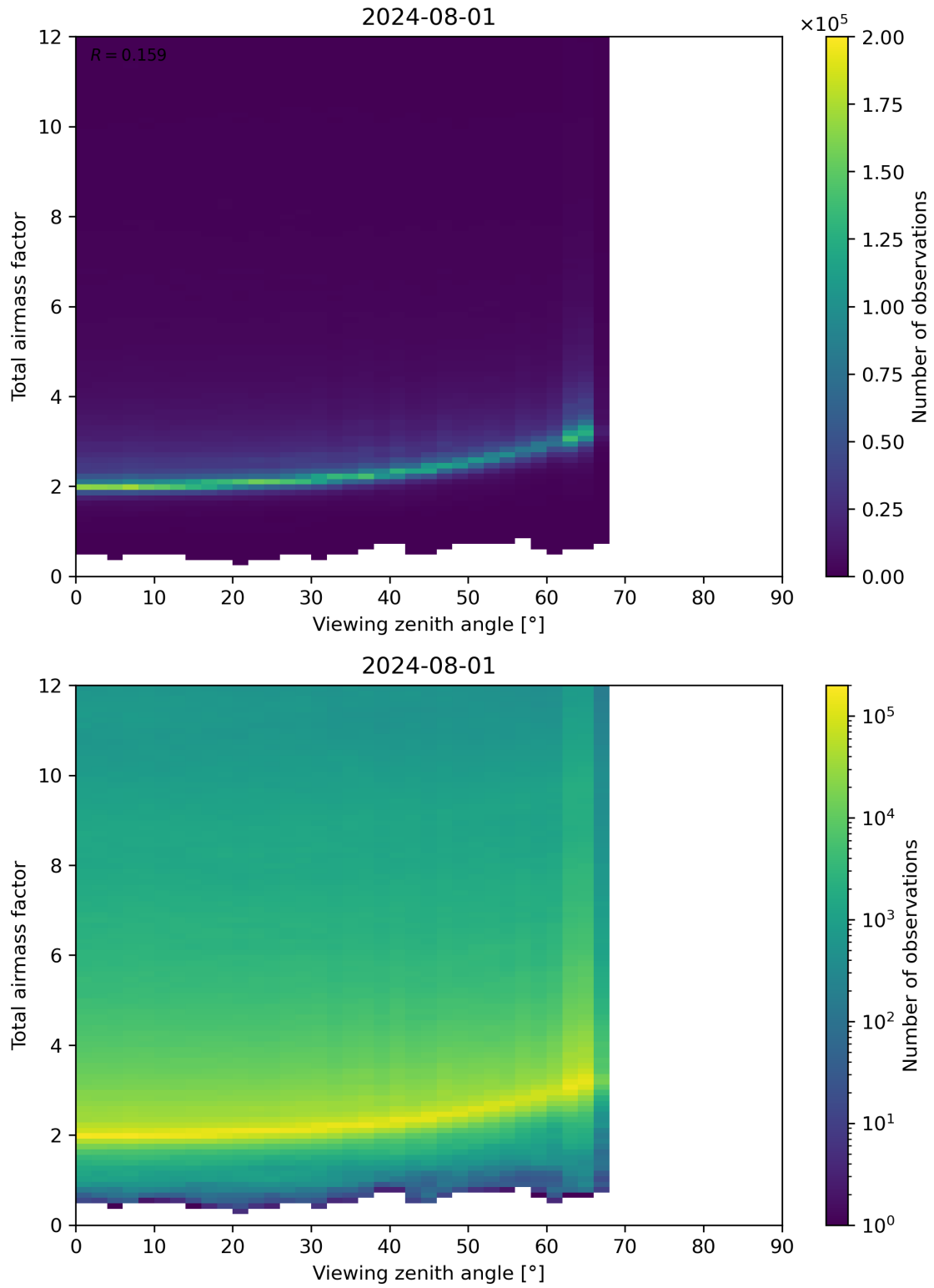
Figure 160: Scatter density plot of “Viewing zenith angle” against “Total airmass factor” for 2024-07-31 to 2024-08-02.
