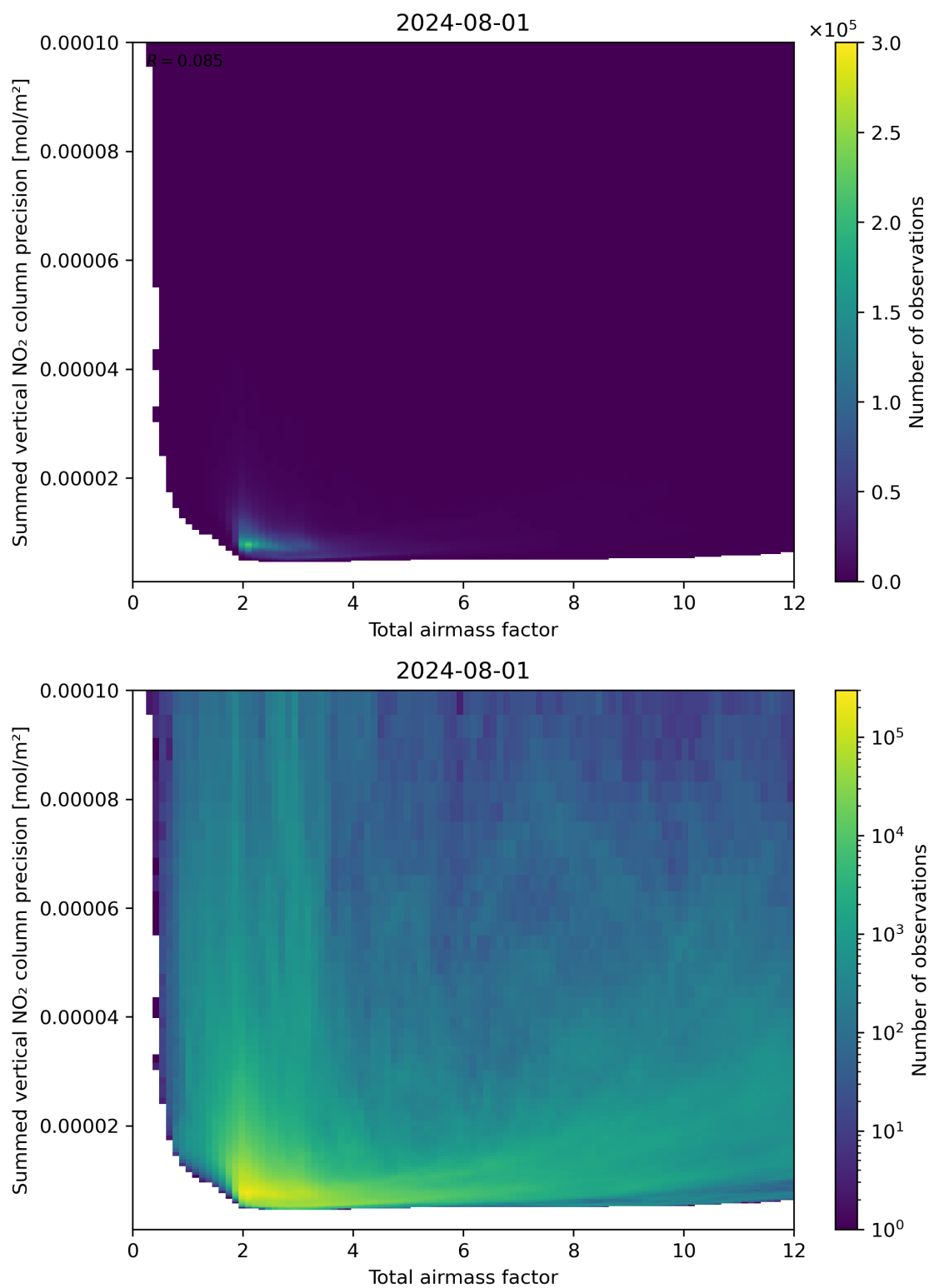
Figure 66: Scatter density plot of “Total airmass factor” against “Summed vertical NO 2 column precision” for 2024-07-31 to 2024-08-02.
