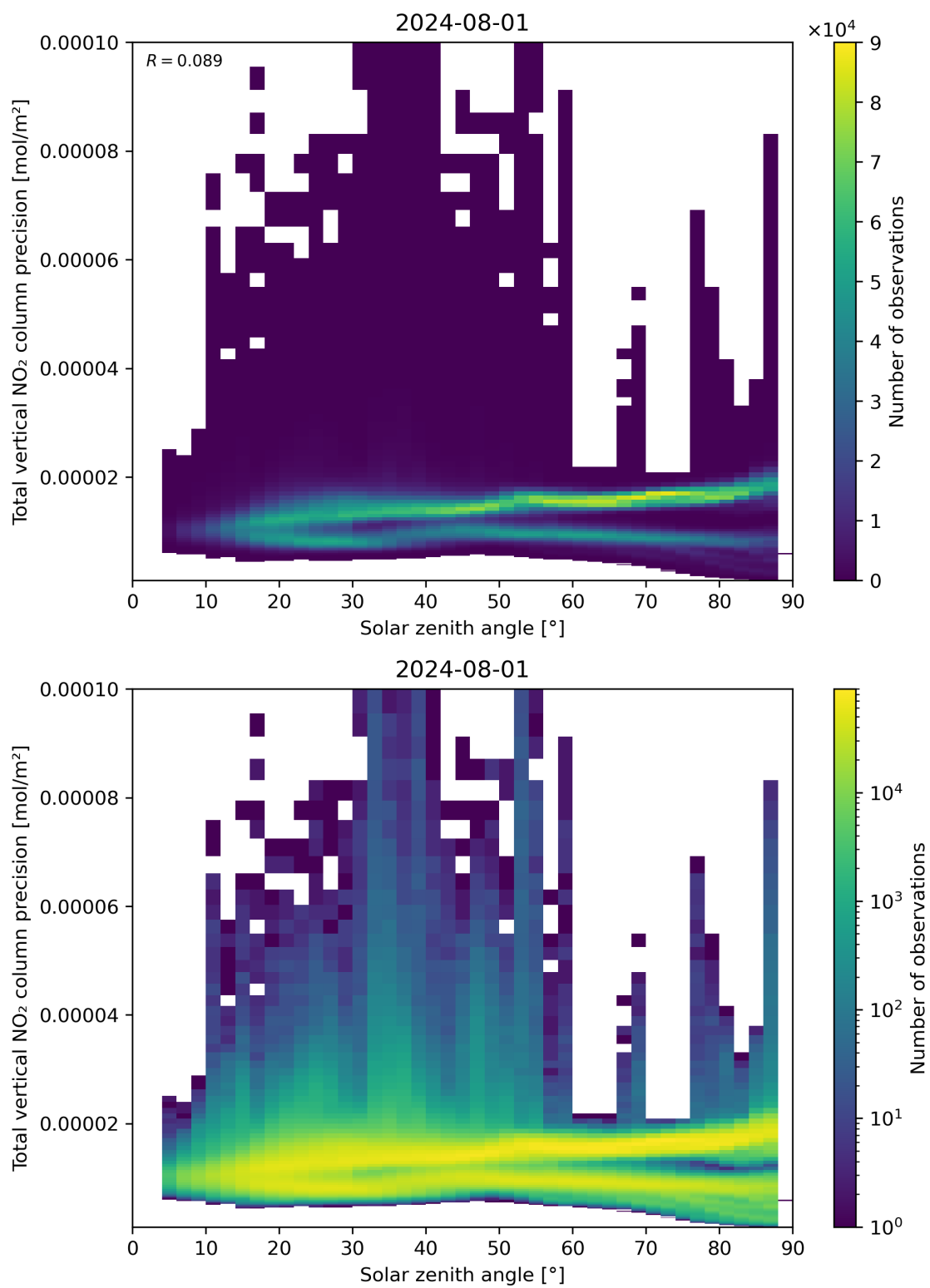
Figure 154: Scatter density plot of “Solar zenith angle” against “Total vertical NO 2 column precision” for 2024-07-31 to 2024-08-02.
