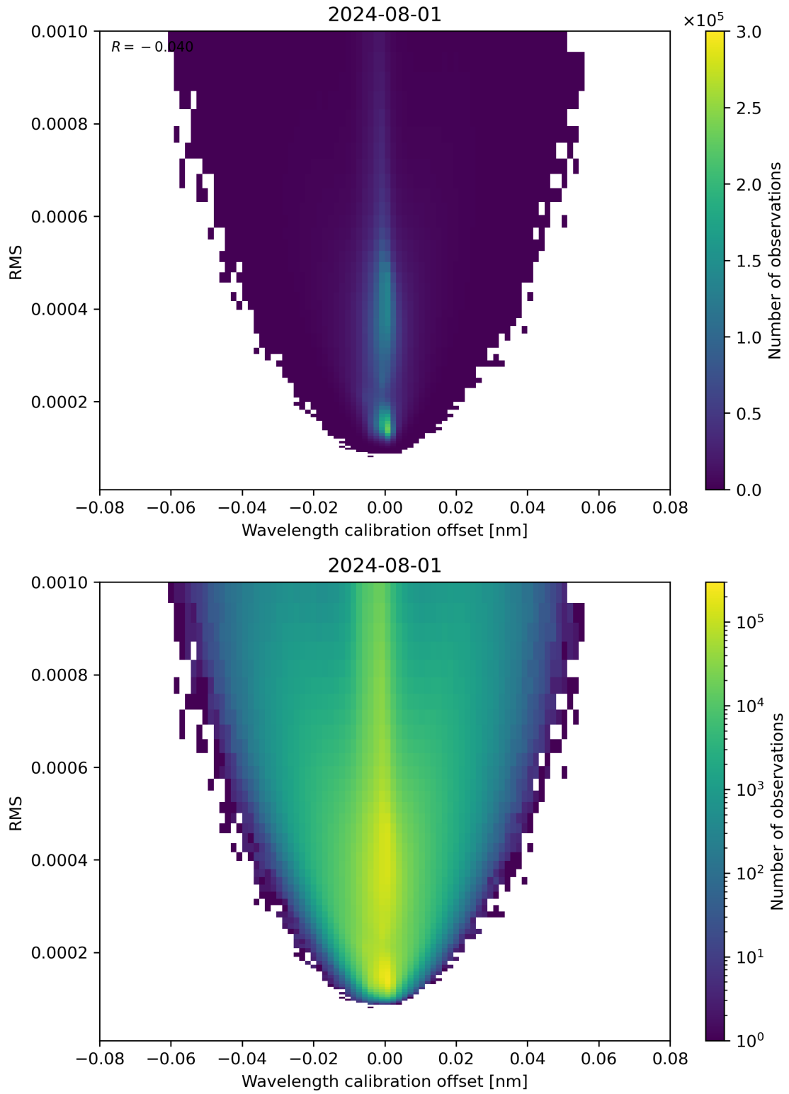
Figure 181: Scatter density plot of “Wavelength calibration offset” against “RMS” for 2024-07-31 to 2024-08-02.
