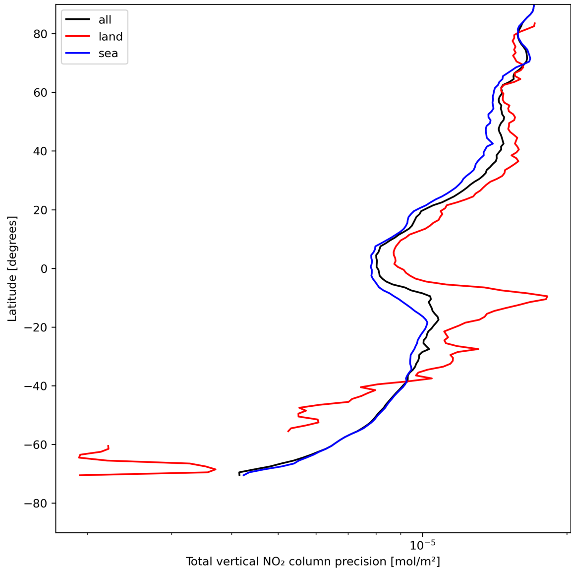
Figure 22: Zonal average of “Total vertical NO 2 column precision” for 2024-07-31 to 2024-08-02.
