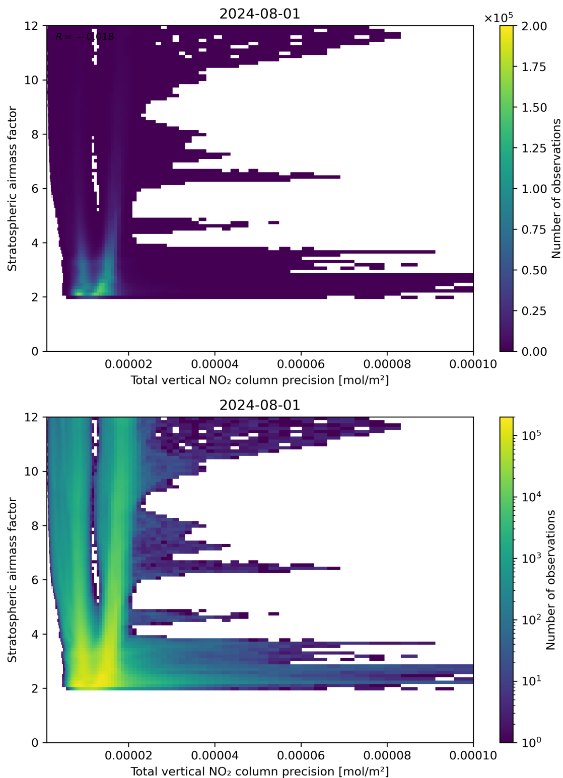
Figure 115: Scatter density plot of “Total vertical NO 2 column precision” against “Stratospheric air mass factor” for 2024-07-31 to 2024-08-02.
