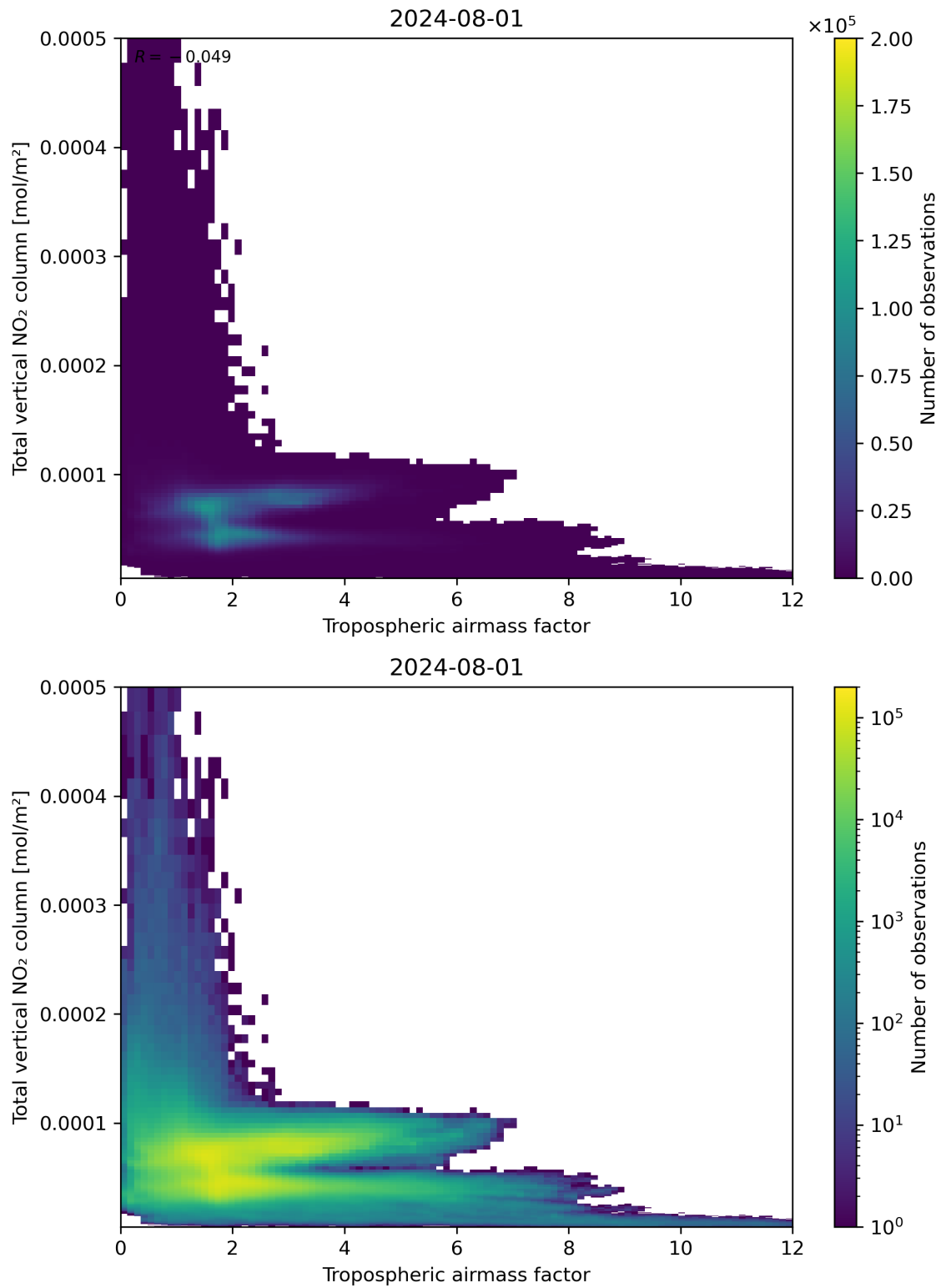
Figure 77: Scatter density plot of “Tropospheric airmass factor” against “Total vertical NO 2 column” for 2024-07-31 to 2024-08-02.
