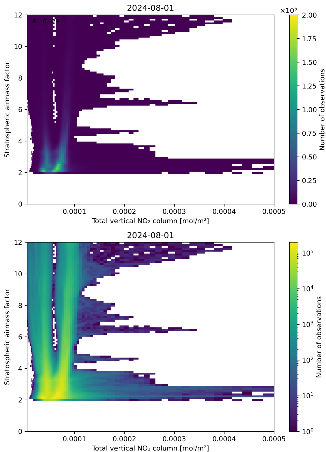
Figure 110: Scatter density plot of “Total vertical NO 2 column” against “Stratospheric airmass factor” for 2024-07-31 to 2024-08-02.
