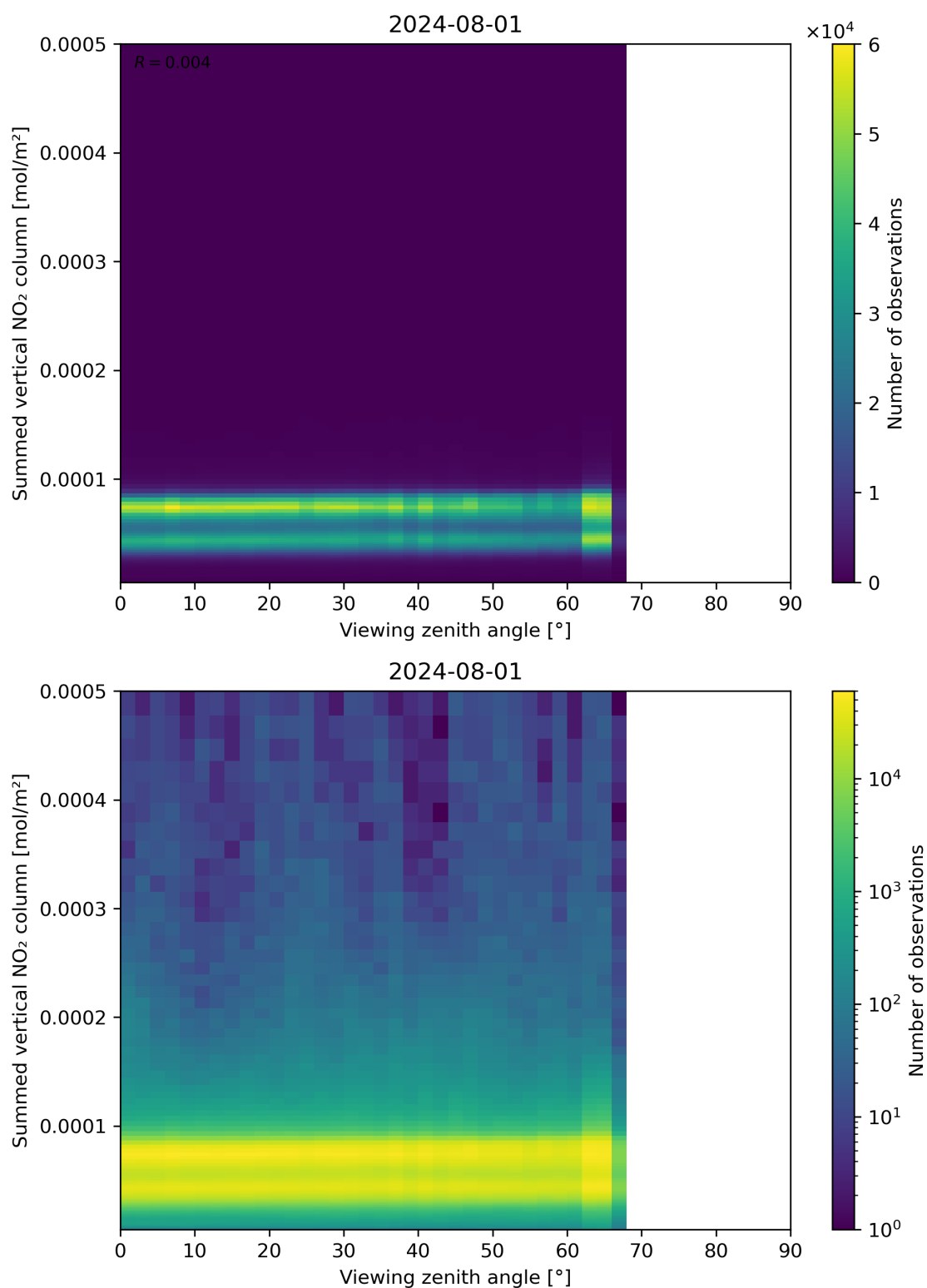
Figure 165: Scatter density plot of “Viewing zenith angle” against “Summed vertical NO 2 column” for 2024-07-31 to 2024-08-02.
