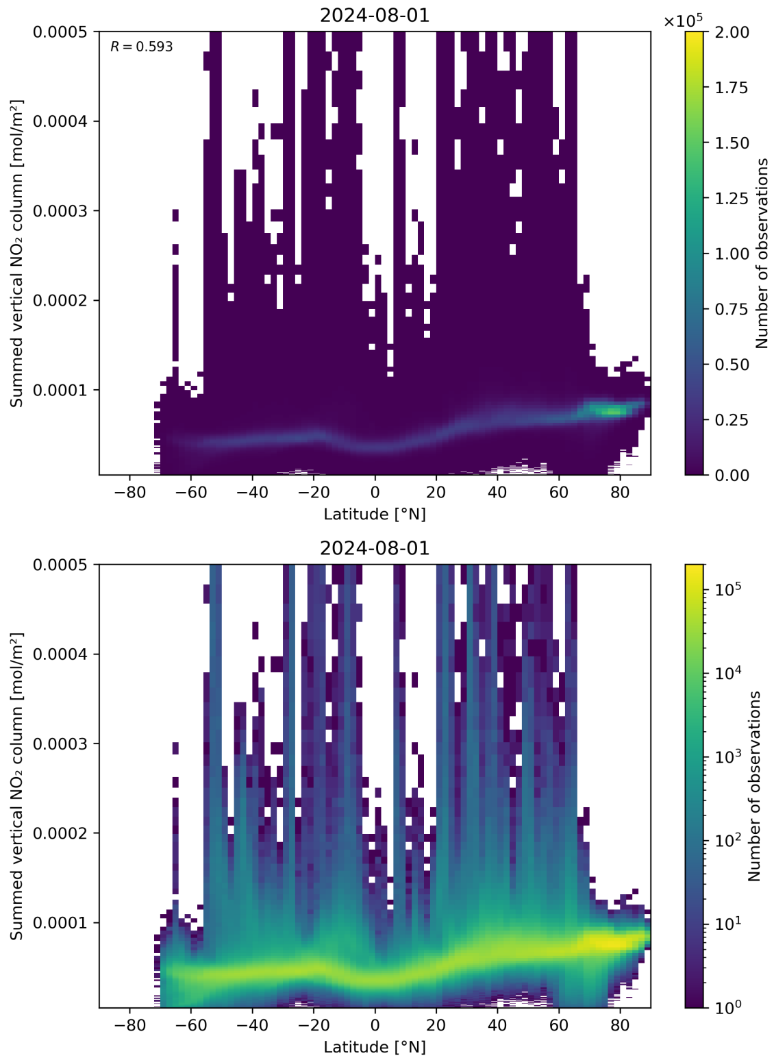
Figure 88: Scatter density plot of “Latitude” against “Summed vertical NO 2 column” for 2024-07-31 to 2024-08-02.
