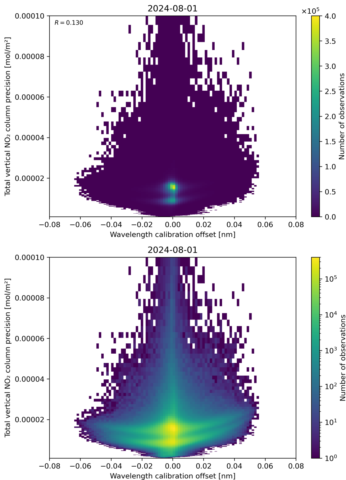
Figure 180: Scatter density plot of “Wavelength calibration offset” against “Total vertical NO 2 column precision” for 2024-07-31 to 2024-08-02.
