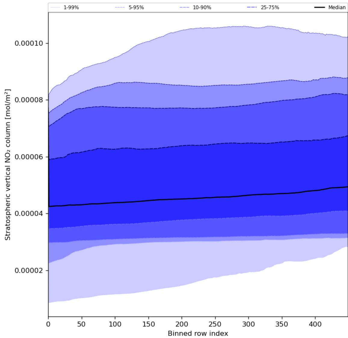
Figure 53: Along track statistics of “Stratospheric vertical NO 2 column” for 2024-07-31 to 2024-08-02
