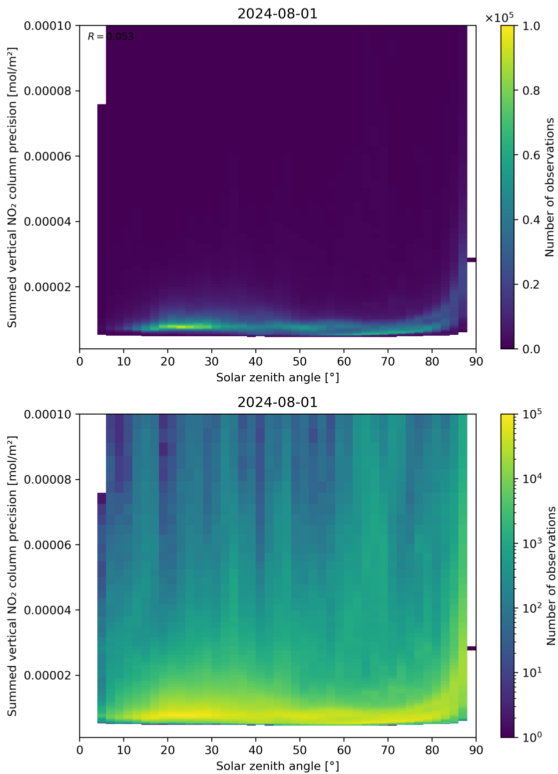
Figure 152: Scatter density plot of “Solar zenith angle” against “Summed vertical NO 2 column precision” for 2024-07-31 to 2024-08-02.
