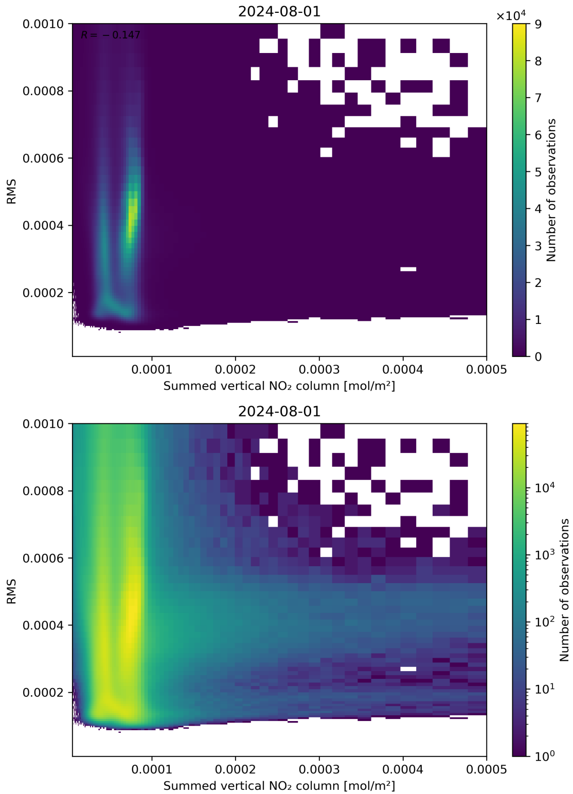
Figure 109: Scatter density plot of “Summed vertical NO 2 column” against “RMS” for 2024-07-31 to 2024-08-02.
