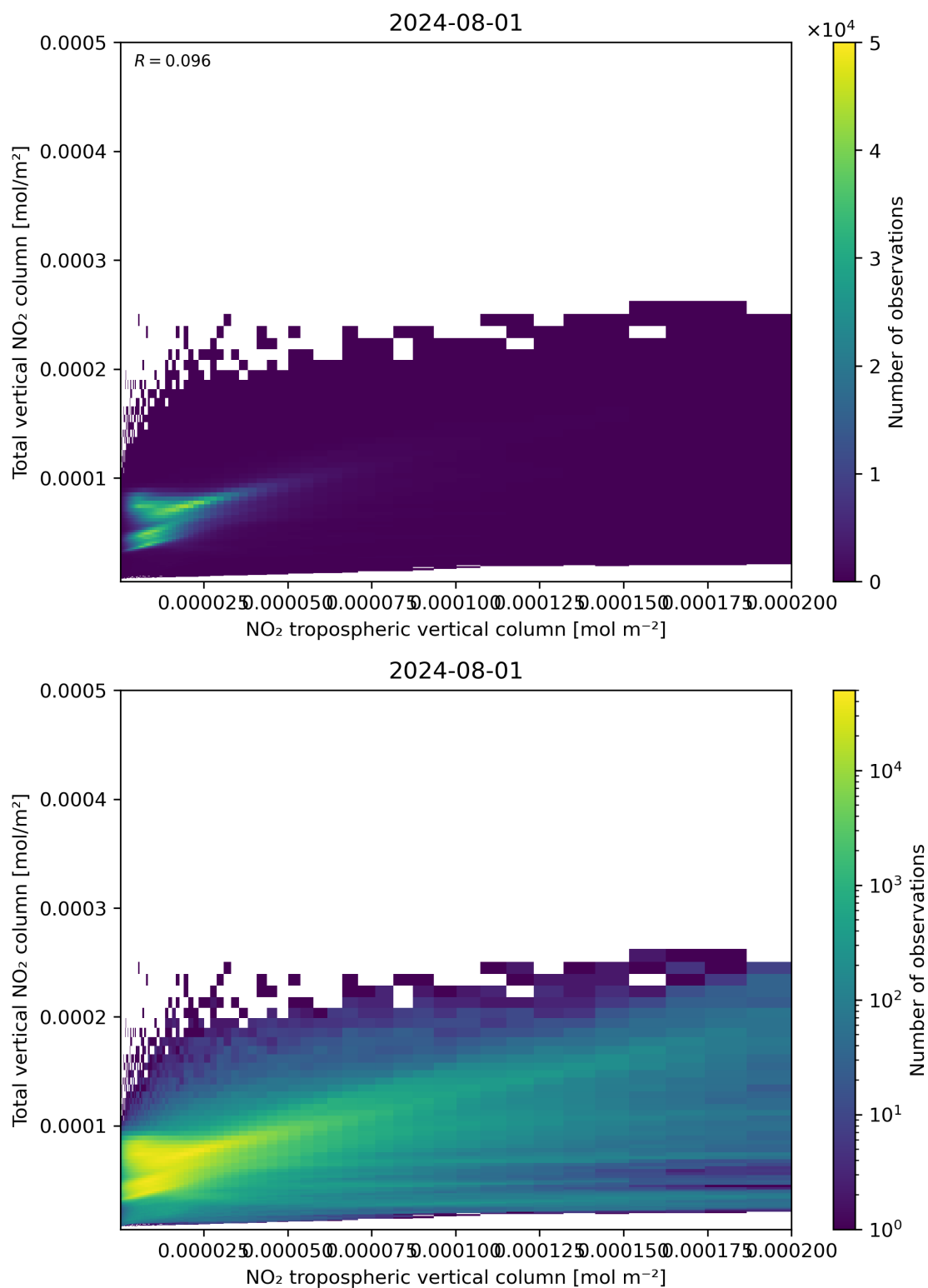
Figure 128: Scatter density plot of “NO 2 tropospheric vertical column” against “Total vertical NO 2 column” for 2024-07-31 to 2024-08-02.
