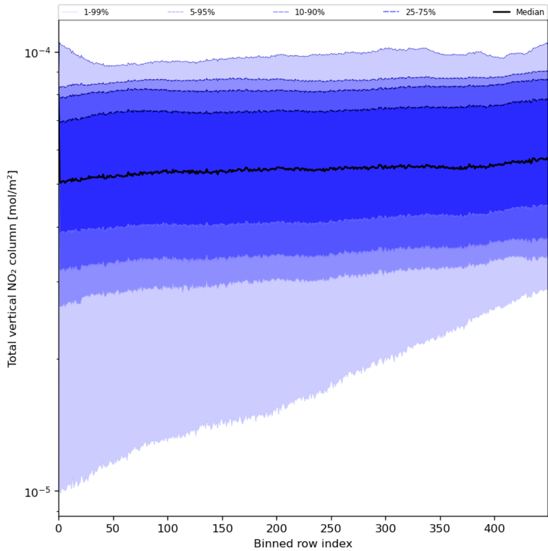
Figure 55: Along track statistics of “Total vertical NO 2 column” for 2024-07-31 to 2024-08-02
