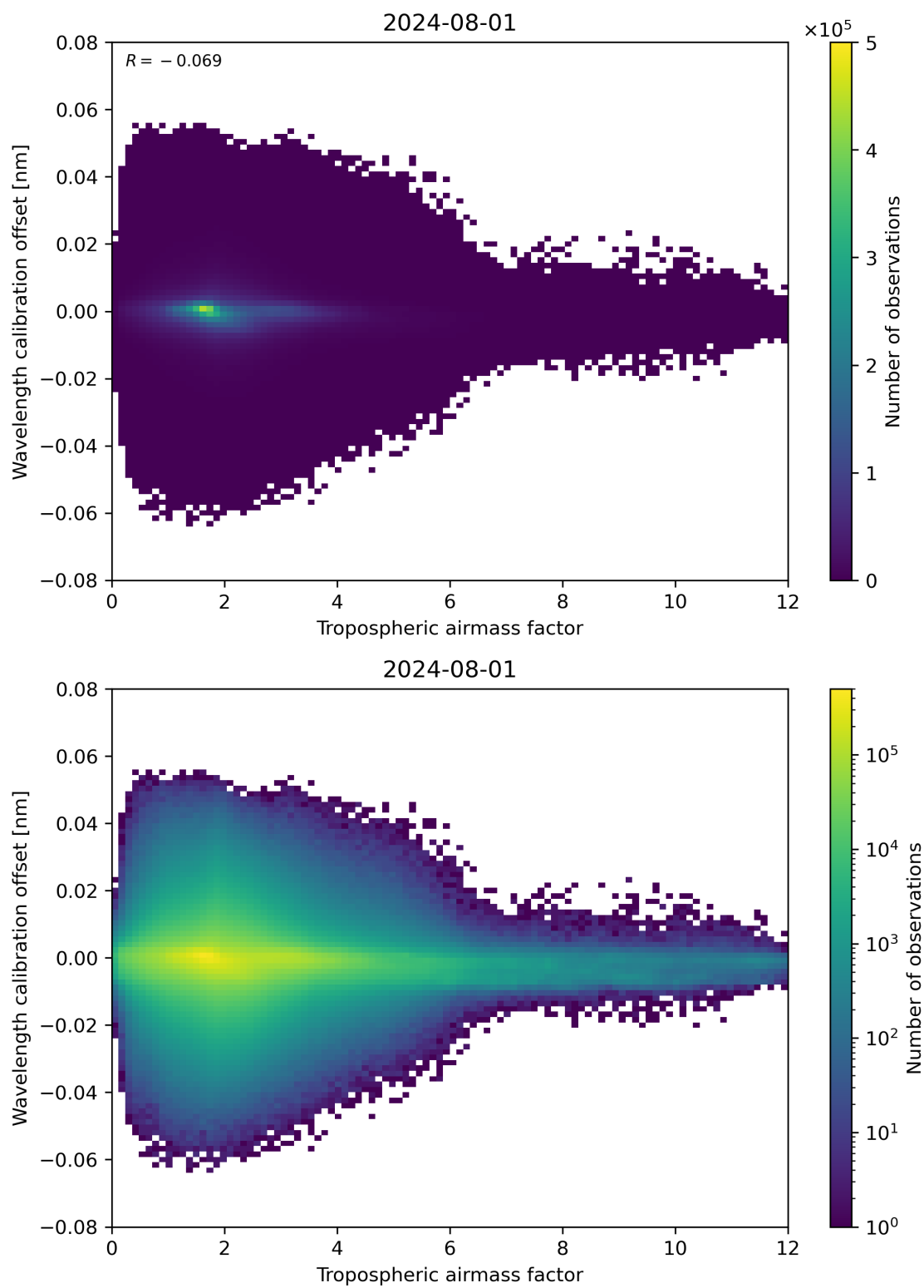
Figure 80: Scatter density plot of “Tropospheric air mass factor” against “Wavelength calibration offset” for 2024-07-31 to 2024-08-02.
