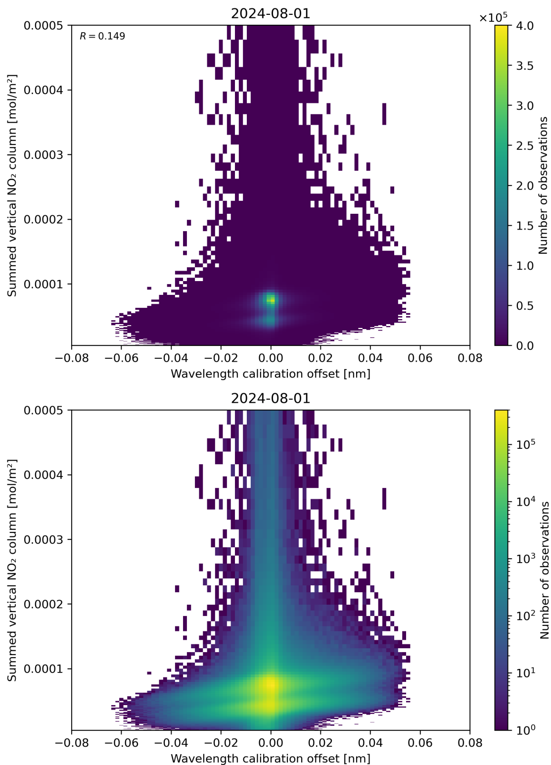
Figure 177: Scatter density plot of “Wavelength calibration offset” against “Summed vertical NO 2 column” for 2024-07-31 to 2024-08-02.
