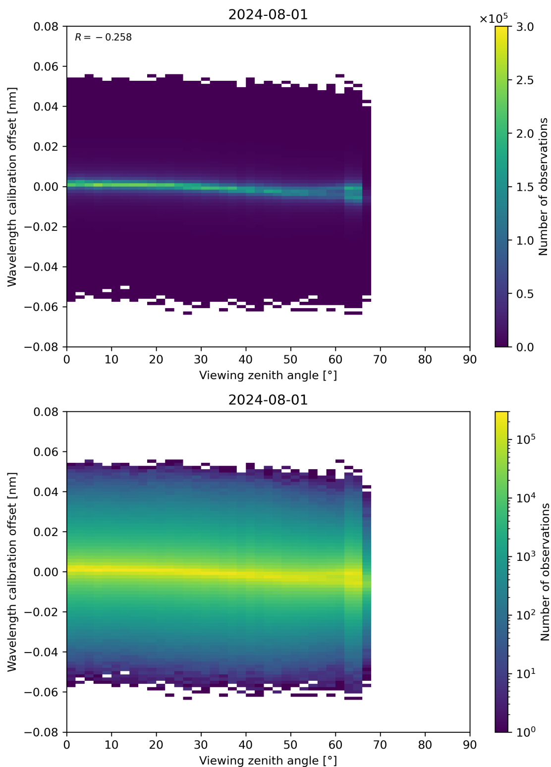
Figure 173: Scatter density plot of “Viewing zenith angle” against “Wavelength calibration offset” for 2024-07-31 to 2024-08-02.
