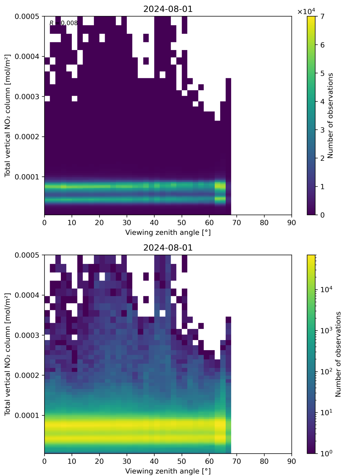
Figure 167: Scatter density plot of “Viewing zenith angle” against “Total vertical NO 2 column” for 2024-07-31 to 2024-08-02.
