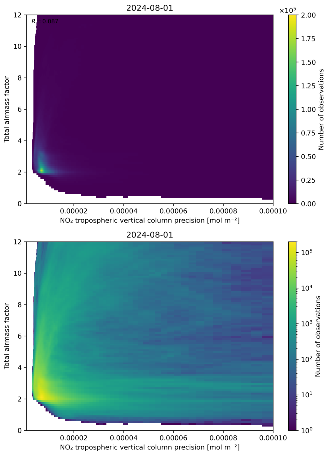
Figure 132: Scatter density plot of “NO 2 tropospheric vertical column precision” against “Total air mass factor” for 2024-07-31 to 2024-08-02.
