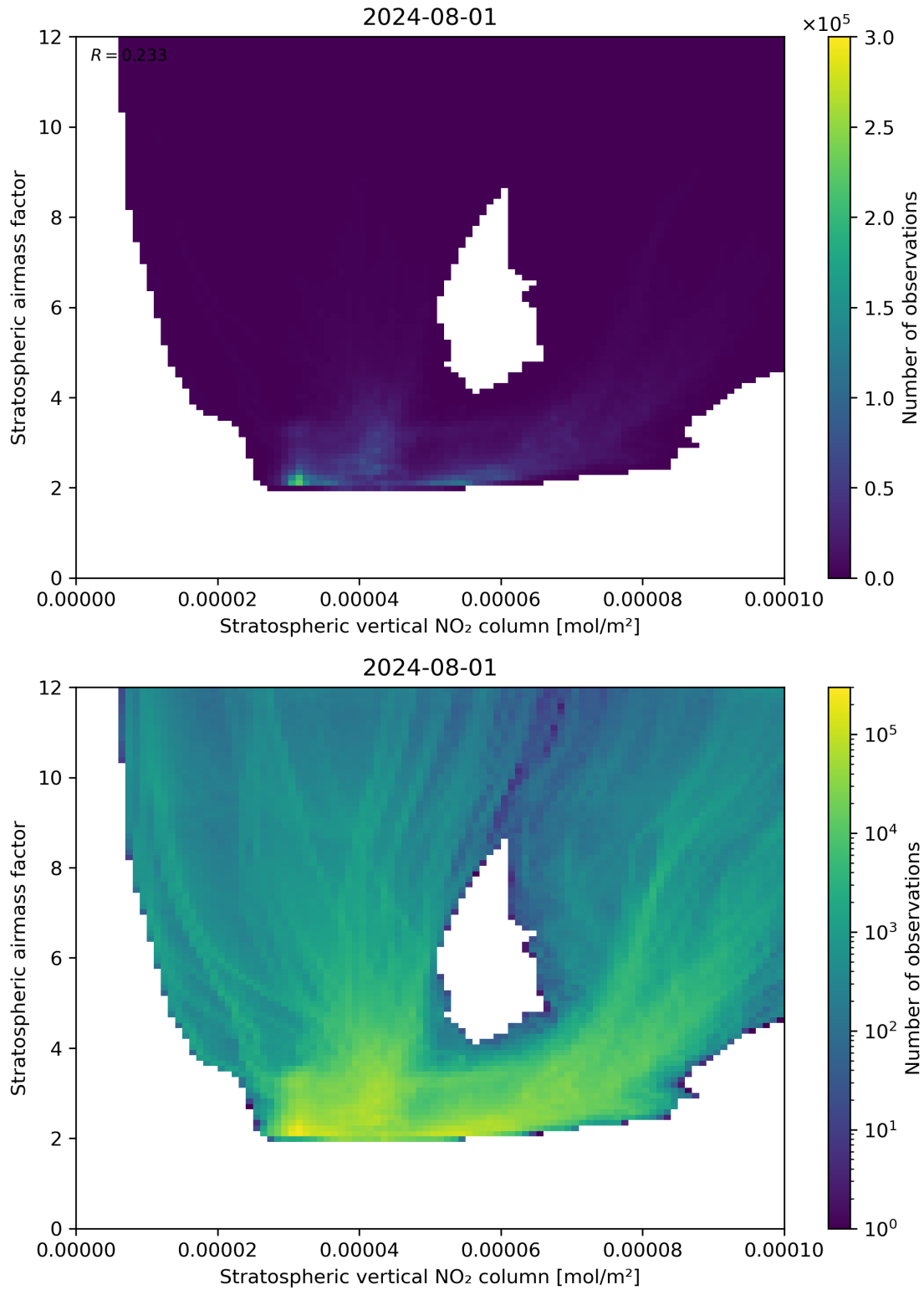
Figure 96: Scatter density plot of “Stratospheric vertical NO 2 column” against “Stratospheric airmass factor” for 2024-07-31 to 2024-08-02.
