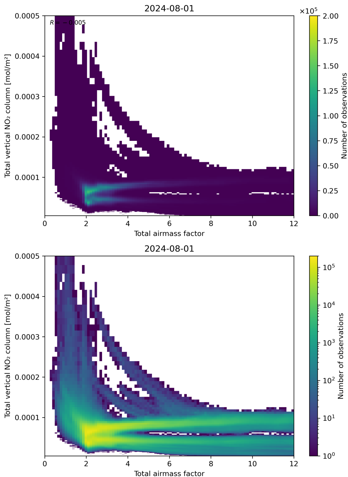
Figure 67: Scatter density plot of “Total airmass factor” against “Total vertical NO 2 column” for 2024-07-31 to 2024-08-02.
