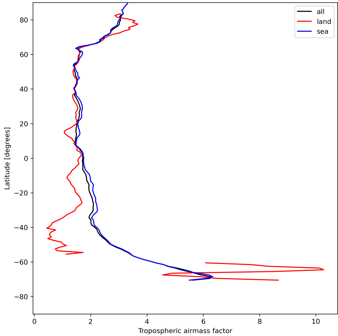
Figure 14: Zonal average of “Tropospheric airmass factor” for 2024-07-31 to 2024-08-02.
