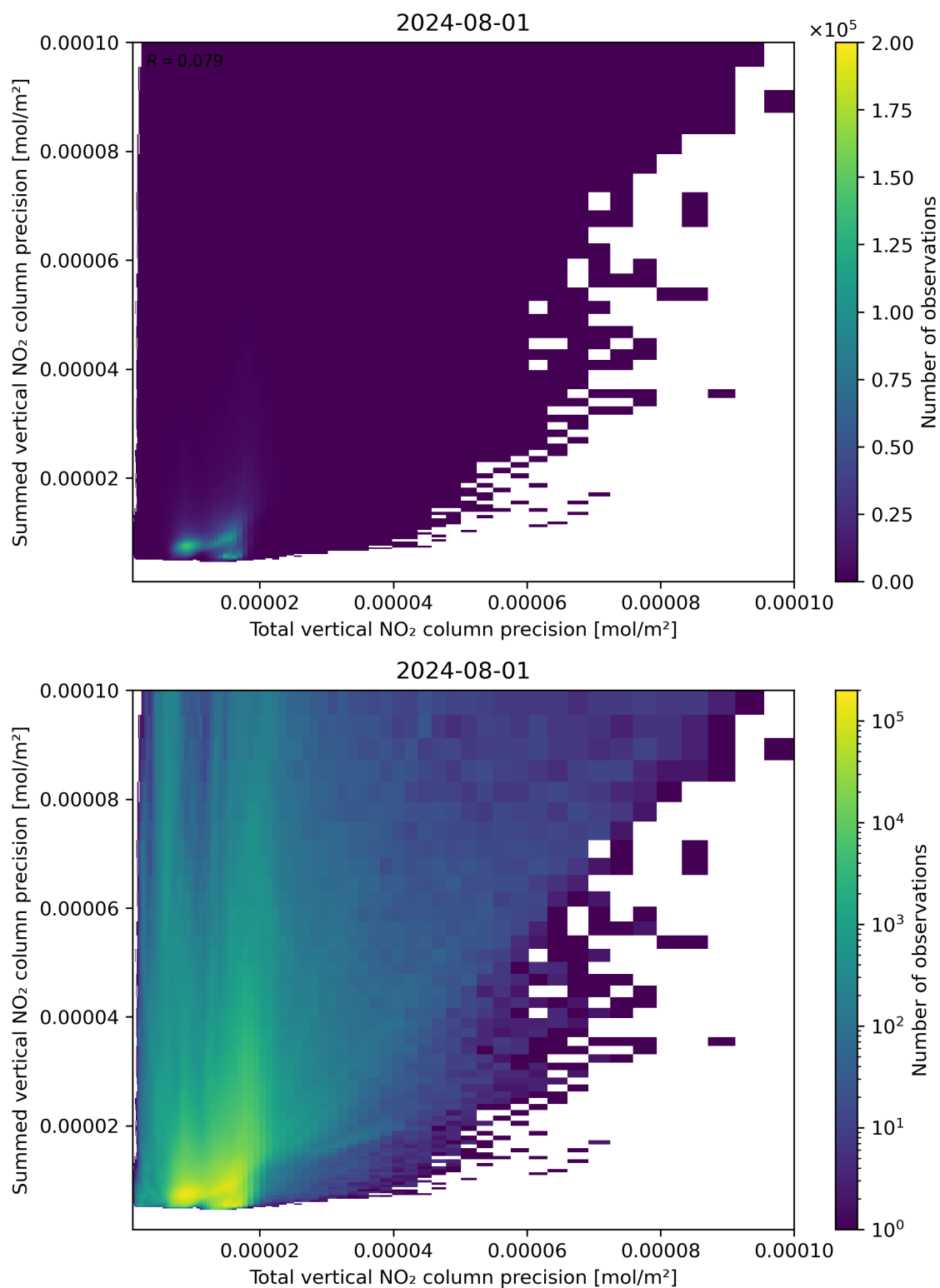
Figure 118: Scatter density plot of “Total vertical NO 2 column precision” against “Summed vertical NO 2 column precision” for 2024-07-31 to 2024-08-02.
