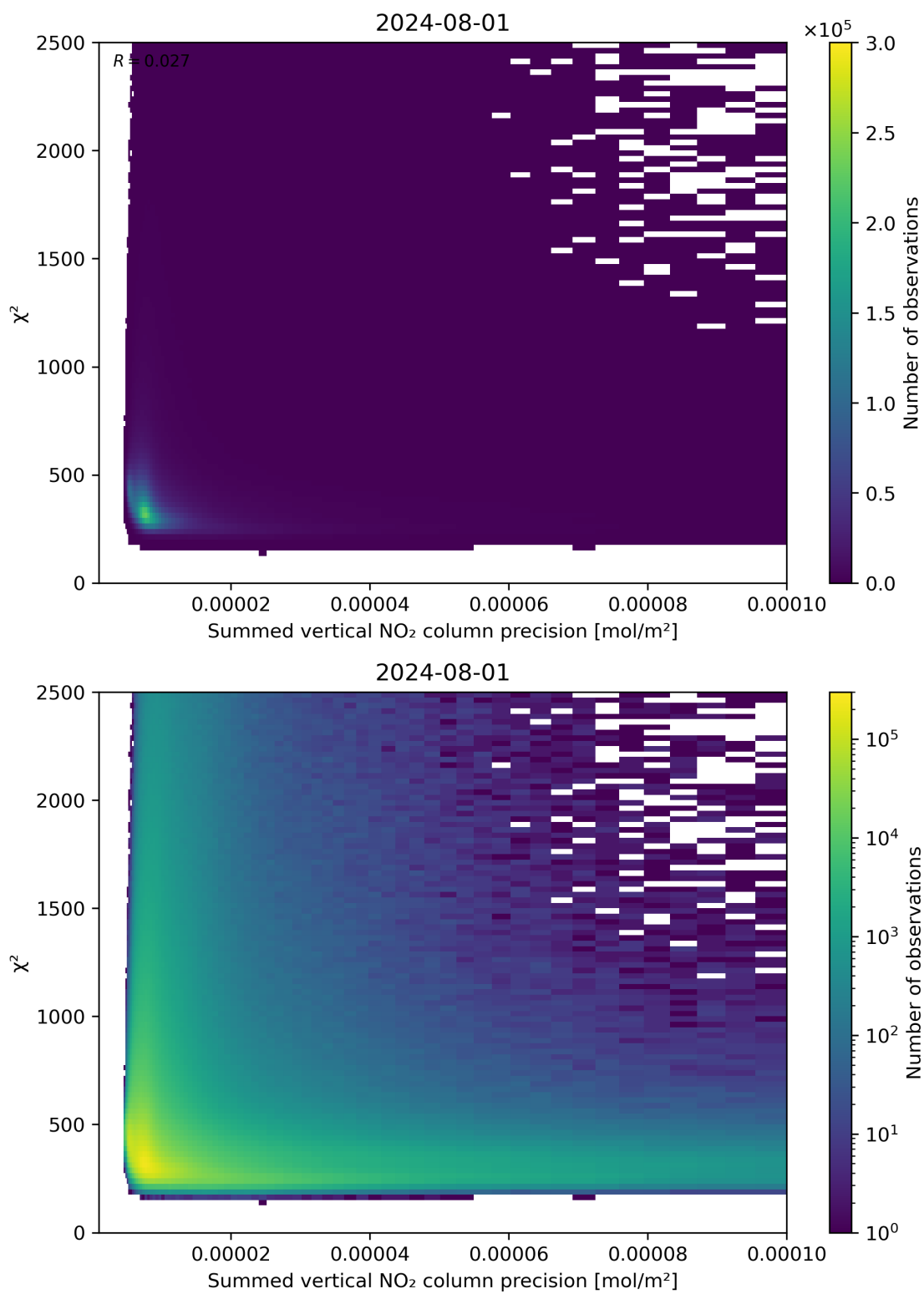
Figure 107: Scatter density plot of “Summed vertical NO 2 column precision” against “ \chi^2 ” for 2024-07-31 to 2024-08-02.
