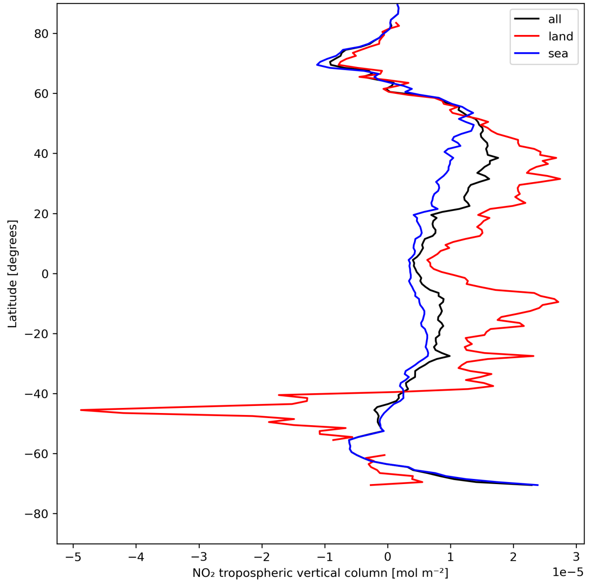
Figure 12: Zonal average of “NO 2 tropospheric vertical column” for 2024-07-31 to 2024-08-02.
