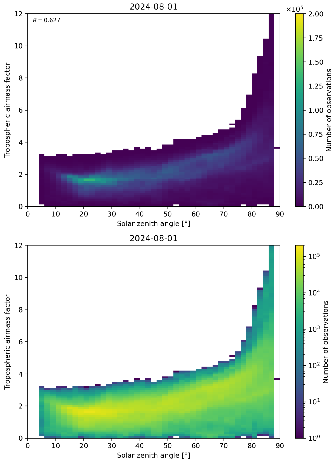
Figure 147: Scatter density plot of “Solar zenith angle” against “Tropospheric airmass factor” for 2024-07-31 to 2024-08-02.
