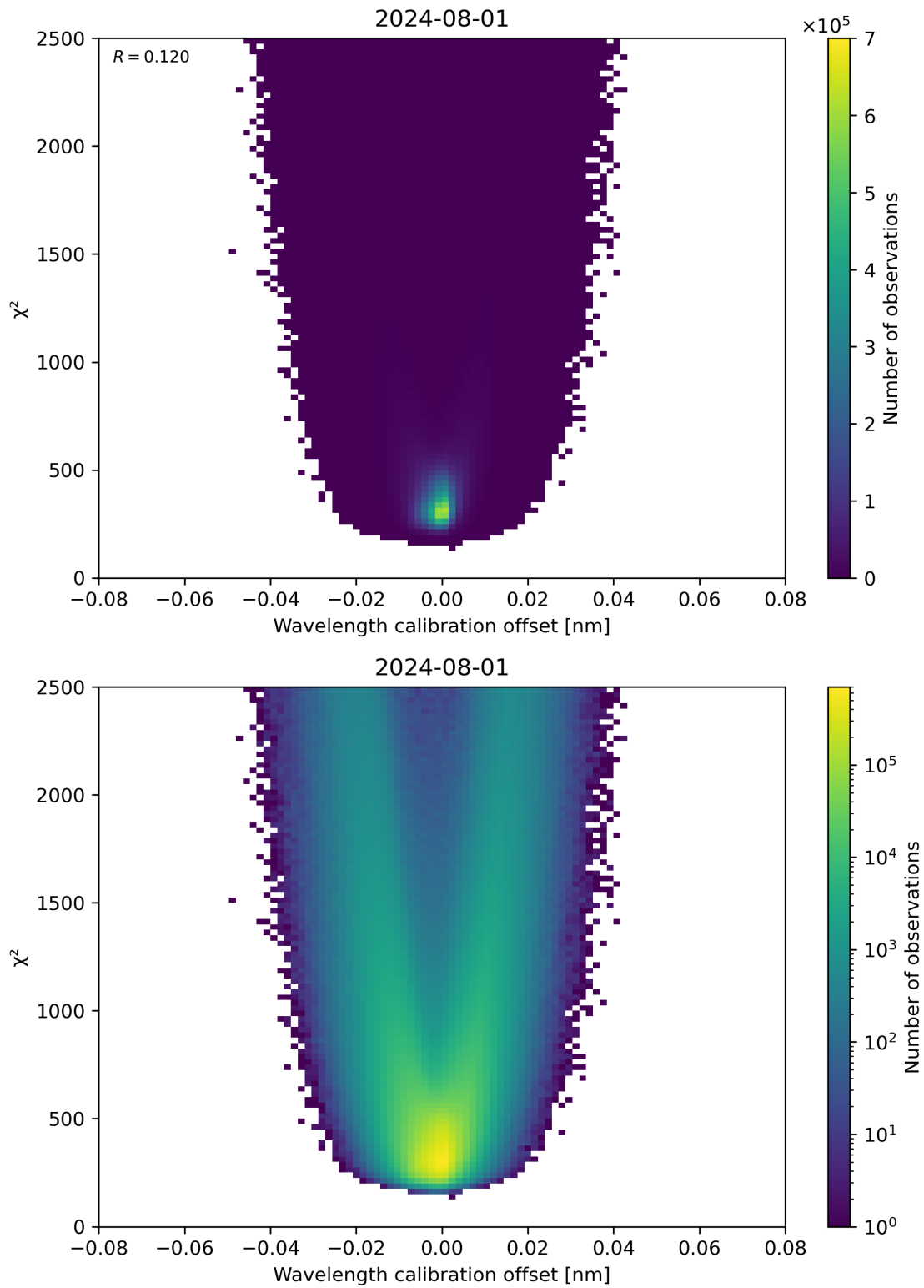
Figure 175: Scatter density plot of “Wavelength calibration offset” against “ \chi^2 ” for 2024-07-31 to 2024-08-02.
