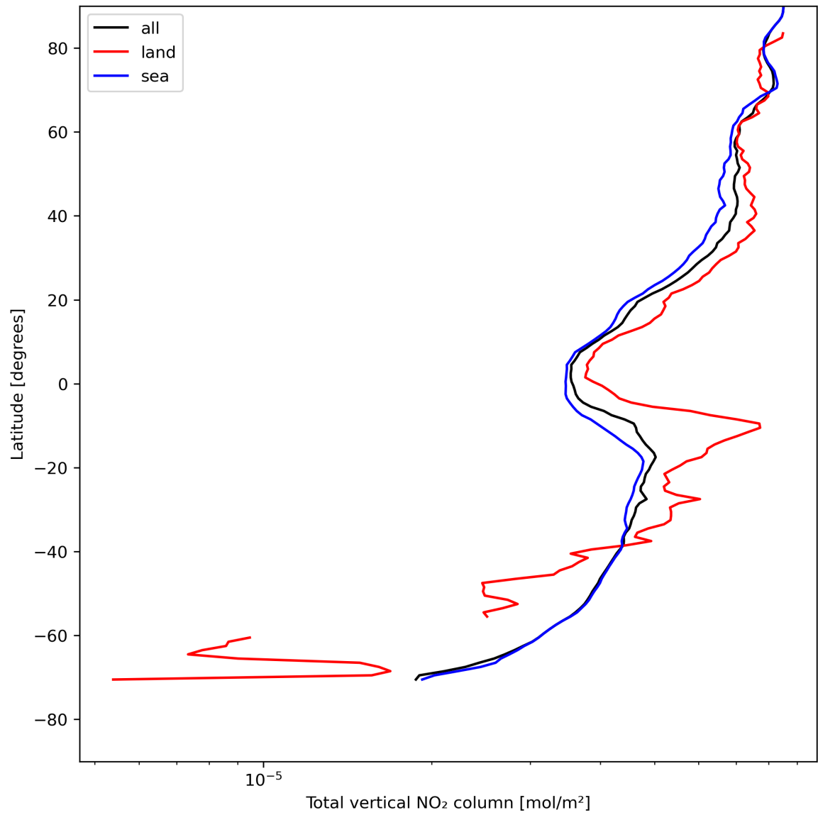
Figure 21: Zonal average of “Total vertical NO 2 column” for 2024-07-31 to 2024-08-02.
