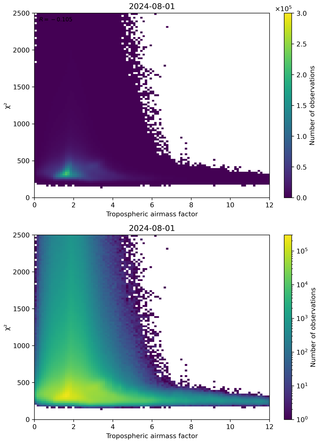
Figure 73: Scatter density plot of “Tropospheric airmass factor” against “ \chi^2 ” for 2024-07-31 to 2024-08-02.
