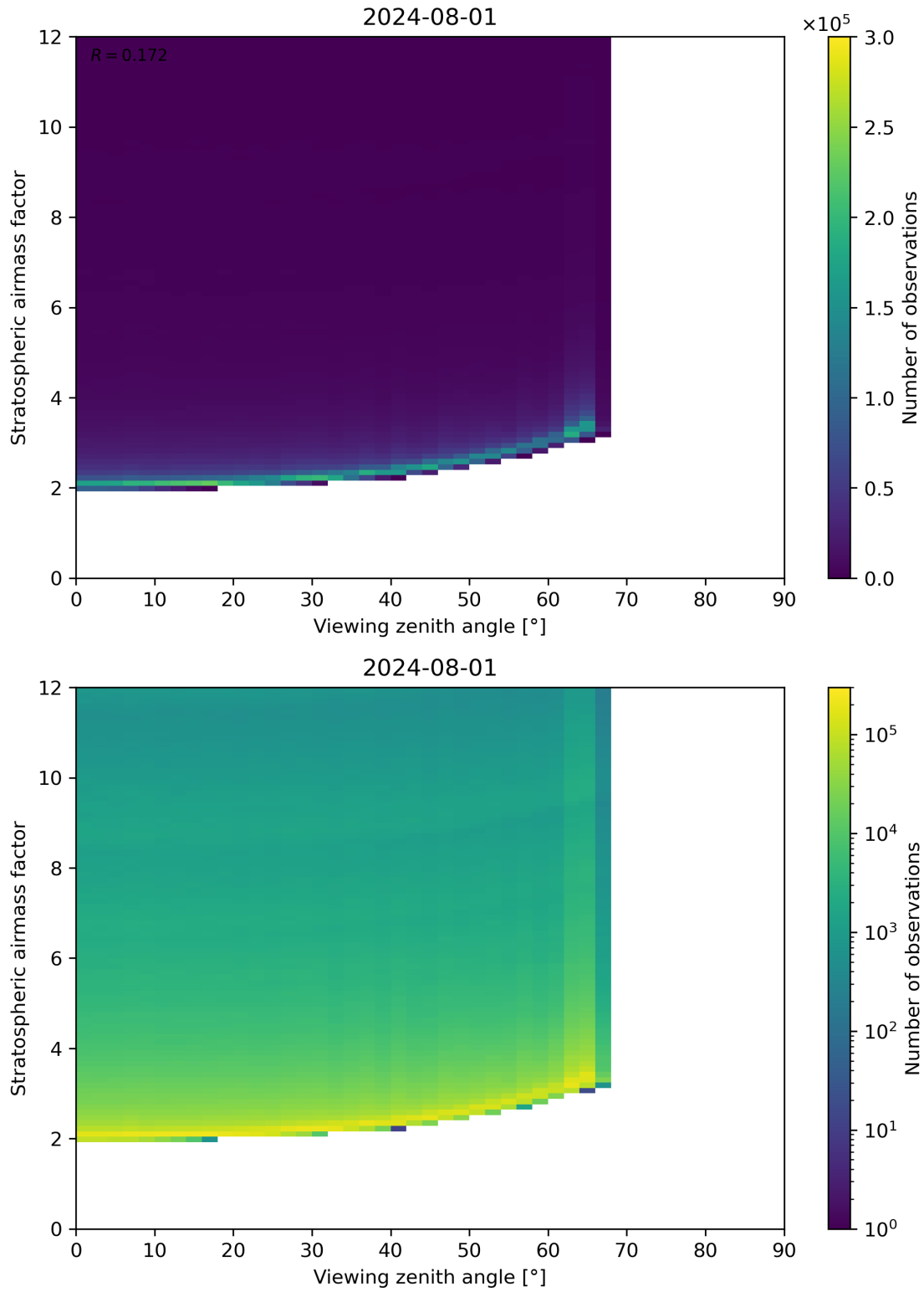
Figure 159: Scatter density plot of “Viewing zenith angle” against “Stratospheric airmass factor” for 2024-07-31 to 2024-08-02.
