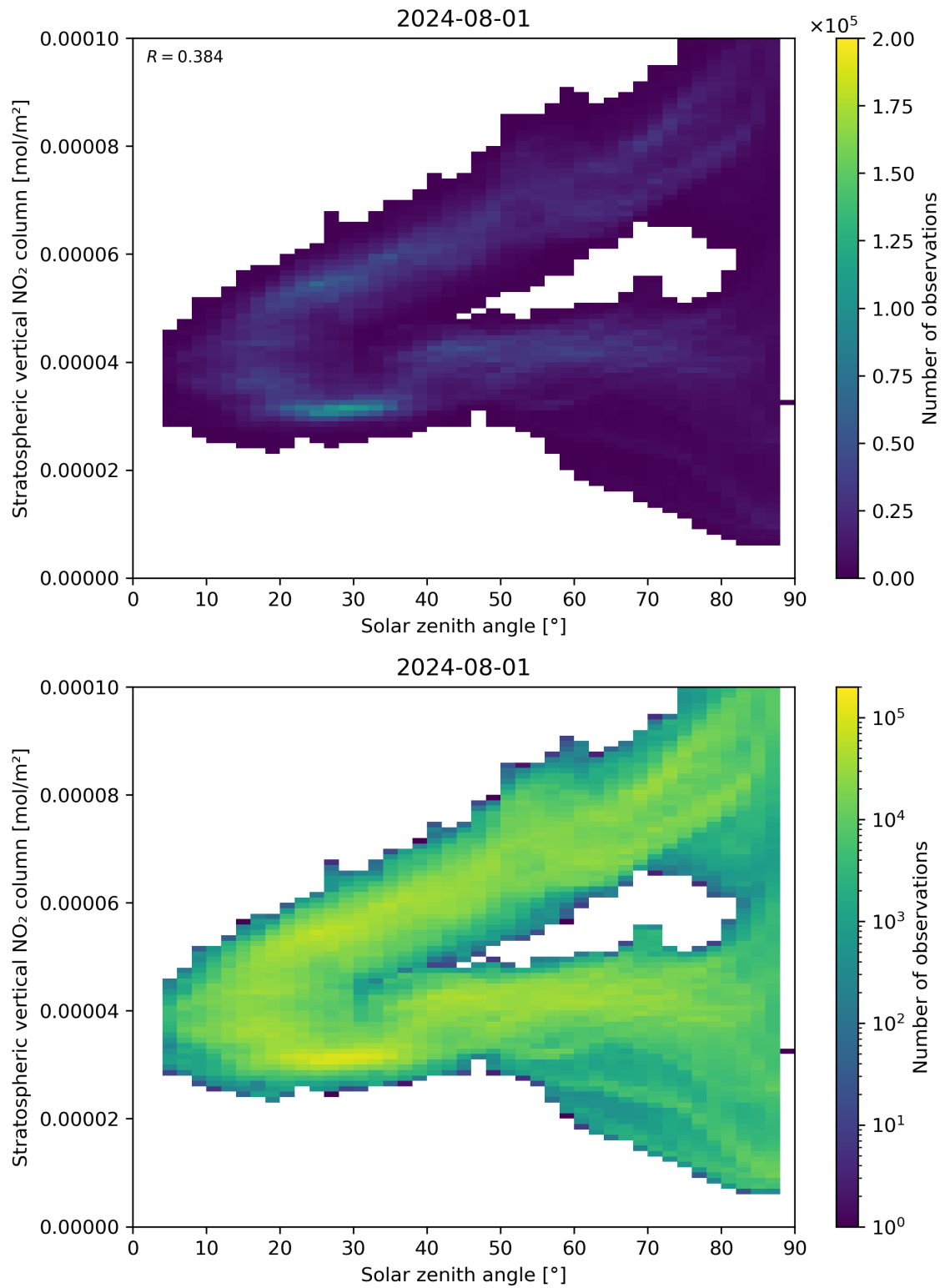
Figure 150: Scatter density plot of “Solar zenith angle” against “Stratospheric vertical NO 2 column” for 2024-07-31 to 2024-08-02.
