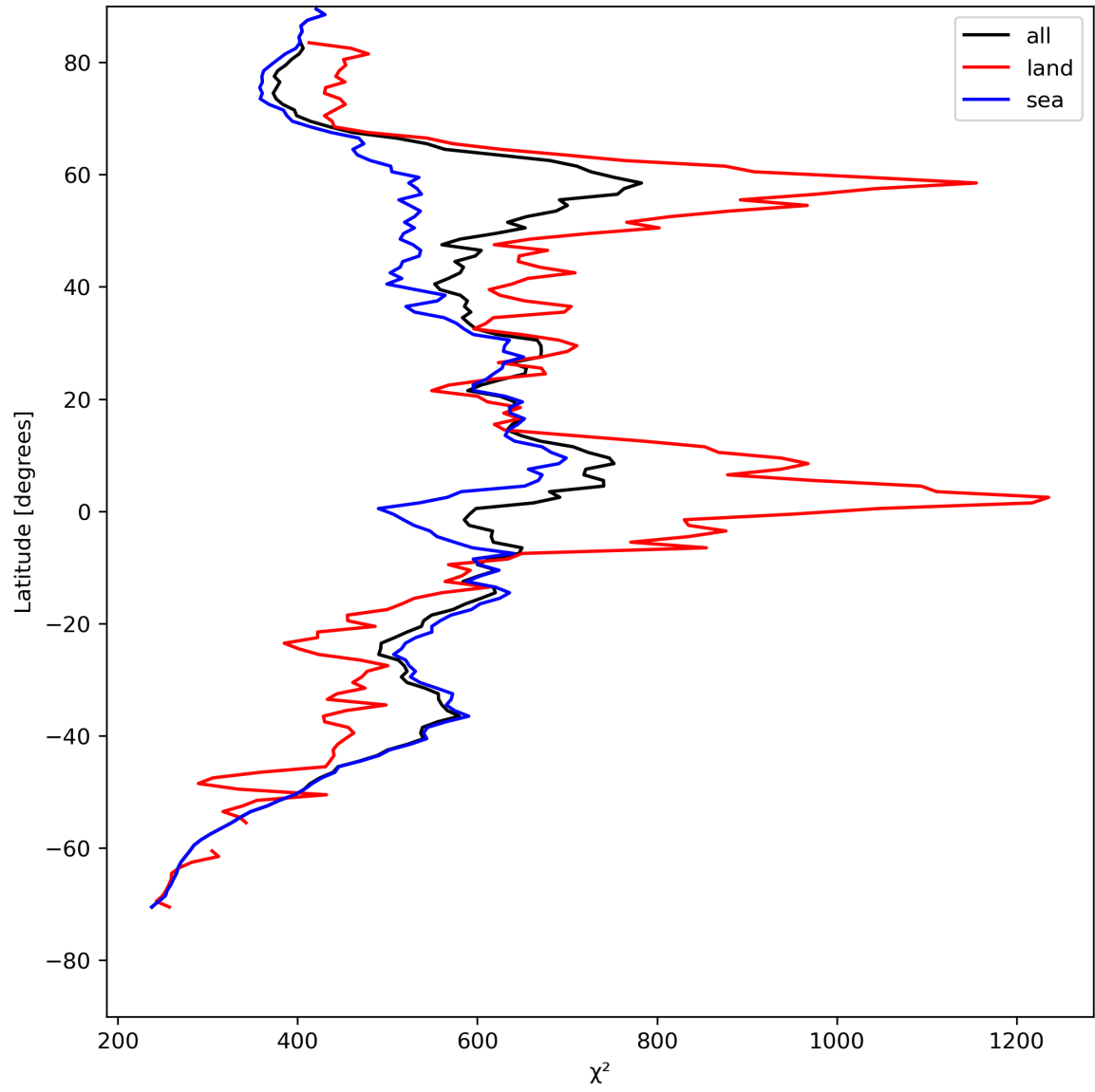
Figure 25: Zonal average of “ \chi^2 ” for 2024-07-31 to 2024-08-02.
