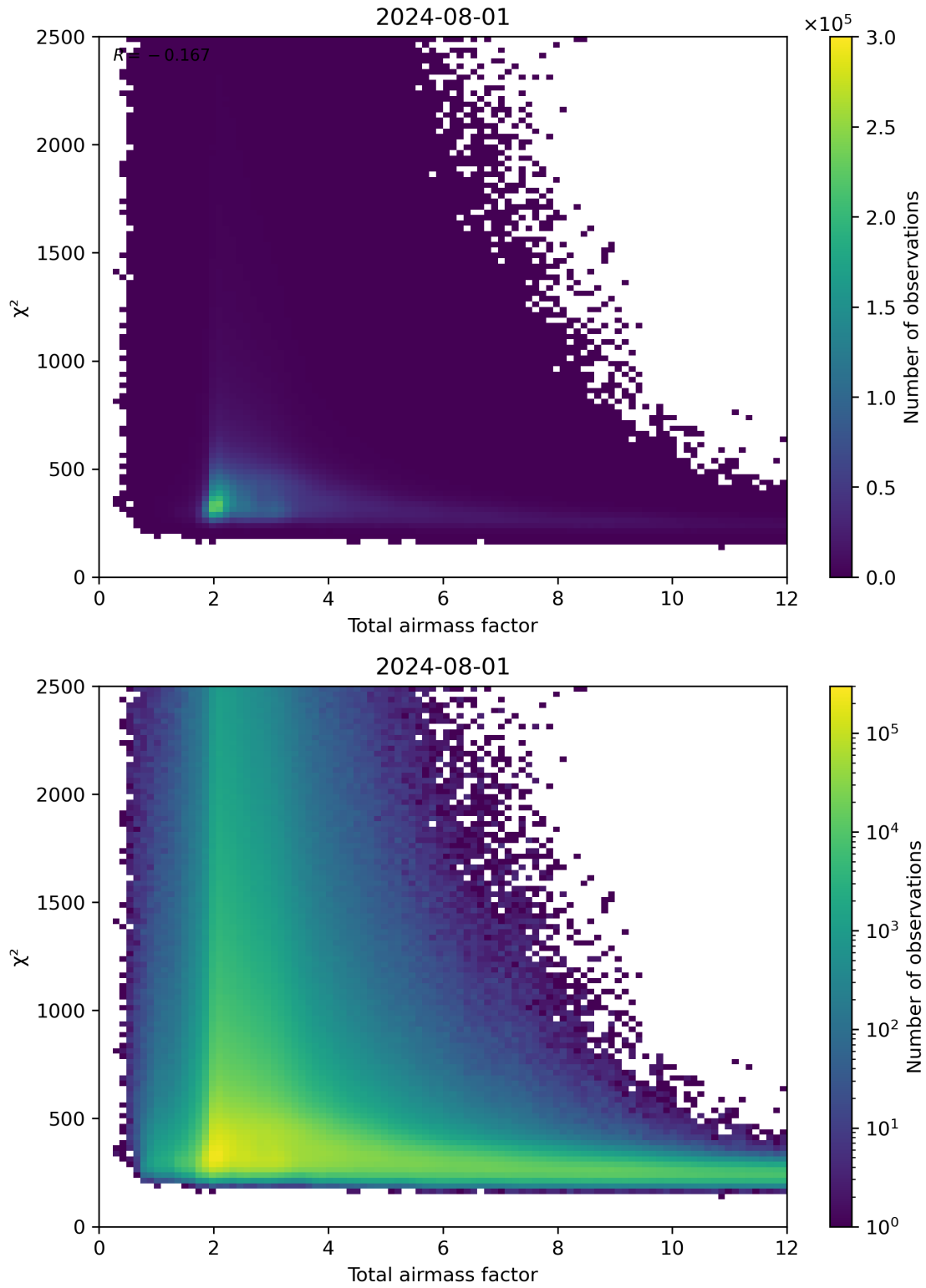
Figure 63: Scatter density plot of “Total airmass factor” against “ \chi^2 ” for 2024-07-31 to 2024-08-02.
