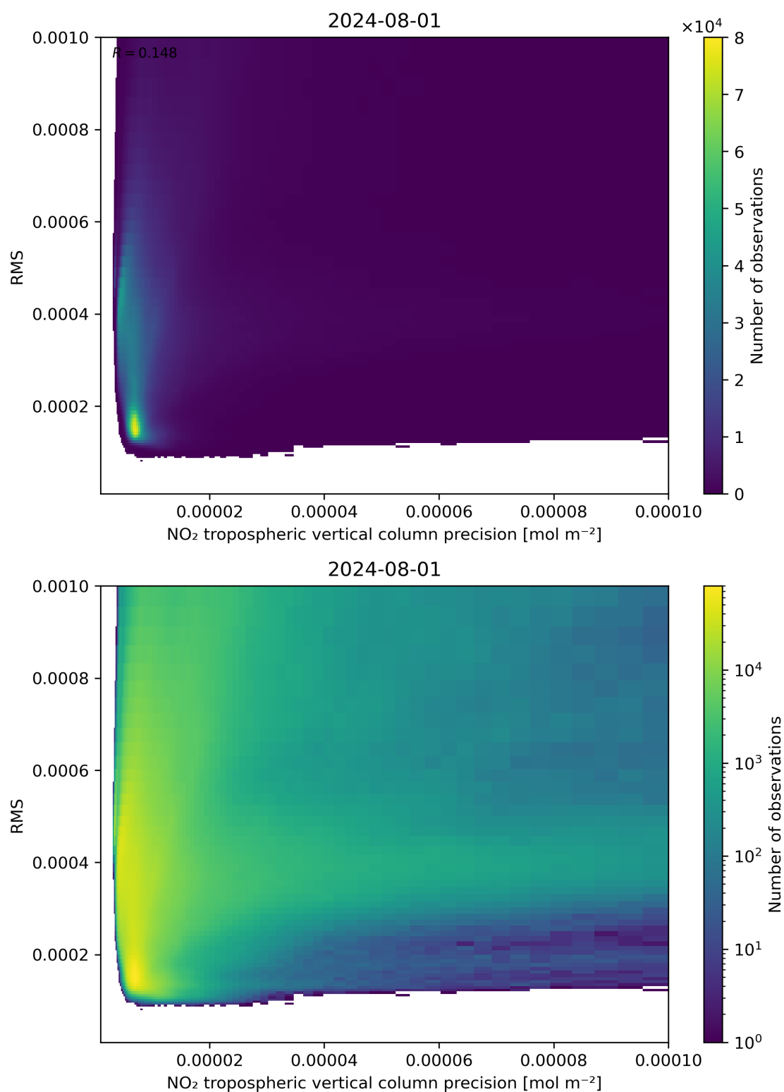
Figure 140: Scatter density plot of “NO 2 tropospheric vertical column precision” against “RMS” for 2024-07-31 to 2024-08-02.
