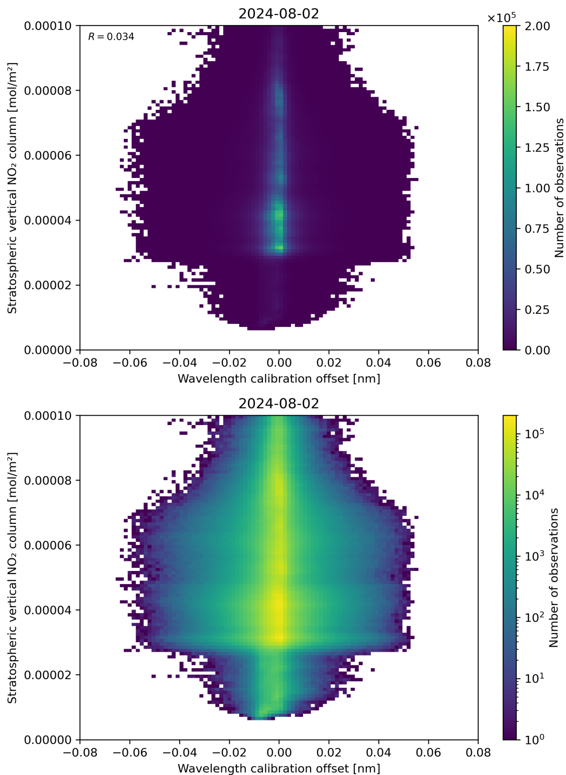
Figure 176: Scatter density plot of “Wavelength calibration offset” against “Stratospheric vertical NO 2 column” for 2024-08-01 to 2024-08-03.
