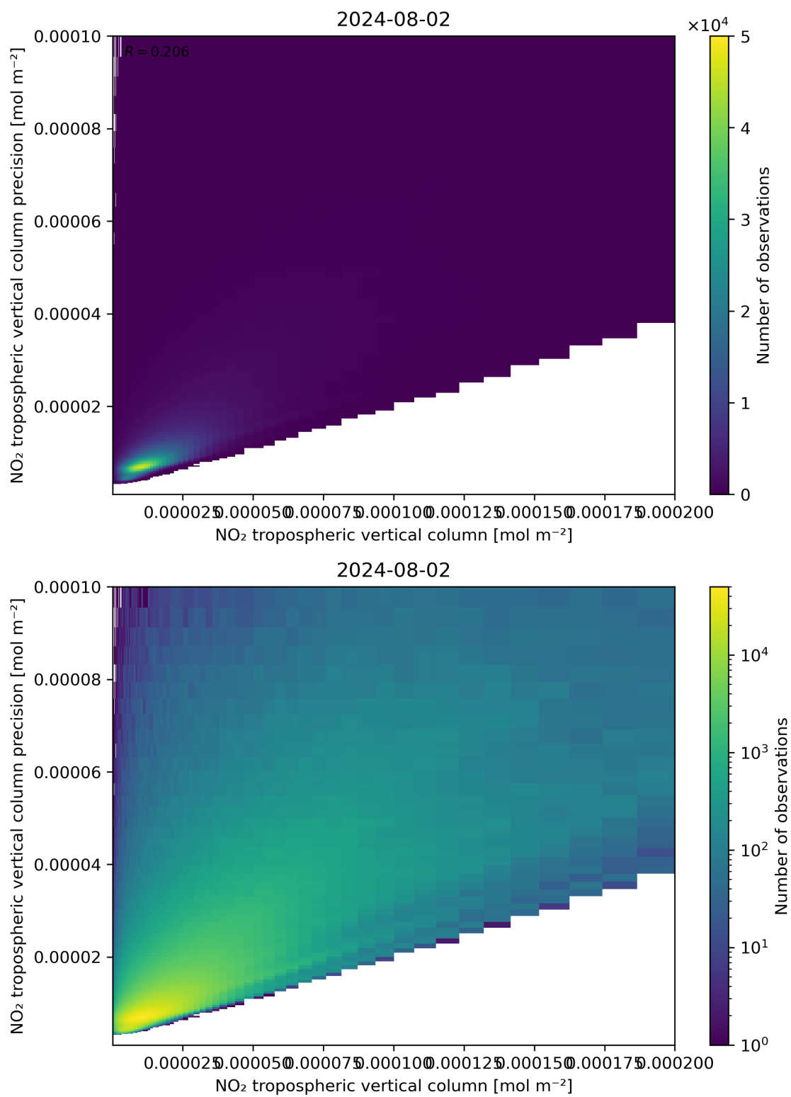
Figure 130: Scatter density plot of “NO 2 tropospheric vertical column” against “NO 2 tropospheric vertical column precision” for 2024-08-01 to 2024-08-03.
