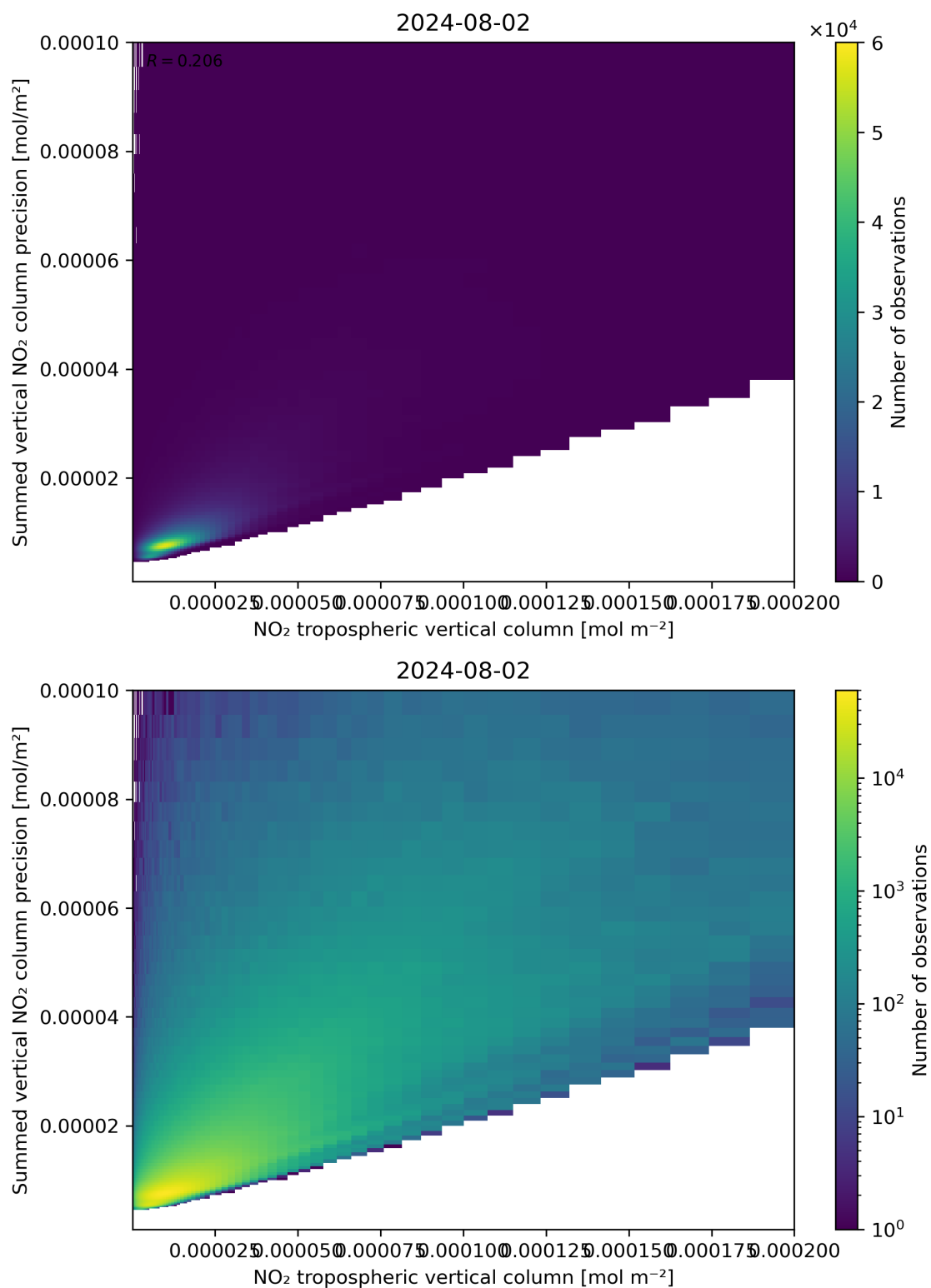
Figure 127: Scatter density plot of “NO 2 tropospheric vertical column” against “Summed vertical NO 2 column precision” for 2024-08-01 to 2024-08-03.
