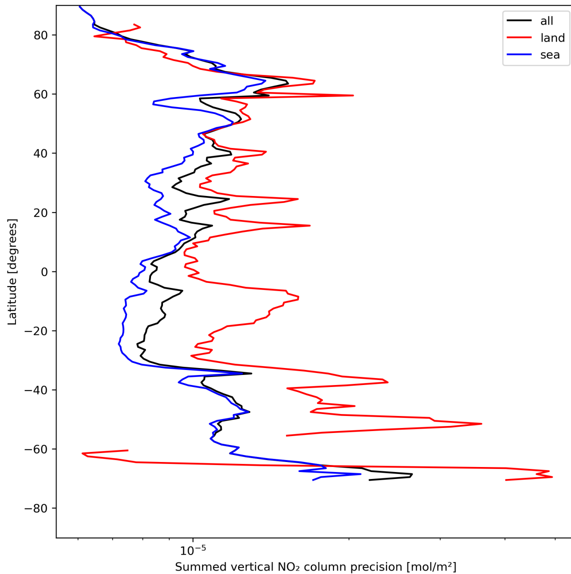
Figure 24: Zonal average of “Summed vertical NO 2 column precision” for 2024-08-01 to 2024-08-03.
