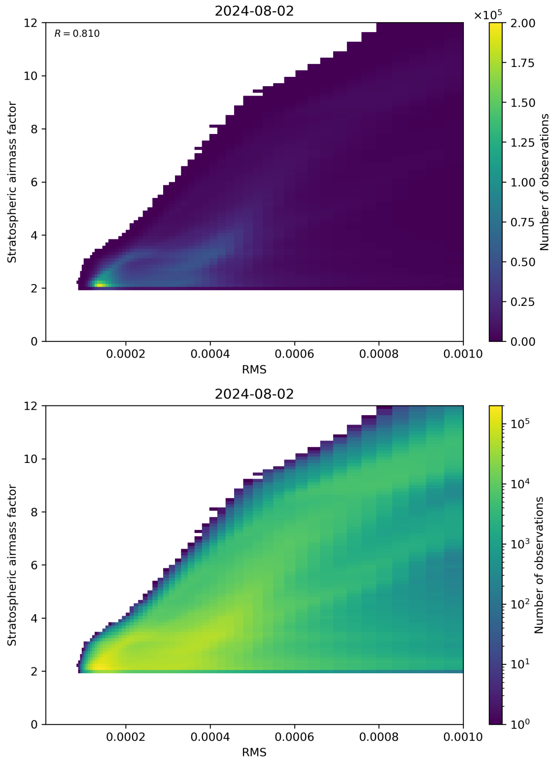
Figure 144: Scatter density plot of “RMS” against “Stratospheric airmass factor” for 2024-08-01 to 2024-08-03.
