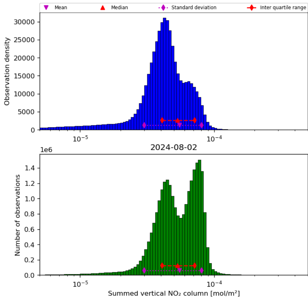
Figure 40: Histogram of “Summed vertical NO 2 column” for 2024-08-01 to 2024-08-03
