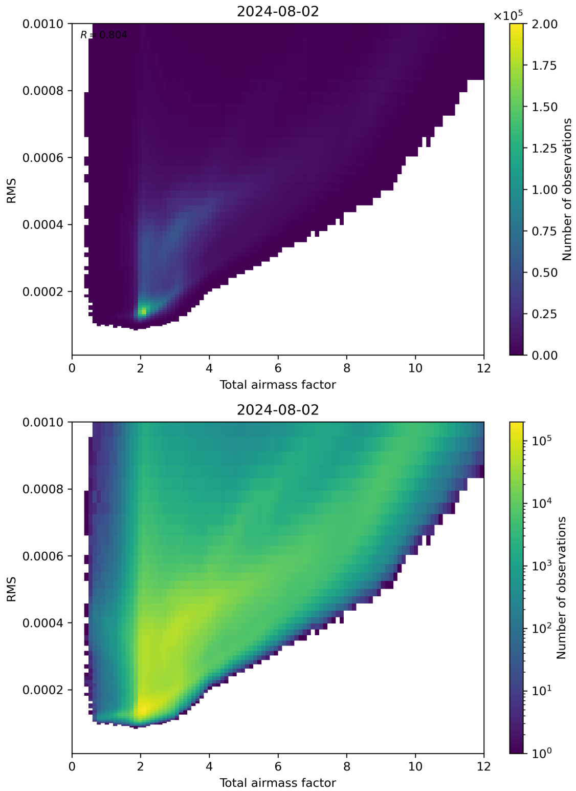
Figure 69: Scatter density plot of “Total airmass factor” against “RMS” for 2024-08-01 to 2024-08-03.
