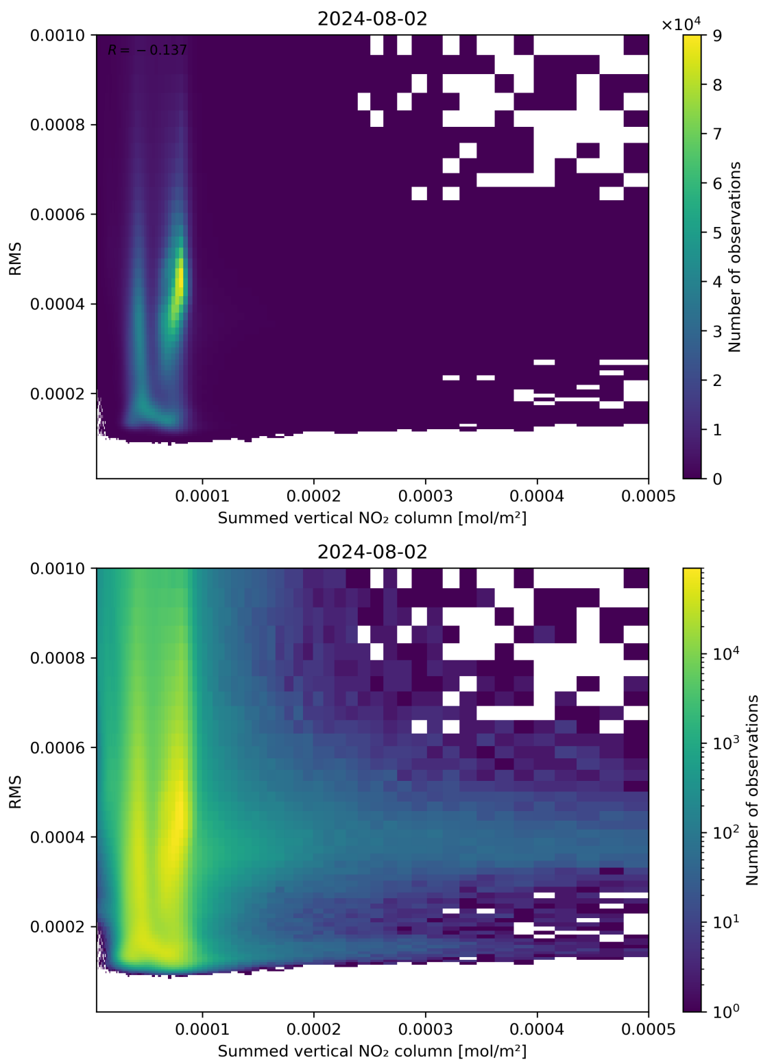
Figure 109: Scatter density plot of “Summed vertical NO 2 column” against “RMS” for 2024-08-01 to 2024-08-03.
