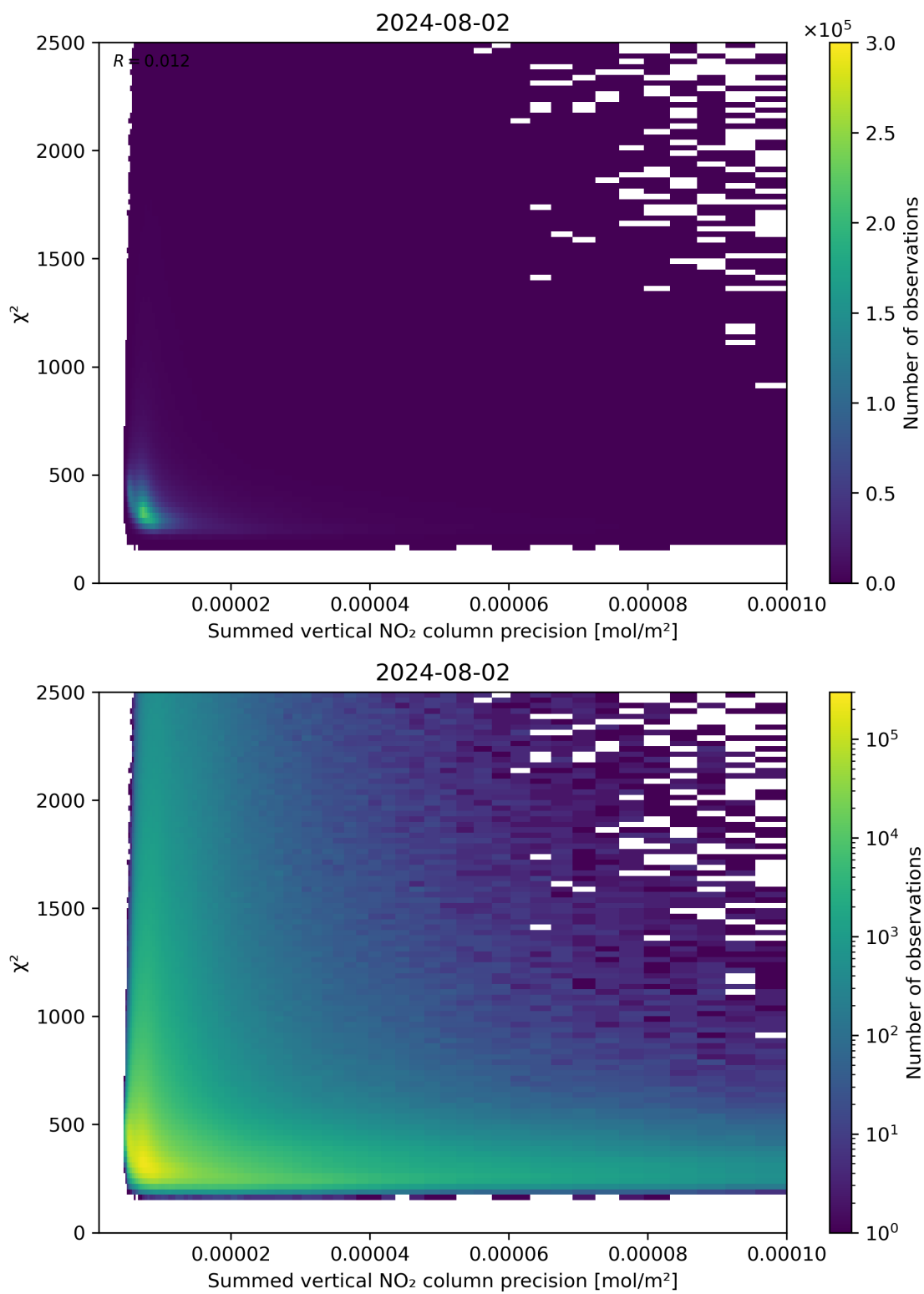
Figure 107: Scatter density plot of “Summed vertical NO 2 column precision” against “ \chi^2 ” for 2024-08-01 to 2024-08-03.
