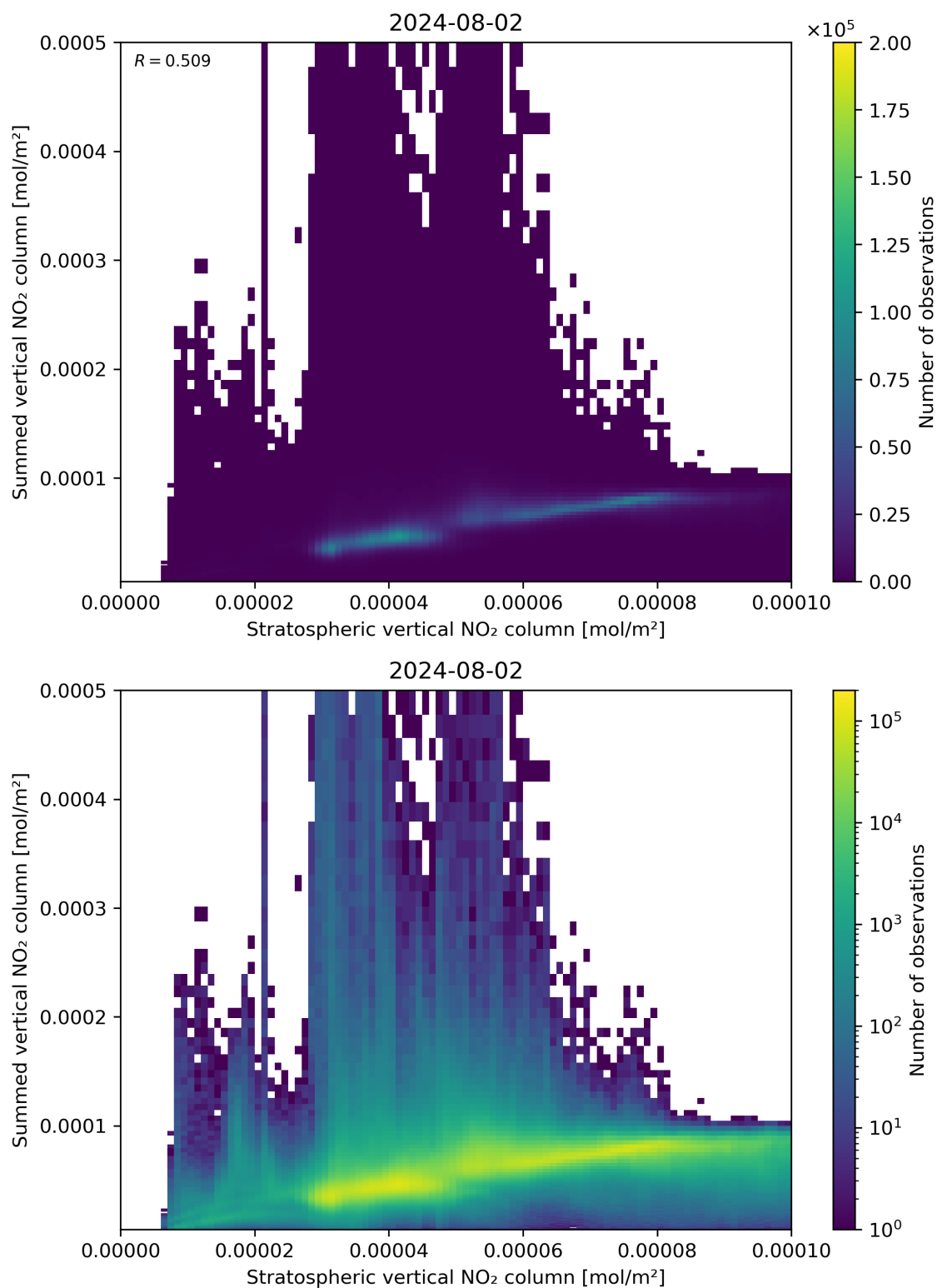
Figure 98: Scatter density plot of “Stratospheric vertical NO 2 column” against “Summed vertical NO 2 column” for 2024-08-01 to 2024-08-03.
