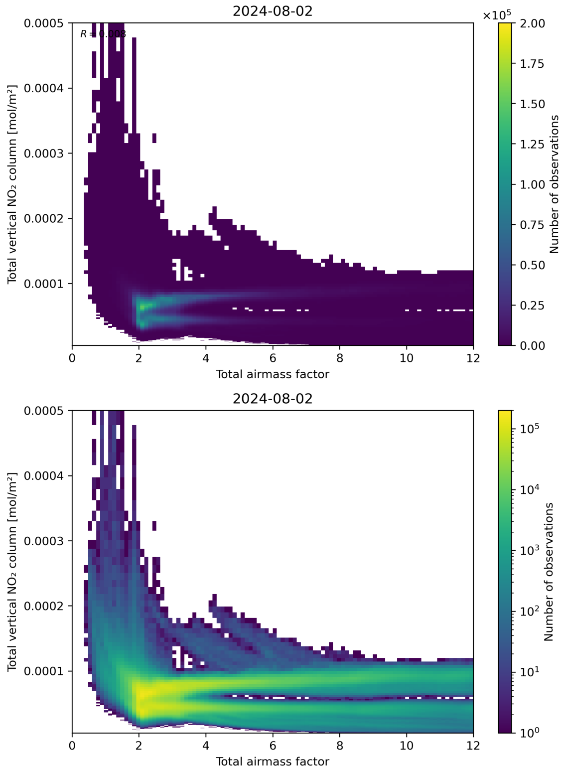
Figure 67: Scatter density plot of “Total air mass factor” against “Total vertical NO 2 column” for 2024-08-01 to 2024-08-03.
