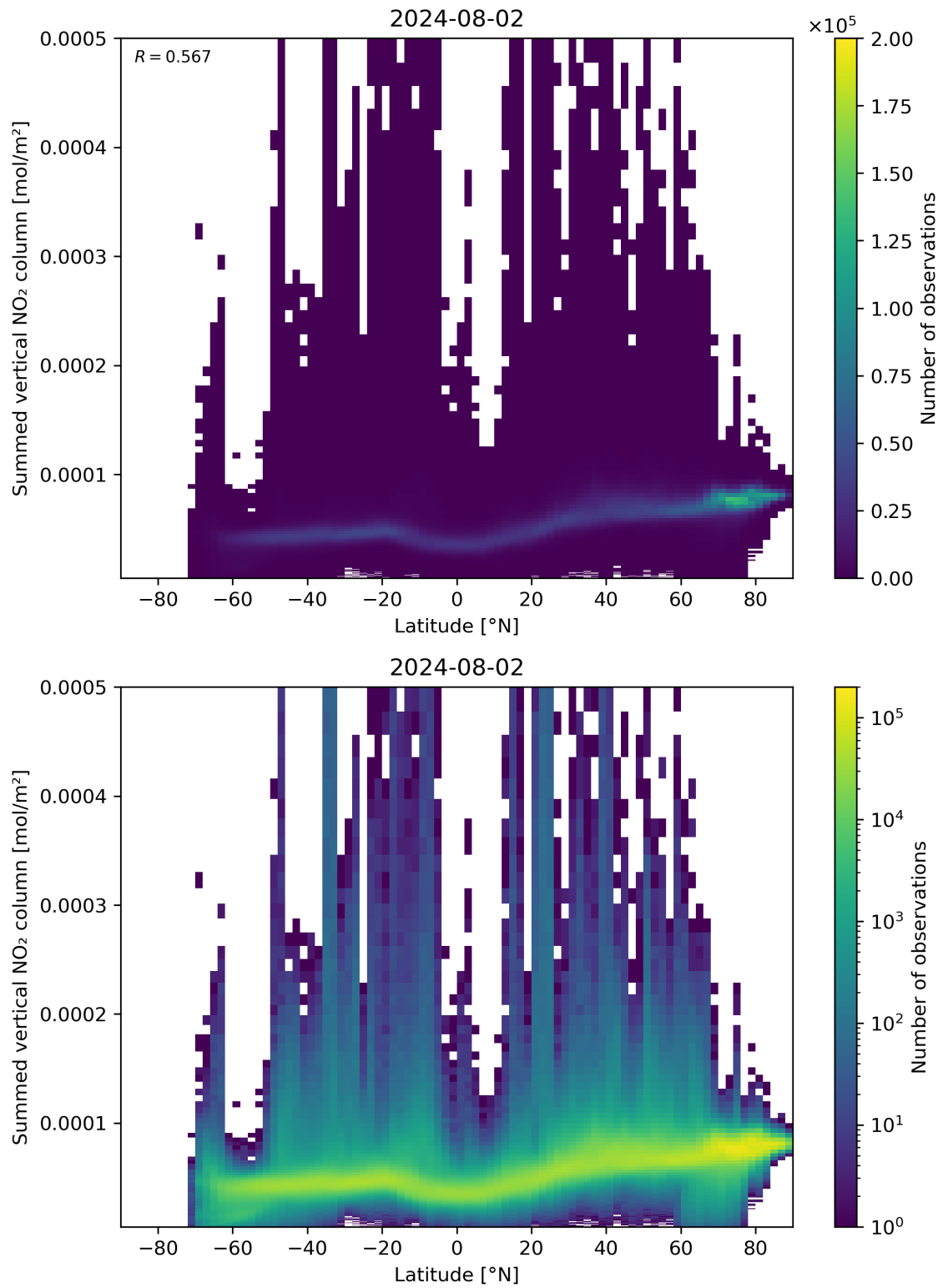
Figure 88: Scatter density plot of “Latitude” against “Summed vertical NO 2 column” for 2024-08-01 to 2024-08-03.
