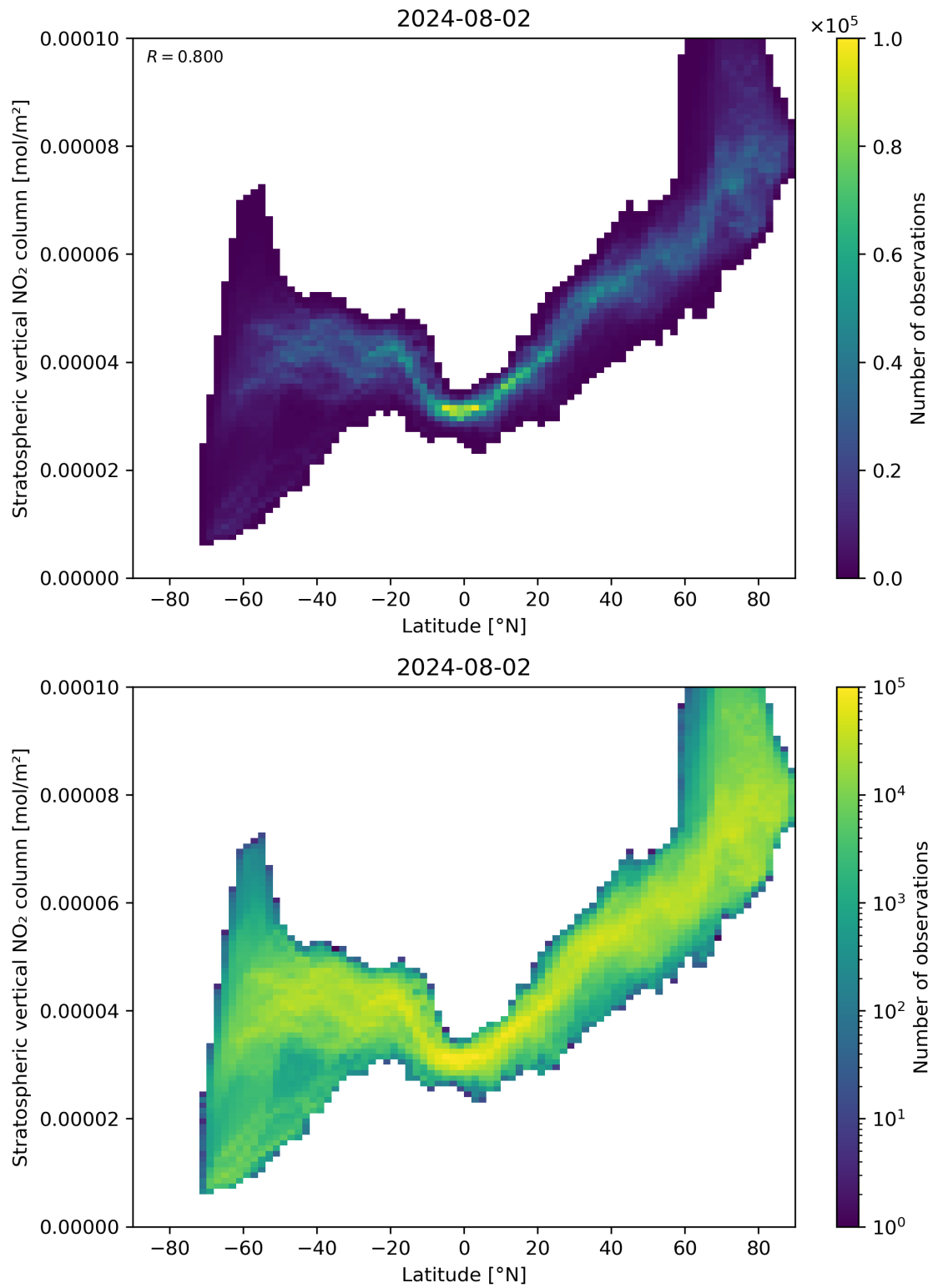
Figure 87: Scatter density plot of “Latitude” against “Stratospheric vertical \text{NO}_2 column” for 2024-08-01 to 2024-08-03.
