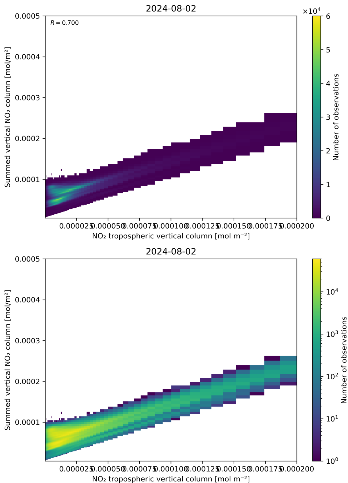
Figure 126: Scatter density plot of “NO 2 tropospheric vertical column” against “Summed vertical NO 2 column” for 2024-08-01 to 2024-08-03.
