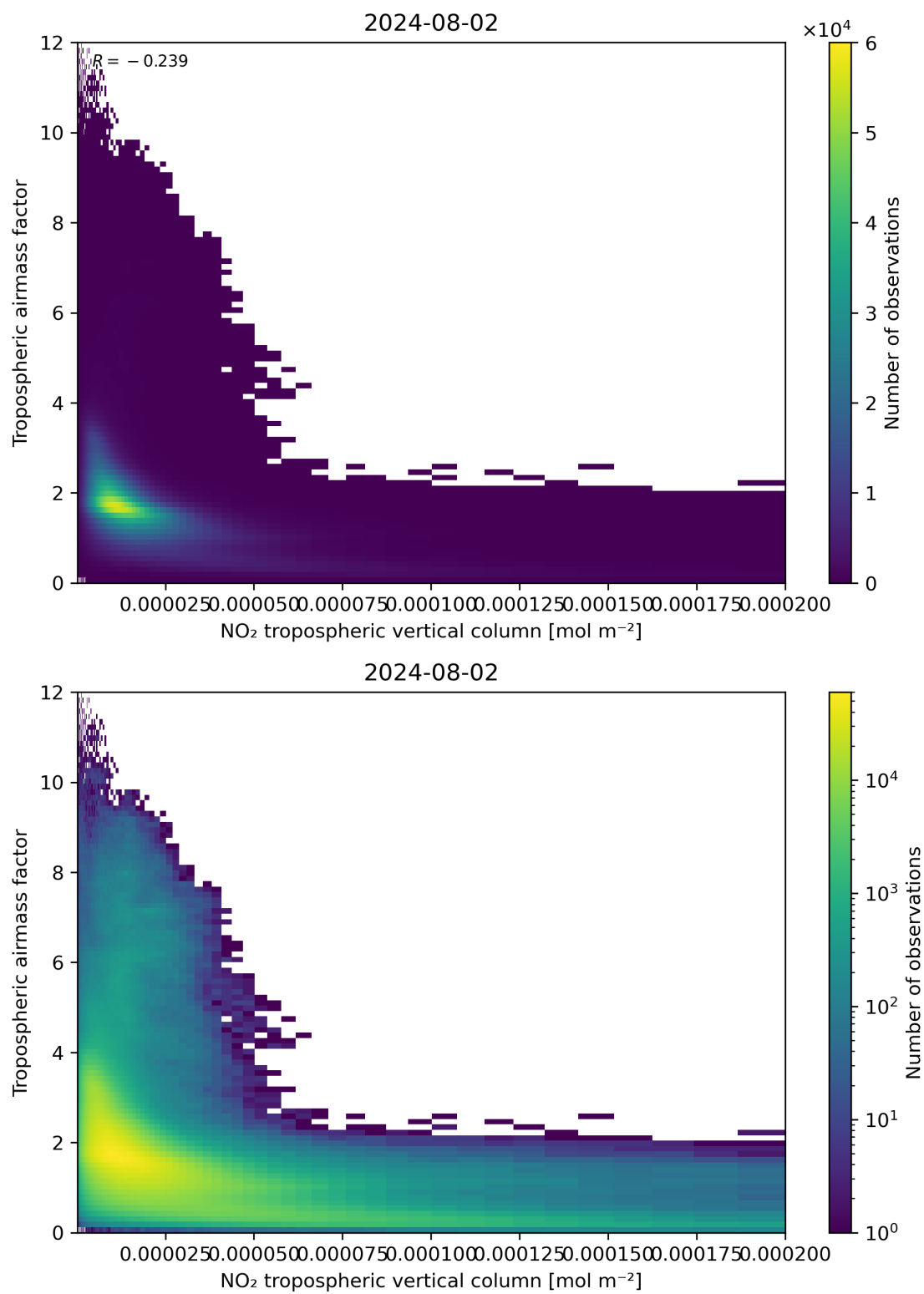
Figure 123: Scatter density plot of “NO 2 tropospheric vertical column” against “Tropospheric air mass factor” for 2024-08-01 to 2024-08-03.
