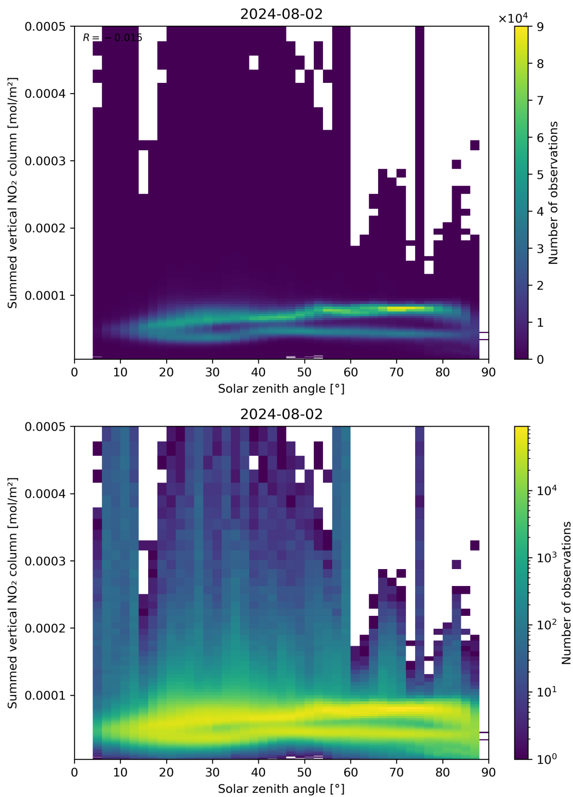
Figure 151: Scatter density plot of “Solar zenith angle” against “Summed vertical NO 2 column” for 2024-08-01 to 2024-08-03.
