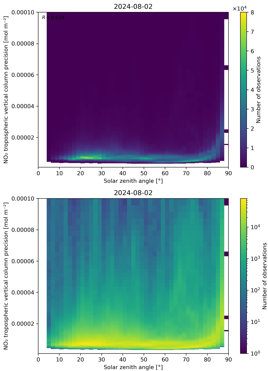
Figure 156: Scatter density plot of “Solar zenith angle” against “NO 2 tropospheric vertical column precision” for 2024-08-01 to 2024-08-03.
