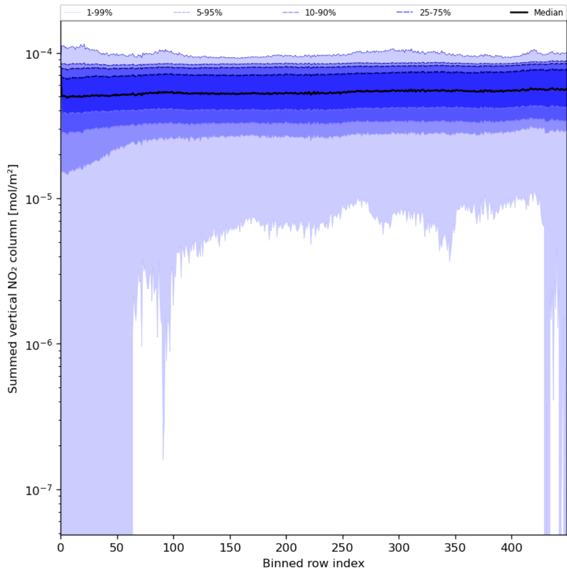
Figure 57: Along track statistics of “Summed vertical NO 2 column” for 2024-08-01 to 2024-08-03
