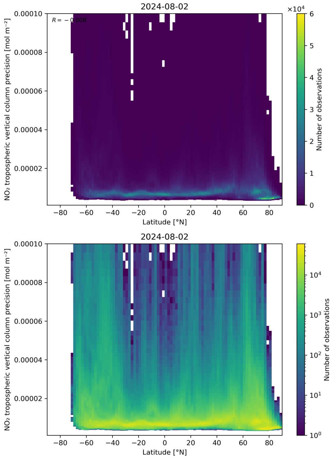
Figure 93: Scatter density plot of “Latitude” against “NO 2 tropospheric vertical column precision” for 2024-08-01 to 2024-08-03.
