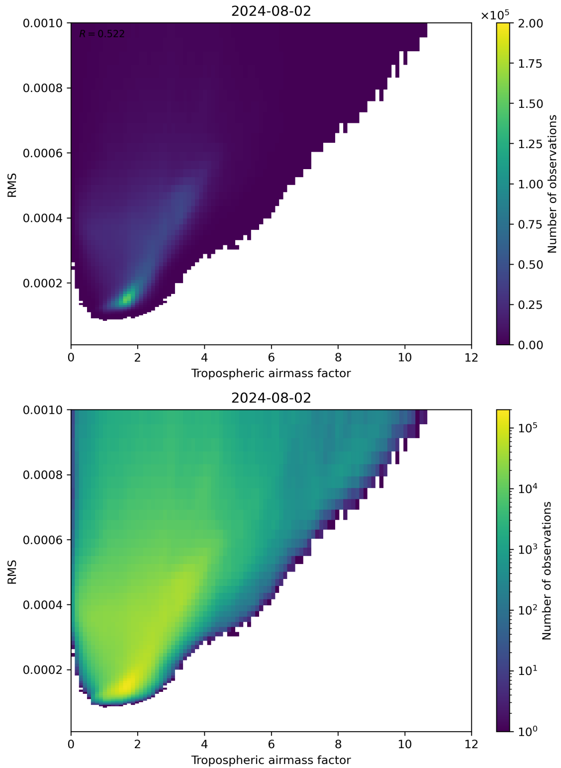
Figure 79: Scatter density plot of “Tropospheric airmass factor” against “RMS” for 2024-08-01 to 2024-08-03.
