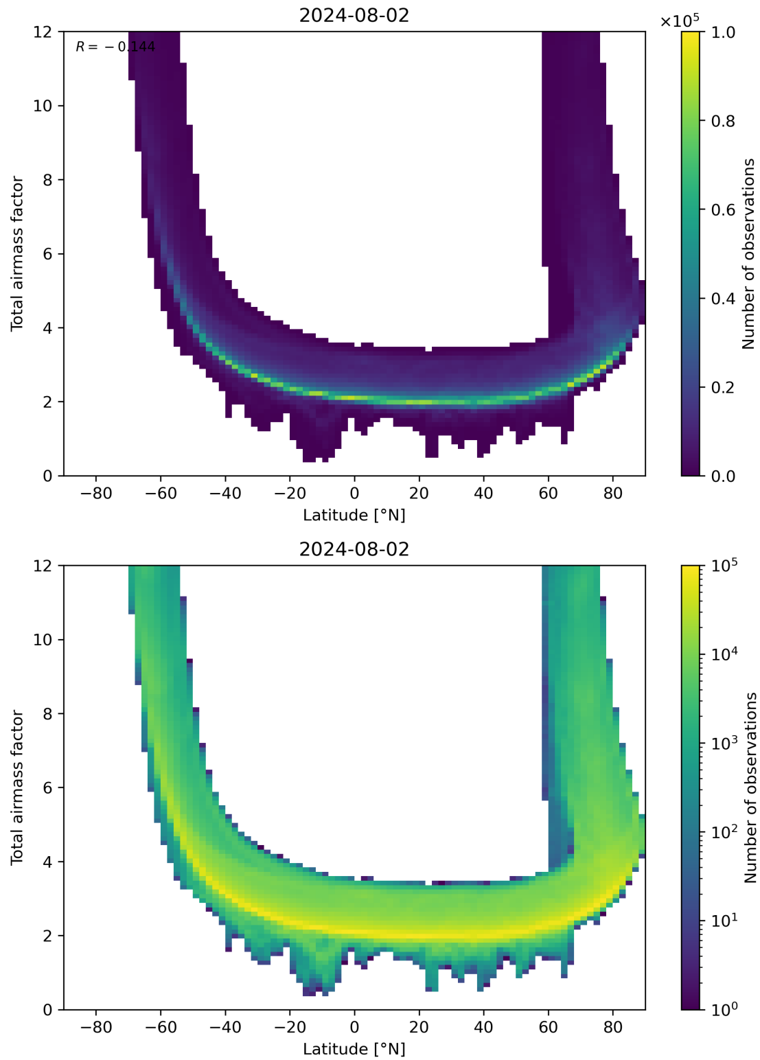
Figure 84: Scatter density plot of “Latitude” against “Total airmass factor” for 2024-08-01 to 2024-08-03.
