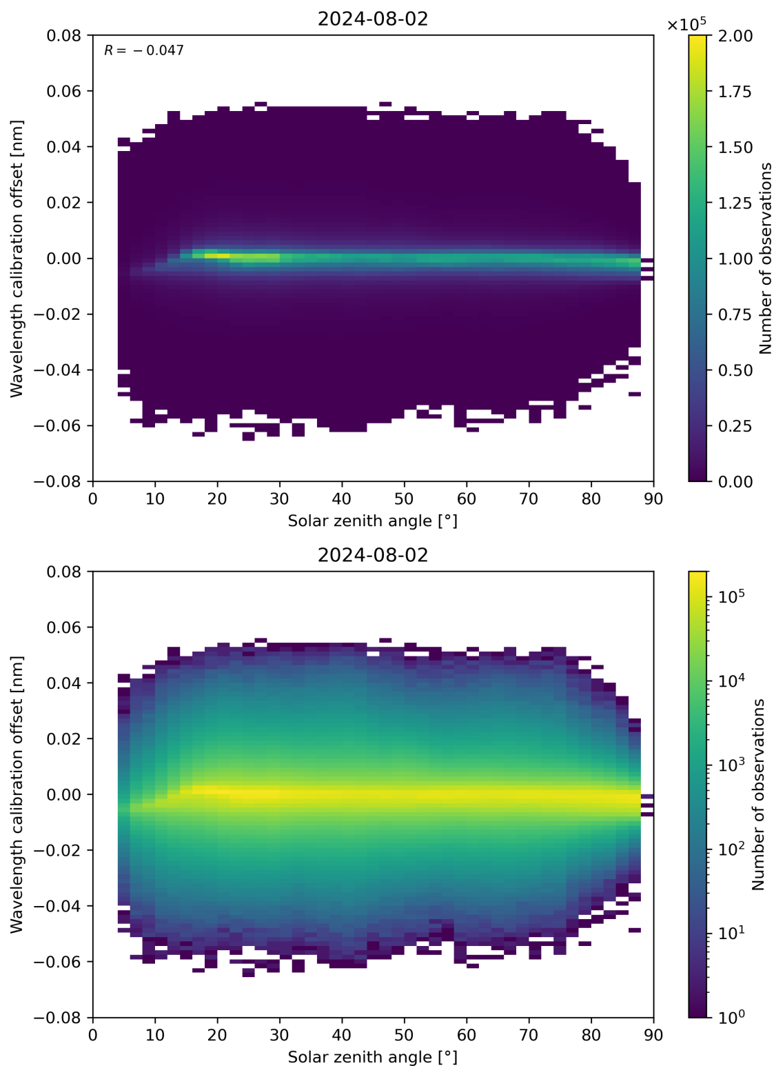
Figure 158: Scatter density plot of “Solar zenith angle” against “Wavelength calibration offset” for 2024-08-01 to 2024-08-03.
