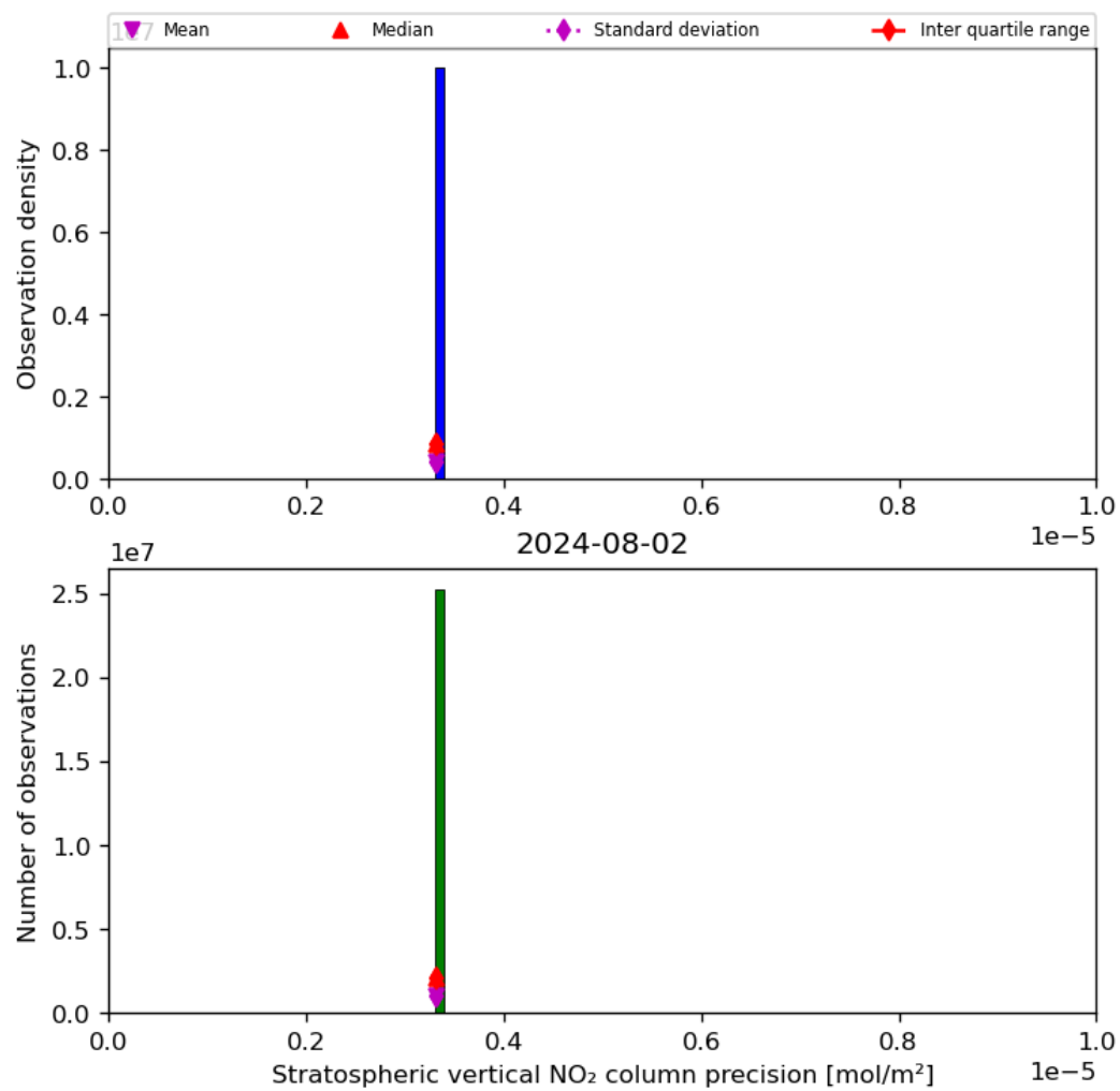
Figure 37: Histogram of “Stratospheric vertical NO 2 column precision” for 2024-08-01 to 2024-08-03
