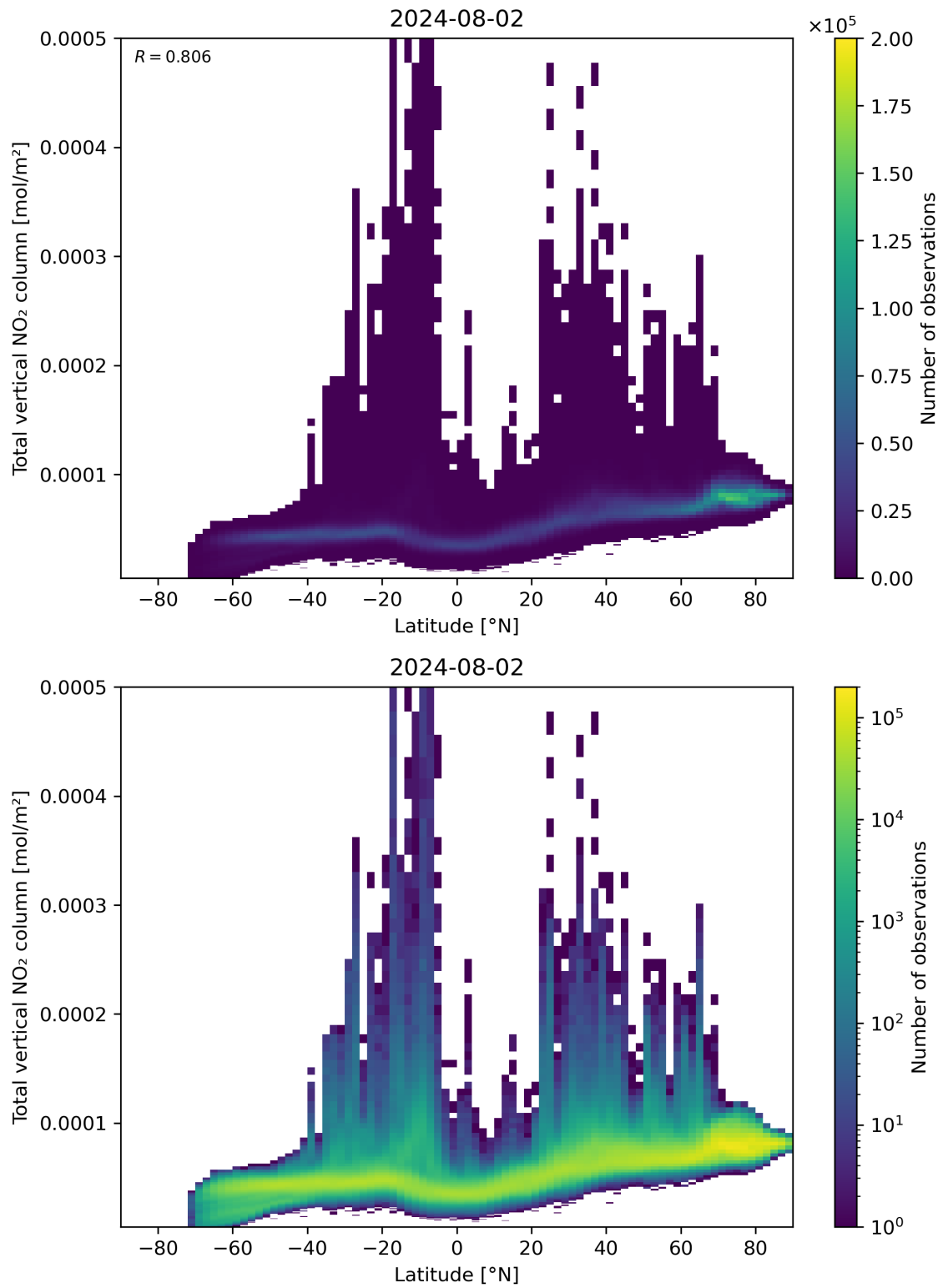
Figure 90: Scatter density plot of “Latitude” against “Total vertical NO 2 column” for 2024-08-01 to 2024-08-03.
