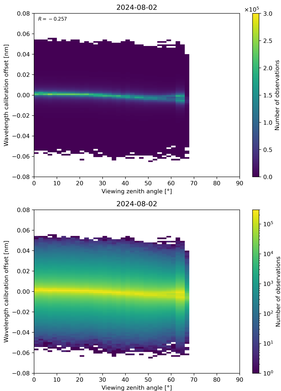
Figure 173: Scatter density plot of “Viewing zenith angle” against “Wavelength calibration offset” for 2024-08-01 to 2024-08-03.
