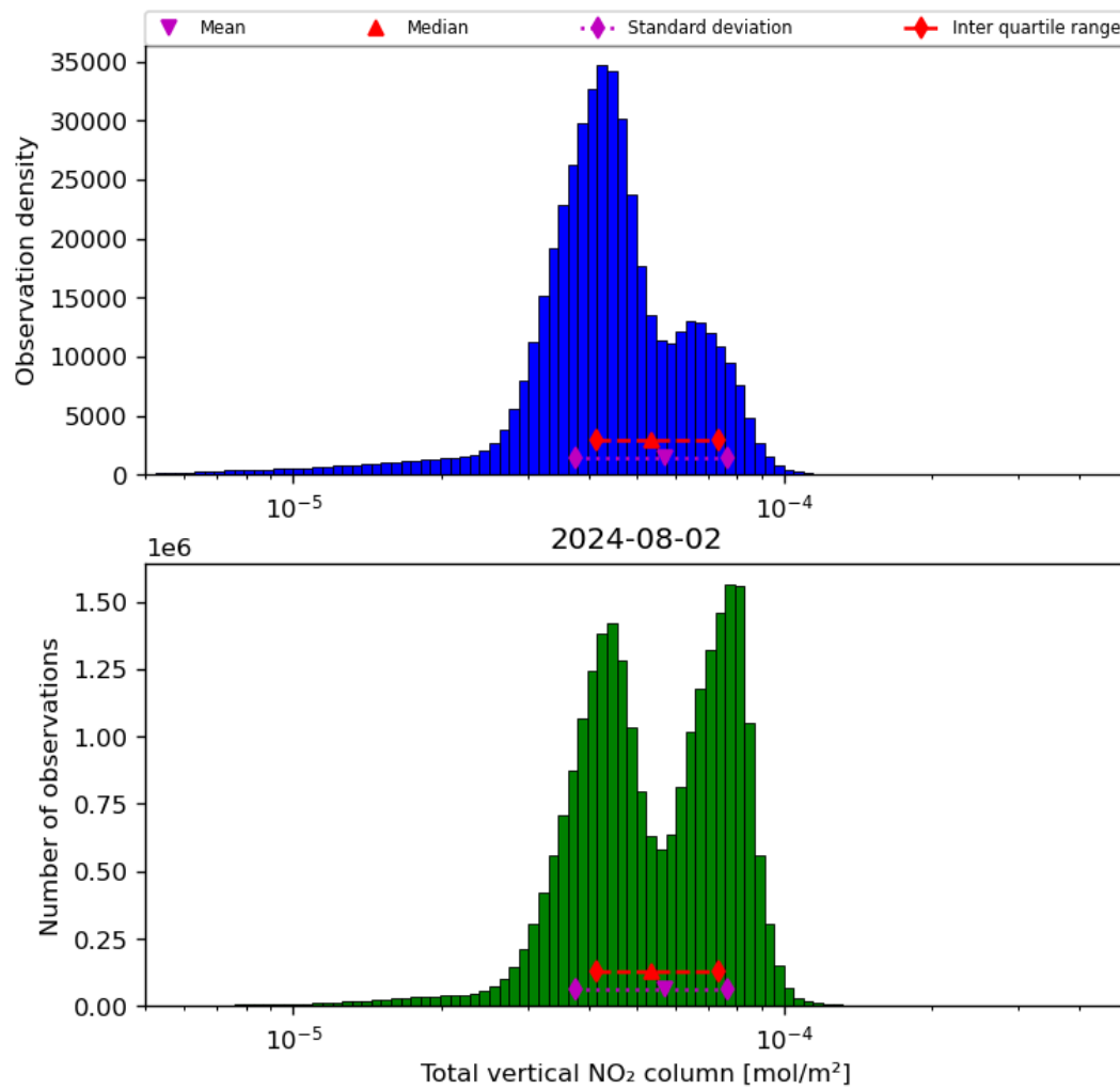
Figure 38: Histogram of “Total vertical NO 2 column” for 2024-08-01 to 2024-08-03
