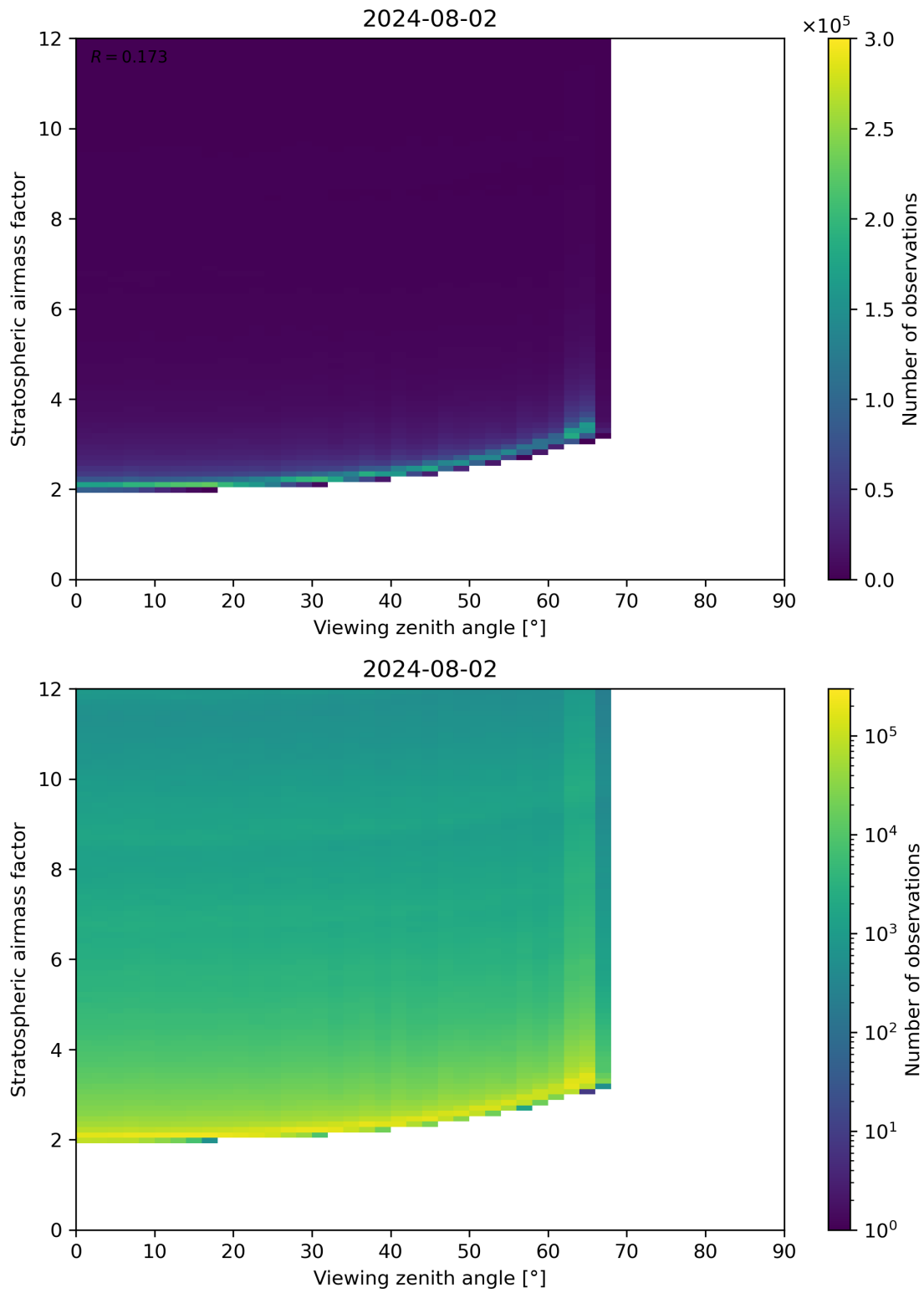
Figure 159: Scatter density plot of “Viewing zenith angle” against “Stratospheric airmass factor” for 2024-08-01 to 2024-08-03.
