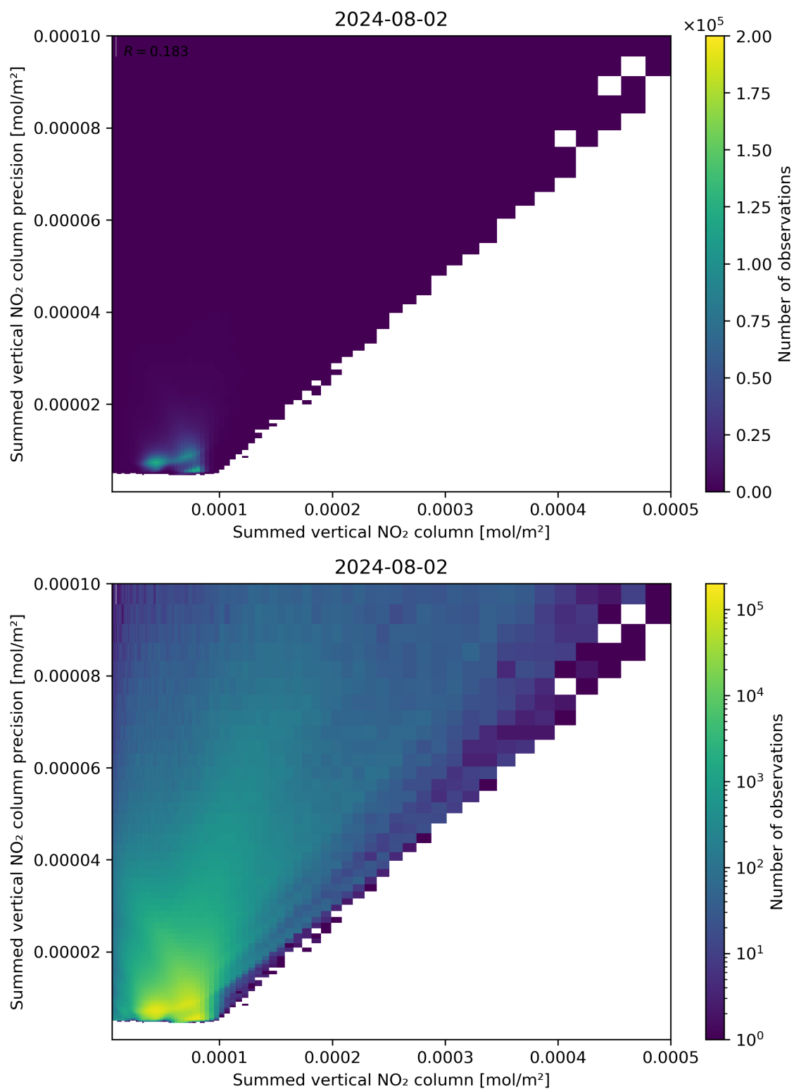
Figure 105: Scatter density plot of “Summed vertical NO 2 column” against “Summed vertical NO 2 column precision” for 2024-08-01 to 2024-08-03.
