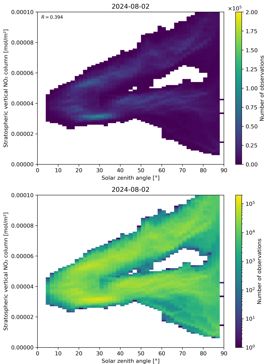
Figure 150: Scatter density plot of “Solar zenith angle” against “Stratospheric vertical NO 2 column” for 2024-08-01 to 2024-08-03.
