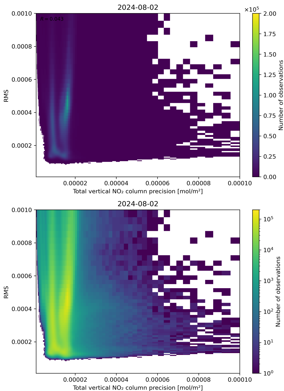
Figure 119: Scatter density plot of “Total vertical NO 2 column precision” against “RMS” for 2024-08-01 to 2024-08-03.
