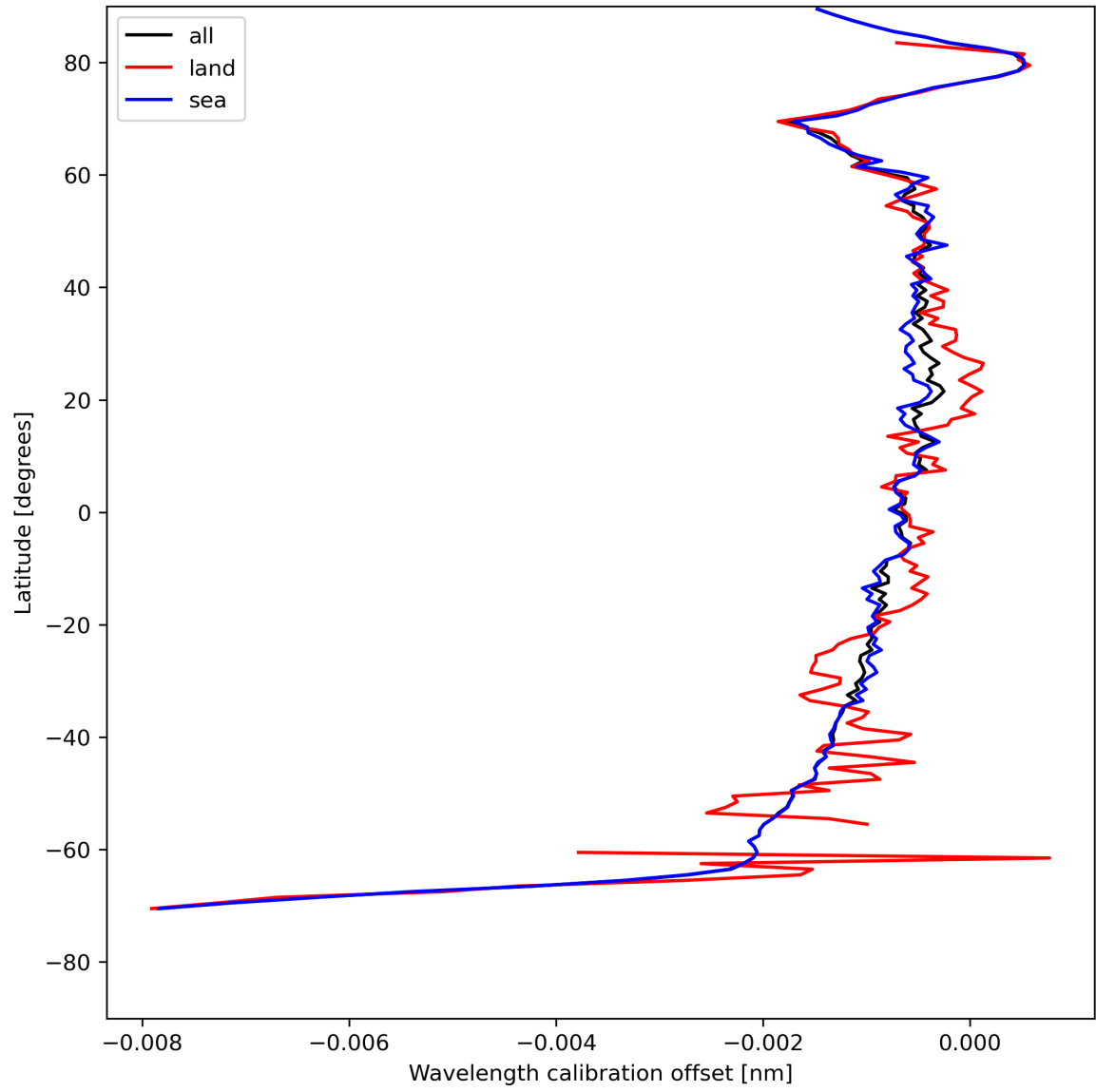
Figure 18: Zonal average of “Wavelength calibration offset” for 2024-08-01 to 2024-08-03.
