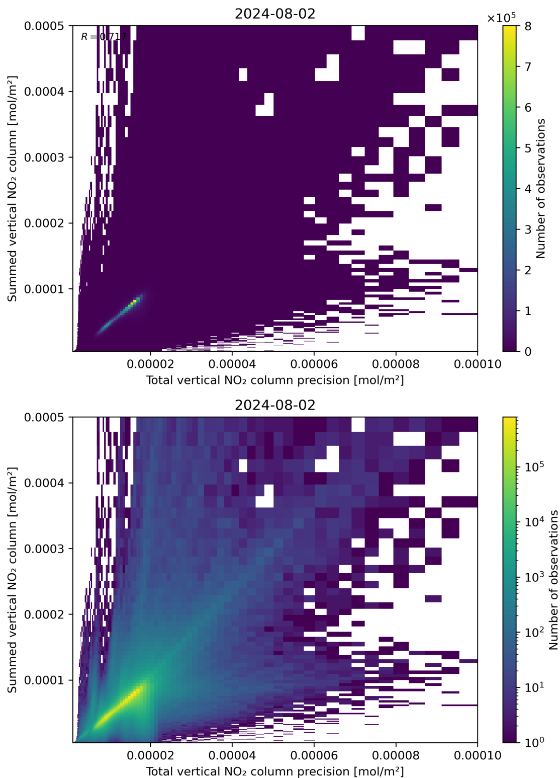
Figure 117: Scatter density plot of “Total vertical NO 2 column precision” against “Summed vertical NO 2 column” for 2024-08-01 to 2024-08-03.
