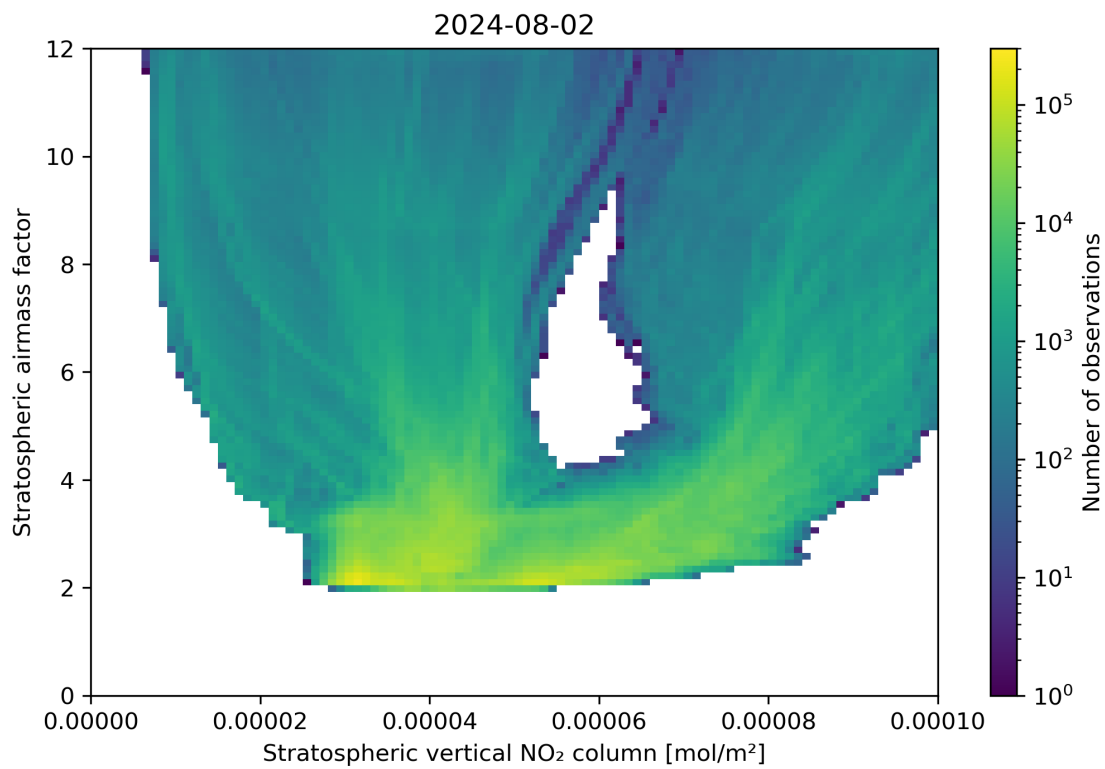
Figure 96: Scatter density plot of “Stratospheric vertical NO 2 column” against “Stratospheric airmass factor” for 2024-08-01 to 2024-08-03.
