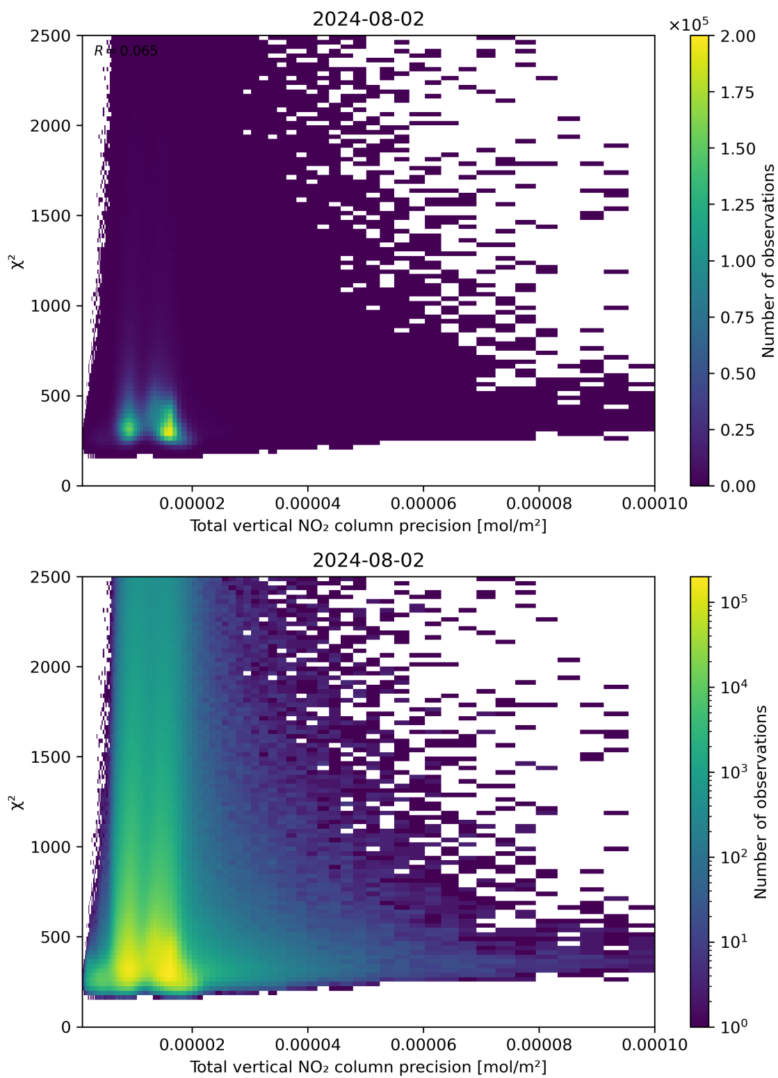
Figure 116: Scatter density plot of “Total vertical NO 2 column precision” against “ \chi^2 ” for 2024-08-01 to 2024-08-03.
