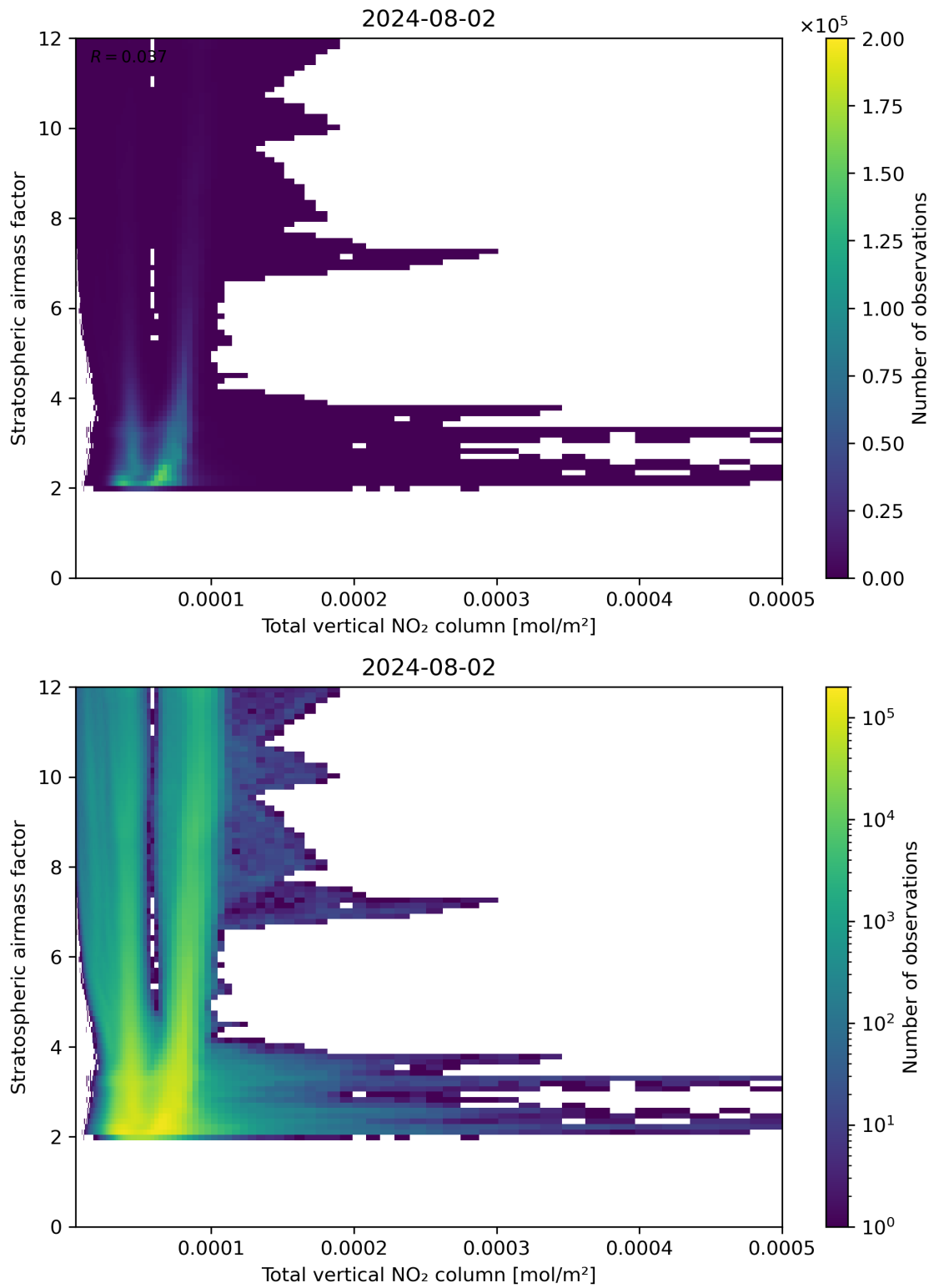
Figure 110: Scatter density plot of “Total vertical NO 2 column” against “Stratospheric airmass factor” for 2024-08-01 to 2024-08-03.
