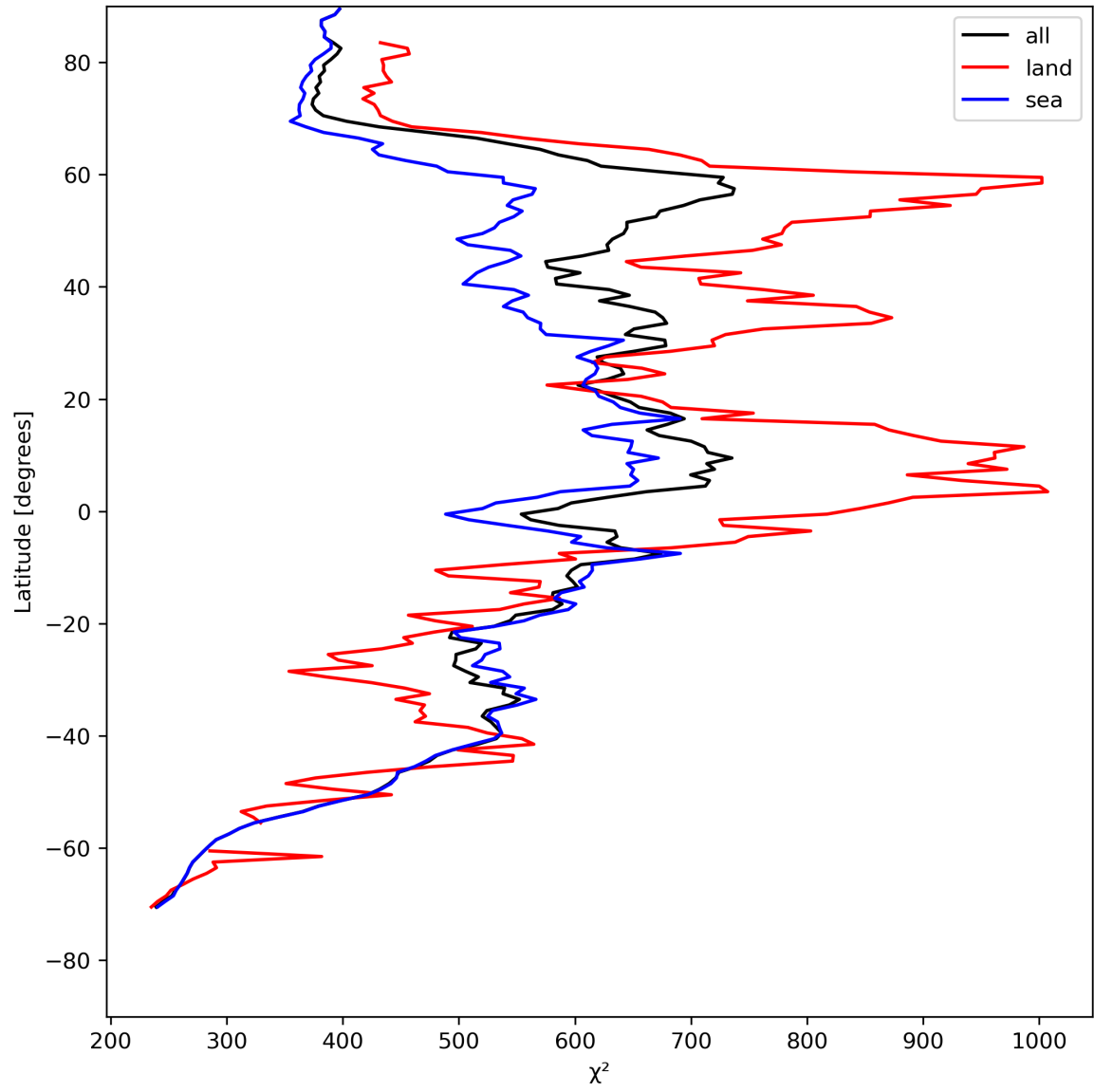
Figure 25: Zonal average of “ \chi^2 ” for 2024-08-01 to 2024-08-03.
