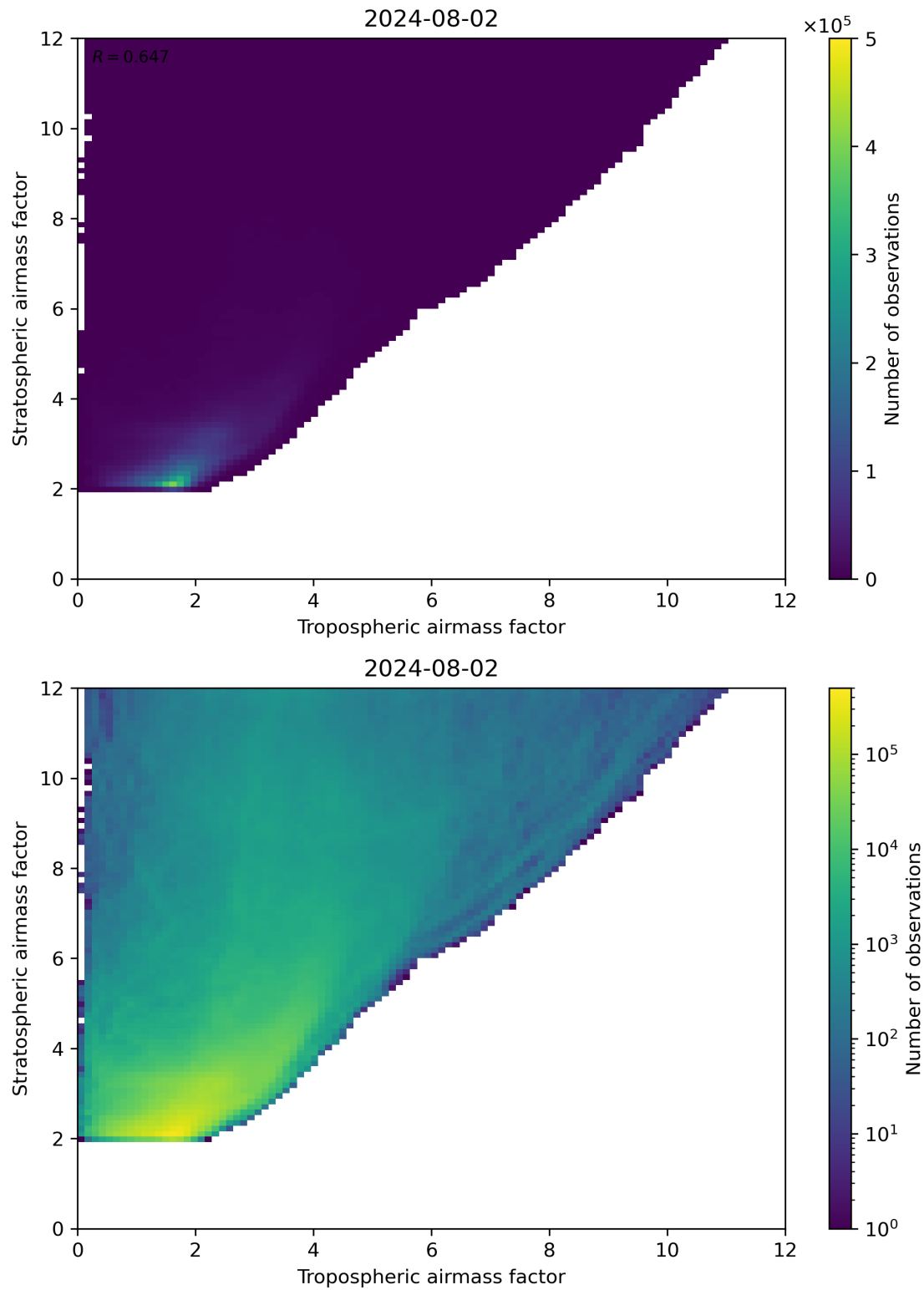
Figure 71: Scatter density plot of “Tropospheric airmass factor” against “Stratospheric airmass factor” for 2024-08-01 to 2024-08-03.
