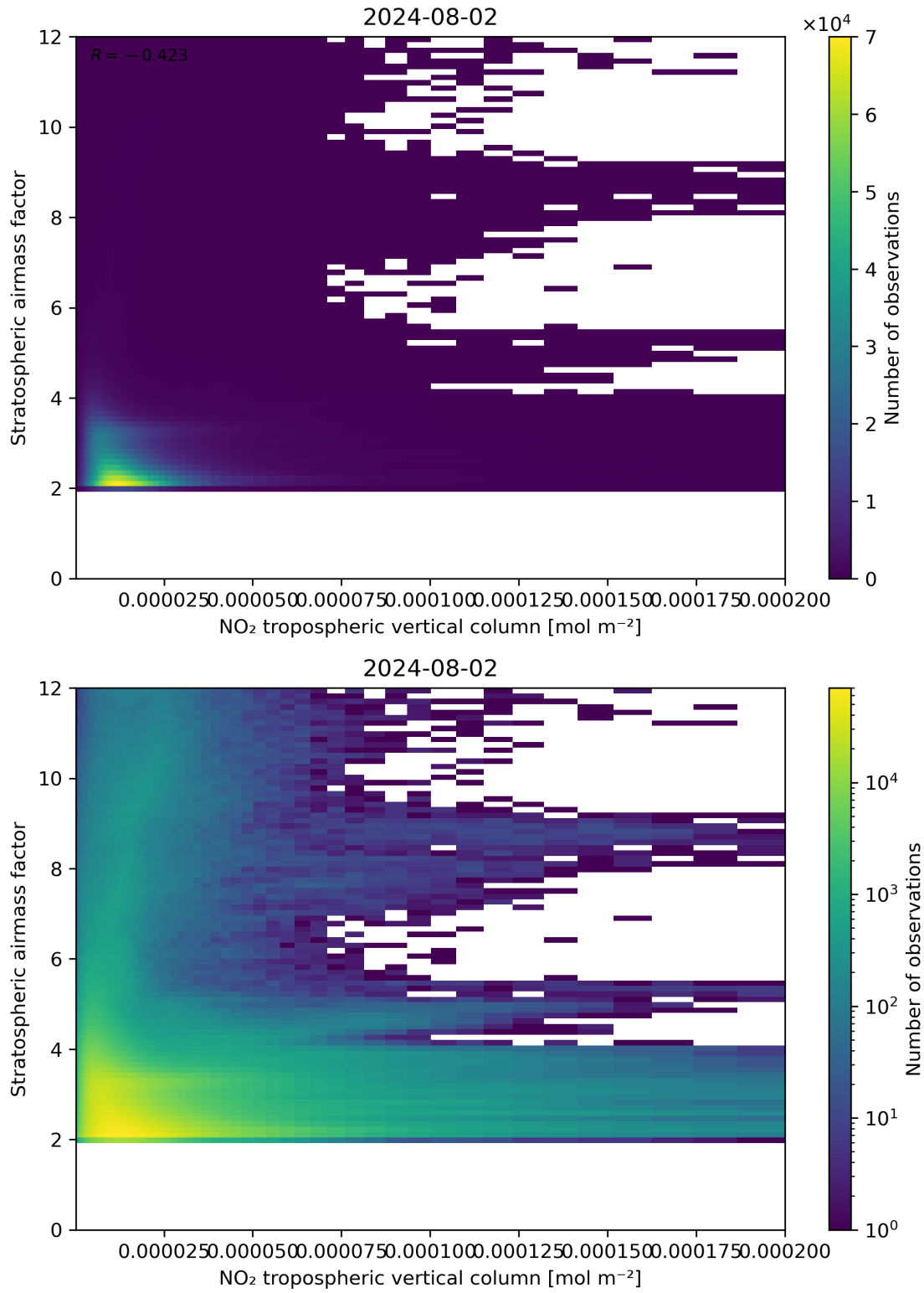
Figure 121: Scatter density plot of “NO 2 tropospheric vertical column” against “Stratospheric air mass factor” for 2024-08-01 to 2024-08-03.
