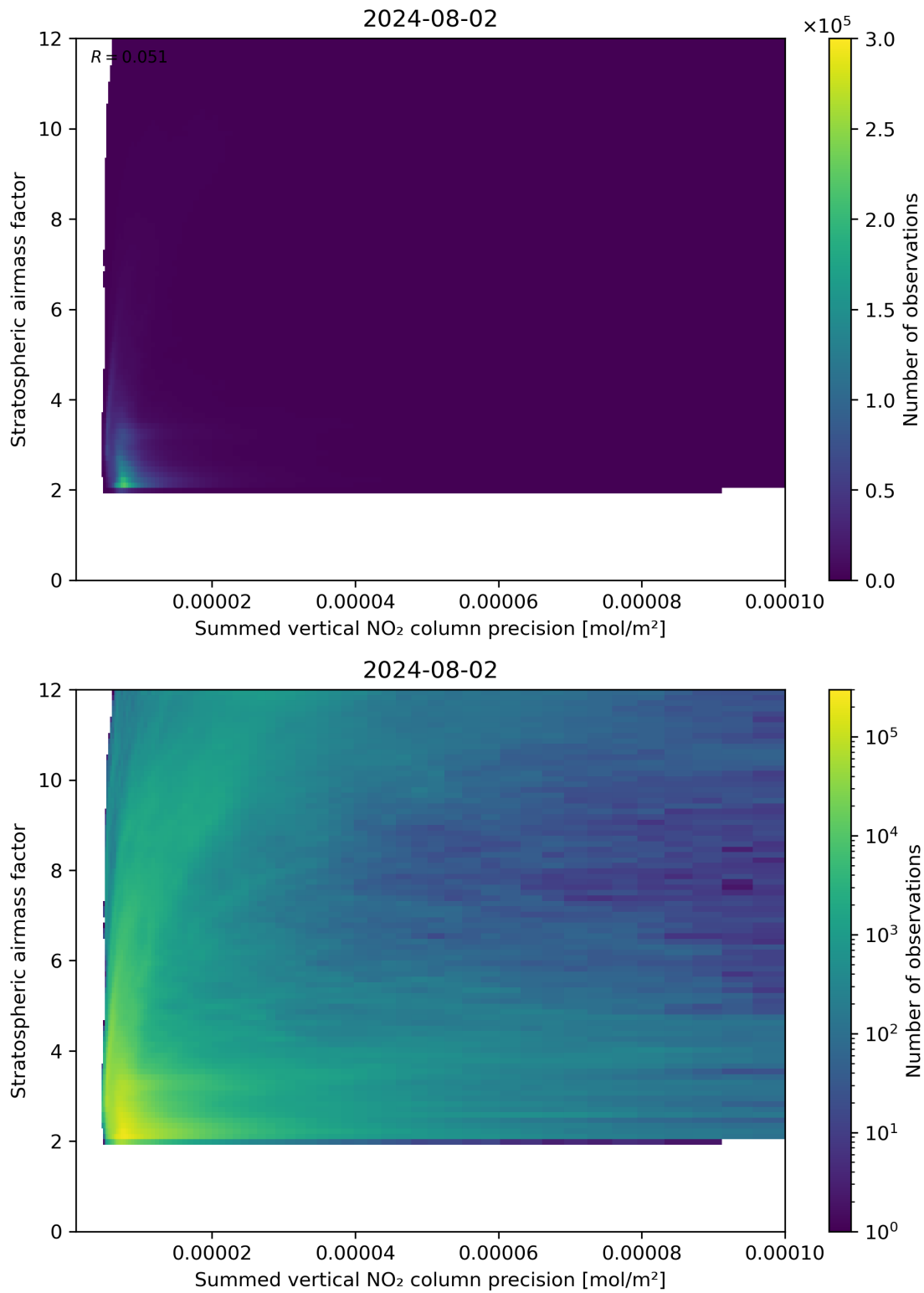
Figure 106: Scatter density plot of “Summed vertical NO 2 column precision” against “Stratospheric airmass factor” for 2024-08-01 to 2024-08-03.
