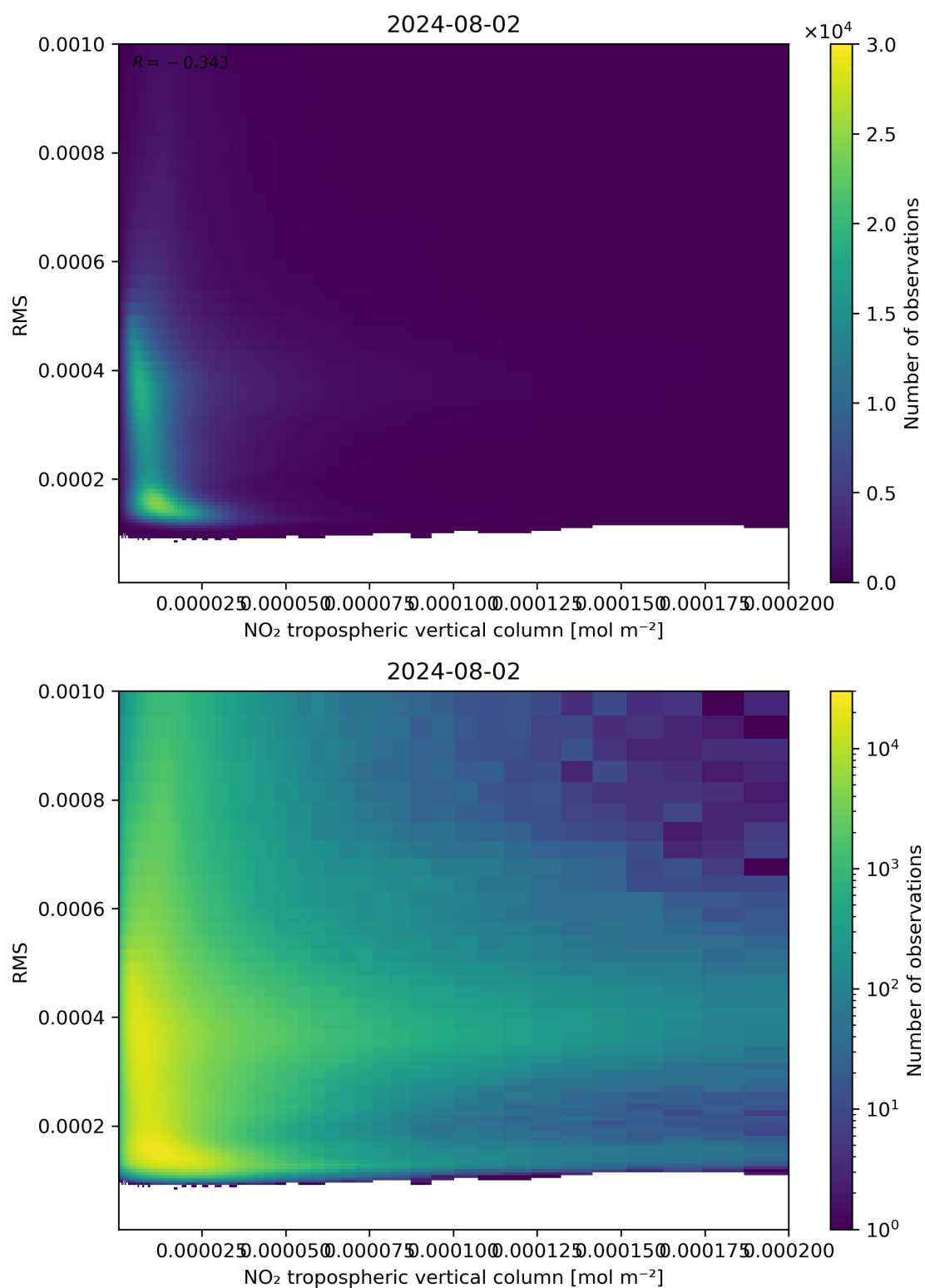
Figure 142: Scatter density plot of “NO 2 tropospheric vertical column” against “RMS” for 2024-08-01 to 2024-08-03.
