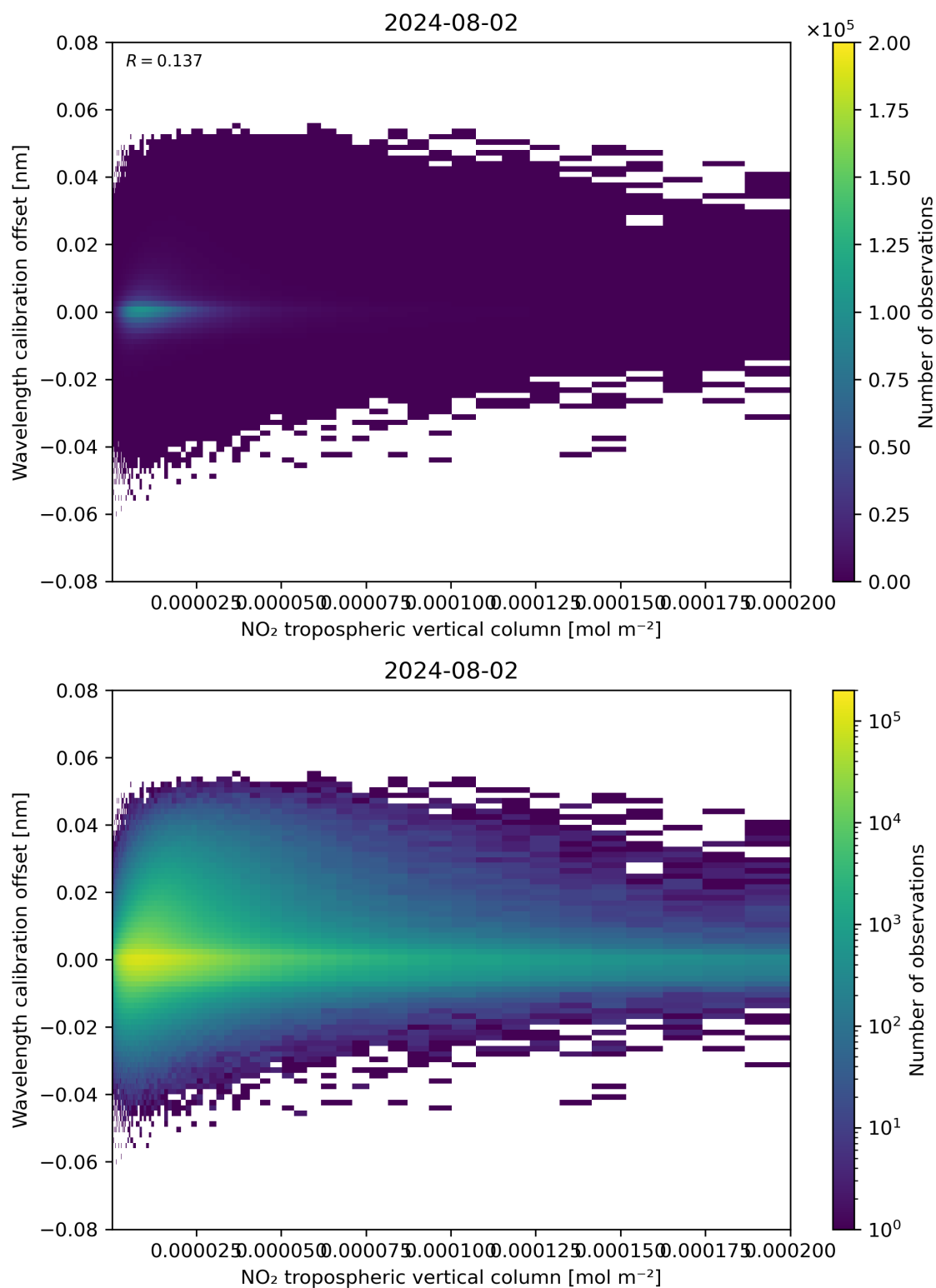
Figure 143: Scatter density plot of “NO 2 tropospheric vertical column” against “Wavelength calibration offset” for 2024-08-01 to 2024-08-03.
