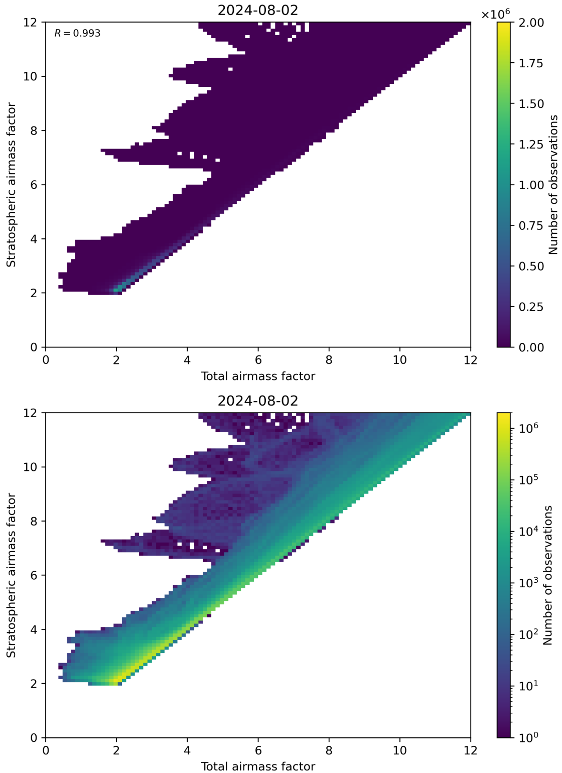
Figure 62: Scatter density plot of “Total airmass factor” against “Stratospheric airmass factor” for 2024-08-01 to 2024-08-03.
