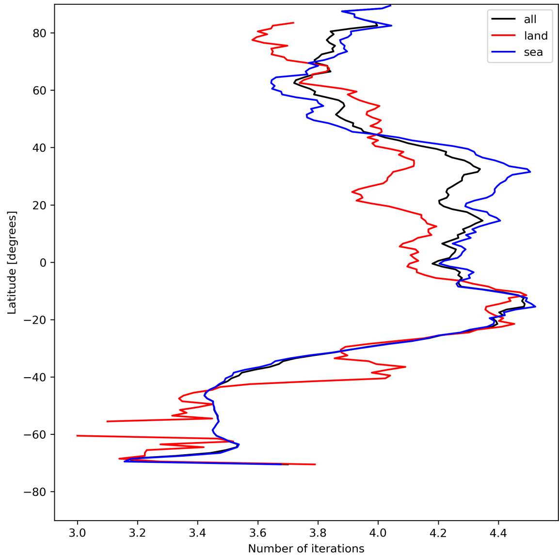
Figure 17: Zonal average of “Number of iterations” for 2024-08-01 to 2024-08-03.
