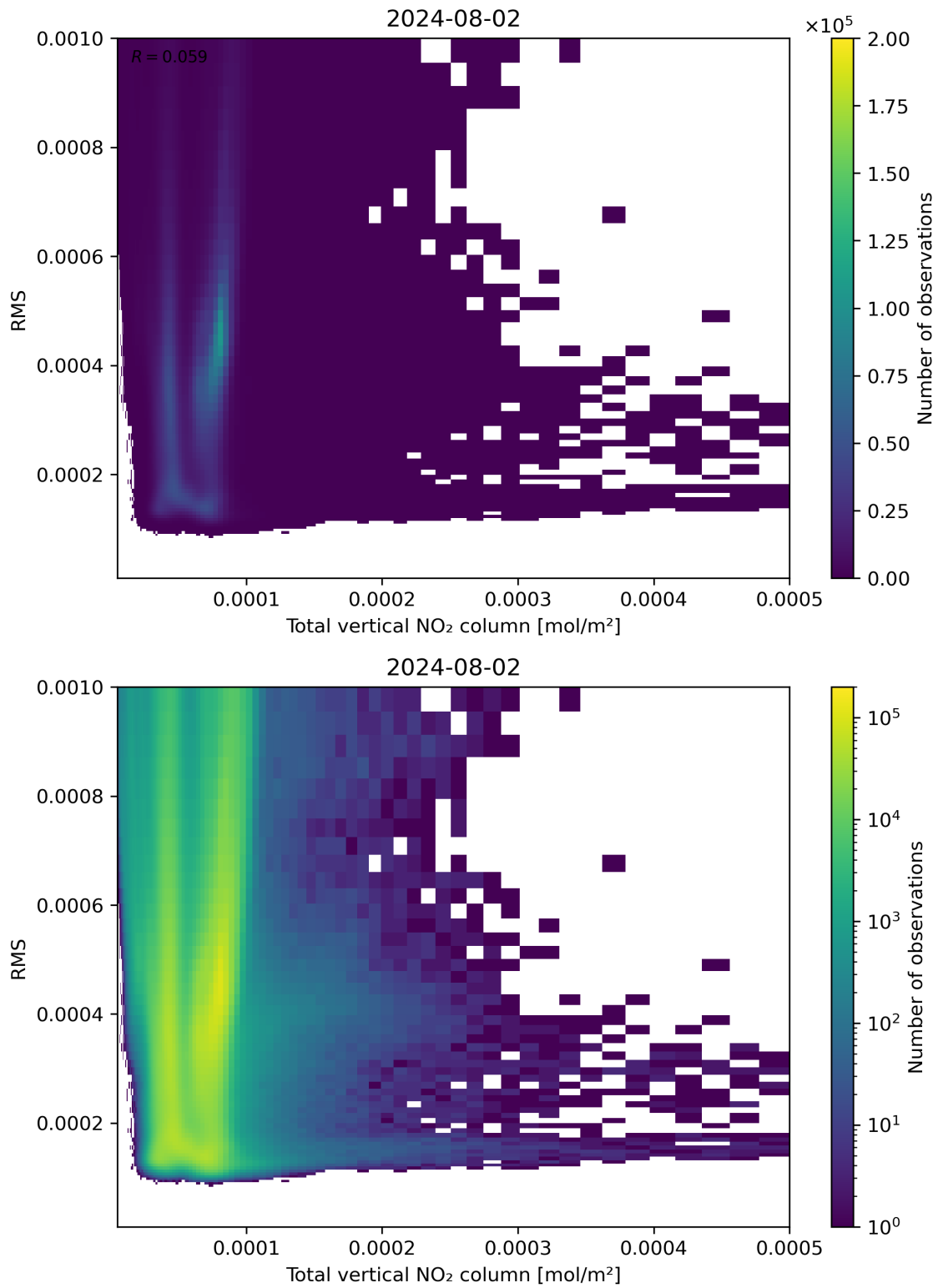
Figure 120: Scatter density plot of “Total vertical NO 2 column” against “RMS” for 2024-08-01 to 2024-08-03.
