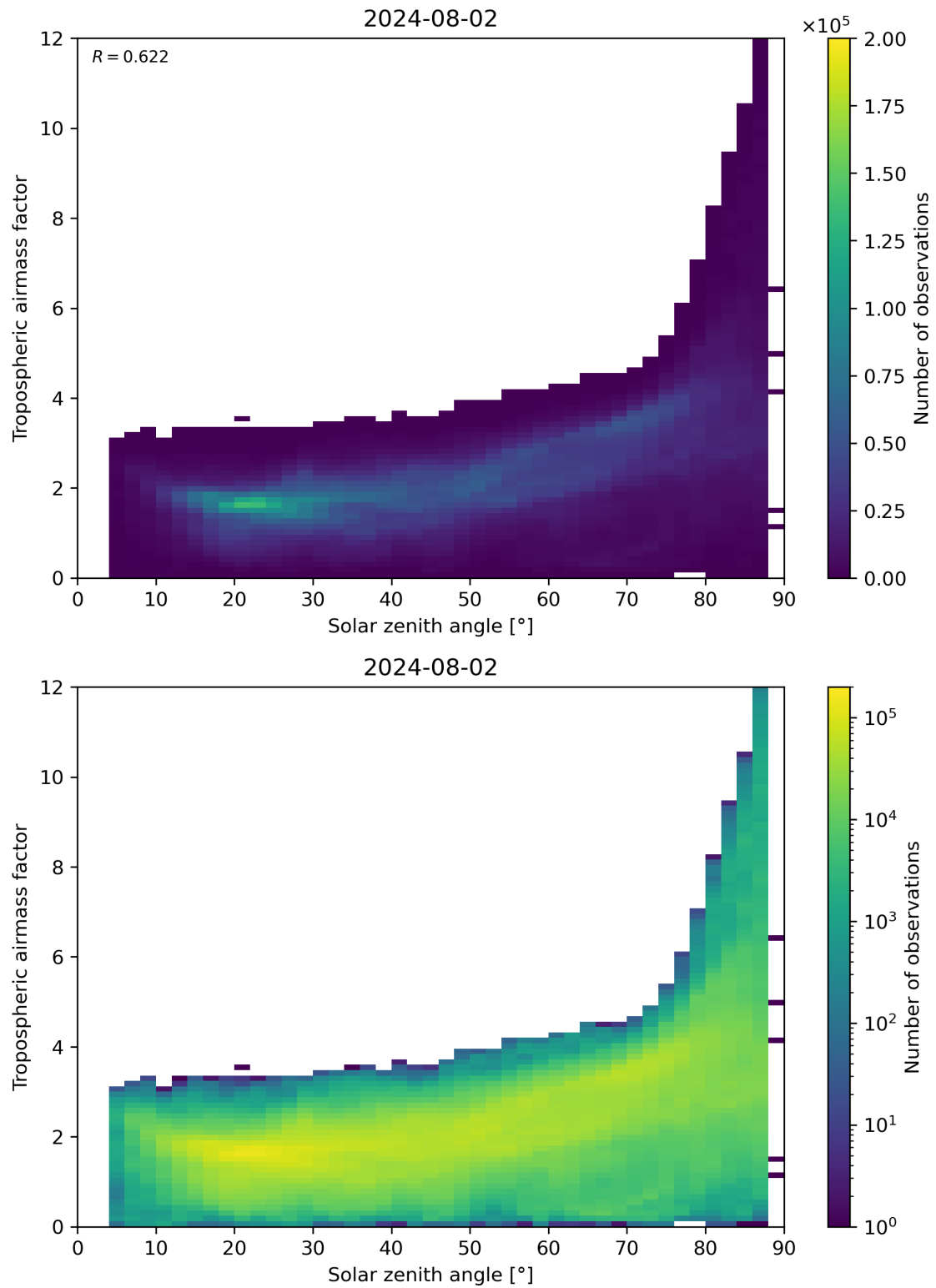
Figure 147: Scatter density plot of “Solar zenith angle” against “Tropospheric airmass factor” for 2024-08-01 to 2024-08-03.
