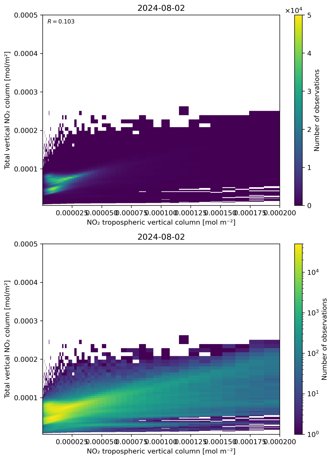
Figure 128: Scatter density plot of “NO 2 tropospheric vertical column” against “Total vertical NO 2 column” for 2024-08-01 to 2024-08-03.
