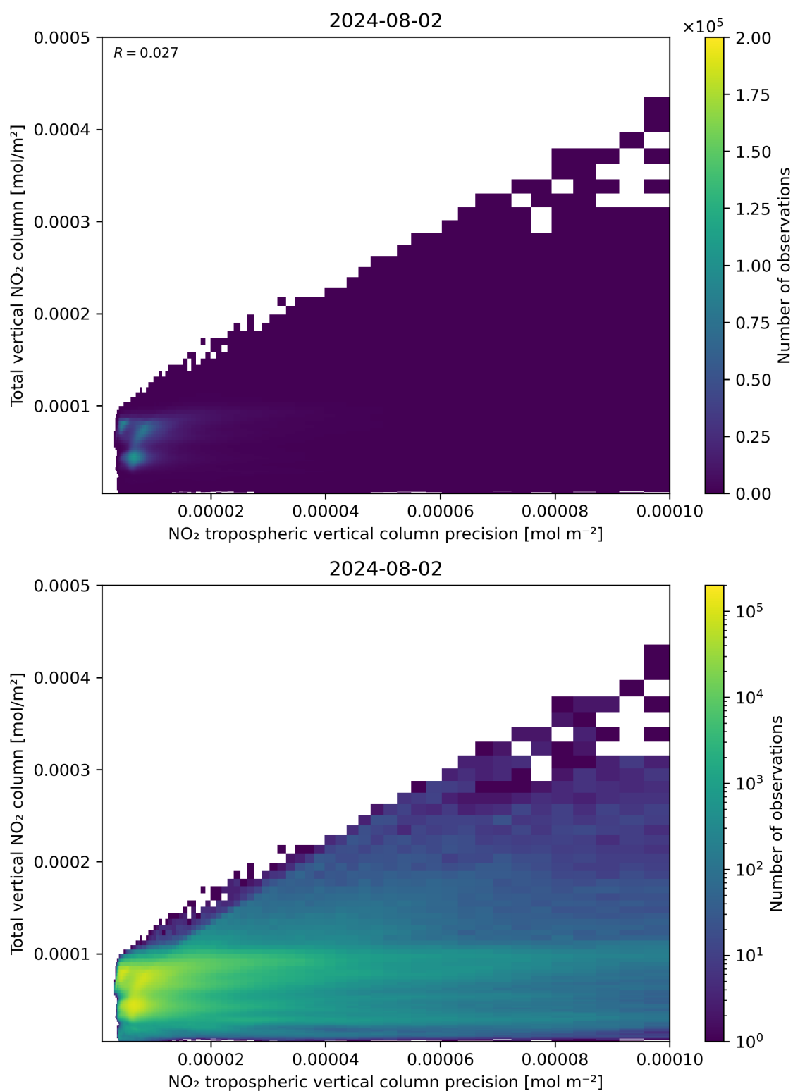
Figure 138: Scatter density plot of “NO 2 tropospheric vertical column precision” against “Total vertical NO 2 column” for 2024-08-01 to 2024-08-03.
