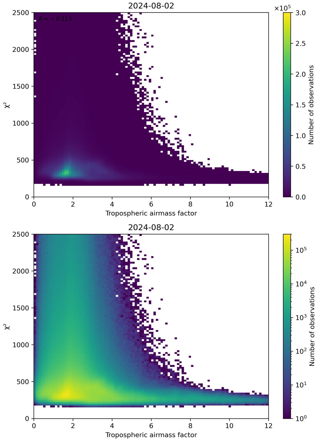
Figure 73: Scatter density plot of “Tropospheric airmass factor” against “ \chi^2 ” for 2024-08-01 to 2024-08-03.
