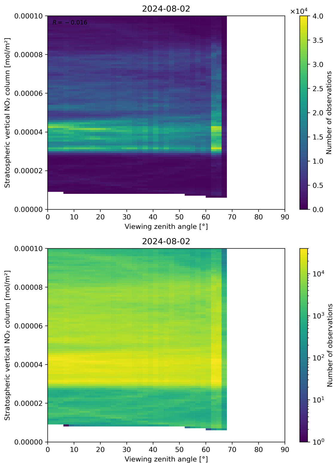
Figure 164: Scatter density plot of “Viewing zenith angle” against “Stratospheric vertical NO 2 column” for 2024-08-01 to 2024-08-03.
