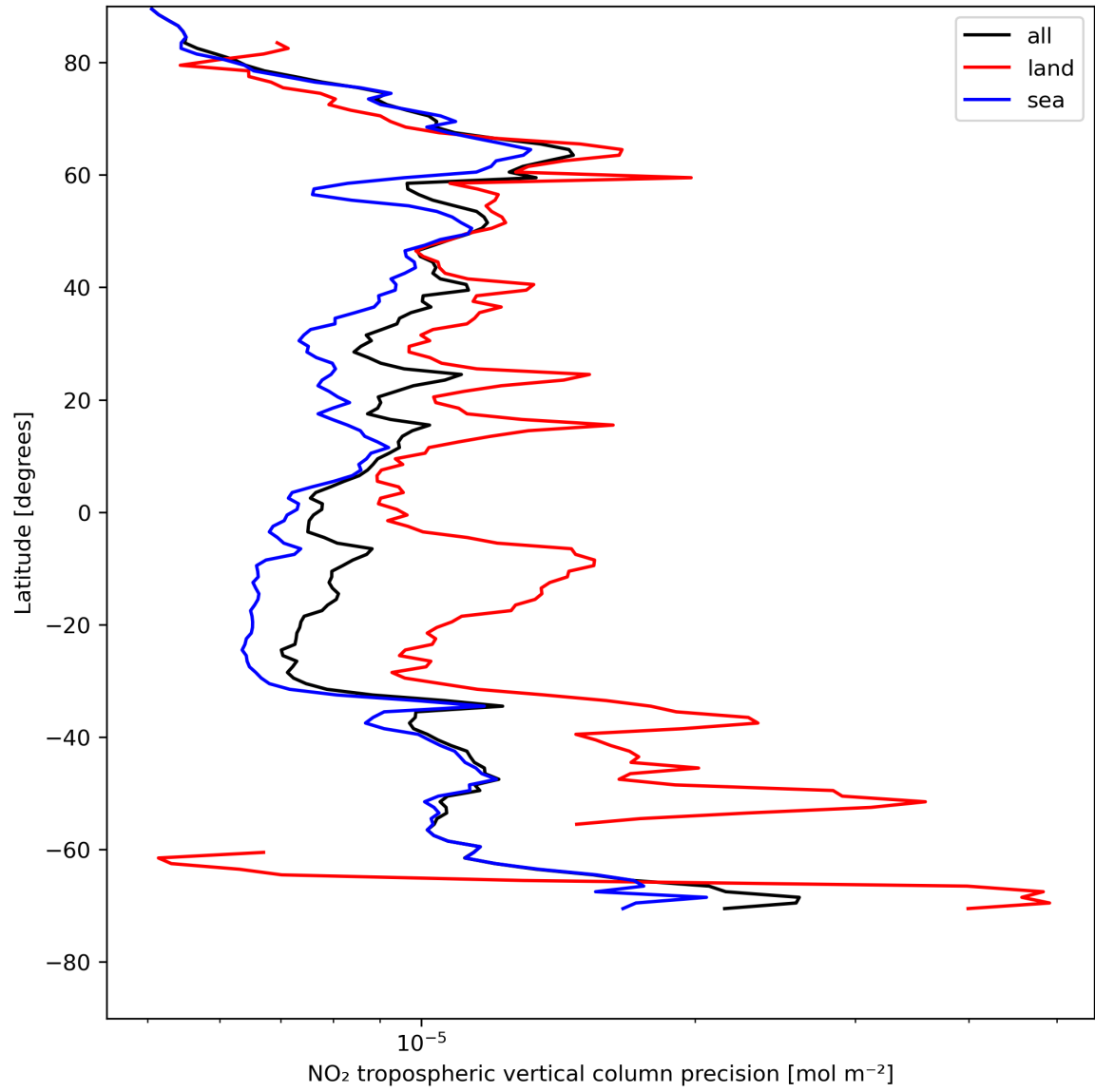
Figure 13: Zonal average of “NO 2 tropospheric vertical column precision” for 2024-08-01 to 2024-08-03.
