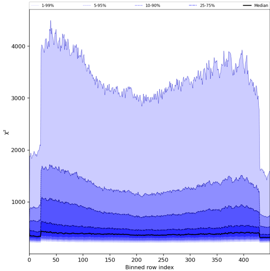
Figure 59: Along track statistics of “ \chi^2 ” for 2024-08-01 to 2024-08-03
