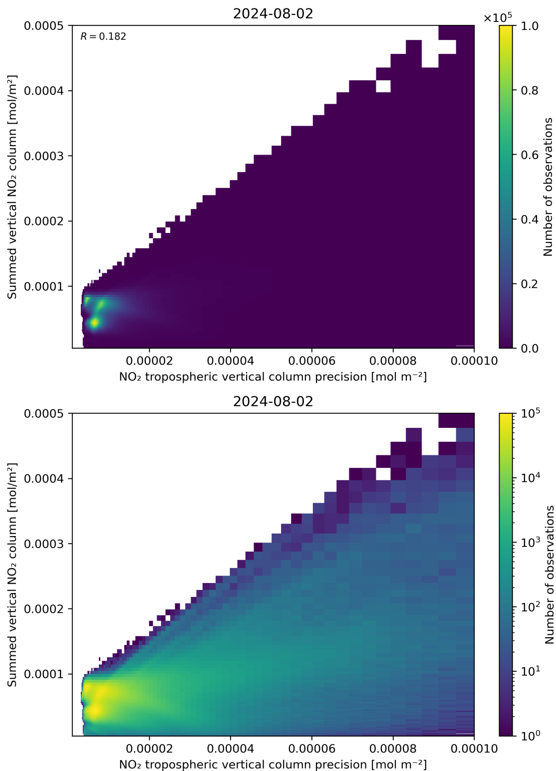
Figure 136: Scatter density plot of “NO 2 tropospheric vertical column precision” against “Summed vertical NO 2 column” for 2024-08-01 to 2024-08-03.
