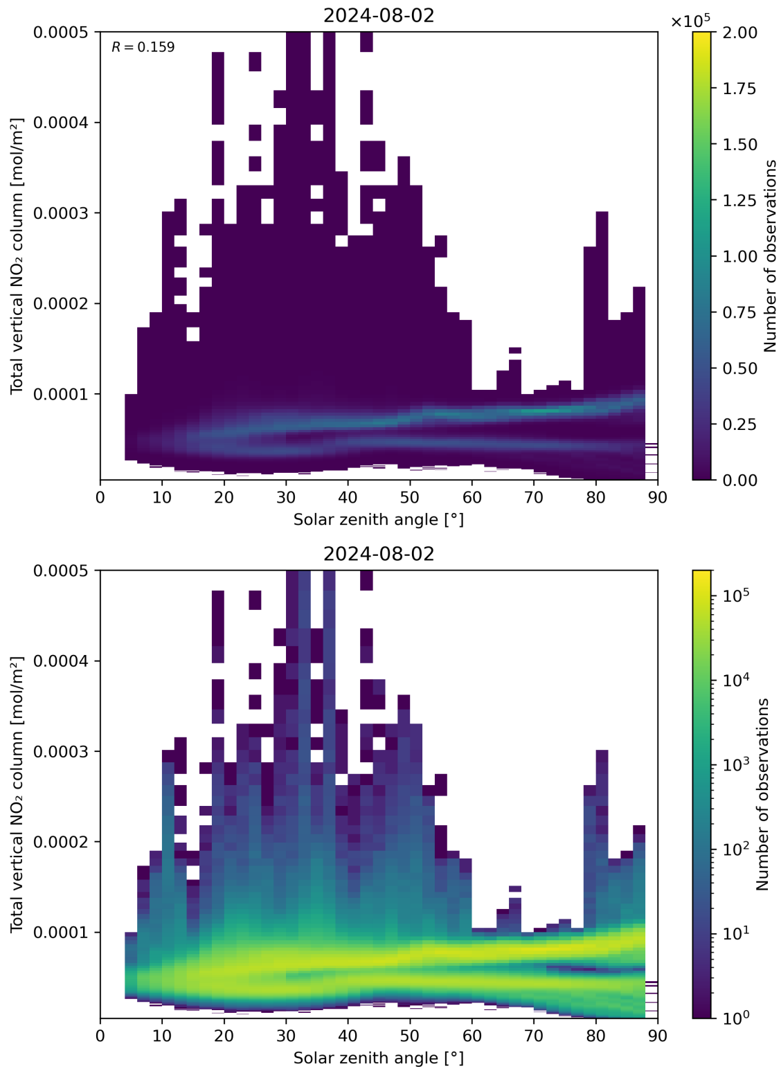
Figure 153: Scatter density plot of “Solar zenith angle” against “Total vertical NO 2 column” for 2024-08-01 to 2024-08-03.
