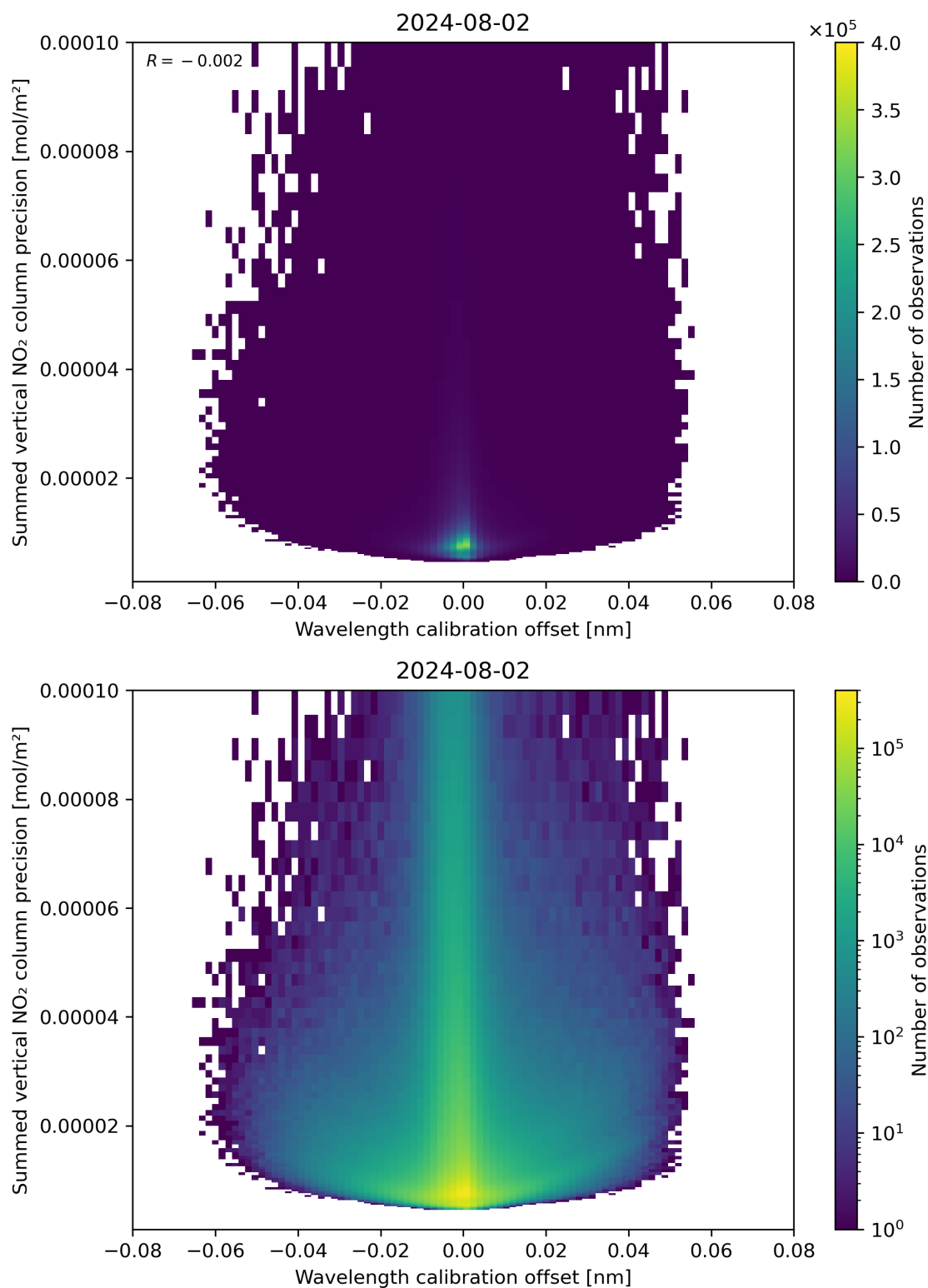
Figure 178: Scatter density plot of “Wavelength calibration offset” against “Summed vertical NO 2 column precision” for 2024-08-01 to 2024-08-03.
