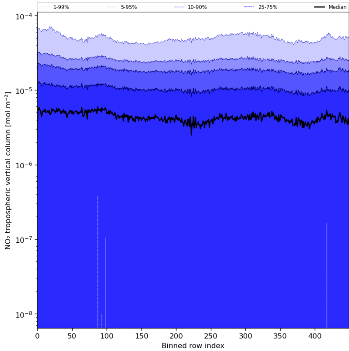
Figure 46: Along track statistics of “NO 2 tropospheric vertical column” for 2024-08-01 to 2024-08-03
