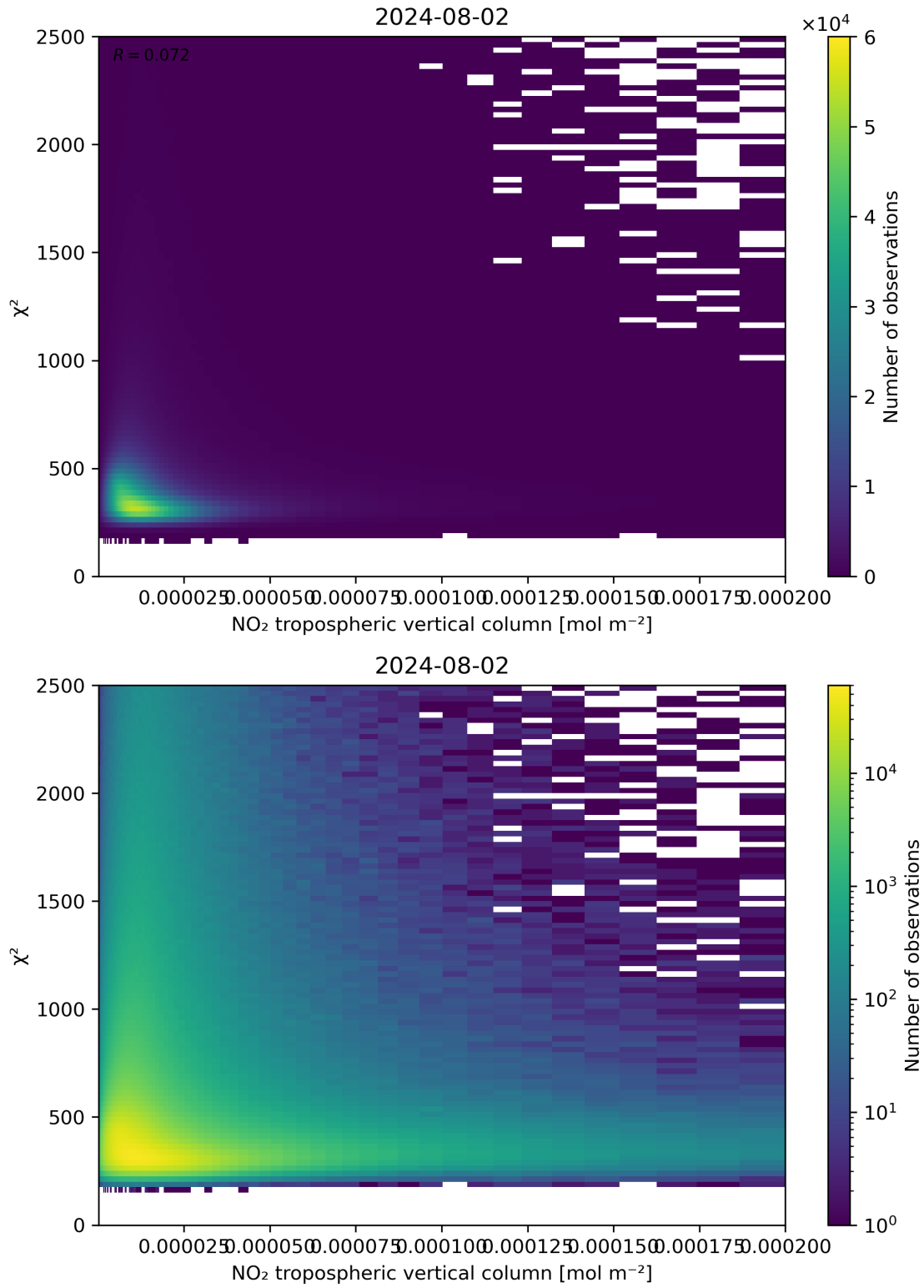
Figure 124: Scatter density plot of “NO 2 tropospheric vertical column” against “ \chi^2 ” for 2024-08-01 to 2024-08-03.
