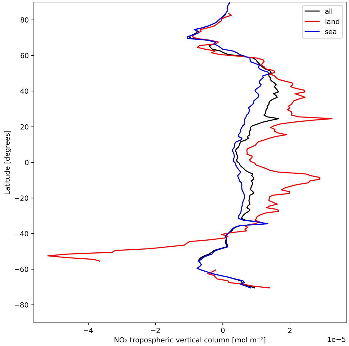
Figure 12: Zonal average of “NO 2 tropospheric vertical column” for 2024-08-01 to 2024-08-03.
