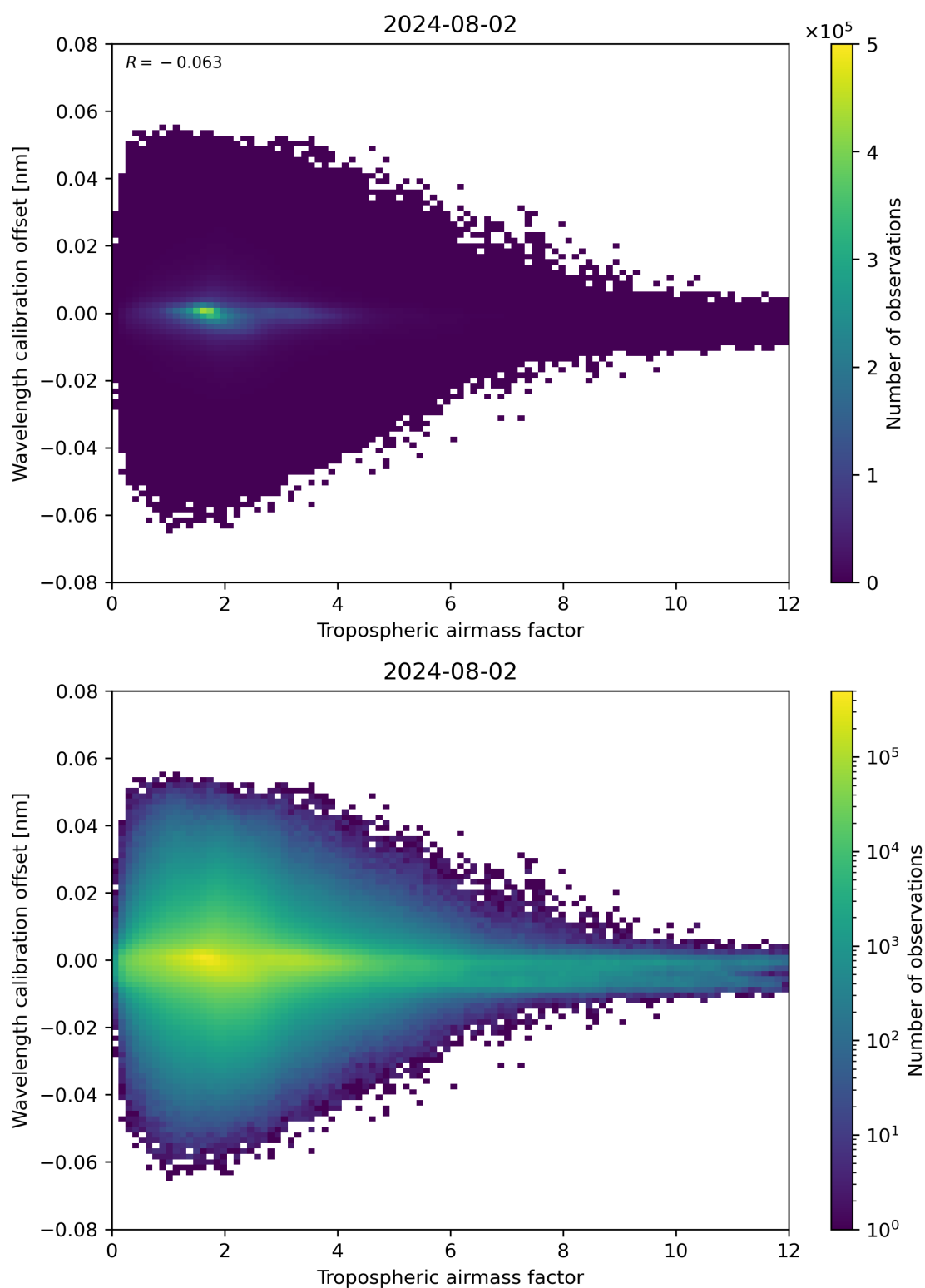
Figure 80: Scatter density plot of “Tropospheric air mass factor” against “Wavelength calibration offset” for 2024-08-01 to 2024-08-03.
