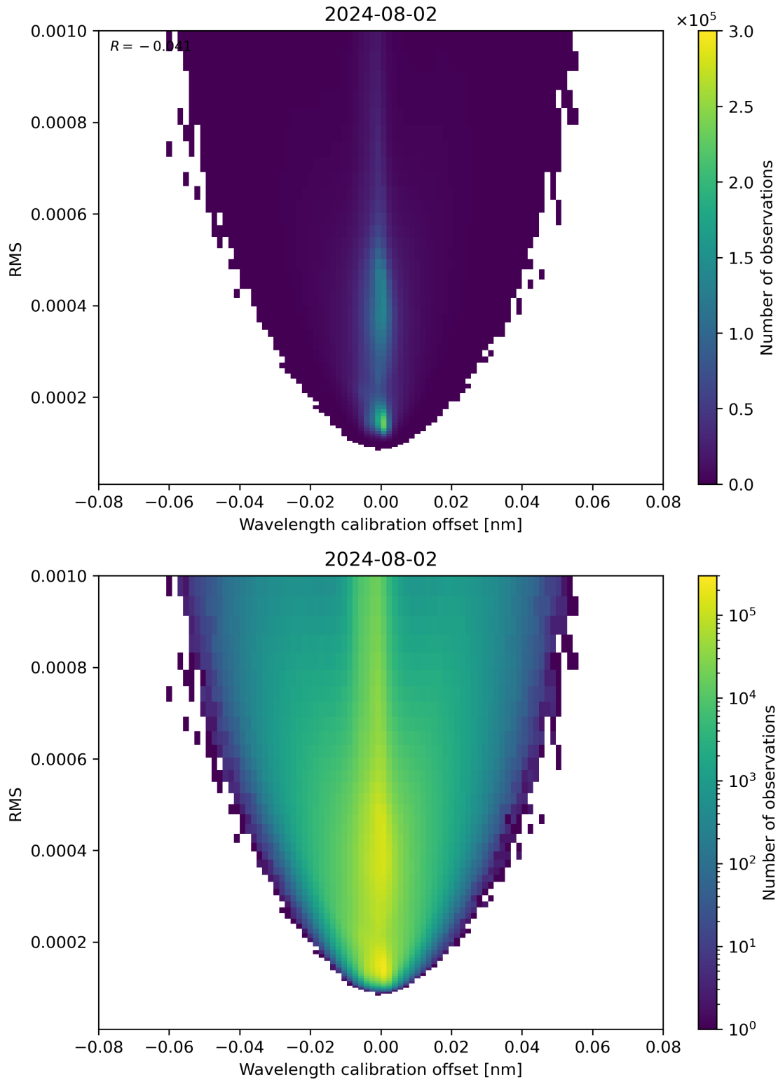
Figure 181: Scatter density plot of “Wavelength calibration offset” against “RMS” for 2024-08-01 to 2024-08-03.
