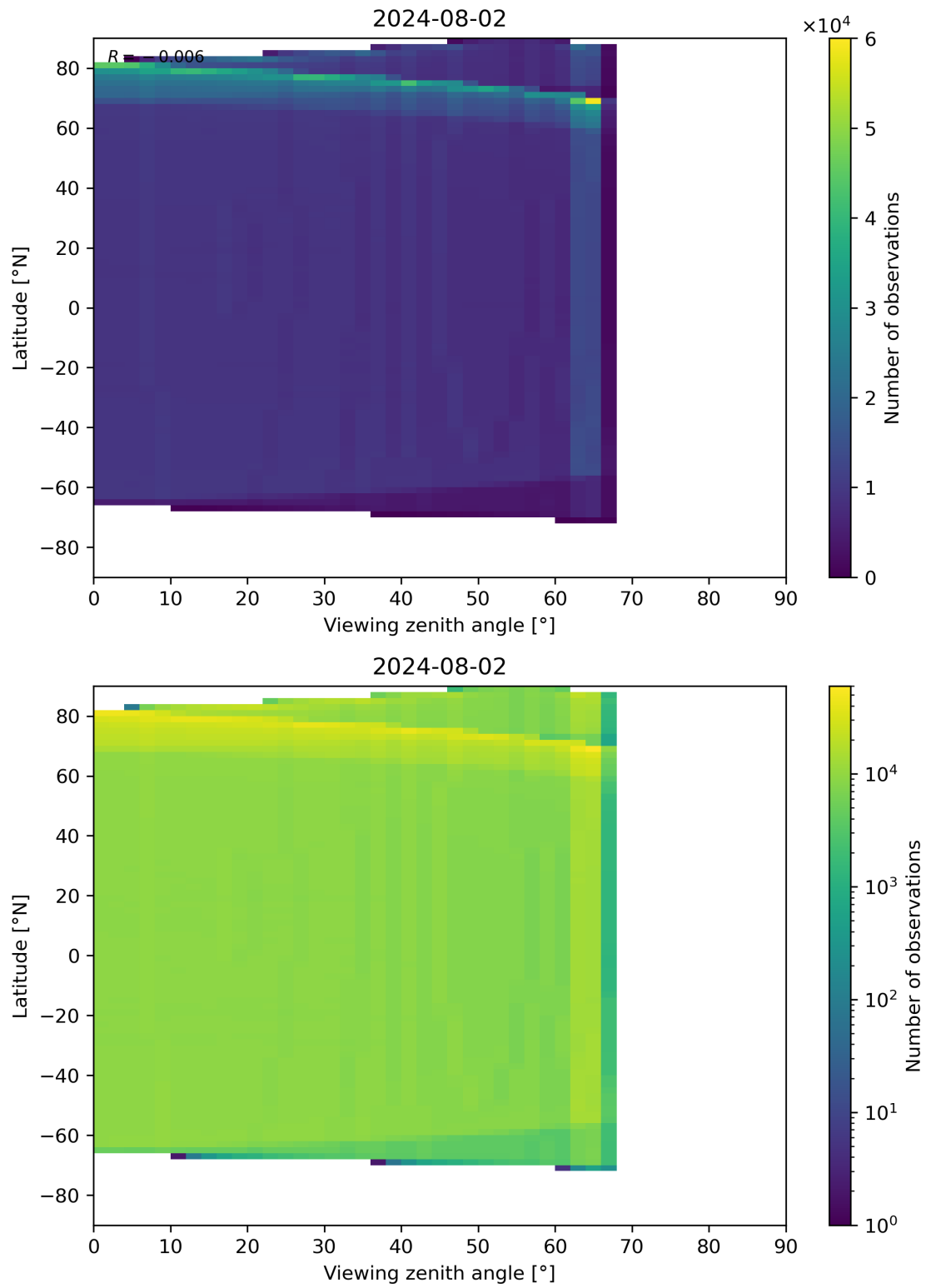
Figure 163: Scatter density plot of “Viewing zenith angle” against “Latitude” for 2024-08-01 to 2024-08-03.
