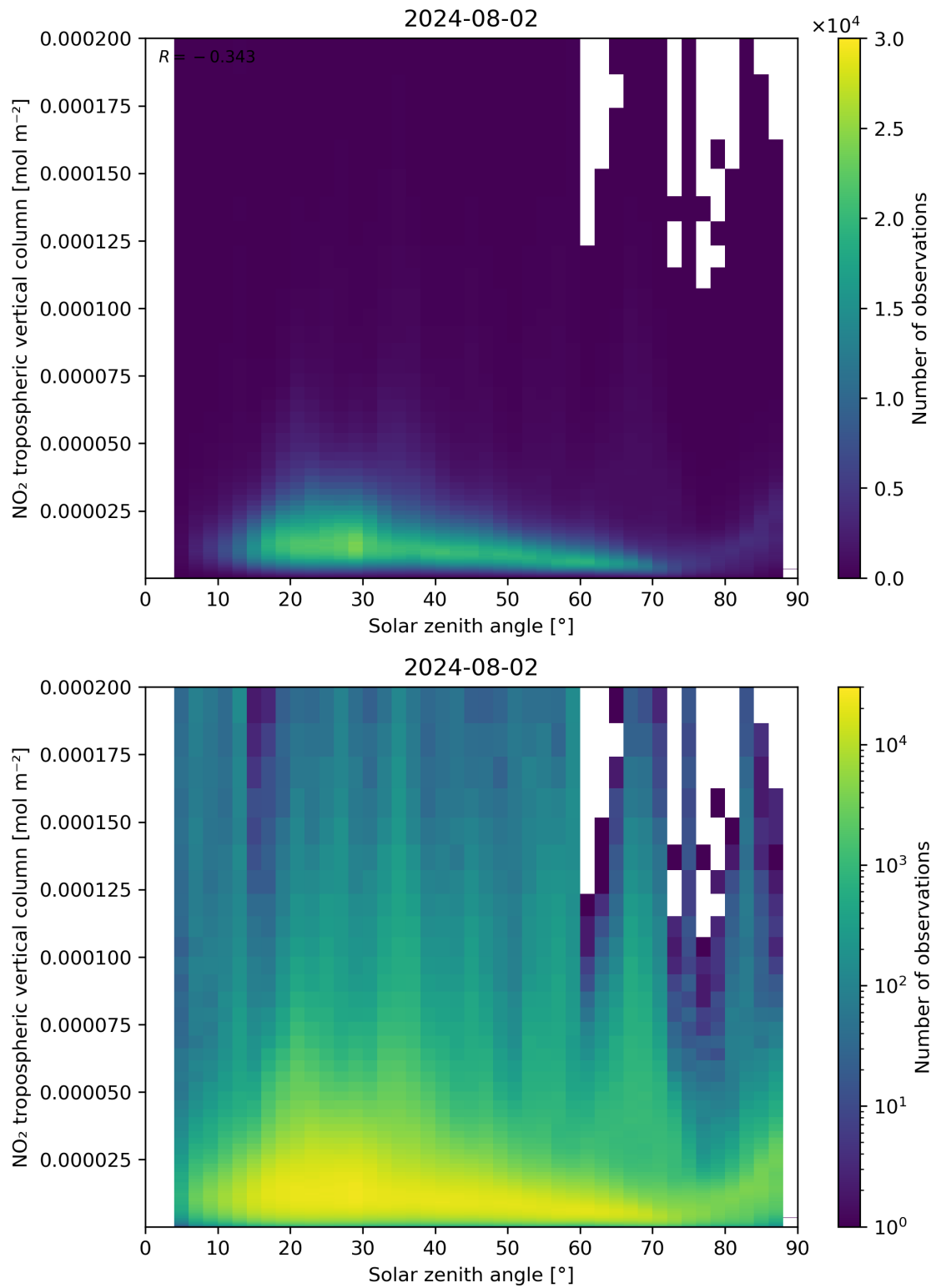
Figure 155: Scatter density plot of “Solar zenith angle” against “NO 2 tropospheric vertical column” for 2024-08-01 to 2024-08-03.
