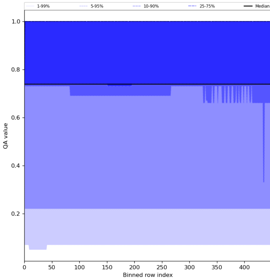
Figure 45: Along track statistics of “QA value” for 2024-08-01 to 2024-08-03
