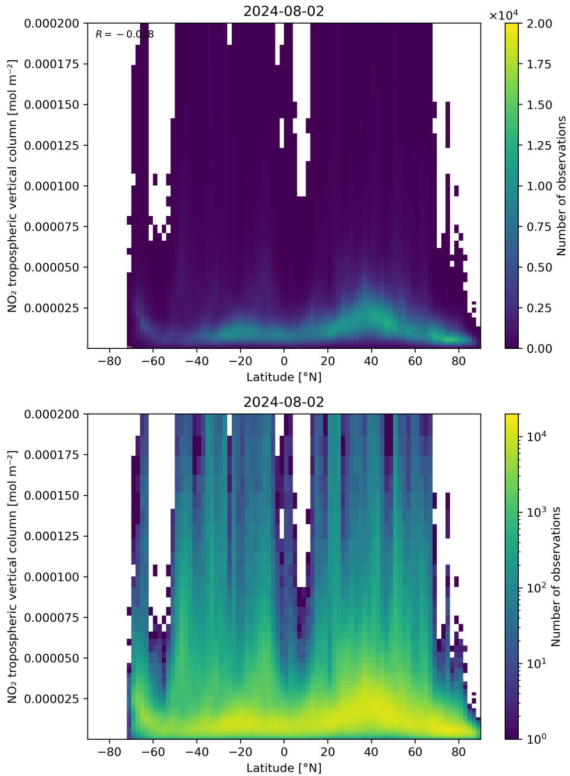
Figure 92: Scatter density plot of “Latitude” against “NO 2 tropospheric vertical column” for 2024-08-01 to 2024-08-03.
