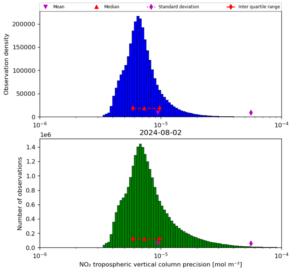
Figure 30: Histogram of “NO 2 tropospheric vertical column precision” for 2024-08-01 to 2024-08-03
