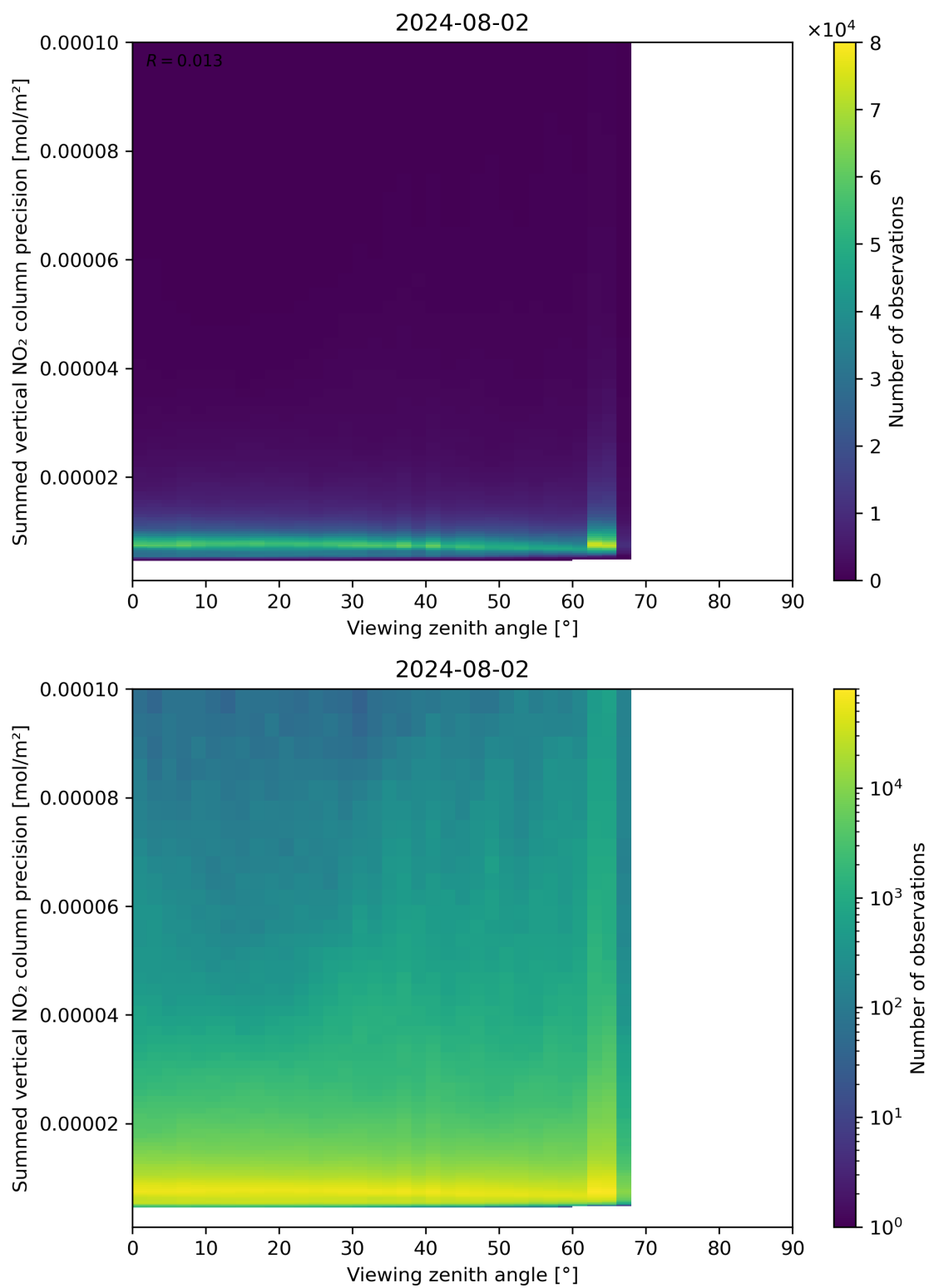
Figure 166: Scatter density plot of “Viewing zenith angle” against “Summed vertical NO 2 column precision” for 2024-08-01 to 2024-08-03.
