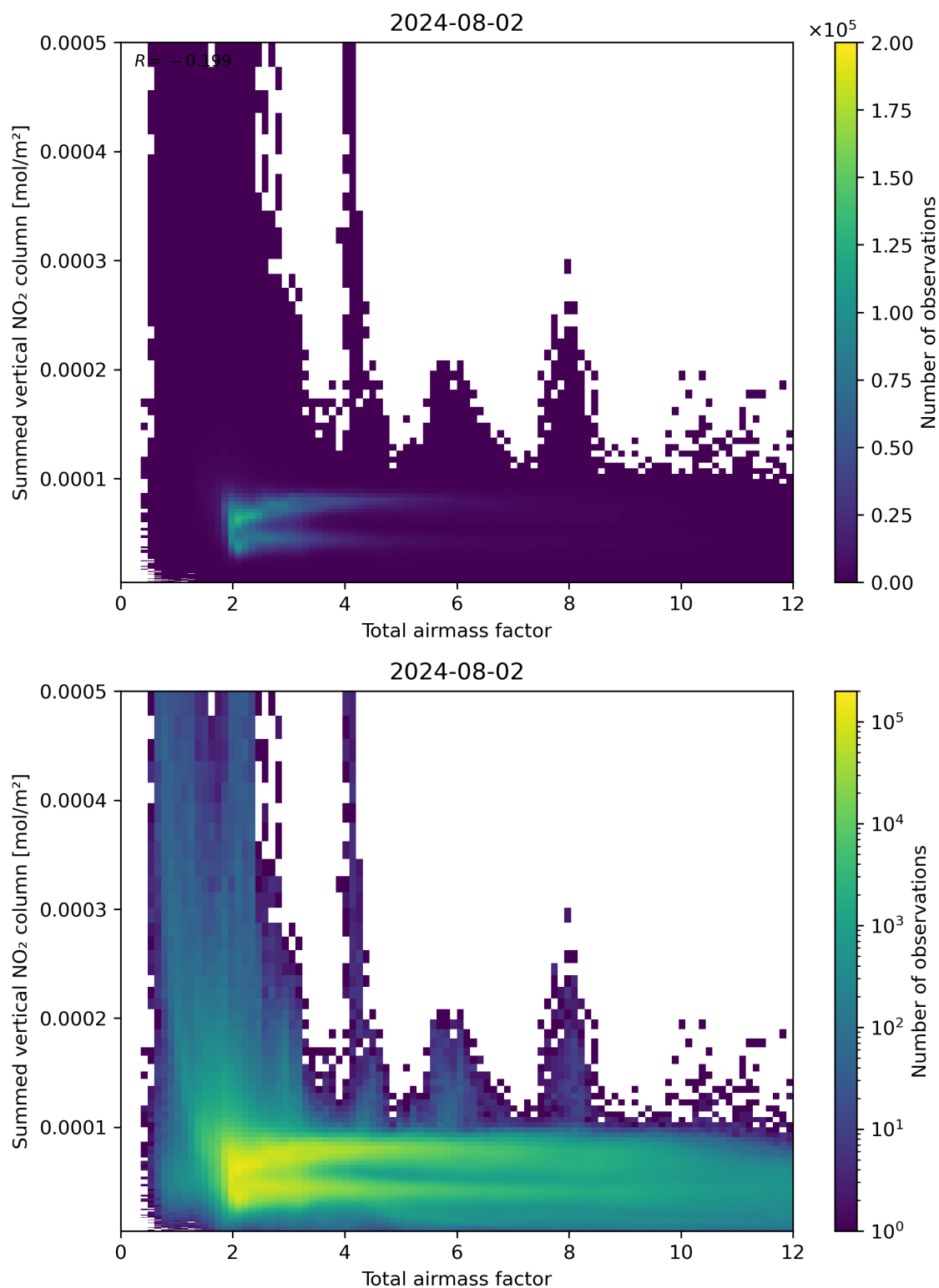
Figure 65: Scatter density plot of “Total airmass factor” against “Summed vertical NO 2 column” for 2024-08-01 to 2024-08-03.
