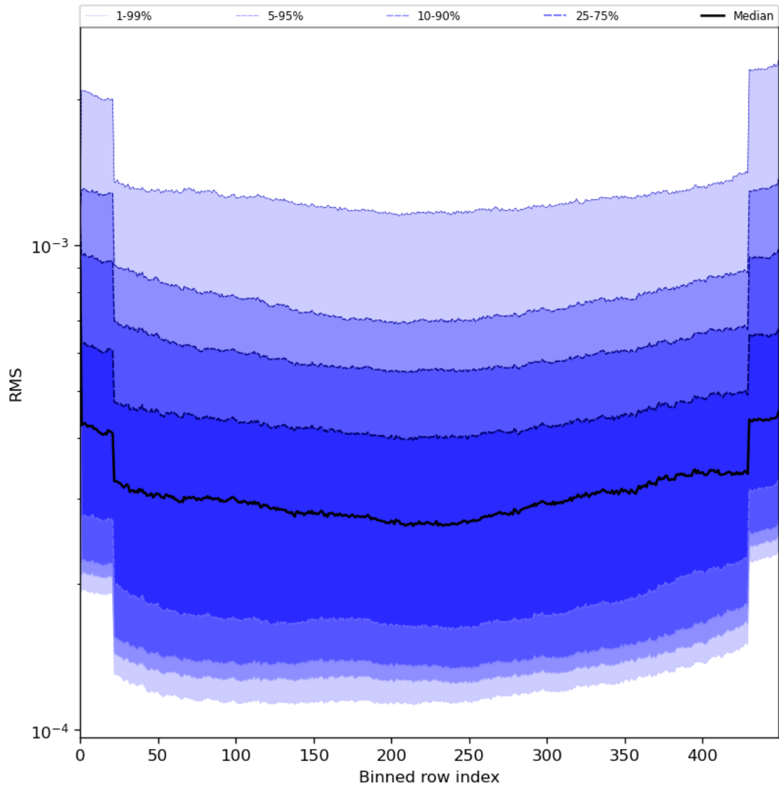
Figure 60: Along track statistics of “RMS” for 2024-08-01 to 2024-08-03
