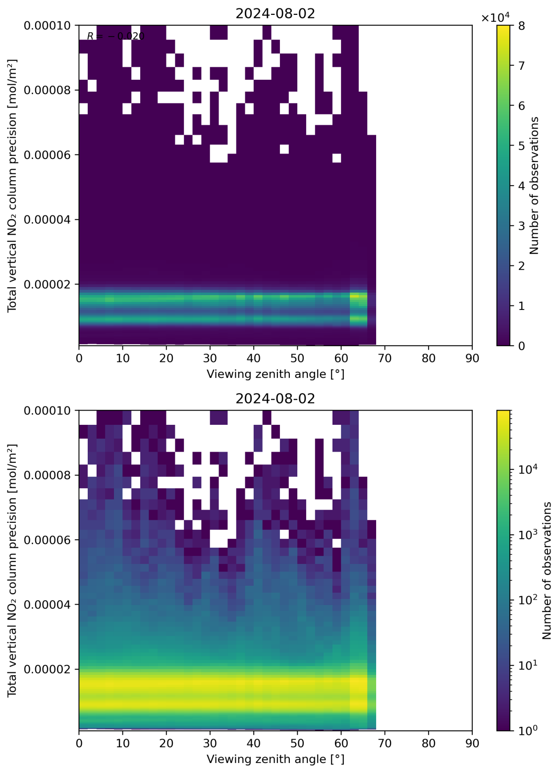
Figure 168: Scatter density plot of “Viewing zenith angle” against “Total vertical NO 2 column precision” for 2024-08-01 to 2024-08-03.
