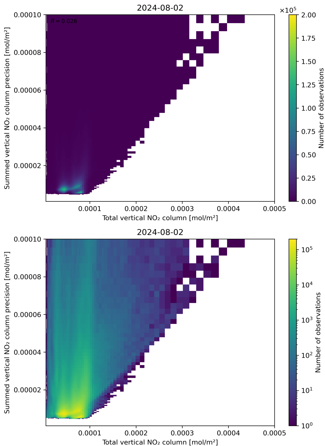
Figure 113: Scatter density plot of “Total vertical NO 2 column” against “Summed vertical NO 2 column precision” for 2024-08-01 to 2024-08-03.
