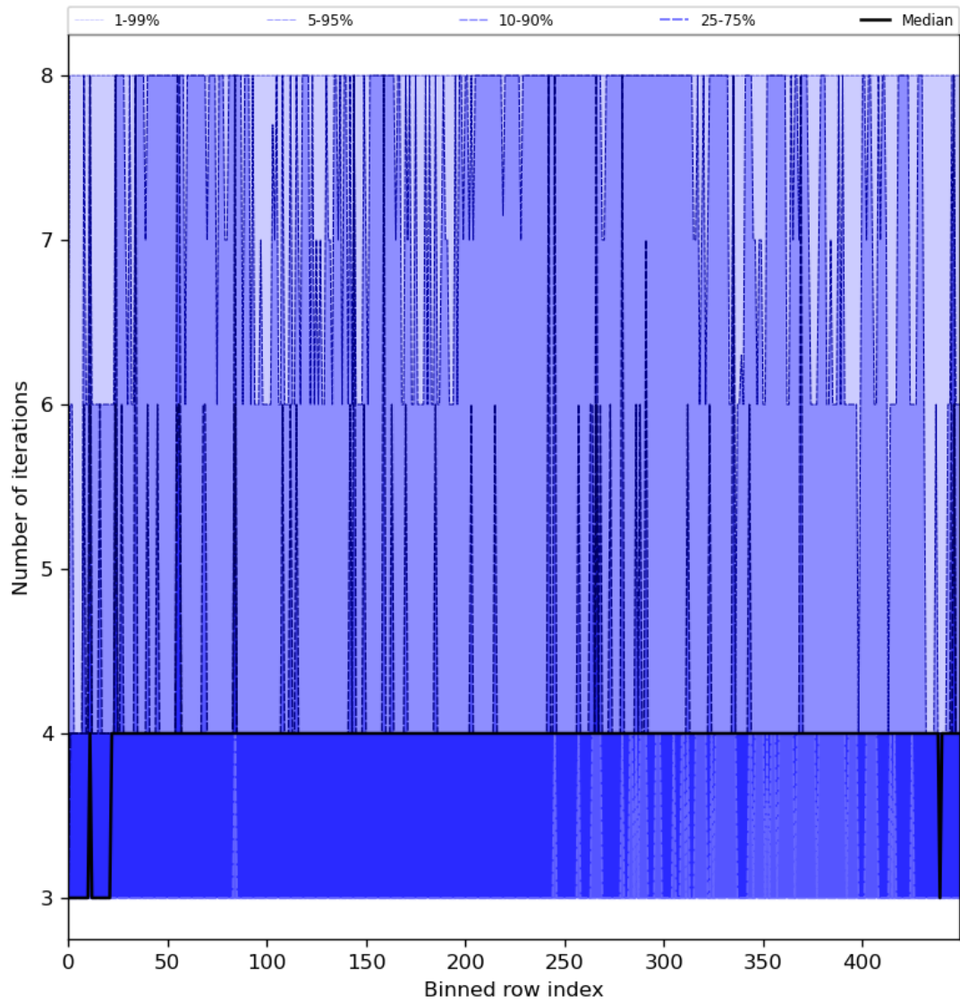
Figure 51: Along track statistics of “Number of iterations” for 2024-08-01 to 2024-08-03
