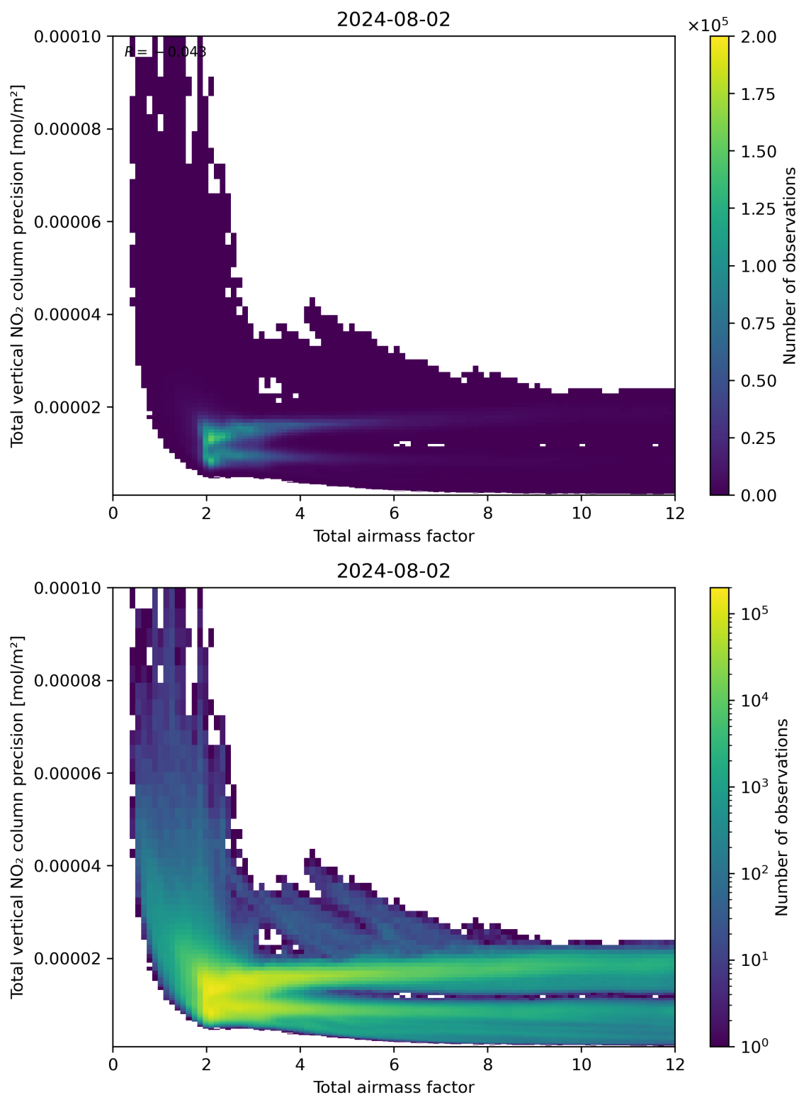
Figure 68: Scatter density plot of “Total airmass factor” against “Total vertical NO 2 column precision” for 2024-08-01 to 2024-08-03.
