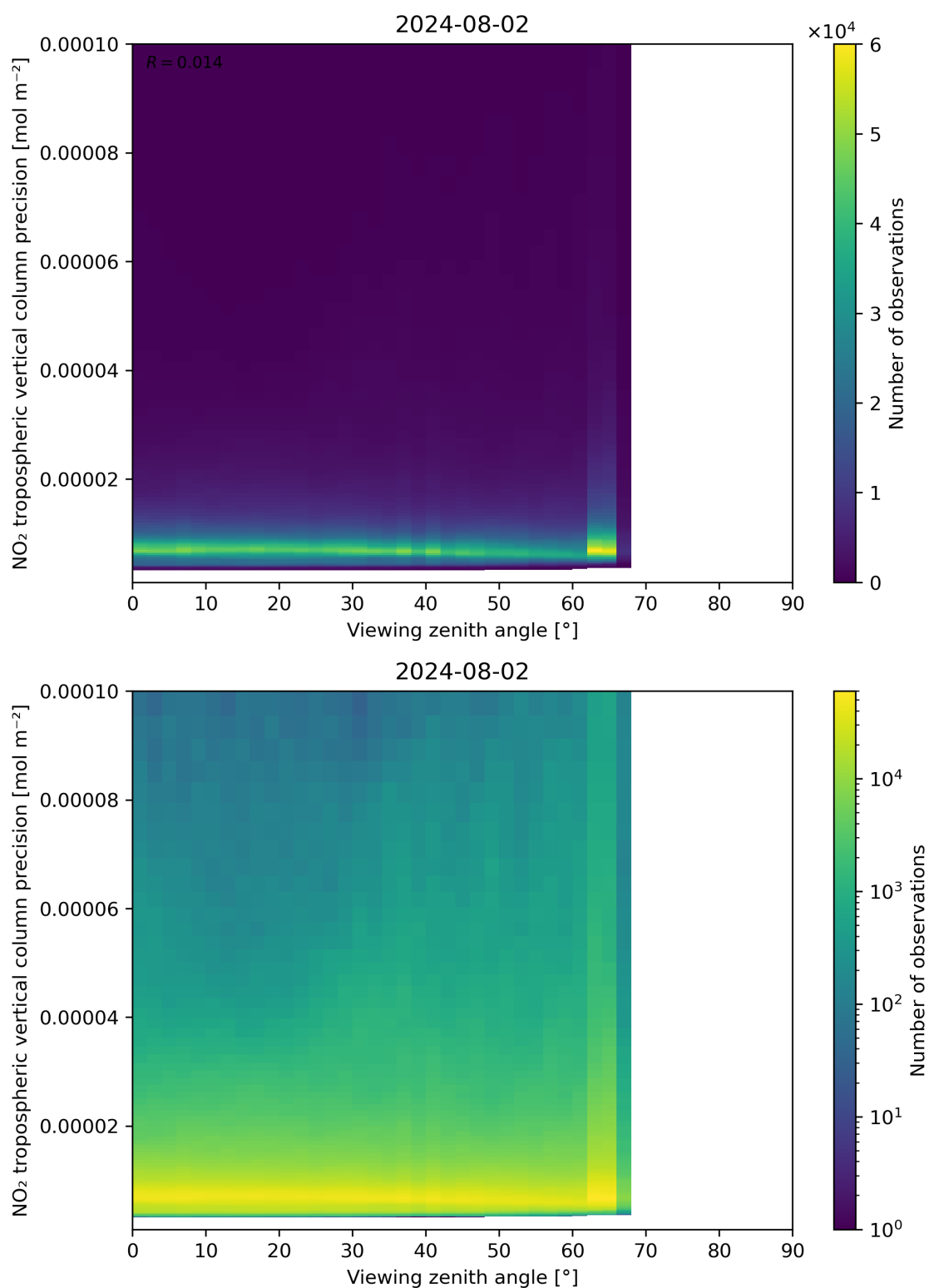
Figure 170: Scatter density plot of “Viewing zenith angle” against “NO 2 tropospheric vertical column precision” for 2024-08-01 to 2024-08-03.
