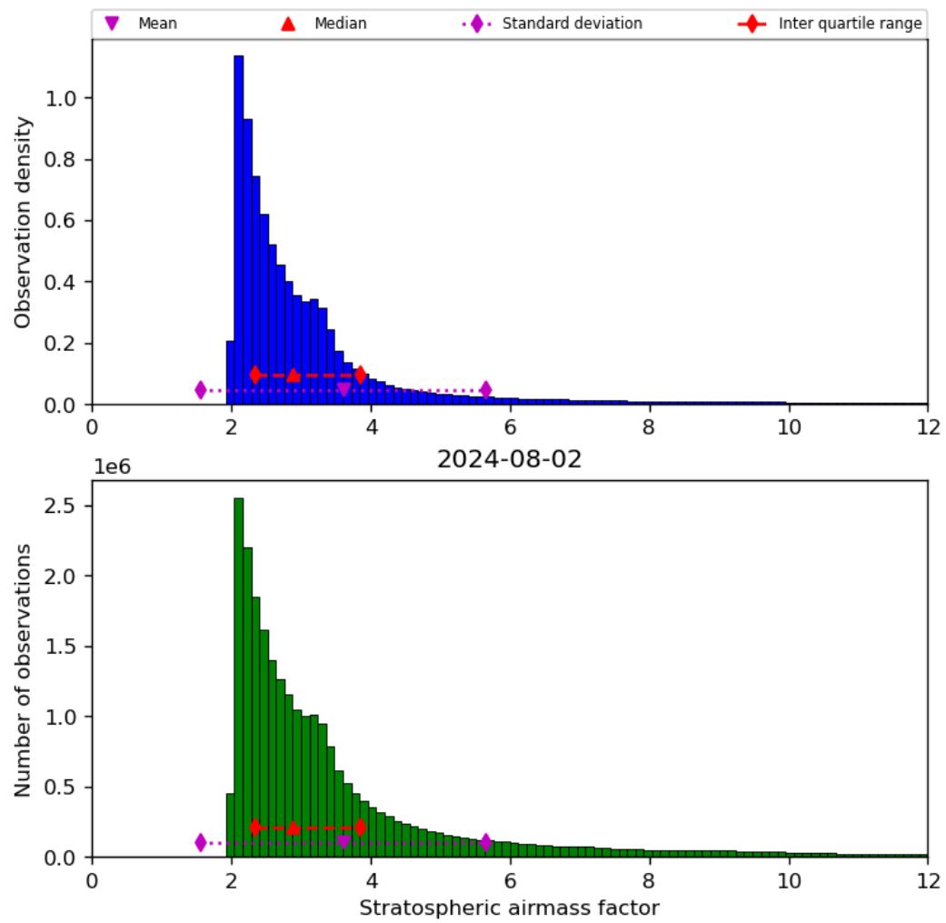
Figure 44: Histogram of “Stratospheric airmass factor” for 2024-08-01 to 2024-08-03
