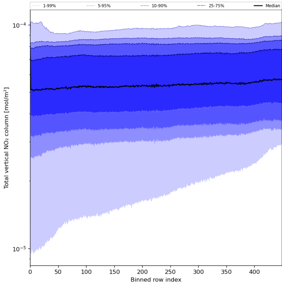
Figure 55: Along track statistics of “Total vertical NO 2 column” for 2024-08-01 to 2024-08-03
