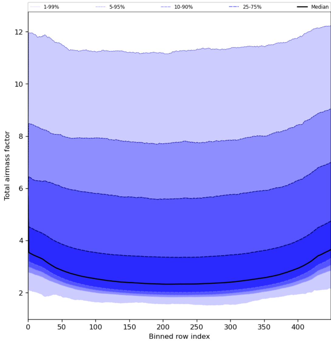
Figure 49: Along track statistics of “Total airmass factor” for 2024-08-01 to 2024-08-03
