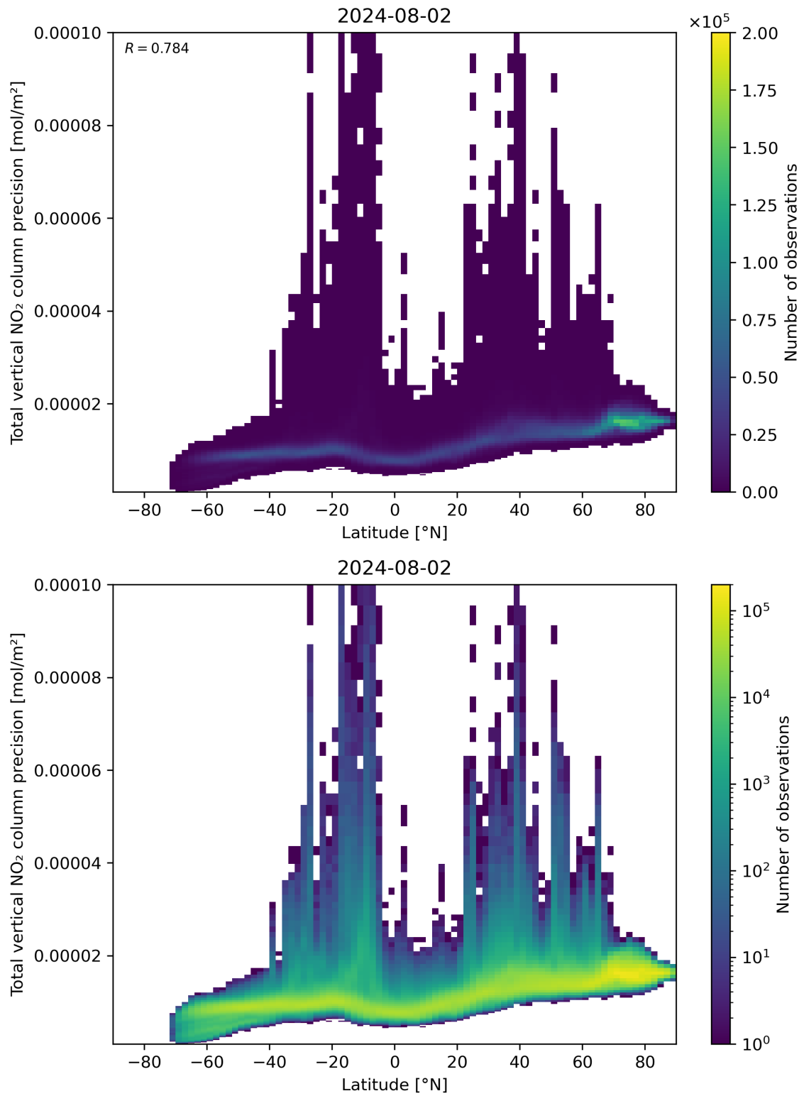
Figure 91: Scatter density plot of “Latitude” against “Total vertical NO 2 column precision” for 2024-08-01 to 2024-08-03.
