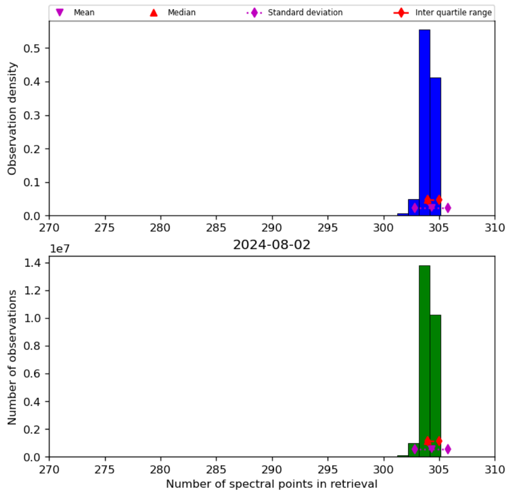
Figure 33: Histogram of “Number of spectral points in retrieval” for 2024-08-01 to 2024-08-03
