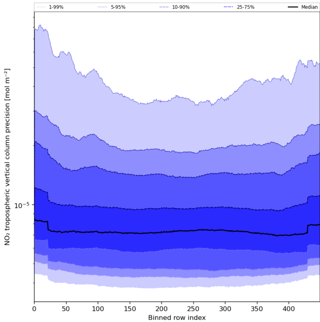
Figure 47: Along track statistics of “NO 2 tropospheric vertical column precision” for 2024-08-01 to 2024-08-03
