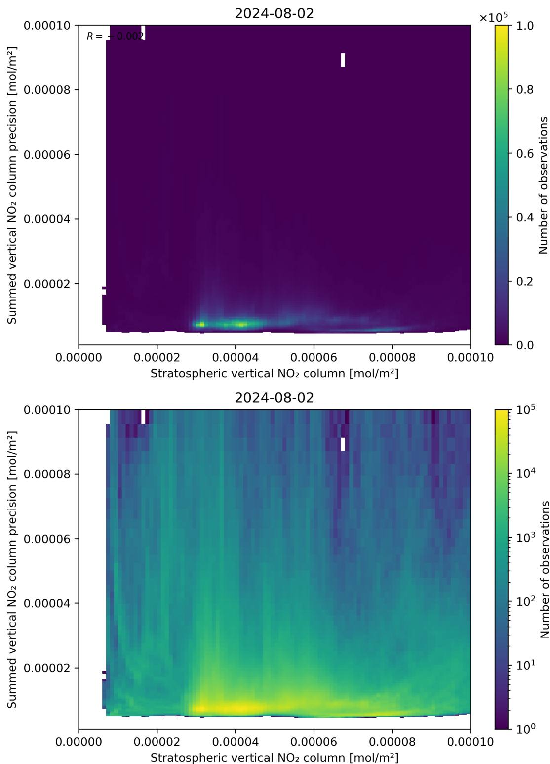
Figure 99: Scatter density plot of “Stratospheric vertical NO 2 column” against “Summed vertical NO 2 column precision” for 2024-08-01 to 2024-08-03.
