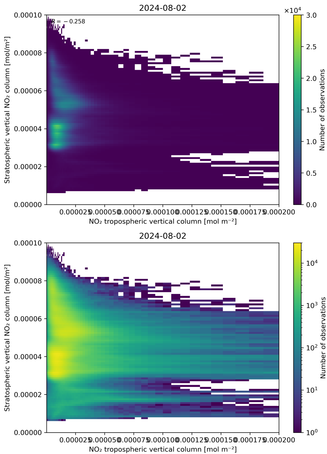
Figure 125: Scatter density plot of “NO 2 tropospheric vertical column” against “Stratospheric vertical NO 2 column” for 2024-08-01 to 2024-08-03.
