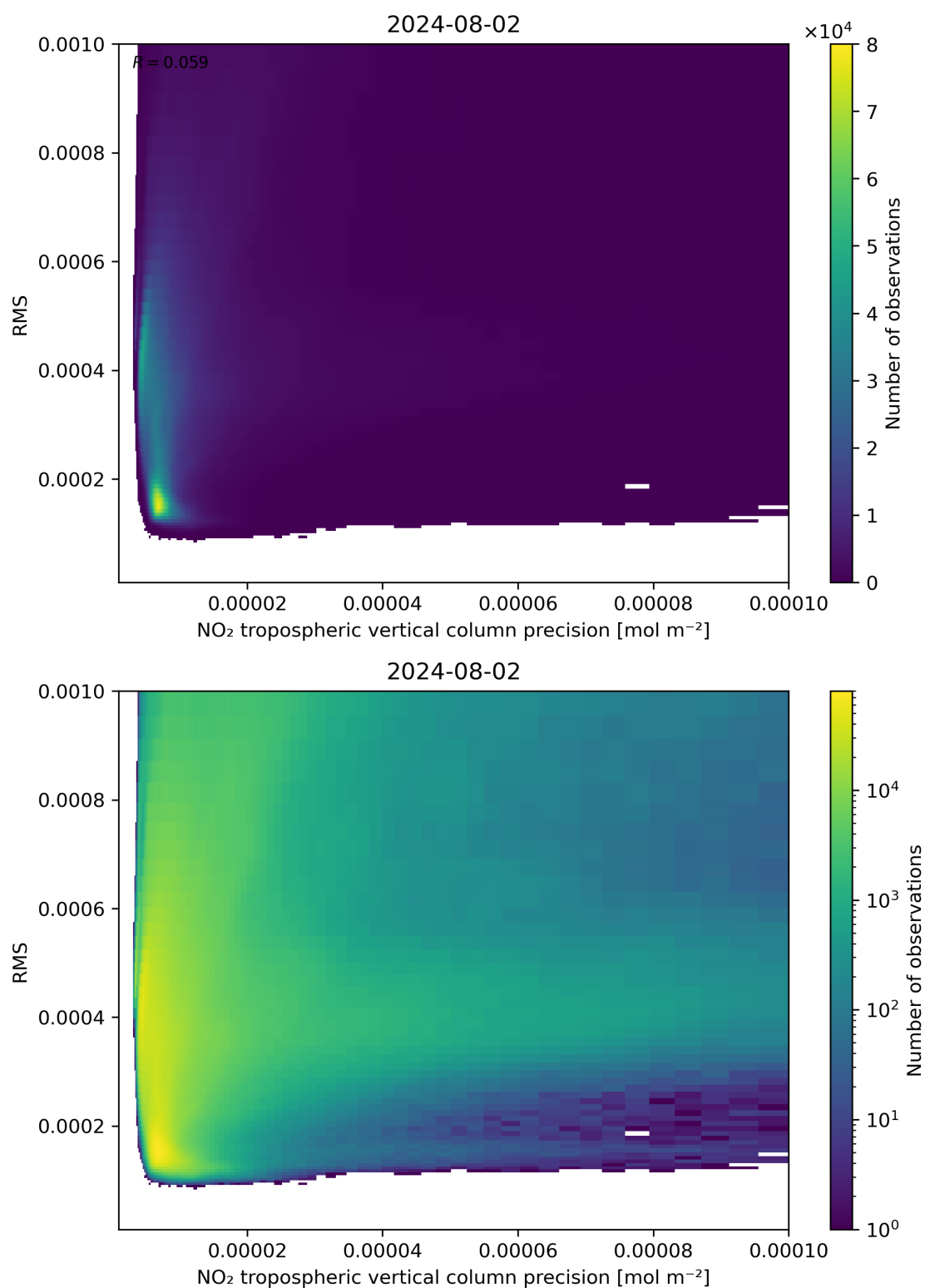
Figure 140: Scatter density plot of “NO 2 tropospheric vertical column precision” against “RMS” for 2024-08-01 to 2024-08-03.
