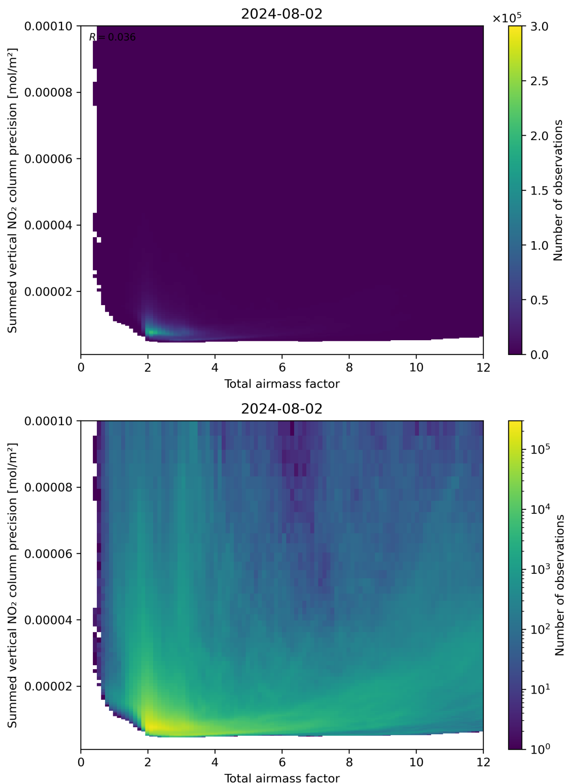
Figure 66: Scatter density plot of “Total airmass factor” against “Summed vertical NO 2 column precision” for 2024-08-01 to 2024-08-03.
