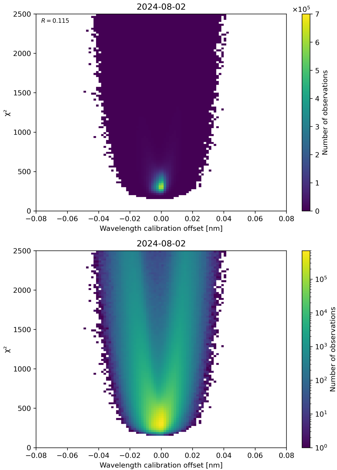
Figure 175: Scatter density plot of “Wavelength calibration offset” against “ \chi^2 ” for 2024-08-01 to 2024-08-03.
