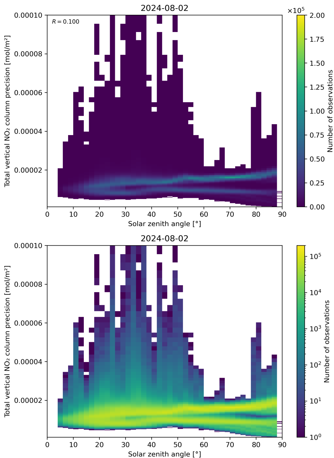
Figure 154: Scatter density plot of “Solar zenith angle” against “Total vertical NO 2 column precision” for 2024-08-01 to 2024-08-03.
