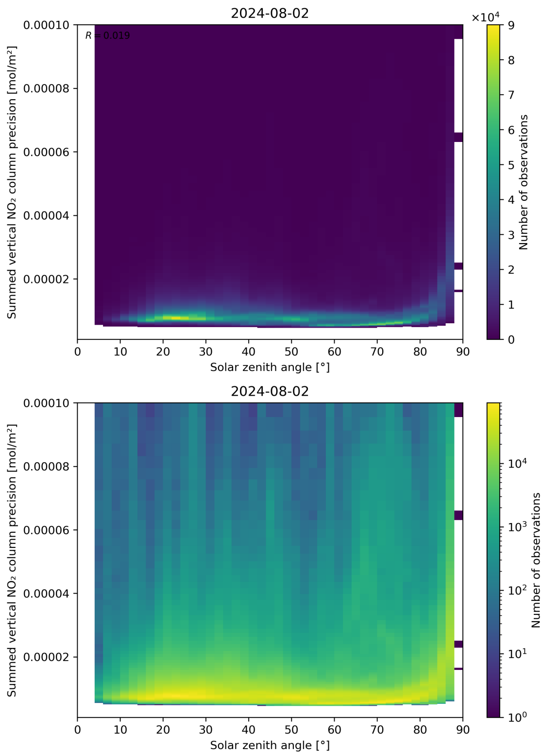
Figure 152: Scatter density plot of “Solar zenith angle” against “Summed vertical NO 2 column precision” for 2024-08-01 to 2024-08-03.
