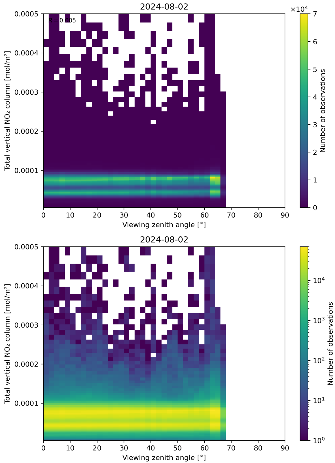
Figure 167: Scatter density plot of “Viewing zenith angle” against “Total vertical NO 2 column” for 2024-08-01 to 2024-08-03.
