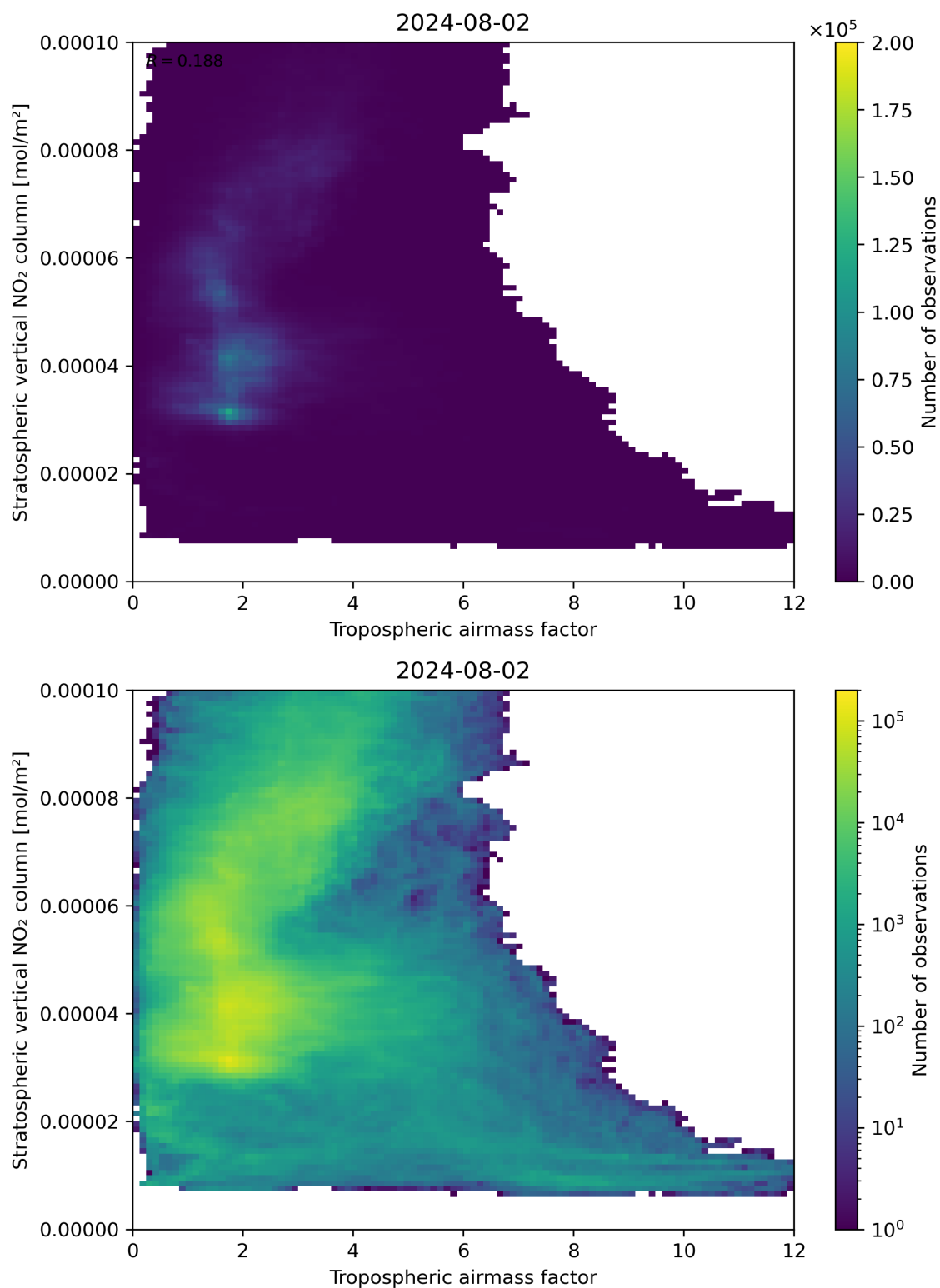
Figure 74: Scatter density plot of “Tropospheric air mass factor” against “Stratospheric vertical NO 2 column” for 2024-08-01 to 2024-08-03.
