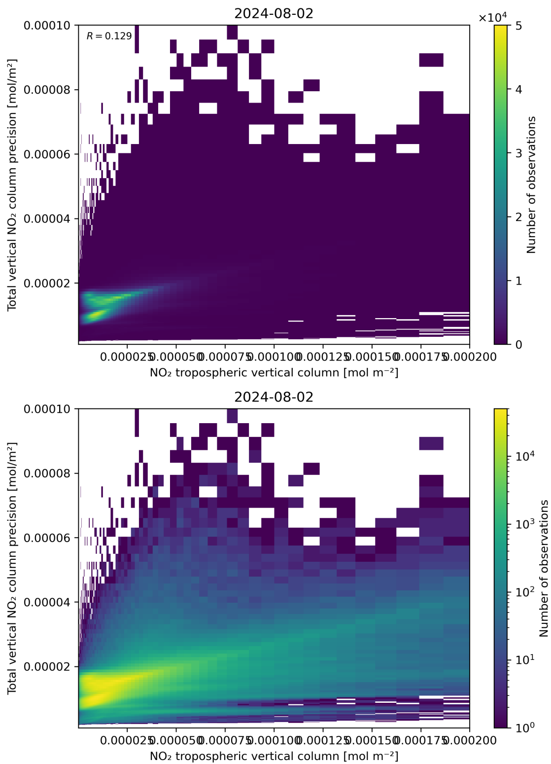
Figure 129: Scatter density plot of “NO 2 tropospheric vertical column” against “Total vertical NO 2 column precision” for 2024-08-01 to 2024-08-03.
