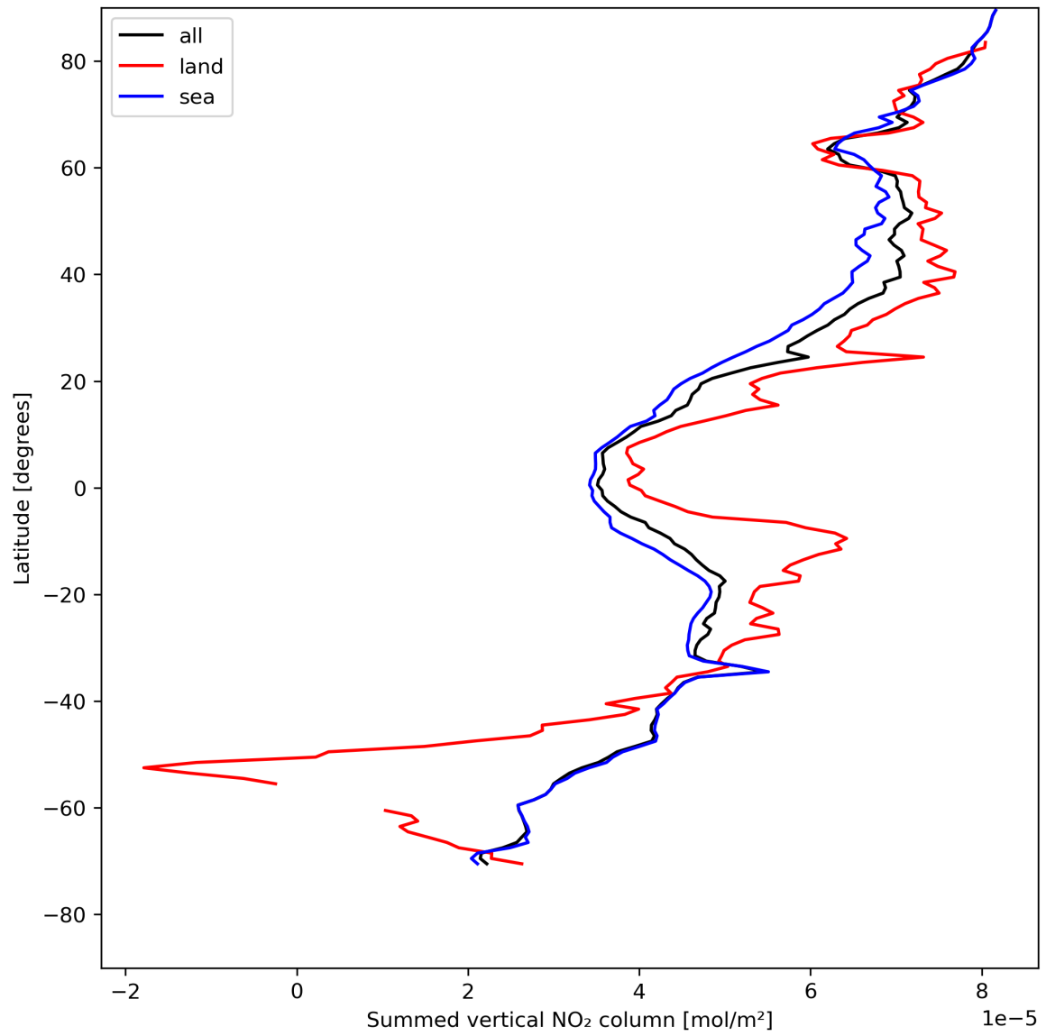
Figure 23: Zonal average of “Summed vertical NO 2 column” for 2024-08-01 to 2024-08-03.
