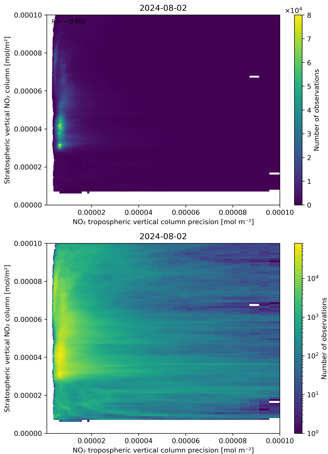
Figure 135: Scatter density plot of “NO 2 tropospheric vertical column precision” against “Stratospheric vertical NO 2 column” for 2024-08-01 to 2024-08-03.
