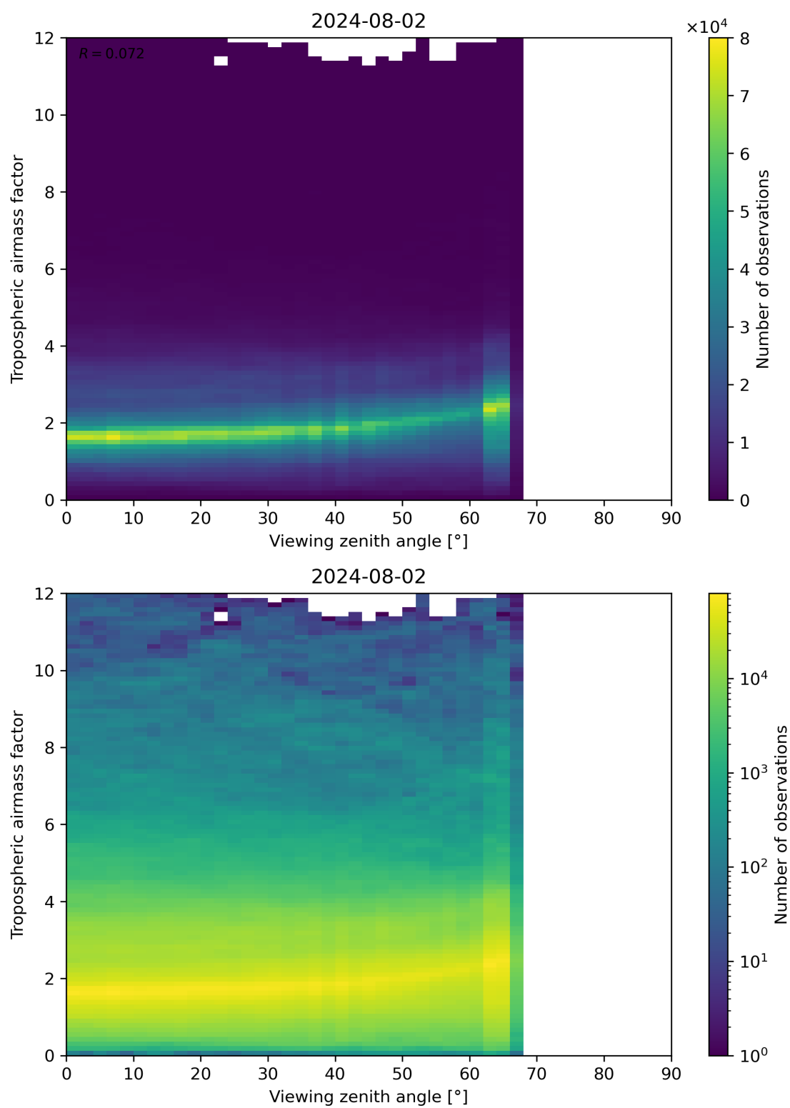
Figure 161: Scatter density plot of “Viewing zenith angle” against “Tropospheric airmass factor” for 2024-08-01 to 2024-08-03.
