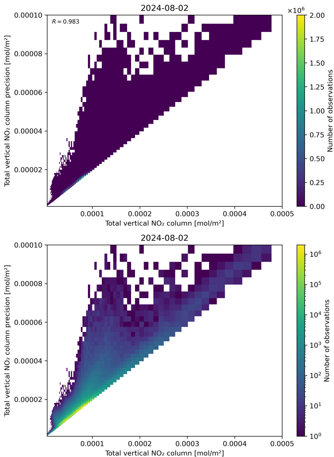
Figure 114: Scatter density plot of “Total vertical NO 2 column” against “Total vertical NO 2 column precision” for 2024-08-01 to 2024-08-03.
