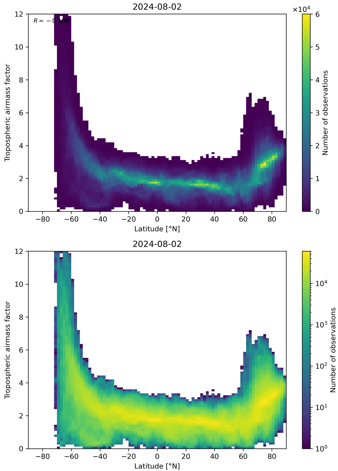
Figure 85: Scatter density plot of “Latitude” against “Tropospheric air mass factor” for 2024-08-01 to 2024-08-03.
