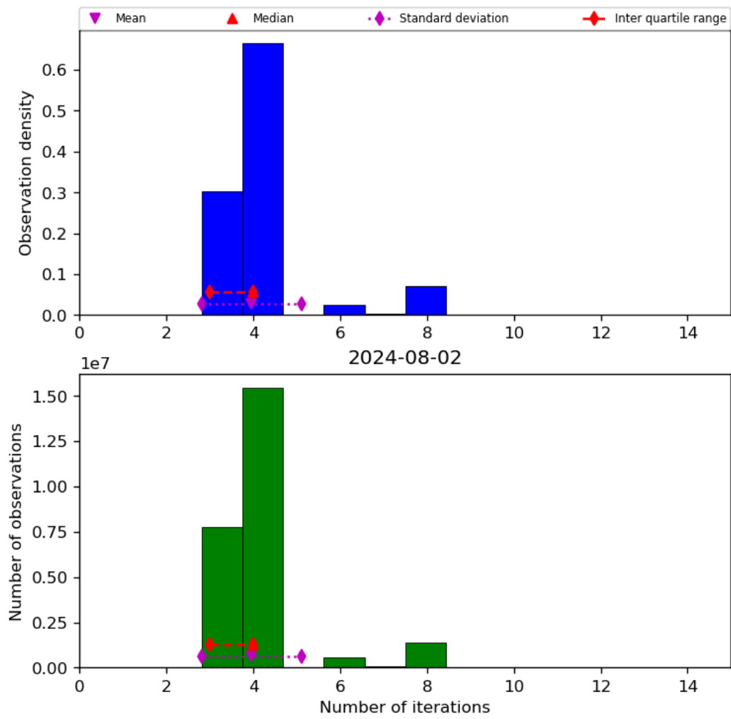
Figure 34: Histogram of “Number of iterations” for 2024-08-01 to 2024-08-03
