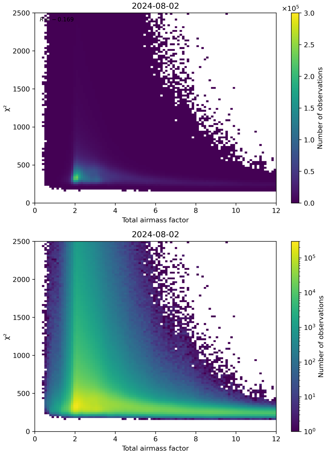
Figure 63: Scatter density plot of “Total airmass factor” against “ \chi^2 ” for 2024-08-01 to 2024-08-03.
