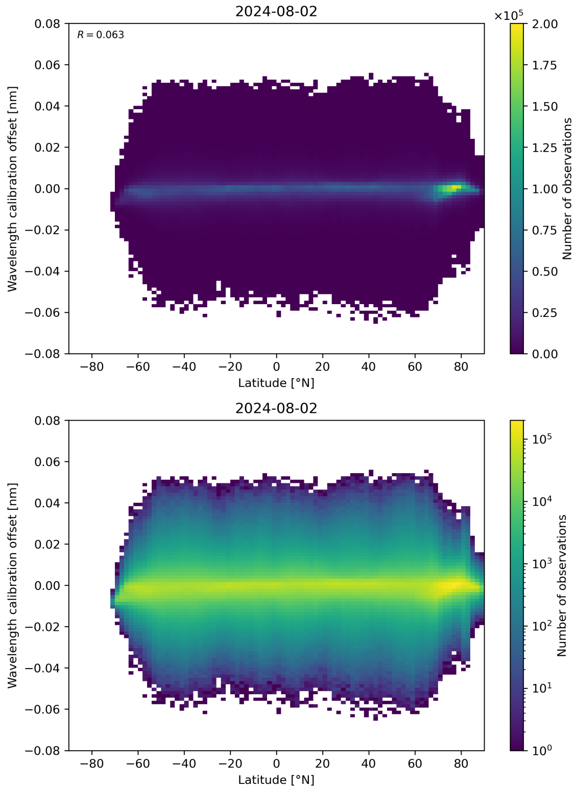
Figure 95: Scatter density plot of “Latitude” against “Wavelength calibration offset” for 2024-08-01 to 2024-08-03.
