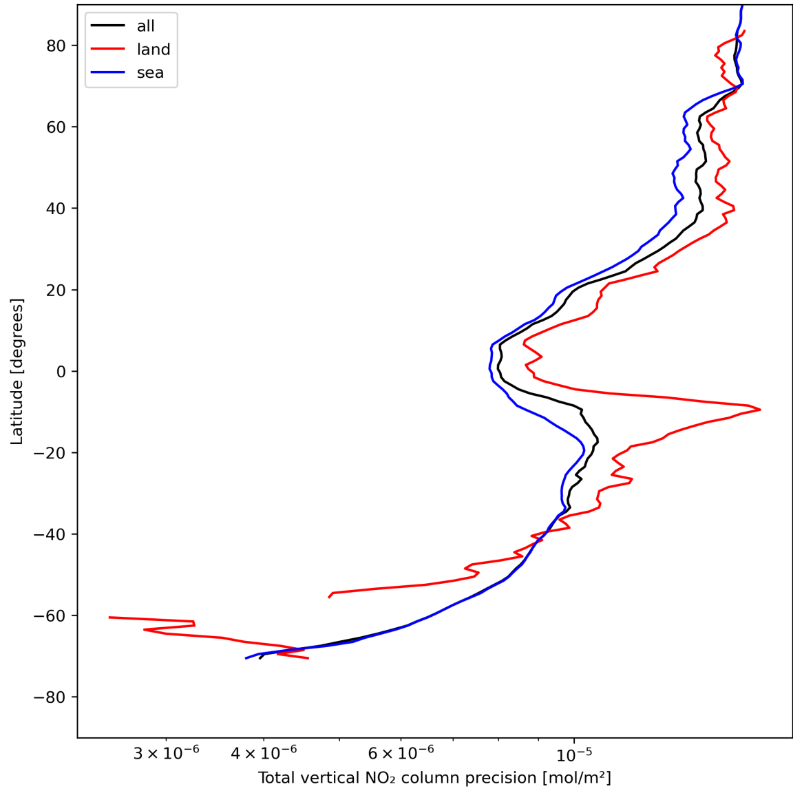
Figure 22: Zonal average of “Total vertical NO 2 column precision” for 2024-08-01 to 2024-08-03.
