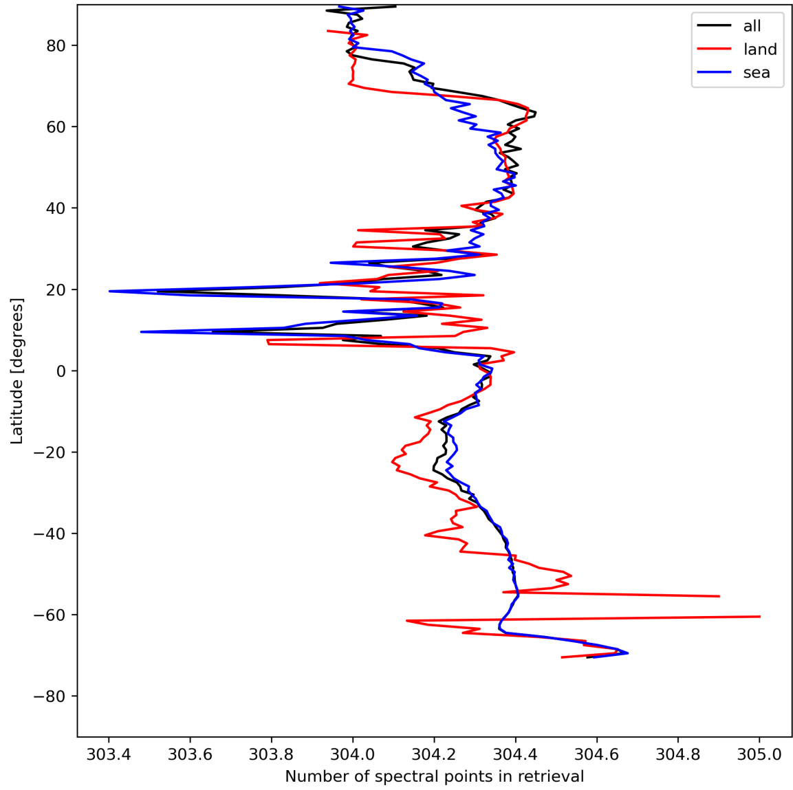
Figure 16: Zonal average of “Number of spectral points in retrieval” for 2024-08-01 to 2024-08-03.
