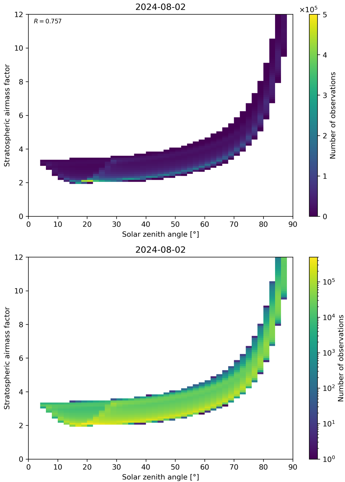
Figure 145: Scatter density plot of “Solar zenith angle” against “Stratospheric airmass factor” for 2024-08-01 to 2024-08-03.
