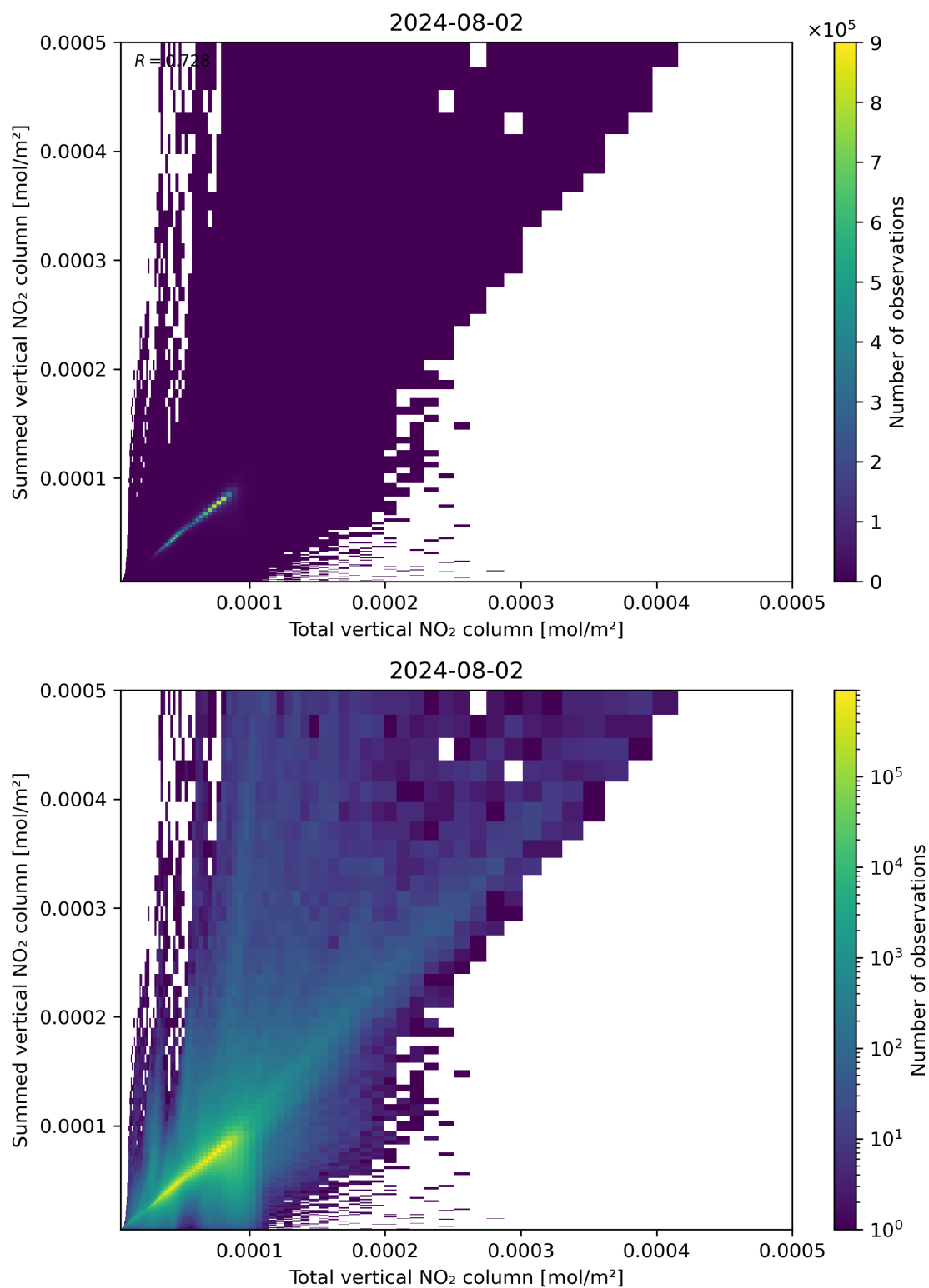
Figure 112: Scatter density plot of “Total vertical NO 2 column” against “Summed vertical NO 2 column” for 2024-08-01 to 2024-08-03.
