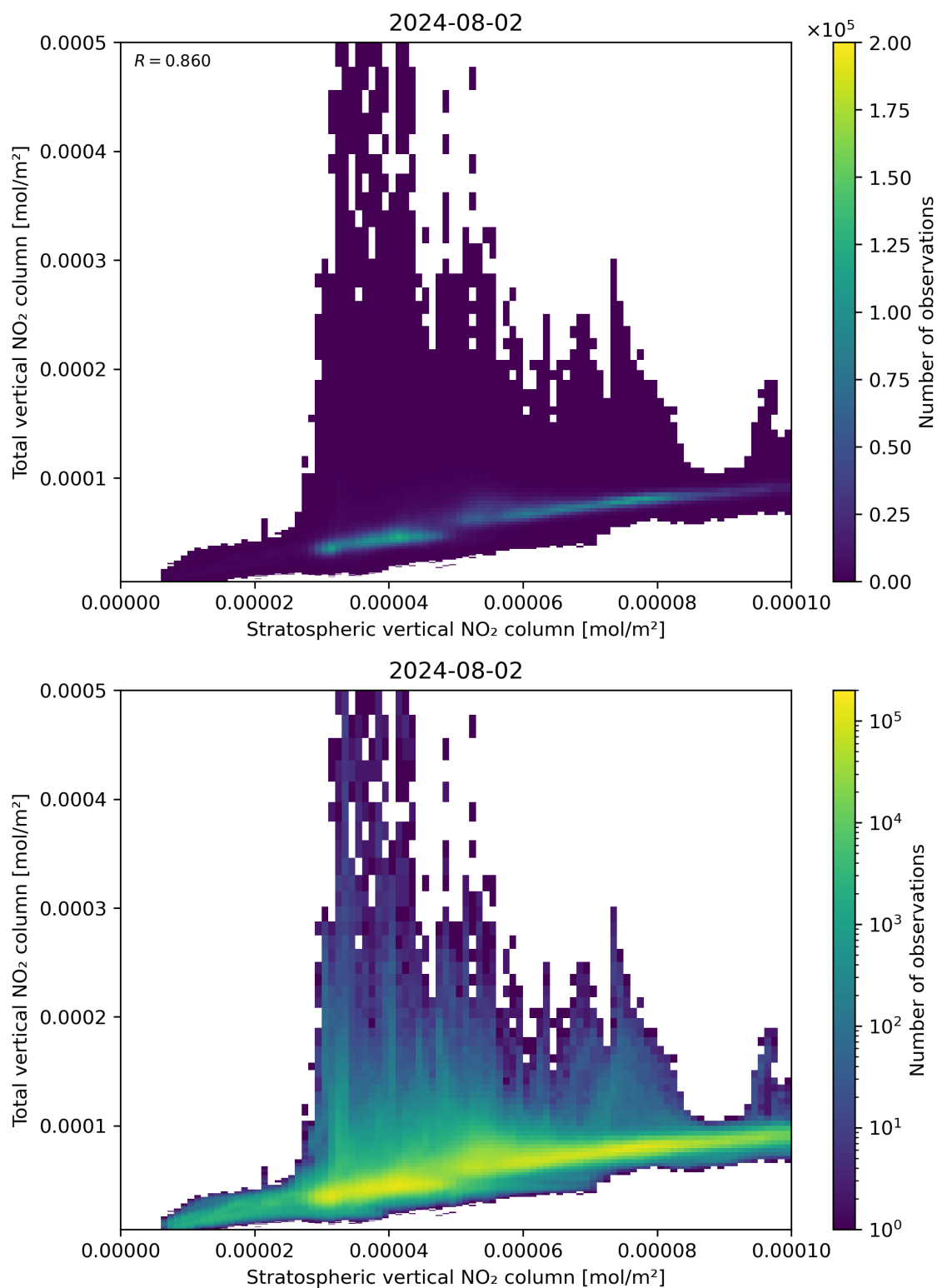
Figure 100: Scatter density plot of “Stratospheric vertical NO 2 column” against “Total vertical NO 2 column” for 2024-08-01 to 2024-08-03.
