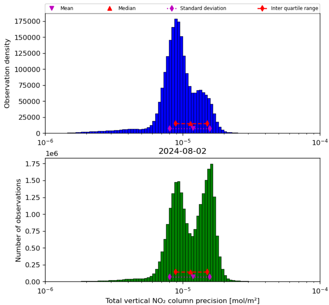
Figure 39: Histogram of “Total vertical NO 2 column precision” for 2024-08-01 to 2024-08-03
