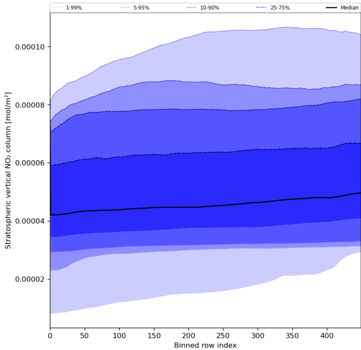
Figure 53: Along track statistics of “Stratospheric vertical NO 2 column” for 2024-08-01 to 2024-08-03
