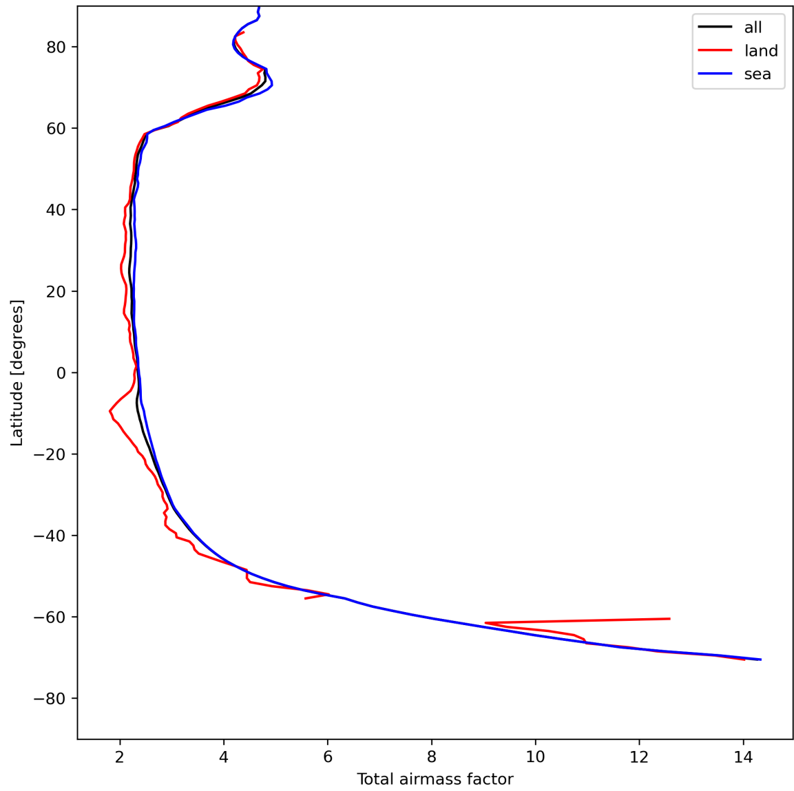
Figure 15: Zonal average of “Total airmass factor” for 2024-08-01 to 2024-08-03.
