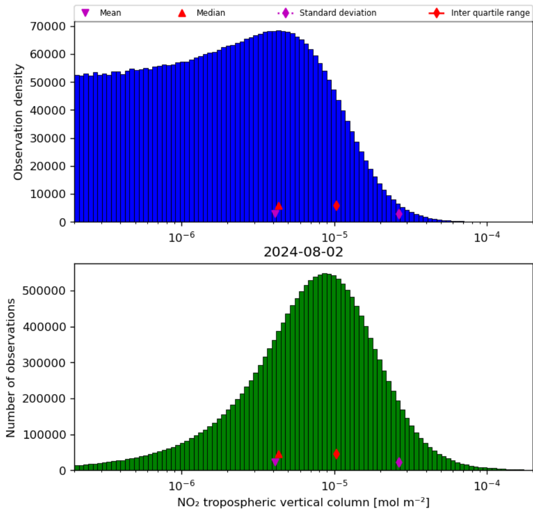
Figure 29: Histogram of “NO 2 tropospheric vertical column” for 2024-08-01 to 2024-08-03
