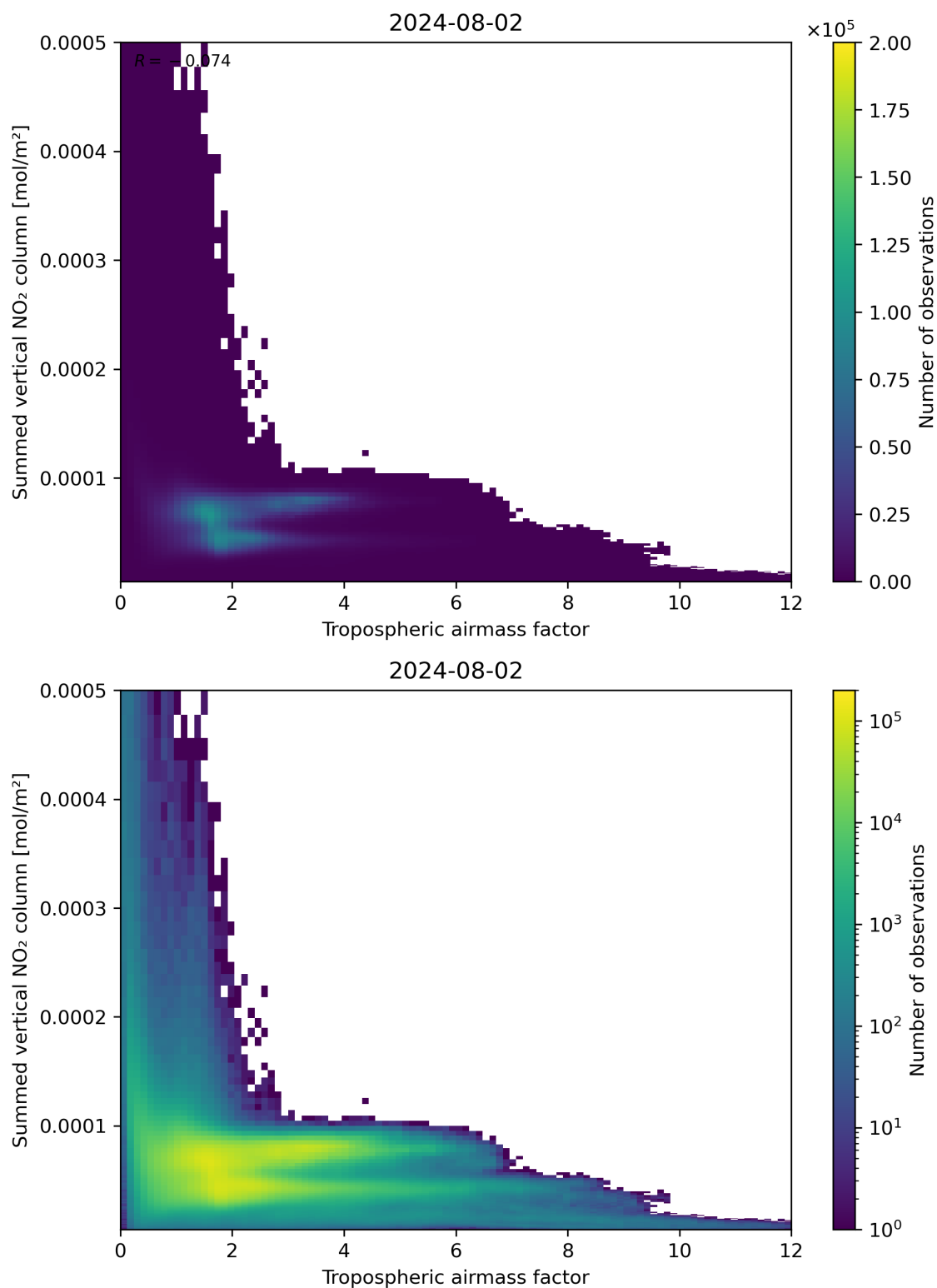
Figure 75: Scatter density plot of “Tropospheric airmass factor” against “Summed vertical NO 2 column” for 2024-08-01 to 2024-08-03.
