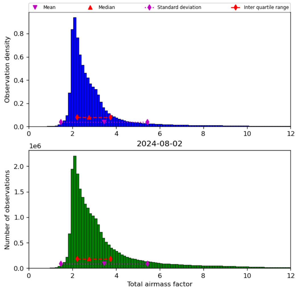
Figure 32: Histogram of “Total airmass factor” for 2024-08-01 to 2024-08-03
