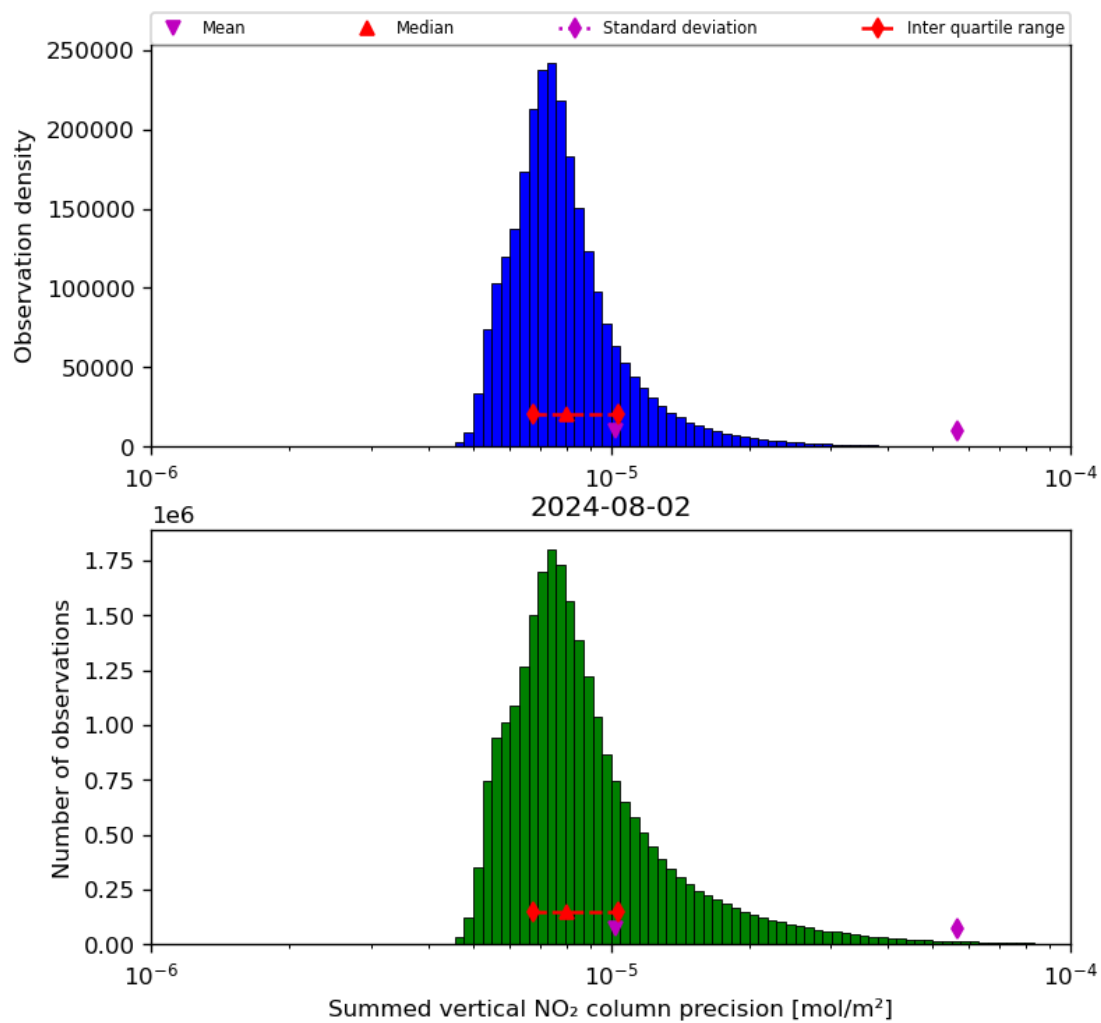
Figure 41: Histogram of “Summed vertical NO 2 column precision” for 2024-08-01 to 2024-08-03
