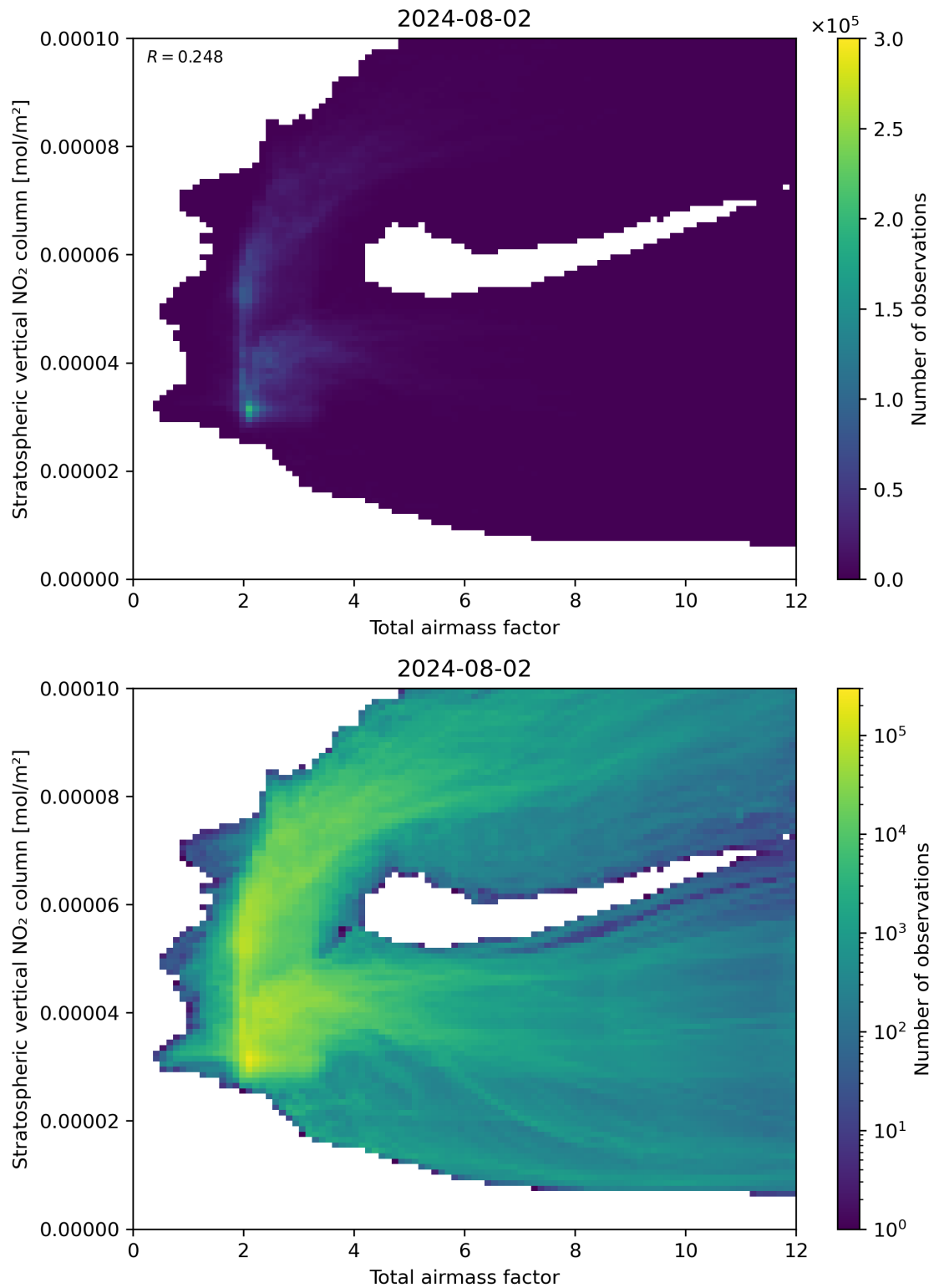
Figure 64: Scatter density plot of “Total airmass factor” against “Stratospheric vertical NO 2 column” for 2024-08-01 to 2024-08-03.
