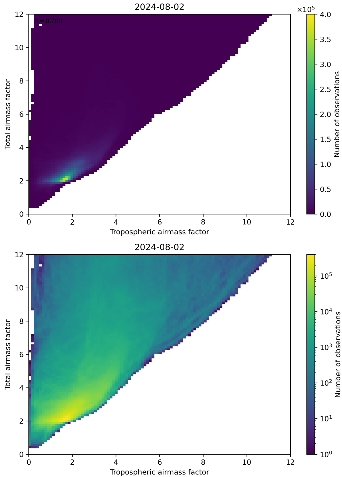
Figure 72: Scatter density plot of “Tropospheric airmass factor” against “Total airmass factor” for 2024-08-01 to 2024-08-03.
