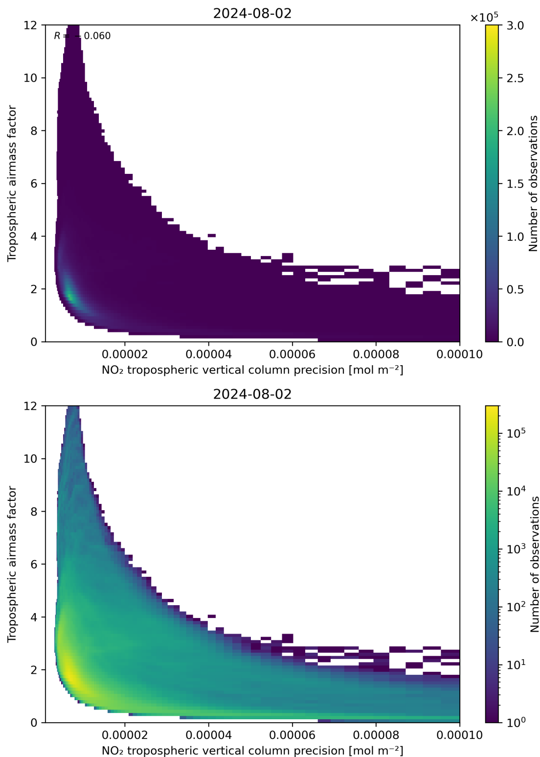
Figure 133: Scatter density plot of “NO 2 tropospheric vertical column precision” against “Tropospheric airmass factor” for 2024-08-01 to 2024-08-03.
