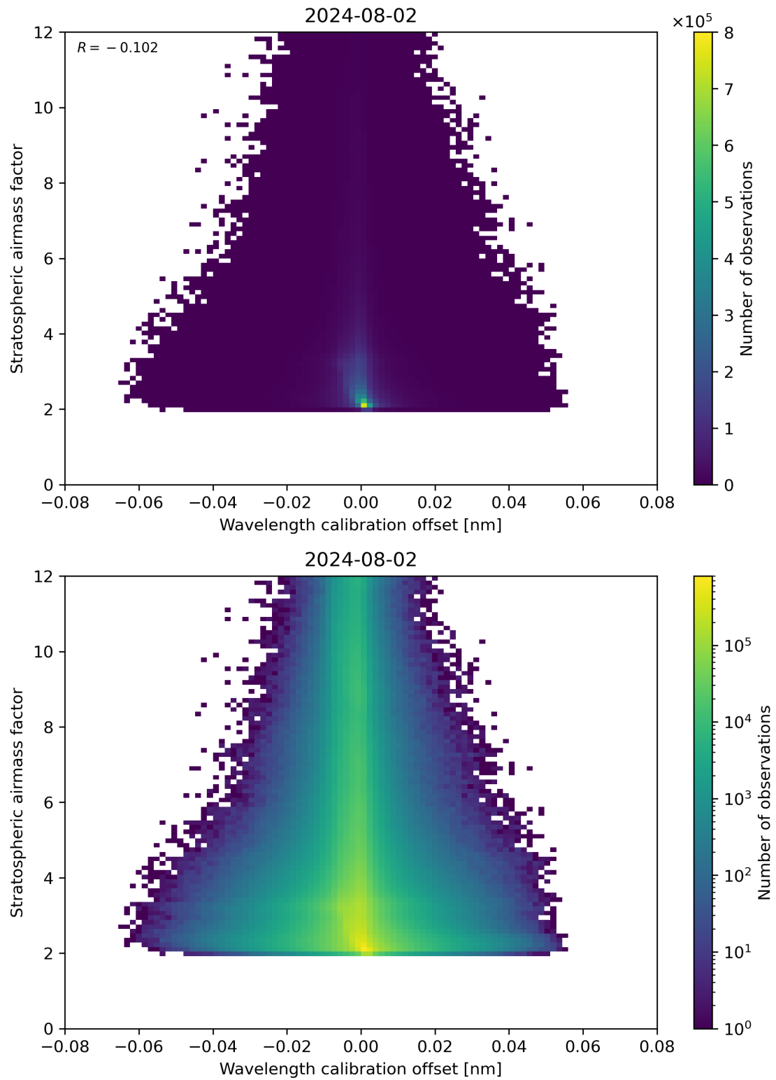
Figure 174: Scatter density plot of “Wavelength calibration offset” against “Stratospheric airmass factor” for 2024-08-01 to 2024-08-03.
