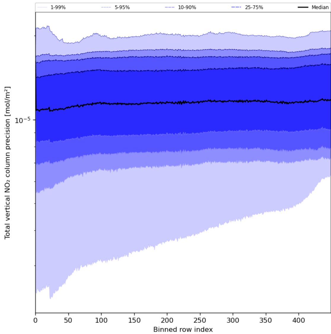
Figure 56: Along track statistics of “Total vertical NO 2 column precision” for 2024-08-01 to 2024-08-03
