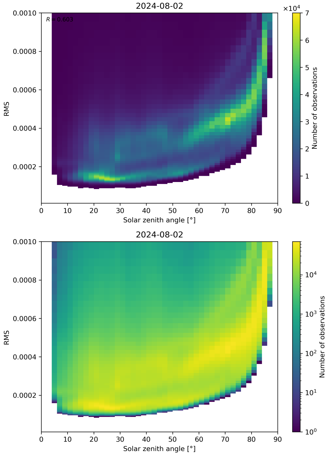
Figure 157: Scatter density plot of “Solar zenith angle” against “RMS” for 2024-08-01 to 2024-08-03.
