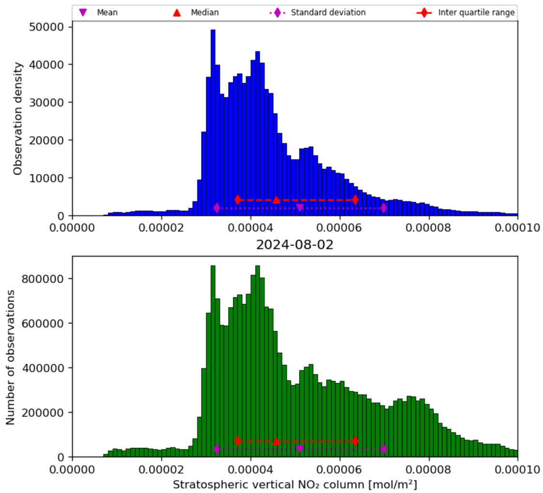
Figure 36: Histogram of “Stratospheric vertical NO 2 column” for 2024-08-01 to 2024-08-03
