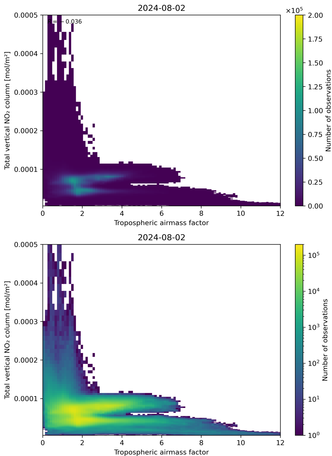
Figure 77: Scatter density plot of “Tropospheric airmass factor” against “Total vertical NO 2 column” for 2024-08-01 to 2024-08-03.
