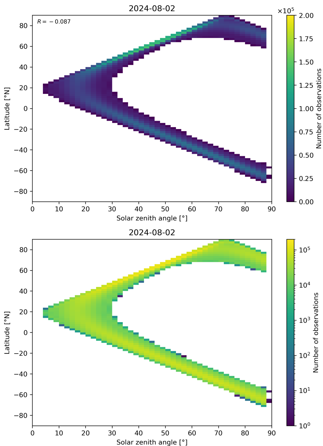
Figure 149: Scatter density plot of “Solar zenith angle” against “Latitude” for 2024-08-01 to 2024-08-03.
