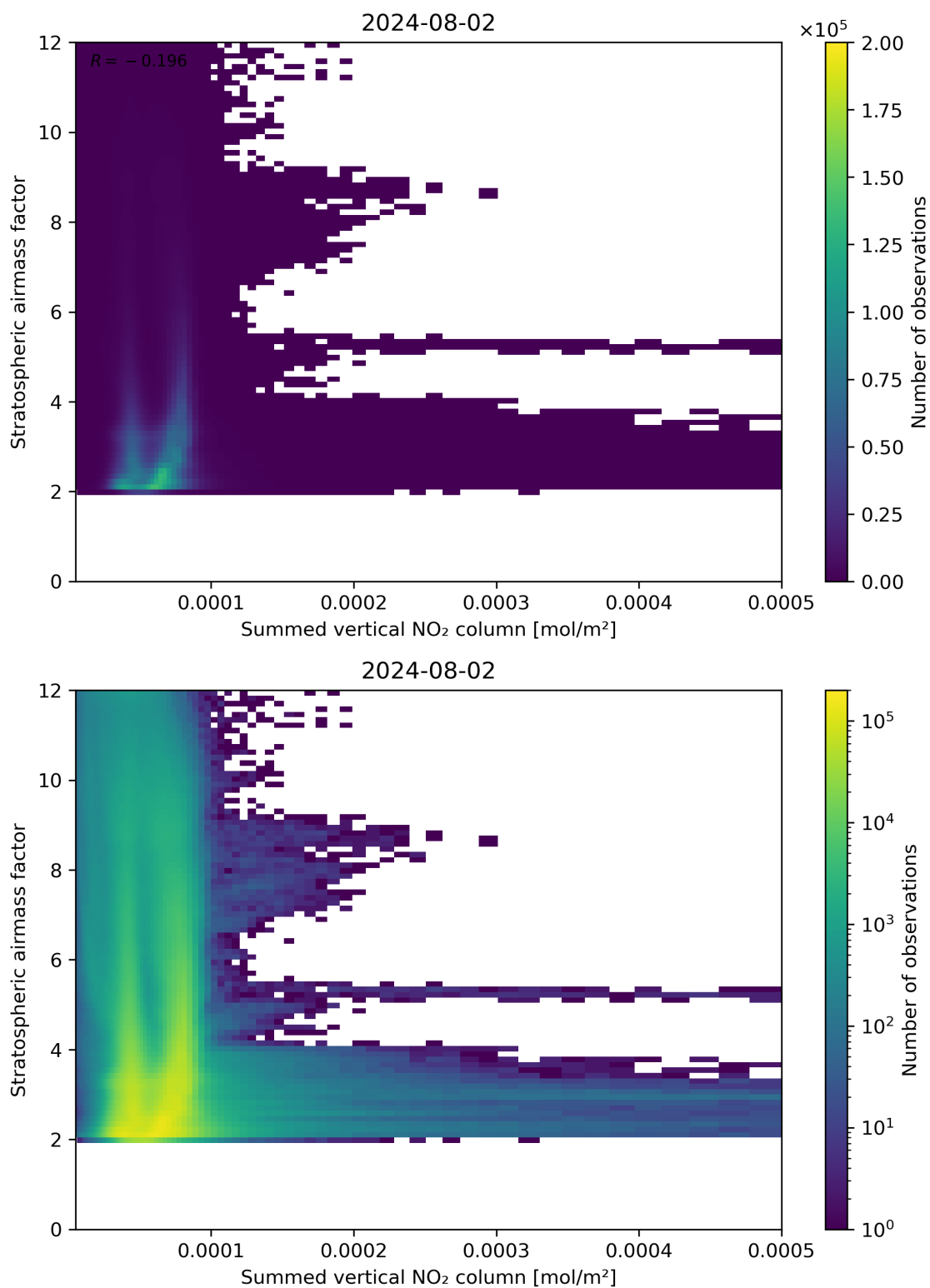
Figure 103: Scatter density plot of “Summed vertical NO 2 column” against “Stratospheric airmass factor” for 2024-08-01 to 2024-08-03.
