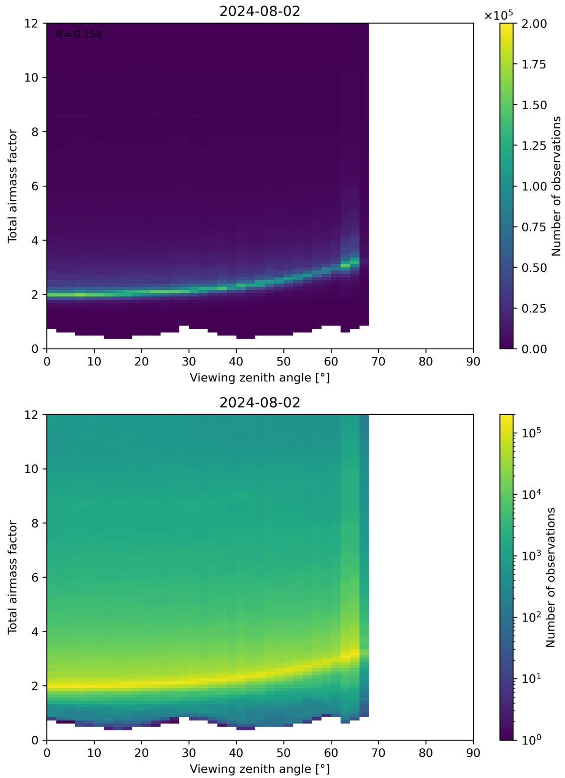
Figure 160: Scatter density plot of “Viewing zenith angle” against “Total airmass factor” for 2024-08-01 to 2024-08-03.
