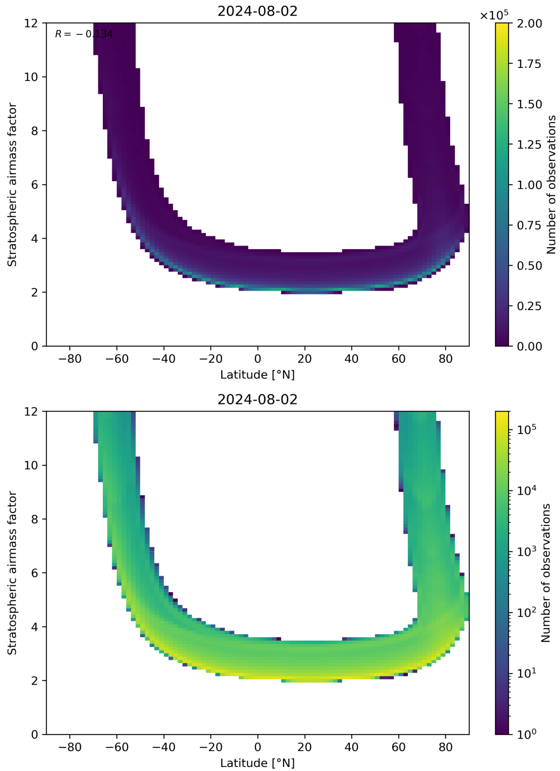
Figure 83: Scatter density plot of “Latitude” against “Stratospheric air mass factor” for 2024-08-01 to 2024-08-03.
