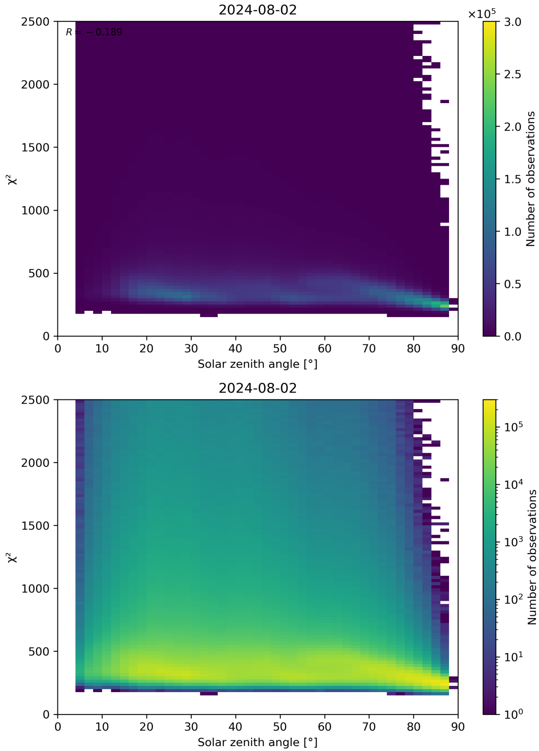
Figure 148: Scatter density plot of “Solar zenith angle” against “ \chi^2 ” for 2024-08-01 to 2024-08-03.
