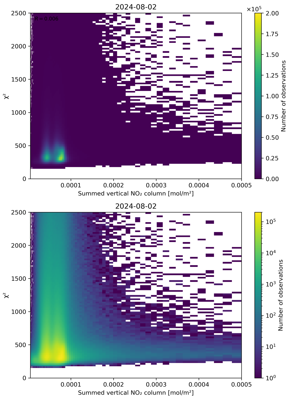
Figure 104: Scatter density plot of “Summed vertical NO 2 column” against “ \chi^2 ” for 2024-08-01 to 2024-08-03.
