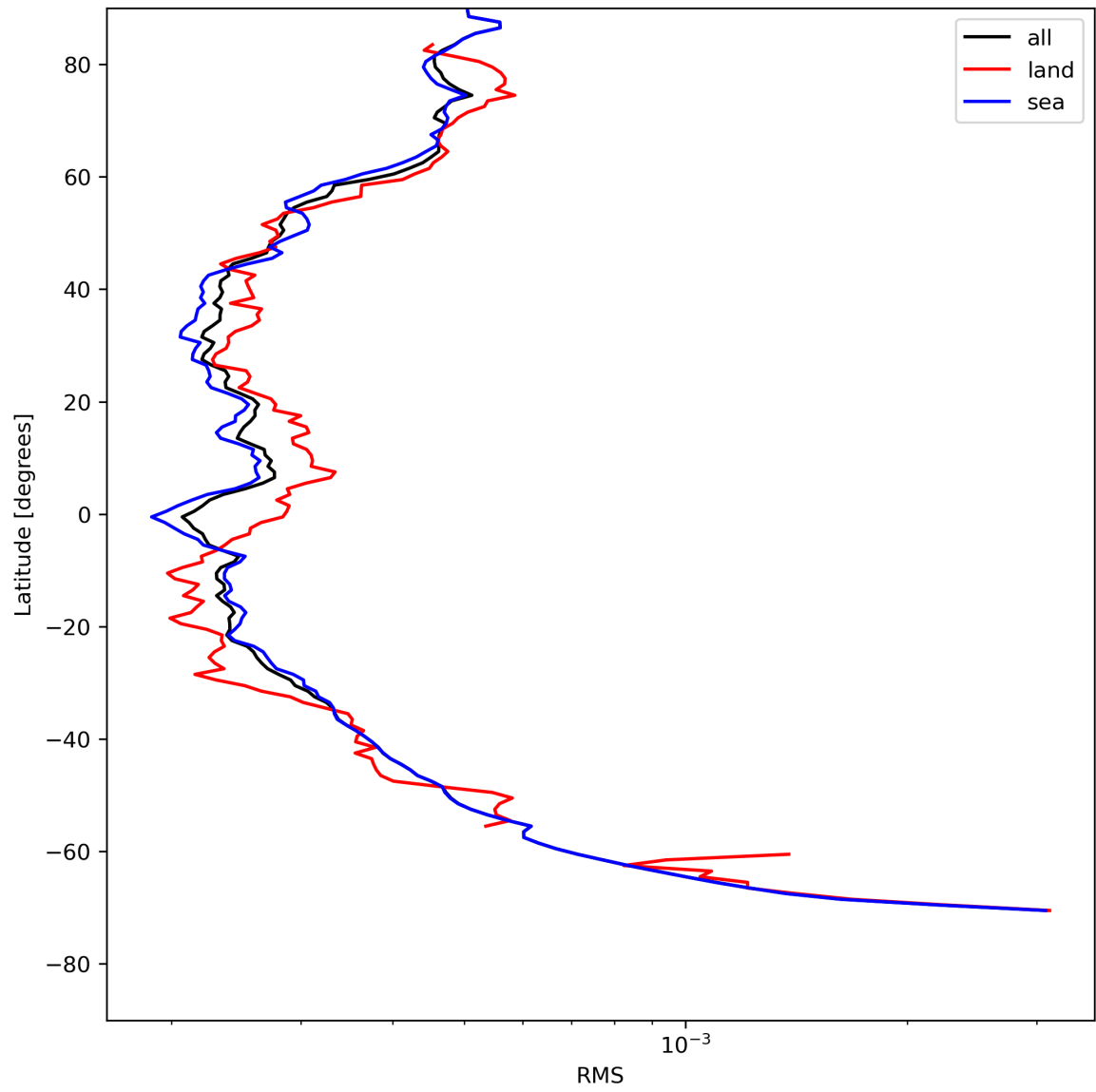
Figure 26: Zonal average of “RMS” for 2024-08-01 to 2024-08-03.
