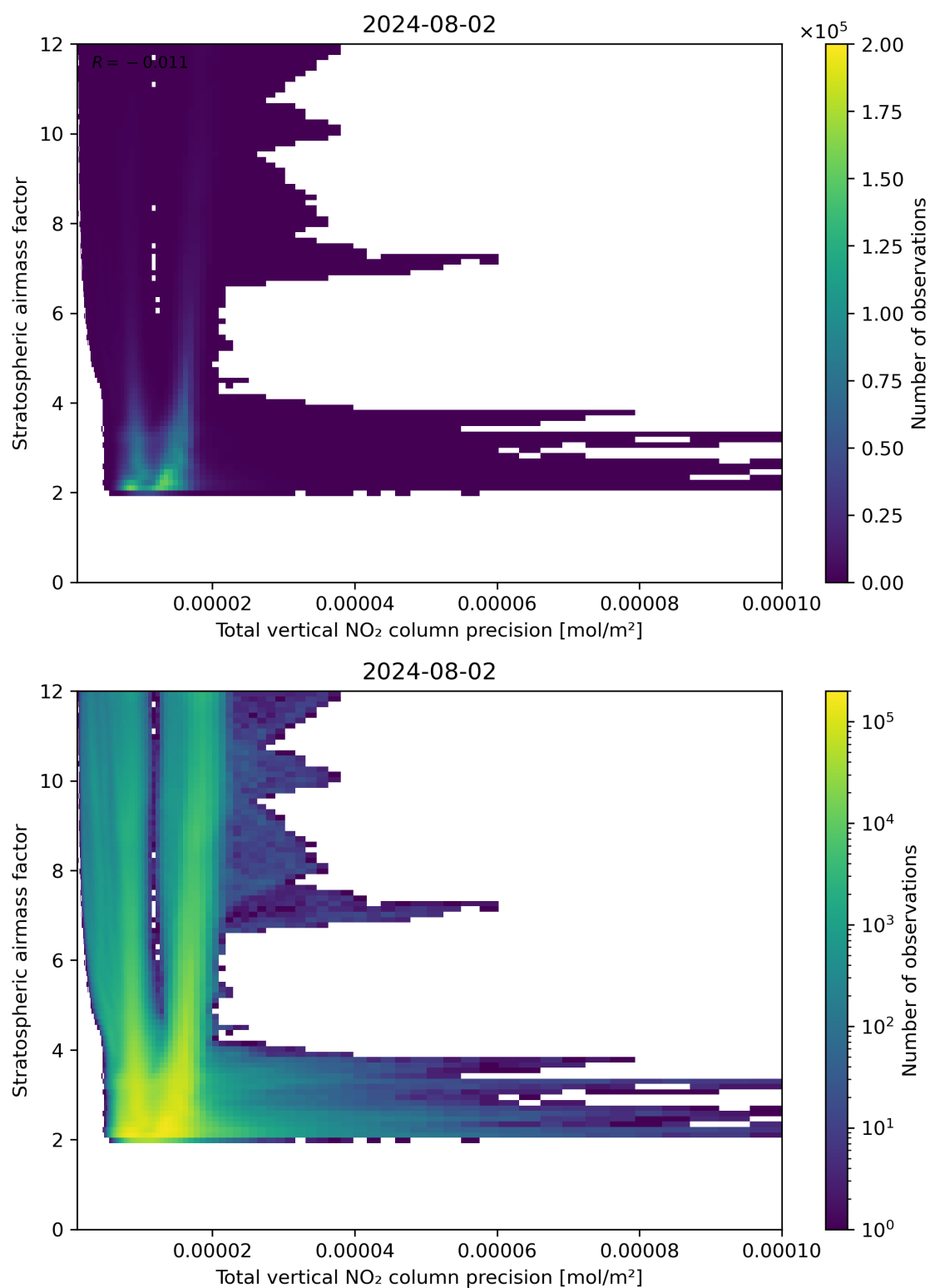
Figure 115: Scatter density plot of “Total vertical NO 2 column precision” against “Stratospheric air mass factor” for 2024-08-01 to 2024-08-03.
