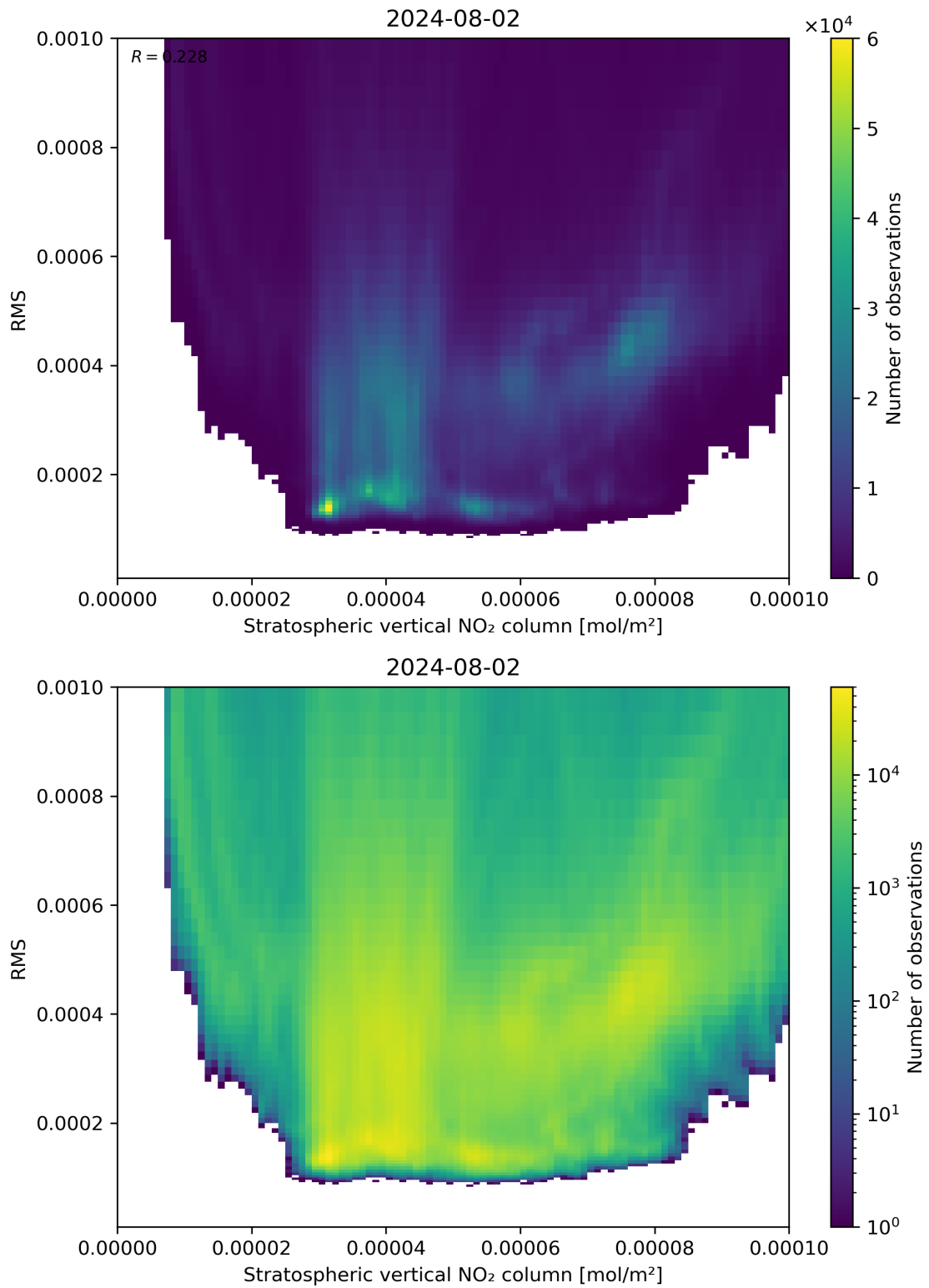
Figure 102: Scatter density plot of “Stratospheric vertical NO 2 column” against “RMS” for 2024-08-01 to 2024-08-03.
