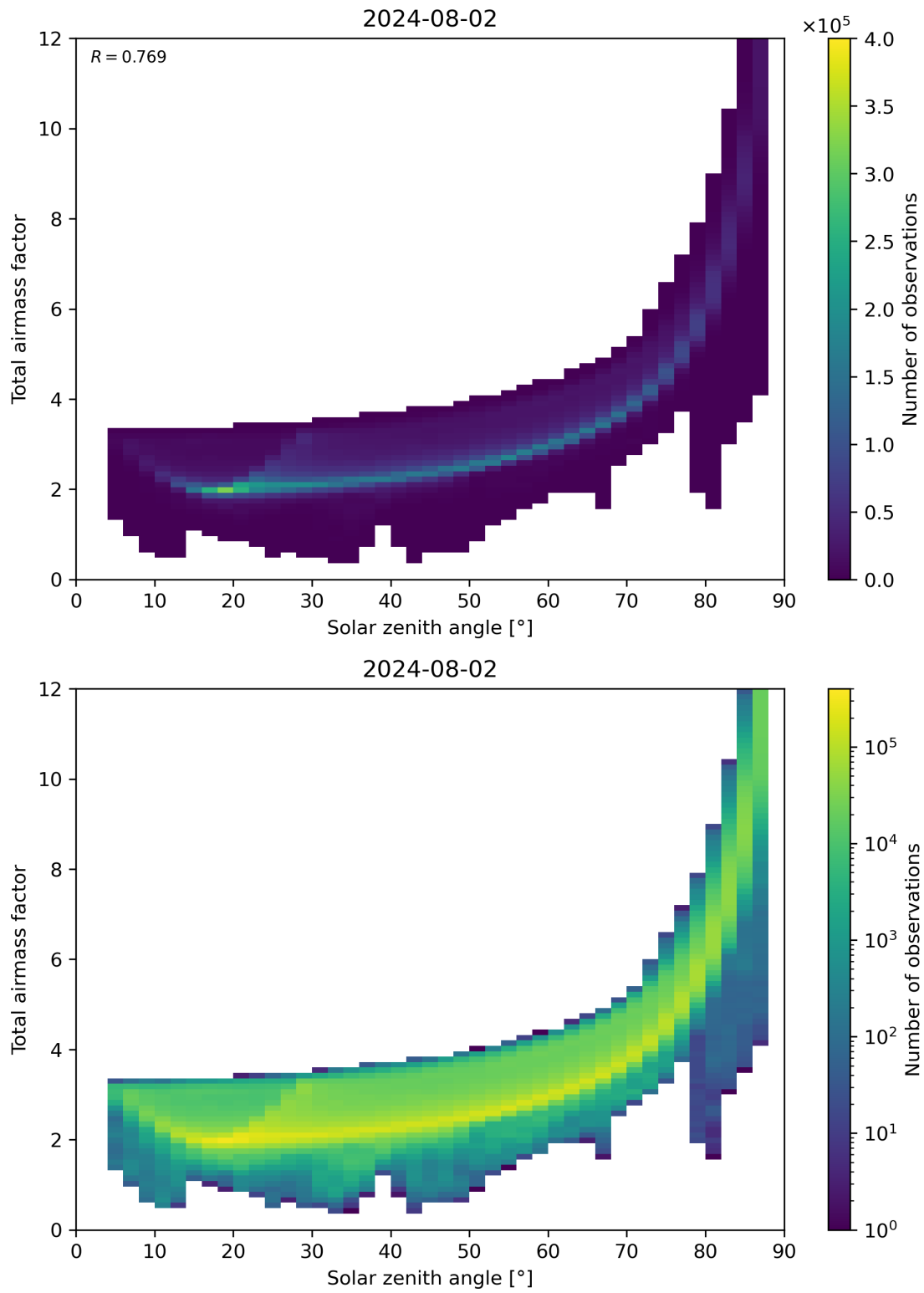
Figure 146: Scatter density plot of “Solar zenith angle” against “Total airmass factor” for 2024-08-01 to 2024-08-03.
