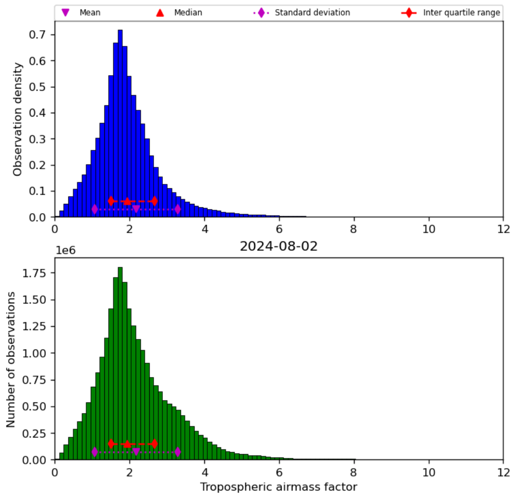
Figure 31: Histogram of “Tropospheric airmass factor” for 2024-08-01 to 2024-08-03
