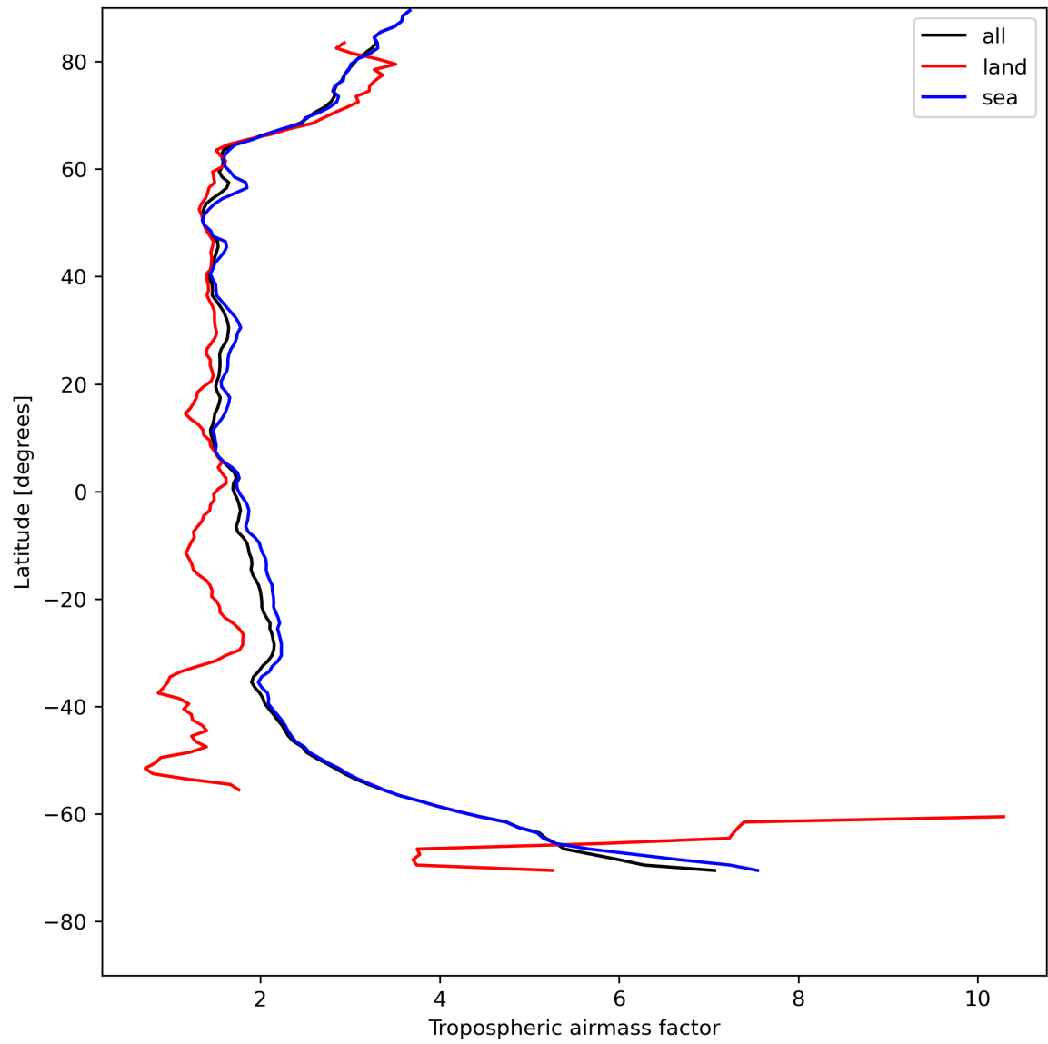
Figure 14: Zonal average of “Tropospheric airmass factor” for 2024-08-01 to 2024-08-03.
