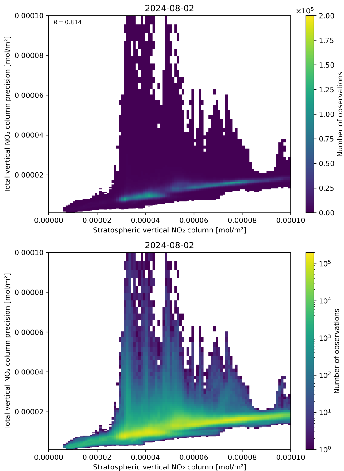
Figure 101: Scatter density plot of “Stratospheric vertical NO 2 column” against “Total vertical NO 2 column precision” for 2024-08-01 to 2024-08-03.
