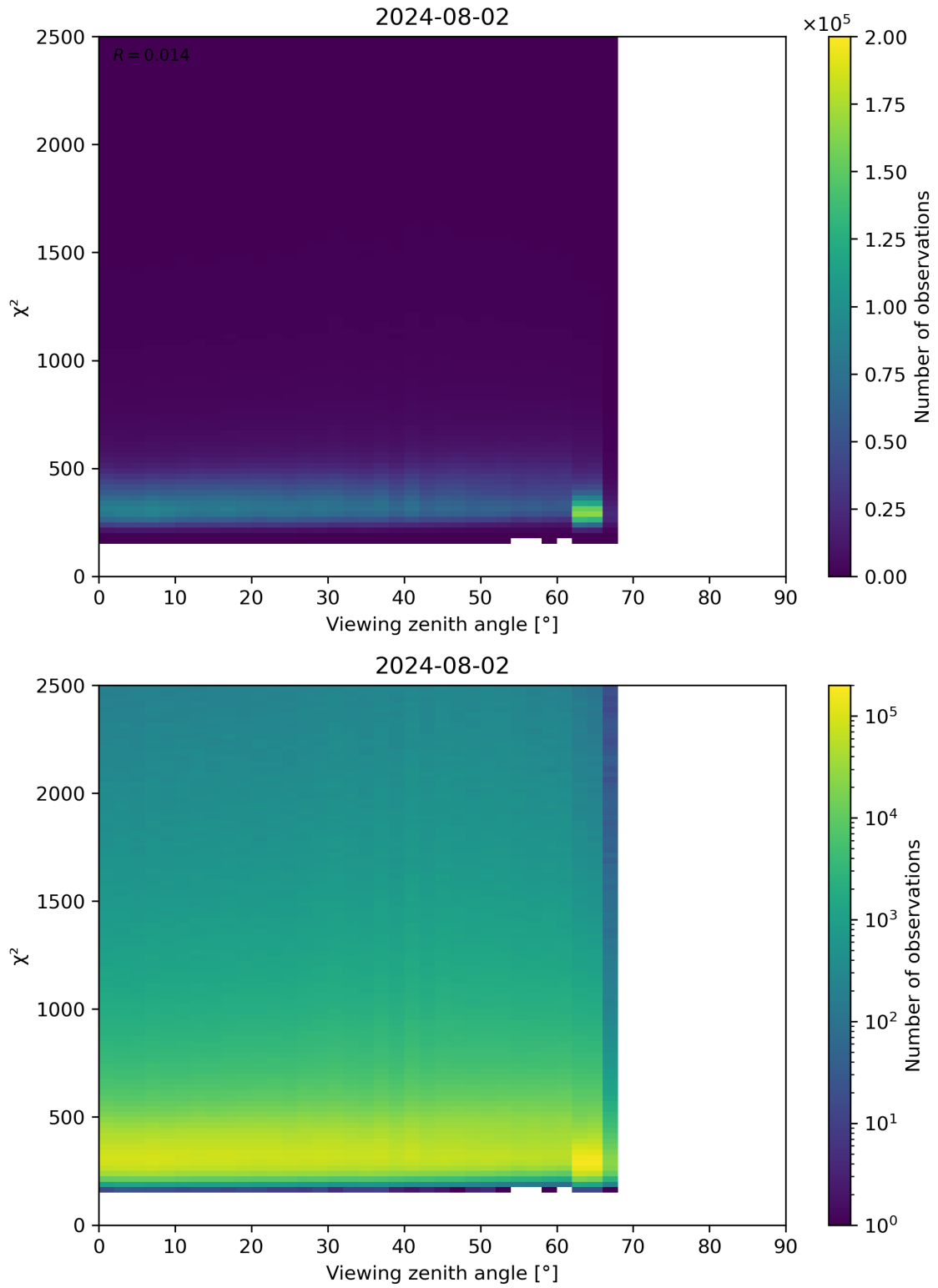
Figure 162: Scatter density plot of “Viewing zenith angle” against “ \chi^2 ” for 2024-08-01 to 2024-08-03.
