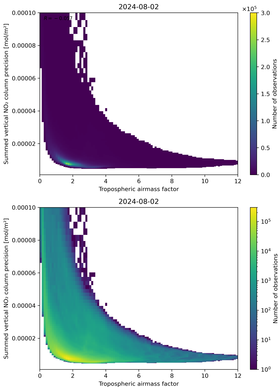
Figure 76: Scatter density plot of “Tropospheric air mass factor” against “Summed vertical NO 2 column precision” for 2024-08-01 to 2024-08-03.
