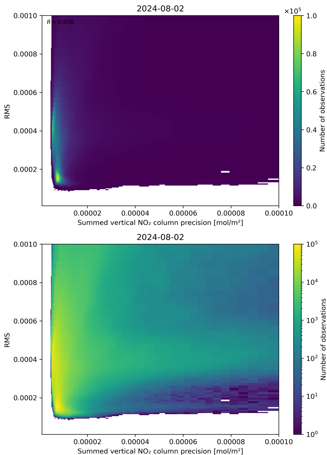
Figure 108: Scatter density plot of “Summed vertical NO 2 column precision” against “RMS” for 2024-08-01 to 2024-08-03.
