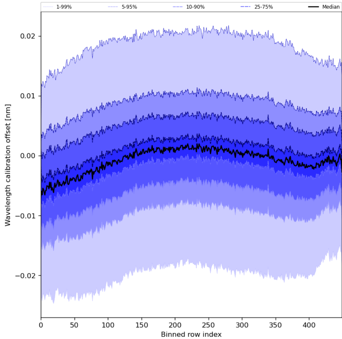
Figure 52: Along track statistics of “Wavelength calibration offset” for 2024-08-01 to 2024-08-03
