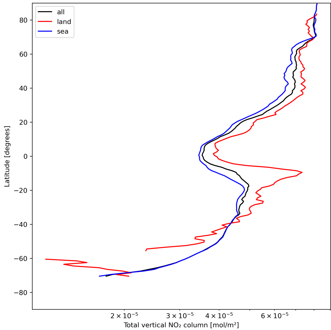
Figure 21: Zonal average of “Total vertical NO 2 column” for 2024-08-01 to 2024-08-03.
