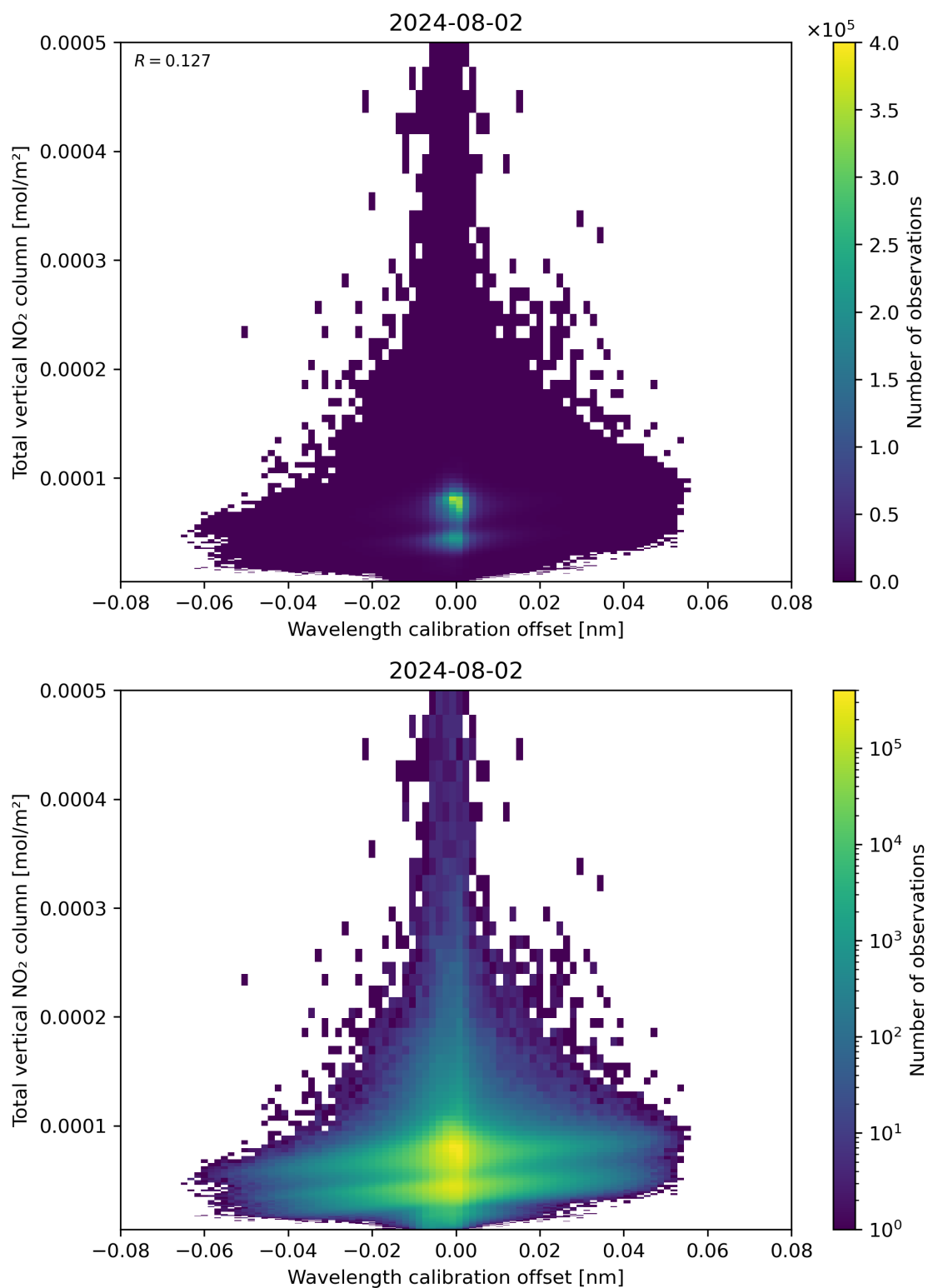
Figure 179: Scatter density plot of “Wavelength calibration offset” against “Total vertical NO 2 column” for 2024-08-01 to 2024-08-03.
