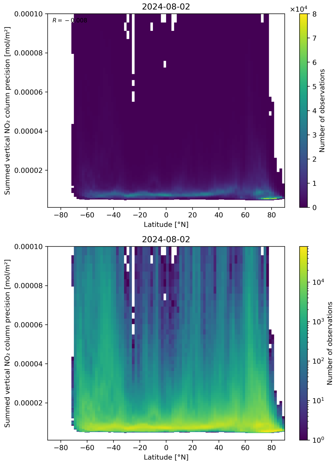
Figure 89: Scatter density plot of “Latitude” against “Summed vertical NO 2 column precision” for 2024-08-01 to 2024-08-03.
