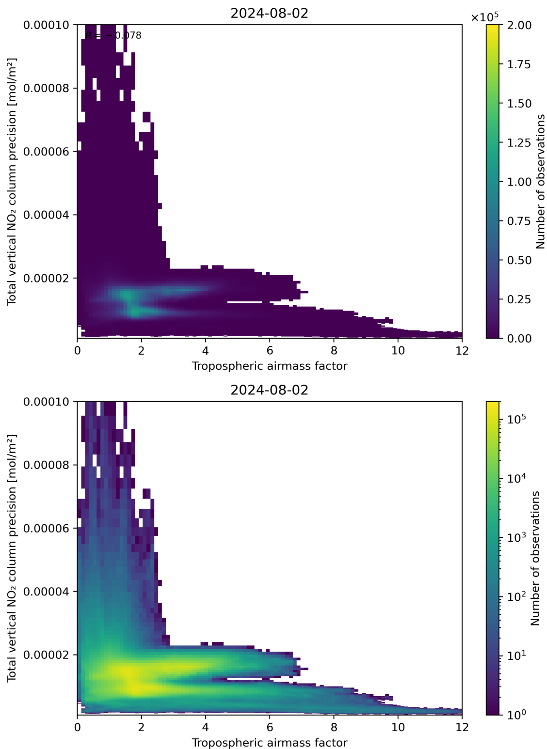
Figure 78: Scatter density plot of “Tropospheric air mass factor” against “Total vertical NO 2 column precision” for 2024-08-01 to 2024-08-03.
