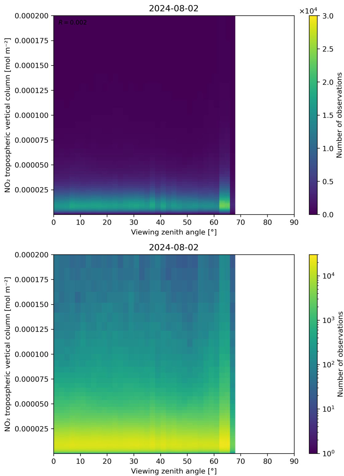
Figure 169: Scatter density plot of “Viewing zenith angle” against “NO 2 tropospheric vertical column” for 2024-08-01 to 2024-08-03.
