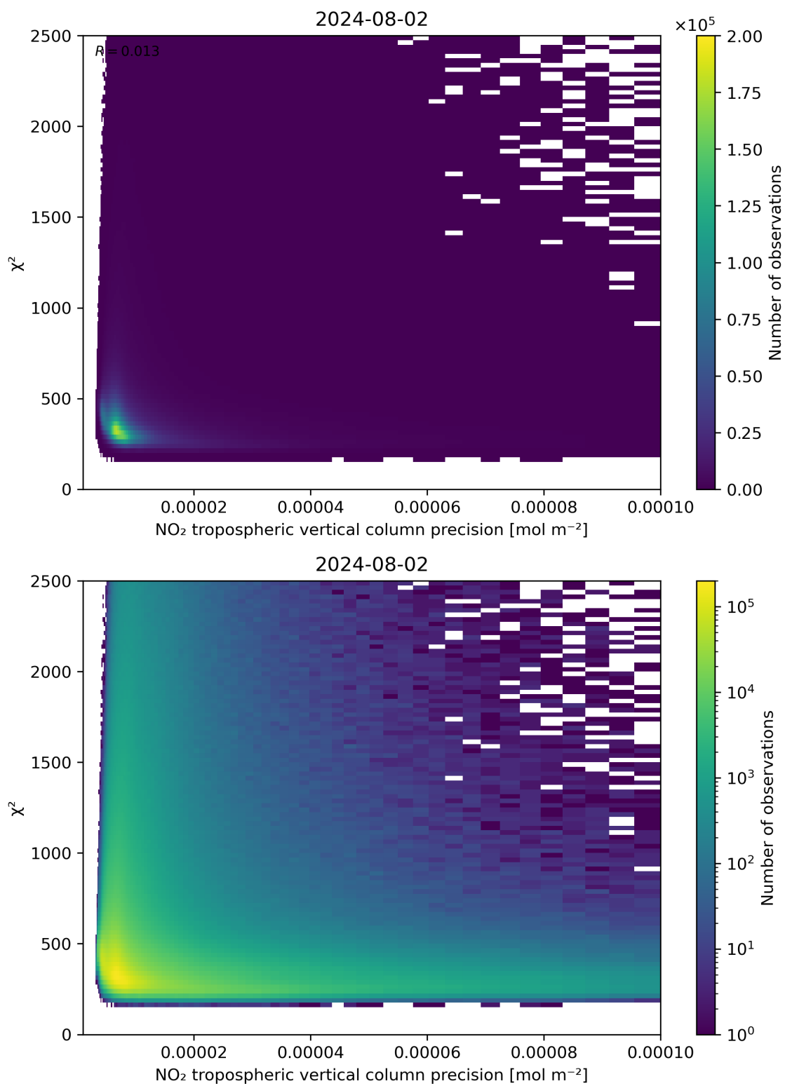
Figure 134: Scatter density plot of “NO 2 tropospheric vertical column precision” against “ \chi^2 ” for 2024-08-01 to 2024-08-03.
