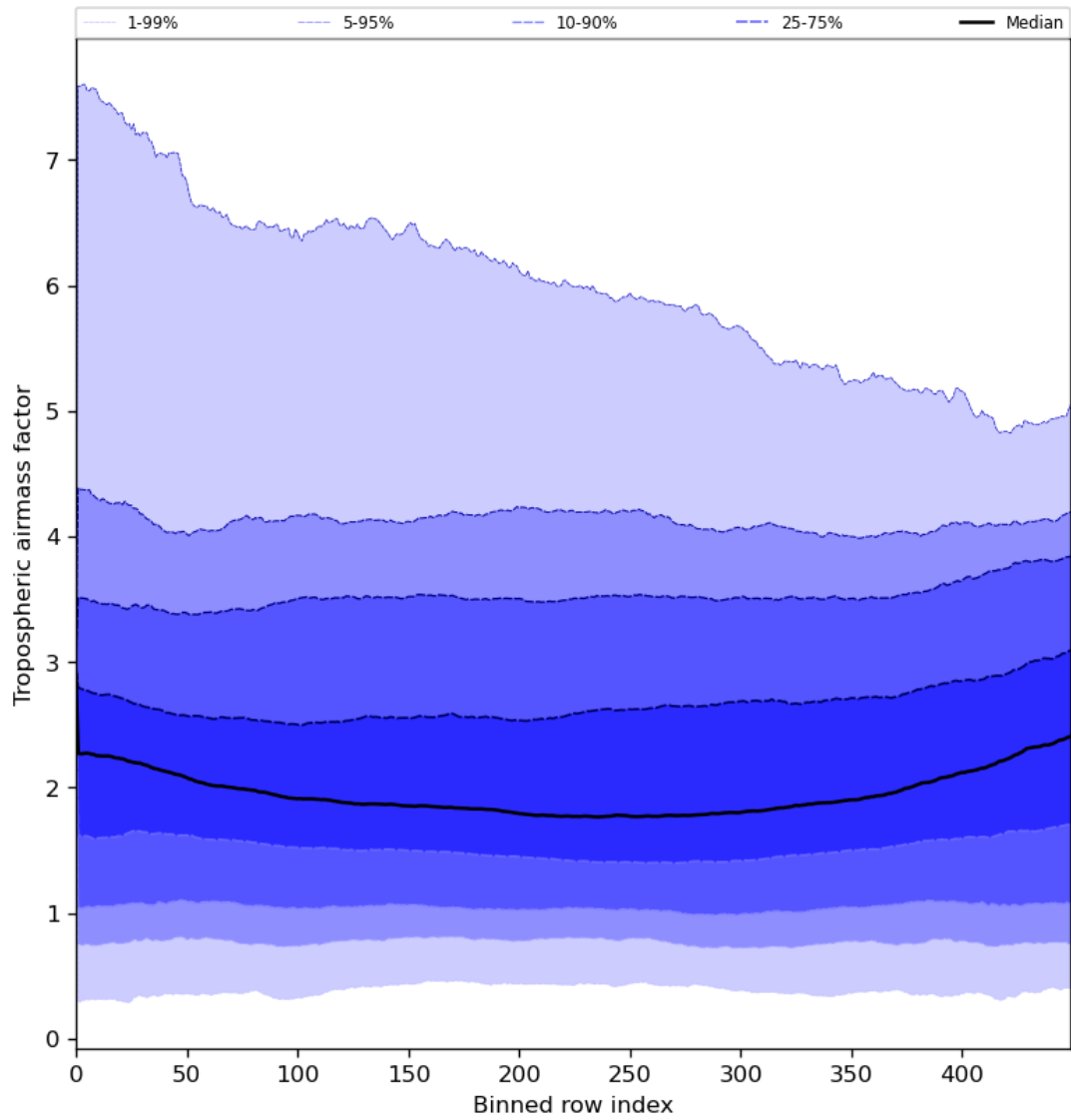
Figure 48: Along track statistics of “Tropospheric airmass factor” for 2024-08-01 to 2024-08-03
