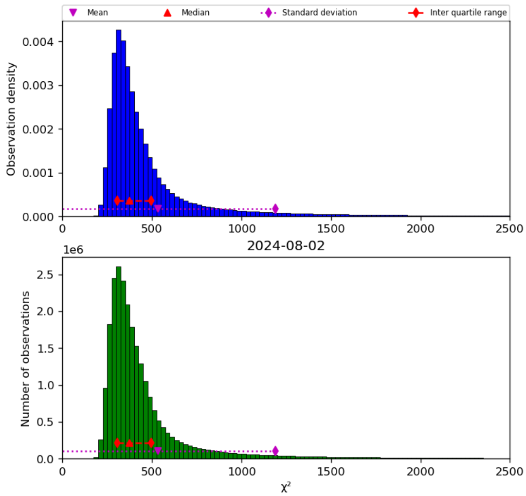
Figure 42: Histogram of “ \chi^2 ” for 2024-08-01 to 2024-08-03
