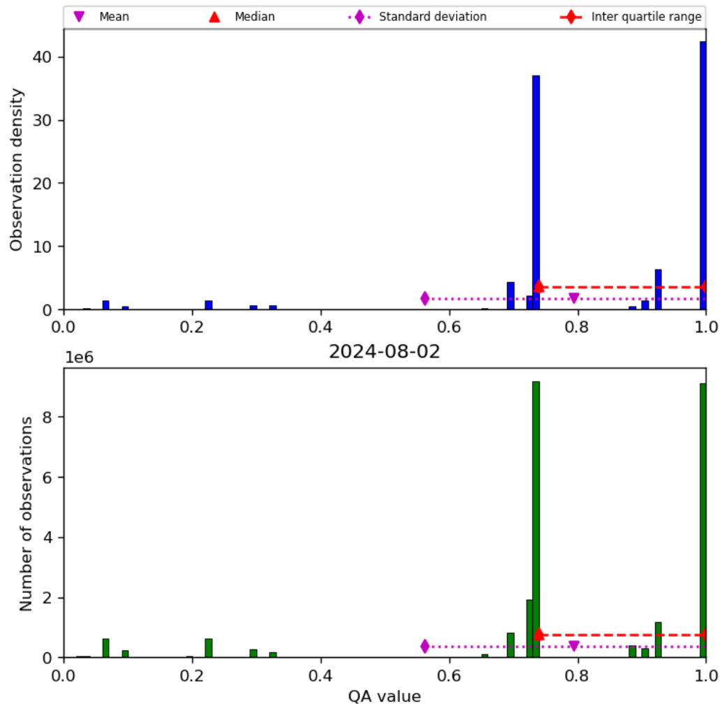
Figure 28: Histogram of “QA value” for 2024-08-01 to 2024-08-03
