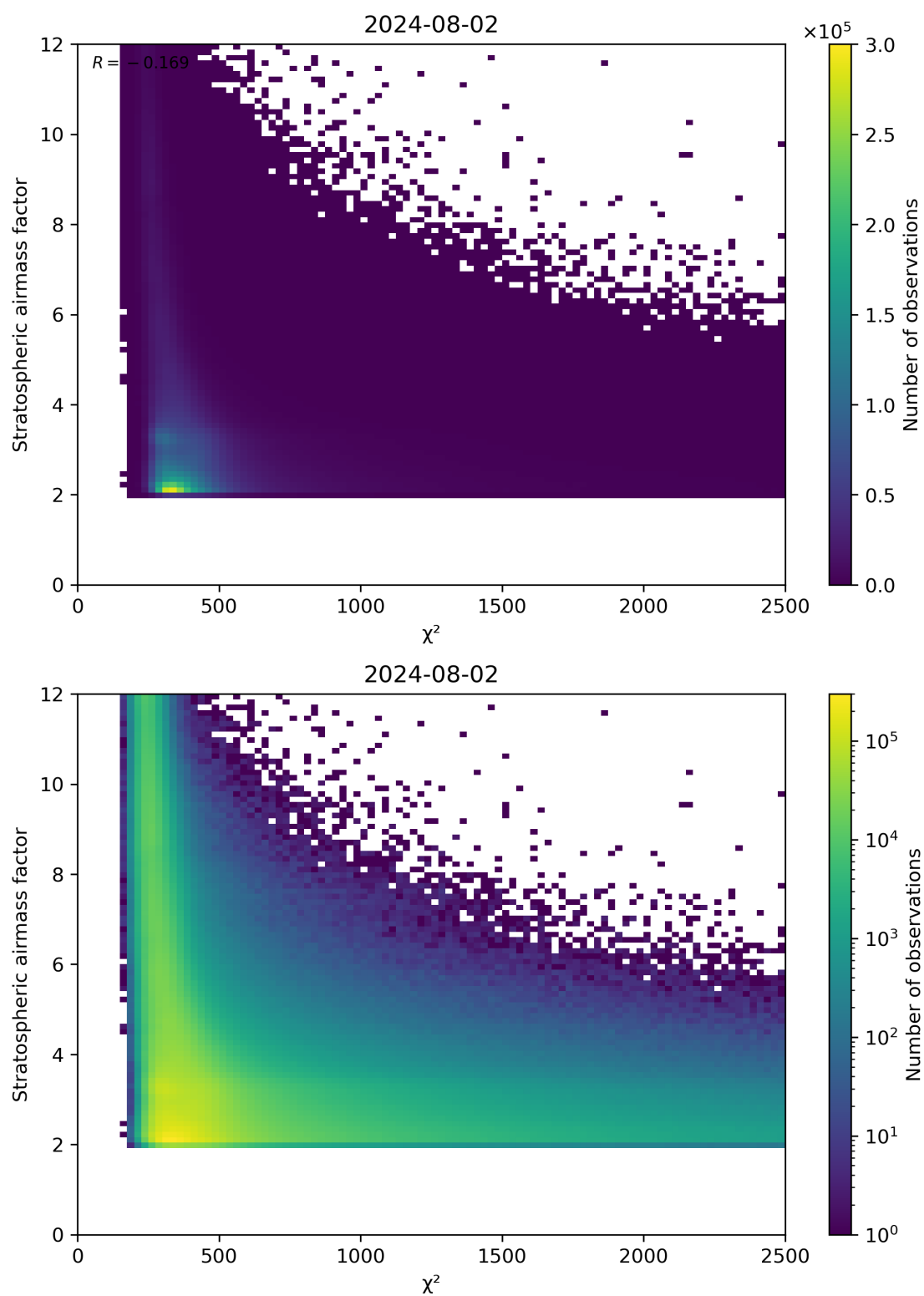
Figure 81: Scatter density plot of “ \chi^2 ” against “Stratospheric airmass factor” for 2024-08-01 to 2024-08-03.
