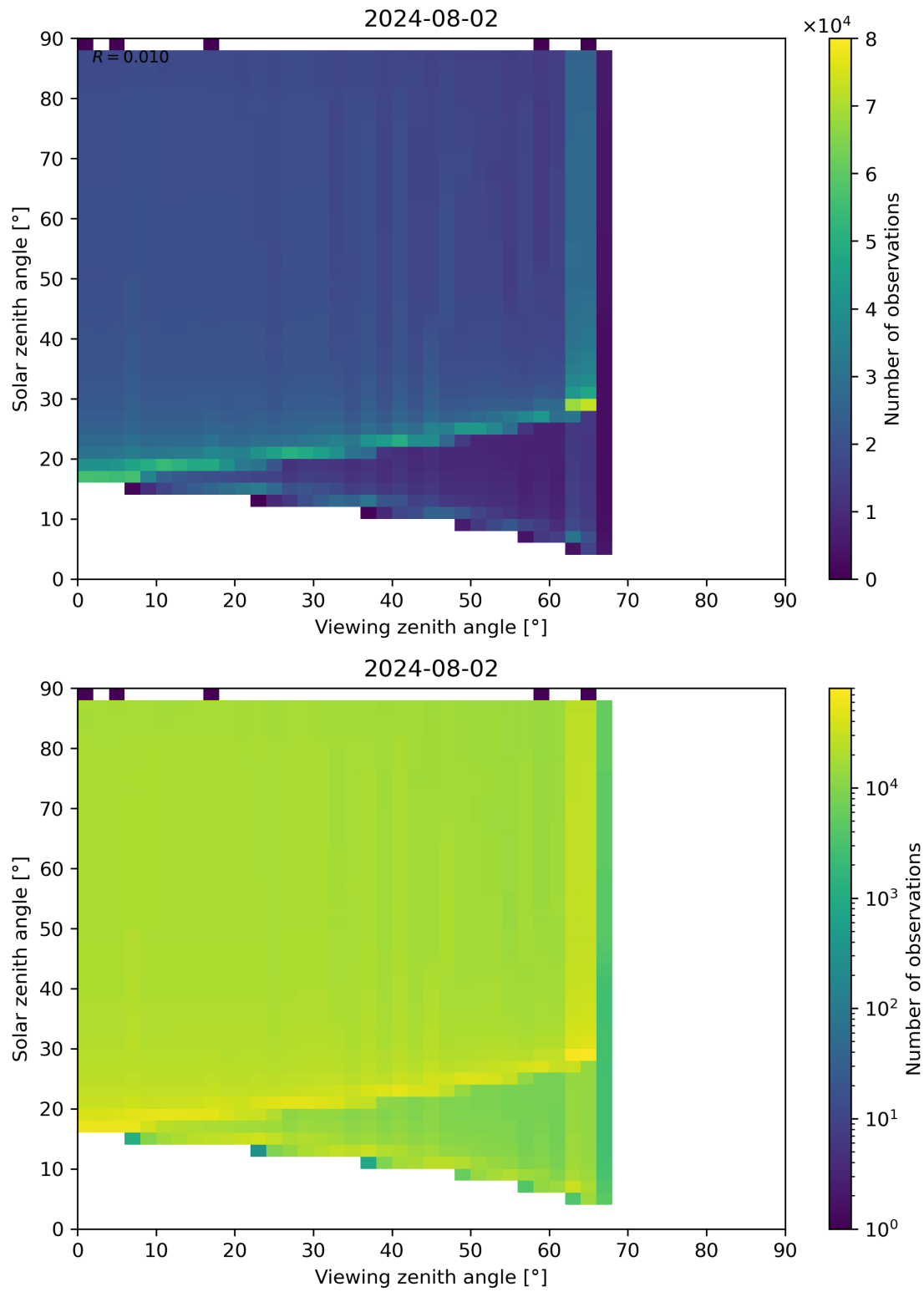
Figure 172: Scatter density plot of “Viewing zenith angle” against “Solar zenith angle” for 2024-08-01 to 2024-08-03.
