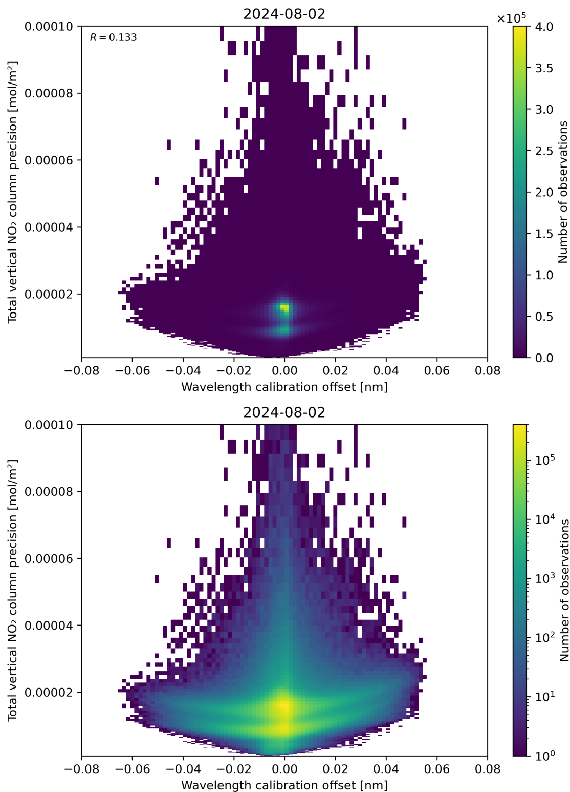
Figure 180: Scatter density plot of “Wavelength calibration offset” against “Total vertical NO 2 column precision” for 2024-08-01 to 2024-08-03.
