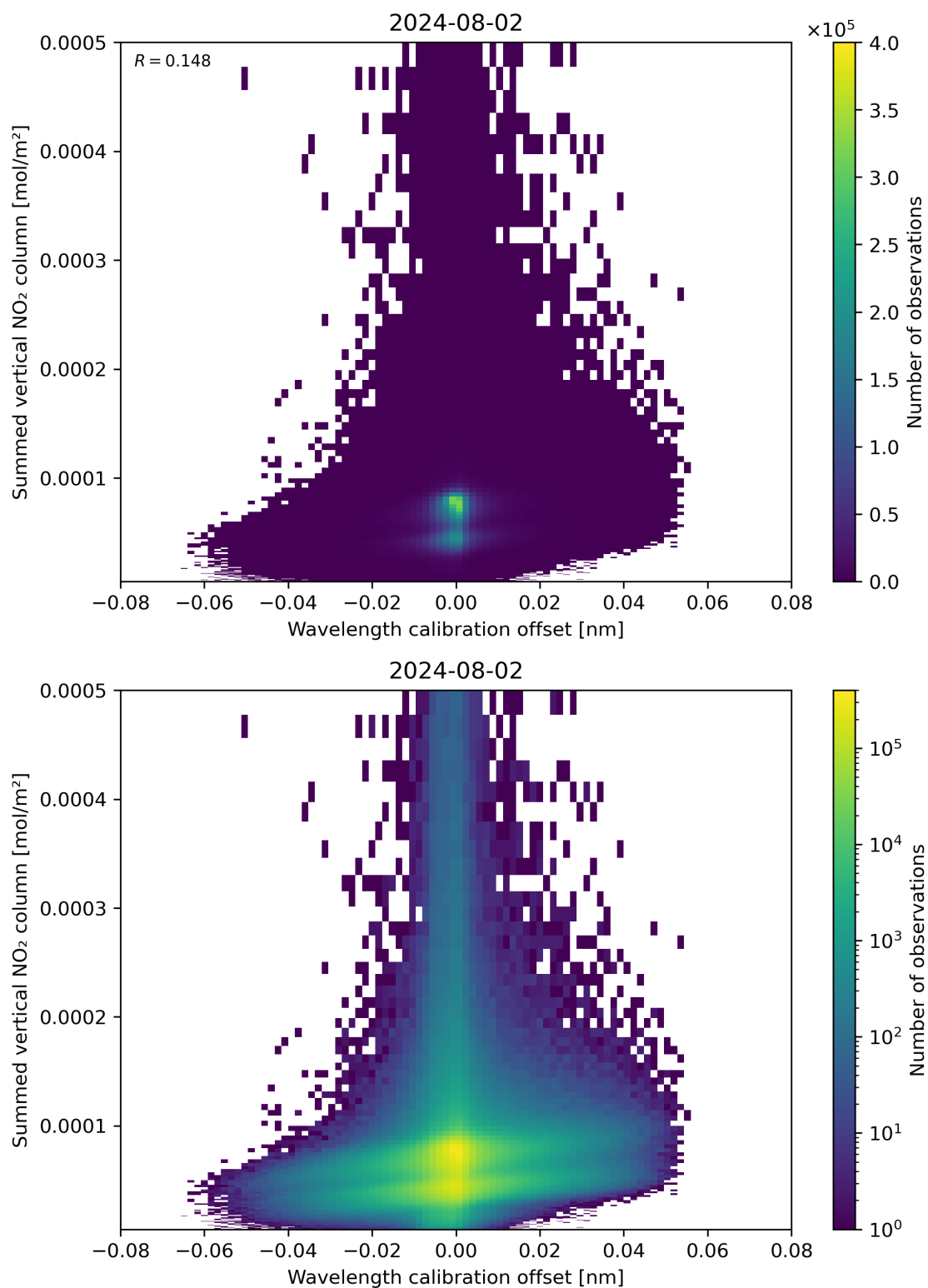
Figure 177: Scatter density plot of “Wavelength calibration offset” against “Summed vertical NO 2 column” for 2024-08-01 to 2024-08-03.
