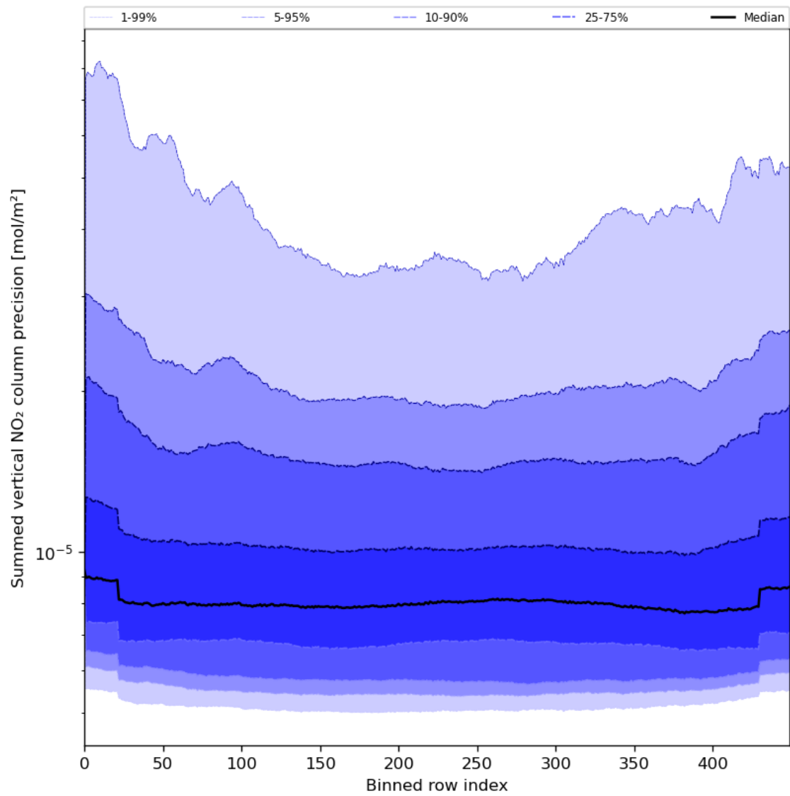
Figure 58: Along track statistics of “Summed vertical NO 2 column precision” for 2024-08-01 to 2024-08-03
