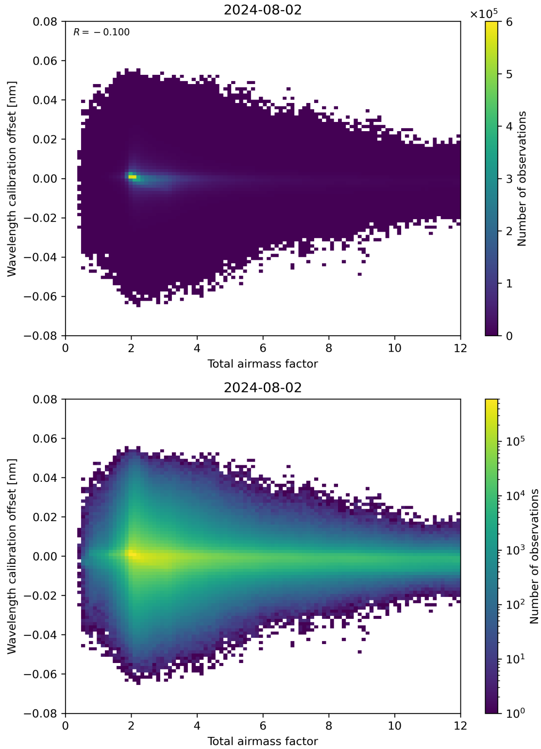
Figure 70: Scatter density plot of “Total airmass factor” against “Wavelength calibration offset” for 2024-08-01 to 2024-08-03.
