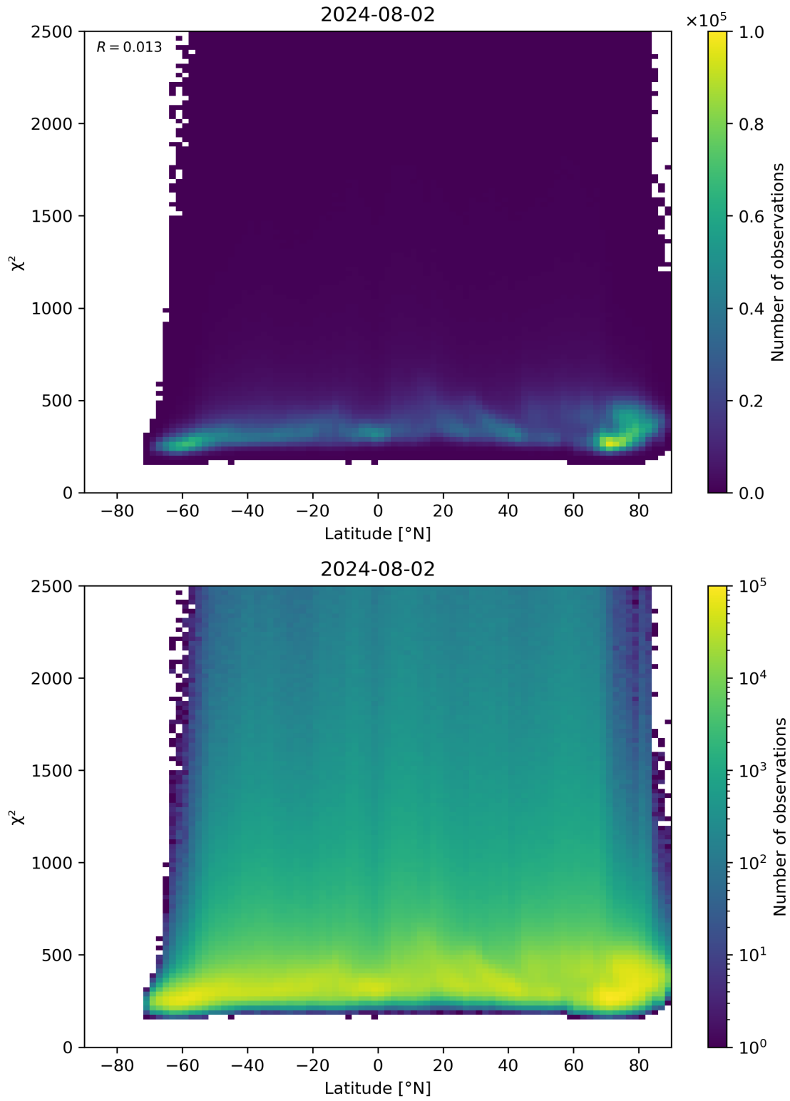
Figure 86: Scatter density plot of “Latitude” against “ \chi^2 ” for 2024-08-01 to 2024-08-03.
