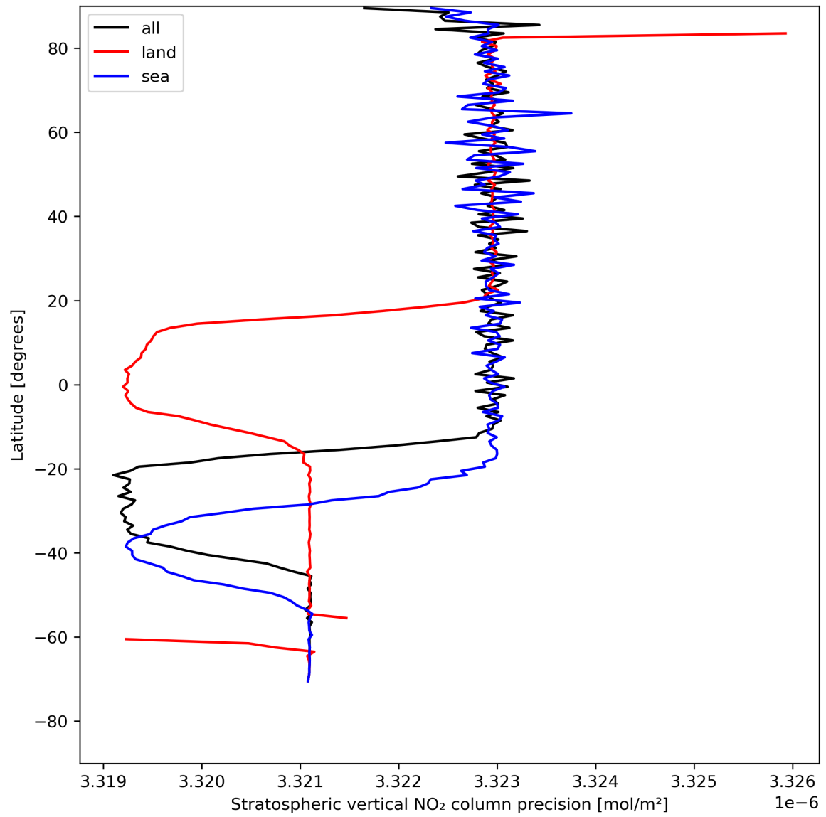
Figure 20: Zonal average of “Stratospheric vertical NO 2 column precision” for 2024-08-01 to 2024-08-03.
