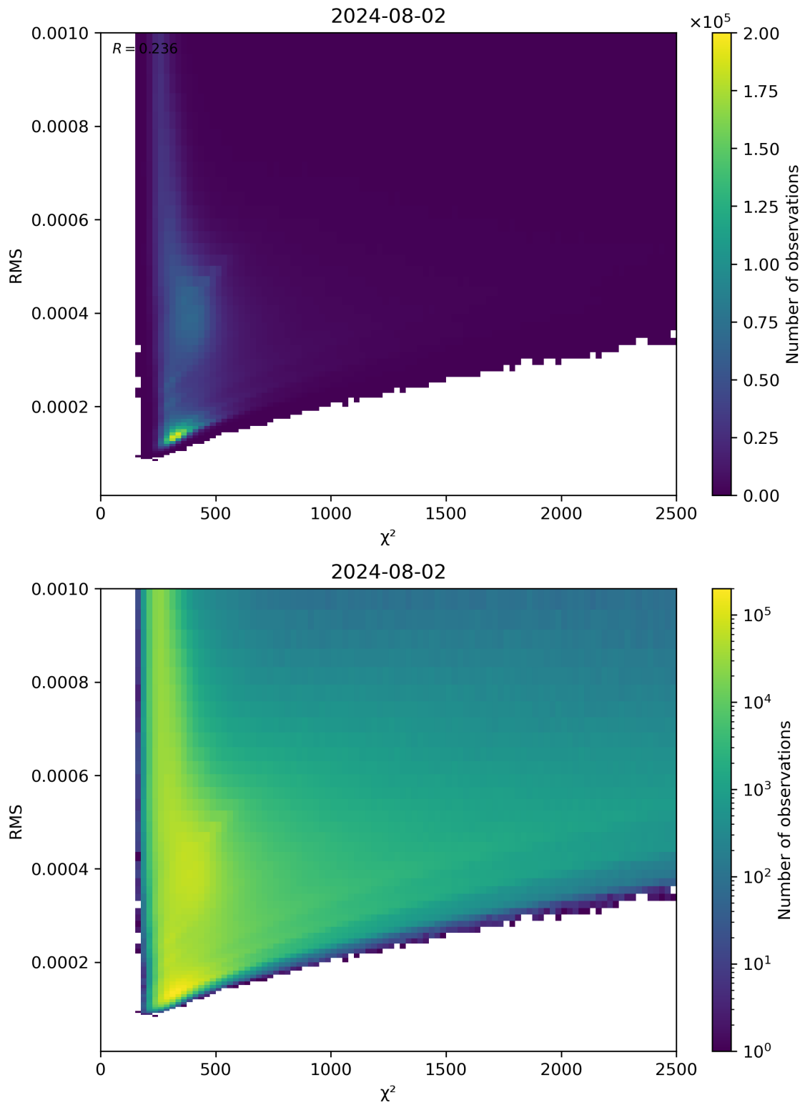
Figure 82: Scatter density plot of “ \chi^2 ” against “RMS” for 2024-08-01 to 2024-08-03.
