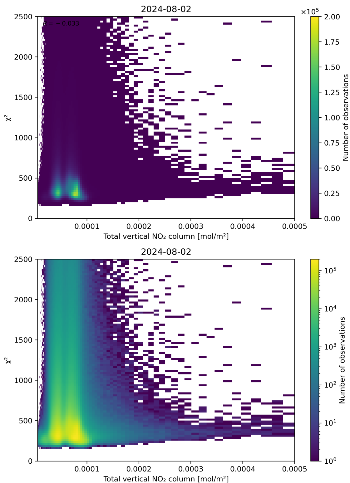
Figure 111: Scatter density plot of “Total vertical NO 2 column” against “ \chi^2 ” for 2024-08-01 to 2024-08-03.
