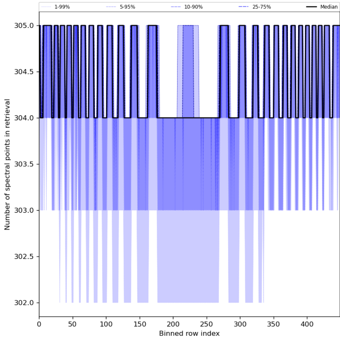
Figure 50: Along track statistics of “Number of spectral points in retrieval” for 2024-08-01 to 2024-08-03
