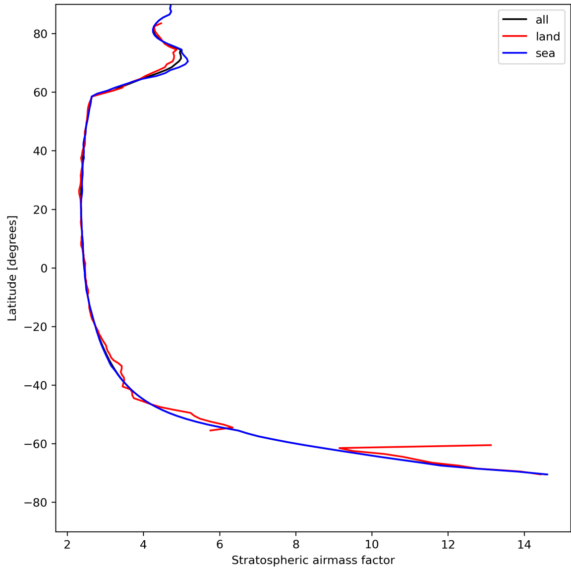
Figure 27: Zonal average of “Stratospheric airmass factor” for 2024-08-01 to 2024-08-03.
