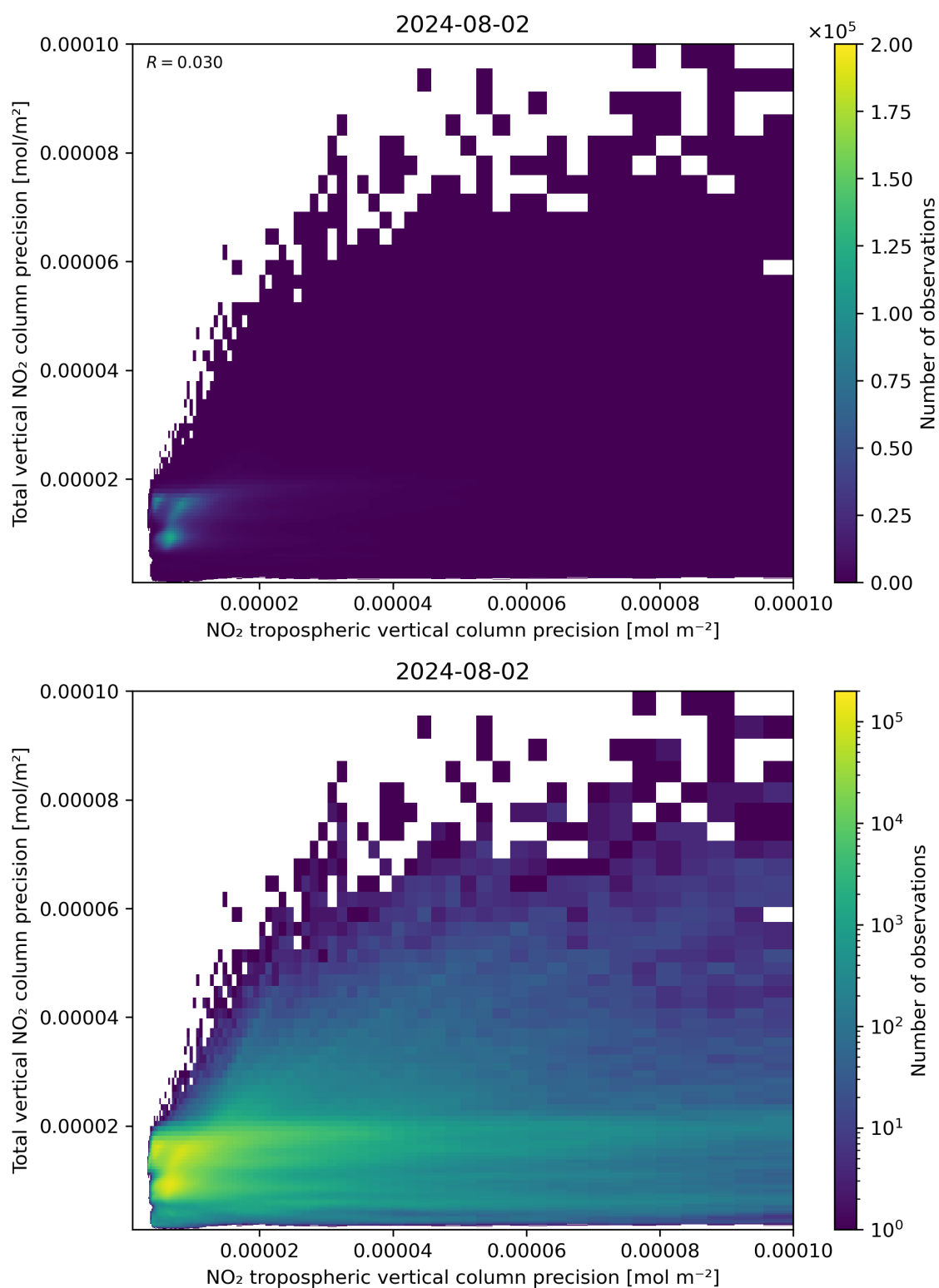
Figure 139: Scatter density plot of “NO 2 tropospheric vertical column precision” against “Total vertical NO 2 column precision” for 2024-08-01 to 2024-08-03.
