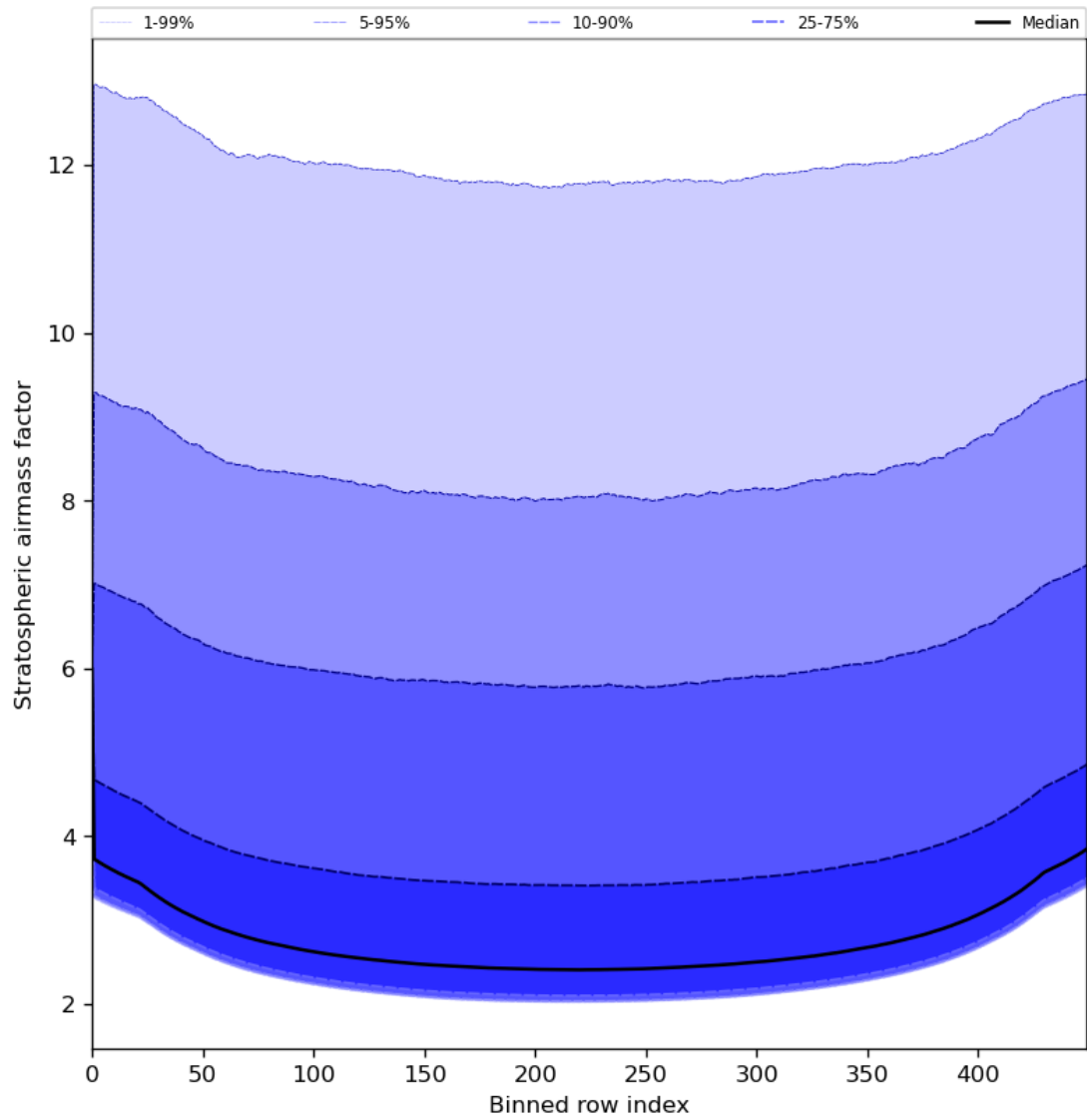
Figure 61: Along track statistics of “Stratospheric airmass factor” for 2024-08-01 to 2024-08-03
