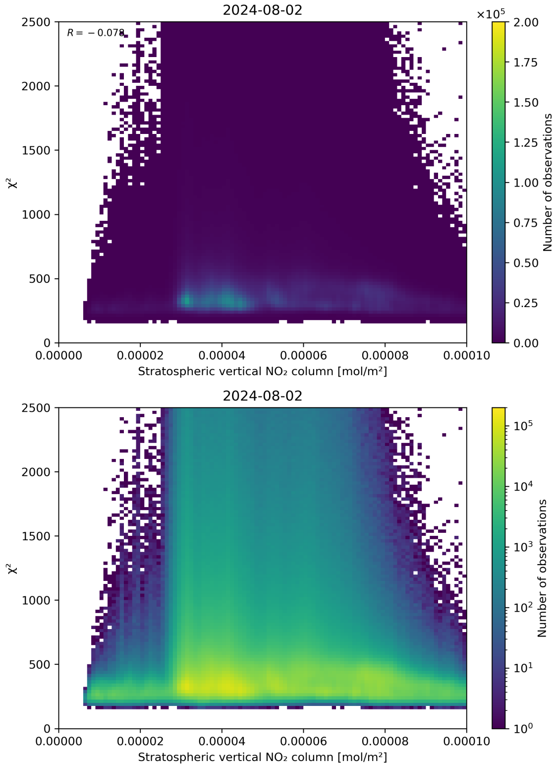
Figure 97: Scatter density plot of “Stratospheric vertical NO 2 column” against “ \chi^2 ” for 2024-08-01 to 2024-08-03.
