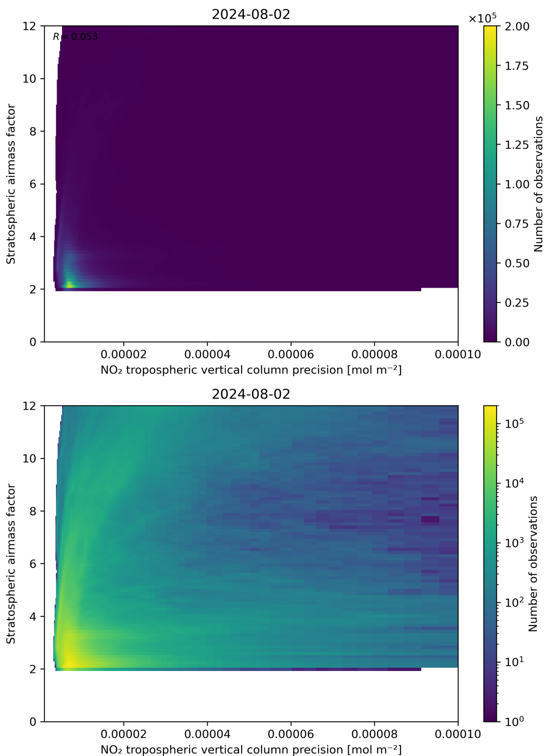
Figure 131: Scatter density plot of “NO 2 tropospheric vertical column precision” against “Stratospheric airmass factor” for 2024-08-01 to 2024-08-03.
