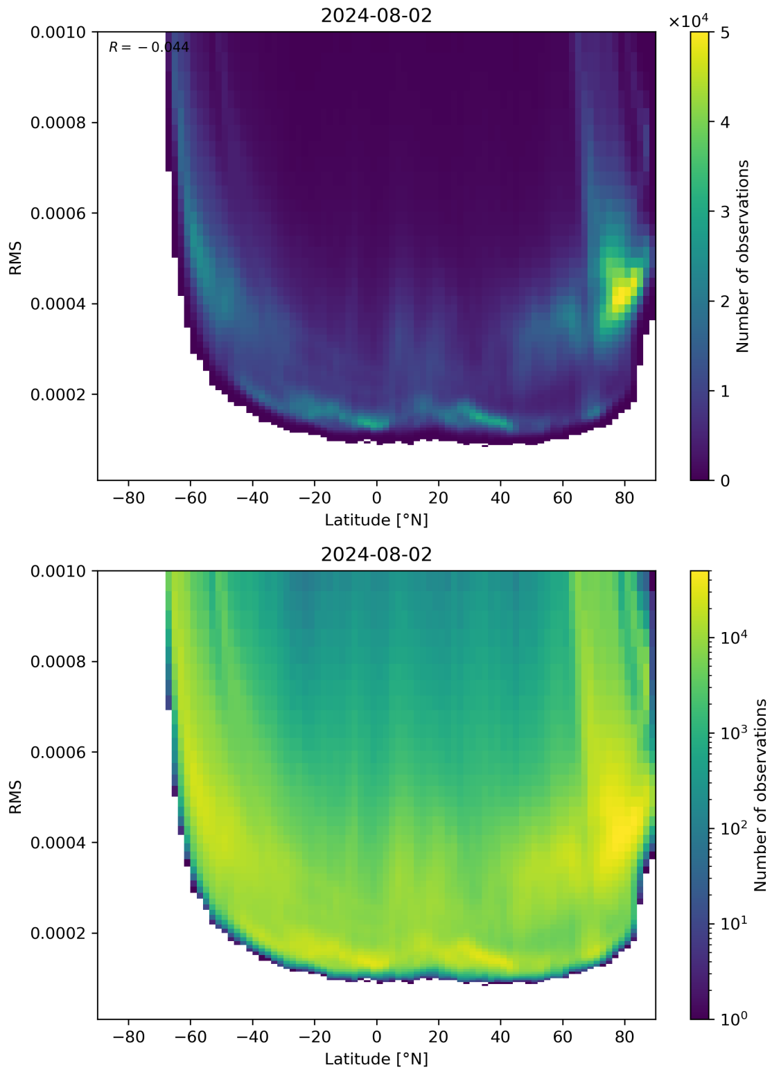
Figure 94: Scatter density plot of “Latitude” against “RMS” for 2024-08-01 to 2024-08-03.
