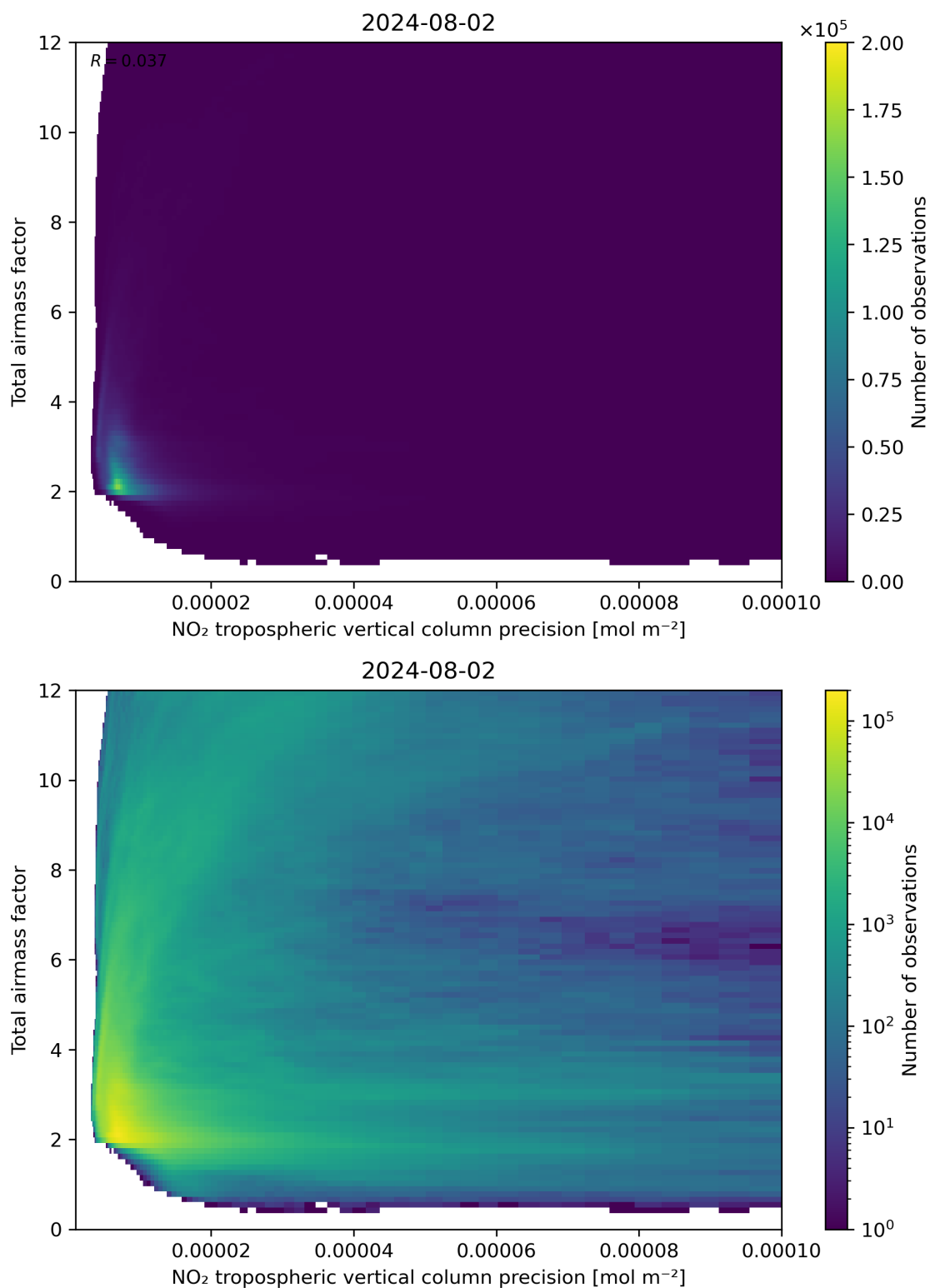
Figure 132: Scatter density plot of “NO 2 tropospheric vertical column precision” against “Total air mass factor” for 2024-08-01 to 2024-08-03.
