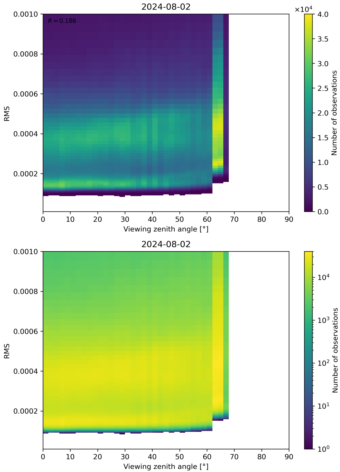
Figure 171: Scatter density plot of “Viewing zenith angle” against “RMS” for 2024-08-01 to 2024-08-03.
