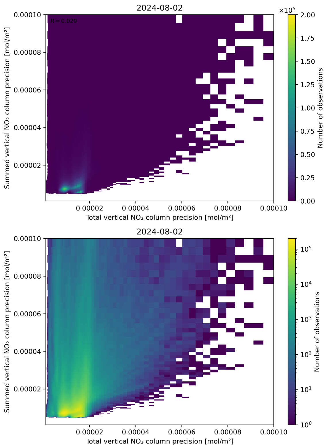
Figure 118: Scatter density plot of “Total vertical NO 2 column precision” against “Summed vertical NO 2 column precision” for 2024-08-01 to 2024-08-03.
