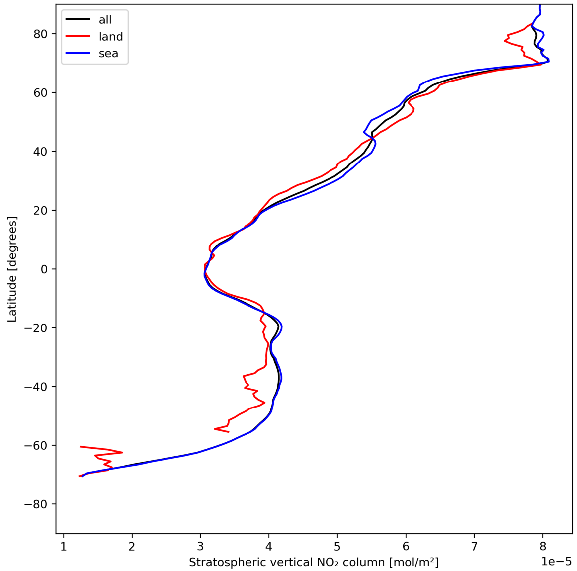
Figure 19: Zonal average of “Stratospheric vertical NO 2 column” for 2024-08-01 to 2024-08-03.
