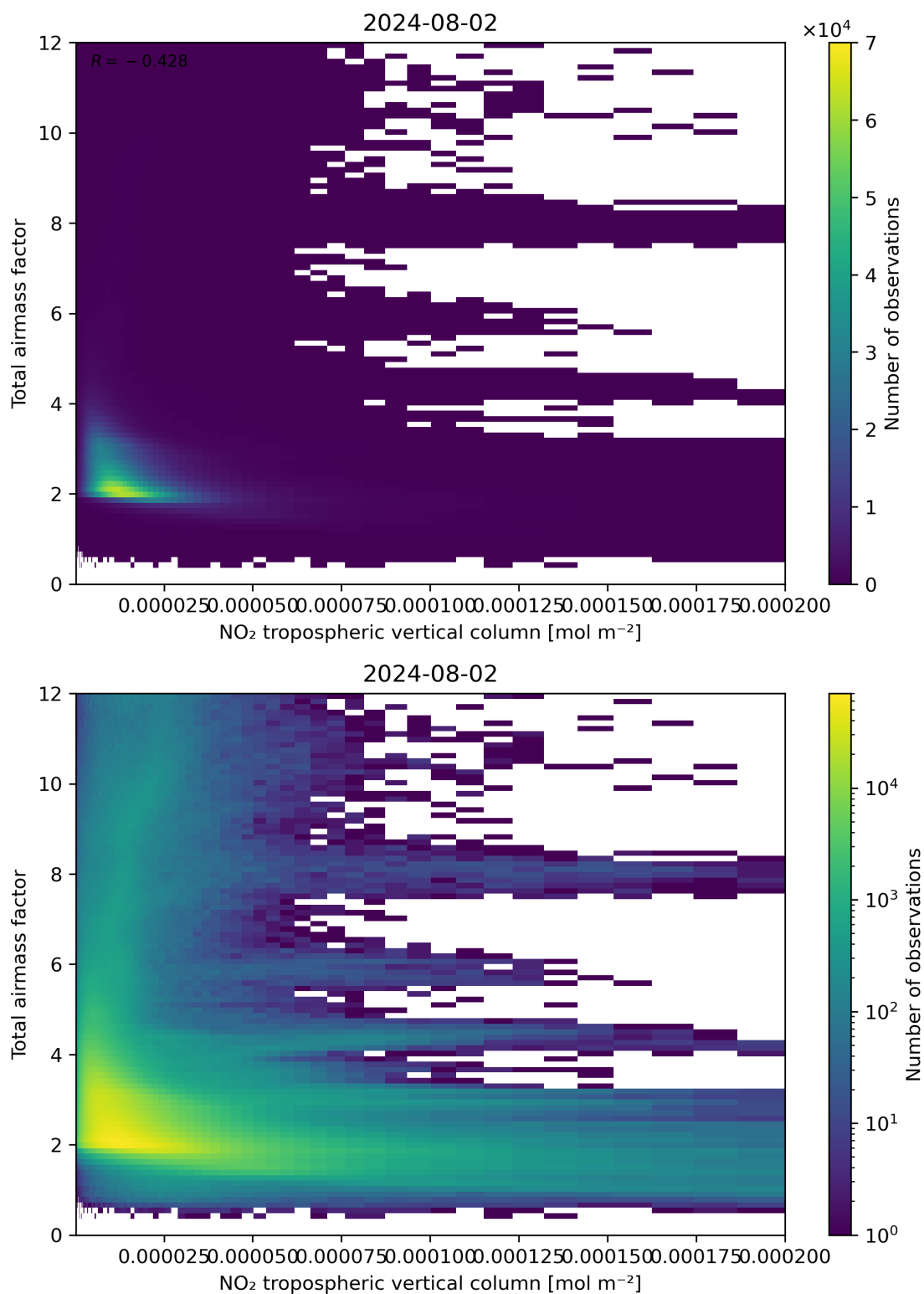
Figure 122: Scatter density plot of “NO 2 tropospheric vertical column” against “Total air mass factor” for 2024-08-01 to 2024-08-03.
