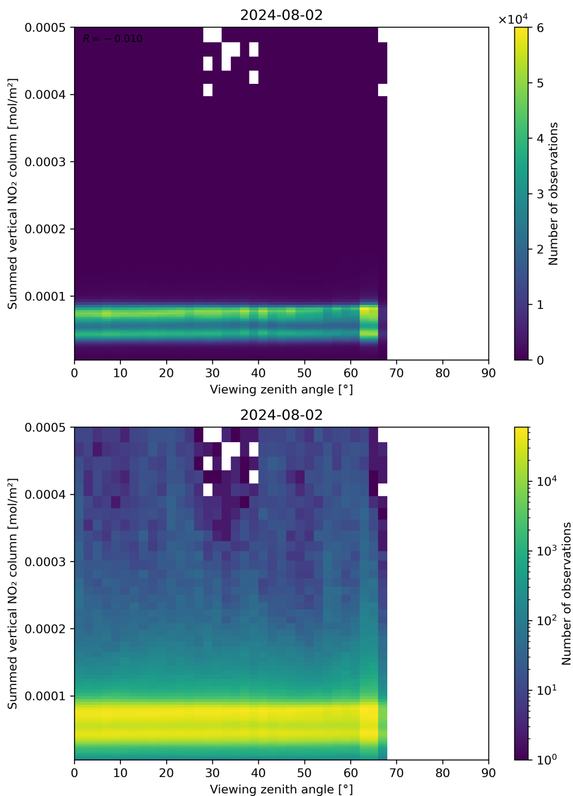
Figure 165: Scatter density plot of “Viewing zenith angle” against “Summed vertical NO 2 column” for 2024-08-01 to 2024-08-03.
