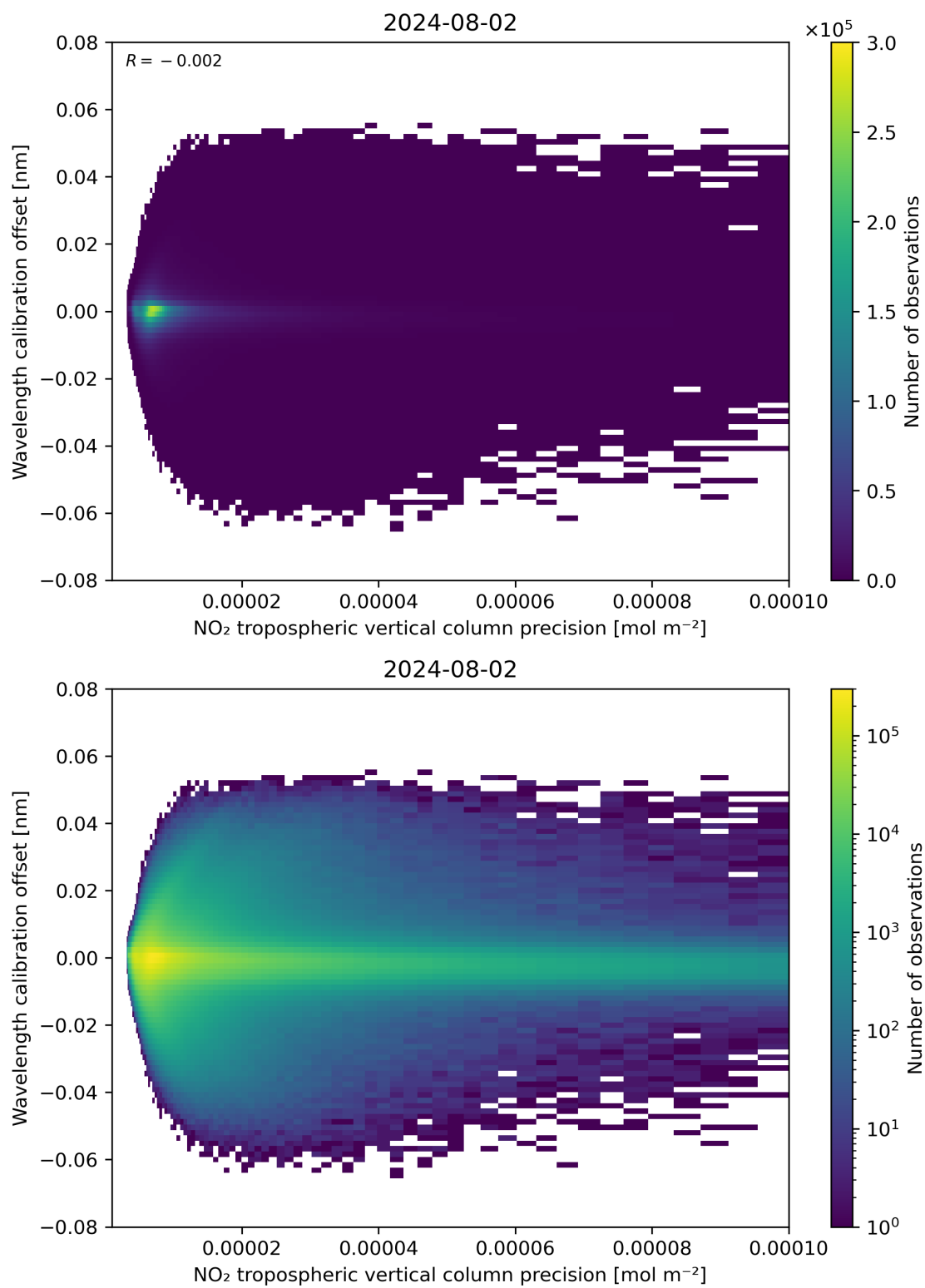
Figure 141: Scatter density plot of “NO 2 tropospheric vertical column precision” against “Wavelength calibration offset” for 2024-08-01 to 2024-08-03.
