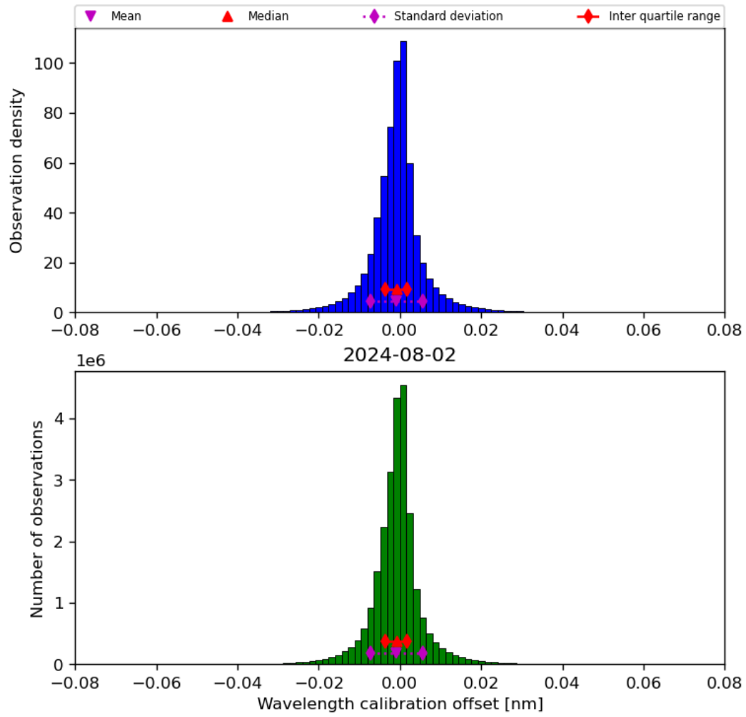
Figure 35: Histogram of “Wavelength calibration offset” for 2024-08-01 to 2024-08-03
