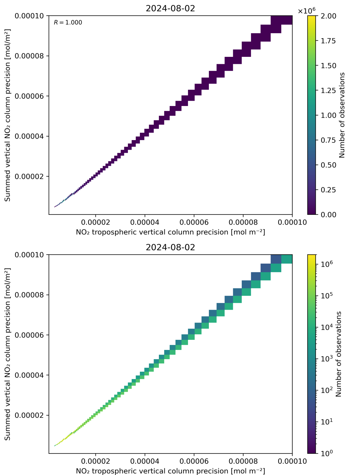
Figure 137: Scatter density plot of “NO 2 tropospheric vertical column precision” against “Summed vertical NO 2 column precision” for 2024-08-01 to 2024-08-03.
