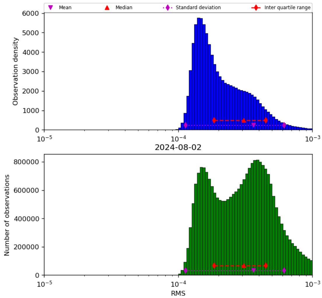
Figure 43: Histogram of “RMS” for 2024-08-01 to 2024-08-03
