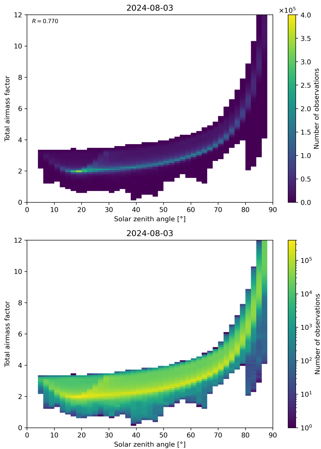
Figure 146: Scatter density plot of “Solar zenith angle” against “Total air mass factor” for 2024-08-02 to 2024-08-04.
