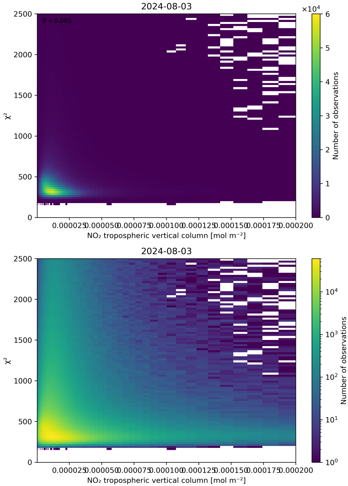
Figure 124: Scatter density plot of “NO 2 tropospheric vertical column” against “ \chi^2 ” for 2024-08-02 to 2024-08-04.
