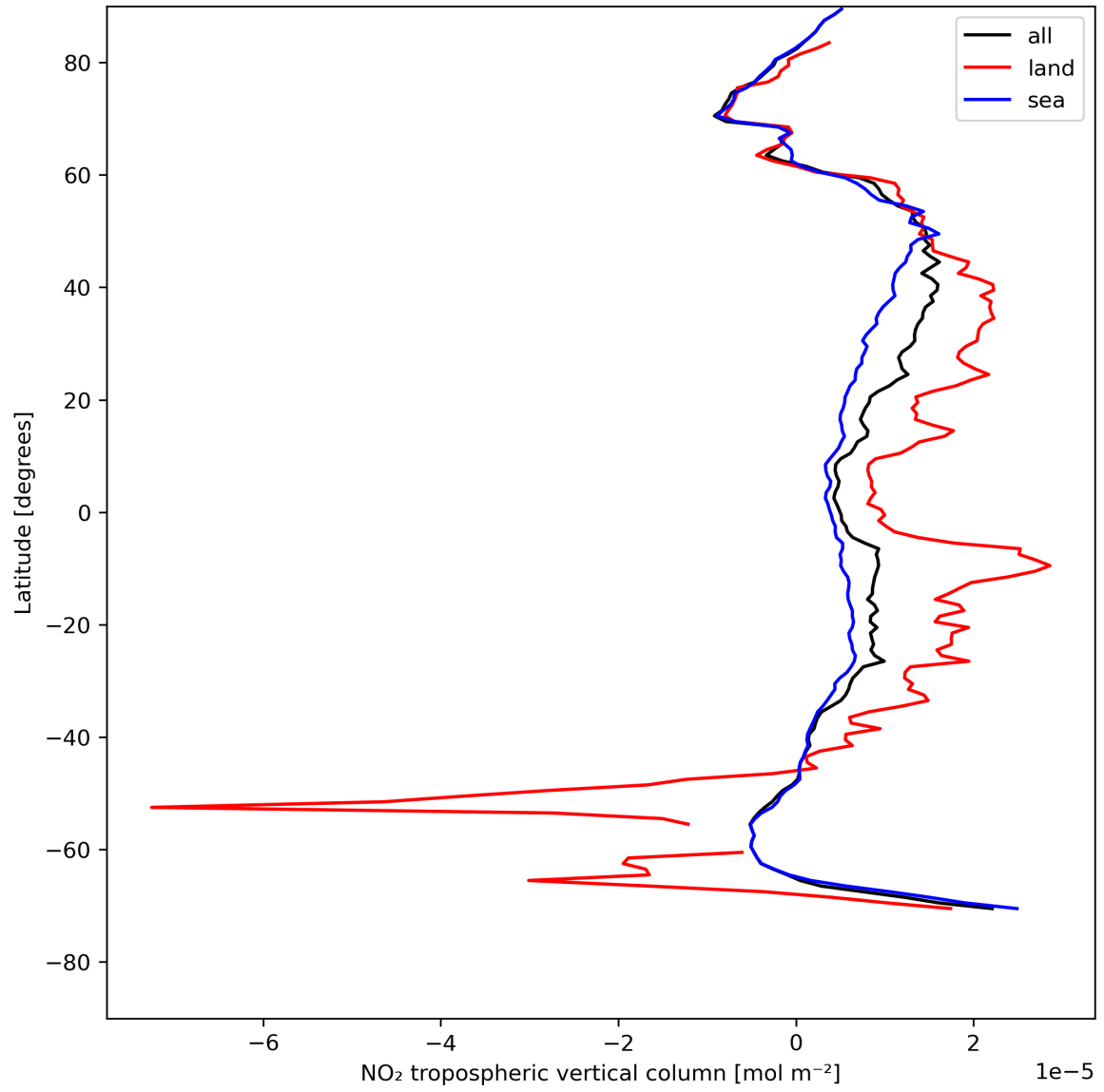
Figure 12: Zonal average of “NO 2 tropospheric vertical column” for 2024-08-02 to 2024-08-04.
