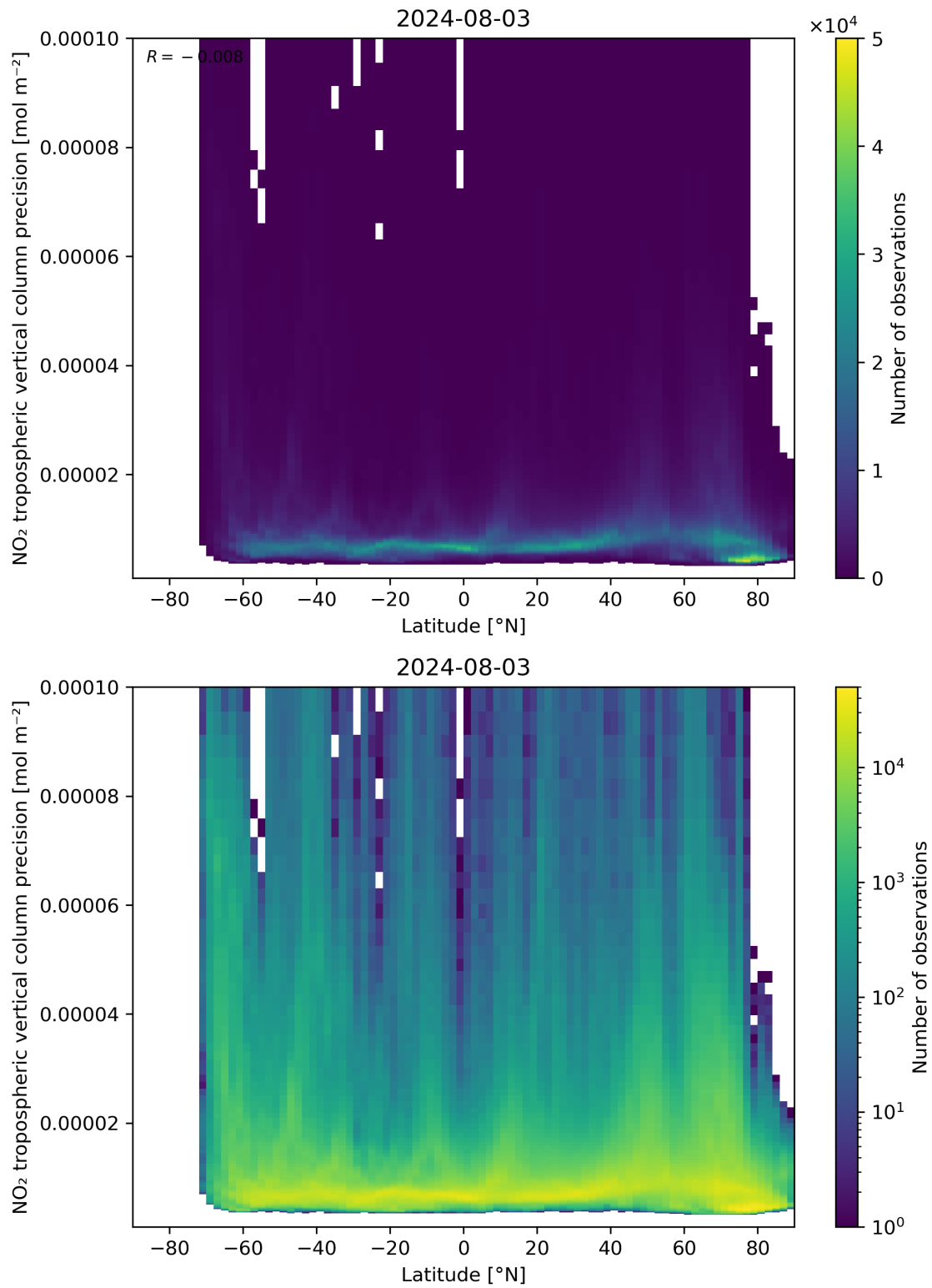
Figure 93: Scatter density plot of “Latitude” against “NO 2 tropospheric vertical column precision” for 2024-08-02 to 2024-08-04.
