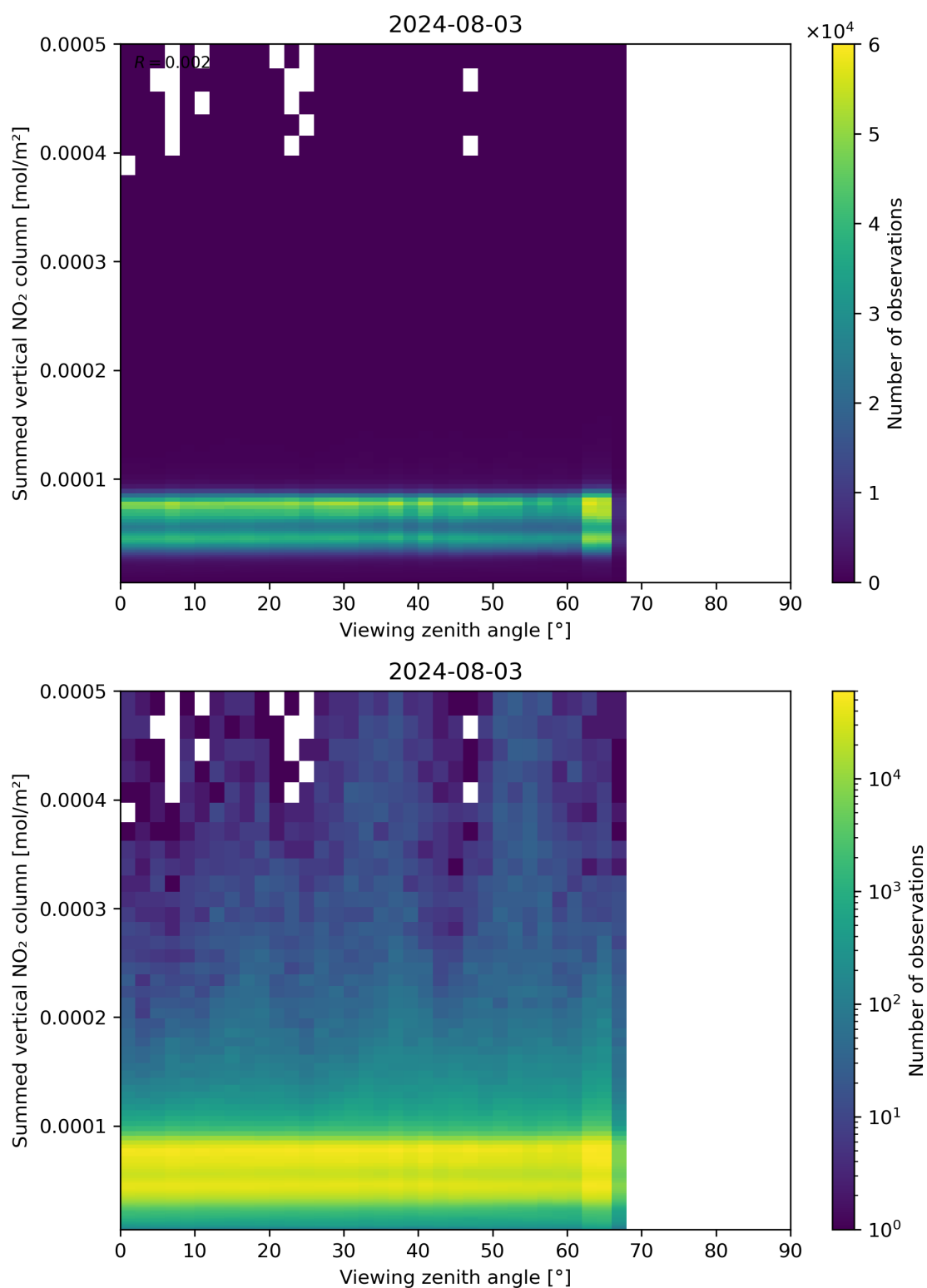
Figure 165: Scatter density plot of “Viewing zenith angle” against “Summed vertical NO 2 column” for 2024-08-02 to 2024-08-04.
