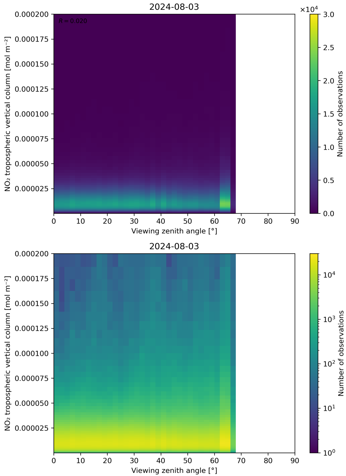
Figure 169: Scatter density plot of “Viewing zenith angle” against “NO 2 tropospheric vertical column” for 2024-08-02 to 2024-08-04.
