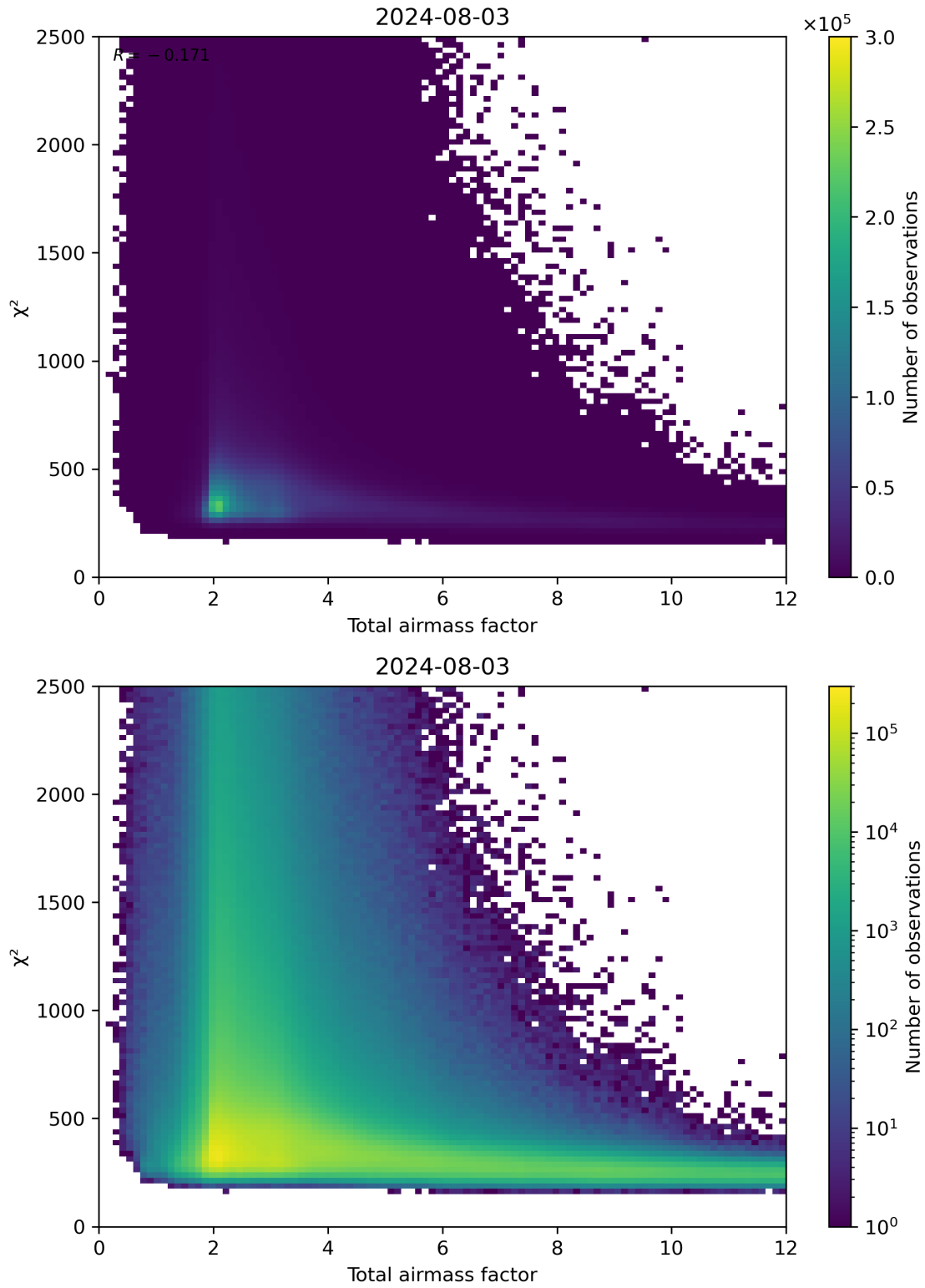
Figure 63: Scatter density plot of “Total airmass factor” against “ \chi^2 ” for 2024-08-02 to 2024-08-04.
