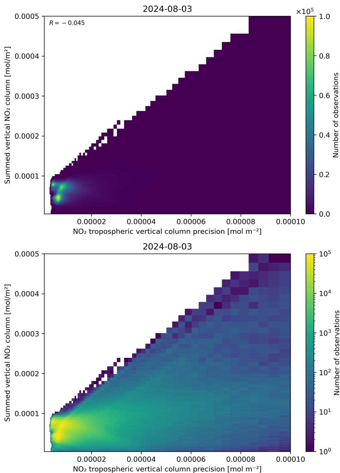
Figure 136: Scatter density plot of “NO 2 tropospheric vertical column precision” against “Summed vertical NO 2 column” for 2024-08-02 to 2024-08-04.
