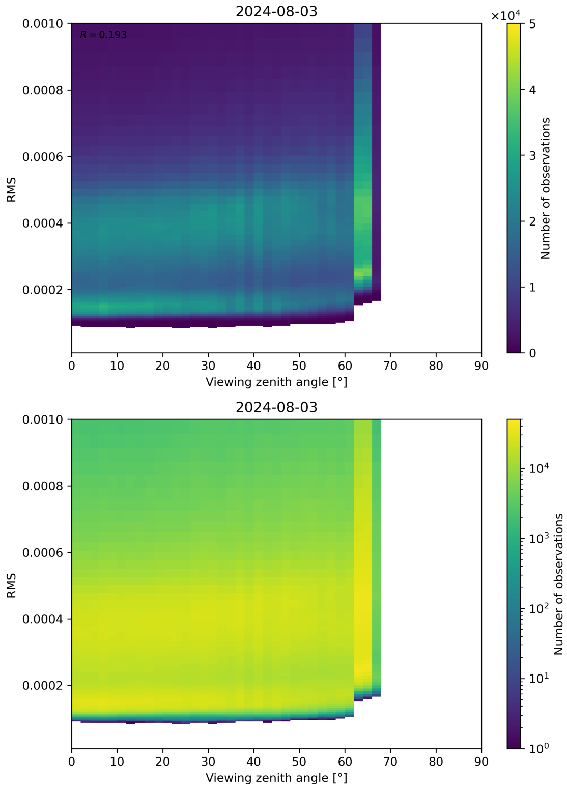
Figure 171: Scatter density plot of “Viewing zenith angle” against “RMS” for 2024-08-02 to 2024-08-04.
