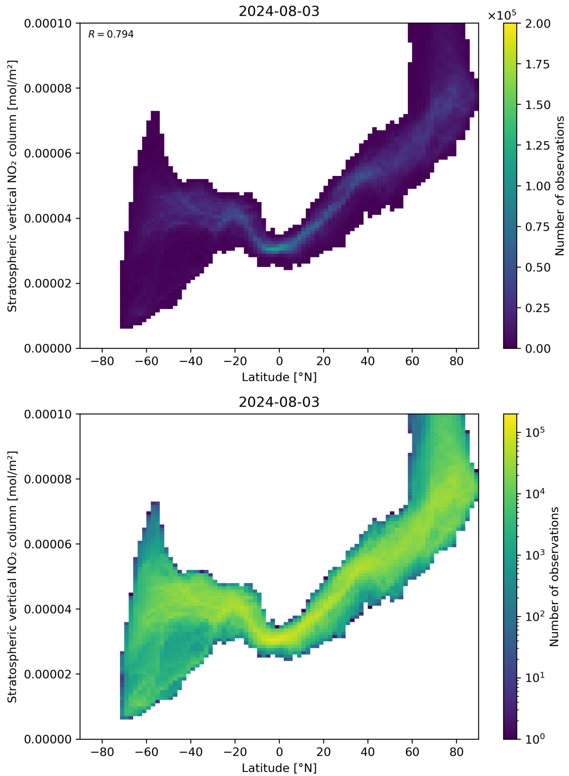
Figure 87: Scatter density plot of “Latitude” against “Stratospheric vertical NO 2 column” for 2024-08-02 to 2024-08-04.
