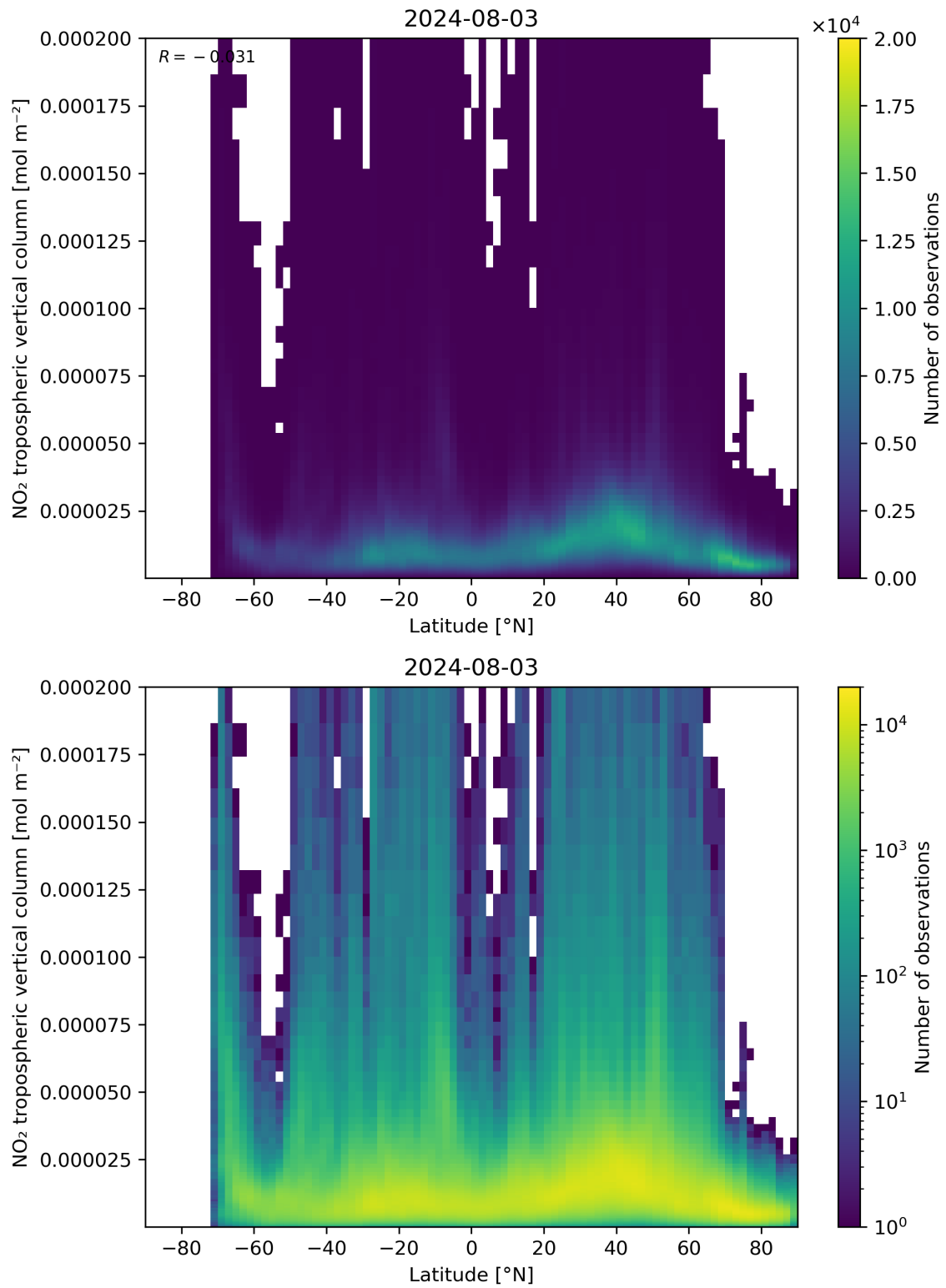
Figure 92: Scatter density plot of “Latitude” against “NO 2 tropospheric vertical column” for 2024-08-02 to 2024-08-04.
