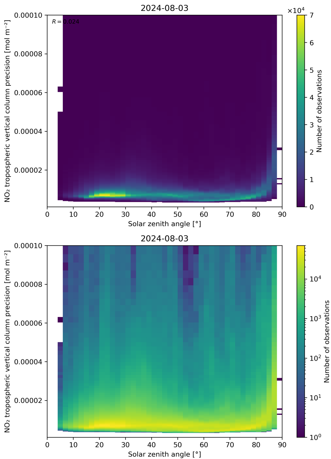
Figure 156: Scatter density plot of “Solar zenith angle” against “NO 2 tropospheric vertical column precision” for 2024-08-02 to 2024-08-04.
