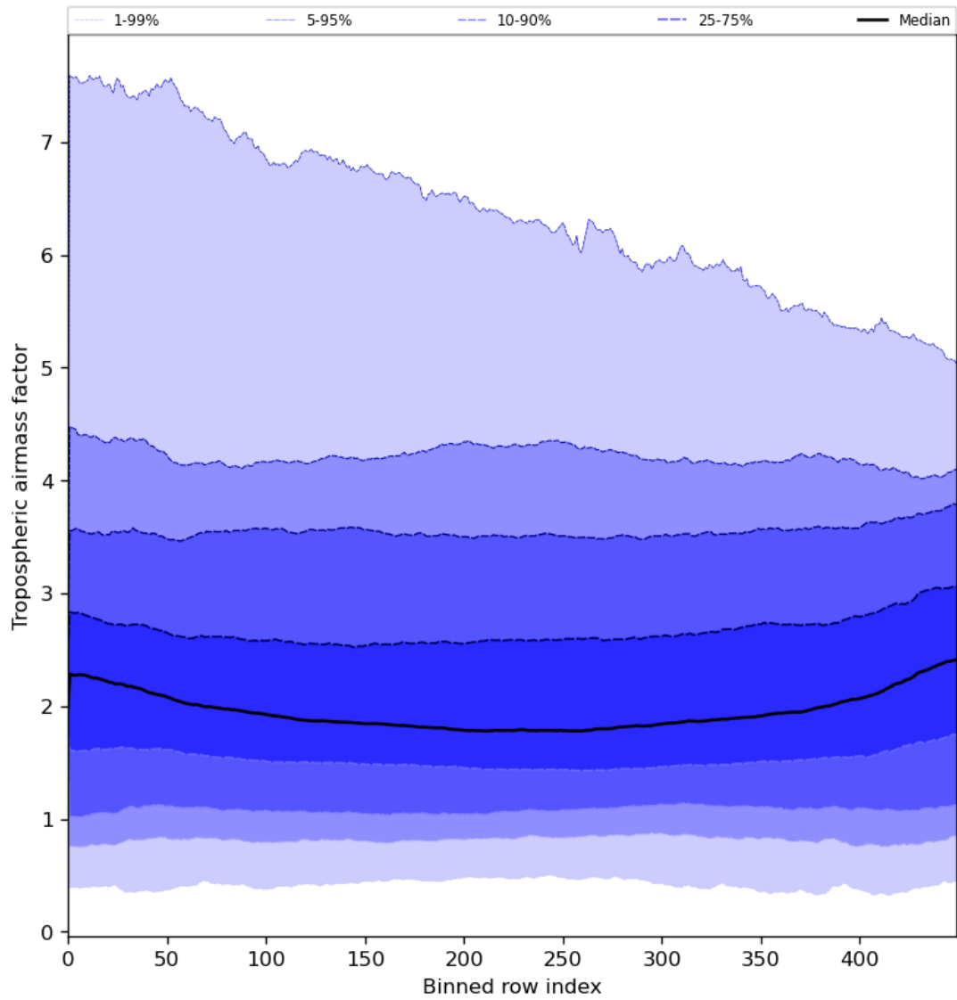
Figure 48: Along track statistics of “Tropospheric airmass factor” for 2024-08-02 to 2024-08-04
