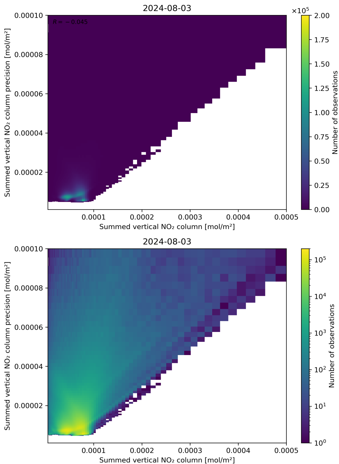
Figure 105: Scatter density plot of “Summed vertical NO 2 column” against “Summed vertical NO 2 column precision” for 2024-08-02 to 2024-08-04.
