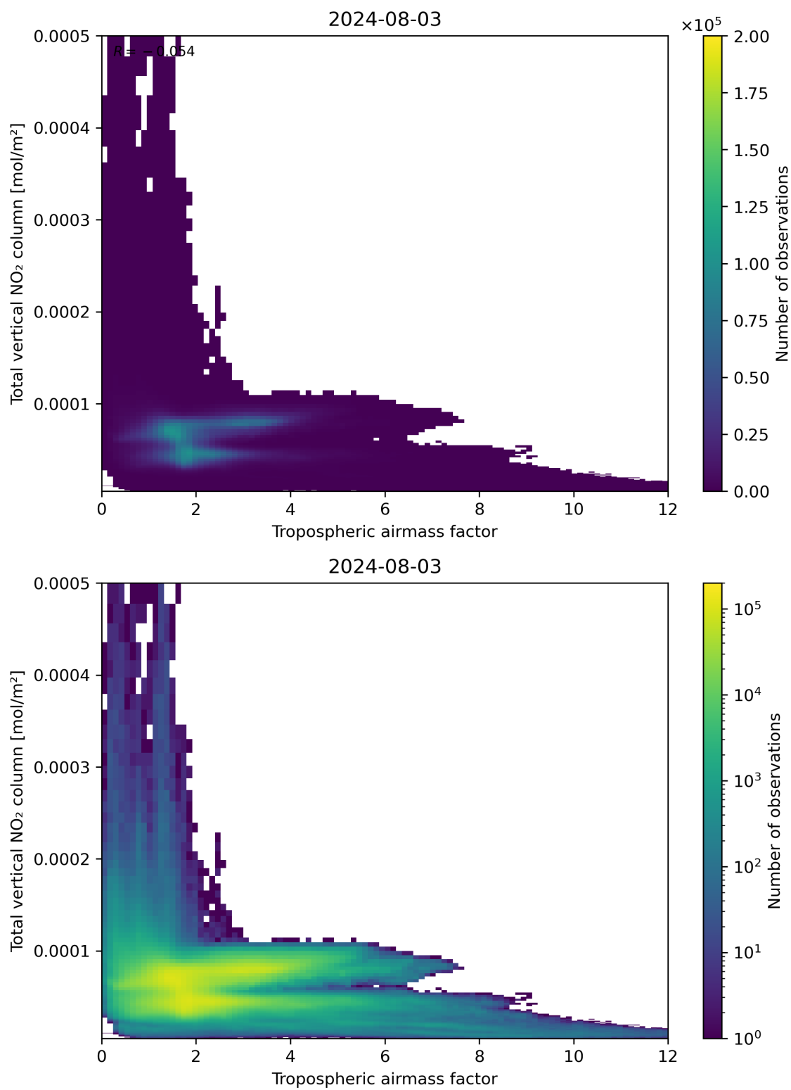
Figure 77: Scatter density plot of “Tropospheric airmass factor” against “Total vertical NO 2 column” for 2024-08-02 to 2024-08-04.
