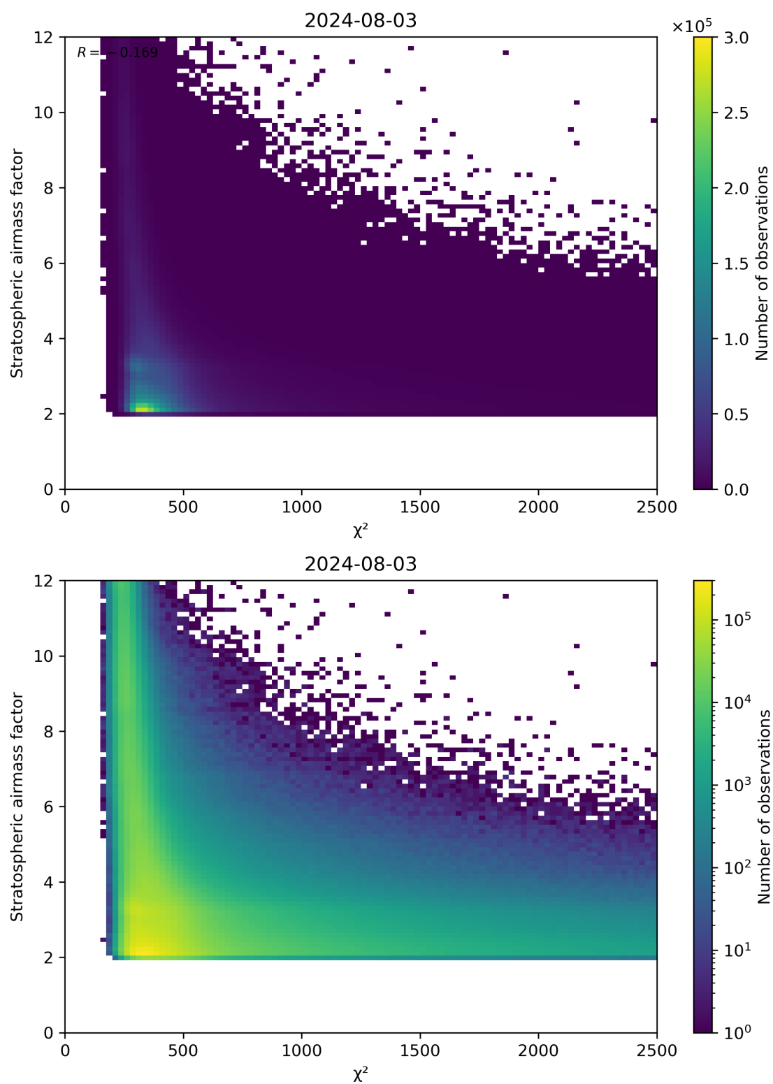
Figure 81: Scatter density plot of “ \chi^2 ” against “Stratospheric airmass factor” for 2024-08-02 to 2024-08-04.
