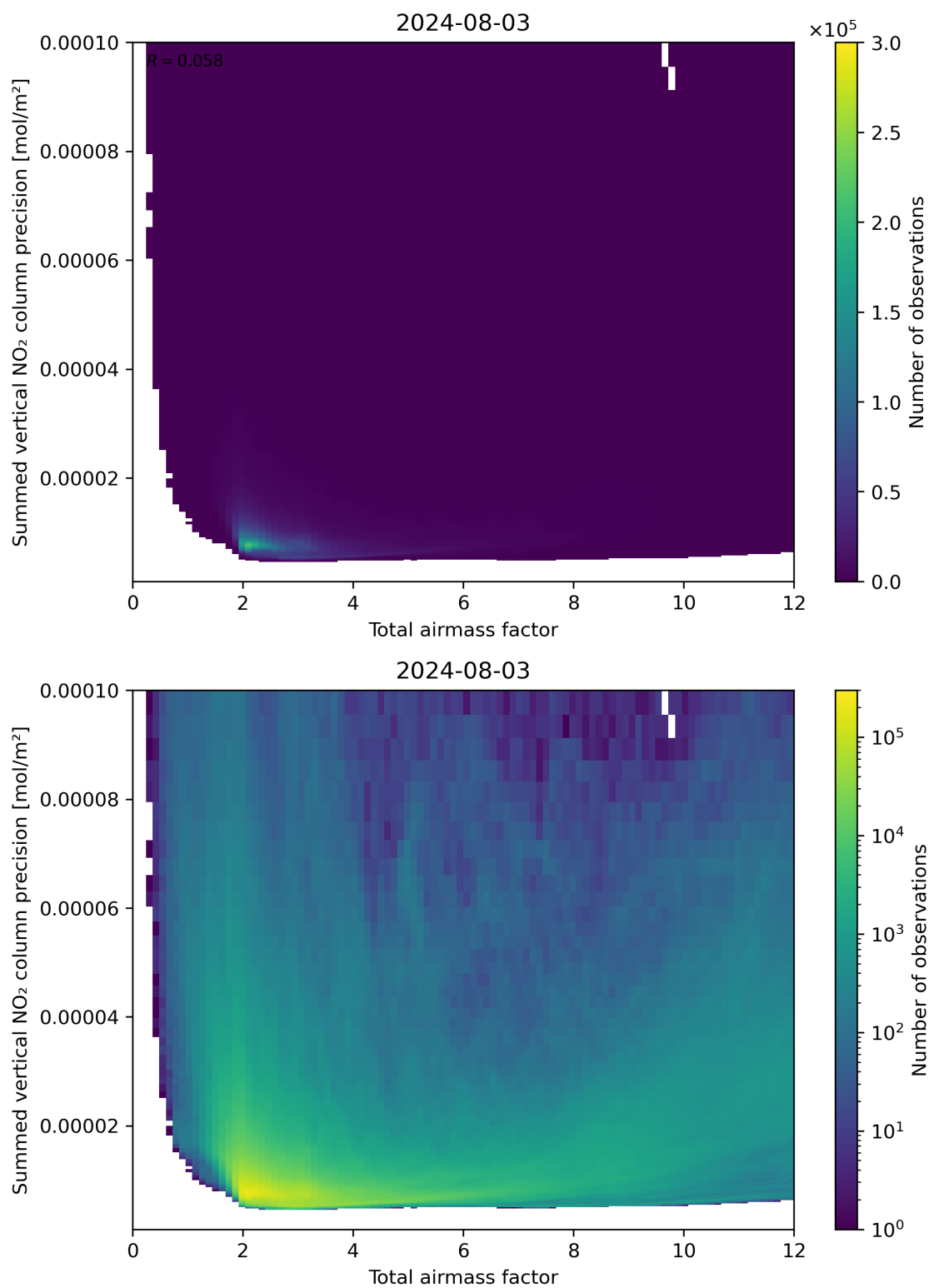
Figure 66: Scatter density plot of “Total airmass factor” against “Summed vertical NO 2 column precision” for 2024-08-02 to 2024-08-04.
