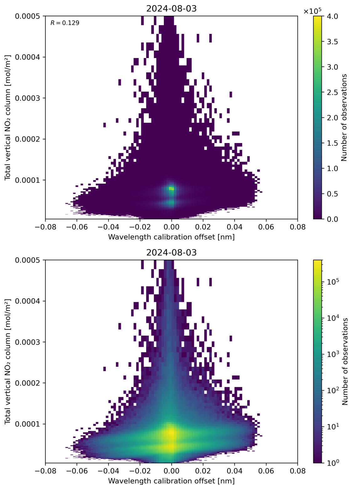
Figure 179: Scatter density plot of “Wavelength calibration offset” against “Total vertical NO 2 column” for 2024-08-02 to 2024-08-04.
