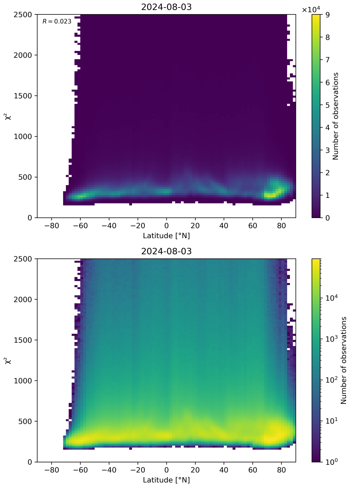
Figure 86: Scatter density plot of “Latitude” against “ \chi^2 ” for 2024-08-02 to 2024-08-04.
