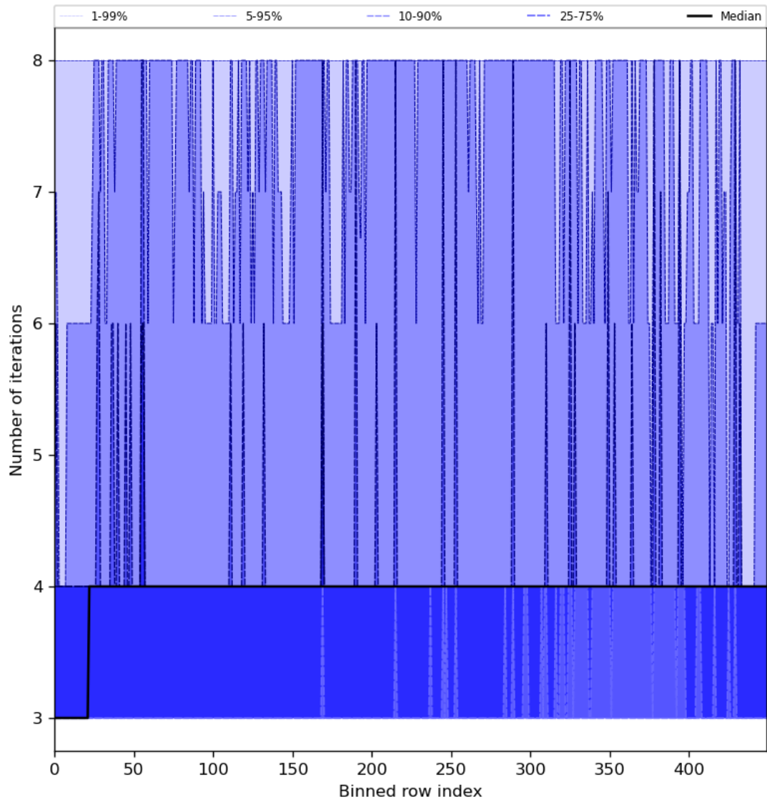
Figure 51: Along track statistics of “Number of iterations” for 2024-08-02 to 2024-08-04
