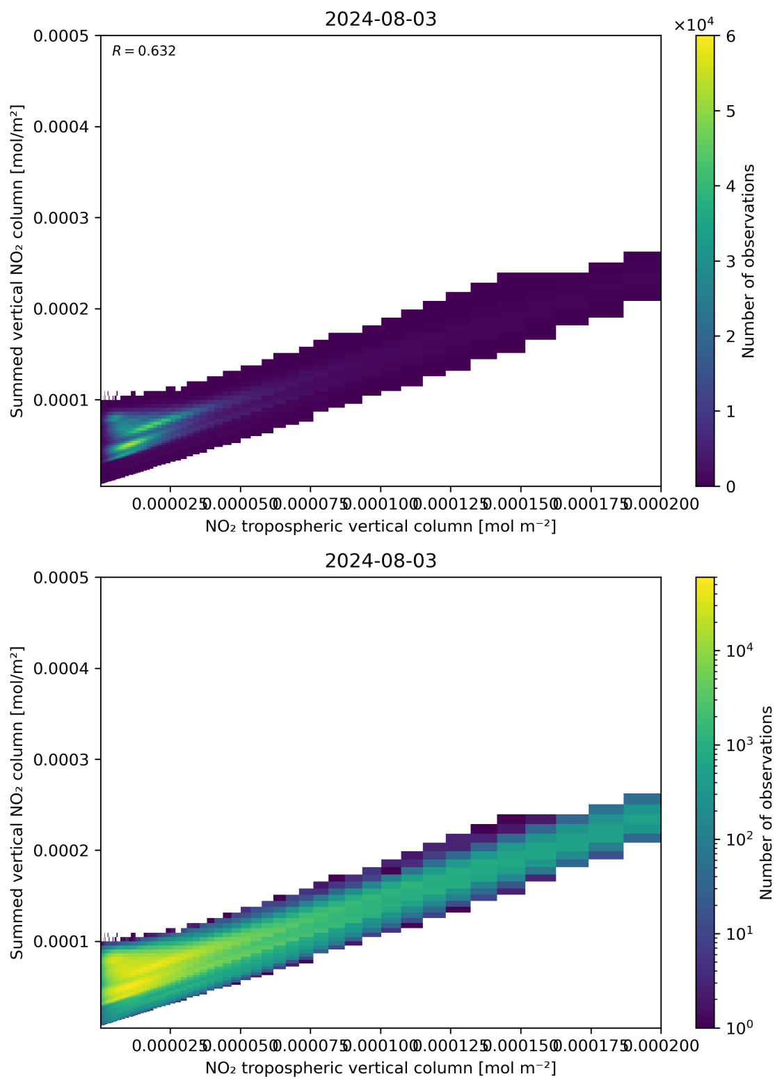
Figure 126: Scatter density plot of “NO 2 tropospheric vertical column” against “Summed vertical NO 2 column” for 2024-08-02 to 2024-08-04.
