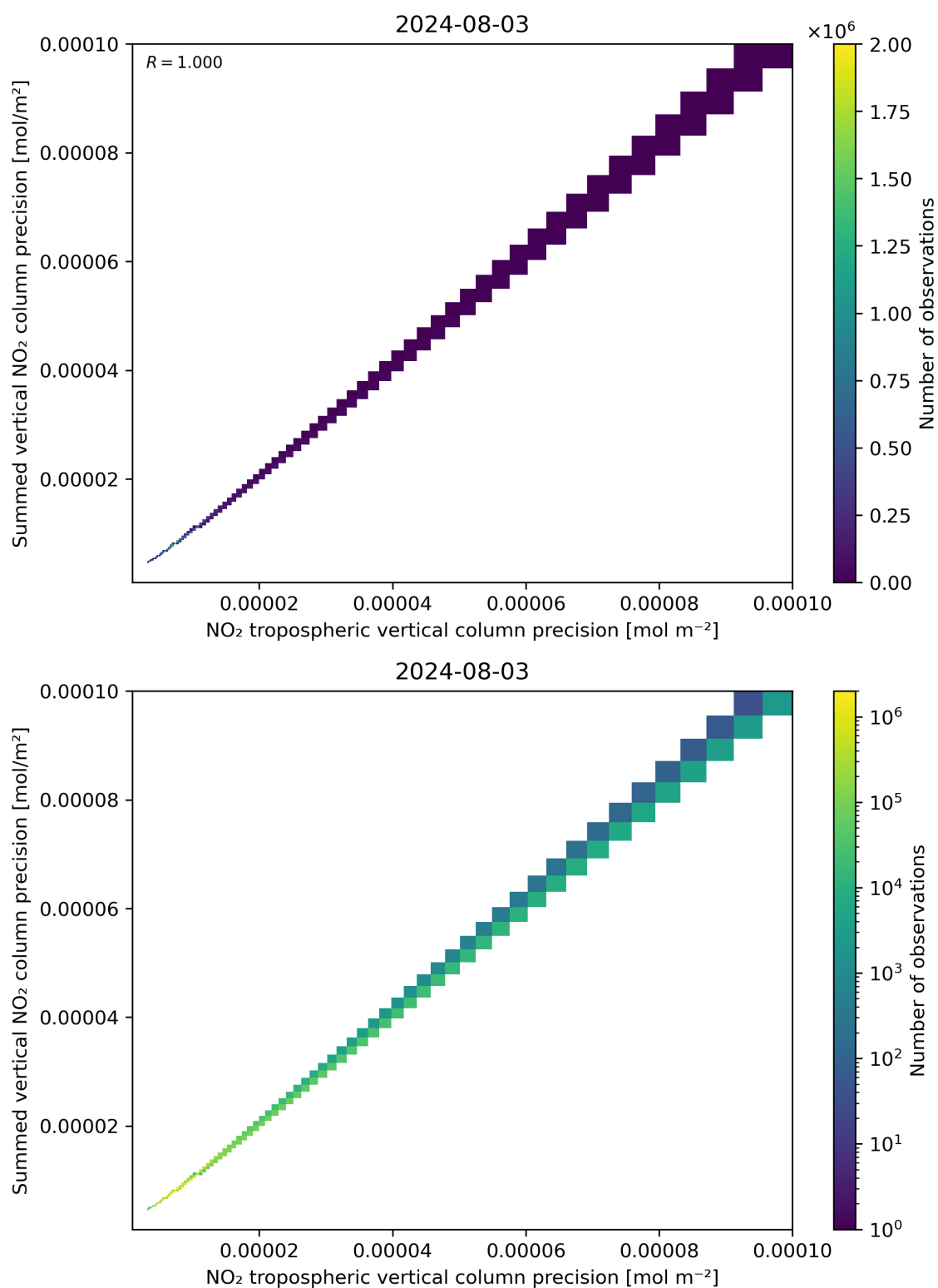
Figure 137: Scatter density plot of “NO 2 tropospheric vertical column precision” against “Summed vertical NO 2 column precision” for 2024-08-02 to 2024-08-04.
