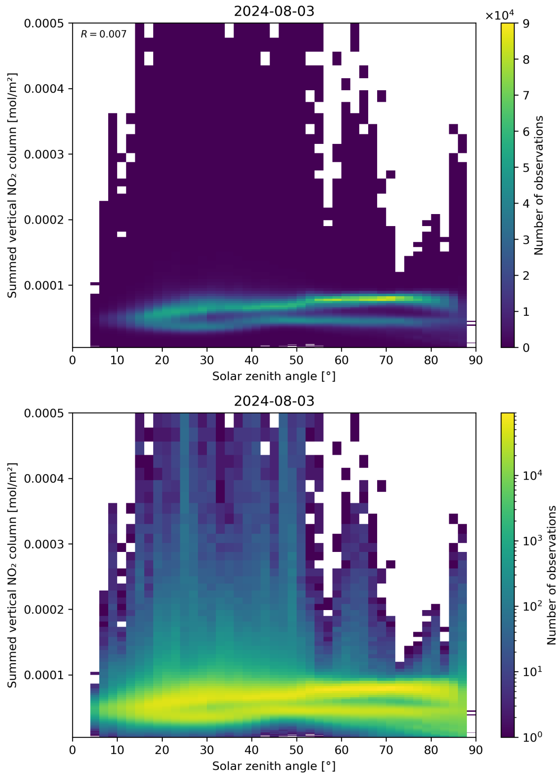
Figure 151: Scatter density plot of “Solar zenith angle” against “Summed vertical NO 2 column” for 2024-08-02 to 2024-08-04.
