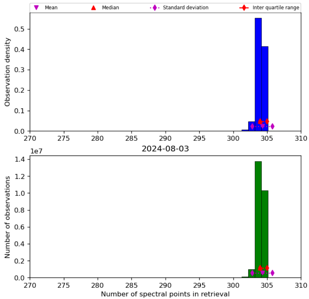
Figure 33: Histogram of “Number of spectral points in retrieval” for 2024-08-02 to 2024-08-04
