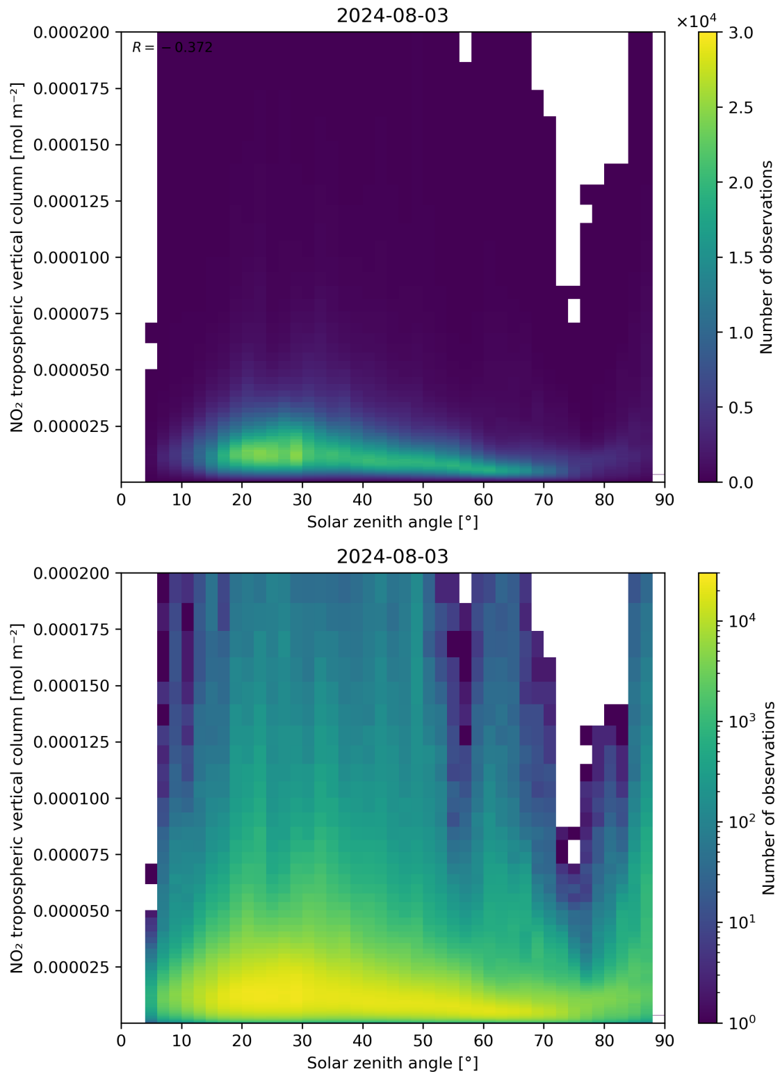
Figure 155: Scatter density plot of “Solar zenith angle” against “NO 2 tropospheric vertical column” for 2024-08-02 to 2024-08-04.
