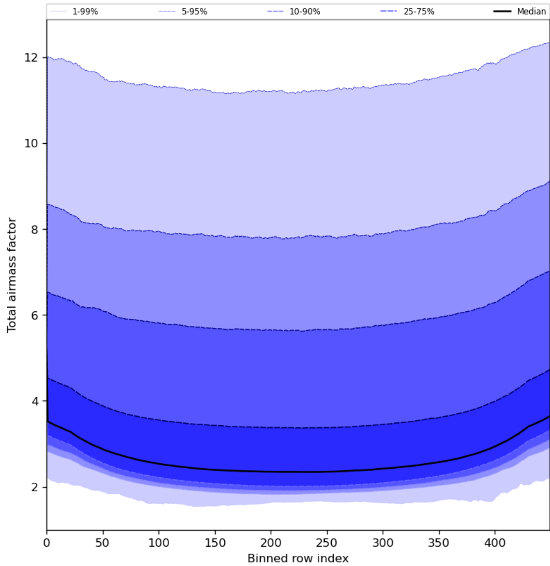
Figure 49: Along track statistics of “Total airmass factor” for 2024-08-02 to 2024-08-04
