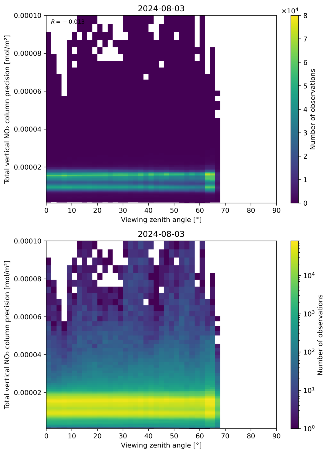
Figure 168: Scatter density plot of “Viewing zenith angle” against “Total vertical NO 2 column precision” for 2024-08-02 to 2024-08-04.
