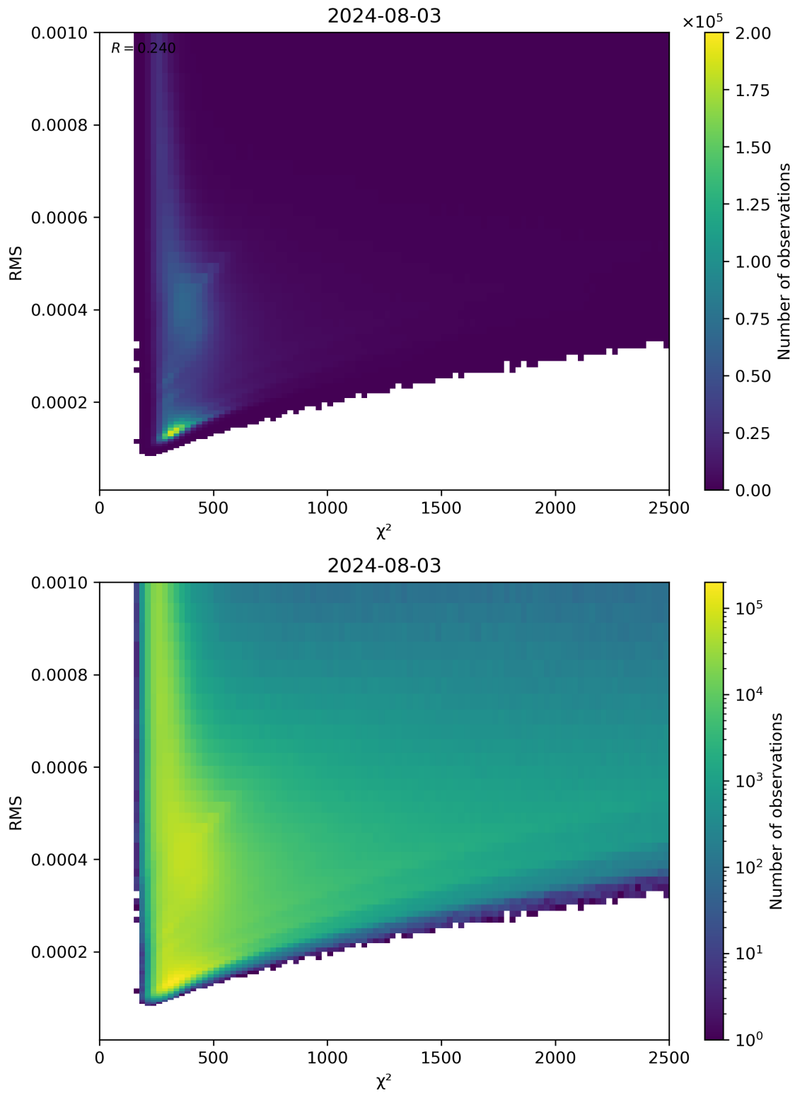
Figure 82: Scatter density plot of “ \chi^2 ” against “RMS” for 2024-08-02 to 2024-08-04.
