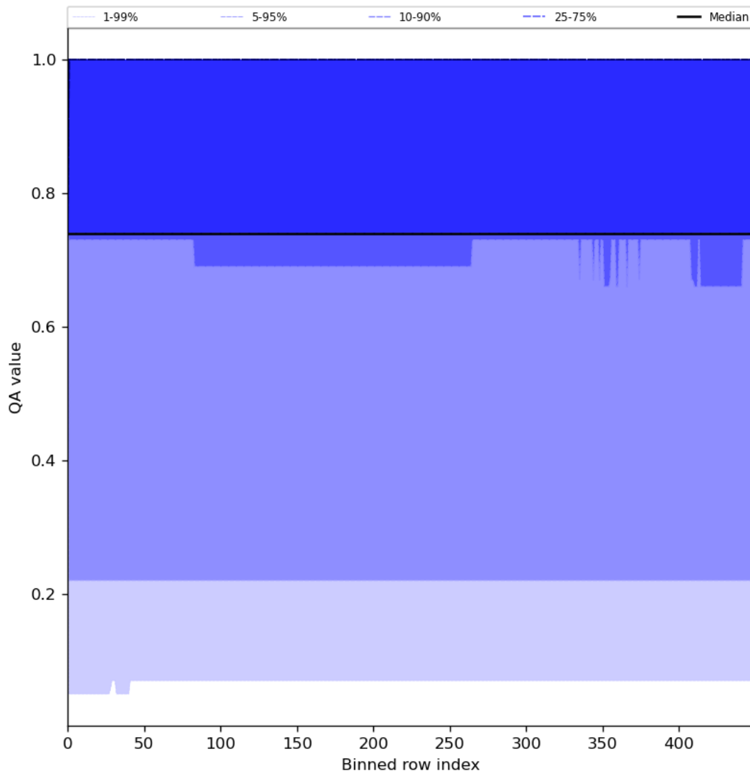
Figure 45: Along track statistics of “QA value” for 2024-08-02 to 2024-08-04
