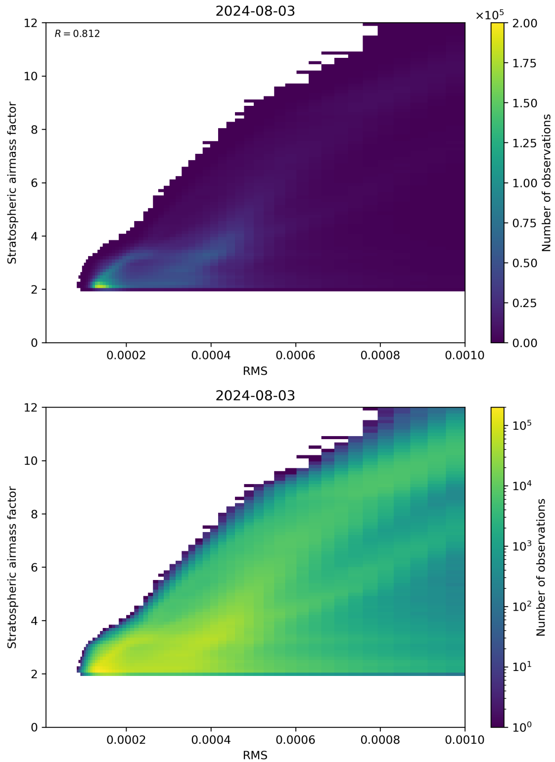
Figure 144: Scatter density plot of “RMS” against “Stratospheric airmass factor” for 2024-08-02 to 2024-08-04.
