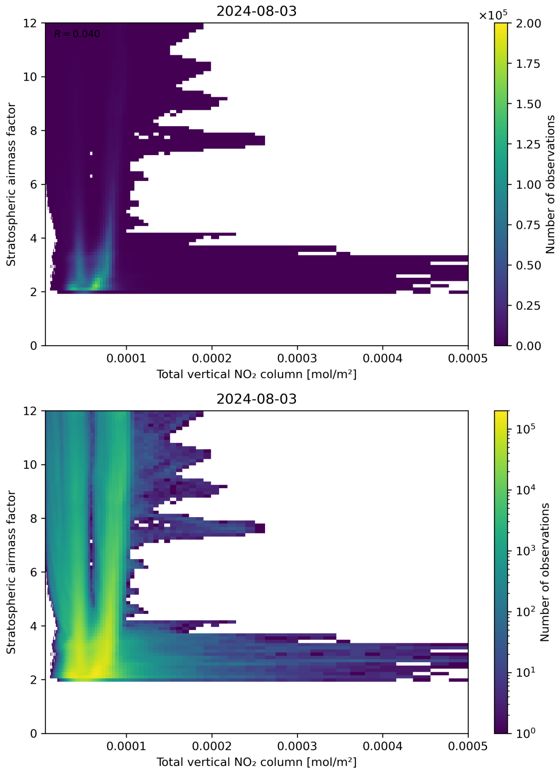
Figure 110: Scatter density plot of “Total vertical NO 2 column” against “Stratospheric airmass factor” for 2024-08-02 to 2024-08-04.
