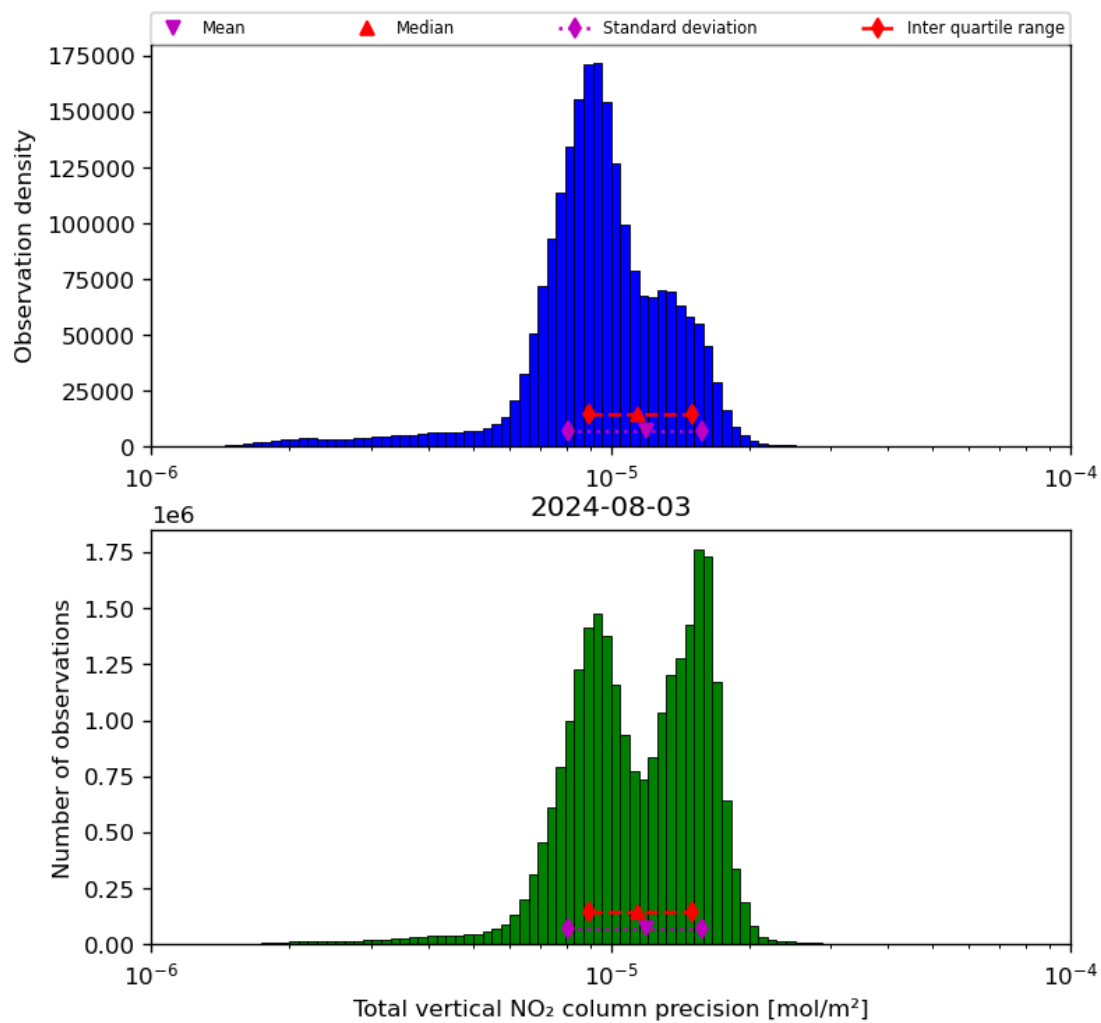
Figure 39: Histogram of "Total vertical NO 2 column precision" for 2024-08-02 to 2024-08-04
