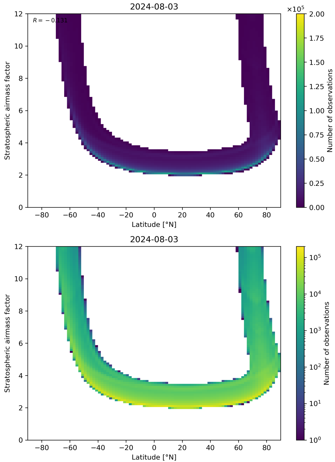
Figure 83: Scatter density plot of “Latitude” against “Stratospheric airmass factor” for 2024-08-02 to 2024-08-04.
