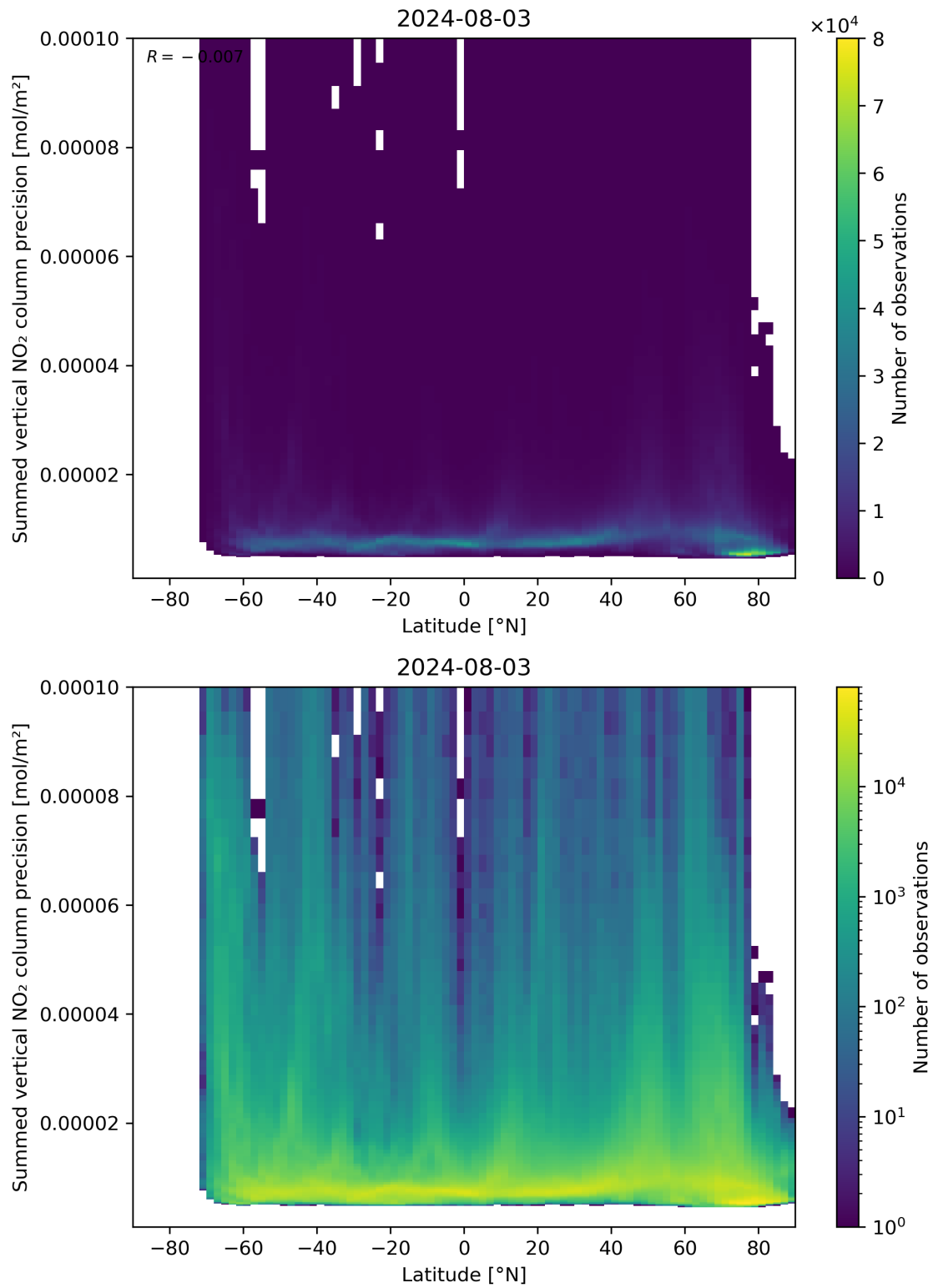
Figure 89: Scatter density plot of “Latitude” against “Summed vertical NO 2 column precision” for 2024-08-02 to 2024-08-04.
