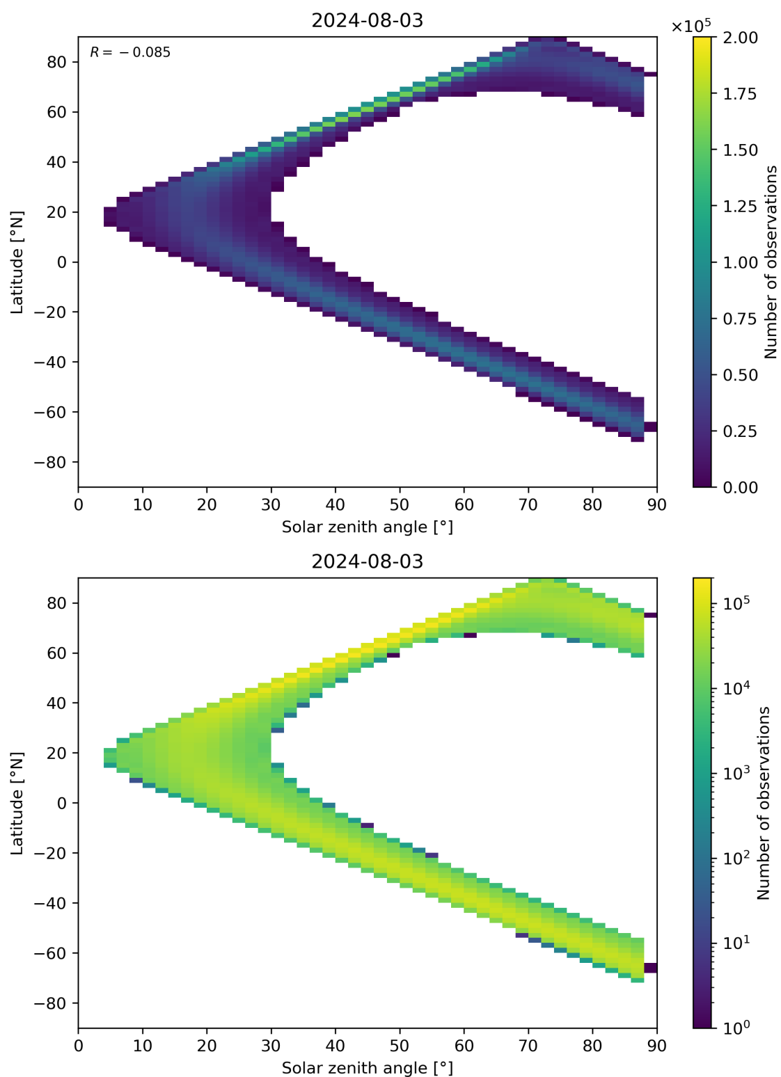
Figure 149: Scatter density plot of “Solar zenith angle” against “Latitude” for 2024-08-02 to 2024-08-04.
