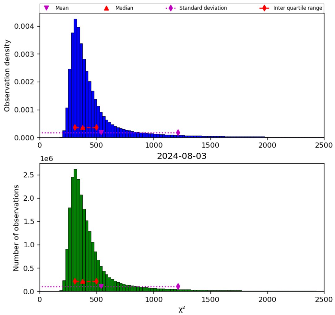
Figure 42: Histogram of “ \chi^2 ” for 2024-08-02 to 2024-08-04
