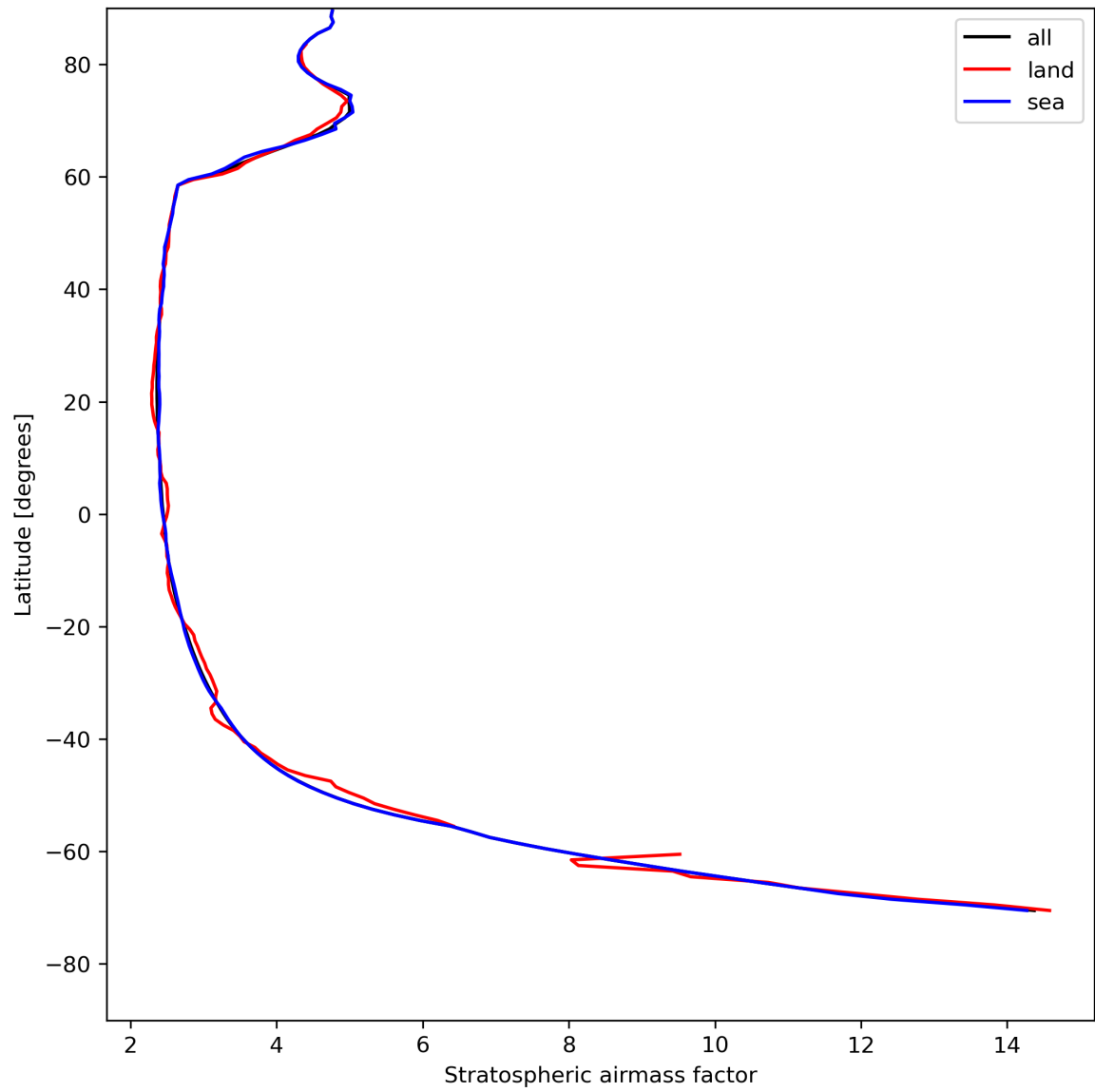
Figure 27: Zonal average of “Stratospheric airmass factor” for 2024-08-02 to 2024-08-04.
