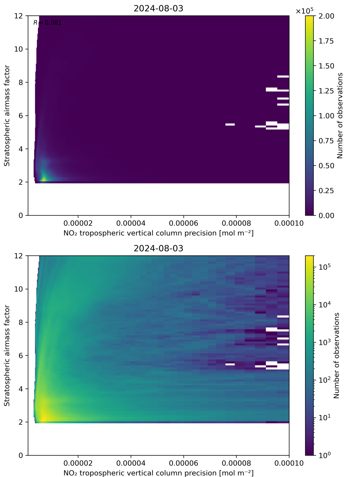
Figure 131: Scatter density plot of “NO 2 tropospheric vertical column precision” against “Stratospheric airmass factor” for 2024-08-02 to 2024-08-04.
