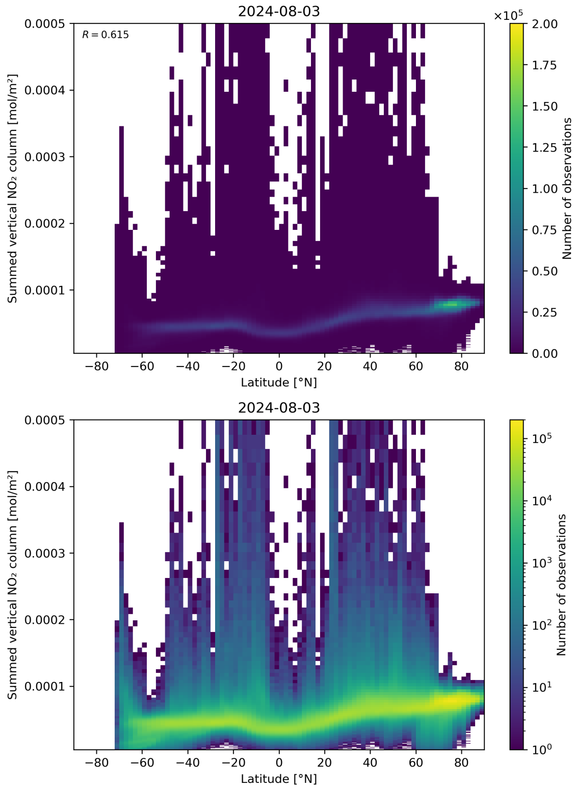
Figure 88: Scatter density plot of “Latitude” against “Summed vertical NO 2 column” for 2024-08-02 to 2024-08-04.
