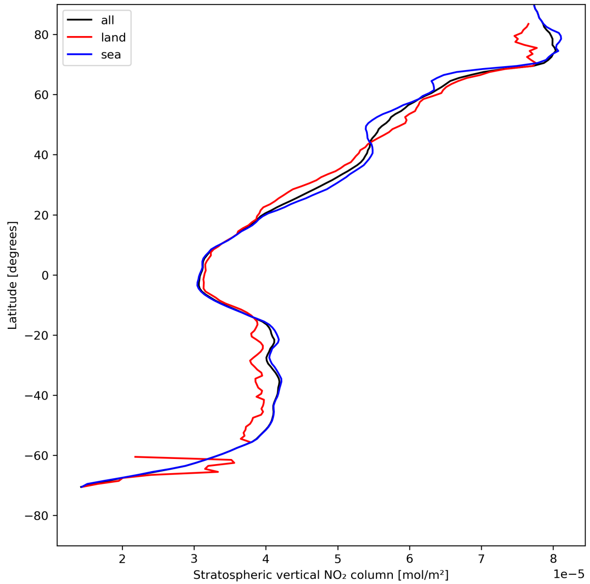
Figure 19: Zonal average of “Stratospheric vertical NO 2 column” for 2024-08-02 to 2024-08-04.
