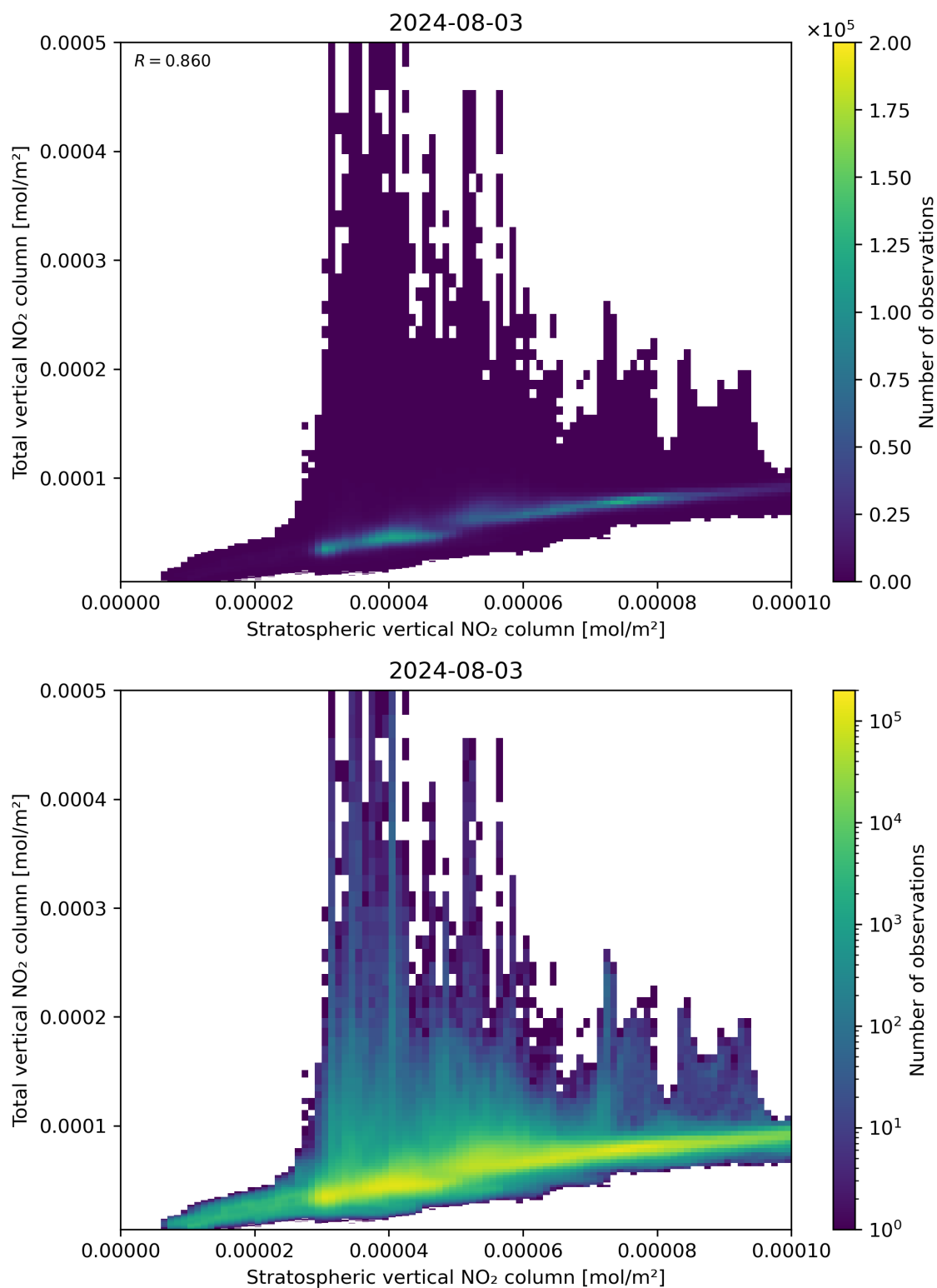
Figure 100: Scatter density plot of “Stratospheric vertical NO 2 column” against “Total vertical NO 2 column” for 2024-08-02 to 2024-08-04.
