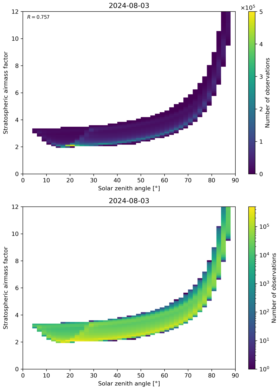
Figure 145: Scatter density plot of “Solar zenith angle” against “Stratospheric airmass factor” for 2024-08-02 to 2024-08-04.
