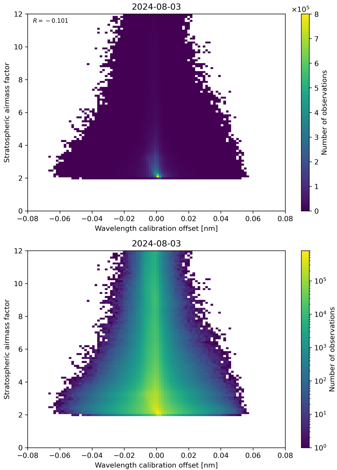
Figure 174: Scatter density plot of “Wavelength calibration offset” against “Stratospheric airmass factor” for 2024-08-02 to 2024-08-04.
