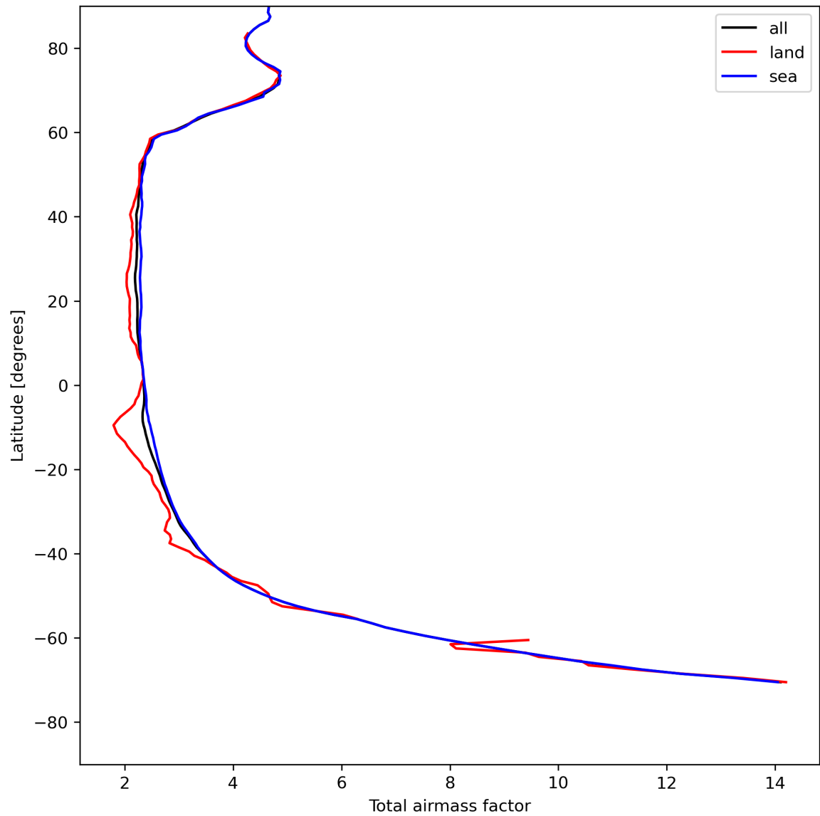
Figure 15: Zonal average of “Total airmass factor” for 2024-08-02 to 2024-08-04.
