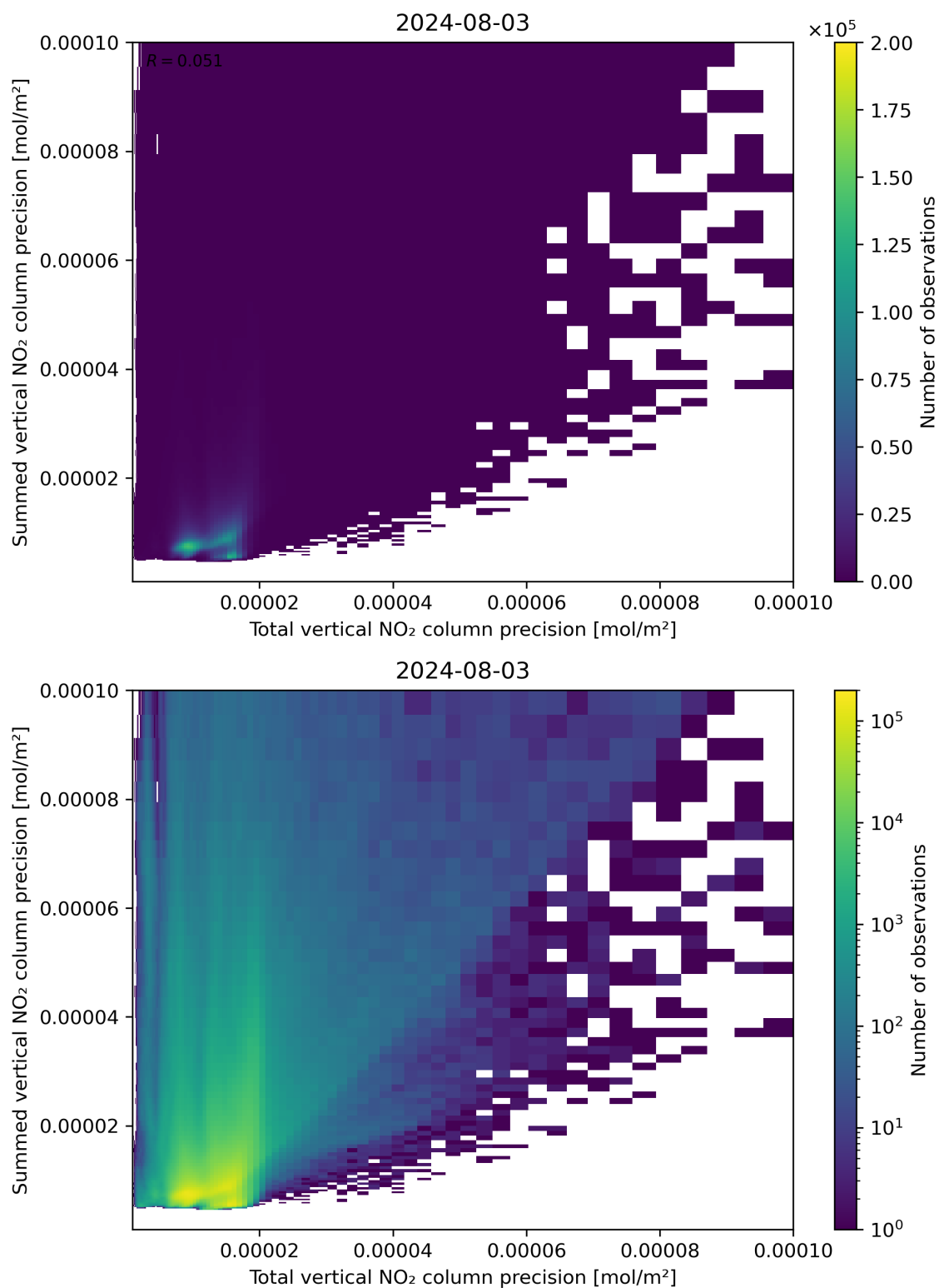
Figure 118: Scatter density plot of “Total vertical NO 2 column precision” against “Summed vertical NO 2 column precision” for 2024-08-02 to 2024-08-04.
