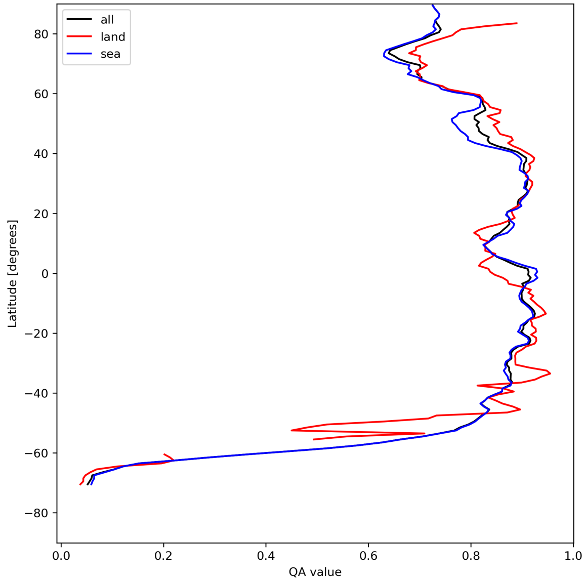
Figure 11: Zonal average of “QA value” for 2024-08-02 to 2024-08-04.
