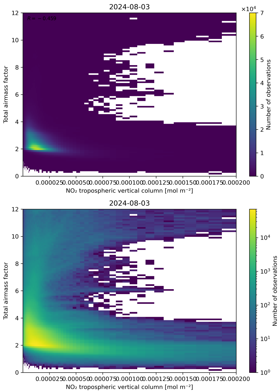
Figure 122: Scatter density plot of “NO 2 tropospheric vertical column” against “Total air mass factor” for 2024-08-02 to 2024-08-04.
