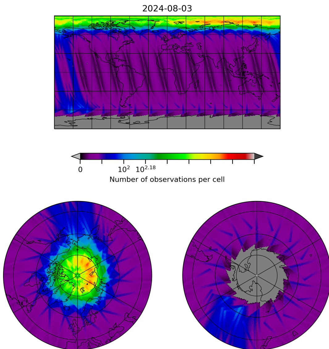
Figure 10: Map of the number of observations for 2024-08-02 to 2024-08-04
