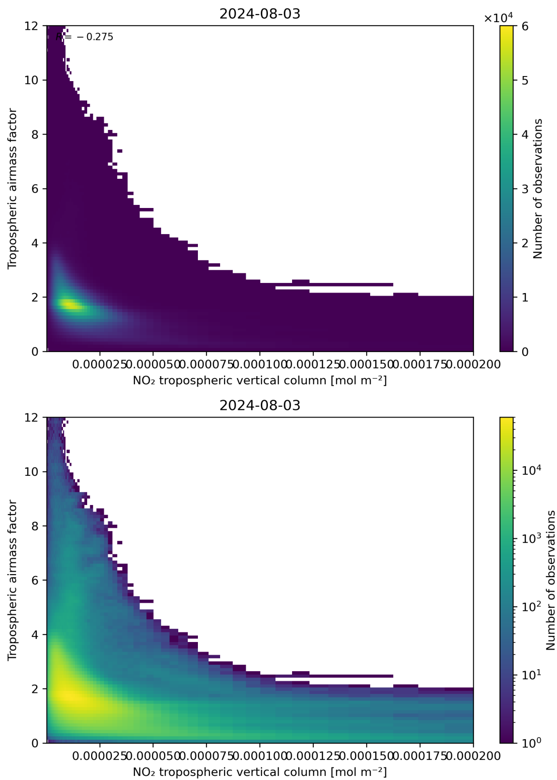
Figure 123: Scatter density plot of “NO 2 tropospheric vertical column” against “Tropospheric air mass factor” for 2024-08-02 to 2024-08-04.
