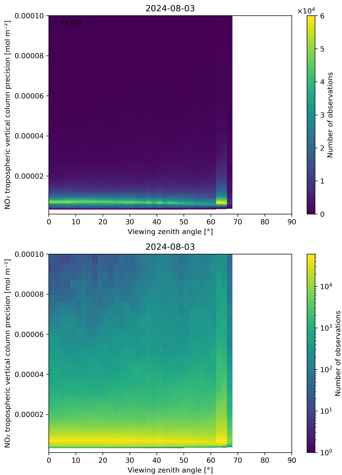
Figure 170: Scatter density plot of “Viewing zenith angle” against “NO 2 tropospheric vertical column precision” for 2024-08-02 to 2024-08-04.
