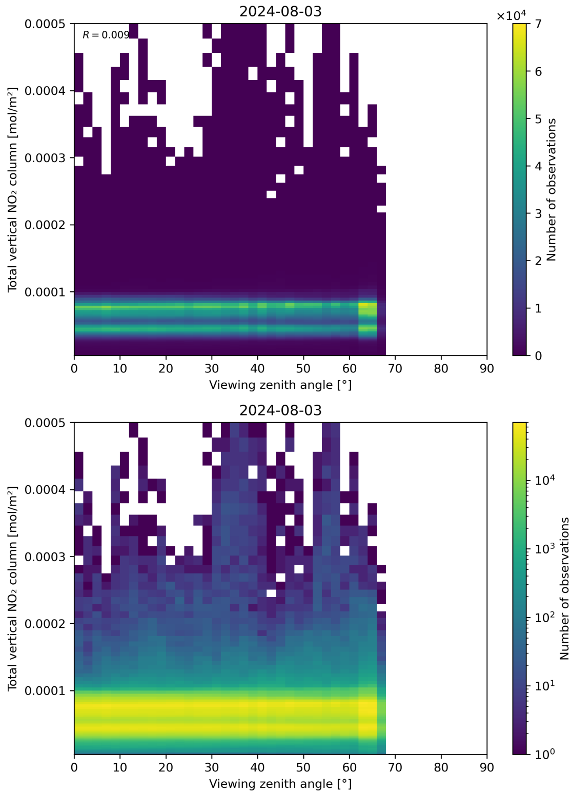
Figure 167: Scatter density plot of “Viewing zenith angle” against “Total vertical NO 2 column” for 2024-08-02 to 2024-08-04.
