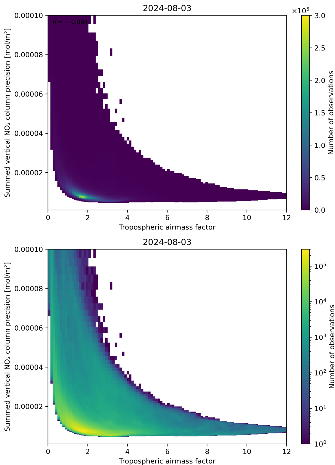
Figure 76: Scatter density plot of “Tropospheric air mass factor” against “Summed vertical NO 2 column precision” for 2024-08-02 to 2024-08-04.
