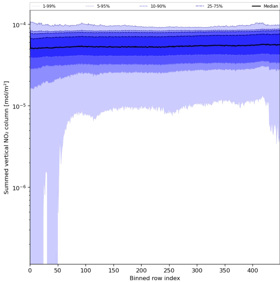
Figure 57: Along track statistics of “Summed vertical NO 2 column” for 2024-08-02 to 2024-08-04
