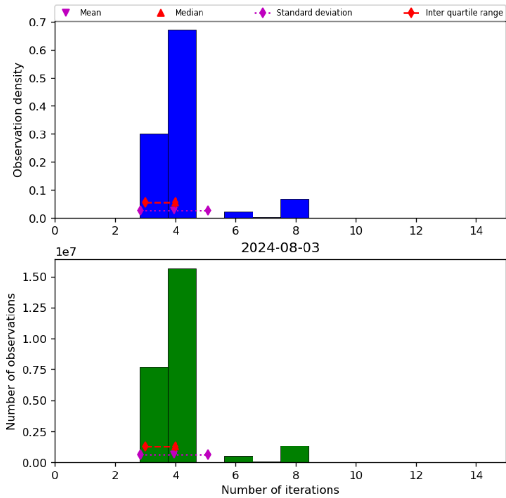
Figure 34: Histogram of “Number of iterations” for 2024-08-02 to 2024-08-04
