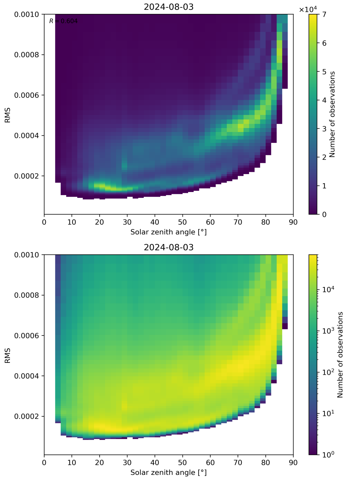
Figure 157: Scatter density plot of “Solar zenith angle” against “RMS” for 2024-08-02 to 2024-08-04.
