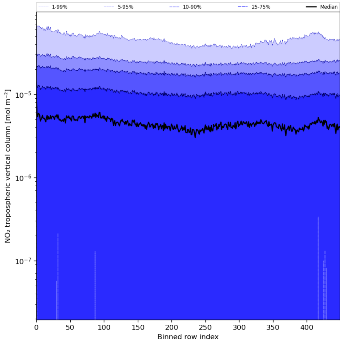
Figure 46: Along track statistics of “NO 2 tropospheric vertical column” for 2024-08-02 to 2024-08-04
