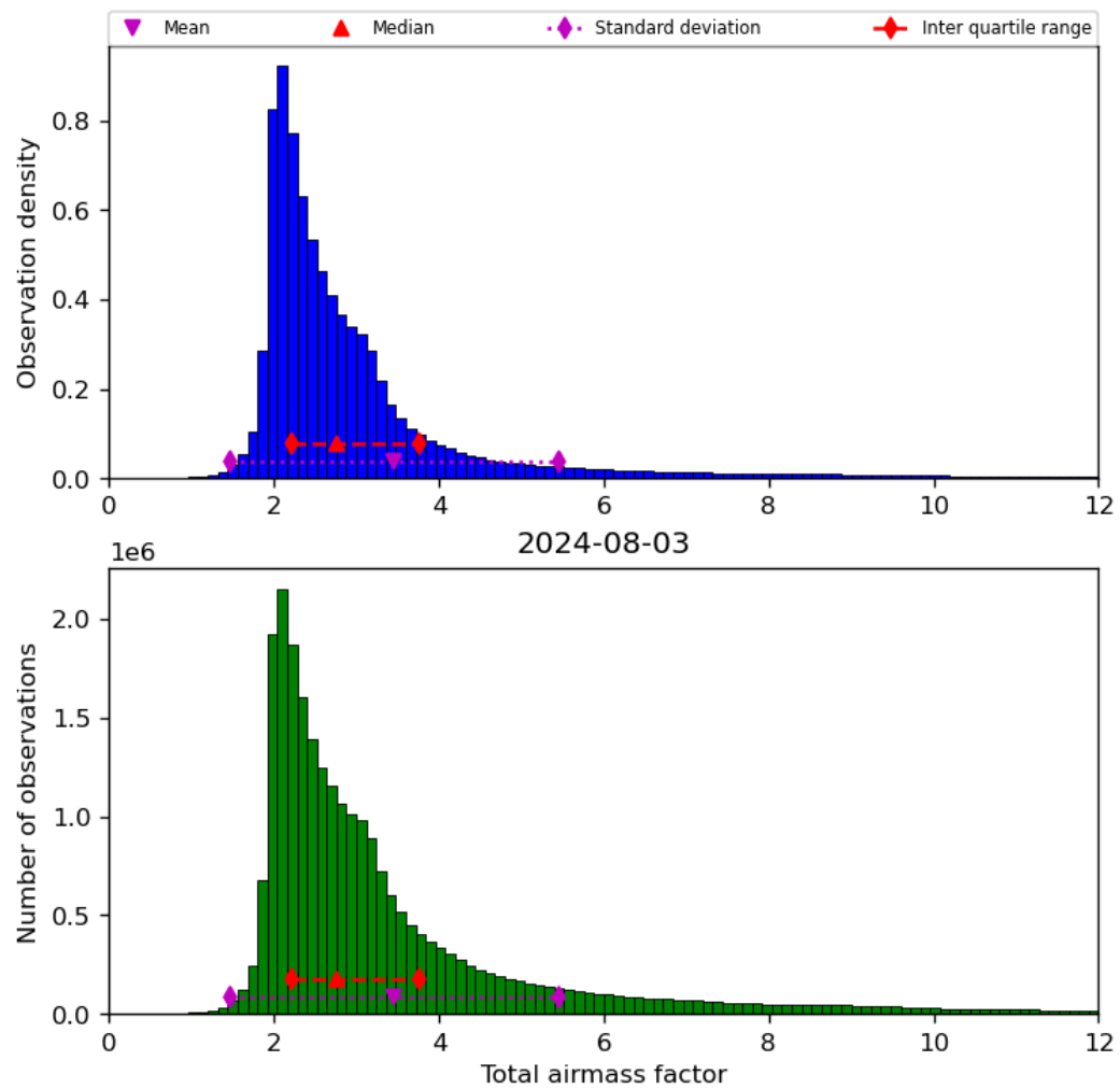
Figure 32: Histogram of “Total airmass factor” for 2024-08-02 to 2024-08-04
