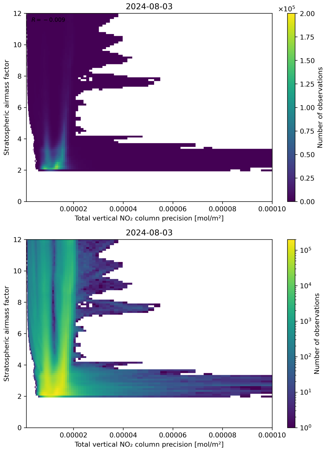
Figure 115: Scatter density plot of “Total vertical NO 2 column precision” against “Stratospheric air mass factor” for 2024-08-02 to 2024-08-04.
