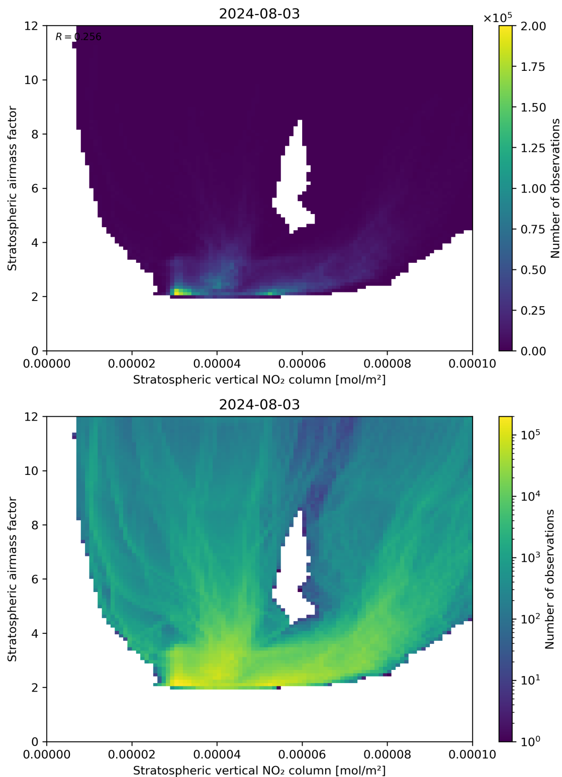
Figure 96: Scatter density plot of “Stratospheric vertical NO 2 column” against “Stratospheric airmass factor” for 2024-08-02 to 2024-08-04.
