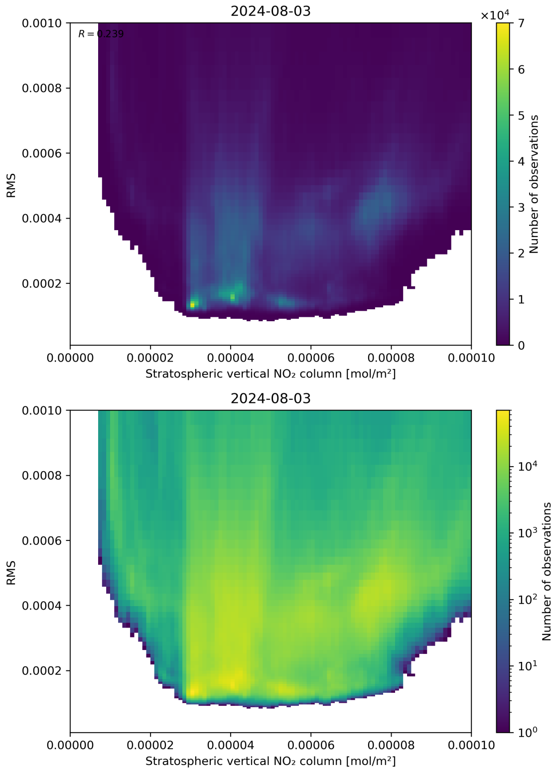
Figure 102: Scatter density plot of “Stratospheric vertical NO 2 column” against “RMS” for 2024-08-02 to 2024-08-04.
