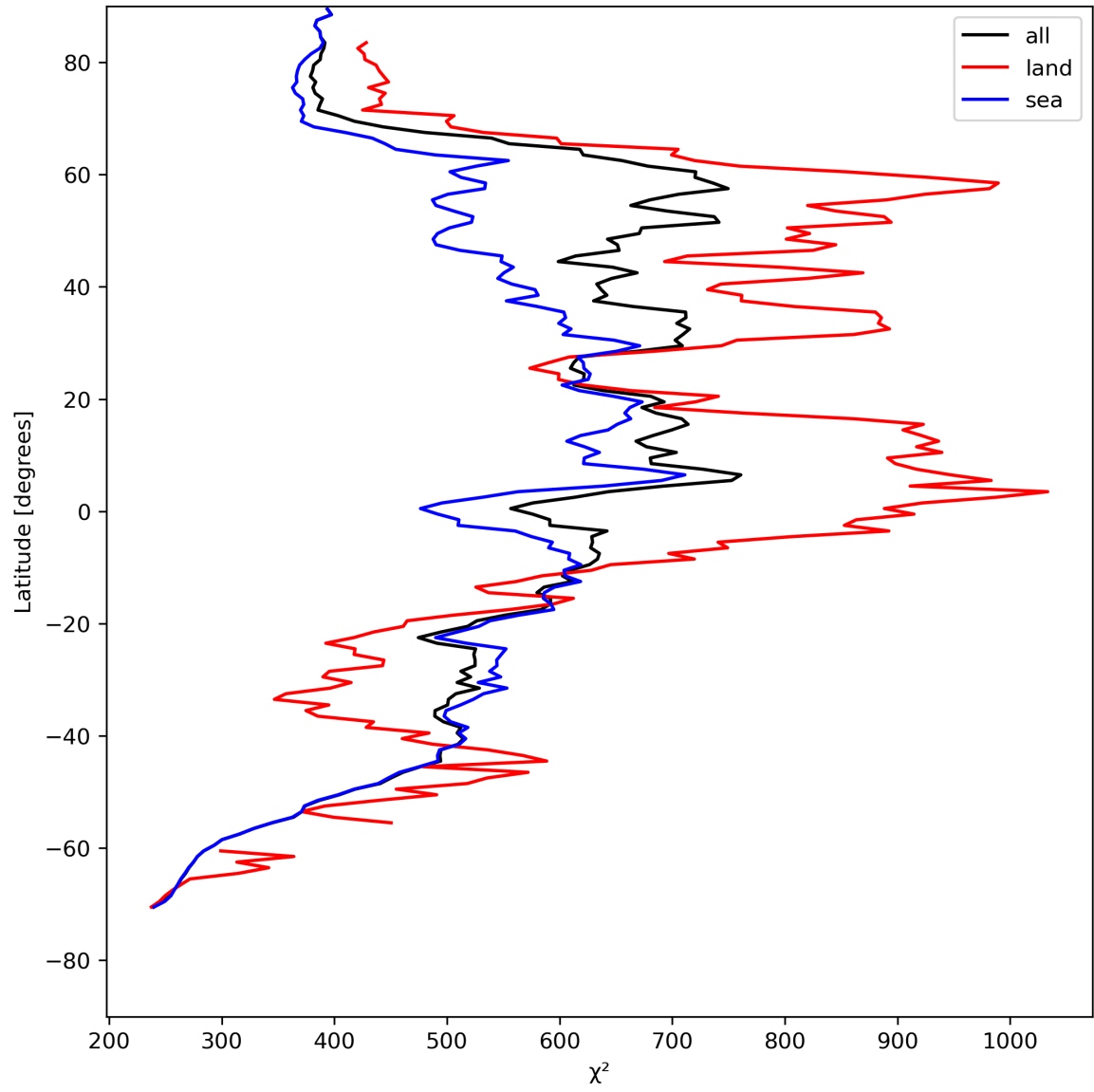
Figure 25: Zonal average of “ \chi^2 ” for 2024-08-02 to 2024-08-04.
