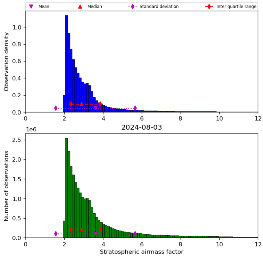
Figure 44: Histogram of “Stratospheric airmass factor” for 2024-08-02 to 2024-08-04
