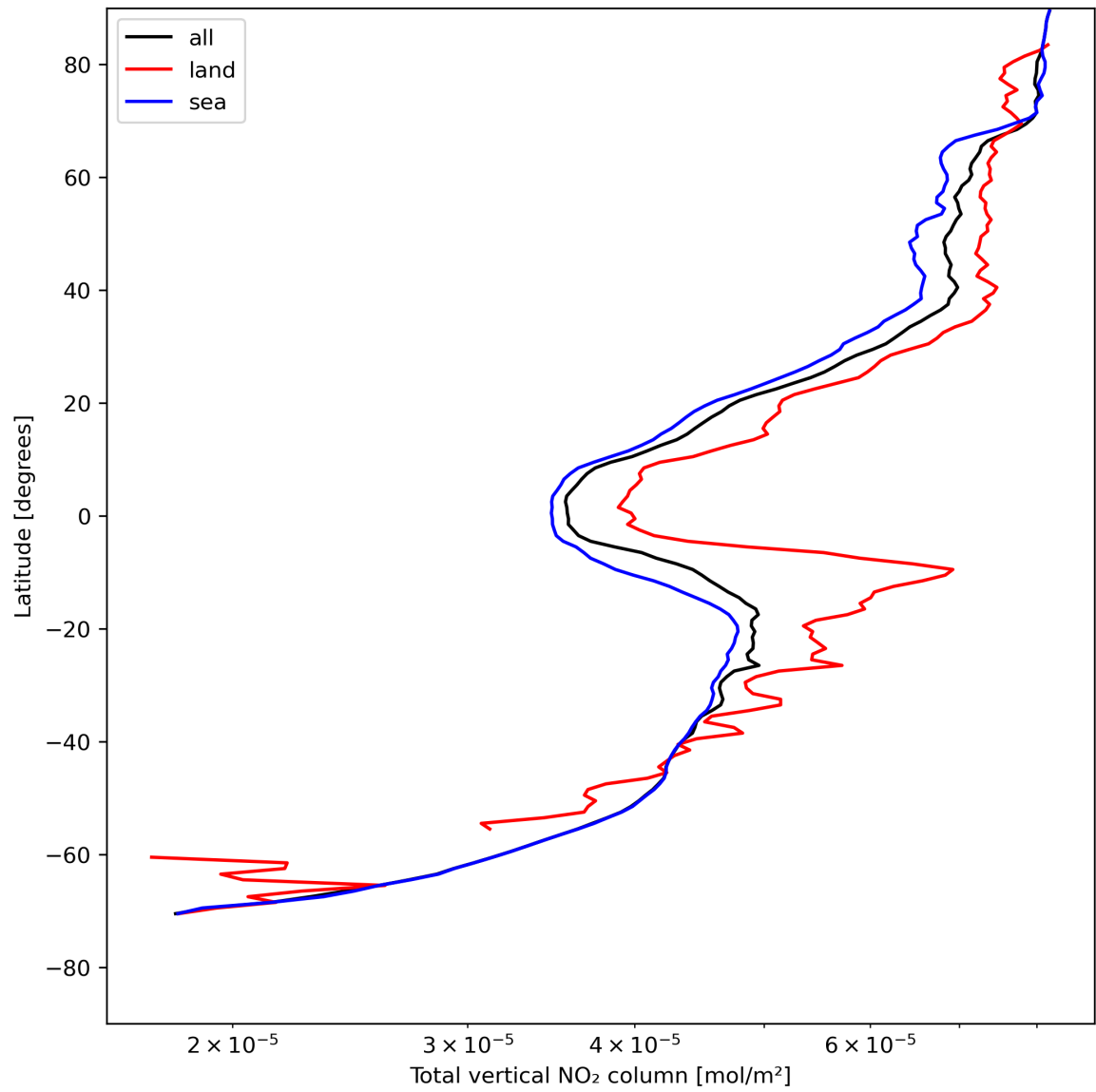
Figure 21: Zonal average of “Total vertical NO 2 column” for 2024-08-02 to 2024-08-04.
