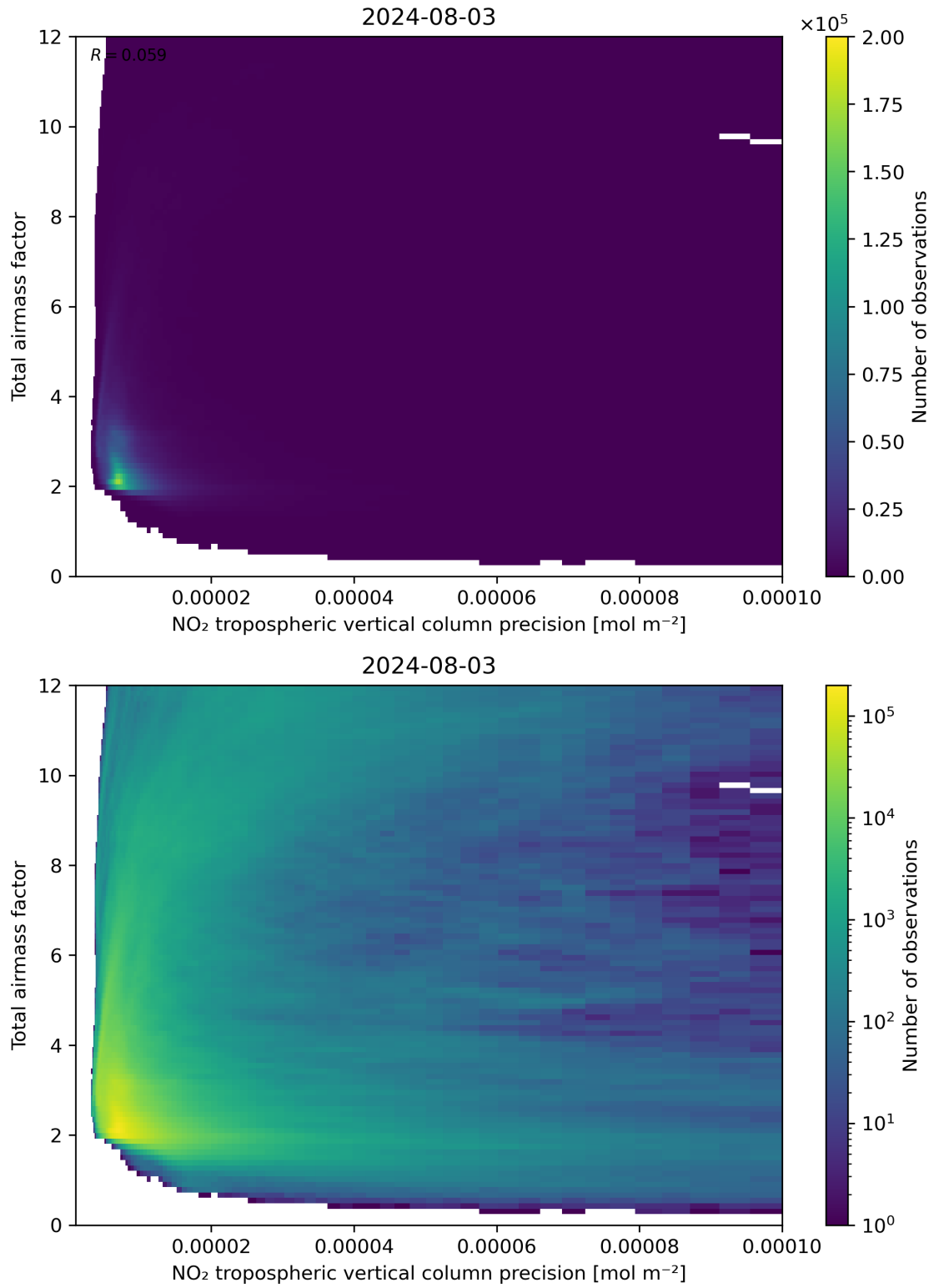
Figure 132: Scatter density plot of “NO 2 tropospheric vertical column precision” against “Total airmass factor” for 2024-08-02 to 2024-08-04.
