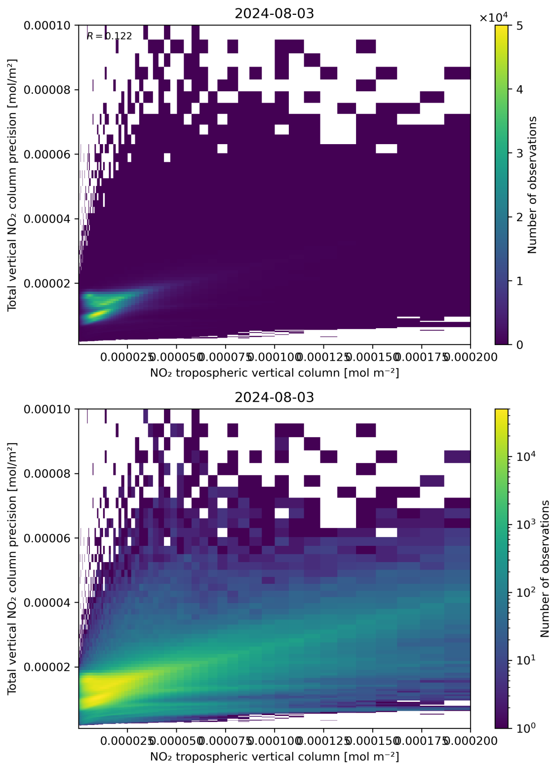
Figure 129: Scatter density plot of “NO 2 tropospheric vertical column” against “Total vertical NO 2 column precision” for 2024-08-02 to 2024-08-04.
