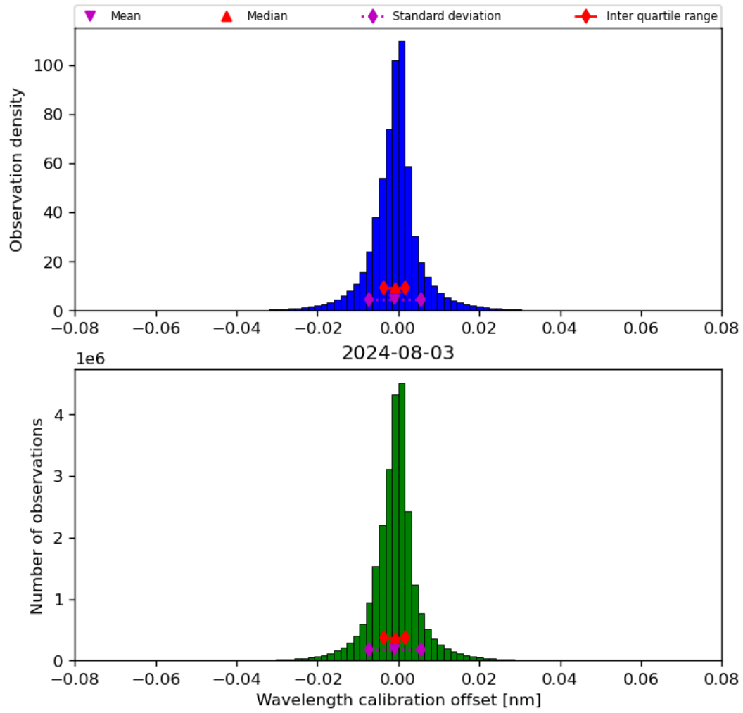
Figure 35: Histogram of “Wavelength calibration offset” for 2024-08-02 to 2024-08-04
