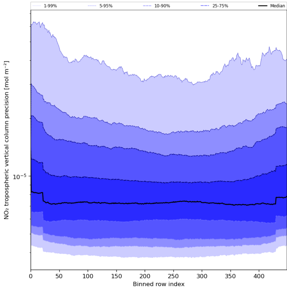
Figure 47: Along track statistics of “NO 2 tropospheric vertical column precision” for 2024-08-02 to 2024-08-04
