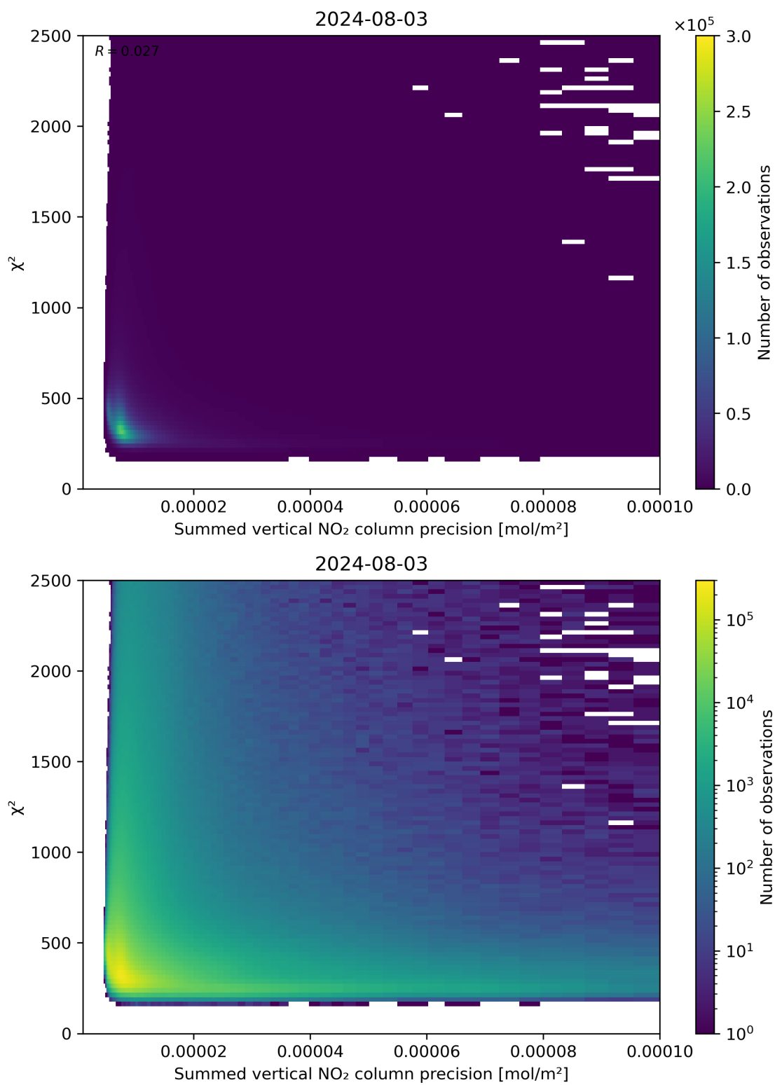
Figure 107: Scatter density plot of “Summed vertical NO 2 column precision” against “ \chi^2 ” for 2024-08-02 to 2024-08-04.
