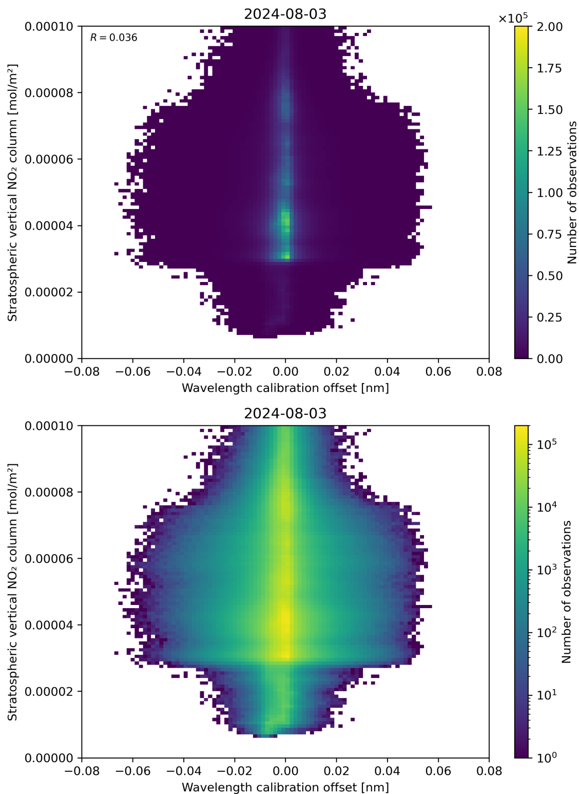
Figure 176: Scatter density plot of “Wavelength calibration offset” against “Stratospheric vertical NO 2 column” for 2024-08-02 to 2024-08-04.
