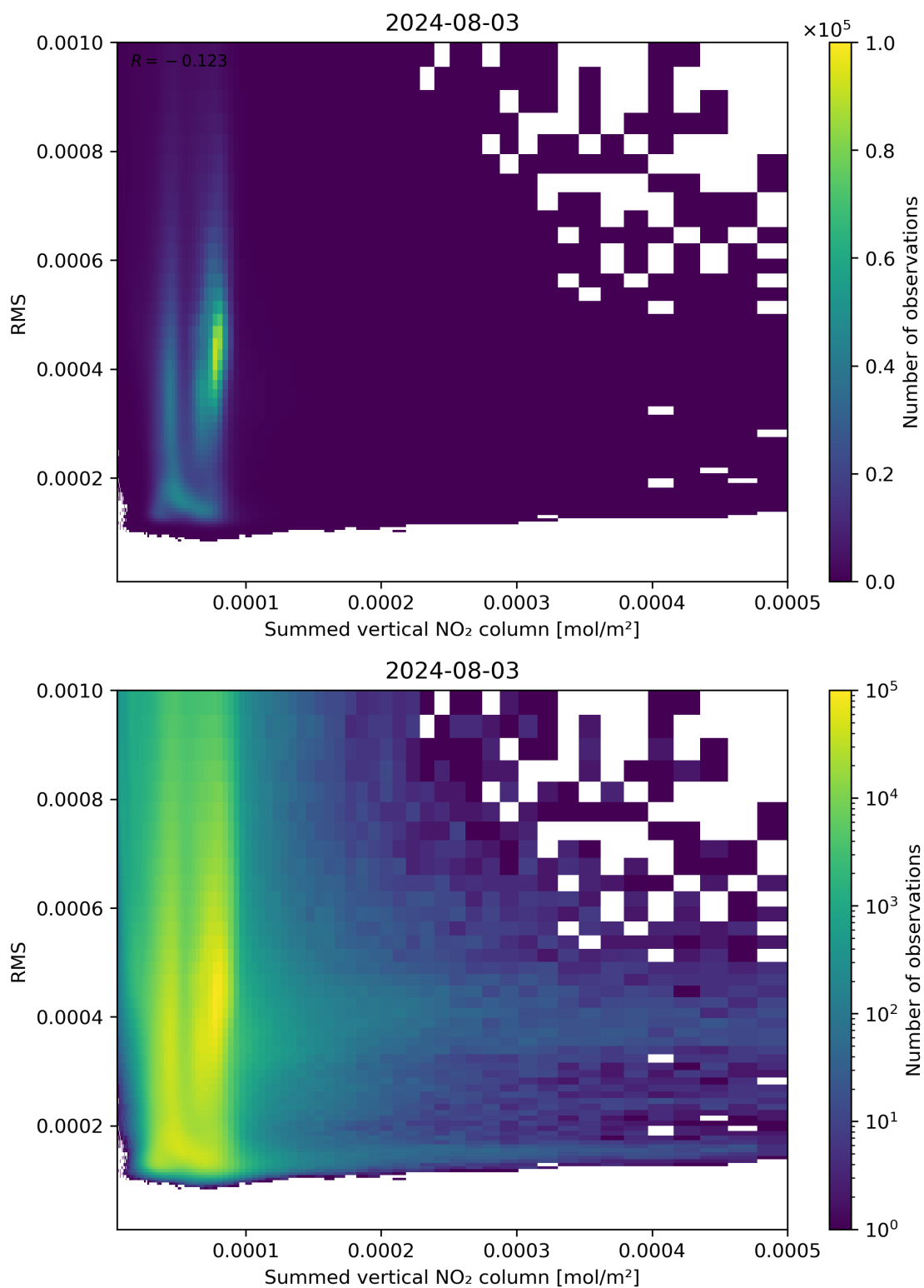
Figure 109: Scatter density plot of “Summed vertical NO 2 column” against “RMS” for 2024-08-02 to 2024-08-04.
