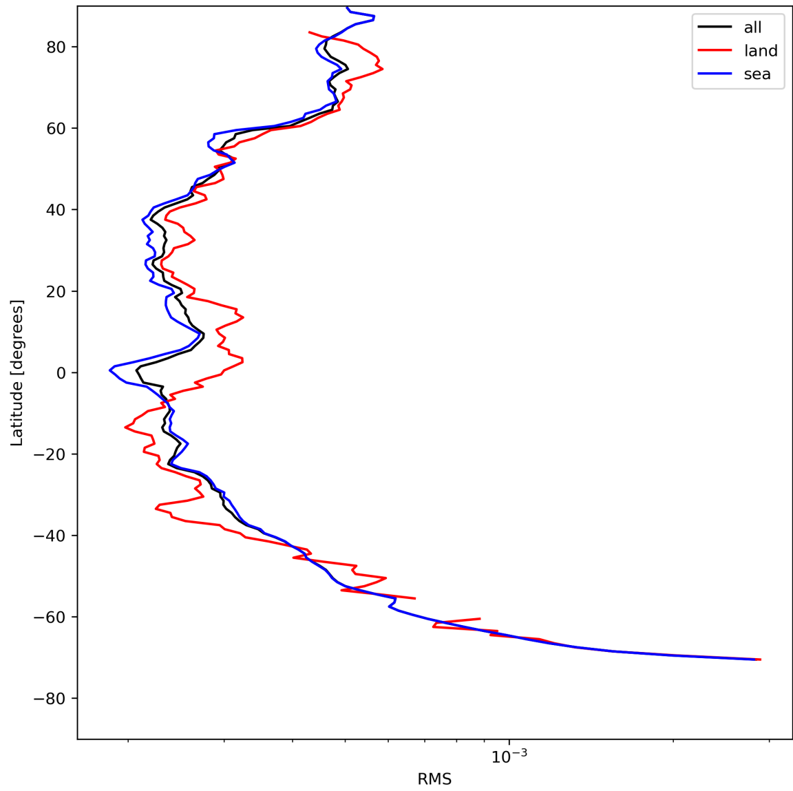
Figure 26: Zonal average of “RMS” for 2024-08-02 to 2024-08-04.
