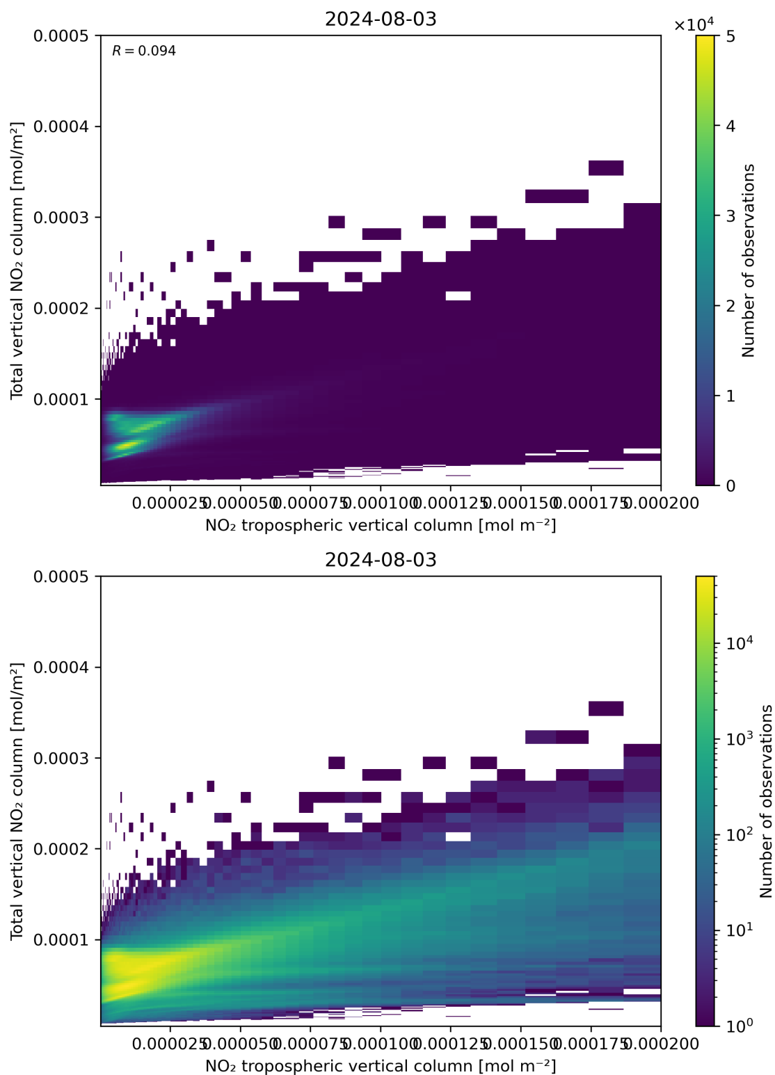
Figure 128: Scatter density plot of “NO 2 tropospheric vertical column” against “Total vertical NO 2 column” for 2024-08-02 to 2024-08-04.
