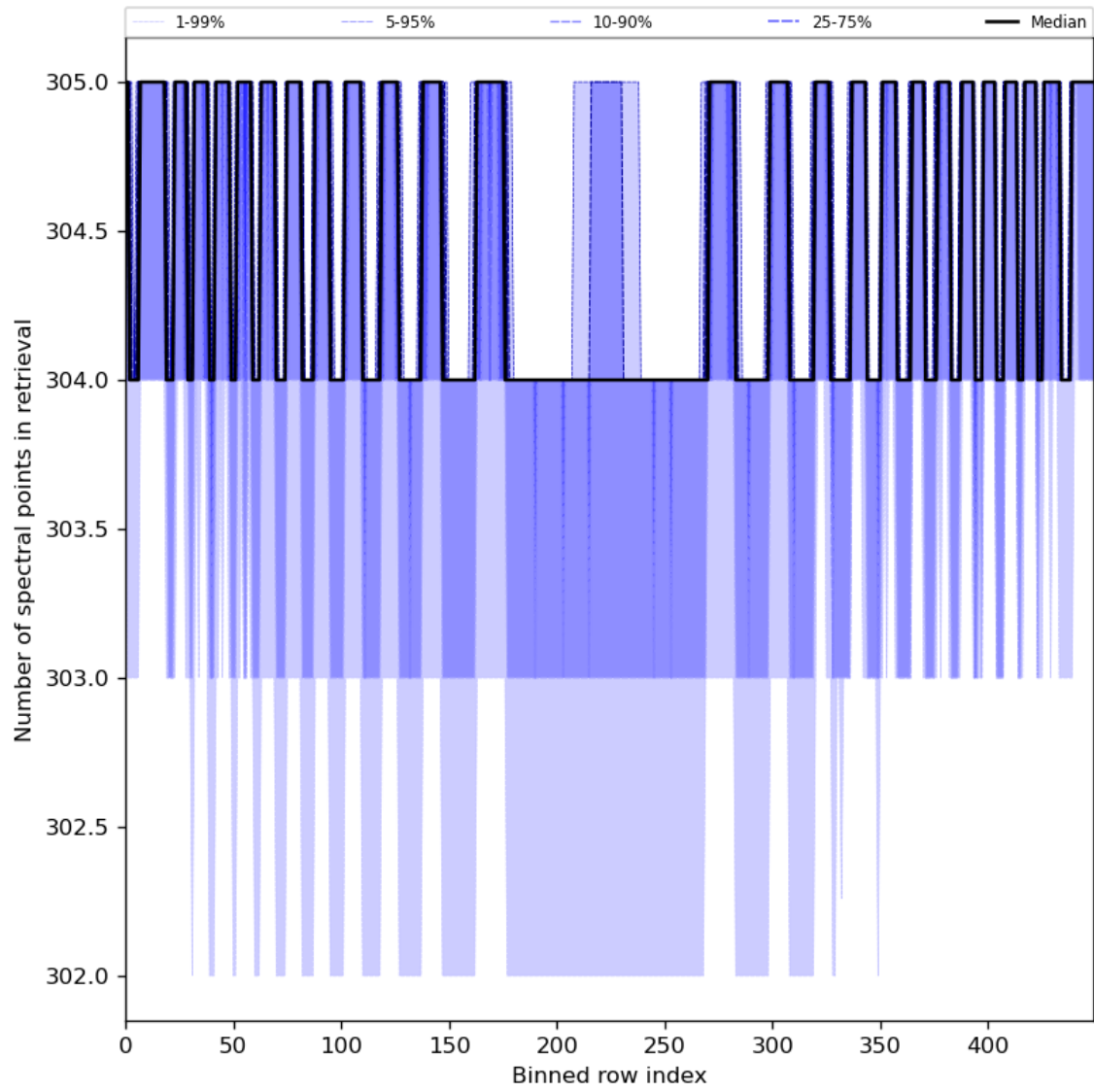
Figure 50: Along track statistics of “Number of spectral points in retrieval” for 2024-08-02 to 2024-08-04
