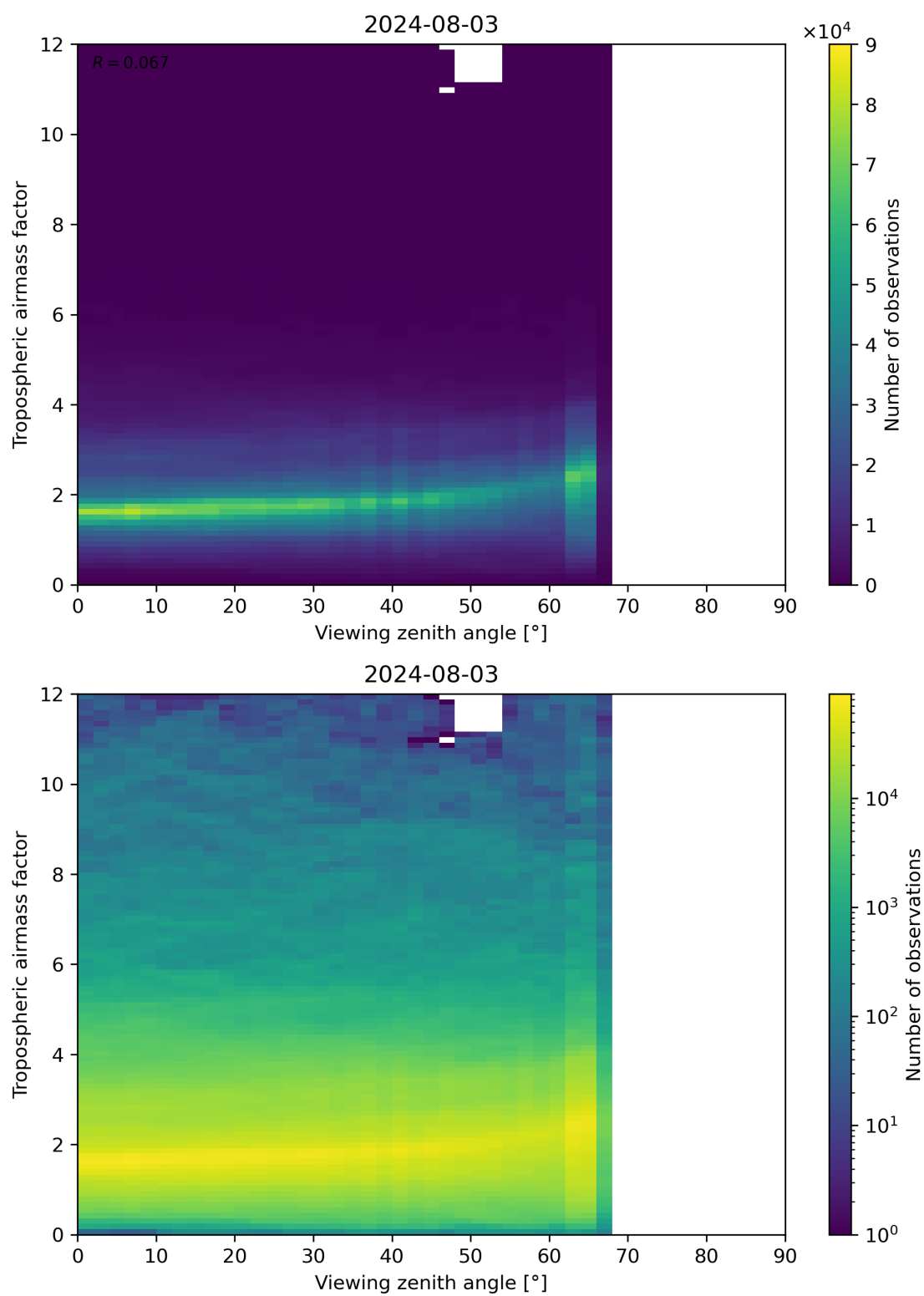
Figure 161: Scatter density plot of “Viewing zenith angle” against “Tropospheric airmass factor” for 2024-08-02 to 2024-08-04.
