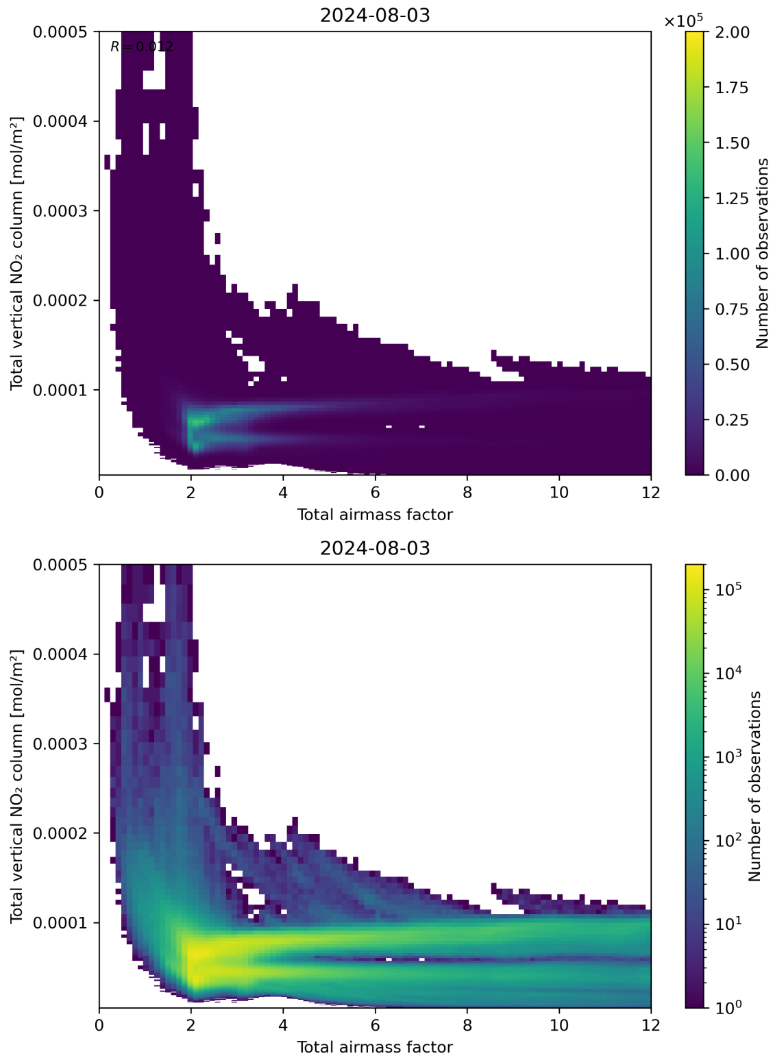
Figure 67: Scatter density plot of “Total airmass factor” against “Total vertical NO 2 column” for 2024-08-02 to 2024-08-04.
