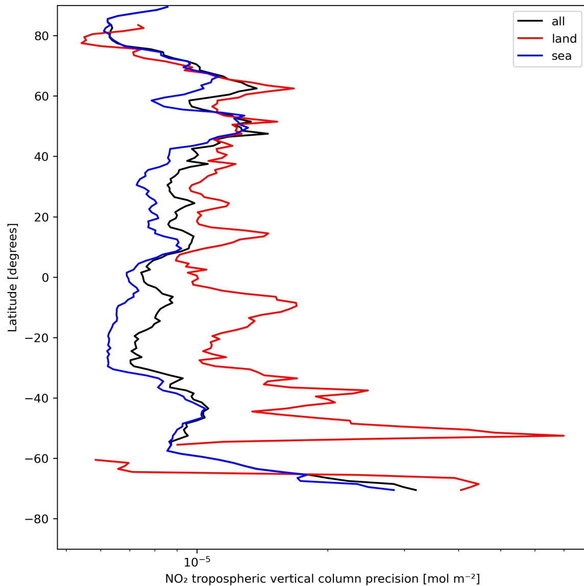
Figure 13: Zonal average of “NO 2 tropospheric vertical column precision” for 2024-08-02 to 2024-08-04.
