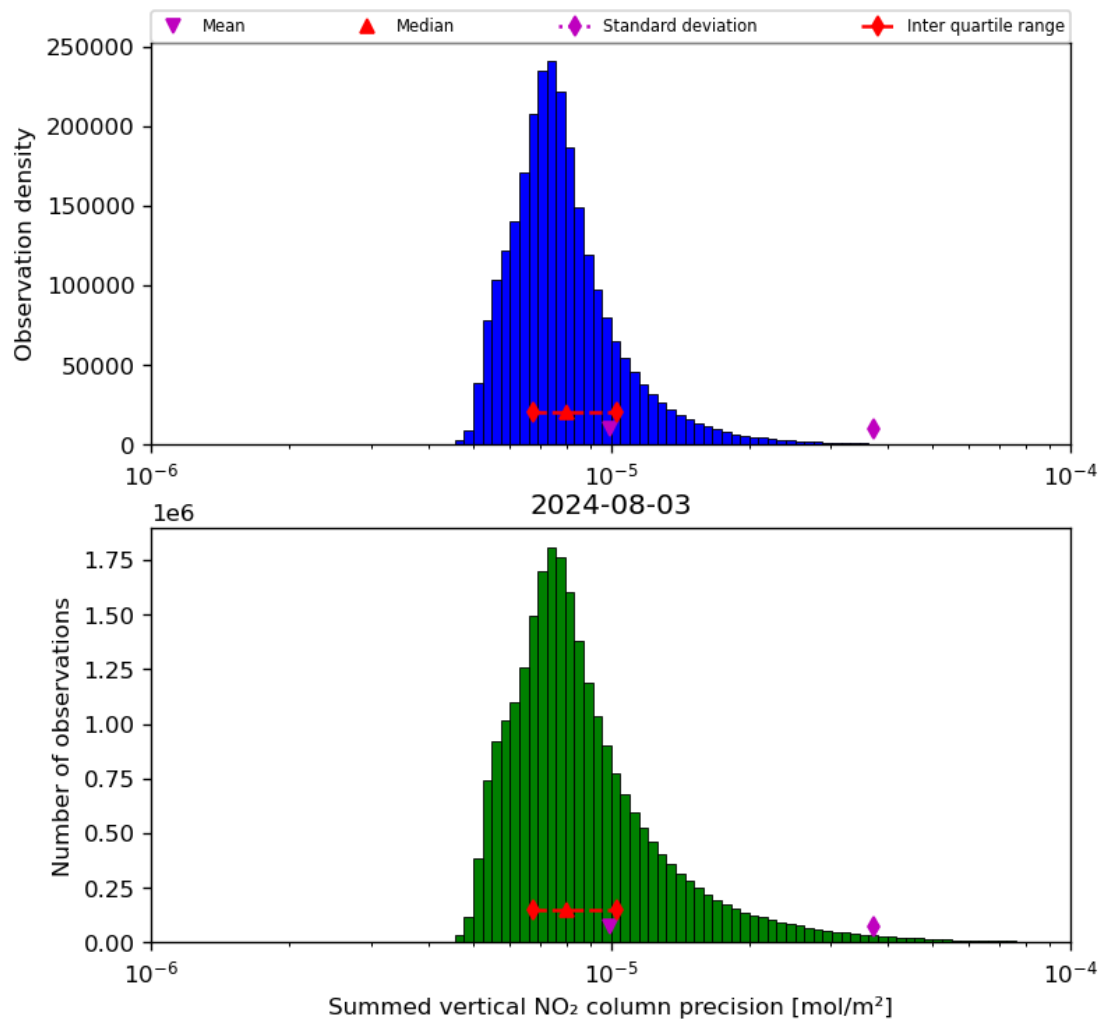
Figure 41: Histogram of "Summed vertical NO 2 column precision" for 2024-08-02 to 2024-08-04
