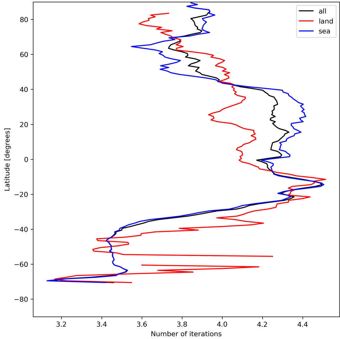
Figure 17: Zonal average of “Number of iterations” for 2024-08-02 to 2024-08-04.
