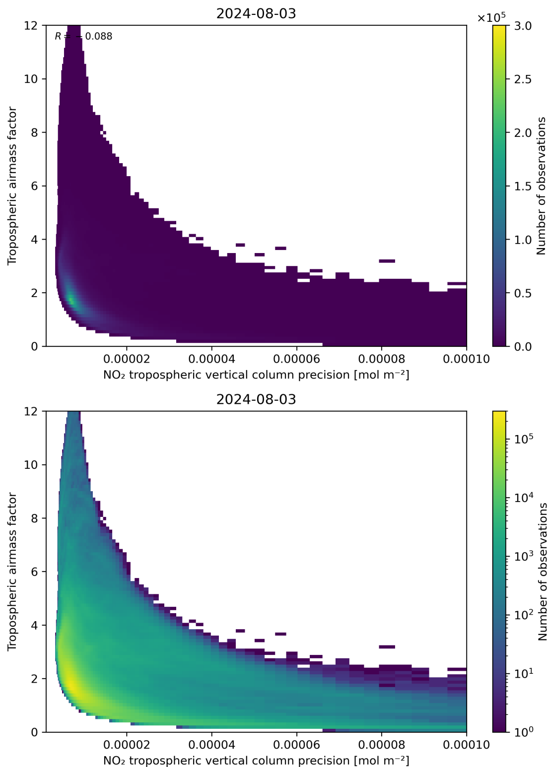
Figure 133: Scatter density plot of “NO 2 tropospheric vertical column precision” against “Tropospheric air mass factor” for 2024-08-02 to 2024-08-04.
