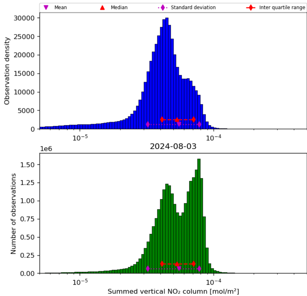
Figure 40: Histogram of "Summed vertical NO 2 column" for 2024-08-02 to 2024-08-04
