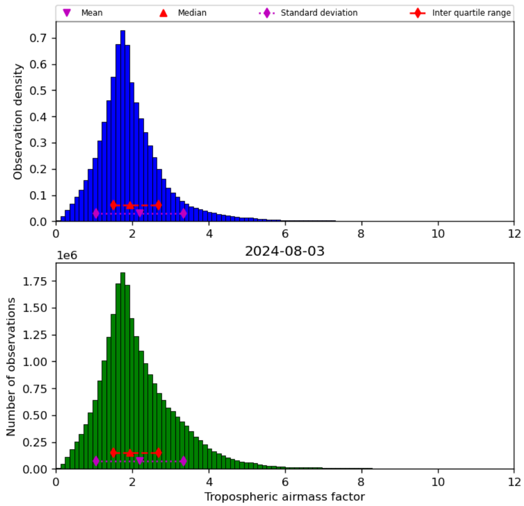
Figure 31: Histogram of “Tropospheric airmass factor” for 2024-08-02 to 2024-08-04
