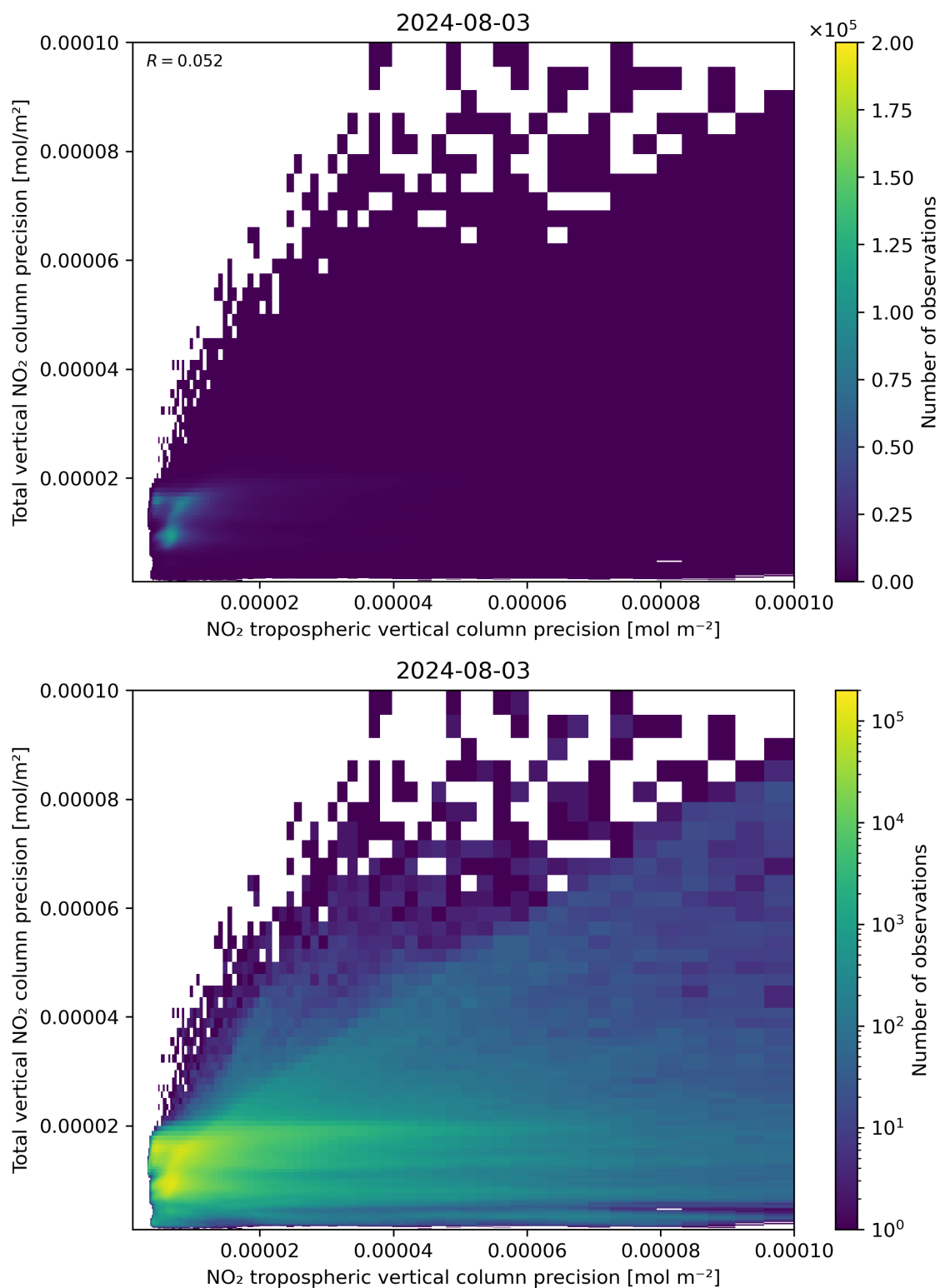
Figure 139: Scatter density plot of “NO 2 tropospheric vertical column precision” against “Total vertical NO 2 column precision” for 2024-08-02 to 2024-08-04.
