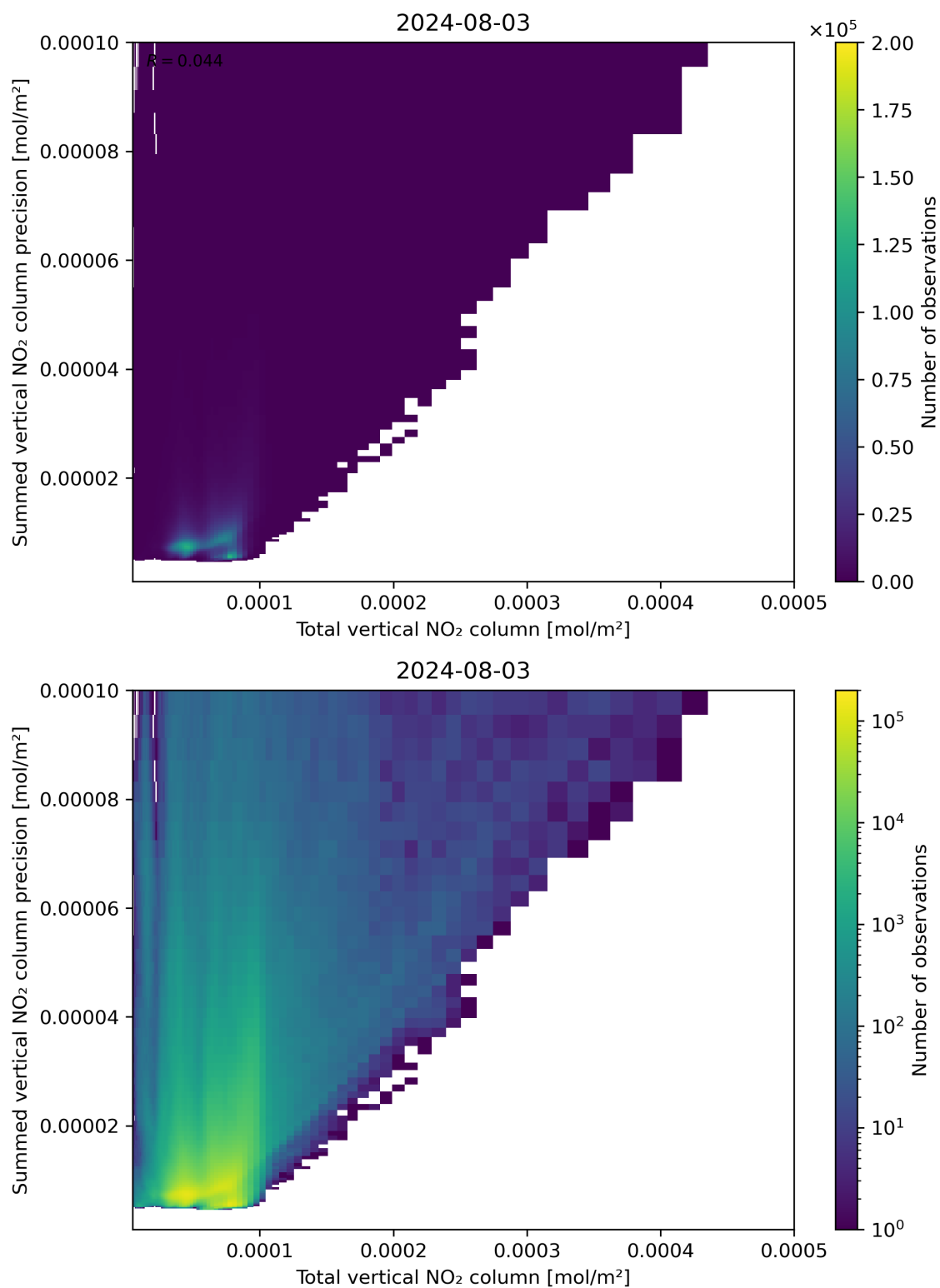
Figure 113: Scatter density plot of “Total vertical NO 2 column” against “Summed vertical NO 2 column precision” for 2024-08-02 to 2024-08-04.
