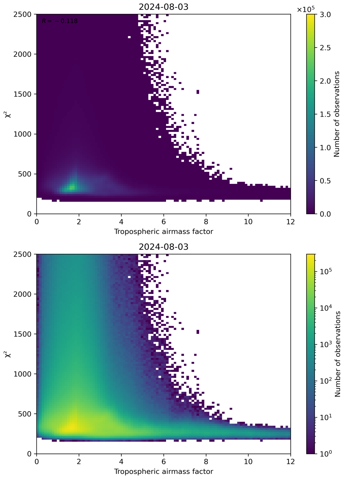
Figure 73: Scatter density plot of “Tropospheric airmass factor” against “ \chi^2 ” for 2024-08-02 to 2024-08-04.
