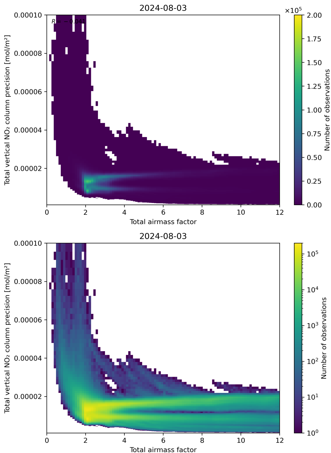
Figure 68: Scatter density plot of “Total airmass factor” against “Total vertical NO 2 column precision” for 2024-08-02 to 2024-08-04.
