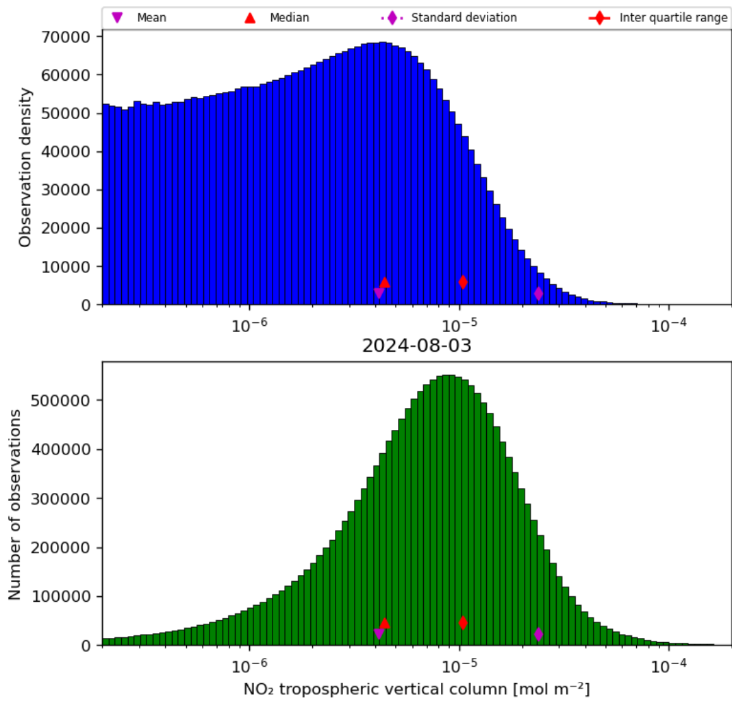
Figure 29: Histogram of “NO 2 tropospheric vertical column” for 2024-08-02 to 2024-08-04
