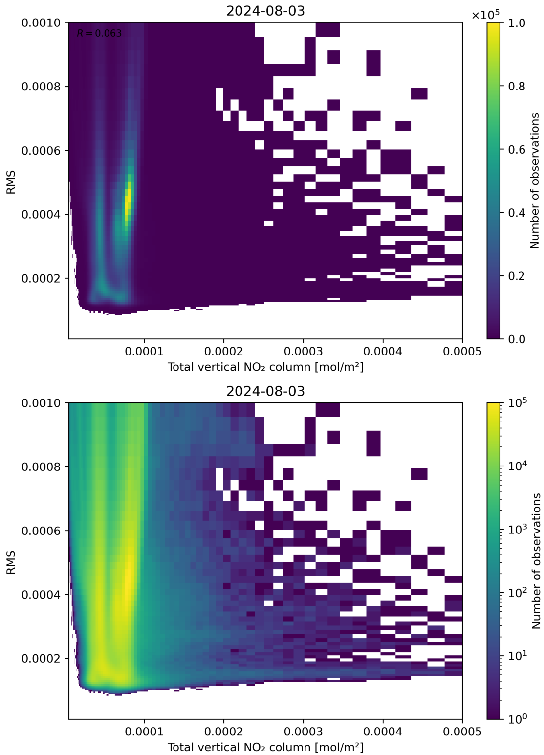
Figure 120: Scatter density plot of “Total vertical NO 2 column” against “RMS” for 2024-08-02 to 2024-08-04.
