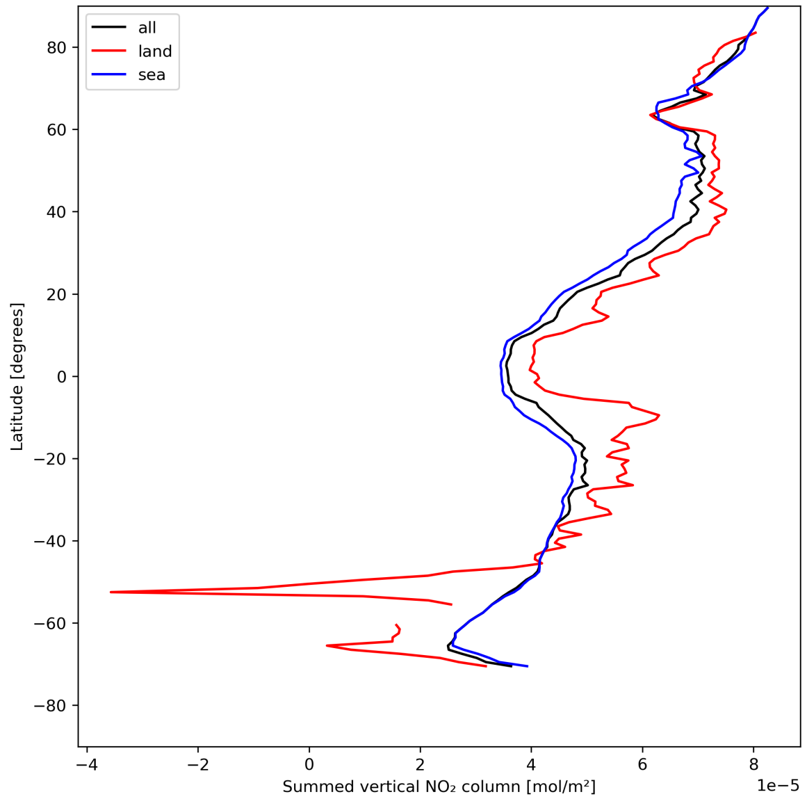
Figure 23: Zonal average of “Summed vertical NO 2 column” for 2024-08-02 to 2024-08-04.
