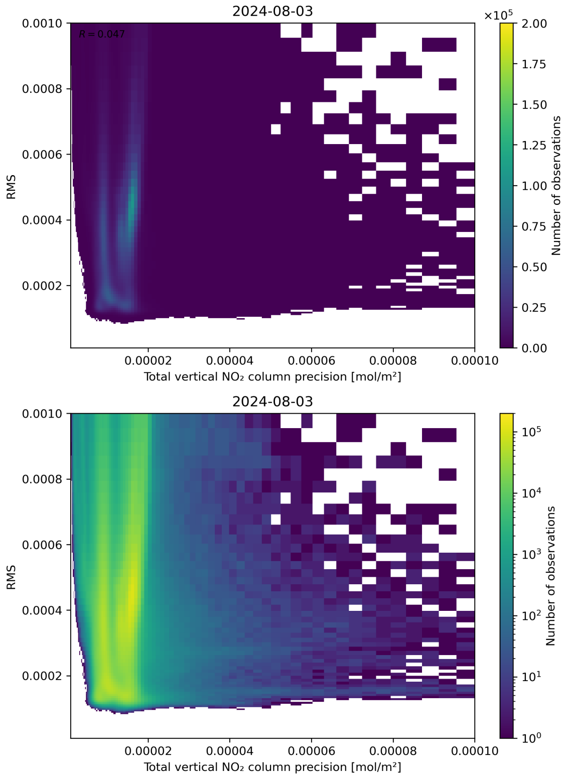
Figure 119: Scatter density plot of “Total vertical NO 2 column precision” against “RMS” for 2024-08-02 to 2024-08-04.
