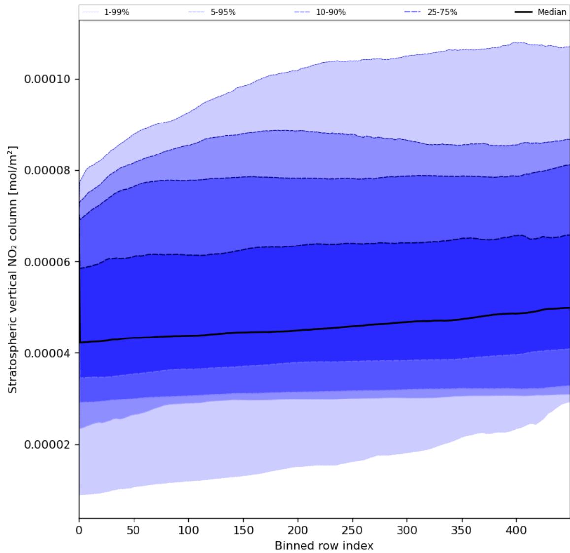
Figure 53: Along track statistics of “Stratospheric vertical NO 2 column” for 2024-08-02 to 2024-08-04
