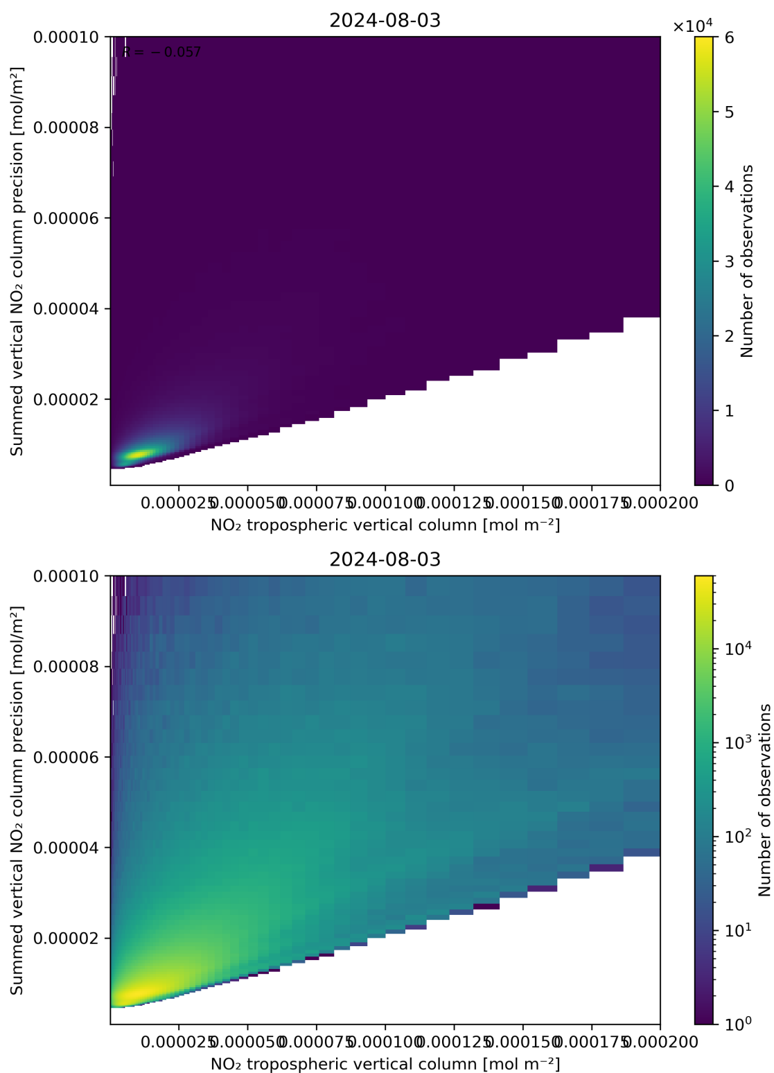
Figure 127: Scatter density plot of “NO 2 tropospheric vertical column” against “Summed vertical NO 2 column precision” for 2024-08-02 to 2024-08-04.
