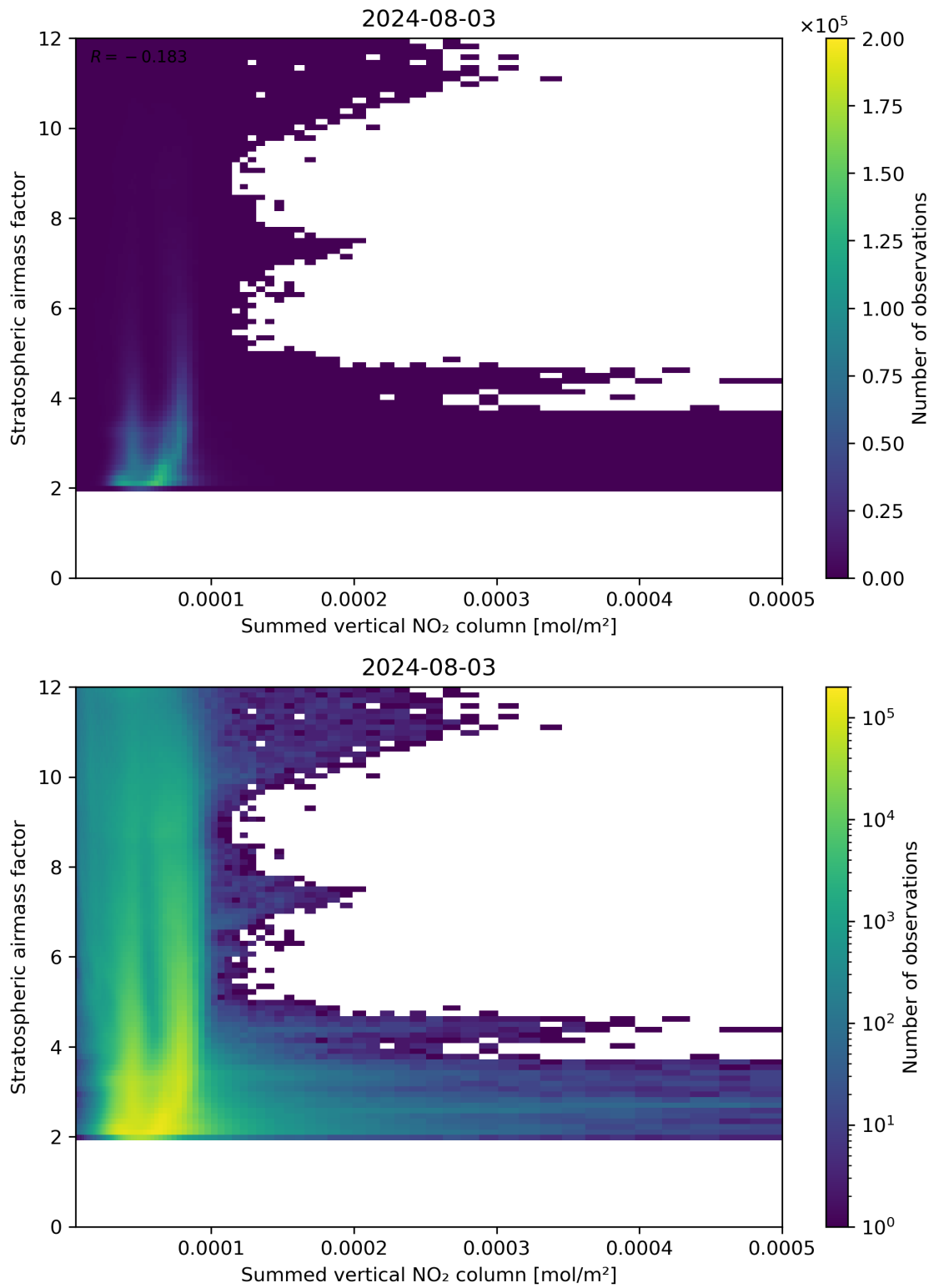
Figure 103: Scatter density plot of “Summed vertical NO 2 column” against “Stratospheric airmass factor” for 2024-08-02 to 2024-08-04.
