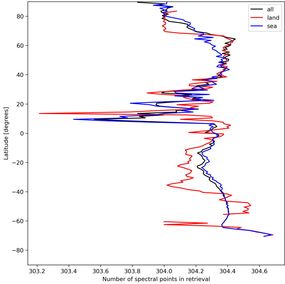
Figure 16: Zonal average of “Number of spectral points in retrieval” for 2024-08-02 to 2024-08-04.
