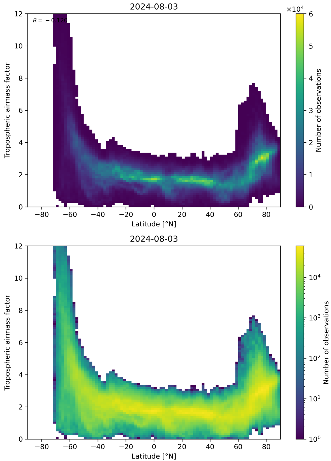
Figure 85: Scatter density plot of “Latitude” against “Tropospheric air mass factor” for 2024-08-02 to 2024-08-04.
