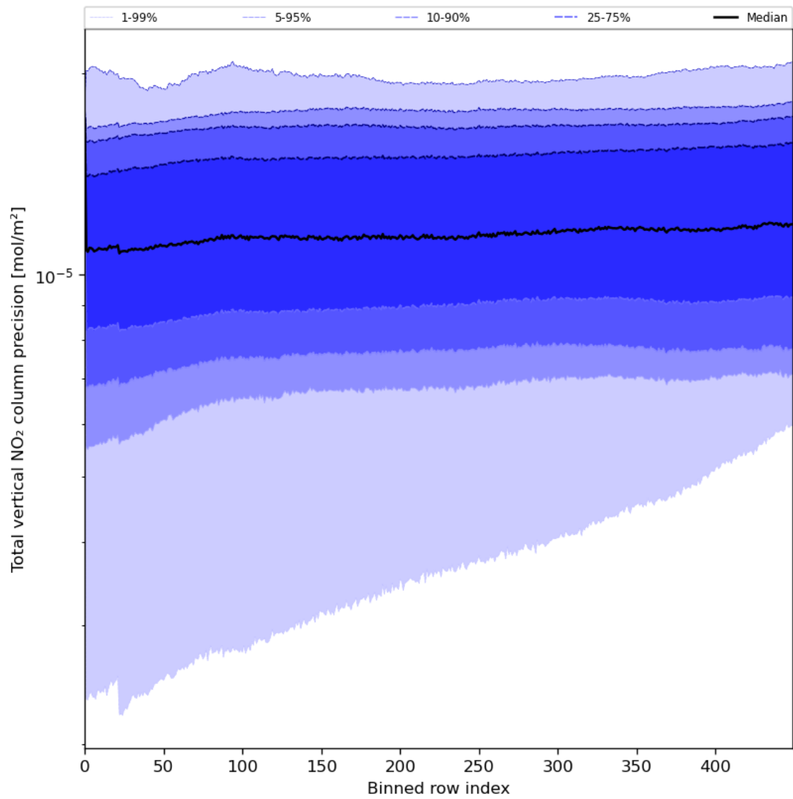
Figure 56: Along track statistics of “Total vertical NO 2 column precision” for 2024-08-02 to 2024-08-04
