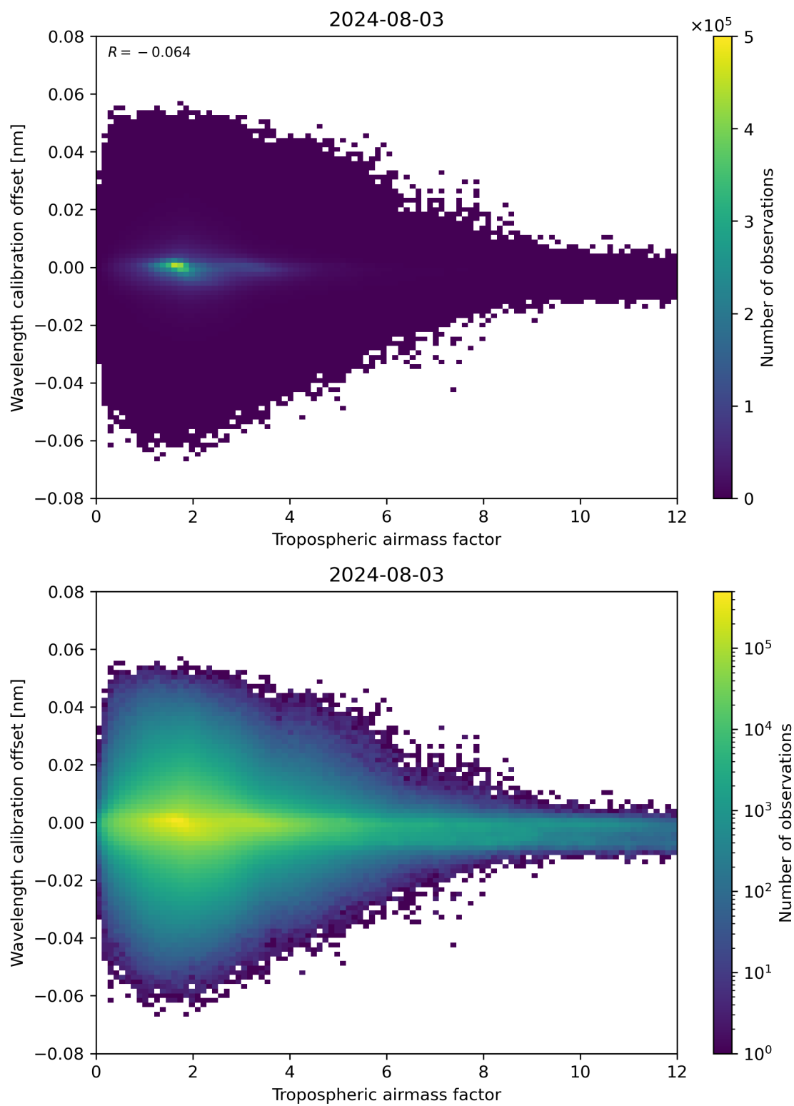
Figure 80: Scatter density plot of “Tropospheric air mass factor” against “Wavelength calibration offset” for 2024-08-02 to 2024-08-04.
