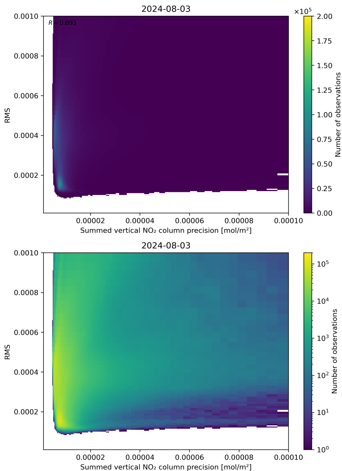
Figure 108: Scatter density plot of “Summed vertical NO 2 column precision” against “RMS” for 2024-08-02 to 2024-08-04.
