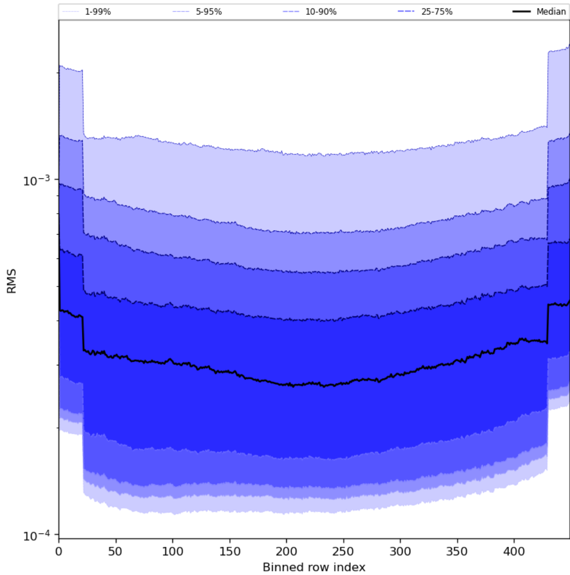
Figure 60: Along track statistics of “RMS” for 2024-08-02 to 2024-08-04
