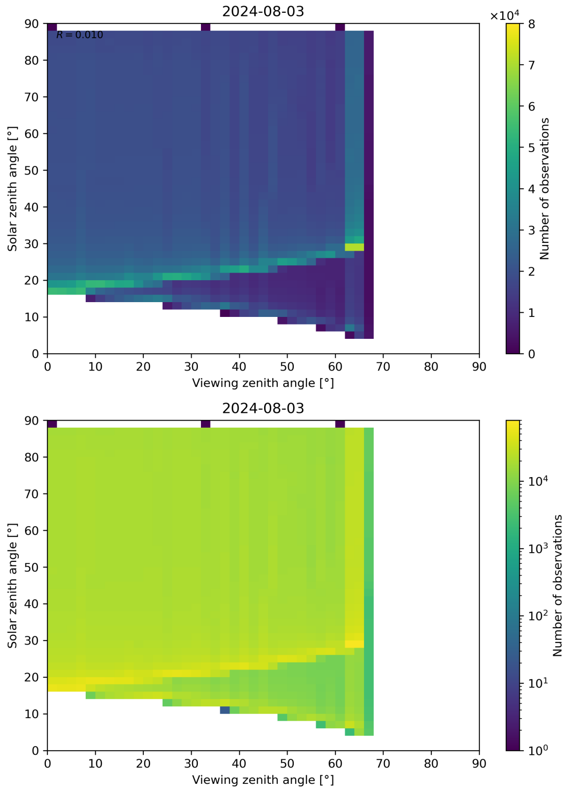
Figure 172: Scatter density plot of “Viewing zenith angle” against “Solar zenith angle” for 2024-08-02 to 2024-08-04.
