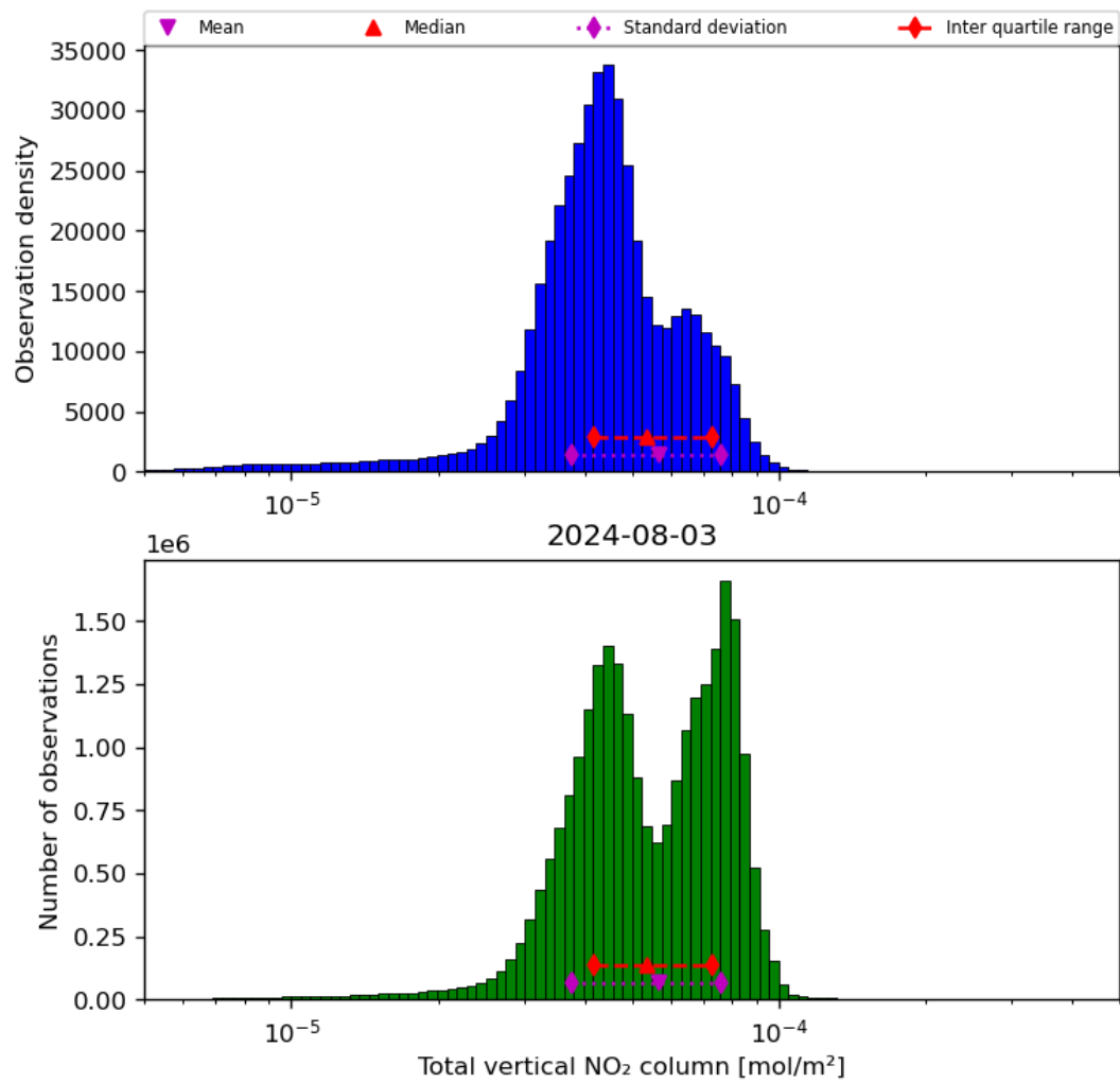
Figure 38: Histogram of “Total vertical NO 2 column” for 2024-08-02 to 2024-08-04
