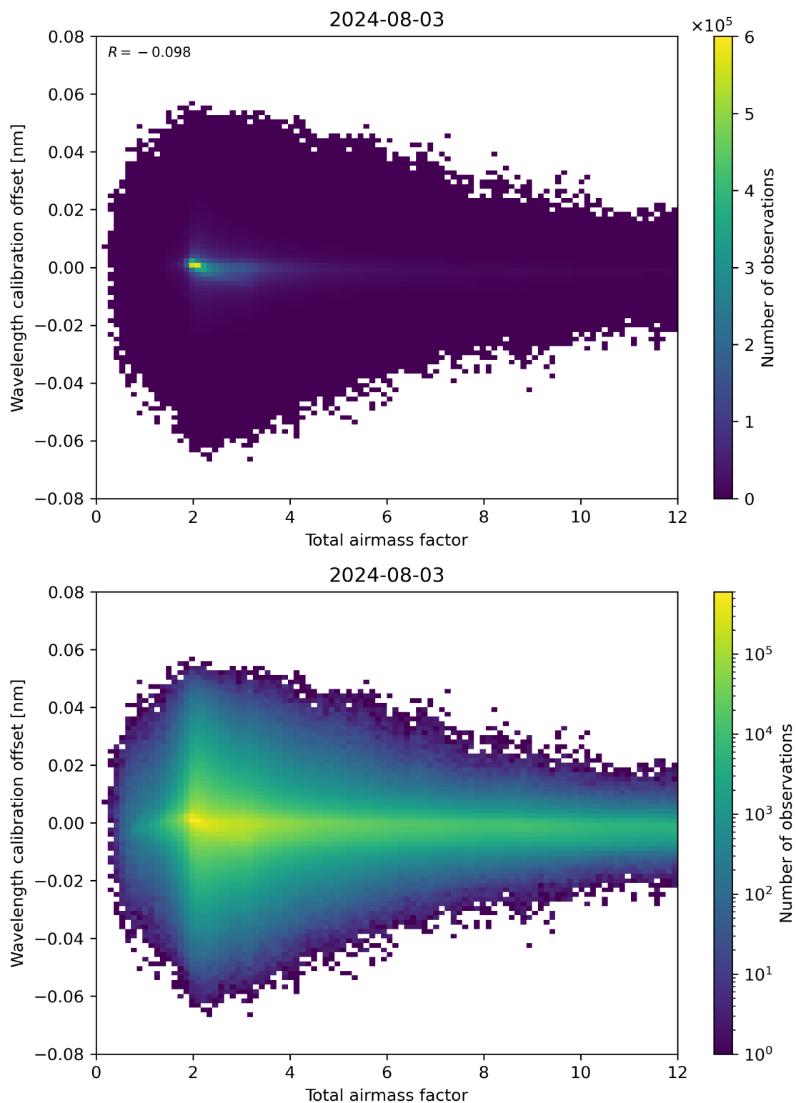
Figure 70: Scatter density plot of “Total airmass factor” against “Wavelength calibration offset” for 2024-08-02 to 2024-08-04.
