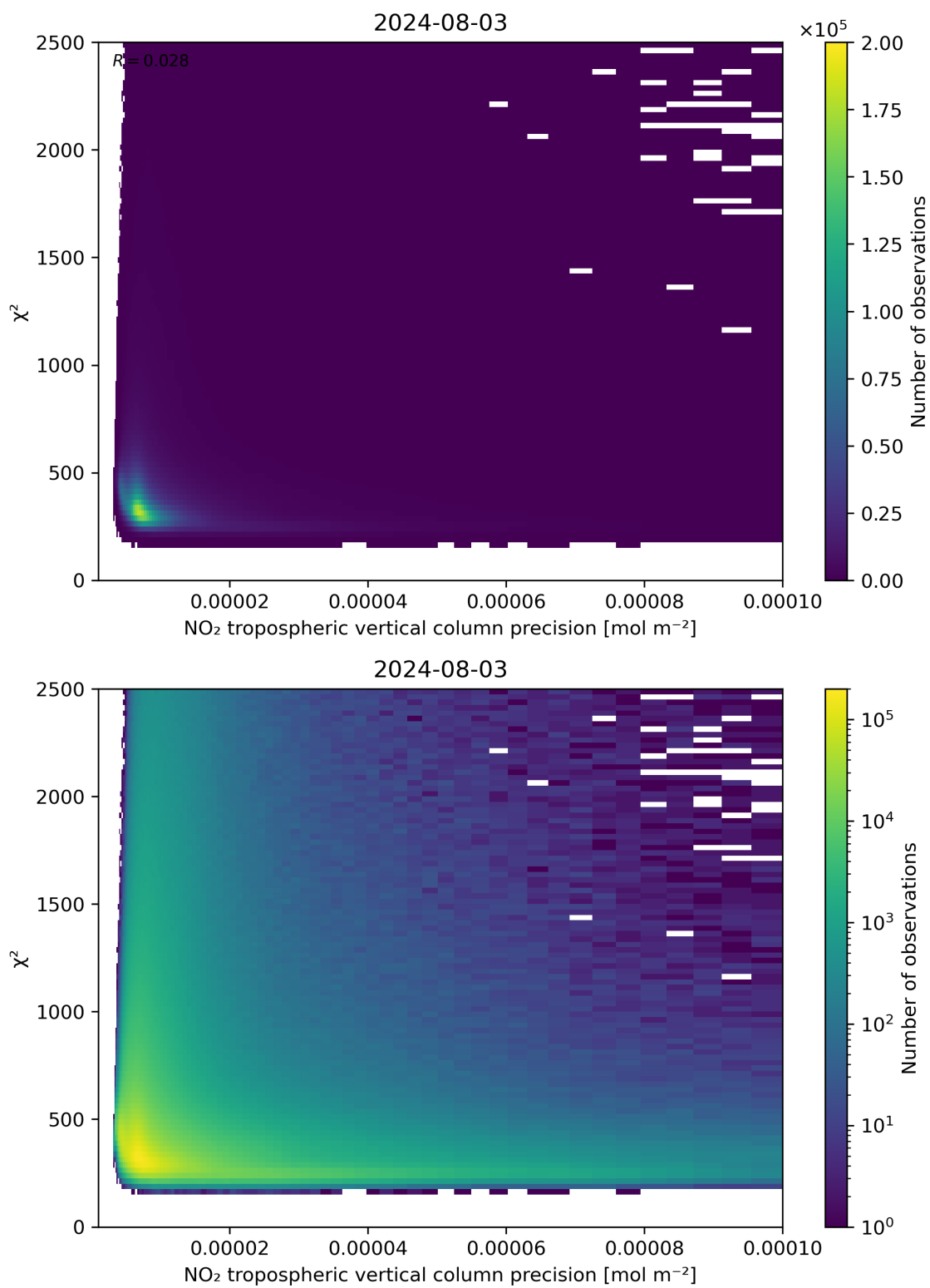
Figure 134: Scatter density plot of “NO 2 tropospheric vertical column precision” against “ \chi^2 ” for 2024-08-02 to 2024-08-04.
