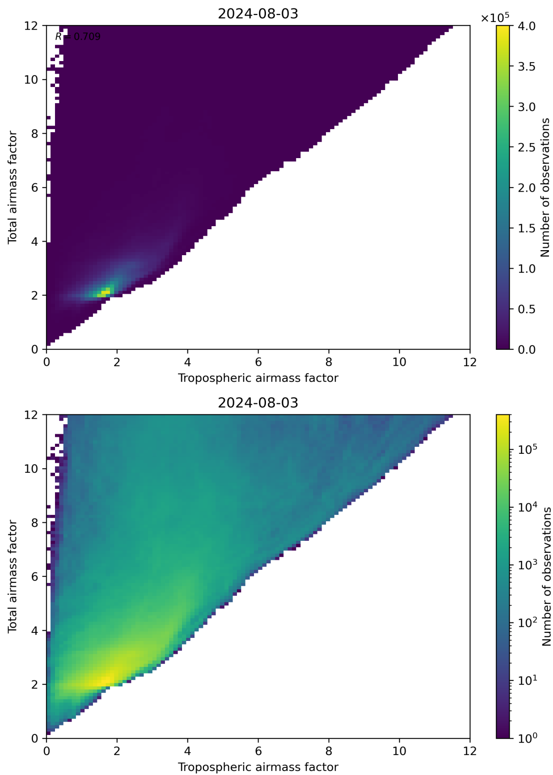
Figure 72: Scatter density plot of “Tropospheric airmass factor” against “Total airmass factor” for 2024-08-02 to 2024-08-04.
