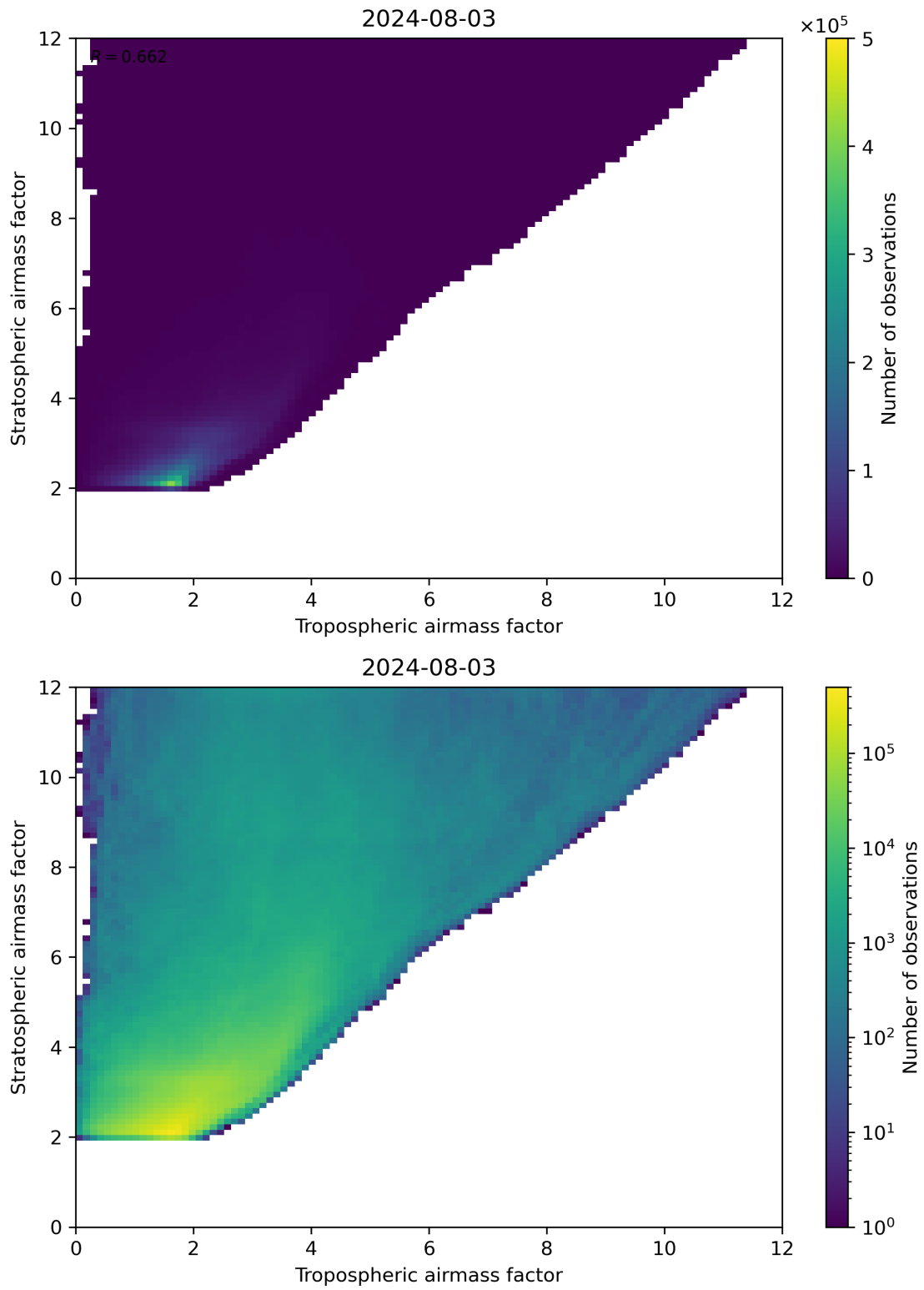
Figure 71: Scatter density plot of “Tropospheric airmass factor” against “Stratospheric airmass factor” for 2024-08-02 to 2024-08-04.
