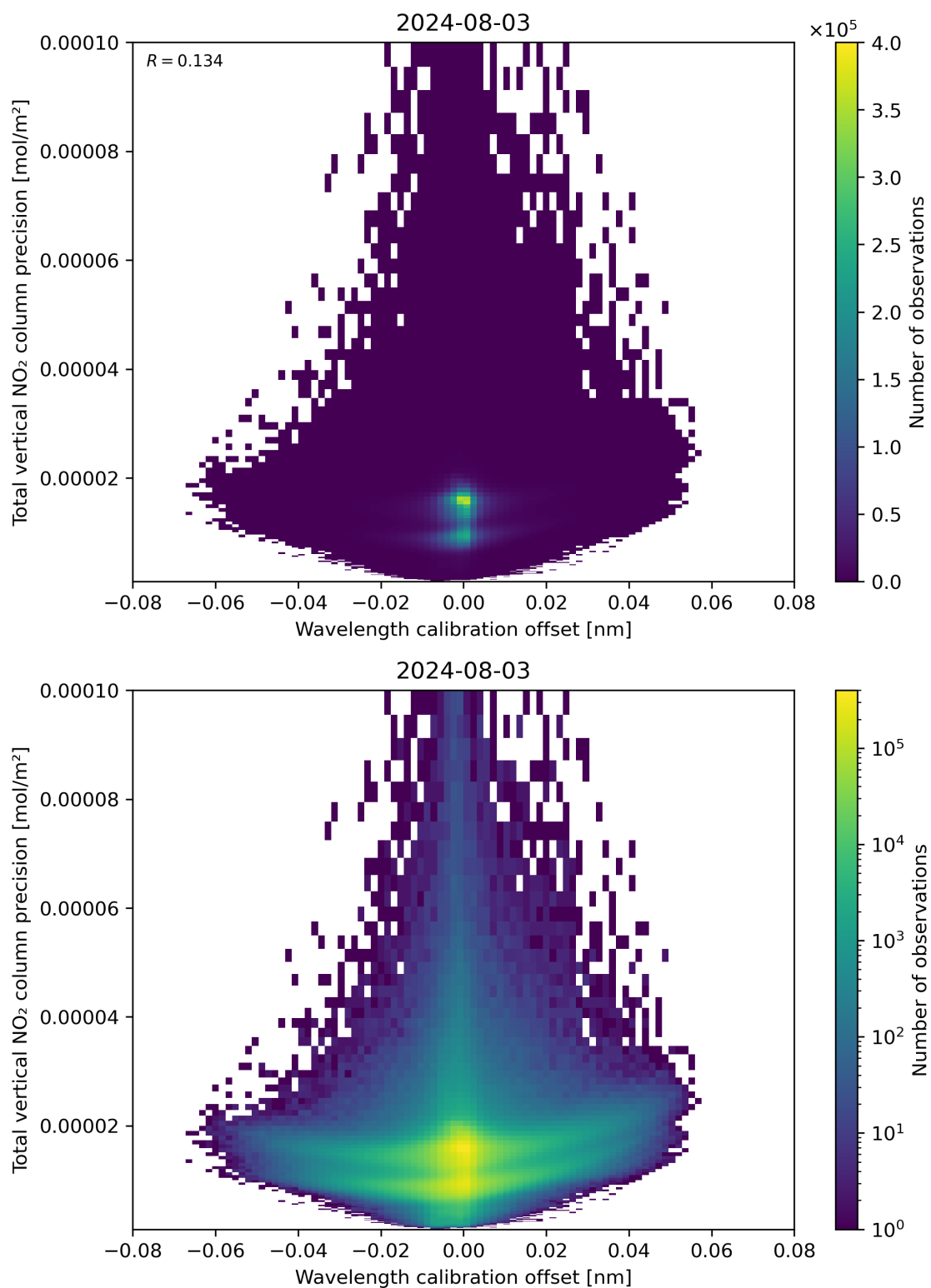
Figure 180: Scatter density plot of “Wavelength calibration offset” against “Total vertical NO 2 column precision” for 2024-08-02 to 2024-08-04.
