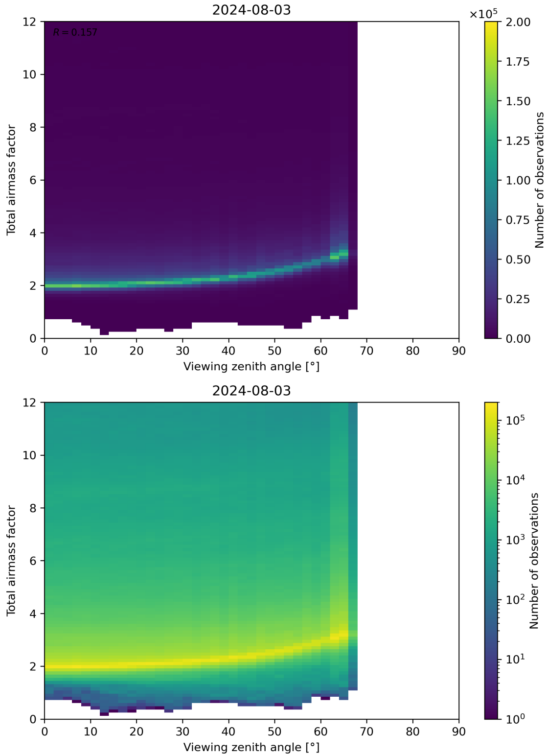
Figure 160: Scatter density plot of “Viewing zenith angle” against “Total airmass factor” for 2024-08-02 to 2024-08-04.
