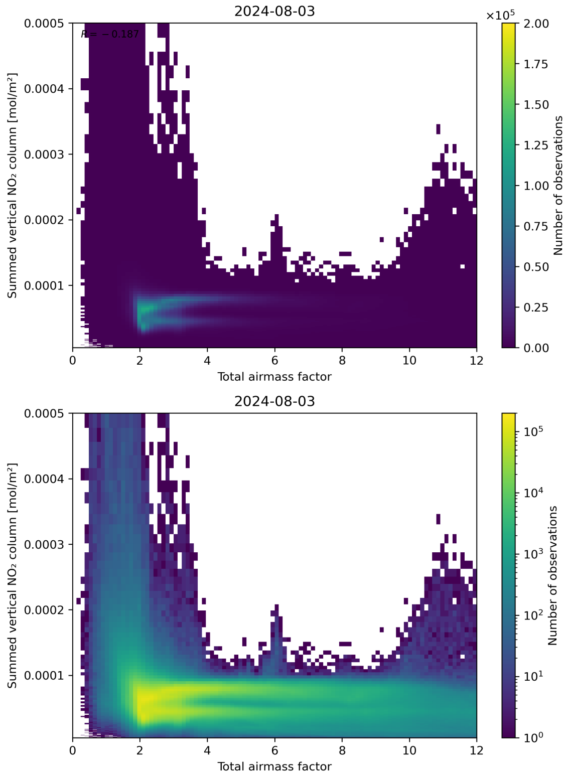
Figure 65: Scatter density plot of “Total airmass factor” against “Summed vertical NO 2 column” for 2024-08-02 to 2024-08-04.
