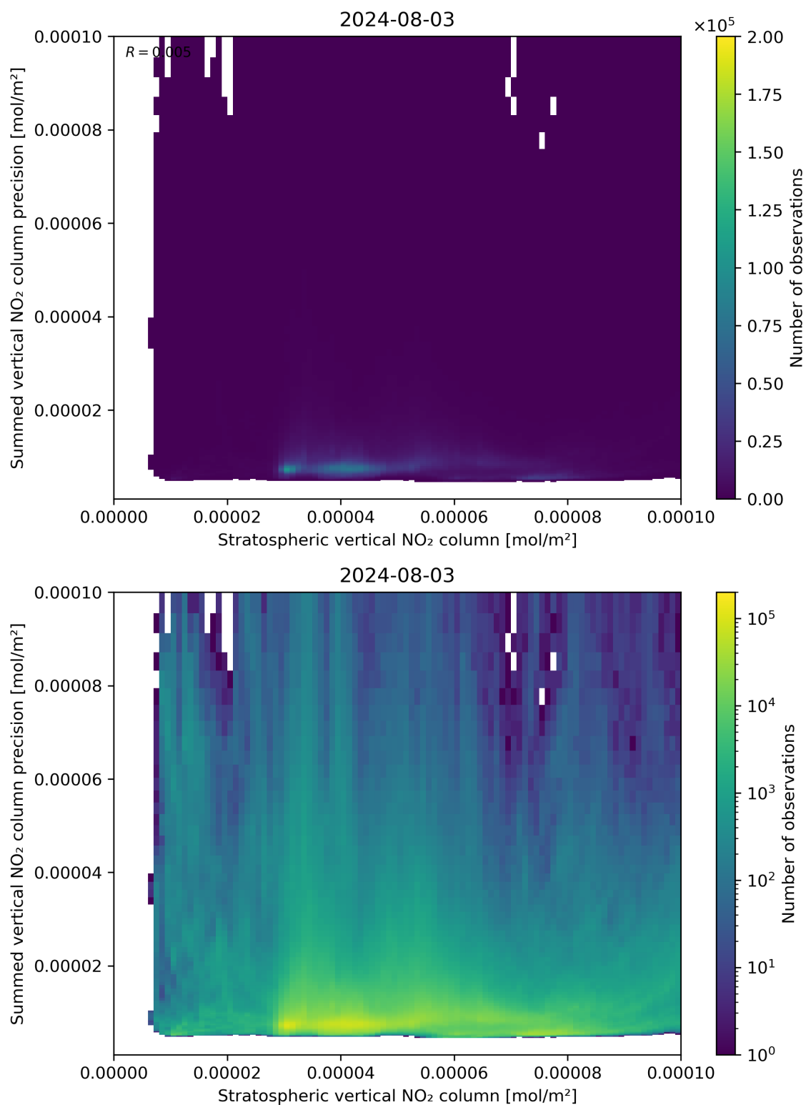
Figure 99: Scatter density plot of “Stratospheric vertical NO 2 column” against “Summed vertical NO 2 column precision” for 2024-08-02 to 2024-08-04.
