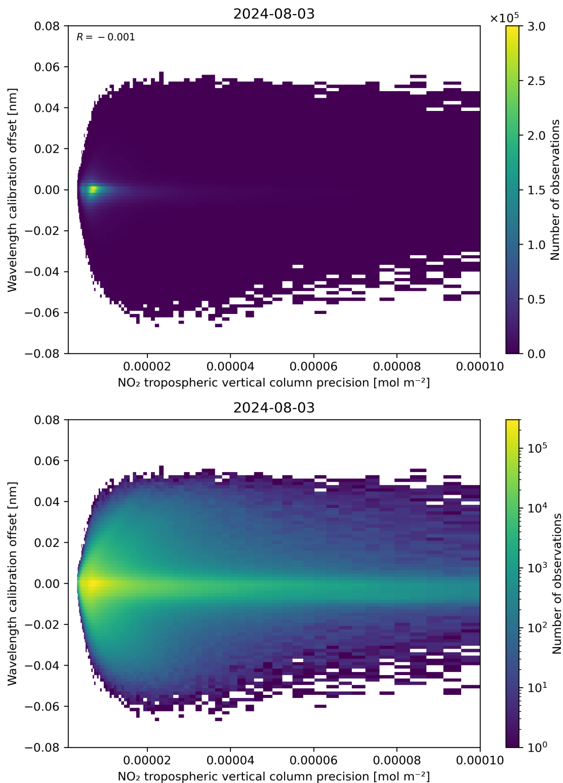
Figure 141: Scatter density plot of “NO 2 tropospheric vertical column precision” against “Wavelength calibration offset” for 2024-08-02 to 2024-08-04.
