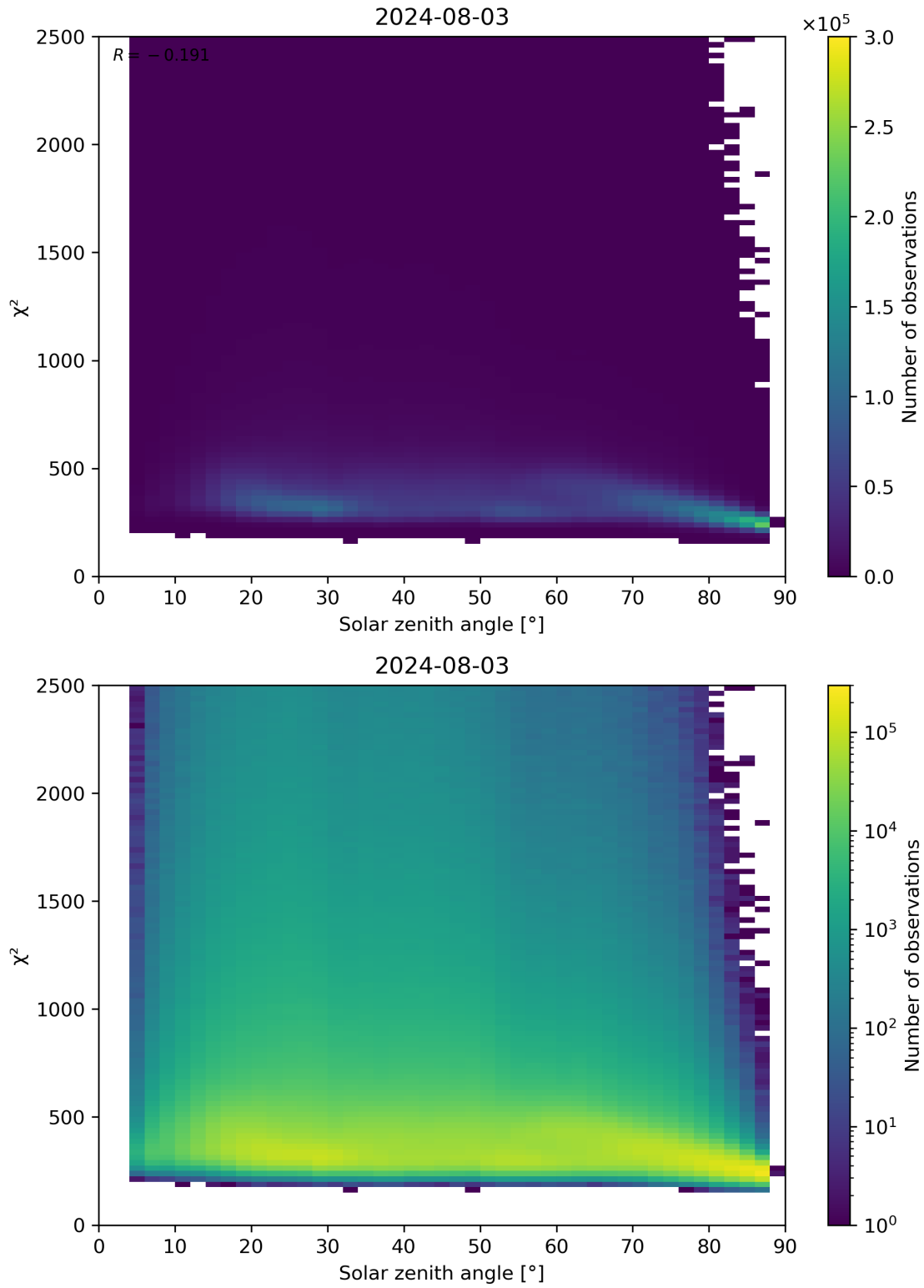
Figure 148: Scatter density plot of “Solar zenith angle” against “ \chi^2 ” for 2024-08-02 to 2024-08-04.
