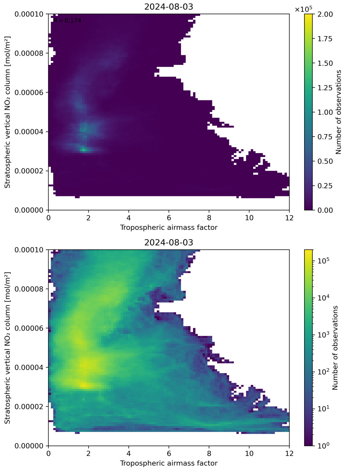
Figure 74: Scatter density plot of “Tropospheric air mass factor” against “Stratospheric vertical NO 2 column” for 2024-08-02 to 2024-08-04.
