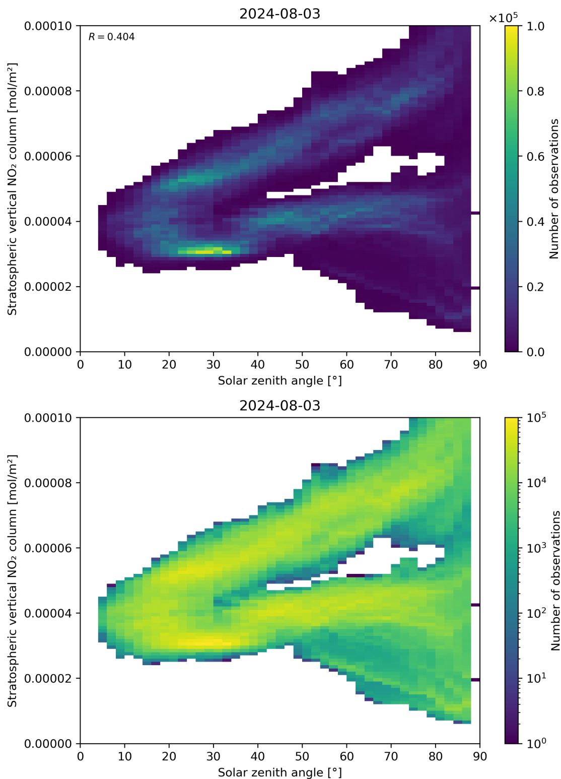
Figure 150: Scatter density plot of “Solar zenith angle” against “Stratospheric vertical NO 2 column” for 2024-08-02 to 2024-08-04.
