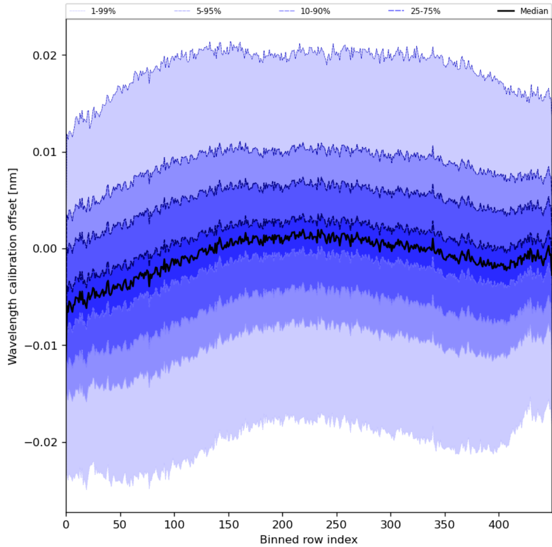
Figure 52: Along track statistics of “Wavelength calibration offset” for 2024-08-02 to 2024-08-04
