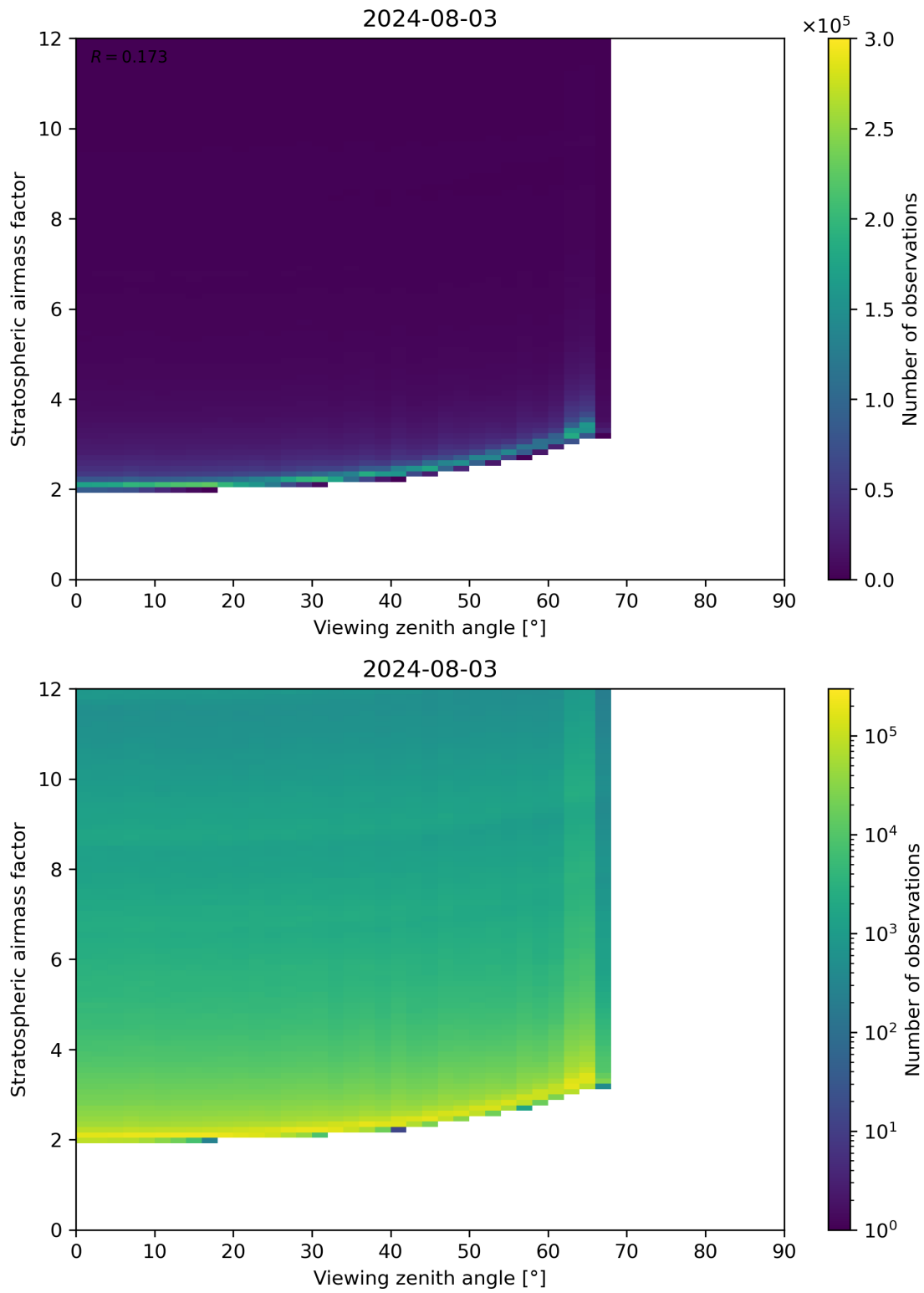
Figure 159: Scatter density plot of “Viewing zenith angle” against “Stratospheric airmass factor” for 2024-08-02 to 2024-08-04.
