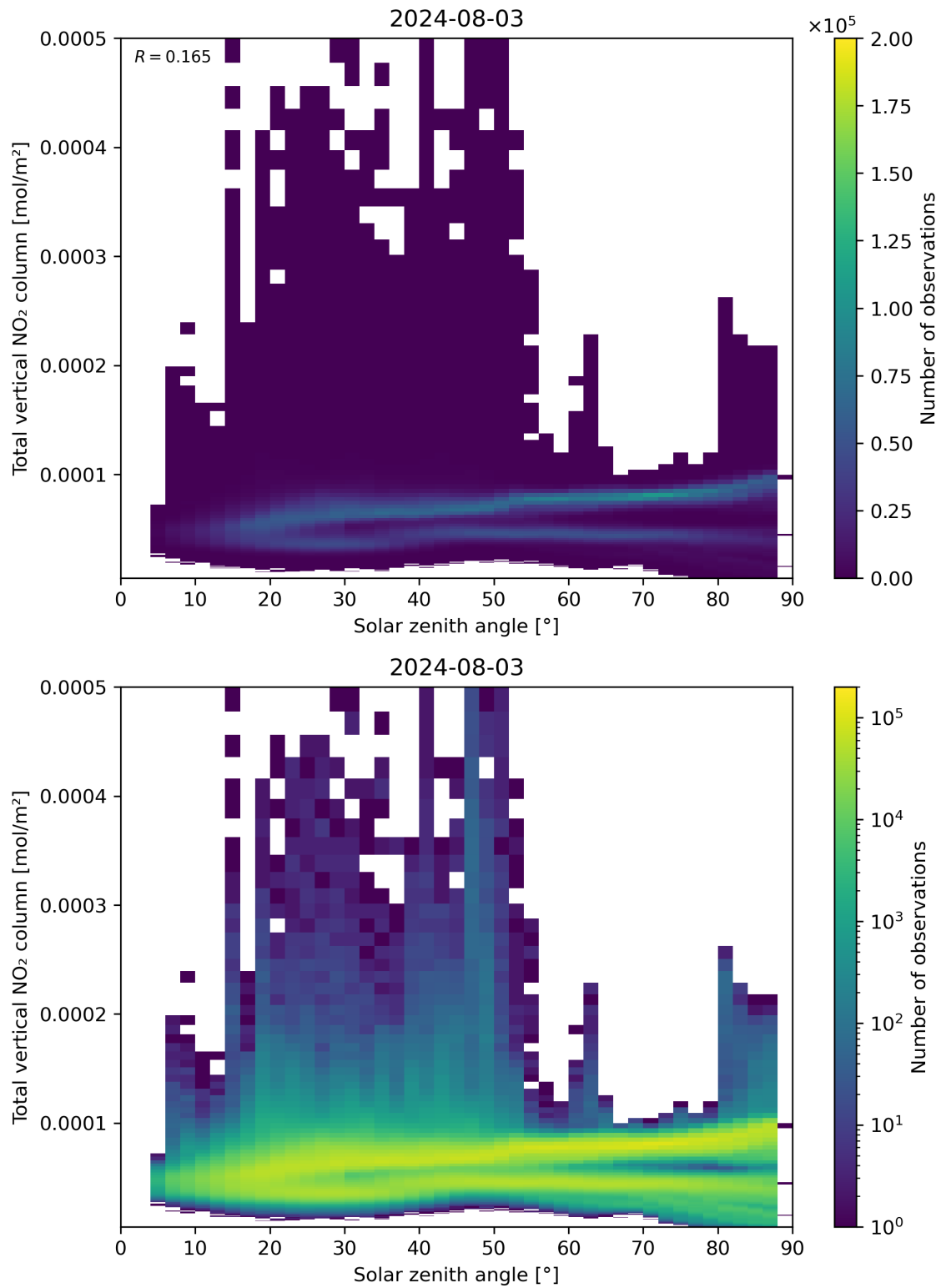
Figure 153: Scatter density plot of “Solar zenith angle” against “Total vertical NO 2 column” for 2024-08-02 to 2024-08-04.
