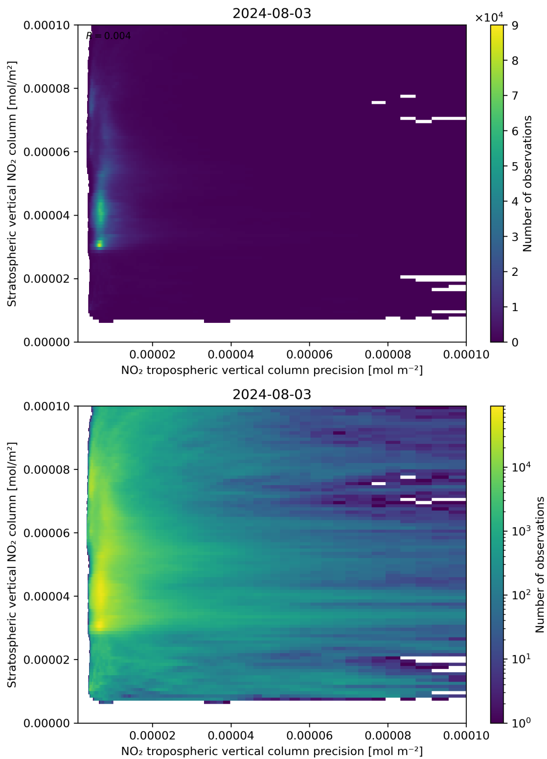
Figure 135: Scatter density plot of “NO 2 tropospheric vertical column precision” against “Stratospheric vertical NO 2 column” for 2024-08-02 to 2024-08-04.
