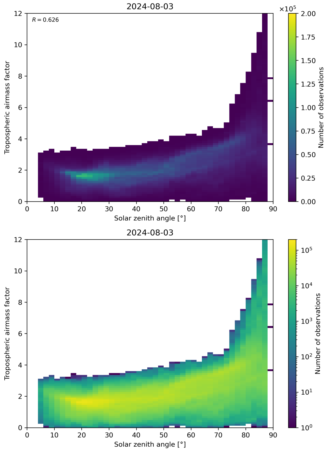
Figure 147: Scatter density plot of “Solar zenith angle” against “Tropospheric airmass factor” for 2024-08-02 to 2024-08-04.
