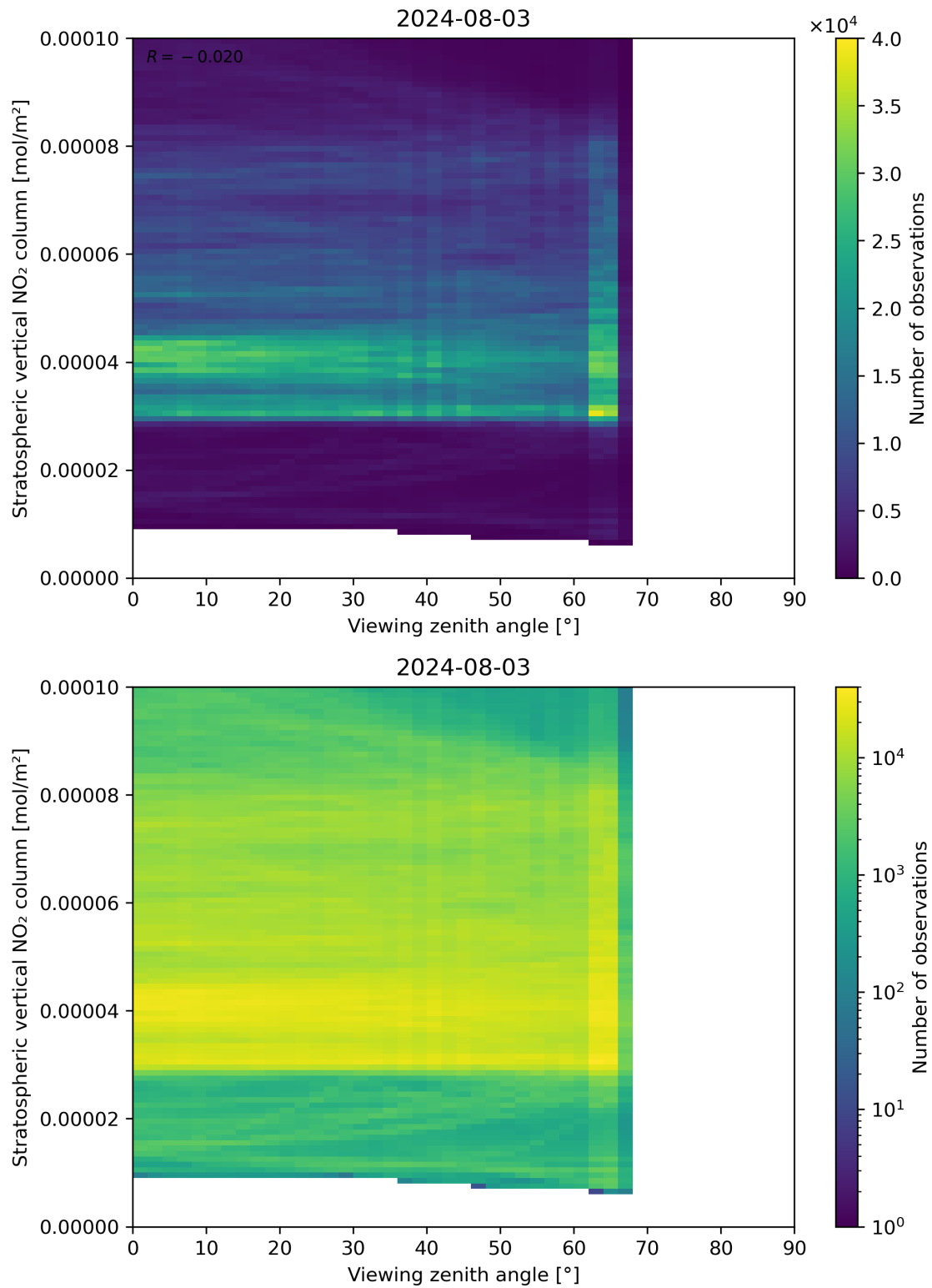
Figure 164: Scatter density plot of “Viewing zenith angle” against “Stratospheric vertical NO 2 column” for 2024-08-02 to 2024-08-04.
