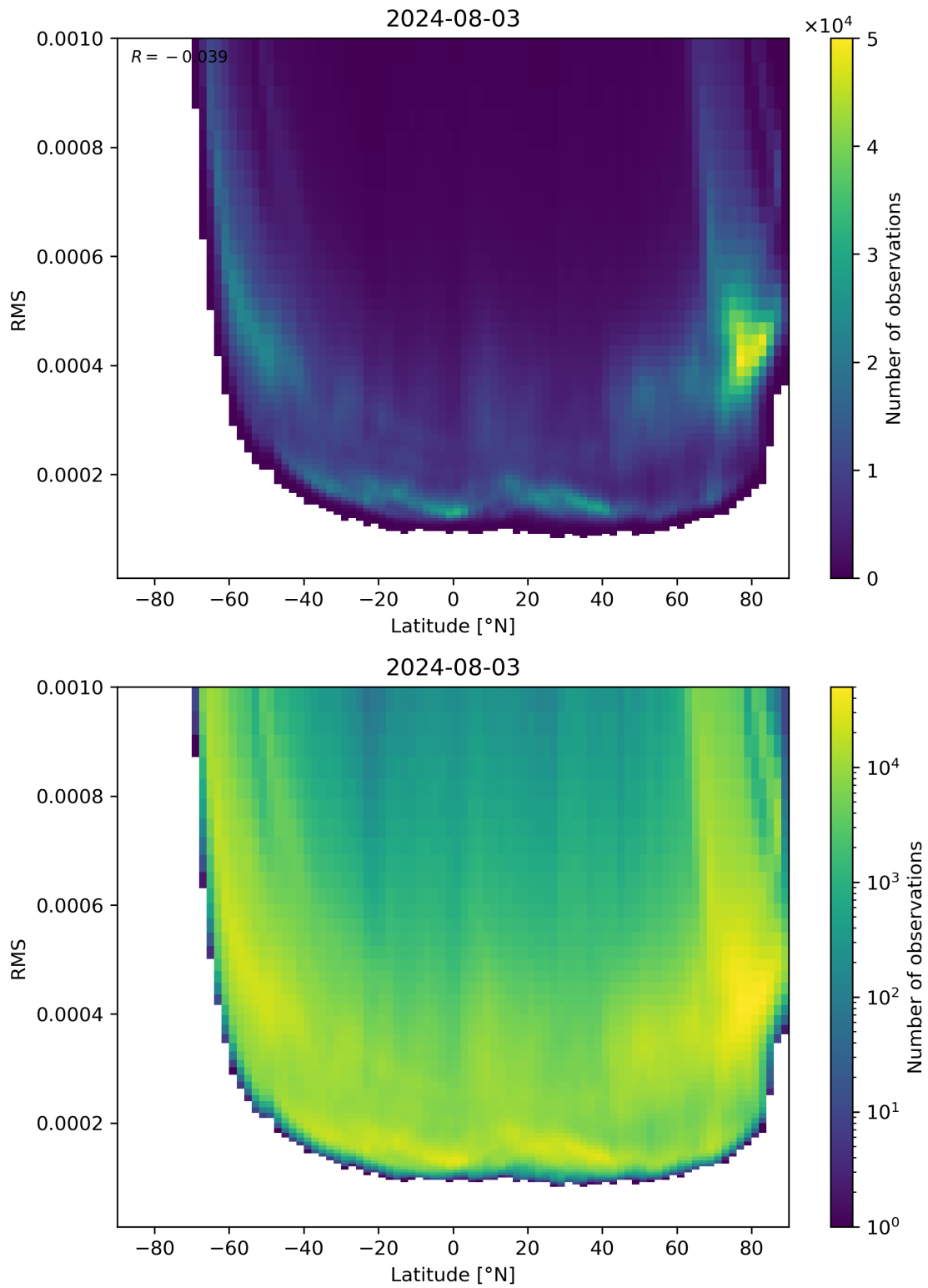
Figure 94: Scatter density plot of “Latitude” against “RMS” for 2024-08-02 to 2024-08-04.
