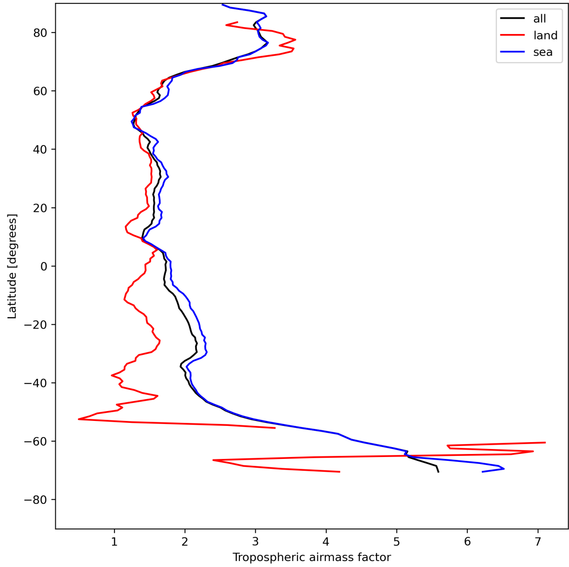
Figure 14: Zonal average of “Tropospheric airmass factor” for 2024-08-02 to 2024-08-04.
