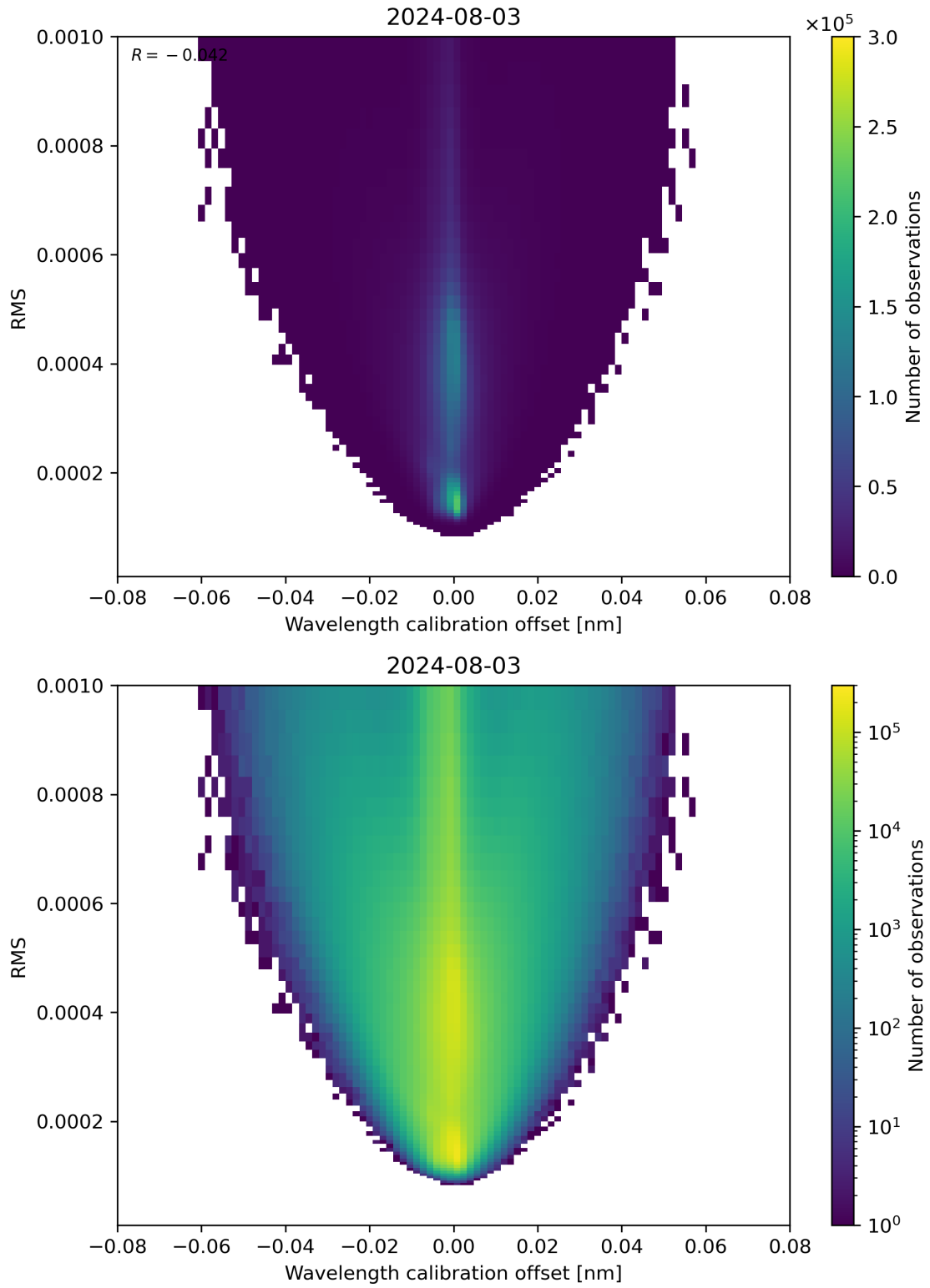
Figure 181: Scatter density plot of “Wavelength calibration offset” against “RMS” for 2024-08-02 to 2024-08-04.
