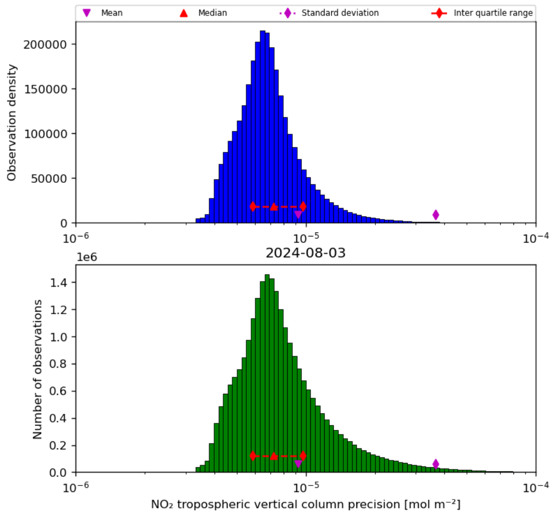
Figure 30: Histogram of “NO 2 tropospheric vertical column precision” for 2024-08-02 to 2024-08-04
