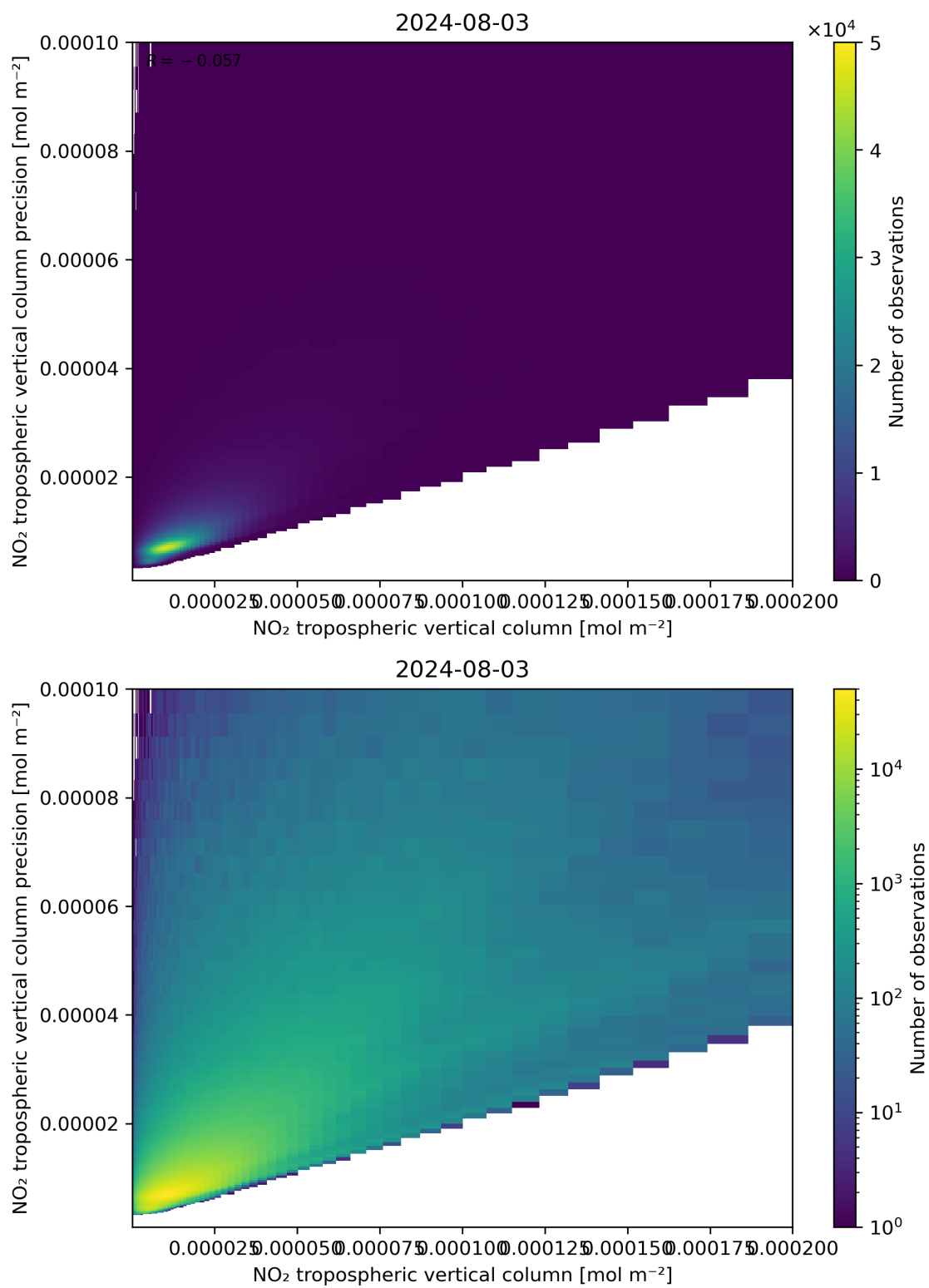
Figure 130: Scatter density plot of “NO 2 tropospheric vertical column” against “NO 2 tropospheric vertical column precision” for 2024-08-02 to 2024-08-04.
