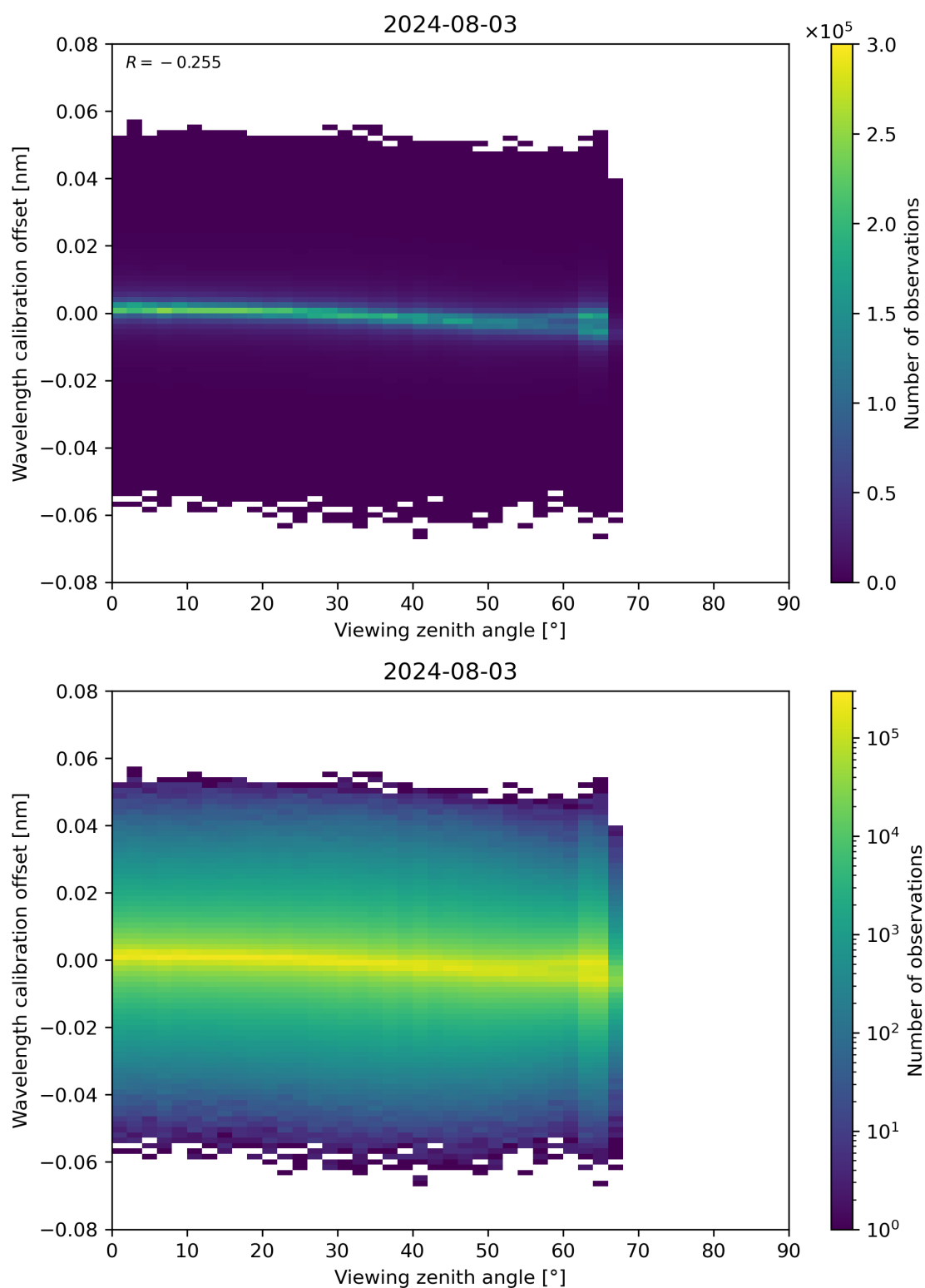
Figure 173: Scatter density plot of “Viewing zenith angle” against “Wavelength calibration offset” for 2024-08-02 to 2024-08-04.
