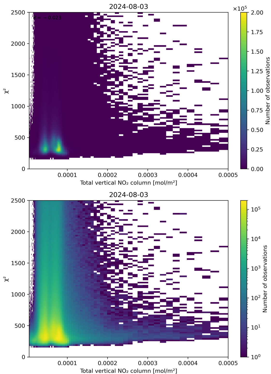
Figure 111: Scatter density plot of “Total vertical NO 2 column” against “ \chi^2 ” for 2024-08-02 to 2024-08-04.
