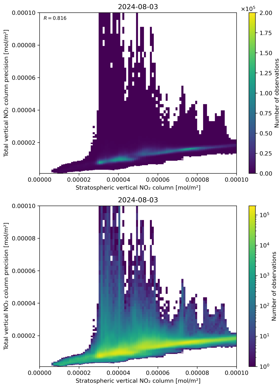
Figure 101: Scatter density plot of “Stratospheric vertical NO 2 column” against “Total vertical NO 2 column precision” for 2024-08-02 to 2024-08-04.
