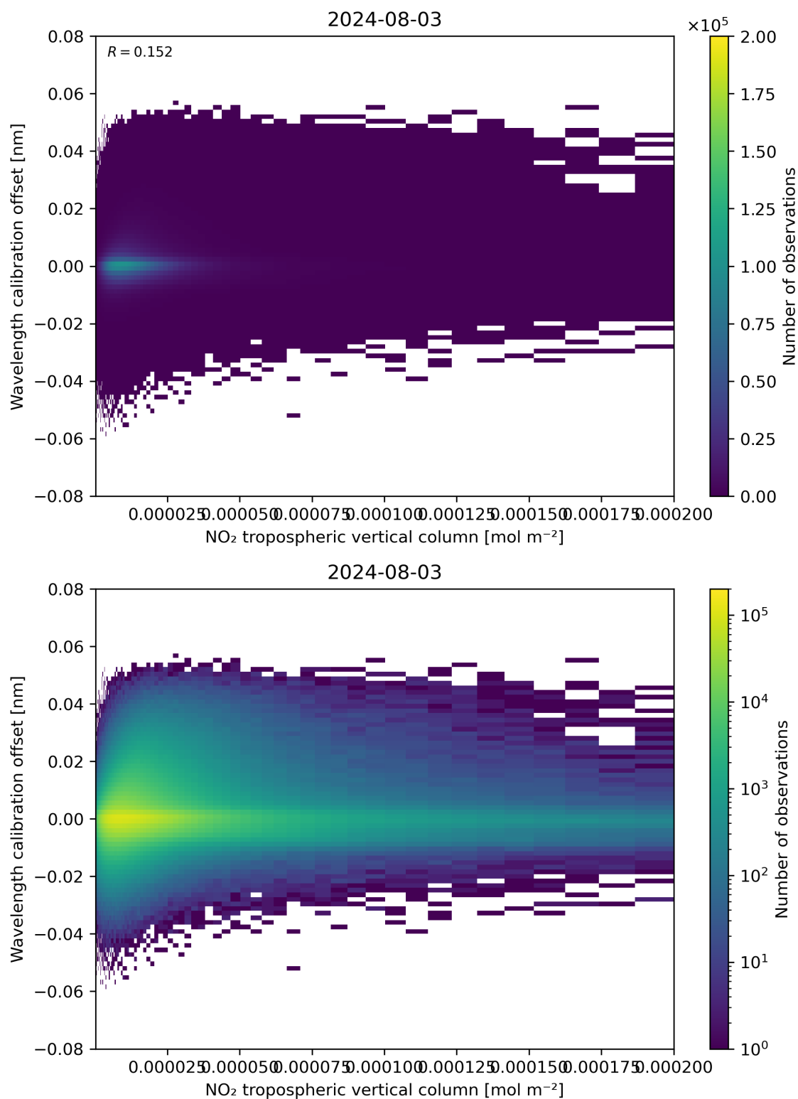
Figure 143: Scatter density plot of “NO 2 tropospheric vertical column” against “Wavelength calibration offset” for 2024-08-02 to 2024-08-04.
