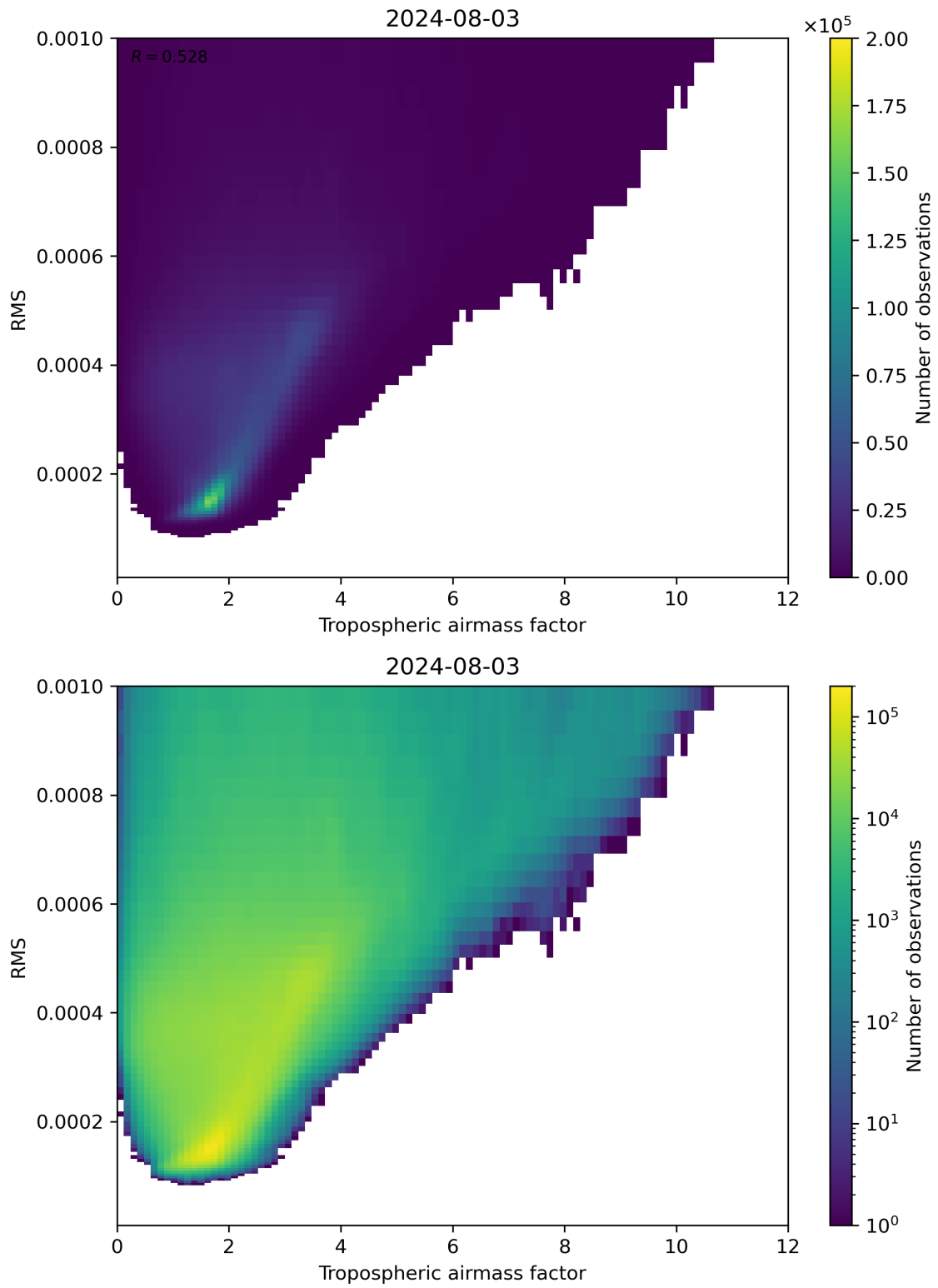
Figure 79: Scatter density plot of “Tropospheric airmass factor” against “RMS” for 2024-08-02 to 2024-08-04.
