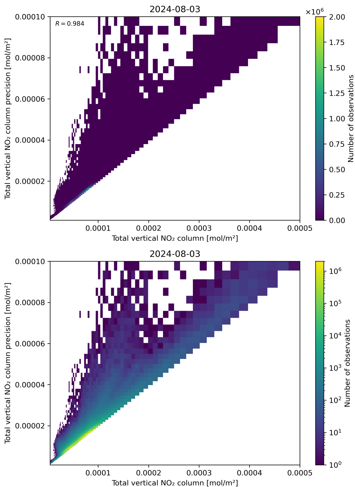
Figure 114: Scatter density plot of “Total vertical NO 2 column” against “Total vertical NO 2 column precision” for 2024-08-02 to 2024-08-04.
