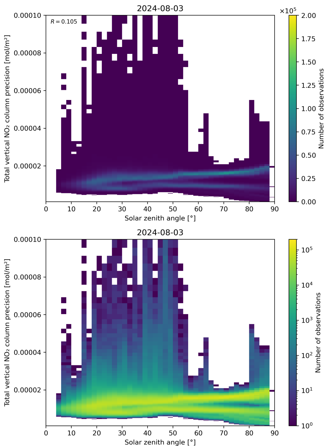
Figure 154: Scatter density plot of “Solar zenith angle” against “Total vertical NO 2 column precision” for 2024-08-02 to 2024-08-04.
