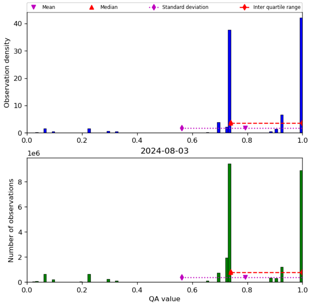
Figure 28: Histogram of “QA value” for 2024-08-02 to 2024-08-04
