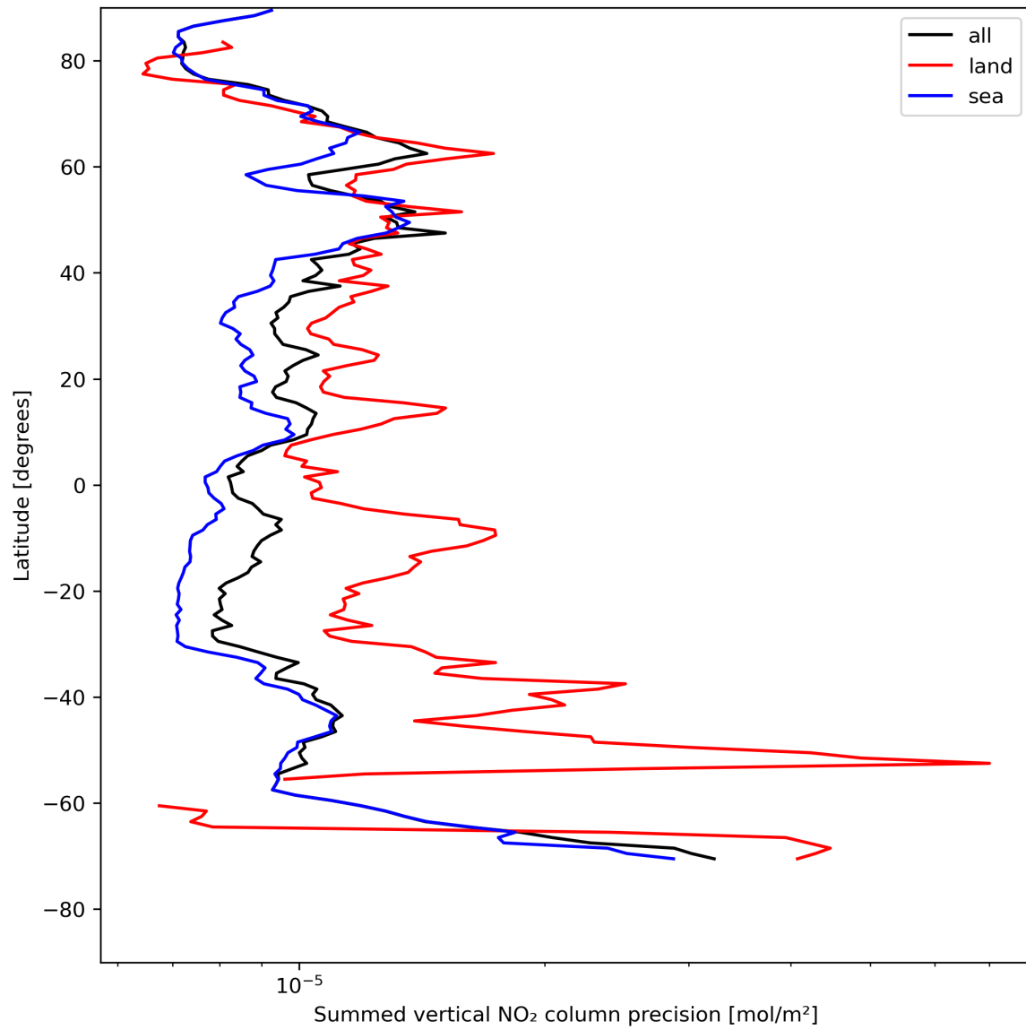
Figure 24: Zonal average of “Summed vertical NO 2 column precision” for 2024-08-02 to 2024-08-04.
