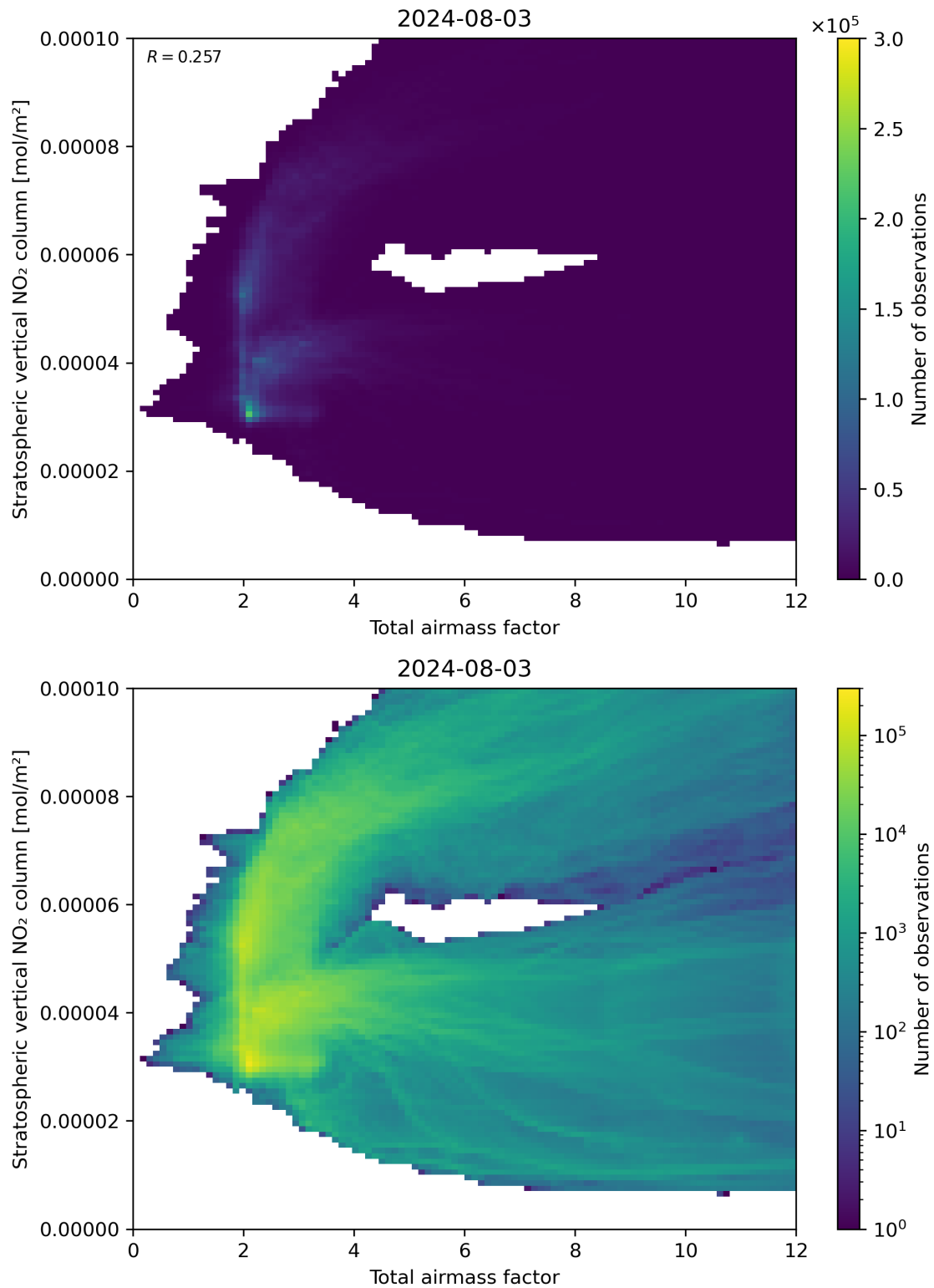
Figure 64: Scatter density plot of “Total airmass factor” against “Stratospheric vertical NO 2 column” for 2024-08-02 to 2024-08-04.
