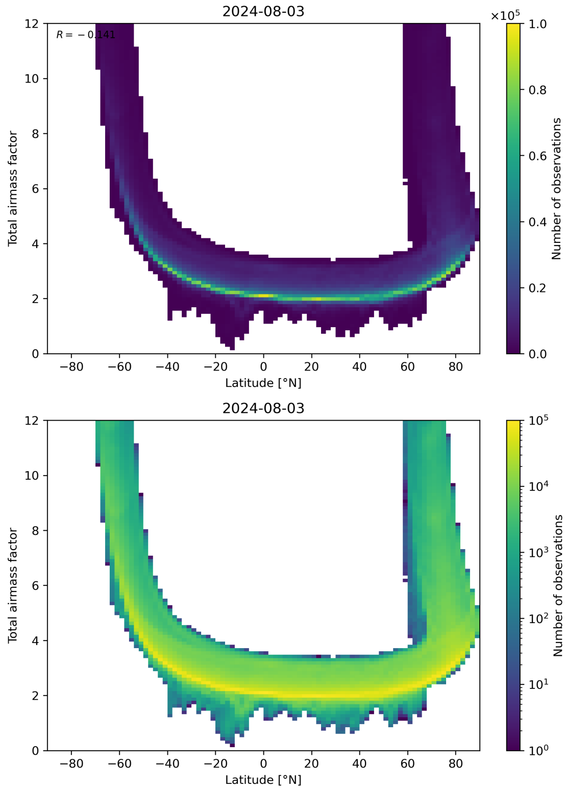
Figure 84: Scatter density plot of “Latitude” against “Total airmass factor” for 2024-08-02 to 2024-08-04.
