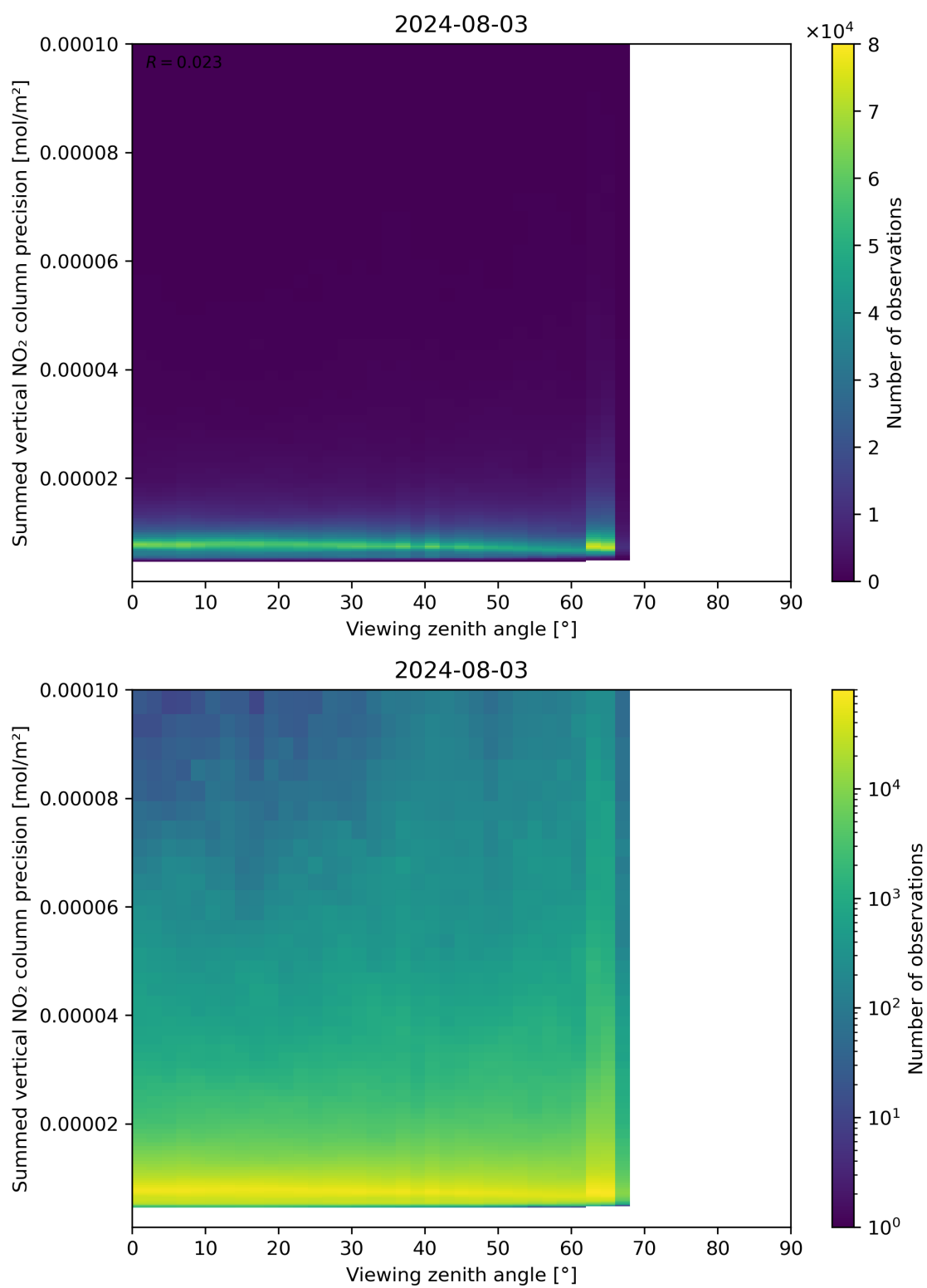
Figure 166: Scatter density plot of “Viewing zenith angle” against “Summed vertical NO 2 column precision” for 2024-08-02 to 2024-08-04.
