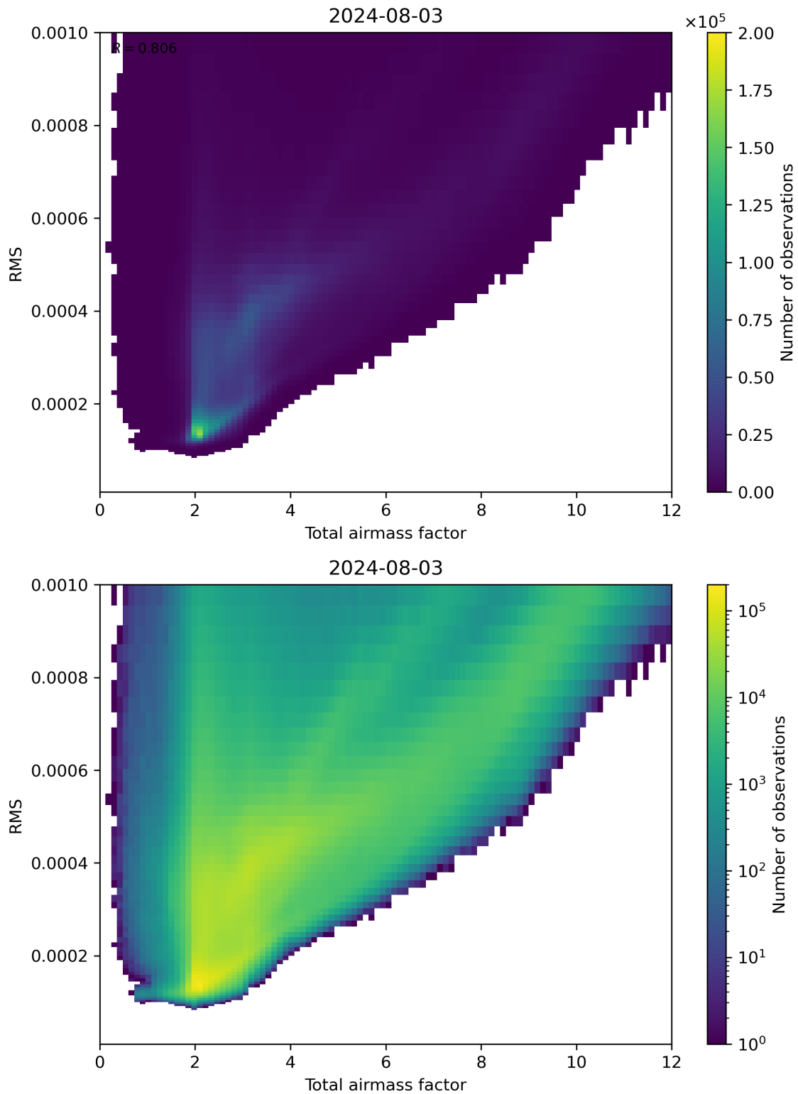
Figure 69: Scatter density plot of “Total airmass factor” against “RMS” for 2024-08-02 to 2024-08-04.
