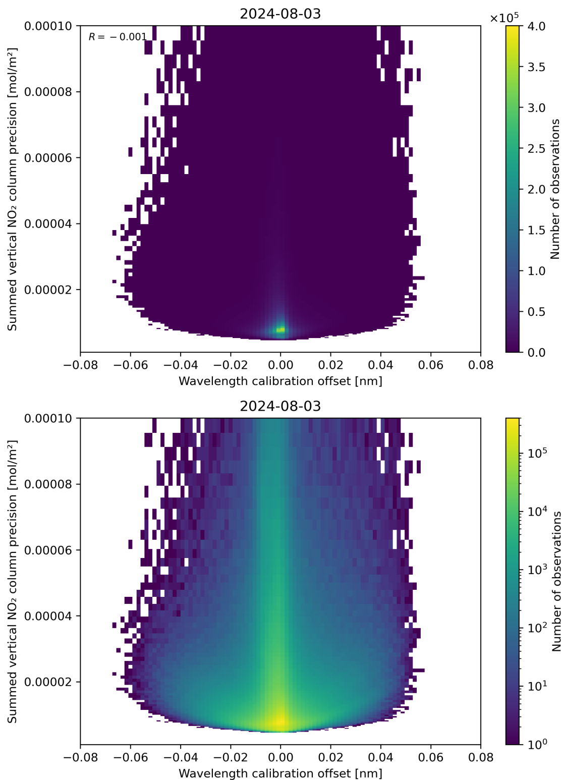
Figure 178: Scatter density plot of “Wavelength calibration offset” against “Summed vertical NO 2 column precision” for 2024-08-02 to 2024-08-04.
