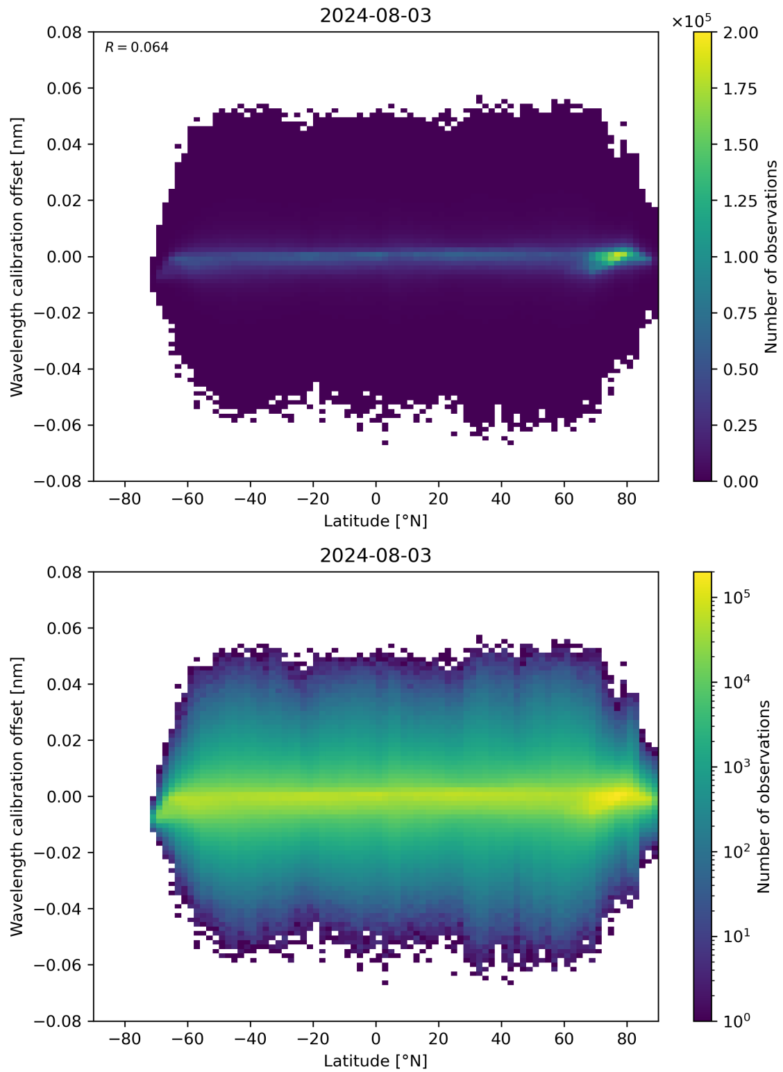
Figure 95: Scatter density plot of “Latitude” against “Wavelength calibration offset” for 2024-08-02 to 2024-08-04.
