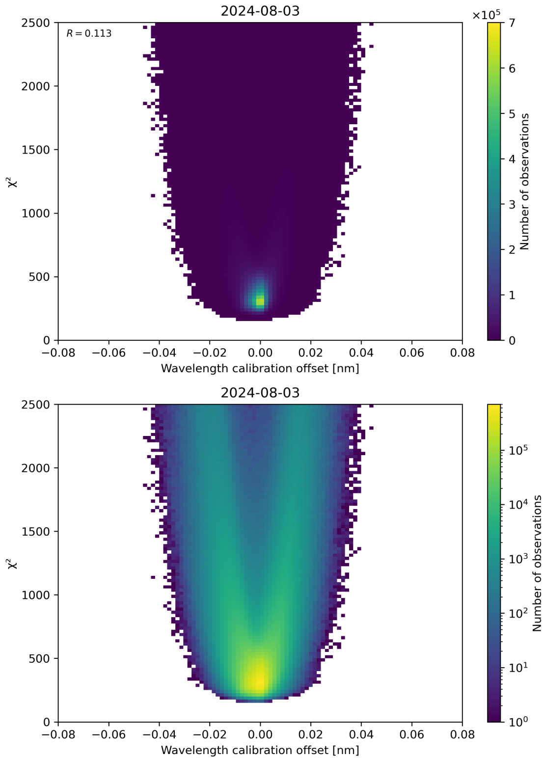
Figure 175: Scatter density plot of “Wavelength calibration offset” against “ \chi^2 ” for 2024-08-02 to 2024-08-04.
