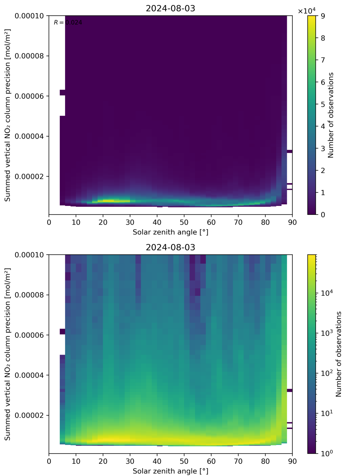
Figure 152: Scatter density plot of “Solar zenith angle” against “Summed vertical NO 2 column precision” for 2024-08-02 to 2024-08-04.
