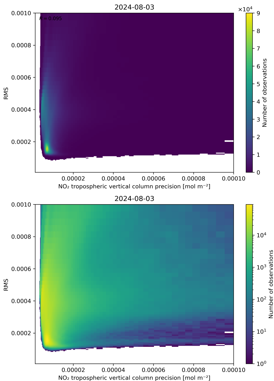
Figure 140: Scatter density plot of “NO 2 tropospheric vertical column precision” against “RMS” for 2024-08-02 to 2024-08-04.
