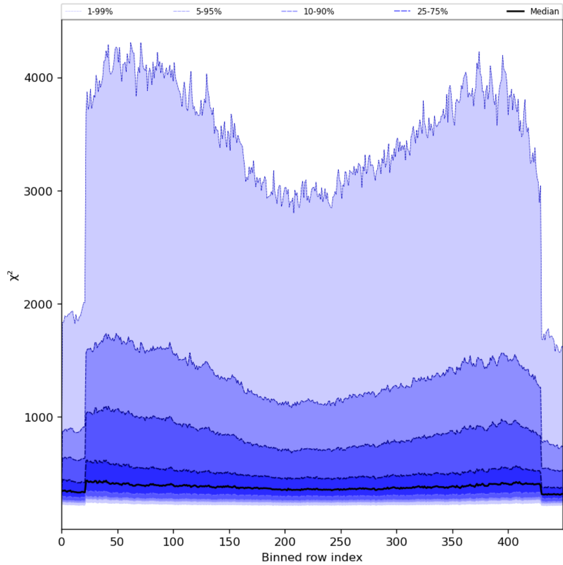
Figure 59: Along track statistics of “ \chi^2 ” for 2024-08-02 to 2024-08-04
