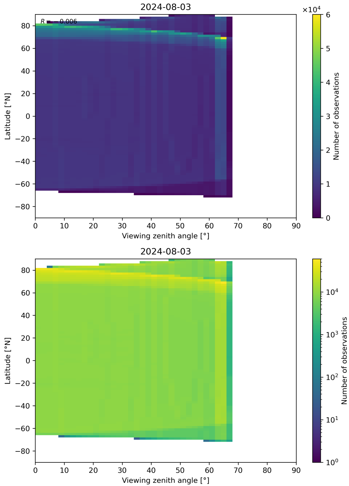
Figure 163: Scatter density plot of “Viewing zenith angle” against “Latitude” for 2024-08-02 to 2024-08-04.
