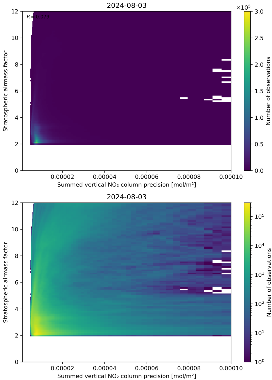
Figure 106: Scatter density plot of “Summed vertical NO 2 column precision” against “Stratospheric airmass factor” for 2024-08-02 to 2024-08-04.
