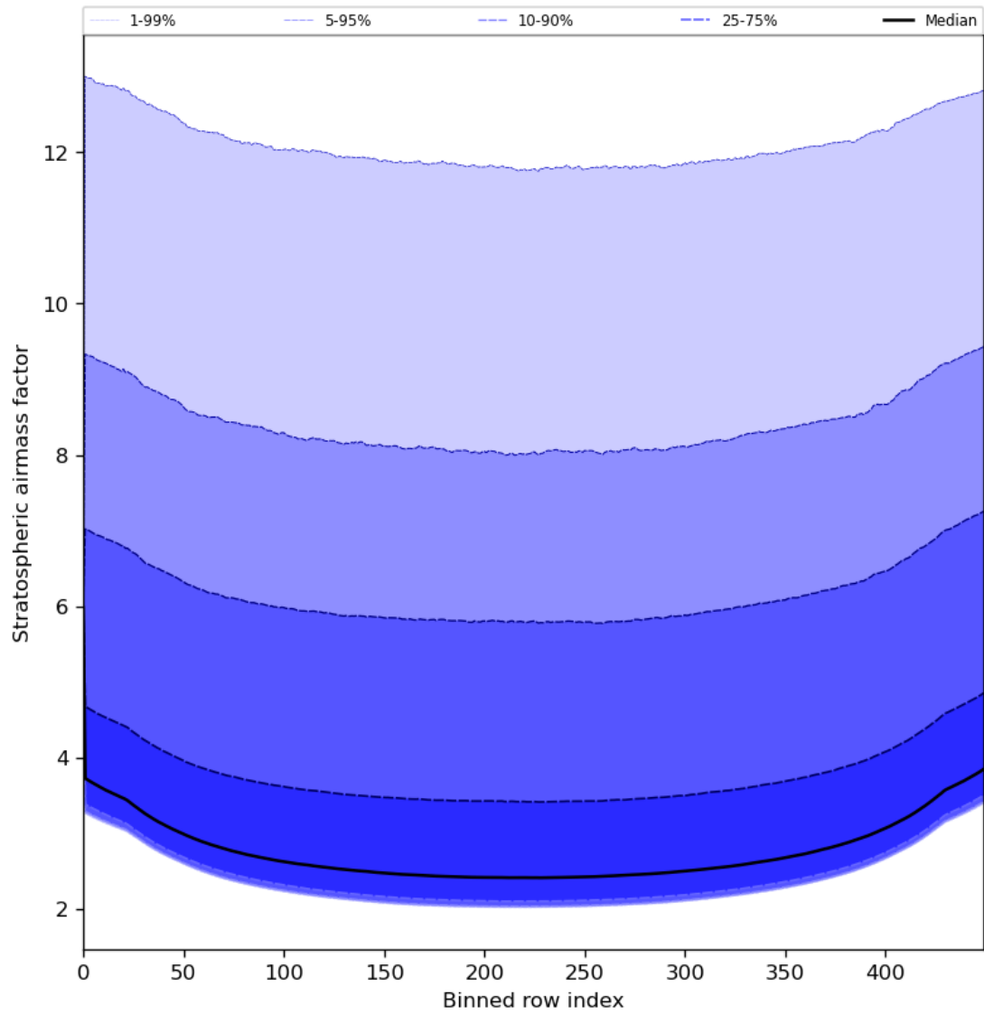
Figure 61: Along track statistics of “Stratospheric airmass factor” for 2024-08-02 to 2024-08-04
