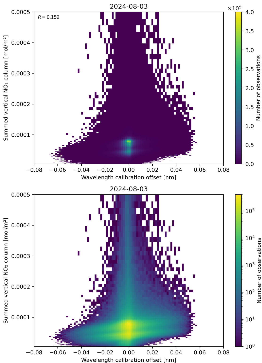
Figure 177: Scatter density plot of “Wavelength calibration offset” against “Summed vertical NO 2 column” for 2024-08-02 to 2024-08-04.
