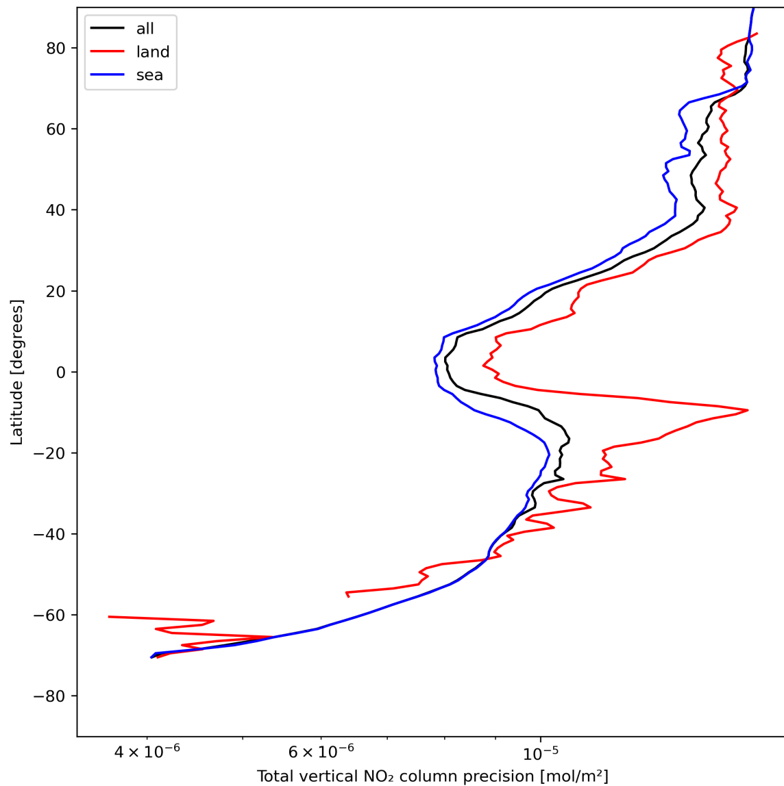
Figure 22: Zonal average of “Total vertical NO 2 column precision” for 2024-08-02 to 2024-08-04.
