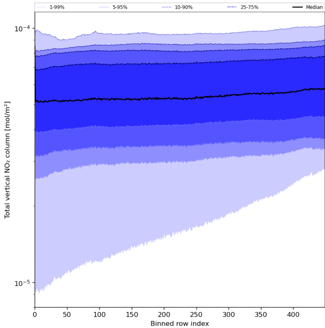
Figure 55: Along track statistics of “Total vertical NO 2 column” for 2024-08-02 to 2024-08-04
