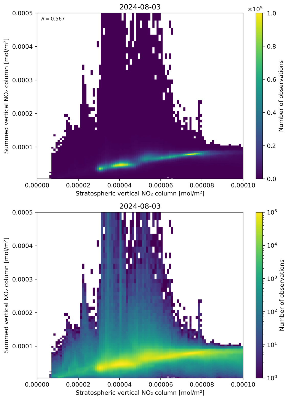
Figure 98: Scatter density plot of “Stratospheric vertical NO 2 column” against “Summed vertical NO 2 column” for 2024-08-02 to 2024-08-04.
