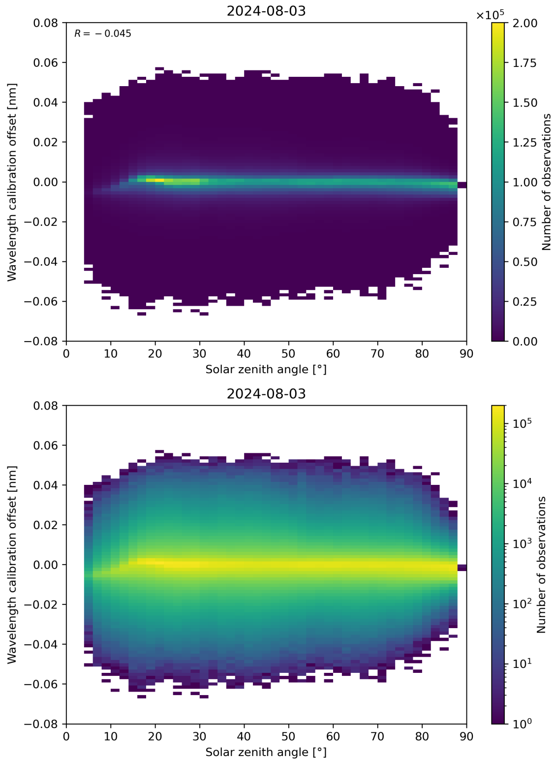
Figure 158: Scatter density plot of “Solar zenith angle” against “Wavelength calibration offset” for 2024-08-02 to 2024-08-04.
