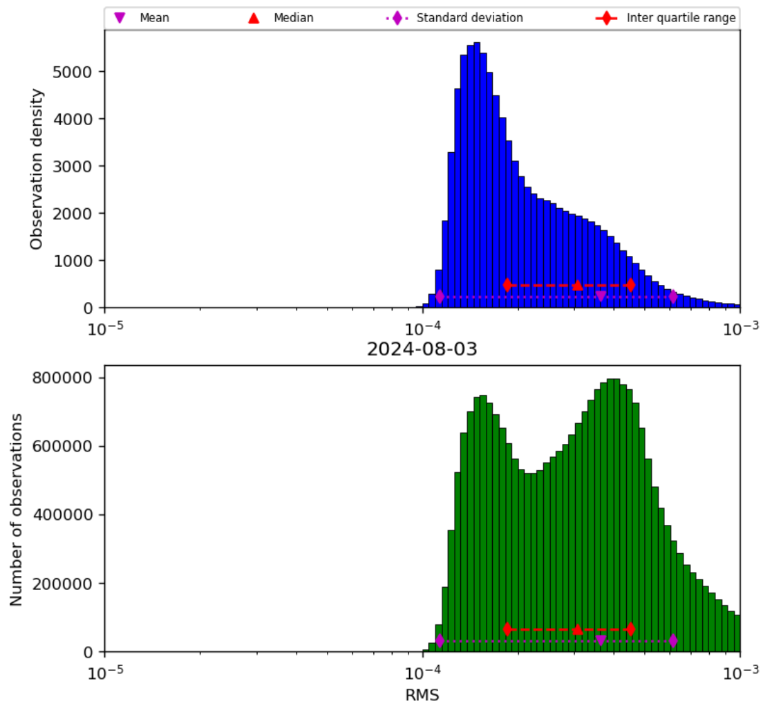
Figure 43: Histogram of “RMS” for 2024-08-02 to 2024-08-04
