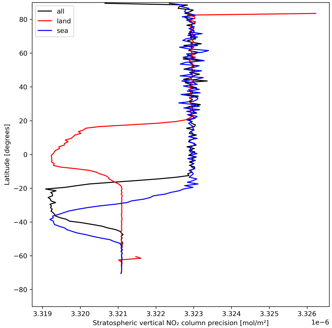
Figure 20: Zonal average of “Stratospheric vertical NO 2 column precision” for 2024-08-02 to 2024-08-04.
