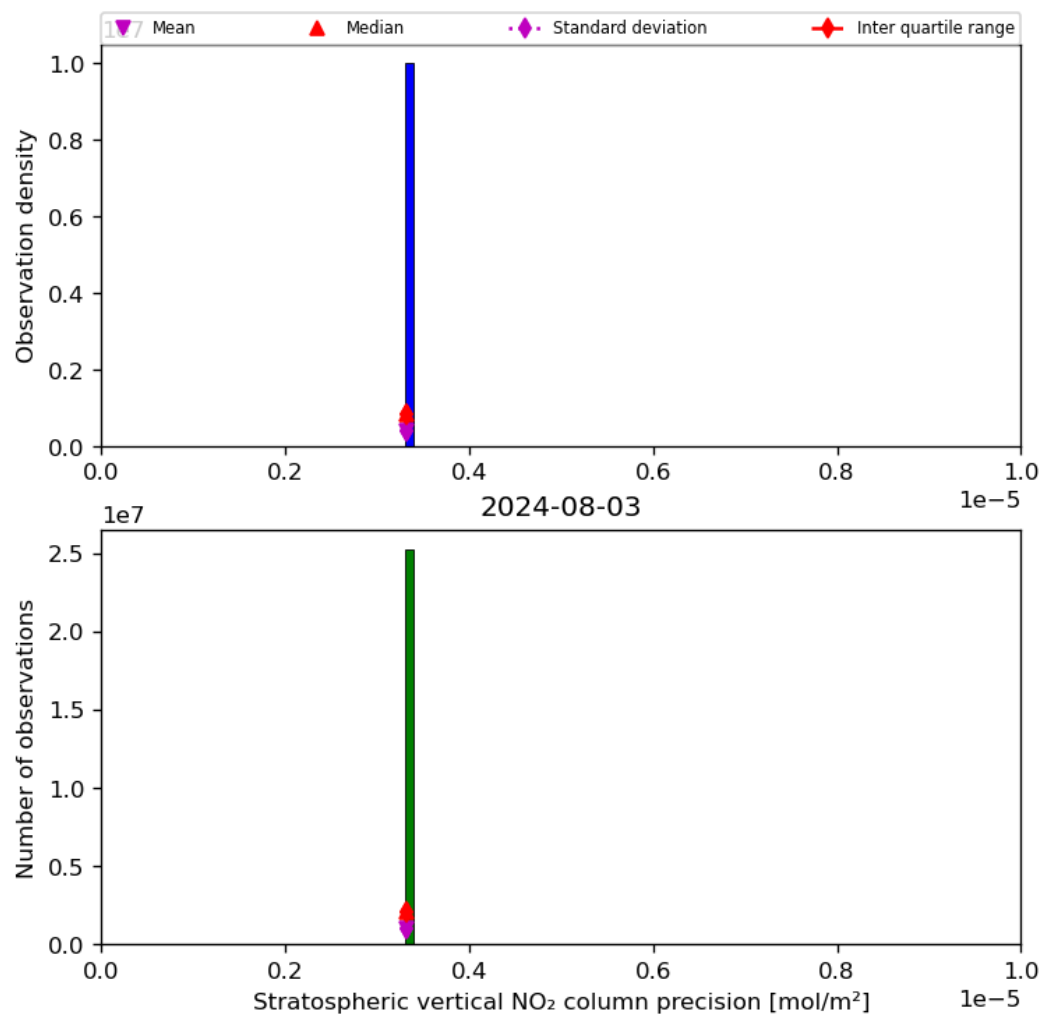
Figure 37: Histogram of “Stratospheric vertical NO 2 column precision” for 2024-08-02 to 2024-08-04
