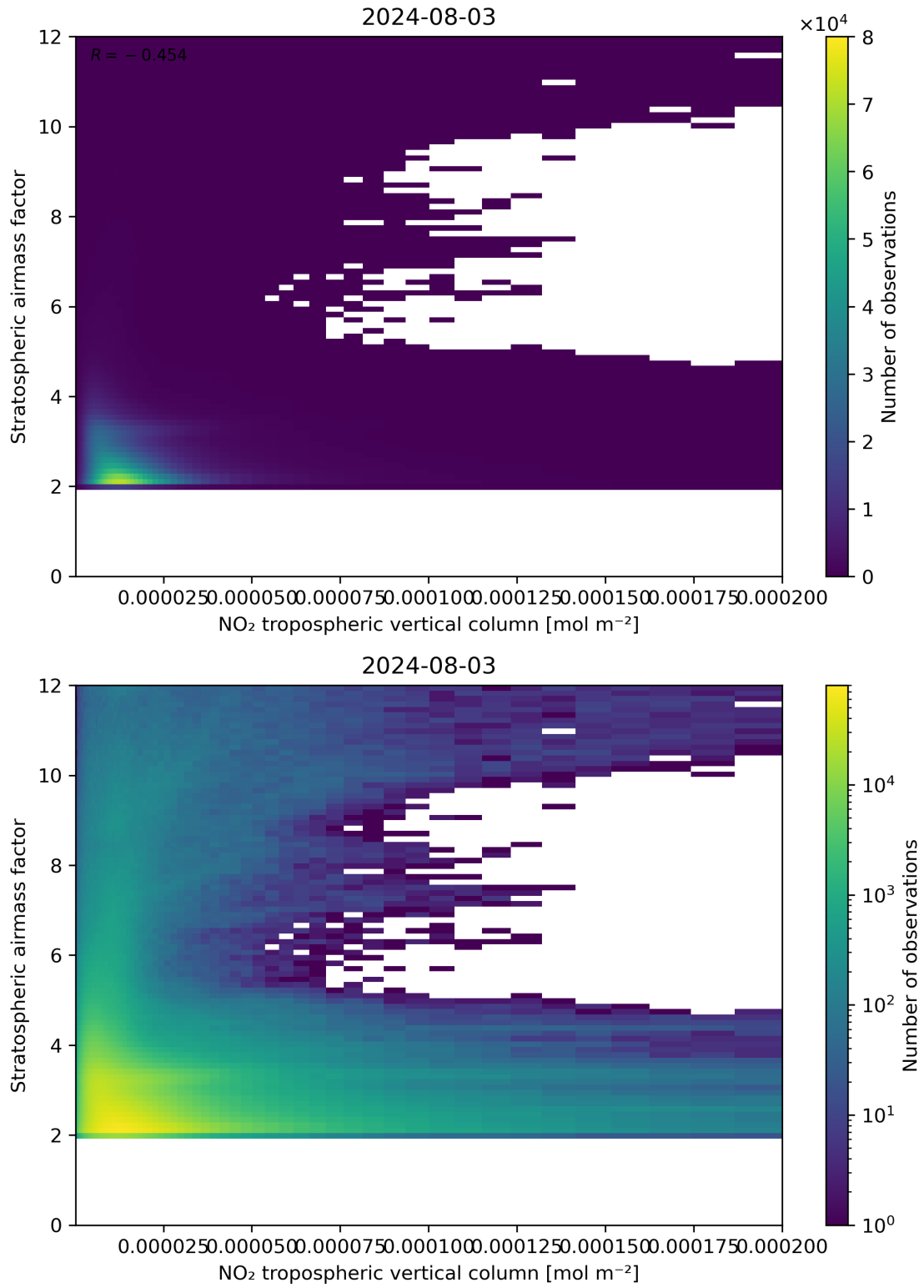
Figure 121: Scatter density plot of “NO 2 tropospheric vertical column” against “Stratospheric air mass factor” for 2024-08-02 to 2024-08-04.
