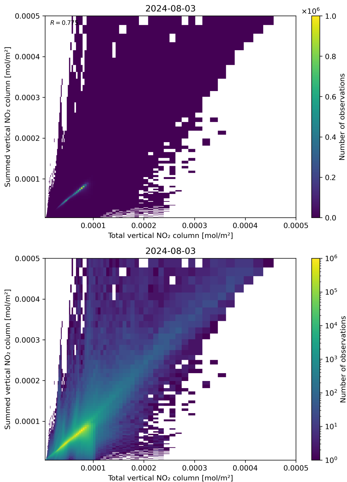
Figure 112: Scatter density plot of “Total vertical NO 2 column” against “Summed vertical NO 2 column” for 2024-08-02 to 2024-08-04.
