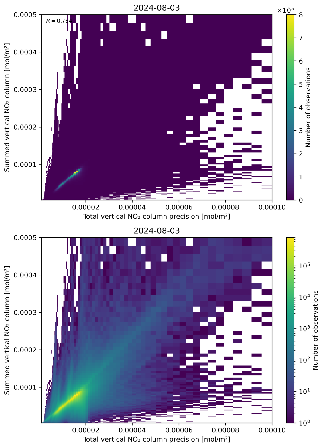
Figure 117: Scatter density plot of “Total vertical NO 2 column precision” against “Summed vertical NO 2 column” for 2024-08-02 to 2024-08-04.
