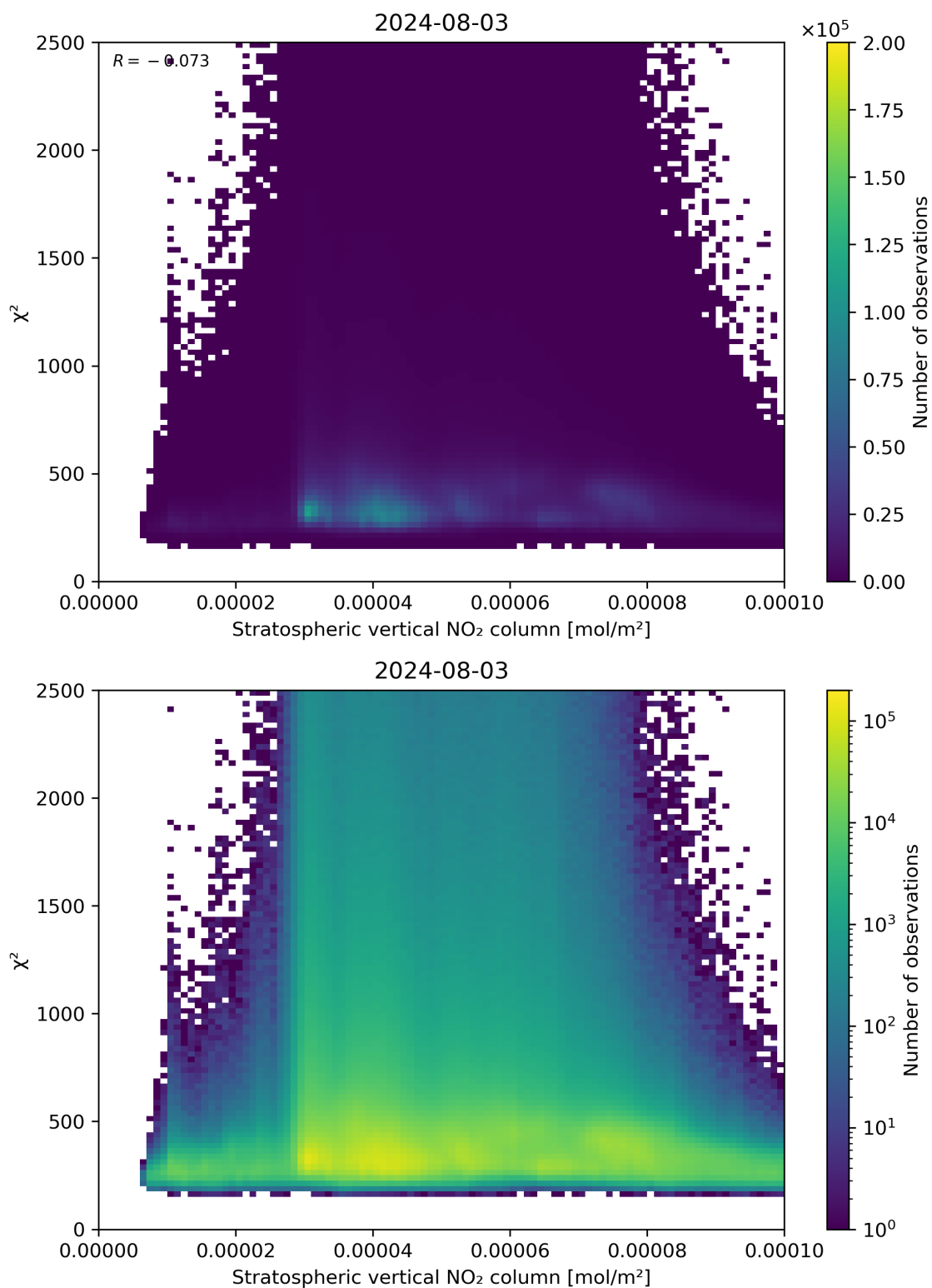
Figure 97: Scatter density plot of “Stratospheric vertical NO 2 column” against “ \chi^2 ” for 2024-08-02 to 2024-08-04.
