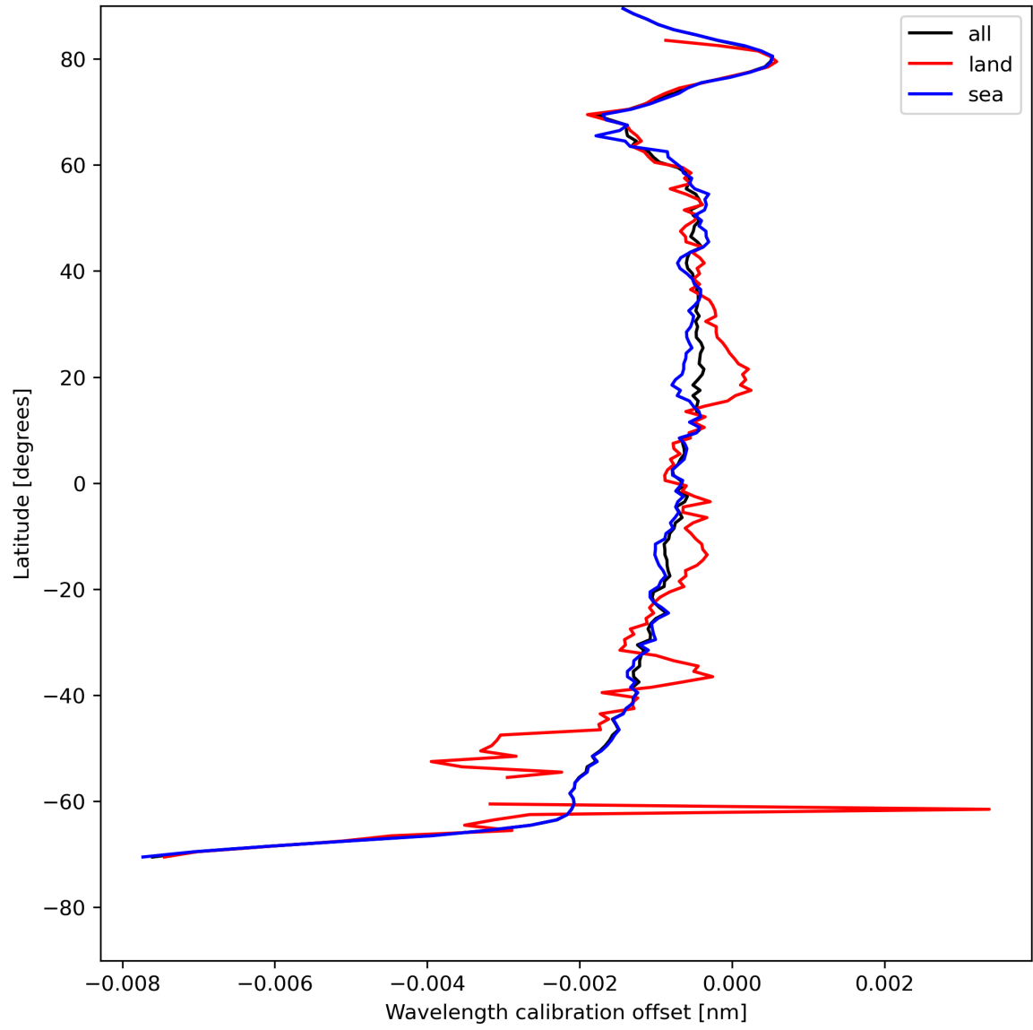
Figure 18: Zonal average of “Wavelength calibration offset” for 2024-08-02 to 2024-08-04.
