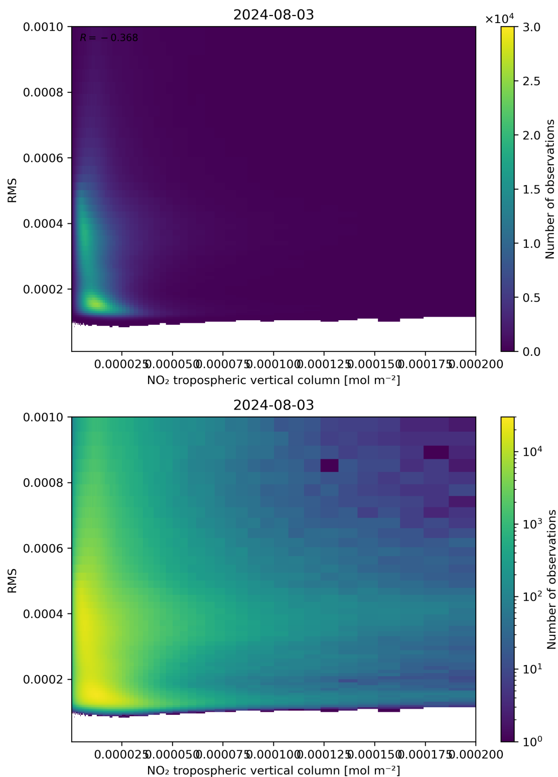
Figure 142: Scatter density plot of “NO 2 tropospheric vertical column” against “RMS” for 2024-08-02 to 2024-08-04.
