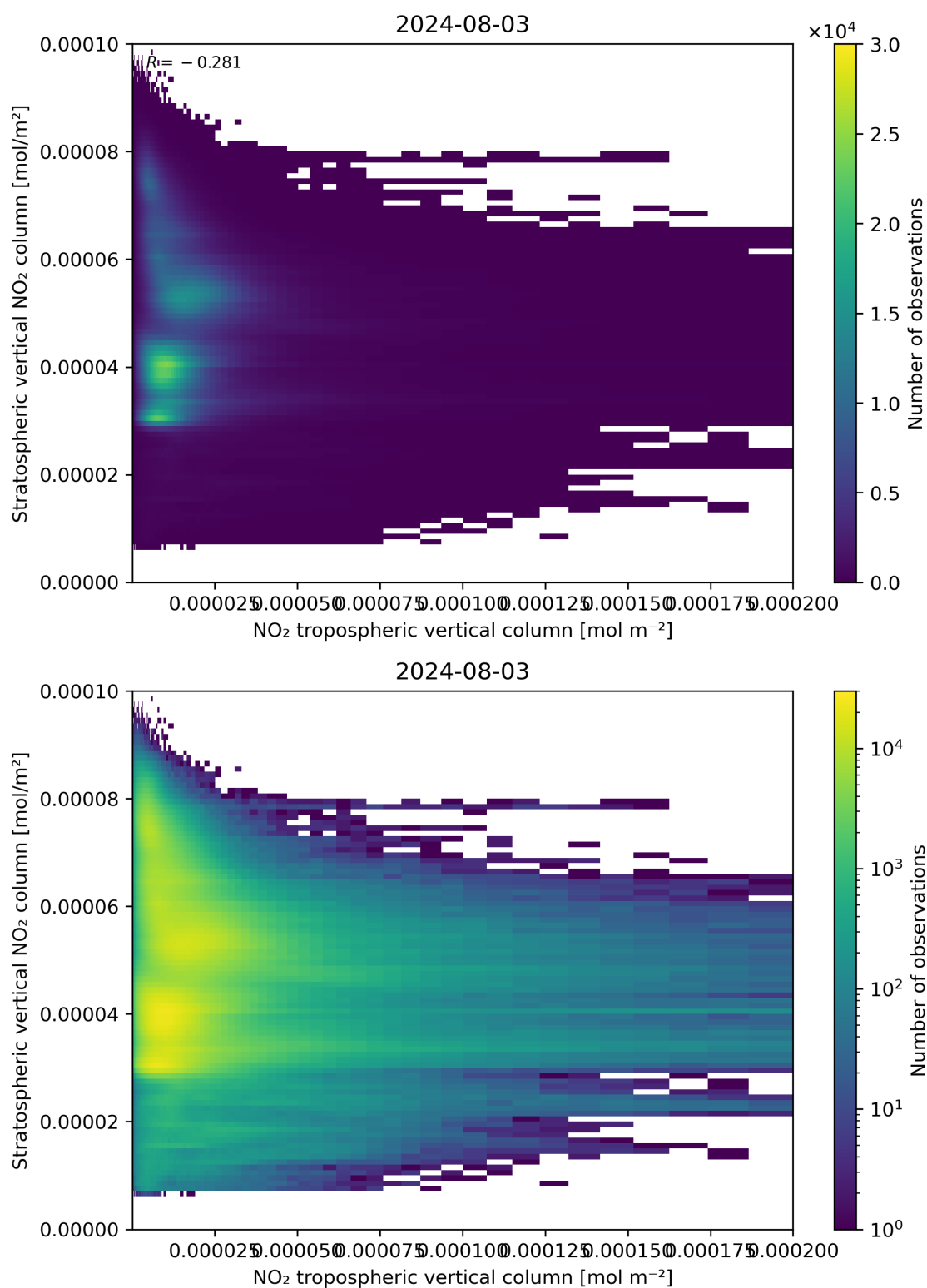
Figure 125: Scatter density plot of “NO 2 tropospheric vertical column” against “Stratospheric vertical NO 2 column” for 2024-08-02 to 2024-08-04.
