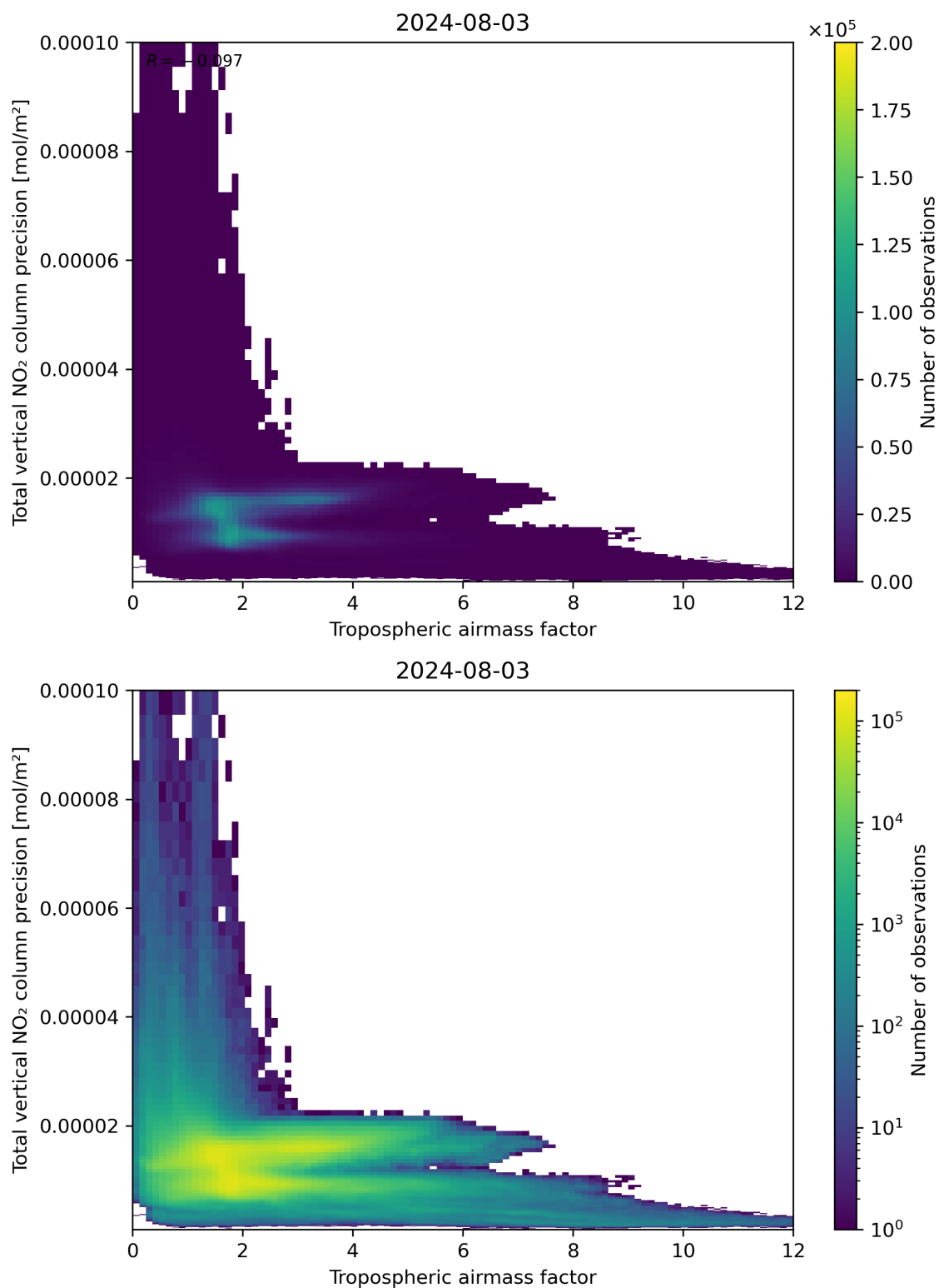
Figure 78: Scatter density plot of “Tropospheric air mass factor” against “Total vertical NO 2 column precision” for 2024-08-02 to 2024-08-04.
