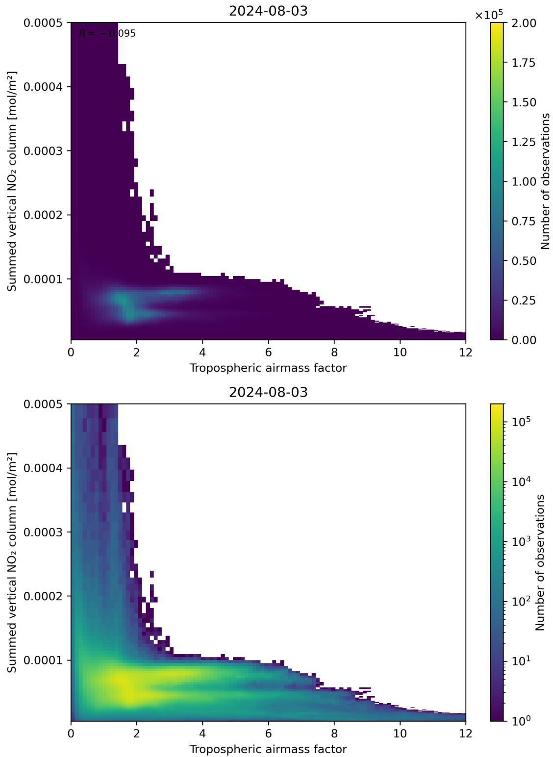
Figure 75: Scatter density plot of “Tropospheric airmass factor” against “Summed vertical NO 2 column” for 2024-08-02 to 2024-08-04.
