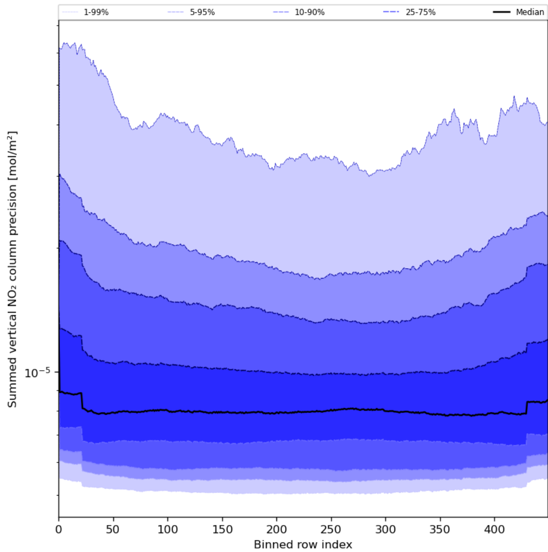
Figure 58: Along track statistics of “Summed vertical NO 2 column precision” for 2024-08-02 to 2024-08-04
