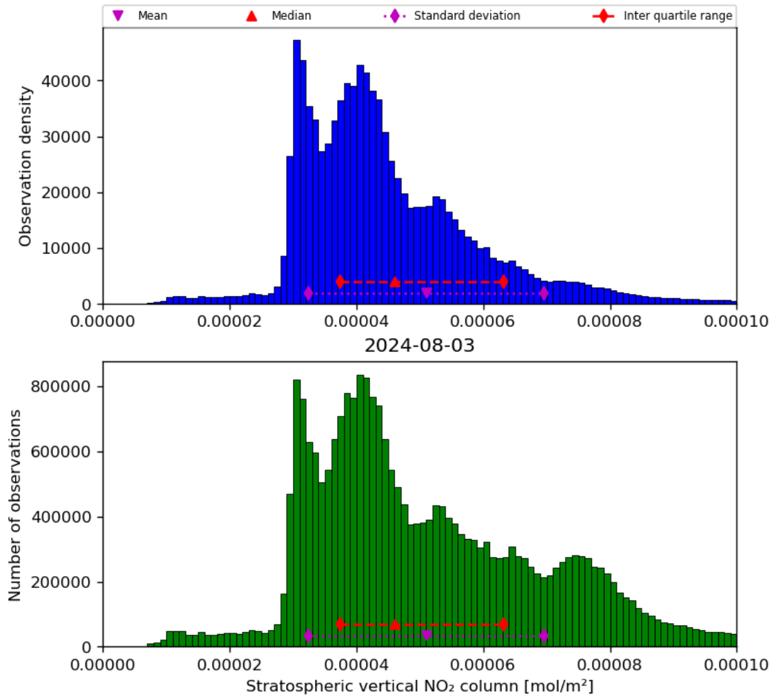
Figure 36: Histogram of “Stratospheric vertical NO 2 column” for 2024-08-02 to 2024-08-04
