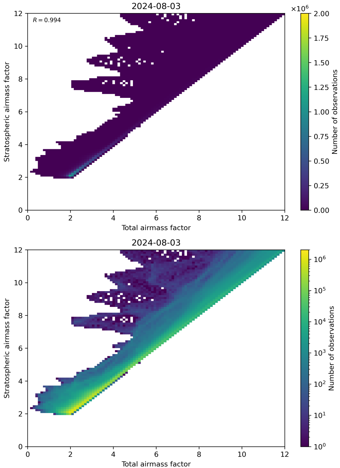
Figure 62: Scatter density plot of “Total airmass factor” against “Stratospheric airmass factor” for 2024-08-02 to 2024-08-04.
