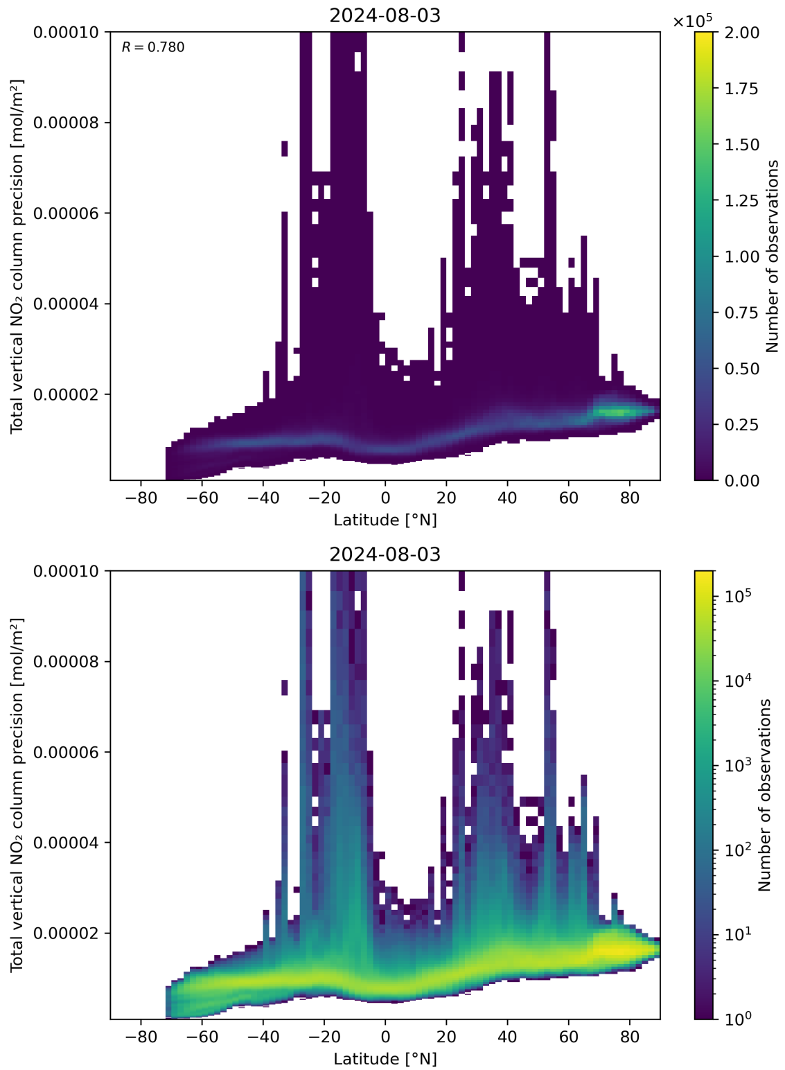
Figure 91: Scatter density plot of “Latitude” against “Total vertical NO 2 column precision” for 2024-08-02 to 2024-08-04.
