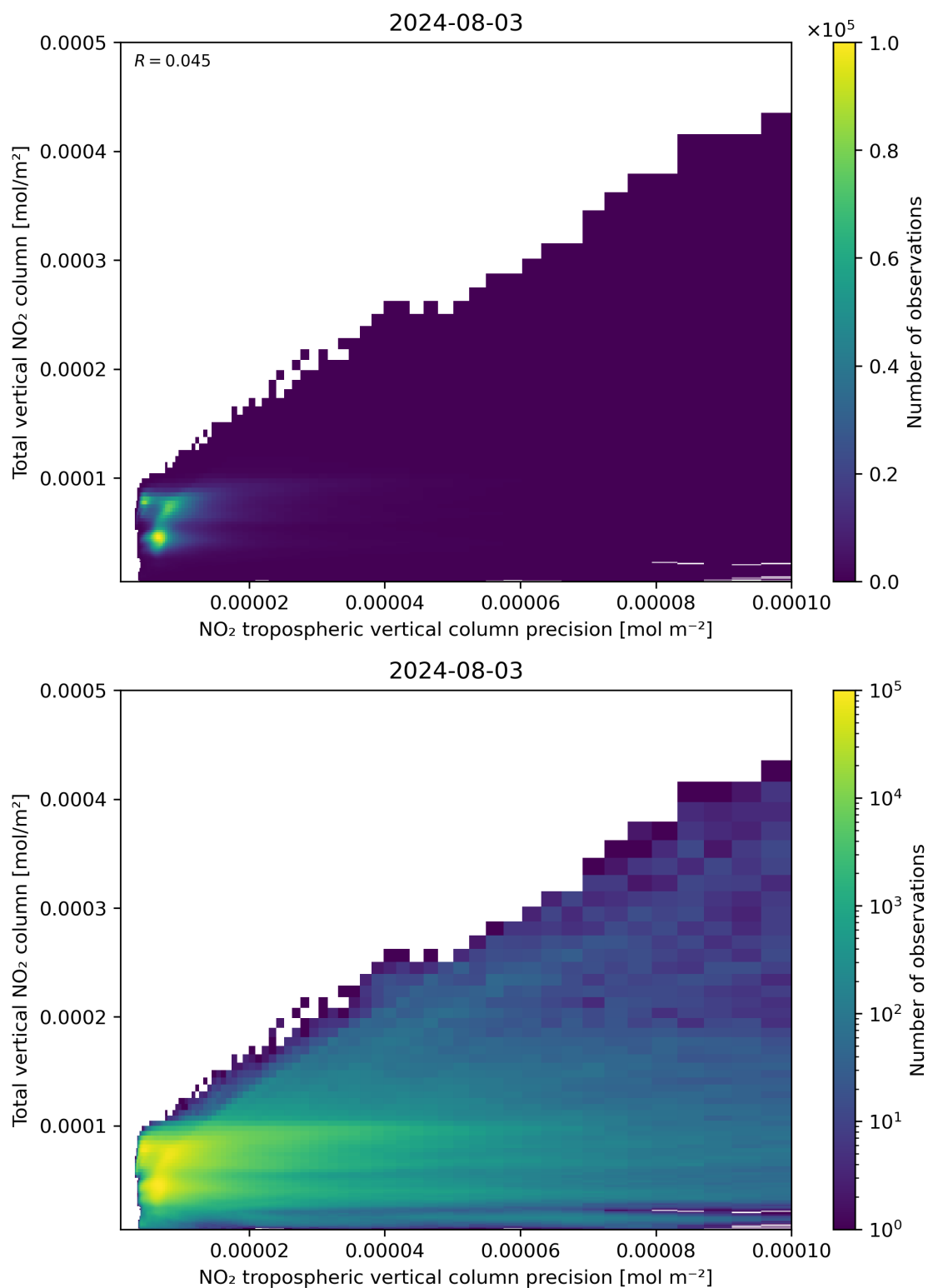
Figure 138: Scatter density plot of “NO 2 tropospheric vertical column precision” against “Total vertical NO 2 column” for 2024-08-02 to 2024-08-04.
