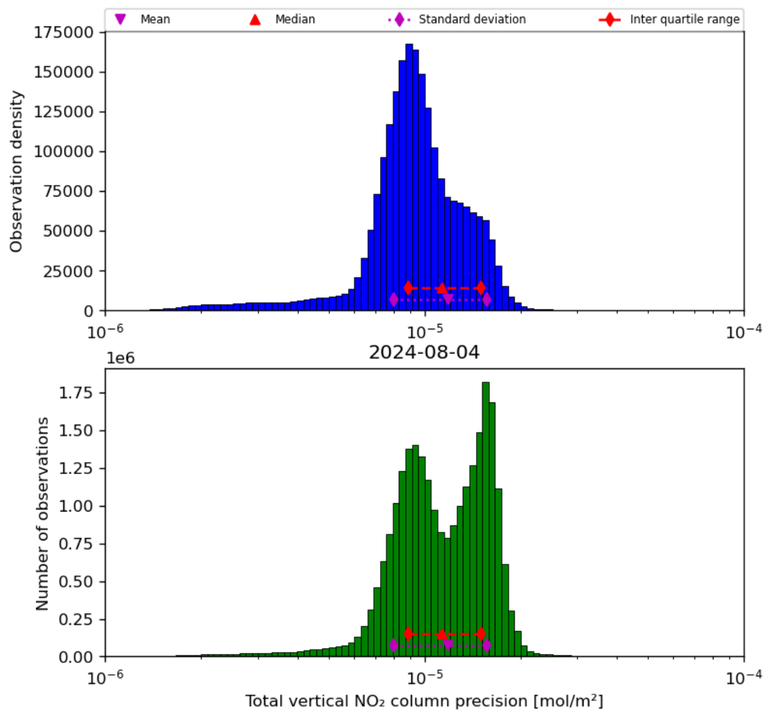
Figure 39: Histogram of “Total vertical NO 2 column precision” for 2024-08-03 to 2024-08-05
