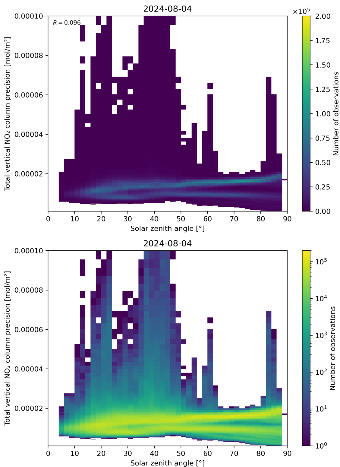
Figure 154: Scatter density plot of “Solar zenith angle” against “Total vertical NO 2 column precision” for 2024-08-03 to 2024-08-05.
