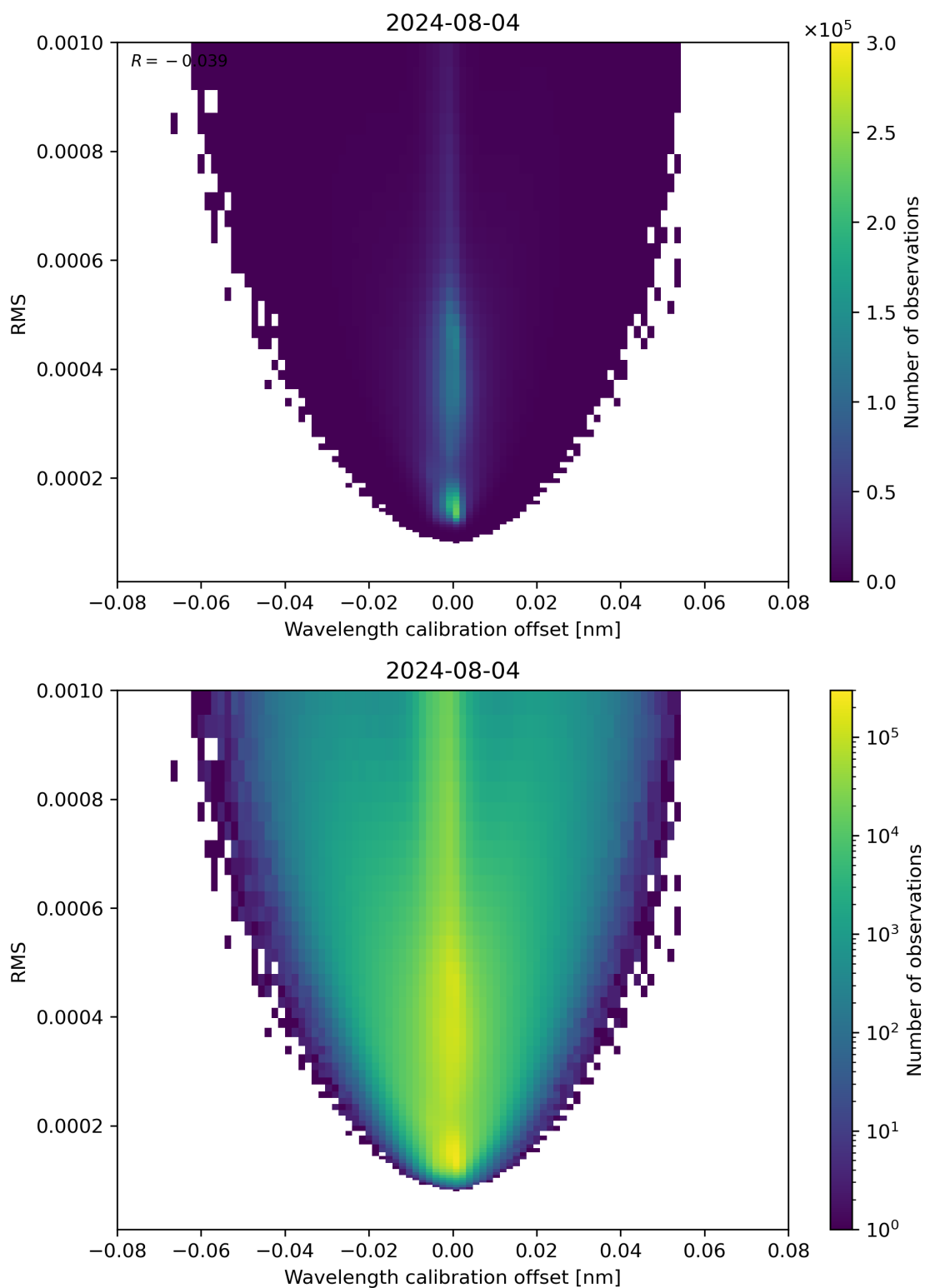
Figure 181: Scatter density plot of “Wavelength calibration offset” against “RMS” for 2024-08-03 to 2024-08-05.
