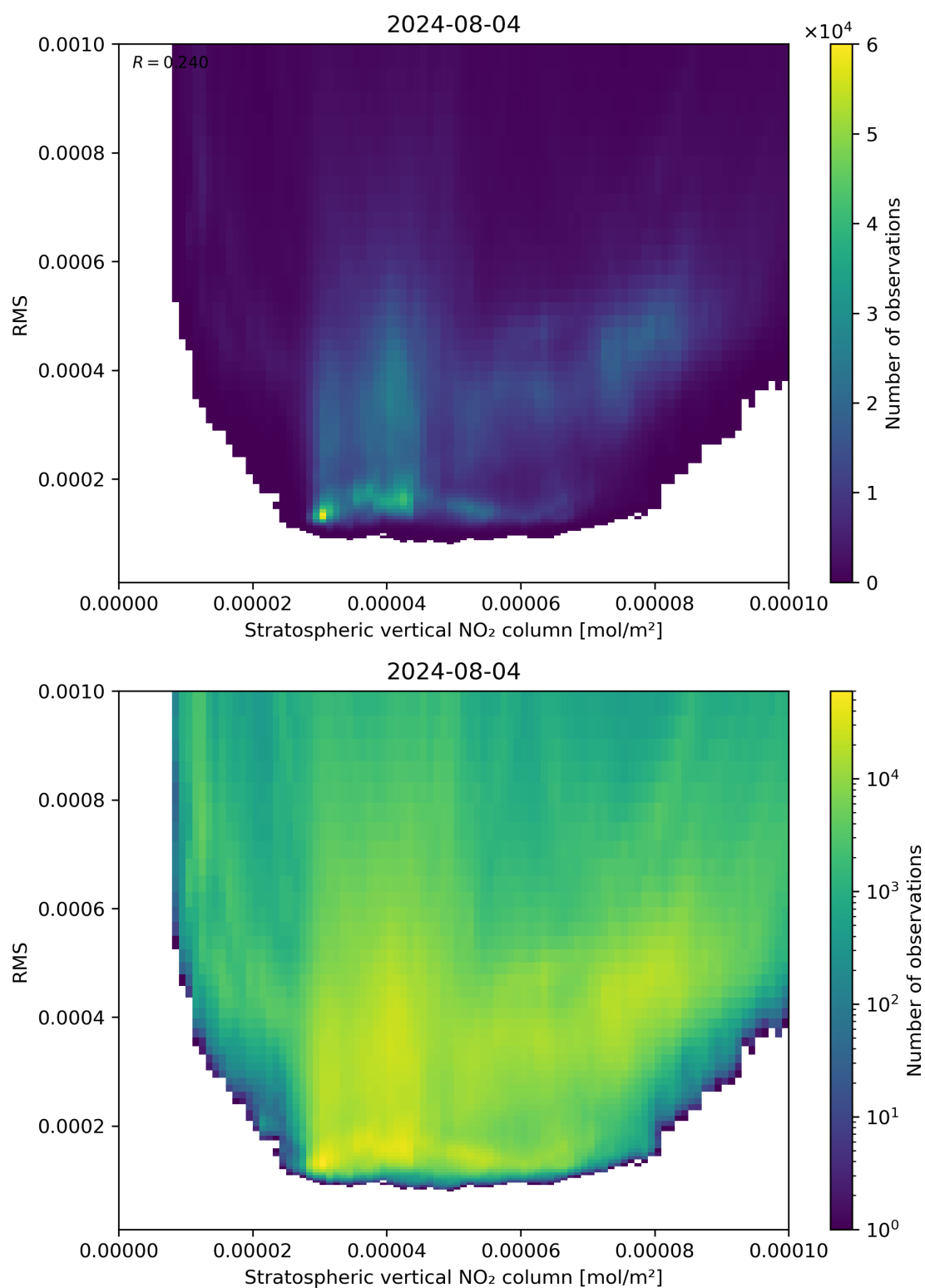
Figure 102: Scatter density plot of “Stratospheric vertical NO 2 column” against “RMS” for 2024-08-03 to 2024-08-05.
