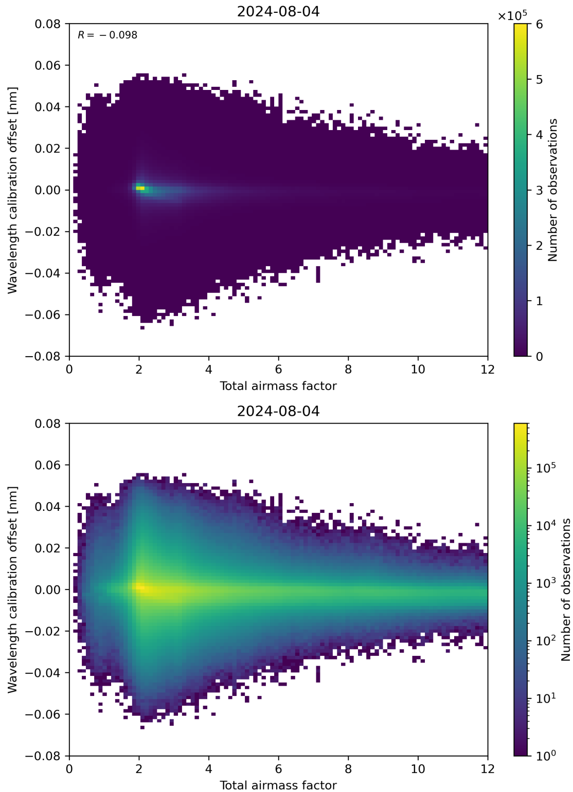
Figure 70: Scatter density plot of “Total airmass factor” against “Wavelength calibration offset” for 2024-08-03 to 2024-08-05.
