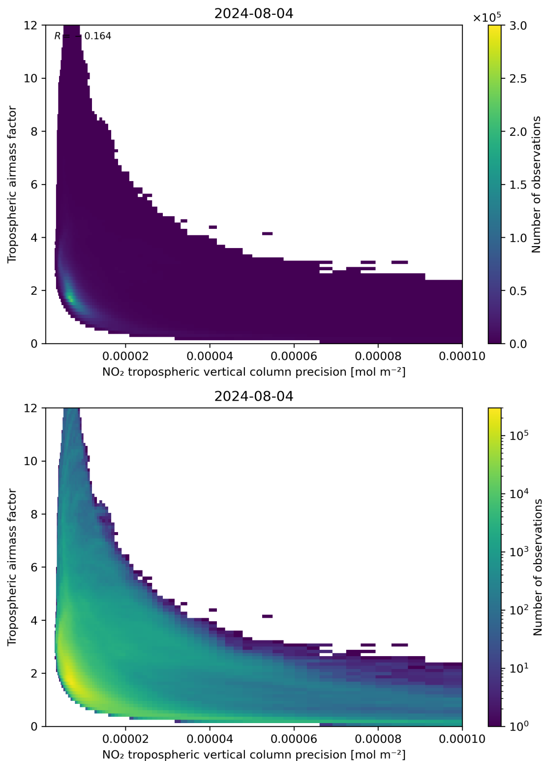
Figure 133: Scatter density plot of “NO 2 tropospheric vertical column precision” against “Tropospheric airmass factor” for 2024-08-03 to 2024-08-05.
