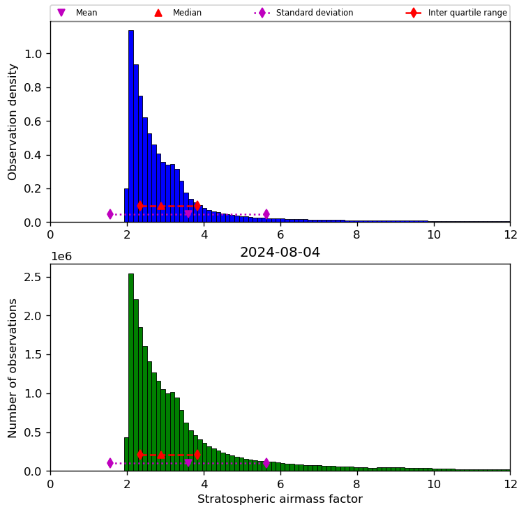
Figure 44: Histogram of “Stratospheric airmass factor” for 2024-08-03 to 2024-08-05
