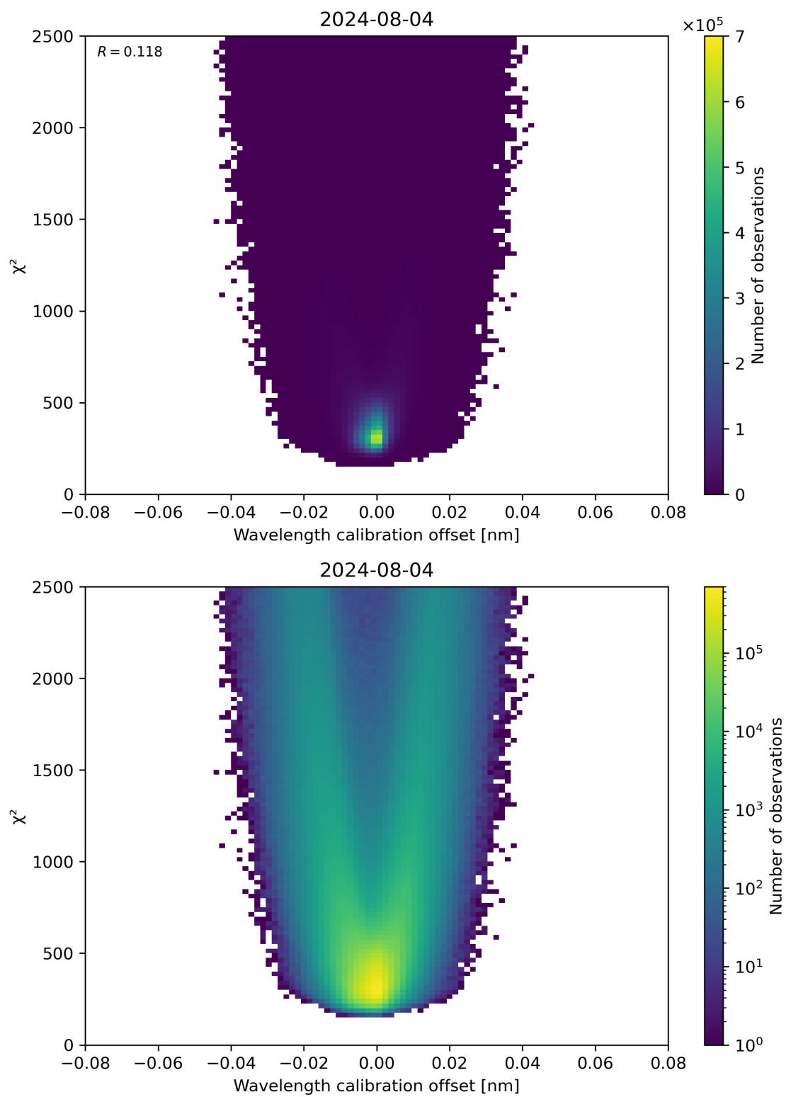
Figure 175: Scatter density plot of “Wavelength calibration offset” against “ \chi^2 ” for 2024-08-03 to 2024-08-05.
