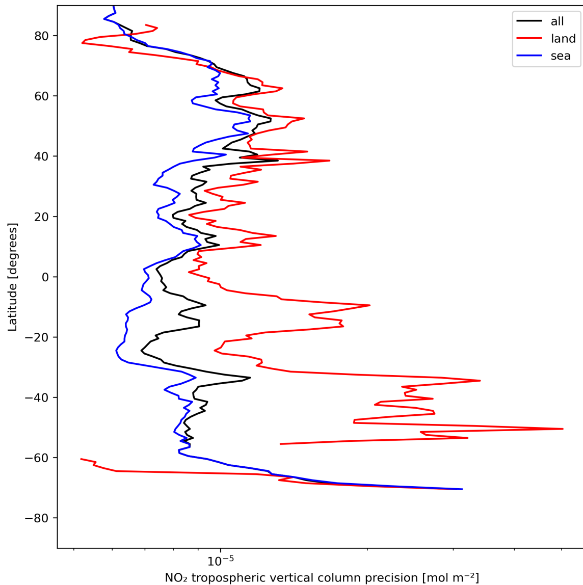
Figure 13: Zonal average of “NO 2 tropospheric vertical column precision” for 2024-08-03 to 2024-08-05.
