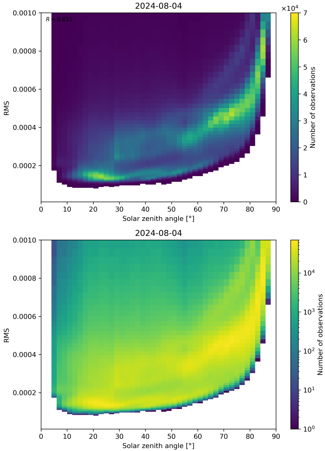
Figure 157: Scatter density plot of “Solar zenith angle” against “RMS” for 2024-08-03 to 2024-08-05.
