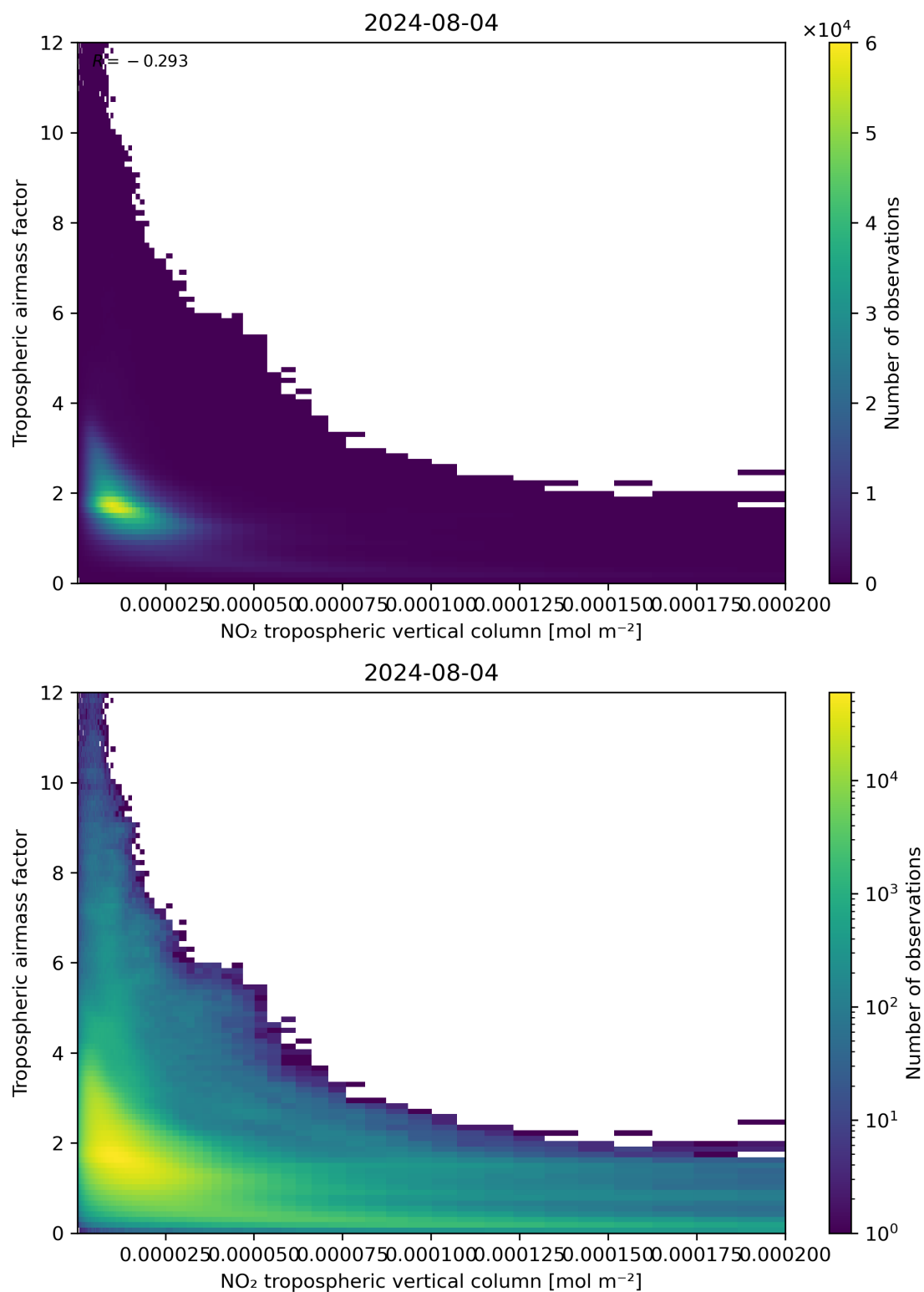
Figure 123: Scatter density plot of “NO 2 tropospheric vertical column” against “Tropospheric air mass factor” for 2024-08-03 to 2024-08-05.
