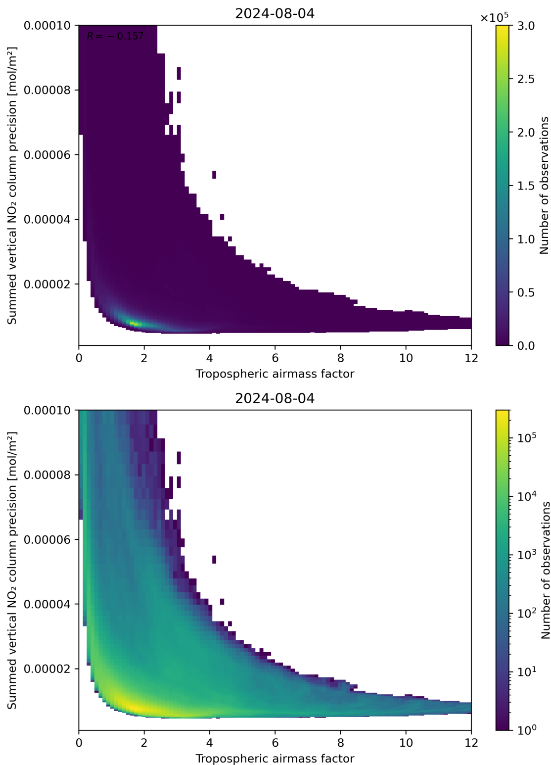
Figure 76: Scatter density plot of “Tropospheric air mass factor” against “Summed vertical NO 2 column precision” for 2024-08-03 to 2024-08-05.
