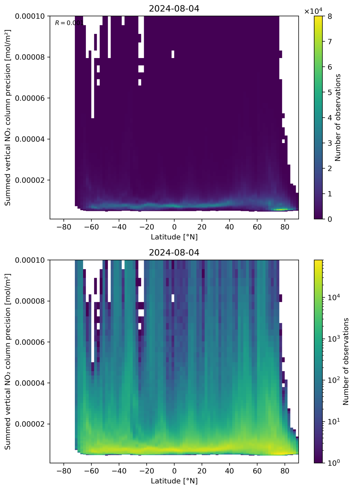
Figure 89: Scatter density plot of “Latitude” against “Summed vertical NO 2 column precision” for 2024-08-03 to 2024-08-05.
