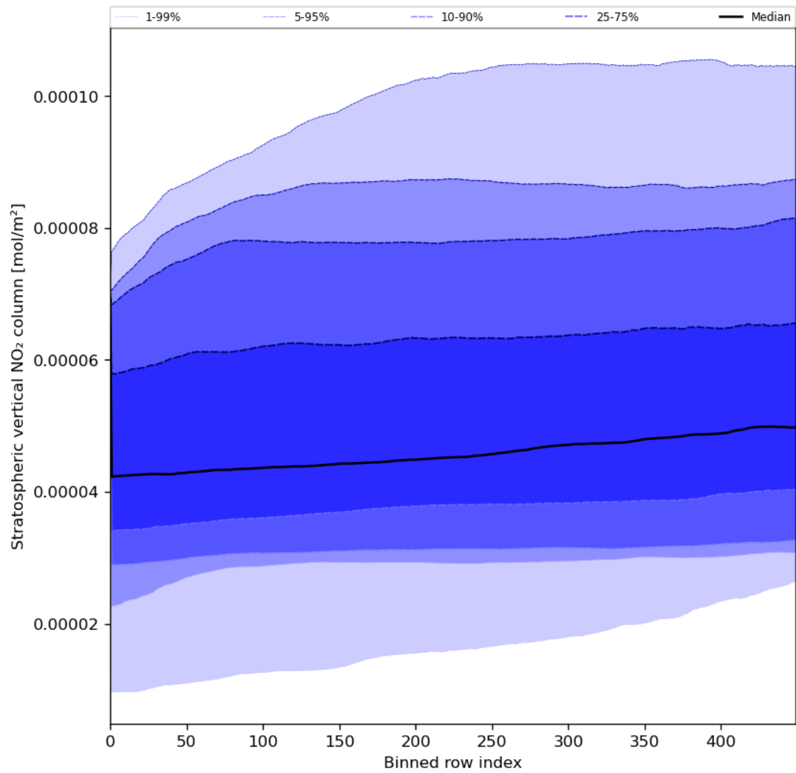
Figure 53: Along track statistics of “Stratospheric vertical NO 2 column” for 2024-08-03 to 2024-08-05
