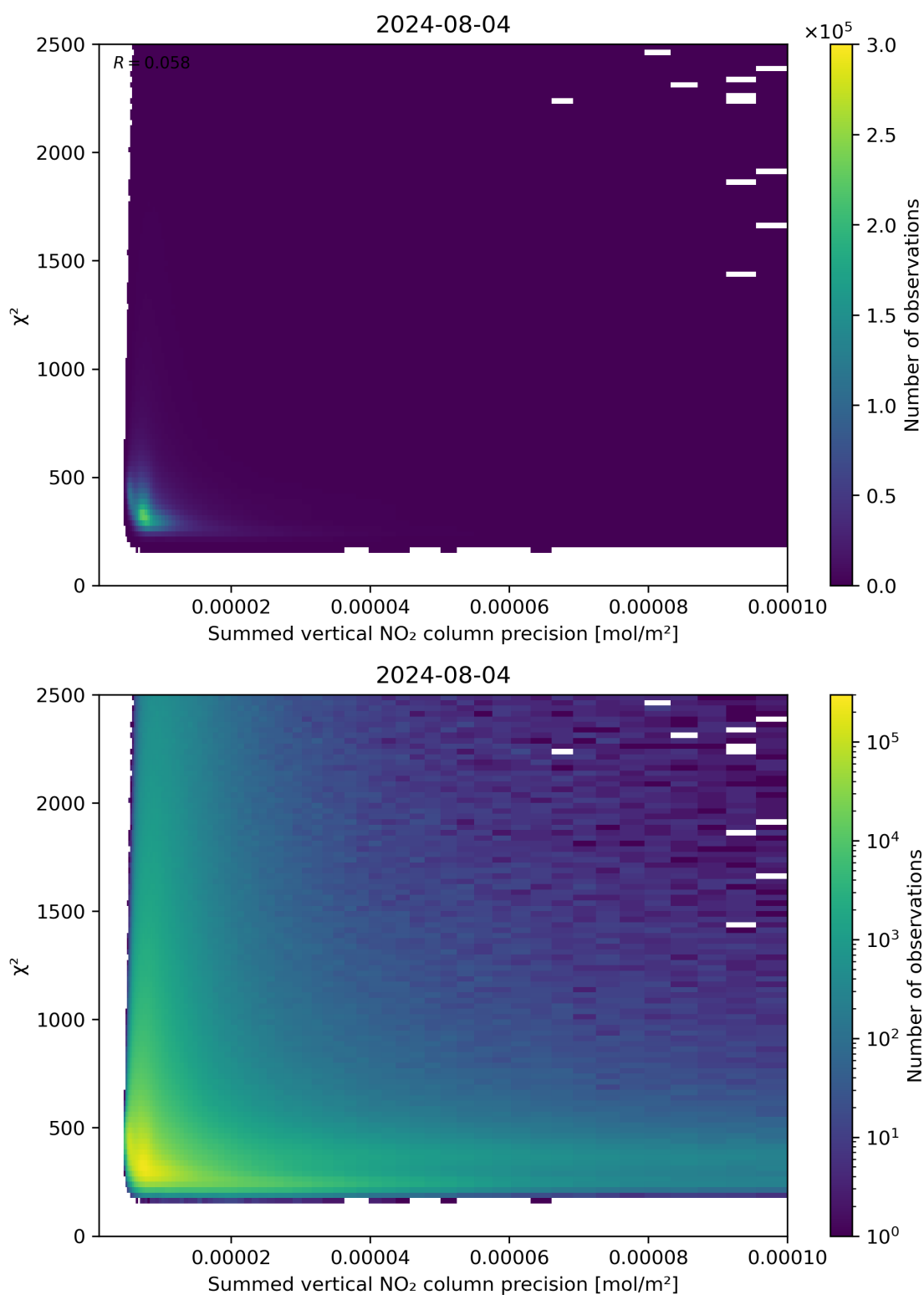
Figure 107: Scatter density plot of “Summed vertical NO 2 column precision” against “ \chi^2 ” for 2024-08-03 to 2024-08-05.
