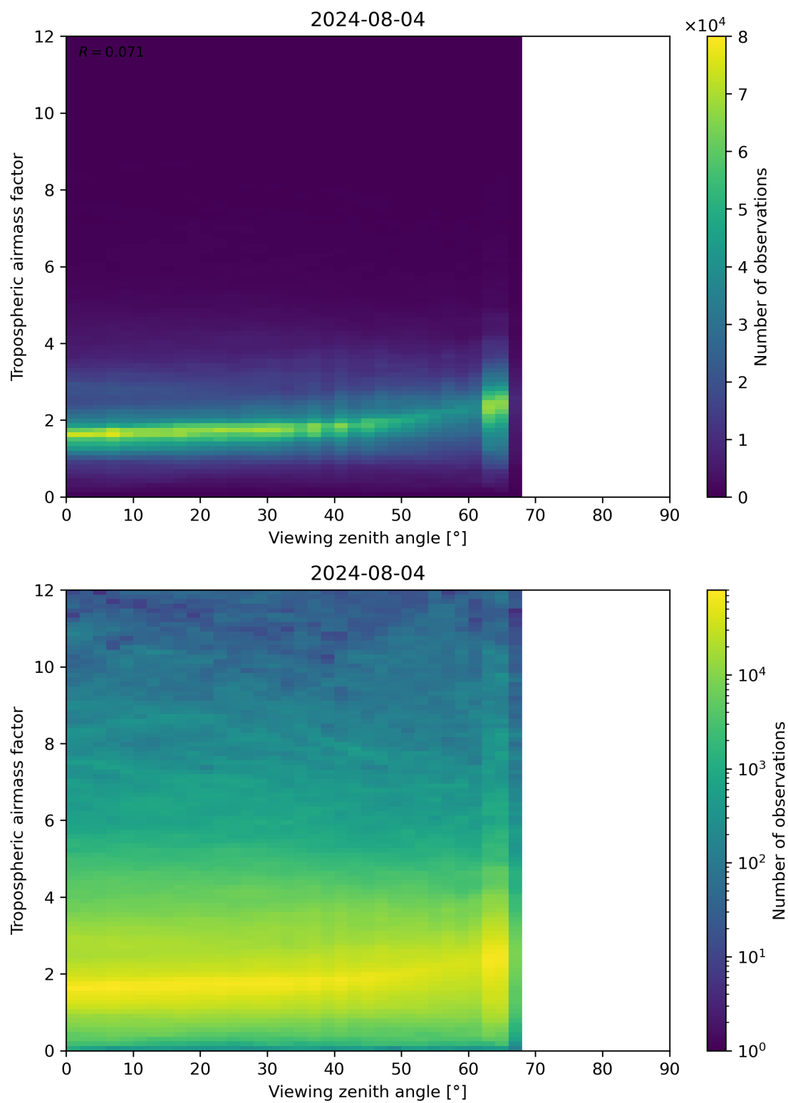
Figure 161: Scatter density plot of “Viewing zenith angle” against “Tropospheric airmass factor” for 2024-08-03 to 2024-08-05.
