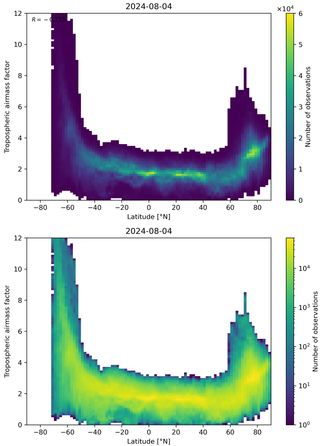
Figure 85: Scatter density plot of “Latitude” against “Tropospheric air mass factor” for 2024-08-03 to 2024-08-05.
