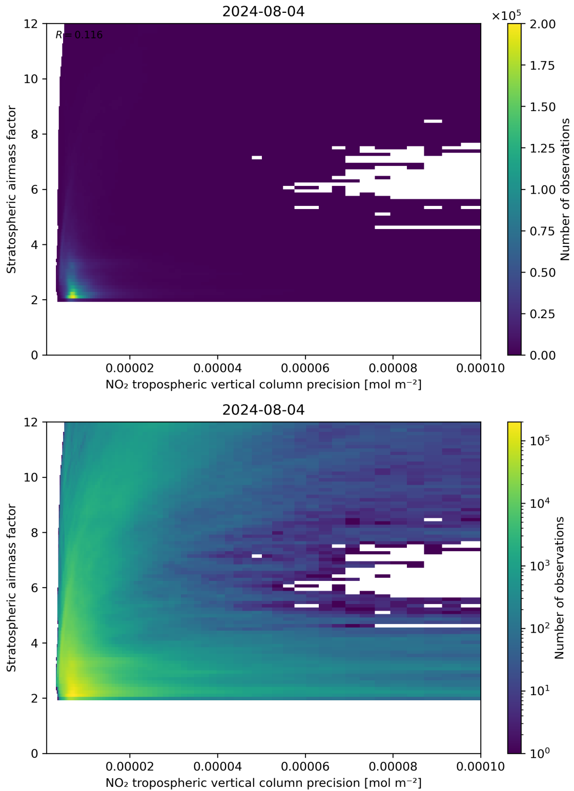
Figure 131: Scatter density plot of “NO 2 tropospheric vertical column precision” against “Stratospheric airmass factor” for 2024-08-03 to 2024-08-05.
