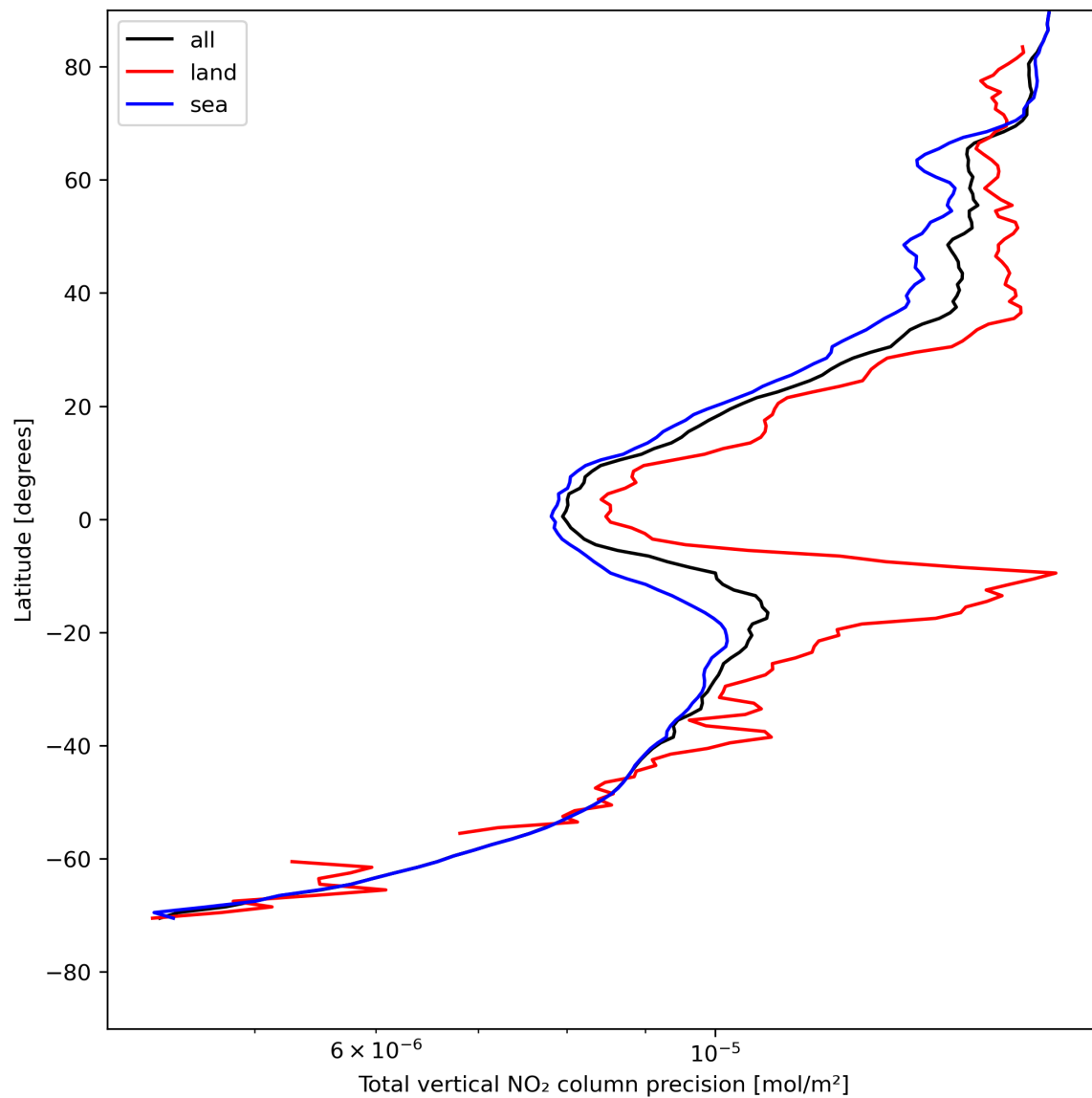
Figure 22: Zonal average of “Total vertical NO 2 column precision” for 2024-08-03 to 2024-08-05.
