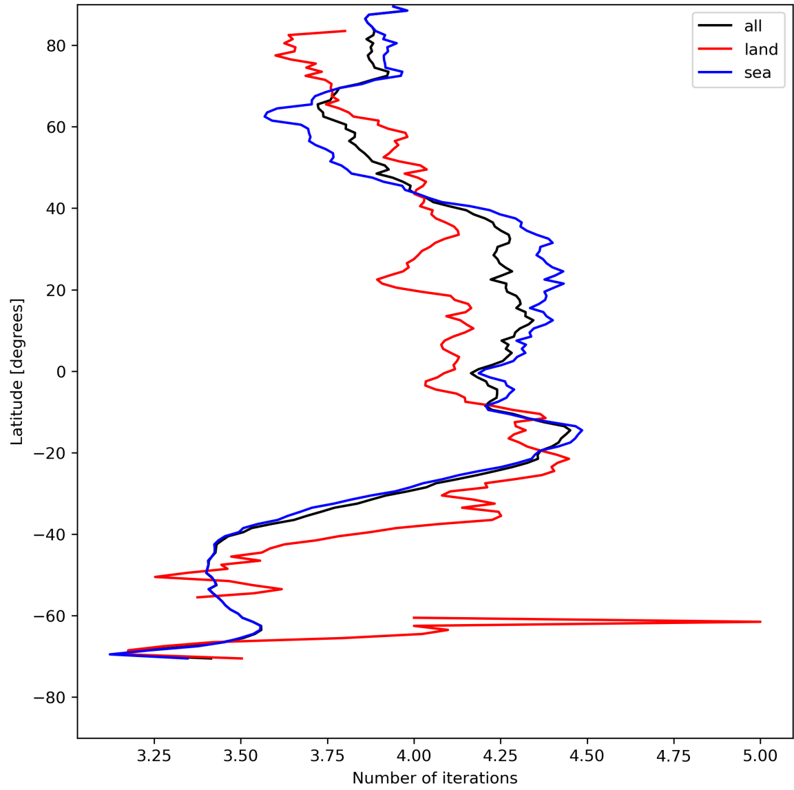
Figure 17: Zonal average of “Number of iterations” for 2024-08-03 to 2024-08-05.
