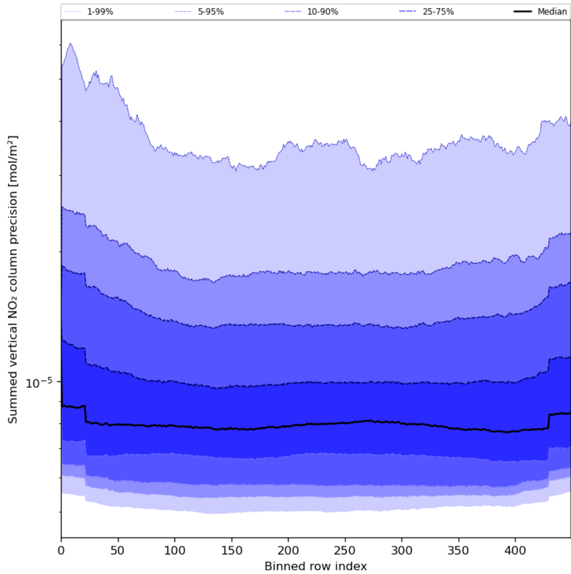
Figure 58: Along track statistics of “Summed vertical NO 2 column precision” for 2024-08-03 to 2024-08-05
