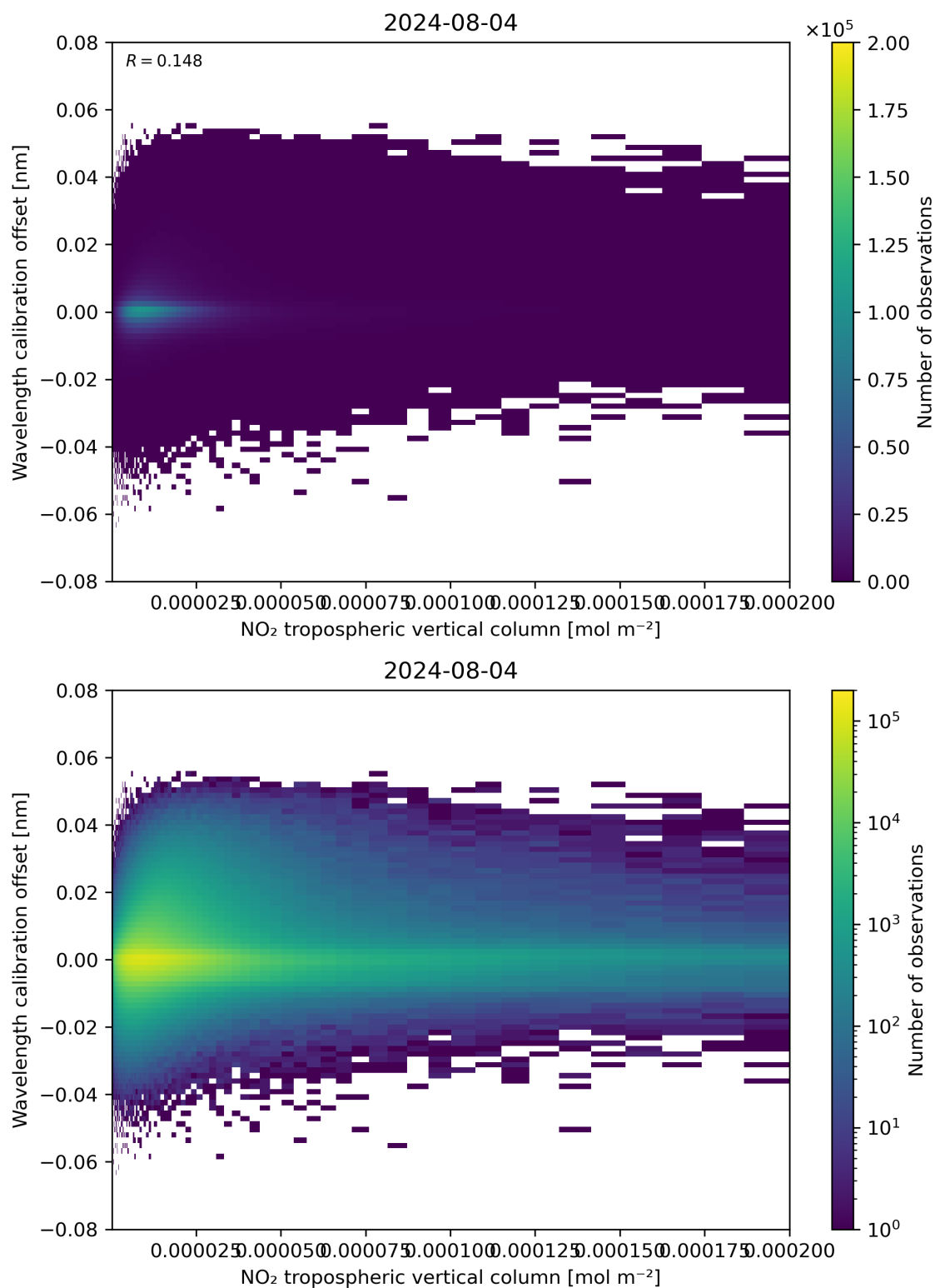
Figure 143: Scatter density plot of “NO 2 tropospheric vertical column” against “Wavelength calibration offset” for 2024-08-03 to 2024-08-05.
