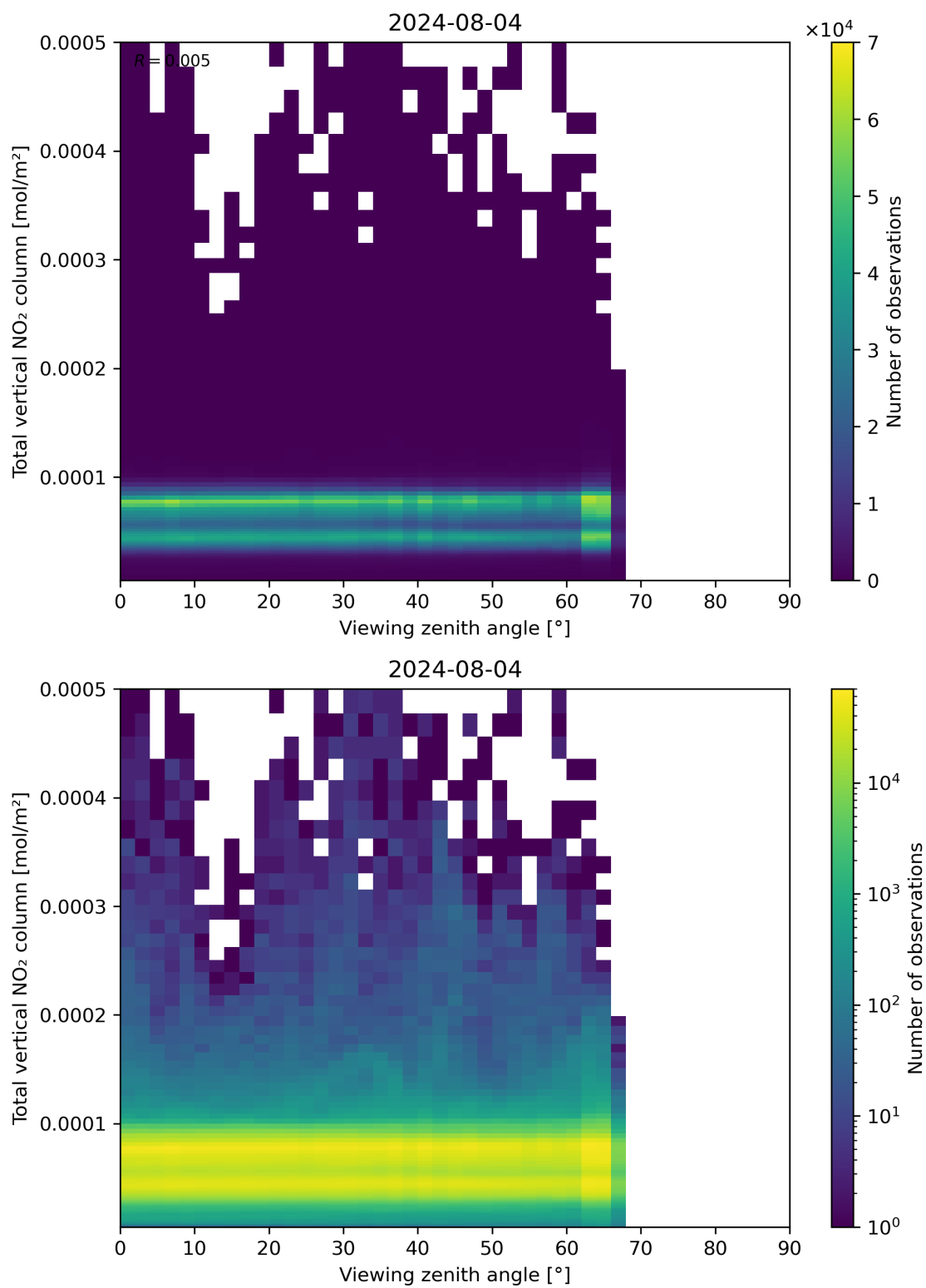
Figure 167: Scatter density plot of “Viewing zenith angle” against “Total vertical NO 2 column” for 2024-08-03 to 2024-08-05.
