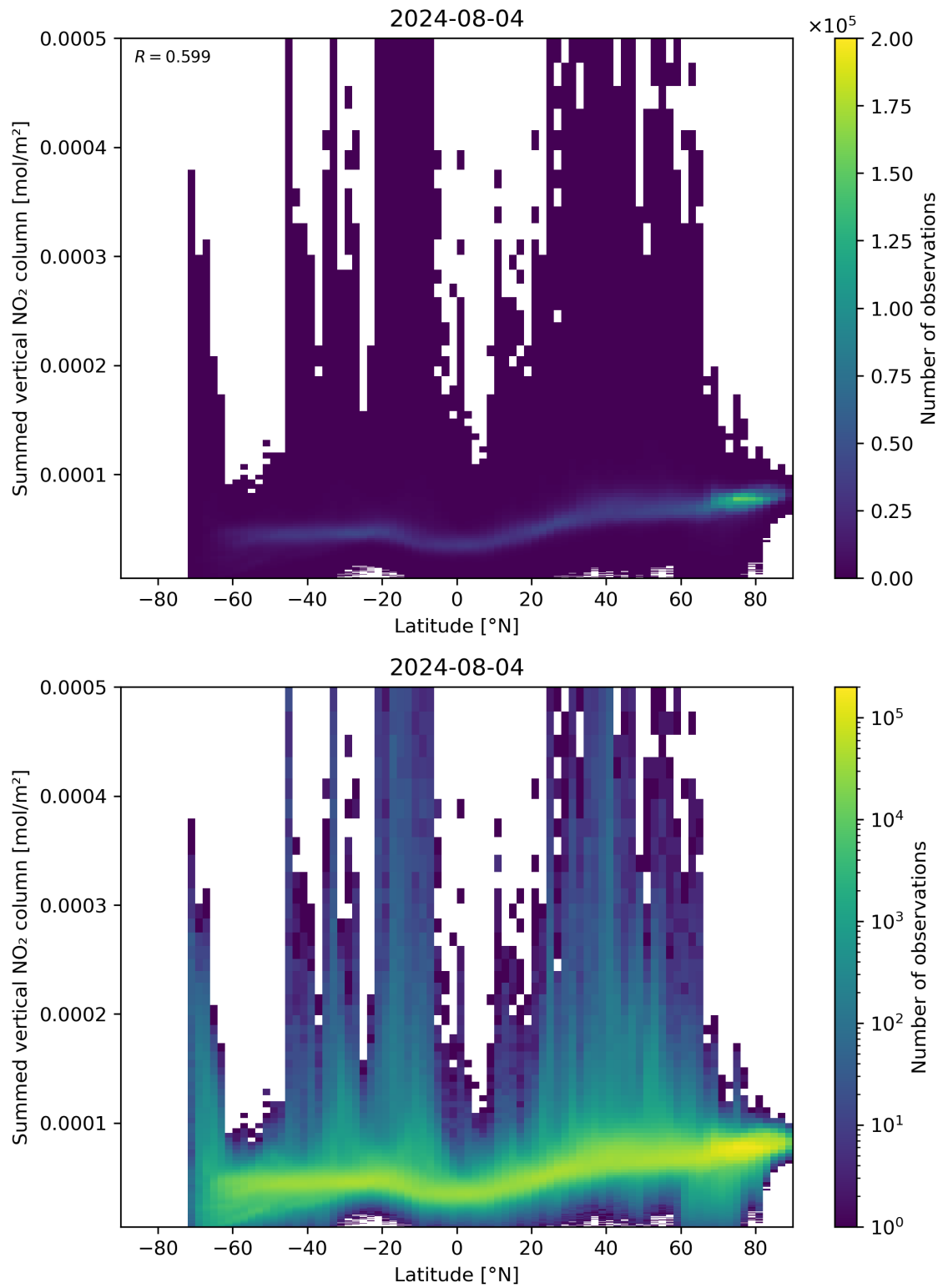
Figure 88: Scatter density plot of “Latitude” against “Summed vertical NO 2 column” for 2024-08-03 to 2024-08-05.
