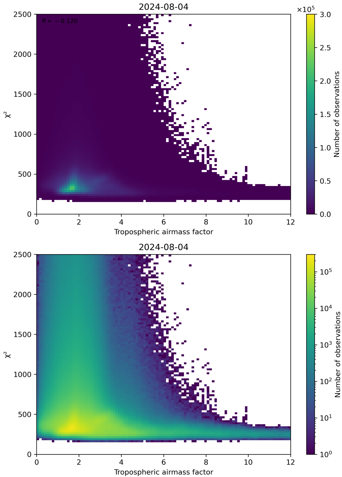
Figure 73: Scatter density plot of “Tropospheric airmass factor” against “ \chi^2 ” for 2024-08-03 to 2024-08-05.
