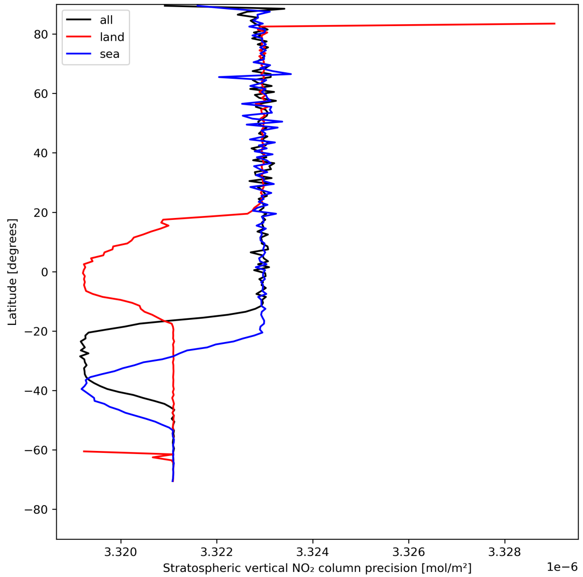
Figure 20: Zonal average of “Stratospheric vertical NO 2 column precision” for 2024-08-03 to 2024-08-05.
