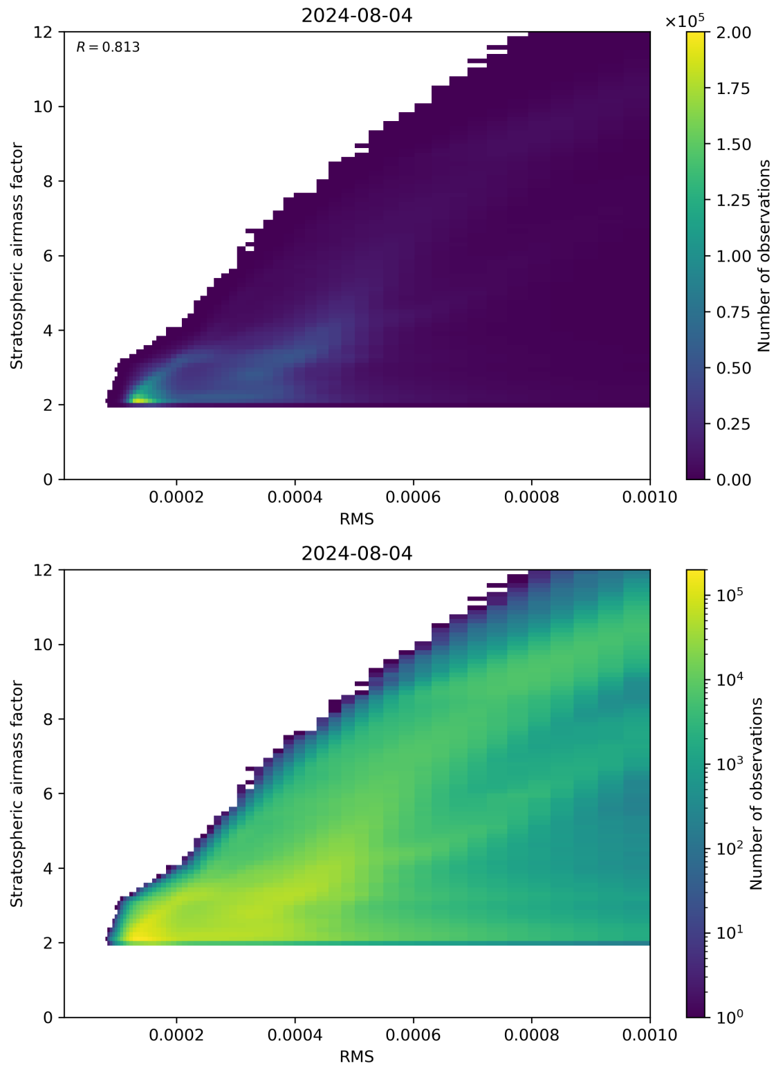
Figure 144: Scatter density plot of “RMS” against “Stratospheric airmass factor” for 2024-08-03 to 2024-08-05.
