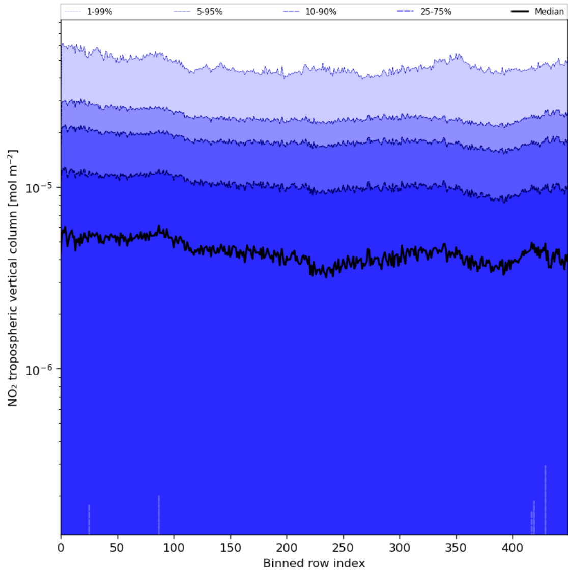
Figure 46: Along track statistics of “NO 2 tropospheric vertical column” for 2024-08-03 to 2024-08-05
