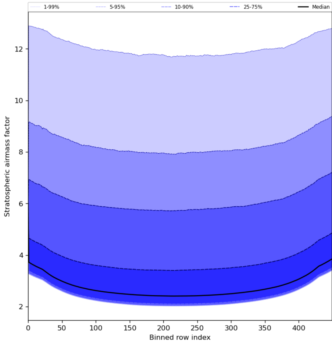
Figure 61: Along track statistics of “Stratospheric airmass factor” for 2024-08-03 to 2024-08-05
