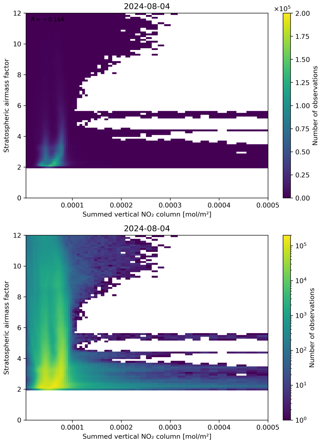
Figure 103: Scatter density plot of “Summed vertical NO 2 column” against “Stratospheric air mass factor” for 2024-08-03 to 2024-08-05.
