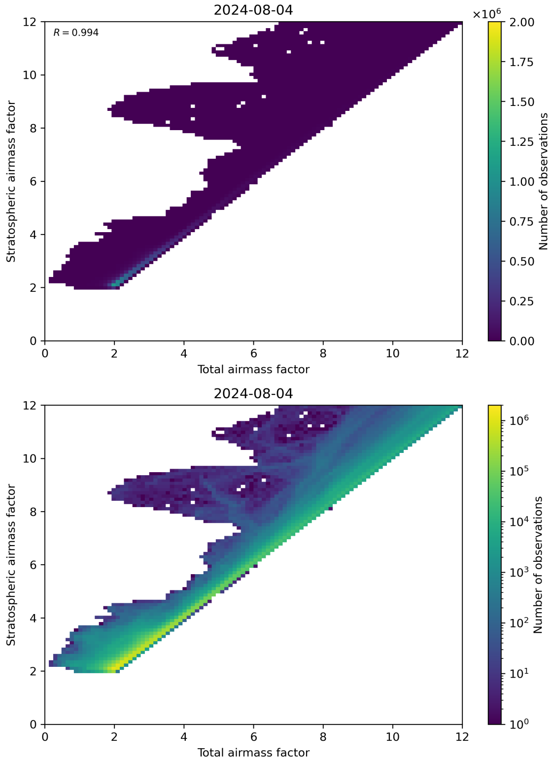
Figure 62: Scatter density plot of “Total airmass factor” against “Stratospheric airmass factor” for 2024-08-03 to 2024-08-05.
