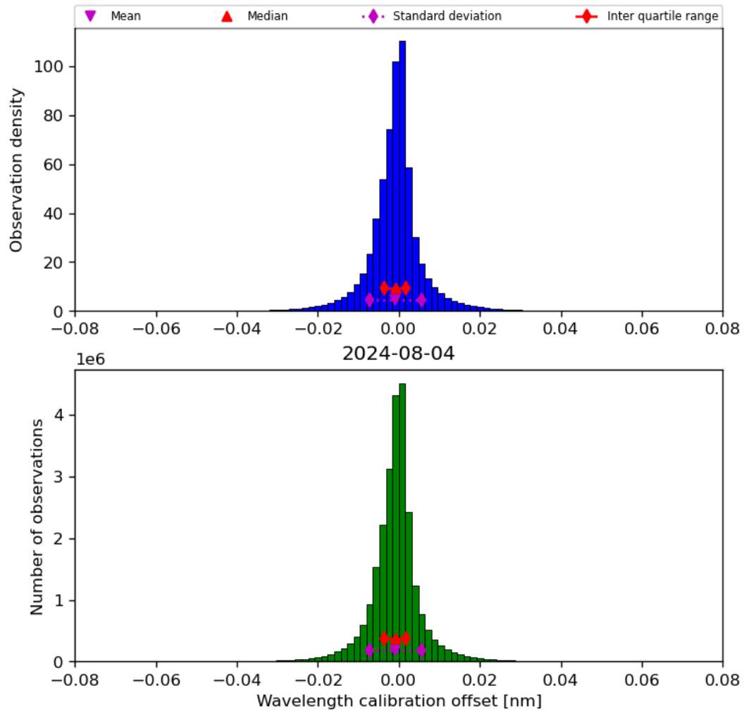
Figure 35: Histogram of “Wavelength calibration offset” for 2024-08-03 to 2024-08-05
