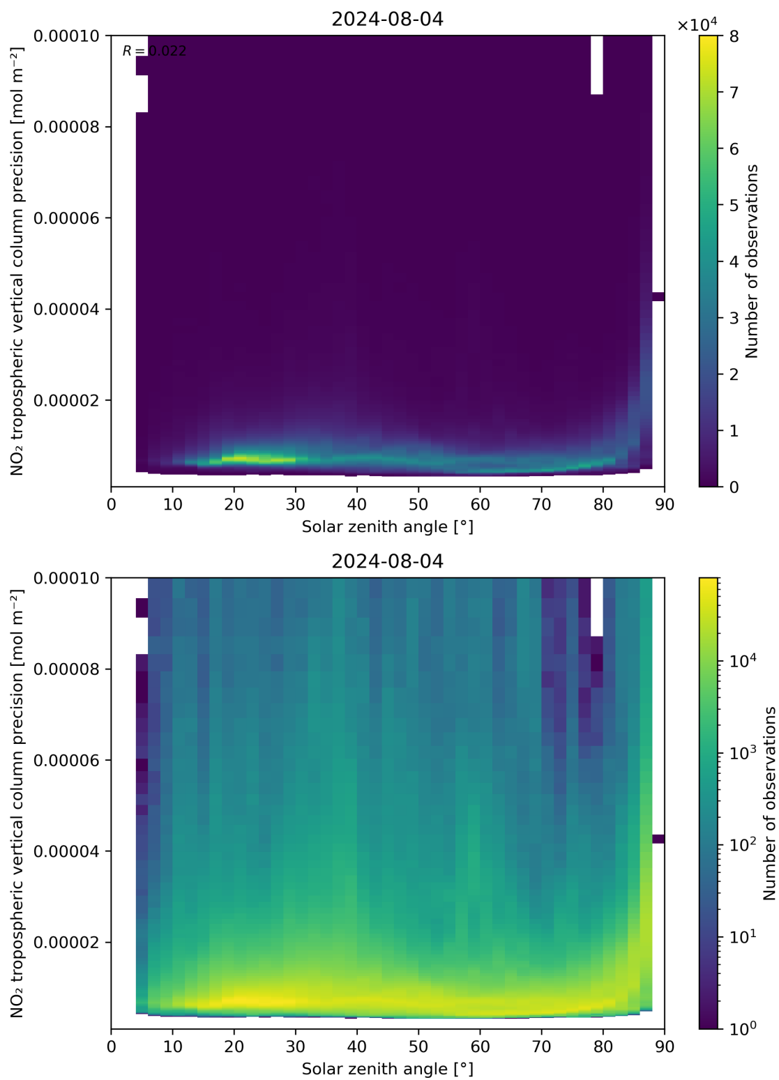
Figure 156: Scatter density plot of “Solar zenith angle” against “NO 2 tropospheric vertical column precision” for 2024-08-03 to 2024-08-05.
