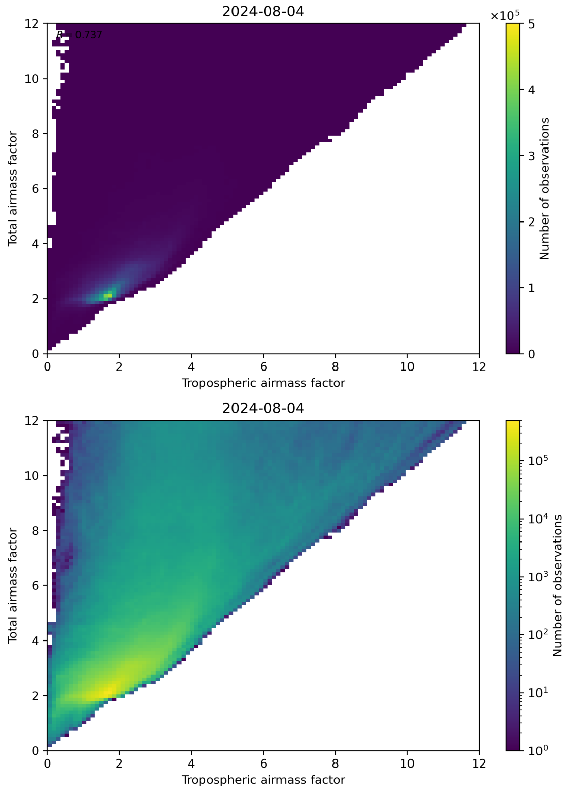
Figure 72: Scatter density plot of “Tropospheric airmass factor” against “Total airmass factor” for 2024-08-03 to 2024-08-05.
