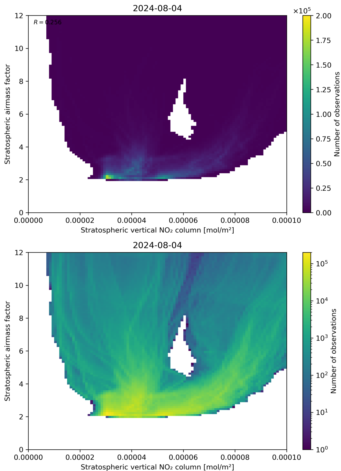
Figure 96: Scatter density plot of “Stratospheric vertical NO 2 column” against “Stratospheric airmass factor” for 2024-08-03 to 2024-08-05.
