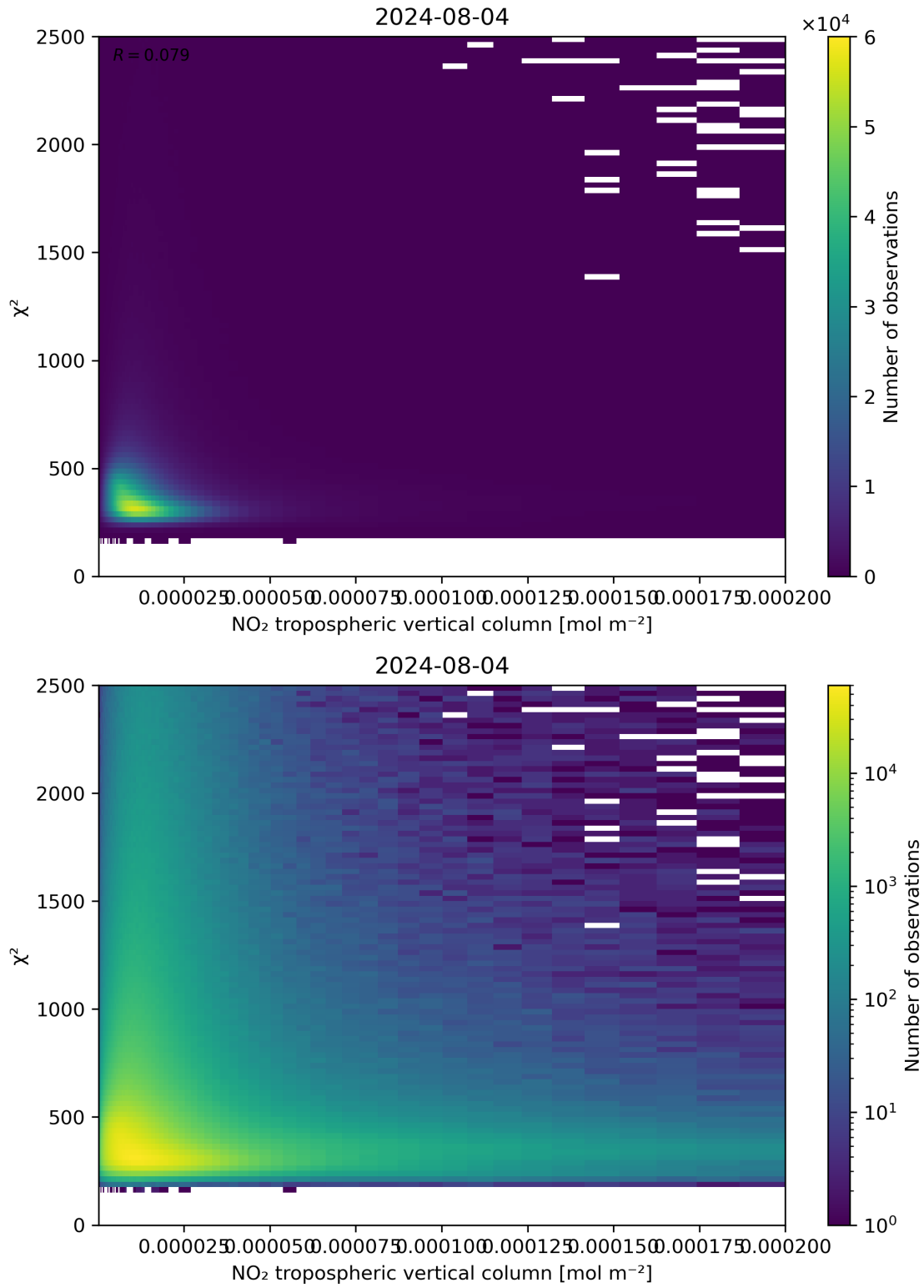
Figure 124: Scatter density plot of “NO 2 tropospheric vertical column” against “ \chi^2 ” for 2024-08-03 to 2024-08-05.
