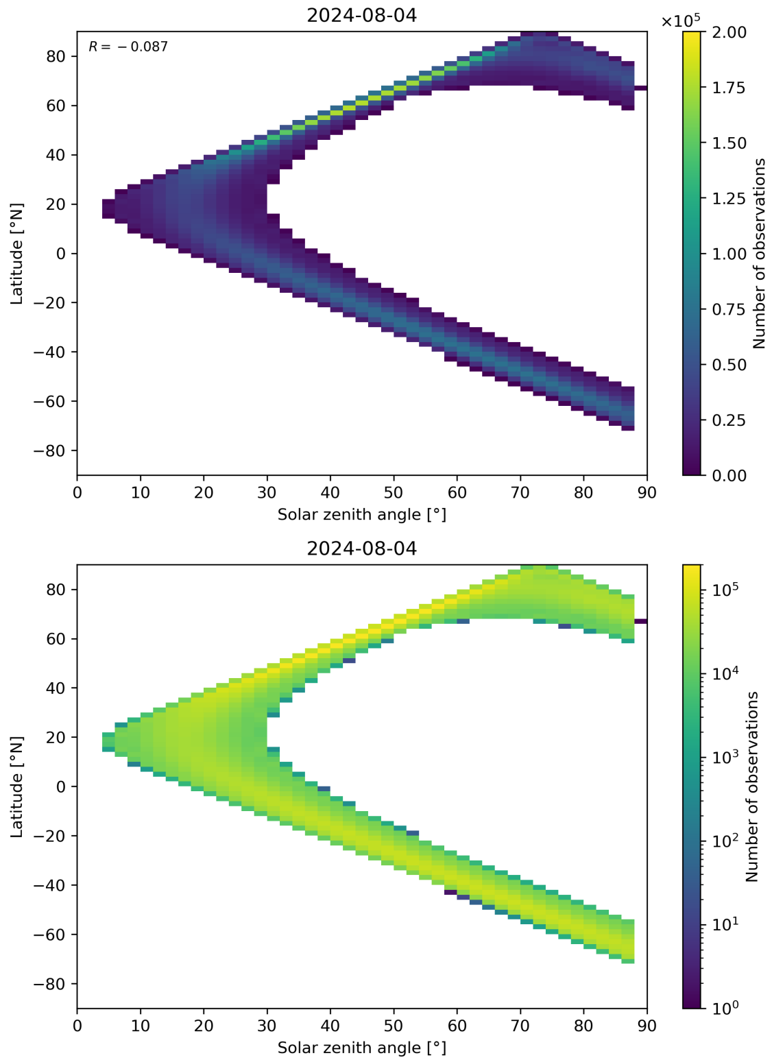
Figure 149: Scatter density plot of “Solar zenith angle” against “Latitude” for 2024-08-03 to 2024-08-05.
