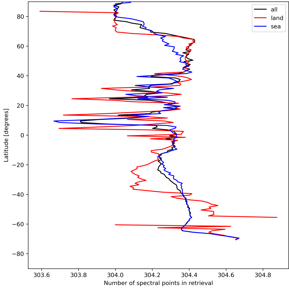
Figure 16: Zonal average of “Number of spectral points in retrieval” for 2024-08-03 to 2024-08-05.
