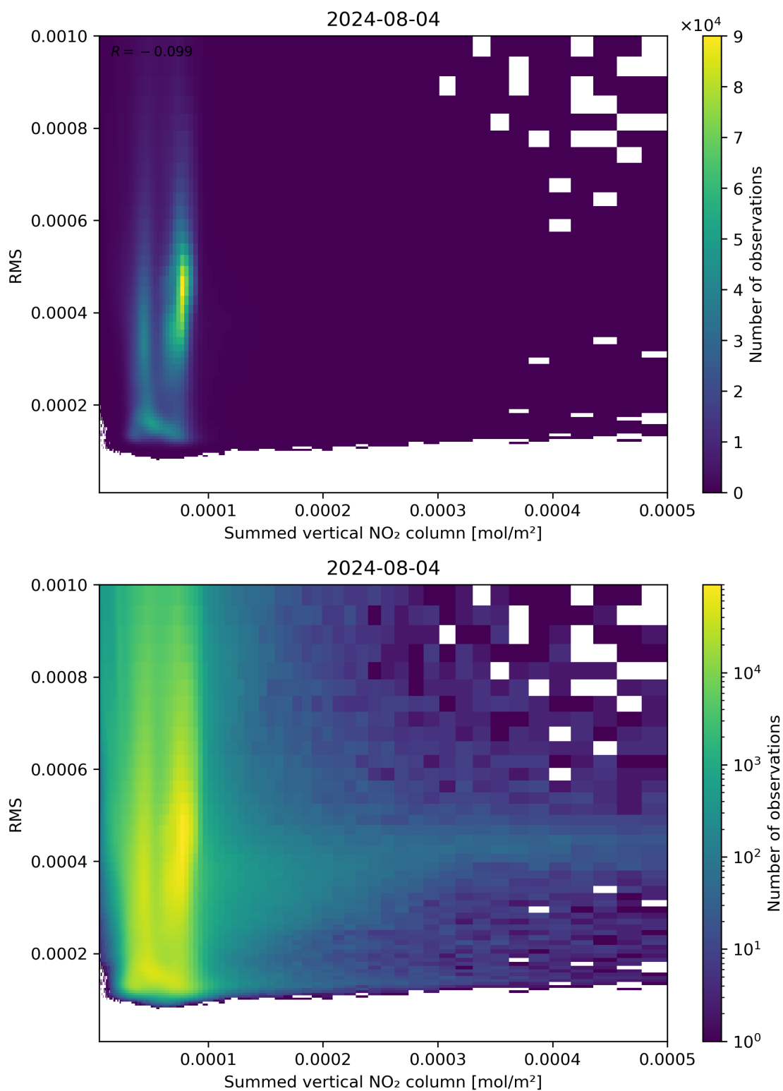
Figure 109: Scatter density plot of “Summed vertical NO 2 column” against “RMS” for 2024-08-03 to 2024-08-05.
