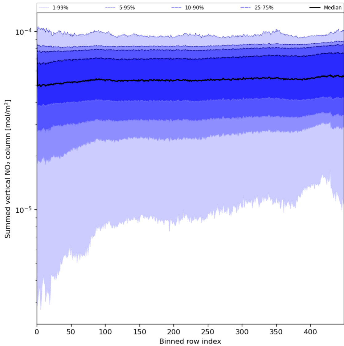
Figure 57: Along track statistics of “Summed vertical NO 2 column” for 2024-08-03 to 2024-08-05
