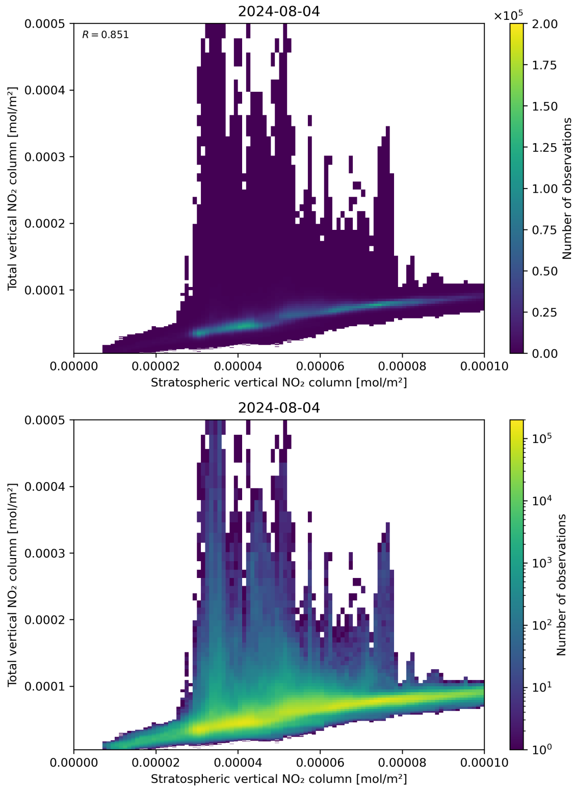
Figure 100: Scatter density plot of “Stratospheric vertical NO 2 column” against “Total vertical NO 2 column” for 2024-08-03 to 2024-08-05.
