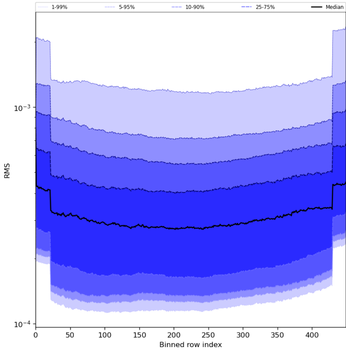
Figure 60: Along track statistics of “RMS” for 2024-08-03 to 2024-08-05
