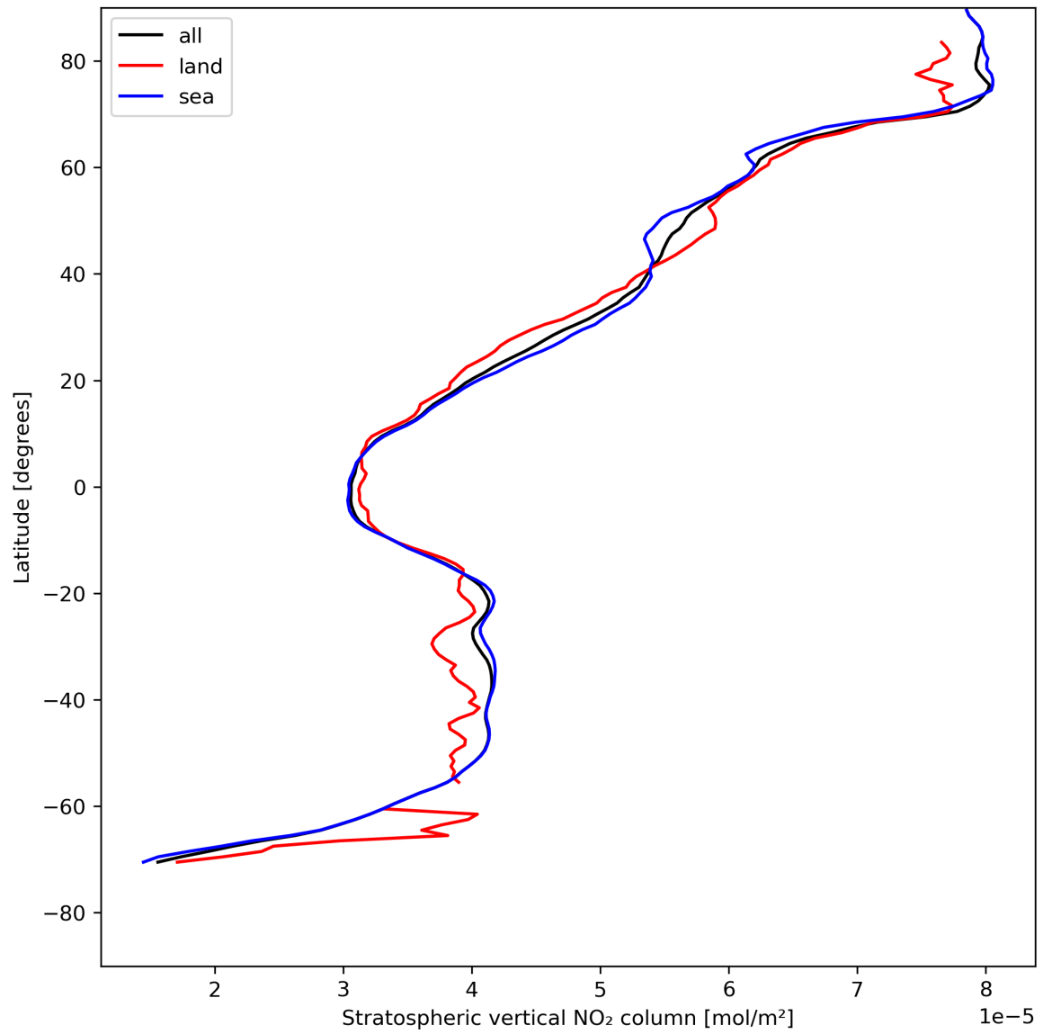
Figure 19: Zonal average of “Stratospheric vertical NO 2 column” for 2024-08-03 to 2024-08-05.
