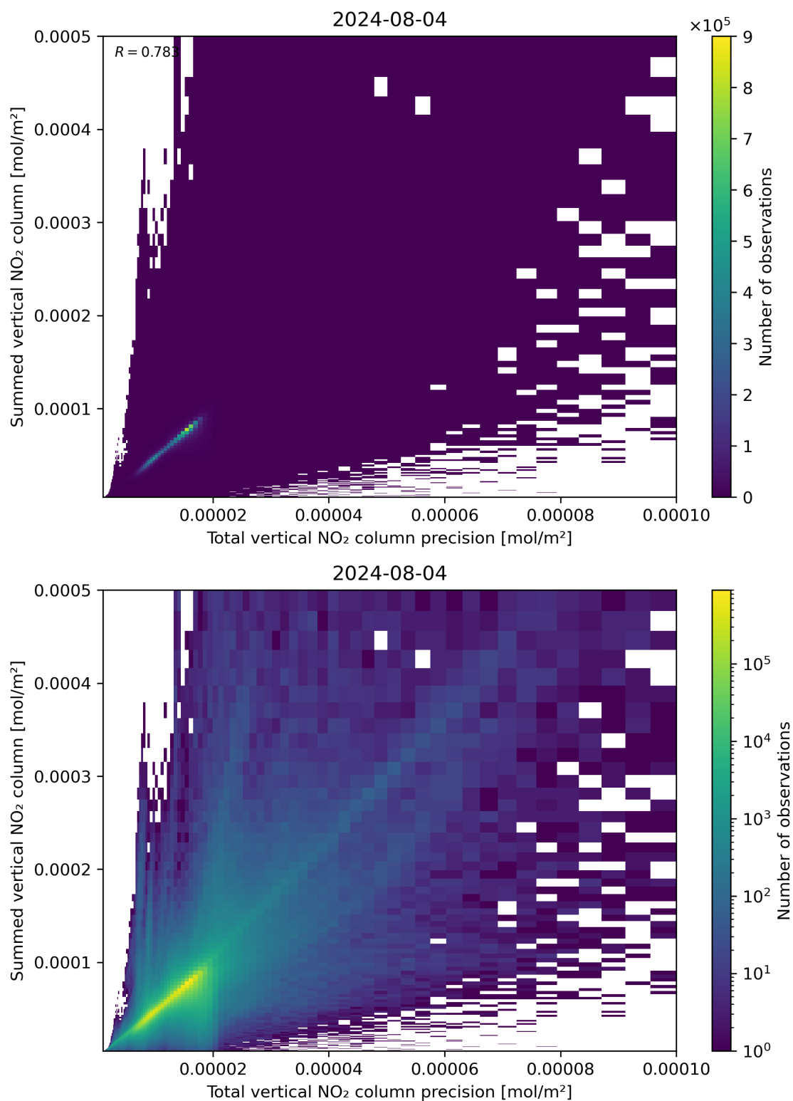
Figure 117: Scatter density plot of “Total vertical NO 2 column precision” against “Summed vertical NO 2 column” for 2024-08-03 to 2024-08-05.
