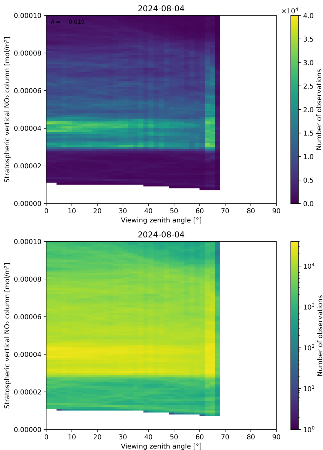
Figure 164: Scatter density plot of “Viewing zenith angle” against “Stratospheric vertical NO 2 column” for 2024-08-03 to 2024-08-05.
