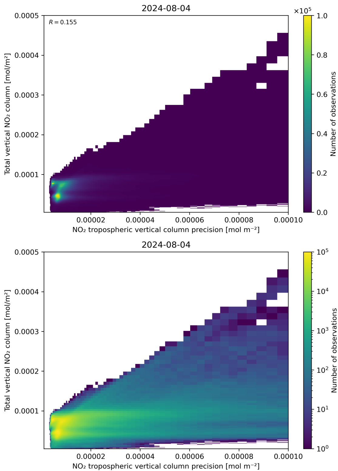
Figure 138: Scatter density plot of “NO 2 tropospheric vertical column precision” against “Total vertical NO 2 column” for 2024-08-03 to 2024-08-05.
