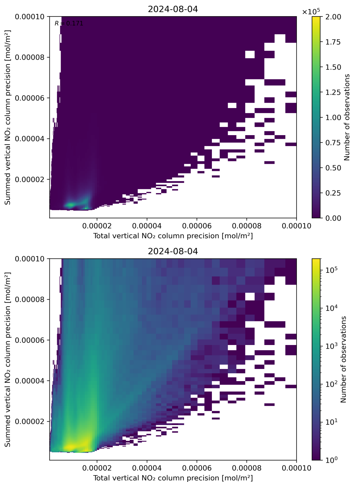
Figure 118: Scatter density plot of “Total vertical NO 2 column precision” against “Summed vertical NO 2 column precision” for 2024-08-03 to 2024-08-05.
