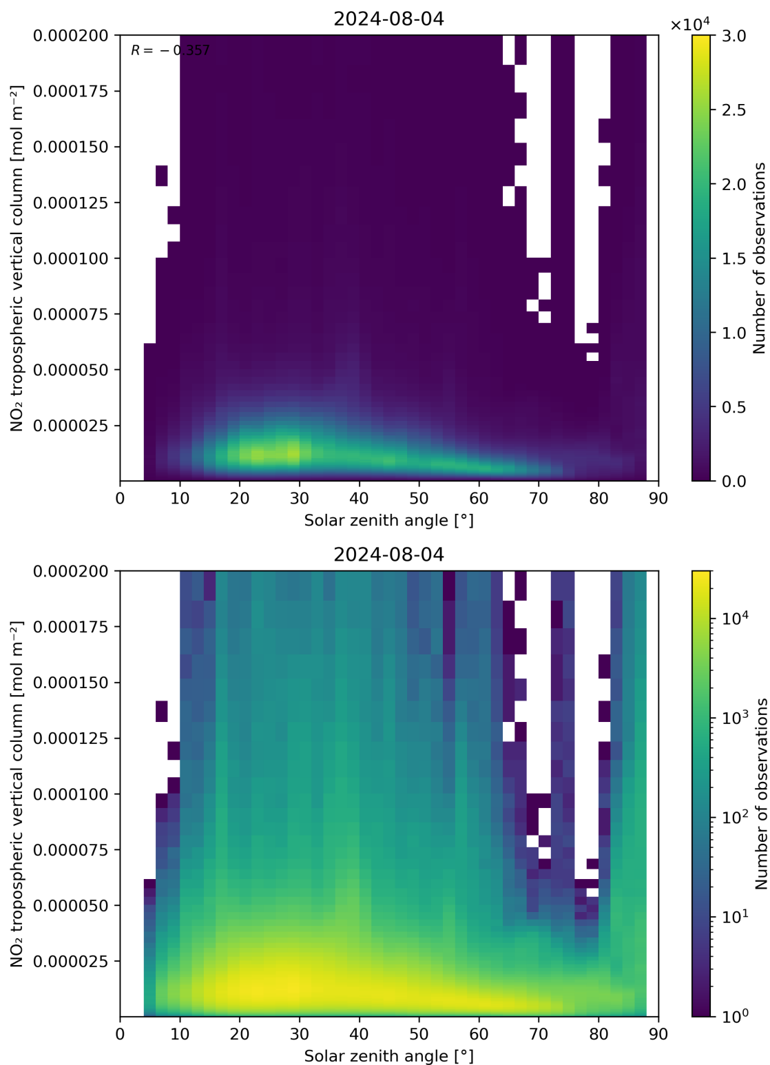
Figure 155: Scatter density plot of “Solar zenith angle” against “NO 2 tropospheric vertical column” for 2024-08-03 to 2024-08-05.
