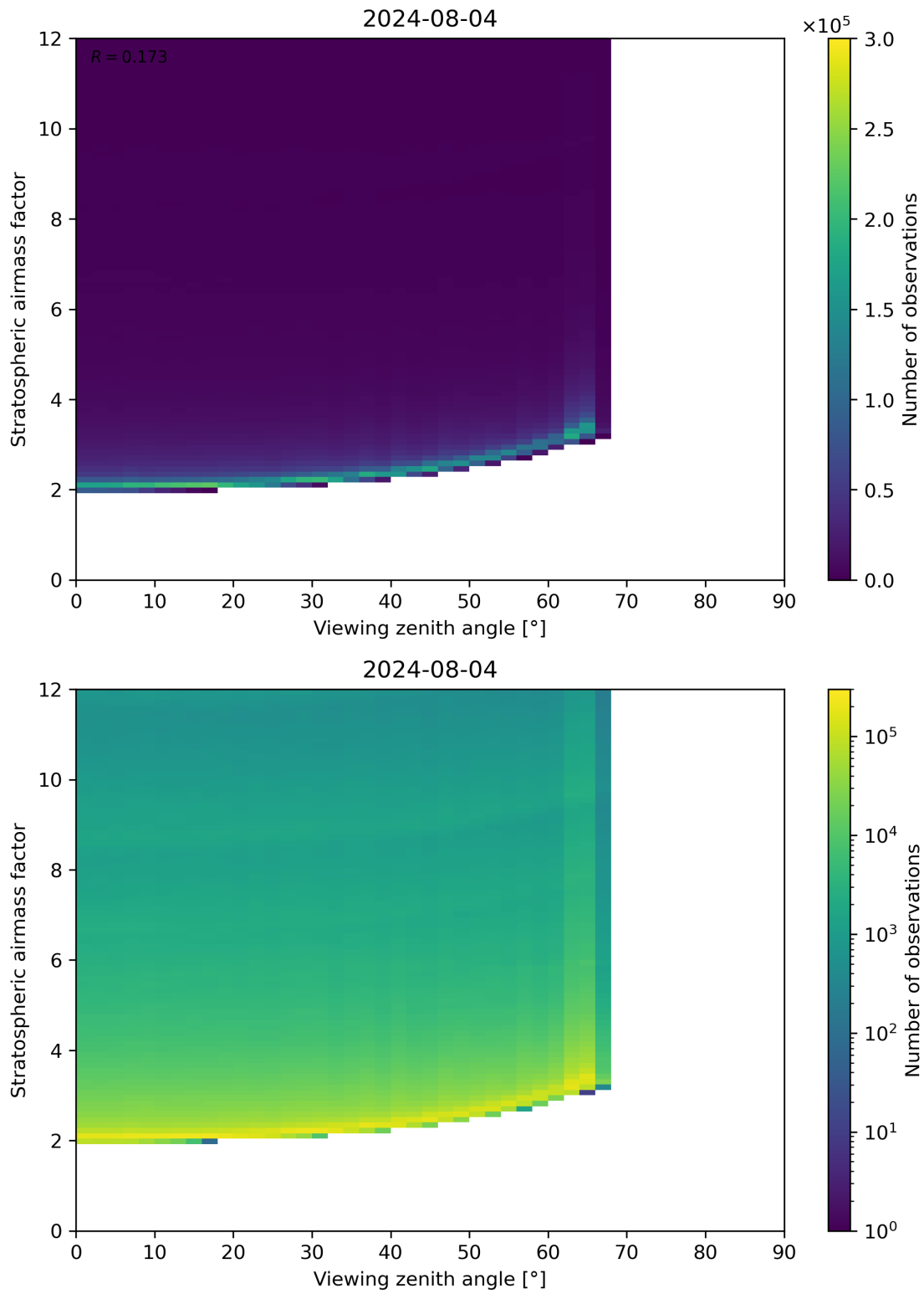
Figure 159: Scatter density plot of “Viewing zenith angle” against “Stratospheric airmass factor” for 2024-08-03 to 2024-08-05.
