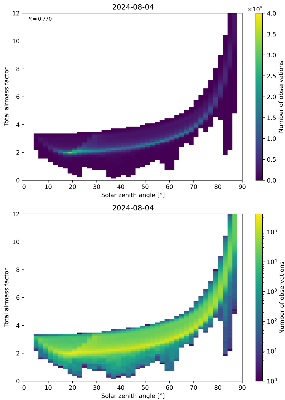
Figure 146: Scatter density plot of “Solar zenith angle” against “Total air mass factor” for 2024-08-03 to 2024-08-05.
