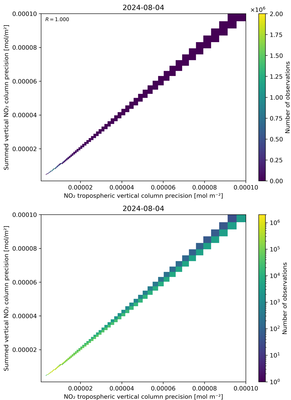
Figure 137: Scatter density plot of “NO 2 tropospheric vertical column precision” against “Summed vertical NO 2 column precision” for 2024-08-03 to 2024-08-05.
