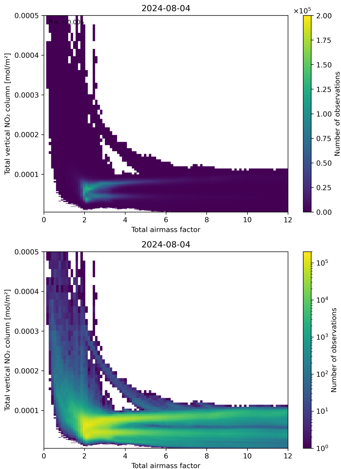
Figure 67: Scatter density plot of “Total airmass factor” against “Total vertical NO 2 column” for 2024-08-03 to 2024-08-05.
