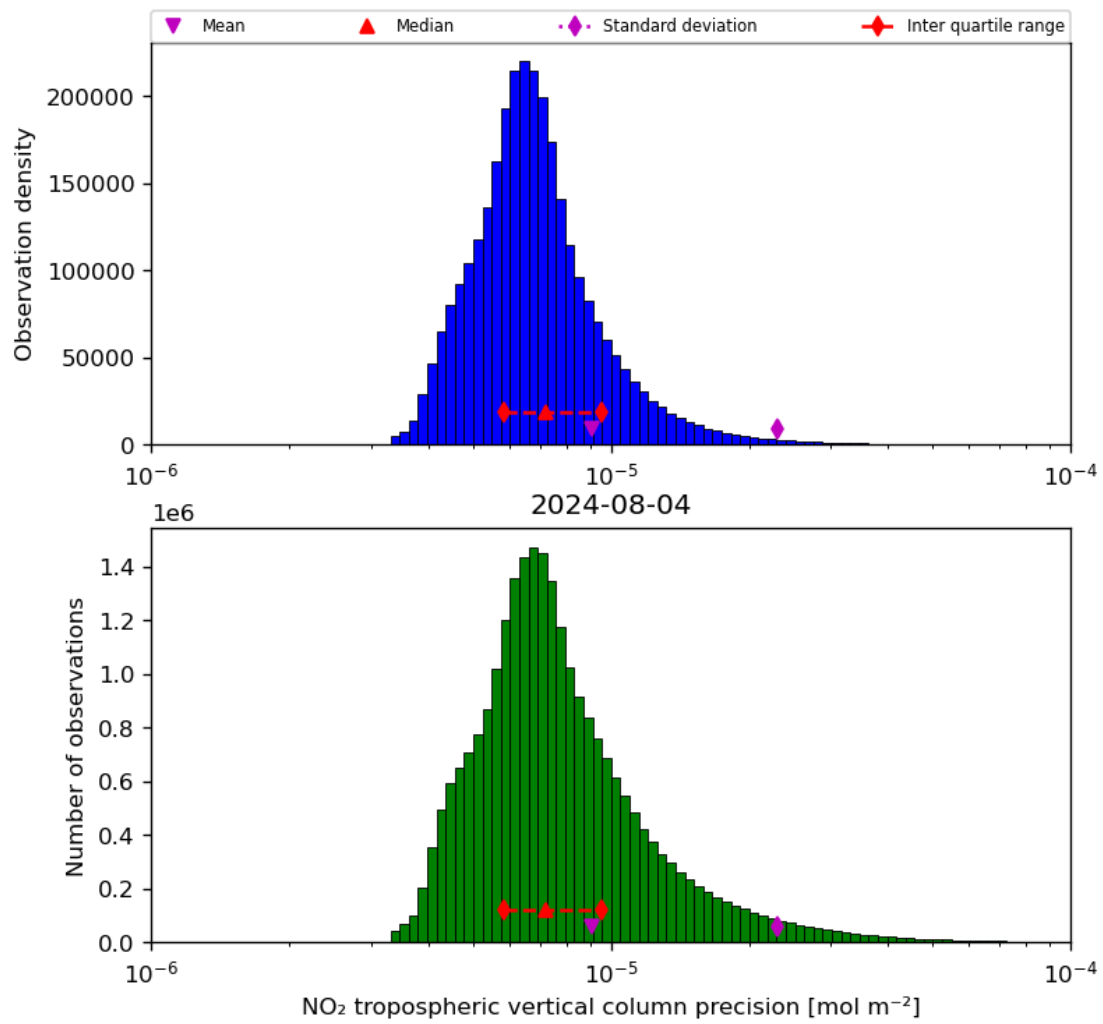
Figure 30: Histogram of “NO 2 tropospheric vertical column precision” for 2024-08-03 to 2024-08-05
