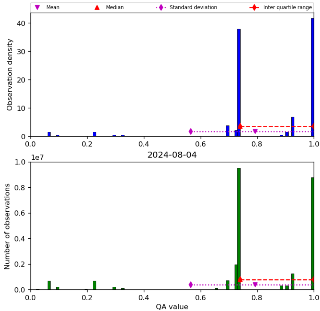
Figure 28: Histogram of “QA value” for 2024-08-03 to 2024-08-05
