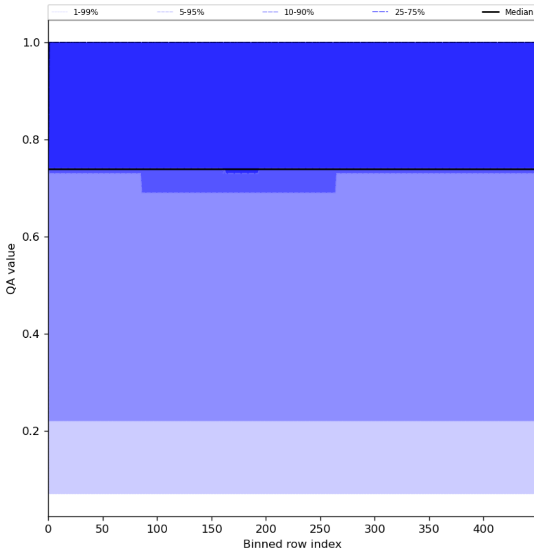
Figure 45: Along track statistics of “QA value” for 2024-08-03 to 2024-08-05
