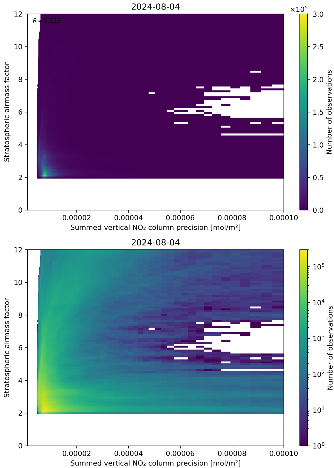
Figure 106: Scatter density plot of “Summed vertical NO 2 column precision” against “Stratospheric airmass factor” for 2024-08-03 to 2024-08-05.
