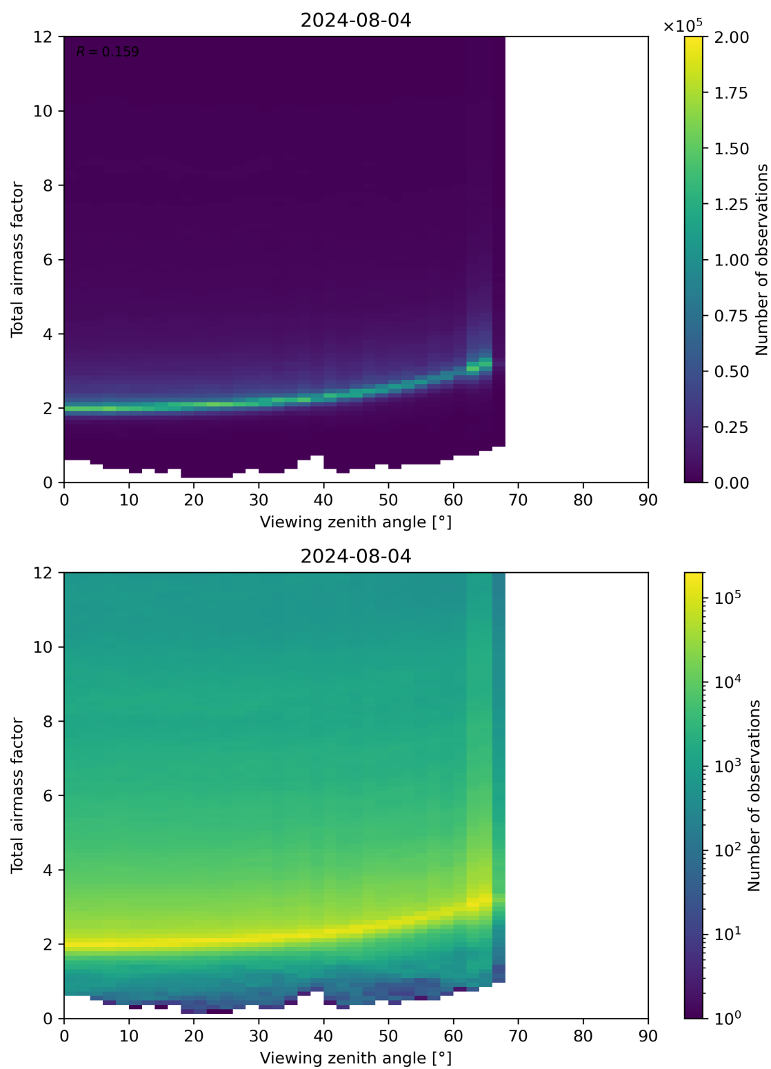
Figure 160: Scatter density plot of “Viewing zenith angle” against “Total airmass factor” for 2024-08-03 to 2024-08-05.
