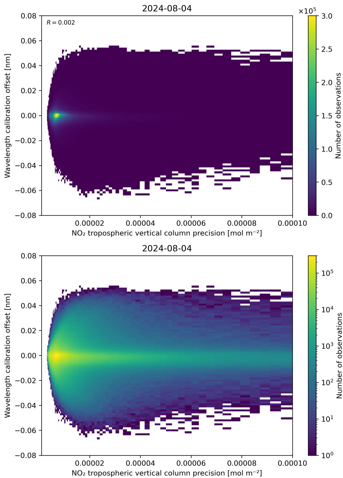
Figure 141: Scatter density plot of “NO 2 tropospheric vertical column precision” against “Wavelength calibration offset” for 2024-08-03 to 2024-08-05.
