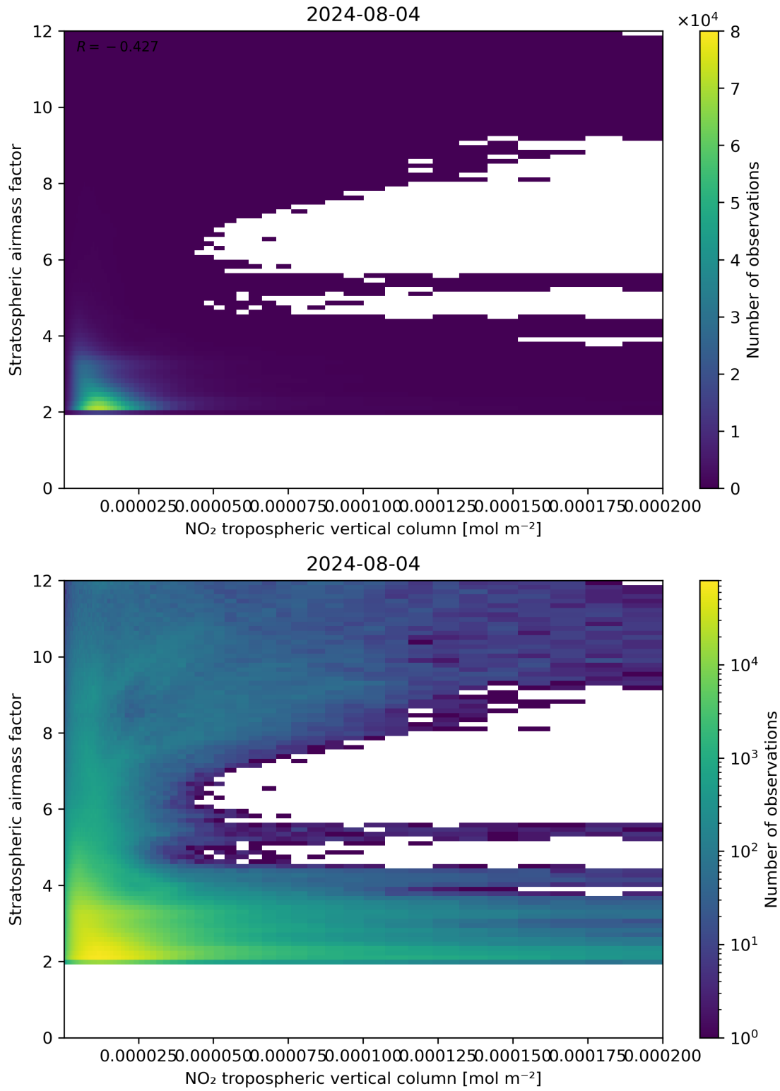
Figure 121: Scatter density plot of “NO 2 tropospheric vertical column” against “Stratospheric air mass factor” for 2024-08-03 to 2024-08-05.
