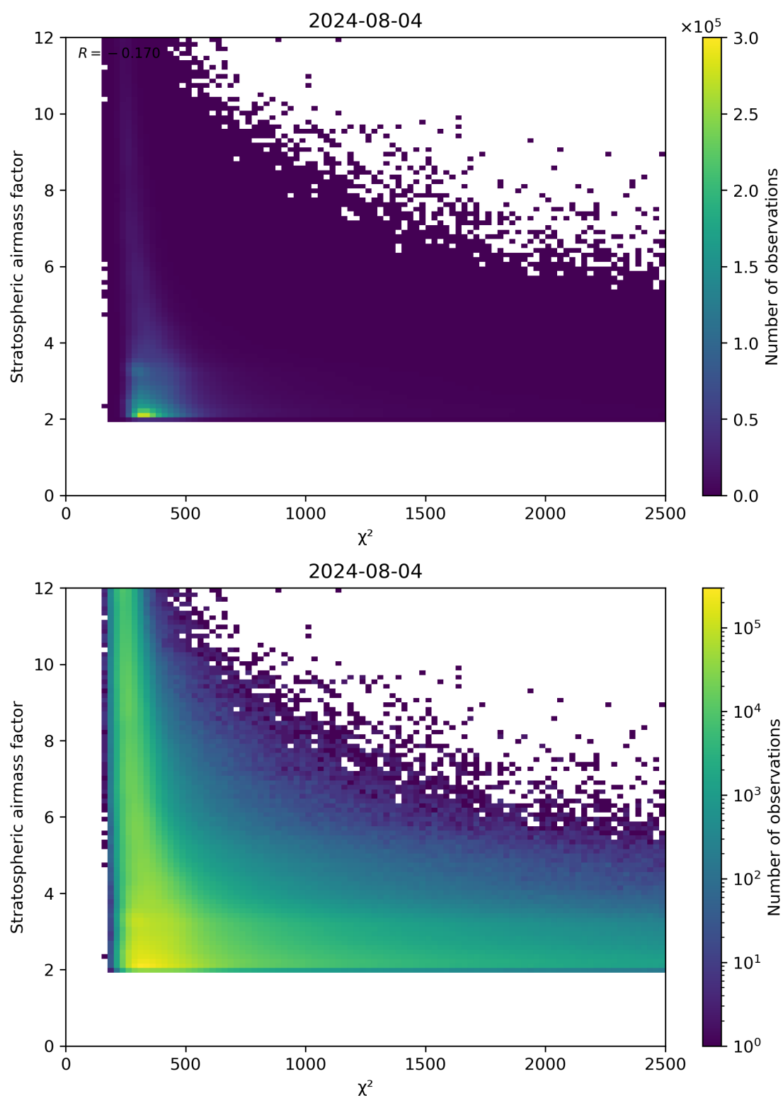
Figure 81: Scatter density plot of “ \chi^2 ” against “Stratospheric airmass factor” for 2024-08-03 to 2024-08-05.
