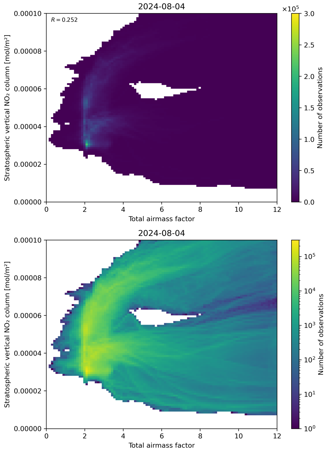
Figure 64: Scatter density plot of “Total airmass factor” against “Stratospheric vertical \text{NO}_2 column” for 2024-08-03 to 2024-08-05.
