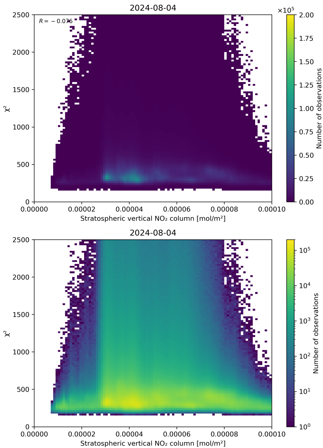
Figure 97: Scatter density plot of “Stratospheric vertical NO 2 column” against “ \chi^2 ” for 2024-08-03 to 2024-08-05.
