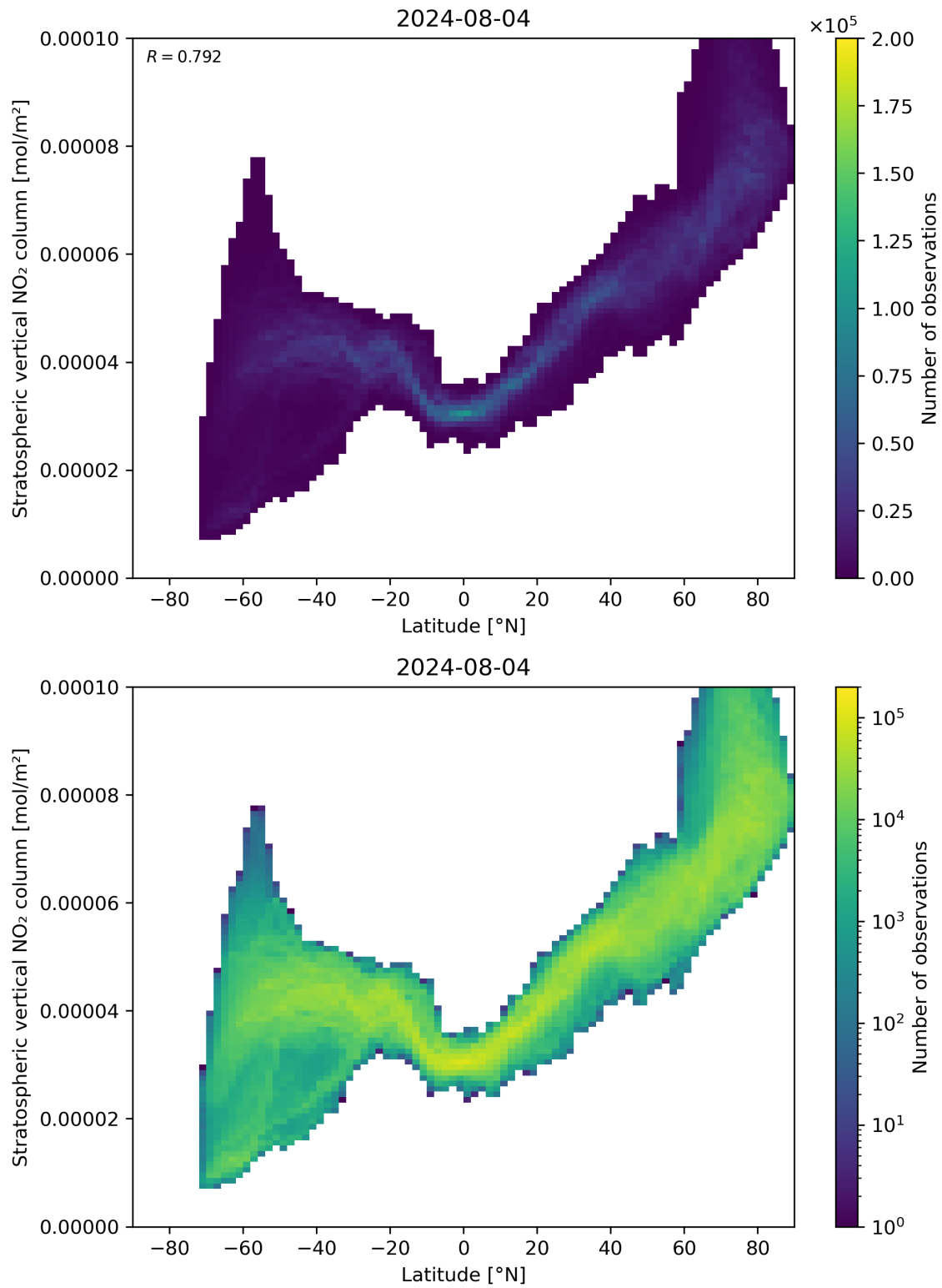
Figure 87: Scatter density plot of “Latitude” against “Stratospheric vertical NO 2 column” for 2024-08-03 to 2024-08-05.
