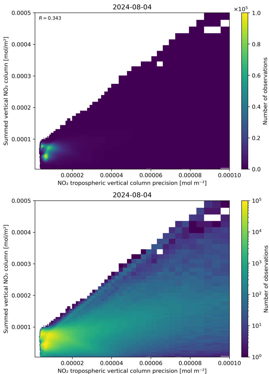
Figure 136: Scatter density plot of “NO 2 tropospheric vertical column precision” against “Summed vertical NO 2 column” for 2024-08-03 to 2024-08-05.
