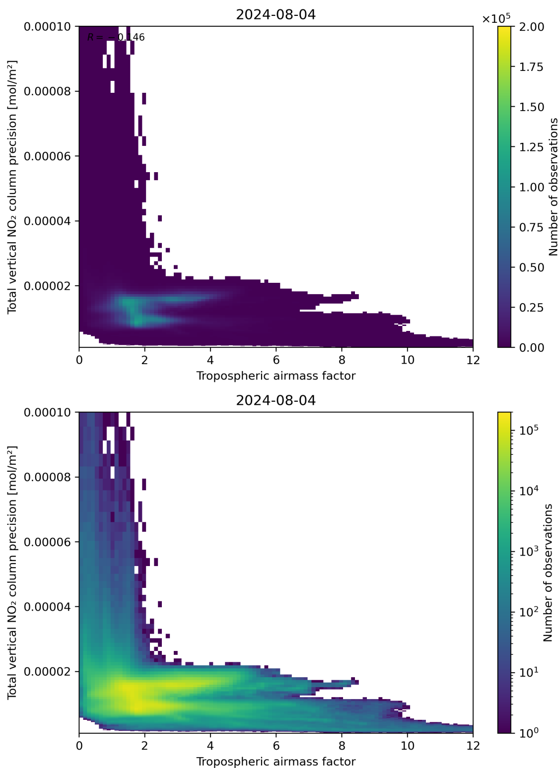
Figure 78: Scatter density plot of “Tropospheric air mass factor” against “Total vertical NO 2 column precision” for 2024-08-03 to 2024-08-05.
