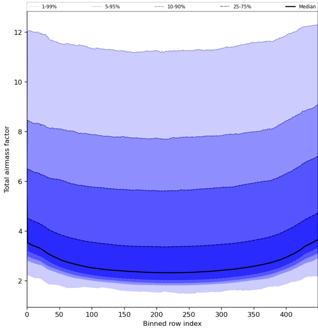
Figure 49: Along track statistics of “Total airmass factor” for 2024-08-03 to 2024-08-05
