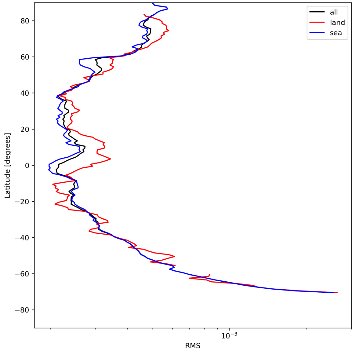
Figure 26: Zonal average of “RMS” for 2024-08-03 to 2024-08-05.
