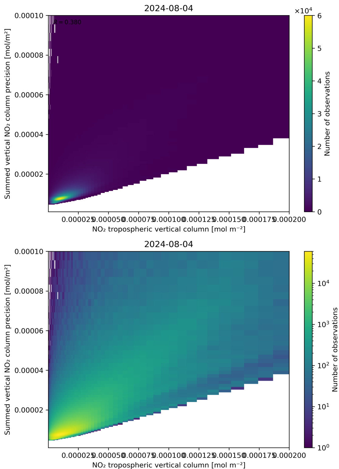
Figure 127: Scatter density plot of “NO 2 tropospheric vertical column” against “Summed vertical NO 2 column precision” for 2024-08-03 to 2024-08-05.
