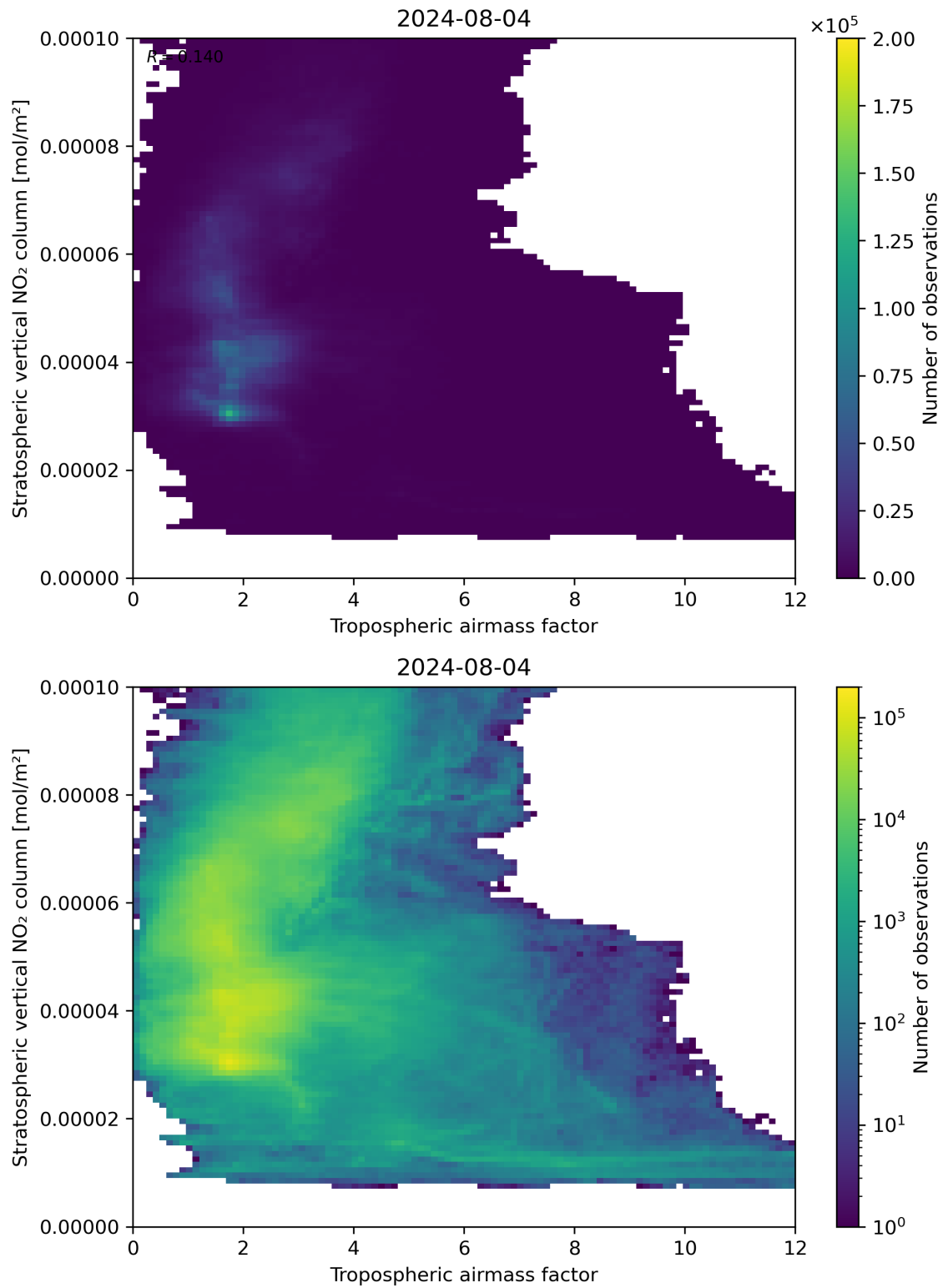
Figure 74: Scatter density plot of “Tropospheric air mass factor” against “Stratospheric vertical NO 2 column” for 2024-08-03 to 2024-08-05.
