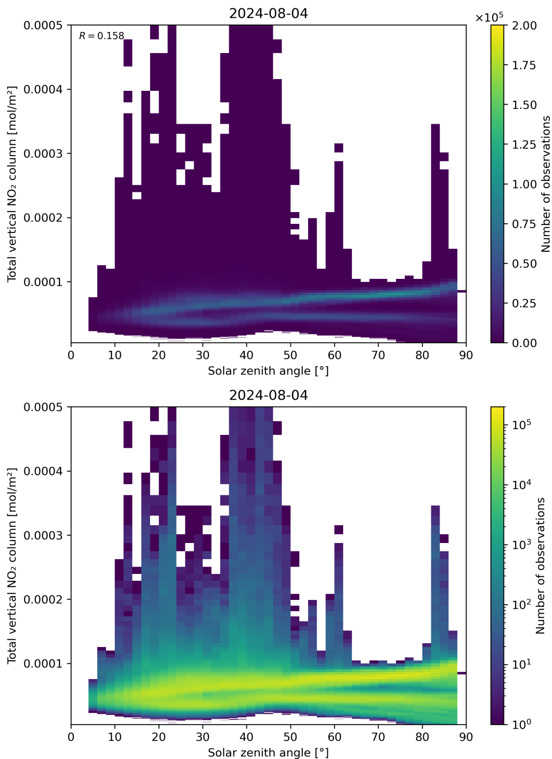
Figure 153: Scatter density plot of “Solar zenith angle” against “Total vertical NO 2 column” for 2024-08-03 to 2024-08-05.
