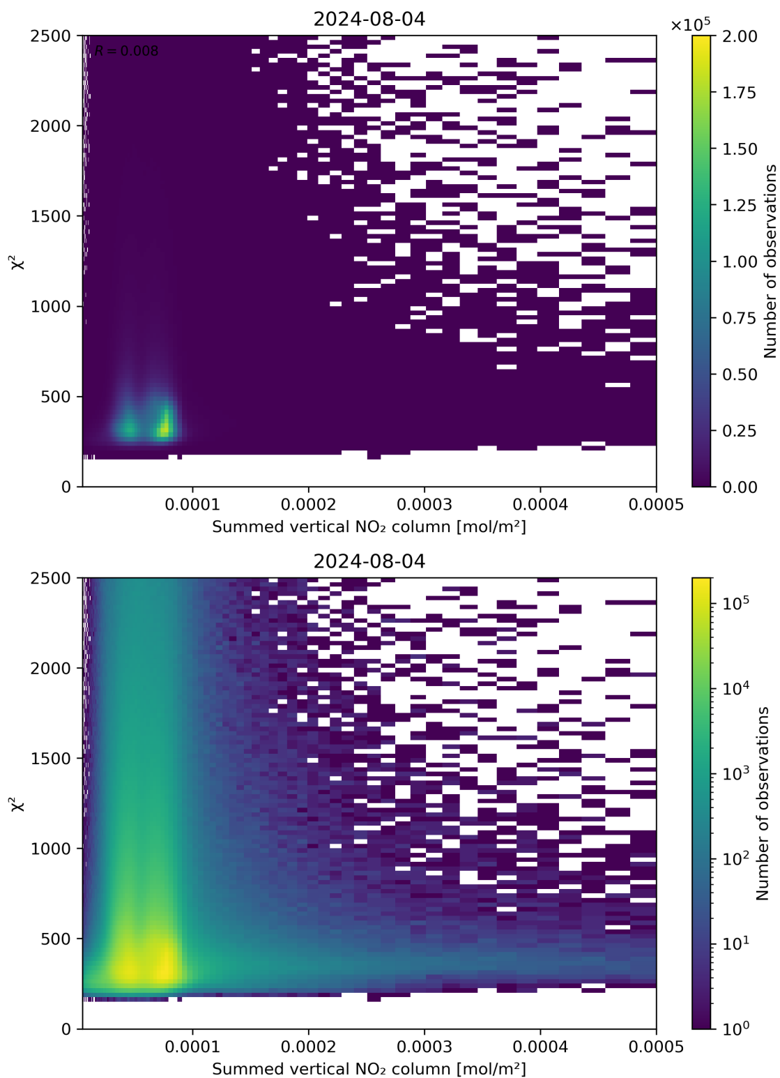
Figure 104: Scatter density plot of “Summed vertical NO 2 column” against “ \chi^2 ” for 2024-08-03 to 2024-08-05.
