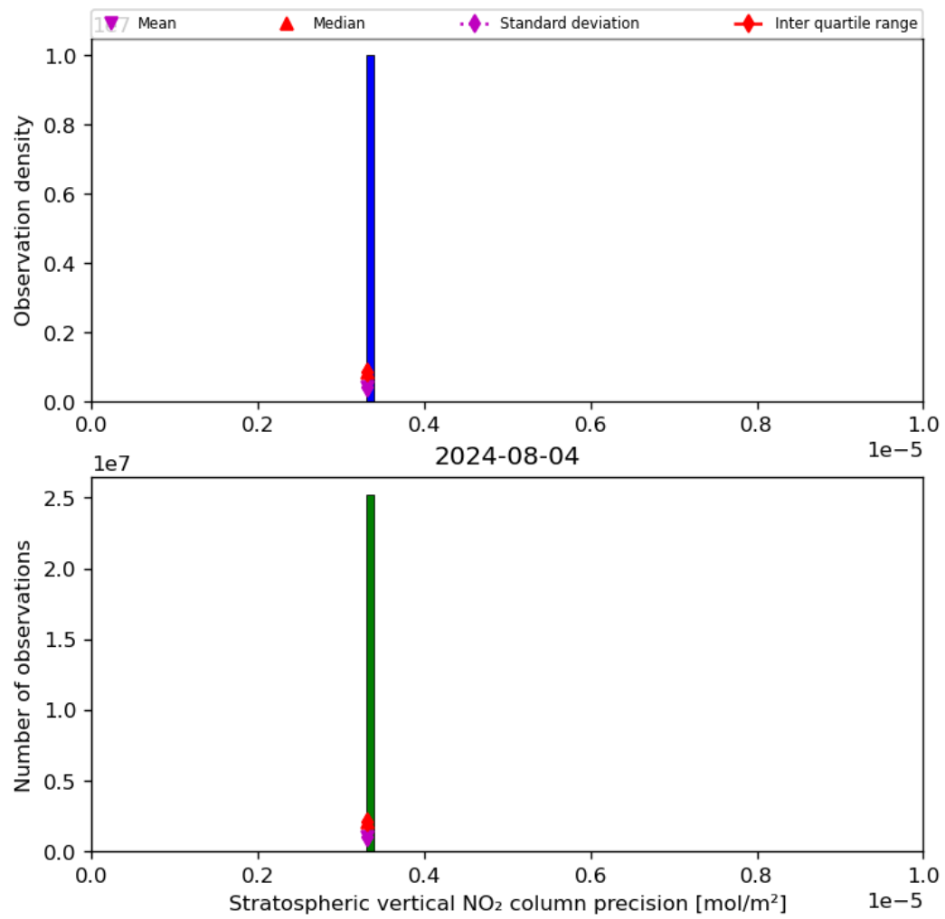
Figure 37: Histogram of “Stratospheric vertical NO 2 column precision” for 2024-08-03 to 2024-08-05
