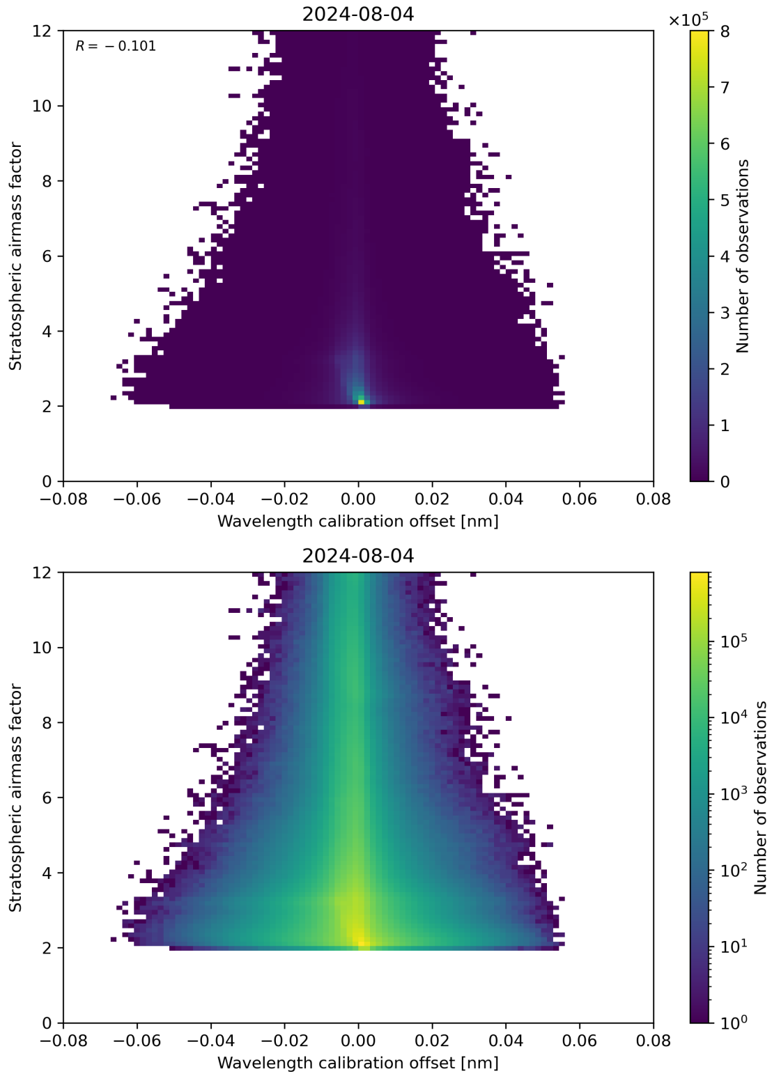
Figure 174: Scatter density plot of “Wavelength calibration offset” against “Stratospheric air mass factor” for 2024-08-03 to 2024-08-05.
