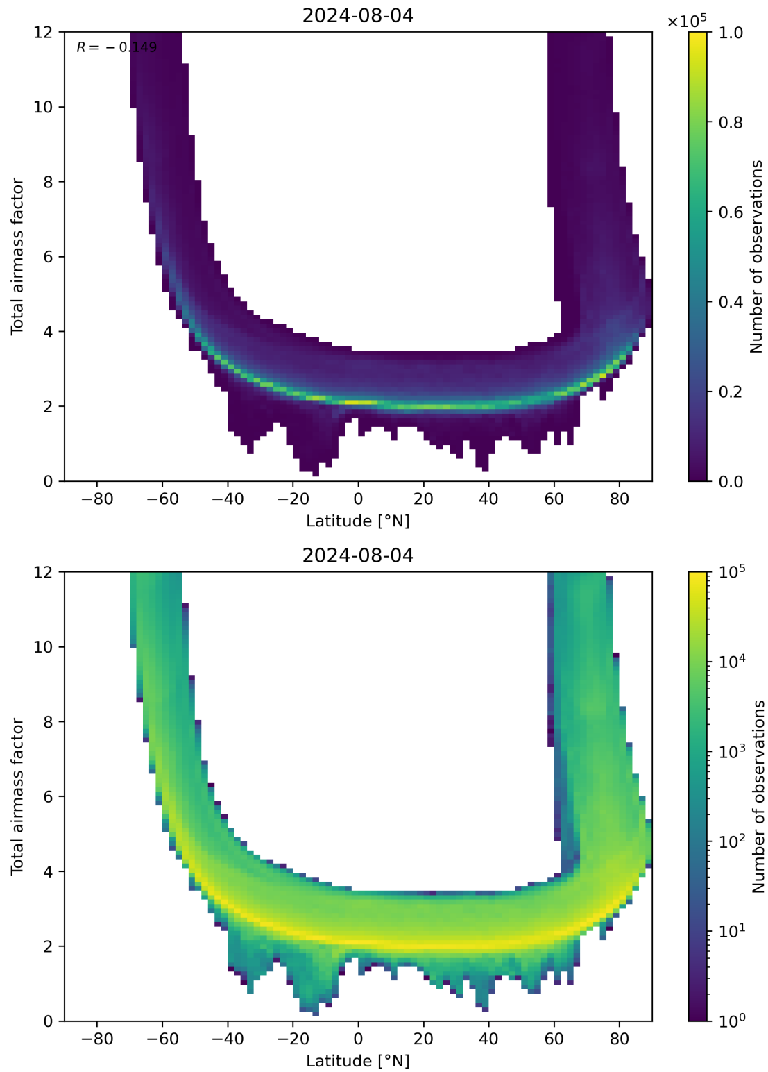
Figure 84: Scatter density plot of “Latitude” against “Total airmass factor” for 2024-08-03 to 2024-08-05.
