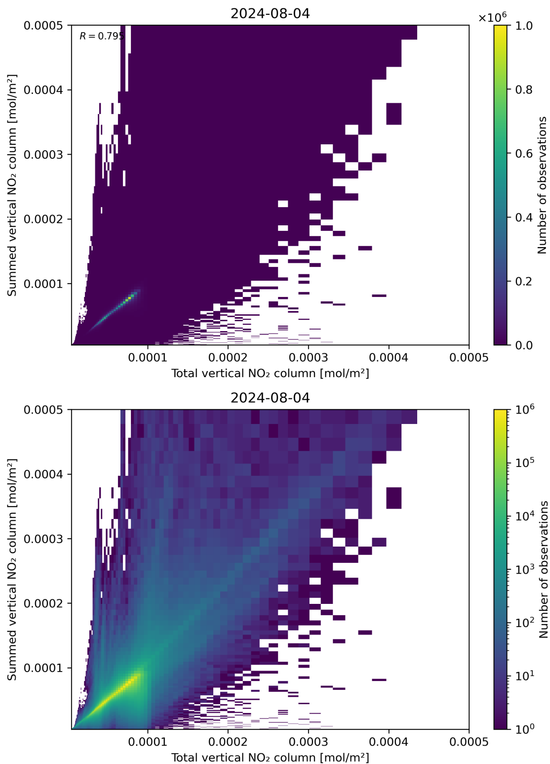
Figure 112: Scatter density plot of “Total vertical NO 2 column” against “Summed vertical NO 2 column” for 2024-08-03 to 2024-08-05.
