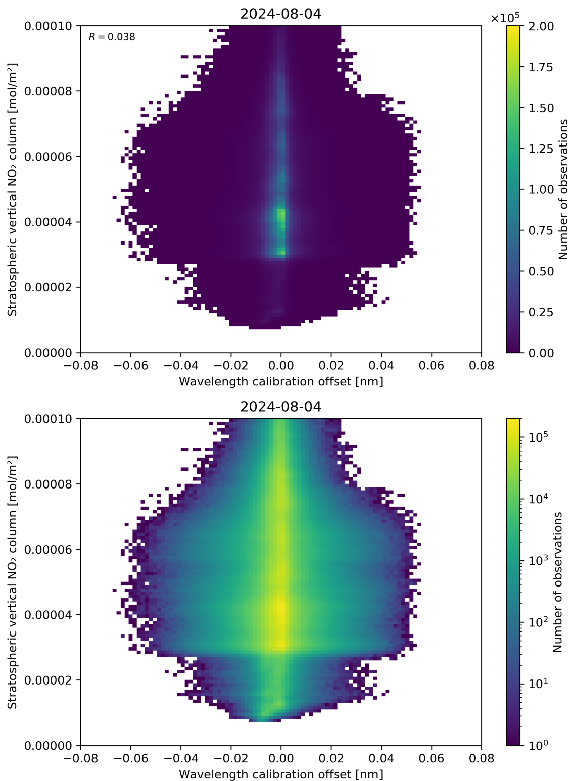
Figure 176: Scatter density plot of “Wavelength calibration offset” against “Stratospheric vertical NO 2 column” for 2024-08-03 to 2024-08-05.
