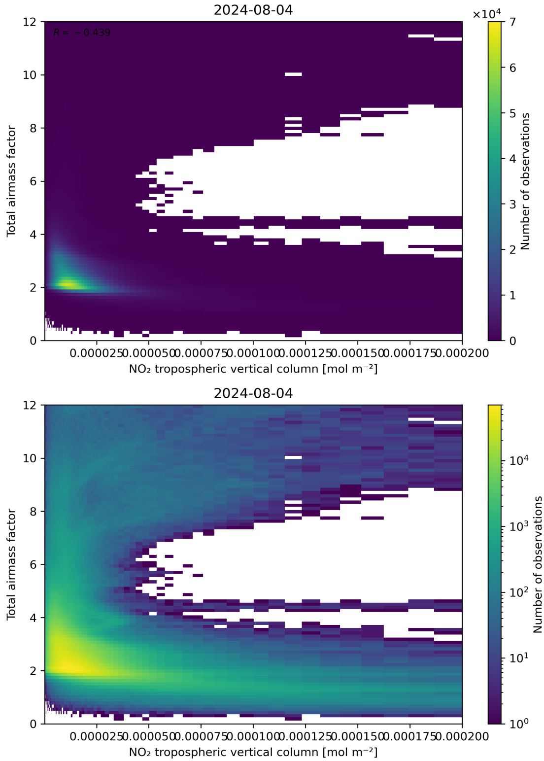
Figure 122: Scatter density plot of “NO 2 tropospheric vertical column” against “Total air mass factor” for 2024-08-03 to 2024-08-05.
