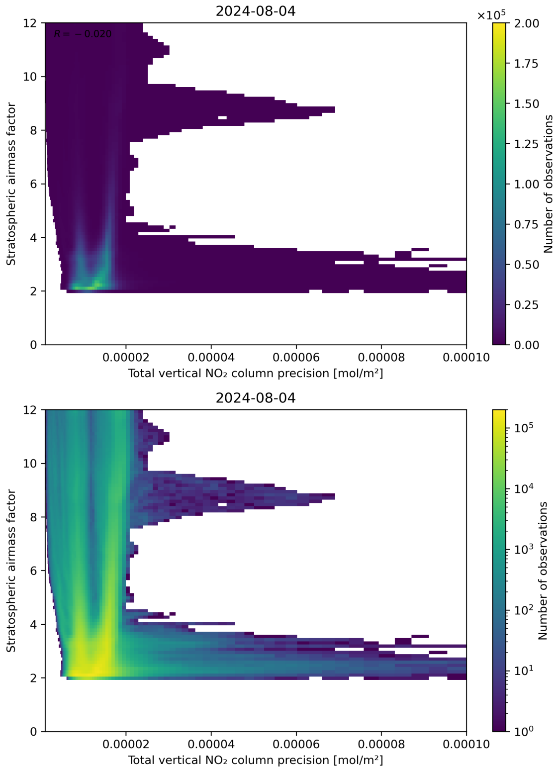
Figure 115: Scatter density plot of “Total vertical NO 2 column precision” against “Stratospheric air mass factor” for 2024-08-03 to 2024-08-05.
