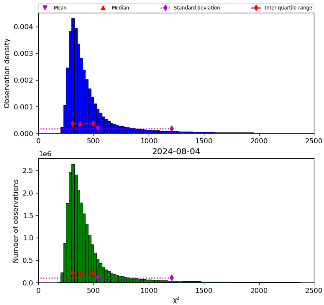
Figure 42: Histogram of “ \chi^2 ” for 2024-08-03 to 2024-08-05
