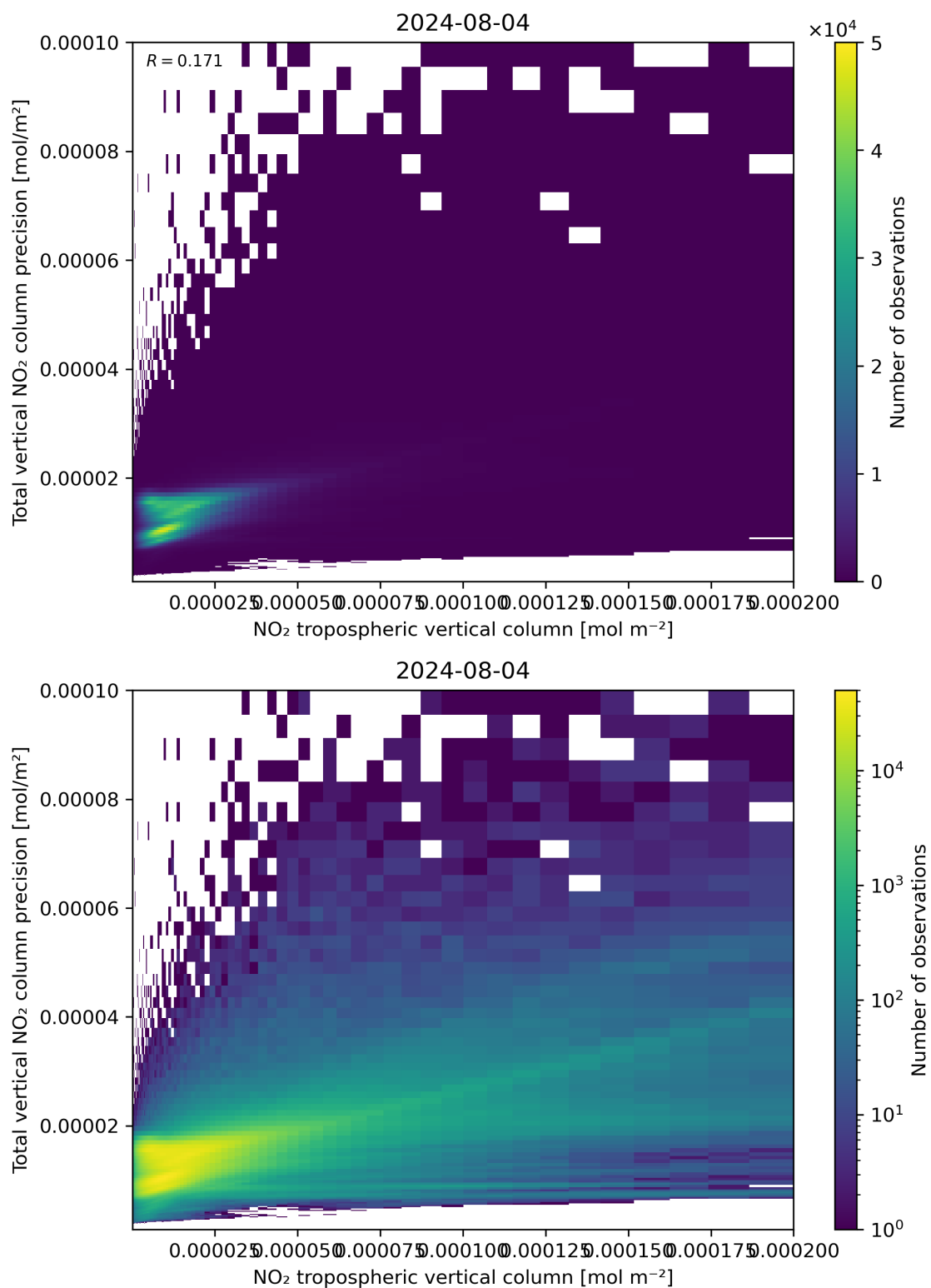
Figure 129: Scatter density plot of “NO 2 tropospheric vertical column” against “Total vertical NO 2 column precision” for 2024-08-03 to 2024-08-05.
