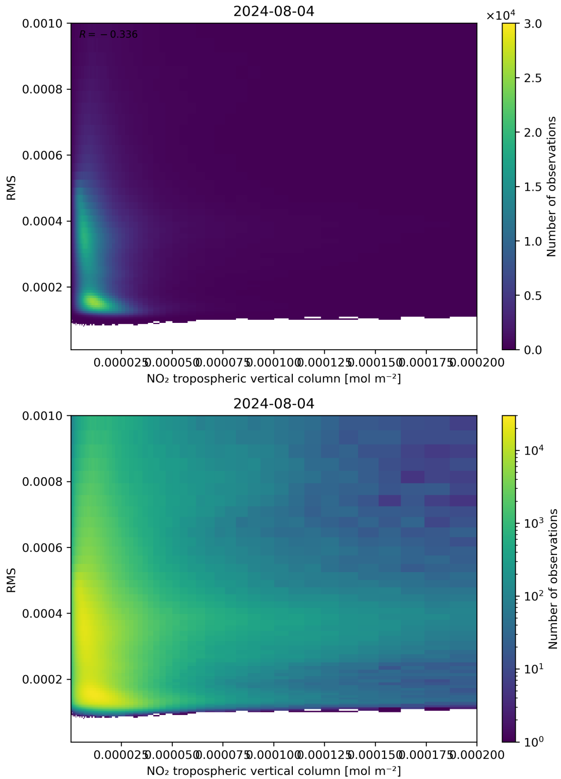
Figure 142: Scatter density plot of “NO 2 tropospheric vertical column” against “RMS” for 2024-08-03 to 2024-08-05.
