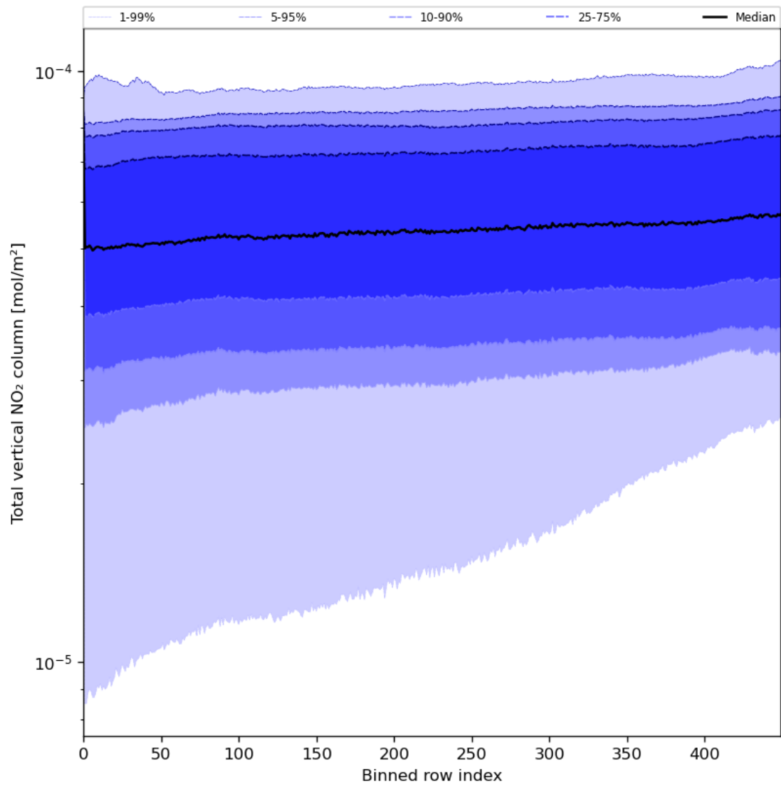
Figure 55: Along track statistics of “Total vertical NO 2 column” for 2024-08-03 to 2024-08-05
