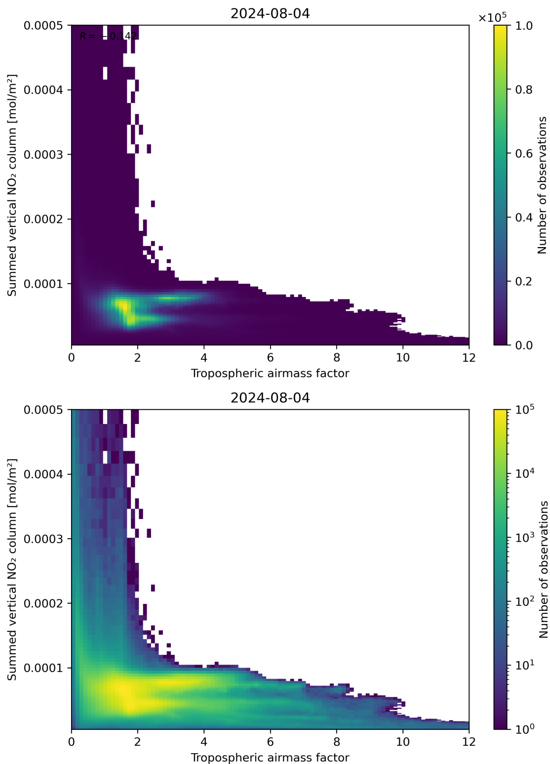
Figure 75: Scatter density plot of “Tropospheric airmass factor” against “Summed vertical NO 2 column” for 2024-08-03 to 2024-08-05.
