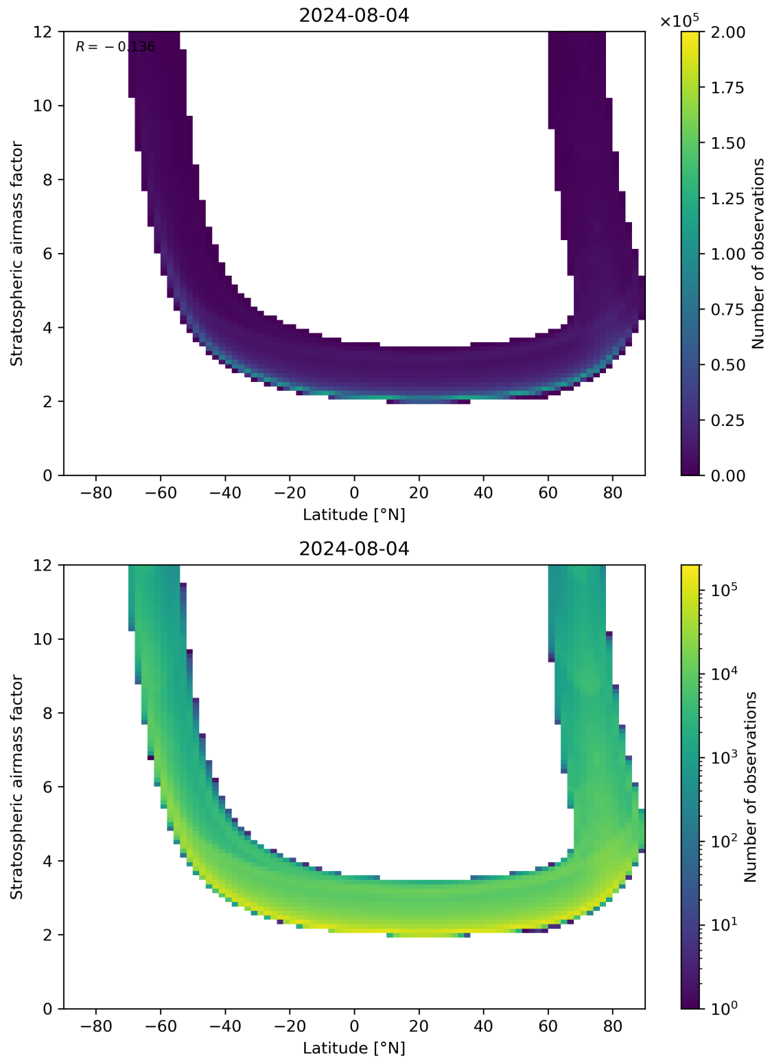
Figure 83: Scatter density plot of “Latitude” against “Stratospheric air mass factor” for 2024-08-03 to 2024-08-05.
