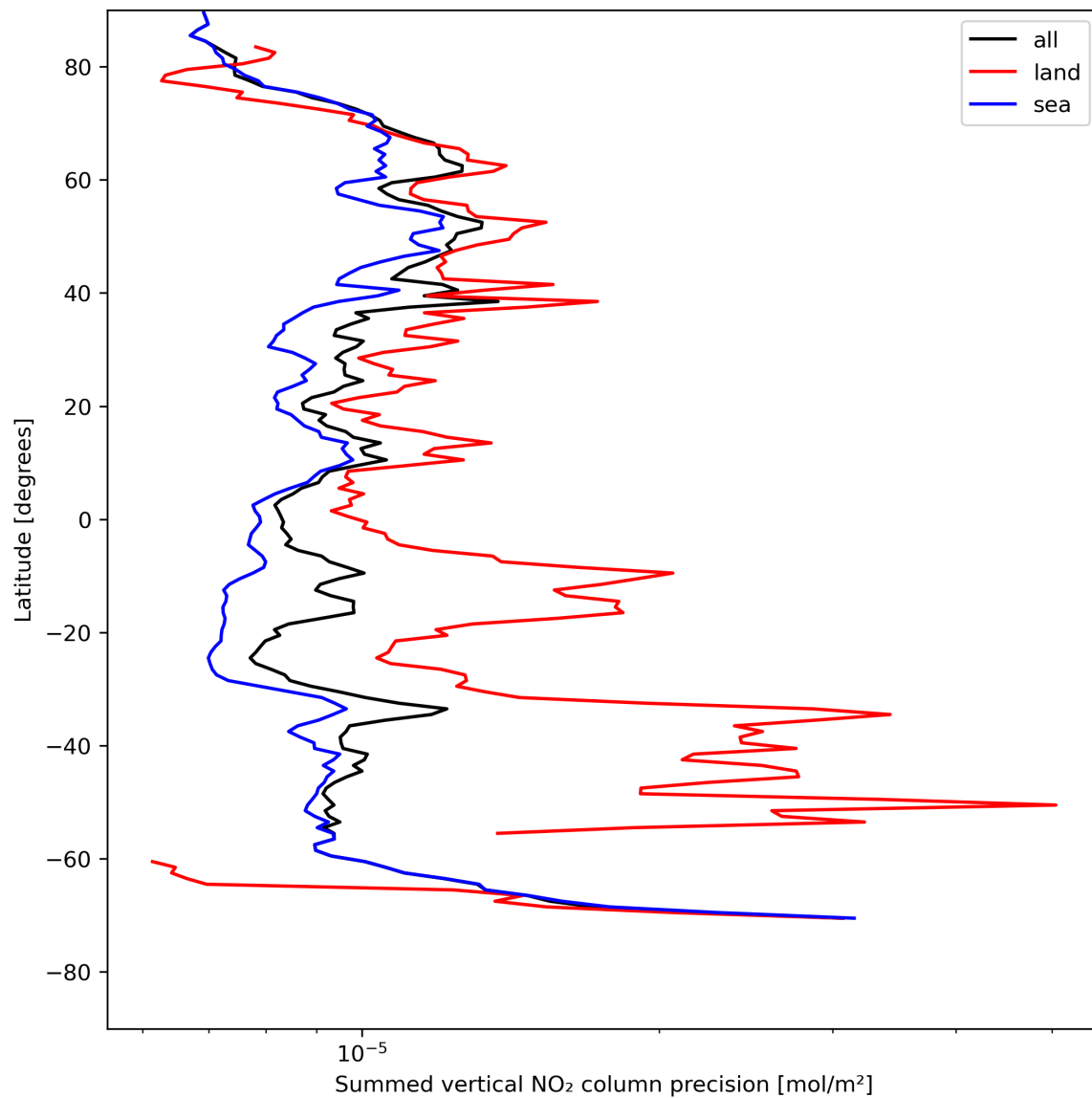
Figure 24: Zonal average of “Summed vertical NO 2 column precision” for 2024-08-03 to 2024-08-05.
