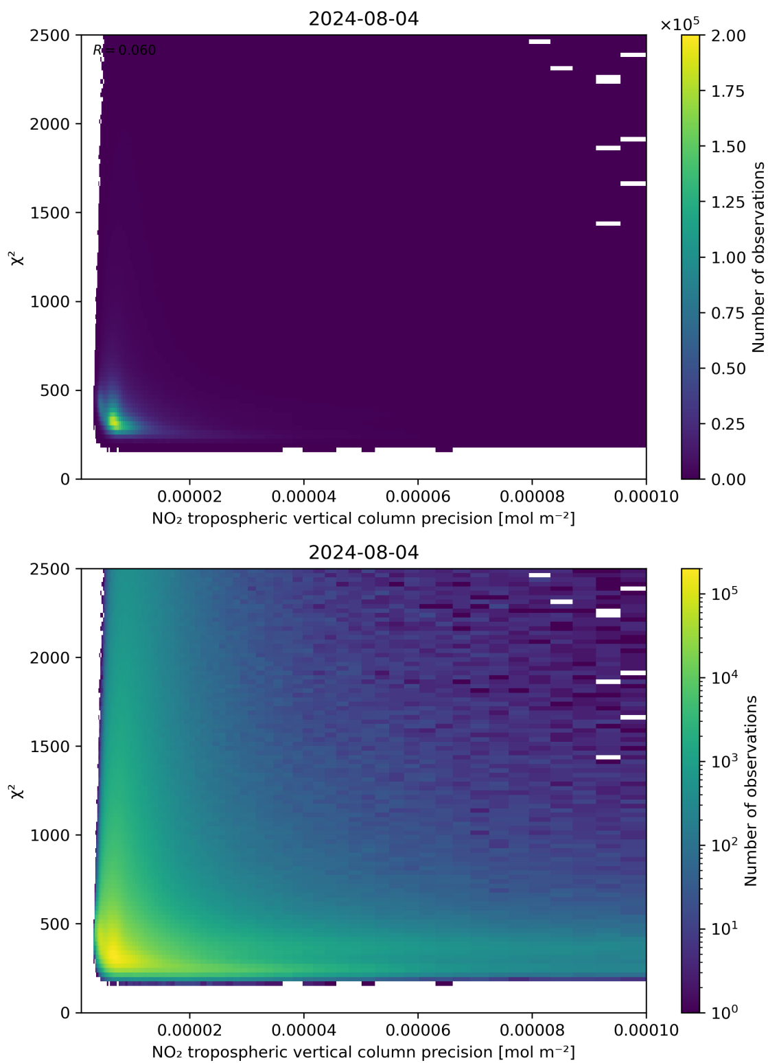
Figure 134: Scatter density plot of “NO 2 tropospheric vertical column precision” against “ \chi^2 ” for 2024-08-03 to 2024-08-05.
