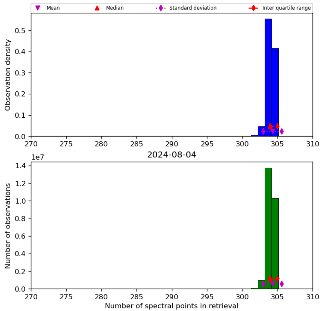
Figure 33: Histogram of “Number of spectral points in retrieval” for 2024-08-03 to 2024-08-05
