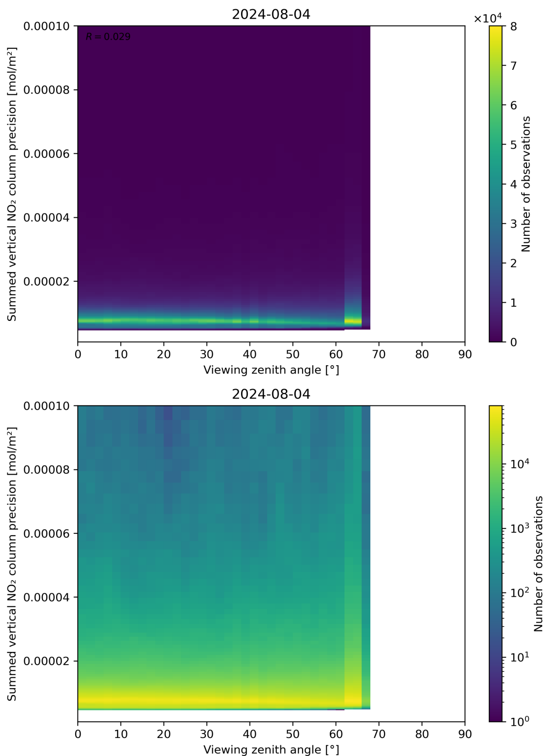
Figure 166: Scatter density plot of “Viewing zenith angle” against “Summed vertical NO 2 column precision” for 2024-08-03 to 2024-08-05.
