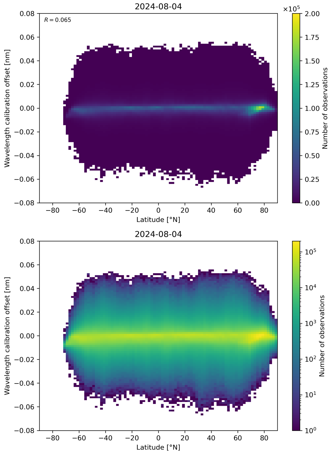
Figure 95: Scatter density plot of “Latitude” against “Wavelength calibration offset” for 2024-08-03 to 2024-08-05.
