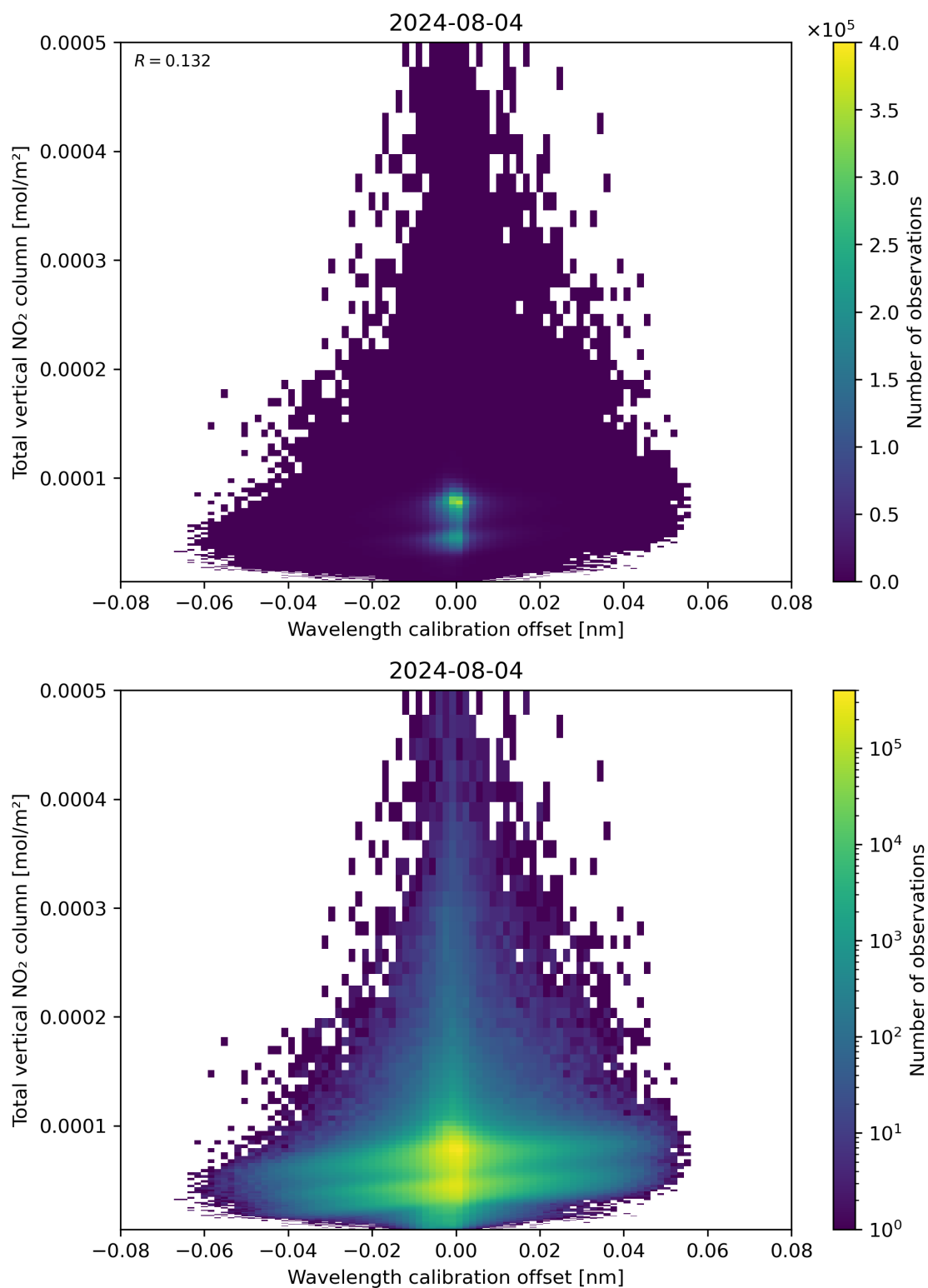
Figure 179: Scatter density plot of “Wavelength calibration offset” against “Total vertical NO 2 column” for 2024-08-03 to 2024-08-05.
