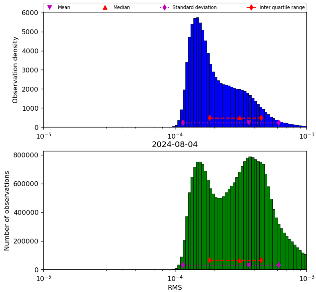
Figure 43: Histogram of “RMS” for 2024-08-03 to 2024-08-05
