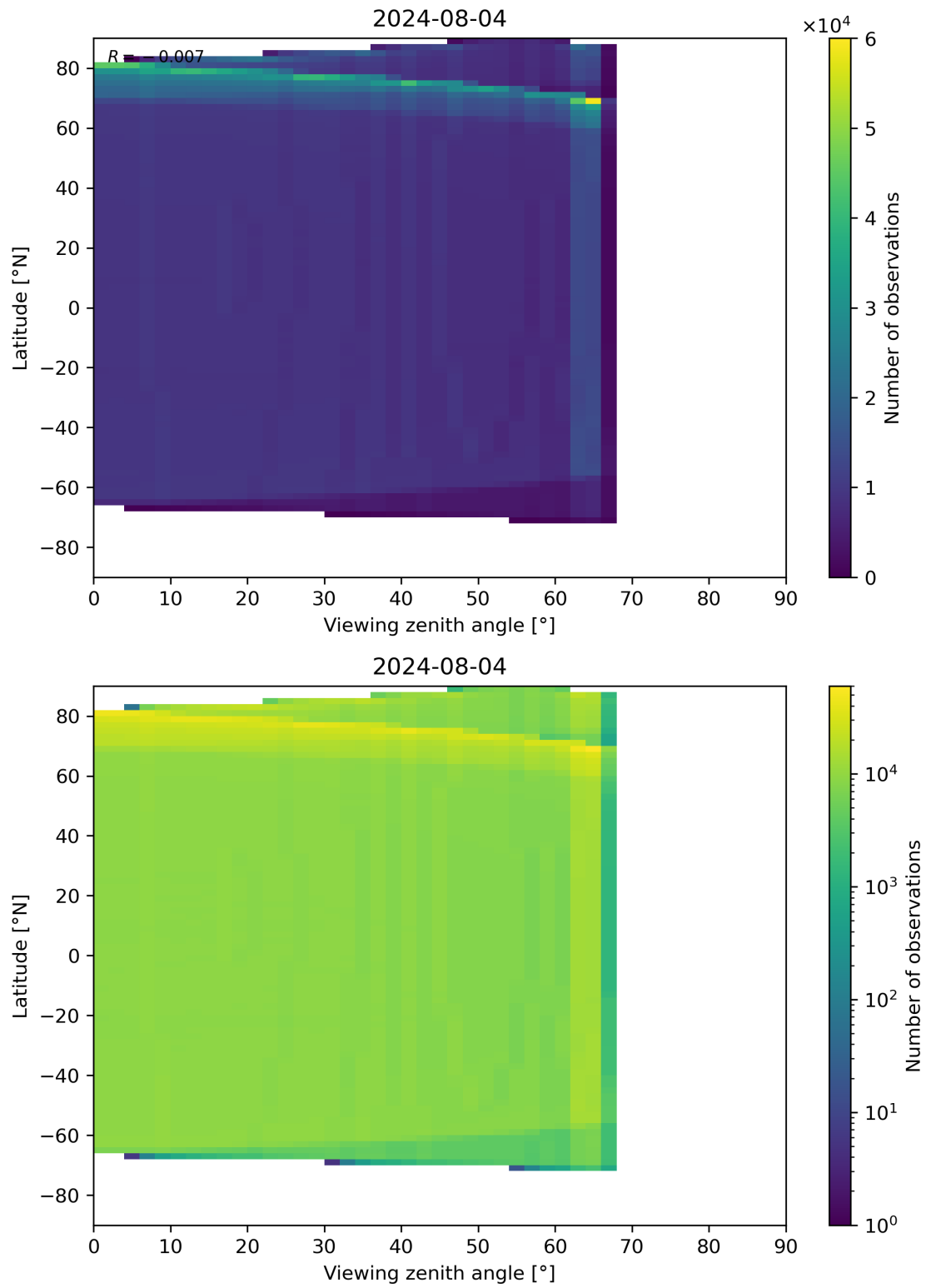
Figure 163: Scatter density plot of “Viewing zenith angle” against “Latitude” for 2024-08-03 to 2024-08-05.
