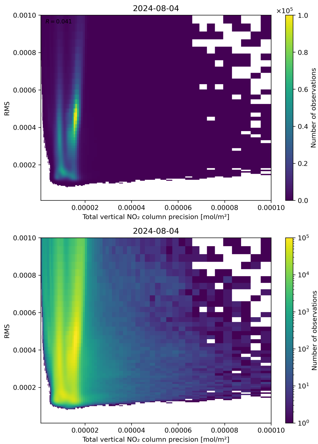
Figure 119: Scatter density plot of “Total vertical NO 2 column precision” against “RMS” for 2024-08-03 to 2024-08-05.
