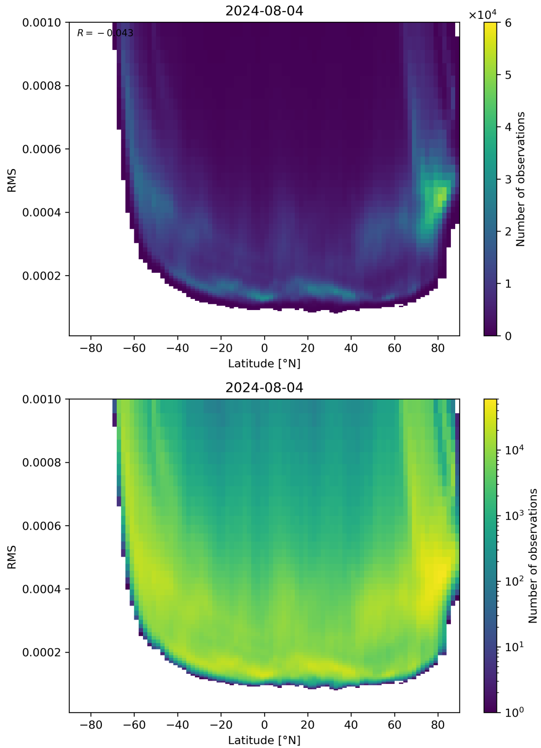
Figure 94: Scatter density plot of “Latitude” against “RMS” for 2024-08-03 to 2024-08-05.
