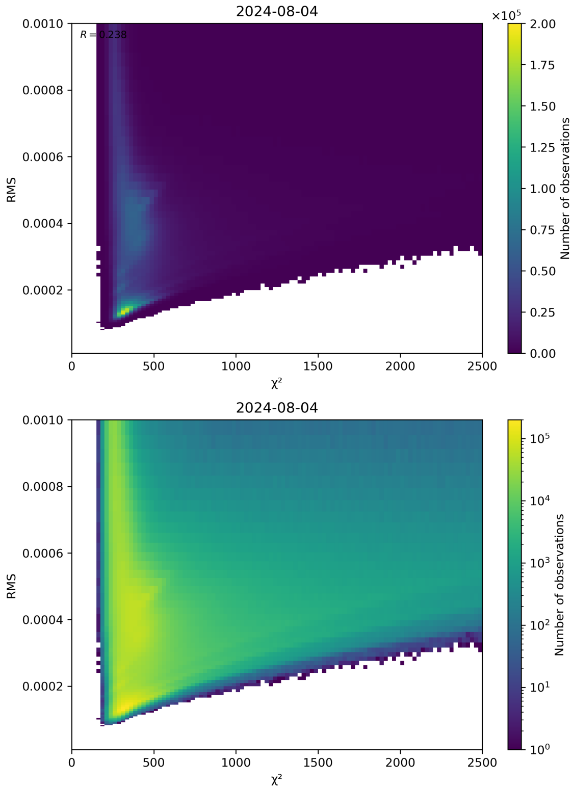
Figure 82: Scatter density plot of “ \chi^2 ” against “RMS” for 2024-08-03 to 2024-08-05.
