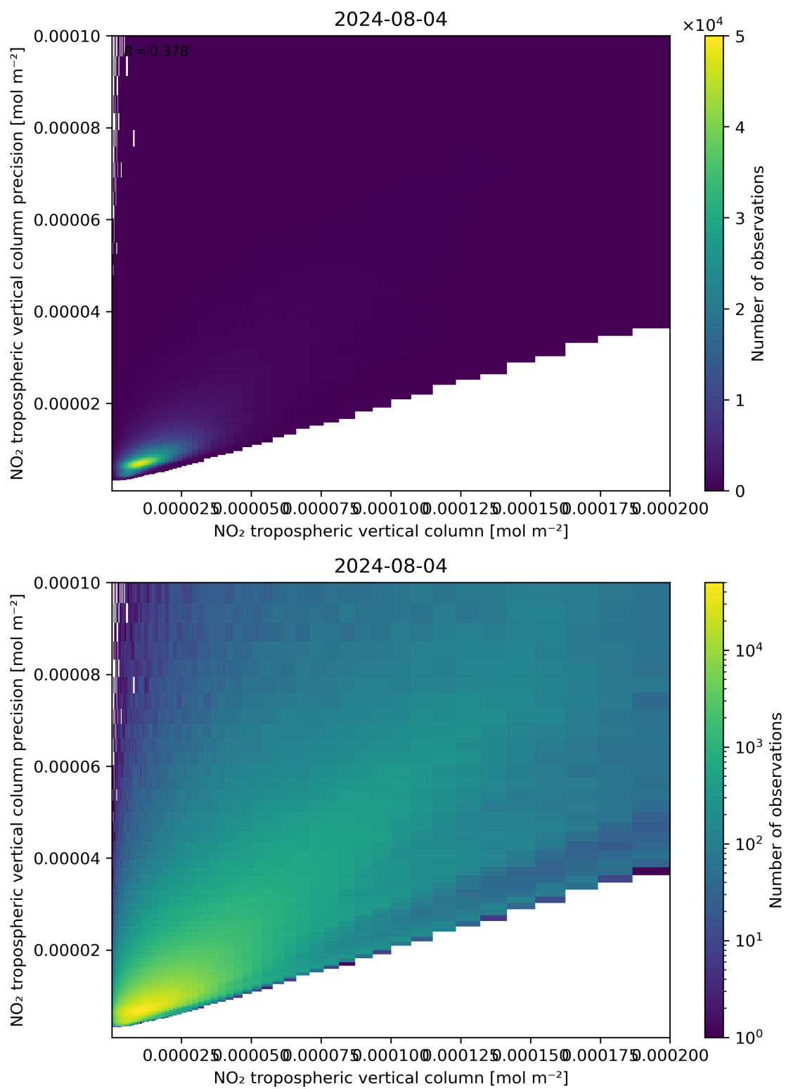
Figure 130: Scatter density plot of “NO 2 tropospheric vertical column” against “NO 2 tropospheric vertical column precision” for 2024-08-03 to 2024-08-05.
