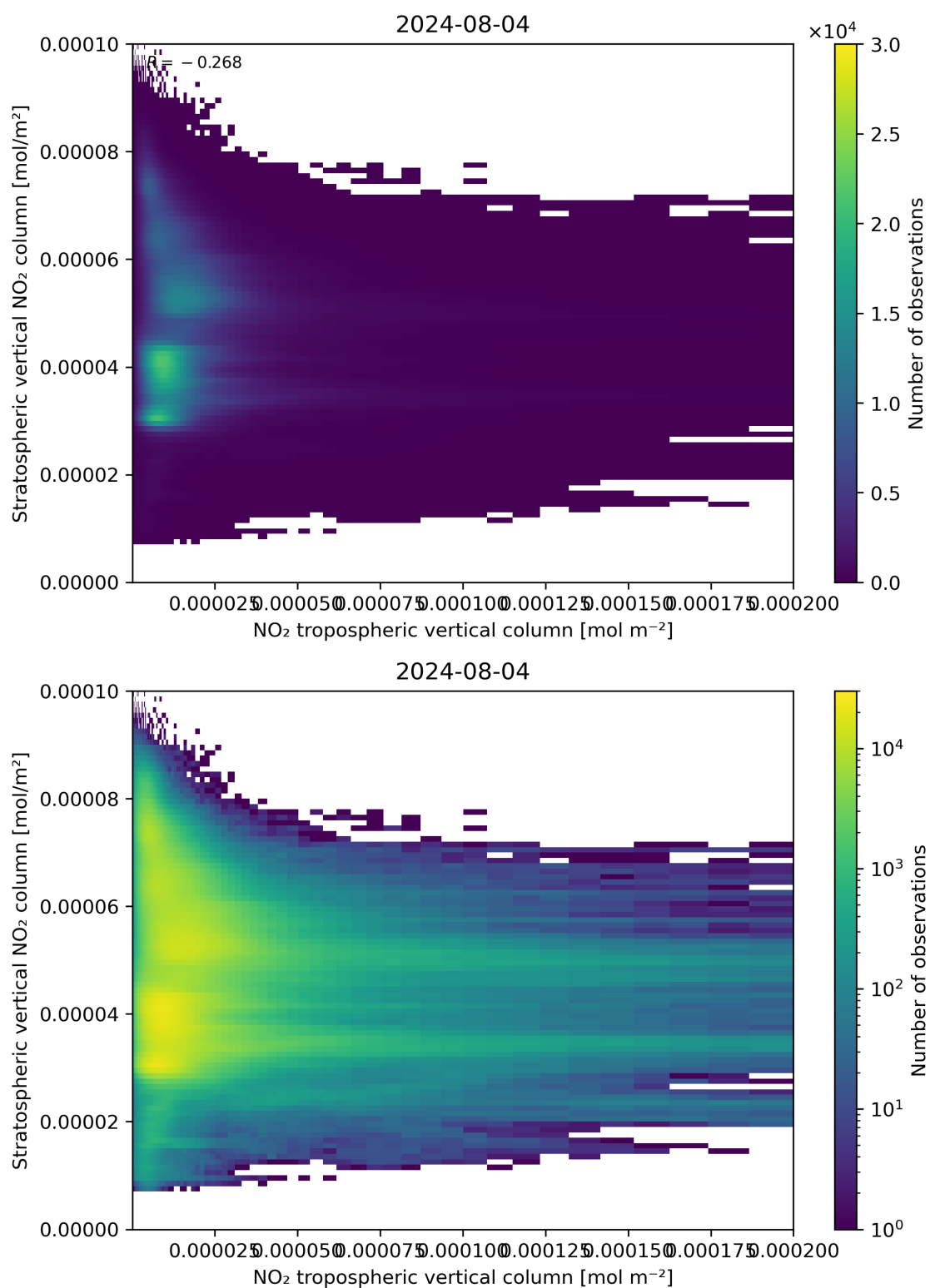
Figure 125: Scatter density plot of “NO 2 tropospheric vertical column” against “Stratospheric vertical NO 2 column” for 2024-08-03 to 2024-08-05.
