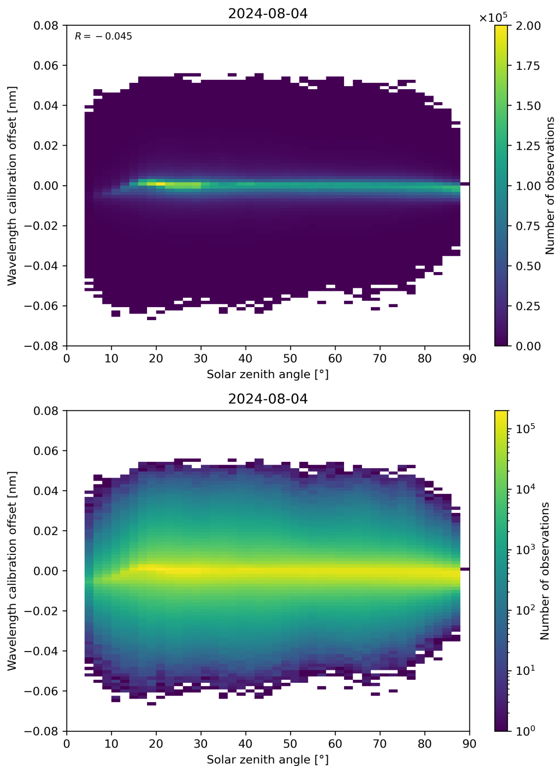
Figure 158: Scatter density plot of “Solar zenith angle” against “Wavelength calibration offset” for 2024-08-03 to 2024-08-05.
