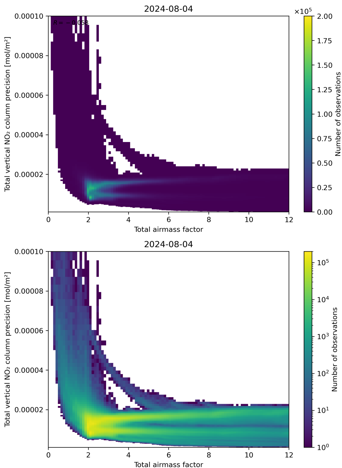
Figure 68: Scatter density plot of “Total airmass factor” against “Total vertical NO 2 column precision” for 2024-08-03 to 2024-08-05.
