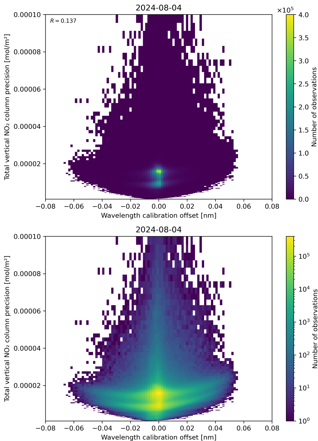
Figure 180: Scatter density plot of “Wavelength calibration offset” against “Total vertical NO 2 column precision” for 2024-08-03 to 2024-08-05.
