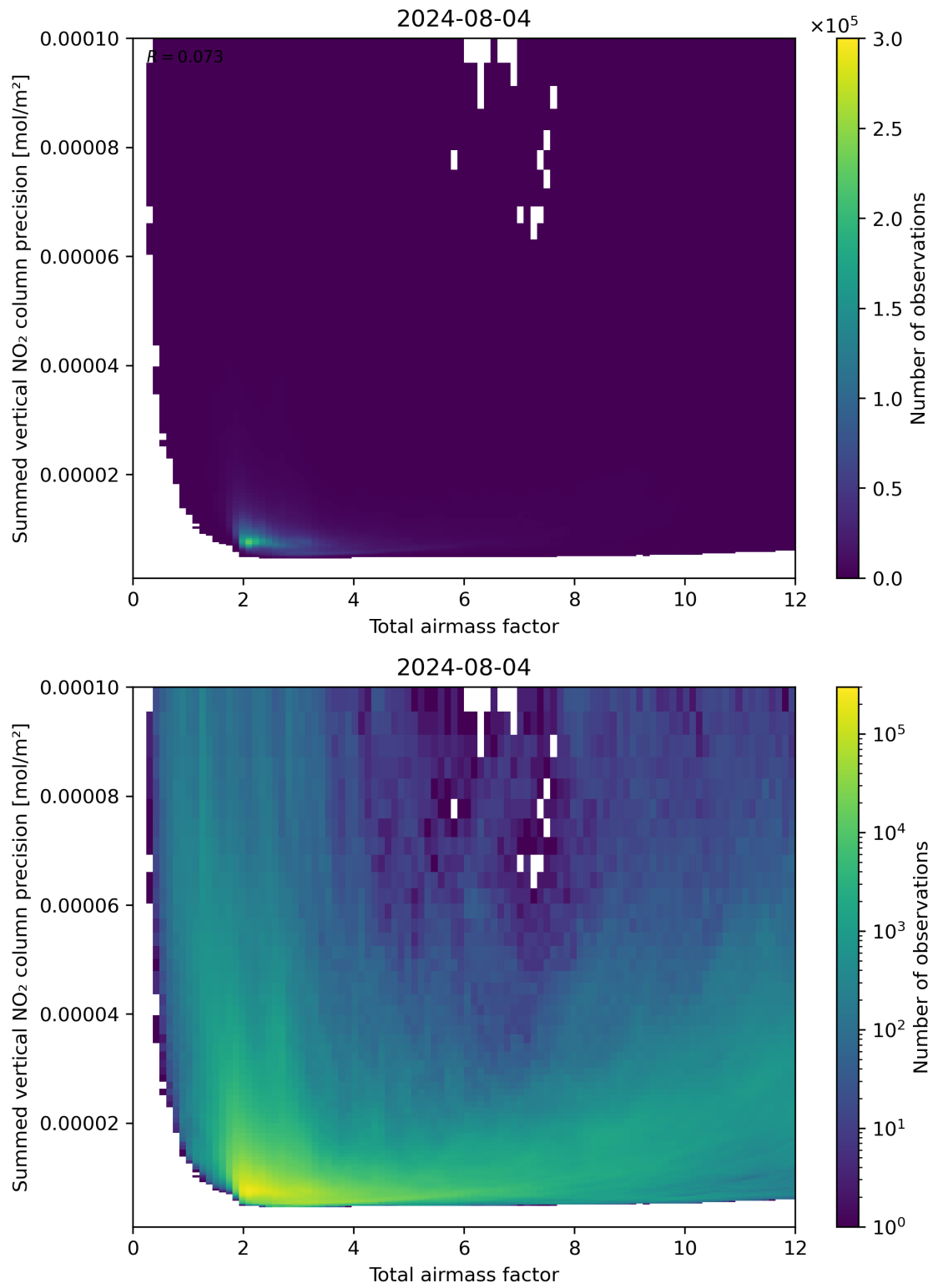
Figure 66: Scatter density plot of “Total airmass factor” against “Summed vertical NO 2 column precision” for 2024-08-03 to 2024-08-05.
