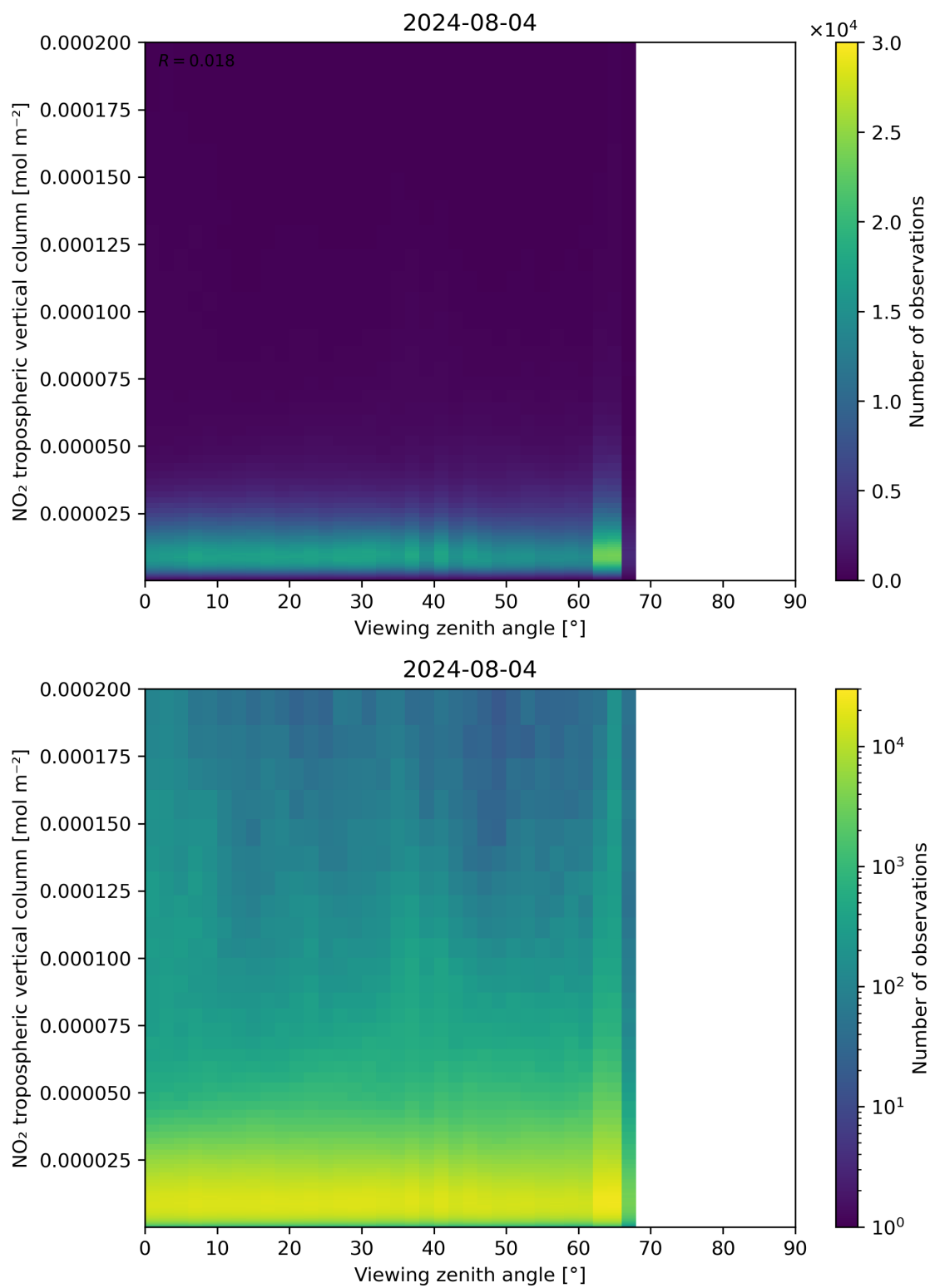
Figure 169: Scatter density plot of “Viewing zenith angle” against “NO 2 tropospheric vertical column” for 2024-08-03 to 2024-08-05.
