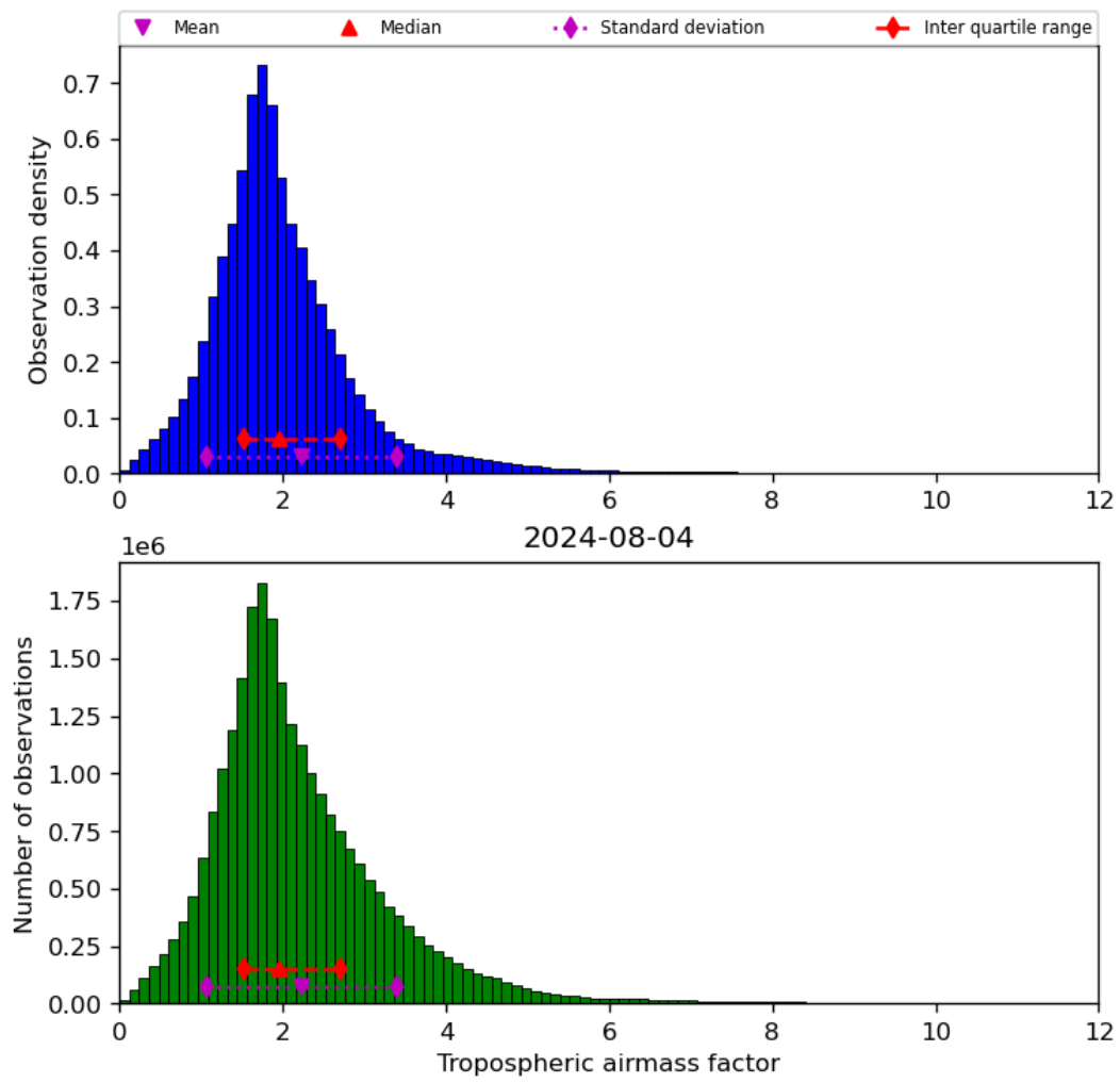
Figure 31: Histogram of “Tropospheric airmass factor” for 2024-08-03 to 2024-08-05
