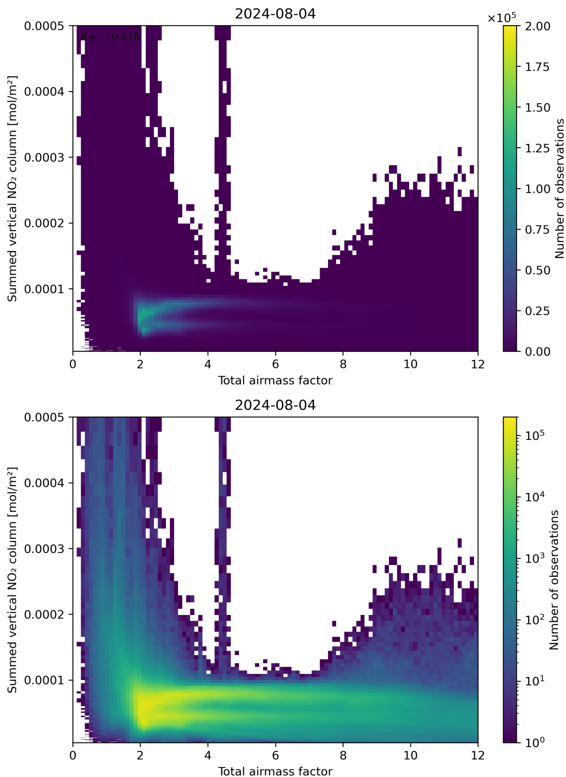
Figure 65: Scatter density plot of “Total air mass factor” against “Summed vertical NO 2 column” for 2024-08-03 to 2024-08-05.
