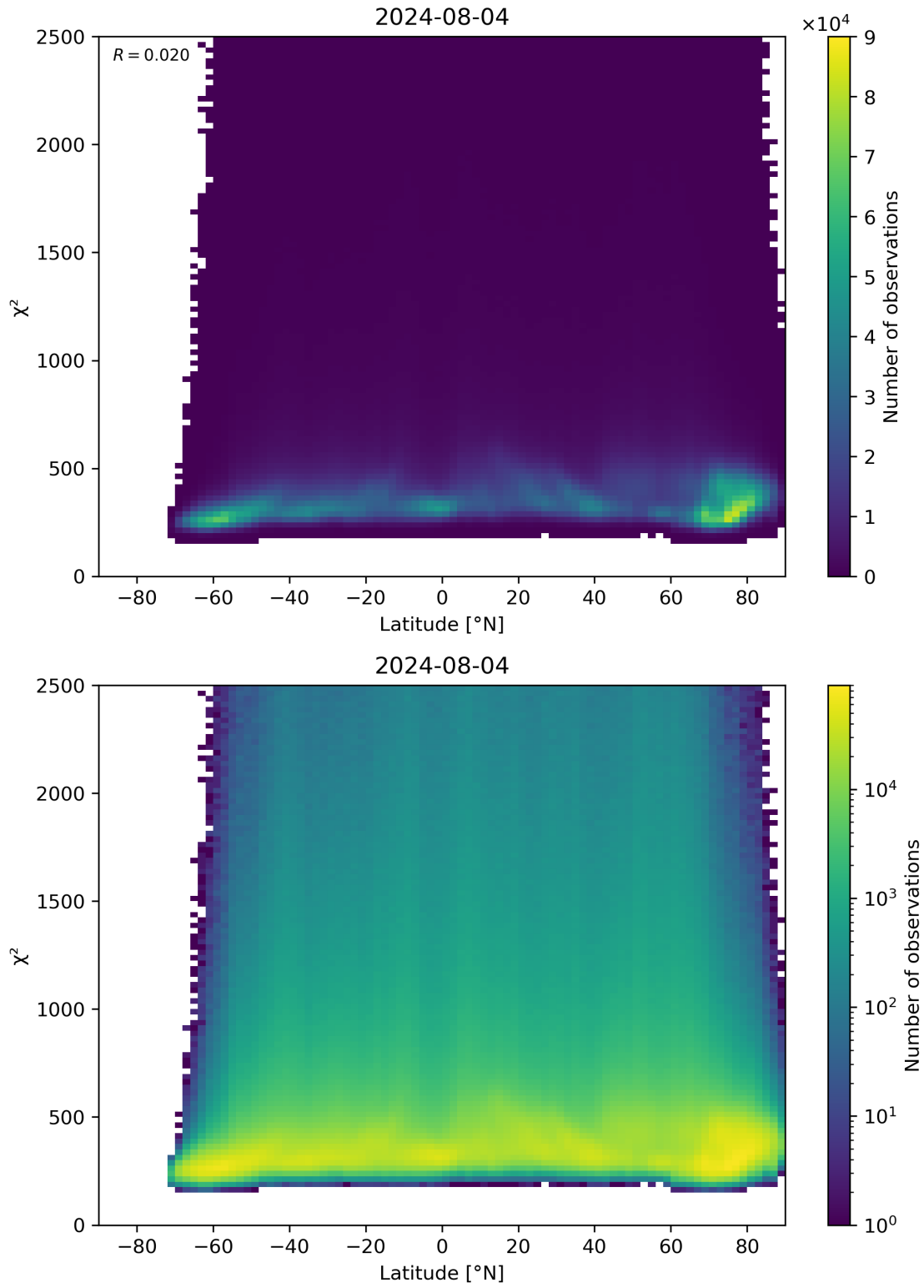
Figure 86: Scatter density plot of “Latitude” against “ \chi^2 ” for 2024-08-03 to 2024-08-05.
