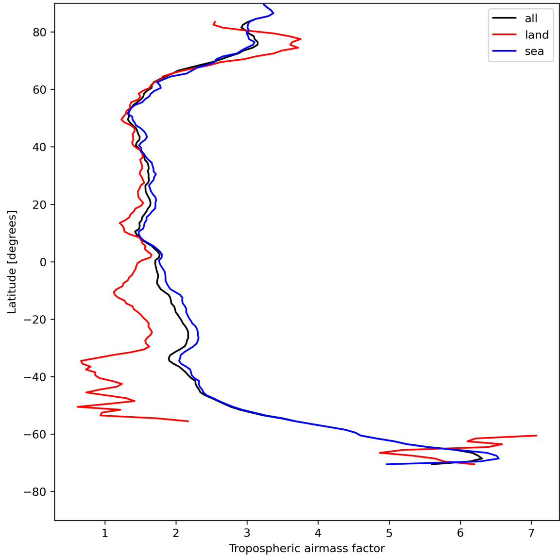
Figure 14: Zonal average of “Tropospheric airmass factor” for 2024-08-03 to 2024-08-05.
