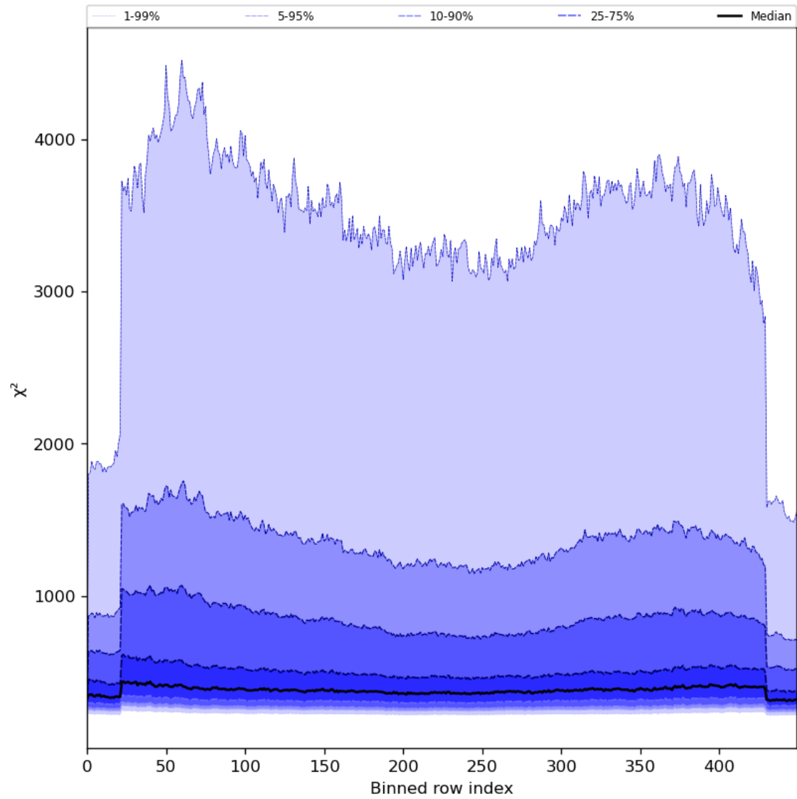
Figure 59: Along track statistics of “ \chi^2 ” for 2024-08-03 to 2024-08-05
