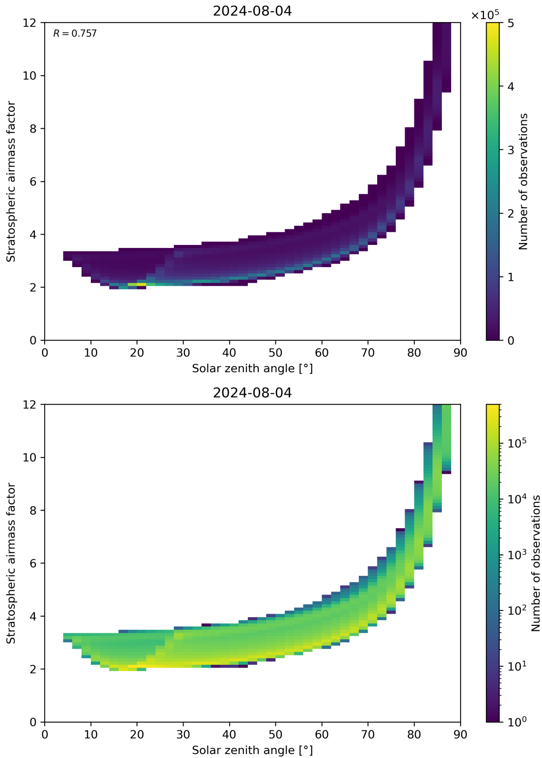
Figure 145: Scatter density plot of “Solar zenith angle” against “Stratospheric airmass factor” for 2024-08-03 to 2024-08-05.
