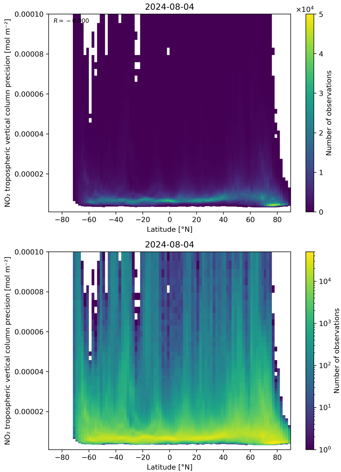
Figure 93: Scatter density plot of “Latitude” against “NO 2 tropospheric vertical column precision” for 2024-08-03 to 2024-08-05.
