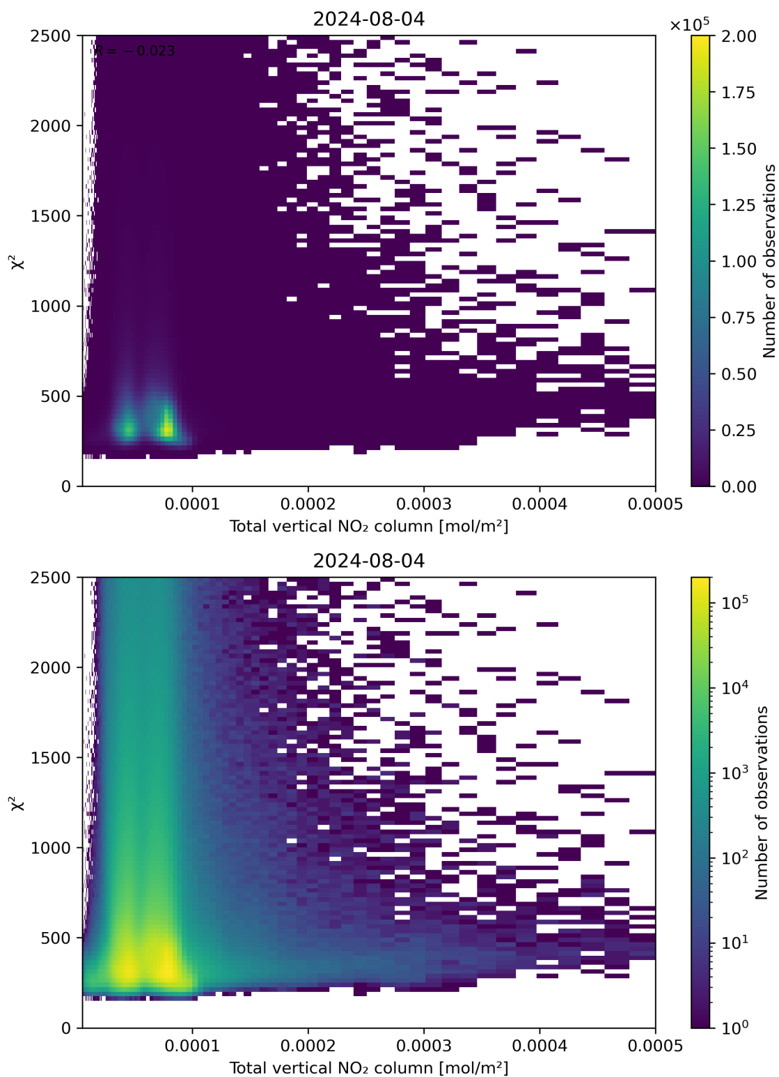
Figure 111: Scatter density plot of “Total vertical NO 2 column” against “ \chi^2 ” for 2024-08-03 to 2024-08-05.
