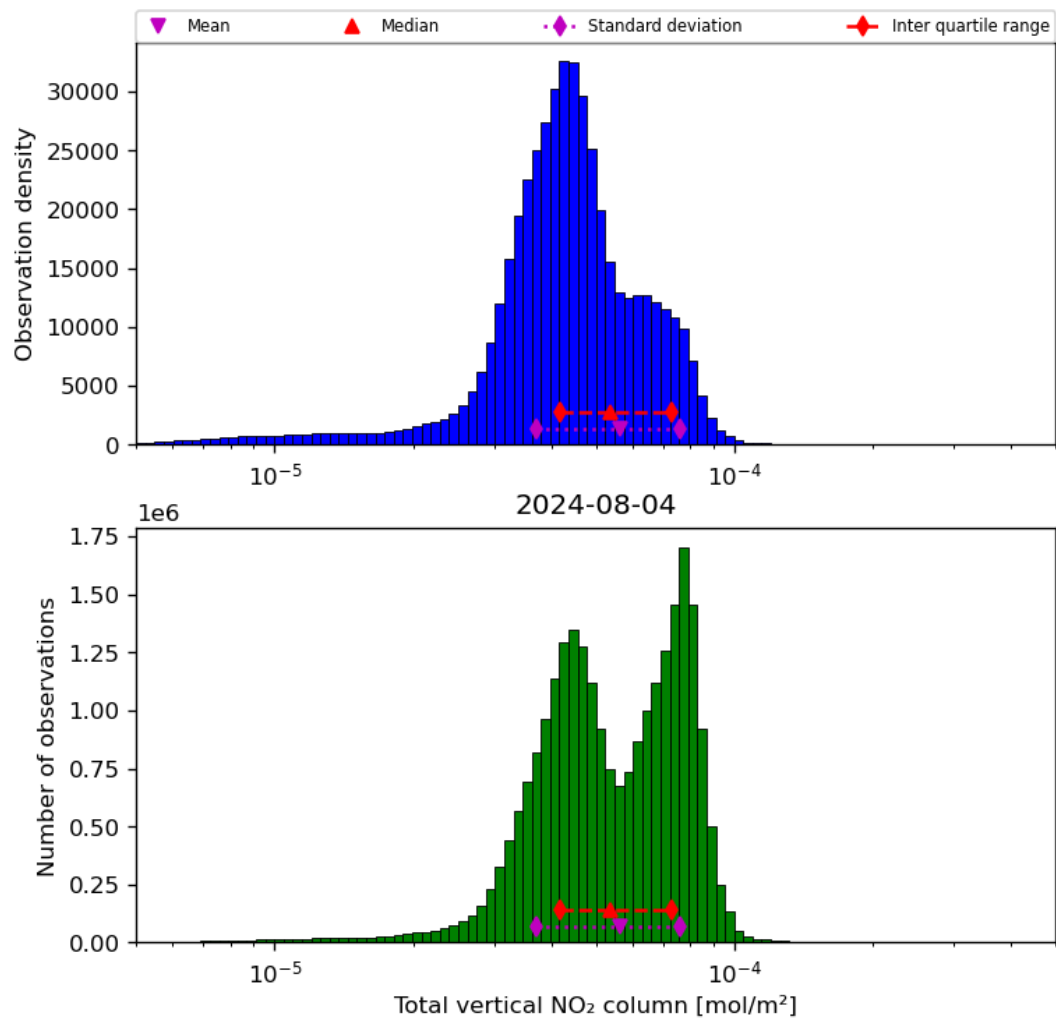
Figure 38: Histogram of "Total vertical NO 2 column" for 2024-08-03 to 2024-08-05
