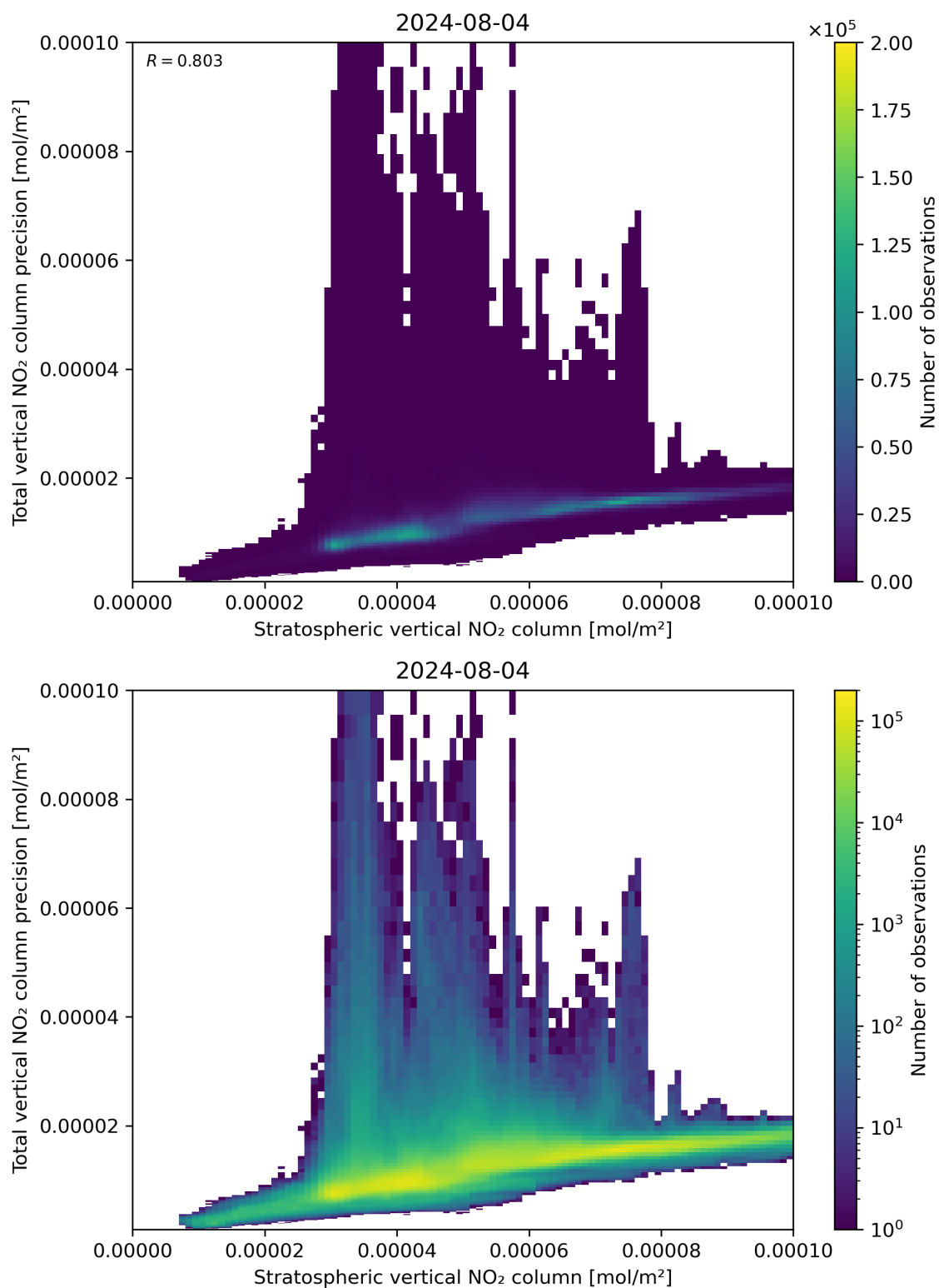
Figure 101: Scatter density plot of “Stratospheric vertical NO 2 column” against “Total vertical NO 2 column precision” for 2024-08-03 to 2024-08-05.
