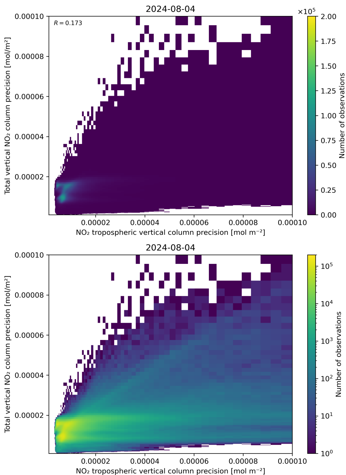
Figure 139: Scatter density plot of “NO 2 tropospheric vertical column precision” against “Total vertical NO 2 column precision” for 2024-08-03 to 2024-08-05.
