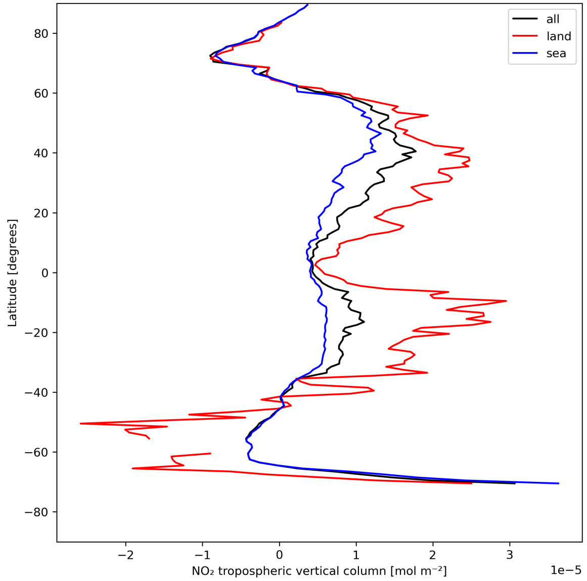
Figure 12: Zonal average of “NO 2 tropospheric vertical column” for 2024-08-03 to 2024-08-05.
