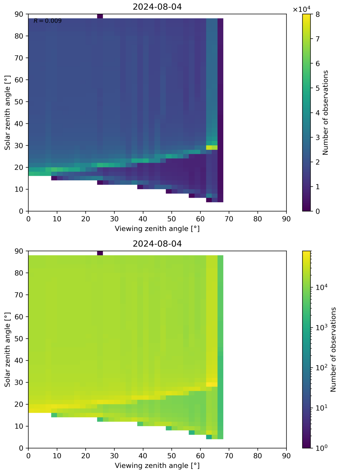
Figure 172: Scatter density plot of “Viewing zenith angle” against “Solar zenith angle” for 2024-08-03 to 2024-08-05.
