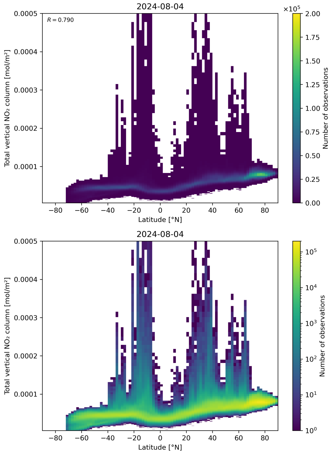
Figure 90: Scatter density plot of “Latitude” against “Total vertical NO 2 column” for 2024-08-03 to 2024-08-05.
