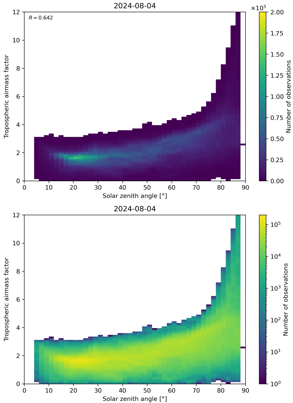
Figure 147: Scatter density plot of “Solar zenith angle” against “Tropospheric airmass factor” for 2024-08-03 to 2024-08-05.
