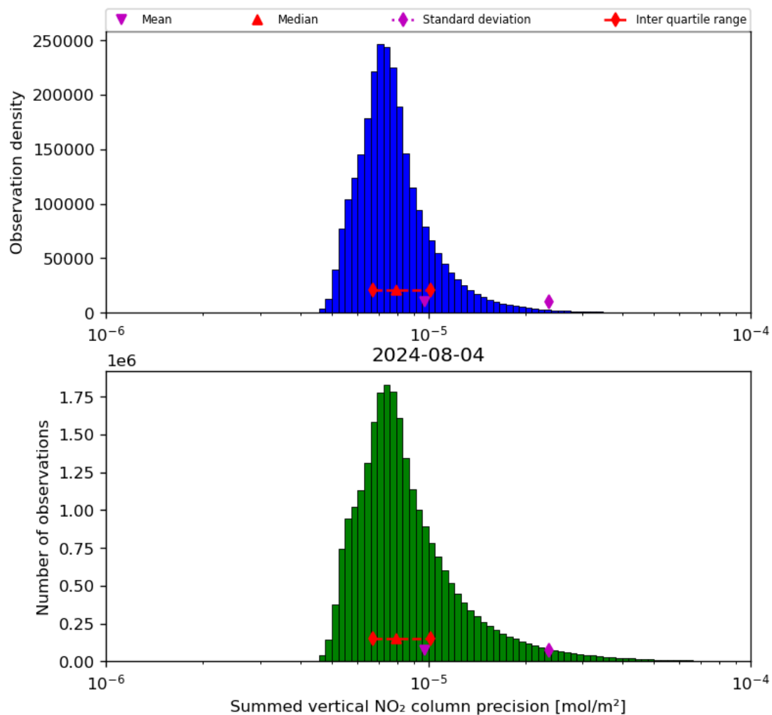
Figure 41: Histogram of "Summed vertical NO 2 column precision" for 2024-08-03 to 2024-08-05
