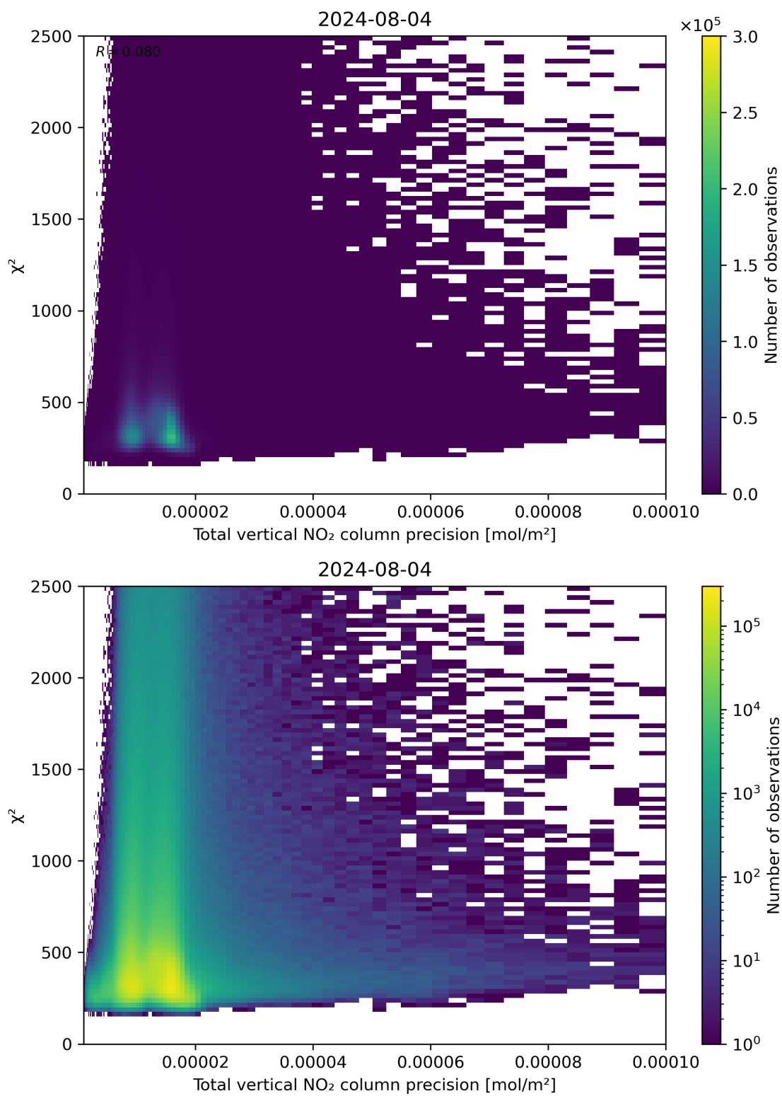
Figure 116: Scatter density plot of “Total vertical NO 2 column precision” against “ \chi^2 ” for 2024-08-03 to 2024-08-05.
