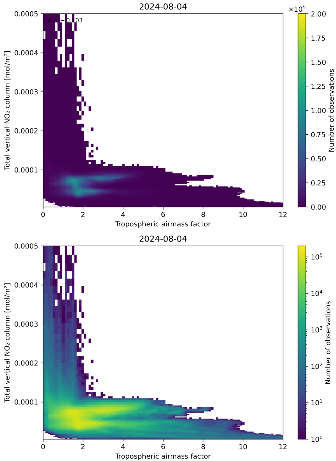
Figure 77: Scatter density plot of “Tropospheric airmass factor” against “Total vertical NO 2 column” for 2024-08-03 to 2024-08-05.
