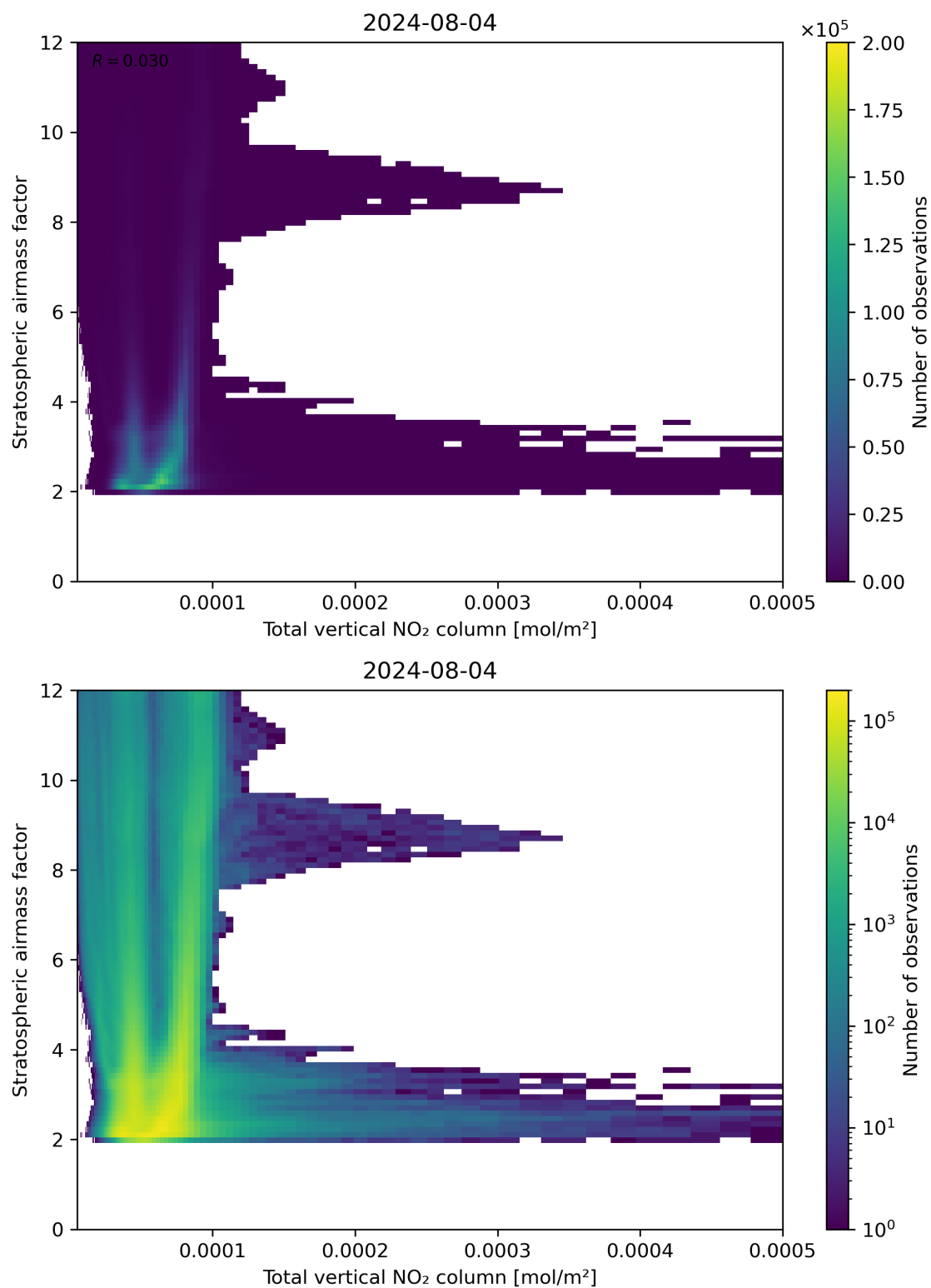
Figure 110: Scatter density plot of “Total vertical NO 2 column” against “Stratospheric airmass factor” for 2024-08-03 to 2024-08-05.
