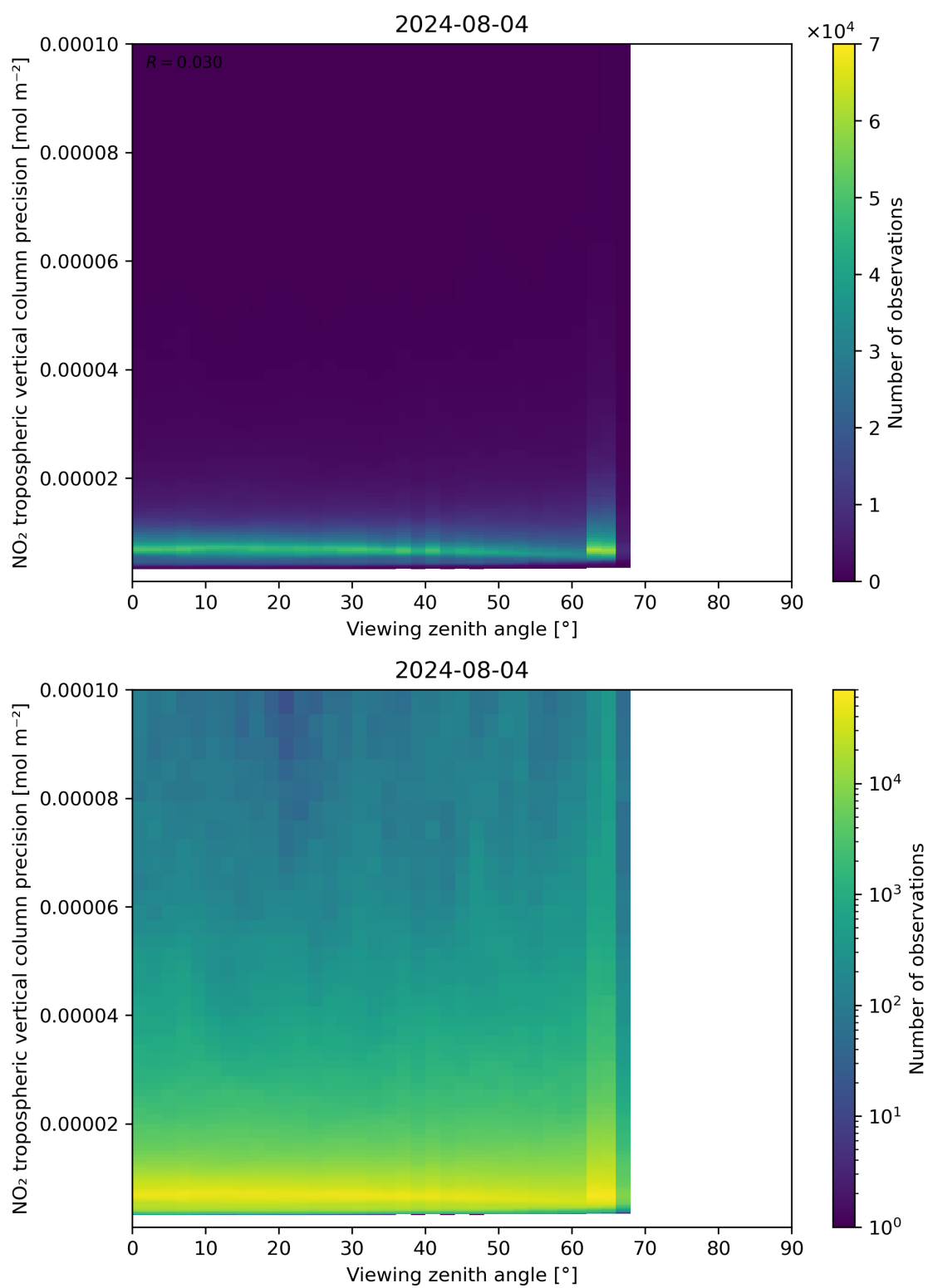
Figure 170: Scatter density plot of “Viewing zenith angle” against “NO 2 tropospheric vertical column precision” for 2024-08-03 to 2024-08-05.
