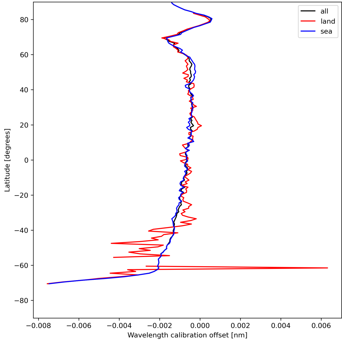
Figure 18: Zonal average of “Wavelength calibration offset” for 2024-08-03 to 2024-08-05.
