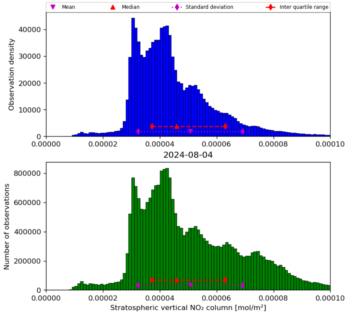
Figure 36: Histogram of “Stratospheric vertical NO 2 column” for 2024-08-03 to 2024-08-05
