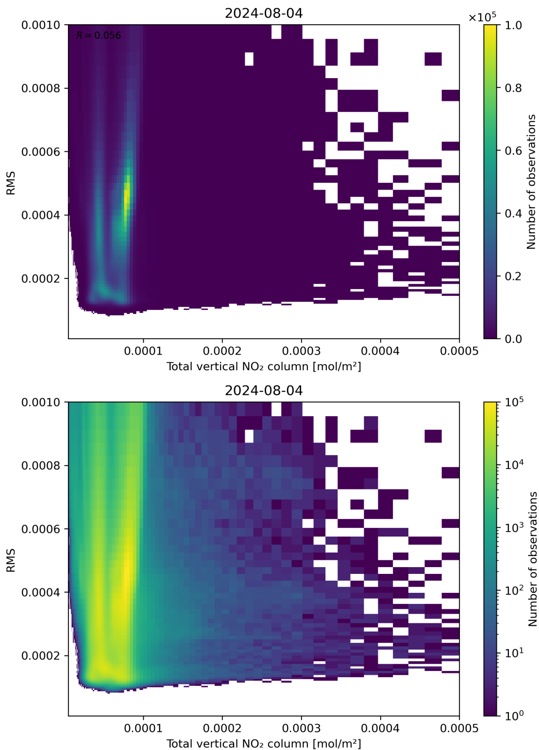
Figure 120: Scatter density plot of “Total vertical NO 2 column” against “RMS” for 2024-08-03 to 2024-08-05.
