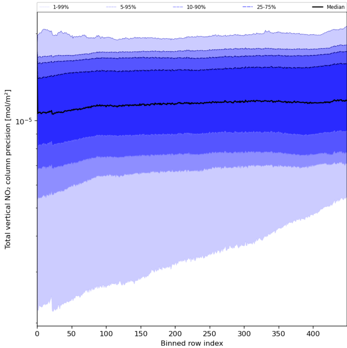
Figure 56: Along track statistics of “Total vertical NO 2 column precision” for 2024-08-03 to 2024-08-05
