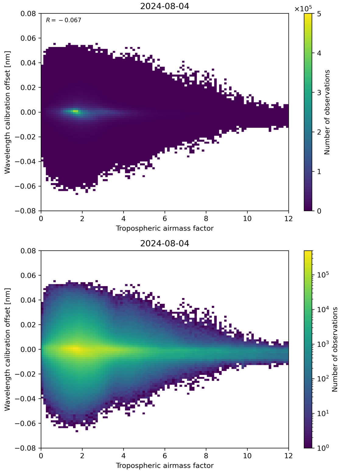
Figure 80: Scatter density plot of “Tropospheric air mass factor” against “Wavelength calibration offset” for 2024-08-03 to 2024-08-05.
