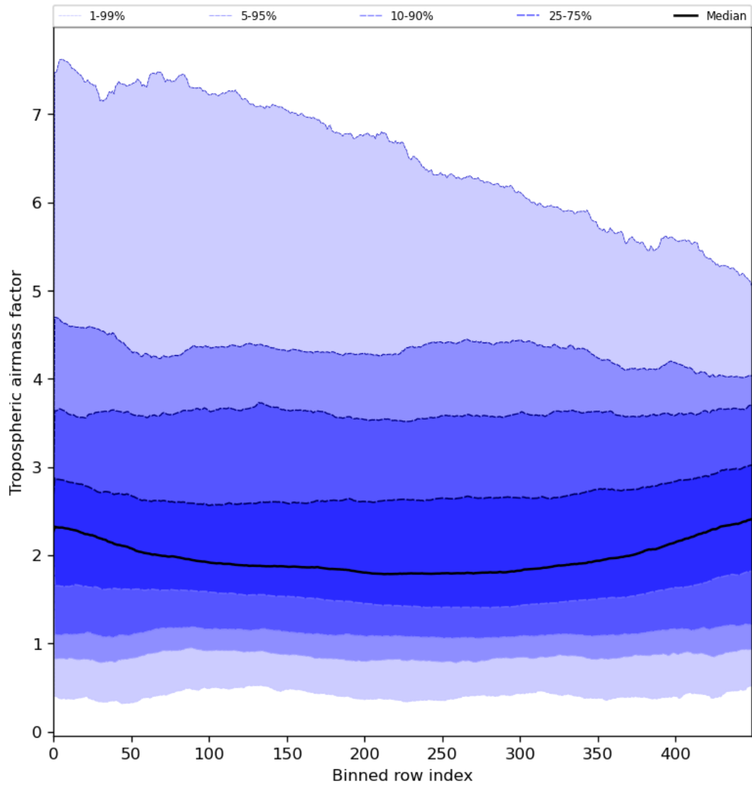
Figure 48: Along track statistics of “Tropospheric airmass factor” for 2024-08-03 to 2024-08-05
