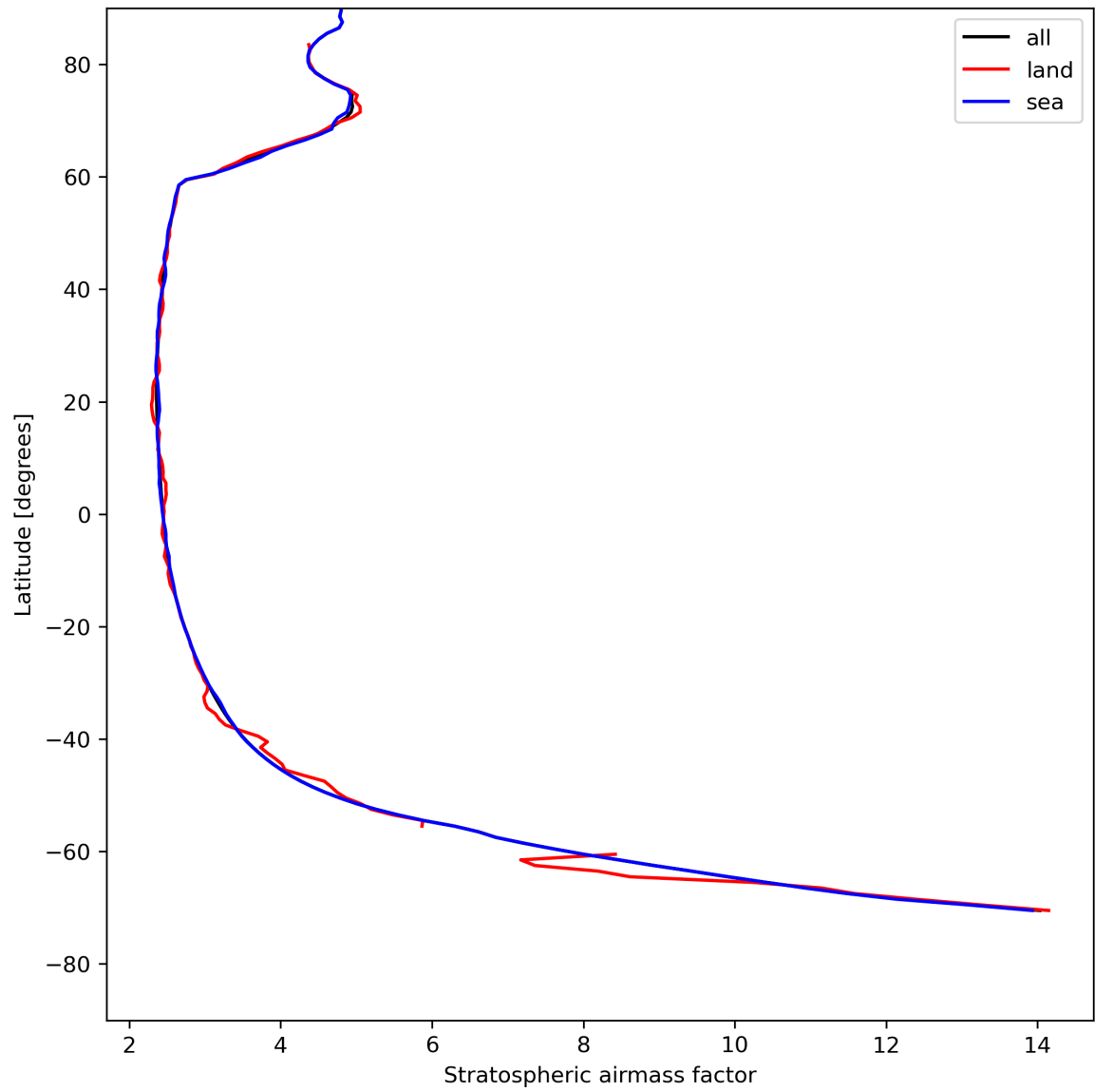
Figure 27: Zonal average of “Stratospheric air mass factor” for 2024-08-03 to 2024-08-05.
