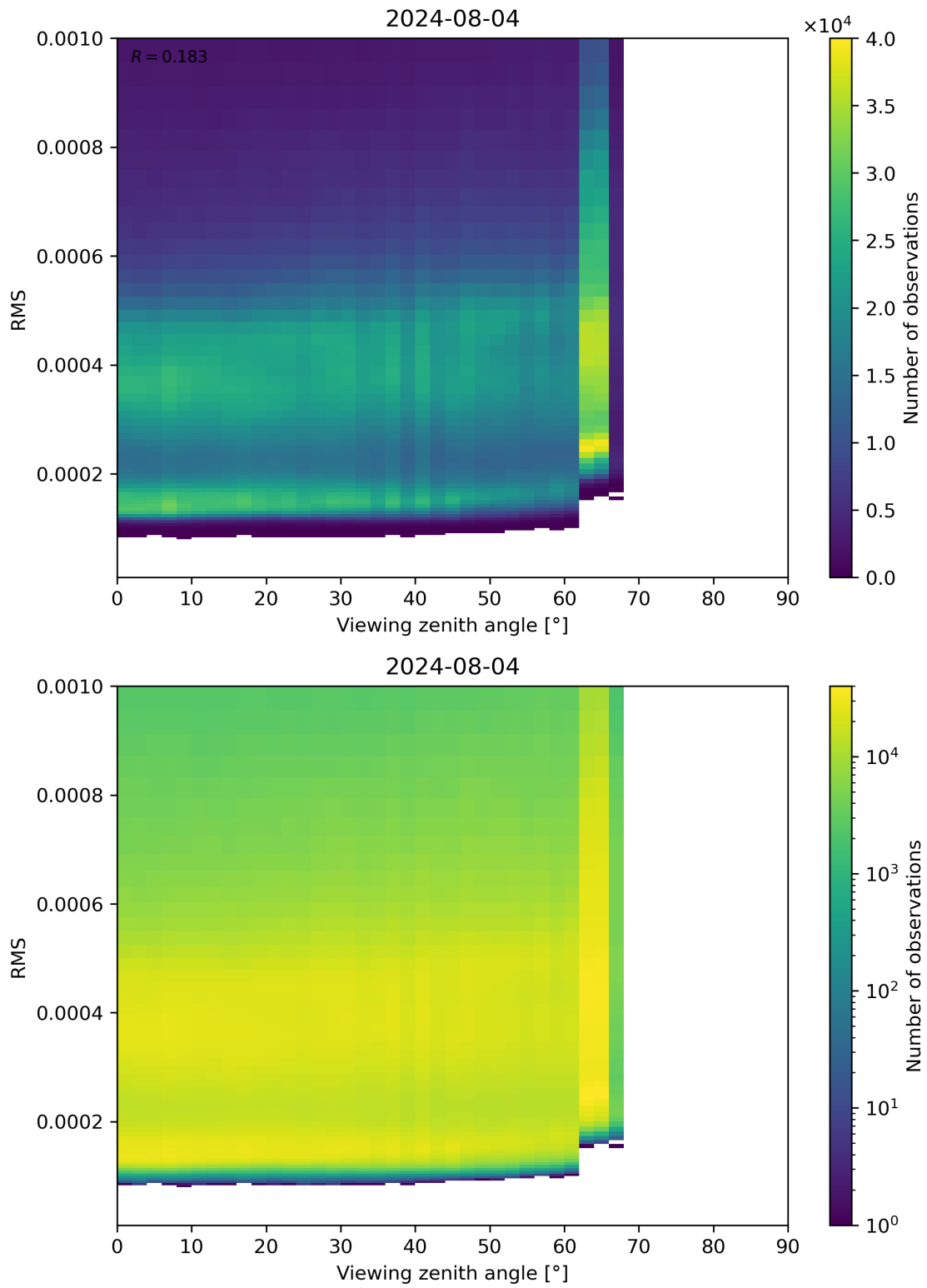
Figure 171: Scatter density plot of “Viewing zenith angle” against “RMS” for 2024-08-03 to 2024-08-05.
