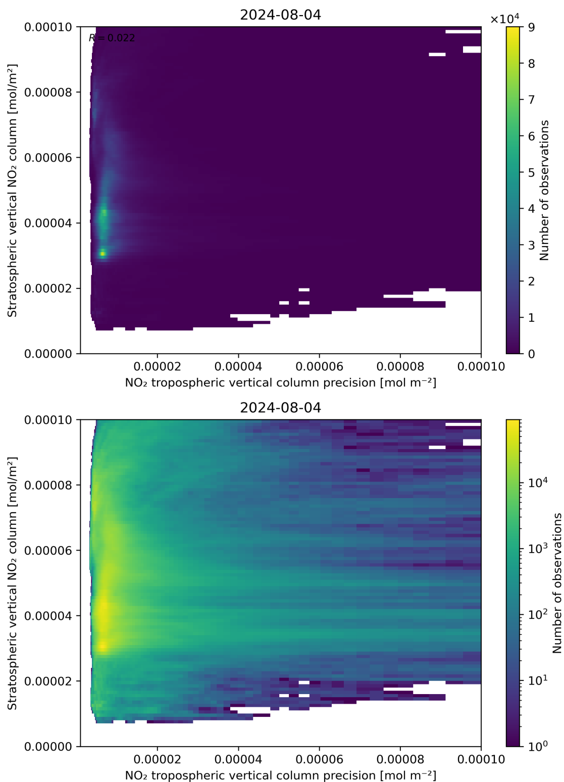
Figure 135: Scatter density plot of “NO 2 tropospheric vertical column precision” against “Stratospheric vertical NO 2 column” for 2024-08-03 to 2024-08-05.
