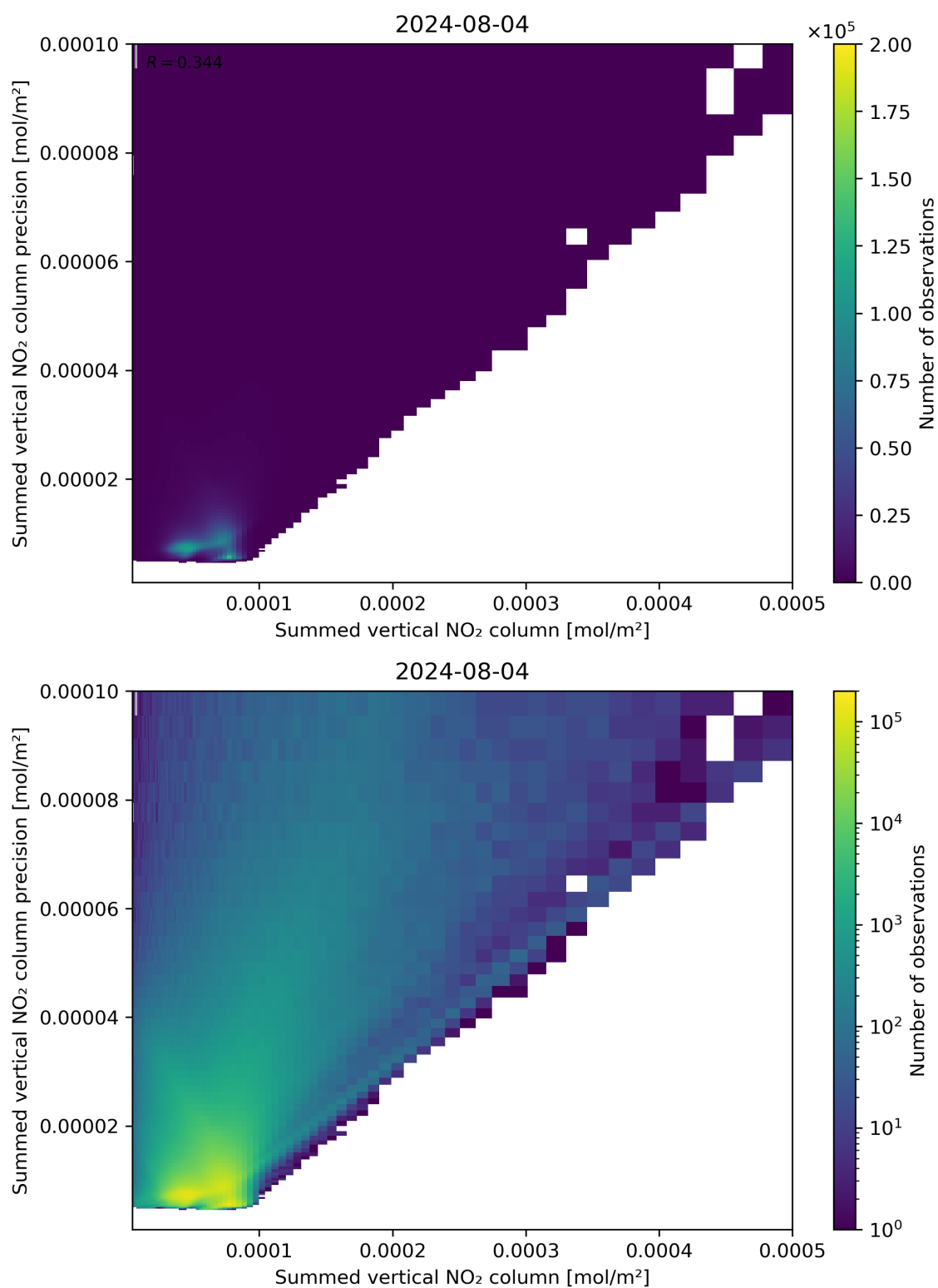
Figure 105: Scatter density plot of “Summed vertical NO 2 column” against “Summed vertical NO 2 column precision” for 2024-08-03 to 2024-08-05.
