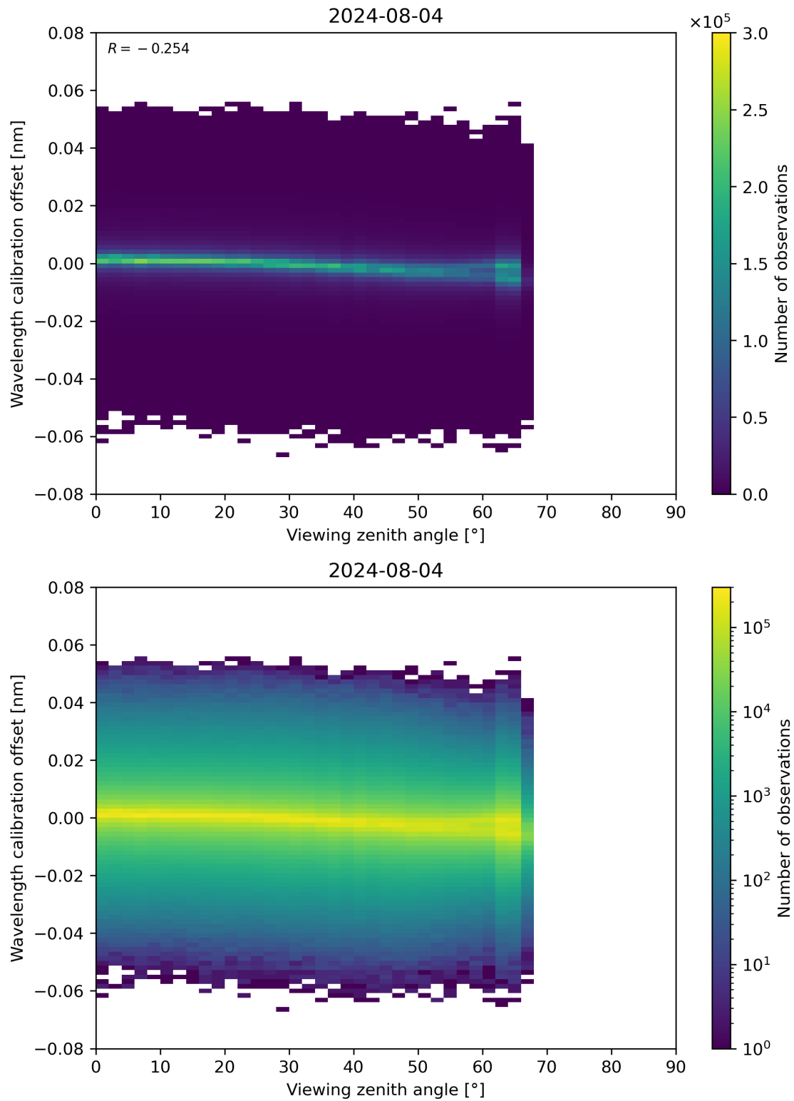
Figure 173: Scatter density plot of “Viewing zenith angle” against “Wavelength calibration offset” for 2024-08-03 to 2024-08-05.
