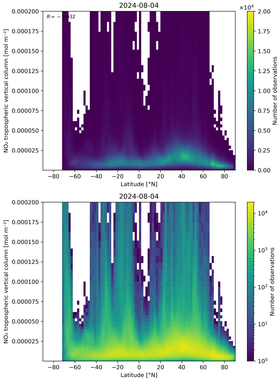
Figure 92: Scatter density plot of “Latitude” against “NO 2 tropospheric vertical column” for 2024-08-03 to 2024-08-05.
