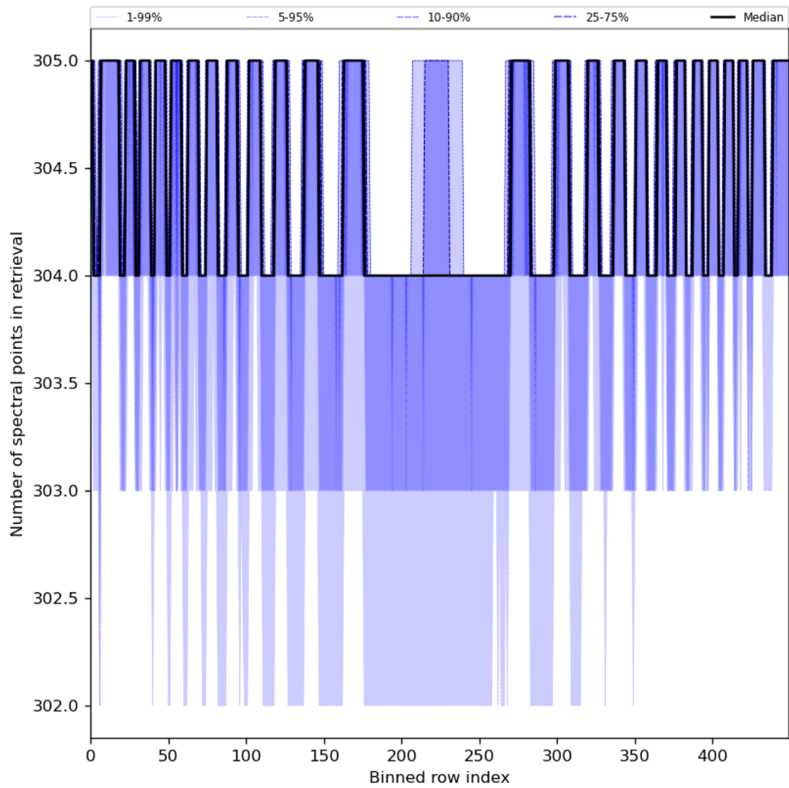
Figure 50: Along track statistics of “Number of spectral points in retrieval” for 2024-08-03 to 2024-08-05
