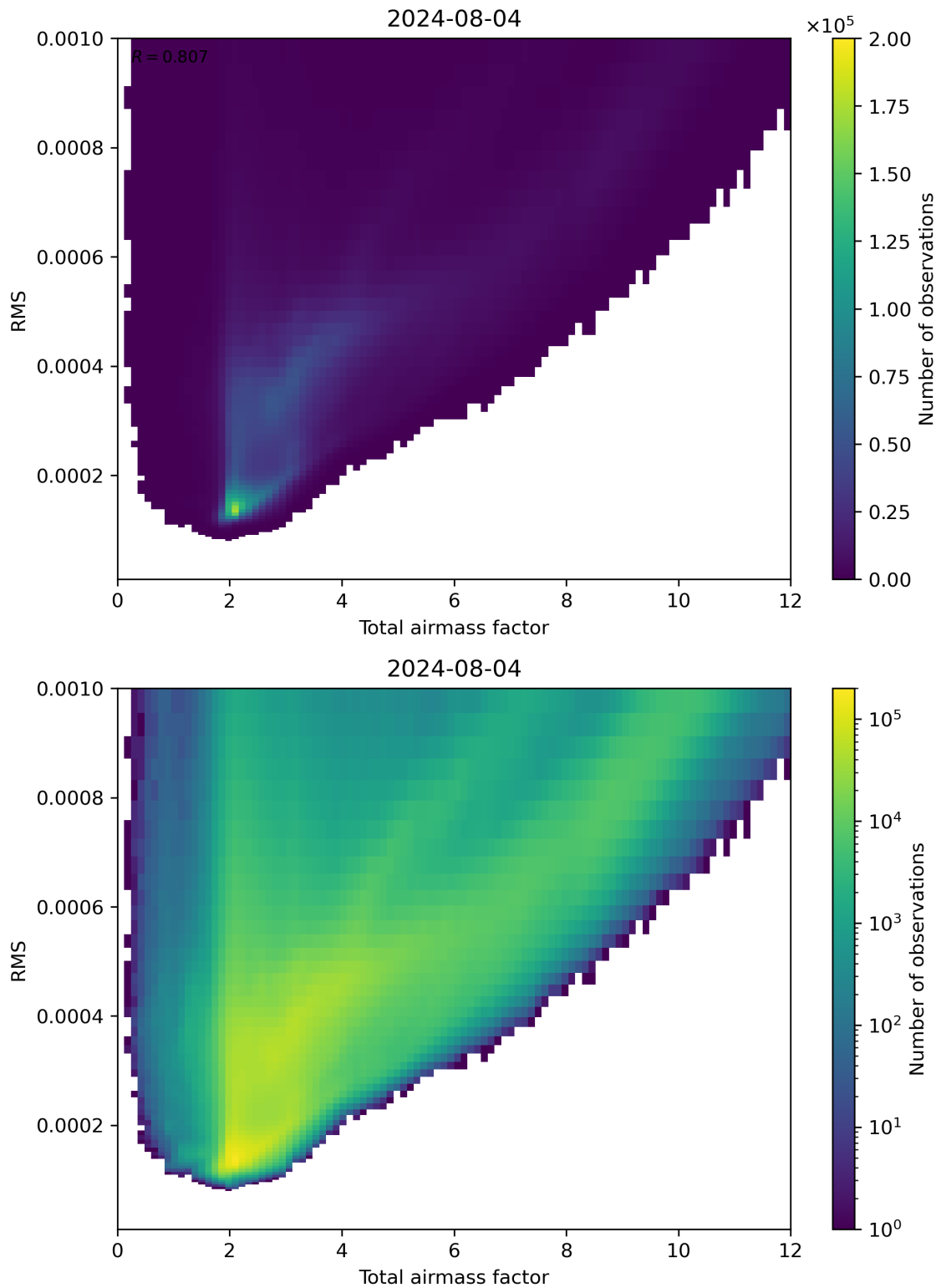
Figure 69: Scatter density plot of “Total airmass factor” against “RMS” for 2024-08-03 to 2024-08-05.
