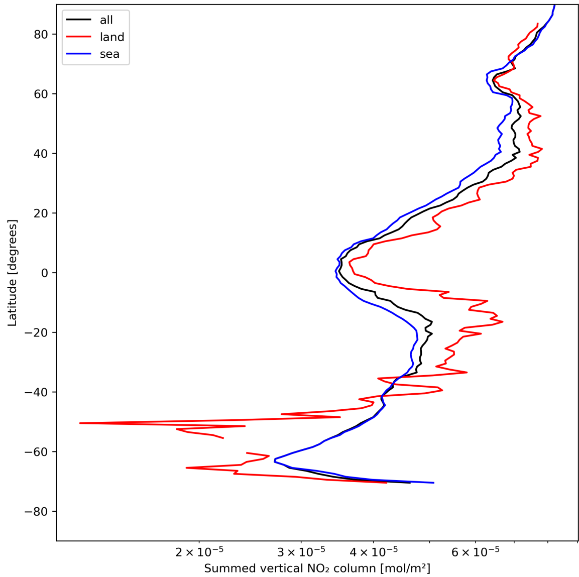
Figure 23: Zonal average of “Summed vertical NO 2 column” for 2024-08-03 to 2024-08-05.
