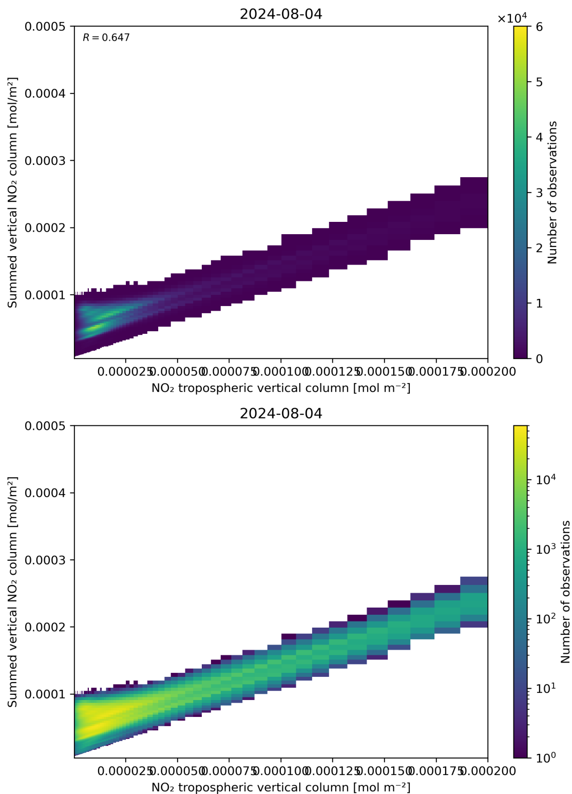
Figure 126: Scatter density plot of “NO 2 tropospheric vertical column” against “Summed vertical NO 2 column” for 2024-08-03 to 2024-08-05.
