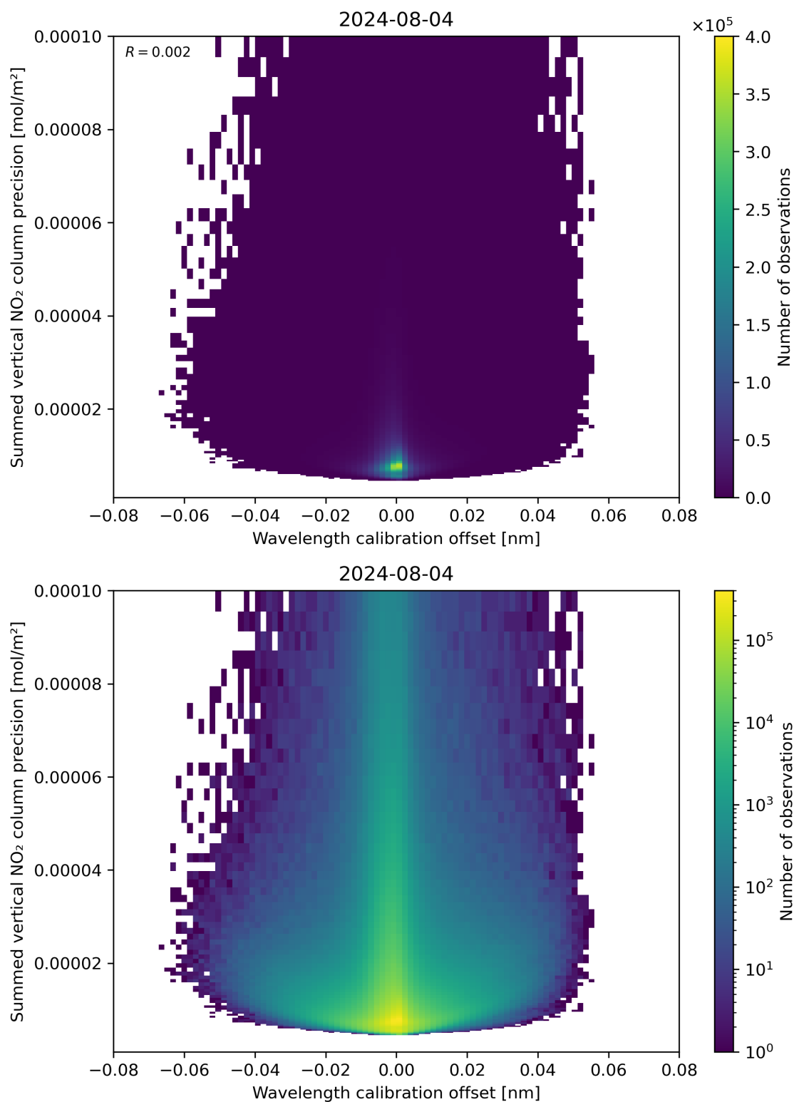
Figure 178: Scatter density plot of “Wavelength calibration offset” against “Summed vertical NO 2 column precision” for 2024-08-03 to 2024-08-05.
