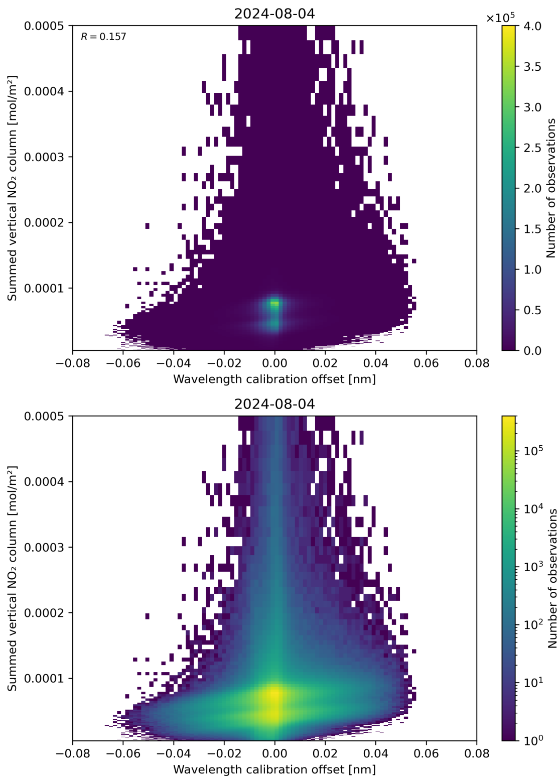
Figure 177: Scatter density plot of “Wavelength calibration offset” against “Summed vertical NO 2 column” for 2024-08-03 to 2024-08-05.
