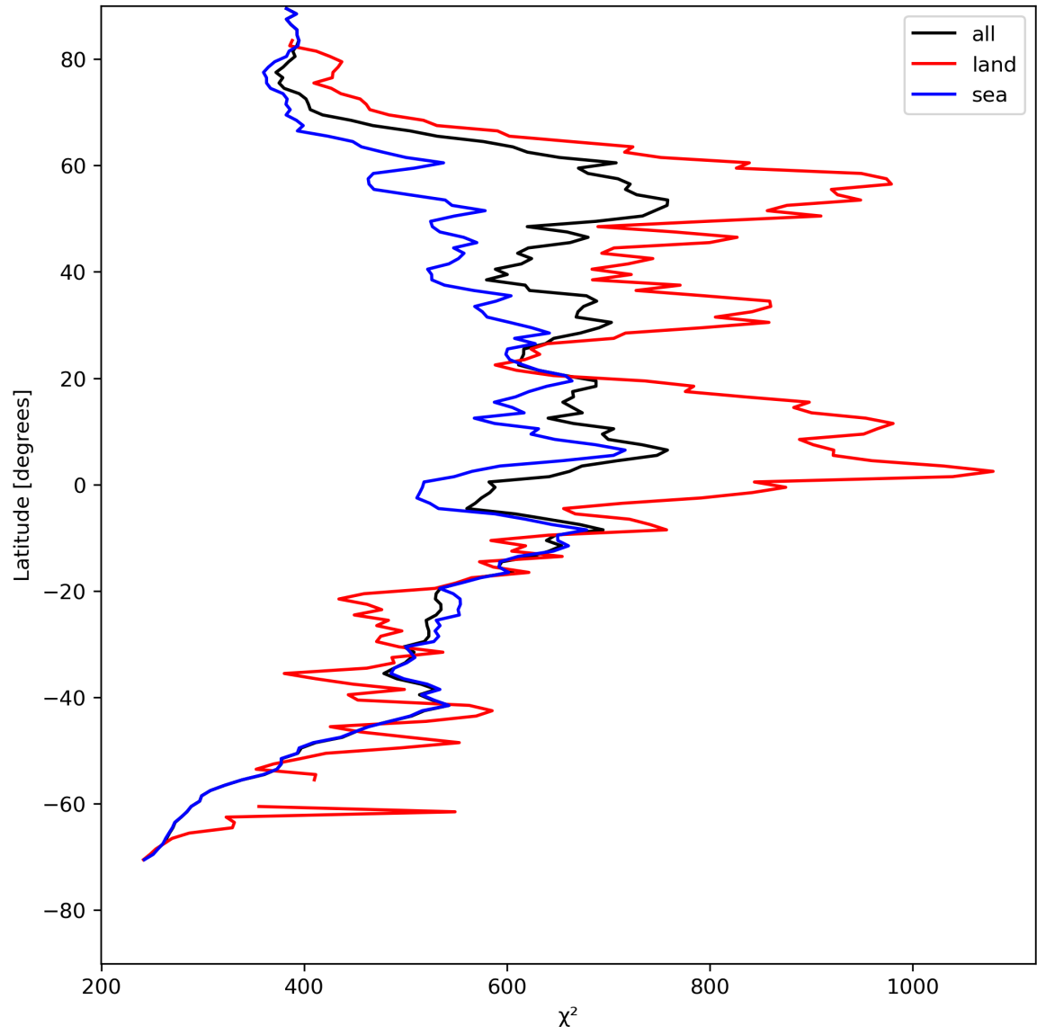
Figure 25: Zonal average of “ \chi^2 ” for 2024-08-03 to 2024-08-05.
