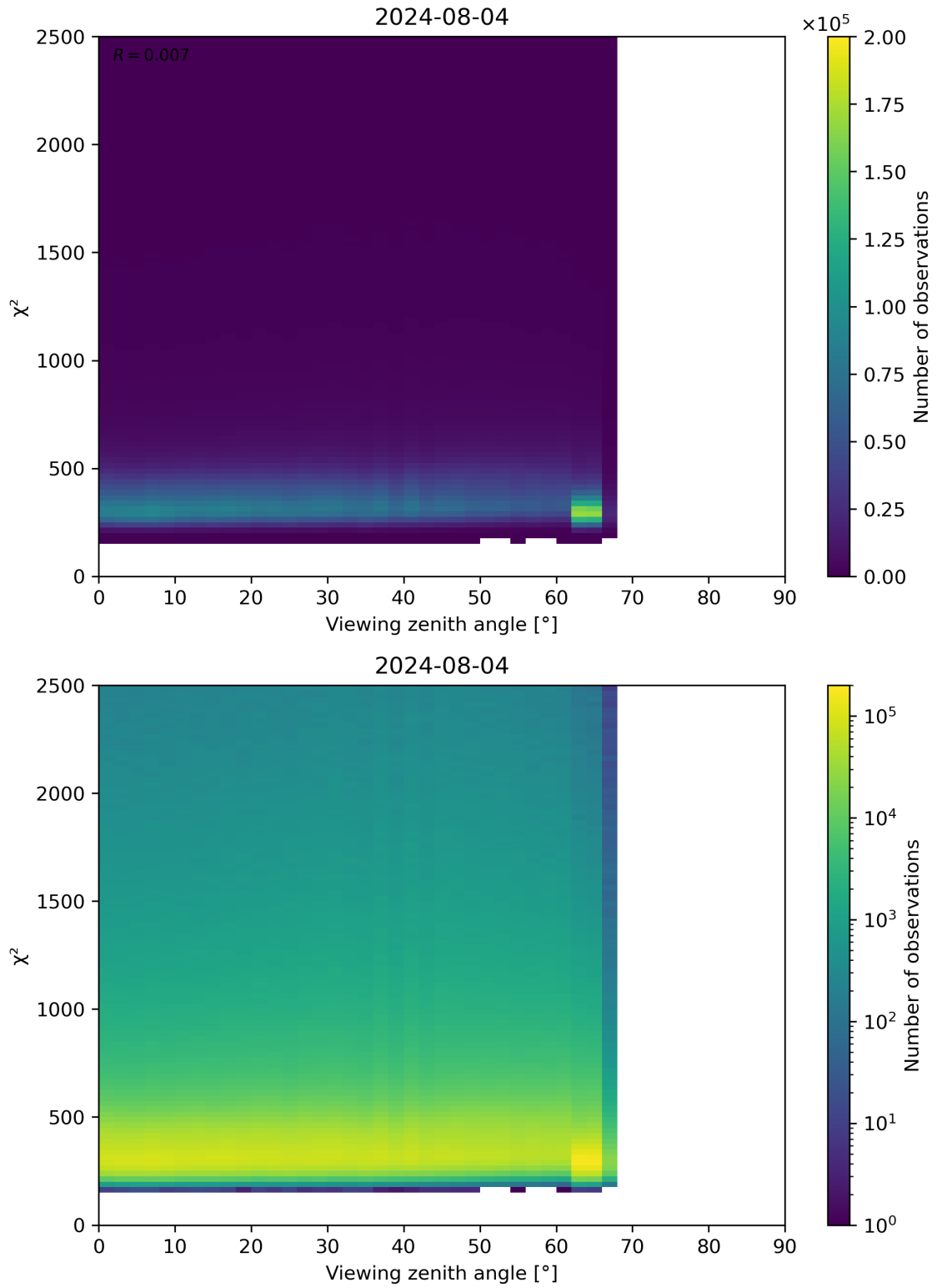
Figure 162: Scatter density plot of “Viewing zenith angle” against “ \chi^2 ” for 2024-08-03 to 2024-08-05.
