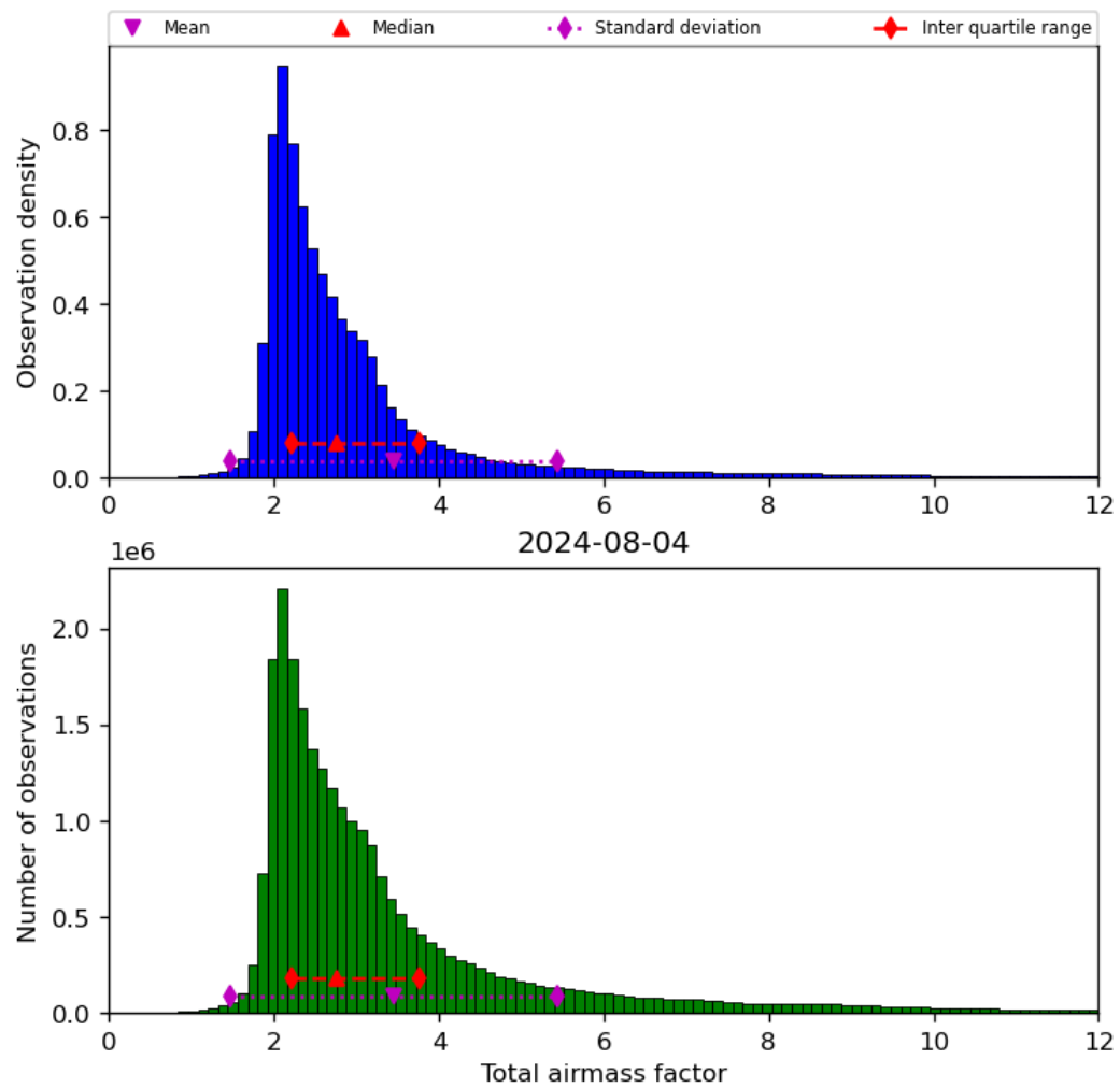
Figure 32: Histogram of “Total airmass factor” for 2024-08-03 to 2024-08-05
