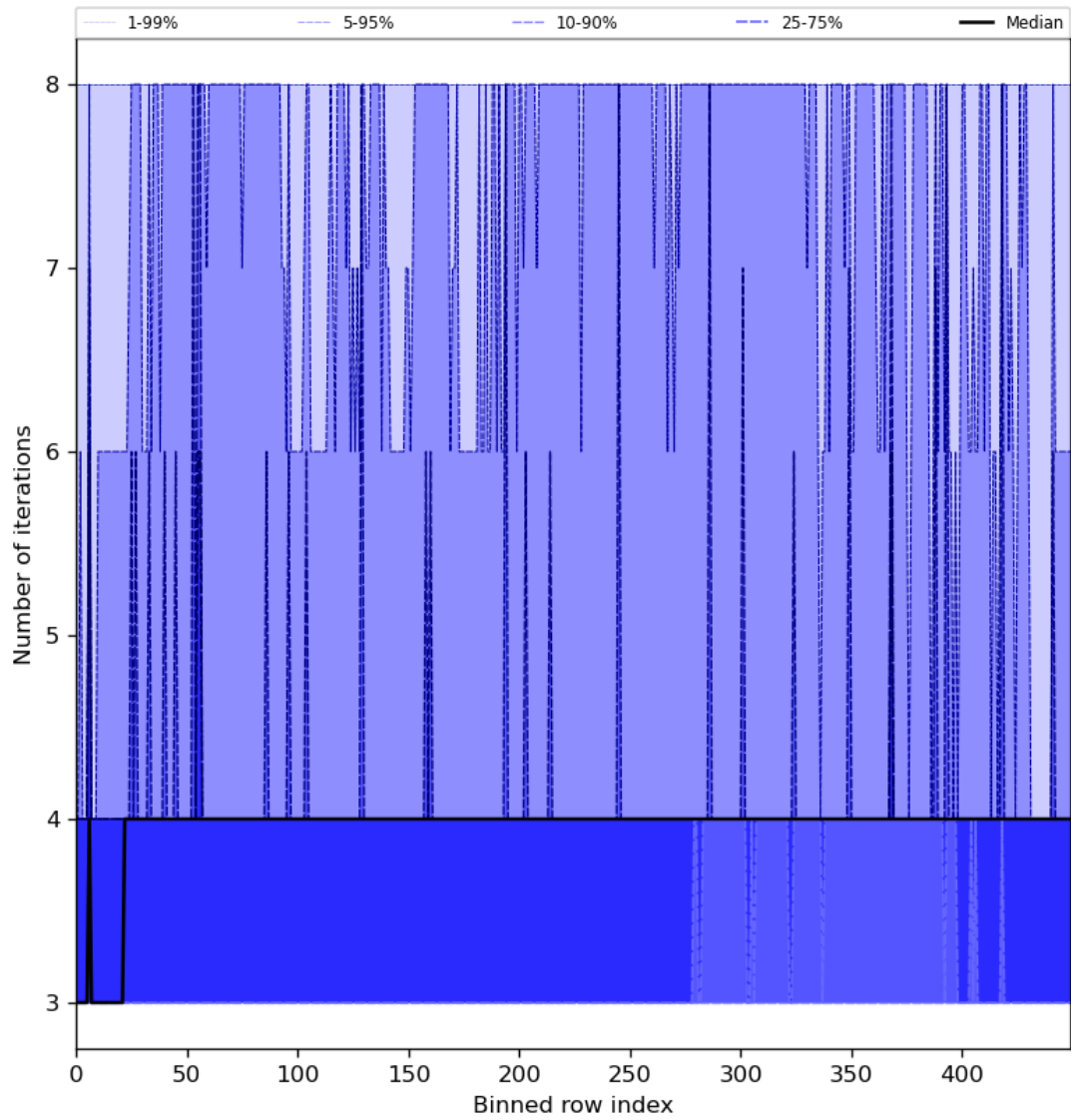
Figure 51: Along track statistics of “Number of iterations” for 2024-08-03 to 2024-08-05
