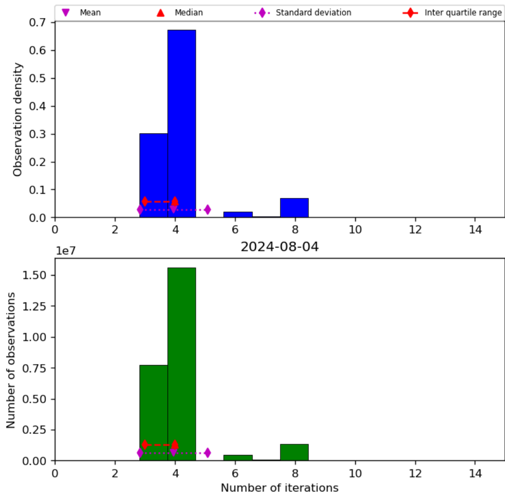
Figure 34: Histogram of “Number of iterations” for 2024-08-03 to 2024-08-05
