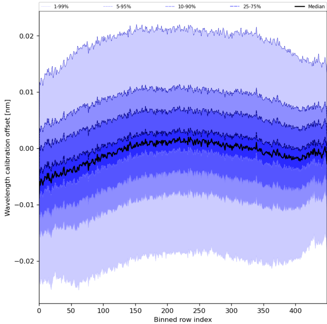
Figure 52: Along track statistics of “Wavelength calibration offset” for 2024-08-03 to 2024-08-05
