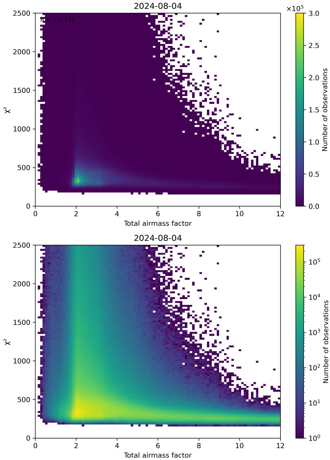
Figure 63: Scatter density plot of “Total airmass factor” against “ \chi^2 ” for 2024-08-03 to 2024-08-05.
