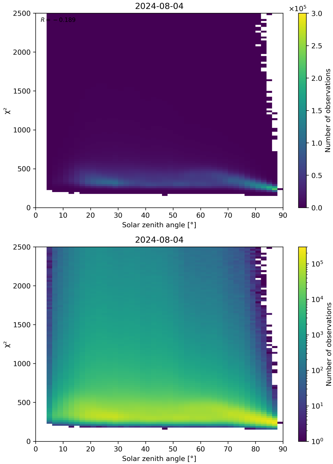
Figure 148: Scatter density plot of “Solar zenith angle” against “ \chi^2 ” for 2024-08-03 to 2024-08-05.
