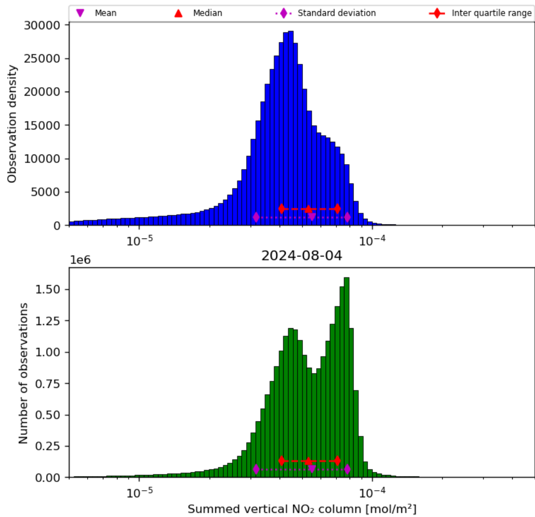
Figure 40: Histogram of “Summed vertical NO 2 column” for 2024-08-03 to 2024-08-05
