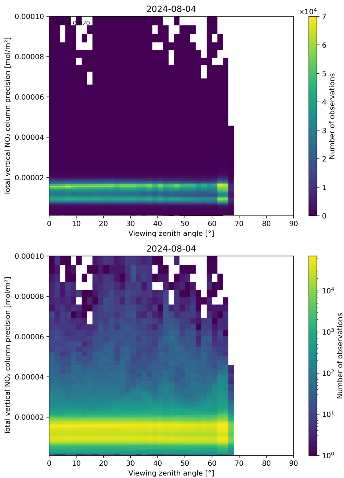
Figure 168: Scatter density plot of “Viewing zenith angle” against “Total vertical NO 2 column precision” for 2024-08-03 to 2024-08-05.
