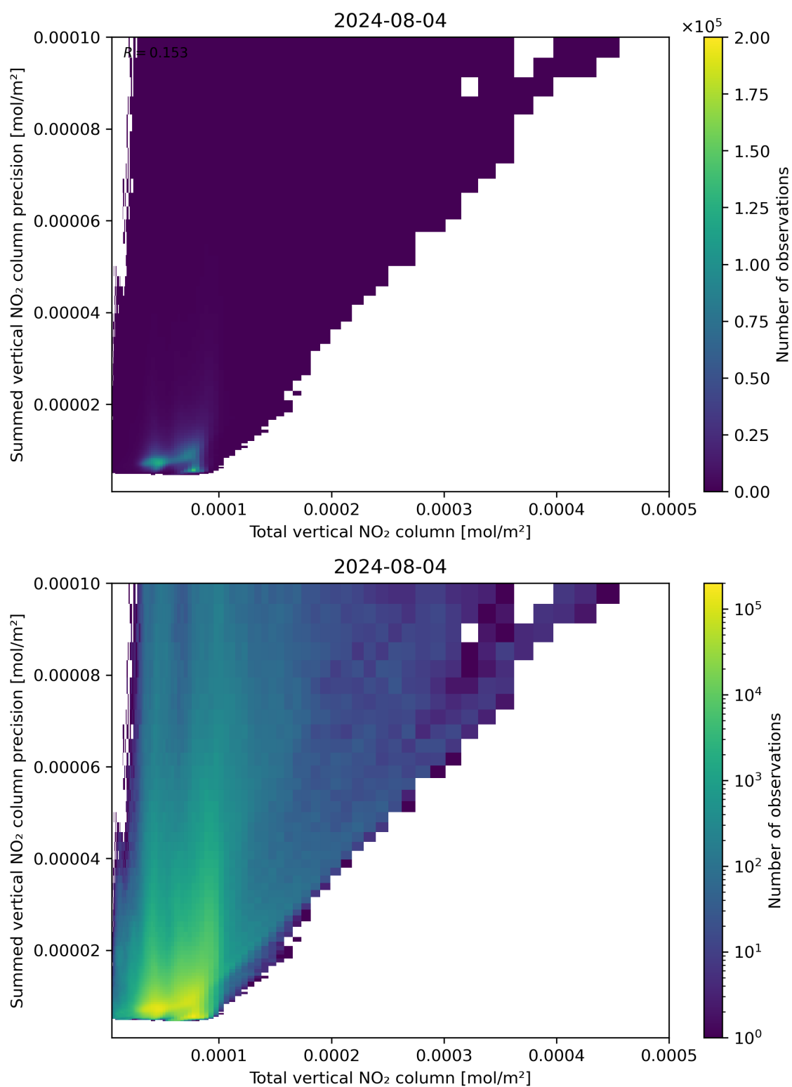
Figure 113: Scatter density plot of “Total vertical NO 2 column” against “Summed vertical NO 2 column precision” for 2024-08-03 to 2024-08-05.
