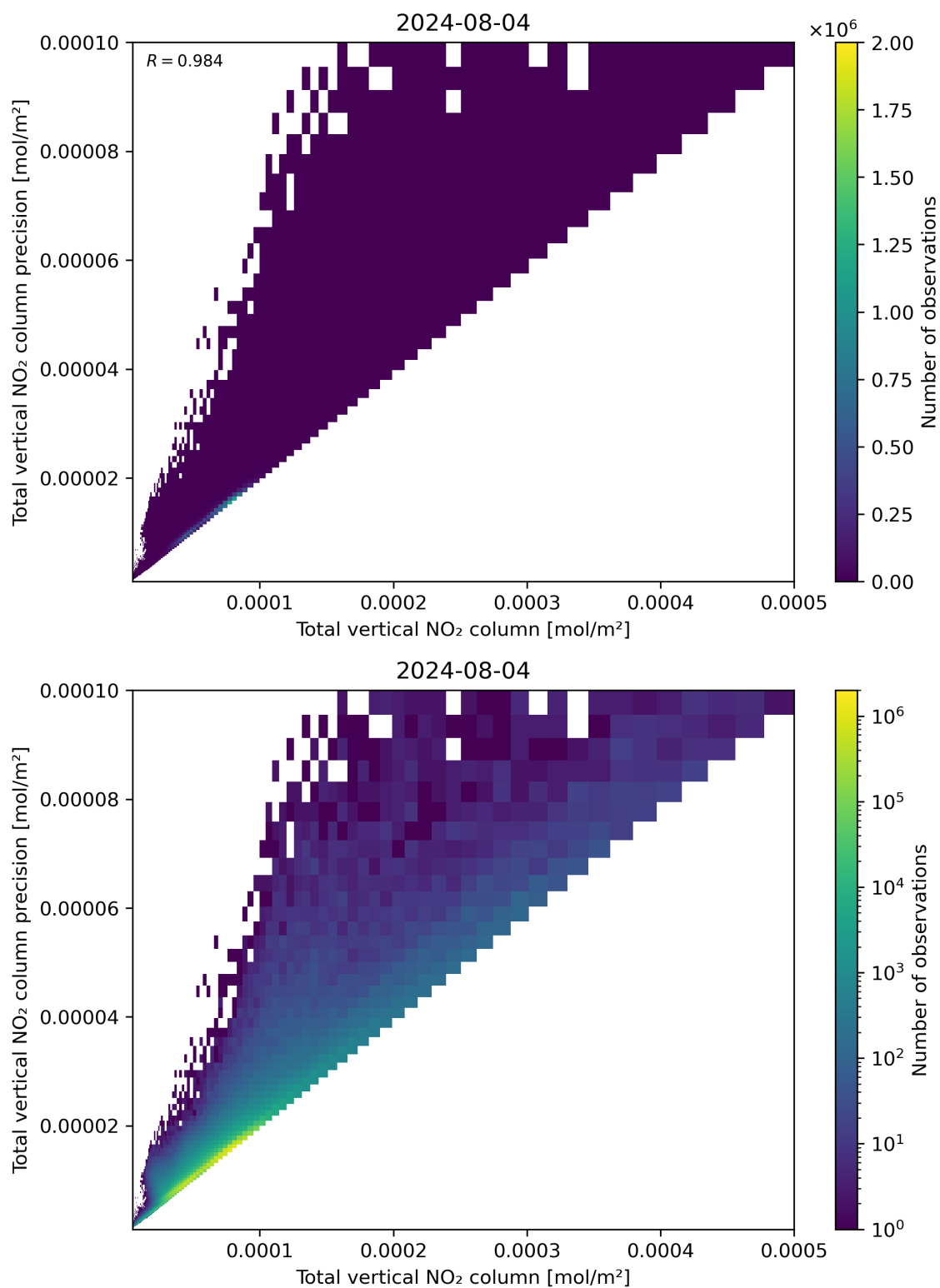
Figure 114: Scatter density plot of “Total vertical NO 2 column” against “Total vertical NO 2 column precision” for 2024-08-03 to 2024-08-05.
