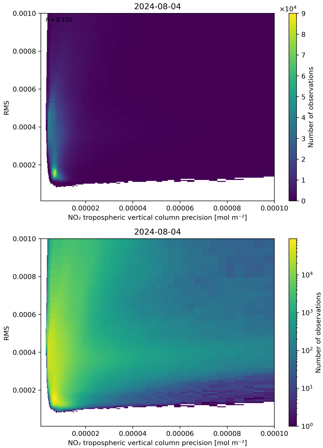
Figure 140: Scatter density plot of “NO 2 tropospheric vertical column precision” against “RMS” for 2024-08-03 to 2024-08-05.
