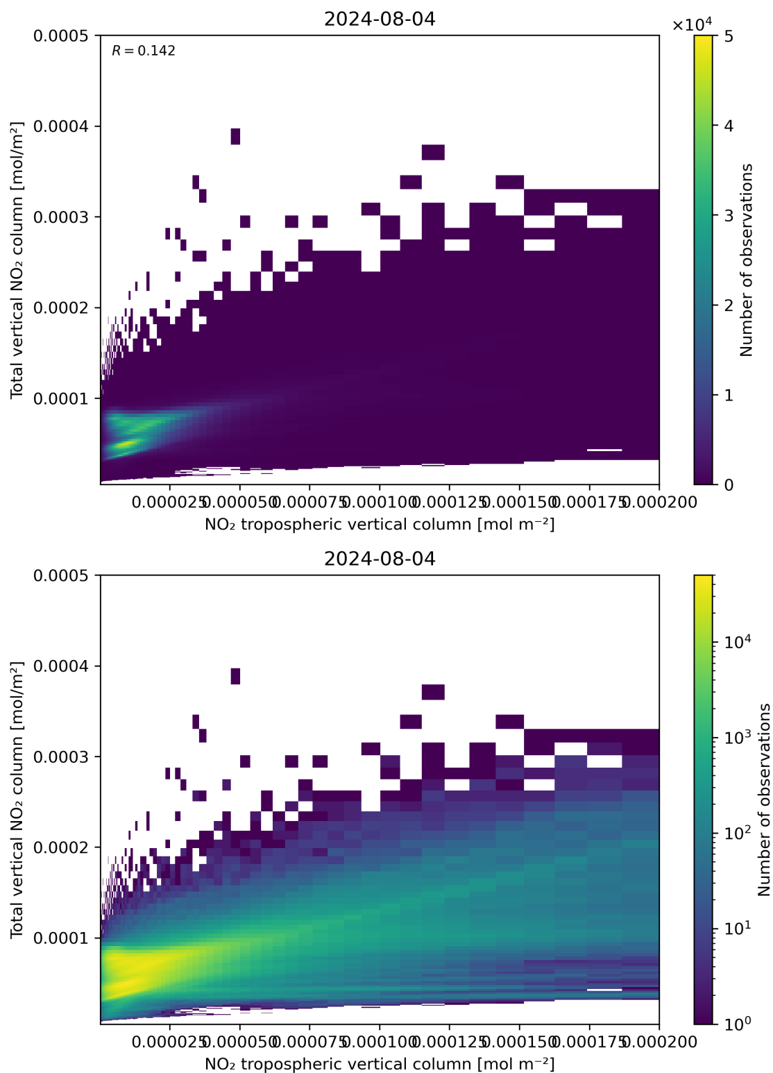
Figure 128: Scatter density plot of “NO 2 tropospheric vertical column” against “Total vertical NO 2 column” for 2024-08-03 to 2024-08-05.
