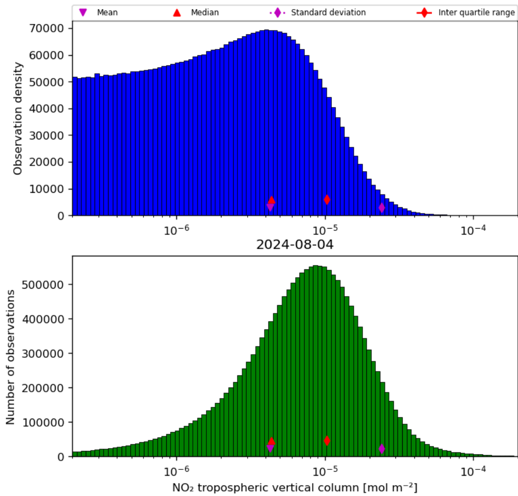
Figure 29: Histogram of “NO 2 tropospheric vertical column” for 2024-08-03 to 2024-08-05
