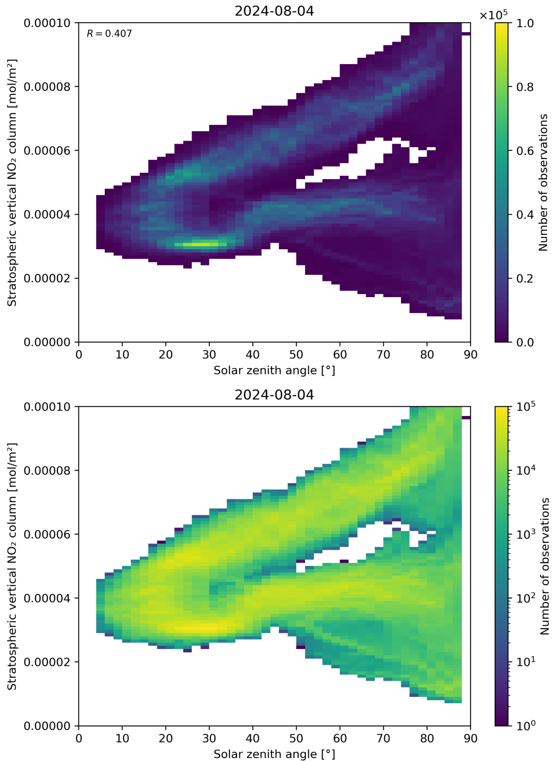
Figure 150: Scatter density plot of “Solar zenith angle” against “Stratospheric vertical NO 2 column” for 2024-08-03 to 2024-08-05.
