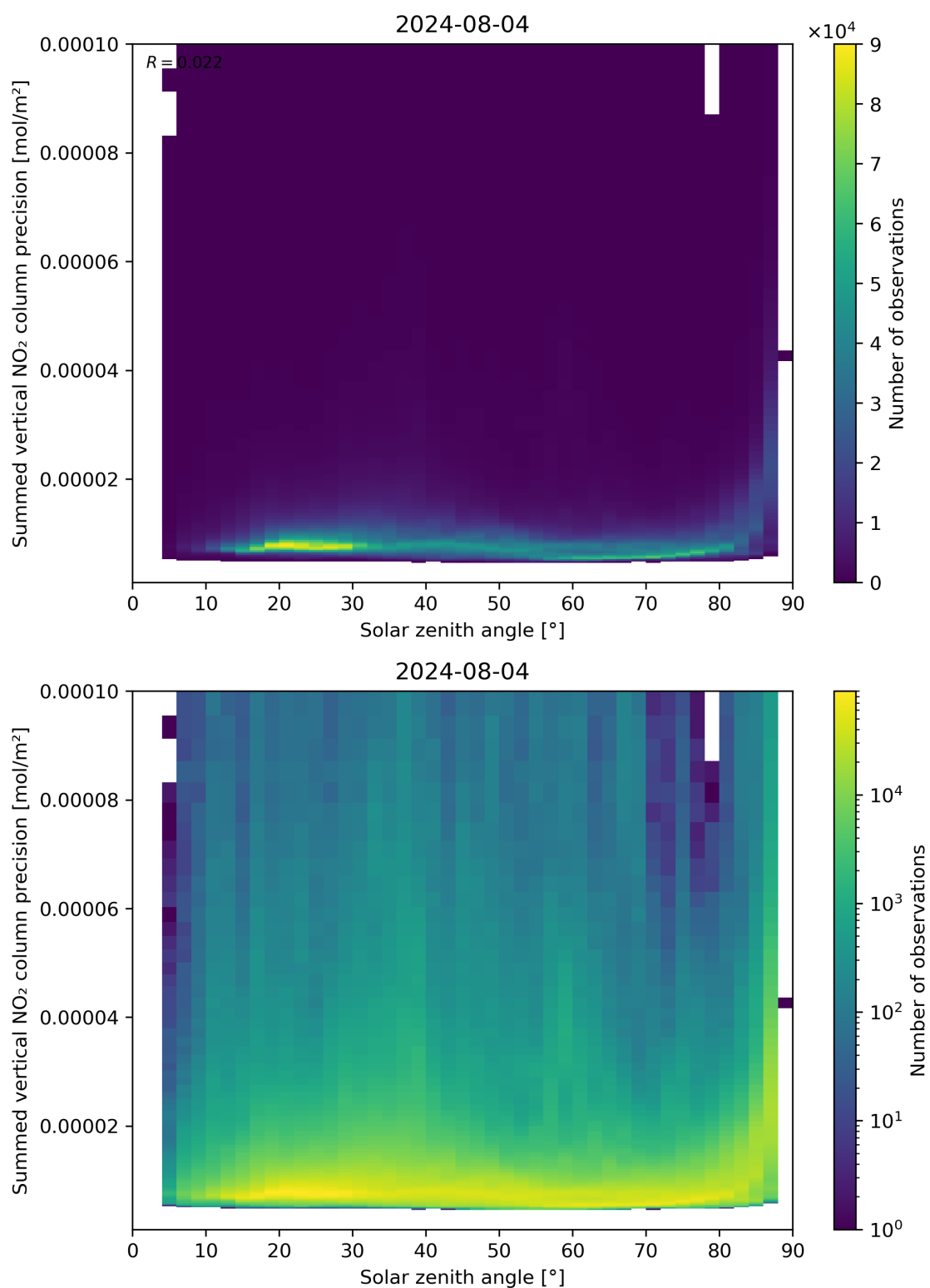
Figure 152: Scatter density plot of “Solar zenith angle” against “Summed vertical NO 2 column precision” for 2024-08-03 to 2024-08-05.
