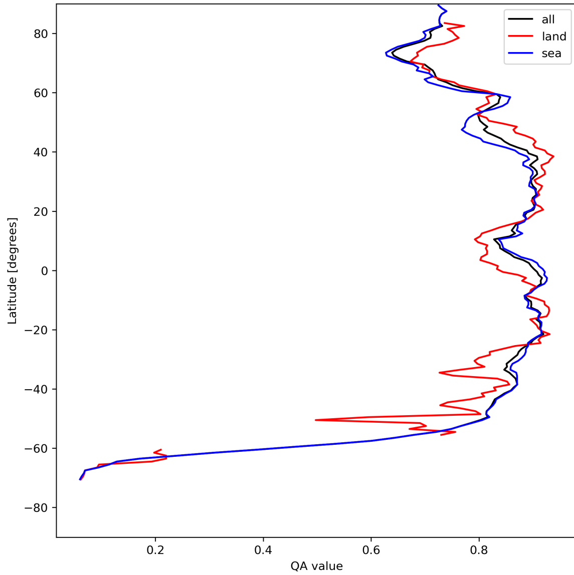
Figure 11: Zonal average of “QA value” for 2024-08-03 to 2024-08-05.
