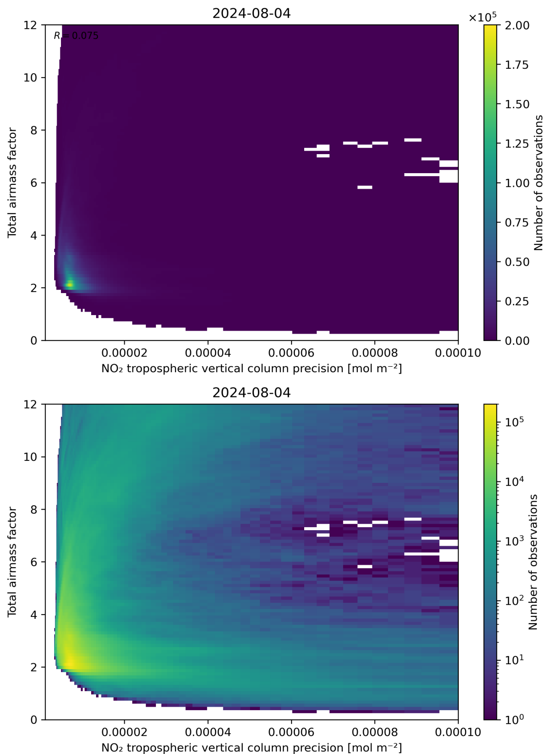
Figure 132: Scatter density plot of “NO 2 tropospheric vertical column precision” against “Total air mass factor” for 2024-08-03 to 2024-08-05.
