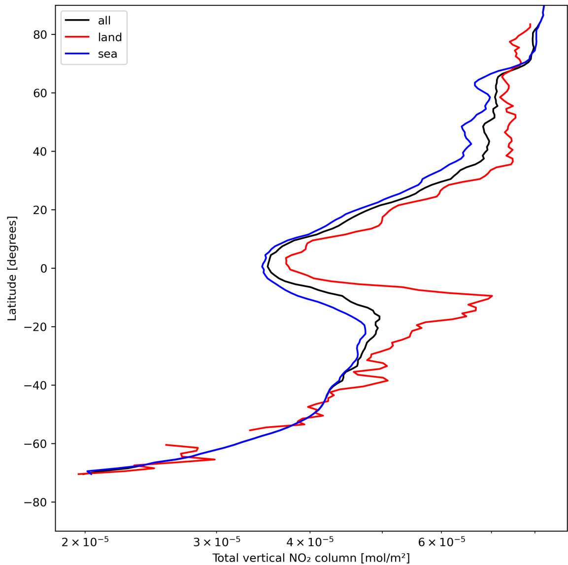
Figure 21: Zonal average of “Total vertical NO 2 column” for 2024-08-03 to 2024-08-05.
