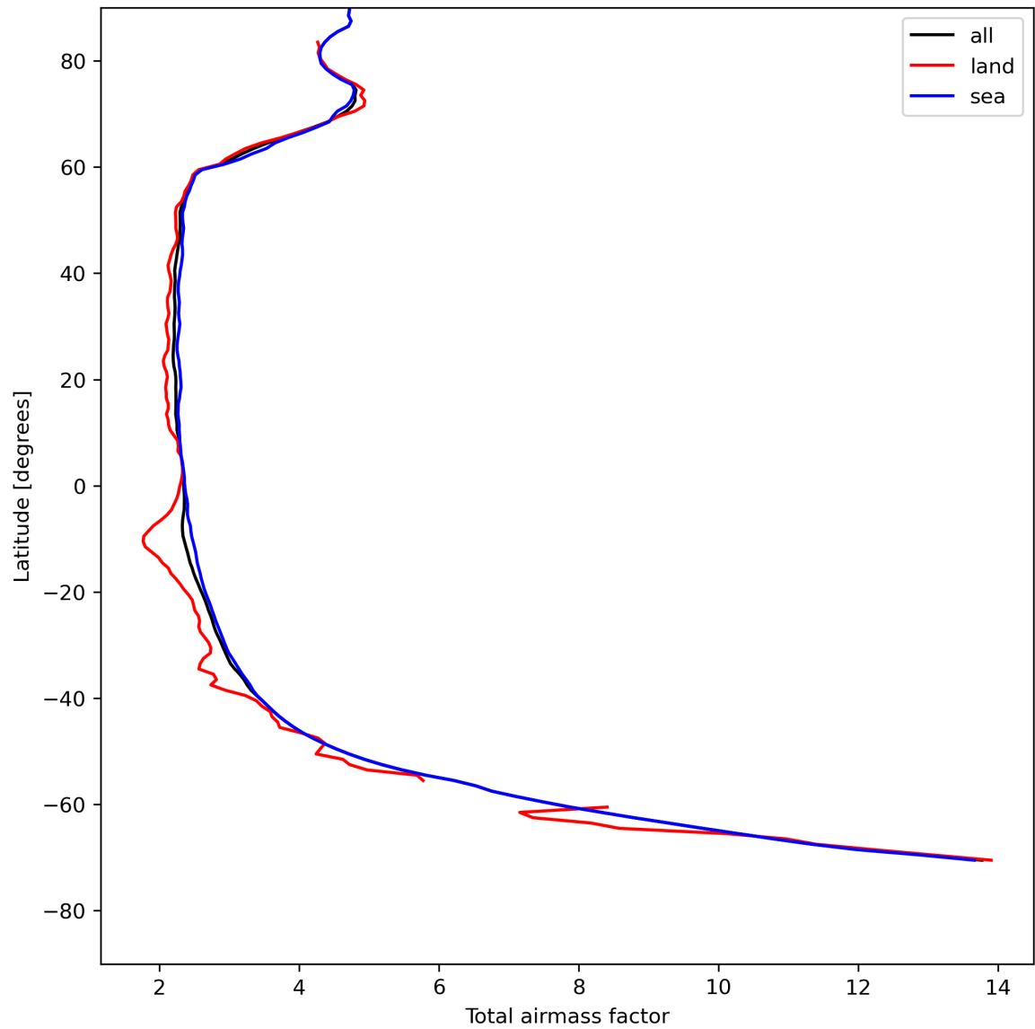
Figure 15: Zonal average of “Total airmass factor” for 2024-08-03 to 2024-08-05.
