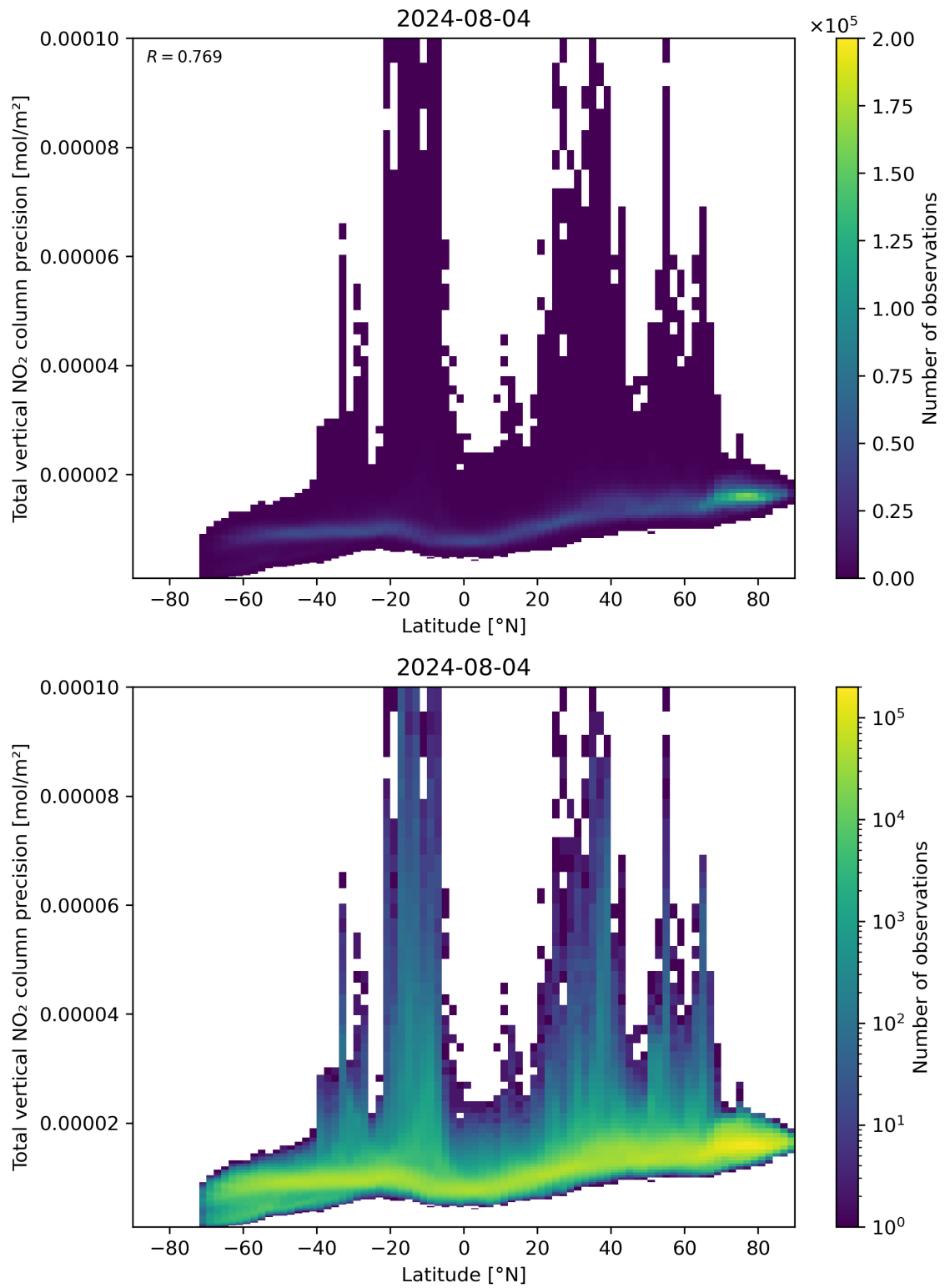
Figure 91: Scatter density plot of “Latitude” against “Total vertical NO 2 column precision” for 2024-08-03 to 2024-08-05.
