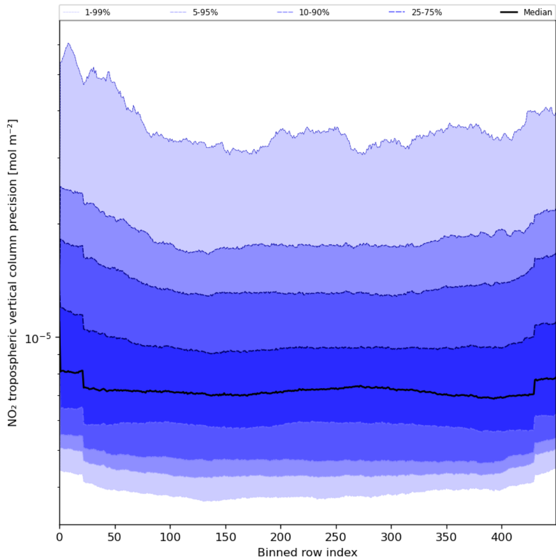
Figure 47: Along track statistics of “NO 2 tropospheric vertical column precision” for 2024-08-03 to 2024-08-05
