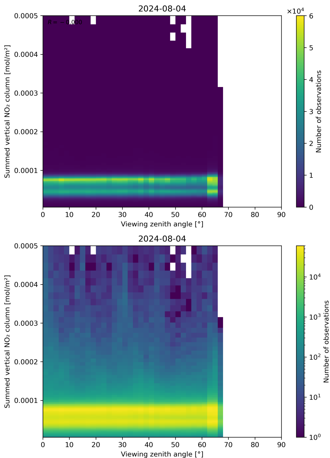
Figure 165: Scatter density plot of “Viewing zenith angle” against “Summed vertical NO 2 column” for 2024-08-03 to 2024-08-05.
