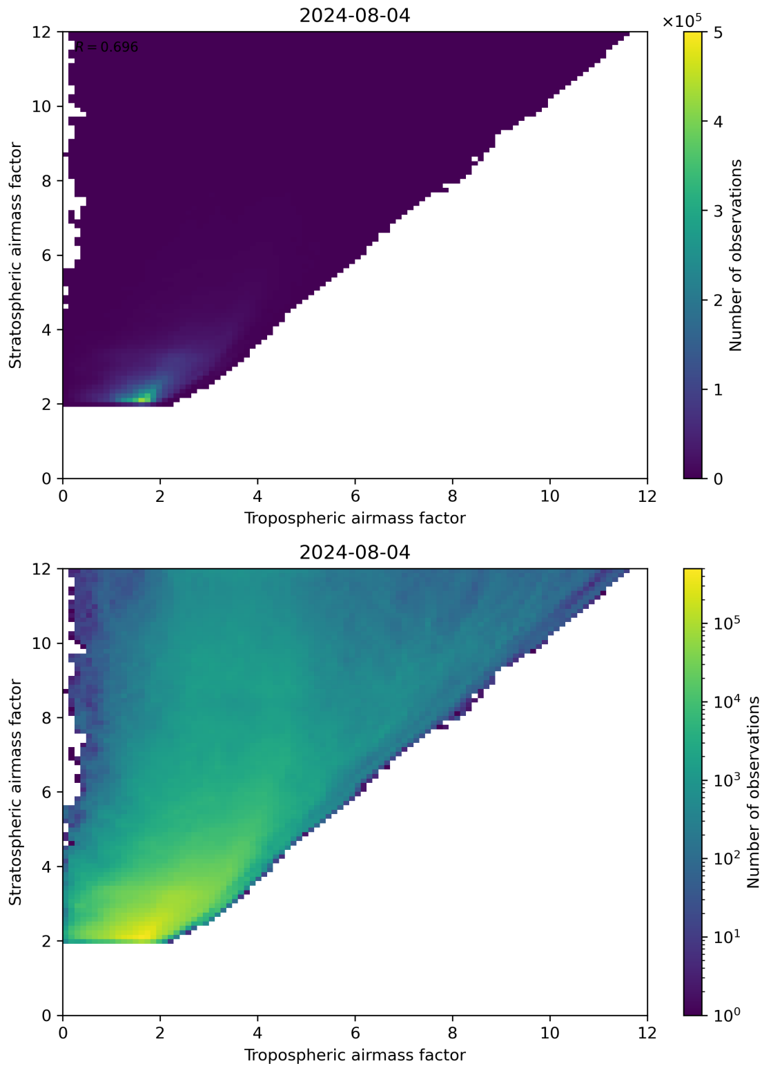
Figure 71: Scatter density plot of “Tropospheric airmass factor” against “Stratospheric airmass factor” for 2024-08-03 to 2024-08-05.
