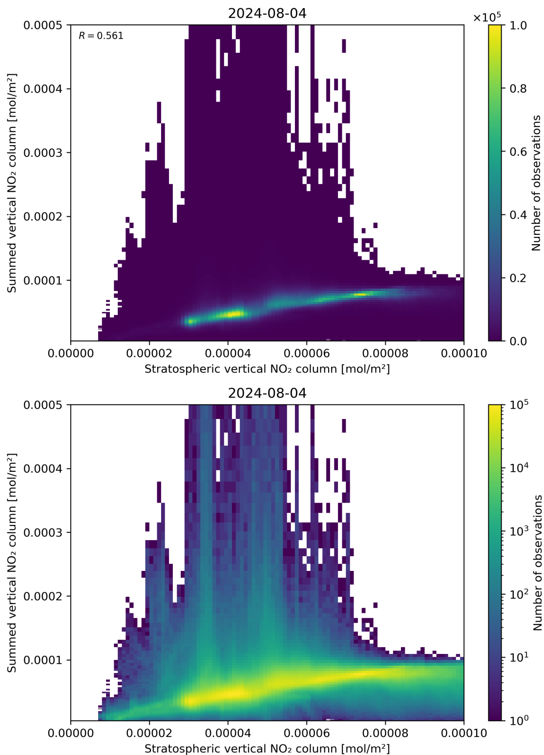
Figure 98: Scatter density plot of “Stratospheric vertical NO 2 column” against “Summed vertical NO 2 column” for 2024-08-03 to 2024-08-05.
