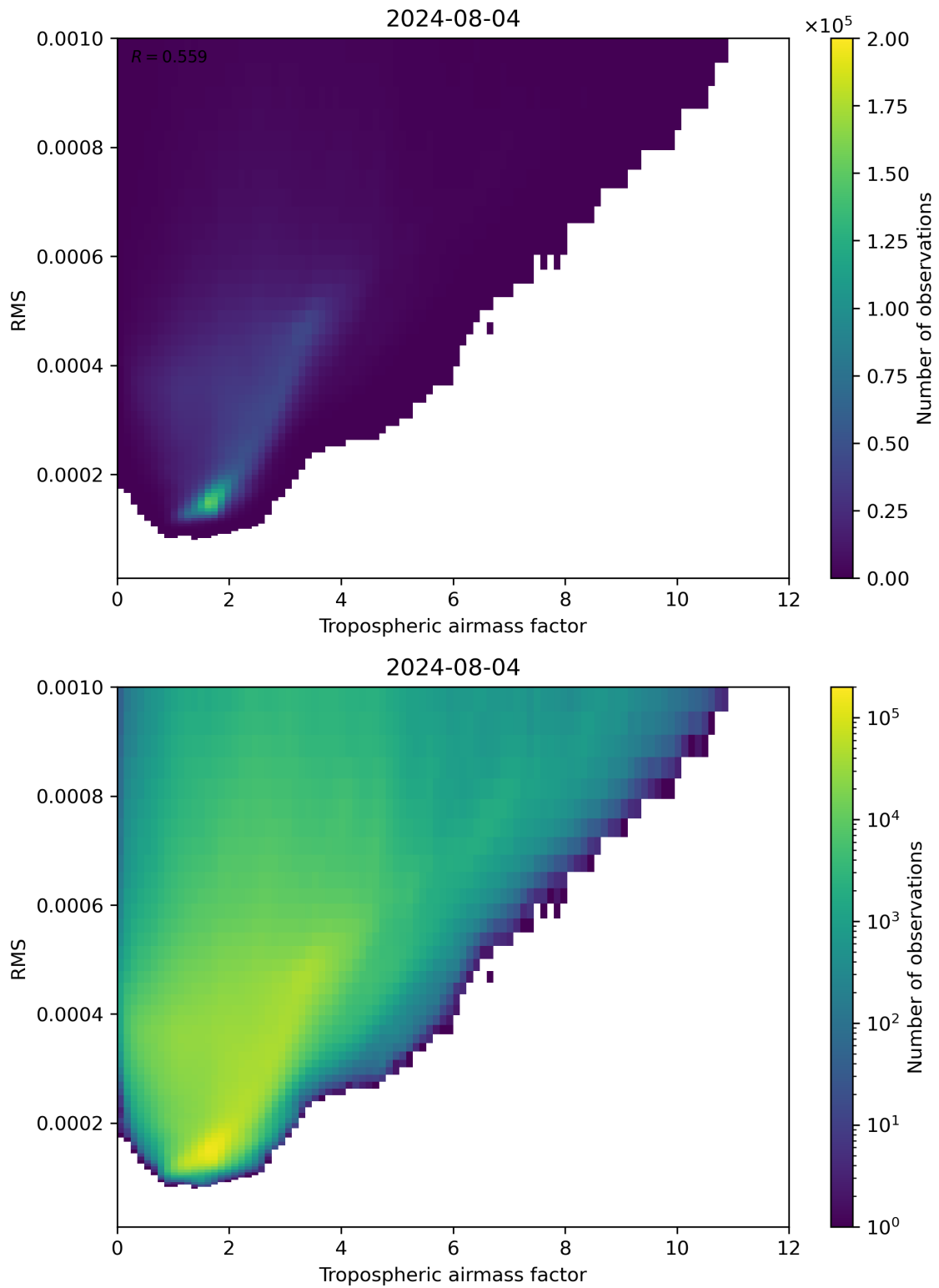
Figure 79: Scatter density plot of “Tropospheric airmass factor” against “RMS” for 2024-08-03 to 2024-08-05.
