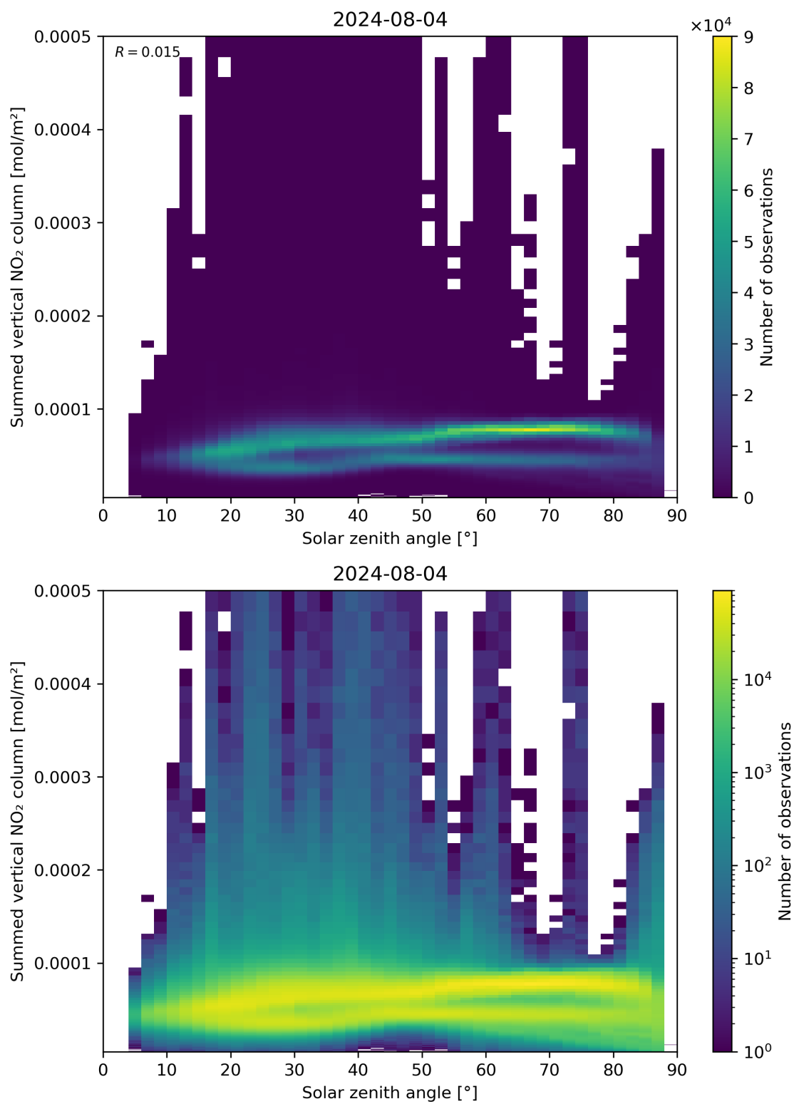
Figure 151: Scatter density plot of “Solar zenith angle” against “Summed vertical NO 2 column” for 2024-08-03 to 2024-08-05.
