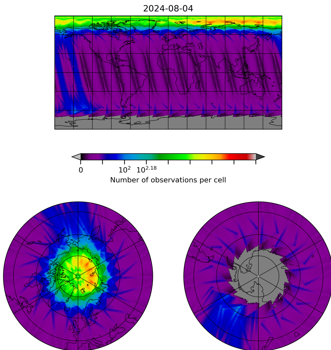
Figure 10: Map of the number of observations for 2024-08-03 to 2024-08-05
