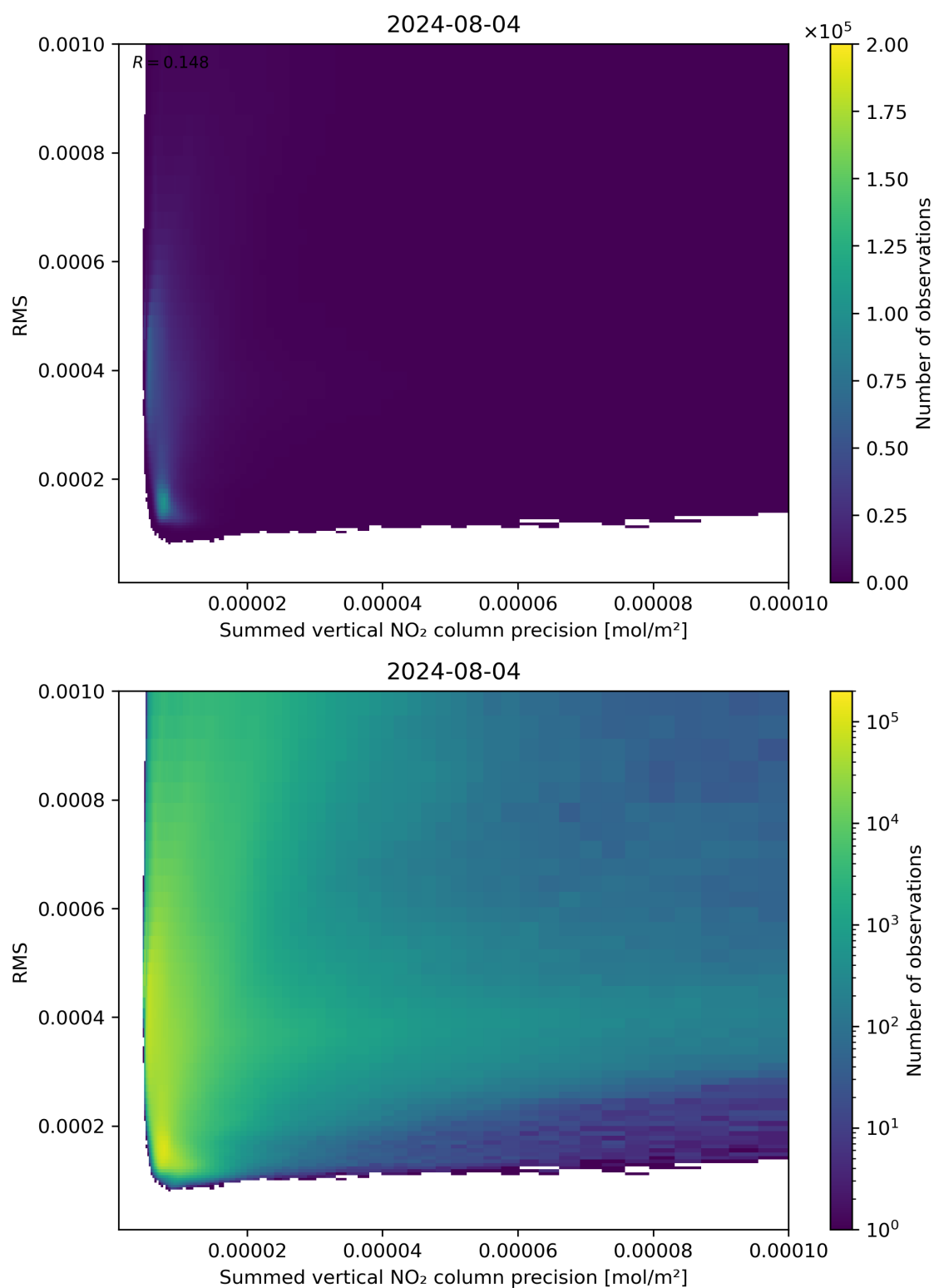
Figure 108: Scatter density plot of “Summed vertical NO 2 column precision” against “RMS” for 2024-08-03 to 2024-08-05.
