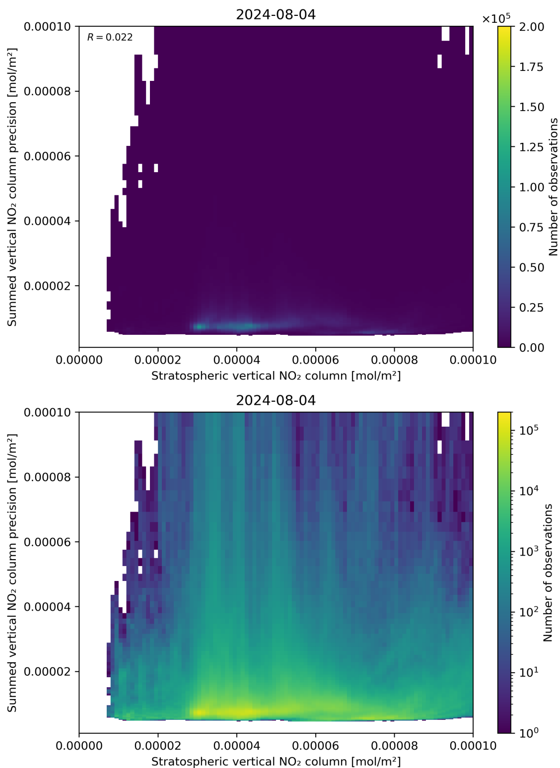
Figure 99: Scatter density plot of “Stratospheric vertical NO 2 column” against “Summed vertical NO 2 column precision” for 2024-08-03 to 2024-08-05.
