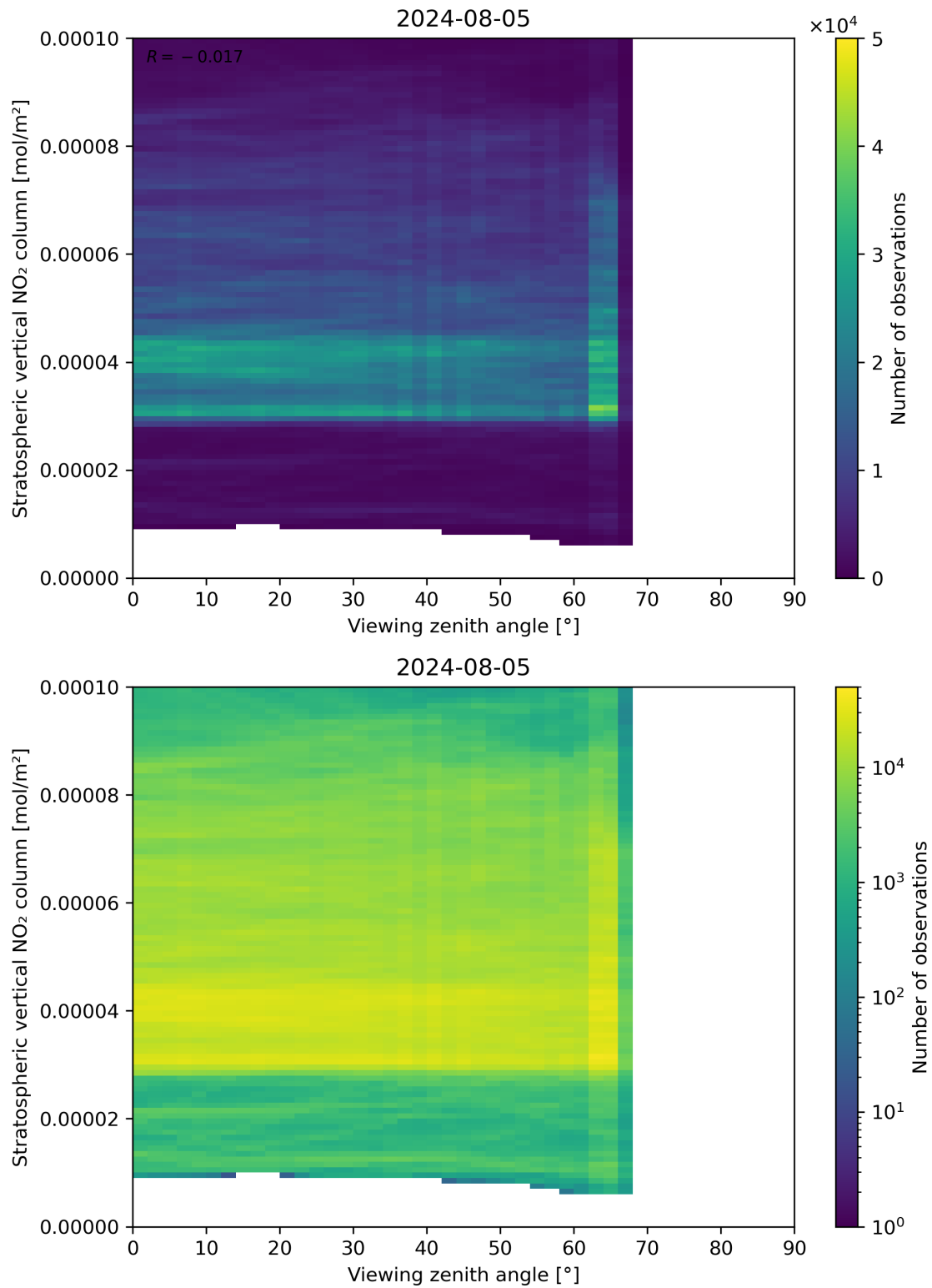
Figure 164: Scatter density plot of “Viewing zenith angle” against “Stratospheric vertical NO 2 column” for 2024-08-04 to 2024-08-06.
