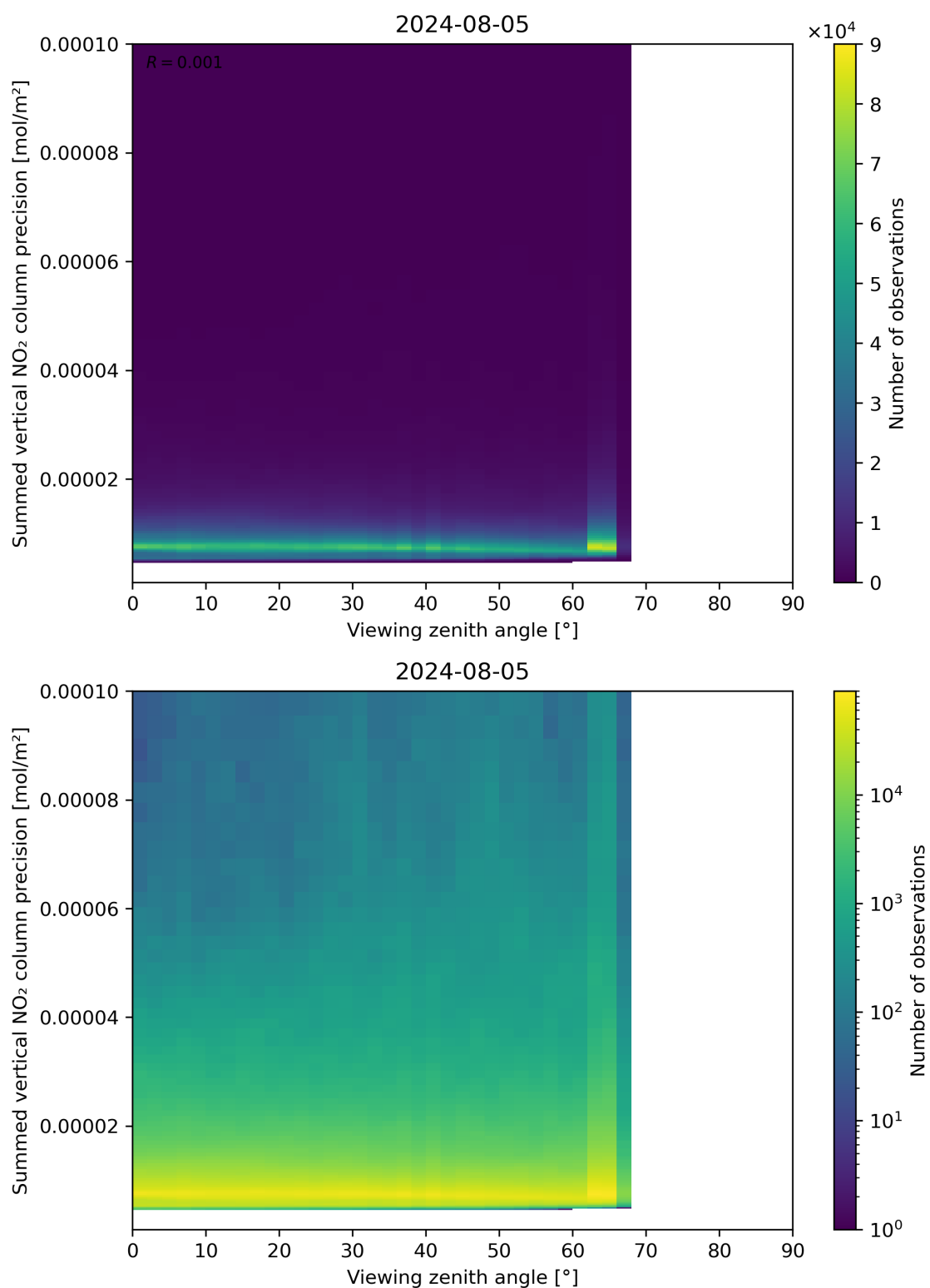
Figure 166: Scatter density plot of “Viewing zenith angle” against “Summed vertical NO 2 column precision” for 2024-08-04 to 2024-08-06.
