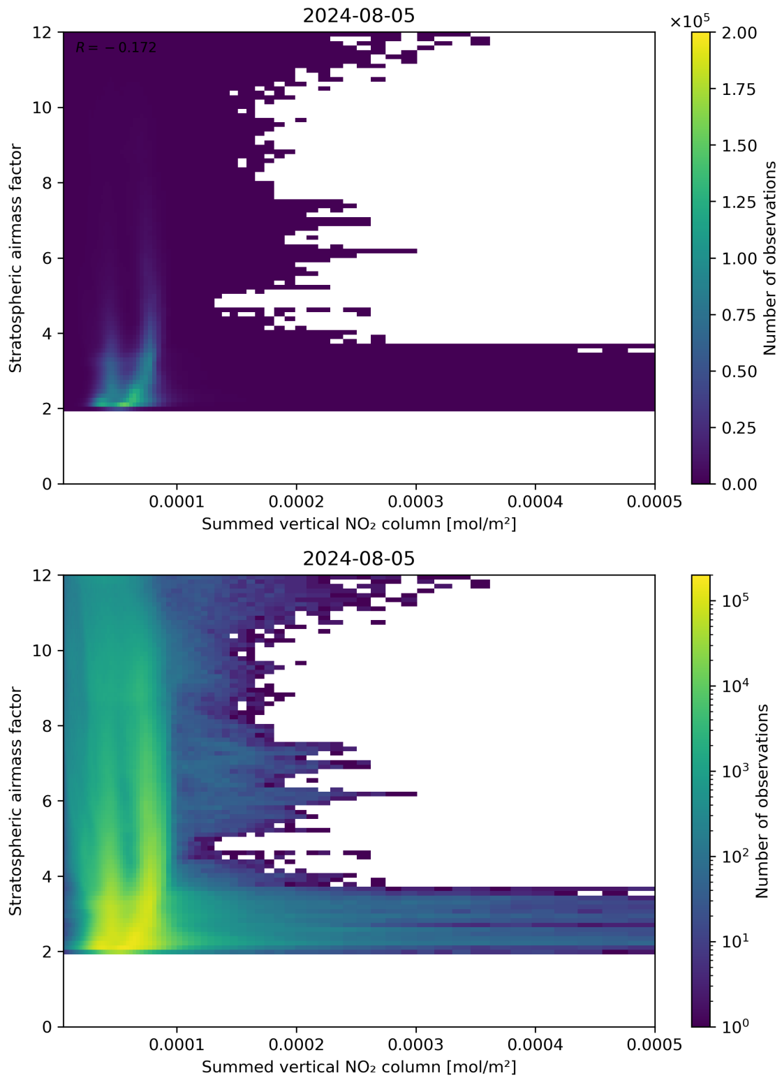
Figure 103: Scatter density plot of “Summed vertical NO 2 column” against “Stratospheric airmass factor” for 2024-08-04 to 2024-08-06.
