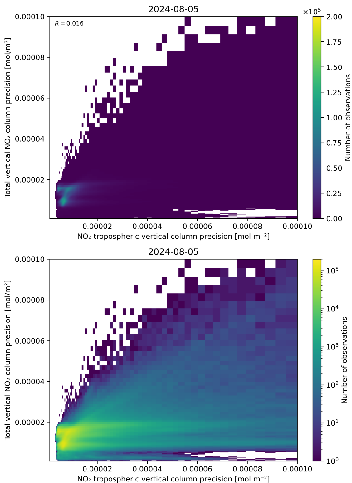
Figure 139: Scatter density plot of “NO 2 tropospheric vertical column precision” against “Total vertical NO 2 column precision” for 2024-08-04 to 2024-08-06.
