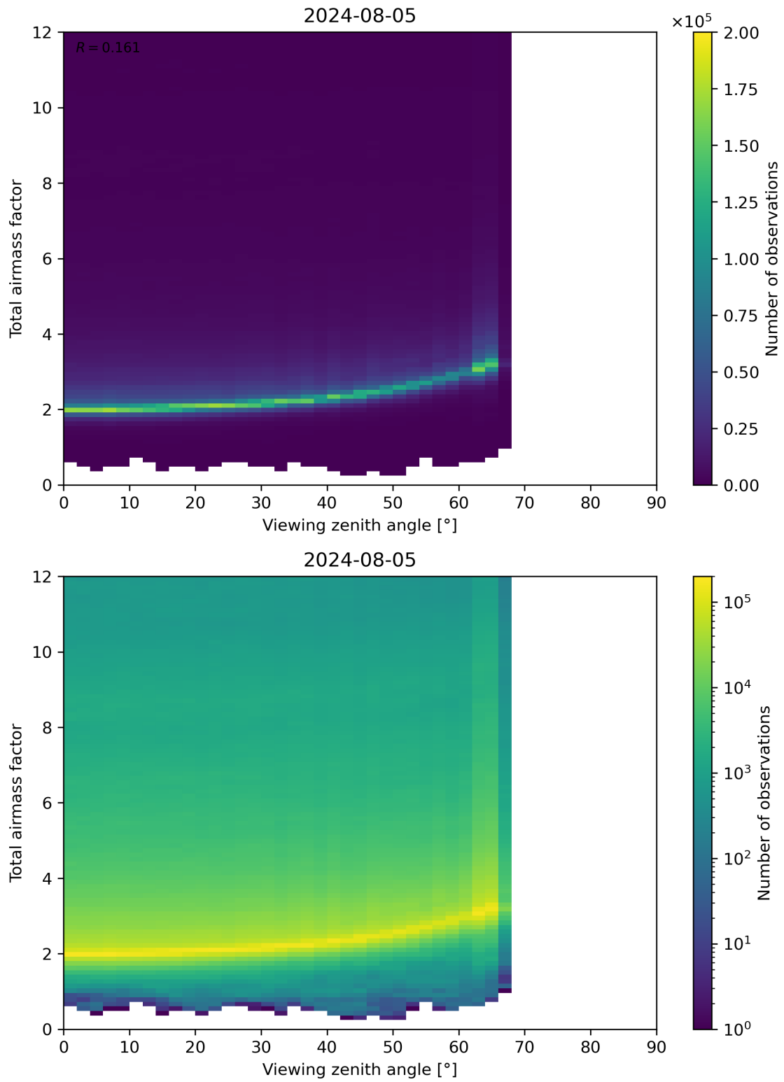
Figure 160: Scatter density plot of “Viewing zenith angle” against “Total airmass factor” for 2024-08-04 to 2024-08-06.
