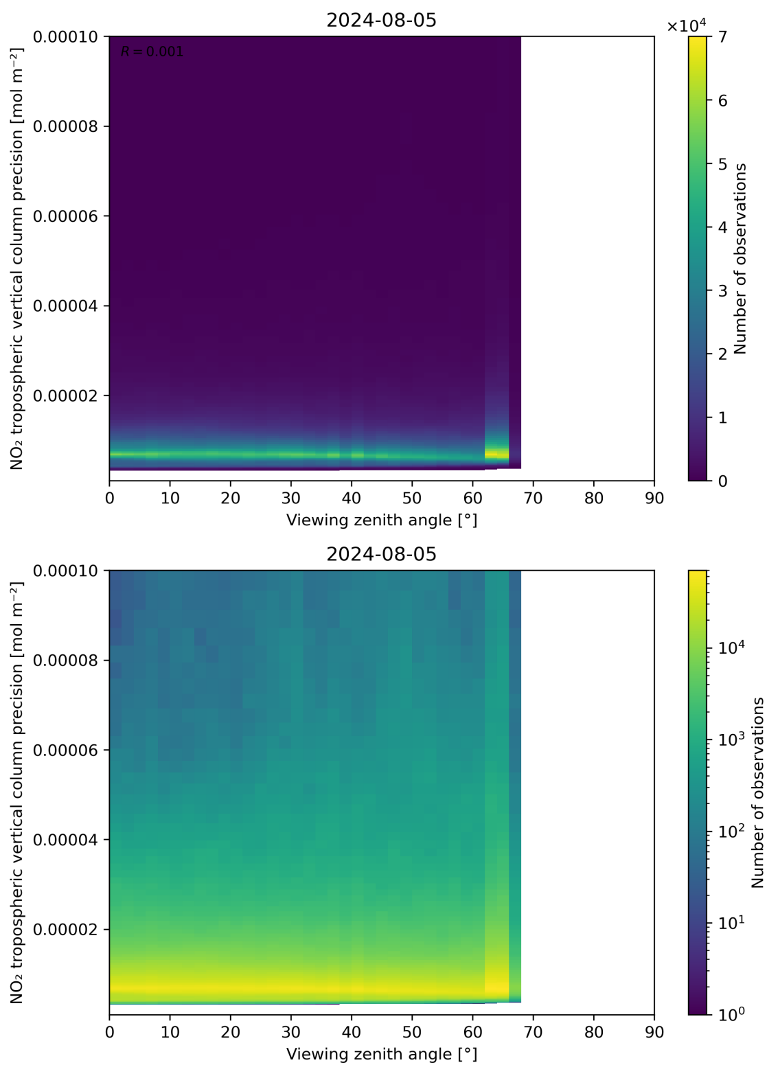
Figure 170: Scatter density plot of “Viewing zenith angle” against “NO 2 tropospheric vertical column precision” for 2024-08-04 to 2024-08-06.
