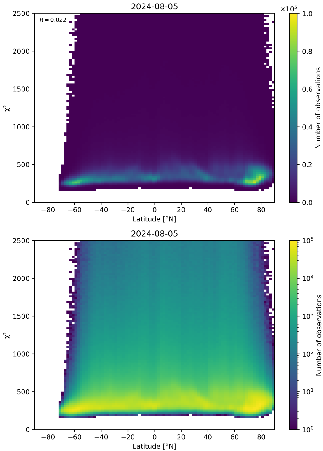
Figure 86: Scatter density plot of “Latitude” against “ \chi^2 ” for 2024-08-04 to 2024-08-06.
