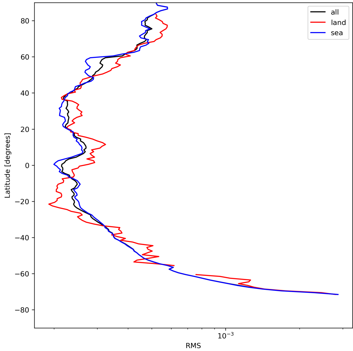
Figure 26: Zonal average of “RMS” for 2024-08-04 to 2024-08-06.
