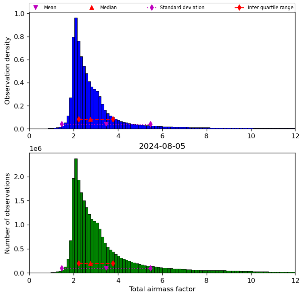
Figure 32: Histogram of “Total airmass factor” for 2024-08-04 to 2024-08-06
