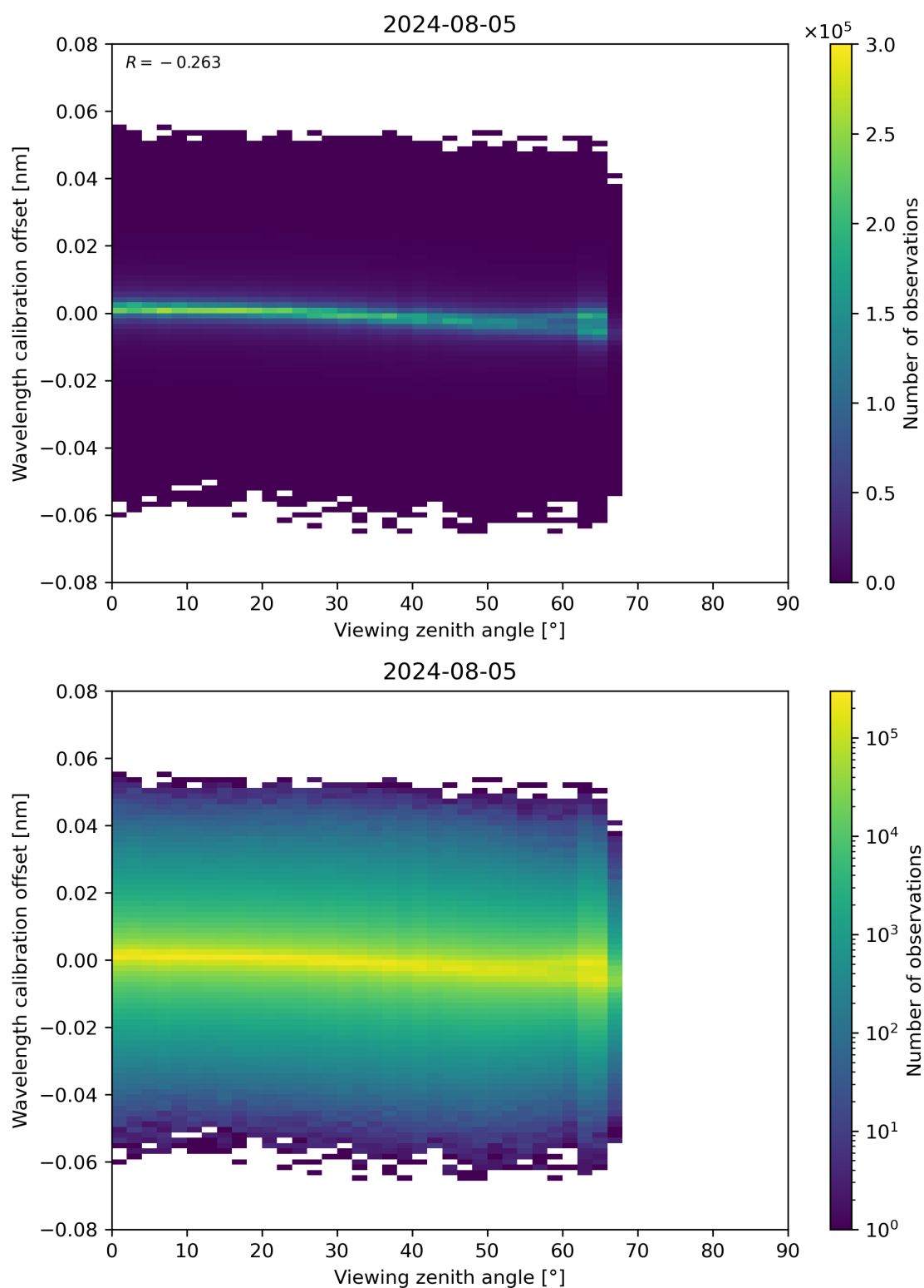
Figure 173: Scatter density plot of “Viewing zenith angle” against “Wavelength calibration offset” for 2024-08-04 to 2024-08-06.
