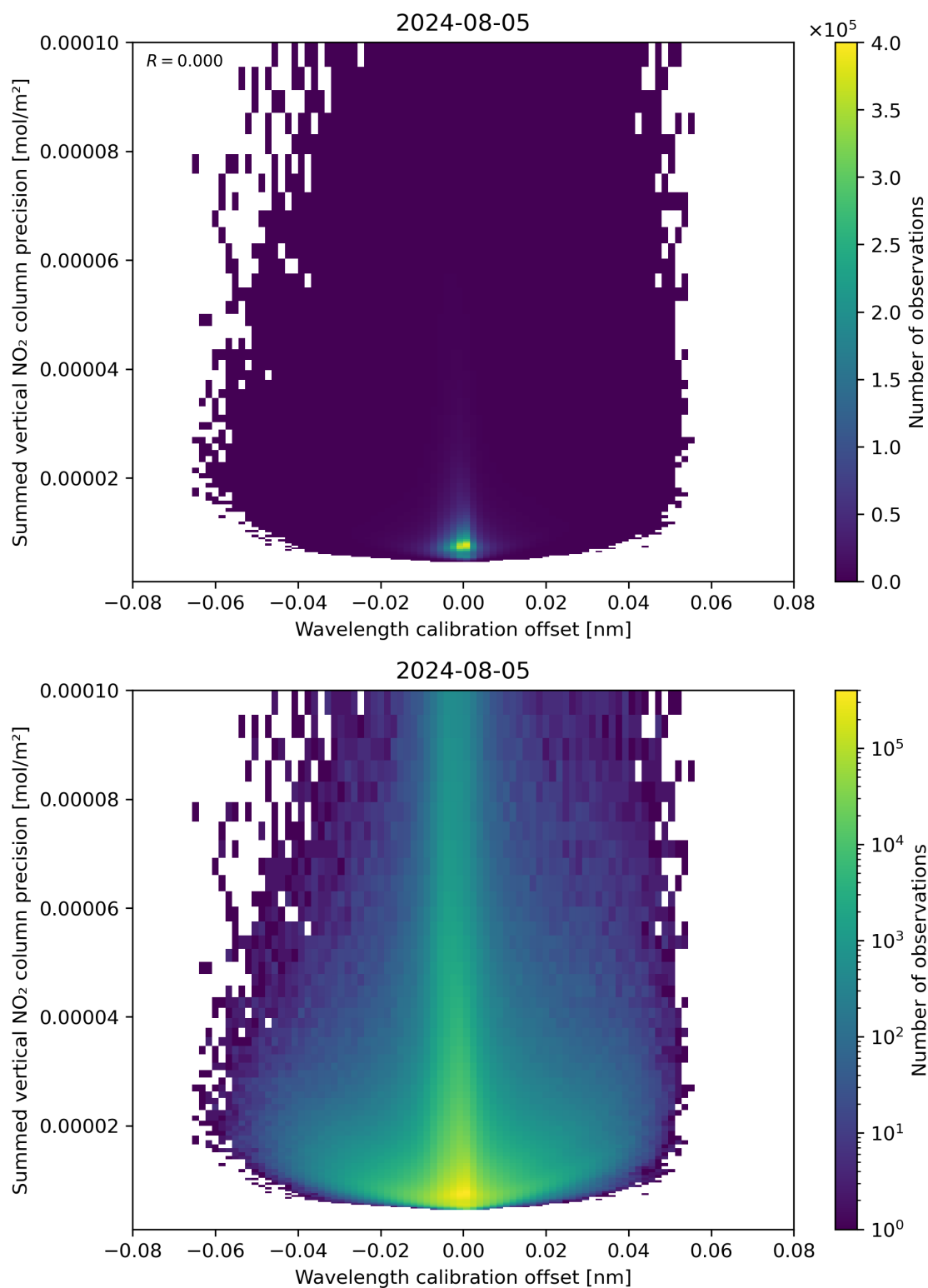
Figure 178: Scatter density plot of “Wavelength calibration offset” against “Summed vertical NO 2 column precision” for 2024-08-04 to 2024-08-06.
