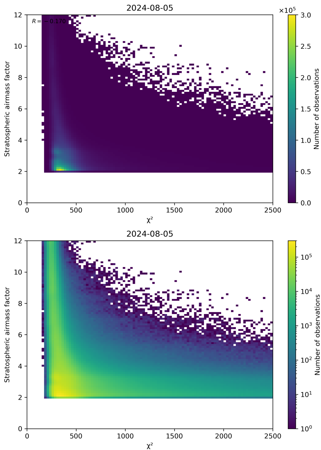
Figure 81: Scatter density plot of “ \chi^2 ” against “Stratospheric airmass factor” for 2024-08-04 to 2024-08-06.
