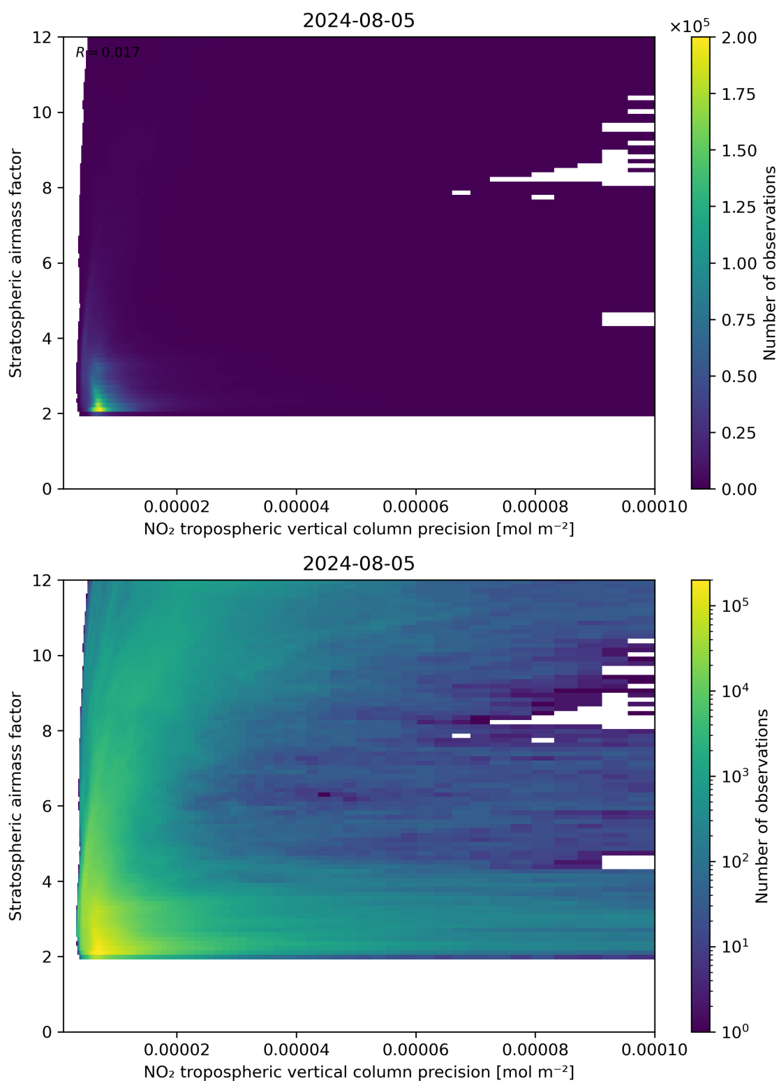
Figure 131: Scatter density plot of “NO 2 tropospheric vertical column precision” against “Stratospheric airmass factor” for 2024-08-04 to 2024-08-06.
