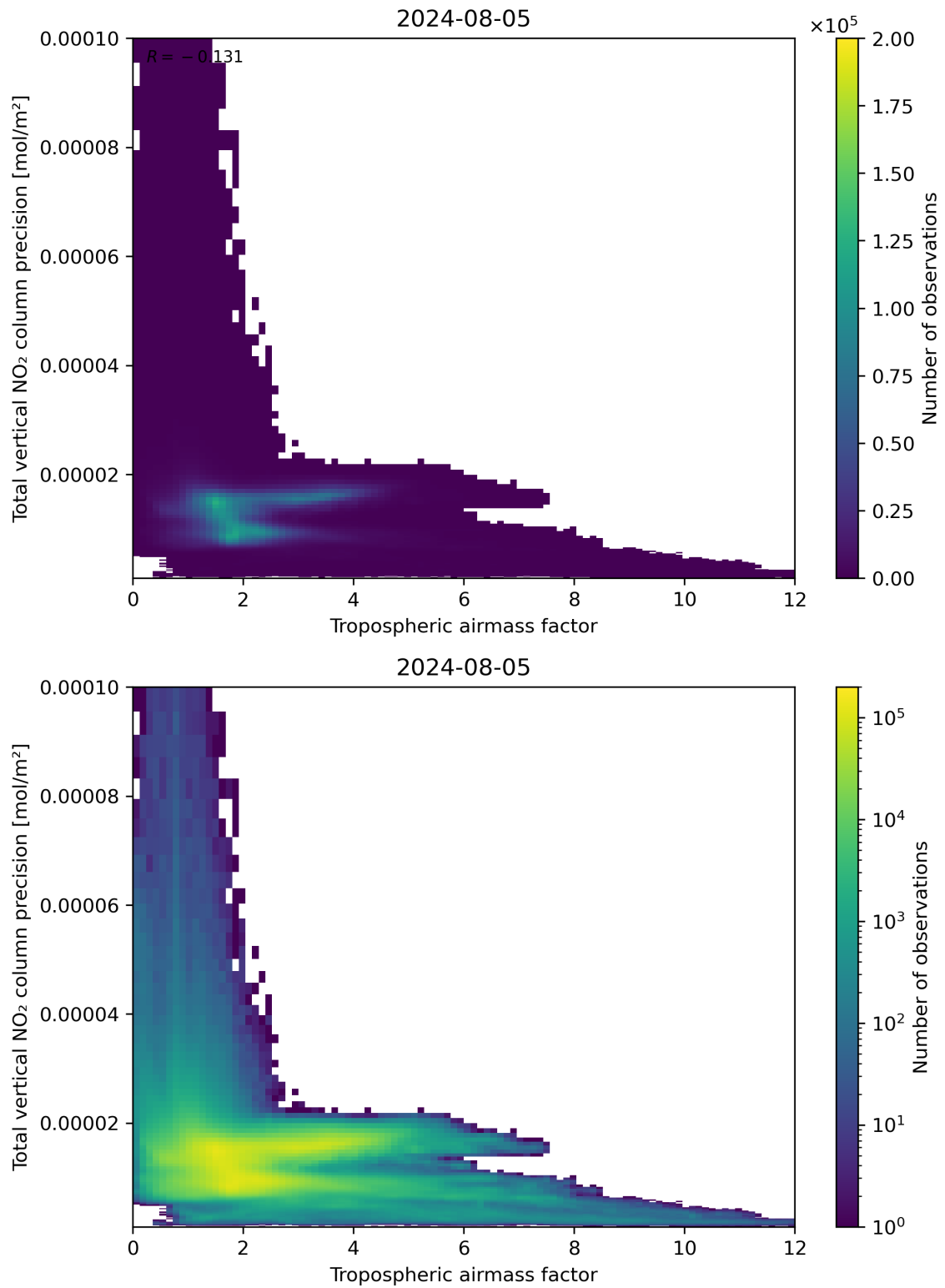
Figure 78: Scatter density plot of “Tropospheric air mass factor” against “Total vertical NO 2 column precision” for 2024-08-04 to 2024-08-06.
