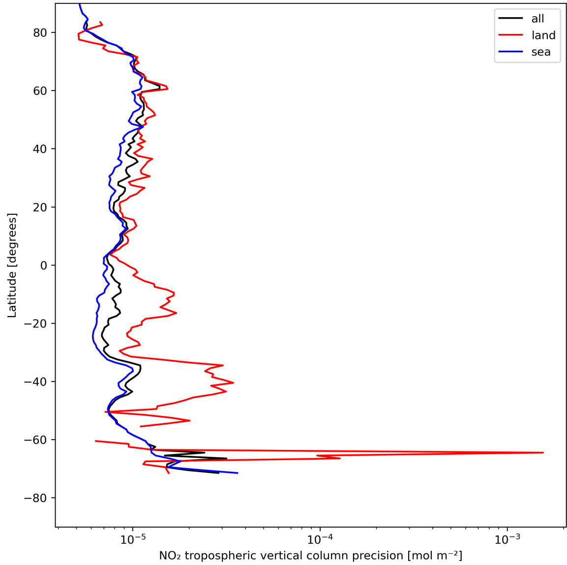
Figure 13: Zonal average of “NO 2 tropospheric vertical column precision” for 2024-08-04 to 2024-08-06.
