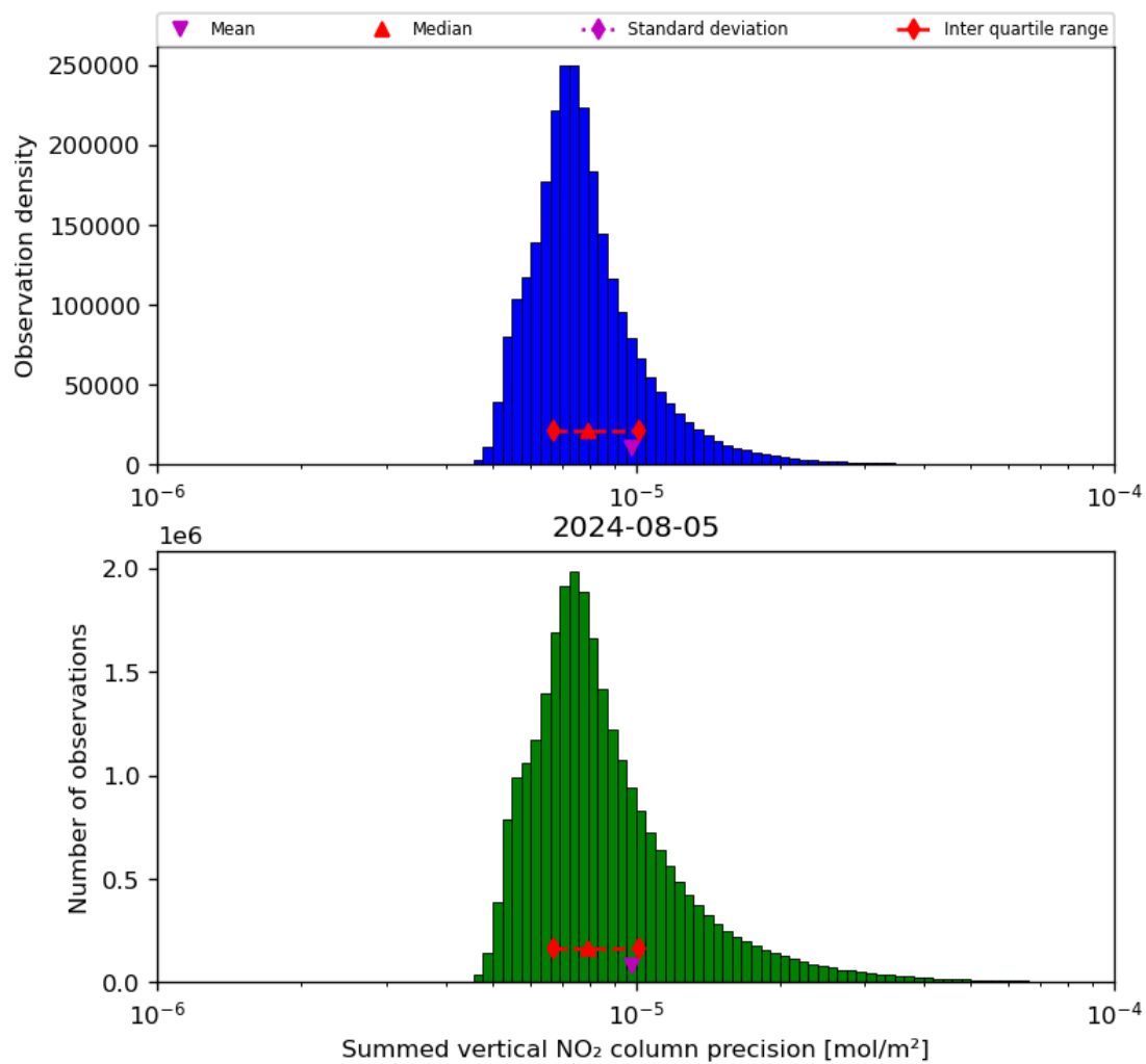
Figure 41: Histogram of "Summed vertical NO 2 column precision" for 2024-08-04 to 2024-08-06
