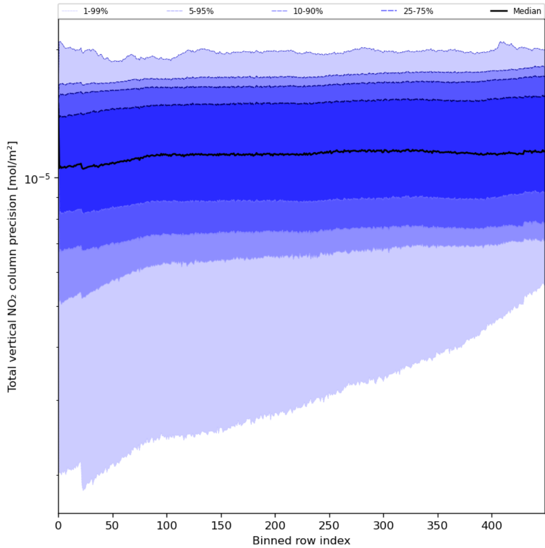
Figure 56: Along track statistics of “Total vertical NO 2 column precision” for 2024-08-04 to 2024-08-06
