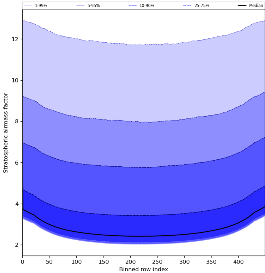
Figure 61: Along track statistics of “Stratospheric airmass factor” for 2024-08-04 to 2024-08-06
