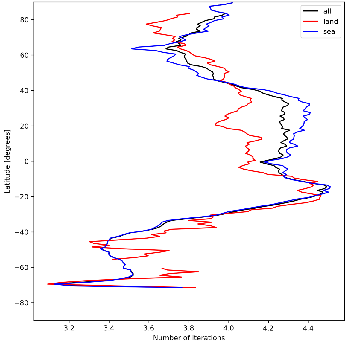
Figure 17: Zonal average of “Number of iterations” for 2024-08-04 to 2024-08-06.
