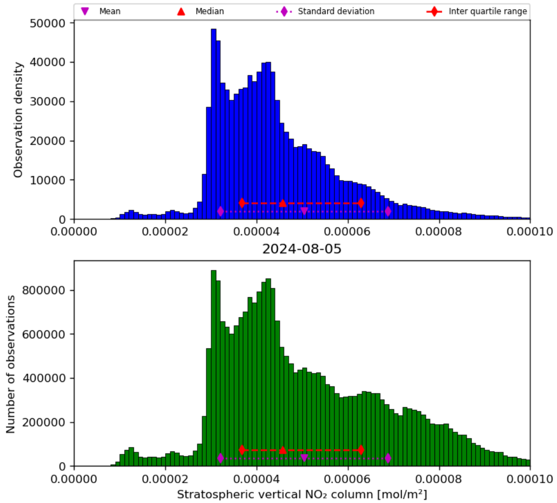
Figure 36: Histogram of “Stratospheric vertical NO 2 column” for 2024-08-04 to 2024-08-06
