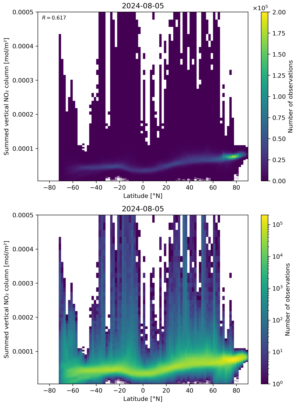
Figure 88: Scatter density plot of “Latitude” against “Summed vertical NO 2 column” for 2024-08-04 to 2024-08-06.
