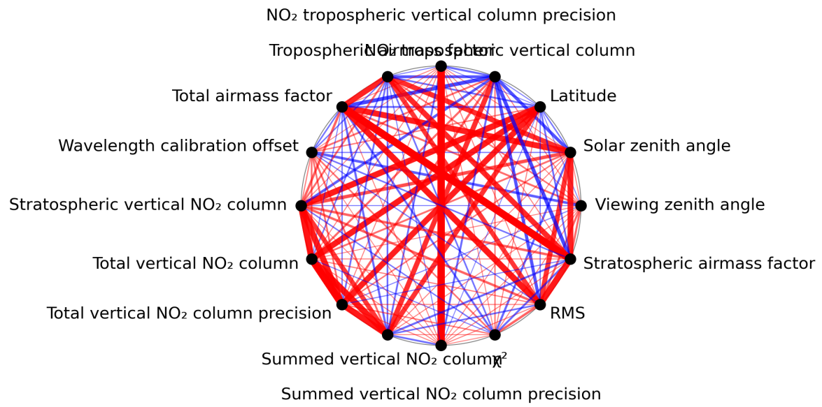
Figure 1: Map of correlation graph for 2024-08-04 to 2024-08-06.
