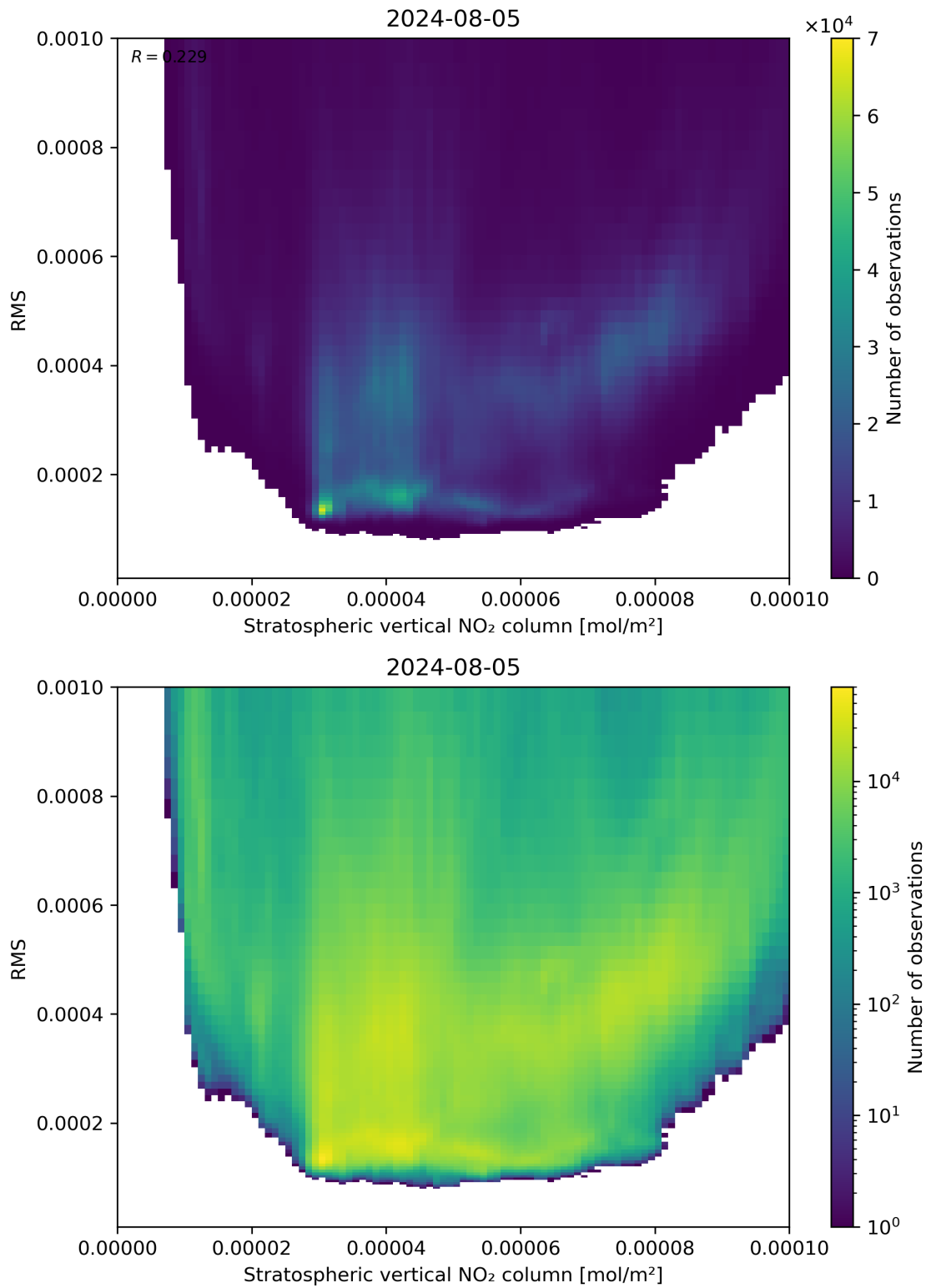
Figure 102: Scatter density plot of “Stratospheric vertical NO 2 column” against “RMS” for 2024-08-04 to 2024-08-06.
