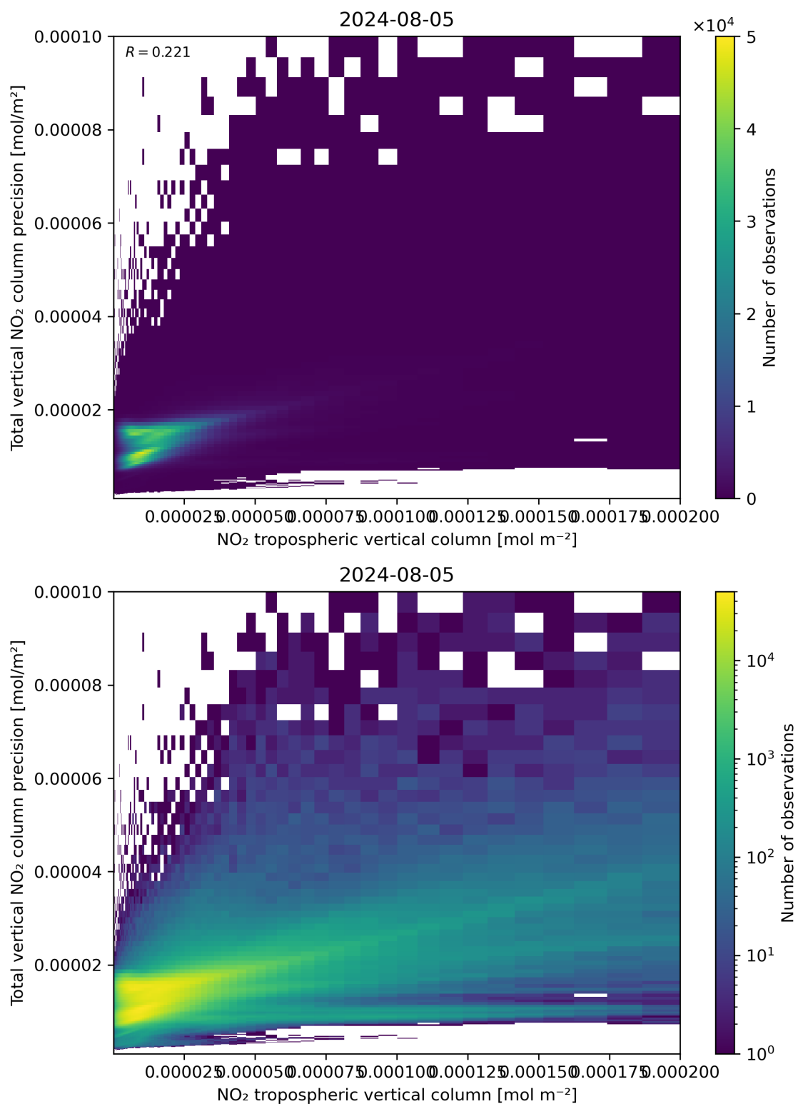
Figure 129: Scatter density plot of “NO 2 tropospheric vertical column” against “Total vertical NO 2 column precision” for 2024-08-04 to 2024-08-06.
