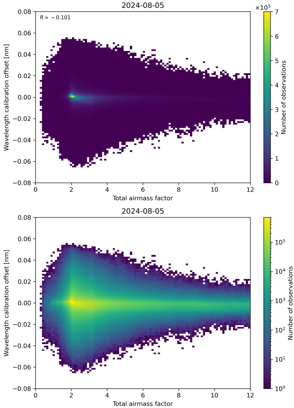
Figure 70: Scatter density plot of “Total airmass factor” against “Wavelength calibration offset” for 2024-08-04 to 2024-08-06.
