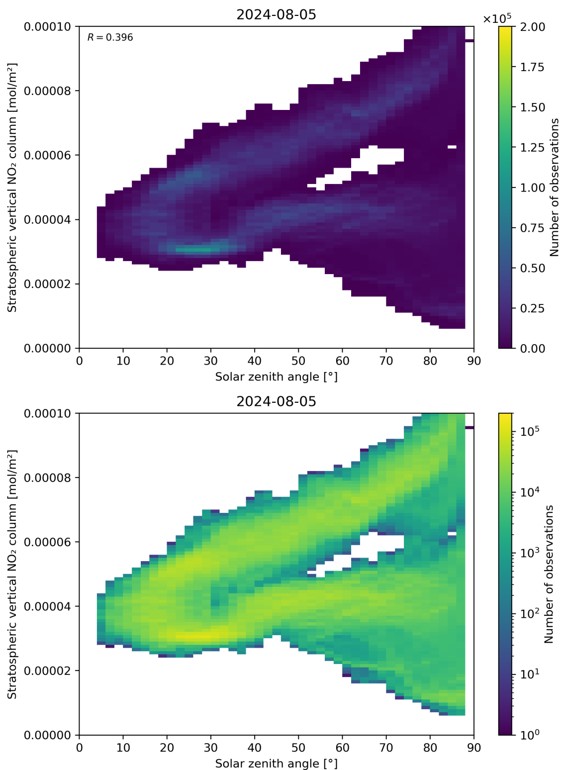
Figure 150: Scatter density plot of “Solar zenith angle” against “Stratospheric vertical NO 2 column” for 2024-08-04 to 2024-08-06.
