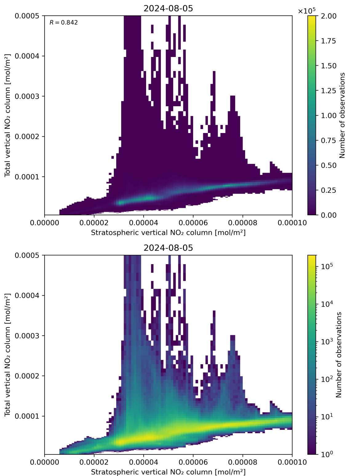
Figure 100: Scatter density plot of “Stratospheric vertical NO 2 column” against “Total vertical NO 2 column” for 2024-08-04 to 2024-08-06.
