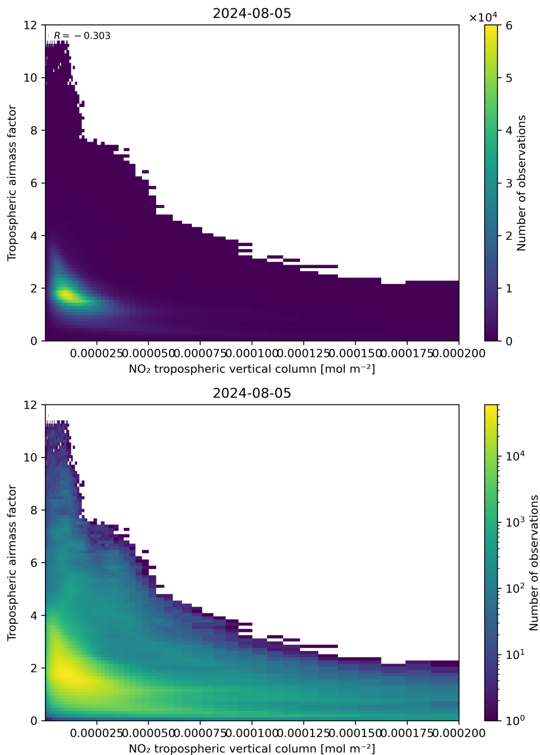
Figure 123: Scatter density plot of “NO 2 tropospheric vertical column” against “Tropospheric air mass factor” for 2024-08-04 to 2024-08-06.
