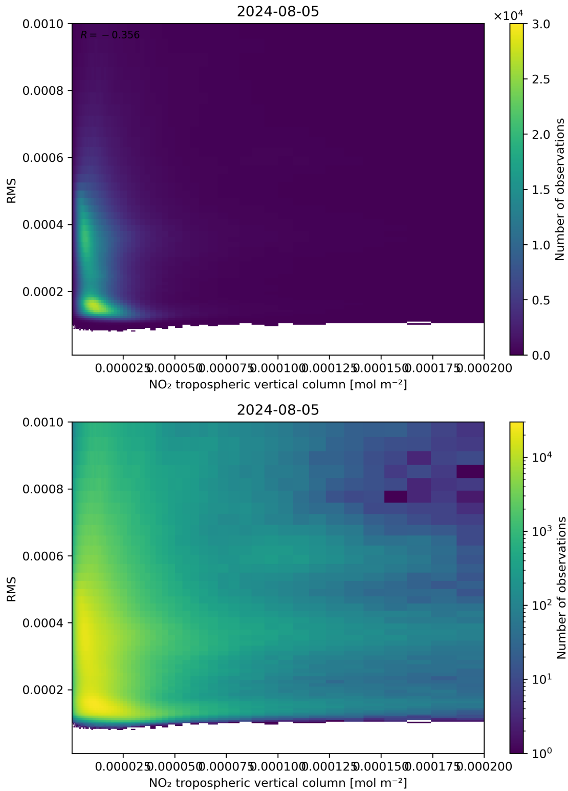
Figure 142: Scatter density plot of “NO 2 tropospheric vertical column” against “RMS” for 2024-08-04 to 2024-08-06.
