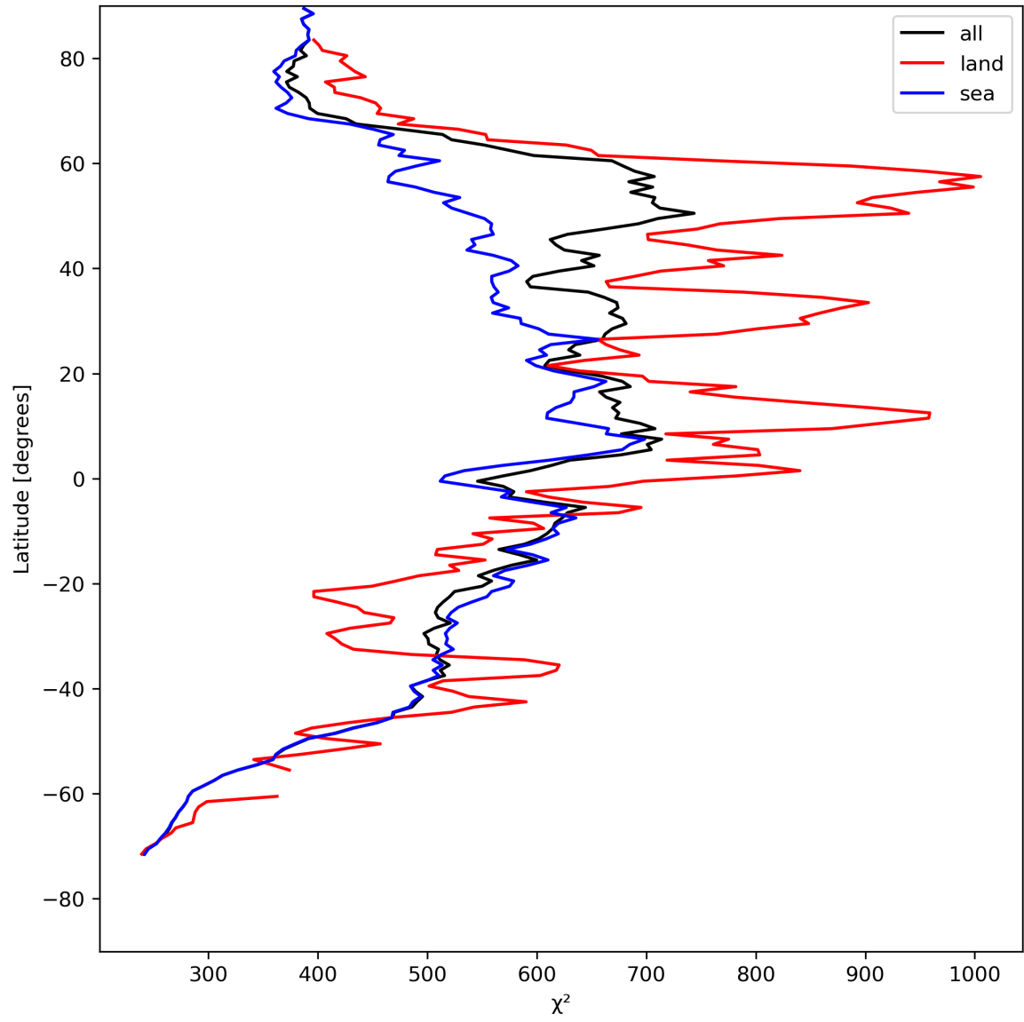
Figure 25: Zonal average of “ \chi^2 ” for 2024-08-04 to 2024-08-06.
