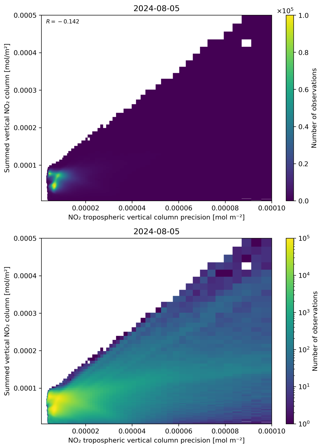
Figure 136: Scatter density plot of “NO 2 tropospheric vertical column precision” against “Summed vertical NO 2 column” for 2024-08-04 to 2024-08-06.
