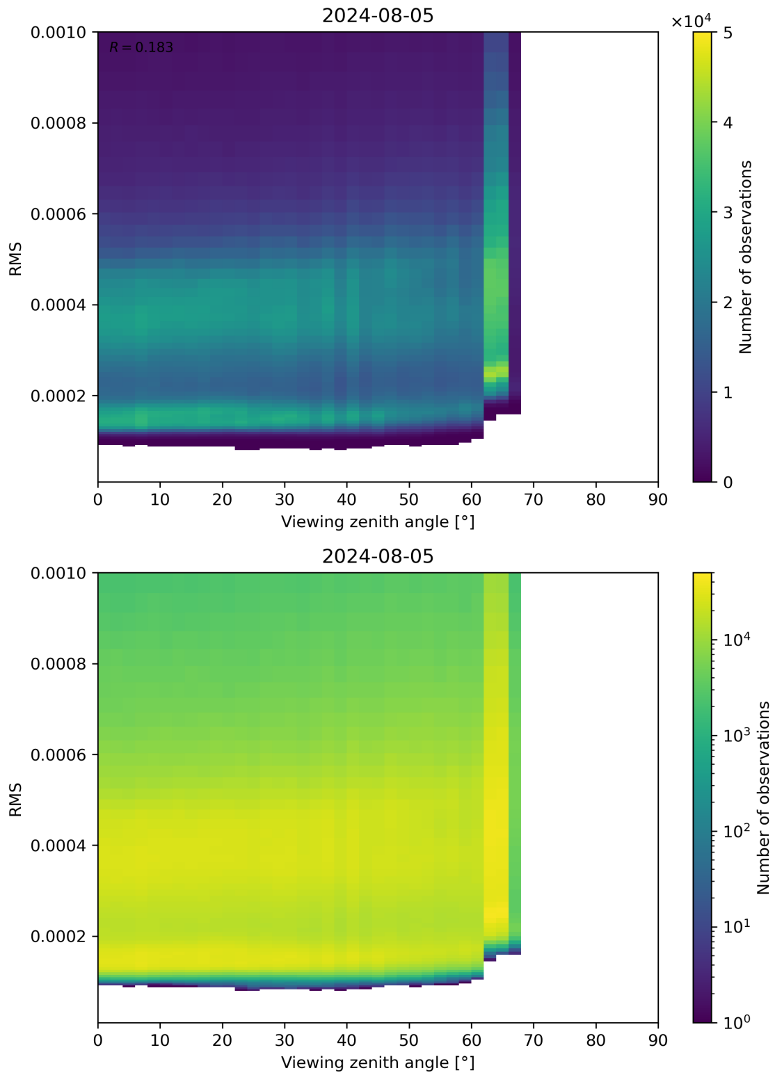
Figure 171: Scatter density plot of “Viewing zenith angle” against “RMS” for 2024-08-04 to 2024-08-06.
