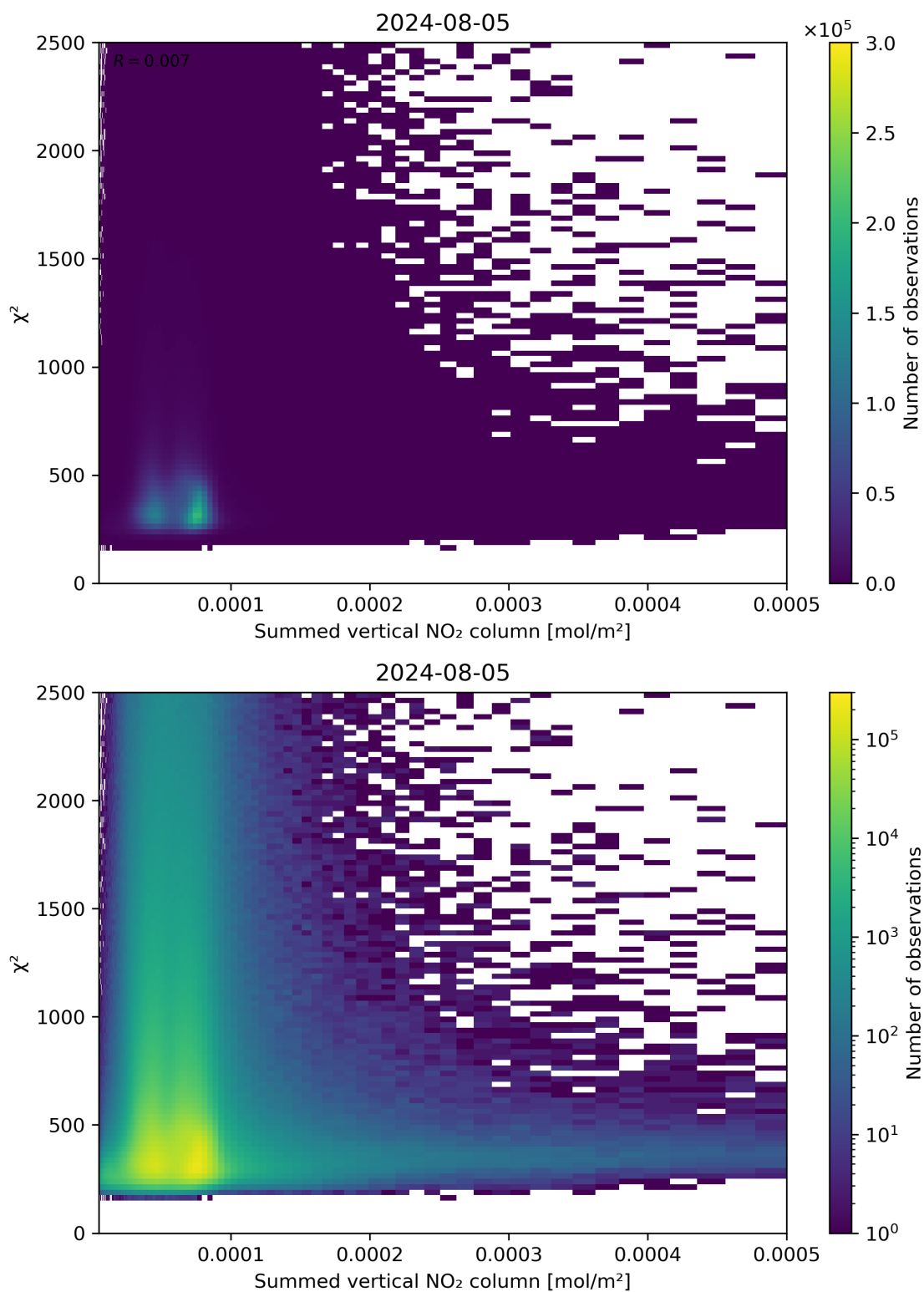
Figure 104: Scatter density plot of “Summed vertical NO 2 column” against “ \chi^2 ” for 2024-08-04 to 2024-08-06.
