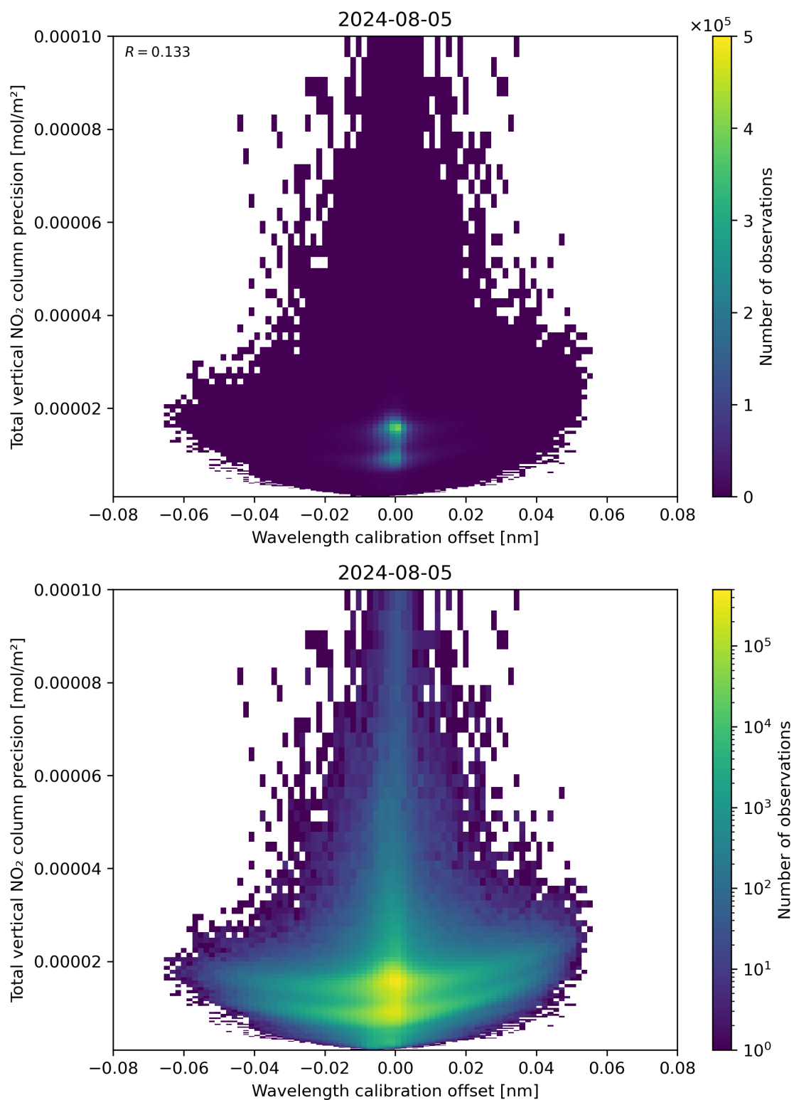
Figure 180: Scatter density plot of “Wavelength calibration offset” against “Total vertical NO 2 column precision” for 2024-08-04 to 2024-08-06.
