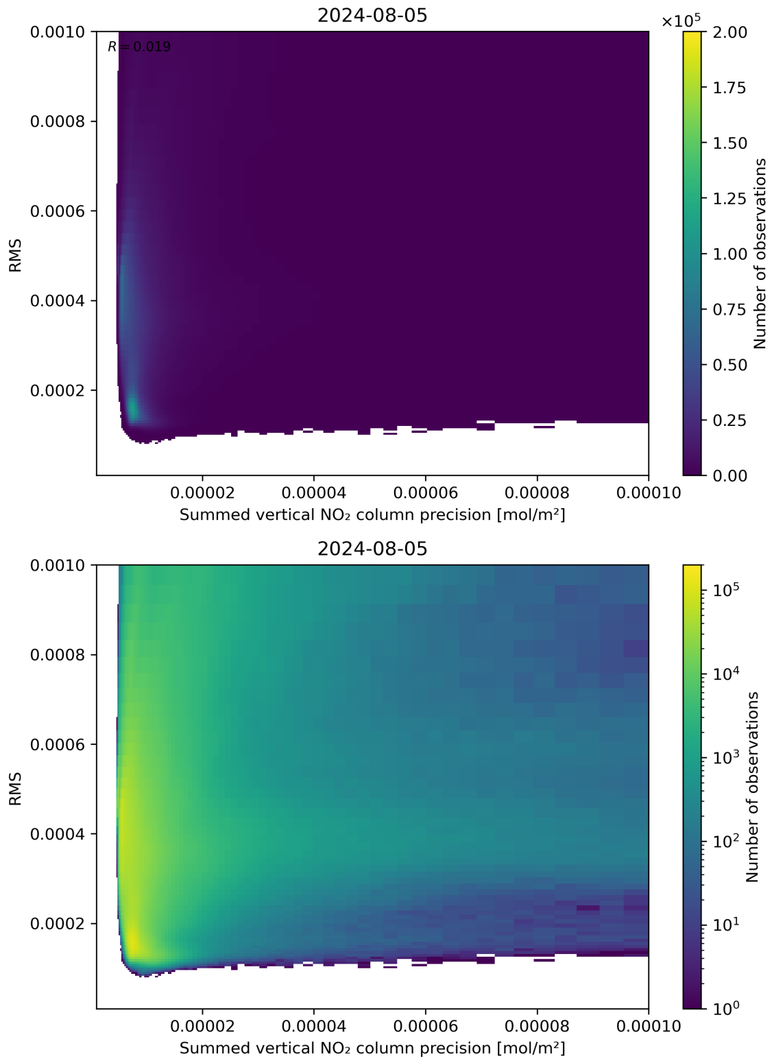
Figure 108: Scatter density plot of “Summed vertical NO 2 column precision” against “RMS” for 2024-08-04 to 2024-08-06.
