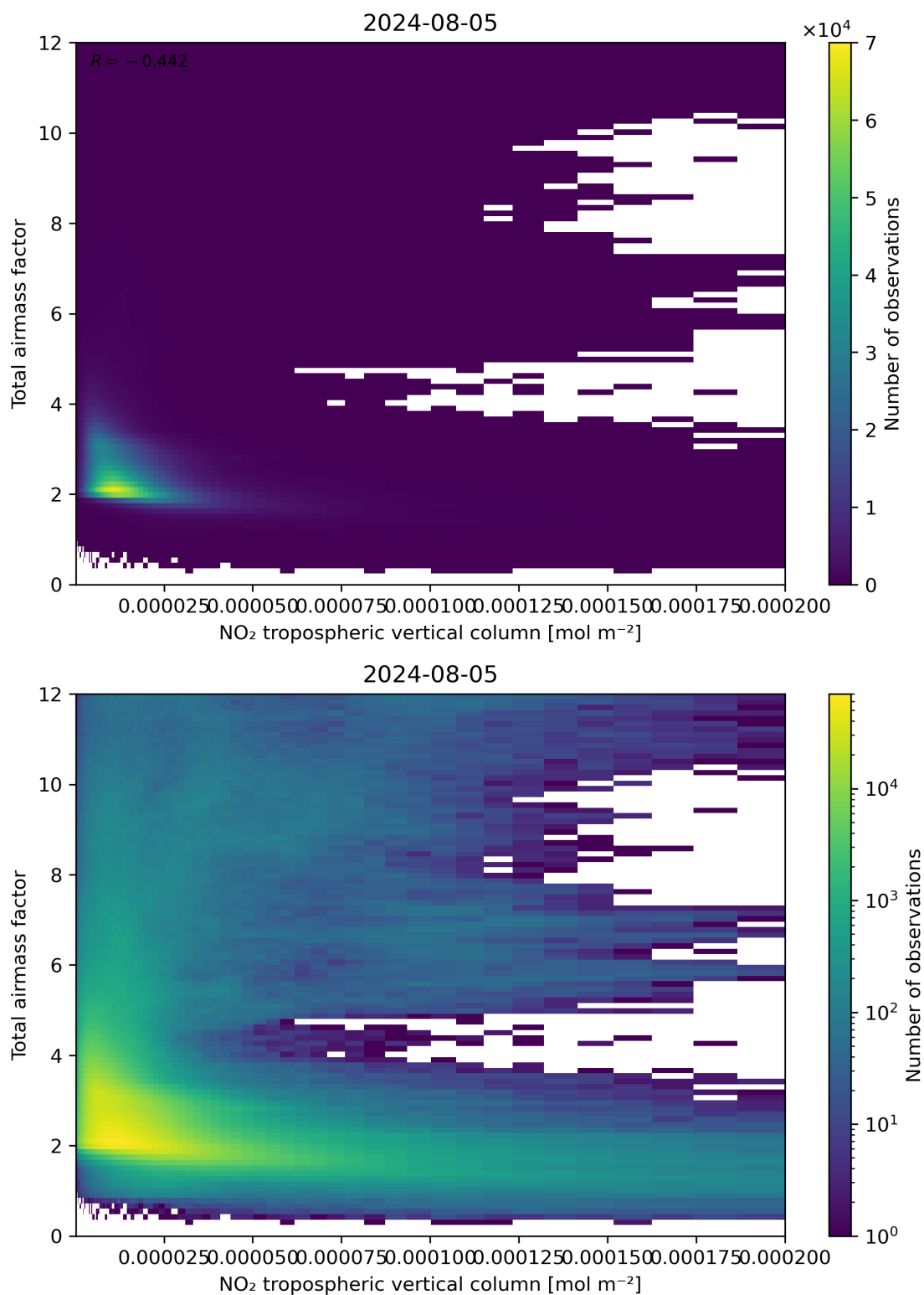
Figure 122: Scatter density plot of “NO 2 tropospheric vertical column” against “Total air mass factor” for 2024-08-04 to 2024-08-06.
