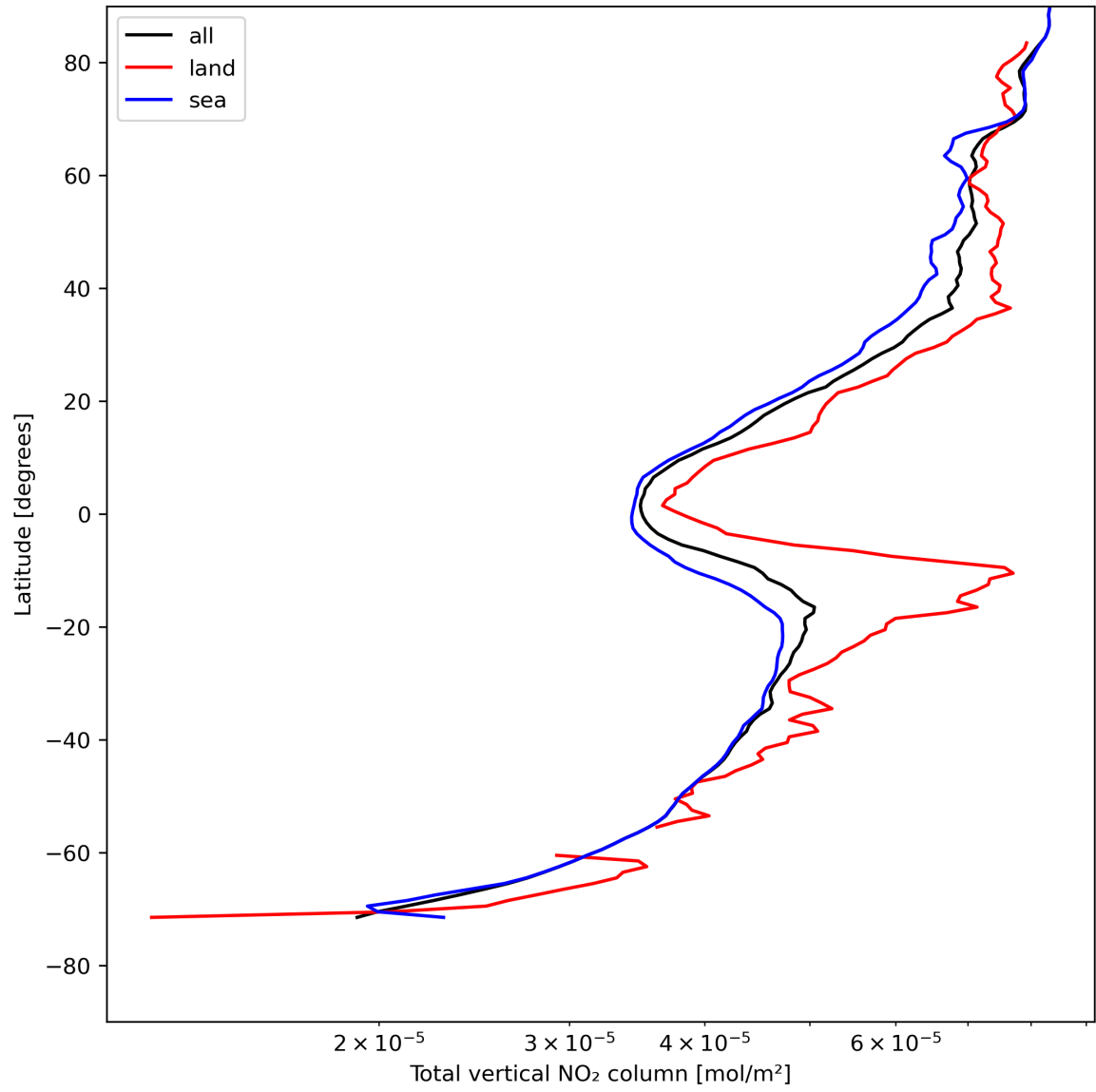
Figure 21: Zonal average of “Total vertical NO 2 column” for 2024-08-04 to 2024-08-06.
