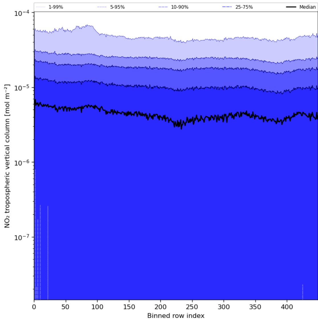
Figure 46: Along track statistics of “NO 2 tropospheric vertical column” for 2024-08-04 to 2024-08-06
