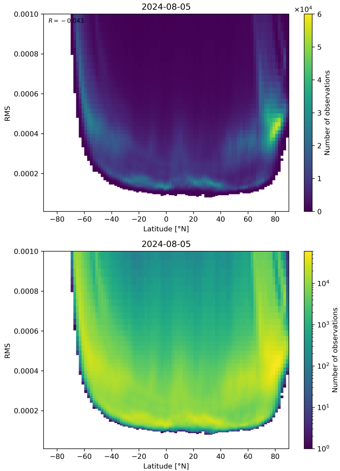
Figure 94: Scatter density plot of “Latitude” against “RMS” for 2024-08-04 to 2024-08-06.
