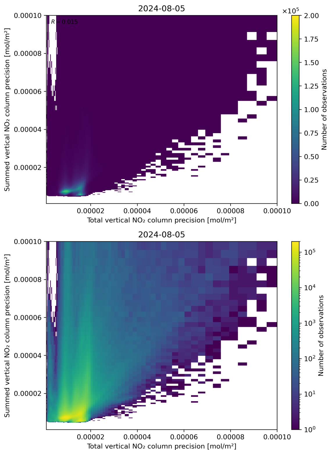
Figure 118: Scatter density plot of “Total vertical NO 2 column precision” against “Summed vertical NO 2 column precision” for 2024-08-04 to 2024-08-06.
