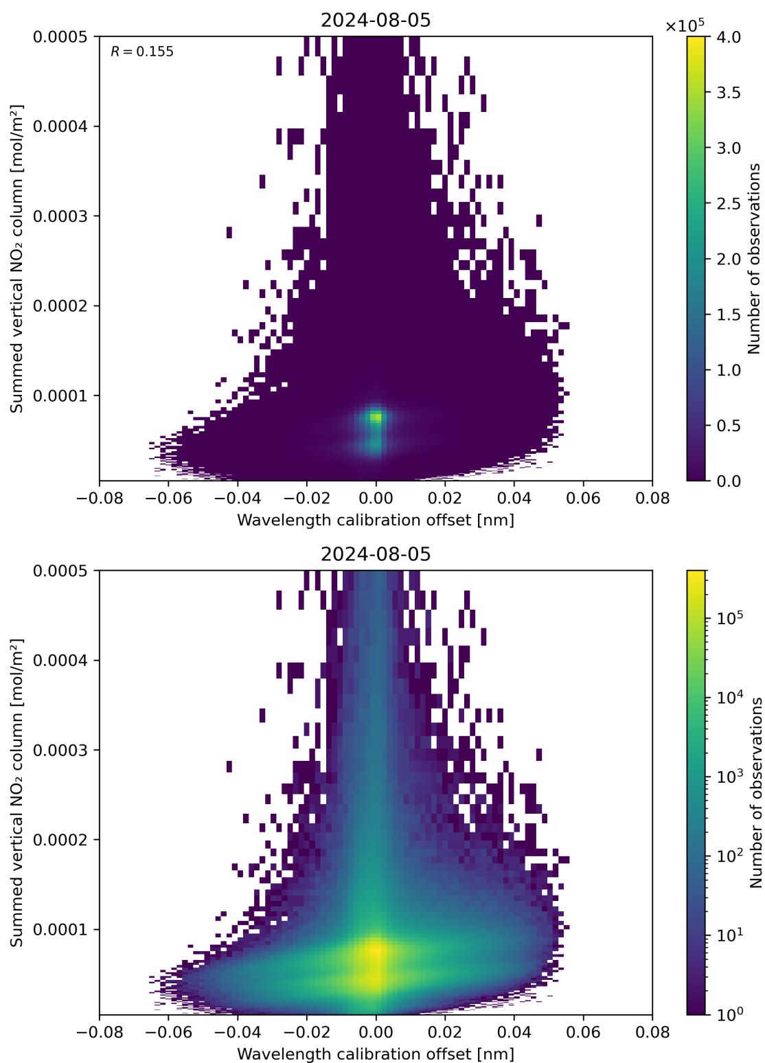
Figure 177: Scatter density plot of “Wavelength calibration offset” against “Summed vertical NO 2 column” for 2024-08-04 to 2024-08-06.
