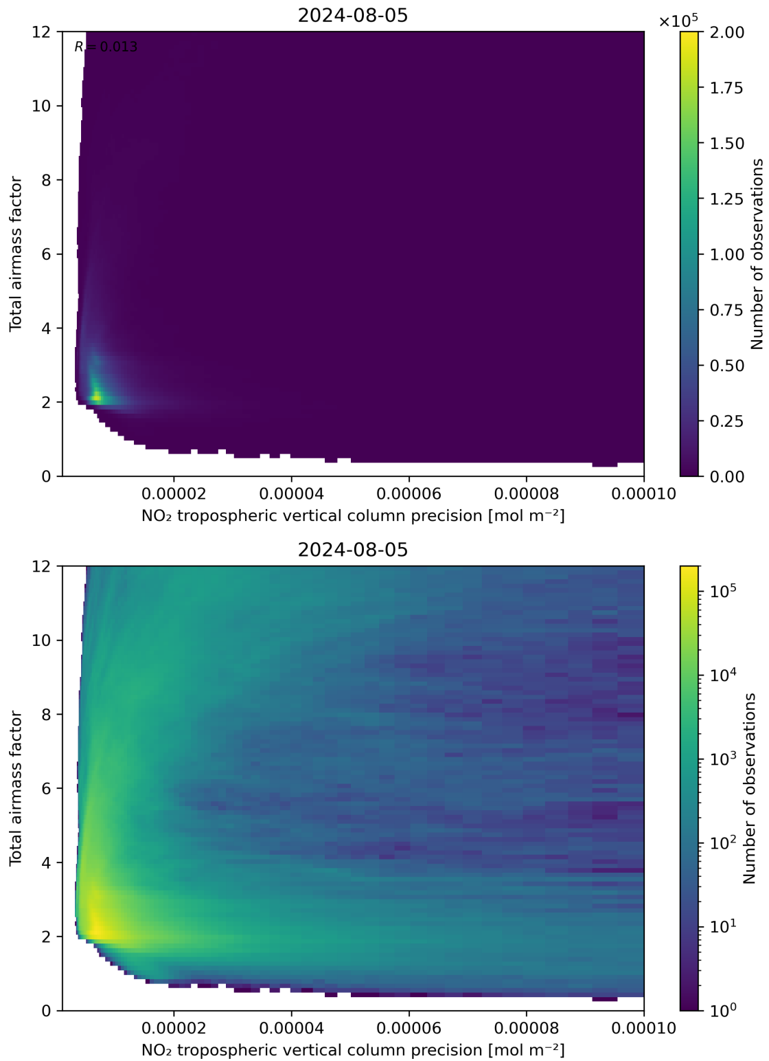
Figure 132: Scatter density plot of “NO 2 tropospheric vertical column precision” against “Total air mass factor” for 2024-08-04 to 2024-08-06.
