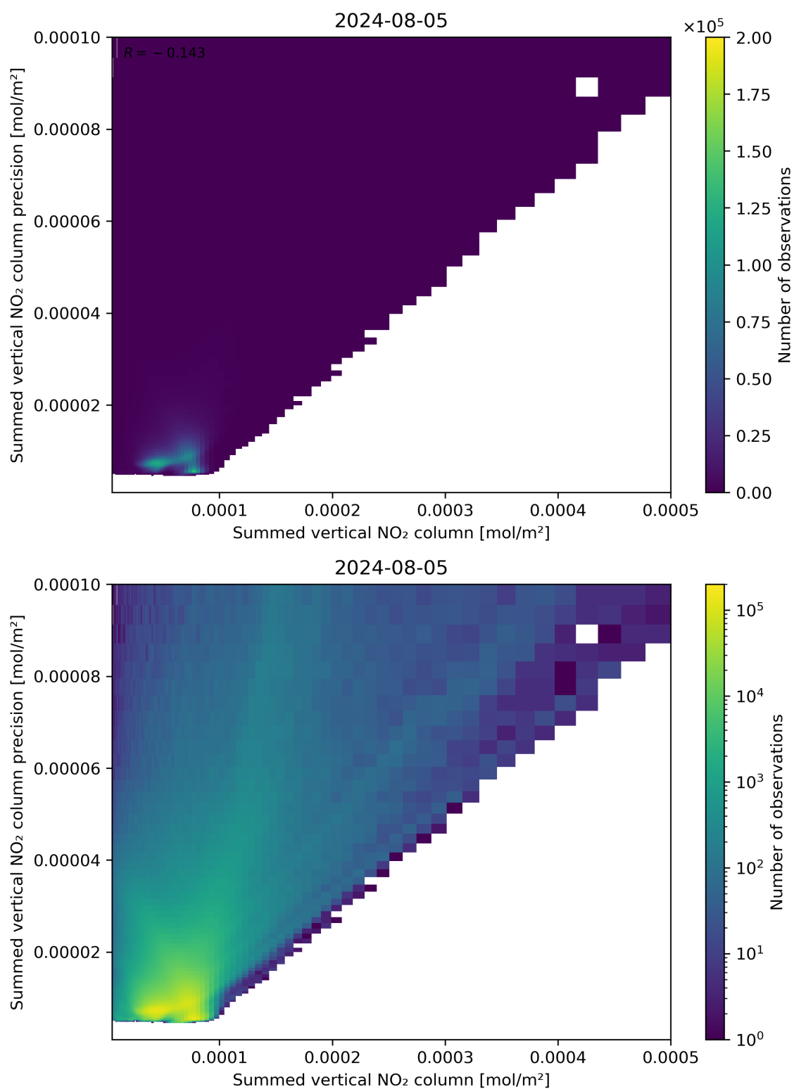
Figure 105: Scatter density plot of “Summed vertical NO 2 column” against “Summed vertical NO 2 column precision” for 2024-08-04 to 2024-08-06.
