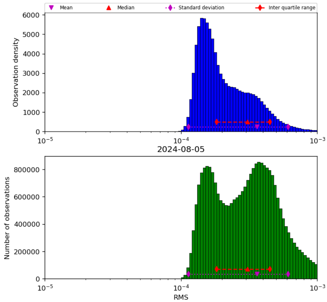
Figure 43: Histogram of “RMS” for 2024-08-04 to 2024-08-06
