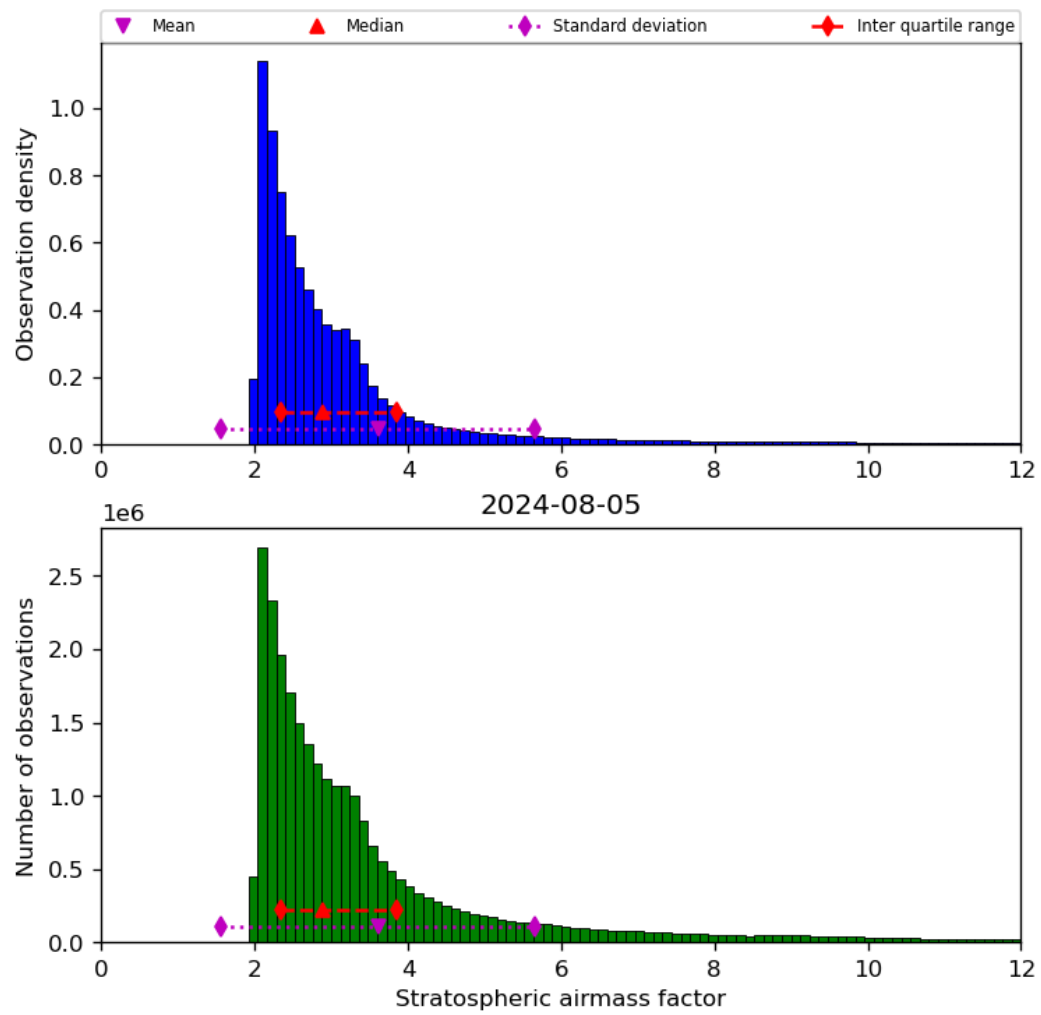
Figure 44: Histogram of “Stratospheric airmass factor” for 2024-08-04 to 2024-08-06
