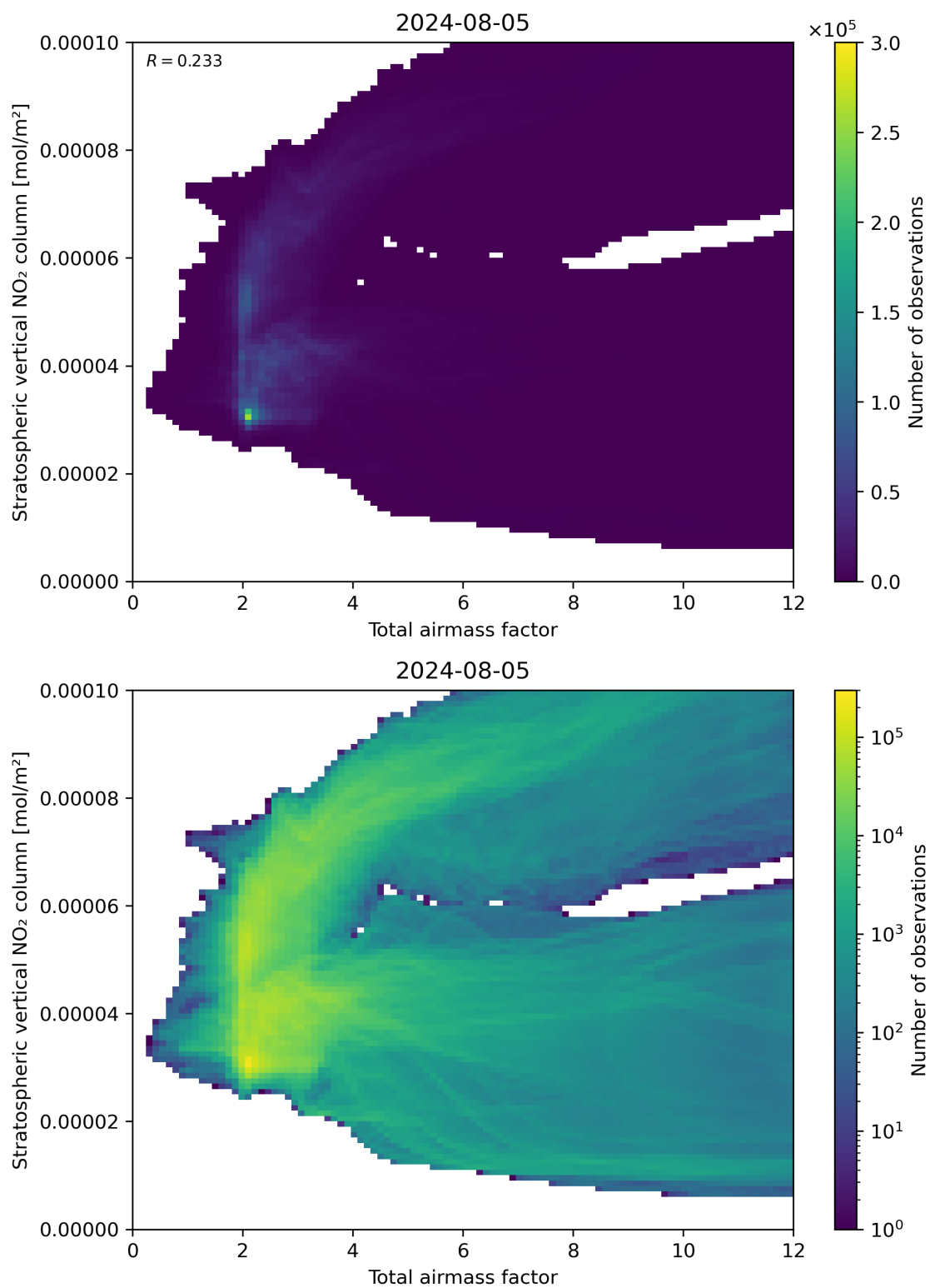
Figure 64: Scatter density plot of “Total airmass factor” against “Stratospheric vertical \text{NO}_2 column” for 2024-08-04 to 2024-08-06.
