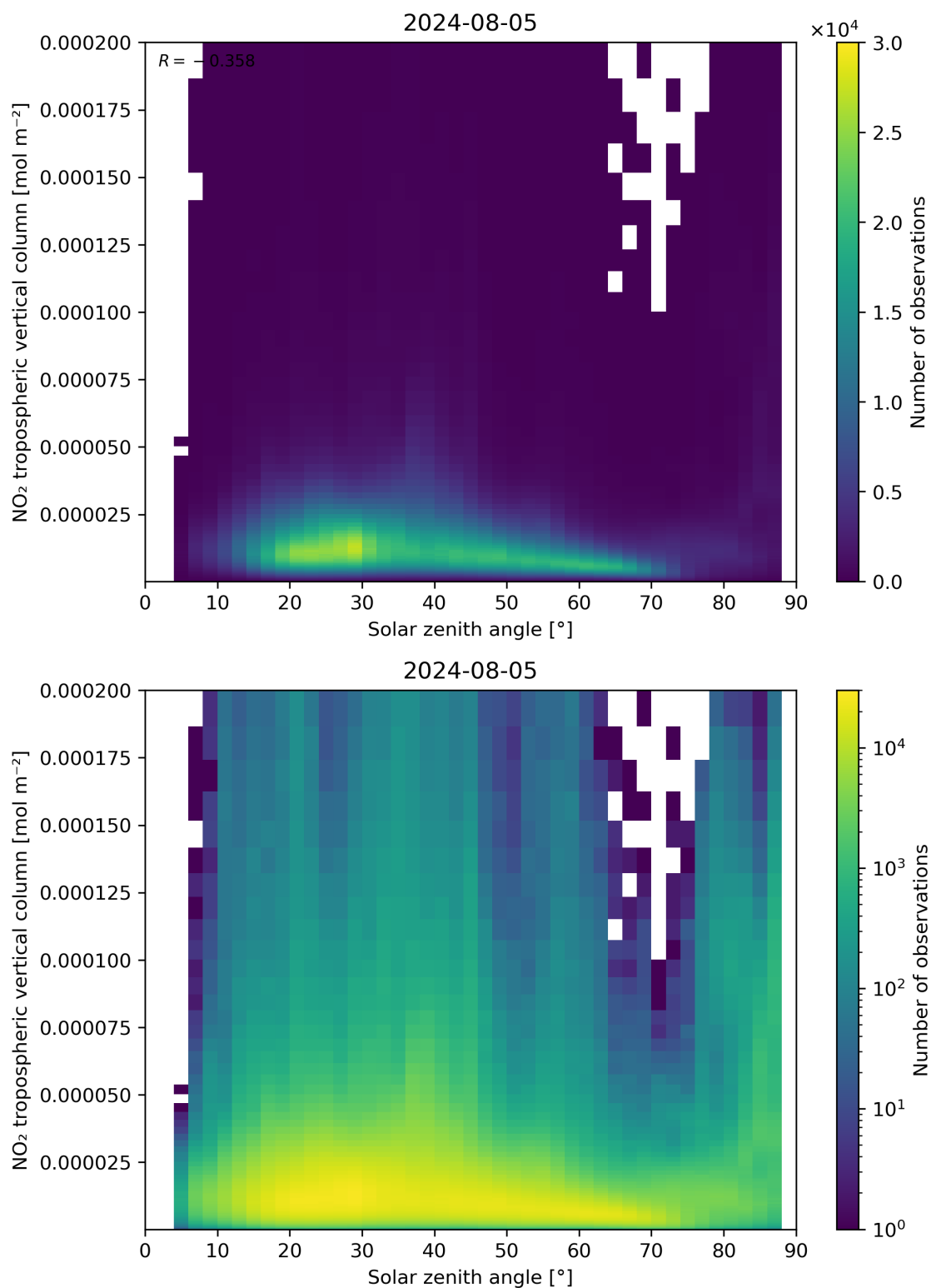
Figure 155: Scatter density plot of “Solar zenith angle” against “NO 2 tropospheric vertical column” for 2024-08-04 to 2024-08-06.
