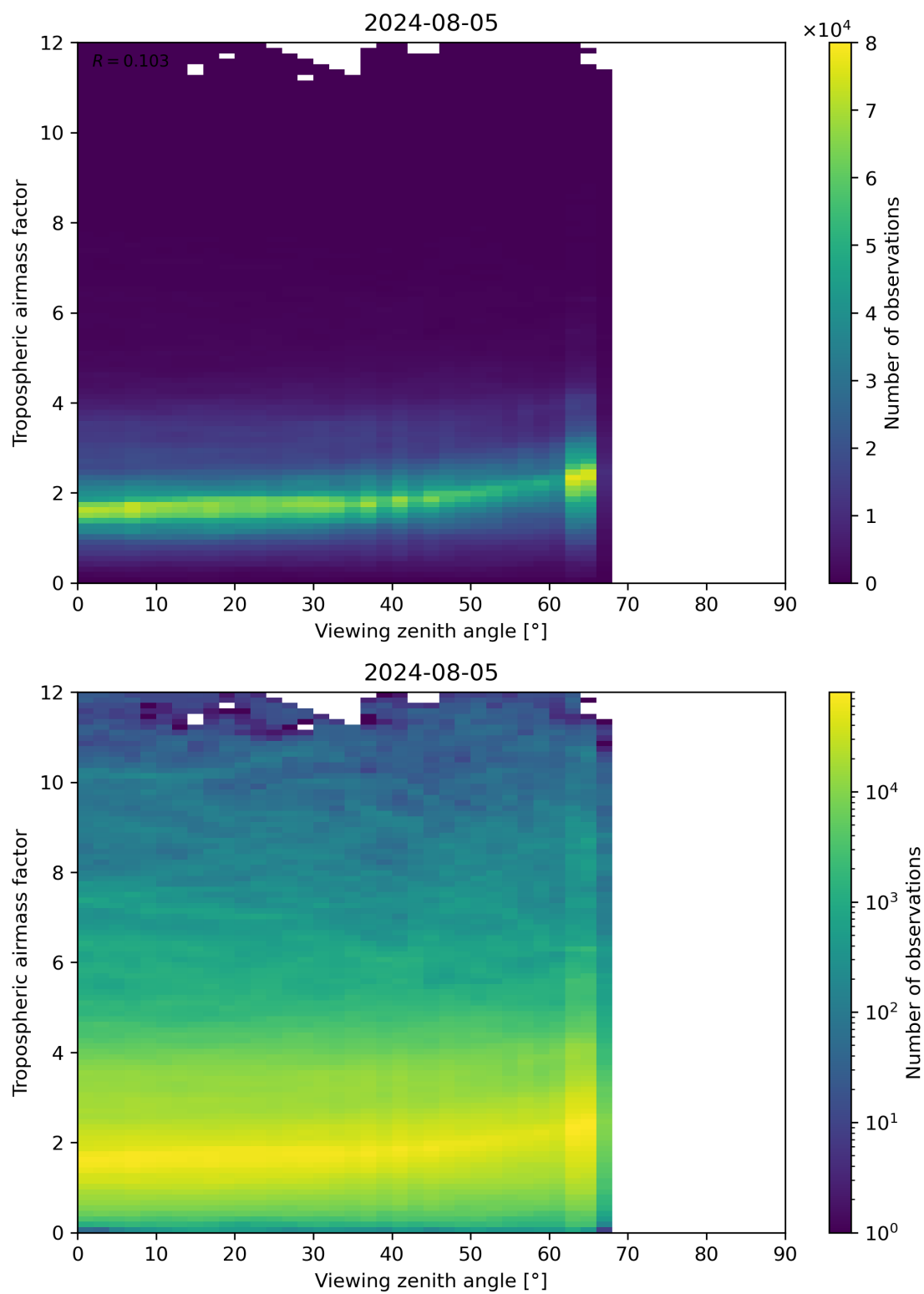
Figure 161: Scatter density plot of “Viewing zenith angle” against “Tropospheric airmass factor” for 2024-08-04 to 2024-08-06.
