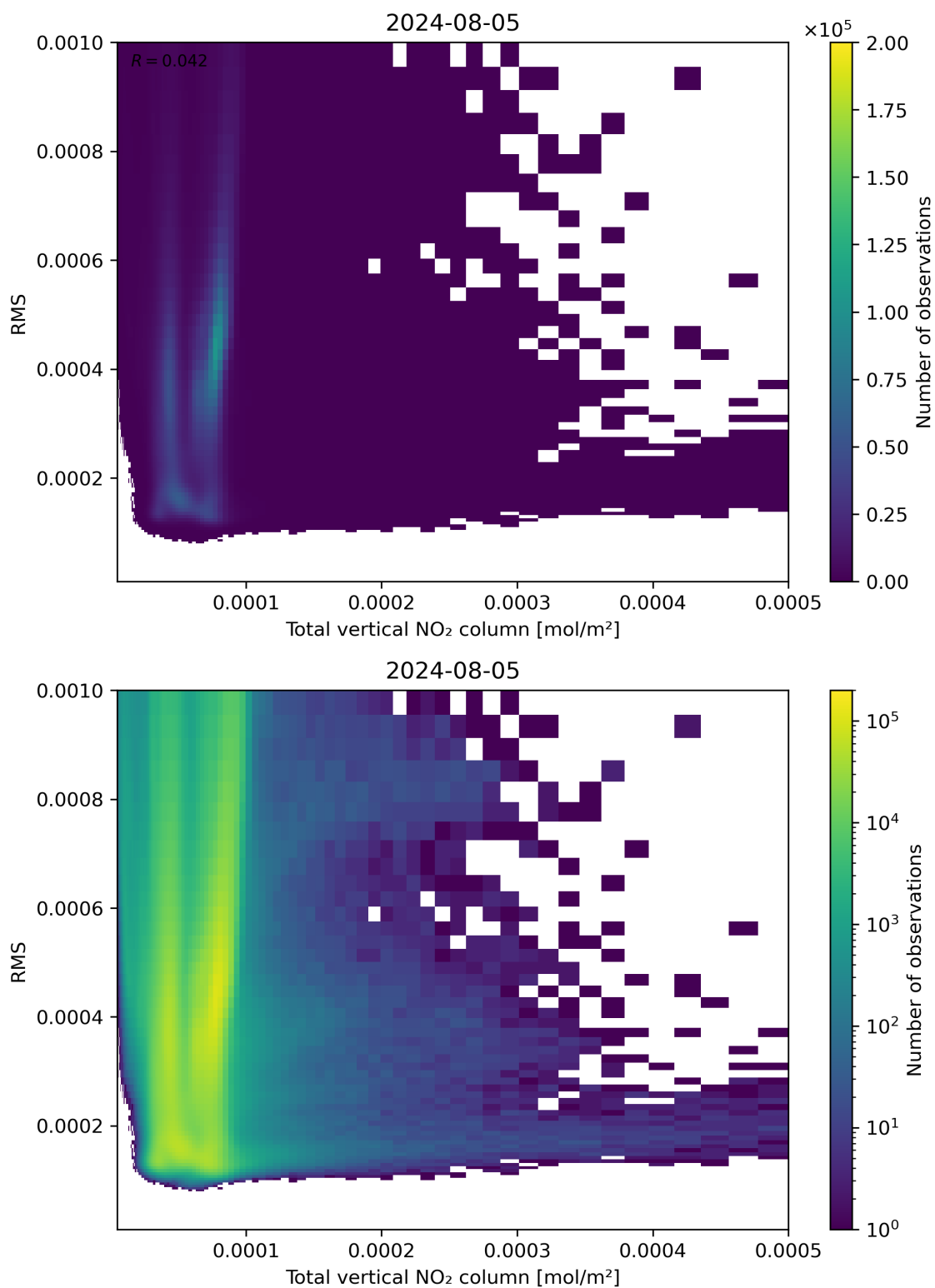
Figure 120: Scatter density plot of “Total vertical NO 2 column” against “RMS” for 2024-08-04 to 2024-08-06.
