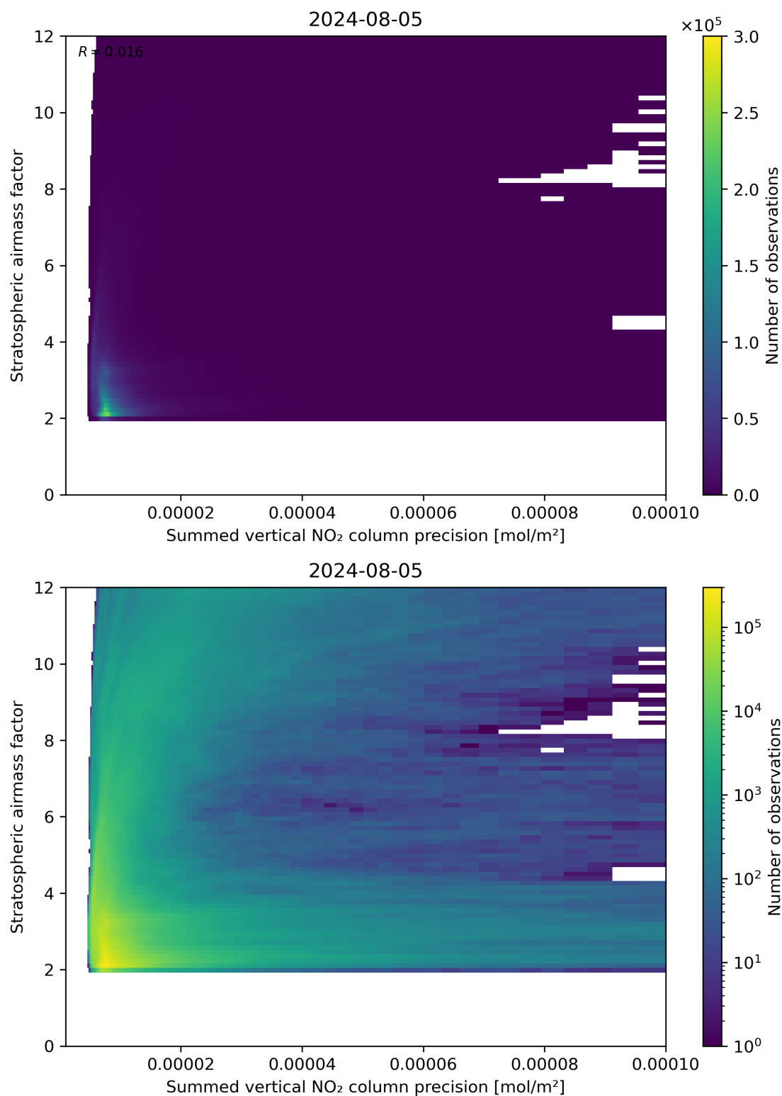
Figure 106: Scatter density plot of “Summed vertical NO 2 column precision” against “Stratospheric airmass factor” for 2024-08-04 to 2024-08-06.
