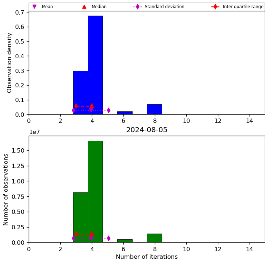
Figure 34: Histogram of “Number of iterations” for 2024-08-04 to 2024-08-06
