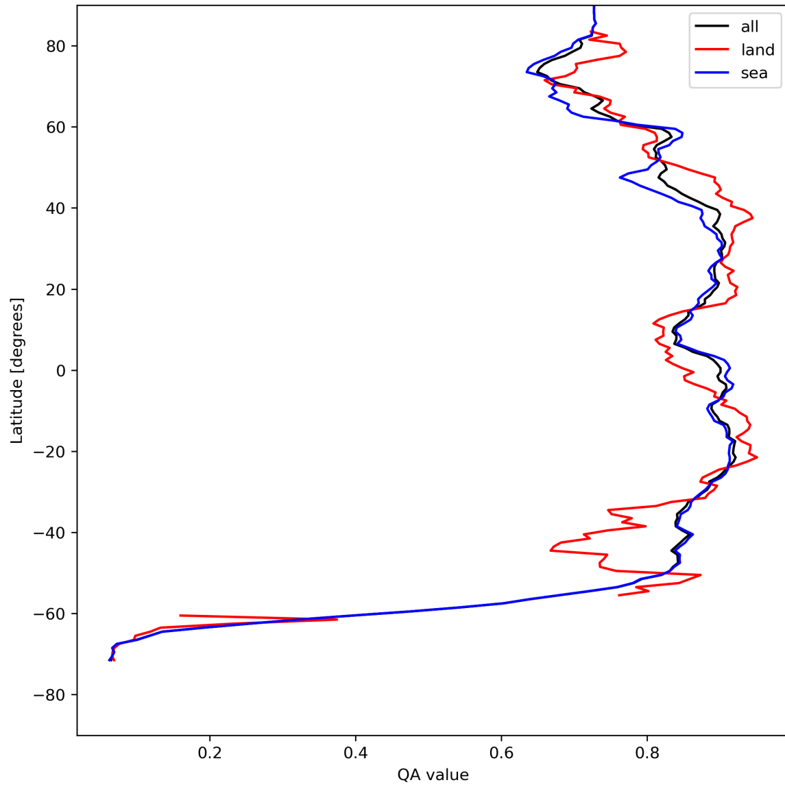
Figure 11: Zonal average of “QA value” for 2024-08-04 to 2024-08-06.
