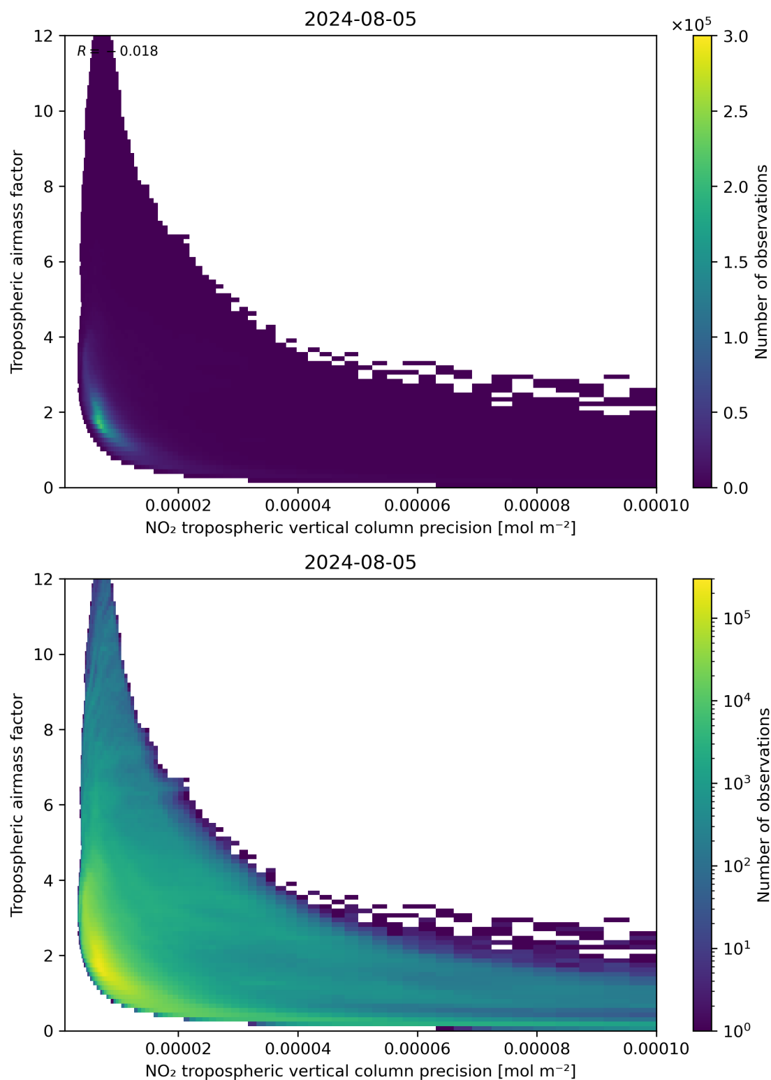
Figure 133: Scatter density plot of “NO 2 tropospheric vertical column precision” against “Tropospheric airmass factor” for 2024-08-04 to 2024-08-06.
