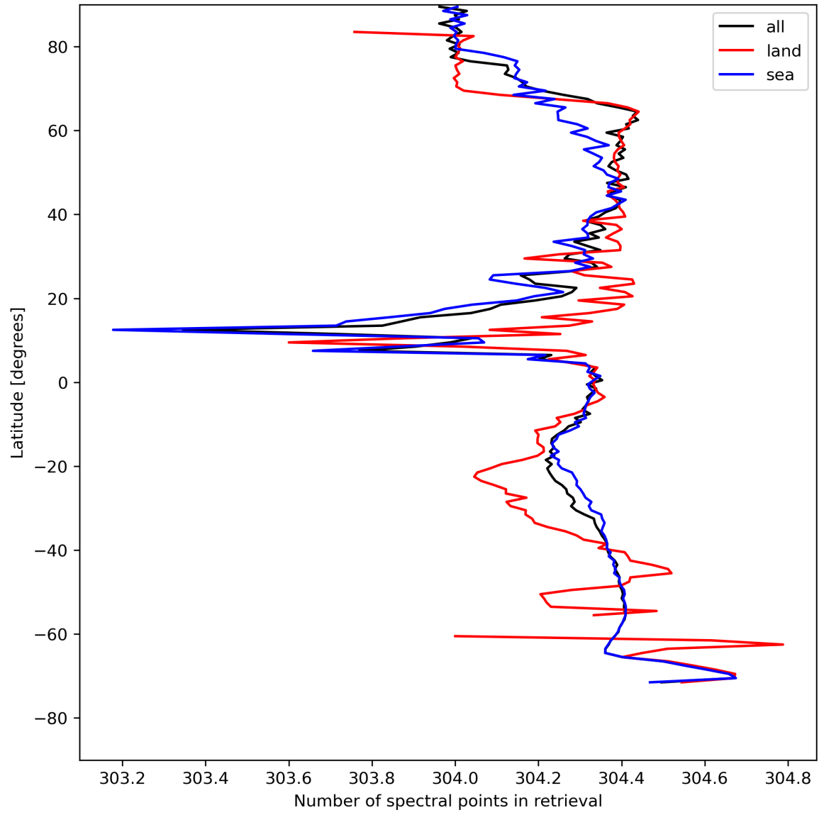
Figure 16: Zonal average of “Number of spectral points in retrieval” for 2024-08-04 to 2024-08-06.
