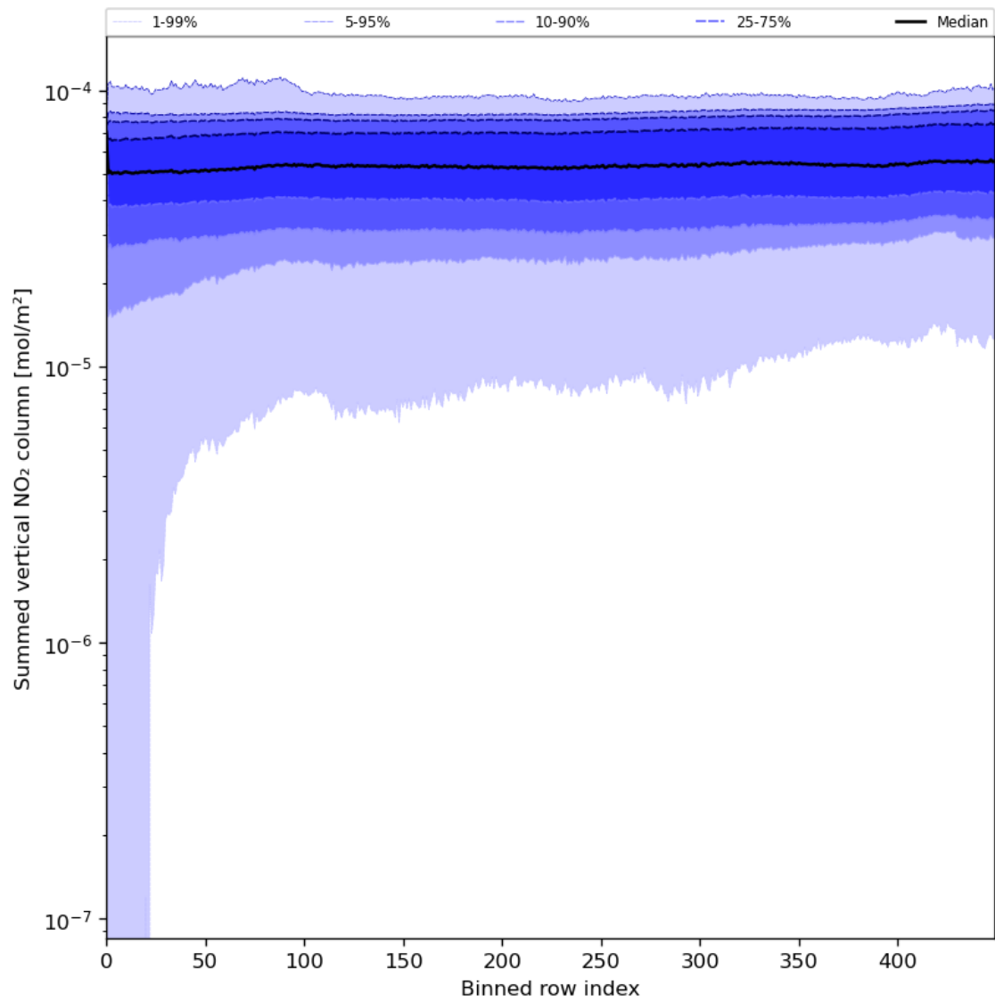
Figure 57: Along track statistics of “Summed vertical NO 2 column” for 2024-08-04 to 2024-08-06
