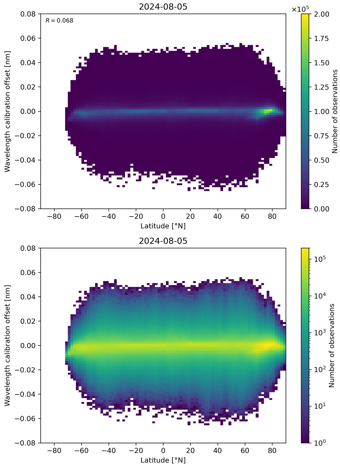
Figure 95: Scatter density plot of “Latitude” against “Wavelength calibration offset” for 2024-08-04 to 2024-08-06.
