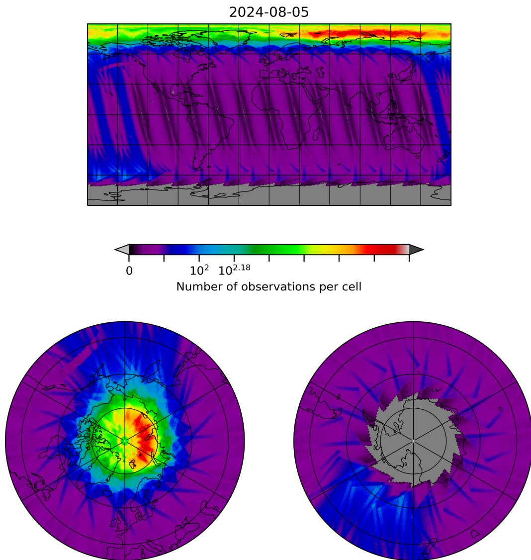
Figure 10: Map of the number of observations for 2024-08-04 to 2024-08-06
