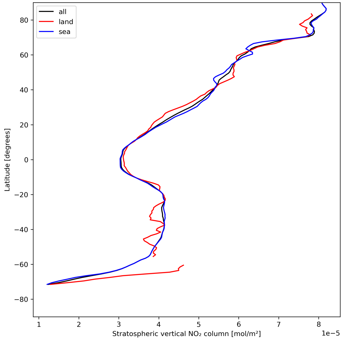
Figure 19: Zonal average of “Stratospheric vertical NO 2 column” for 2024-08-04 to 2024-08-06.
