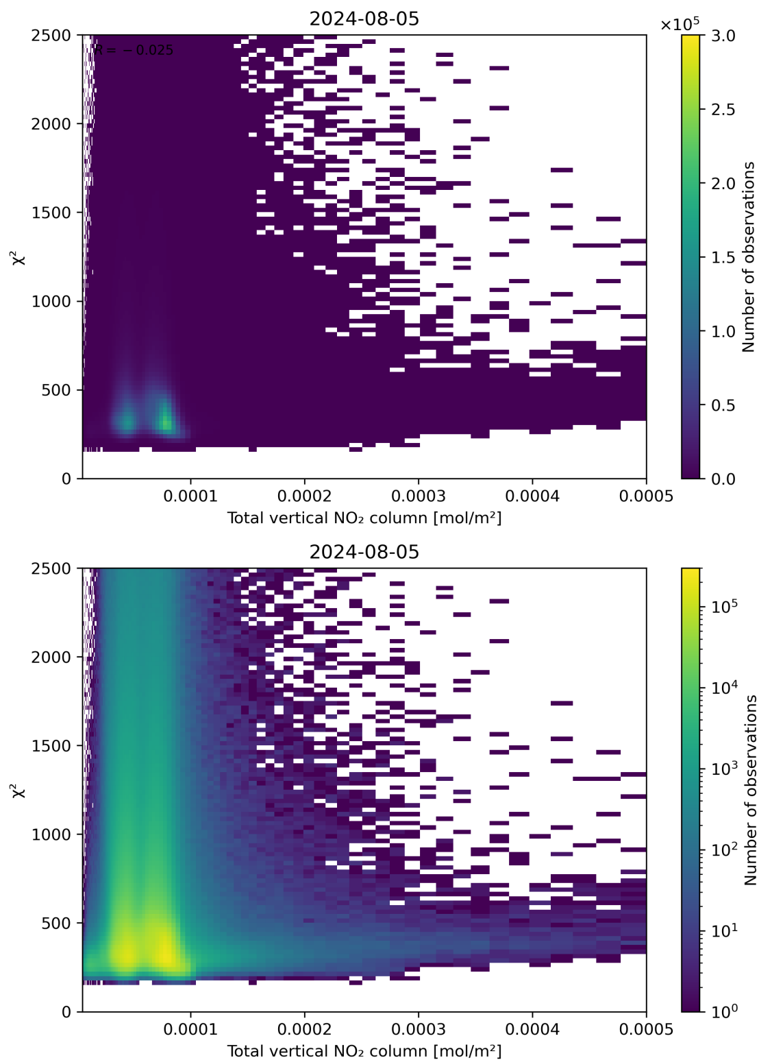
Figure 111: Scatter density plot of “Total vertical NO 2 column” against “ \chi^2 ” for 2024-08-04 to 2024-08-06.
