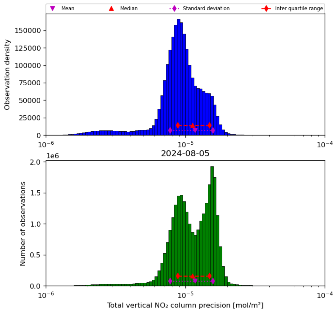
Figure 39: Histogram of “Total vertical NO 2 column precision” for 2024-08-04 to 2024-08-06
