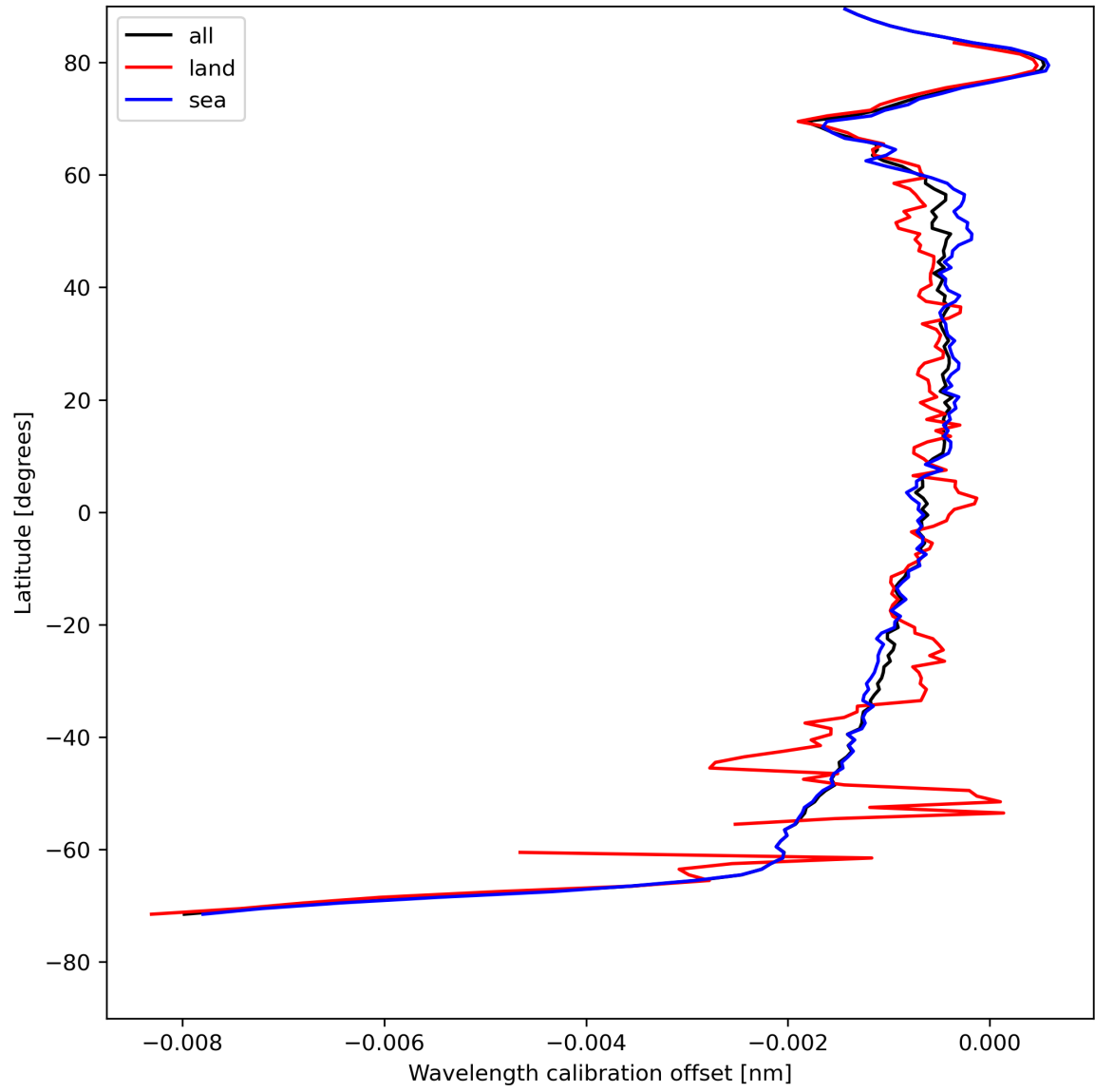
Figure 18: Zonal average of “Wavelength calibration offset” for 2024-08-04 to 2024-08-06.
