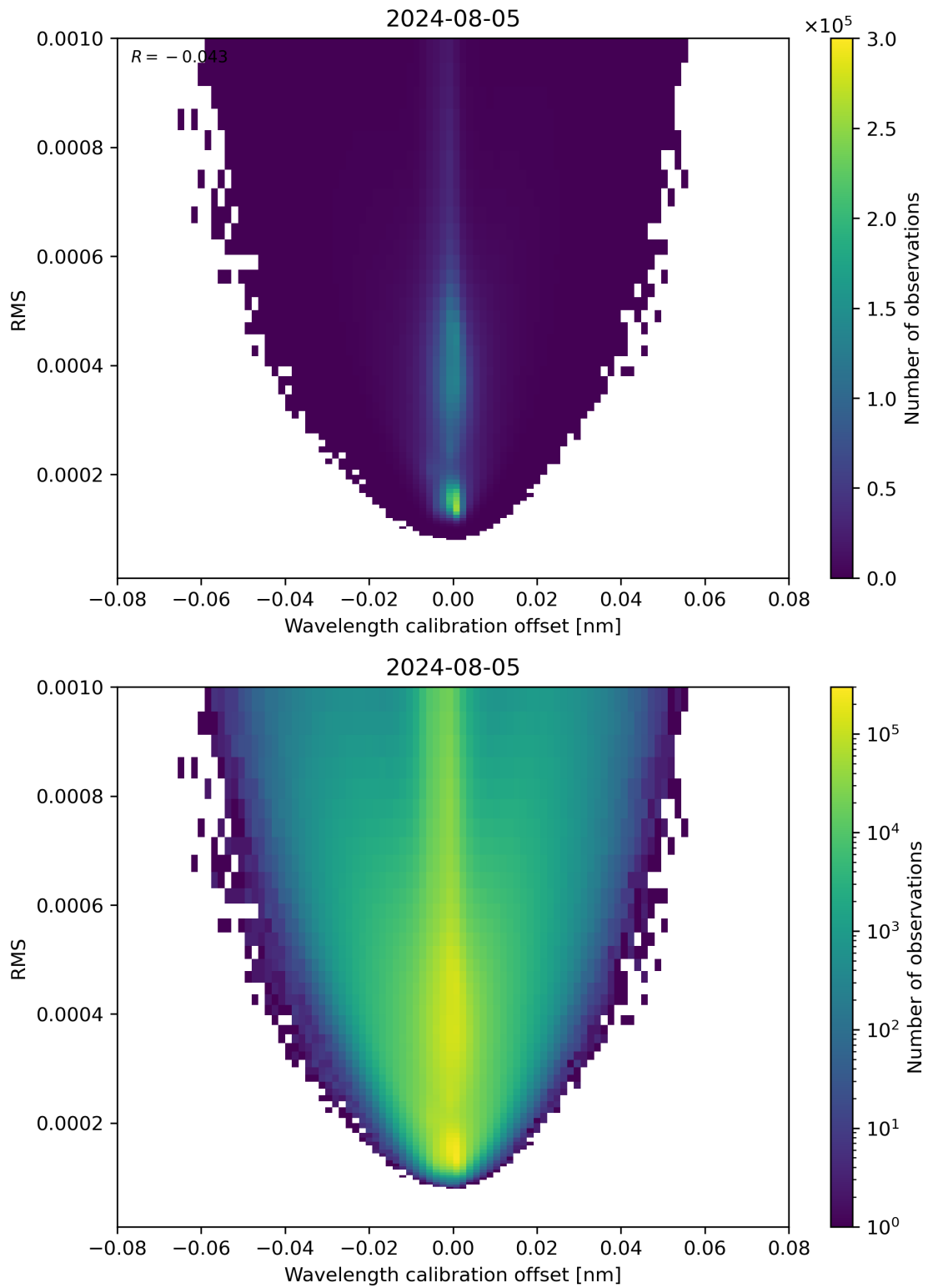
Figure 181: Scatter density plot of “Wavelength calibration offset” against “RMS” for 2024-08-04 to 2024-08-06.
