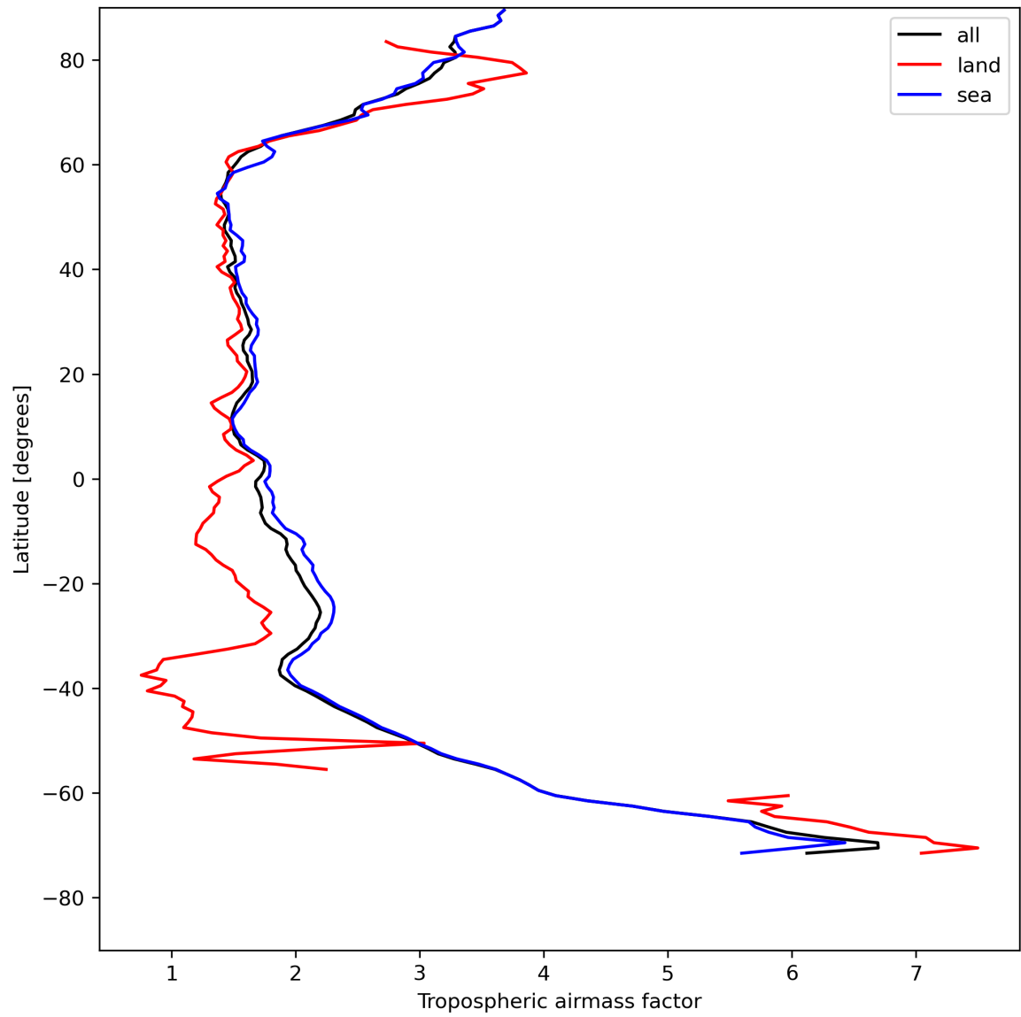
Figure 14: Zonal average of “Tropospheric airmass factor” for 2024-08-04 to 2024-08-06.
