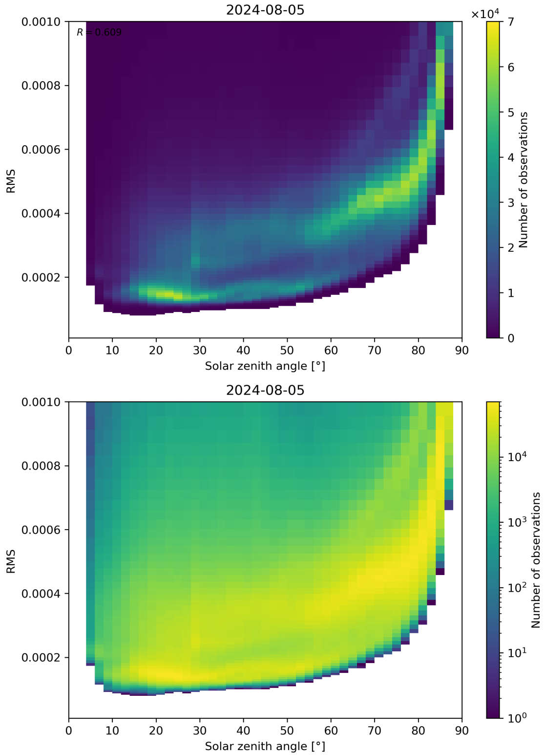
Figure 157: Scatter density plot of “Solar zenith angle” against “RMS” for 2024-08-04 to 2024-08-06.
