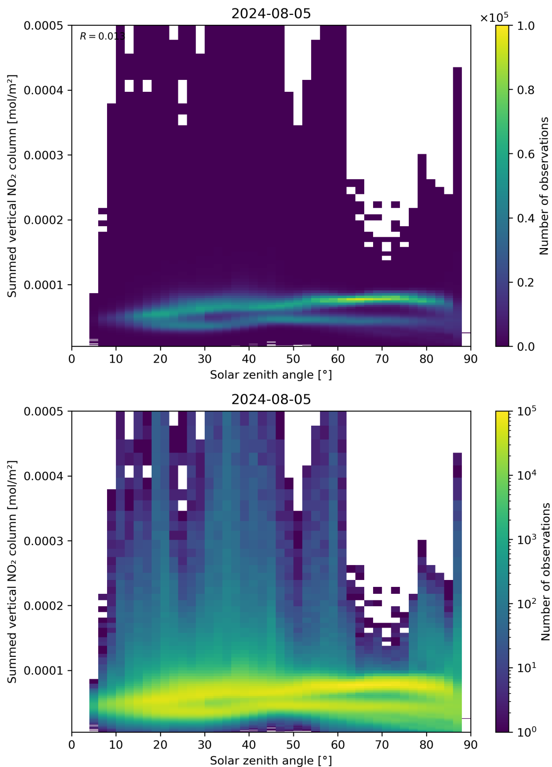
Figure 151: Scatter density plot of “Solar zenith angle” against “Summed vertical NO 2 column” for 2024-08-04 to 2024-08-06.
