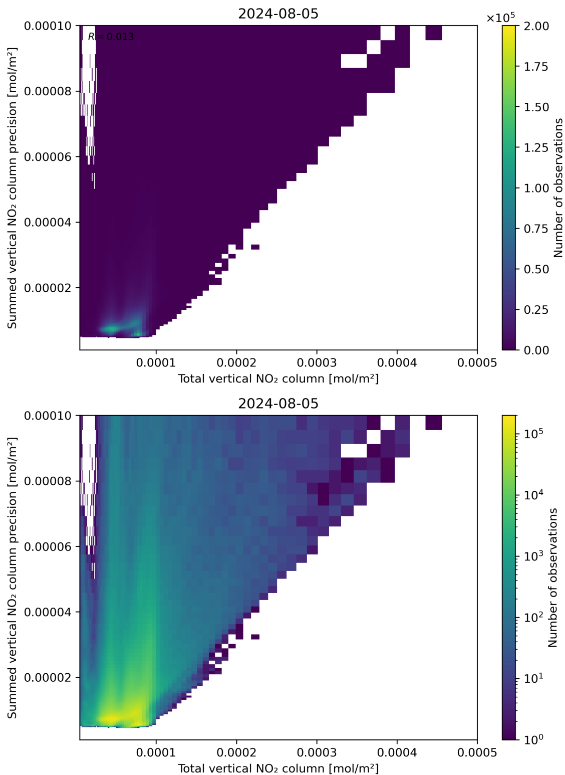
Figure 113: Scatter density plot of “Total vertical NO 2 column” against “Summed vertical NO 2 column precision” for 2024-08-04 to 2024-08-06.
