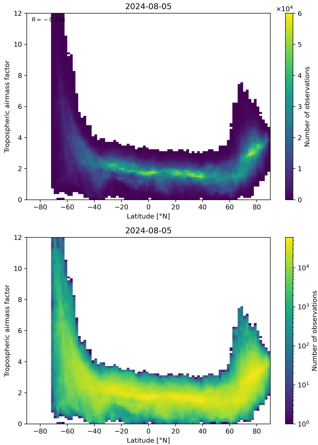
Figure 85: Scatter density plot of “Latitude” against “Tropospheric air mass factor” for 2024-08-04 to 2024-08-06.
