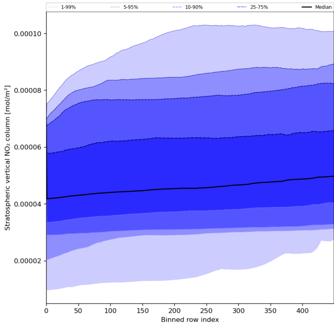
Figure 53: Along track statistics of “Stratospheric vertical NO 2 column” for 2024-08-04 to 2024-08-06
