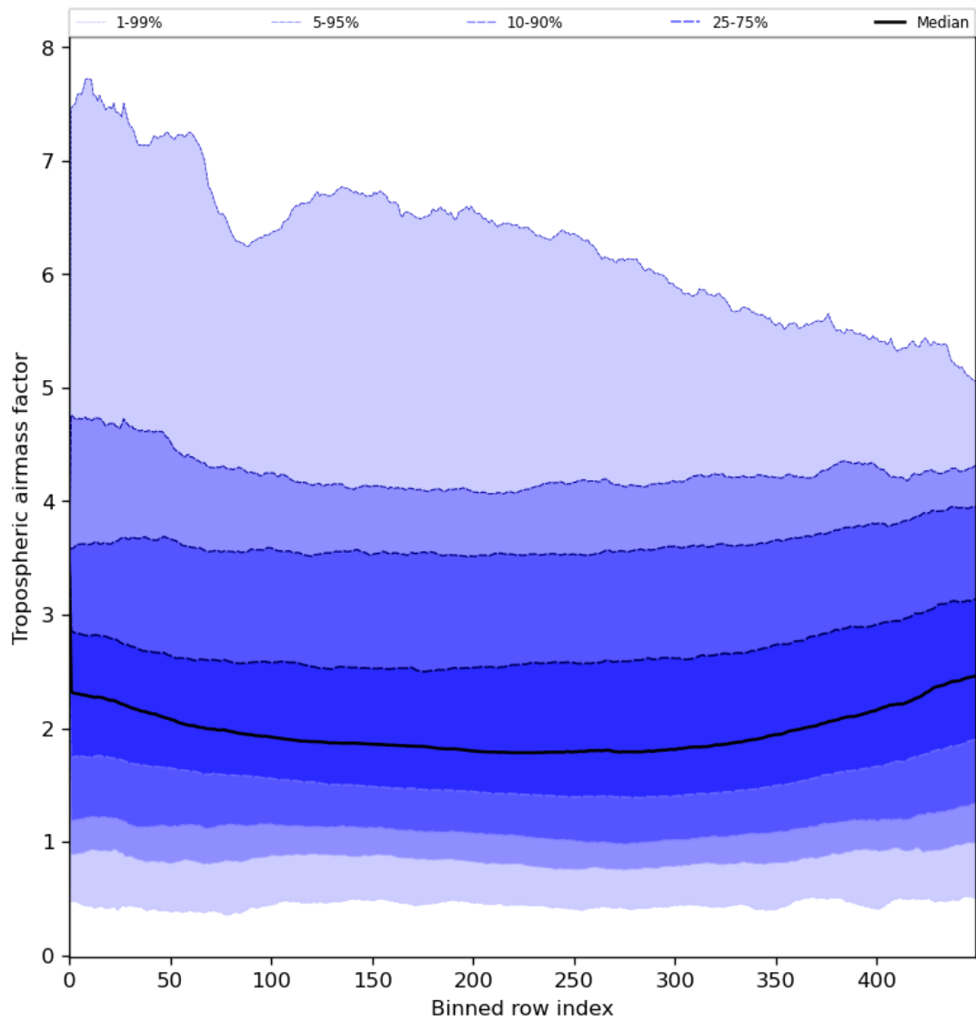
Figure 48: Along track statistics of “Tropospheric airmass factor” for 2024-08-04 to 2024-08-06
