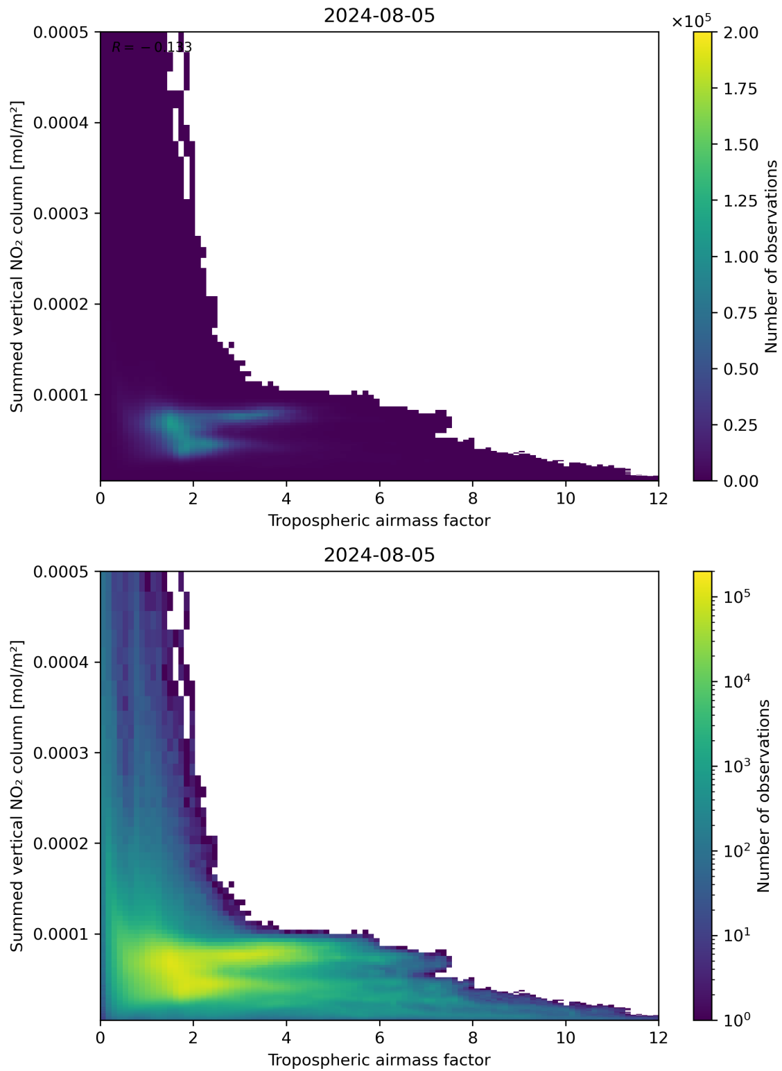
Figure 75: Scatter density plot of “Tropospheric air mass factor” against “Summed vertical NO 2 column” for 2024-08-04 to 2024-08-06.
