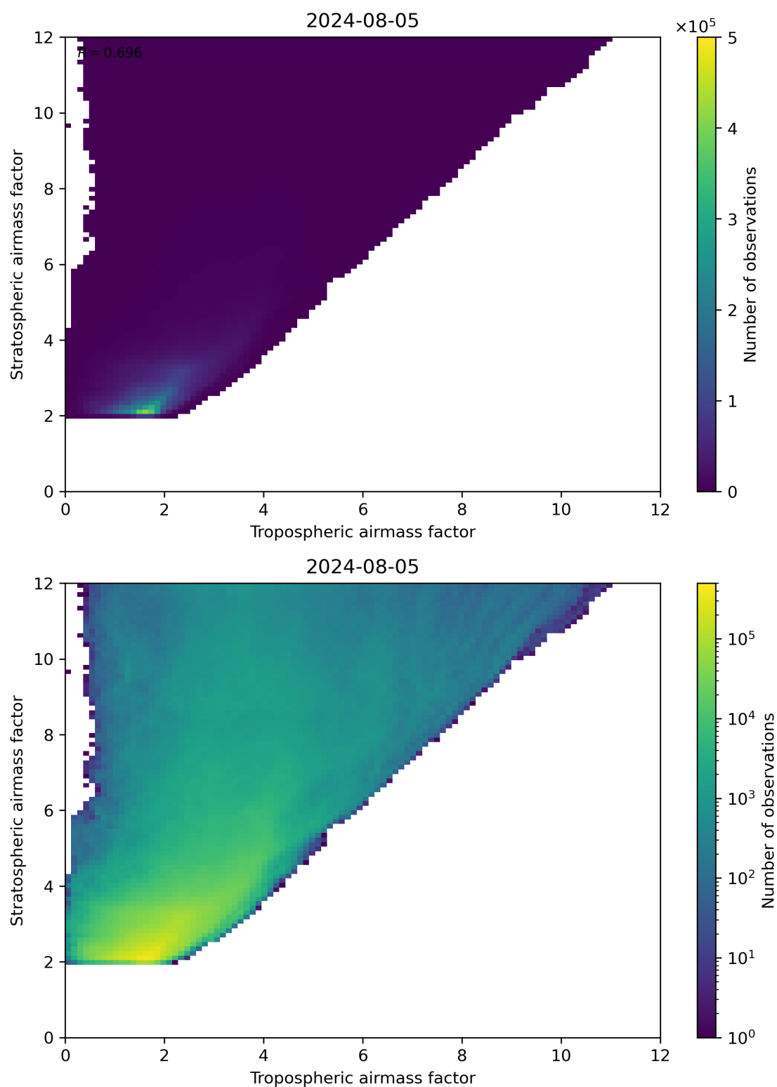
Figure 71: Scatter density plot of “Tropospheric airmass factor” against “Stratospheric airmass factor” for 2024-08-04 to 2024-08-06.
