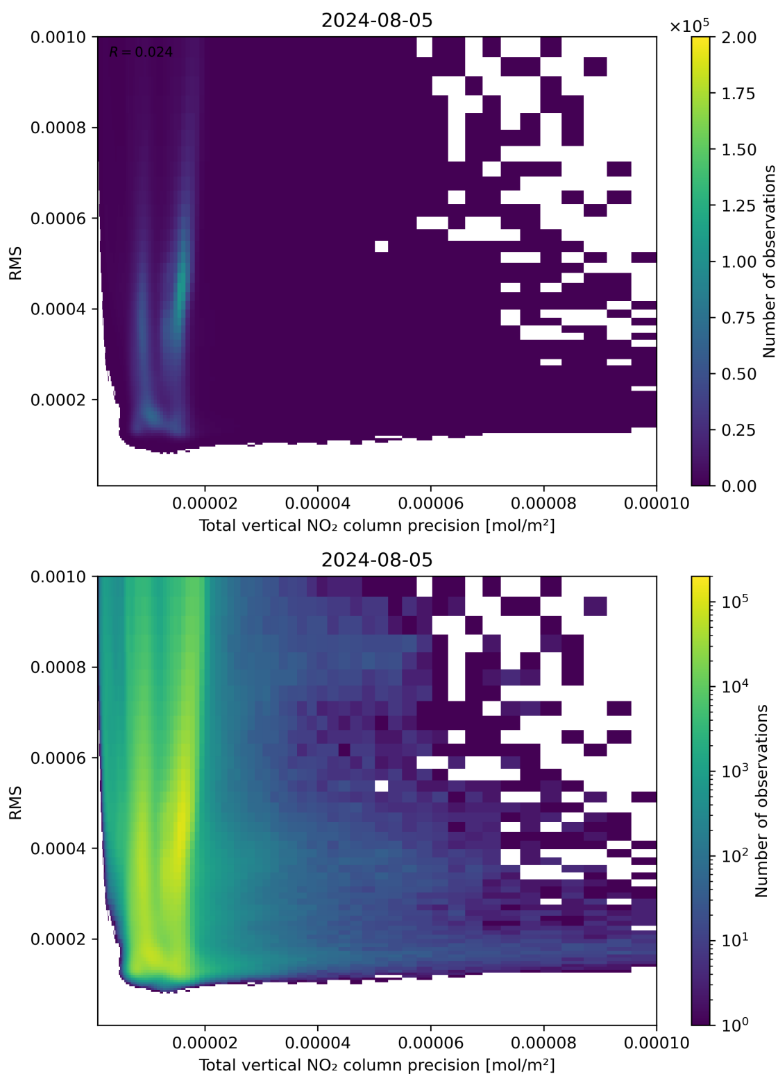
Figure 119: Scatter density plot of “Total vertical NO 2 column precision” against “RMS” for 2024-08-04 to 2024-08-06.
