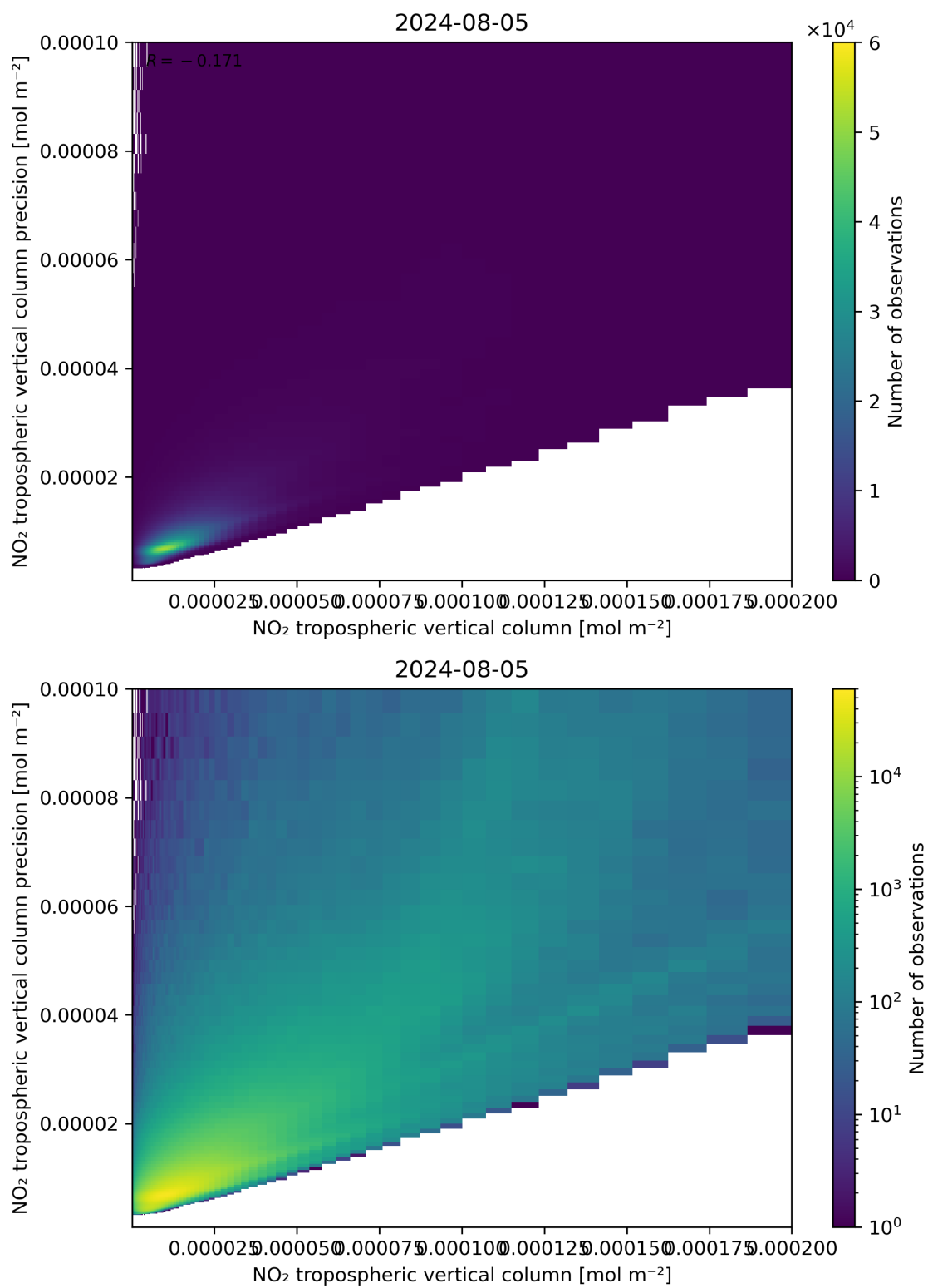
Figure 130: Scatter density plot of “NO 2 tropospheric vertical column” against “NO 2 tropospheric vertical column precision” for 2024-08-04 to 2024-08-06.
