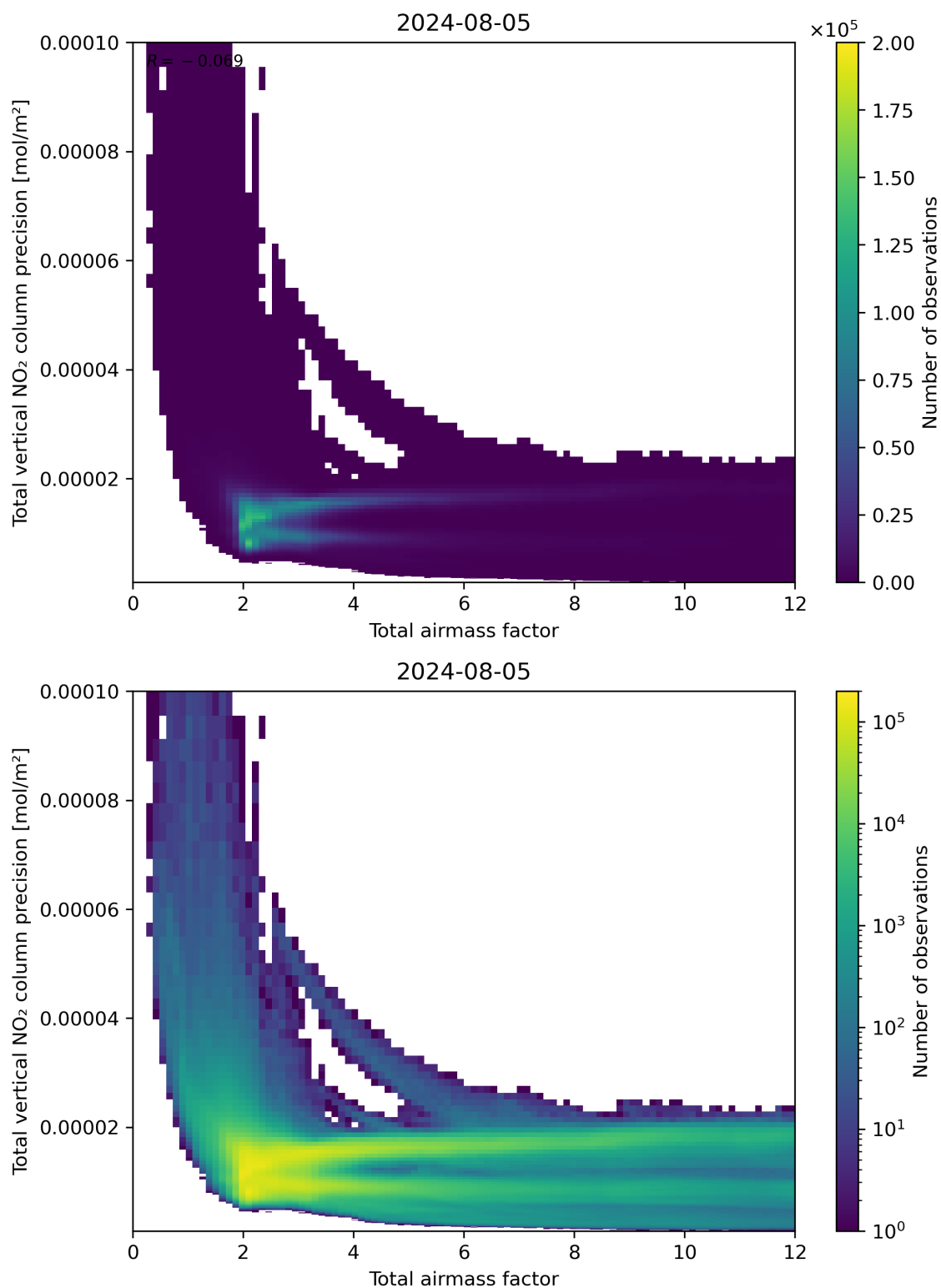
Figure 68: Scatter density plot of “Total airmass factor” against “Total vertical NO 2 column precision” for 2024-08-04 to 2024-08-06.
