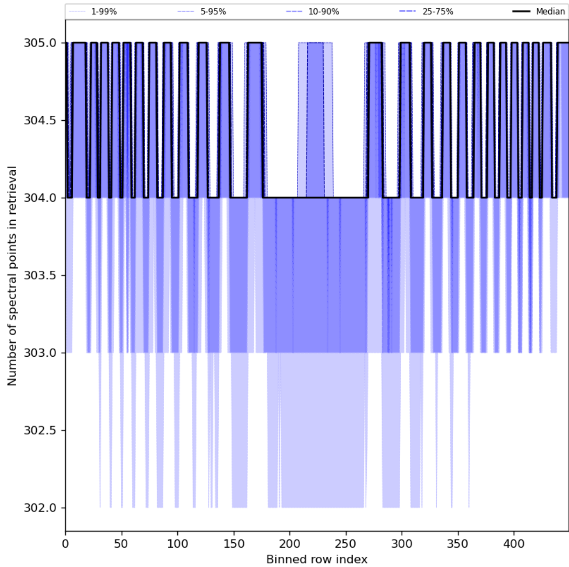
Figure 50: Along track statistics of “Number of spectral points in retrieval” for 2024-08-04 to 2024-08-06
