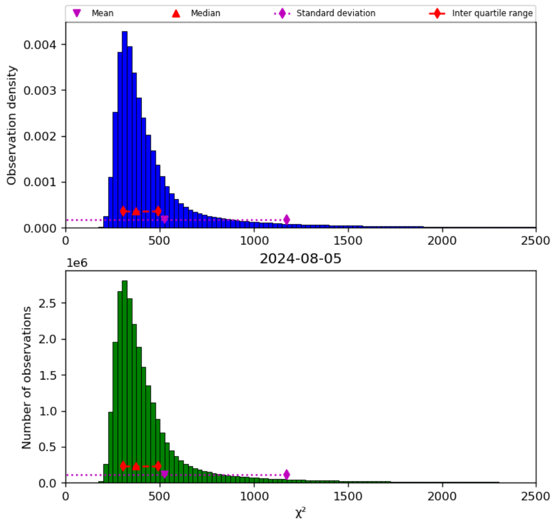
Figure 42: Histogram of “ \chi^2 ” for 2024-08-04 to 2024-08-06
