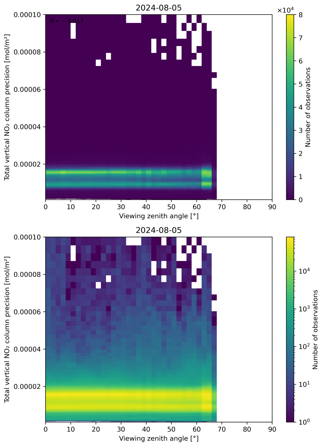
Figure 168: Scatter density plot of “Viewing zenith angle” against “Total vertical NO 2 column precision” for 2024-08-04 to 2024-08-06.
