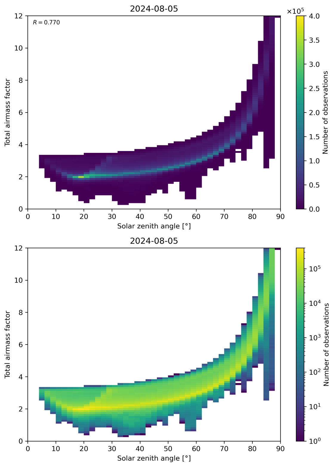
Figure 146: Scatter density plot of “Solar zenith angle” against “Total airmass factor” for 2024-08-04 to 2024-08-06.
