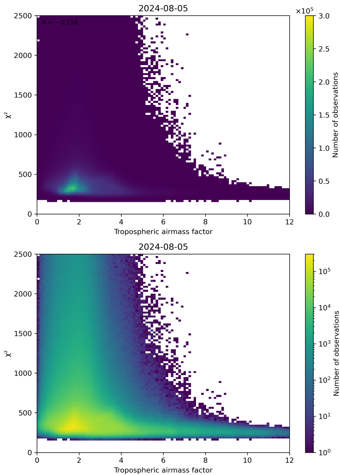
Figure 73: Scatter density plot of “Tropospheric airmass factor” against “ \chi^2 ” for 2024-08-04 to 2024-08-06.
