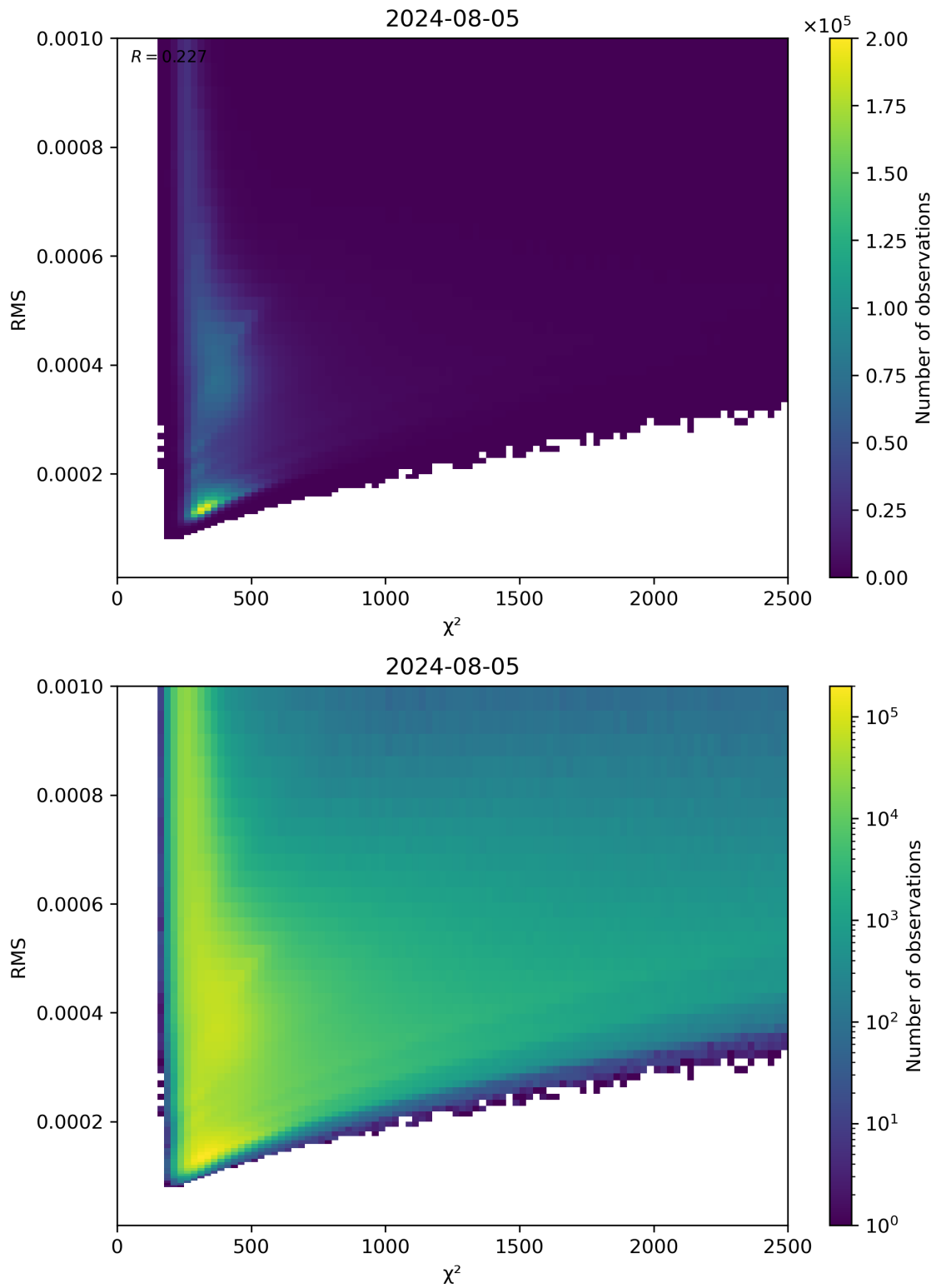
Figure 82: Scatter density plot of “ \chi^2 ” against “RMS” for 2024-08-04 to 2024-08-06.
