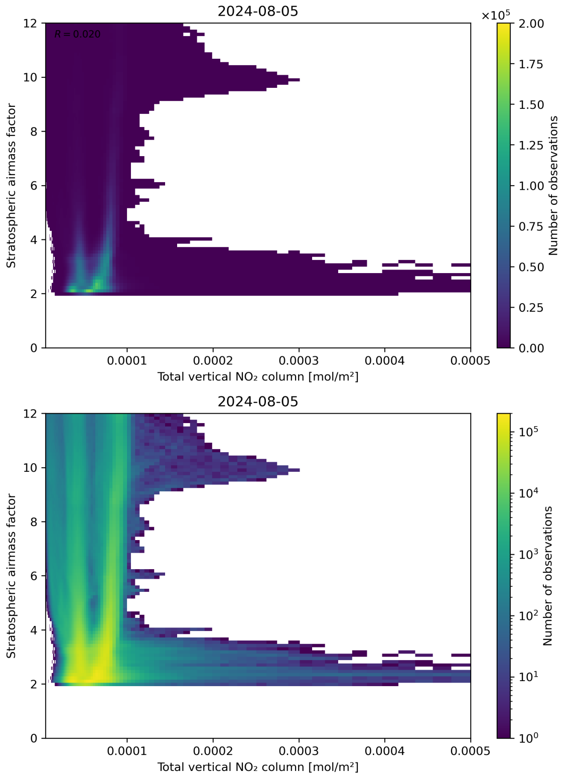
Figure 110: Scatter density plot of “Total vertical NO 2 column” against “Stratospheric airmass factor” for 2024-08-04 to 2024-08-06.
