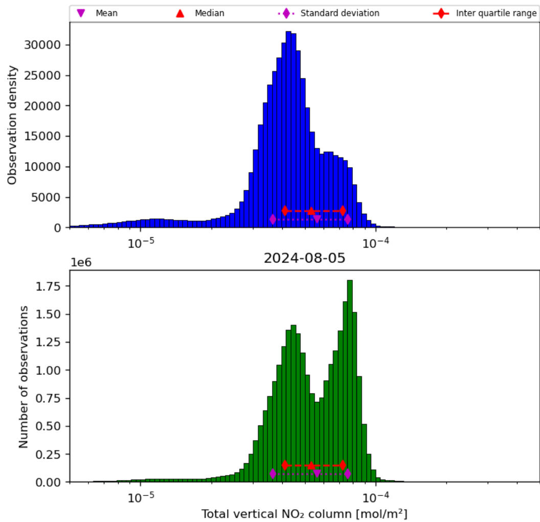
Figure 38: Histogram of “Total vertical NO 2 column” for 2024-08-04 to 2024-08-06
