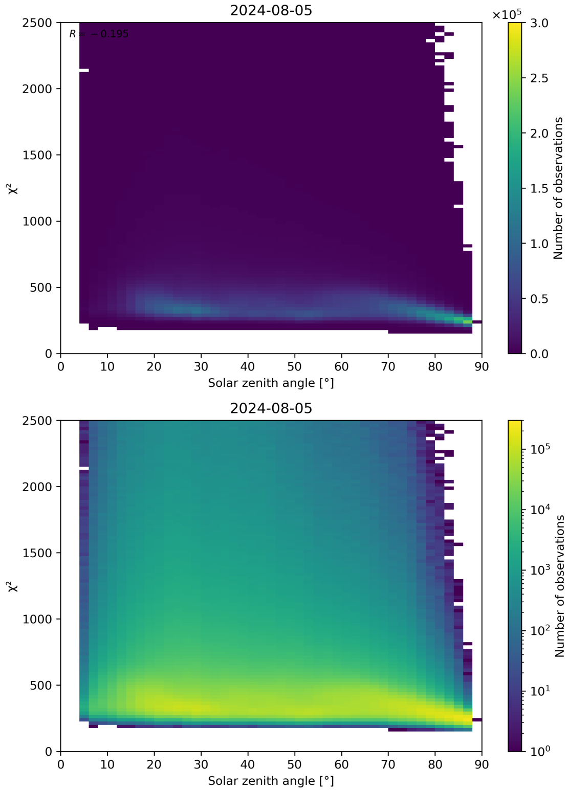
Figure 148: Scatter density plot of “Solar zenith angle” against “ \chi^2 ” for 2024-08-04 to 2024-08-06.
