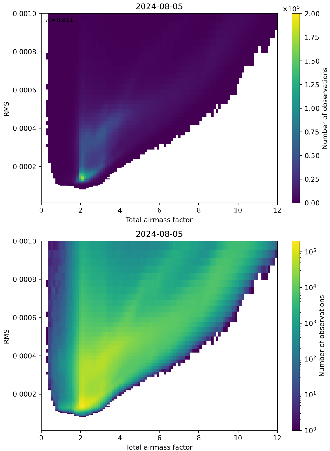
Figure 69: Scatter density plot of “Total airmass factor” against “RMS” for 2024-08-04 to 2024-08-06.
