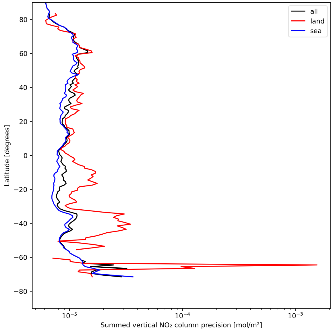
Figure 24: Zonal average of “Summed vertical NO 2 column precision” for 2024-08-04 to 2024-08-06.
