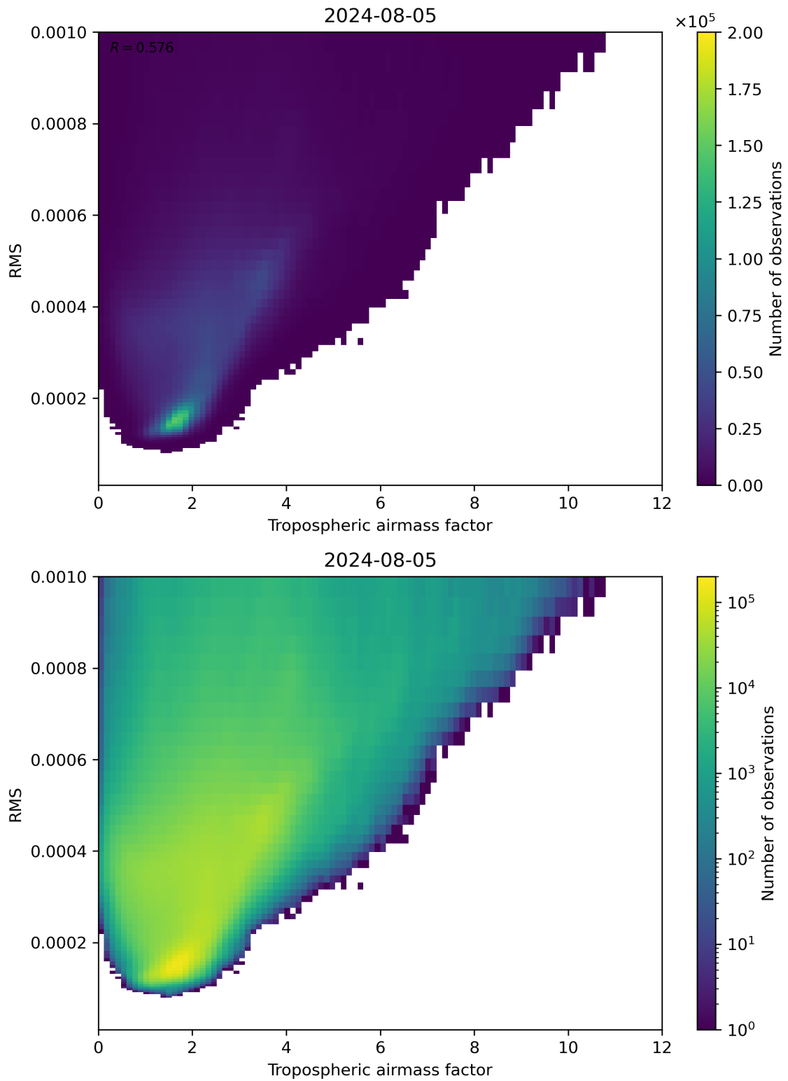
Figure 79: Scatter density plot of “Tropospheric airmass factor” against “RMS” for 2024-08-04 to 2024-08-06.
