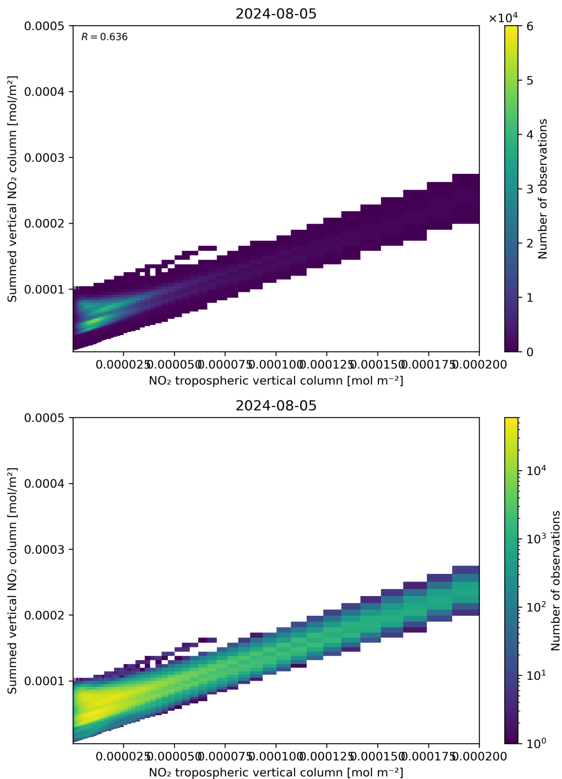
Figure 126: Scatter density plot of “NO 2 tropospheric vertical column” against “Summed vertical NO 2 column” for 2024-08-04 to 2024-08-06.
