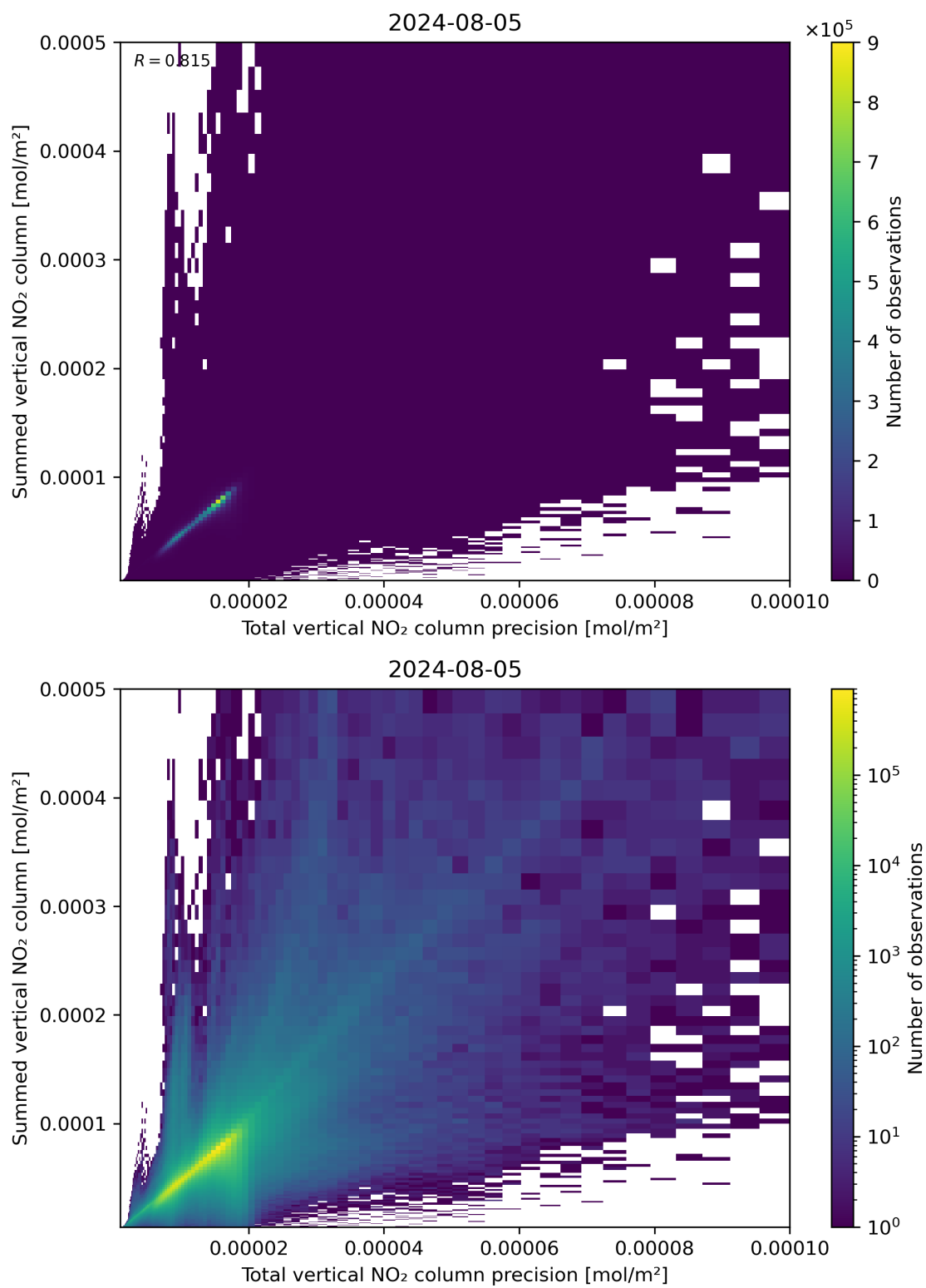
Figure 117: Scatter density plot of “Total vertical NO 2 column precision” against “Summed vertical NO 2 column” for 2024-08-04 to 2024-08-06.
