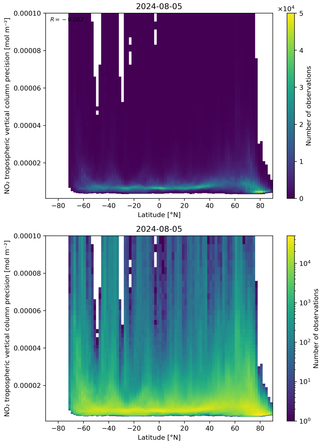
Figure 93: Scatter density plot of “Latitude” against “NO 2 tropospheric vertical column precision” for 2024-08-04 to 2024-08-06.
