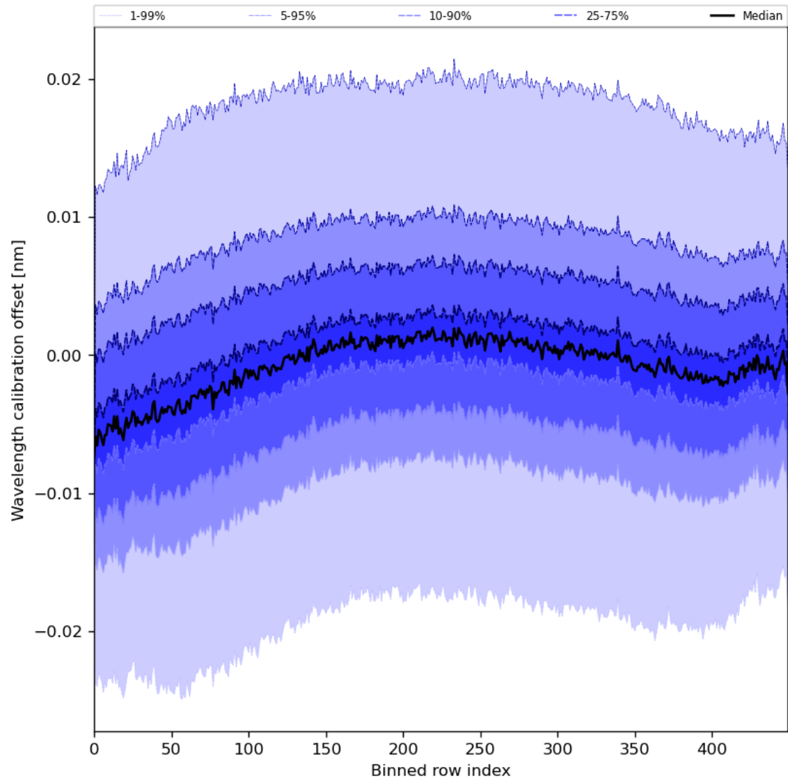
Figure 52: Along track statistics of “Wavelength calibration offset” for 2024-08-04 to 2024-08-06
