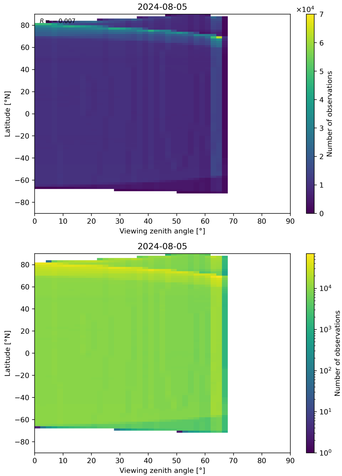
Figure 163: Scatter density plot of “Viewing zenith angle” against “Latitude” for 2024-08-04 to 2024-08-06.
