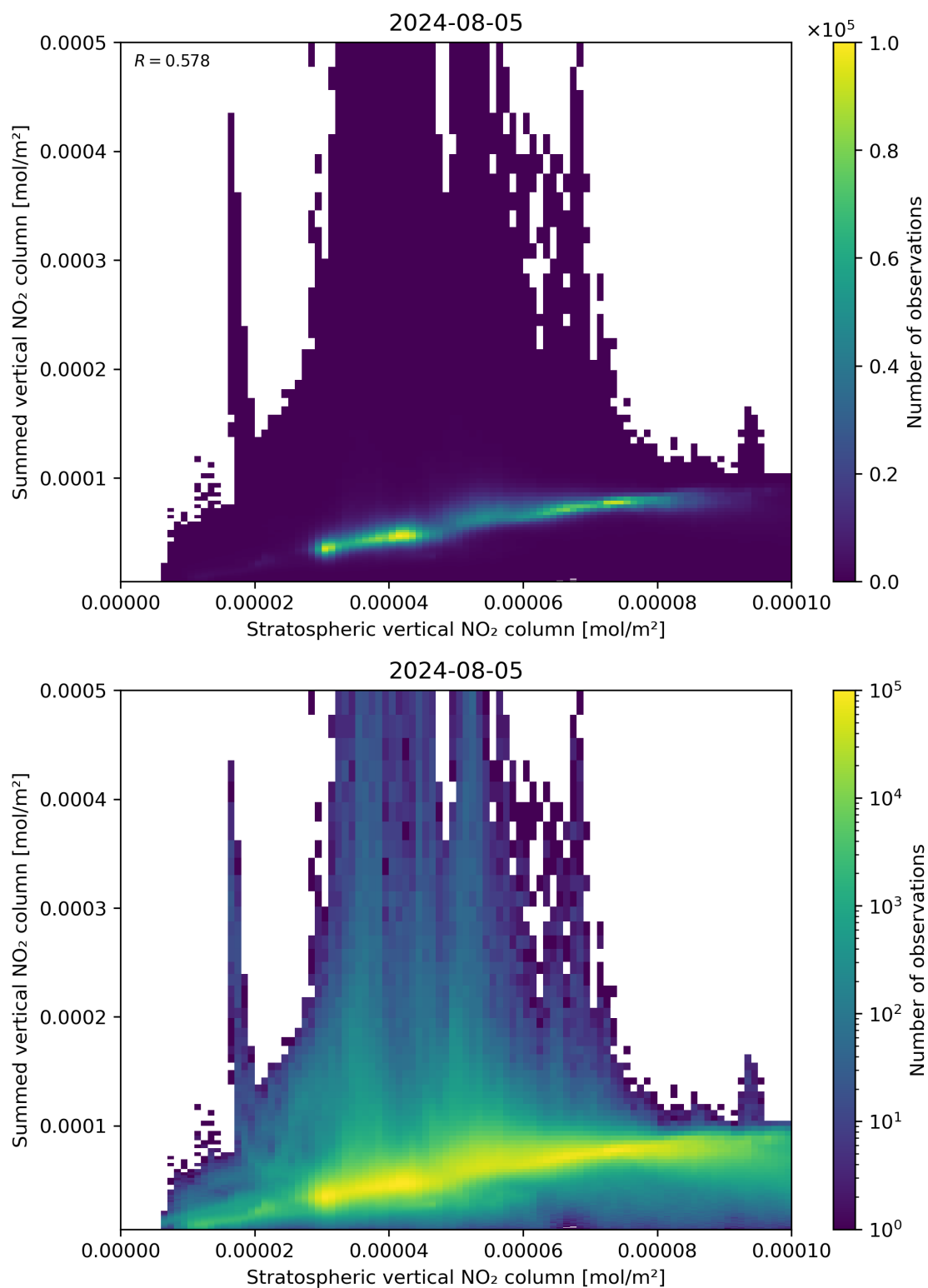
Figure 98: Scatter density plot of “Stratospheric vertical NO 2 column” against “Summed vertical NO 2 column” for 2024-08-04 to 2024-08-06.
