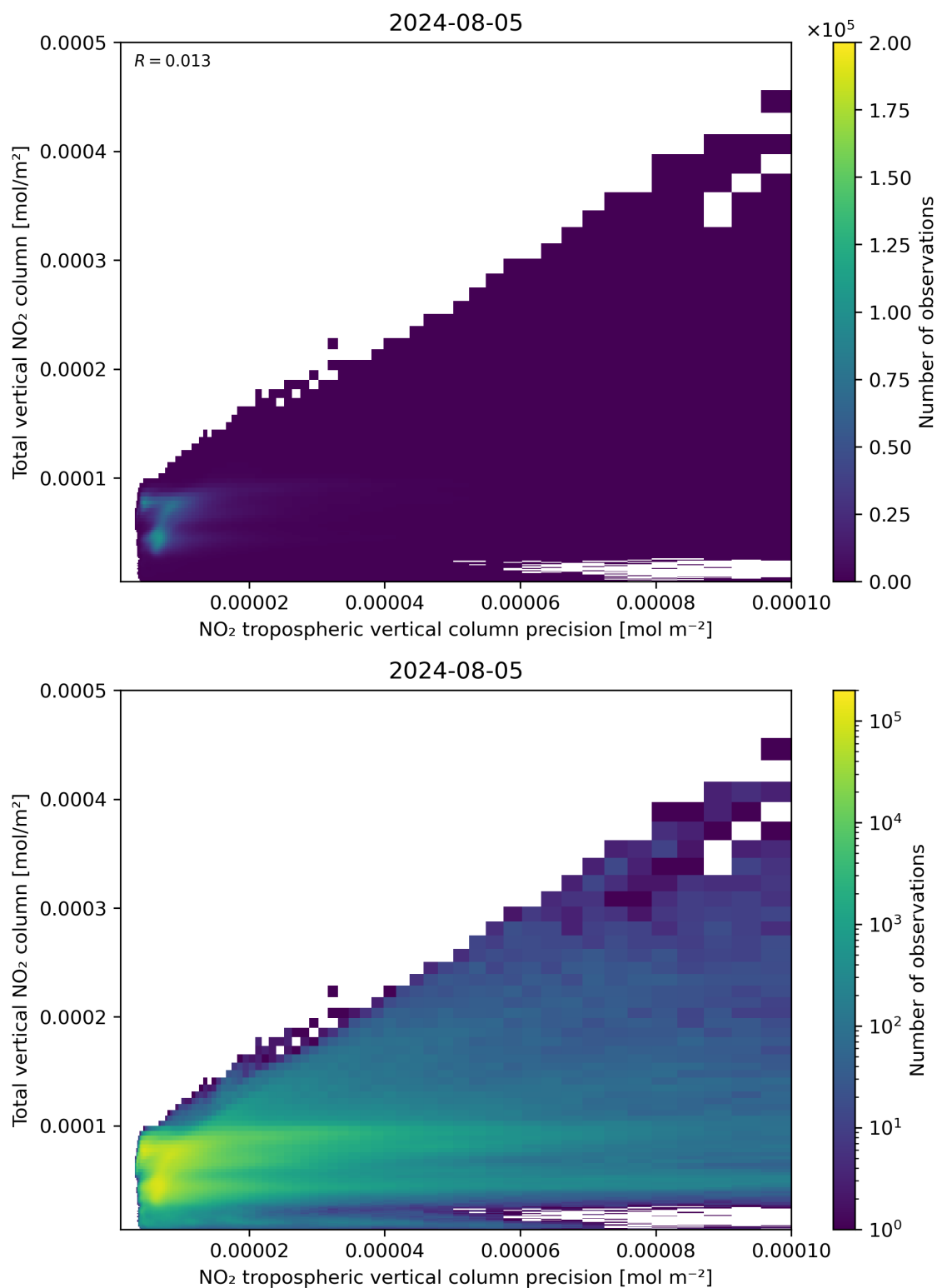
Figure 138: Scatter density plot of “NO 2 tropospheric vertical column precision” against “Total vertical NO 2 column” for 2024-08-04 to 2024-08-06.
