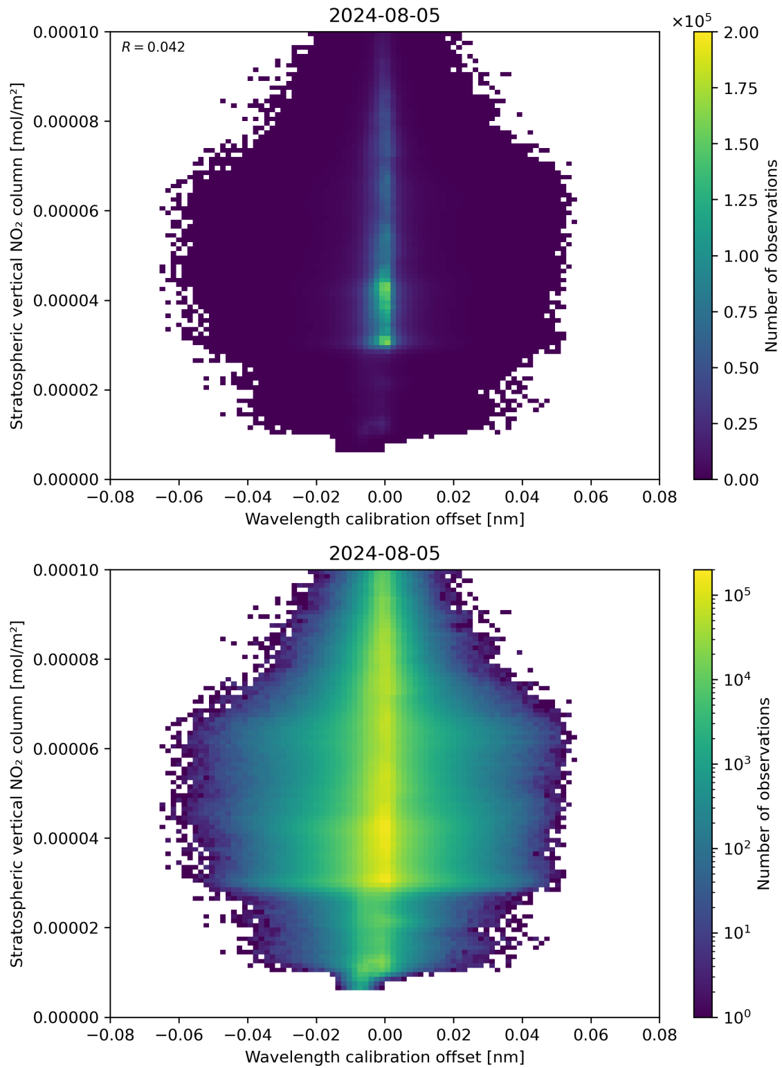
Figure 176: Scatter density plot of “Wavelength calibration offset” against “Stratospheric vertical NO 2 column” for 2024-08-04 to 2024-08-06.
