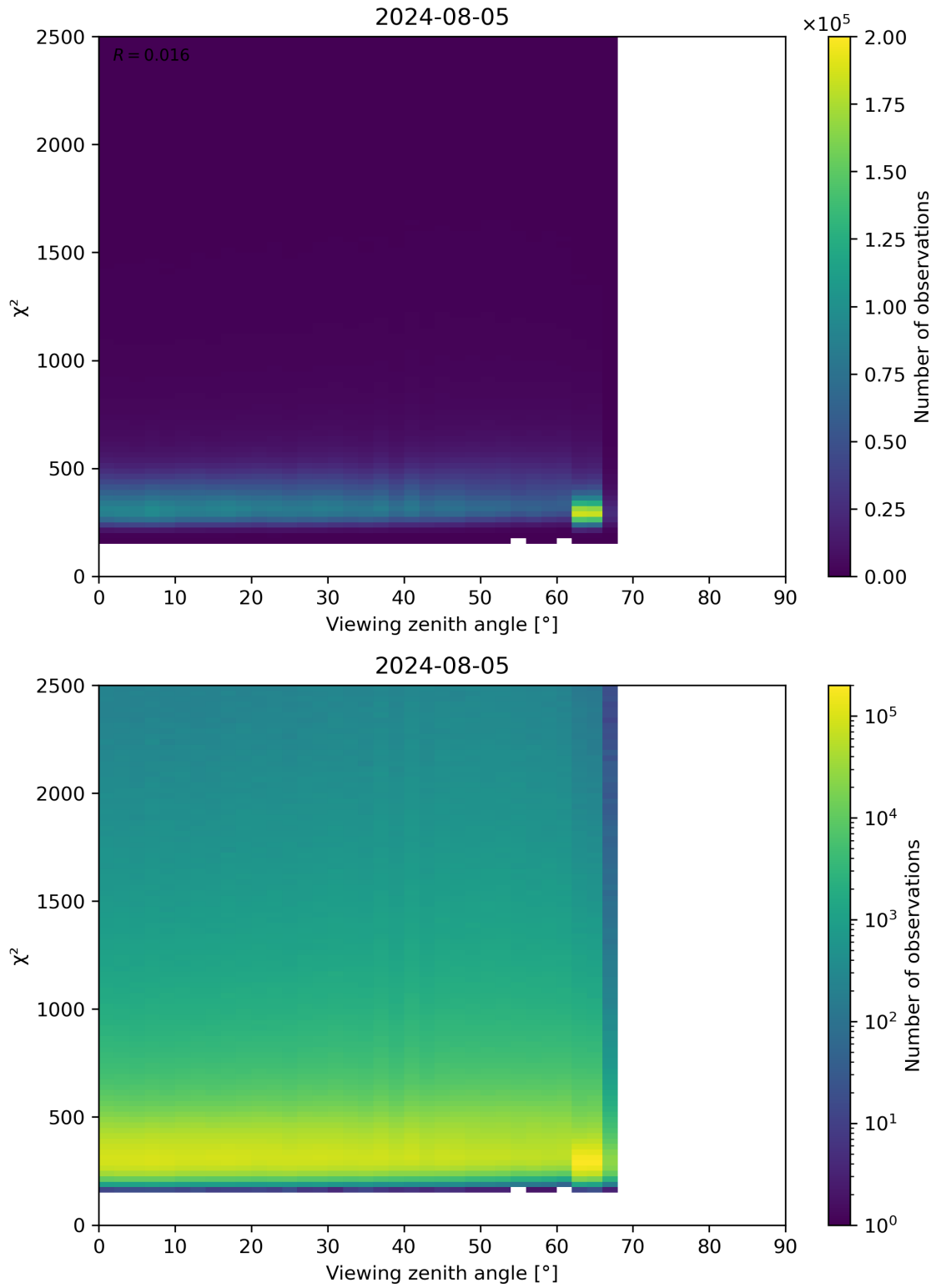
Figure 162: Scatter density plot of “Viewing zenith angle” against “ \chi^2 ” for 2024-08-04 to 2024-08-06.
