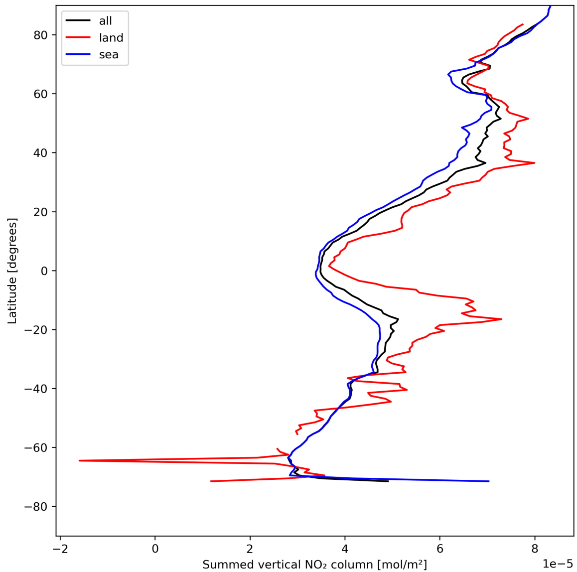
Figure 23: Zonal average of “Summed vertical NO 2 column” for 2024-08-04 to 2024-08-06.
