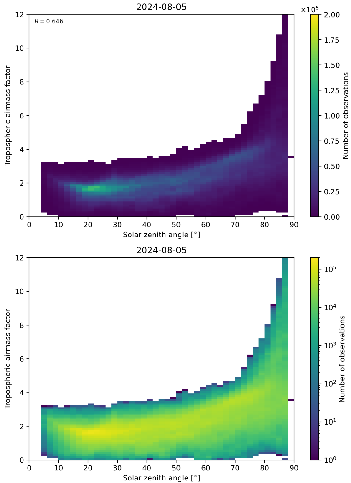
Figure 147: Scatter density plot of “Solar zenith angle” against “Tropospheric airmass factor” for 2024-08-04 to 2024-08-06.
