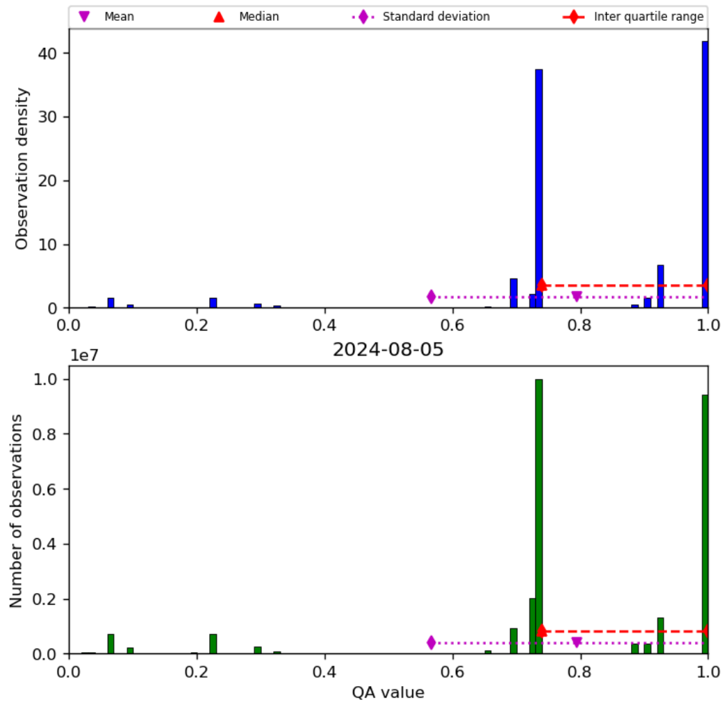
Figure 28: Histogram of “QA value” for 2024-08-04 to 2024-08-06
