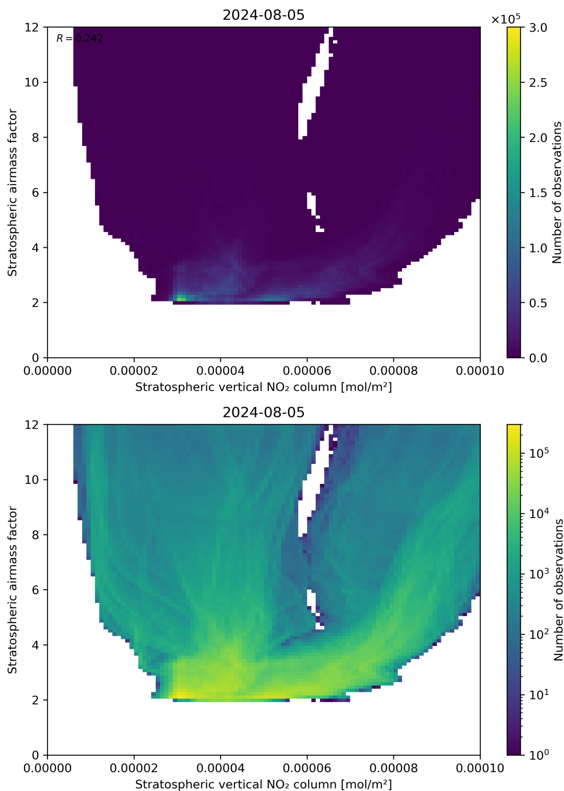
Figure 96: Scatter density plot of “Stratospheric vertical NO 2 column” against “Stratospheric airmass factor” for 2024-08-04 to 2024-08-06.
