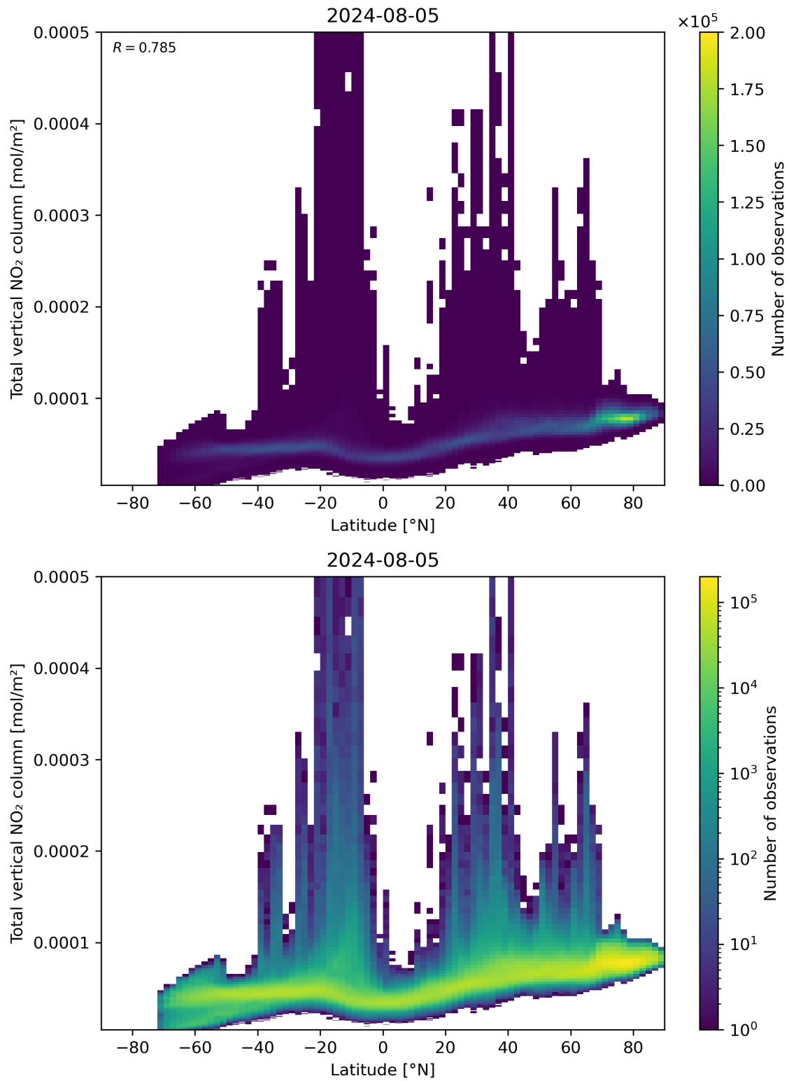
Figure 90: Scatter density plot of “Latitude” against “Total vertical NO 2 column” for 2024-08-04 to 2024-08-06.
