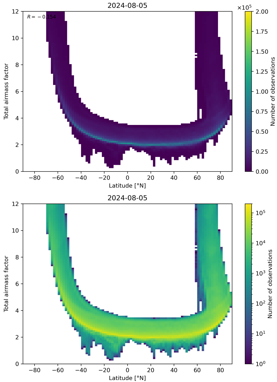
Figure 84: Scatter density plot of “Latitude” against “Total airmass factor” for 2024-08-04 to 2024-08-06.
