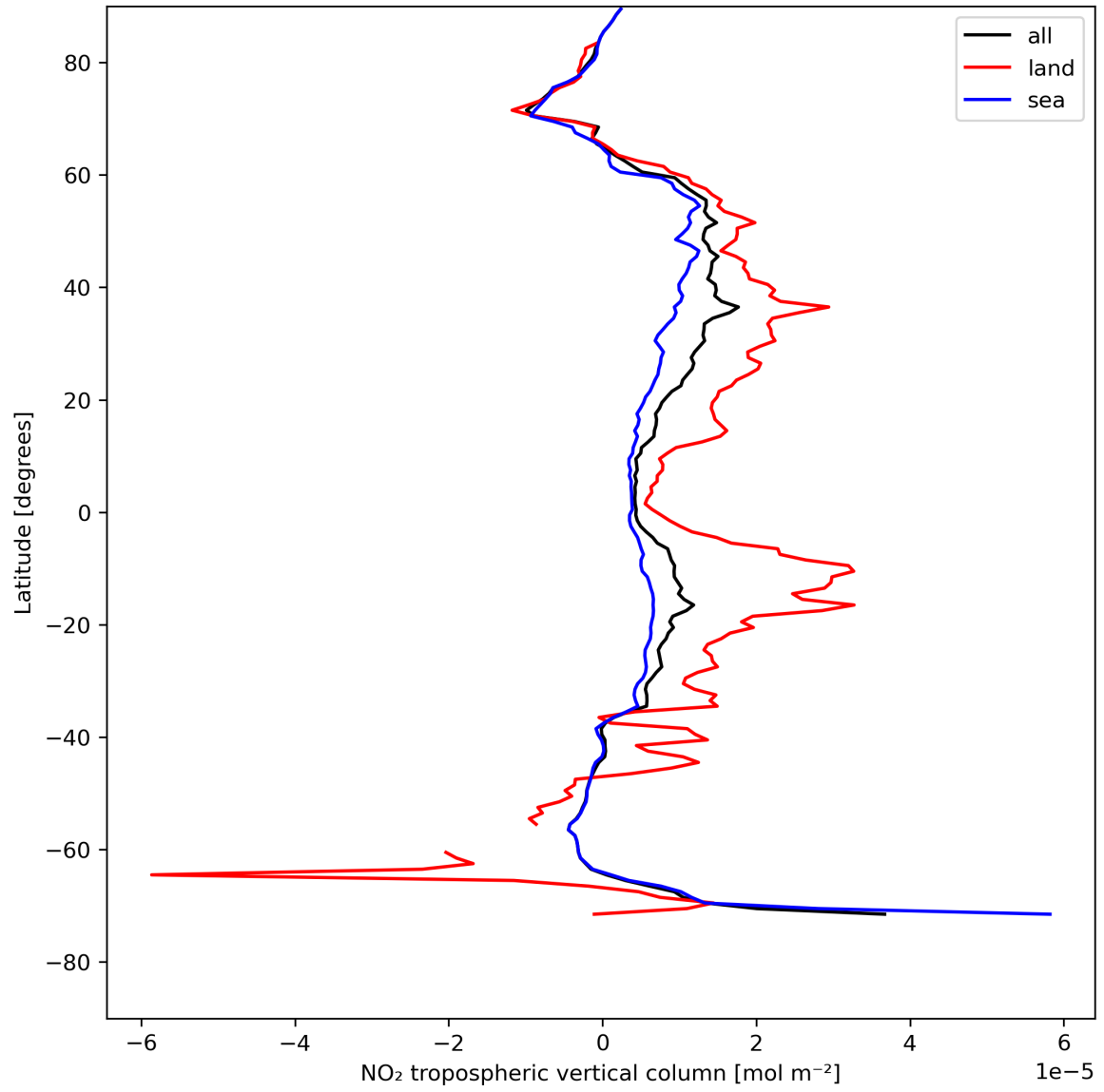
Figure 12: Zonal average of “NO 2 tropospheric vertical column” for 2024-08-04 to 2024-08-06.
