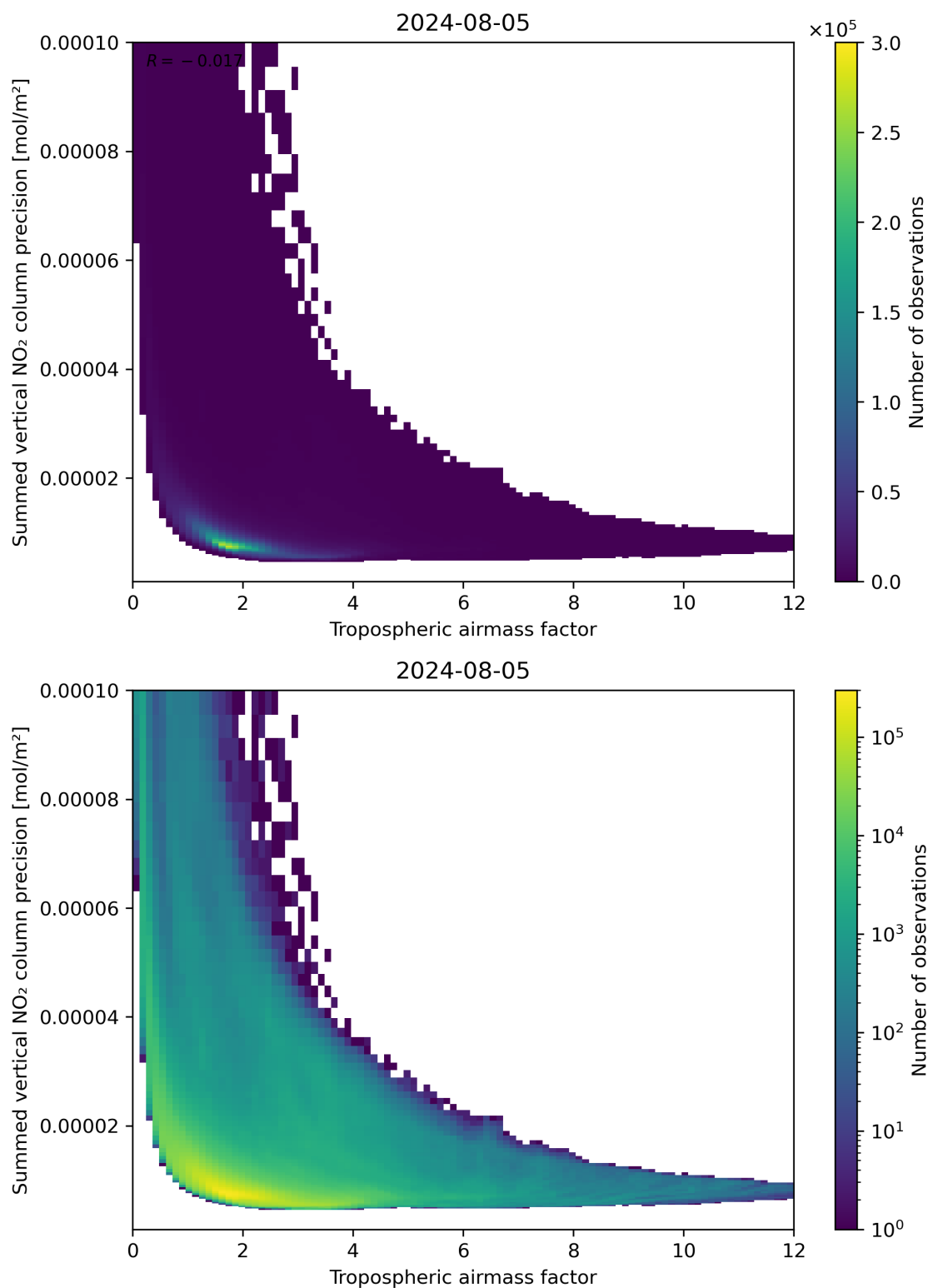
Figure 76: Scatter density plot of “Tropospheric air mass factor” against “Summed vertical NO 2 column precision” for 2024-08-04 to 2024-08-06.
