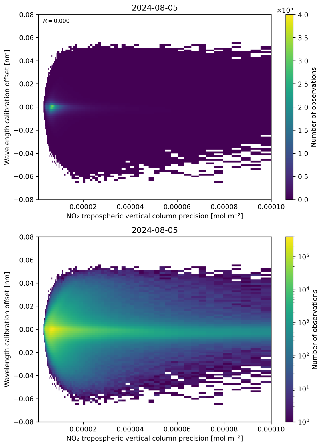
Figure 141: Scatter density plot of “NO 2 tropospheric vertical column precision” against “Wavelength calibration offset” for 2024-08-04 to 2024-08-06.
