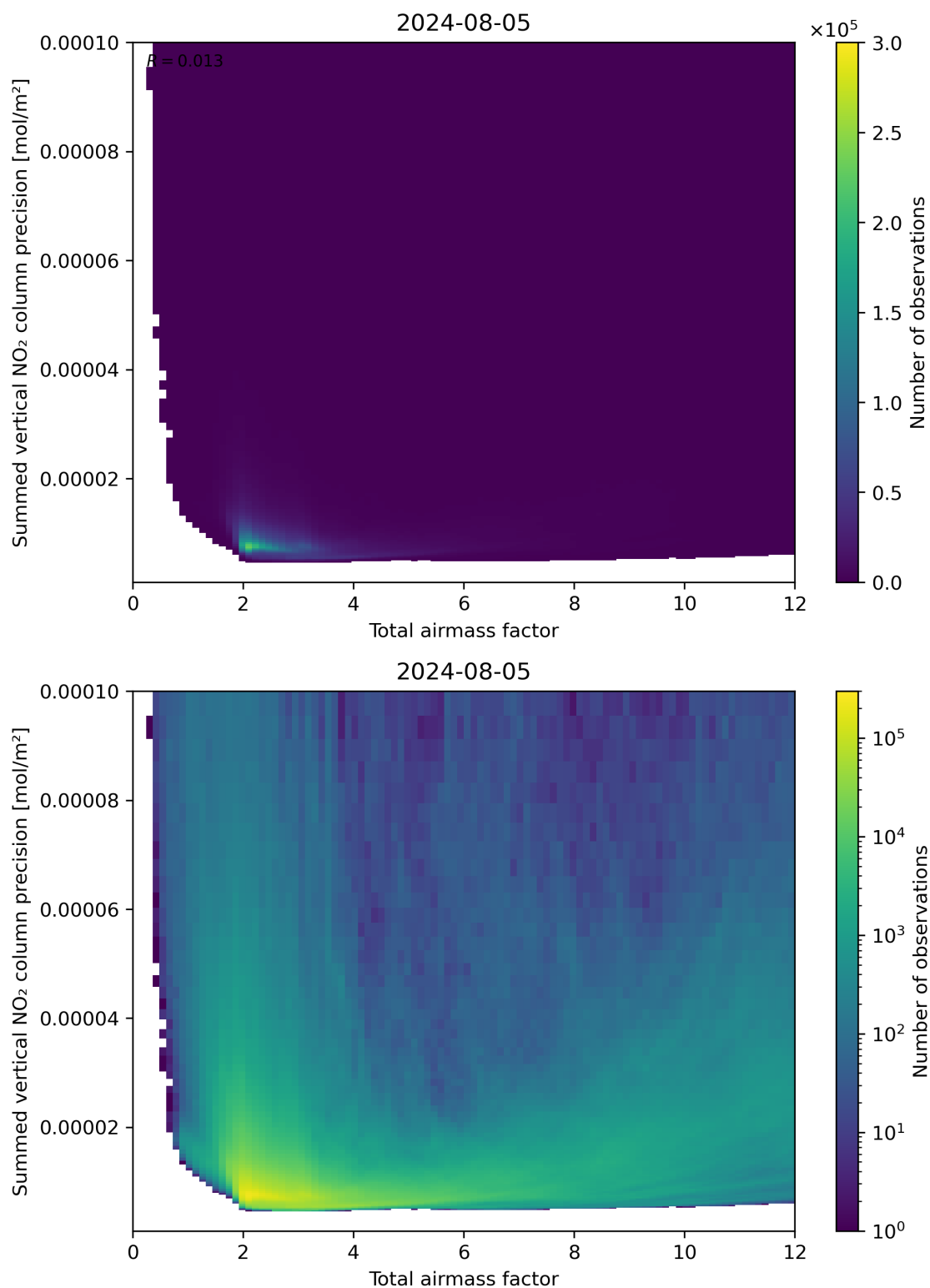
Figure 66: Scatter density plot of “Total airmass factor” against “Summed vertical NO 2 column precision” for 2024-08-04 to 2024-08-06.
