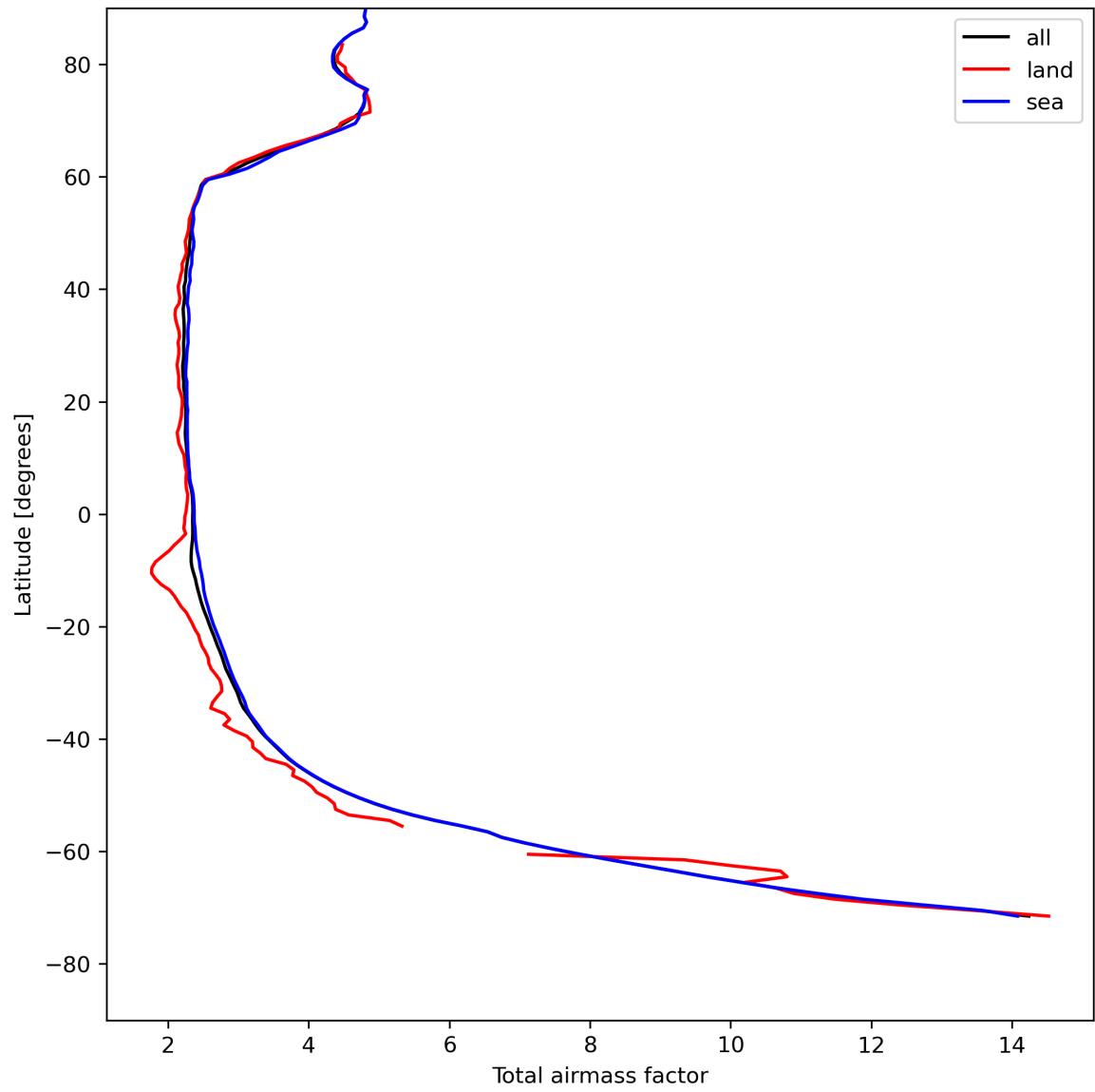
Figure 15: Zonal average of “Total airmass factor” for 2024-08-04 to 2024-08-06.
