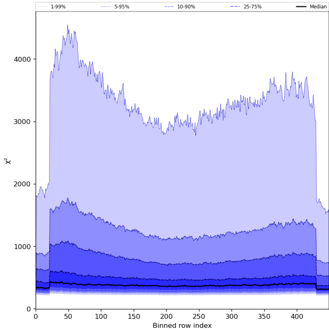
Figure 59: Along track statistics of “ \chi^2 ” for 2024-08-04 to 2024-08-06
