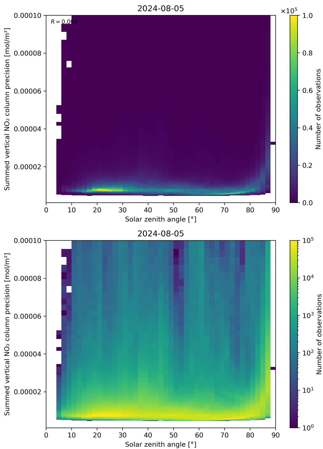
Figure 152: Scatter density plot of “Solar zenith angle” against “Summed vertical NO 2 column precision” for 2024-08-04 to 2024-08-06.
