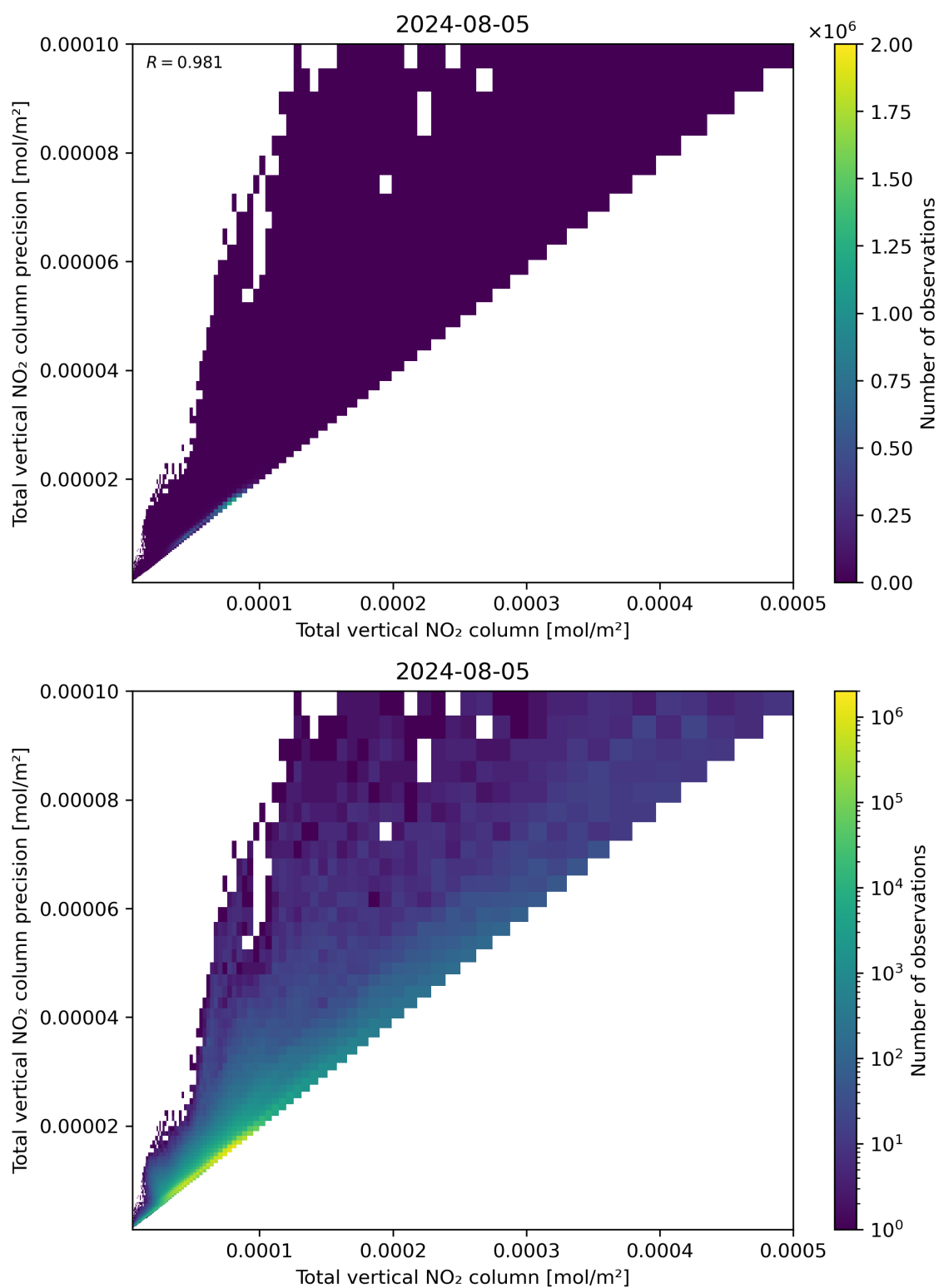
Figure 114: Scatter density plot of “Total vertical NO 2 column” against “Total vertical NO 2 column precision” for 2024-08-04 to 2024-08-06.
