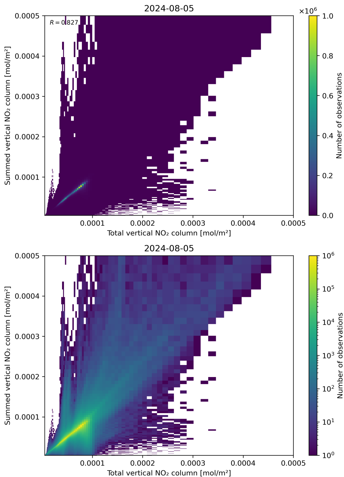
Figure 112: Scatter density plot of “Total vertical NO 2 column” against “Summed vertical NO 2 column” for 2024-08-04 to 2024-08-06.
