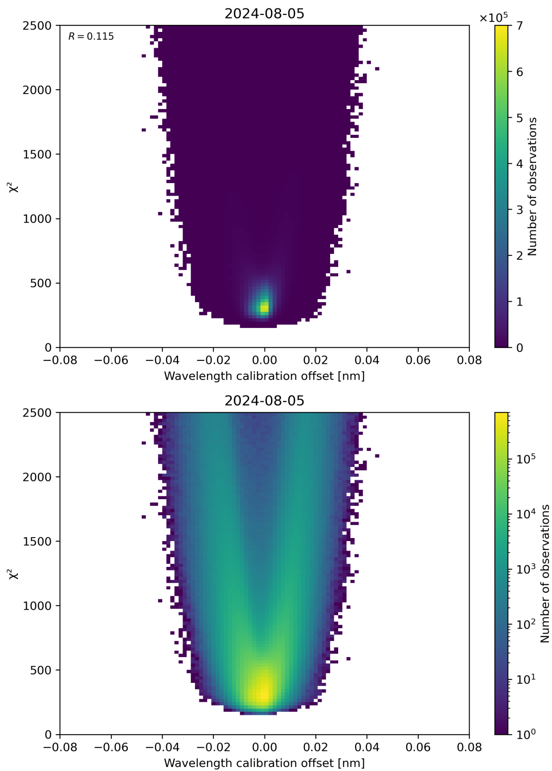
Figure 175: Scatter density plot of “Wavelength calibration offset” against “ \chi^2 ” for 2024-08-04 to 2024-08-06.
