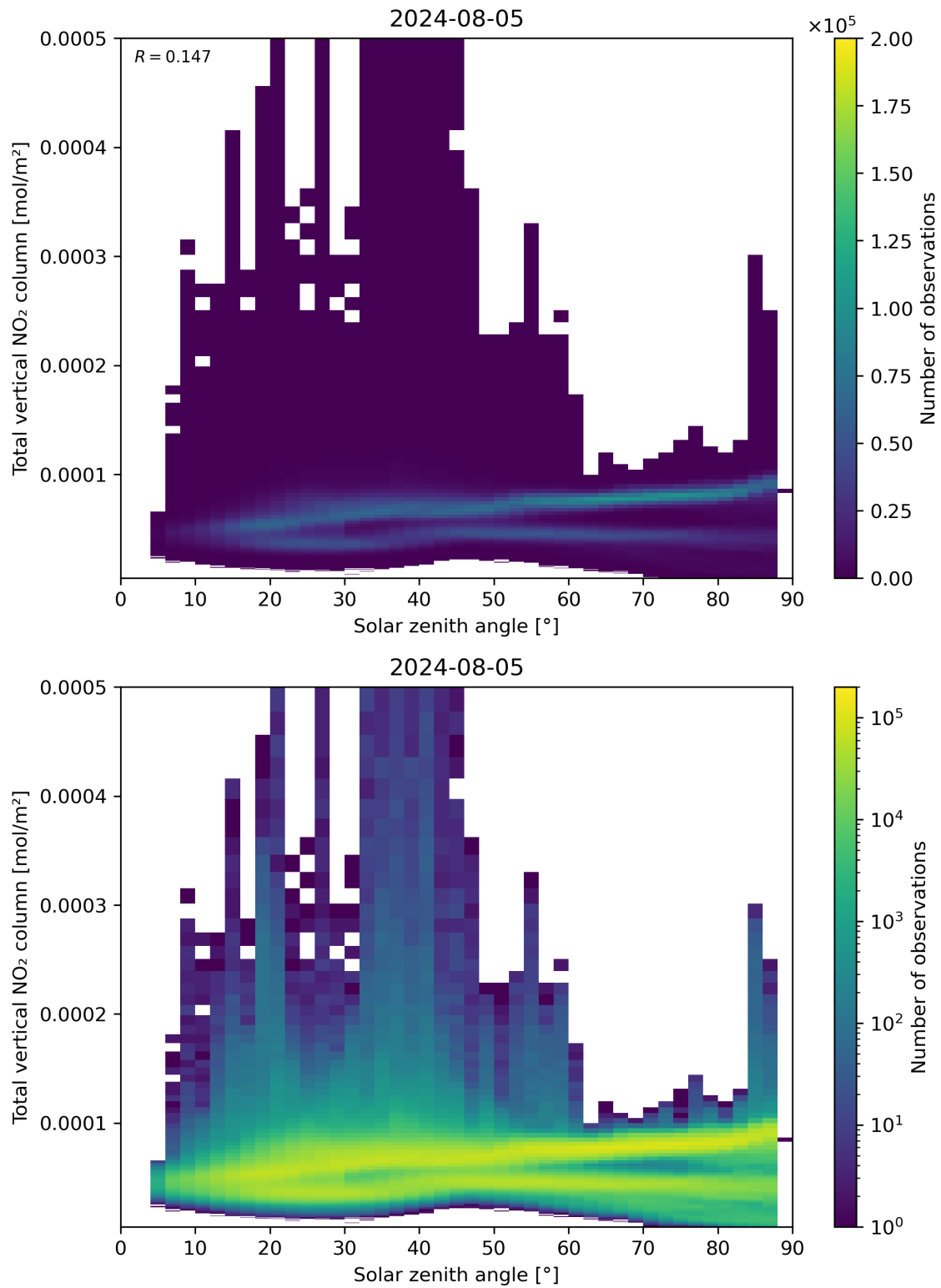
Figure 153: Scatter density plot of “Solar zenith angle” against “Total vertical NO 2 column” for 2024-08-04 to 2024-08-06.
