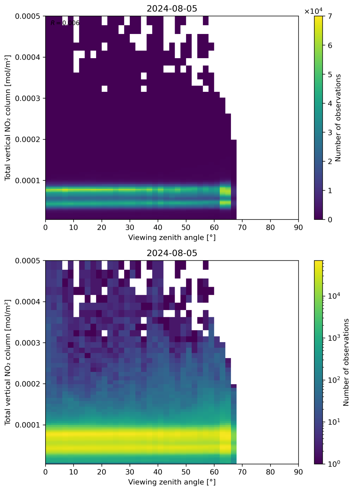
Figure 167: Scatter density plot of “Viewing zenith angle” against “Total vertical NO 2 column” for 2024-08-04 to 2024-08-06.
