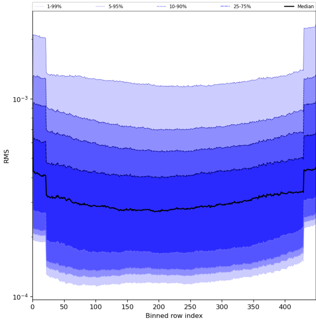
Figure 60: Along track statistics of “RMS” for 2024-08-04 to 2024-08-06
