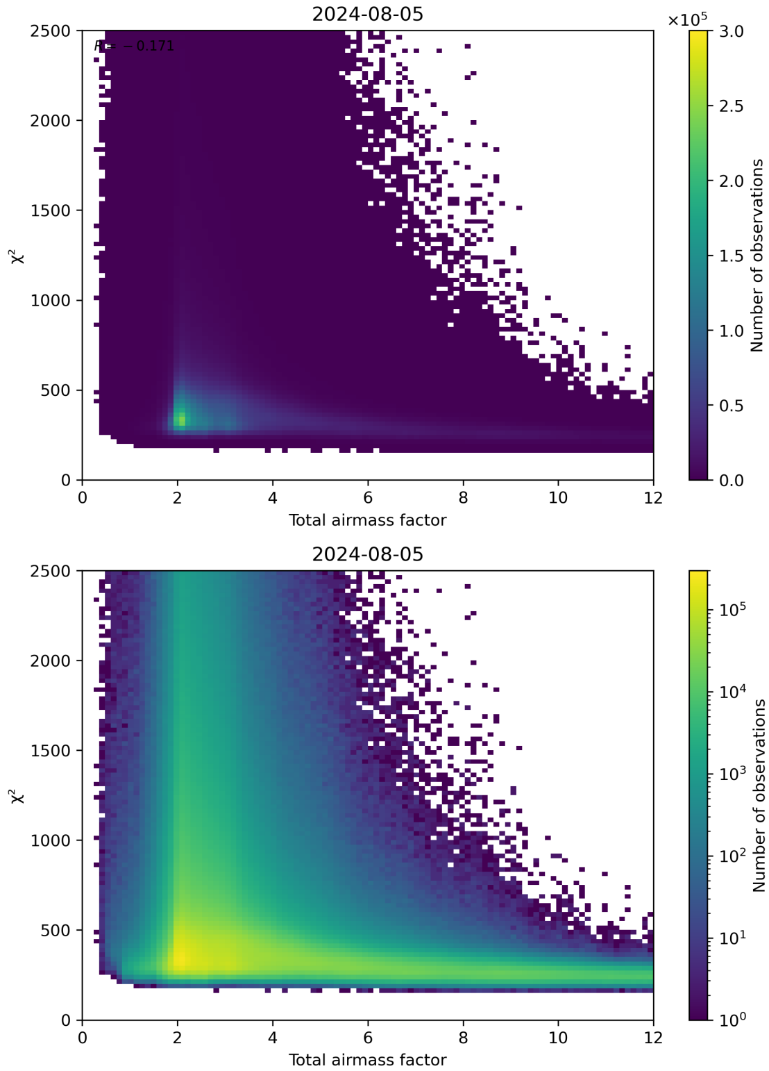
Figure 63: Scatter density plot of “Total airmass factor” against “ \chi^2 ” for 2024-08-04 to 2024-08-06.
