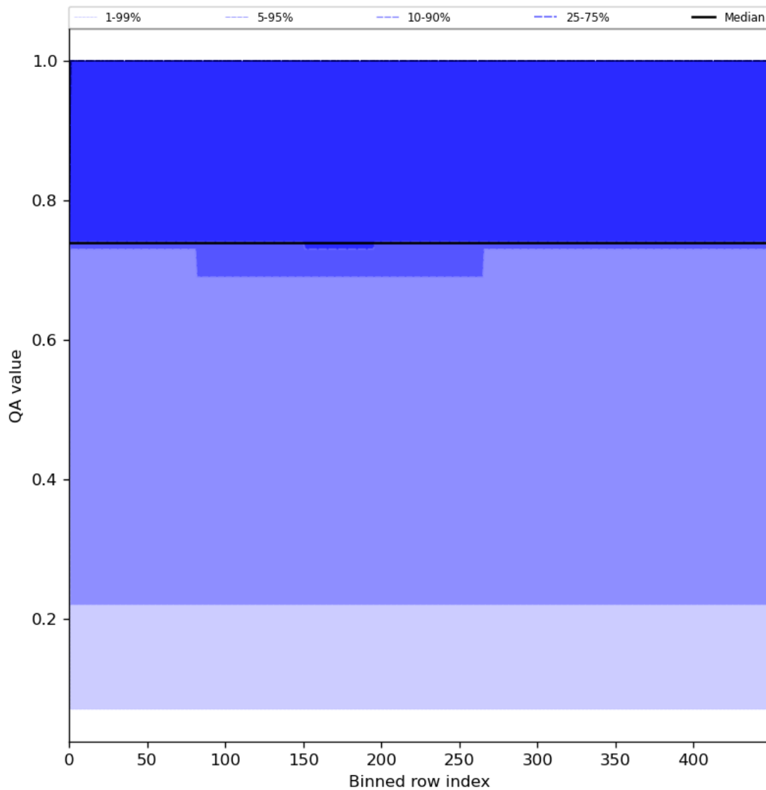
Figure 45: Along track statistics of “QA value” for 2024-08-04 to 2024-08-06
