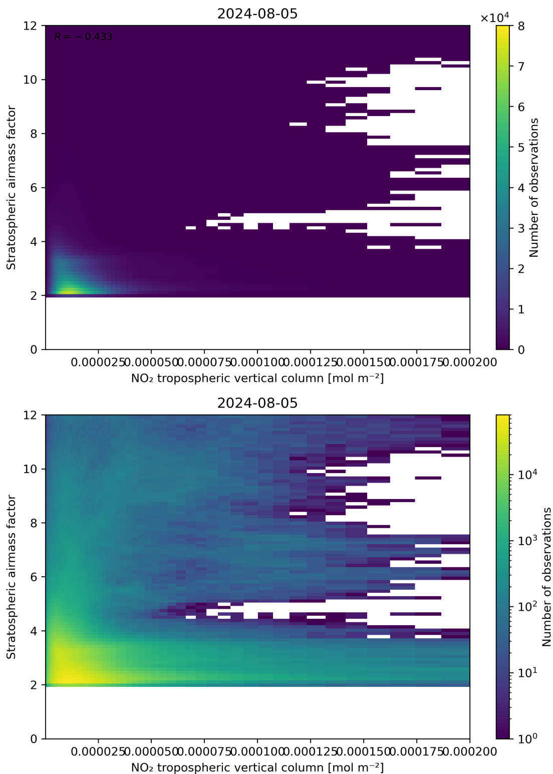
Figure 121: Scatter density plot of “NO 2 tropospheric vertical column” against “Stratospheric air mass factor” for 2024-08-04 to 2024-08-06.
