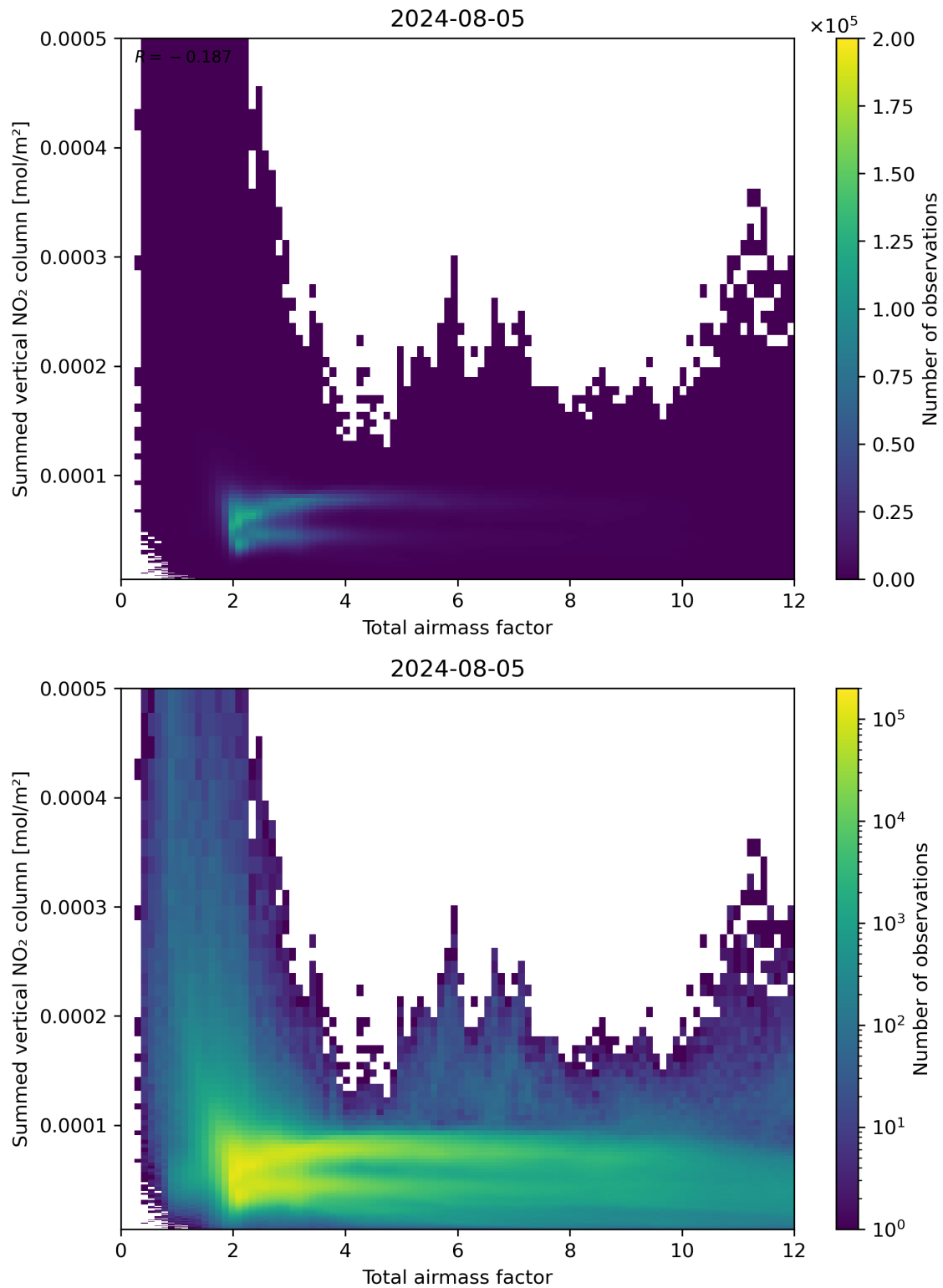
Figure 65: Scatter density plot of “Total airmass factor” against “Summed vertical NO 2 column” for 2024-08-04 to 2024-08-06.
