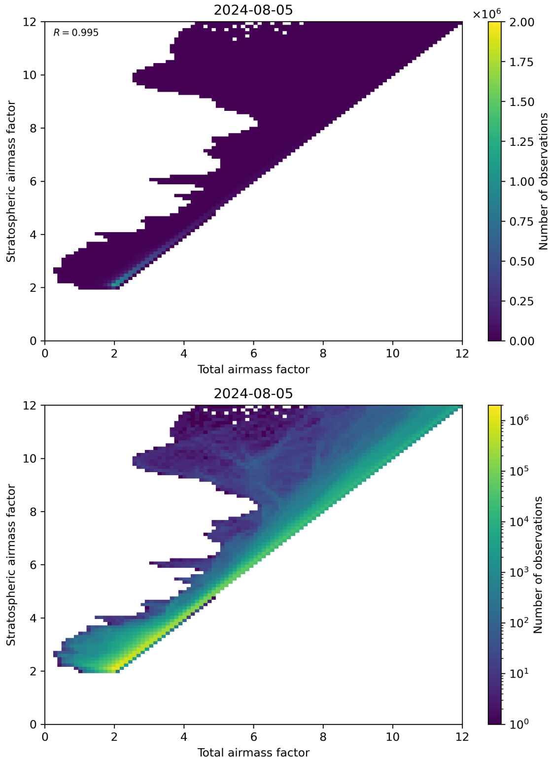
Figure 62: Scatter density plot of “Total airmass factor” against “Stratospheric airmass factor” for 2024-08-04 to 2024-08-06.
