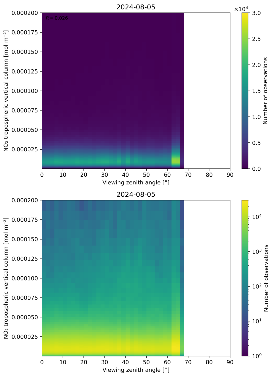
Figure 169: Scatter density plot of “Viewing zenith angle” against “NO 2 tropospheric vertical column” for 2024-08-04 to 2024-08-06.
