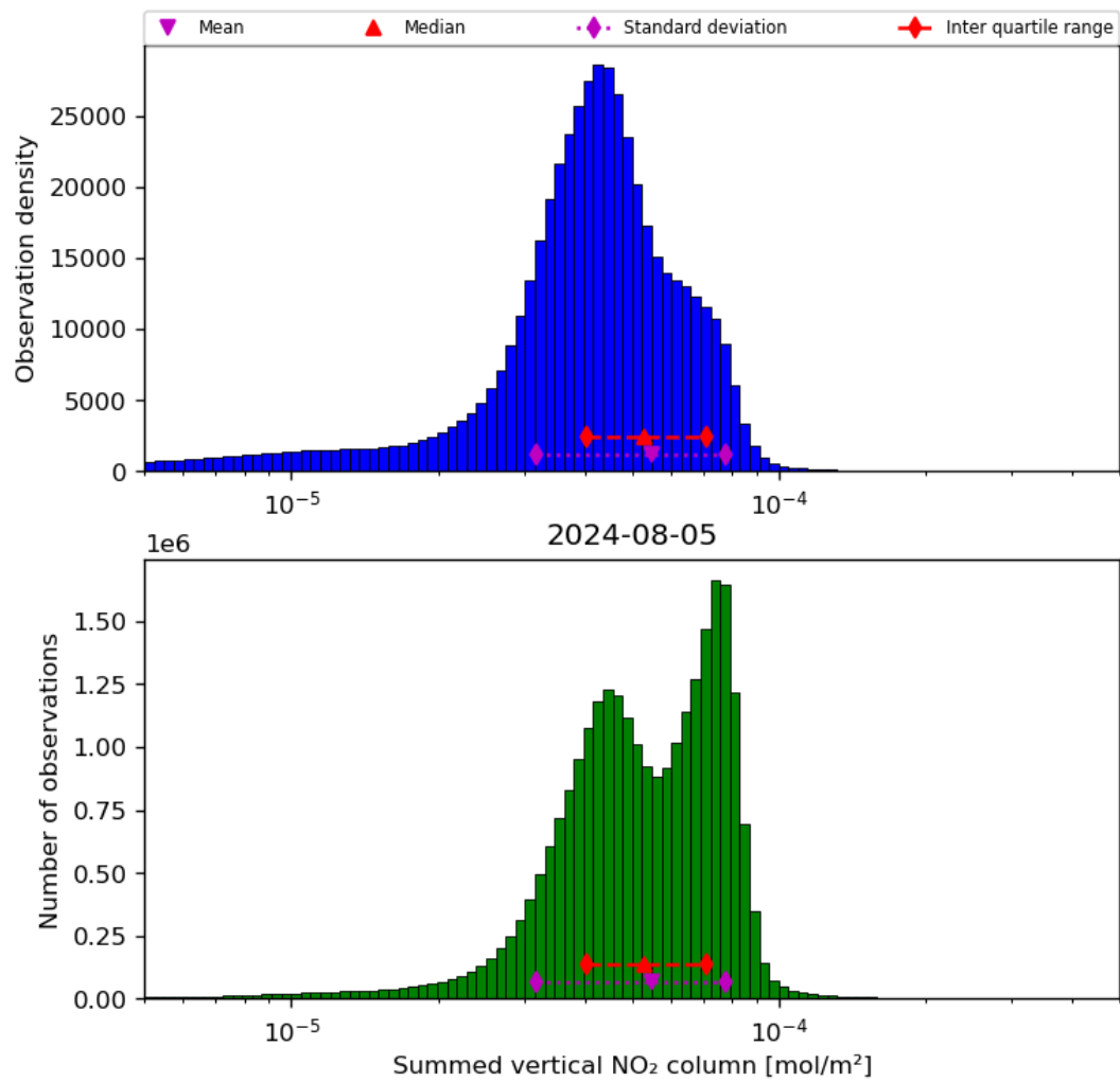
Figure 40: Histogram of “Summed vertical NO 2 column” for 2024-08-04 to 2024-08-06
