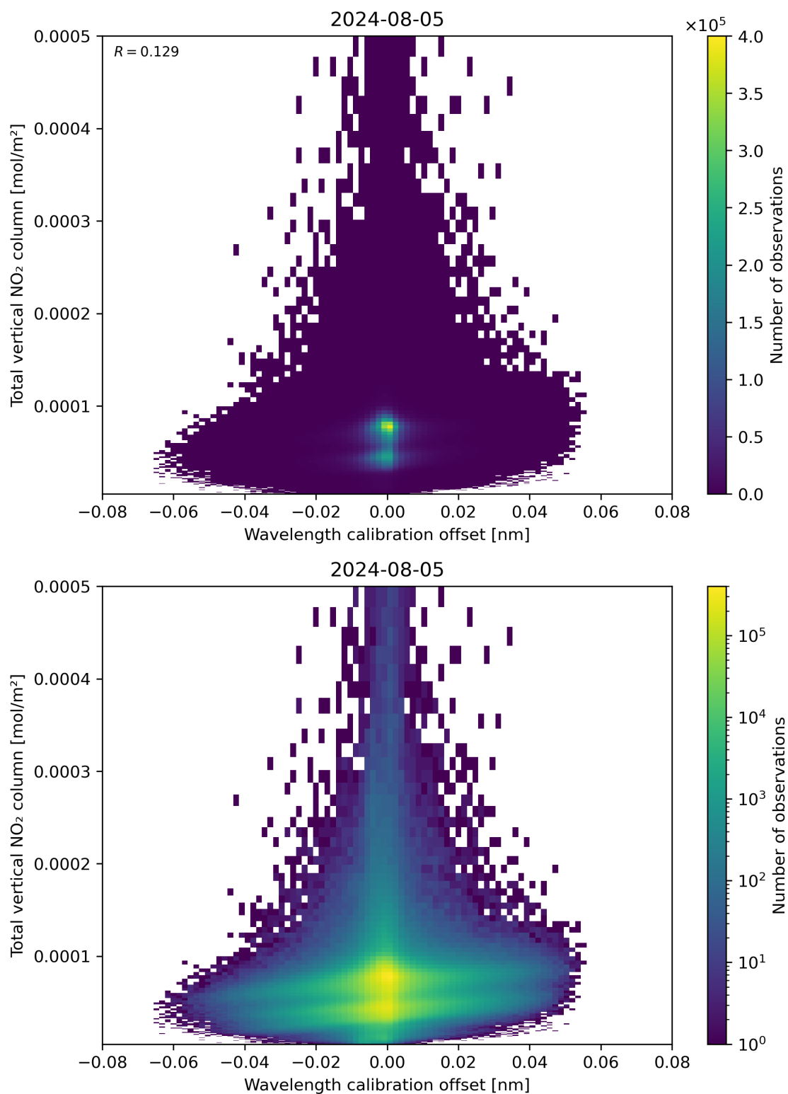
Figure 179: Scatter density plot of “Wavelength calibration offset” against “Total vertical NO 2 column” for 2024-08-04 to 2024-08-06.
