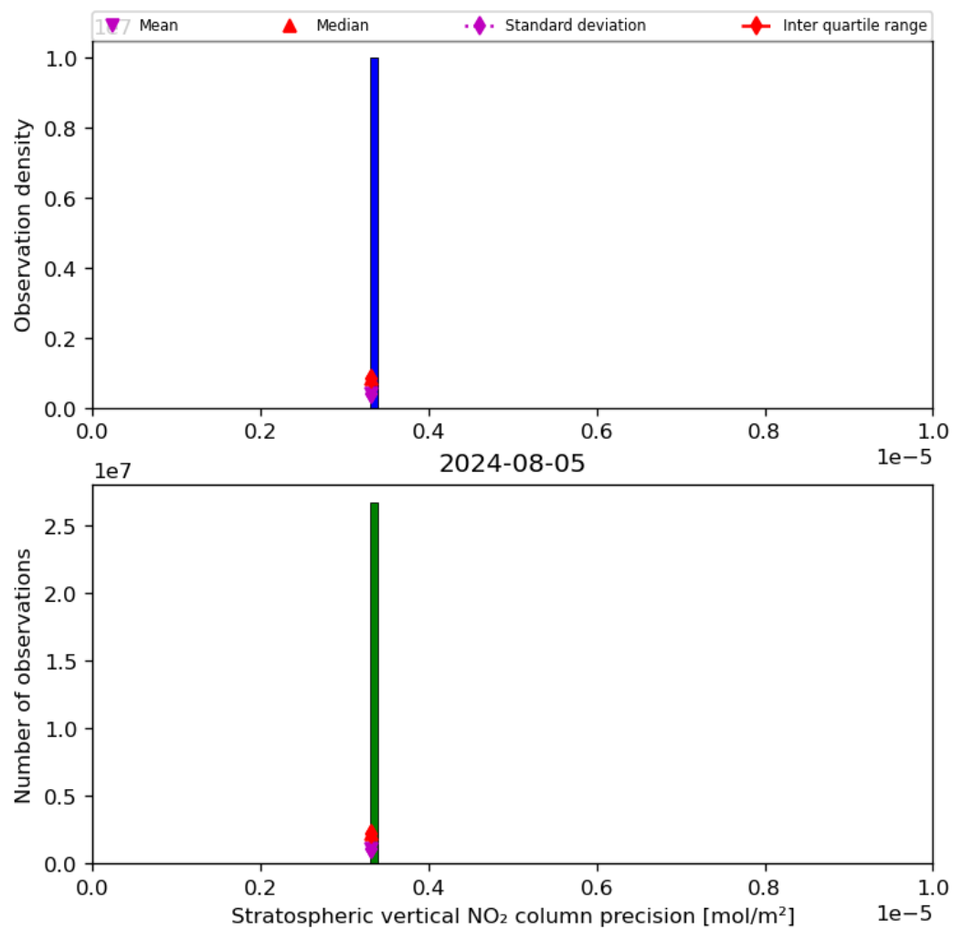
Figure 37: Histogram of “Stratospheric vertical NO 2 column precision” for 2024-08-04 to 2024-08-06
