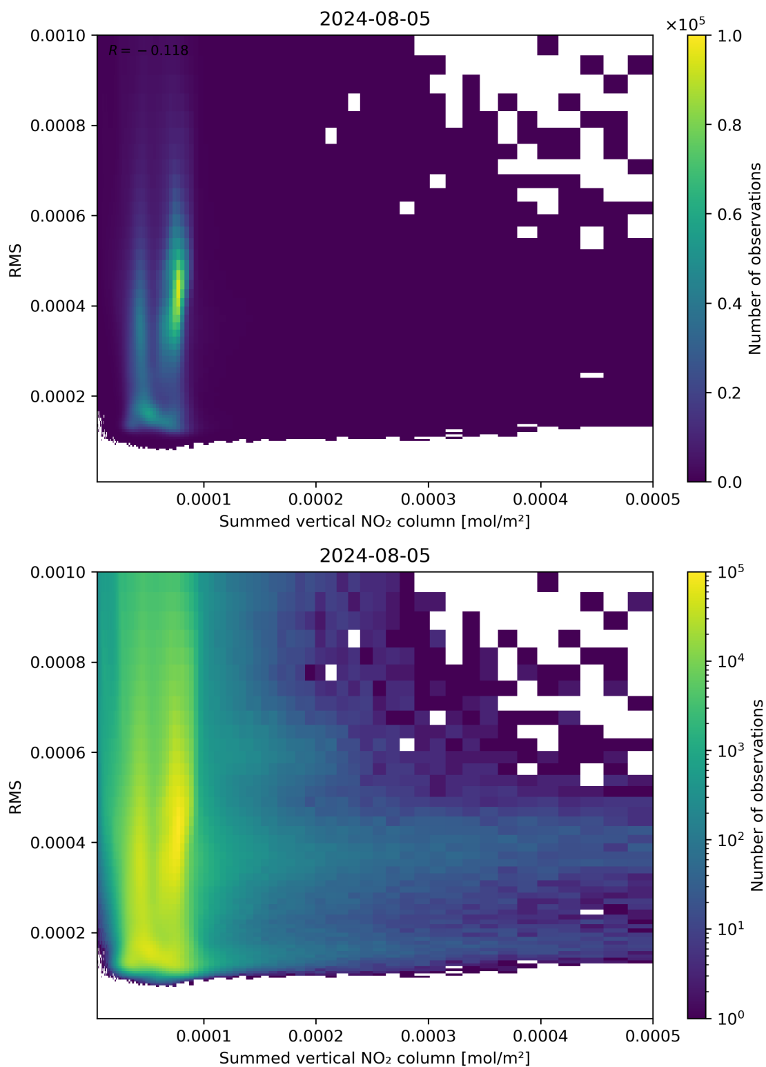
Figure 109: Scatter density plot of “Summed vertical NO 2 column” against “RMS” for 2024-08-04 to 2024-08-06.
