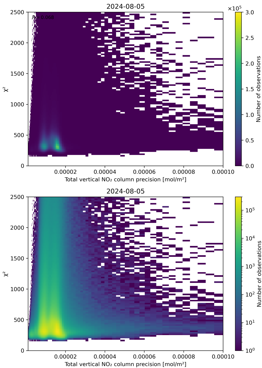
Figure 116: Scatter density plot of “Total vertical NO 2 column precision” against “ \chi^2 ” for 2024-08-04 to 2024-08-06.
