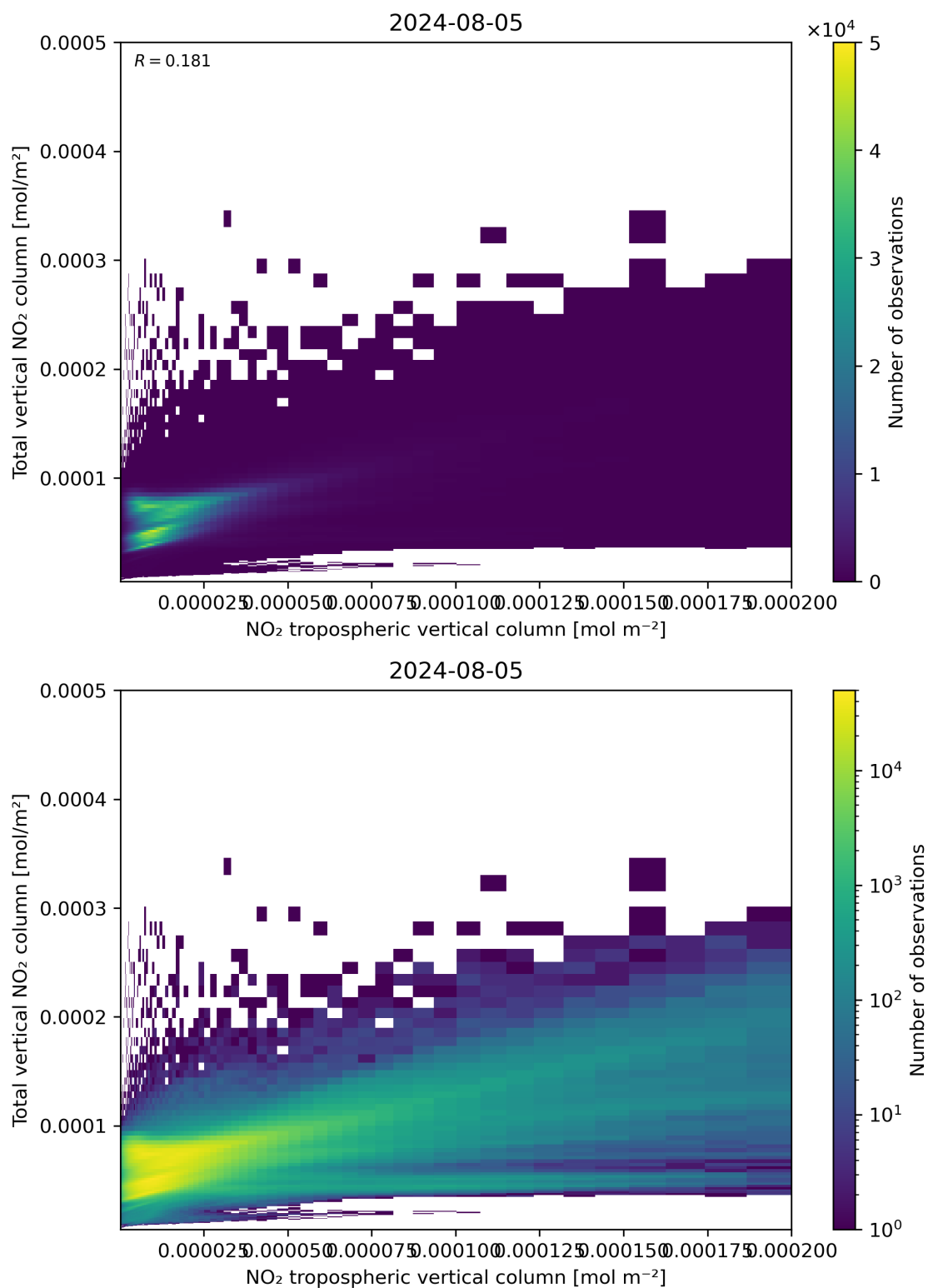
Figure 128: Scatter density plot of “NO 2 tropospheric vertical column” against “Total vertical NO 2 column” for 2024-08-04 to 2024-08-06.
