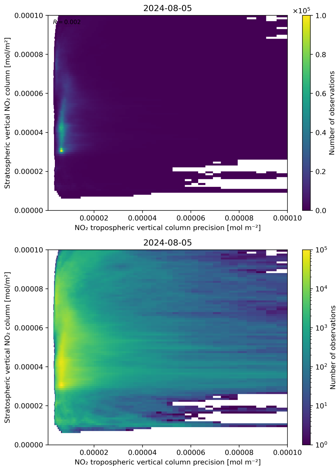
Figure 135: Scatter density plot of “NO 2 tropospheric vertical column precision” against “Stratospheric vertical NO 2 column” for 2024-08-04 to 2024-08-06.
