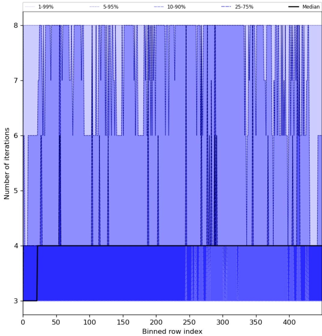
Figure 51: Along track statistics of "Number of iterations" for 2024-08-04 to 2024-08-06
