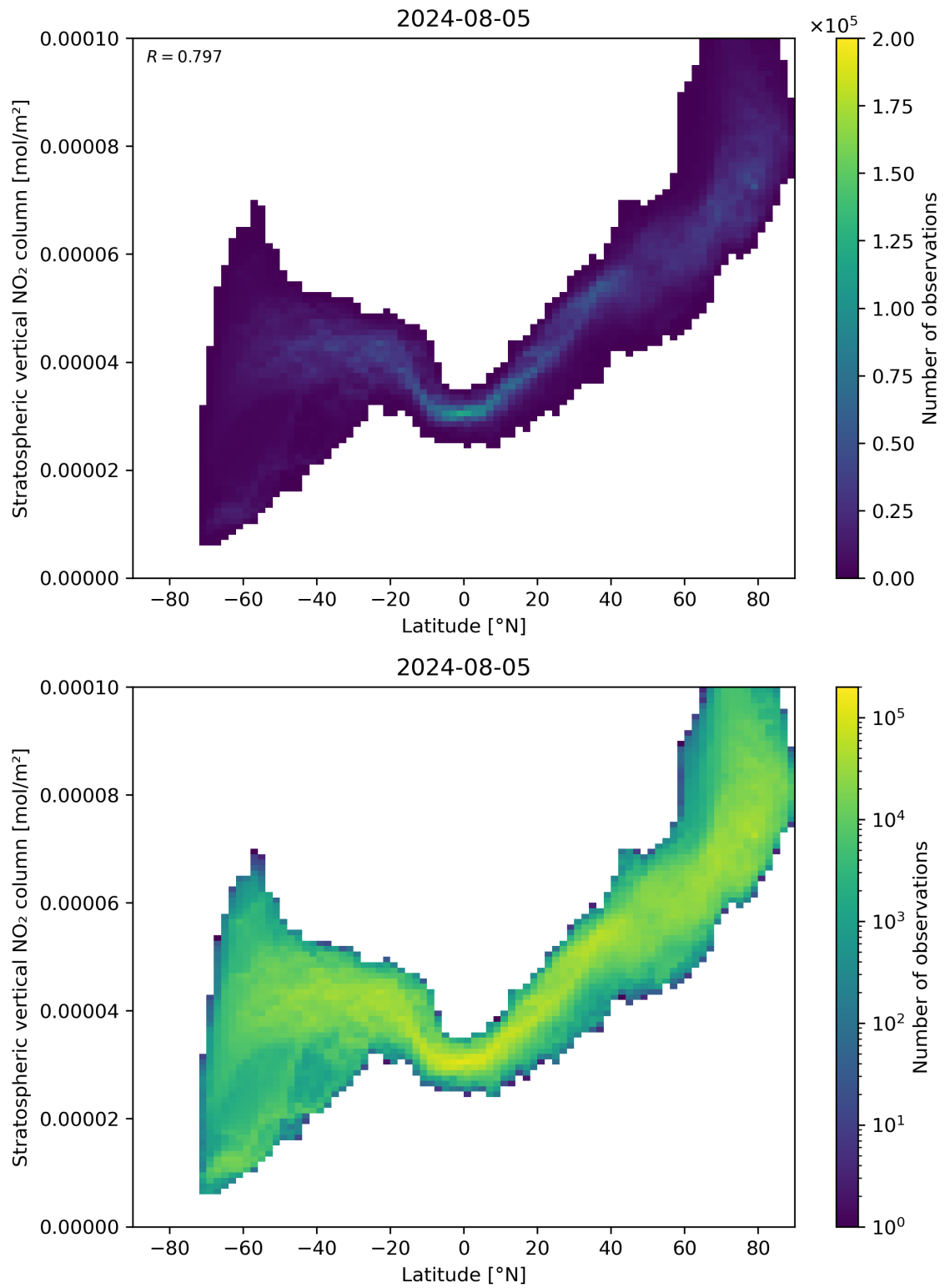
Figure 87: Scatter density plot of “Latitude” against “Stratospheric vertical \text{NO}_2 column” for 2024-08-04 to 2024-08-06.
