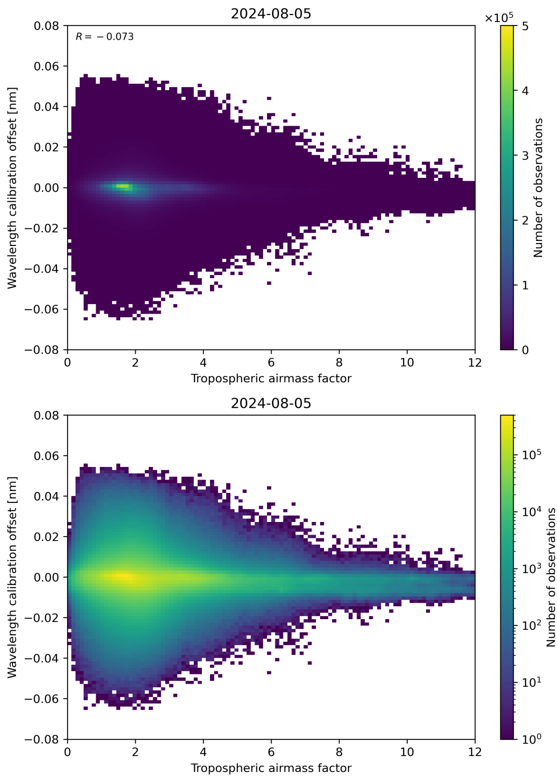
Figure 80: Scatter density plot of “Tropospheric airmass factor” against “Wavelength calibration offset” for 2024-08-04 to 2024-08-06.
