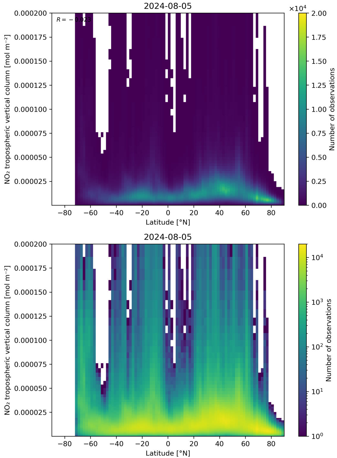
Figure 92: Scatter density plot of “Latitude” against “NO 2 tropospheric vertical column” for 2024-08-04 to 2024-08-06.
