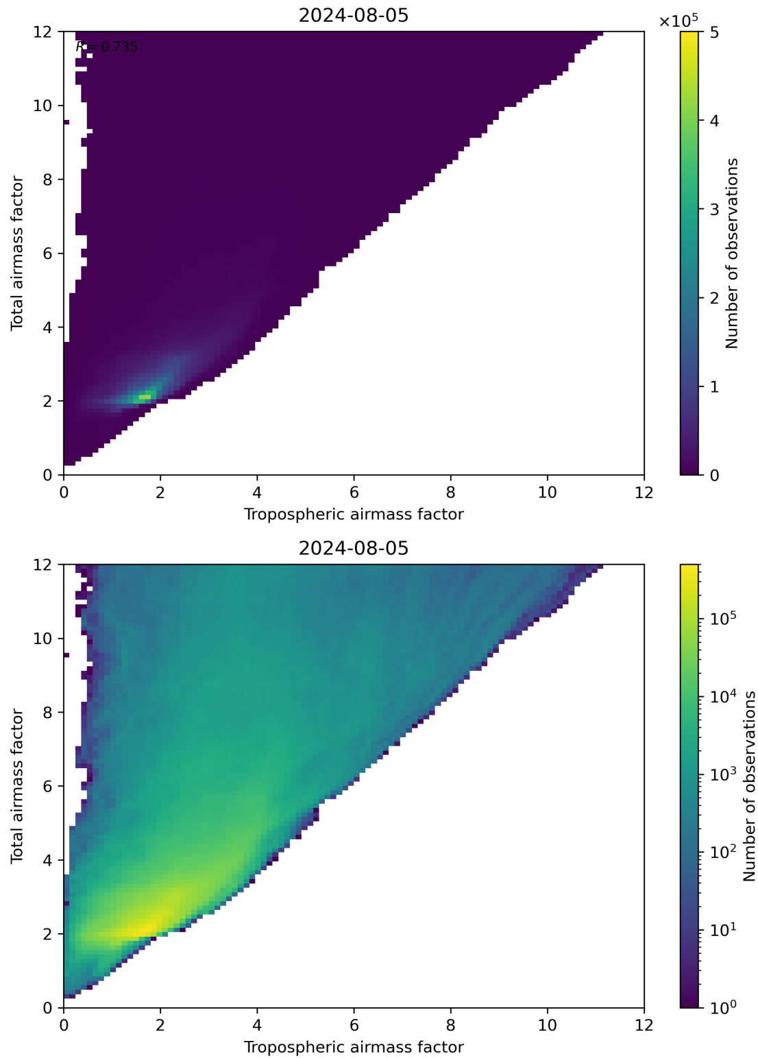
Figure 72: Scatter density plot of “Tropospheric airmass factor” against “Total airmass factor” for 2024-08-04 to 2024-08-06.
