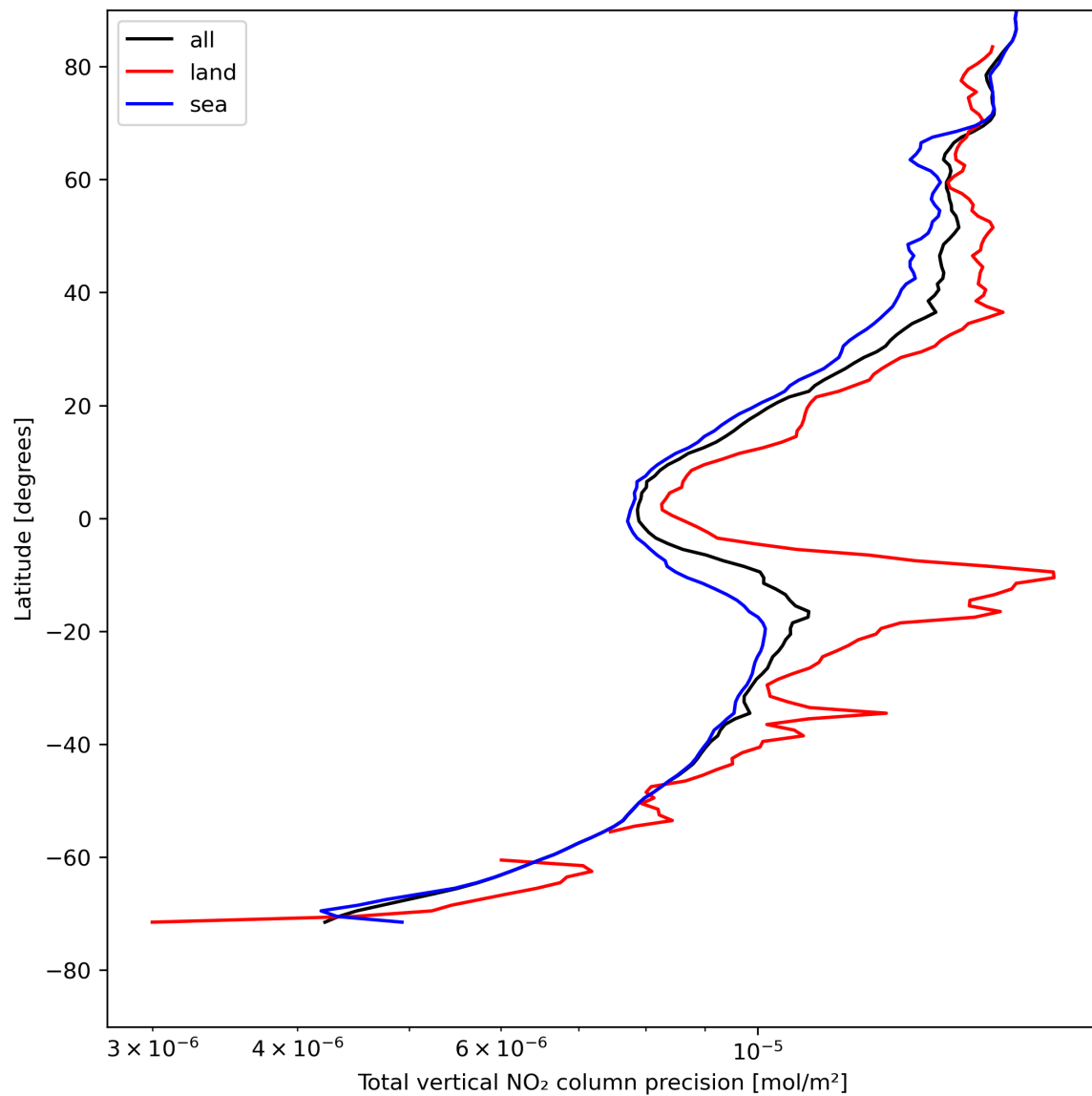
Figure 22: Zonal average of “Total vertical NO 2 column precision” for 2024-08-04 to 2024-08-06.
