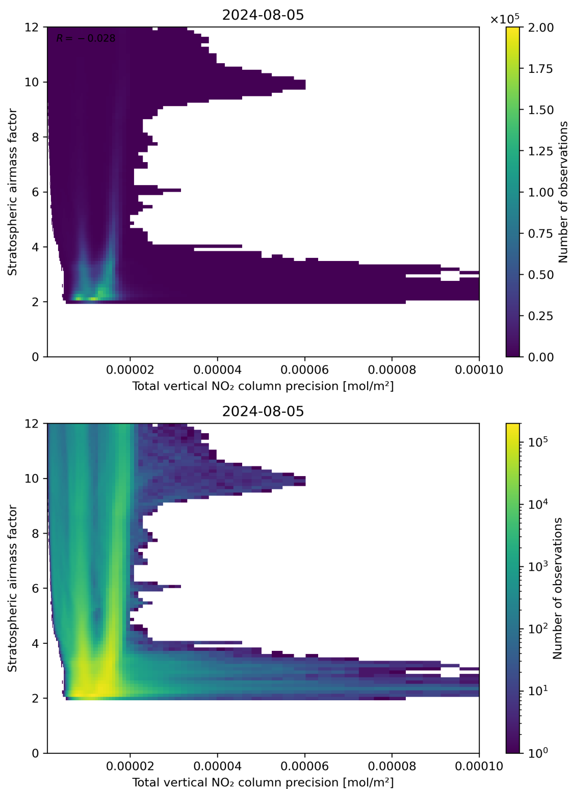
Figure 115: Scatter density plot of “Total vertical NO 2 column precision” against “Stratospheric air mass factor” for 2024-08-04 to 2024-08-06.
