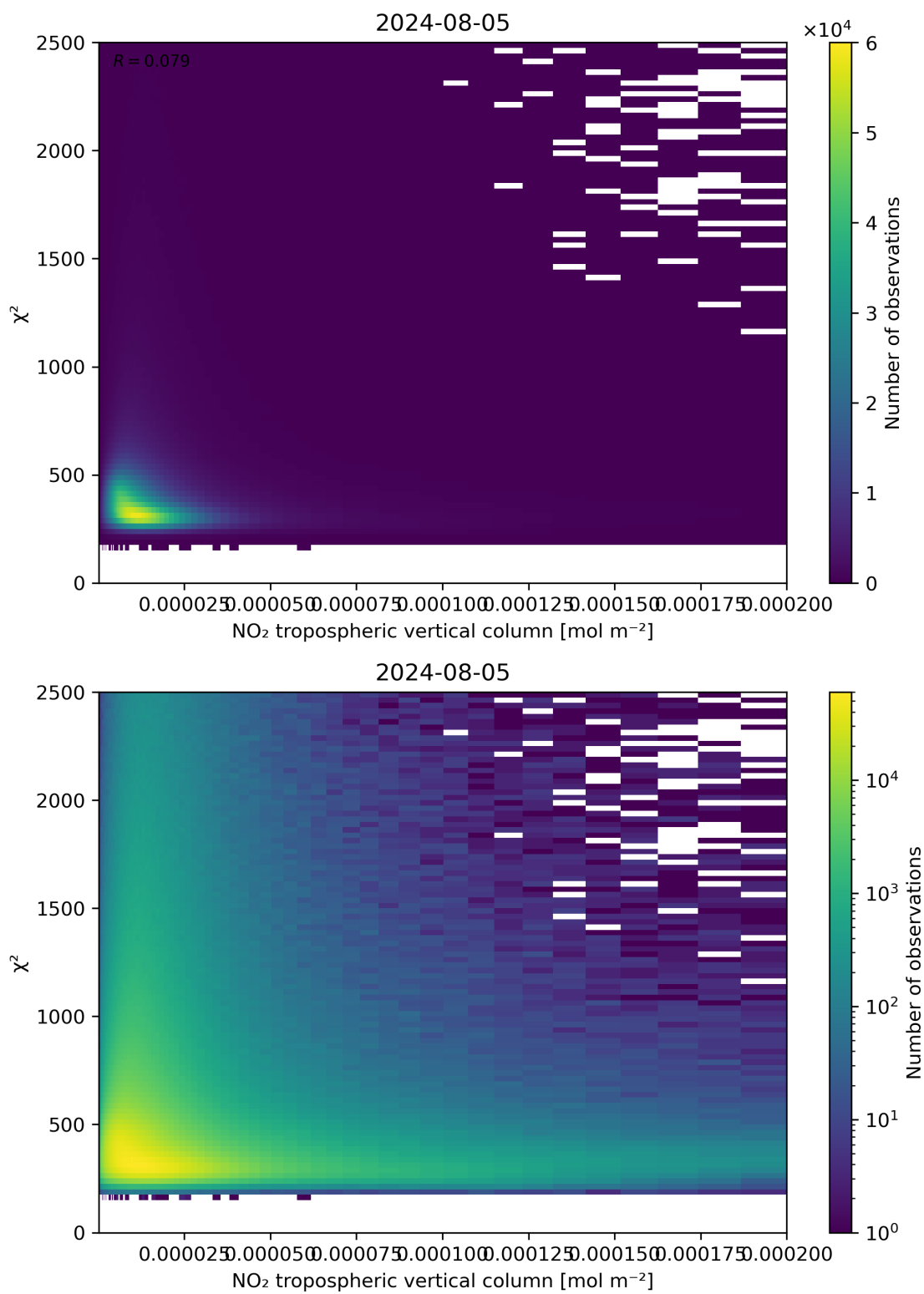
Figure 124: Scatter density plot of “NO 2 tropospheric vertical column” against “ \chi^2 ” for 2024-08-04 to 2024-08-06.
