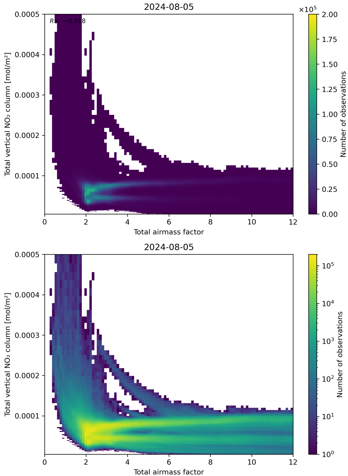
Figure 67: Scatter density plot of “Total airmass factor” against “Total vertical NO 2 column” for 2024-08-04 to 2024-08-06.
