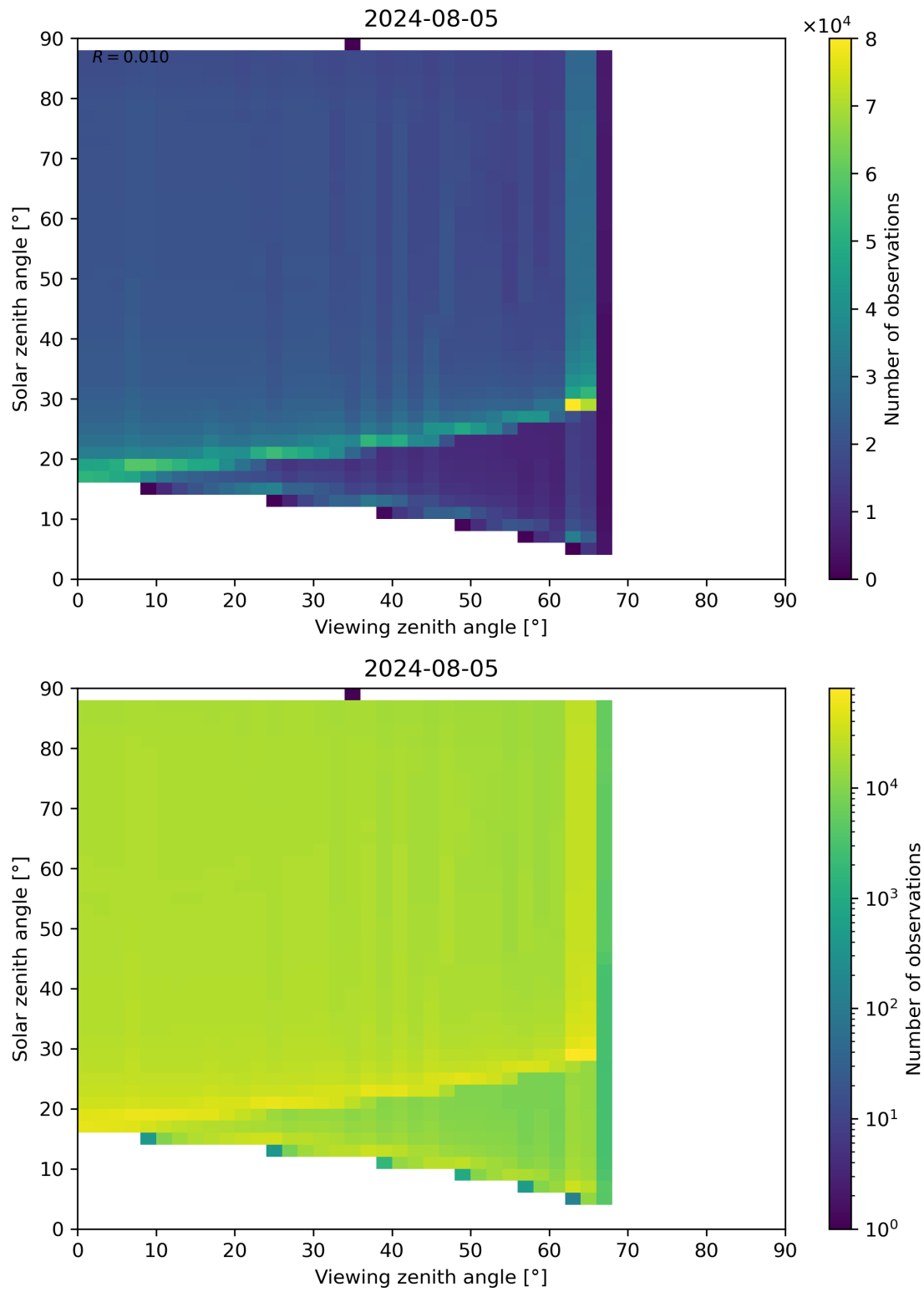
Figure 172: Scatter density plot of “Viewing zenith angle” against “Solar zenith angle” for 2024-08-04 to 2024-08-06.
