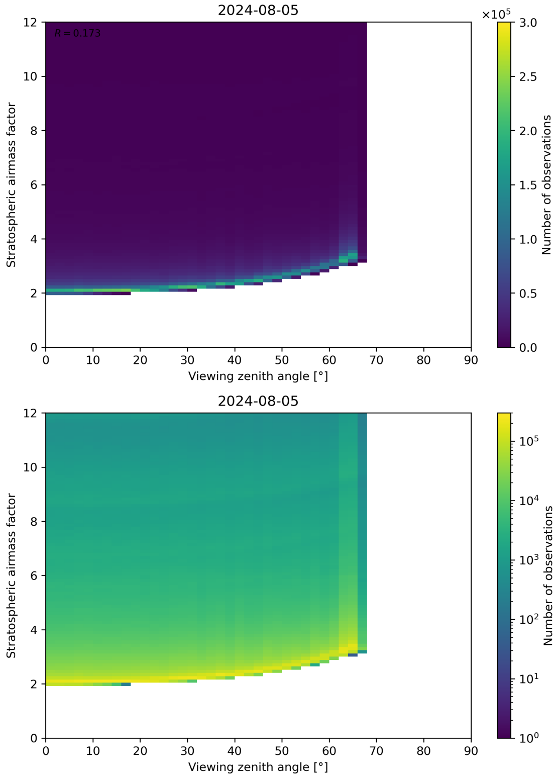
Figure 159: Scatter density plot of “Viewing zenith angle” against “Stratospheric airmass factor” for 2024-08-04 to 2024-08-06.
