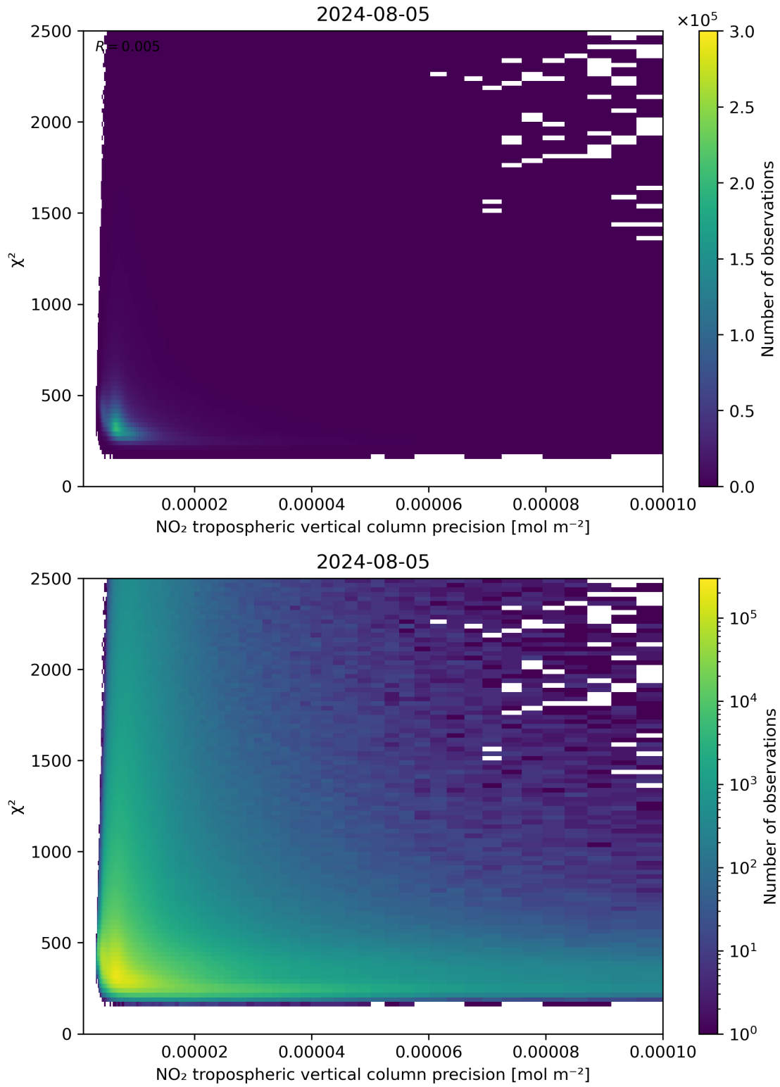
Figure 134: Scatter density plot of “NO 2 tropospheric vertical column precision” against “ \chi^2 ” for 2024-08-04 to 2024-08-06.
