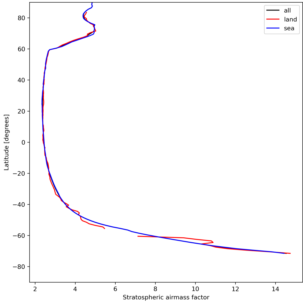
Figure 27: Zonal average of “Stratospheric air mass factor” for 2024-08-04 to 2024-08-06.
