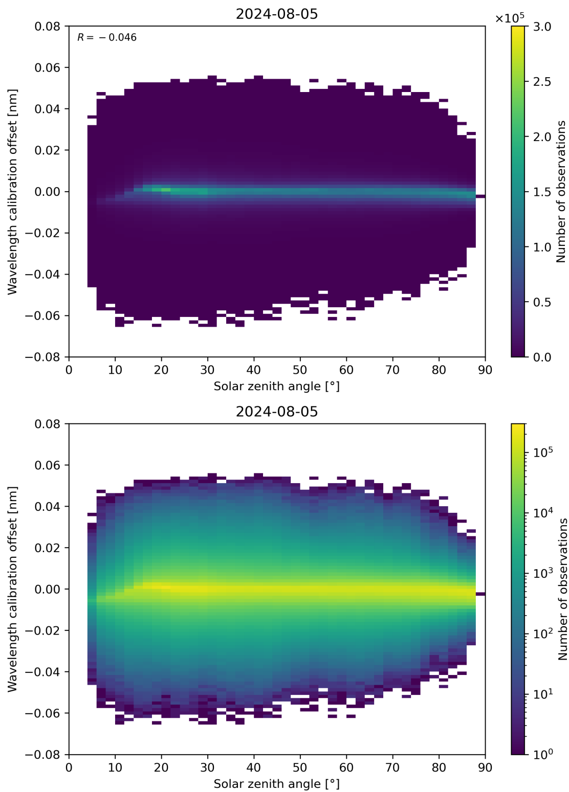
Figure 158: Scatter density plot of “Solar zenith angle” against “Wavelength calibration offset” for 2024-08-04 to 2024-08-06.
