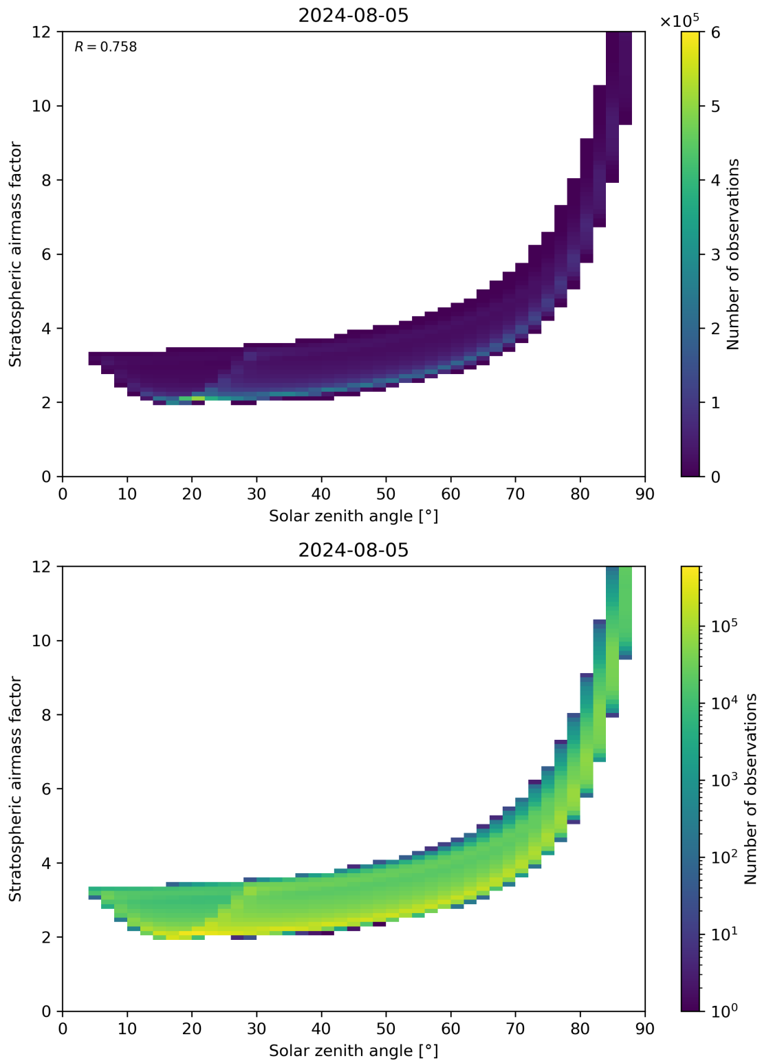
Figure 145: Scatter density plot of “Solar zenith angle” against “Stratospheric airmass factor” for 2024-08-04 to 2024-08-06.
