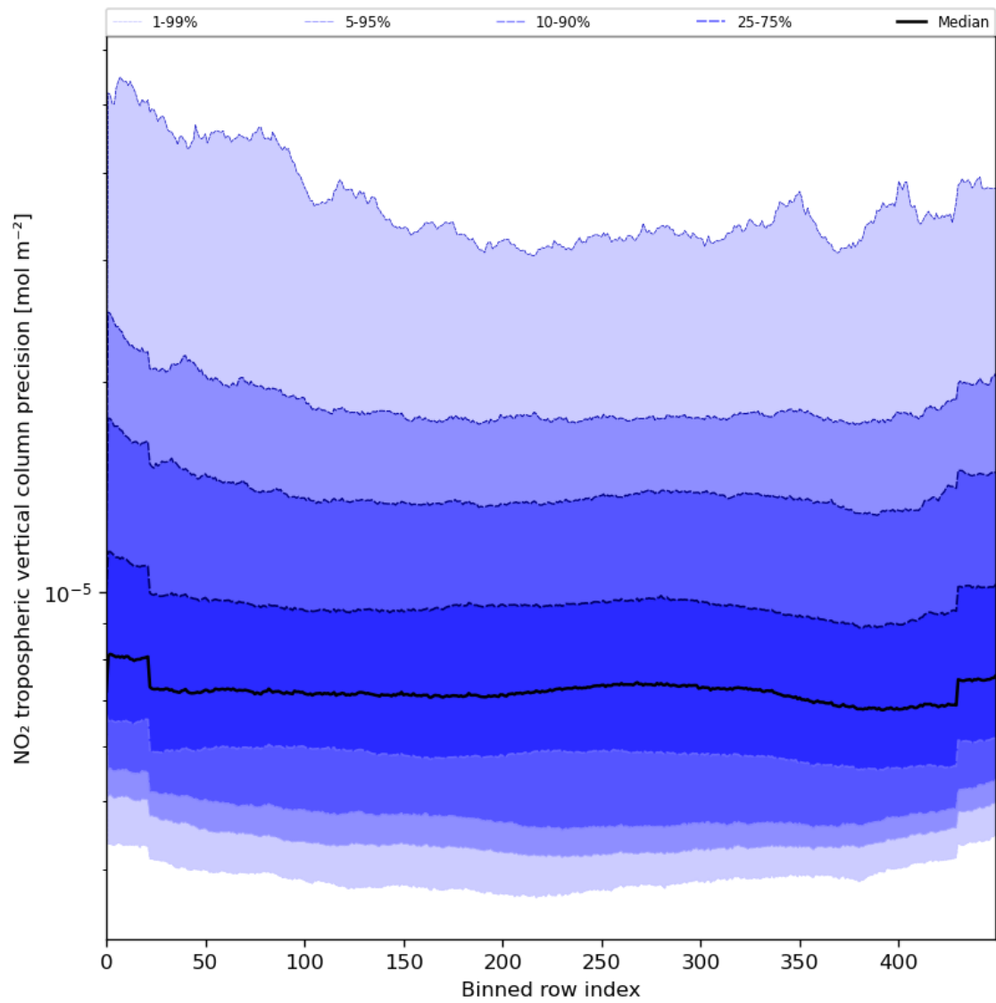
Figure 47: Along track statistics of “NO 2 tropospheric vertical column precision” for 2024-08-04 to 2024-08-06
