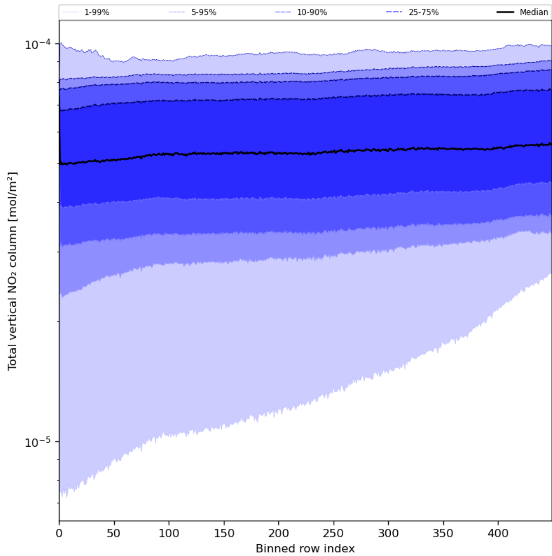
Figure 55: Along track statistics of “Total vertical NO 2 column” for 2024-08-04 to 2024-08-06
