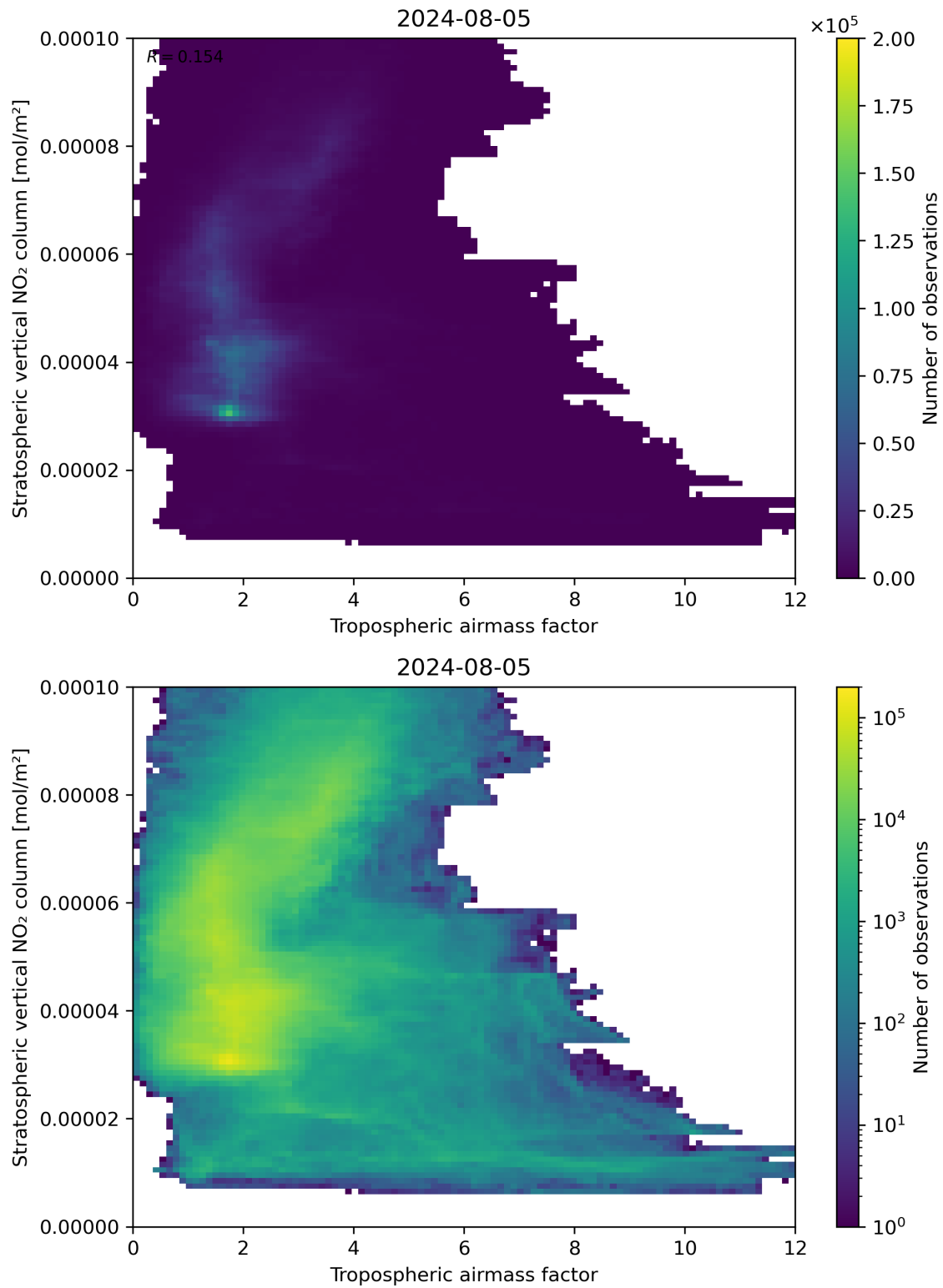
Figure 74: Scatter density plot of “Tropospheric air mass factor” against “Stratospheric vertical NO 2 column” for 2024-08-04 to 2024-08-06.
