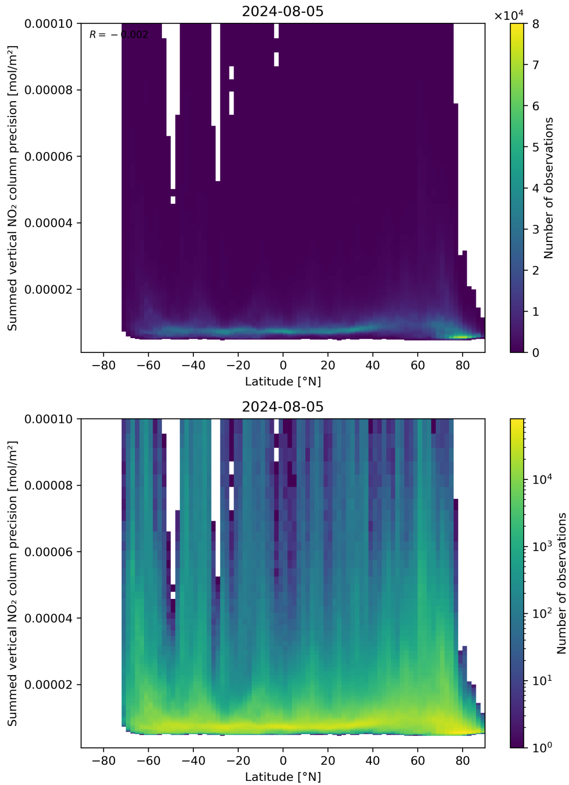
Figure 89: Scatter density plot of “Latitude” against “Summed vertical NO 2 column precision” for 2024-08-04 to 2024-08-06.
