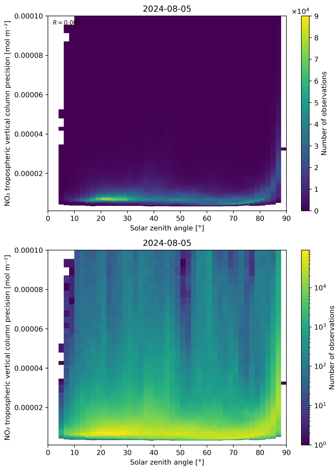
Figure 156: Scatter density plot of “Solar zenith angle” against “NO 2 tropospheric vertical column precision” for 2024-08-04 to 2024-08-06.
