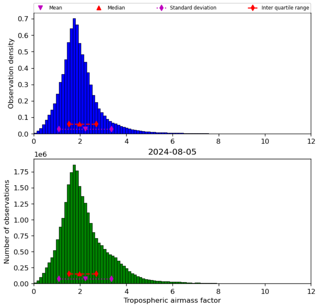
Figure 31: Histogram of “Tropospheric airmass factor” for 2024-08-04 to 2024-08-06
