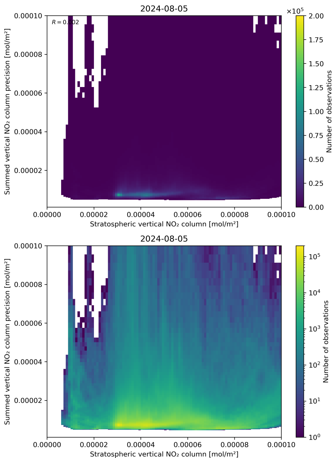
Figure 99: Scatter density plot of “Stratospheric vertical NO 2 column” against “Summed vertical NO 2 column precision” for 2024-08-04 to 2024-08-06.
