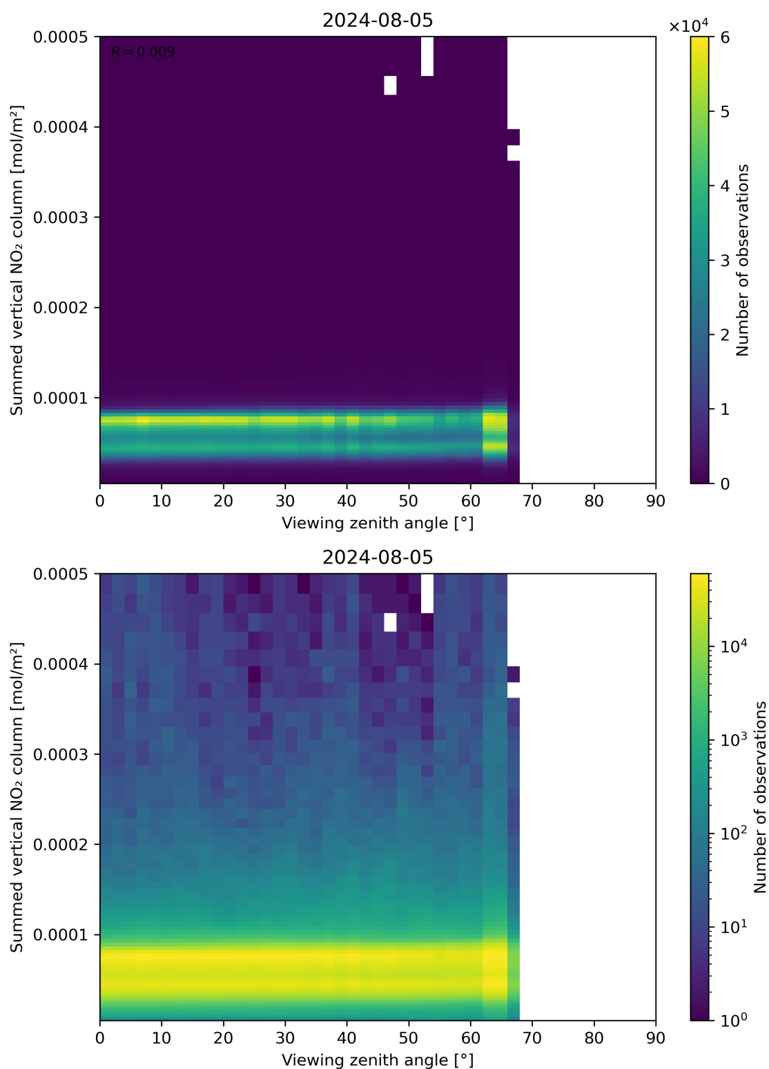
Figure 165: Scatter density plot of “Viewing zenith angle” against “Summed vertical NO 2 column” for 2024-08-04 to 2024-08-06.
