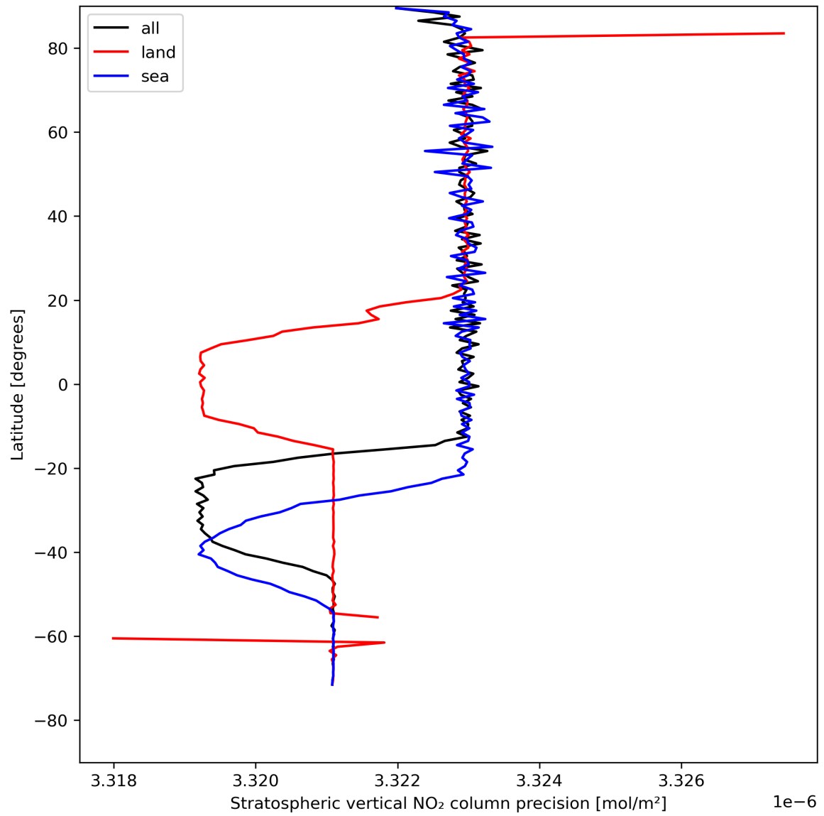
Figure 20: Zonal average of “Stratospheric vertical NO 2 column precision” for 2024-08-04 to 2024-08-06.
