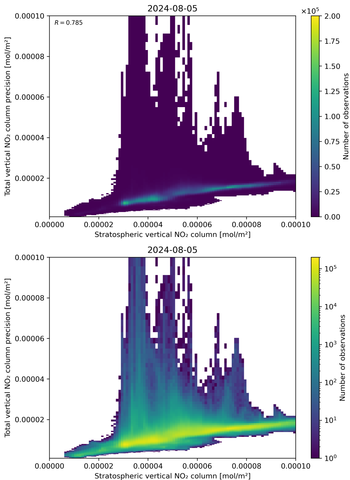
Figure 101: Scatter density plot of “Stratospheric vertical NO 2 column” against “Total vertical NO 2 column precision” for 2024-08-04 to 2024-08-06.
