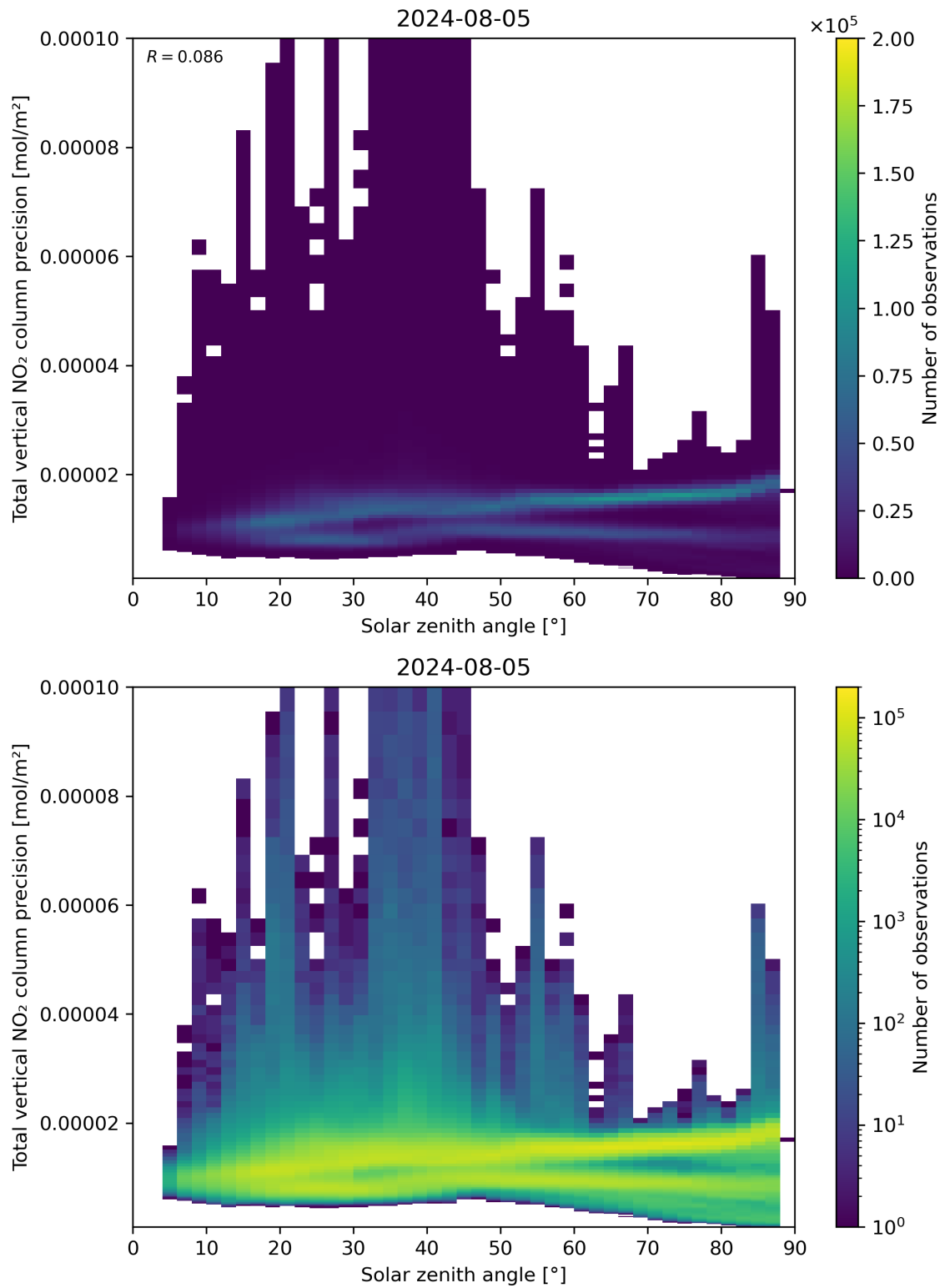
Figure 154: Scatter density plot of “Solar zenith angle” against “Total vertical NO 2 column precision” for 2024-08-04 to 2024-08-06.
