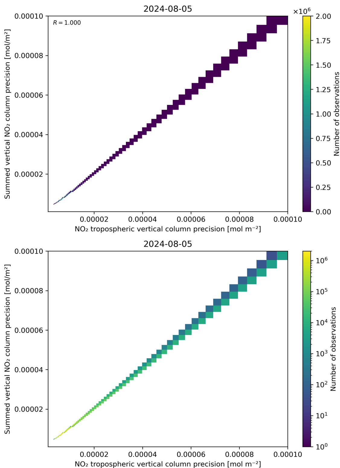
Figure 137: Scatter density plot of “NO 2 tropospheric vertical column precision” against “Summed vertical NO 2 column precision” for 2024-08-04 to 2024-08-06.
