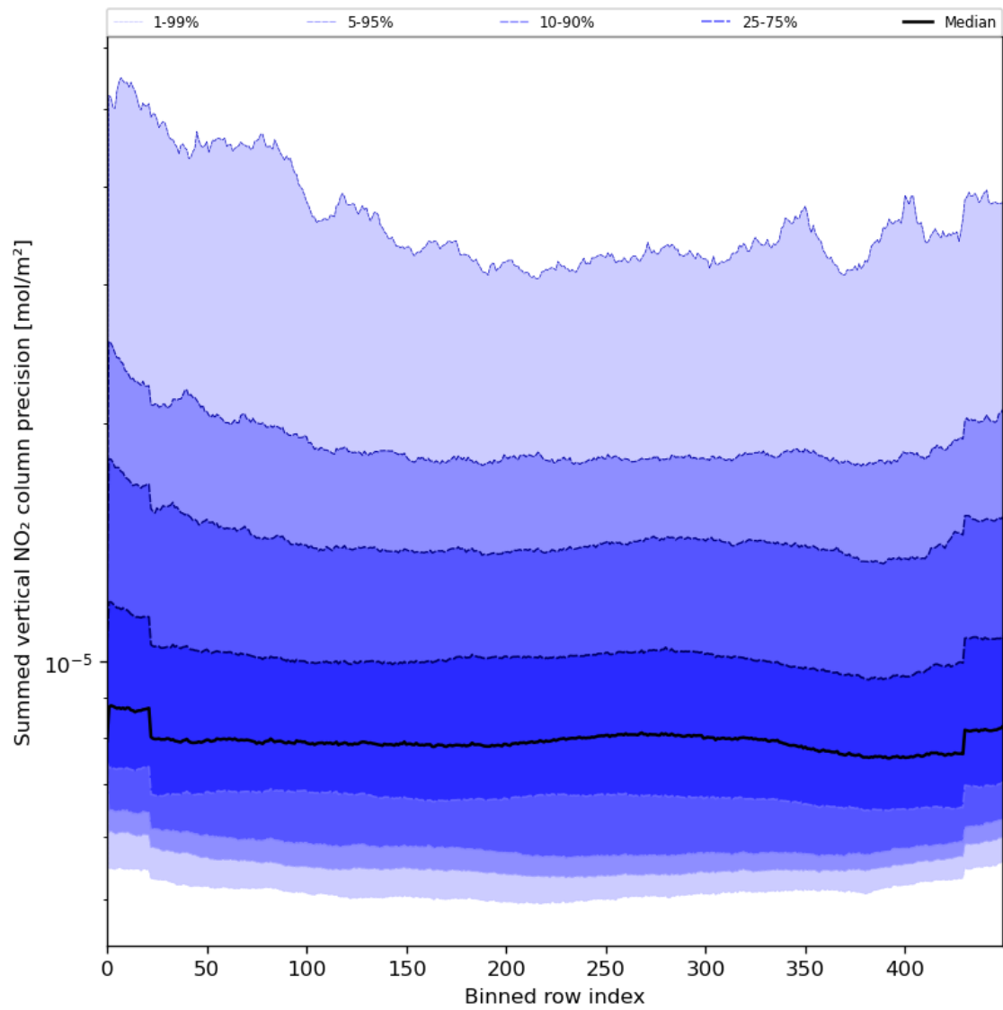
Figure 58: Along track statistics of “Summed vertical NO 2 column precision” for 2024-08-04 to 2024-08-06
