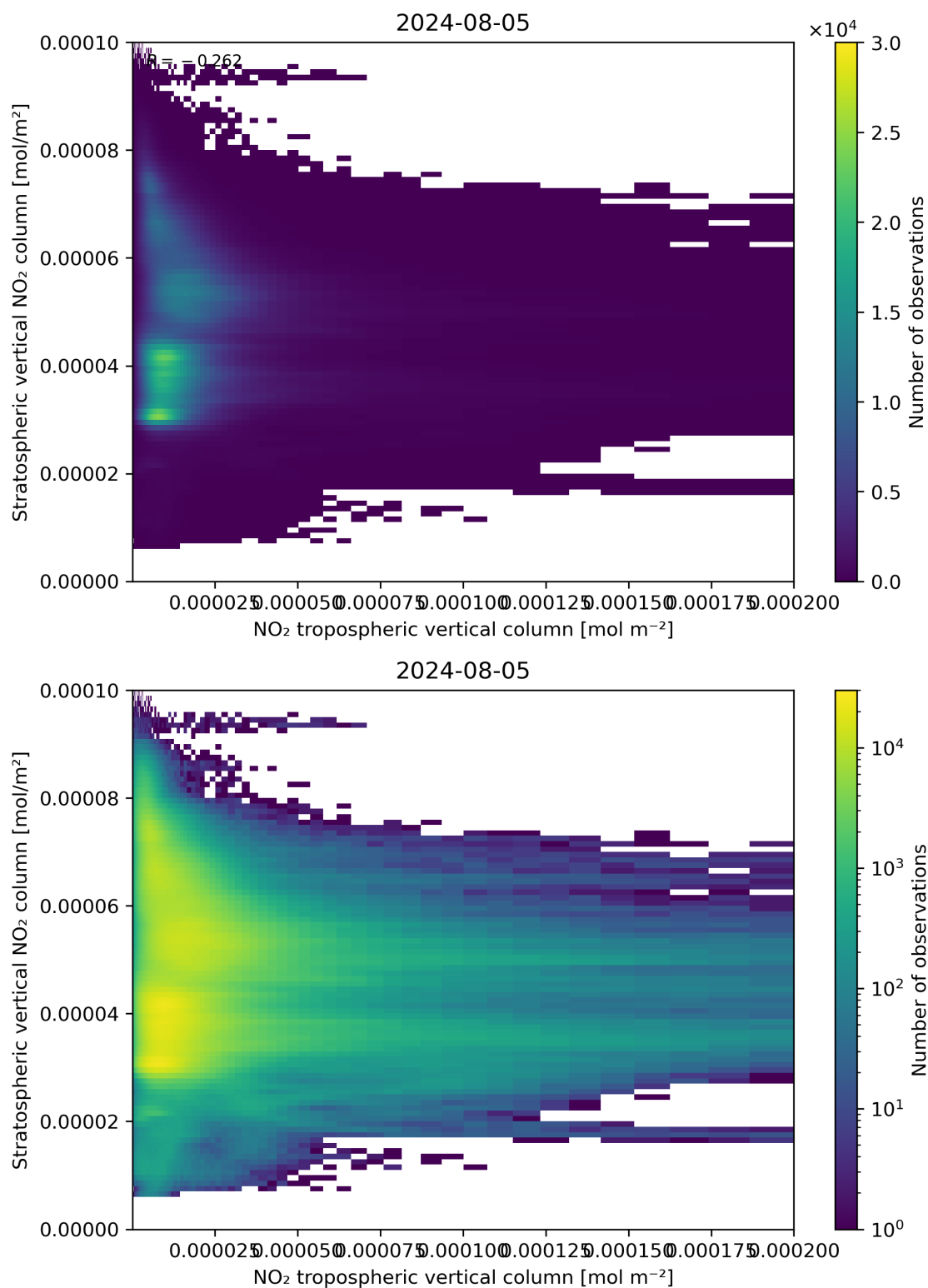
Figure 125: Scatter density plot of “NO 2 tropospheric vertical column” against “Stratospheric vertical NO 2 column” for 2024-08-04 to 2024-08-06.
