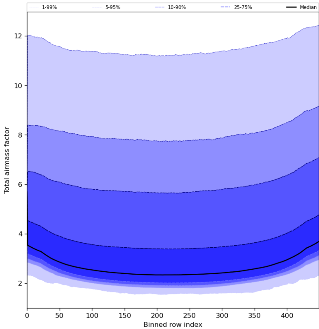
Figure 49: Along track statistics of “Total airmass factor” for 2024-08-04 to 2024-08-06
