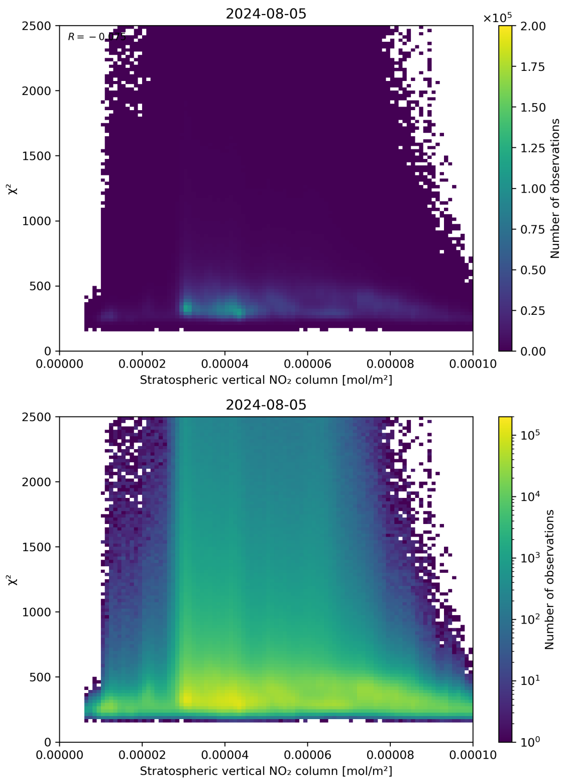
Figure 97: Scatter density plot of “Stratospheric vertical NO 2 column” against “ \chi^2 ” for 2024-08-04 to 2024-08-06.
