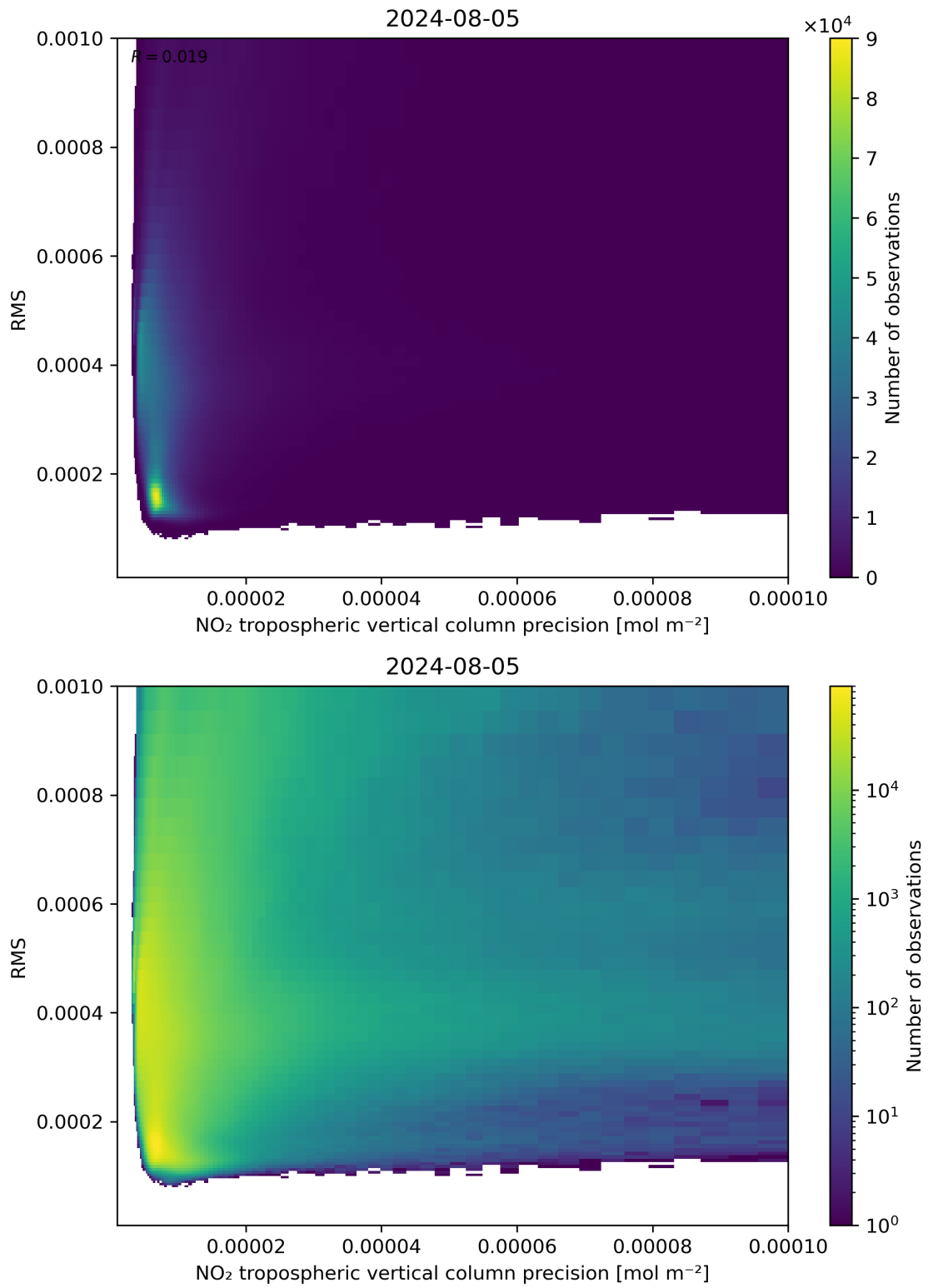
Figure 140: Scatter density plot of “NO 2 tropospheric vertical column precision” against “RMS” for 2024-08-04 to 2024-08-06.
