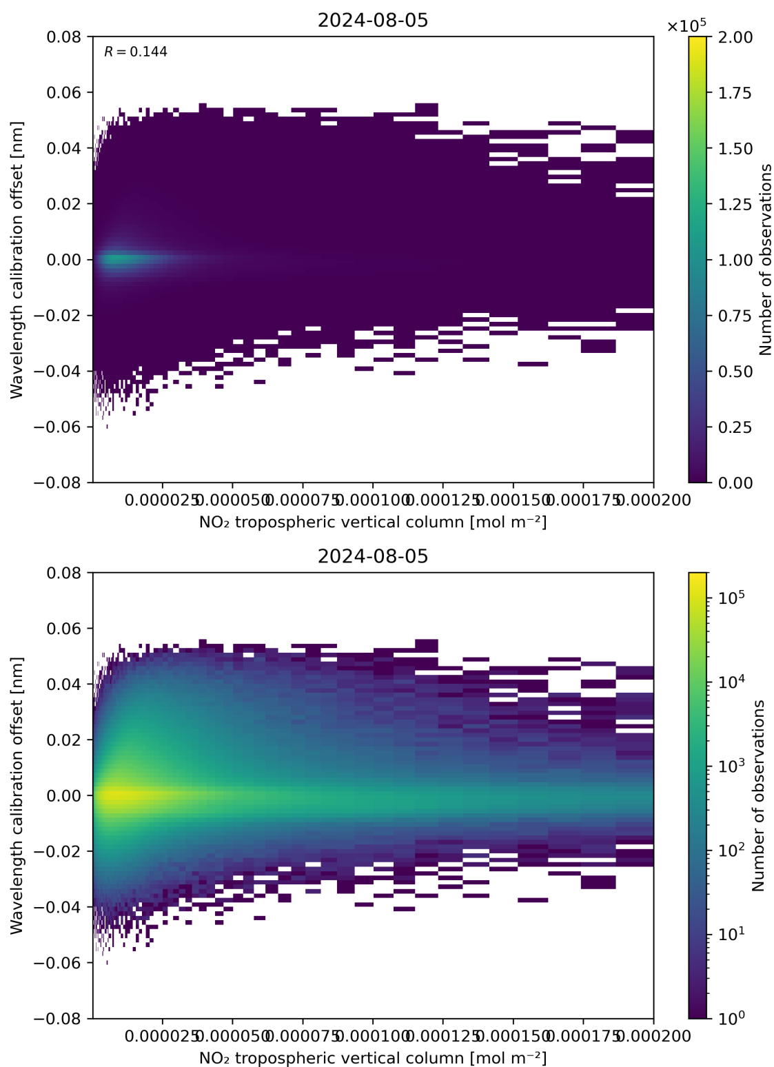
Figure 143: Scatter density plot of “NO 2 tropospheric vertical column” against “Wavelength calibration offset” for 2024-08-04 to 2024-08-06.
