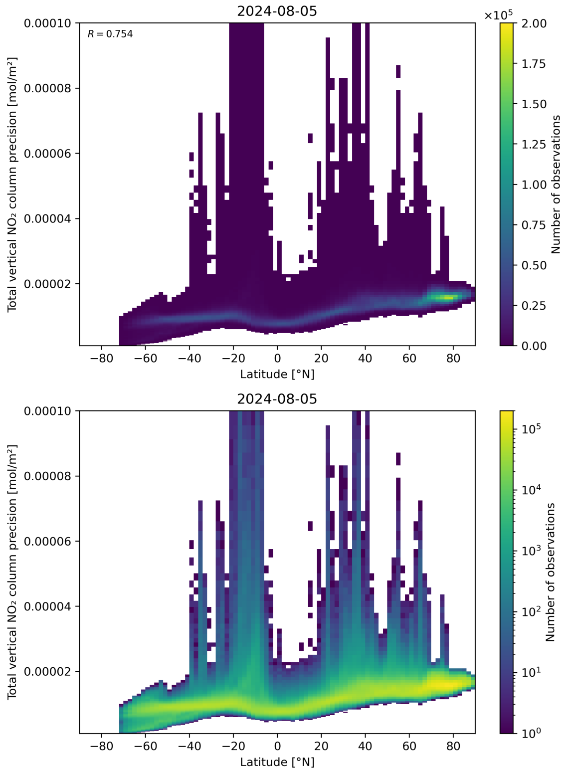
Figure 91: Scatter density plot of “Latitude” against “Total vertical NO 2 column precision” for 2024-08-04 to 2024-08-06.
