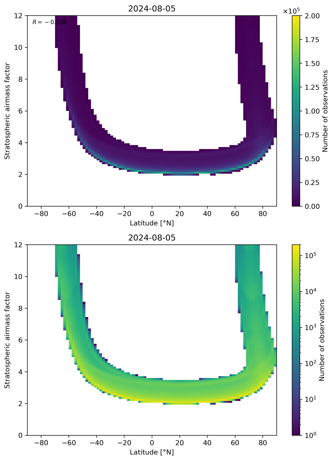
Figure 83: Scatter density plot of “Latitude” against “Stratospheric air mass factor” for 2024-08-04 to 2024-08-06.
