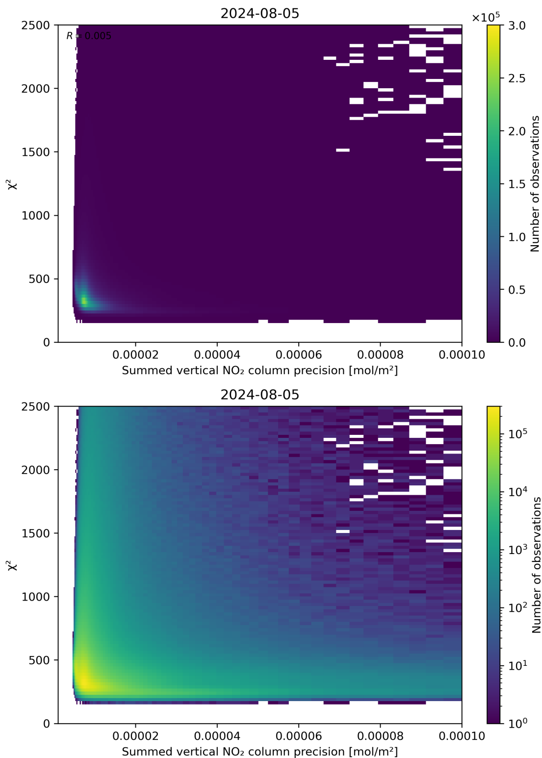
Figure 107: Scatter density plot of “Summed vertical NO 2 column precision” against “ \chi^2 ” for 2024-08-04 to 2024-08-06.
