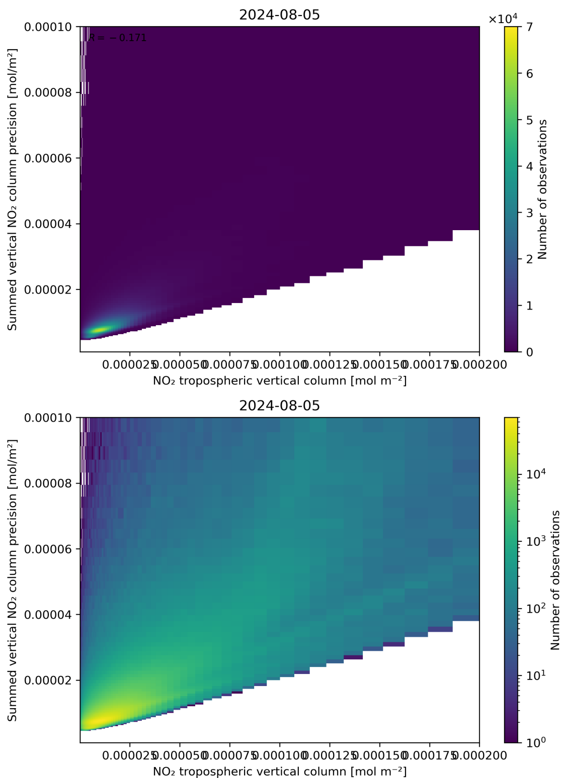
Figure 127: Scatter density plot of “NO 2 tropospheric vertical column” against “Summed vertical NO 2 column precision” for 2024-08-04 to 2024-08-06.
