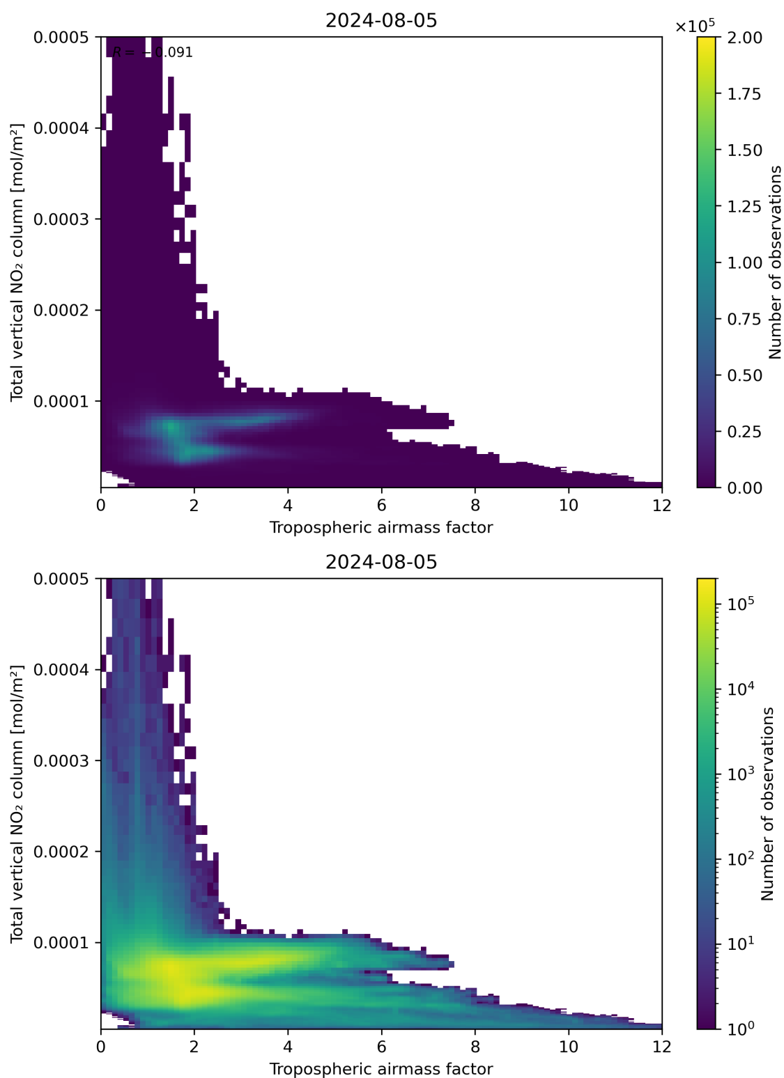
Figure 77: Scatter density plot of “Tropospheric airmass factor” against “Total vertical NO 2 column” for 2024-08-04 to 2024-08-06.
