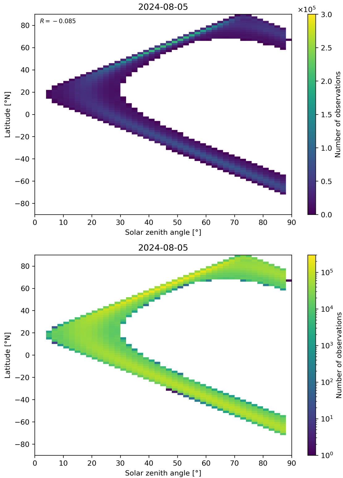
Figure 149: Scatter density plot of “Solar zenith angle” against “Latitude” for 2024-08-04 to 2024-08-06.
