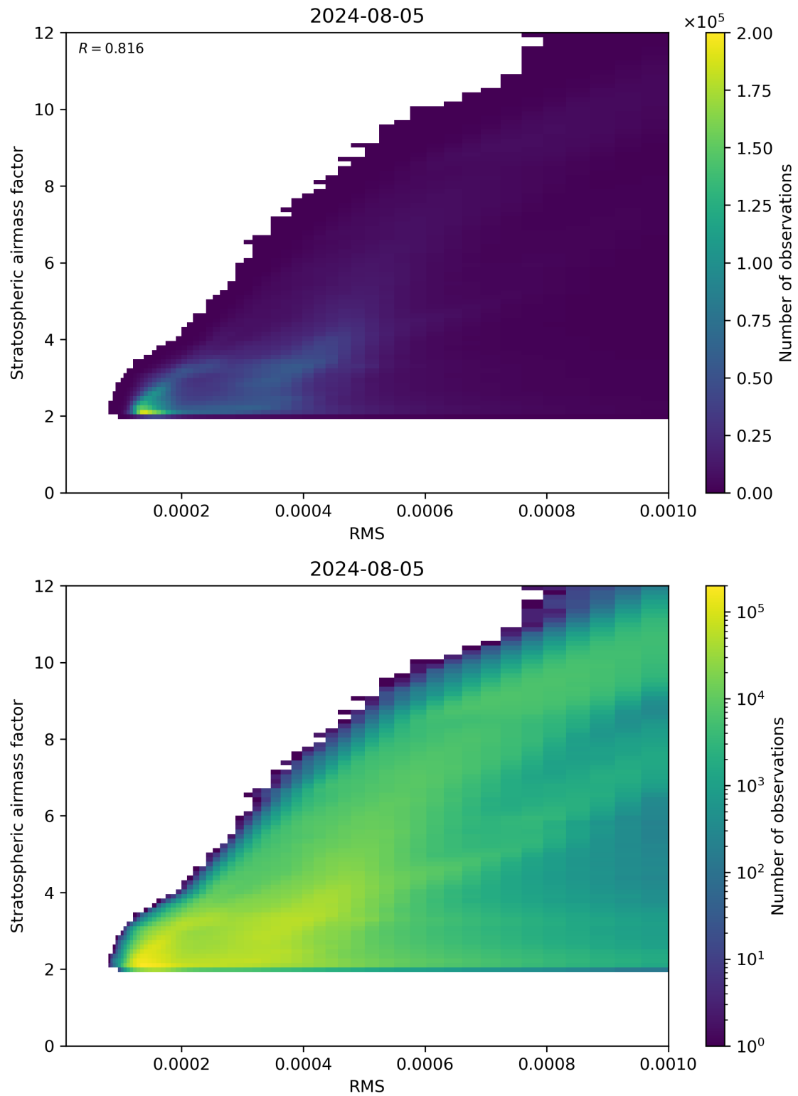
Figure 144: Scatter density plot of “RMS” against “Stratospheric airmass factor” for 2024-08-04 to 2024-08-06.
