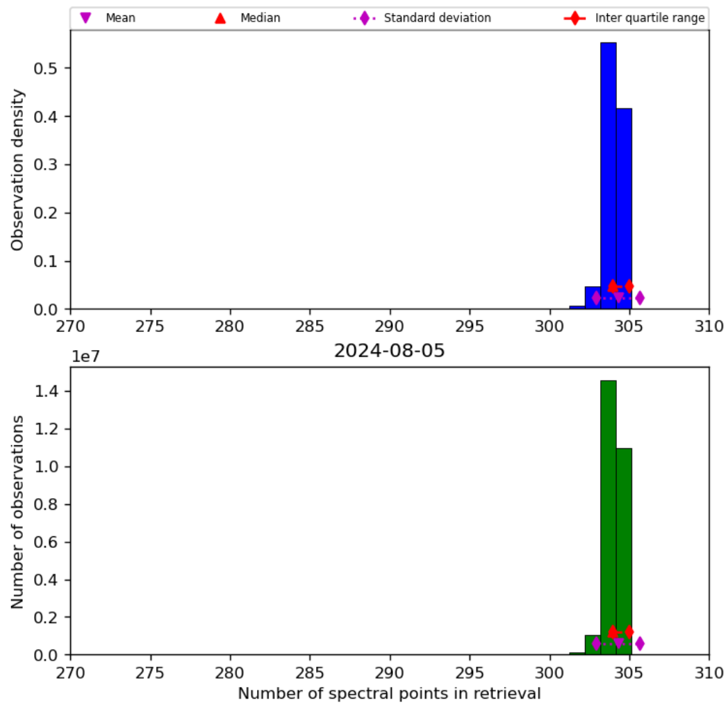
Figure 33: Histogram of “Number of spectral points in retrieval” for 2024-08-04 to 2024-08-06
