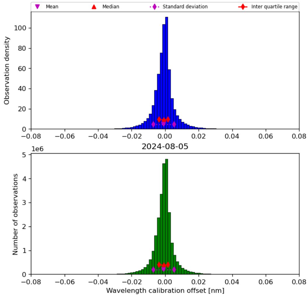
Figure 35: Histogram of “Wavelength calibration offset” for 2024-08-04 to 2024-08-06
