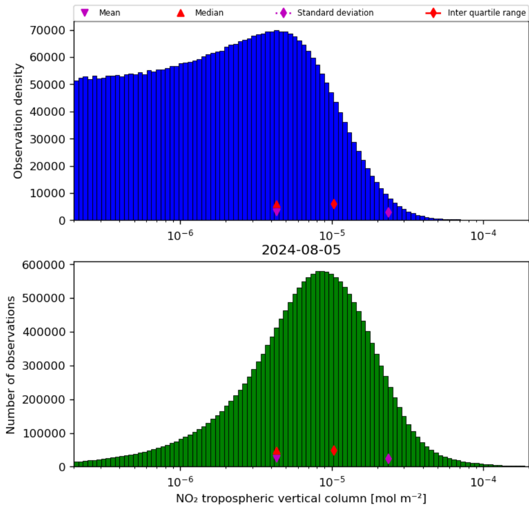
Figure 29: Histogram of “NO 2 tropospheric vertical column” for 2024-08-04 to 2024-08-06
