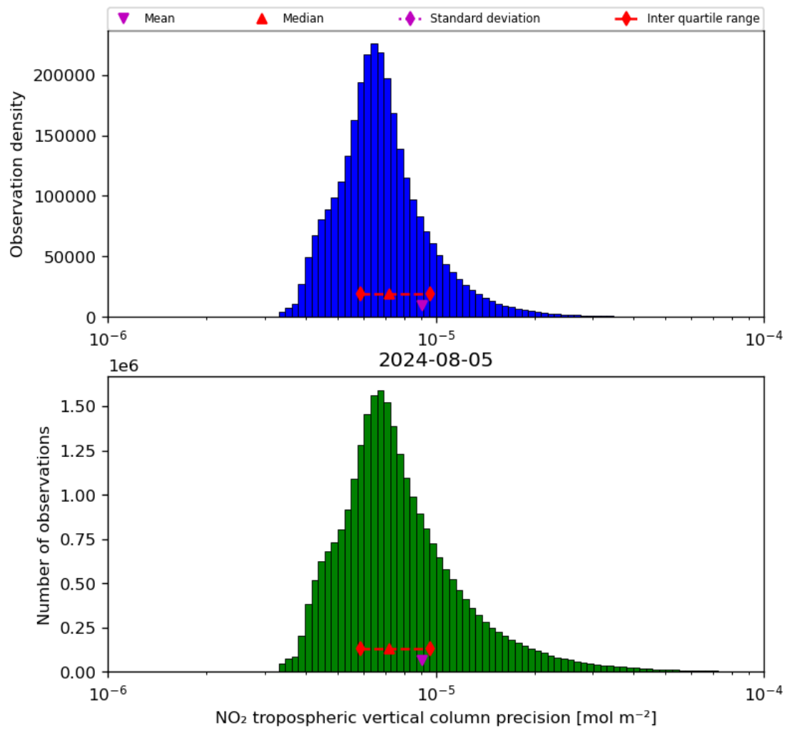
Figure 30: Histogram of “NO 2 tropospheric vertical column precision” for 2024-08-04 to 2024-08-06
