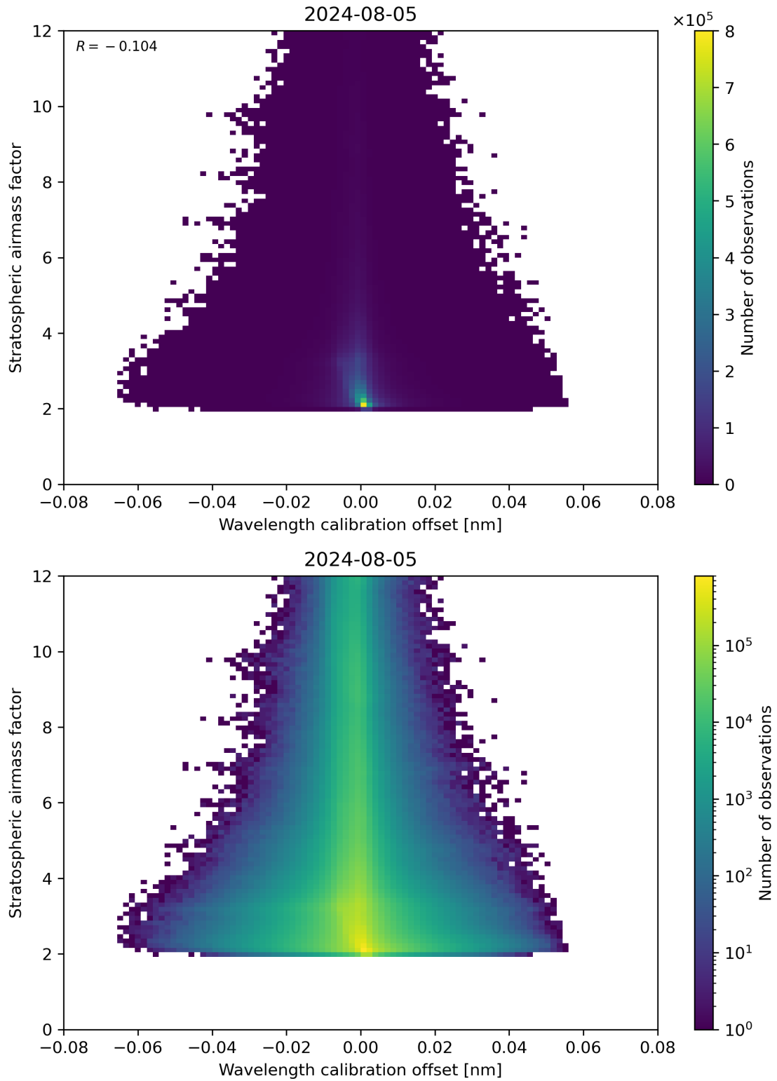
Figure 174: Scatter density plot of “Wavelength calibration offset” against “Stratospheric airmass factor” for 2024-08-04 to 2024-08-06.
