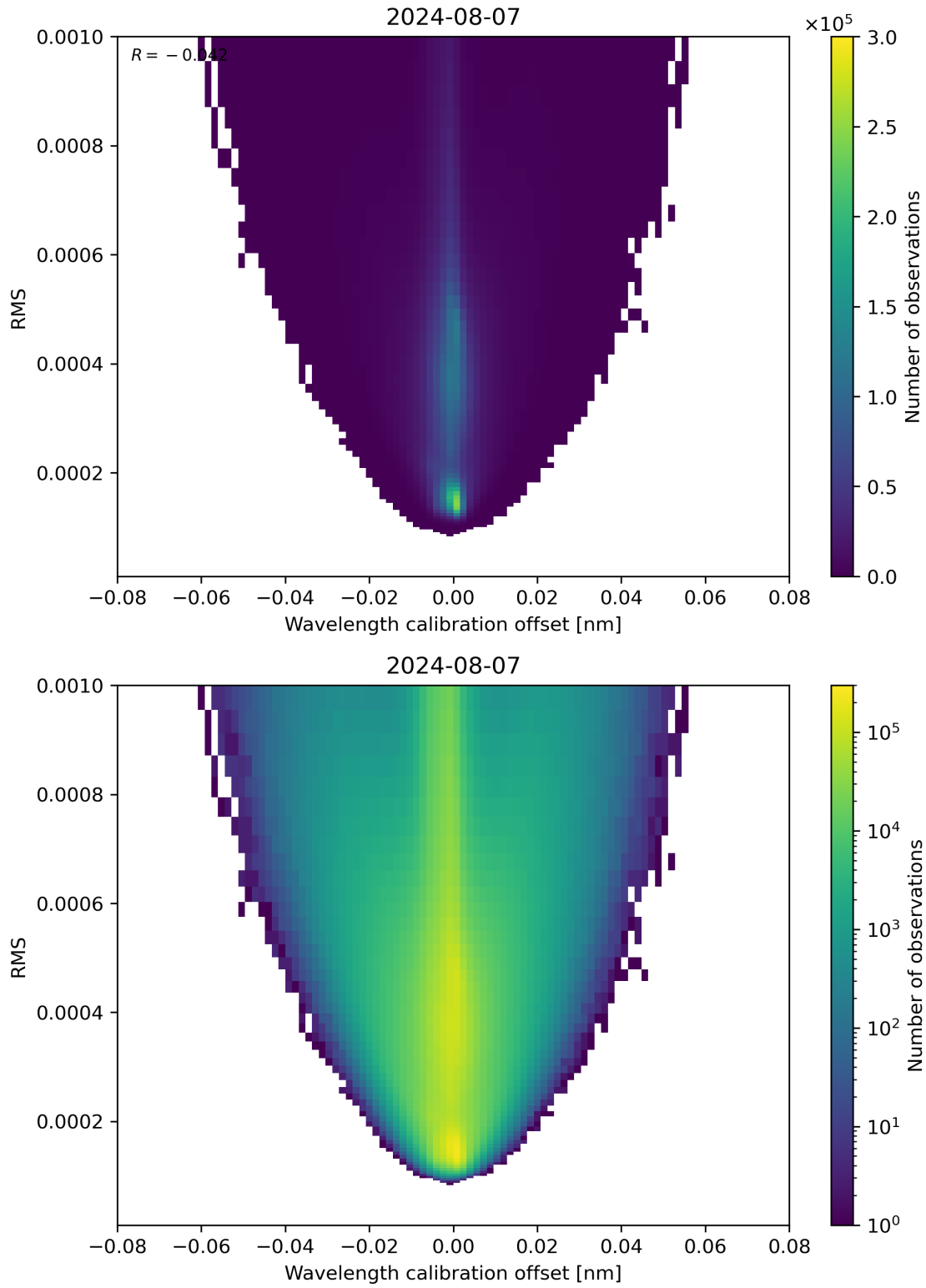
Figure 181: Scatter density plot of “Wavelength calibration offset” against “RMS” for 2024-08-06 to 2024-08-08.
