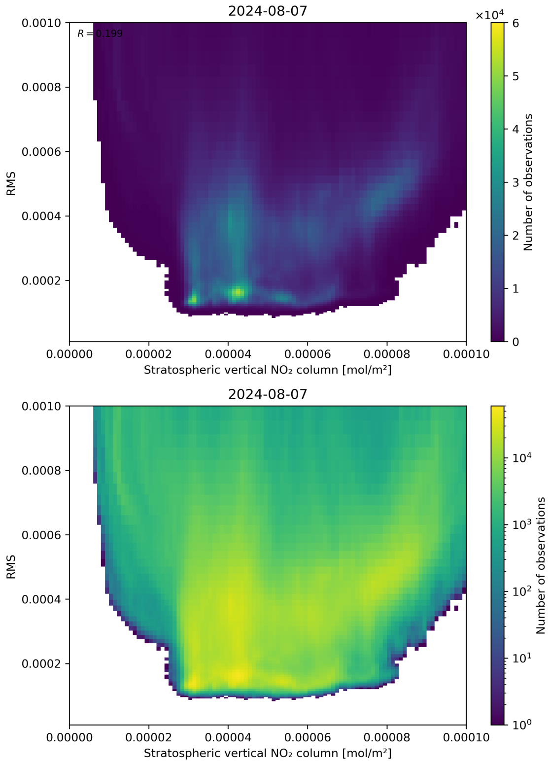
Figure 102: Scatter density plot of “Stratospheric vertical NO 2 column” against “RMS” for 2024-08-06 to 2024-08-08.
