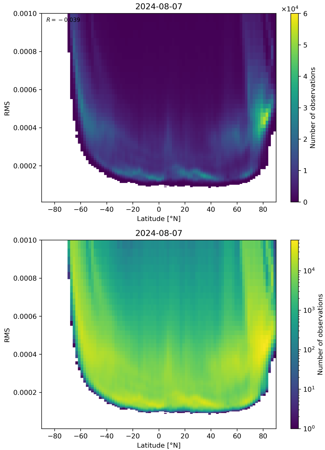
Figure 94: Scatter density plot of “Latitude” against “RMS” for 2024-08-06 to 2024-08-08.
