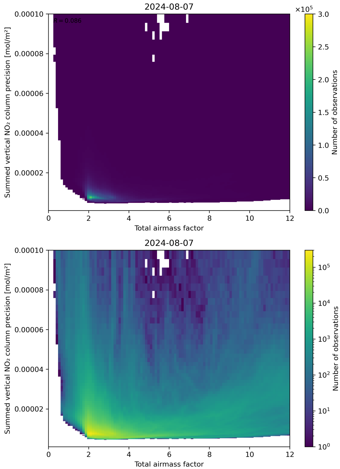
Figure 66: Scatter density plot of “Total airmass factor” against “Summed vertical NO 2 column precision” for 2024-08-06 to 2024-08-08.
