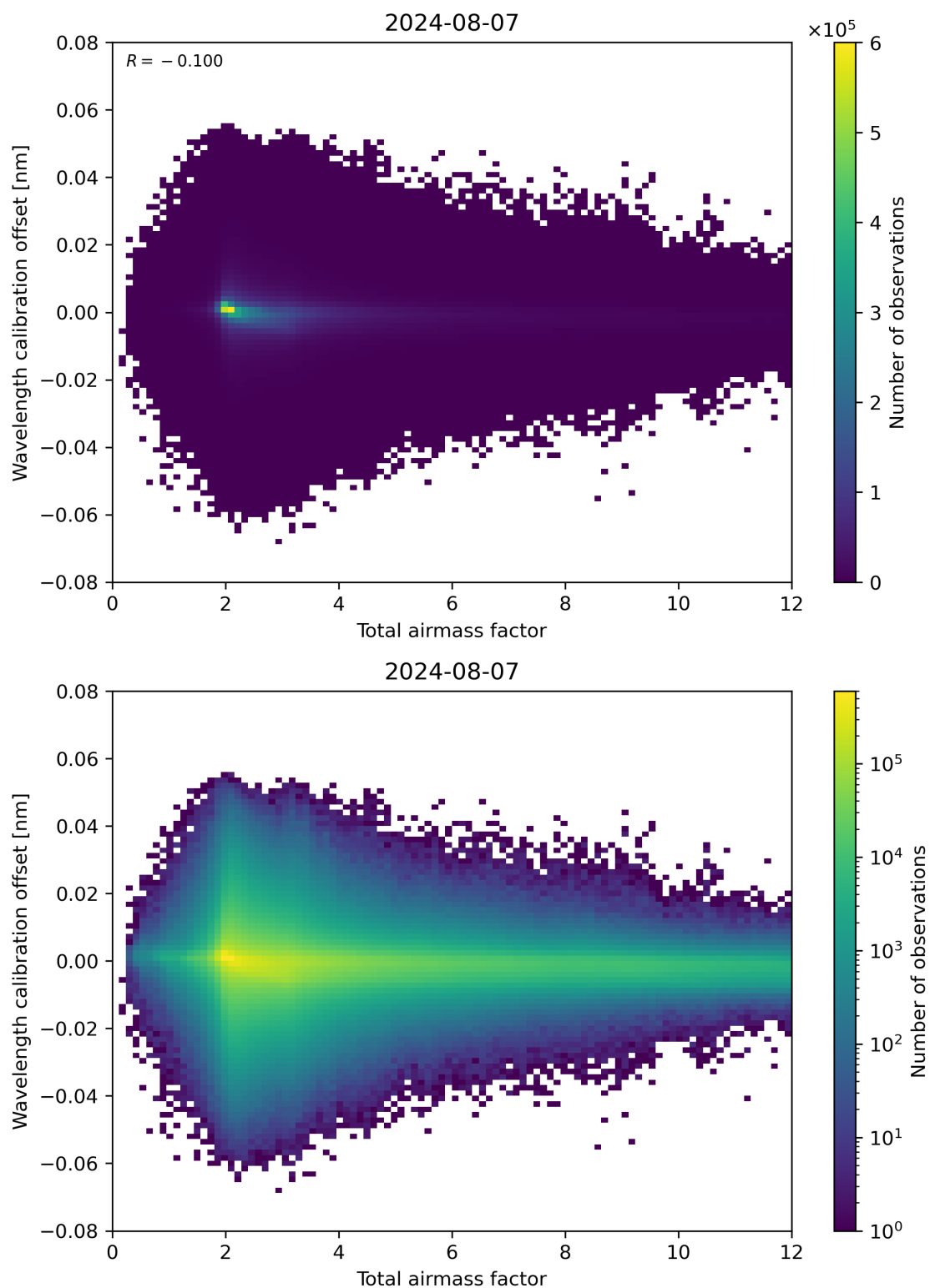
Figure 70: Scatter density plot of “Total airmass factor” against “Wavelength calibration offset” for 2024-08-06 to 2024-08-08.
