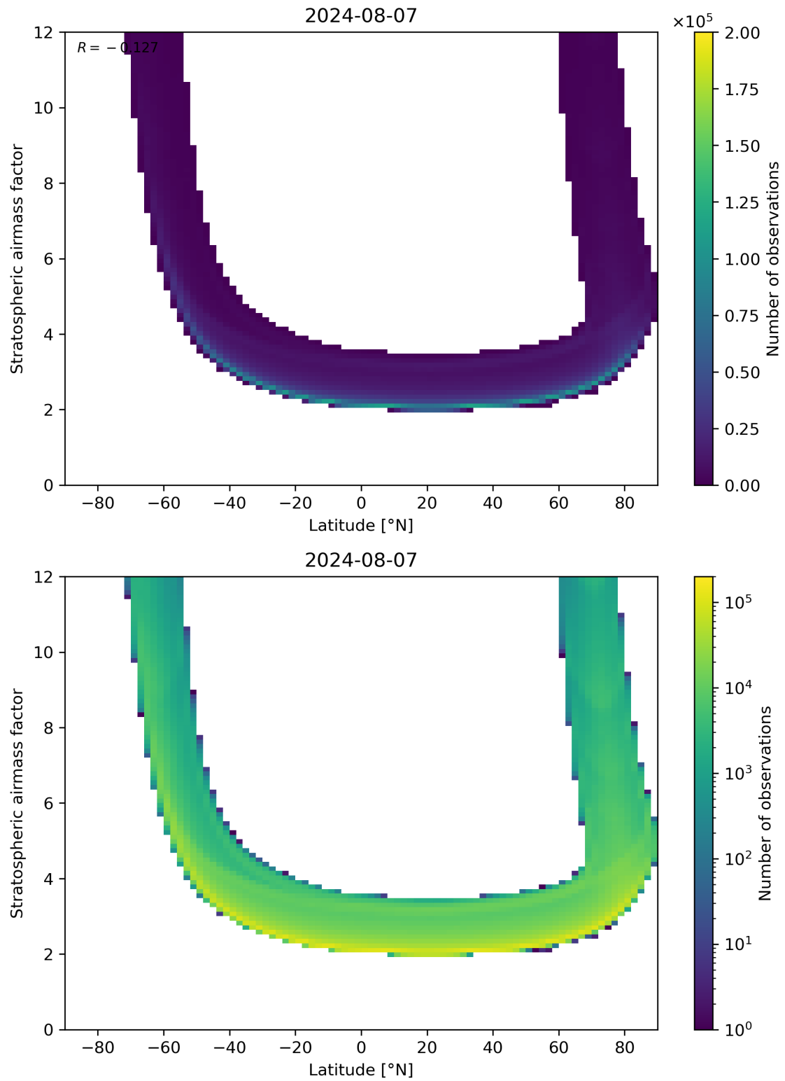
Figure 83: Scatter density plot of “Latitude” against “Stratospheric airmass factor” for 2024-08-06 to 2024-08-08.
