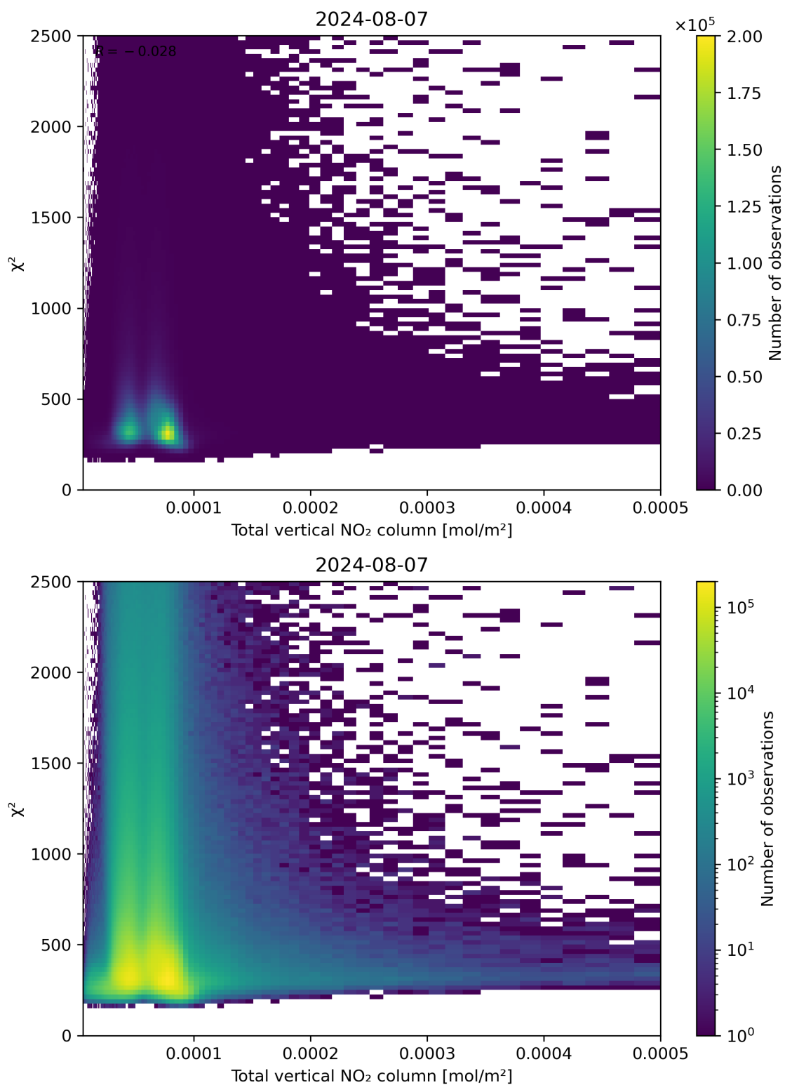
Figure 111: Scatter density plot of “Total vertical NO 2 column” against “ \chi^2 ” for 2024-08-06 to 2024-08-08.
