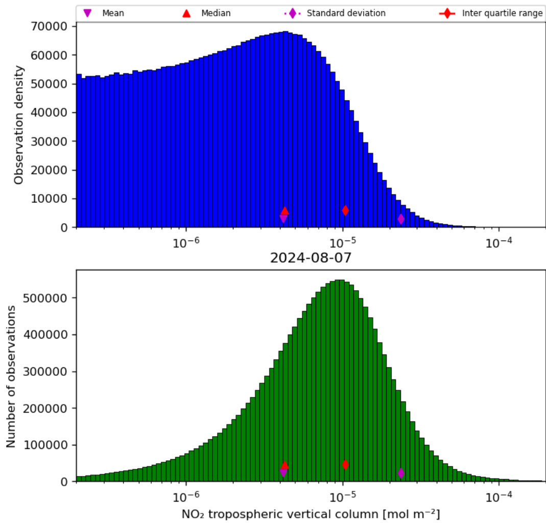
Figure 29: Histogram of “NO 2 tropospheric vertical column” for 2024-08-06 to 2024-08-08
