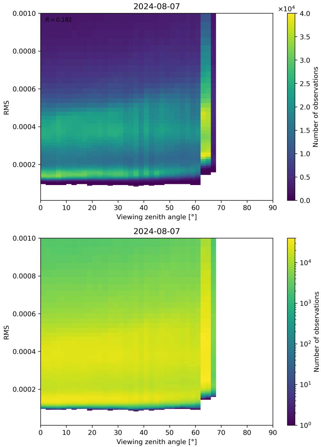
Figure 171: Scatter density plot of “Viewing zenith angle” against “RMS” for 2024-08-06 to 2024-08-08.
