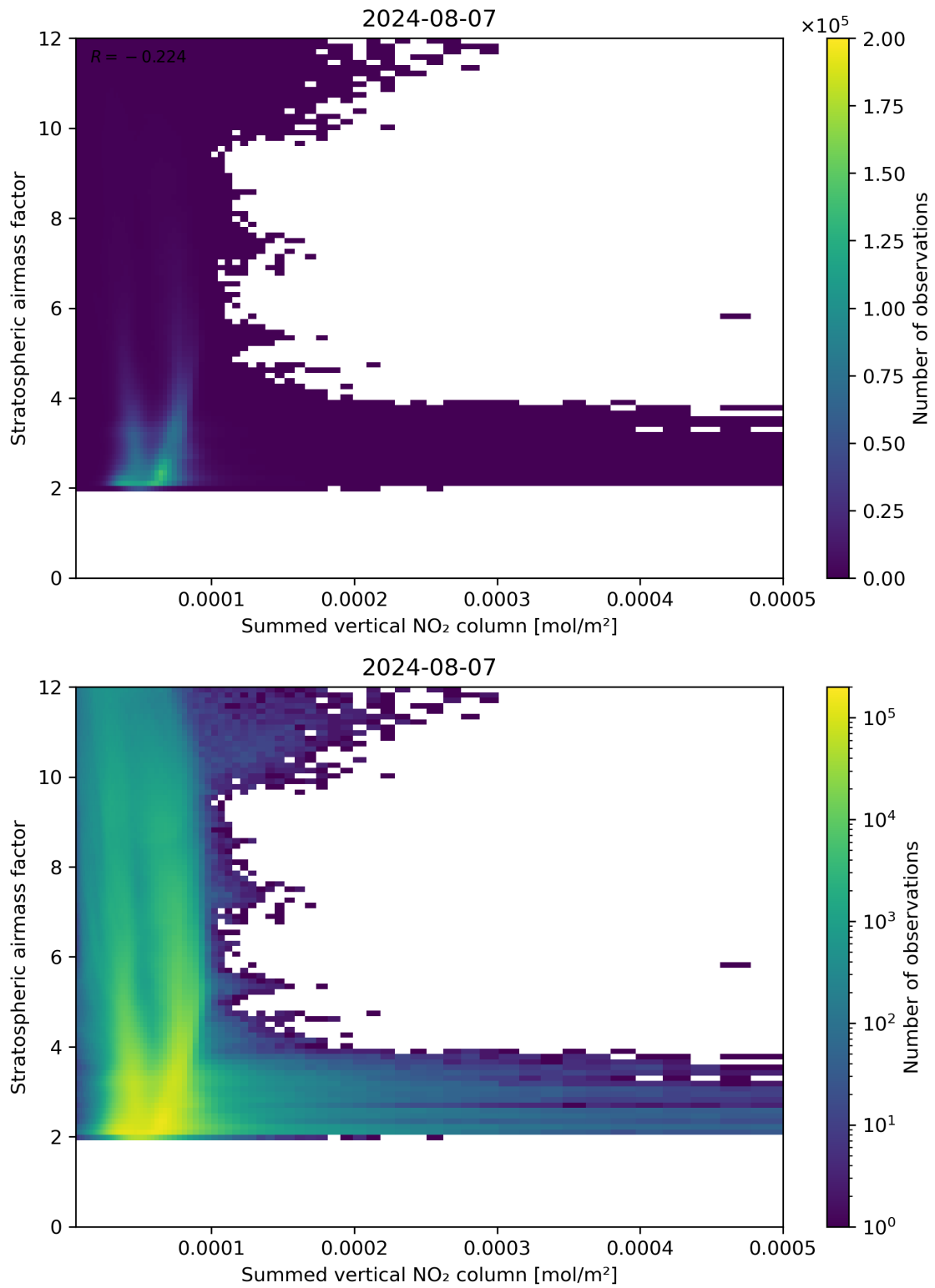
Figure 103: Scatter density plot of “Summed vertical NO 2 column” against “Stratospheric airmass factor” for 2024-08-06 to 2024-08-08.
