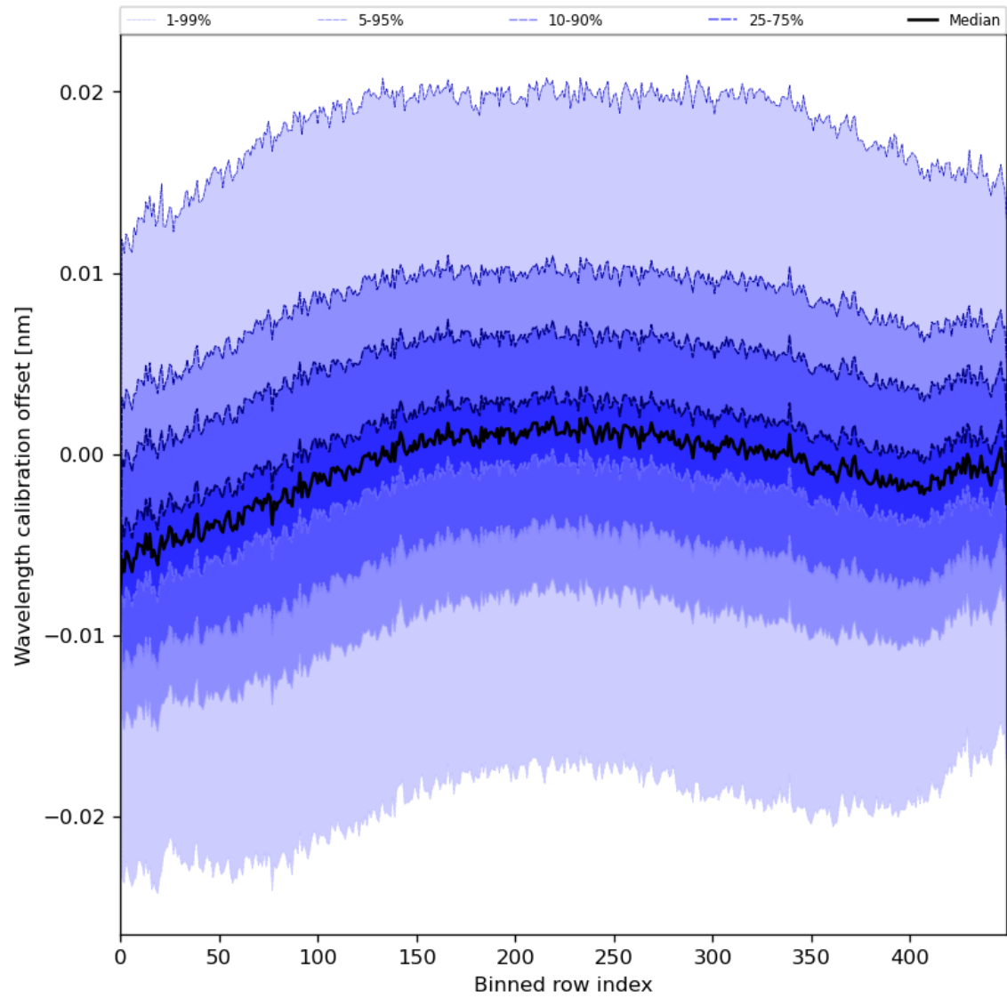
Figure 52: Along track statistics of “Wavelength calibration offset” for 2024-08-06 to 2024-08-08
