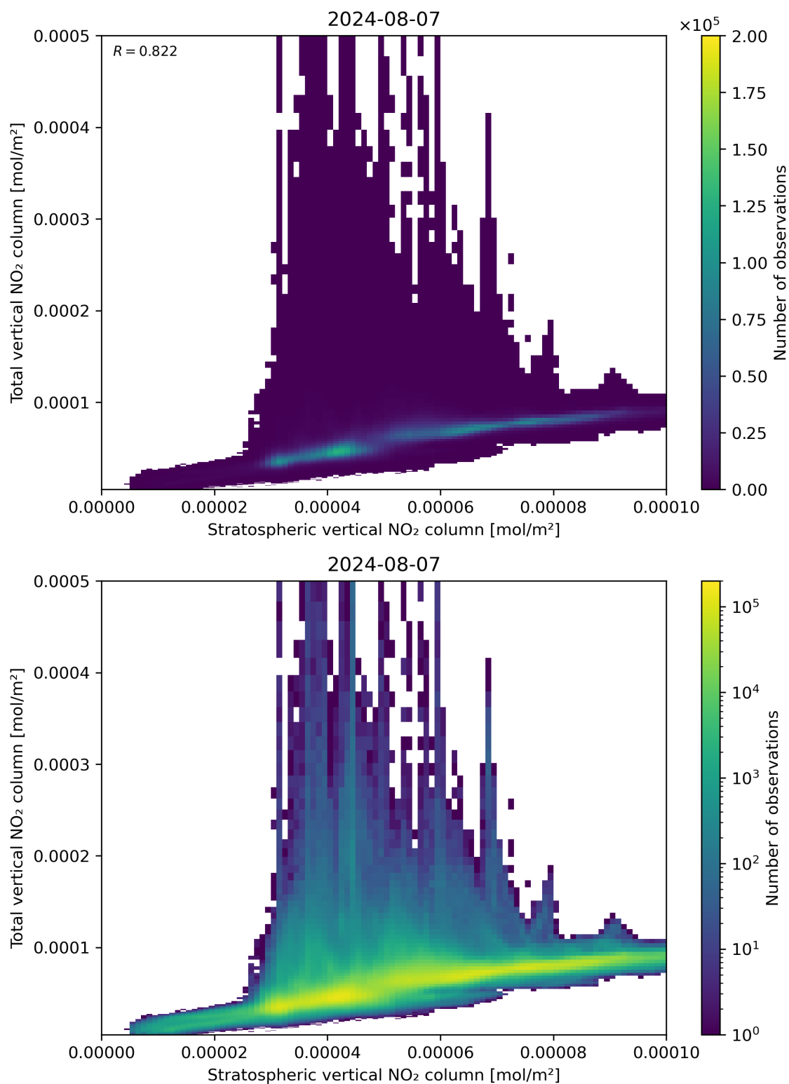
Figure 100: Scatter density plot of “Stratospheric vertical NO 2 column” against “Total vertical NO 2 column” for 2024-08-06 to 2024-08-08.
