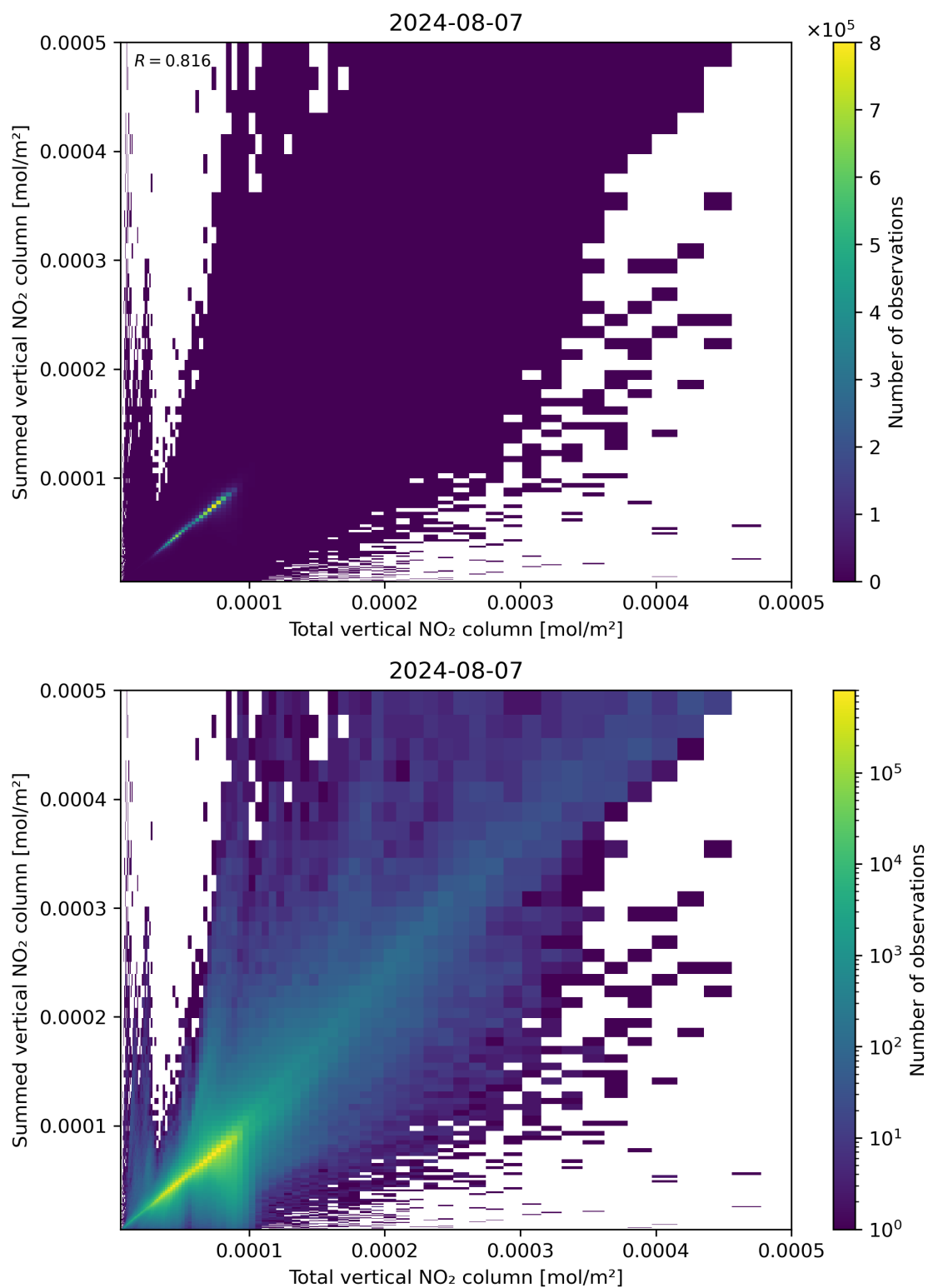
Figure 112: Scatter density plot of “Total vertical NO 2 column” against “Summed vertical NO 2 column” for 2024-08-06 to 2024-08-08.
