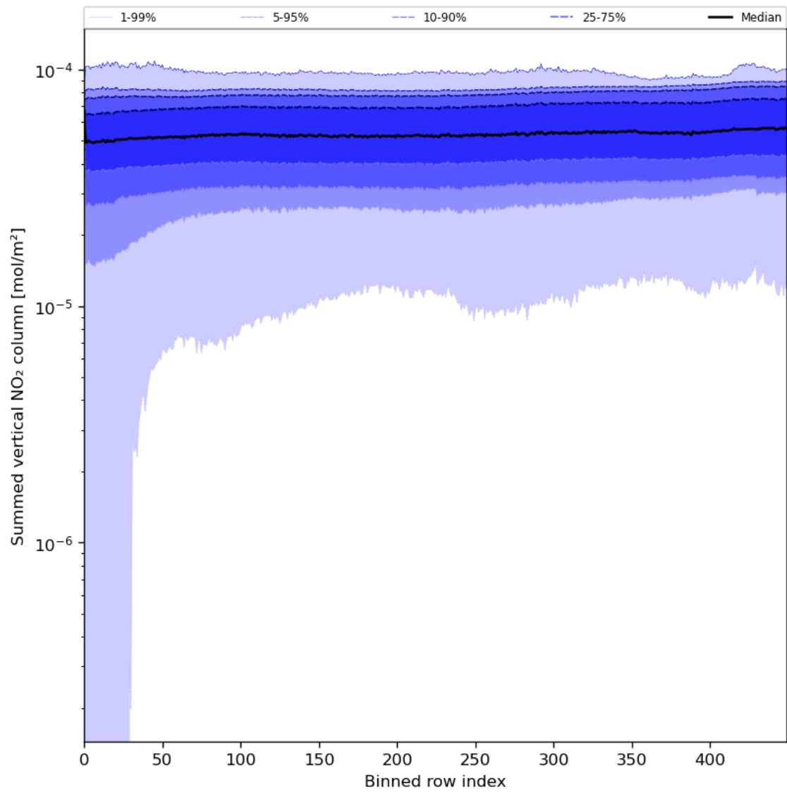
Figure 57: Along track statistics of “Summed vertical NO 2 column” for 2024-08-06 to 2024-08-08
