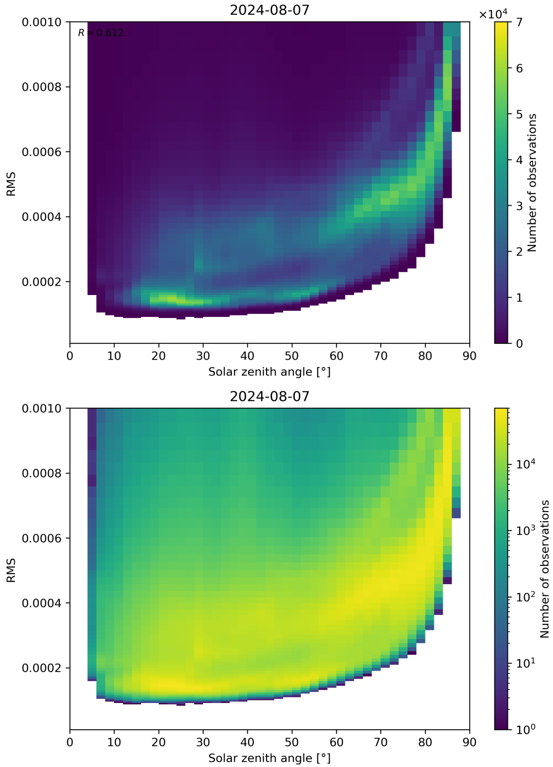
Figure 157: Scatter density plot of “Solar zenith angle” against “RMS” for 2024-08-06 to 2024-08-08.
