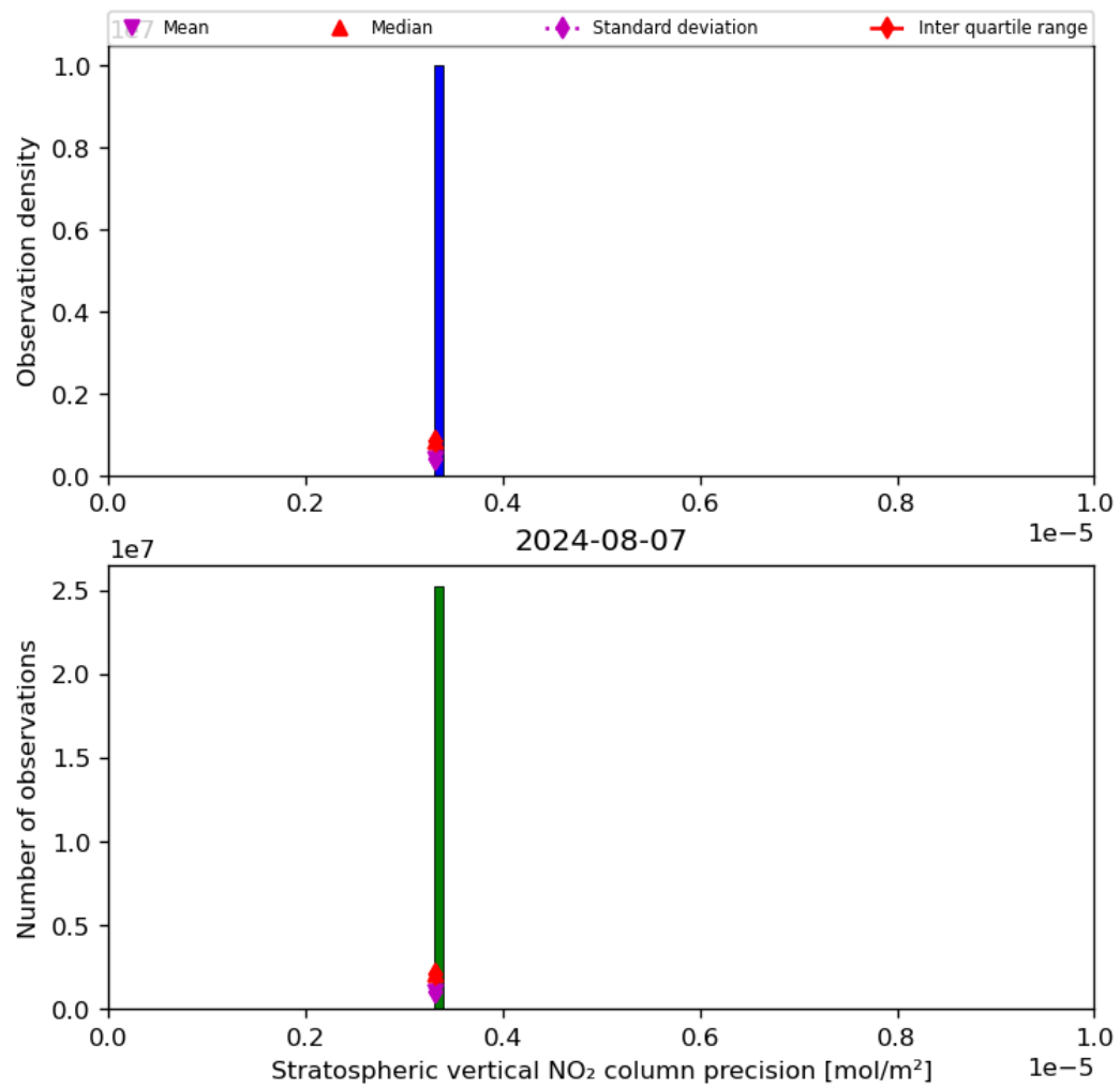
Figure 37: Histogram of “Stratospheric vertical NO 2 column precision” for 2024-08-06 to 2024-08-08
