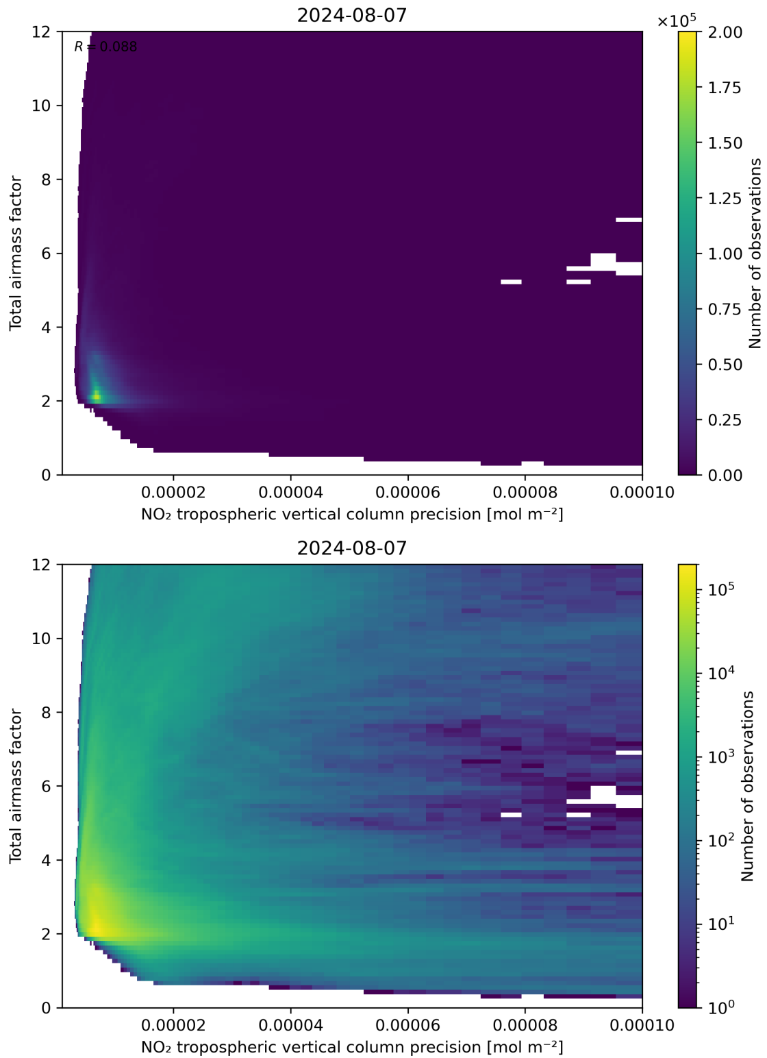
Figure 132: Scatter density plot of “NO 2 tropospheric vertical column precision” against “Total air mass factor” for 2024-08-06 to 2024-08-08.
