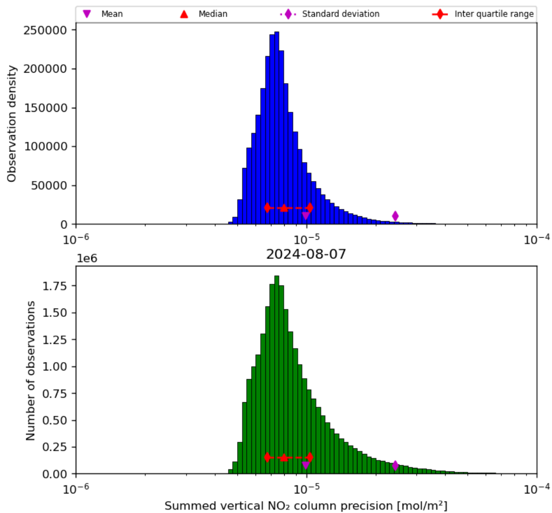
Figure 41: Histogram of “Summed vertical NO 2 column precision” for 2024-08-06 to 2024-08-08
