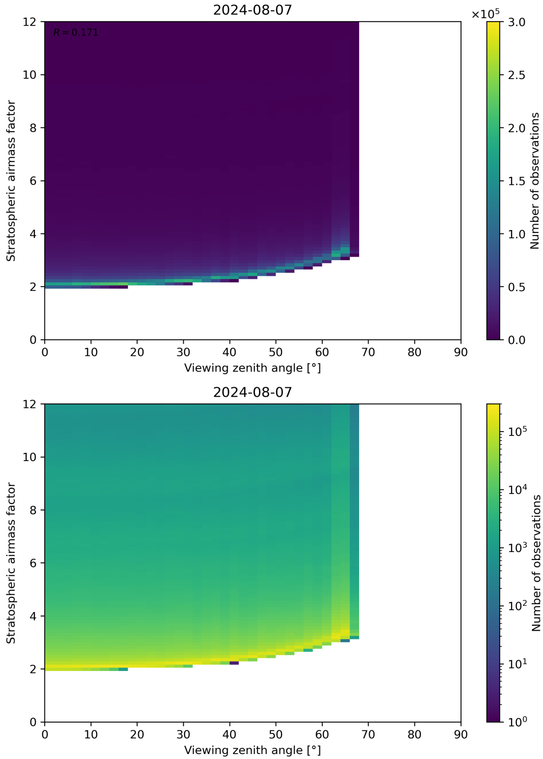
Figure 159: Scatter density plot of “Viewing zenith angle” against “Stratospheric airmass factor” for 2024-08-06 to 2024-08-08.
