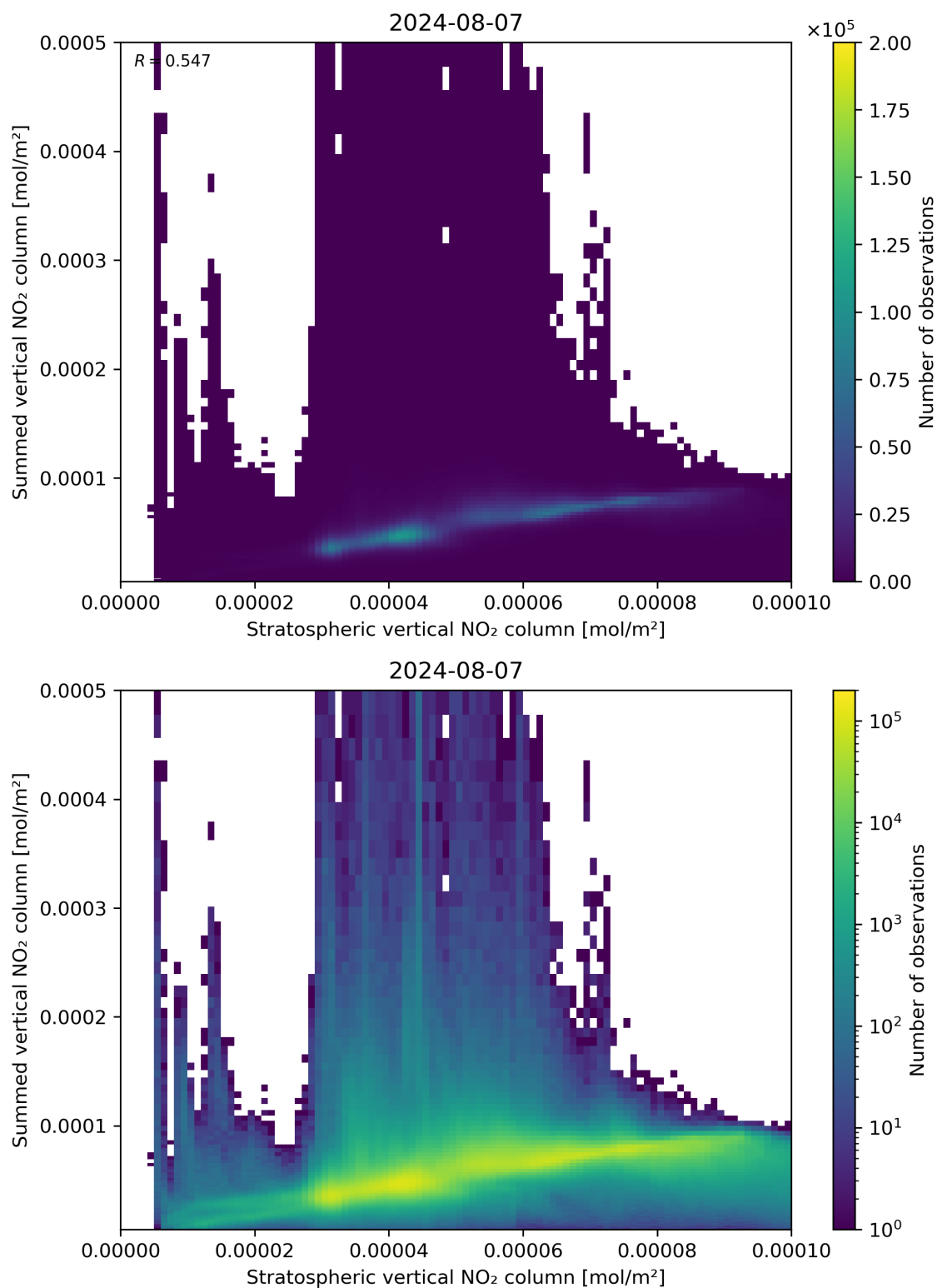
Figure 98: Scatter density plot of “Stratospheric vertical NO 2 column” against “Summed vertical NO 2 column” for 2024-08-06 to 2024-08-08.
