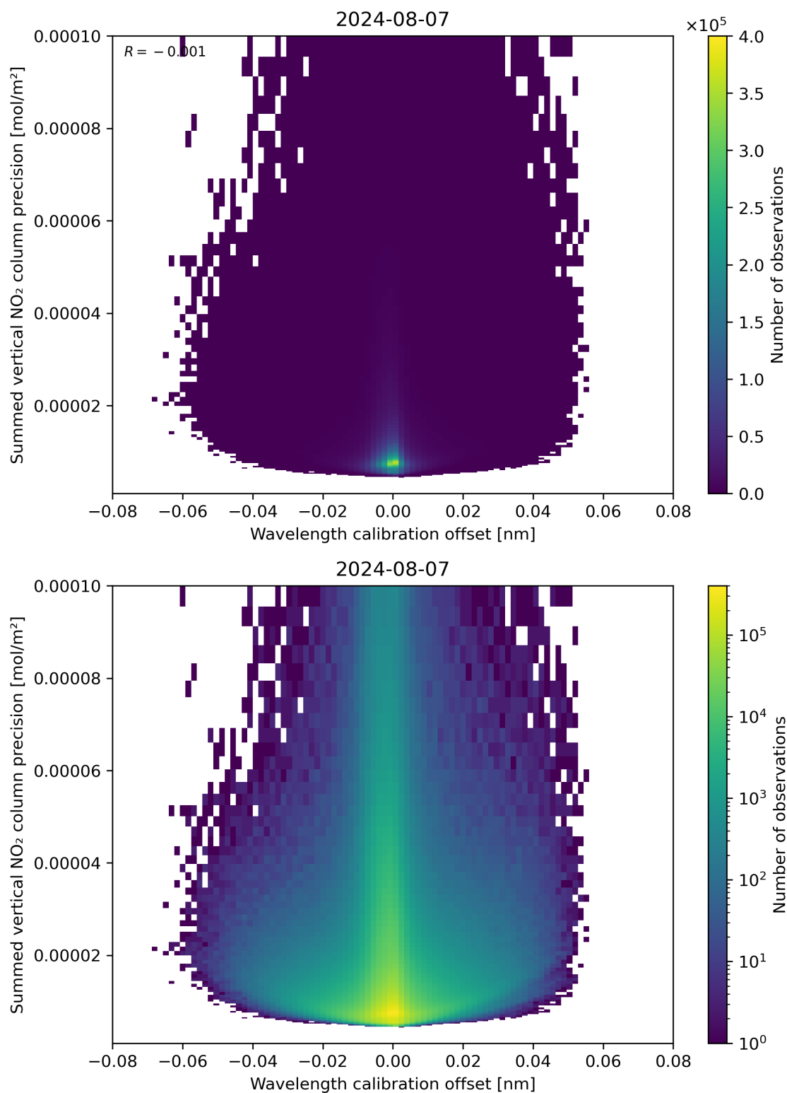
Figure 178: Scatter density plot of “Wavelength calibration offset” against “Summed vertical NO 2 column precision” for 2024-08-06 to 2024-08-08.
