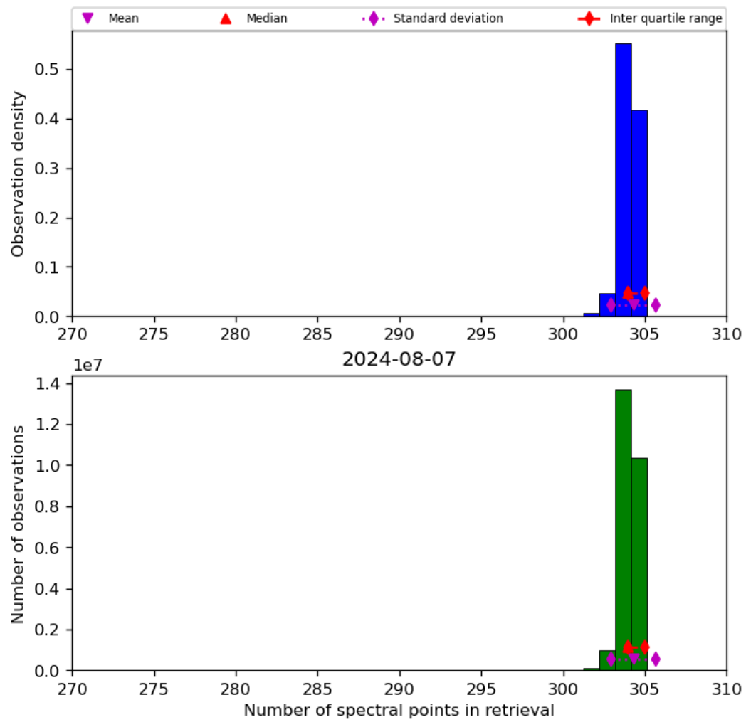
Figure 33: Histogram of “Number of spectral points in retrieval” for 2024-08-06 to 2024-08-08
