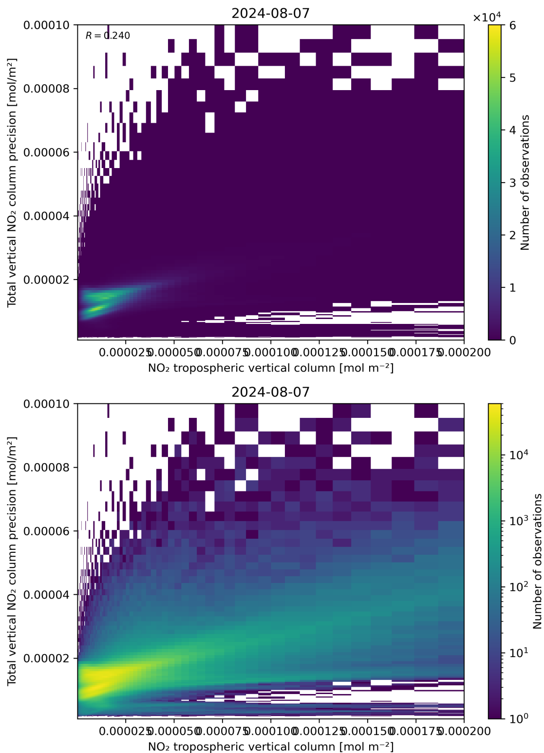
Figure 129: Scatter density plot of “NO 2 tropospheric vertical column” against “Total vertical NO 2 column precision” for 2024-08-06 to 2024-08-08.
