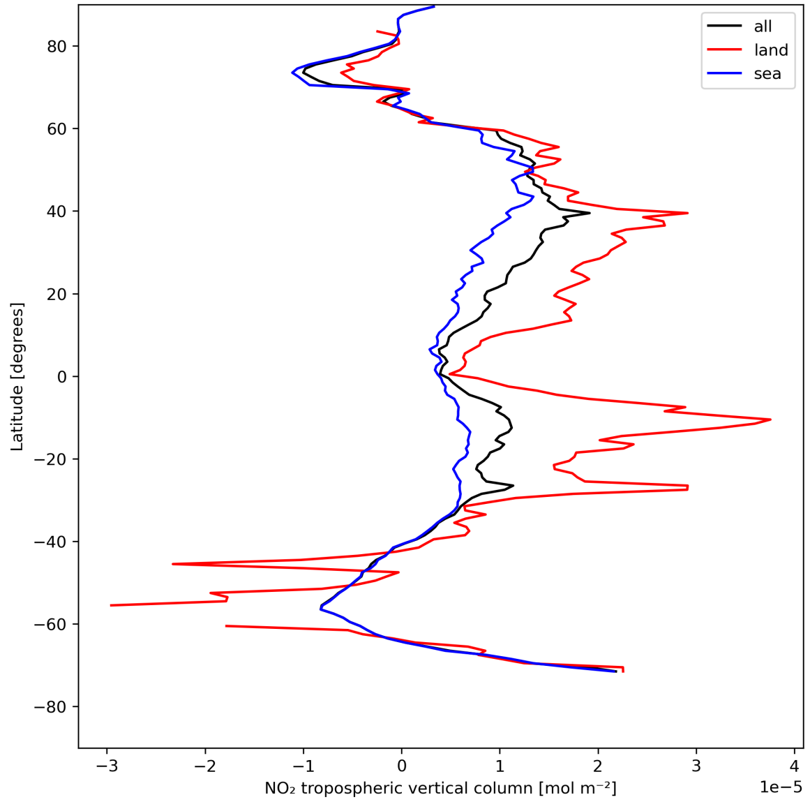
Figure 12: Zonal average of “NO 2 tropospheric vertical column” for 2024-08-06 to 2024-08-08.
