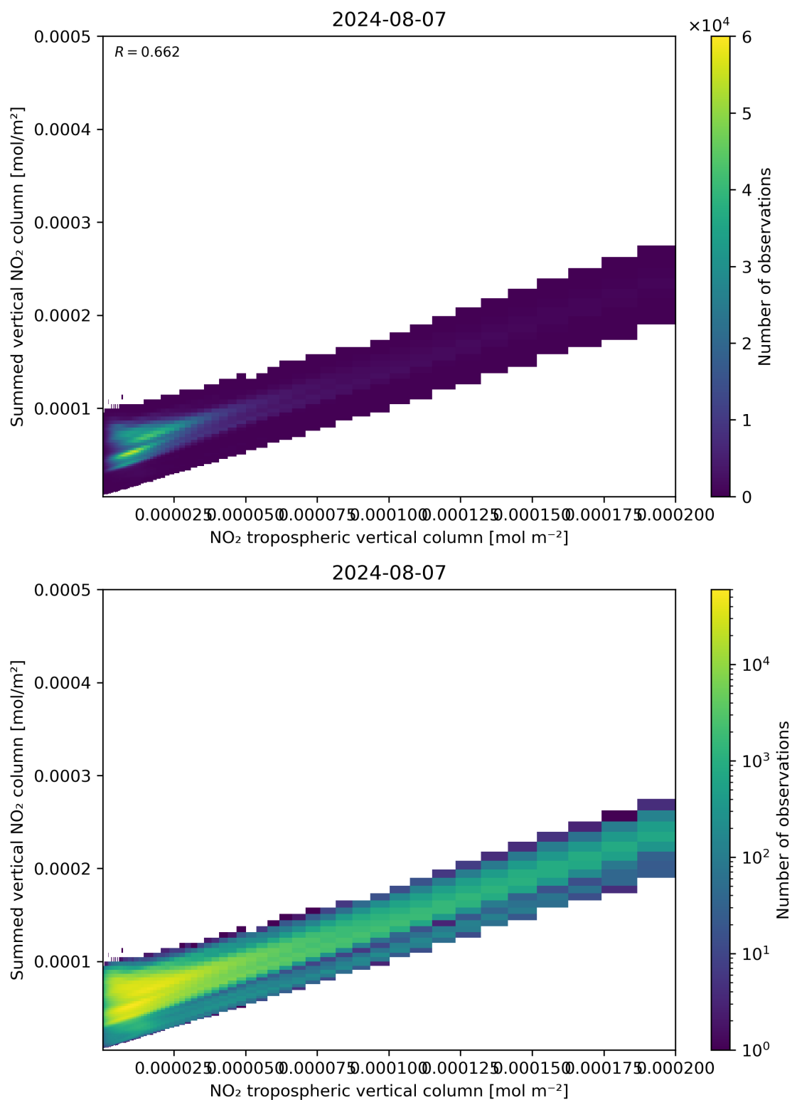
Figure 126: Scatter density plot of “NO 2 tropospheric vertical column” against “Summed vertical NO 2 column” for 2024-08-06 to 2024-08-08.
