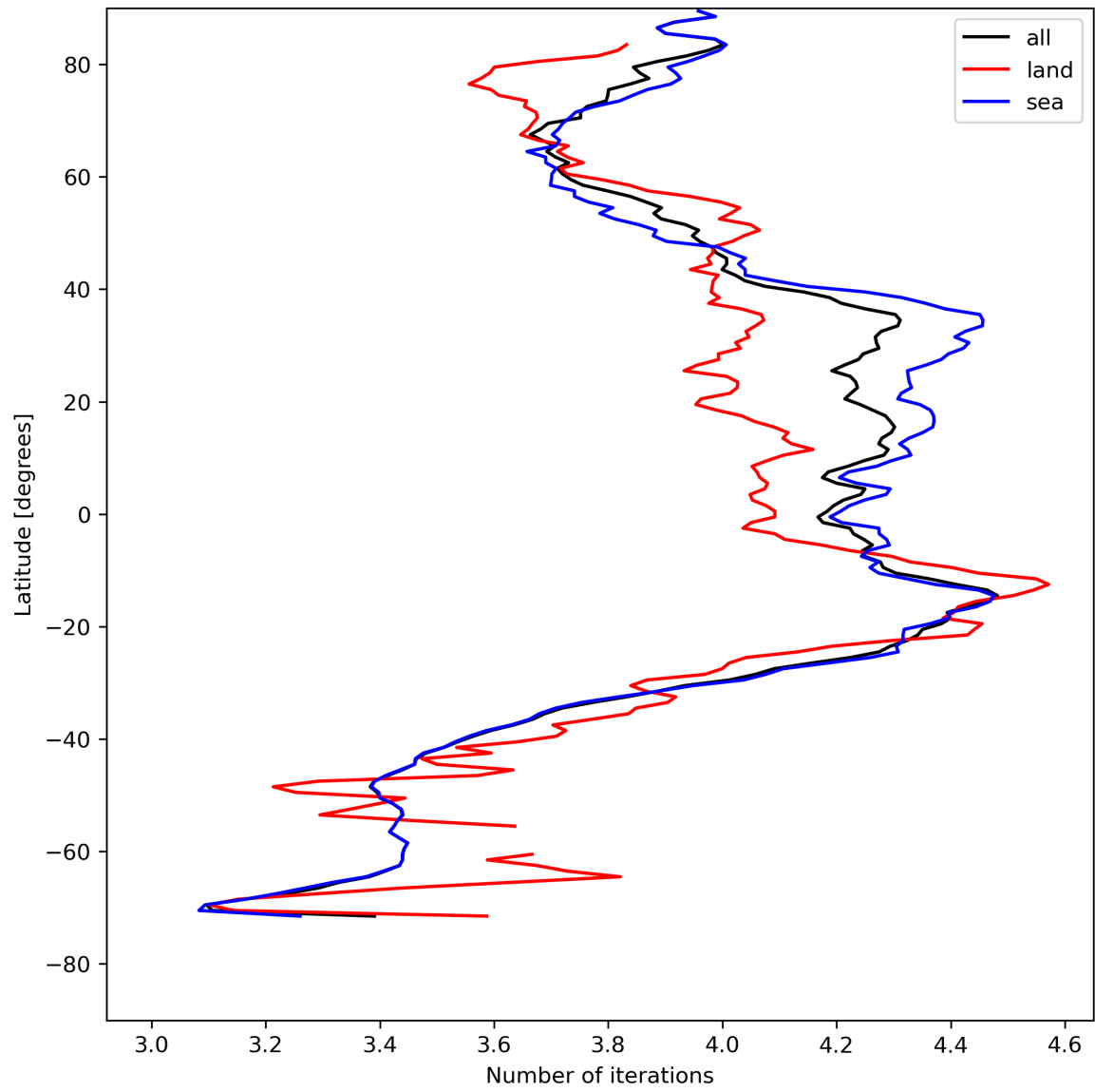
Figure 17: Zonal average of “Number of iterations” for 2024-08-06 to 2024-08-08.
