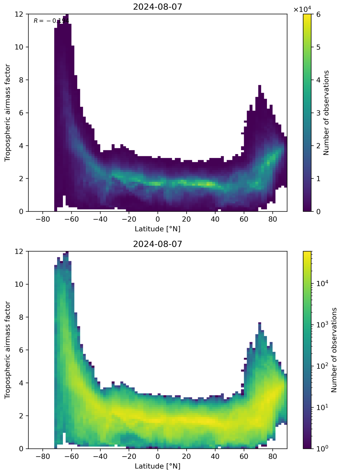
Figure 85: Scatter density plot of “Latitude” against “Tropospheric airmass factor” for 2024-08-06 to 2024-08-08.
