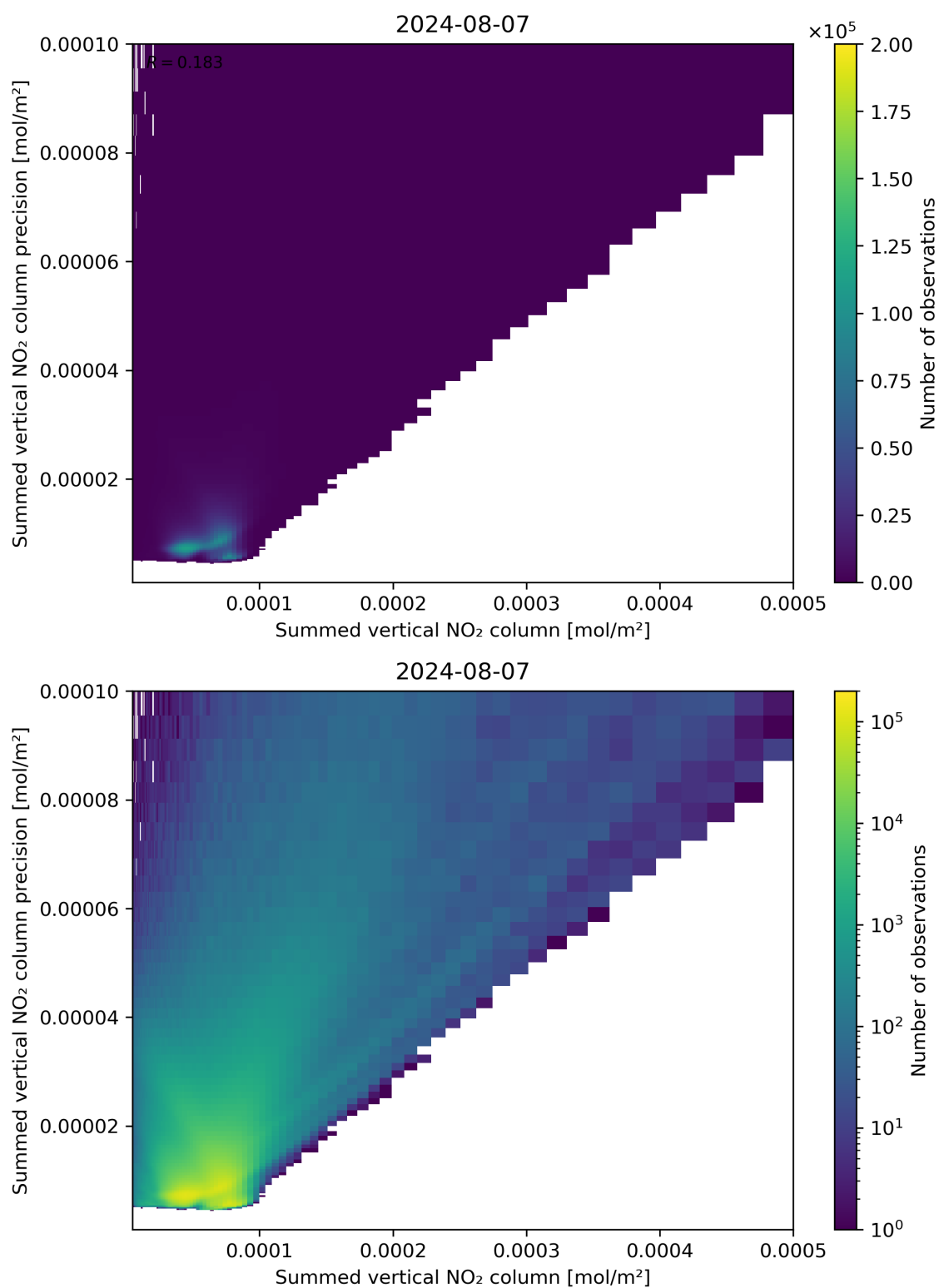
Figure 105: Scatter density plot of “Summed vertical NO 2 column” against “Summed vertical NO 2 column precision” for 2024-08-06 to 2024-08-08.
