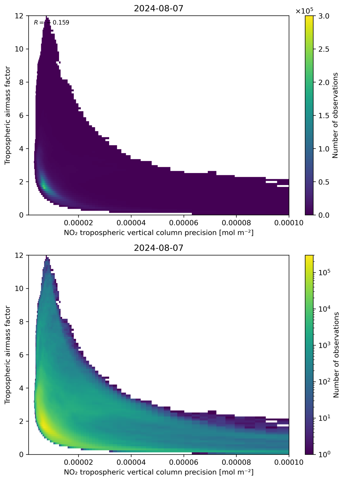
Figure 133: Scatter density plot of “NO 2 tropospheric vertical column precision” against “Tropospheric airmass factor” for 2024-08-06 to 2024-08-08.
