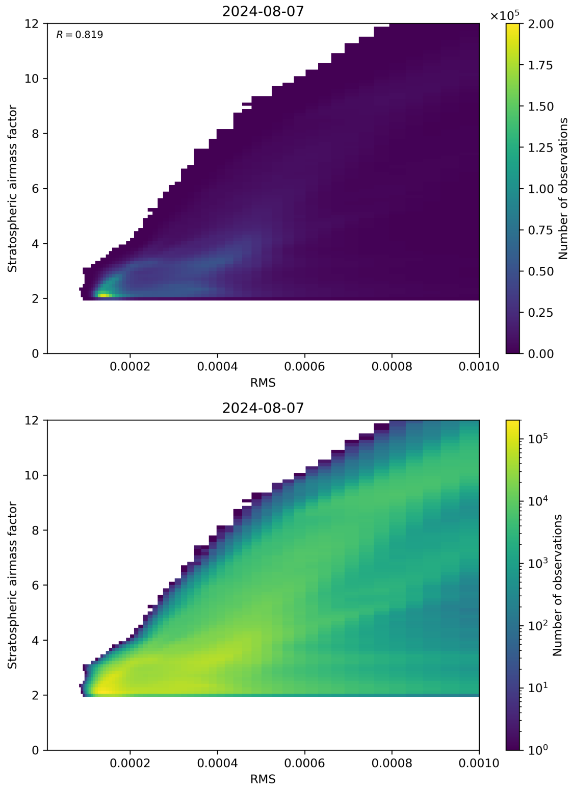
Figure 144: Scatter density plot of “RMS” against “Stratospheric airmass factor” for 2024-08-06 to 2024-08-08.
