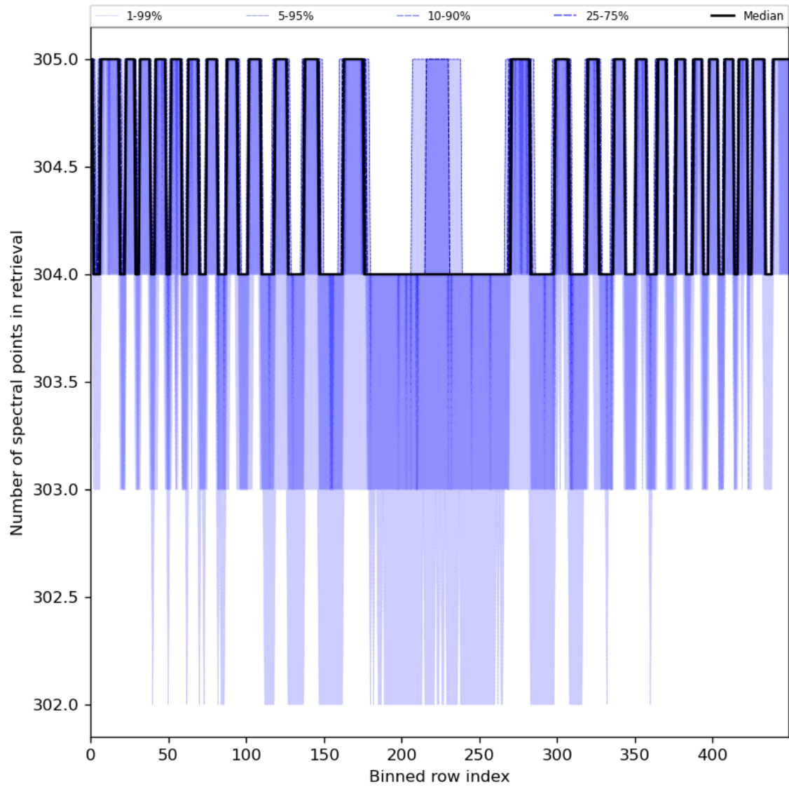
Figure 50: Along track statistics of “Number of spectral points in retrieval” for 2024-08-06 to 2024-08-08
