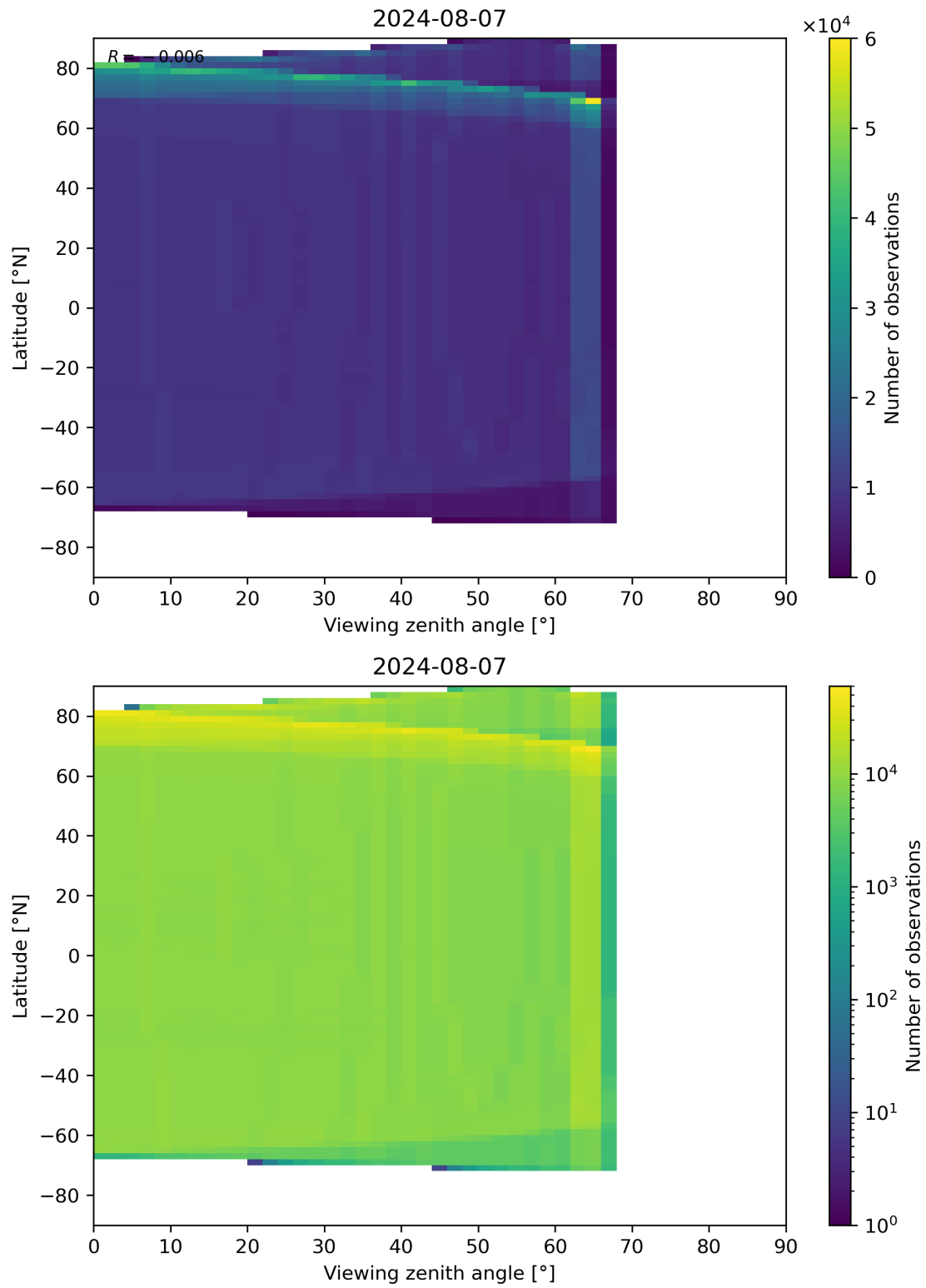
Figure 163: Scatter density plot of “Viewing zenith angle” against “Latitude” for 2024-08-06 to 2024-08-08.
