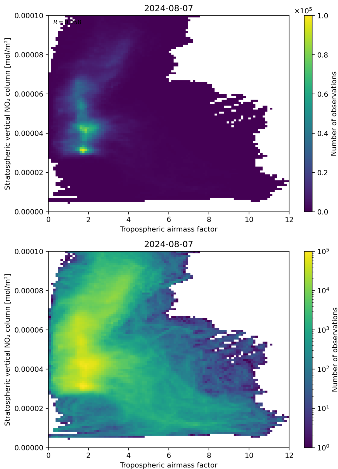
Figure 74: Scatter density plot of “Tropospheric air mass factor” against “Stratospheric vertical NO 2 column” for 2024-08-06 to 2024-08-08.
