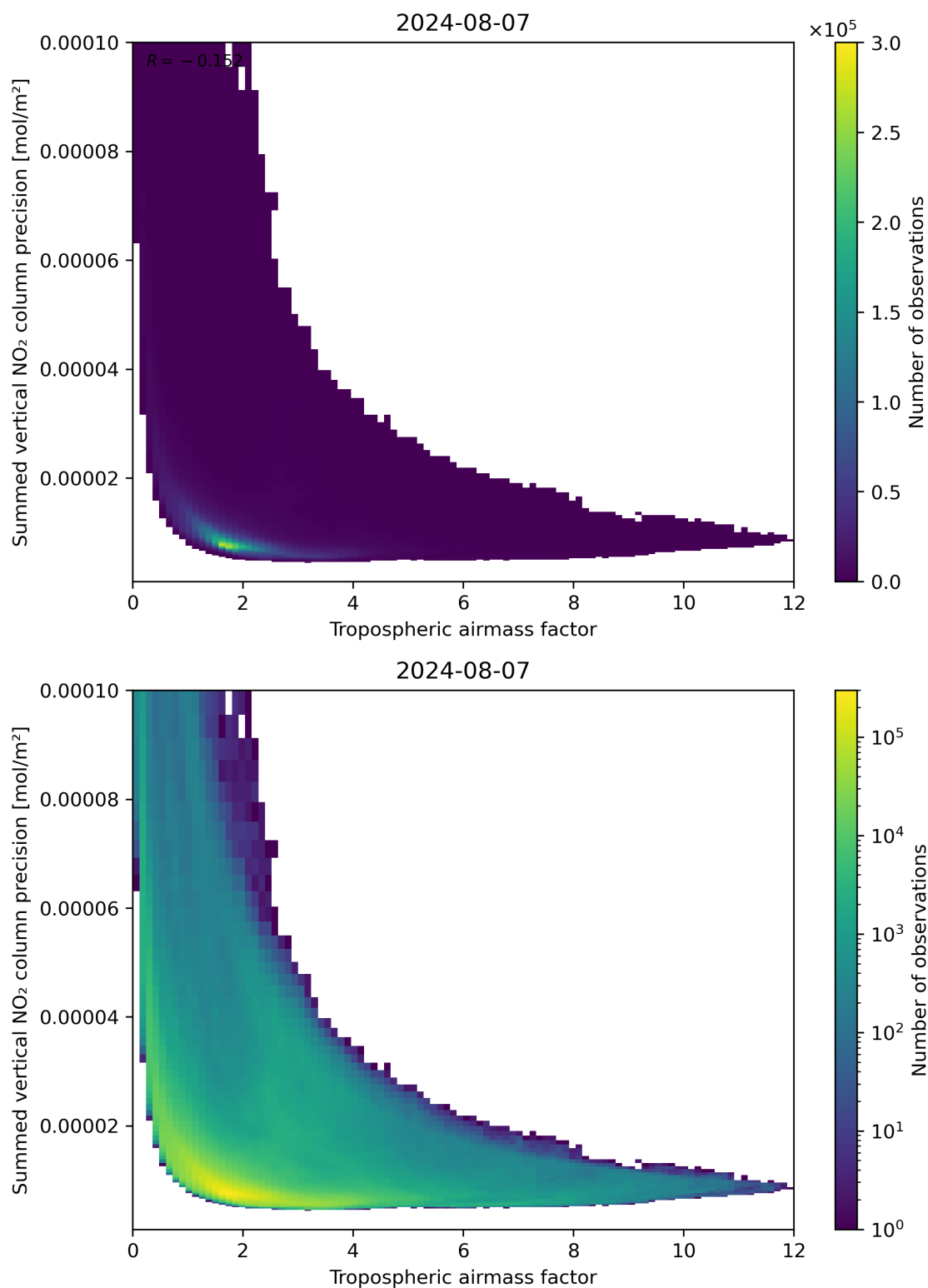
Figure 76: Scatter density plot of “Tropospheric air mass factor” against “Summed vertical NO 2 column precision” for 2024-08-06 to 2024-08-08.
