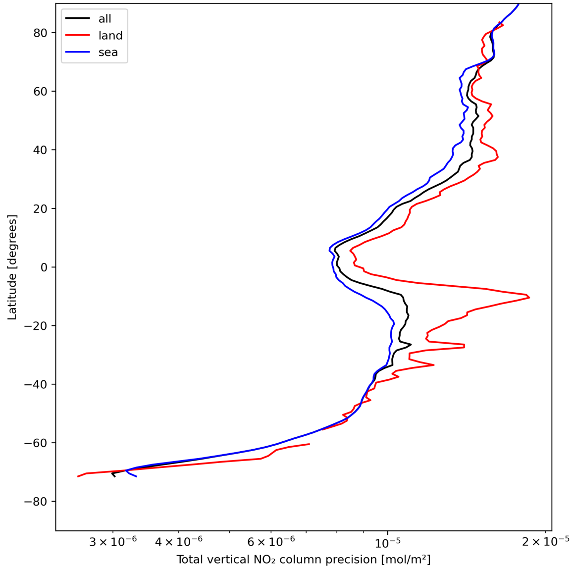
Figure 22: Zonal average of “Total vertical NO 2 column precision” for 2024-08-06 to 2024-08-08.
