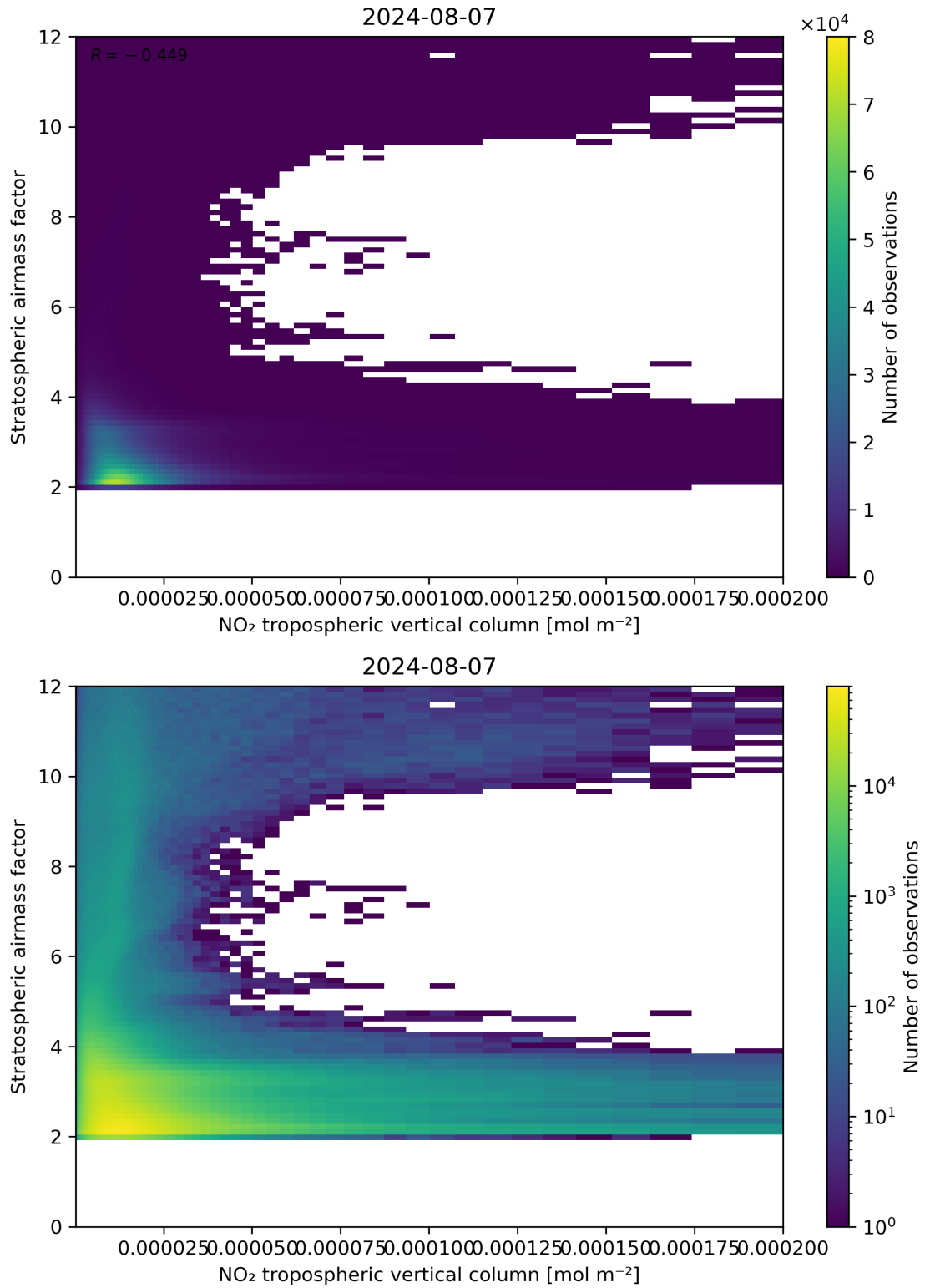
Figure 121: Scatter density plot of “NO 2 tropospheric vertical column” against “Stratospheric air mass factor” for 2024-08-06 to 2024-08-08.
