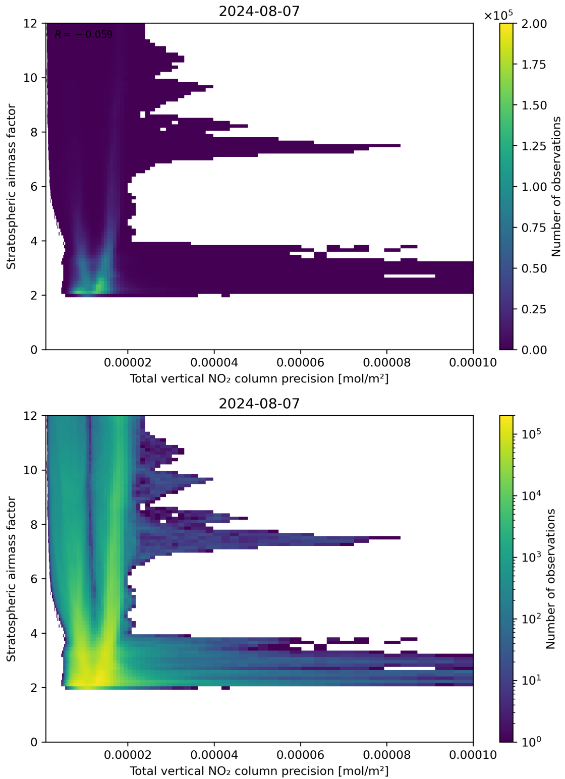
Figure 115: Scatter density plot of “Total vertical NO 2 column precision” against “Stratospheric air mass factor” for 2024-08-06 to 2024-08-08.
