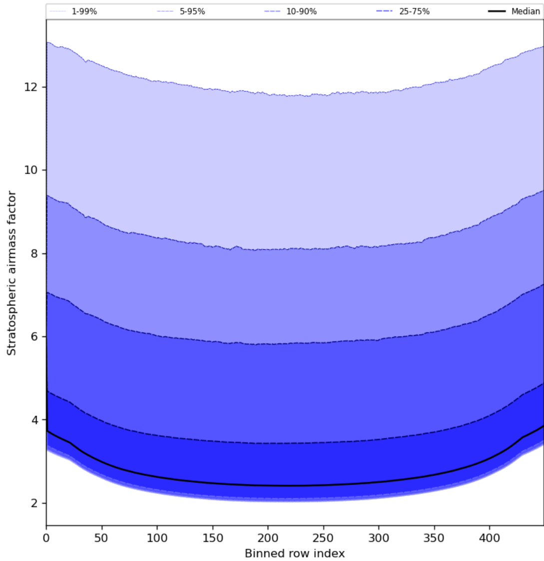
Figure 61: Along track statistics of “Stratospheric airmass factor” for 2024-08-06 to 2024-08-08
