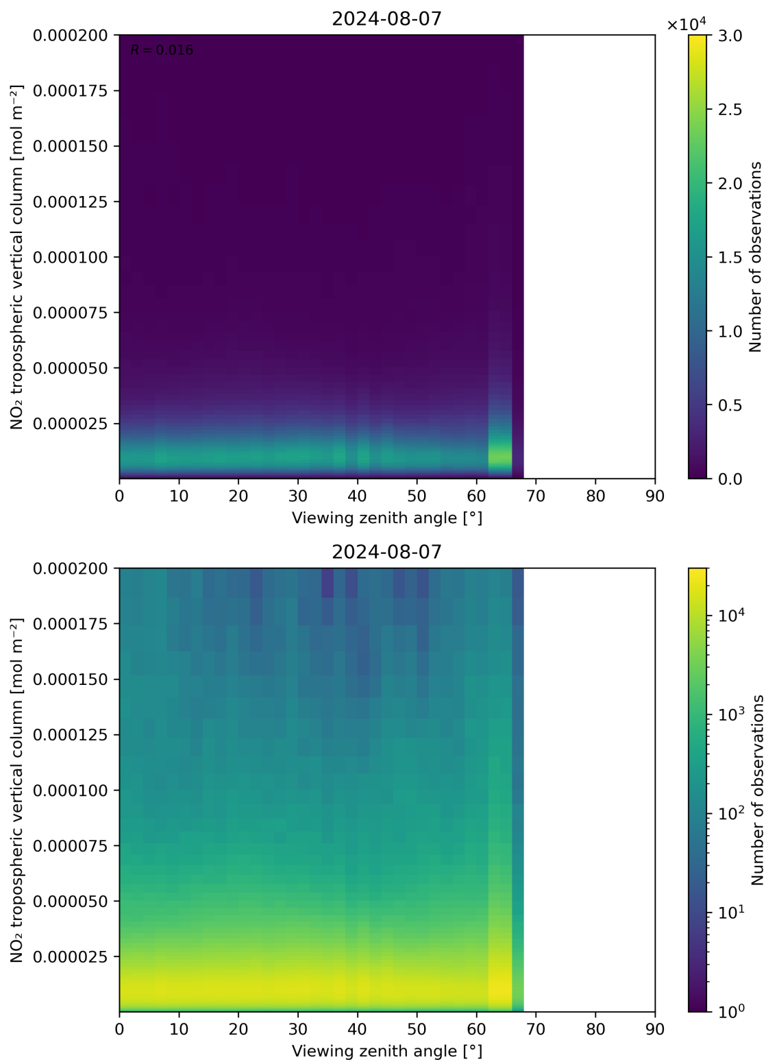
Figure 169: Scatter density plot of “Viewing zenith angle” against “NO 2 tropospheric vertical column” for 2024-08-06 to 2024-08-08.
