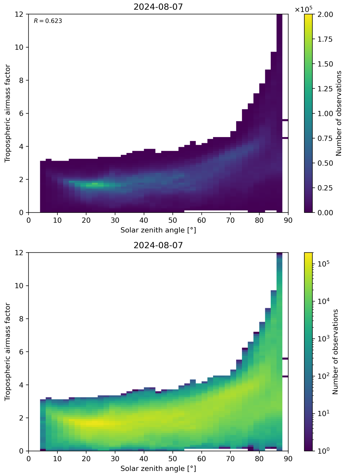
Figure 147: Scatter density plot of “Solar zenith angle” against “Tropospheric airmass factor” for 2024-08-06 to 2024-08-08.
