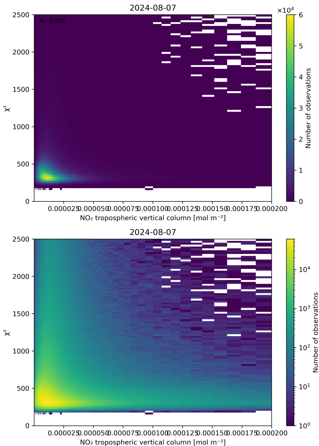
Figure 124: Scatter density plot of “NO 2 tropospheric vertical column” against “ \chi^2 ” for 2024-08-06 to 2024-08-08.
