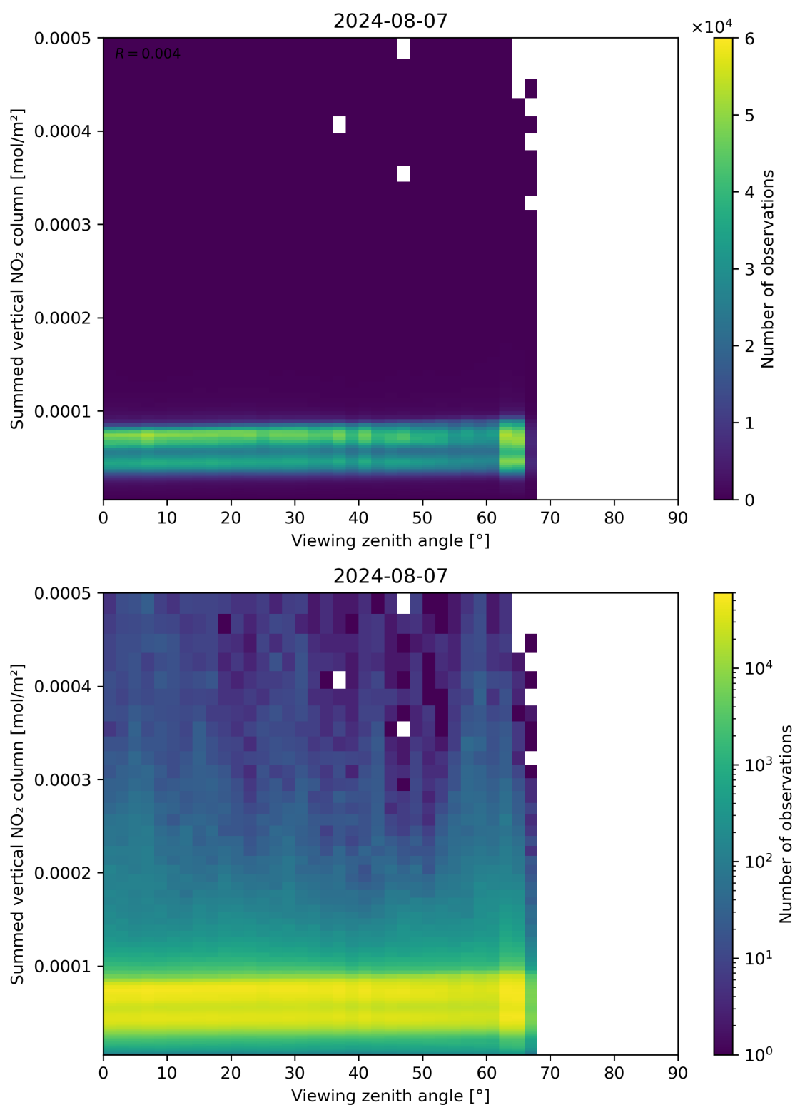
Figure 165: Scatter density plot of “Viewing zenith angle” against “Summed vertical NO 2 column” for 2024-08-06 to 2024-08-08.
