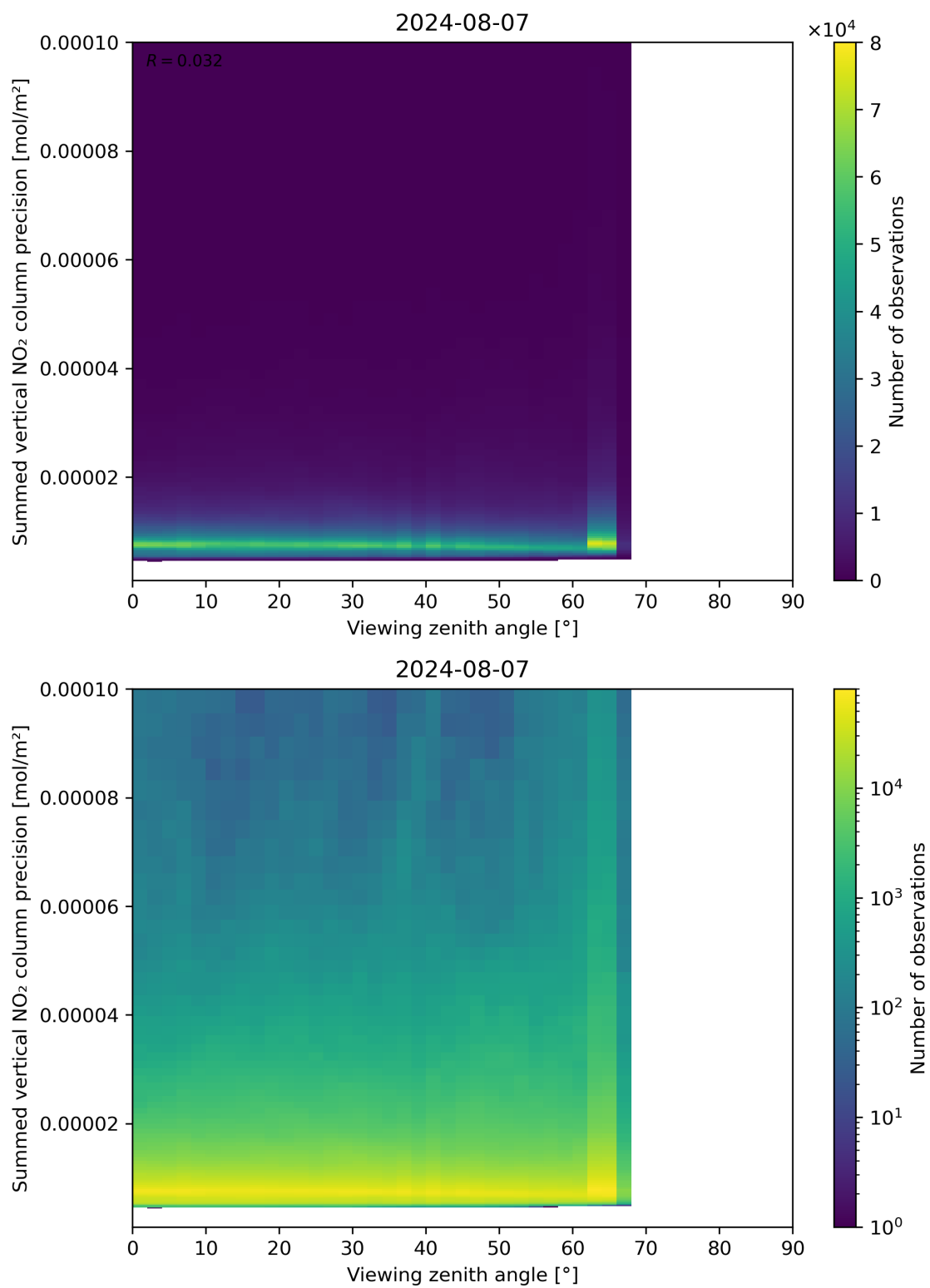
Figure 166: Scatter density plot of “Viewing zenith angle” against “Summed vertical NO 2 column precision” for 2024-08-06 to 2024-08-08.
