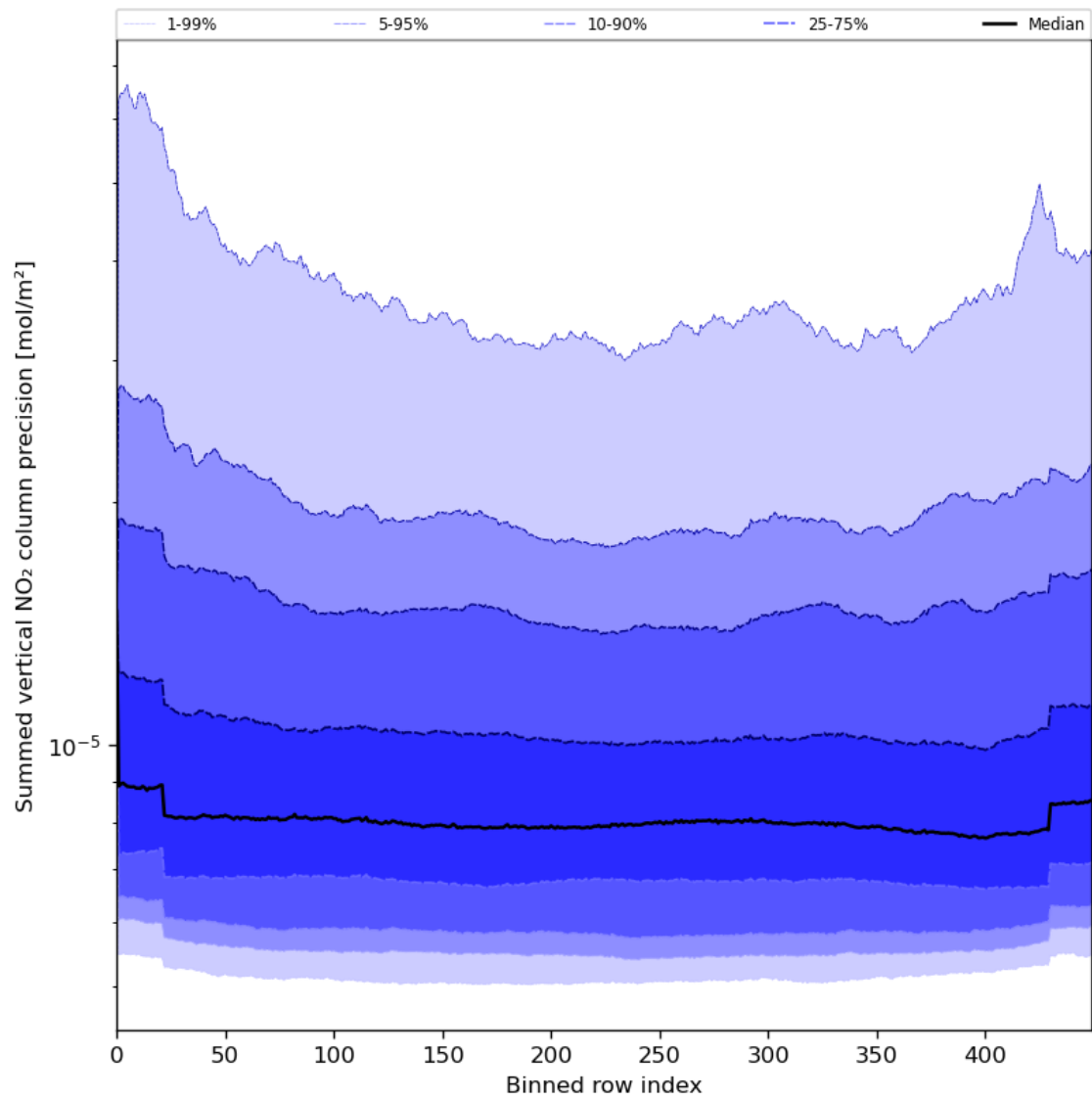
Figure 58: Along track statistics of “Summed vertical NO 2 column precision” for 2024-08-06 to 2024-08-08
