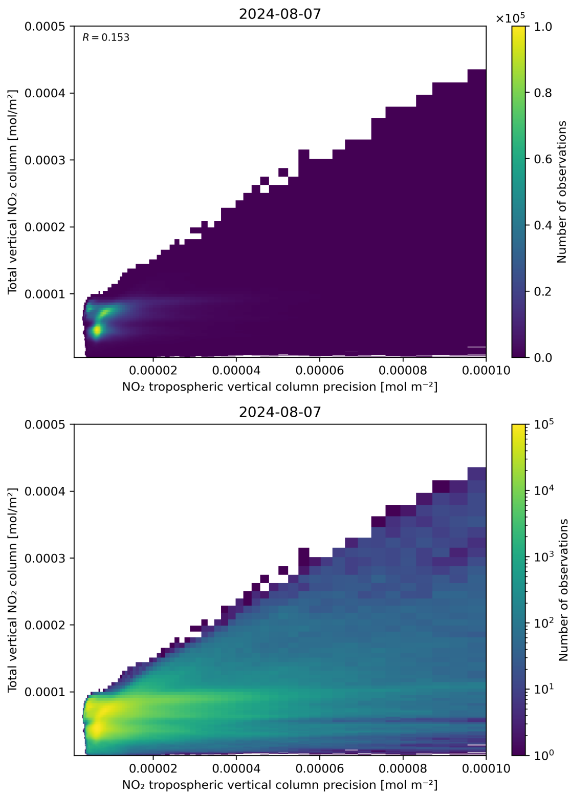
Figure 138: Scatter density plot of “NO 2 tropospheric vertical column precision” against “Total vertical NO 2 column” for 2024-08-06 to 2024-08-08.
