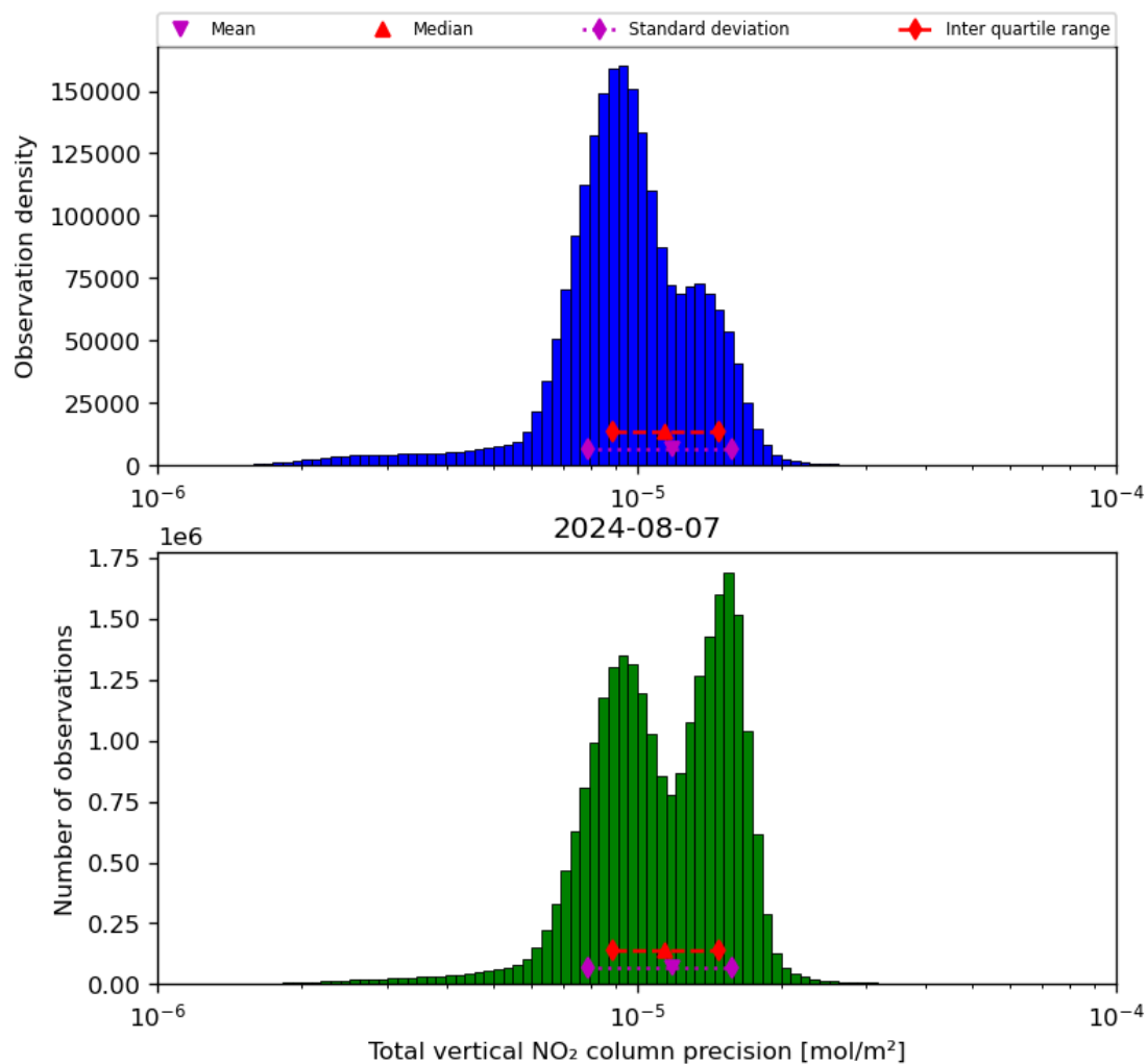
Figure 39: Histogram of “Total vertical NO 2 column precision” for 2024-08-06 to 2024-08-08
