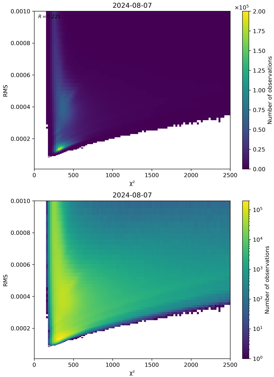
Figure 82: Scatter density plot of “ \chi^2 ” against “RMS” for 2024-08-06 to 2024-08-08.
