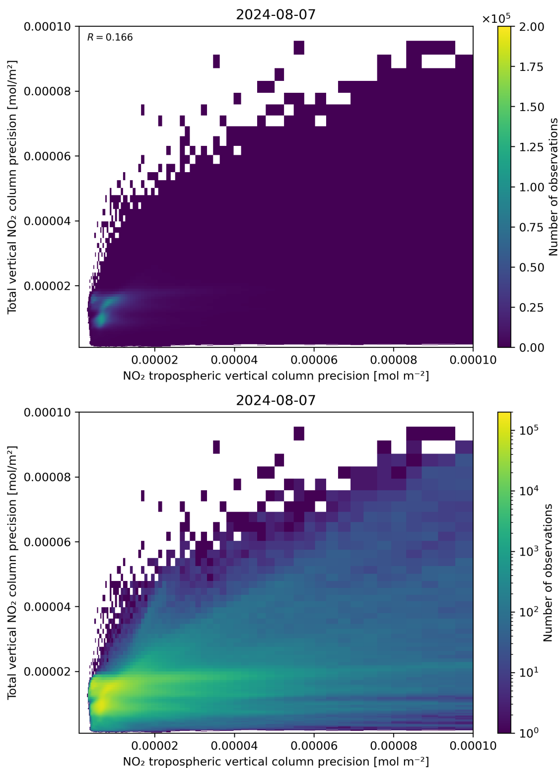
Figure 139: Scatter density plot of “NO 2 tropospheric vertical column precision” against “Total vertical NO 2 column precision” for 2024-08-06 to 2024-08-08.
