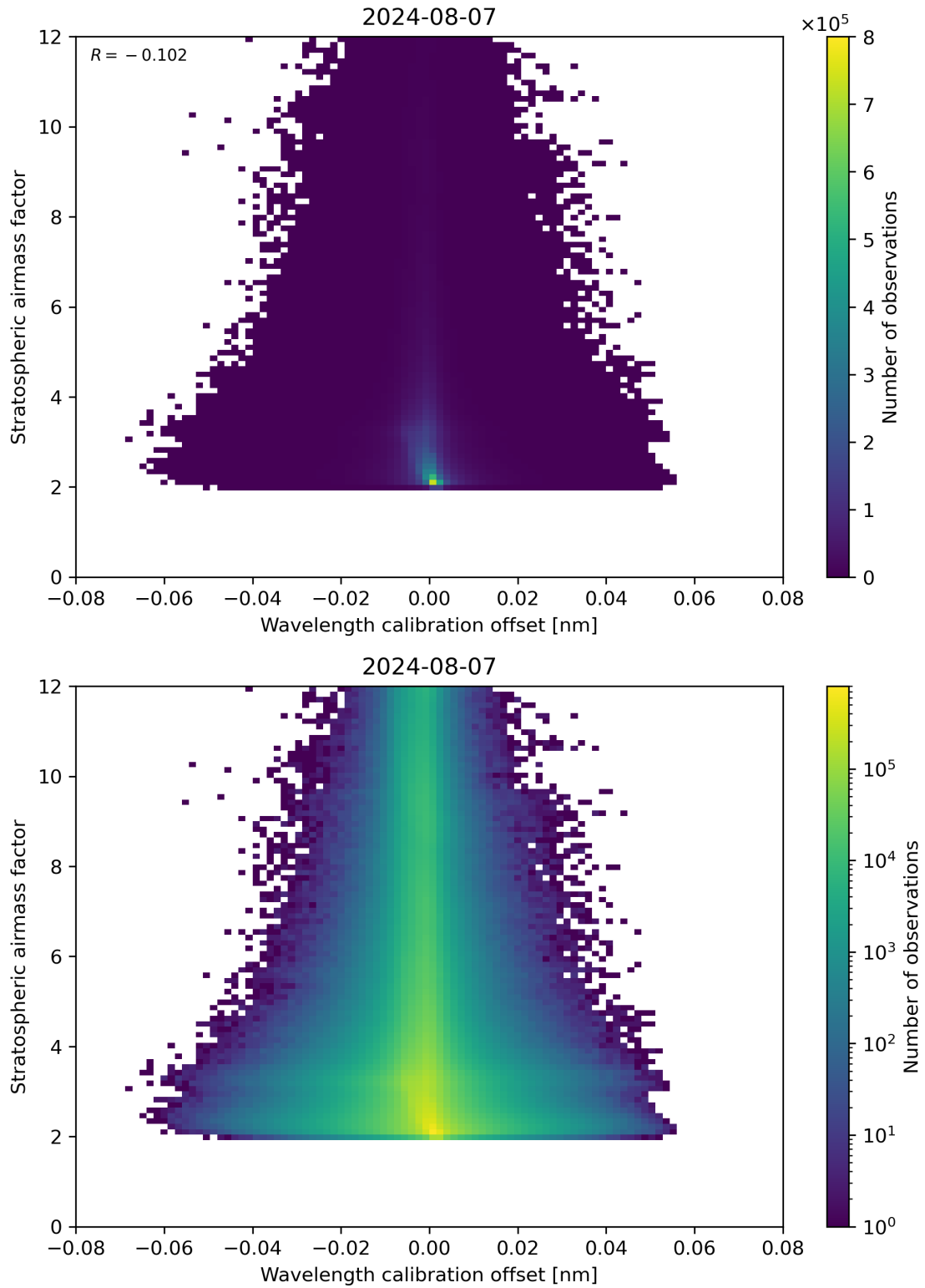
Figure 174: Scatter density plot of “Wavelength calibration offset” against “Stratospheric air mass factor” for 2024-08-06 to 2024-08-08.
