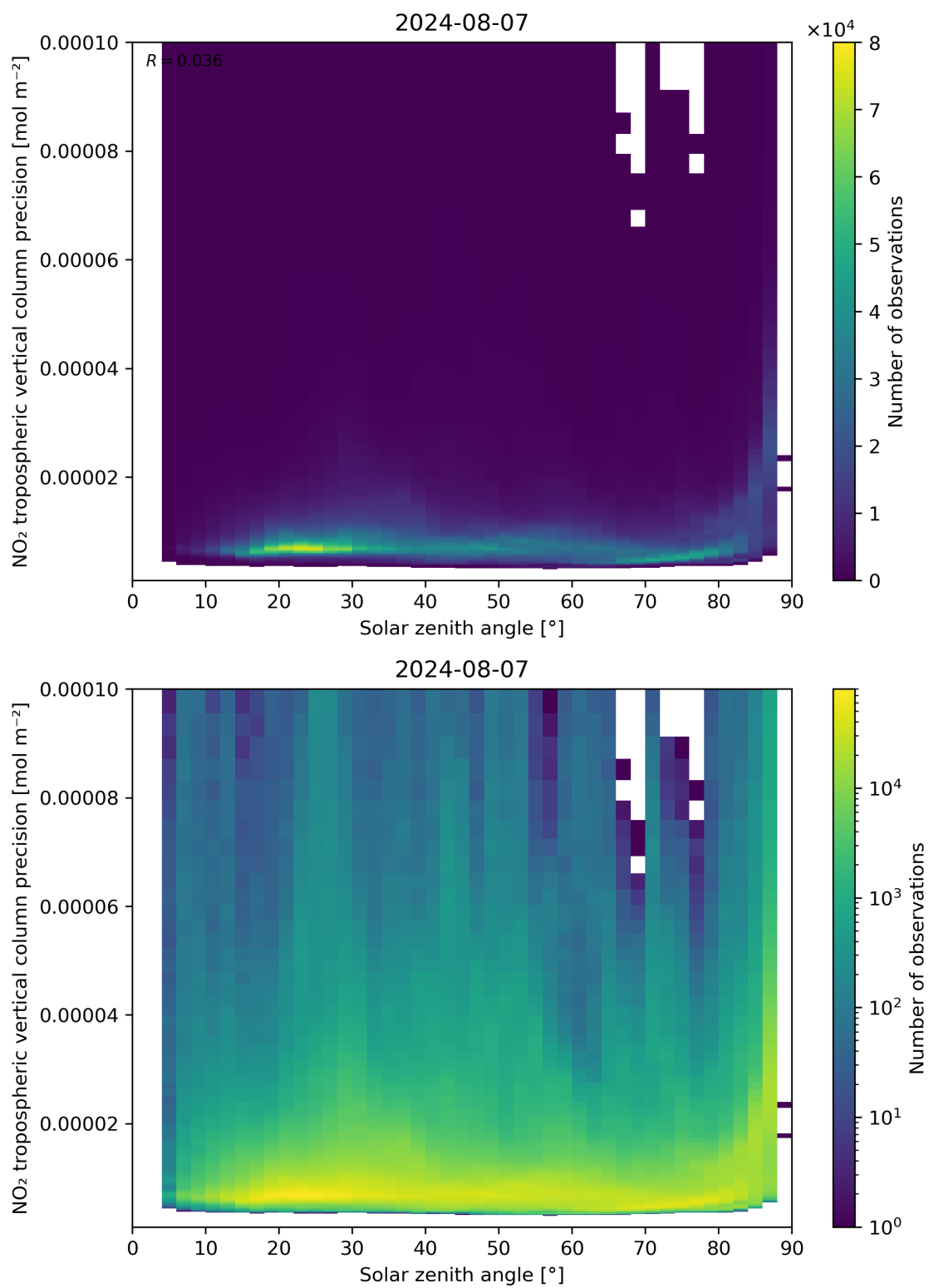
Figure 156: Scatter density plot of “Solar zenith angle” against “NO 2 tropospheric vertical column precision” for 2024-08-06 to 2024-08-08.
