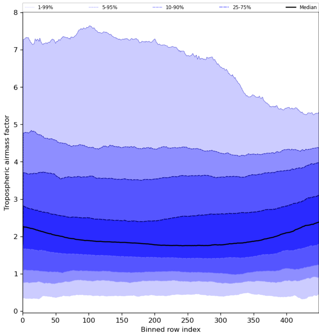
Figure 48: Along track statistics of “Tropospheric airmass factor” for 2024-08-06 to 2024-08-08
