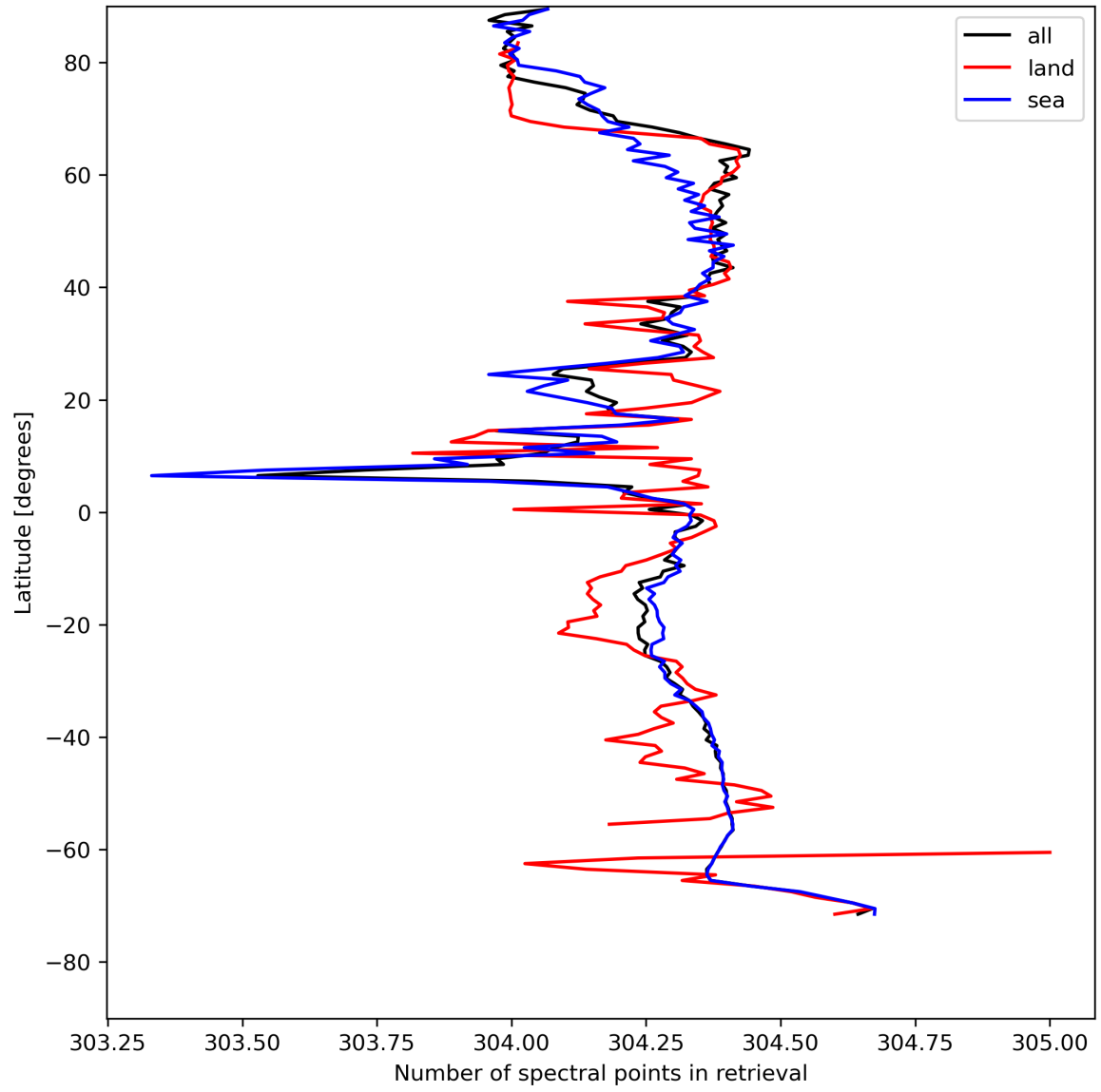
Figure 16: Zonal average of “Number of spectral points in retrieval” for 2024-08-06 to 2024-08-08.
