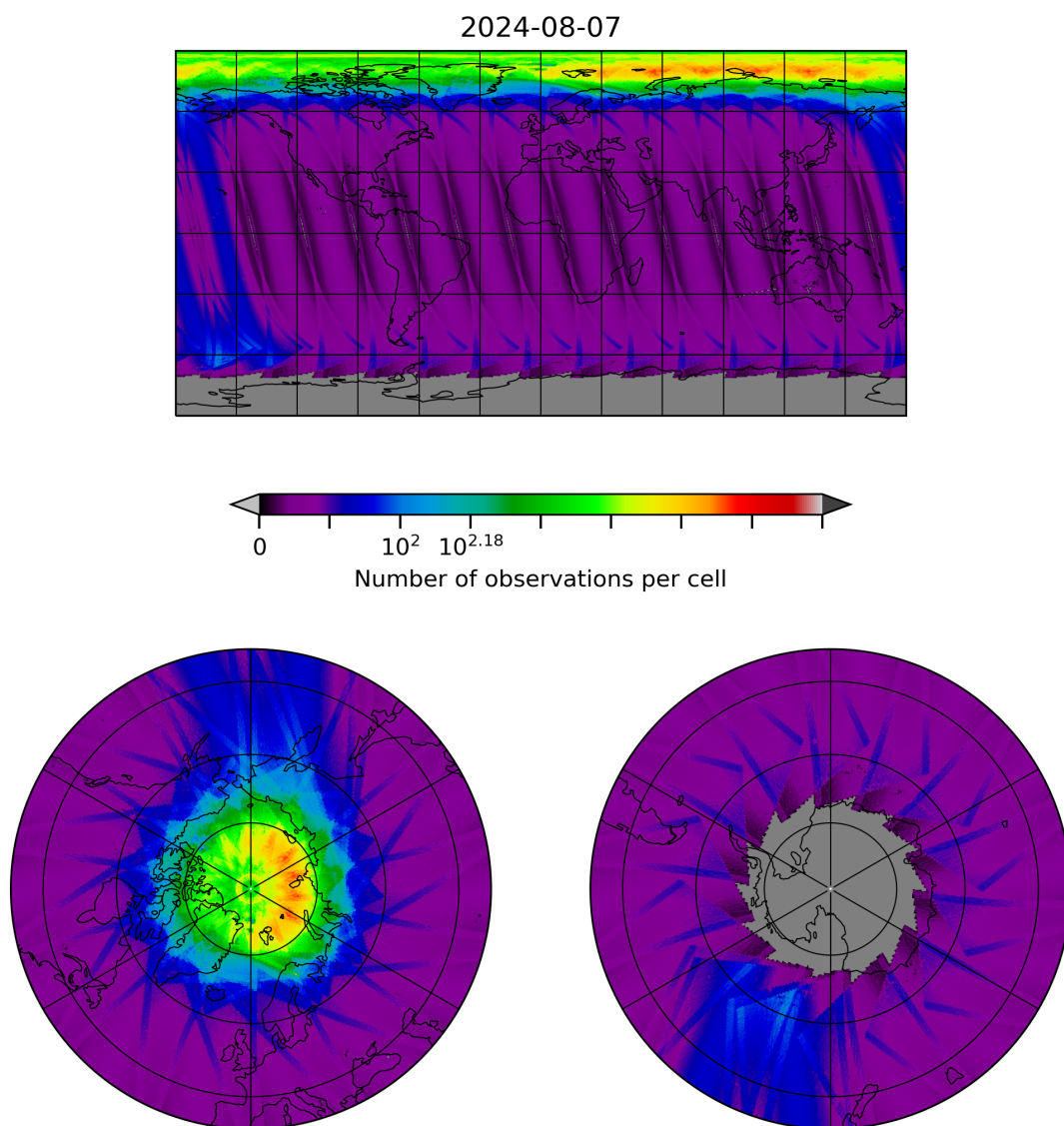
Figure 10: Map of the number of observations for 2024-08-06 to 2024-08-08
