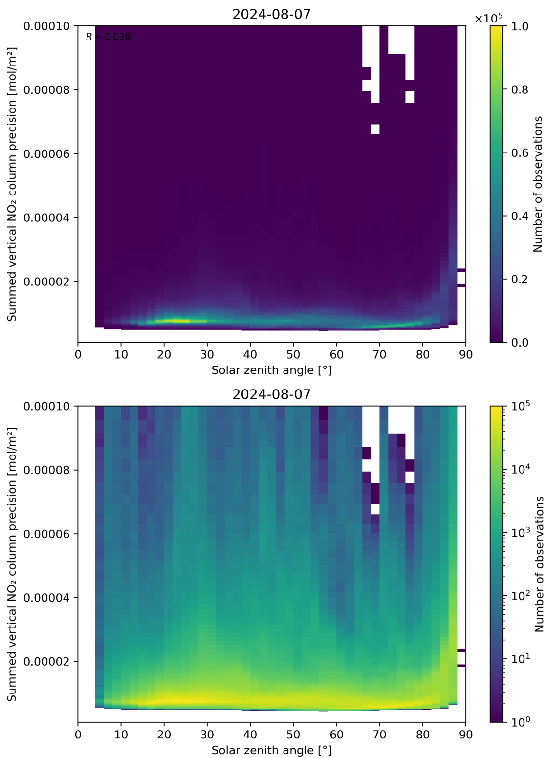
Figure 152: Scatter density plot of “Solar zenith angle” against “Summed vertical NO 2 column precision” for 2024-08-06 to 2024-08-08.
