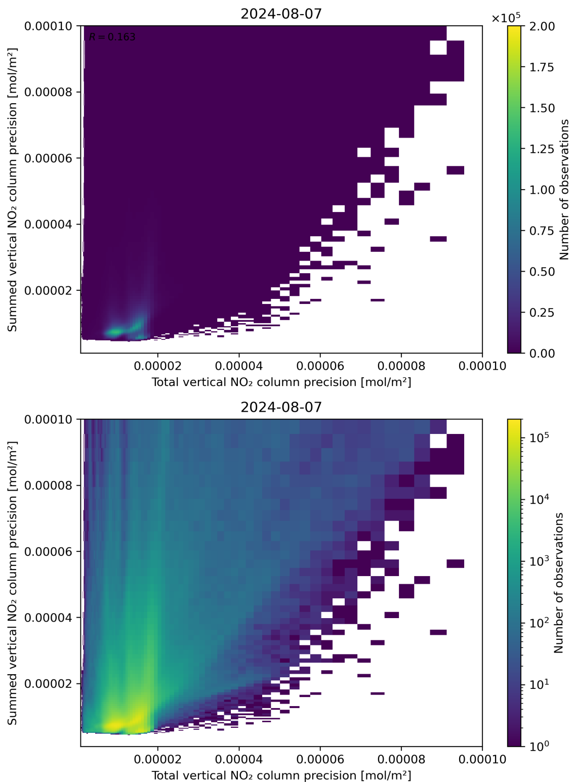
Figure 118: Scatter density plot of “Total vertical NO 2 column precision” against “Summed vertical NO 2 column precision” for 2024-08-06 to 2024-08-08.
