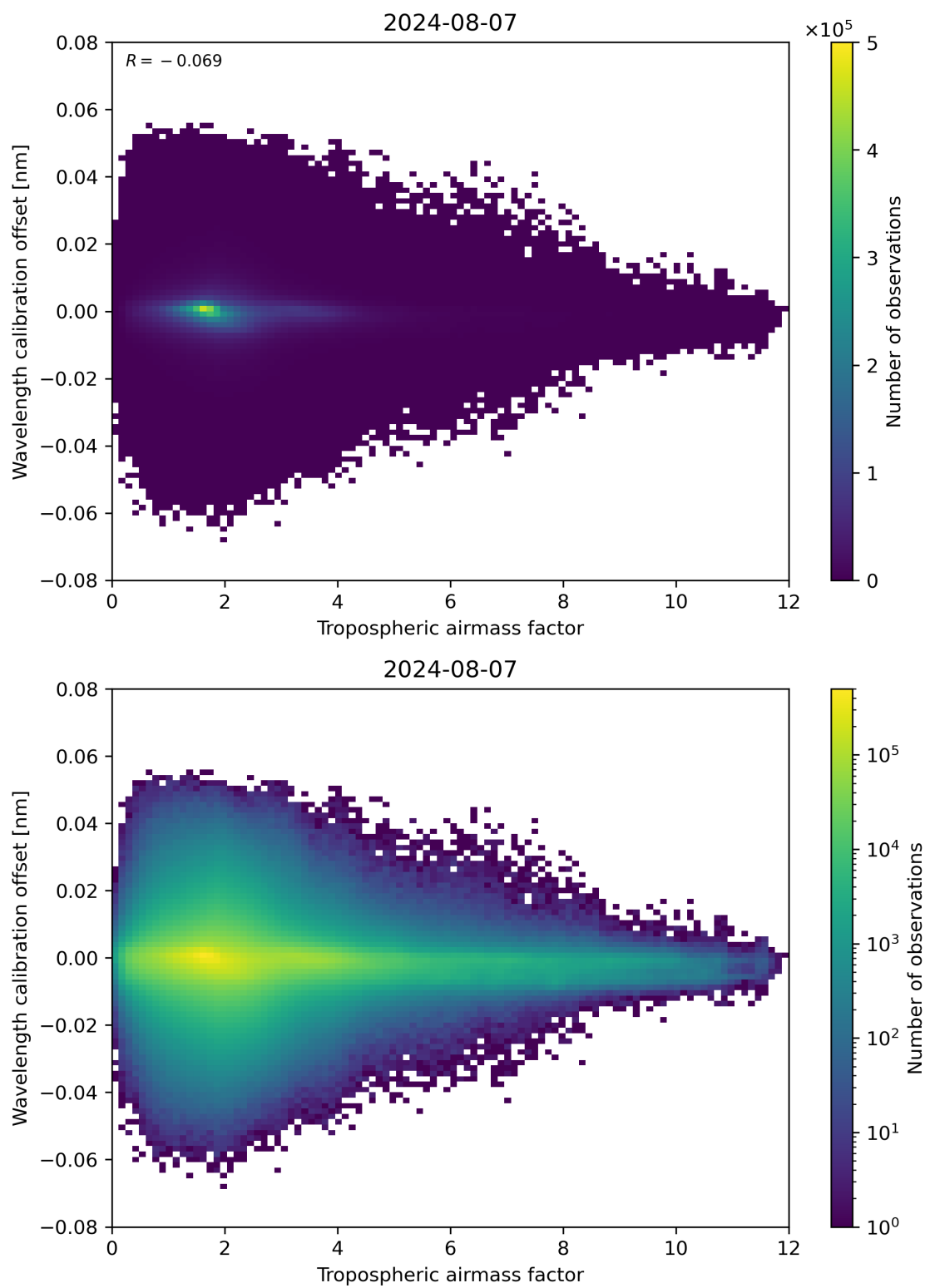
Figure 80: Scatter density plot of “Tropospheric airmass factor” against “Wavelength calibration offset” for 2024-08-06 to 2024-08-08.
