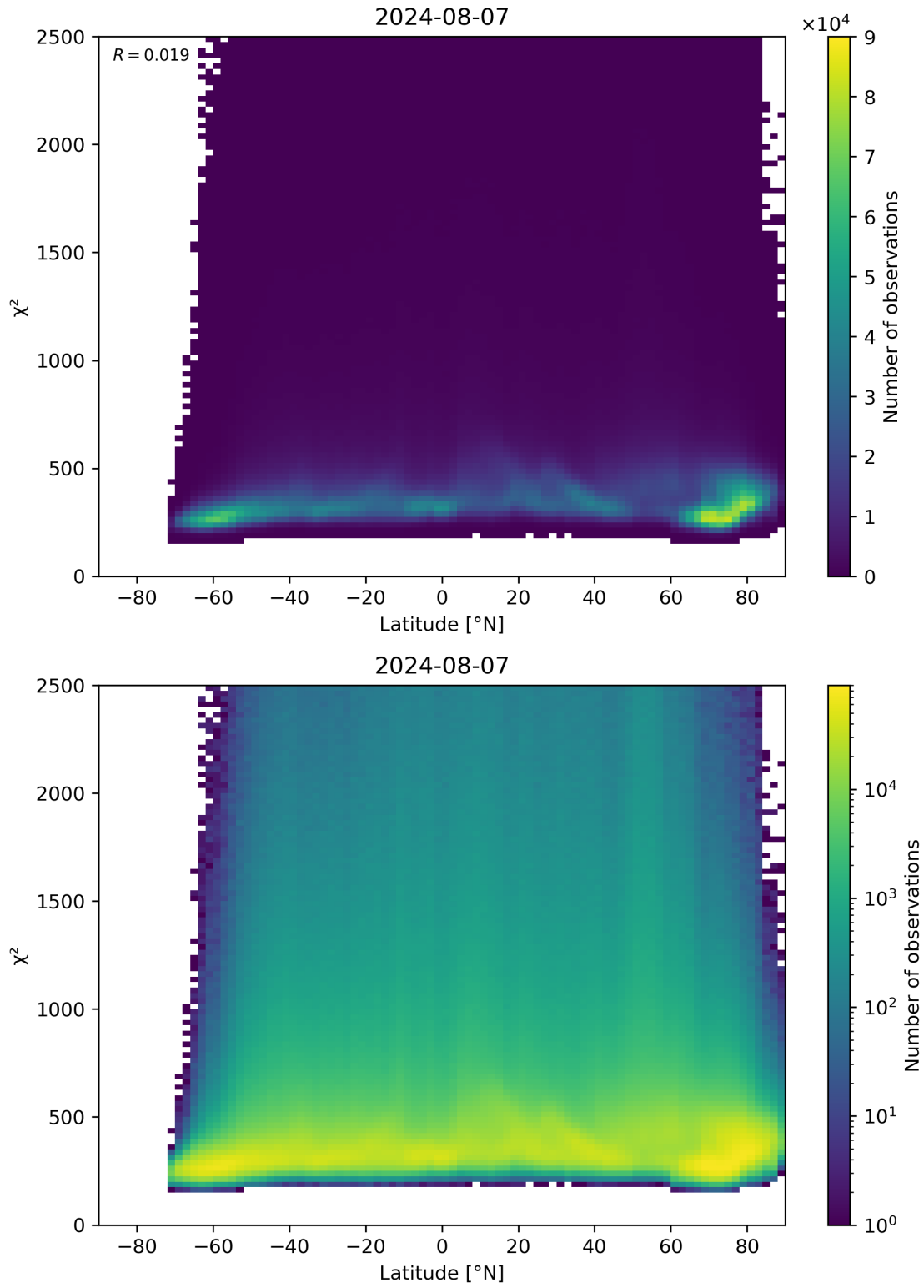
Figure 86: Scatter density plot of “Latitude” against “ \chi^2 ” for 2024-08-06 to 2024-08-08.
