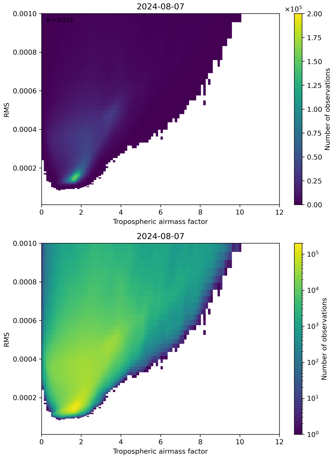
Figure 79: Scatter density plot of “Tropospheric airmass factor” against “RMS” for 2024-08-06 to 2024-08-08.
