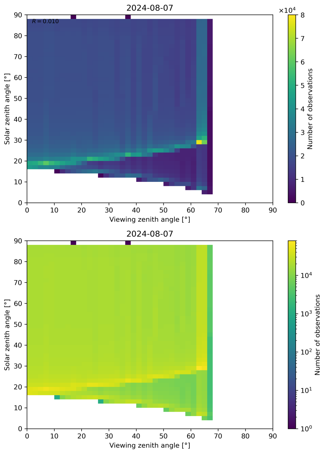
Figure 172: Scatter density plot of “Viewing zenith angle” against “Solar zenith angle” for 2024-08-06 to 2024-08-08.
