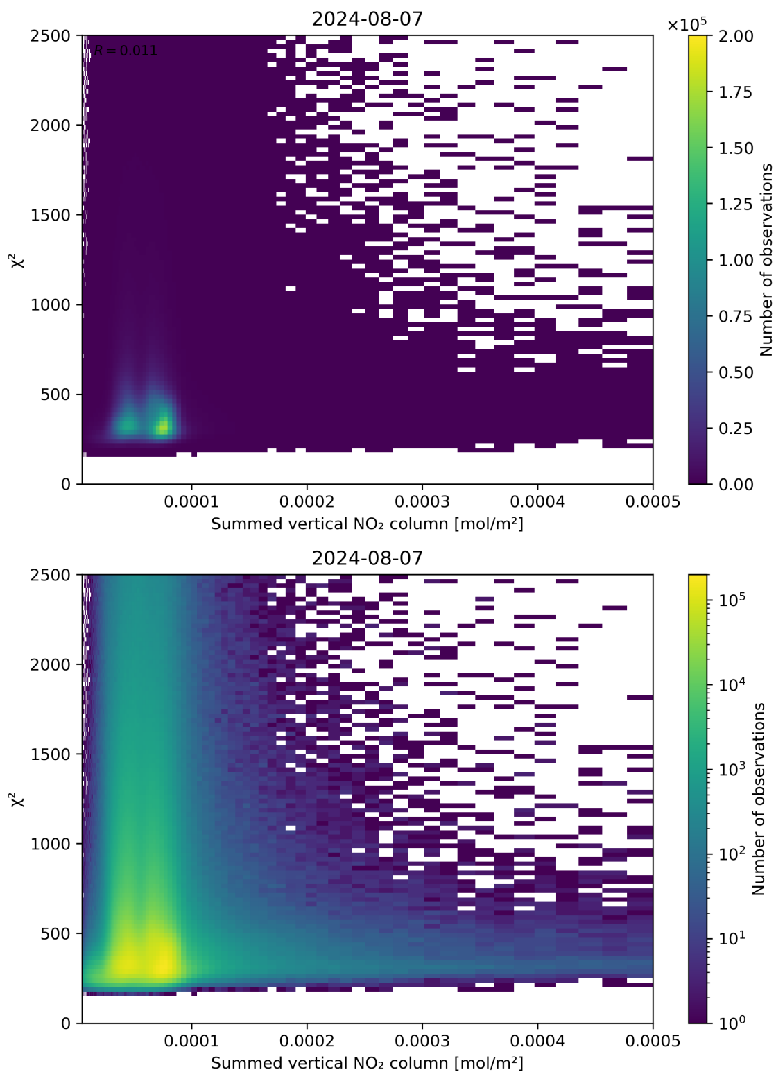
Figure 104: Scatter density plot of “Summed vertical NO 2 column” against “ \chi^2 ” for 2024-08-06 to 2024-08-08.
