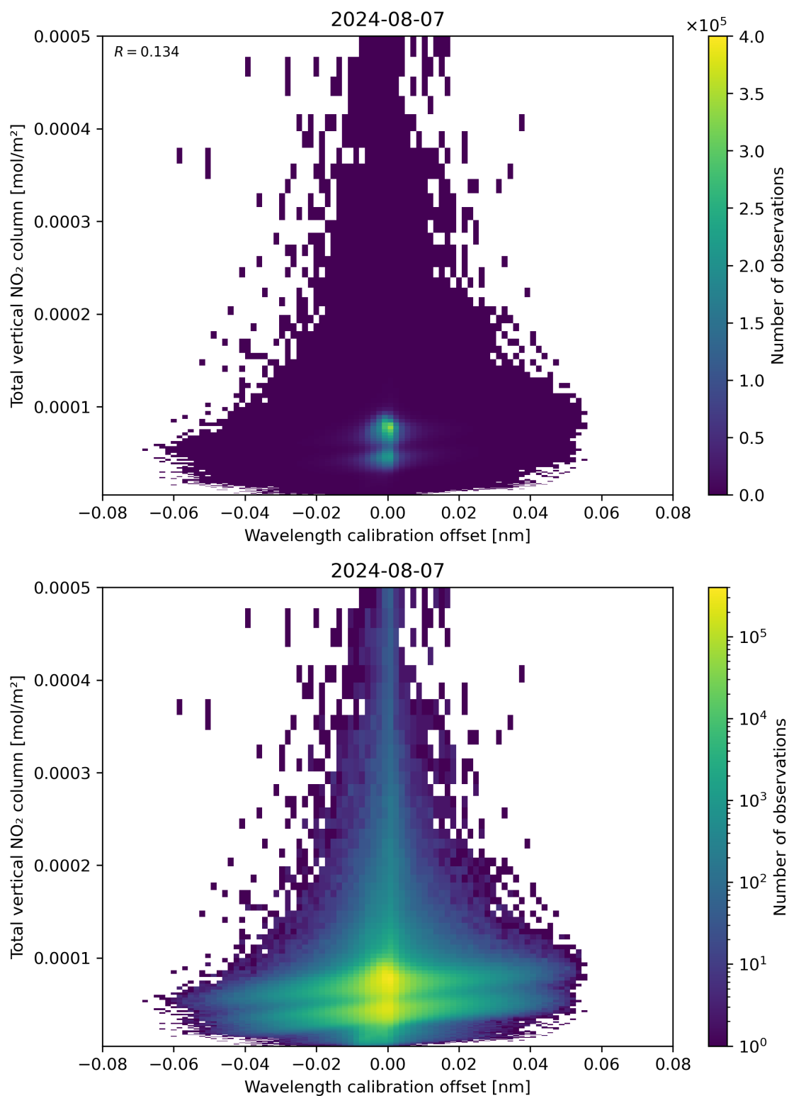
Figure 179: Scatter density plot of “Wavelength calibration offset” against “Total vertical NO 2 column” for 2024-08-06 to 2024-08-08.
