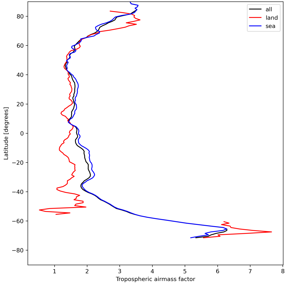
Figure 14: Zonal average of “Tropospheric airmass factor” for 2024-08-06 to 2024-08-08.
