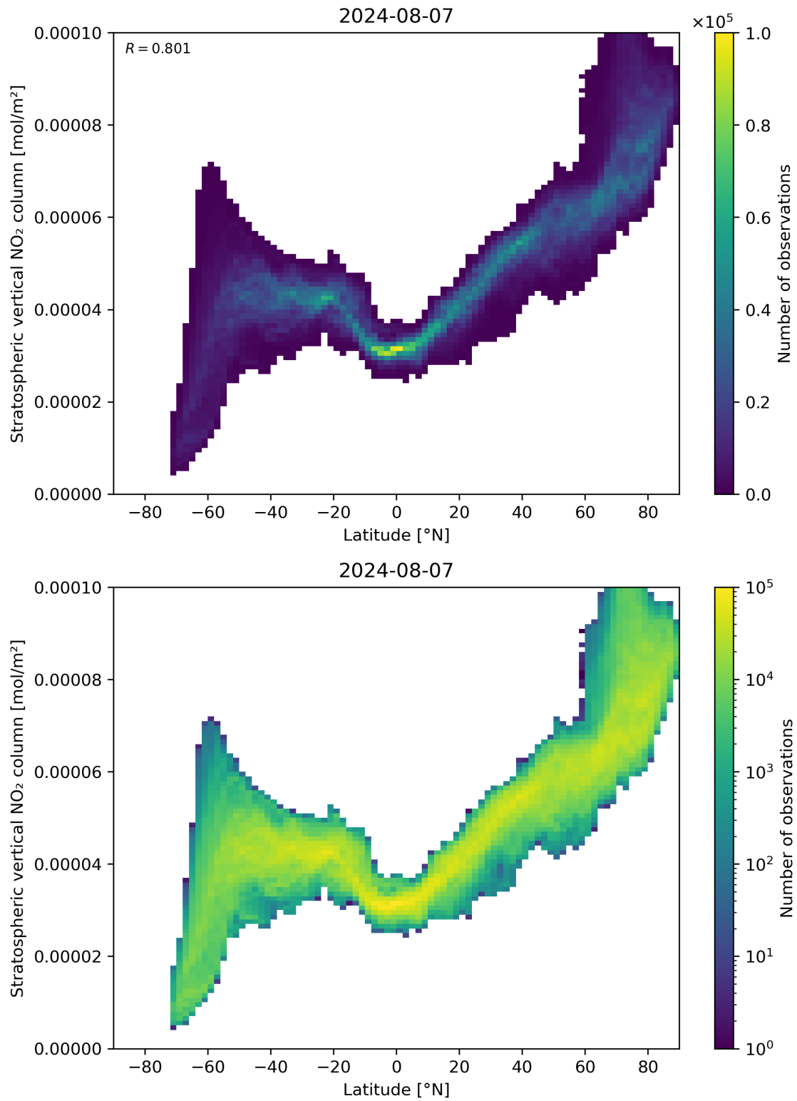
Figure 87: Scatter density plot of “Latitude” against “Stratospheric vertical NO 2 column” for 2024-08-06 to 2024-08-08.
