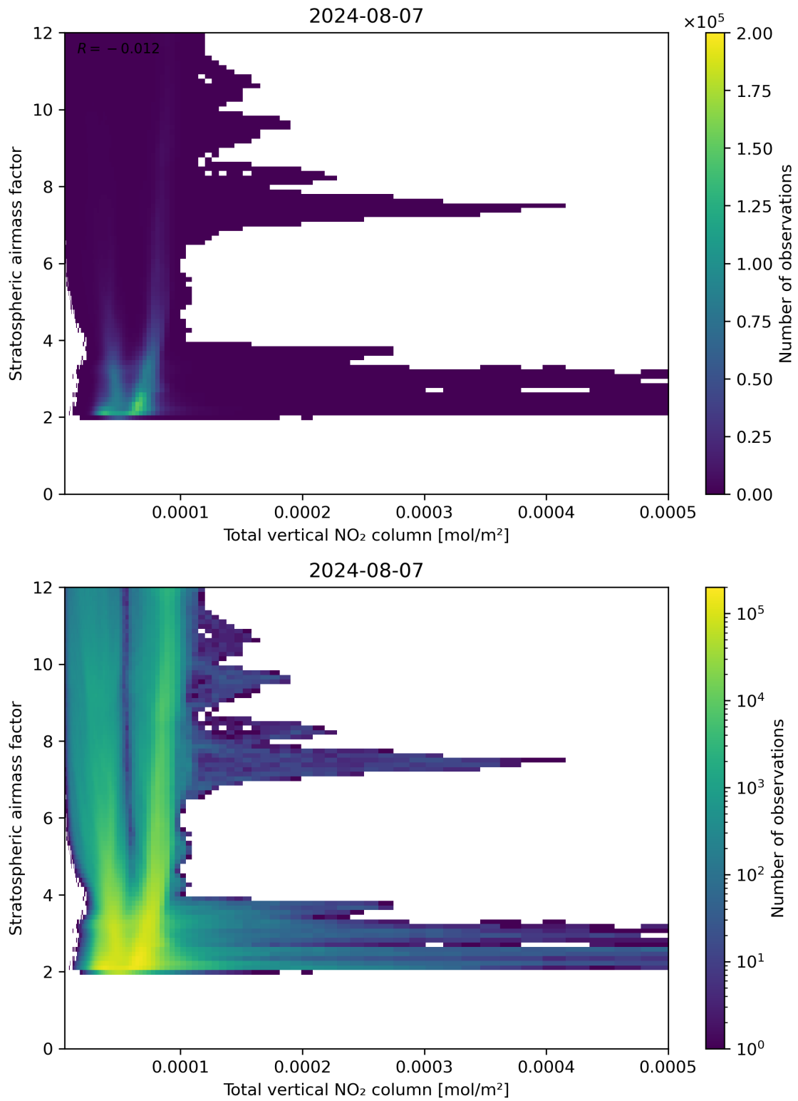
Figure 110: Scatter density plot of “Total vertical NO 2 column” against “Stratospheric airmass factor” for 2024-08-06 to 2024-08-08.
