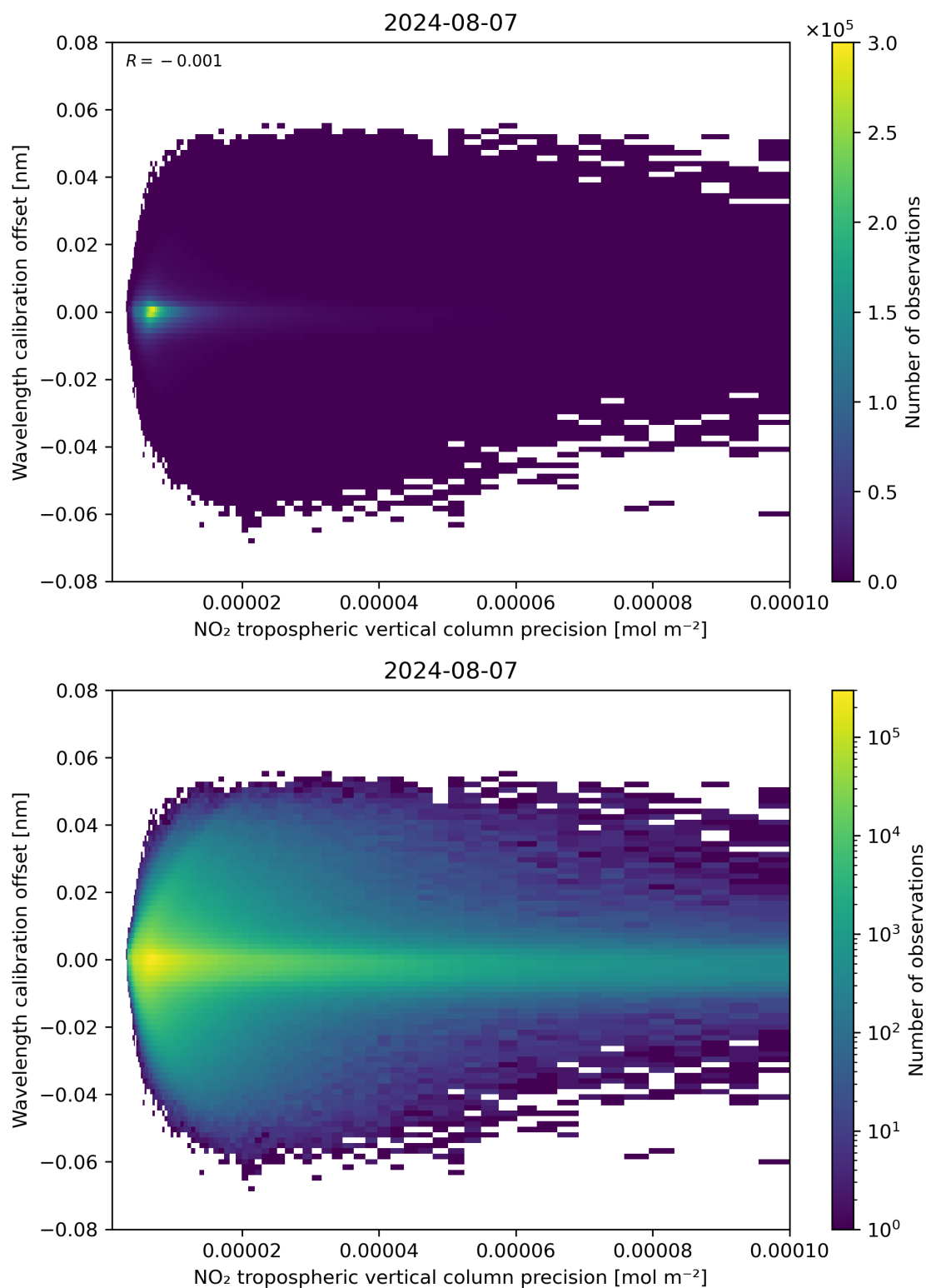
Figure 141: Scatter density plot of “NO 2 tropospheric vertical column precision” against “Wavelength calibration offset” for 2024-08-06 to 2024-08-08.
