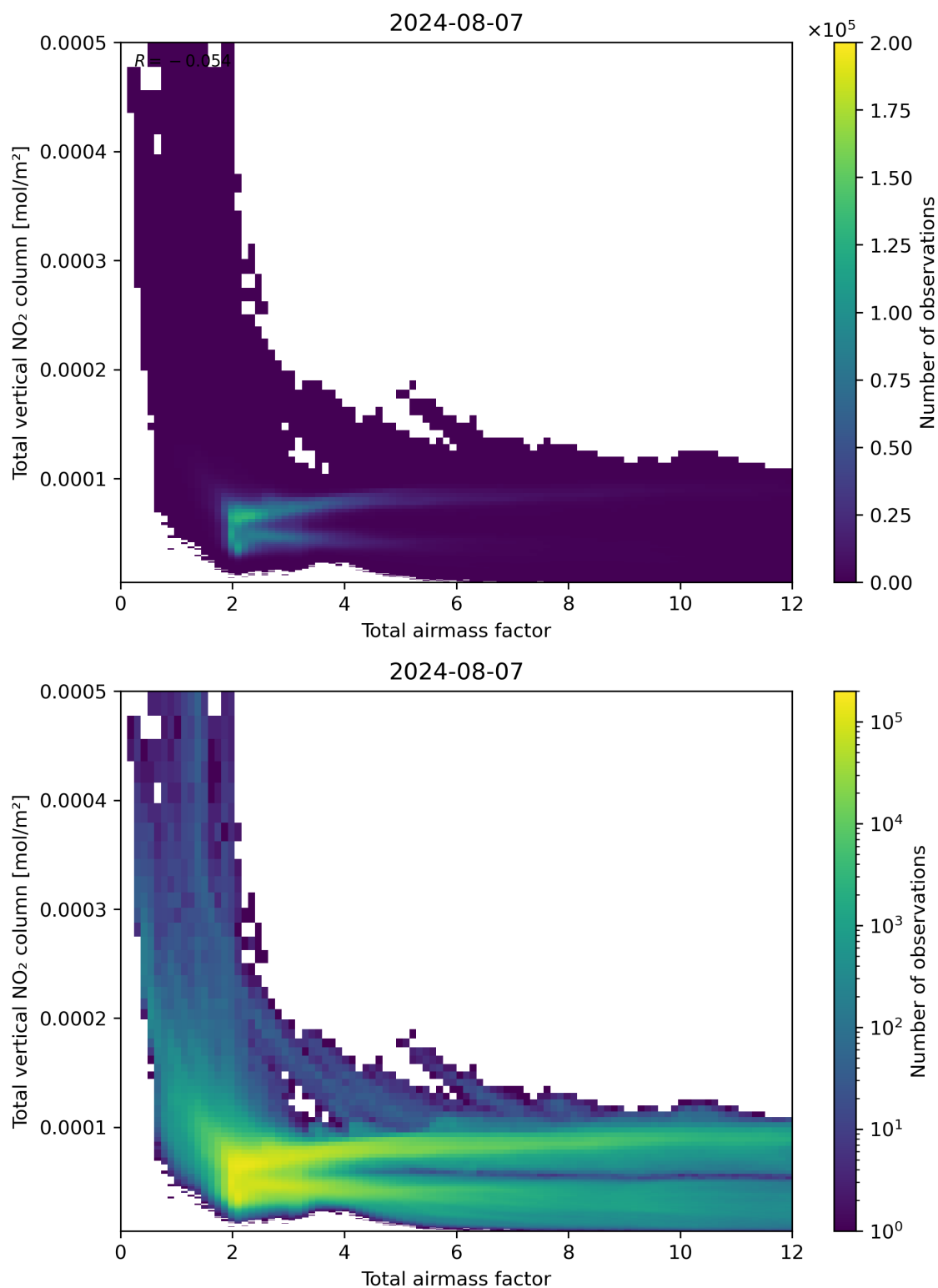
Figure 67: Scatter density plot of “Total airmass factor” against “Total vertical NO 2 column” for 2024-08-06 to 2024-08-08.
