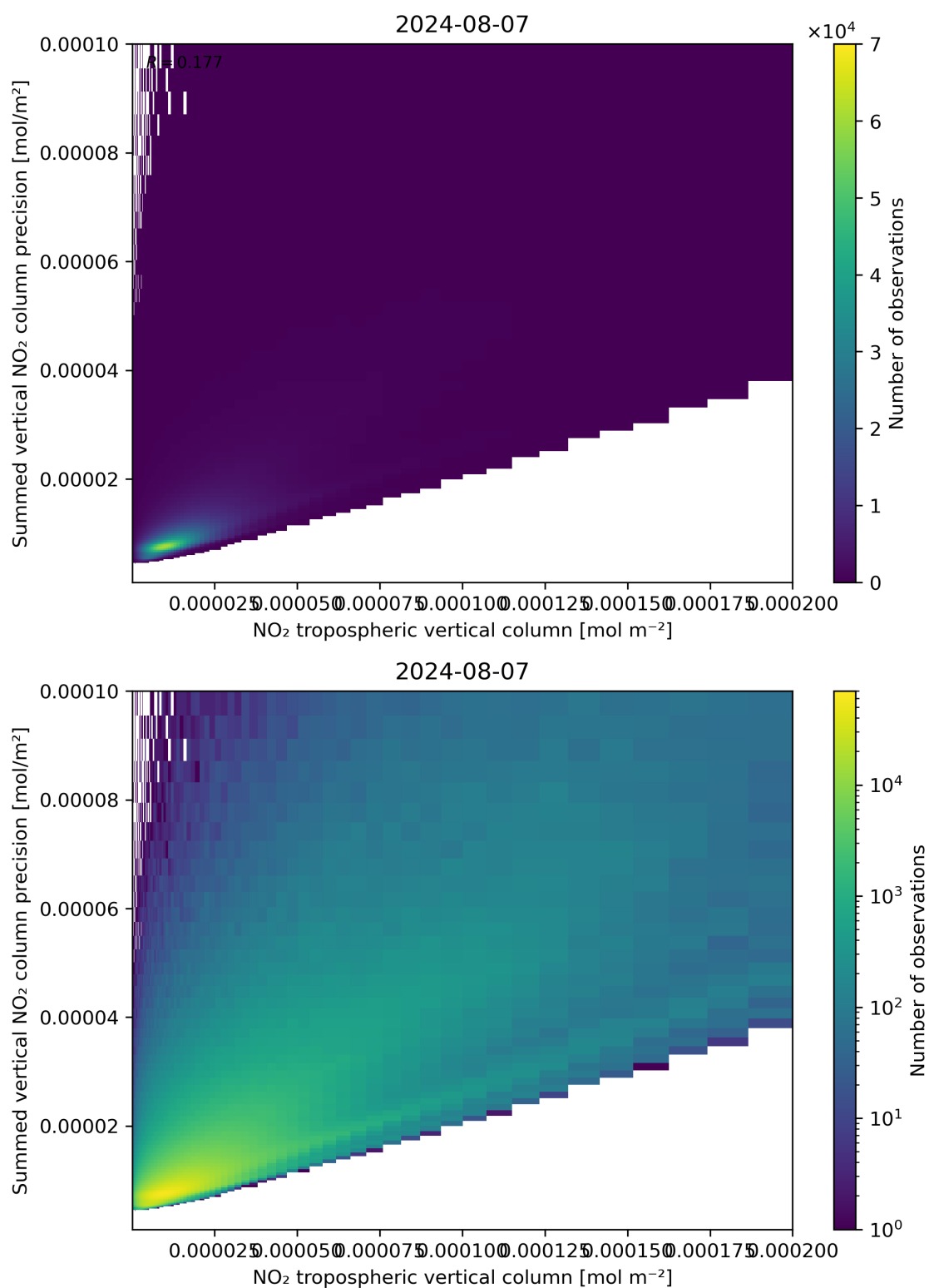
Figure 127: Scatter density plot of “NO 2 tropospheric vertical column” against “Summed vertical NO 2 column precision” for 2024-08-06 to 2024-08-08.
