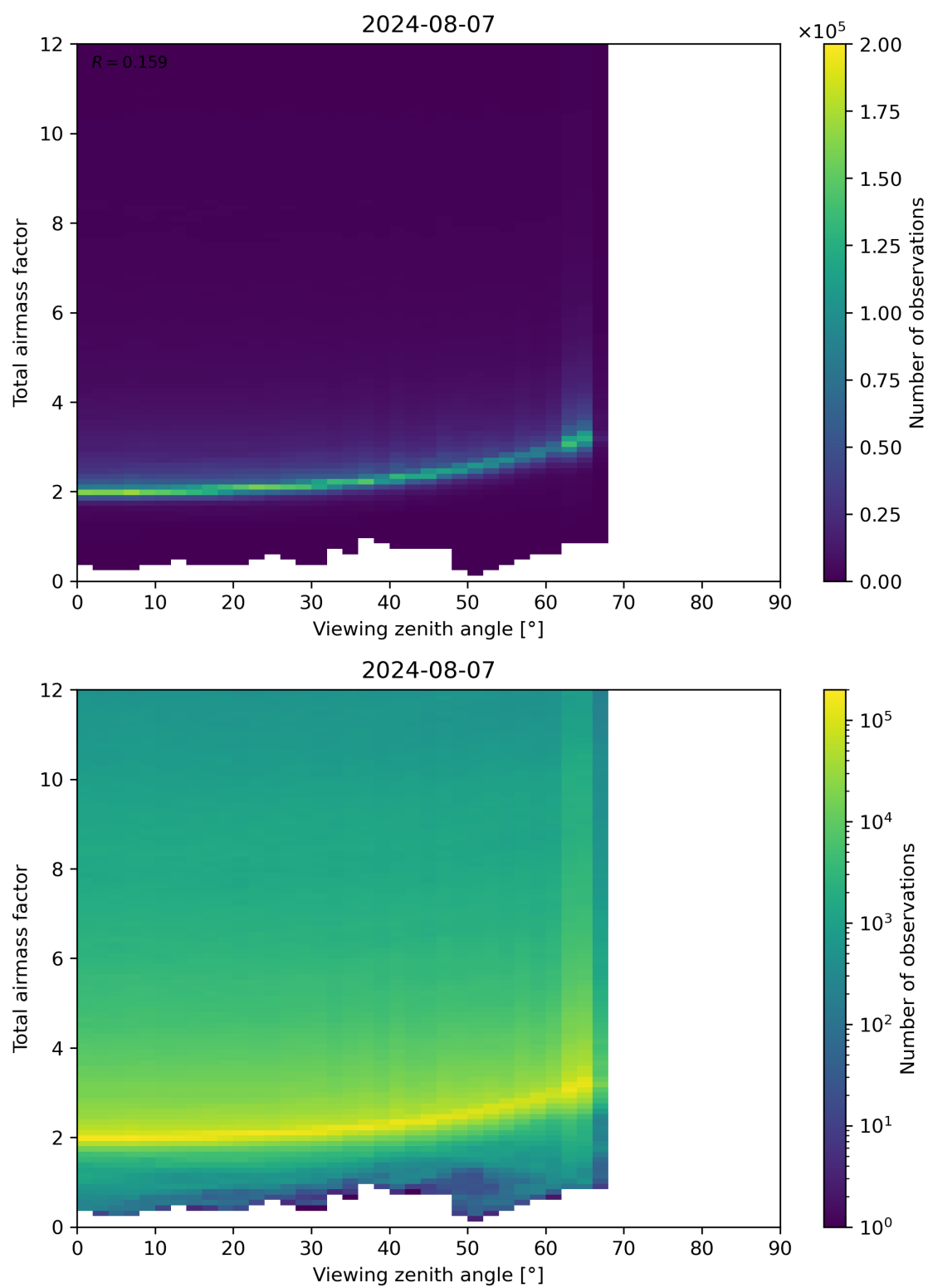
Figure 160: Scatter density plot of “Viewing zenith angle” against “Total airmass factor” for 2024-08-06 to 2024-08-08.
