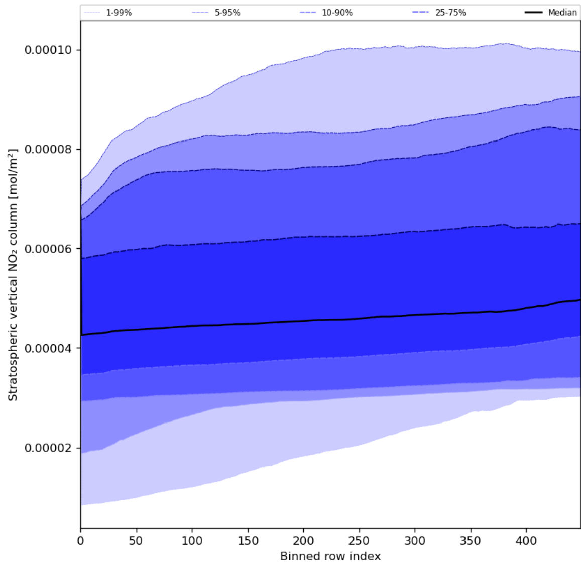
Figure 53: Along track statistics of “Stratospheric vertical NO 2 column” for 2024-08-06 to 2024-08-08
