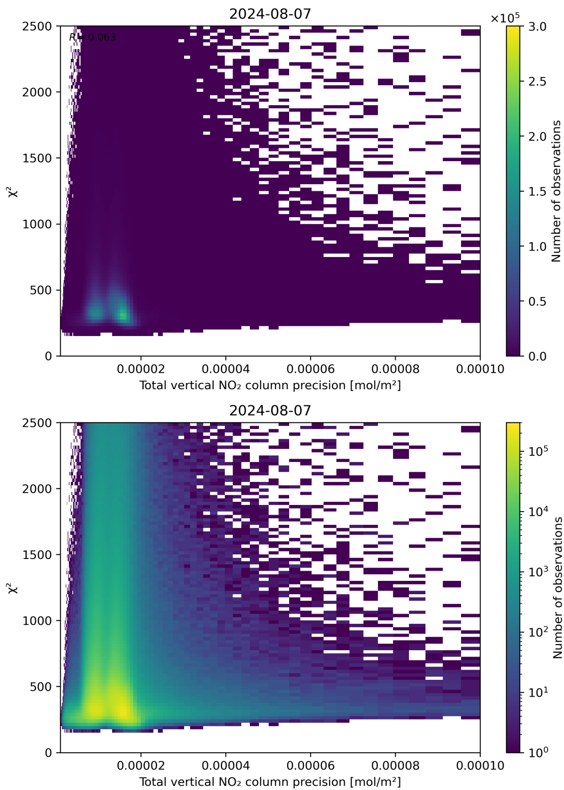
Figure 116: Scatter density plot of “Total vertical NO 2 column precision” against “ \chi^2 ” for 2024-08-06 to 2024-08-08.
