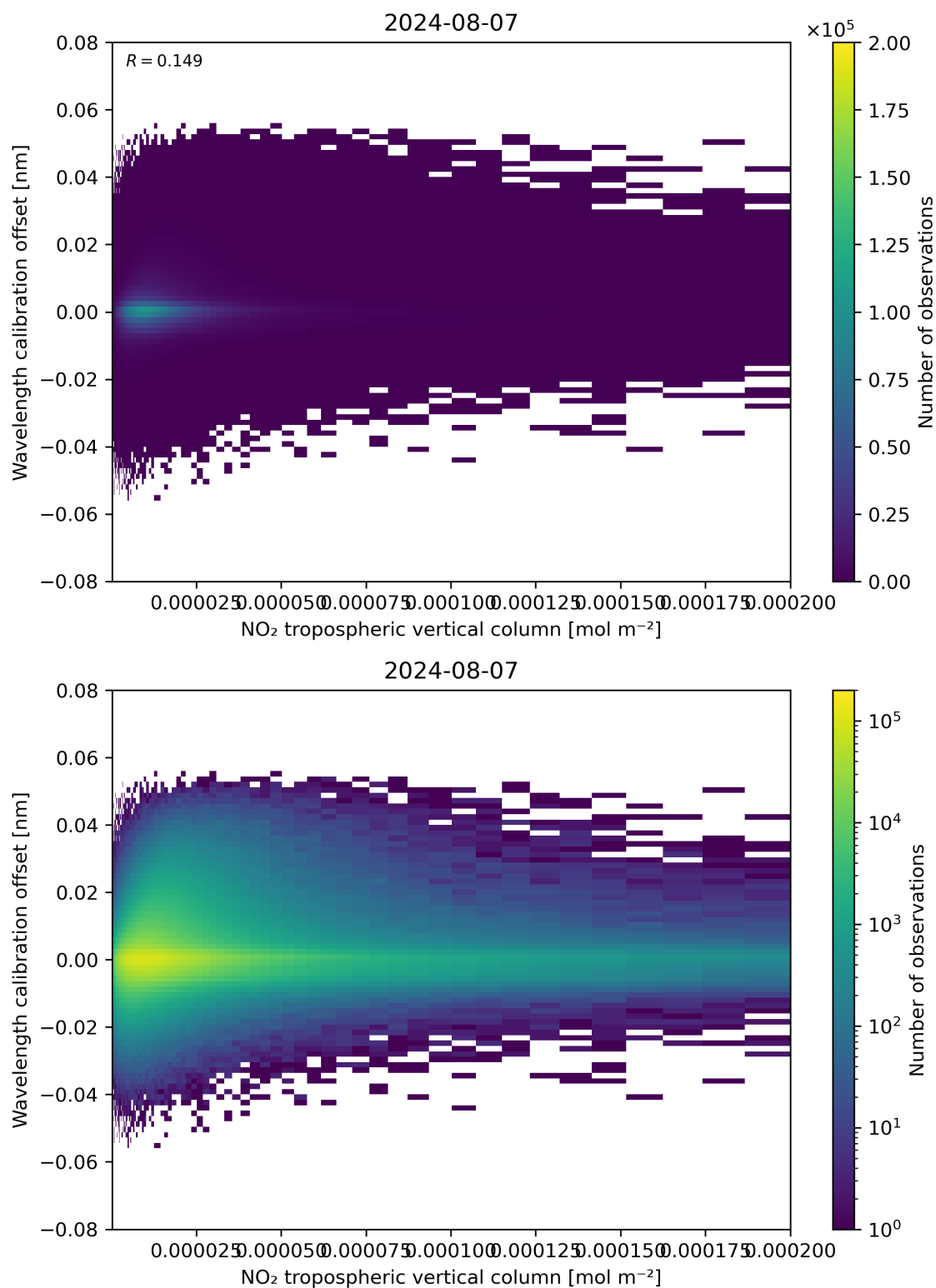
Figure 143: Scatter density plot of “NO 2 tropospheric vertical column” against “Wavelength calibration offset” for 2024-08-06 to 2024-08-08.
