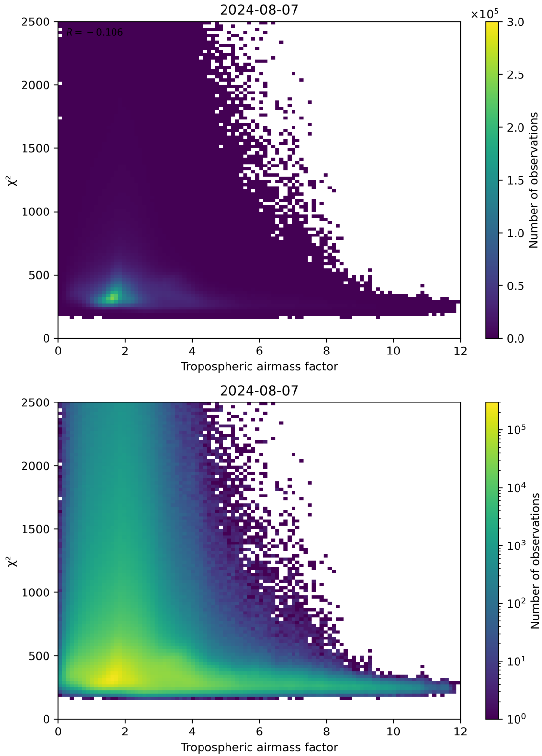
Figure 73: Scatter density plot of “Tropospheric airmass factor” against “ \chi^2 ” for 2024-08-06 to 2024-08-08.
