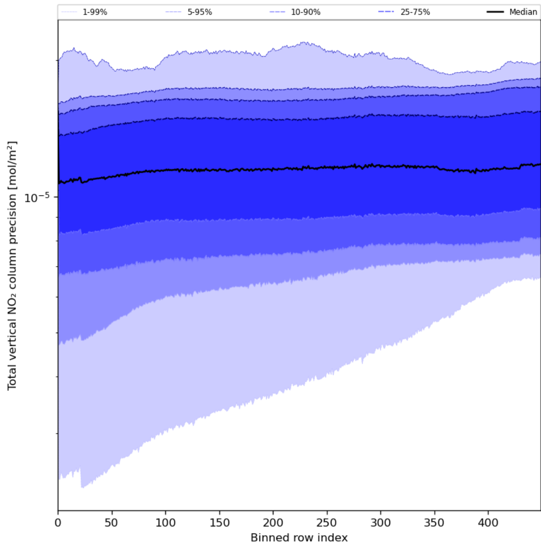
Figure 56: Along track statistics of “Total vertical NO 2 column precision” for 2024-08-06 to 2024-08-08
