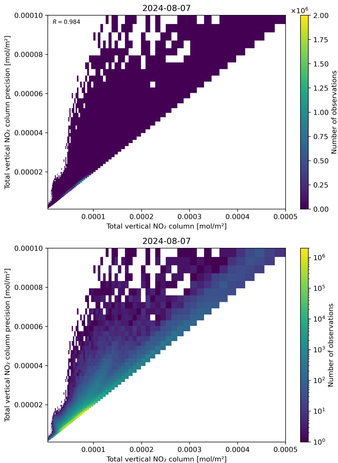
Figure 114: Scatter density plot of “Total vertical NO 2 column” against “Total vertical NO 2 column precision” for 2024-08-06 to 2024-08-08.
