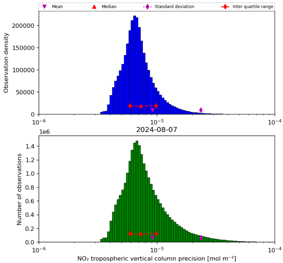
Figure 30: Histogram of “NO 2 tropospheric vertical column precision” for 2024-08-06 to 2024-08-08
