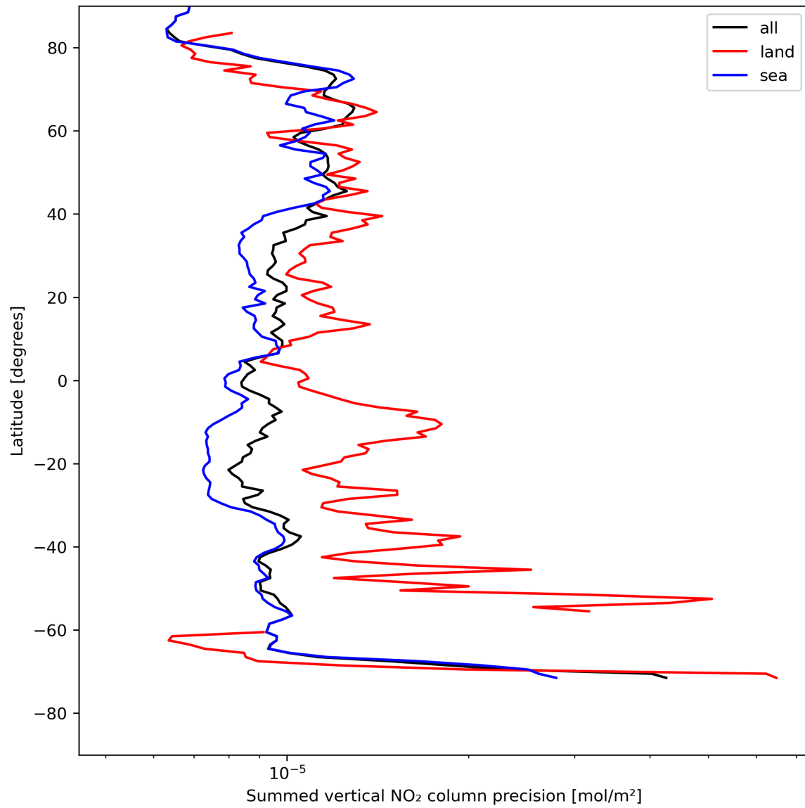
Figure 24: Zonal average of “Summed vertical NO 2 column precision” for 2024-08-06 to 2024-08-08.
