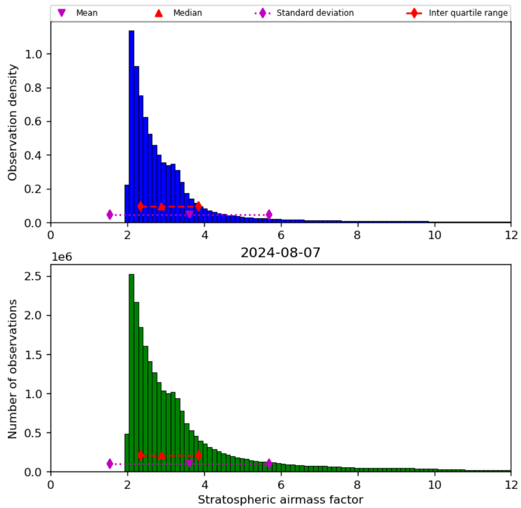
Figure 44: Histogram of “Stratospheric airmass factor” for 2024-08-06 to 2024-08-08
