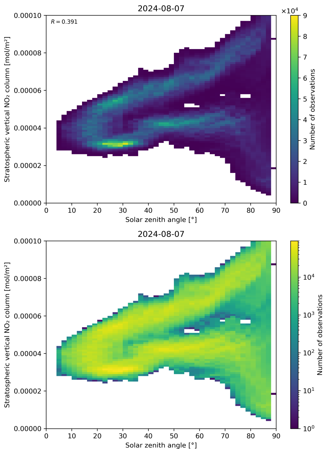
Figure 150: Scatter density plot of “Solar zenith angle” against “Stratospheric vertical NO 2 column” for 2024-08-06 to 2024-08-08.
