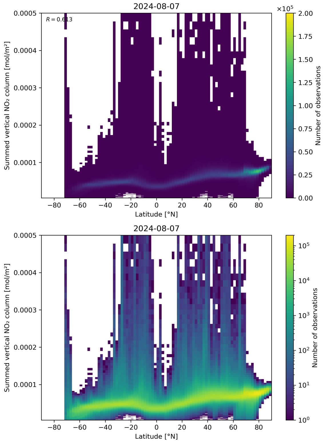
Figure 88: Scatter density plot of “Latitude” against “Summed vertical NO 2 column” for 2024-08-06 to 2024-08-08.
