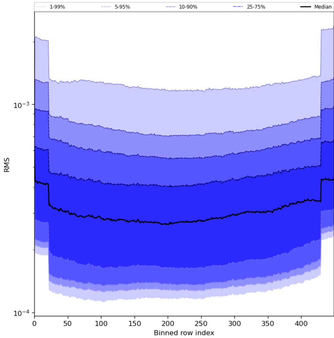
Figure 60: Along track statistics of “RMS” for 2024-08-06 to 2024-08-08
