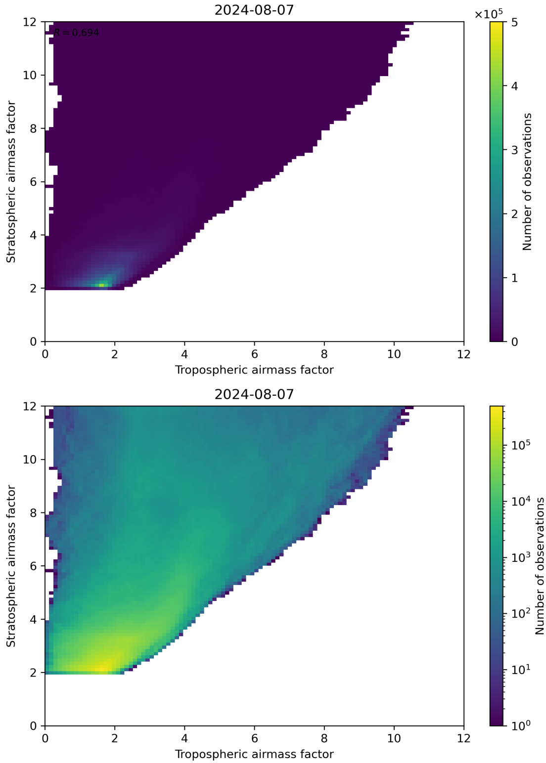
Figure 71: Scatter density plot of “Tropospheric airmass factor” against “Stratospheric airmass factor” for 2024-08-06 to 2024-08-08.
