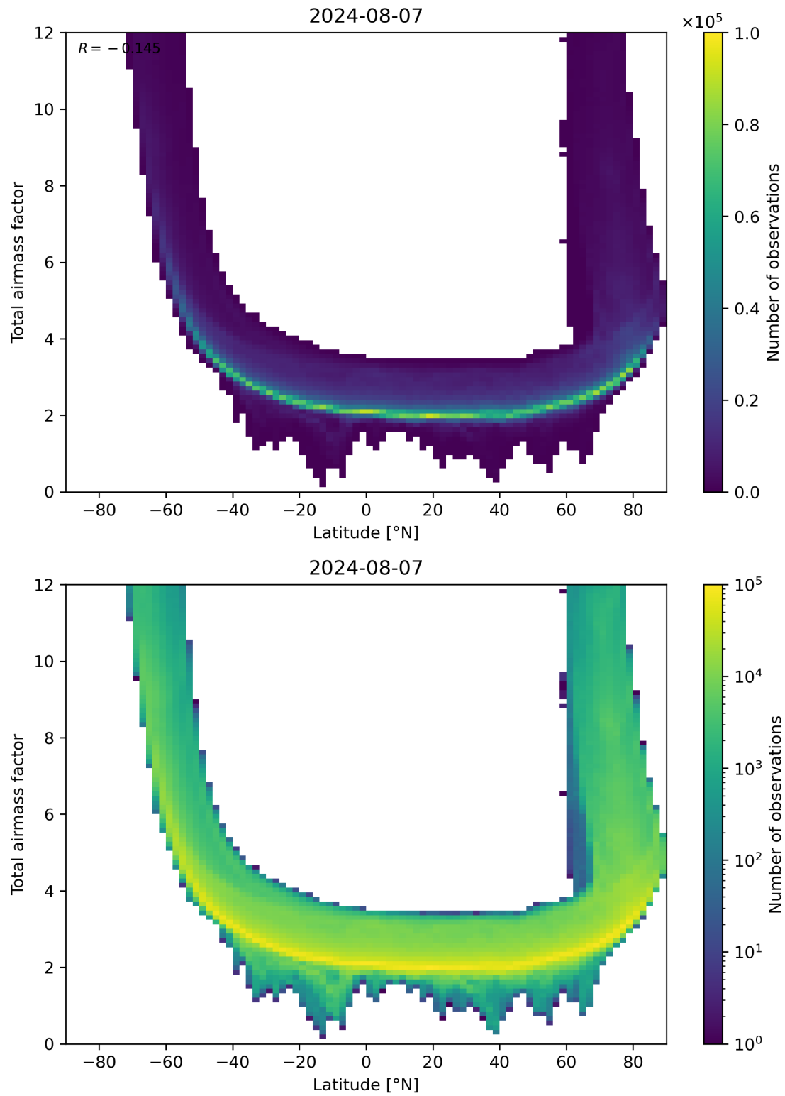
Figure 84: Scatter density plot of “Latitude” against “Total airmass factor” for 2024-08-06 to 2024-08-08.
