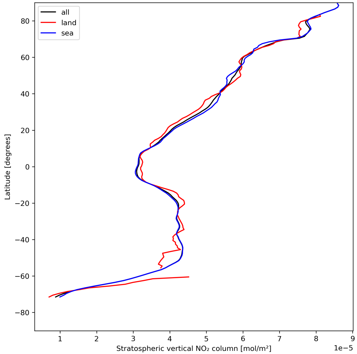
Figure 19: Zonal average of “Stratospheric vertical NO 2 column” for 2024-08-06 to 2024-08-08.
