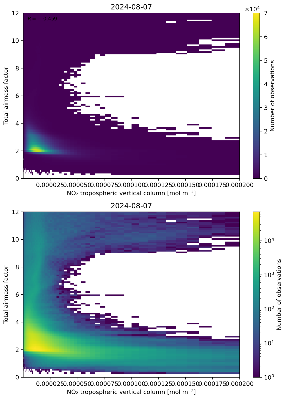
Figure 122: Scatter density plot of “NO 2 tropospheric vertical column” against “Total air mass factor” for 2024-08-06 to 2024-08-08.
