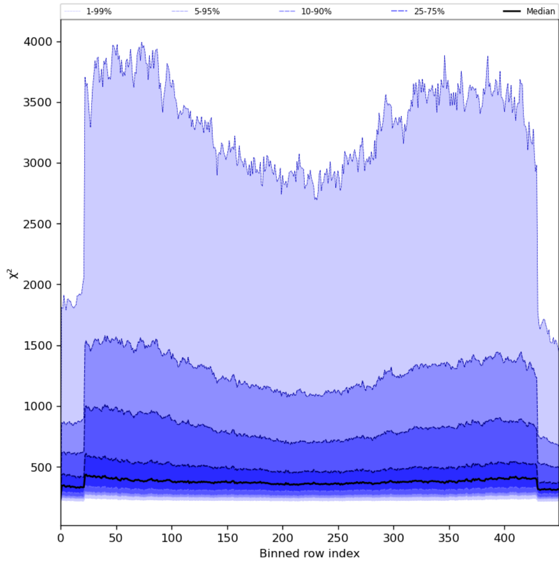
Figure 59: Along track statistics of “ \chi^2 ” for 2024-08-06 to 2024-08-08
