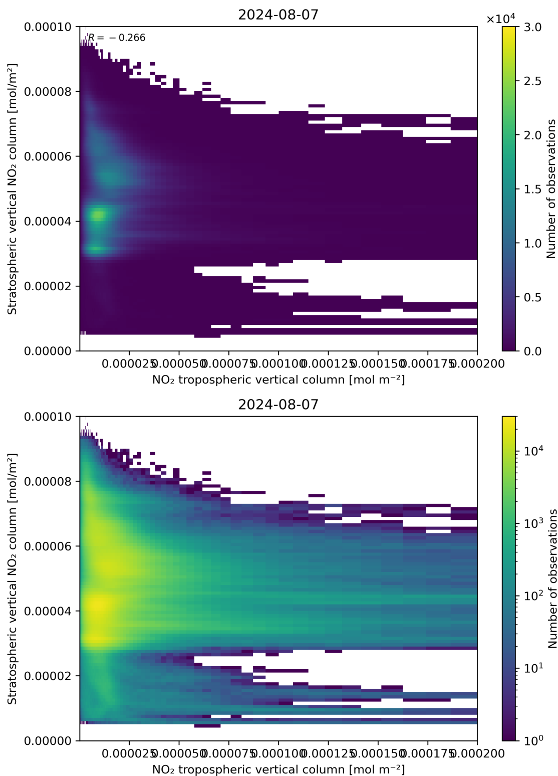
Figure 125: Scatter density plot of “NO 2 tropospheric vertical column” against “Stratospheric vertical NO 2 column” for 2024-08-06 to 2024-08-08.
