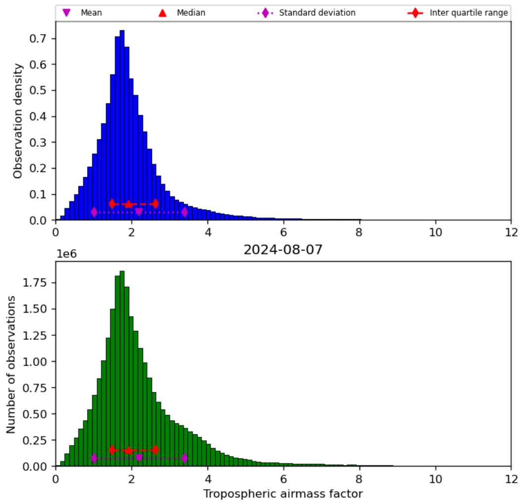
Figure 31: Histogram of “Tropospheric airmass factor” for 2024-08-06 to 2024-08-08
