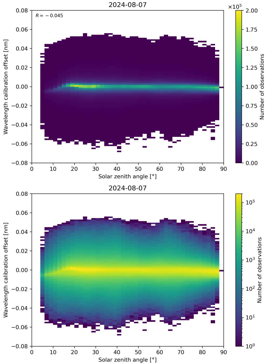
Figure 158: Scatter density plot of “Solar zenith angle” against “Wavelength calibration offset” for 2024-08-06 to 2024-08-08.
