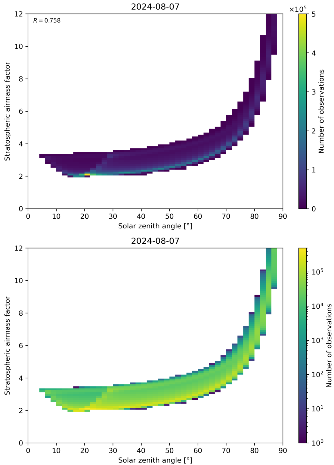
Figure 145: Scatter density plot of “Solar zenith angle” against “Stratospheric airmass factor” for 2024-08-06 to 2024-08-08.
