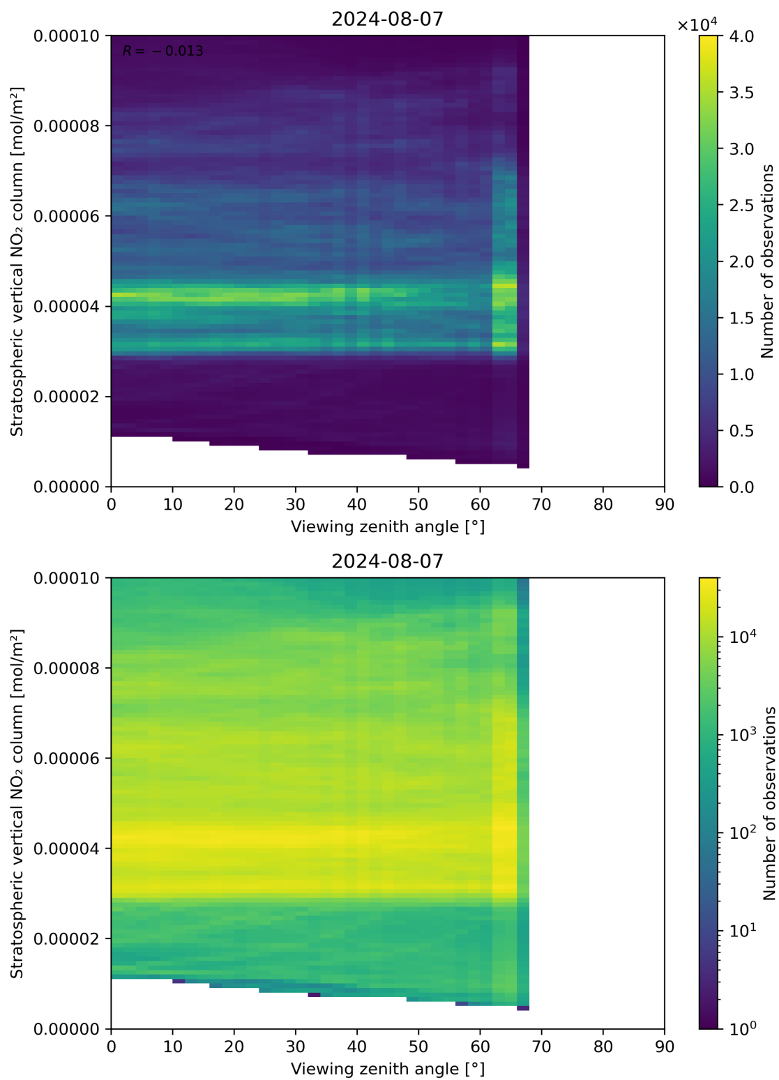
Figure 164: Scatter density plot of “Viewing zenith angle” against “Stratospheric vertical NO 2 column” for 2024-08-06 to 2024-08-08.
