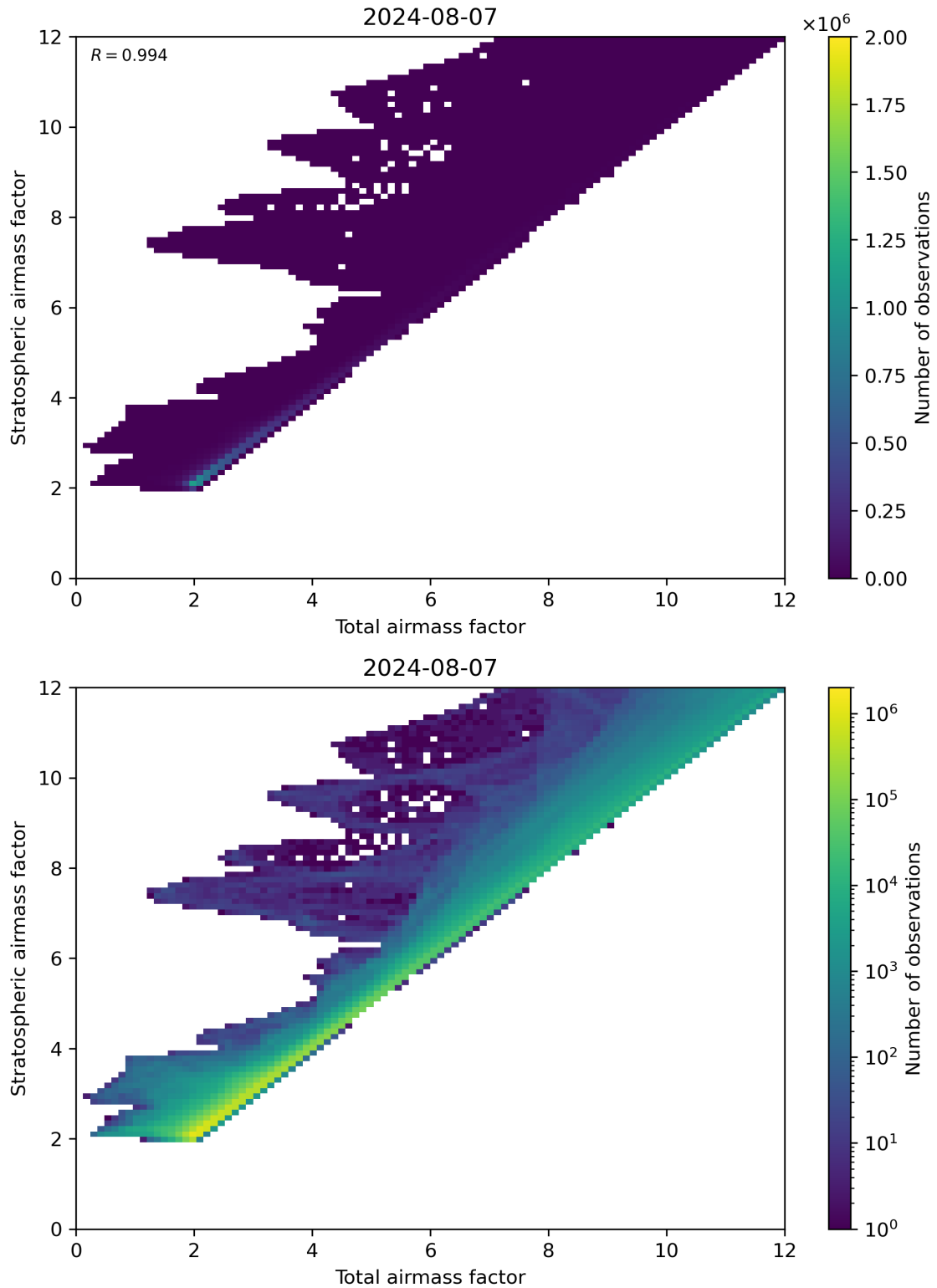
Figure 62: Scatter density plot of “Total airmass factor” against “Stratospheric airmass factor” for 2024-08-06 to 2024-08-08.
