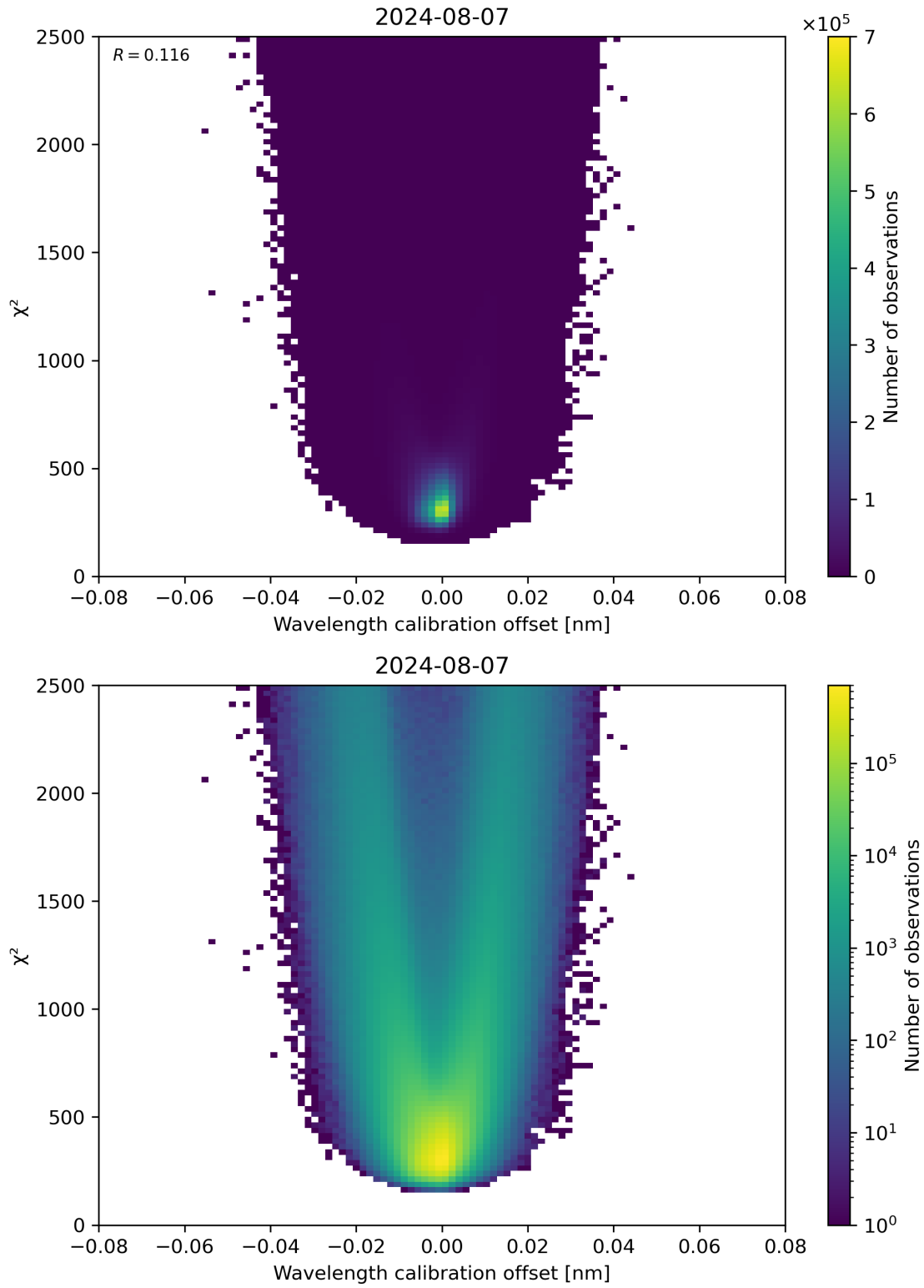
Figure 175: Scatter density plot of “Wavelength calibration offset” against “ \chi^2 ” for 2024-08-06 to 2024-08-08.
