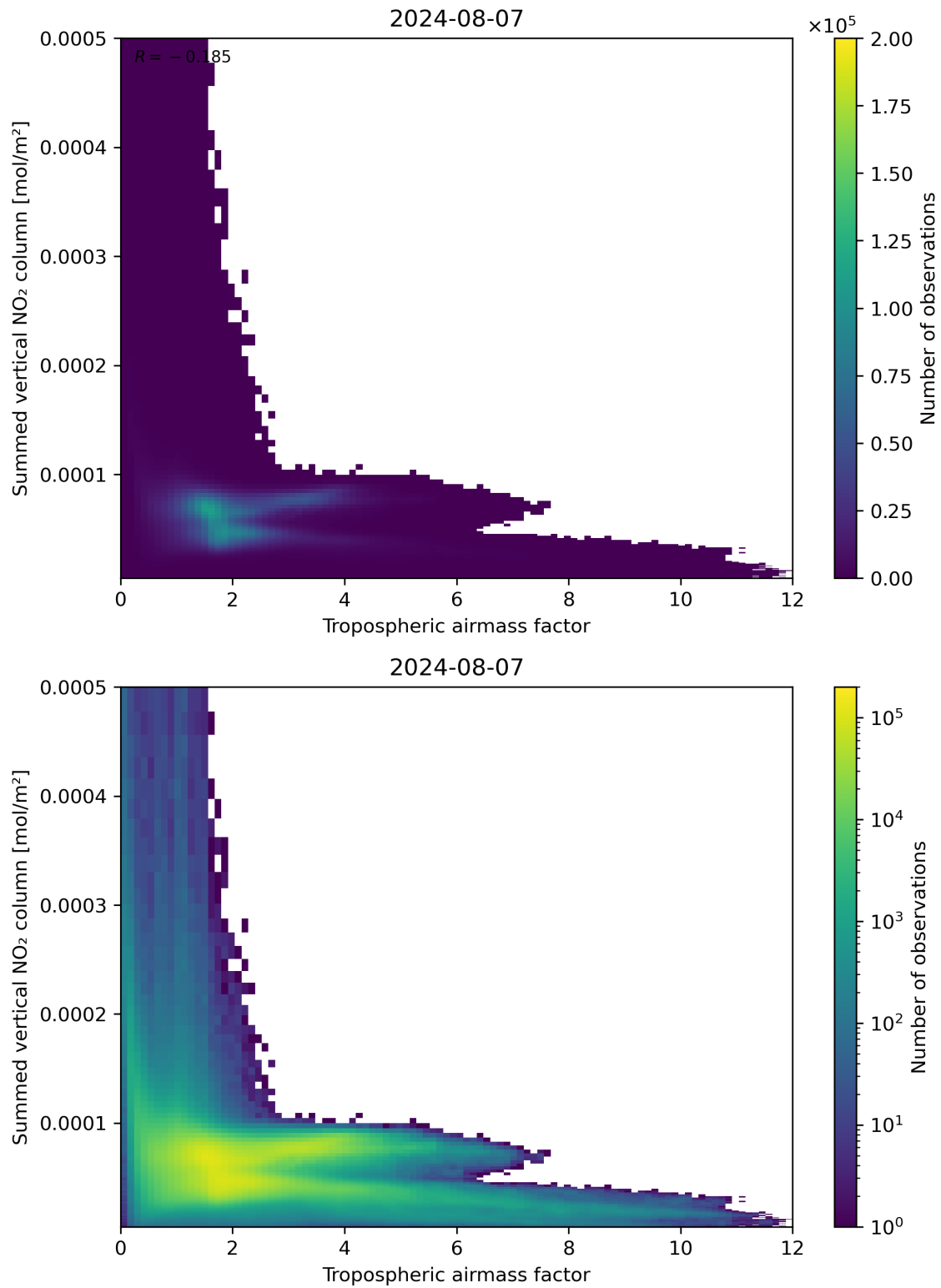
Figure 75: Scatter density plot of “Tropospheric airmass factor” against “Summed vertical NO 2 column” for 2024-08-06 to 2024-08-08.
