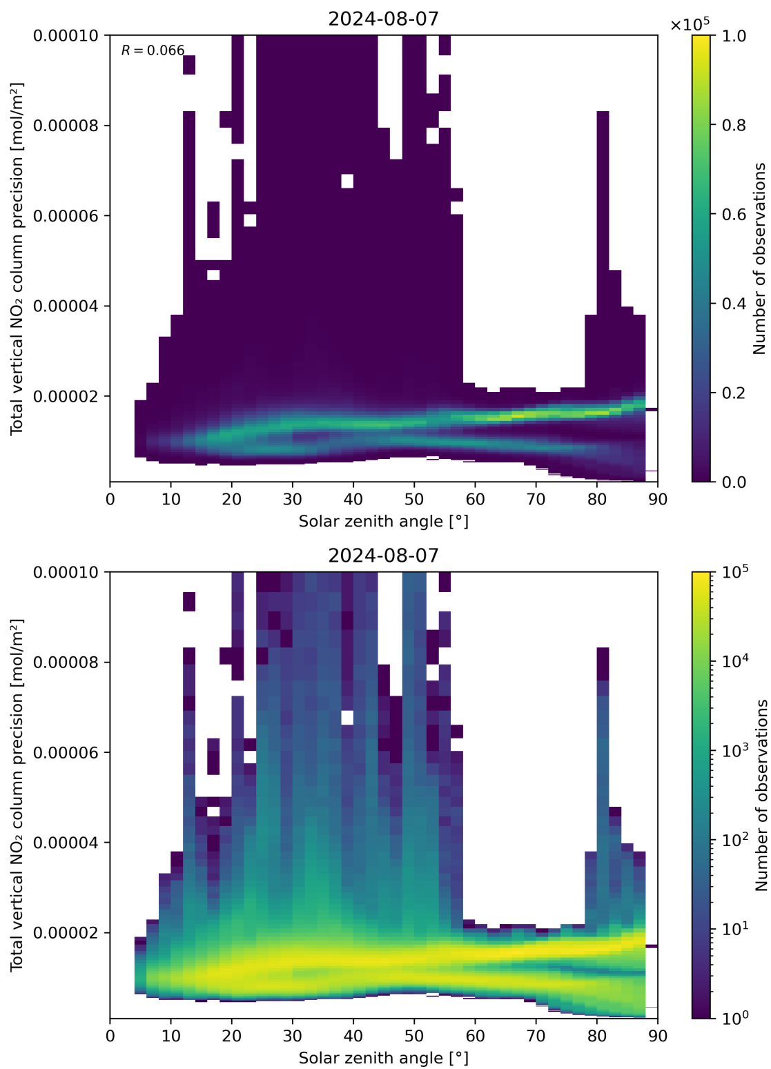
Figure 154: Scatter density plot of “Solar zenith angle” against “Total vertical NO 2 column precision” for 2024-08-06 to 2024-08-08.
