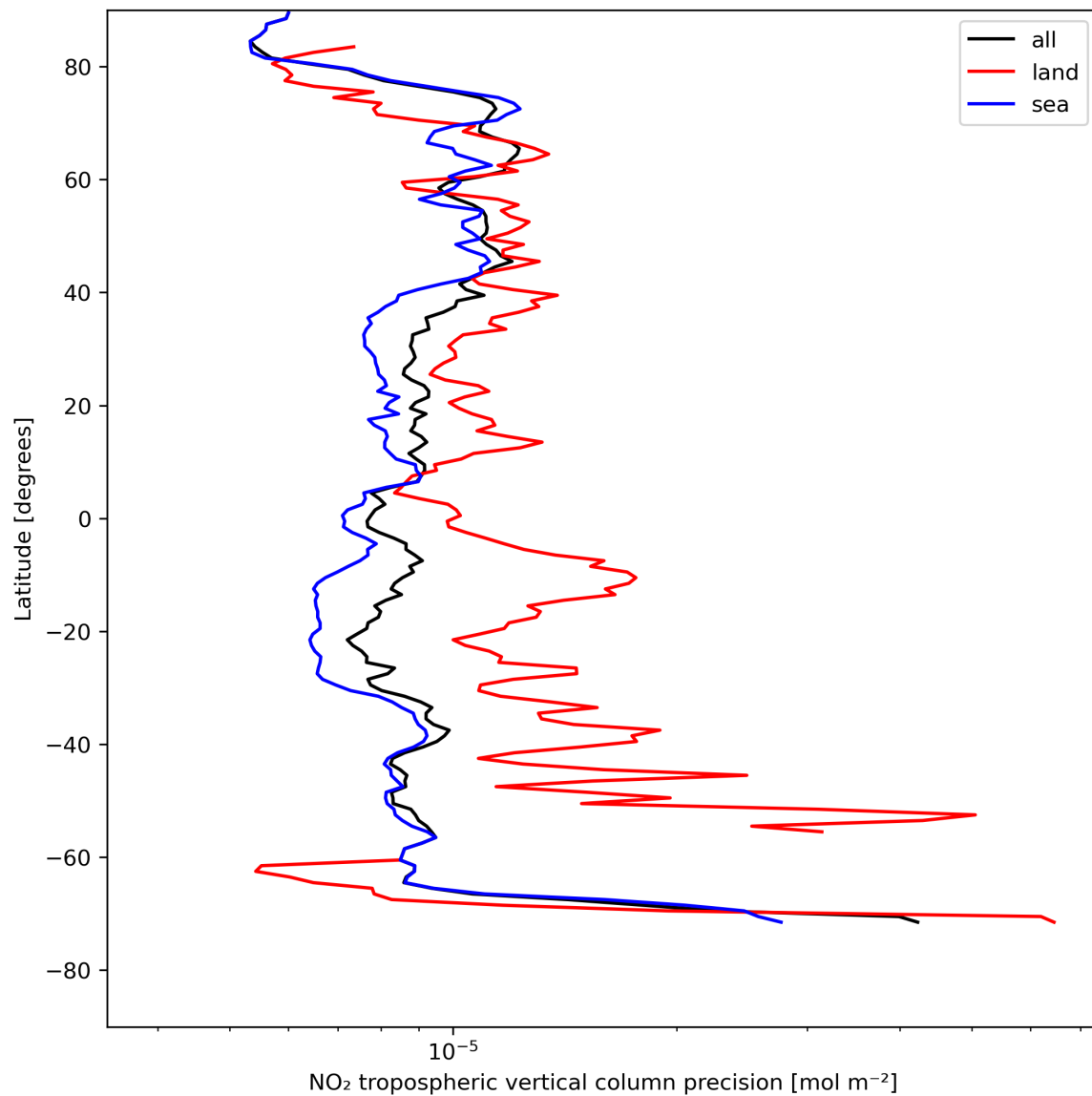
Figure 13: Zonal average of “NO 2 tropospheric vertical column precision” for 2024-08-06 to 2024-08-08.
