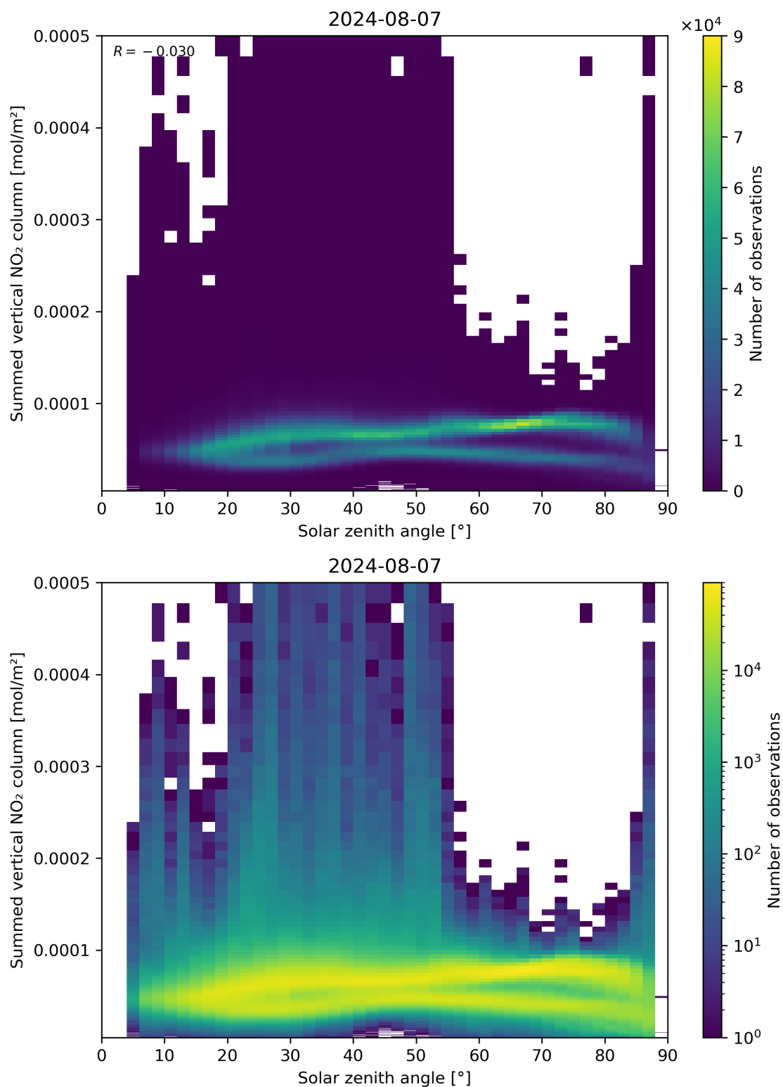
Figure 151: Scatter density plot of “Solar zenith angle” against “Summed vertical NO 2 column” for 2024-08-06 to 2024-08-08.
