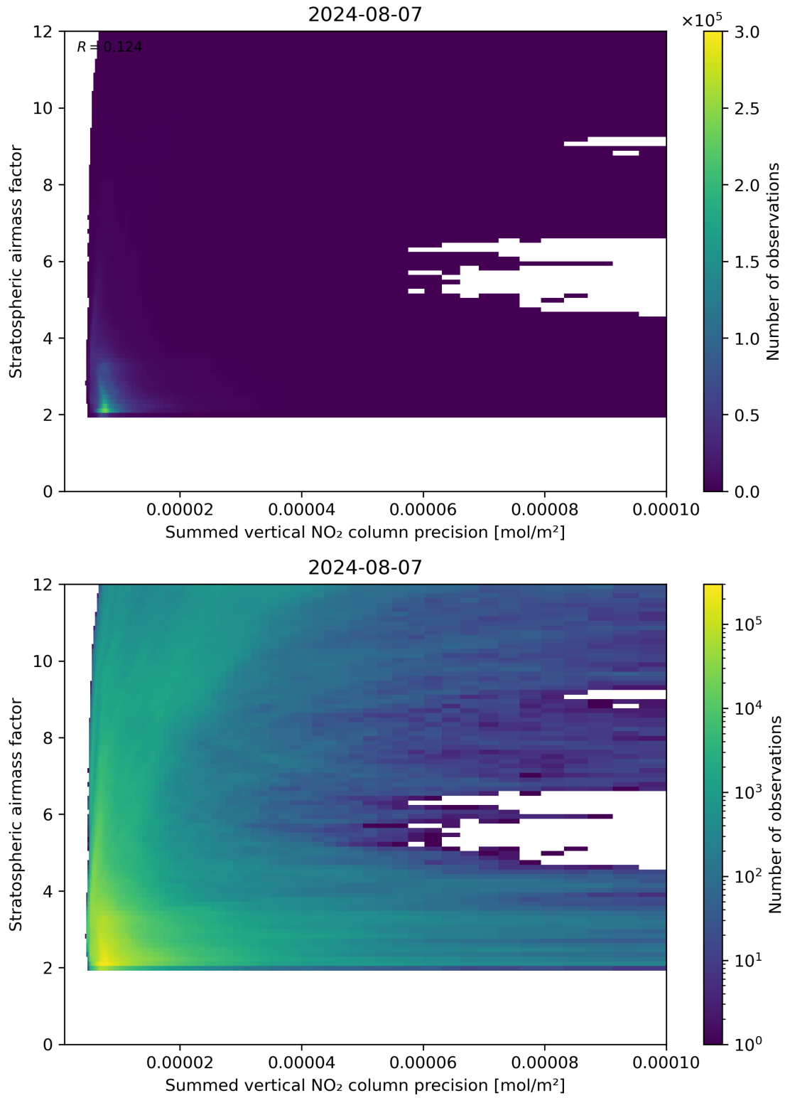
Figure 106: Scatter density plot of “Summed vertical NO 2 column precision” against “Stratospheric airmass factor” for 2024-08-06 to 2024-08-08.
