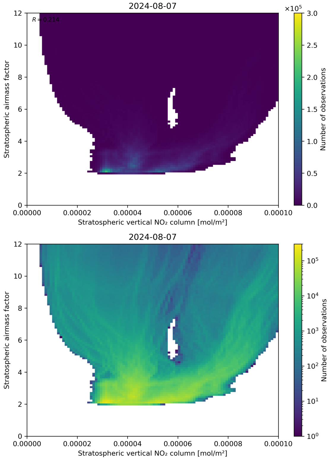
Figure 96: Scatter density plot of “Stratospheric vertical NO 2 column” against “Stratospheric airmass factor” for 2024-08-06 to 2024-08-08.
