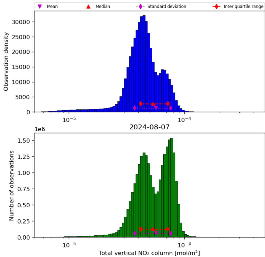
Figure 38: Histogram of “Total vertical NO 2 column” for 2024-08-06 to 2024-08-08
