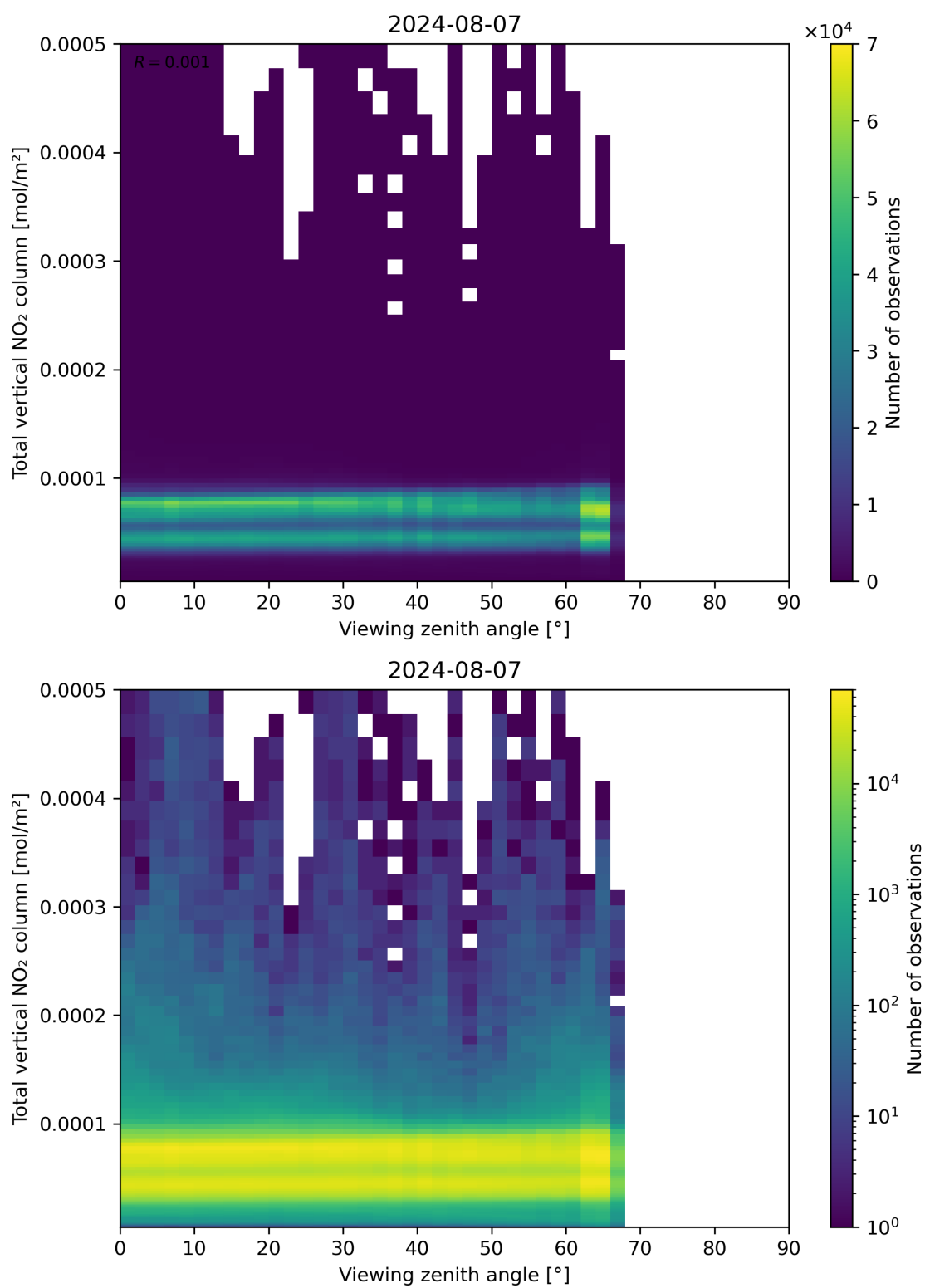
Figure 167: Scatter density plot of “Viewing zenith angle” against “Total vertical NO 2 column” for 2024-08-06 to 2024-08-08.
