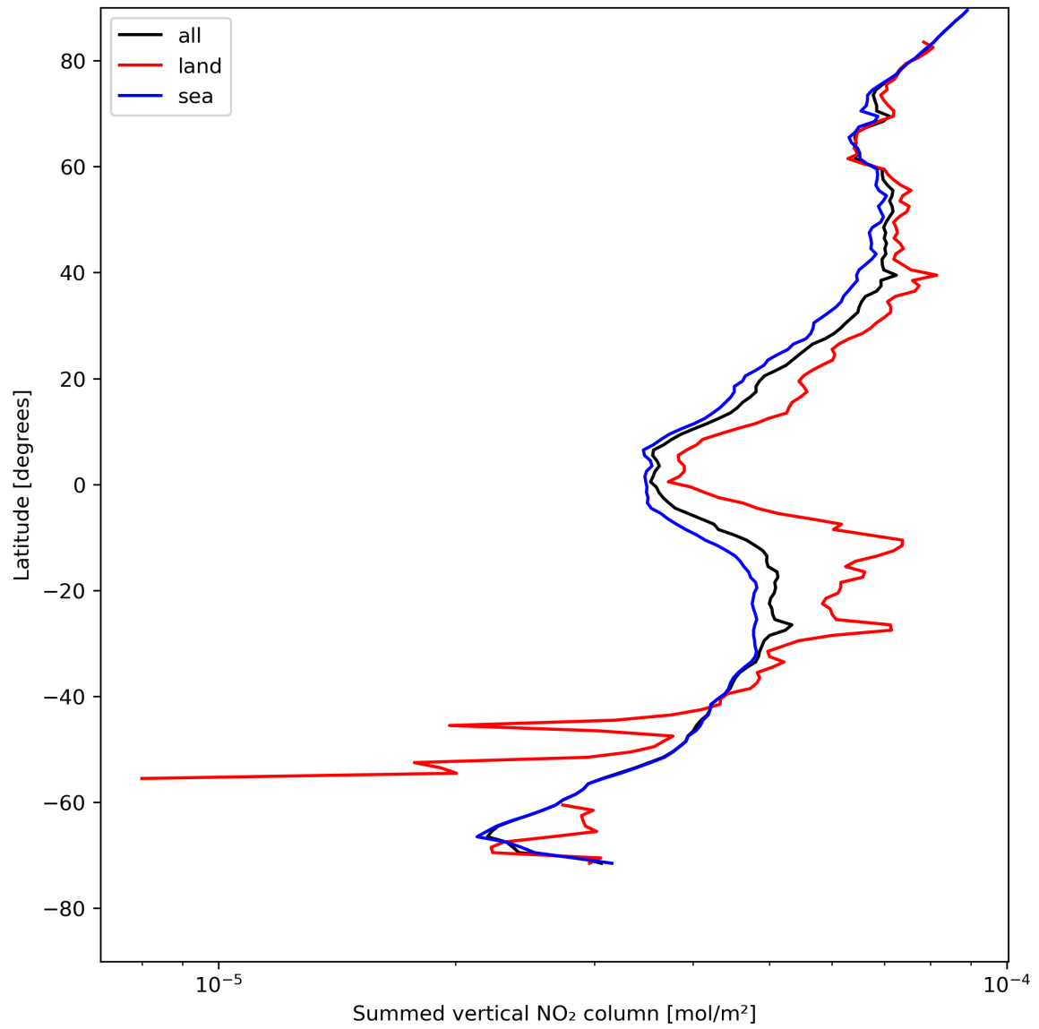
Figure 23: Zonal average of “Summed vertical NO 2 column” for 2024-08-06 to 2024-08-08.
