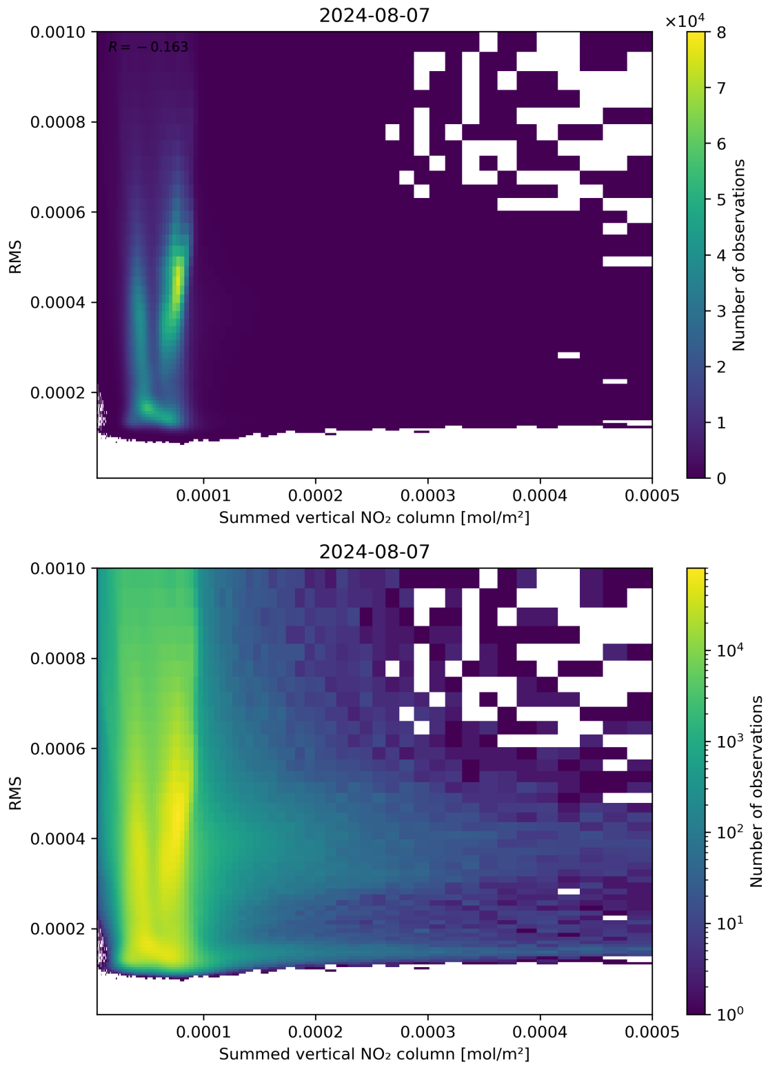
Figure 109: Scatter density plot of “Summed vertical NO 2 column” against “RMS” for 2024-08-06 to 2024-08-08.
