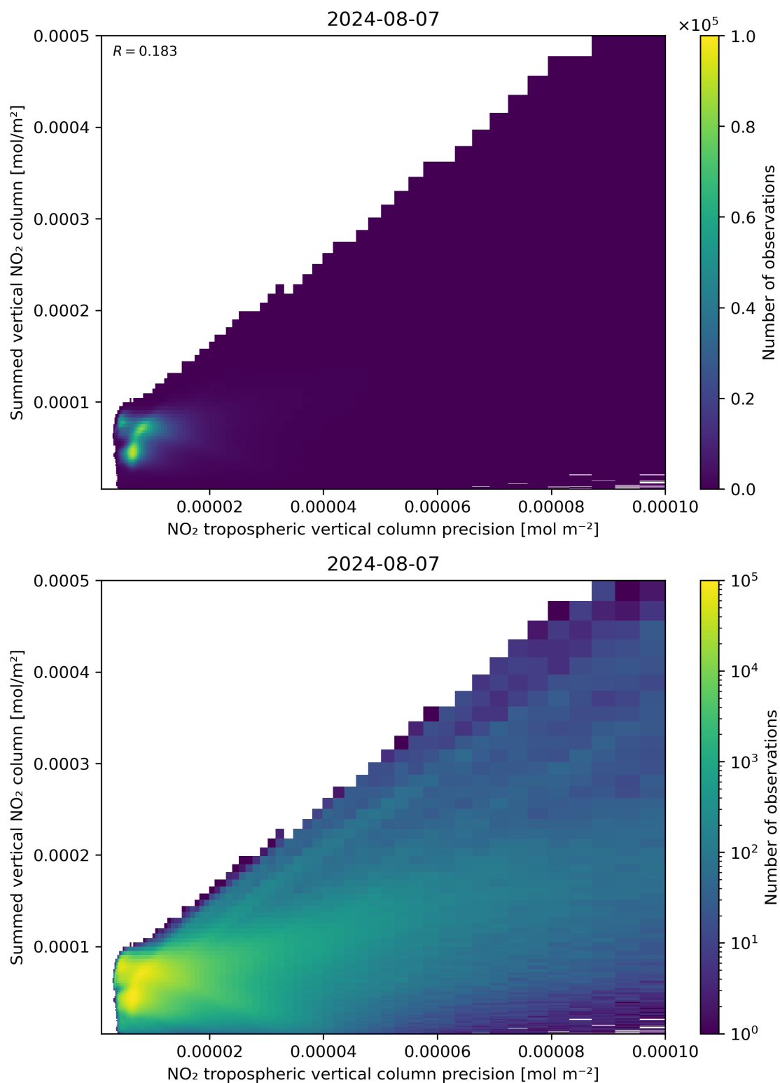
Figure 136: Scatter density plot of “NO 2 tropospheric vertical column precision” against “Summed vertical NO 2 column” for 2024-08-06 to 2024-08-08.
