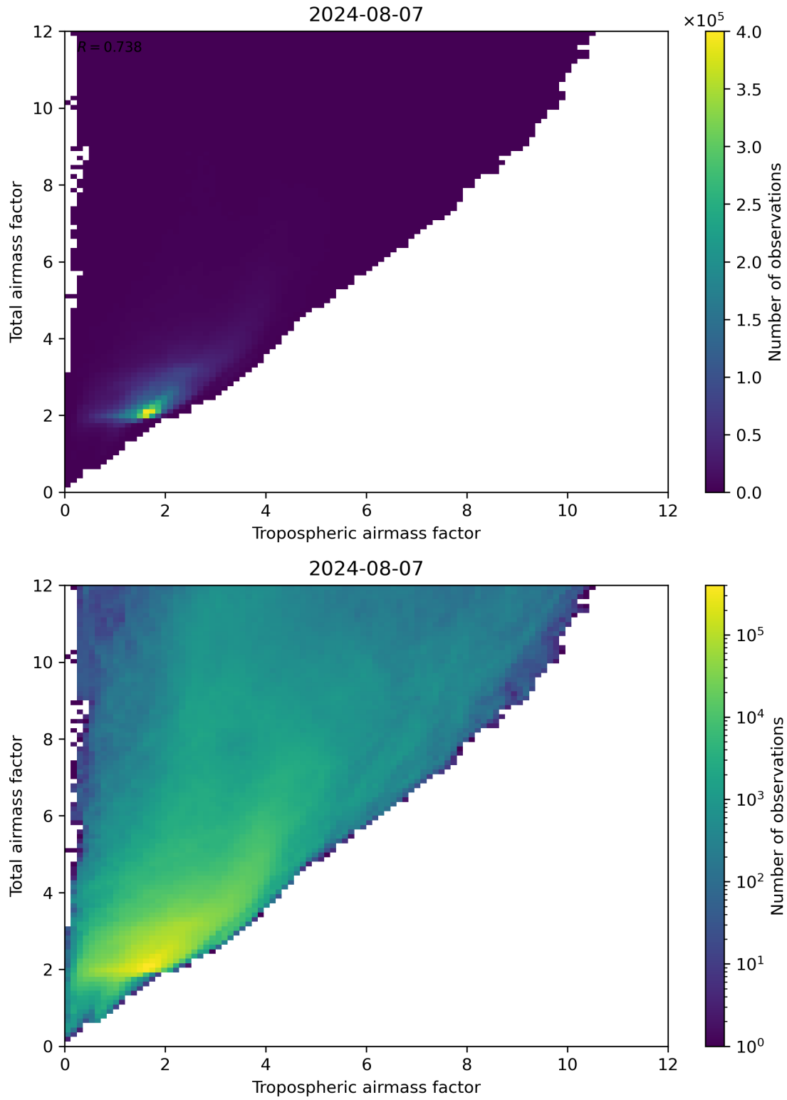
Figure 72: Scatter density plot of “Tropospheric airmass factor” against “Total airmass factor” for 2024-08-06 to 2024-08-08.
