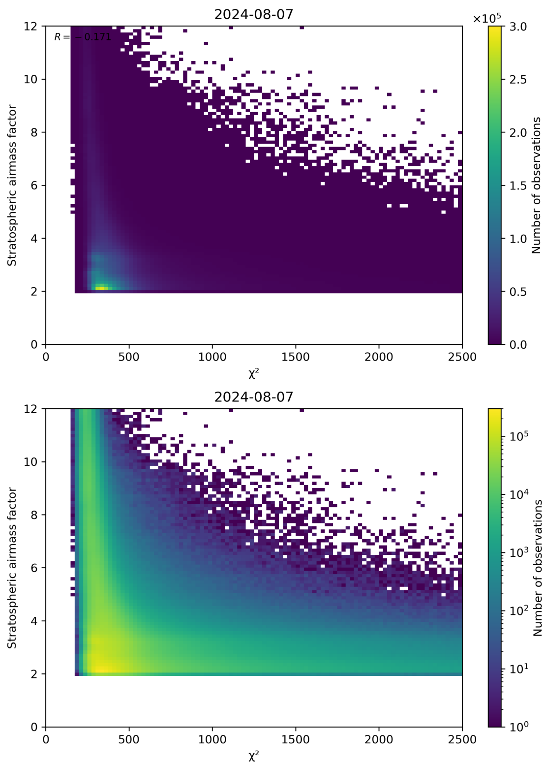
Figure 81: Scatter density plot of “ \chi^2 ” against “Stratospheric airmass factor” for 2024-08-06 to 2024-08-08.
