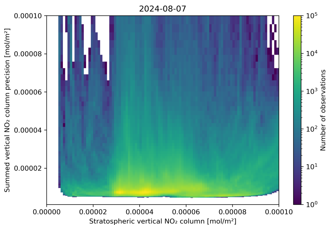
Figure 99: Scatter density plot of “Stratospheric vertical NO 2 column” against “Summed vertical NO 2 column precision” for 2024-08-06 to 2024-08-08.
