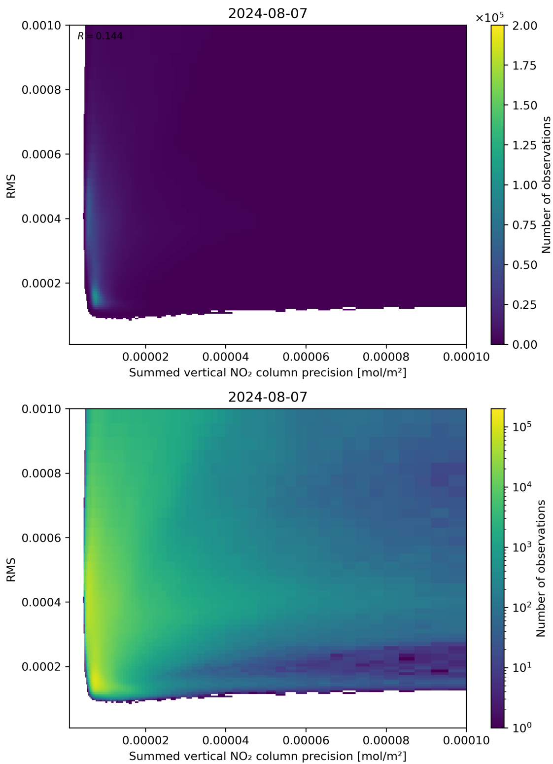
Figure 108: Scatter density plot of “Summed vertical NO 2 column precision” against “RMS” for 2024-08-06 to 2024-08-08.
