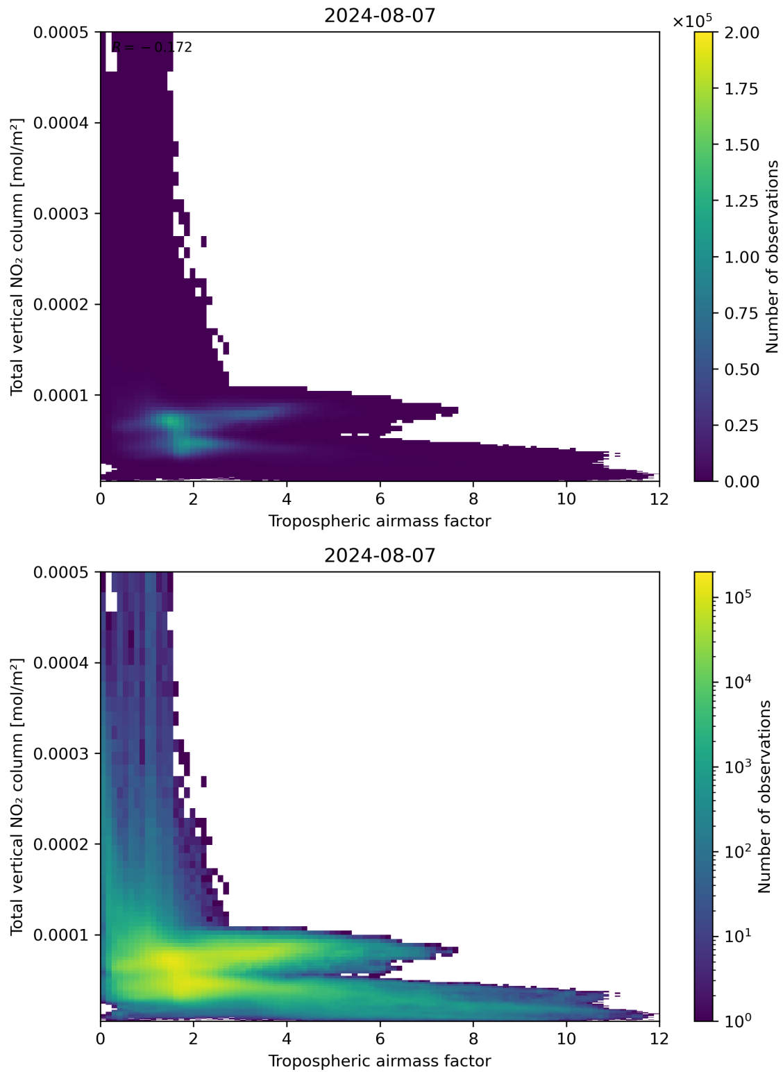
Figure 77: Scatter density plot of “Tropospheric airmass factor” against “Total vertical NO 2 column” for 2024-08-06 to 2024-08-08.
