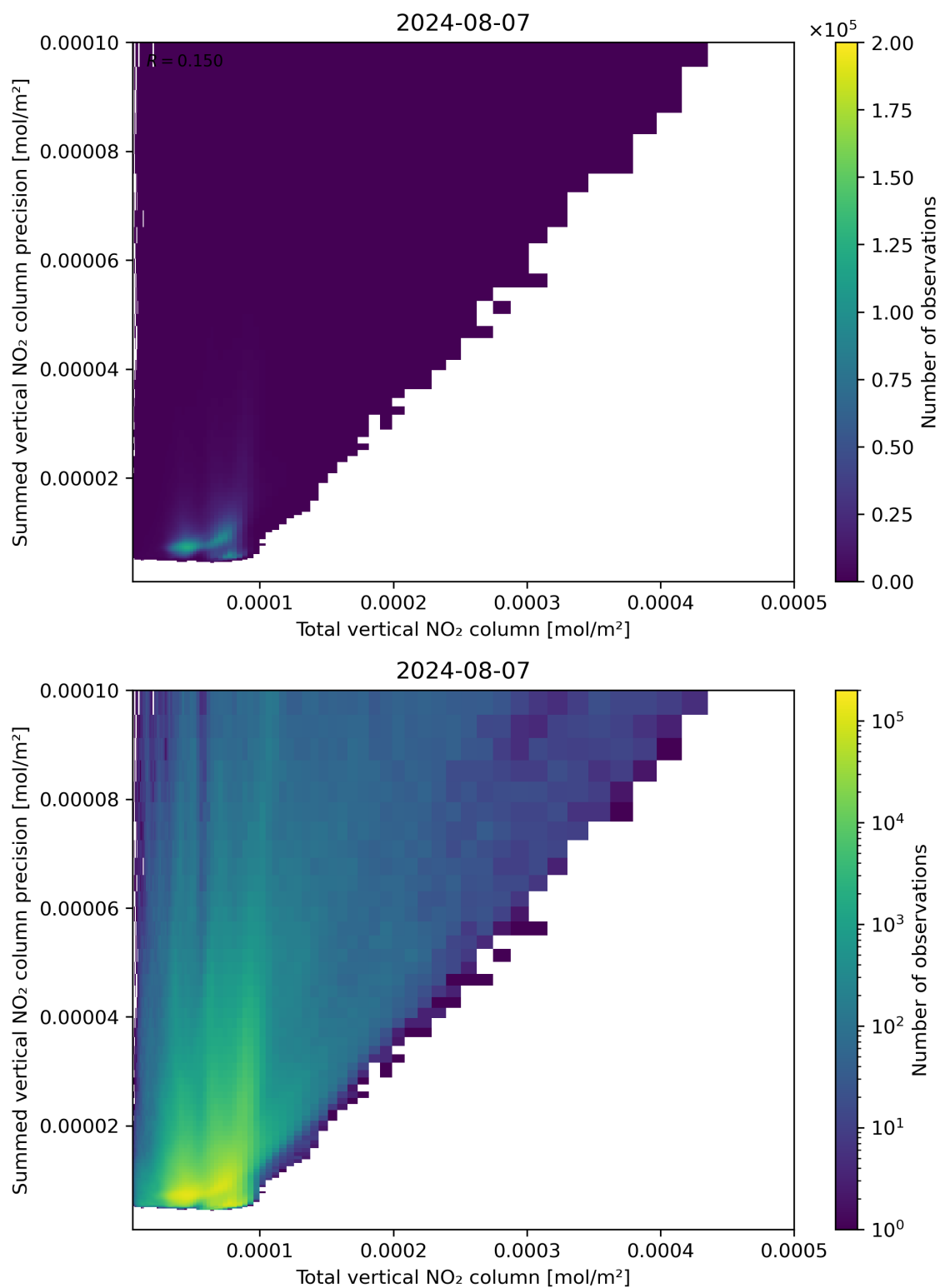
Figure 113: Scatter density plot of “Total vertical NO 2 column” against “Summed vertical NO 2 column precision” for 2024-08-06 to 2024-08-08.
