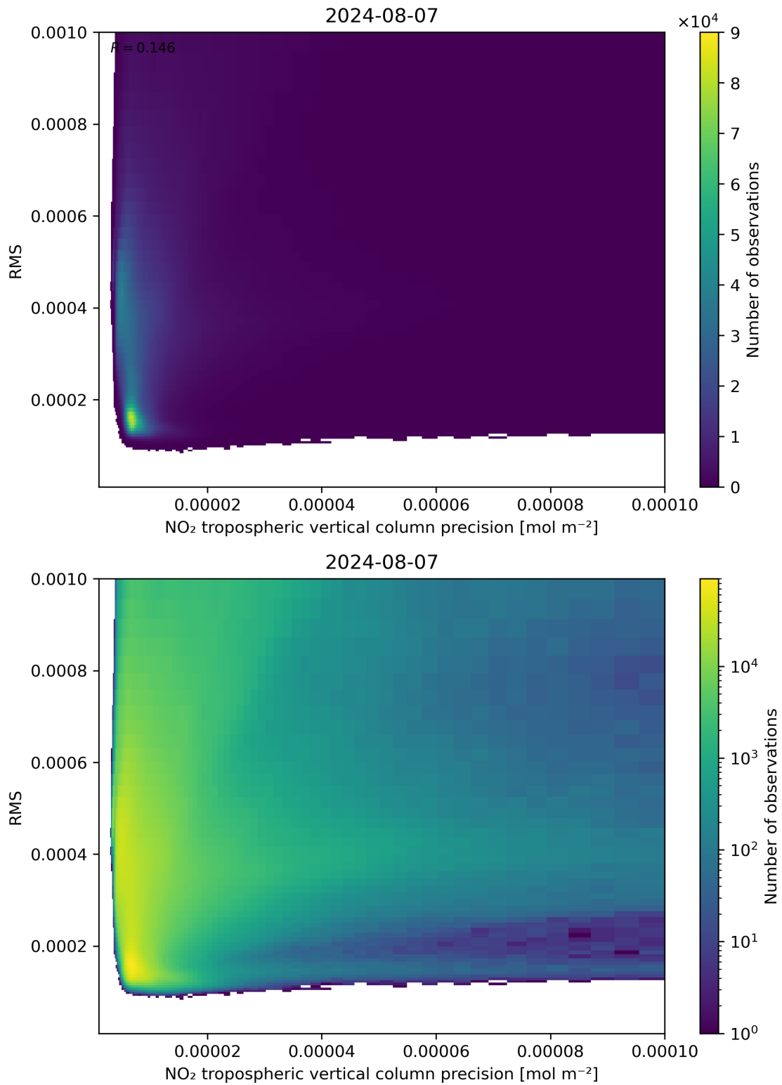
Figure 140: Scatter density plot of “NO 2 tropospheric vertical column precision” against “RMS” for 2024-08-06 to 2024-08-08.
