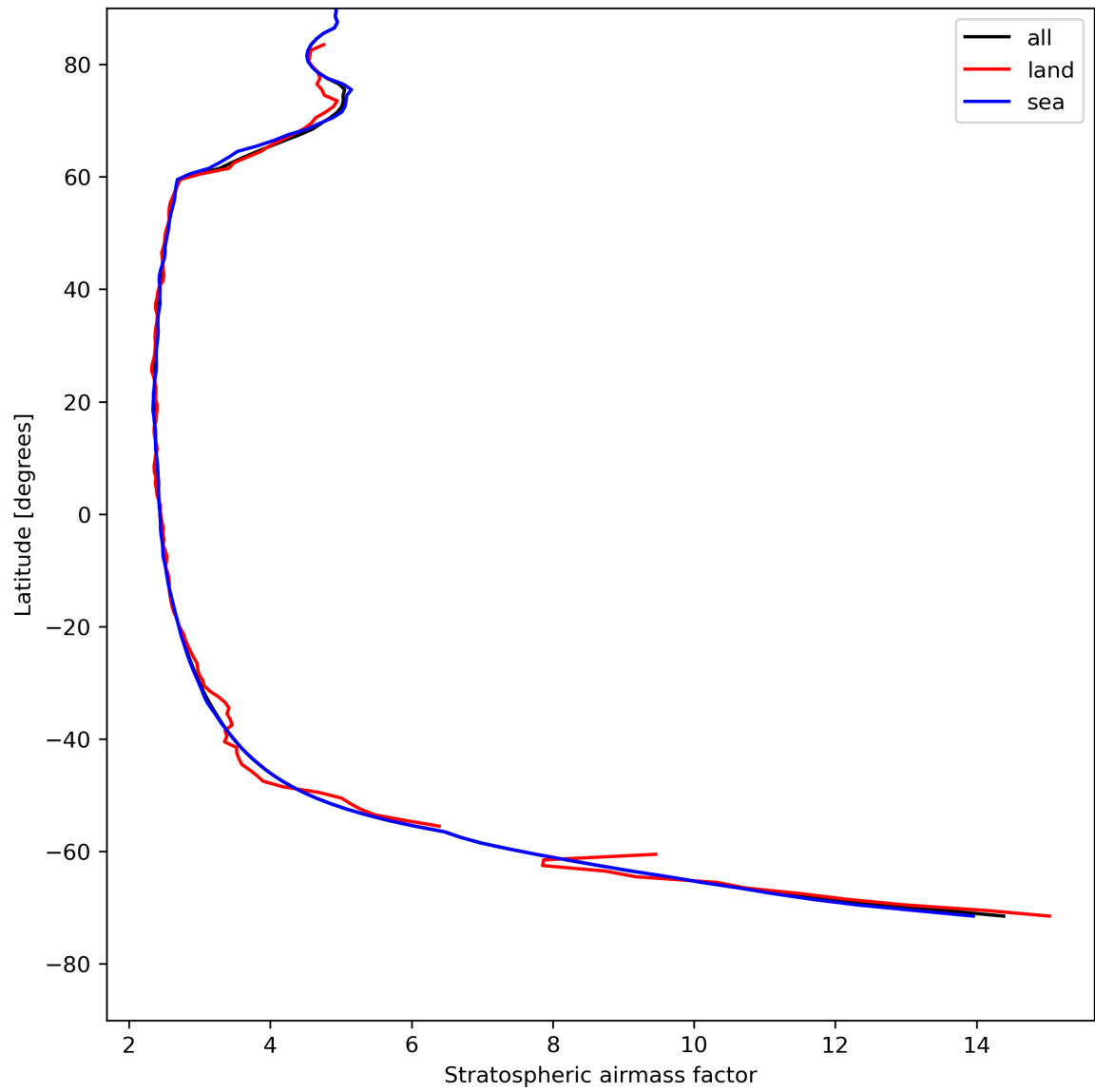
Figure 27: Zonal average of “Stratospheric air mass factor” for 2024-08-06 to 2024-08-08.
