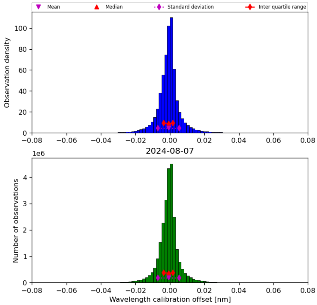
Figure 35: Histogram of “Wavelength calibration offset” for 2024-08-06 to 2024-08-08
