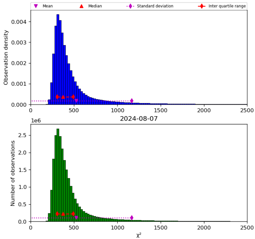
Figure 42: Histogram of “ \chi^2 ” for 2024-08-06 to 2024-08-08
