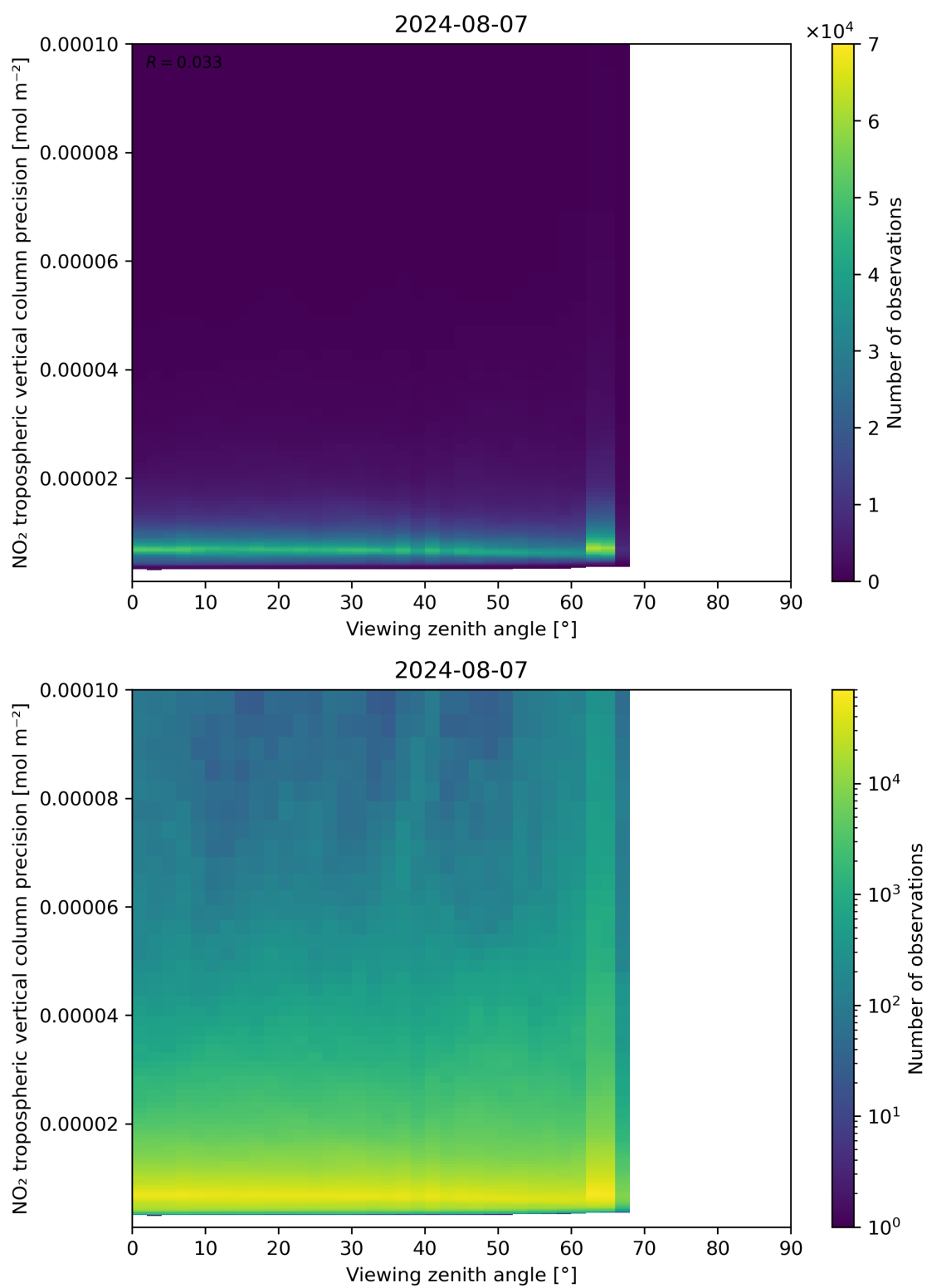
Figure 170: Scatter density plot of “Viewing zenith angle” against “NO 2 tropospheric vertical column precision” for 2024-08-06 to 2024-08-08.
