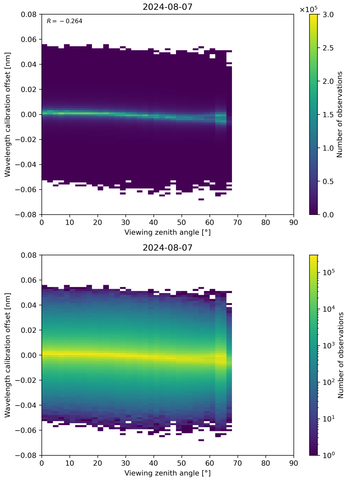
Figure 173: Scatter density plot of “Viewing zenith angle” against “Wavelength calibration offset” for 2024-08-06 to 2024-08-08.
