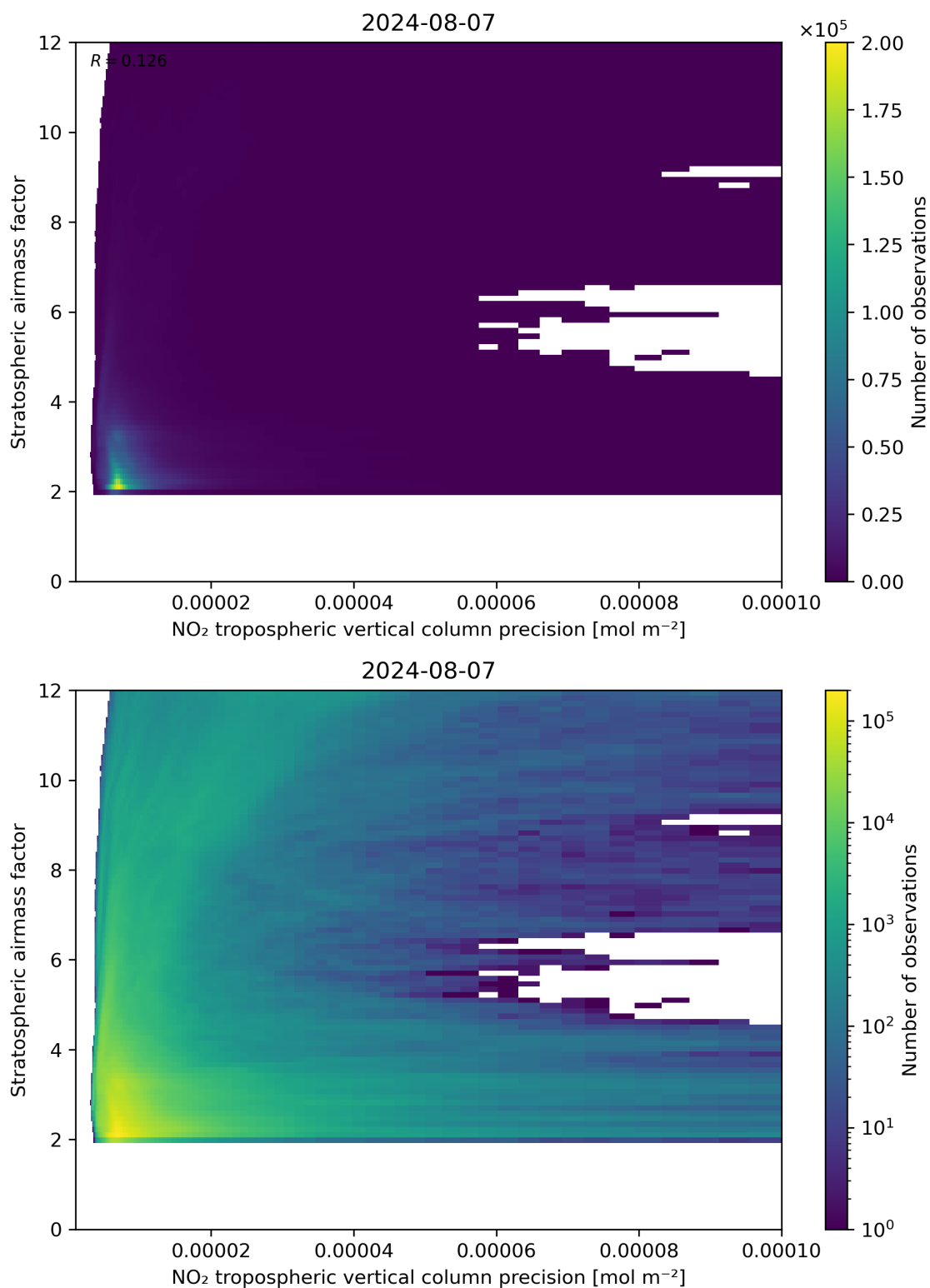
Figure 131: Scatter density plot of “NO 2 tropospheric vertical column precision” against “Stratospheric airmass factor” for 2024-08-06 to 2024-08-08.
