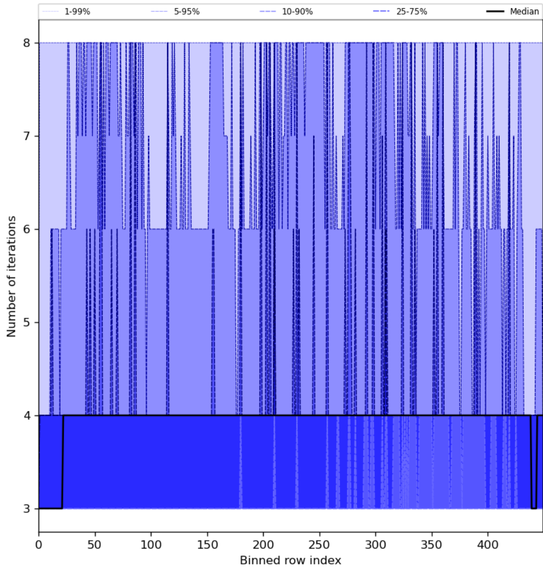
Figure 51: Along track statistics of “Number of iterations” for 2024-08-06 to 2024-08-08
