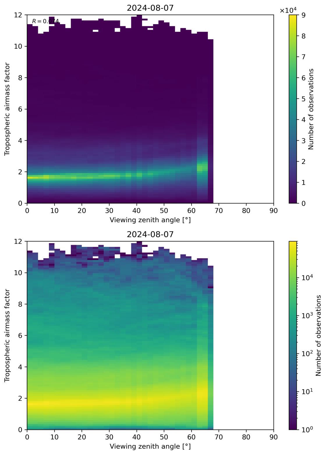
Figure 161: Scatter density plot of “Viewing zenith angle” against “Tropospheric airmass factor” for 2024-08-06 to 2024-08-08.
