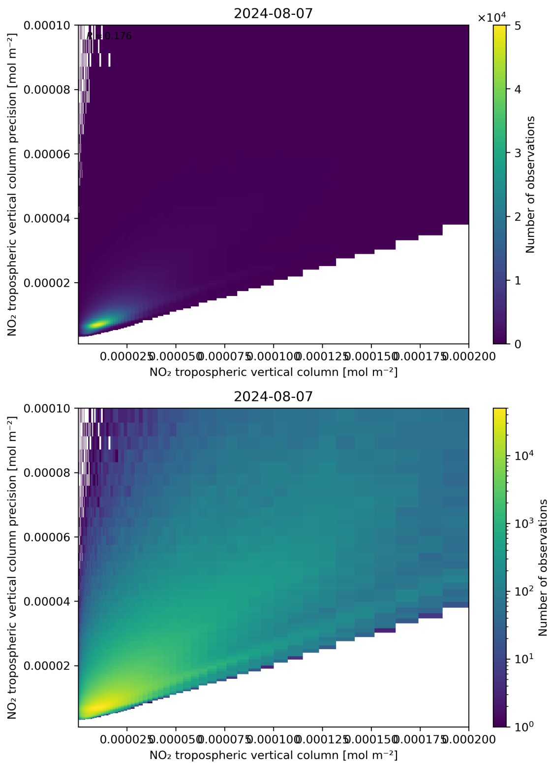
Figure 130: Scatter density plot of “NO 2 tropospheric vertical column” against “NO 2 tropospheric vertical column precision” for 2024-08-06 to 2024-08-08.
