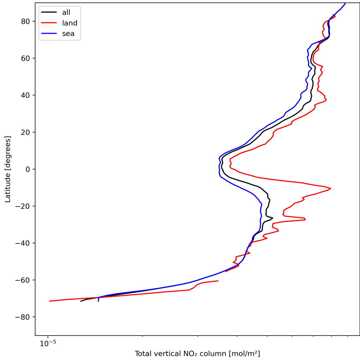
Figure 21: Zonal average of “Total vertical NO 2 column” for 2024-08-06 to 2024-08-08.
