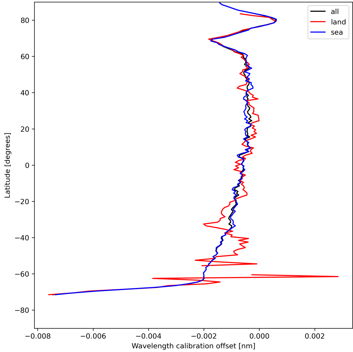
Figure 18: Zonal average of “Wavelength calibration offset” for 2024-08-06 to 2024-08-08.
