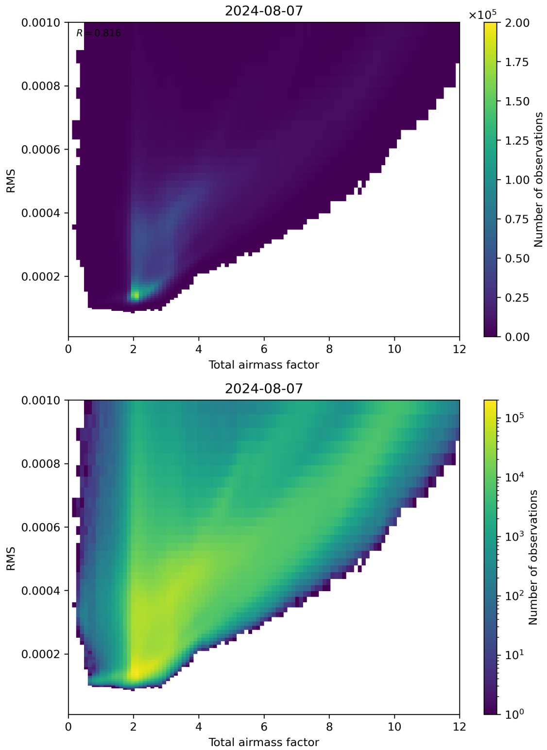
Figure 69: Scatter density plot of “Total airmass factor” against “RMS” for 2024-08-06 to 2024-08-08.
