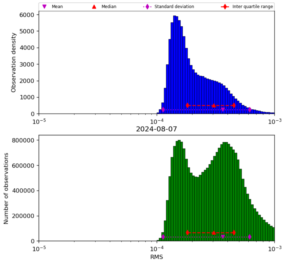
Figure 43: Histogram of “RMS” for 2024-08-06 to 2024-08-08
