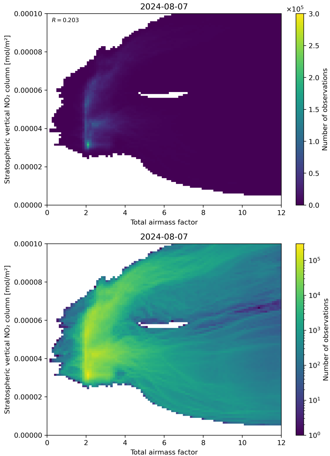
Figure 64: Scatter density plot of “Total airmass factor” against “Stratospheric vertical NO 2 column” for 2024-08-06 to 2024-08-08.
