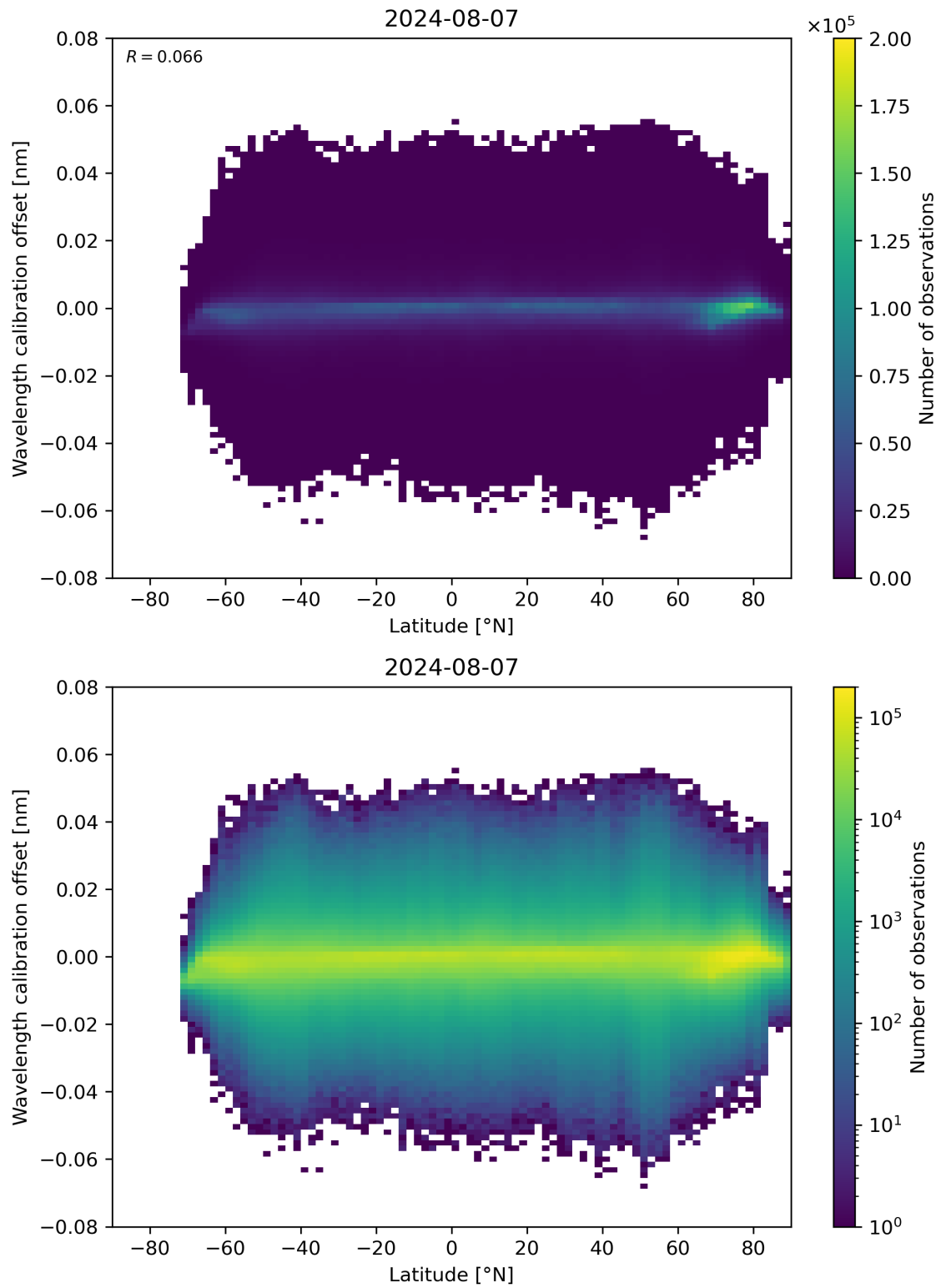
Figure 95: Scatter density plot of “Latitude” against “Wavelength calibration offset” for 2024-08-06 to 2024-08-08.
