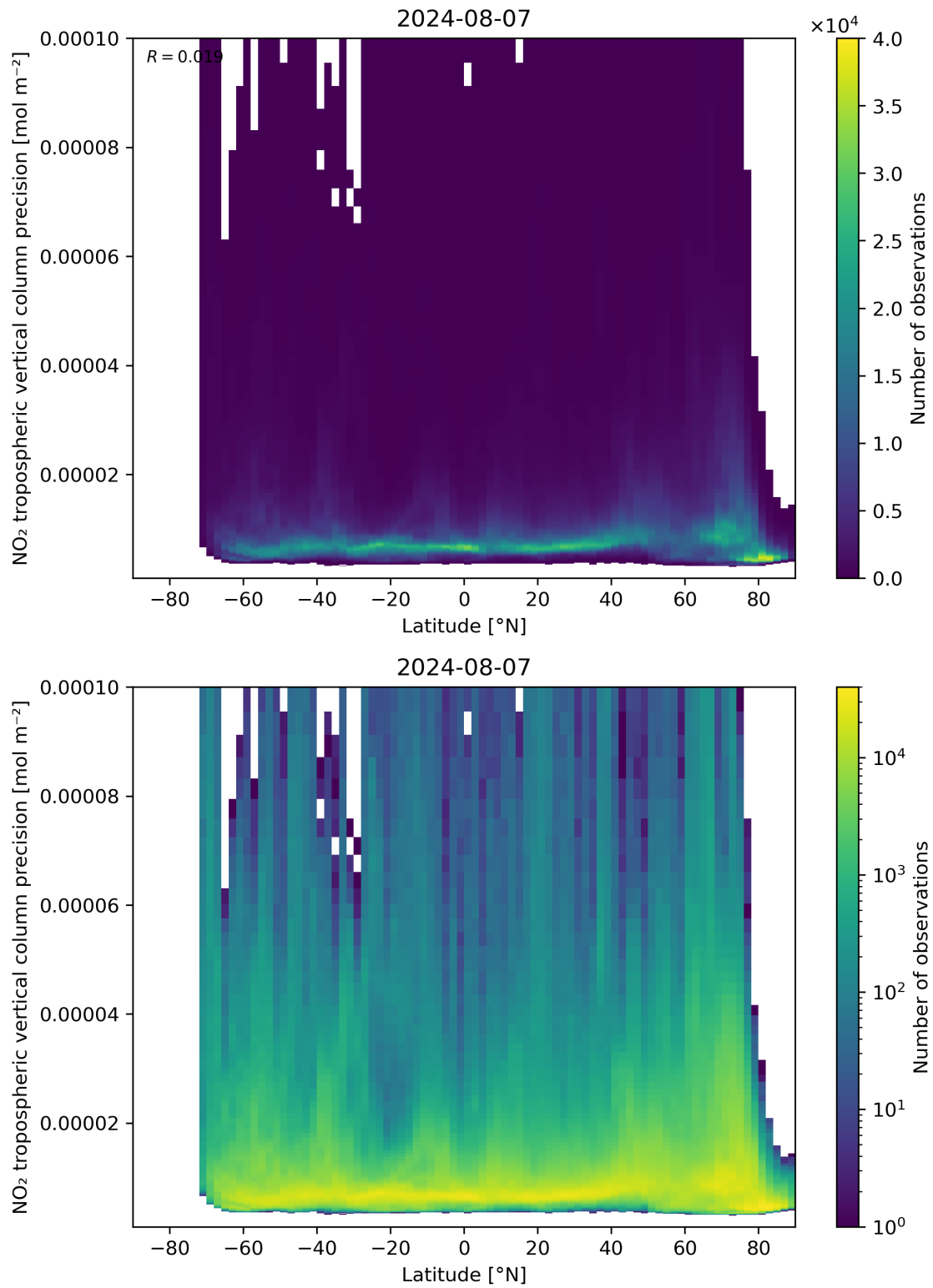
Figure 93: Scatter density plot of “Latitude” against “NO 2 tropospheric vertical column precision” for 2024-08-06 to 2024-08-08.
