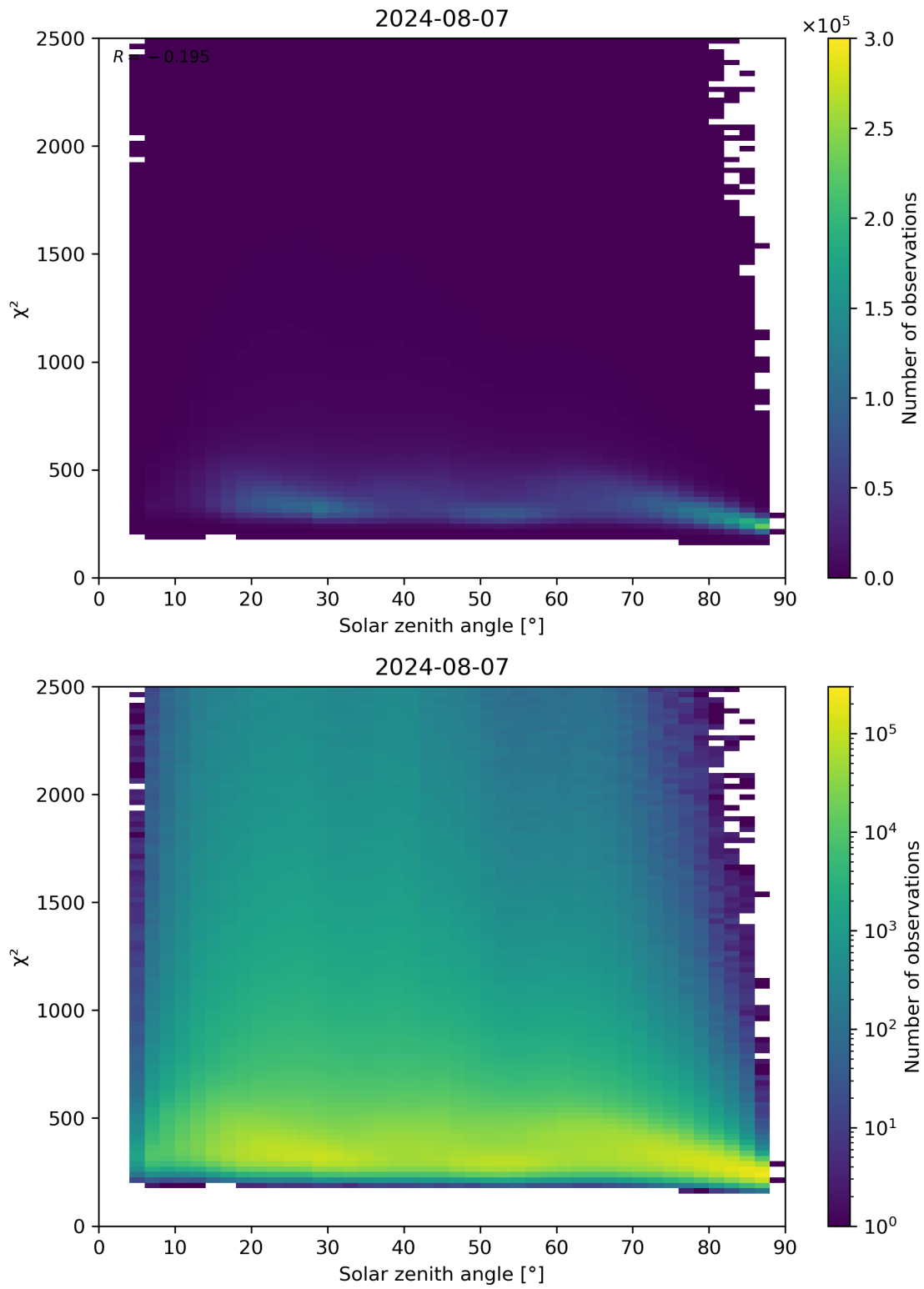
Figure 148: Scatter density plot of “Solar zenith angle” against “ \chi^2 ” for 2024-08-06 to 2024-08-08.
