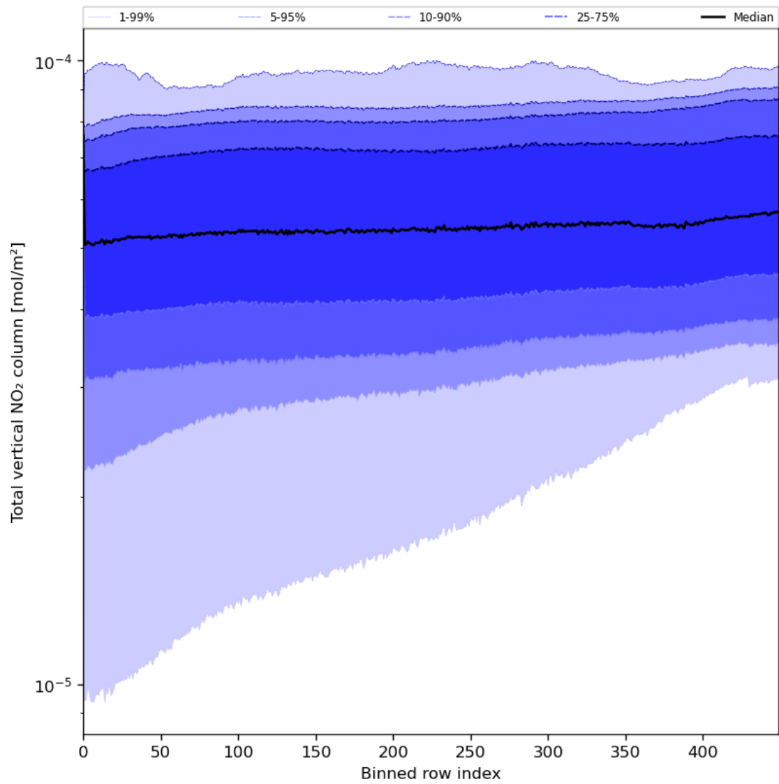
Figure 55: Along track statistics of “Total vertical NO 2 column” for 2024-08-06 to 2024-08-08
