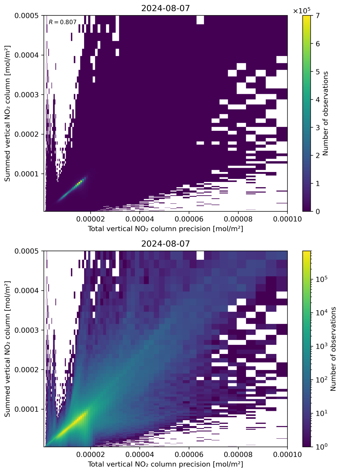
Figure 117: Scatter density plot of “Total vertical NO 2 column precision” against “Summed vertical NO 2 column” for 2024-08-06 to 2024-08-08.
