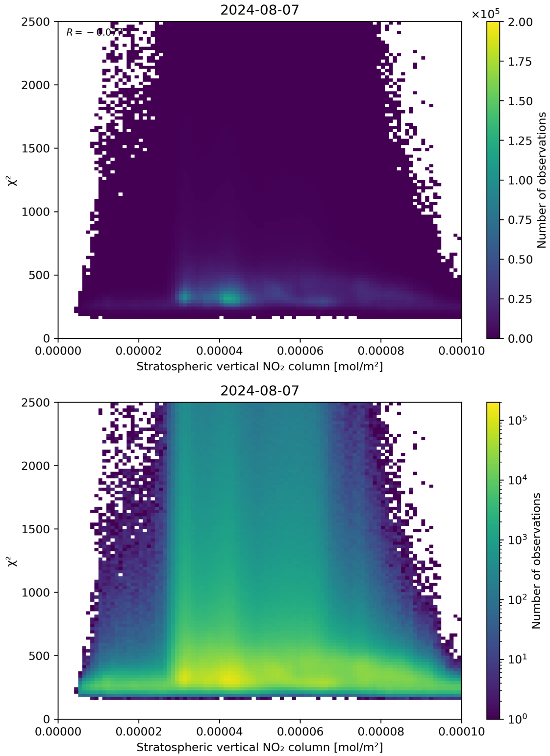
Figure 97: Scatter density plot of “Stratospheric vertical NO 2 column” against “ \chi^2 ” for 2024-08-06 to 2024-08-08.
