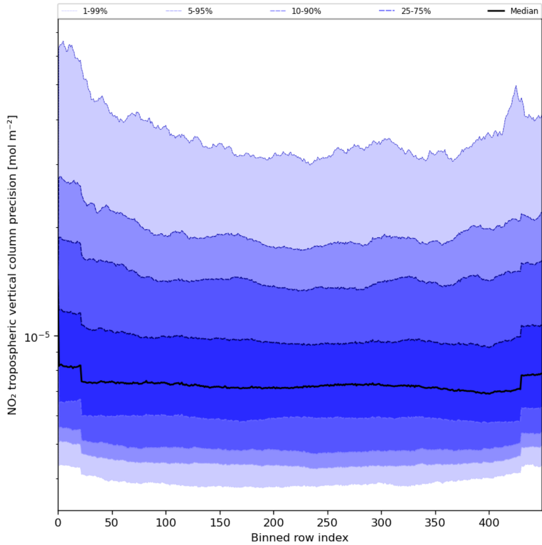
Figure 47: Along track statistics of “NO 2 tropospheric vertical column precision” for 2024-08-06 to 2024-08-08
