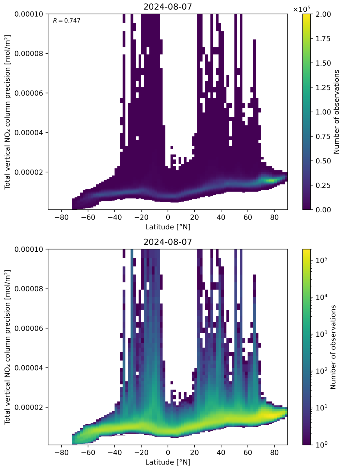
Figure 91: Scatter density plot of “Latitude” against “Total vertical NO 2 column precision” for 2024-08-06 to 2024-08-08.
