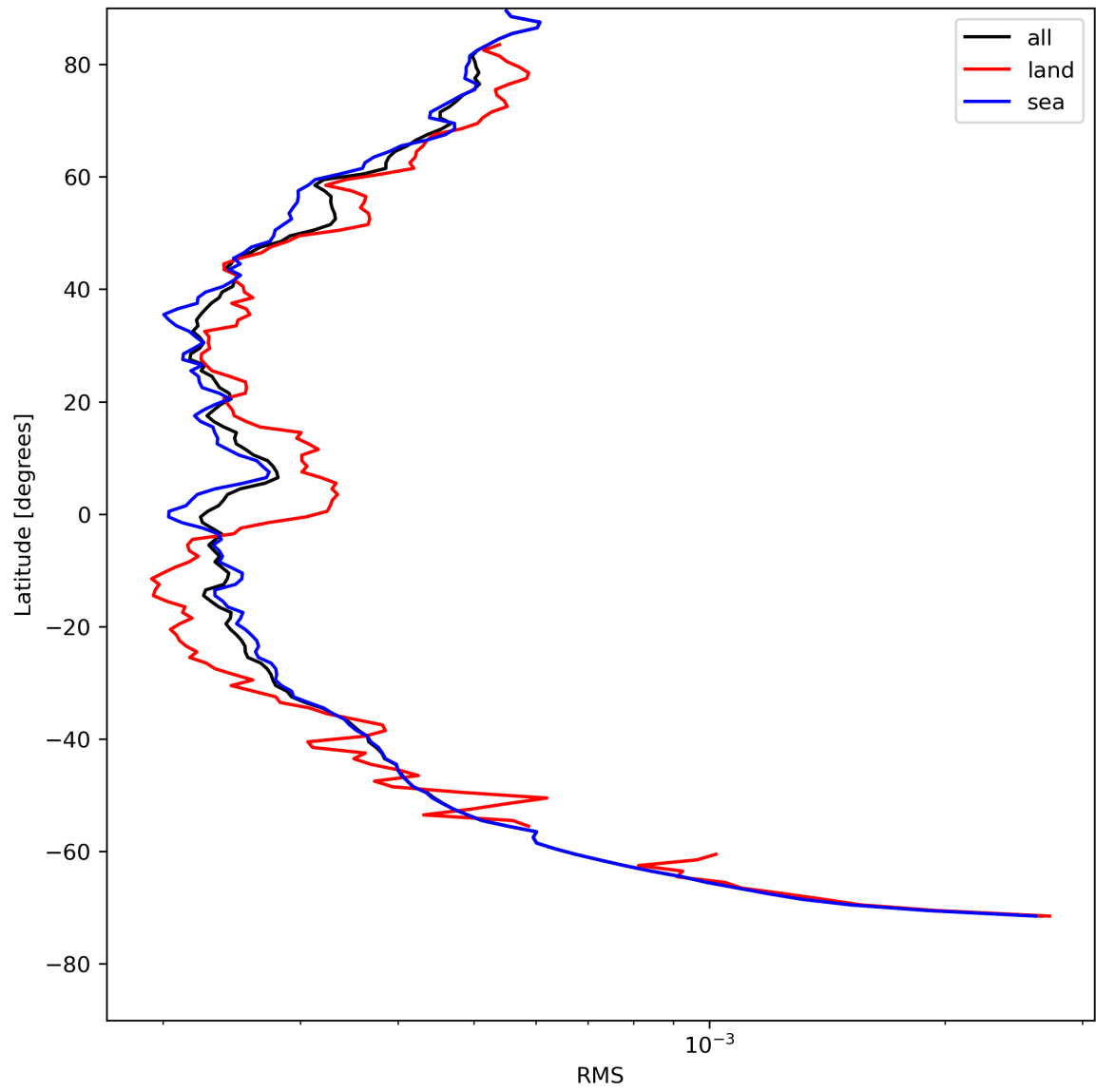
Figure 26: Zonal average of “RMS” for 2024-08-06 to 2024-08-08.
