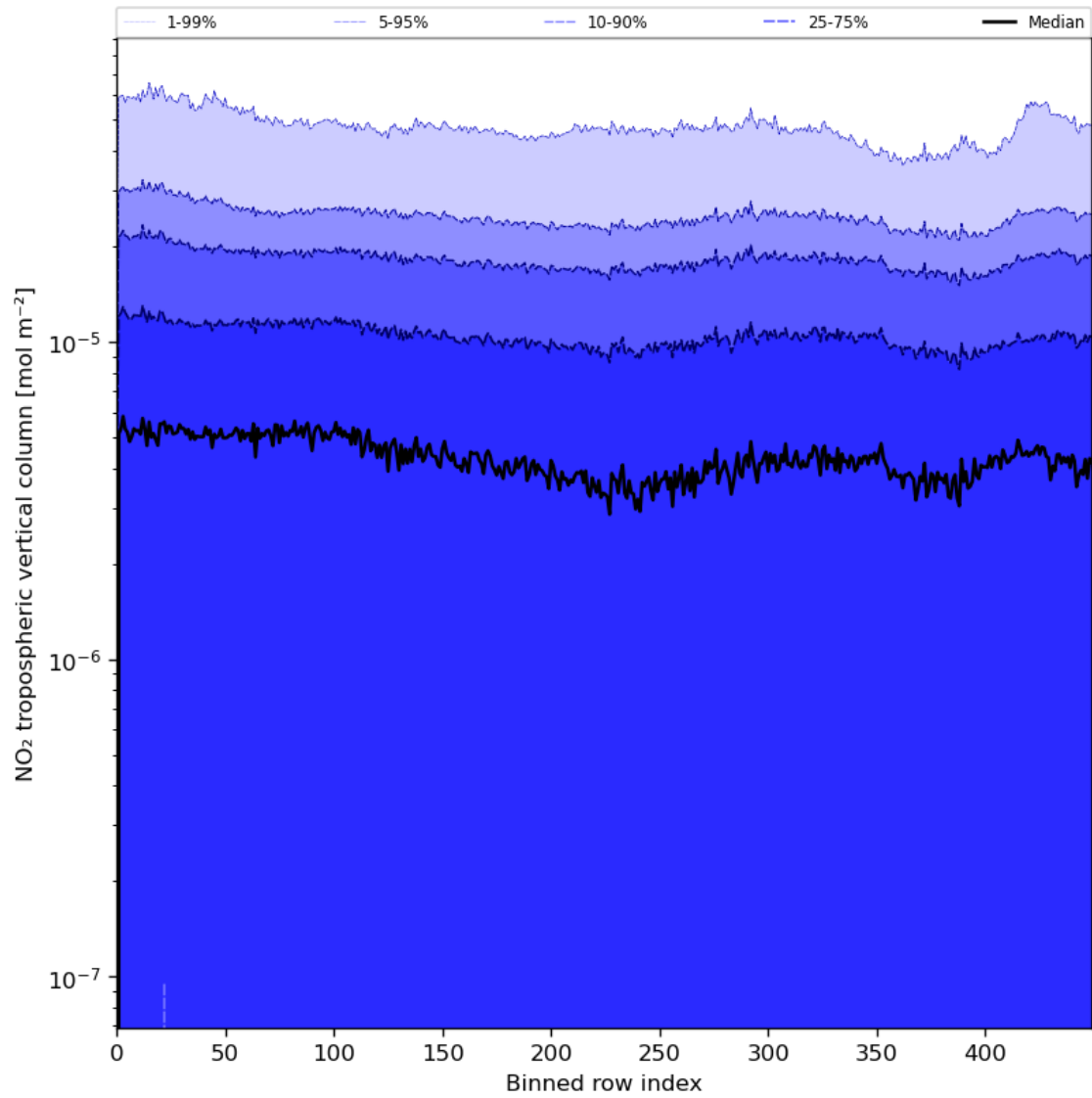
Figure 46: Along track statistics of “NO 2 tropospheric vertical column” for 2024-08-06 to 2024-08-08
