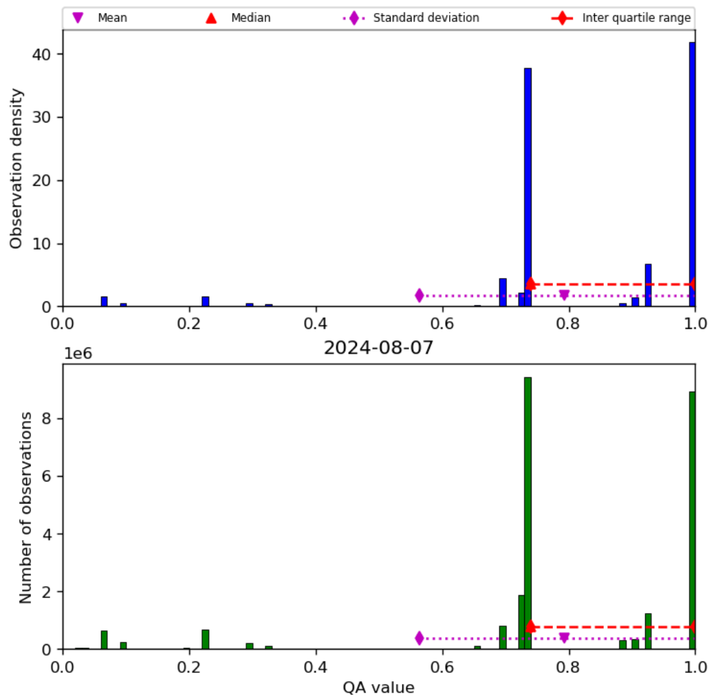
Figure 28: Histogram of “QA value” for 2024-08-06 to 2024-08-08
