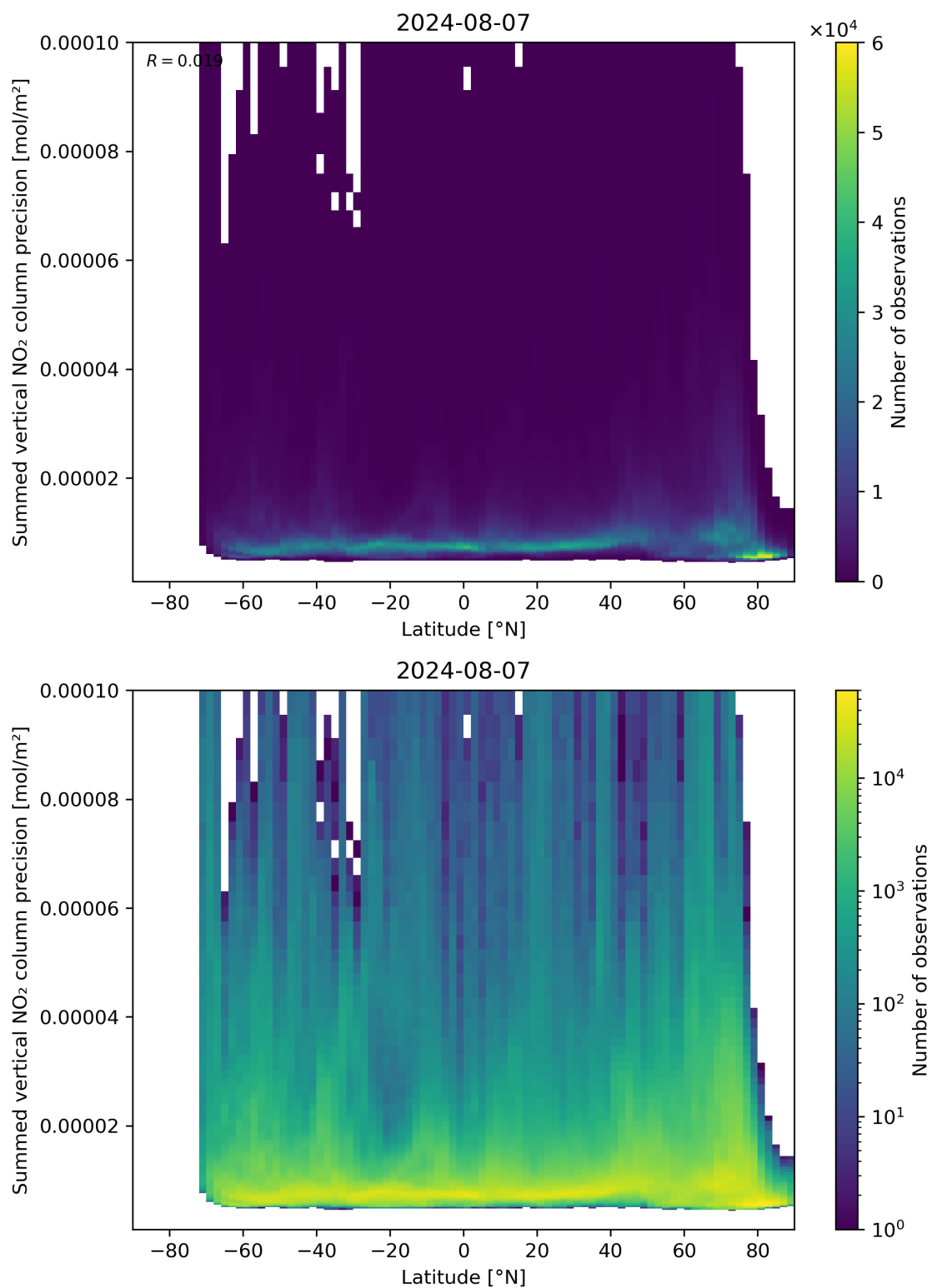
Figure 89: Scatter density plot of “Latitude” against “Summed vertical NO 2 column precision” for 2024-08-06 to 2024-08-08.
