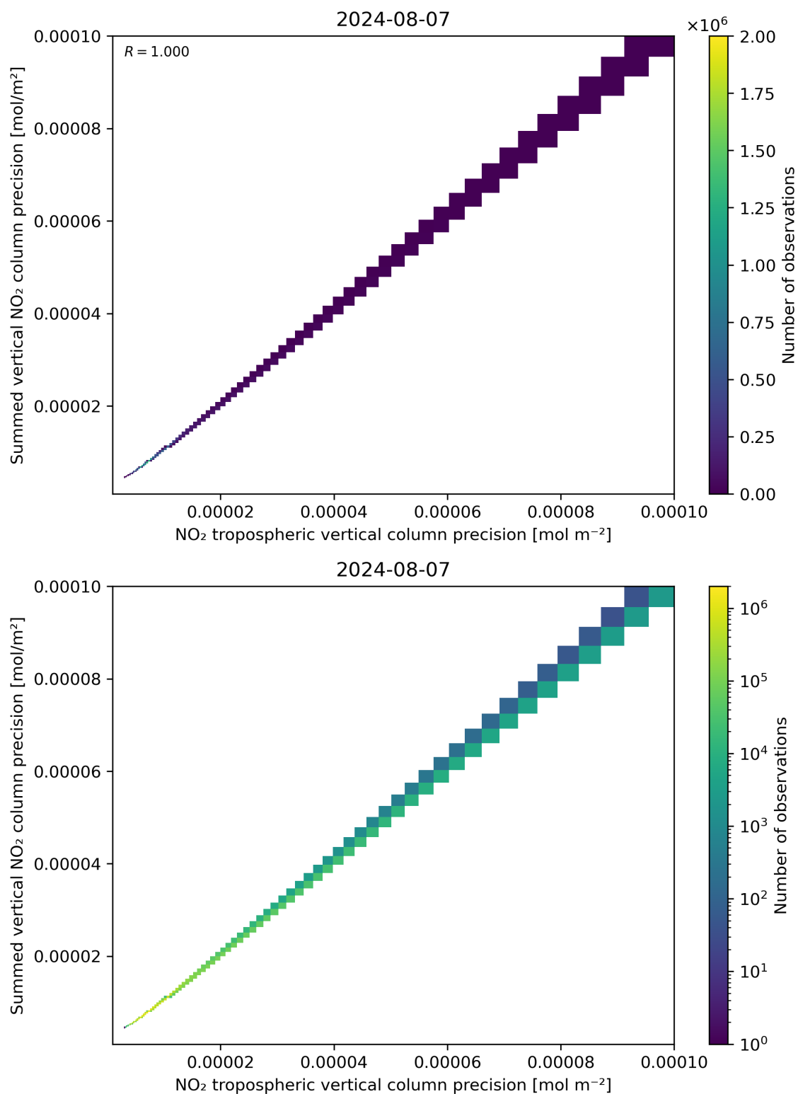
Figure 137: Scatter density plot of “NO 2 tropospheric vertical column precision” against “Summed vertical NO 2 column precision” for 2024-08-06 to 2024-08-08.
