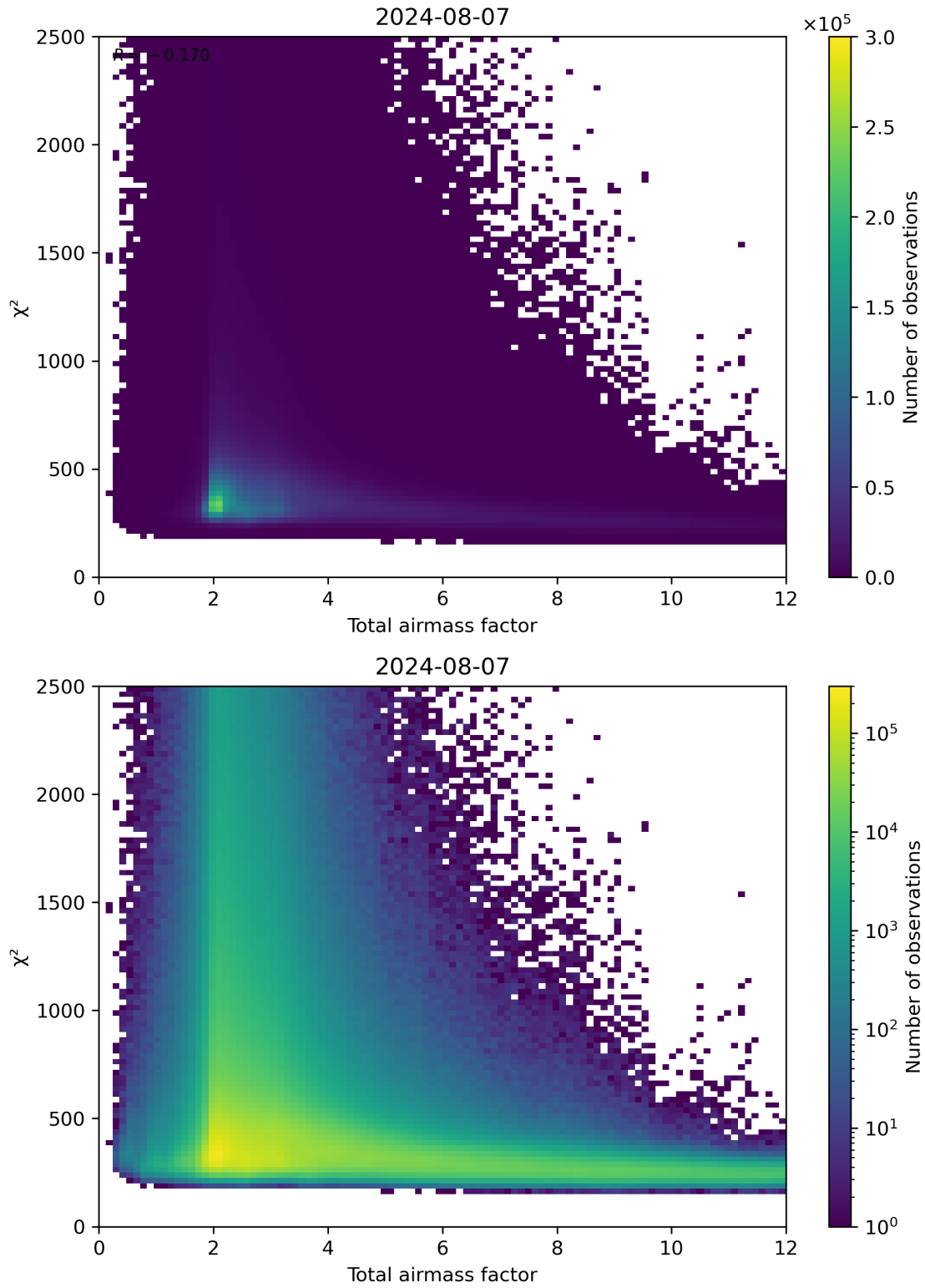
Figure 63: Scatter density plot of “Total airmass factor” against “ \chi^2 ” for 2024-08-06 to 2024-08-08.
