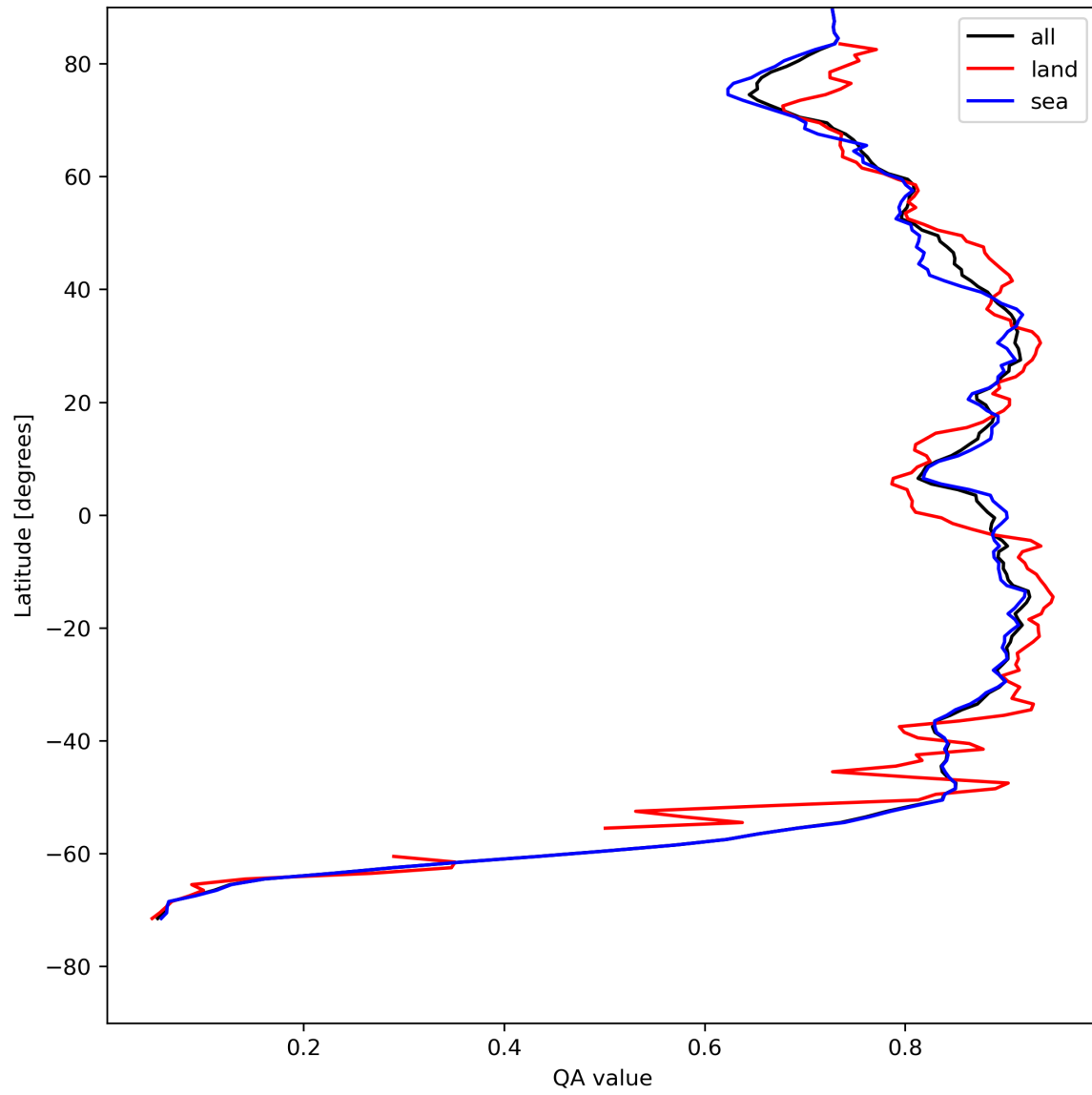
Figure 11: Zonal average of “QA value” for 2024-08-06 to 2024-08-08.
