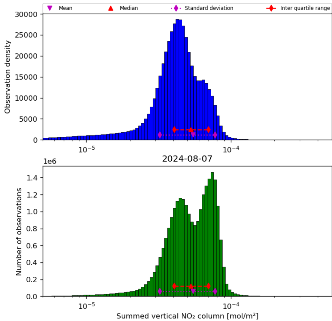
Figure 40: Histogram of “Summed vertical NO 2 column” for 2024-08-06 to 2024-08-08
