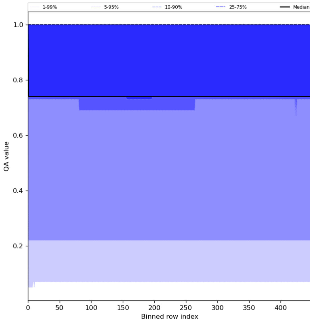
Figure 45: Along track statistics of “QA value” for 2024-08-06 to 2024-08-08
