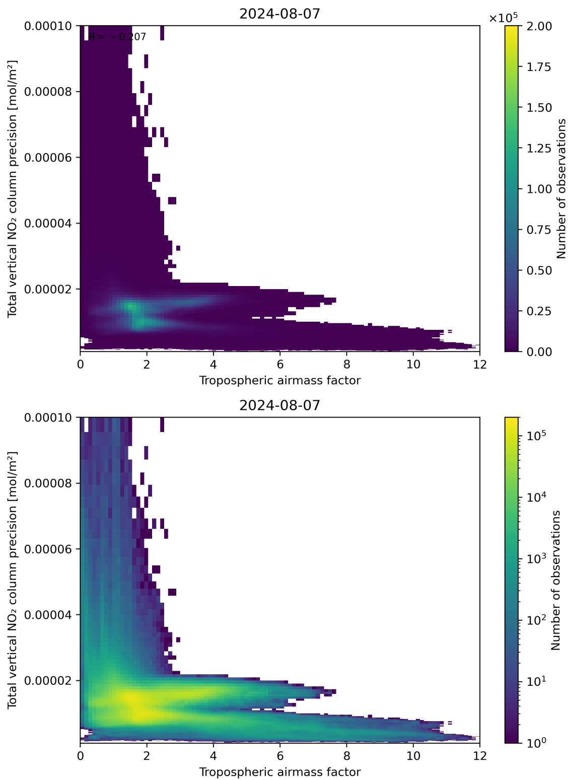
Figure 78: Scatter density plot of “Tropospheric airmass factor” against “Total vertical NO 2 column precision” for 2024-08-06 to 2024-08-08.
