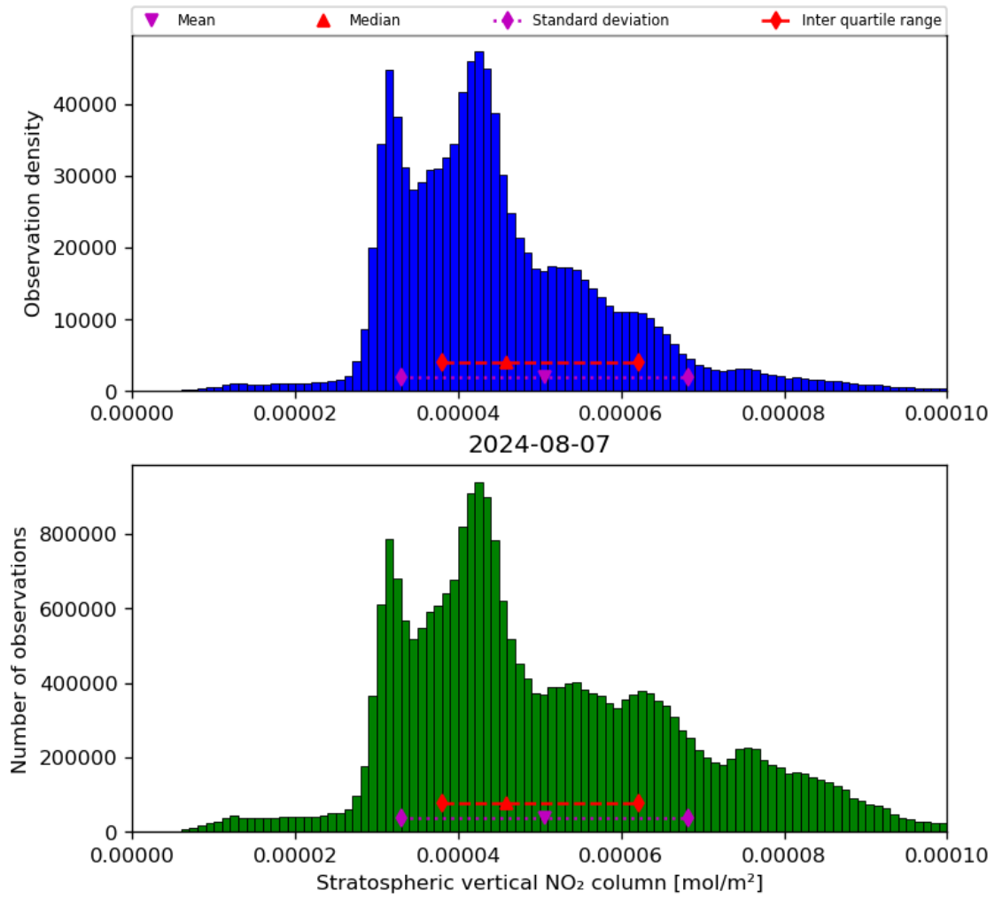
Figure 36: Histogram of “Stratospheric vertical NO 2 column” for 2024-08-06 to 2024-08-08
