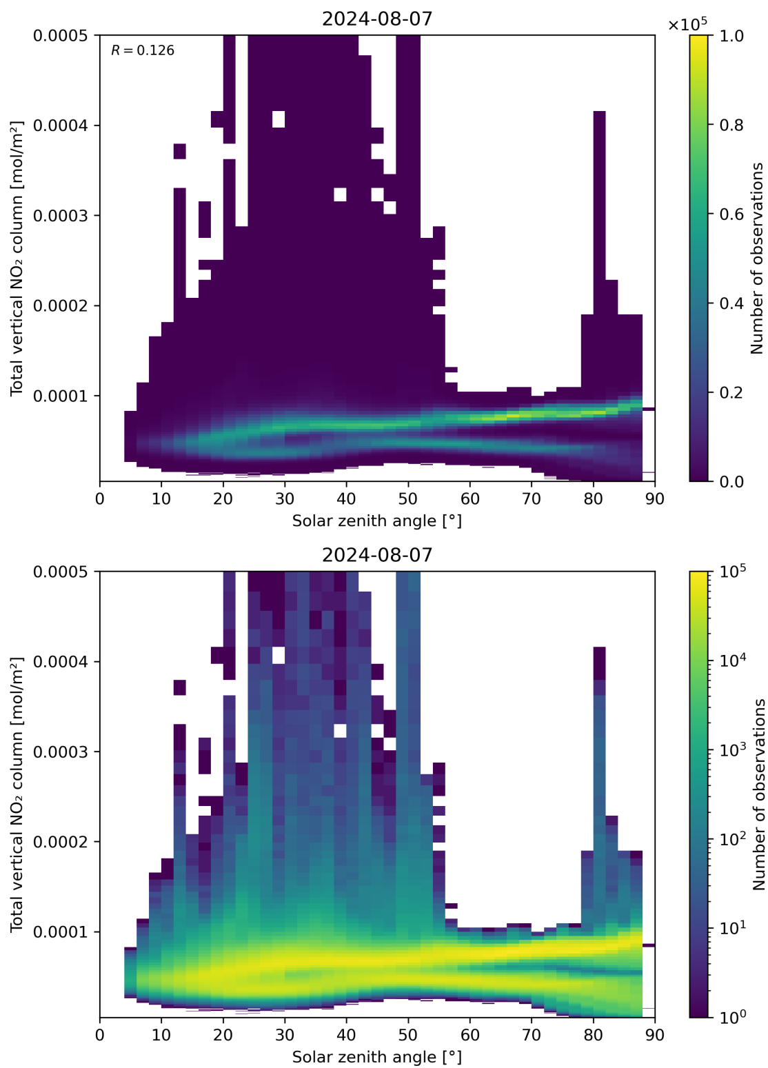
Figure 153: Scatter density plot of “Solar zenith angle” against “Total vertical NO 2 column” for 2024-08-06 to 2024-08-08.
