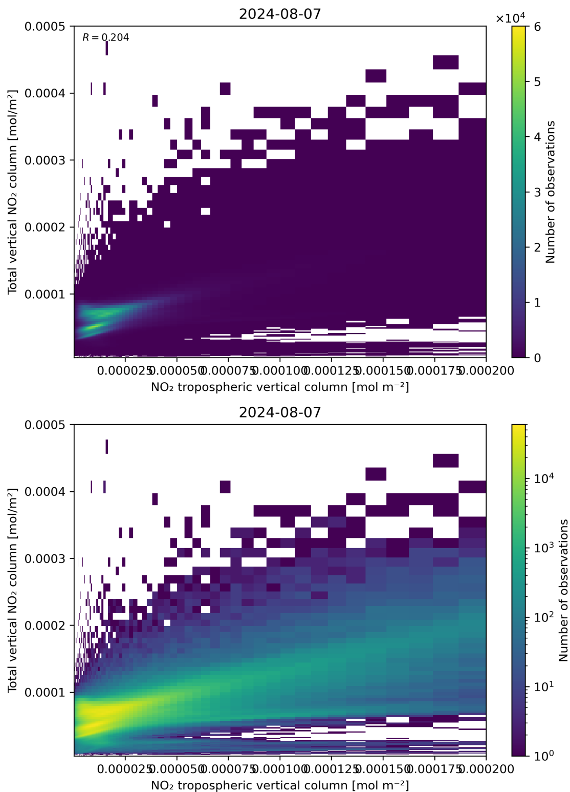
Figure 128: Scatter density plot of “NO 2 tropospheric vertical column” against “Total vertical NO 2 column” for 2024-08-06 to 2024-08-08.
