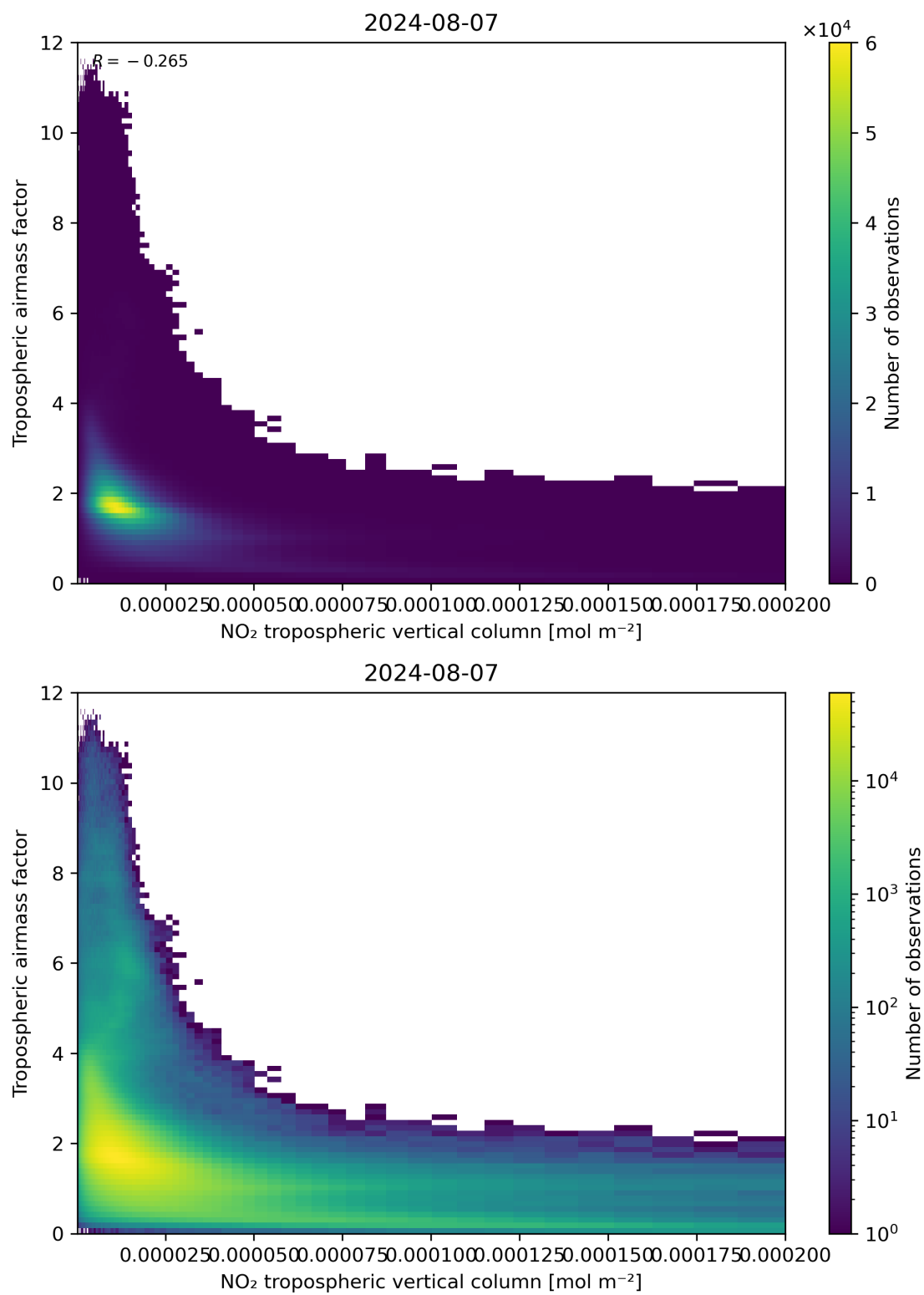
Figure 123: Scatter density plot of “NO 2 tropospheric vertical column” against “Tropospheric airmass factor” for 2024-08-06 to 2024-08-08.
