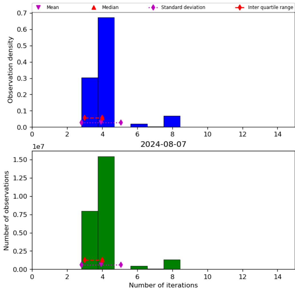
Figure 34: Histogram of “Number of iterations” for 2024-08-06 to 2024-08-08
