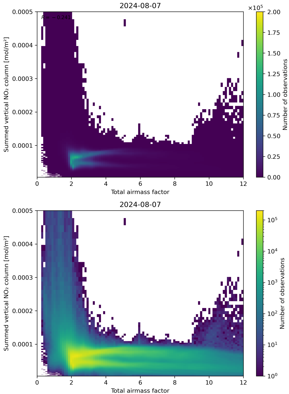
Figure 65: Scatter density plot of “Total airmass factor” against “Summed vertical NO 2 column” for 2024-08-06 to 2024-08-08.
