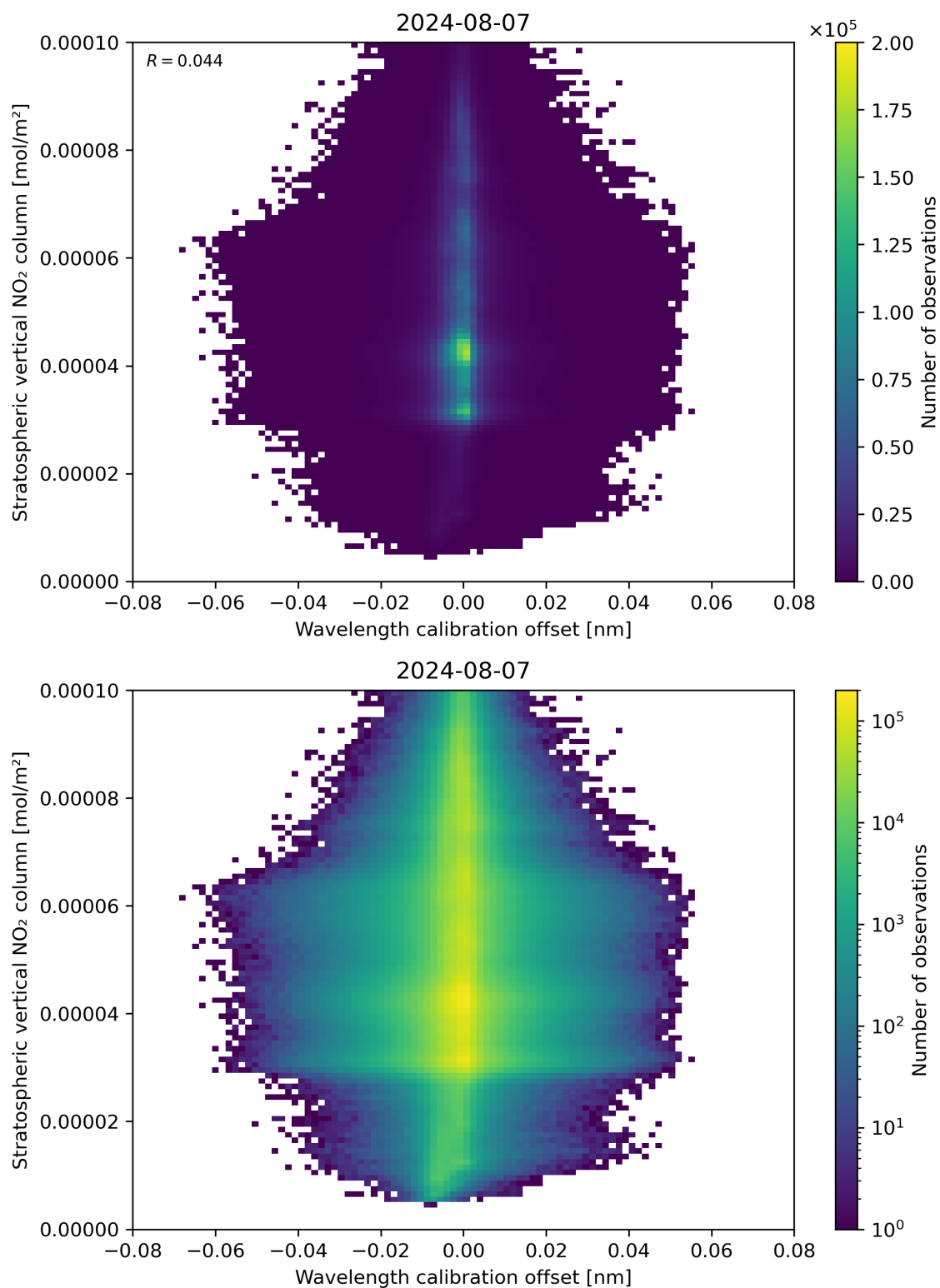
Figure 176: Scatter density plot of “Wavelength calibration offset” against “Stratospheric vertical NO 2 column” for 2024-08-06 to 2024-08-08.
