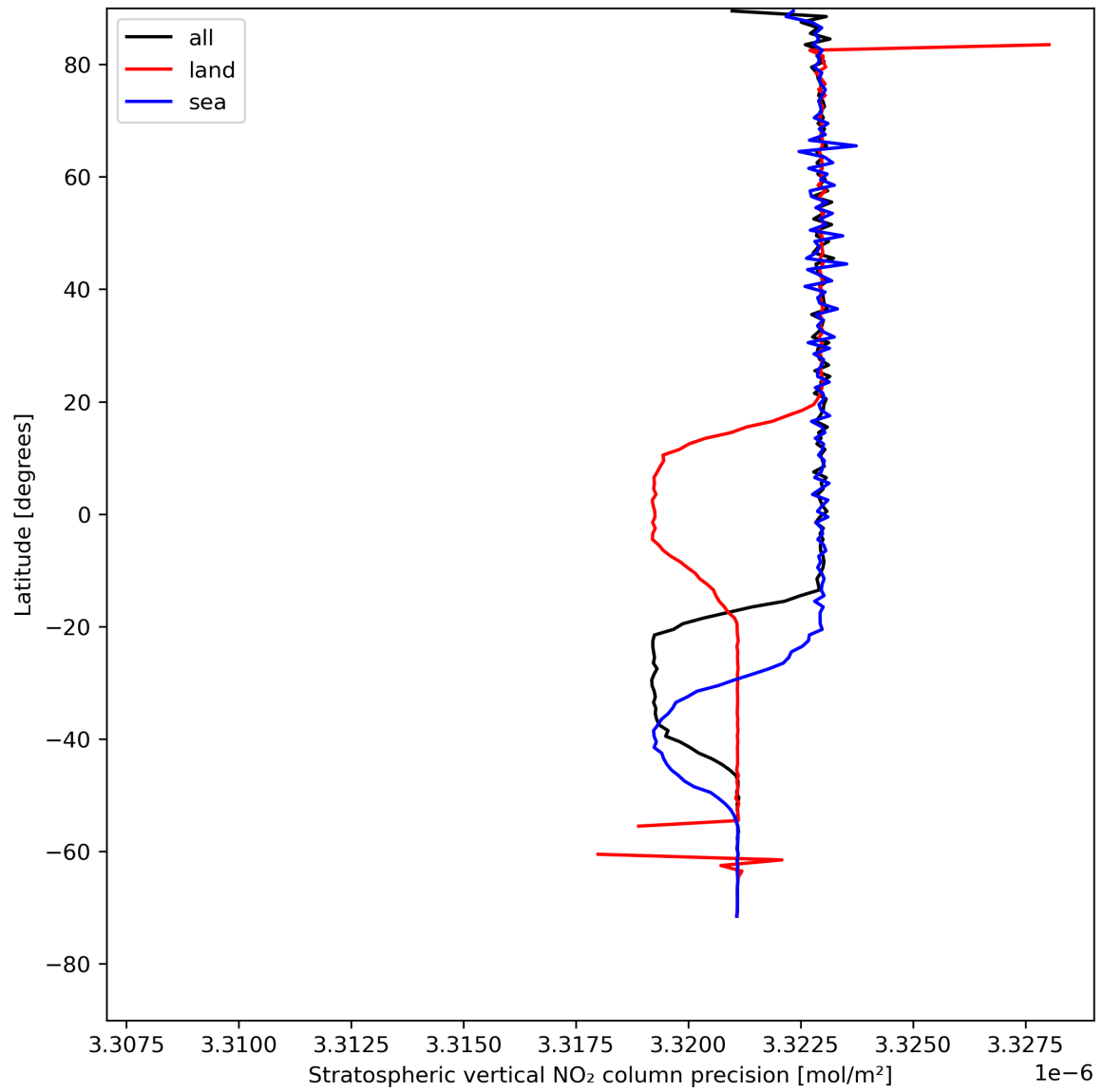
Figure 20: Zonal average of “Stratospheric vertical NO 2 column precision” for 2024-08-06 to 2024-08-08.
