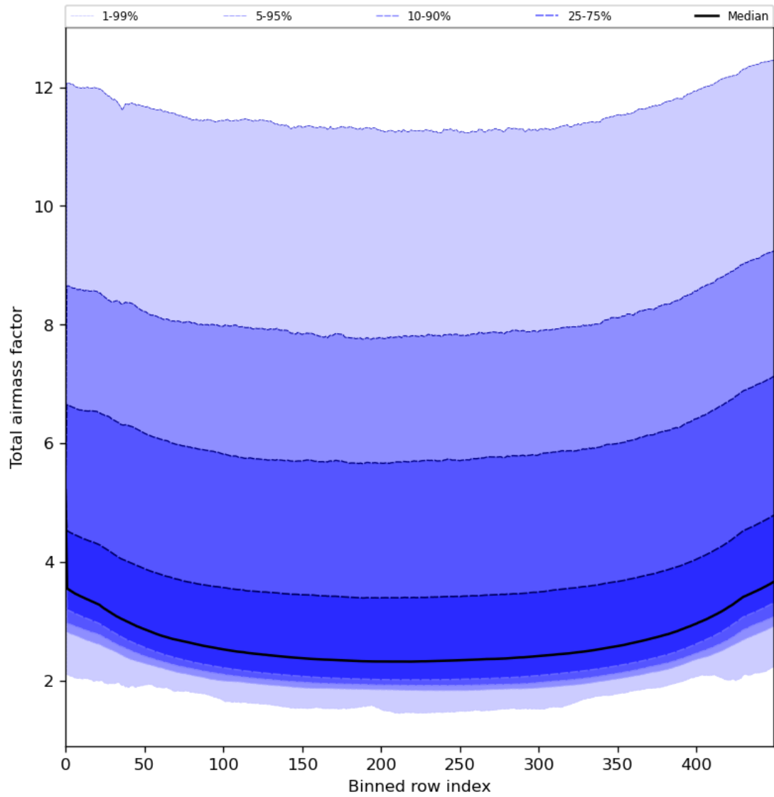
Figure 49: Along track statistics of “Total airmass factor” for 2024-08-06 to 2024-08-08
