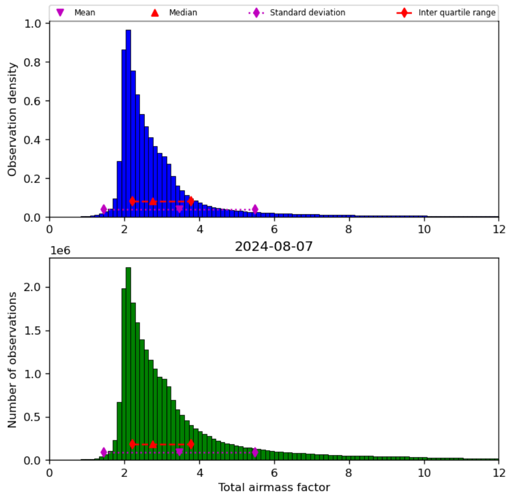
Figure 32: Histogram of “Total airmass factor” for 2024-08-06 to 2024-08-08
