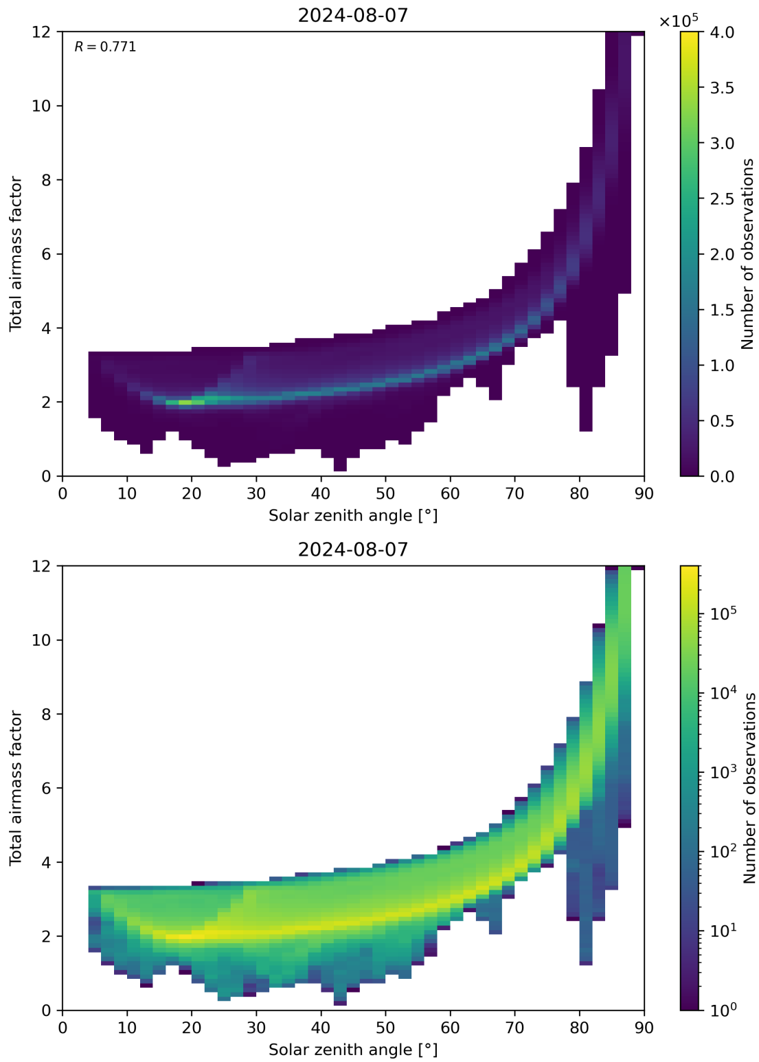
Figure 146: Scatter density plot of “Solar zenith angle” against “Total air mass factor” for 2024-08-06 to 2024-08-08.
