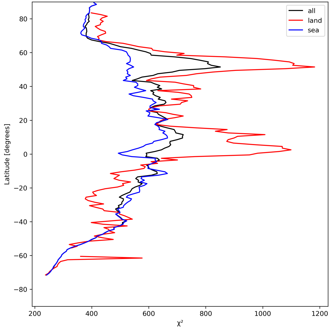
Figure 25: Zonal average of “ \chi^2 ” for 2024-08-06 to 2024-08-08.
