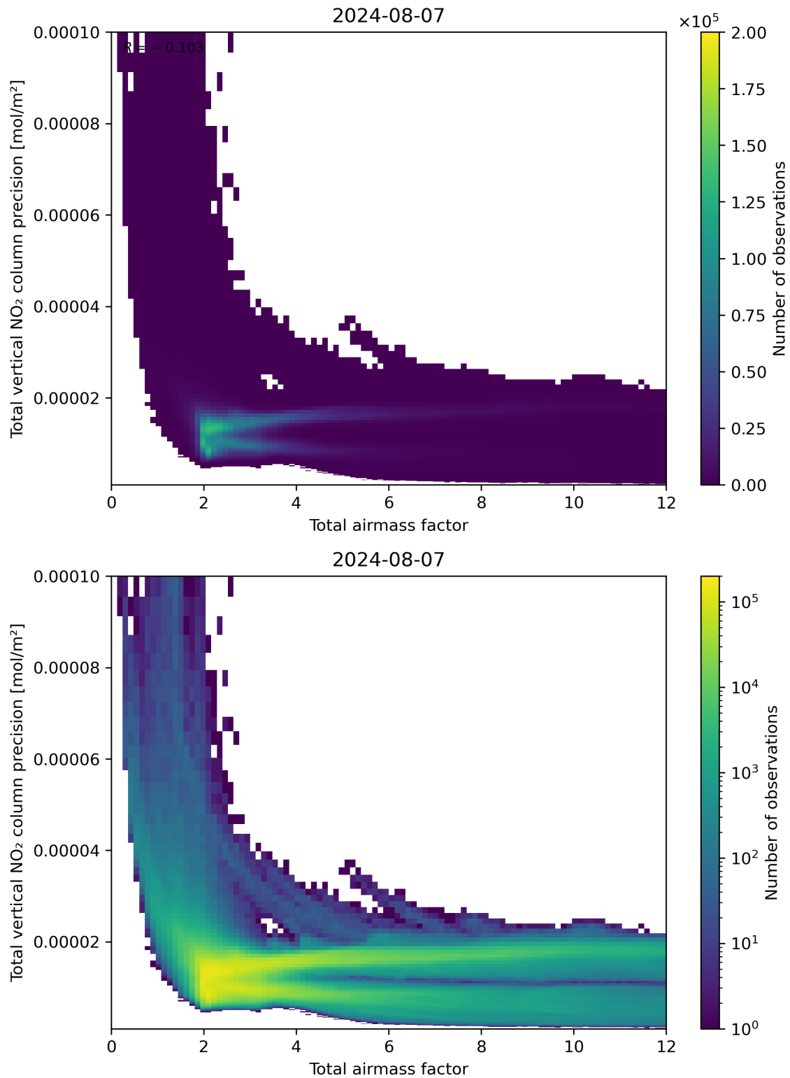
Figure 68: Scatter density plot of “Total airmass factor” against “Total vertical NO 2 column precision” for 2024-08-06 to 2024-08-08.
