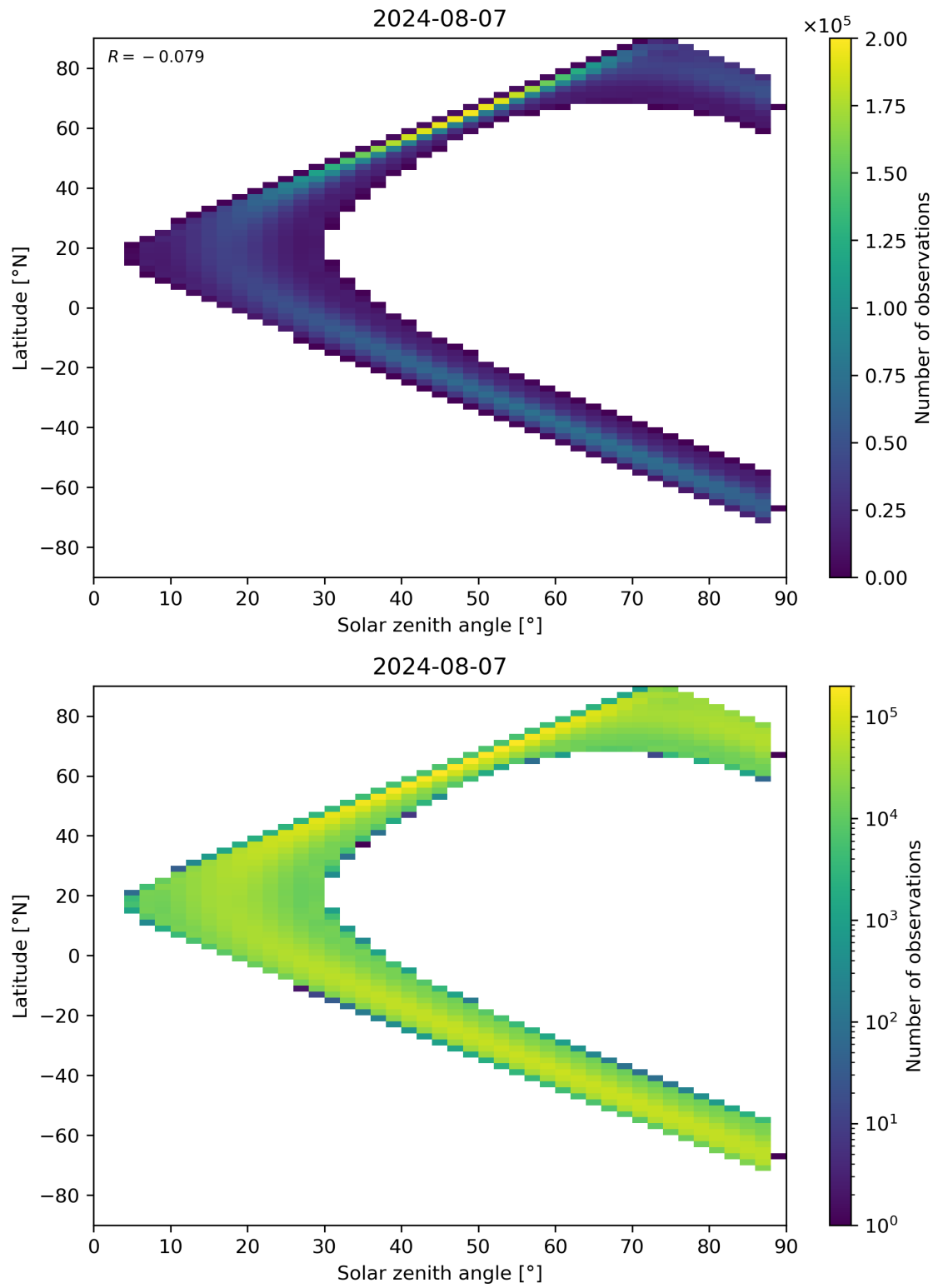
Figure 149: Scatter density plot of “Solar zenith angle” against “Latitude” for 2024-08-06 to 2024-08-08.
