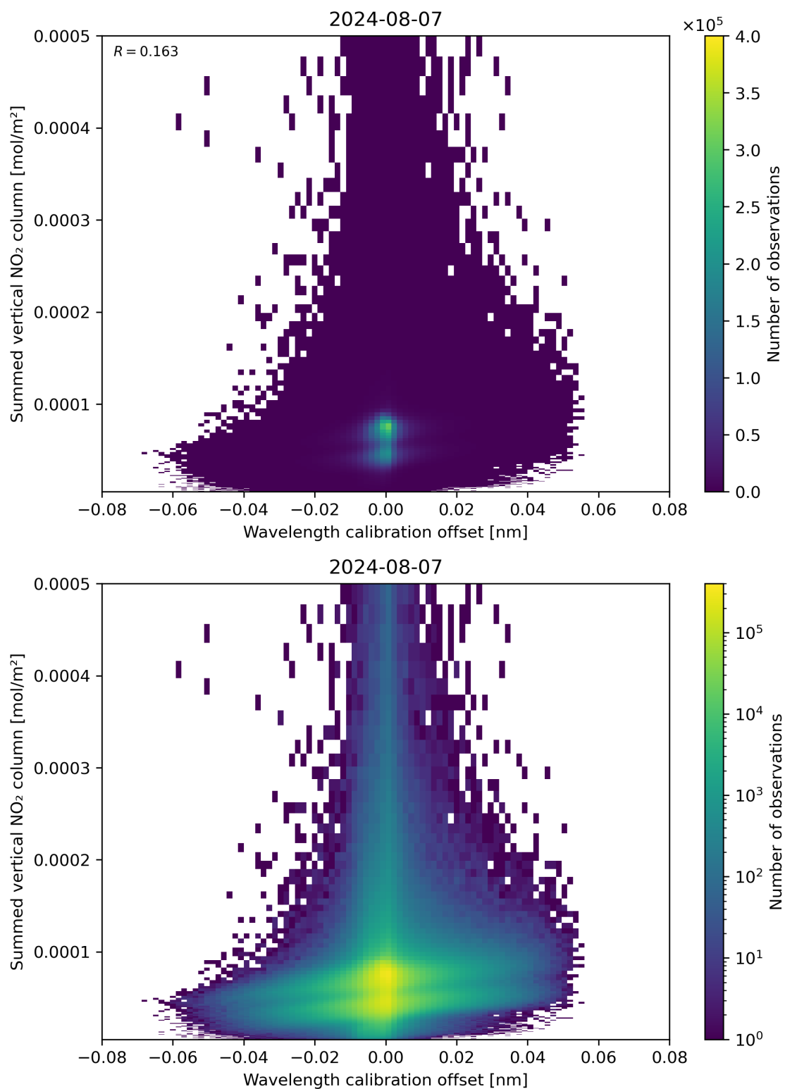
Figure 177: Scatter density plot of “Wavelength calibration offset” against “Summed vertical NO 2 column” for 2024-08-06 to 2024-08-08.
