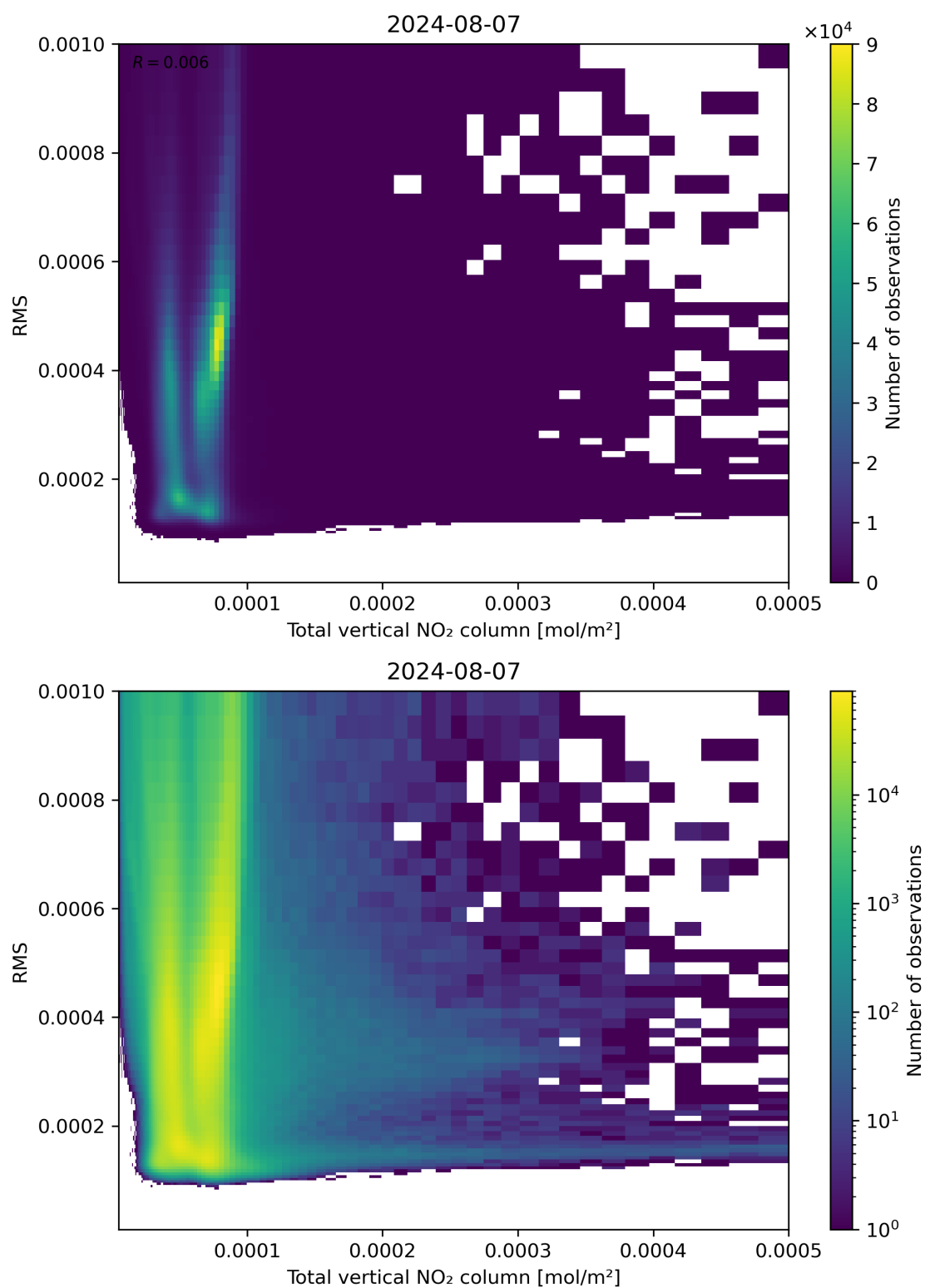
Figure 120: Scatter density plot of “Total vertical NO 2 column” against “RMS” for 2024-08-06 to 2024-08-08.
