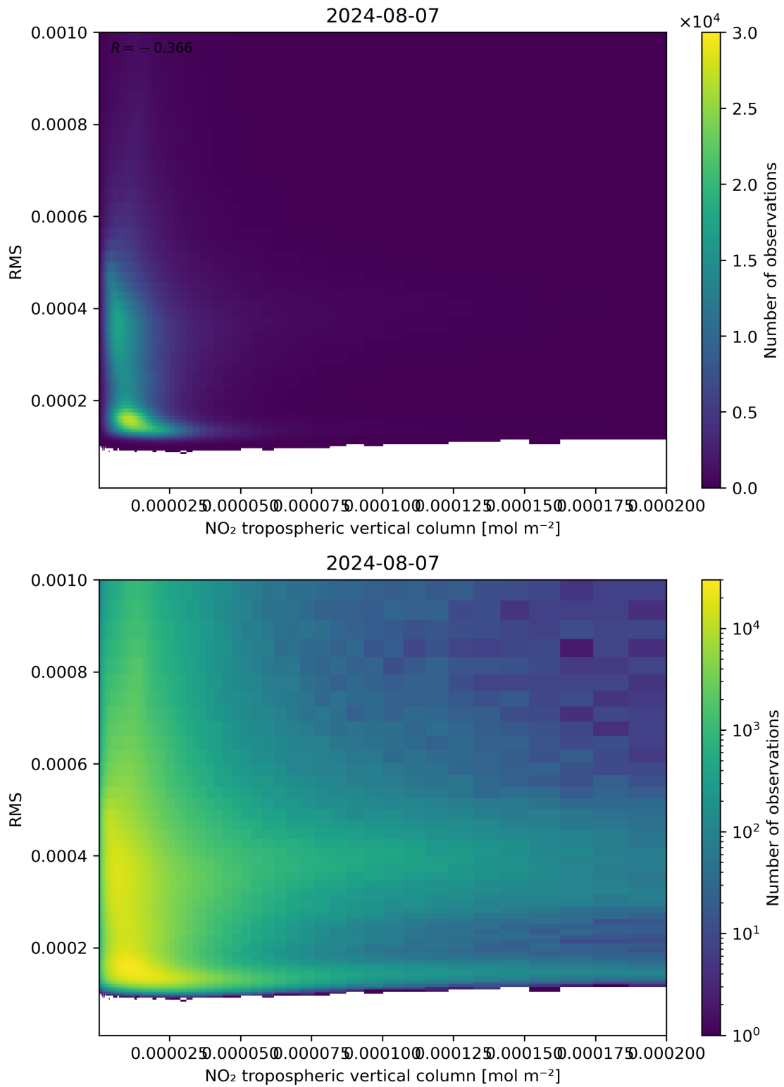
Figure 142: Scatter density plot of “NO 2 tropospheric vertical column” against “RMS” for 2024-08-06 to 2024-08-08.
