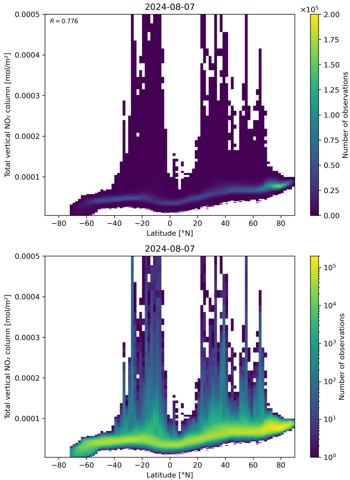
Figure 90: Scatter density plot of “Latitude” against “Total vertical NO 2 column” for 2024-08-06 to 2024-08-08.
