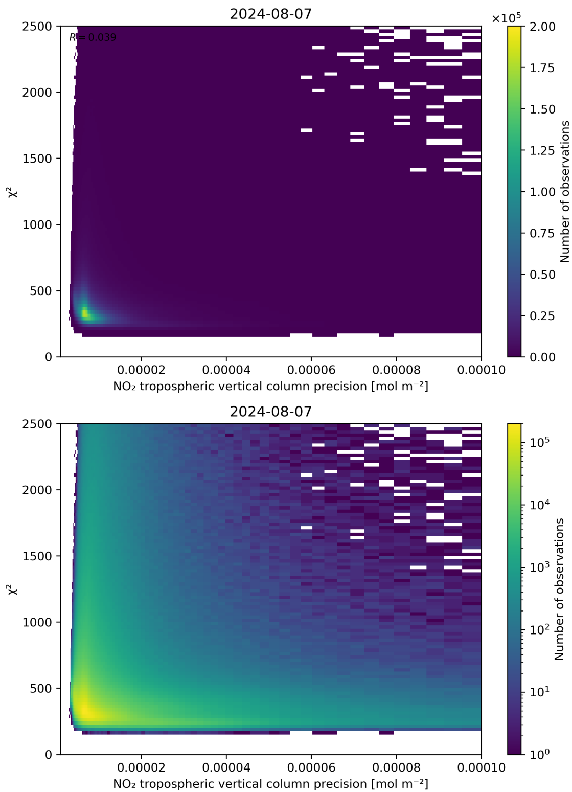
Figure 134: Scatter density plot of “NO 2 tropospheric vertical column precision” against “ \chi^2 ” for 2024-08-06 to 2024-08-08.
