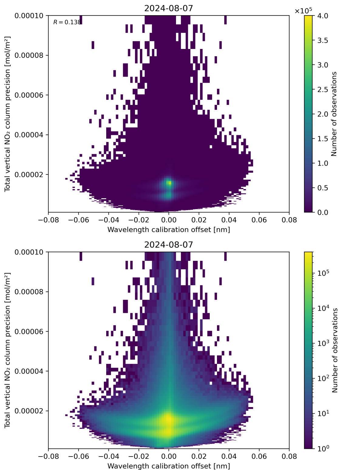
Figure 180: Scatter density plot of “Wavelength calibration offset” against “Total vertical NO 2 column precision” for 2024-08-06 to 2024-08-08.
