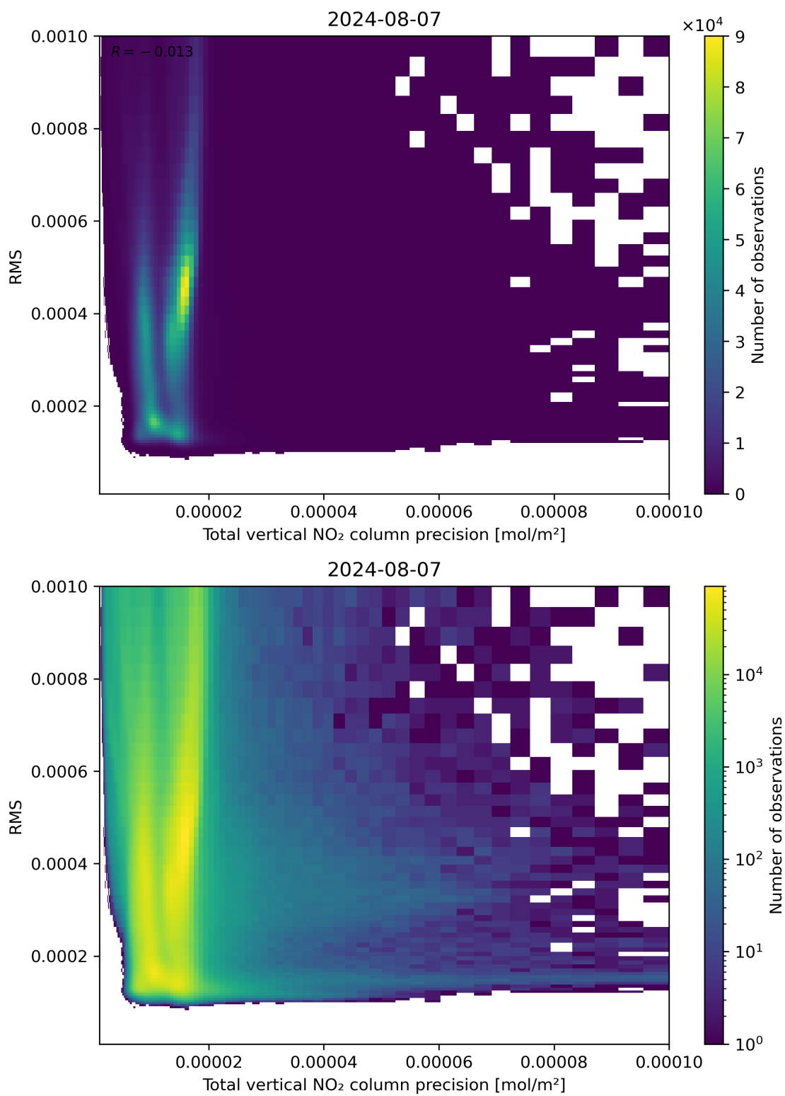
Figure 119: Scatter density plot of “Total vertical NO 2 column precision” against “RMS” for 2024-08-06 to 2024-08-08.
