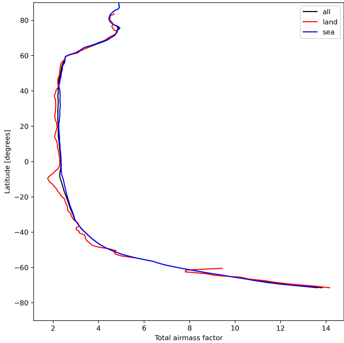
Figure 15: Zonal average of “Total airmass factor” for 2024-08-06 to 2024-08-08.
