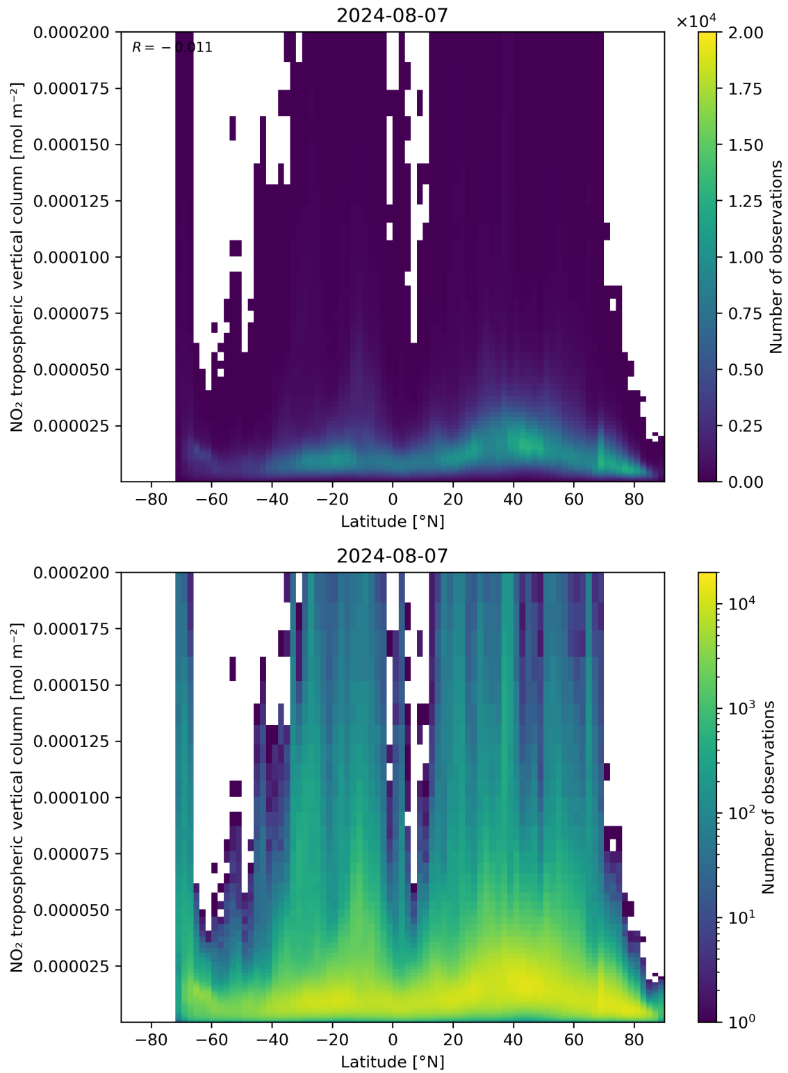
Figure 92: Scatter density plot of “Latitude” against “NO 2 tropospheric vertical column” for 2024-08-06 to 2024-08-08.
