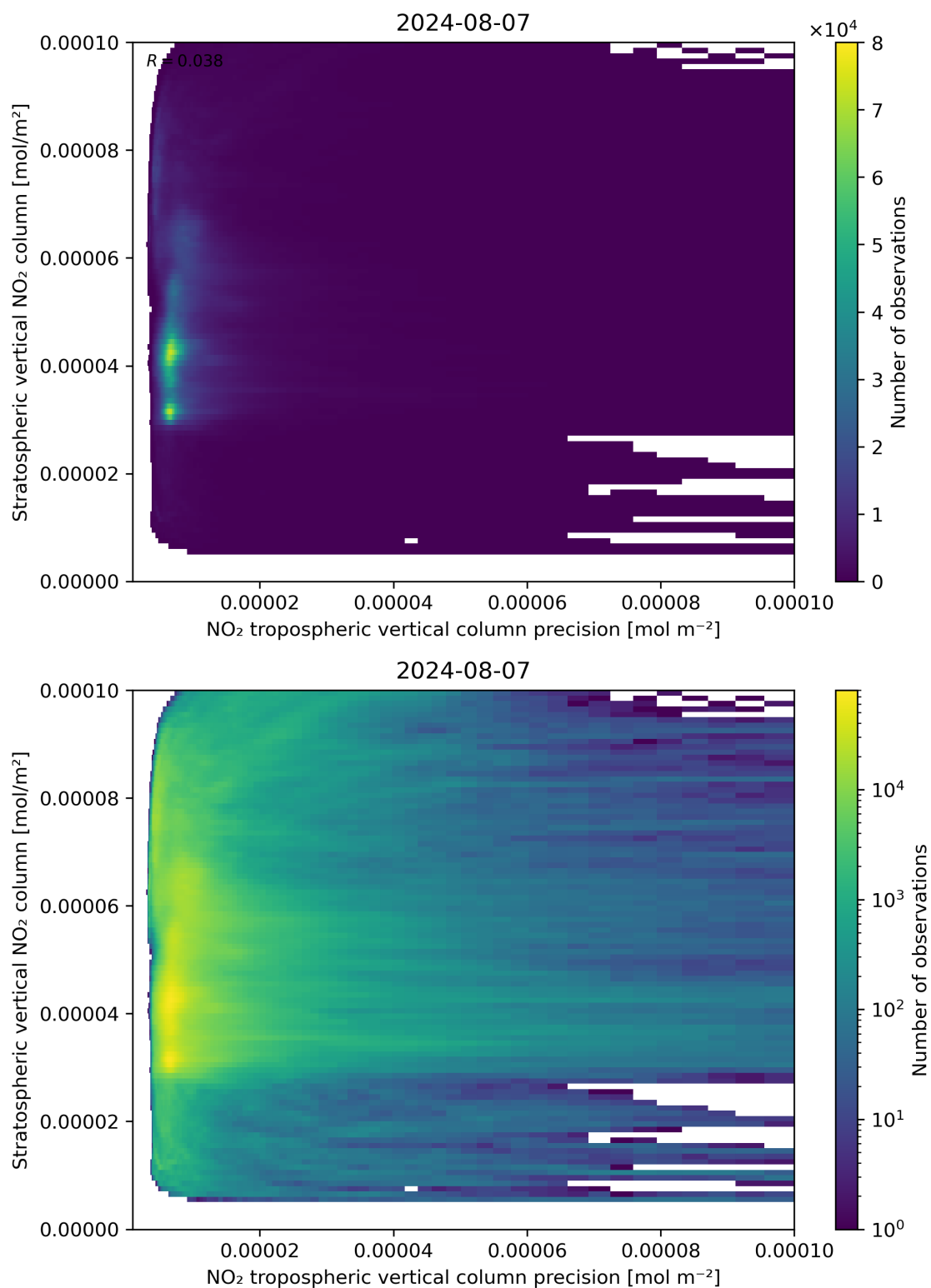
Figure 135: Scatter density plot of “NO 2 tropospheric vertical column precision” against “Stratospheric vertical NO 2 column” for 2024-08-06 to 2024-08-08.
