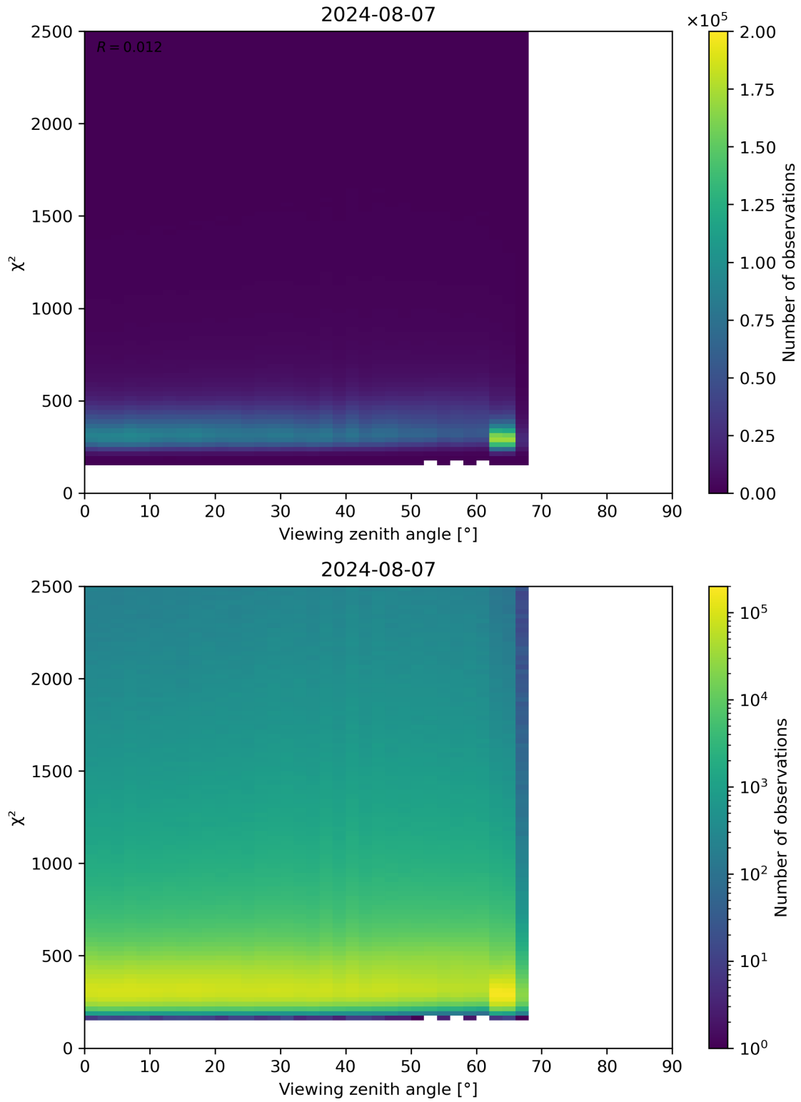
Figure 162: Scatter density plot of “Viewing zenith angle” against “ \chi^2 ” for 2024-08-06 to 2024-08-08.
