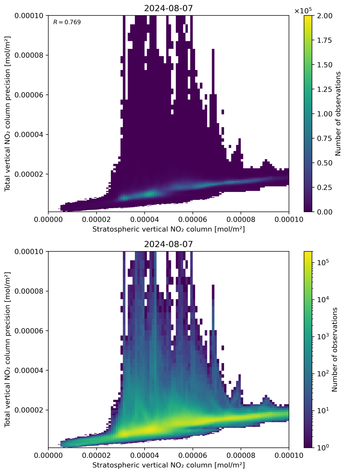
Figure 101: Scatter density plot of “Stratospheric vertical NO 2 column” against “Total vertical NO 2 column precision” for 2024-08-06 to 2024-08-08.
