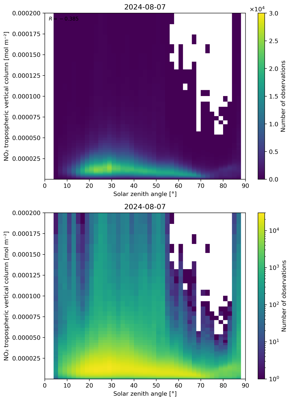
Figure 155: Scatter density plot of “Solar zenith angle” against “NO 2 tropospheric vertical column” for 2024-08-06 to 2024-08-08.
