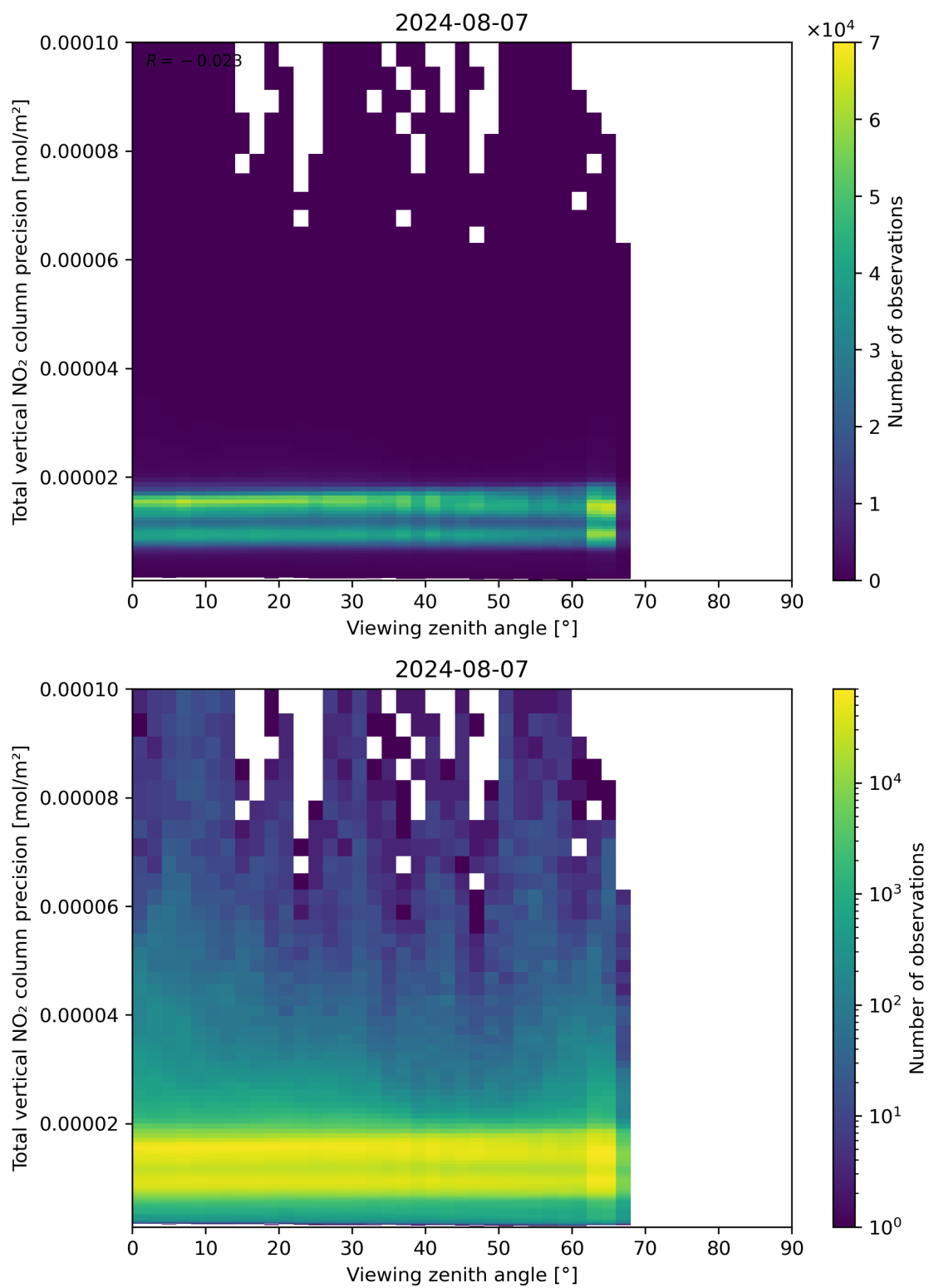
Figure 168: Scatter density plot of “Viewing zenith angle” against “Total vertical NO 2 column precision” for 2024-08-06 to 2024-08-08.
