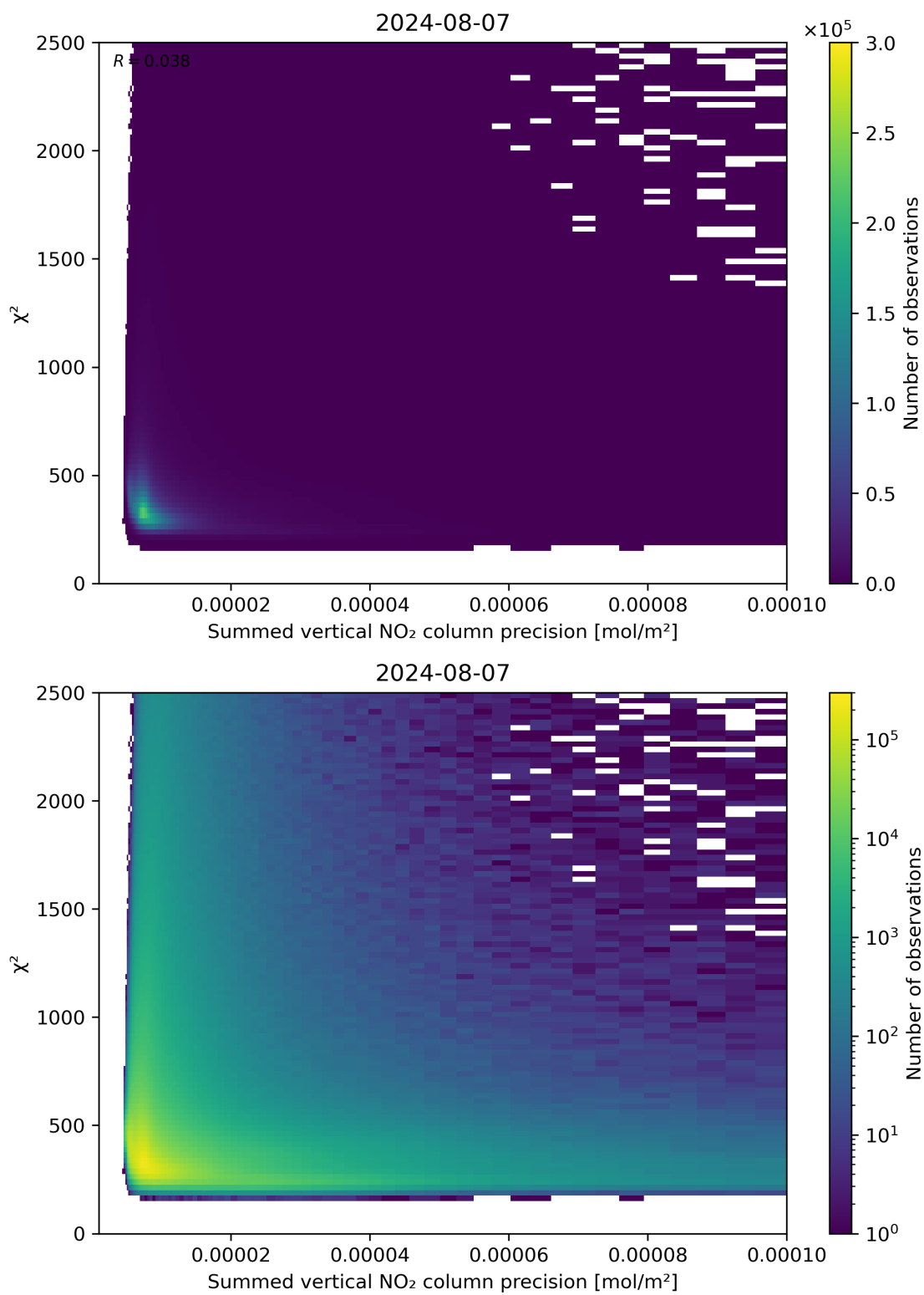
Figure 107: Scatter density plot of “Summed vertical NO 2 column precision” against “ \chi^2 ” for 2024-08-06 to 2024-08-08.
