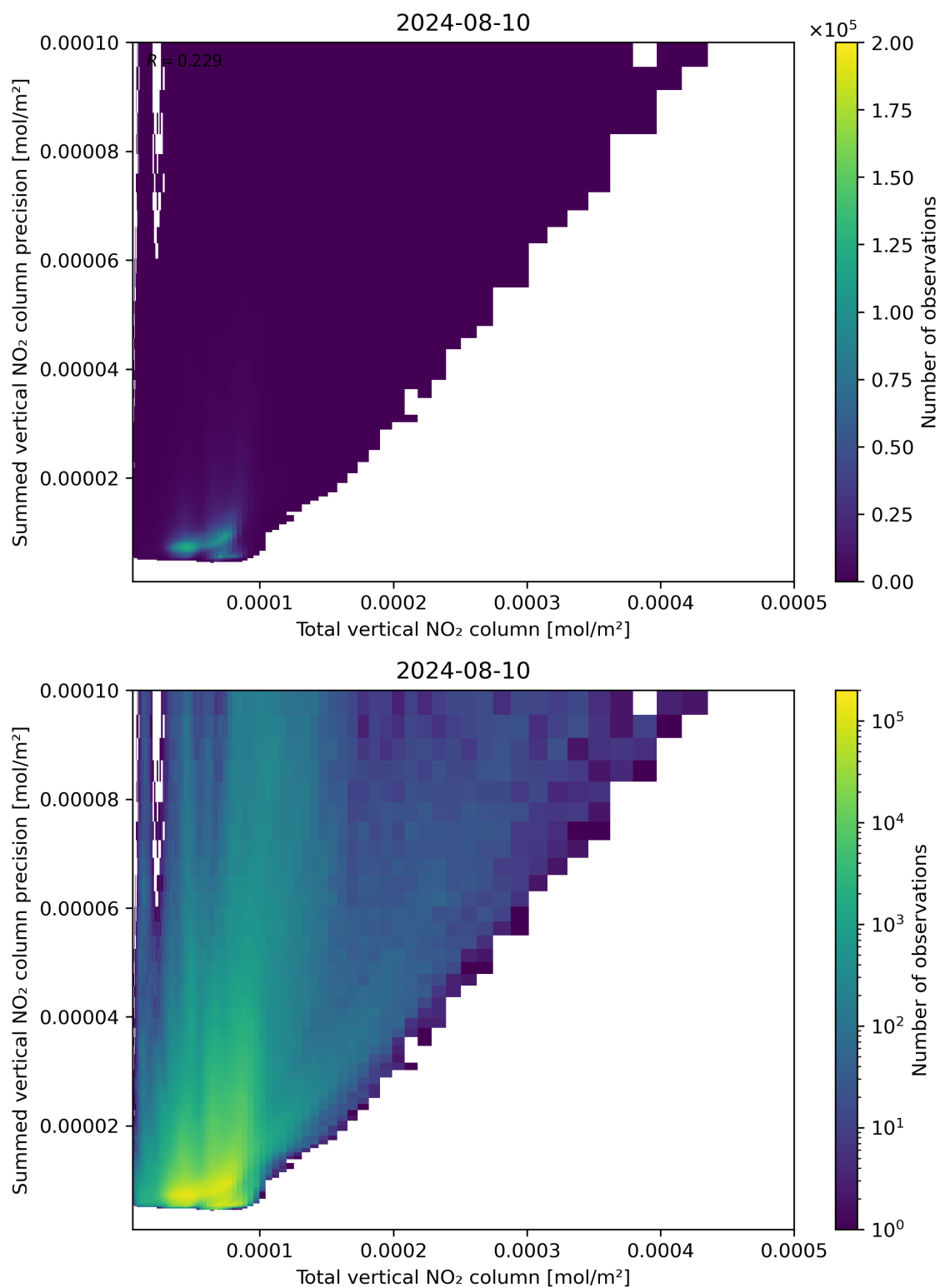
Figure 113: Scatter density plot of “Total vertical NO 2 column” against “Summed vertical NO 2 column precision” for 2024-08-09 to 2024-08-11.
