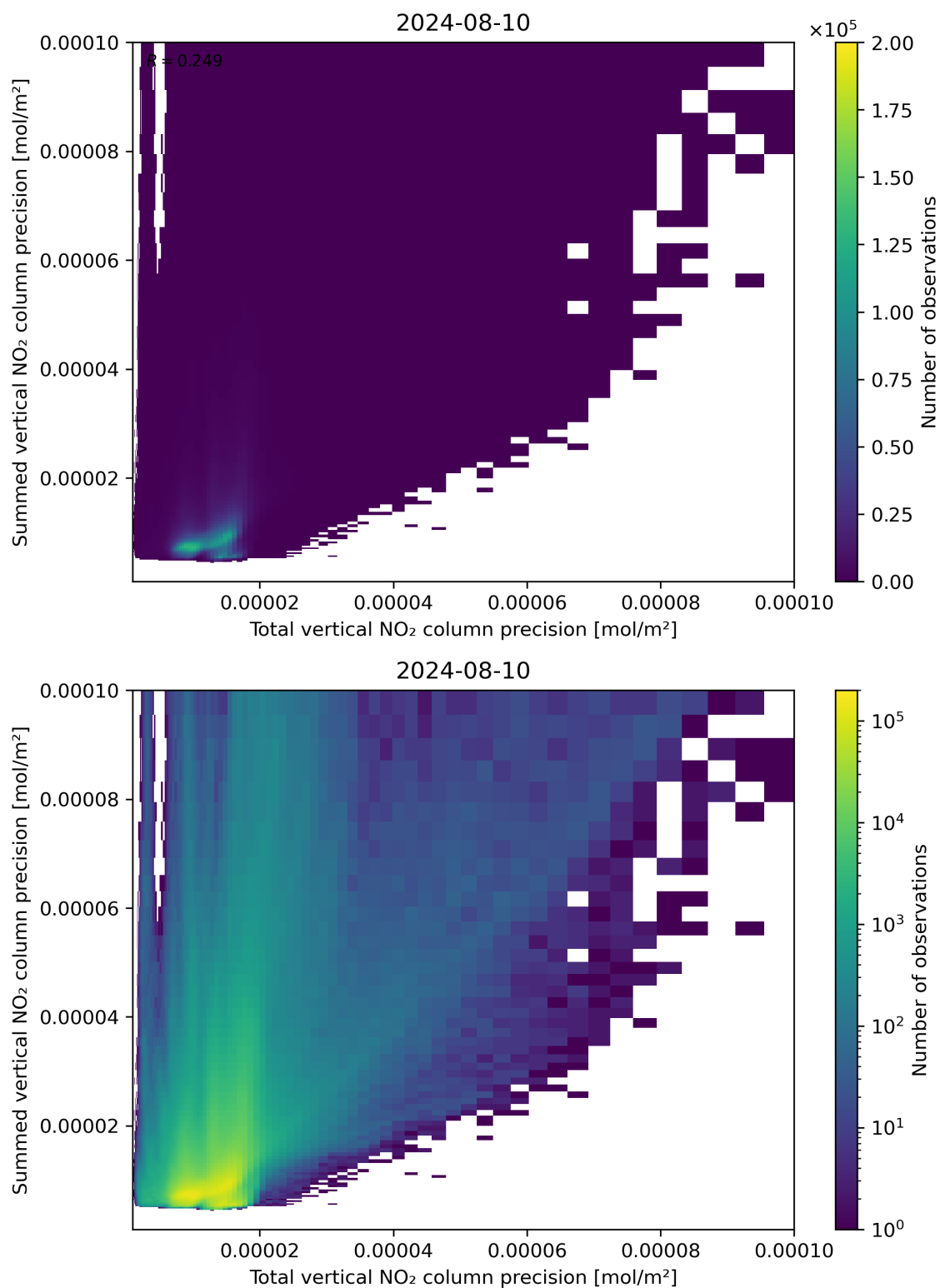
Figure 118: Scatter density plot of “Total vertical NO 2 column precision” against “Summed vertical NO 2 column precision” for 2024-08-09 to 2024-08-11.
