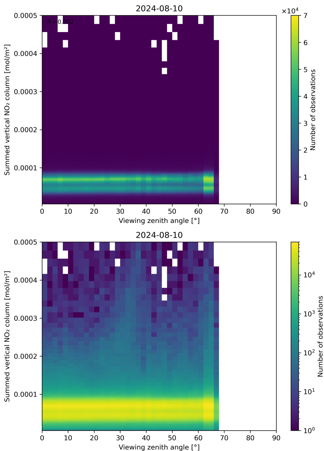
Figure 165: Scatter density plot of “Viewing zenith angle” against “Summed vertical NO 2 column” for 2024-08-09 to 2024-08-11.
