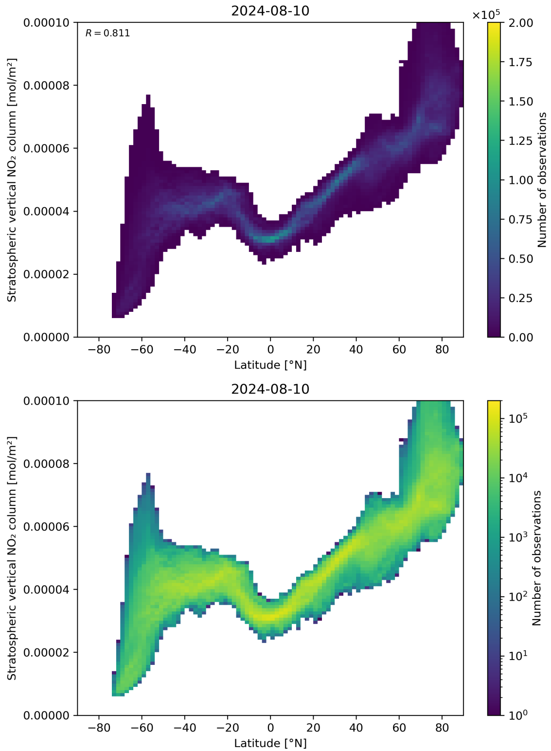
Figure 87: Scatter density plot of “Latitude” against “Stratospheric vertical NO 2 column” for 2024-08-09 to 2024-08-11.
