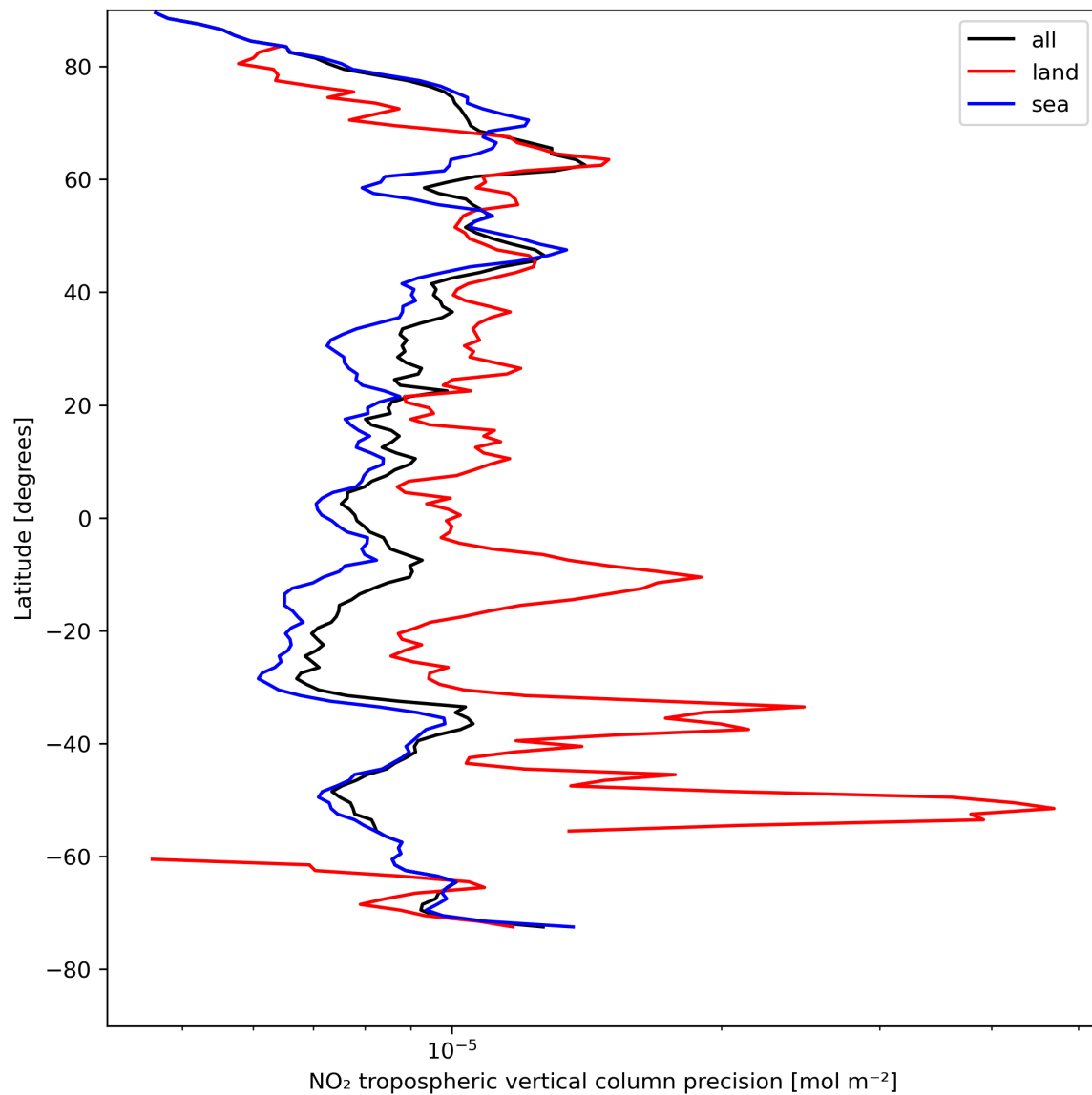
Figure 13: Zonal average of “NO 2 tropospheric vertical column precision” for 2024-08-09 to 2024-08-11.
