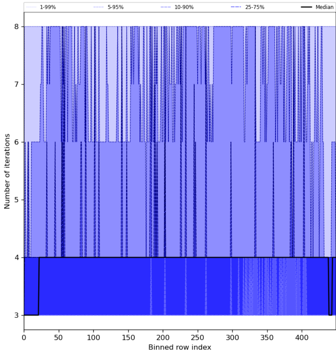
Figure 51: Along track statistics of “Number of iterations” for 2024-08-09 to 2024-08-11
