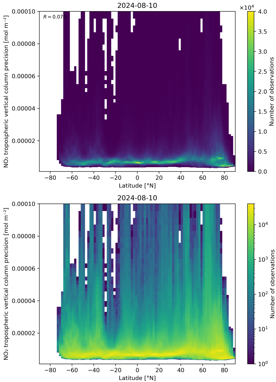
Figure 93: Scatter density plot of “Latitude” against “NO 2 tropospheric vertical column precision” for 2024-08-09 to 2024-08-11.
