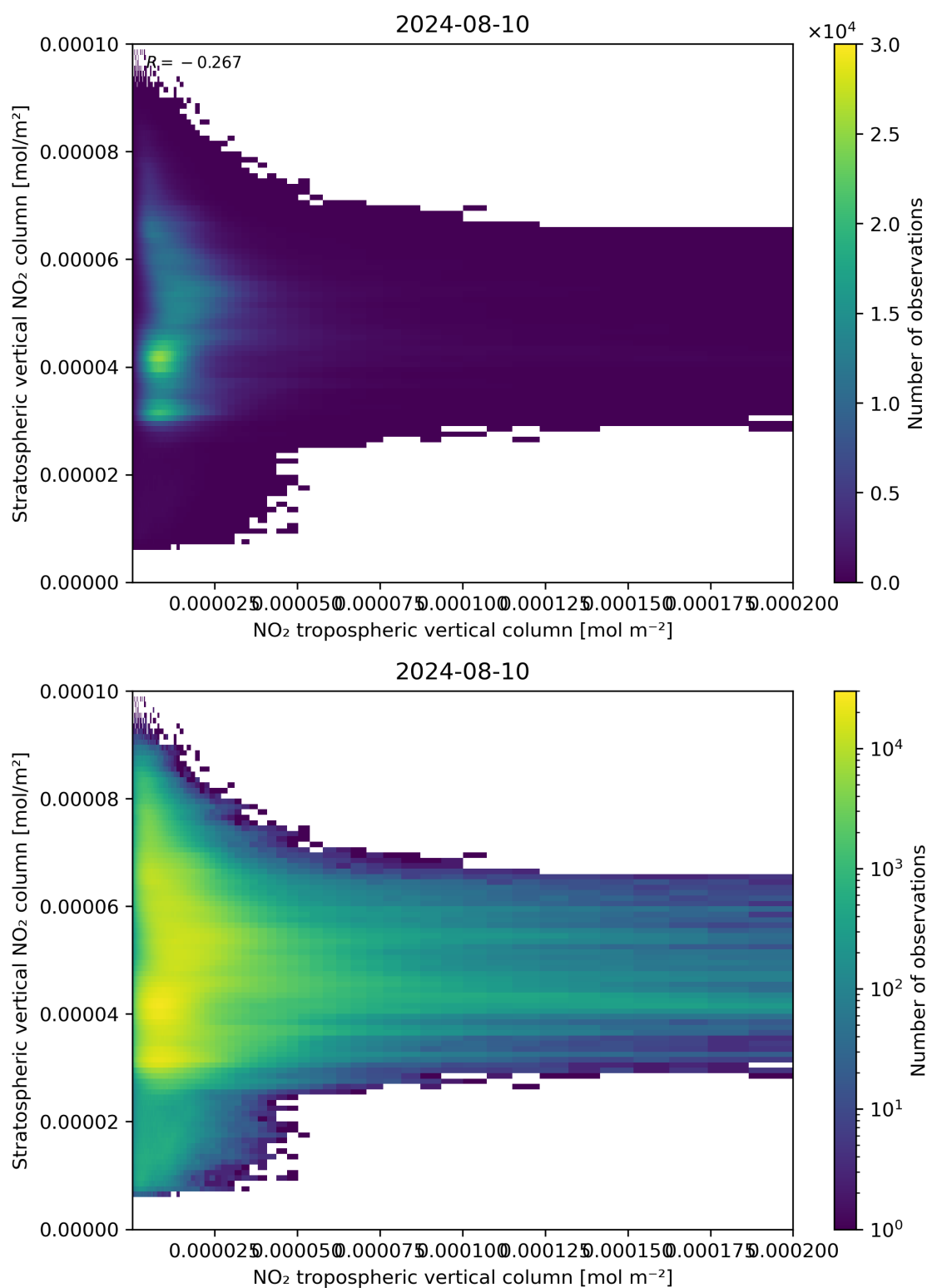
Figure 125: Scatter density plot of “NO 2 tropospheric vertical column” against “Stratospheric vertical NO 2 column” for 2024-08-09 to 2024-08-11.
