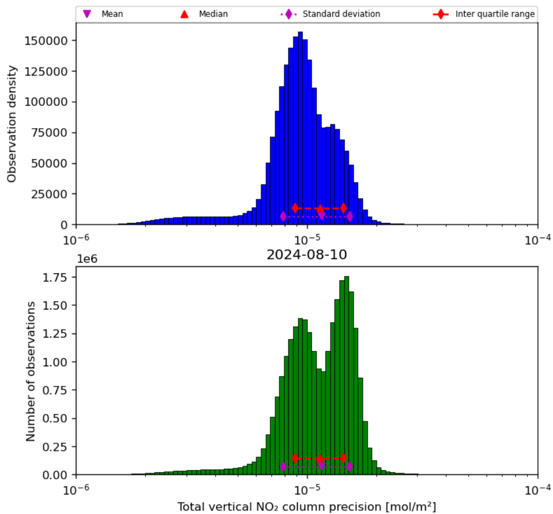
Figure 39: Histogram of "Total vertical NO 2 column precision" for 2024-08-09 to 2024-08-11
