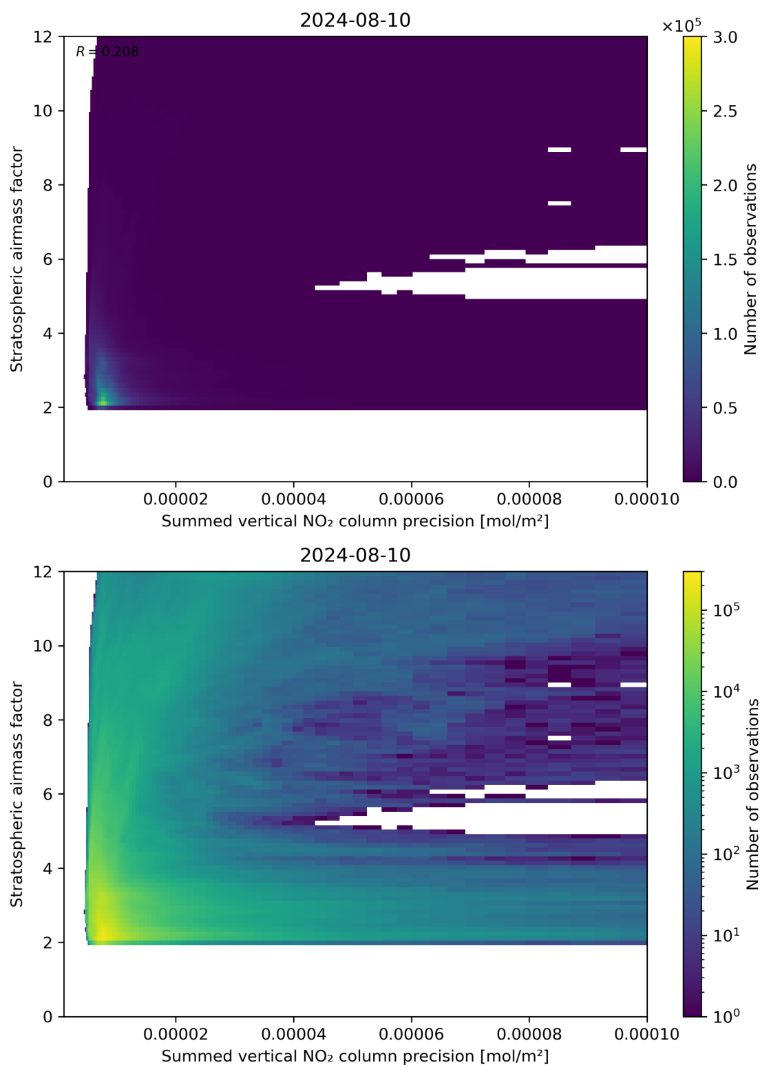
Figure 106: Scatter density plot of “Summed vertical NO 2 column precision” against “Stratospheric airmass factor” for 2024-08-09 to 2024-08-11.
