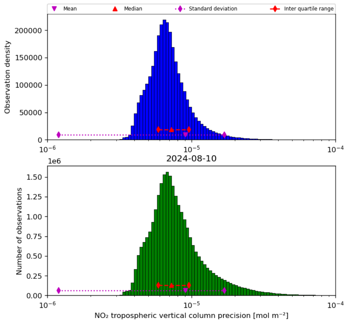
Figure 30: Histogram of “NO 2 tropospheric vertical column precision” for 2024-08-09 to 2024-08-11
