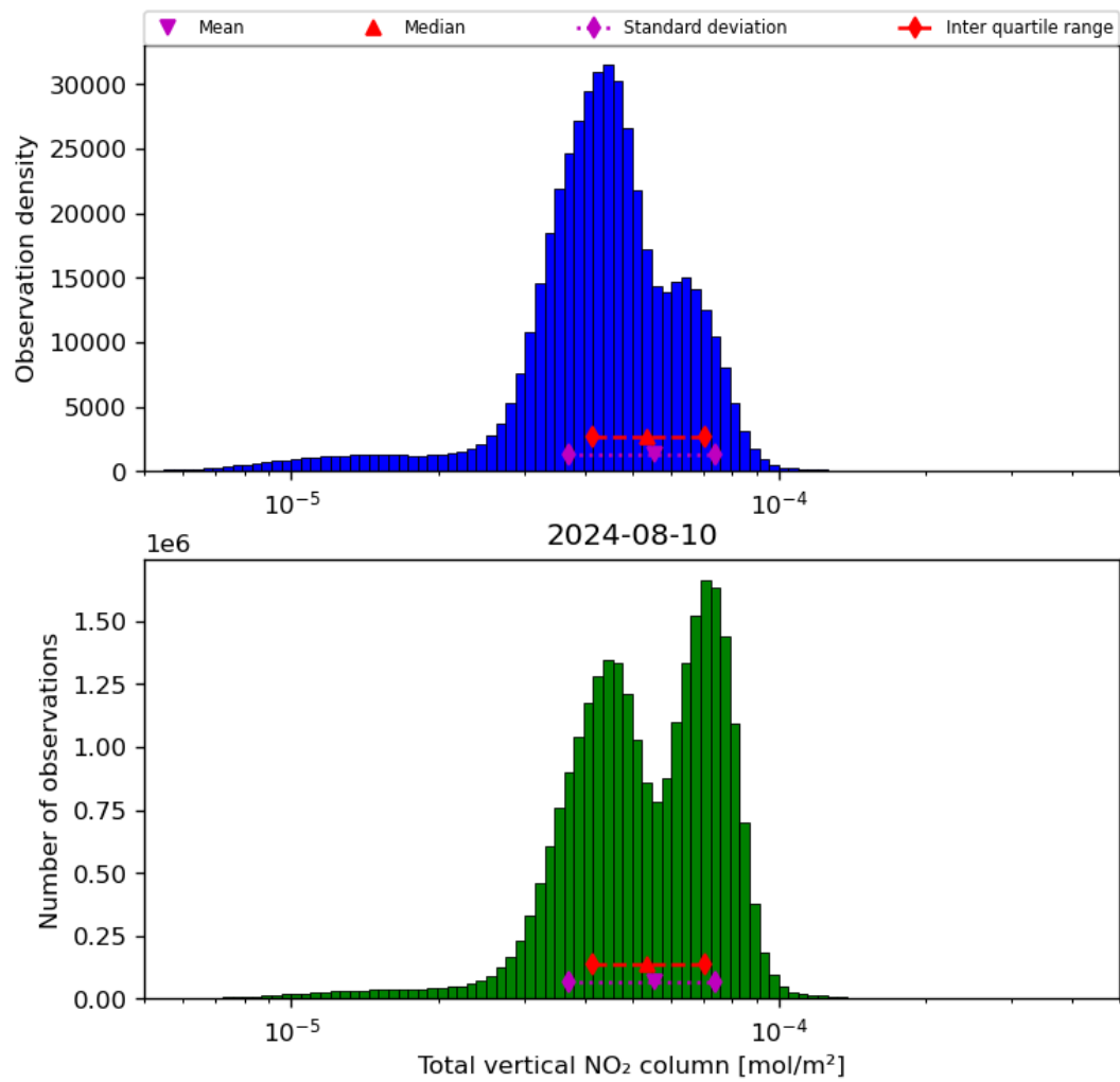
Figure 38: Histogram of “Total vertical NO 2 column” for 2024-08-09 to 2024-08-11
