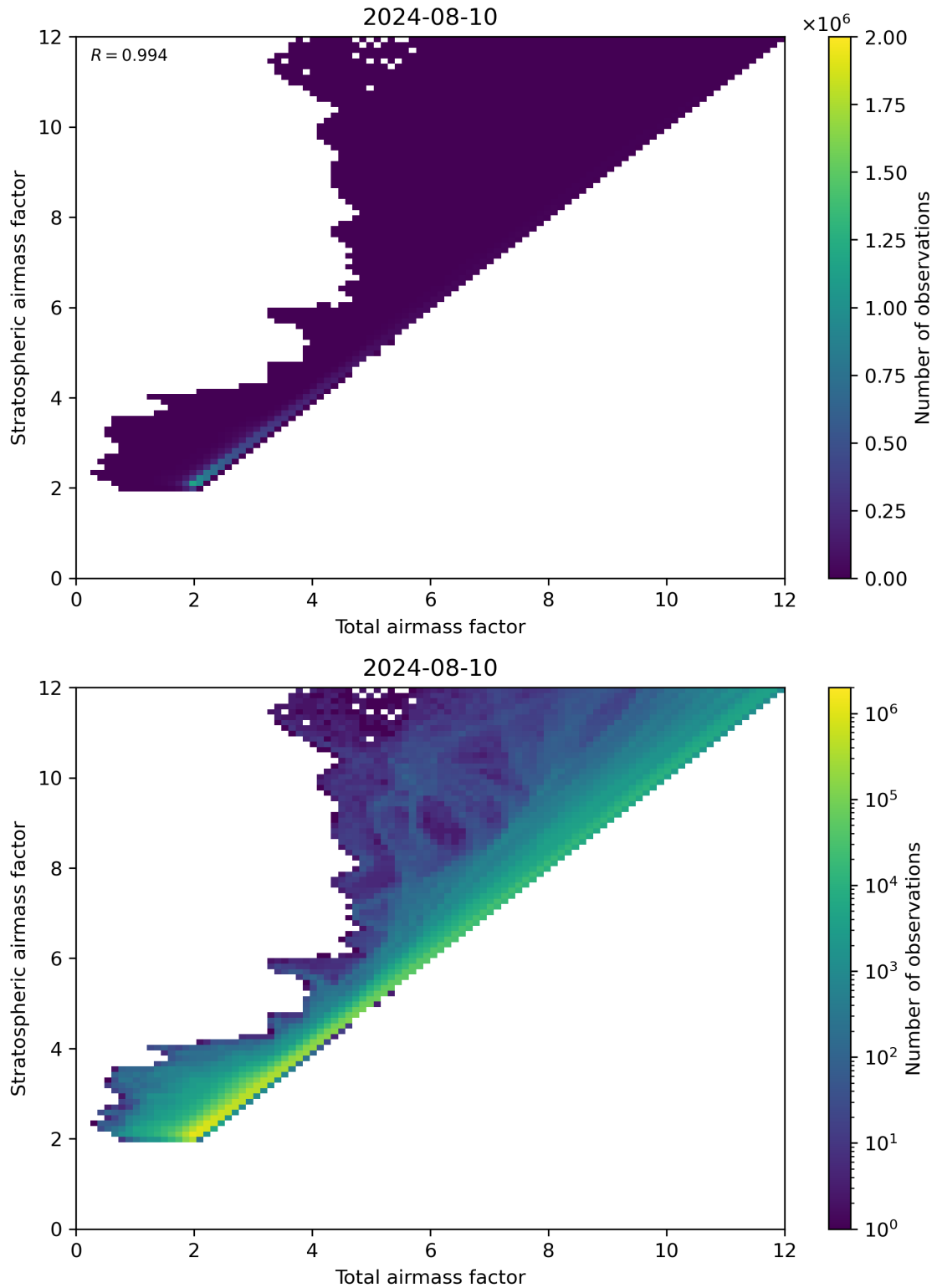
Figure 62: Scatter density plot of “Total airmass factor” against “Stratospheric airmass factor” for 2024-08-09 to 2024-08-11.
