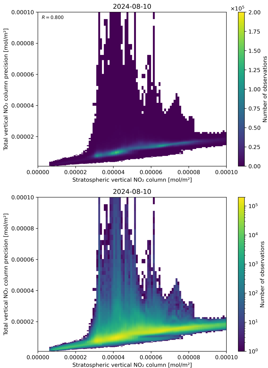
Figure 101: Scatter density plot of “Stratospheric vertical NO 2 column” against “Total vertical NO 2 column precision” for 2024-08-09 to 2024-08-11.
