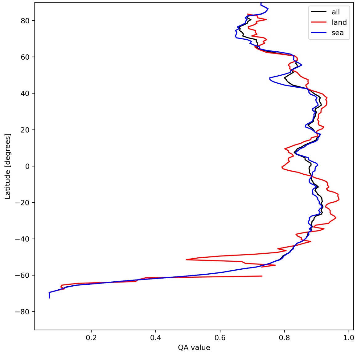
Figure 11: Zonal average of “QA value” for 2024-08-09 to 2024-08-11.
