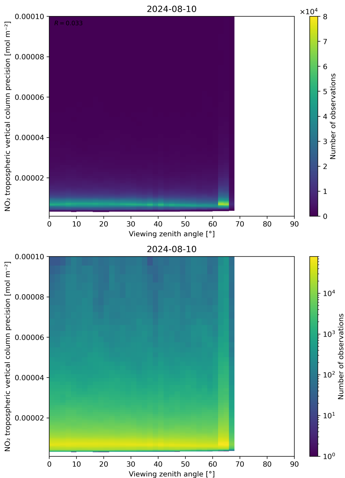
Figure 170: Scatter density plot of “Viewing zenith angle” against “NO 2 tropospheric vertical column precision” for 2024-08-09 to 2024-08-11.
