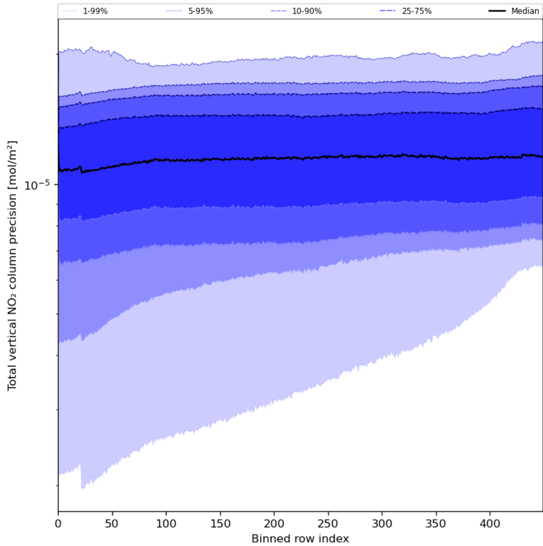
Figure 56: Along track statistics of “Total vertical NO 2 column precision” for 2024-08-09 to 2024-08-11
