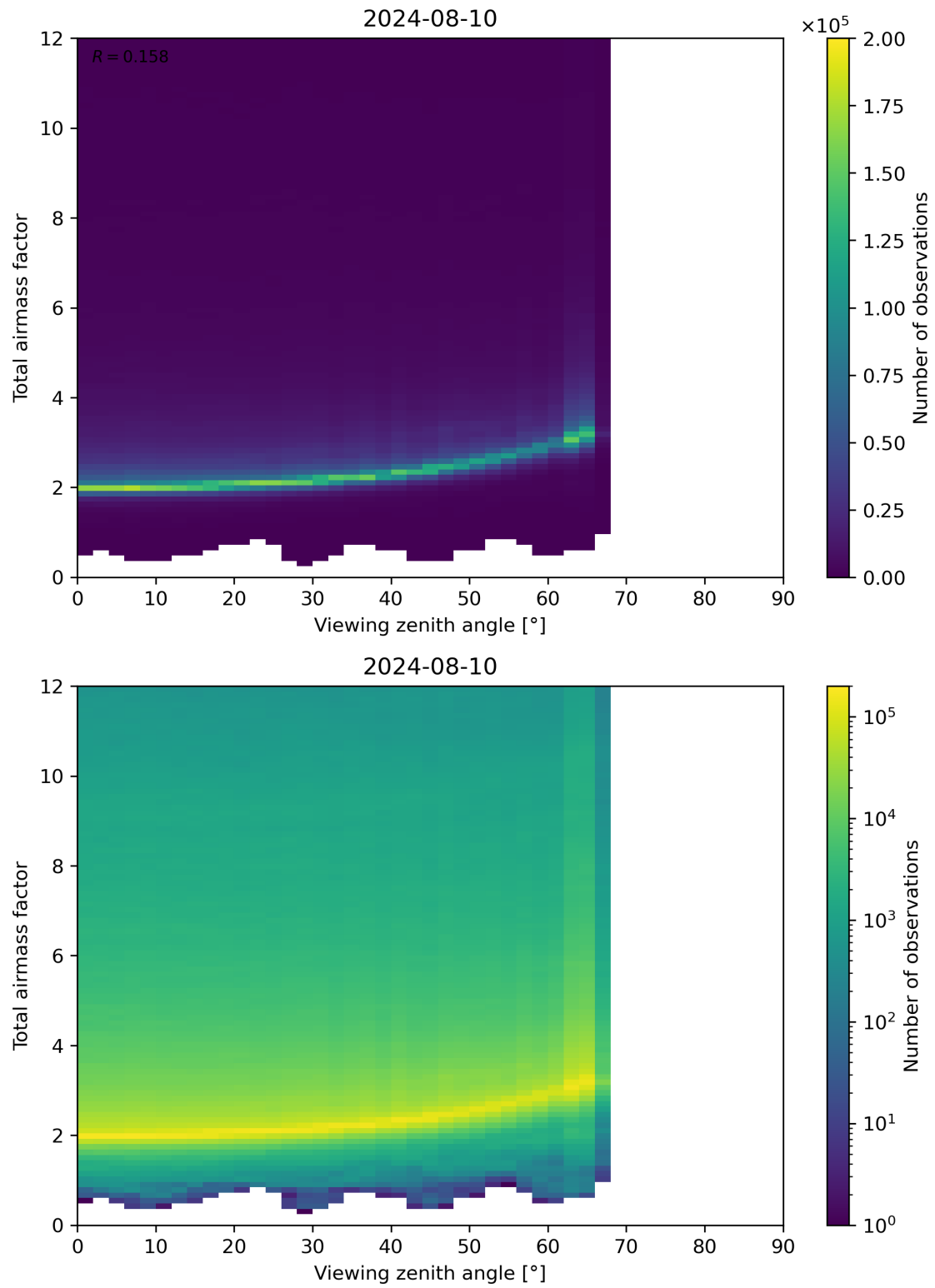
Figure 160: Scatter density plot of “Viewing zenith angle” against “Total airmass factor” for 2024-08-09 to 2024-08-11.
