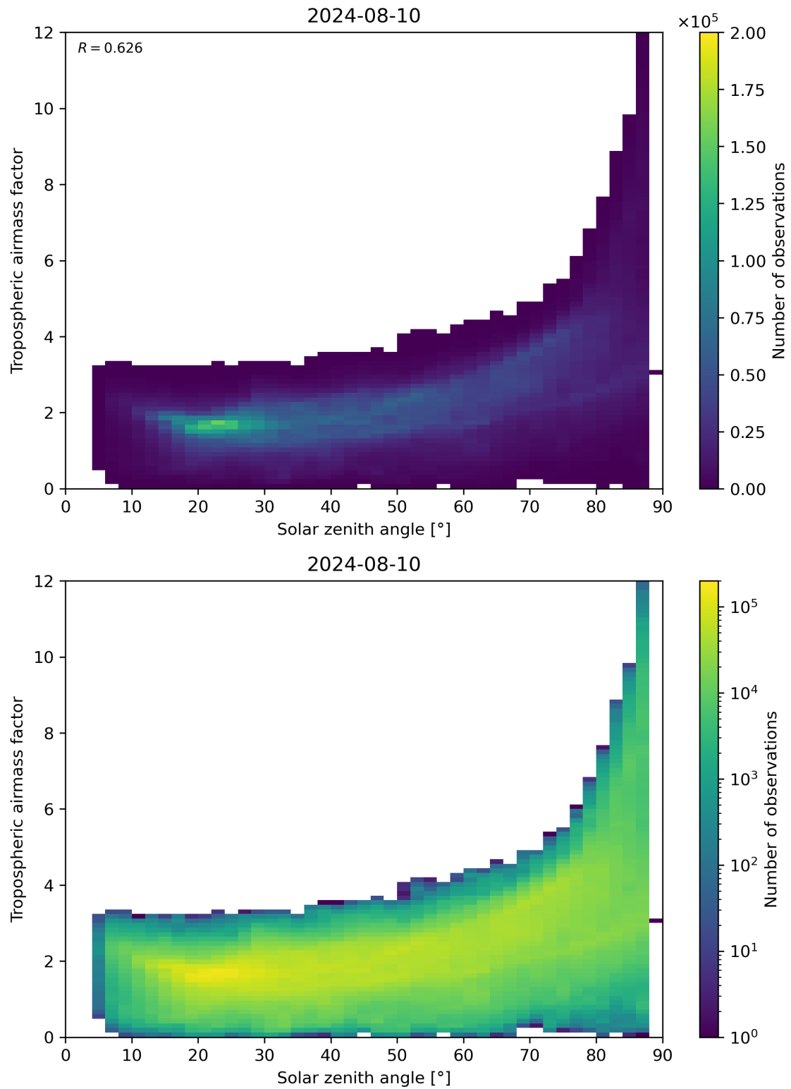
Figure 147: Scatter density plot of “Solar zenith angle” against “Tropospheric airmass factor” for 2024-08-09 to 2024-08-11.
