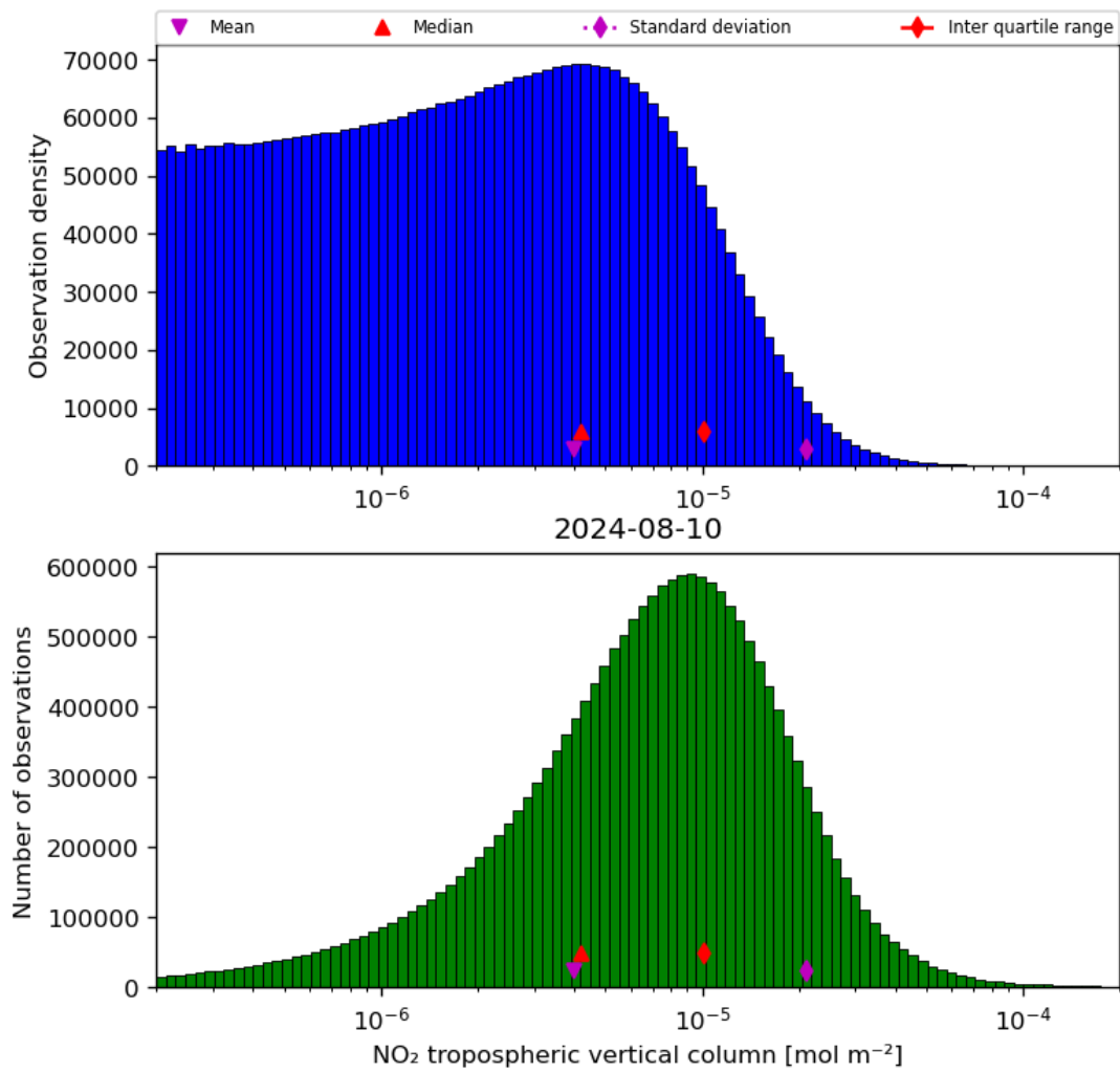
Figure 29: Histogram of “NO 2 tropospheric vertical column” for 2024-08-09 to 2024-08-11
