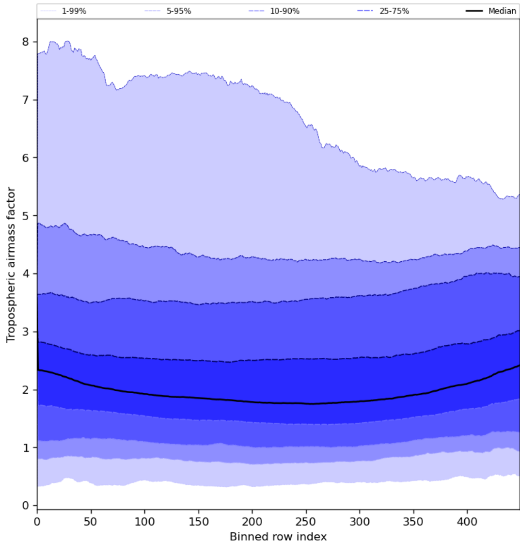
Figure 48: Along track statistics of “Tropospheric airmass factor” for 2024-08-09 to 2024-08-11
