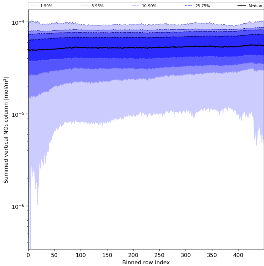
Figure 57: Along track statistics of “Summed vertical NO 2 column” for 2024-08-09 to 2024-08-11
