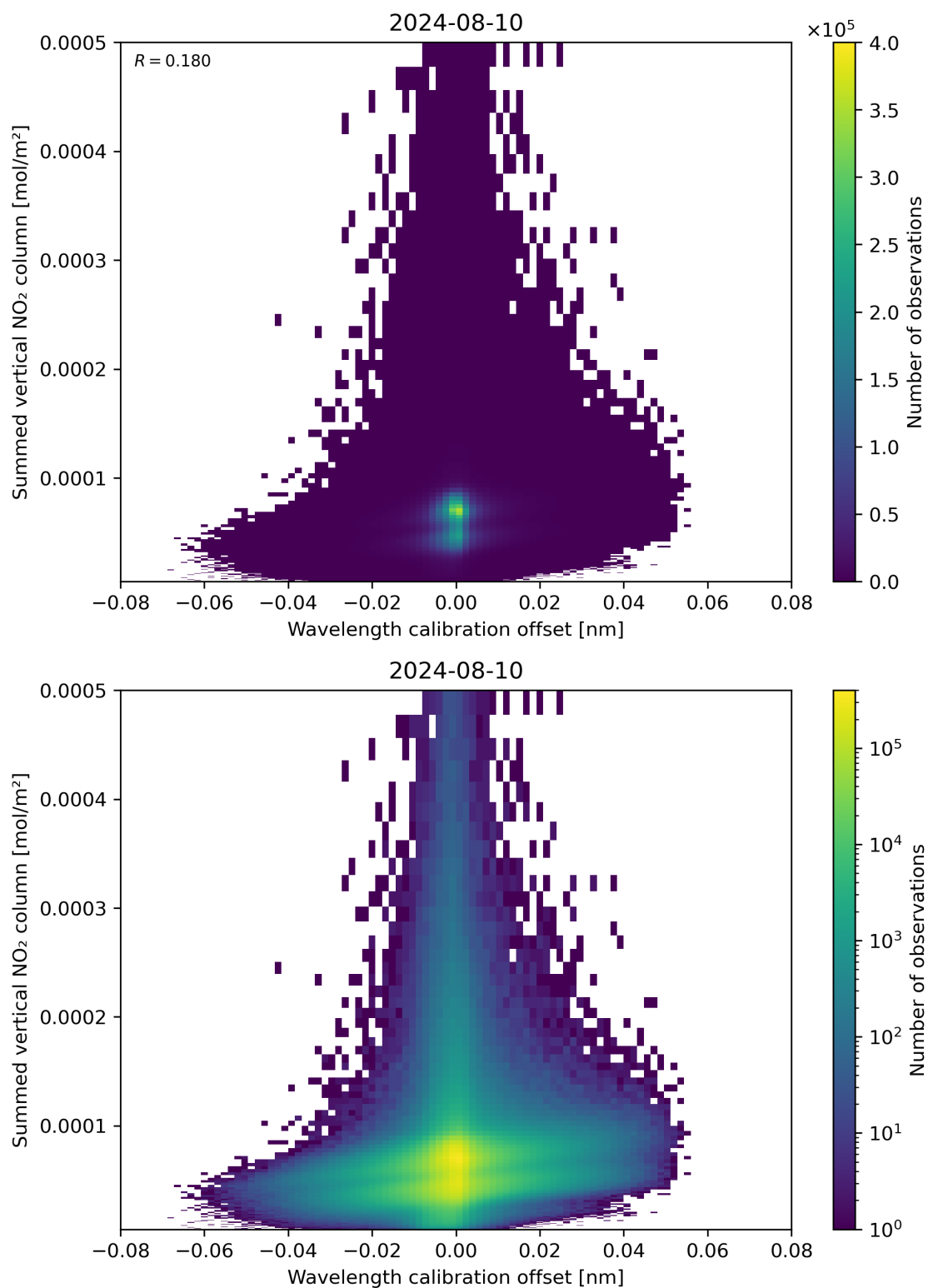
Figure 177: Scatter density plot of “Wavelength calibration offset” against “Summed vertical NO 2 column” for 2024-08-09 to 2024-08-11.
