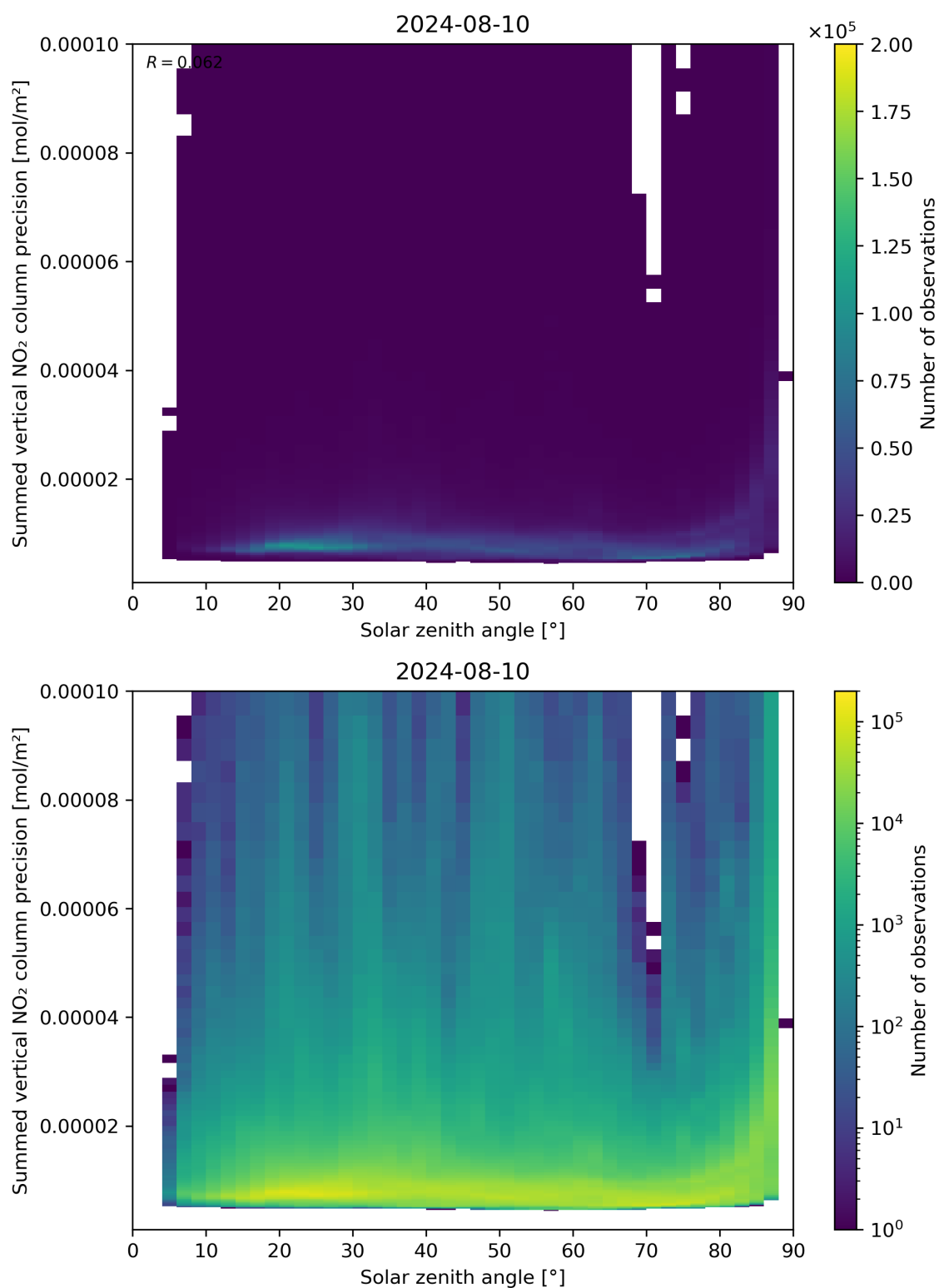
Figure 152: Scatter density plot of “Solar zenith angle” against “Summed vertical NO 2 column precision” for 2024-08-09 to 2024-08-11.
