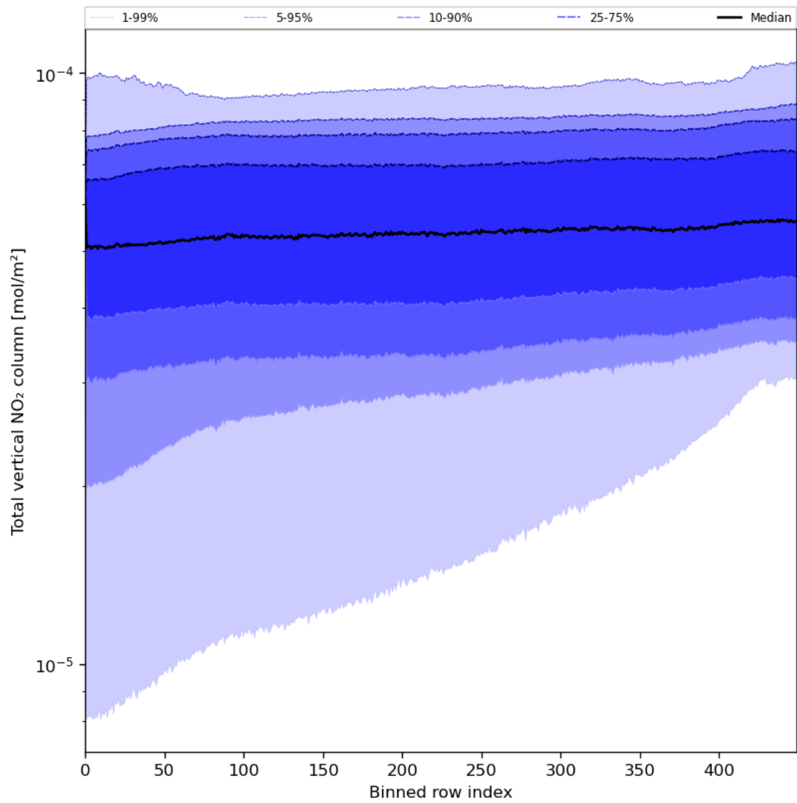
Figure 55: Along track statistics of “Total vertical NO 2 column” for 2024-08-09 to 2024-08-11
