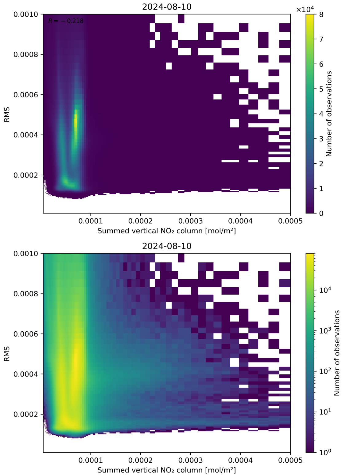
Figure 109: Scatter density plot of “Summed vertical NO 2 column” against “RMS” for 2024-08-09 to 2024-08-11.
