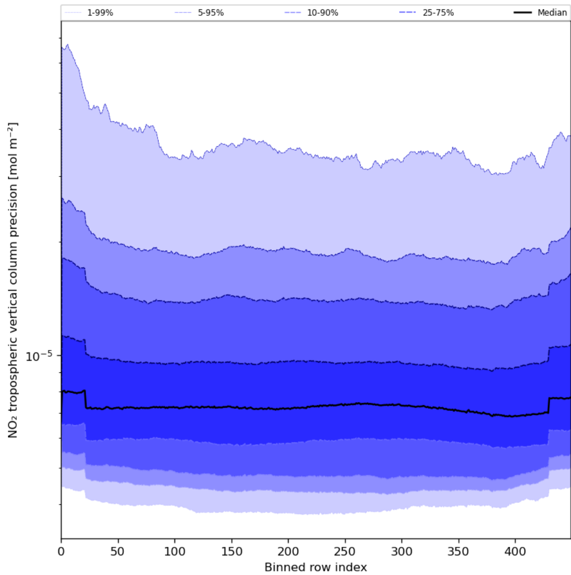
Figure 47: Along track statistics of “NO 2 tropospheric vertical column precision” for 2024-08-09 to 2024-08-11
