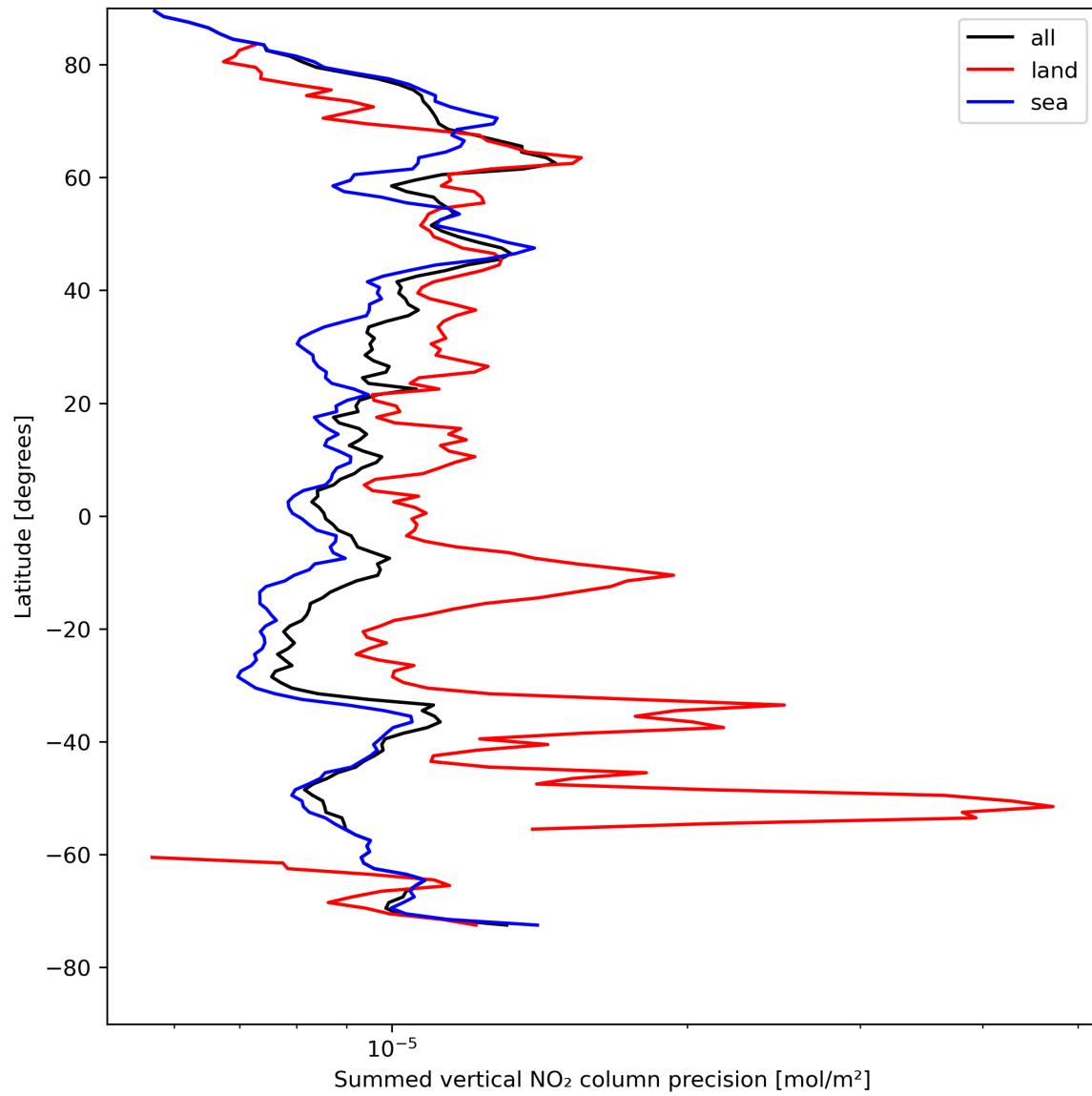
Figure 24: Zonal average of “Summed vertical NO 2 column precision” for 2024-08-09 to 2024-08-11.
