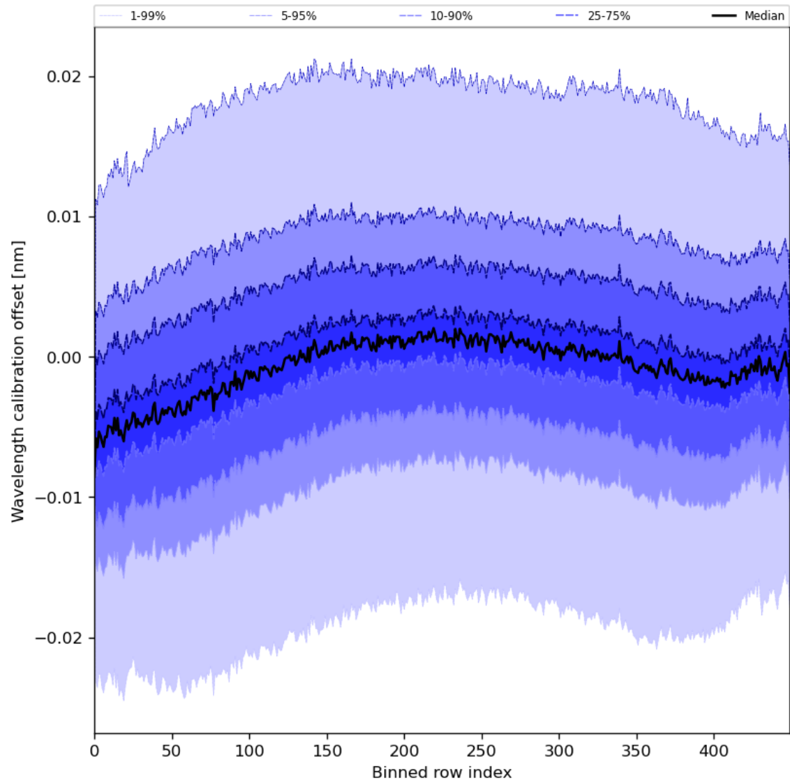
Figure 52: Along track statistics of “Wavelength calibration offset” for 2024-08-09 to 2024-08-11
