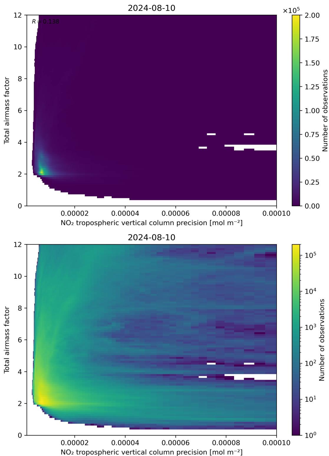
Figure 132: Scatter density plot of “NO 2 tropospheric vertical column precision” against “Total air mass factor” for 2024-08-09 to 2024-08-11.
