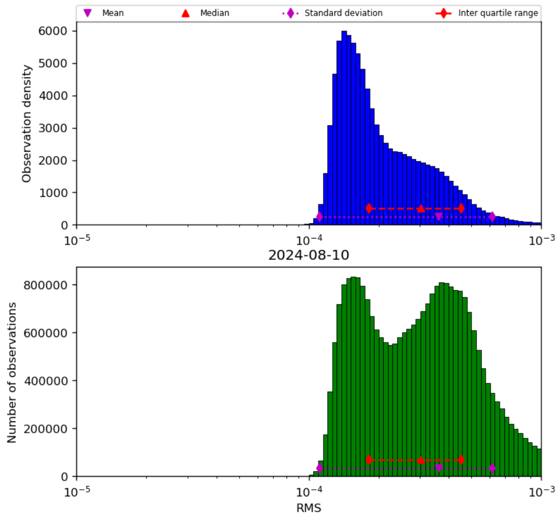
Figure 43: Histogram of “RMS” for 2024-08-09 to 2024-08-11
