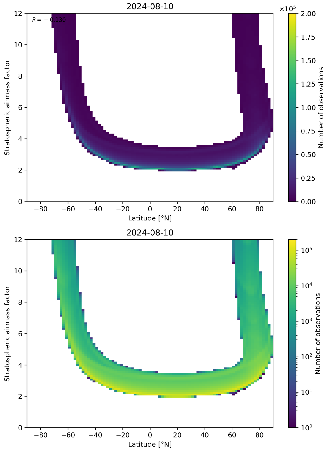
Figure 83: Scatter density plot of “Latitude” against “Stratospheric air mass factor” for 2024-08-09 to 2024-08-11.
