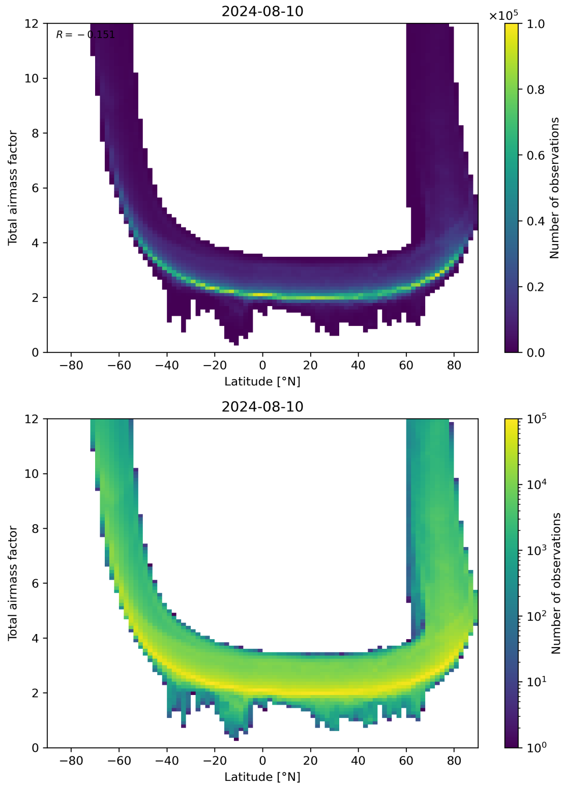
Figure 84: Scatter density plot of “Latitude” against “Total airmass factor” for 2024-08-09 to 2024-08-11.
