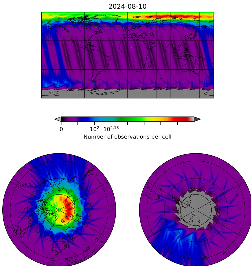
Figure 10: Map of the number of observations for 2024-08-09 to 2024-08-11
