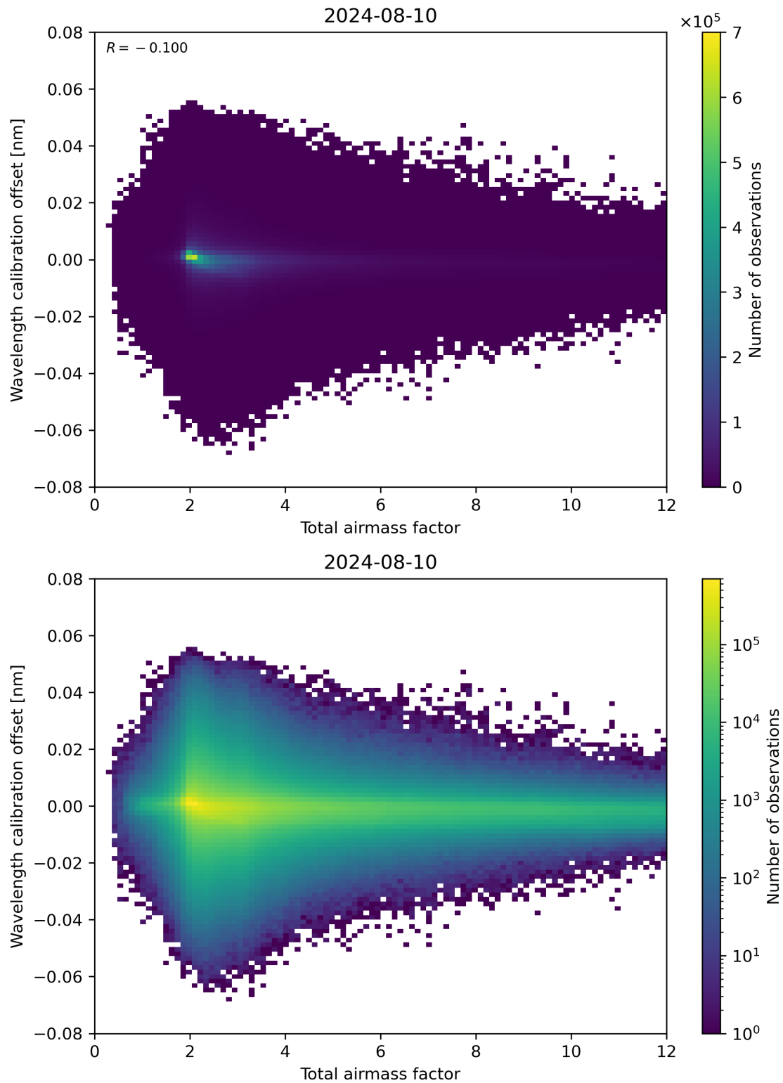
Figure 70: Scatter density plot of “Total airmass factor” against “Wavelength calibration offset” for 2024-08-09 to 2024-08-11.
