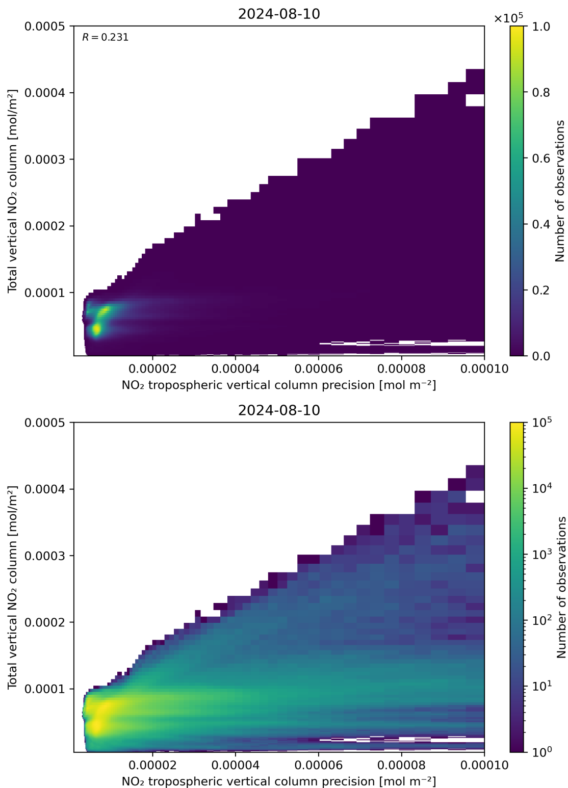
Figure 138: Scatter density plot of “NO 2 tropospheric vertical column precision” against “Total vertical NO 2 column” for 2024-08-09 to 2024-08-11.
