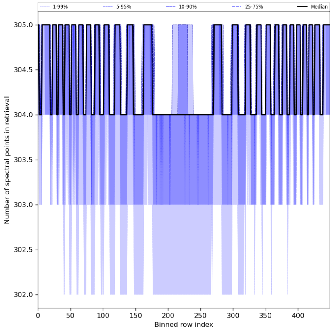
Figure 50: Along track statistics of “Number of spectral points in retrieval” for 2024-08-09 to 2024-08-11
