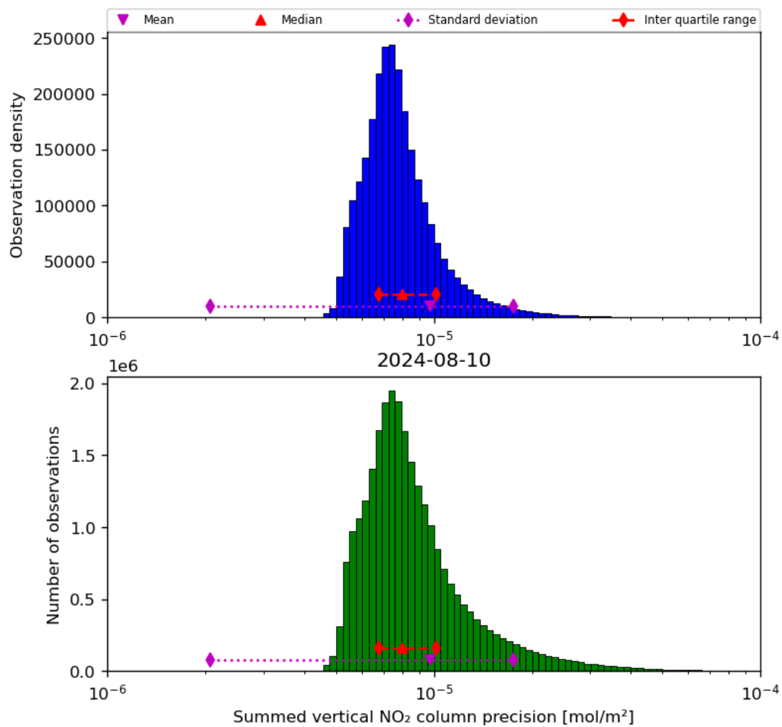
Figure 41: Histogram of "Summed vertical NO 2 column precision" for 2024-08-09 to 2024-08-11
