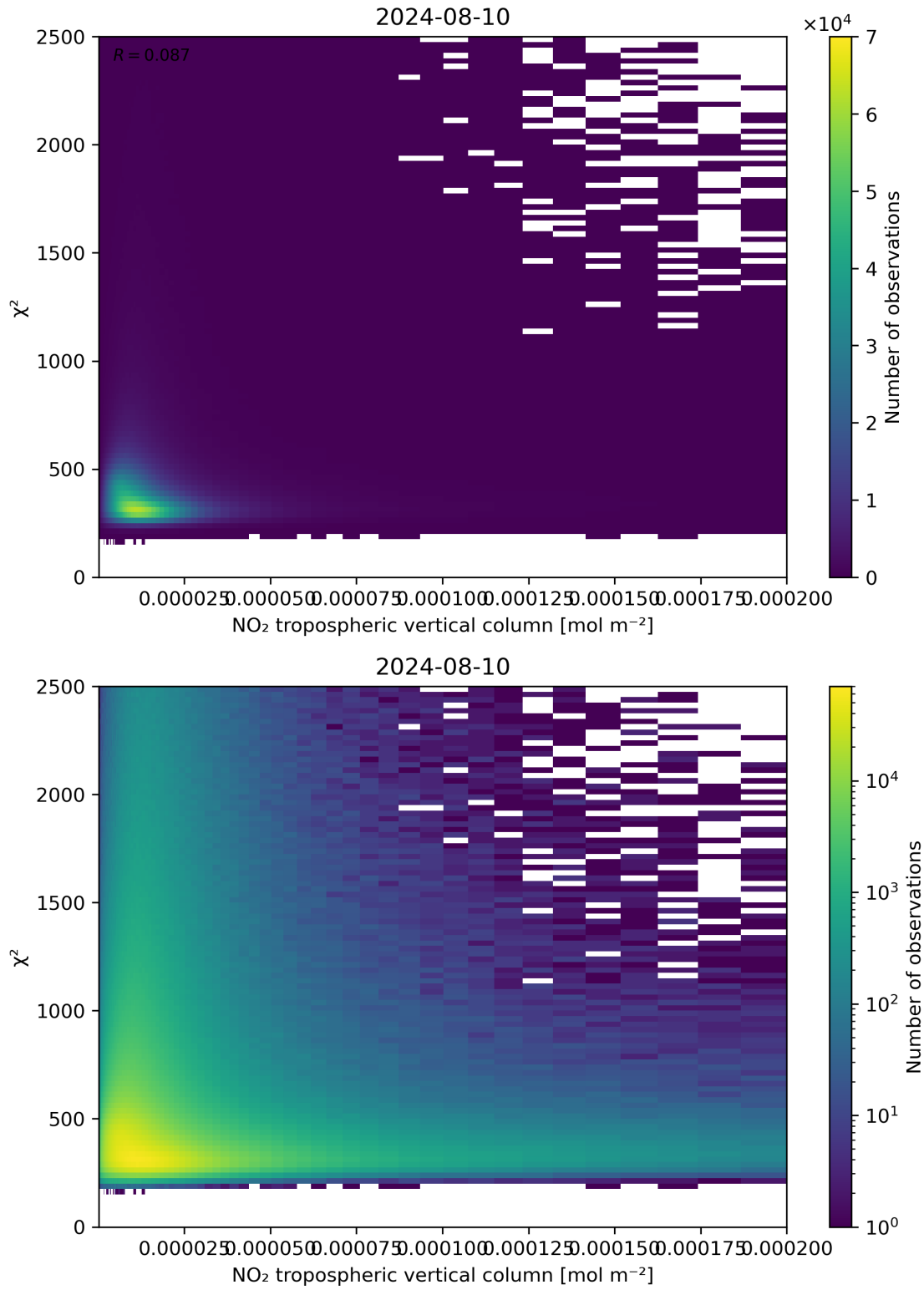
Figure 124: Scatter density plot of “NO 2 tropospheric vertical column” against “ \chi^2 ” for 2024-08-09 to 2024-08-11.
