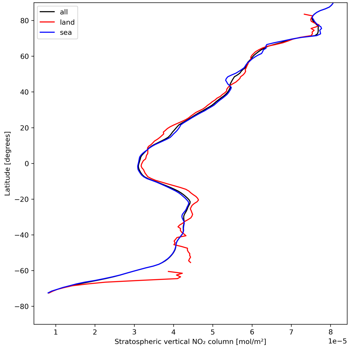
Figure 19: Zonal average of “Stratospheric vertical NO 2 column” for 2024-08-09 to 2024-08-11.
