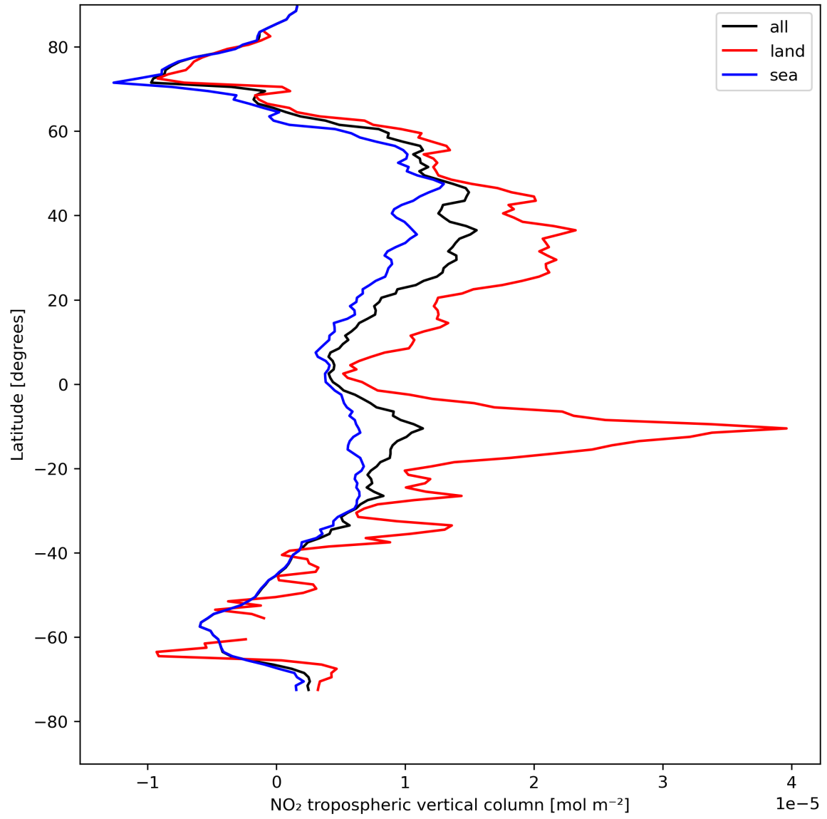
Figure 12: Zonal average of “NO 2 tropospheric vertical column” for 2024-08-09 to 2024-08-11.
