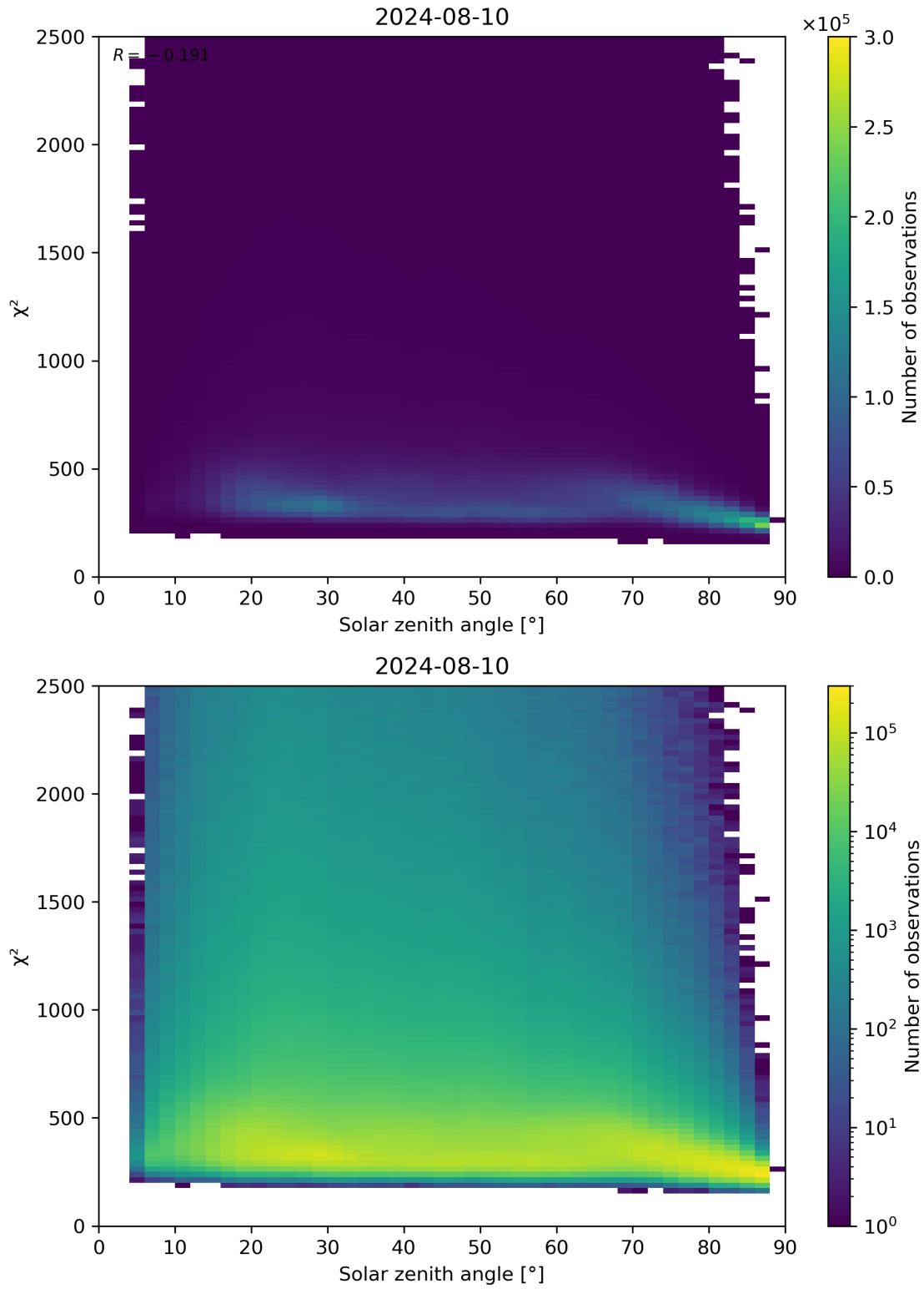
Figure 148: Scatter density plot of “Solar zenith angle” against “ \chi^2 ” for 2024-08-09 to 2024-08-11.
