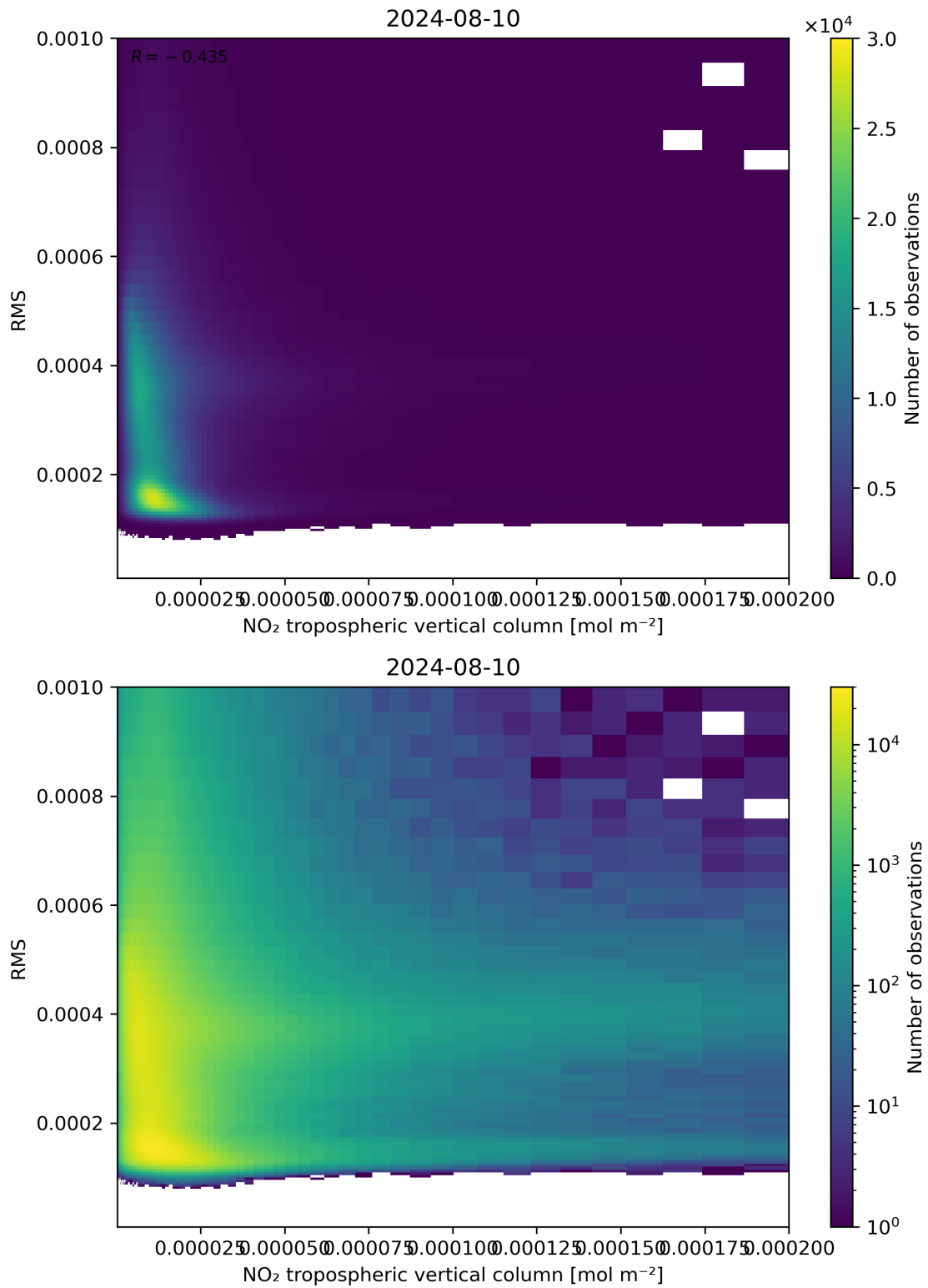
Figure 142: Scatter density plot of “NO 2 tropospheric vertical column” against “RMS” for 2024-08-09 to 2024-08-11.
