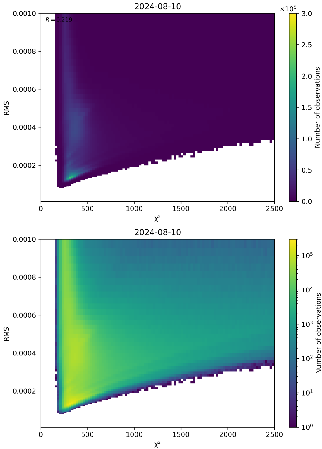
Figure 82: Scatter density plot of “ \chi^2 ” against “RMS” for 2024-08-09 to 2024-08-11.
