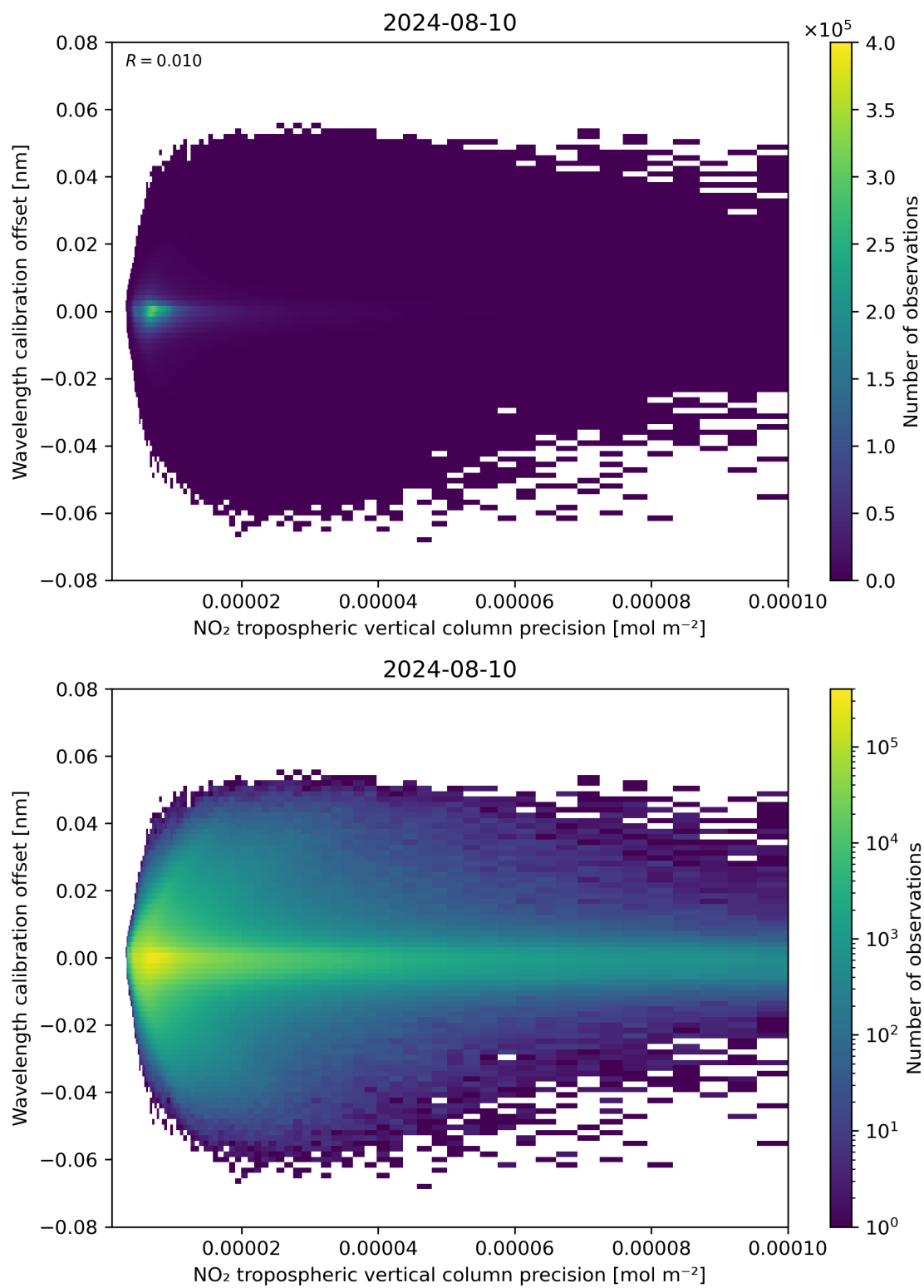
Figure 141: Scatter density plot of “NO 2 tropospheric vertical column precision” against “Wavelength calibration offset” for 2024-08-09 to 2024-08-11.
