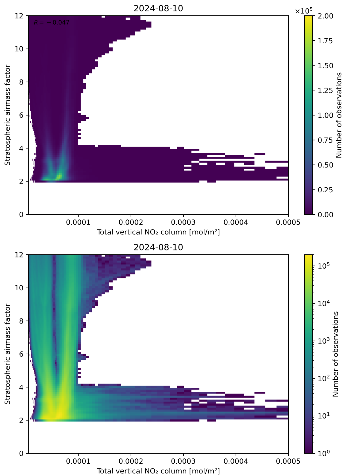
Figure 110: Scatter density plot of “Total vertical NO 2 column” against “Stratospheric airmass factor” for 2024-08-09 to 2024-08-11.
