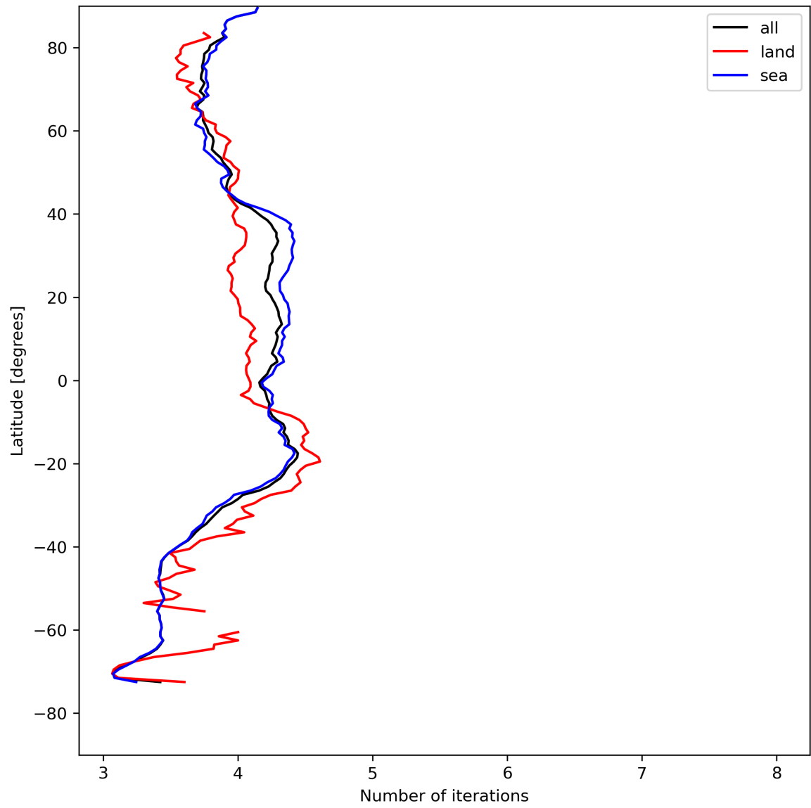
Figure 17: Zonal average of “Number of iterations” for 2024-08-09 to 2024-08-11.
