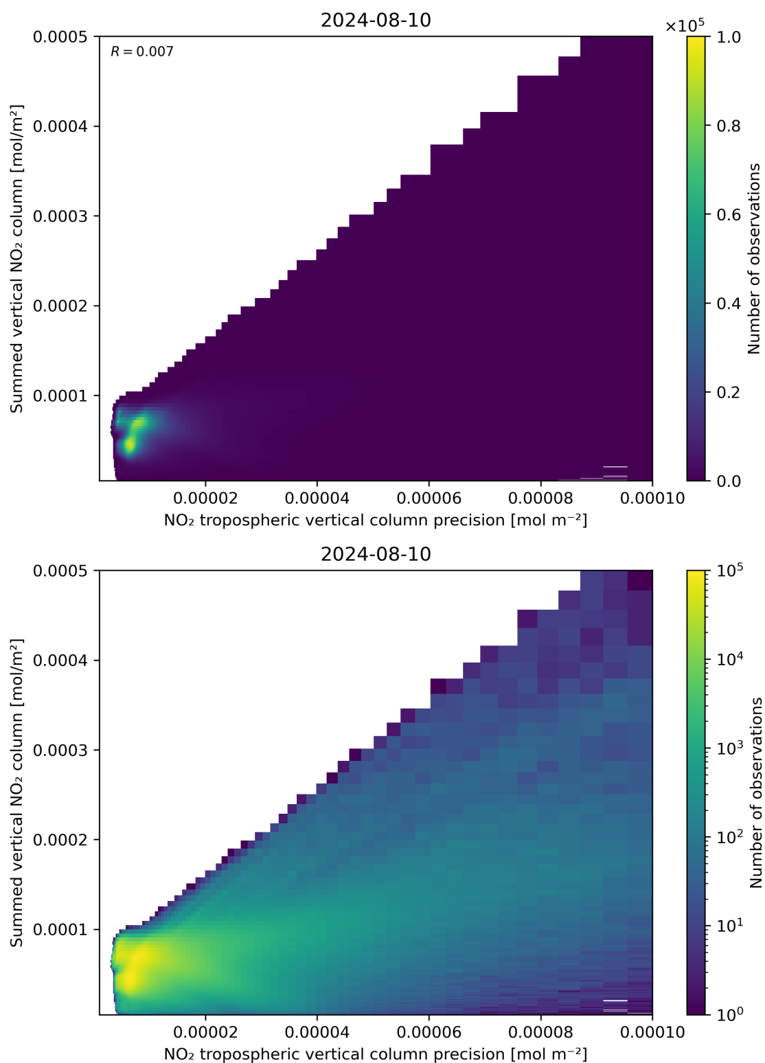
Figure 136: Scatter density plot of “NO 2 tropospheric vertical column precision” against “Summed vertical NO 2 column” for 2024-08-09 to 2024-08-11.
