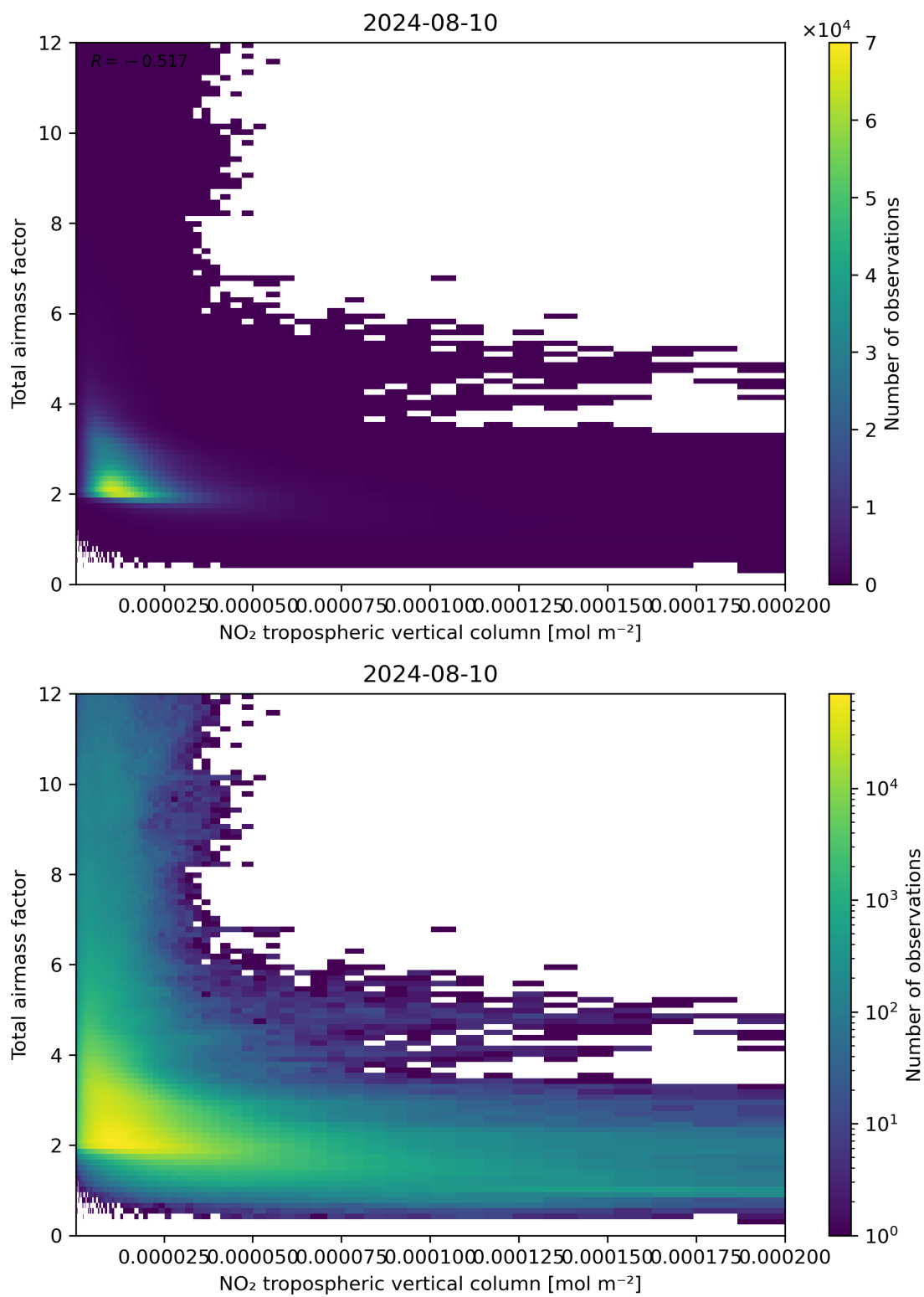
Figure 122: Scatter density plot of “NO 2 tropospheric vertical column” against “Total air mass factor” for 2024-08-09 to 2024-08-11.
