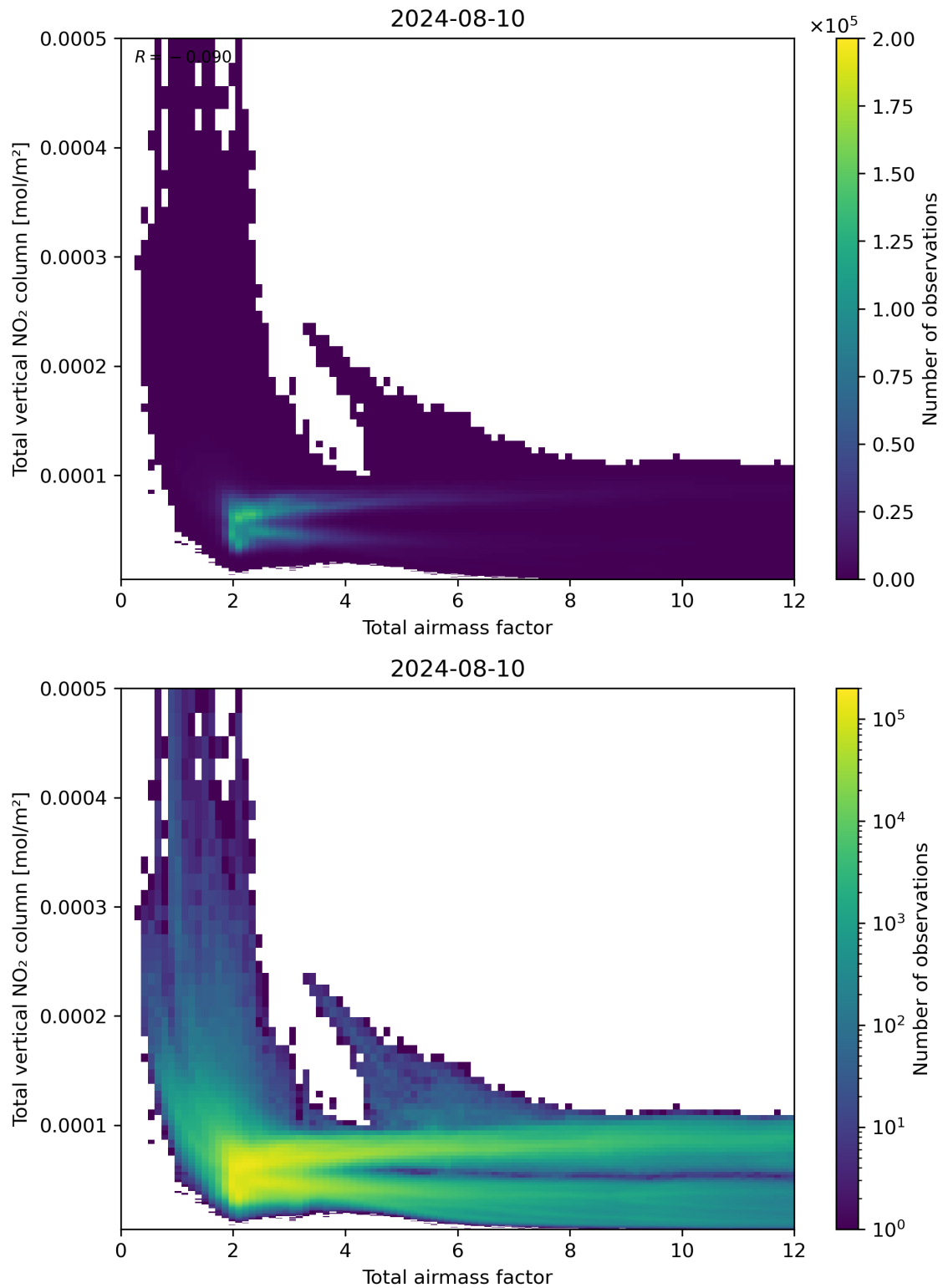
Figure 67: Scatter density plot of “Total airmass factor” against “Total vertical NO 2 column” for 2024-08-09 to 2024-08-11.
