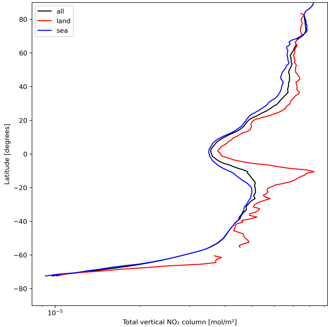
Figure 21: Zonal average of “Total vertical NO 2 column” for 2024-08-09 to 2024-08-11.
