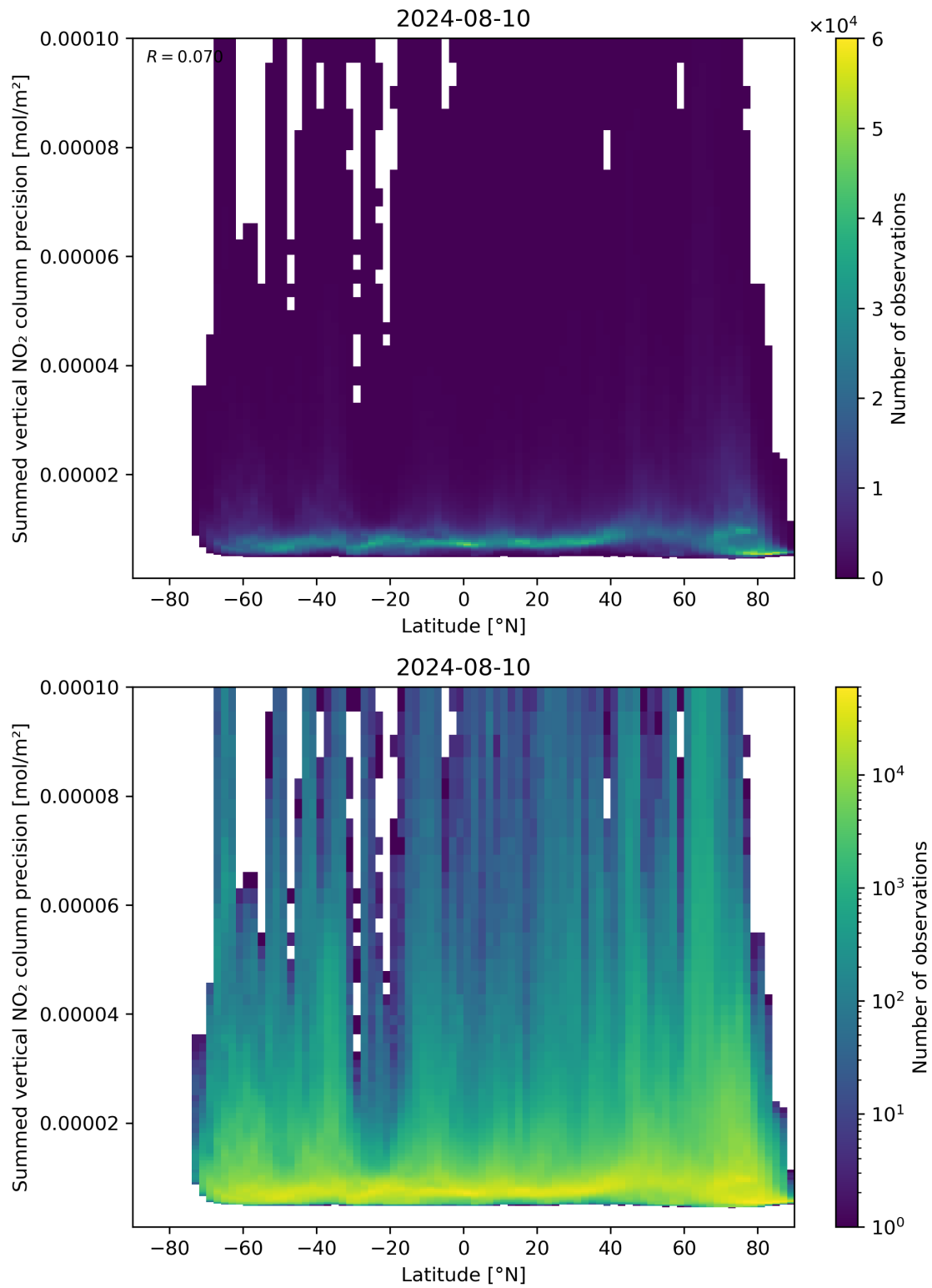
Figure 89: Scatter density plot of “Latitude” against “Summed vertical NO 2 column precision” for 2024-08-09 to 2024-08-11.
