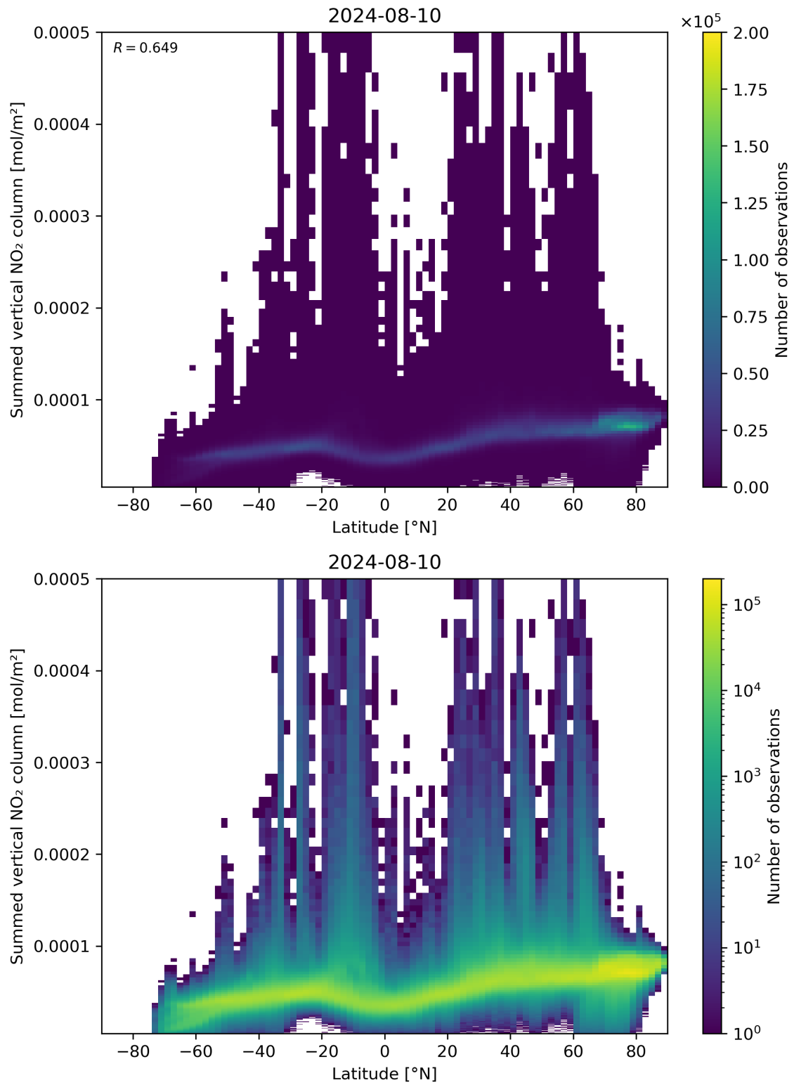
Figure 88: Scatter density plot of “Latitude” against “Summed vertical NO 2 column” for 2024-08-09 to 2024-08-11.
