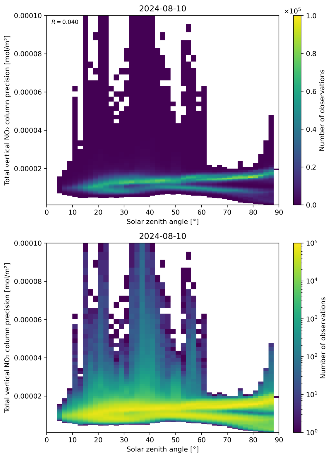
Figure 154: Scatter density plot of “Solar zenith angle” against “Total vertical NO 2 column precision” for 2024-08-09 to 2024-08-11.
