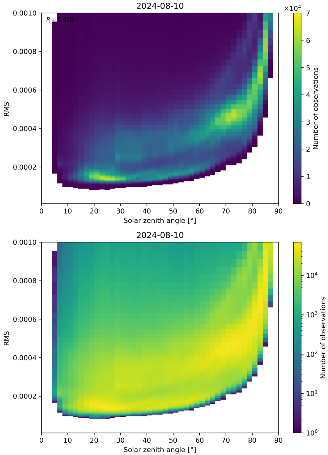
Figure 157: Scatter density plot of “Solar zenith angle” against “RMS” for 2024-08-09 to 2024-08-11.
