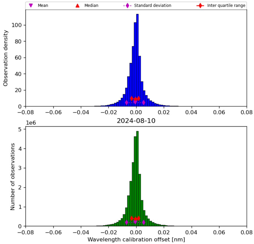
Figure 35: Histogram of “Wavelength calibration offset” for 2024-08-09 to 2024-08-11
