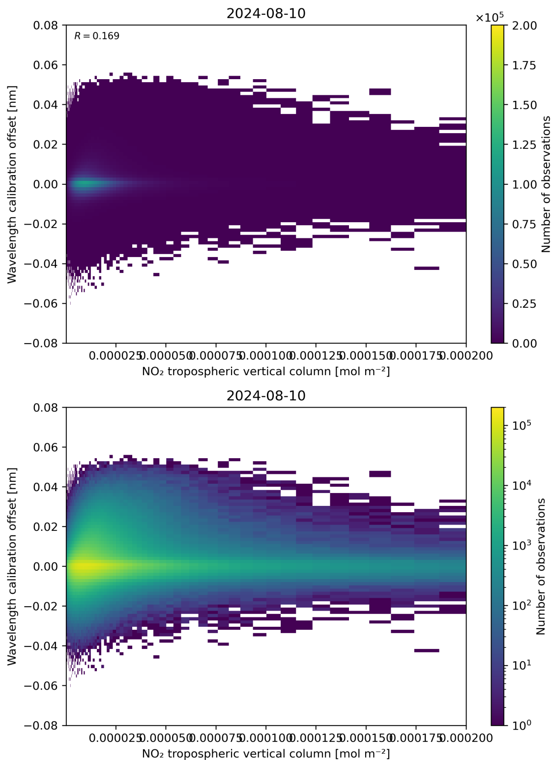
Figure 143: Scatter density plot of “NO 2 tropospheric vertical column” against “Wavelength calibration offset” for 2024-08-09 to 2024-08-11.
