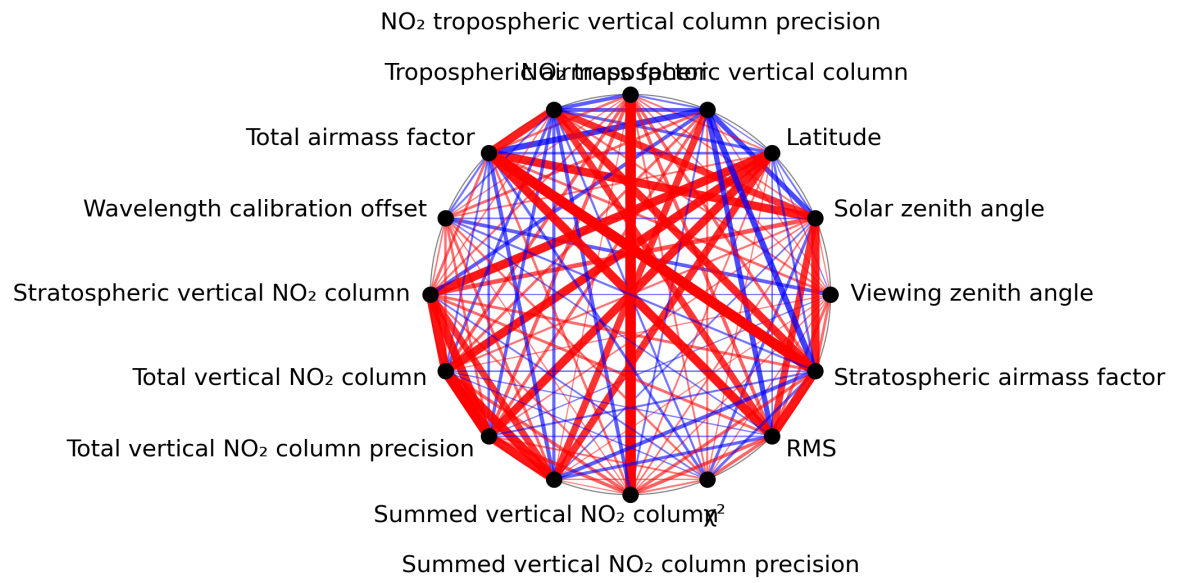
Figure 1: Map of correlation graph for 2024-08-09 to 2024-08-11.
