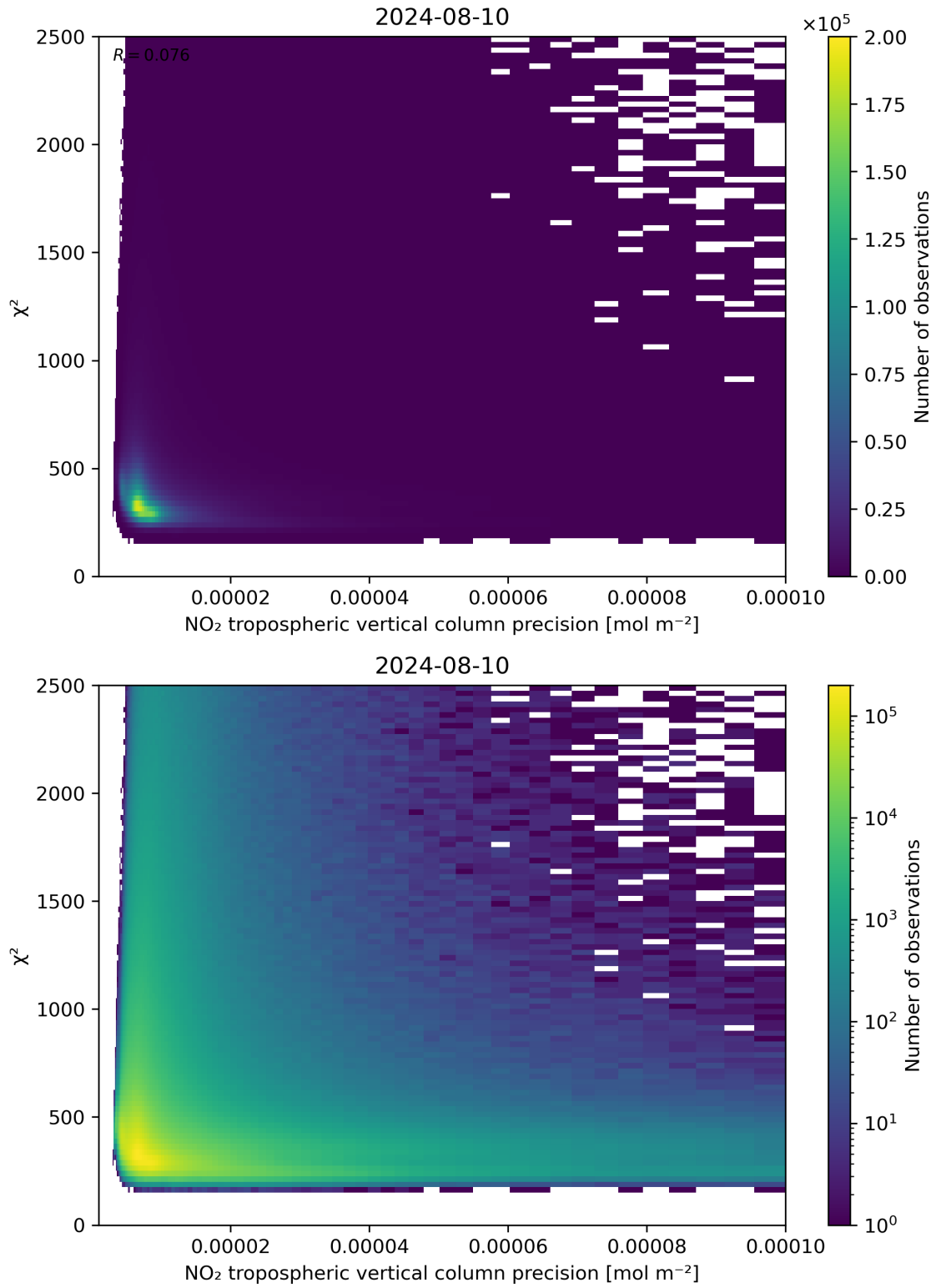
Figure 134: Scatter density plot of “NO 2 tropospheric vertical column precision” against “ \chi^2 ” for 2024-08-09 to 2024-08-11.
