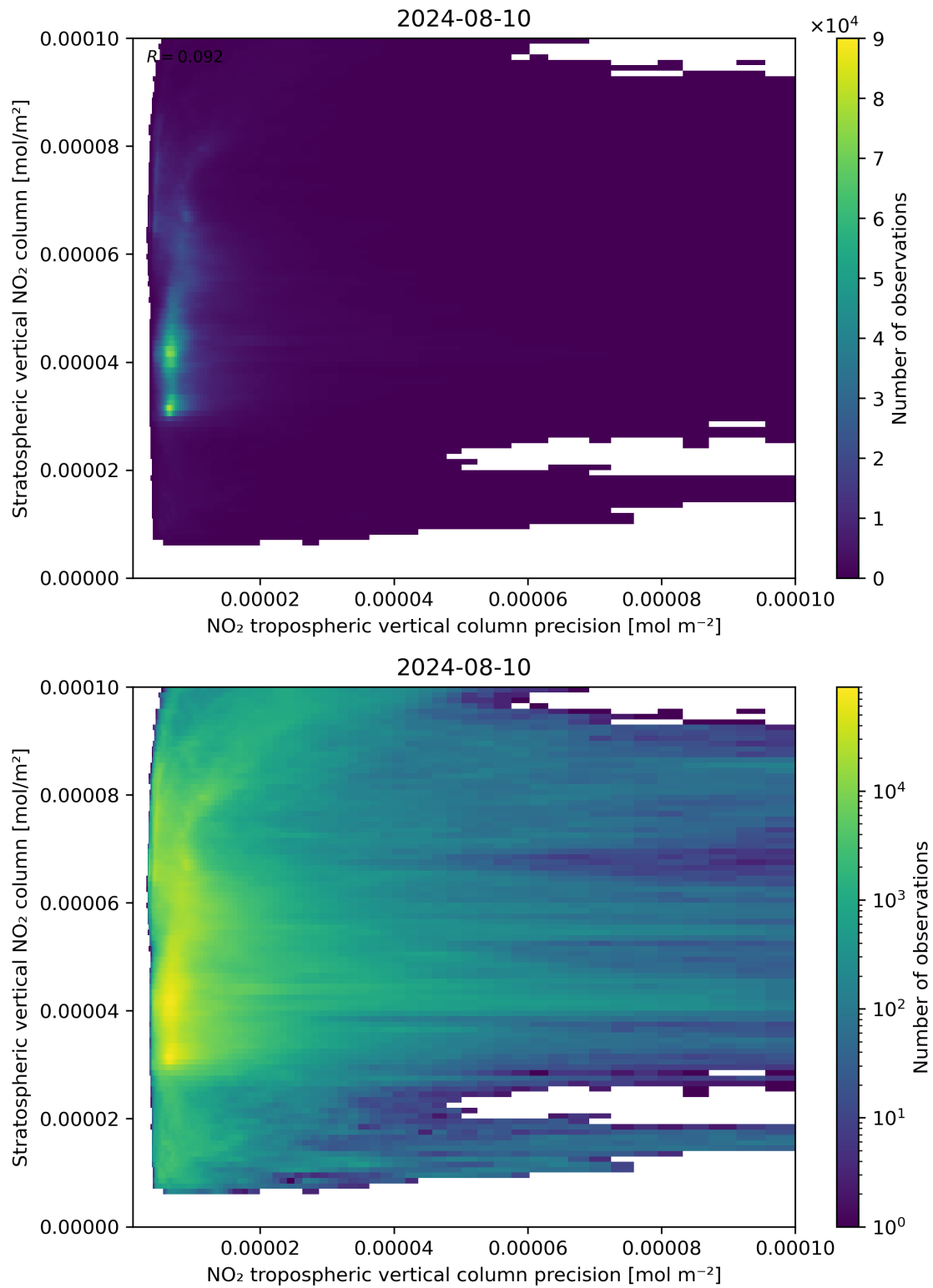
Figure 135: Scatter density plot of “NO 2 tropospheric vertical column precision” against “Stratospheric vertical NO 2 column” for 2024-08-09 to 2024-08-11.
