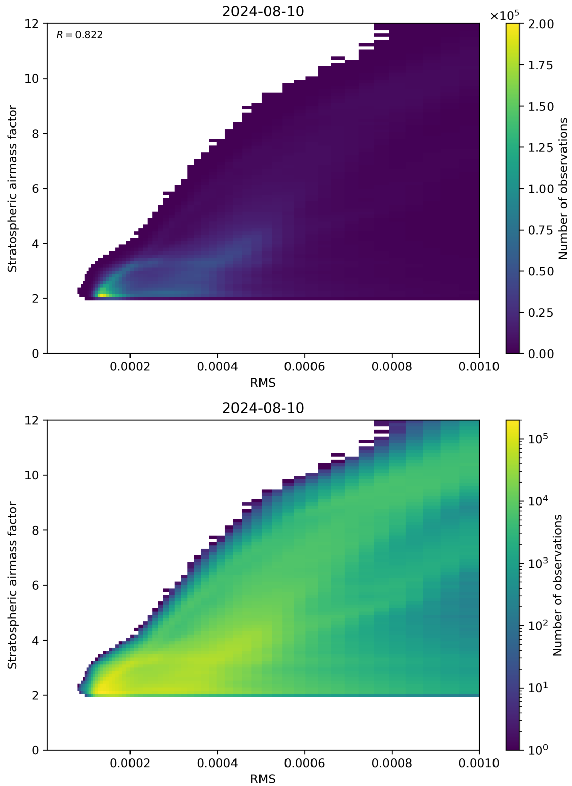
Figure 144: Scatter density plot of “RMS” against “Stratospheric airmass factor” for 2024-08-09 to 2024-08-11.
