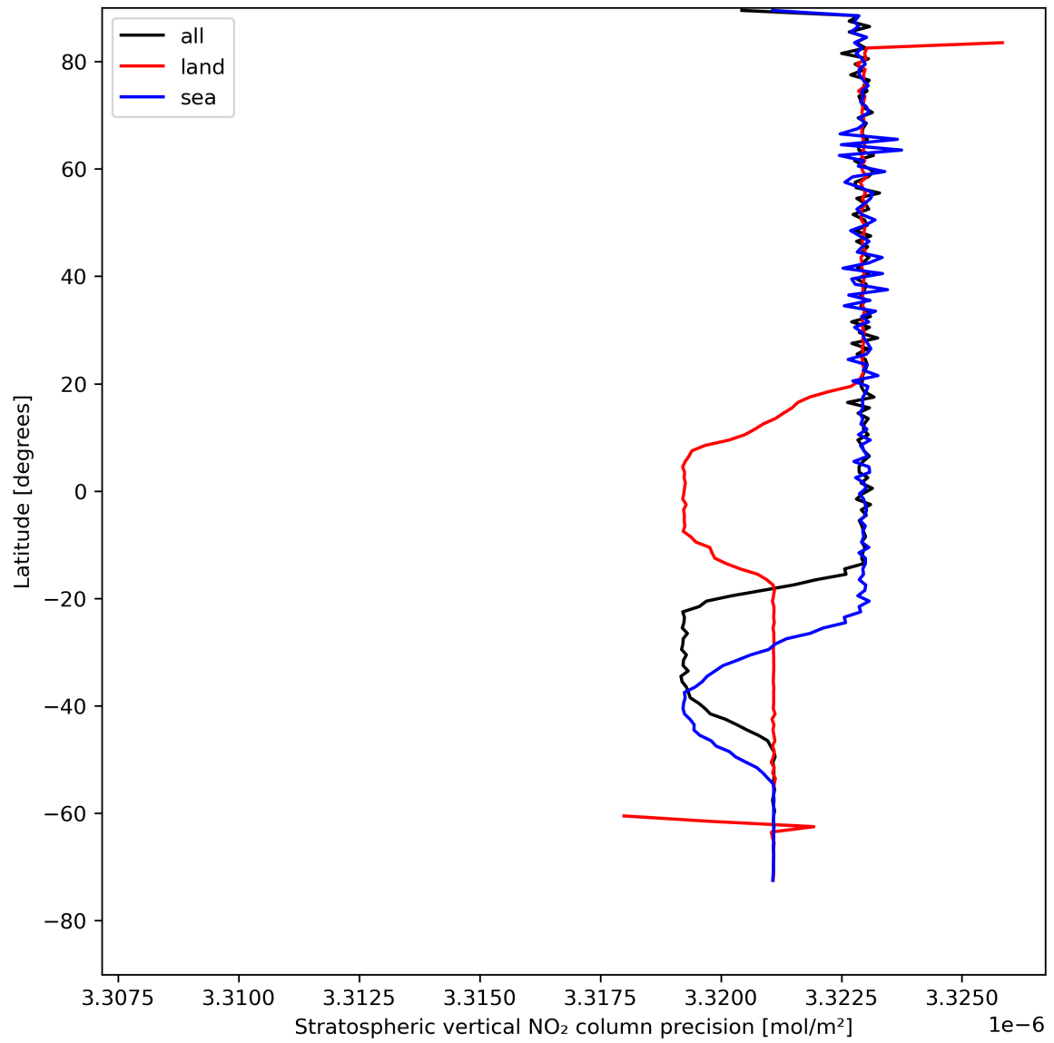
Figure 20: Zonal average of “Stratospheric vertical NO 2 column precision” for 2024-08-09 to 2024-08-11.
