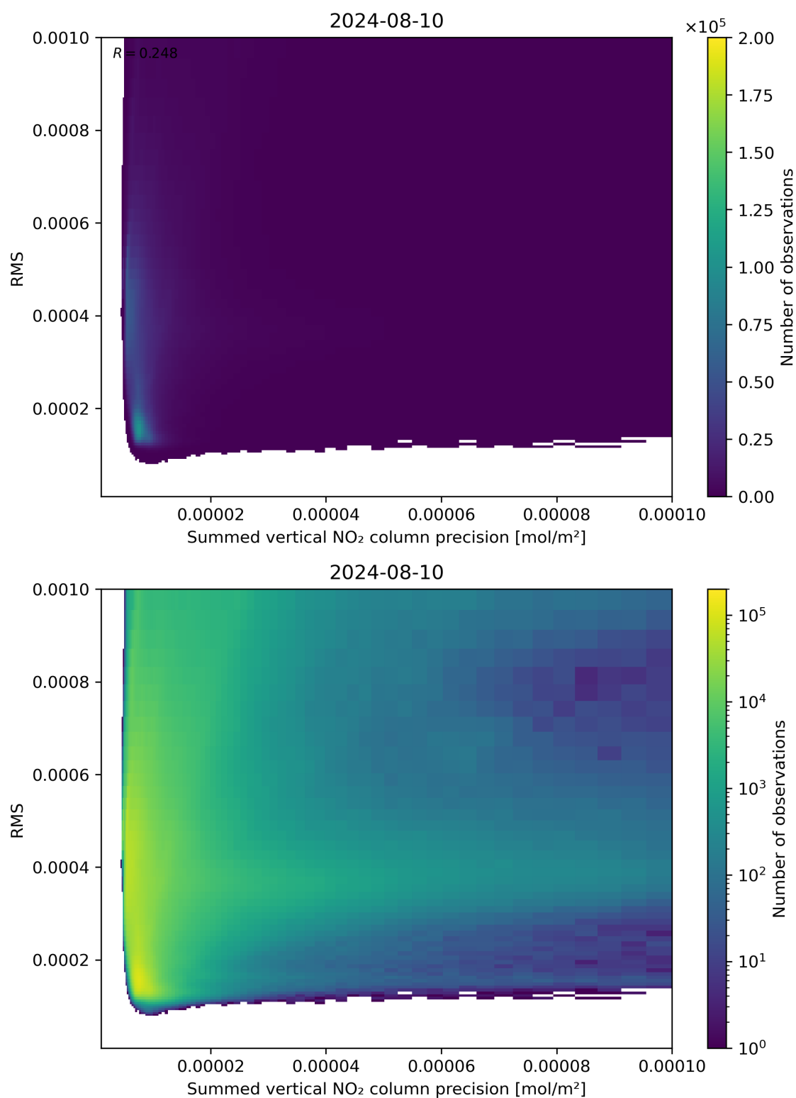
Figure 108: Scatter density plot of “Summed vertical NO 2 column precision” against “RMS” for 2024-08-09 to 2024-08-11.
