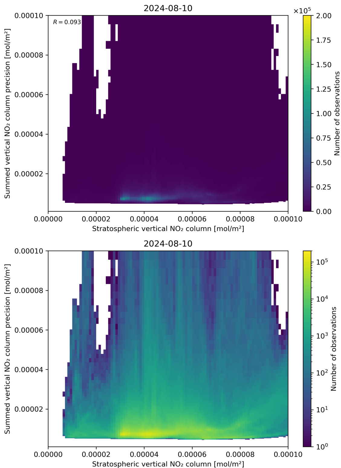
Figure 99: Scatter density plot of “Stratospheric vertical NO 2 column” against “Summed vertical NO 2 column precision” for 2024-08-09 to 2024-08-11.
