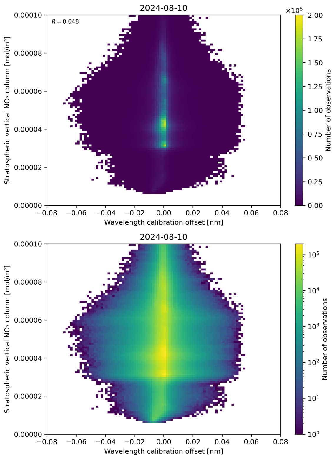
Figure 176: Scatter density plot of “Wavelength calibration offset” against “Stratospheric vertical NO 2 column” for 2024-08-09 to 2024-08-11.
