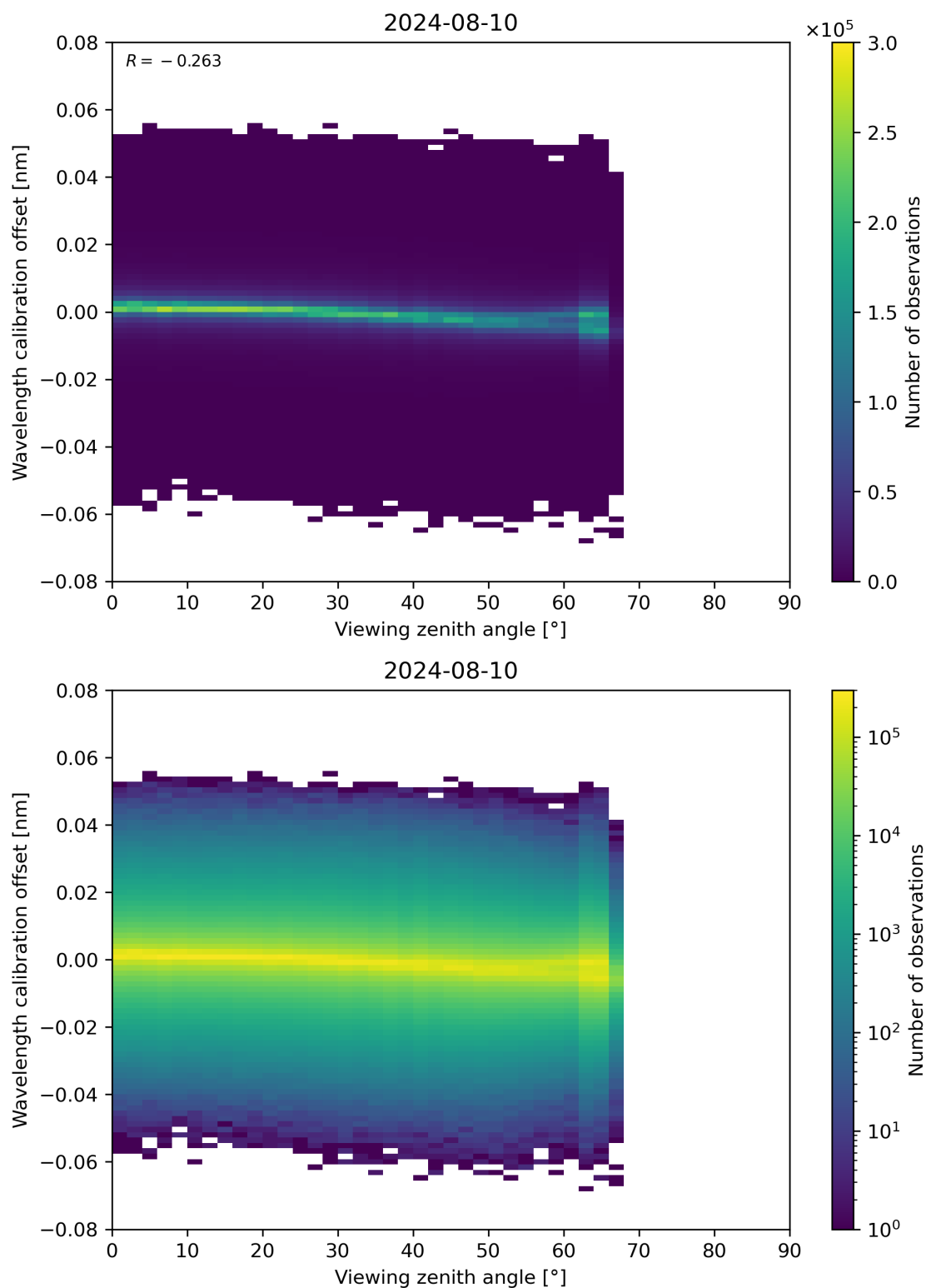
Figure 173: Scatter density plot of “Viewing zenith angle” against “Wavelength calibration offset” for 2024-08-09 to 2024-08-11.
