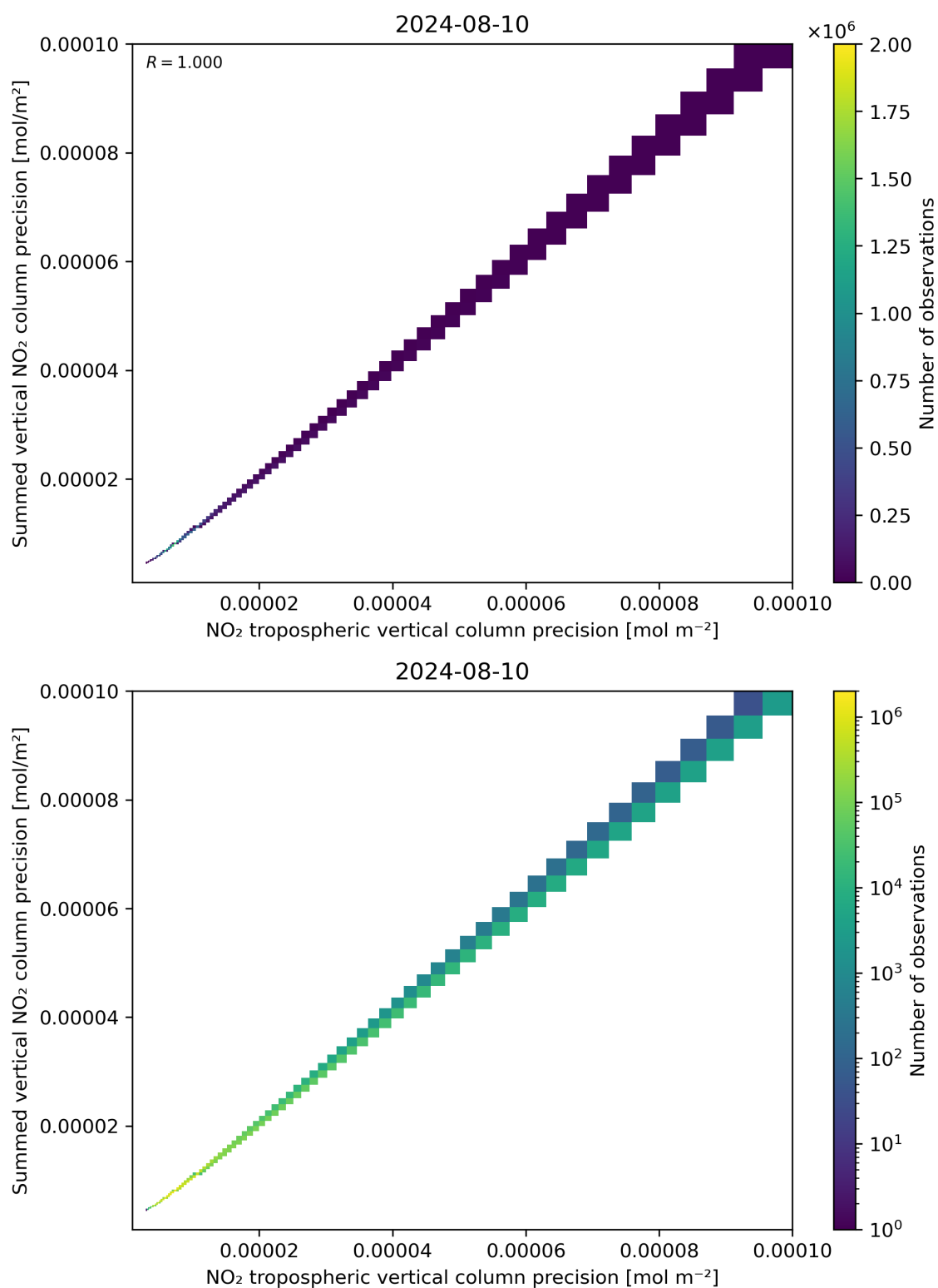
Figure 137: Scatter density plot of “NO 2 tropospheric vertical column precision” against “Summed vertical NO 2 column precision” for 2024-08-09 to 2024-08-11.
