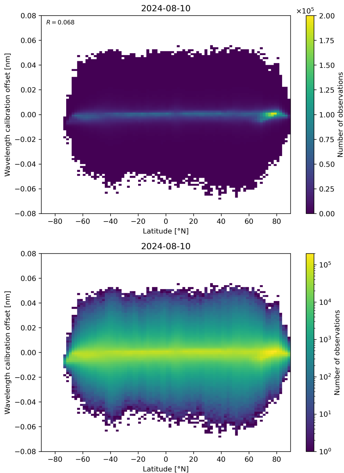
Figure 95: Scatter density plot of “Latitude” against “Wavelength calibration offset” for 2024-08-09 to 2024-08-11.
