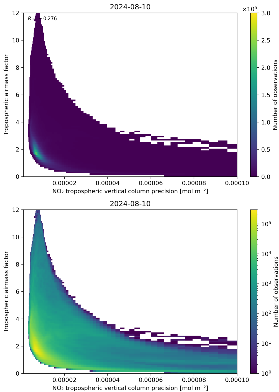
Figure 133: Scatter density plot of “NO 2 tropospheric vertical column precision” against “Tropospheric airmass factor” for 2024-08-09 to 2024-08-11.
