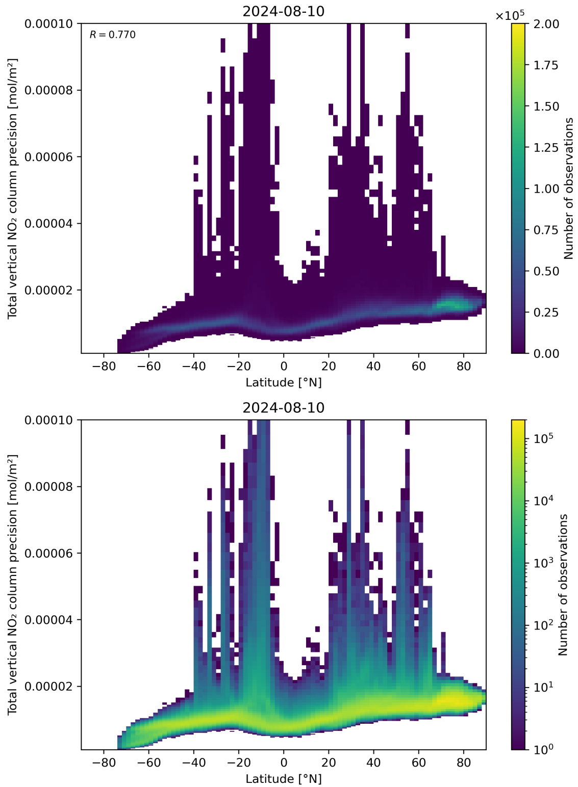
Figure 91: Scatter density plot of “Latitude” against “Total vertical NO 2 column precision” for 2024-08-09 to 2024-08-11.
