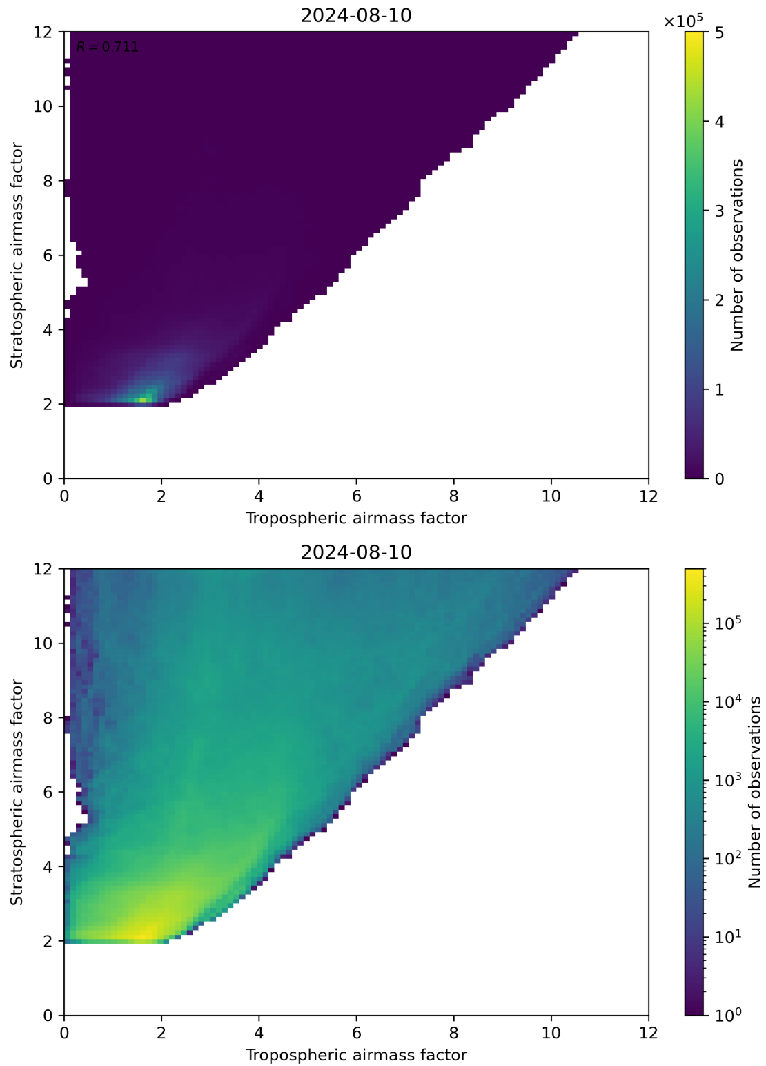
Figure 71: Scatter density plot of “Tropospheric airmass factor” against “Stratospheric airmass factor” for 2024-08-09 to 2024-08-11.
