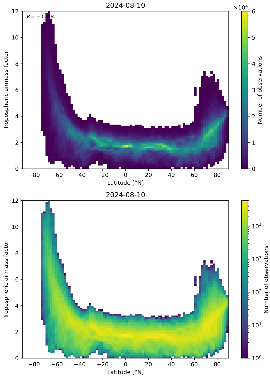
Figure 85: Scatter density plot of “Latitude” against “Tropospheric airmass factor” for 2024-08-09 to 2024-08-11.
