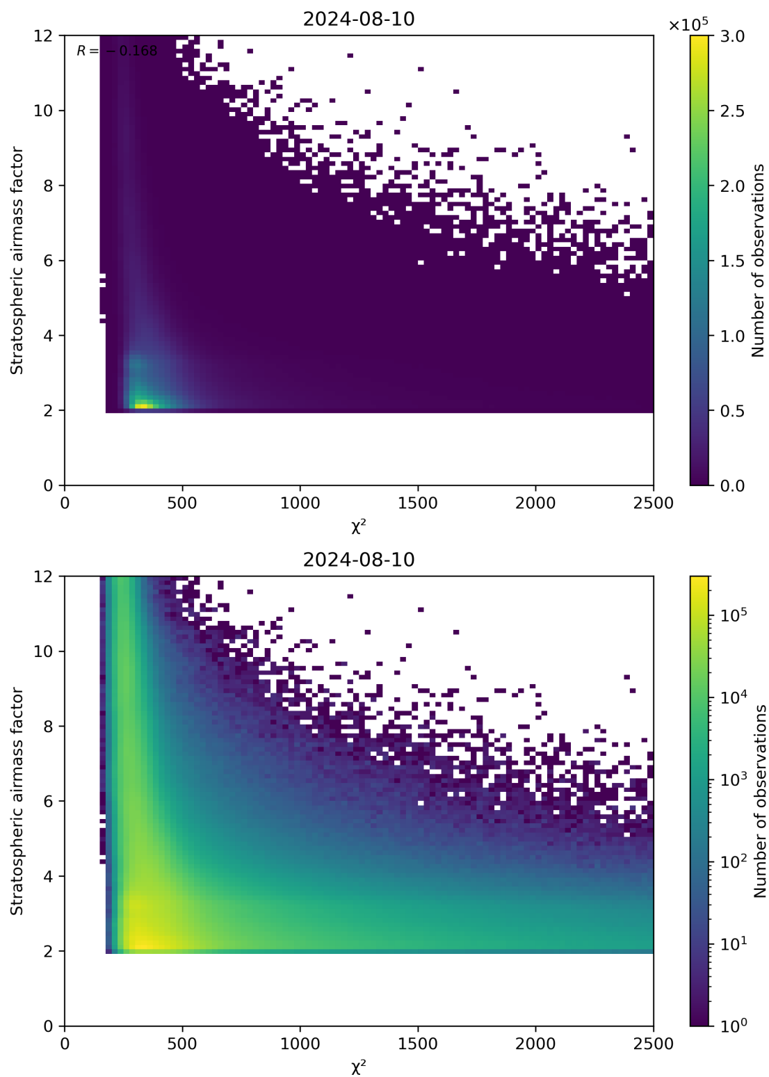
Figure 81: Scatter density plot of “ \chi^2 ” against “Stratospheric airmass factor” for 2024-08-09 to 2024-08-11.
