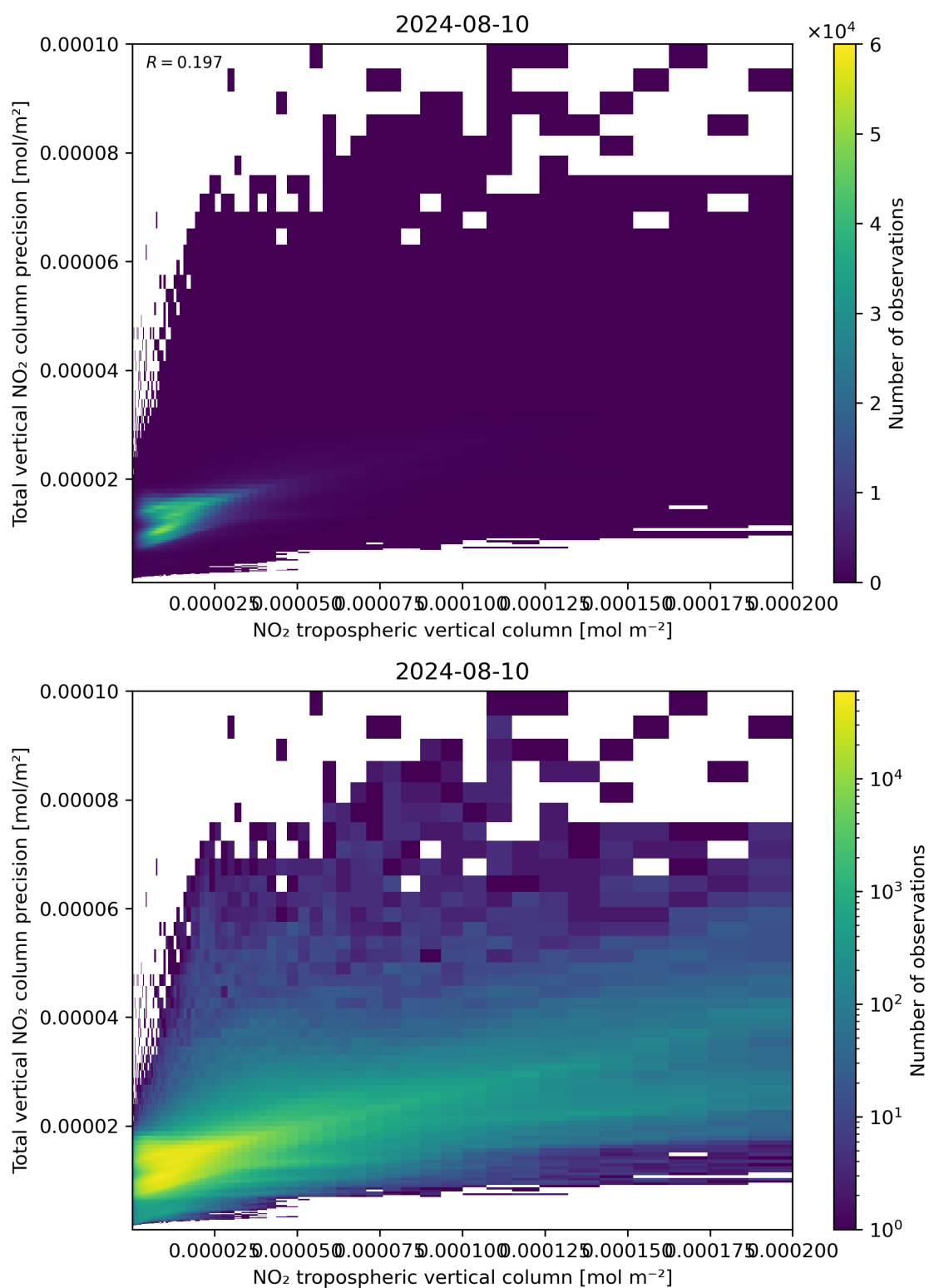
Figure 129: Scatter density plot of “NO 2 tropospheric vertical column” against “Total vertical NO 2 column precision” for 2024-08-09 to 2024-08-11.
