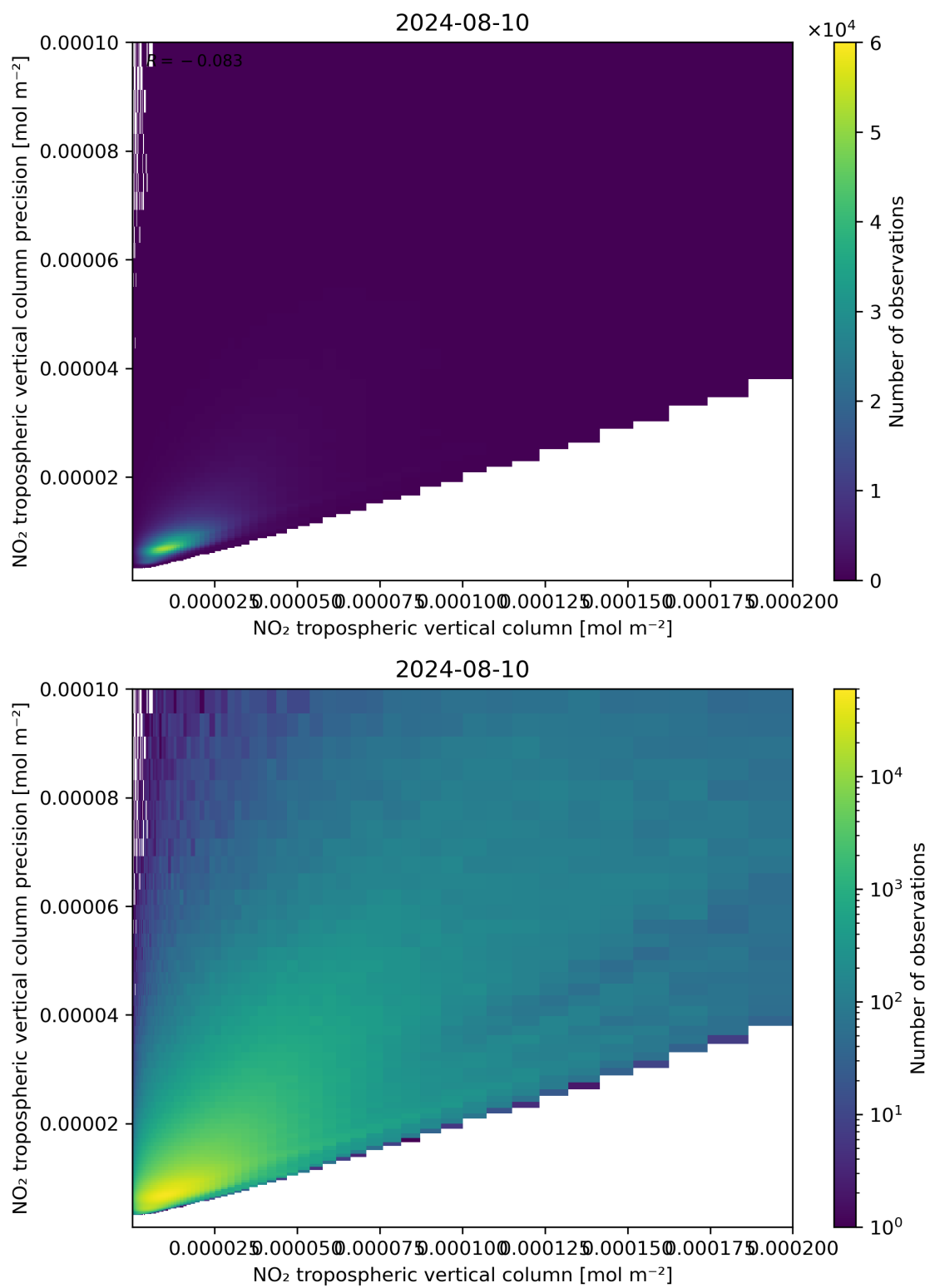
Figure 130: Scatter density plot of “NO 2 tropospheric vertical column” against “NO 2 tropospheric vertical column precision” for 2024-08-09 to 2024-08-11.
