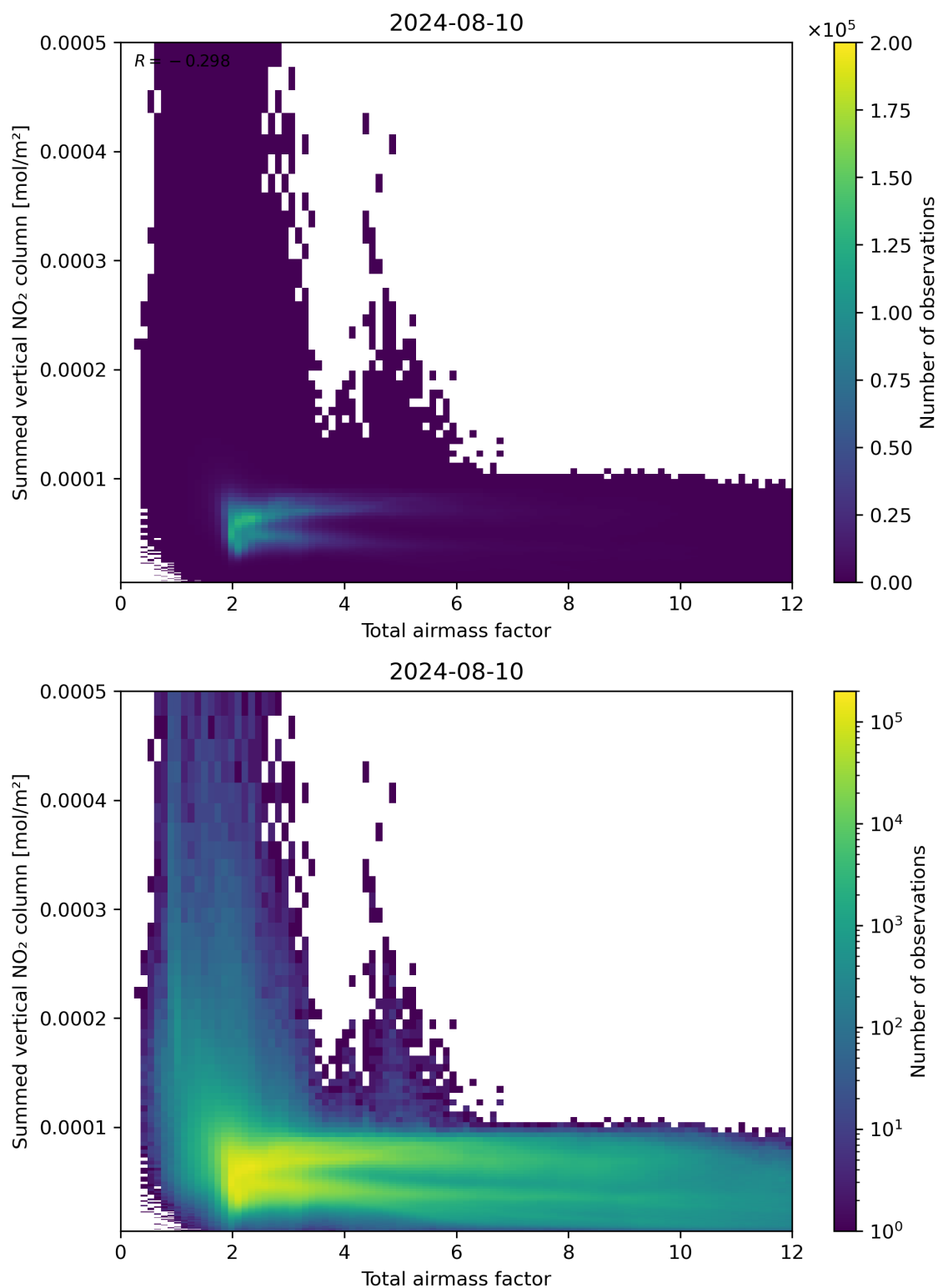
Figure 65: Scatter density plot of “Total airmass factor” against “Summed vertical NO 2 column” for 2024-08-09 to 2024-08-11.
