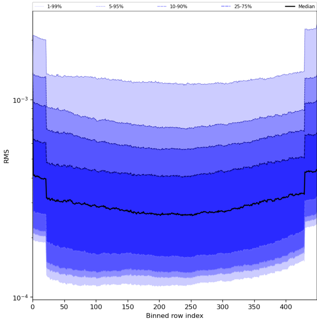
Figure 60: Along track statistics of “RMS” for 2024-08-11 to 2024-08-11
