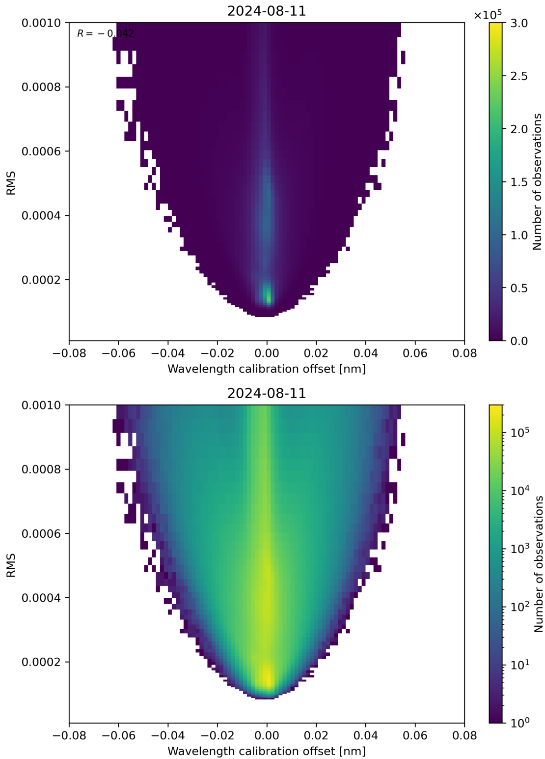
Figure 181: Scatter density plot of “Wavelength calibration offset” against “RMS” for 2024-08-11 to 2024-08-11.
