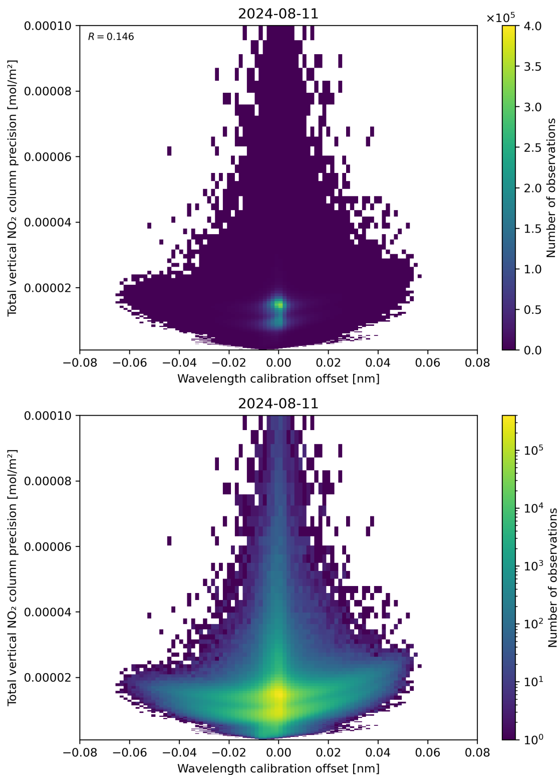
Figure 180: Scatter density plot of “Wavelength calibration offset” against “Total vertical NO 2 column precision” for 2024-08-11 to 2024-08-11.
