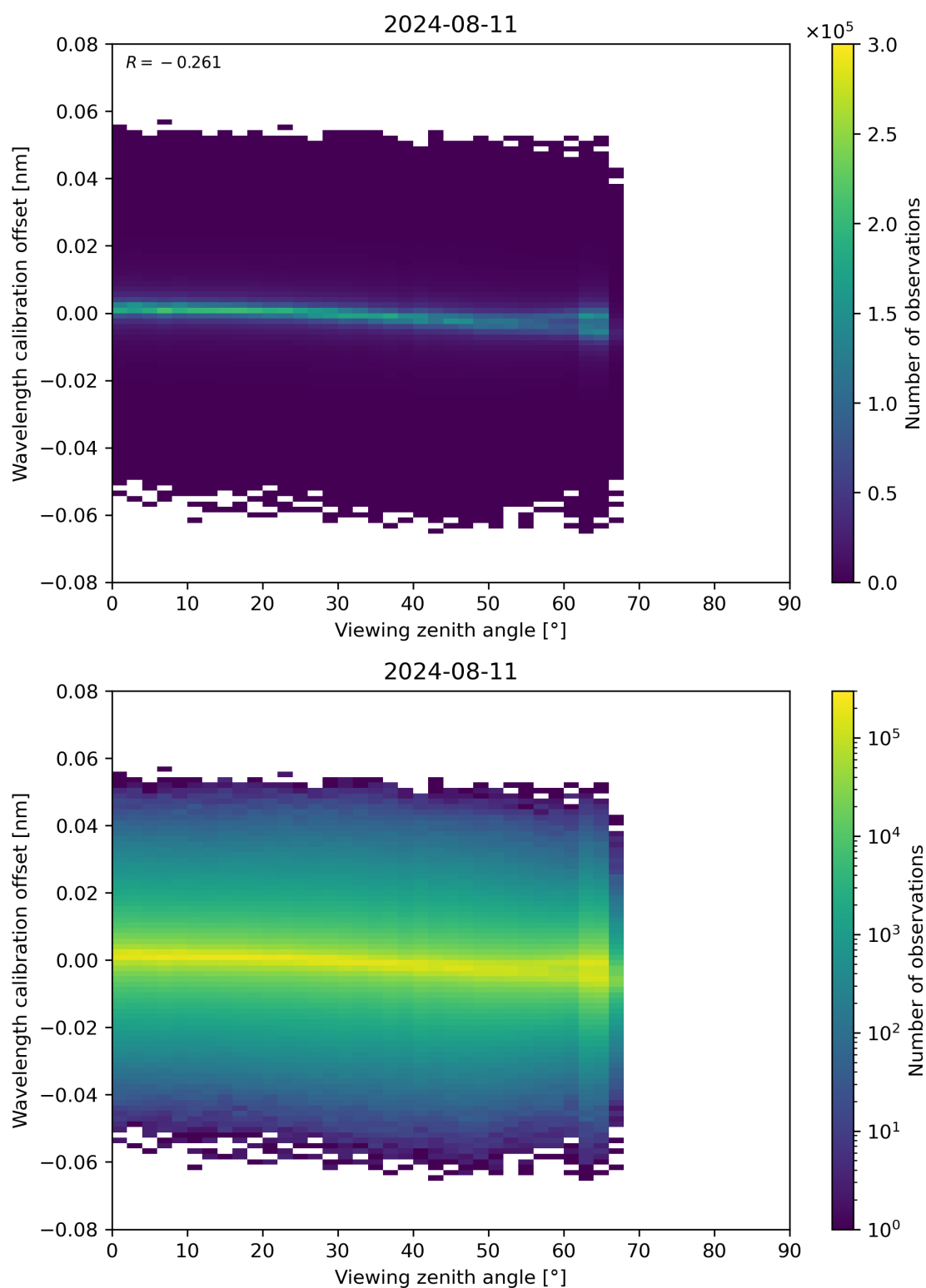
Figure 173: Scatter density plot of “Viewing zenith angle” against “Wavelength calibration offset” for 2024-08-11 to 2024-08-11.
