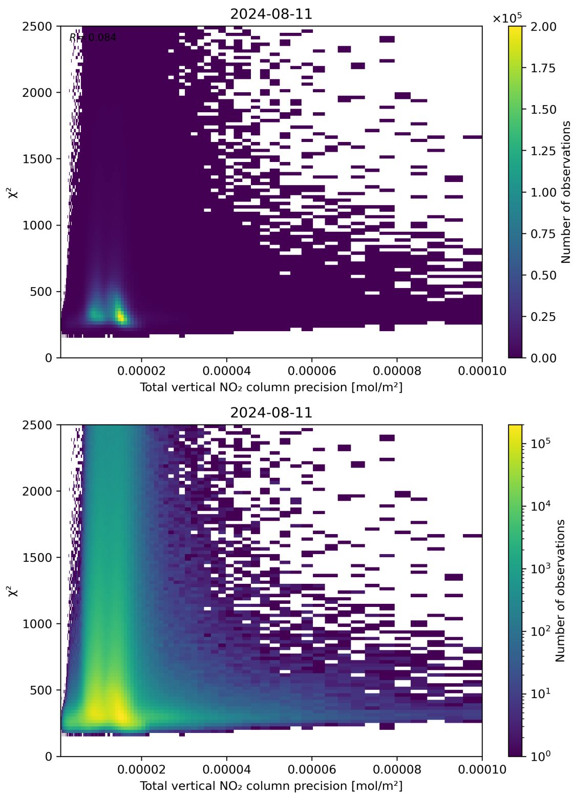
Figure 116: Scatter density plot of “Total vertical NO 2 column precision” against “ \chi^2 ” for 2024-08-11 to 2024-08-11.
