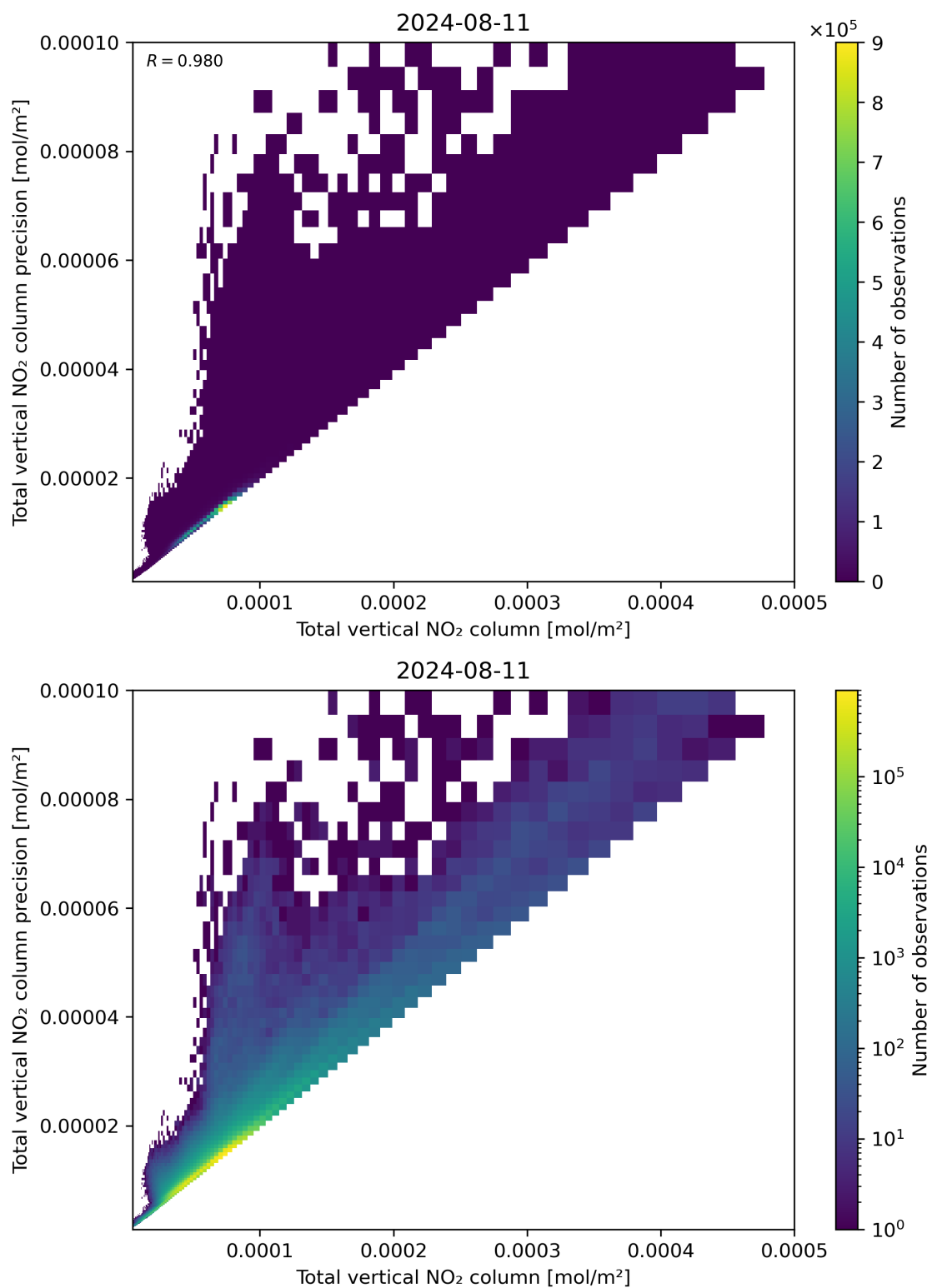
Figure 114: Scatter density plot of “Total vertical NO 2 column” against “Total vertical NO 2 column precision” for 2024-08-11 to 2024-08-11.
