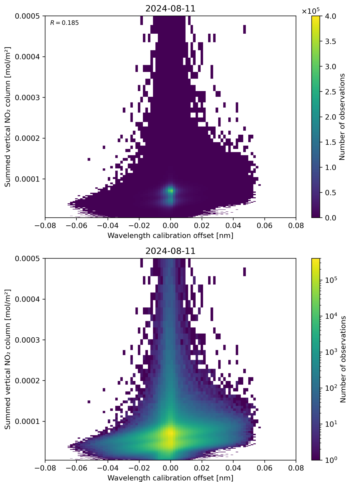
Figure 177: Scatter density plot of “Wavelength calibration offset” against “Summed vertical NO 2 column” for 2024-08-11 to 2024-08-11.
