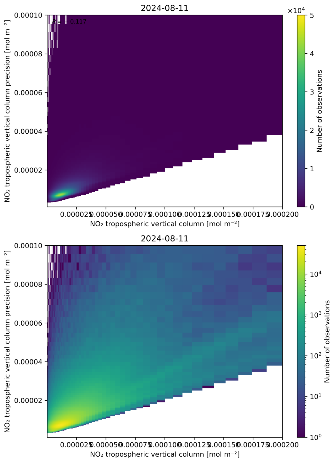
Figure 130: Scatter density plot of “NO 2 tropospheric vertical column” against “NO 2 tropospheric vertical column precision” for 2024-08-11 to 2024-08-11.
