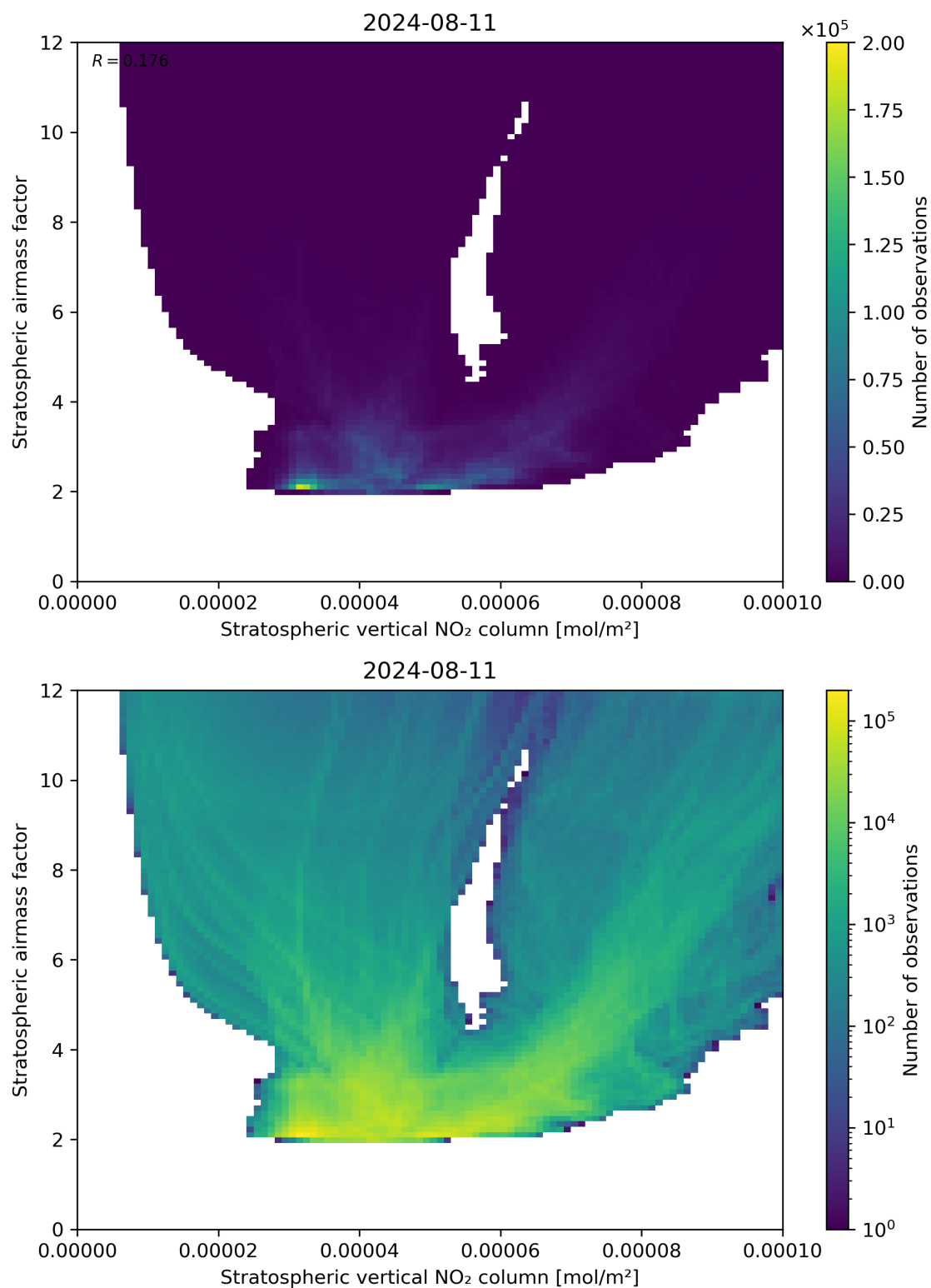
Figure 96: Scatter density plot of “Stratospheric vertical NO 2 column” against “Stratospheric airmass factor” for 2024-08-11 to 2024-08-11.
