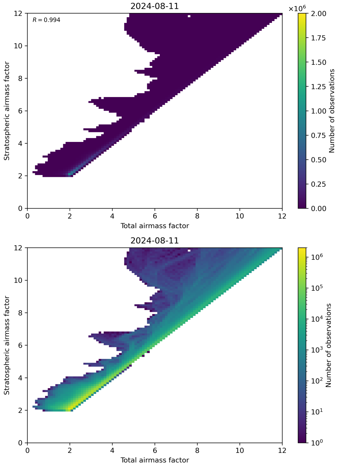
Figure 62: Scatter density plot of “Total airmass factor” against “Stratospheric airmass factor” for 2024-08-11 to 2024-08-11.
