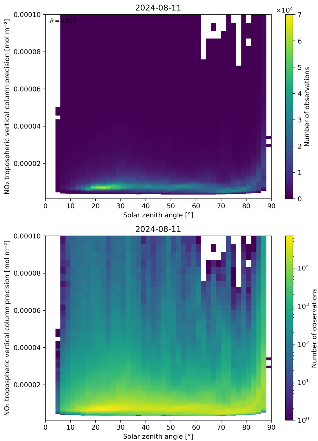
Figure 156: Scatter density plot of “Solar zenith angle” against “NO 2 tropospheric vertical column precision” for 2024-08-11 to 2024-08-11.
