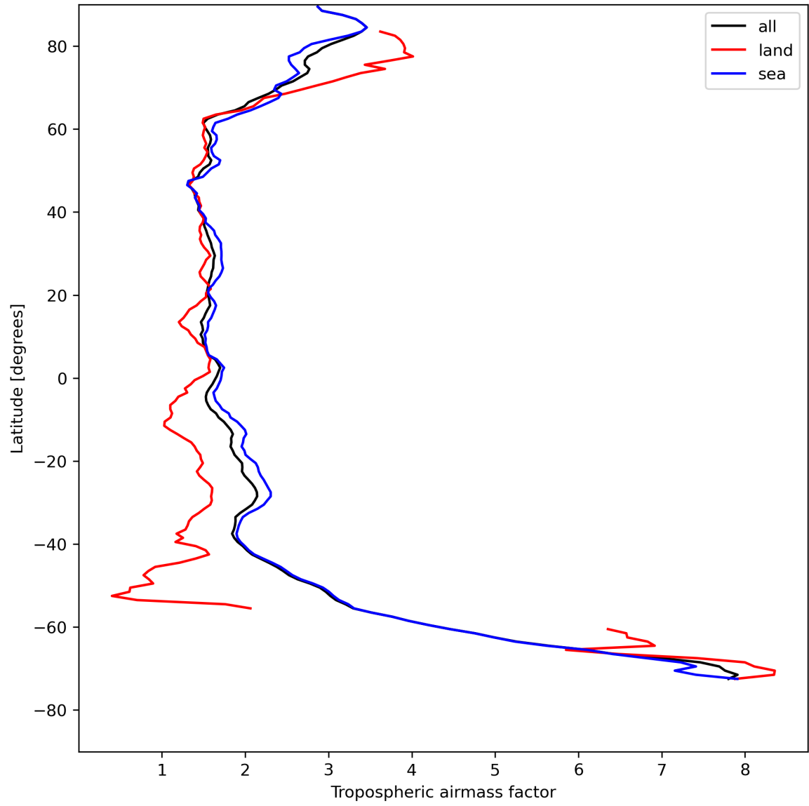
Figure 14: Zonal average of “Tropospheric airmass factor” for 2024-08-11 to 2024-08-11.
