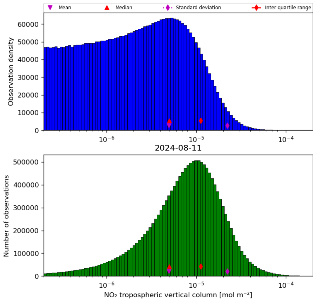
Figure 29: Histogram of “NO 2 tropospheric vertical column” for 2024-08-11 to 2024-08-11
