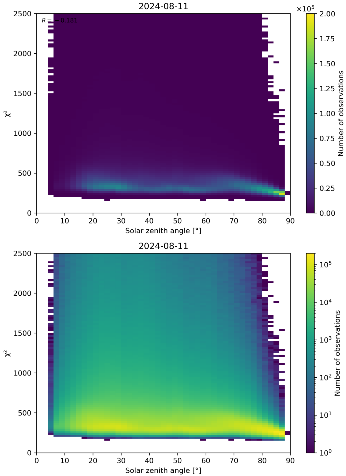
Figure 148: Scatter density plot of “Solar zenith angle” against “ \chi^2 ” for 2024-08-11 to 2024-08-11.
