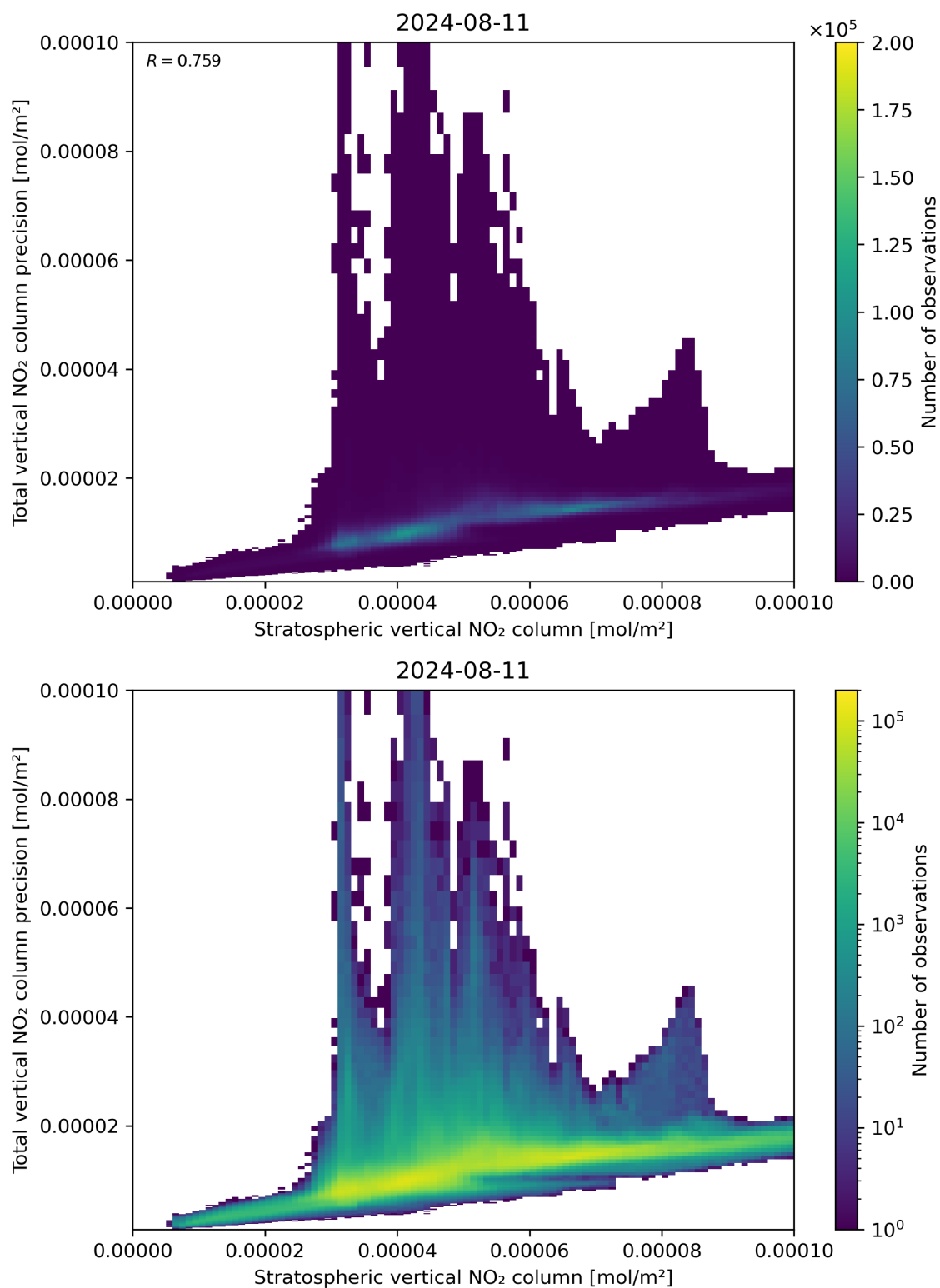
Figure 101: Scatter density plot of “Stratospheric vertical NO 2 column” against “Total vertical NO 2 column precision” for 2024-08-11 to 2024-08-11.
