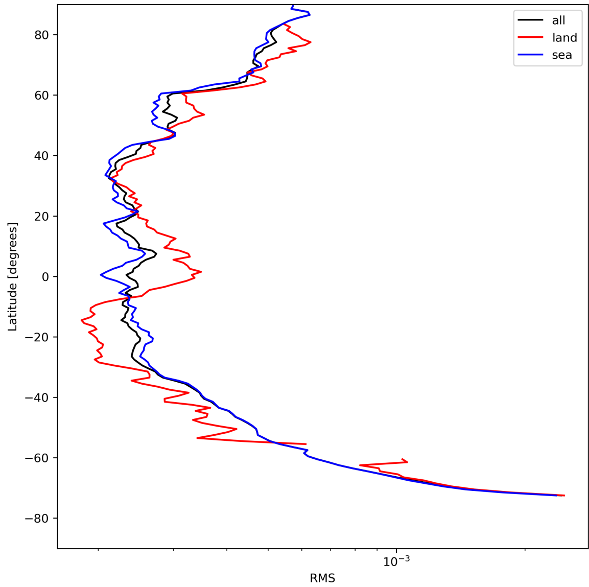
Figure 26: Zonal average of “RMS” for 2024-08-11 to 2024-08-11.
