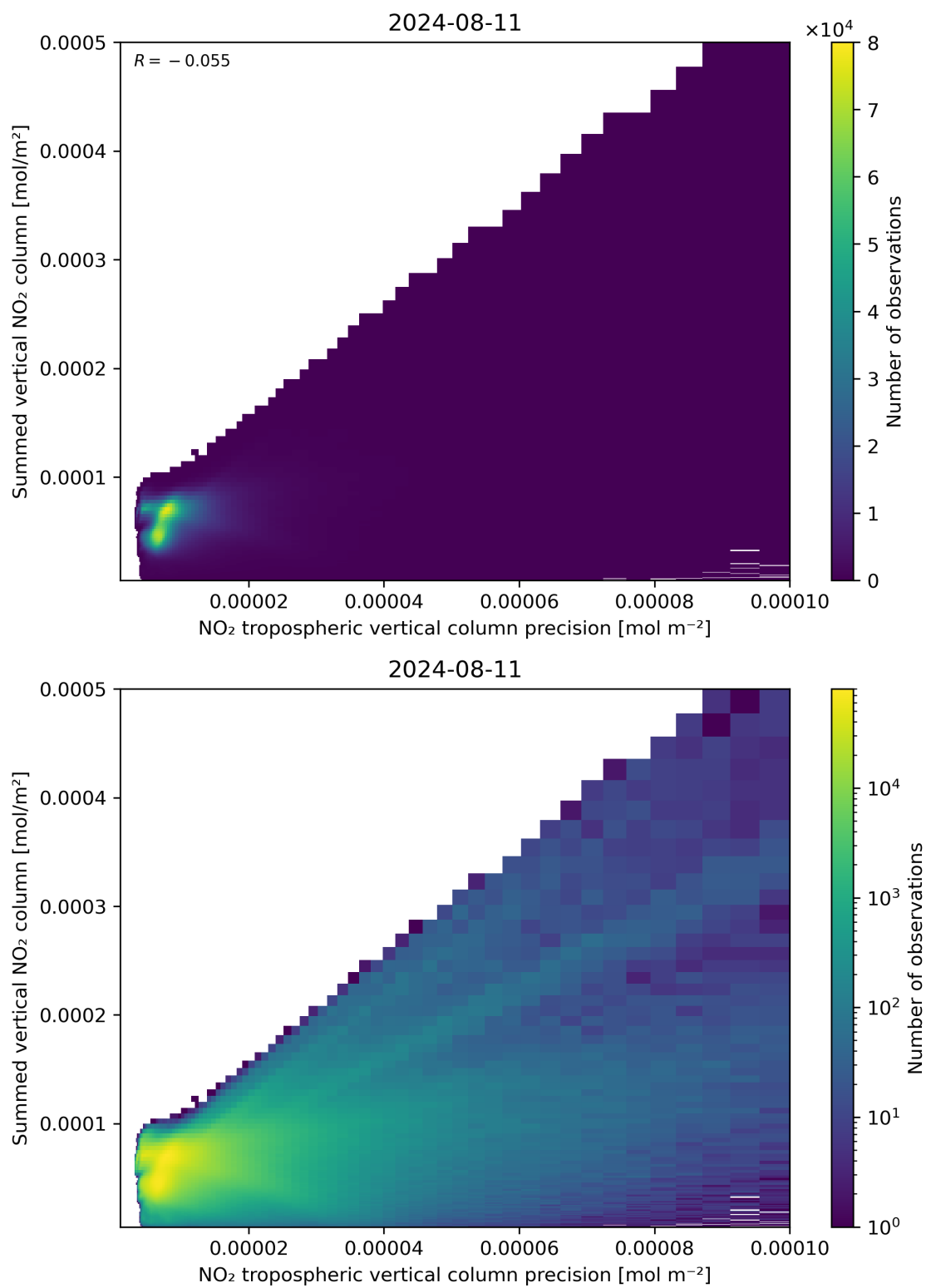
Figure 136: Scatter density plot of “NO 2 tropospheric vertical column precision” against “Summed vertical NO 2 column” for 2024-08-11 to 2024-08-11.
