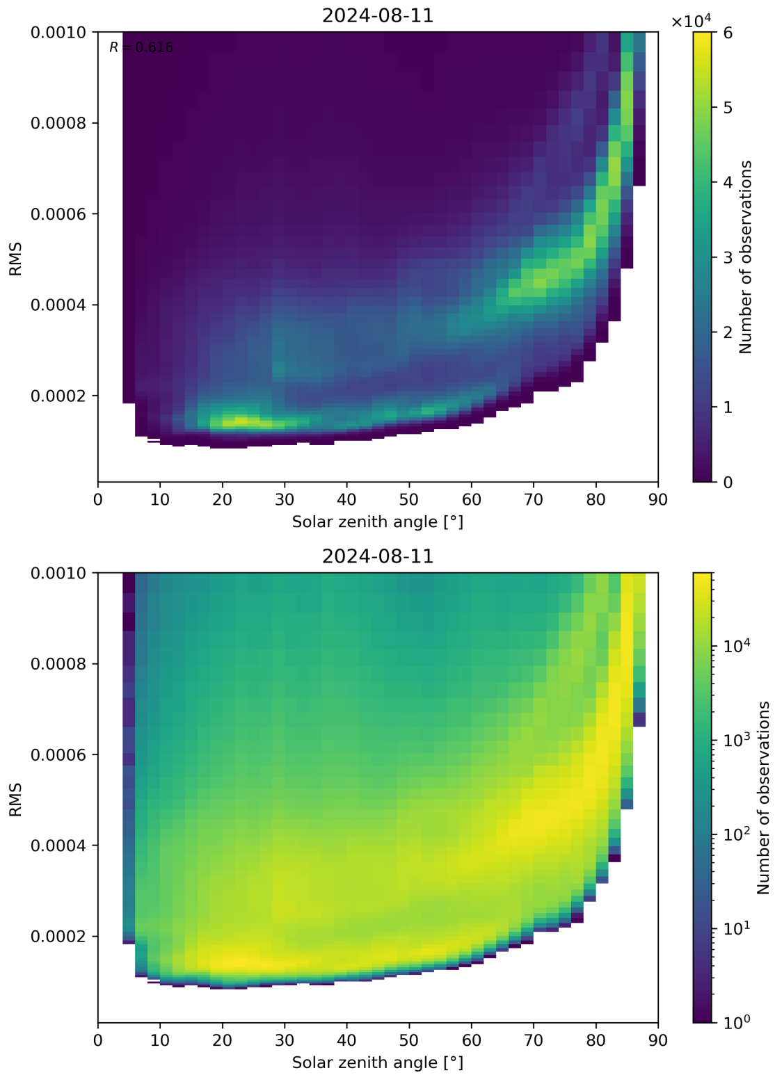
Figure 157: Scatter density plot of “Solar zenith angle” against “RMS” for 2024-08-11 to 2024-08-11.
