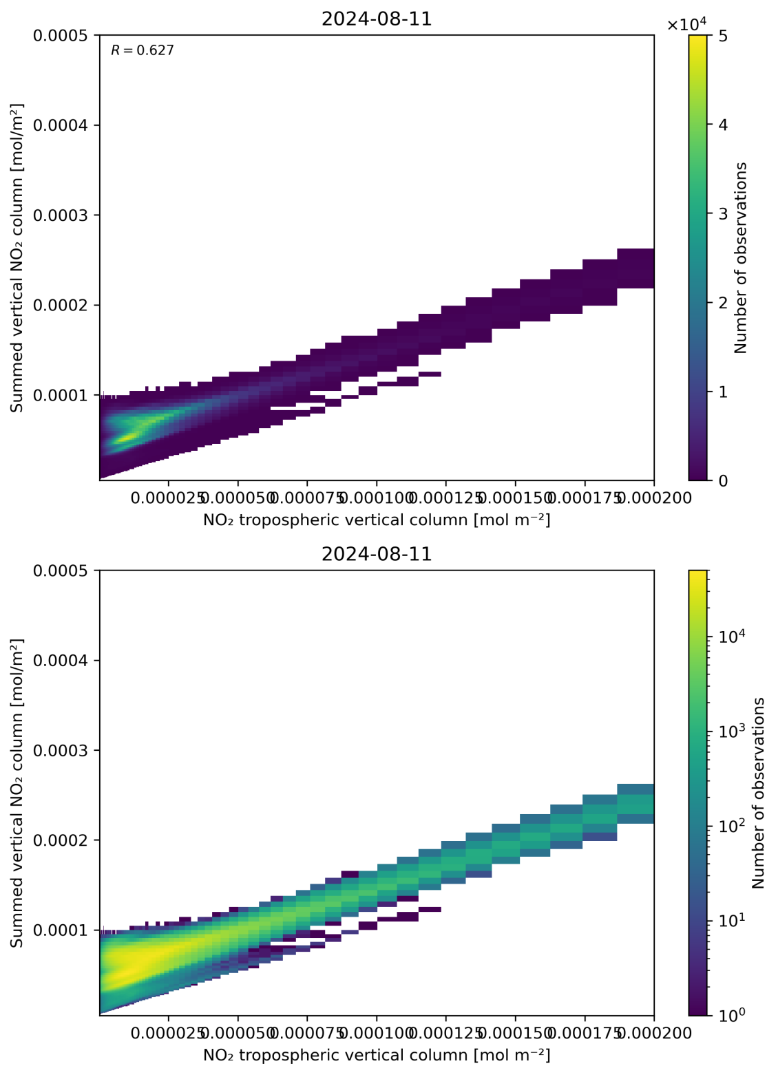
Figure 126: Scatter density plot of “NO 2 tropospheric vertical column” against “Summed vertical NO 2 column” for 2024-08-11 to 2024-08-11.
