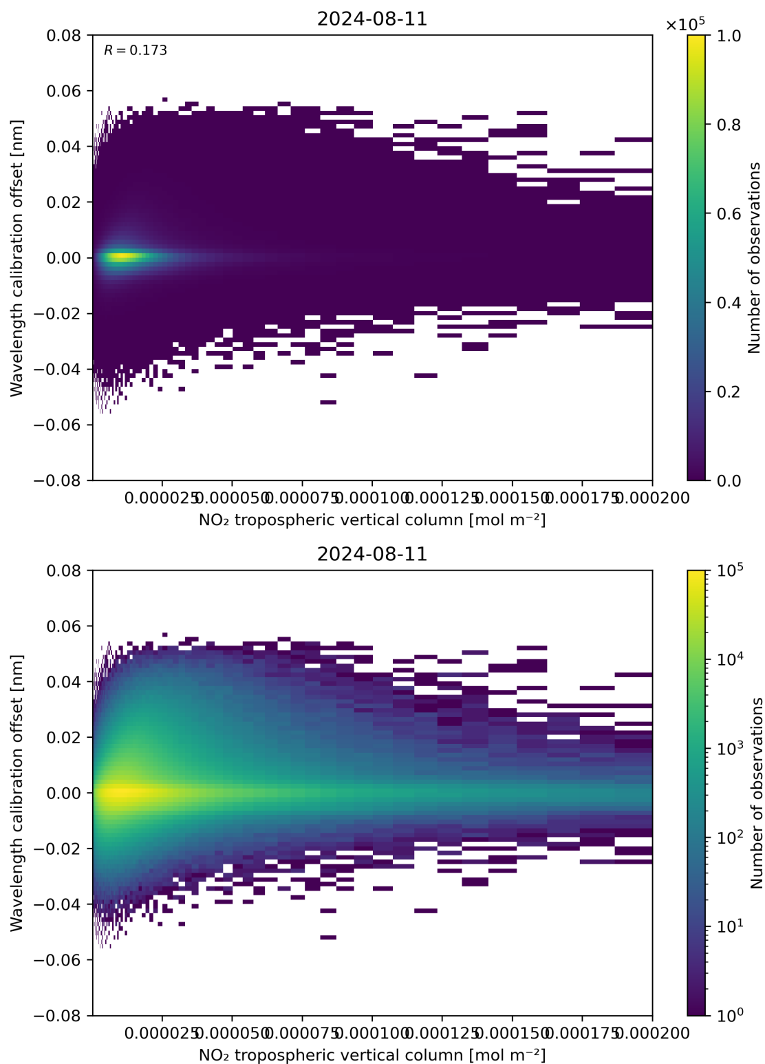
Figure 143: Scatter density plot of “NO 2 tropospheric vertical column” against “Wavelength calibration offset” for 2024-08-11 to 2024-08-11.
