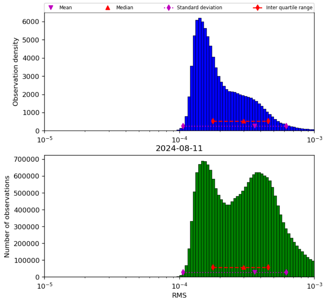
Figure 43: Histogram of “RMS” for 2024-08-11 to 2024-08-11
