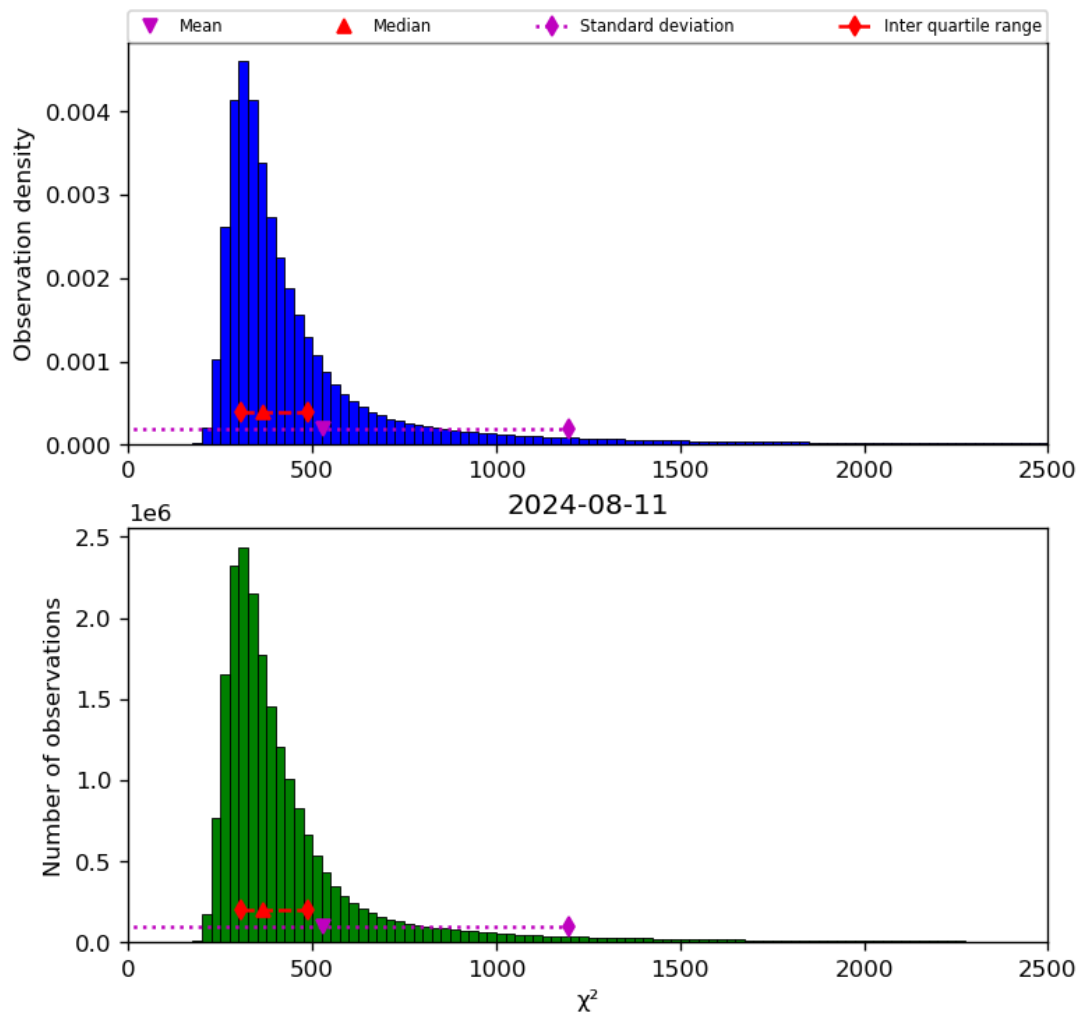
Figure 42: Histogram of “ \chi^2 ” for 2024-08-11 to 2024-08-11
