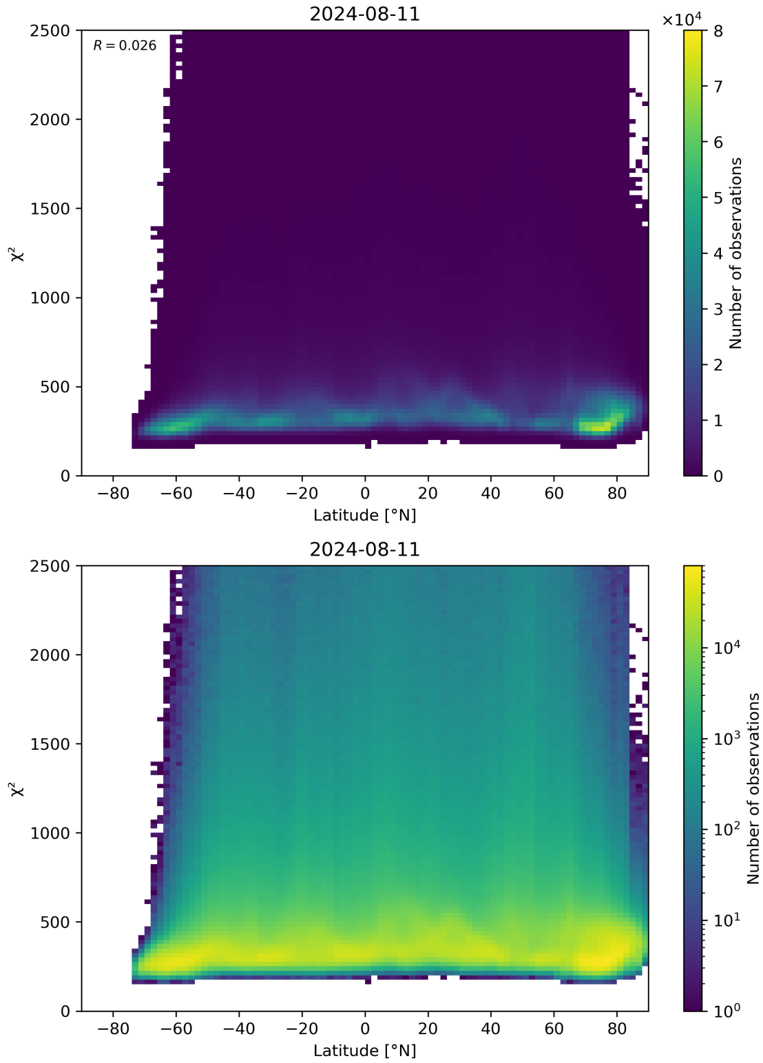
Figure 86: Scatter density plot of “Latitude” against “ \chi^2 ” for 2024-08-11 to 2024-08-11.
