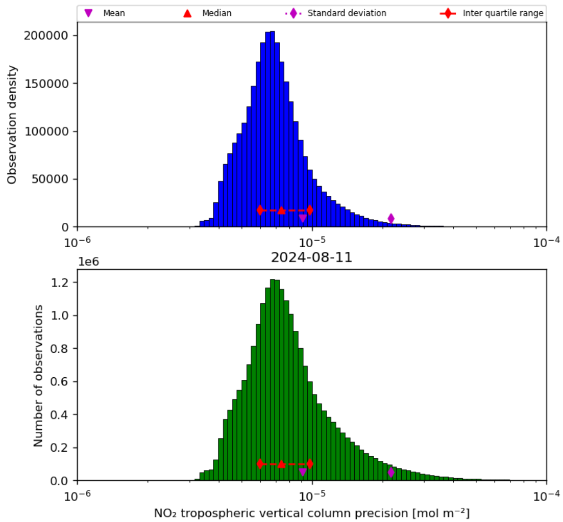
Figure 30: Histogram of “NO 2 tropospheric vertical column precision” for 2024-08-11 to 2024-08-11
