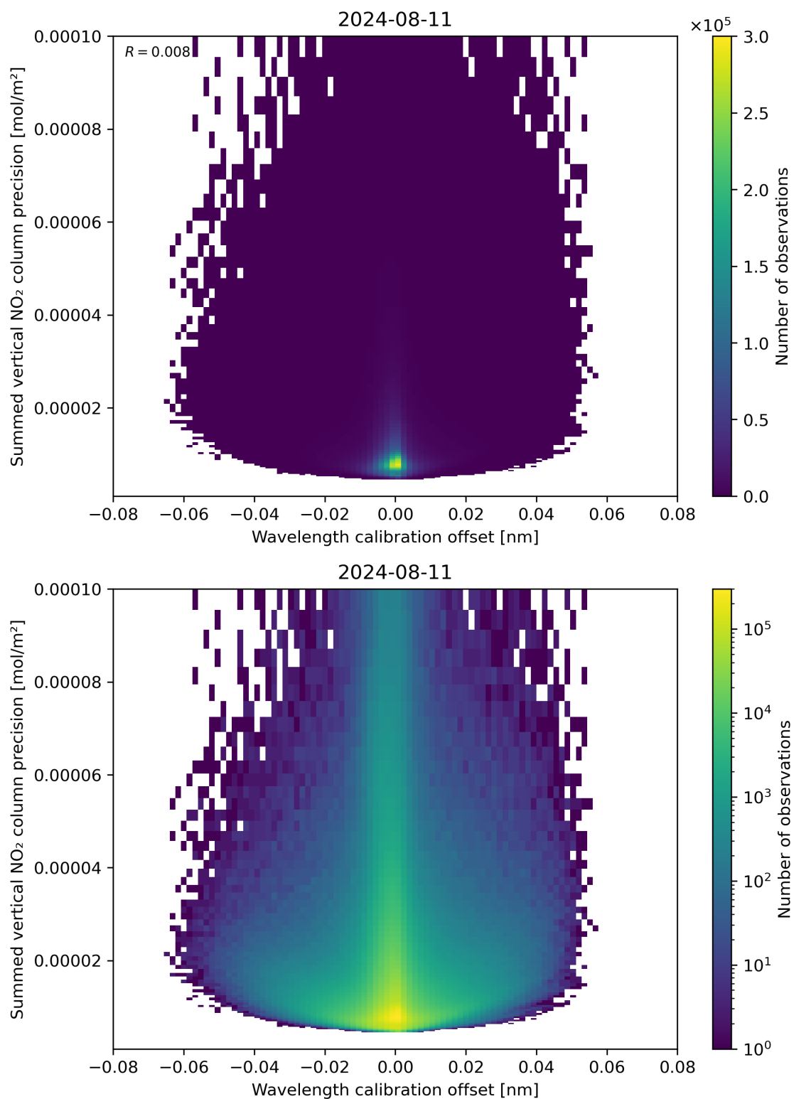
Figure 178: Scatter density plot of “Wavelength calibration offset” against “Summed vertical NO 2 column precision” for 2024-08-11 to 2024-08-11.
