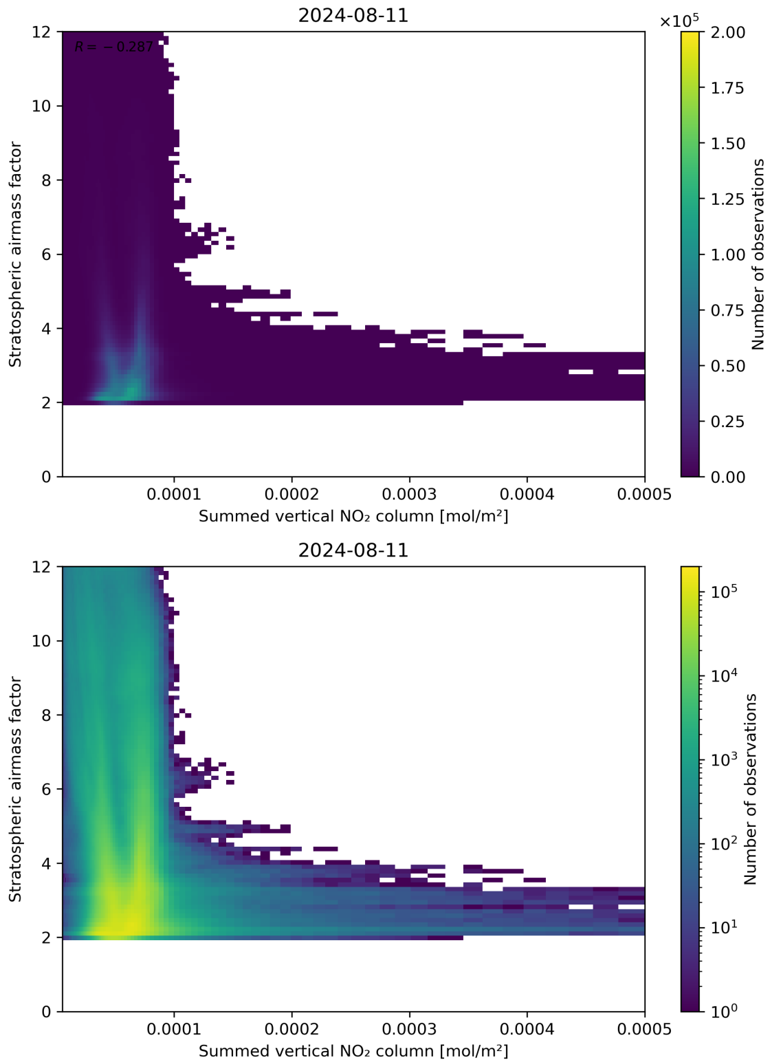
Figure 103: Scatter density plot of “Summed vertical NO 2 column” against “Stratospheric airmass factor” for 2024-08-11 to 2024-08-11.
