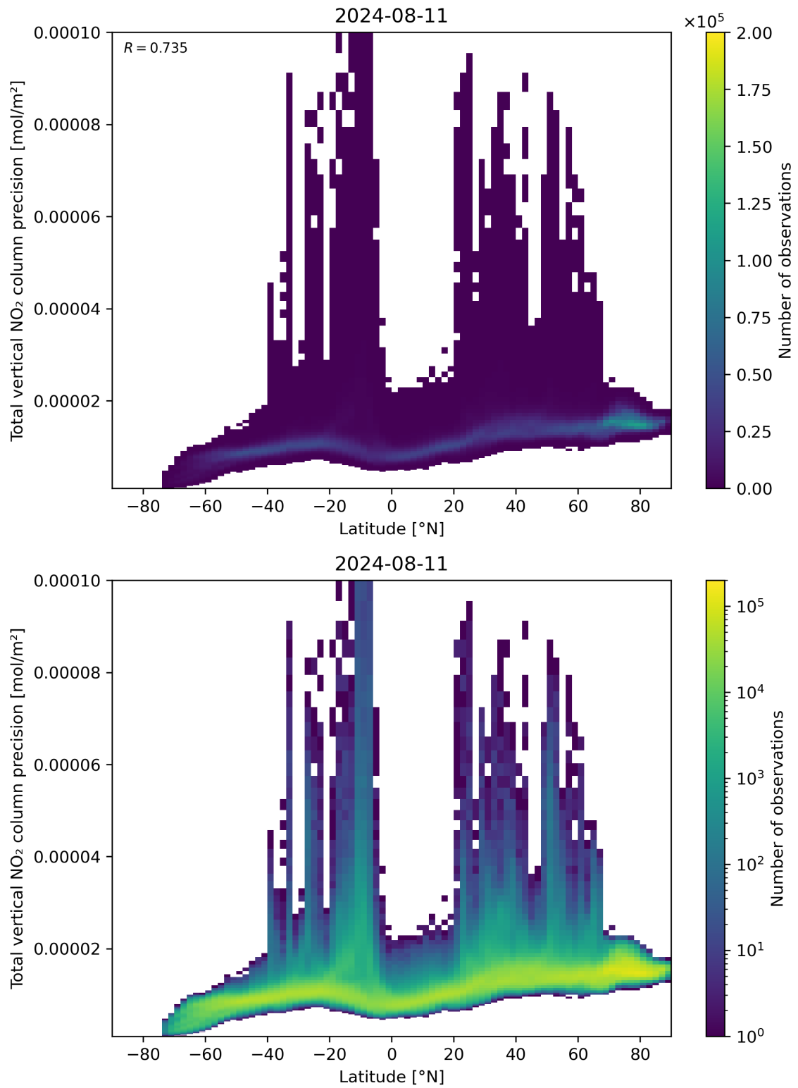
Figure 91: Scatter density plot of “Latitude” against “Total vertical NO 2 column precision” for 2024-08-11 to 2024-08-11.
