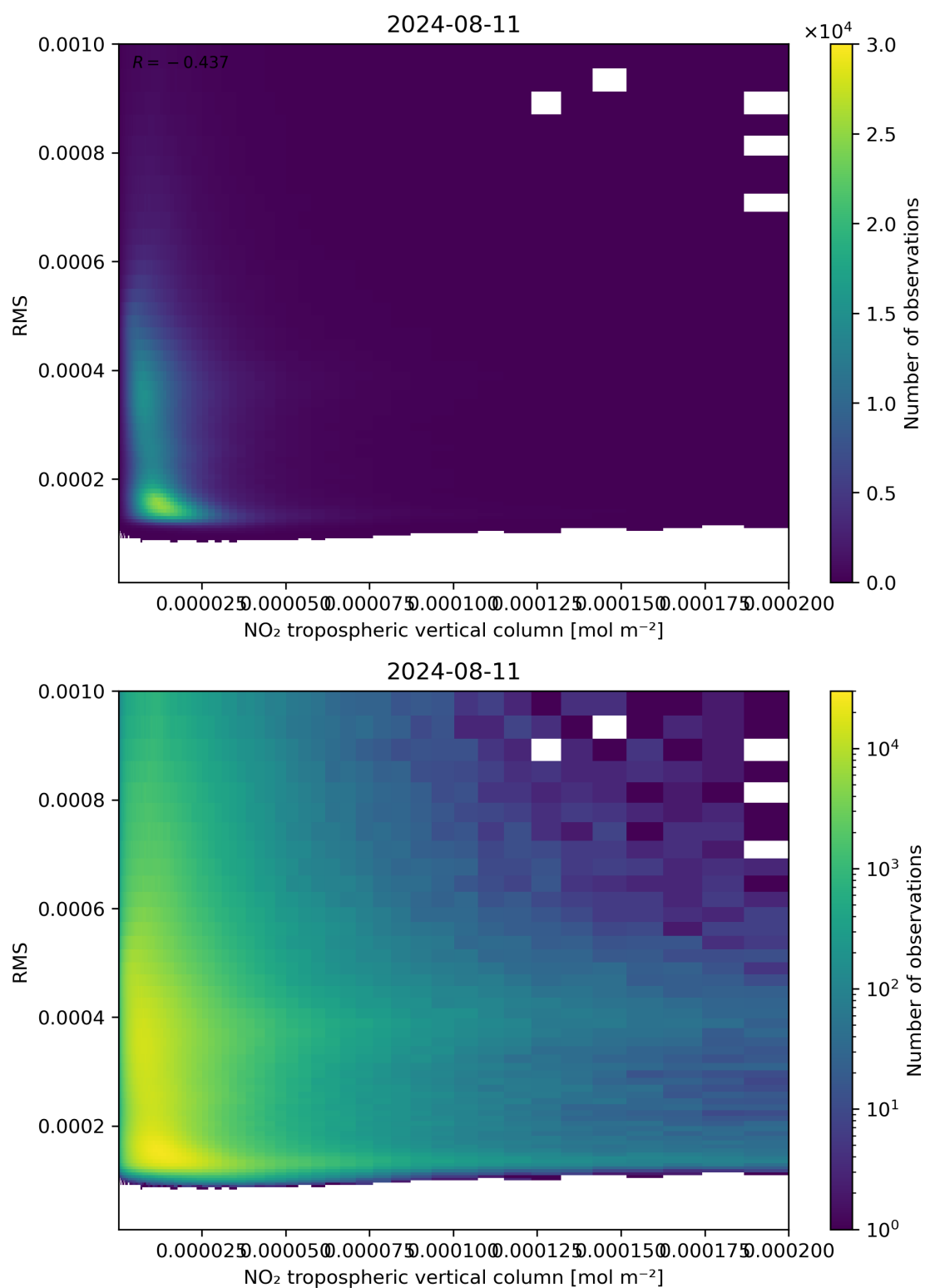
Figure 142: Scatter density plot of “NO 2 tropospheric vertical column” against “RMS” for 2024-08-11 to 2024-08-11.
