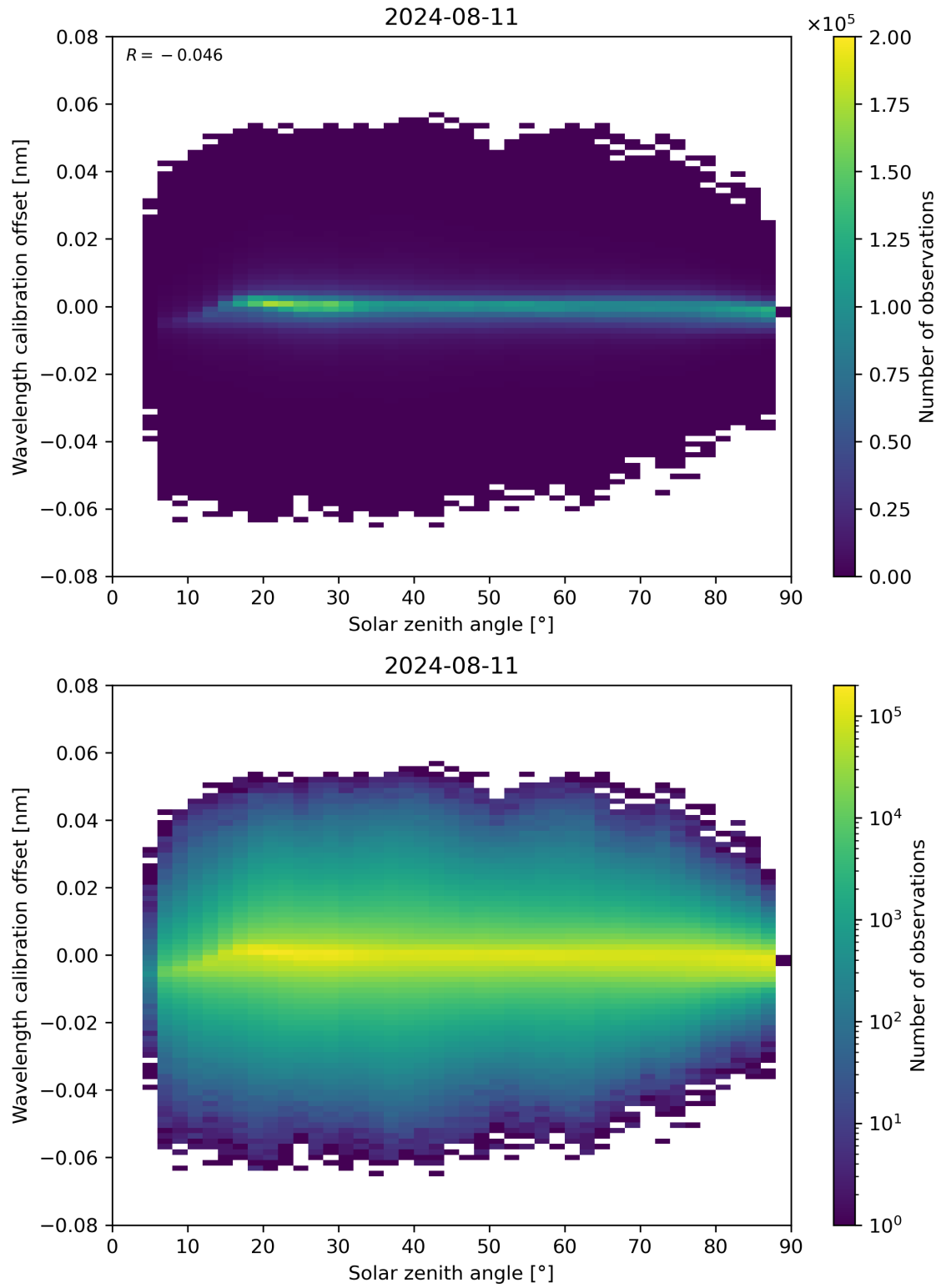
Figure 158: Scatter density plot of “Solar zenith angle” against “Wavelength calibration offset” for 2024-08-11 to 2024-08-11.
