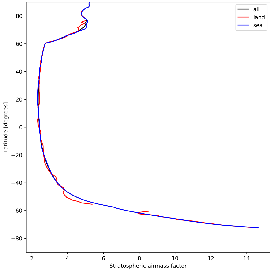
Figure 27: Zonal average of “Stratospheric air mass factor” for 2024-08-11 to 2024-08-11.
