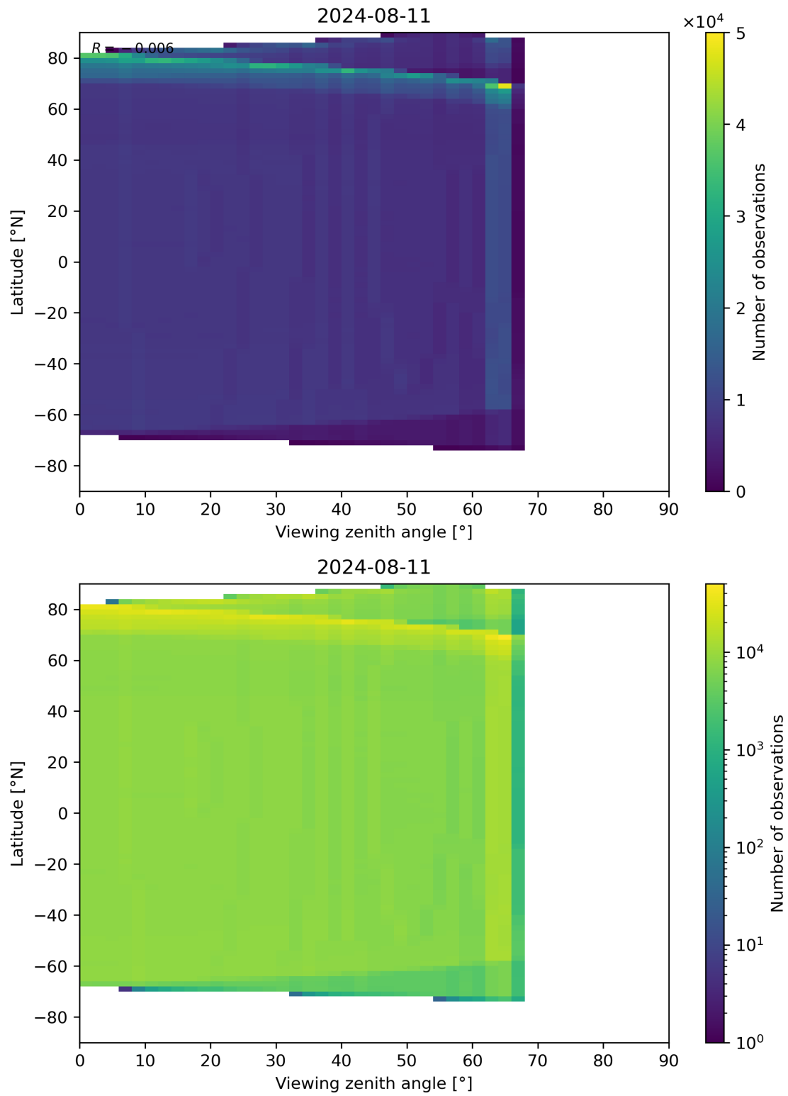
Figure 163: Scatter density plot of “Viewing zenith angle” against “Latitude” for 2024-08-11 to 2024-08-11.
