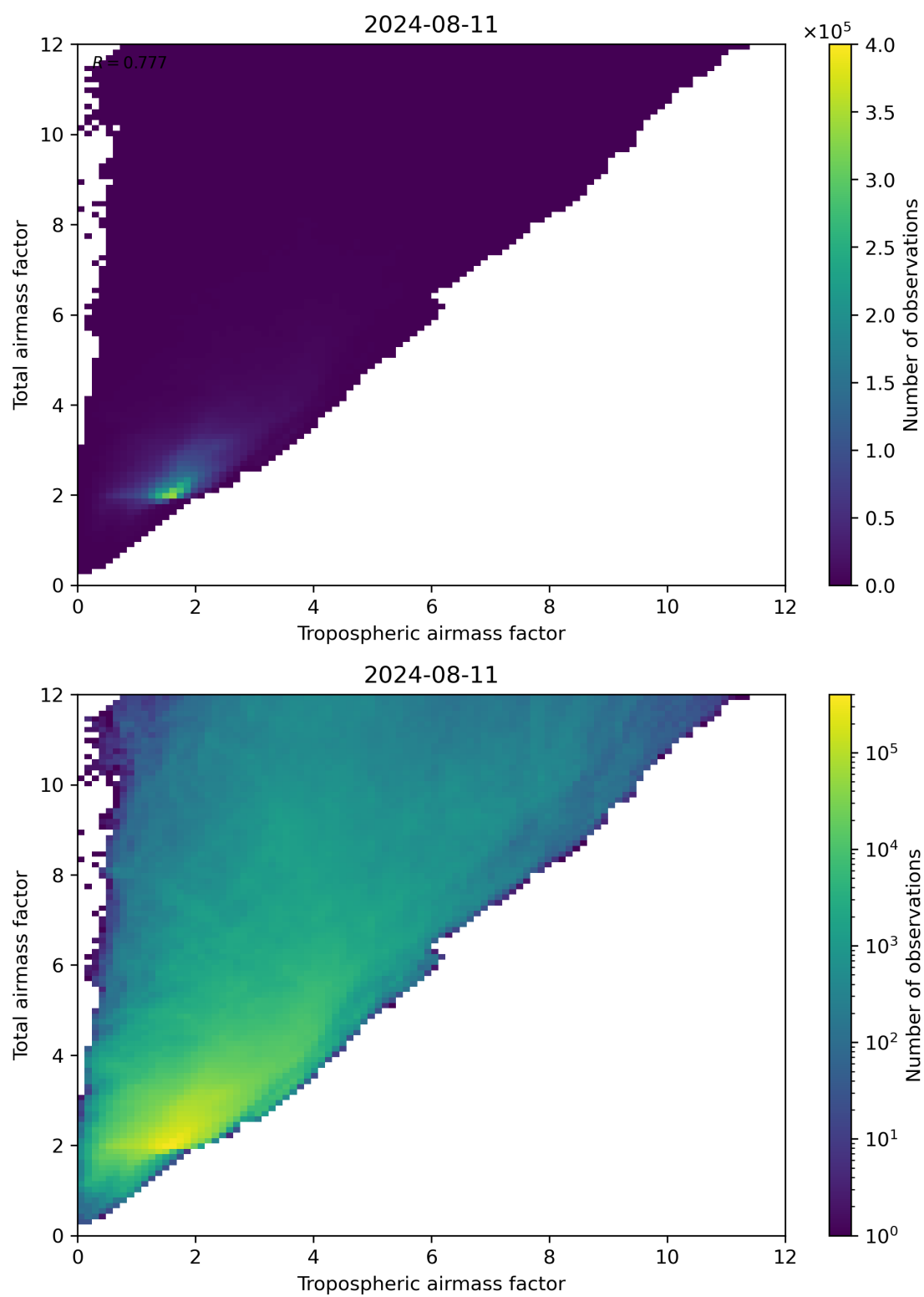
Figure 72: Scatter density plot of “Tropospheric airmass factor” against “Total airmass factor” for 2024-08-11 to 2024-08-11.
