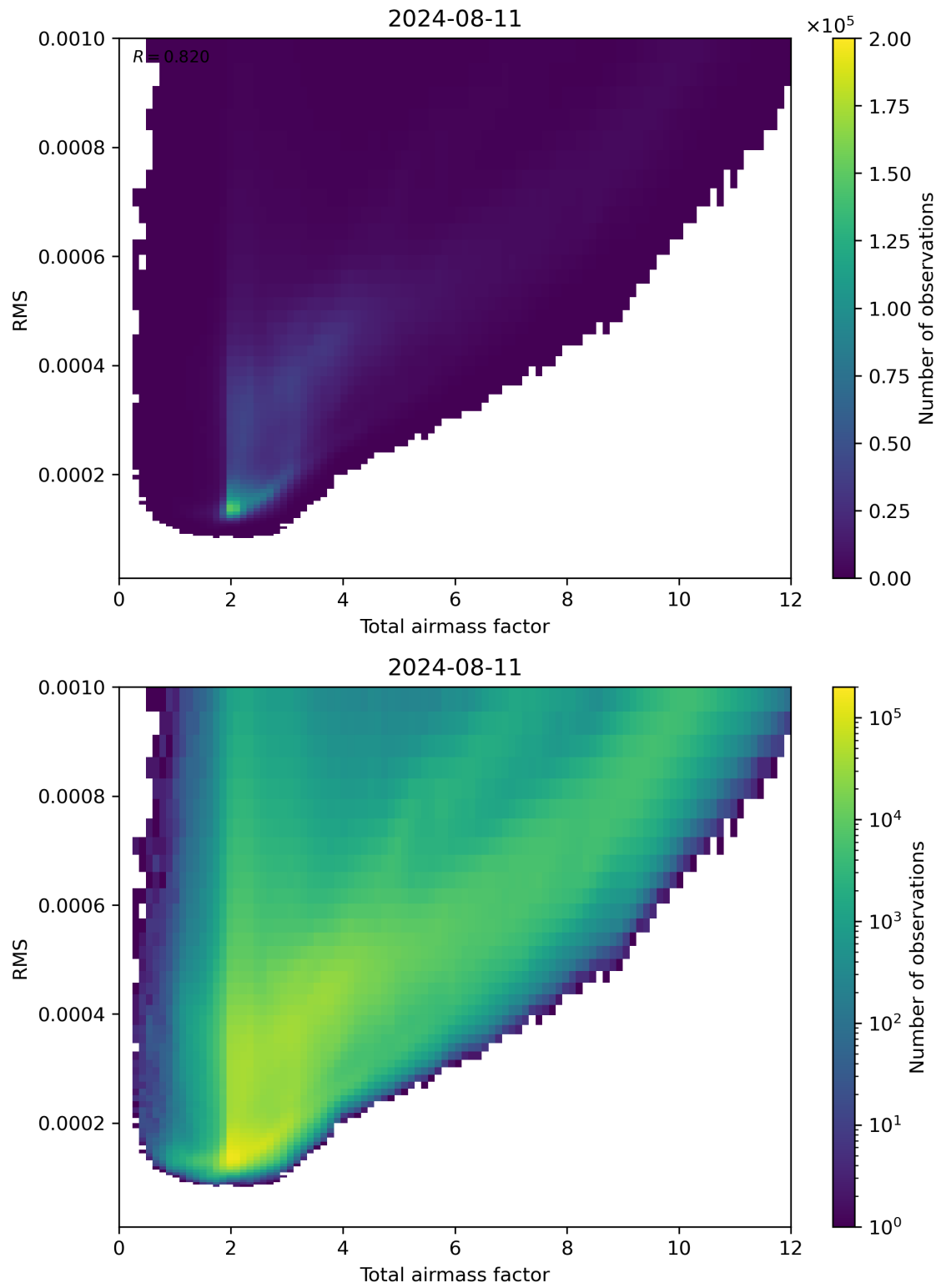
Figure 69: Scatter density plot of “Total airmass factor” against “RMS” for 2024-08-11 to 2024-08-11.
