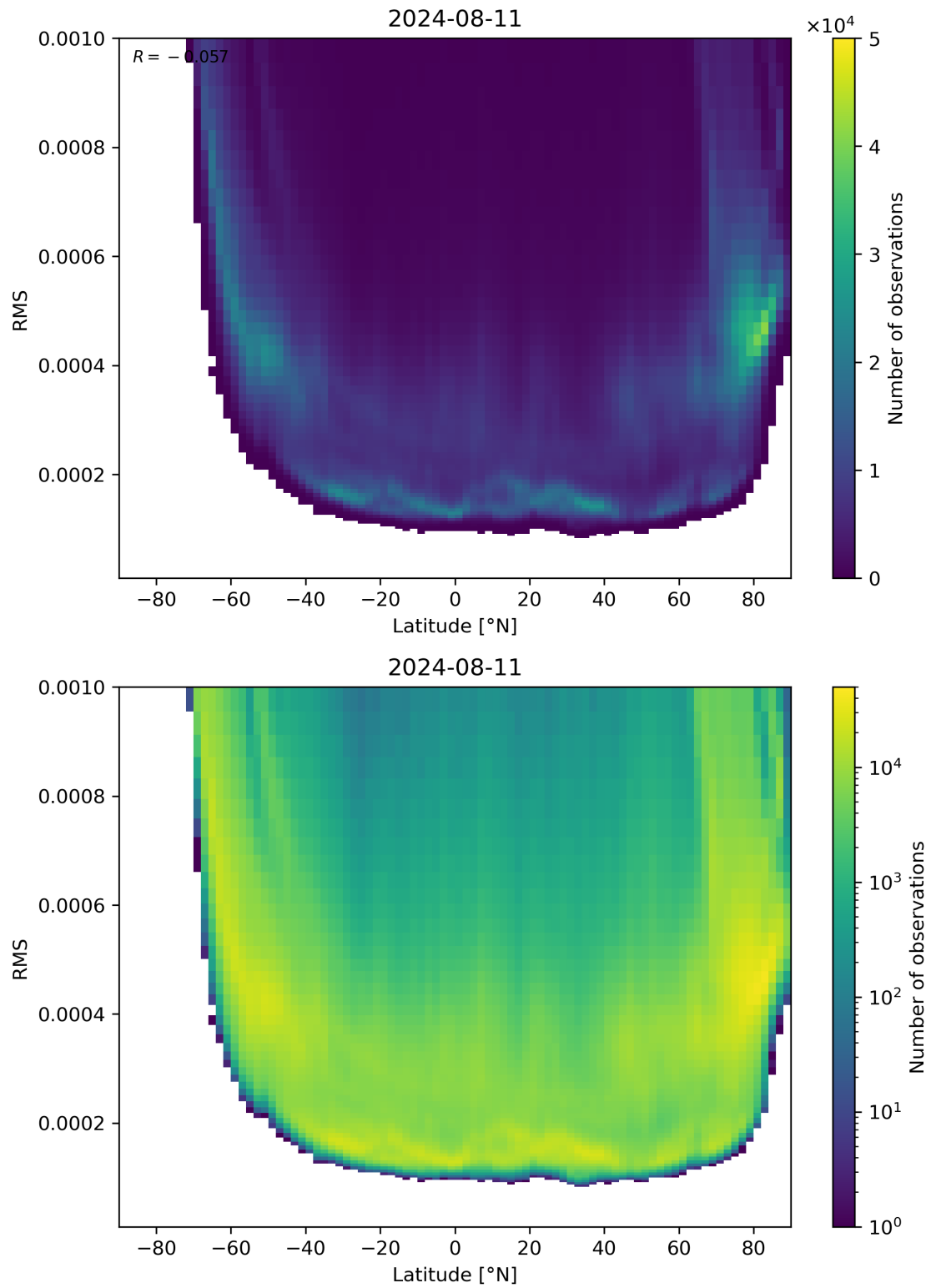
Figure 94: Scatter density plot of “Latitude” against “RMS” for 2024-08-11 to 2024-08-11.
