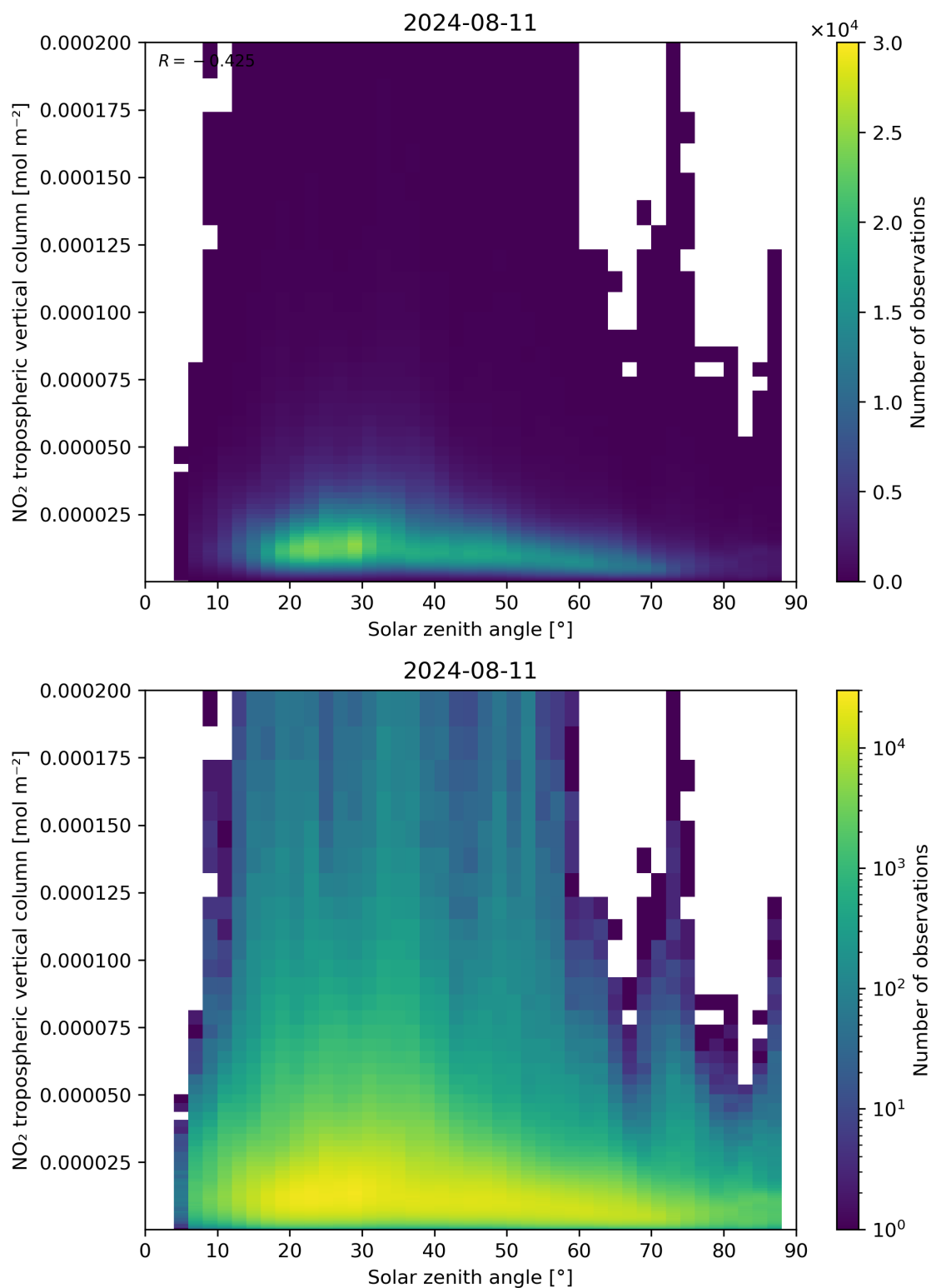
Figure 155: Scatter density plot of “Solar zenith angle” against “NO 2 tropospheric vertical column” for 2024-08-11 to 2024-08-11.
