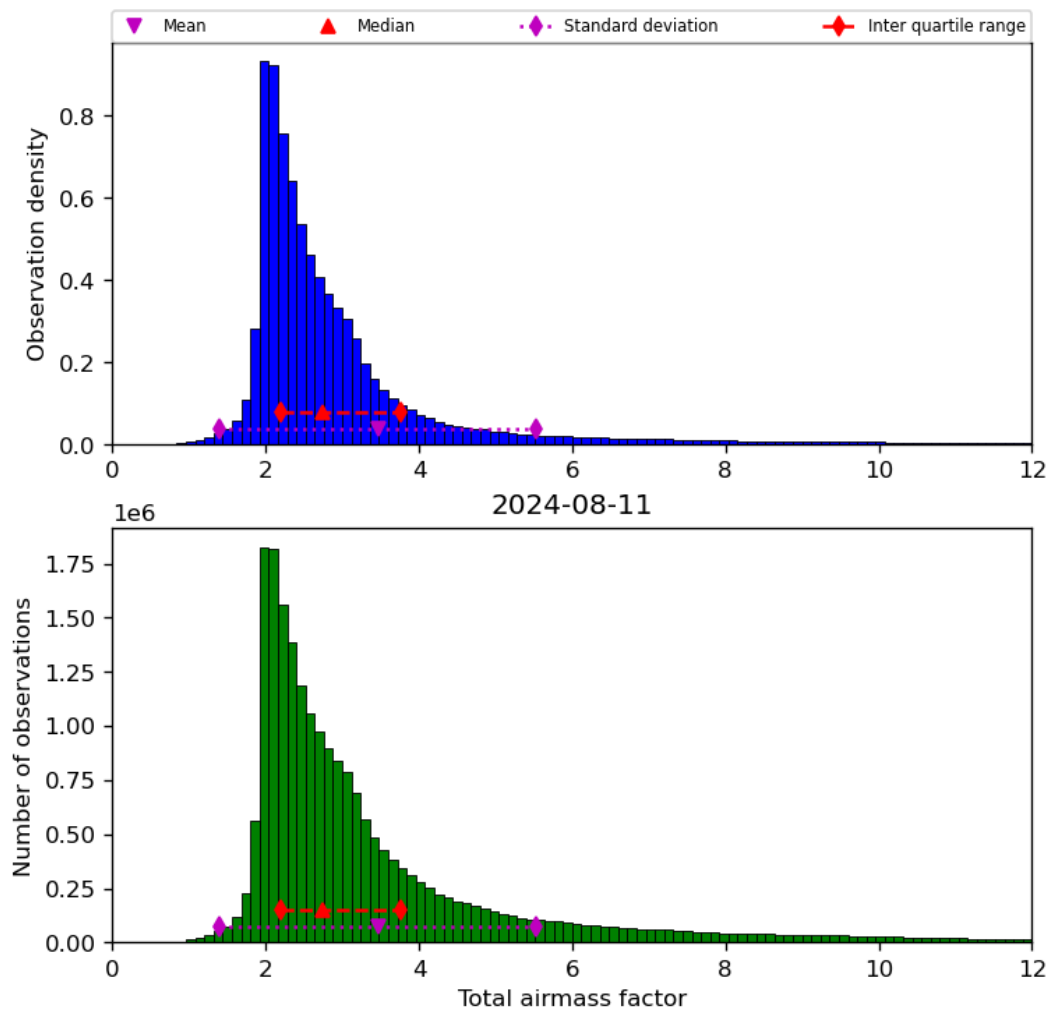
Figure 32: Histogram of “Total airmass factor” for 2024-08-11 to 2024-08-11
