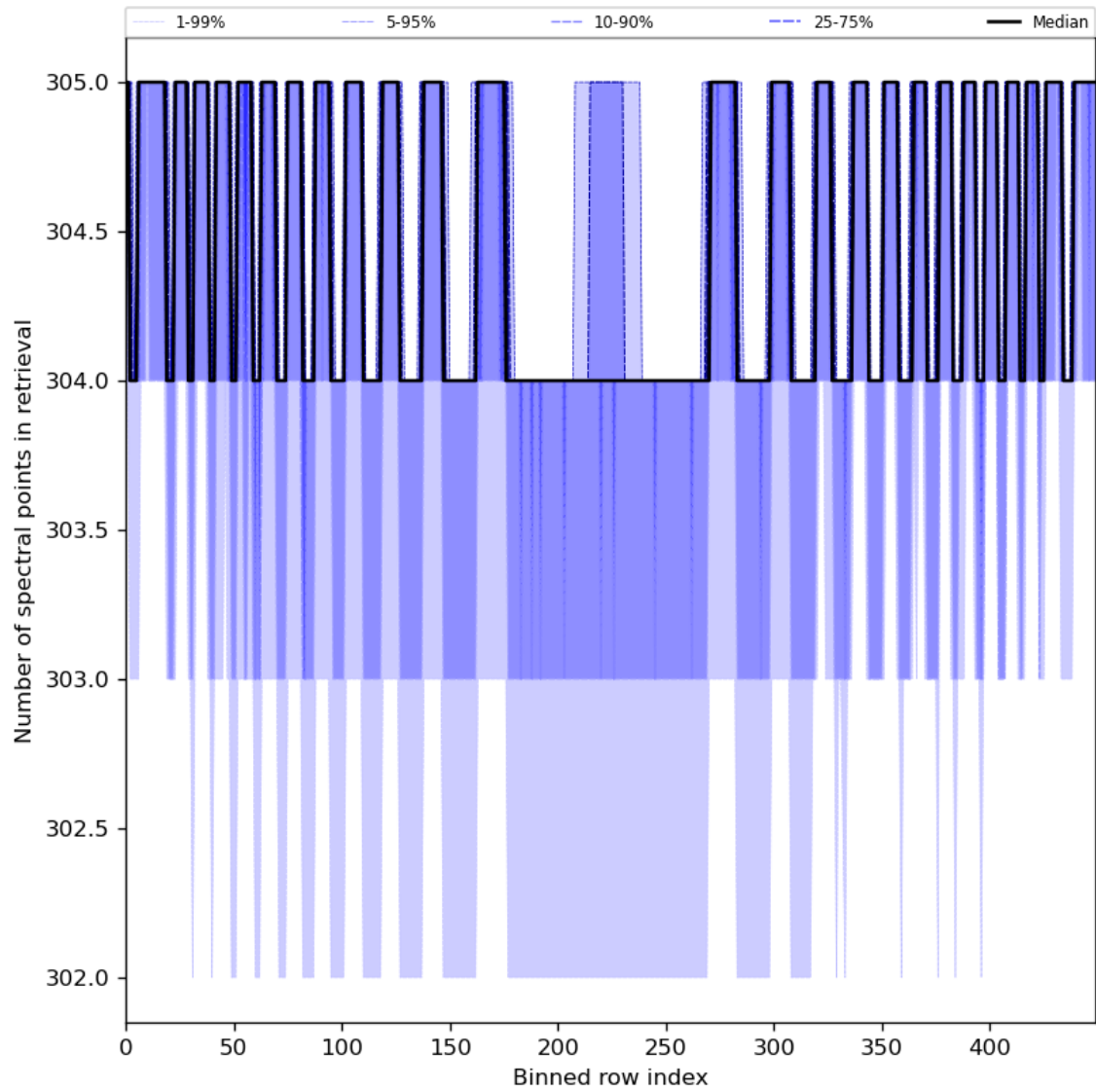
Figure 50: Along track statistics of “Number of spectral points in retrieval” for 2024-08-11 to 2024-08-11
