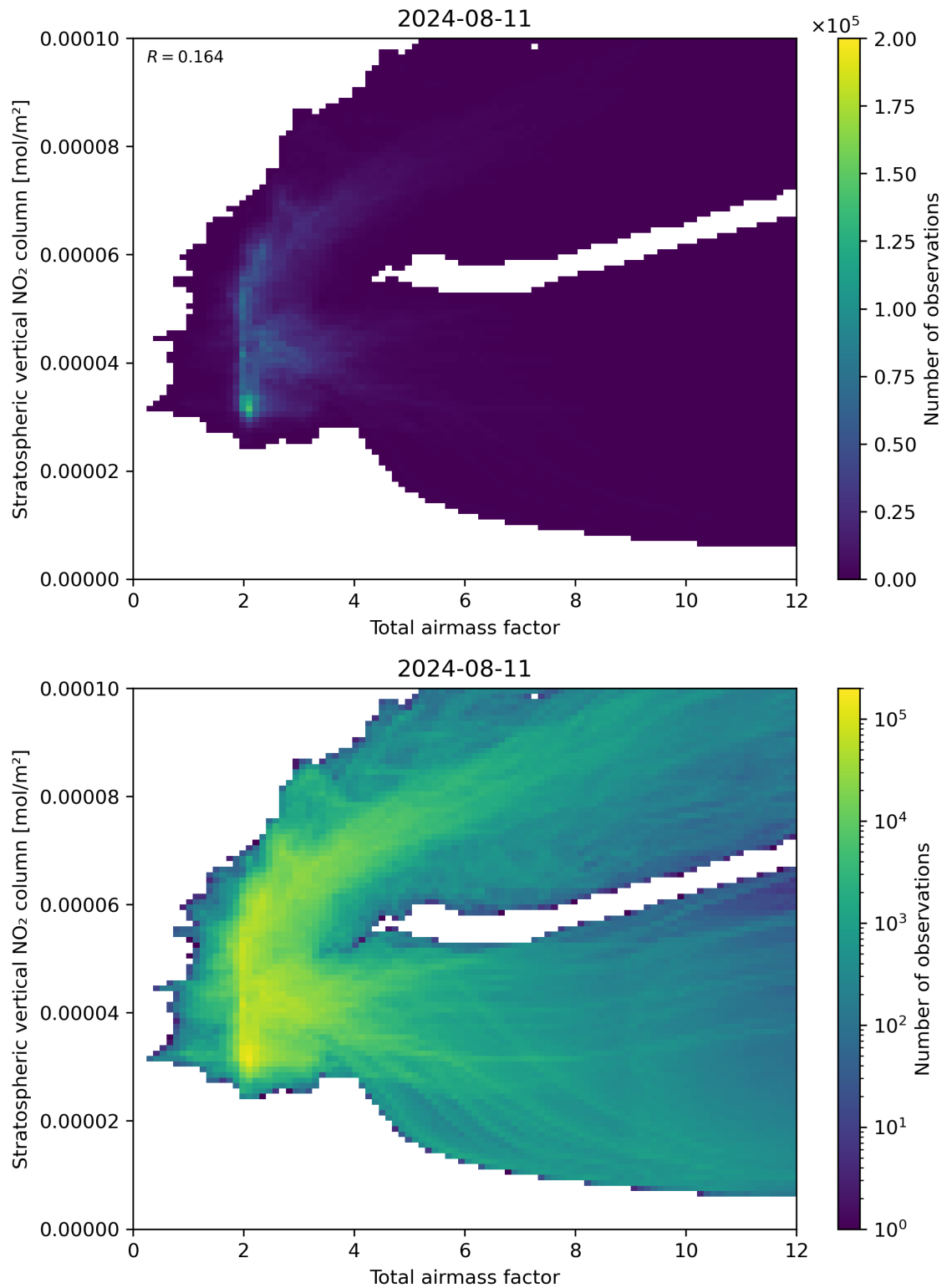
Figure 64: Scatter density plot of “Total airmass factor” against “Stratospheric vertical NO 2 column” for 2024-08-11 to 2024-08-11.
