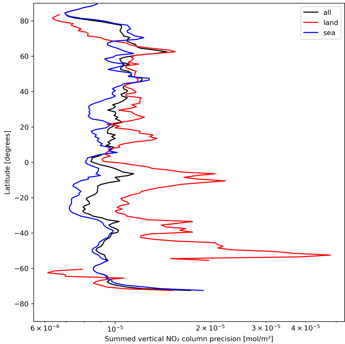
Figure 24: Zonal average of “Summed vertical NO 2 column precision” for 2024-08-11 to 2024-08-11.
