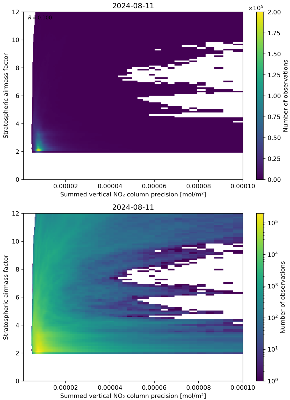
Figure 106: Scatter density plot of “Summed vertical NO 2 column precision” against “Stratospheric airmass factor” for 2024-08-11 to 2024-08-11.
