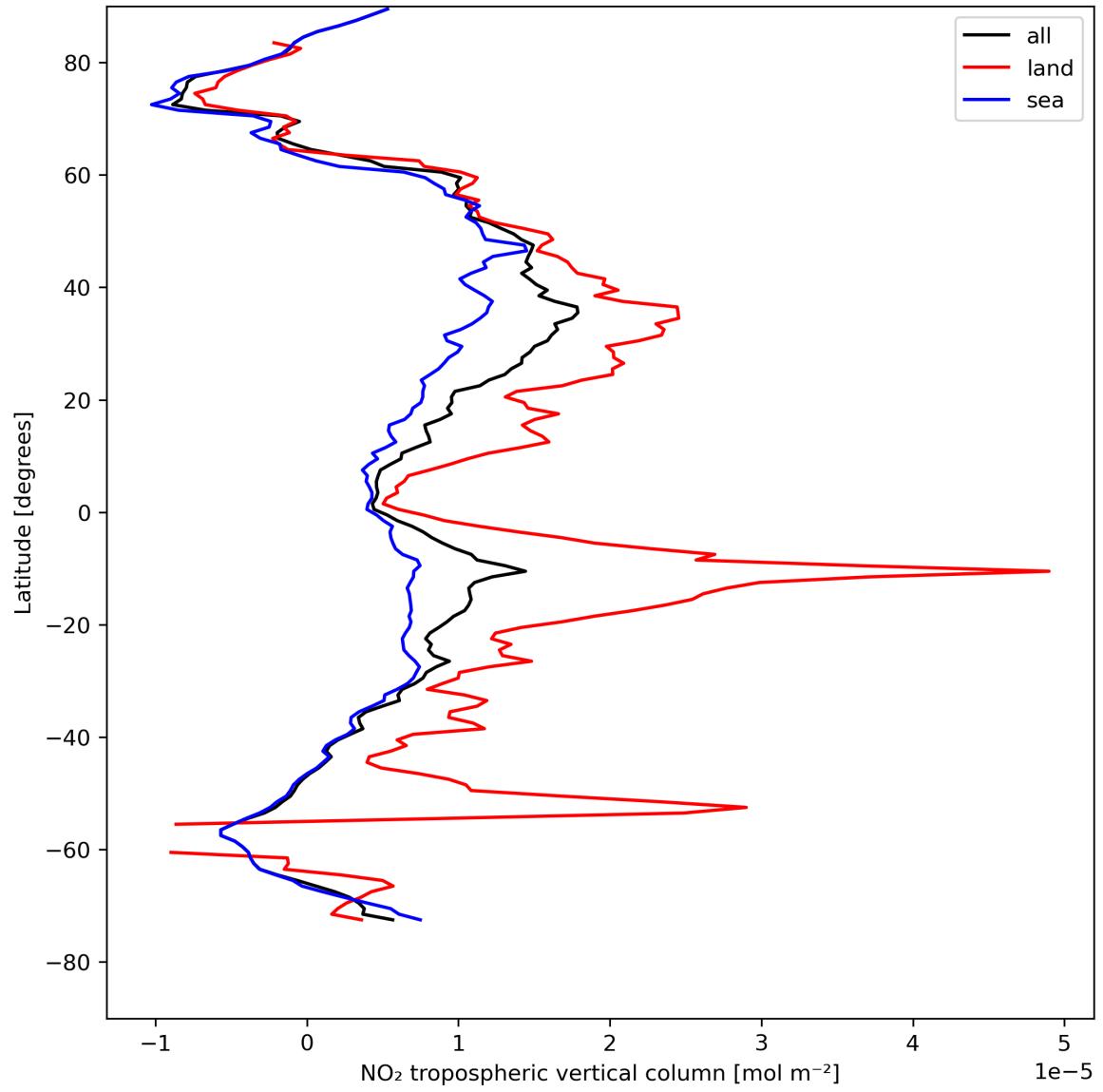
Figure 12: Zonal average of “NO 2 tropospheric vertical column” for 2024-08-11 to 2024-08-11.
