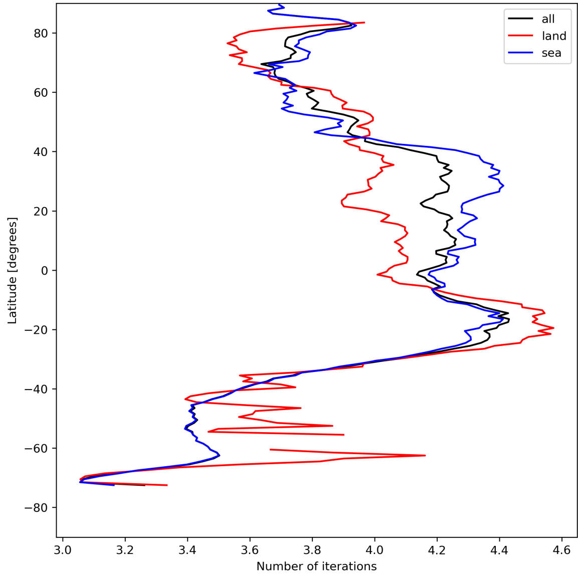
Figure 17: Zonal average of “Number of iterations” for 2024-08-11 to 2024-08-11.
