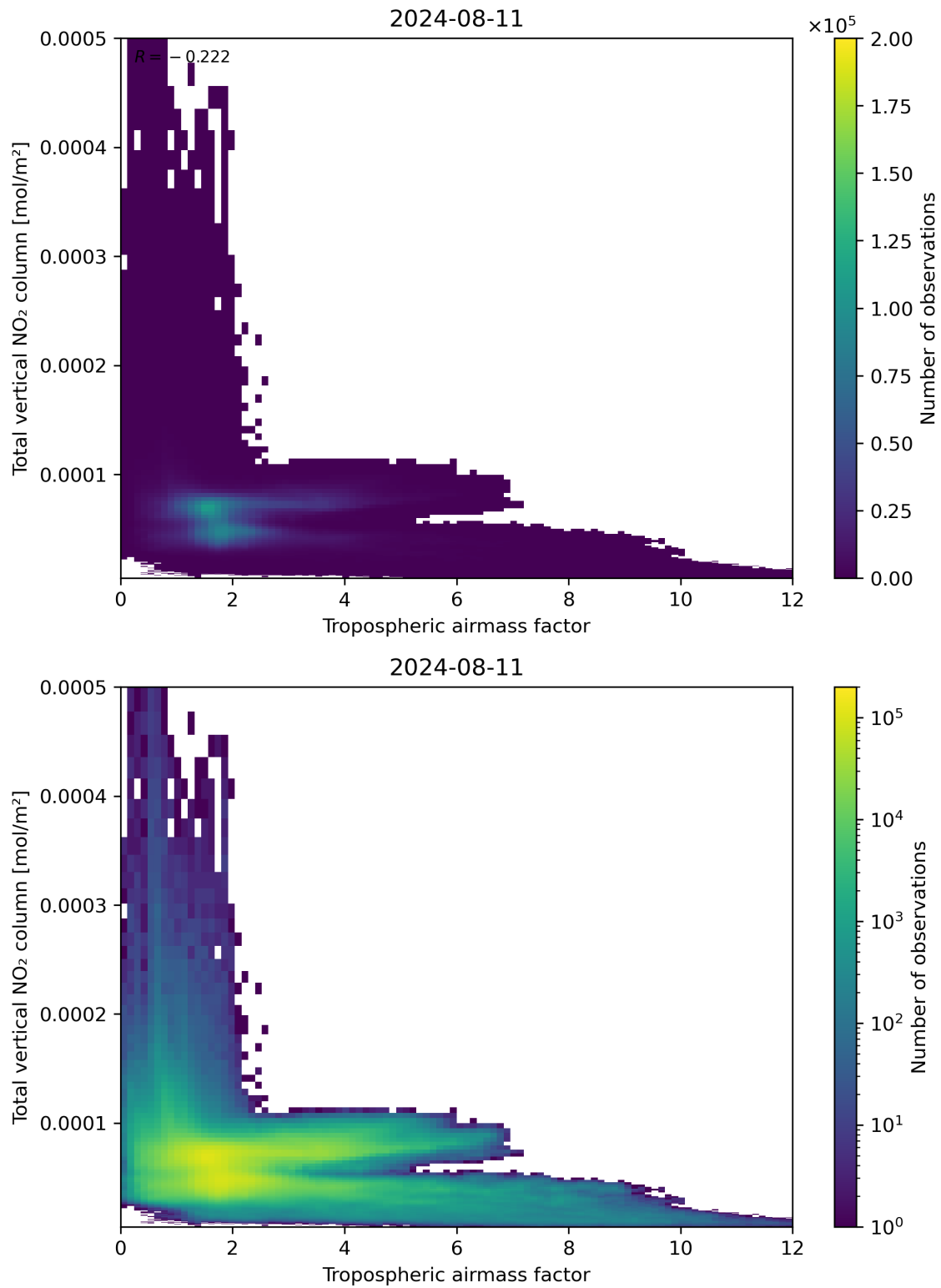
Figure 77: Scatter density plot of “Tropospheric airmass factor” against “Total vertical NO 2 column” for 2024-08-11 to 2024-08-11.
