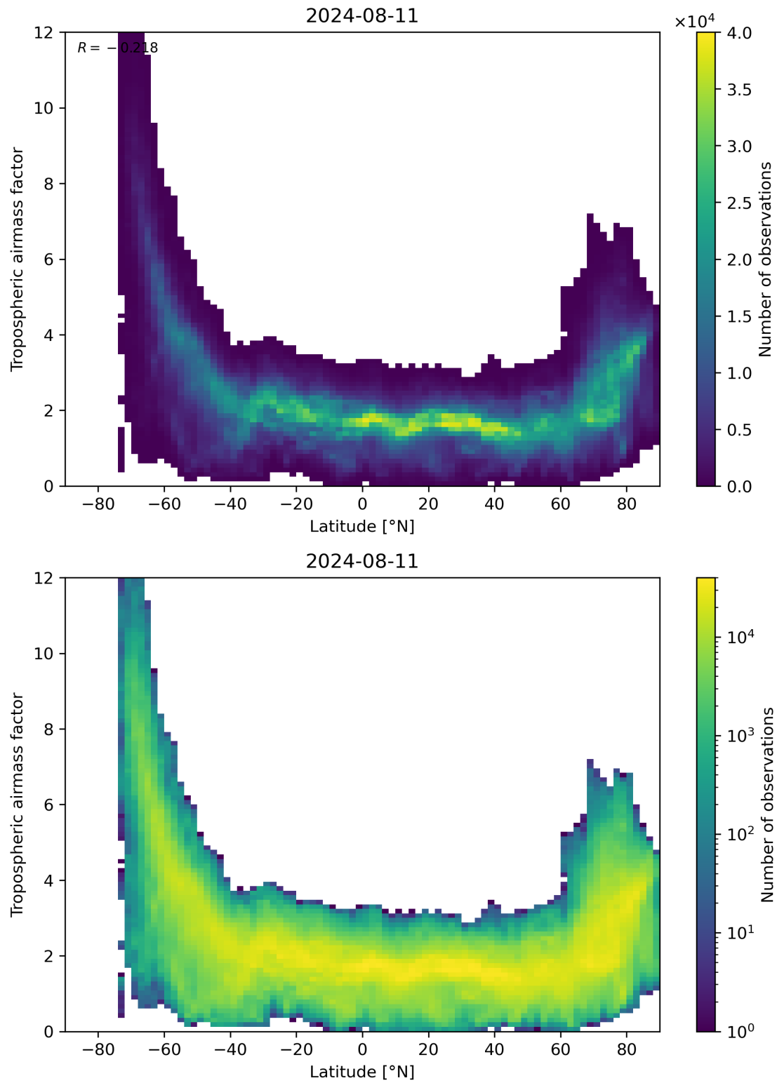
Figure 85: Scatter density plot of “Latitude” against “Tropospheric airmass factor” for 2024-08-11 to 2024-08-11.
