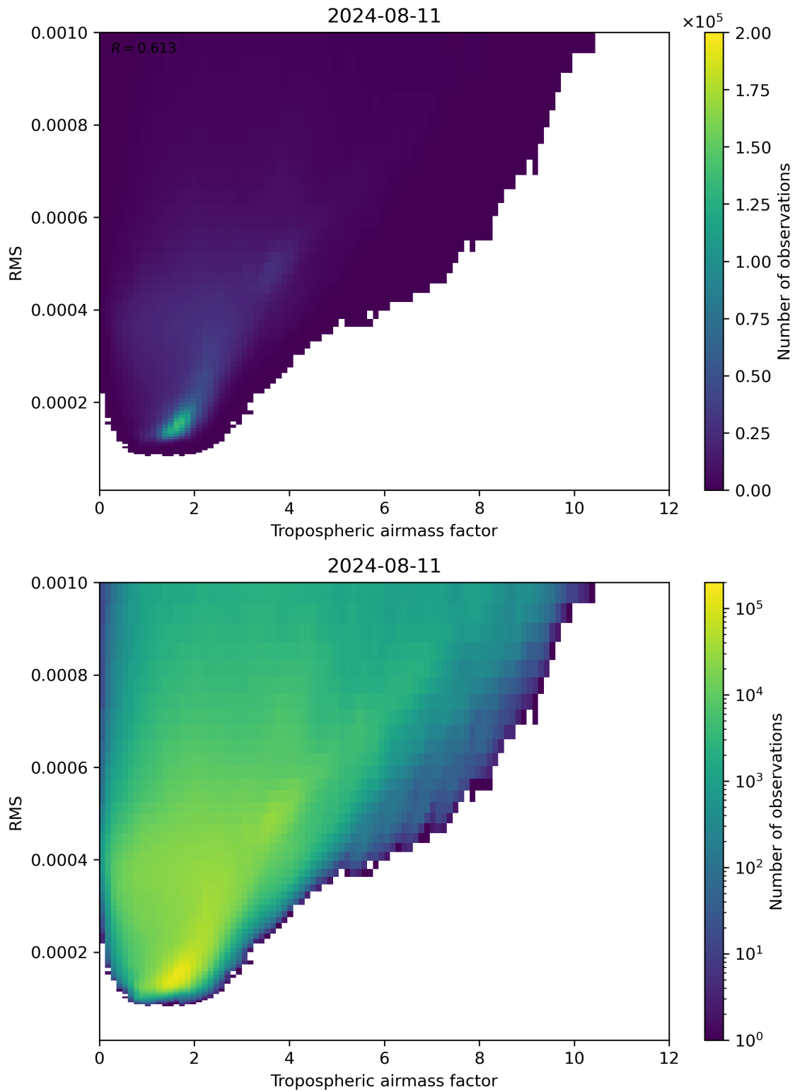
Figure 79: Scatter density plot of “Tropospheric airmass factor” against “RMS” for 2024-08-11 to 2024-08-11.
