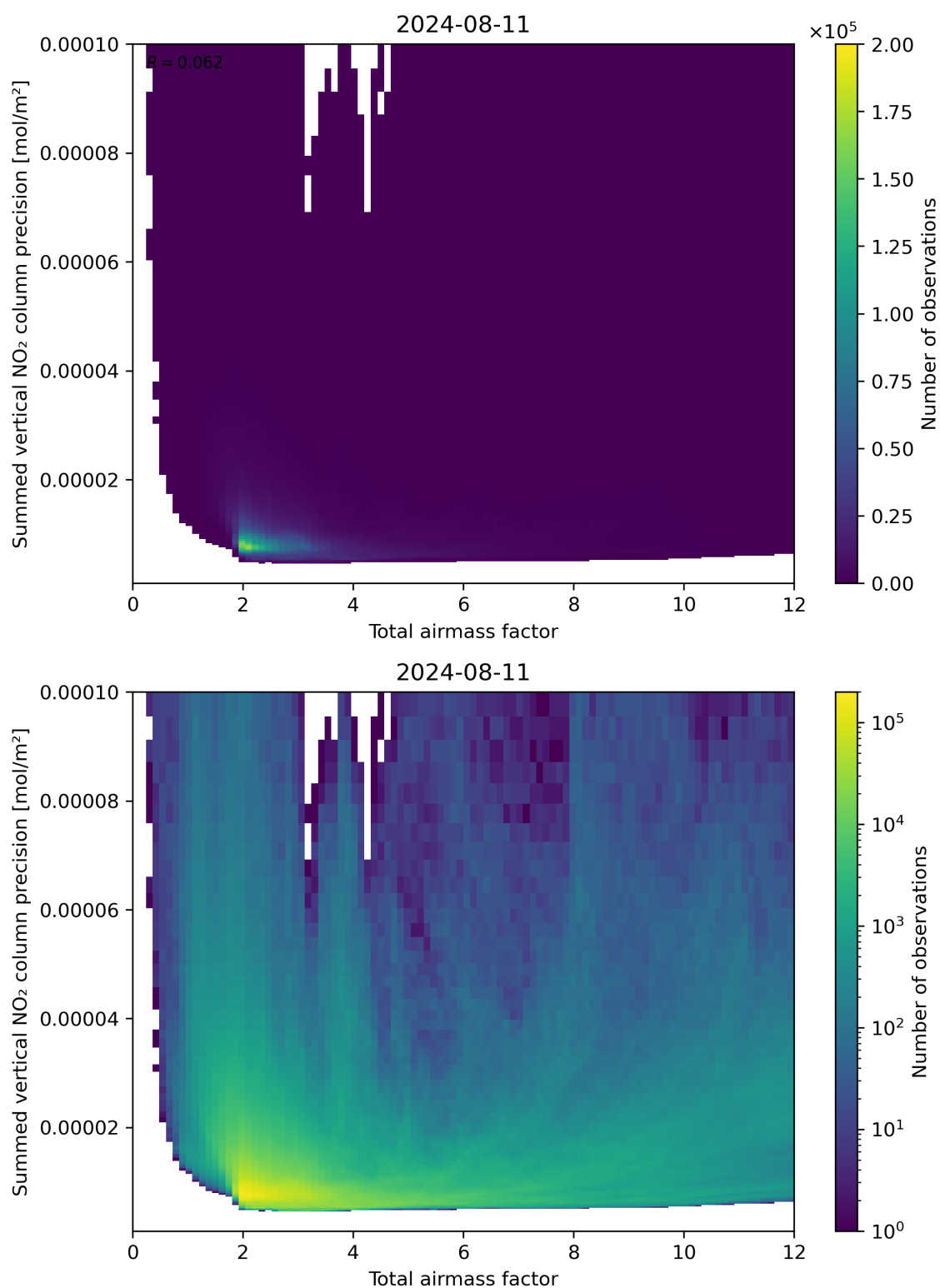
Figure 66: Scatter density plot of “Total airmass factor” against “Summed vertical NO 2 column precision” for 2024-08-11 to 2024-08-11.
