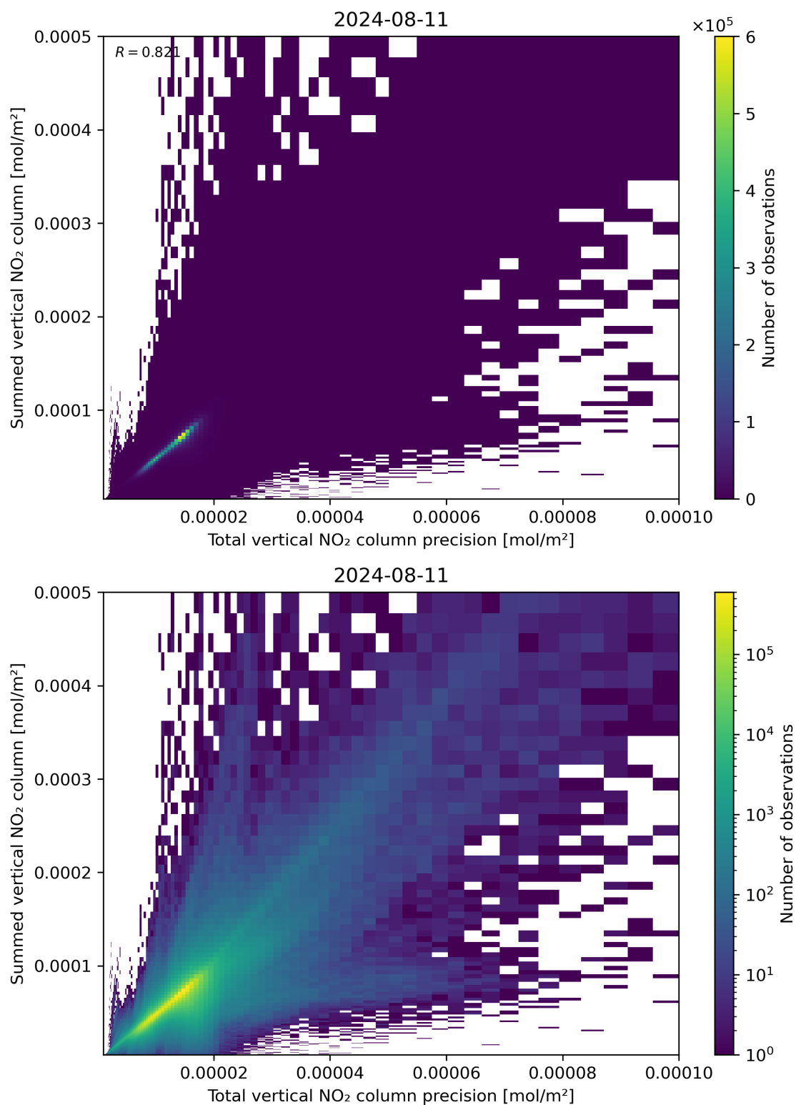
Figure 117: Scatter density plot of “Total vertical NO 2 column precision” against “Summed vertical NO 2 column” for 2024-08-11 to 2024-08-11.
