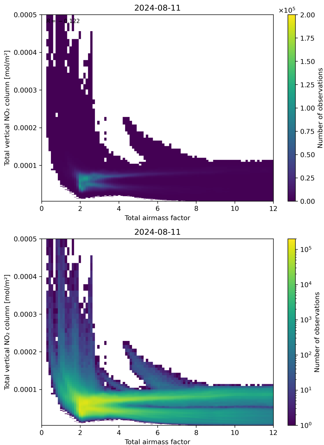
Figure 67: Scatter density plot of “Total airmass factor” against “Total vertical NO 2 column” for 2024-08-11 to 2024-08-11.
