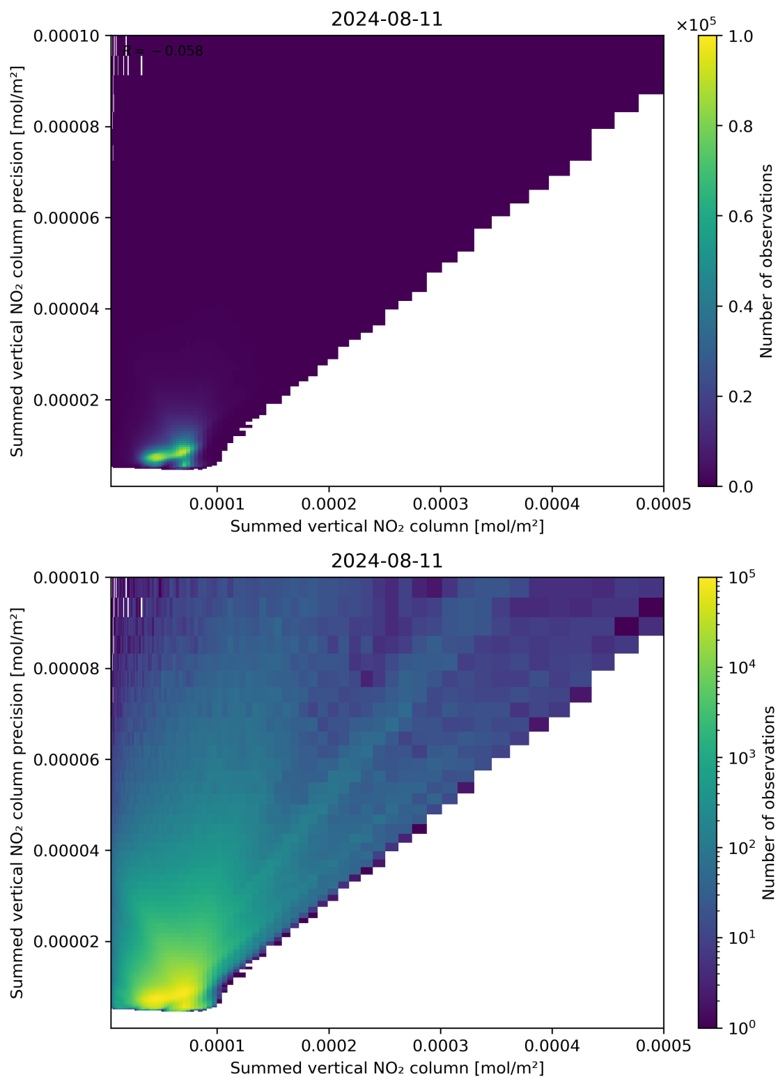
Figure 105: Scatter density plot of “Summed vertical NO 2 column” against “Summed vertical NO 2 column precision” for 2024-08-11 to 2024-08-11.
