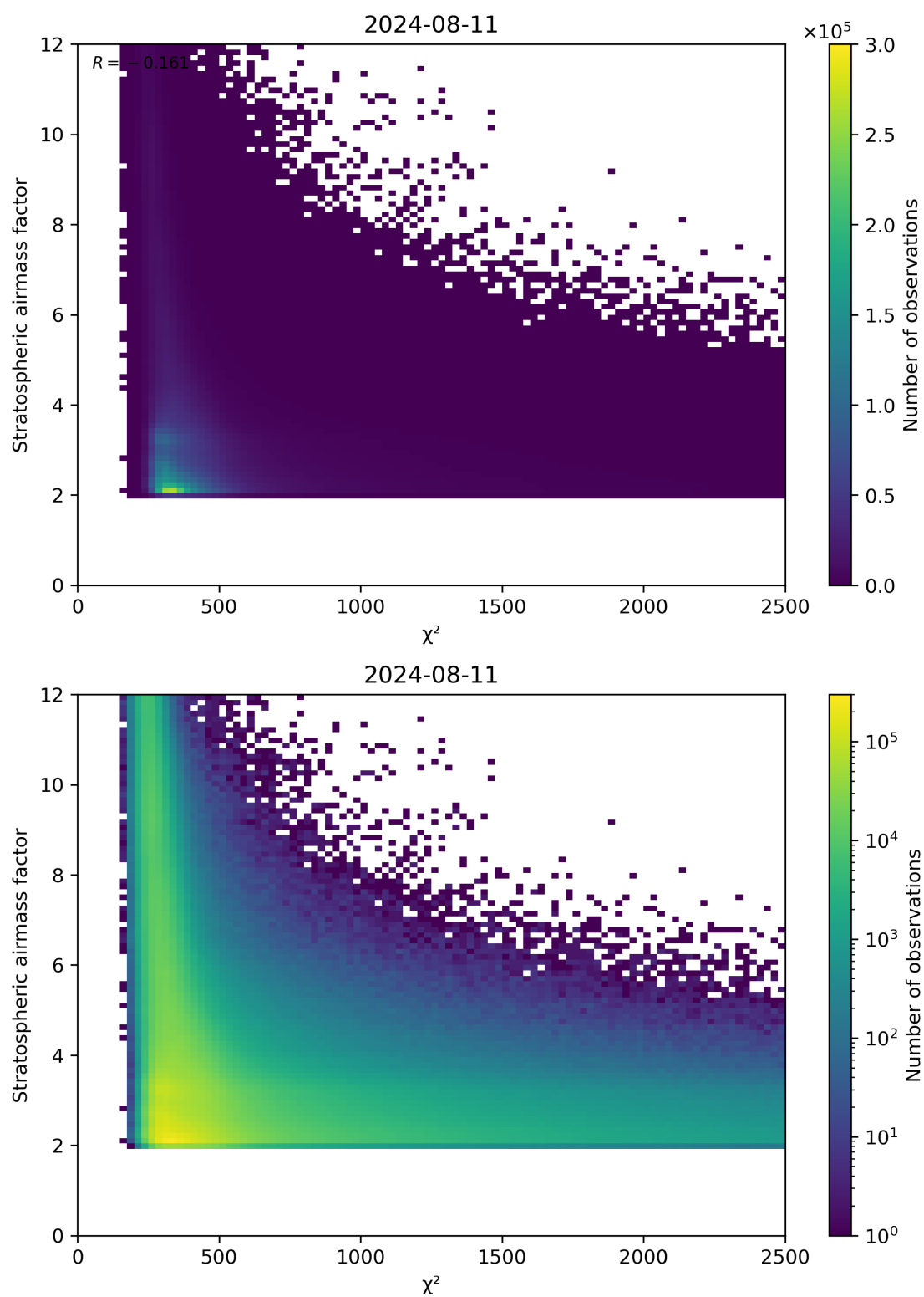
Figure 81: Scatter density plot of “ \chi^2 ” against “Stratospheric airmass factor” for 2024-08-11 to 2024-08-11.
