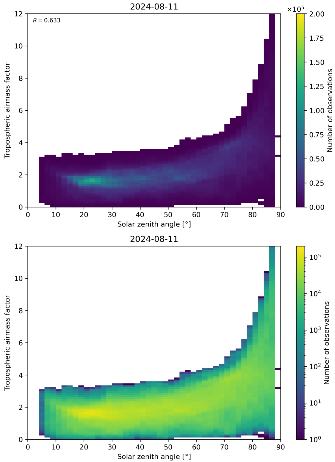
Figure 147: Scatter density plot of “Solar zenith angle” against “Tropospheric airmass factor” for 2024-08-11 to 2024-08-11.
