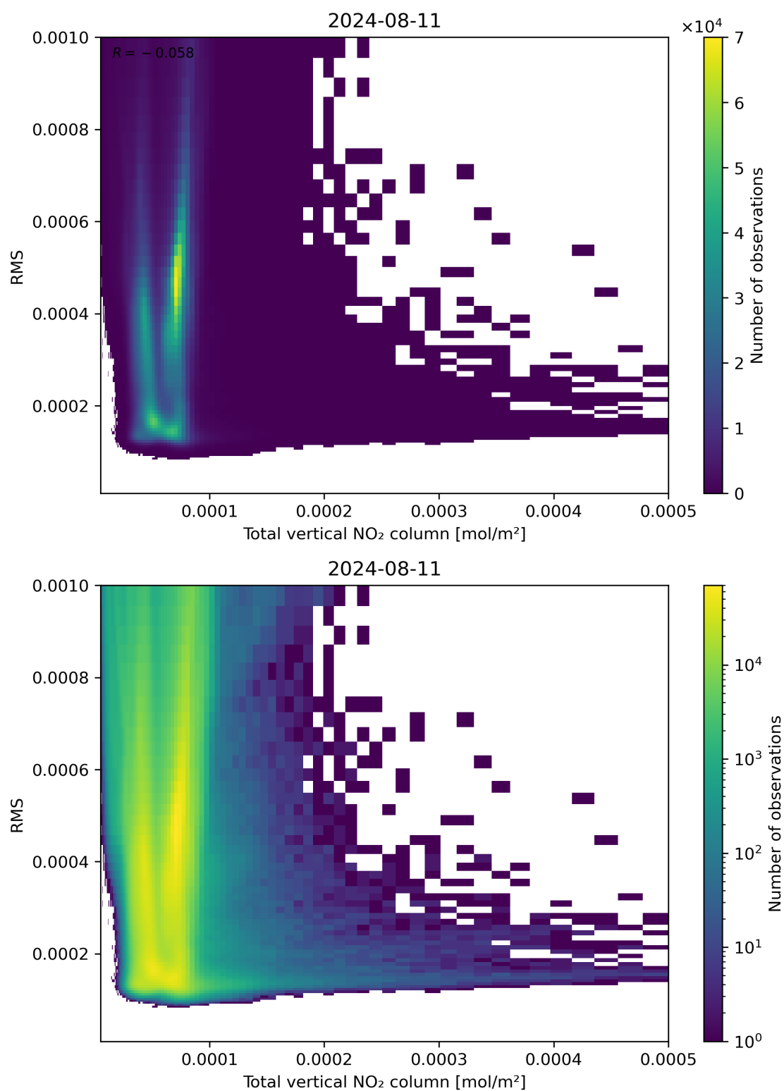
Figure 120: Scatter density plot of “Total vertical NO 2 column” against “RMS” for 2024-08-11 to 2024-08-11.
