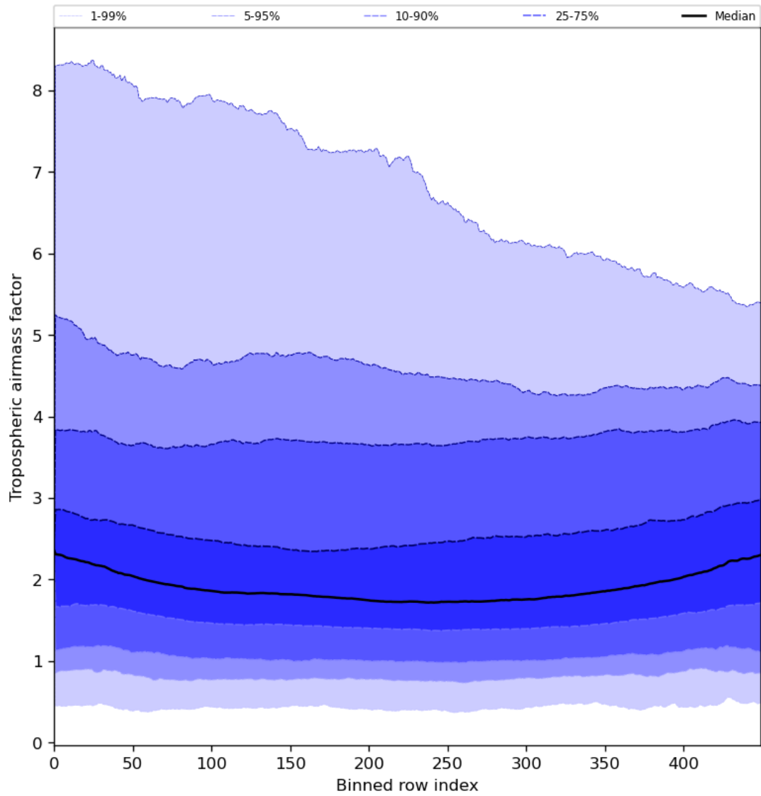
Figure 48: Along track statistics of “Tropospheric airmass factor” for 2024-08-11 to 2024-08-11
