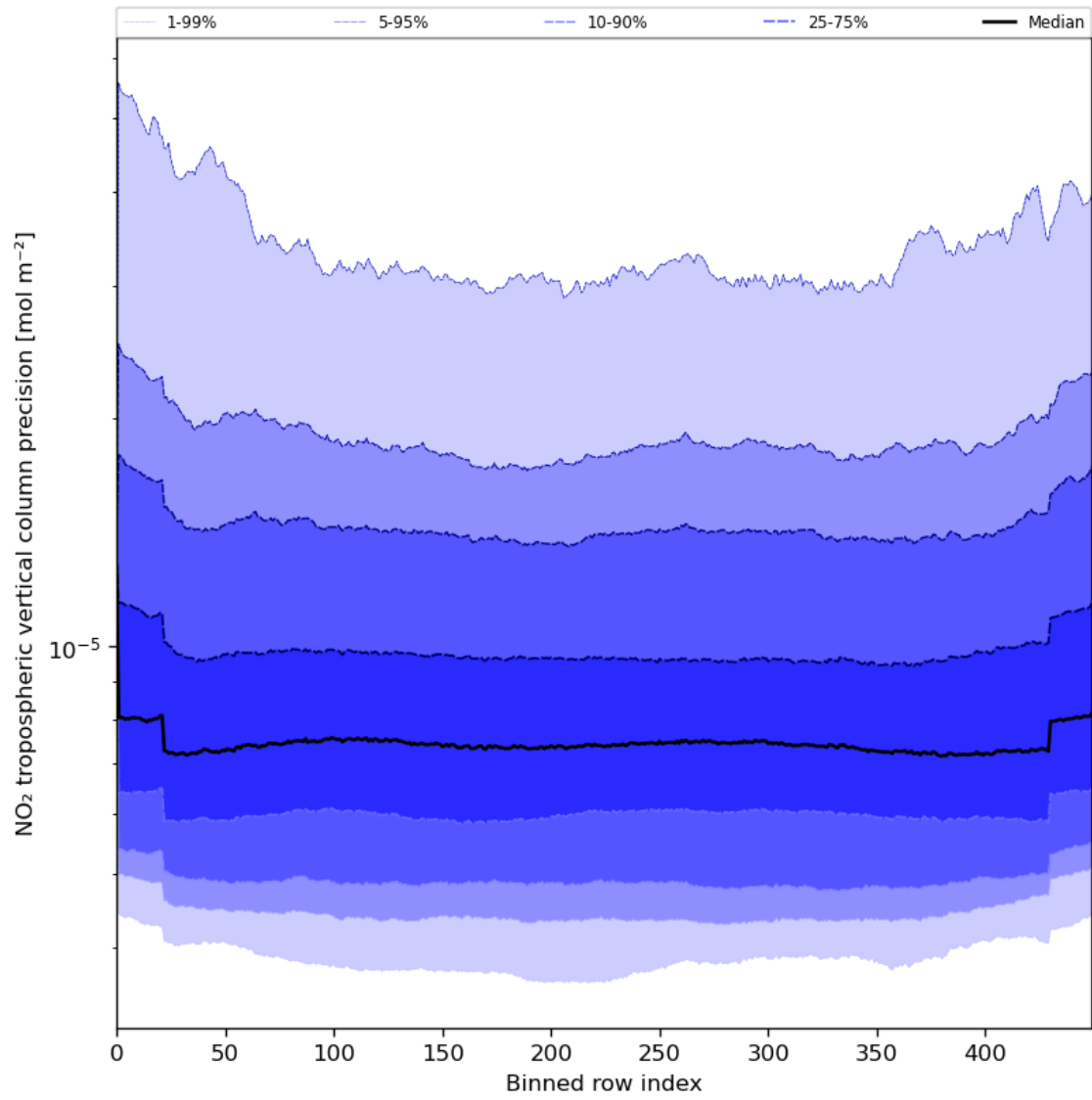
Figure 47: Along track statistics of “NO 2 tropospheric vertical column precision” for 2024-08-11 to 2024-08-11
