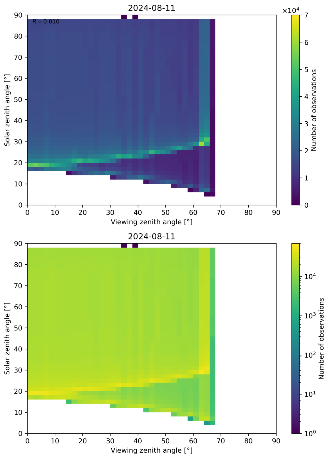
Figure 172: Scatter density plot of “Viewing zenith angle” against “Solar zenith angle” for 2024-08-11 to 2024-08-11.
