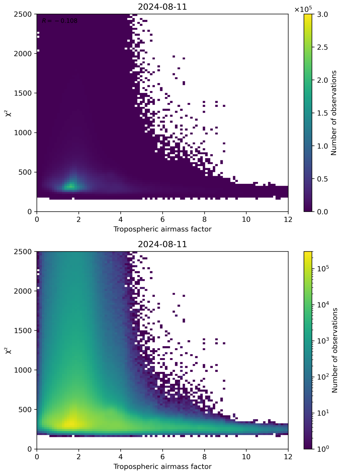
Figure 73: Scatter density plot of “Tropospheric airmass factor” against “ \chi^2 ” for 2024-08-11 to 2024-08-11.
