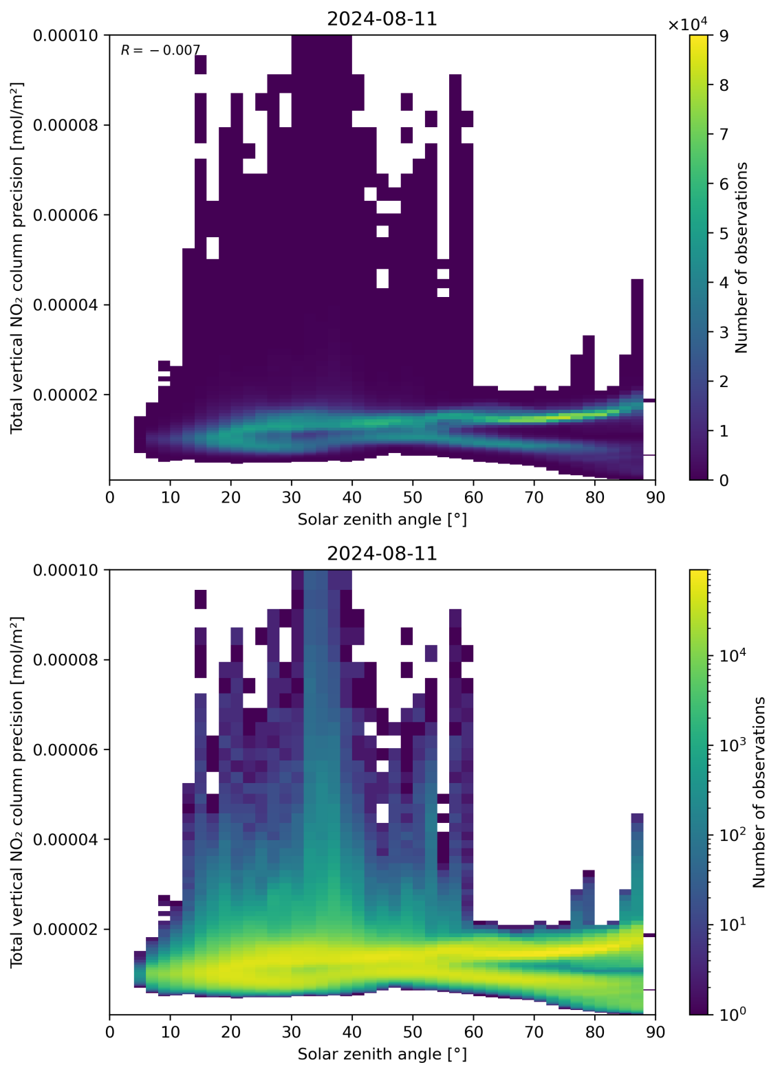
Figure 154: Scatter density plot of “Solar zenith angle” against “Total vertical NO 2 column precision” for 2024-08-11 to 2024-08-11.
