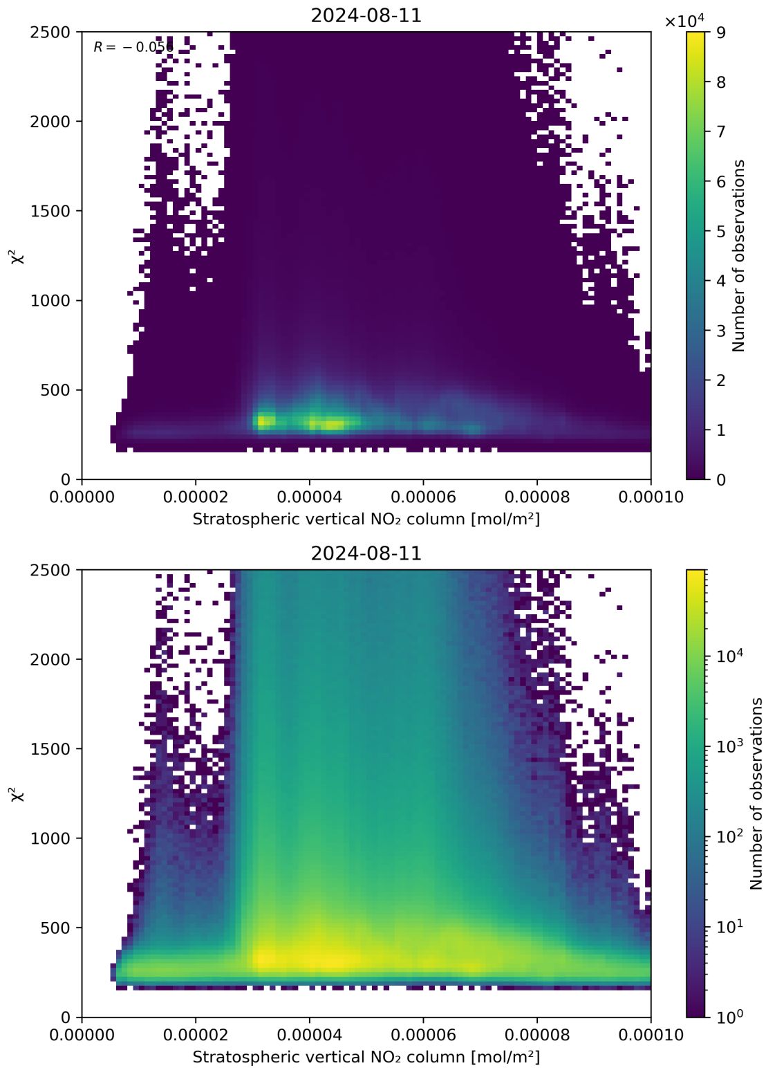
Figure 97: Scatter density plot of “Stratospheric vertical NO 2 column” against “ \chi^2 ” for 2024-08-11 to 2024-08-11.
