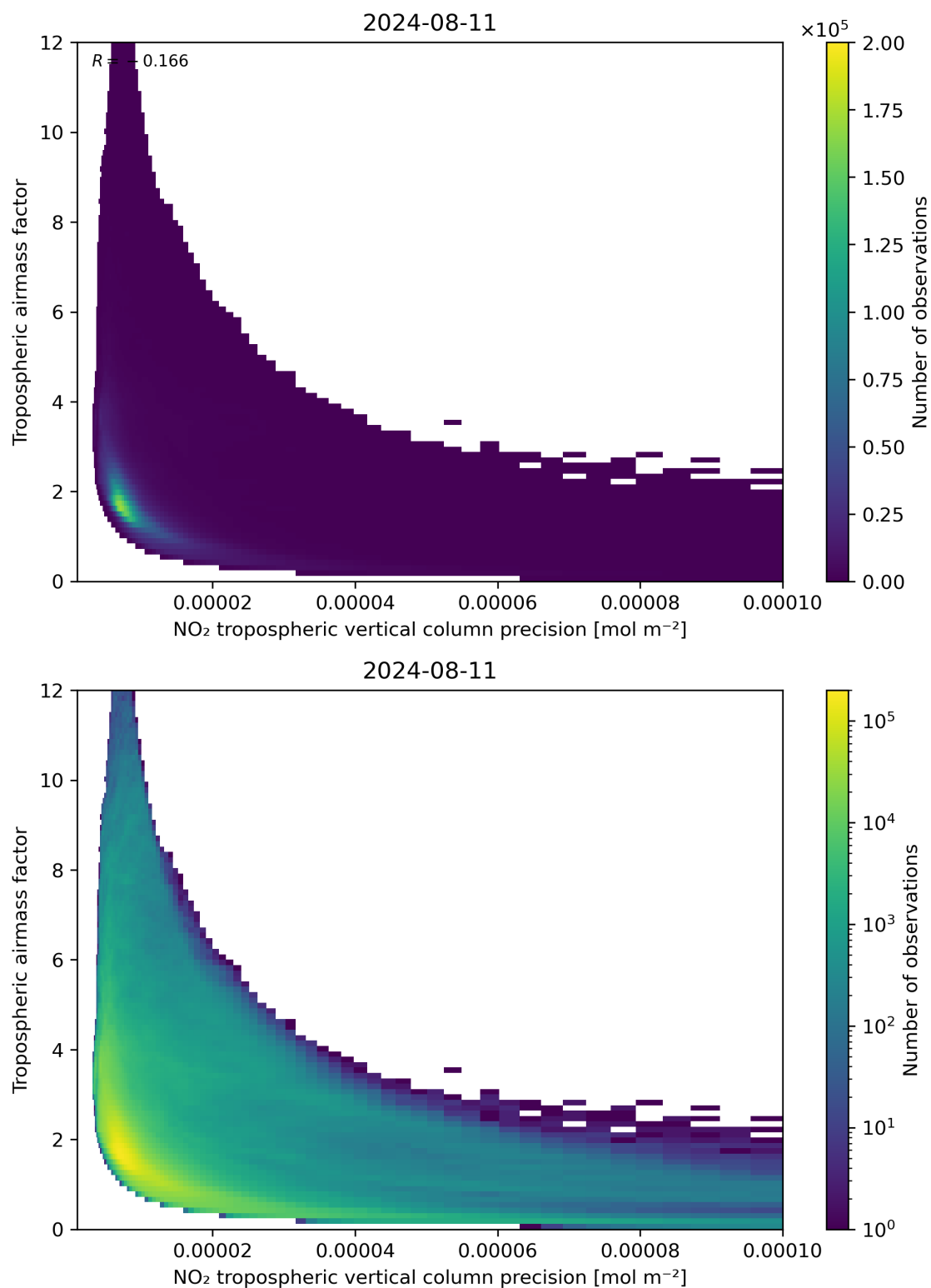
Figure 133: Scatter density plot of “NO 2 tropospheric vertical column precision” against “Tropospheric airmass factor” for 2024-08-11 to 2024-08-11.
