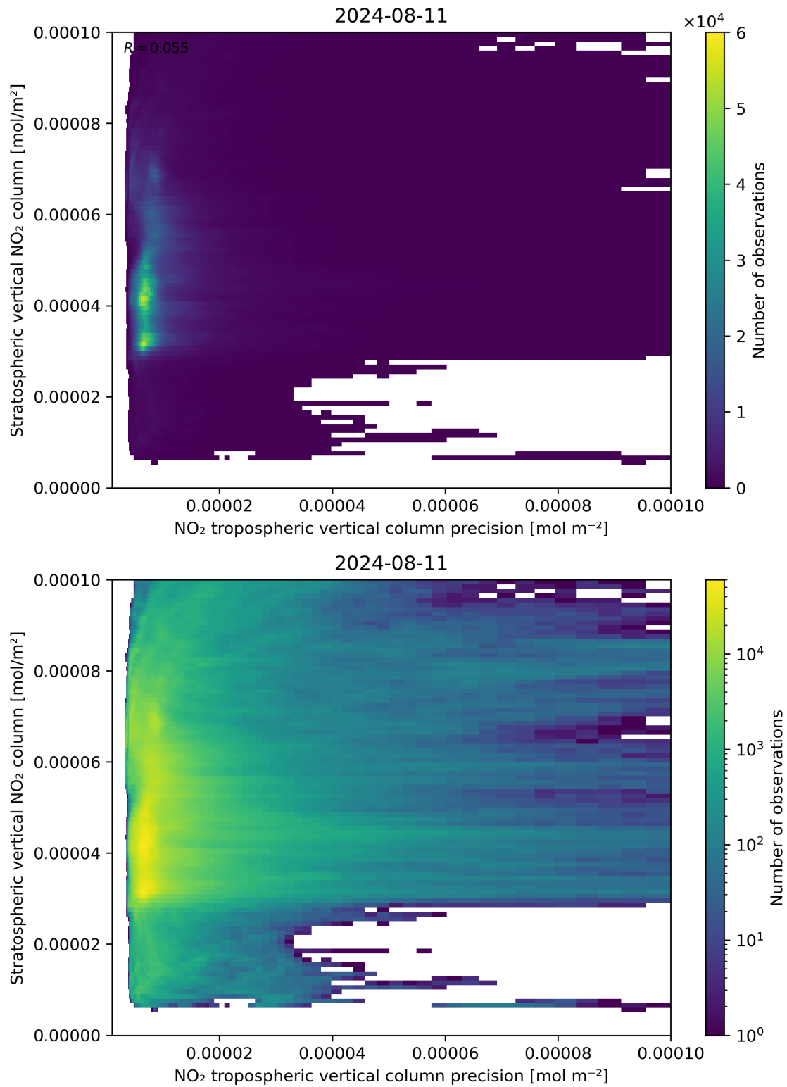
Figure 135: Scatter density plot of “NO 2 tropospheric vertical column precision” against “Stratospheric vertical NO 2 column” for 2024-08-11 to 2024-08-11.
