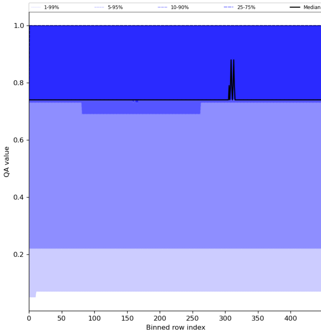
Figure 45: Along track statistics of “QA value” for 2024-08-11 to 2024-08-11
