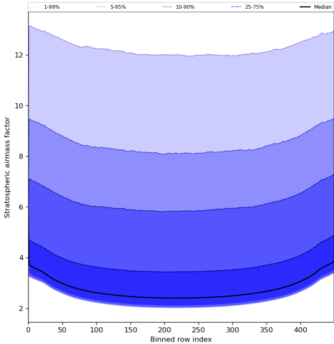
Figure 61: Along track statistics of “Stratospheric airmass factor” for 2024-08-11 to 2024-08-11
