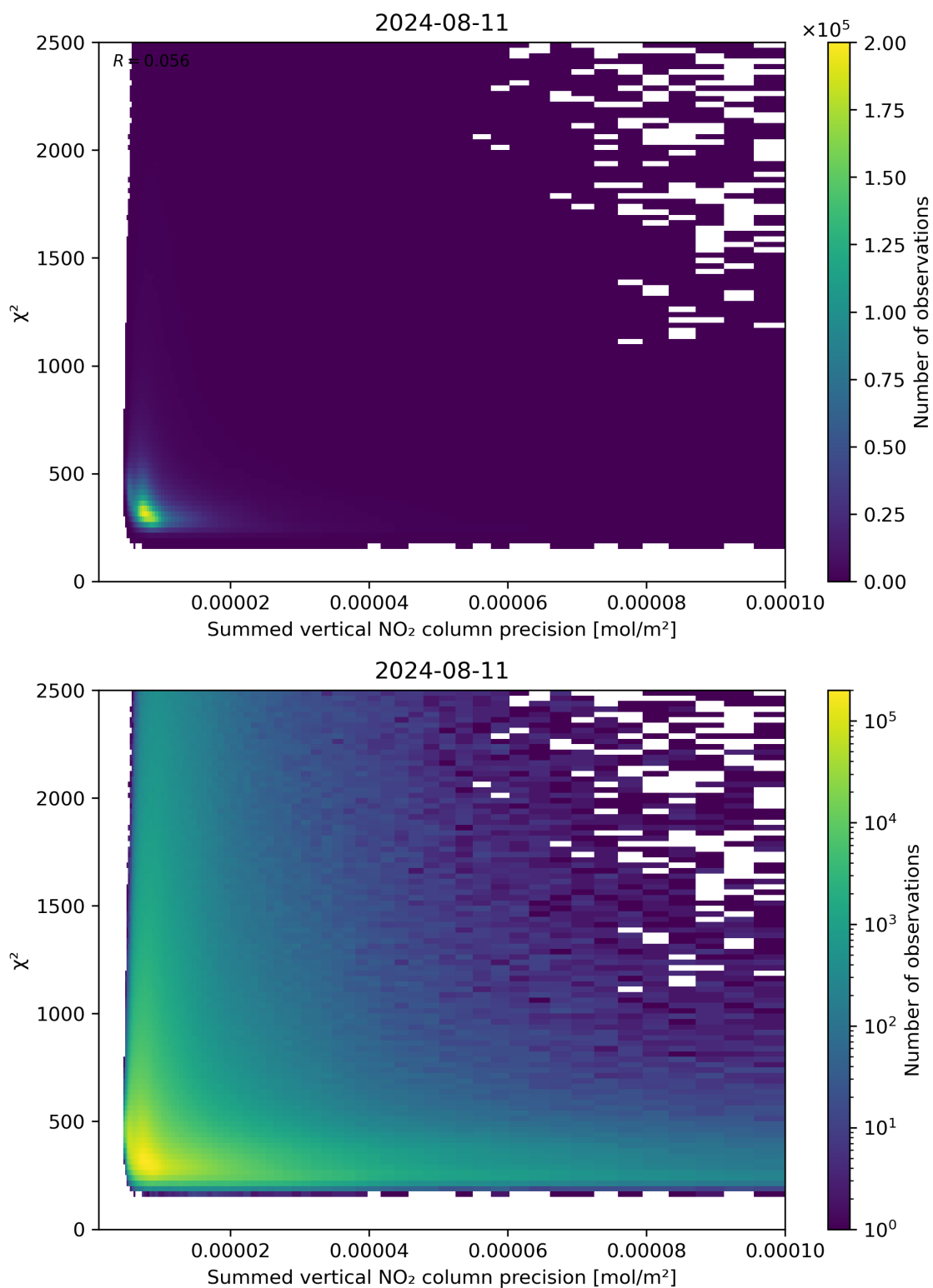
Figure 107: Scatter density plot of “Summed vertical NO 2 column precision” against “ \chi^2 ” for 2024-08-11 to 2024-08-11.
