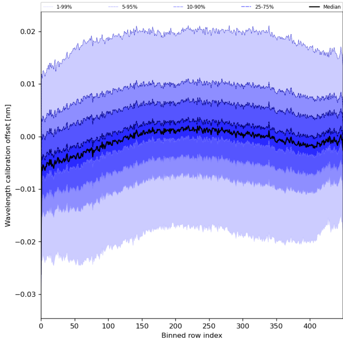
Figure 52: Along track statistics of “Wavelength calibration offset” for 2024-08-11 to 2024-08-11
