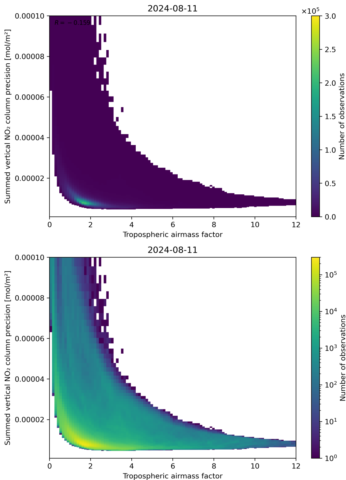
Figure 76: Scatter density plot of “Tropospheric air mass factor” against “Summed vertical NO 2 column precision” for 2024-08-11 to 2024-08-11.
