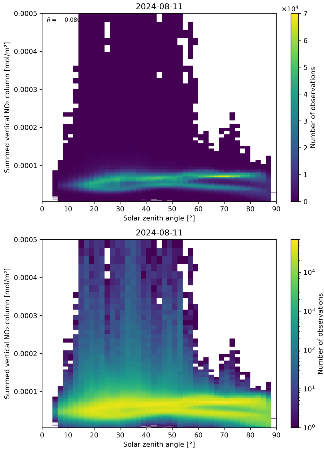
Figure 151: Scatter density plot of “Solar zenith angle” against “Summed vertical NO 2 column” for 2024-08-11 to 2024-08-11.
