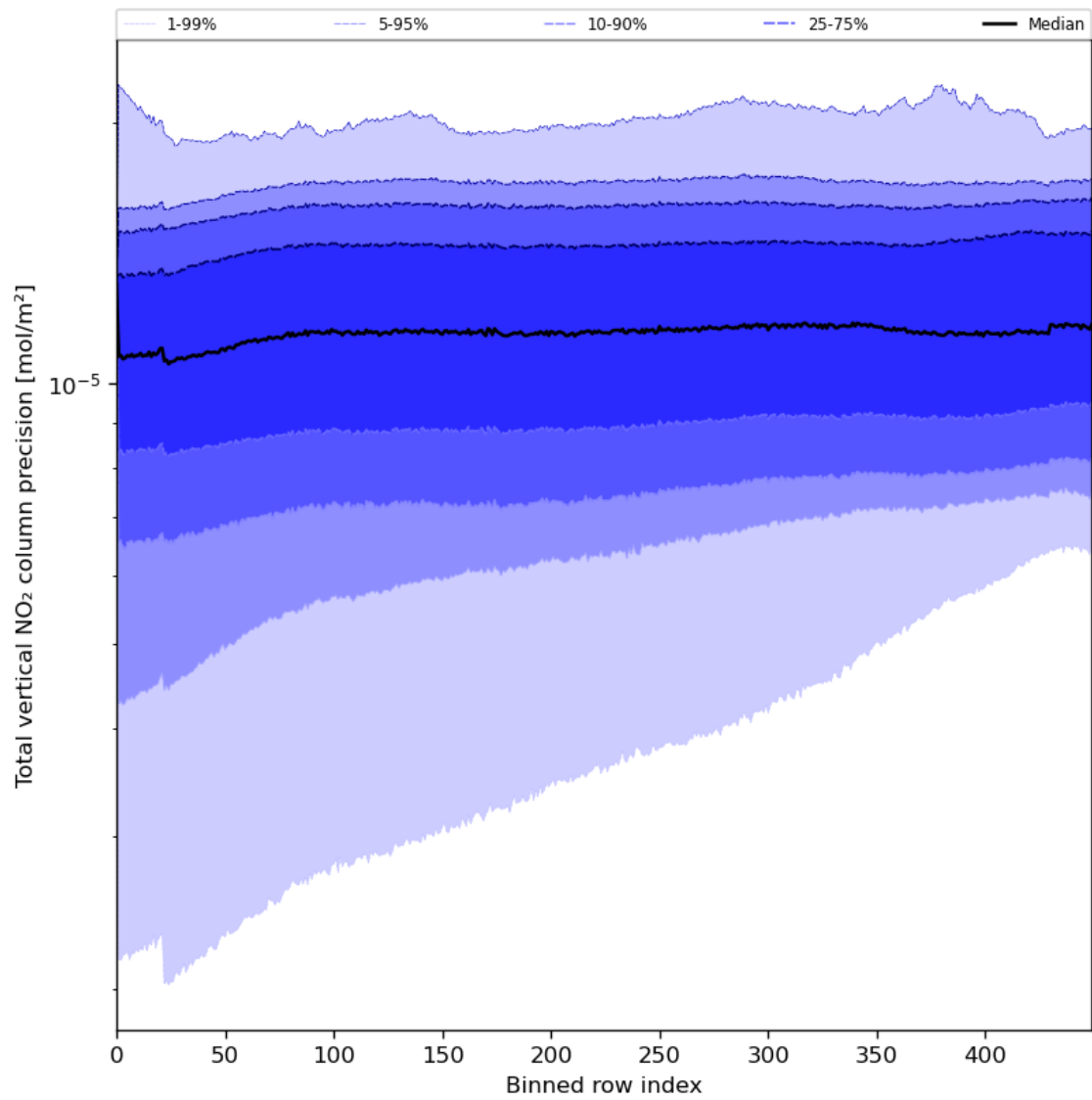
Figure 56: Along track statistics of “Total vertical NO 2 column precision” for 2024-08-11 to 2024-08-11
