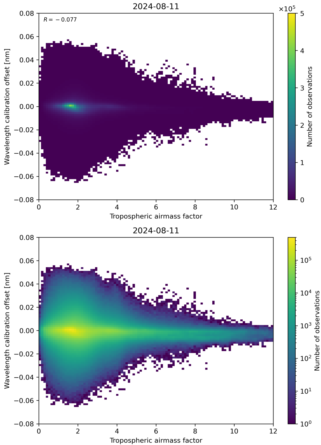
Figure 80: Scatter density plot of “Tropospheric air mass factor” against “Wavelength calibration offset” for 2024-08-11 to 2024-08-11.
