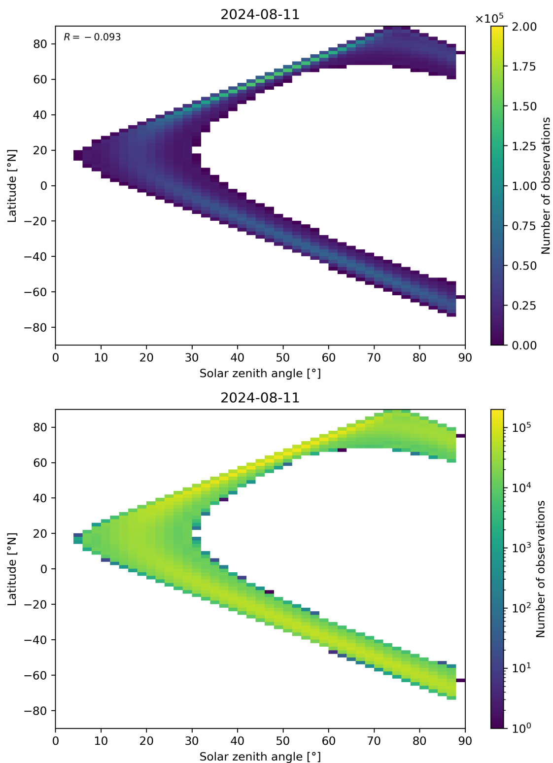
Figure 149: Scatter density plot of “Solar zenith angle” against “Latitude” for 2024-08-11 to 2024-08-11.
