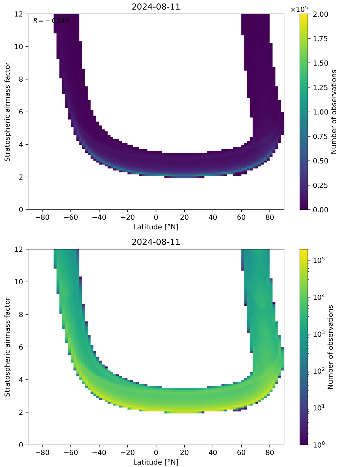
Figure 83: Scatter density plot of “Latitude” against “Stratospheric air mass factor” for 2024-08-11 to 2024-08-11.
