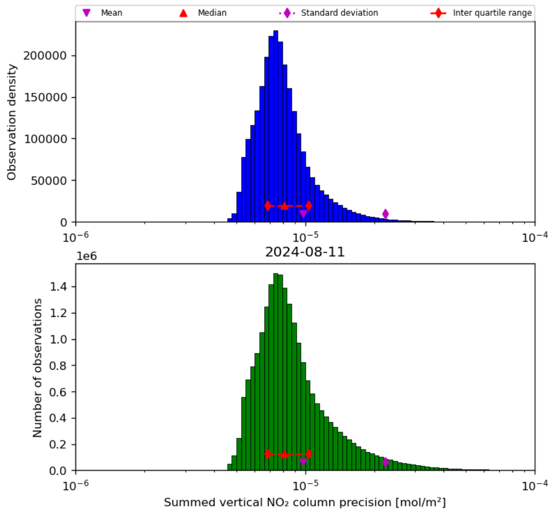
Figure 41: Histogram of "Summed vertical NO 2 column precision" for 2024-08-11 to 2024-08-11
