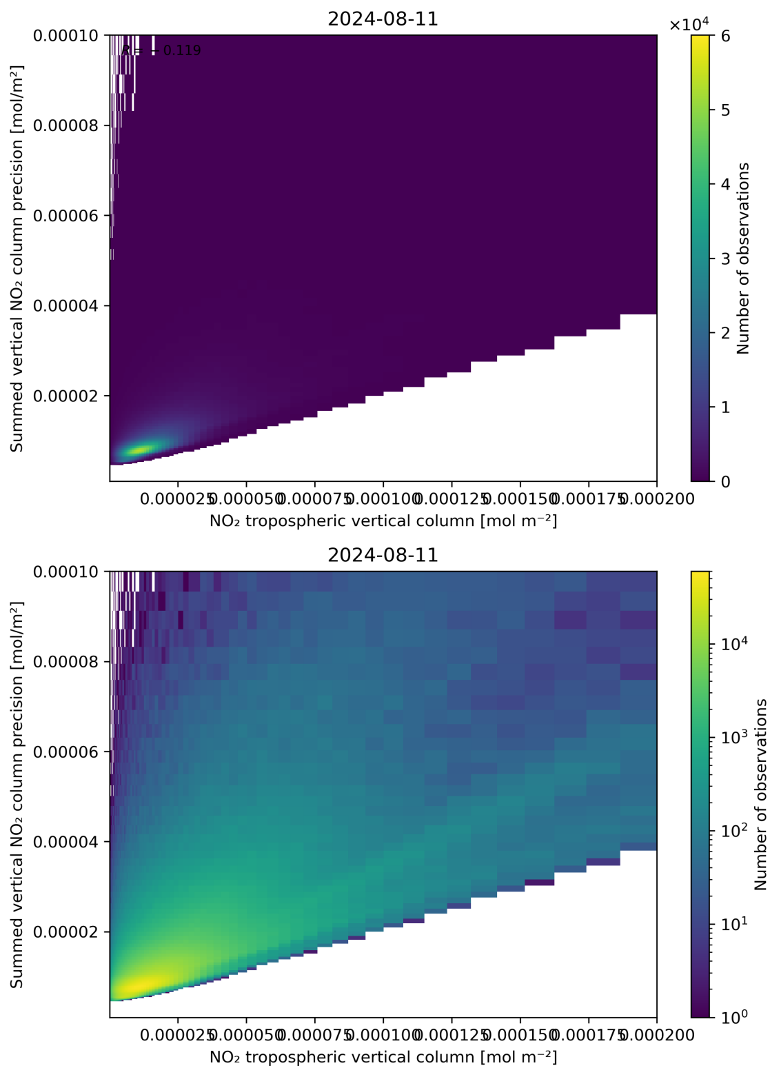
Figure 127: Scatter density plot of “NO 2 tropospheric vertical column” against “Summed vertical NO 2 column precision” for 2024-08-11 to 2024-08-11.
