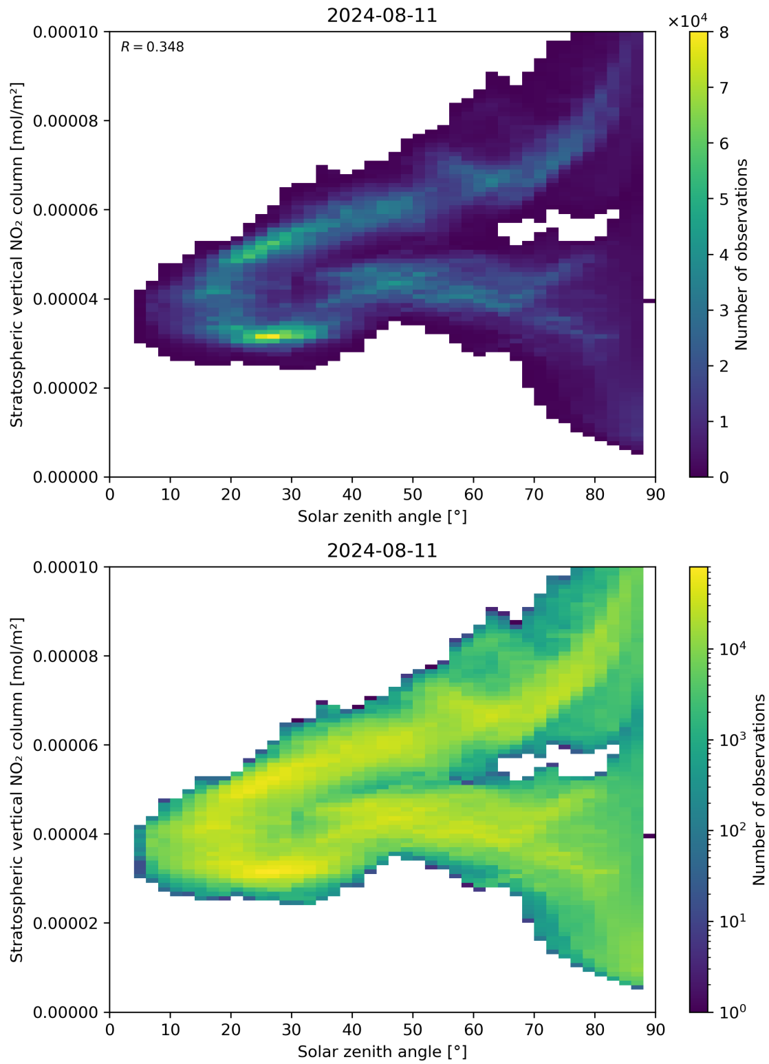
Figure 150: Scatter density plot of “Solar zenith angle” against “Stratospheric vertical NO 2 column” for 2024-08-11 to 2024-08-11.
