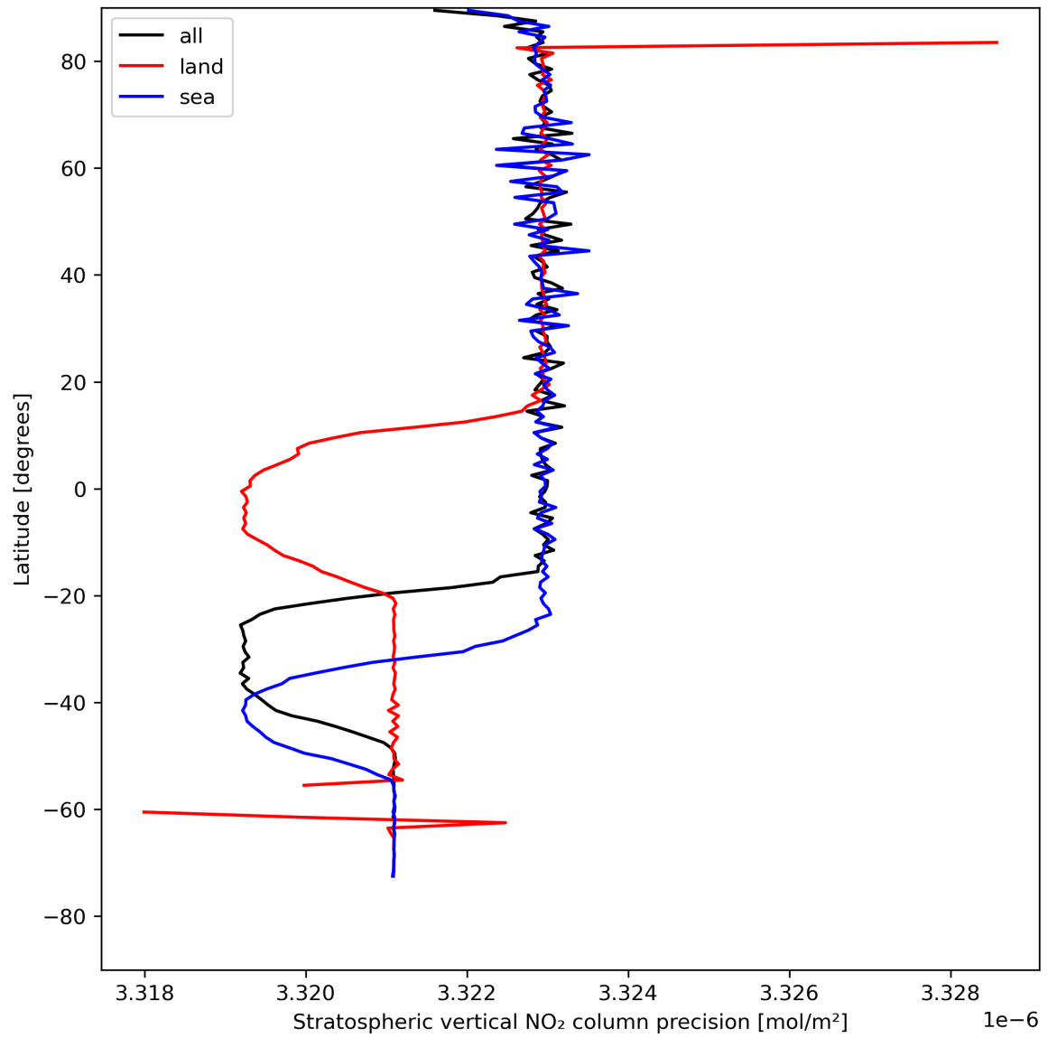
Figure 20: Zonal average of “Stratospheric vertical NO 2 column precision” for 2024-08-11 to 2024-08-11.
