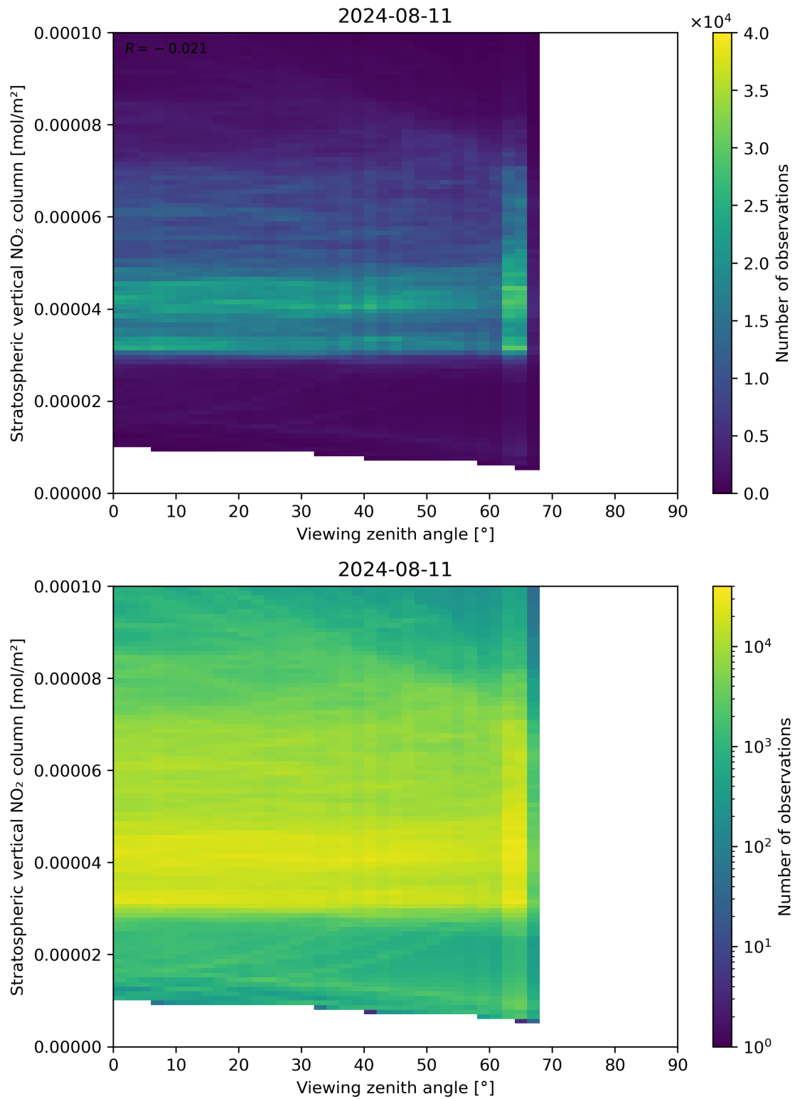
Figure 164: Scatter density plot of “Viewing zenith angle” against “Stratospheric vertical NO 2 column” for 2024-08-11 to 2024-08-11.
