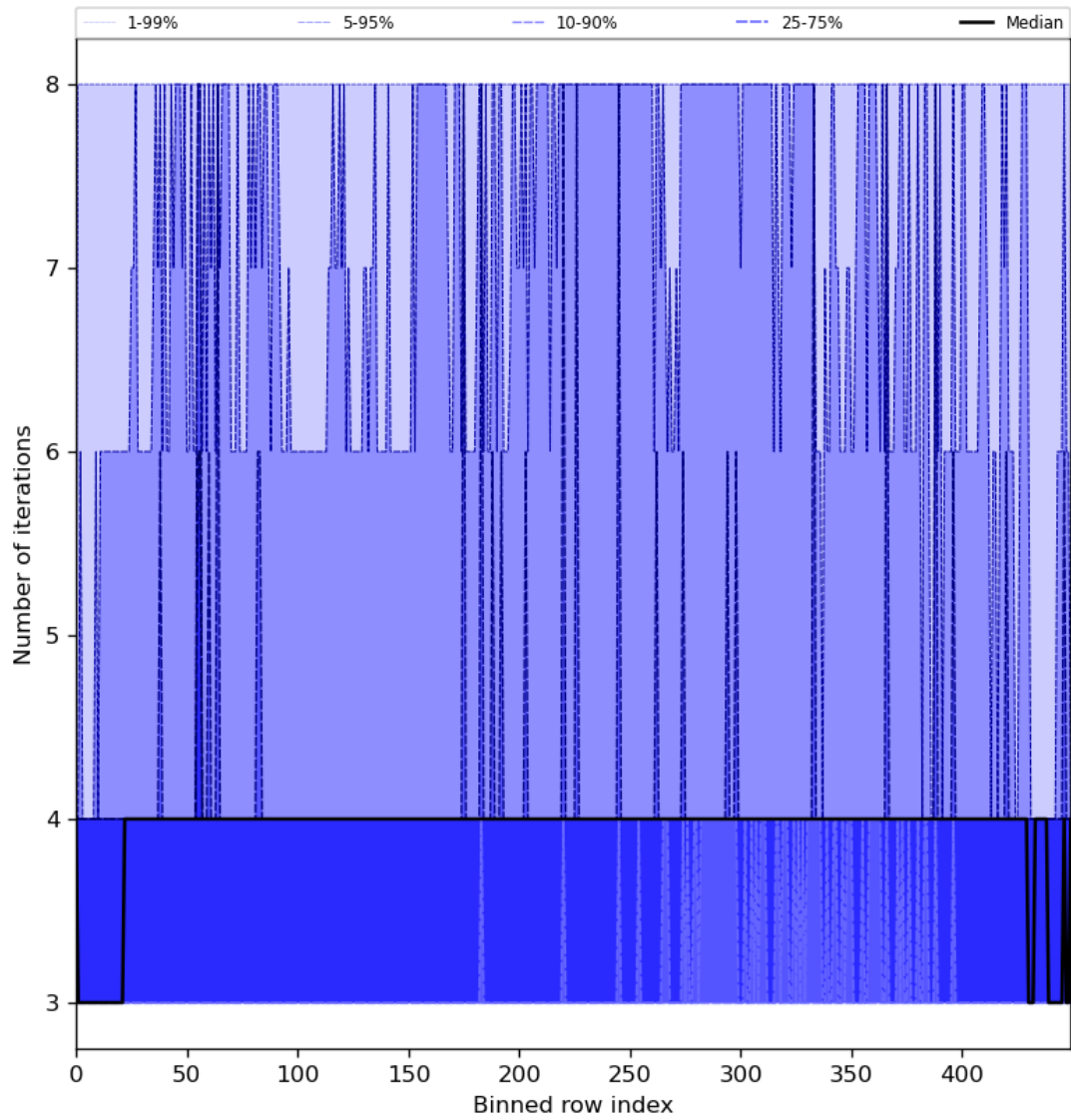
Figure 51: Along track statistics of “Number of iterations” for 2024-08-11 to 2024-08-11
