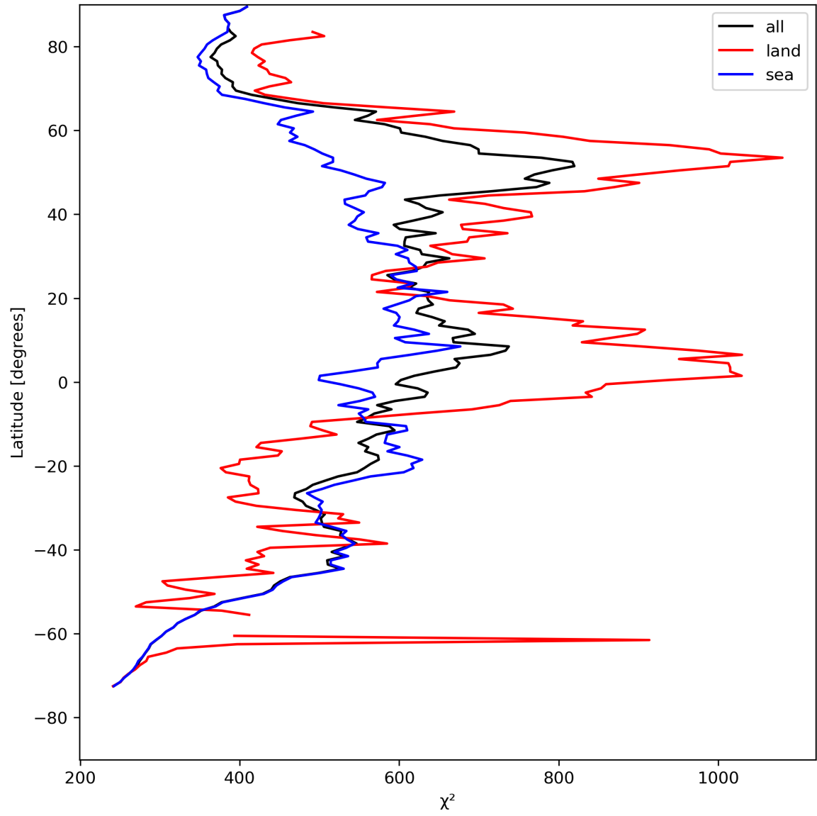
Figure 25: Zonal average of “ \chi^2 ” for 2024-08-11 to 2024-08-11.
