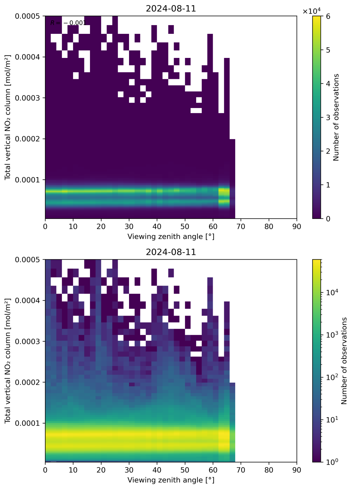
Figure 167: Scatter density plot of “Viewing zenith angle” against “Total vertical NO 2 column” for 2024-08-11 to 2024-08-11.
