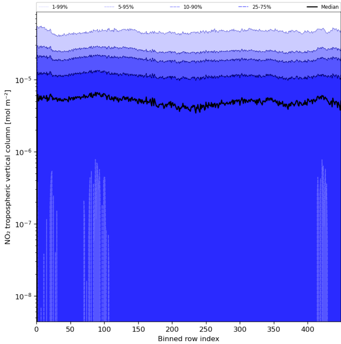
Figure 46: Along track statistics of “NO 2 tropospheric vertical column” for 2024-08-11 to 2024-08-11
