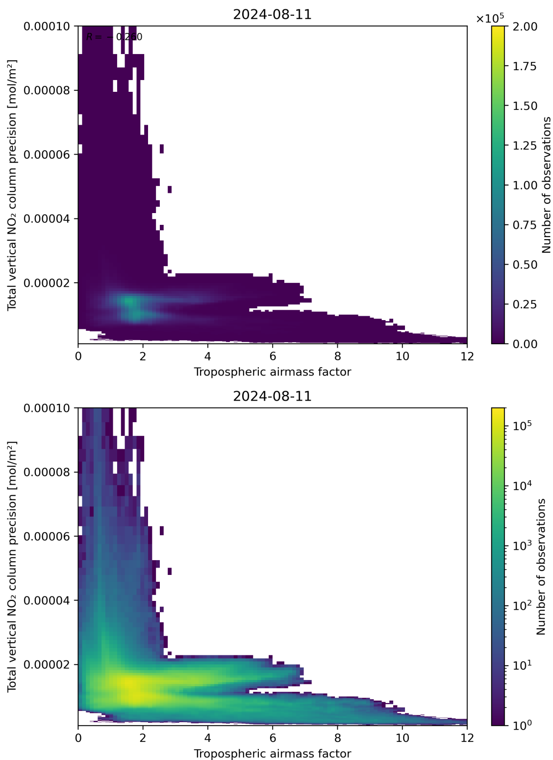
Figure 78: Scatter density plot of “Tropospheric air mass factor” against “Total vertical NO 2 column precision” for 2024-08-11 to 2024-08-11.
