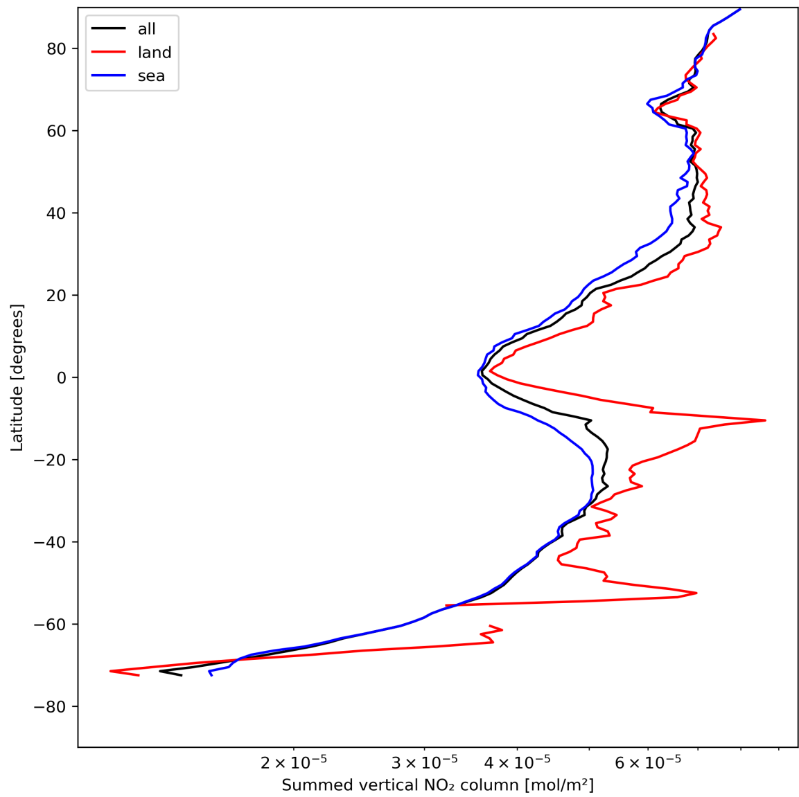
Figure 23: Zonal average of “Summed vertical NO 2 column” for 2024-08-11 to 2024-08-11.
