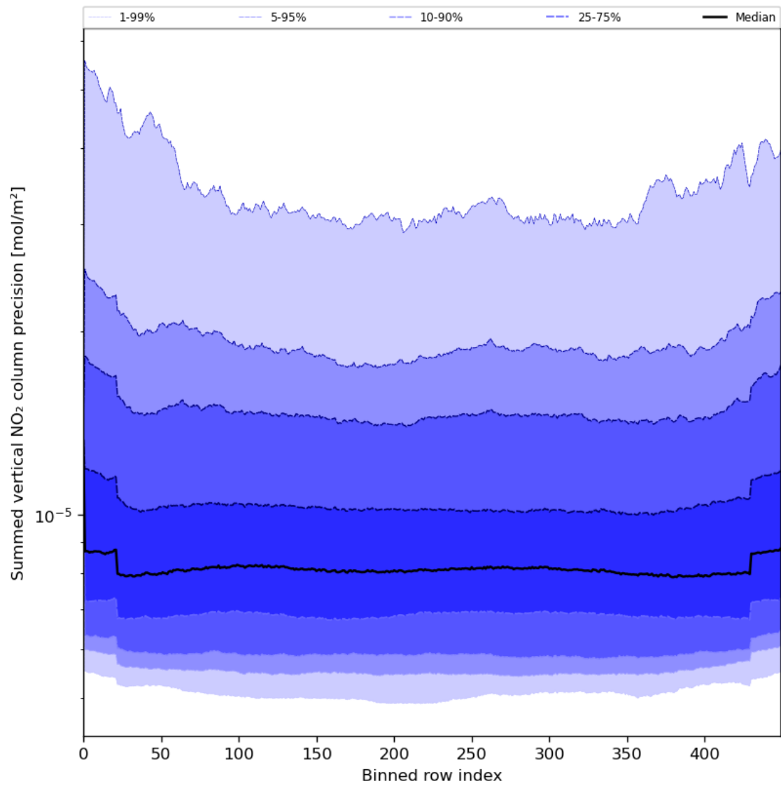
Figure 58: Along track statistics of “Summed vertical NO 2 column precision” for 2024-08-11 to 2024-08-11
