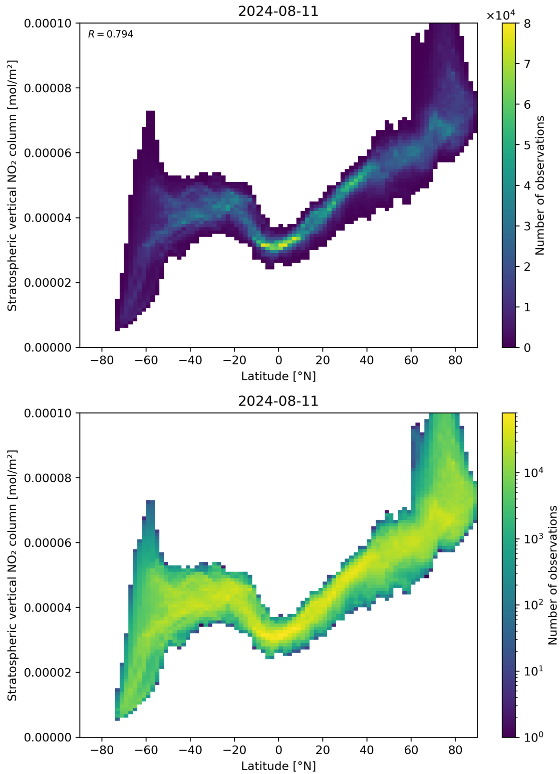
Figure 87: Scatter density plot of “Latitude” against “Stratospheric vertical \text{NO}_2 column” for 2024-08-11 to 2024-08-11.
