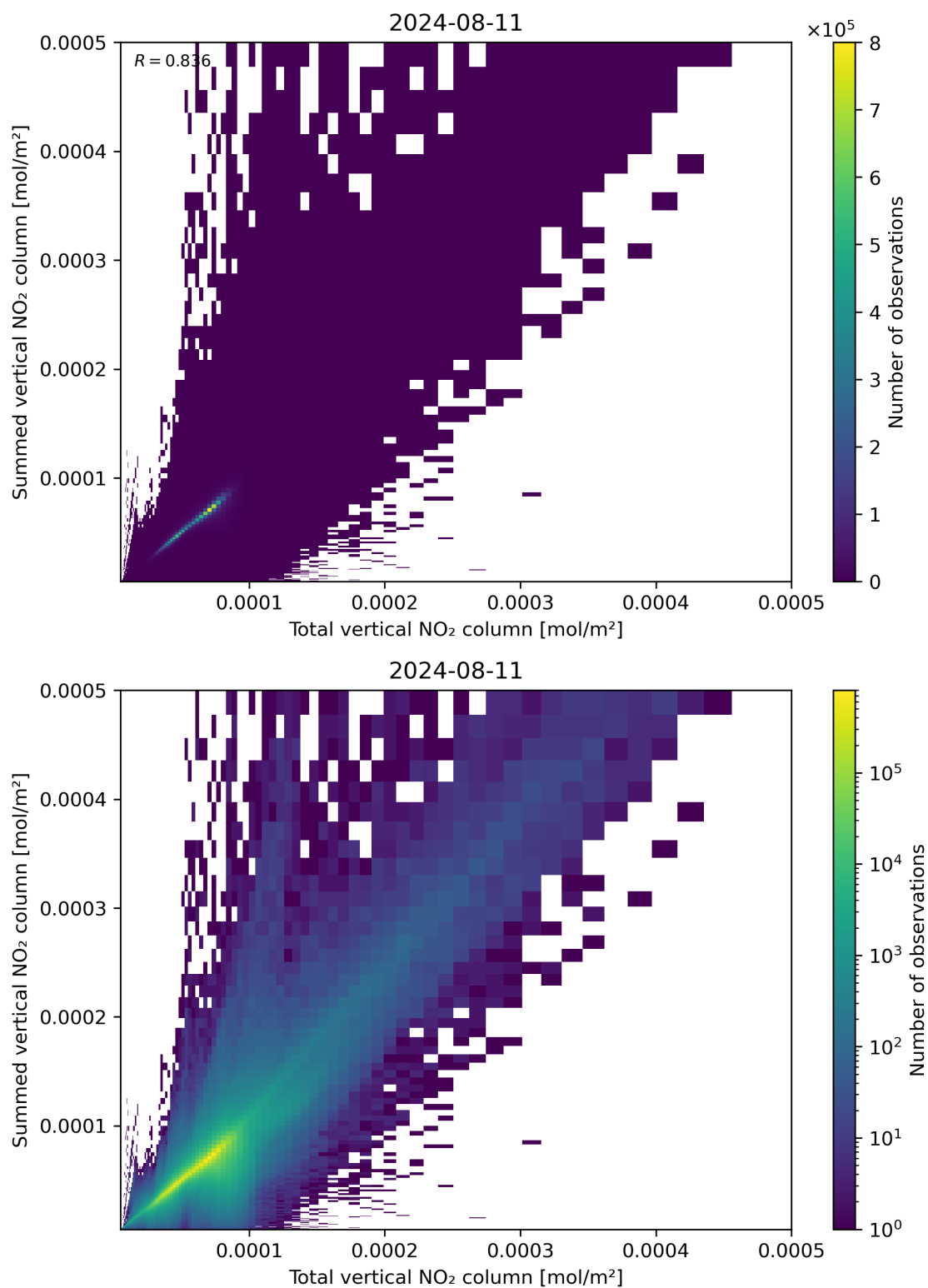
Figure 112: Scatter density plot of “Total vertical NO 2 column” against “Summed vertical NO 2 column” for 2024-08-11 to 2024-08-11.
