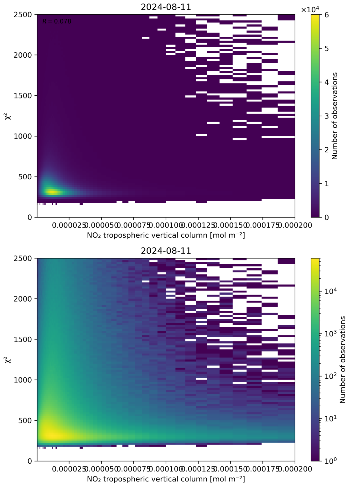
Figure 124: Scatter density plot of “NO 2 tropospheric vertical column” against “ \chi^2 ” for 2024-08-11 to 2024-08-11.
