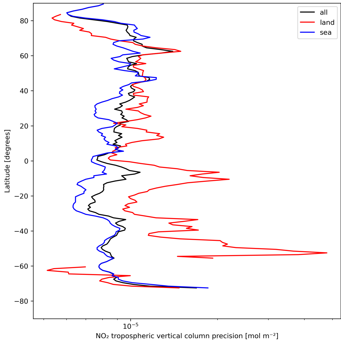
Figure 13: Zonal average of “NO 2 tropospheric vertical column precision” for 2024-08-11 to 2024-08-11.
