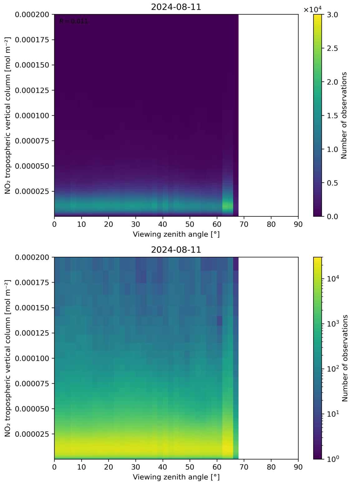
Figure 169: Scatter density plot of “Viewing zenith angle” against “NO 2 tropospheric vertical column” for 2024-08-11 to 2024-08-11.
