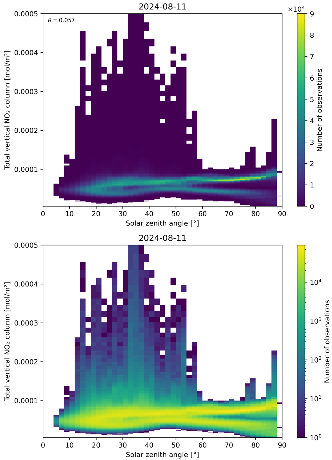
Figure 153: Scatter density plot of “Solar zenith angle” against “Total vertical NO 2 column” for 2024-08-11 to 2024-08-11.
