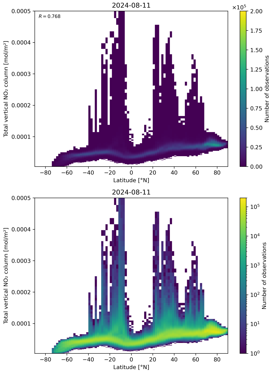
Figure 90: Scatter density plot of “Latitude” against “Total vertical NO 2 column” for 2024-08-11 to 2024-08-11.
