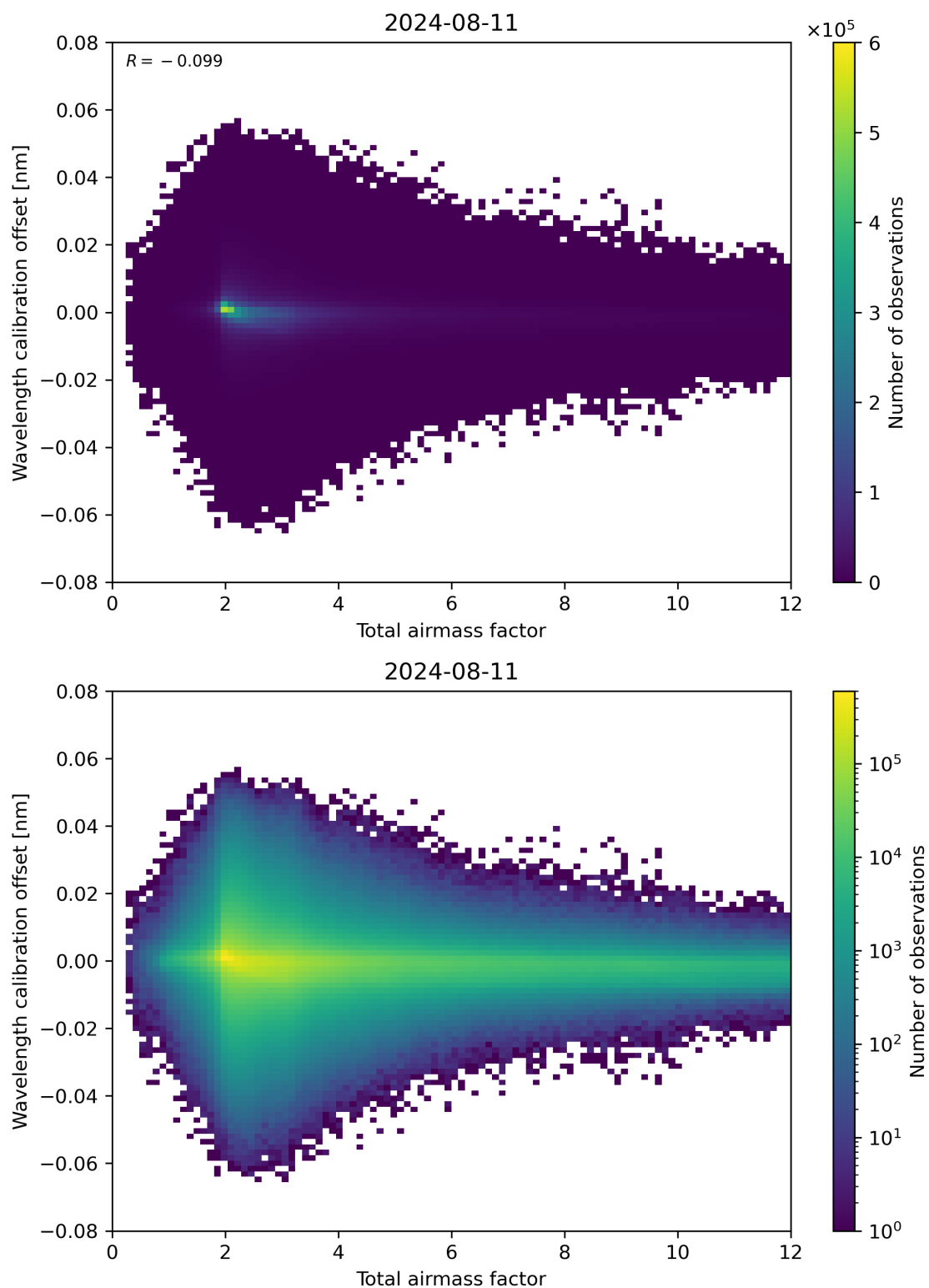
Figure 70: Scatter density plot of “Total airmass factor” against “Wavelength calibration offset” for 2024-08-11 to 2024-08-11.
