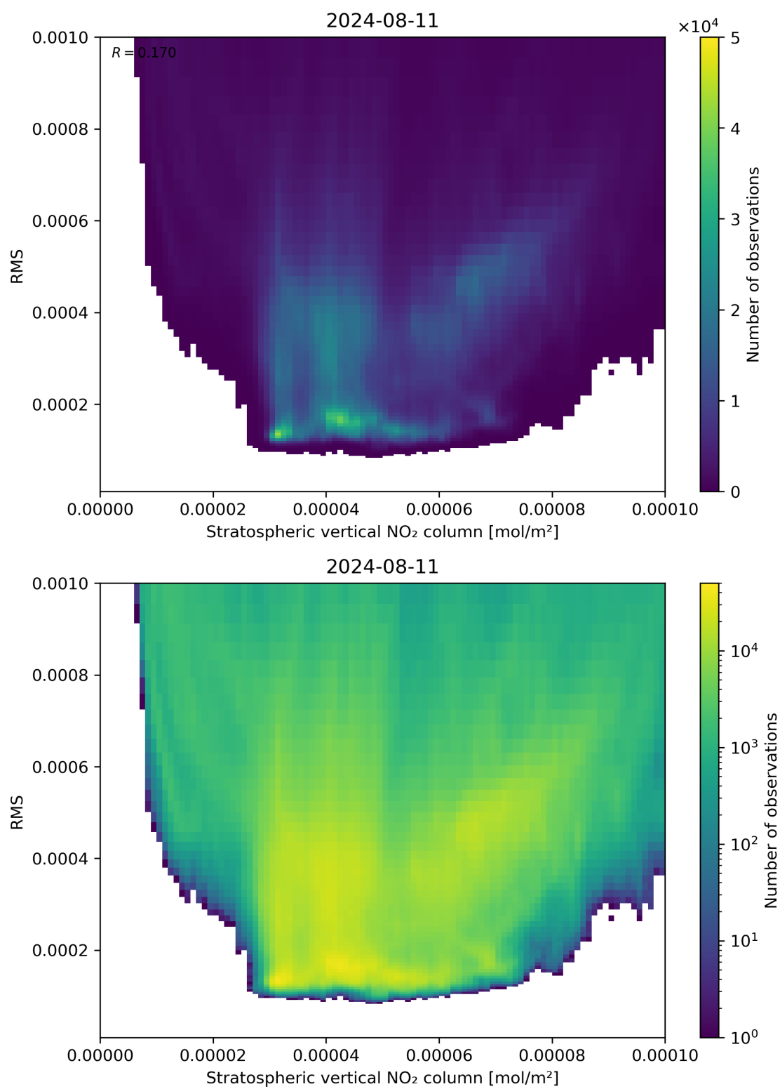
Figure 102: Scatter density plot of “Stratospheric vertical NO 2 column” against “RMS” for 2024-08-11 to 2024-08-11.
