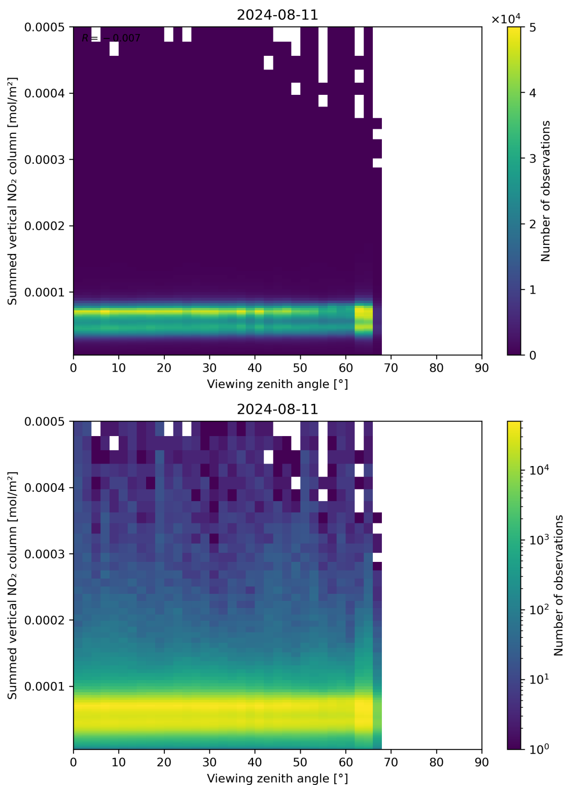
Figure 165: Scatter density plot of “Viewing zenith angle” against “Summed vertical NO 2 column” for 2024-08-11 to 2024-08-11.
