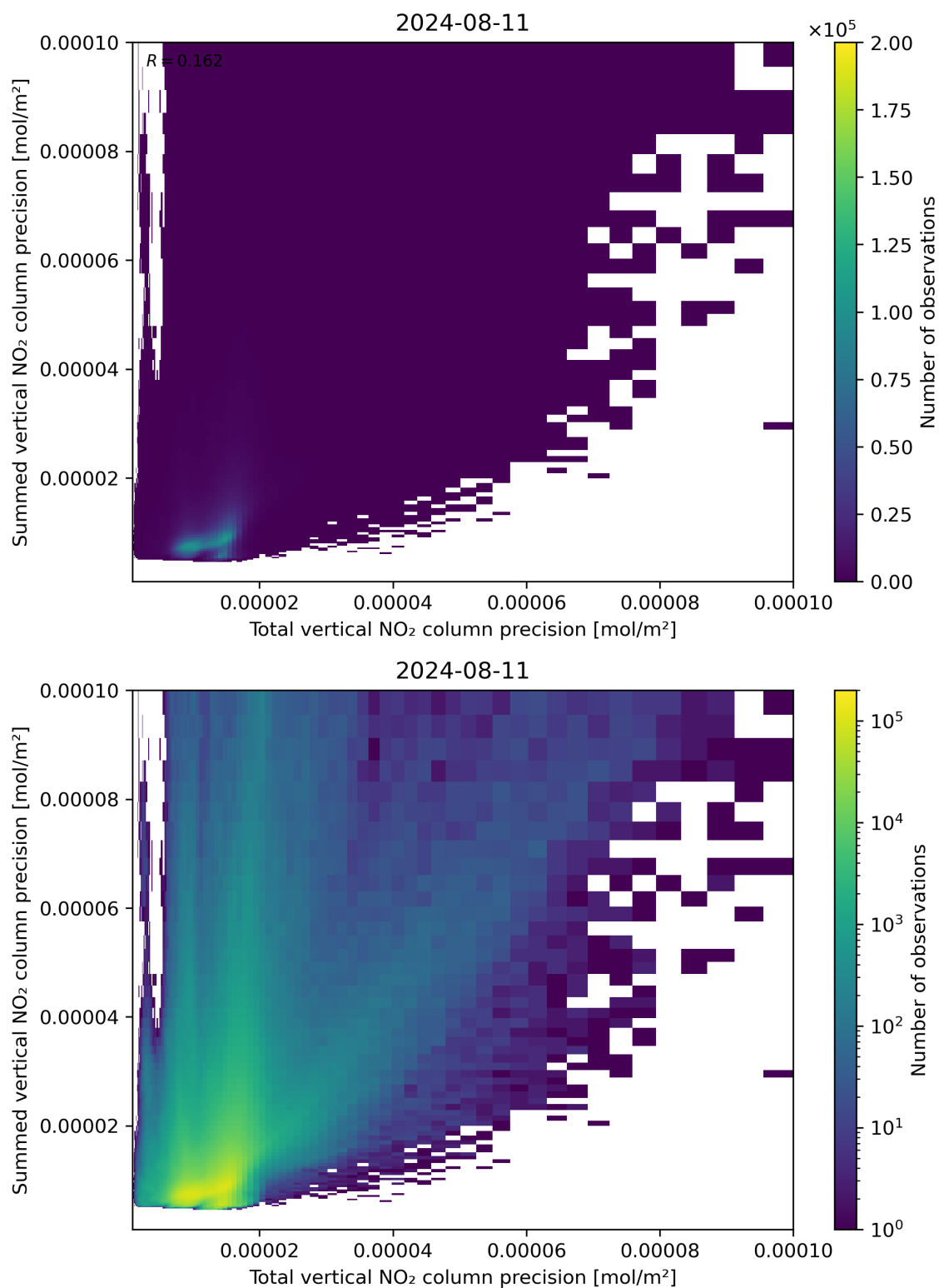
Figure 118: Scatter density plot of “Total vertical NO 2 column precision” against “Summed vertical NO 2 column precision” for 2024-08-11 to 2024-08-11.
