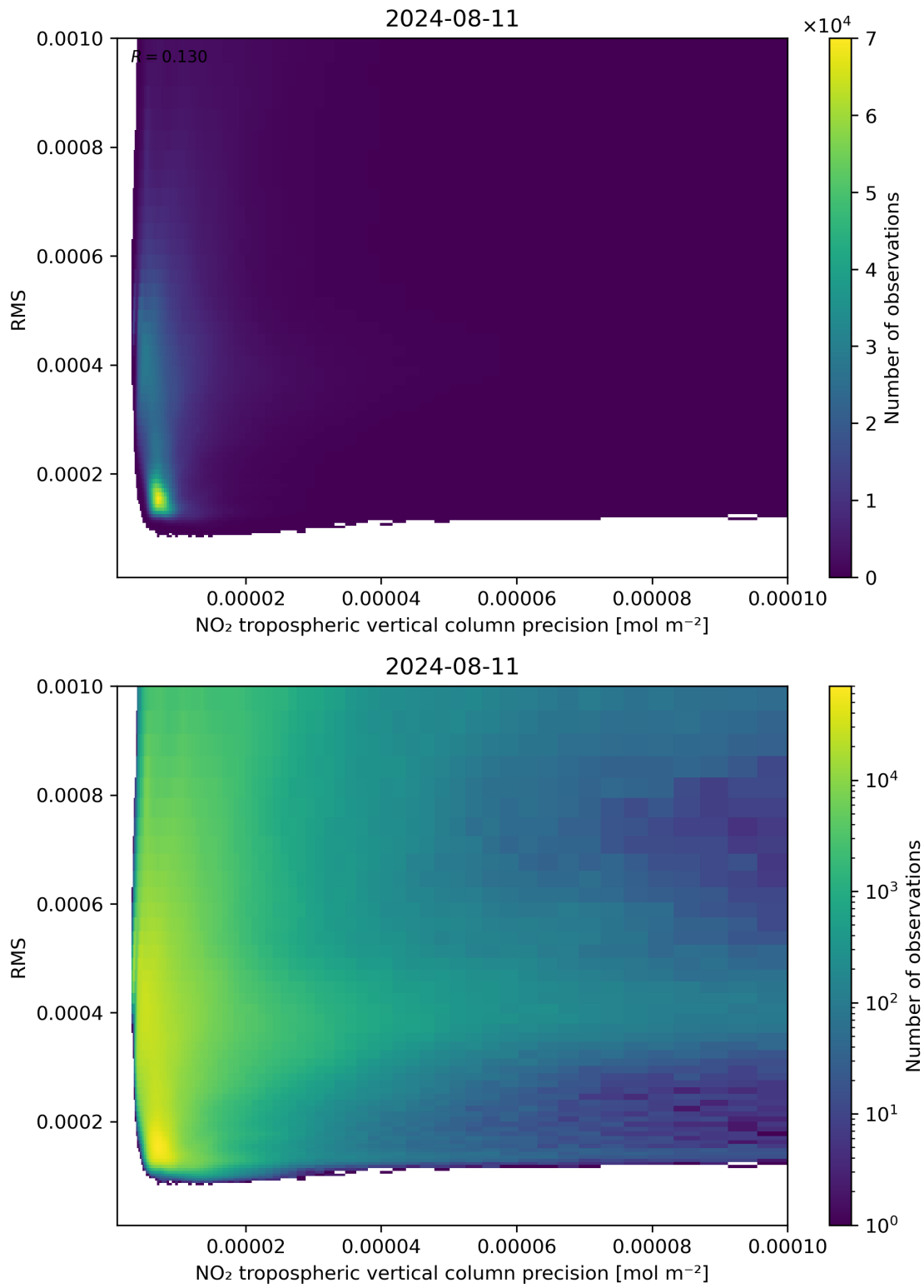
Figure 140: Scatter density plot of “NO 2 tropospheric vertical column precision” against “RMS” for 2024-08-11 to 2024-08-11.
