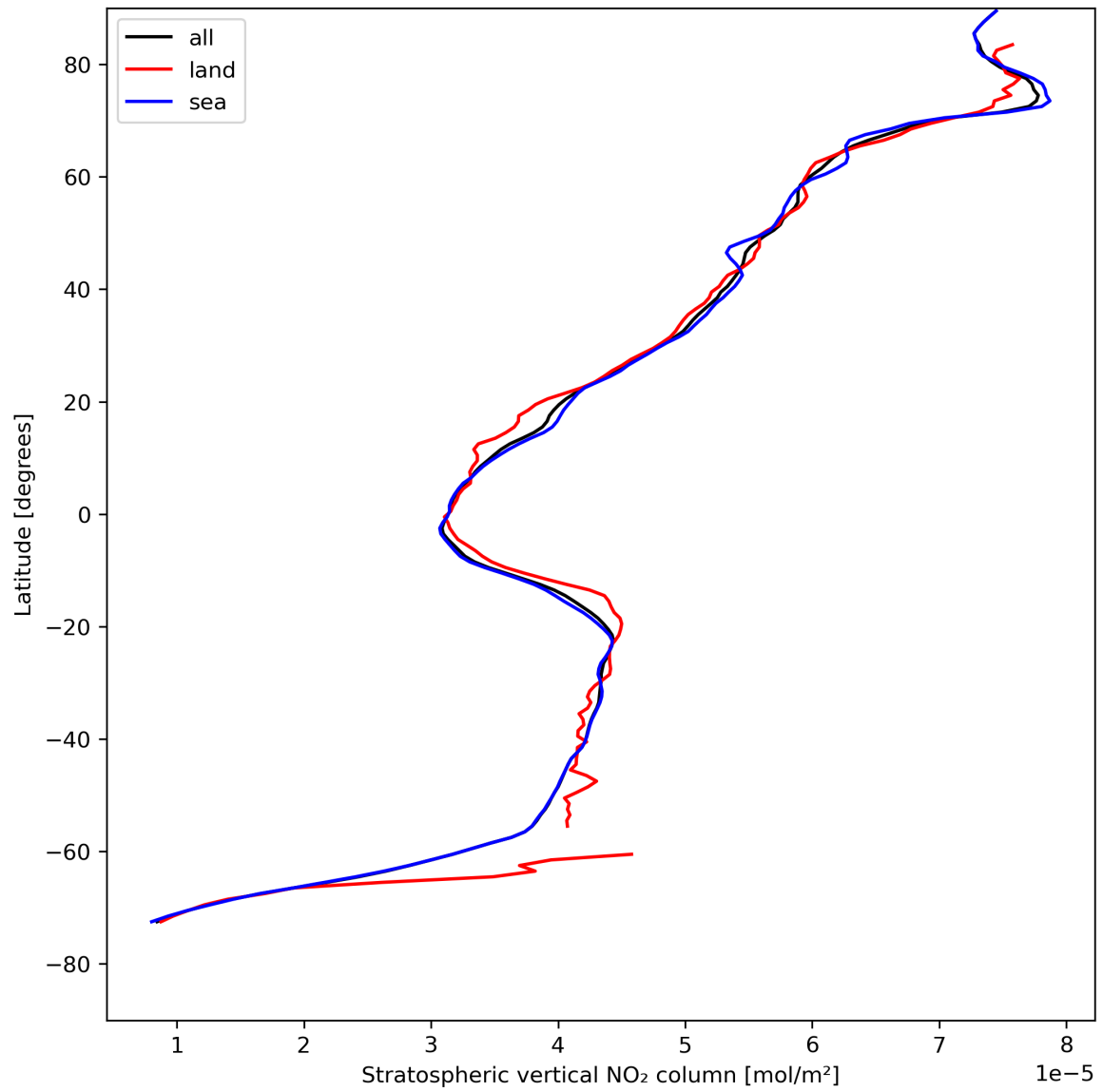
Figure 19: Zonal average of “Stratospheric vertical NO 2 column” for 2024-08-11 to 2024-08-11.
