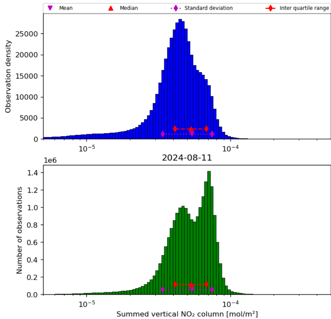
Figure 40: Histogram of "Summed vertical NO 2 column" for 2024-08-11 to 2024-08-11
