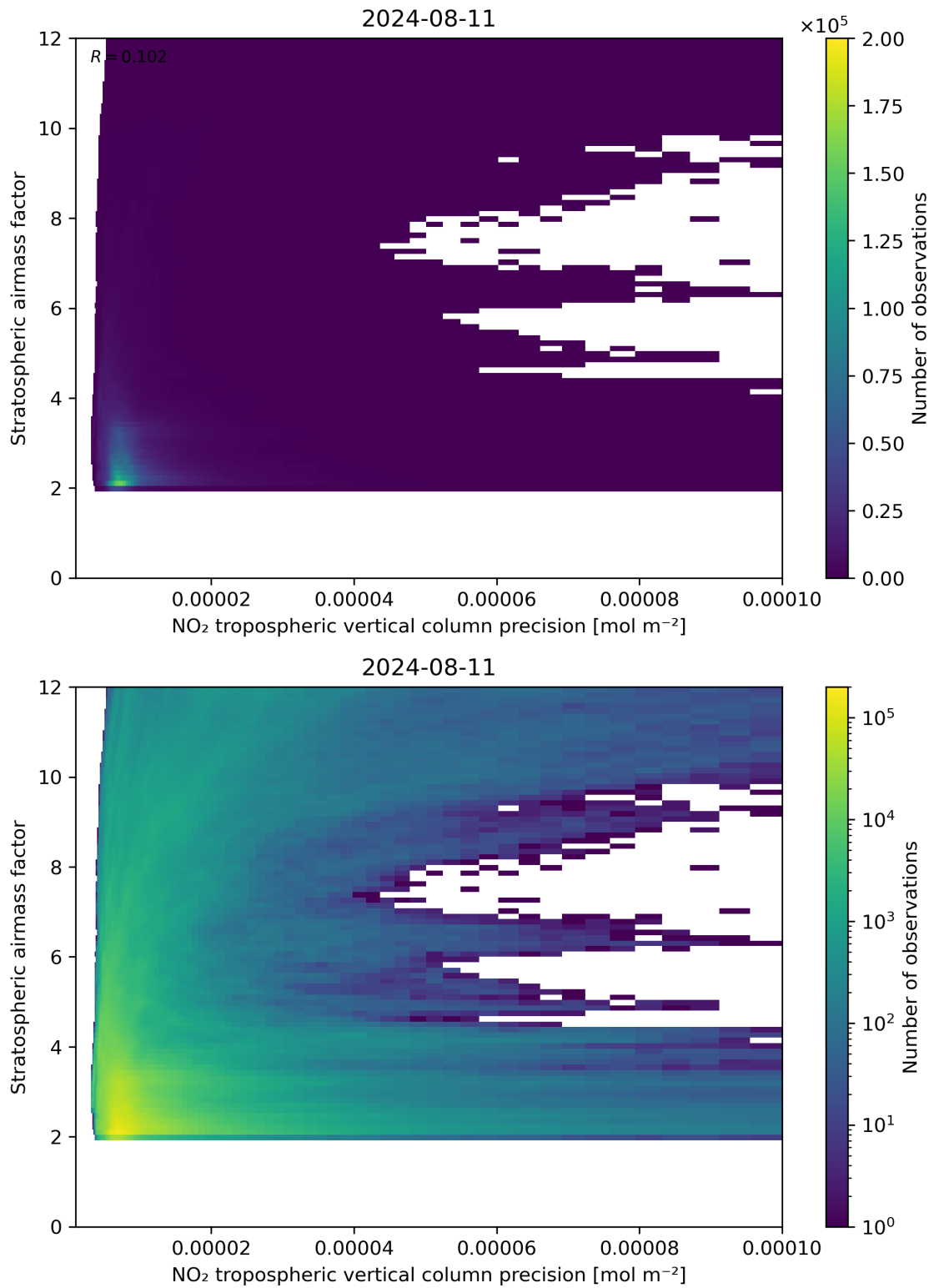
Figure 131: Scatter density plot of “NO 2 tropospheric vertical column precision” against “Stratospheric airmass factor” for 2024-08-11 to 2024-08-11.
