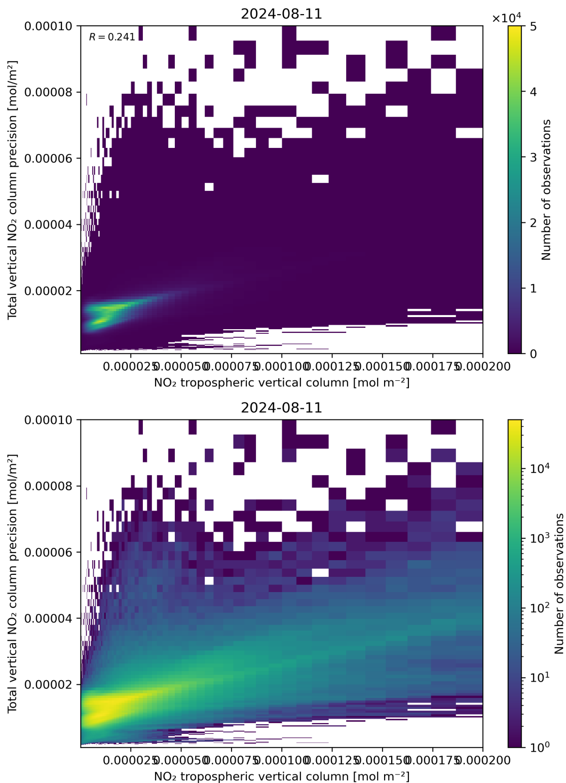
Figure 129: Scatter density plot of “NO 2 tropospheric vertical column” against “Total vertical NO 2 column precision” for 2024-08-11 to 2024-08-11.
