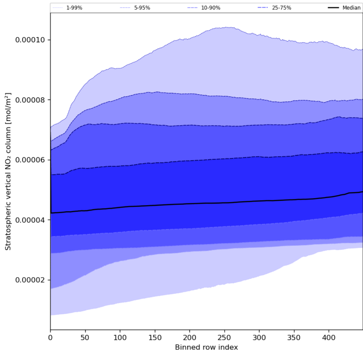
Figure 53: Along track statistics of “Stratospheric vertical NO 2 column” for 2024-08-11 to 2024-08-11
