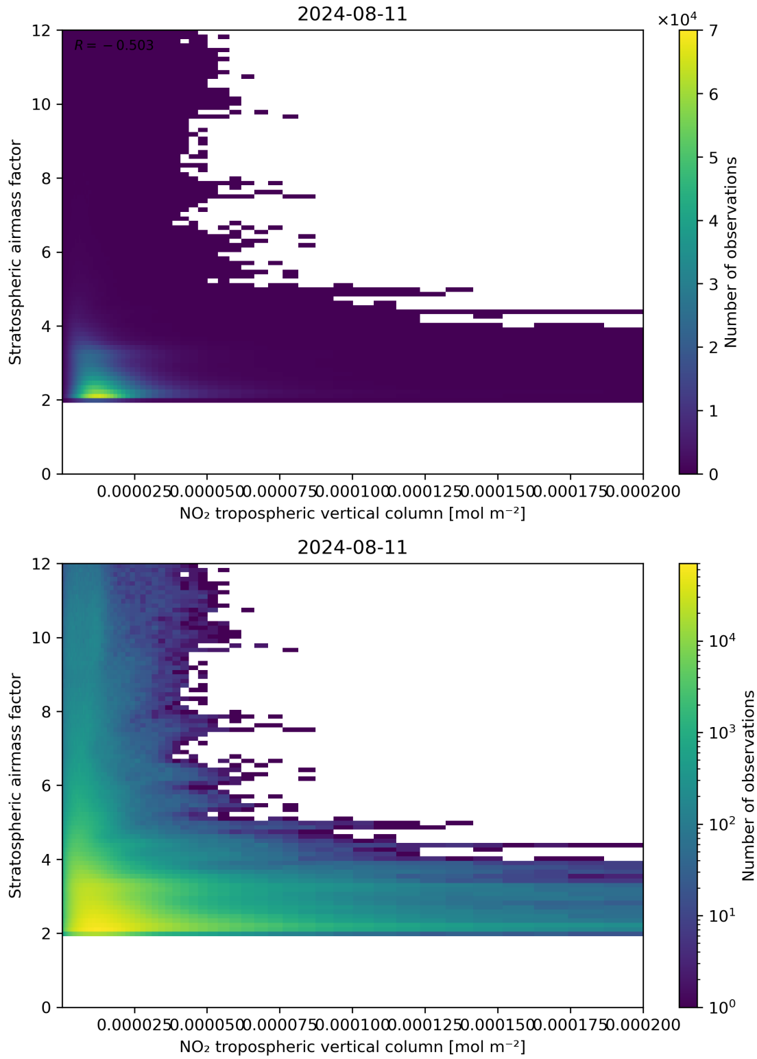
Figure 121: Scatter density plot of “NO 2 tropospheric vertical column” against “Stratospheric airmass factor” for 2024-08-11 to 2024-08-11.
