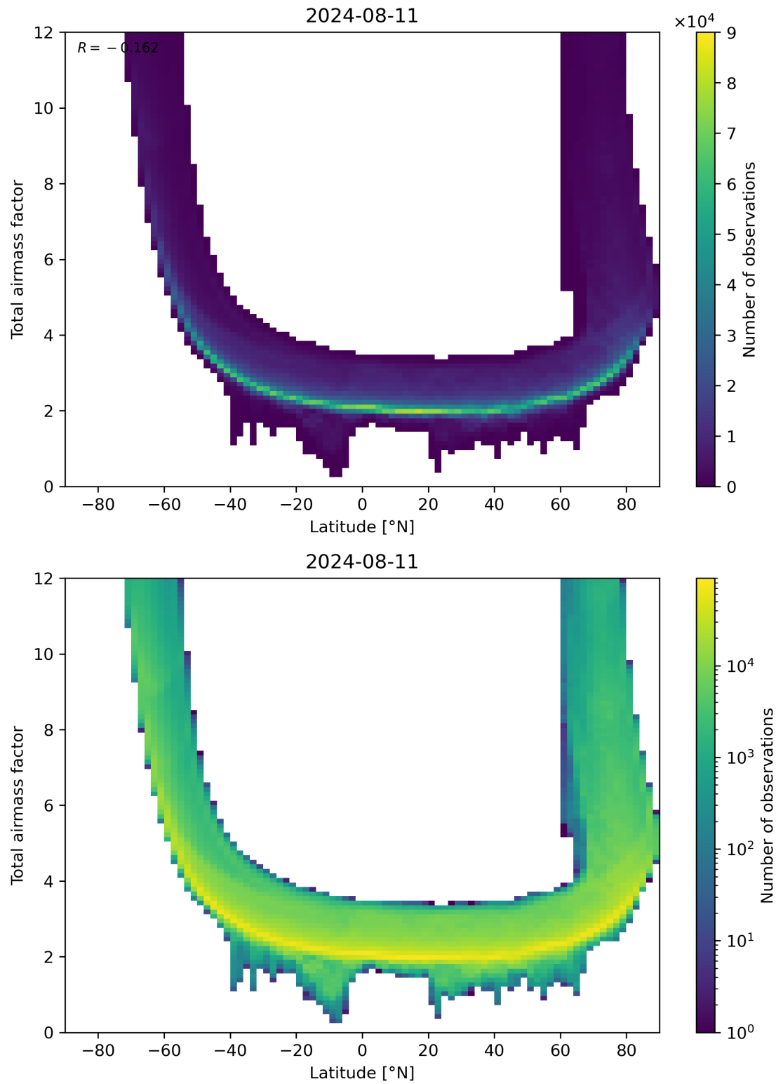
Figure 84: Scatter density plot of “Latitude” against “Total airmass factor” for 2024-08-11 to 2024-08-11.
