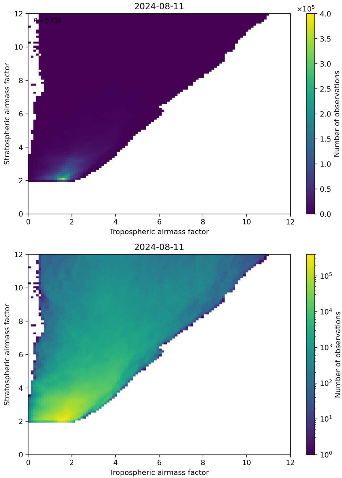
Figure 71: Scatter density plot of “Tropospheric airmass factor” against “Stratospheric airmass factor” for 2024-08-11 to 2024-08-11.
