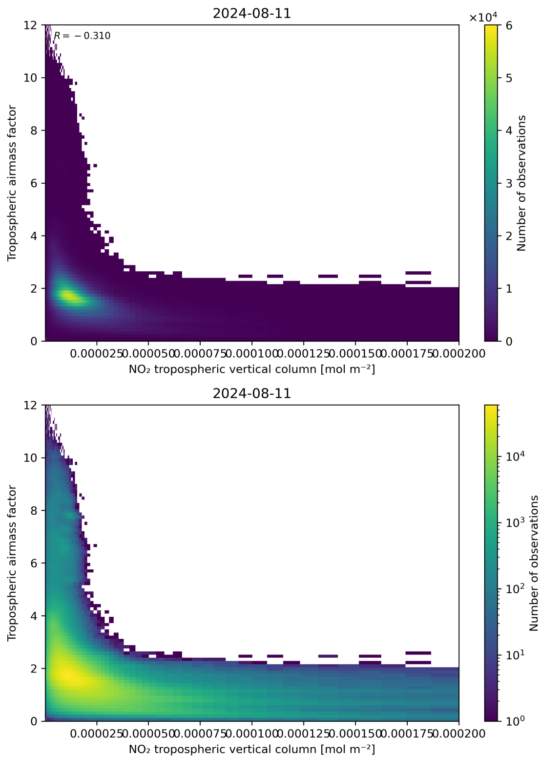
Figure 123: Scatter density plot of “NO 2 tropospheric vertical column” against “Tropospheric air mass factor” for 2024-08-11 to 2024-08-11.
