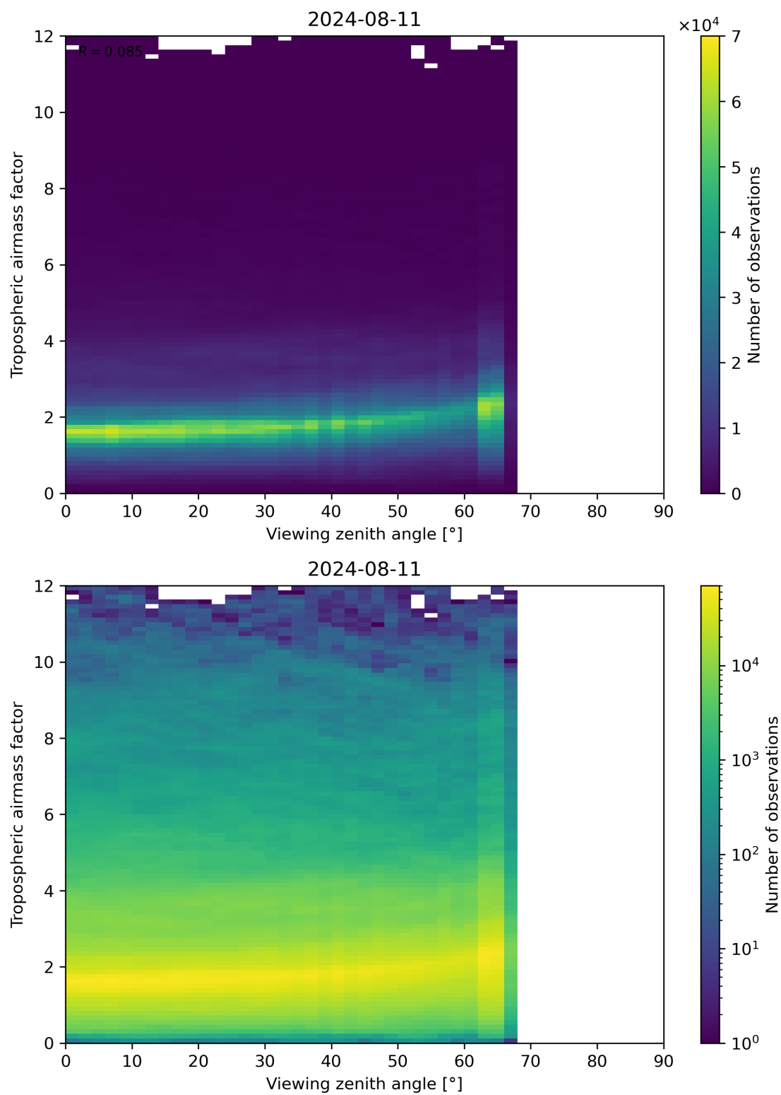
Figure 161: Scatter density plot of “Viewing zenith angle” against “Tropospheric airmass factor” for 2024-08-11 to 2024-08-11.
