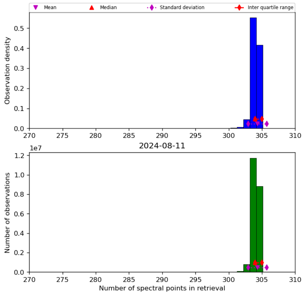
Figure 33: Histogram of “Number of spectral points in retrieval” for 2024-08-11 to 2024-08-11
