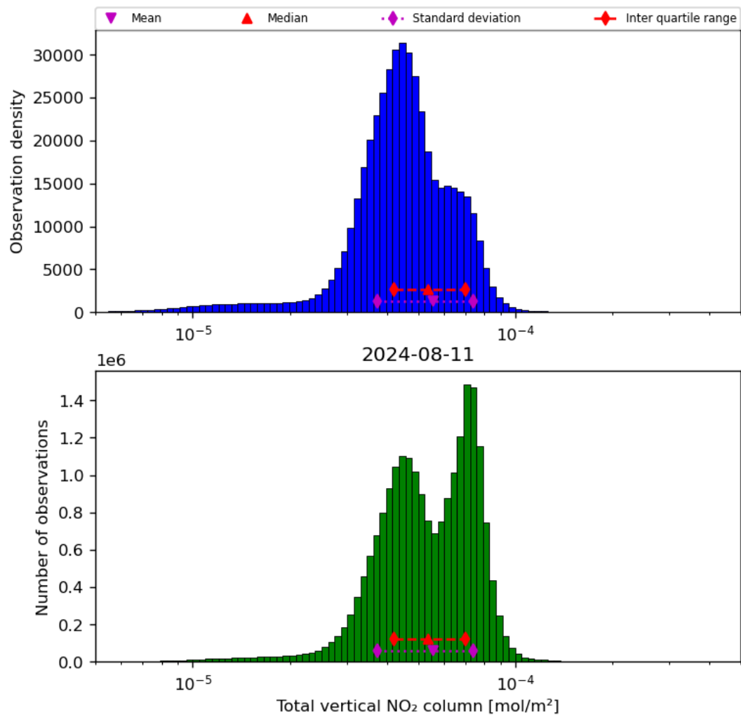
Figure 38: Histogram of "Total vertical NO 2 column" for 2024-08-11 to 2024-08-11
