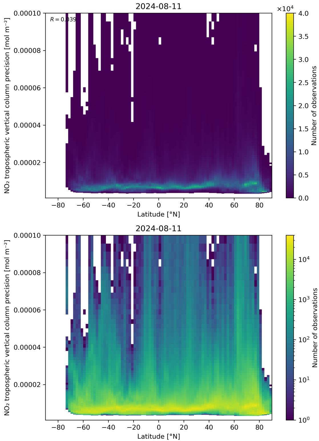
Figure 93: Scatter density plot of “Latitude” against “NO 2 tropospheric vertical column precision” for 2024-08-11 to 2024-08-11.
