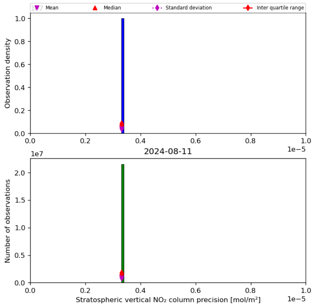
Figure 37: Histogram of “Stratospheric vertical NO 2 column precision” for 2024-08-11 to 2024-08-11
