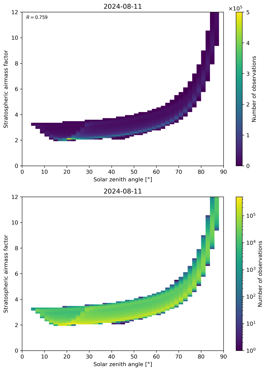
Figure 145: Scatter density plot of “Solar zenith angle” against “Stratospheric airmass factor” for 2024-08-11 to 2024-08-11.
