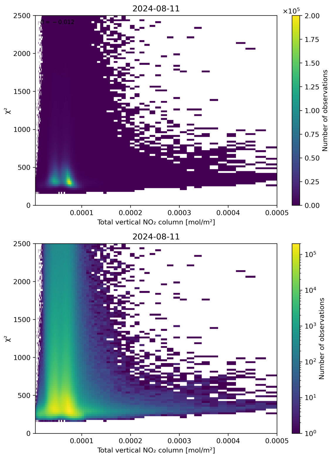
Figure 111: Scatter density plot of “Total vertical NO 2 column” against “ \chi^2 ” for 2024-08-11 to 2024-08-11.
