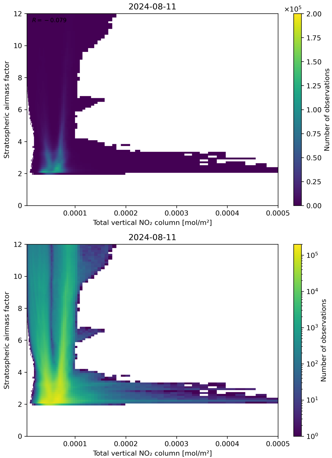
Figure 110: Scatter density plot of “Total vertical NO 2 column” against “Stratospheric airmass factor” for 2024-08-11 to 2024-08-11.
