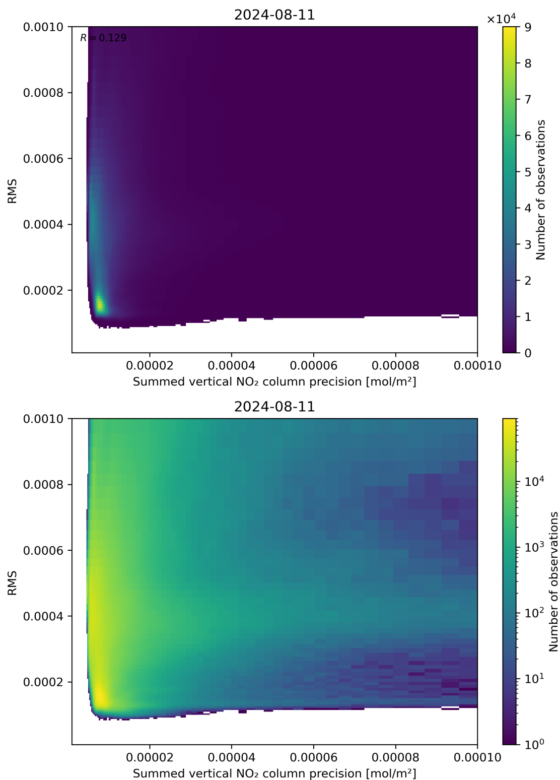
Figure 108: Scatter density plot of “Summed vertical NO 2 column precision” against “RMS” for 2024-08-11 to 2024-08-11.
