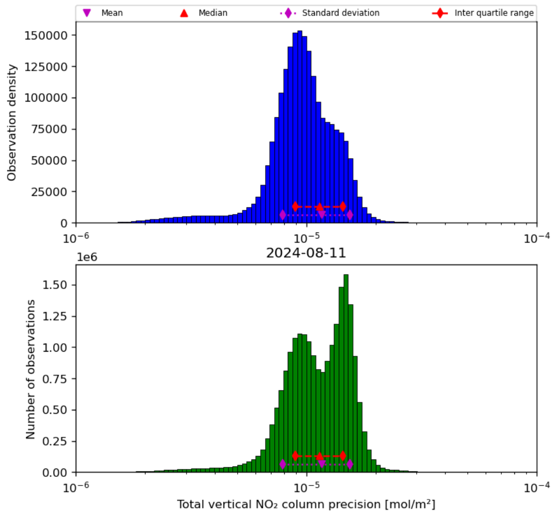
Figure 39: Histogram of "Total vertical NO 2 column precision" for 2024-08-11 to 2024-08-11
