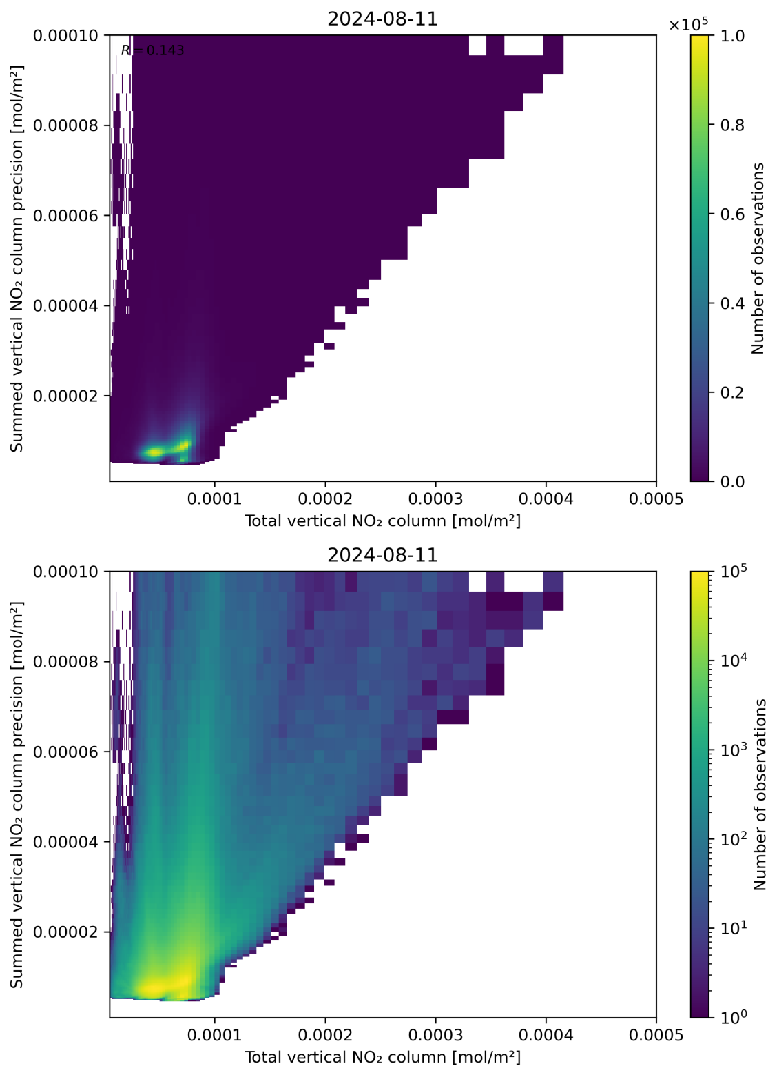
Figure 113: Scatter density plot of “Total vertical NO 2 column” against “Summed vertical NO 2 column precision” for 2024-08-11 to 2024-08-11.
