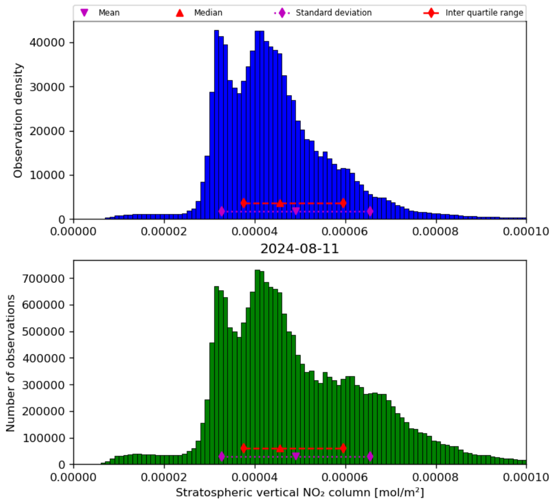
Figure 36: Histogram of “Stratospheric vertical NO 2 column” for 2024-08-11 to 2024-08-11
