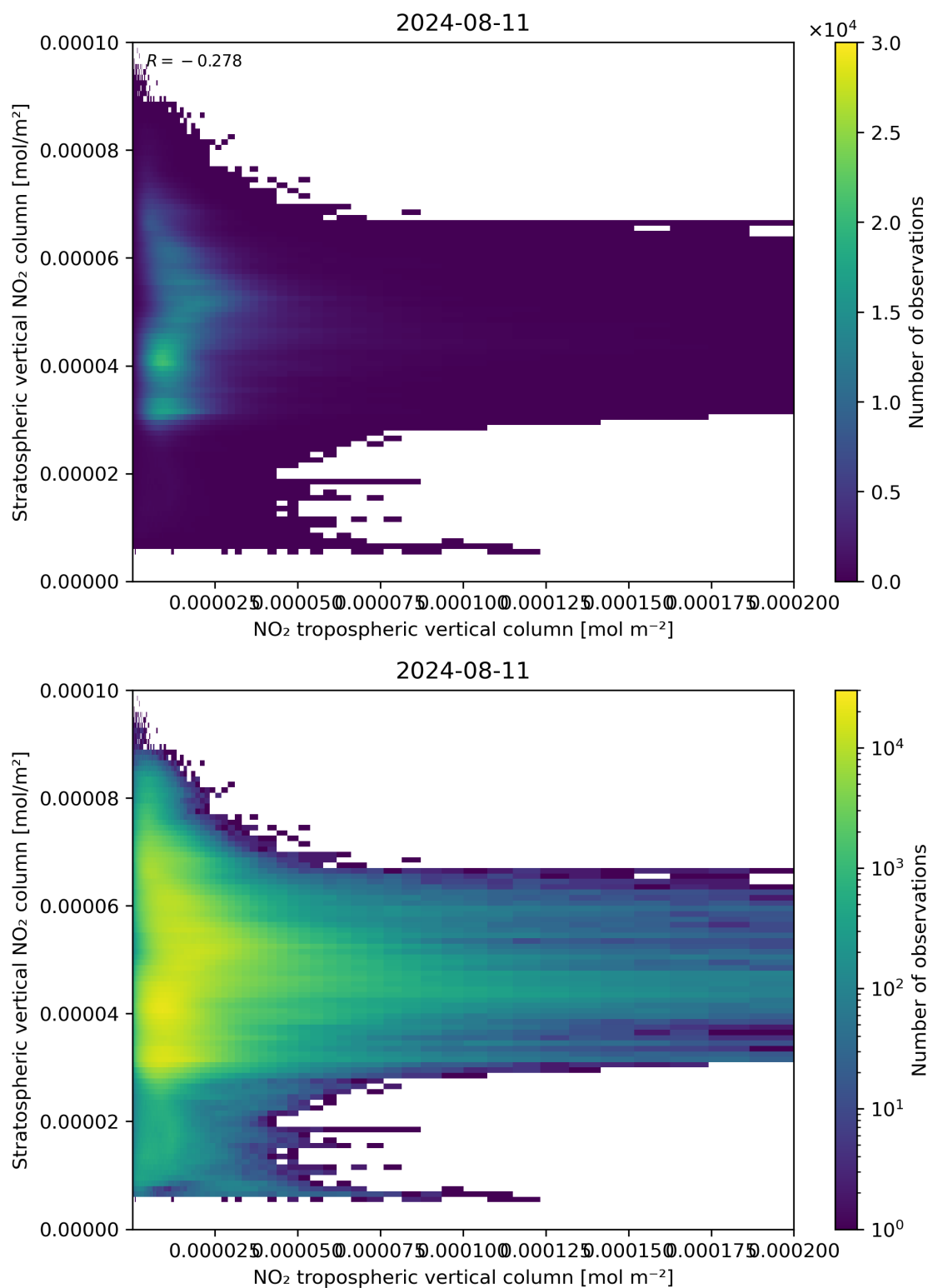
Figure 125: Scatter density plot of “NO 2 tropospheric vertical column” against “Stratospheric vertical NO 2 column” for 2024-08-11 to 2024-08-11.
