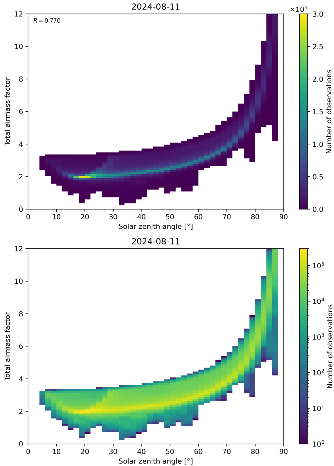
Figure 146: Scatter density plot of “Solar zenith angle” against “Total air mass factor” for 2024-08-11 to 2024-08-11.
