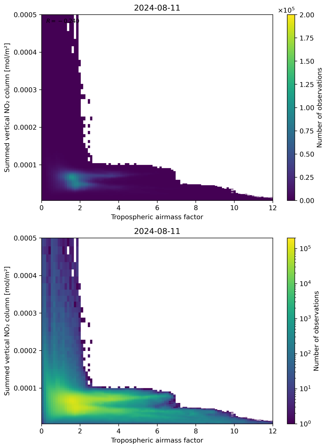
Figure 75: Scatter density plot of “Tropospheric airmass factor” against “Summed vertical NO 2 column” for 2024-08-11 to 2024-08-11.
