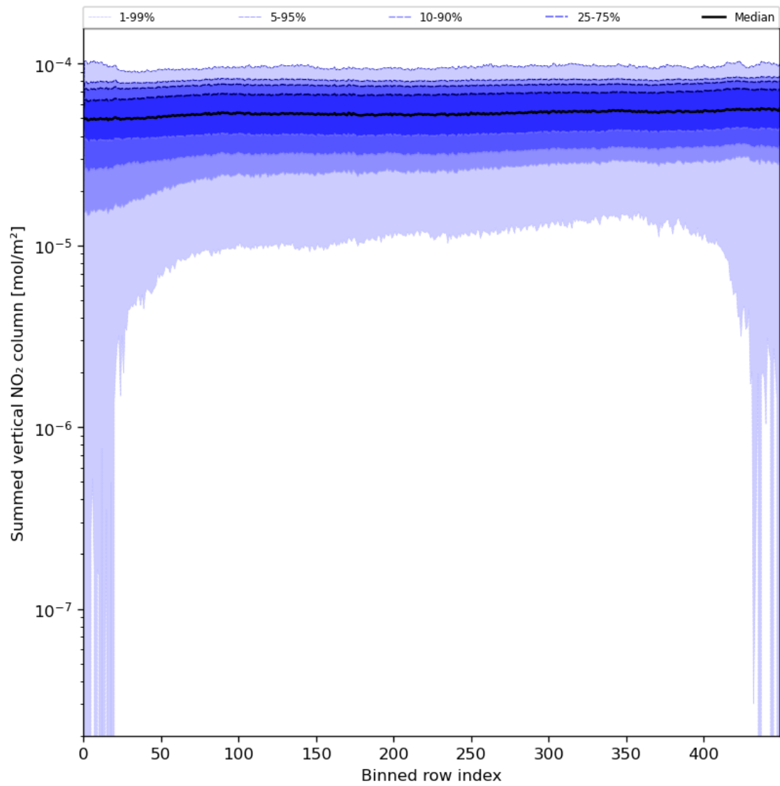
Figure 57: Along track statistics of “Summed vertical NO 2 column” for 2024-08-11 to 2024-08-11
