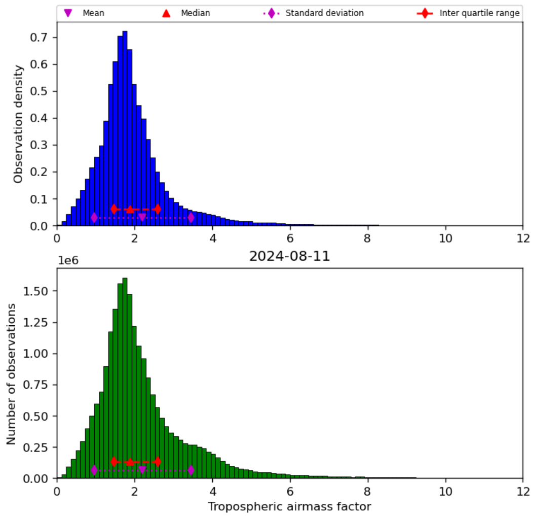
Figure 31: Histogram of “Tropospheric airmass factor” for 2024-08-11 to 2024-08-11
