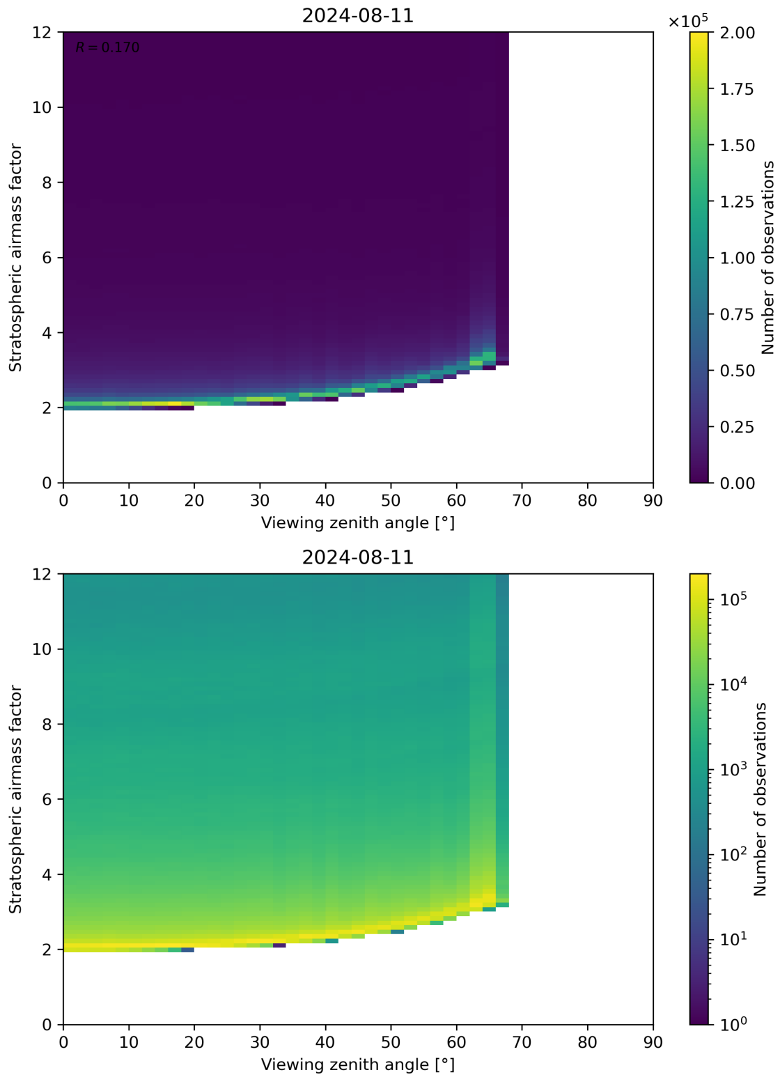
Figure 159: Scatter density plot of “Viewing zenith angle” against “Stratospheric airmass factor” for 2024-08-11 to 2024-08-11.
