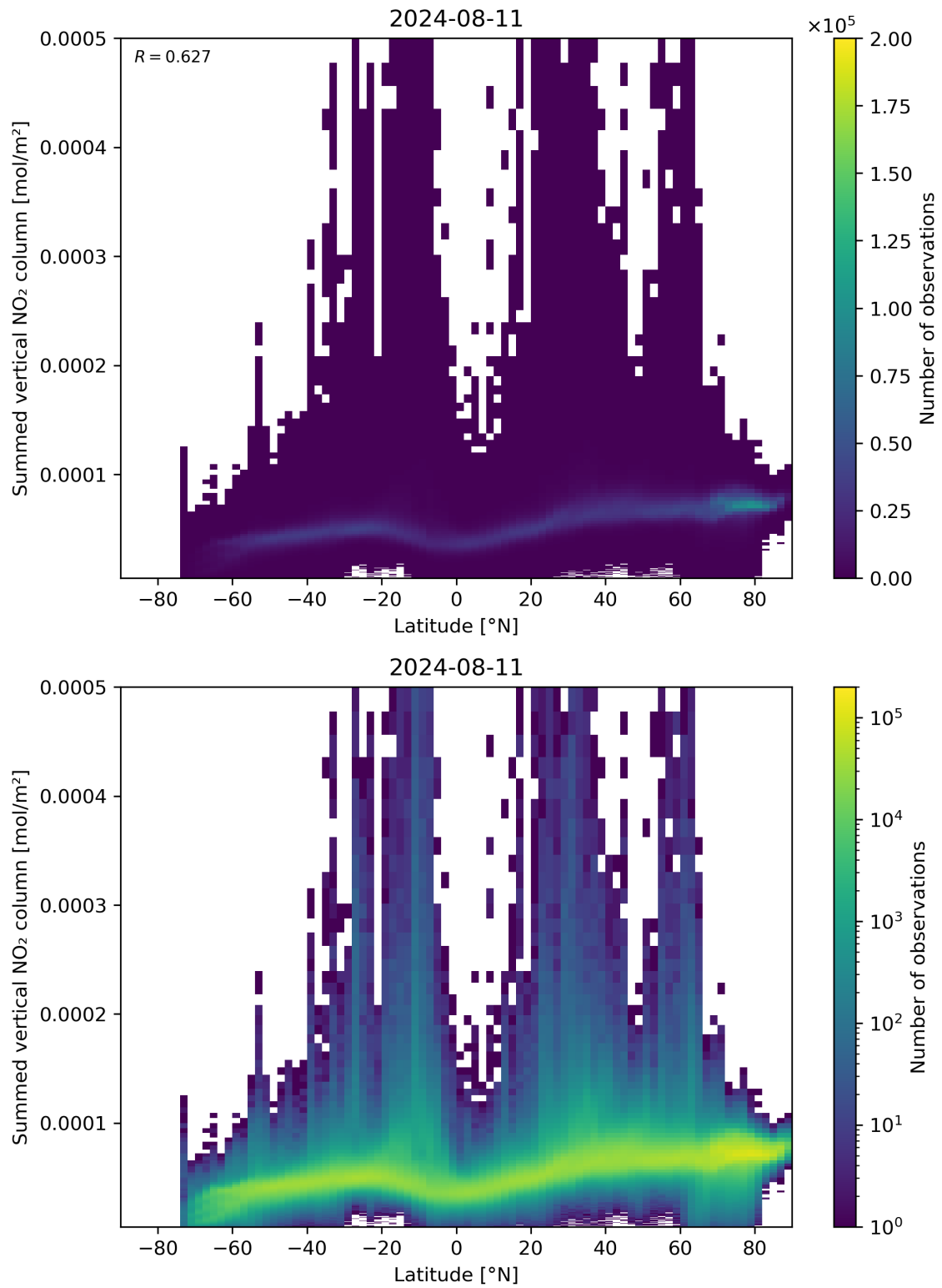
Figure 88: Scatter density plot of “Latitude” against “Summed vertical NO 2 column” for 2024-08-11 to 2024-08-11.
