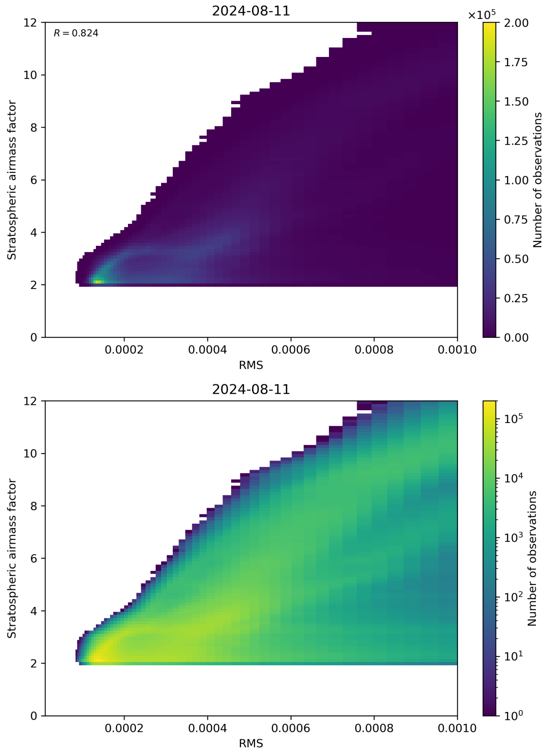
Figure 144: Scatter density plot of “RMS” against “Stratospheric airmass factor” for 2024-08-11 to 2024-08-11.
