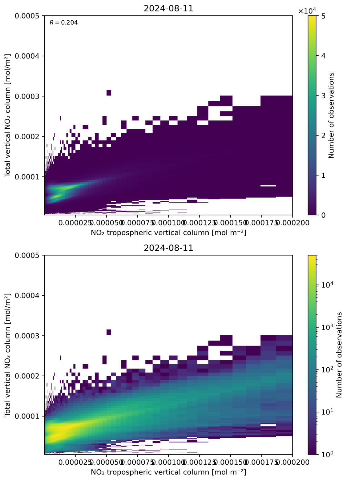
Figure 128: Scatter density plot of “NO 2 tropospheric vertical column” against “Total vertical NO 2 column” for 2024-08-11 to 2024-08-11.
