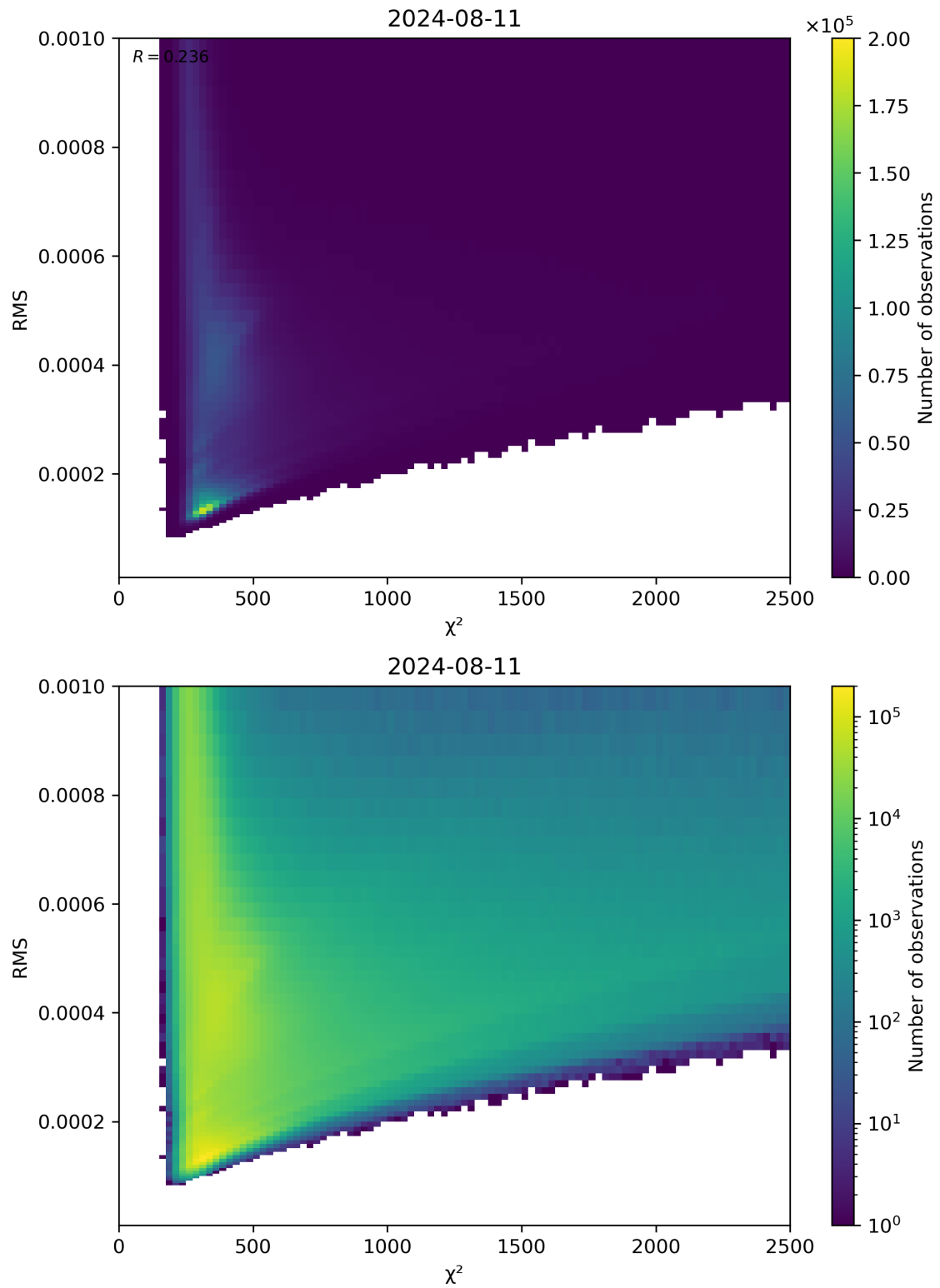
Figure 82: Scatter density plot of “ \chi^2 ” against “RMS” for 2024-08-11 to 2024-08-11.
