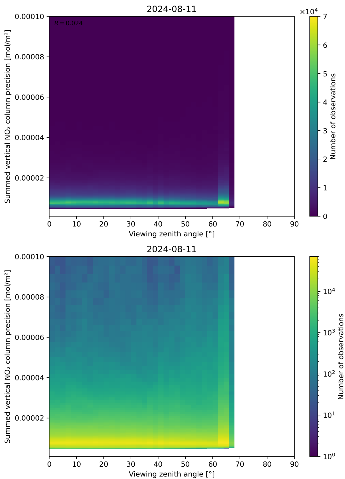
Figure 166: Scatter density plot of “Viewing zenith angle” against “Summed vertical NO 2 column precision” for 2024-08-11 to 2024-08-11.
