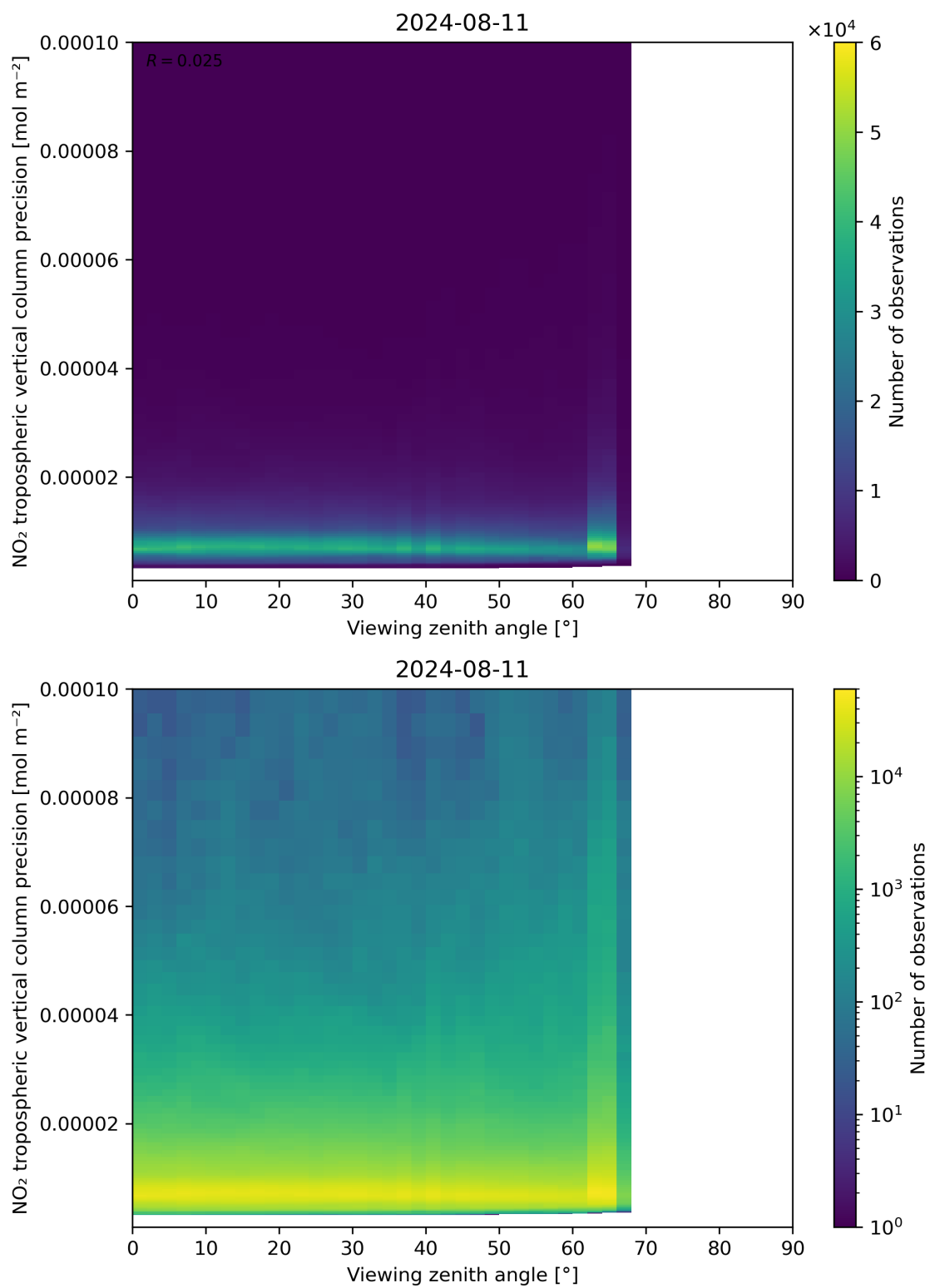
Figure 170: Scatter density plot of “Viewing zenith angle” against “NO 2 tropospheric vertical column precision” for 2024-08-11 to 2024-08-11.
