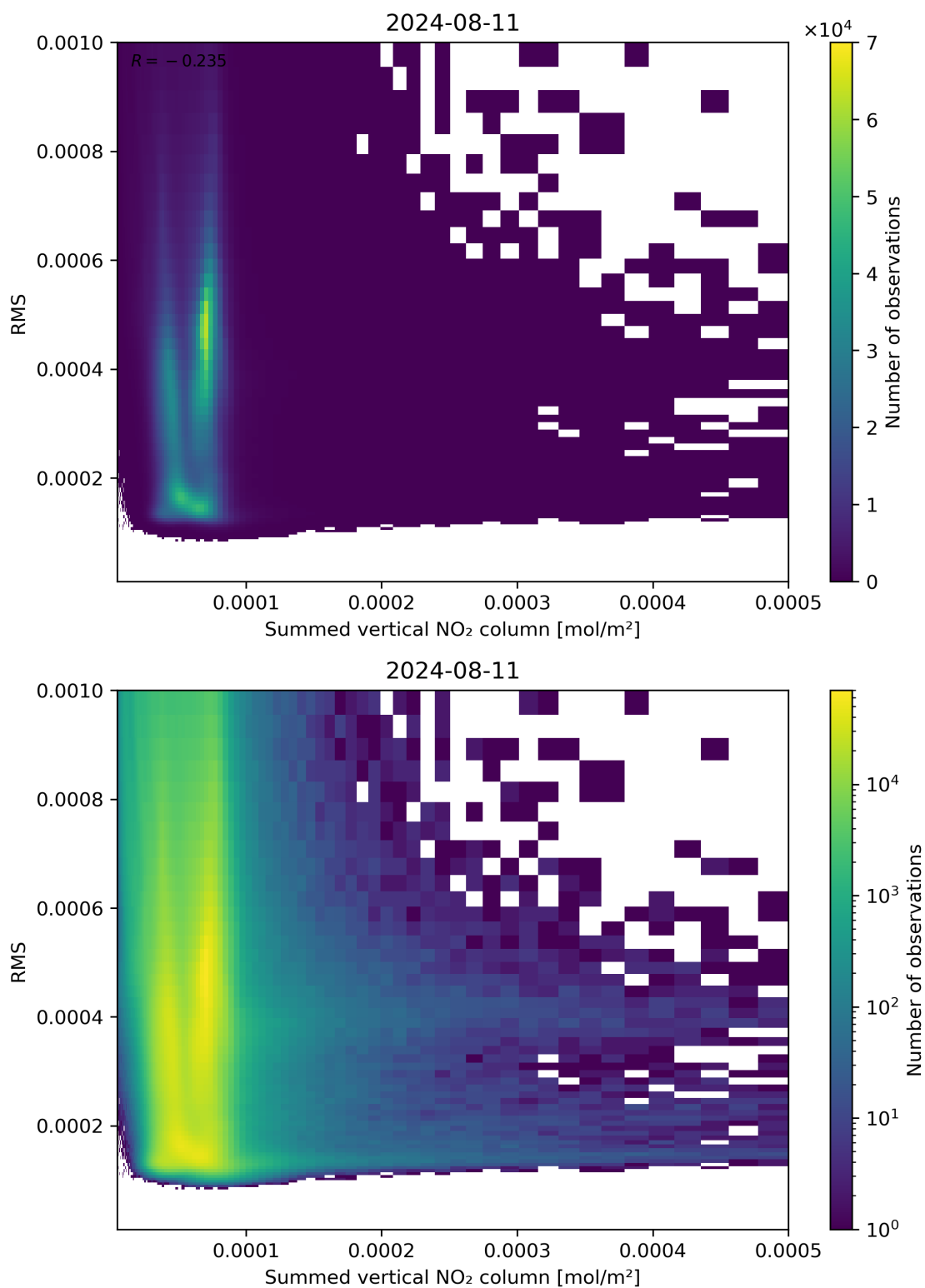
Figure 109: Scatter density plot of “Summed vertical NO 2 column” against “RMS” for 2024-08-11 to 2024-08-11.
