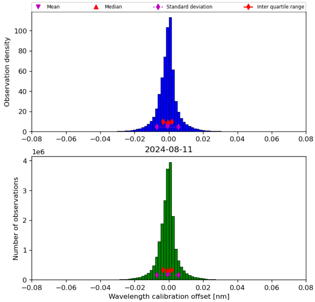
Figure 35: Histogram of “Wavelength calibration offset” for 2024-08-11 to 2024-08-11
