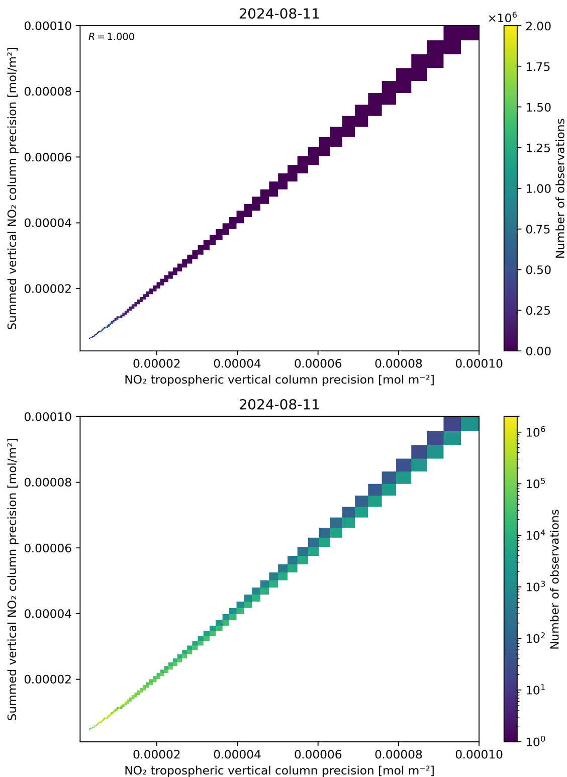
Figure 137: Scatter density plot of “NO 2 tropospheric vertical column precision” against “Summed vertical NO 2 column precision” for 2024-08-11 to 2024-08-11.
