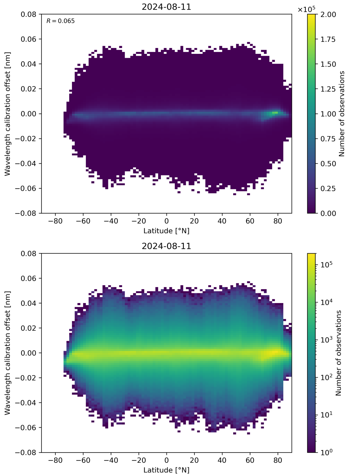
Figure 95: Scatter density plot of “Latitude” against “Wavelength calibration offset” for 2024-08-11 to 2024-08-11.
