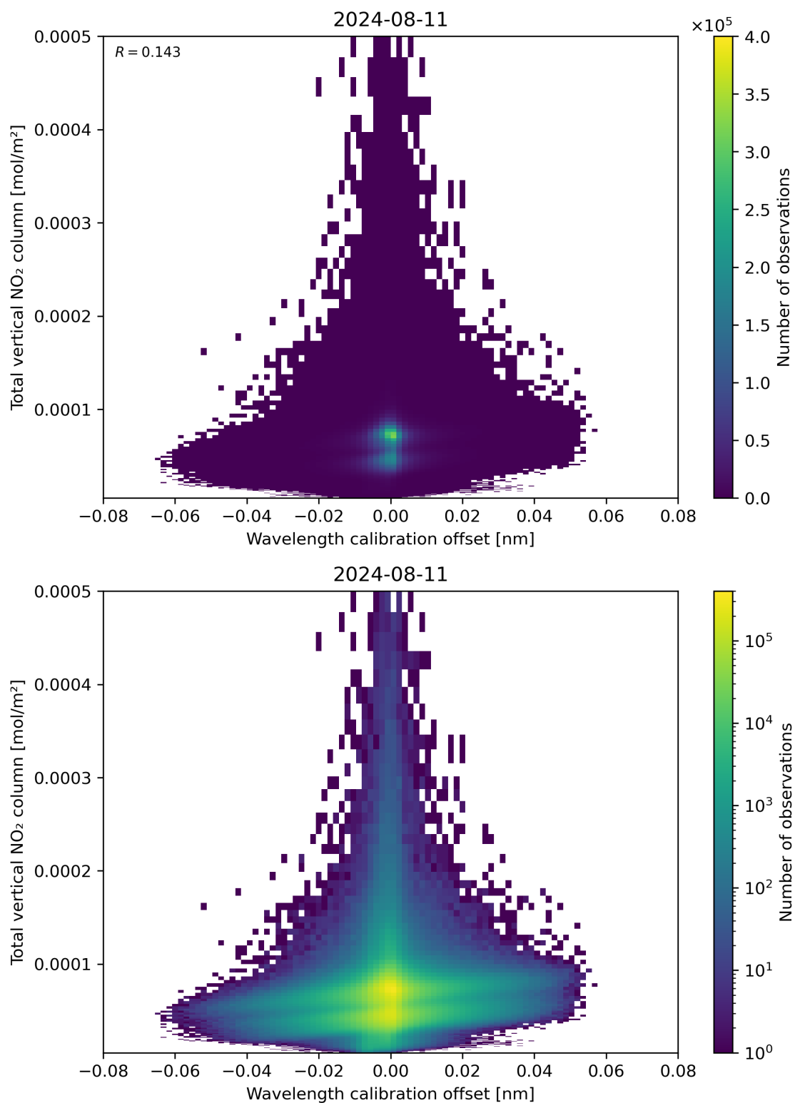
Figure 179: Scatter density plot of “Wavelength calibration offset” against “Total vertical NO 2 column” for 2024-08-11 to 2024-08-11.
