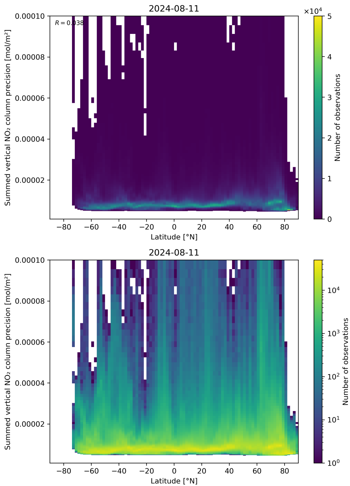
Figure 89: Scatter density plot of “Latitude” against “Summed vertical NO 2 column precision” for 2024-08-11 to 2024-08-11.
