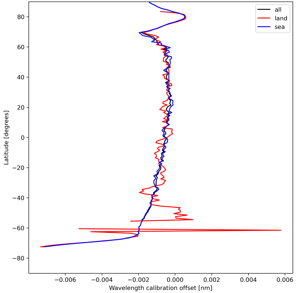
Figure 18: Zonal average of “Wavelength calibration offset” for 2024-08-11 to 2024-08-11.
