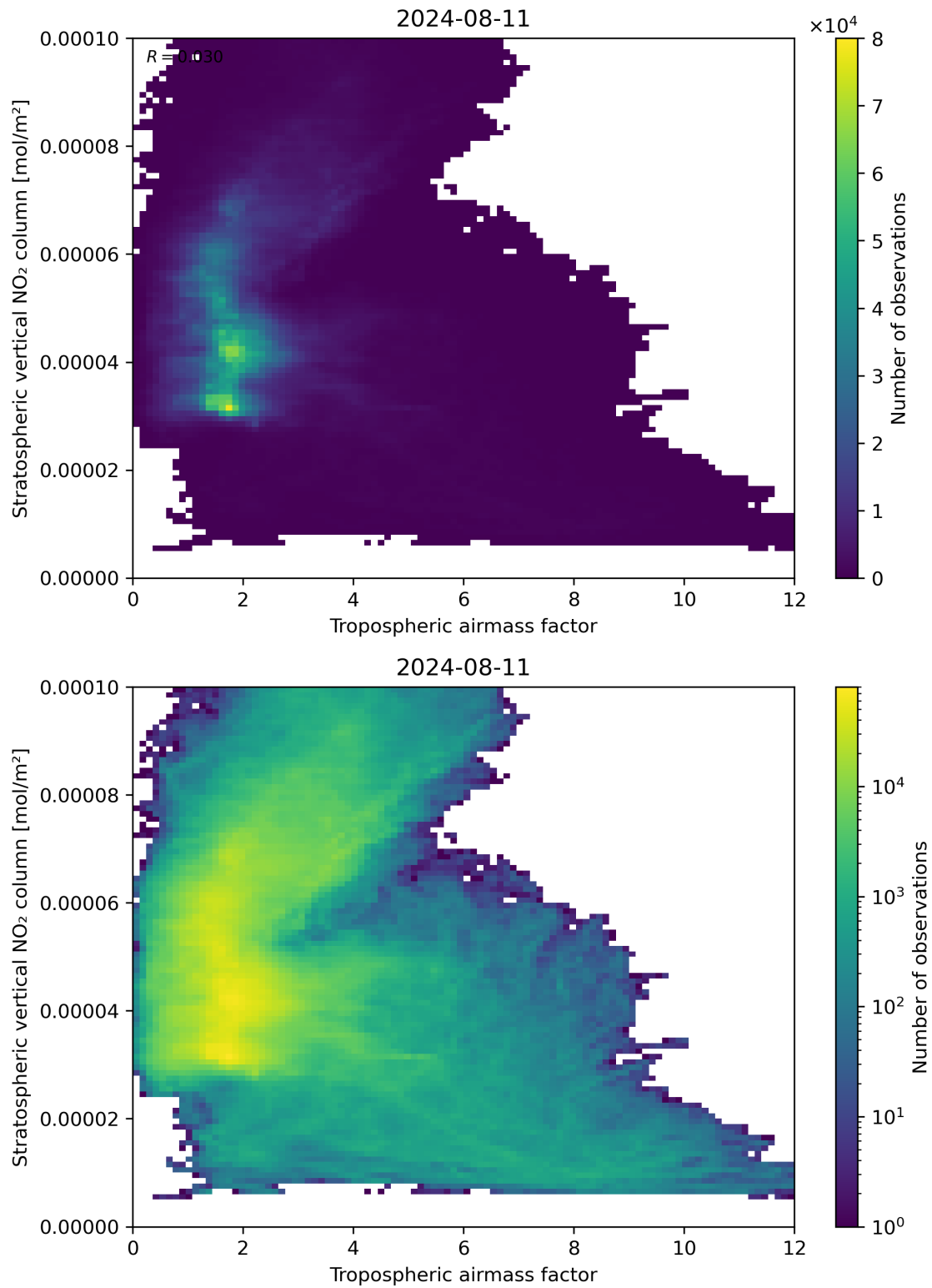
Figure 74: Scatter density plot of “Tropospheric air mass factor” against “Stratospheric vertical NO 2 column” for 2024-08-11 to 2024-08-11.
