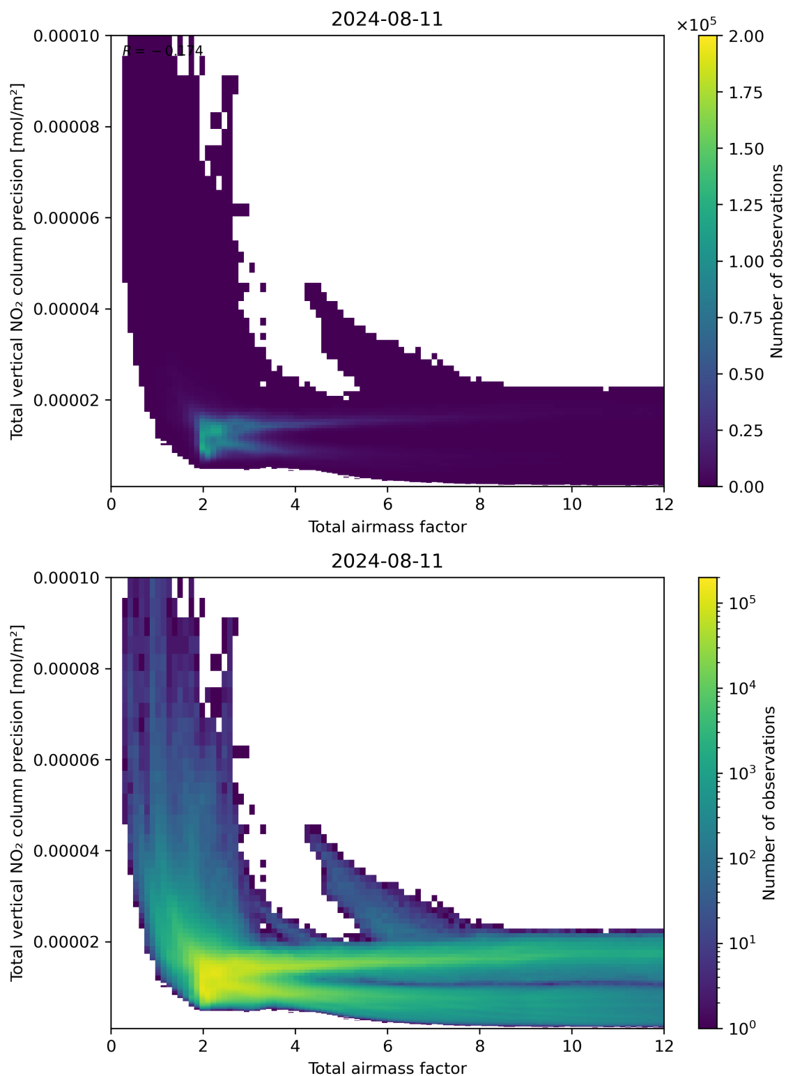
Figure 68: Scatter density plot of “Total airmass factor” against “Total vertical NO 2 column precision” for 2024-08-11 to 2024-08-11.
