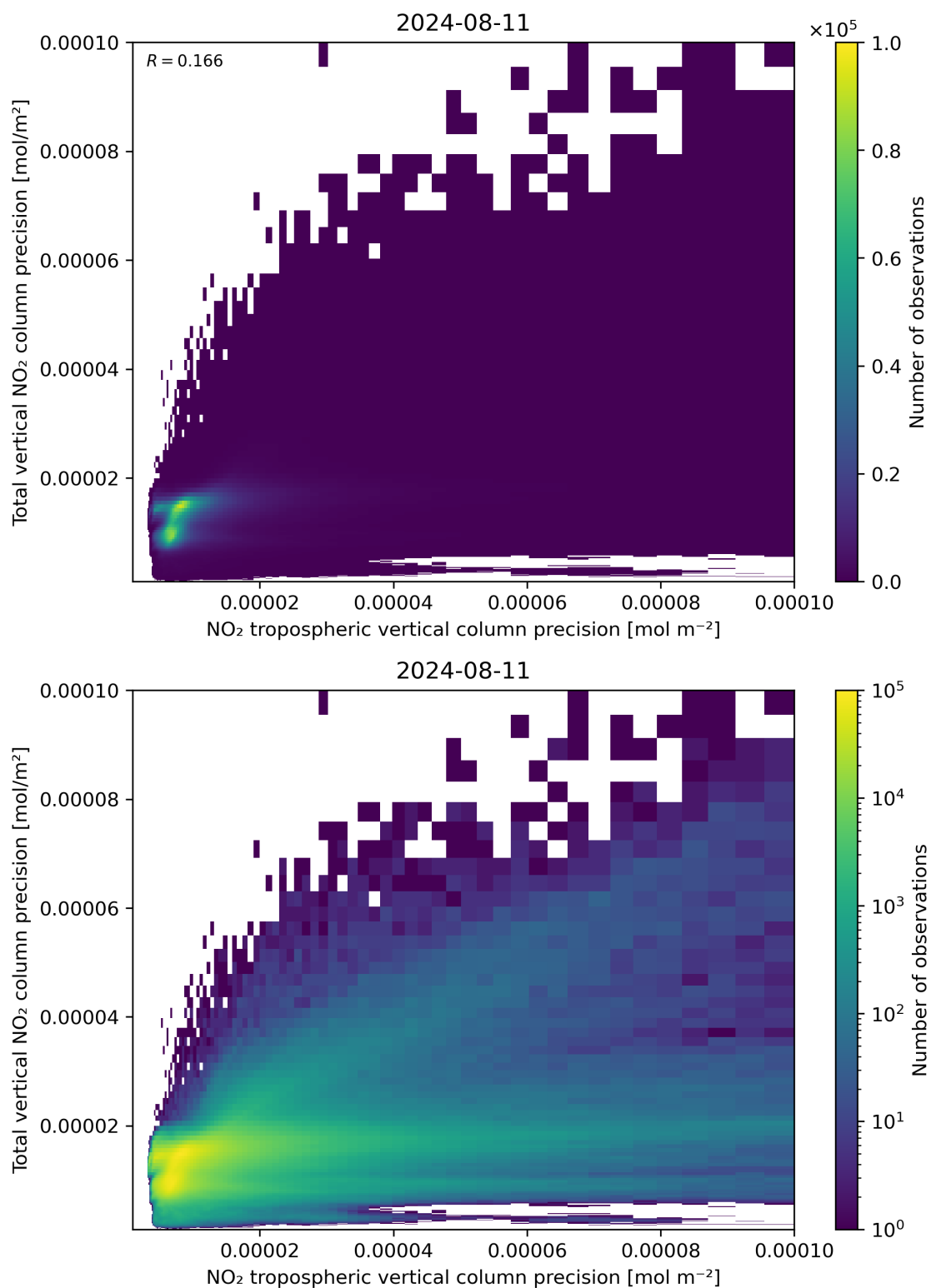
Figure 139: Scatter density plot of “NO 2 tropospheric vertical column precision” against “Total vertical NO 2 column precision” for 2024-08-11 to 2024-08-11.
