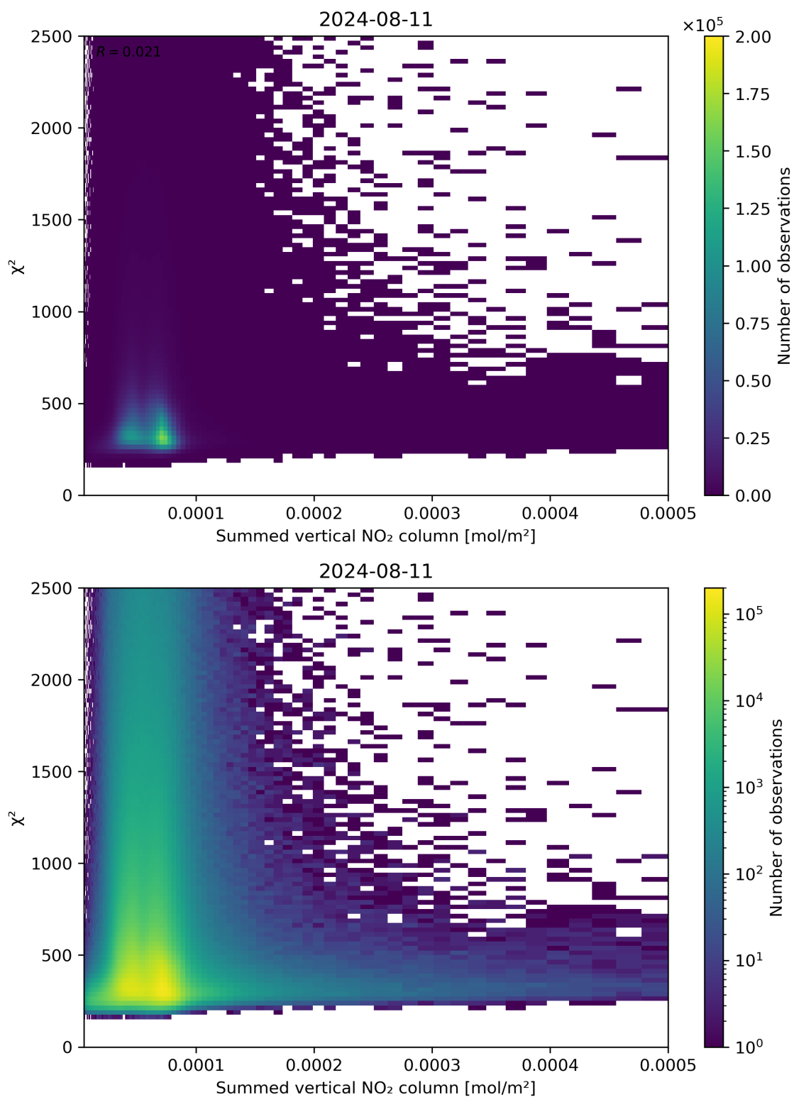
Figure 104: Scatter density plot of “Summed vertical NO 2 column” against “ \chi^2 ” for 2024-08-11 to 2024-08-11.
