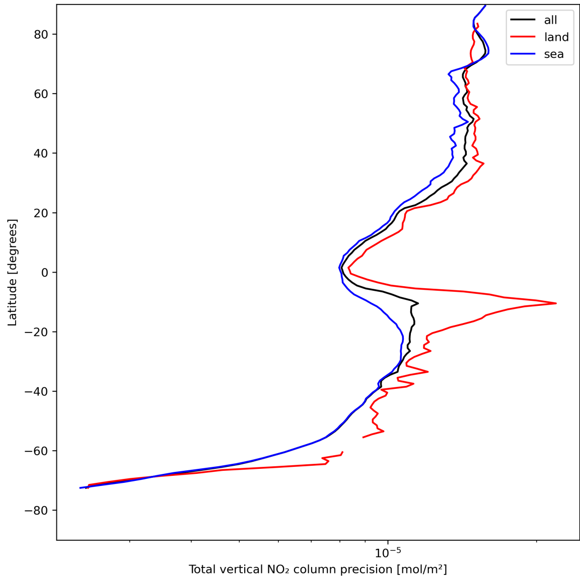
Figure 22: Zonal average of “Total vertical NO 2 column precision” for 2024-08-11 to 2024-08-11.
