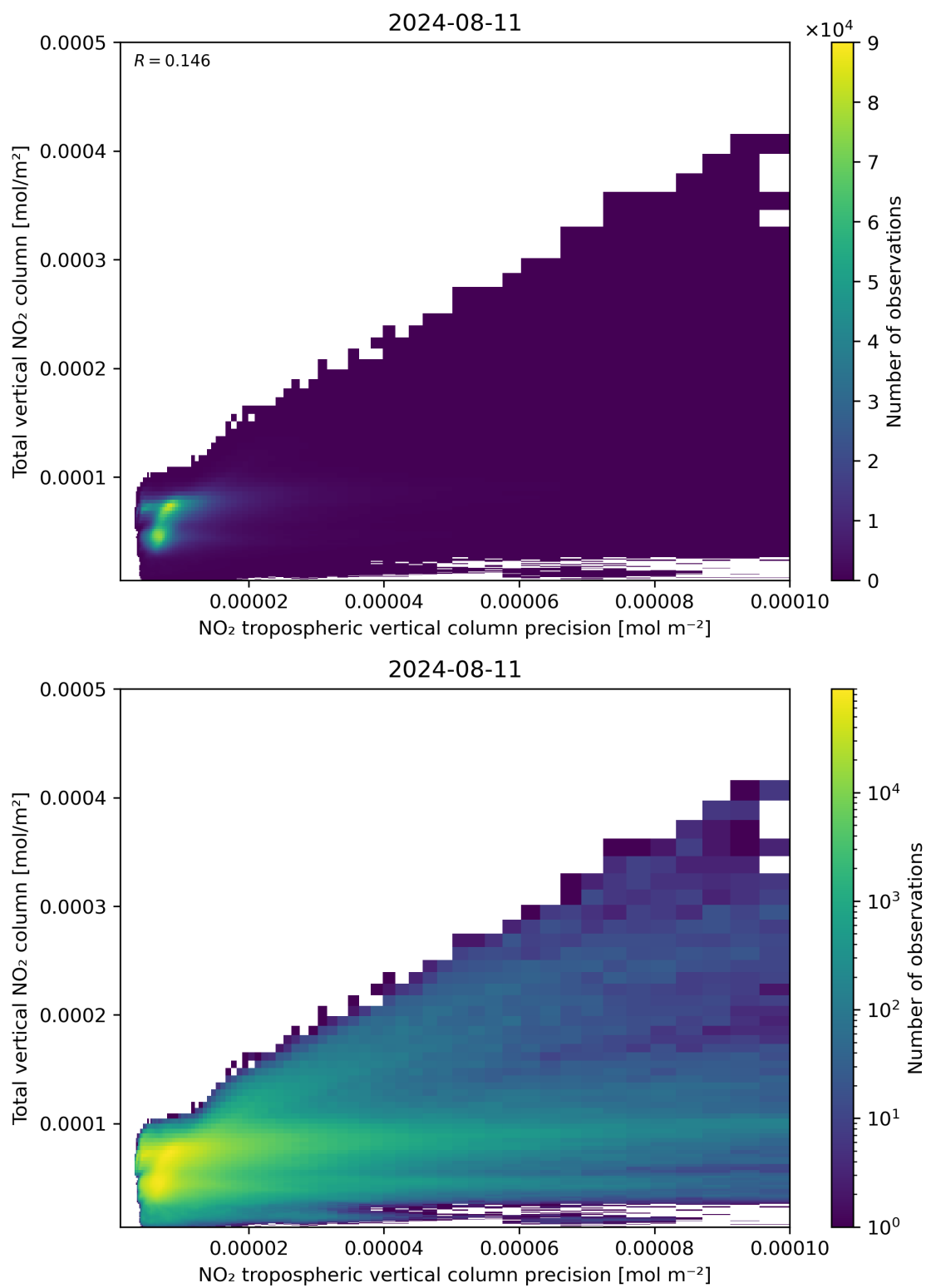
Figure 138: Scatter density plot of “NO 2 tropospheric vertical column precision” against “Total vertical NO 2 column” for 2024-08-11 to 2024-08-11.
