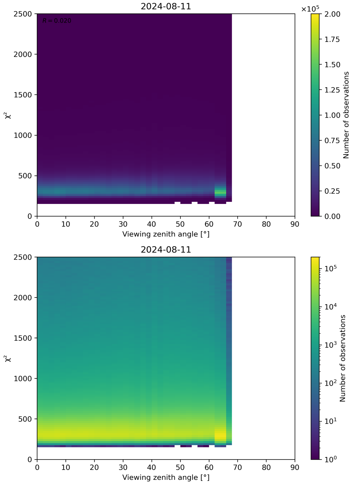
Figure 162: Scatter density plot of “Viewing zenith angle” against “ \chi^2 ” for 2024-08-11 to 2024-08-11.
