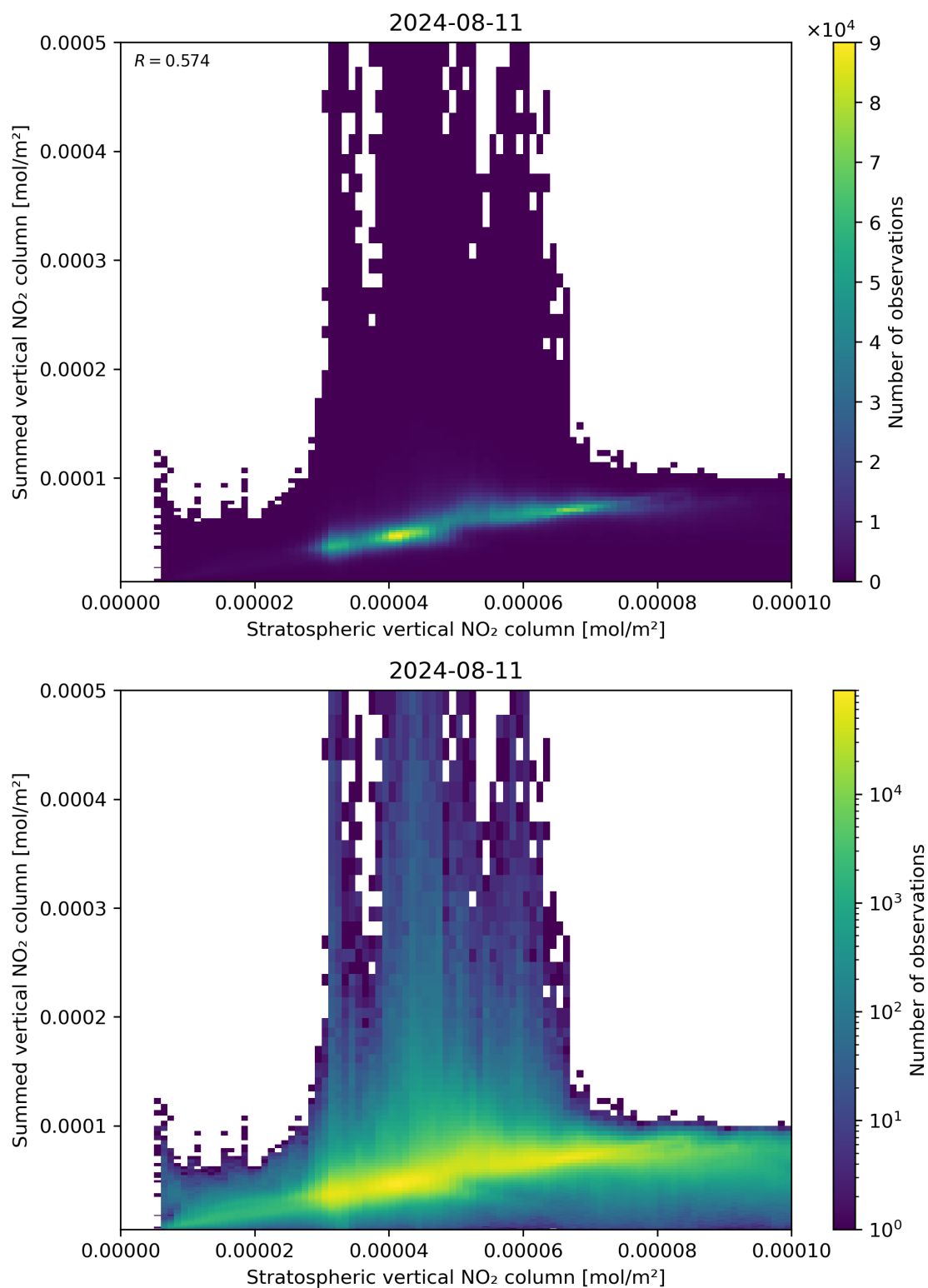
Figure 98: Scatter density plot of “Stratospheric vertical NO 2 column” against “Summed vertical NO 2 column” for 2024-08-11 to 2024-08-11.
