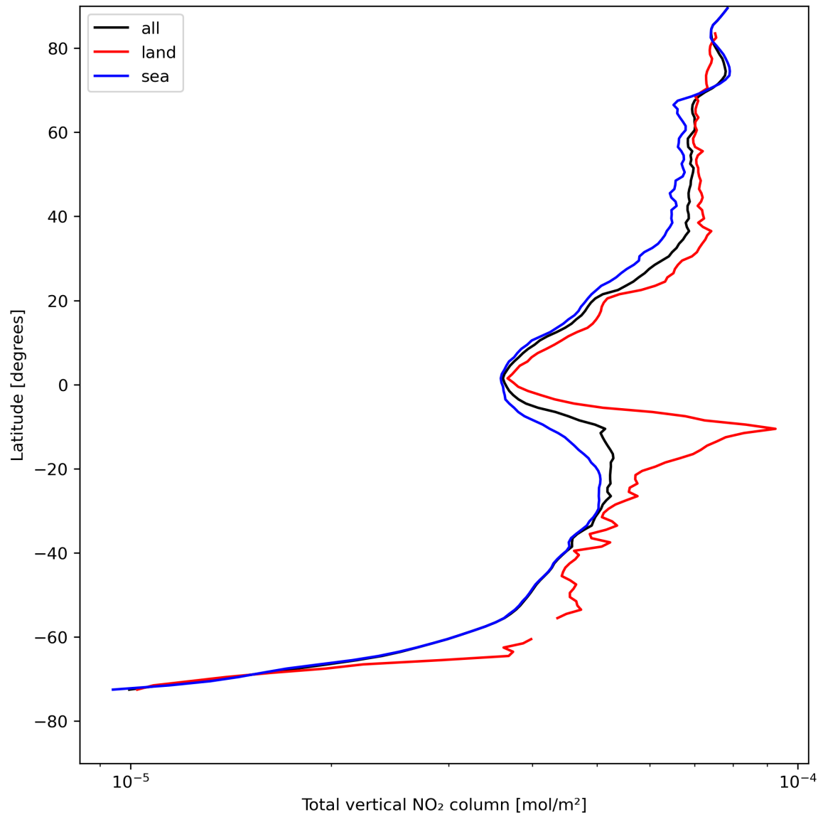
Figure 21: Zonal average of “Total vertical NO 2 column” for 2024-08-11 to 2024-08-11.
