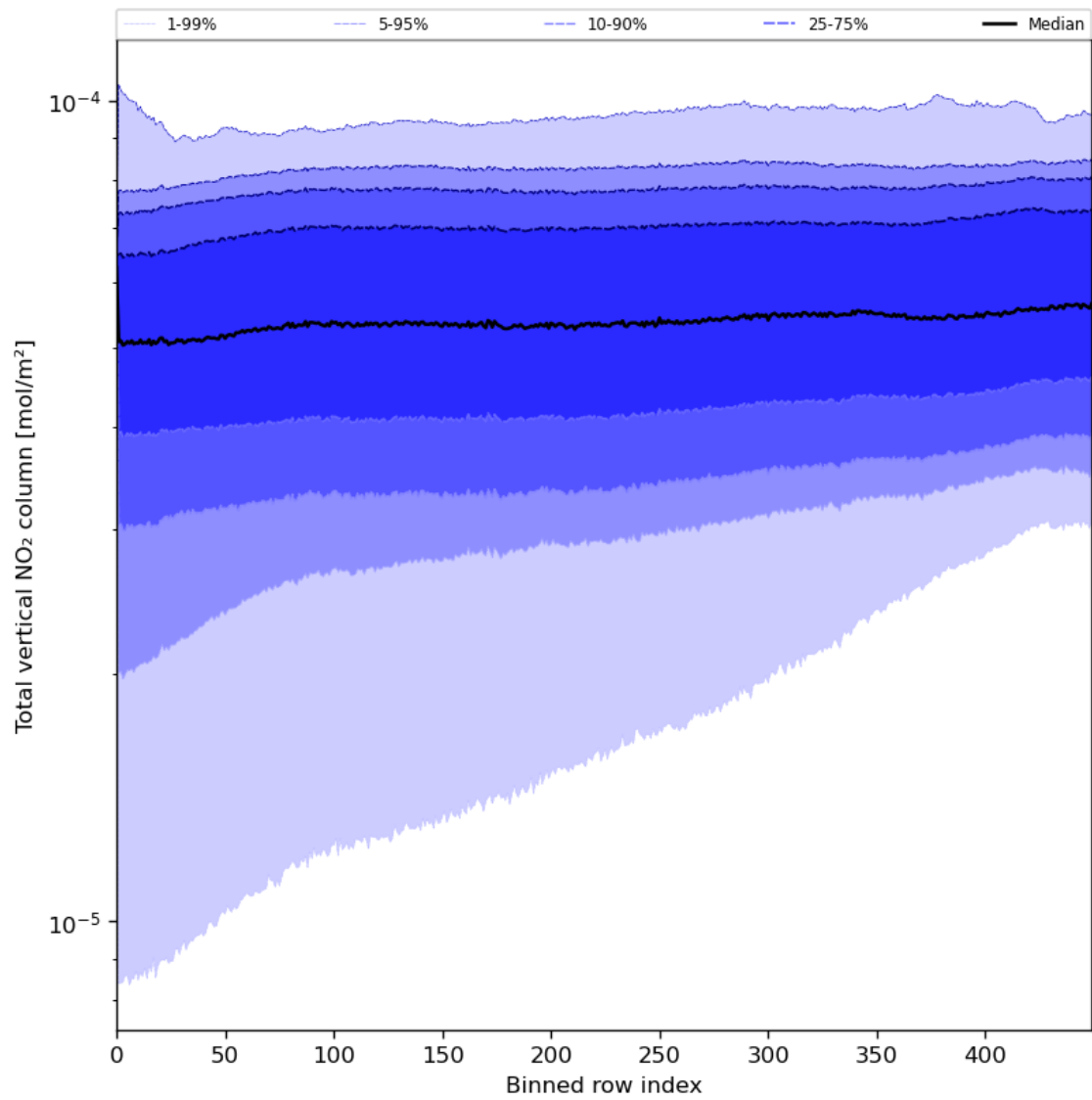
Figure 55: Along track statistics of “Total vertical NO 2 column” for 2024-08-11 to 2024-08-11
