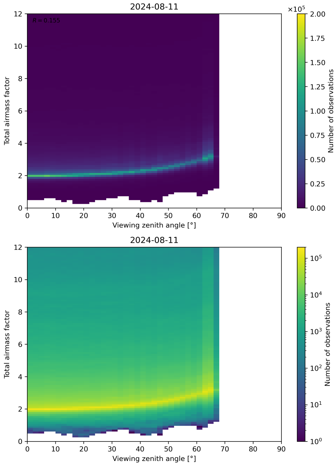
Figure 160: Scatter density plot of “Viewing zenith angle” against “Total airmass factor” for 2024-08-11 to 2024-08-11.
