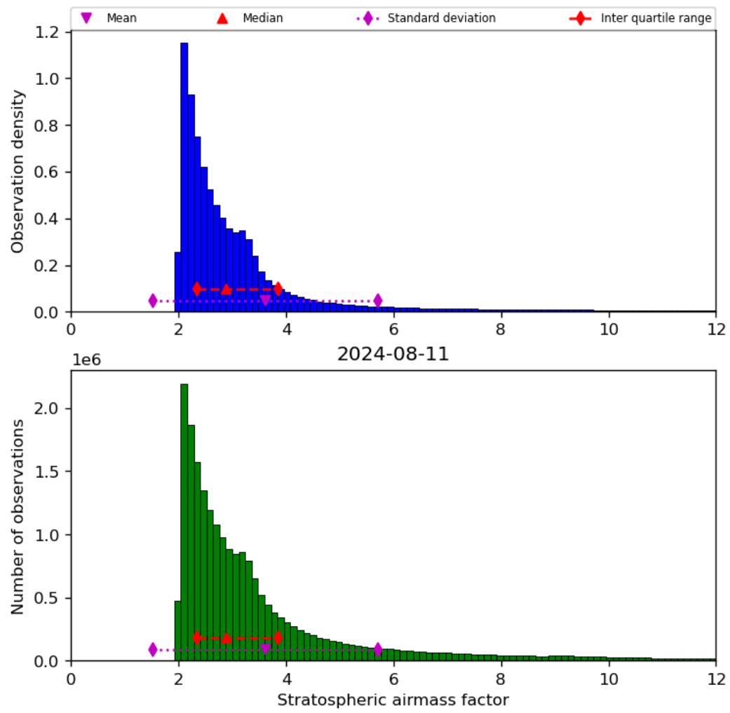
Figure 44: Histogram of “Stratospheric airmass factor” for 2024-08-11 to 2024-08-11
