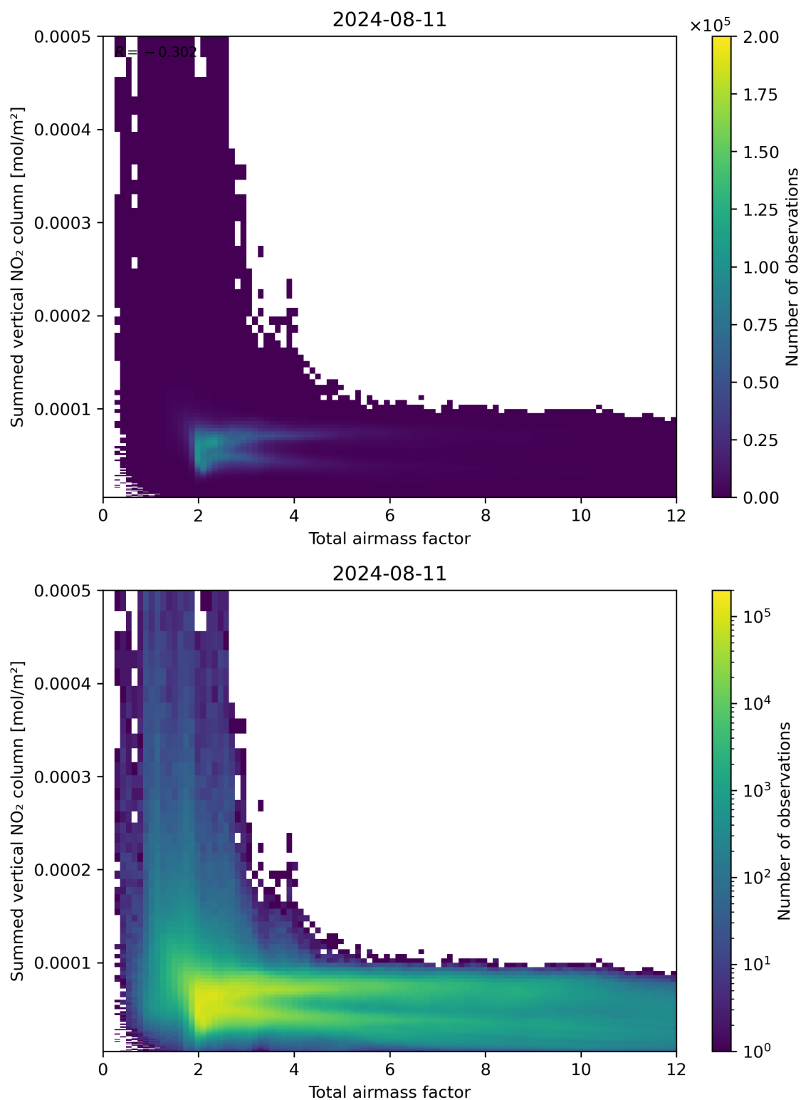
Figure 65: Scatter density plot of “Total airmass factor” against “Summed vertical NO 2 column” for 2024-08-11 to 2024-08-11.
