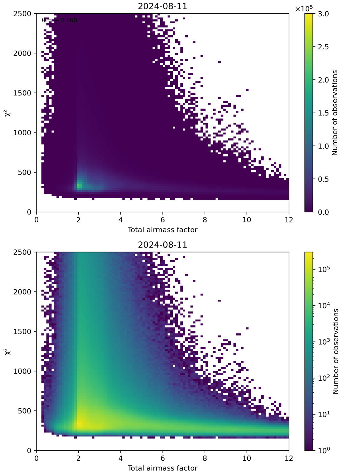
Figure 63: Scatter density plot of “Total airmass factor” against “ \chi^2 ” for 2024-08-11 to 2024-08-11.
