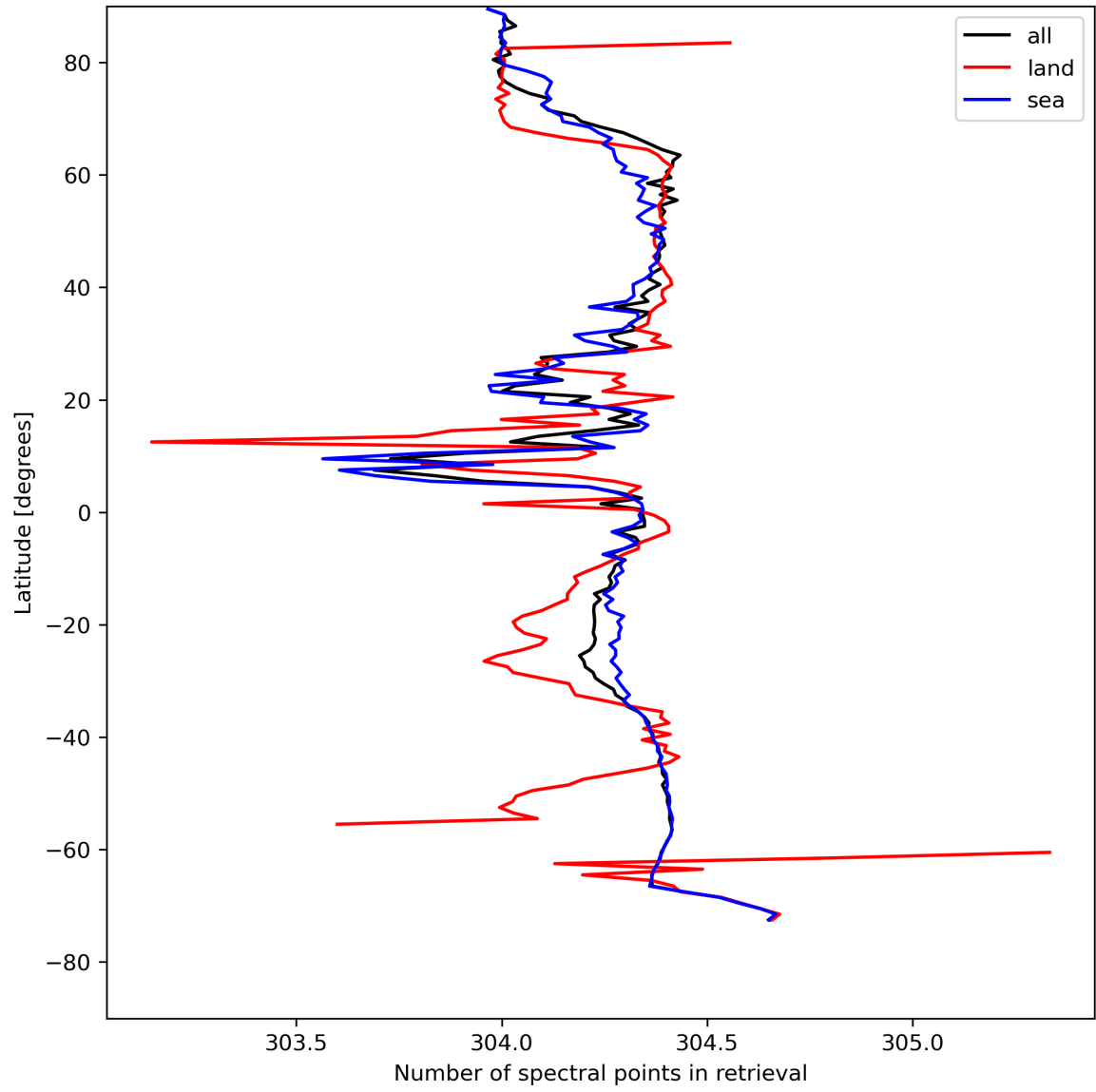
Figure 16: Zonal average of “Number of spectral points in retrieval” for 2024-08-11 to 2024-08-11.
