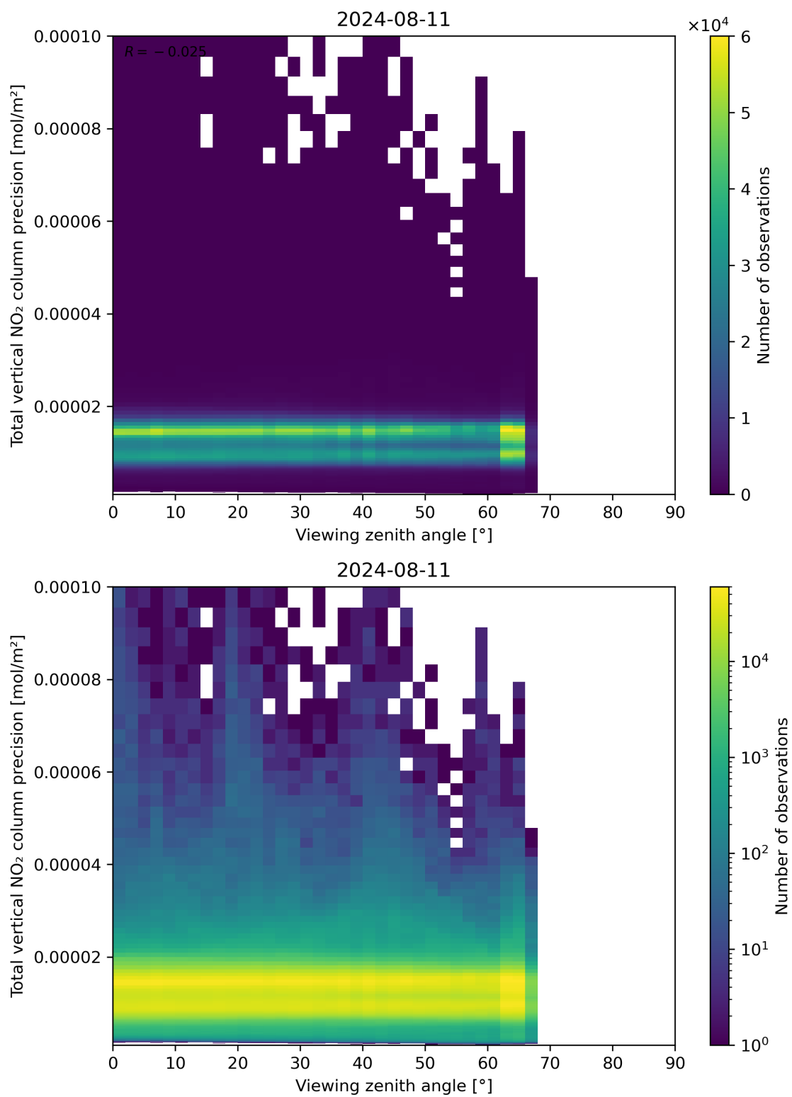
Figure 168: Scatter density plot of “Viewing zenith angle” against “Total vertical NO 2 column precision” for 2024-08-11 to 2024-08-11.
