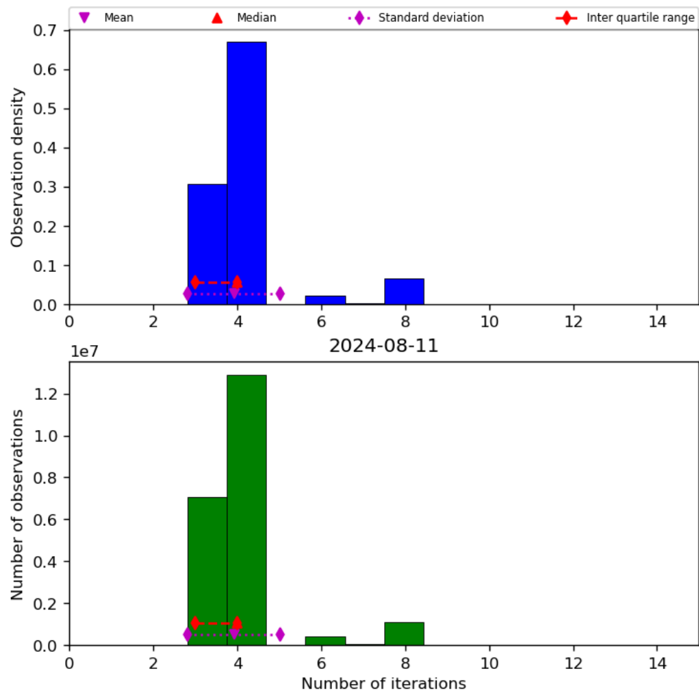
Figure 34: Histogram of “Number of iterations” for 2024-08-11 to 2024-08-11
