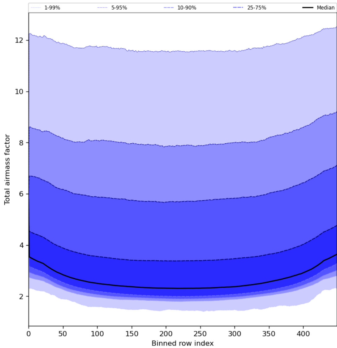
Figure 49: Along track statistics of “Total airmass factor” for 2024-08-11 to 2024-08-11
