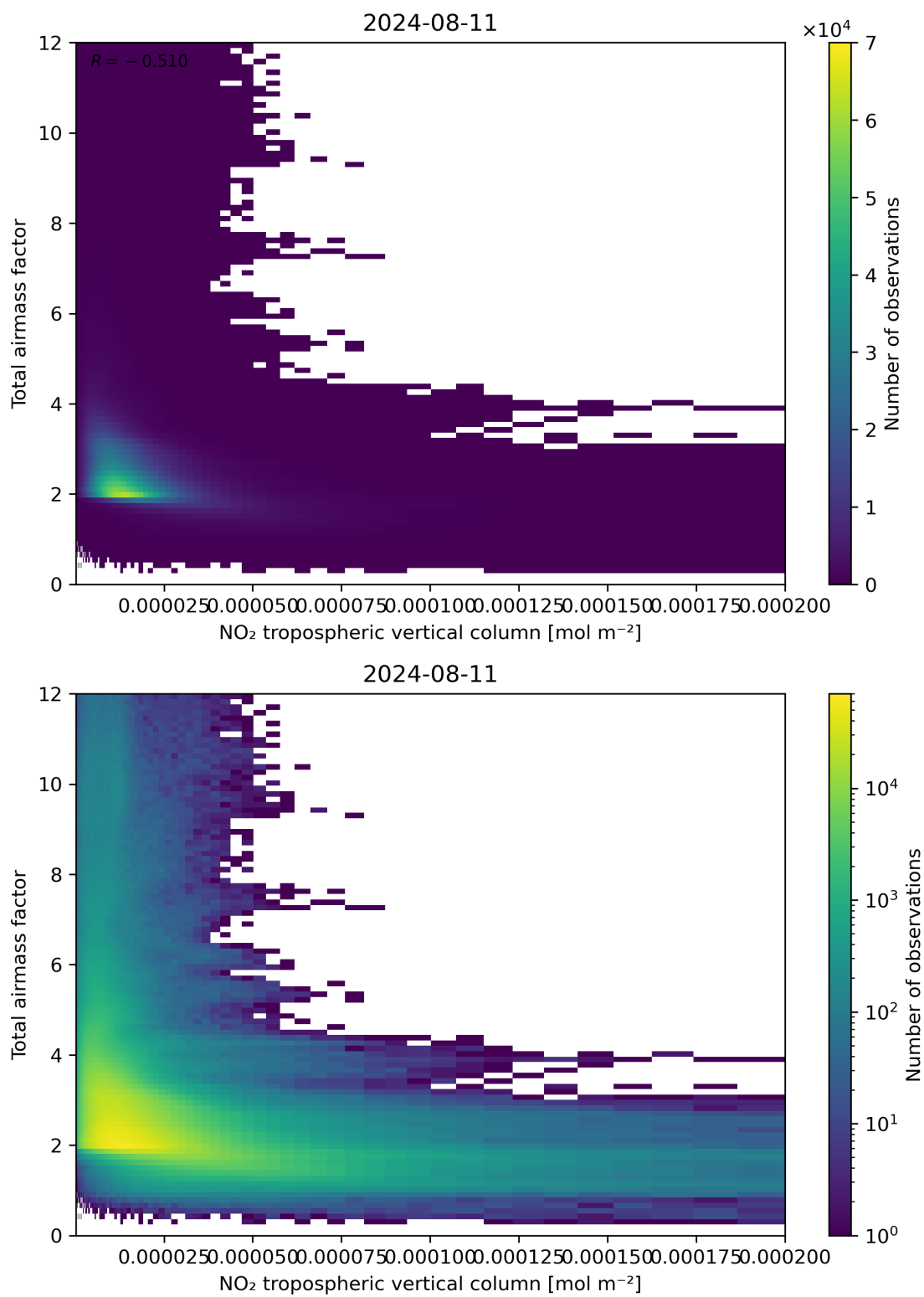
Figure 122: Scatter density plot of “NO 2 tropospheric vertical column” against “Total air mass factor” for 2024-08-11 to 2024-08-11.
