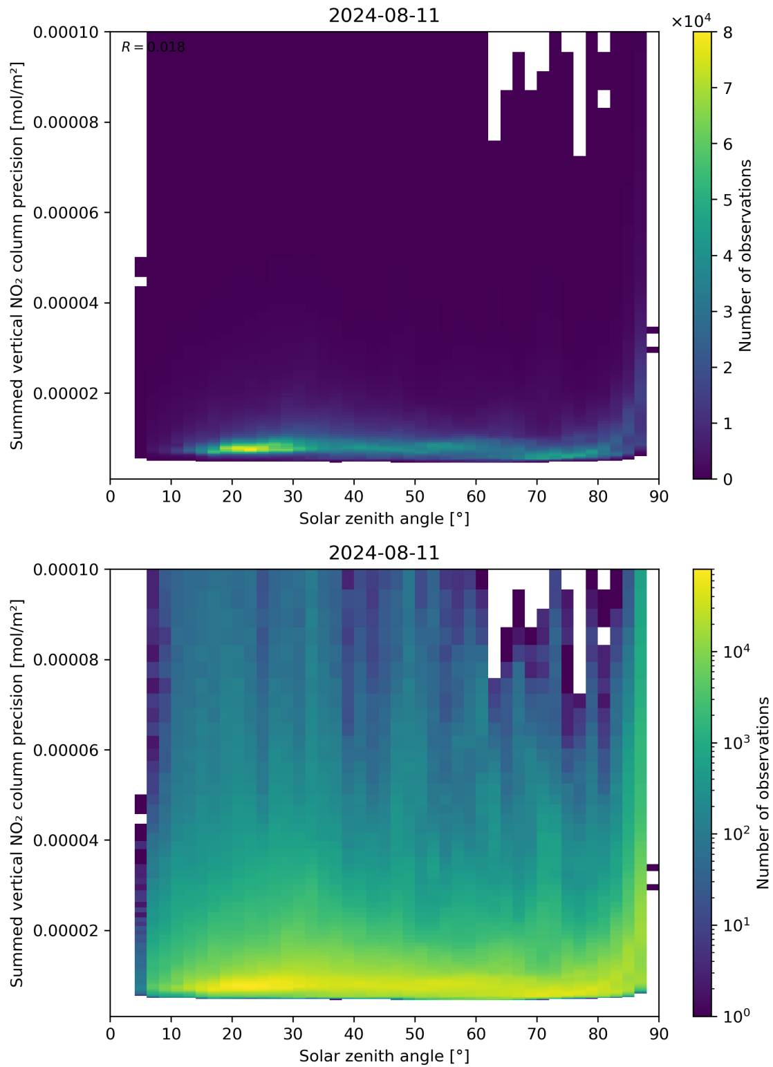
Figure 152: Scatter density plot of “Solar zenith angle” against “Summed vertical NO 2 column precision” for 2024-08-11 to 2024-08-11.
