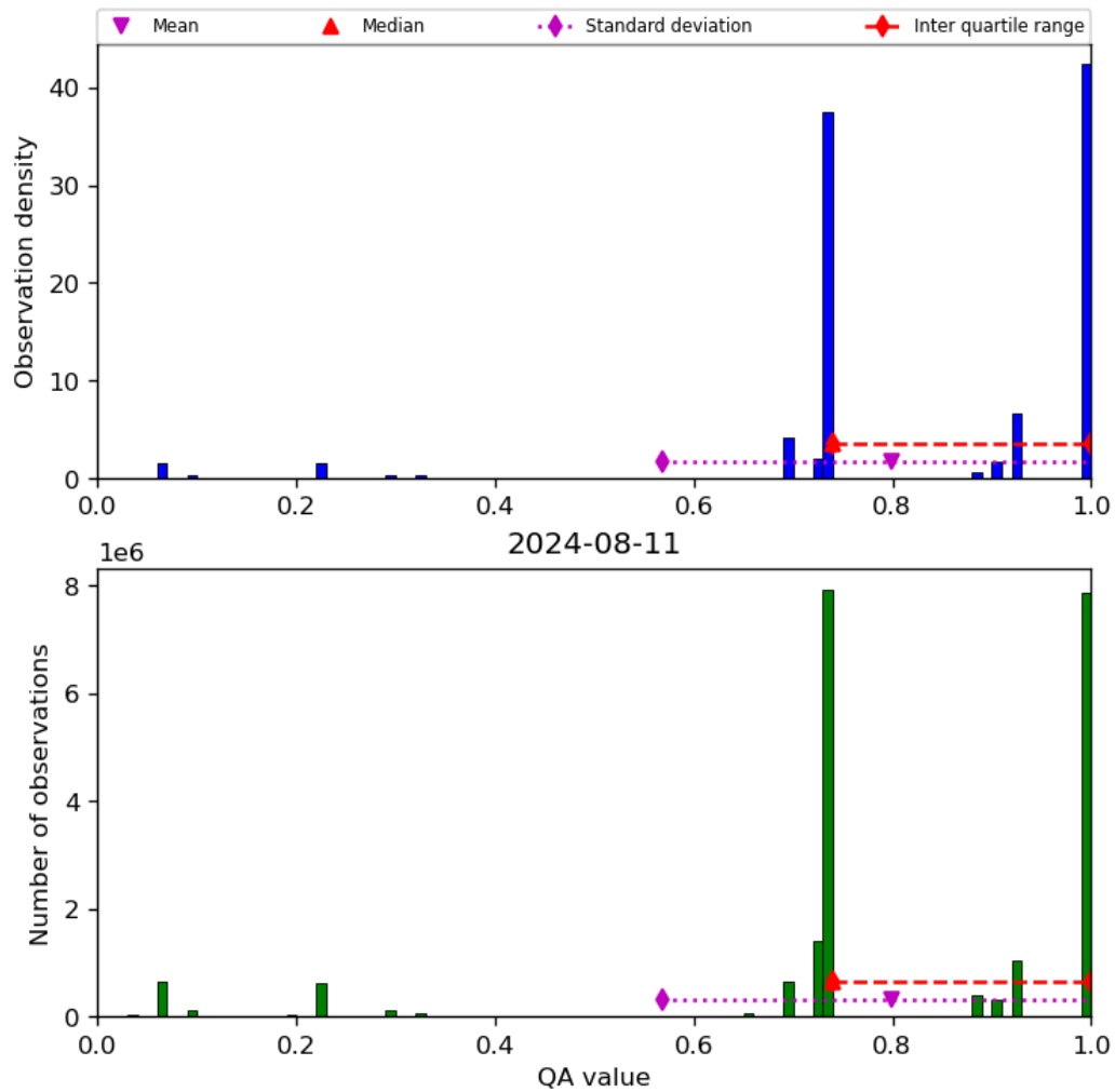
Figure 28: Histogram of “QA value” for 2024-08-11 to 2024-08-11
