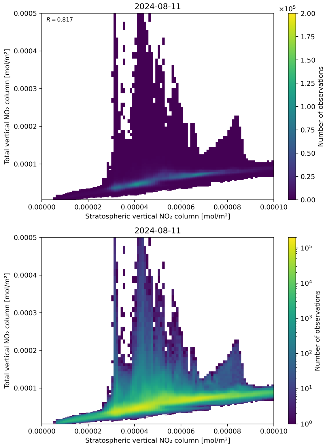
Figure 100: Scatter density plot of “Stratospheric vertical NO 2 column” against “Total vertical NO 2 column” for 2024-08-11 to 2024-08-11.
