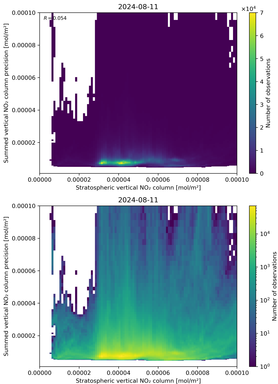
Figure 99: Scatter density plot of “Stratospheric vertical NO 2 column” against “Summed vertical NO 2 column precision” for 2024-08-11 to 2024-08-11.
