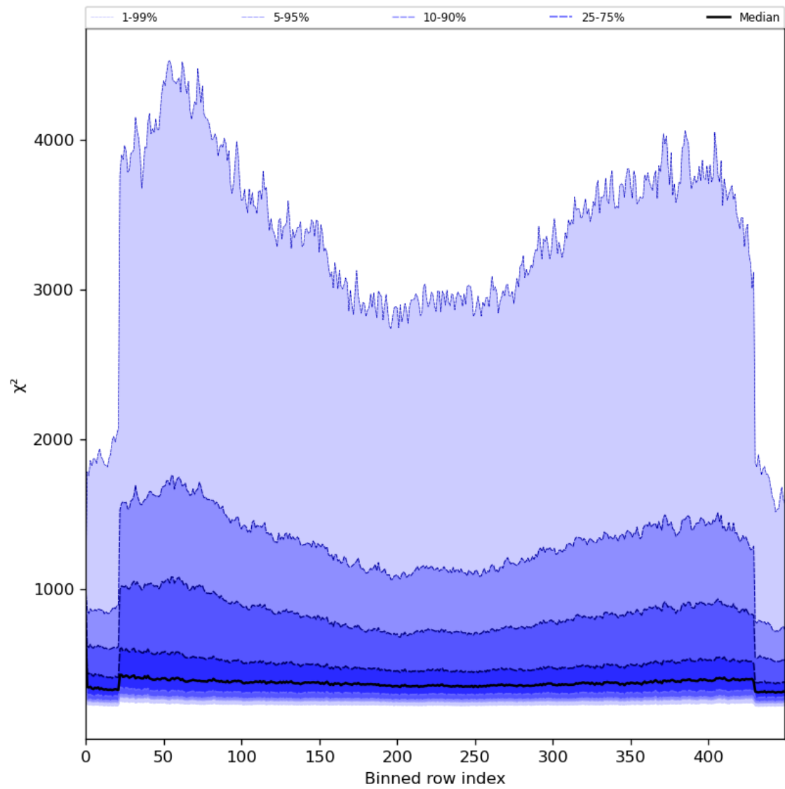
Figure 59: Along track statistics of “ \chi^2 ” for 2024-08-11 to 2024-08-11
