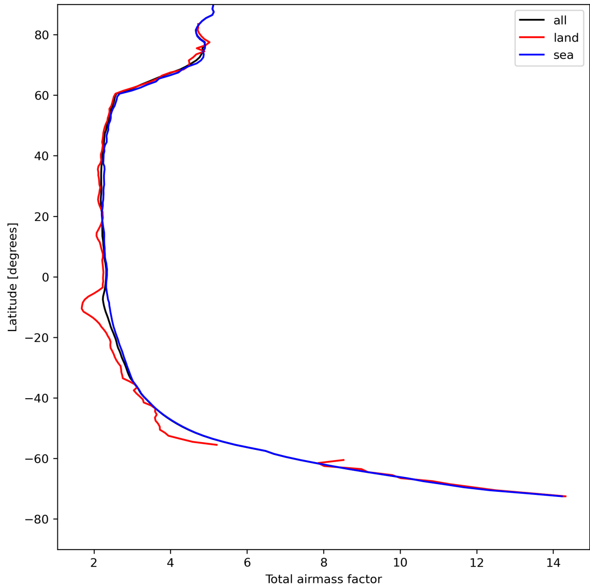
Figure 15: Zonal average of “Total airmass factor” for 2024-08-11 to 2024-08-11.
