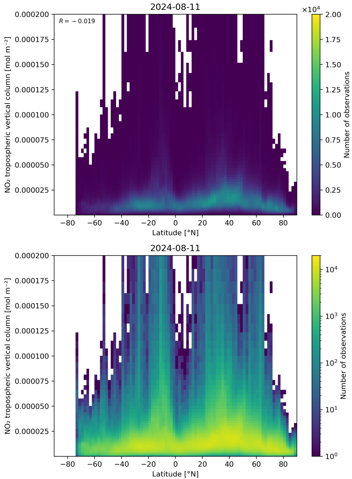
Figure 92: Scatter density plot of “Latitude” against “NO 2 tropospheric vertical column” for 2024-08-11 to 2024-08-11.
