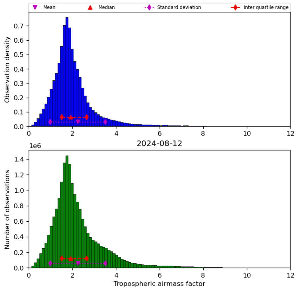
Figure 31: Histogram of “Tropospheric airmass factor” for 2024-08-12 to 2024-08-13
