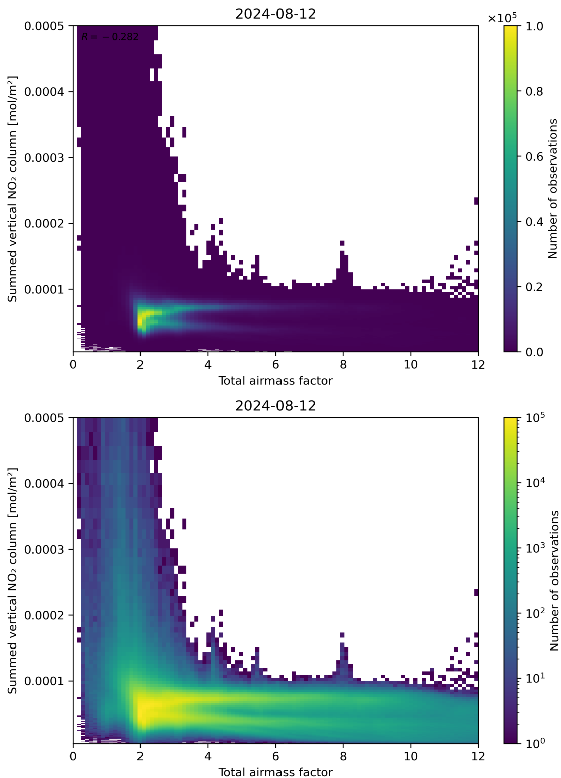
Figure 65: Scatter density plot of “Total airmass factor” against “Summed vertical NO 2 column” for 2024-08-12 to 2024-08-13.
