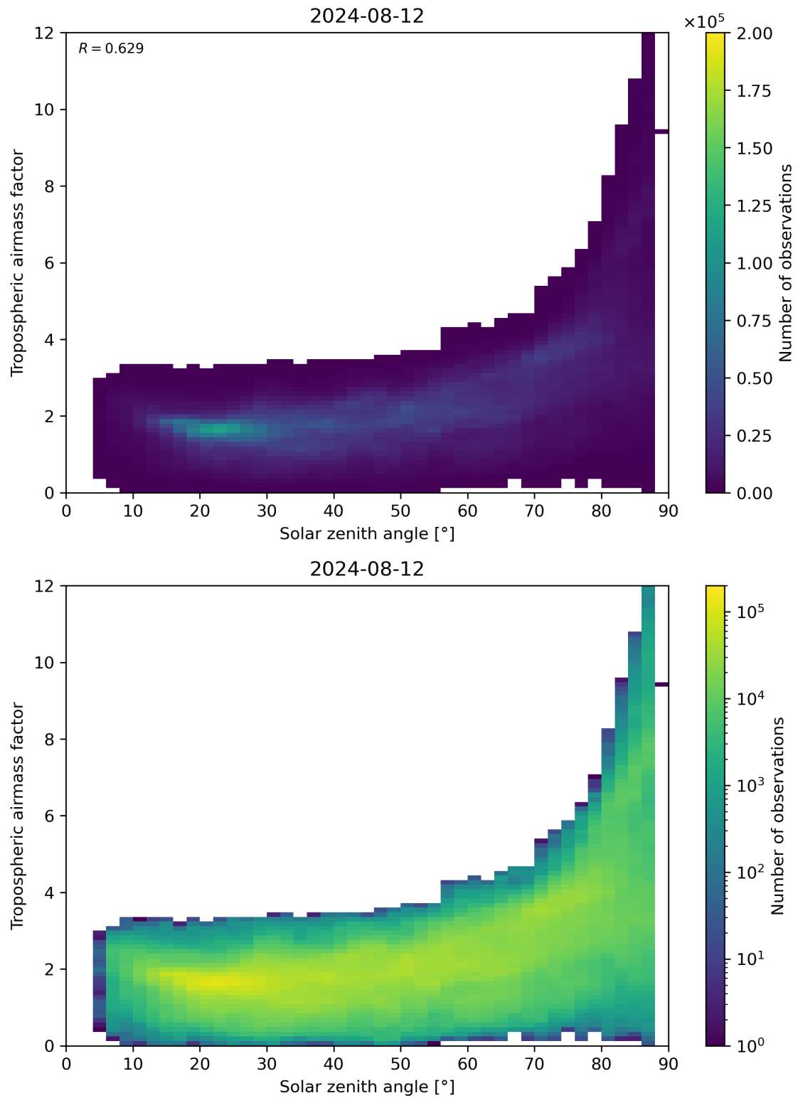
Figure 147: Scatter density plot of “Solar zenith angle” against “Tropospheric airmass factor” for 2024-08-12 to 2024-08-13.
