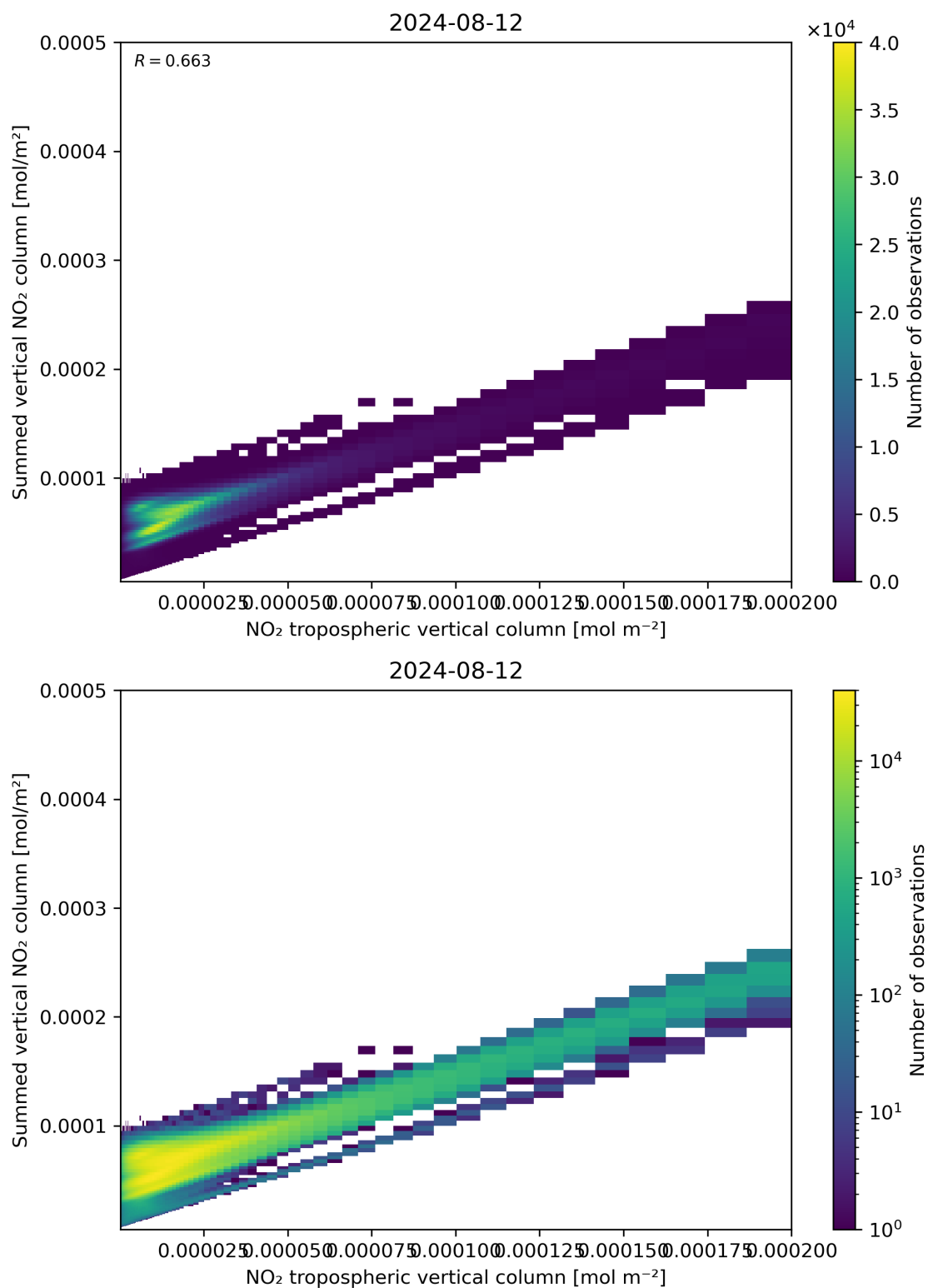
Figure 126: Scatter density plot of “NO 2 tropospheric vertical column” against “Summed vertical NO 2 column” for 2024-08-12 to 2024-08-13.
