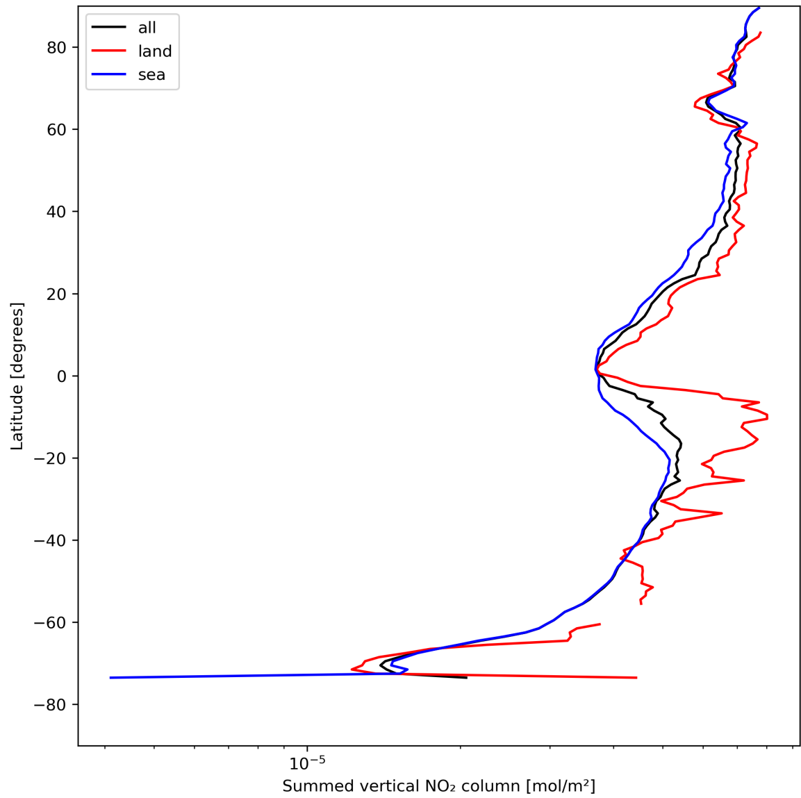
Figure 23: Zonal average of “Summed vertical NO 2 column” for 2024-08-12 to 2024-08-13.
