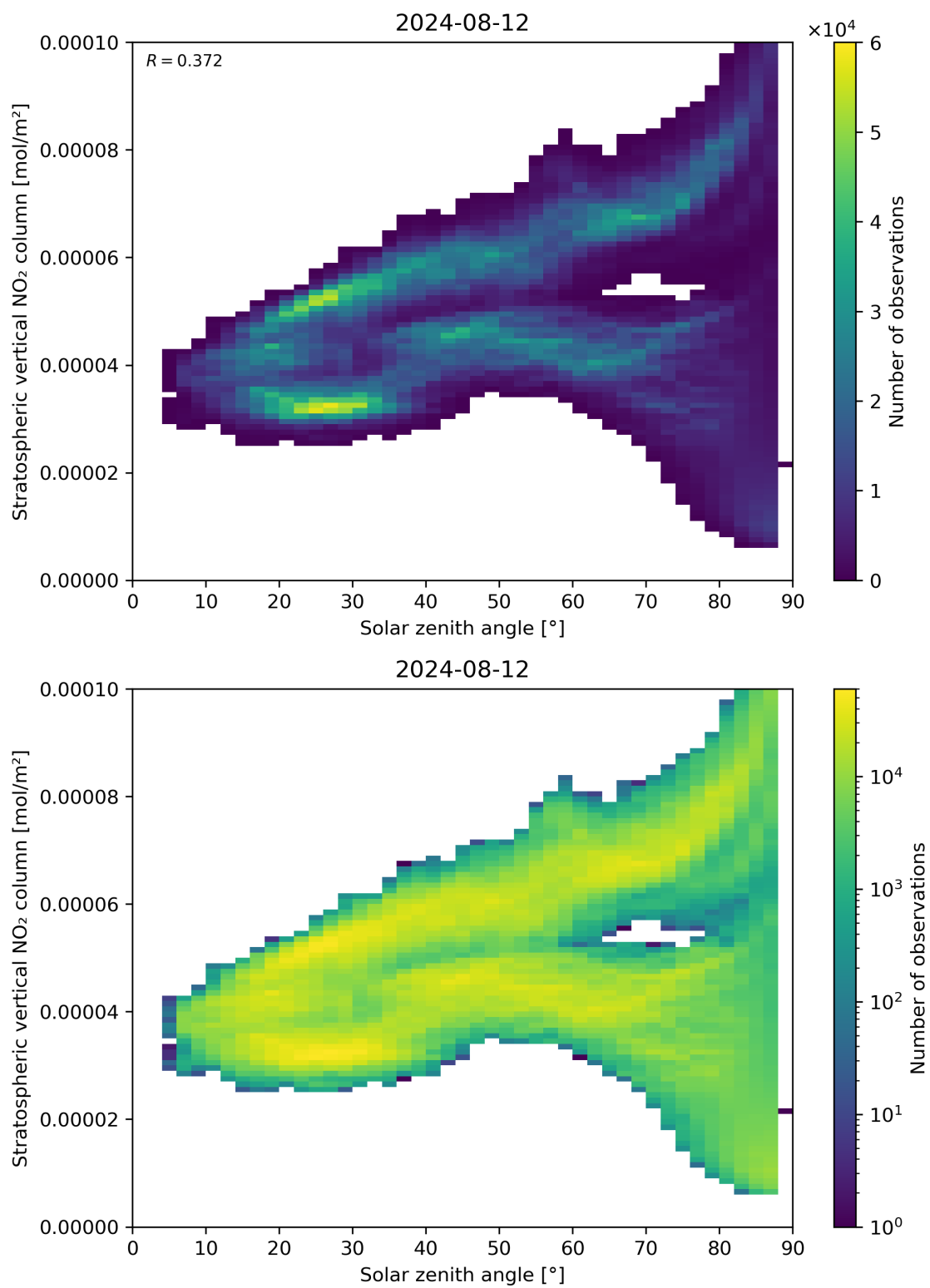
Figure 150: Scatter density plot of “Solar zenith angle” against “Stratospheric vertical NO 2 column” for 2024-08-12 to 2024-08-13.
