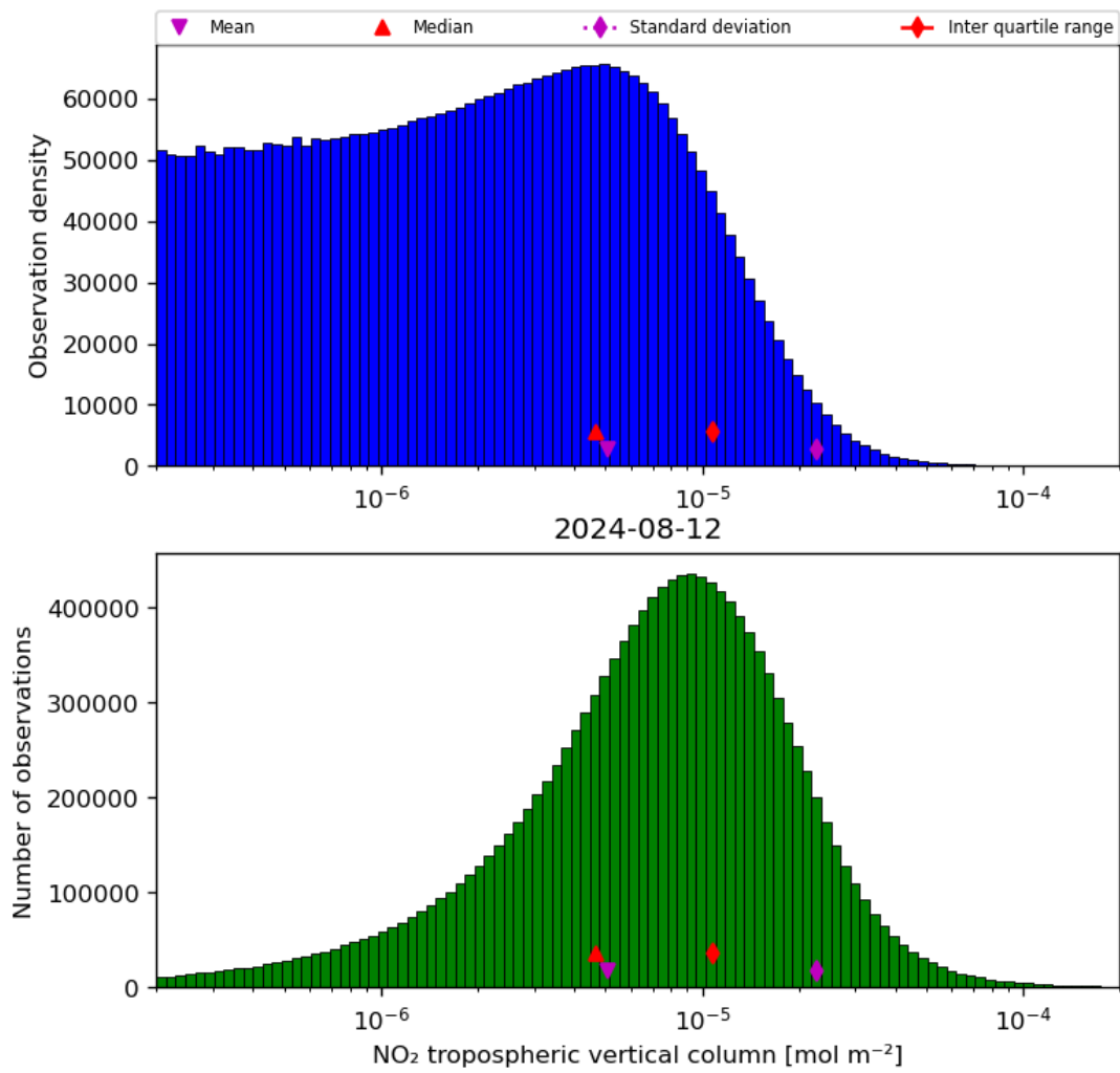
Figure 29: Histogram of “NO 2 tropospheric vertical column” for 2024-08-12 to 2024-08-13
