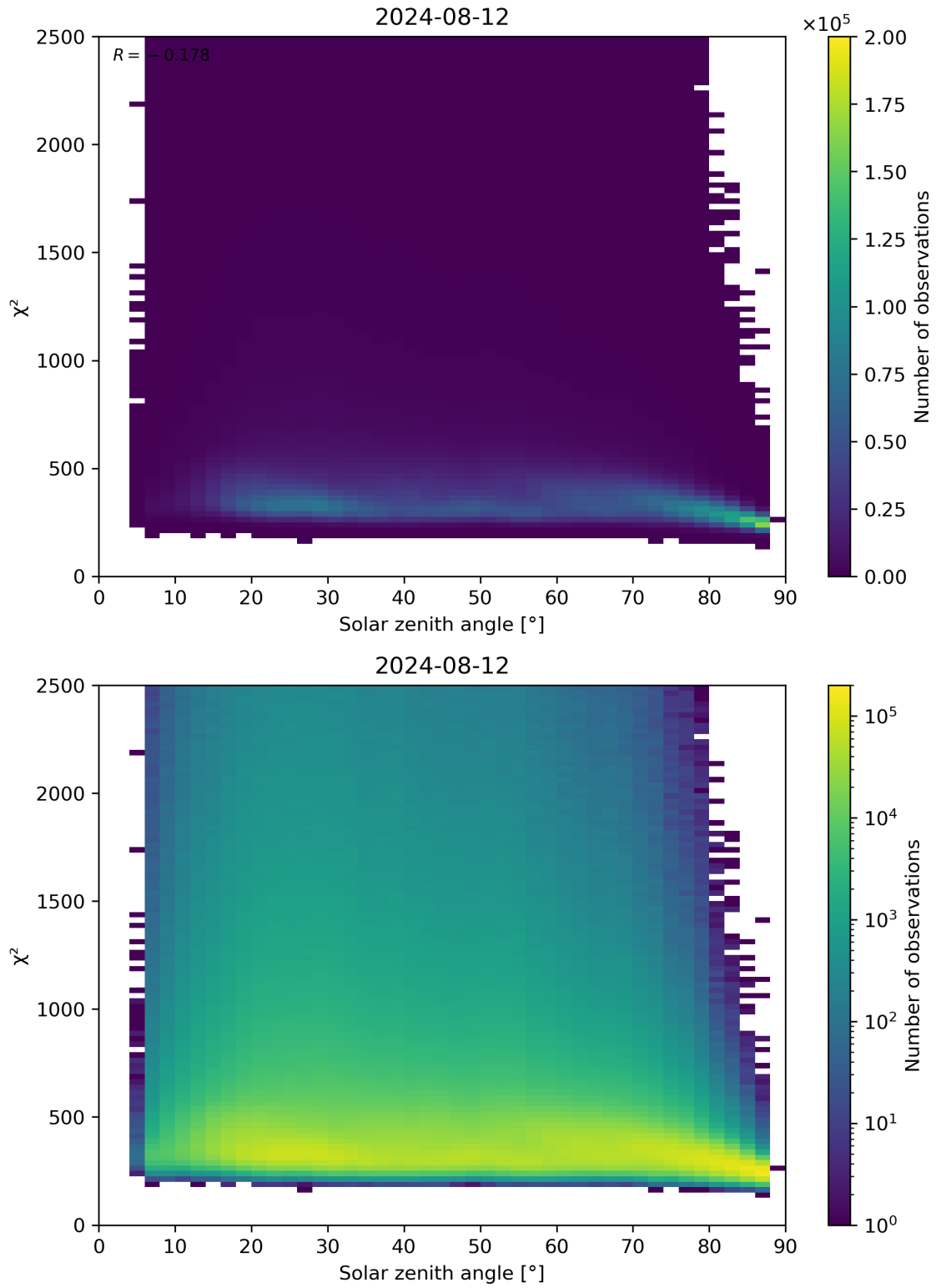
Figure 148: Scatter density plot of “Solar zenith angle” against “ \chi^2 ” for 2024-08-12 to 2024-08-13.
