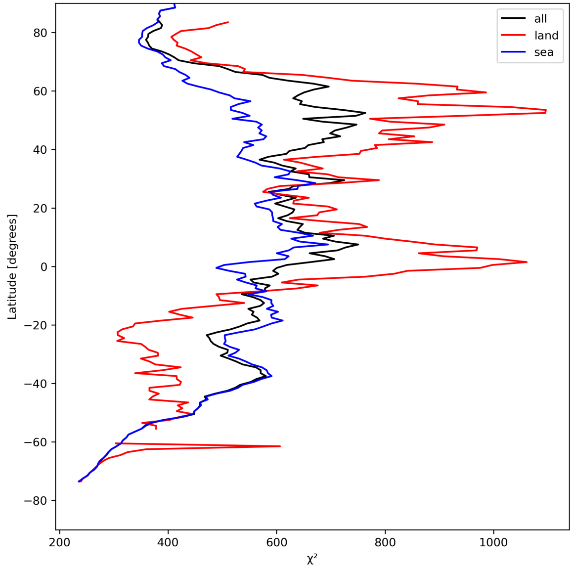
Figure 25: Zonal average of “ \chi^2 ” for 2024-08-12 to 2024-08-13.
