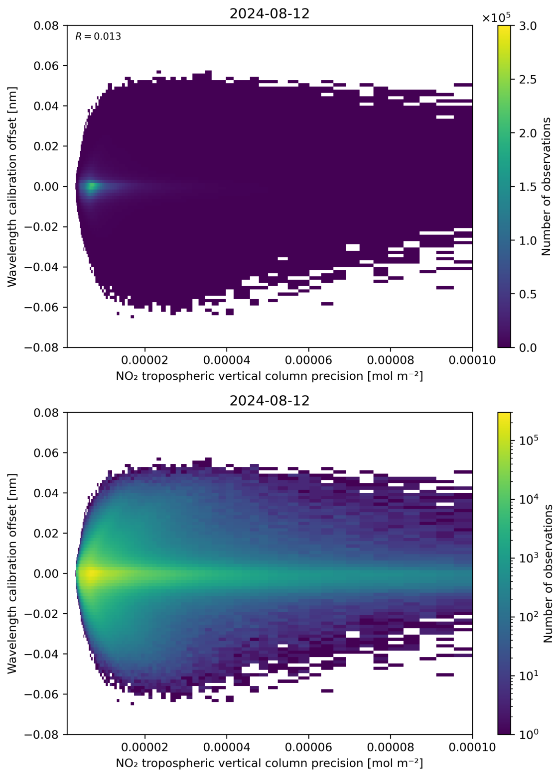
Figure 141: Scatter density plot of “NO 2 tropospheric vertical column precision” against “Wavelength calibration offset” for 2024-08-12 to 2024-08-13.
