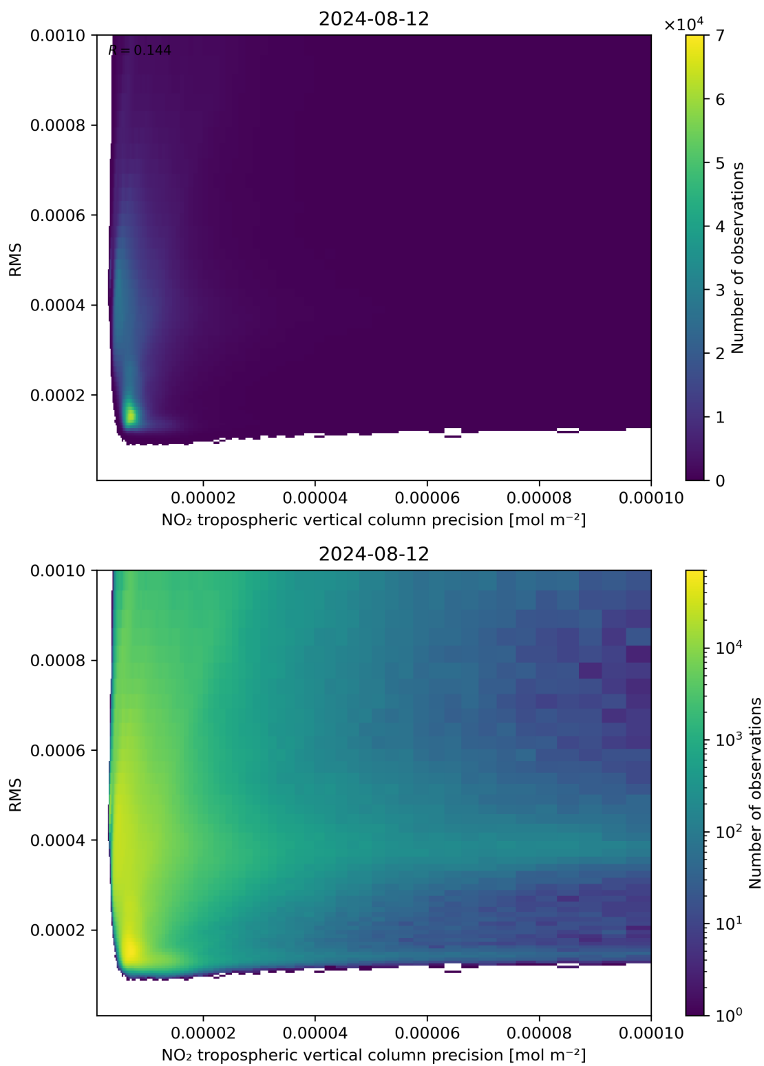
Figure 140: Scatter density plot of “NO 2 tropospheric vertical column precision” against “RMS” for 2024-08-12 to 2024-08-13.
