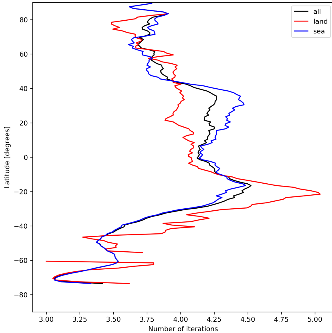
Figure 17: Zonal average of “Number of iterations” for 2024-08-12 to 2024-08-13.
