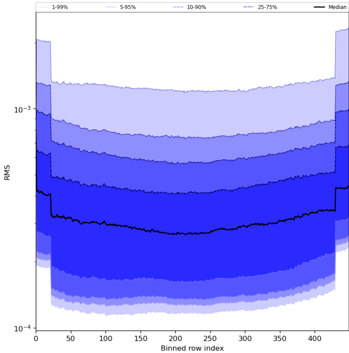
Figure 60: Along track statistics of “RMS” for 2024-08-12 to 2024-08-13
