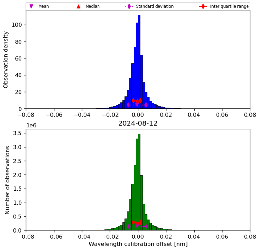
Figure 35: Histogram of “Wavelength calibration offset” for 2024-08-12 to 2024-08-13
