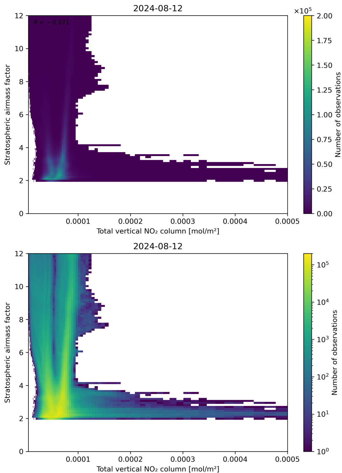
Figure 110: Scatter density plot of “Total vertical NO 2 column” against “Stratospheric airmass factor” for 2024-08-12 to 2024-08-13.
