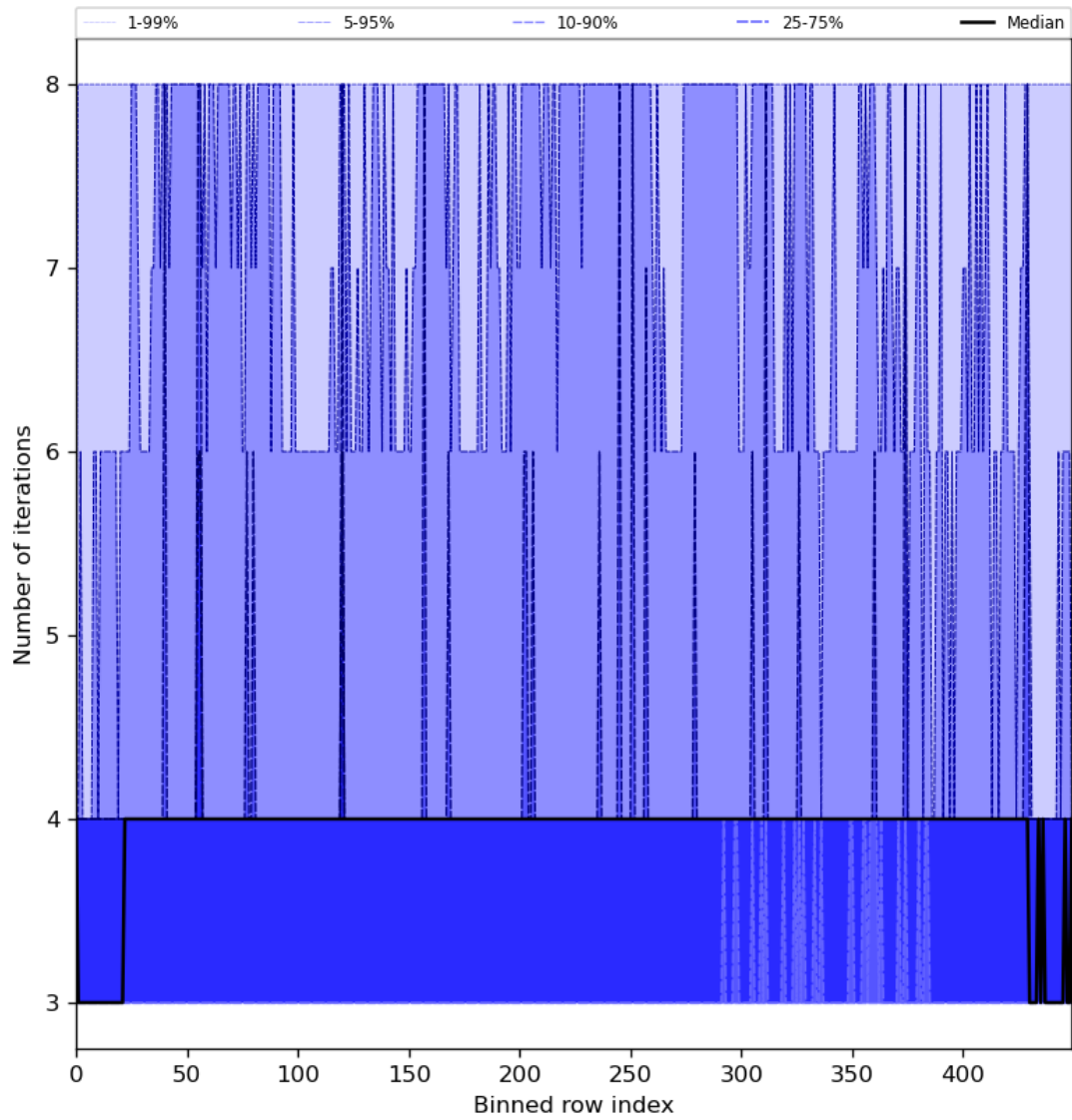
Figure 51: Along track statistics of “Number of iterations” for 2024-08-12 to 2024-08-13
