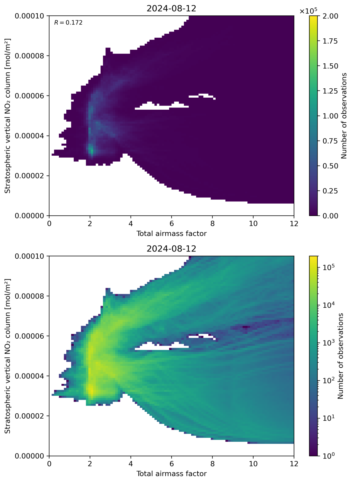
Figure 64: Scatter density plot of “Total airmass factor” against “Stratospheric vertical \text{NO}_2 column” for 2024-08-12 to 2024-08-13.
