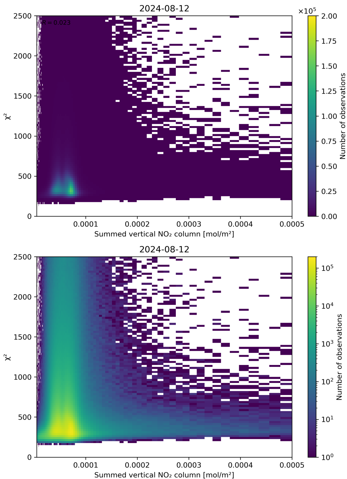
Figure 104: Scatter density plot of “Summed vertical NO 2 column” against “ \chi^2 ” for 2024-08-12 to 2024-08-13.
