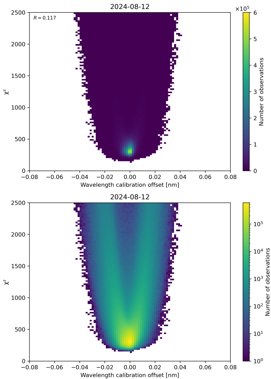
Figure 175: Scatter density plot of “Wavelength calibration offset” against “ \chi^2 ” for 2024-08-12 to 2024-08-13.
