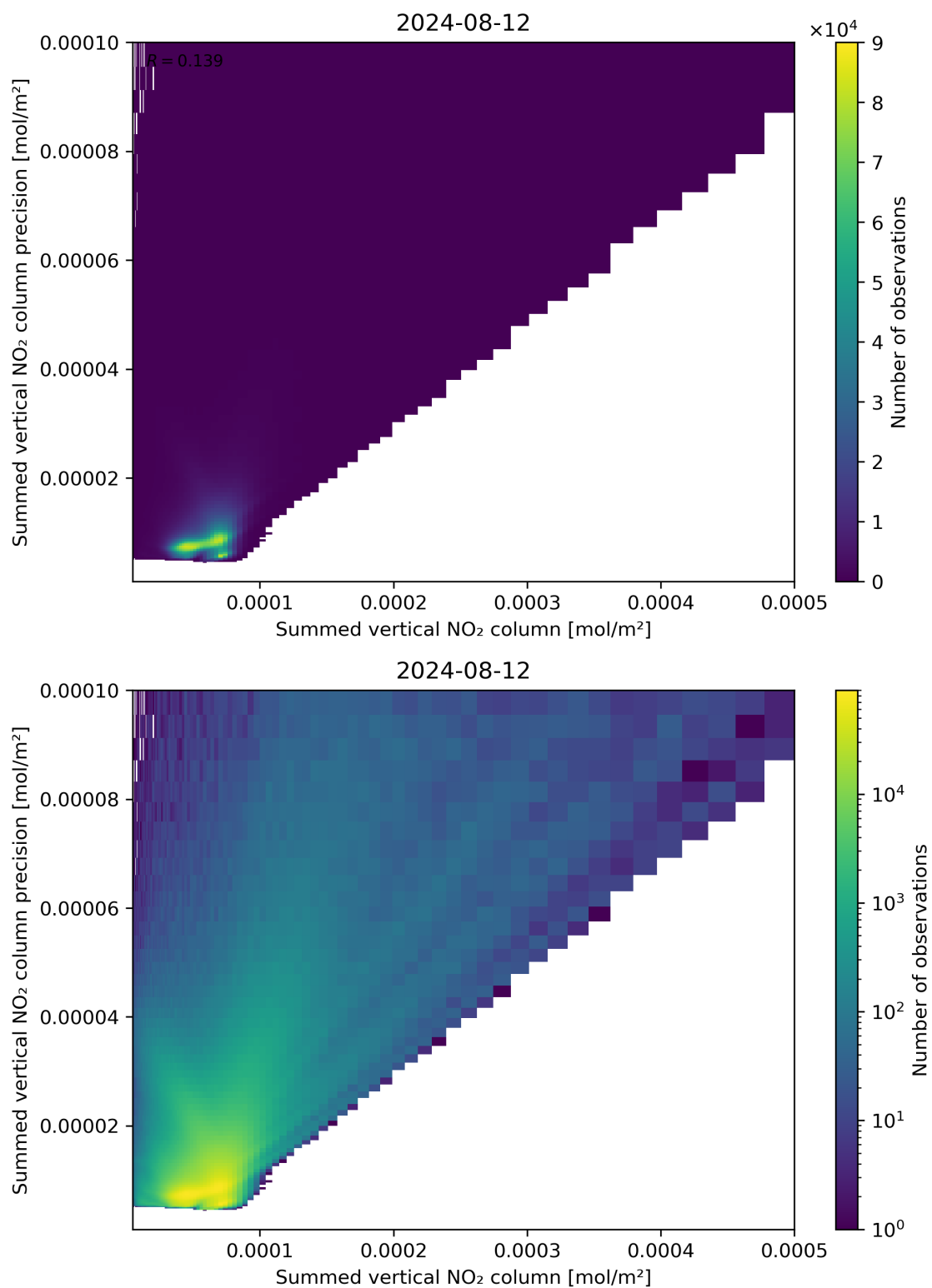
Figure 105: Scatter density plot of “Summed vertical NO 2 column” against “Summed vertical NO 2 column precision” for 2024-08-12 to 2024-08-13.
