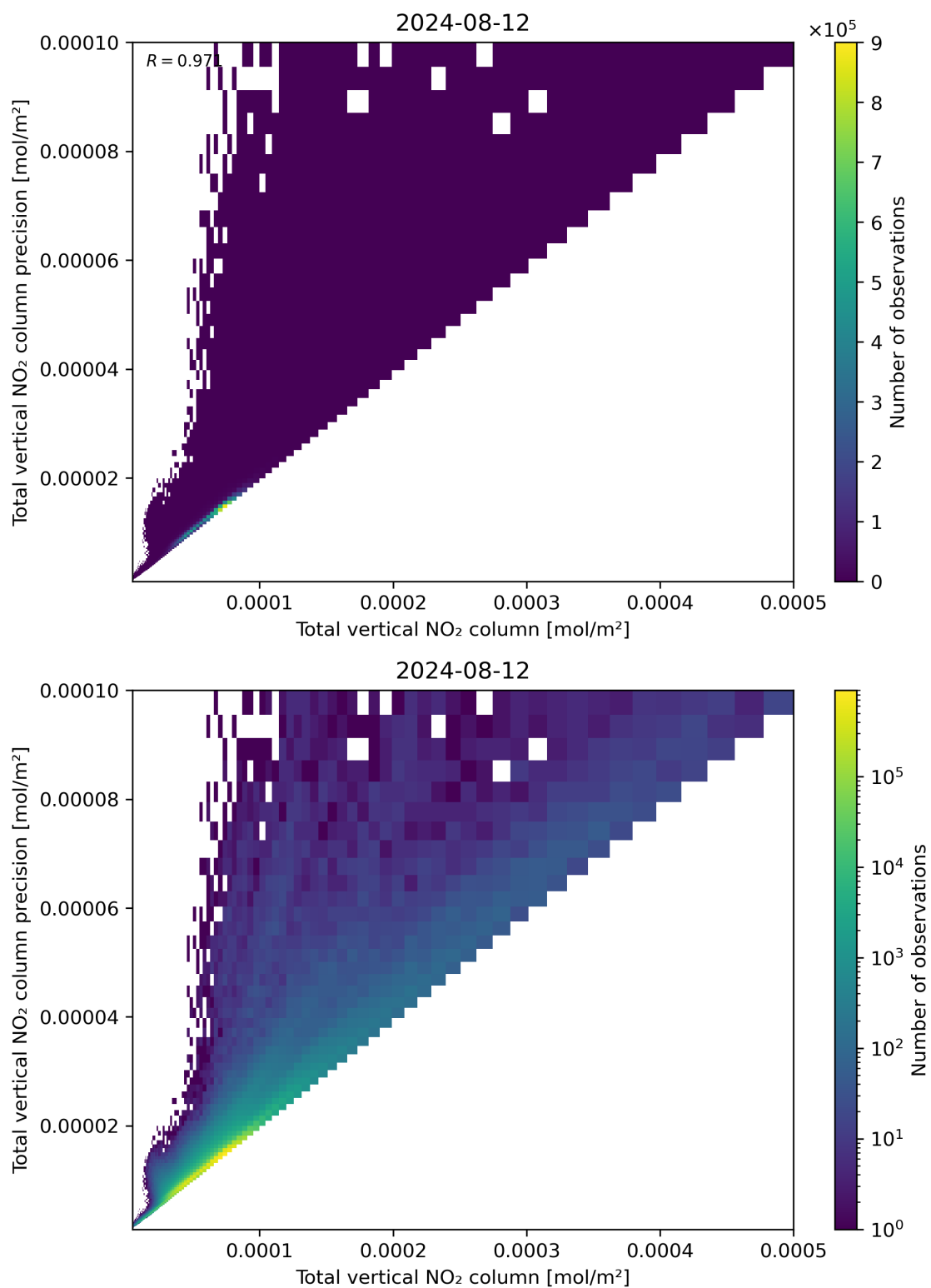
Figure 114: Scatter density plot of “Total vertical NO 2 column” against “Total vertical NO 2 column precision” for 2024-08-12 to 2024-08-13.
