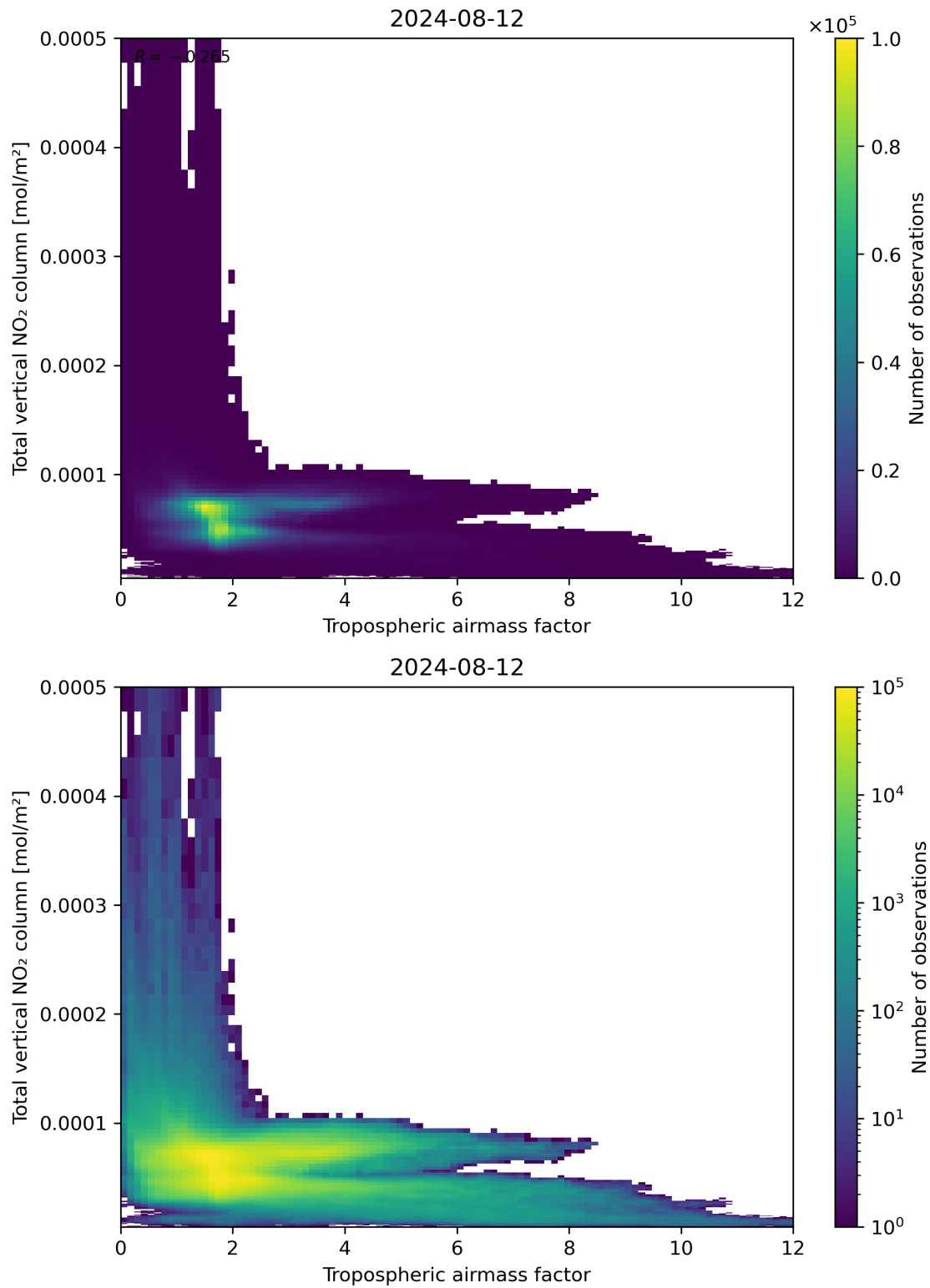
Figure 77: Scatter density plot of “Tropospheric airmass factor” against “Total vertical NO 2 column” for 2024-08-12 to 2024-08-13.
