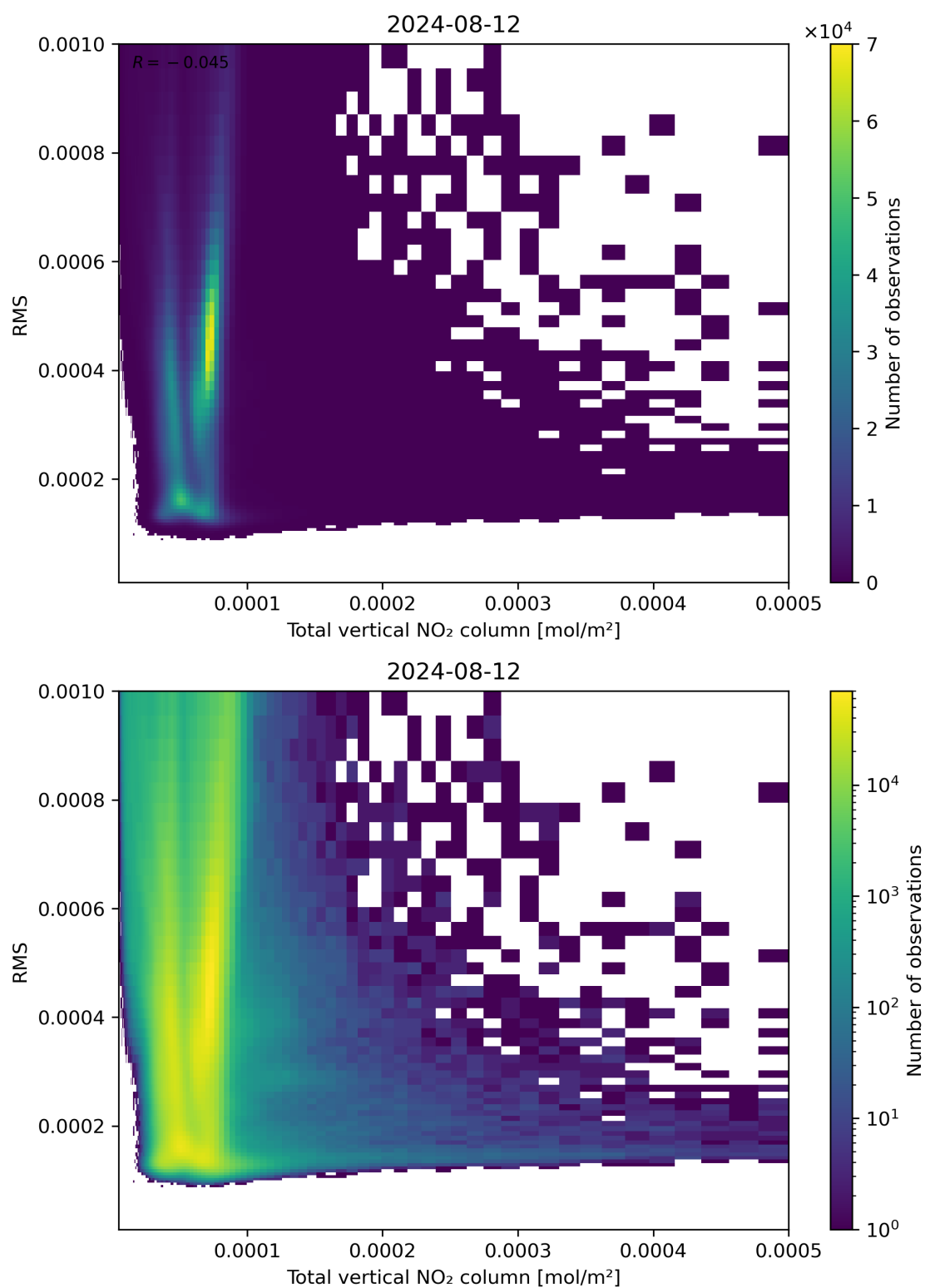
Figure 120: Scatter density plot of “Total vertical NO 2 column” against “RMS” for 2024-08-12 to 2024-08-13.
