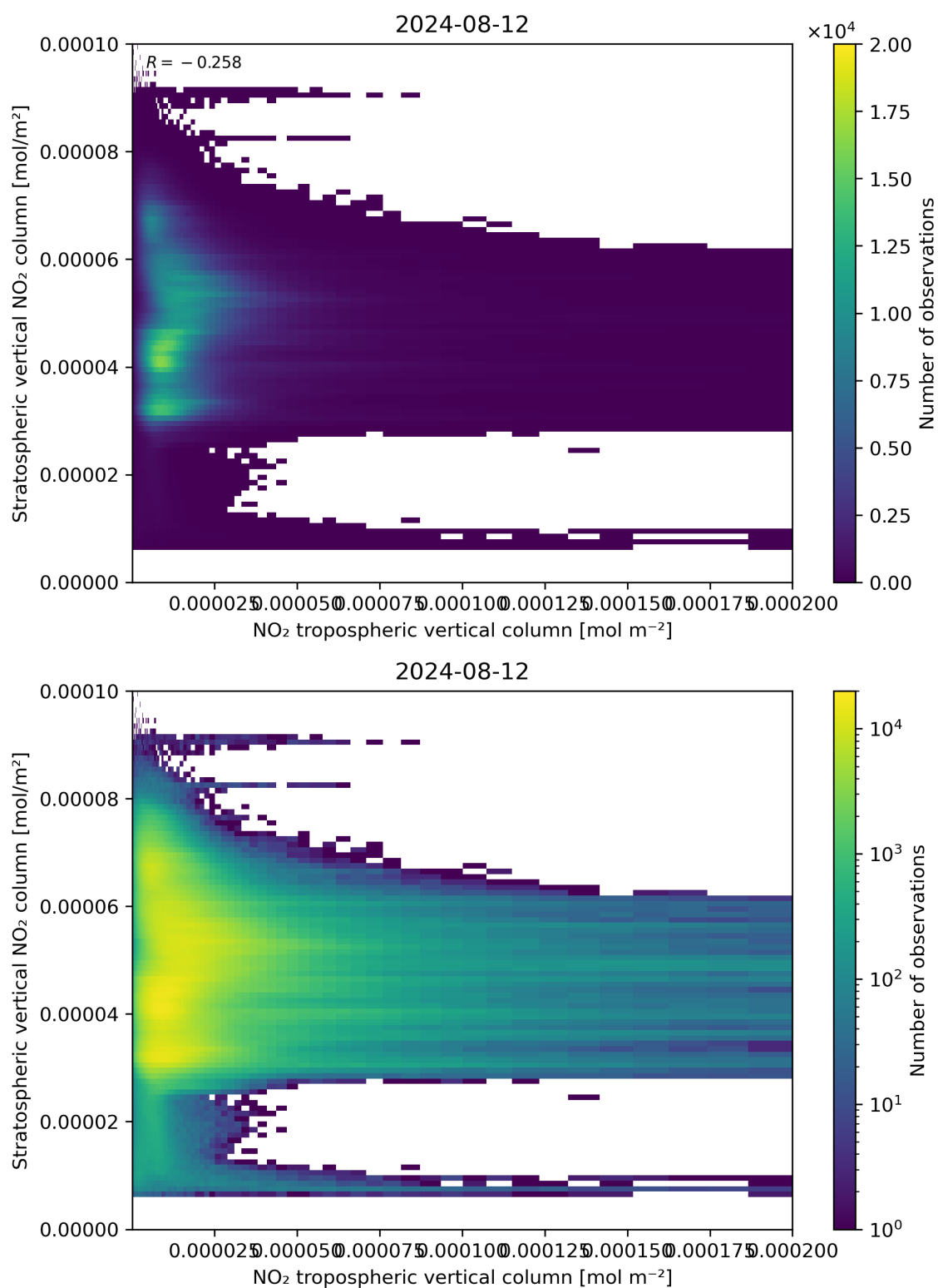
Figure 125: Scatter density plot of “NO 2 tropospheric vertical column” against “Stratospheric vertical NO 2 column” for 2024-08-12 to 2024-08-13.
