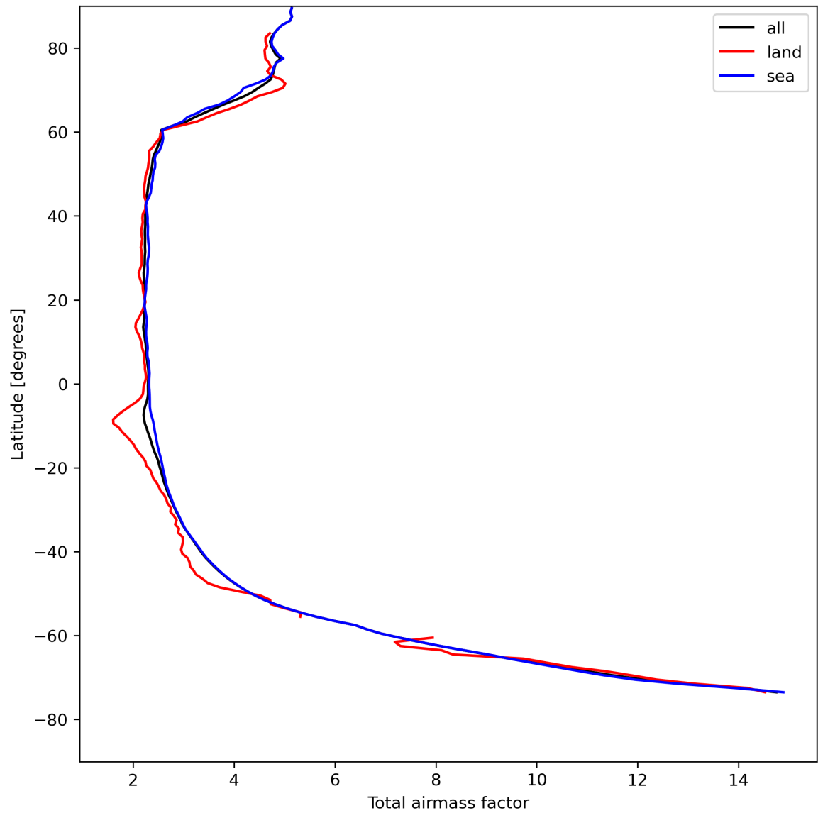
Figure 15: Zonal average of “Total airmass factor” for 2024-08-12 to 2024-08-13.
