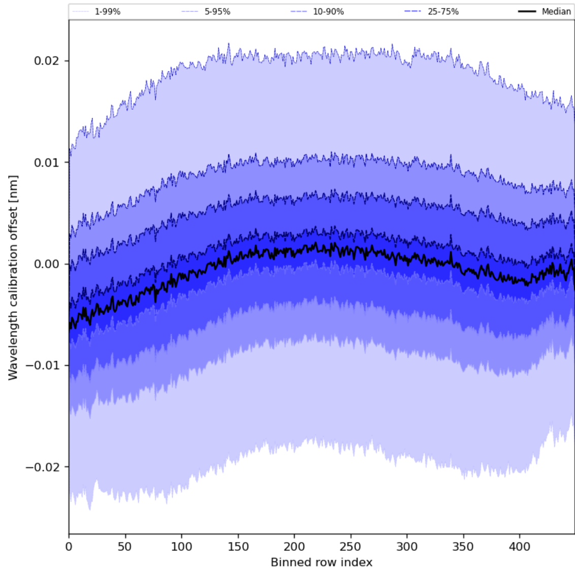
Figure 52: Along track statistics of “Wavelength calibration offset” for 2024-08-12 to 2024-08-13
