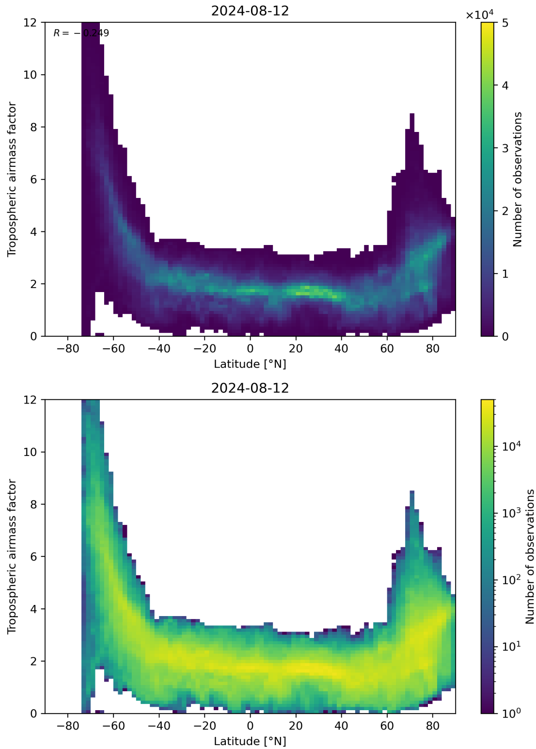
Figure 85: Scatter density plot of “Latitude” against “Tropospheric air mass factor” for 2024-08-12 to 2024-08-13.
