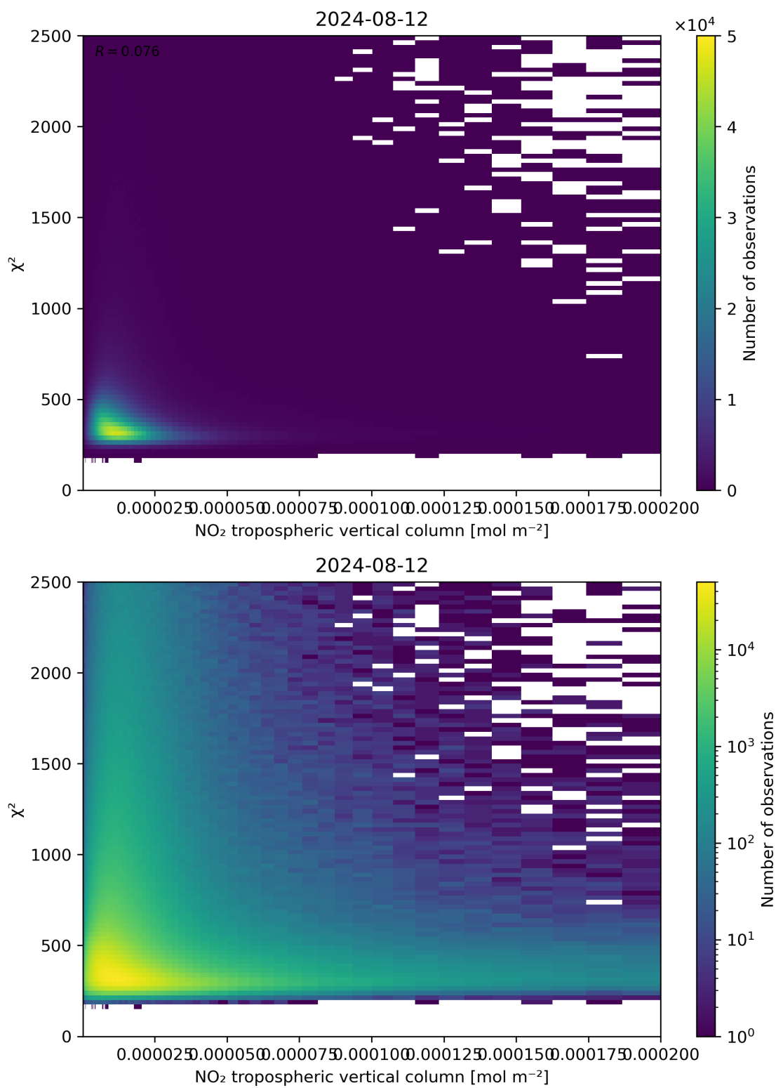
Figure 124: Scatter density plot of “NO 2 tropospheric vertical column” against “ \chi^2 ” for 2024-08-12 to 2024-08-13.
