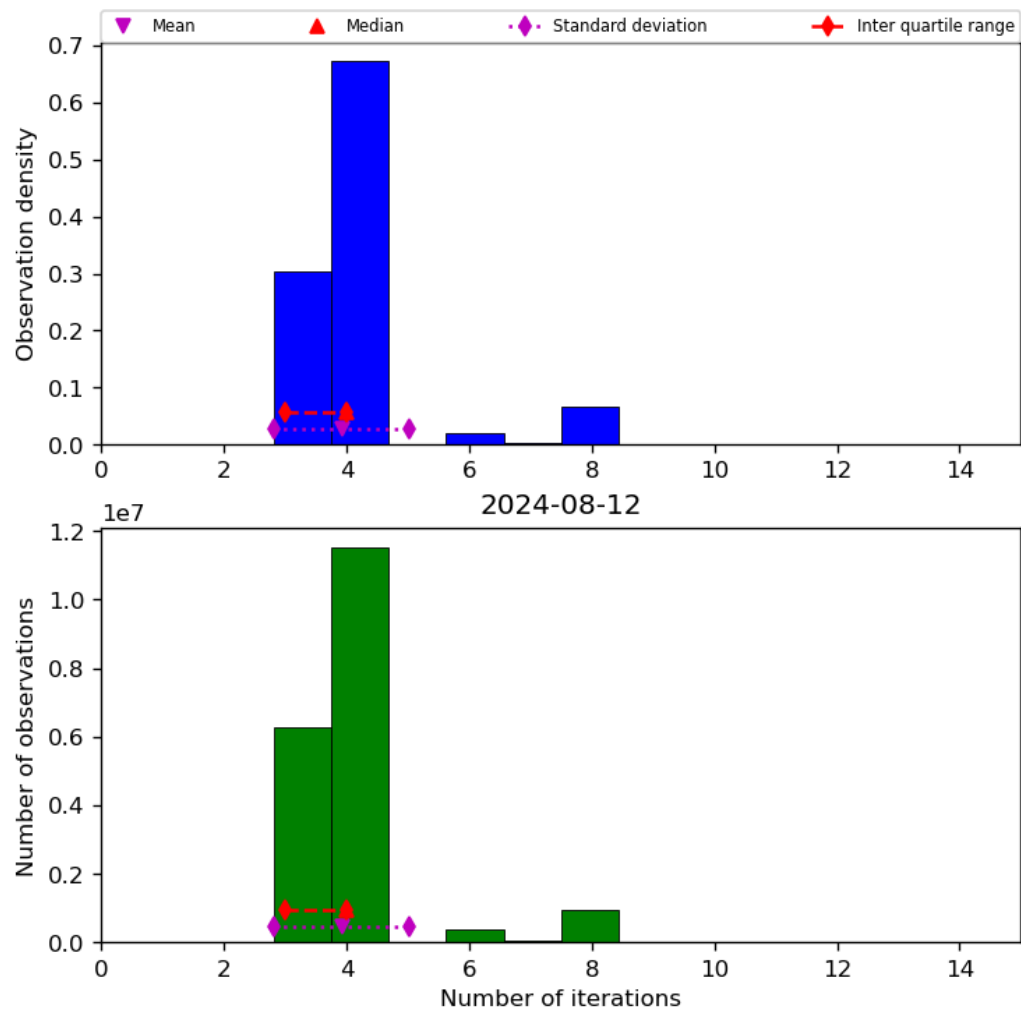
Figure 34: Histogram of “Number of iterations” for 2024-08-12 to 2024-08-13
