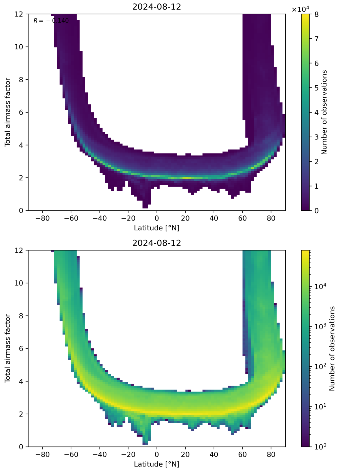
Figure 84: Scatter density plot of “Latitude” against “Total airmass factor” for 2024-08-12 to 2024-08-13.
