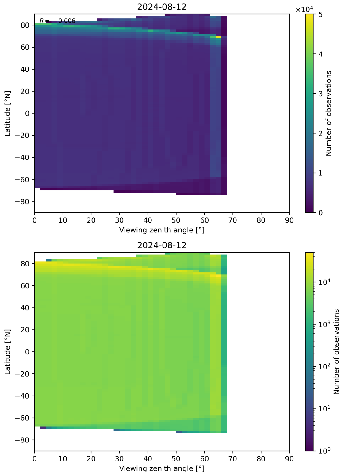
Figure 163: Scatter density plot of “Viewing zenith angle” against “Latitude” for 2024-08-12 to 2024-08-13.
