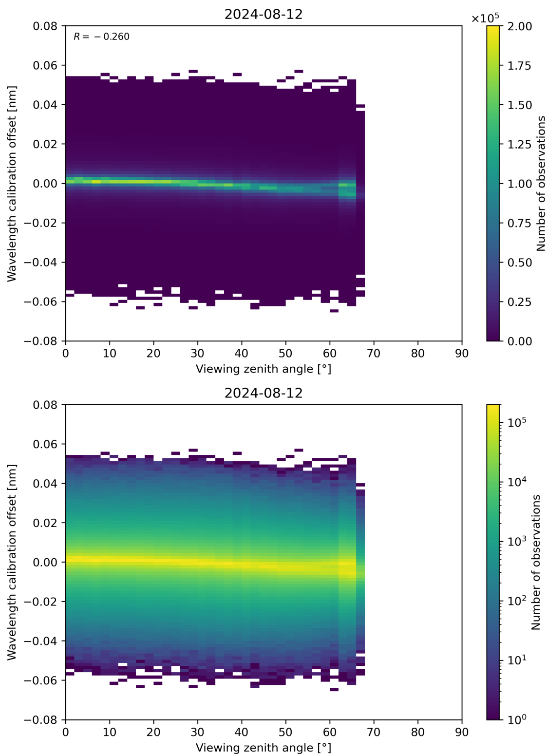
Figure 173: Scatter density plot of “Viewing zenith angle” against “Wavelength calibration offset” for 2024-08-12 to 2024-08-13.
