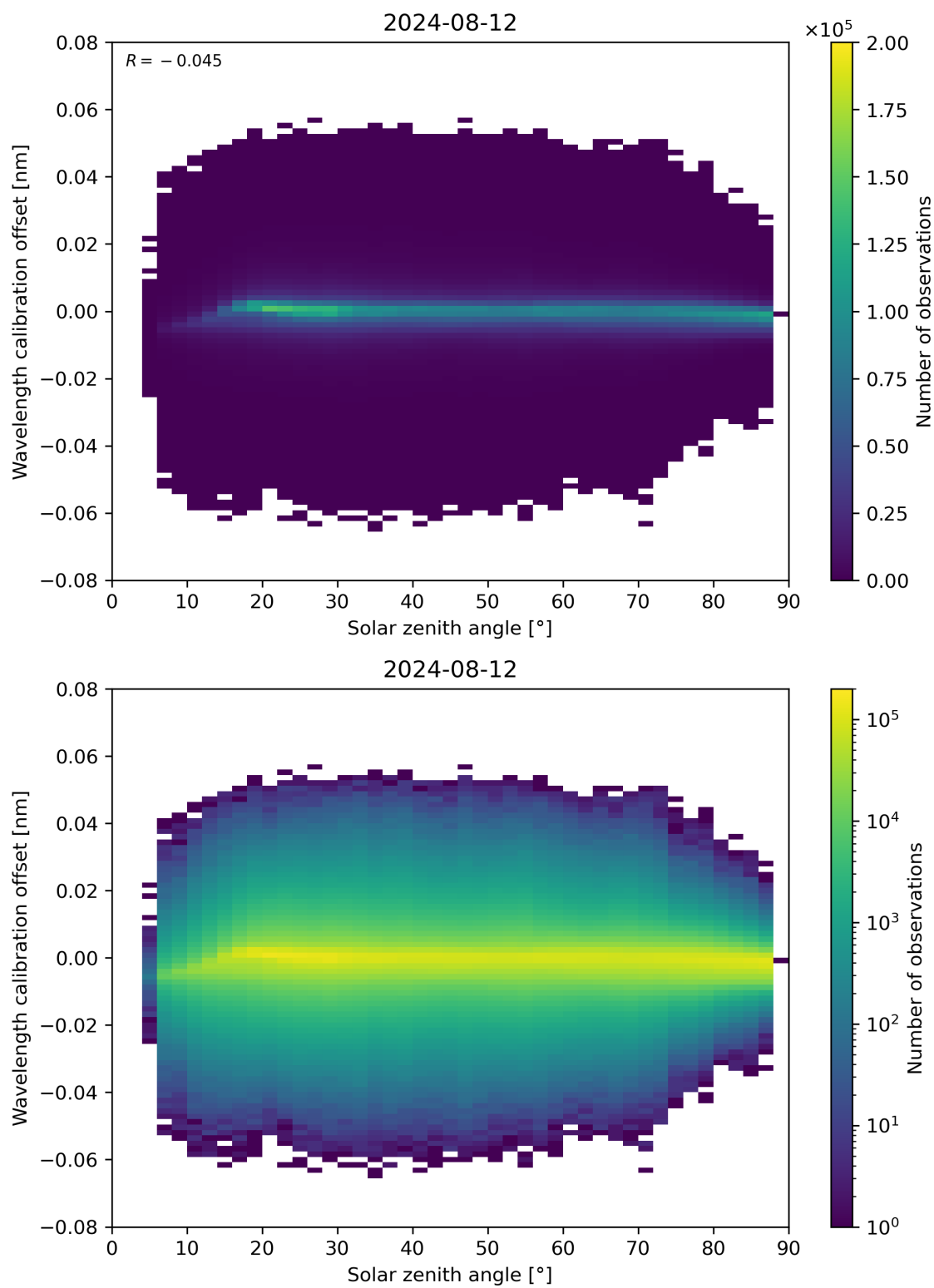
Figure 158: Scatter density plot of “Solar zenith angle” against “Wavelength calibration offset” for 2024-08-12 to 2024-08-13.
