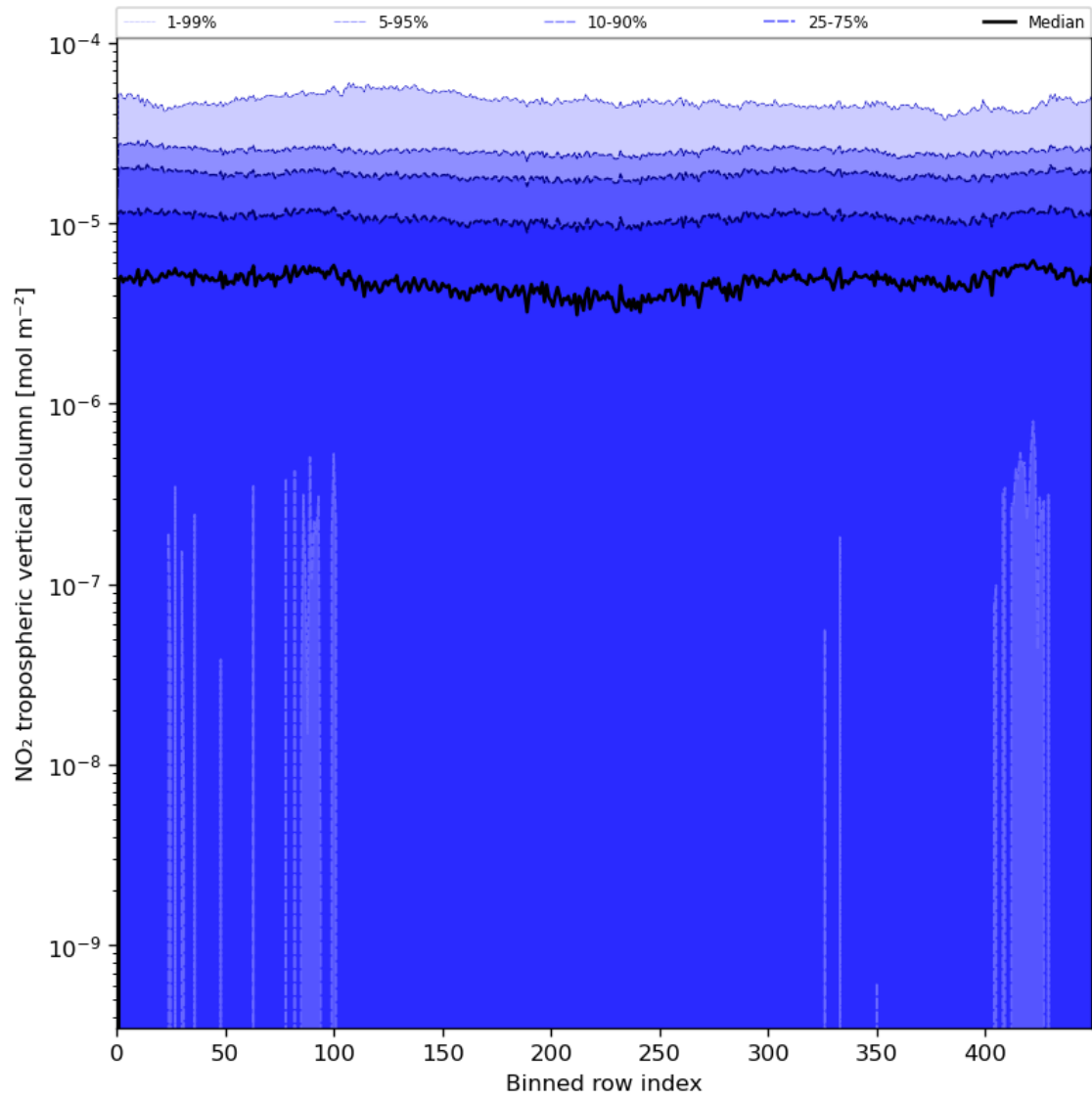
Figure 46: Along track statistics of “ \text{NO}_2 tropospheric vertical column” for 2024-08-12 to 2024-08-13
