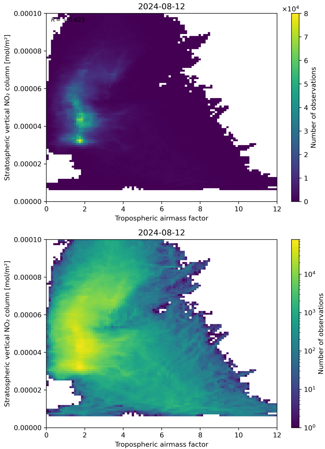
Figure 74: Scatter density plot of “Tropospheric air mass factor” against “Stratospheric vertical NO 2 column” for 2024-08-12 to 2024-08-13.
