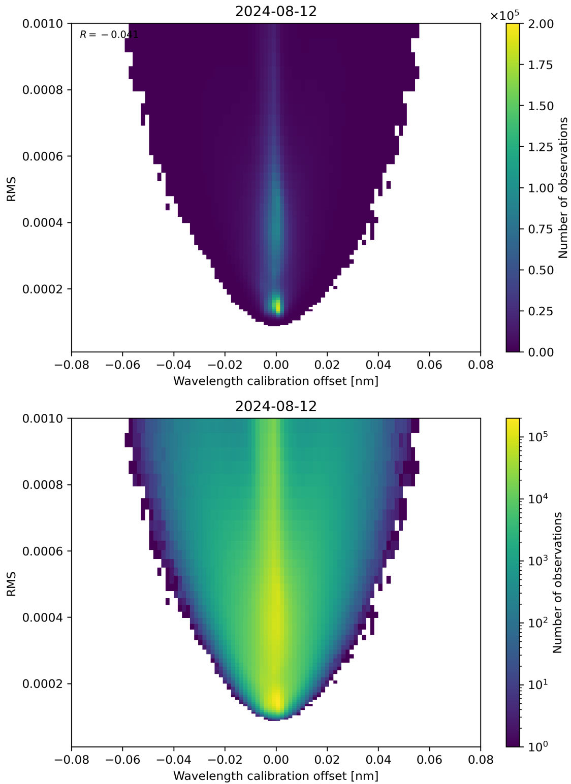
Figure 181: Scatter density plot of “Wavelength calibration offset” against “RMS” for 2024-08-12 to 2024-08-13.
