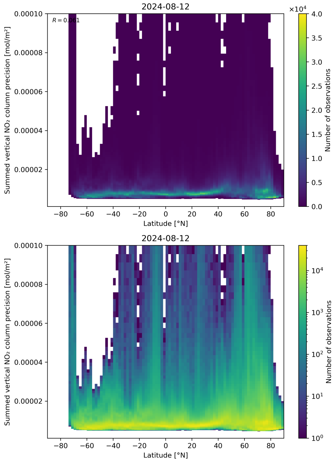
Figure 89: Scatter density plot of “Latitude” against “Summed vertical NO 2 column precision” for 2024-08-12 to 2024-08-13.
