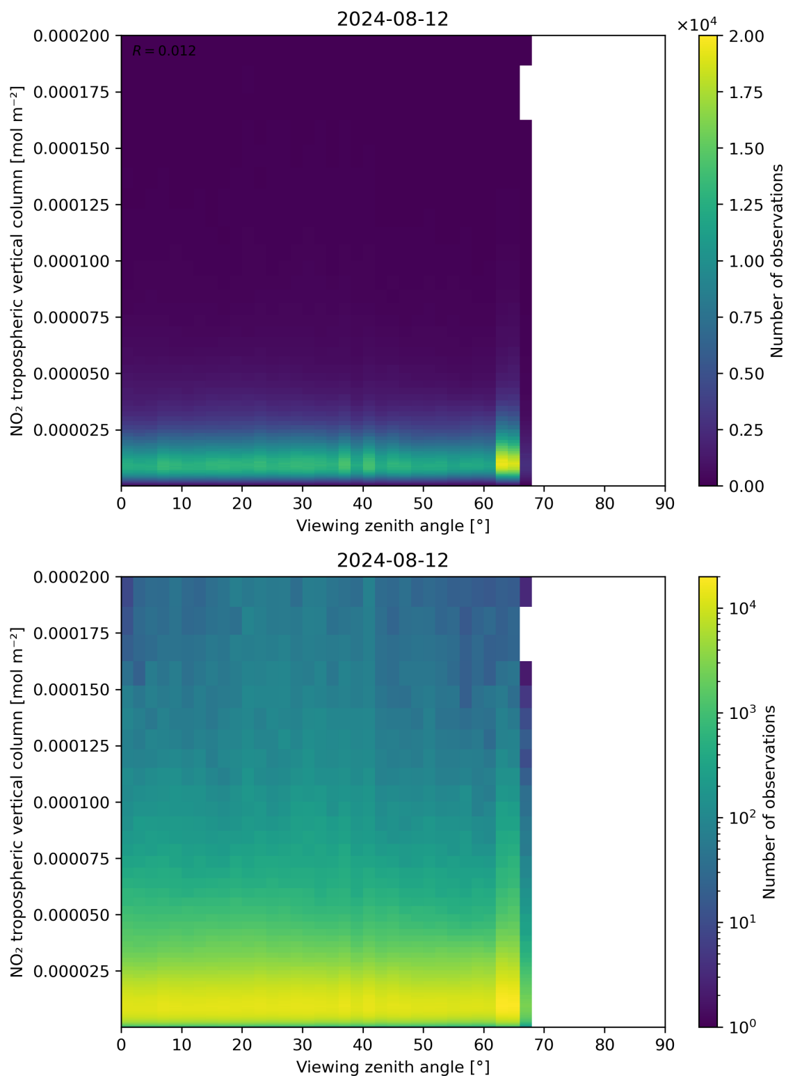
Figure 169: Scatter density plot of “Viewing zenith angle” against “NO 2 tropospheric vertical column” for 2024-08-12 to 2024-08-13.
