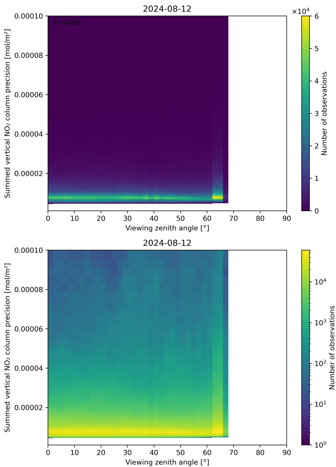
Figure 166: Scatter density plot of “Viewing zenith angle” against “Summed vertical NO 2 column precision” for 2024-08-12 to 2024-08-13.
