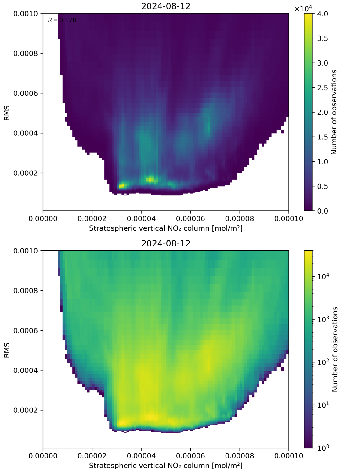
Figure 102: Scatter density plot of “Stratospheric vertical NO 2 column” against “RMS” for 2024-08-12 to 2024-08-13.
