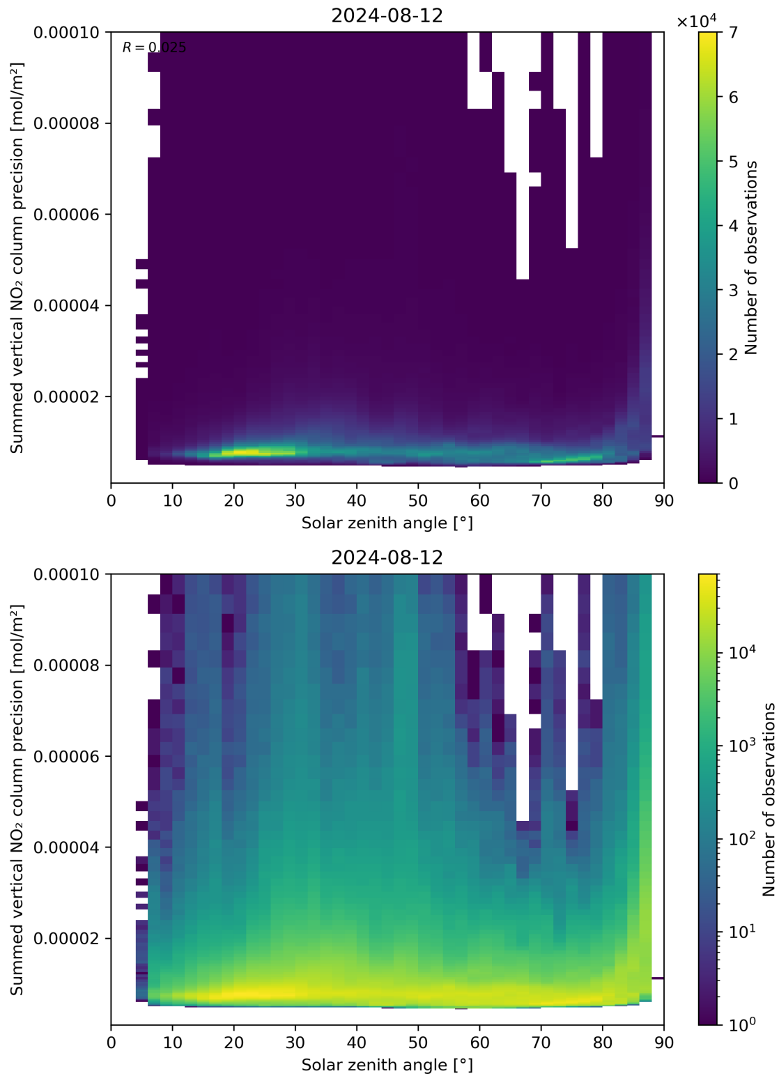
Figure 152: Scatter density plot of “Solar zenith angle” against “Summed vertical NO 2 column precision” for 2024-08-12 to 2024-08-13.
