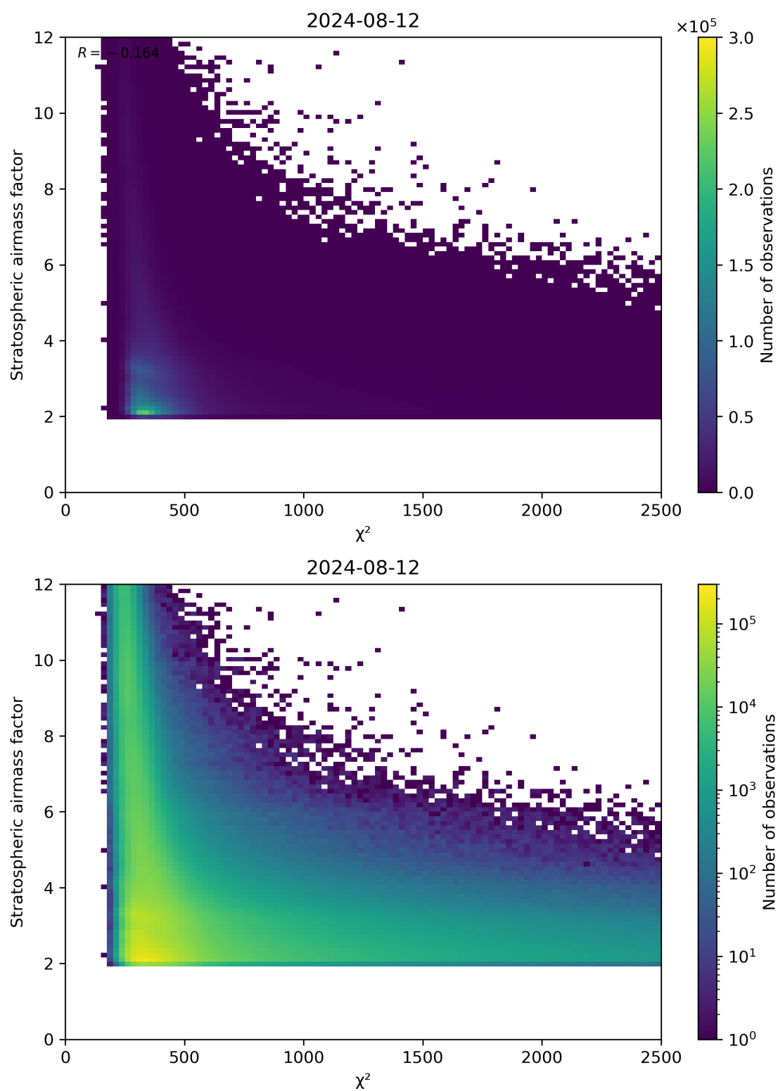
Figure 81: Scatter density plot of “ \chi^2 ” against “Stratospheric airmass factor” for 2024-08-12 to 2024-08-13.
