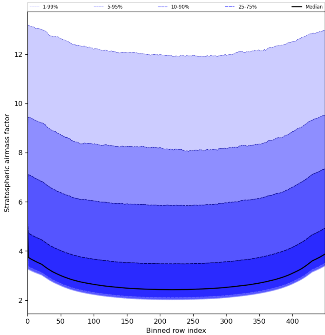
Figure 61: Along track statistics of “Stratospheric airmass factor” for 2024-08-12 to 2024-08-13
