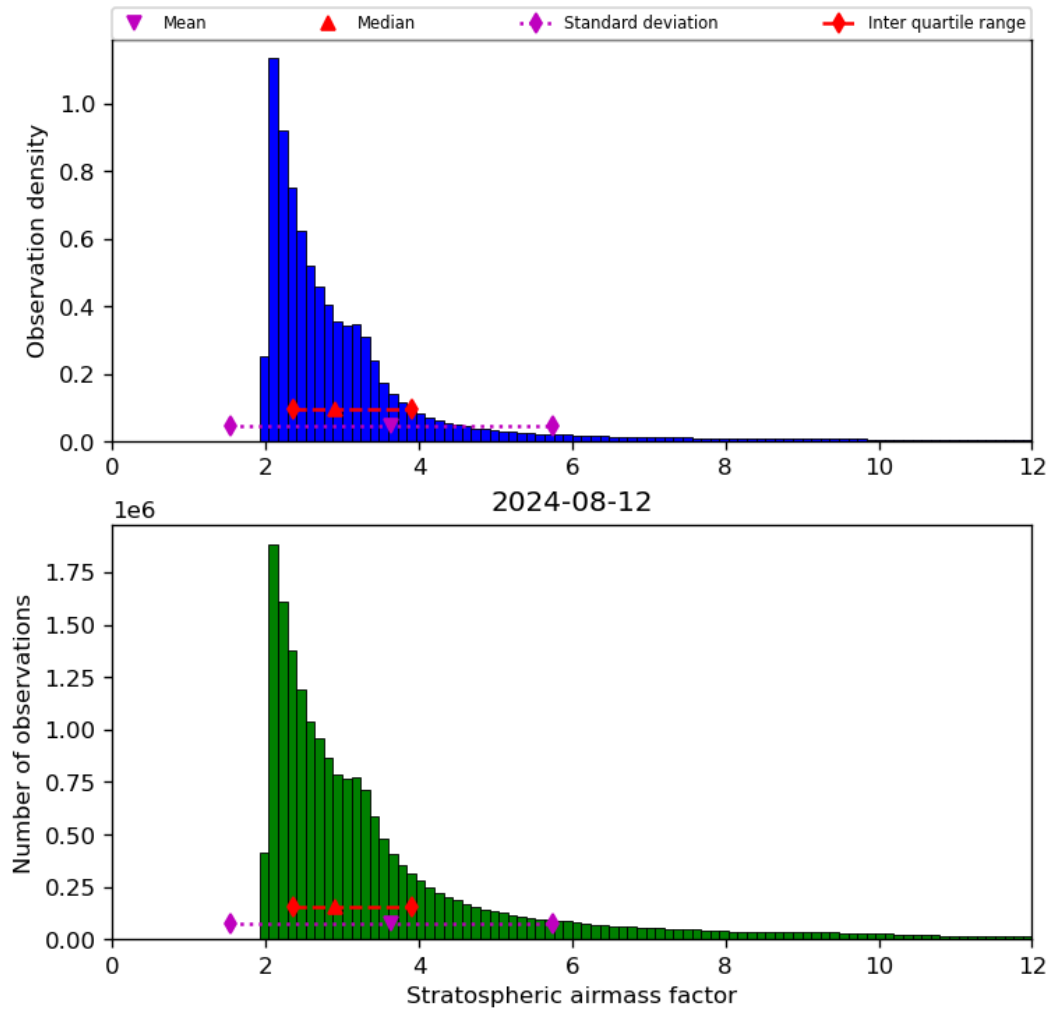
Figure 44: Histogram of “Stratospheric airmass factor” for 2024-08-12 to 2024-08-13
