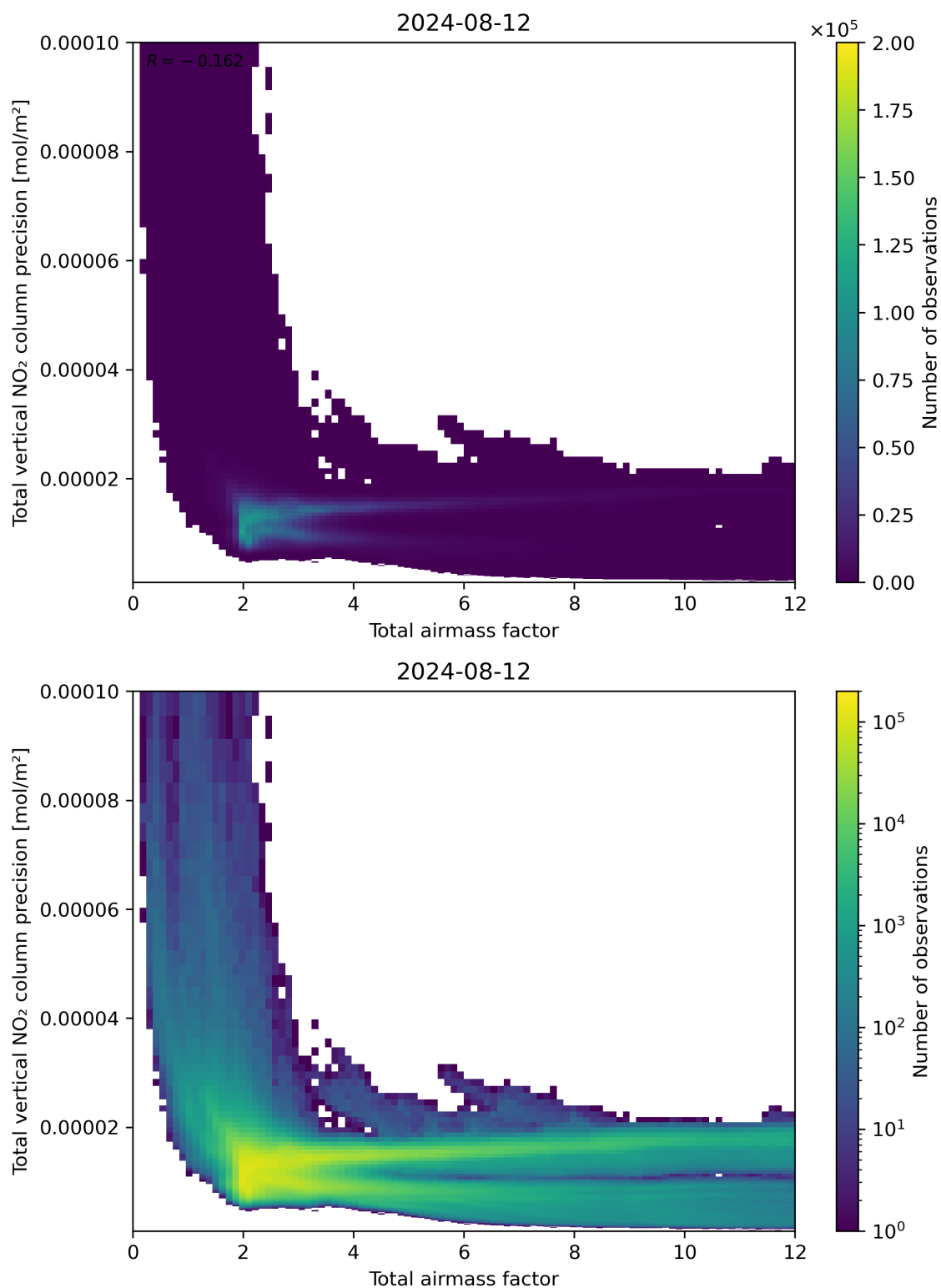
Figure 68: Scatter density plot of “Total airmass factor” against “Total vertical NO 2 column precision” for 2024-08-12 to 2024-08-13.
