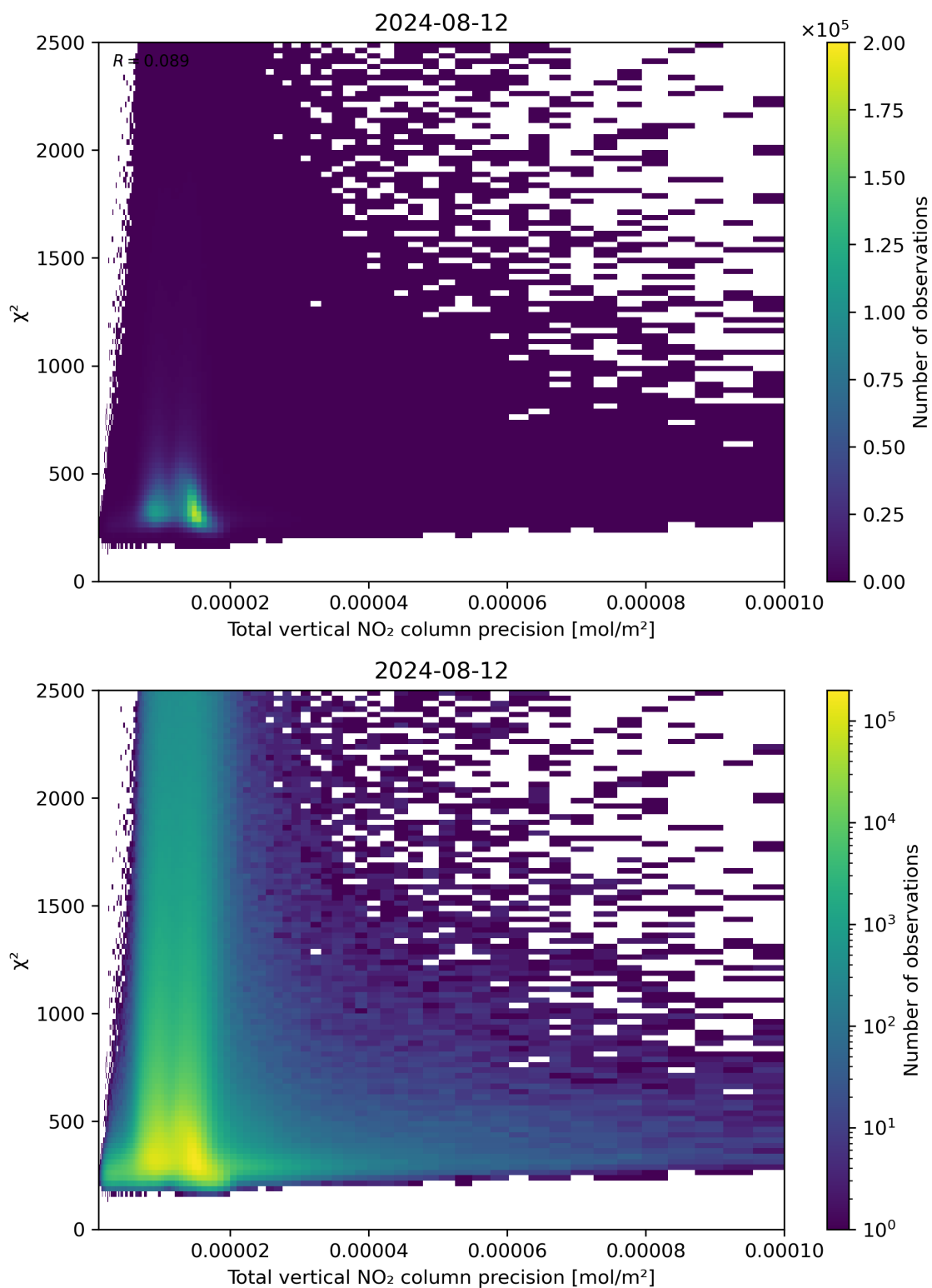
Figure 116: Scatter density plot of “Total vertical NO 2 column precision” against “ \chi^2 ” for 2024-08-12 to 2024-08-13.
