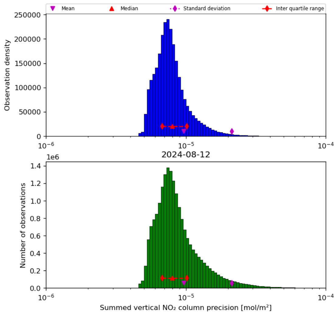
Figure 41: Histogram of “Summed vertical NO 2 column precision” for 2024-08-12 to 2024-08-13
