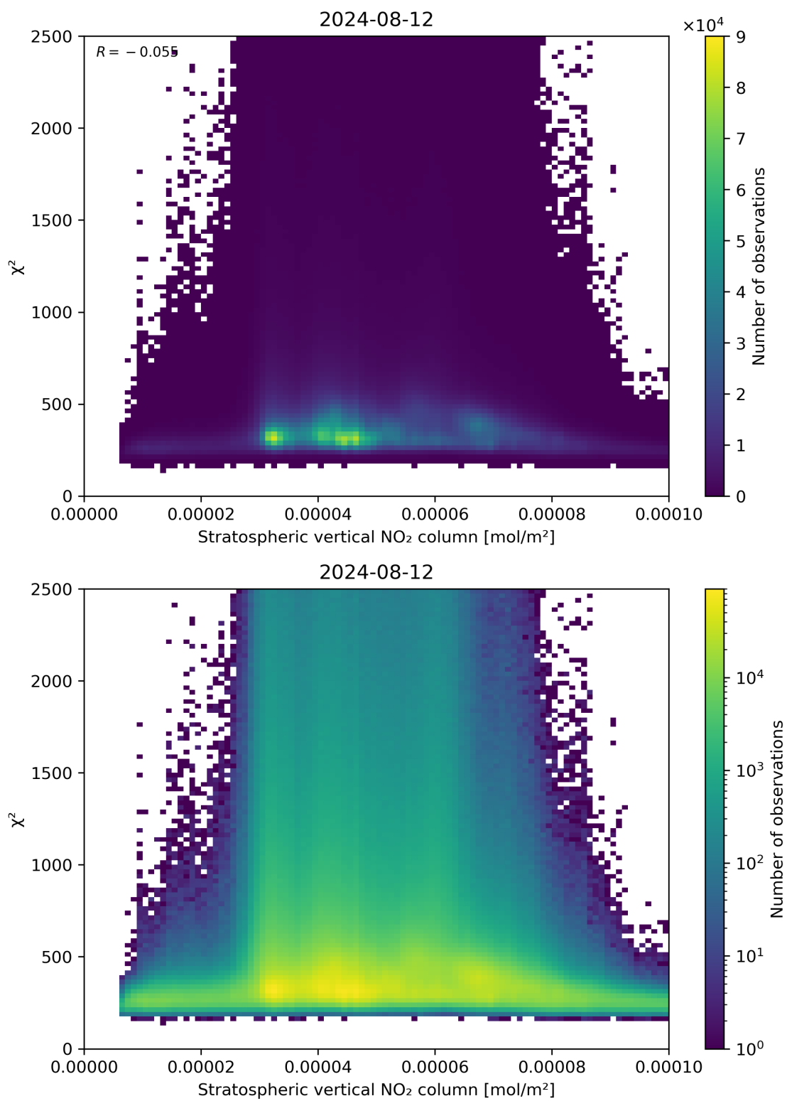
Figure 97: Scatter density plot of “Stratospheric vertical NO 2 column” against “ \chi^2 ” for 2024-08-12 to 2024-08-13.
