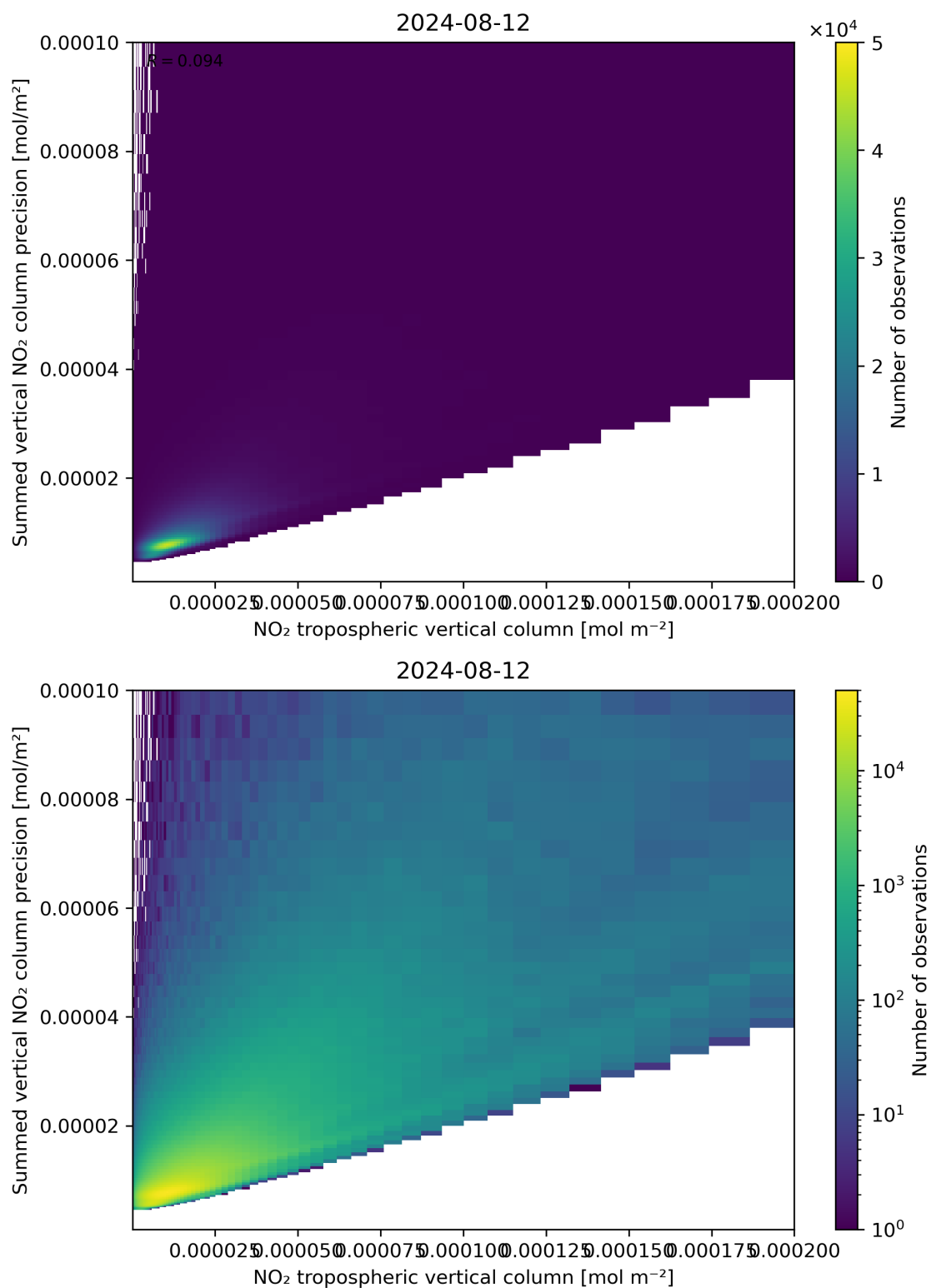
Figure 127: Scatter density plot of “NO 2 tropospheric vertical column” against “Summed vertical NO 2 column precision” for 2024-08-12 to 2024-08-13.
