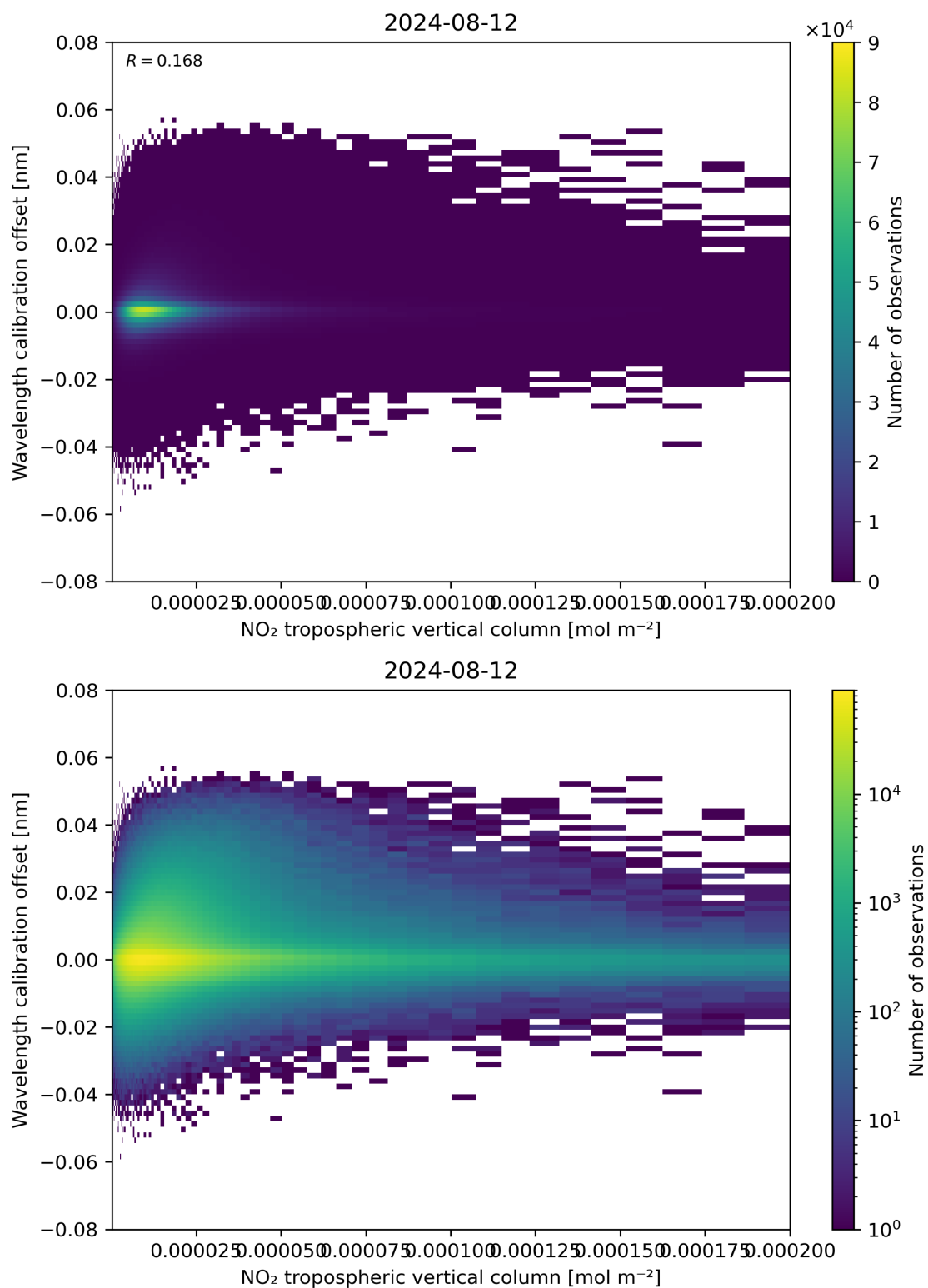
Figure 143: Scatter density plot of “NO 2 tropospheric vertical column” against “Wavelength calibration offset” for 2024-08-12 to 2024-08-13.
