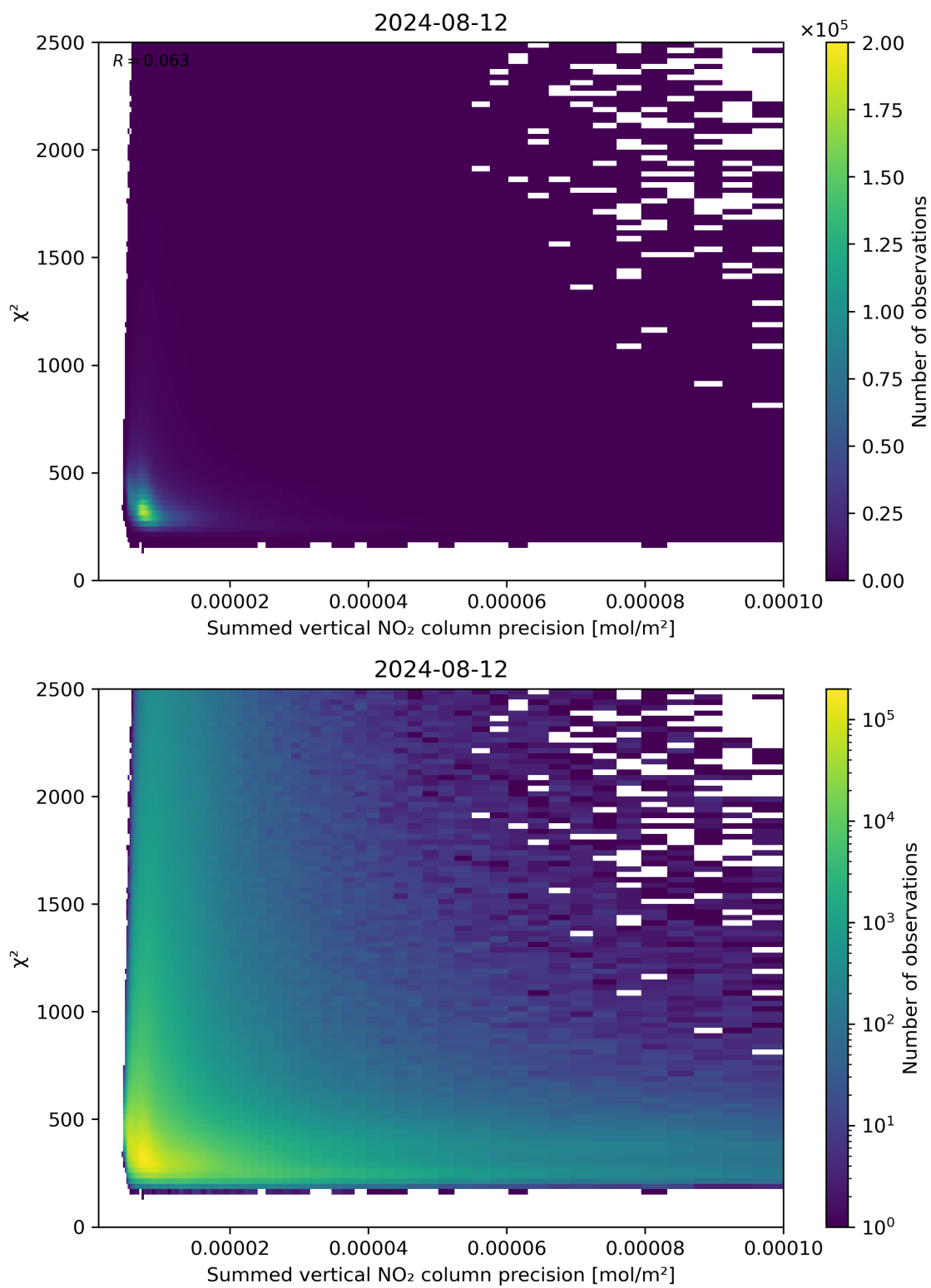
Figure 107: Scatter density plot of “Summed vertical NO 2 column precision” against “ \chi^2 ” for 2024-08-12 to 2024-08-13.
