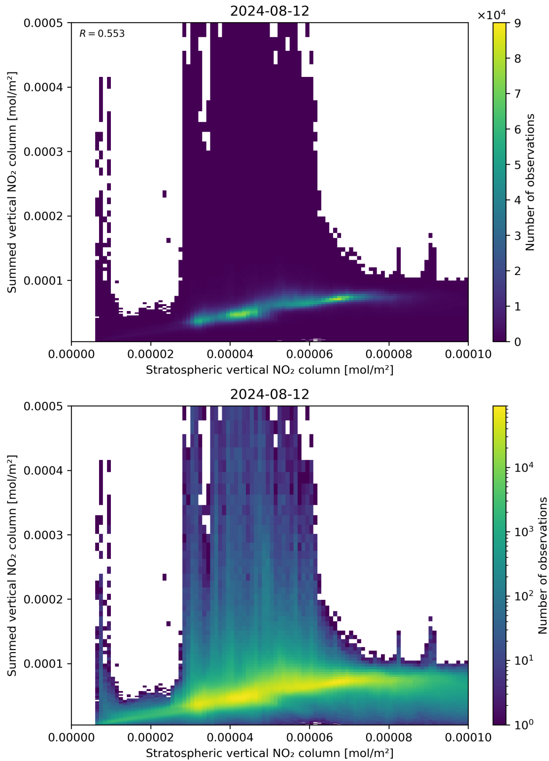
Figure 98: Scatter density plot of “Stratospheric vertical NO 2 column” against “Summed vertical NO 2 column” for 2024-08-12 to 2024-08-13.
