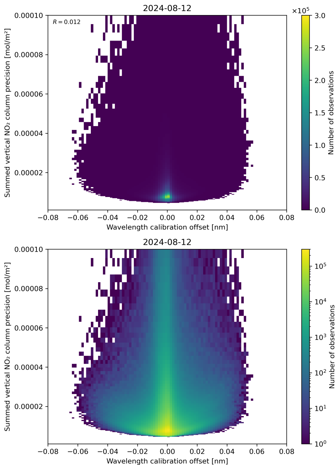
Figure 178: Scatter density plot of “Wavelength calibration offset” against “Summed vertical NO 2 column precision” for 2024-08-12 to 2024-08-13.
