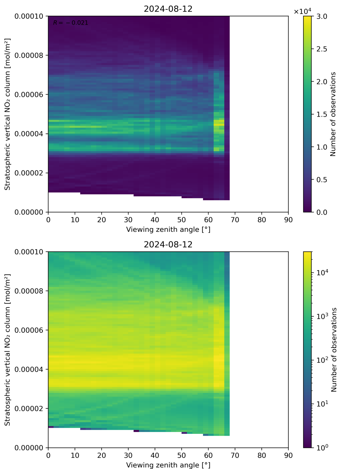
Figure 164: Scatter density plot of “Viewing zenith angle” against “Stratospheric vertical NO 2 column” for 2024-08-12 to 2024-08-13.
