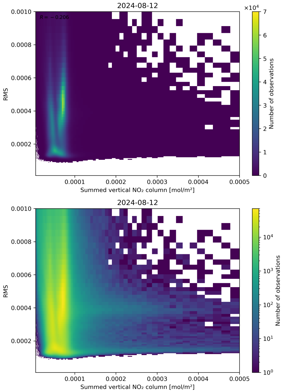
Figure 109: Scatter density plot of “Summed vertical NO 2 column” against “RMS” for 2024-08-12 to 2024-08-13.
