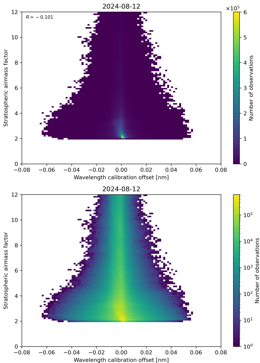
Figure 174: Scatter density plot of “Wavelength calibration offset” against “Stratospheric airmass factor” for 2024-08-12 to 2024-08-13.
