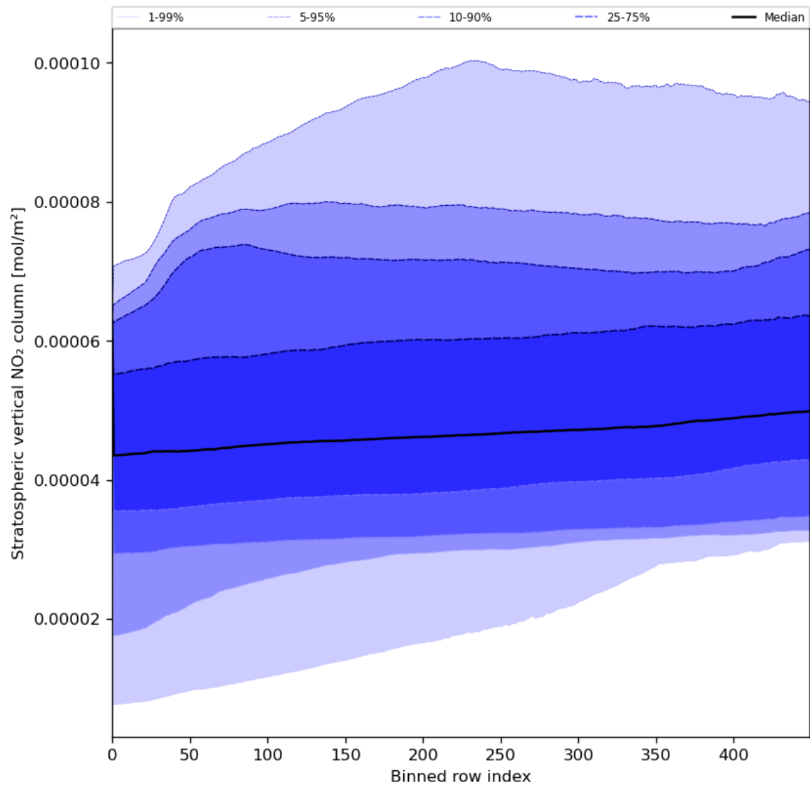
Figure 53: Along track statistics of “Stratospheric vertical NO 2 column” for 2024-08-12 to 2024-08-13
