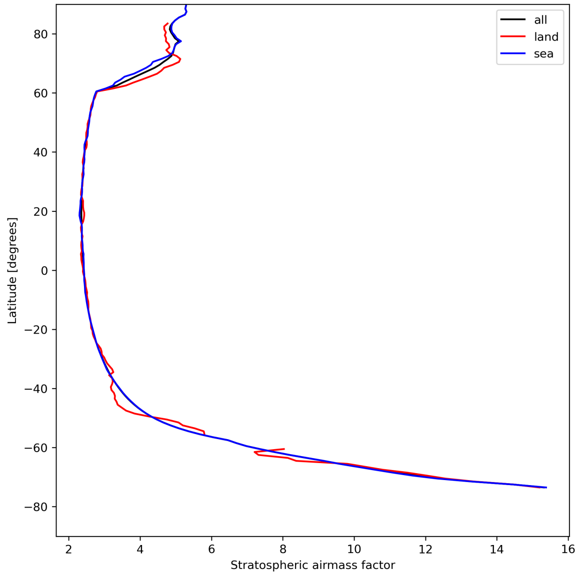
Figure 27: Zonal average of “Stratospheric airmass factor” for 2024-08-12 to 2024-08-13.
