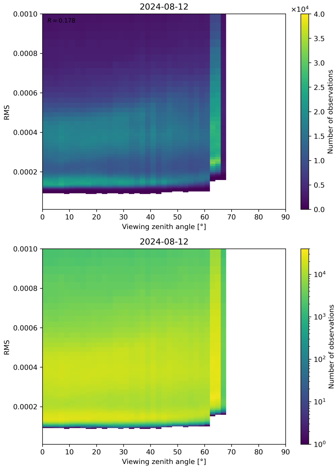
Figure 171: Scatter density plot of “Viewing zenith angle” against “RMS” for 2024-08-12 to 2024-08-13.
