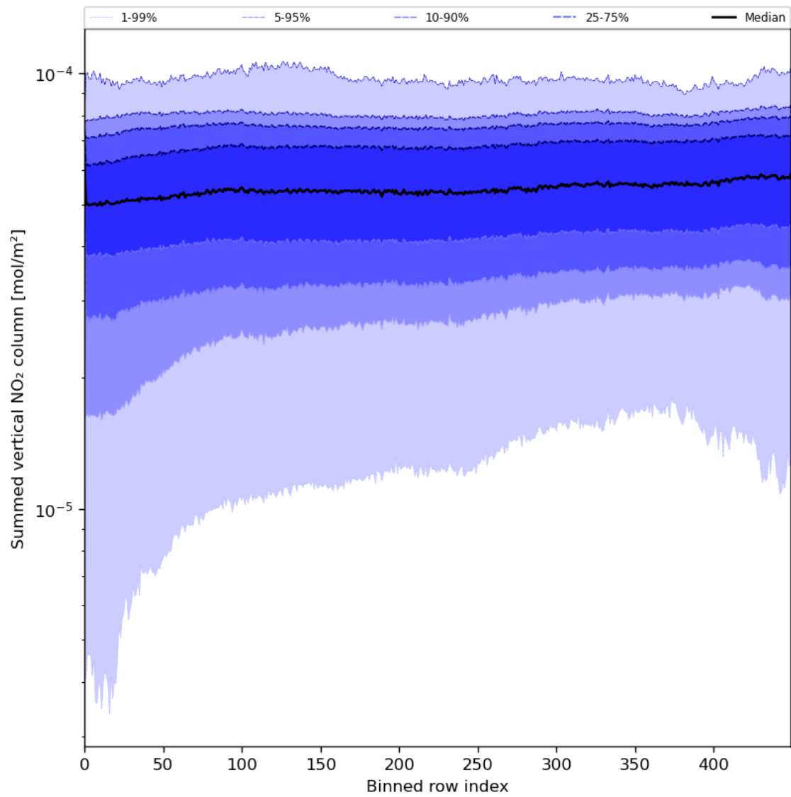
Figure 57: Along track statistics of “Summed vertical NO 2 column” for 2024-08-12 to 2024-08-13
