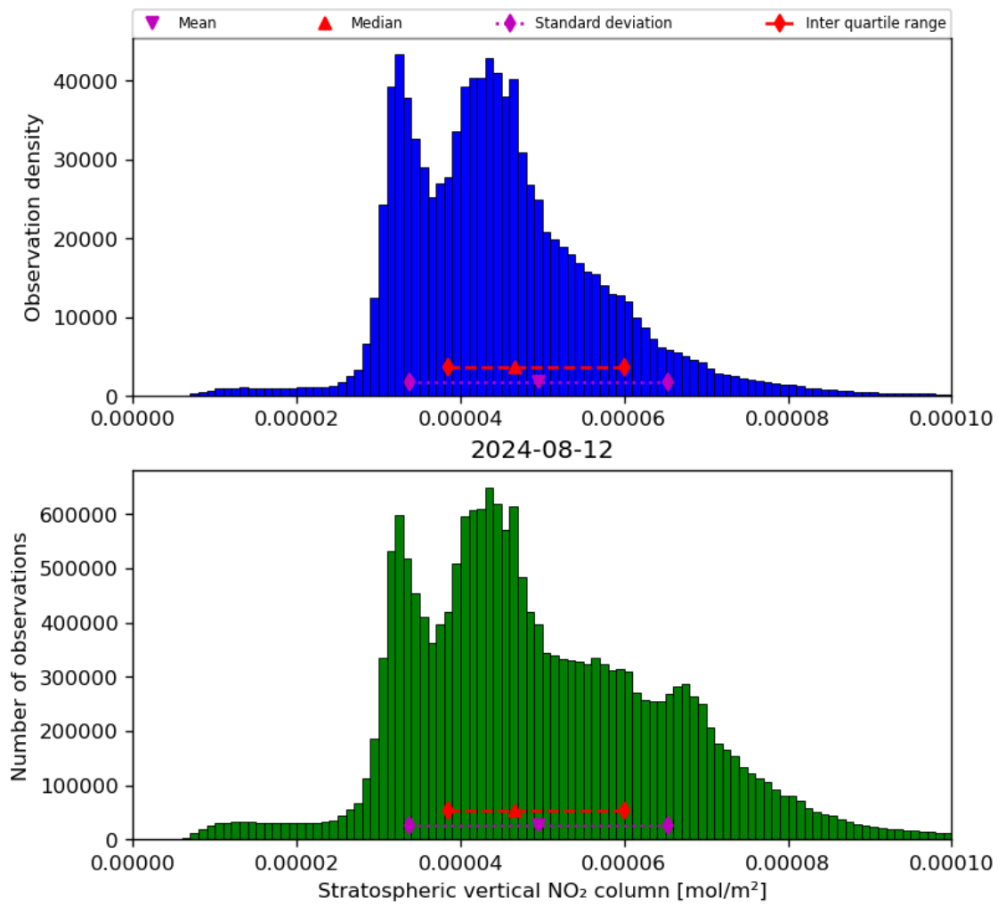
Figure 36: Histogram of “Stratospheric vertical NO 2 column” for 2024-08-12 to 2024-08-13
