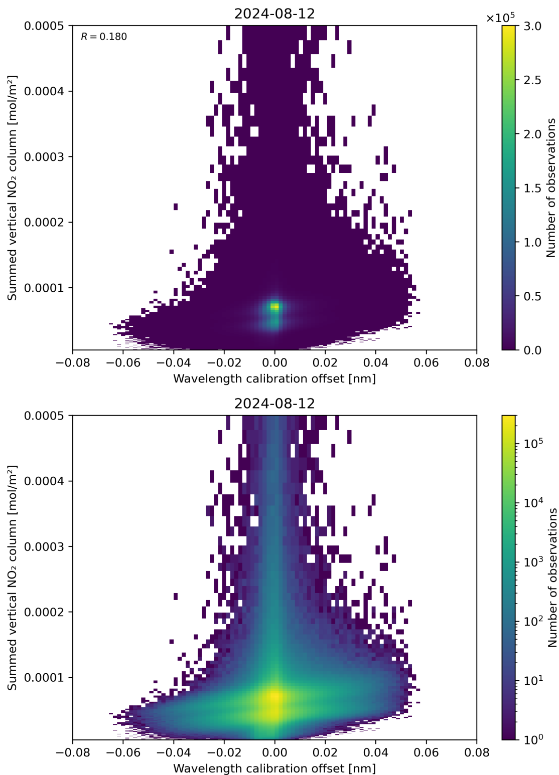
Figure 177: Scatter density plot of “Wavelength calibration offset” against “Summed vertical NO 2 column” for 2024-08-12 to 2024-08-13.
