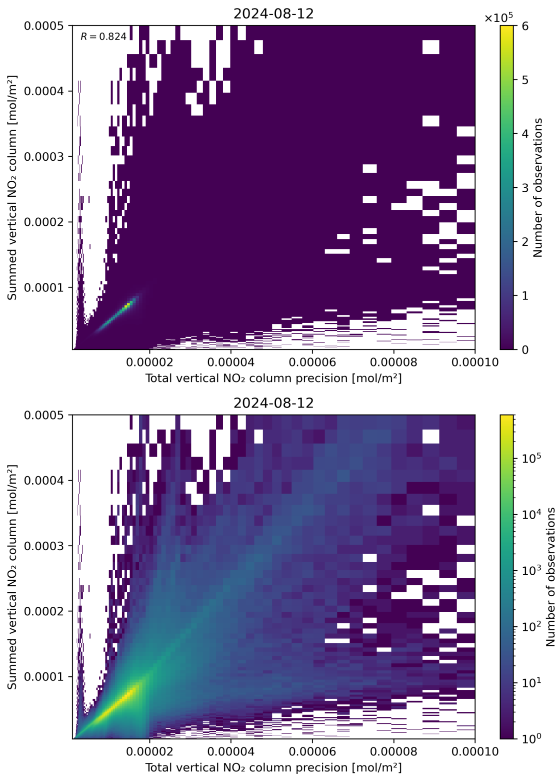
Figure 117: Scatter density plot of “Total vertical NO 2 column precision” against “Summed vertical NO 2 column” for 2024-08-12 to 2024-08-13.
