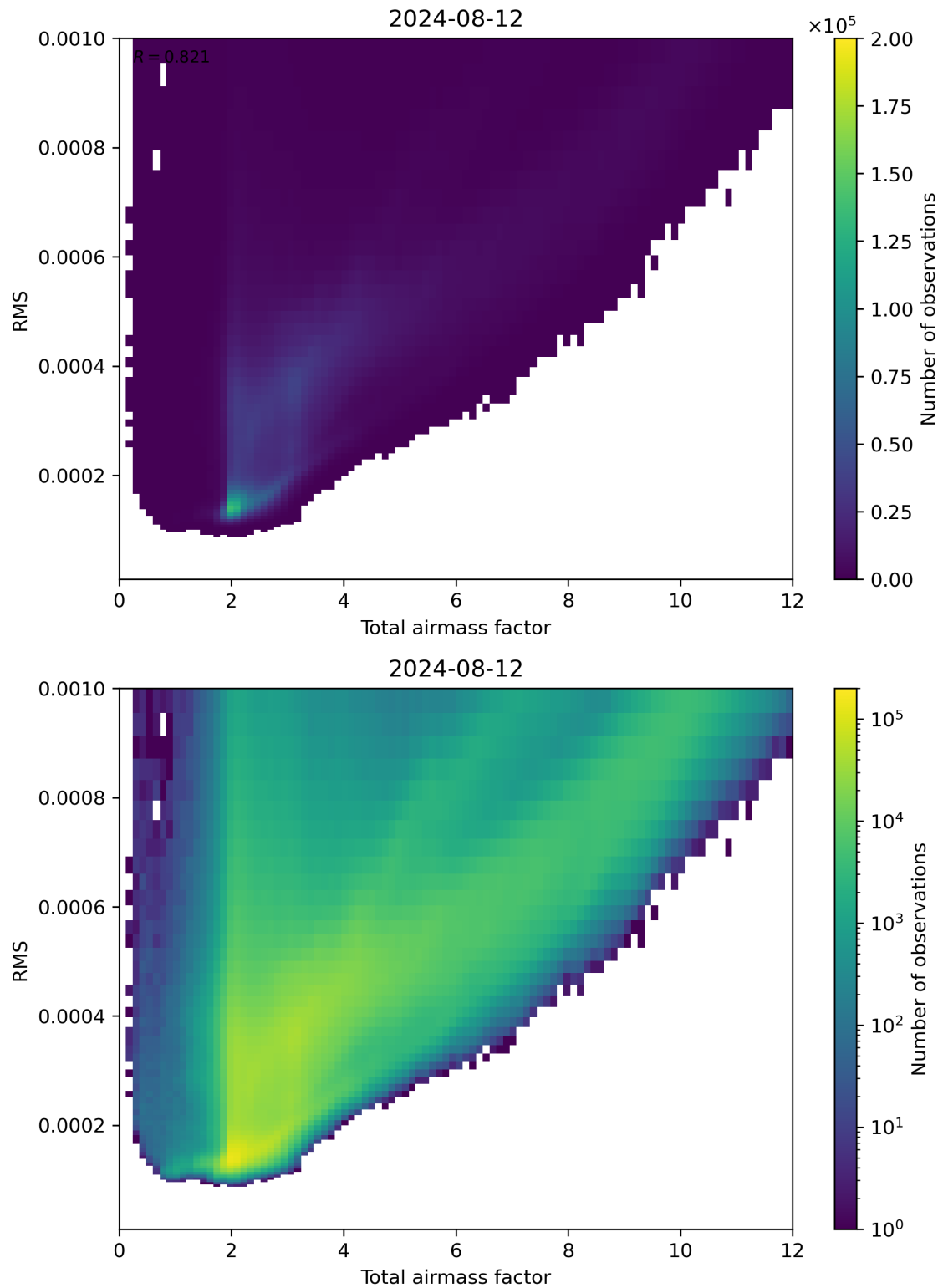
Figure 69: Scatter density plot of “Total airmass factor” against “RMS” for 2024-08-12 to 2024-08-13.
