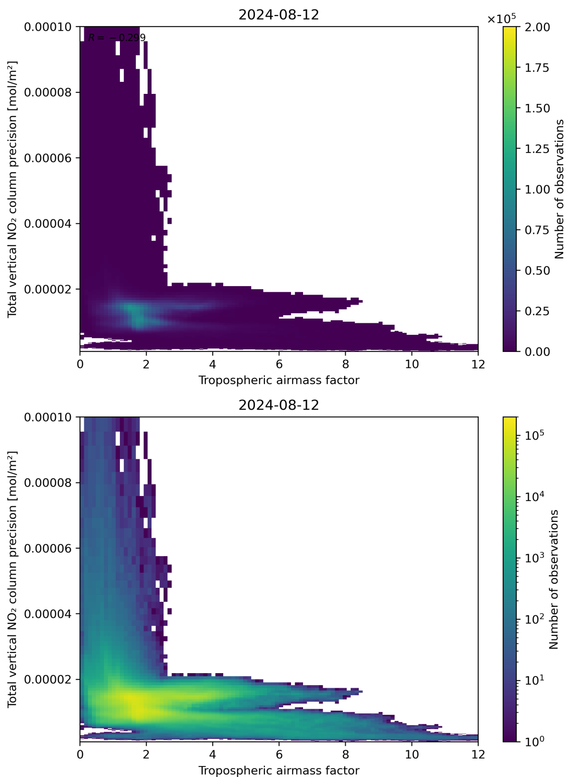
Figure 78: Scatter density plot of “Tropospheric air mass factor” against “Total vertical NO 2 column precision” for 2024-08-12 to 2024-08-13.
