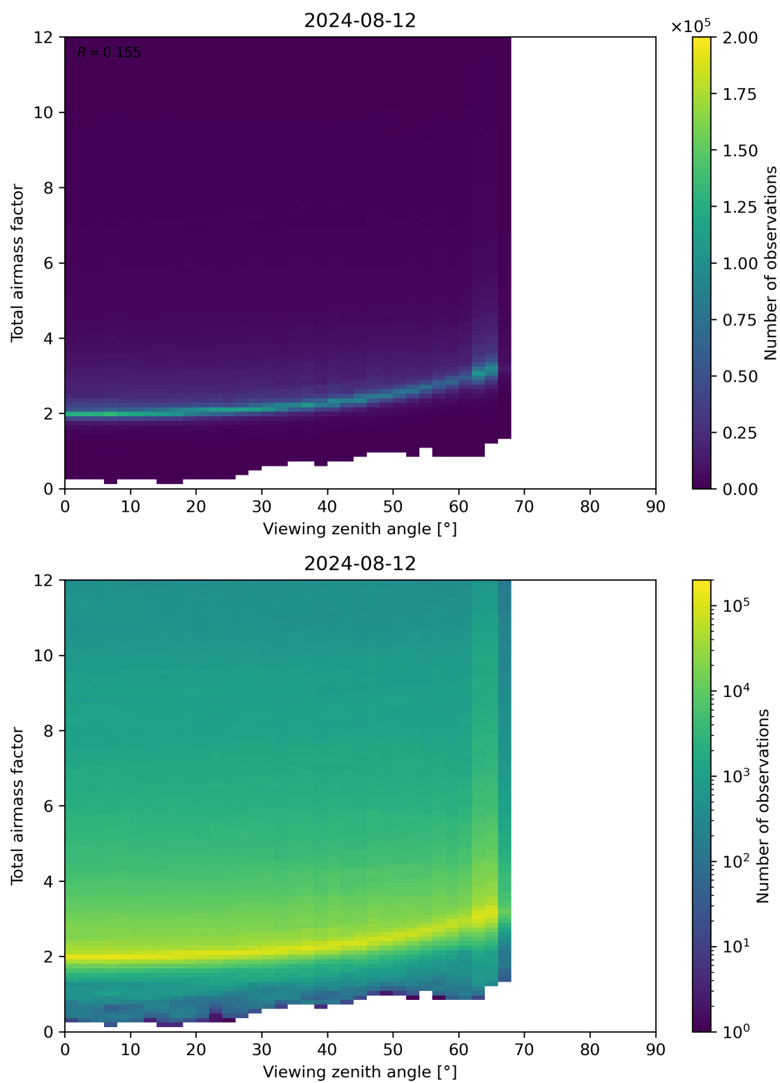
Figure 160: Scatter density plot of “Viewing zenith angle” against “Total airmass factor” for 2024-08-12 to 2024-08-13.
