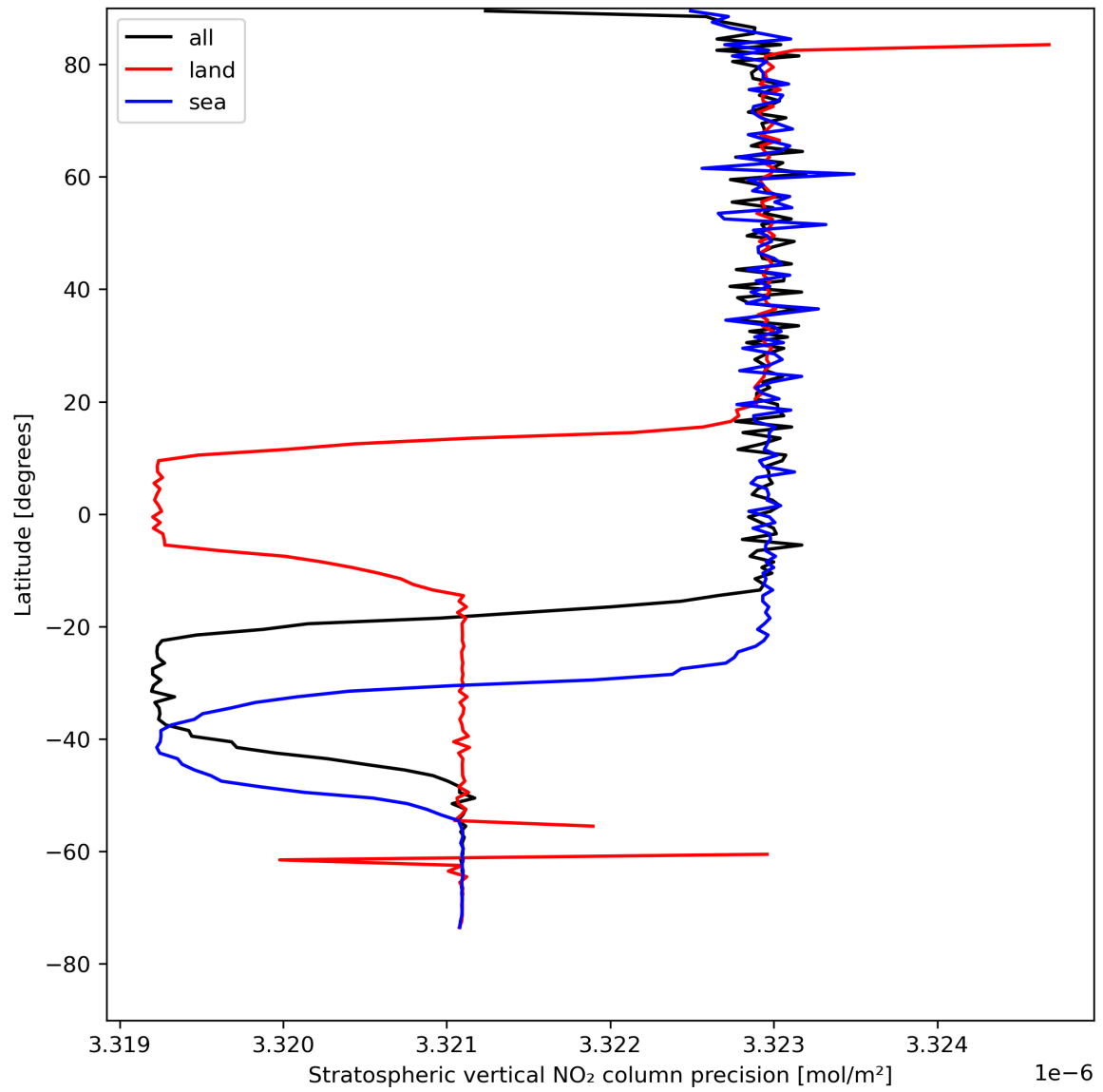
Figure 20: Zonal average of “Stratospheric vertical NO 2 column precision” for 2024-08-12 to 2024-08-13.
