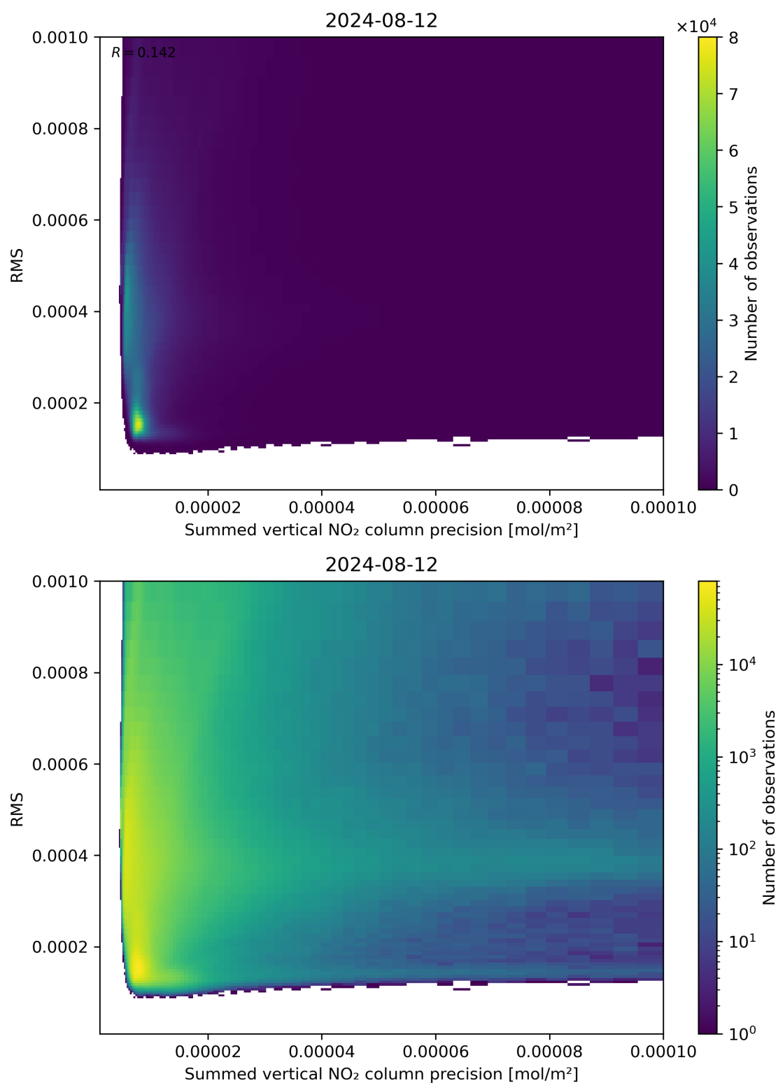
Figure 108: Scatter density plot of “Summed vertical NO 2 column precision” against “RMS” for 2024-08-12 to 2024-08-13.
