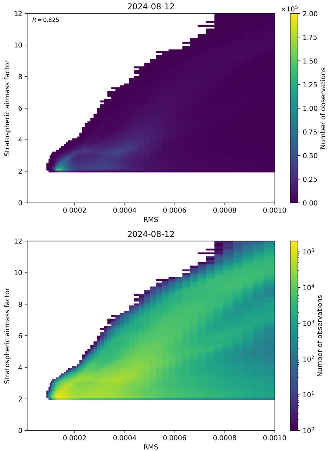
Figure 144: Scatter density plot of “RMS” against “Stratospheric airmass factor” for 2024-08-12 to 2024-08-13.
