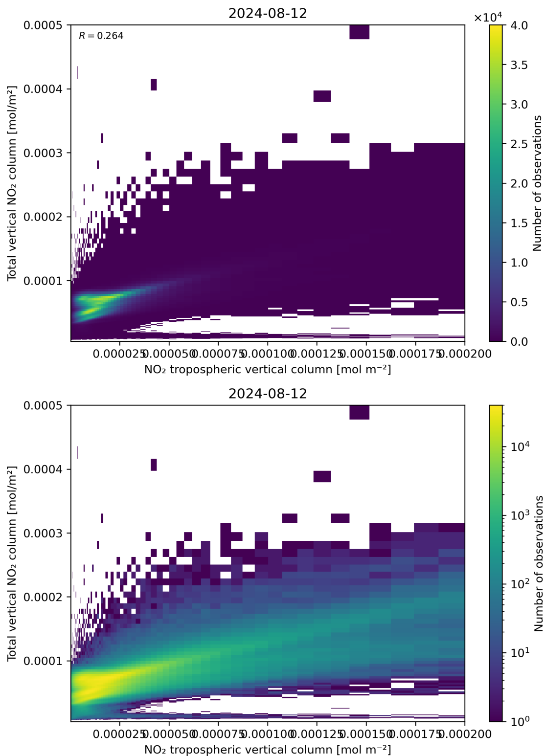
Figure 128: Scatter density plot of “NO 2 tropospheric vertical column” against “Total vertical NO 2 column” for 2024-08-12 to 2024-08-13.
