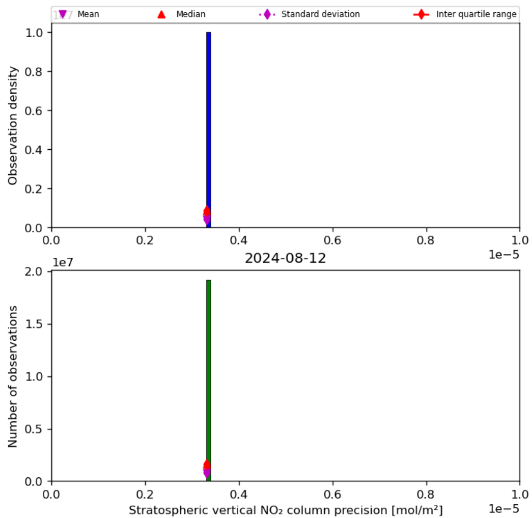
Figure 37: Histogram of “Stratospheric vertical NO 2 column precision” for 2024-08-12 to 2024-08-13
