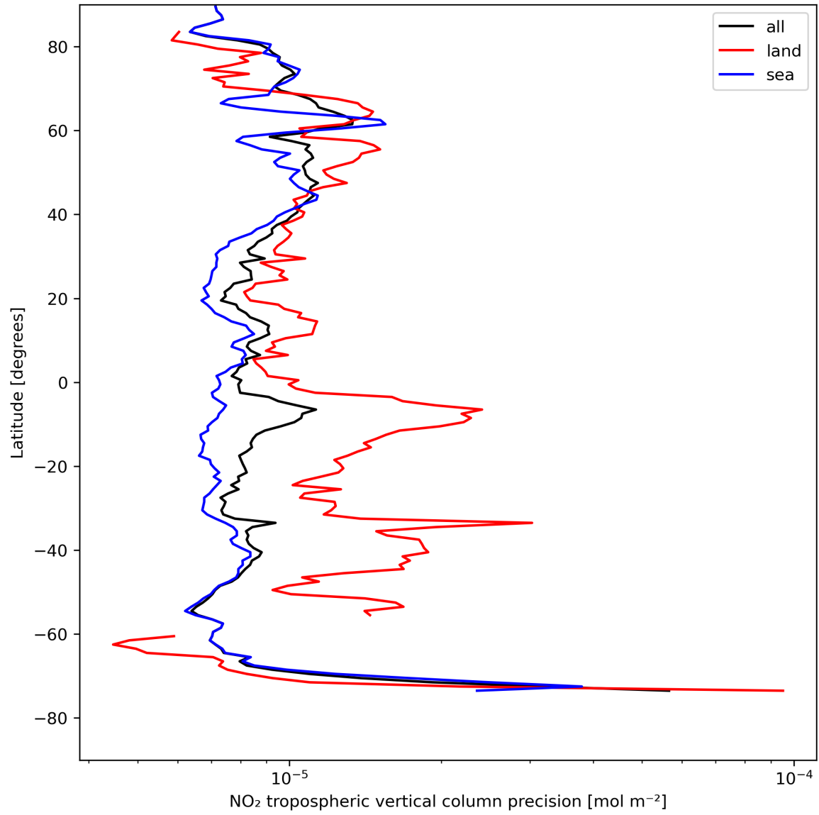
Figure 13: Zonal average of “NO 2 tropospheric vertical column precision” for 2024-08-12 to 2024-08-13.
