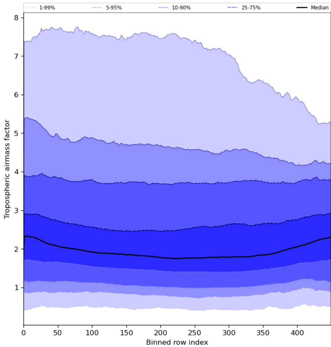
Figure 48: Along track statistics of “Tropospheric airmass factor” for 2024-08-12 to 2024-08-13
