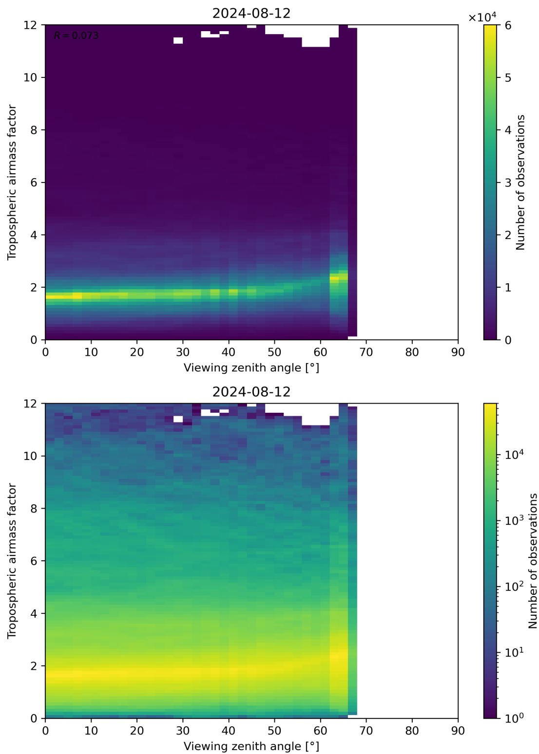
Figure 161: Scatter density plot of “Viewing zenith angle” against “Tropospheric airmass factor” for 2024-08-12 to 2024-08-13.
