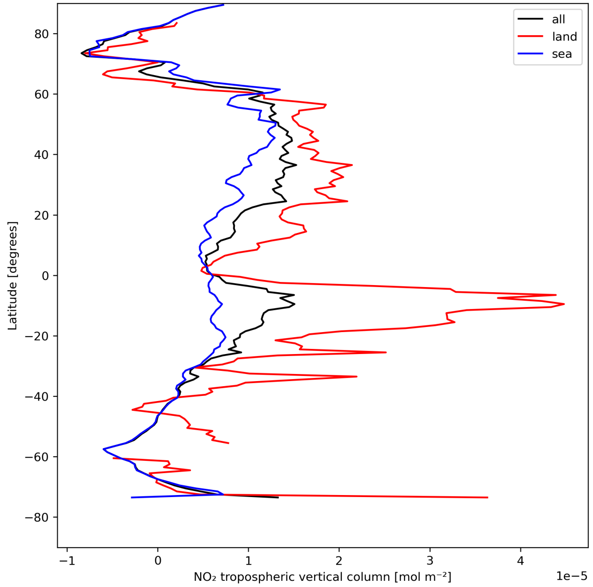
Figure 12: Zonal average of “NO 2 tropospheric vertical column” for 2024-08-12 to 2024-08-13.
