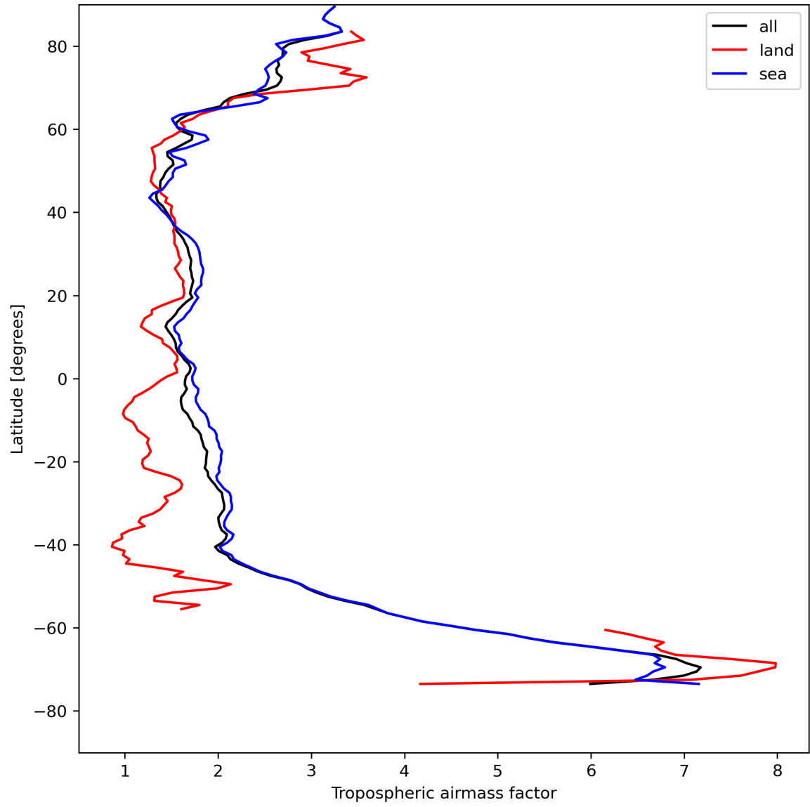
Figure 14: Zonal average of “Tropospheric airmass factor” for 2024-08-12 to 2024-08-13.
