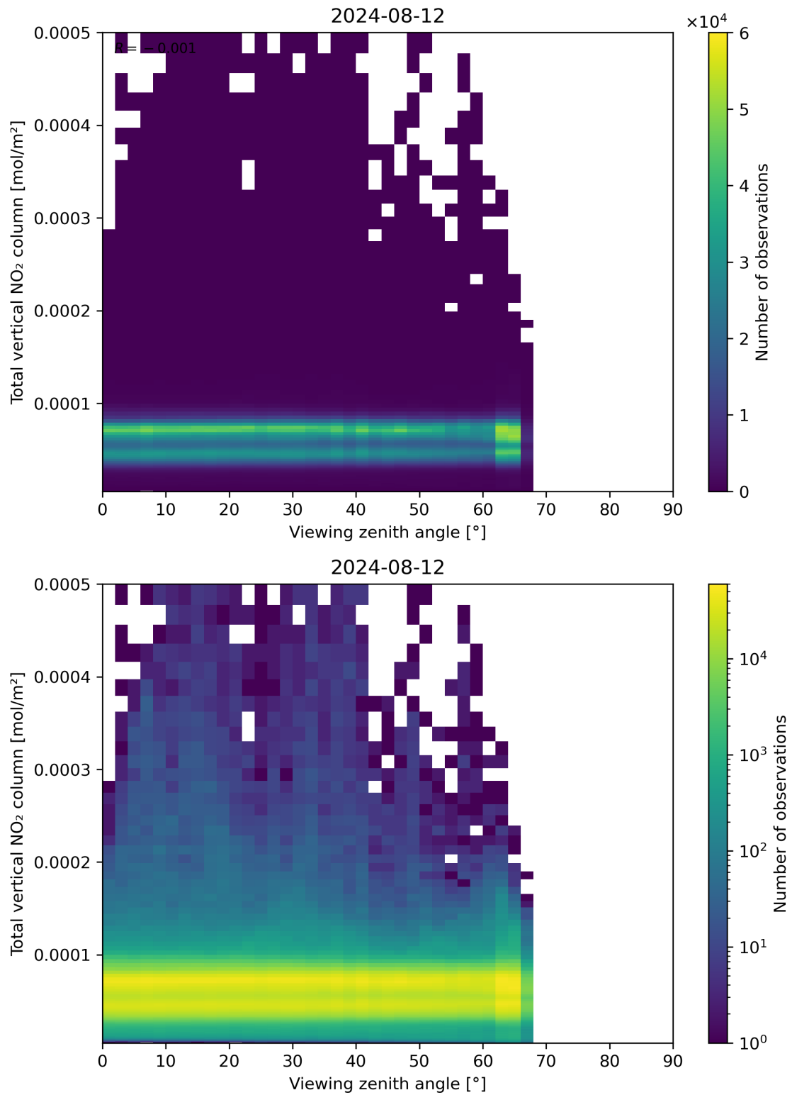
Figure 167: Scatter density plot of “Viewing zenith angle” against “Total vertical NO 2 column” for 2024-08-12 to 2024-08-13.
