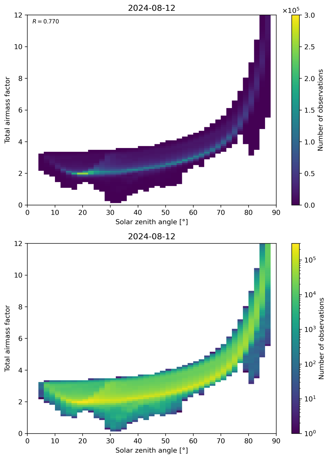
Figure 146: Scatter density plot of “Solar zenith angle” against “Total air mass factor” for 2024-08-12 to 2024-08-13.
