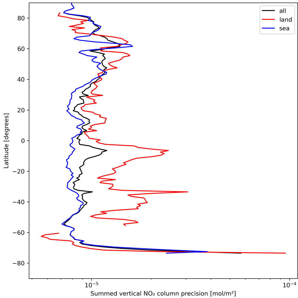
Figure 24: Zonal average of “Summed vertical NO 2 column precision” for 2024-08-12 to 2024-08-13.
