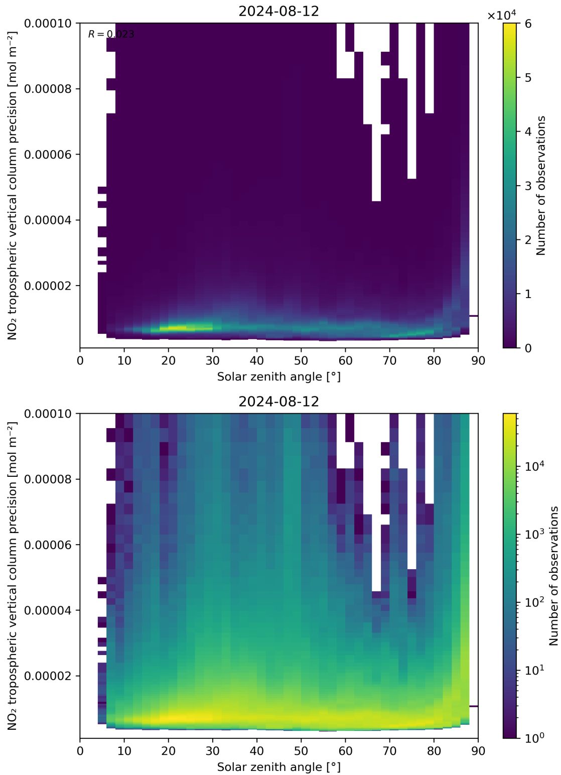
Figure 156: Scatter density plot of “Solar zenith angle” against “NO 2 tropospheric vertical column precision” for 2024-08-12 to 2024-08-13.
