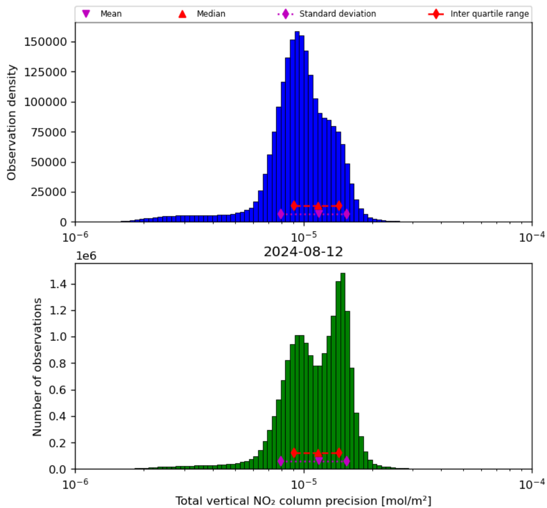
Figure 39: Histogram of “Total vertical NO 2 column precision” for 2024-08-12 to 2024-08-13
