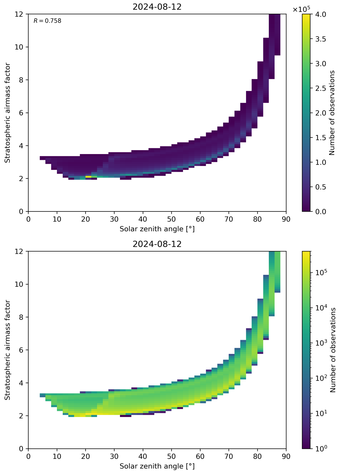
Figure 145: Scatter density plot of “Solar zenith angle” against “Stratospheric airmass factor” for 2024-08-12 to 2024-08-13.
