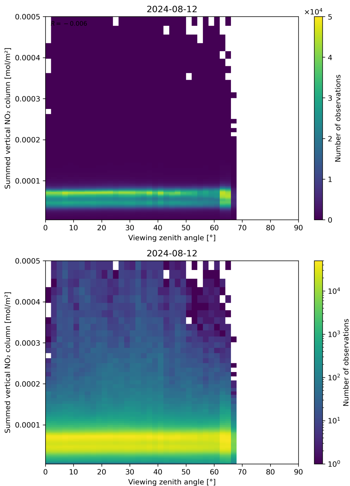
Figure 165: Scatter density plot of “Viewing zenith angle” against “Summed vertical NO 2 column” for 2024-08-12 to 2024-08-13.
