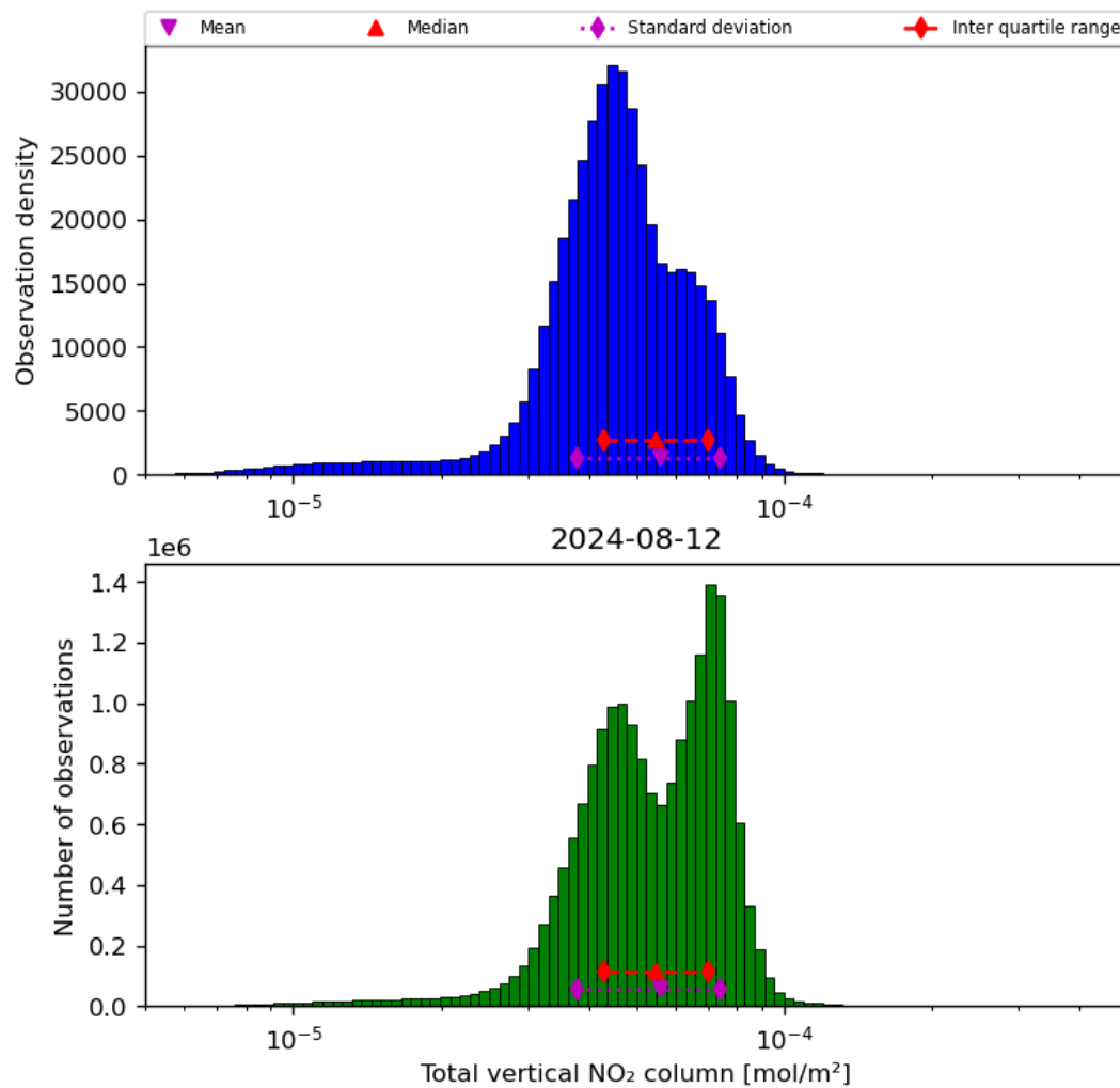
Figure 38: Histogram of “Total vertical NO 2 column” for 2024-08-12 to 2024-08-13
