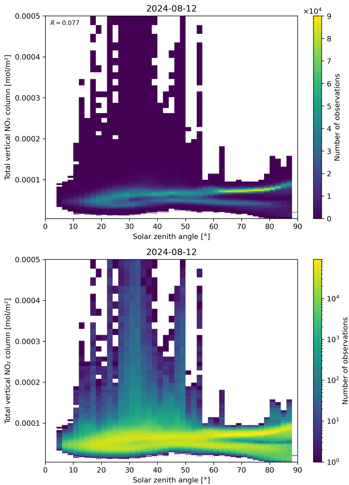
Figure 153: Scatter density plot of “Solar zenith angle” against “Total vertical NO 2 column” for 2024-08-12 to 2024-08-13.
