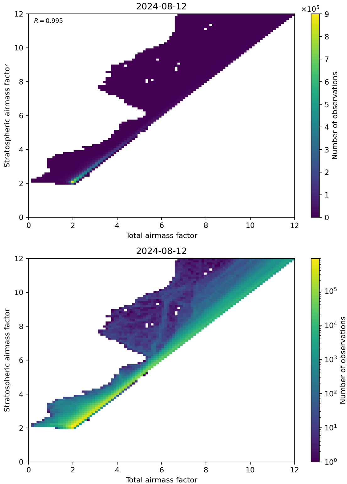
Figure 62: Scatter density plot of “Total airmass factor” against “Stratospheric airmass factor” for 2024-08-12 to 2024-08-13.
