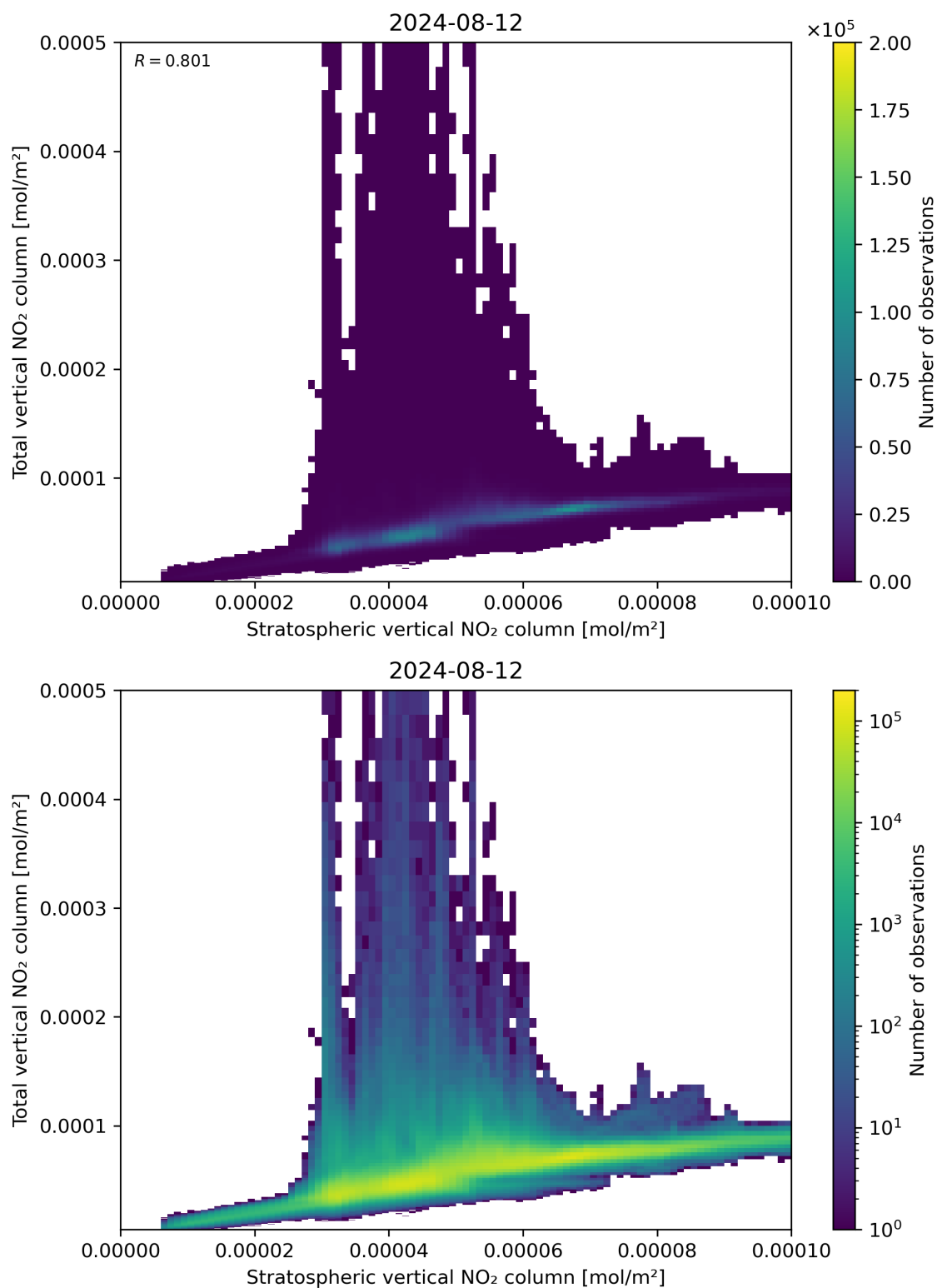
Figure 100: Scatter density plot of “Stratospheric vertical NO 2 column” against “Total vertical NO 2 column” for 2024-08-12 to 2024-08-13.
