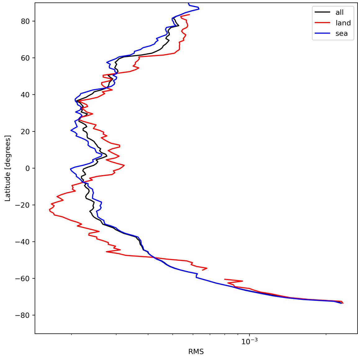
Figure 26: Zonal average of “RMS” for 2024-08-12 to 2024-08-13.
