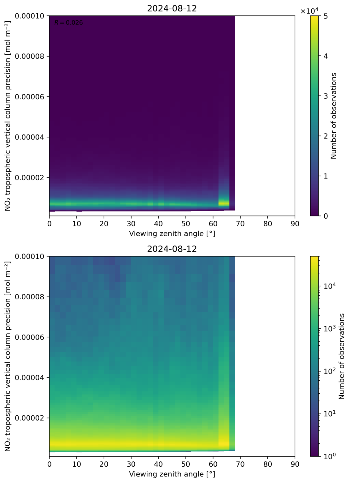
Figure 170: Scatter density plot of “Viewing zenith angle” against “NO 2 tropospheric vertical column precision” for 2024-08-12 to 2024-08-13.
