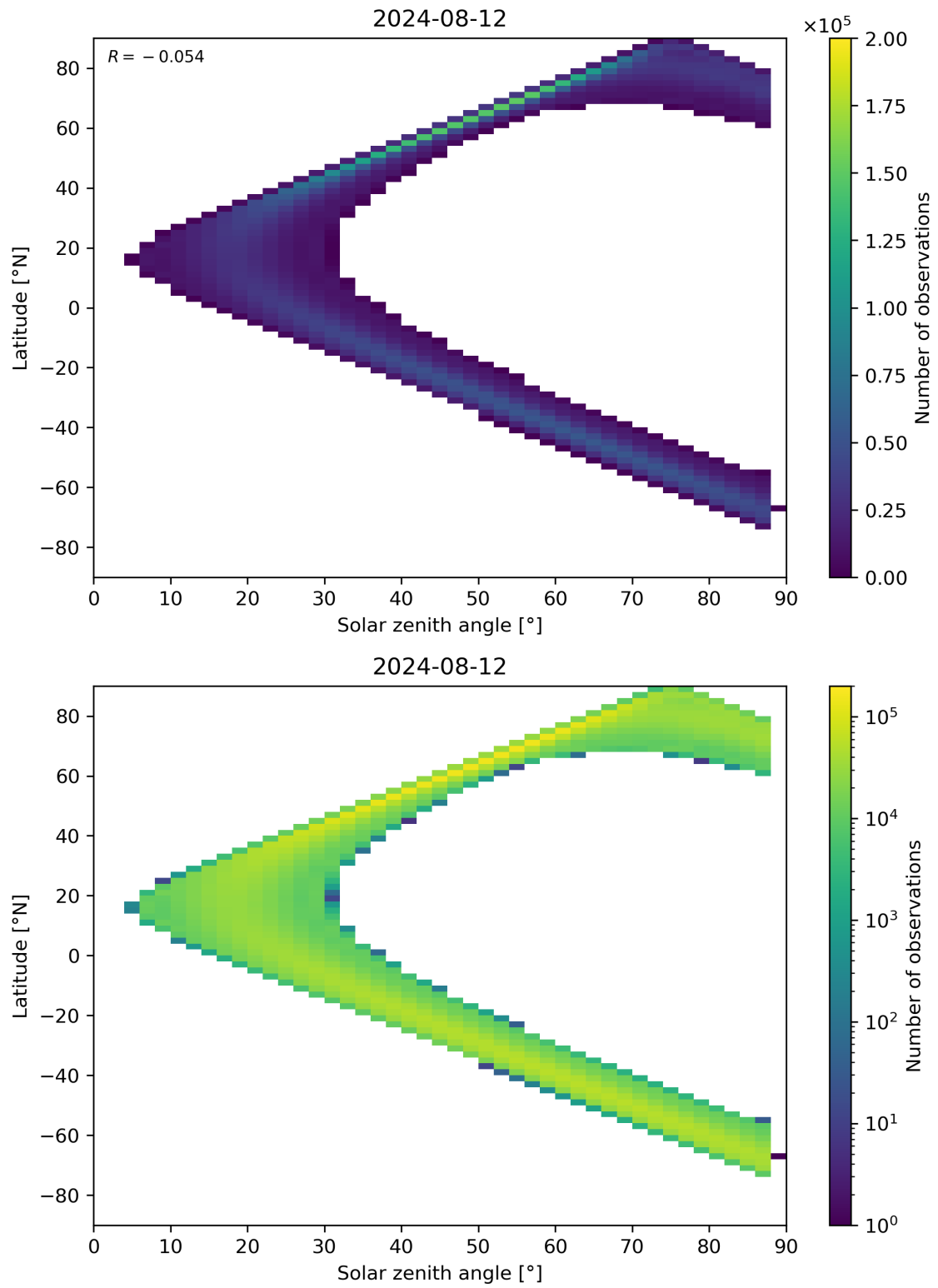
Figure 149: Scatter density plot of “Solar zenith angle” against “Latitude” for 2024-08-12 to 2024-08-13.
