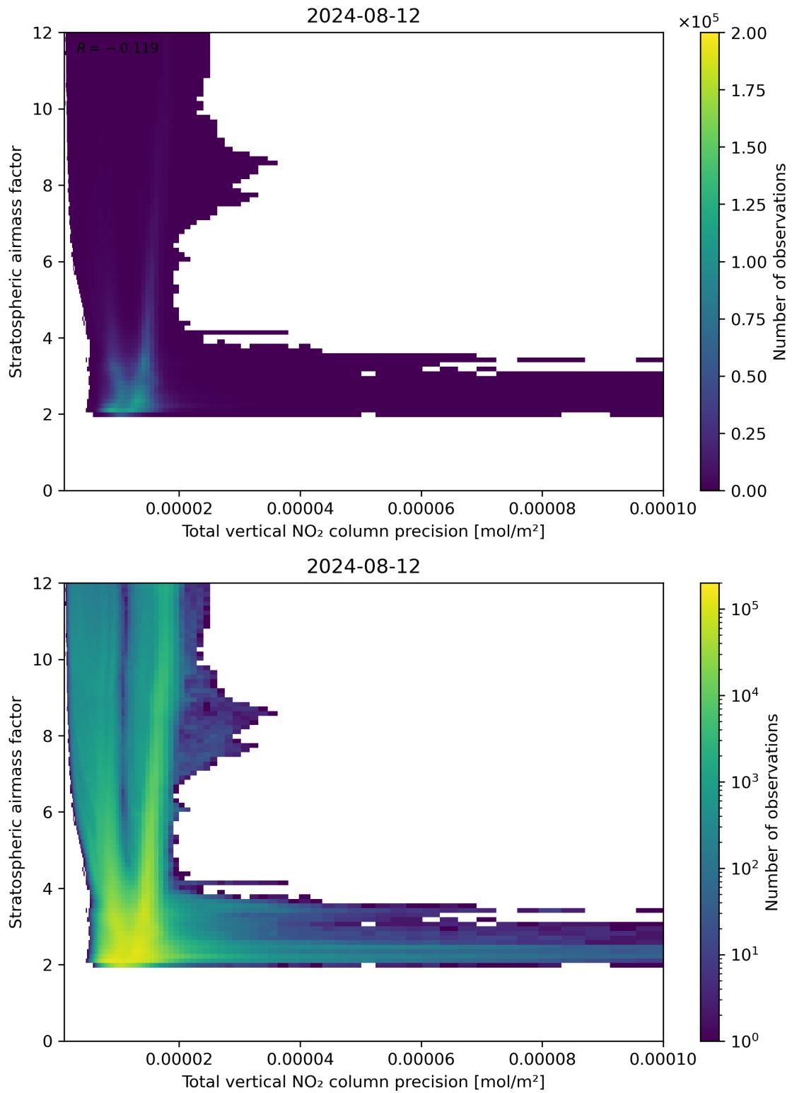
Figure 115: Scatter density plot of “Total vertical NO 2 column precision” against “Stratospheric air mass factor” for 2024-08-12 to 2024-08-13.
