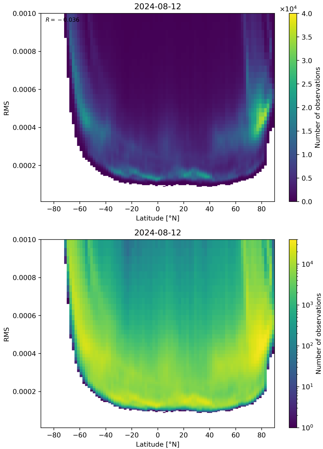
Figure 94: Scatter density plot of “Latitude” against “RMS” for 2024-08-12 to 2024-08-13.
