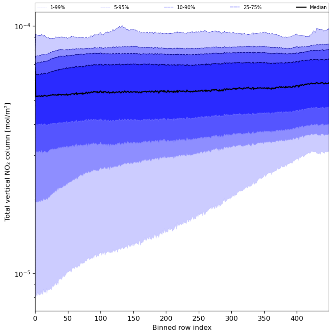
Figure 55: Along track statistics of “Total vertical NO 2 column” for 2024-08-12 to 2024-08-13
