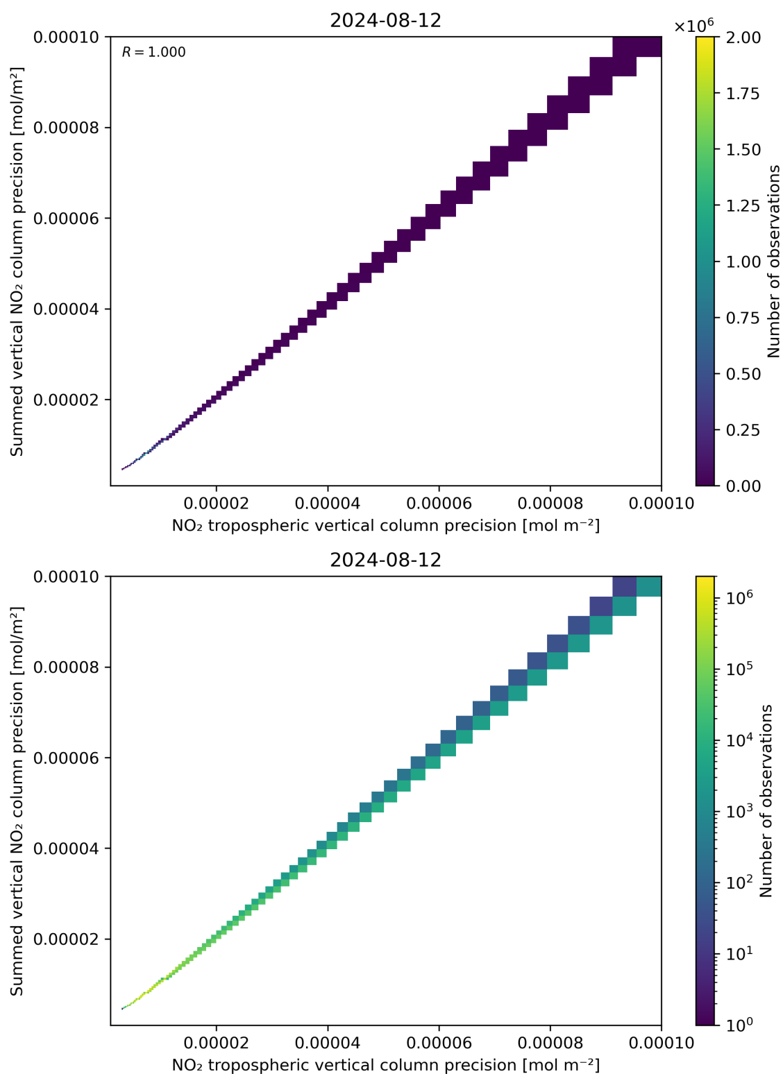
Figure 137: Scatter density plot of “NO 2 tropospheric vertical column precision” against “Summed vertical NO 2 column precision” for 2024-08-12 to 2024-08-13.
