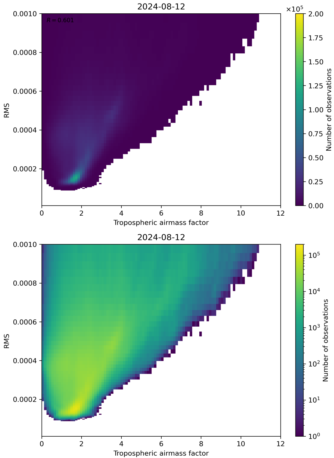
Figure 79: Scatter density plot of “Tropospheric airmass factor” against “RMS” for 2024-08-12 to 2024-08-13.
