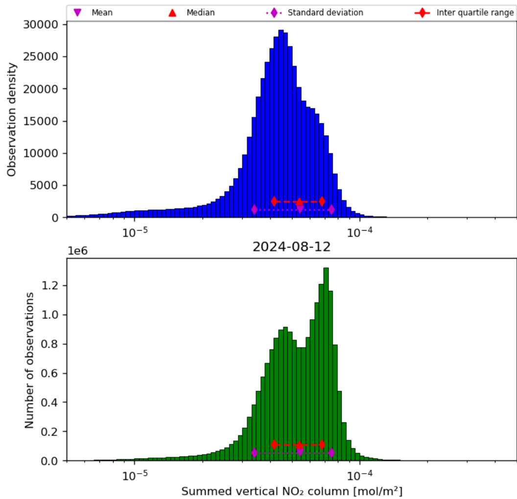
Figure 40: Histogram of “Summed vertical NO 2 column” for 2024-08-12 to 2024-08-13
