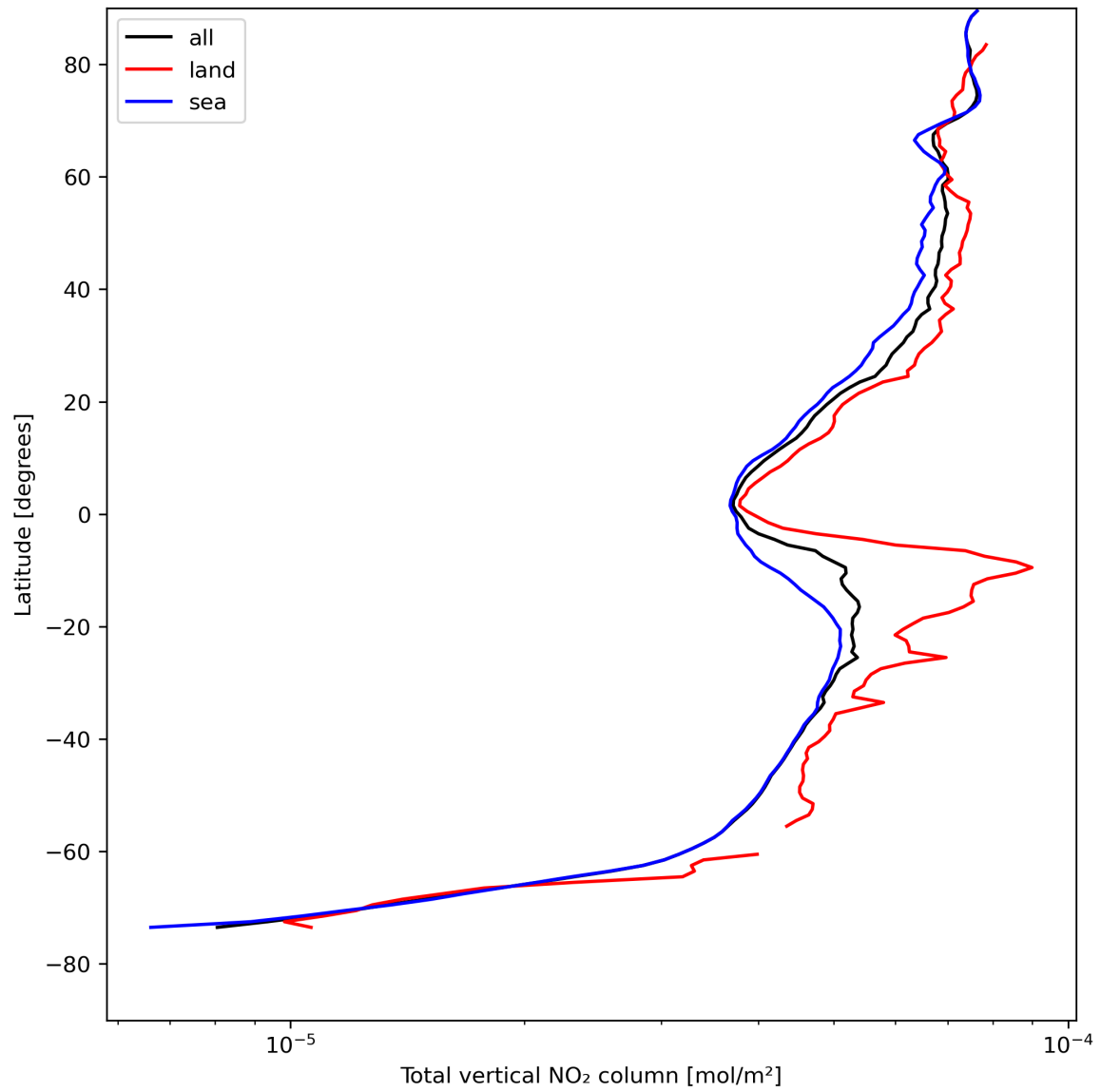
Figure 21: Zonal average of “Total vertical NO 2 column” for 2024-08-12 to 2024-08-13.
