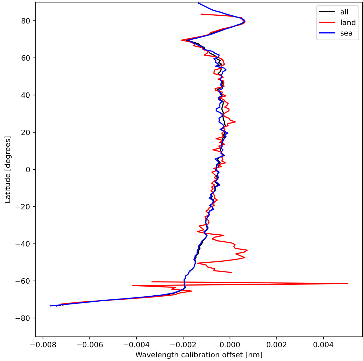
Figure 18: Zonal average of “Wavelength calibration offset” for 2024-08-12 to 2024-08-13.
