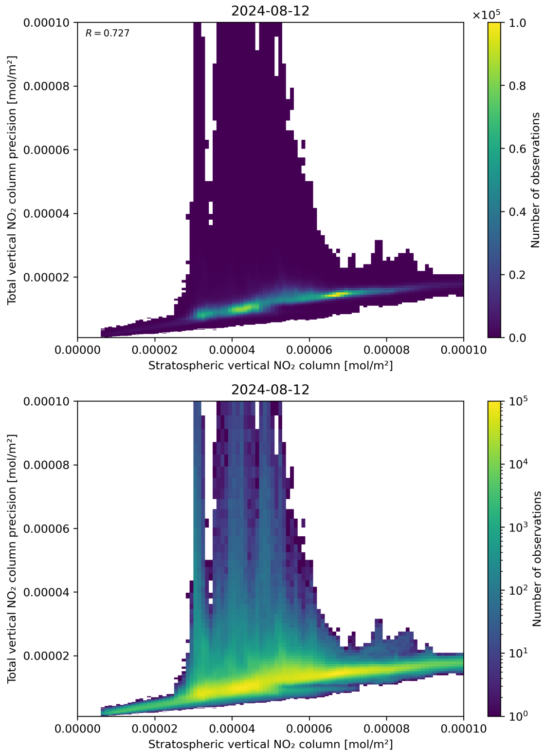
Figure 101: Scatter density plot of “Stratospheric vertical NO 2 column” against “Total vertical NO 2 column precision” for 2024-08-12 to 2024-08-13.
