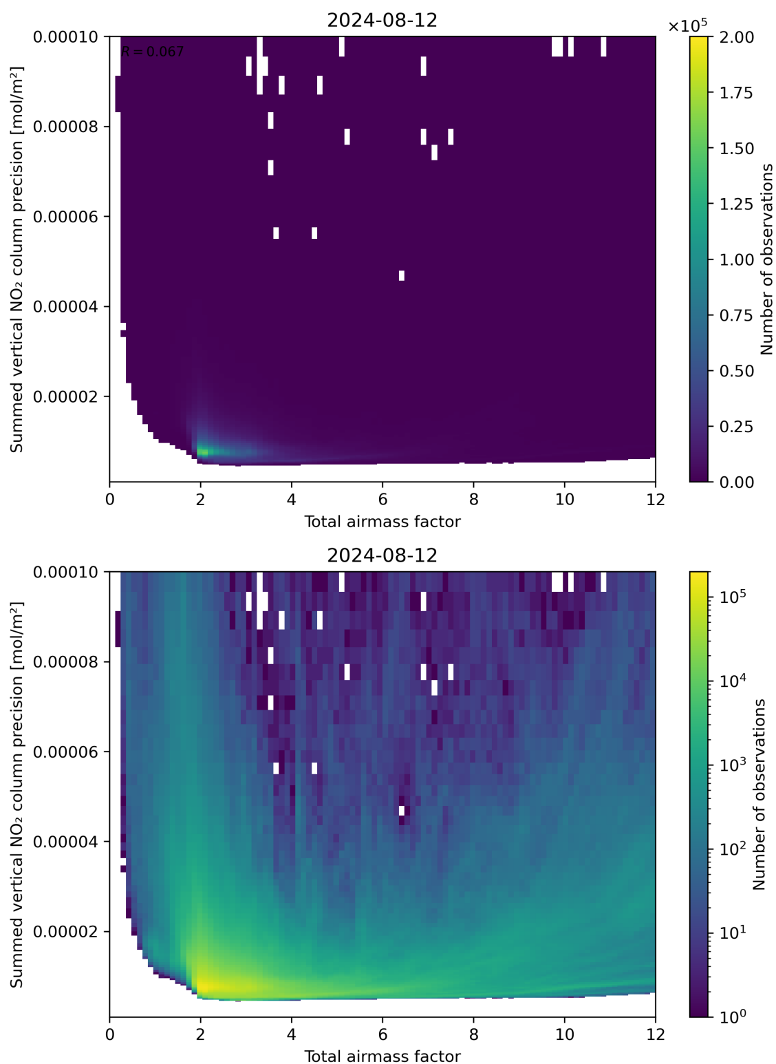
Figure 66: Scatter density plot of “Total airmass factor” against “Summed vertical NO 2 column precision” for 2024-08-12 to 2024-08-13.
