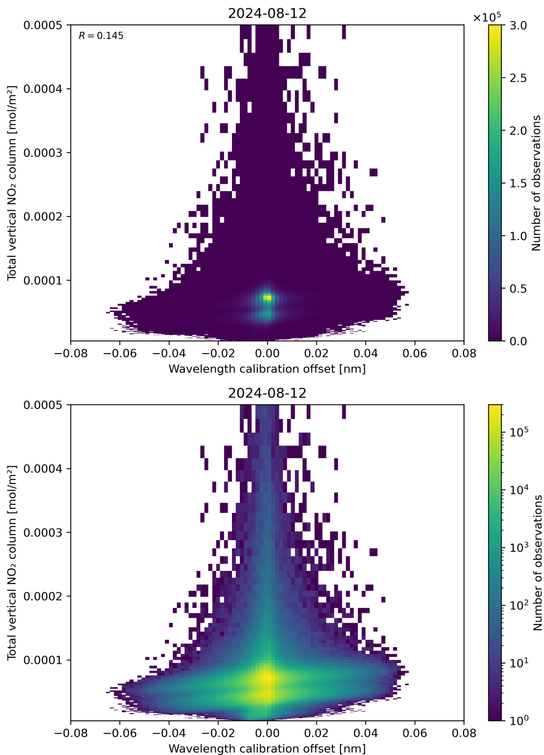
Figure 179: Scatter density plot of “Wavelength calibration offset” against “Total vertical NO 2 column” for 2024-08-12 to 2024-08-13.
