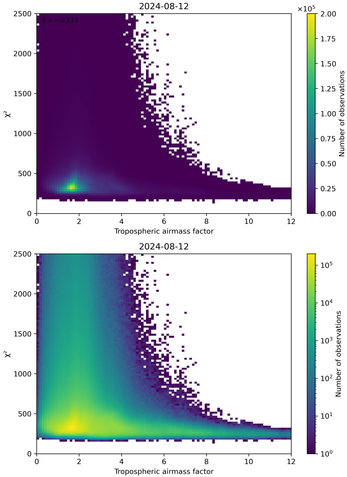
Figure 73: Scatter density plot of “Tropospheric airmass factor” against “ \chi^2 ” for 2024-08-12 to 2024-08-13.
