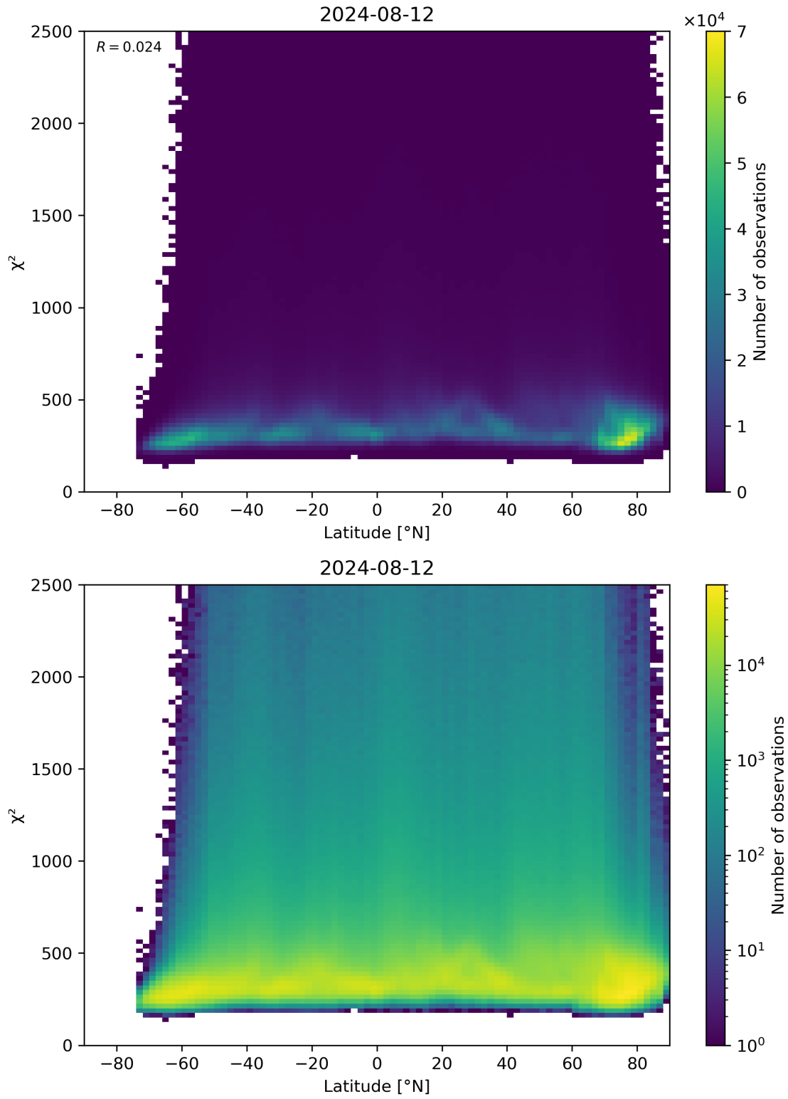
Figure 86: Scatter density plot of “Latitude” against “ \chi^2 ” for 2024-08-12 to 2024-08-13.
