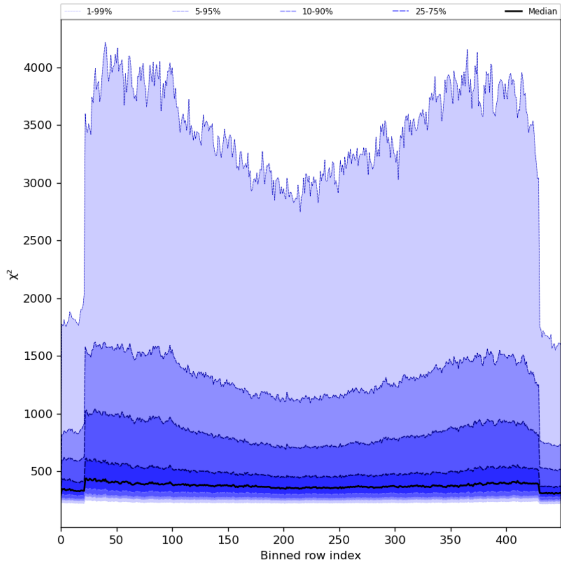
Figure 59: Along track statistics of “ \chi^2 ” for 2024-08-12 to 2024-08-13
