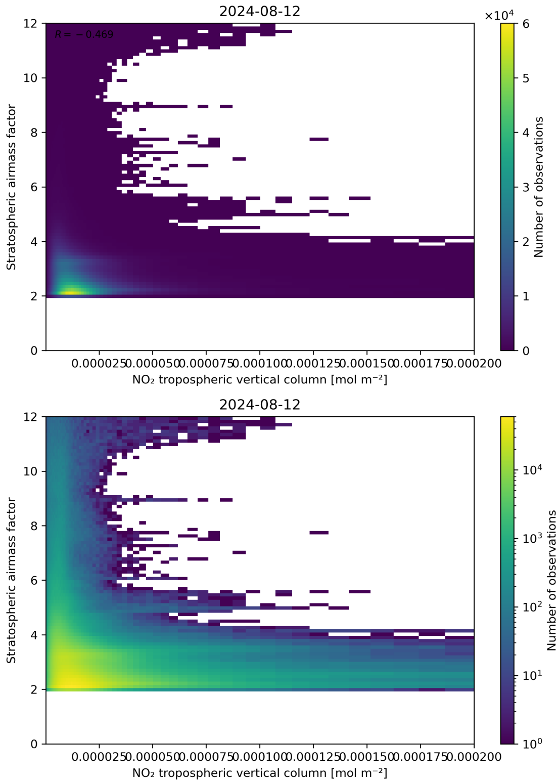
Figure 121: Scatter density plot of “NO 2 tropospheric vertical column” against “Stratospheric airmass factor” for 2024-08-12 to 2024-08-13.
