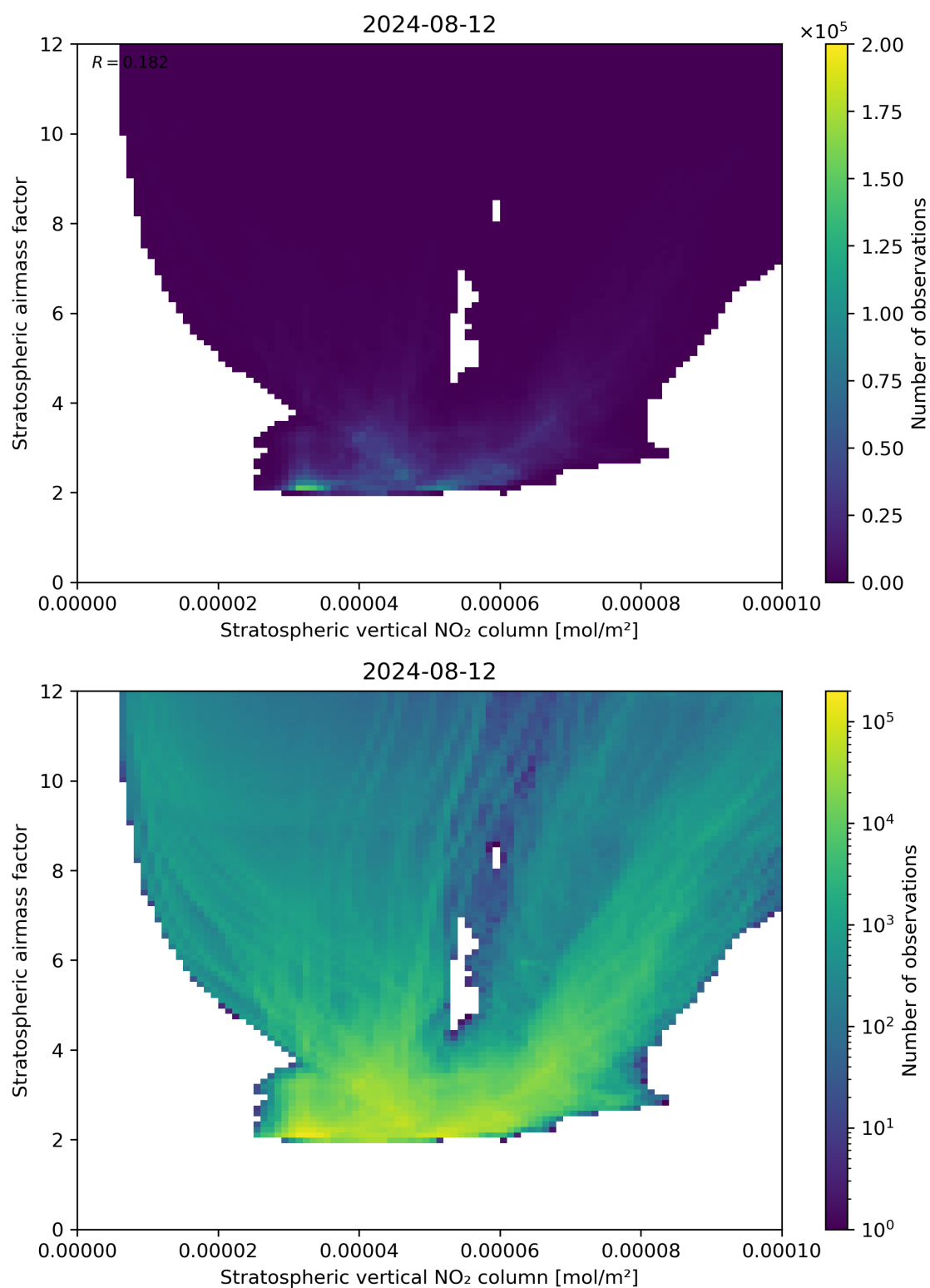
Figure 96: Scatter density plot of “Stratospheric vertical NO 2 column” against “Stratospheric airmass factor” for 2024-08-12 to 2024-08-13.
