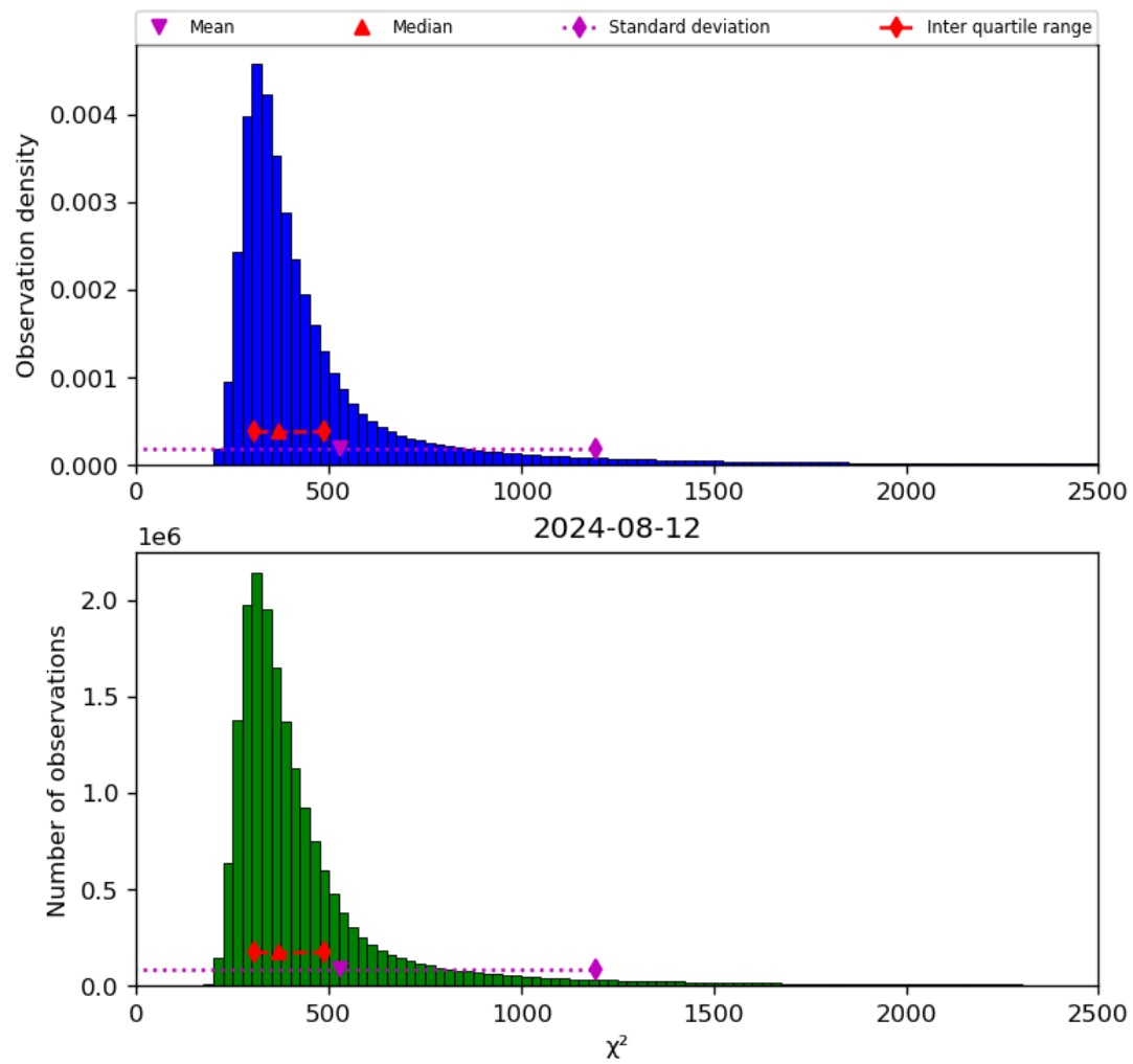
Figure 42: Histogram of “ \chi^2 ” for 2024-08-12 to 2024-08-13
