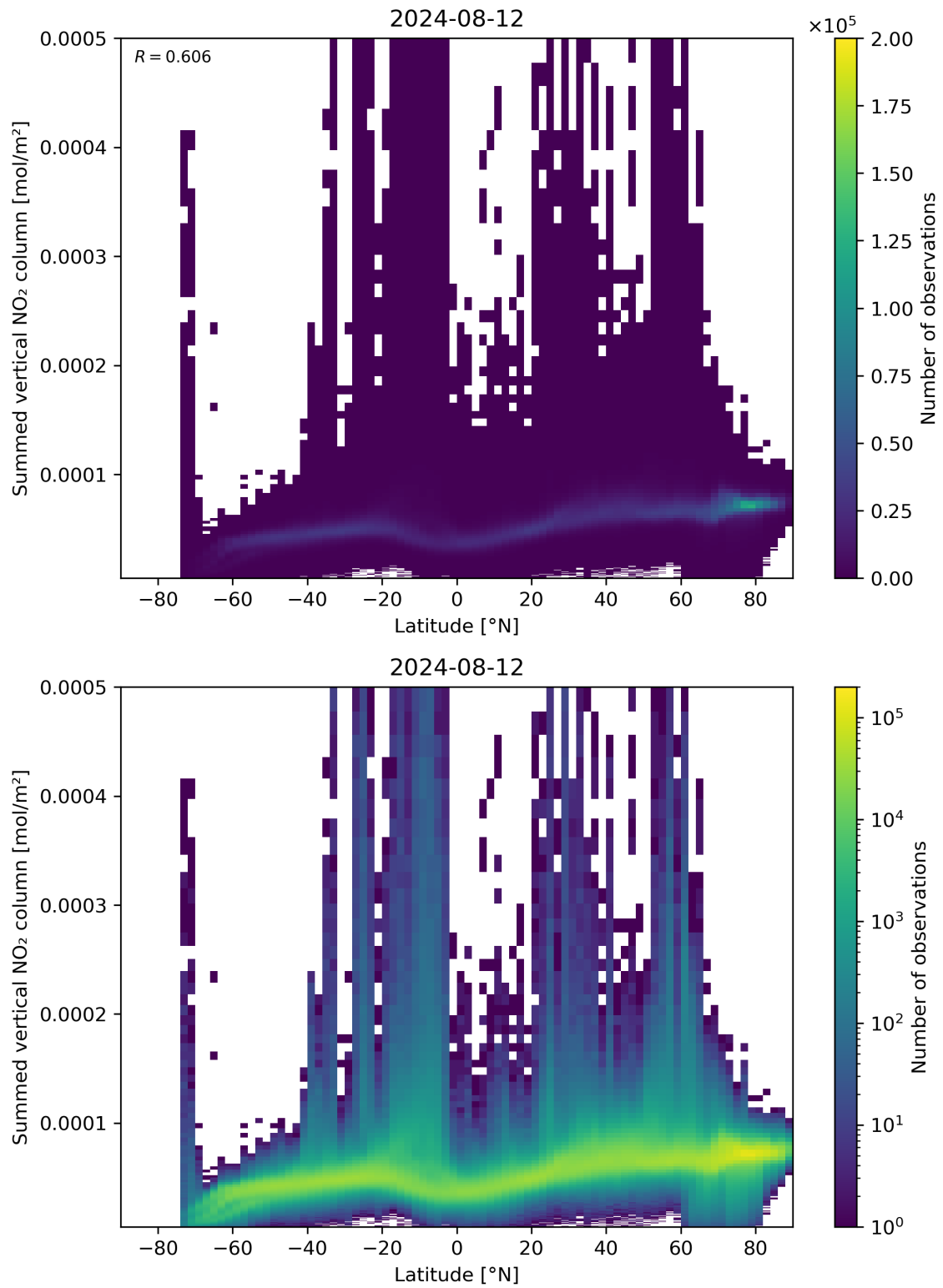
Figure 88: Scatter density plot of “Latitude” against “Summed vertical NO 2 column” for 2024-08-12 to 2024-08-13.
