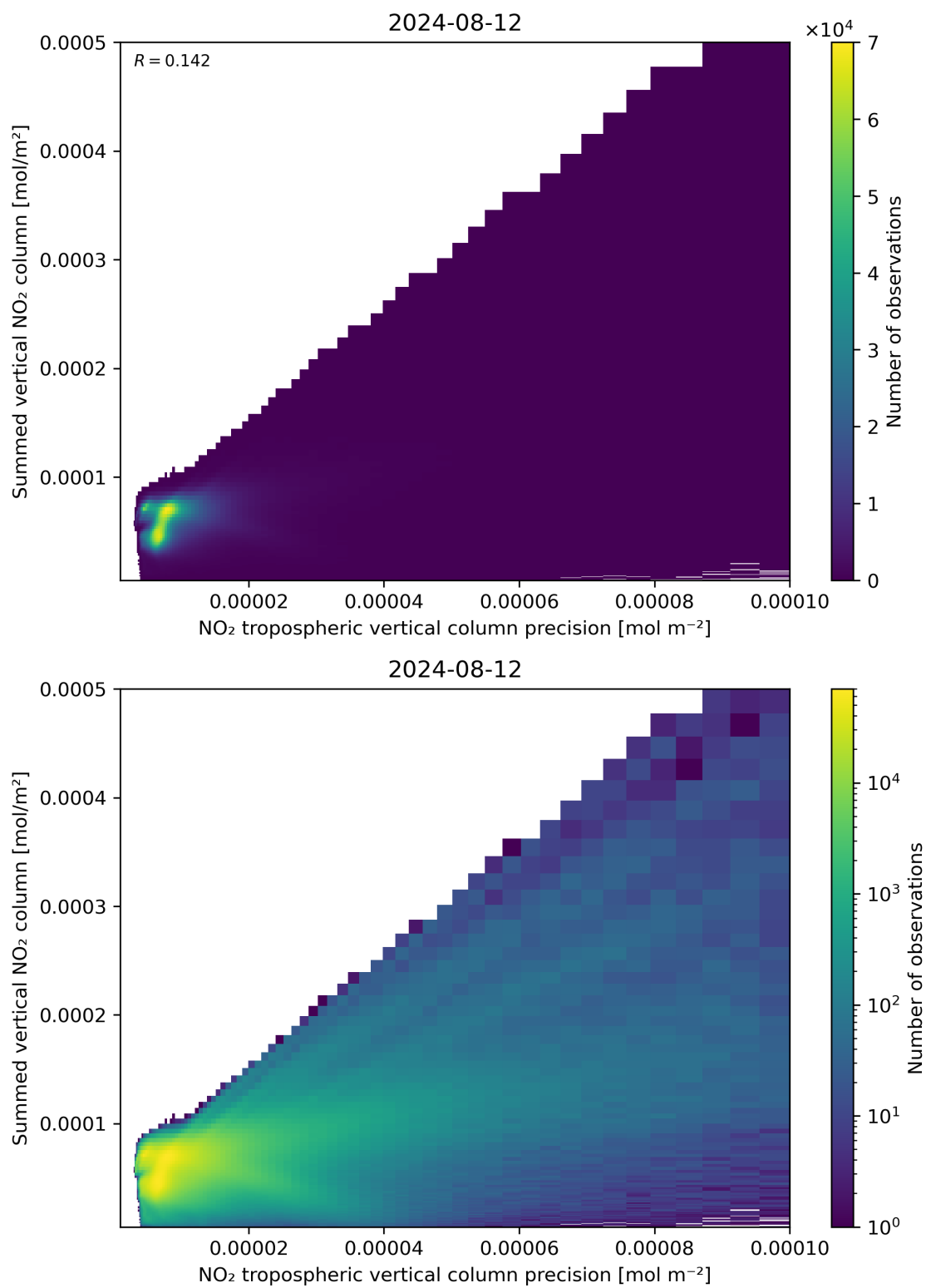
Figure 136: Scatter density plot of “NO 2 tropospheric vertical column precision” against “Summed vertical NO 2 column” for 2024-08-12 to 2024-08-13.
