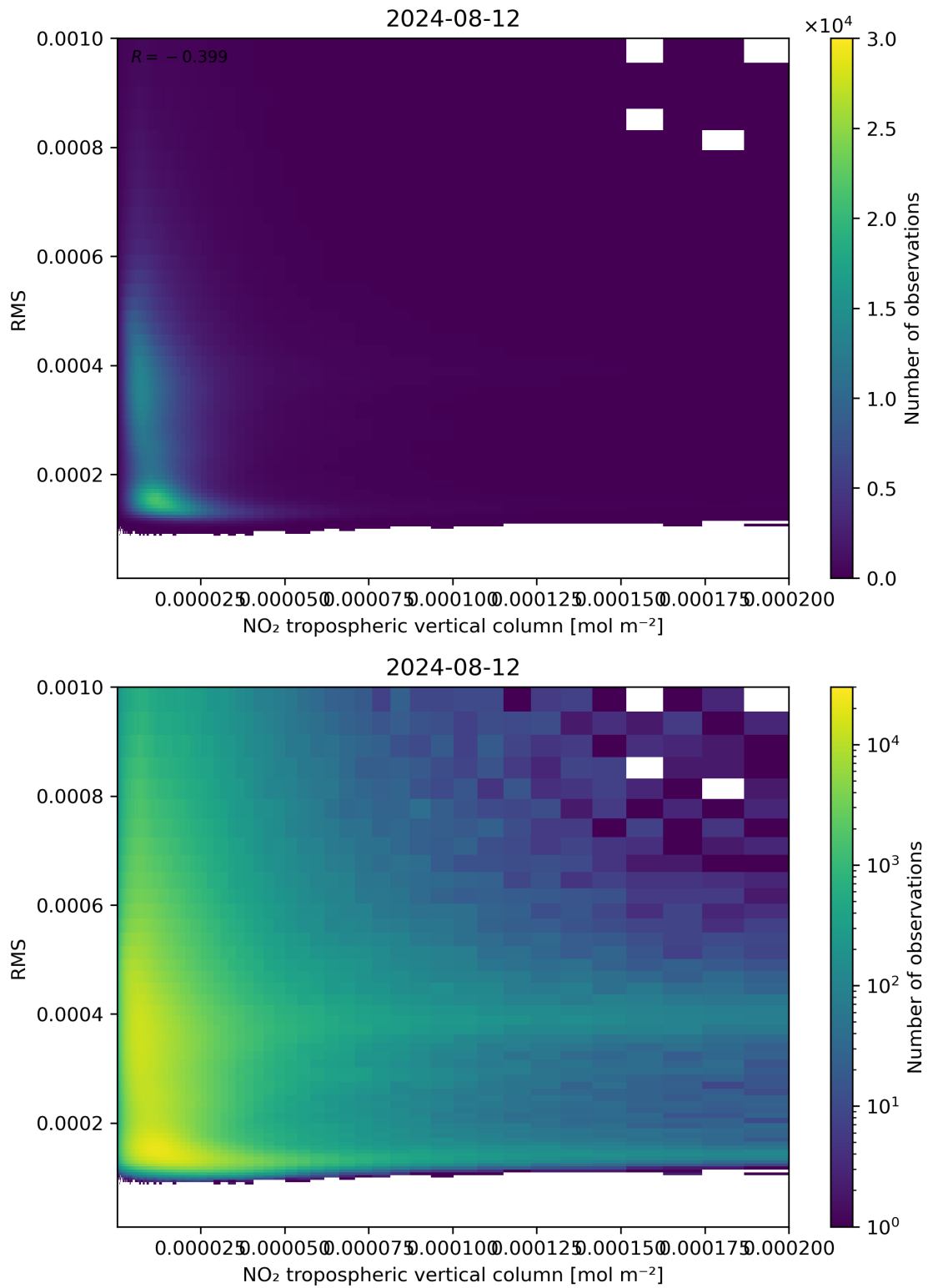
Figure 142: Scatter density plot of “NO 2 tropospheric vertical column” against “RMS” for 2024-08-12 to 2024-08-13.
