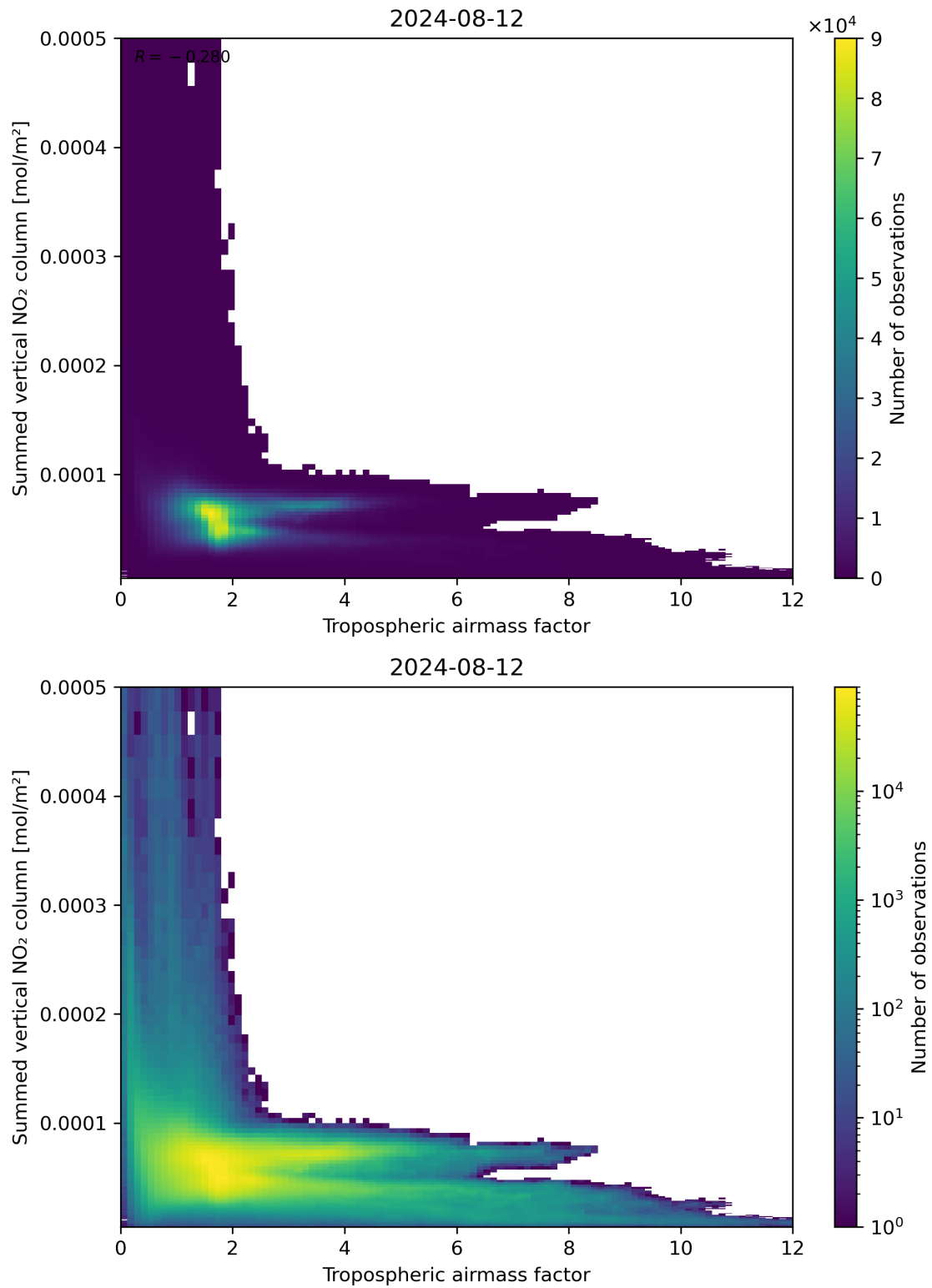
Figure 75: Scatter density plot of “Tropospheric air mass factor” against “Summed vertical NO 2 column” for 2024-08-12 to 2024-08-13.
