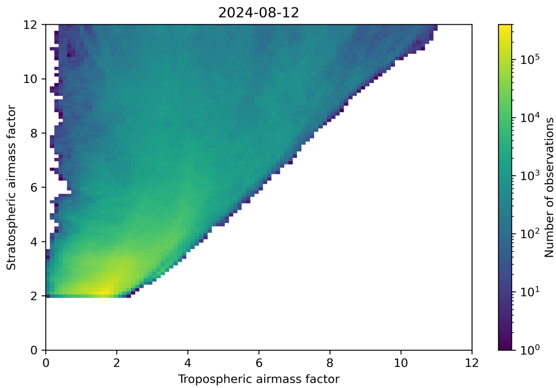
Figure 71: Scatter density plot of “Tropospheric airmass factor” against “Stratospheric airmass factor” for 2024-08-12 to 2024-08-13.
