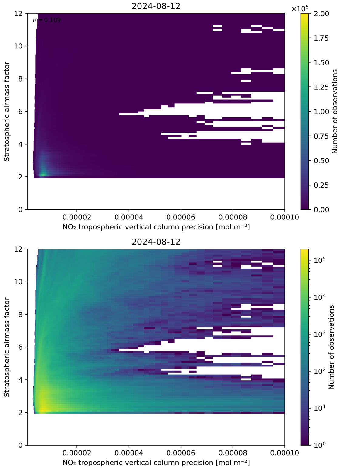
Figure 131: Scatter density plot of “NO 2 tropospheric vertical column precision” against “Stratospheric airmass factor” for 2024-08-12 to 2024-08-13.
