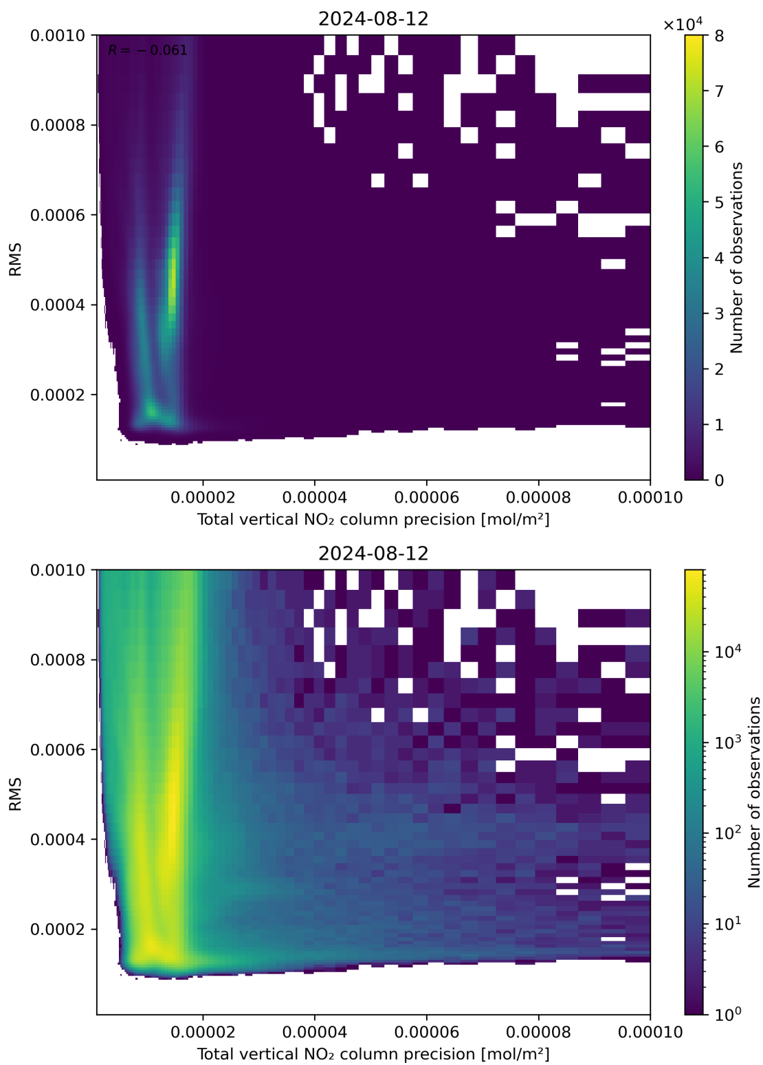
Figure 119: Scatter density plot of “Total vertical NO 2 column precision” against “RMS” for 2024-08-12 to 2024-08-13.
