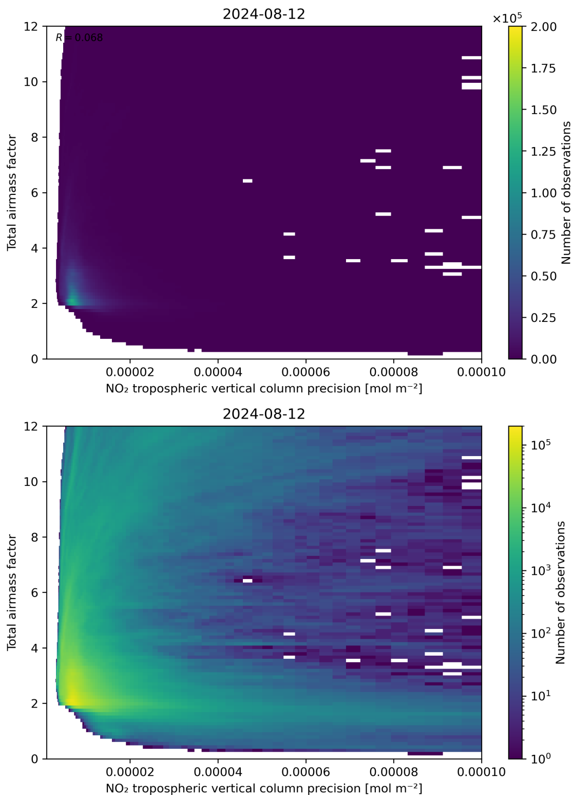
Figure 132: Scatter density plot of “NO 2 tropospheric vertical column precision” against “Total air mass factor” for 2024-08-12 to 2024-08-13.
