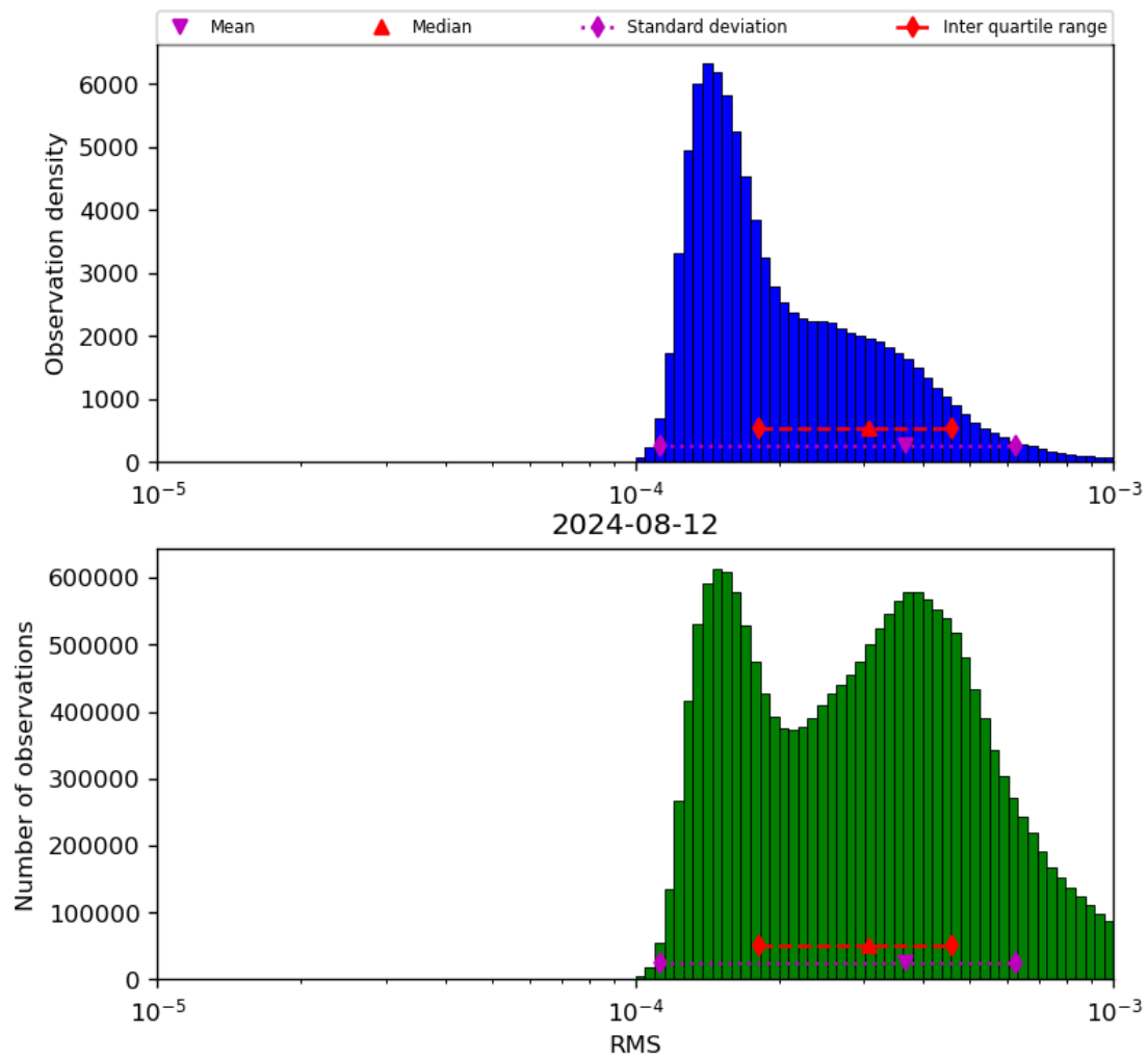
Figure 43: Histogram of “RMS” for 2024-08-12 to 2024-08-13
