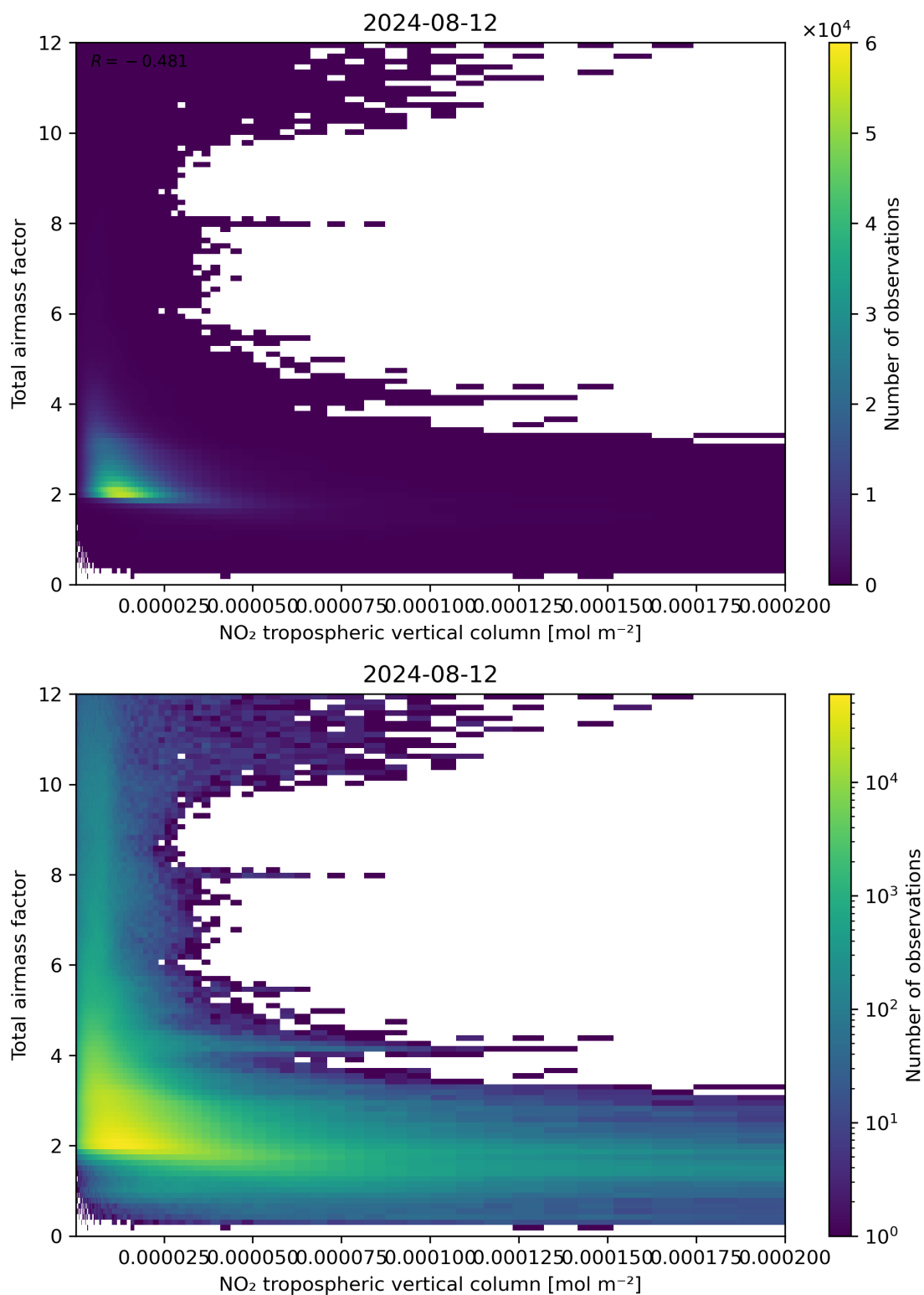
Figure 122: Scatter density plot of “NO 2 tropospheric vertical column” against “Total air mass factor” for 2024-08-12 to 2024-08-13.
