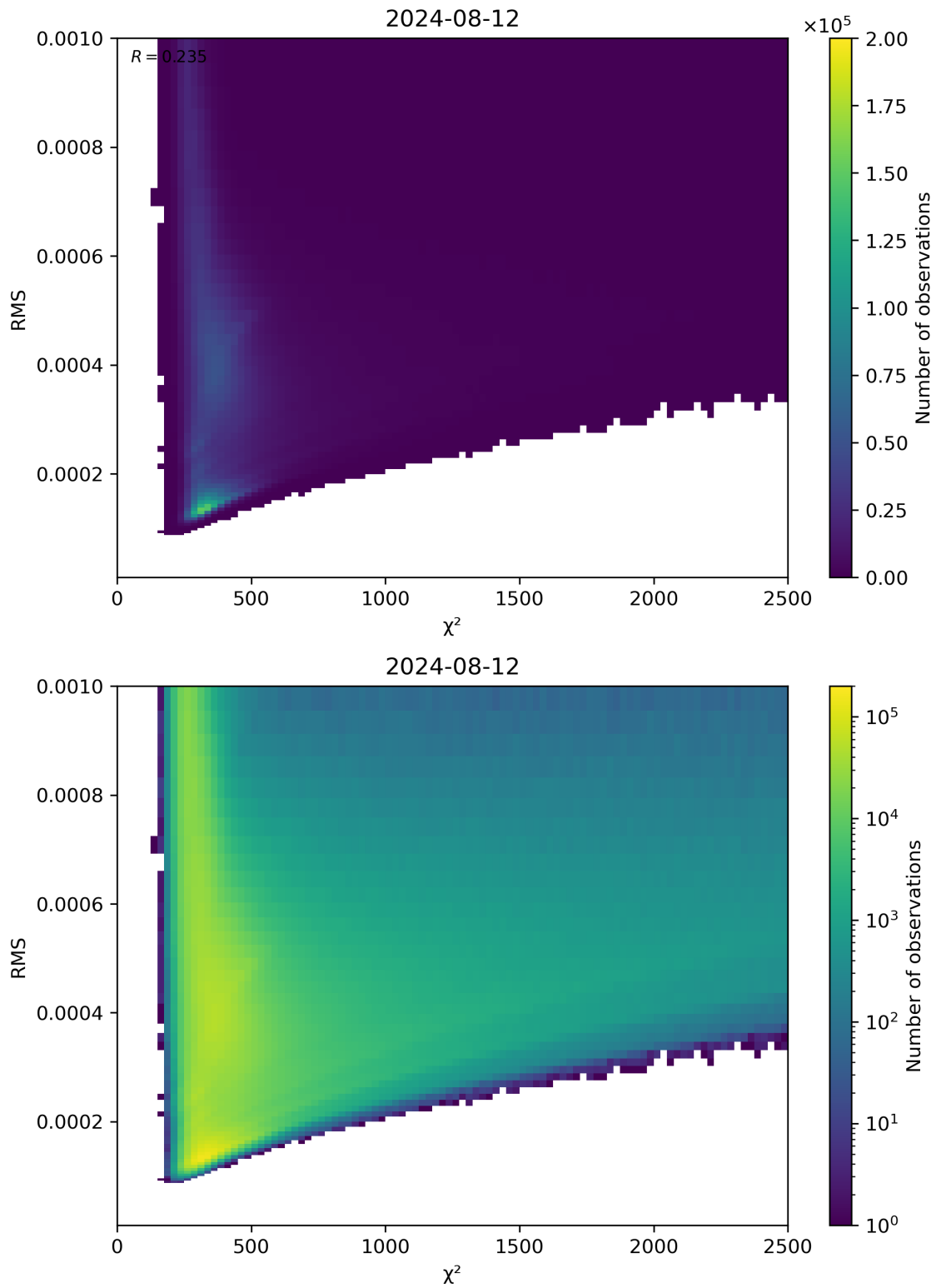
Figure 82: Scatter density plot of “ \chi^2 ” against “RMS” for 2024-08-12 to 2024-08-13.
