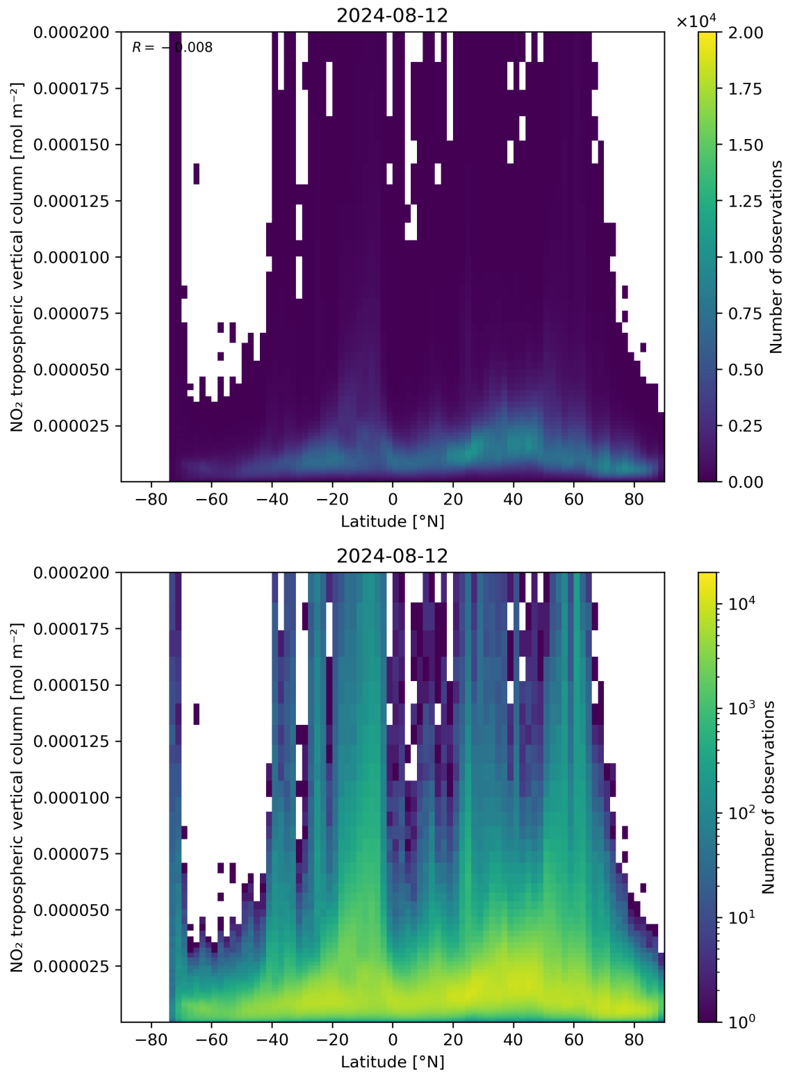
Figure 92: Scatter density plot of “Latitude” against “NO 2 tropospheric vertical column” for 2024-08-12 to 2024-08-13.
