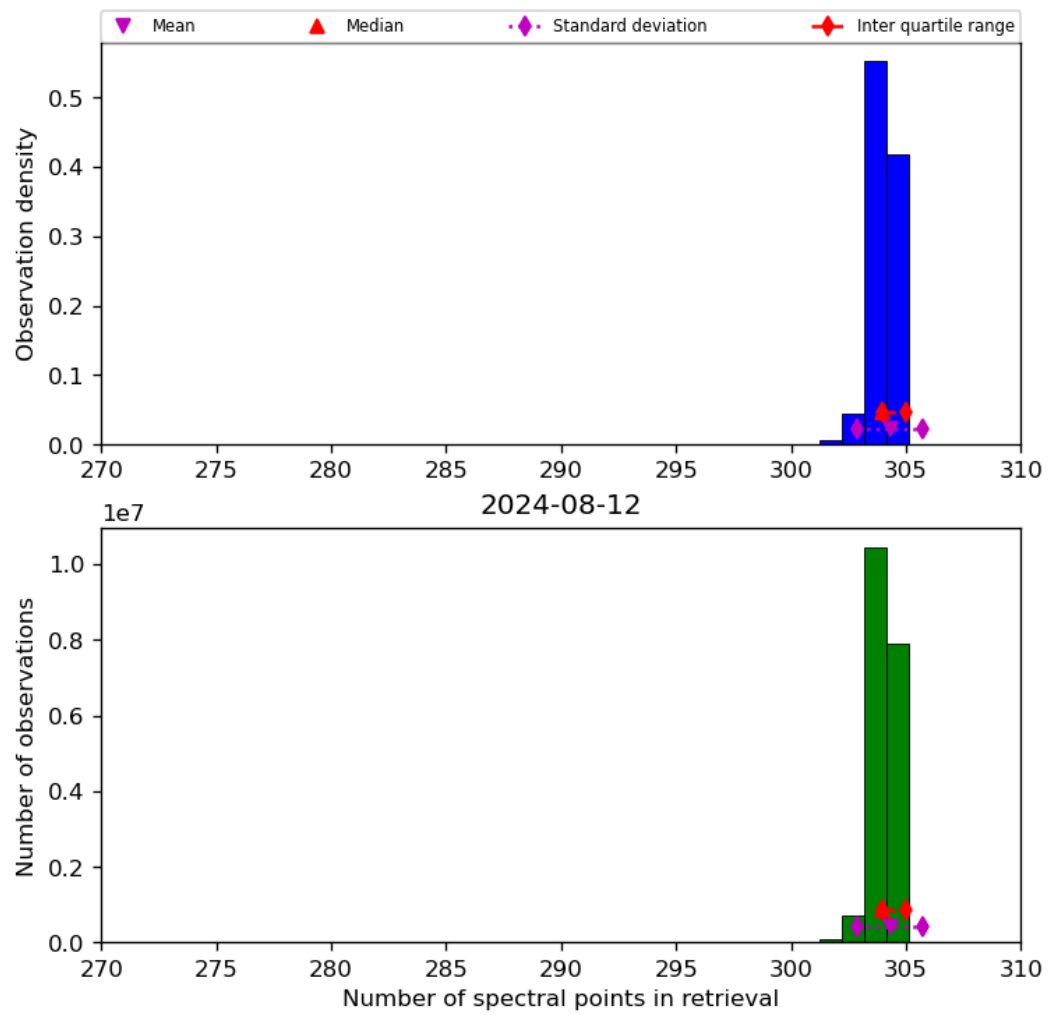
Figure 33: Histogram of “Number of spectral points in retrieval” for 2024-08-12 to 2024-08-13
