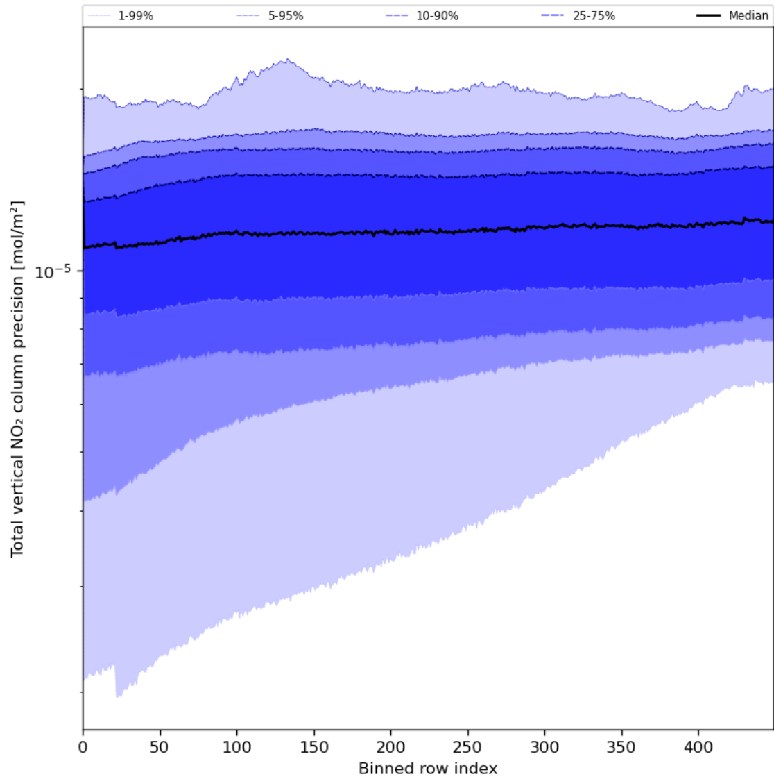
Figure 56: Along track statistics of “Total vertical NO 2 column precision” for 2024-08-12 to 2024-08-13
