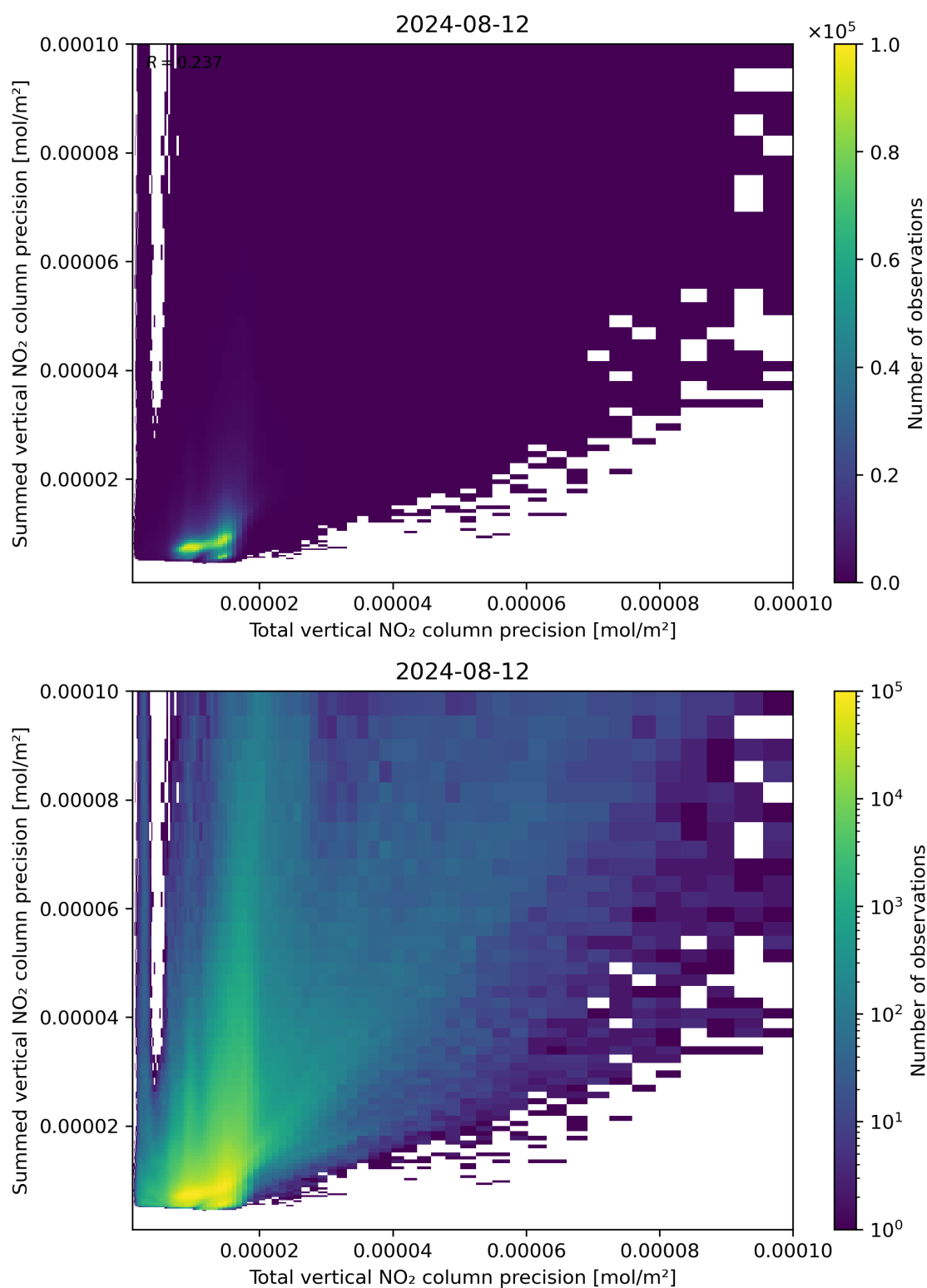
Figure 118: Scatter density plot of “Total vertical NO 2 column precision” against “Summed vertical NO 2 column precision” for 2024-08-12 to 2024-08-13.
