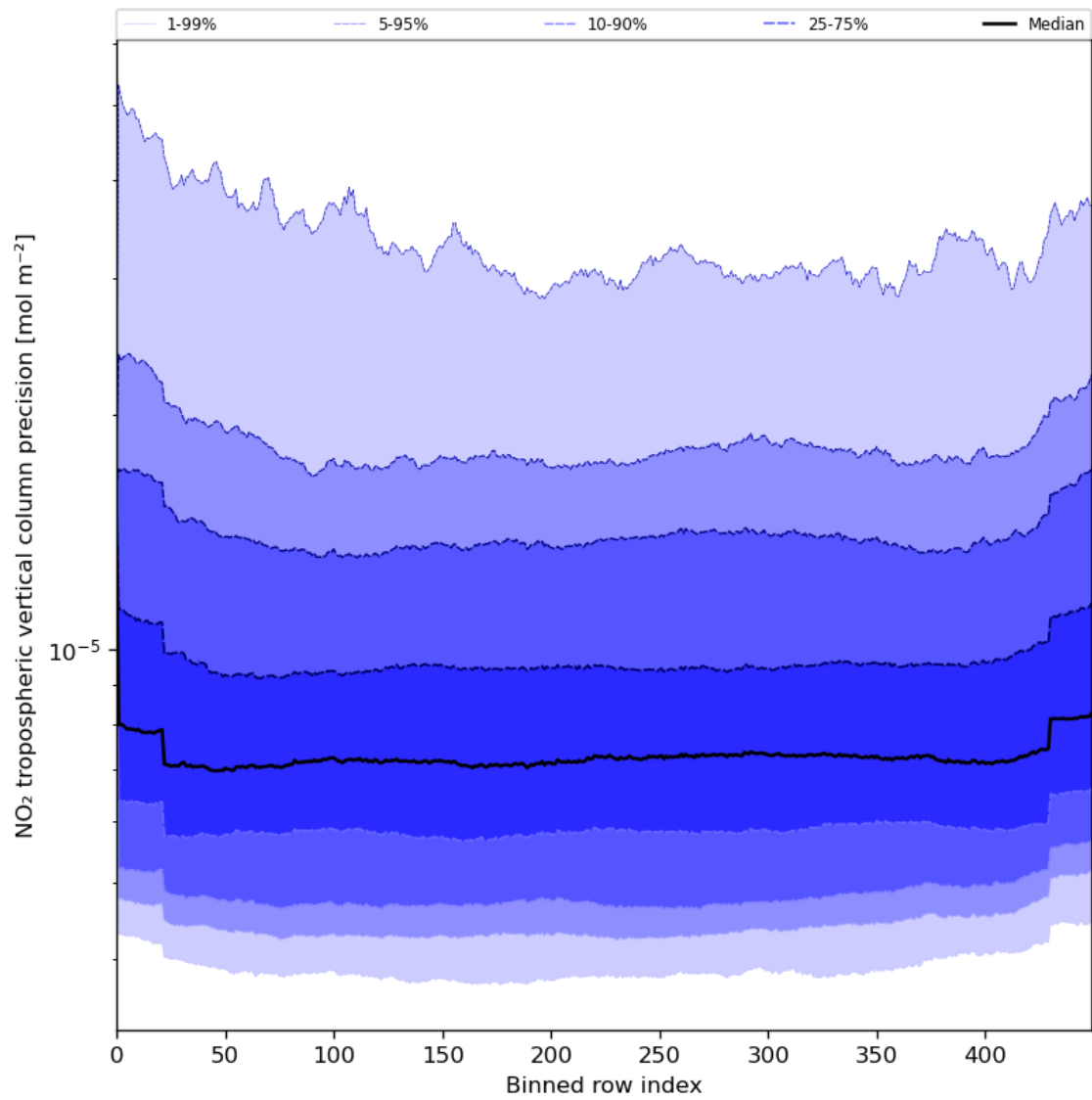
Figure 47: Along track statistics of “NO 2 tropospheric vertical column precision” for 2024-08-12 to 2024-08-13
