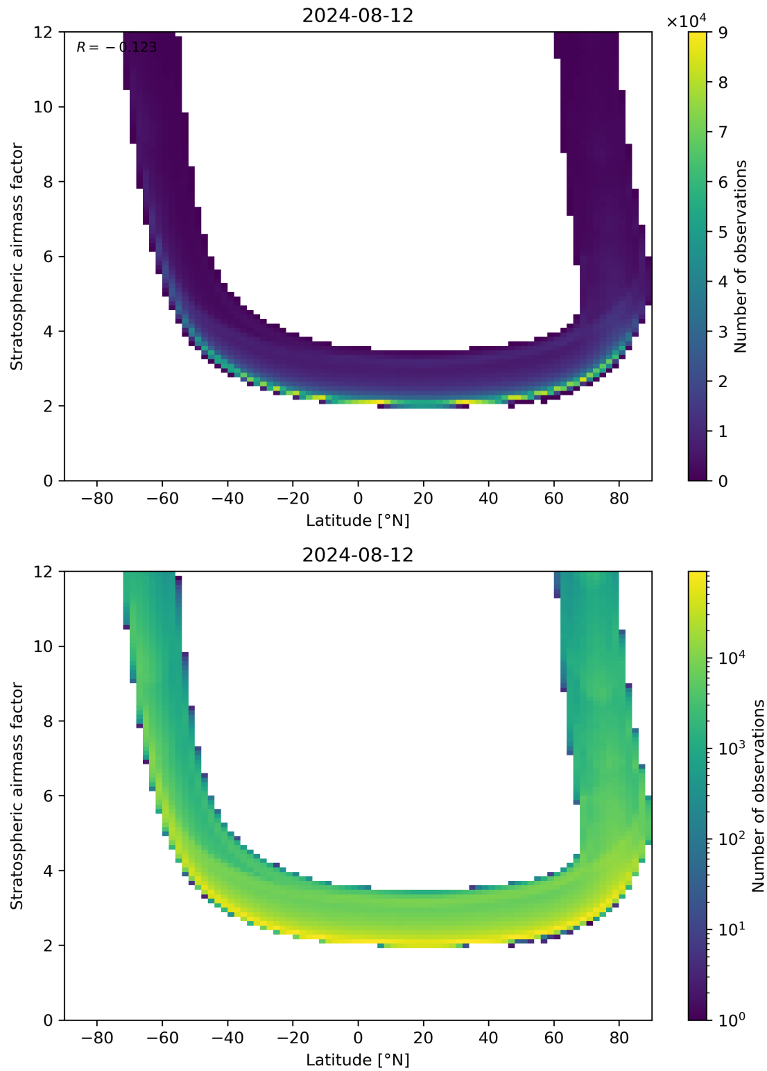
Figure 83: Scatter density plot of “Latitude” against “Stratospheric airmass factor” for 2024-08-12 to 2024-08-13.
