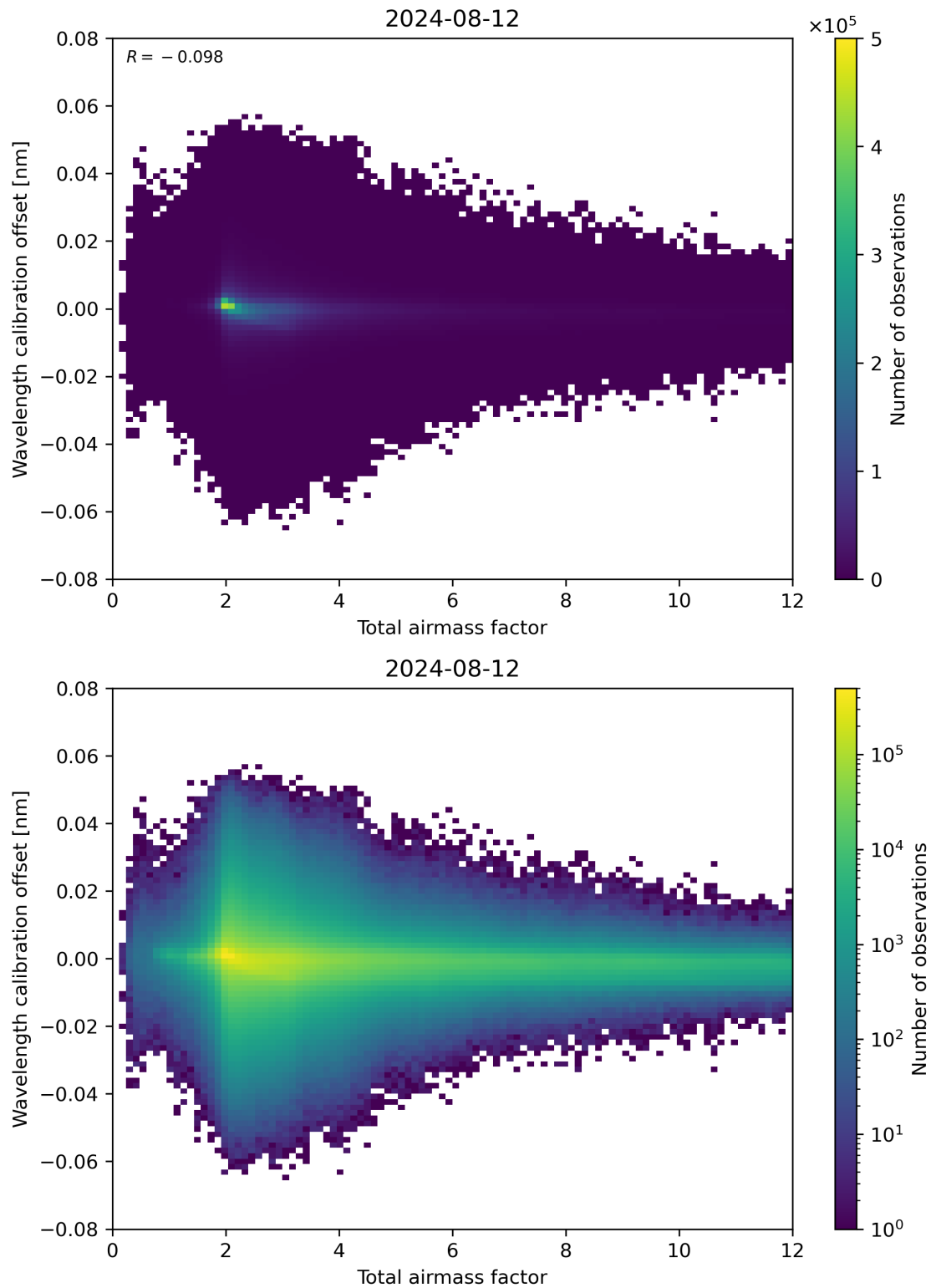
Figure 70: Scatter density plot of “Total airmass factor” against “Wavelength calibration offset” for 2024-08-12 to 2024-08-13.
