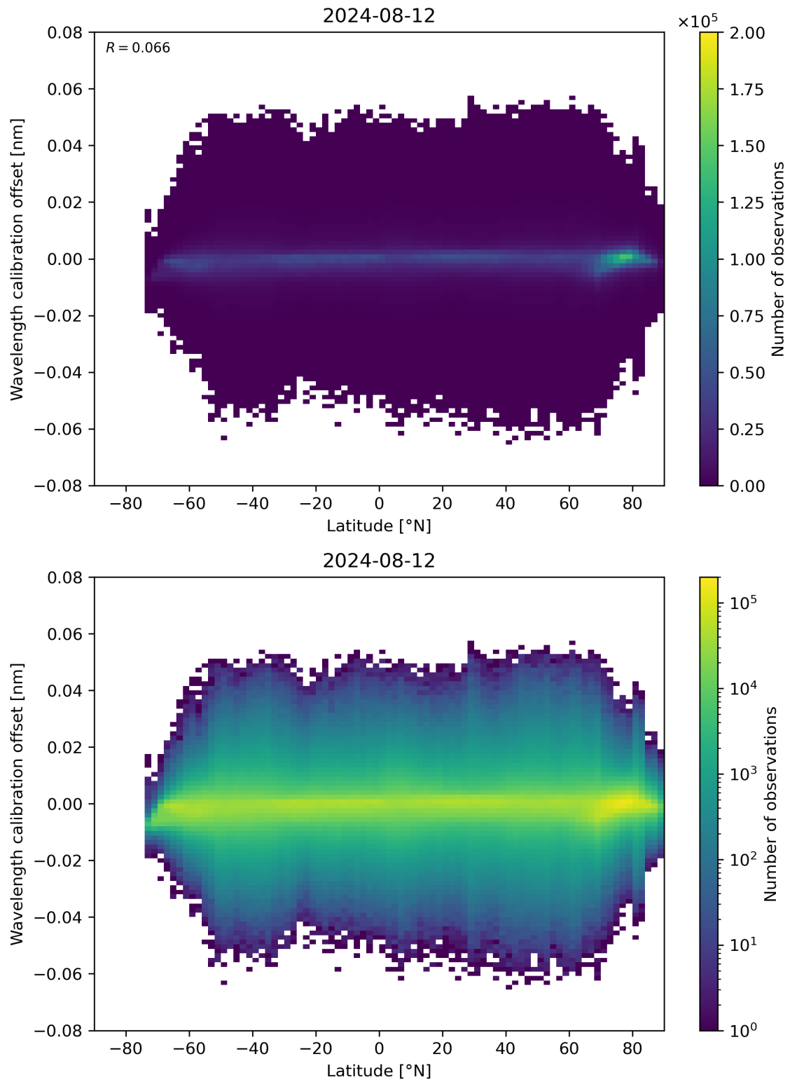
Figure 95: Scatter density plot of “Latitude” against “Wavelength calibration offset” for 2024-08-12 to 2024-08-13.
