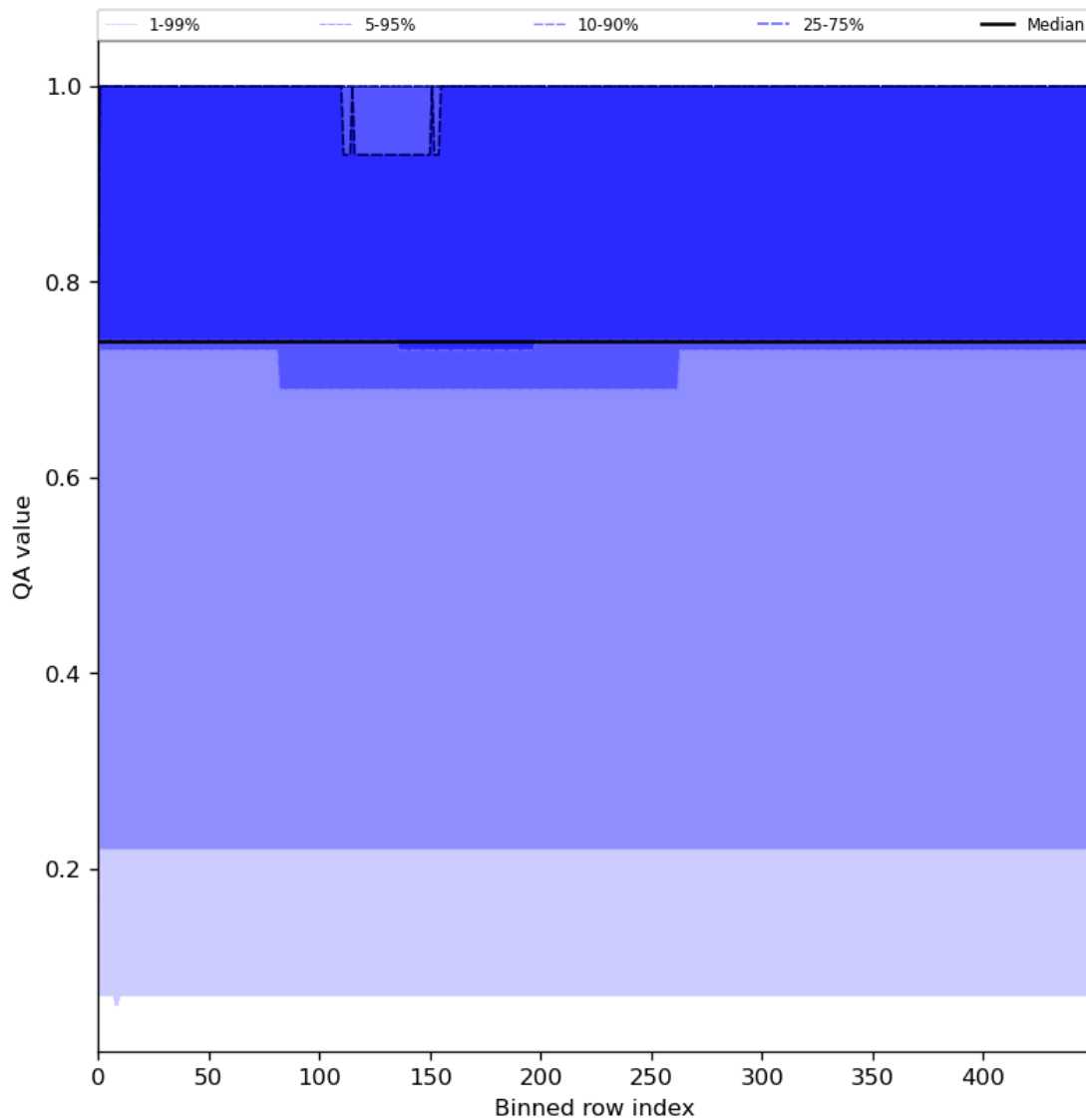
Figure 45: Along track statistics of "QA value" for 2024-08-12 to 2024-08-13
