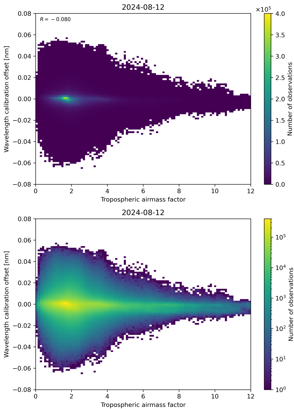
Figure 80: Scatter density plot of “Tropospheric airmass factor” against “Wavelength calibration offset” for 2024-08-12 to 2024-08-13.
