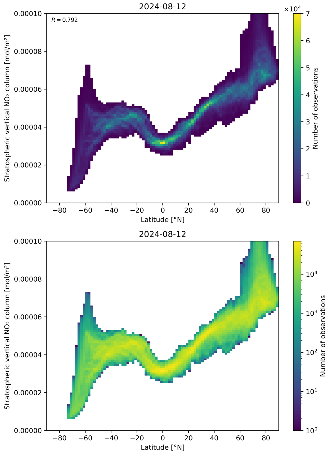
Figure 87: Scatter density plot of “Latitude” against “Stratospheric vertical NO 2 column” for 2024-08-12 to 2024-08-13.
