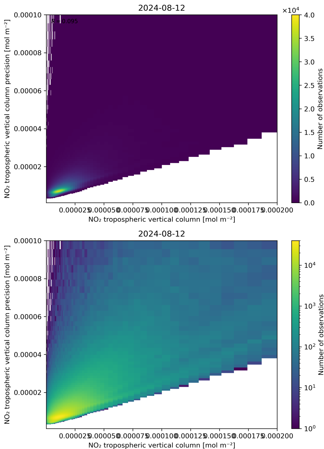
Figure 130: Scatter density plot of “NO 2 tropospheric vertical column” against “NO 2 tropospheric vertical column precision” for 2024-08-12 to 2024-08-13.
