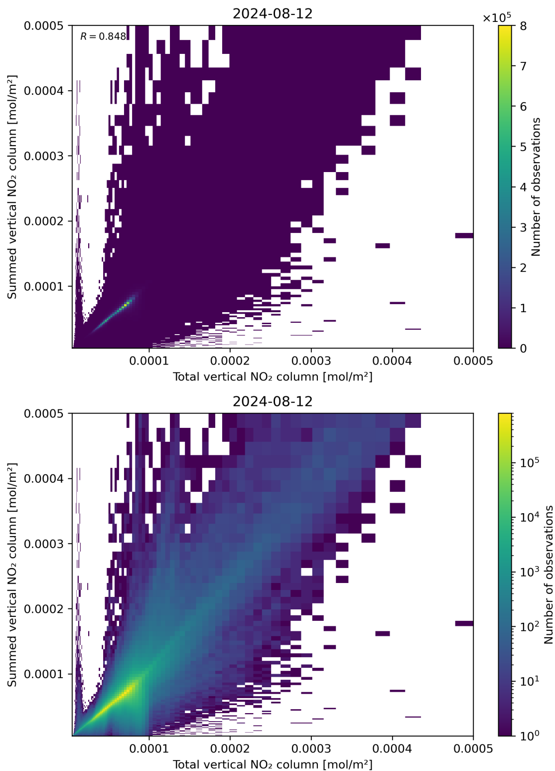
Figure 112: Scatter density plot of “Total vertical NO 2 column” against “Summed vertical NO 2 column” for 2024-08-12 to 2024-08-13.
