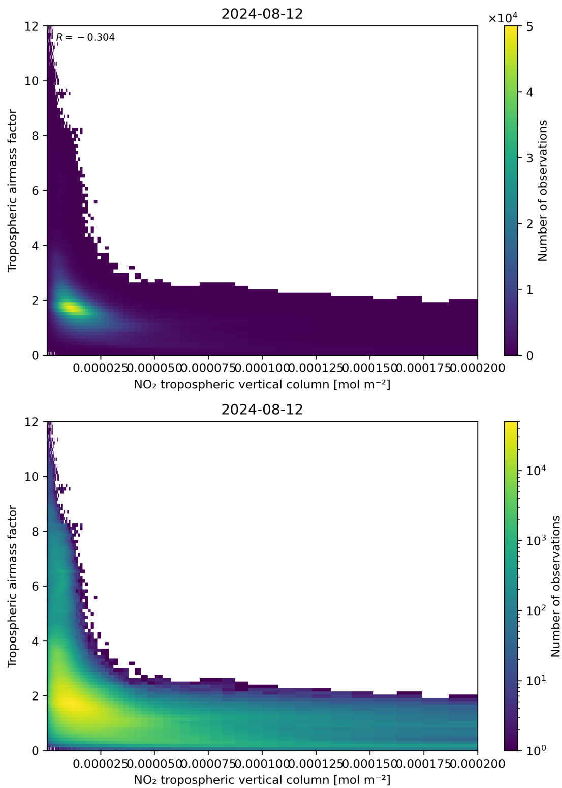
Figure 123: Scatter density plot of “NO 2 tropospheric vertical column” against “Tropospheric air mass factor” for 2024-08-12 to 2024-08-13.
