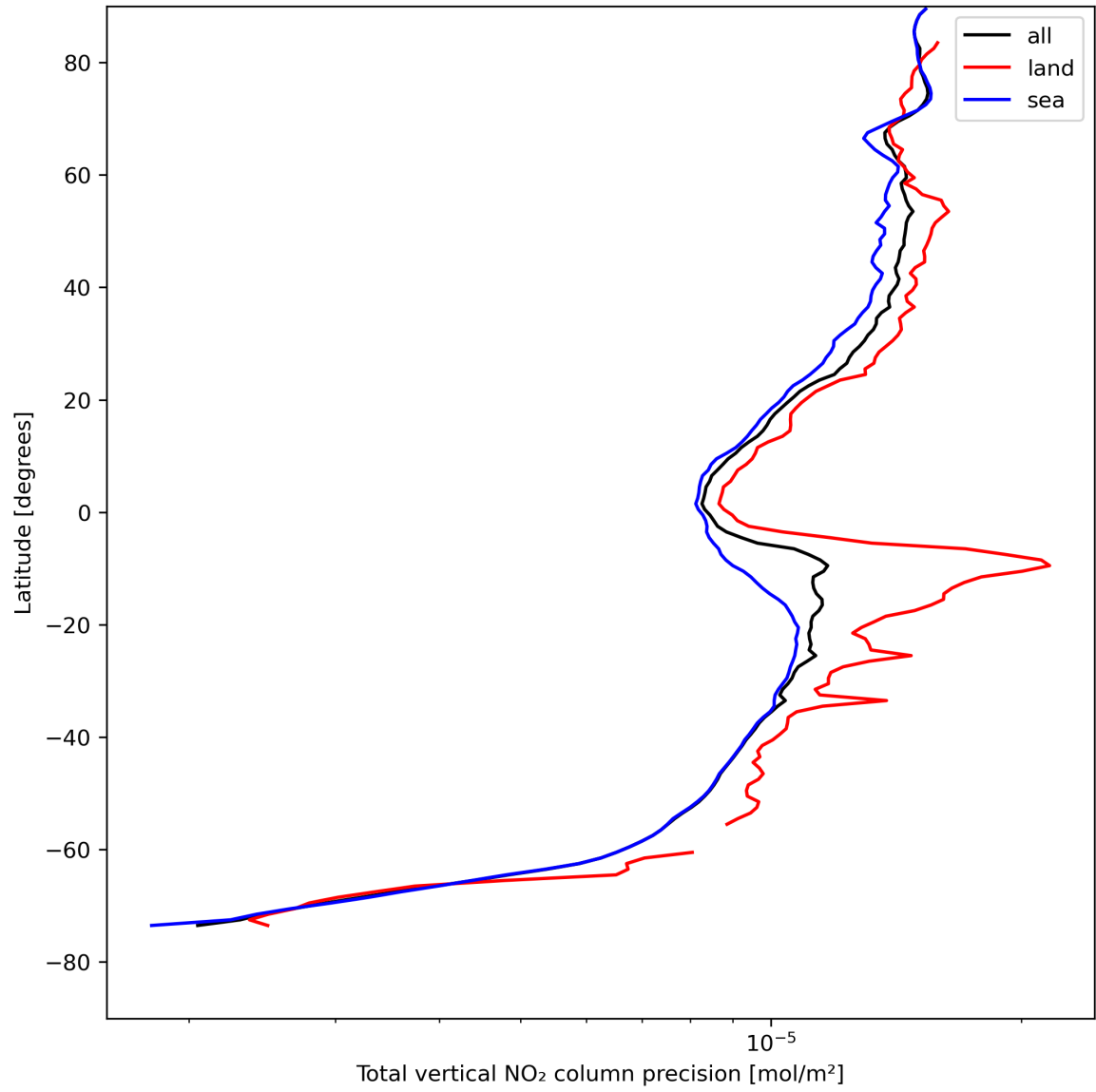
Figure 22: Zonal average of “Total vertical NO 2 column precision” for 2024-08-12 to 2024-08-13.
