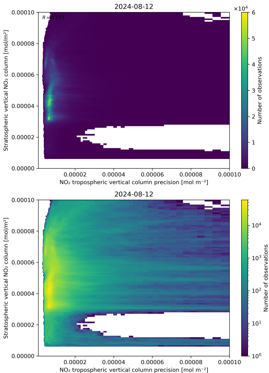
Figure 135: Scatter density plot of “NO 2 tropospheric vertical column precision” against “Stratospheric vertical NO 2 column” for 2024-08-12 to 2024-08-13.
