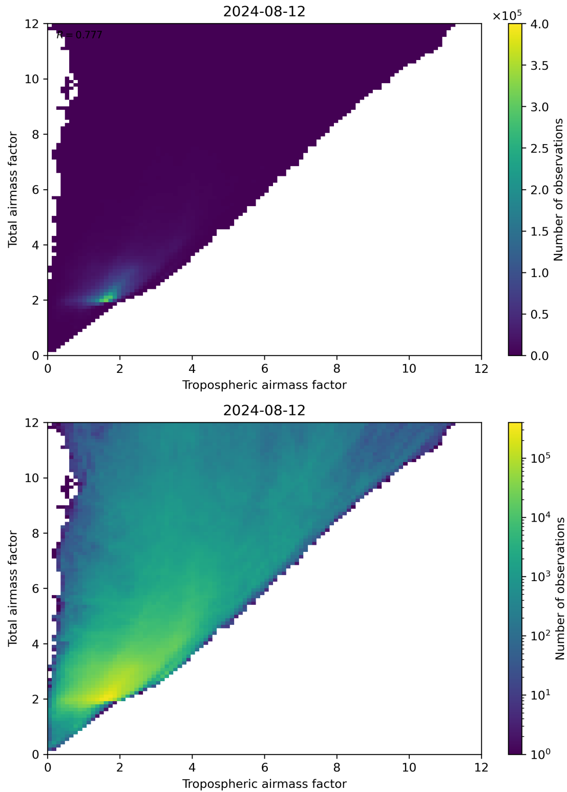
Figure 72: Scatter density plot of “Tropospheric airmass factor” against “Total airmass factor” for 2024-08-12 to 2024-08-13.
