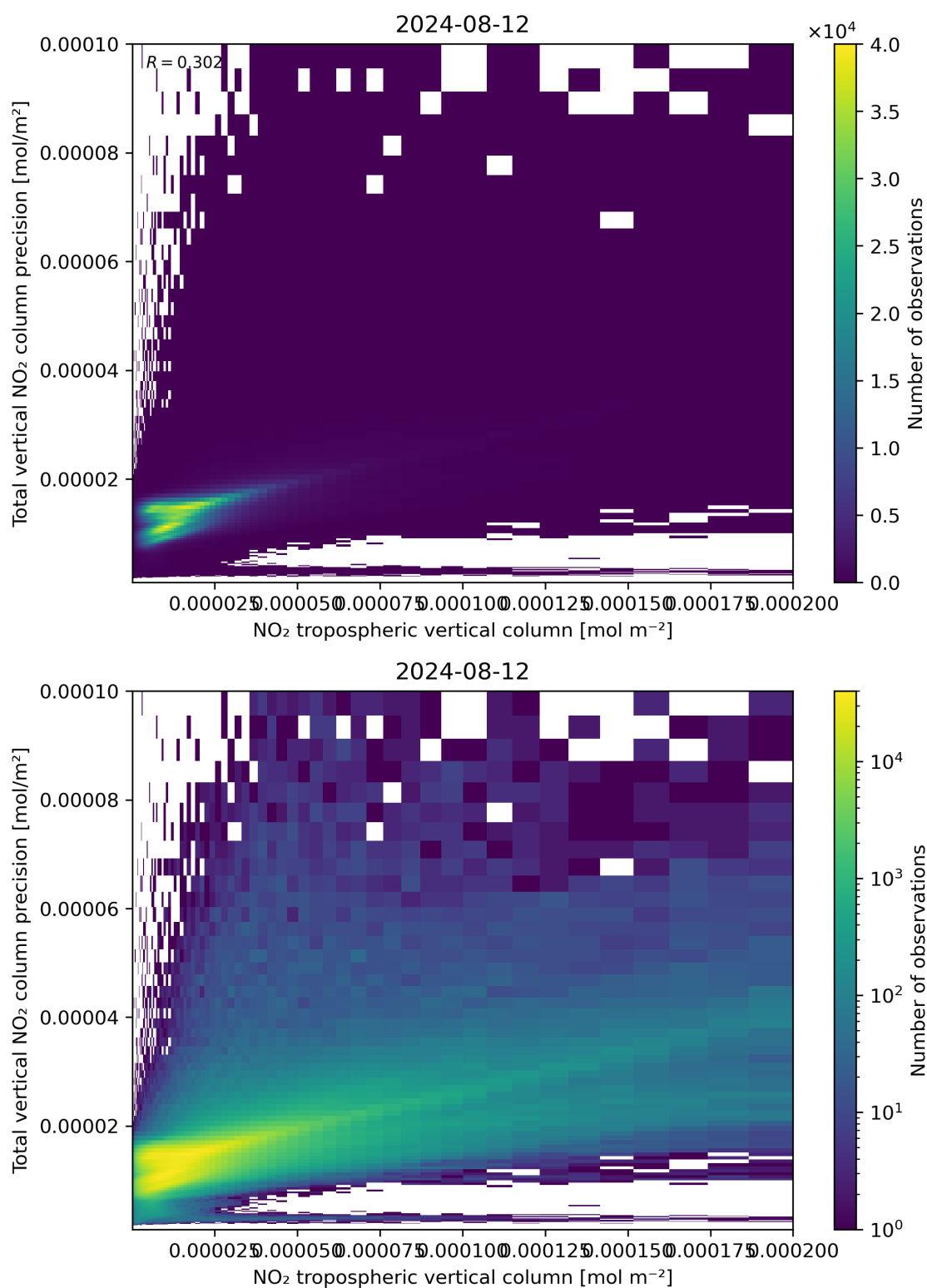
Figure 129: Scatter density plot of “NO 2 tropospheric vertical column” against “Total vertical NO 2 column precision” for 2024-08-12 to 2024-08-13.
