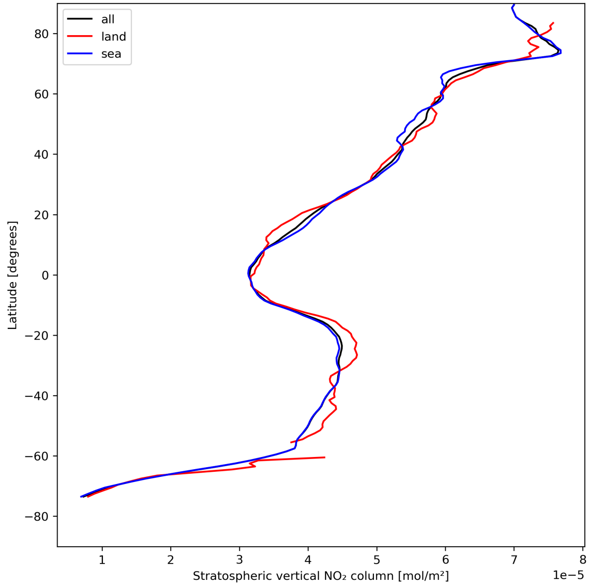
Figure 19: Zonal average of “Stratospheric vertical NO 2 column” for 2024-08-12 to 2024-08-13.
