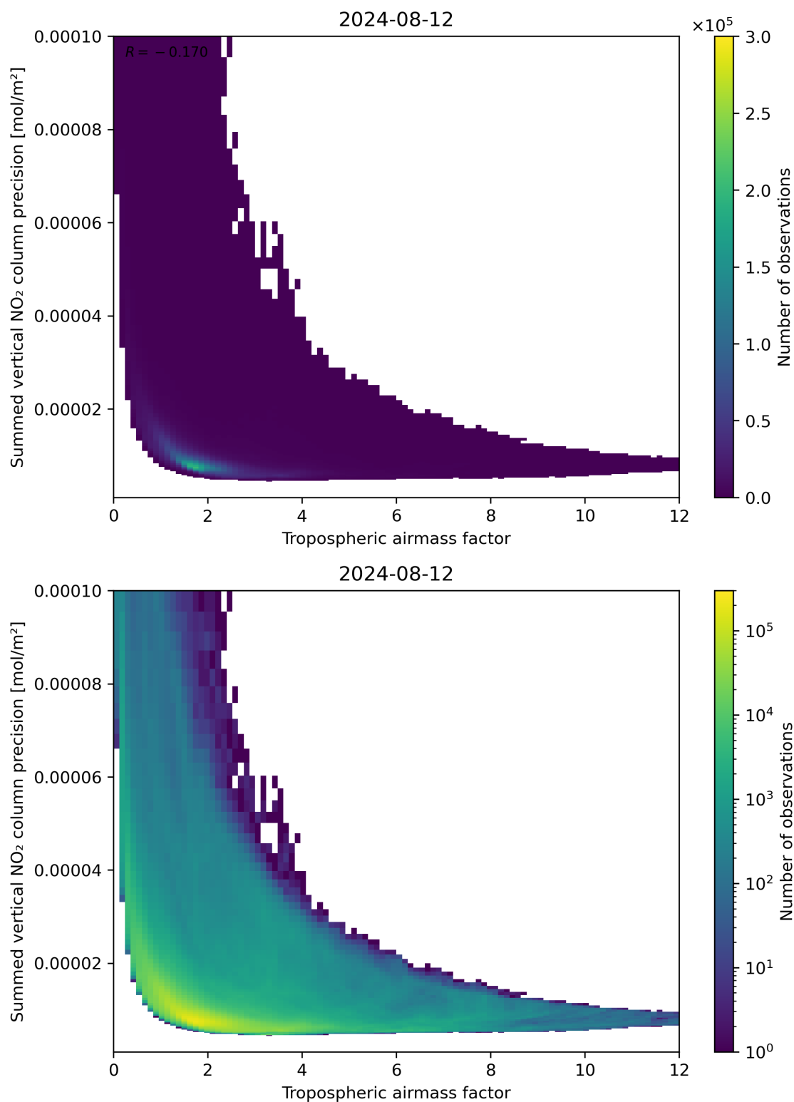
Figure 76: Scatter density plot of “Tropospheric air mass factor” against “Summed vertical NO 2 column precision” for 2024-08-12 to 2024-08-13.
