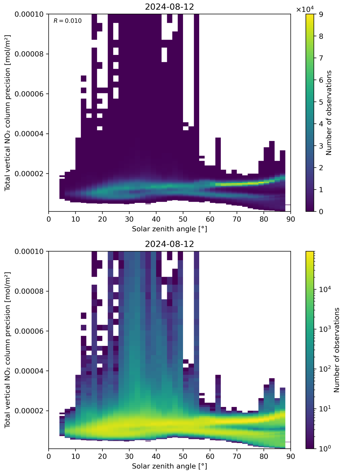
Figure 154: Scatter density plot of “Solar zenith angle” against “Total vertical NO 2 column precision” for 2024-08-12 to 2024-08-13.
