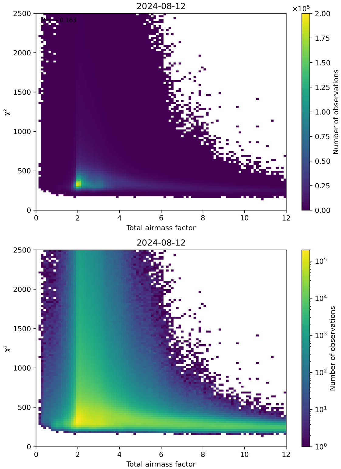
Figure 63: Scatter density plot of “Total airmass factor” against “ \chi^2 ” for 2024-08-12 to 2024-08-13.
