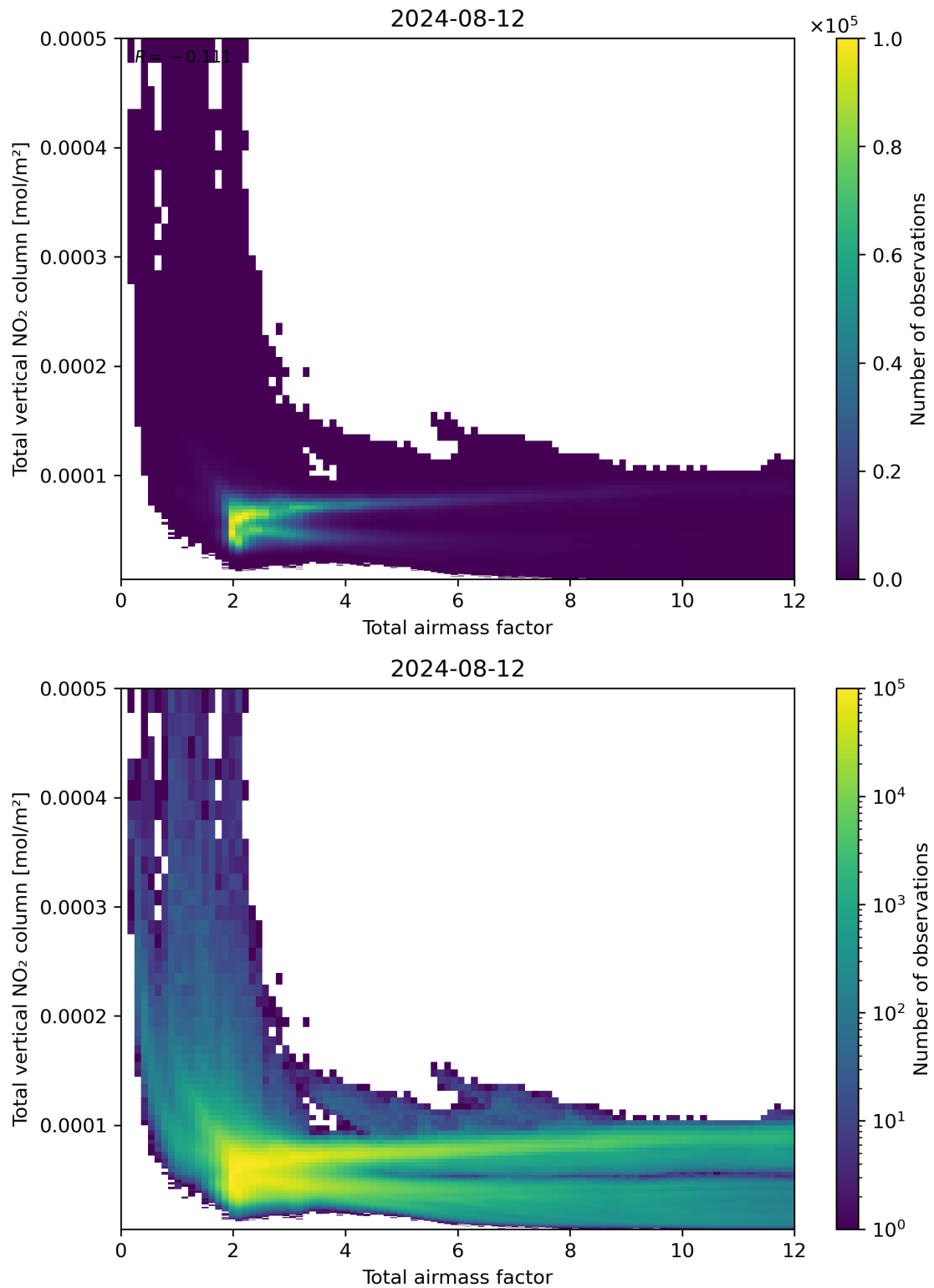
Figure 67: Scatter density plot of “Total airmass factor” against “Total vertical NO 2 column” for 2024-08-12 to 2024-08-13.
