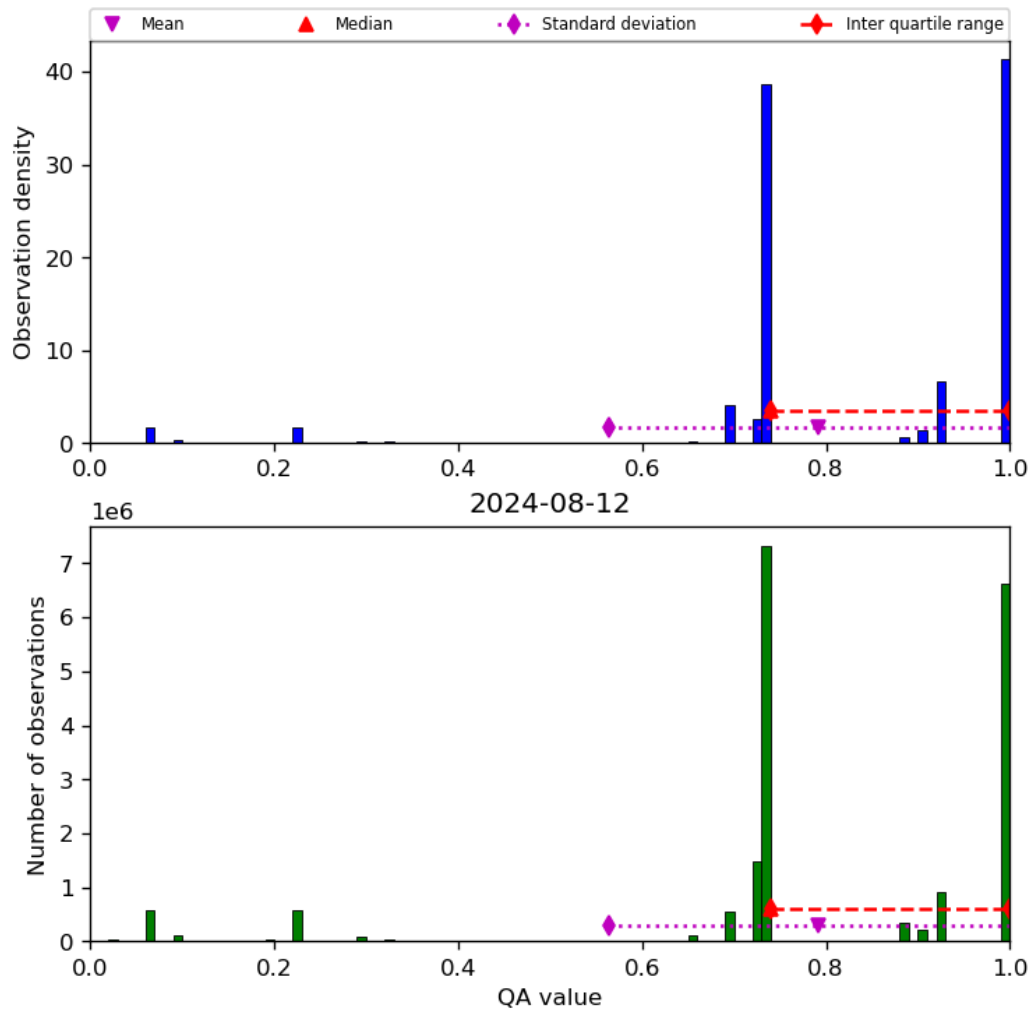
Figure 28: Histogram of “QA value” for 2024-08-12 to 2024-08-13
