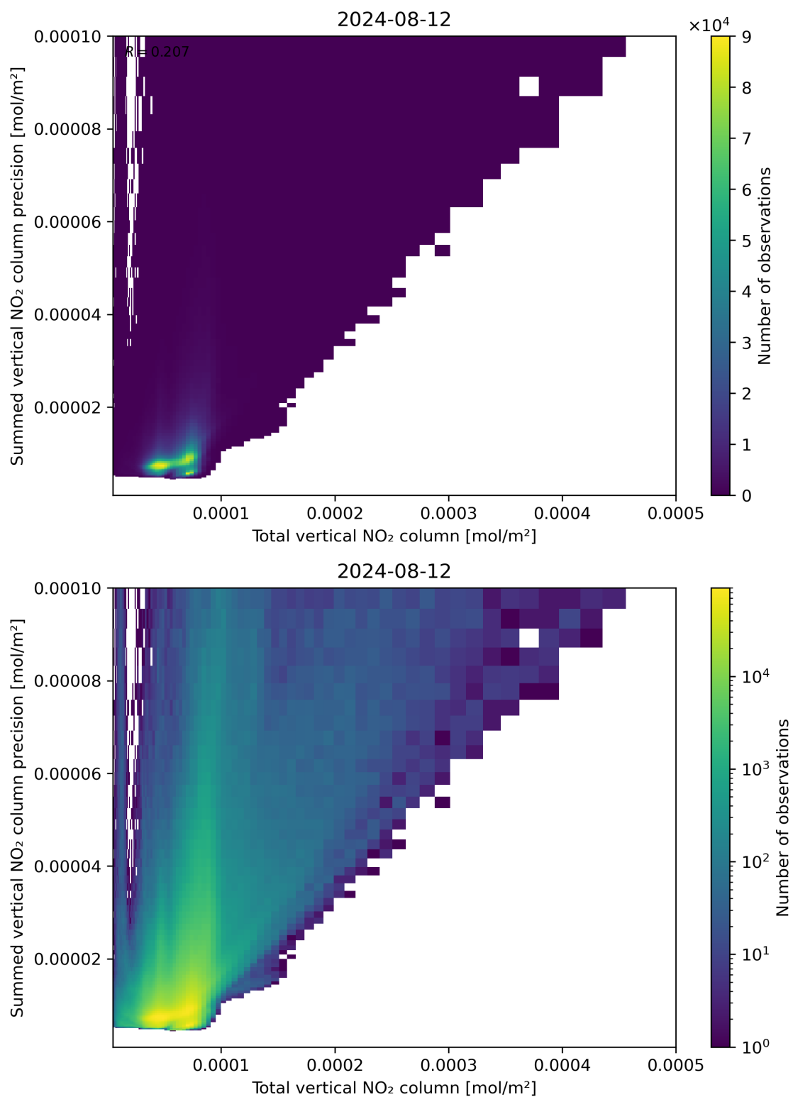
Figure 113: Scatter density plot of “Total vertical NO 2 column” against “Summed vertical NO 2 column precision” for 2024-08-12 to 2024-08-13.
