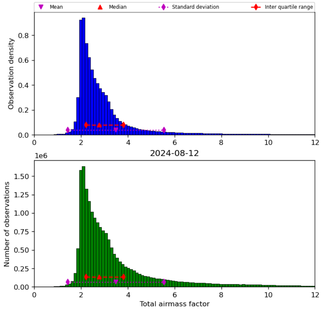
Figure 32: Histogram of “Total airmass factor” for 2024-08-12 to 2024-08-13
