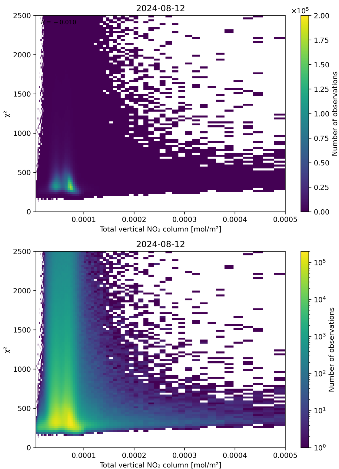
Figure 111: Scatter density plot of “Total vertical NO 2 column” against “ \chi^2 ” for 2024-08-12 to 2024-08-13.
