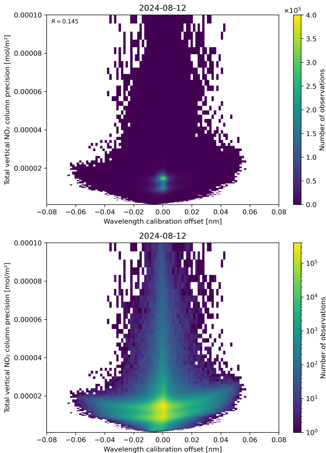
Figure 180: Scatter density plot of “Wavelength calibration offset” against “Total vertical NO 2 column precision” for 2024-08-12 to 2024-08-13.
