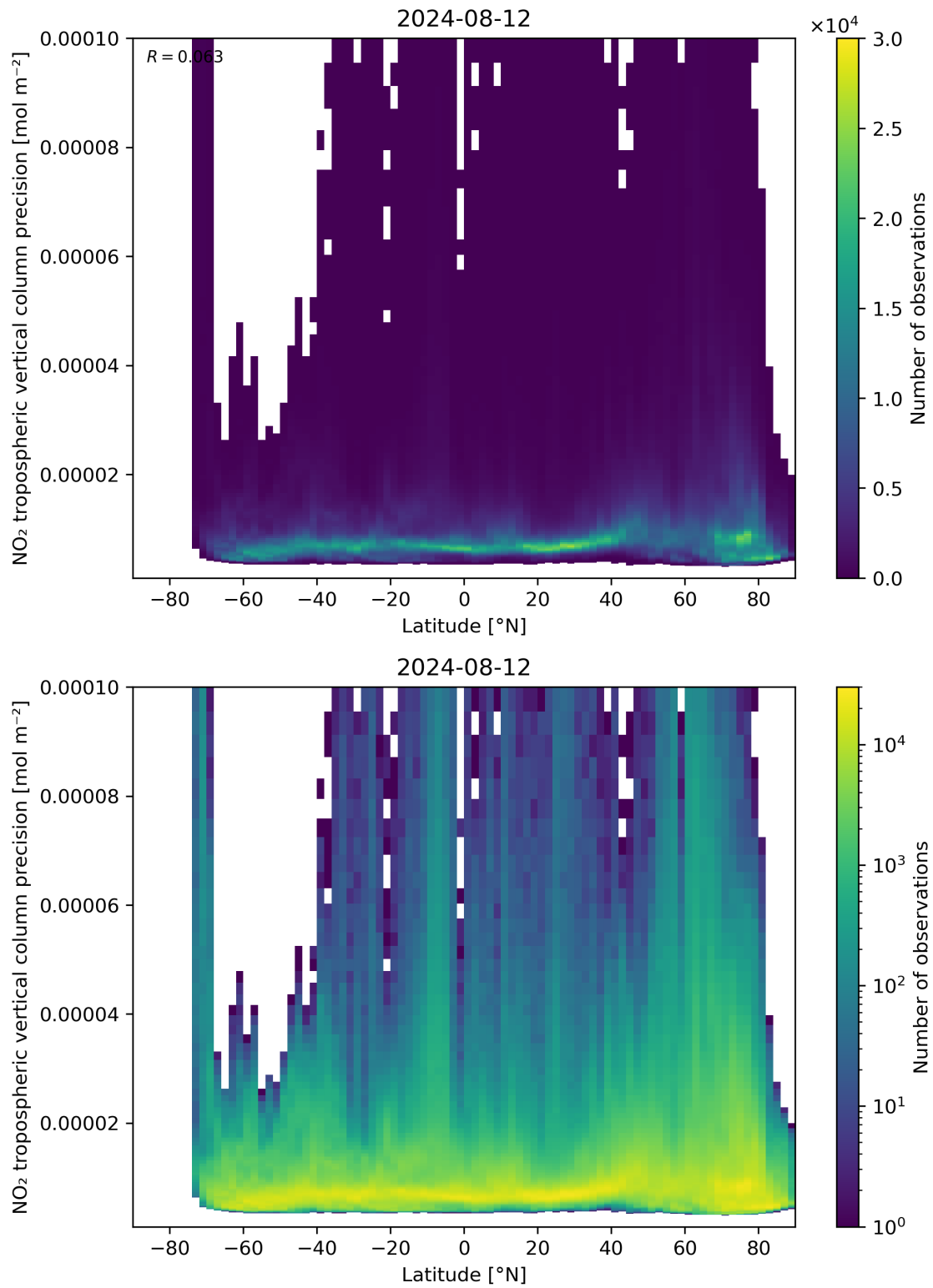
Figure 93: Scatter density plot of “Latitude” against “NO 2 tropospheric vertical column precision” for 2024-08-12 to 2024-08-13.
