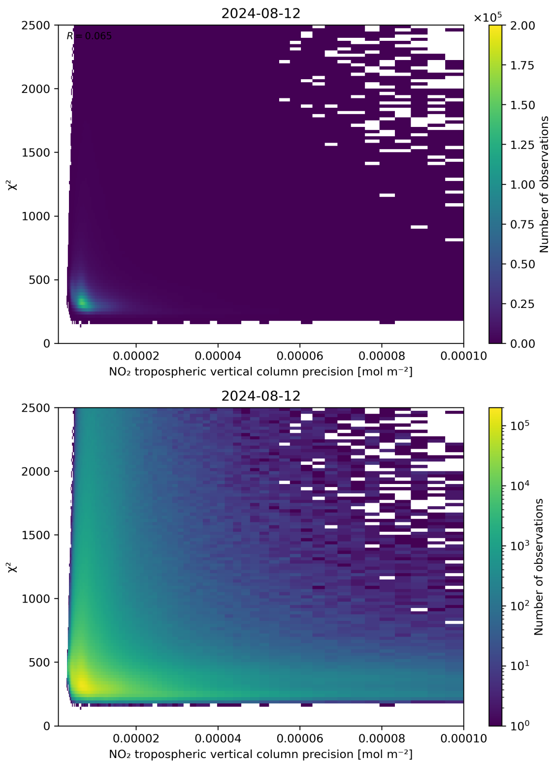
Figure 134: Scatter density plot of “NO 2 tropospheric vertical column precision” against “ \chi^2 ” for 2024-08-12 to 2024-08-13.
