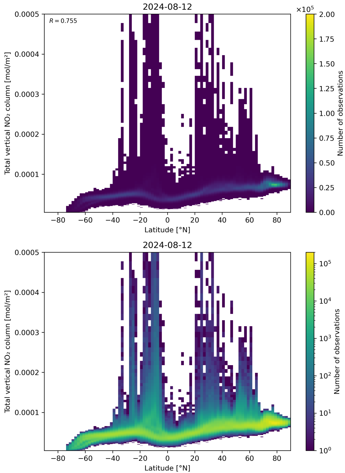
Figure 90: Scatter density plot of “Latitude” against “Total vertical NO 2 column” for 2024-08-12 to 2024-08-13.
