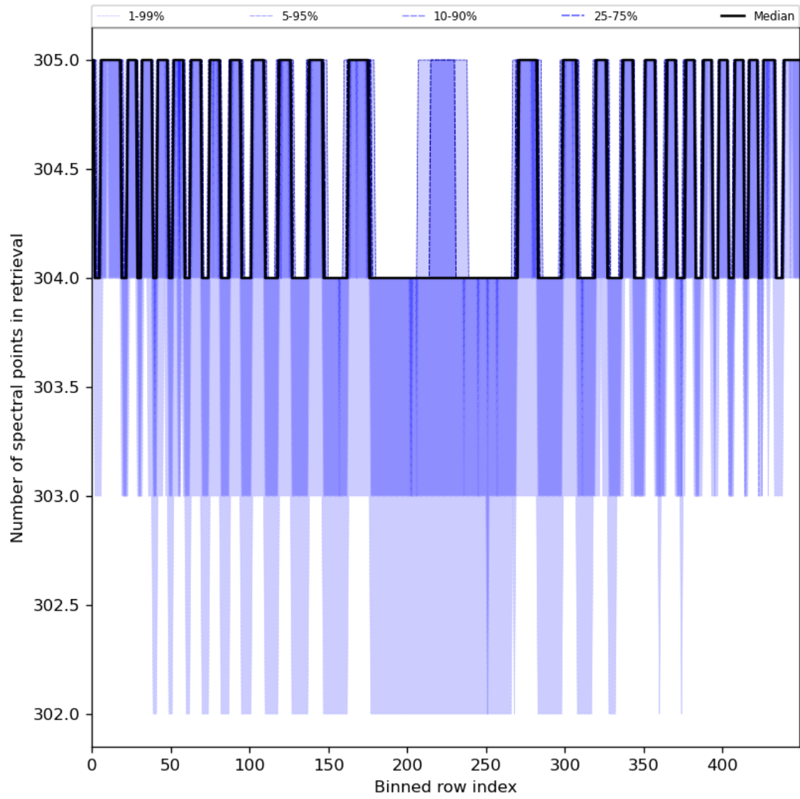
Figure 50: Along track statistics of “Number of spectral points in retrieval” for 2024-08-12 to 2024-08-13
