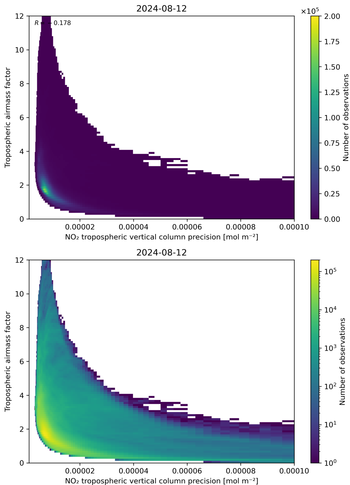
Figure 133: Scatter density plot of “NO 2 tropospheric vertical column precision” against “Tropospheric airmass factor” for 2024-08-12 to 2024-08-13.
