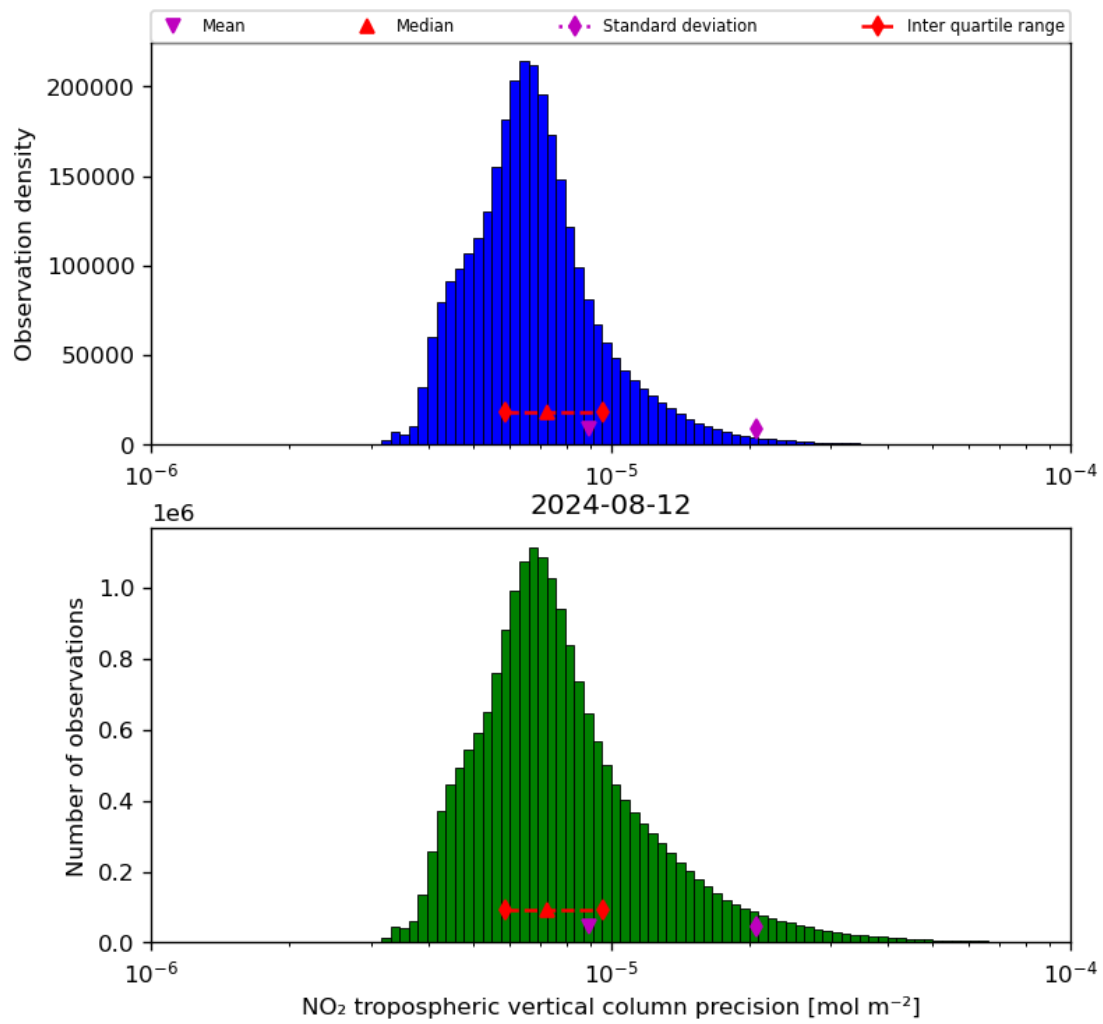
Figure 30: Histogram of “NO 2 tropospheric vertical column precision” for 2024-08-12 to 2024-08-13
