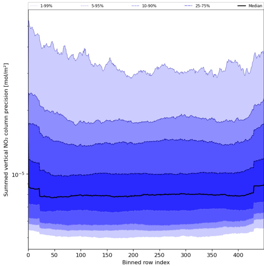
Figure 58: Along track statistics of “Summed vertical NO 2 column precision” for 2024-08-12 to 2024-08-13
