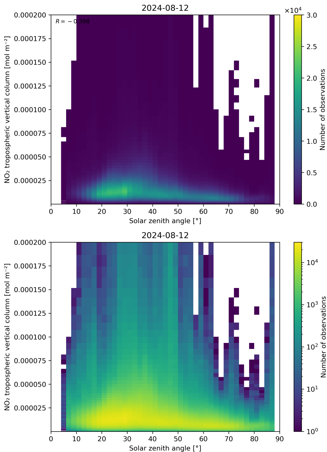
Figure 155: Scatter density plot of “Solar zenith angle” against “NO 2 tropospheric vertical column” for 2024-08-12 to 2024-08-13.
