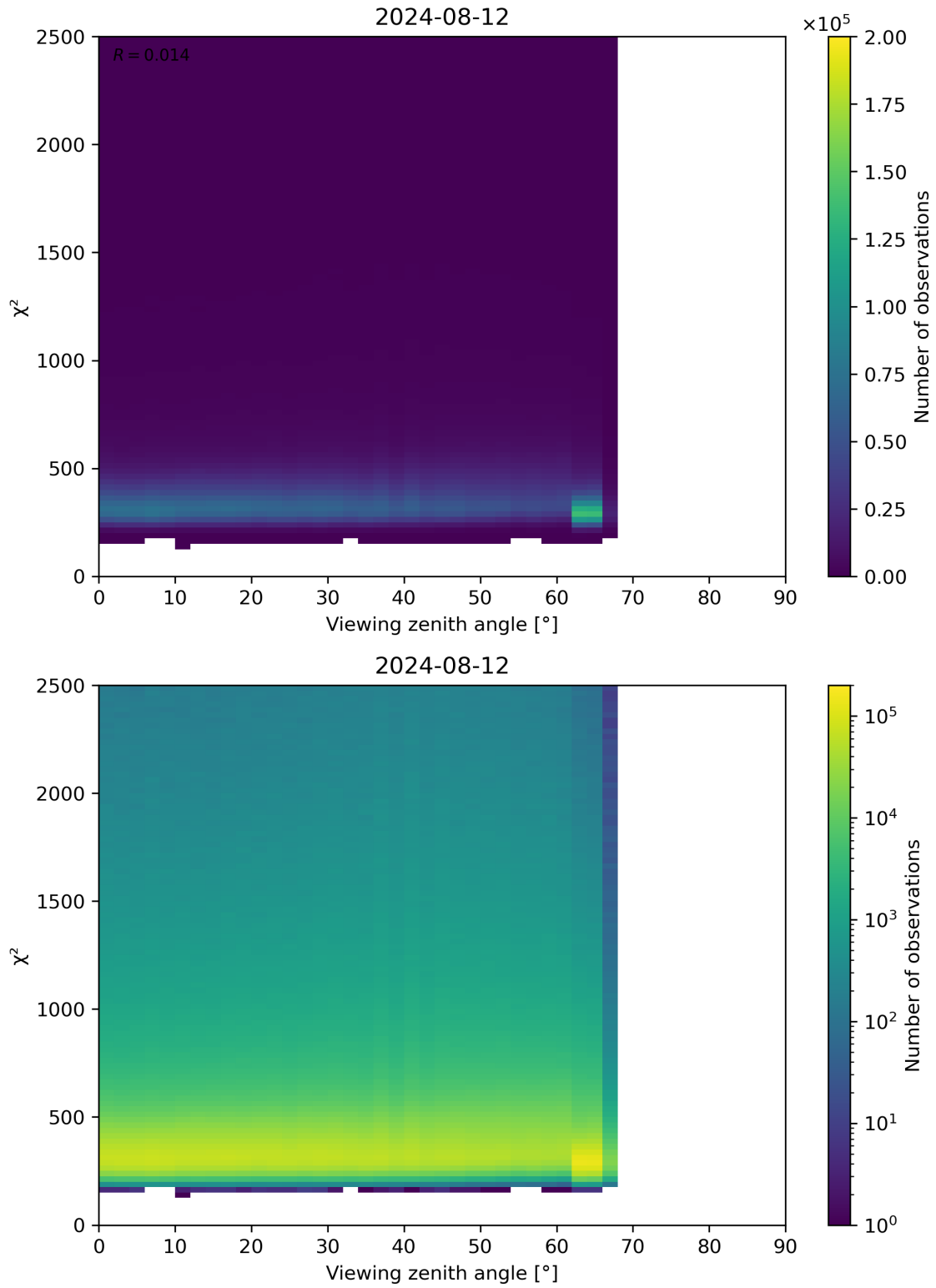
Figure 162: Scatter density plot of “Viewing zenith angle” against “ \chi^2 ” for 2024-08-12 to 2024-08-13.
