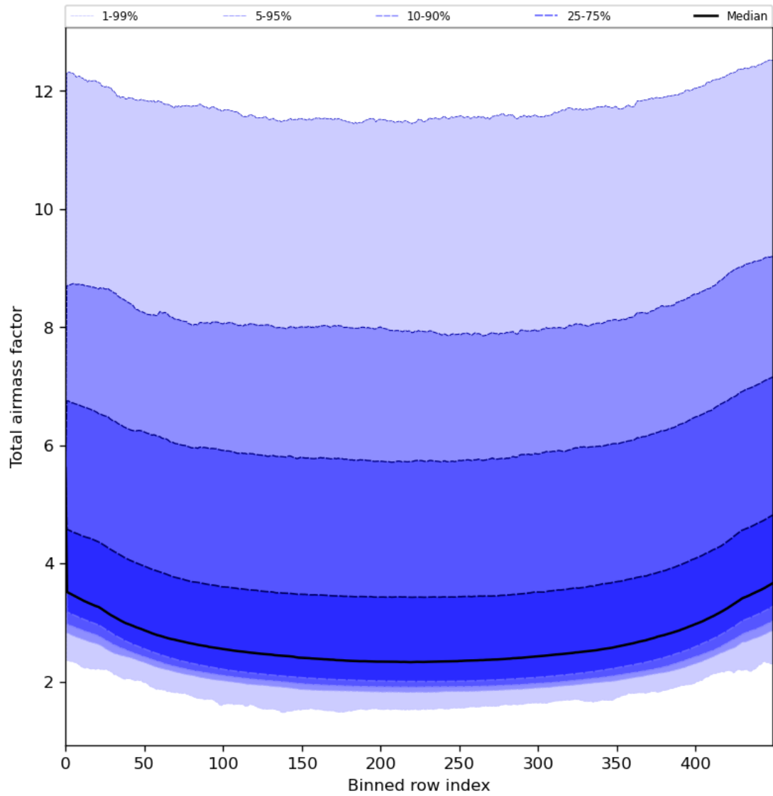
Figure 49: Along track statistics of “Total airmass factor” for 2024-08-12 to 2024-08-13
