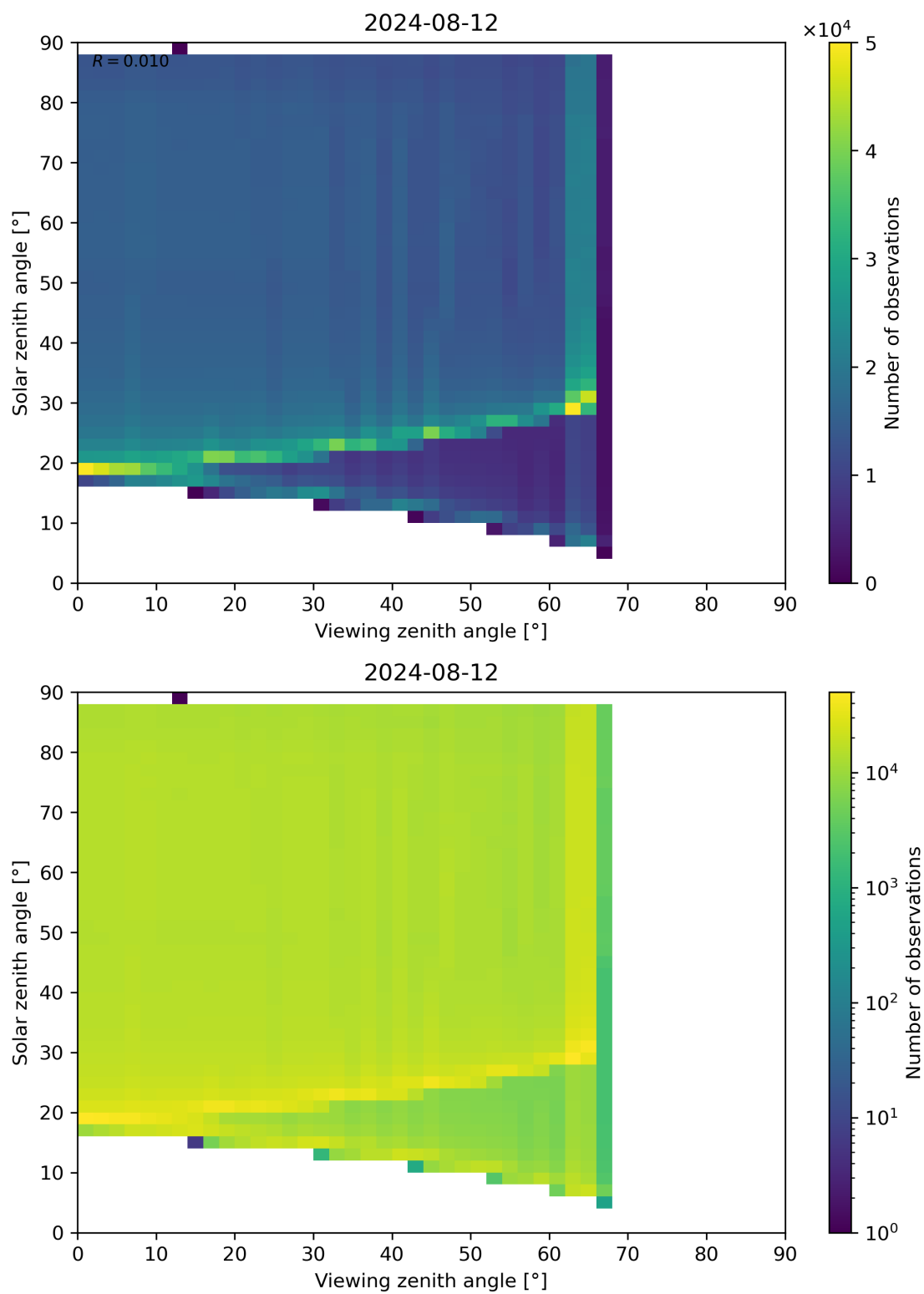
Figure 172: Scatter density plot of “Viewing zenith angle” against “Solar zenith angle” for 2024-08-12 to 2024-08-13.
