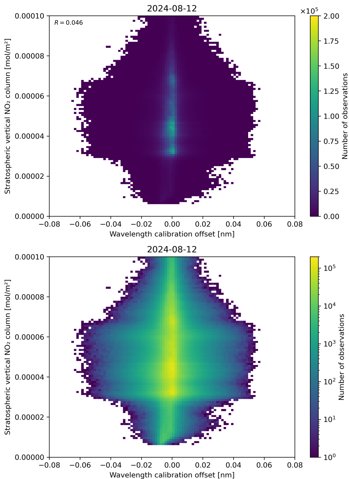
Figure 176: Scatter density plot of “Wavelength calibration offset” against “Stratospheric vertical NO 2 column” for 2024-08-12 to 2024-08-13.
