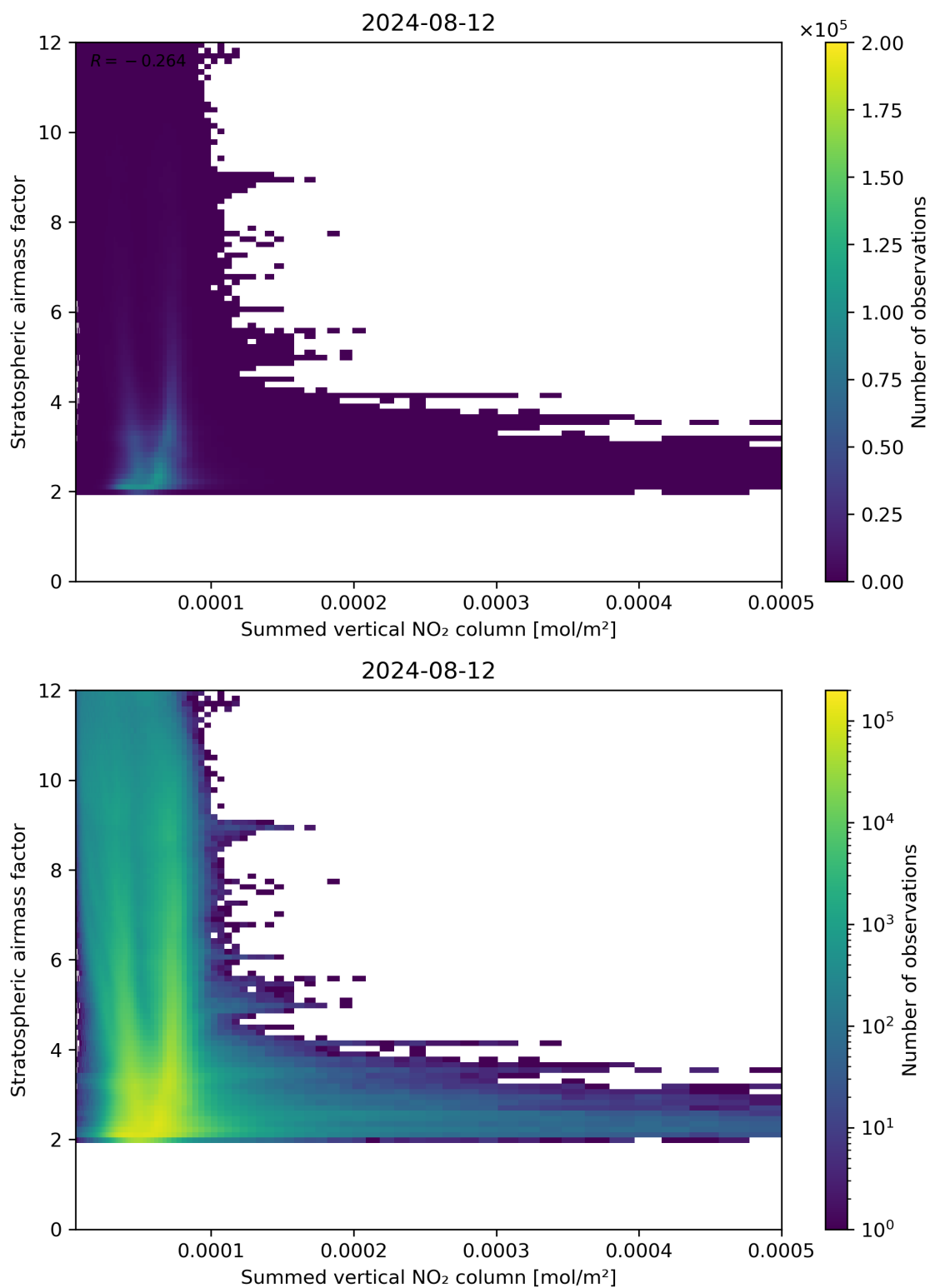
Figure 103: Scatter density plot of “Summed vertical NO 2 column” against “Stratospheric airmass factor” for 2024-08-12 to 2024-08-13.
