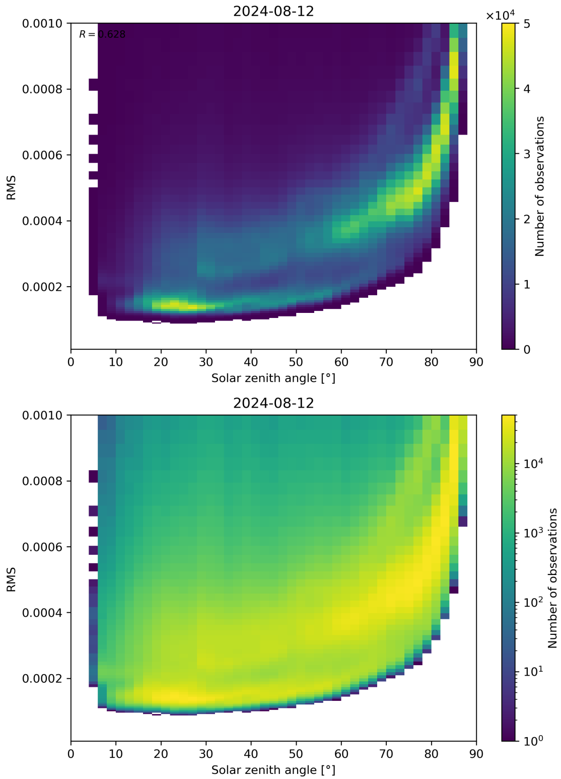
Figure 157: Scatter density plot of “Solar zenith angle” against “RMS” for 2024-08-12 to 2024-08-13.
