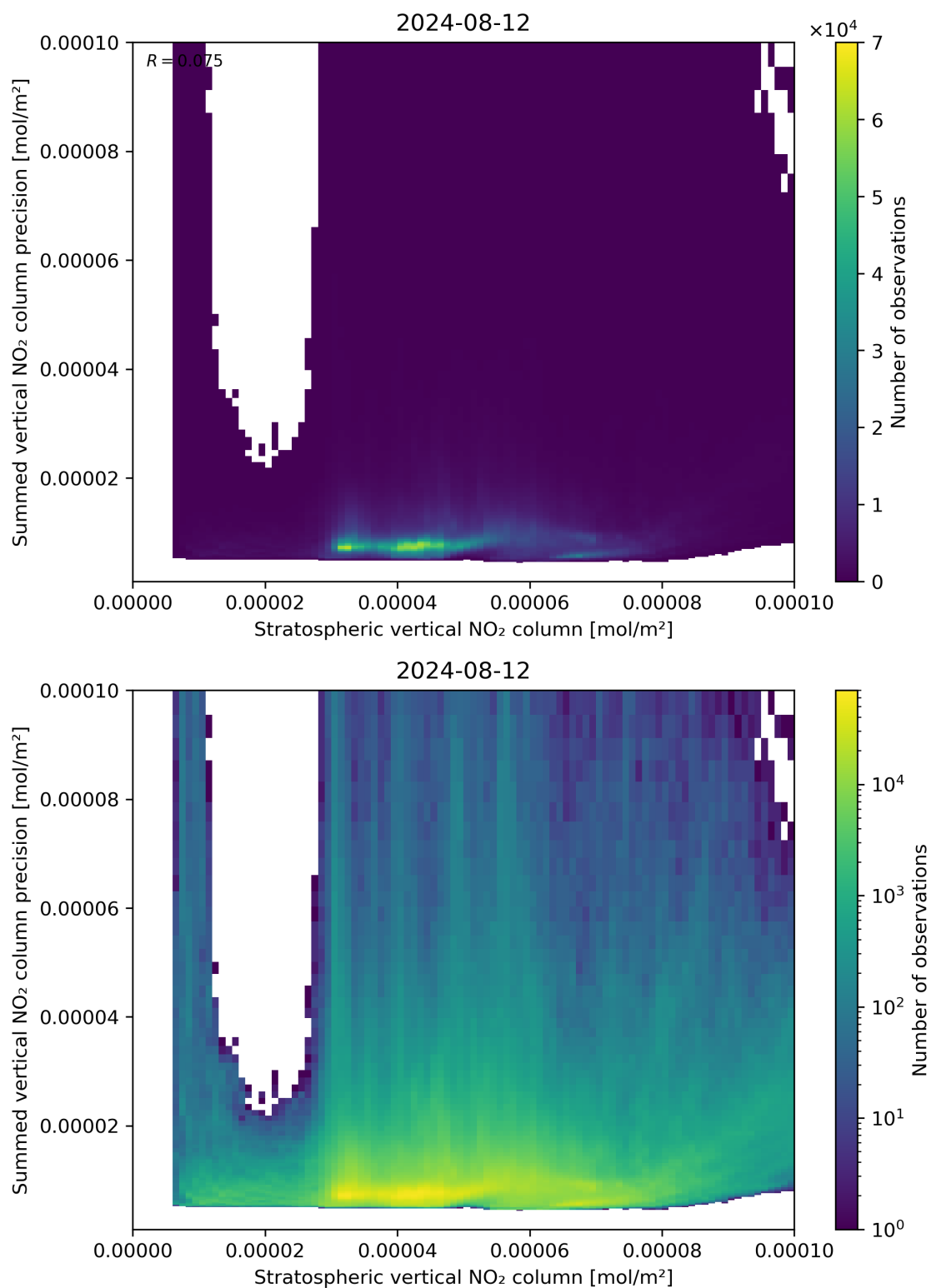
Figure 99: Scatter density plot of “Stratospheric vertical NO 2 column” against “Summed vertical NO 2 column precision” for 2024-08-12 to 2024-08-13.
