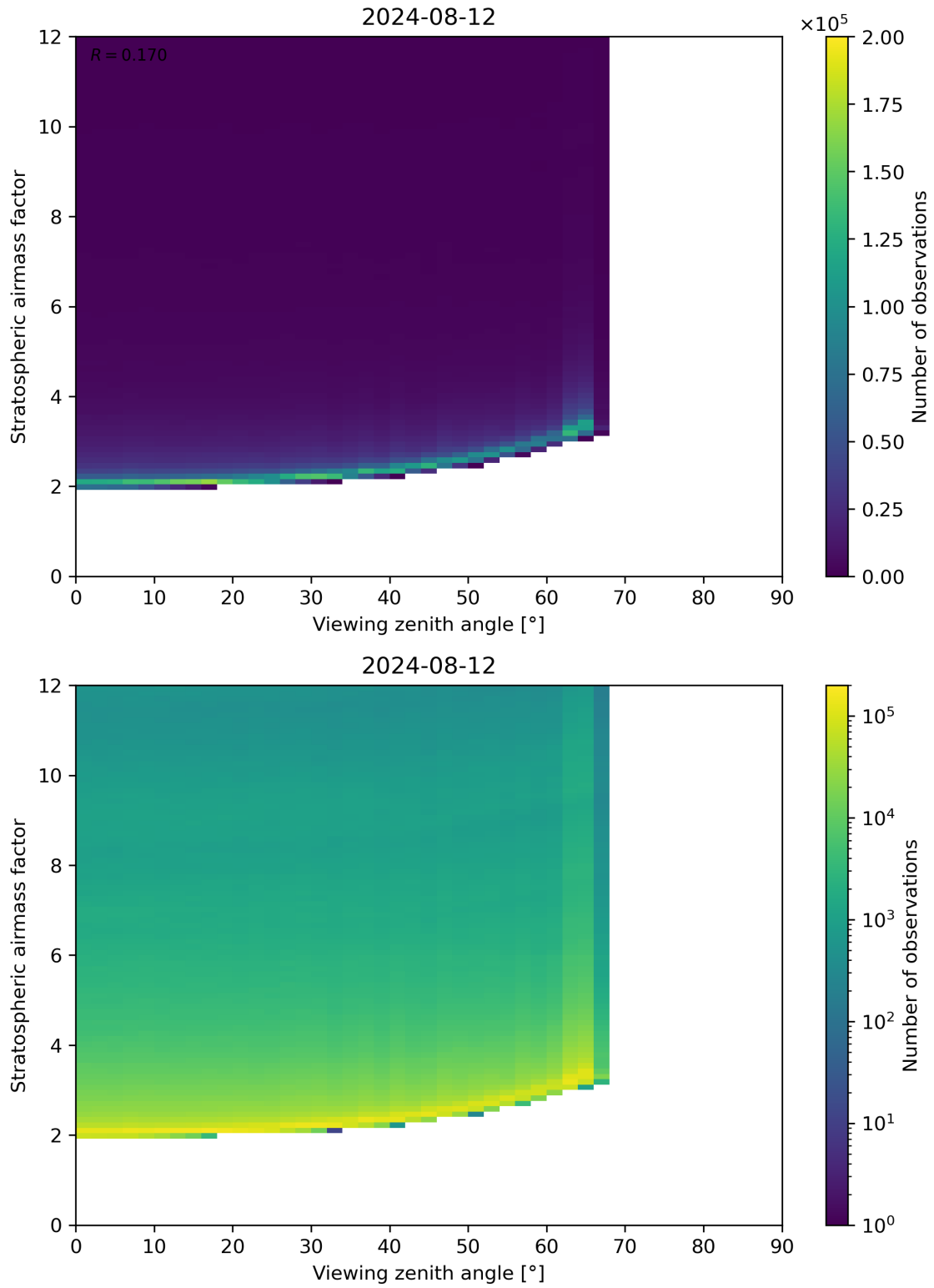
Figure 159: Scatter density plot of “Viewing zenith angle” against “Stratospheric airmass factor” for 2024-08-12 to 2024-08-13.
