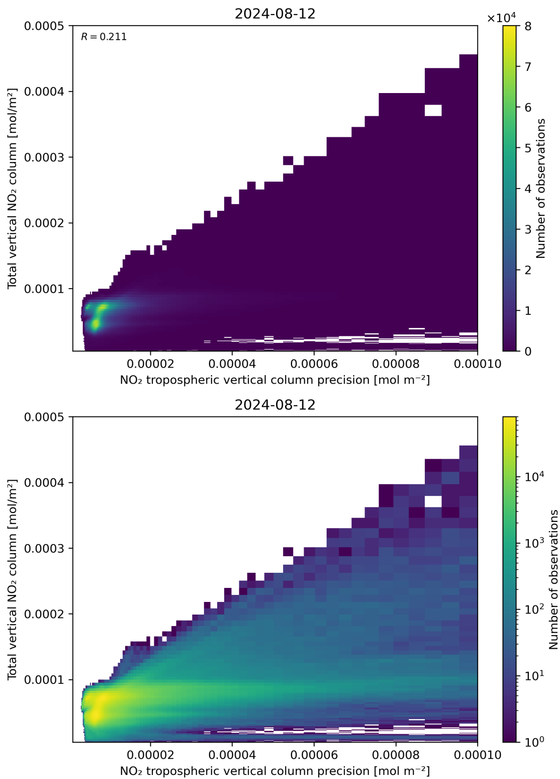
Figure 138: Scatter density plot of “NO 2 tropospheric vertical column precision” against “Total vertical NO 2 column” for 2024-08-12 to 2024-08-13.
