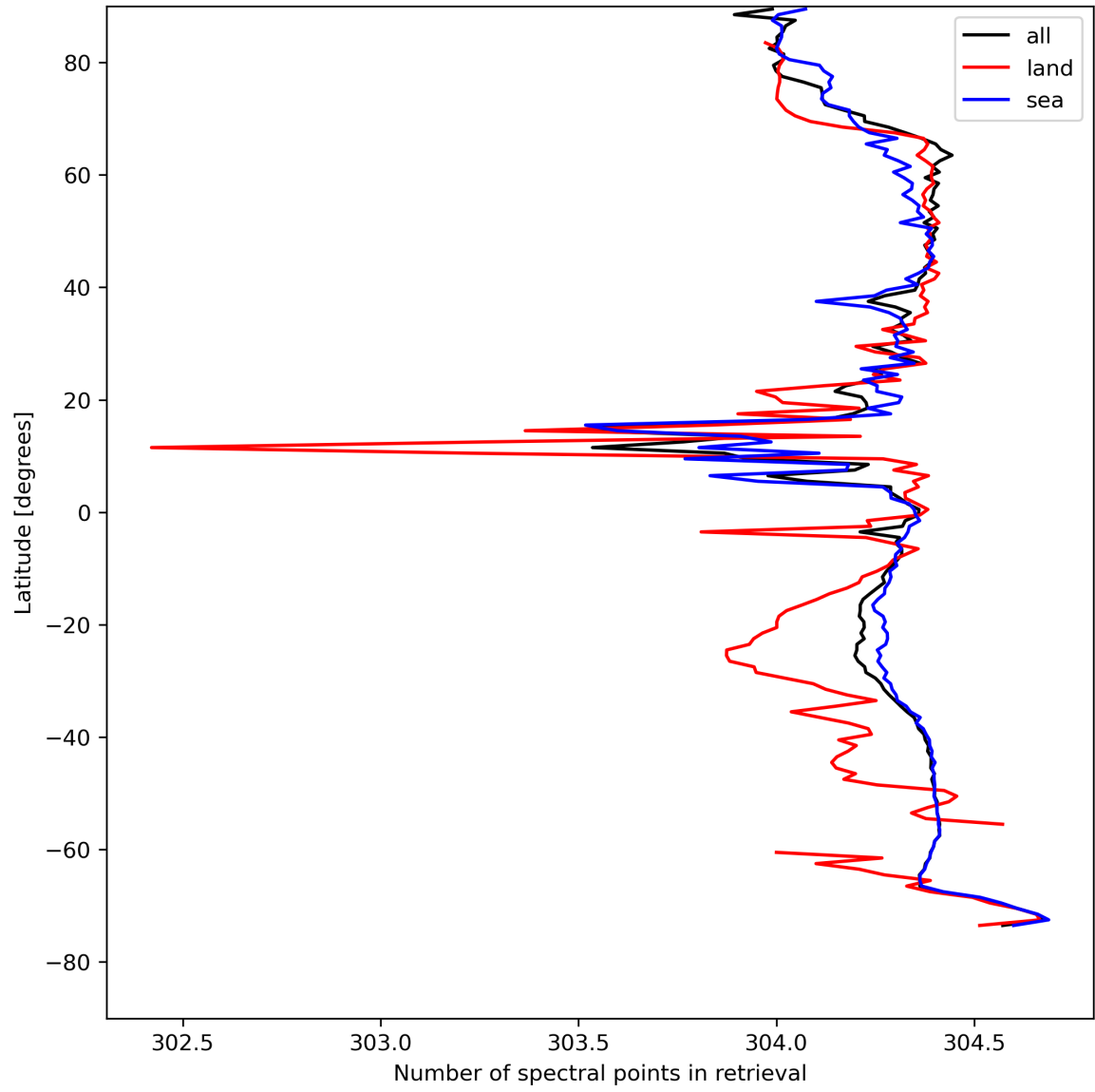
Figure 16: Zonal average of “Number of spectral points in retrieval” for 2024-08-12 to 2024-08-13.
