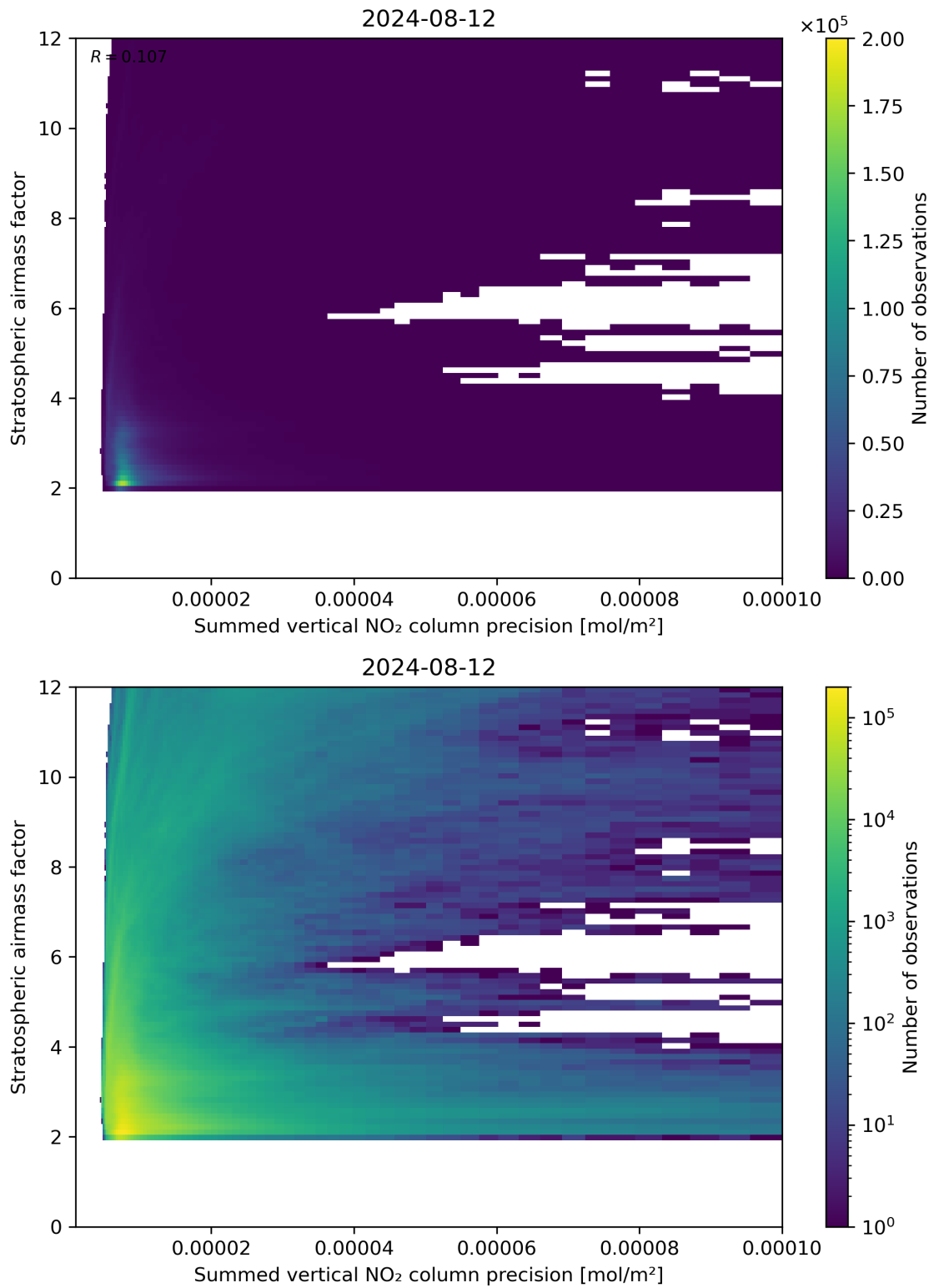
Figure 106: Scatter density plot of “Summed vertical NO 2 column precision” against “Stratospheric airmass factor” for 2024-08-12 to 2024-08-13.
