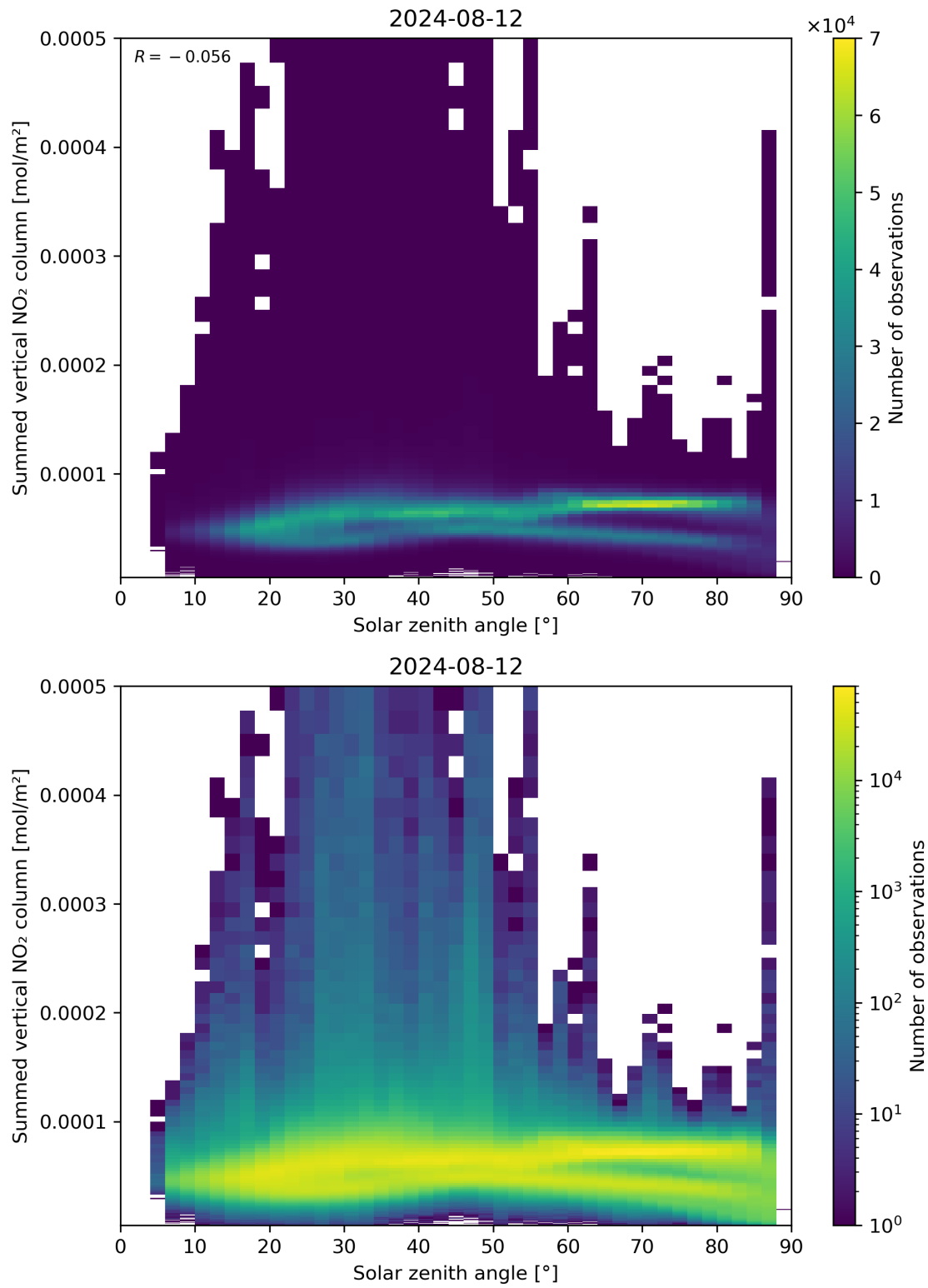
Figure 151: Scatter density plot of “Solar zenith angle” against “Summed vertical NO 2 column” for 2024-08-12 to 2024-08-13.
