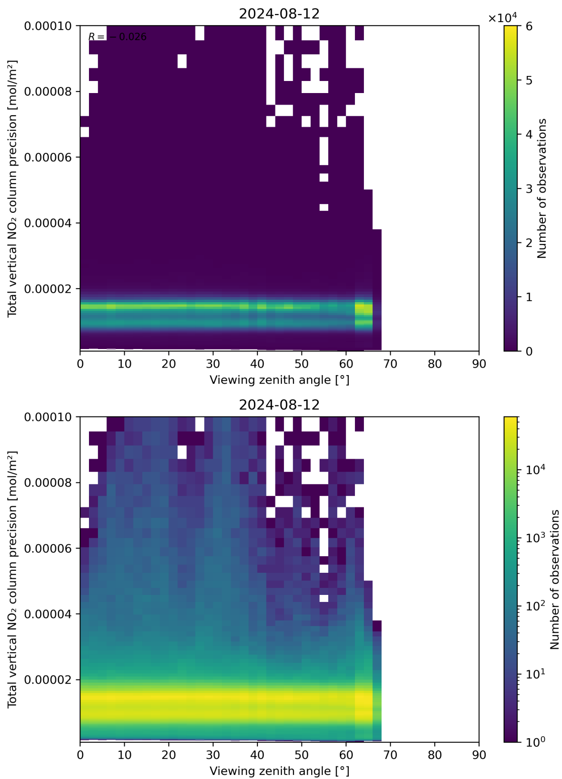
Figure 168: Scatter density plot of “Viewing zenith angle” against “Total vertical NO 2 column precision” for 2024-08-12 to 2024-08-13.
