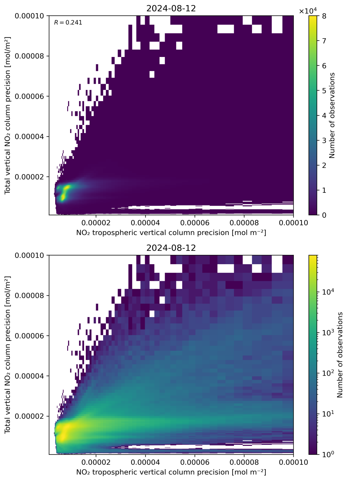
Figure 139: Scatter density plot of “NO 2 tropospheric vertical column precision” against “Total vertical NO 2 column precision” for 2024-08-12 to 2024-08-13.
