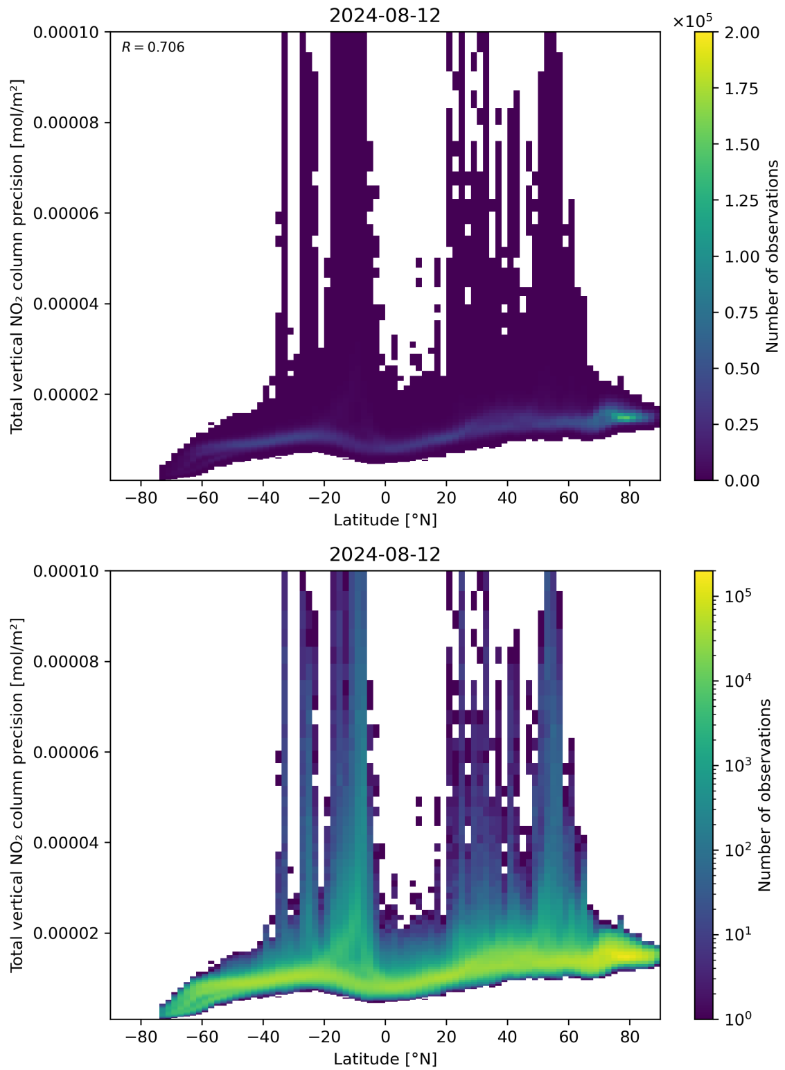
Figure 91: Scatter density plot of “Latitude” against “Total vertical NO 2 column precision” for 2024-08-12 to 2024-08-13.
