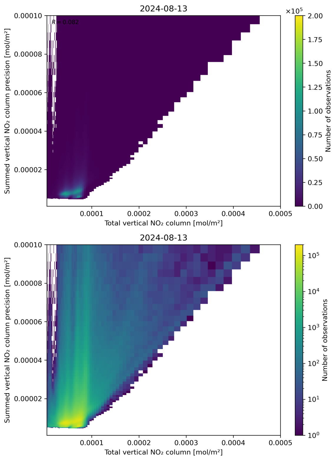
Figure 113: Scatter density plot of “Total vertical NO 2 column” against “Summed vertical NO 2 column precision” for 2024-08-12 to 2024-08-14.
