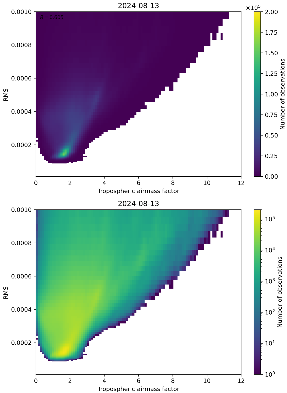
Figure 79: Scatter density plot of “Tropospheric airmass factor” against “RMS” for 2024-08-12 to 2024-08-14.
