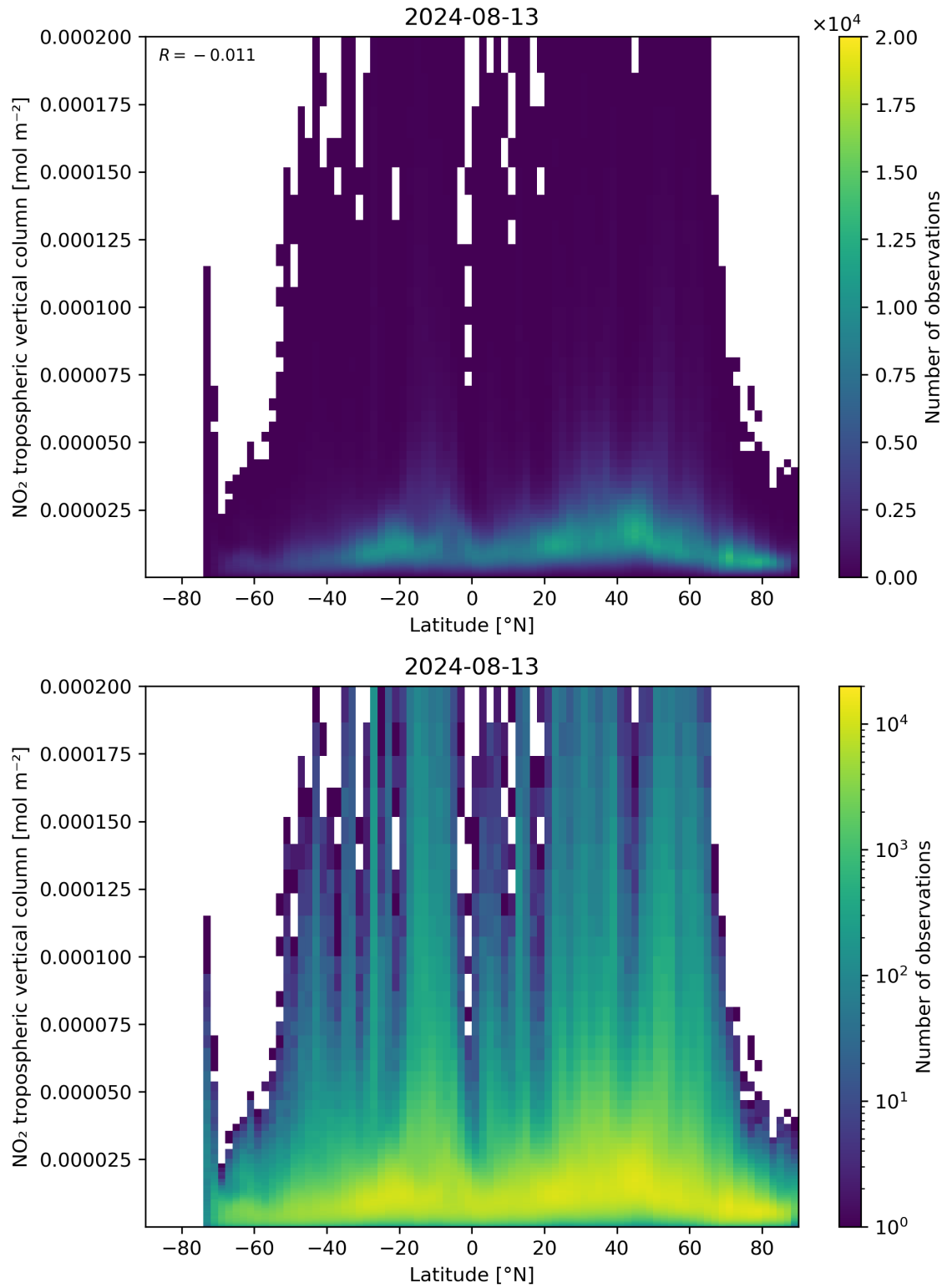
Figure 92: Scatter density plot of “Latitude” against “NO 2 tropospheric vertical column” for 2024-08-12 to 2024-08-14.
