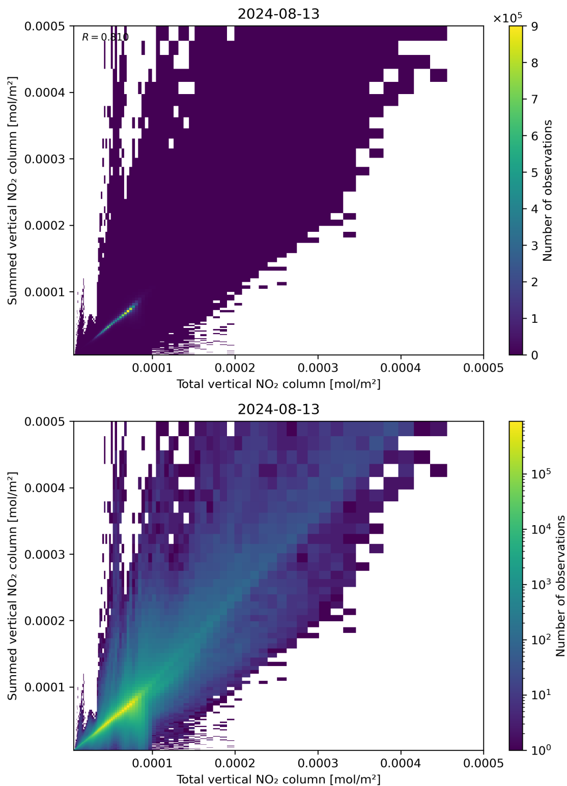
Figure 112: Scatter density plot of “Total vertical NO 2 column” against “Summed vertical NO 2 column” for 2024-08-12 to 2024-08-14.
