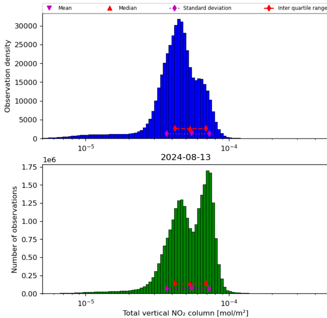
Figure 38: Histogram of “Total vertical NO 2 column” for 2024-08-12 to 2024-08-14
