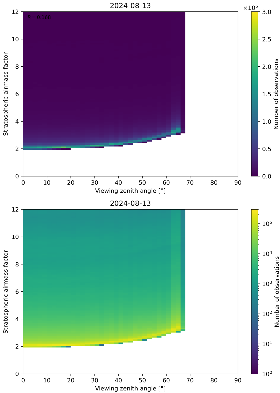
Figure 159: Scatter density plot of “Viewing zenith angle” against “Stratospheric airmass factor” for 2024-08-12 to 2024-08-14.
