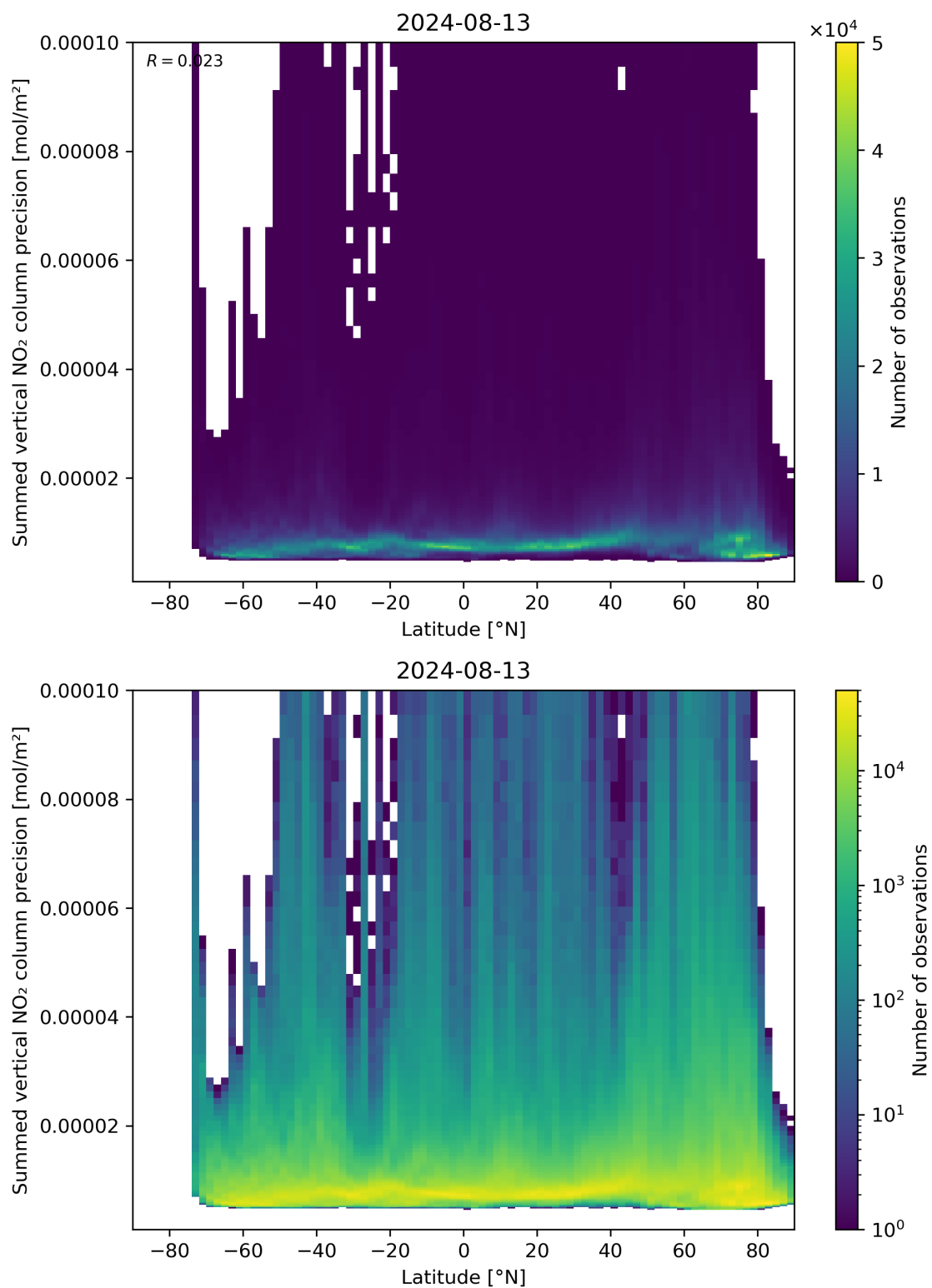
Figure 89: Scatter density plot of “Latitude” against “Summed vertical NO 2 column precision” for 2024-08-12 to 2024-08-14.
