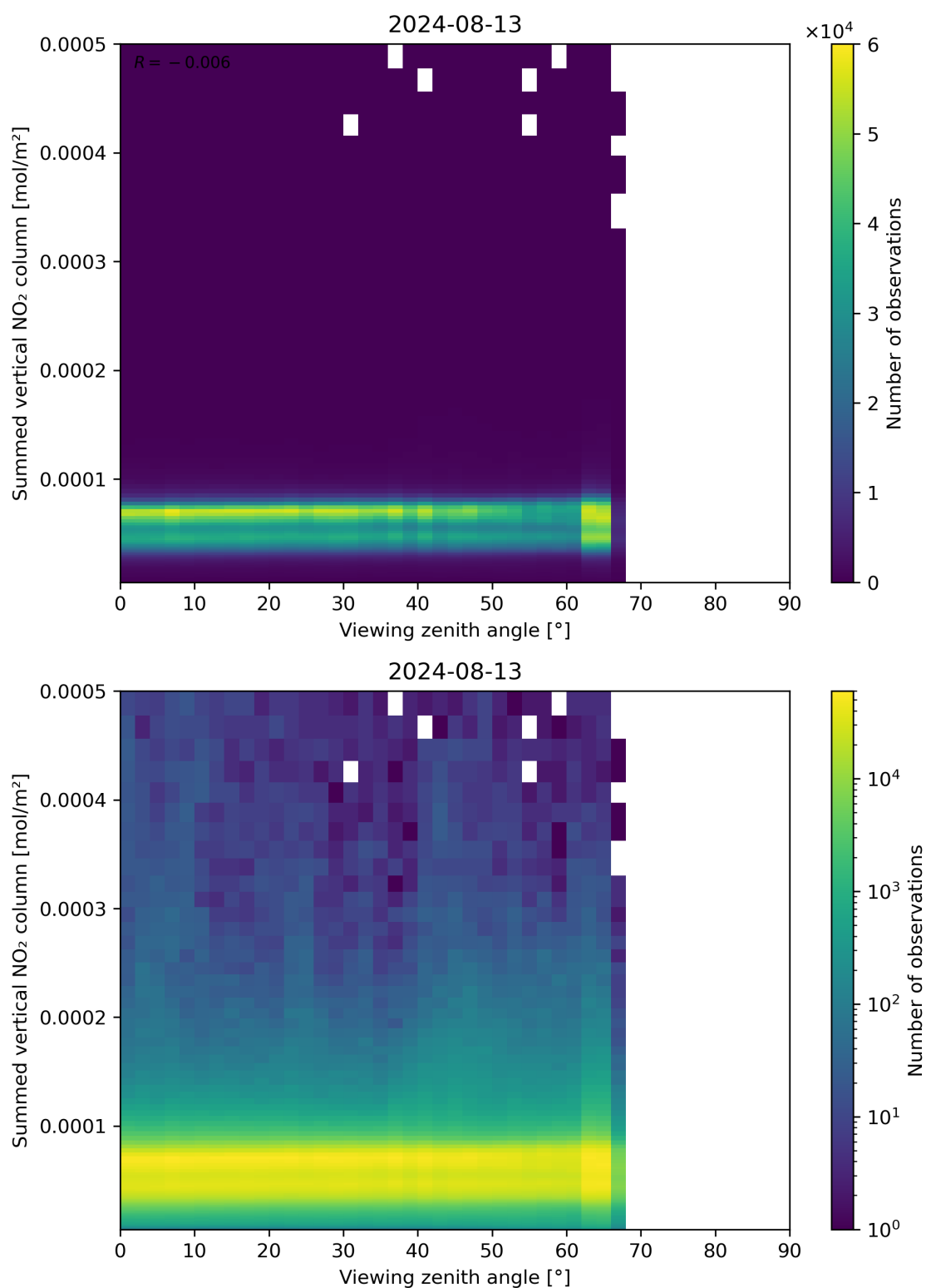
Figure 165: Scatter density plot of “Viewing zenith angle” against “Summed vertical NO 2 column” for 2024-08-12 to 2024-08-14.
