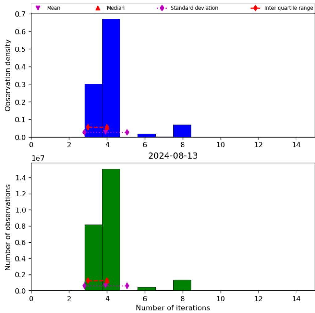
Figure 34: Histogram of “Number of iterations” for 2024-08-12 to 2024-08-14
