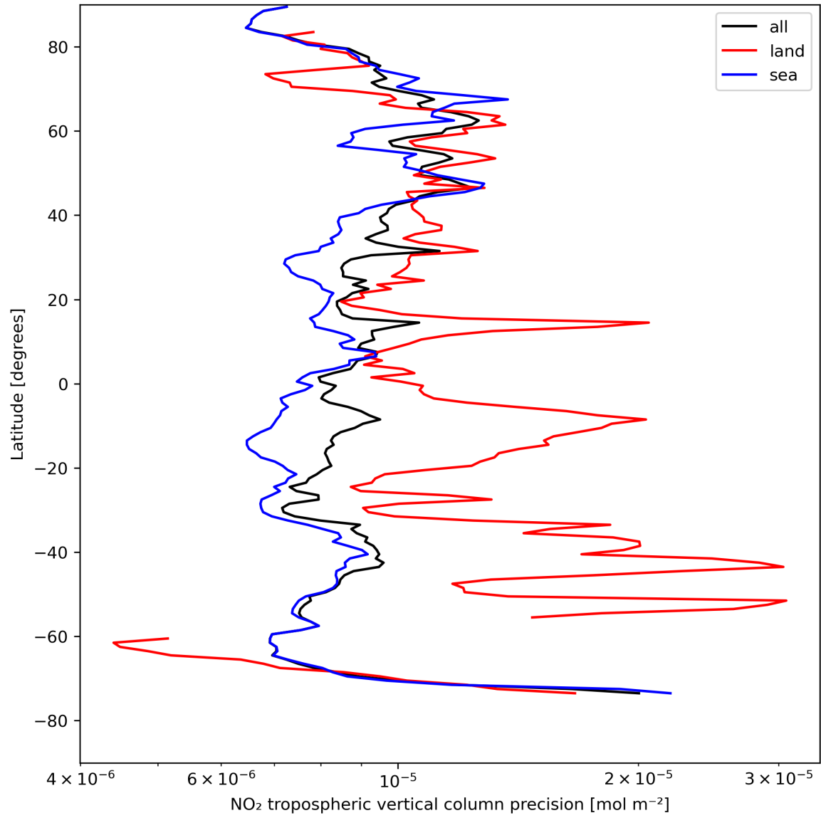
Figure 13: Zonal average of “NO 2 tropospheric vertical column precision” for 2024-08-12 to 2024-08-14.
