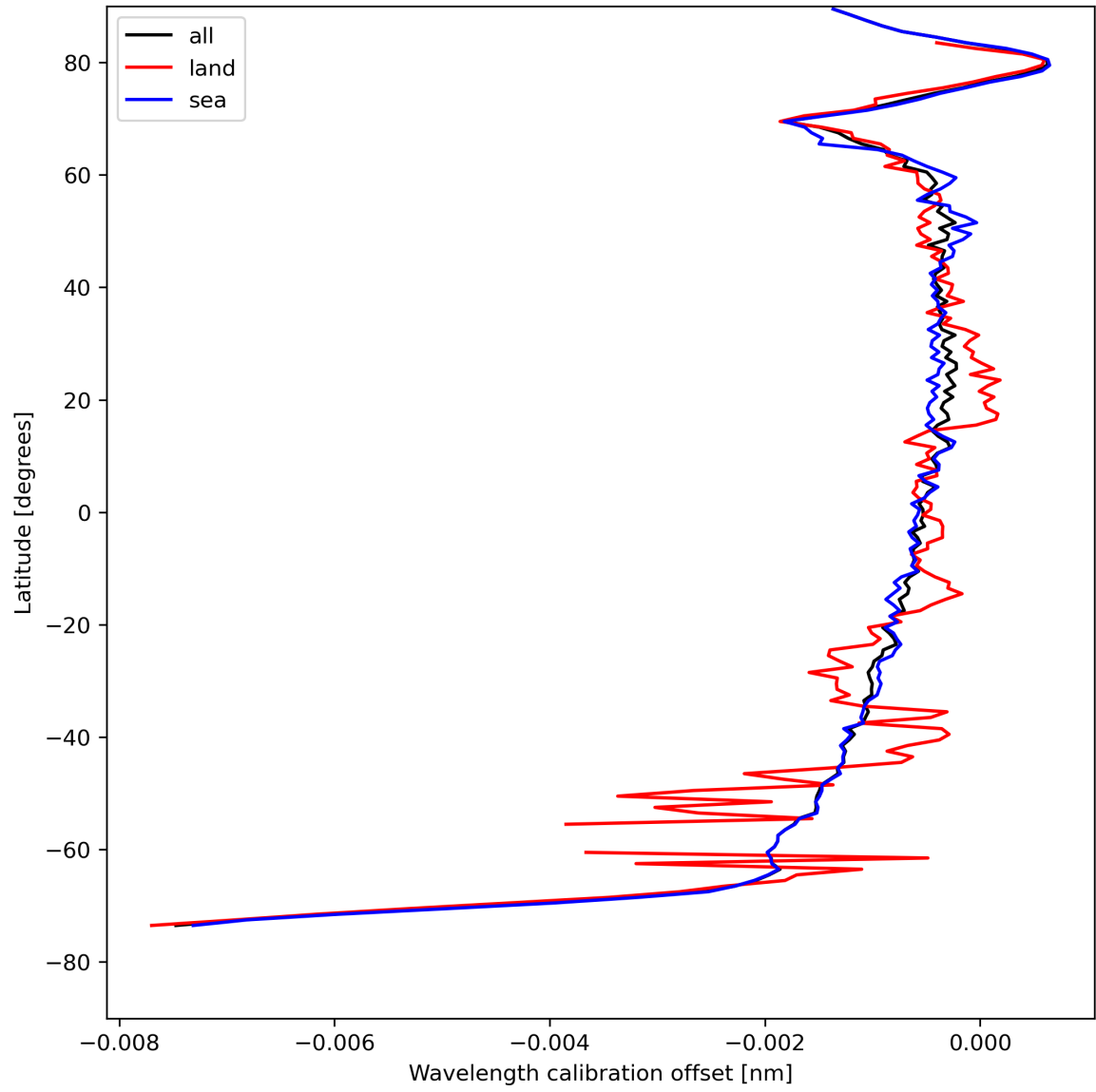
Figure 18: Zonal average of “Wavelength calibration offset” for 2024-08-12 to 2024-08-14.
