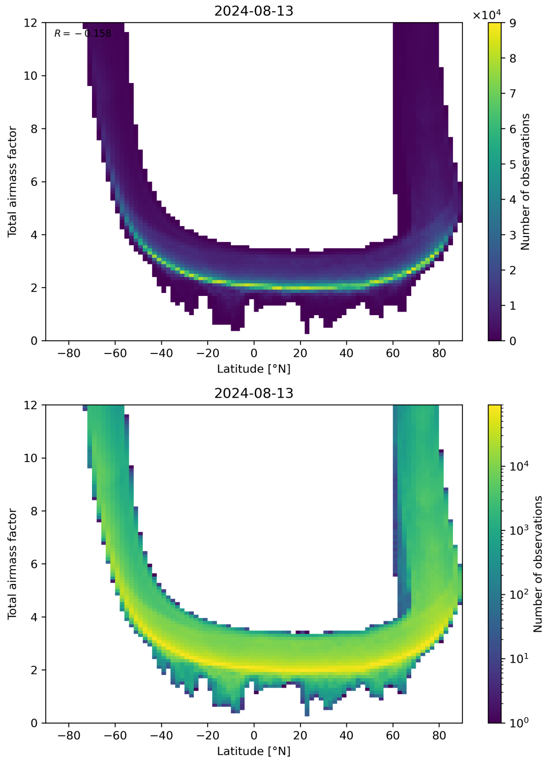
Figure 84: Scatter density plot of “Latitude” against “Total airmass factor” for 2024-08-12 to 2024-08-14.
