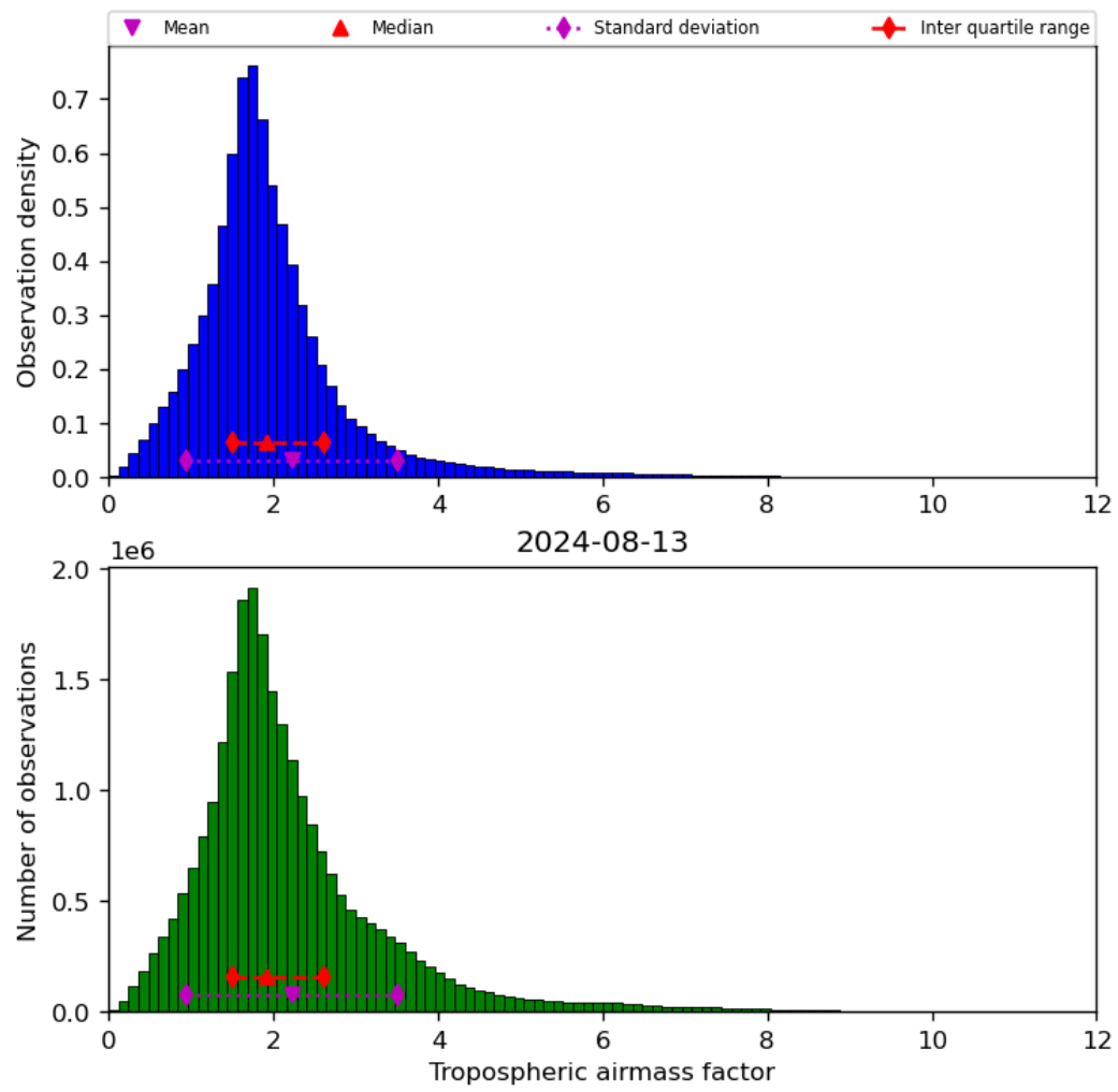
Figure 31: Histogram of “Tropospheric airmass factor” for 2024-08-12 to 2024-08-14
