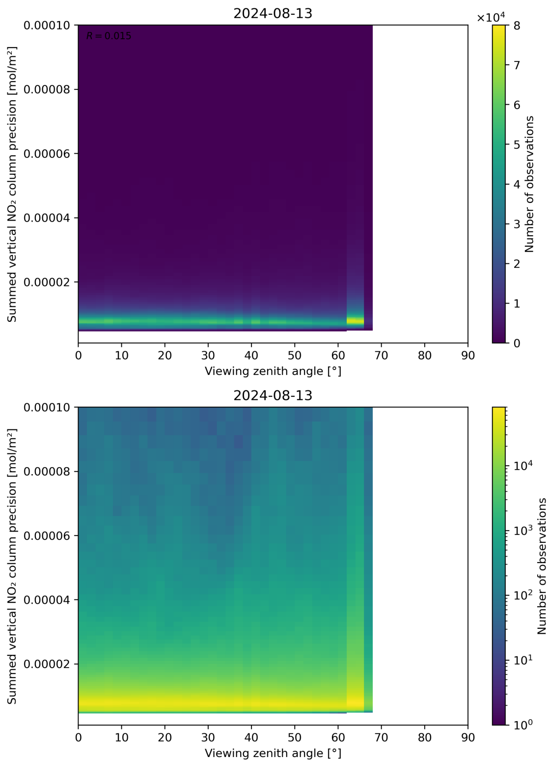
Figure 166: Scatter density plot of “Viewing zenith angle” against “Summed vertical NO 2 column precision” for 2024-08-12 to 2024-08-14.
