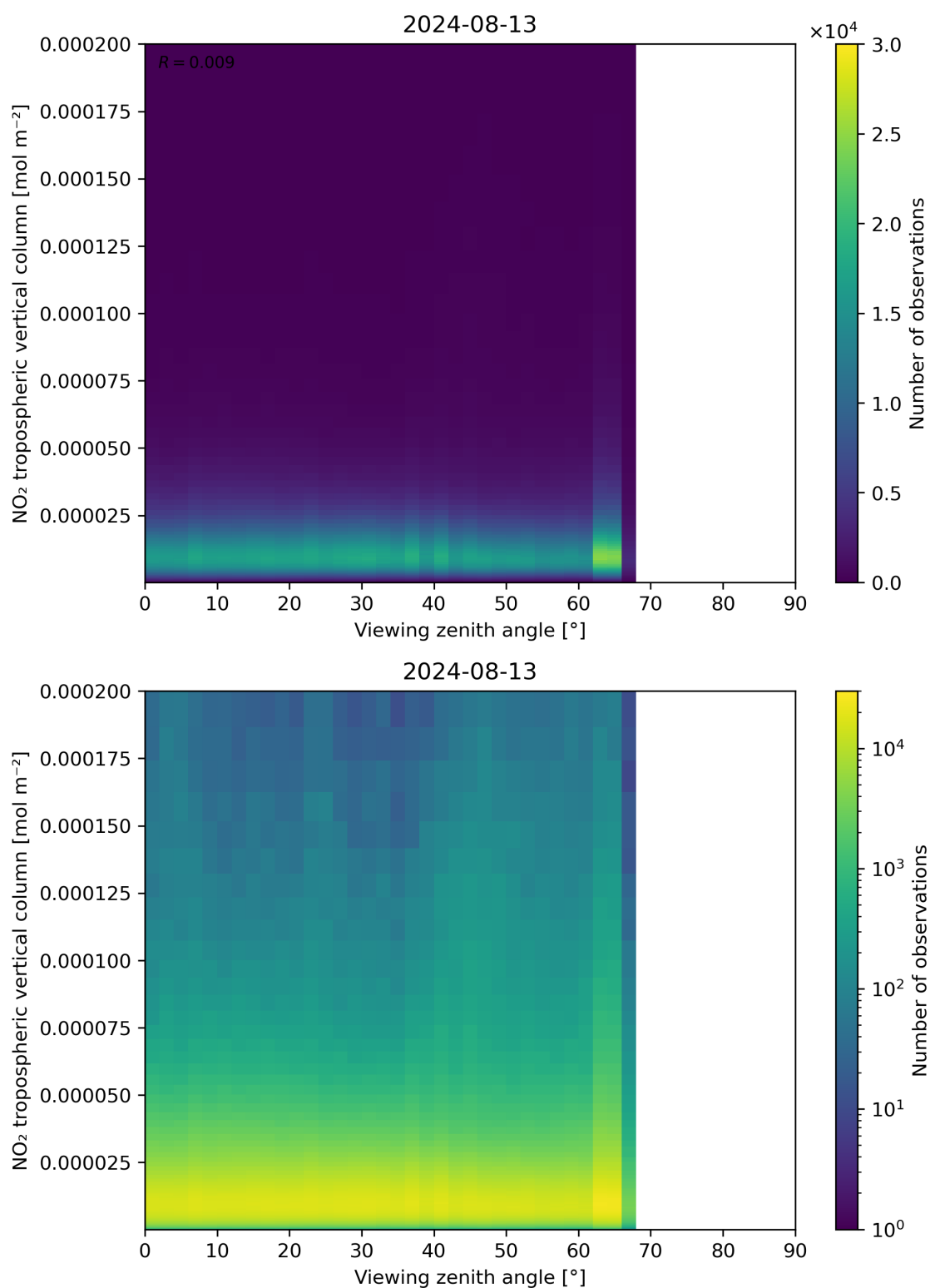
Figure 169: Scatter density plot of “Viewing zenith angle” against “NO 2 tropospheric vertical column” for 2024-08-12 to 2024-08-14.
