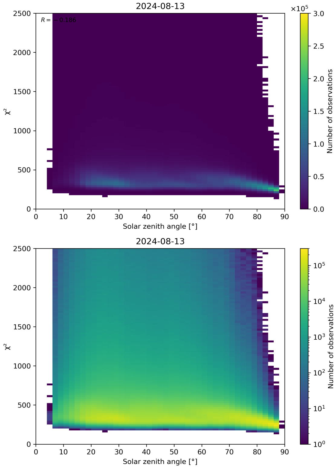
Figure 148: Scatter density plot of “Solar zenith angle” against “ \chi^2 ” for 2024-08-12 to 2024-08-14.
