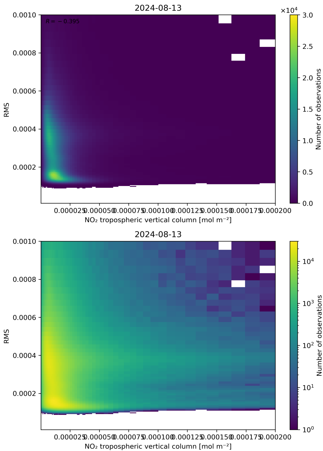
Figure 142: Scatter density plot of “NO 2 tropospheric vertical column” against “RMS” for 2024-08-12 to 2024-08-14.
