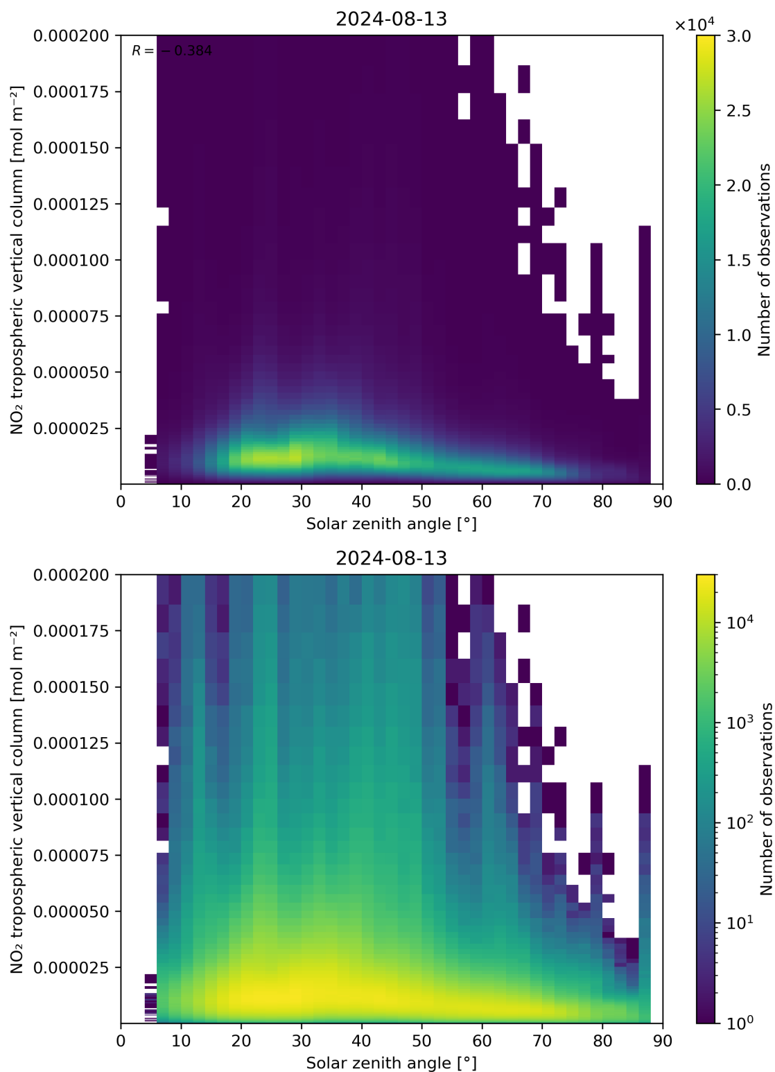
Figure 155: Scatter density plot of “Solar zenith angle” against “NO 2 tropospheric vertical column” for 2024-08-12 to 2024-08-14.
