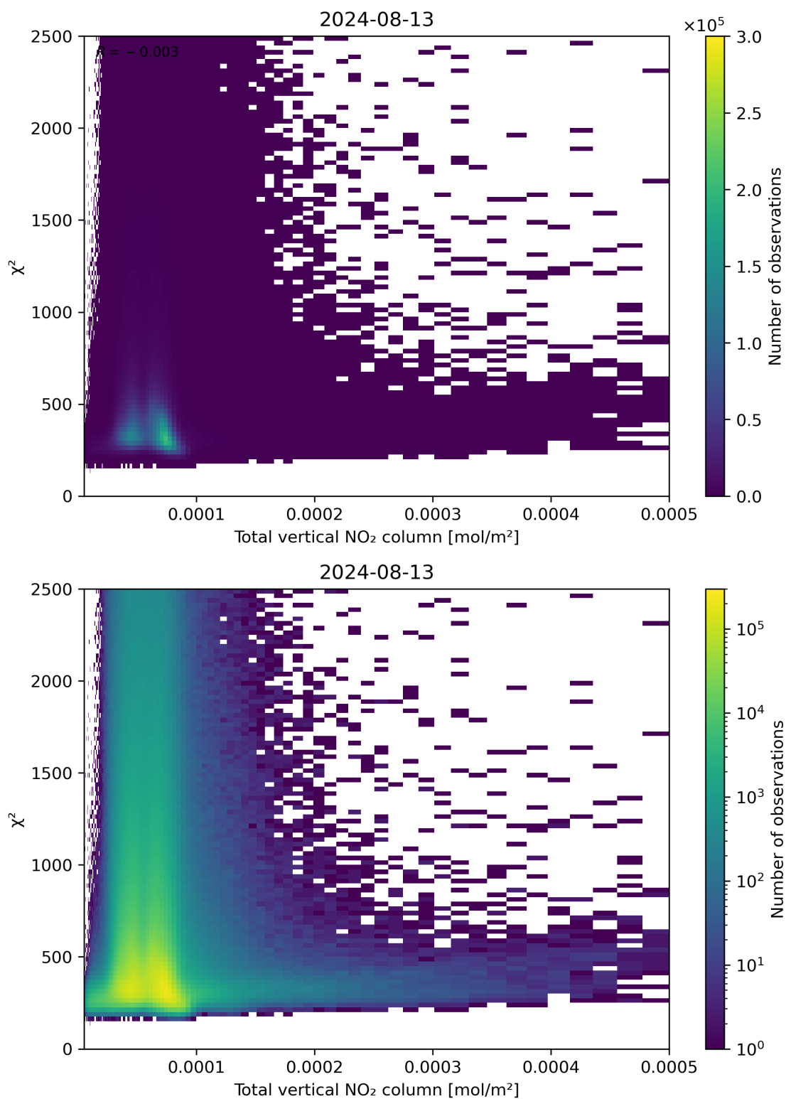
Figure 111: Scatter density plot of “Total vertical NO 2 column” against “ \chi^2 ” for 2024-08-12 to 2024-08-14.
