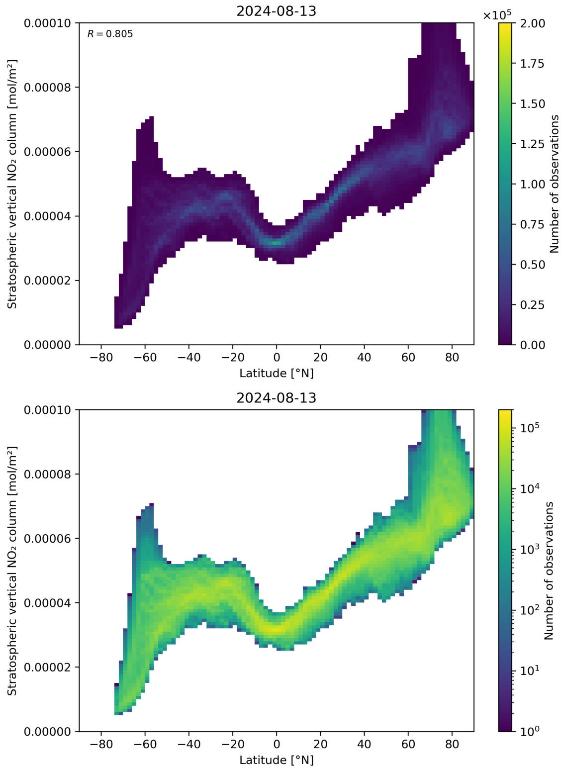
Figure 87: Scatter density plot of “Latitude” against “Stratospheric vertical \text{NO}_2 column” for 2024-08-12 to 2024-08-14.
