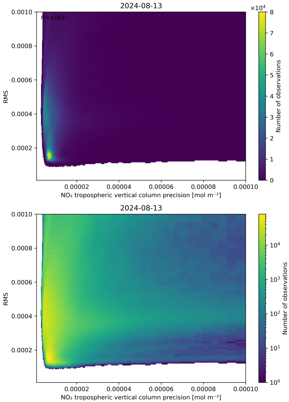
Figure 140: Scatter density plot of “NO 2 tropospheric vertical column precision” against “RMS” for 2024-08-12 to 2024-08-14.
