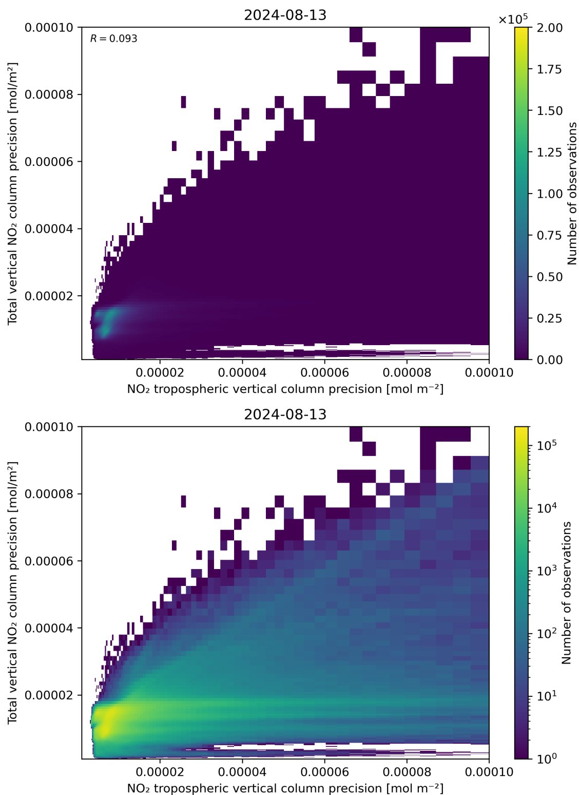
Figure 139: Scatter density plot of “NO 2 tropospheric vertical column precision” against “Total vertical NO 2 column precision” for 2024-08-12 to 2024-08-14.
