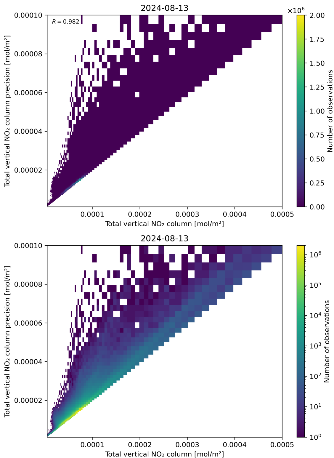
Figure 114: Scatter density plot of “Total vertical NO 2 column” against “Total vertical NO 2 column precision” for 2024-08-12 to 2024-08-14.
