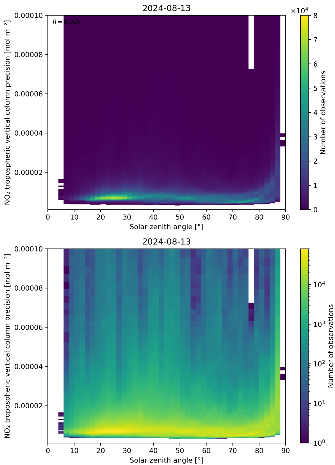
Figure 156: Scatter density plot of “Solar zenith angle” against “NO 2 tropospheric vertical column precision” for 2024-08-12 to 2024-08-14.
