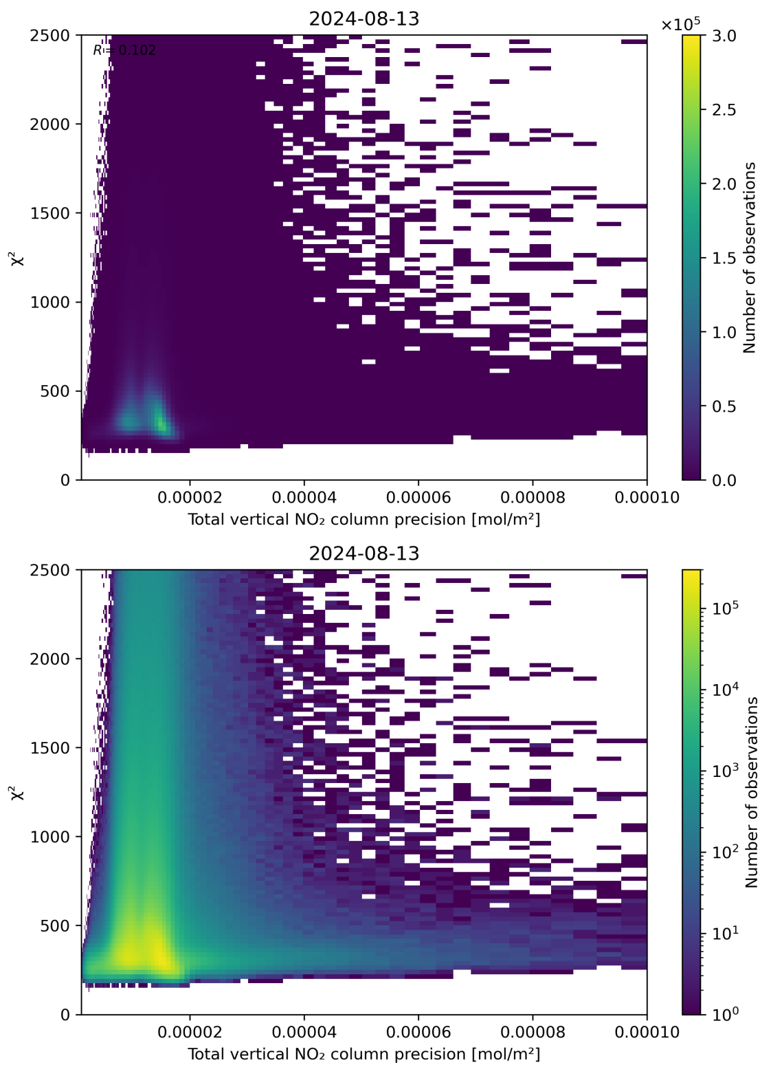
Figure 116: Scatter density plot of “Total vertical NO 2 column precision” against “ \chi^2 ” for 2024-08-12 to 2024-08-14.
