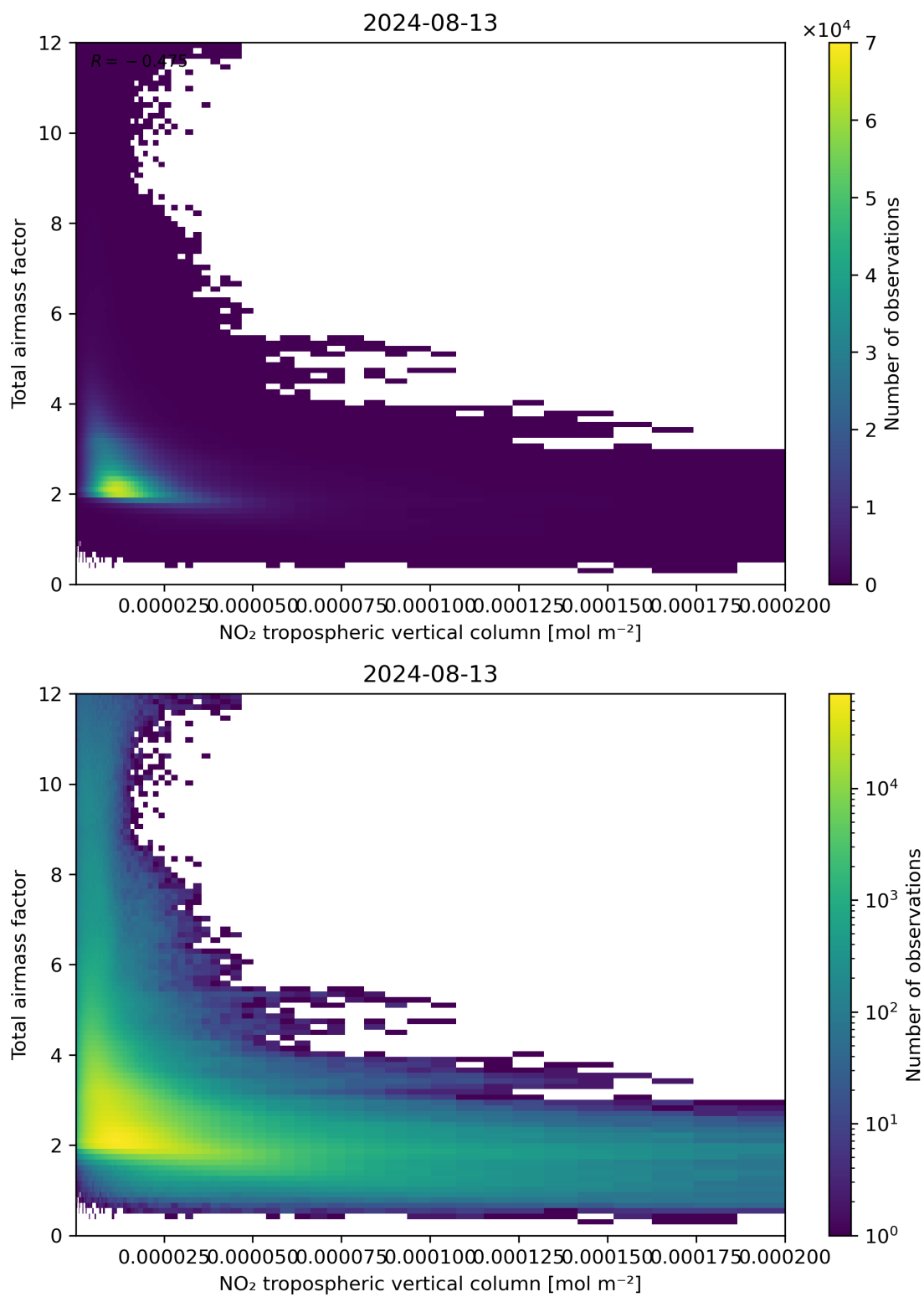
Figure 122: Scatter density plot of “NO 2 tropospheric vertical column” against “Total airmass factor” for 2024-08-12 to 2024-08-14.
