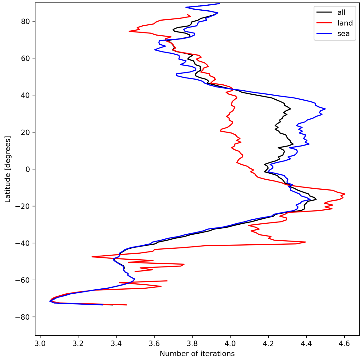
Figure 17: Zonal average of “Number of iterations” for 2024-08-12 to 2024-08-14.
