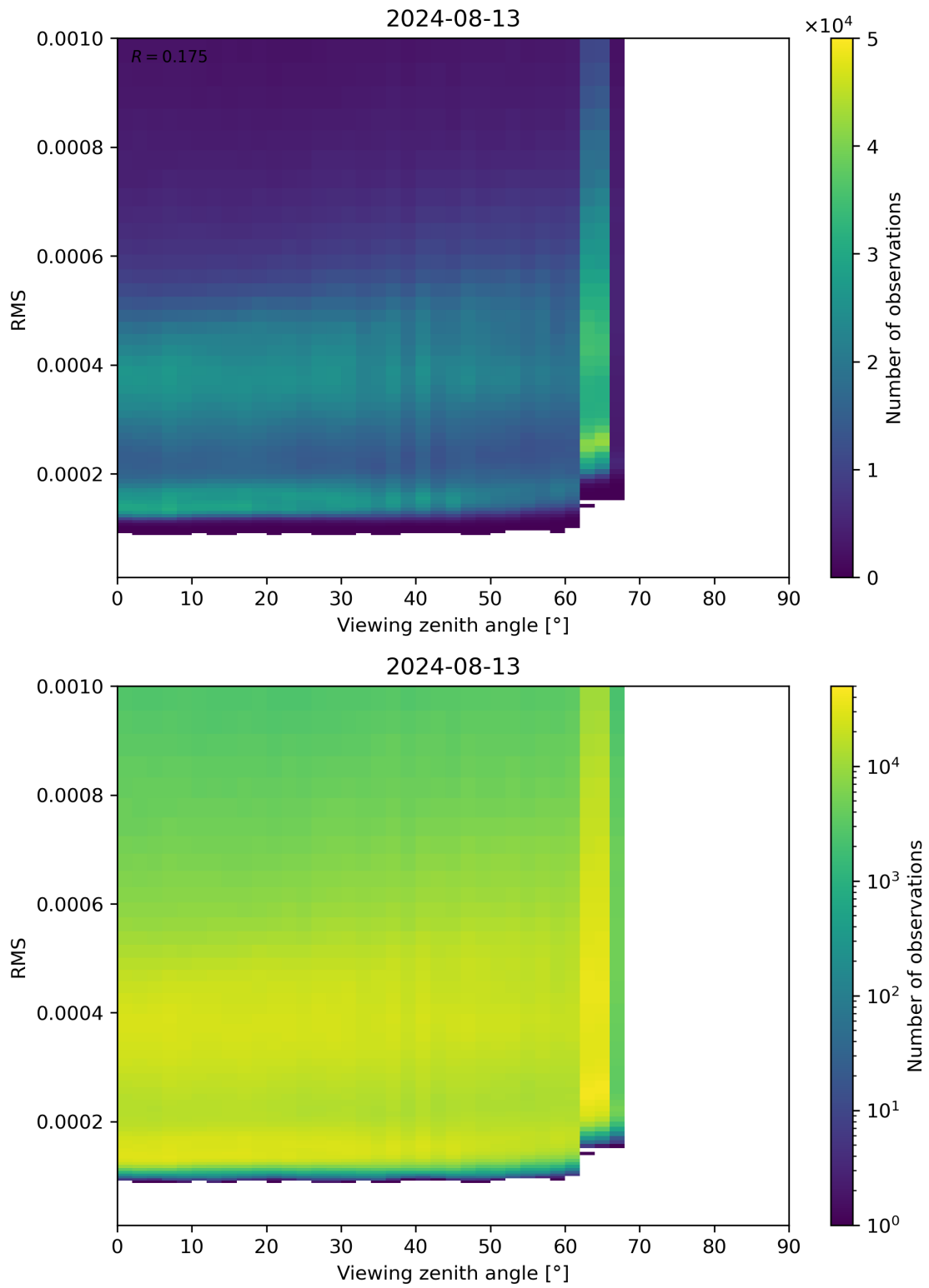
Figure 171: Scatter density plot of “Viewing zenith angle” against “RMS” for 2024-08-12 to 2024-08-14.
