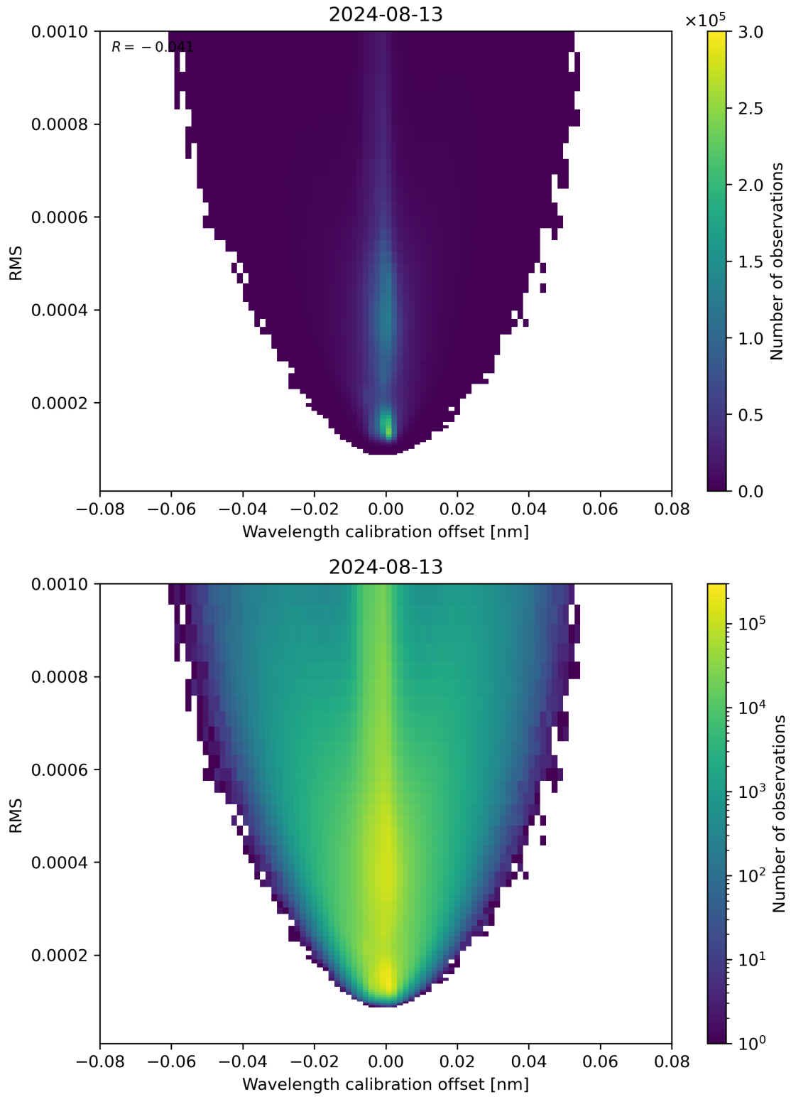
Figure 181: Scatter density plot of “Wavelength calibration offset” against “RMS” for 2024-08-12 to 2024-08-14.
