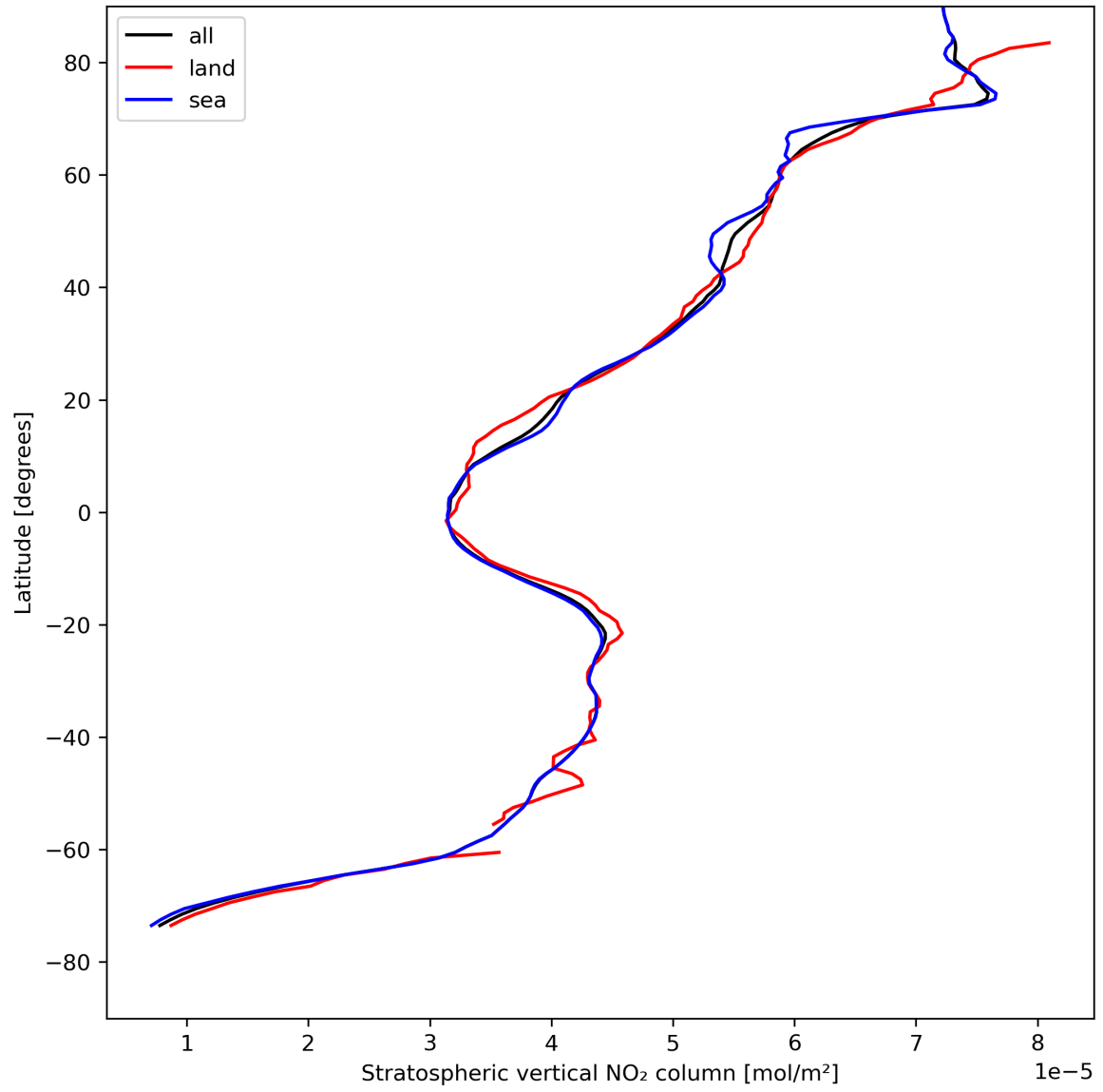
Figure 19: Zonal average of “Stratospheric vertical NO 2 column” for 2024-08-12 to 2024-08-14.
