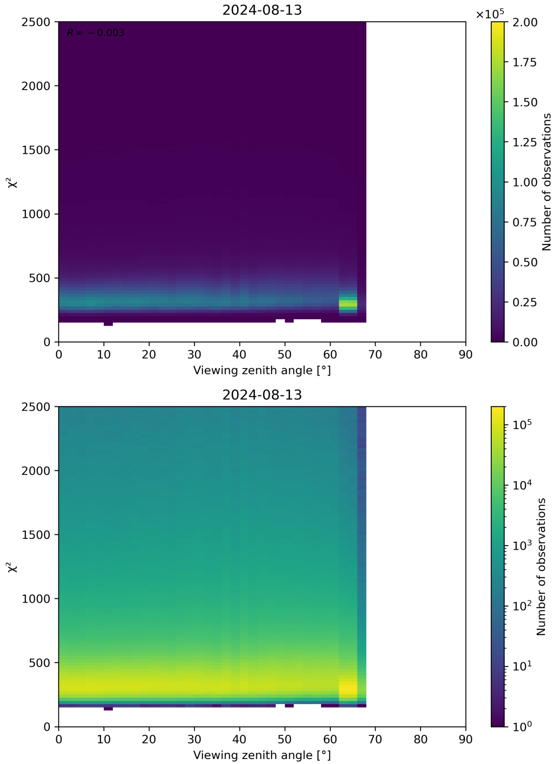
Figure 162: Scatter density plot of “Viewing zenith angle” against “ \chi^2 ” for 2024-08-12 to 2024-08-14.
