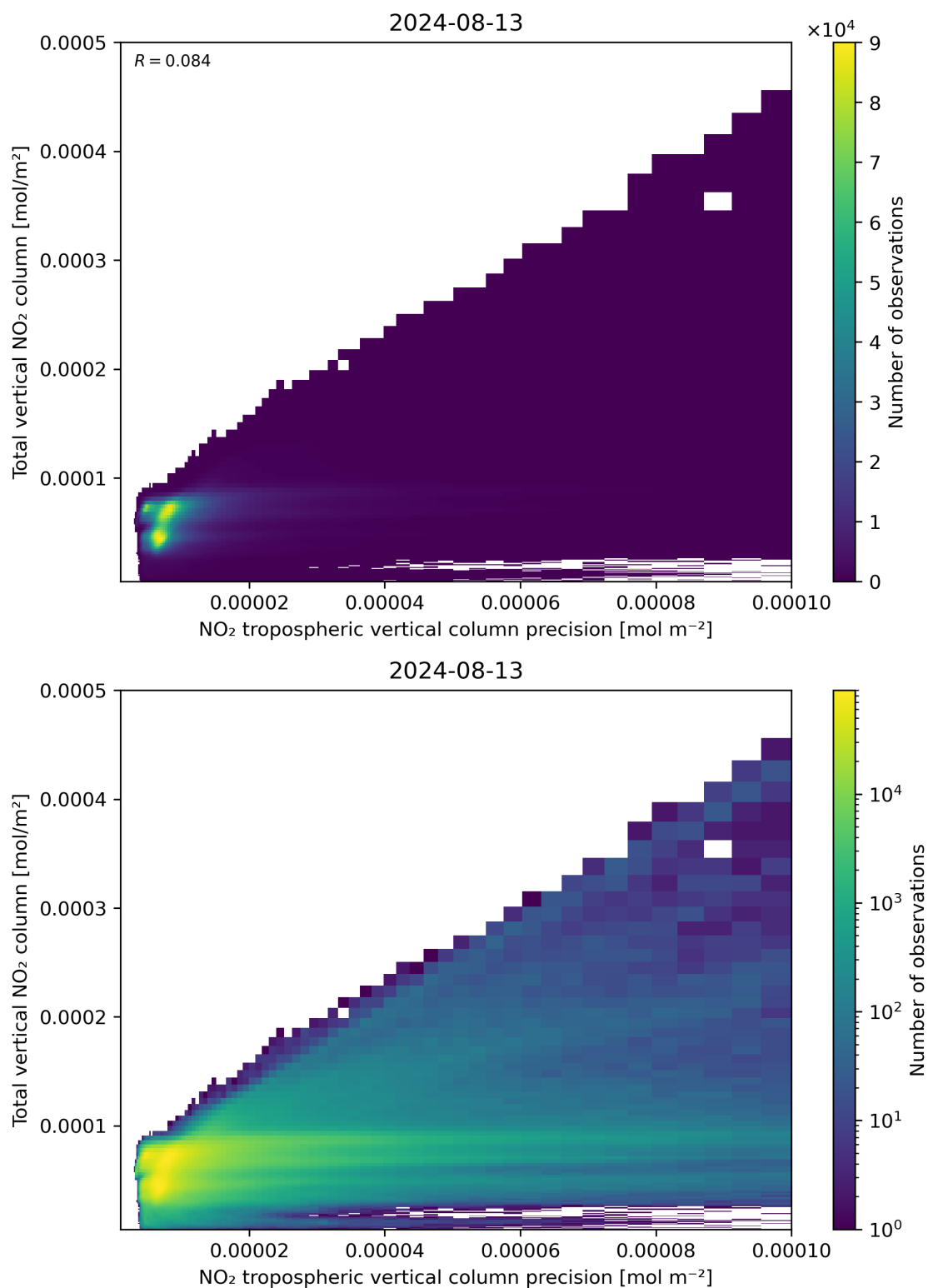
Figure 138: Scatter density plot of “NO 2 tropospheric vertical column precision” against “Total vertical NO 2 column” for 2024-08-12 to 2024-08-14.
