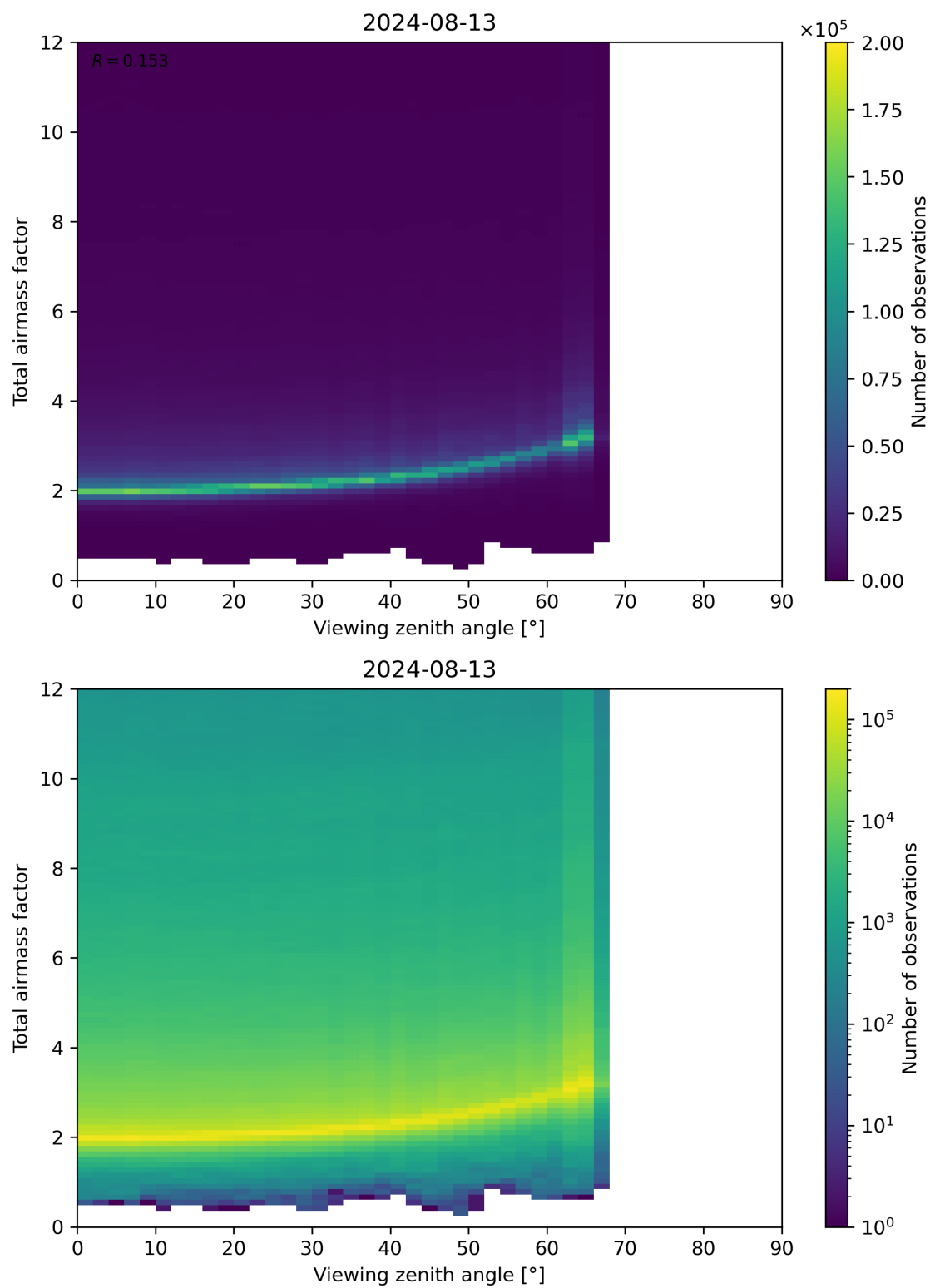
Figure 160: Scatter density plot of “Viewing zenith angle” against “Total airmass factor” for 2024-08-12 to 2024-08-14.
