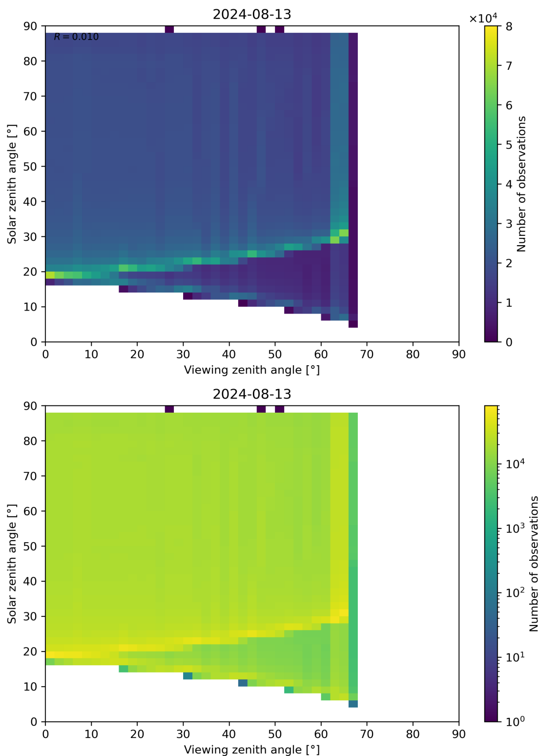
Figure 172: Scatter density plot of “Viewing zenith angle” against “Solar zenith angle” for 2024-08-12 to 2024-08-14.
