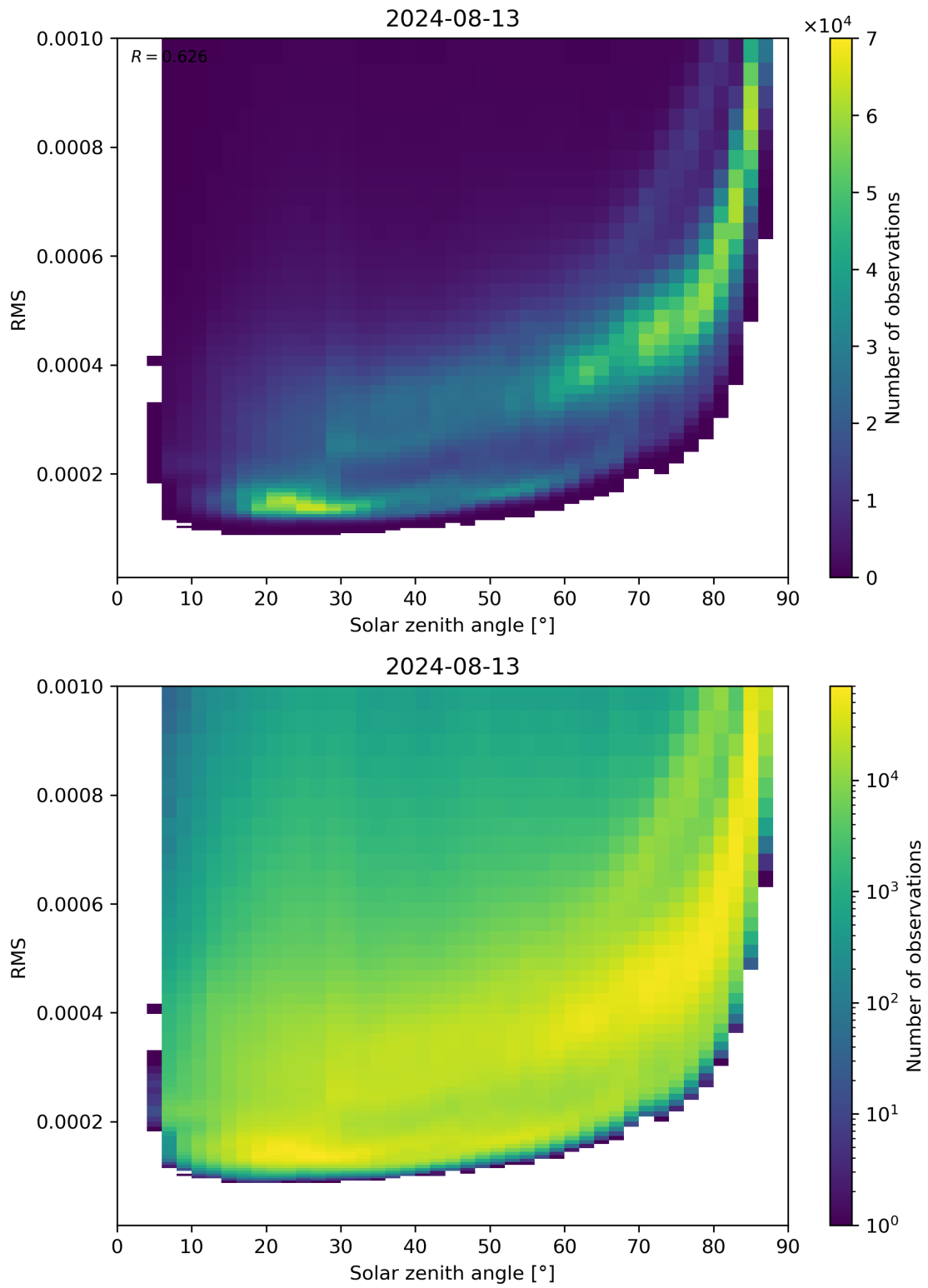
Figure 157: Scatter density plot of “Solar zenith angle” against “RMS” for 2024-08-12 to 2024-08-14.
