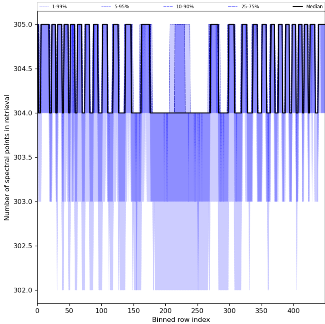
Figure 50: Along track statistics of “Number of spectral points in retrieval” for 2024-08-12 to 2024-08-14
