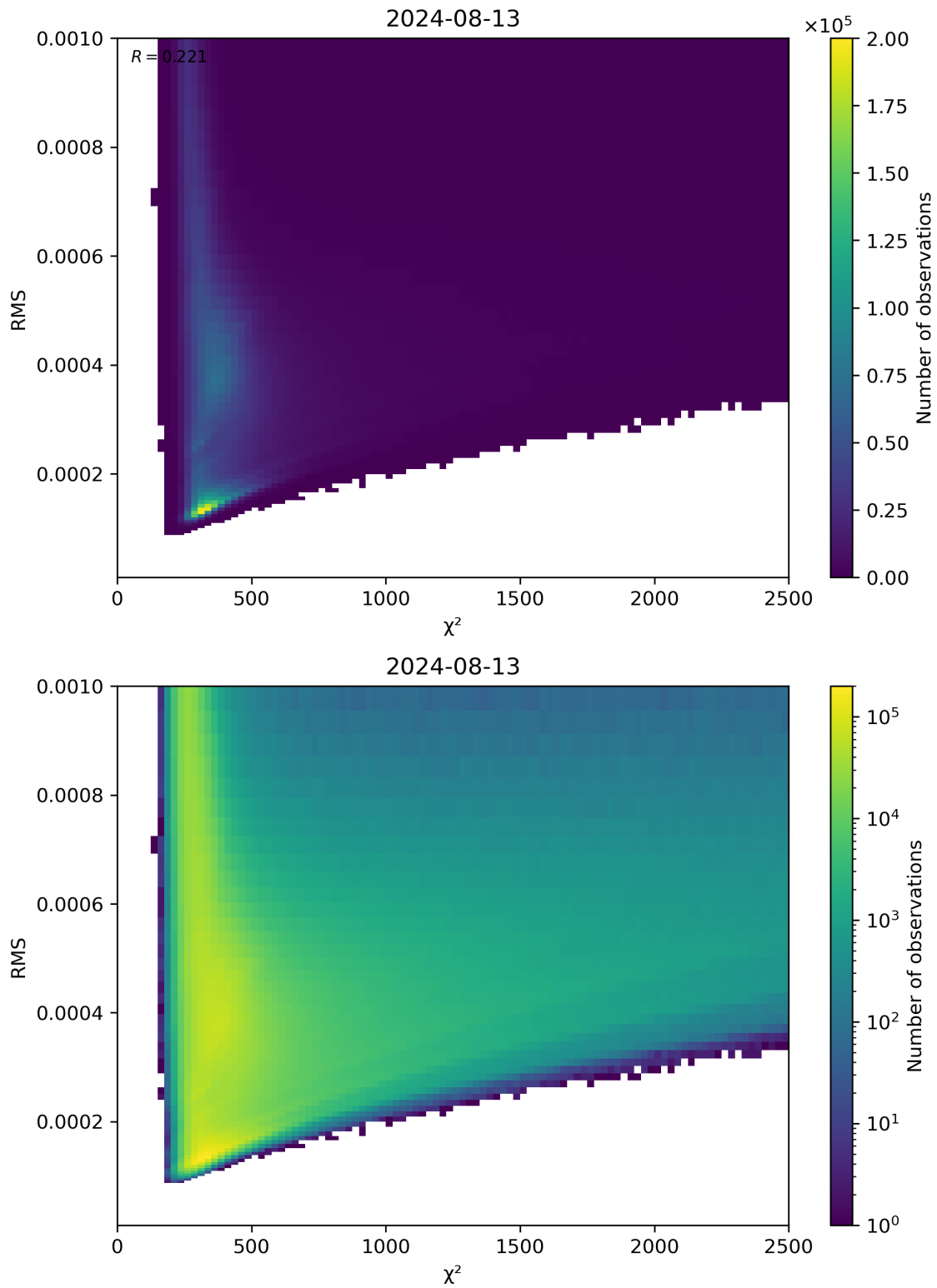
Figure 82: Scatter density plot of “ \chi^2 ” against “RMS” for 2024-08-12 to 2024-08-14.
