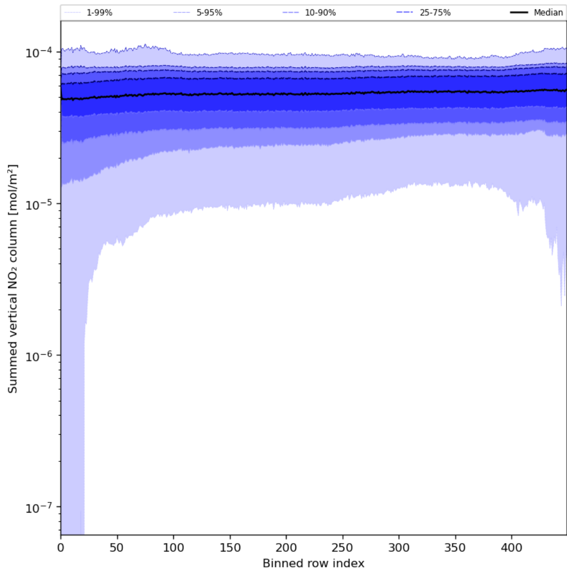
Figure 57: Along track statistics of “Summed vertical NO 2 column” for 2024-08-12 to 2024-08-14
