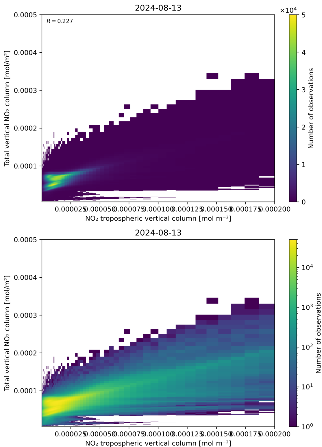
Figure 128: Scatter density plot of “NO 2 tropospheric vertical column” against “Total vertical NO 2 column” for 2024-08-12 to 2024-08-14.
