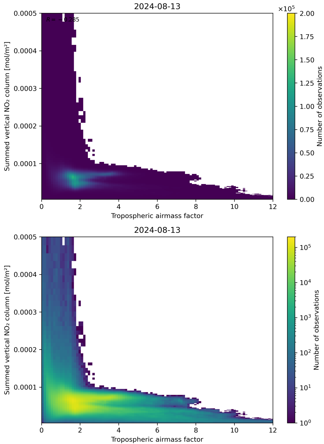
Figure 75: Scatter density plot of “Tropospheric airmass factor” against “Summed vertical NO 2 column” for 2024-08-12 to 2024-08-14.
