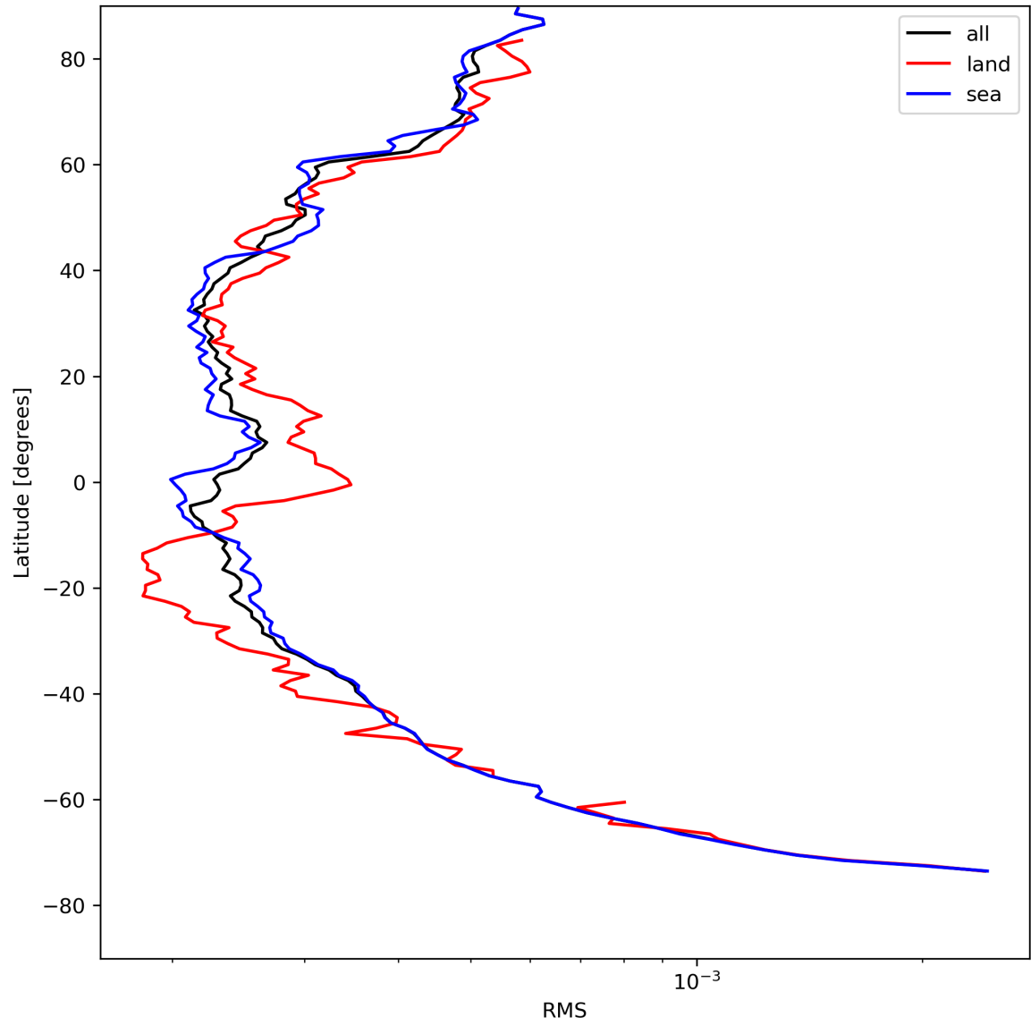
Figure 26: Zonal average of “RMS” for 2024-08-12 to 2024-08-14.
