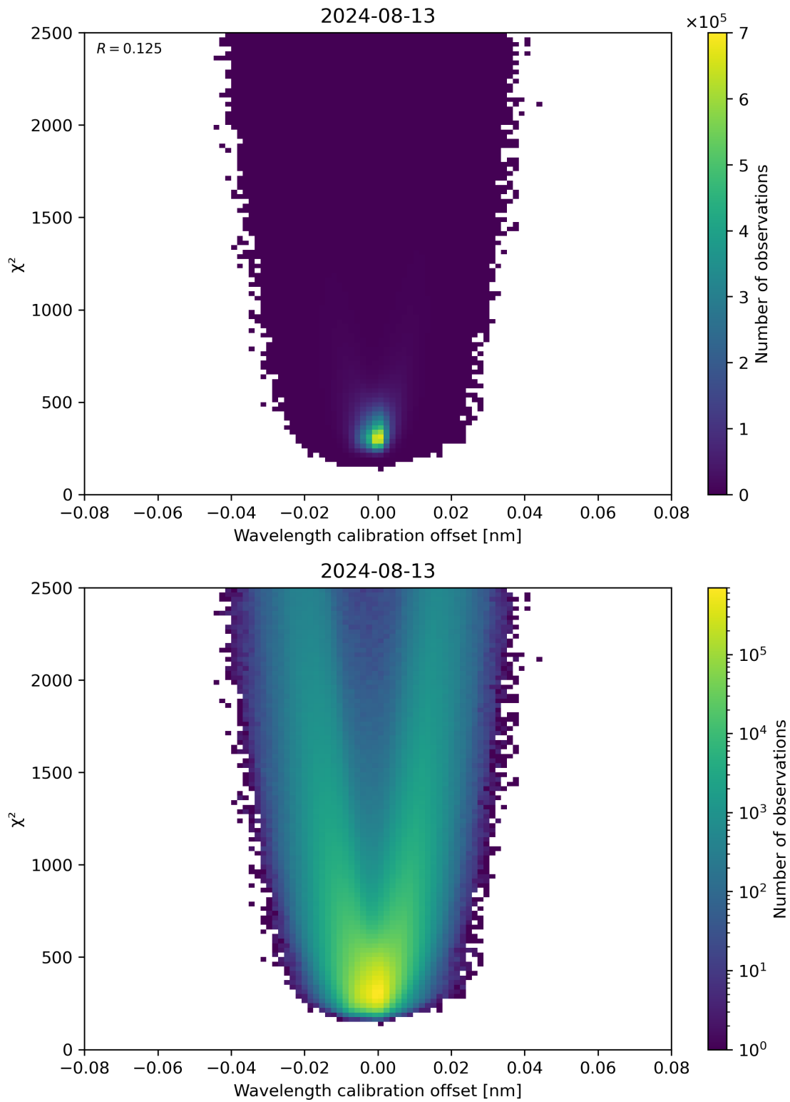
Figure 175: Scatter density plot of “Wavelength calibration offset” against “ \chi^2 ” for 2024-08-12 to 2024-08-14.
