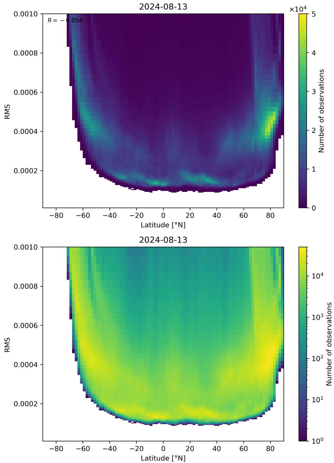
Figure 94: Scatter density plot of “Latitude” against “RMS” for 2024-08-12 to 2024-08-14.
