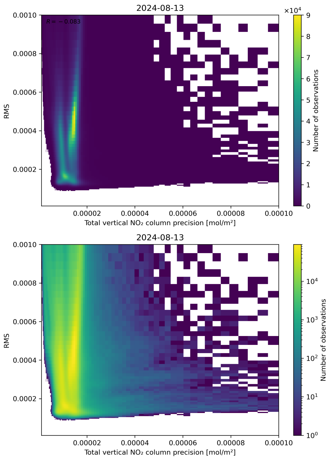
Figure 119: Scatter density plot of “Total vertical NO 2 column precision” against “RMS” for 2024-08-12 to 2024-08-14.
