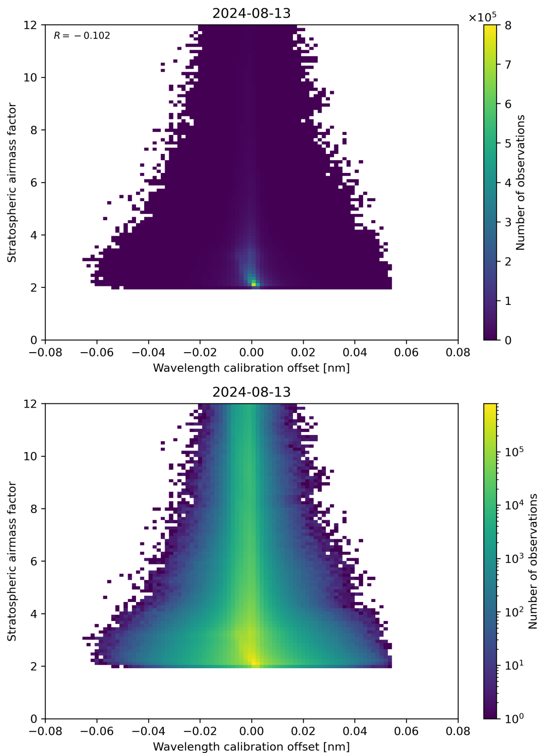
Figure 174: Scatter density plot of “Wavelength calibration offset” against “Stratospheric air mass factor” for 2024-08-12 to 2024-08-14.
