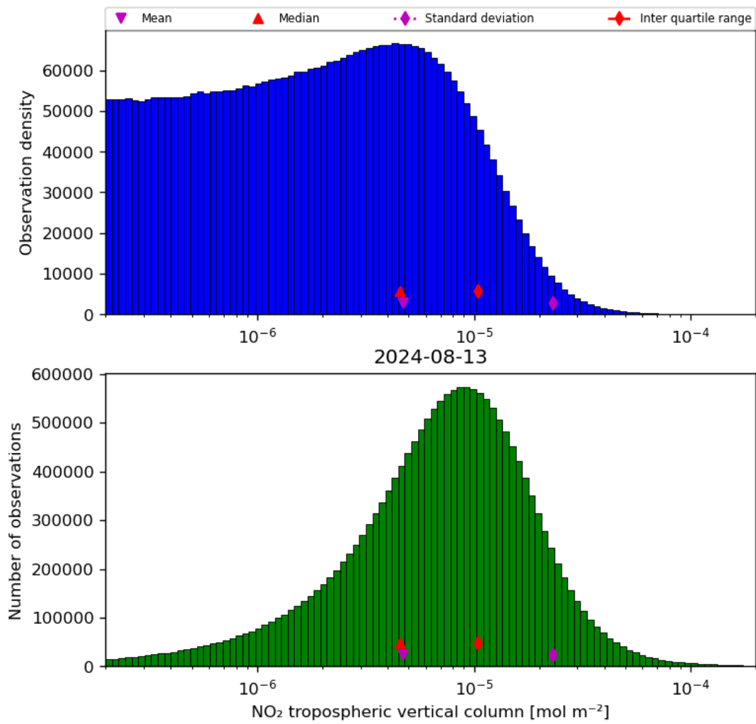
Figure 29: Histogram of “NO 2 tropospheric vertical column” for 2024-08-12 to 2024-08-14
