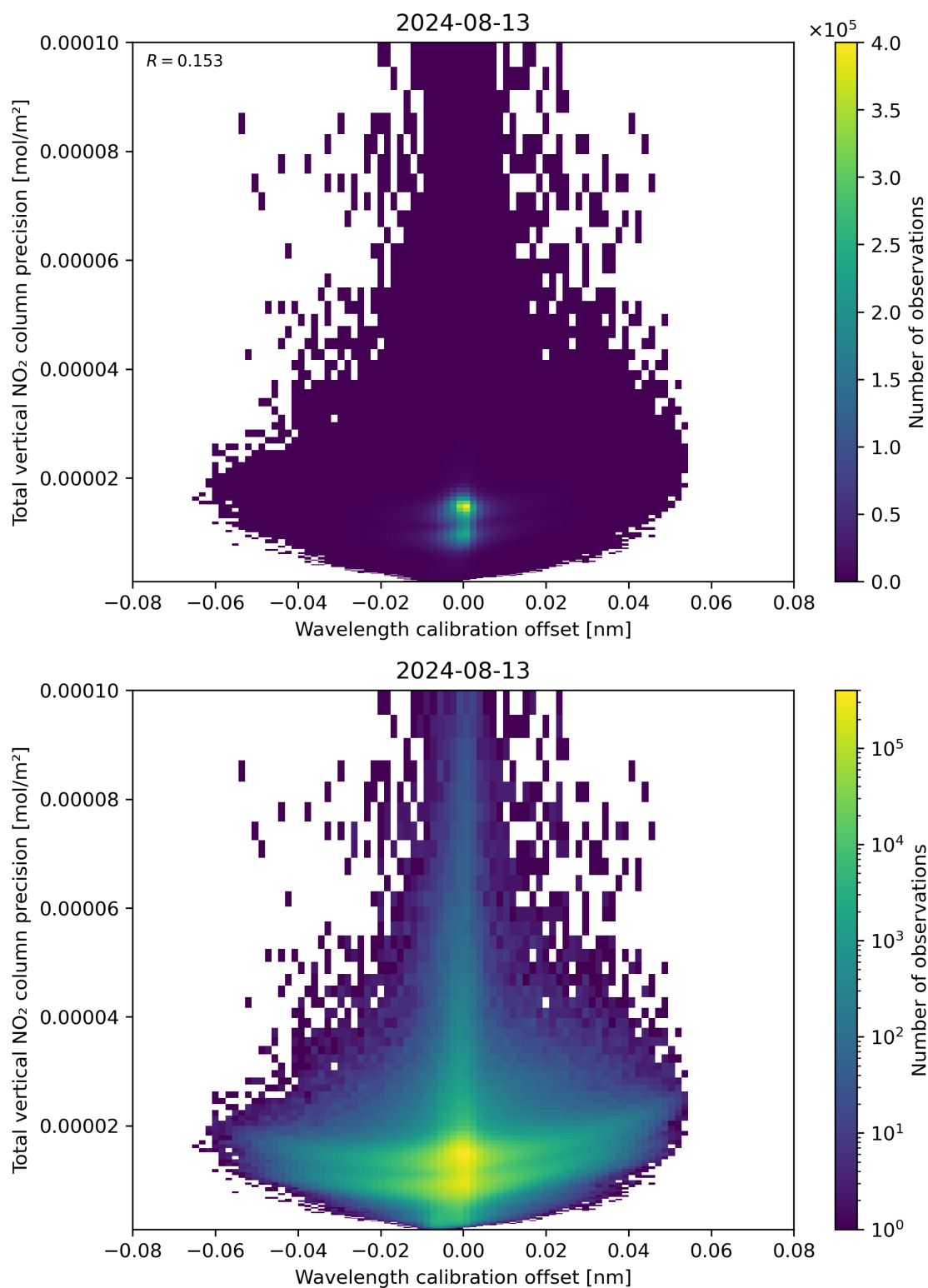
Figure 180: Scatter density plot of “Wavelength calibration offset” against “Total vertical NO 2 column precision” for 2024-08-12 to 2024-08-14.
