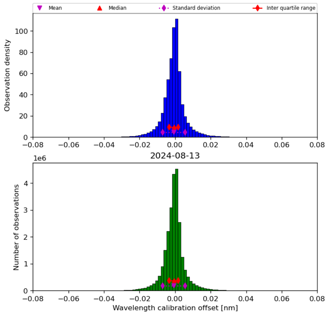
Figure 35: Histogram of “Wavelength calibration offset” for 2024-08-12 to 2024-08-14
