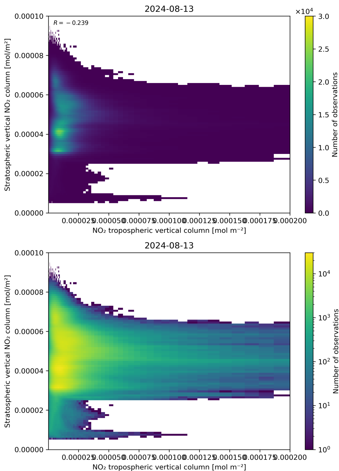
Figure 125: Scatter density plot of “NO 2 tropospheric vertical column” against “Stratospheric vertical NO 2 column” for 2024-08-12 to 2024-08-14.
