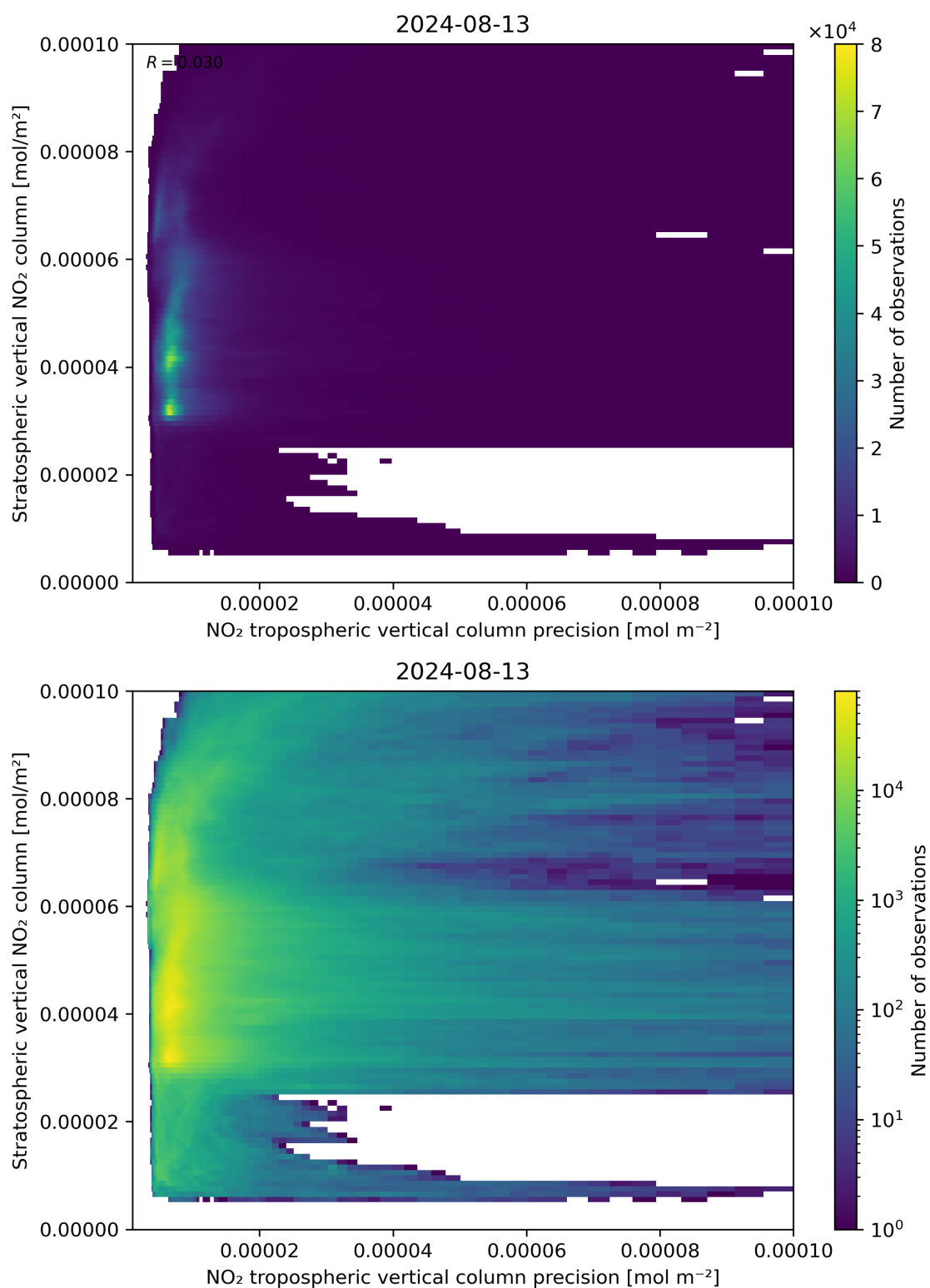
Figure 135: Scatter density plot of “NO 2 tropospheric vertical column precision” against “Stratospheric vertical NO 2 column” for 2024-08-12 to 2024-08-14.
