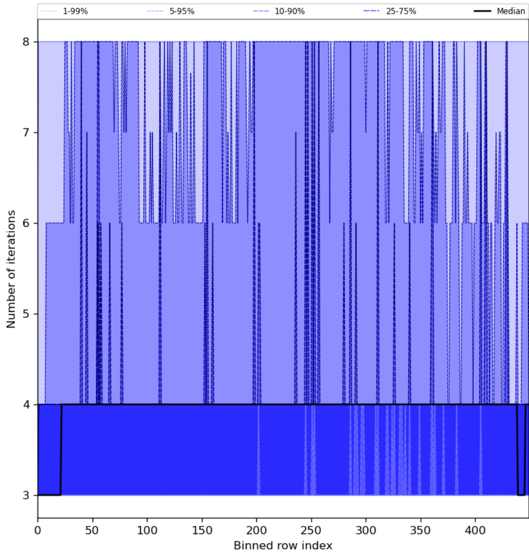
Figure 51: Along track statistics of “Number of iterations” for 2024-08-12 to 2024-08-14
