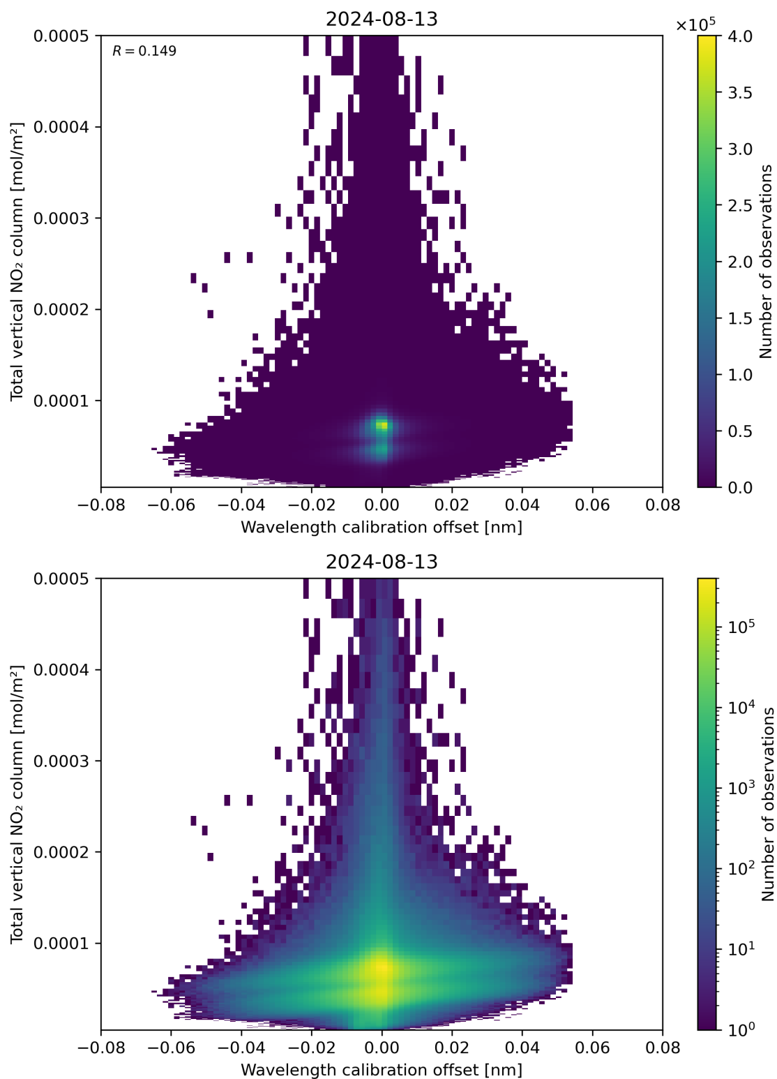
Figure 179: Scatter density plot of “Wavelength calibration offset” against “Total vertical NO 2 column” for 2024-08-12 to 2024-08-14.
