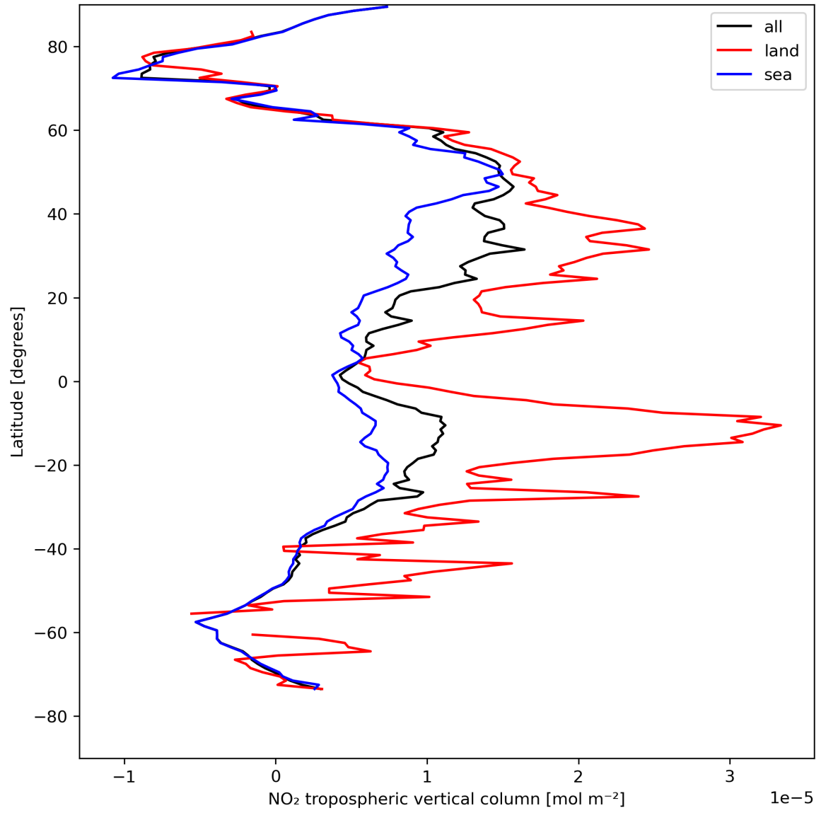
Figure 12: Zonal average of “NO 2 tropospheric vertical column” for 2024-08-12 to 2024-08-14.
