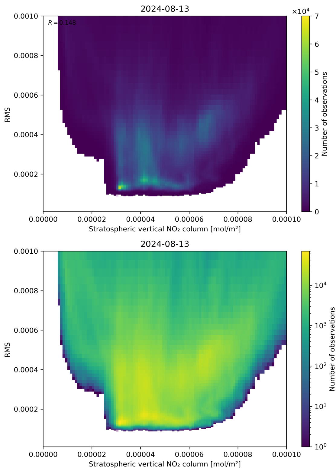
Figure 102: Scatter density plot of “Stratospheric vertical NO 2 column” against “RMS” for 2024-08-12 to 2024-08-14.
