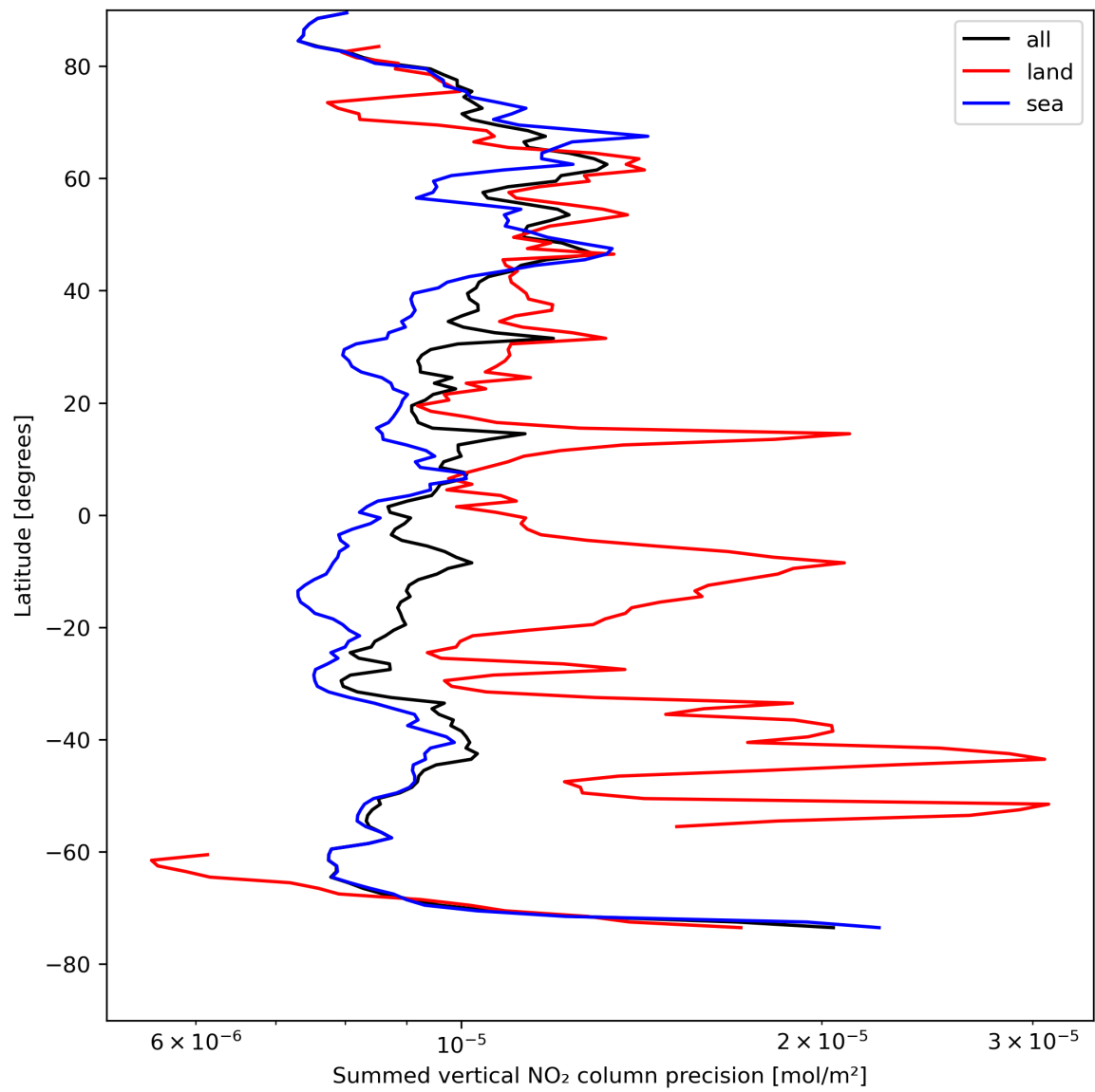
Figure 24: Zonal average of “Summed vertical NO 2 column precision” for 2024-08-12 to 2024-08-14.
