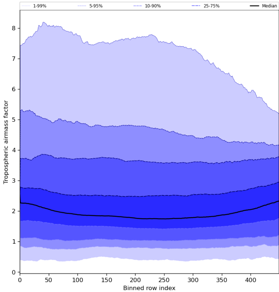
Figure 48: Along track statistics of “Tropospheric airmass factor” for 2024-08-12 to 2024-08-14
