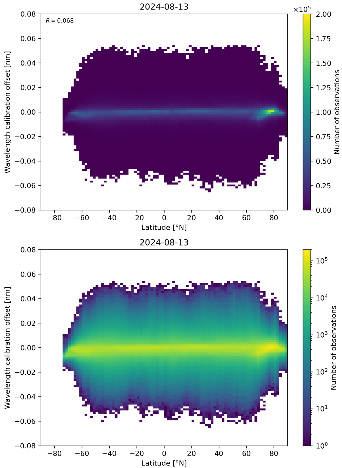
Figure 95: Scatter density plot of “Latitude” against “Wavelength calibration offset” for 2024-08-12 to 2024-08-14.
