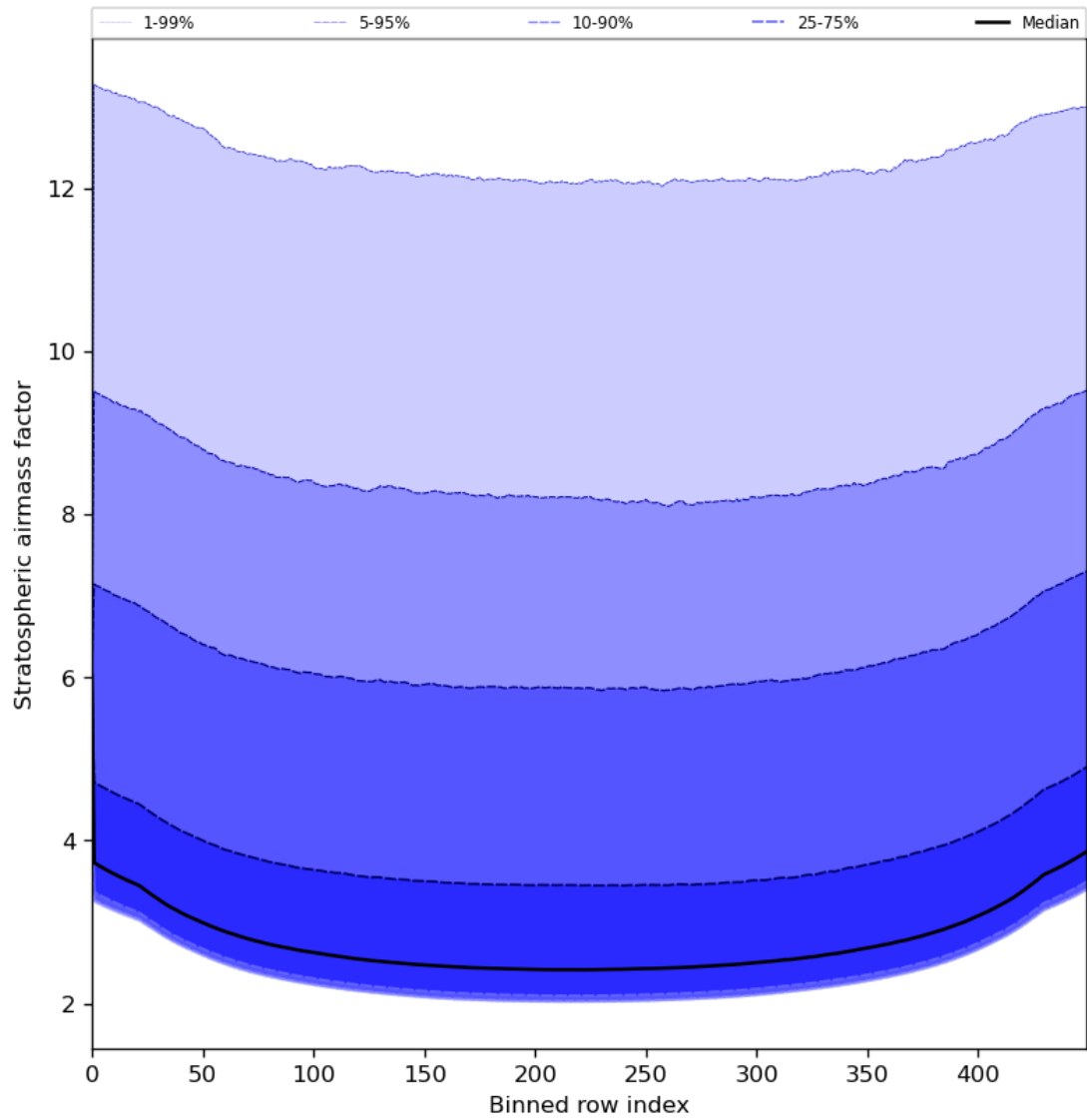
Figure 61: Along track statistics of “Stratospheric airmass factor” for 2024-08-12 to 2024-08-14
