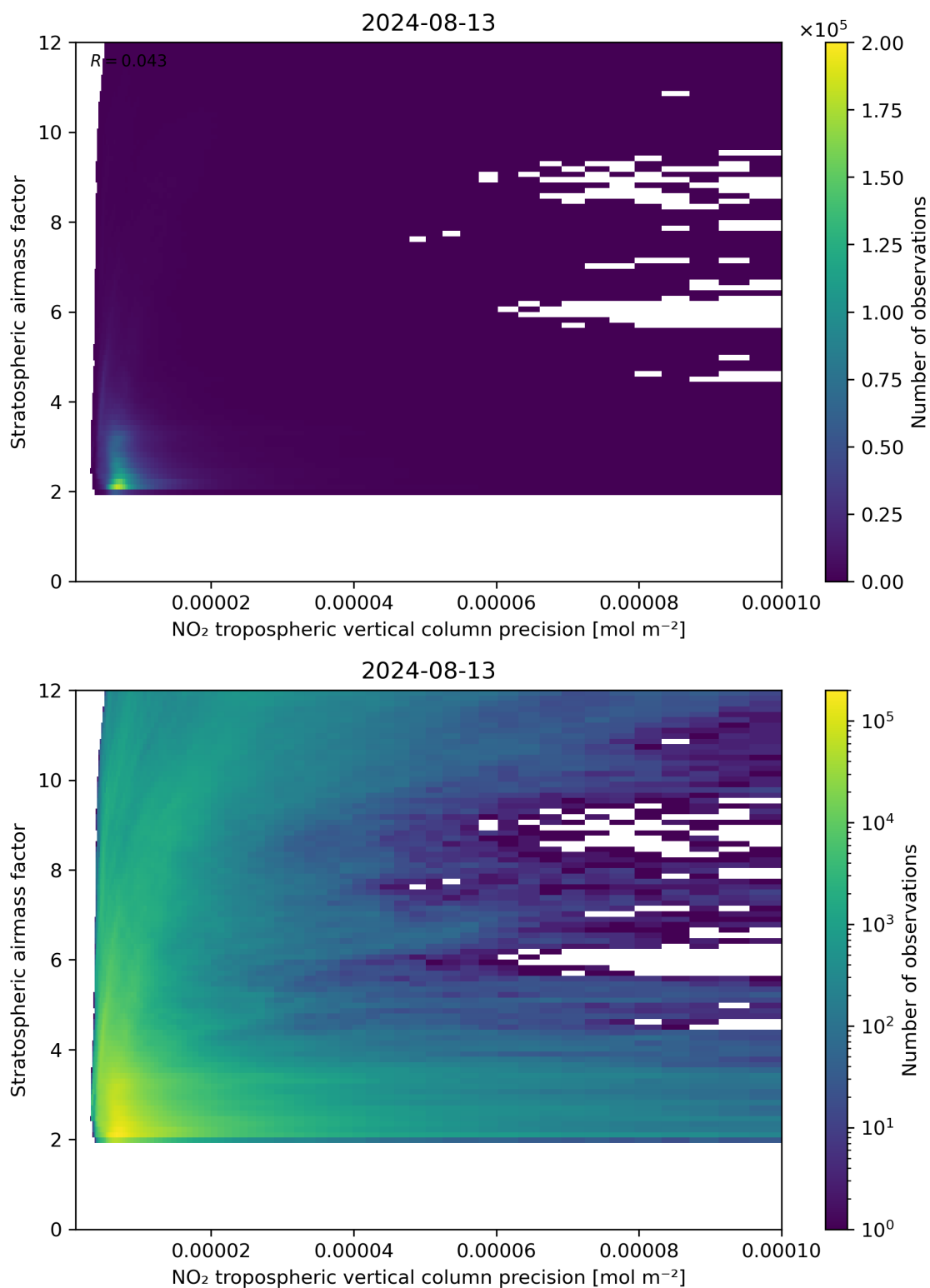
Figure 131: Scatter density plot of “NO 2 tropospheric vertical column precision” against “Stratospheric airmass factor” for 2024-08-12 to 2024-08-14.
