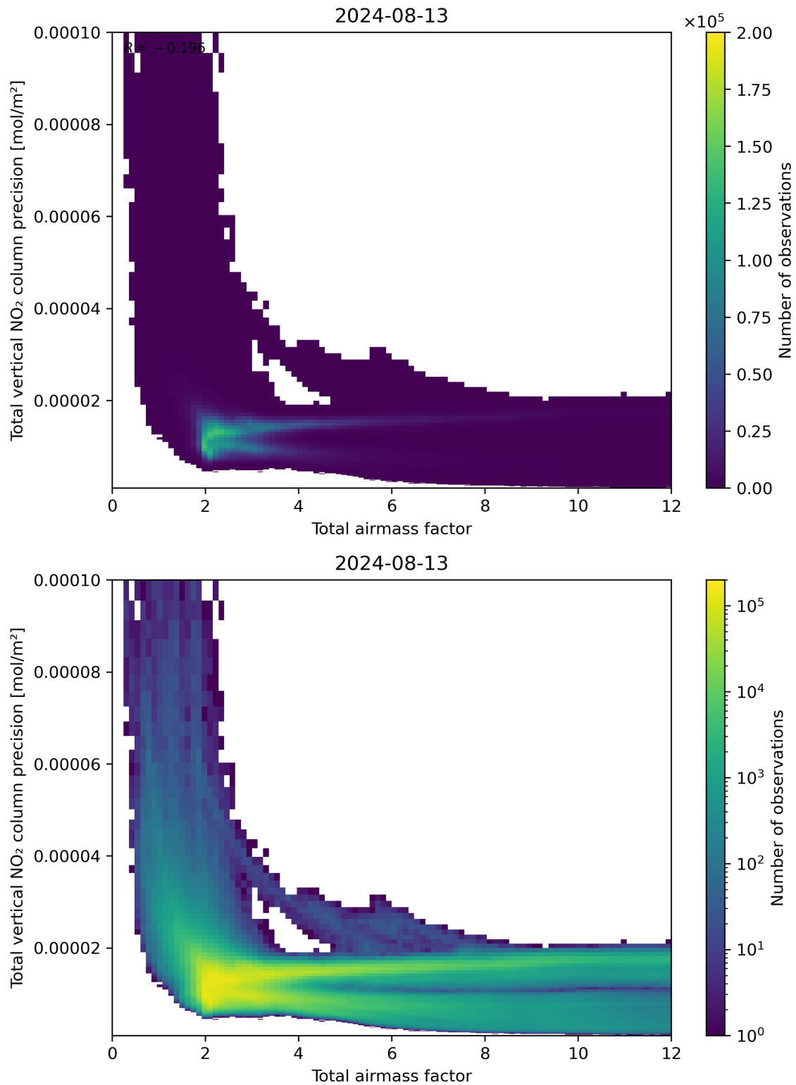
Figure 68: Scatter density plot of “Total airmass factor” against “Total vertical NO 2 column precision” for 2024-08-12 to 2024-08-14.
