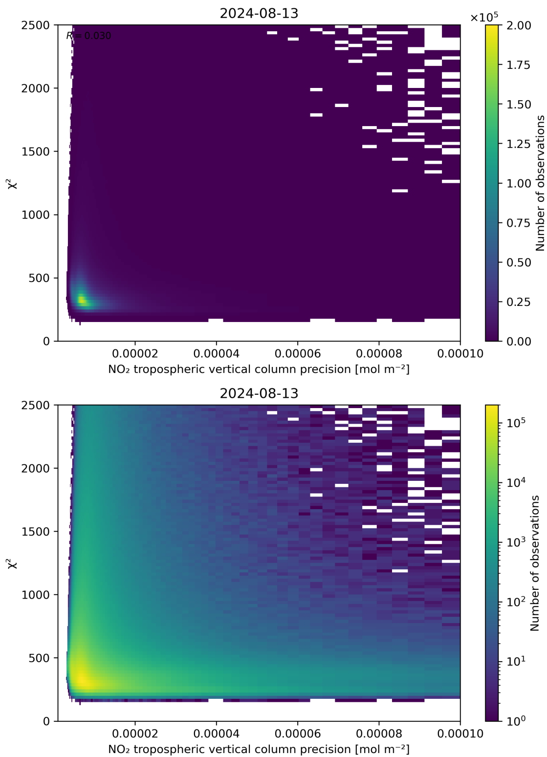
Figure 134: Scatter density plot of “NO 2 tropospheric vertical column precision” against “ \chi^2 ” for 2024-08-12 to 2024-08-14.
