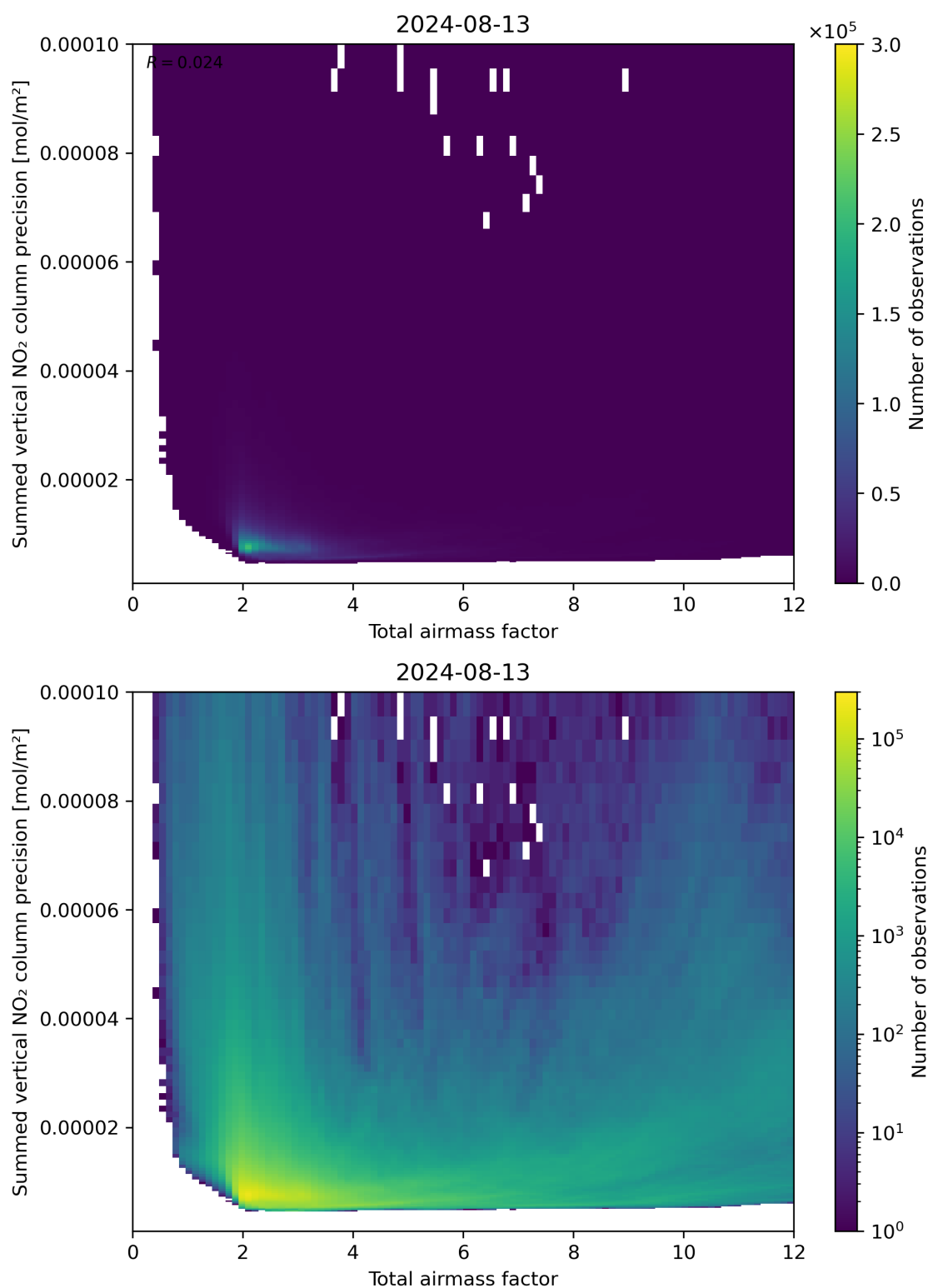
Figure 66: Scatter density plot of “Total airmass factor” against “Summed vertical NO 2 column precision” for 2024-08-12 to 2024-08-14.
