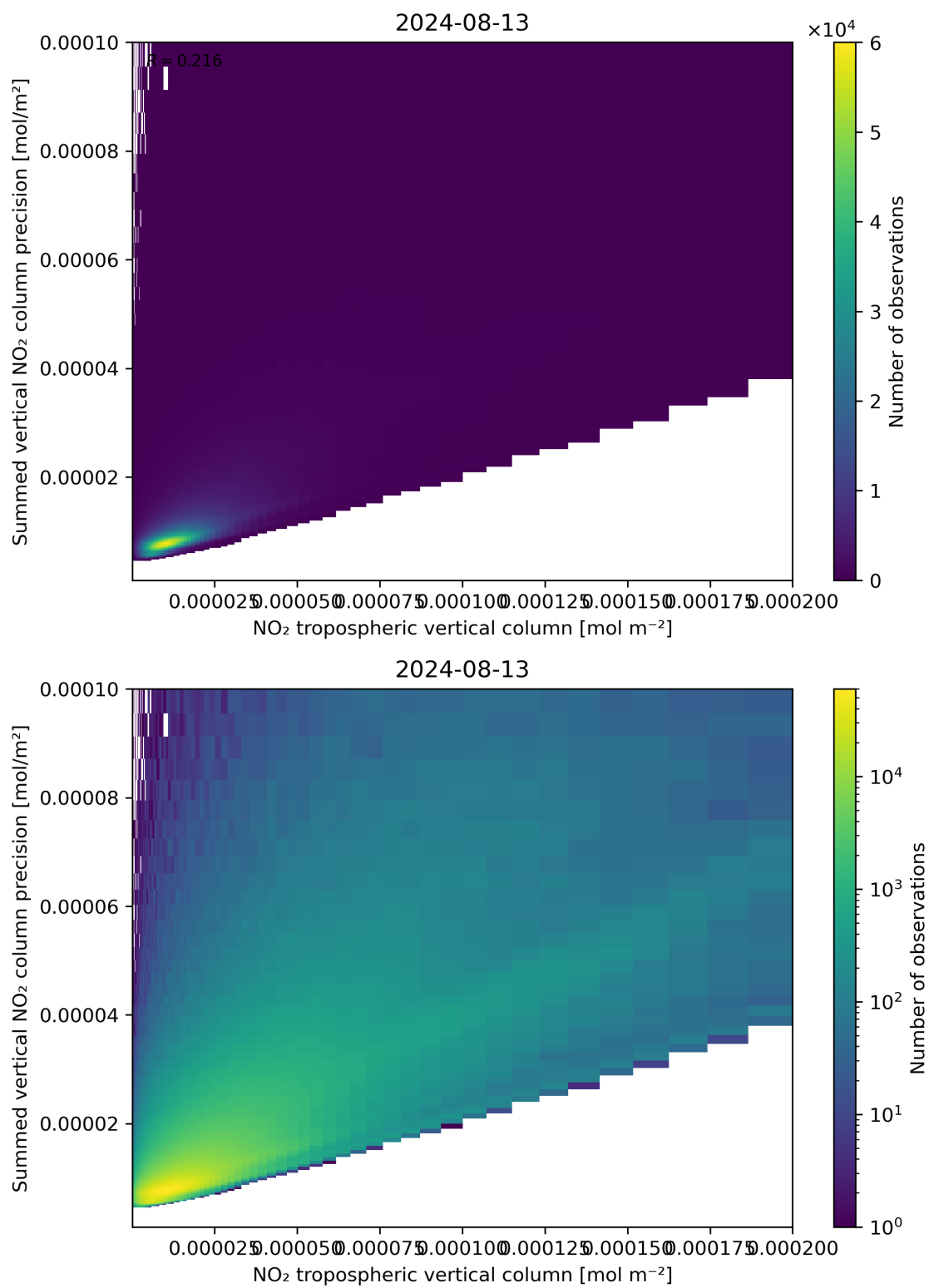
Figure 127: Scatter density plot of “NO 2 tropospheric vertical column” against “Summed vertical NO 2 column precision” for 2024-08-12 to 2024-08-14.
