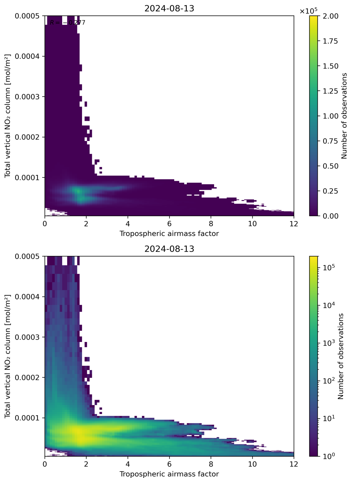
Figure 77: Scatter density plot of “Tropospheric airmass factor” against “Total vertical NO 2 column” for 2024-08-12 to 2024-08-14.
