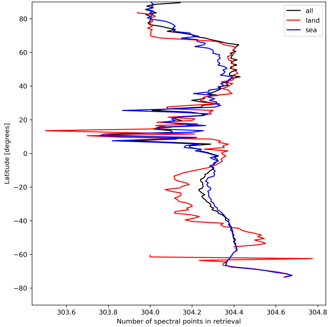
Figure 16: Zonal average of “Number of spectral points in retrieval” for 2024-08-12 to 2024-08-14.
