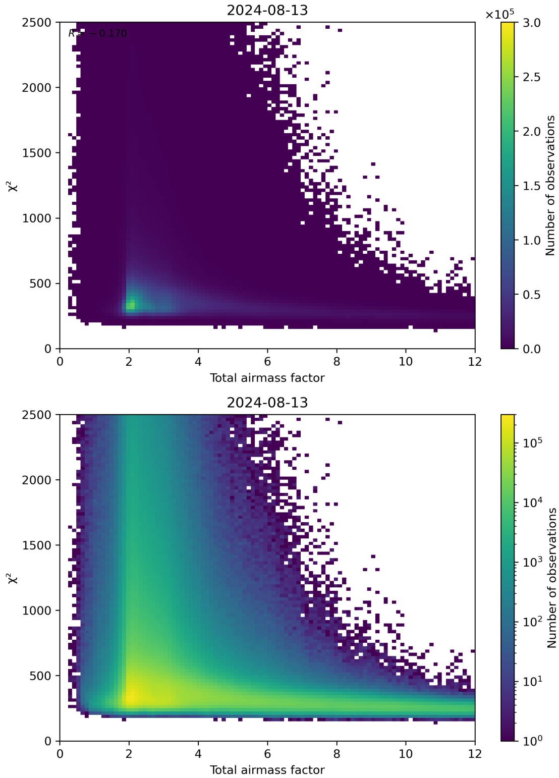
Figure 63: Scatter density plot of “Total airmass factor” against “ \chi^2 ” for 2024-08-12 to 2024-08-14.
