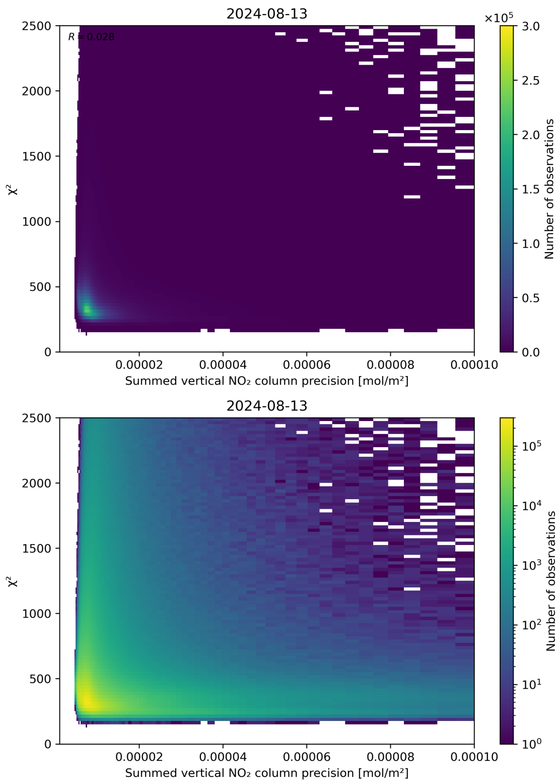
Figure 107: Scatter density plot of “Summed vertical NO 2 column precision” against “ \chi^2 ” for 2024-08-12 to 2024-08-14.
