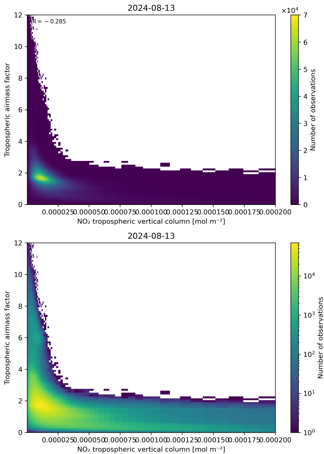
Figure 123: Scatter density plot of “NO 2 tropospheric vertical column” against “Tropospheric air mass factor” for 2024-08-12 to 2024-08-14.
