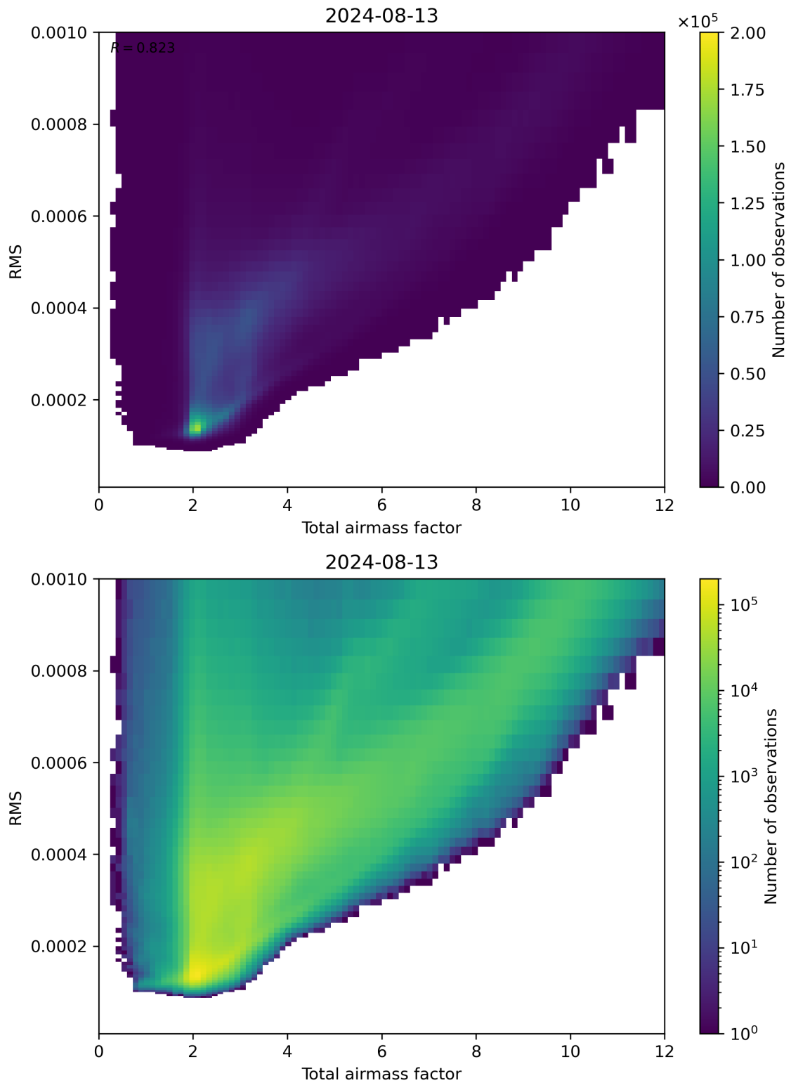
Figure 69: Scatter density plot of “Total airmass factor” against “RMS” for 2024-08-12 to 2024-08-14.
