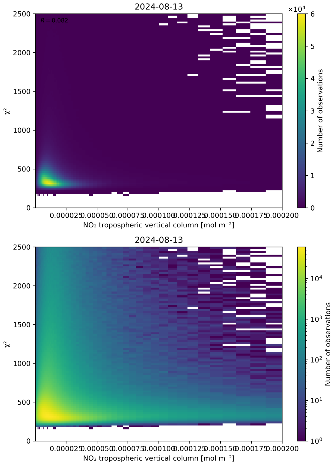
Figure 124: Scatter density plot of “NO 2 tropospheric vertical column” against “ \chi^2 ” for 2024-08-12 to 2024-08-14.
