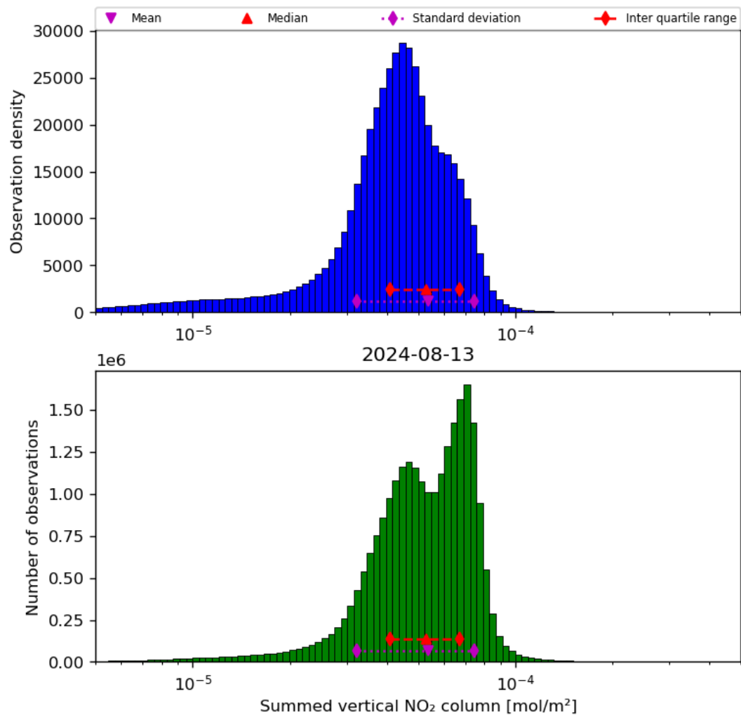
Figure 40: Histogram of “Summed vertical NO 2 column” for 2024-08-12 to 2024-08-14
