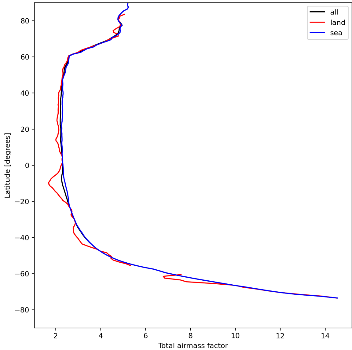
Figure 15: Zonal average of “Total airmass factor” for 2024-08-12 to 2024-08-14.
