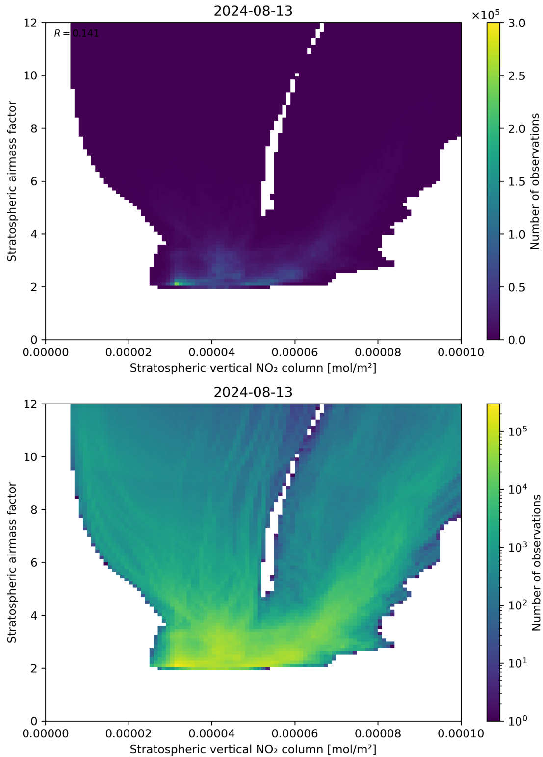
Figure 96: Scatter density plot of “Stratospheric vertical NO 2 column” against “Stratospheric airmass factor” for 2024-08-12 to 2024-08-14.
