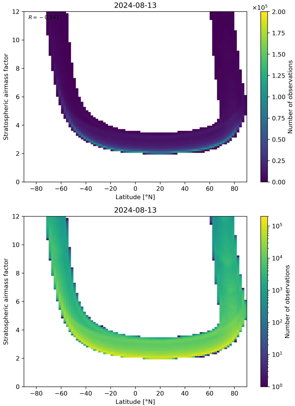
Figure 83: Scatter density plot of “Latitude” against “Stratospheric air mass factor” for 2024-08-12 to 2024-08-14.
