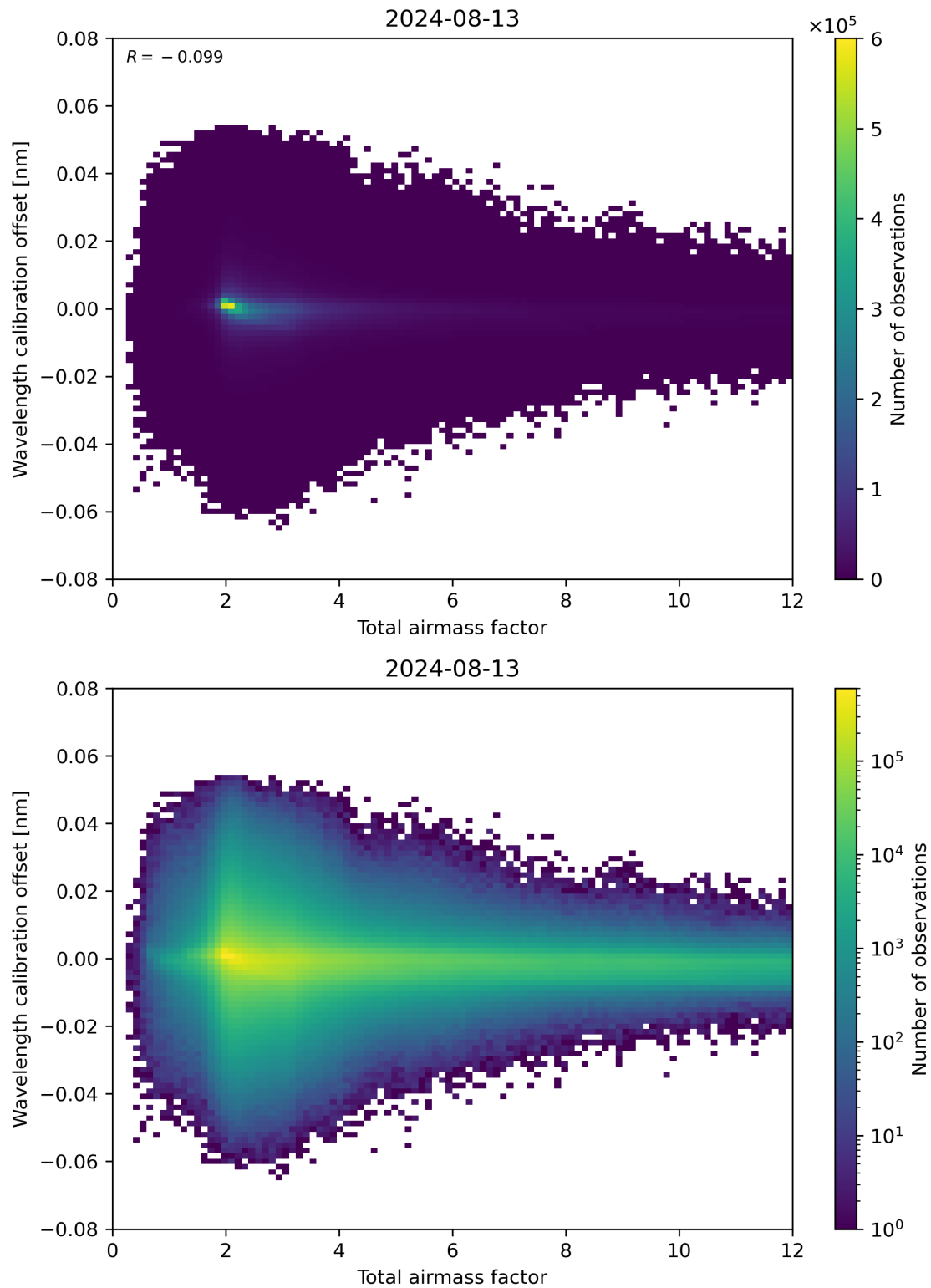
Figure 70: Scatter density plot of “Total airmass factor” against “Wavelength calibration offset” for 2024-08-12 to 2024-08-14.
