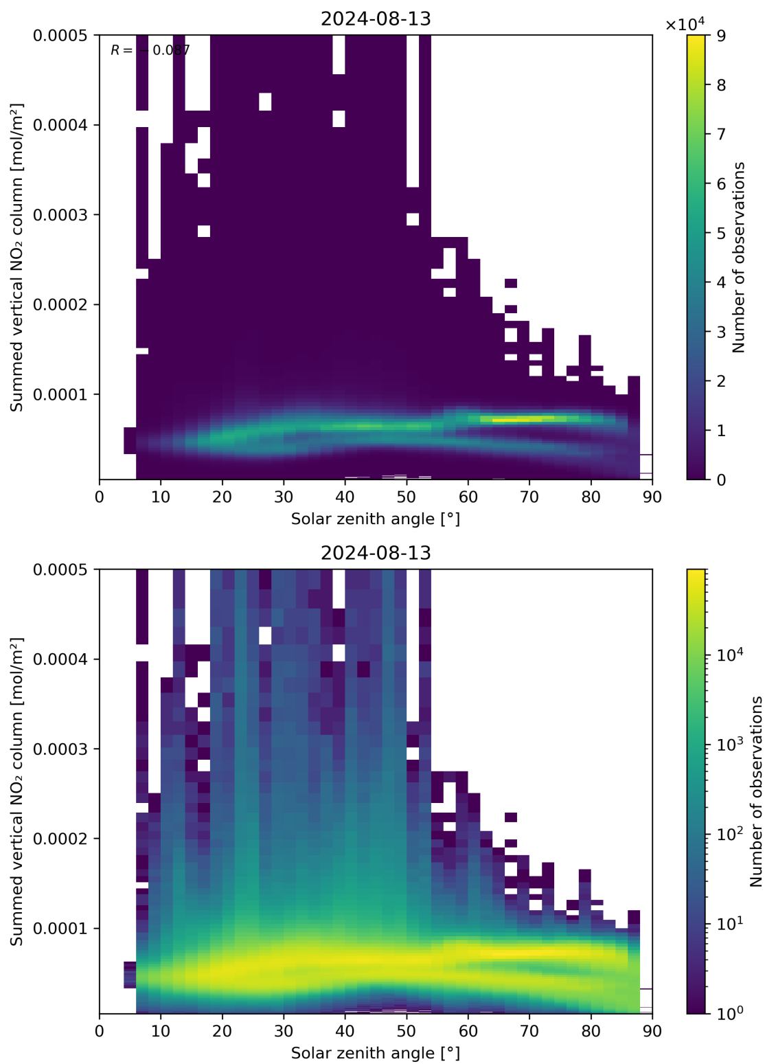
Figure 151: Scatter density plot of “Solar zenith angle” against “Summed vertical NO 2 column” for 2024-08-12 to 2024-08-14.
