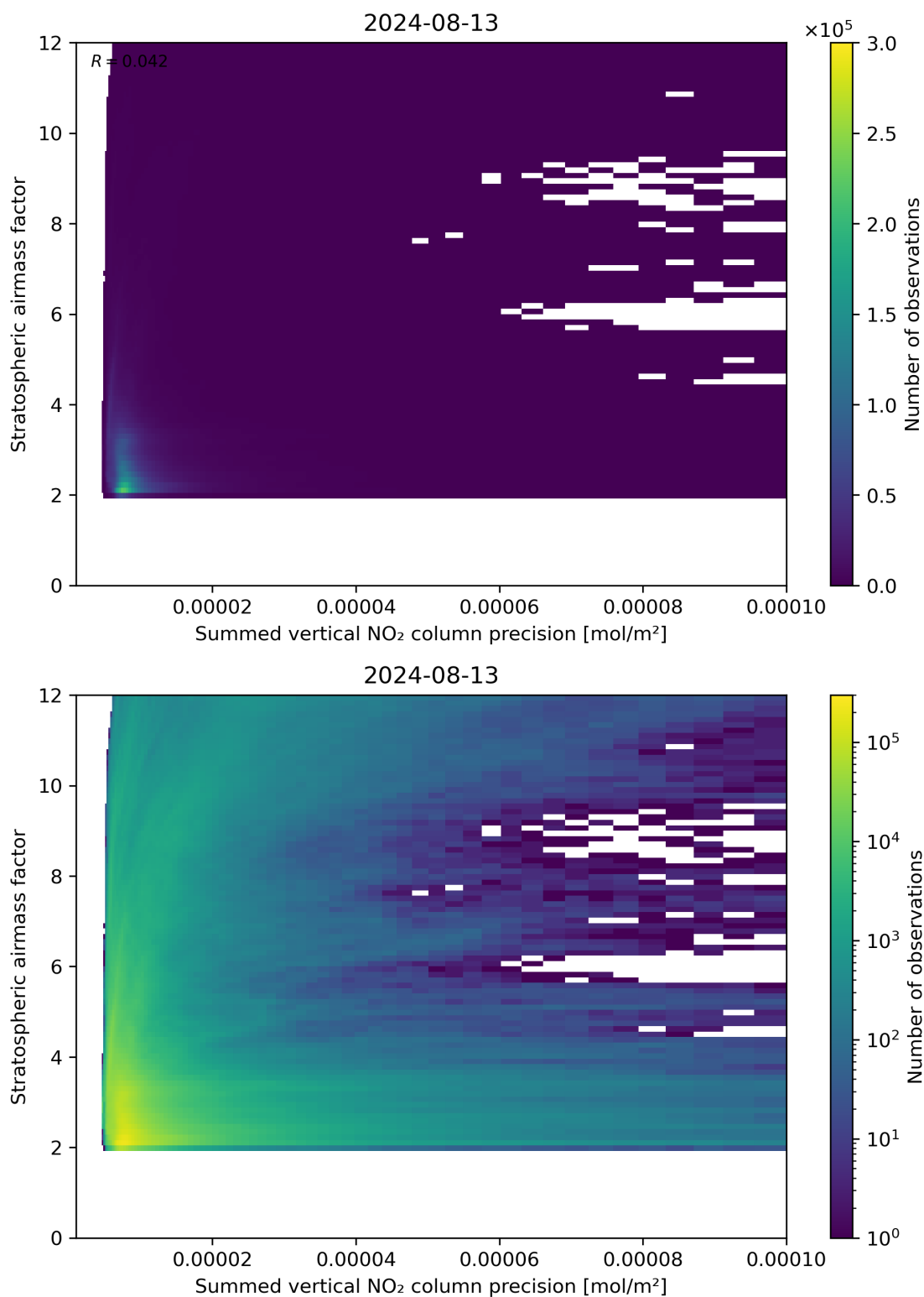
Figure 106: Scatter density plot of “Summed vertical NO 2 column precision” against “Stratospheric airmass factor” for 2024-08-12 to 2024-08-14.
