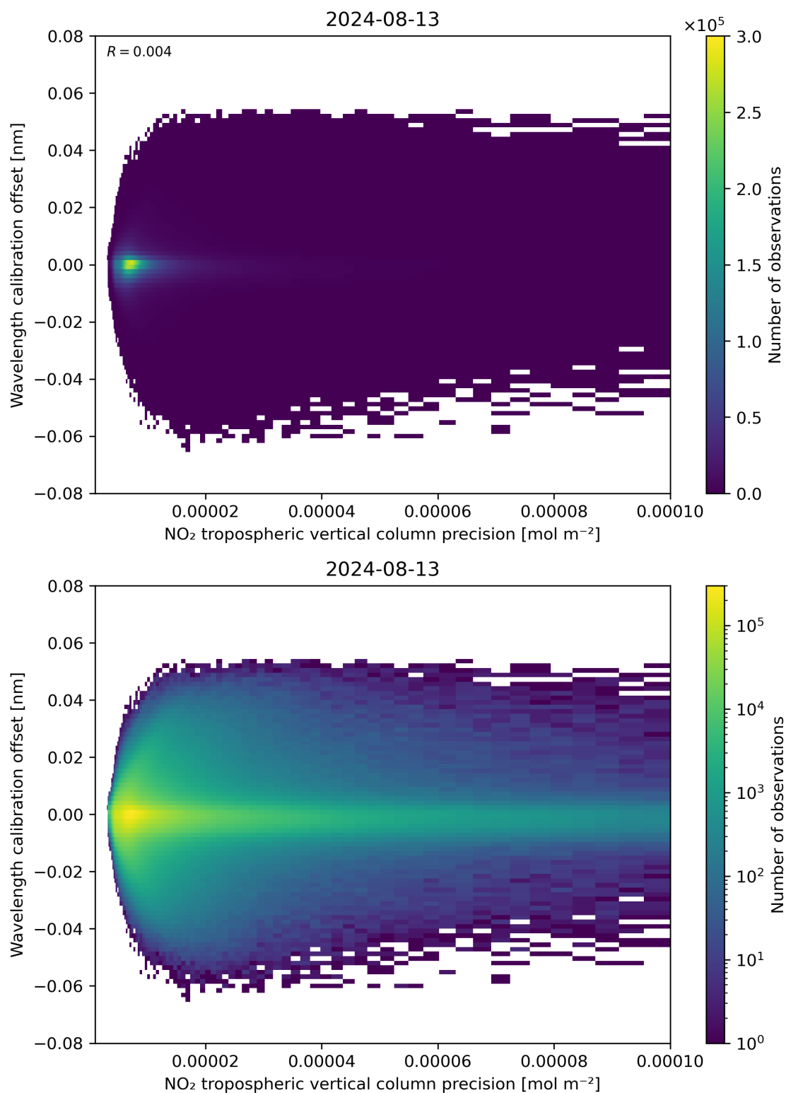
Figure 141: Scatter density plot of “NO 2 tropospheric vertical column precision” against “Wavelength calibration offset” for 2024-08-12 to 2024-08-14.
