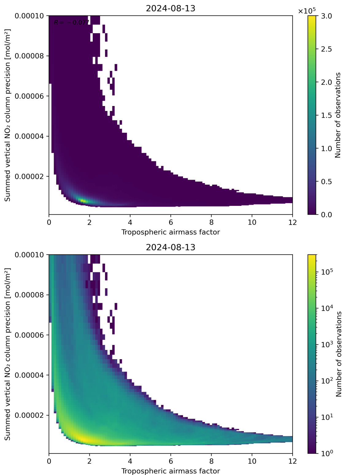
Figure 76: Scatter density plot of “Tropospheric air mass factor” against “Summed vertical NO 2 column precision” for 2024-08-12 to 2024-08-14.
