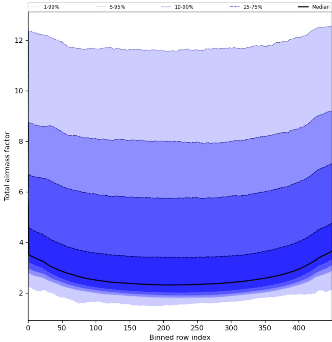
Figure 49: Along track statistics of “Total airmass factor” for 2024-08-12 to 2024-08-14
