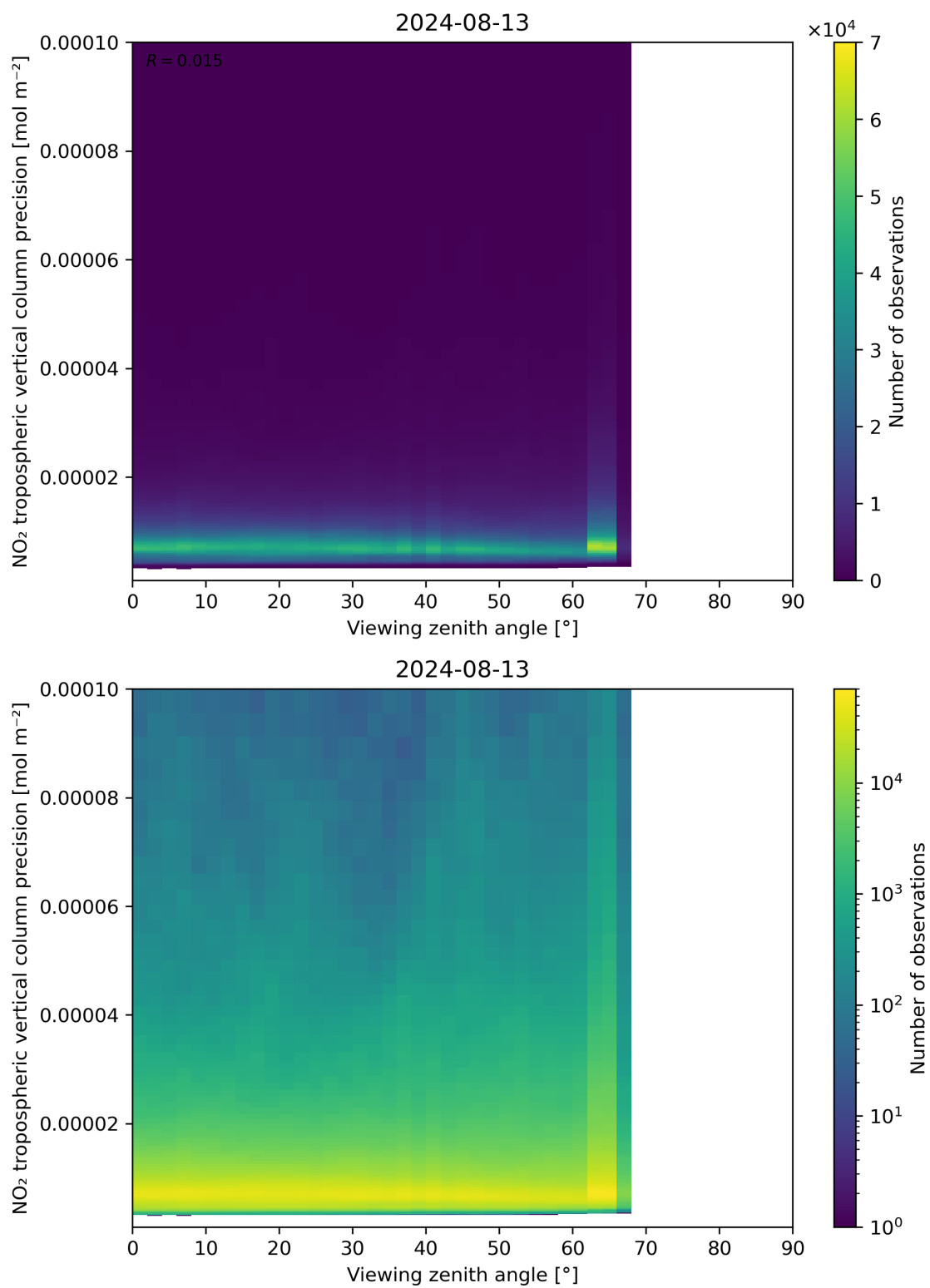
Figure 170: Scatter density plot of “Viewing zenith angle” against “NO 2 tropospheric vertical column precision” for 2024-08-12 to 2024-08-14.
