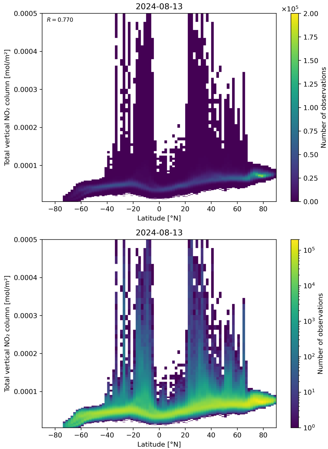
Figure 90: Scatter density plot of “Latitude” against “Total vertical NO 2 column” for 2024-08-12 to 2024-08-14.
