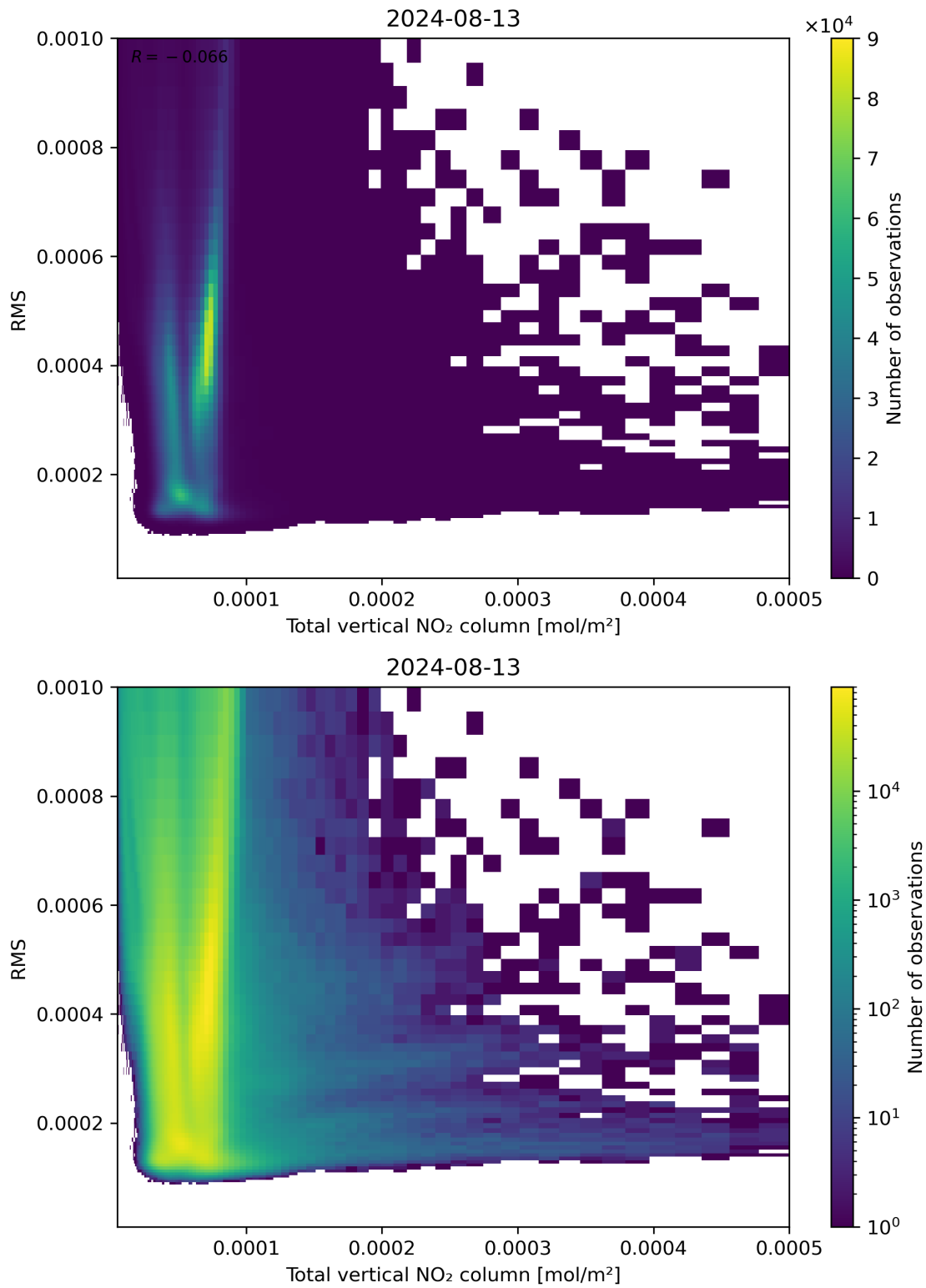
Figure 120: Scatter density plot of “Total vertical NO 2 column” against “RMS” for 2024-08-12 to 2024-08-14.
