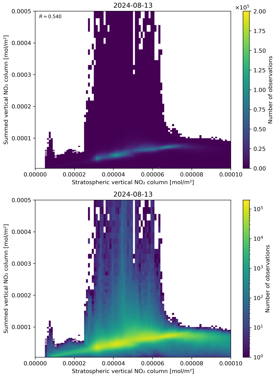
Figure 98: Scatter density plot of “Stratospheric vertical NO 2 column” against “Summed vertical NO 2 column” for 2024-08-12 to 2024-08-14.
