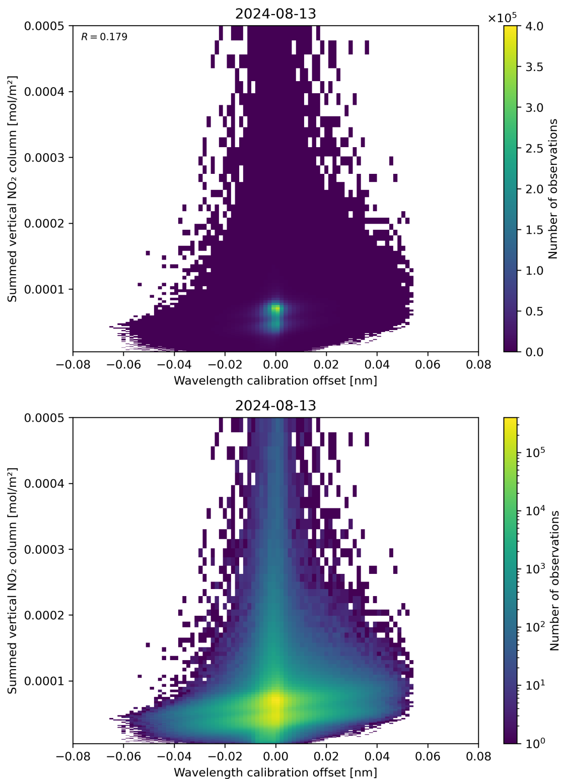
Figure 177: Scatter density plot of “Wavelength calibration offset” against “Summed vertical NO 2 column” for 2024-08-12 to 2024-08-14.
