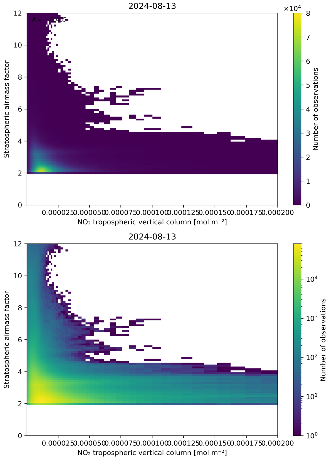
Figure 121: Scatter density plot of “NO 2 tropospheric vertical column” against “Stratospheric air mass factor” for 2024-08-12 to 2024-08-14.
