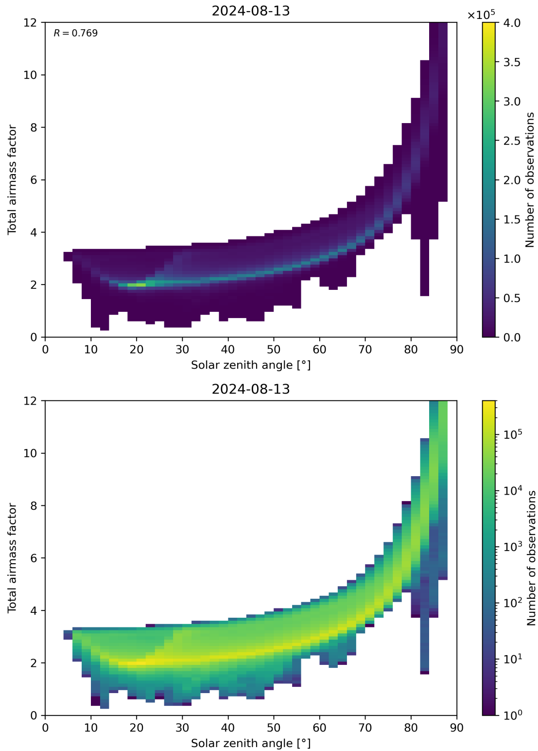
Figure 146: Scatter density plot of “Solar zenith angle” against “Total airmass factor” for 2024-08-12 to 2024-08-14.
