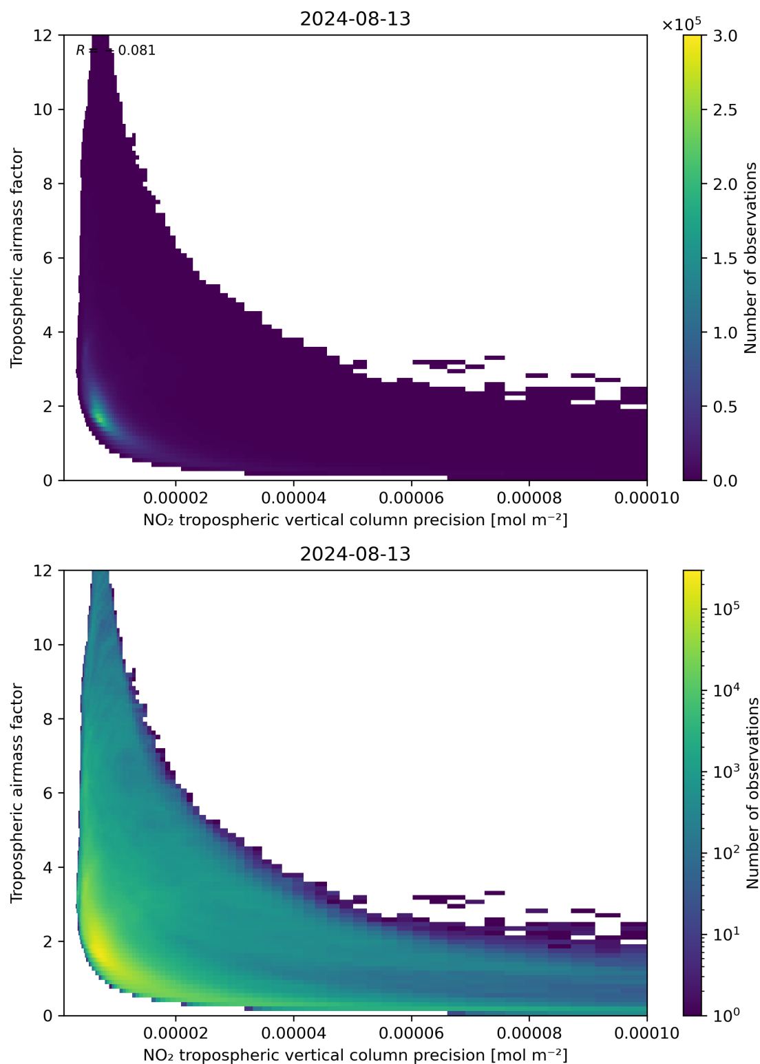
Figure 133: Scatter density plot of “NO 2 tropospheric vertical column precision” against “Tropospheric airmass factor” for 2024-08-12 to 2024-08-14.
