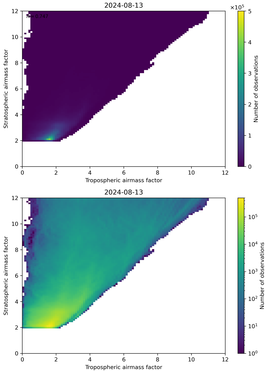
Figure 71: Scatter density plot of “Tropospheric airmass factor” against “Stratospheric airmass factor” for 2024-08-12 to 2024-08-14.
