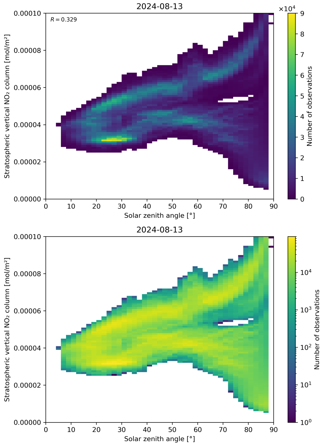
Figure 150: Scatter density plot of “Solar zenith angle” against “Stratospheric vertical NO 2 column” for 2024-08-12 to 2024-08-14.
