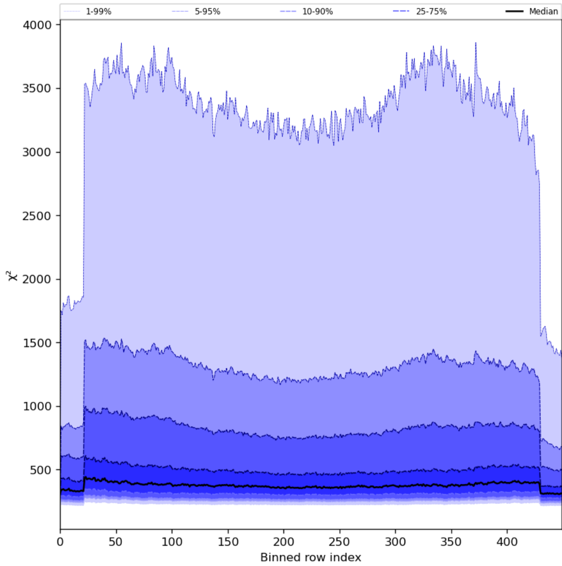
Figure 59: Along track statistics of “ \chi^2 ” for 2024-08-12 to 2024-08-14
