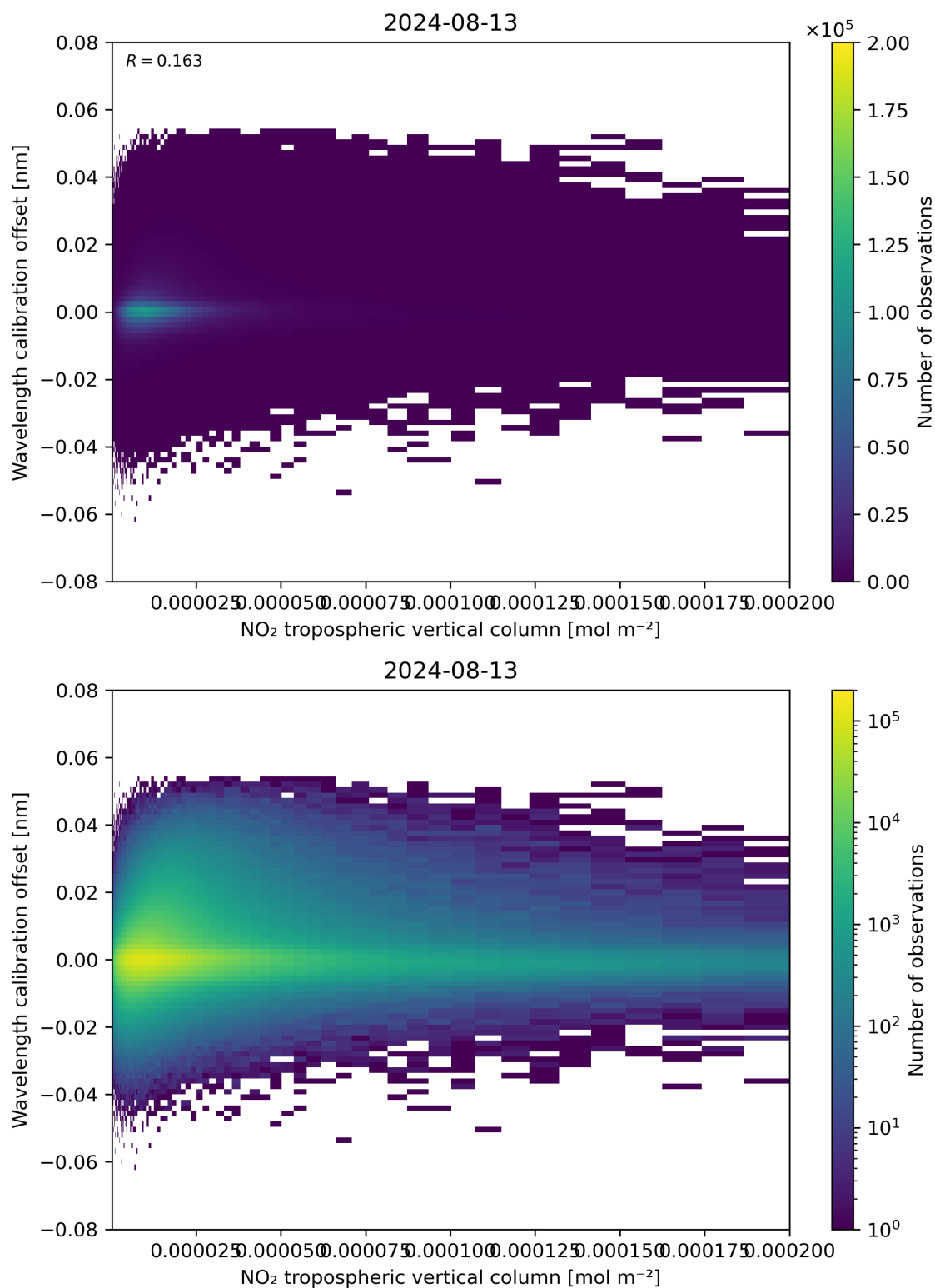
Figure 143: Scatter density plot of “NO 2 tropospheric vertical column” against “Wavelength calibration offset” for 2024-08-12 to 2024-08-14.
