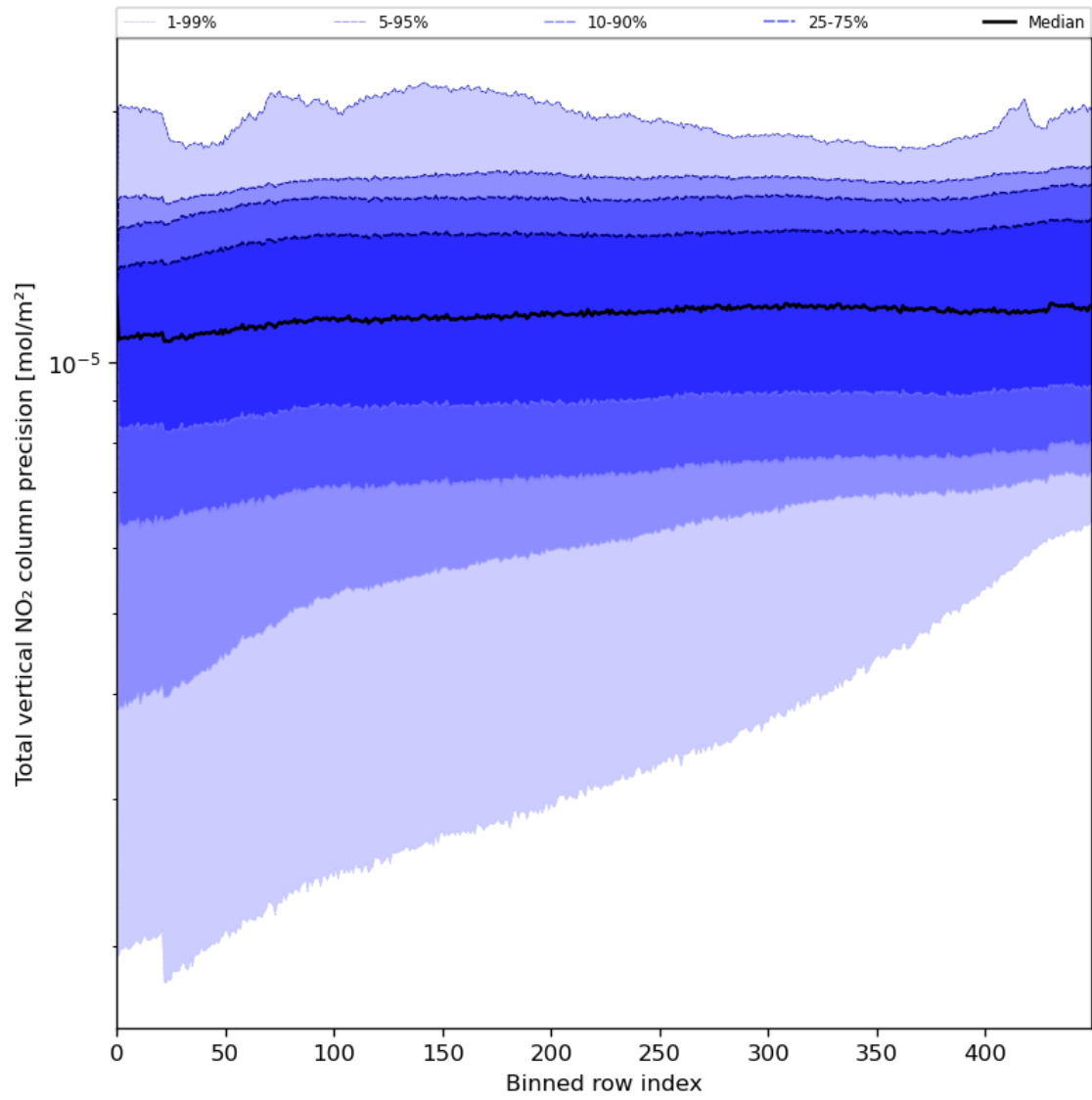
Figure 56: Along track statistics of “Total vertical NO 2 column precision” for 2024-08-12 to 2024-08-14
