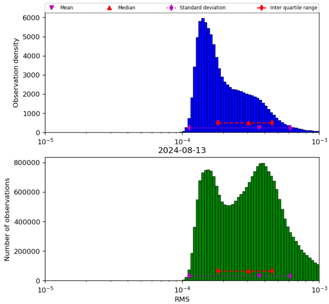
Figure 43: Histogram of “RMS” for 2024-08-12 to 2024-08-14
