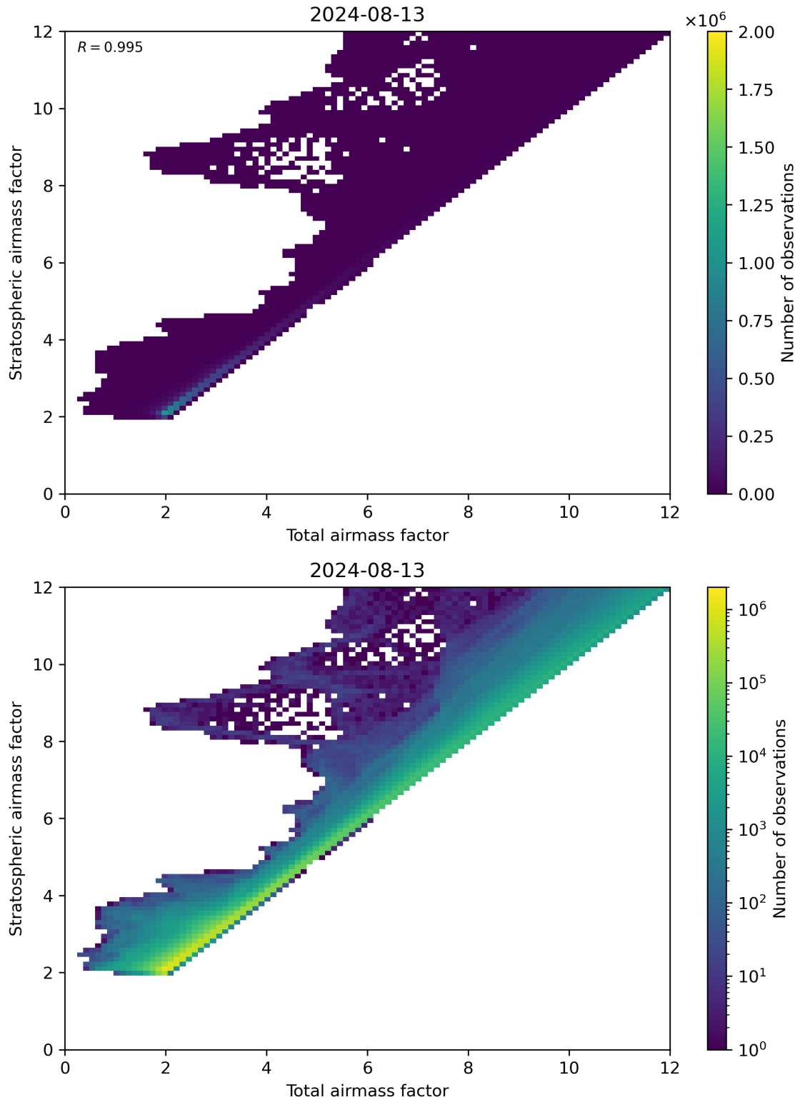
Figure 62: Scatter density plot of “Total airmass factor” against “Stratospheric airmass factor” for 2024-08-12 to 2024-08-14.
