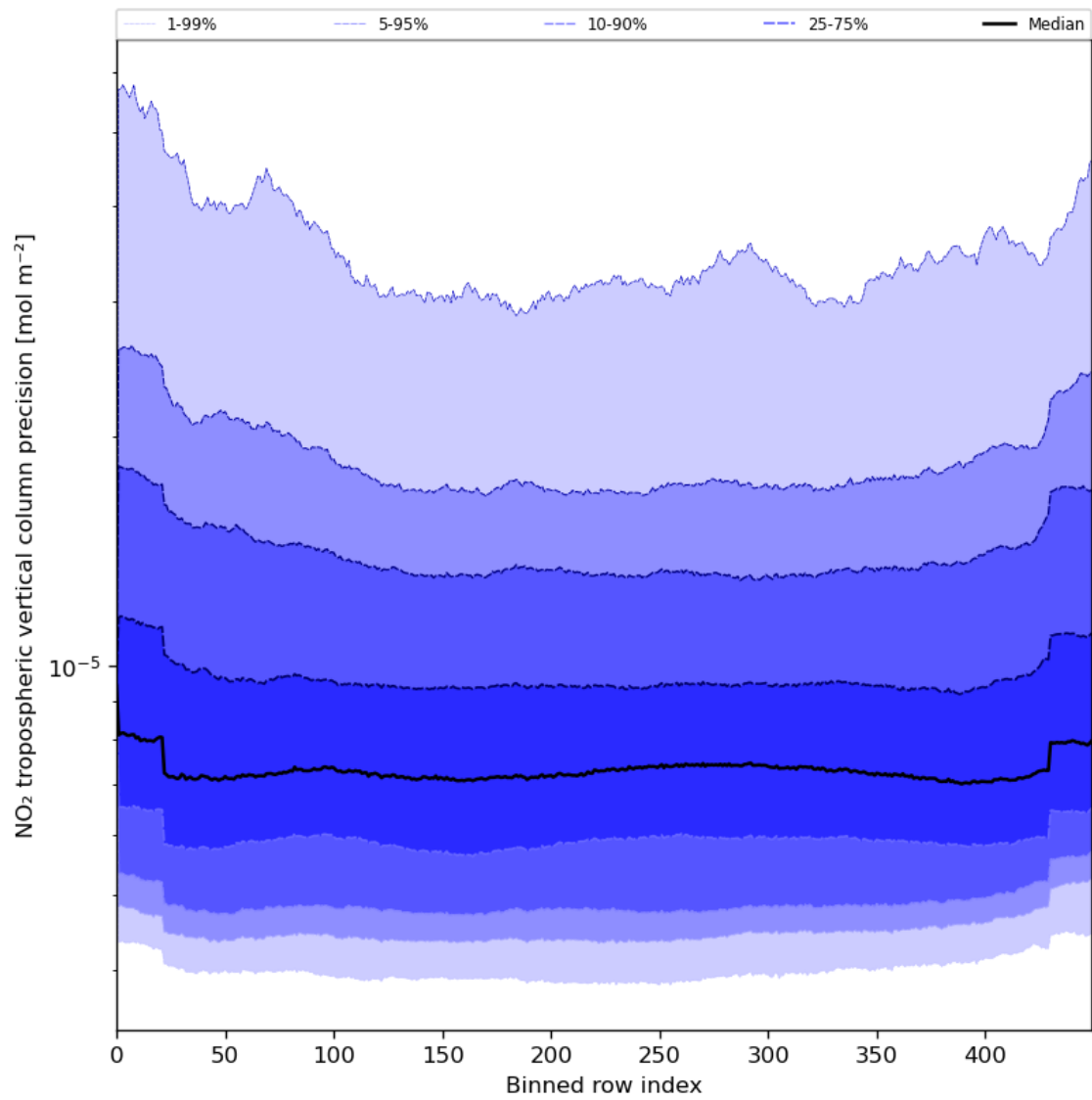
Figure 47: Along track statistics of “NO 2 tropospheric vertical column precision” for 2024-08-12 to 2024-08-14
