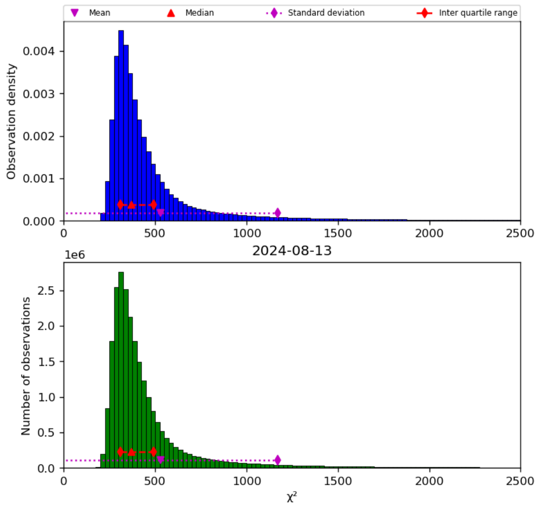
Figure 42: Histogram of “ \chi^2 ” for 2024-08-12 to 2024-08-14
