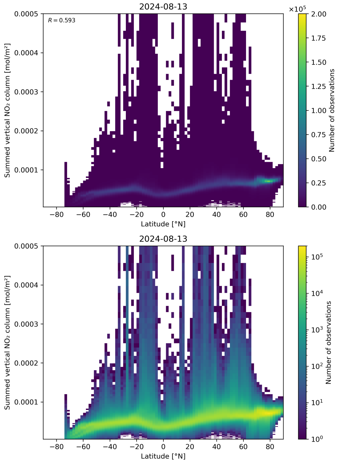
Figure 88: Scatter density plot of “Latitude” against “Summed vertical NO 2 column” for 2024-08-12 to 2024-08-14.
