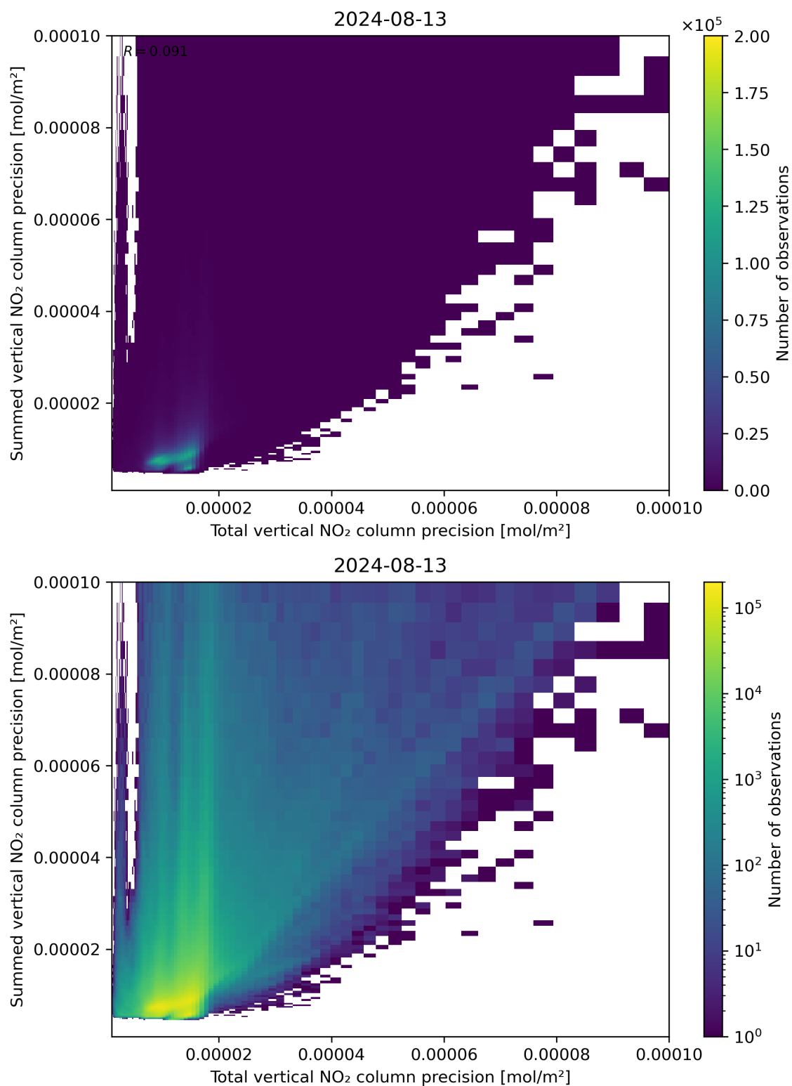
Figure 118: Scatter density plot of “Total vertical NO 2 column precision” against “Summed vertical NO 2 column precision” for 2024-08-12 to 2024-08-14.
