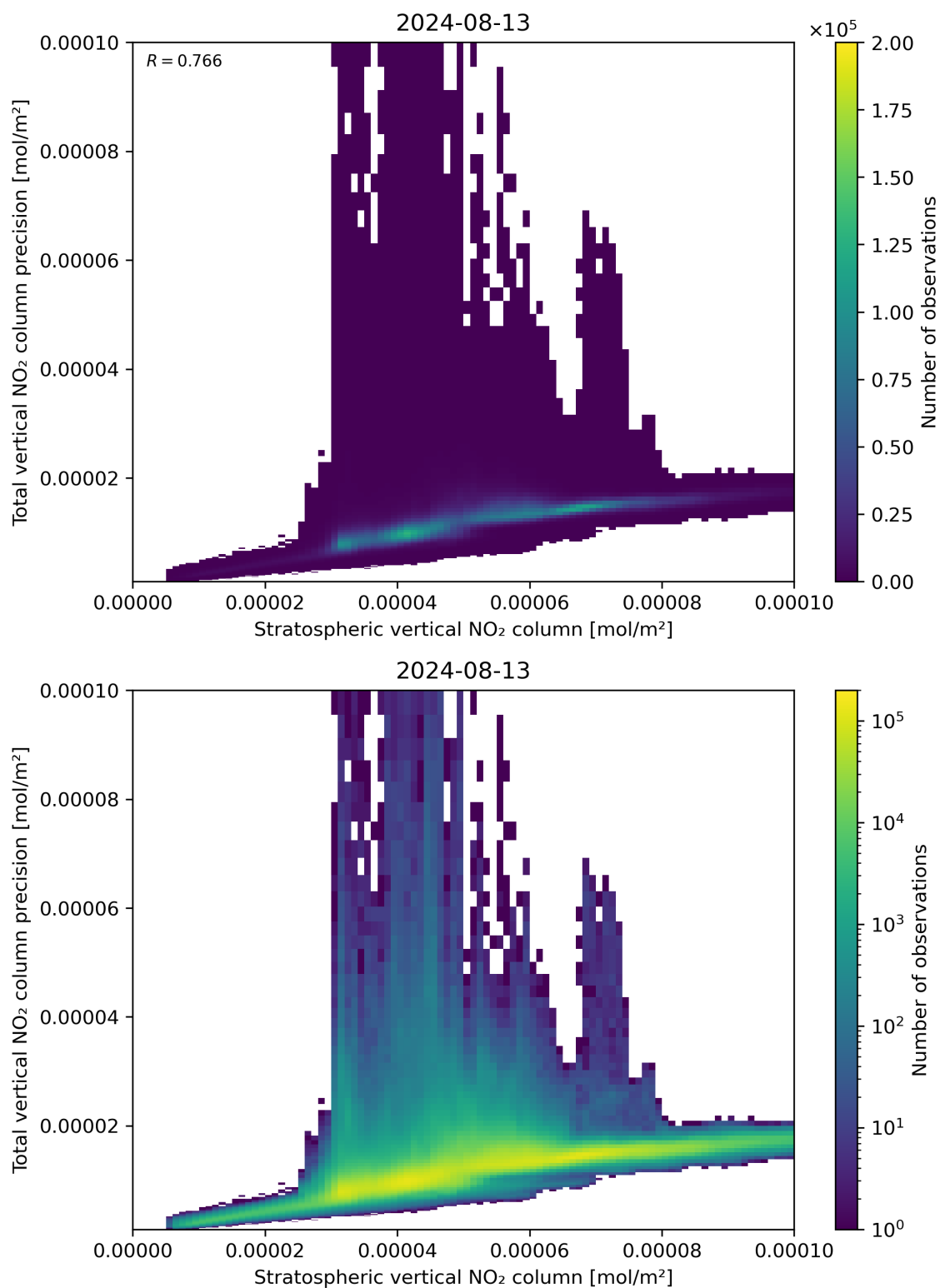
Figure 101: Scatter density plot of “Stratospheric vertical NO 2 column” against “Total vertical NO 2 column precision” for 2024-08-12 to 2024-08-14.
