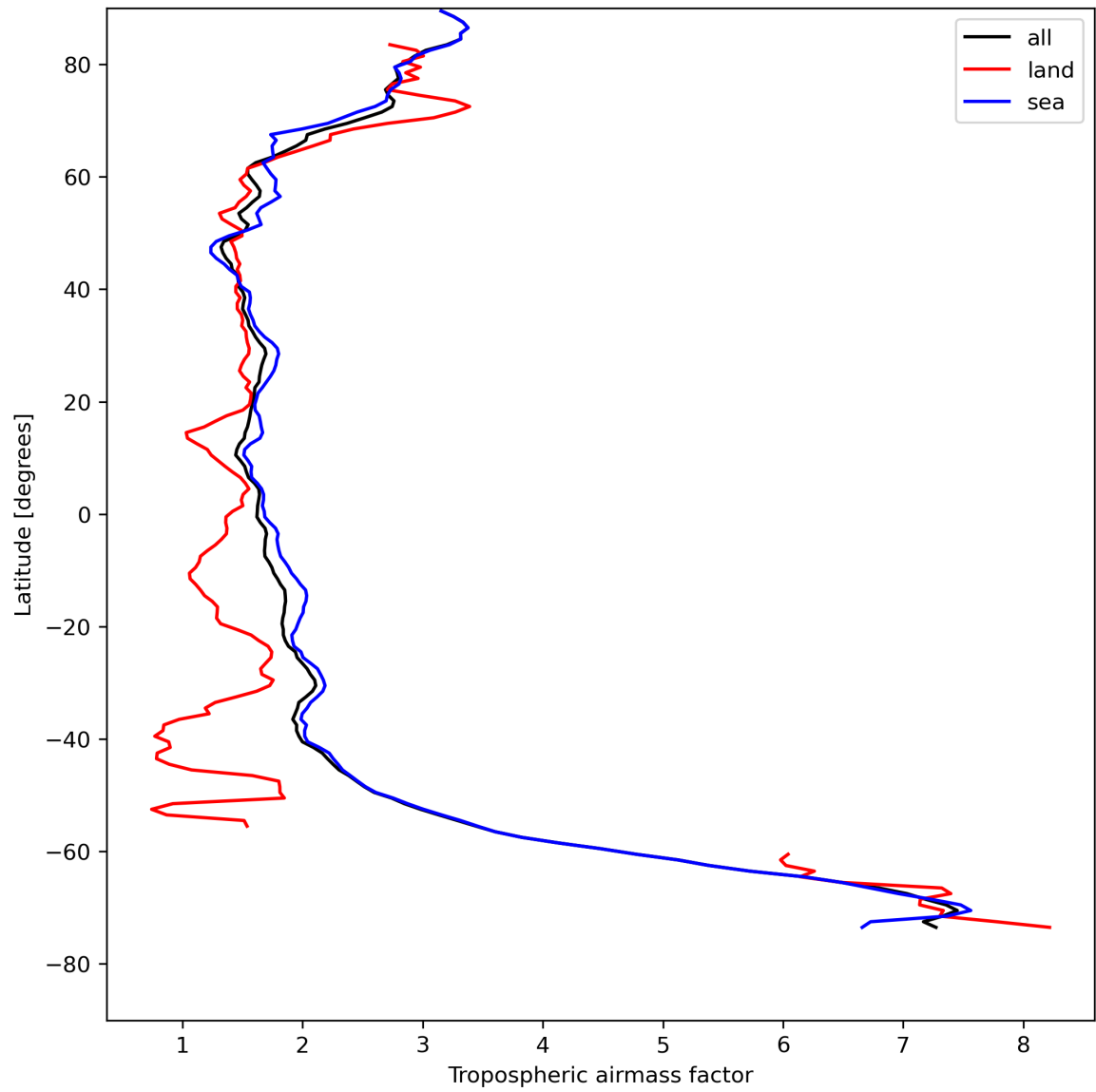
Figure 14: Zonal average of “Tropospheric airmass factor” for 2024-08-12 to 2024-08-14.
