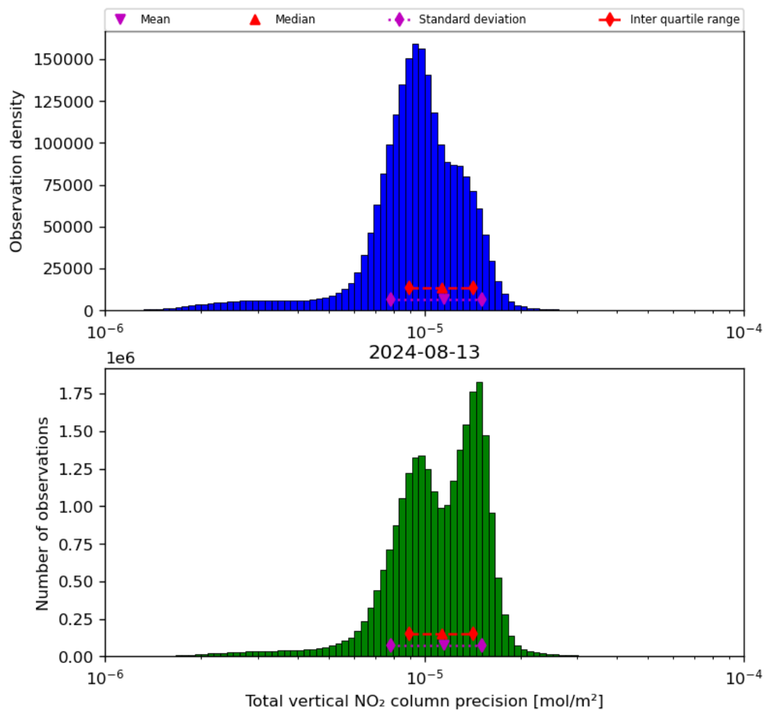
Figure 39: Histogram of “Total vertical NO 2 column precision” for 2024-08-12 to 2024-08-14
