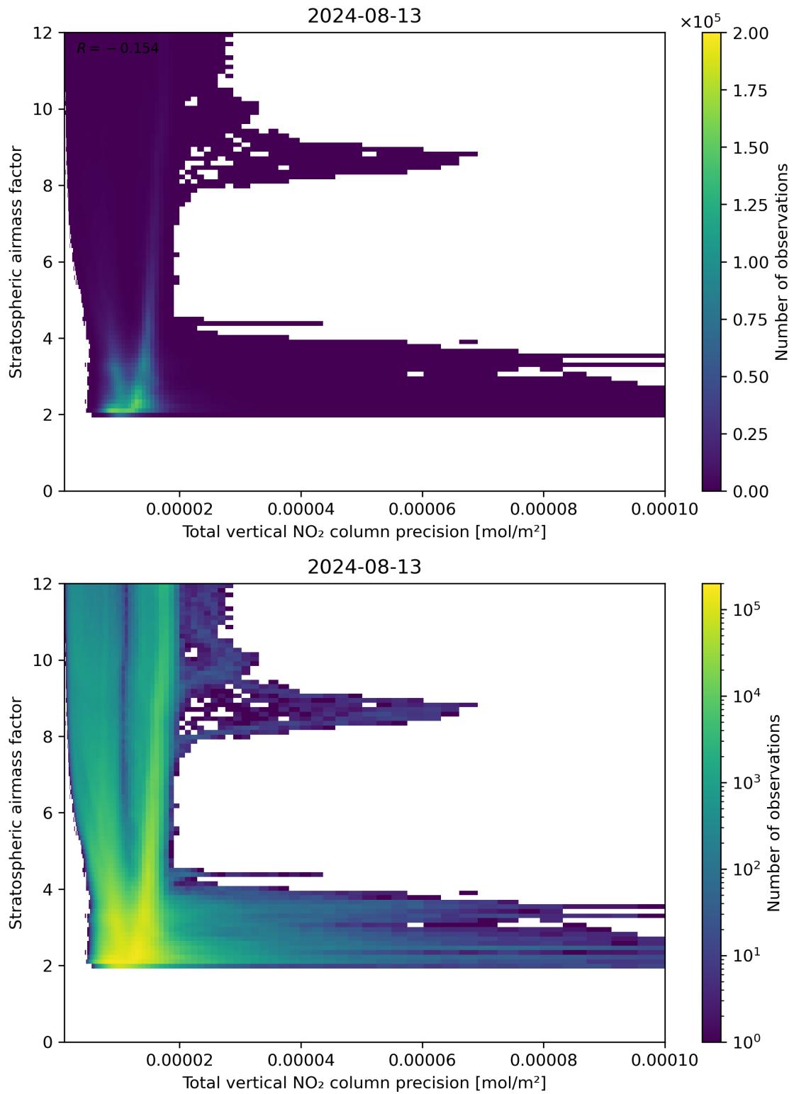
Figure 115: Scatter density plot of “Total vertical NO 2 column precision” against “Stratospheric airmass factor” for 2024-08-12 to 2024-08-14.
