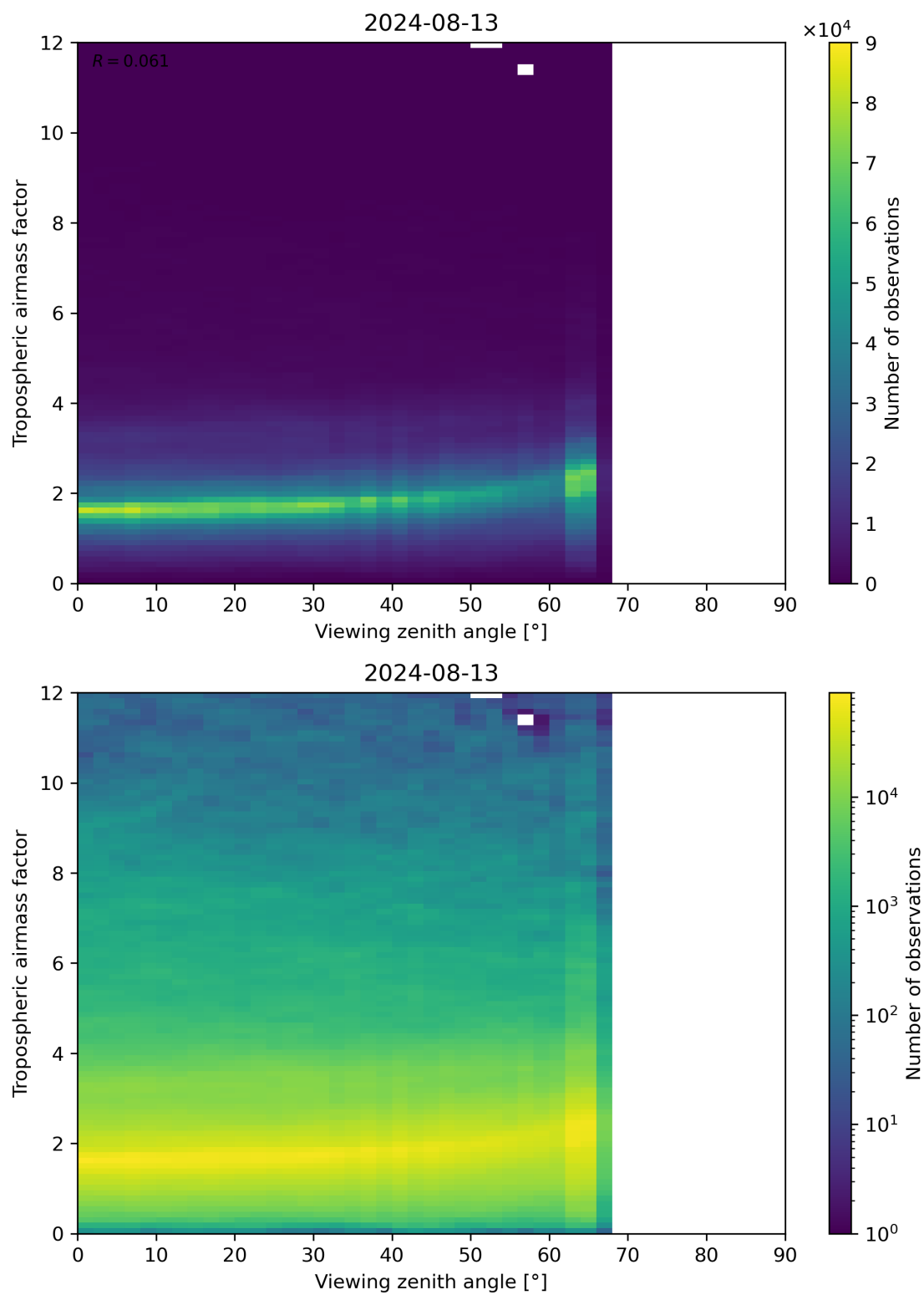
Figure 161: Scatter density plot of “Viewing zenith angle” against “Tropospheric airmass factor” for 2024-08-12 to 2024-08-14.
