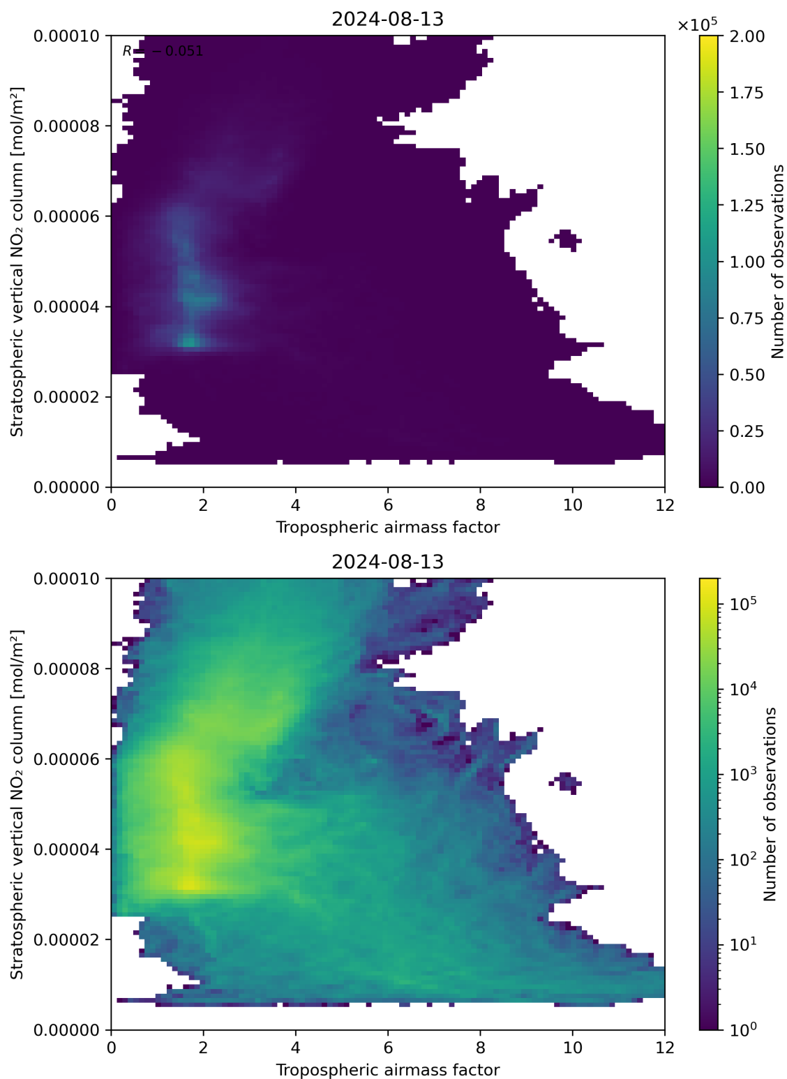
Figure 74: Scatter density plot of “Tropospheric air mass factor” against “Stratospheric vertical NO 2 column” for 2024-08-12 to 2024-08-14.
