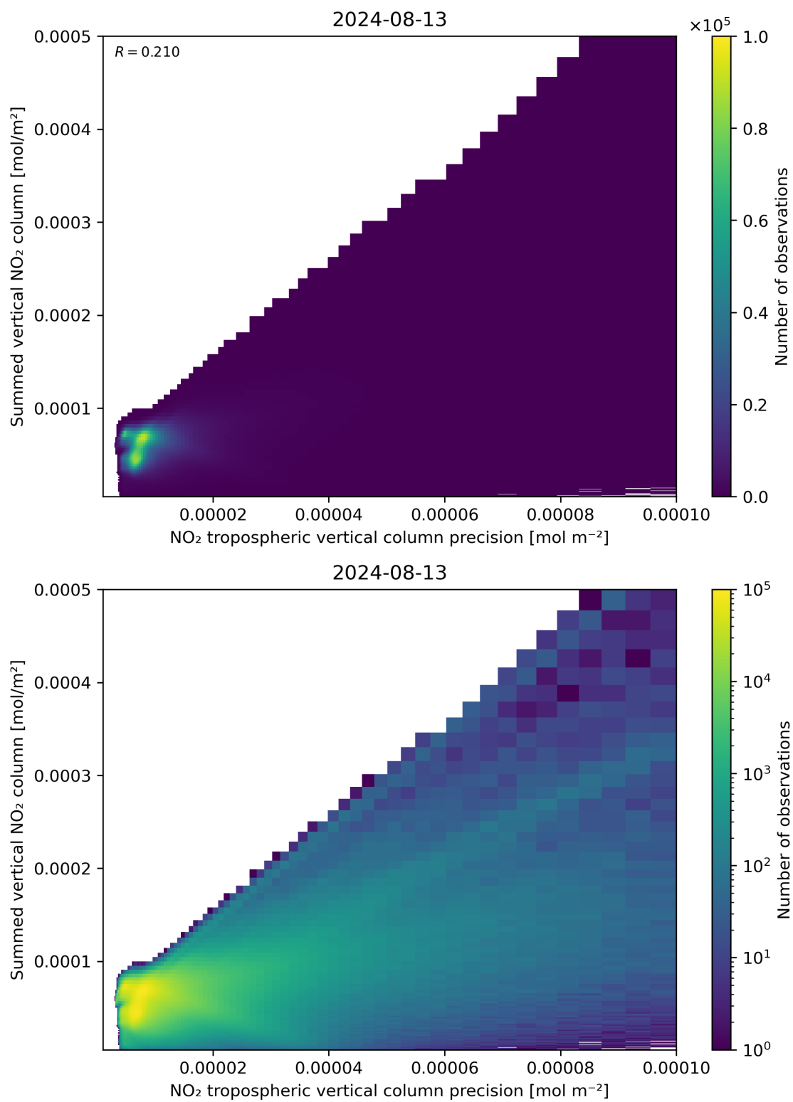
Figure 136: Scatter density plot of “NO 2 tropospheric vertical column precision” against “Summed vertical NO 2 column” for 2024-08-12 to 2024-08-14.
