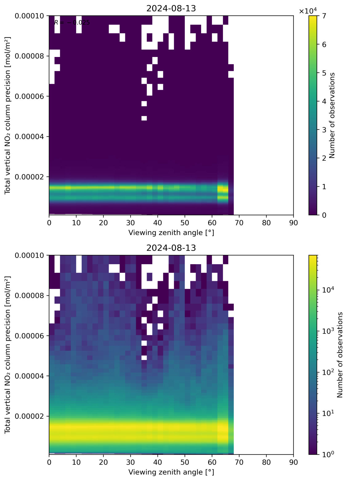
Figure 168: Scatter density plot of “Viewing zenith angle” against “Total vertical NO 2 column precision” for 2024-08-12 to 2024-08-14.
