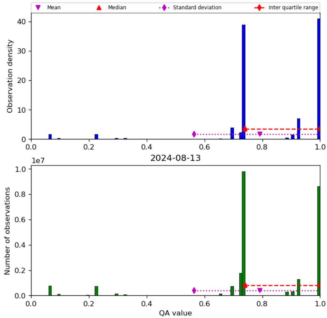
Figure 28: Histogram of “QA value” for 2024-08-12 to 2024-08-14
