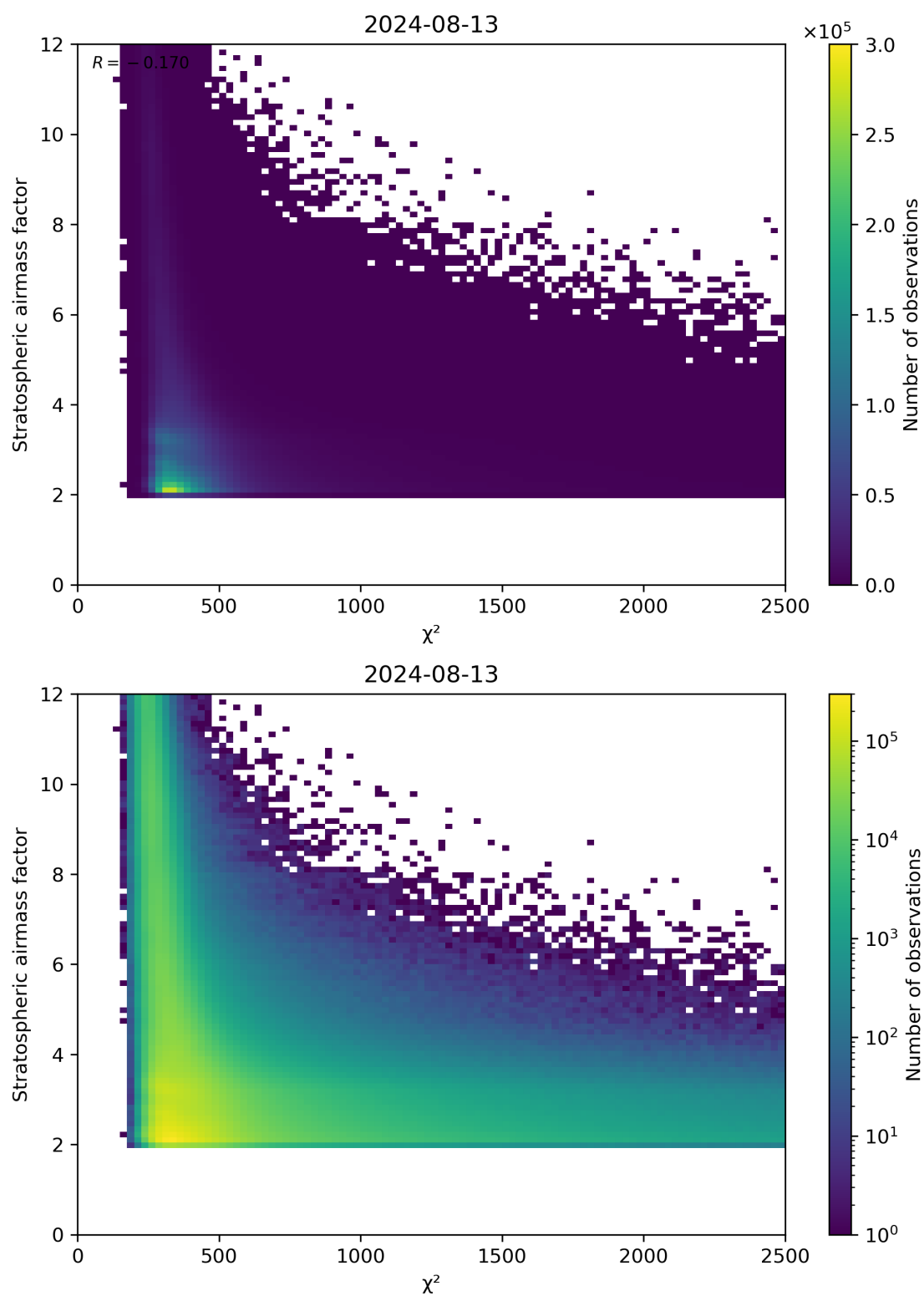
Figure 81: Scatter density plot of “ \chi^2 ” against “Stratospheric airmass factor” for 2024-08-12 to 2024-08-14.
