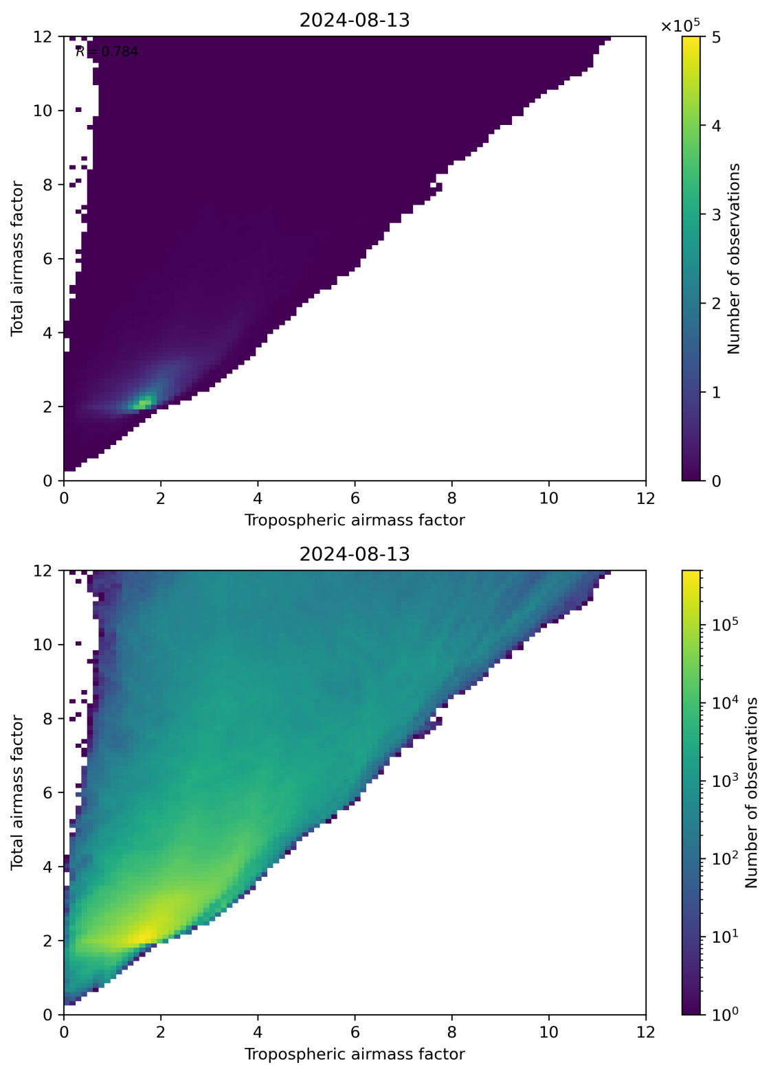
Figure 72: Scatter density plot of “Tropospheric airmass factor” against “Total airmass factor” for 2024-08-12 to 2024-08-14.
