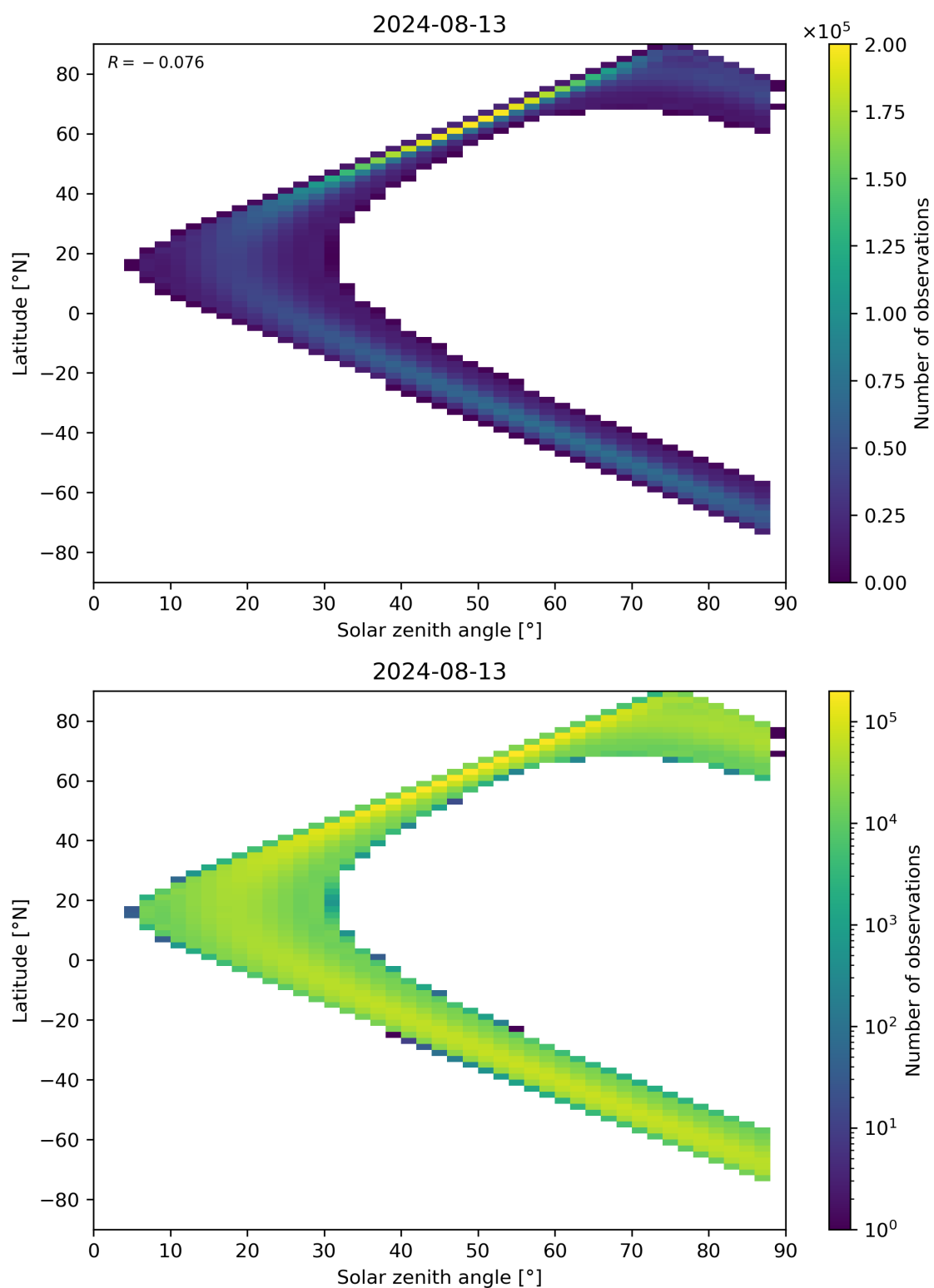
Figure 149: Scatter density plot of “Solar zenith angle” against “Latitude” for 2024-08-12 to 2024-08-14.
