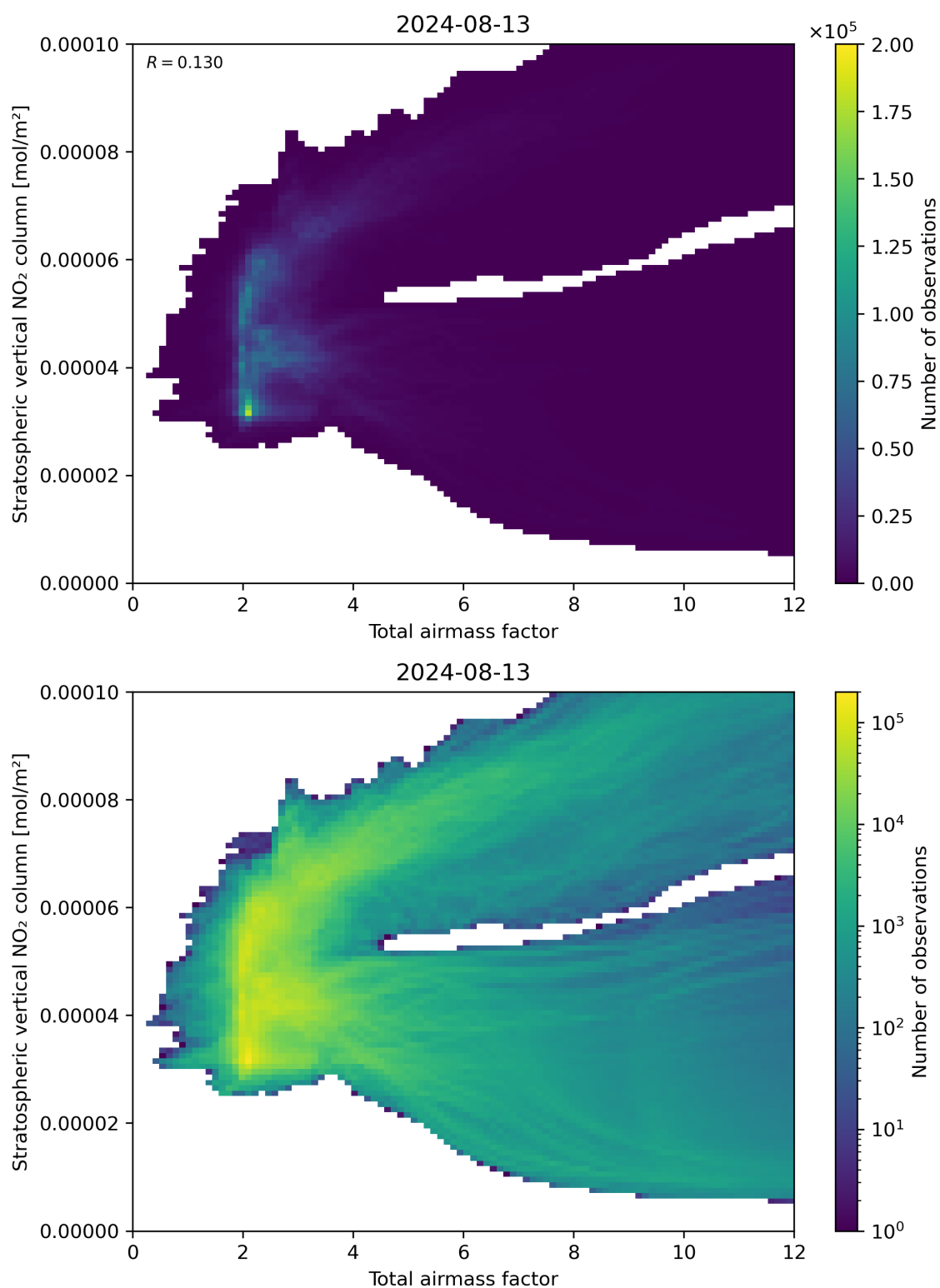
Figure 64: Scatter density plot of “Total airmass factor” against “Stratospheric vertical NO 2 column” for 2024-08-12 to 2024-08-14.
