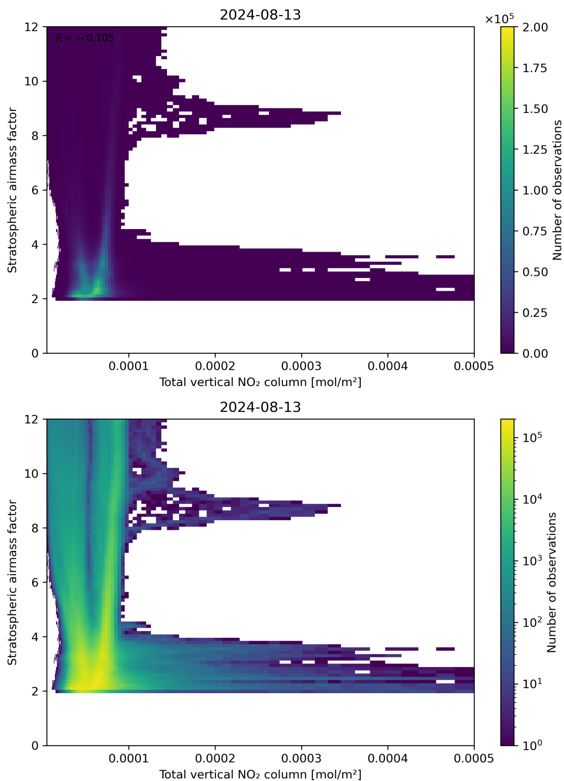
Figure 110: Scatter density plot of “Total vertical NO 2 column” against “Stratospheric airmass factor” for 2024-08-12 to 2024-08-14.
