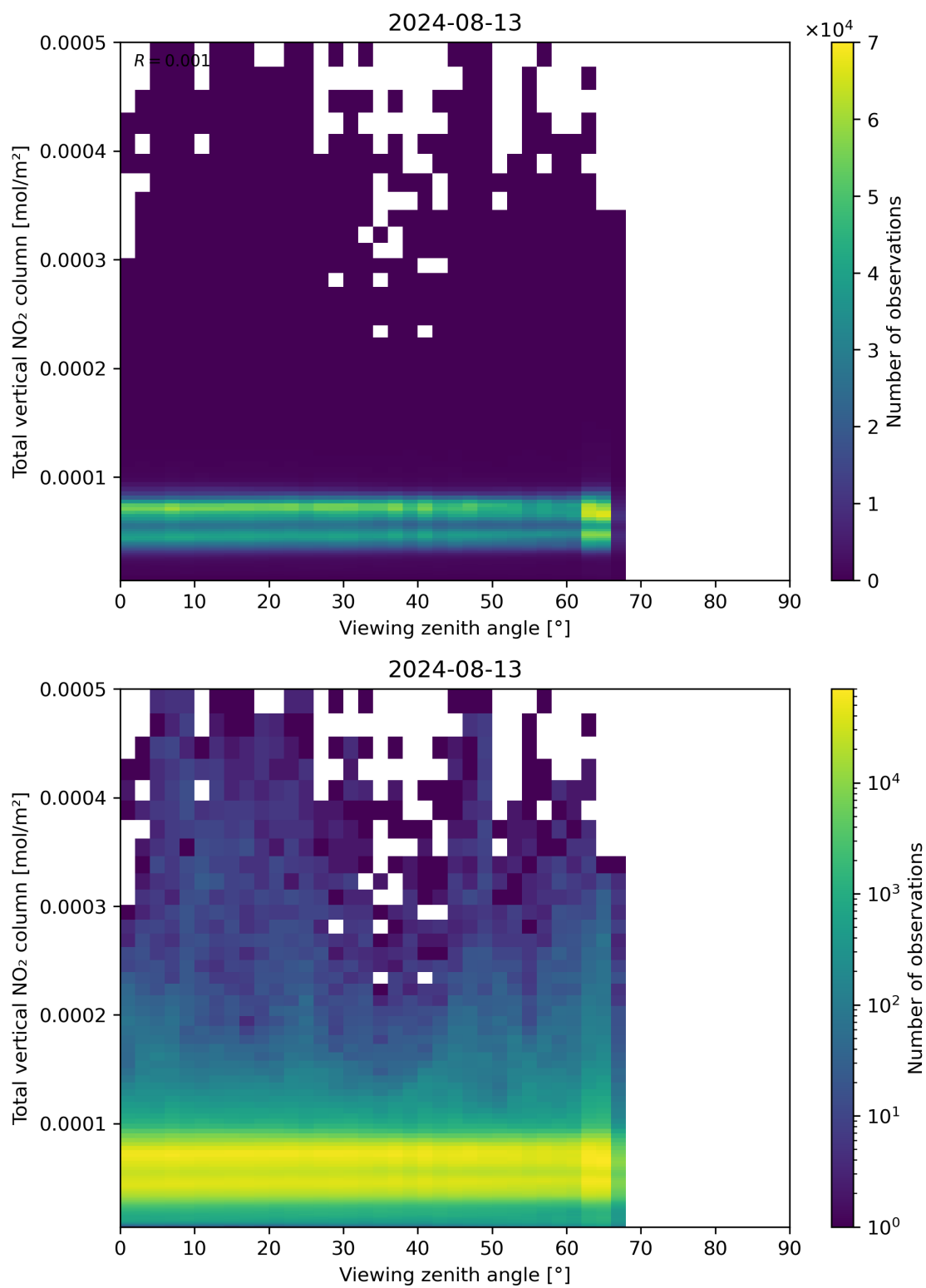
Figure 167: Scatter density plot of “Viewing zenith angle” against “Total vertical NO 2 column” for 2024-08-12 to 2024-08-14.
