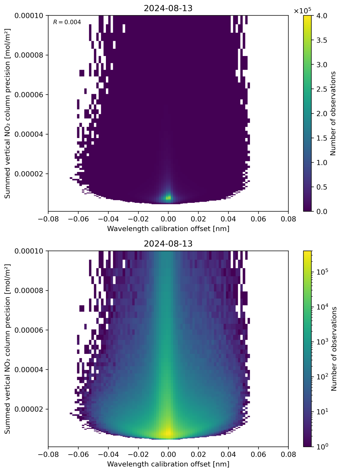
Figure 178: Scatter density plot of “Wavelength calibration offset” against “Summed vertical NO 2 column precision” for 2024-08-12 to 2024-08-14.
