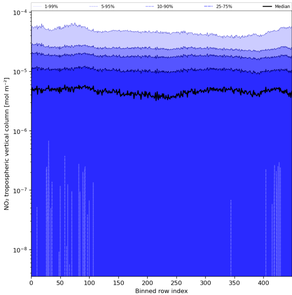
Figure 46: Along track statistics of “ \text{NO}_2 tropospheric vertical column” for 2024-08-12 to 2024-08-14
