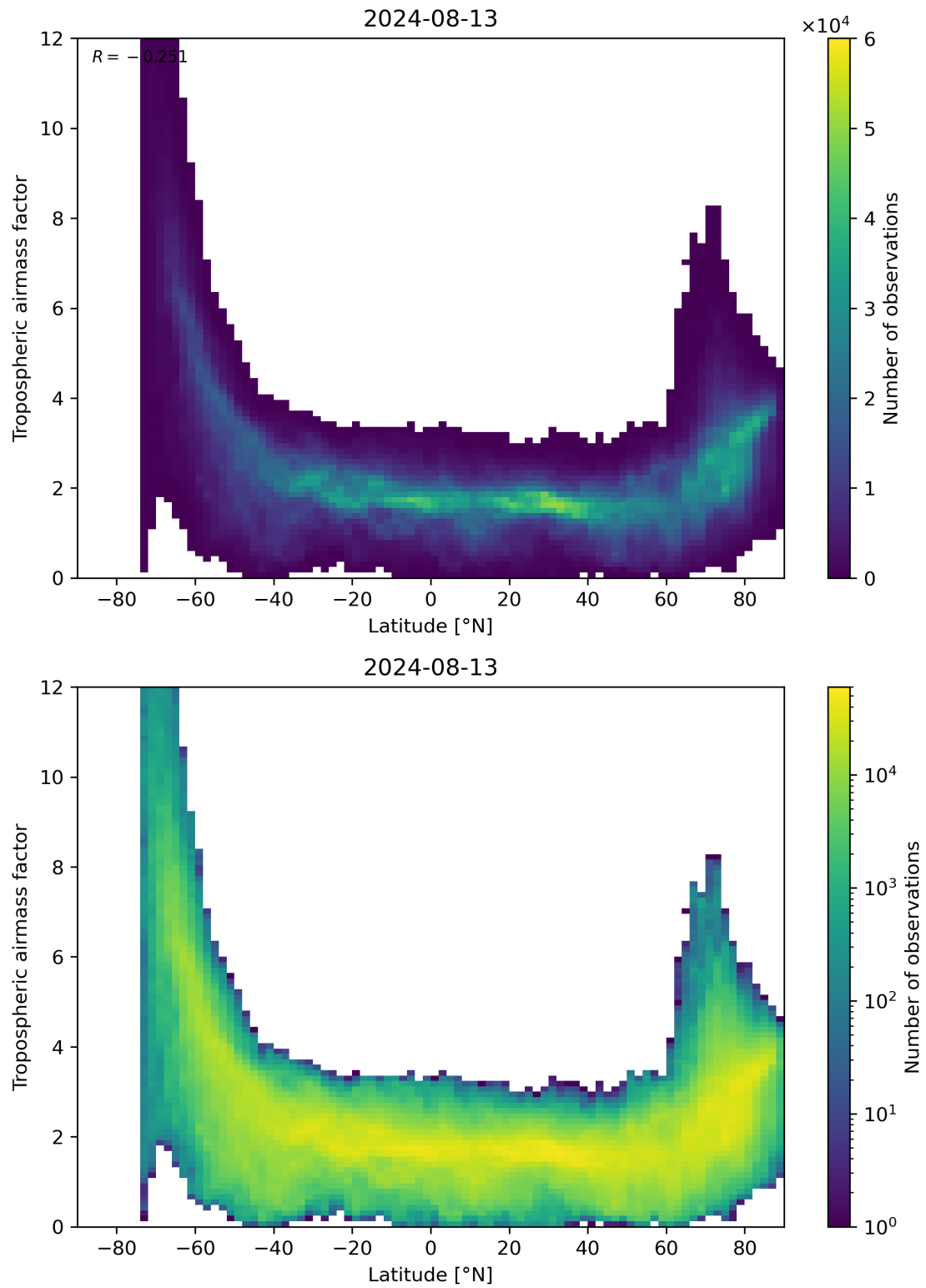
Figure 85: Scatter density plot of “Latitude” against “Tropospheric airmass factor” for 2024-08-12 to 2024-08-14.
