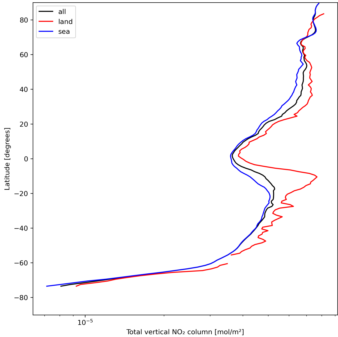
Figure 21: Zonal average of “Total vertical NO 2 column” for 2024-08-12 to 2024-08-14.
