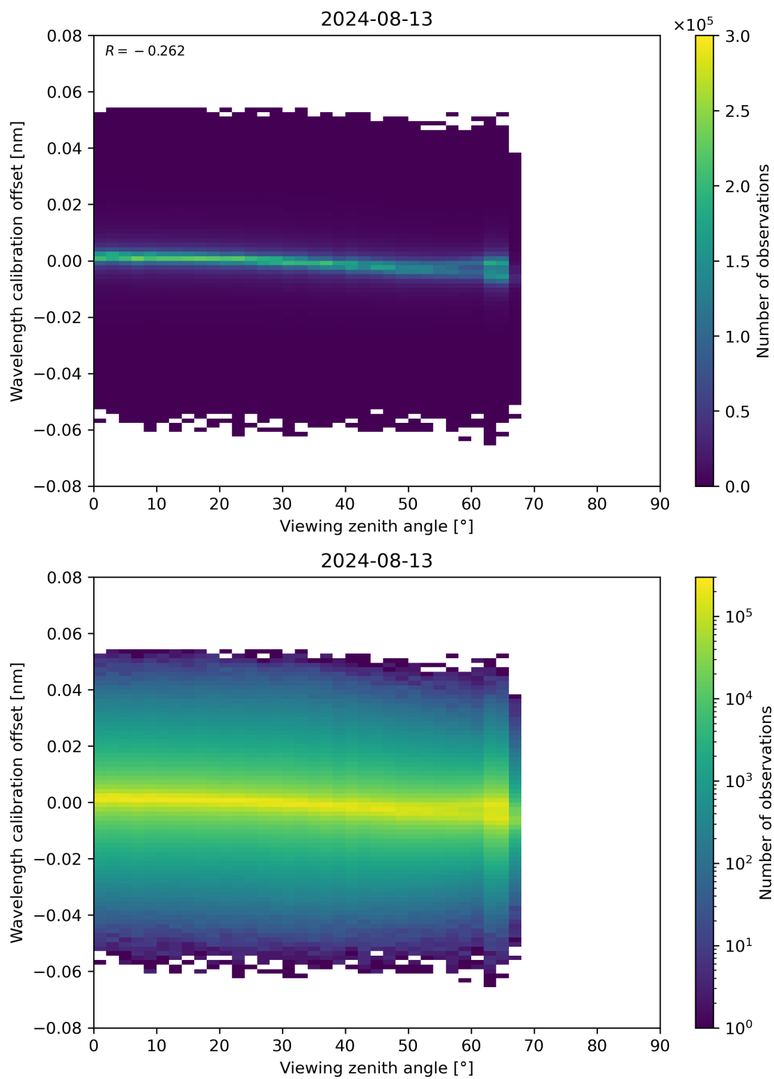
Figure 173: Scatter density plot of “Viewing zenith angle” against “Wavelength calibration offset” for 2024-08-12 to 2024-08-14.
