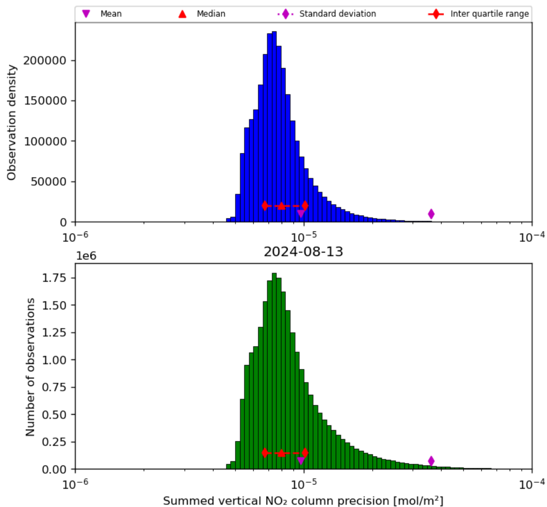
Figure 41: Histogram of “Summed vertical NO 2 column precision” for 2024-08-12 to 2024-08-14
