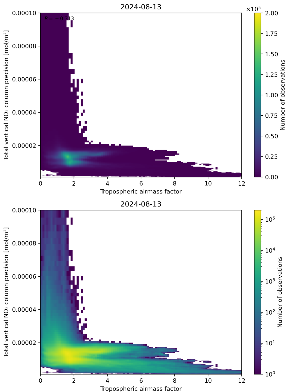
Figure 78: Scatter density plot of “Tropospheric air mass factor” against “Total vertical NO 2 column precision” for 2024-08-12 to 2024-08-14.
