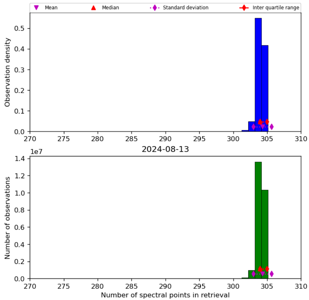
Figure 33: Histogram of “Number of spectral points in retrieval” for 2024-08-12 to 2024-08-14
