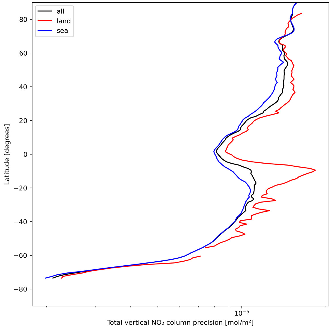
Figure 22: Zonal average of “Total vertical NO 2 column precision” for 2024-08-12 to 2024-08-14.
