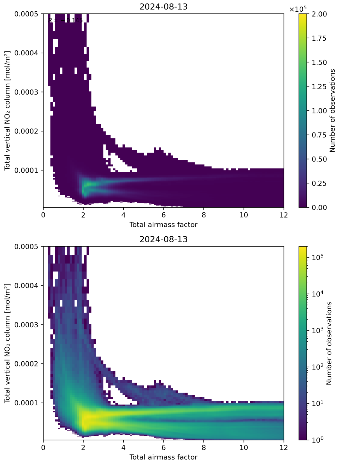
Figure 67: Scatter density plot of “Total airmass factor” against “Total vertical NO 2 column” for 2024-08-12 to 2024-08-14.
