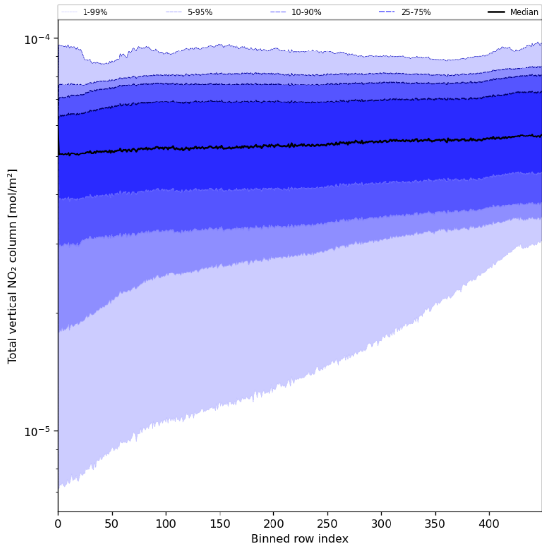
Figure 55: Along track statistics of “Total vertical NO 2 column” for 2024-08-12 to 2024-08-14
