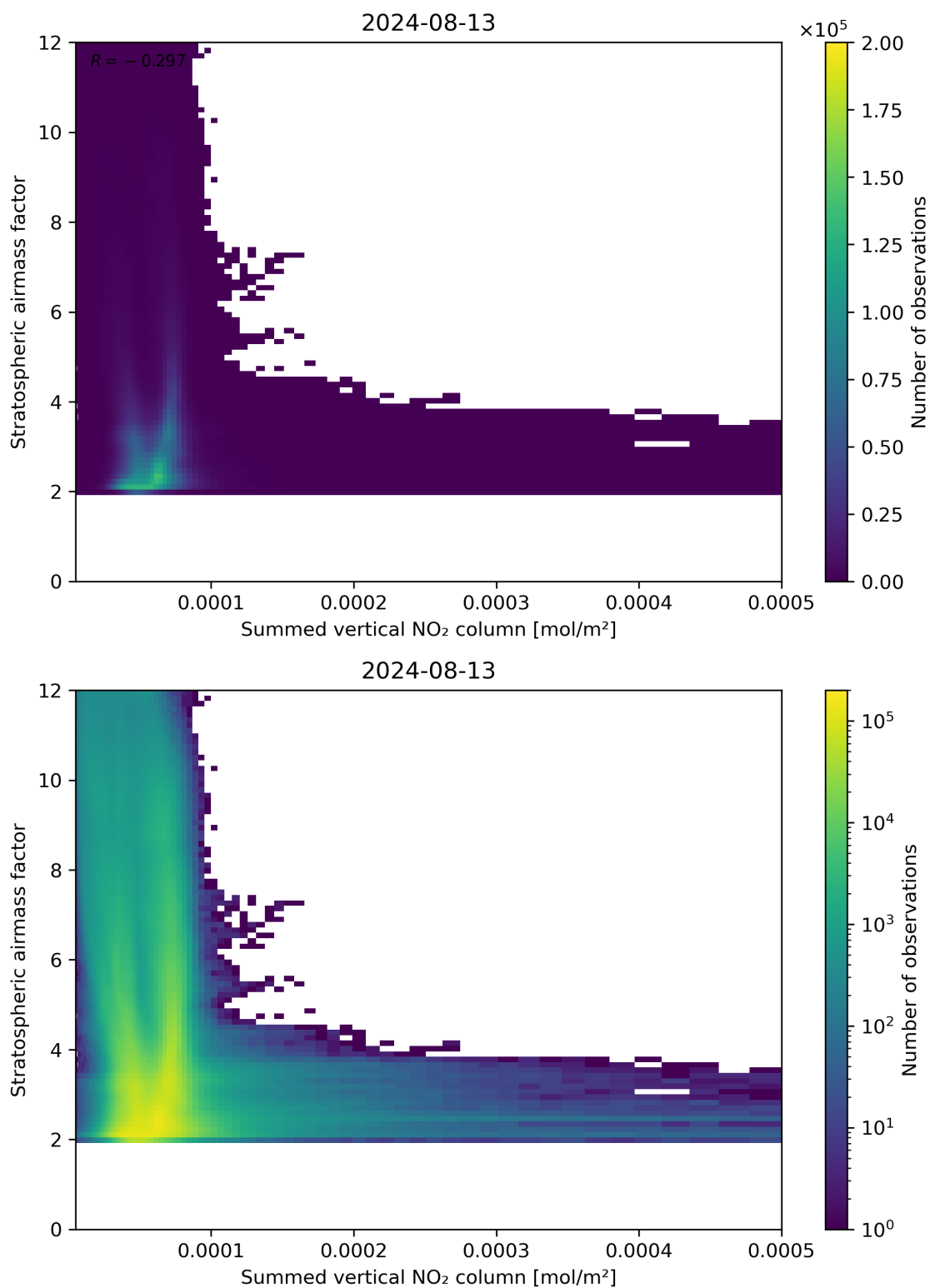
Figure 103: Scatter density plot of “Summed vertical NO 2 column” against “Stratospheric air mass factor” for 2024-08-12 to 2024-08-14.
