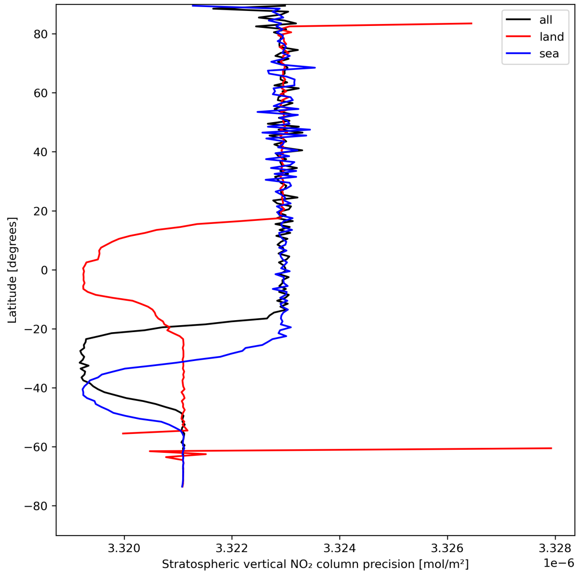
Figure 20: Zonal average of “Stratospheric vertical NO 2 column precision” for 2024-08-12 to 2024-08-14.
