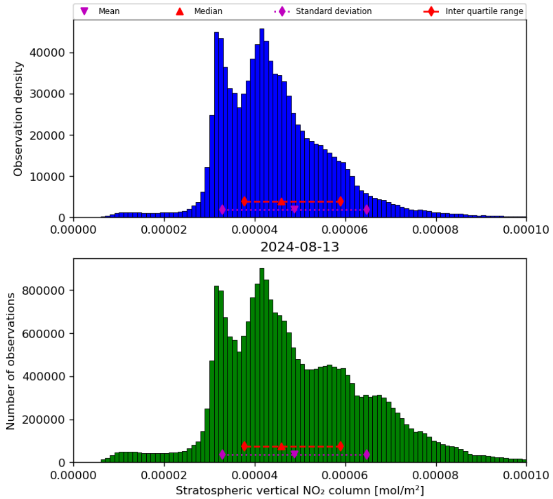
Figure 36: Histogram of “Stratospheric vertical NO 2 column” for 2024-08-12 to 2024-08-14
