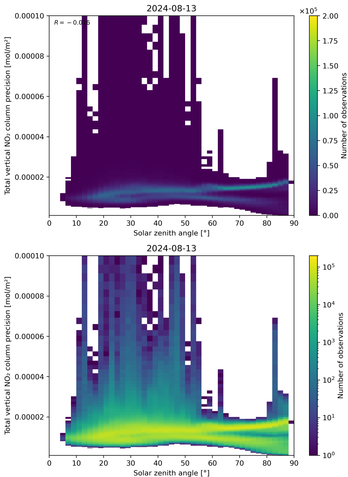
Figure 154: Scatter density plot of “Solar zenith angle” against “Total vertical NO 2 column precision” for 2024-08-12 to 2024-08-14.
