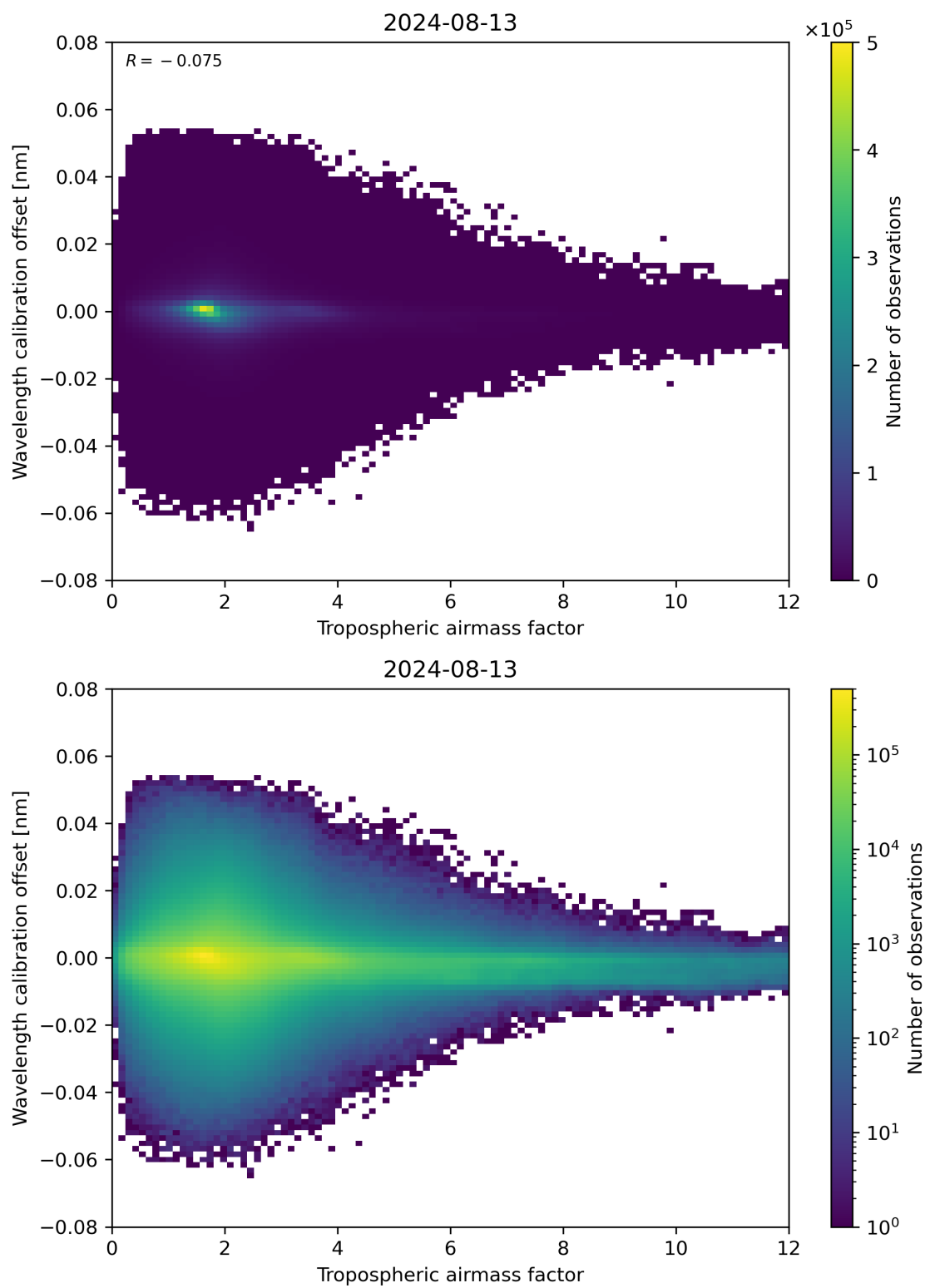
Figure 80: Scatter density plot of “Tropospheric air mass factor” against “Wavelength calibration offset” for 2024-08-12 to 2024-08-14.
