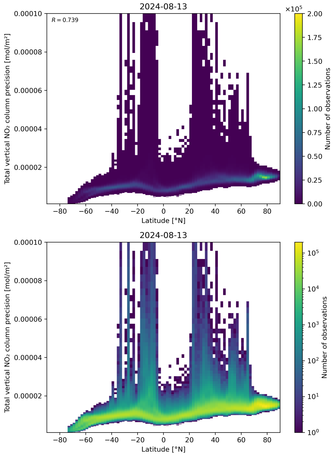
Figure 91: Scatter density plot of “Latitude” against “Total vertical NO 2 column precision” for 2024-08-12 to 2024-08-14.
