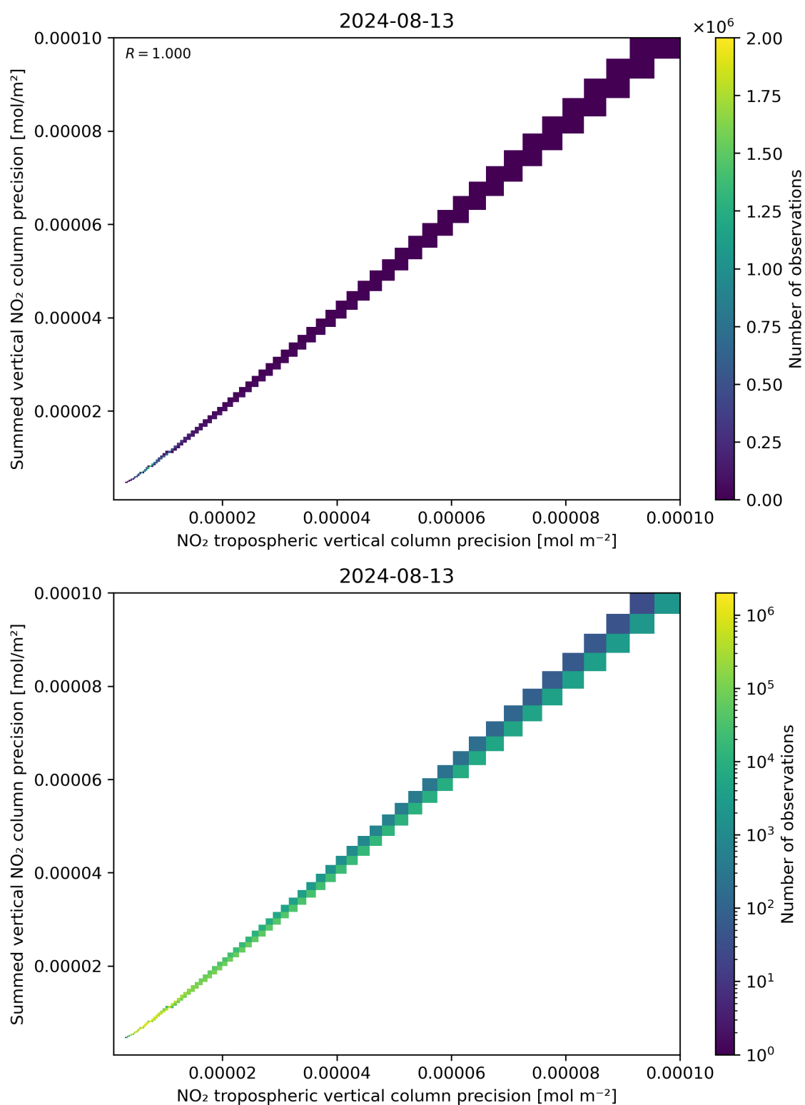
Figure 137: Scatter density plot of “NO 2 tropospheric vertical column precision” against “Summed vertical NO 2 column precision” for 2024-08-12 to 2024-08-14.
