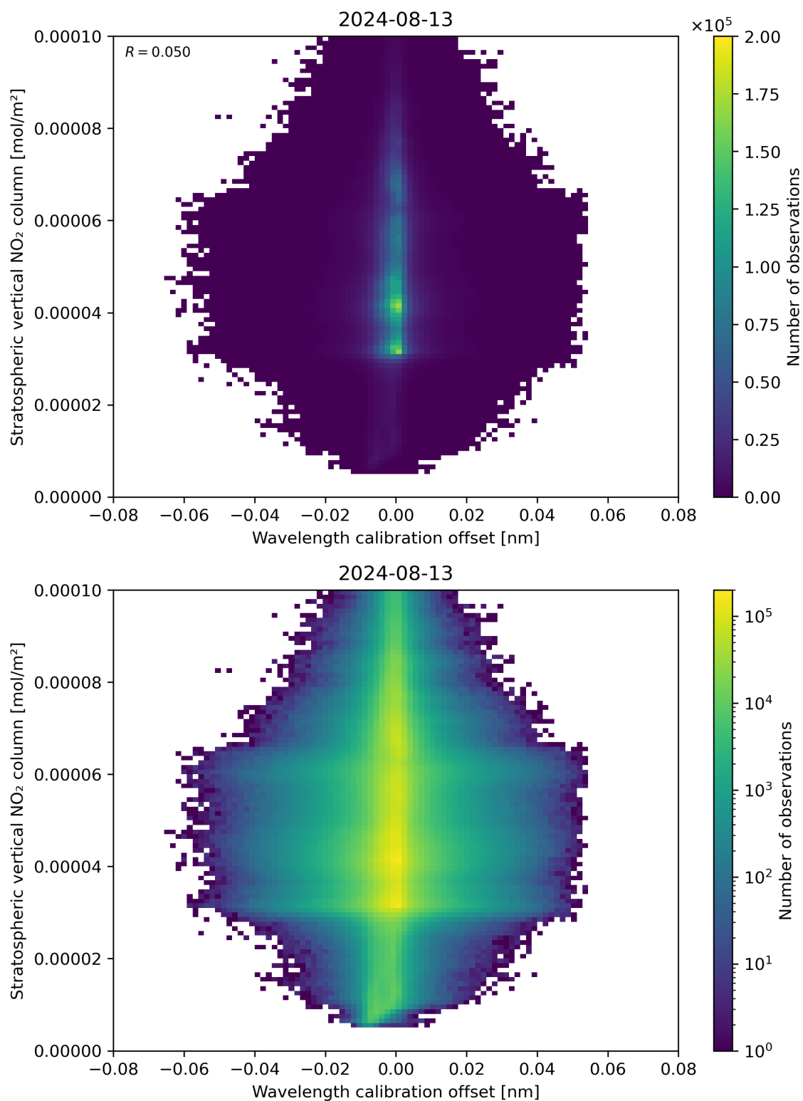
Figure 176: Scatter density plot of “Wavelength calibration offset” against “Stratospheric vertical NO 2 column” for 2024-08-12 to 2024-08-14.
