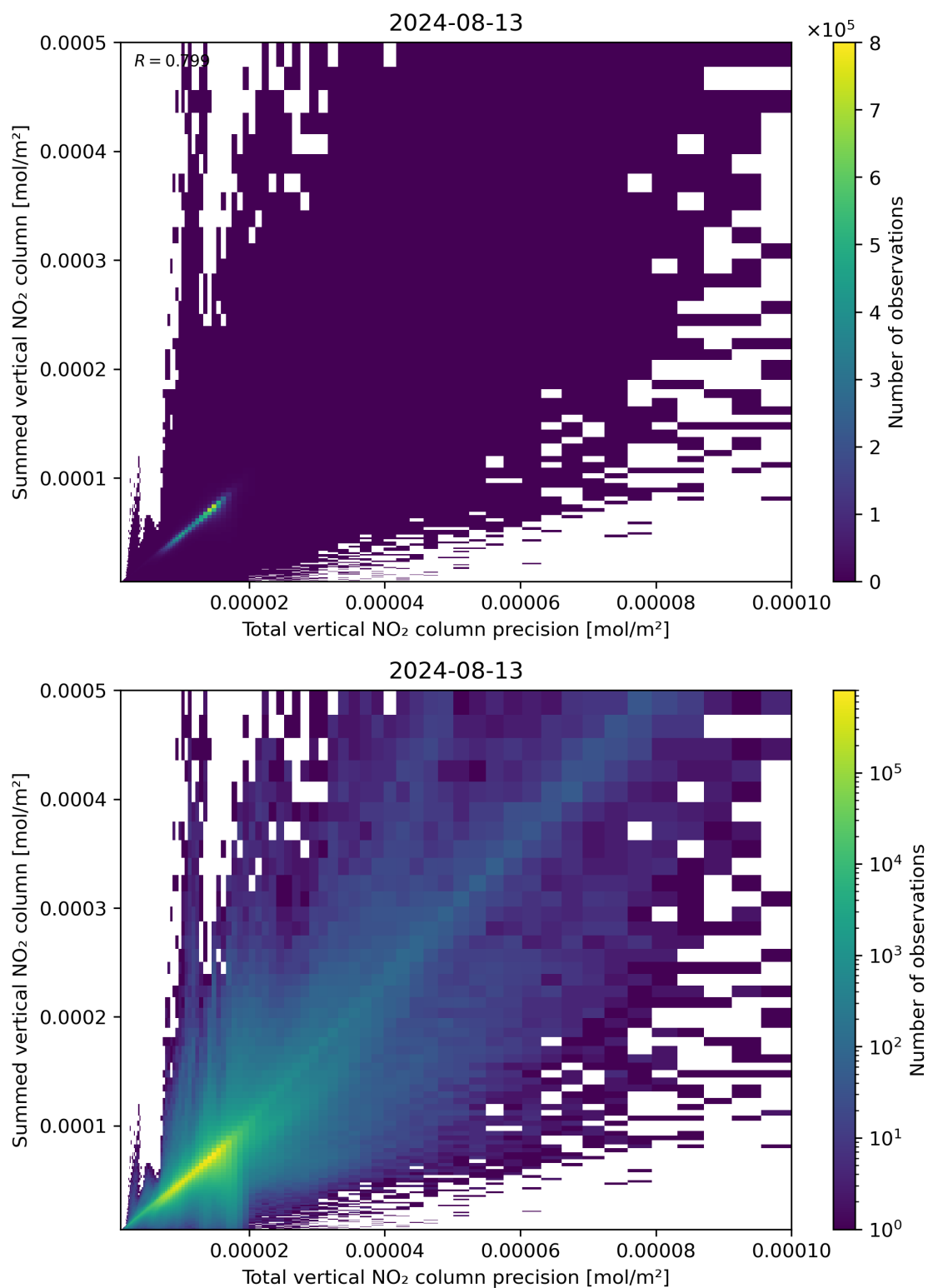
Figure 117: Scatter density plot of “Total vertical NO 2 column precision” against “Summed vertical NO 2 column” for 2024-08-12 to 2024-08-14.
