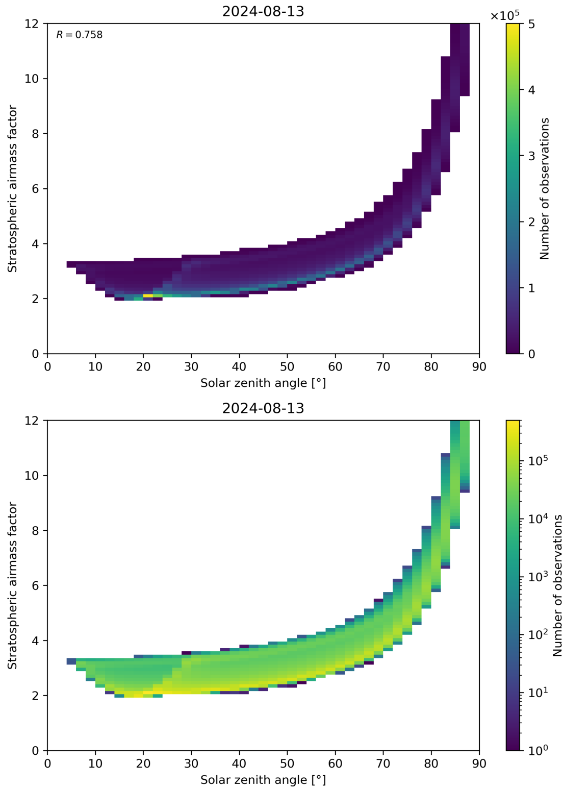
Figure 145: Scatter density plot of “Solar zenith angle” against “Stratospheric airmass factor” for 2024-08-12 to 2024-08-14.
