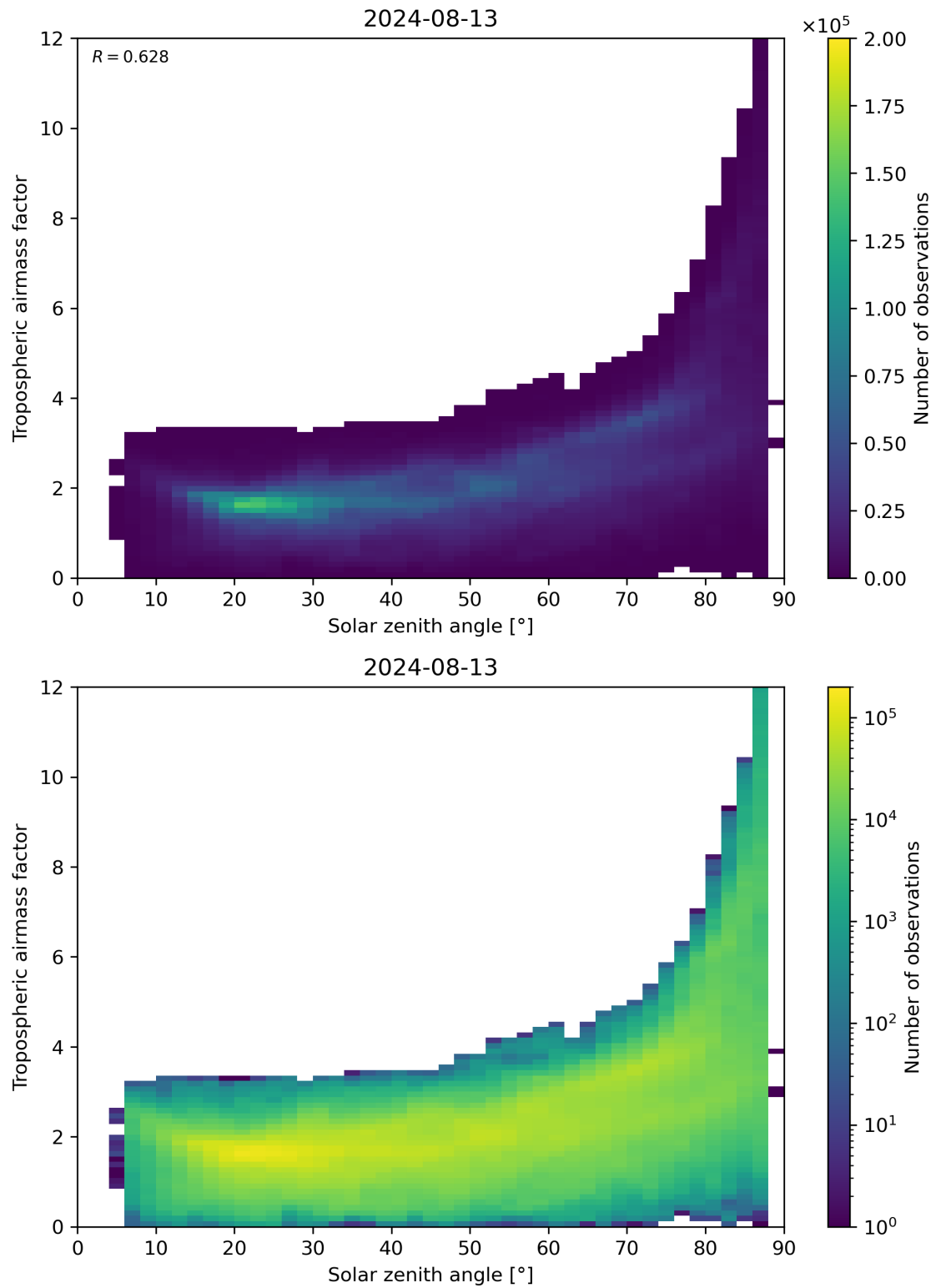
Figure 147: Scatter density plot of “Solar zenith angle” against “Tropospheric airmass factor” for 2024-08-12 to 2024-08-14.
