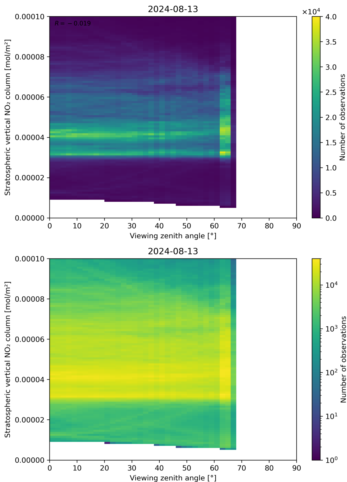
Figure 164: Scatter density plot of “Viewing zenith angle” against “Stratospheric vertical NO 2 column” for 2024-08-12 to 2024-08-14.
