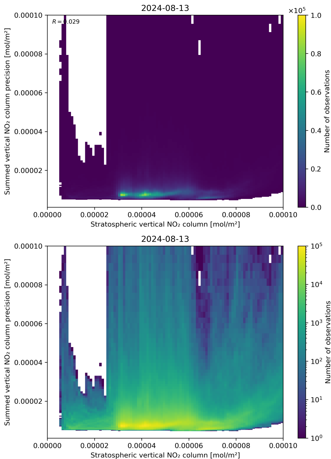
Figure 99: Scatter density plot of “Stratospheric vertical NO 2 column” against “Summed vertical NO 2 column precision” for 2024-08-12 to 2024-08-14.
