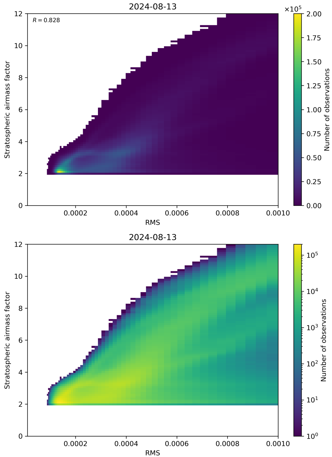
Figure 144: Scatter density plot of “RMS” against “Stratospheric airmass factor” for 2024-08-12 to 2024-08-14.
