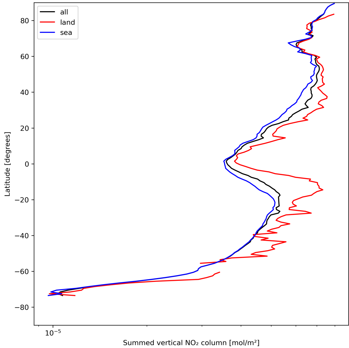
Figure 23: Zonal average of “Summed vertical NO 2 column” for 2024-08-12 to 2024-08-14.
