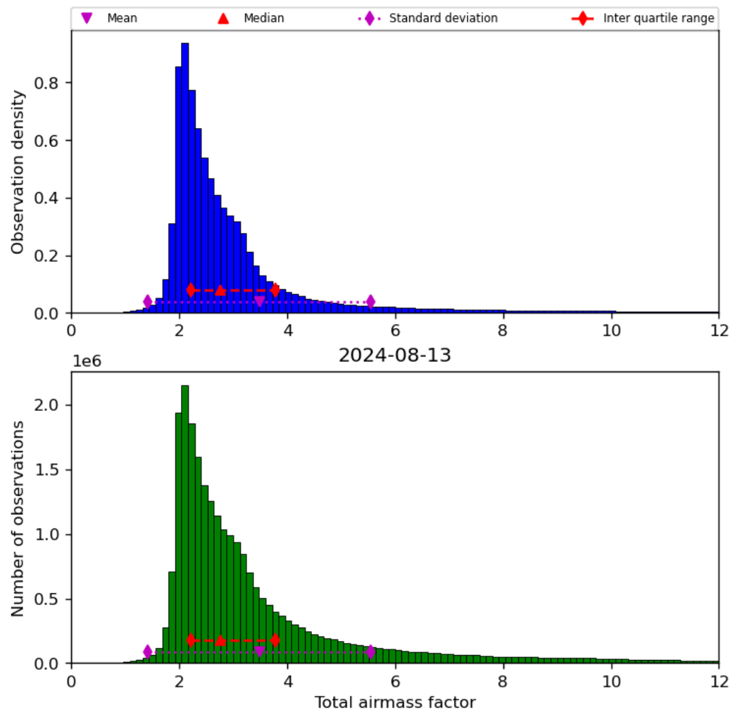
Figure 32: Histogram of “Total airmass factor” for 2024-08-12 to 2024-08-14
