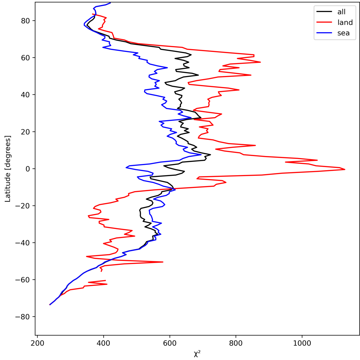
Figure 25: Zonal average of “ \chi^2 ” for 2024-08-12 to 2024-08-14.
