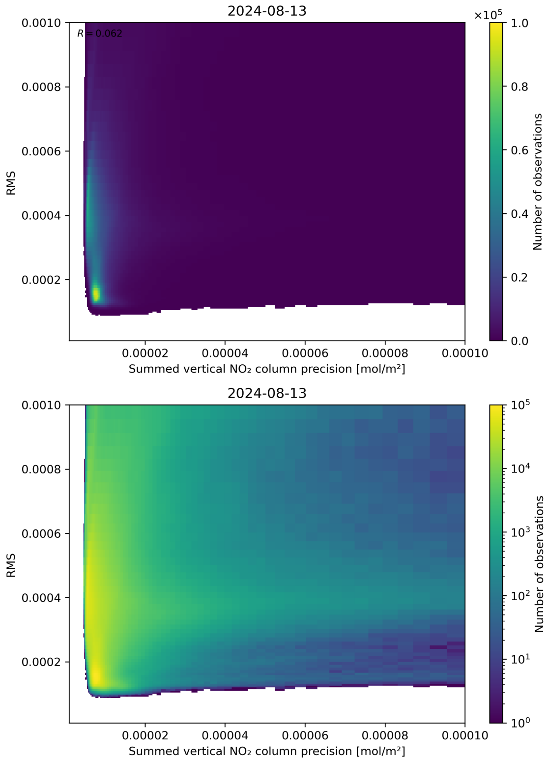
Figure 108: Scatter density plot of “Summed vertical NO 2 column precision” against “RMS” for 2024-08-12 to 2024-08-14.
