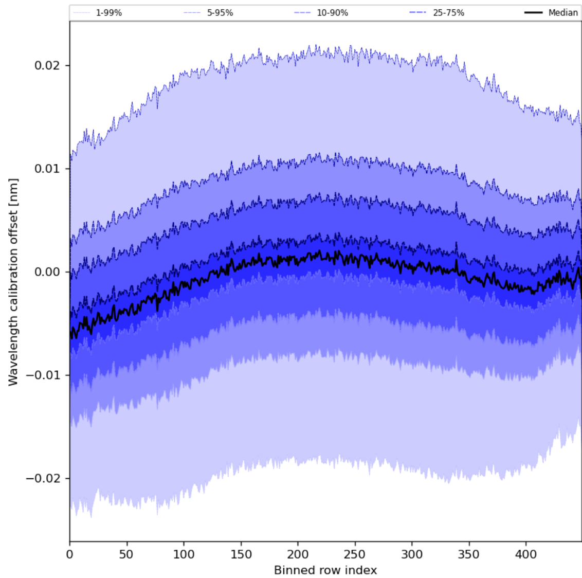
Figure 52: Along track statistics of “Wavelength calibration offset” for 2024-08-12 to 2024-08-14
