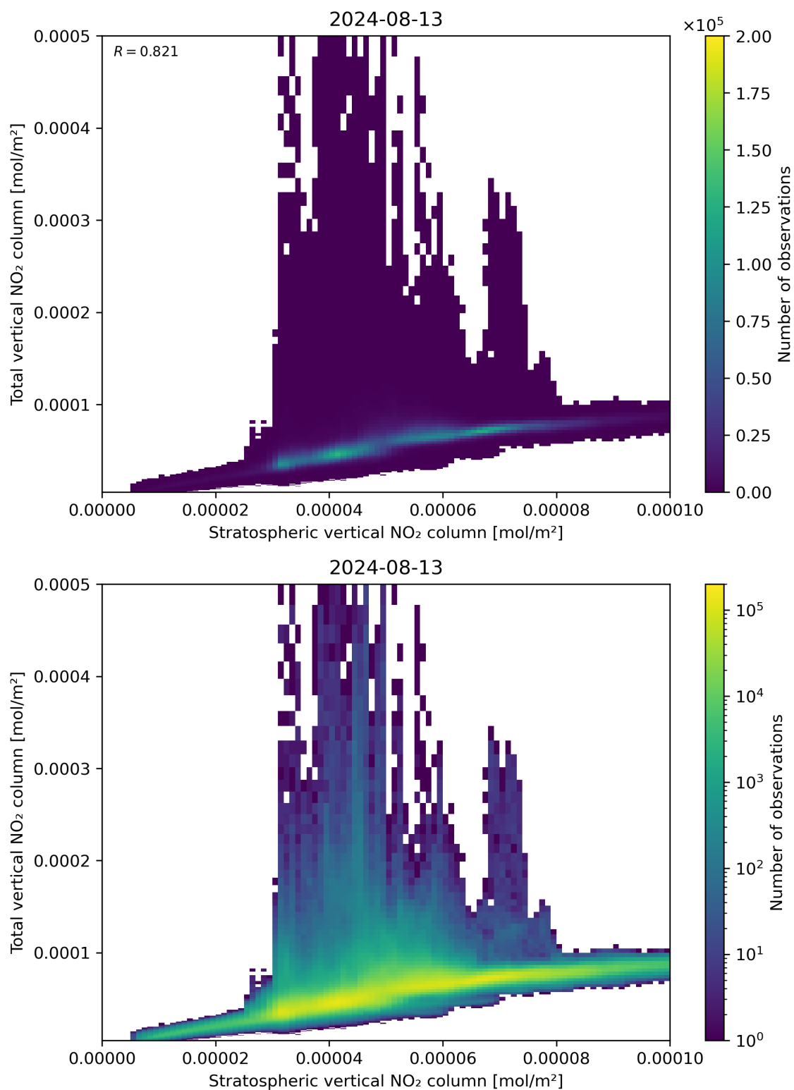
Figure 100: Scatter density plot of “Stratospheric vertical NO 2 column” against “Total vertical NO 2 column” for 2024-08-12 to 2024-08-14.
