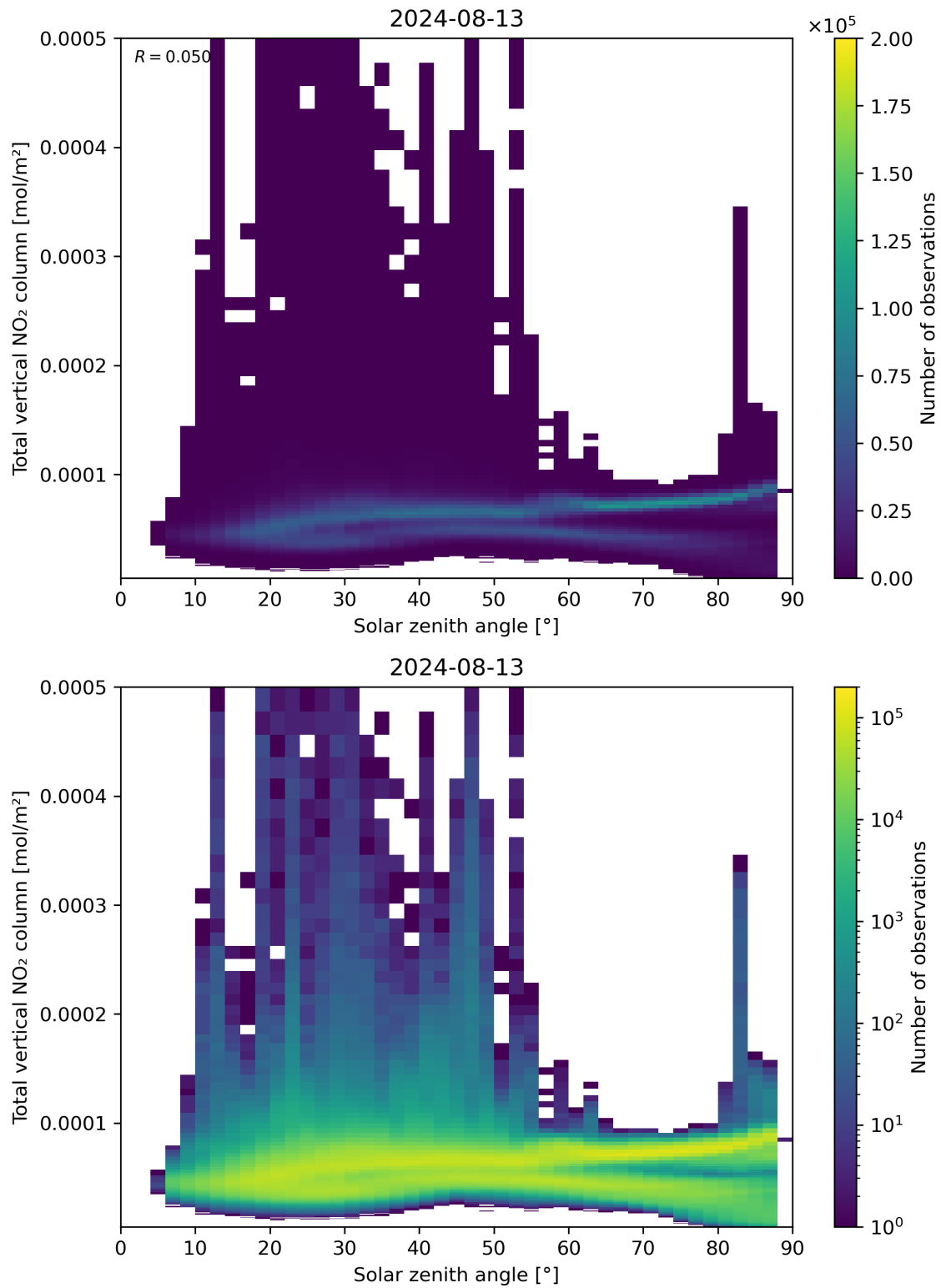
Figure 153: Scatter density plot of “Solar zenith angle” against “Total vertical NO 2 column” for 2024-08-12 to 2024-08-14.
