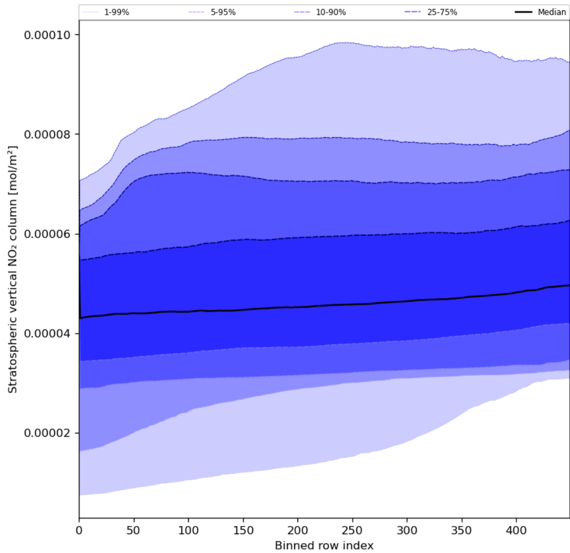
Figure 53: Along track statistics of “Stratospheric vertical NO 2 column” for 2024-08-12 to 2024-08-14
