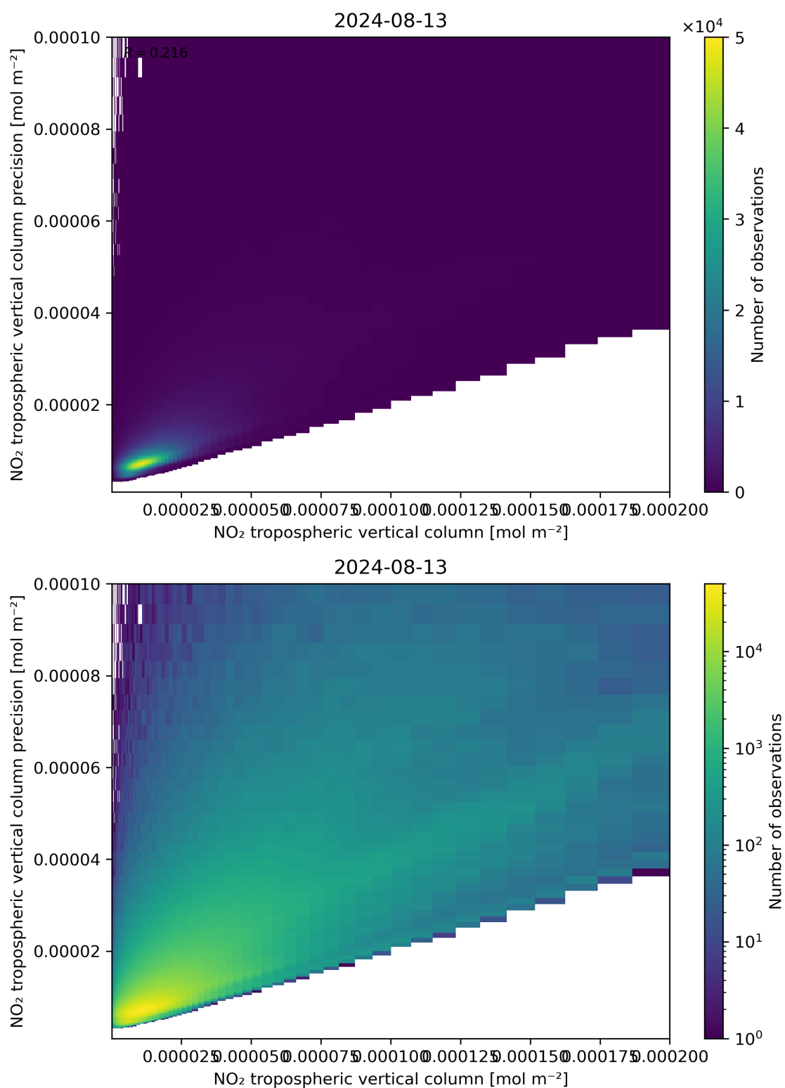
Figure 130: Scatter density plot of “NO 2 tropospheric vertical column” against “NO 2 tropospheric vertical column precision” for 2024-08-12 to 2024-08-14.
