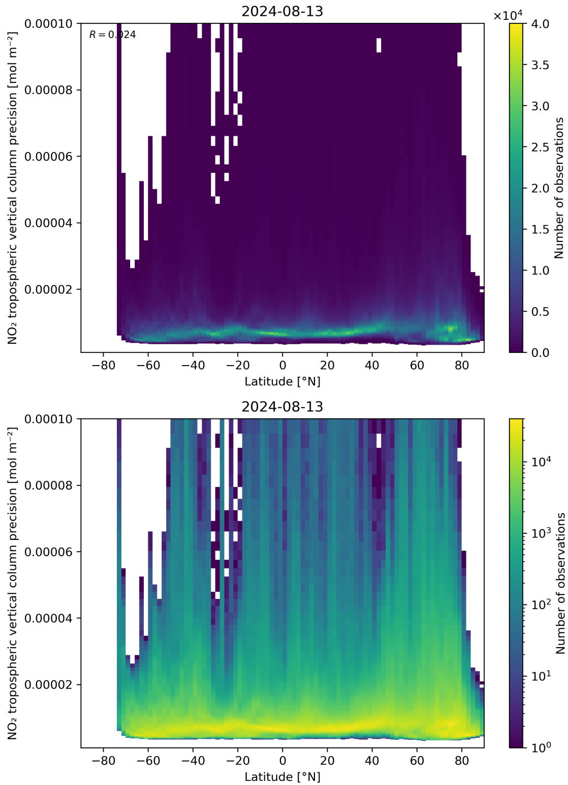
Figure 93: Scatter density plot of “Latitude” against “NO 2 tropospheric vertical column precision” for 2024-08-12 to 2024-08-14.
