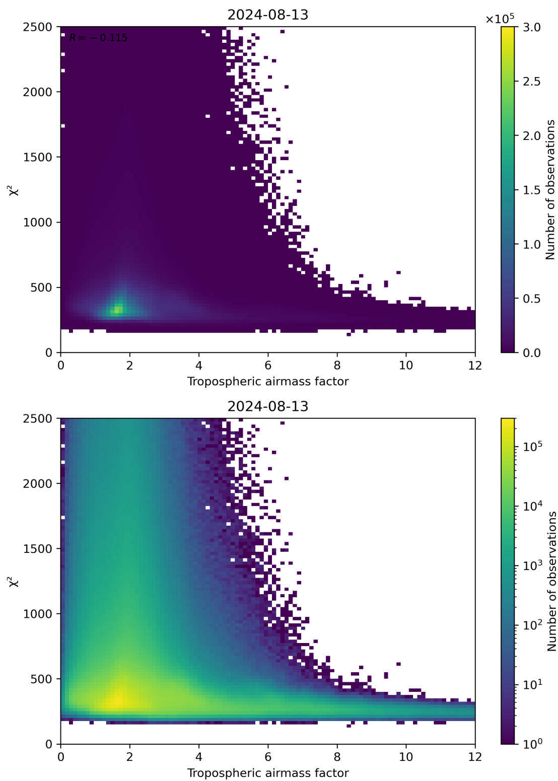
Figure 73: Scatter density plot of “Tropospheric airmass factor” against “ \chi^2 ” for 2024-08-12 to 2024-08-14.
