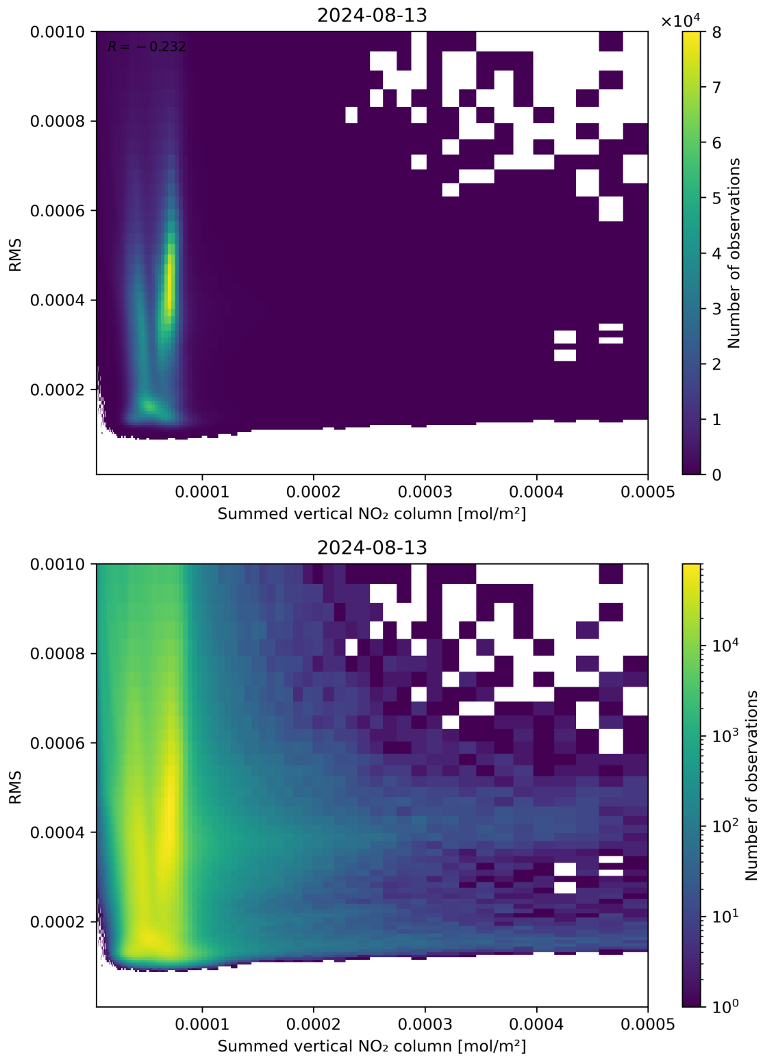
Figure 109: Scatter density plot of “Summed vertical NO 2 column” against “RMS” for 2024-08-12 to 2024-08-14.
