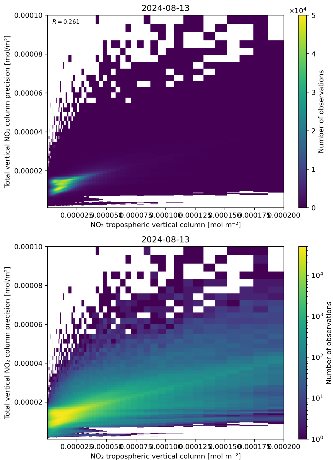
Figure 129: Scatter density plot of “NO 2 tropospheric vertical column” against “Total vertical NO 2 column precision” for 2024-08-12 to 2024-08-14.
