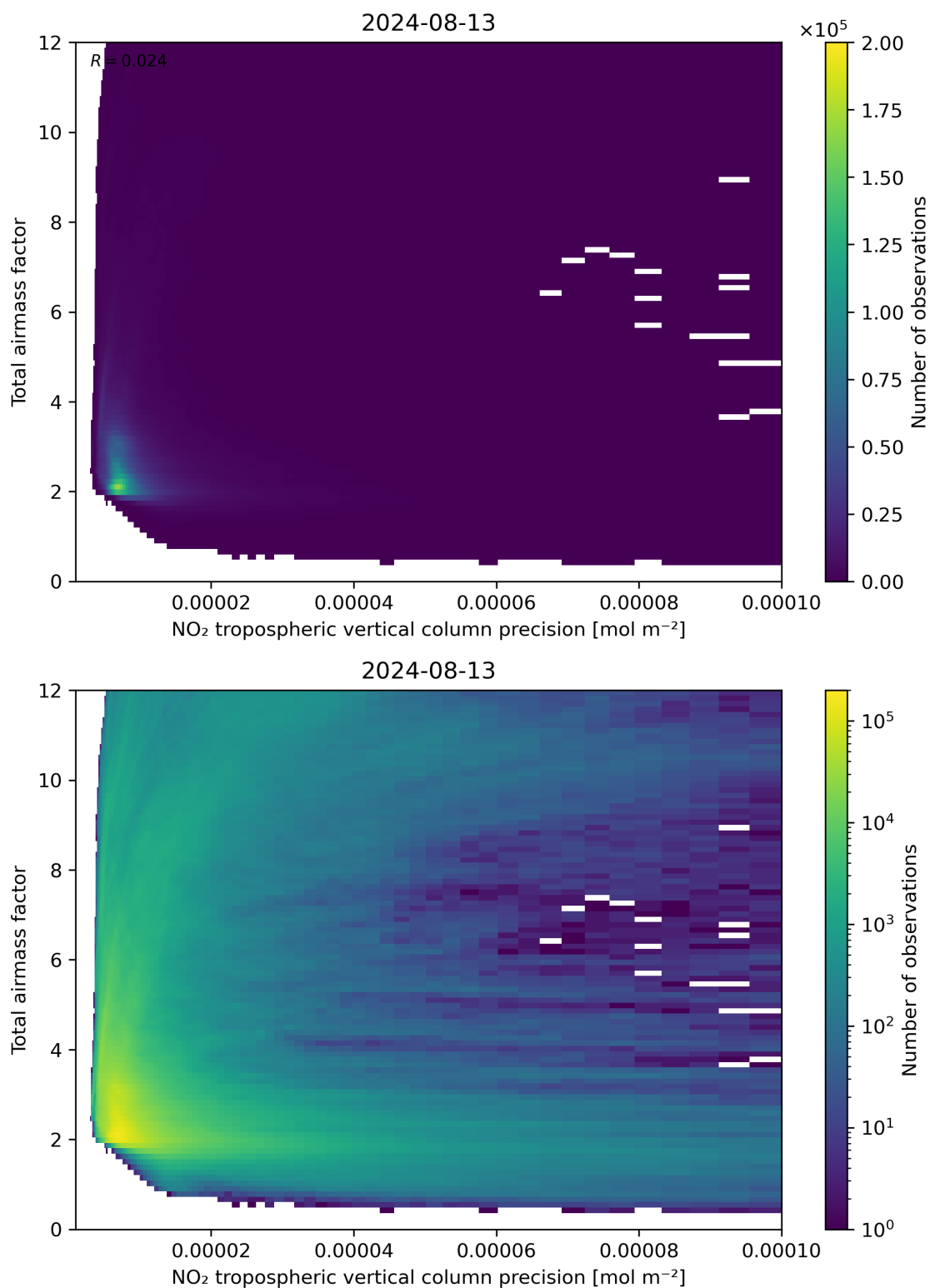
Figure 132: Scatter density plot of “NO 2 tropospheric vertical column precision” against “Total air mass factor” for 2024-08-12 to 2024-08-14.
