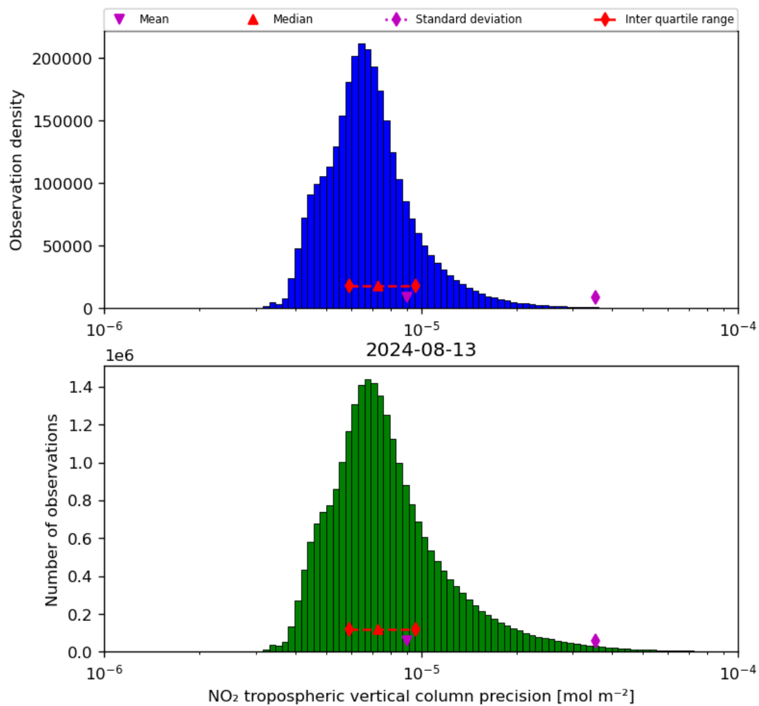
Figure 30: Histogram of “NO 2 tropospheric vertical column precision” for 2024-08-12 to 2024-08-14
