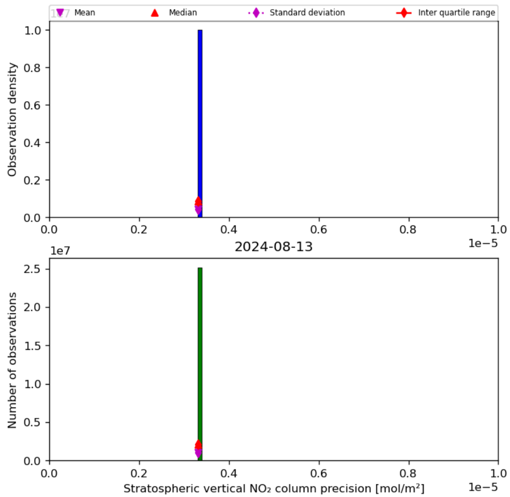
Figure 37: Histogram of “Stratospheric vertical NO 2 column precision” for 2024-08-12 to 2024-08-14
