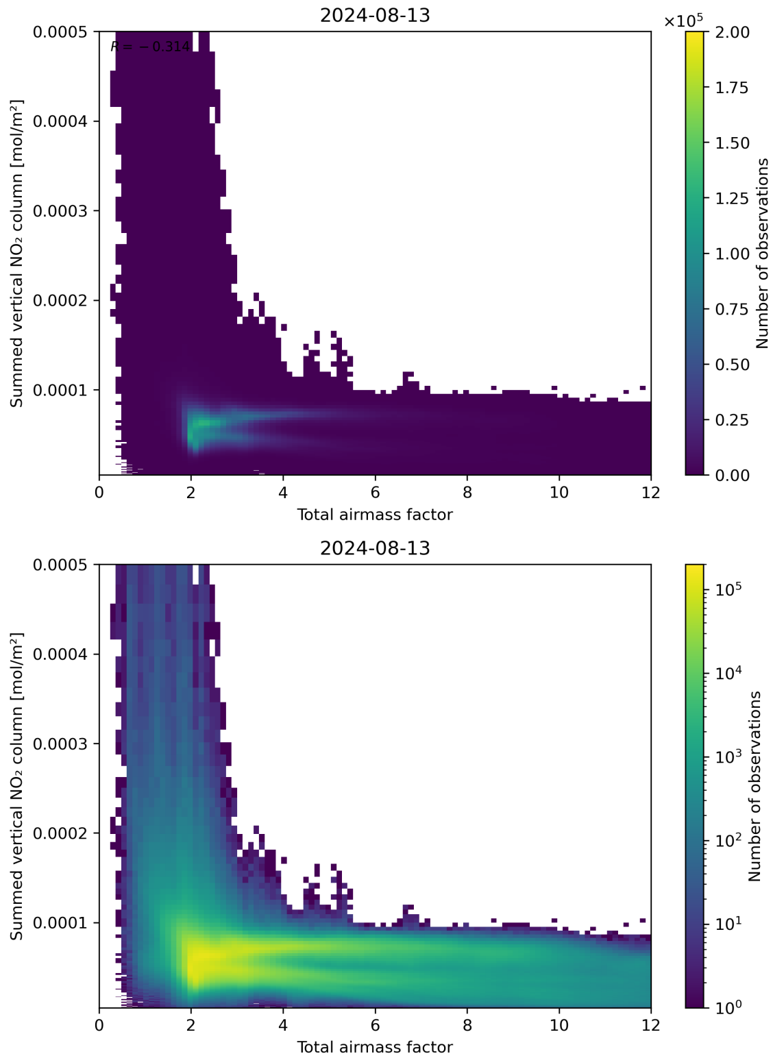
Figure 65: Scatter density plot of “Total airmass factor” against “Summed vertical NO 2 column” for 2024-08-12 to 2024-08-14.
