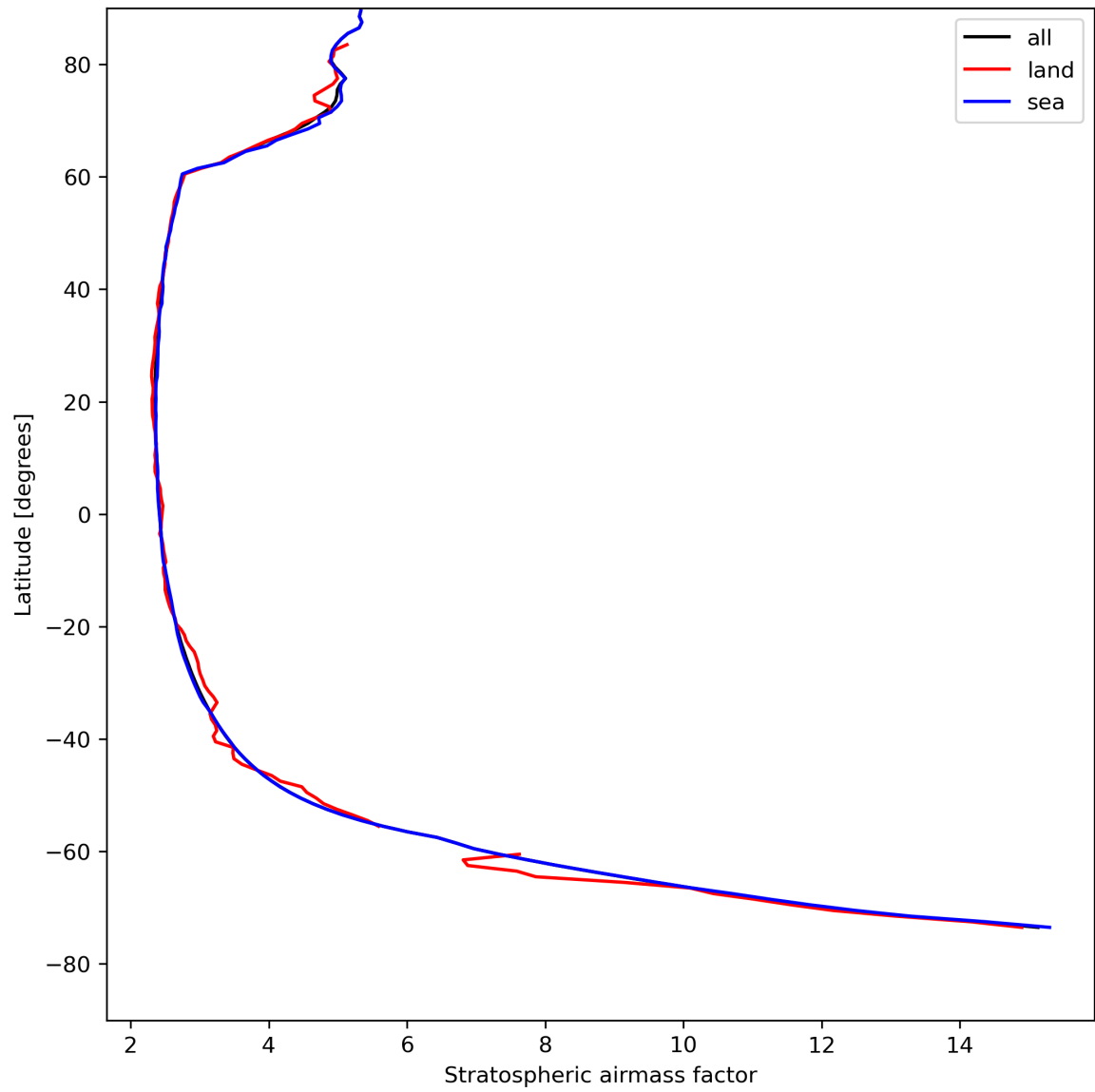
Figure 27: Zonal average of “Stratospheric airmass factor” for 2024-08-12 to 2024-08-14.
