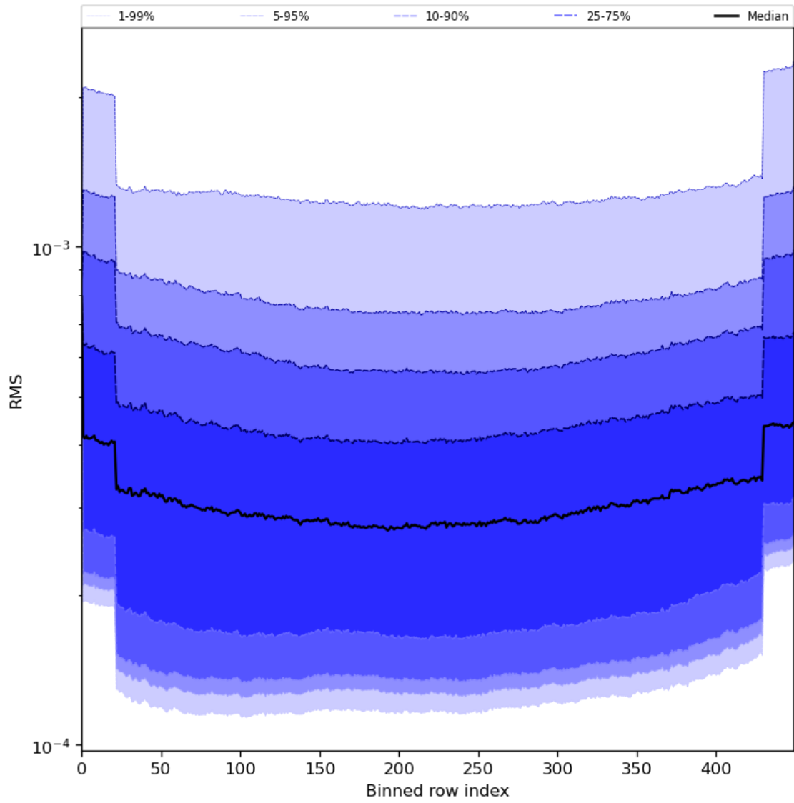
Figure 60: Along track statistics of “RMS” for 2024-08-12 to 2024-08-14
