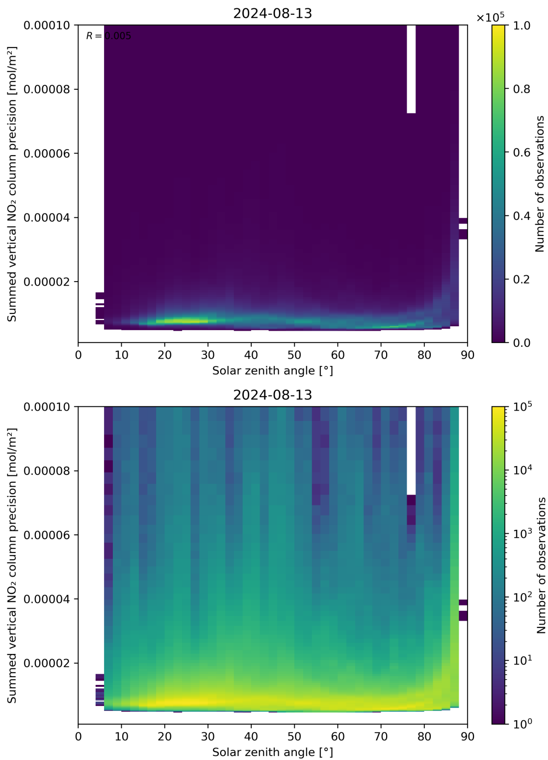
Figure 152: Scatter density plot of “Solar zenith angle” against “Summed vertical NO 2 column precision” for 2024-08-12 to 2024-08-14.
