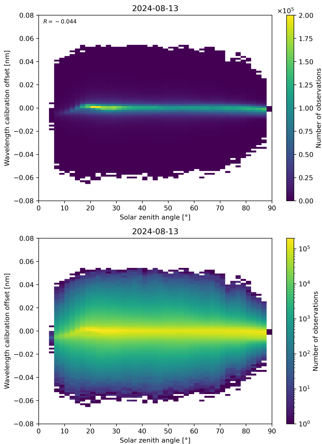
Figure 158: Scatter density plot of “Solar zenith angle” against “Wavelength calibration offset” for 2024-08-12 to 2024-08-14.
