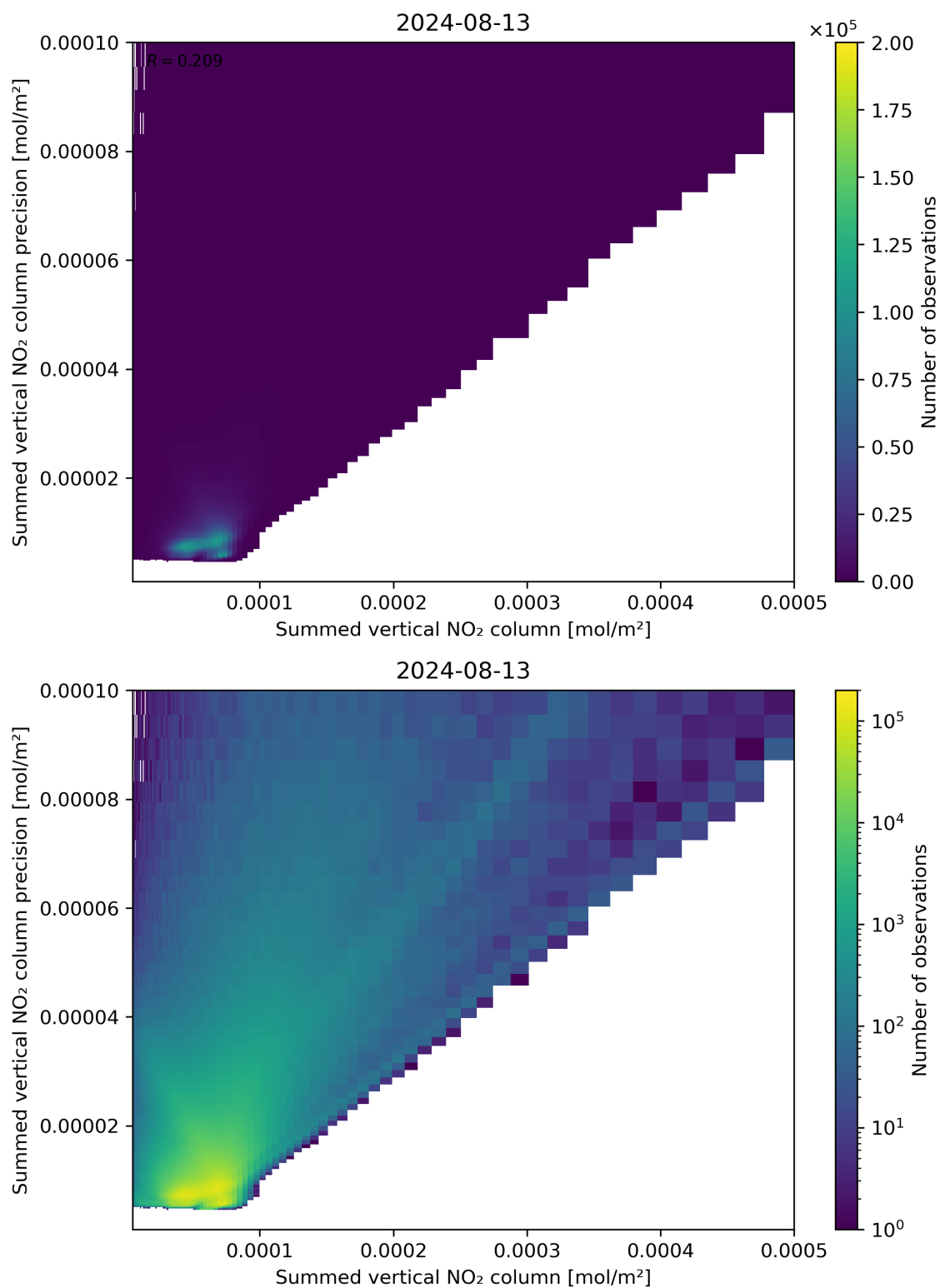
Figure 105: Scatter density plot of “Summed vertical NO 2 column” against “Summed vertical NO 2 column precision” for 2024-08-12 to 2024-08-14.
