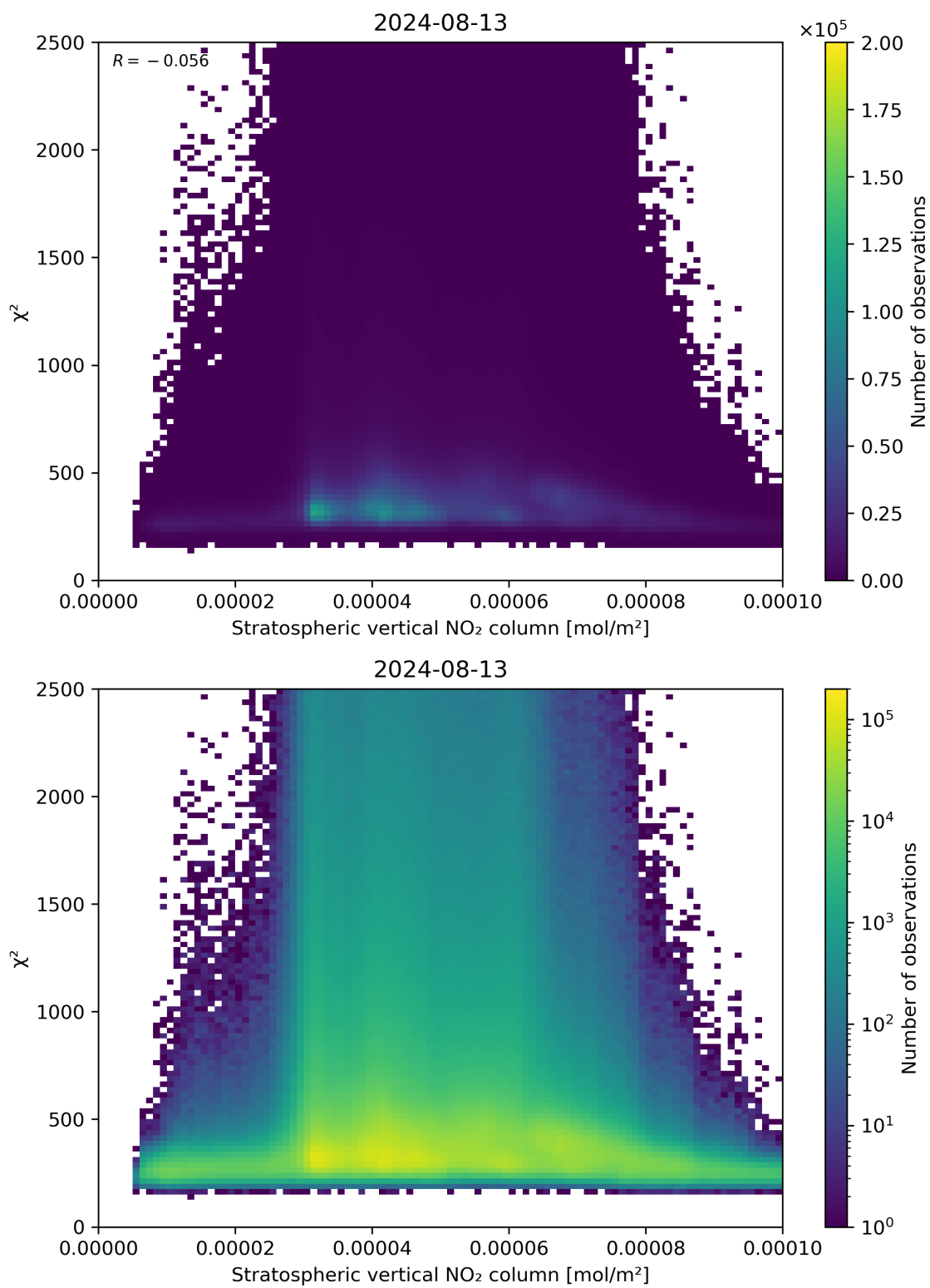
Figure 97: Scatter density plot of “Stratospheric vertical NO 2 column” against “ \chi^2 ” for 2024-08-12 to 2024-08-14.
