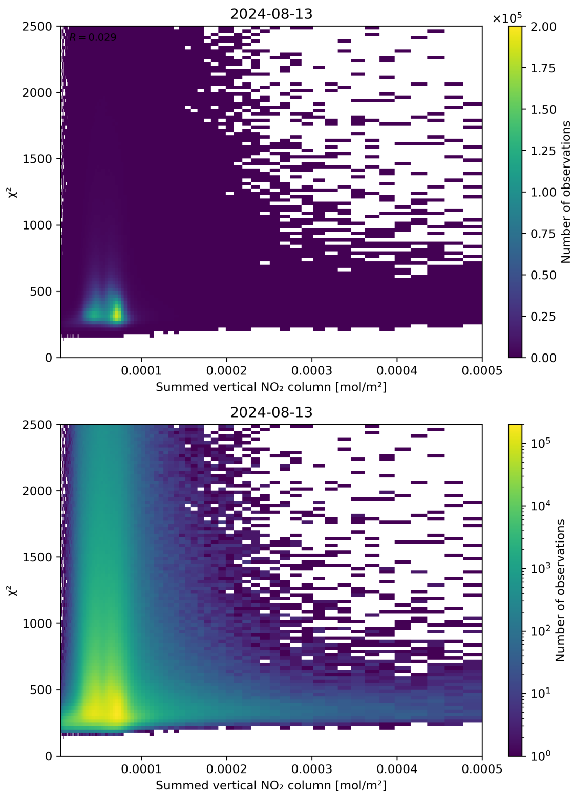
Figure 104: Scatter density plot of “Summed vertical NO 2 column” against “ \chi^2 ” for 2024-08-12 to 2024-08-14.
