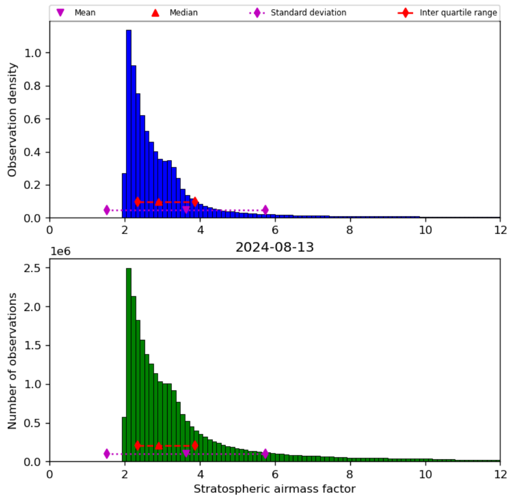
Figure 44: Histogram of “Stratospheric airmass factor” for 2024-08-12 to 2024-08-14
