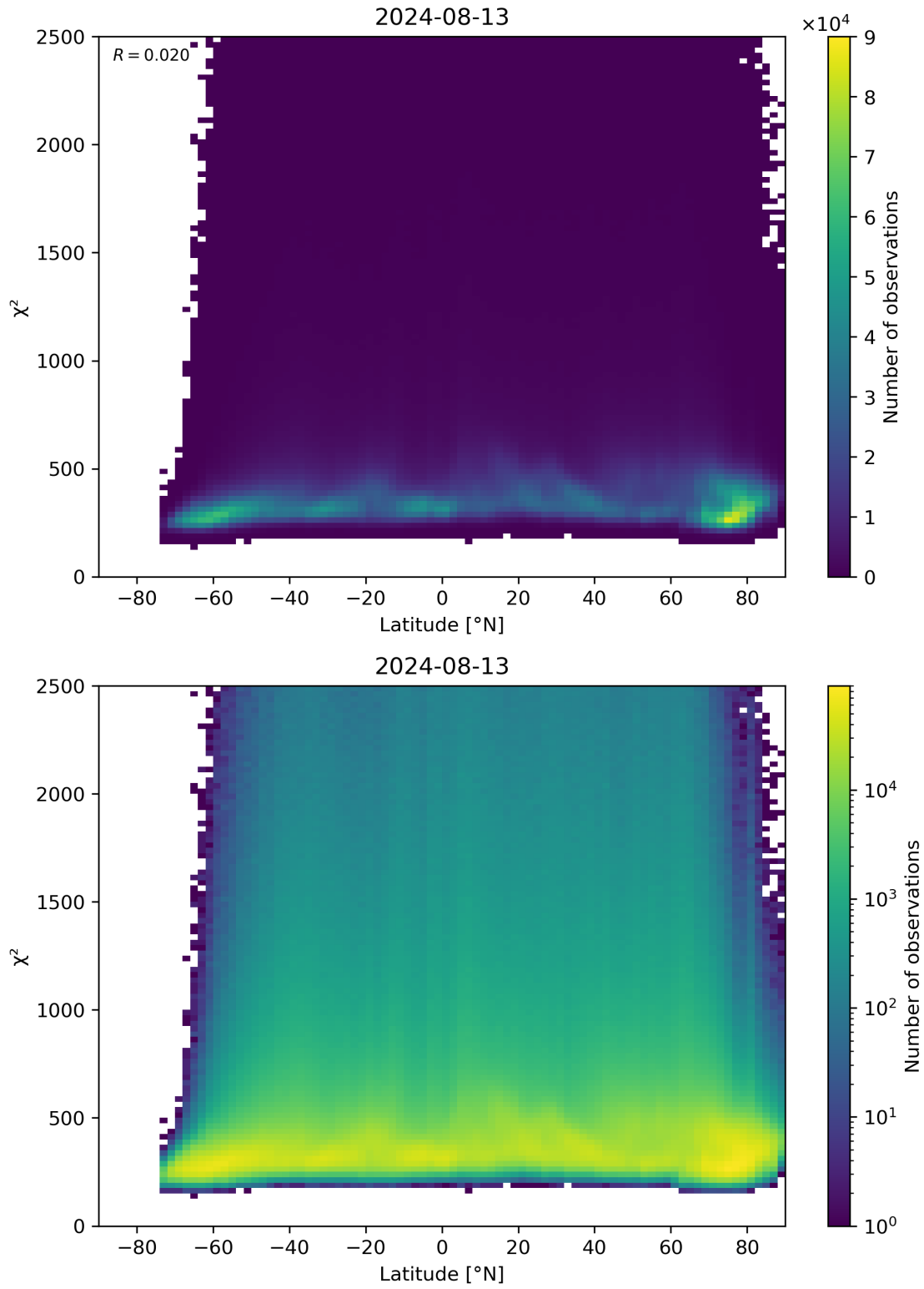
Figure 86: Scatter density plot of “Latitude” against “ \chi^2 ” for 2024-08-12 to 2024-08-14.
