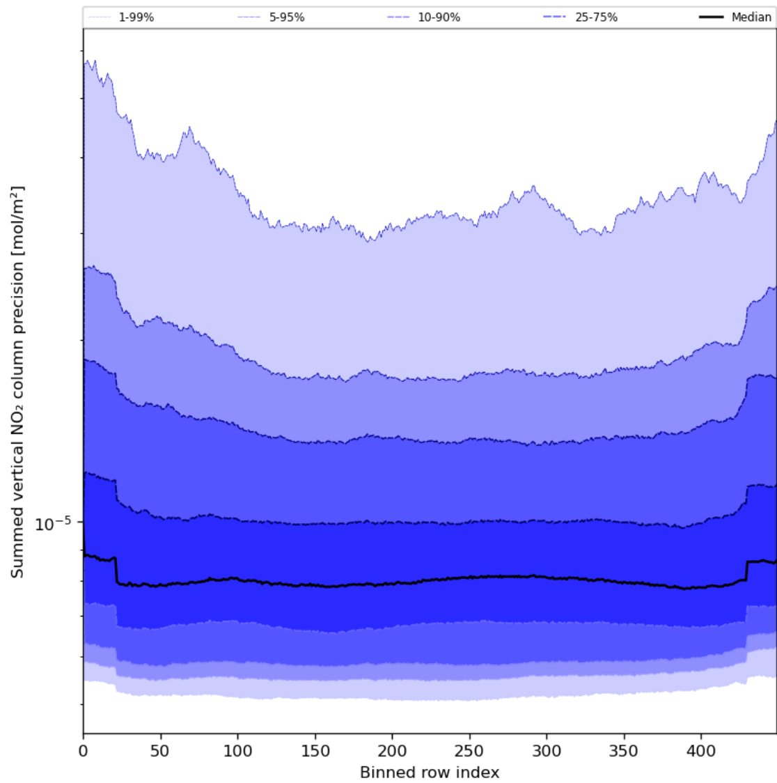
Figure 58: Along track statistics of “Summed vertical NO 2 column precision” for 2024-08-12 to 2024-08-14
