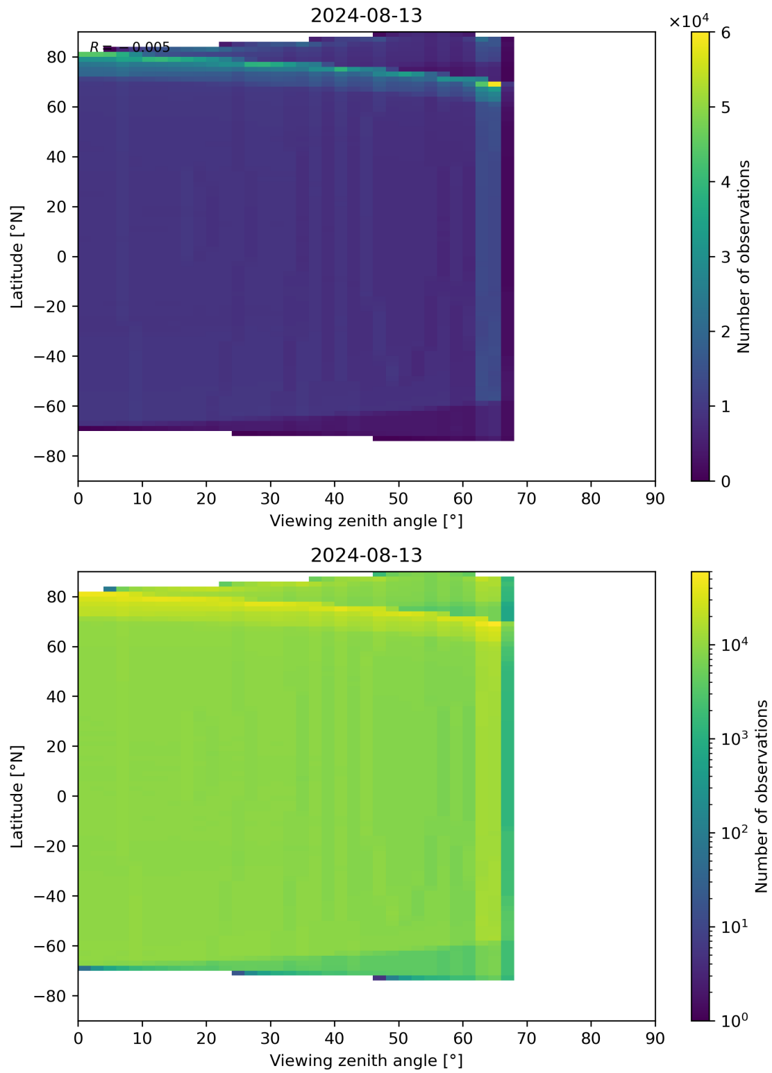
Figure 163: Scatter density plot of “Viewing zenith angle” against “Latitude” for 2024-08-12 to 2024-08-14.
