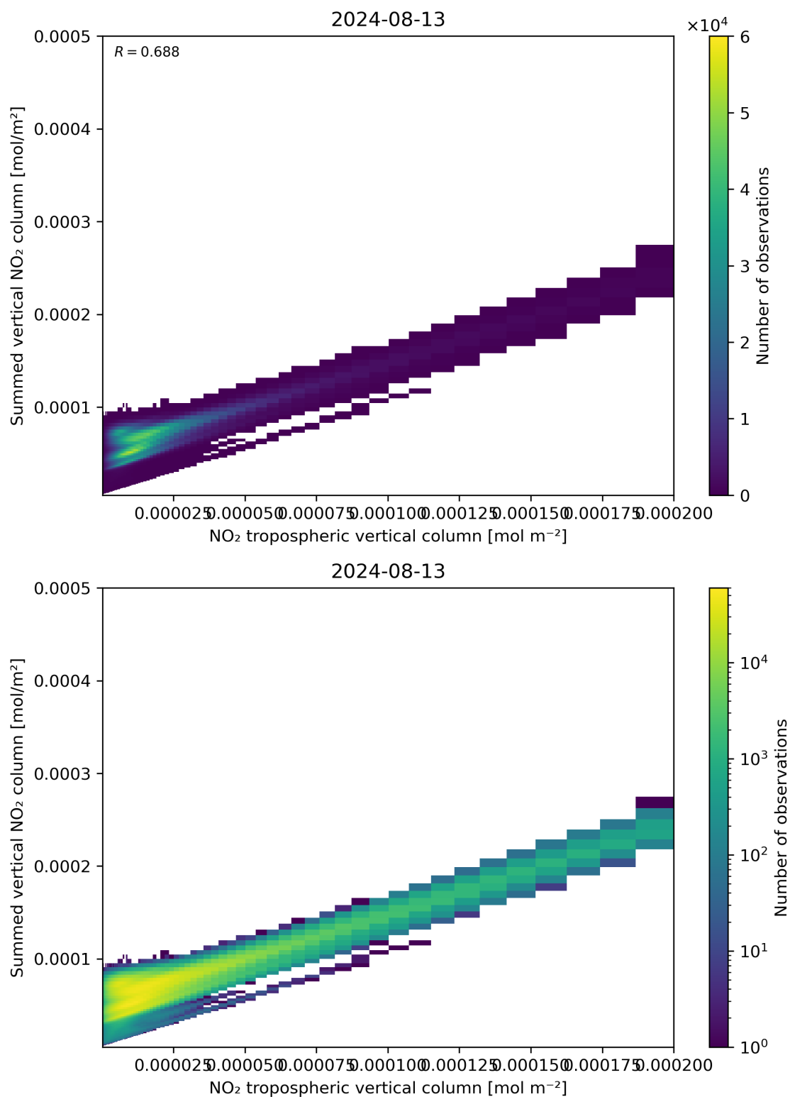
Figure 126: Scatter density plot of “NO 2 tropospheric vertical column” against “Summed vertical NO 2 column” for 2024-08-12 to 2024-08-14.
