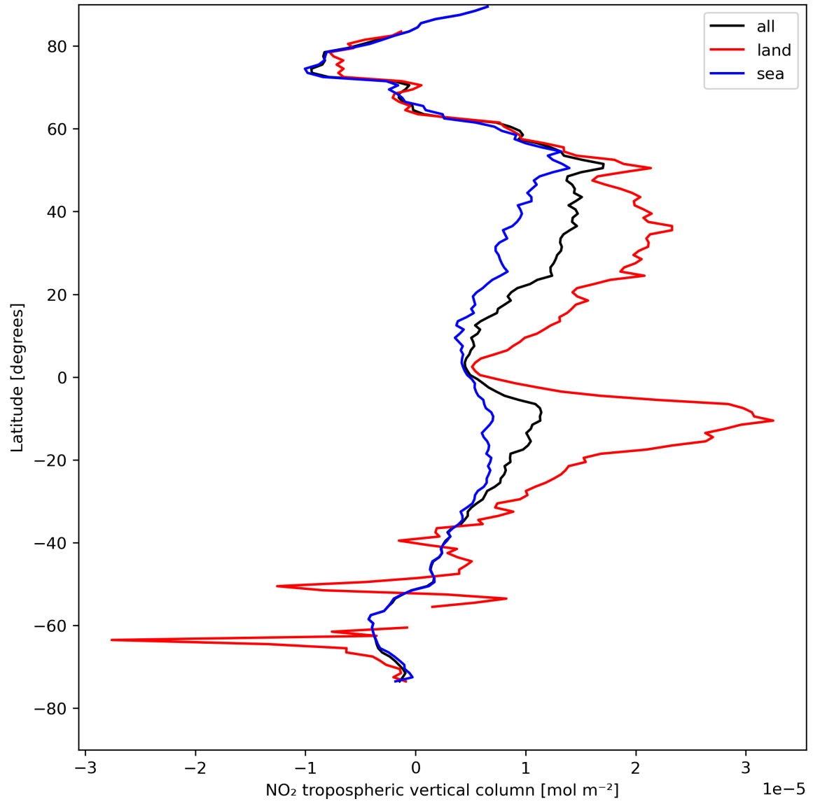
Figure 12: Zonal average of “NO 2 tropospheric vertical column” for 2024-08-13 to 2024-08-15.
