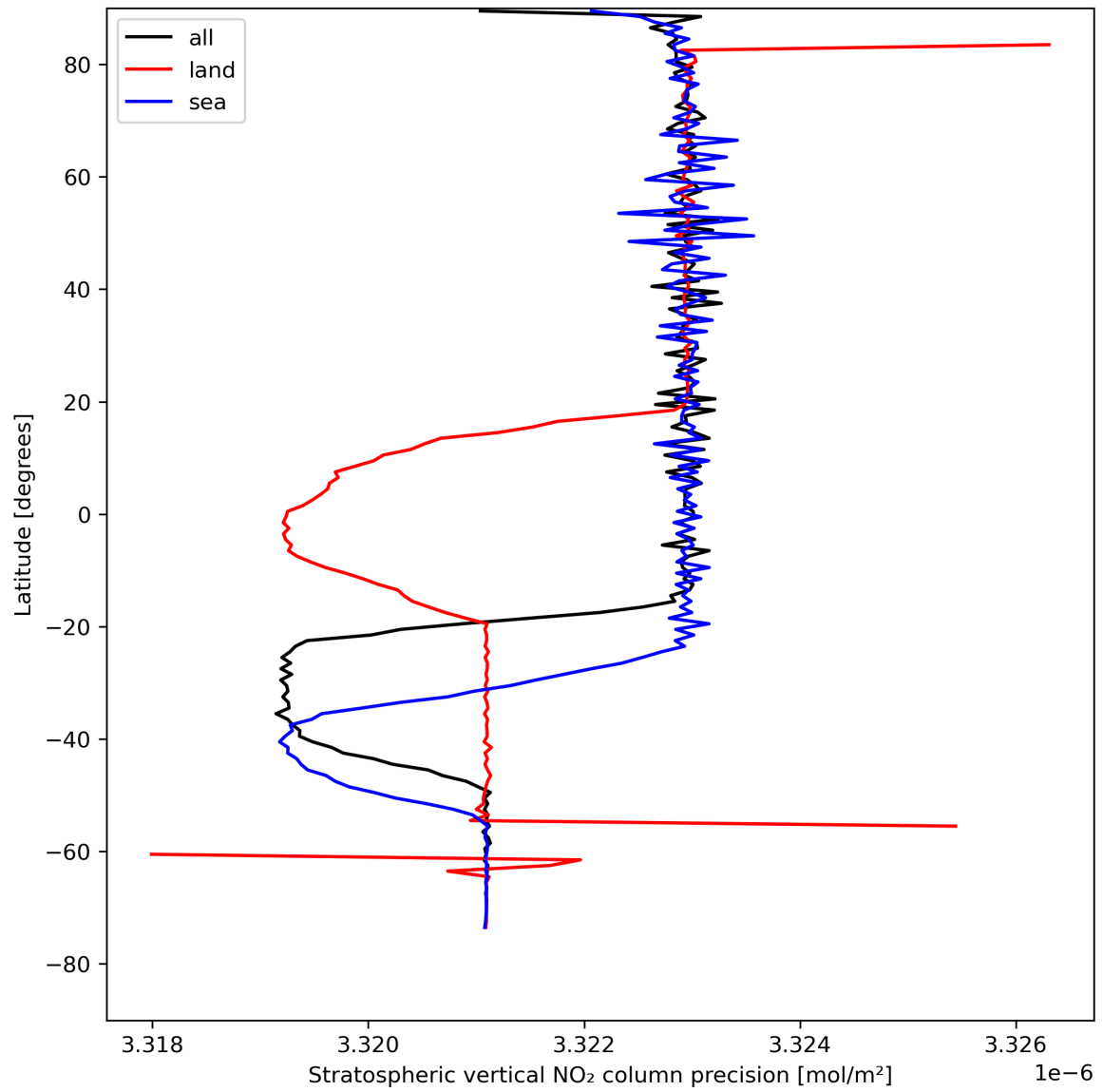
Figure 20: Zonal average of “Stratospheric vertical NO 2 column precision” for 2024-08-13 to 2024-08-15.
