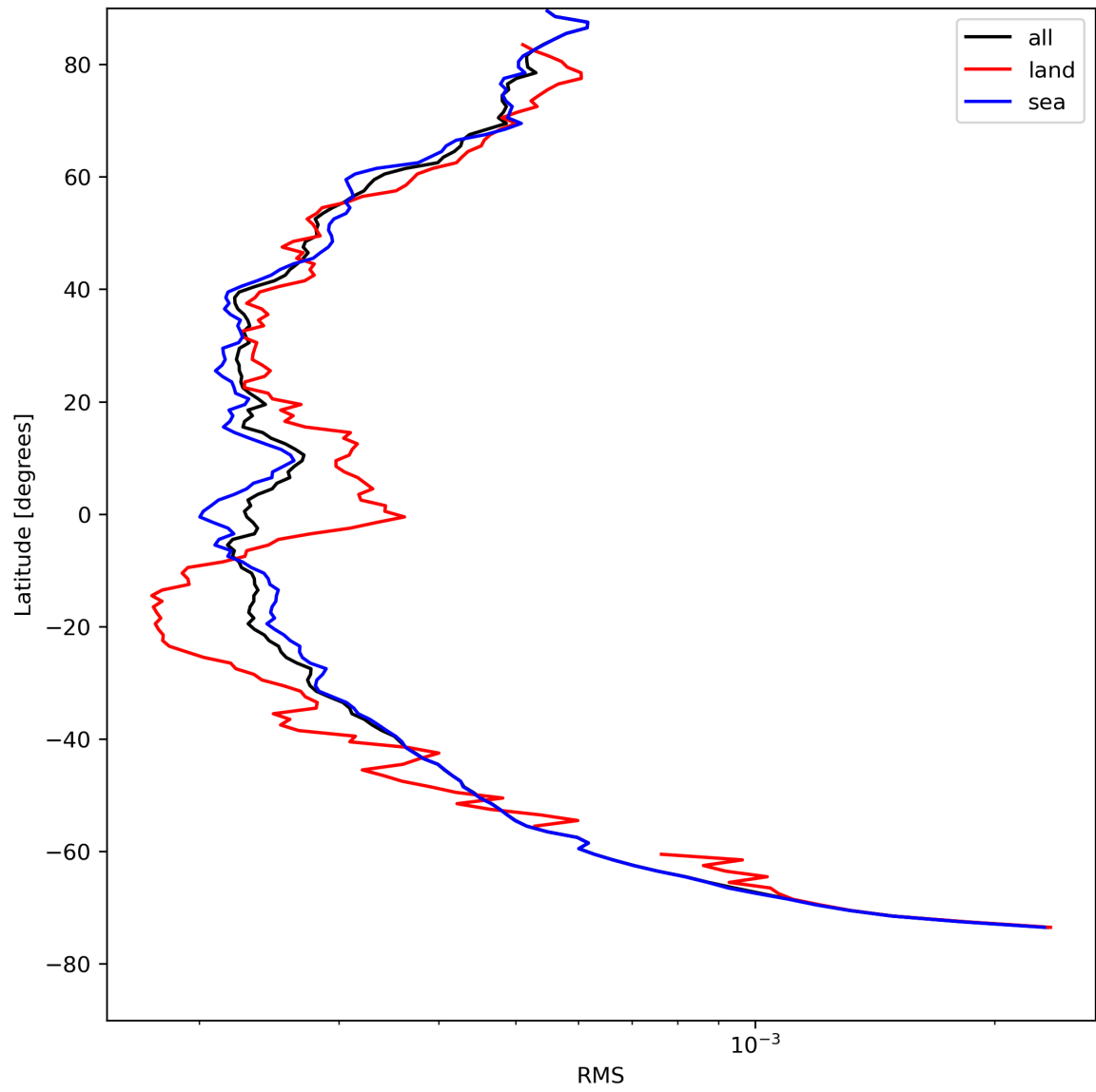
Figure 26: Zonal average of “RMS” for 2024-08-13 to 2024-08-15.
