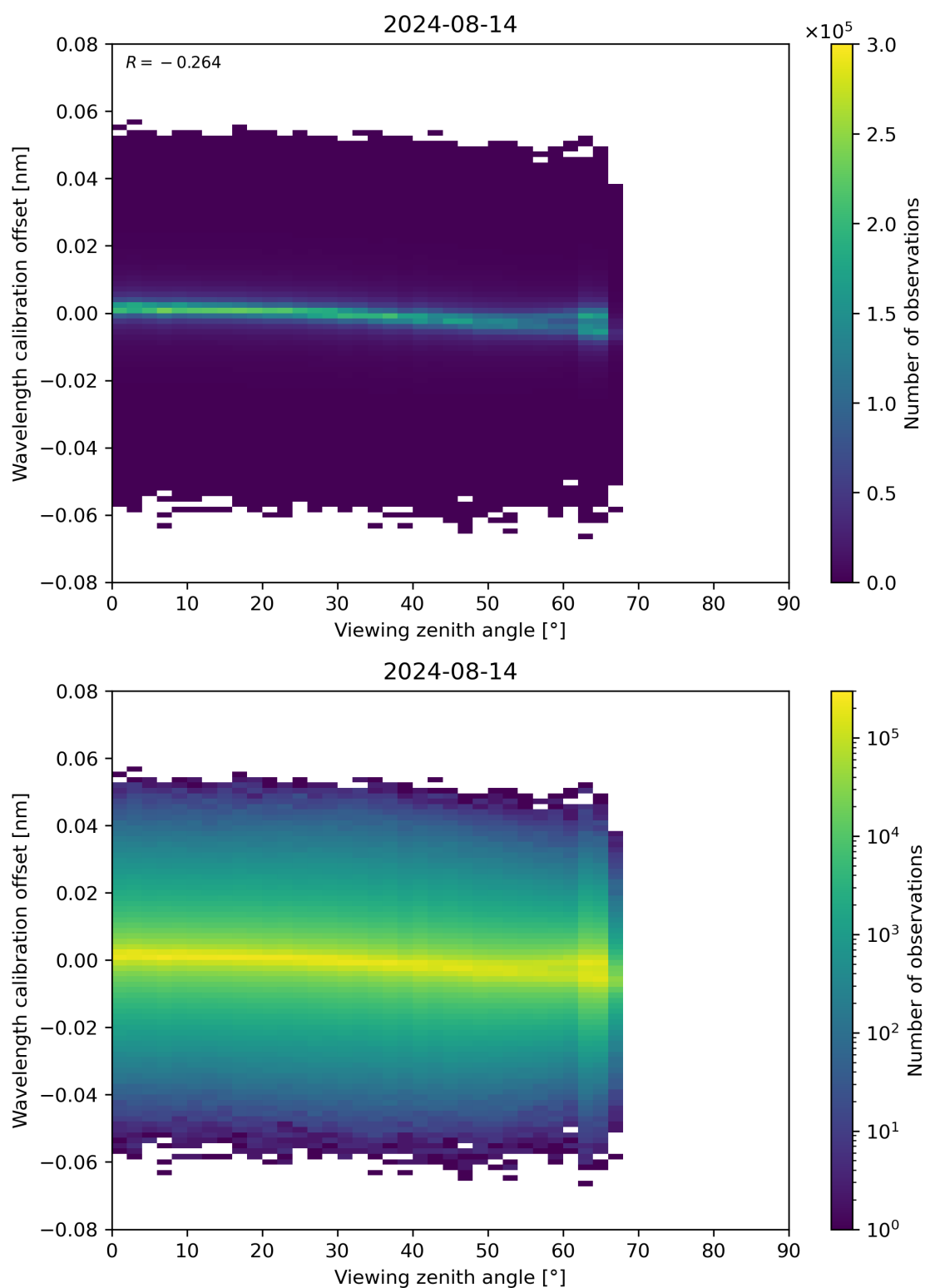
Figure 173: Scatter density plot of “Viewing zenith angle” against “Wavelength calibration offset” for 2024-08-13 to 2024-08-15.
