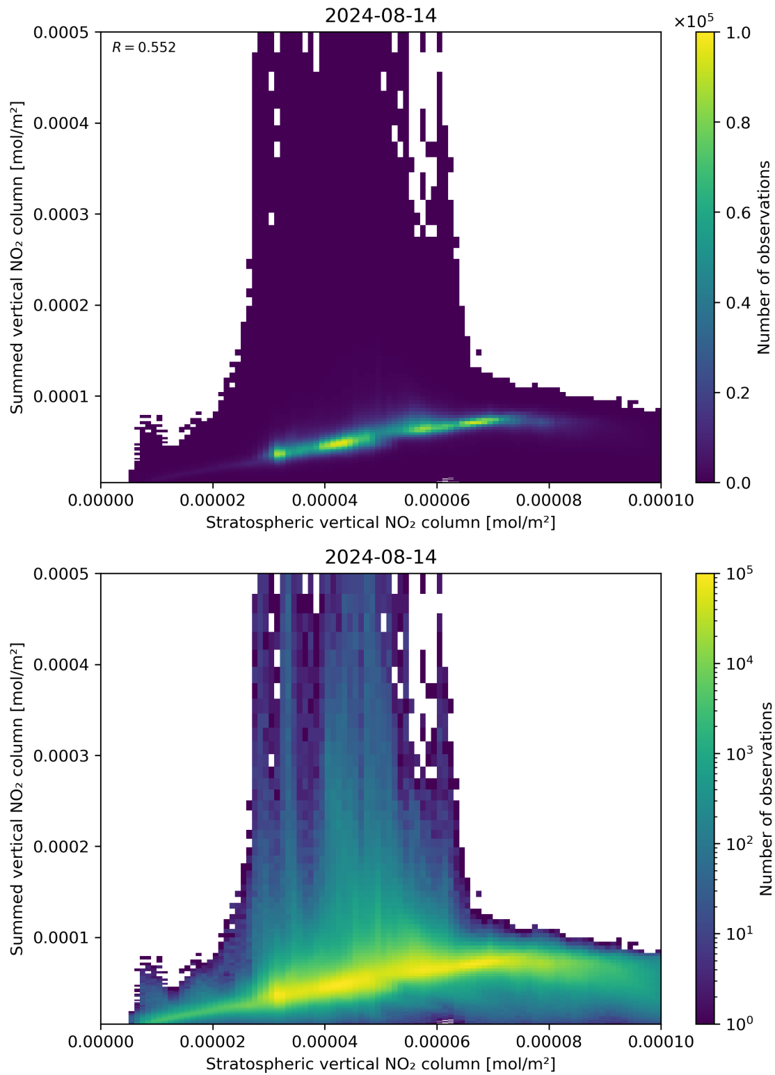
Figure 98: Scatter density plot of “Stratospheric vertical NO 2 column” against “Summed vertical NO 2 column” for 2024-08-13 to 2024-08-15.
