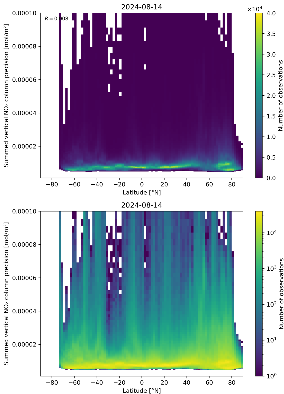
Figure 89: Scatter density plot of “Latitude” against “Summed vertical NO 2 column precision” for 2024-08-13 to 2024-08-15.
