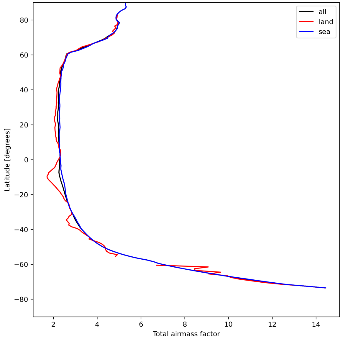
Figure 15: Zonal average of “Total airmass factor” for 2024-08-13 to 2024-08-15.
