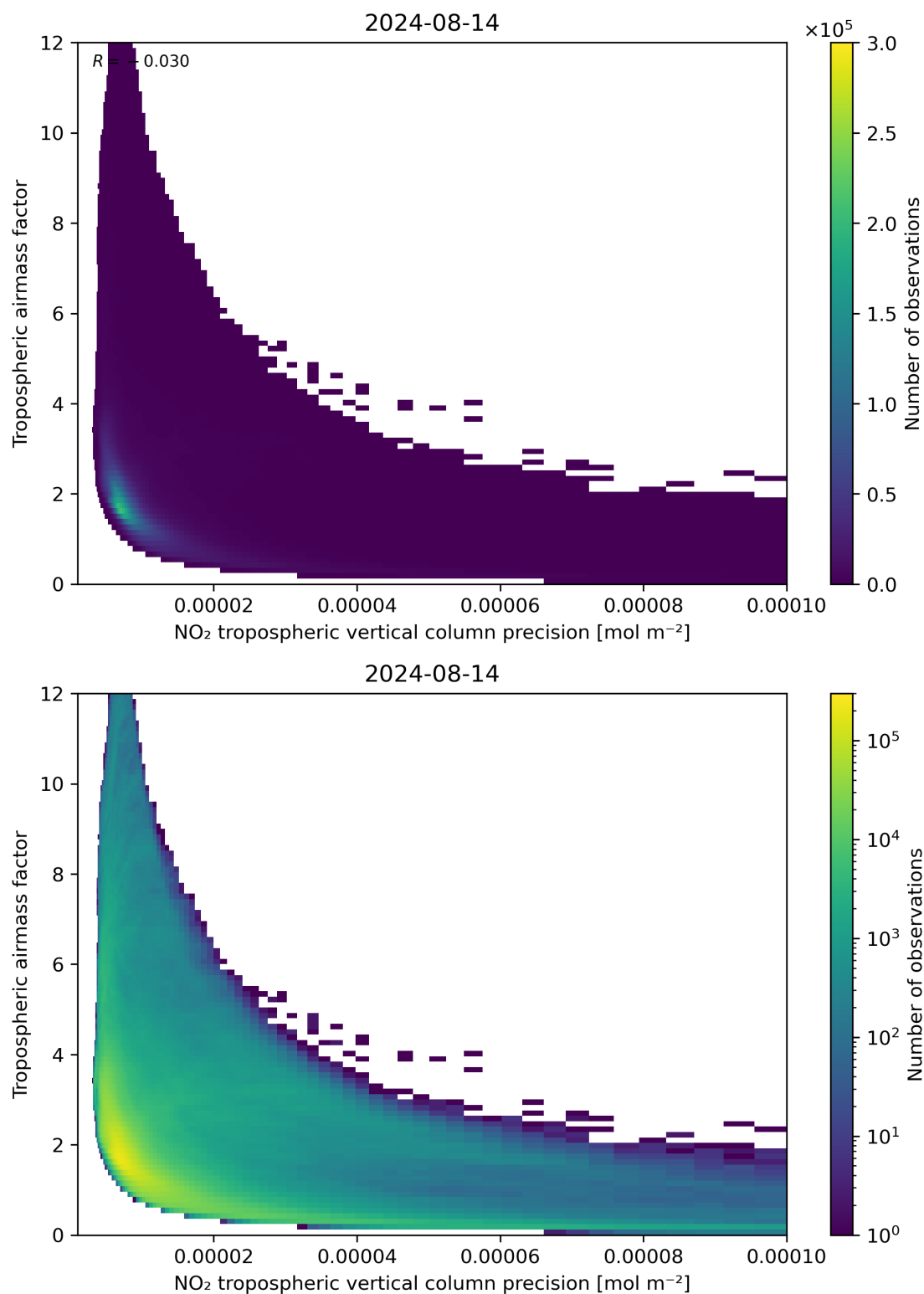
Figure 133: Scatter density plot of “NO 2 tropospheric vertical column precision” against “Tropospheric airmass factor” for 2024-08-13 to 2024-08-15.
