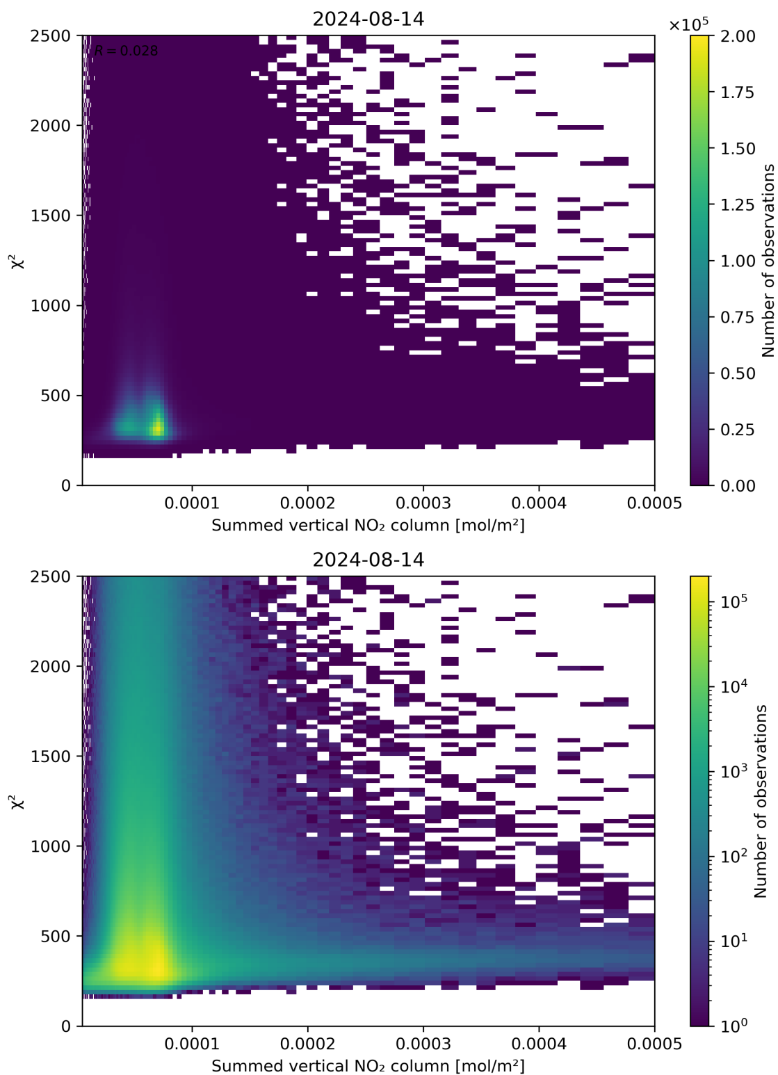
Figure 104: Scatter density plot of “Summed vertical NO 2 column” against “ \chi^2 ” for 2024-08-13 to 2024-08-15.
