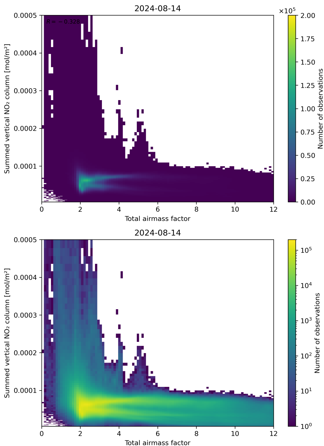
Figure 65: Scatter density plot of “Total airmass factor” against “Summed vertical NO 2 column” for 2024-08-13 to 2024-08-15.
