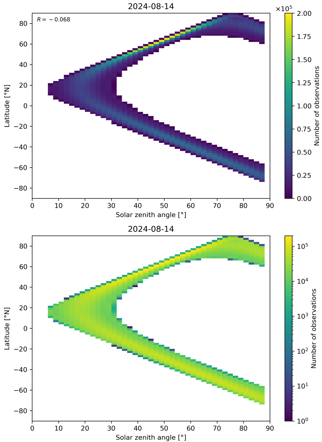
Figure 149: Scatter density plot of “Solar zenith angle” against “Latitude” for 2024-08-13 to 2024-08-15.
