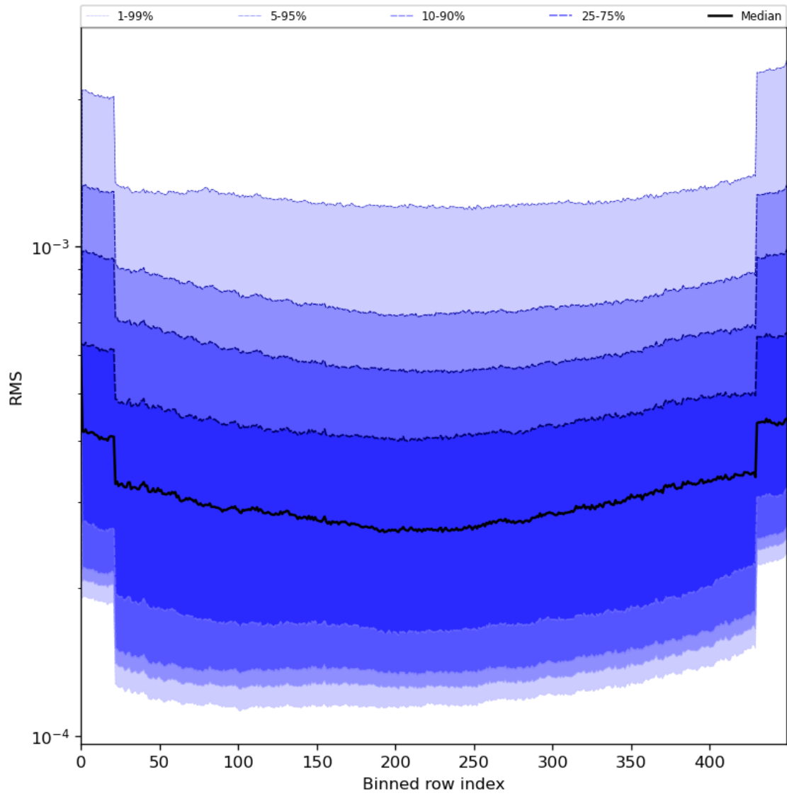
Figure 60: Along track statistics of “RMS” for 2024-08-13 to 2024-08-15
