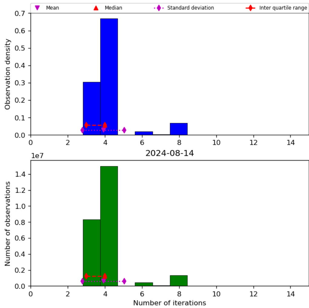
Figure 34: Histogram of “Number of iterations” for 2024-08-13 to 2024-08-15
