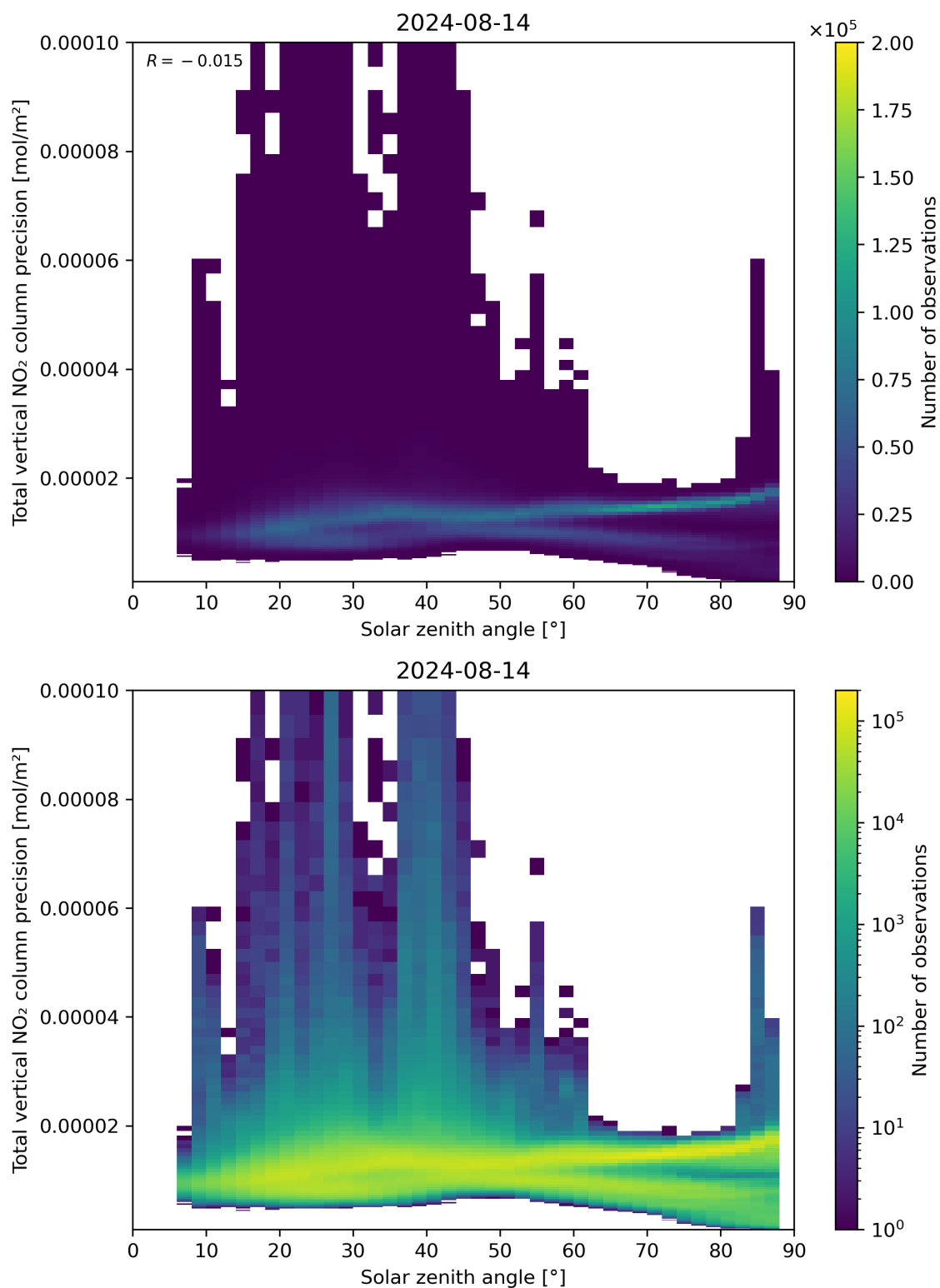
Figure 154: Scatter density plot of “Solar zenith angle” against “Total vertical NO 2 column precision” for 2024-08-13 to 2024-08-15.
