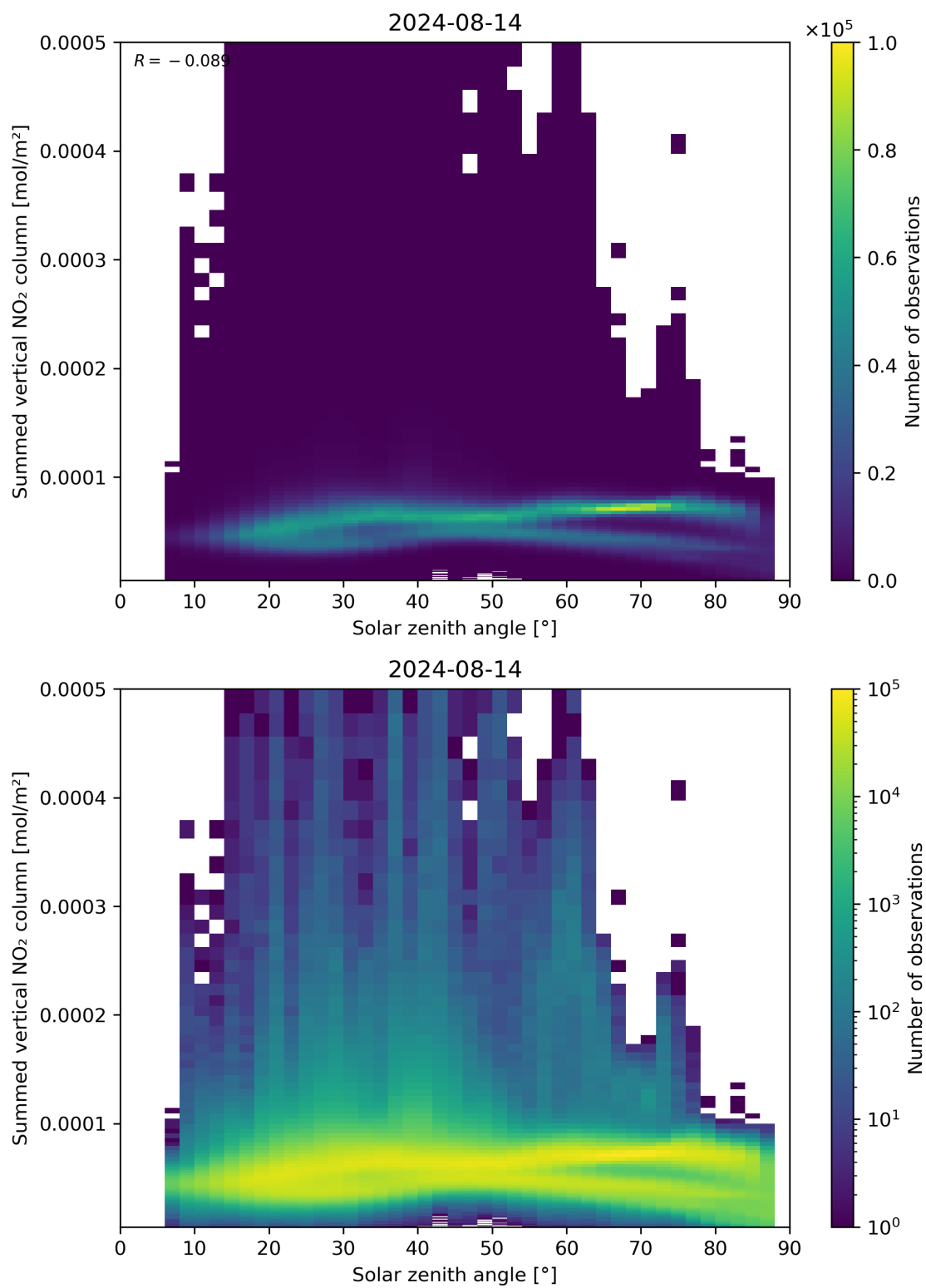
Figure 151: Scatter density plot of “Solar zenith angle” against “Summed vertical NO 2 column” for 2024-08-13 to 2024-08-15.
