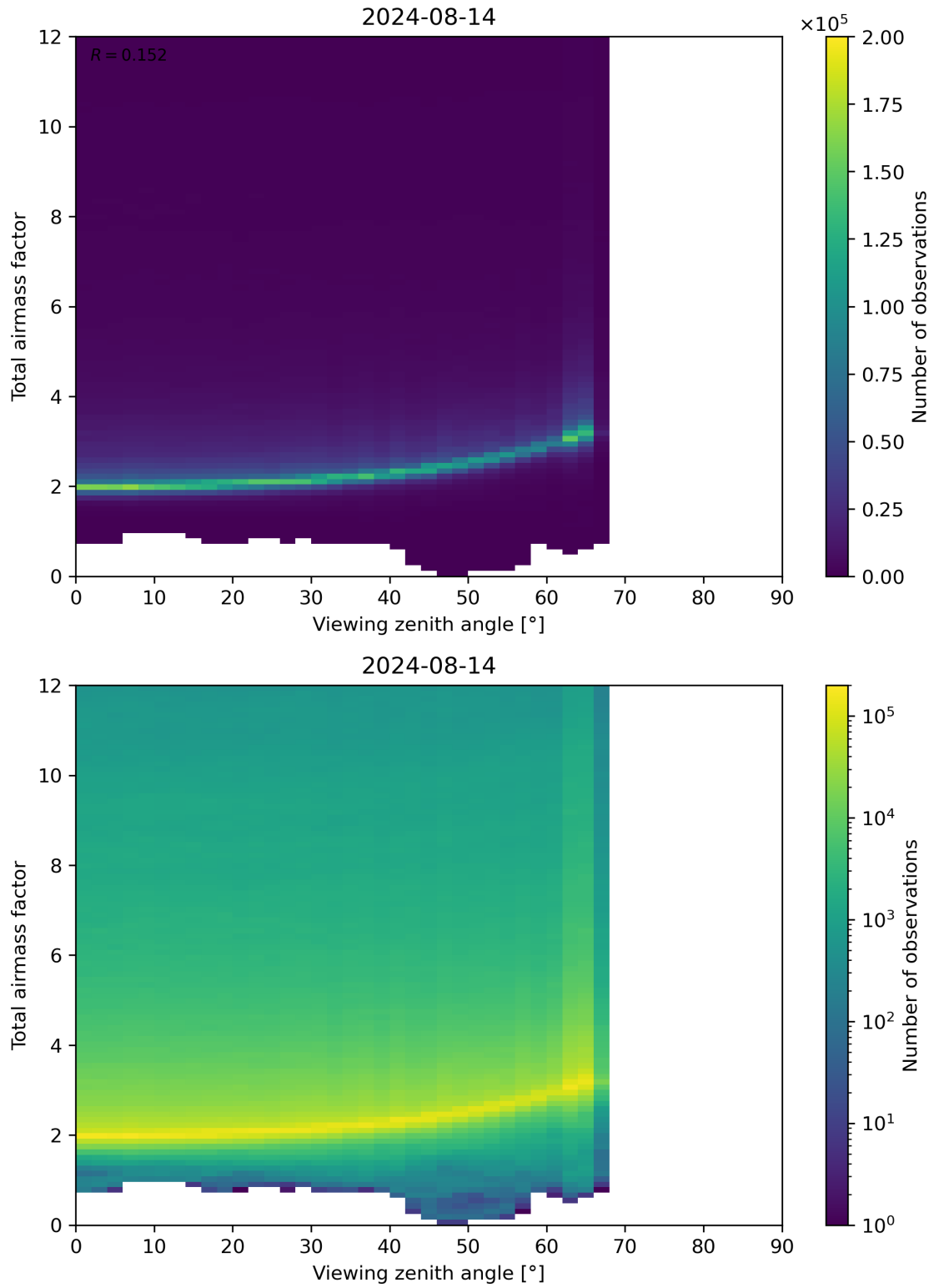
Figure 160: Scatter density plot of “Viewing zenith angle” against “Total airmass factor” for 2024-08-13 to 2024-08-15.
