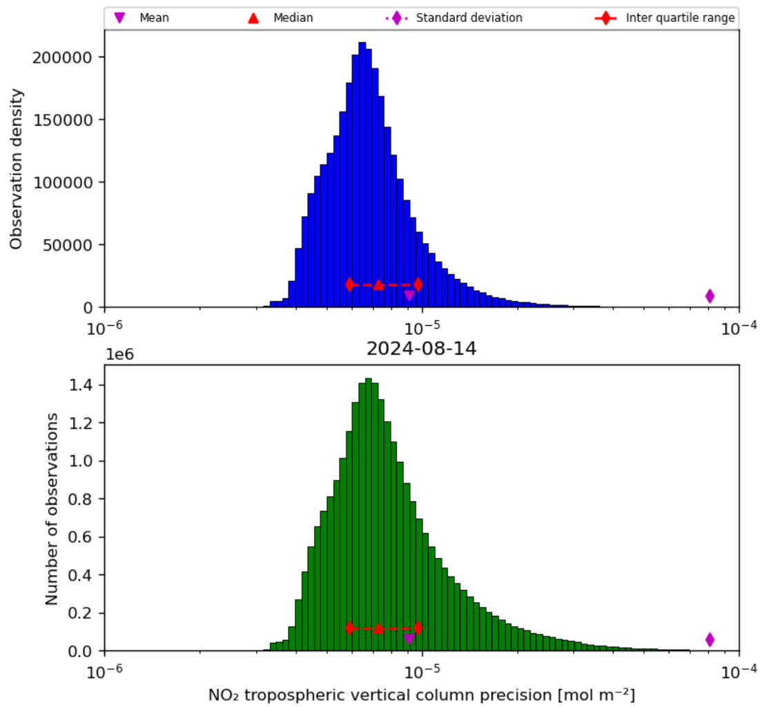
Figure 30: Histogram of “NO 2 tropospheric vertical column precision” for 2024-08-13 to 2024-08-15
