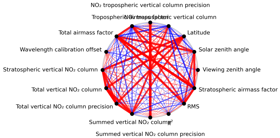
Figure 1: Map of correlation graph for 2024-08-13 to 2024-08-15.
