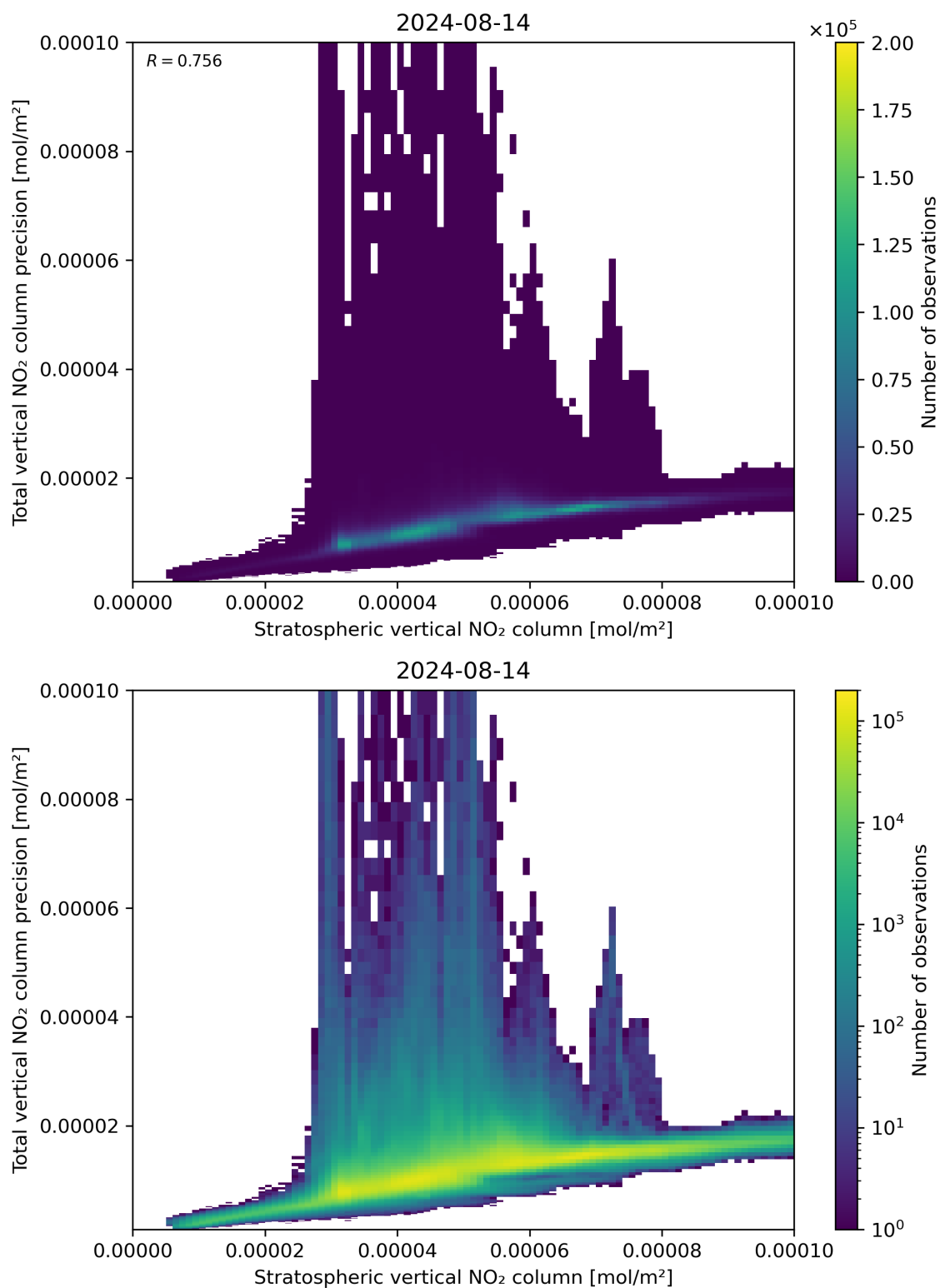
Figure 101: Scatter density plot of “Stratospheric vertical NO 2 column” against “Total vertical NO 2 column precision” for 2024-08-13 to 2024-08-15.
