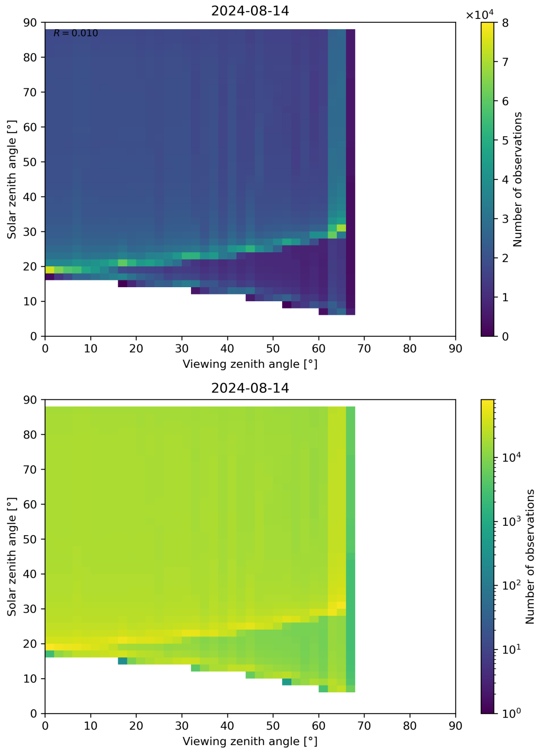
Figure 172: Scatter density plot of “Viewing zenith angle” against “Solar zenith angle” for 2024-08-13 to 2024-08-15.
