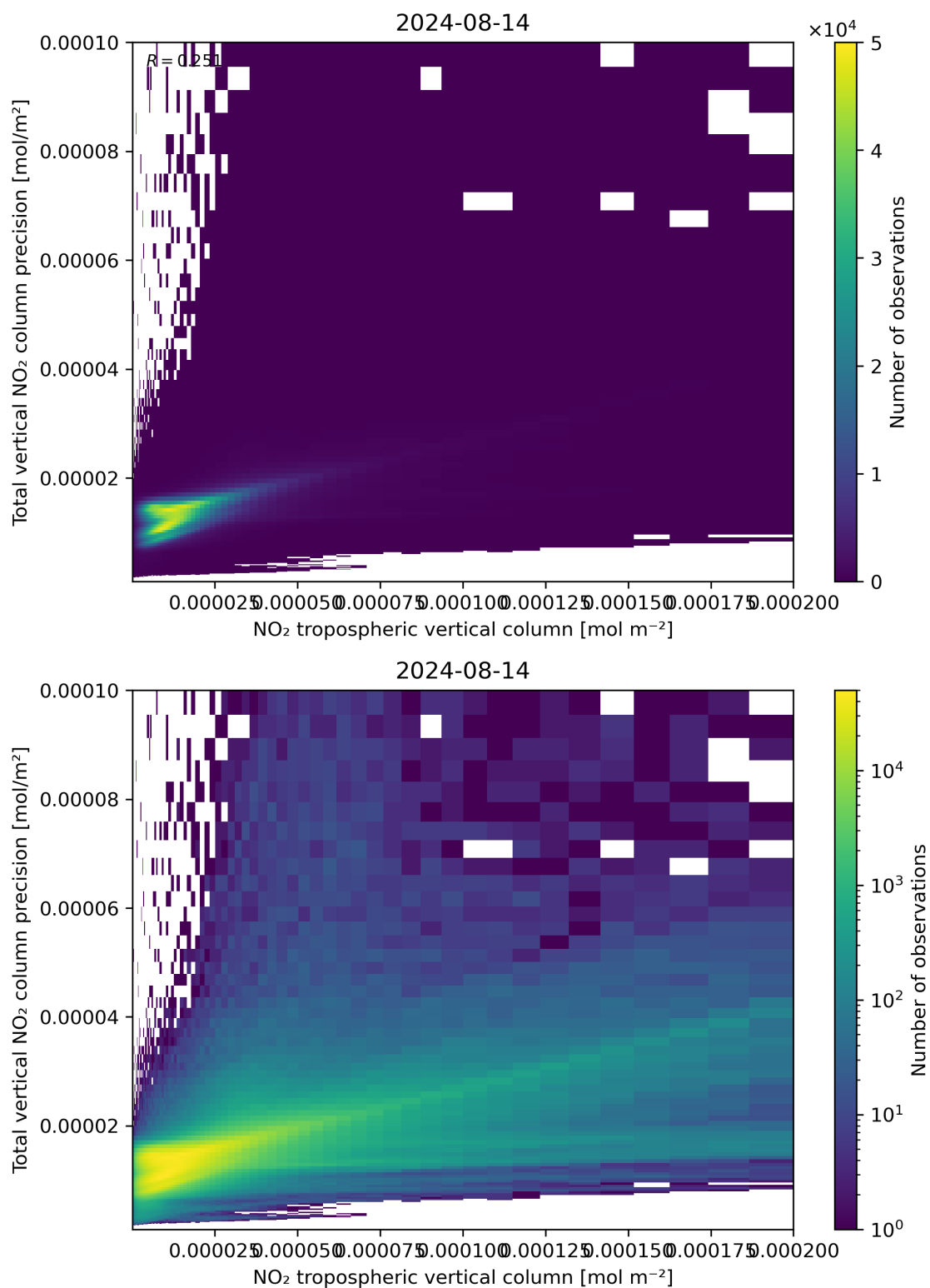
Figure 129: Scatter density plot of “NO 2 tropospheric vertical column” against “Total vertical NO 2 column precision” for 2024-08-13 to 2024-08-15.
