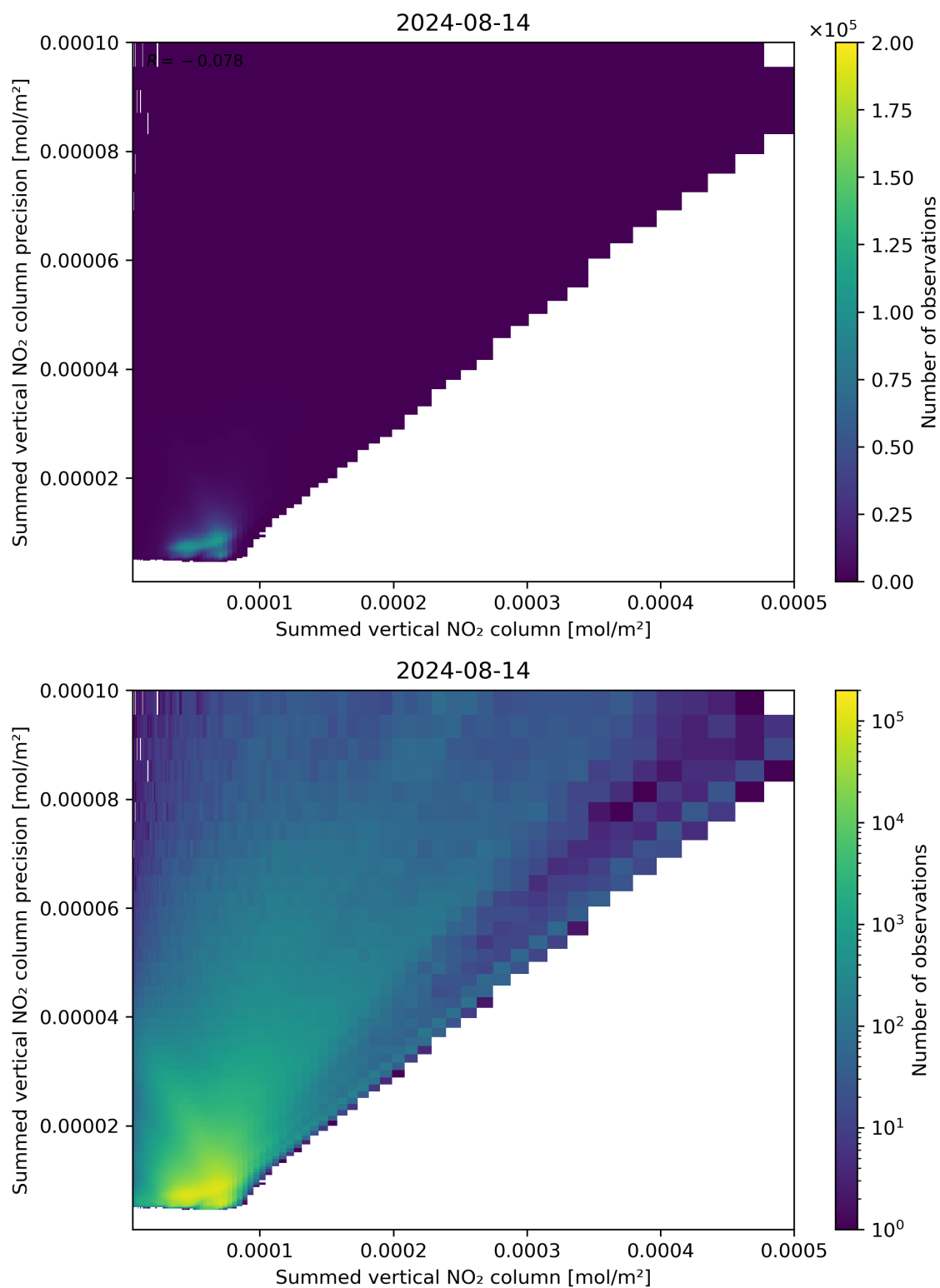
Figure 105: Scatter density plot of “Summed vertical NO 2 column” against “Summed vertical NO 2 column precision” for 2024-08-13 to 2024-08-15.
