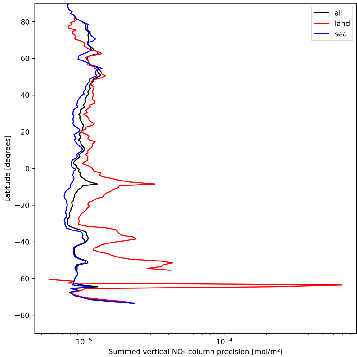
Figure 24: Zonal average of “Summed vertical NO 2 column precision” for 2024-08-13 to 2024-08-15.
