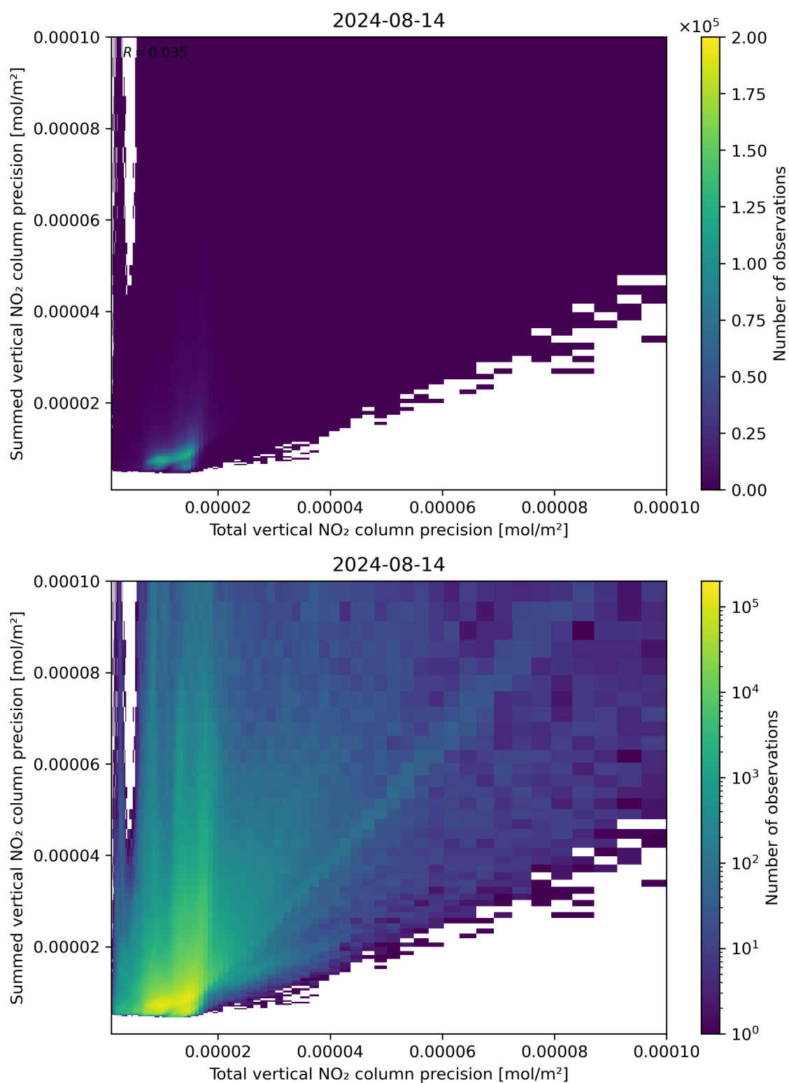
Figure 118: Scatter density plot of “Total vertical NO 2 column precision” against “Summed vertical NO 2 column precision” for 2024-08-13 to 2024-08-15.
