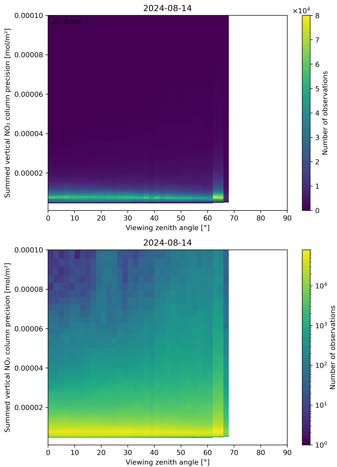
Figure 166: Scatter density plot of “Viewing zenith angle” against “Summed vertical NO 2 column precision” for 2024-08-13 to 2024-08-15.
