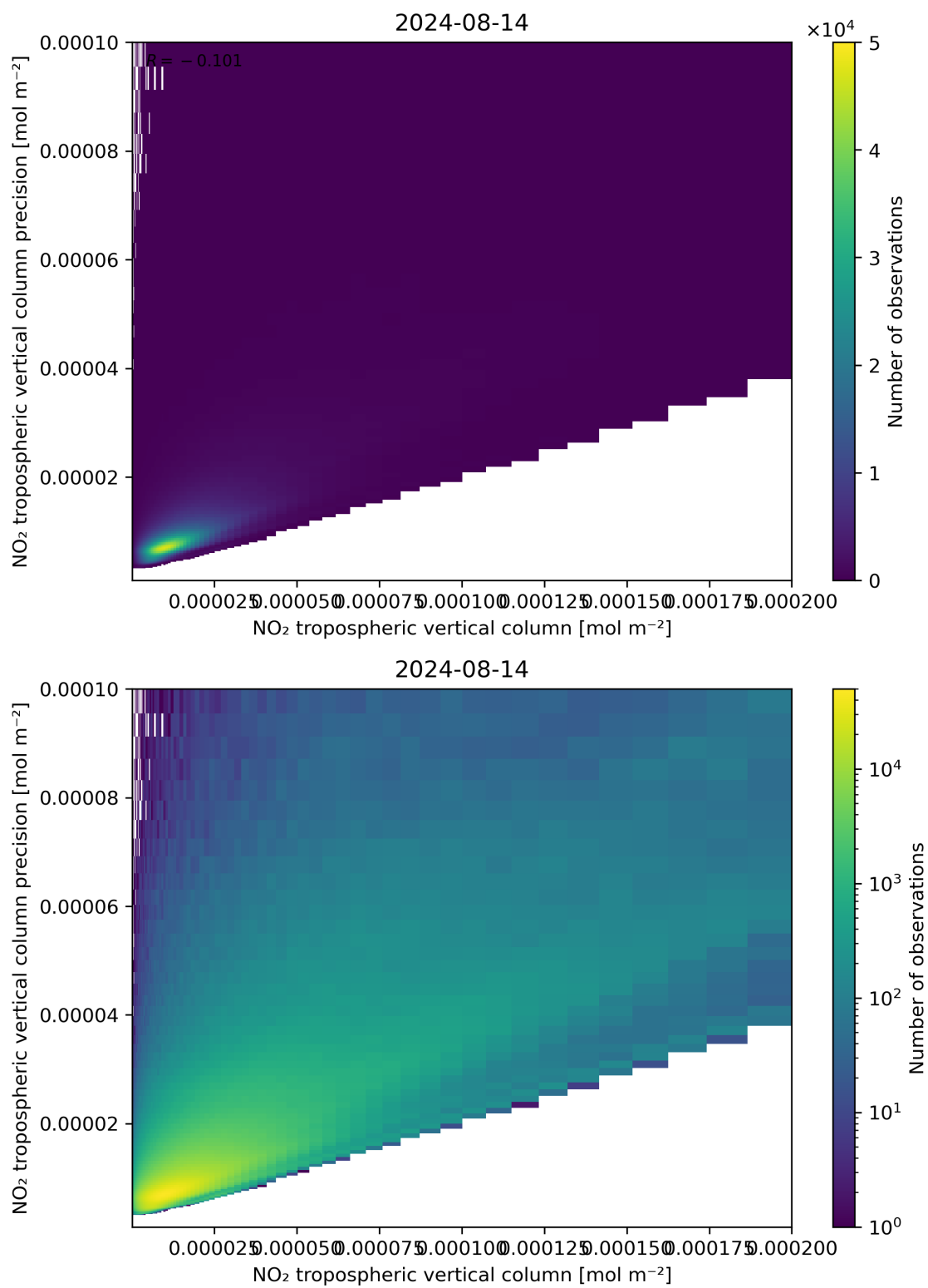
Figure 130: Scatter density plot of “NO 2 tropospheric vertical column” against “NO 2 tropospheric vertical column precision” for 2024-08-13 to 2024-08-15.
