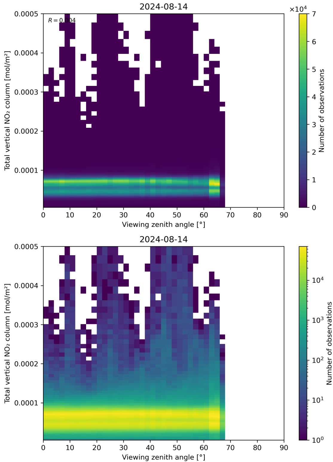
Figure 167: Scatter density plot of “Viewing zenith angle” against “Total vertical NO 2 column” for 2024-08-13 to 2024-08-15.
