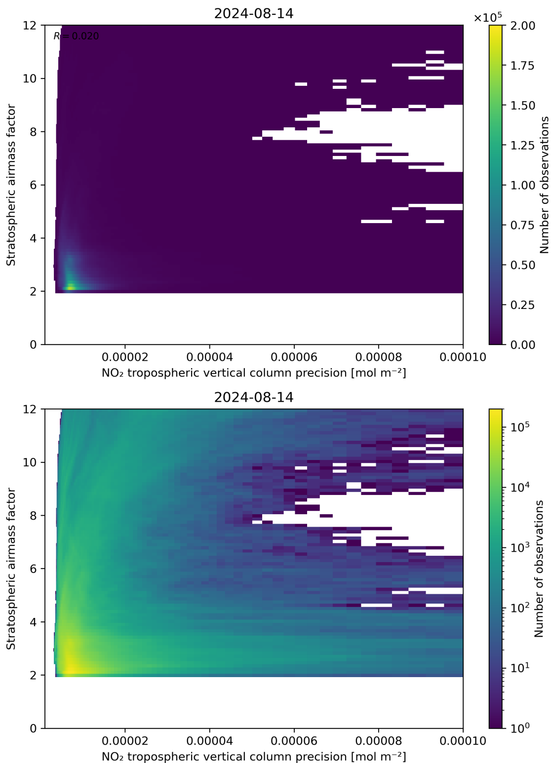
Figure 131: Scatter density plot of “NO 2 tropospheric vertical column precision” against “Stratospheric airmass factor” for 2024-08-13 to 2024-08-15.
