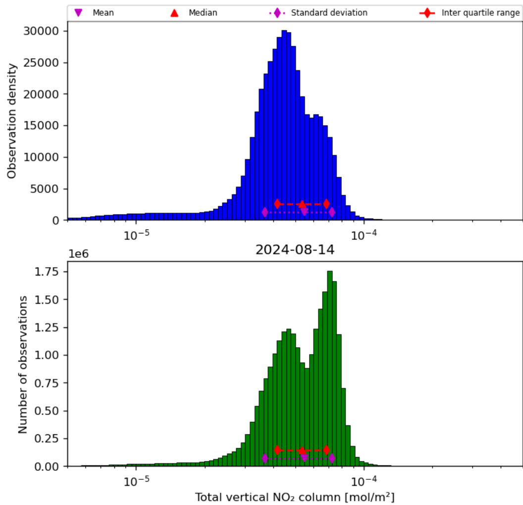
Figure 38: Histogram of “Total vertical NO 2 column” for 2024-08-13 to 2024-08-15
