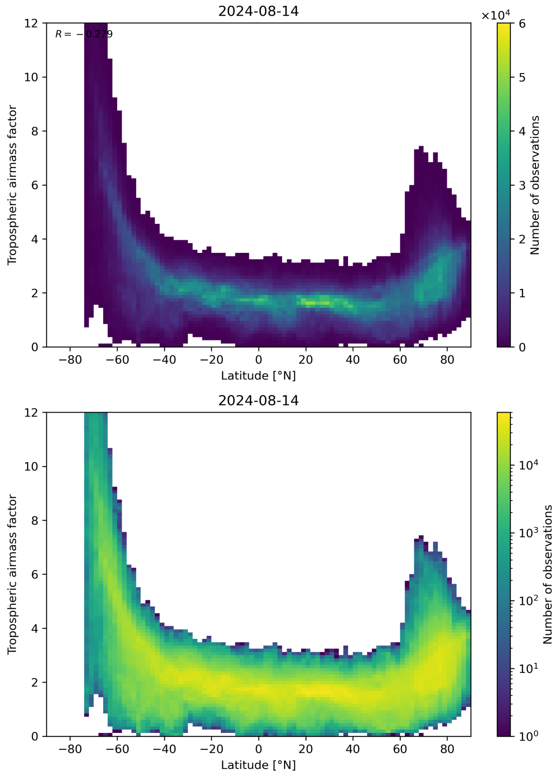
Figure 85: Scatter density plot of “Latitude” against “Tropospheric airmass factor” for 2024-08-13 to 2024-08-15.
