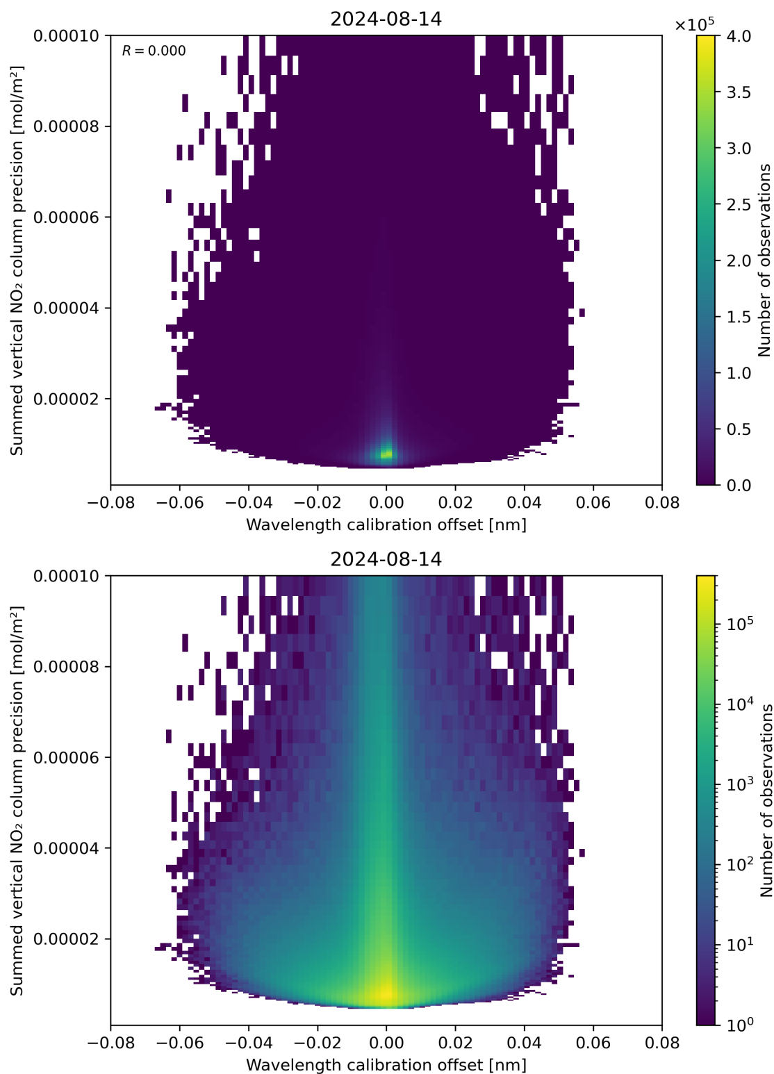
Figure 178: Scatter density plot of “Wavelength calibration offset” against “Summed vertical NO 2 column precision” for 2024-08-13 to 2024-08-15.
