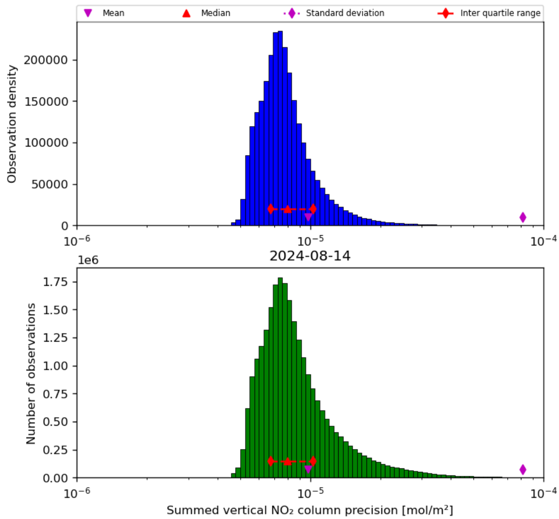
Figure 41: Histogram of "Summed vertical NO 2 column precision" for 2024-08-13 to 2024-08-15
