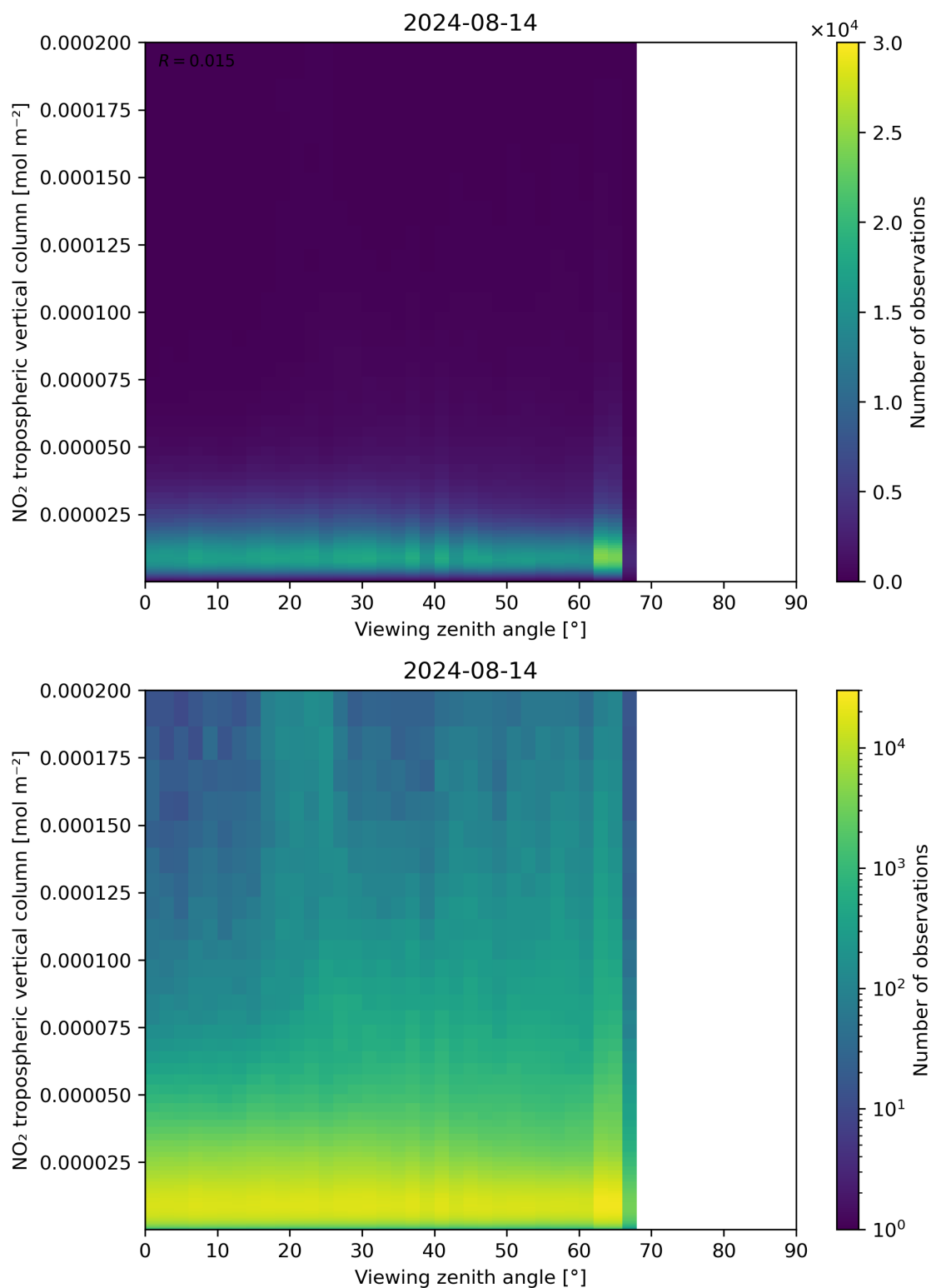
Figure 169: Scatter density plot of “Viewing zenith angle” against “NO 2 tropospheric vertical column” for 2024-08-13 to 2024-08-15.
