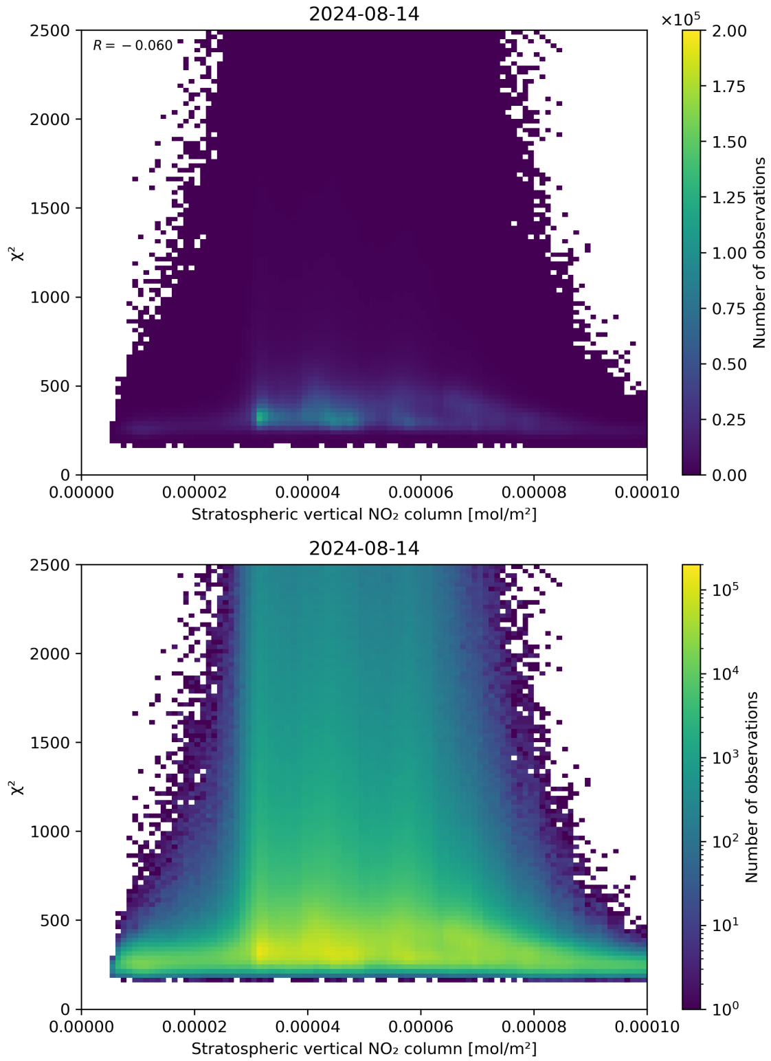
Figure 97: Scatter density plot of “Stratospheric vertical NO 2 column” against “ \chi^2 ” for 2024-08-13 to 2024-08-15.
