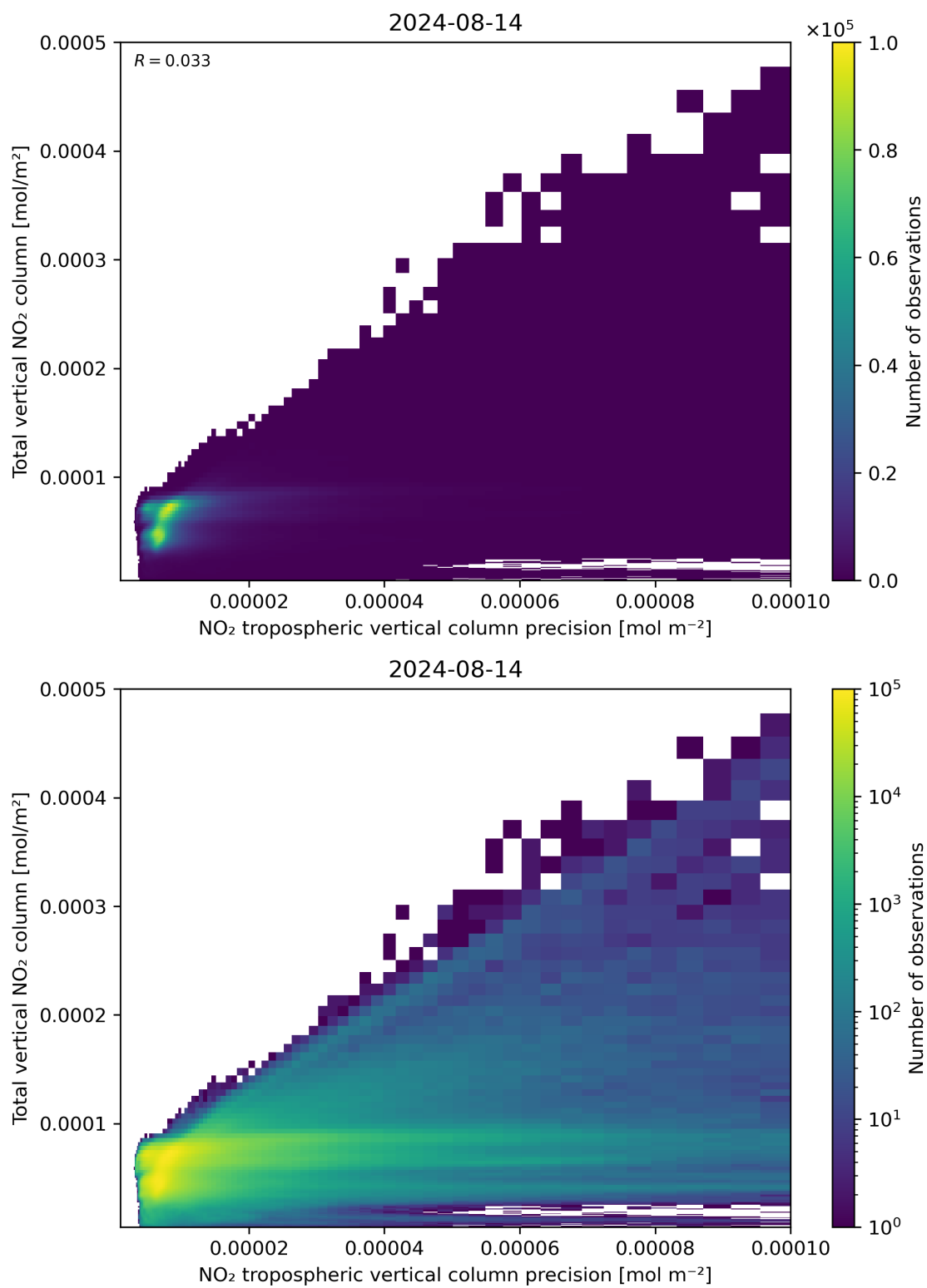
Figure 138: Scatter density plot of “NO 2 tropospheric vertical column precision” against “Total vertical NO 2 column” for 2024-08-13 to 2024-08-15.
