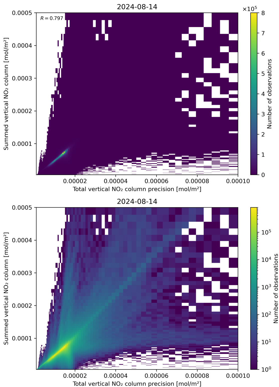
Figure 117: Scatter density plot of “Total vertical NO 2 column precision” against “Summed vertical NO 2 column” for 2024-08-13 to 2024-08-15.
