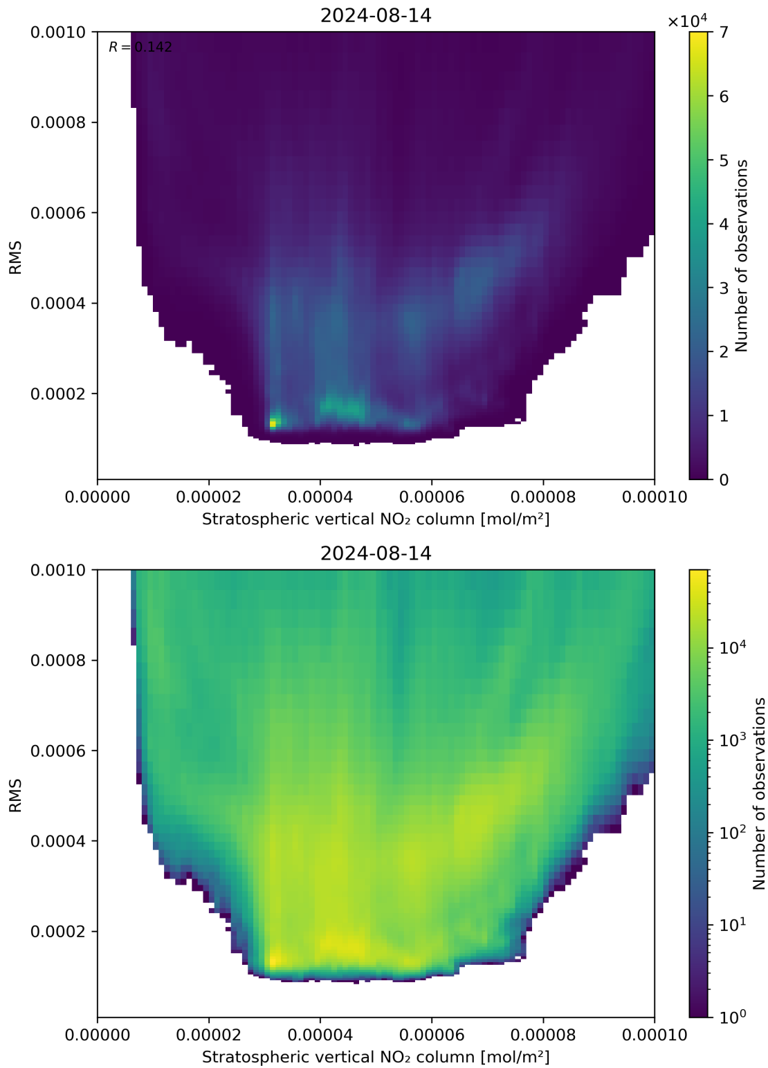
Figure 102: Scatter density plot of “Stratospheric vertical NO 2 column” against “RMS” for 2024-08-13 to 2024-08-15.
