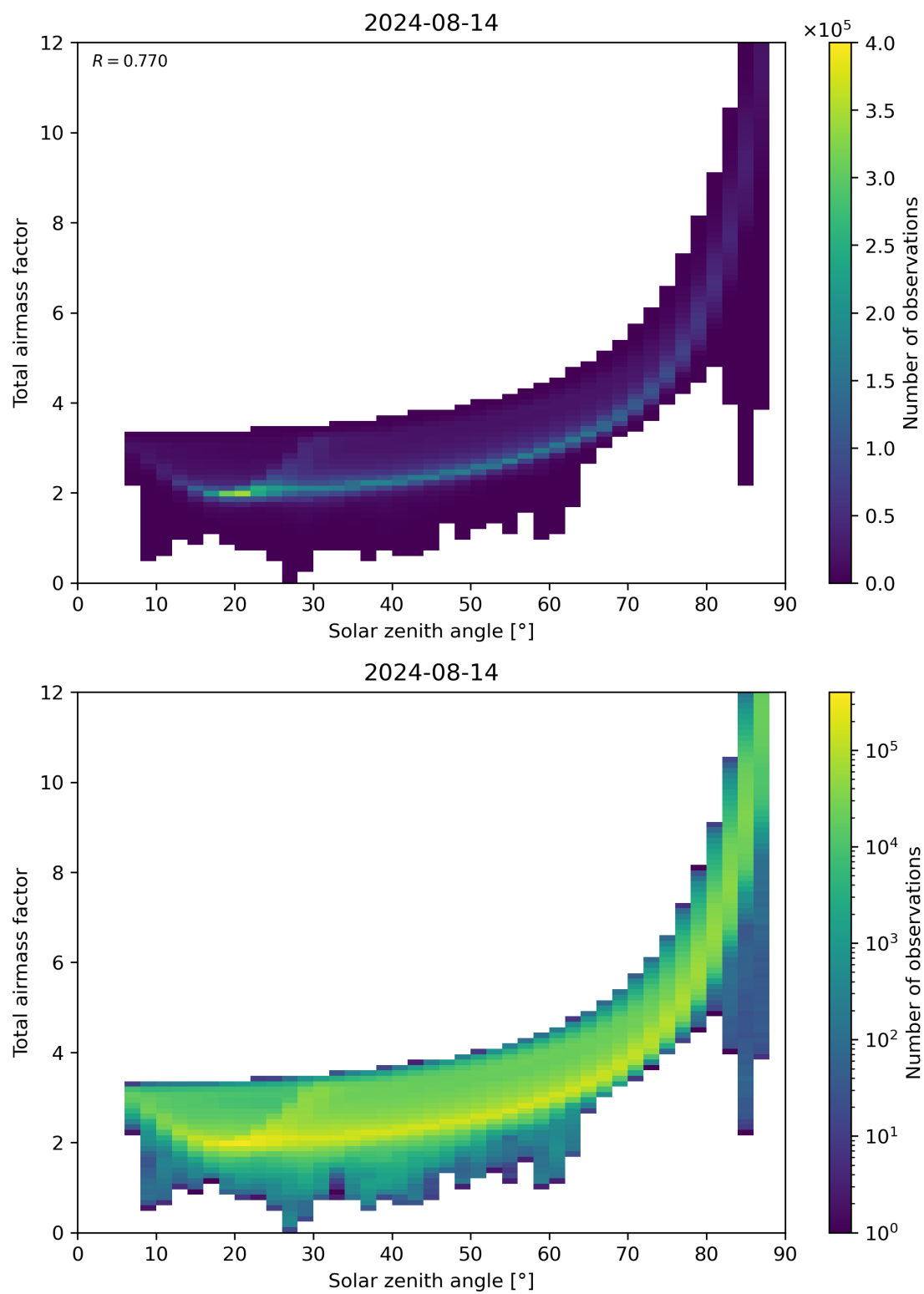
Figure 146: Scatter density plot of “Solar zenith angle” against “Total air mass factor” for 2024-08-13 to 2024-08-15.
