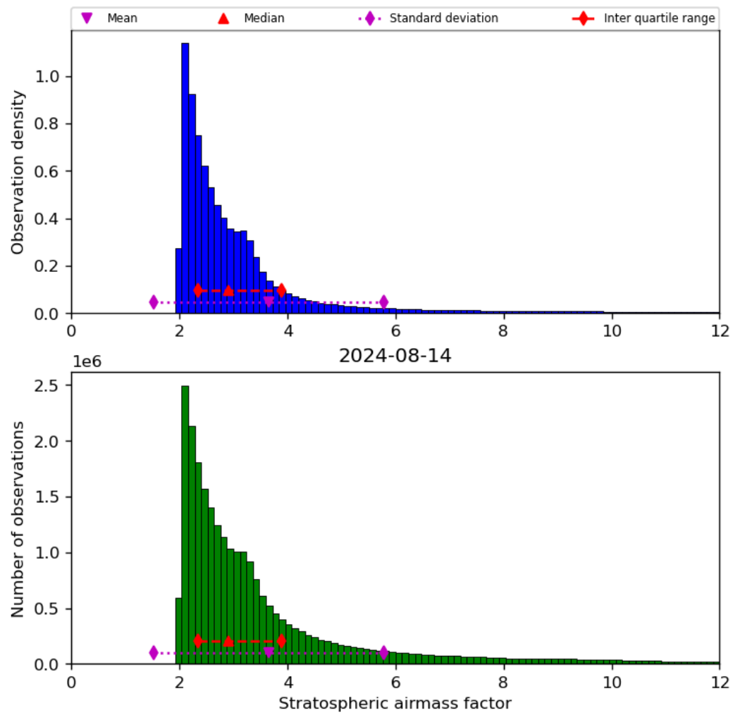
Figure 44: Histogram of “Stratospheric airmass factor” for 2024-08-13 to 2024-08-15
