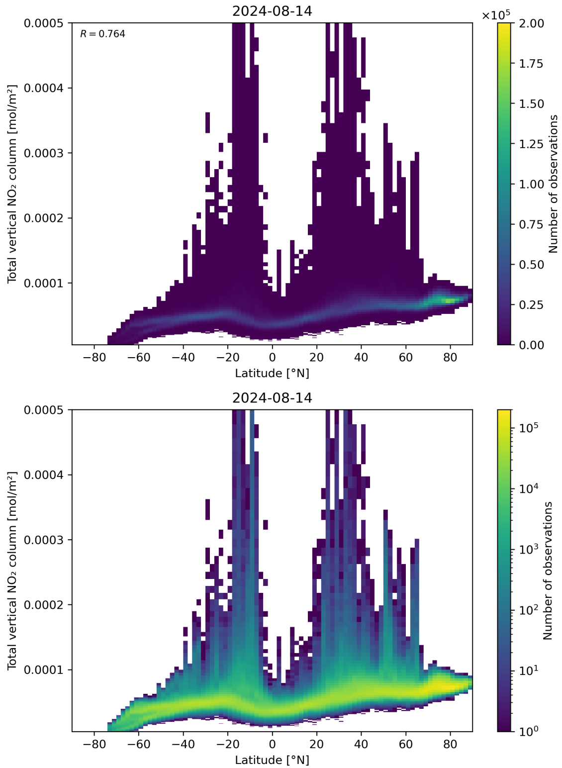
Figure 90: Scatter density plot of “Latitude” against “Total vertical NO 2 column” for 2024-08-13 to 2024-08-15.
