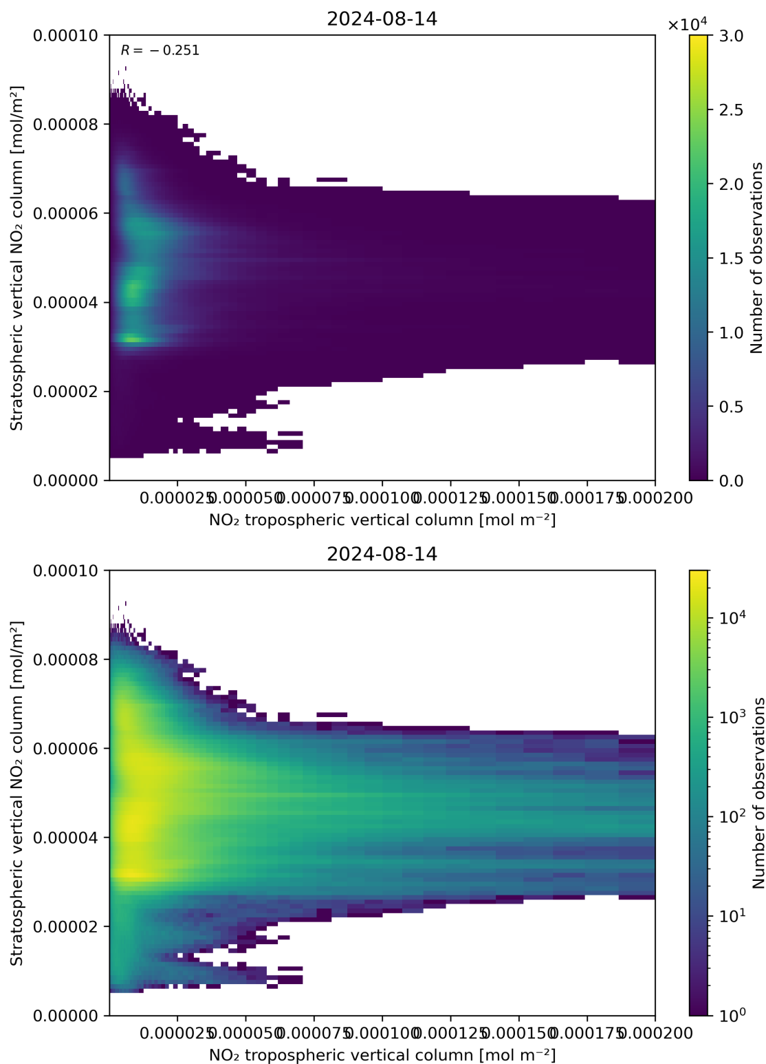
Figure 125: Scatter density plot of “NO 2 tropospheric vertical column” against “Stratospheric vertical NO 2 column” for 2024-08-13 to 2024-08-15.
