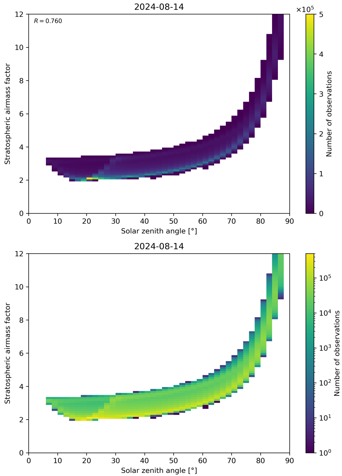
Figure 145: Scatter density plot of “Solar zenith angle” against “Stratospheric airmass factor” for 2024-08-13 to 2024-08-15.
