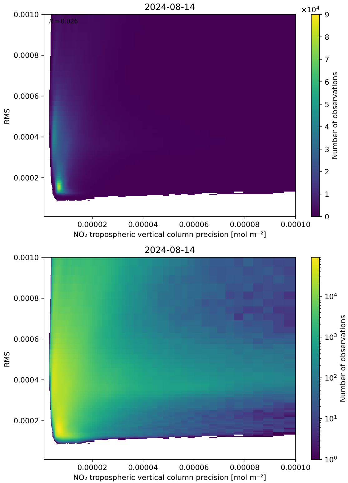
Figure 140: Scatter density plot of “NO 2 tropospheric vertical column precision” against “RMS” for 2024-08-13 to 2024-08-15.
