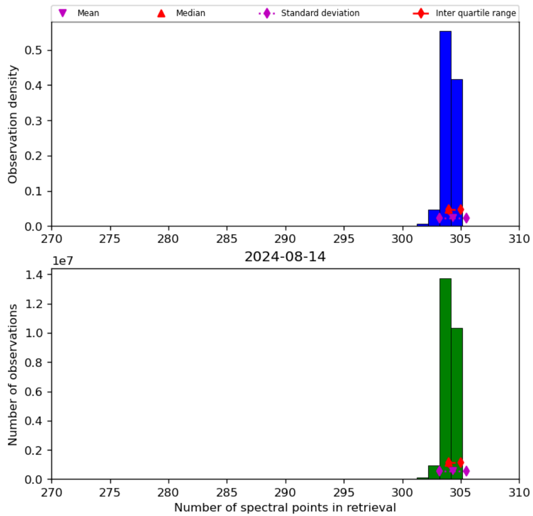
Figure 33: Histogram of “Number of spectral points in retrieval” for 2024-08-13 to 2024-08-15
