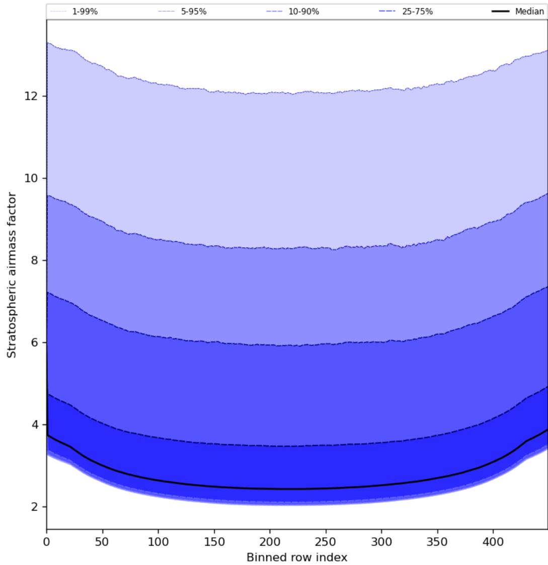
Figure 61: Along track statistics of “Stratospheric airmass factor” for 2024-08-13 to 2024-08-15
