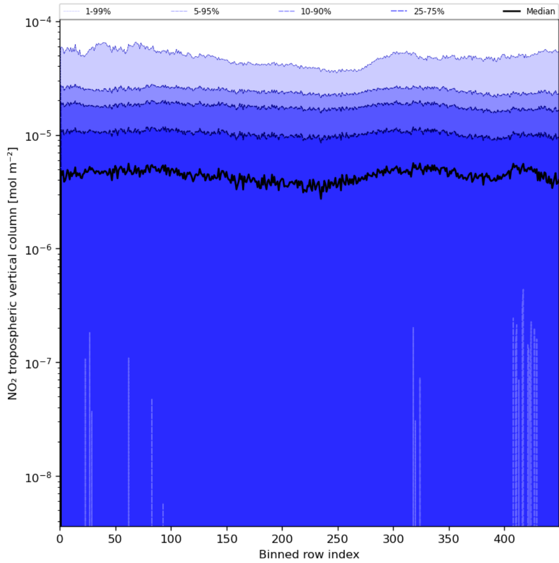
Figure 46: Along track statistics of “NO 2 tropospheric vertical column” for 2024-08-13 to 2024-08-15
