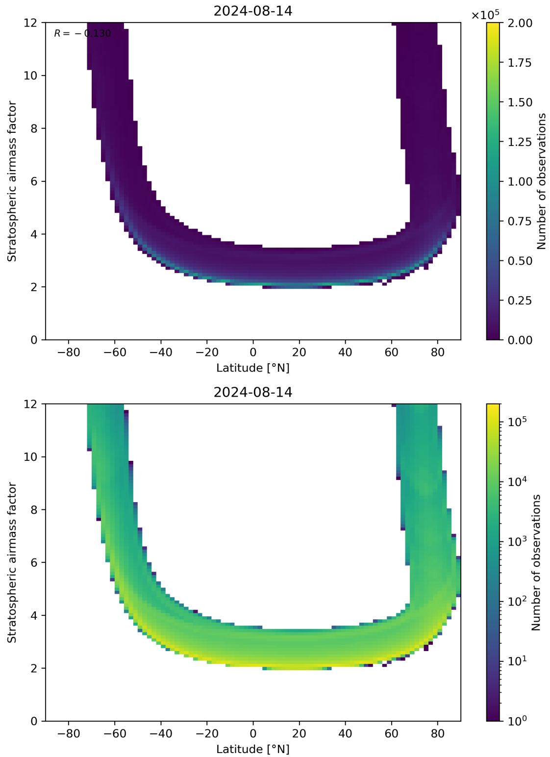
Figure 83: Scatter density plot of “Latitude” against “Stratospheric airmass factor” for 2024-08-13 to 2024-08-15.
