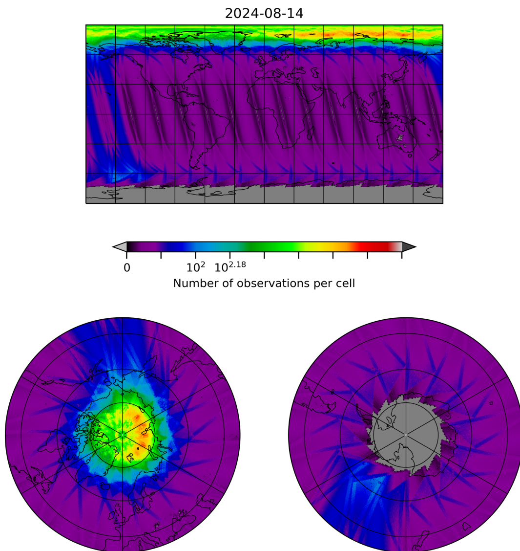
Figure 10: Map of the number of observations for 2024-08-13 to 2024-08-15
