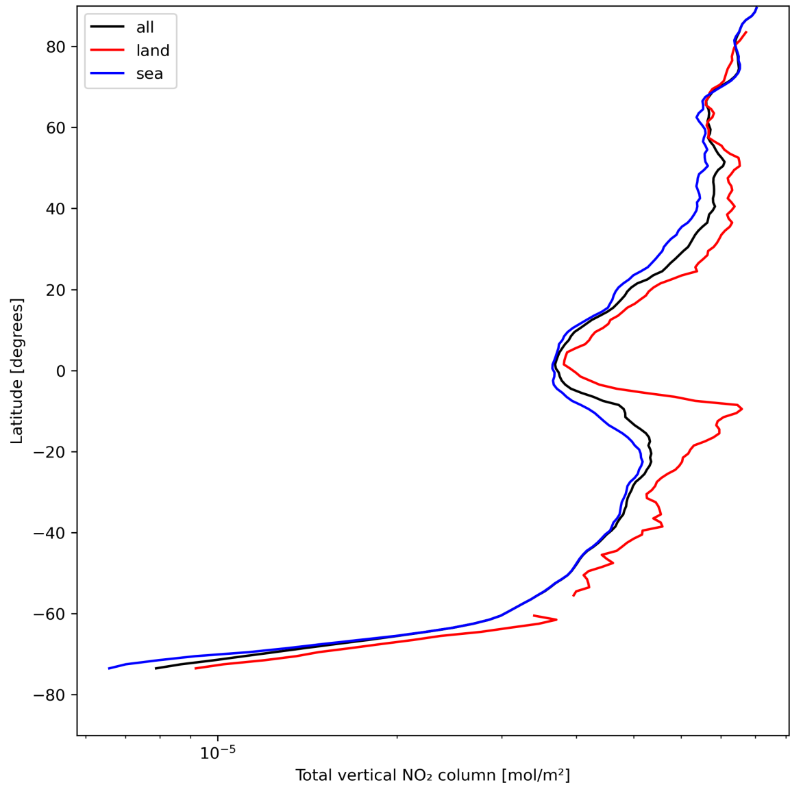
Figure 21: Zonal average of “Total vertical NO 2 column” for 2024-08-13 to 2024-08-15.
