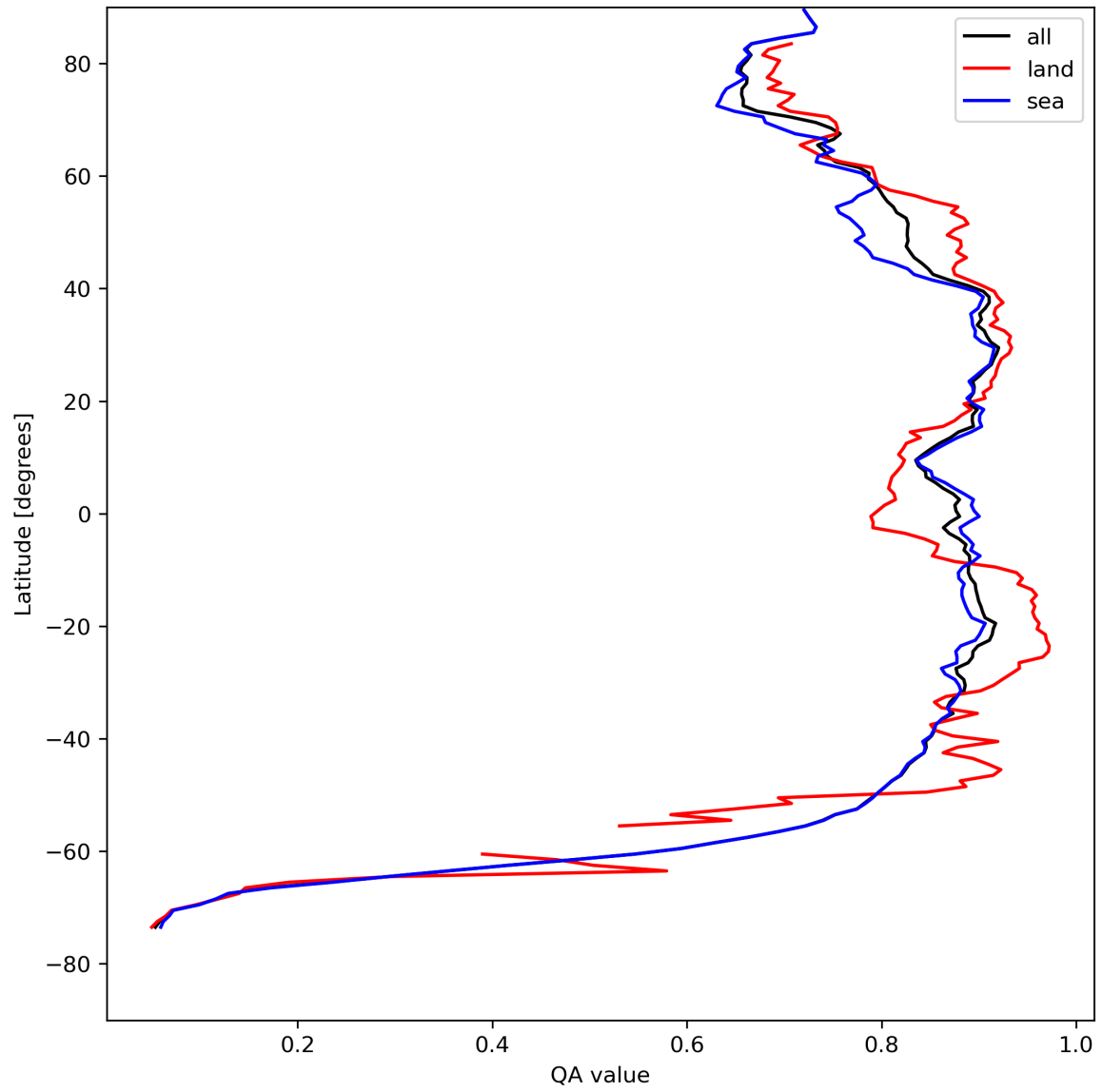
Figure 11: Zonal average of “QA value” for 2024-08-13 to 2024-08-15.
