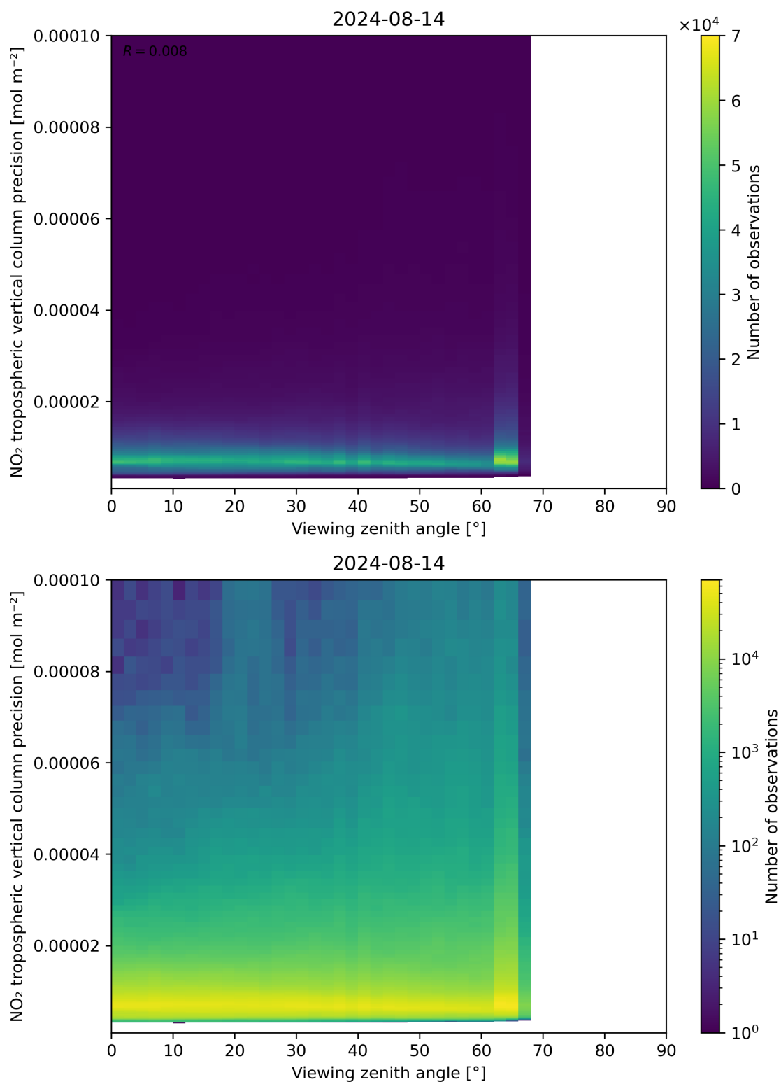
Figure 170: Scatter density plot of “Viewing zenith angle” against “NO 2 tropospheric vertical column precision” for 2024-08-13 to 2024-08-15.
