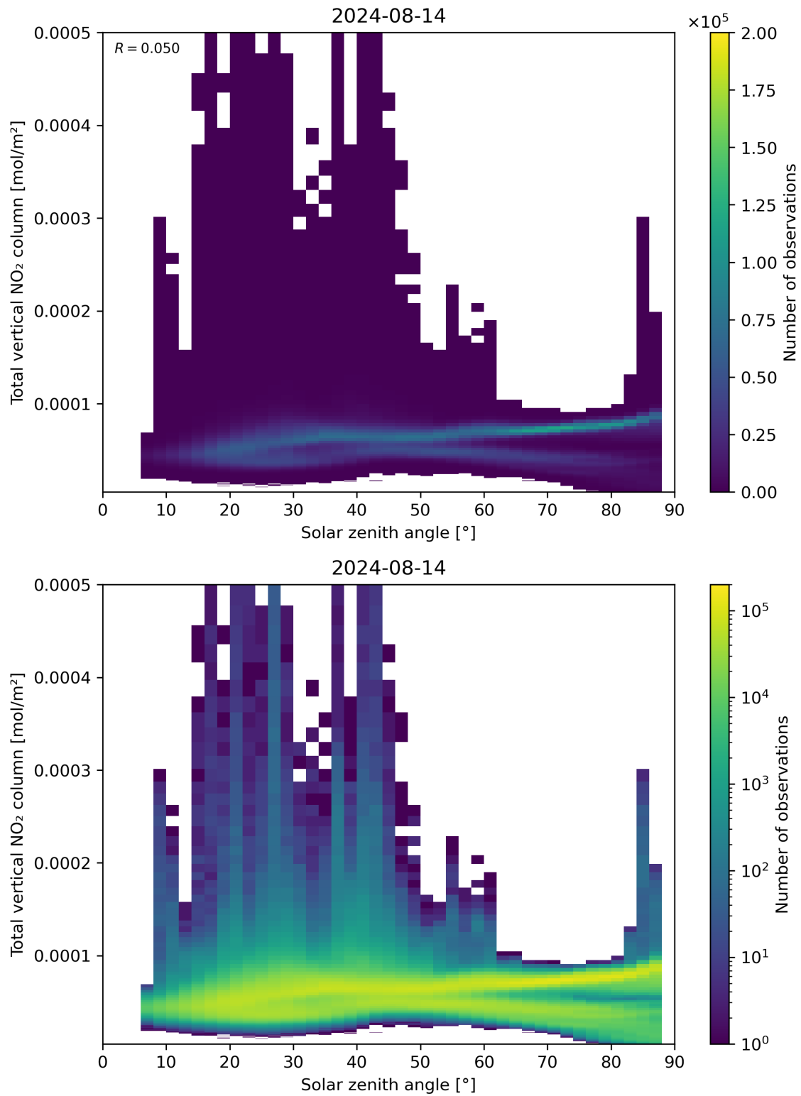
Figure 153: Scatter density plot of “Solar zenith angle” against “Total vertical NO 2 column” for 2024-08-13 to 2024-08-15.
