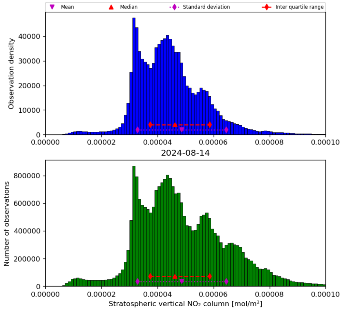
Figure 36: Histogram of “Stratospheric vertical NO 2 column” for 2024-08-13 to 2024-08-15
