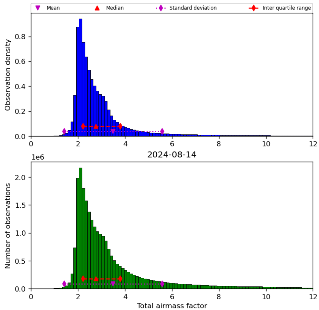
Figure 32: Histogram of “Total airmass factor” for 2024-08-13 to 2024-08-15
