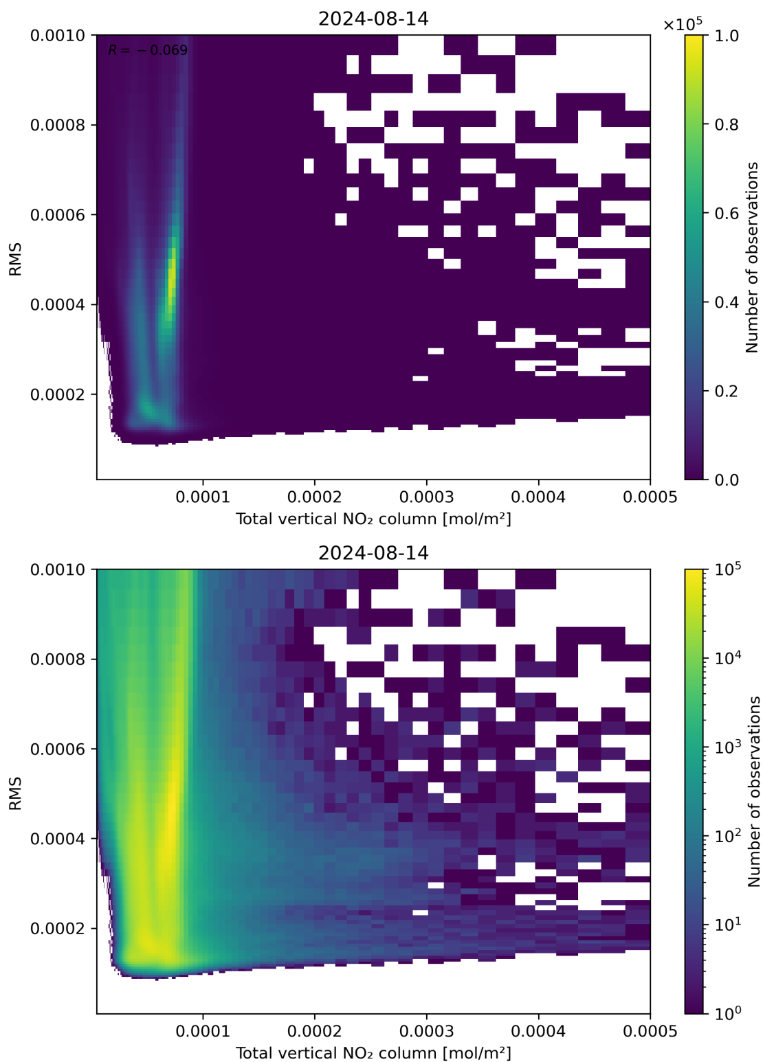
Figure 120: Scatter density plot of “Total vertical NO 2 column” against “RMS” for 2024-08-13 to 2024-08-15.
