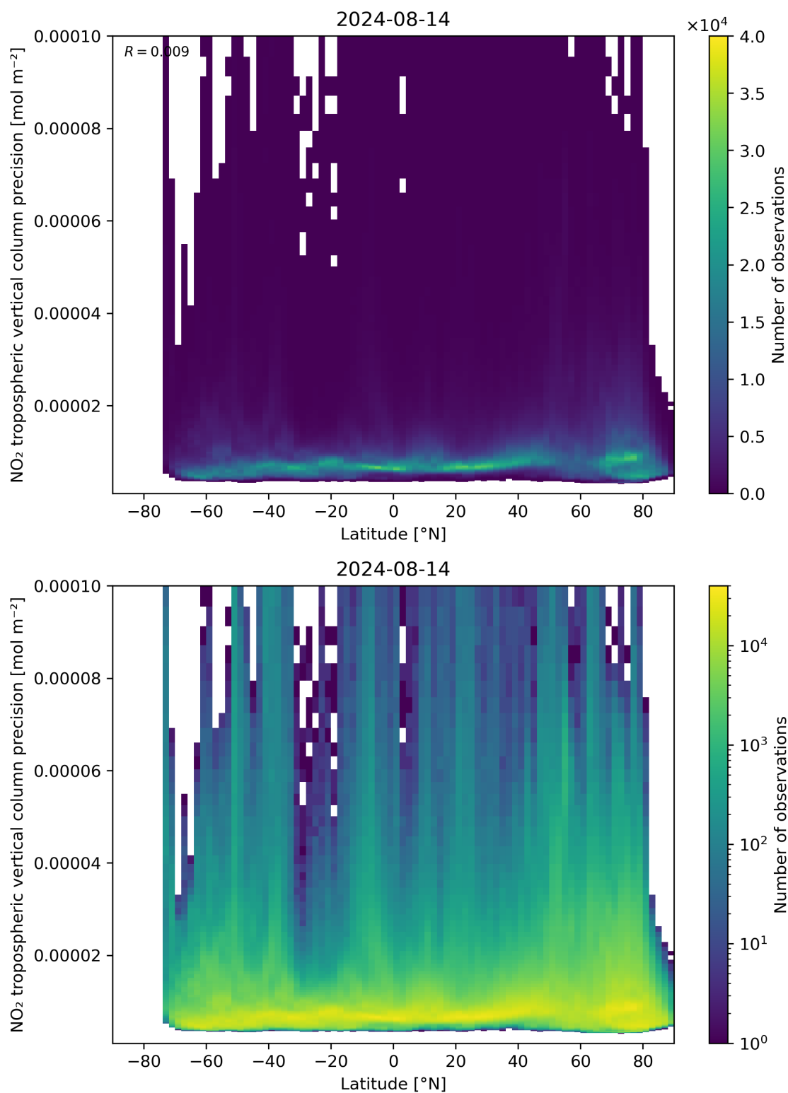
Figure 93: Scatter density plot of “Latitude” against “NO 2 tropospheric vertical column precision” for 2024-08-13 to 2024-08-15.
