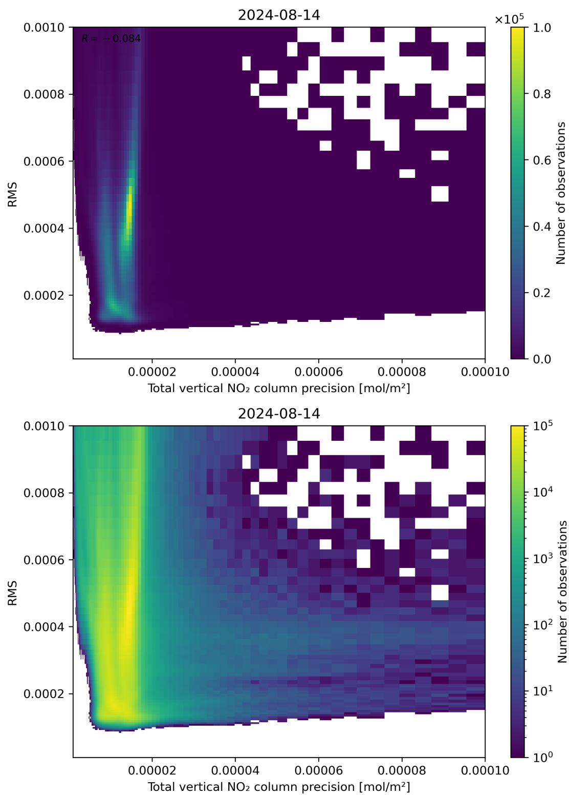
Figure 119: Scatter density plot of “Total vertical NO 2 column precision” against “RMS” for 2024-08-13 to 2024-08-15.
