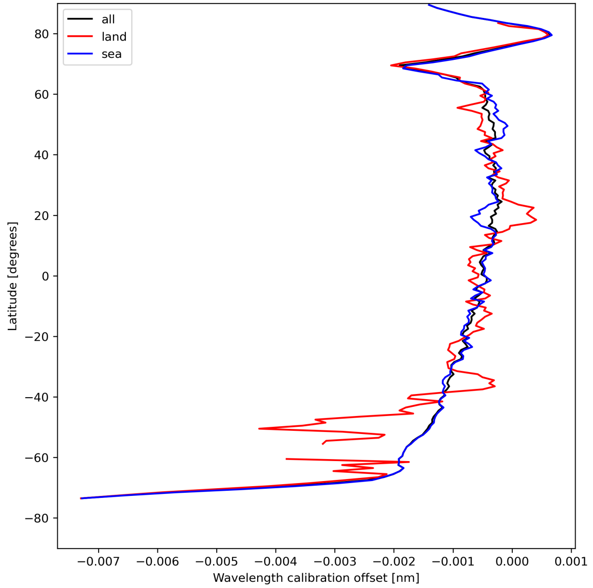
Figure 18: Zonal average of “Wavelength calibration offset” for 2024-08-13 to 2024-08-15.
