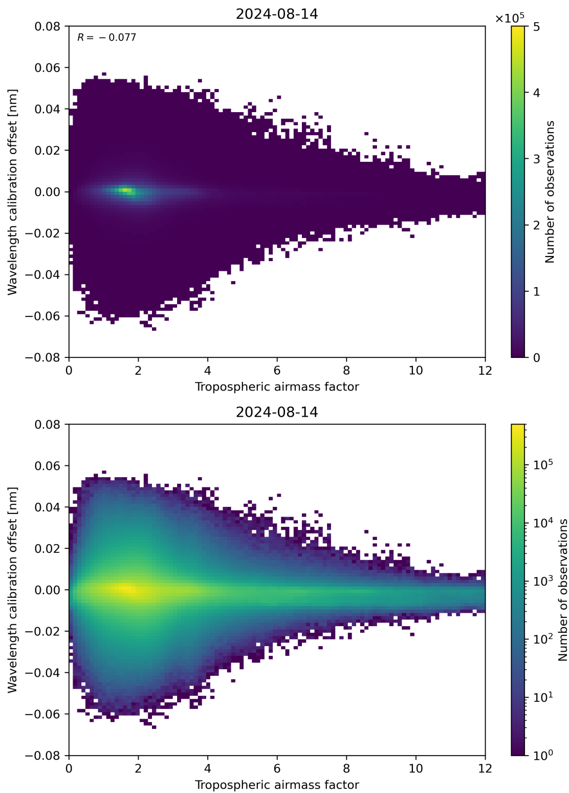
Figure 80: Scatter density plot of “Tropospheric air mass factor” against “Wavelength calibration offset” for 2024-08-13 to 2024-08-15.
