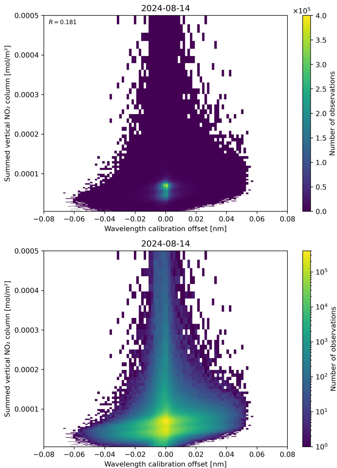
Figure 177: Scatter density plot of “Wavelength calibration offset” against “Summed vertical NO 2 column” for 2024-08-13 to 2024-08-15.
