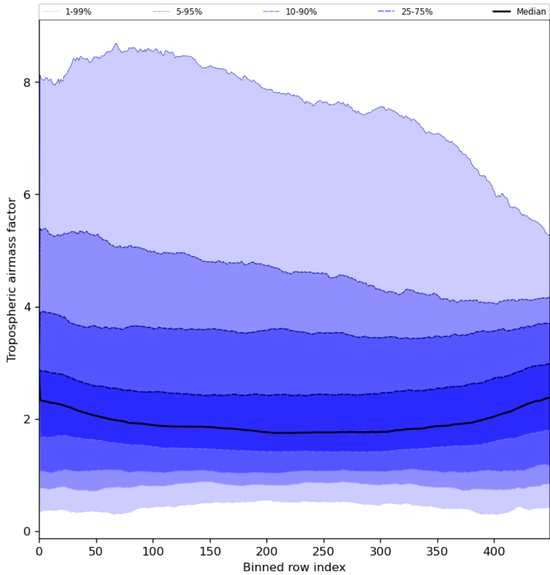
Figure 48: Along track statistics of “Tropospheric airmass factor” for 2024-08-13 to 2024-08-15
