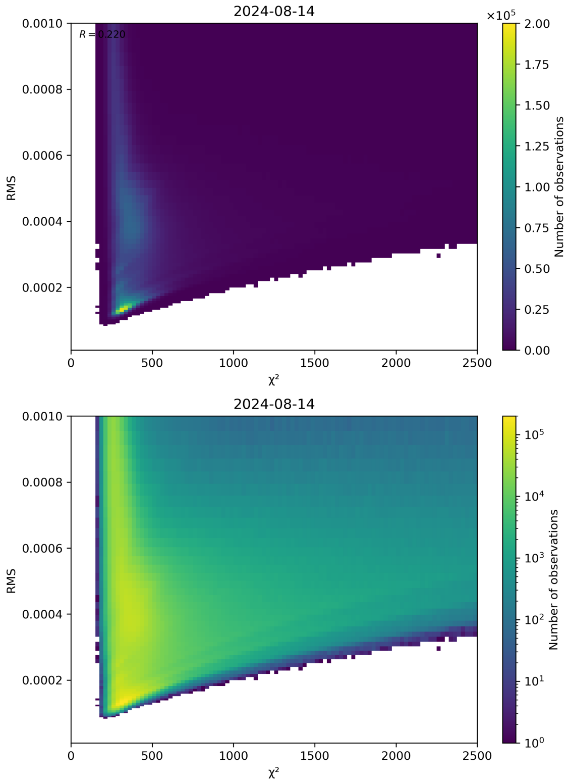
Figure 82: Scatter density plot of " \chi^2 " against "RMS" for 2024-08-13 to 2024-08-15.
