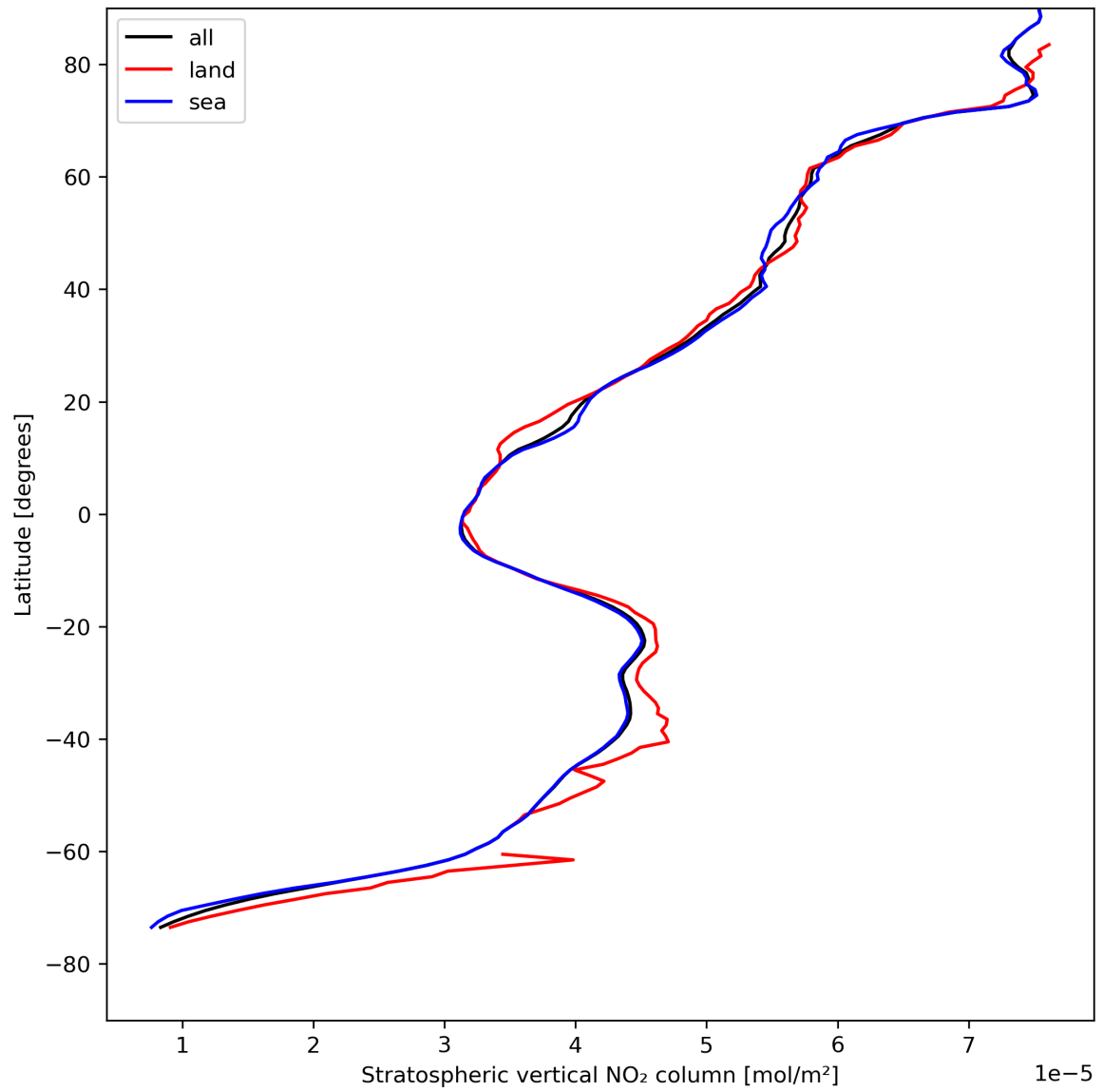
Figure 19: Zonal average of “Stratospheric vertical NO 2 column” for 2024-08-13 to 2024-08-15.
