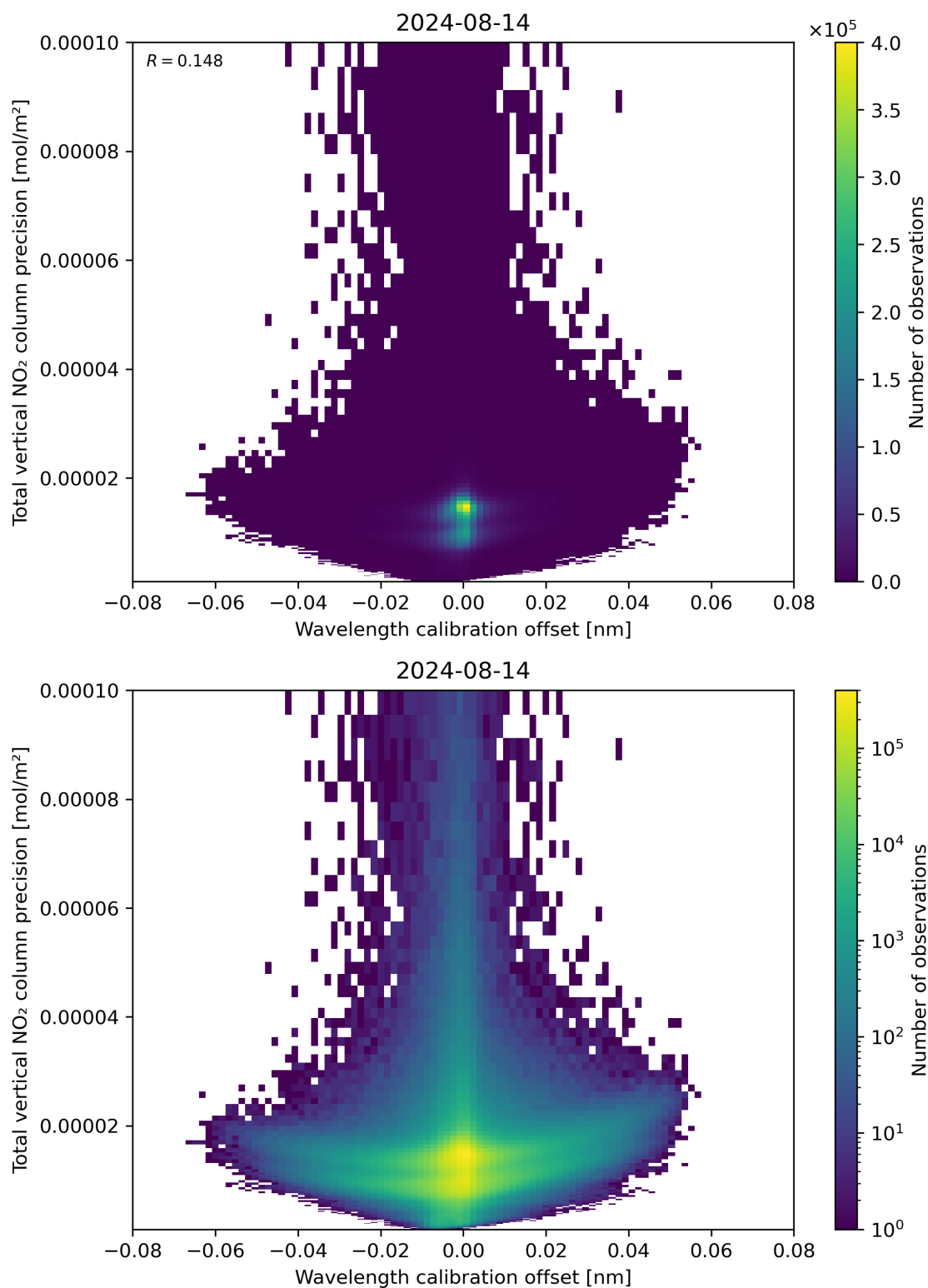
Figure 180: Scatter density plot of “Wavelength calibration offset” against “Total vertical NO 2 column precision” for 2024-08-13 to 2024-08-15.
