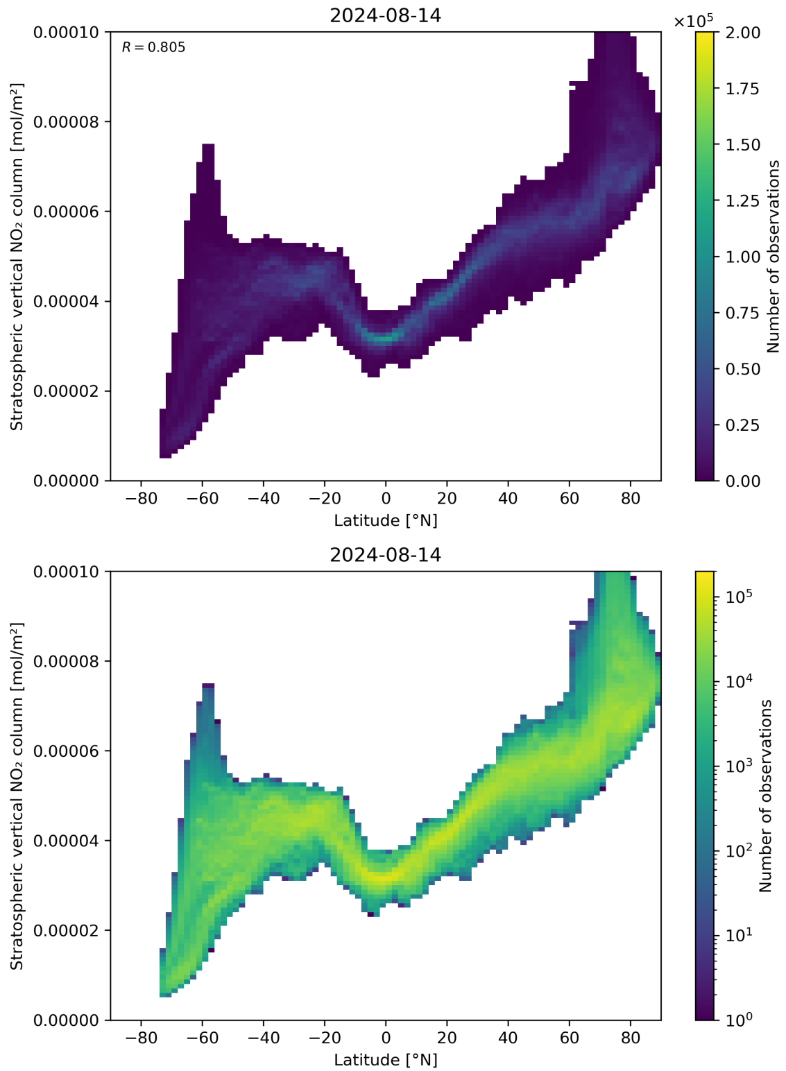
Figure 87: Scatter density plot of “Latitude” against “Stratospheric vertical \text{NO}_2 column” for 2024-08-13 to 2024-08-15.
