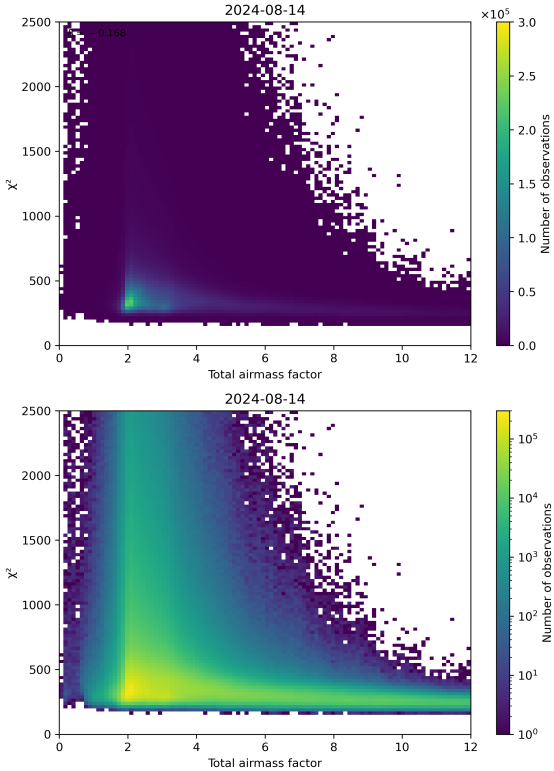
Figure 63: Scatter density plot of “Total airmass factor” against “ \chi^2 ” for 2024-08-13 to 2024-08-15.
