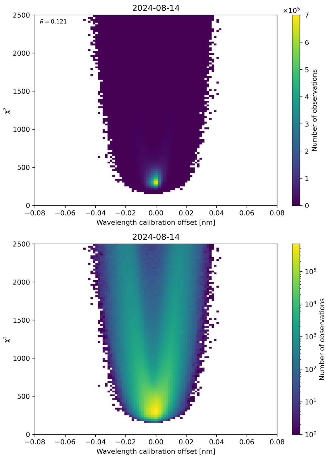
Figure 175: Scatter density plot of “Wavelength calibration offset” against “ \chi^2 ” for 2024-08-13 to 2024-08-15.
