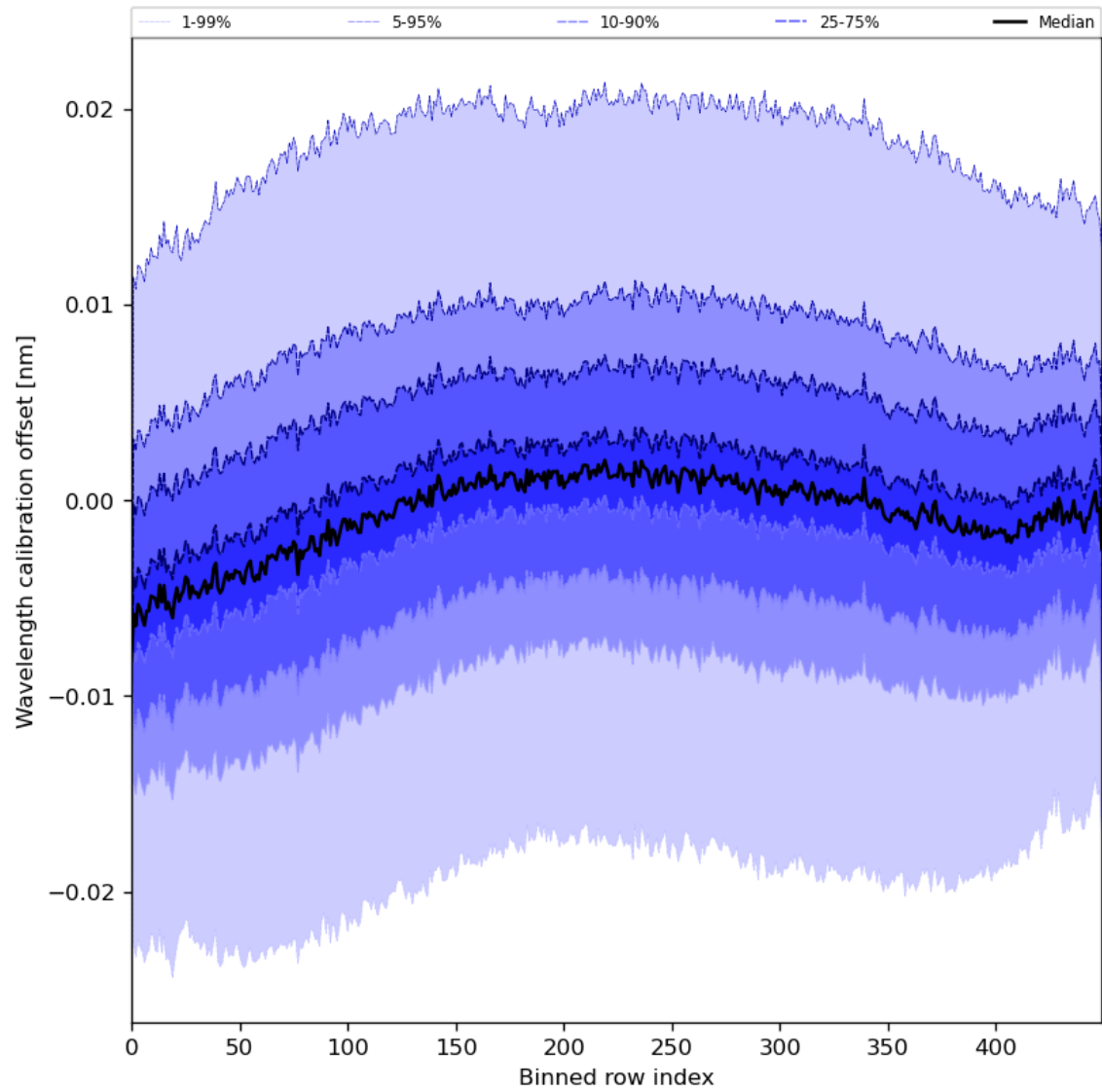
Figure 52: Along track statistics of “Wavelength calibration offset” for 2024-08-13 to 2024-08-15
