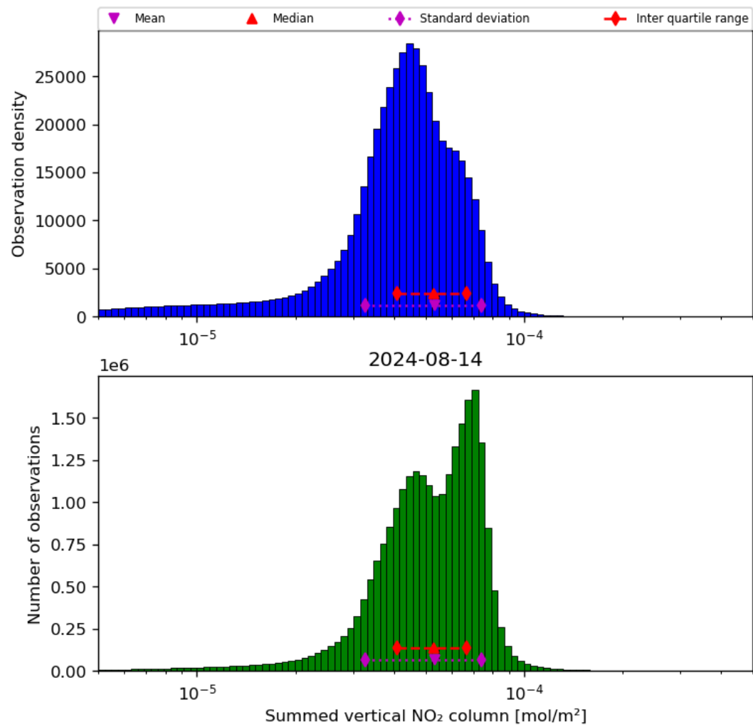
Figure 40: Histogram of “Summed vertical NO 2 column” for 2024-08-13 to 2024-08-15
