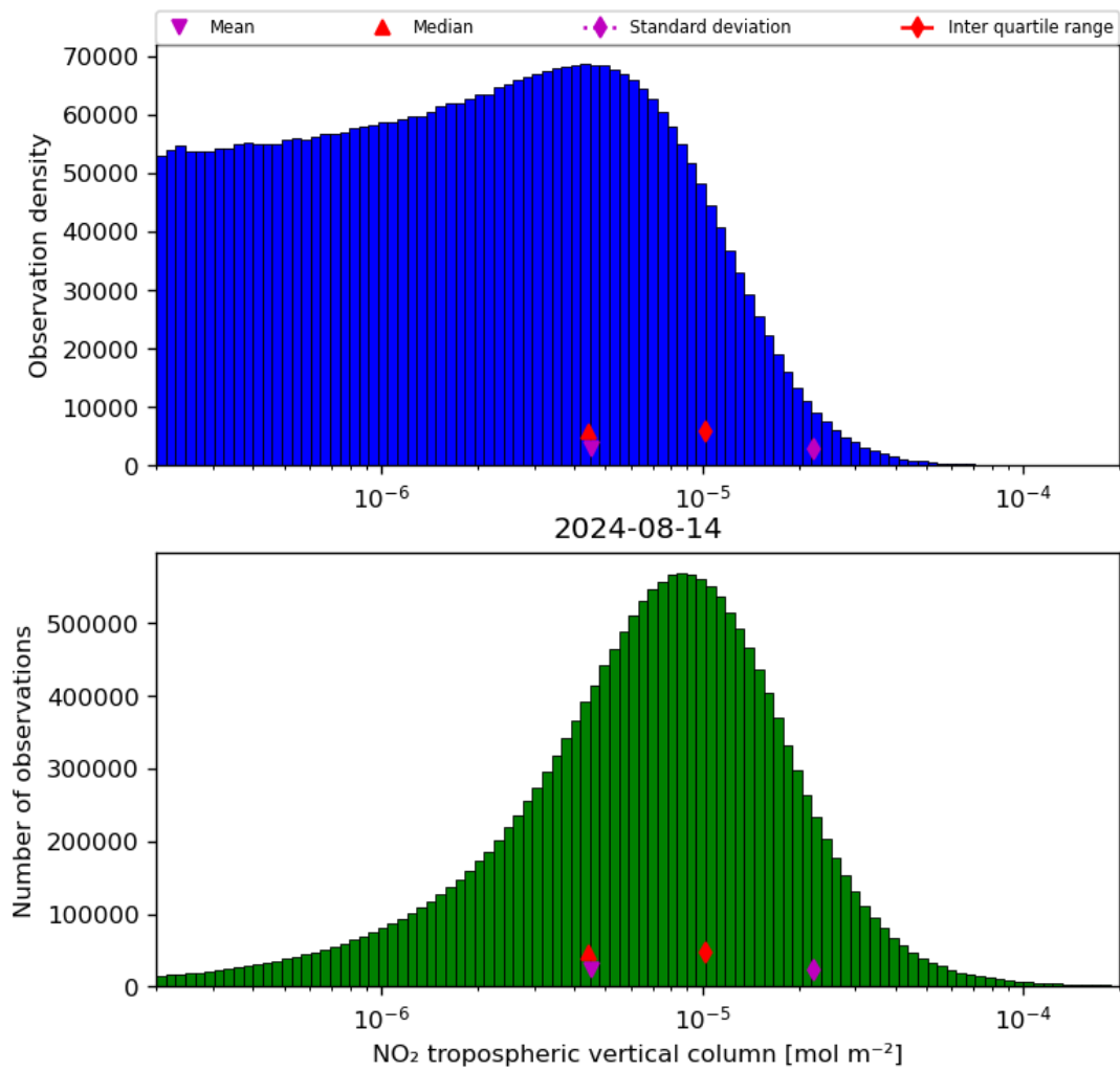
Figure 29: Histogram of “NO 2 tropospheric vertical column” for 2024-08-13 to 2024-08-15
