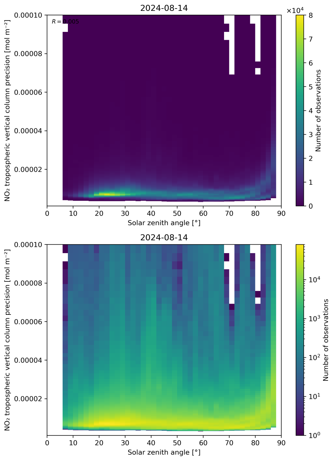
Figure 156: Scatter density plot of “Solar zenith angle” against “NO 2 tropospheric vertical column precision” for 2024-08-13 to 2024-08-15.
