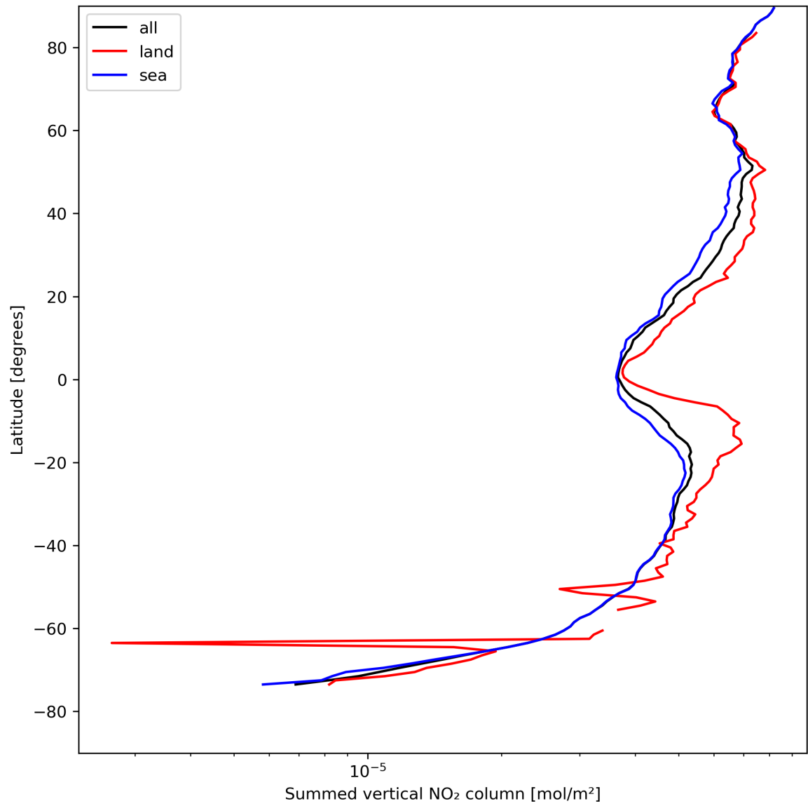
Figure 23: Zonal average of “Summed vertical NO 2 column” for 2024-08-13 to 2024-08-15.
