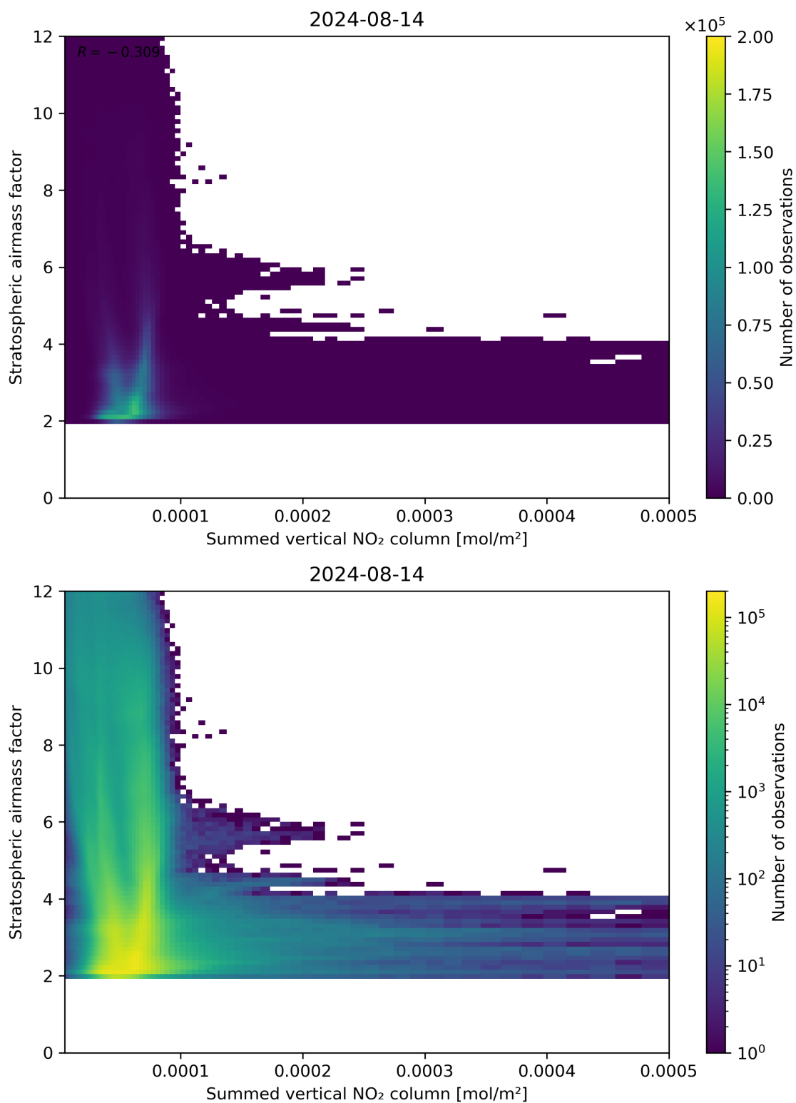
Figure 103: Scatter density plot of “Summed vertical NO 2 column” against “Stratospheric airmass factor” for 2024-08-13 to 2024-08-15.
