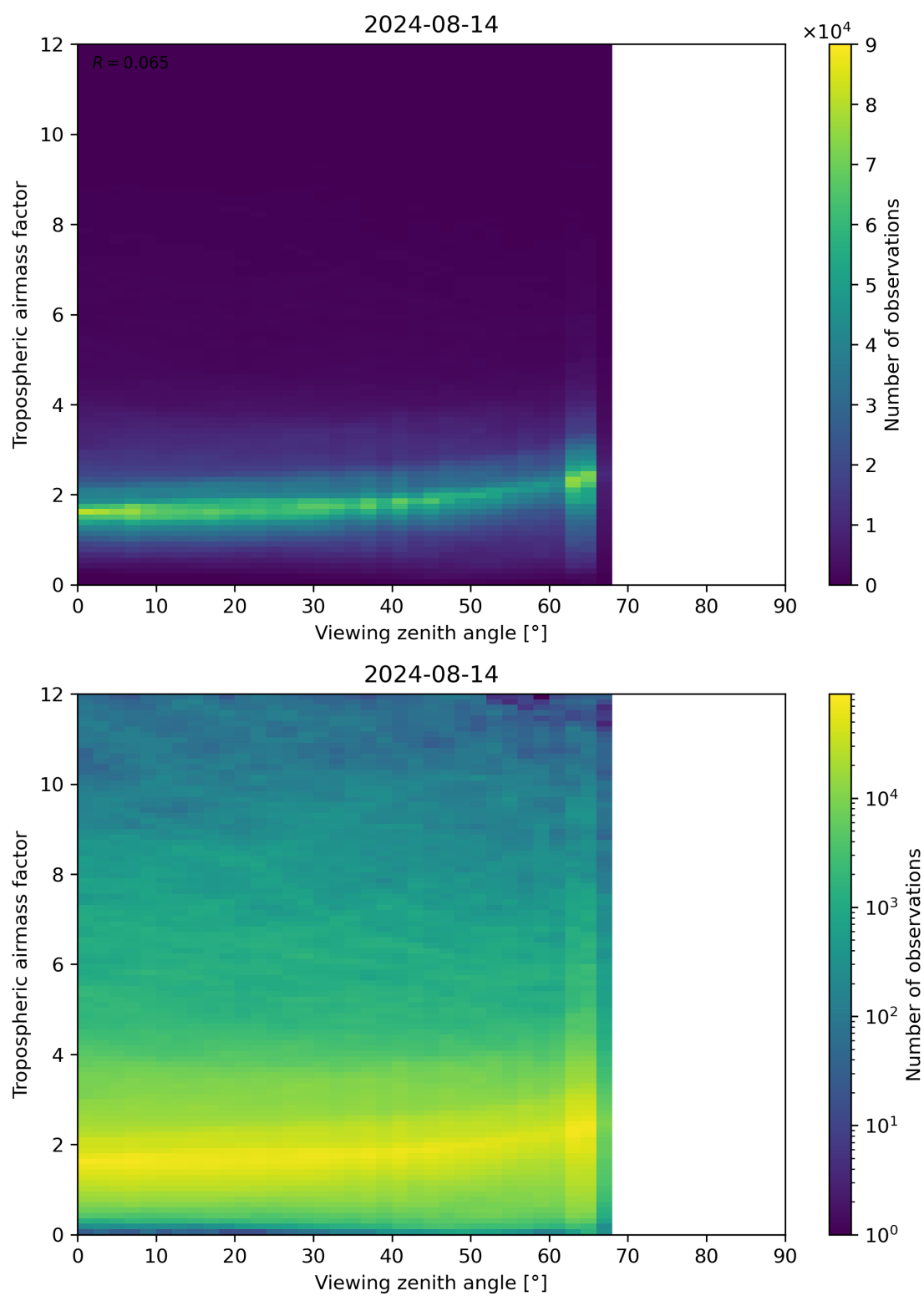
Figure 161: Scatter density plot of “Viewing zenith angle” against “Tropospheric airmass factor” for 2024-08-13 to 2024-08-15.
