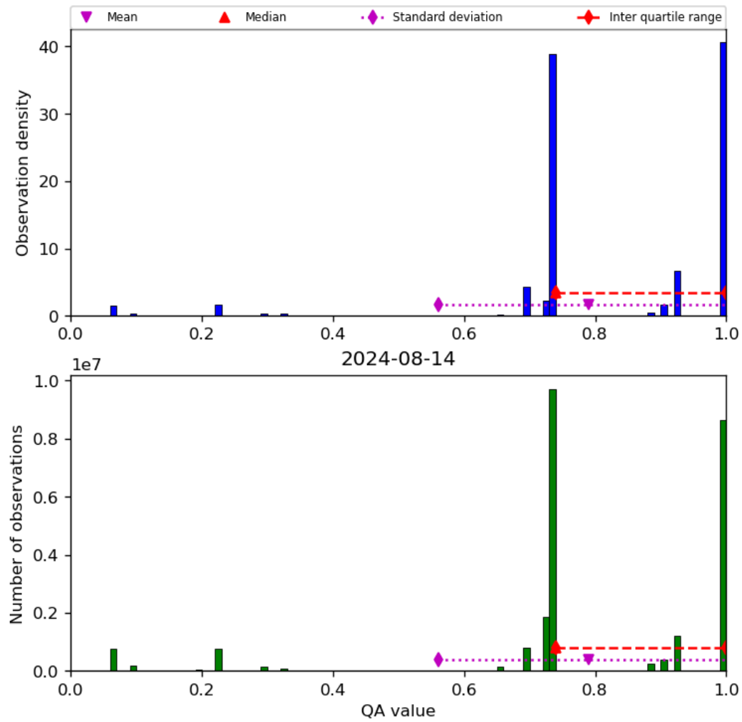
Figure 28: Histogram of “QA value” for 2024-08-13 to 2024-08-15
