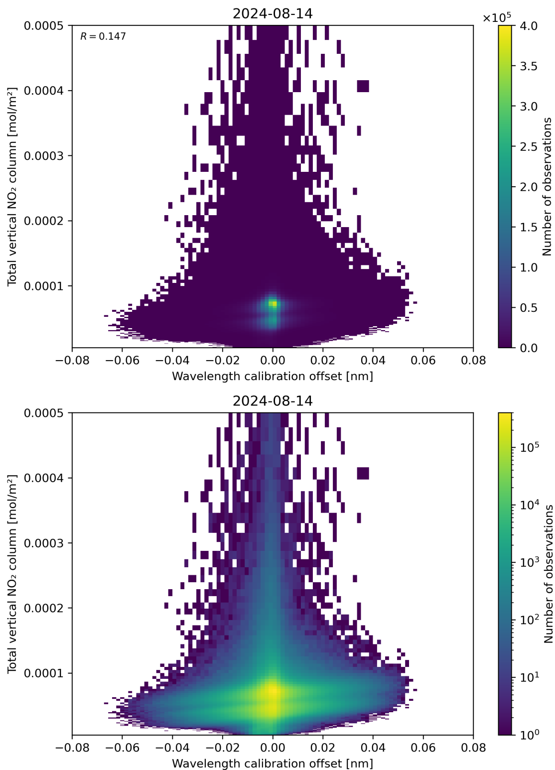
Figure 179: Scatter density plot of “Wavelength calibration offset” against “Total vertical NO 2 column” for 2024-08-13 to 2024-08-15.
