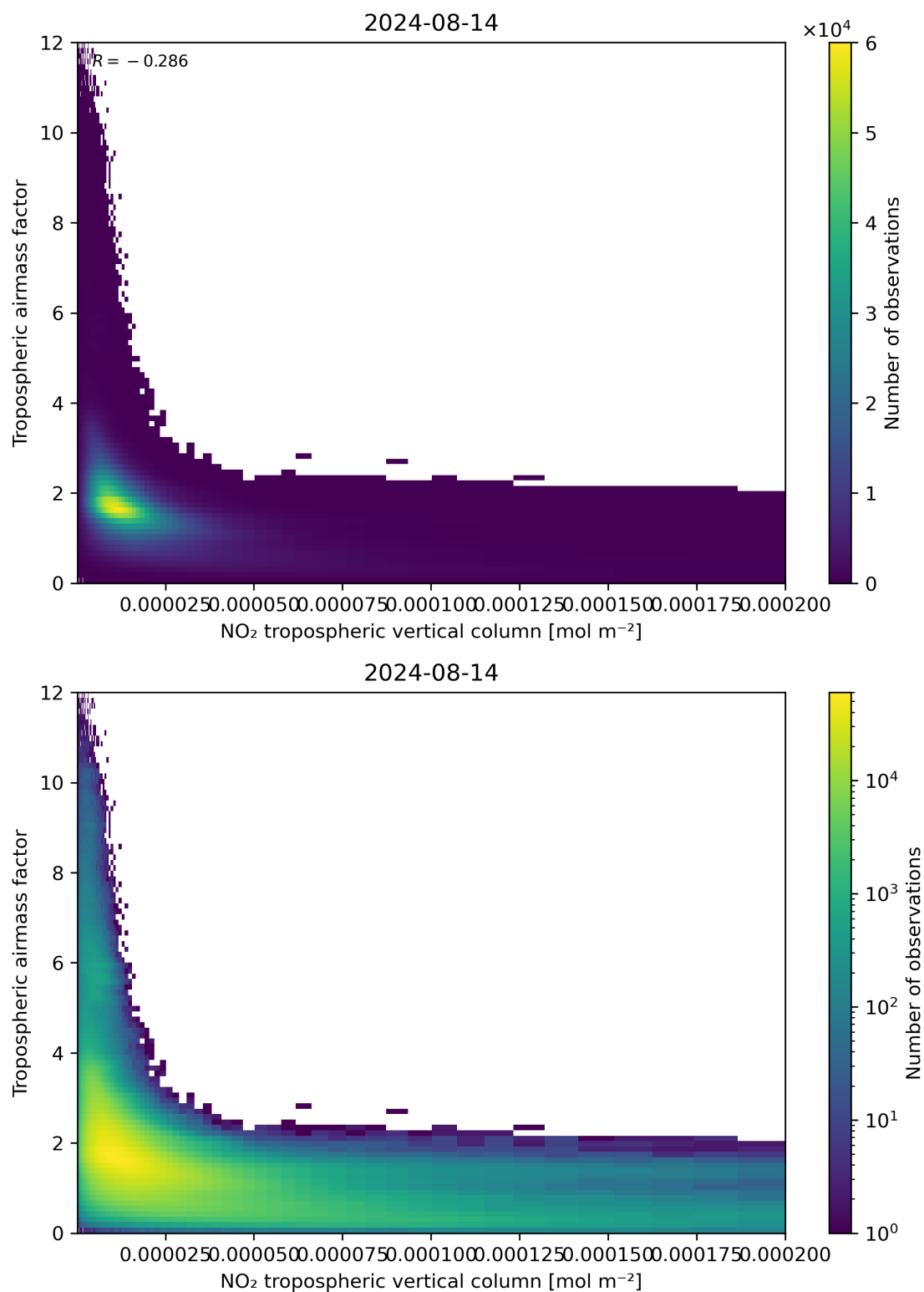
Figure 123: Scatter density plot of “NO 2 tropospheric vertical column” against “Tropospheric airmass factor” for 2024-08-13 to 2024-08-15.
