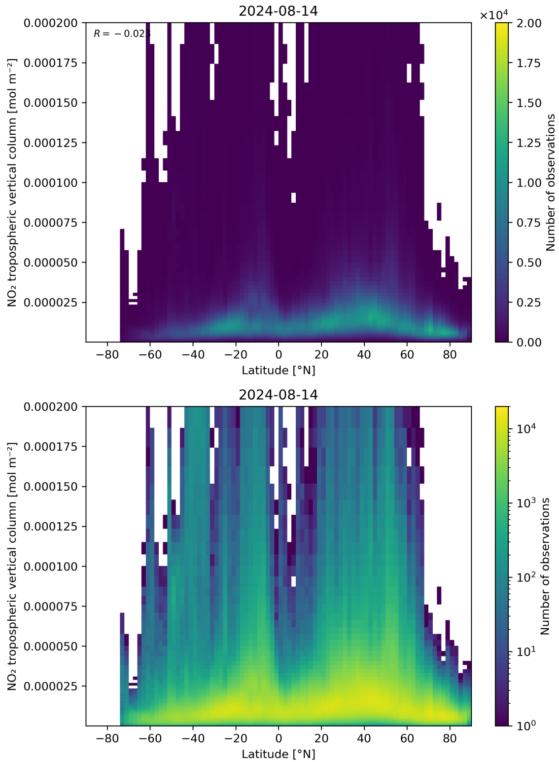
Figure 92: Scatter density plot of “Latitude” against “NO 2 tropospheric vertical column” for 2024-08-13 to 2024-08-15.
