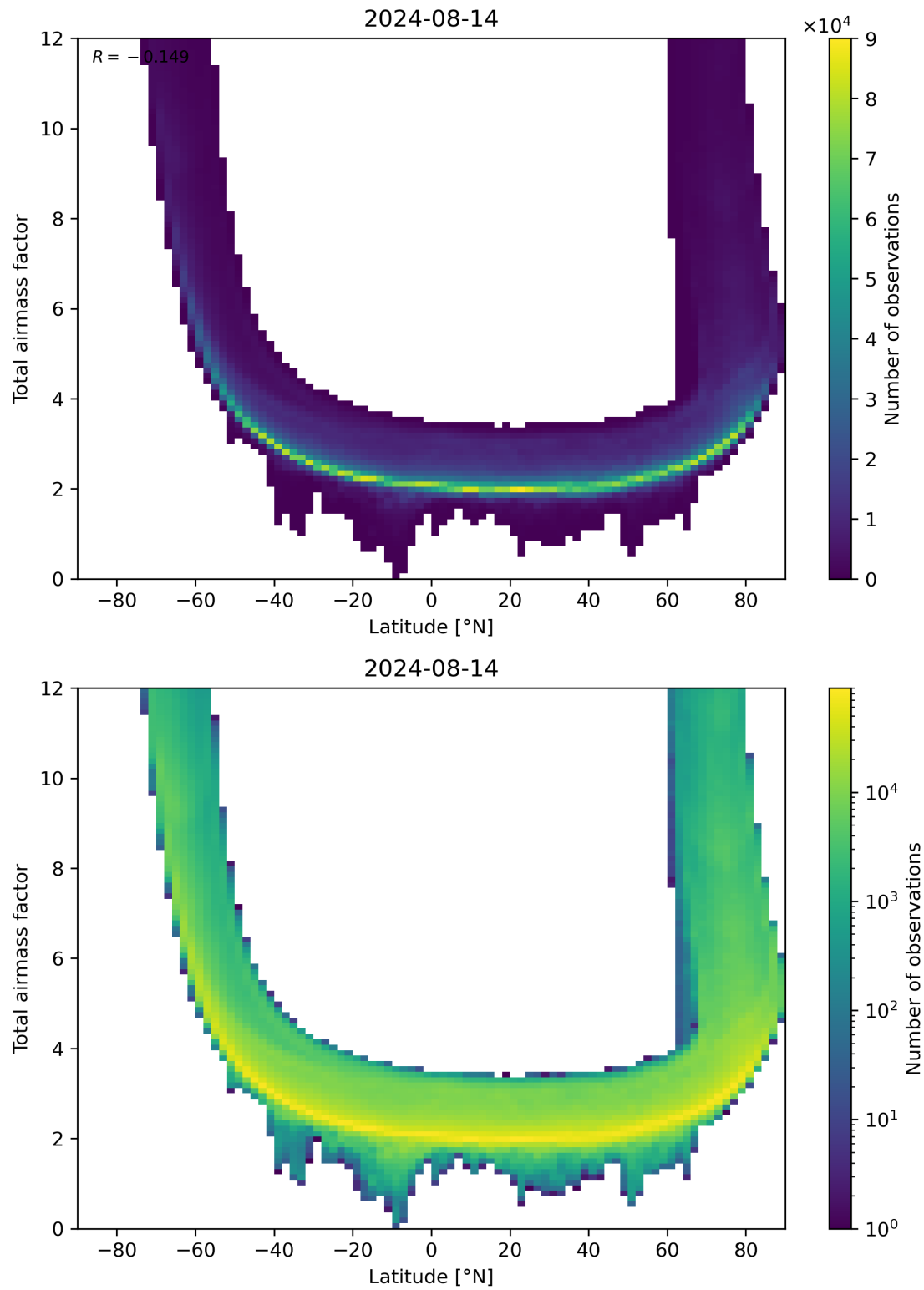
Figure 84: Scatter density plot of “Latitude” against “Total airmass factor” for 2024-08-13 to 2024-08-15.
