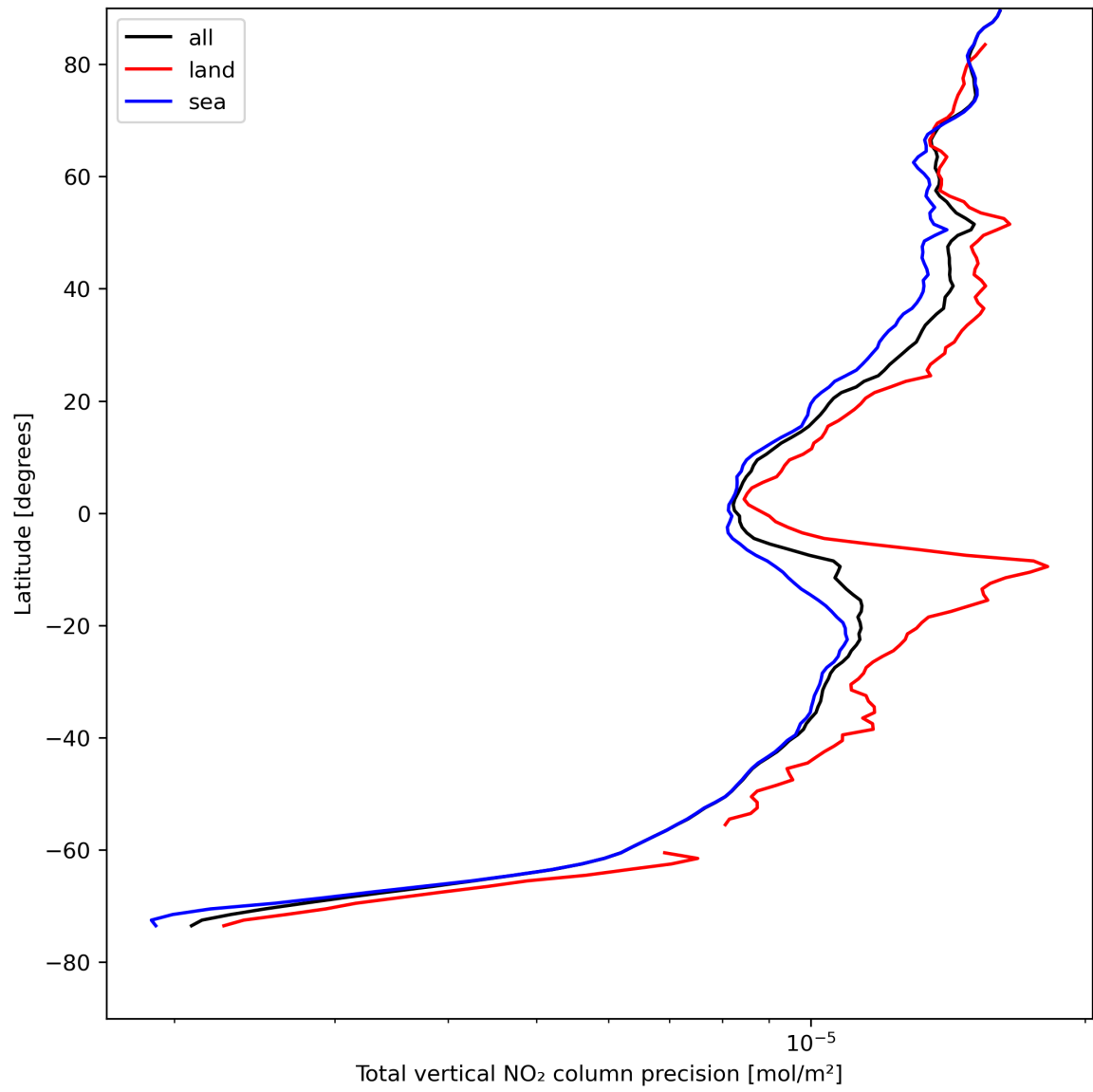
Figure 22: Zonal average of “Total vertical NO 2 column precision” for 2024-08-13 to 2024-08-15.
