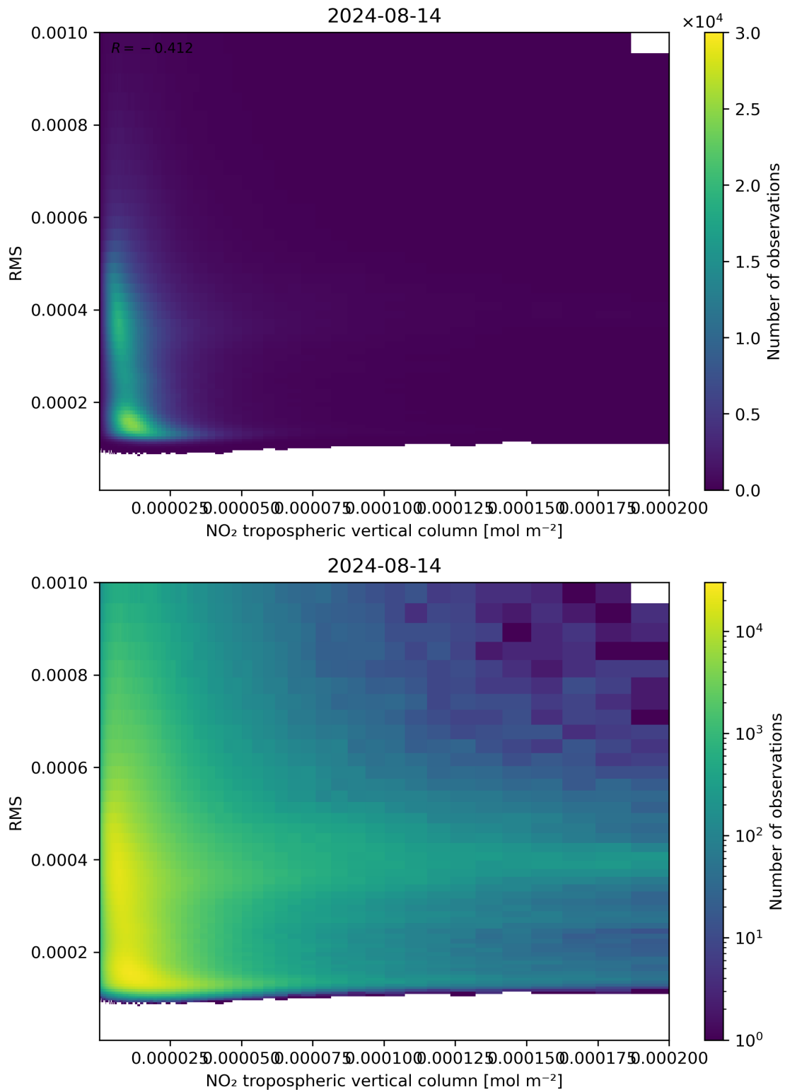
Figure 142: Scatter density plot of “NO 2 tropospheric vertical column” against “RMS” for 2024-08-13 to 2024-08-15.
