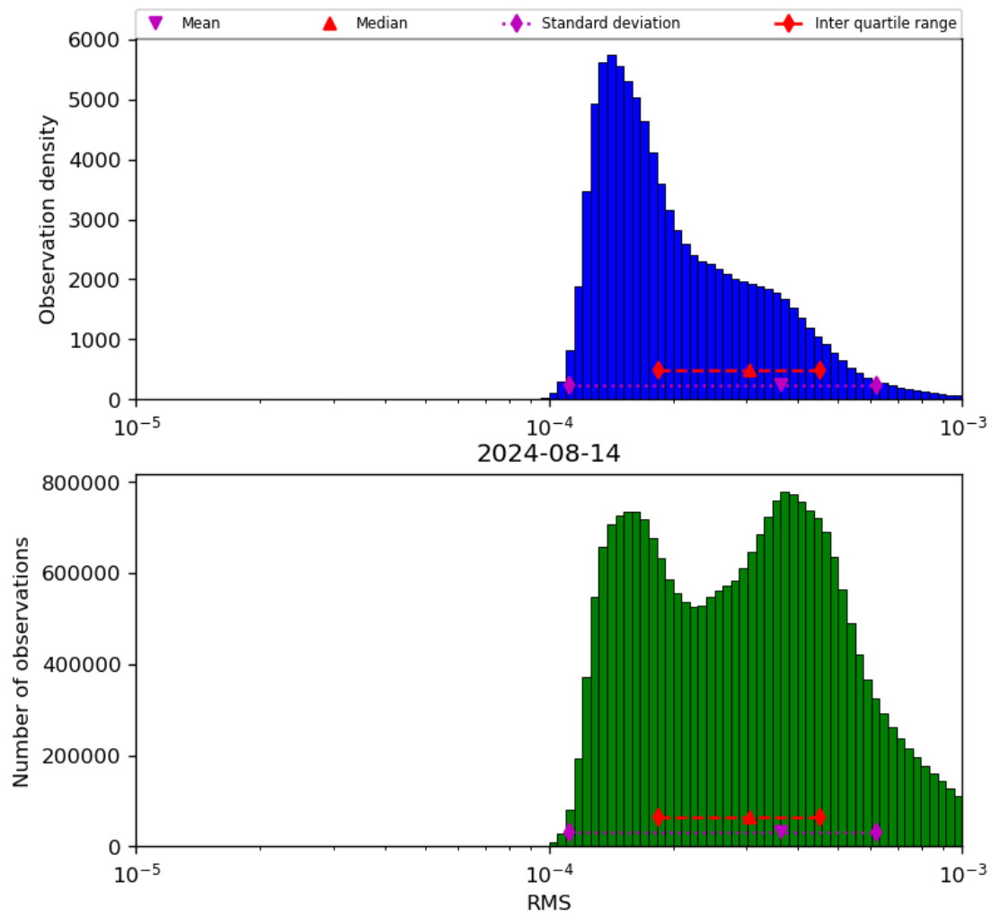
Figure 43: Histogram of “RMS” for 2024-08-13 to 2024-08-15
