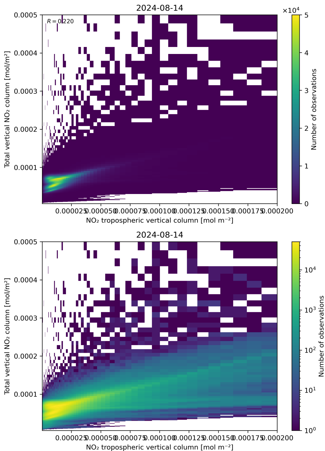
Figure 128: Scatter density plot of “NO 2 tropospheric vertical column” against “Total vertical NO 2 column” for 2024-08-13 to 2024-08-15.
