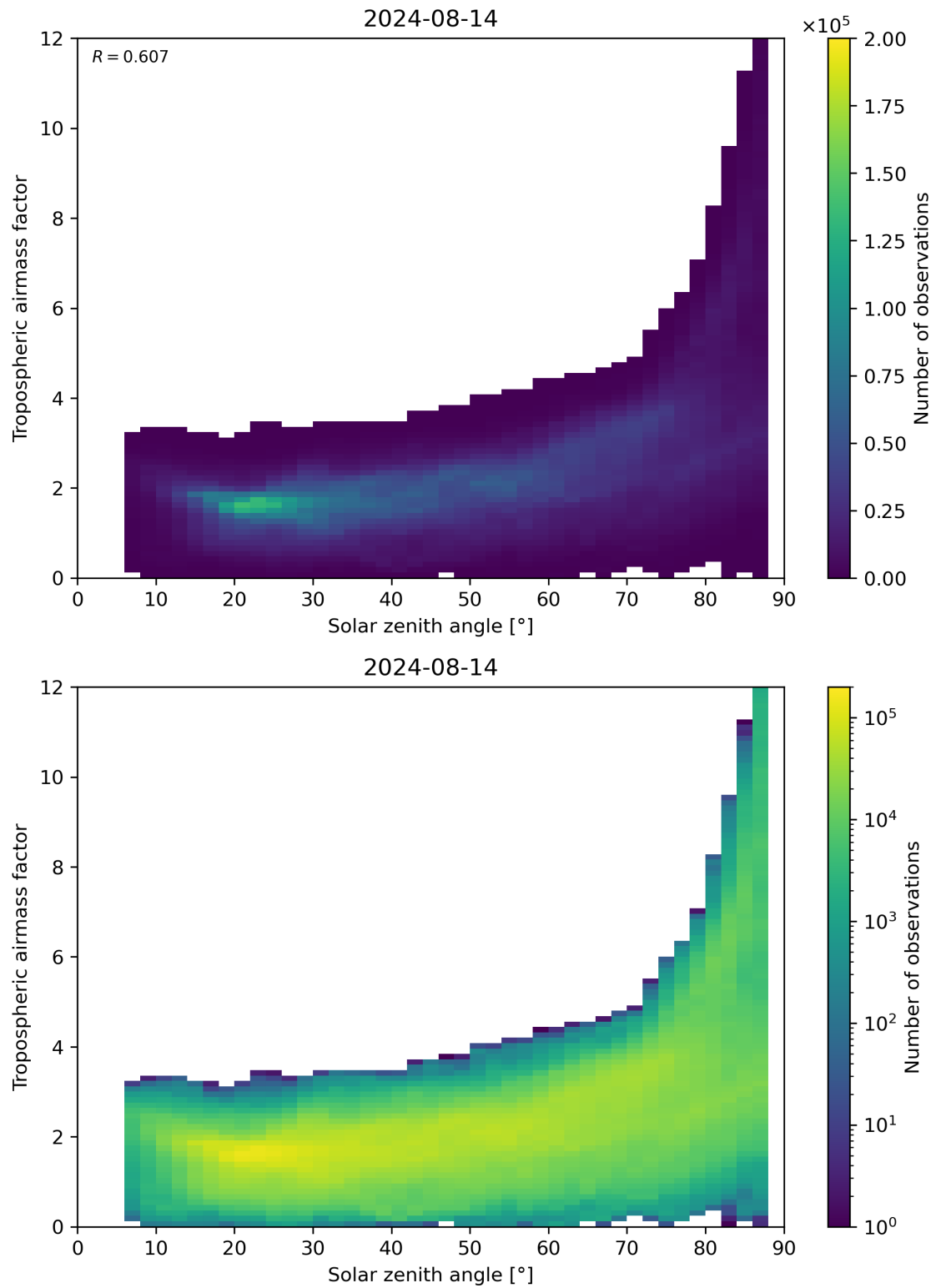
Figure 147: Scatter density plot of “Solar zenith angle” against “Tropospheric airmass factor” for 2024-08-13 to 2024-08-15.
