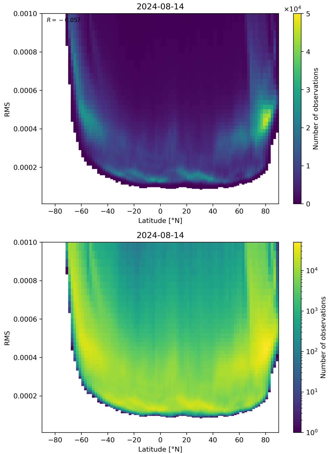
Figure 94: Scatter density plot of “Latitude” against “RMS” for 2024-08-13 to 2024-08-15.
