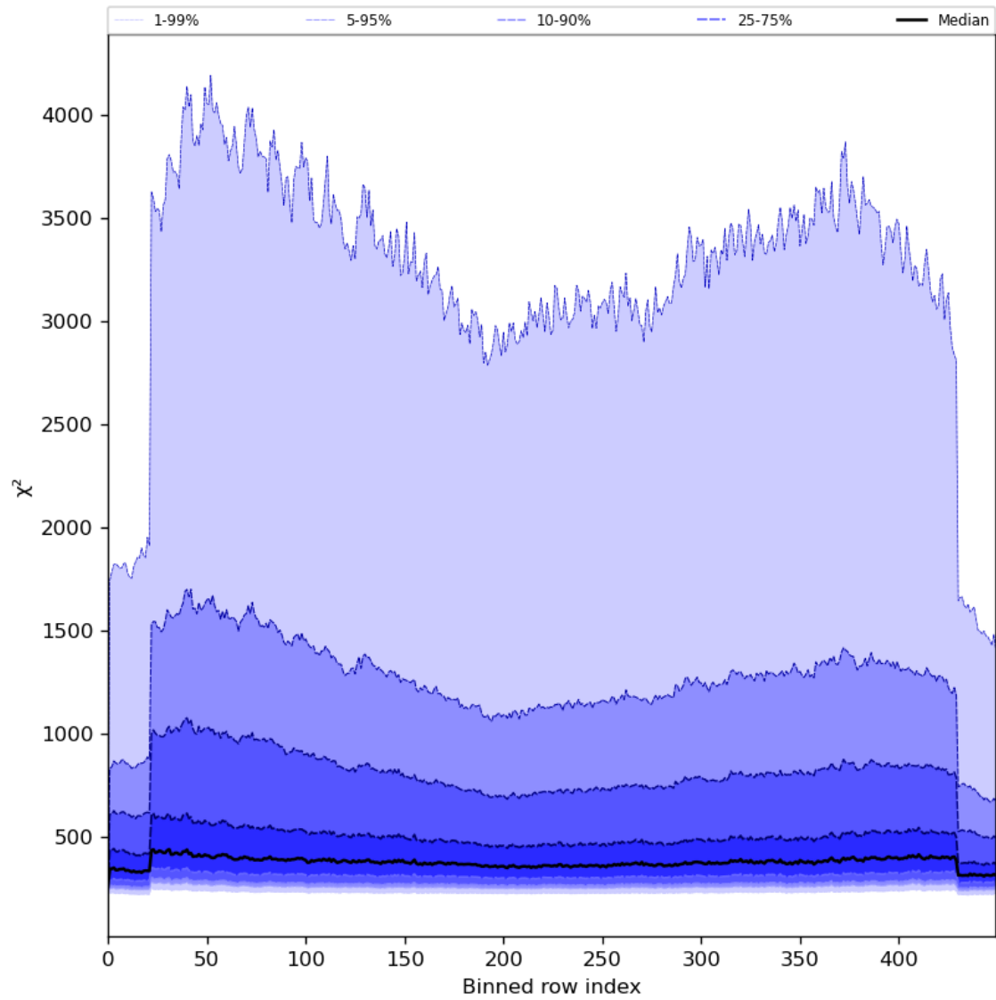
Figure 59: Along track statistics of “ \chi^2 ” for 2024-08-13 to 2024-08-15
