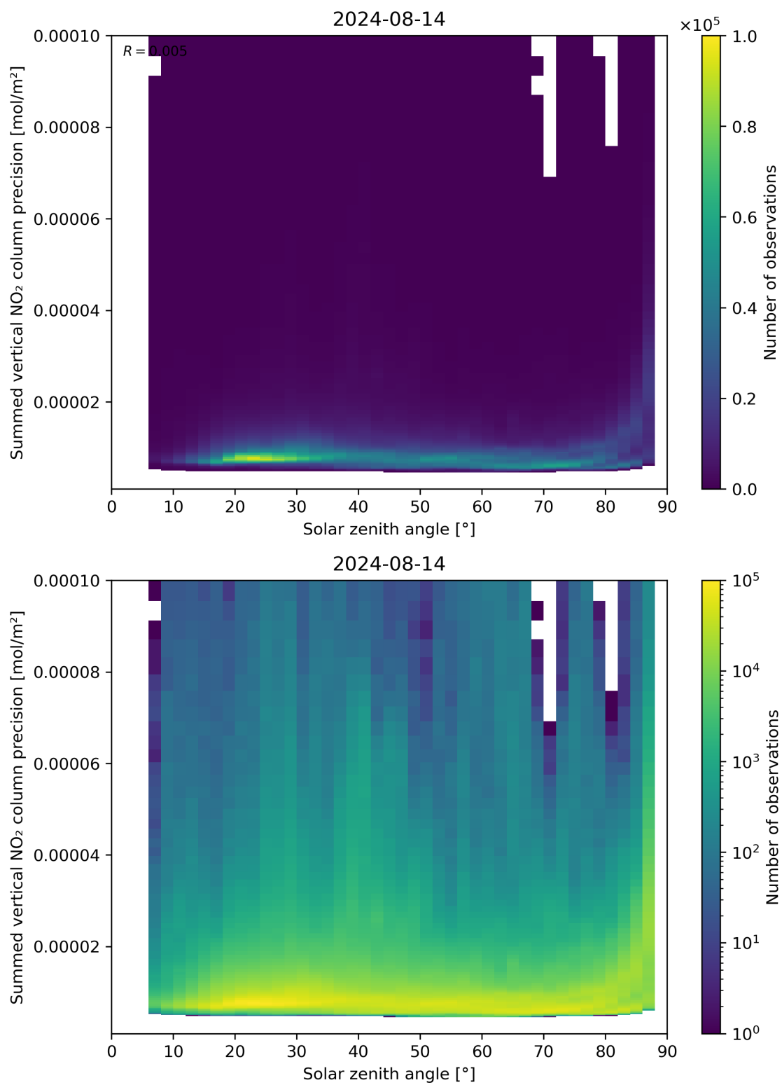
Figure 152: Scatter density plot of “Solar zenith angle” against “Summed vertical NO 2 column precision” for 2024-08-13 to 2024-08-15.
