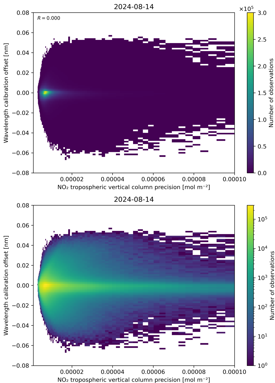
Figure 141: Scatter density plot of “NO 2 tropospheric vertical column precision” against “Wavelength calibration offset” for 2024-08-13 to 2024-08-15.
