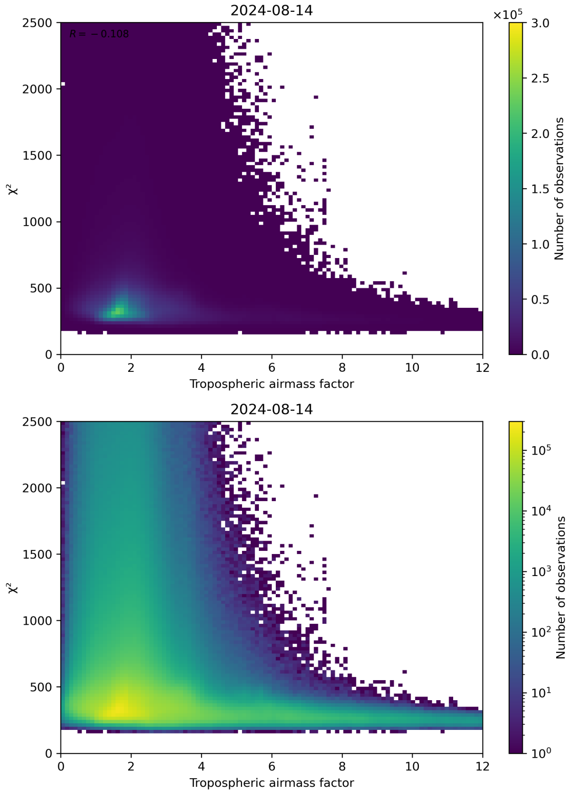
Figure 73: Scatter density plot of “Tropospheric airmass factor” against “ \chi^2 ” for 2024-08-13 to 2024-08-15.
