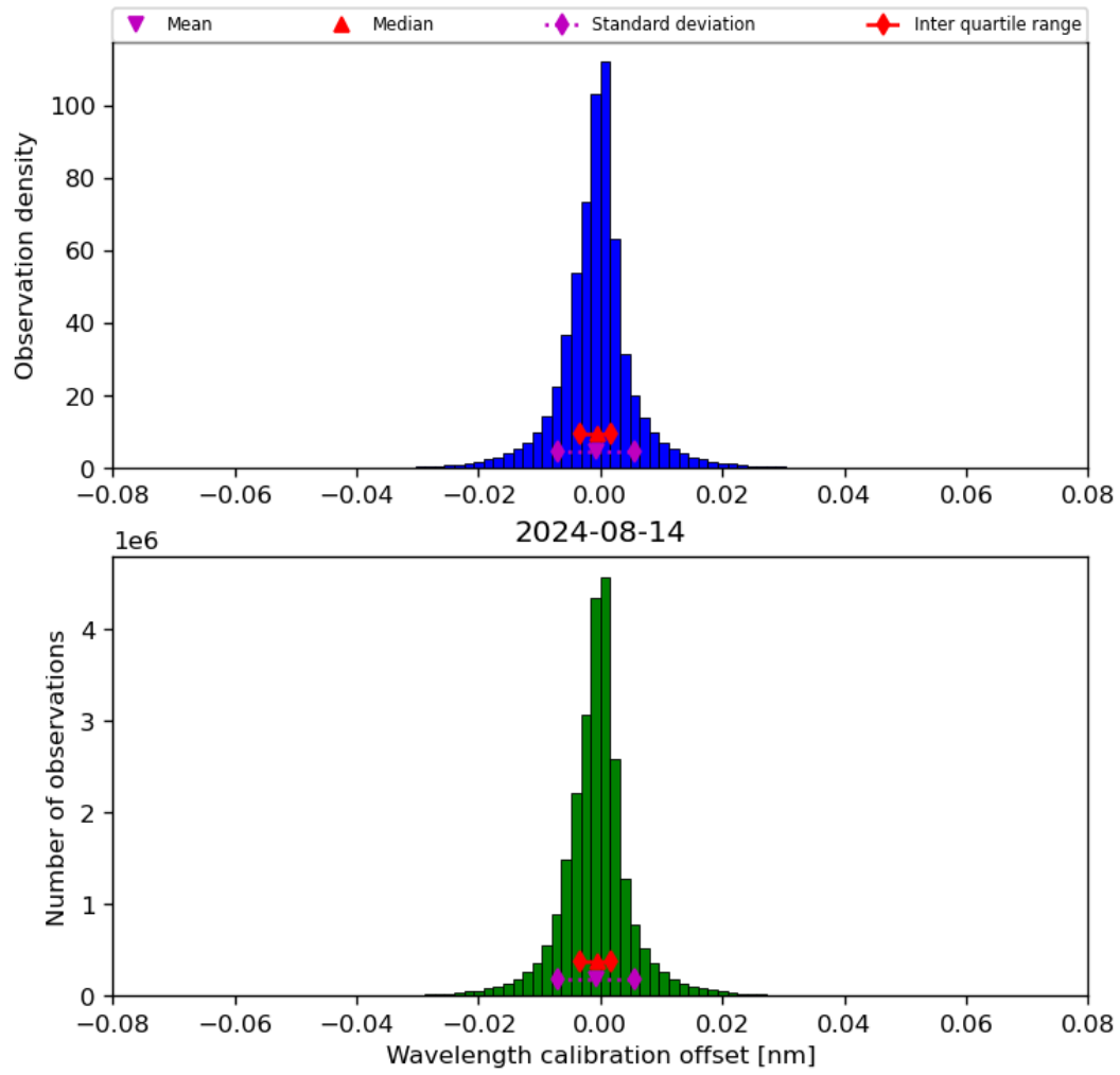
Figure 35: Histogram of “Wavelength calibration offset” for 2024-08-13 to 2024-08-15
