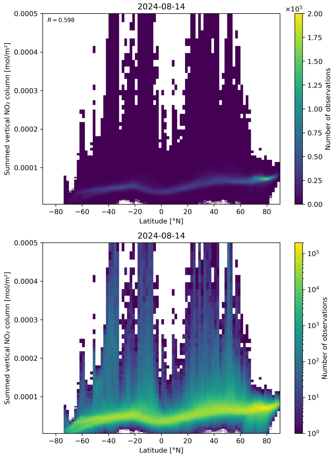
Figure 88: Scatter density plot of “Latitude” against “Summed vertical NO 2 column” for 2024-08-13 to 2024-08-15.
