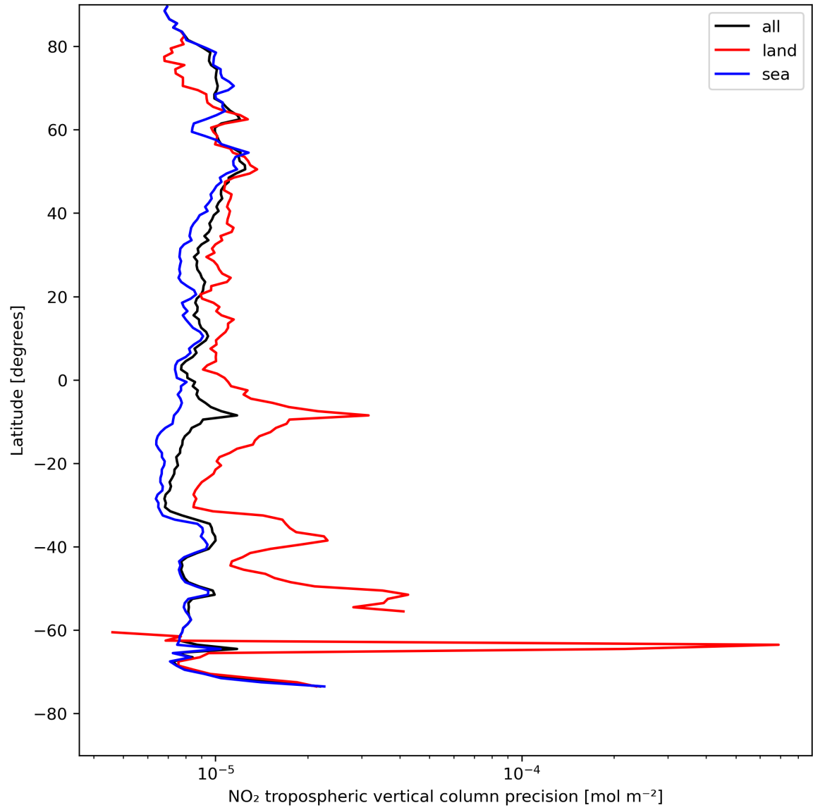
Figure 13: Zonal average of “NO 2 tropospheric vertical column precision” for 2024-08-13 to 2024-08-15.
