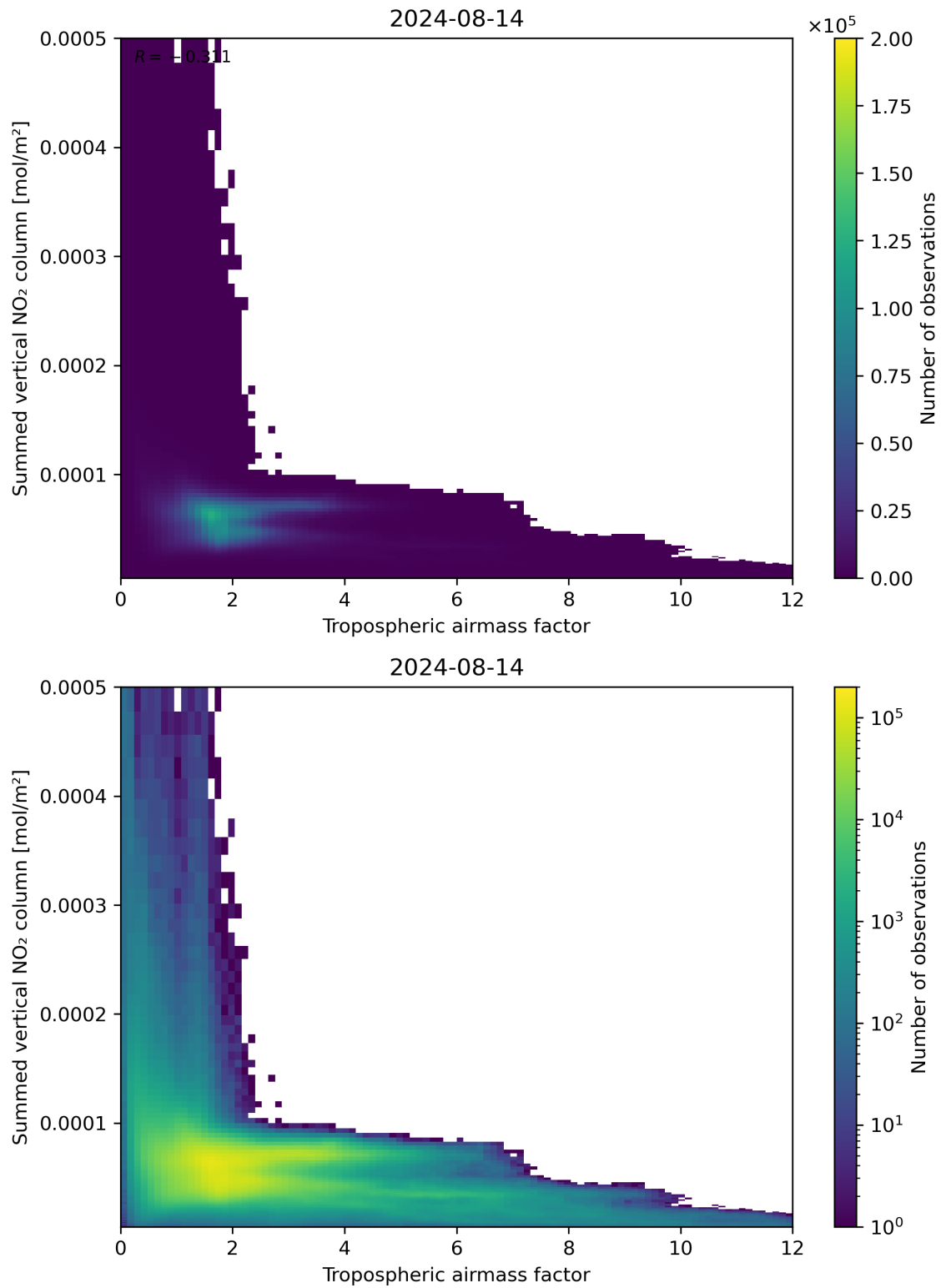
Figure 75: Scatter density plot of “Tropospheric airmass factor” against “Summed vertical NO 2 column” for 2024-08-13 to 2024-08-15.
