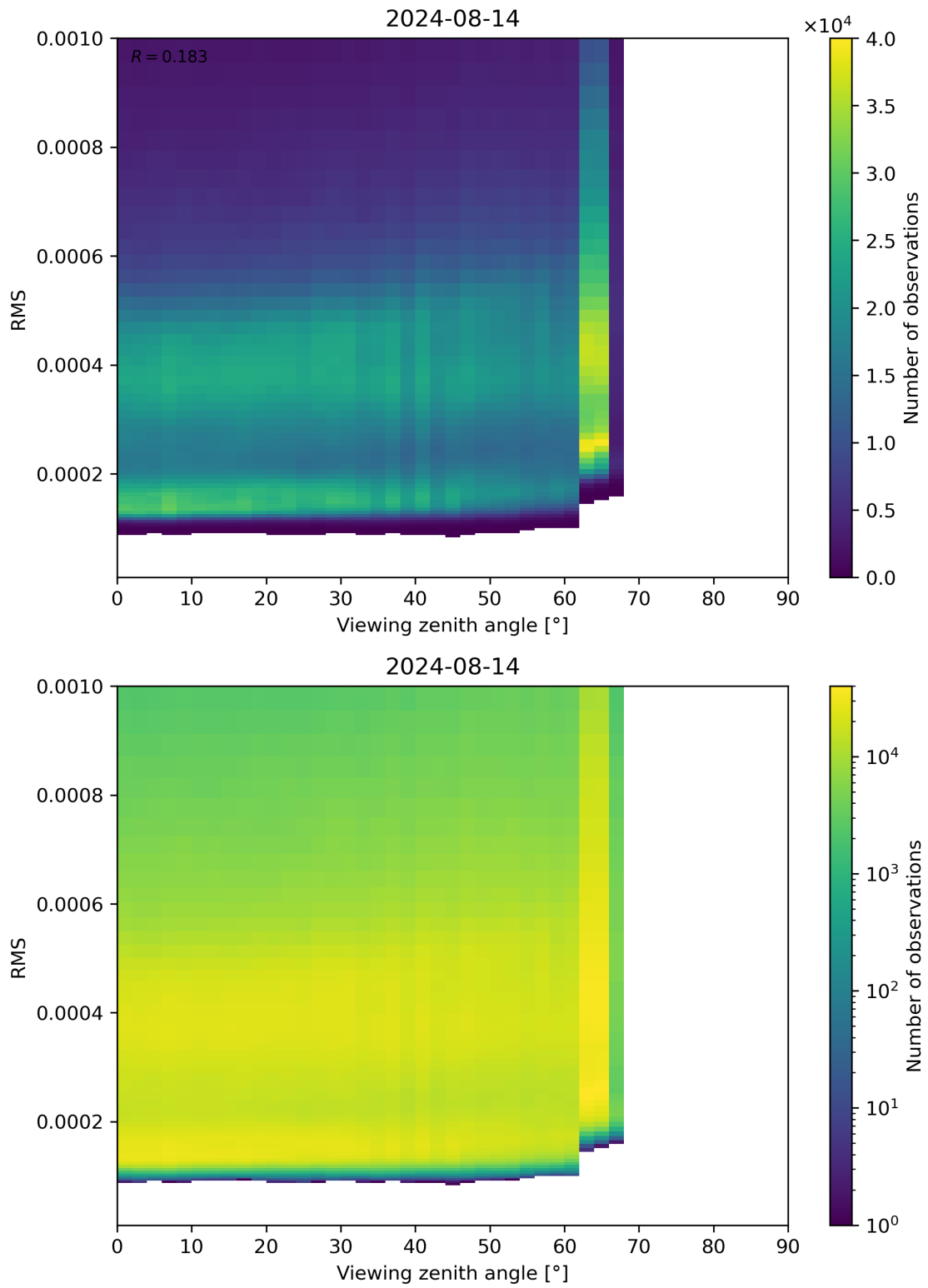
Figure 171: Scatter density plot of “Viewing zenith angle” against “RMS” for 2024-08-13 to 2024-08-15.
