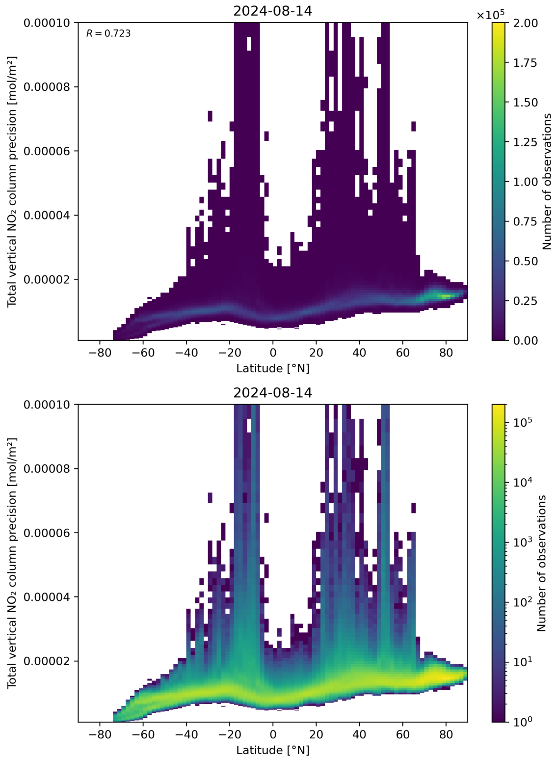
Figure 91: Scatter density plot of “Latitude” against “Total vertical NO 2 column precision” for 2024-08-13 to 2024-08-15.
