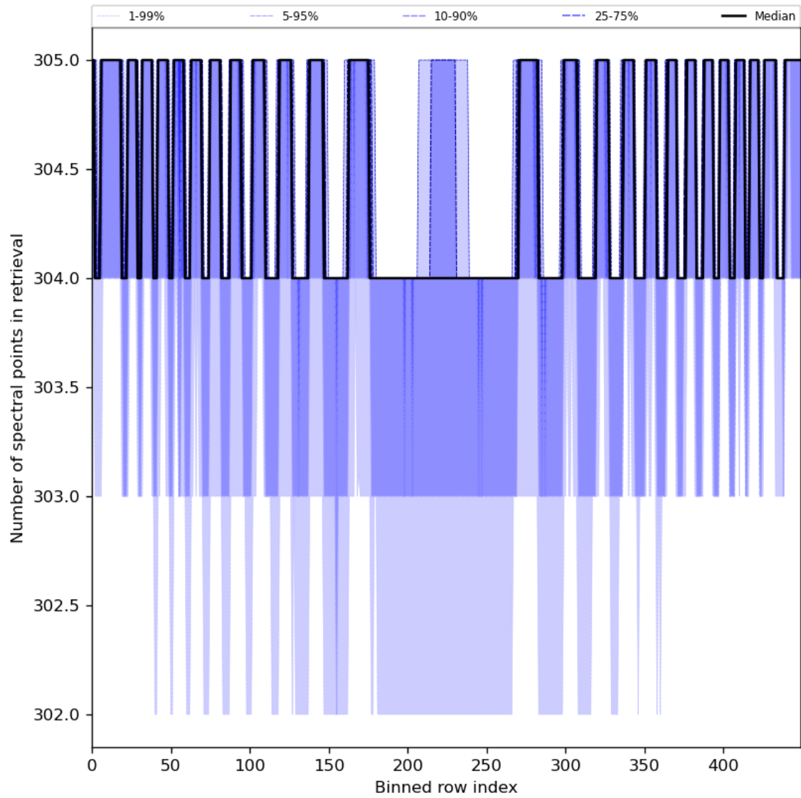
Figure 50: Along track statistics of “Number of spectral points in retrieval” for 2024-08-13 to 2024-08-15
