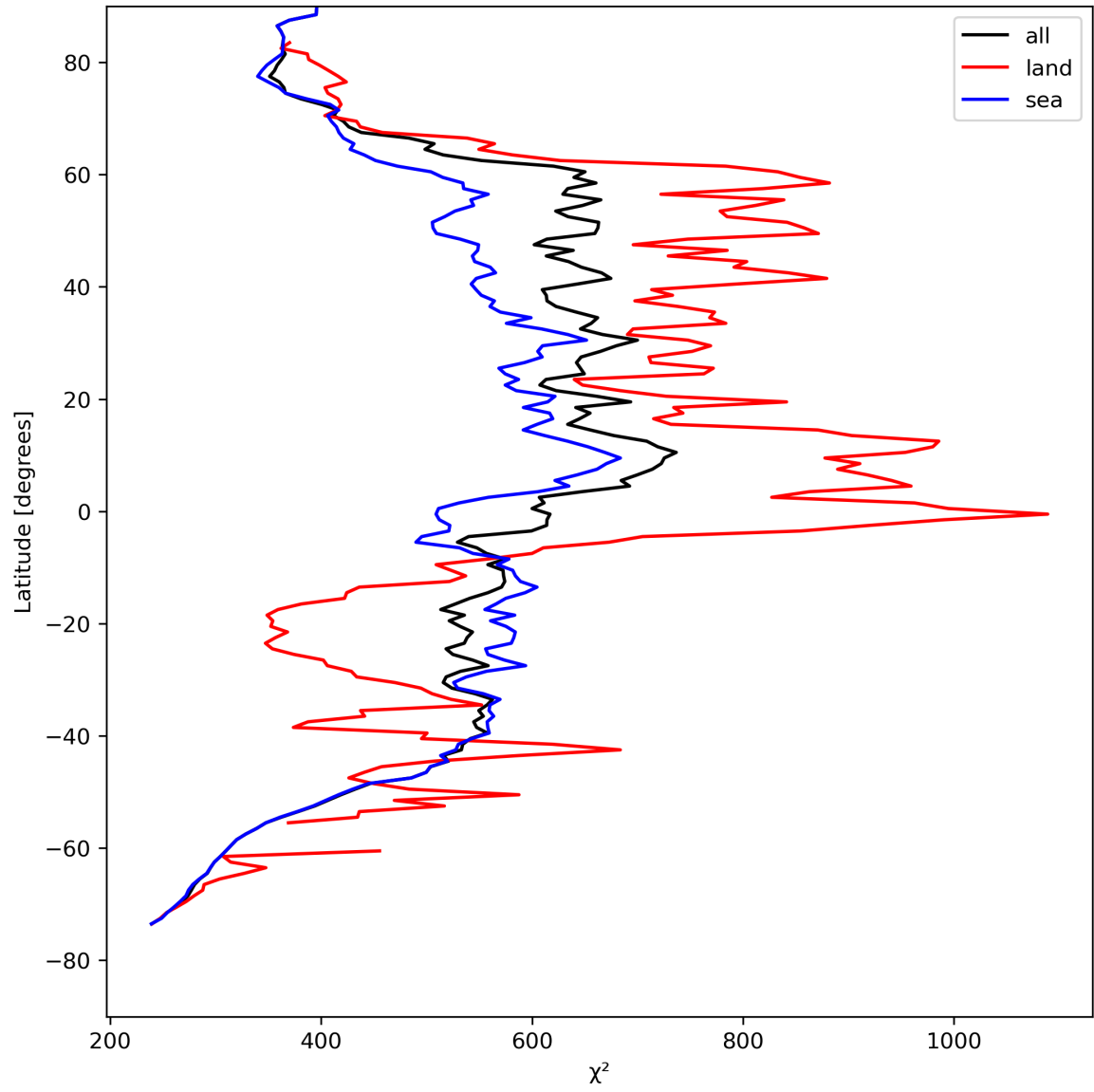
Figure 25: Zonal average of “ \chi^2 ” for 2024-08-13 to 2024-08-15.
