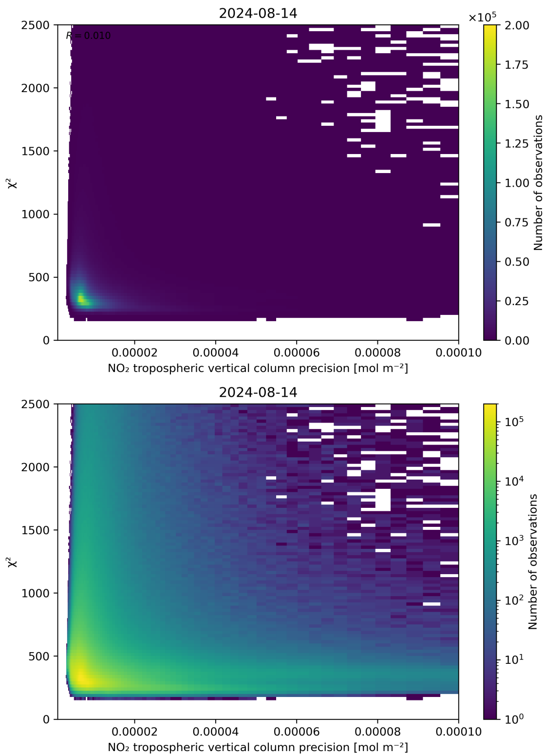
Figure 134: Scatter density plot of “NO 2 tropospheric vertical column precision” against “ \chi^2 ” for 2024-08-13 to 2024-08-15.
