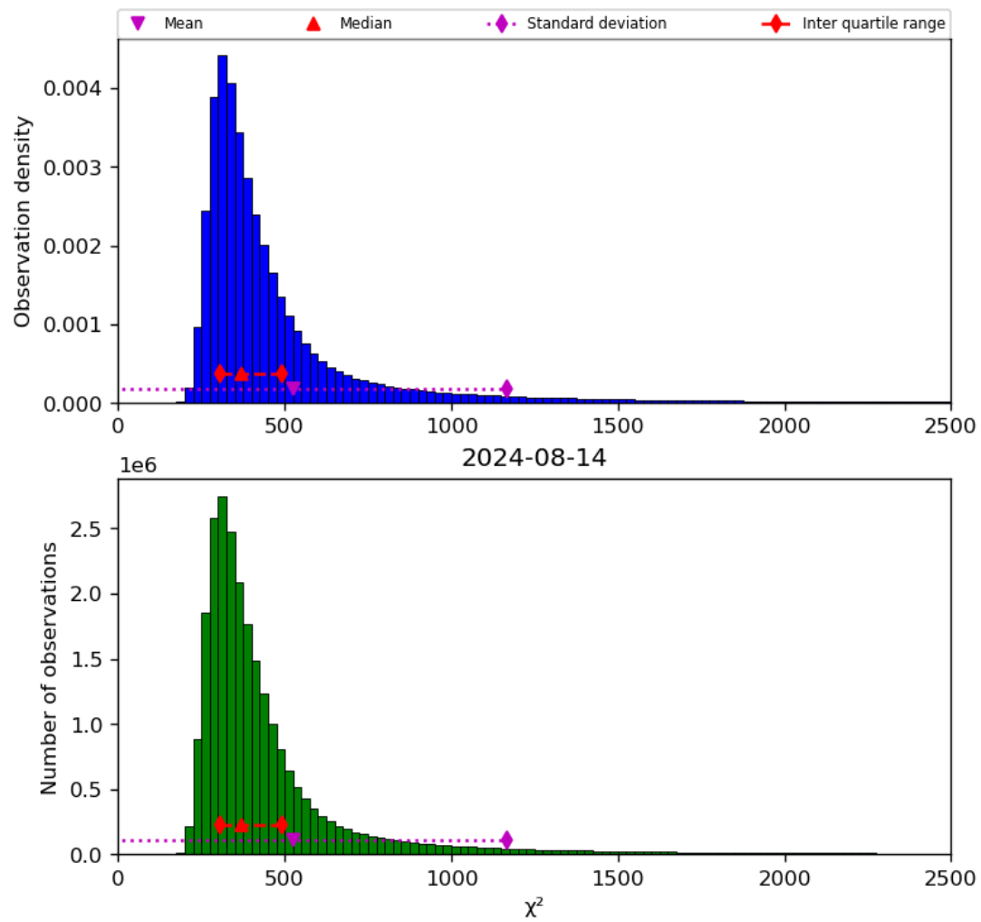
Figure 42: Histogram of “ \chi^2 ” for 2024-08-13 to 2024-08-15
