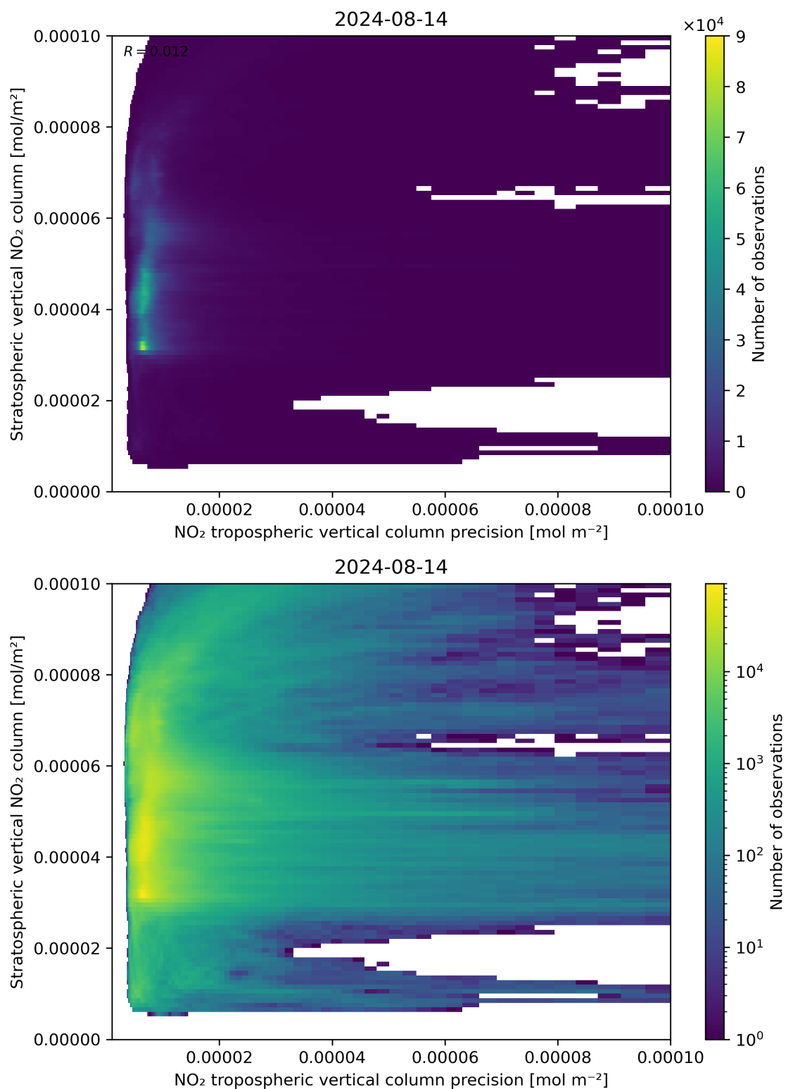
Figure 135: Scatter density plot of “NO 2 tropospheric vertical column precision” against “Stratospheric vertical NO 2 column” for 2024-08-13 to 2024-08-15.
