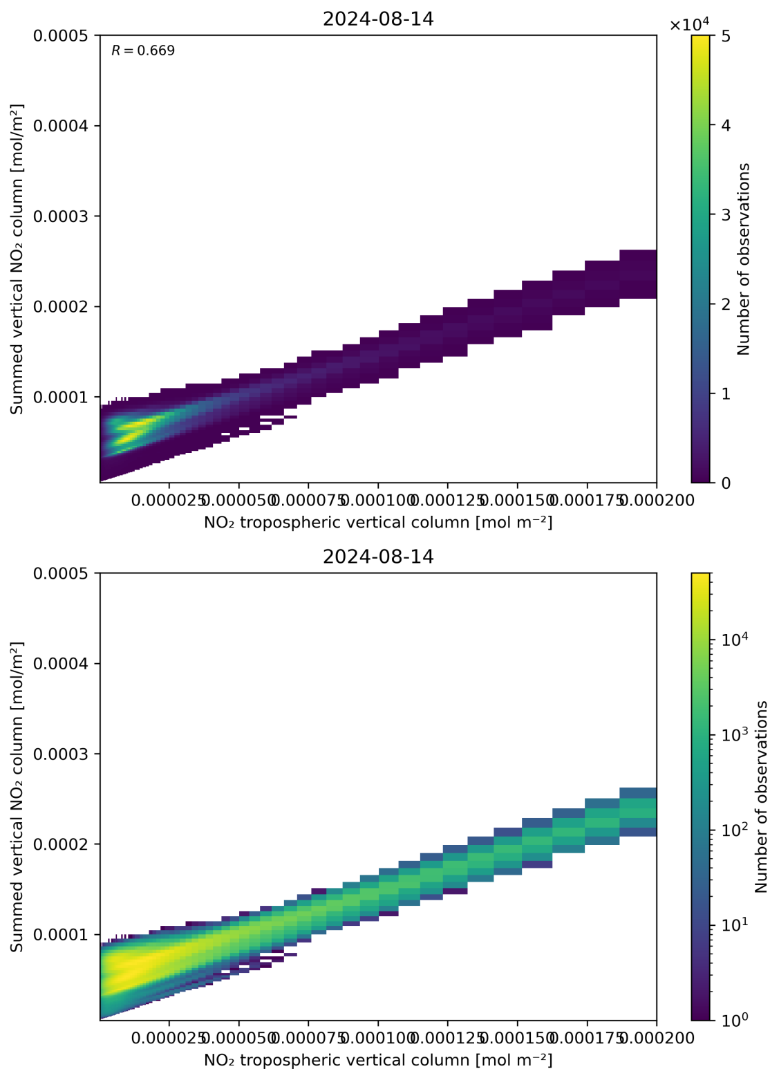
Figure 126: Scatter density plot of “NO 2 tropospheric vertical column” against “Summed vertical NO 2 column” for 2024-08-13 to 2024-08-15.
