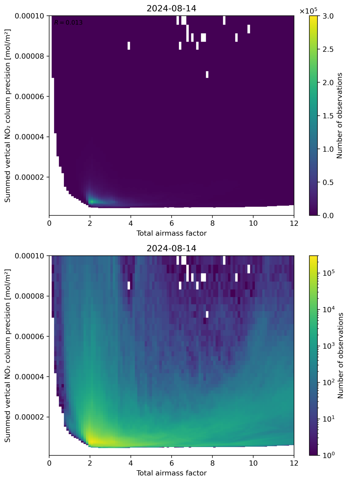
Figure 66: Scatter density plot of “Total airmass factor” against “Summed vertical NO 2 column precision” for 2024-08-13 to 2024-08-15.
