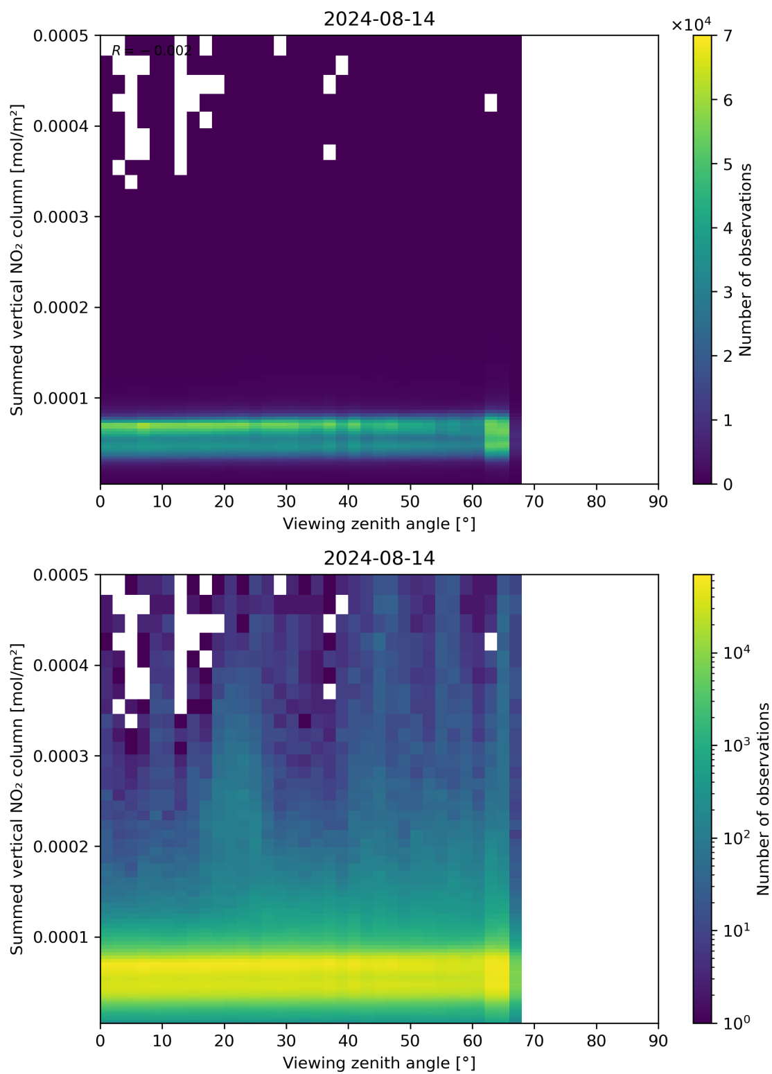
Figure 165: Scatter density plot of “Viewing zenith angle” against “Summed vertical NO 2 column” for 2024-08-13 to 2024-08-15.
