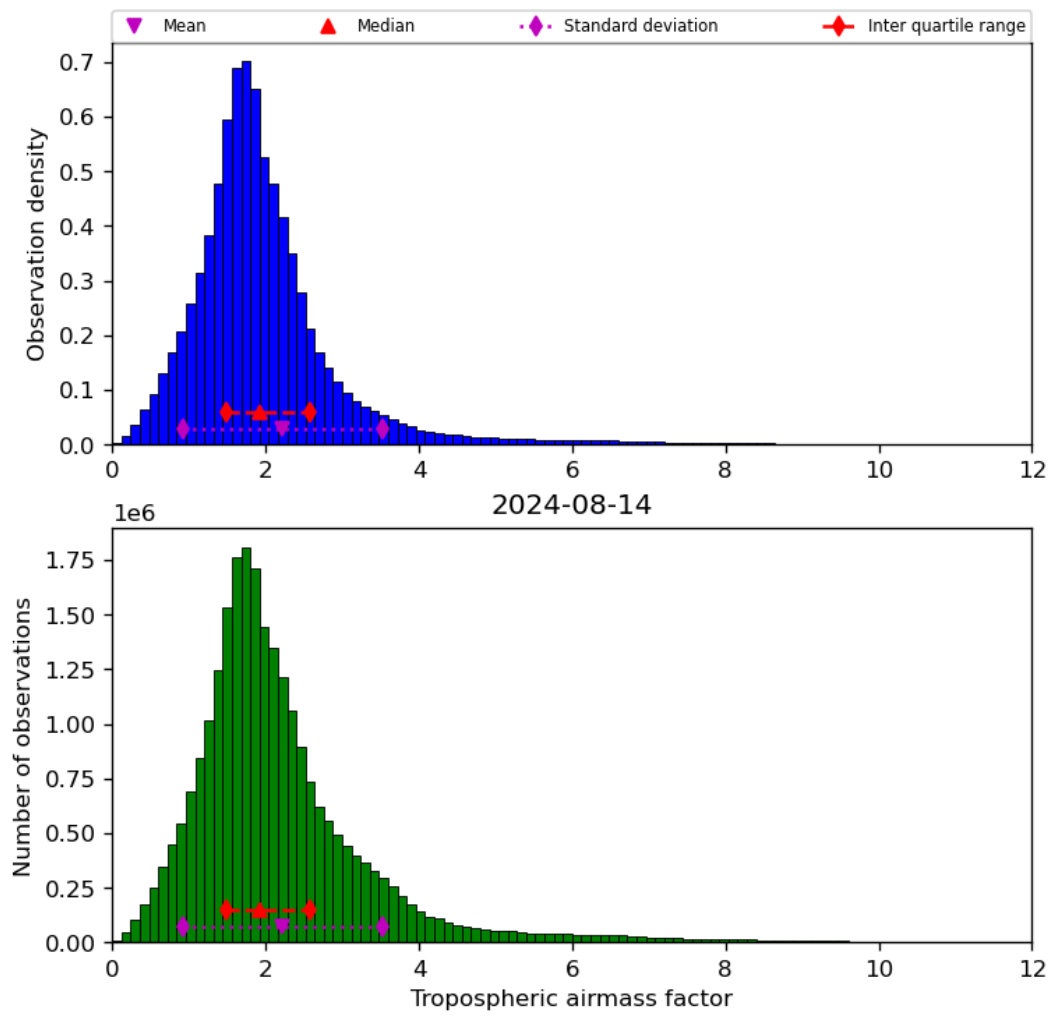
Figure 31: Histogram of “Tropospheric airmass factor” for 2024-08-13 to 2024-08-15
