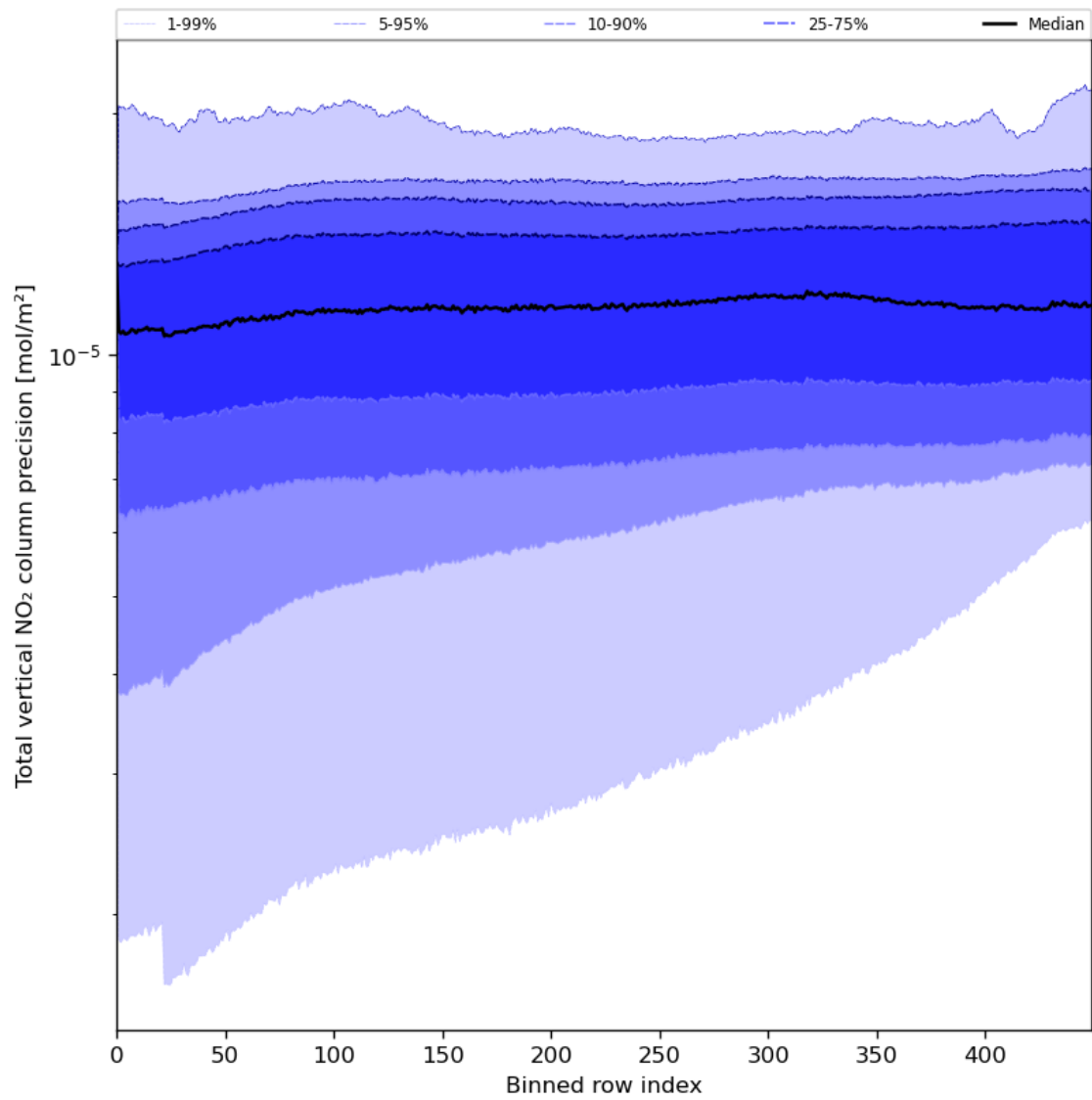
Figure 56: Along track statistics of “Total vertical NO 2 column precision” for 2024-08-13 to 2024-08-15
