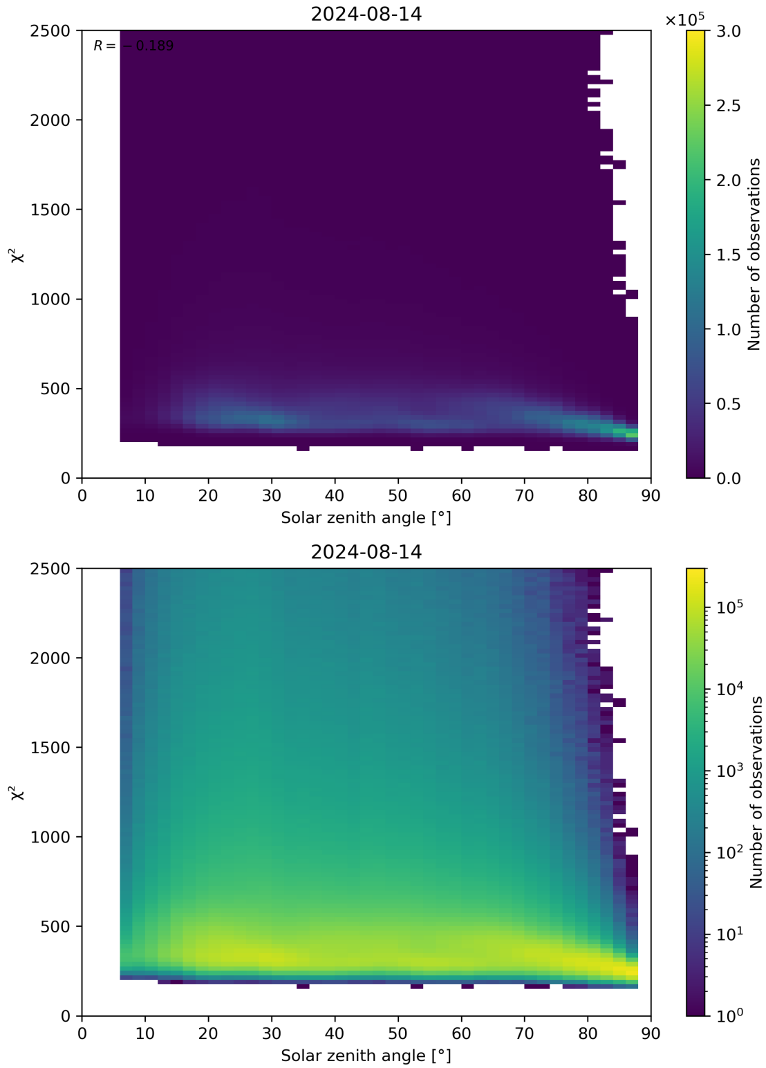
Figure 148: Scatter density plot of “Solar zenith angle” against “ \chi^2 ” for 2024-08-13 to 2024-08-15.
