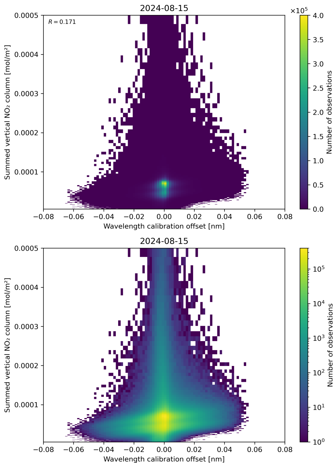
Figure 177: Scatter density plot of “Wavelength calibration offset” against “Summed vertical NO 2 column” for 2024-08-14 to 2024-08-16.
