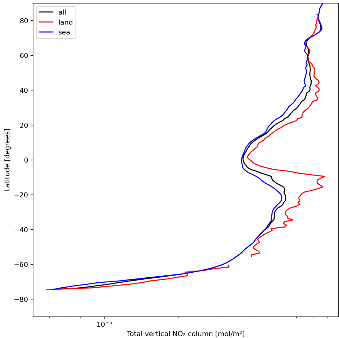
Figure 21: Zonal average of “Total vertical NO 2 column” for 2024-08-14 to 2024-08-16.
