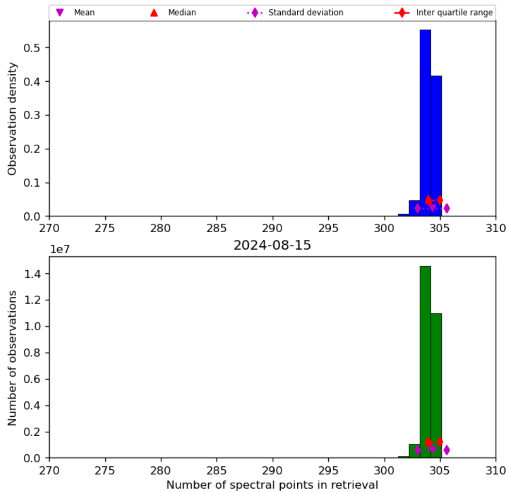
Figure 33: Histogram of “Number of spectral points in retrieval” for 2024-08-14 to 2024-08-16
