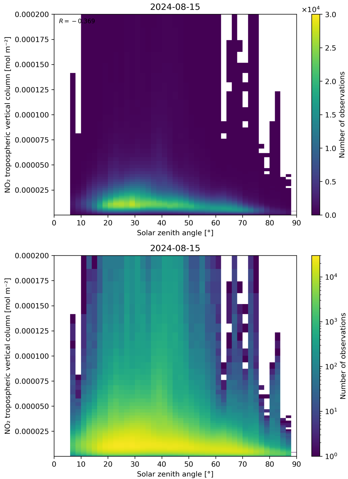
Figure 155: Scatter density plot of “Solar zenith angle” against “NO 2 tropospheric vertical column” for 2024-08-14 to 2024-08-16.
