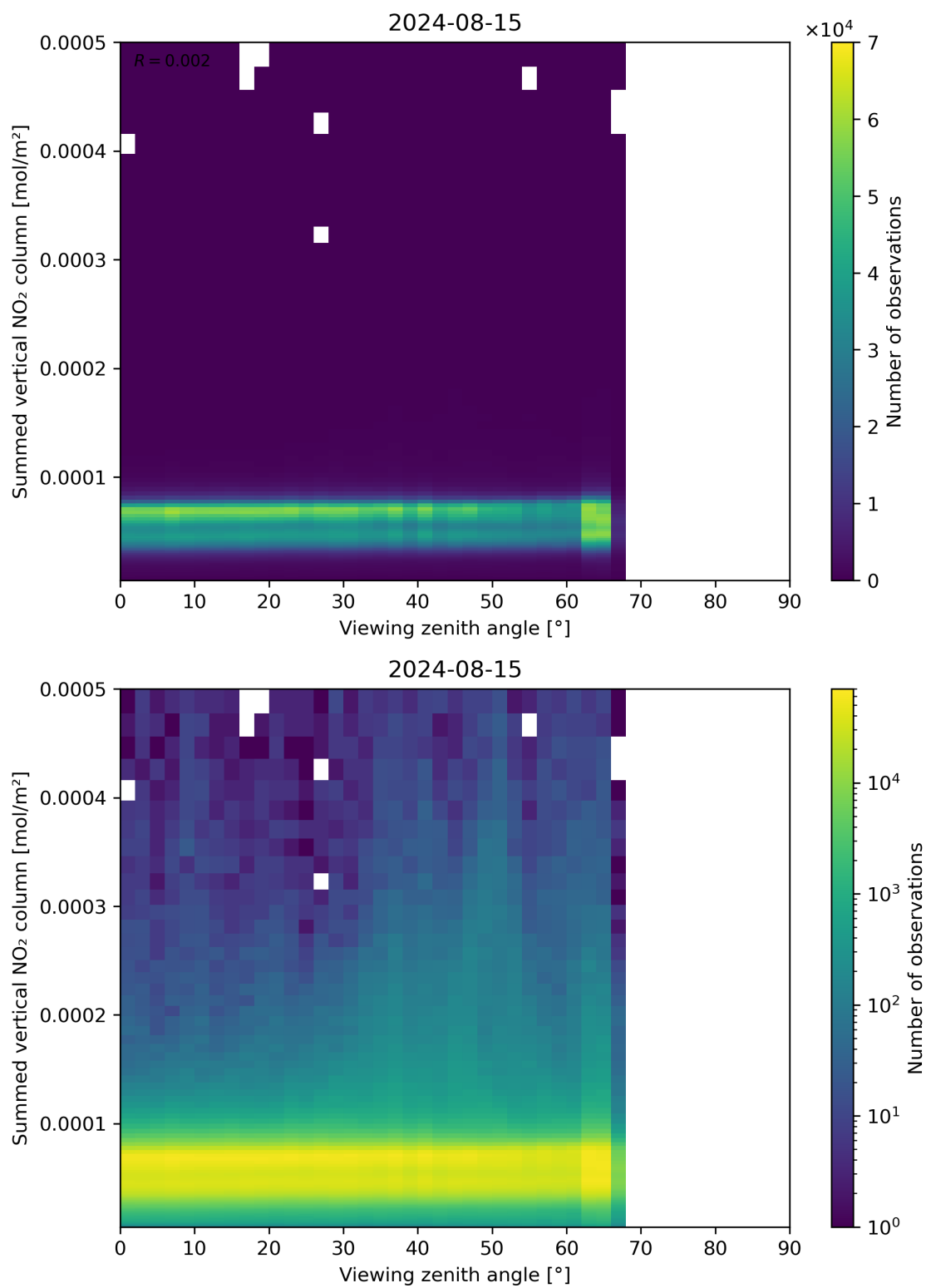
Figure 165: Scatter density plot of “Viewing zenith angle” against “Summed vertical NO 2 column” for 2024-08-14 to 2024-08-16.
