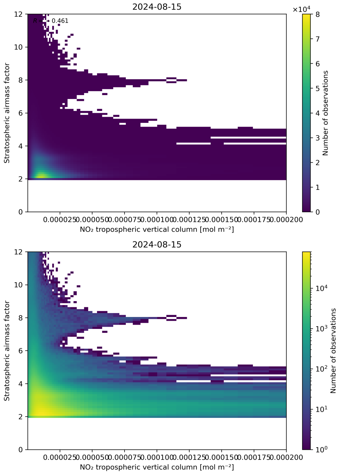
Figure 121: Scatter density plot of “NO 2 tropospheric vertical column” against “Stratospheric air mass factor” for 2024-08-14 to 2024-08-16.
