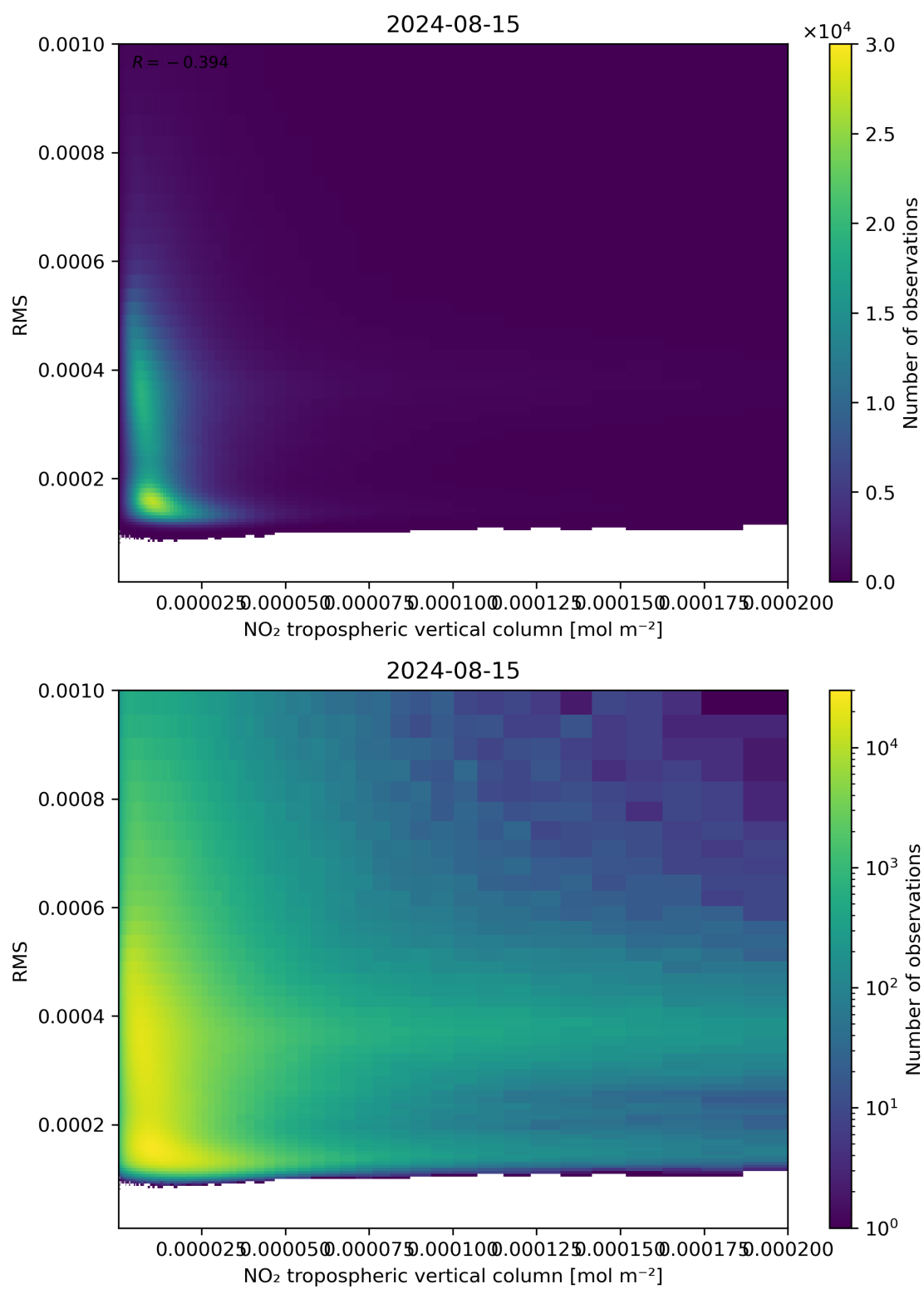
Figure 142: Scatter density plot of “NO 2 tropospheric vertical column” against “RMS” for 2024-08-14 to 2024-08-16.
