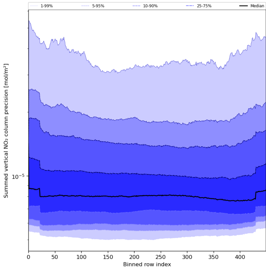
Figure 58: Along track statistics of “Summed vertical NO 2 column precision” for 2024-08-14 to 2024-08-16
