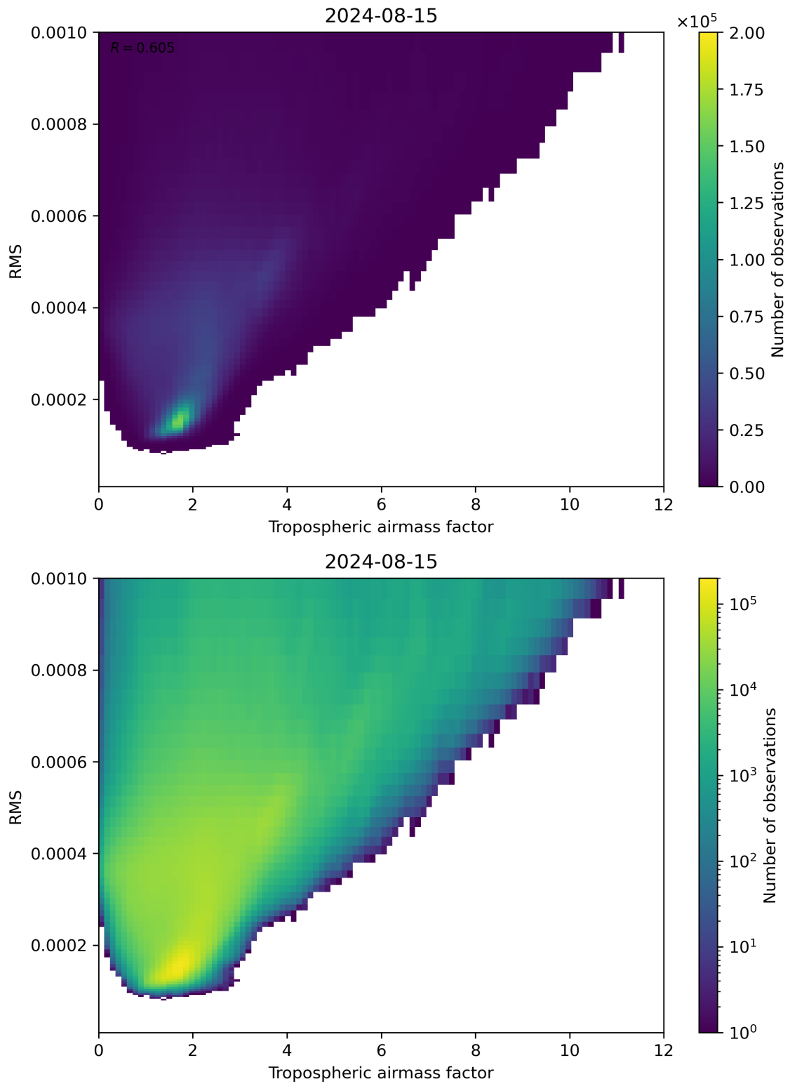
Figure 79: Scatter density plot of “Tropospheric airmass factor” against “RMS” for 2024-08-14 to 2024-08-16.
