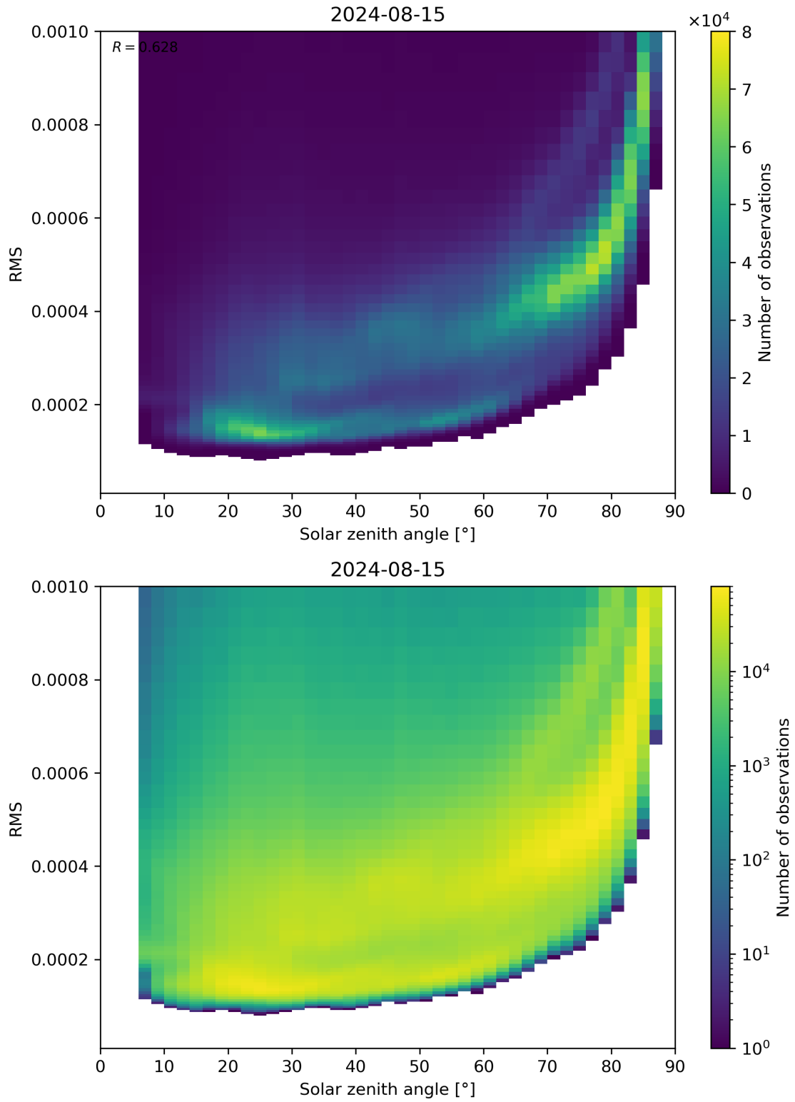
Figure 157: Scatter density plot of “Solar zenith angle” against “RMS” for 2024-08-14 to 2024-08-16.
