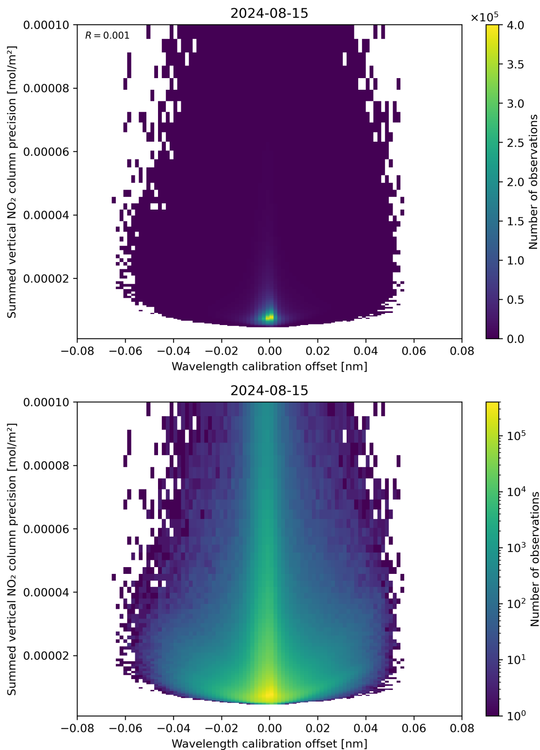
Figure 178: Scatter density plot of “Wavelength calibration offset” against “Summed vertical NO 2 column precision” for 2024-08-14 to 2024-08-16.
