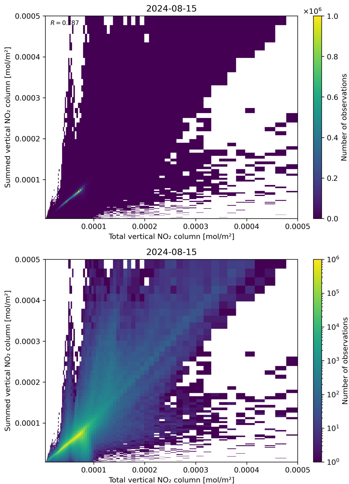
Figure 112: Scatter density plot of “Total vertical NO 2 column” against “Summed vertical NO 2 column” for 2024-08-14 to 2024-08-16.
