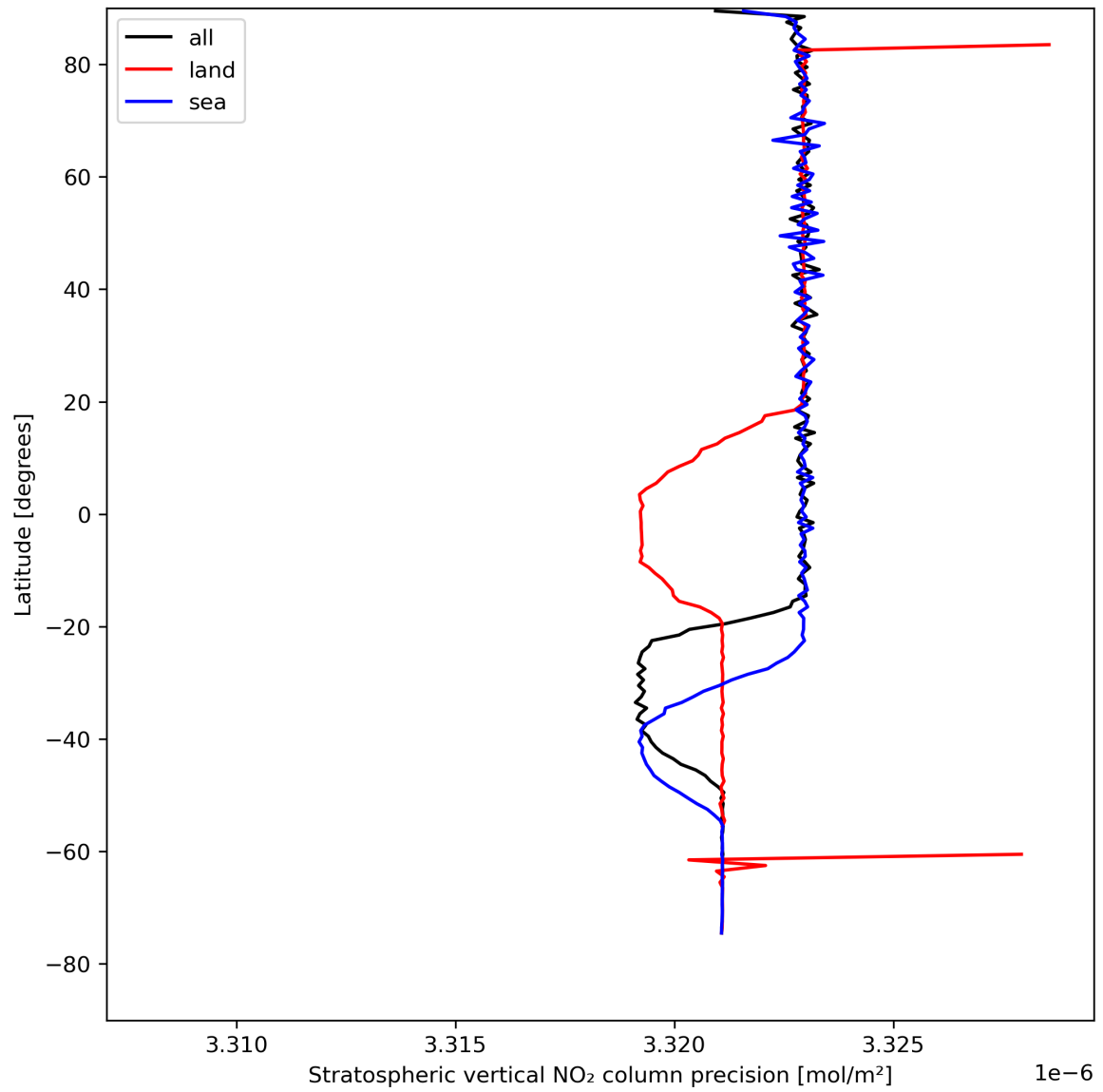
Figure 20: Zonal average of “Stratospheric vertical NO 2 column precision” for 2024-08-14 to 2024-08-16.
