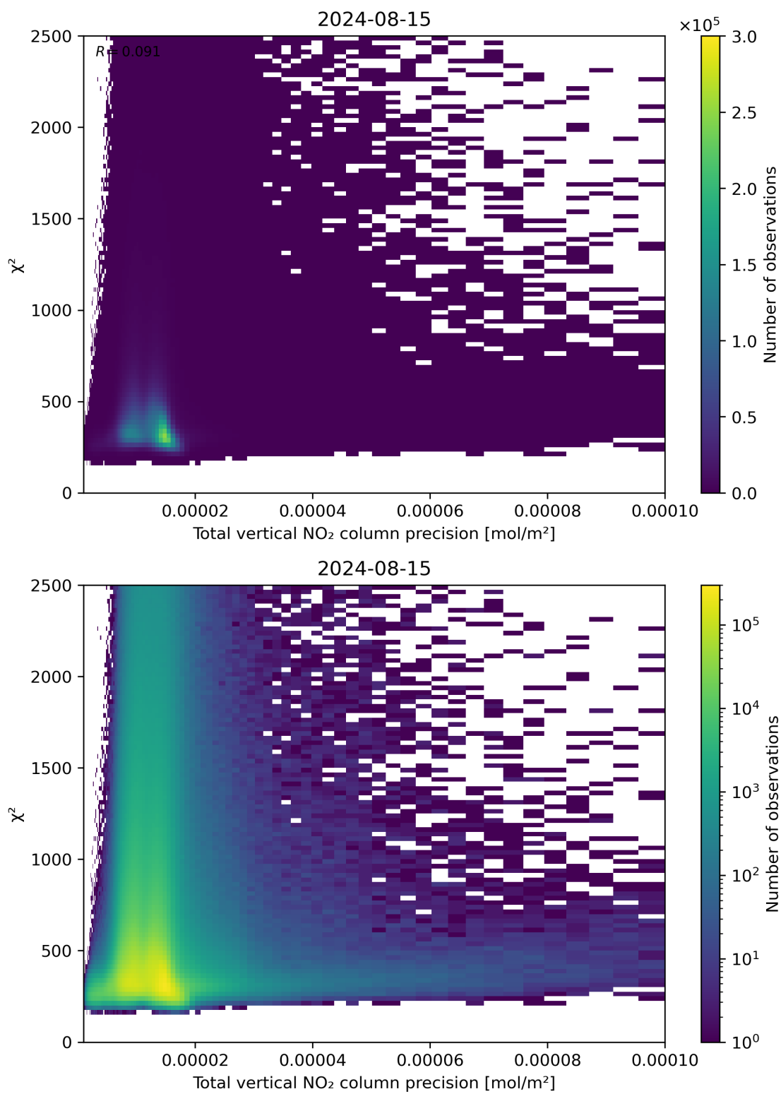
Figure 116: Scatter density plot of “Total vertical NO 2 column precision” against “ \chi^2 ” for 2024-08-14 to 2024-08-16.
