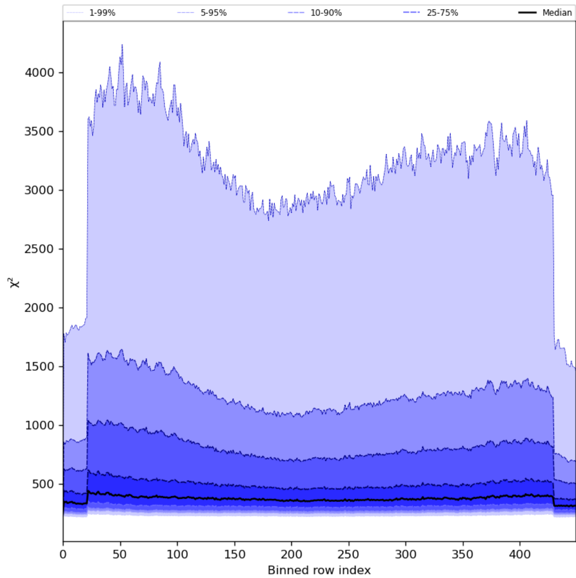
Figure 59: Along track statistics of “ \chi^2 ” for 2024-08-14 to 2024-08-16
