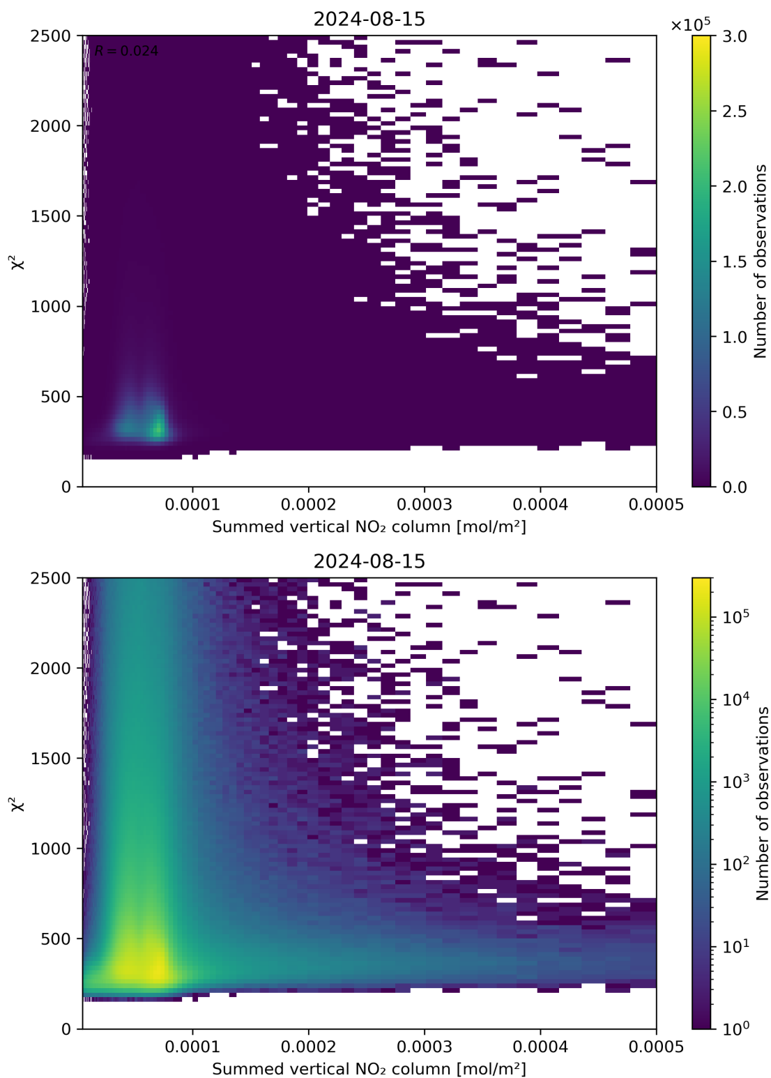
Figure 104: Scatter density plot of “Summed vertical NO 2 column” against “ \chi^2 ” for 2024-08-14 to 2024-08-16.
