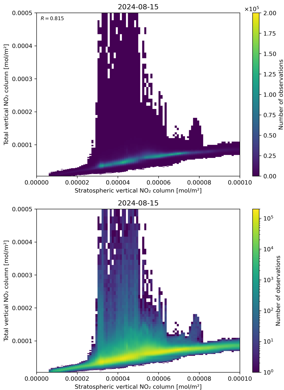
Figure 100: Scatter density plot of “Stratospheric vertical NO 2 column” against “Total vertical NO 2 column” for 2024-08-14 to 2024-08-16.
