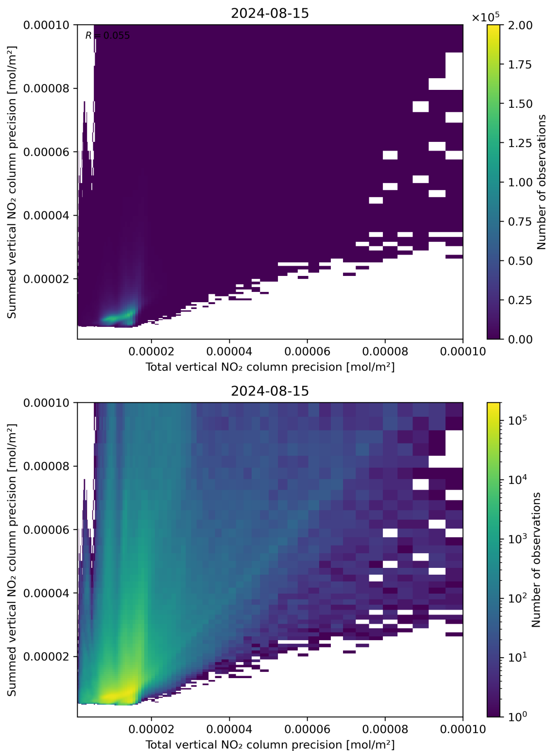
Figure 118: Scatter density plot of “Total vertical NO 2 column precision” against “Summed vertical NO 2 column precision” for 2024-08-14 to 2024-08-16.
