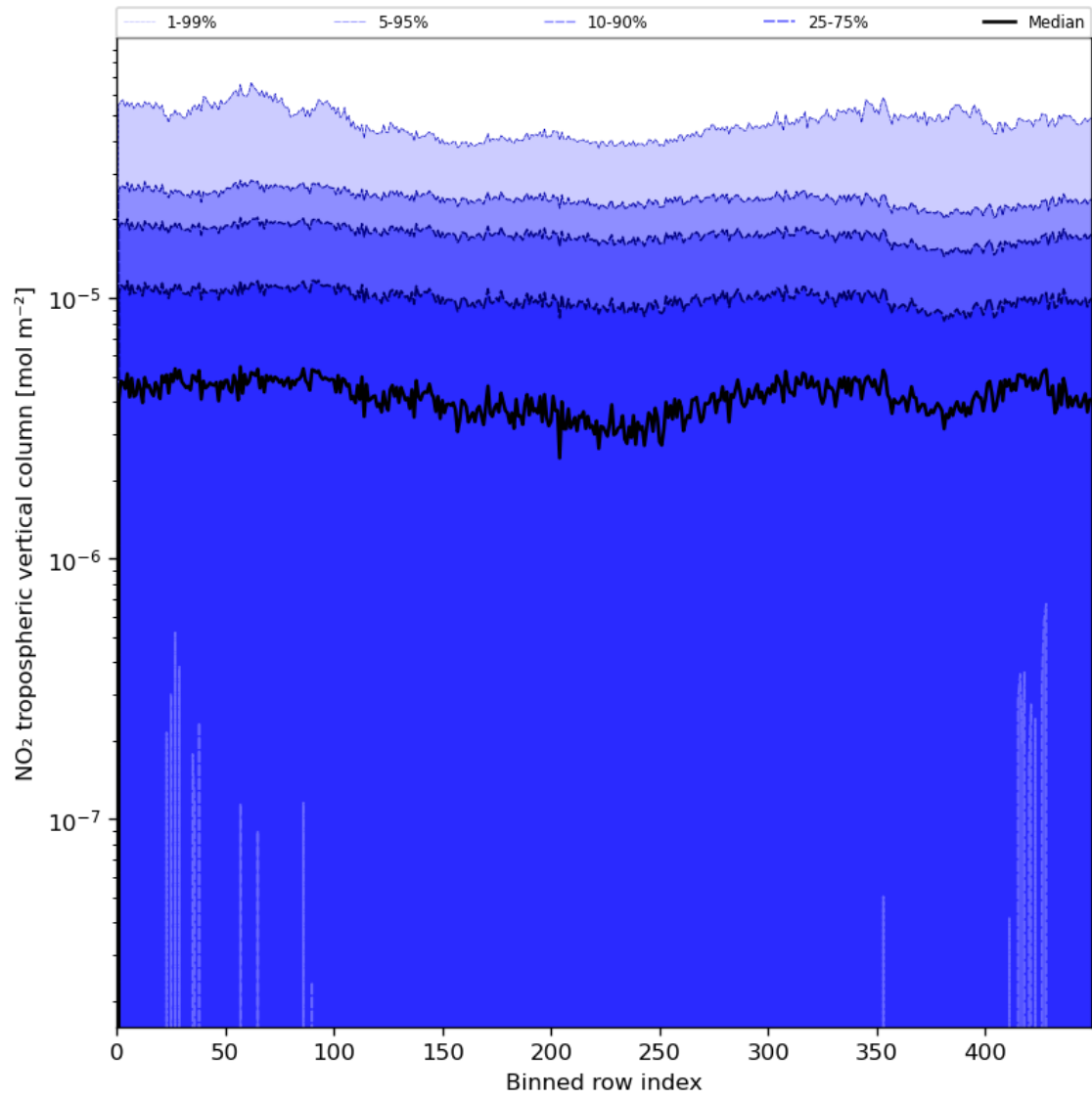
Figure 46: Along track statistics of “NO 2 tropospheric vertical column” for 2024-08-14 to 2024-08-16
