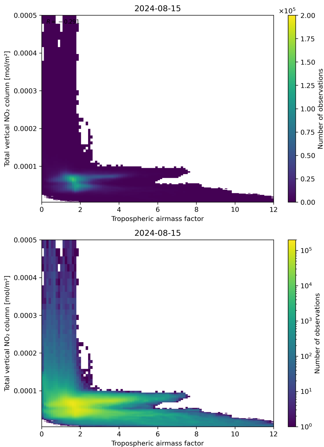
Figure 77: Scatter density plot of “Tropospheric airmass factor” against “Total vertical NO 2 column” for 2024-08-14 to 2024-08-16.
