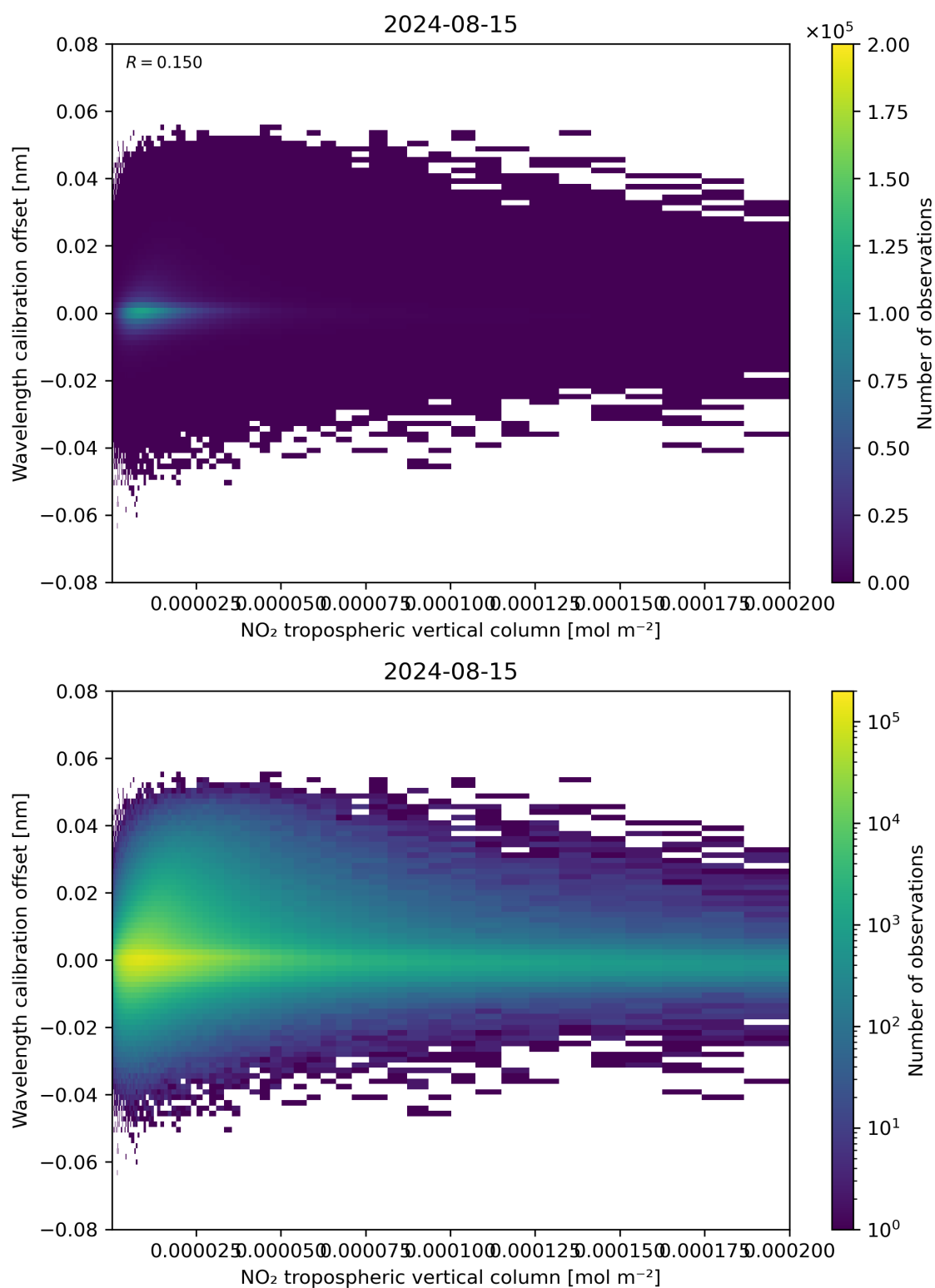
Figure 143: Scatter density plot of “NO 2 tropospheric vertical column” against “Wavelength calibration offset” for 2024-08-14 to 2024-08-16.
