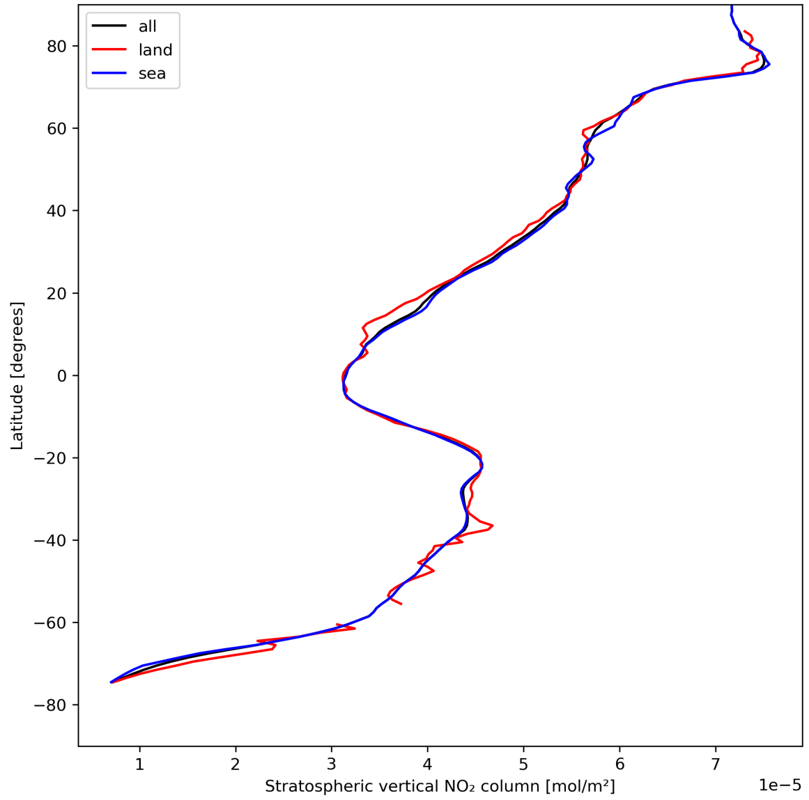
Figure 19: Zonal average of “Stratospheric vertical NO 2 column” for 2024-08-14 to 2024-08-16.
