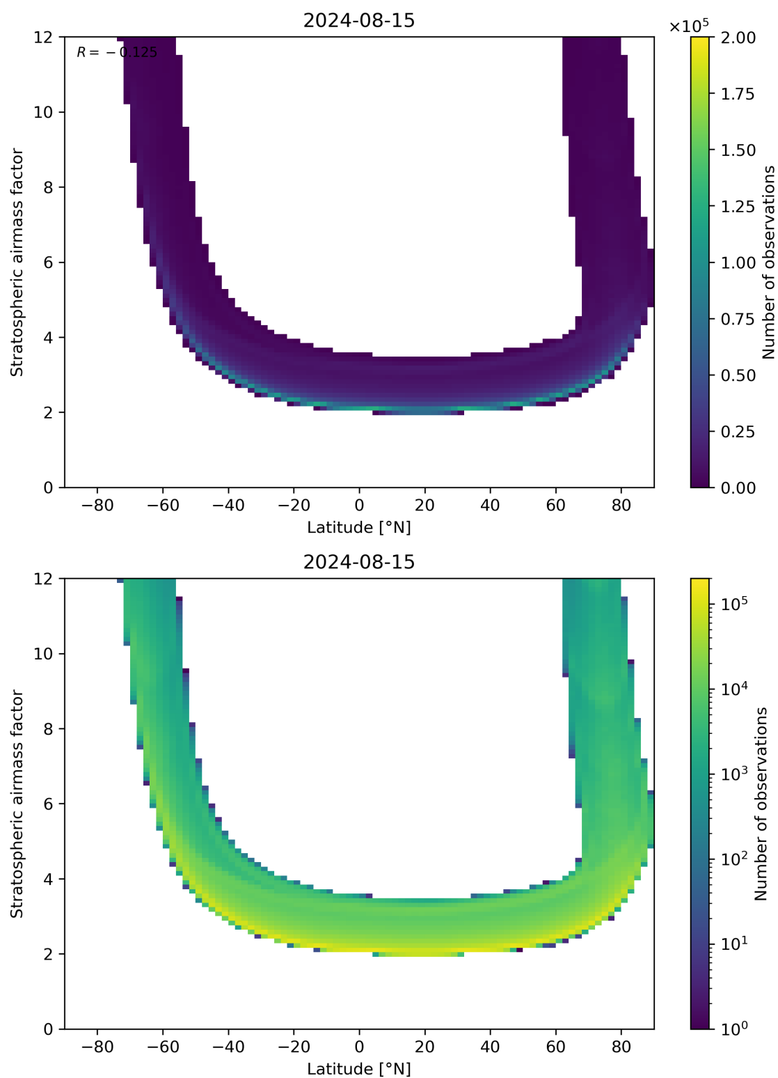
Figure 83: Scatter density plot of “Latitude” against “Stratospheric air mass factor” for 2024-08-14 to 2024-08-16.
