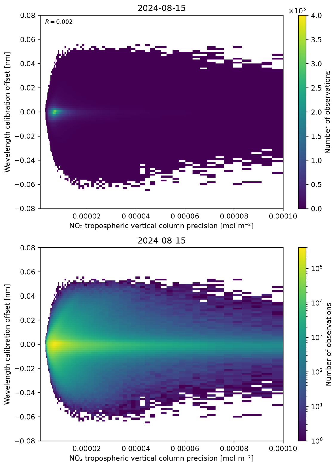
Figure 141: Scatter density plot of “NO 2 tropospheric vertical column precision” against “Wavelength calibration offset” for 2024-08-14 to 2024-08-16.
