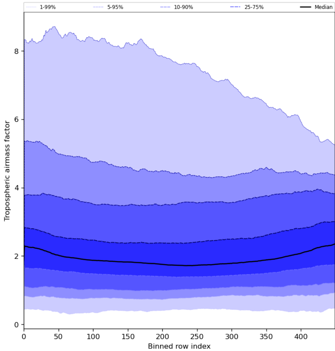
Figure 48: Along track statistics of “Tropospheric airmass factor” for 2024-08-14 to 2024-08-16
