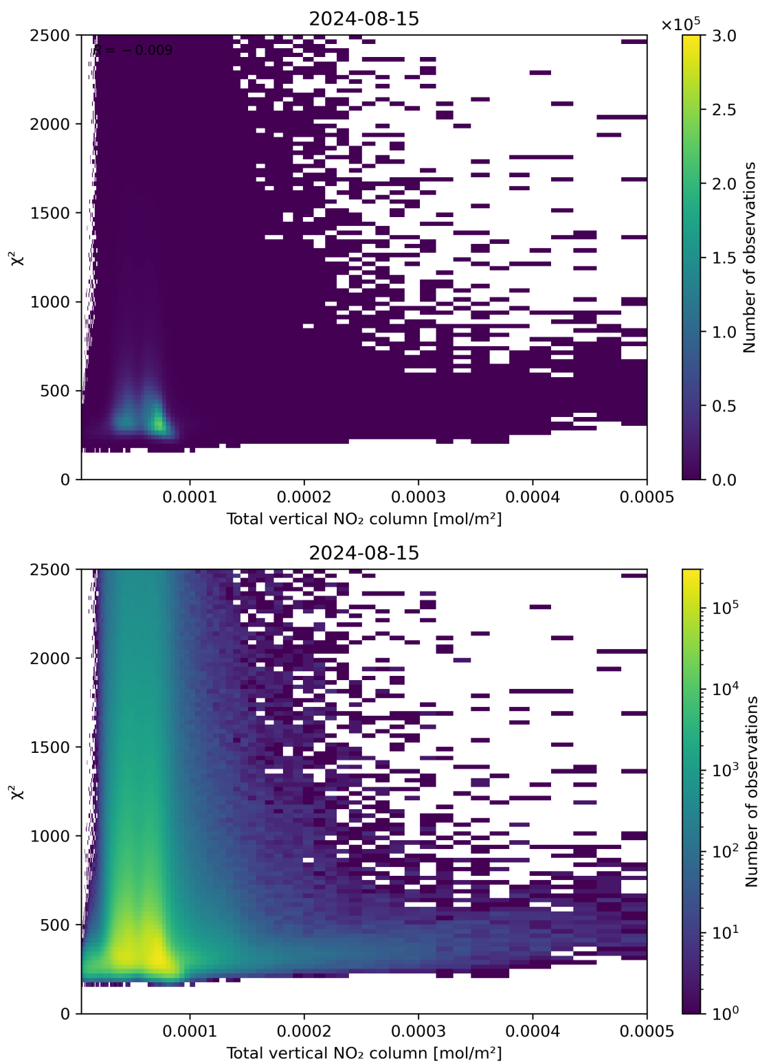
Figure 111: Scatter density plot of “Total vertical NO 2 column” against “ \chi^2 ” for 2024-08-14 to 2024-08-16.
