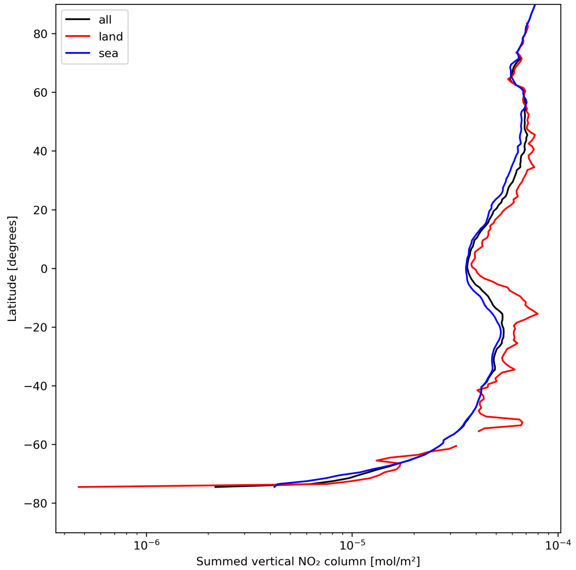
Figure 23: Zonal average of “Summed vertical NO 2 column” for 2024-08-14 to 2024-08-16.
