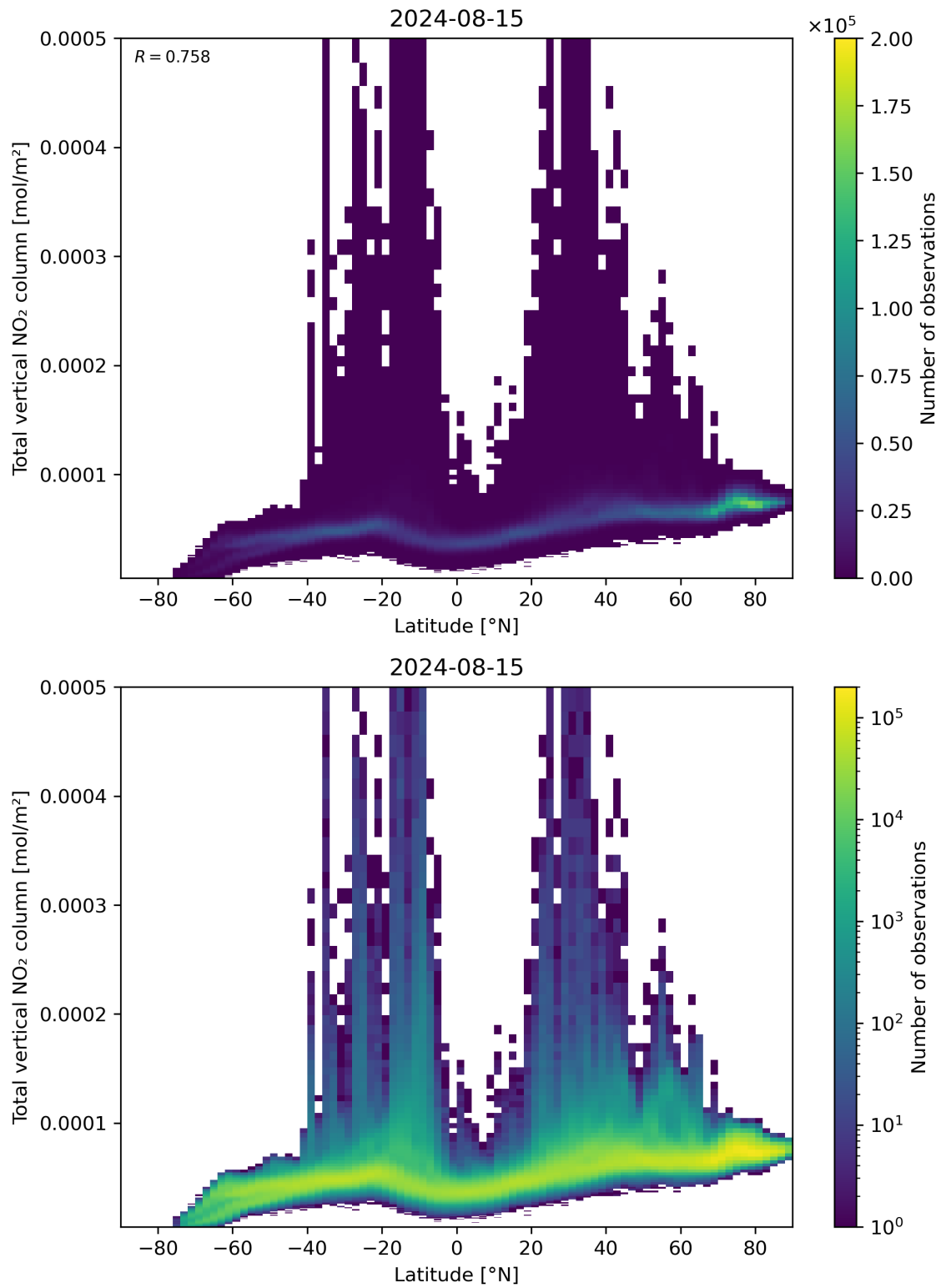
Figure 90: Scatter density plot of “Latitude” against “Total vertical NO 2 column” for 2024-08-14 to 2024-08-16.
