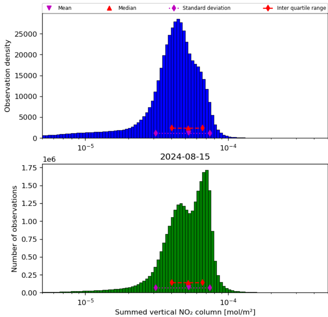
Figure 40: Histogram of “Summed vertical NO 2 column” for 2024-08-14 to 2024-08-16
