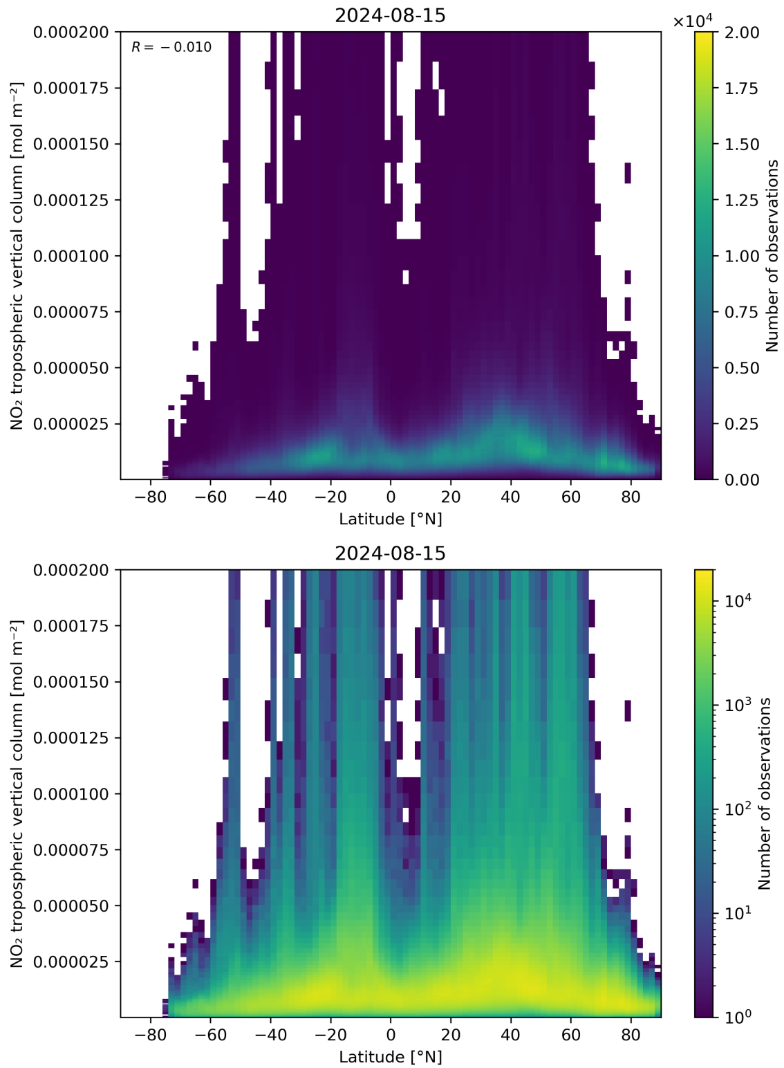
Figure 92: Scatter density plot of “Latitude” against “NO 2 tropospheric vertical column” for 2024-08-14 to 2024-08-16.
