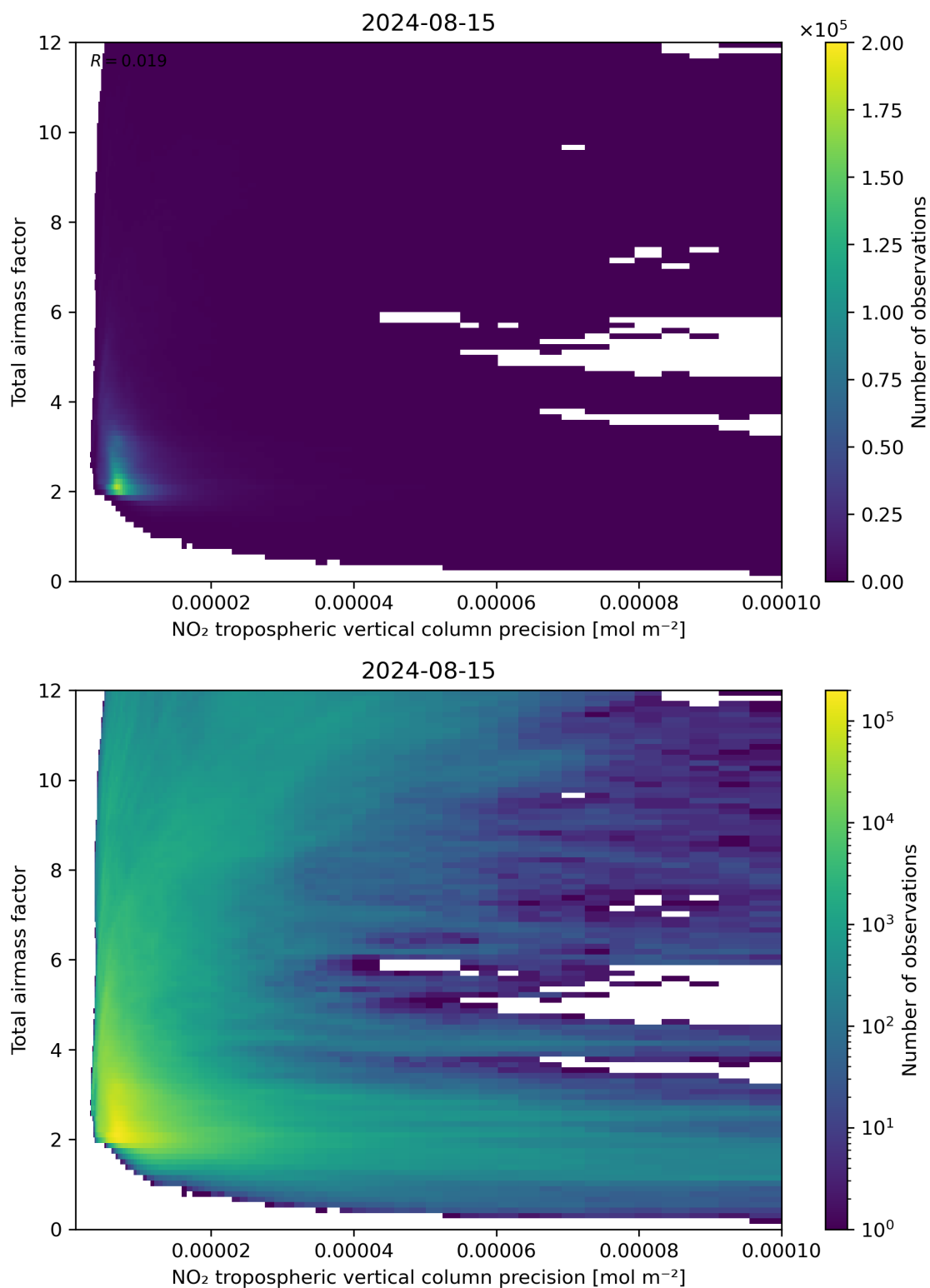
Figure 132: Scatter density plot of “NO 2 tropospheric vertical column precision” against “Total air mass factor” for 2024-08-14 to 2024-08-16.
