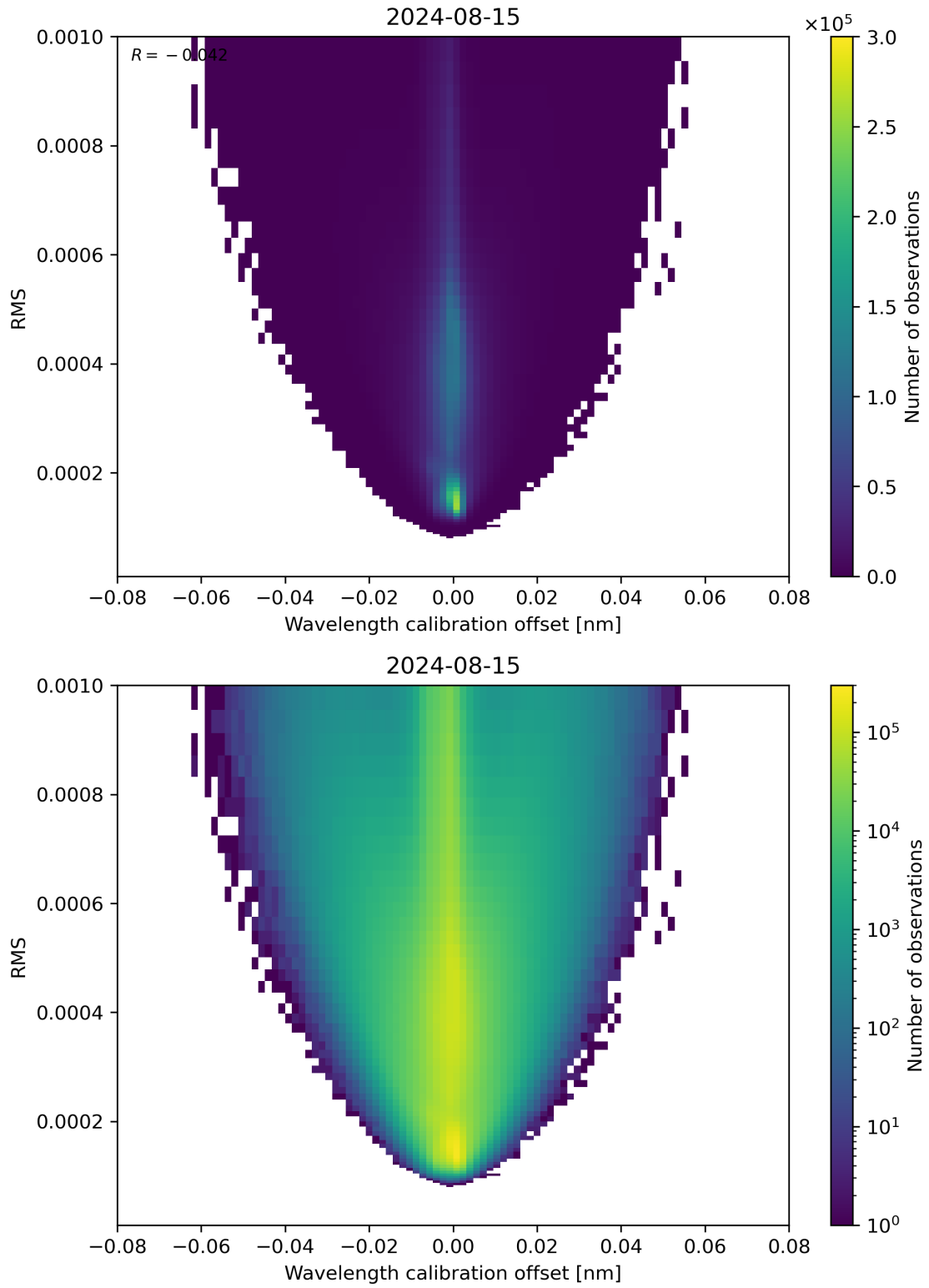
Figure 181: Scatter density plot of “Wavelength calibration offset” against “RMS” for 2024-08-14 to 2024-08-16.
