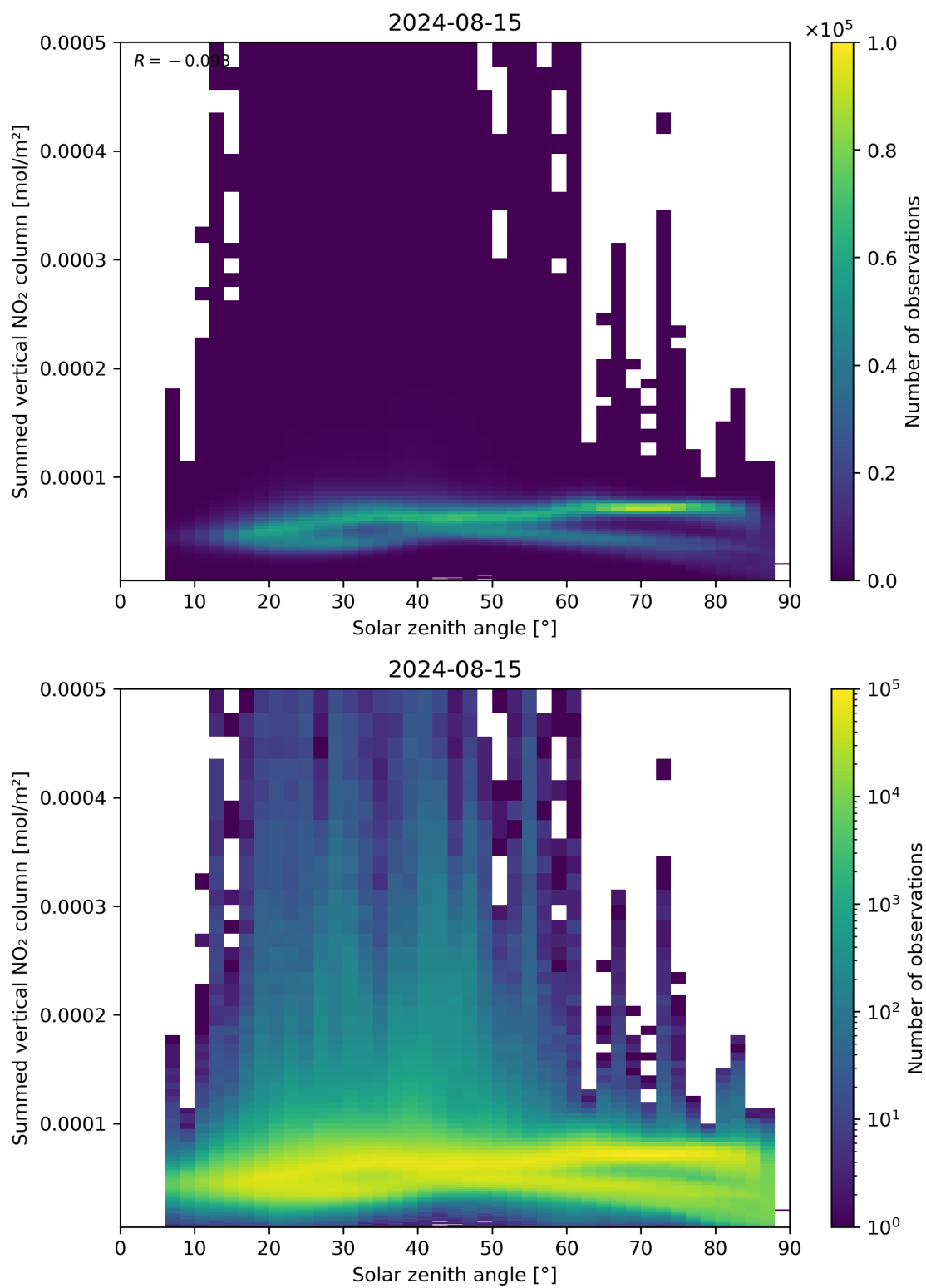
Figure 151: Scatter density plot of “Solar zenith angle” against “Summed vertical NO 2 column” for 2024-08-14 to 2024-08-16.
