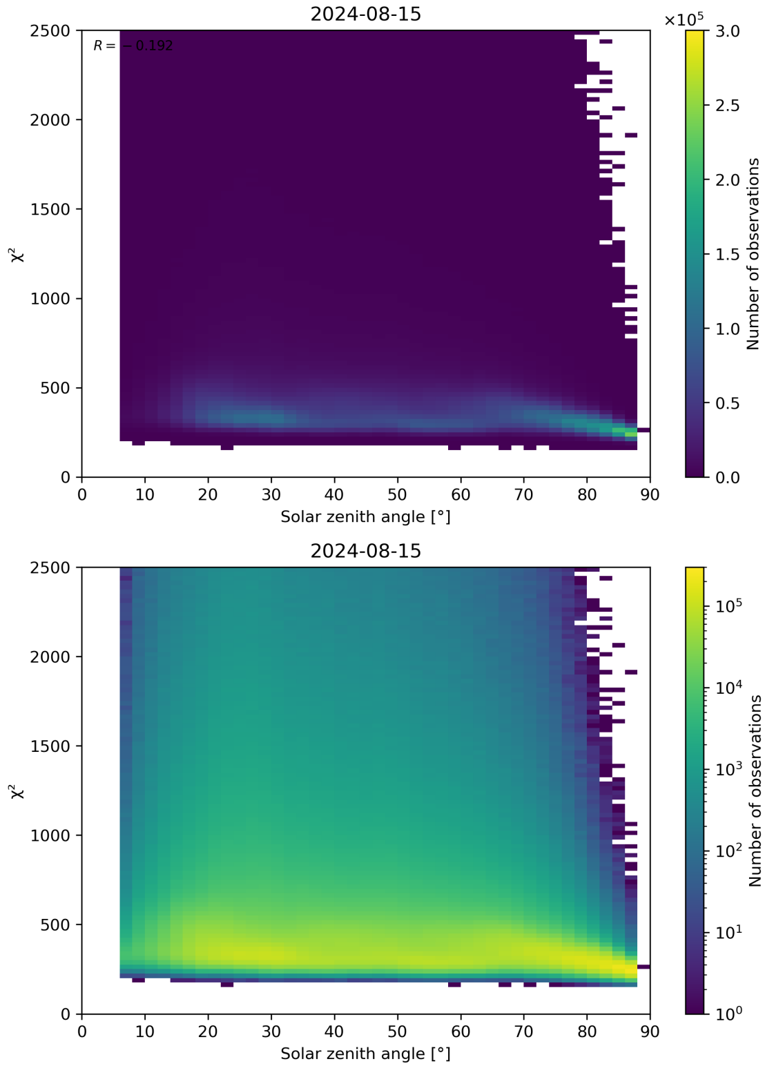
Figure 148: Scatter density plot of “Solar zenith angle” against “ \chi^2 ” for 2024-08-14 to 2024-08-16.
