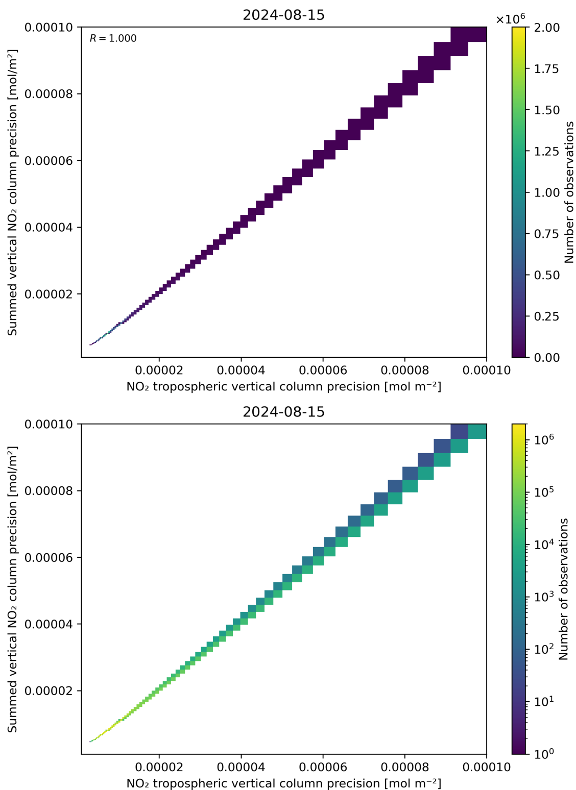
Figure 137: Scatter density plot of “NO 2 tropospheric vertical column precision” against “Summed vertical NO 2 column precision” for 2024-08-14 to 2024-08-16.
