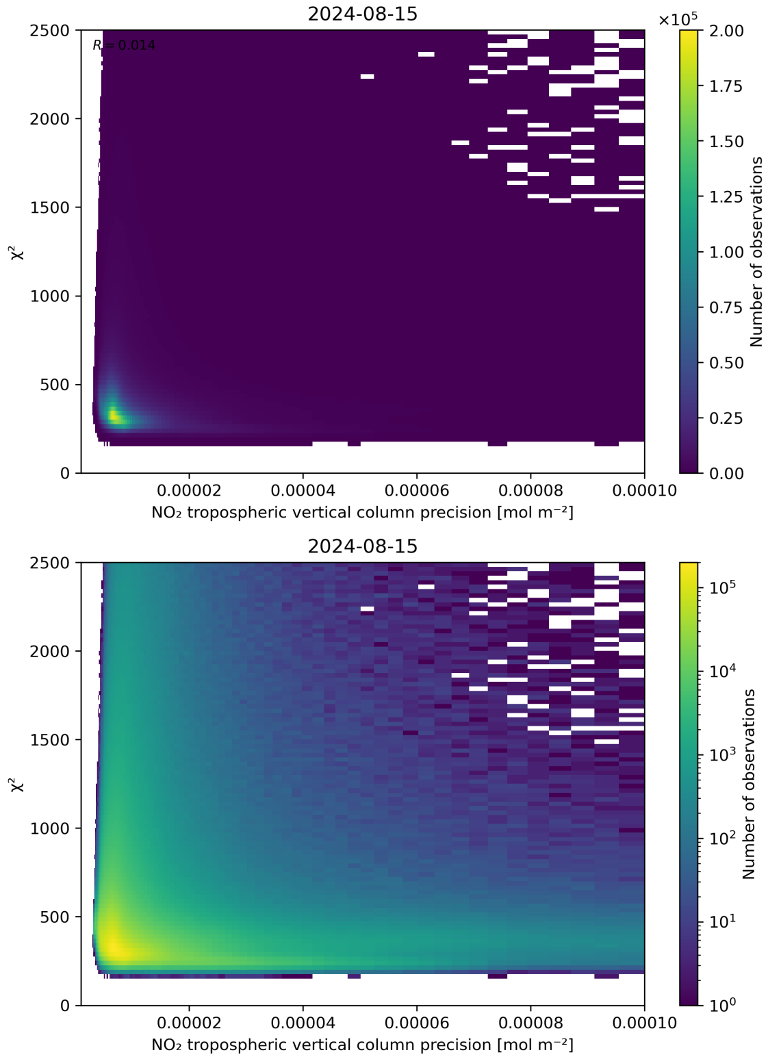
Figure 134: Scatter density plot of “NO 2 tropospheric vertical column precision” against “ \chi^2 ” for 2024-08-14 to 2024-08-16.
