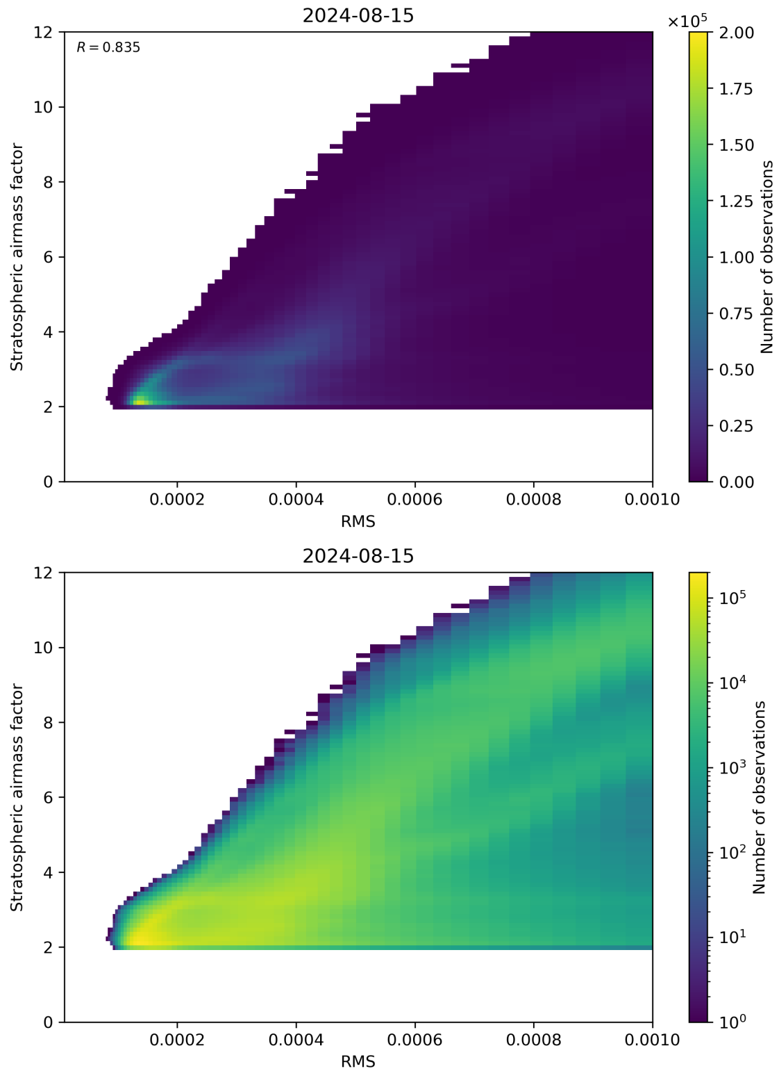
Figure 144: Scatter density plot of “RMS” against “Stratospheric airmass factor” for 2024-08-14 to 2024-08-16.
