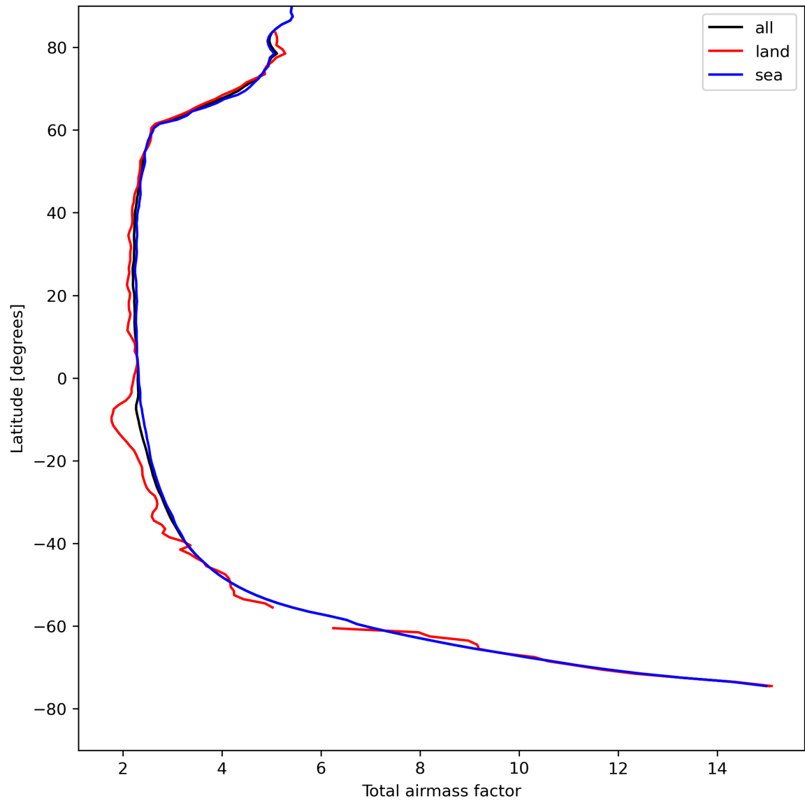
Figure 15: Zonal average of “Total airmass factor” for 2024-08-14 to 2024-08-16.
