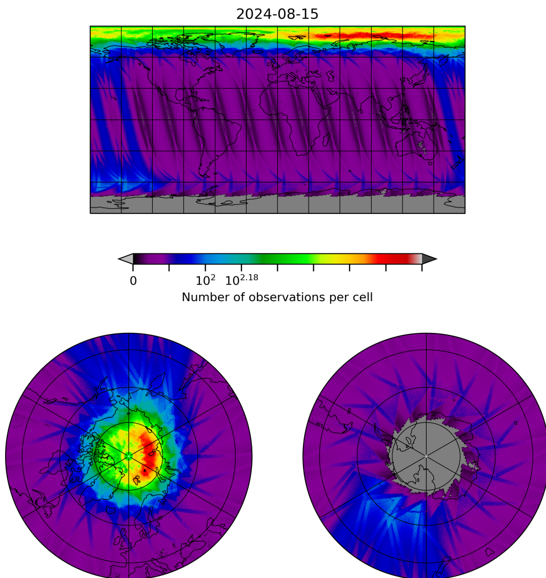
Figure 10: Map of the number of observations for 2024-08-14 to 2024-08-16
