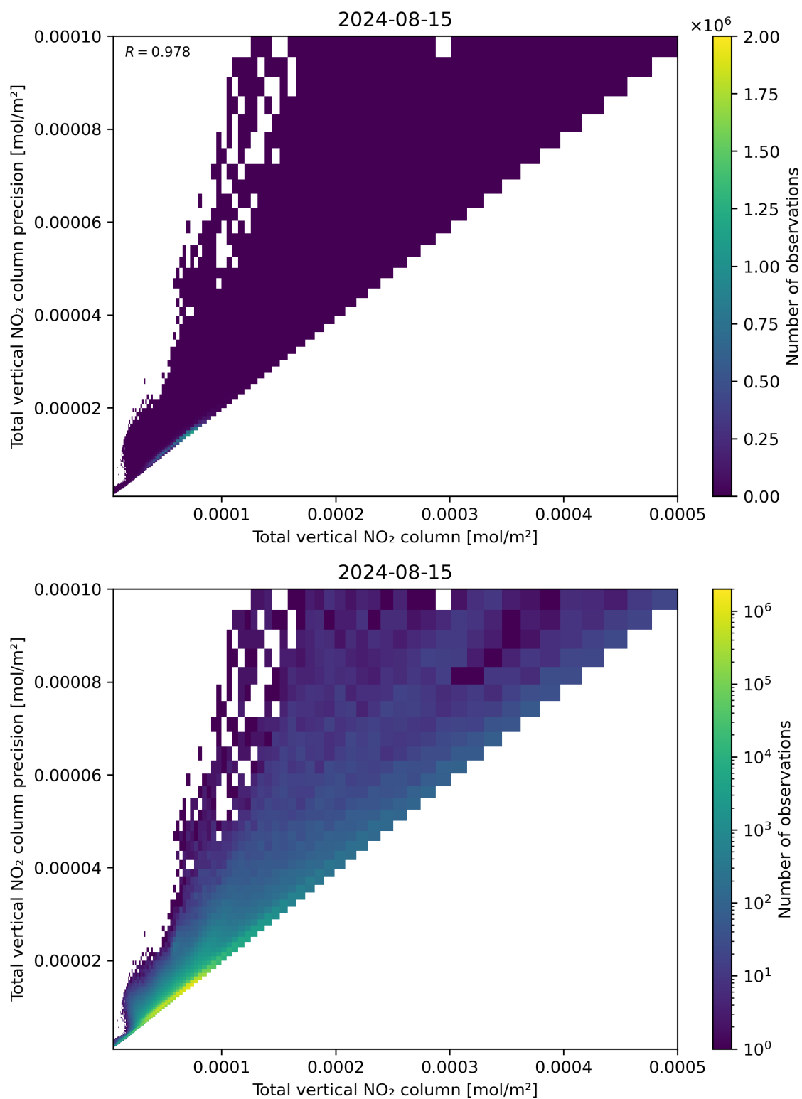
Figure 114: Scatter density plot of “Total vertical NO 2 column” against “Total vertical NO 2 column precision” for 2024-08-14 to 2024-08-16.
