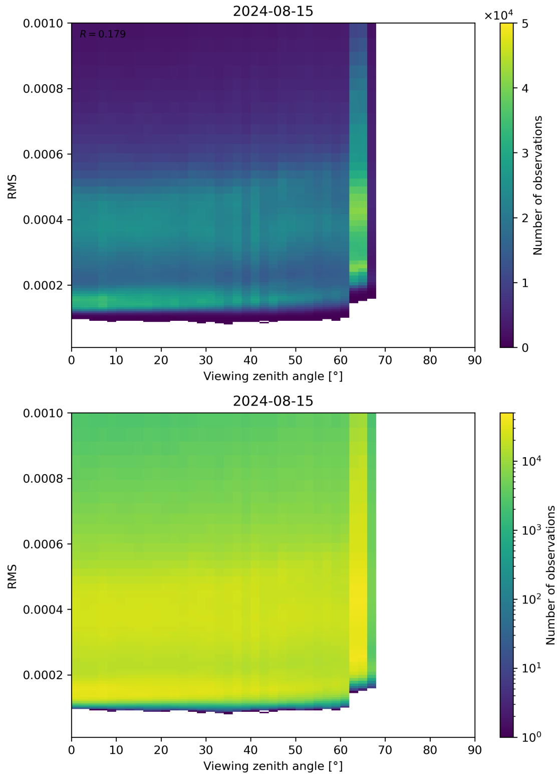
Figure 171: Scatter density plot of “Viewing zenith angle” against “RMS” for 2024-08-14 to 2024-08-16.
