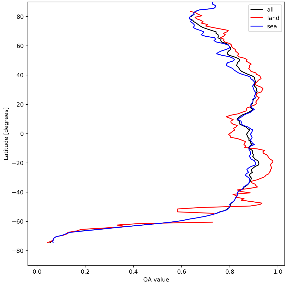
Figure 11: Zonal average of “QA value” for 2024-08-14 to 2024-08-16.
