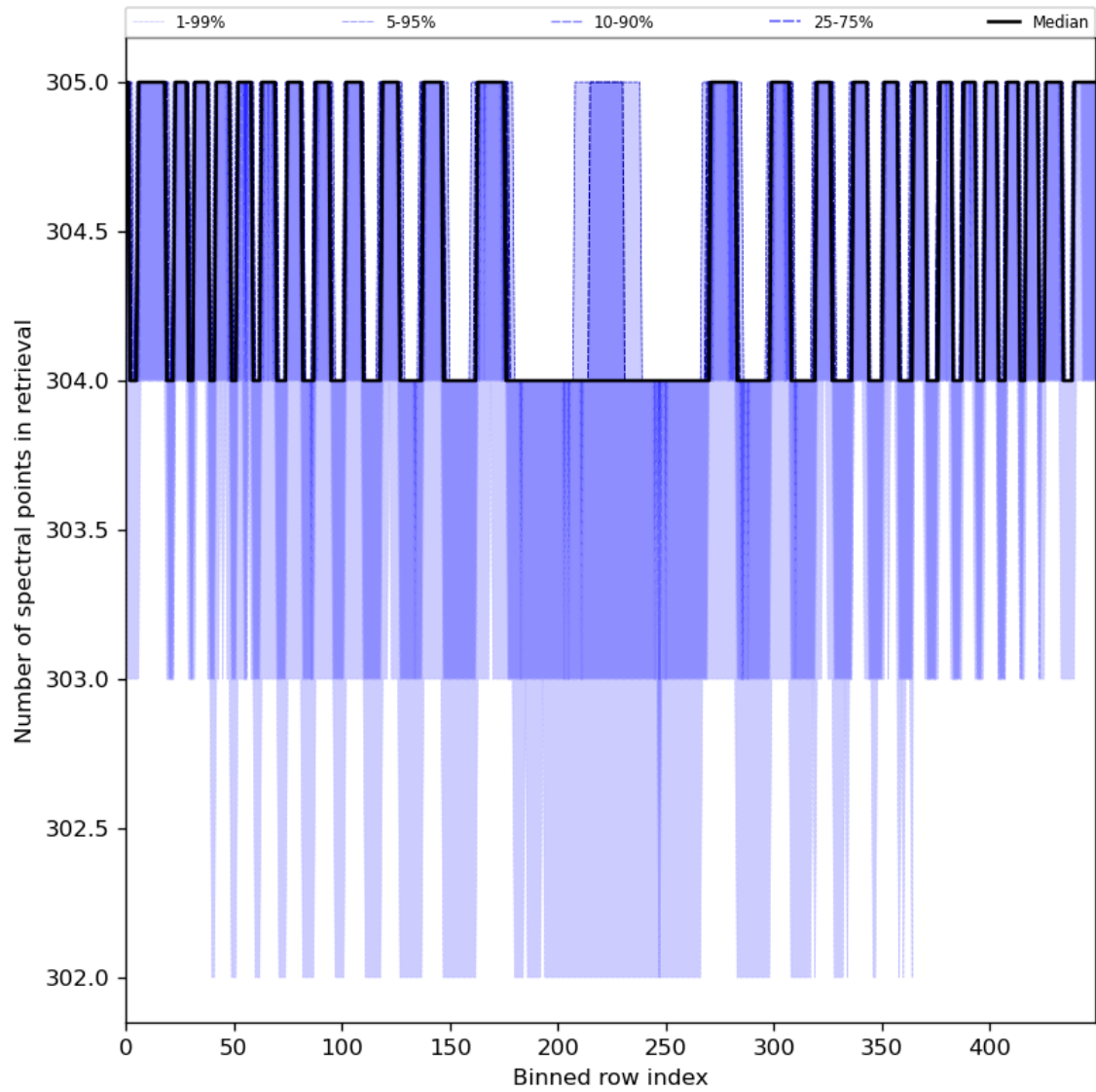
Figure 50: Along track statistics of “Number of spectral points in retrieval” for 2024-08-14 to 2024-08-16
