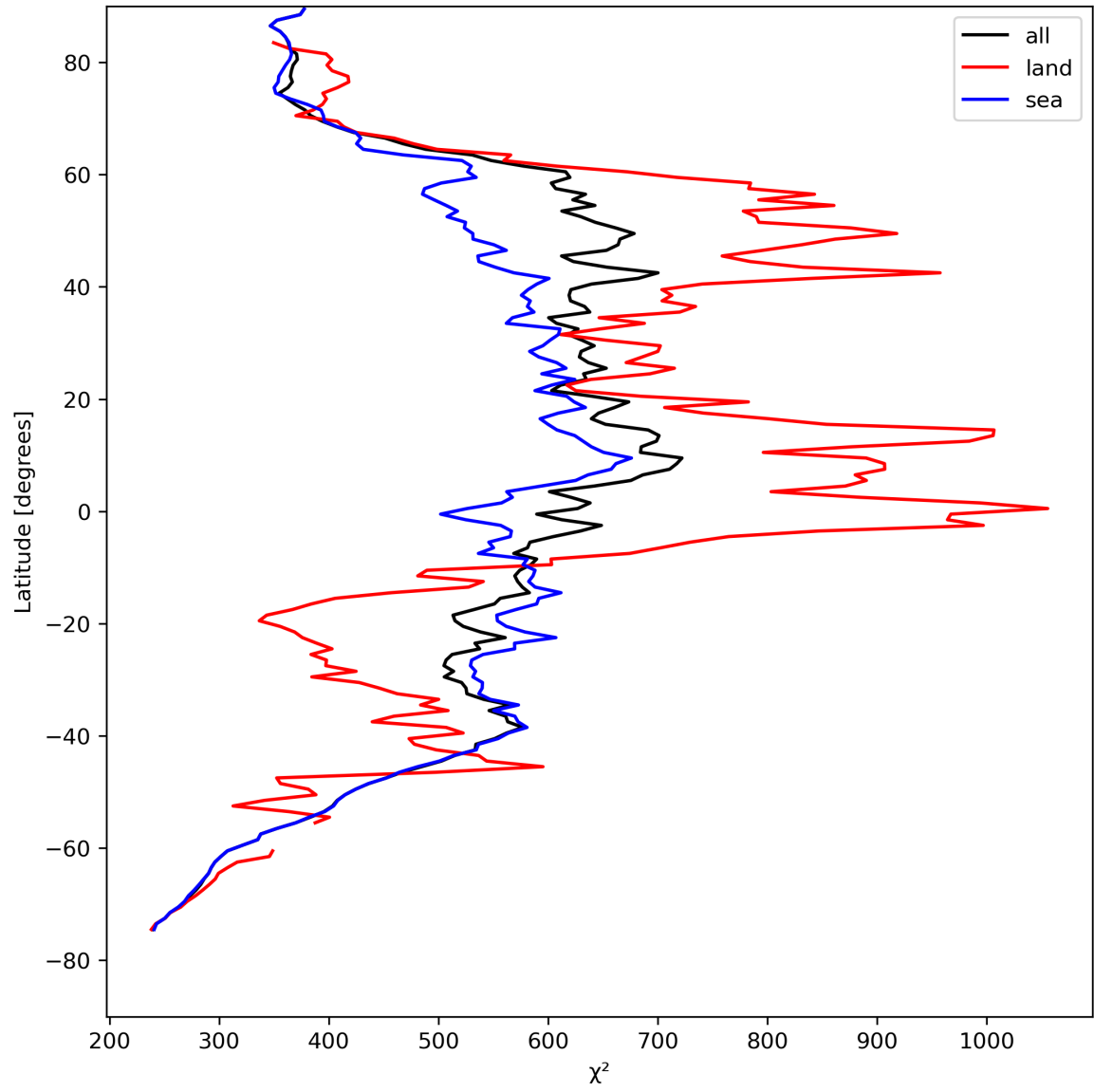
Figure 25: Zonal average of “ \chi^2 ” for 2024-08-14 to 2024-08-16.
