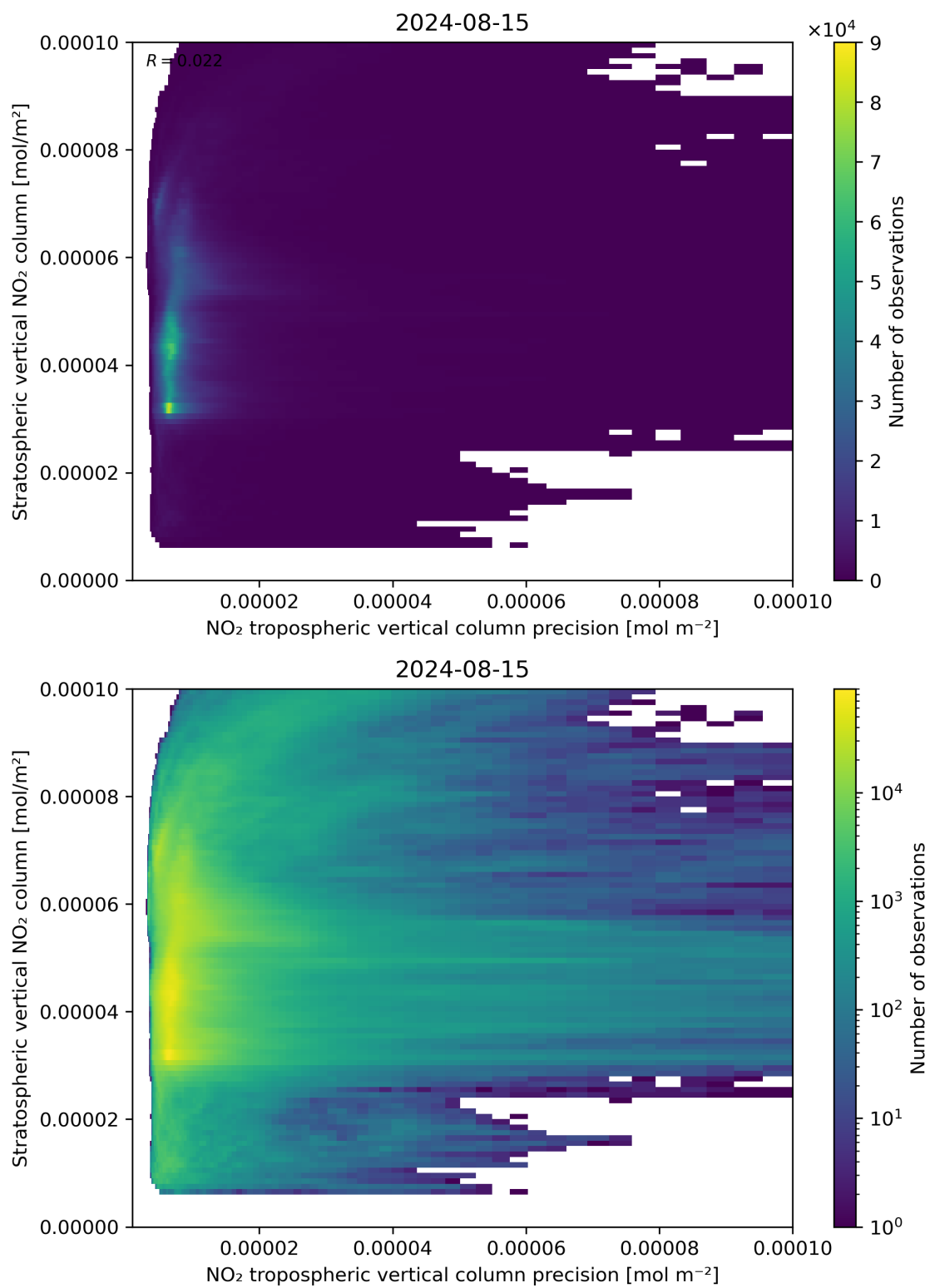
Figure 135: Scatter density plot of “NO 2 tropospheric vertical column precision” against “Stratospheric vertical NO 2 column” for 2024-08-14 to 2024-08-16.
