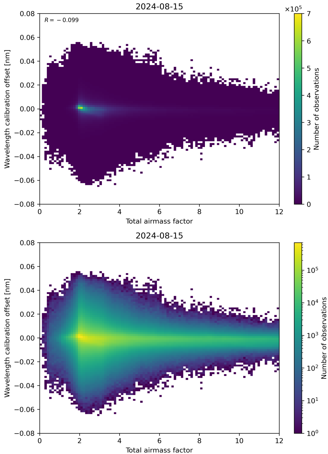
Figure 70: Scatter density plot of “Total airmass factor” against “Wavelength calibration offset” for 2024-08-14 to 2024-08-16.
