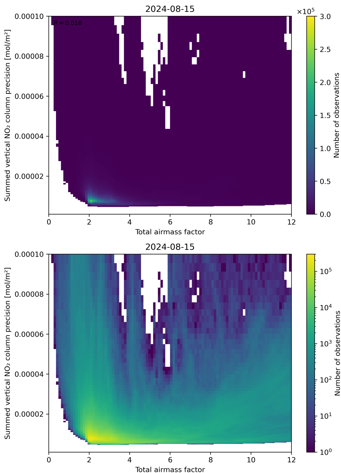
Figure 66: Scatter density plot of “Total airmass factor” against “Summed vertical NO 2 column precision” for 2024-08-14 to 2024-08-16.
