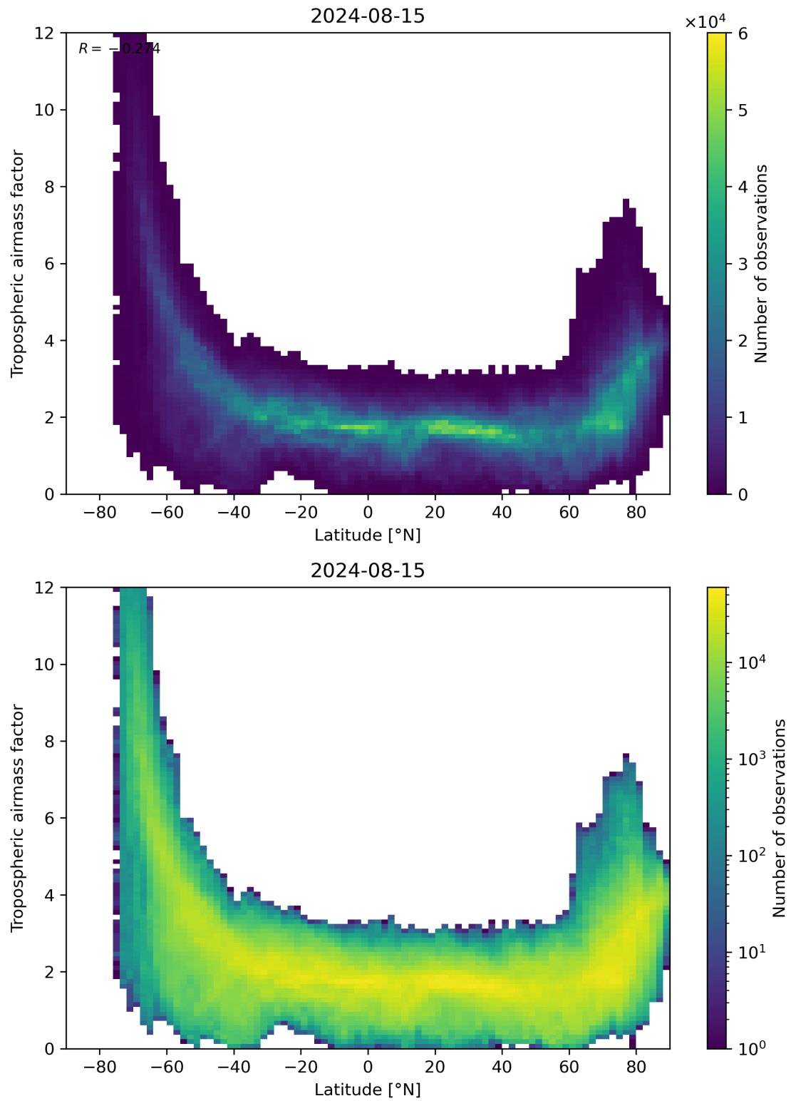
Figure 85: Scatter density plot of “Latitude” against “Tropospheric airmass factor” for 2024-08-14 to 2024-08-16.
