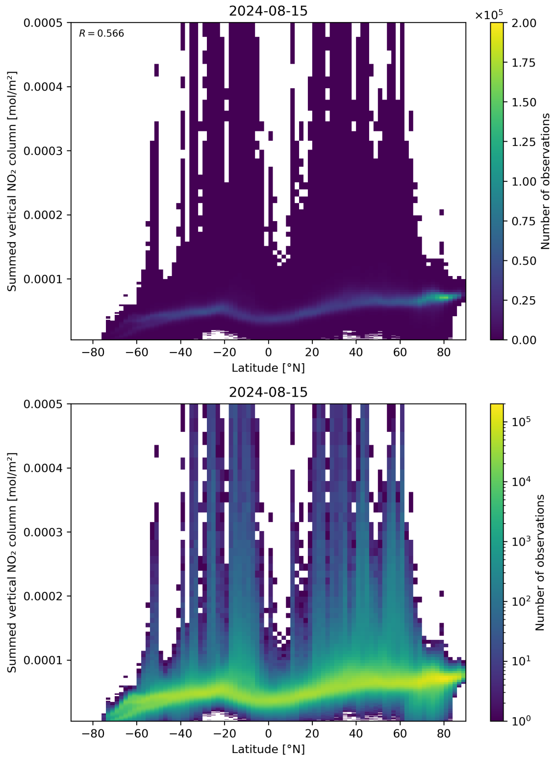
Figure 88: Scatter density plot of “Latitude” against “Summed vertical NO 2 column” for 2024-08-14 to 2024-08-16.
