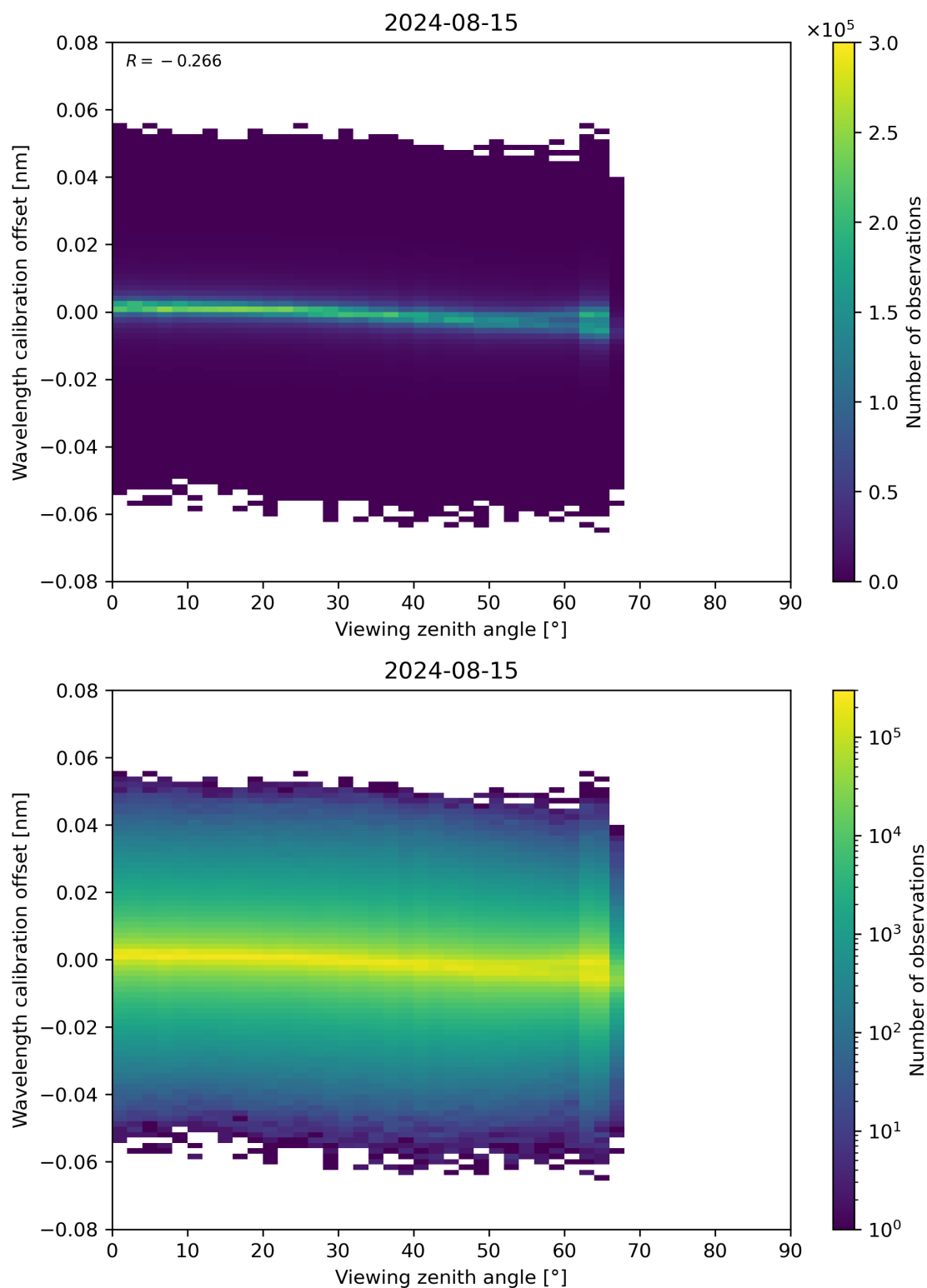
Figure 173: Scatter density plot of “Viewing zenith angle” against “Wavelength calibration offset” for 2024-08-14 to 2024-08-16.
