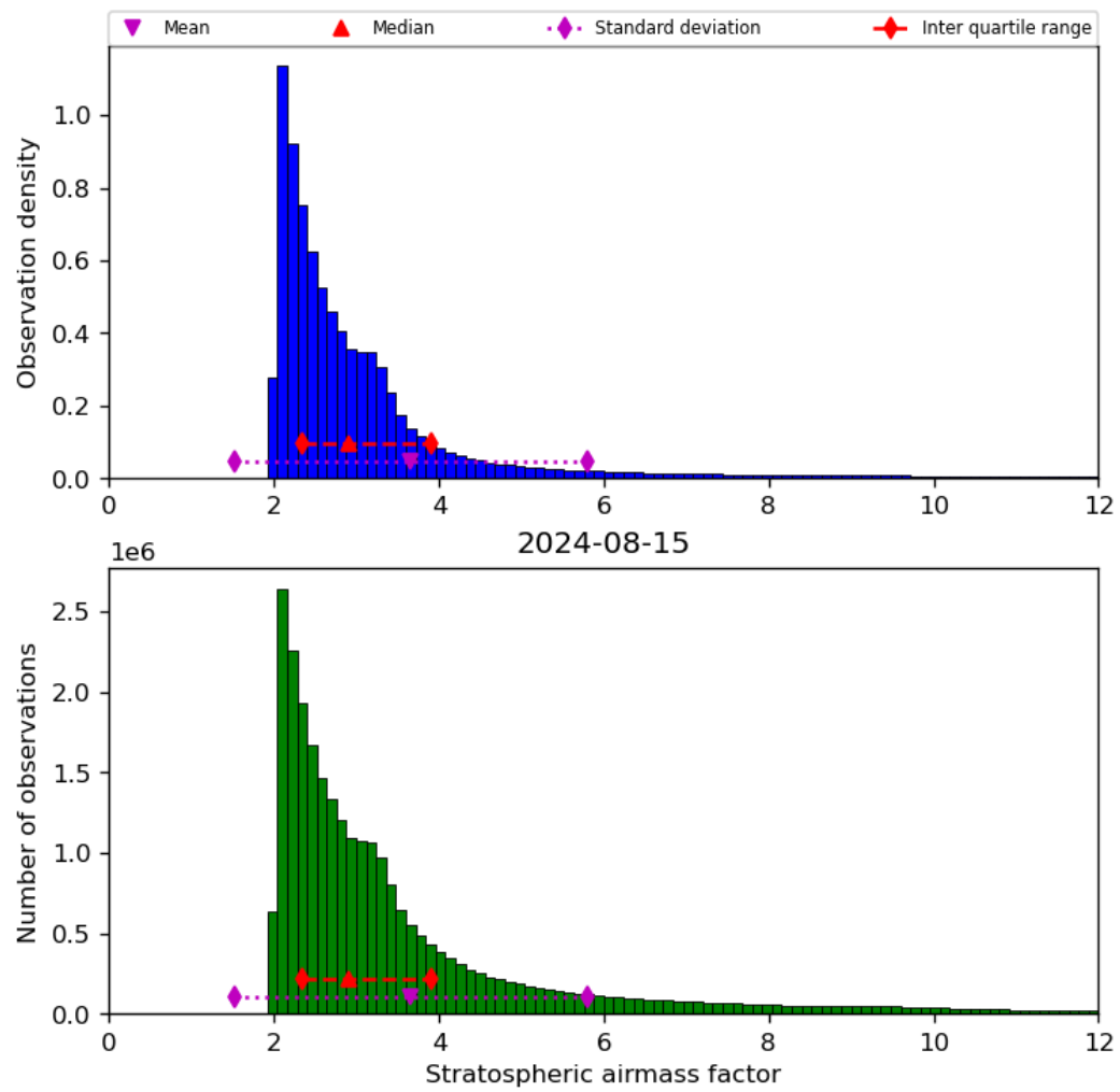
Figure 44: Histogram of “Stratospheric airmass factor” for 2024-08-14 to 2024-08-16
