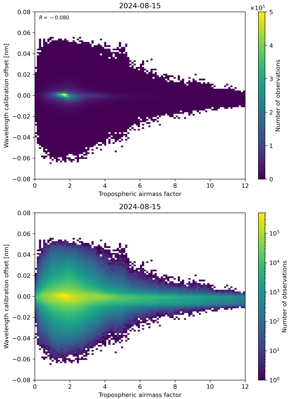
Figure 80: Scatter density plot of “Tropospheric airmass factor” against “Wavelength calibration offset” for 2024-08-14 to 2024-08-16.
