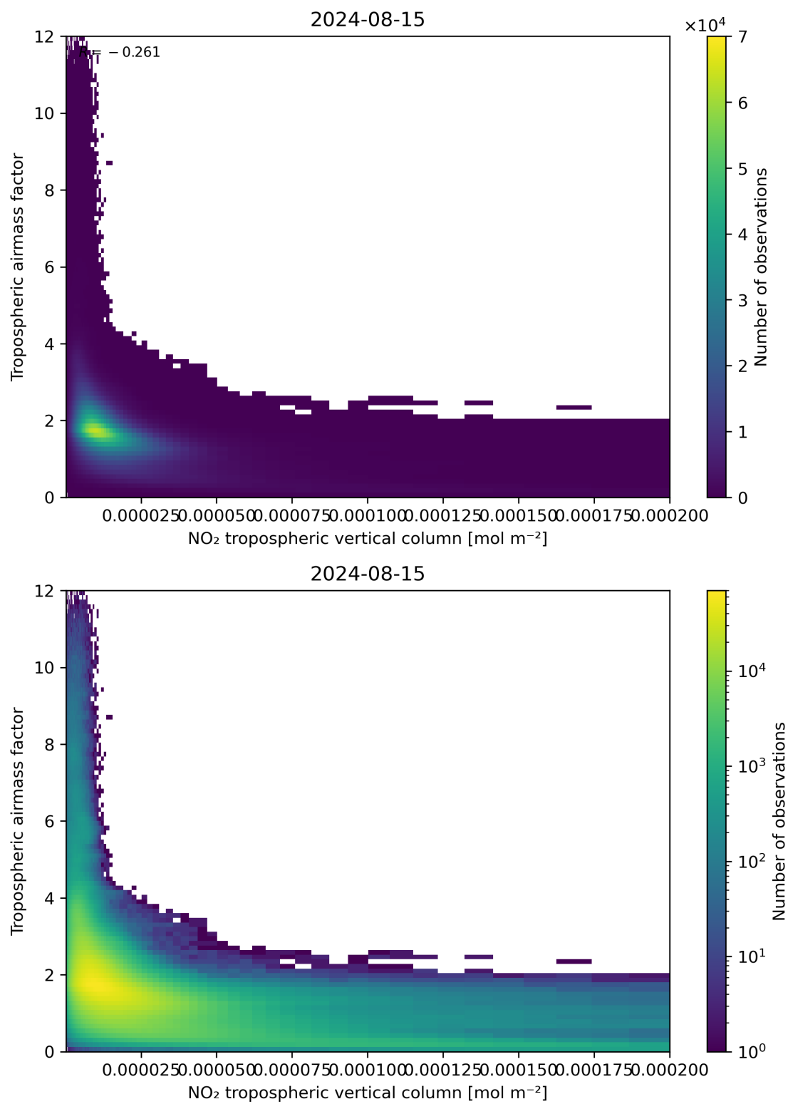
Figure 123: Scatter density plot of “NO 2 tropospheric vertical column” against “Tropospheric air mass factor” for 2024-08-14 to 2024-08-16.
