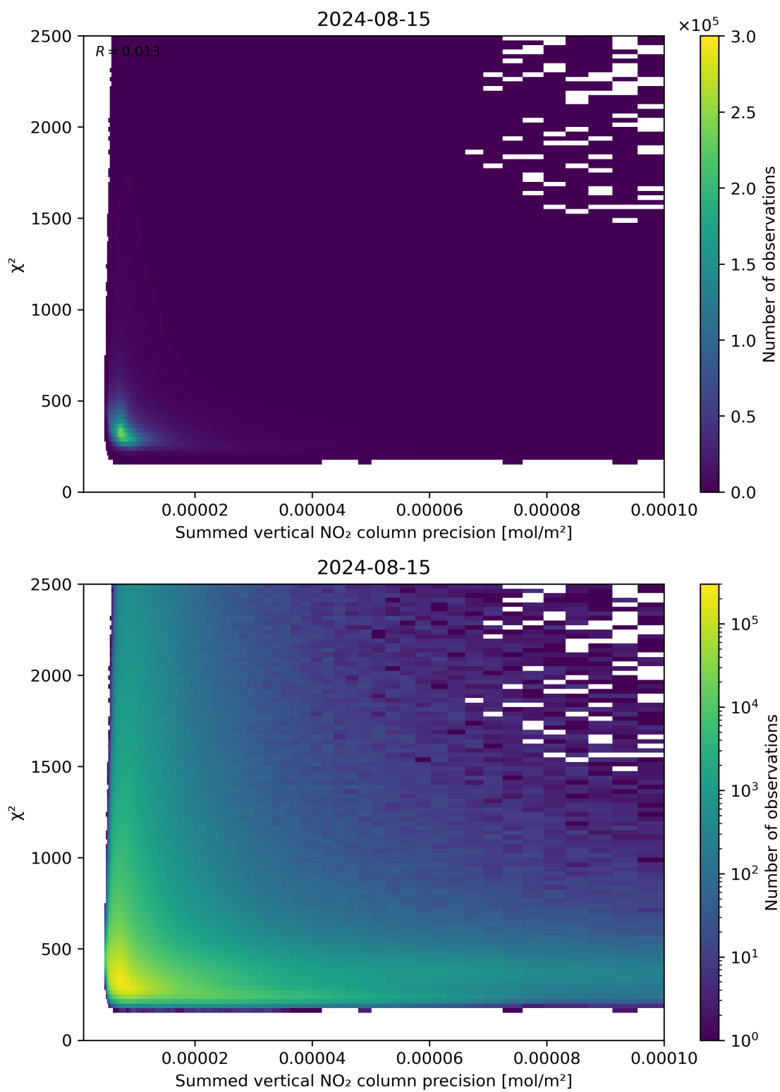
Figure 107: Scatter density plot of “Summed vertical NO 2 column precision” against “ \chi^2 ” for 2024-08-14 to 2024-08-16.
