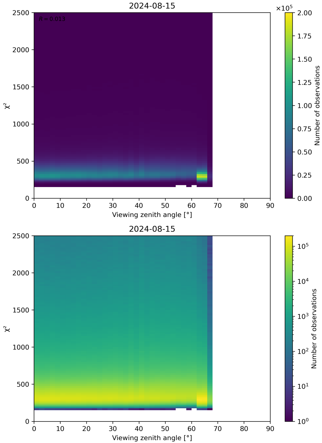
Figure 162: Scatter density plot of “Viewing zenith angle” against “ \chi^2 ” for 2024-08-14 to 2024-08-16.
