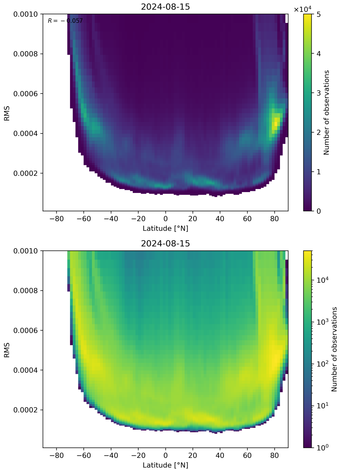
Figure 94: Scatter density plot of “Latitude” against “RMS” for 2024-08-14 to 2024-08-16.
