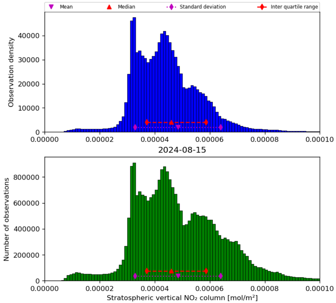
Figure 36: Histogram of “Stratospheric vertical NO 2 column” for 2024-08-14 to 2024-08-16
