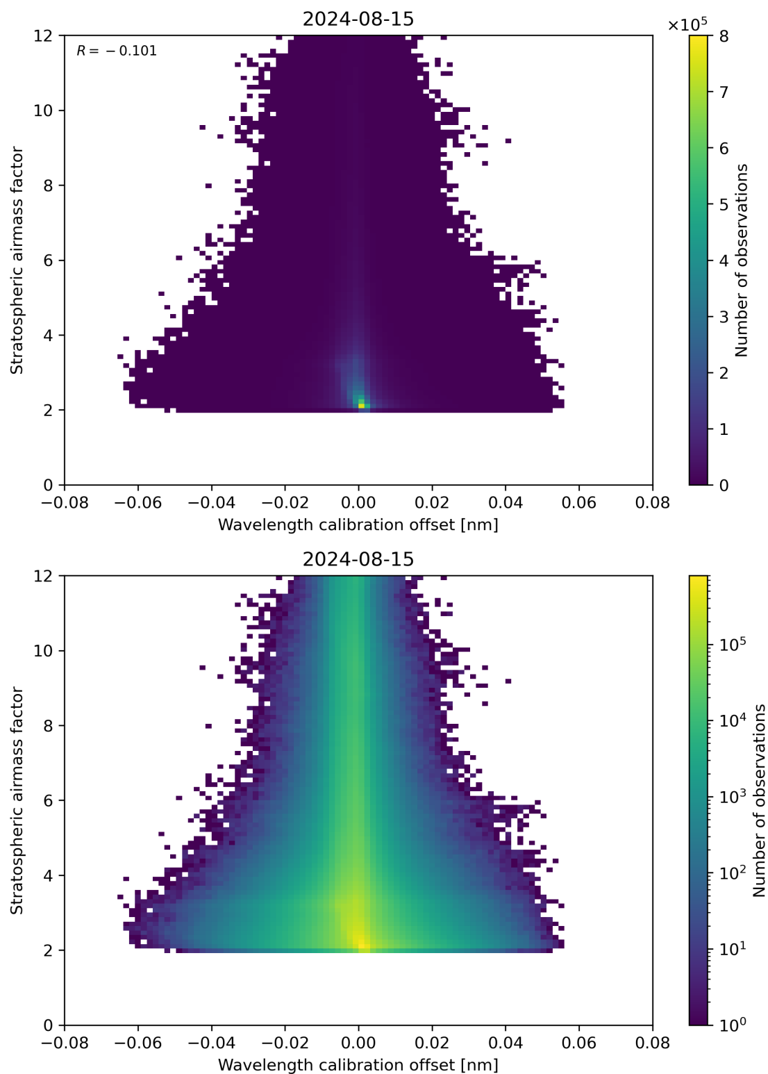
Figure 174: Scatter density plot of “Wavelength calibration offset” against “Stratospheric air mass factor” for 2024-08-14 to 2024-08-16.
