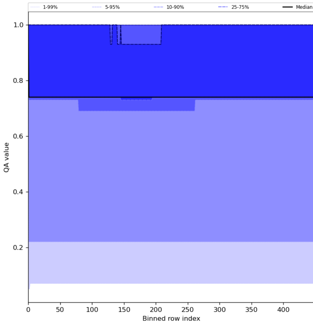
Figure 45: Along track statistics of “QA value” for 2024-08-14 to 2024-08-16
