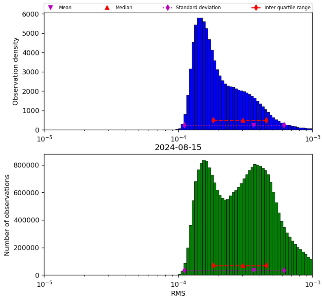
Figure 43: Histogram of “RMS” for 2024-08-14 to 2024-08-16
