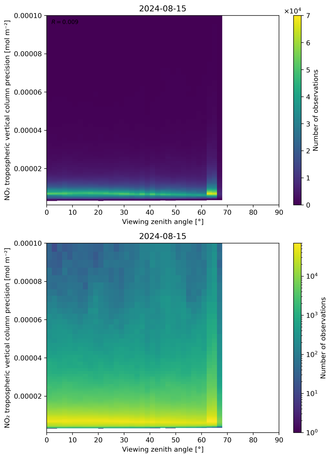
Figure 170: Scatter density plot of “Viewing zenith angle” against “NO 2 tropospheric vertical column precision” for 2024-08-14 to 2024-08-16.
