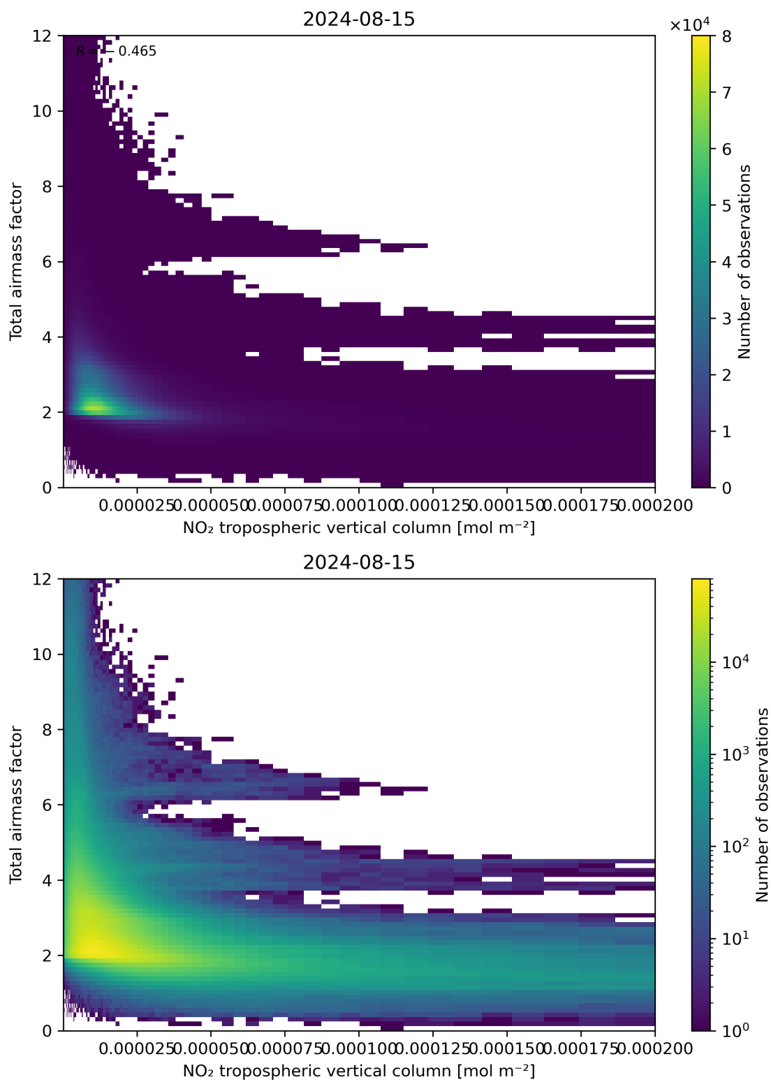
Figure 122: Scatter density plot of “NO 2 tropospheric vertical column” against “Total air mass factor” for 2024-08-14 to 2024-08-16.
