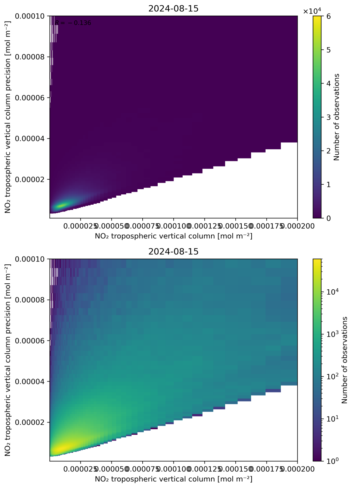
Figure 130: Scatter density plot of “NO 2 tropospheric vertical column” against “NO 2 tropospheric vertical column precision” for 2024-08-14 to 2024-08-16.
