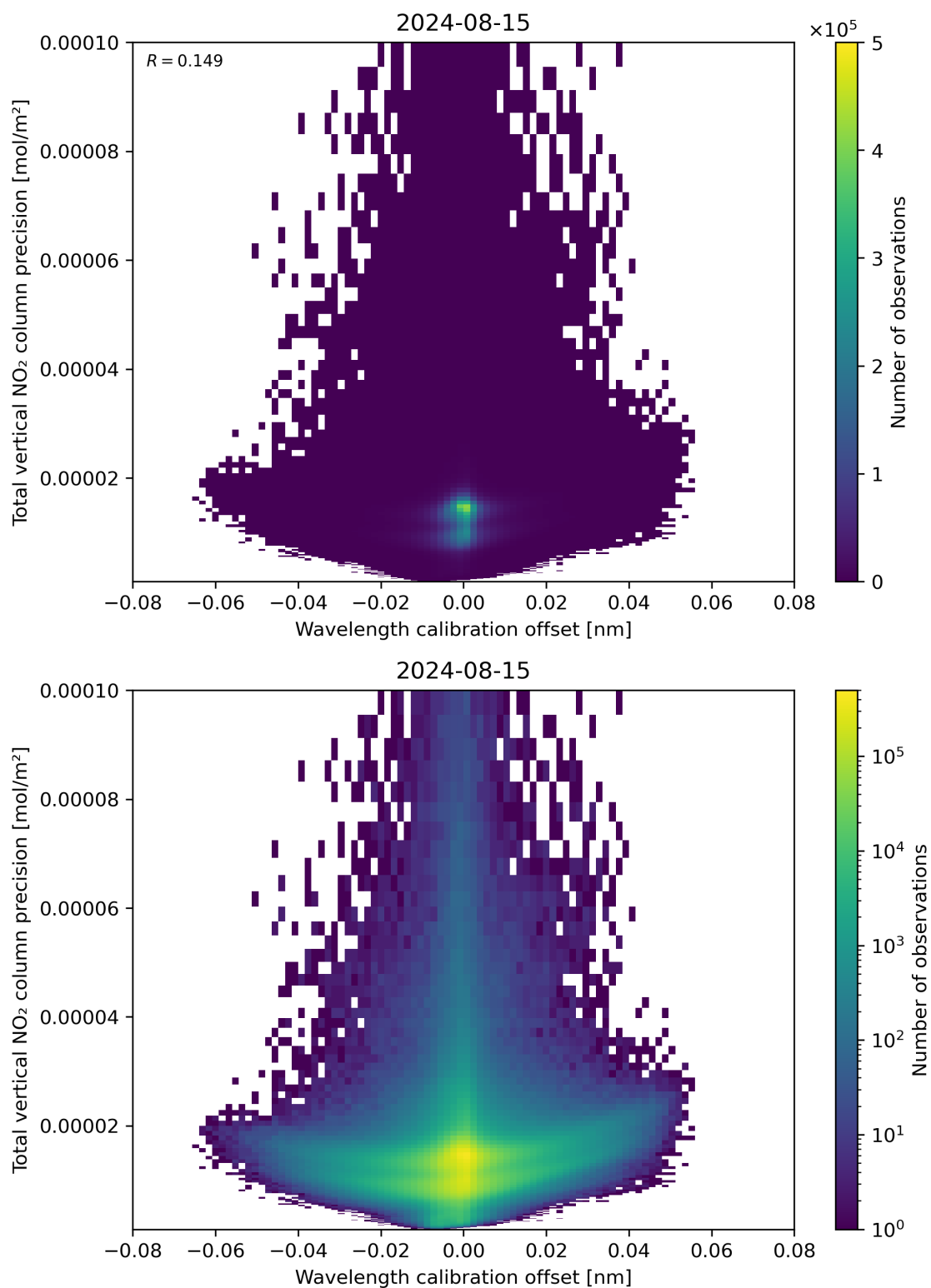
Figure 180: Scatter density plot of “Wavelength calibration offset” against “Total vertical NO 2 column precision” for 2024-08-14 to 2024-08-16.
