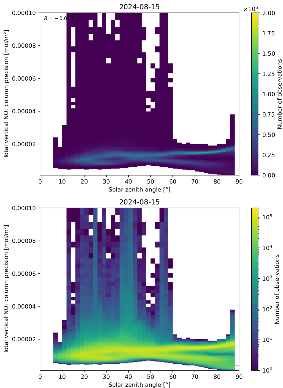
Figure 154: Scatter density plot of “Solar zenith angle” against “Total vertical NO 2 column precision” for 2024-08-14 to 2024-08-16.
