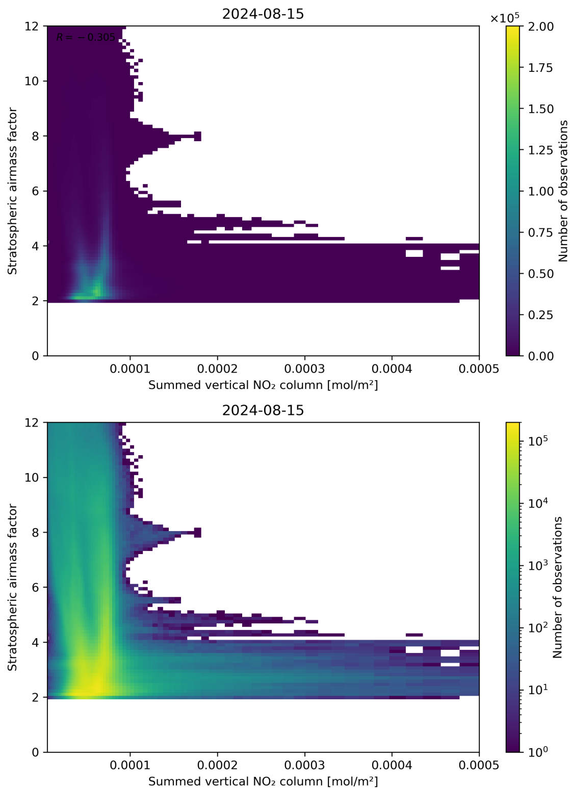
Figure 103: Scatter density plot of “Summed vertical NO 2 column” against “Stratospheric airmass factor” for 2024-08-14 to 2024-08-16.
