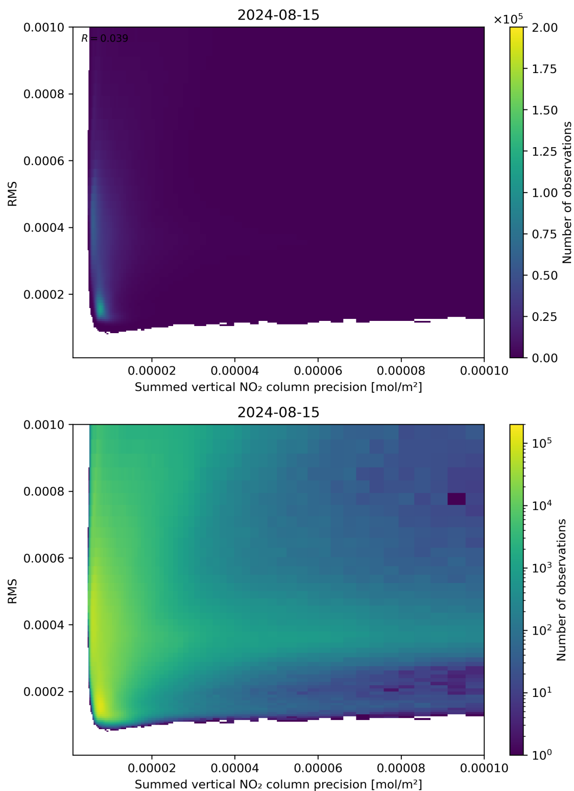
Figure 108: Scatter density plot of “Summed vertical NO 2 column precision” against “RMS” for 2024-08-14 to 2024-08-16.
