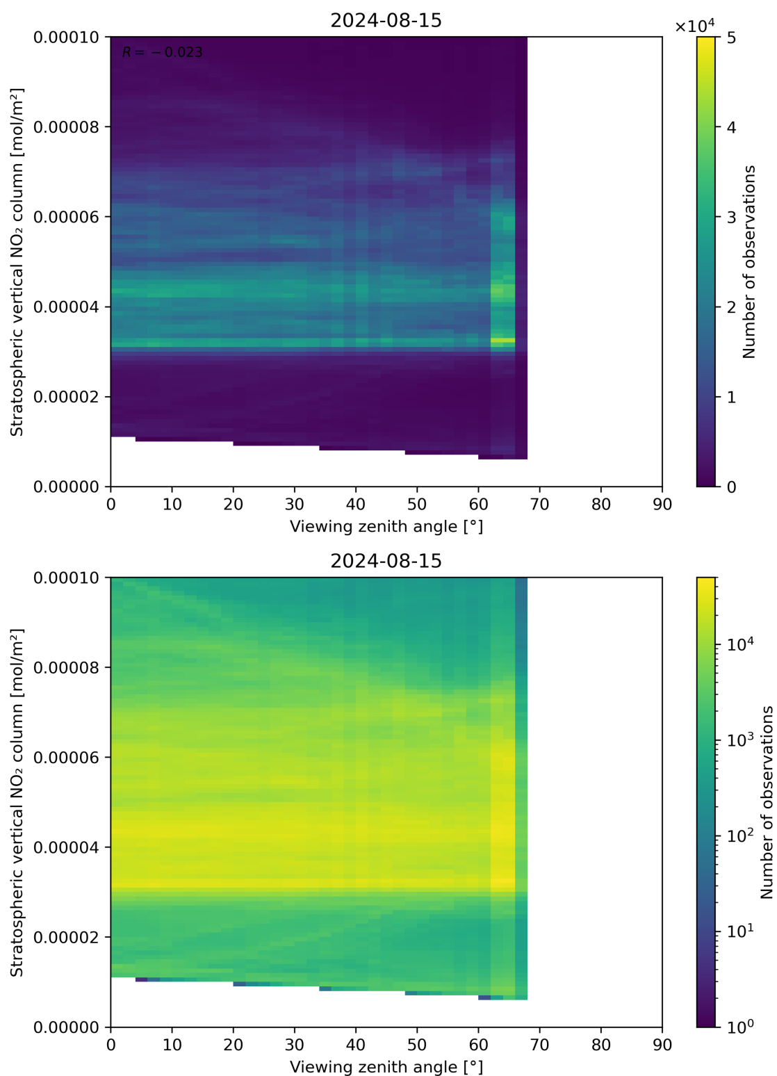
Figure 164: Scatter density plot of “Viewing zenith angle” against “Stratospheric vertical NO 2 column” for 2024-08-14 to 2024-08-16.
