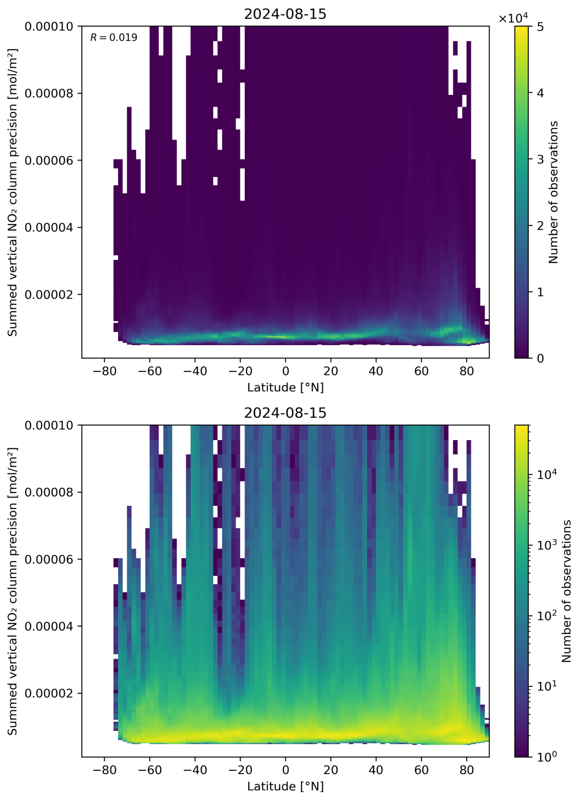
Figure 89: Scatter density plot of “Latitude” against “Summed vertical NO 2 column precision” for 2024-08-14 to 2024-08-16.
