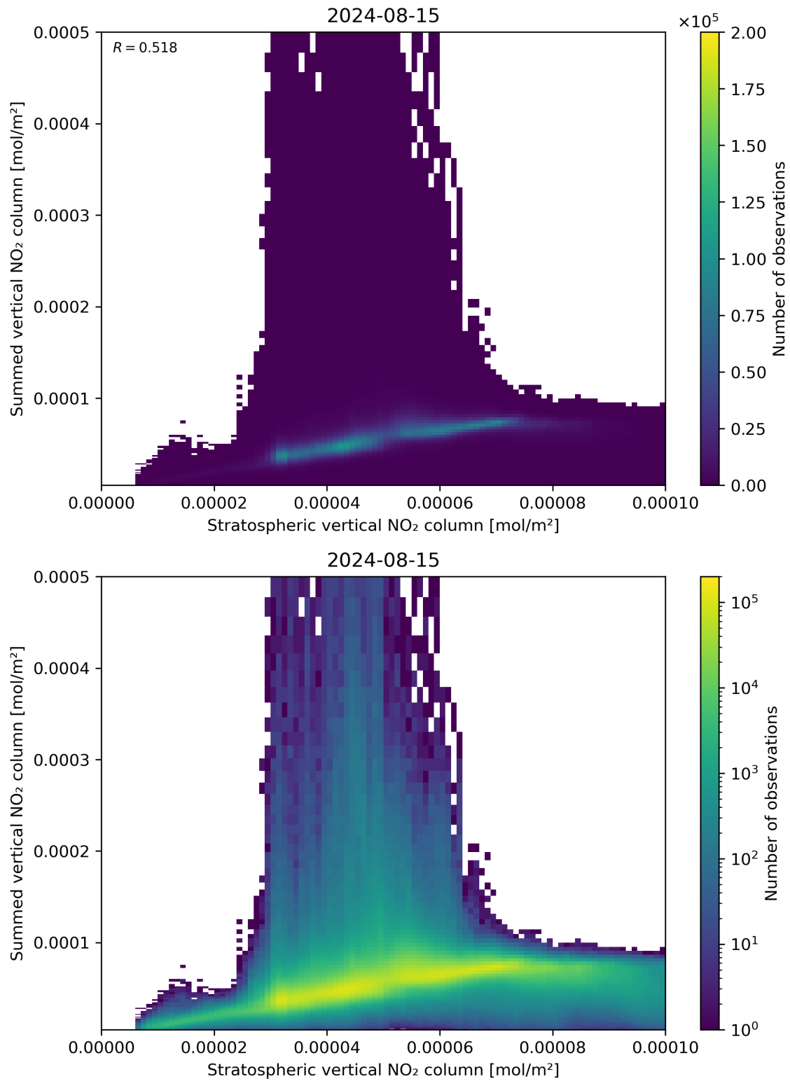
Figure 98: Scatter density plot of “Stratospheric vertical NO 2 column” against “Summed vertical NO 2 column” for 2024-08-14 to 2024-08-16.
