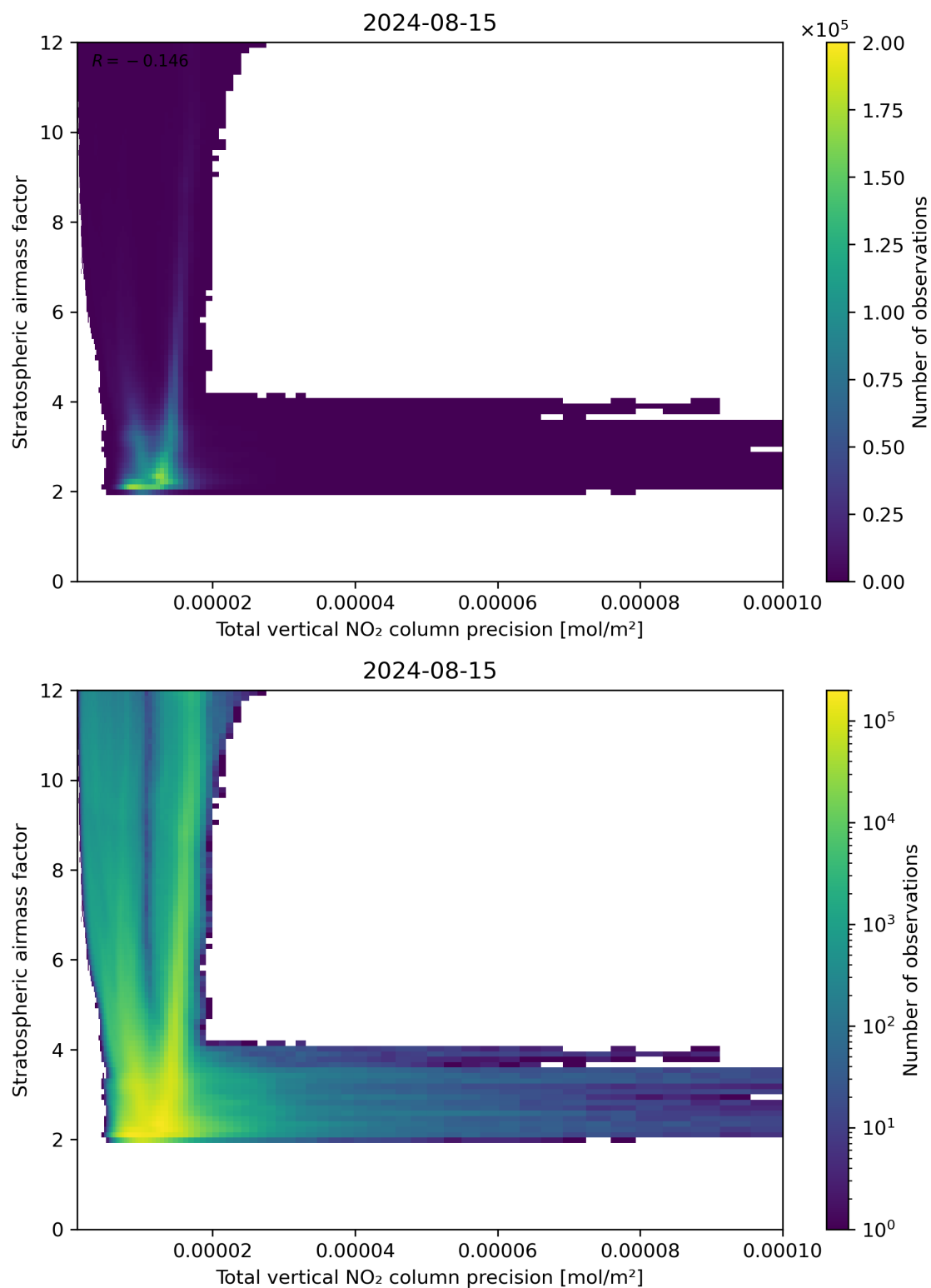
Figure 115: Scatter density plot of “Total vertical NO 2 column precision” against “Stratospheric air mass factor” for 2024-08-14 to 2024-08-16.
