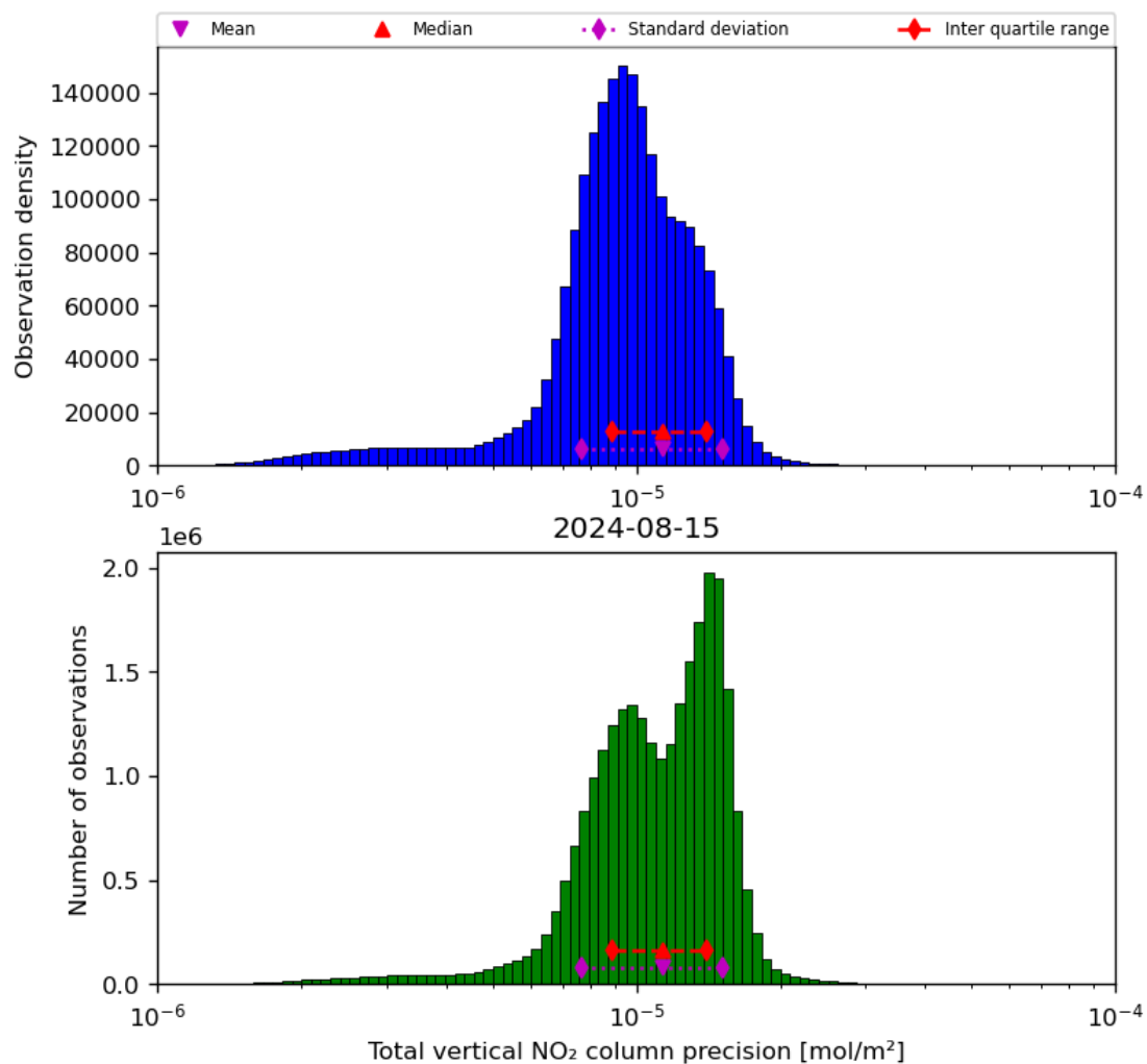
Figure 39: Histogram of “Total vertical NO 2 column precision” for 2024-08-14 to 2024-08-16
