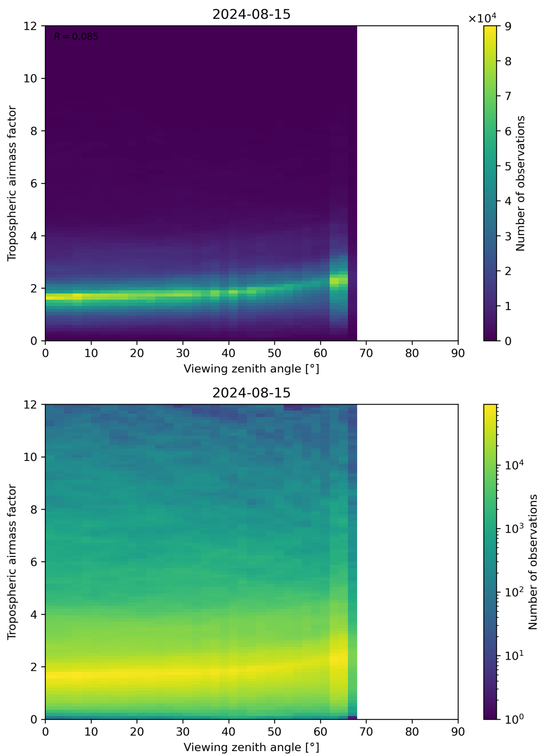
Figure 161: Scatter density plot of “Viewing zenith angle” against “Tropospheric airmass factor” for 2024-08-14 to 2024-08-16.
