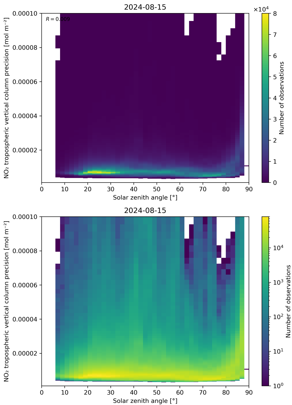
Figure 156: Scatter density plot of “Solar zenith angle” against “NO 2 tropospheric vertical column precision” for 2024-08-14 to 2024-08-16.
