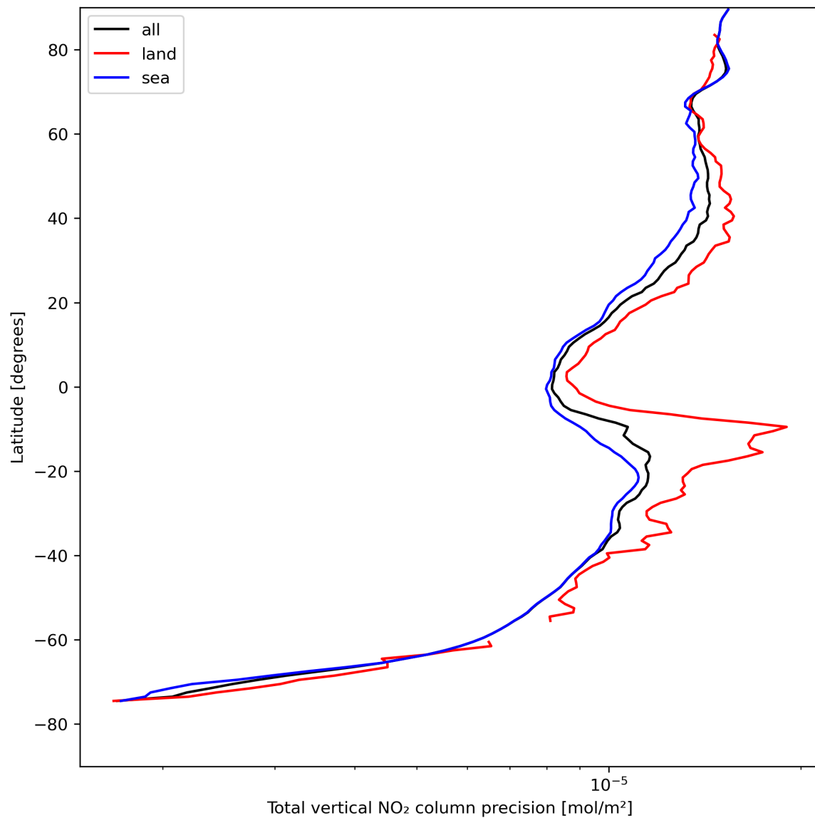
Figure 22: Zonal average of “Total vertical NO 2 column precision” for 2024-08-14 to 2024-08-16.
