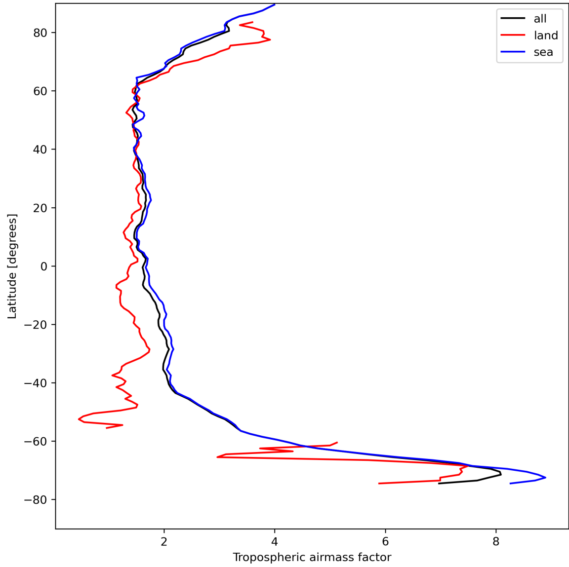
Figure 14: Zonal average of “Tropospheric airmass factor” for 2024-08-14 to 2024-08-16.
