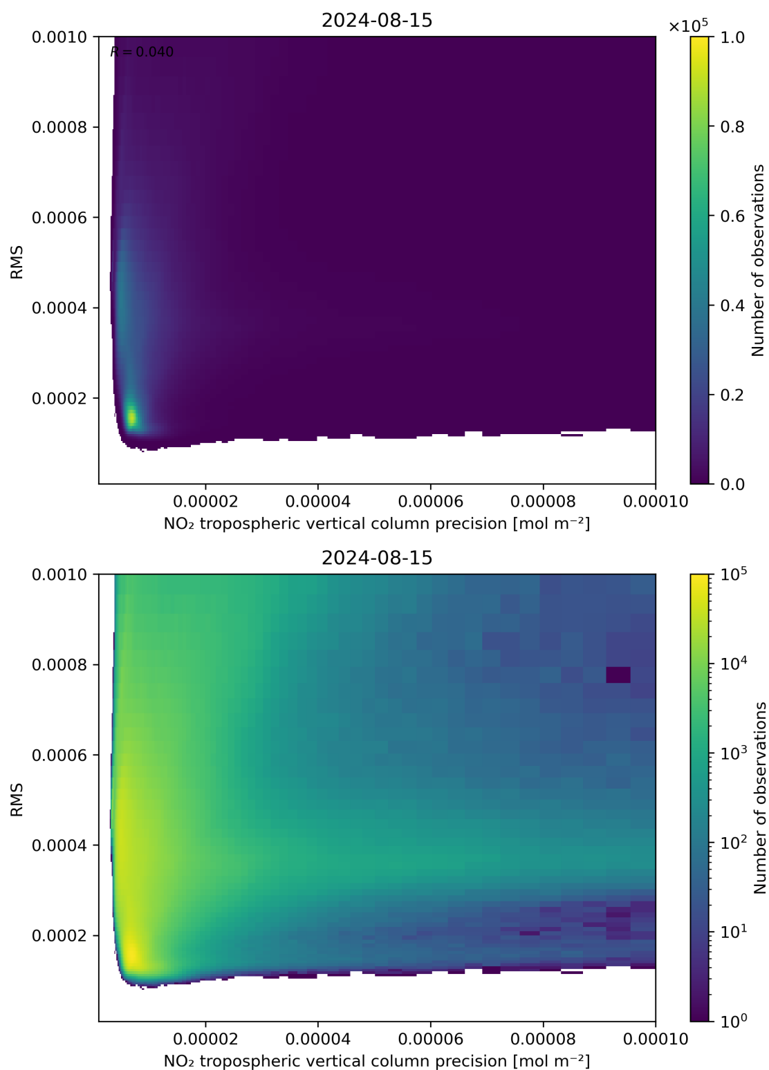
Figure 140: Scatter density plot of “NO 2 tropospheric vertical column precision” against “RMS” for 2024-08-14 to 2024-08-16.
