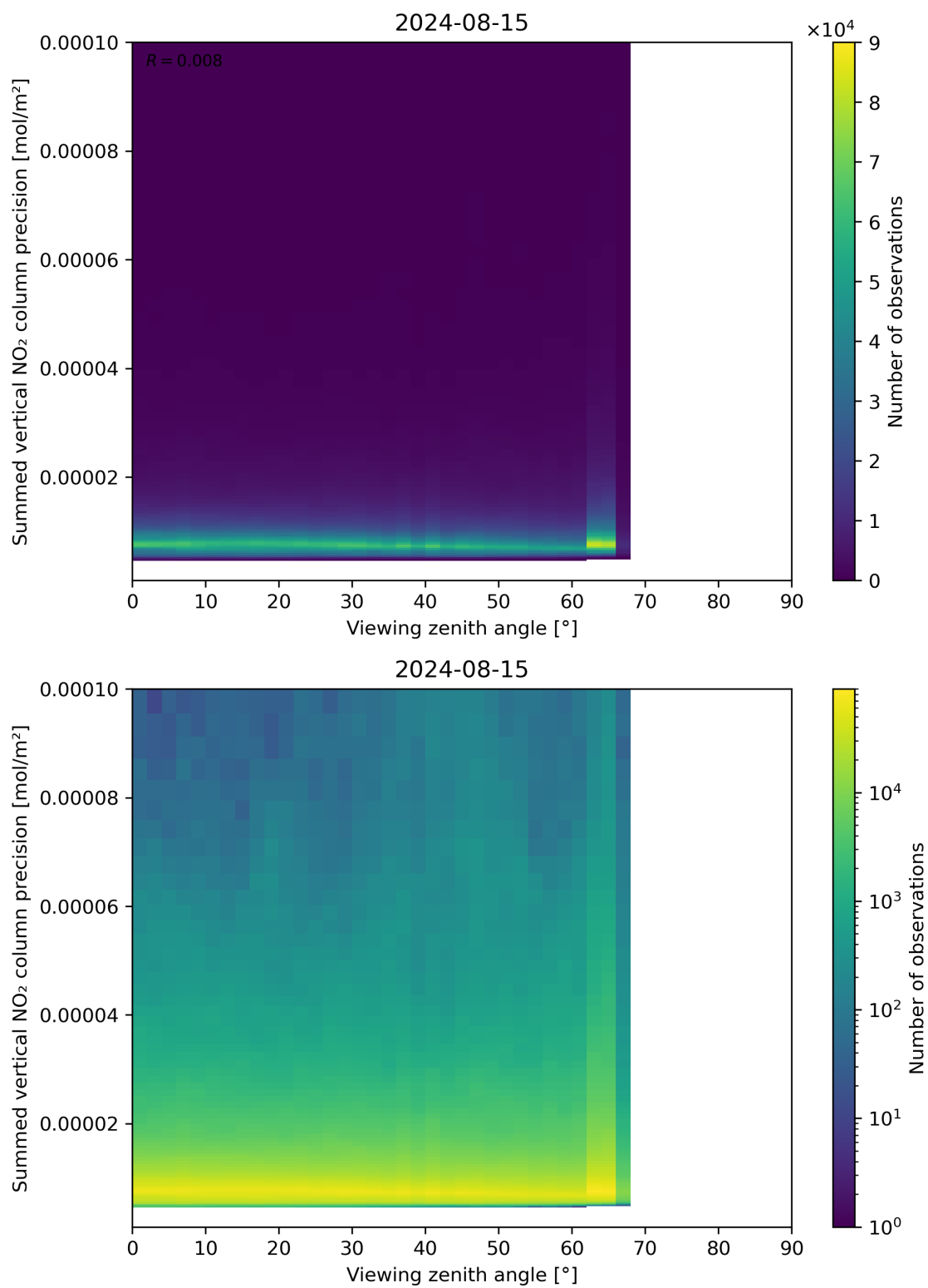
Figure 166: Scatter density plot of “Viewing zenith angle” against “Summed vertical NO 2 column precision” for 2024-08-14 to 2024-08-16.
