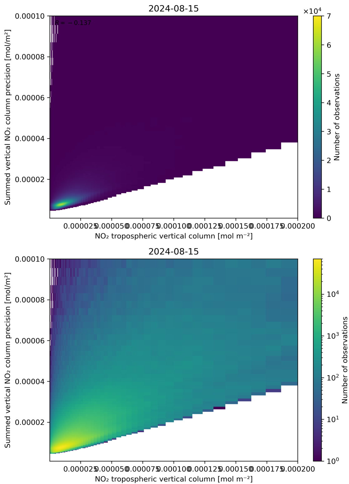
Figure 127: Scatter density plot of “NO 2 tropospheric vertical column” against “Summed vertical NO 2 column precision” for 2024-08-14 to 2024-08-16.
