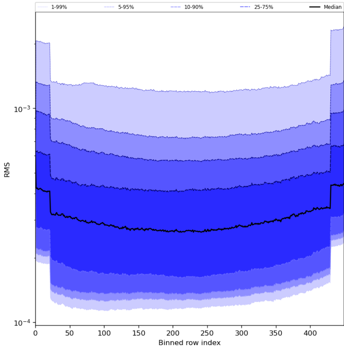
Figure 60: Along track statistics of “RMS” for 2024-08-14 to 2024-08-16
