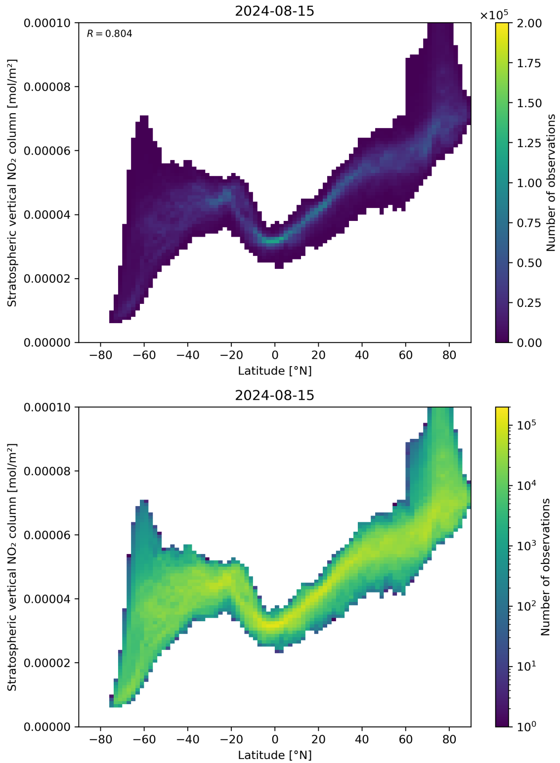
Figure 87: Scatter density plot of “Latitude” against “Stratospheric vertical \text{NO}_2 column” for 2024-08-14 to 2024-08-16.
