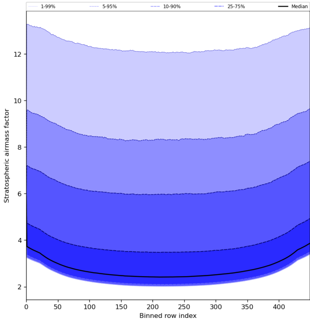
Figure 61: Along track statistics of “Stratospheric airmass factor” for 2024-08-14 to 2024-08-16
