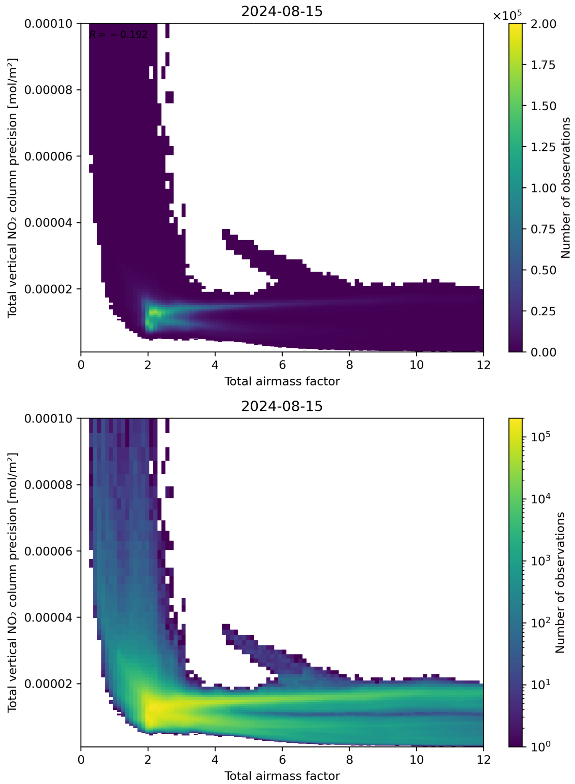
Figure 68: Scatter density plot of “Total airmass factor” against “Total vertical NO 2 column precision” for 2024-08-14 to 2024-08-16.
