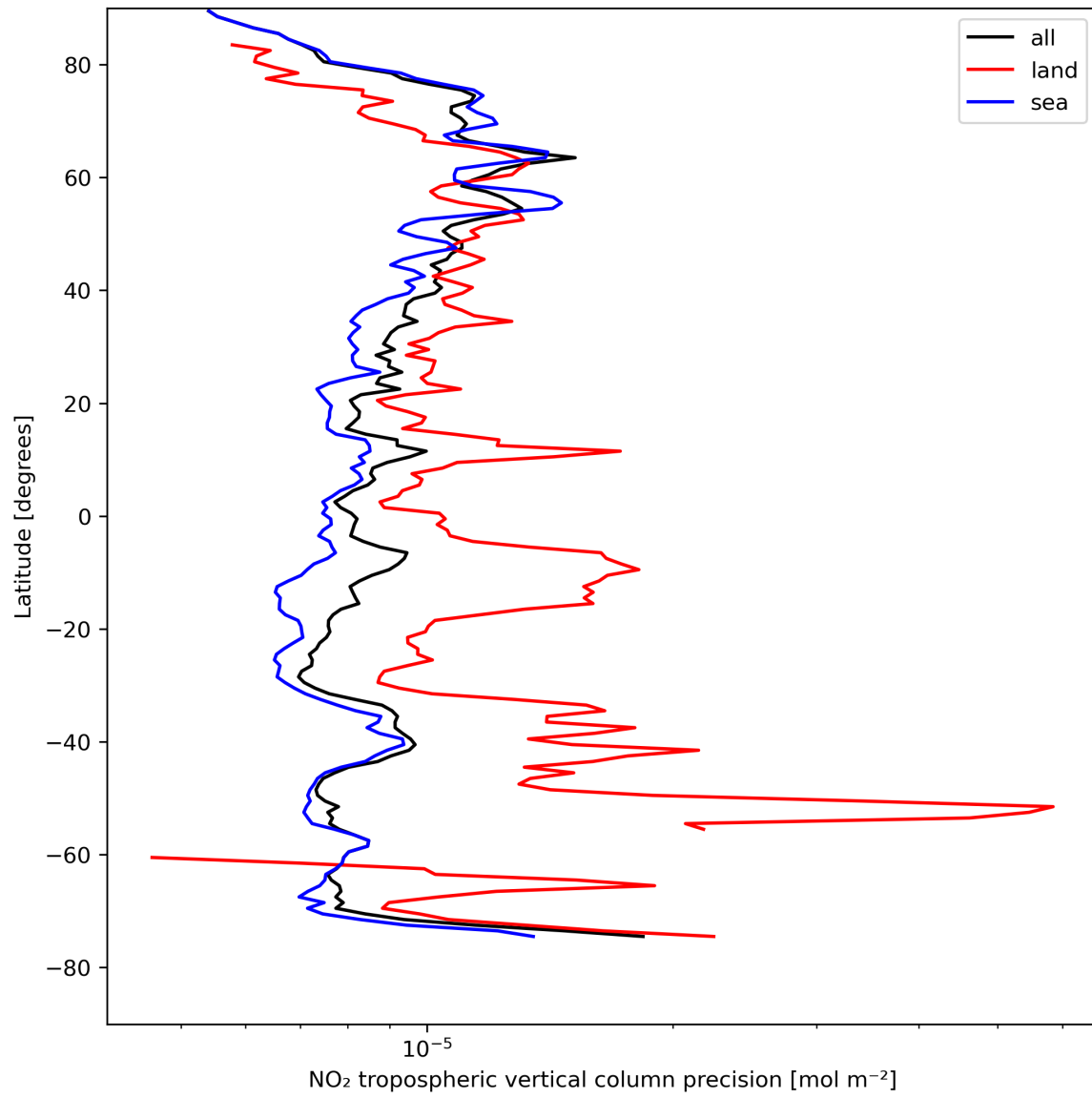
Figure 13: Zonal average of “NO 2 tropospheric vertical column precision” for 2024-08-14 to 2024-08-16.
