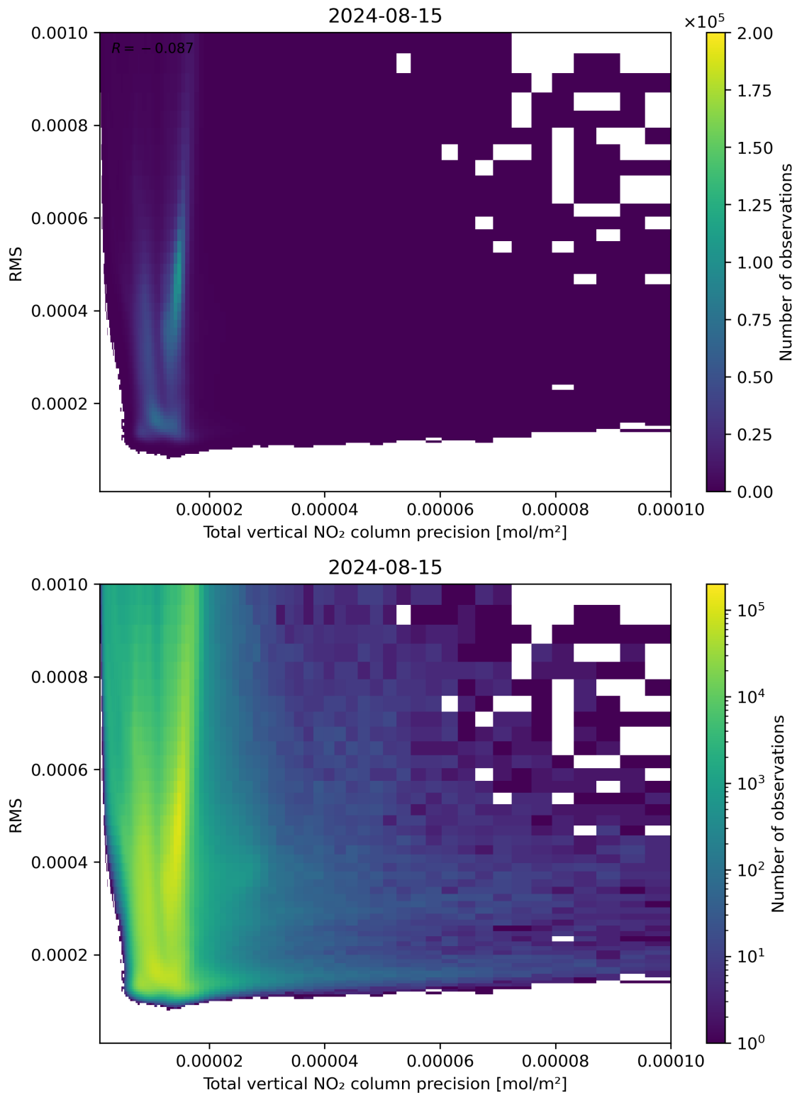
Figure 119: Scatter density plot of “Total vertical NO 2 column precision” against “RMS” for 2024-08-14 to 2024-08-16.
