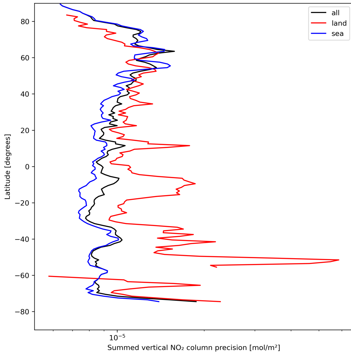
Figure 24: Zonal average of “Summed vertical NO 2 column precision” for 2024-08-14 to 2024-08-16.
