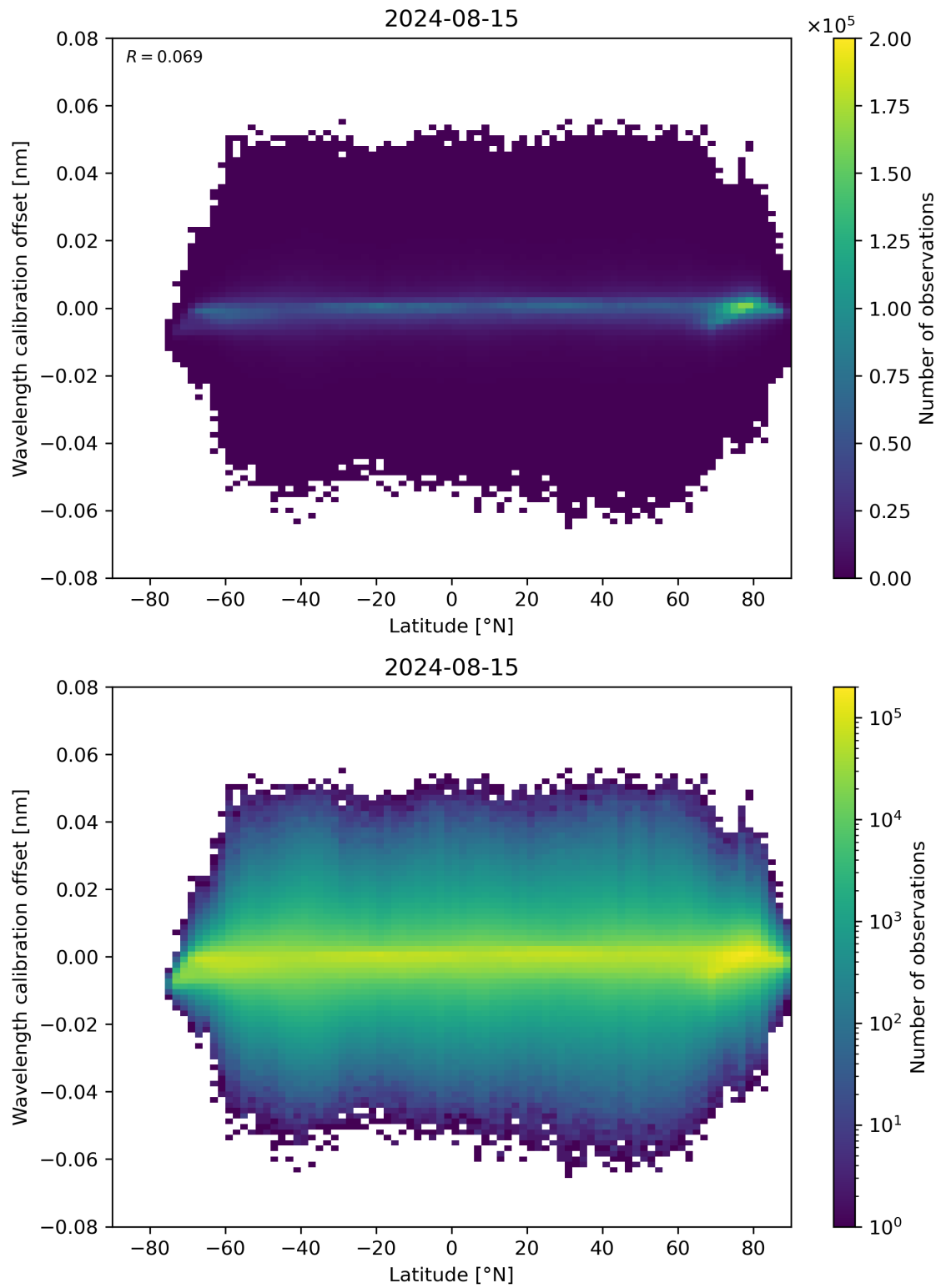
Figure 95: Scatter density plot of “Latitude” against “Wavelength calibration offset” for 2024-08-14 to 2024-08-16.
