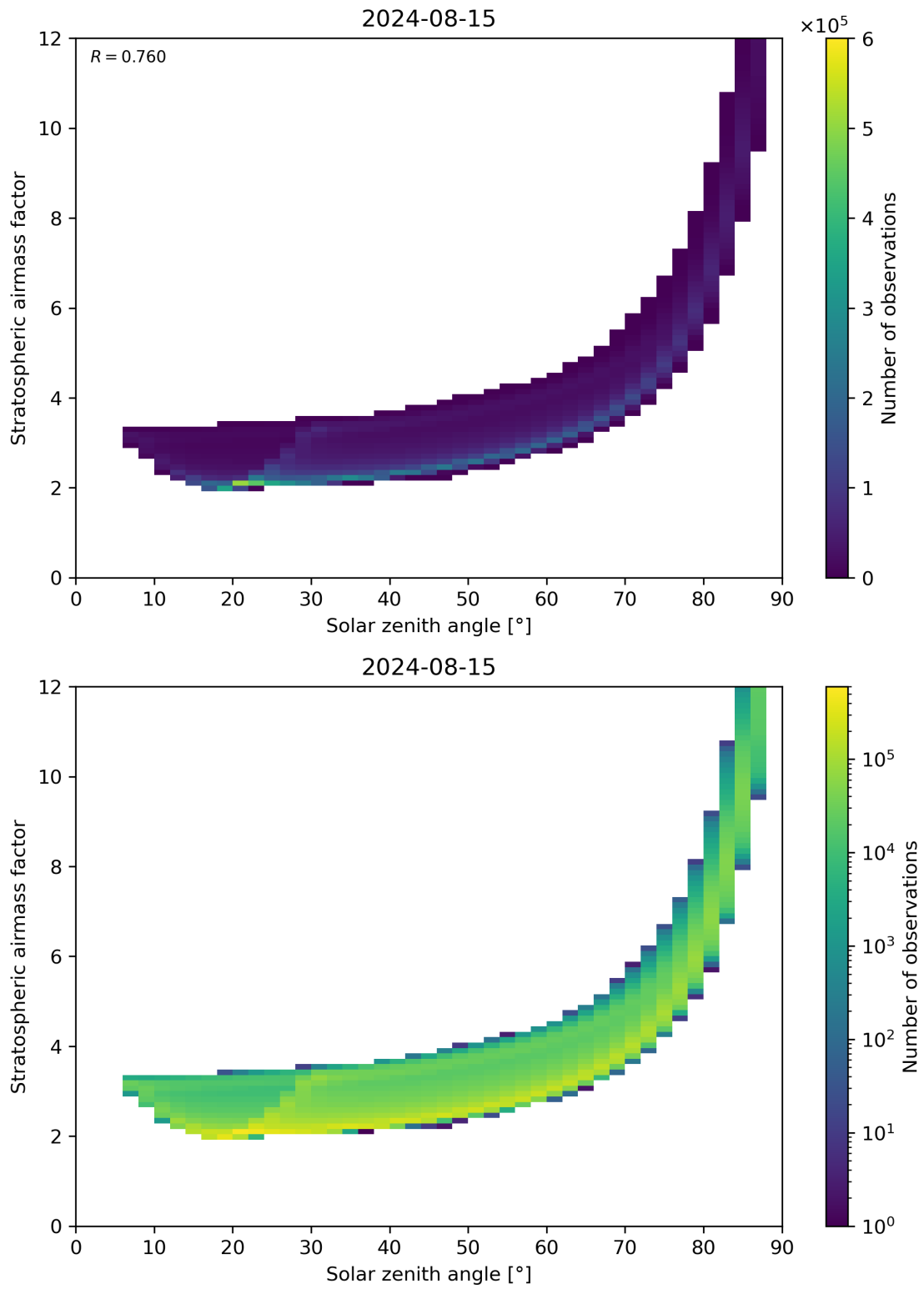
Figure 145: Scatter density plot of “Solar zenith angle” against “Stratospheric airmass factor” for 2024-08-14 to 2024-08-16.
