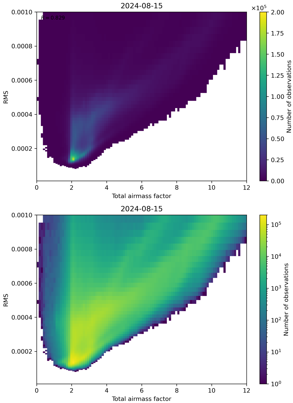
Figure 69: Scatter density plot of “Total airmass factor” against “RMS” for 2024-08-14 to 2024-08-16.
