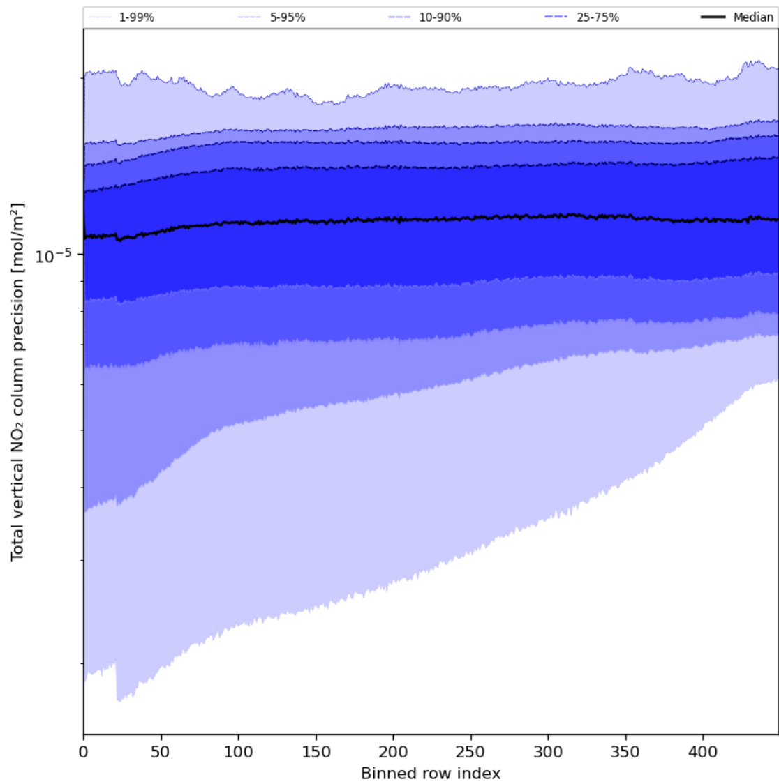
Figure 56: Along track statistics of “Total vertical NO 2 column precision” for 2024-08-14 to 2024-08-16
