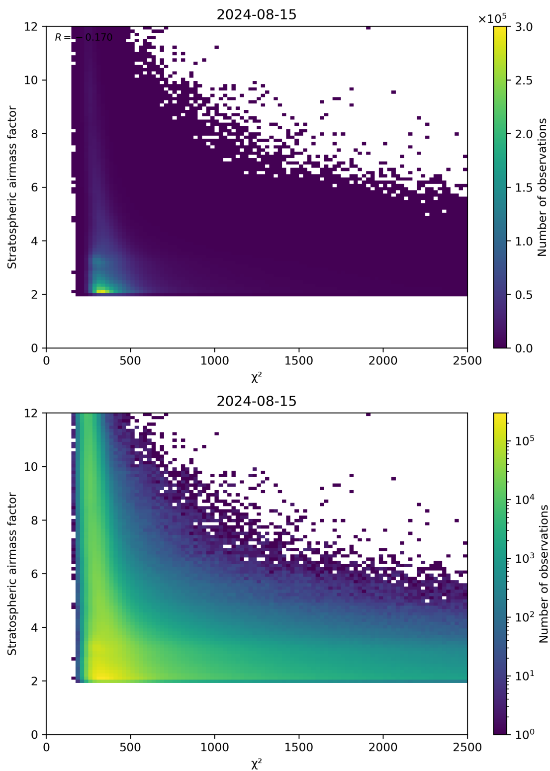
Figure 81: Scatter density plot of “ \chi^2 ” against “Stratospheric airmass factor” for 2024-08-14 to 2024-08-16.
