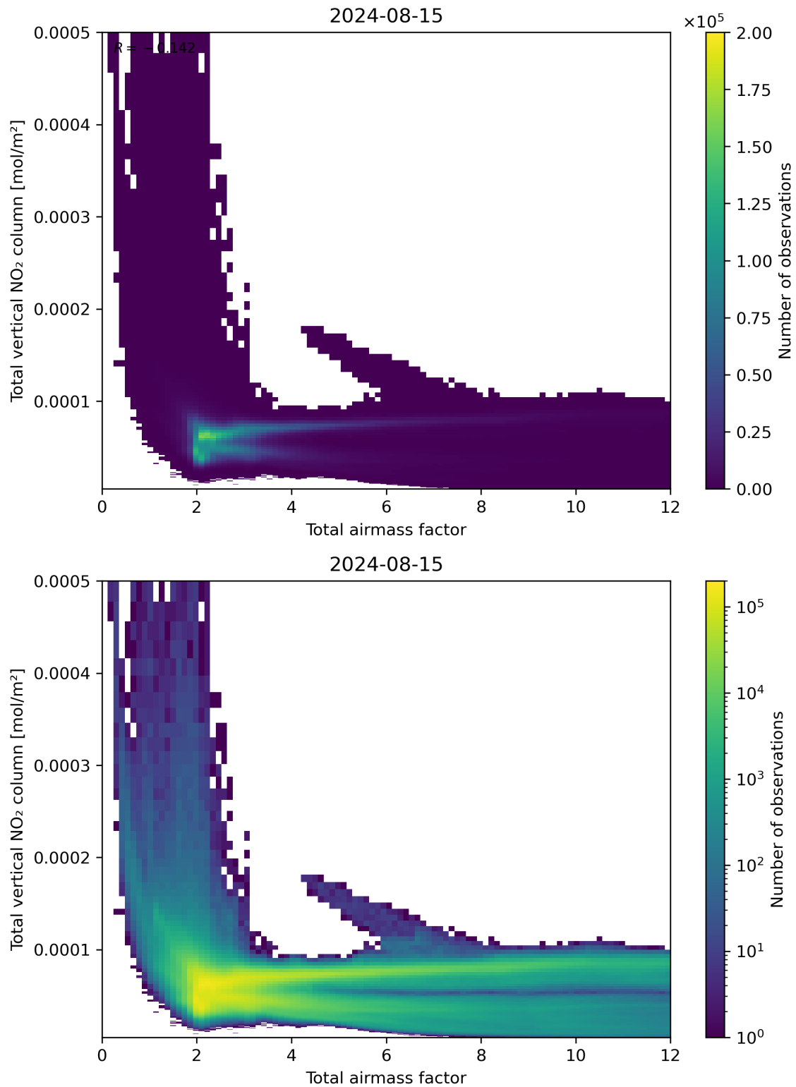
Figure 67: Scatter density plot of “Total airmass factor” against “Total vertical NO 2 column” for 2024-08-14 to 2024-08-16.
