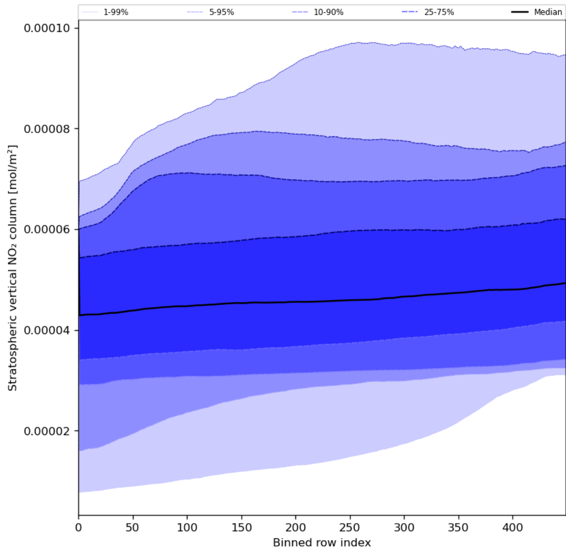
Figure 53: Along track statistics of “Stratospheric vertical NO 2 column” for 2024-08-14 to 2024-08-16
