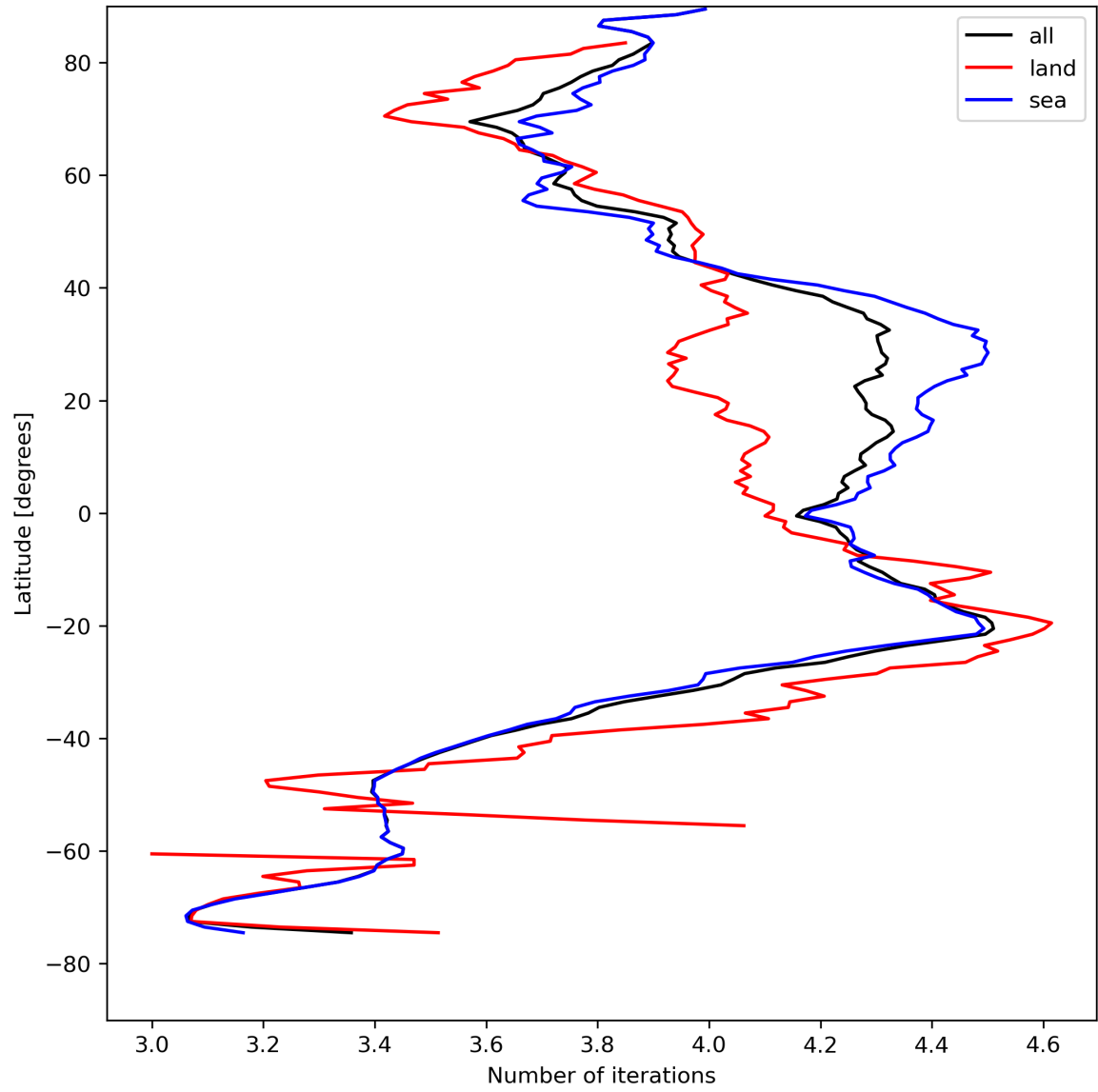
Figure 17: Zonal average of “Number of iterations” for 2024-08-14 to 2024-08-16.
