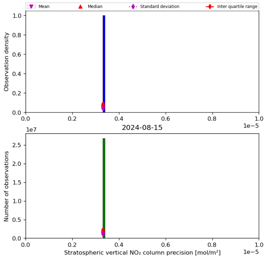
Figure 37: Histogram of “Stratospheric vertical NO 2 column precision” for 2024-08-14 to 2024-08-16
