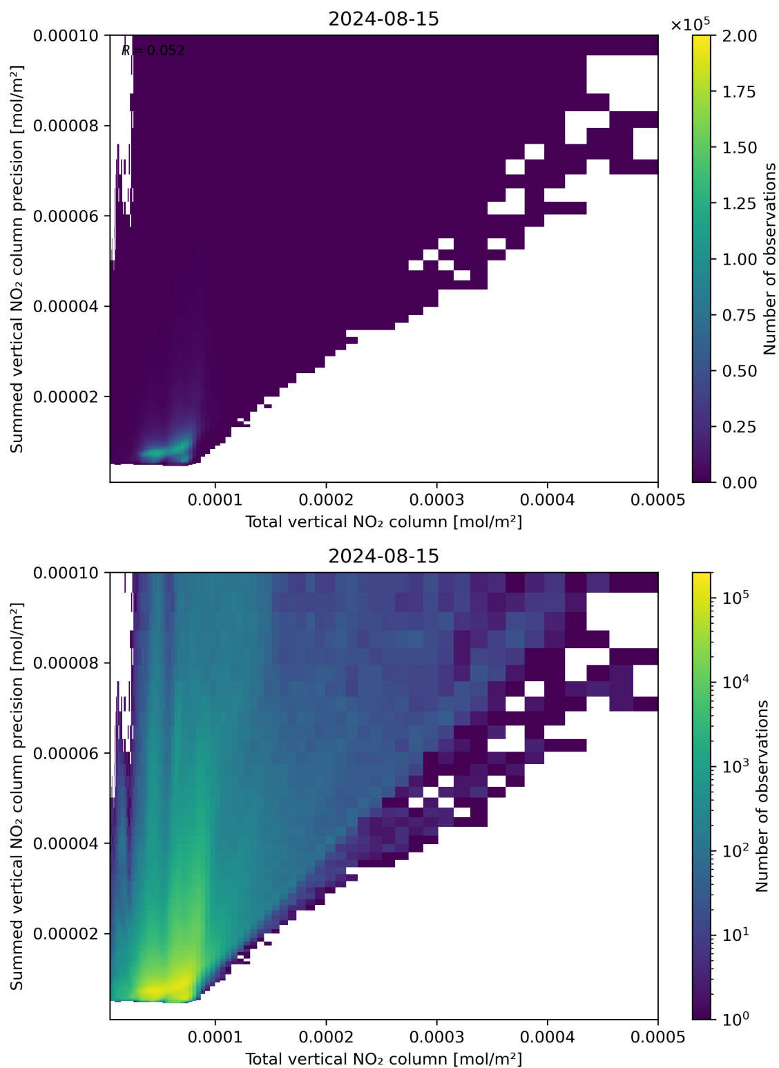
Figure 113: Scatter density plot of “Total vertical NO 2 column” against “Summed vertical NO 2 column precision” for 2024-08-14 to 2024-08-16.
