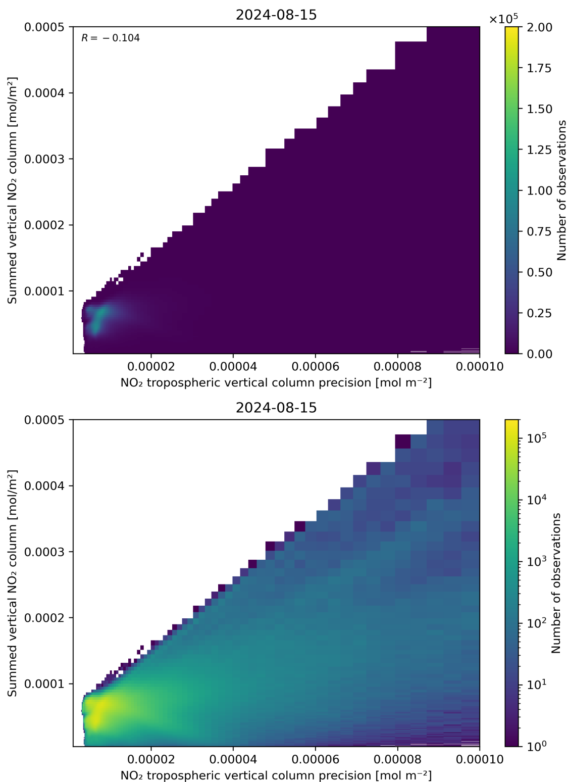
Figure 136: Scatter density plot of “NO 2 tropospheric vertical column precision” against “Summed vertical NO 2 column” for 2024-08-14 to 2024-08-16.
