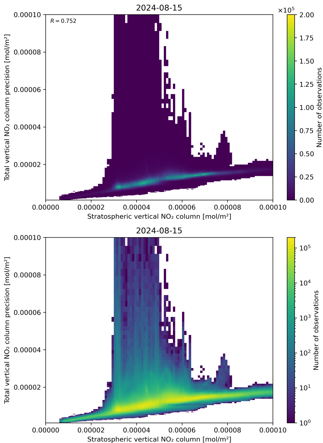
Figure 101: Scatter density plot of “Stratospheric vertical NO 2 column” against “Total vertical NO 2 column precision” for 2024-08-14 to 2024-08-16.
