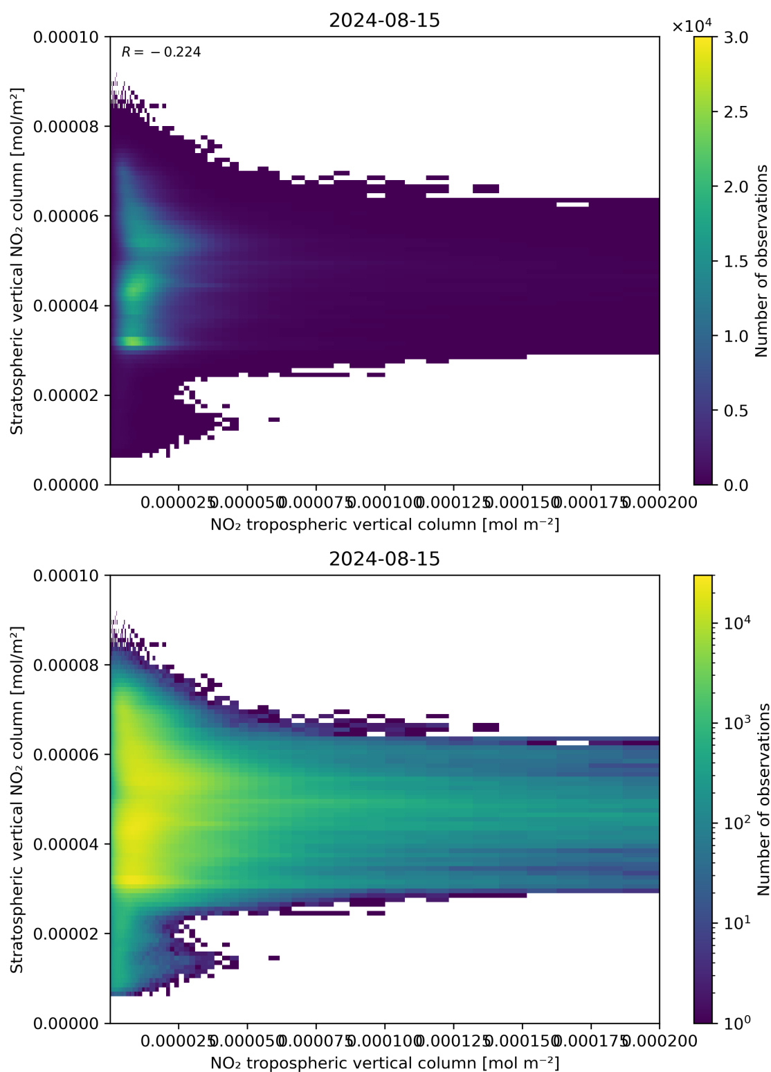
Figure 125: Scatter density plot of “NO 2 tropospheric vertical column” against “Stratospheric vertical NO 2 column” for 2024-08-14 to 2024-08-16.
