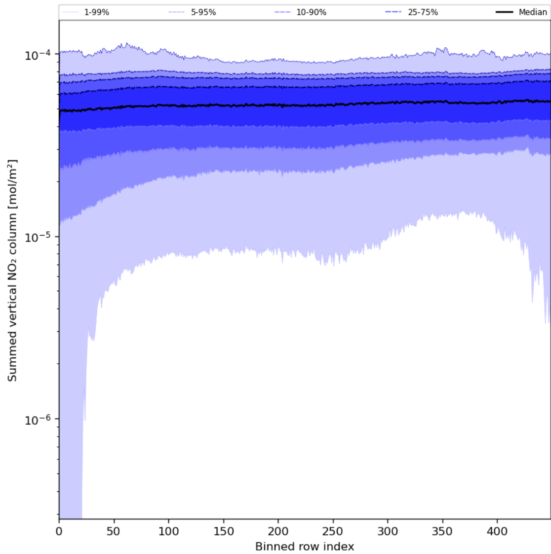
Figure 57: Along track statistics of “Summed vertical NO 2 column” for 2024-08-14 to 2024-08-16
