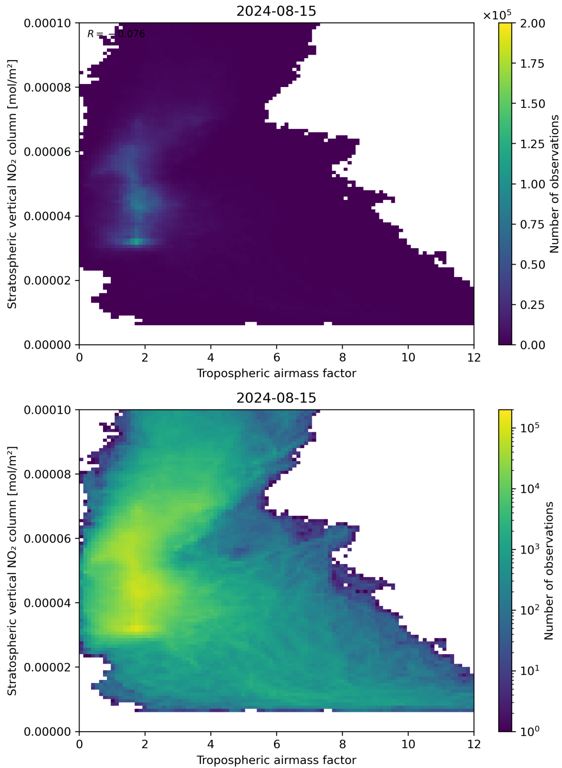
Figure 74: Scatter density plot of “Tropospheric air mass factor” against “Stratospheric vertical NO 2 column” for 2024-08-14 to 2024-08-16.
