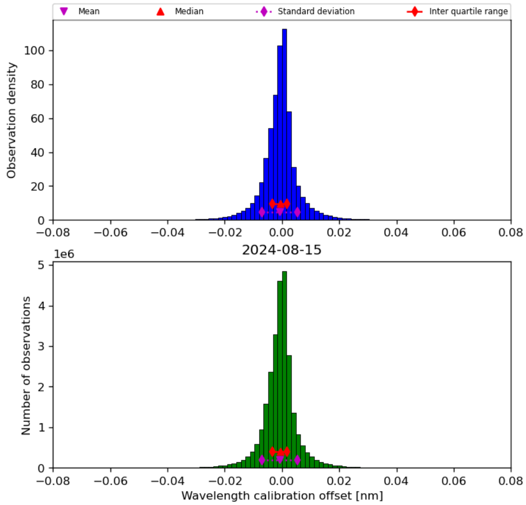
Figure 35: Histogram of “Wavelength calibration offset” for 2024-08-14 to 2024-08-16
