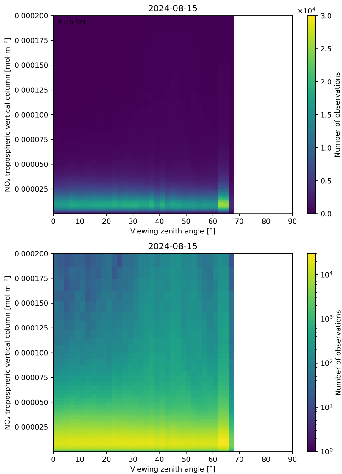
Figure 169: Scatter density plot of “Viewing zenith angle” against “NO 2 tropospheric vertical column” for 2024-08-14 to 2024-08-16.
