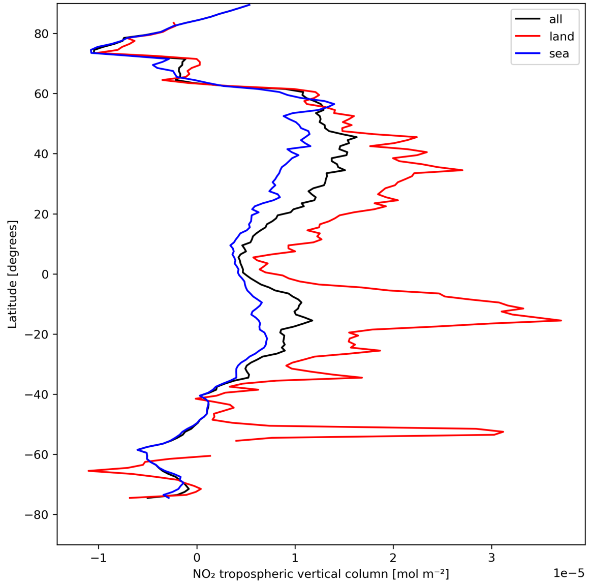
Figure 12: Zonal average of “NO 2 tropospheric vertical column” for 2024-08-14 to 2024-08-16.
