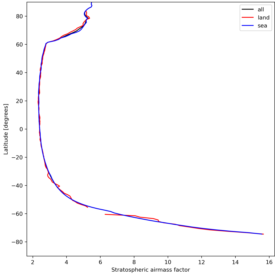
Figure 27: Zonal average of “Stratospheric airmass factor” for 2024-08-14 to 2024-08-16.
