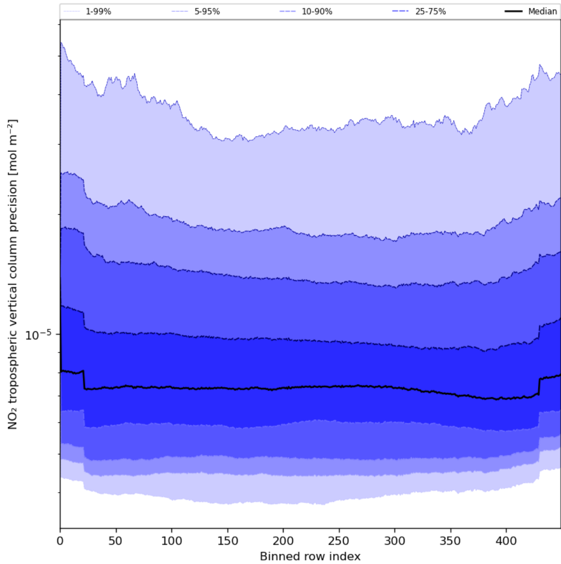
Figure 47: Along track statistics of “NO 2 tropospheric vertical column precision” for 2024-08-14 to 2024-08-16
