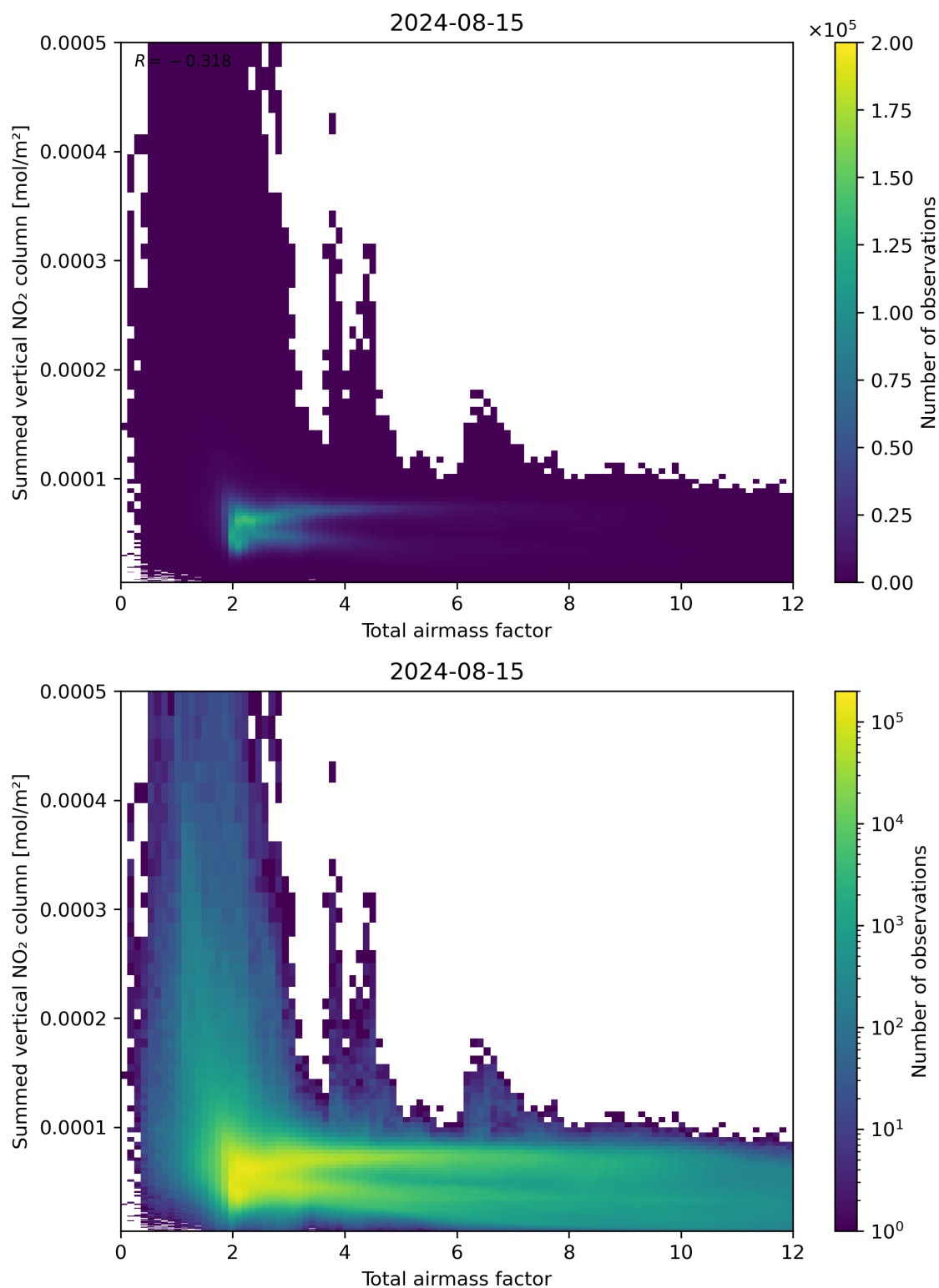
Figure 65: Scatter density plot of “Total airmass factor” against “Summed vertical NO 2 column” for 2024-08-14 to 2024-08-16.
