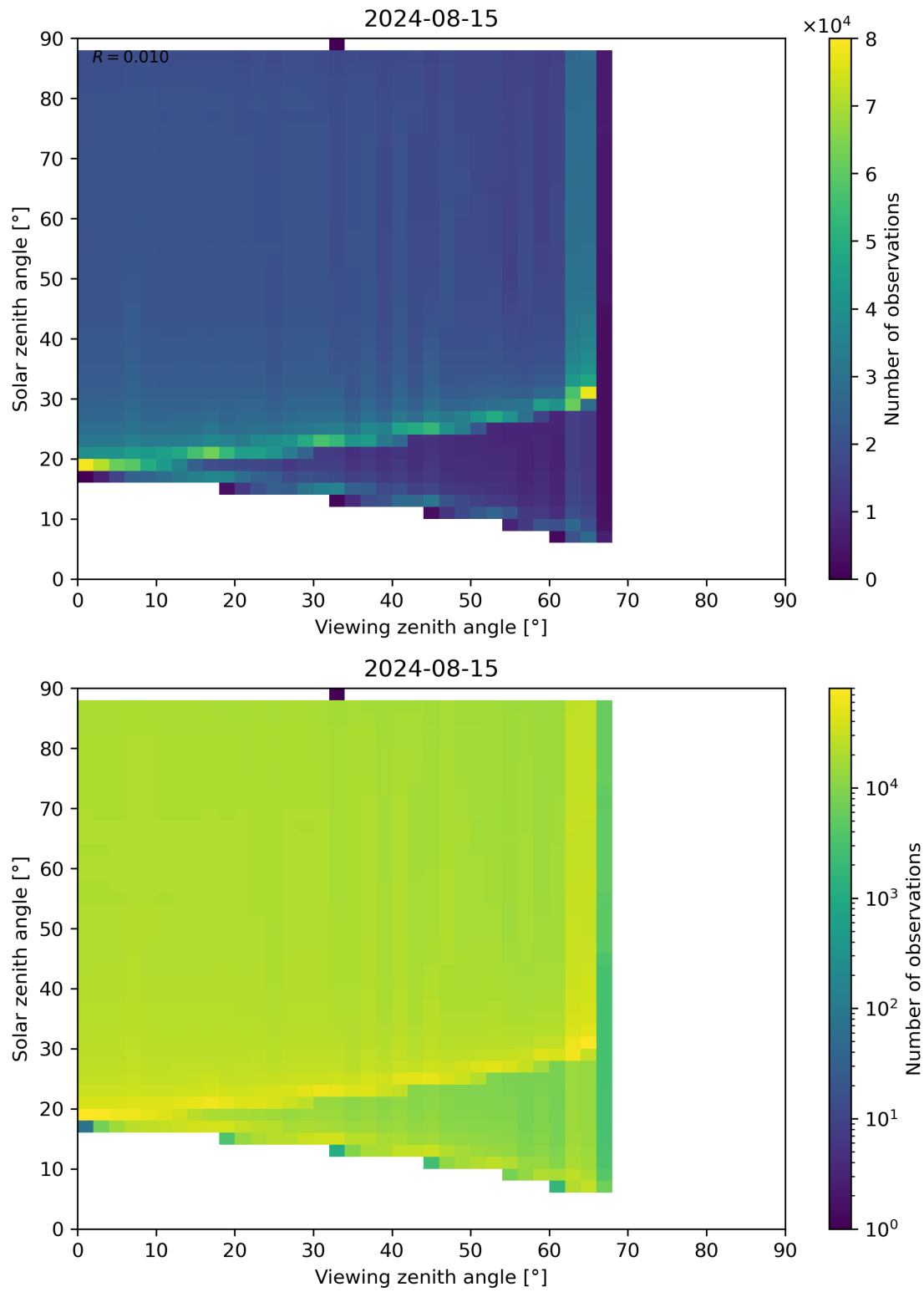
Figure 172: Scatter density plot of “Viewing zenith angle” against “Solar zenith angle” for 2024-08-14 to 2024-08-16.
