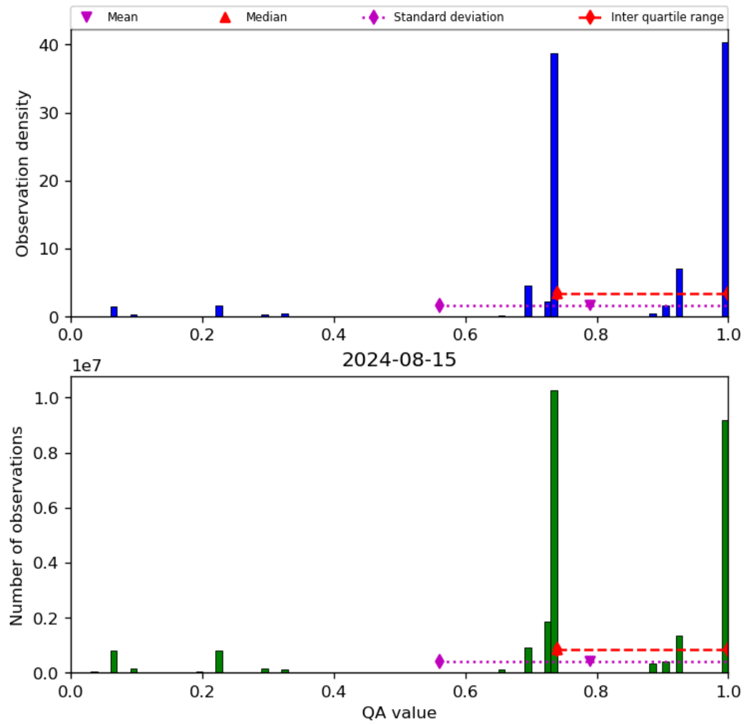
Figure 28: Histogram of “QA value” for 2024-08-14 to 2024-08-16
