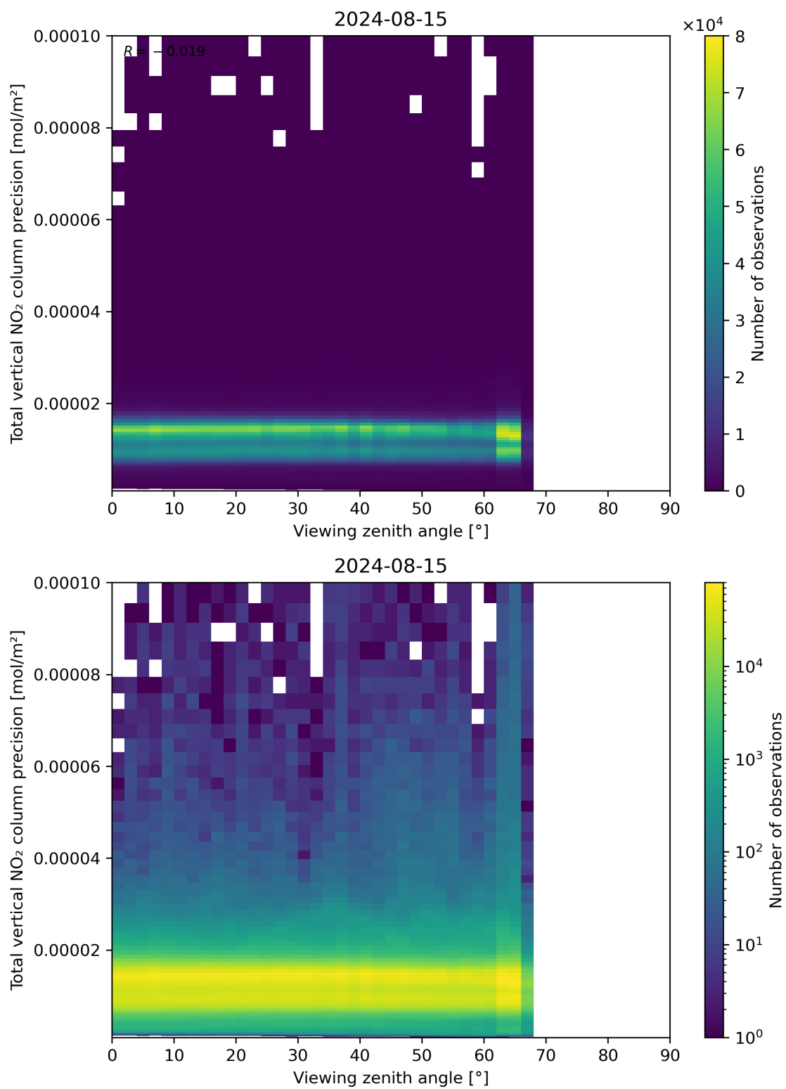
Figure 168: Scatter density plot of “Viewing zenith angle” against “Total vertical NO 2 column precision” for 2024-08-14 to 2024-08-16.
