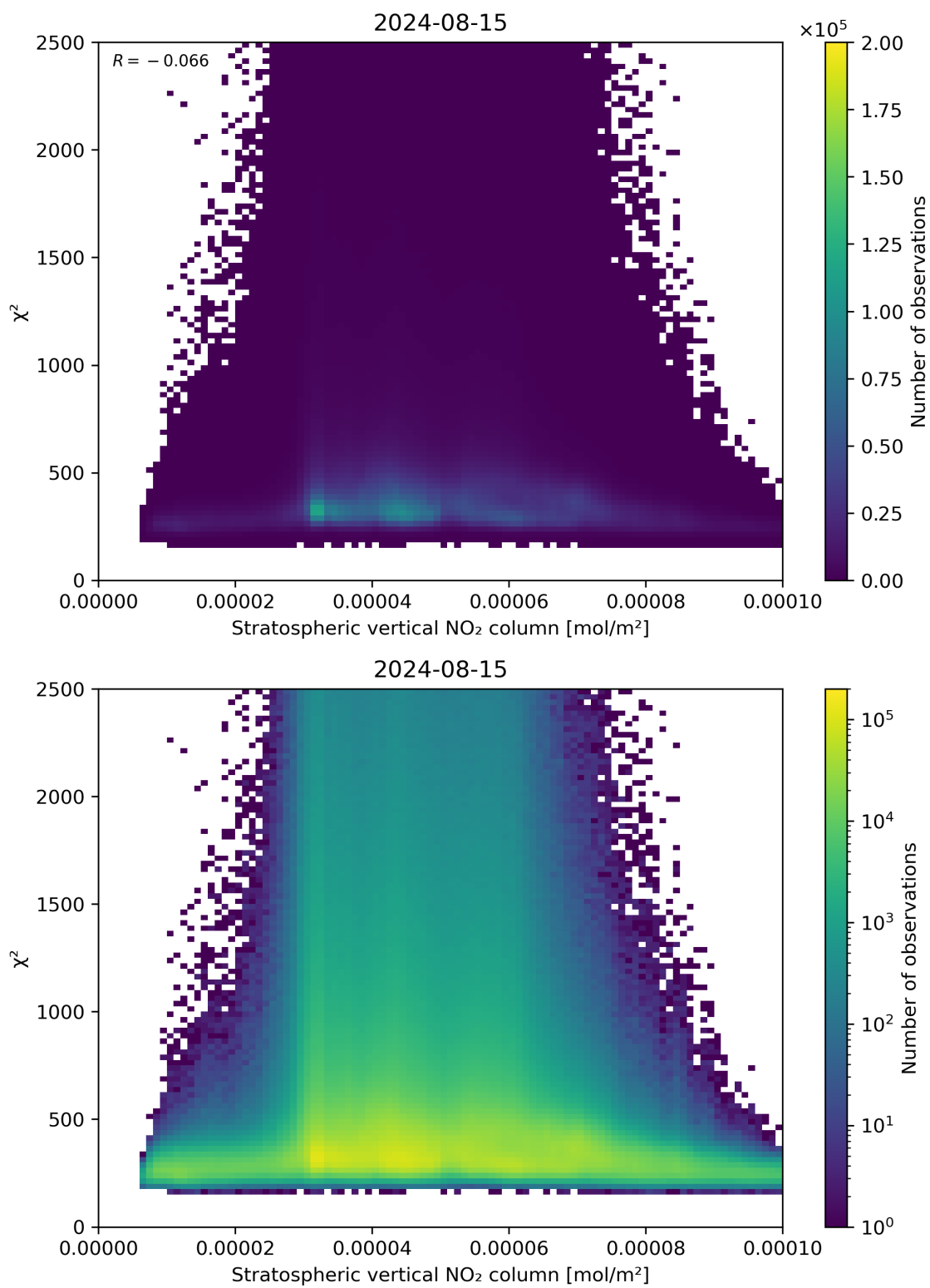
Figure 97: Scatter density plot of “Stratospheric vertical NO 2 column” against “ \chi^2 ” for 2024-08-14 to 2024-08-16.
