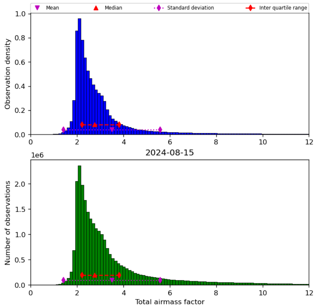
Figure 32: Histogram of “Total airmass factor” for 2024-08-14 to 2024-08-16
