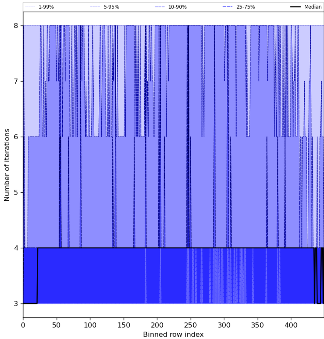
Figure 51: Along track statistics of “Number of iterations” for 2024-08-14 to 2024-08-16
