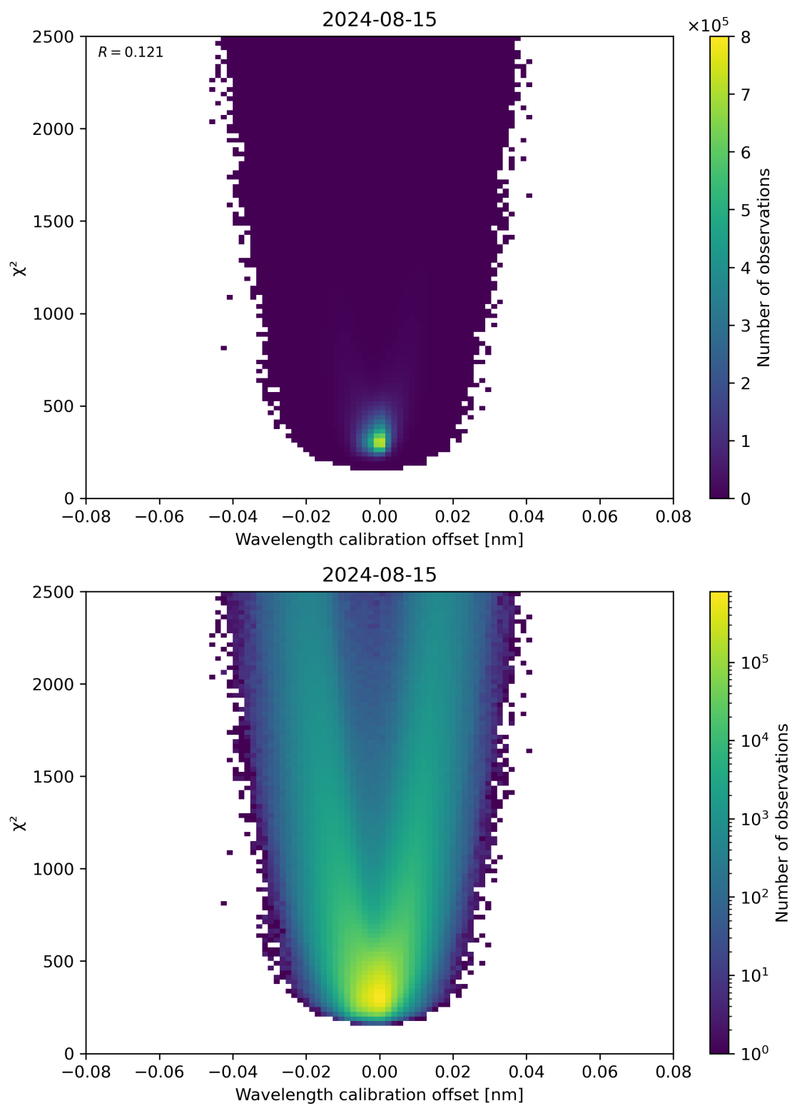
Figure 175: Scatter density plot of “Wavelength calibration offset” against “ \chi^2 ” for 2024-08-14 to 2024-08-16.
