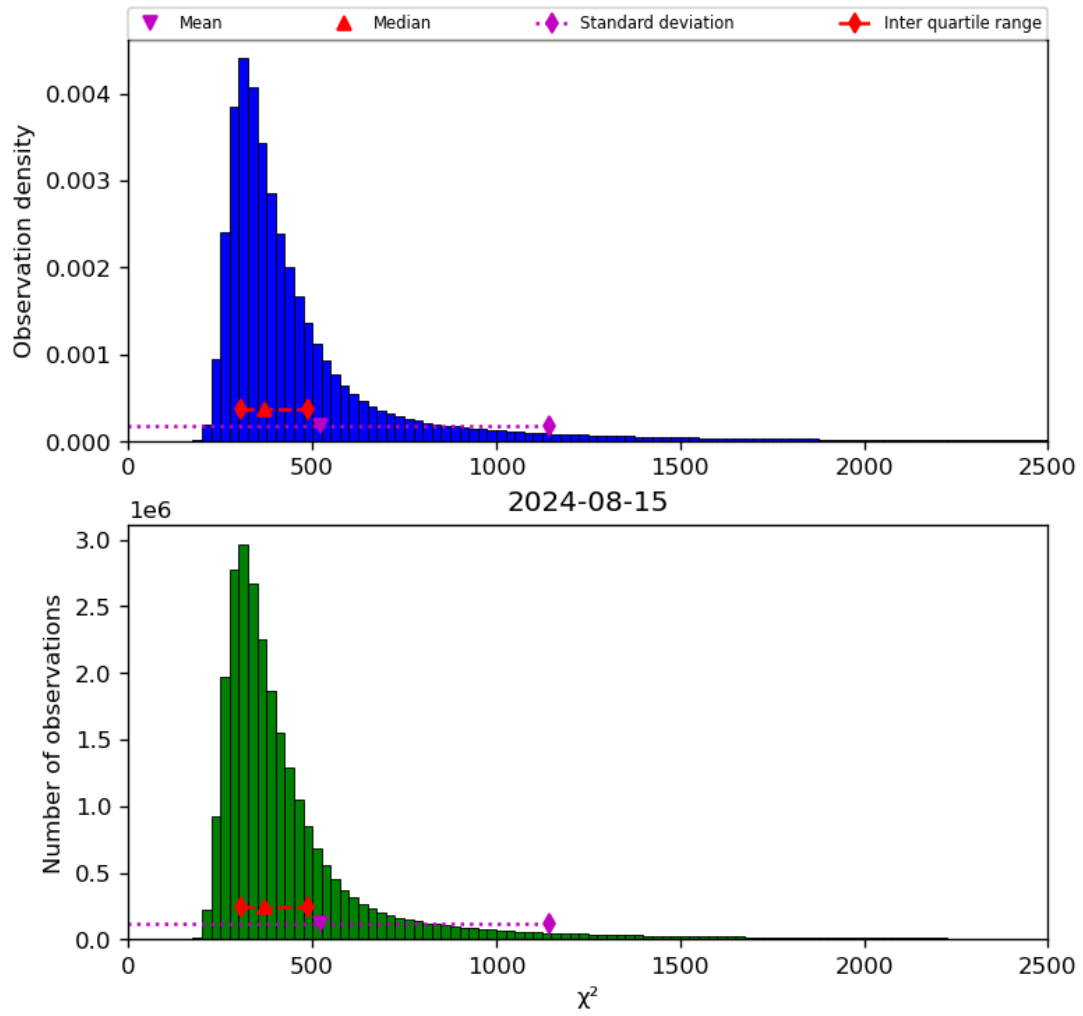
Figure 42: Histogram of “ \chi^2 ” for 2024-08-14 to 2024-08-16
