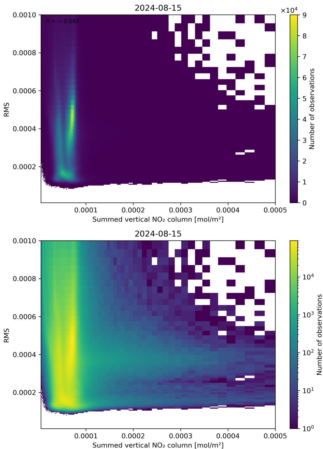
Figure 109: Scatter density plot of “Summed vertical NO 2 column” against “RMS” for 2024-08-14 to 2024-08-16.
