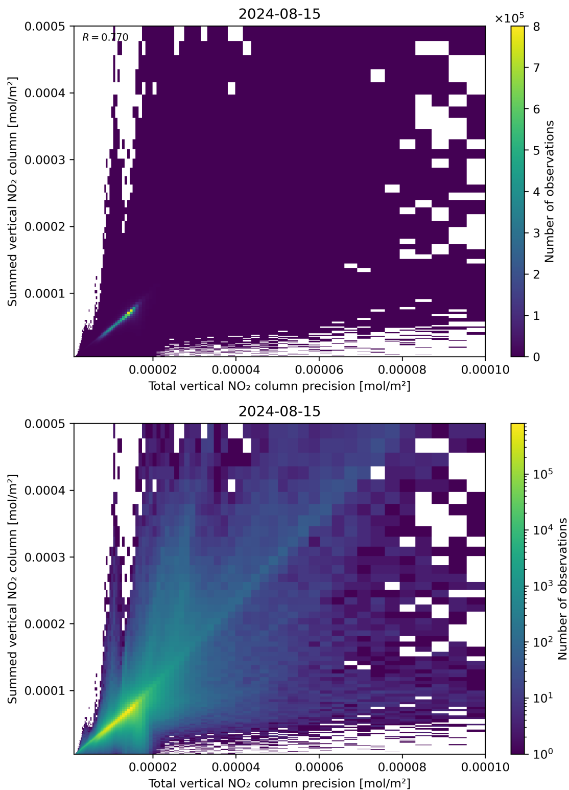
Figure 117: Scatter density plot of “Total vertical NO 2 column precision” against “Summed vertical NO 2 column” for 2024-08-14 to 2024-08-16.
