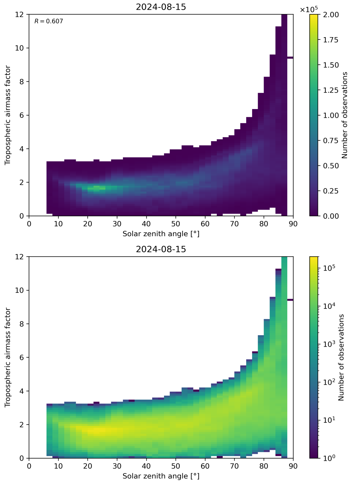
Figure 147: Scatter density plot of “Solar zenith angle” against “Tropospheric airmass factor” for 2024-08-14 to 2024-08-16.
