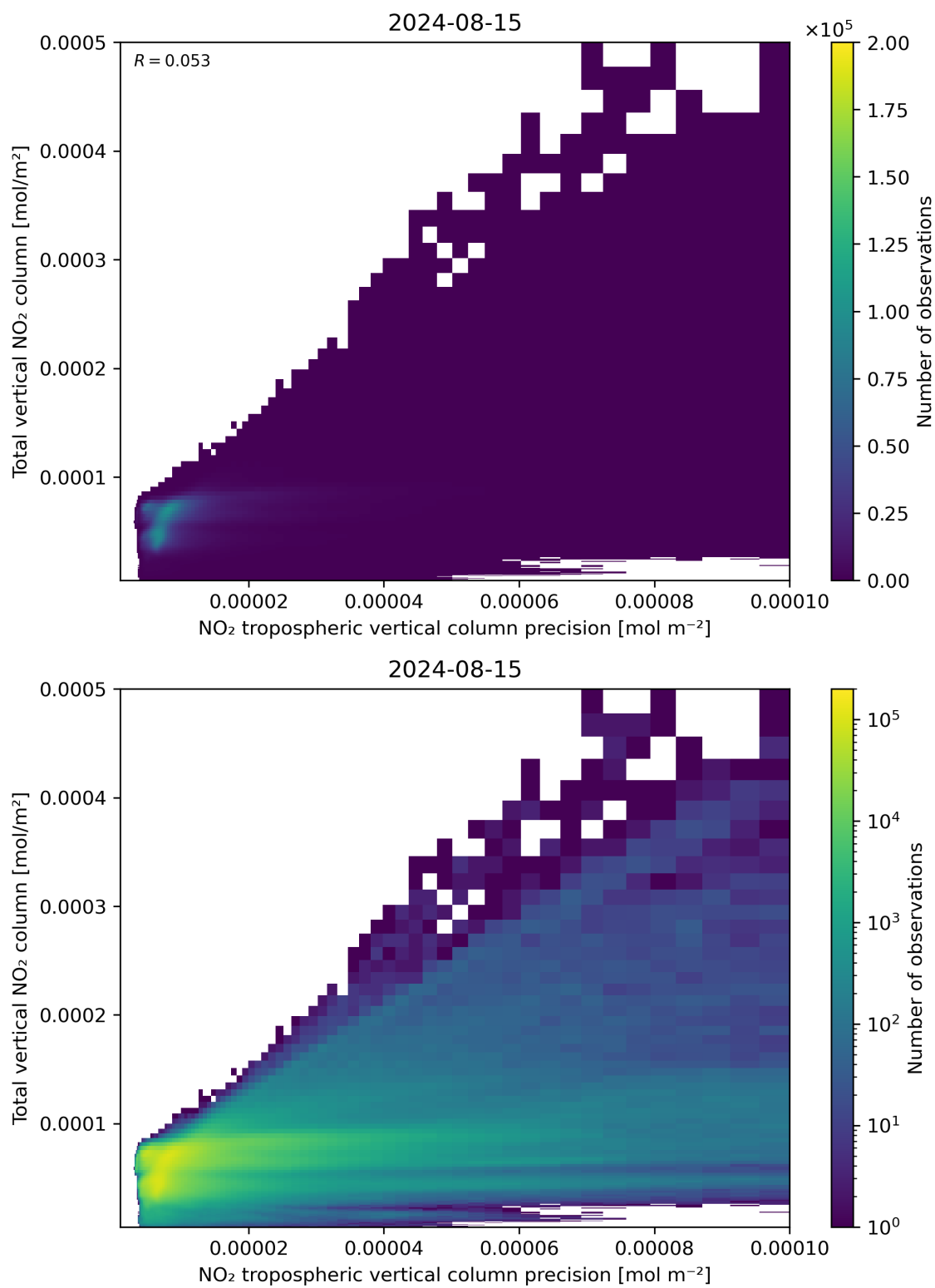
Figure 138: Scatter density plot of “NO 2 tropospheric vertical column precision” against “Total vertical NO 2 column” for 2024-08-14 to 2024-08-16.
