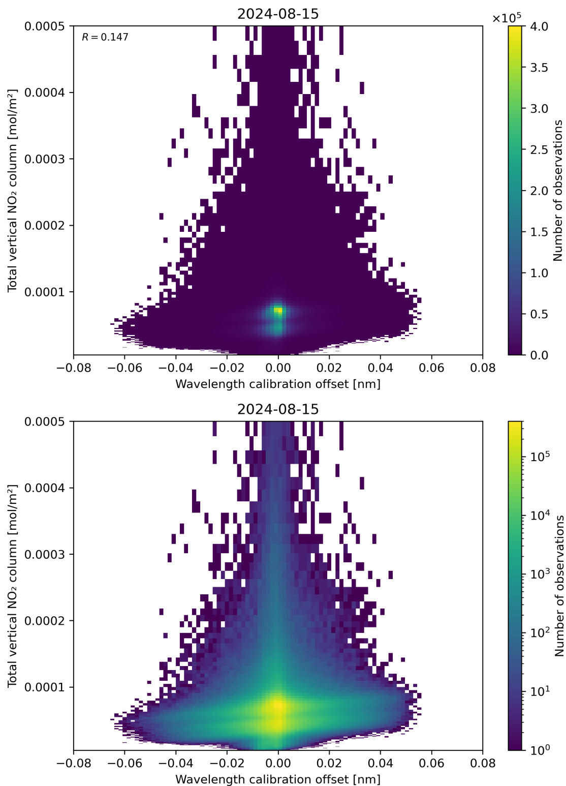
Figure 179: Scatter density plot of “Wavelength calibration offset” against “Total vertical NO 2 column” for 2024-08-14 to 2024-08-16.
