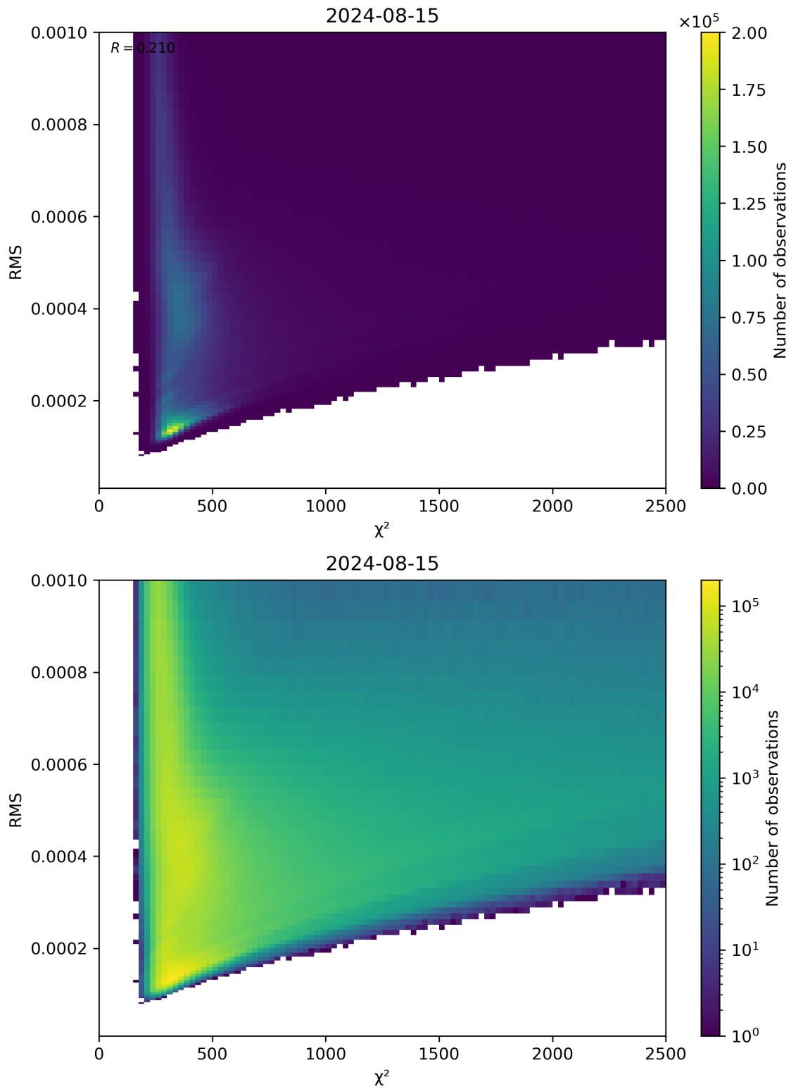
Figure 82: Scatter density plot of “ \chi^2 ” against “RMS” for 2024-08-14 to 2024-08-16.
