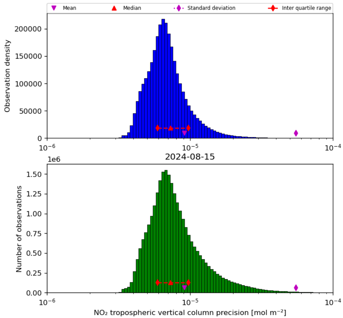
Figure 30: Histogram of “NO 2 tropospheric vertical column precision” for 2024-08-14 to 2024-08-16
