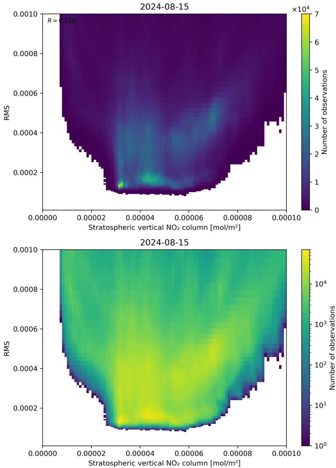
Figure 102: Scatter density plot of “Stratospheric vertical NO 2 column” against “RMS” for 2024-08-14 to 2024-08-16.
