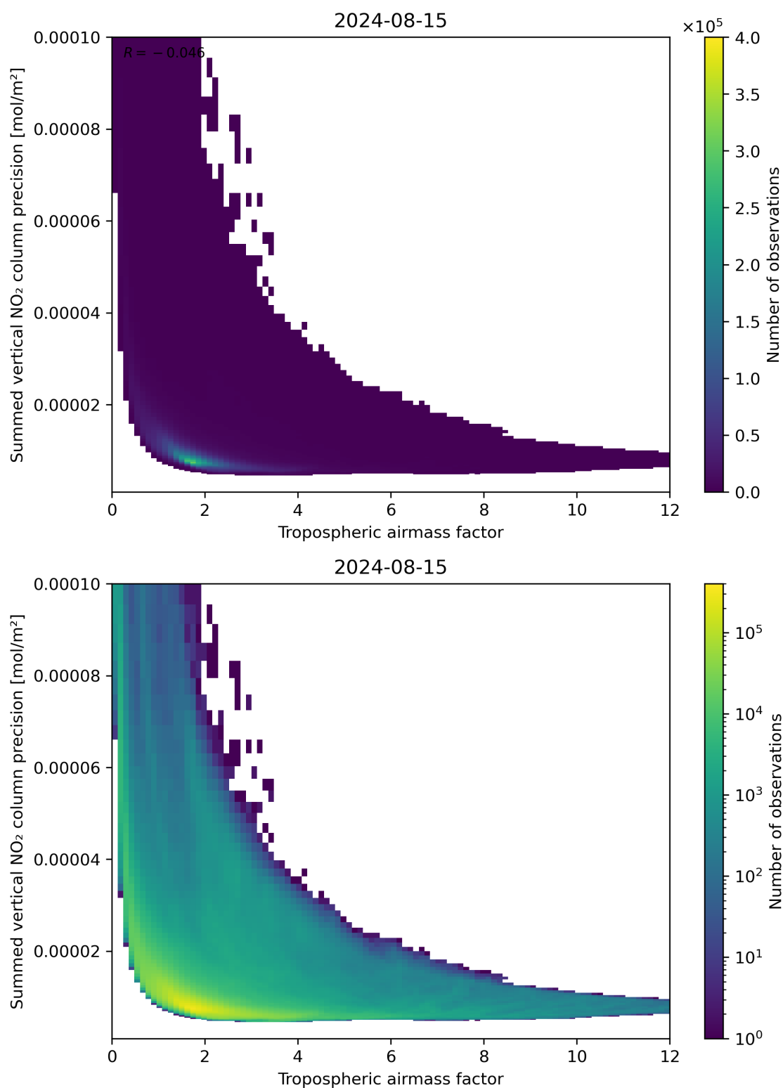
Figure 76: Scatter density plot of “Tropospheric air mass factor” against “Summed vertical NO 2 column precision” for 2024-08-14 to 2024-08-16.
