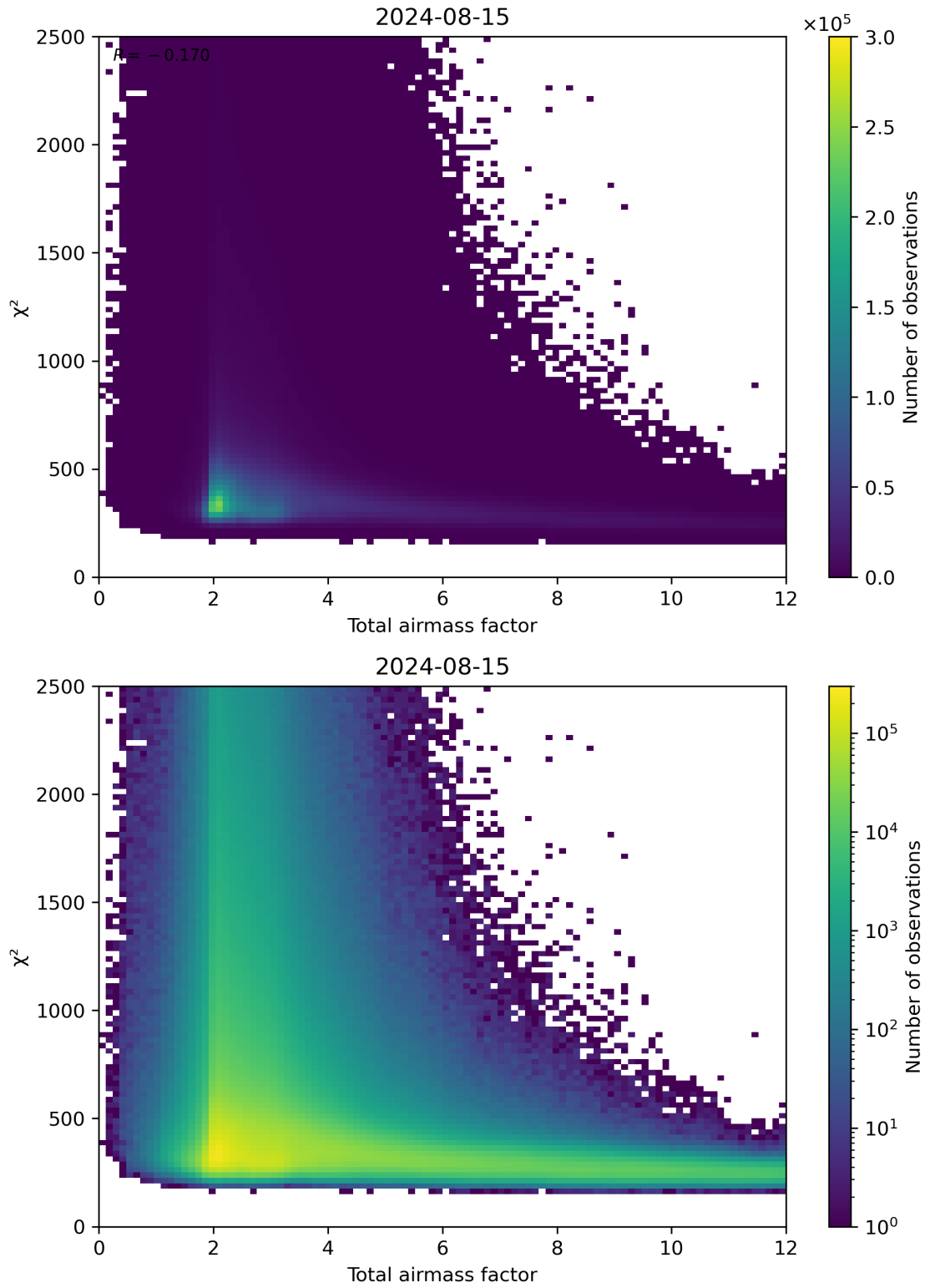
Figure 63: Scatter density plot of “Total airmass factor” against “ \chi^2 ” for 2024-08-14 to 2024-08-16.
