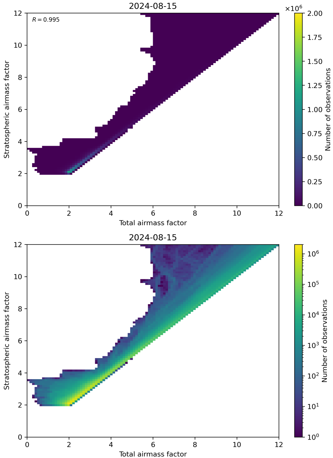
Figure 62: Scatter density plot of “Total airmass factor” against “Stratospheric airmass factor” for 2024-08-14 to 2024-08-16.
