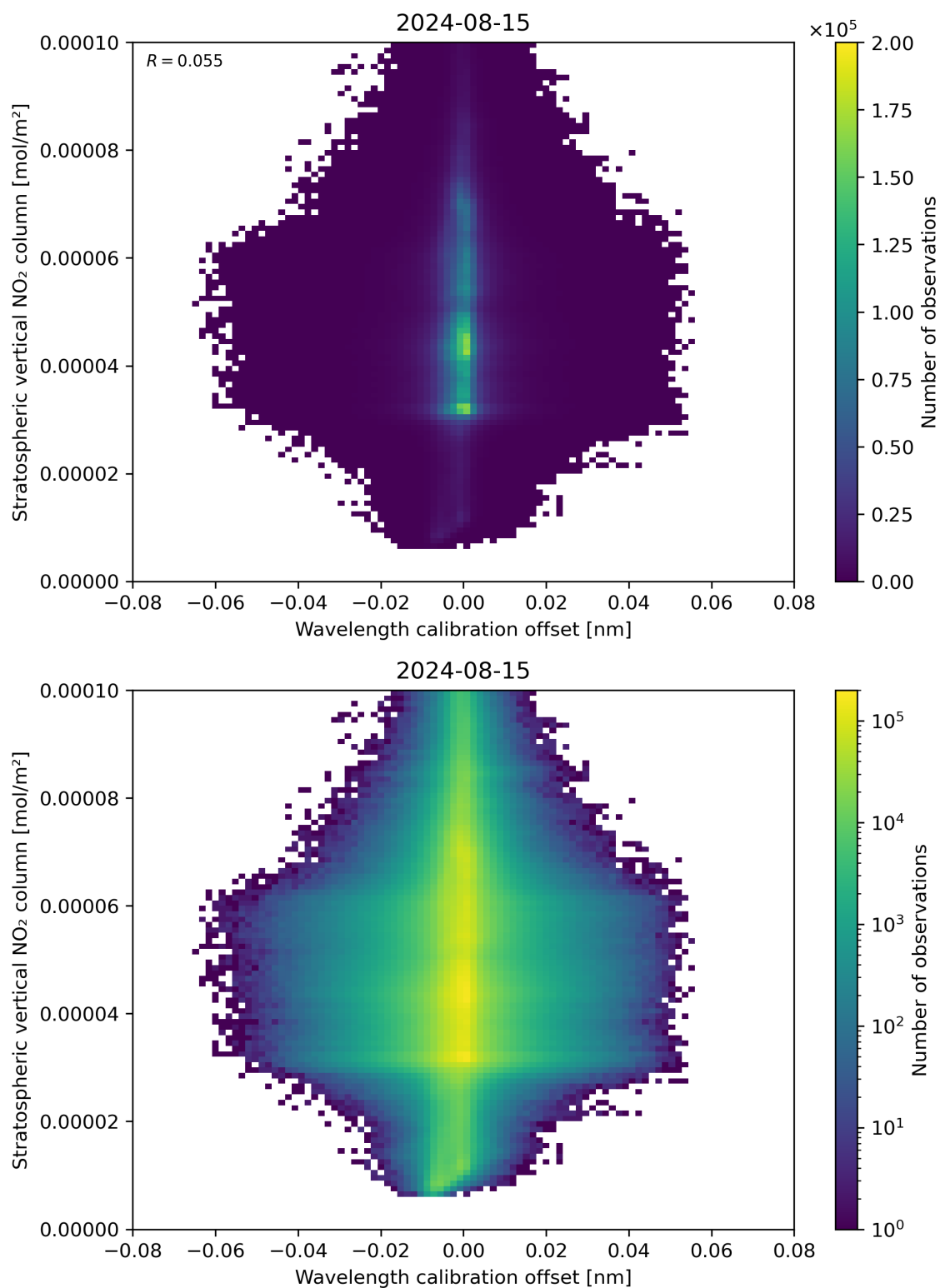
Figure 176: Scatter density plot of “Wavelength calibration offset” against “Stratospheric vertical NO 2 column” for 2024-08-14 to 2024-08-16.
