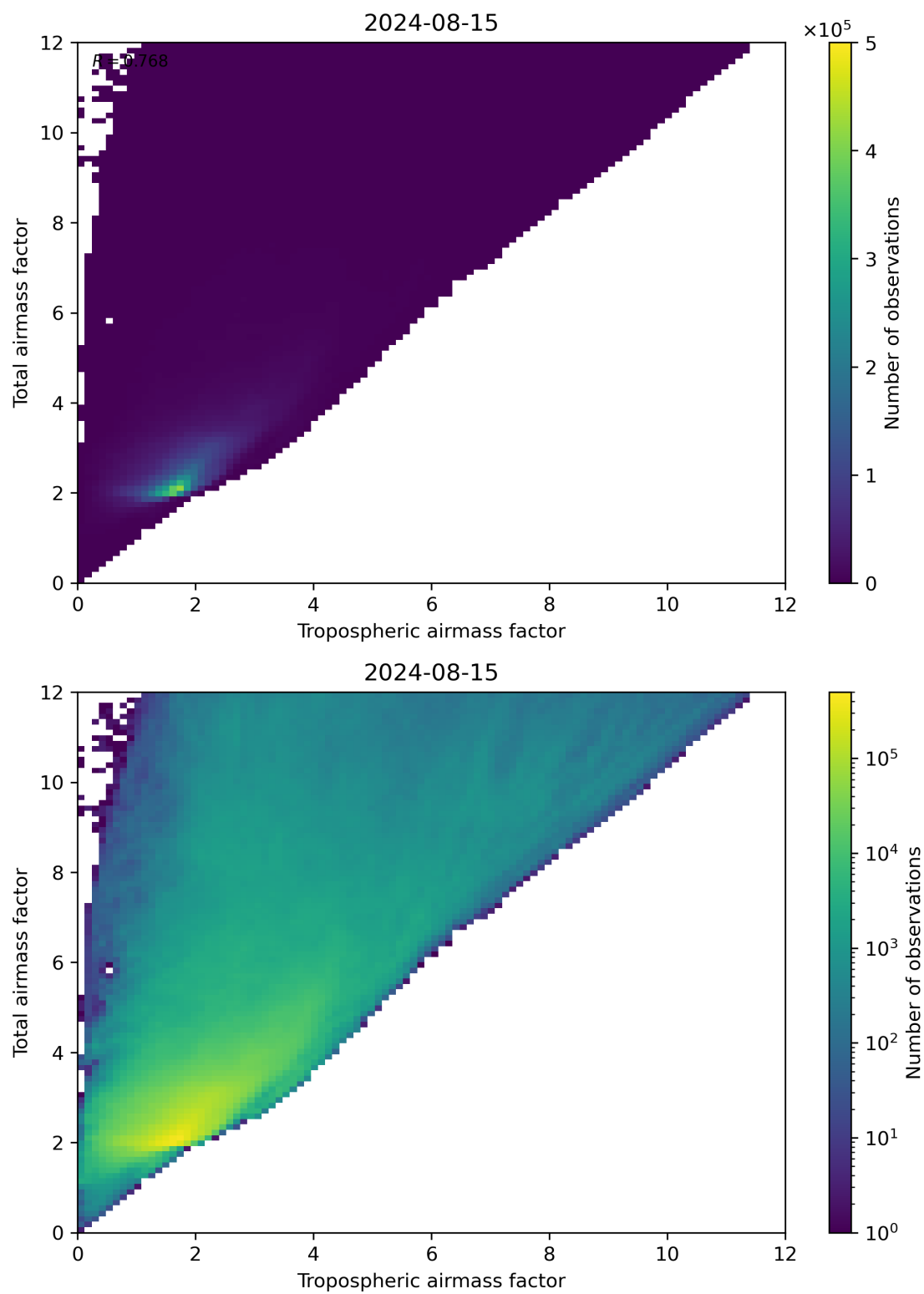
Figure 72: Scatter density plot of “Tropospheric airmass factor” against “Total airmass factor” for 2024-08-14 to 2024-08-16.
