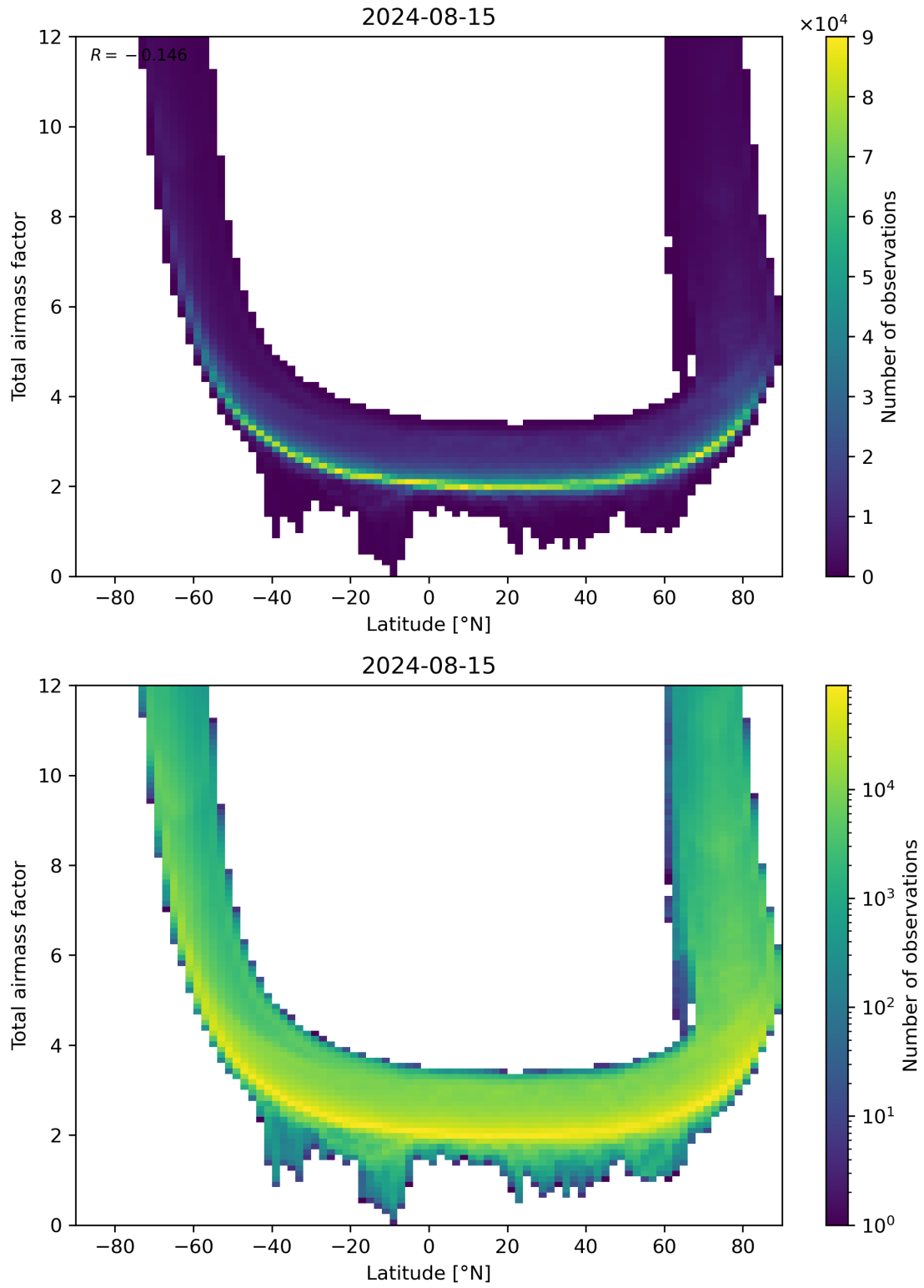
Figure 84: Scatter density plot of “Latitude” against “Total airmass factor” for 2024-08-14 to 2024-08-16.
