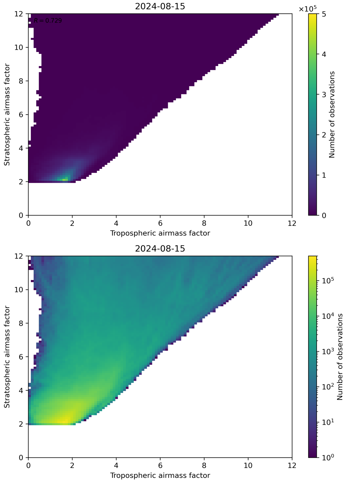
Figure 71: Scatter density plot of “Tropospheric airmass factor” against “Stratospheric airmass factor” for 2024-08-14 to 2024-08-16.
