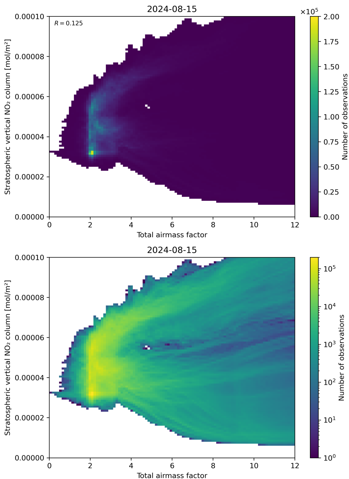
Figure 64: Scatter density plot of “Total airmass factor” against “Stratospheric vertical \text{NO}_2 column” for 2024-08-14 to 2024-08-16.
