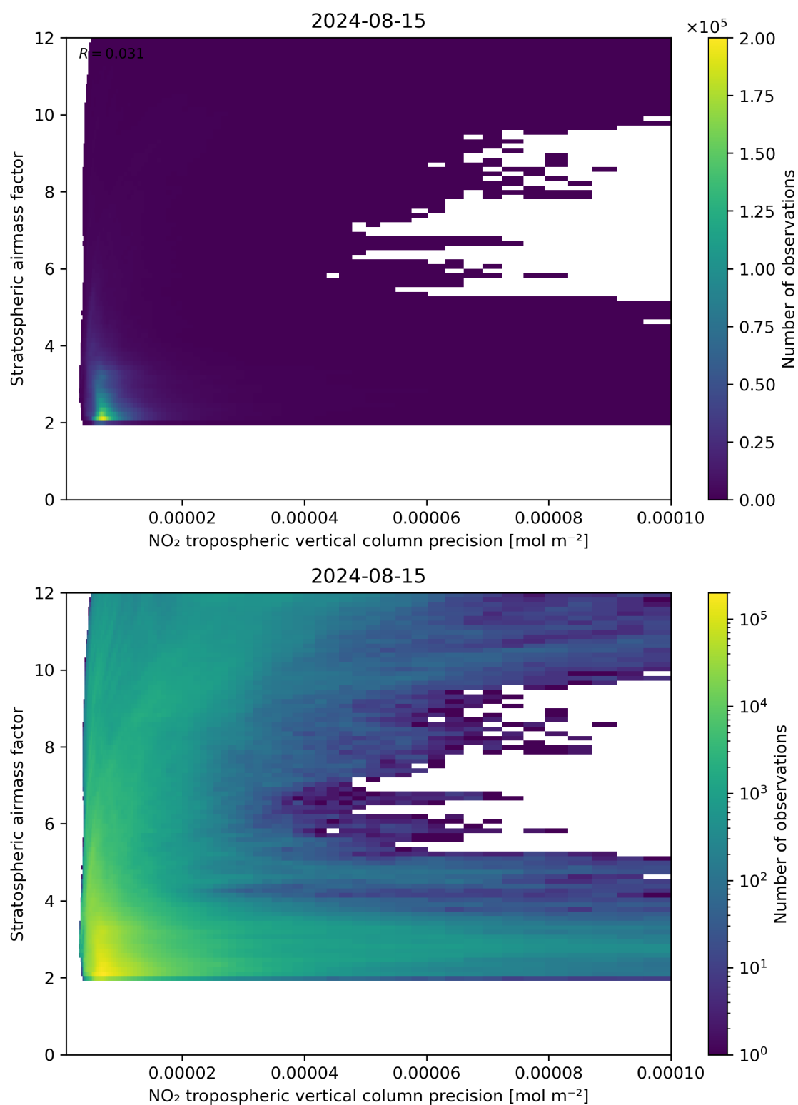
Figure 131: Scatter density plot of “NO 2 tropospheric vertical column precision” against “Stratospheric airmass factor” for 2024-08-14 to 2024-08-16.
