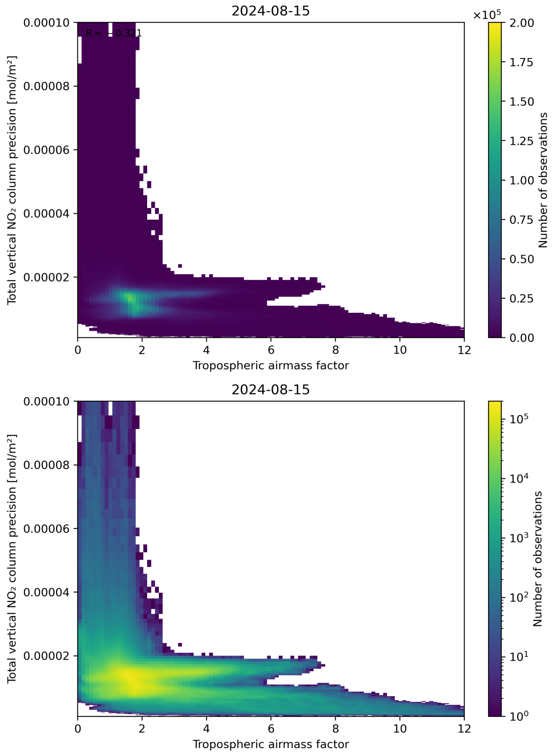
Figure 78: Scatter density plot of “Tropospheric air mass factor” against “Total vertical NO 2 column precision” for 2024-08-14 to 2024-08-16.
