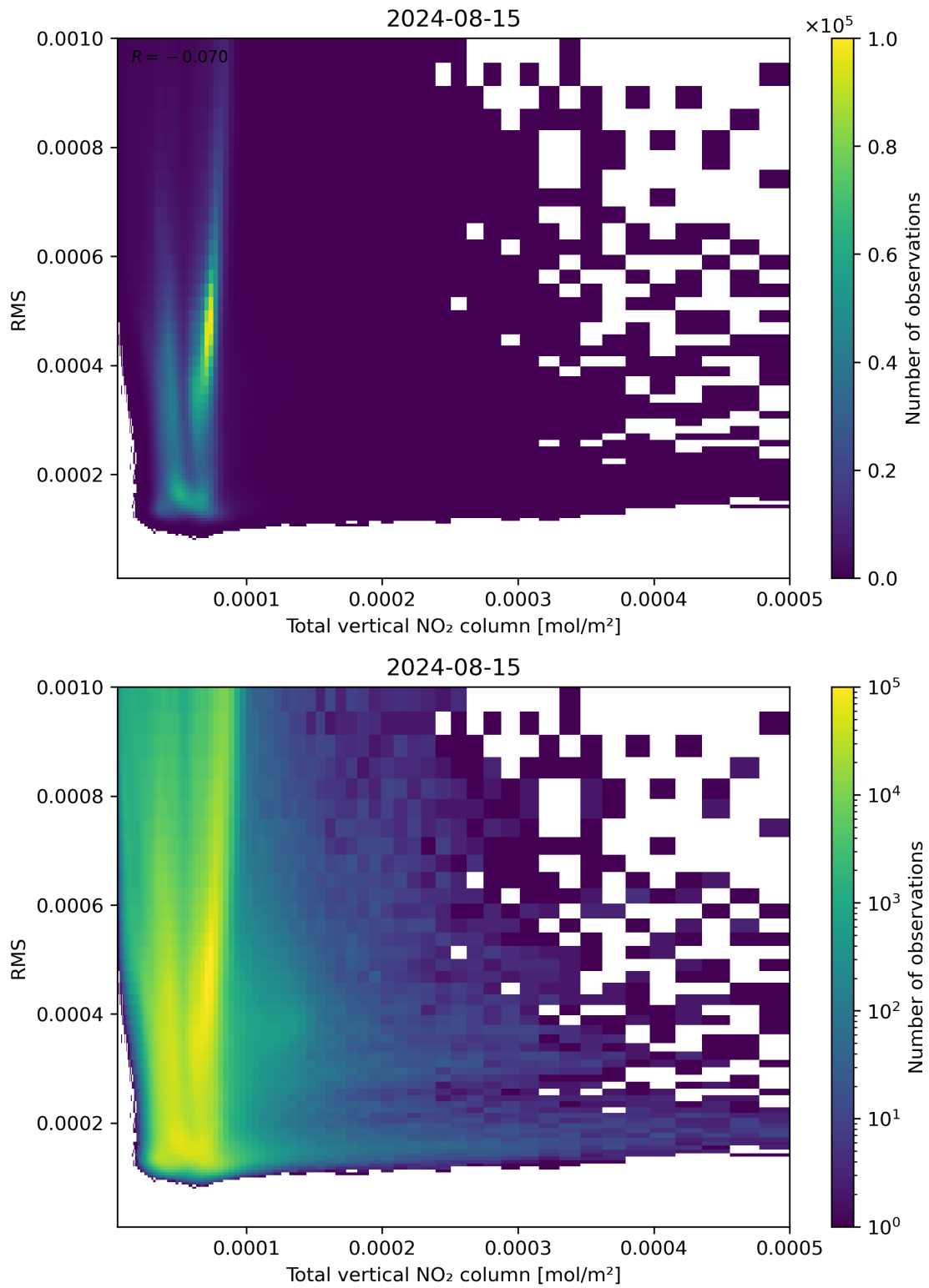
Figure 120: Scatter density plot of “Total vertical NO 2 column” against “RMS” for 2024-08-14 to 2024-08-16.
