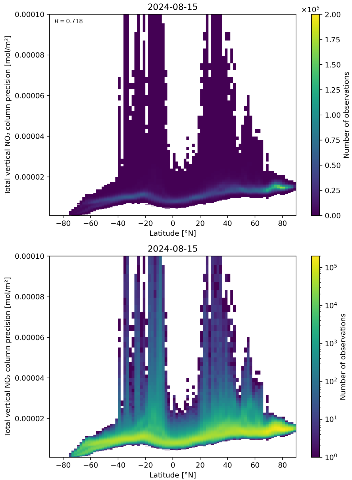
Figure 91: Scatter density plot of “Latitude” against “Total vertical NO 2 column precision” for 2024-08-14 to 2024-08-16.
