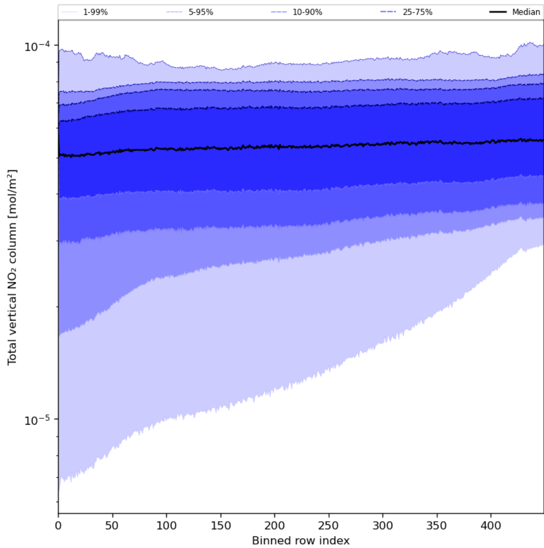
Figure 55: Along track statistics of “Total vertical NO 2 column” for 2024-08-14 to 2024-08-16
