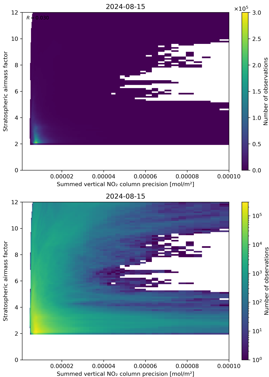
Figure 106: Scatter density plot of “Summed vertical NO 2 column precision” against “Stratospheric airmass factor” for 2024-08-14 to 2024-08-16.
