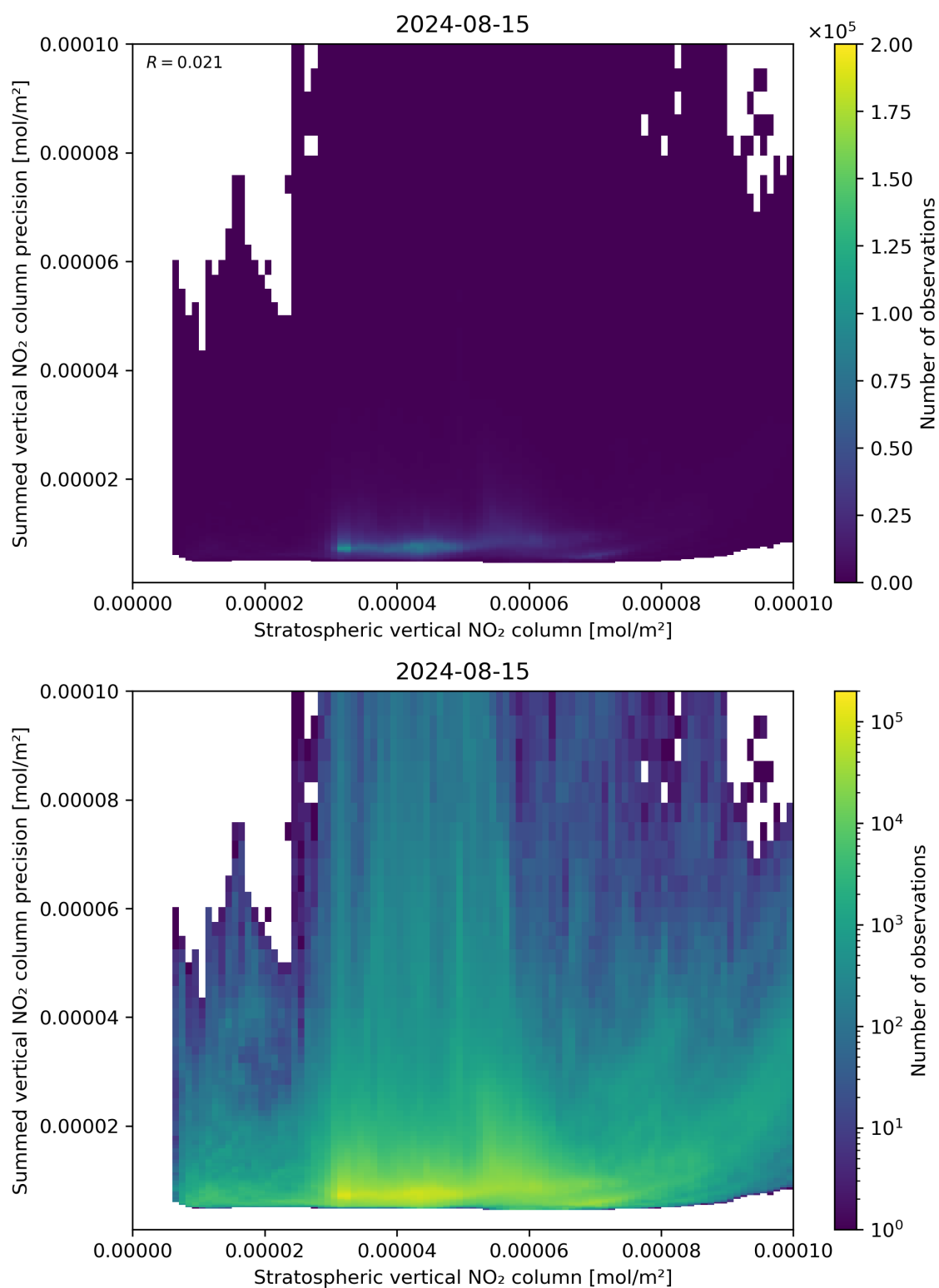
Figure 99: Scatter density plot of “Stratospheric vertical NO 2 column” against “Summed vertical NO 2 column precision” for 2024-08-14 to 2024-08-16.
