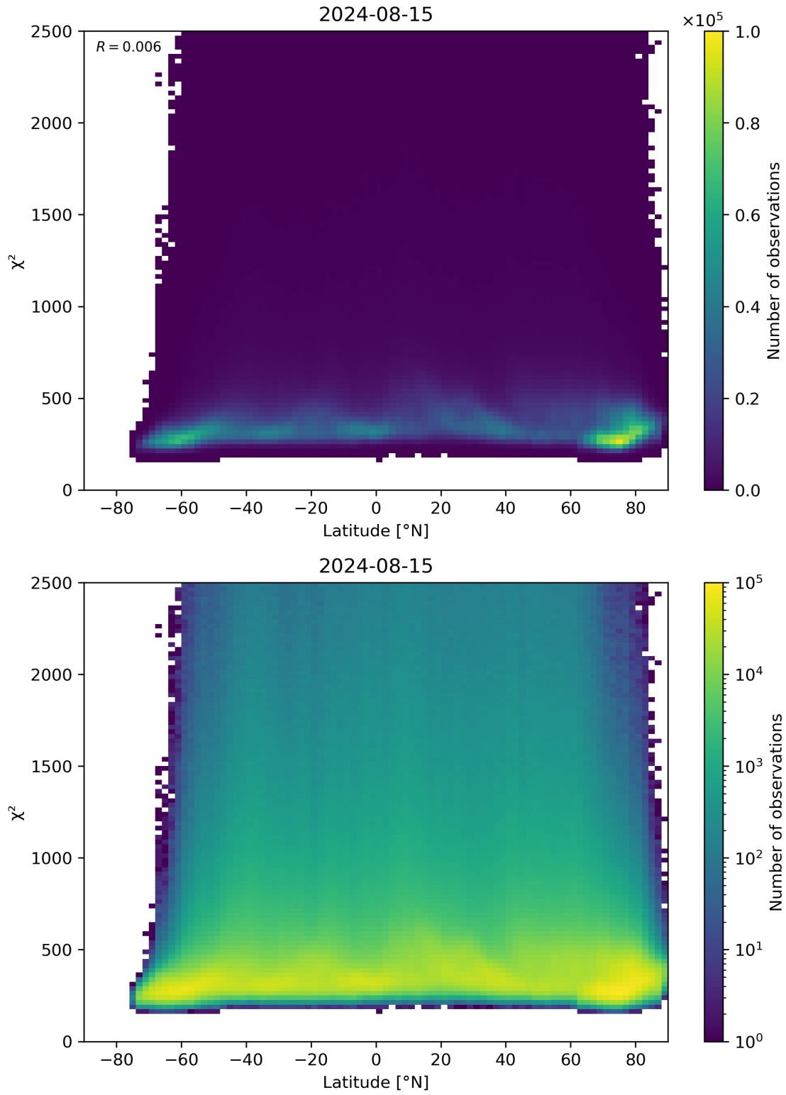
Figure 86: Scatter density plot of “Latitude” against “ \chi^2 ” for 2024-08-14 to 2024-08-16.
