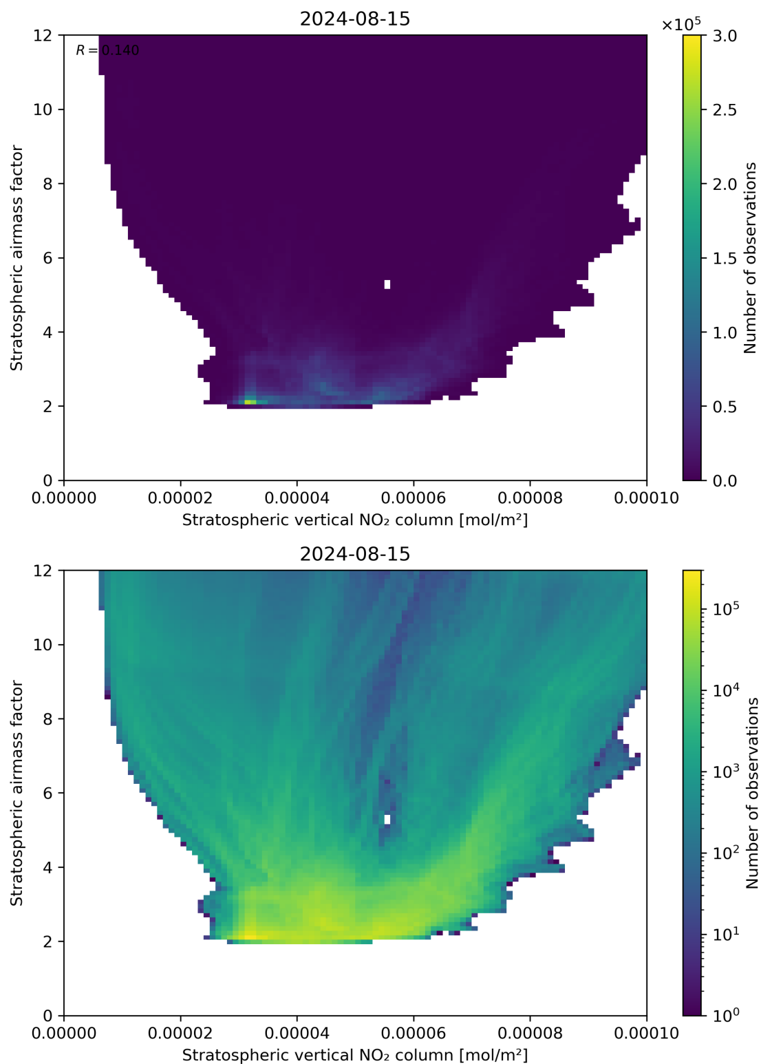
Figure 96: Scatter density plot of “Stratospheric vertical NO 2 column” against “Stratospheric airmass factor” for 2024-08-14 to 2024-08-16.
