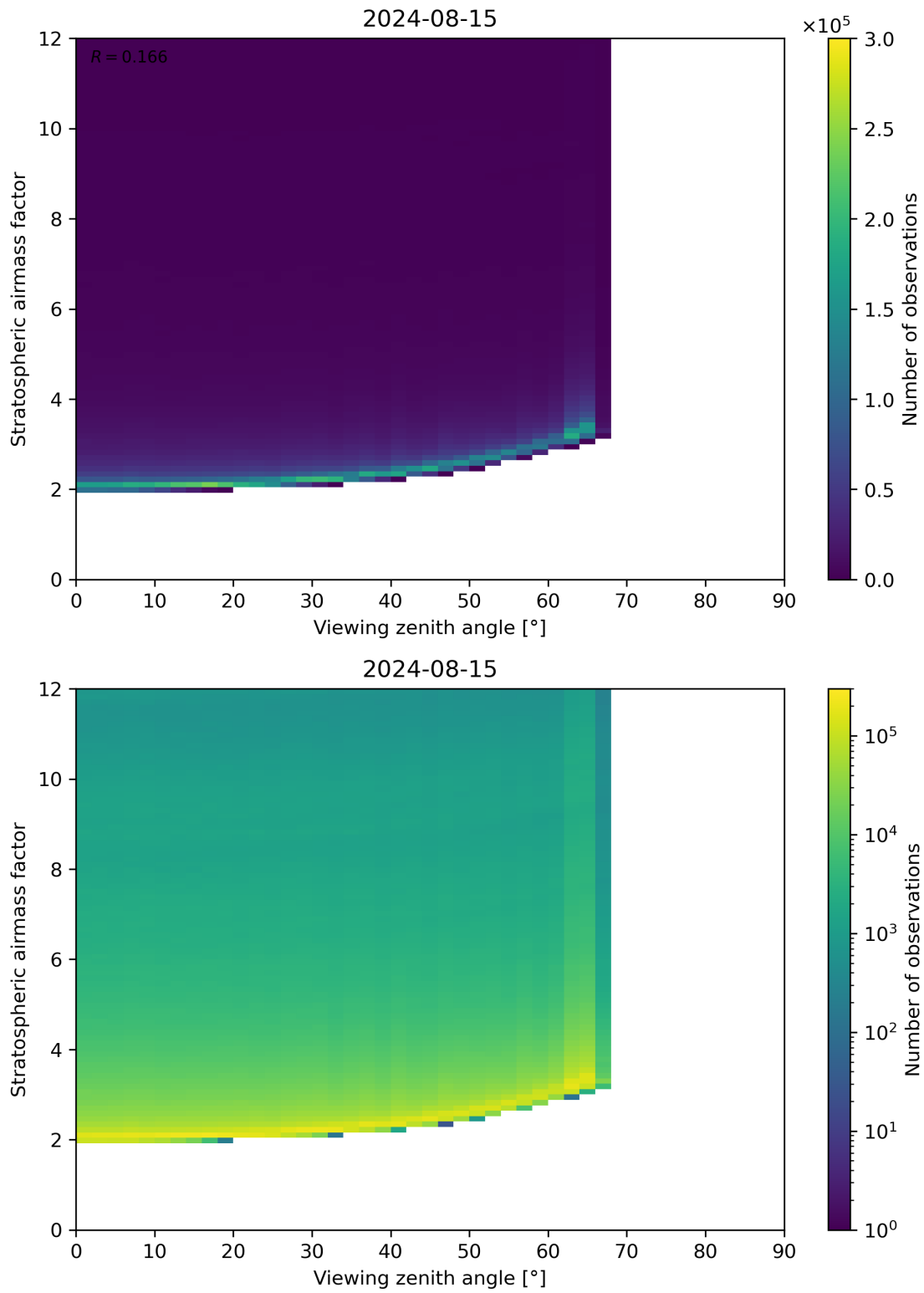
Figure 159: Scatter density plot of “Viewing zenith angle” against “Stratospheric airmass factor” for 2024-08-14 to 2024-08-16.
