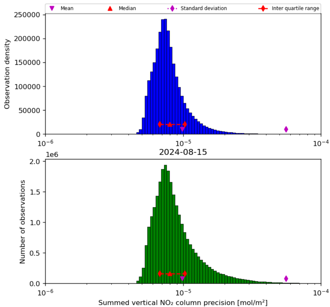
Figure 41: Histogram of "Summed vertical NO 2 column precision" for 2024-08-14 to 2024-08-16
