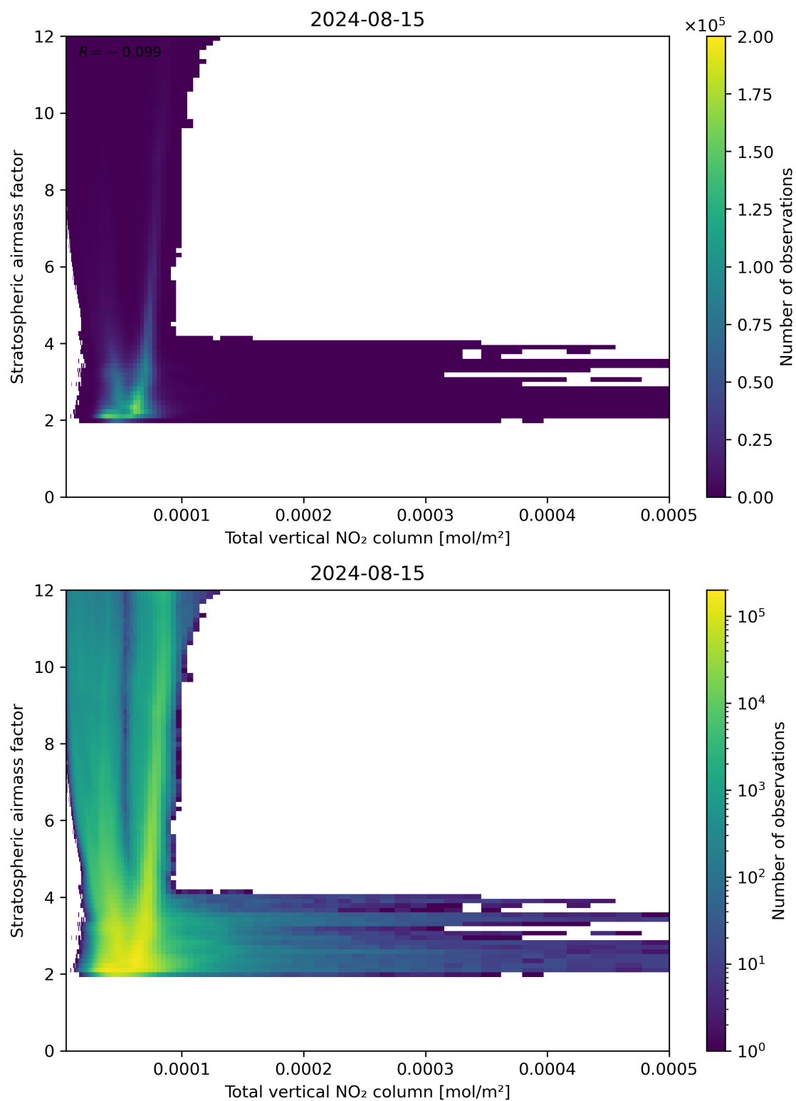
Figure 110: Scatter density plot of “Total vertical NO 2 column” against “Stratospheric airmass factor” for 2024-08-14 to 2024-08-16.
