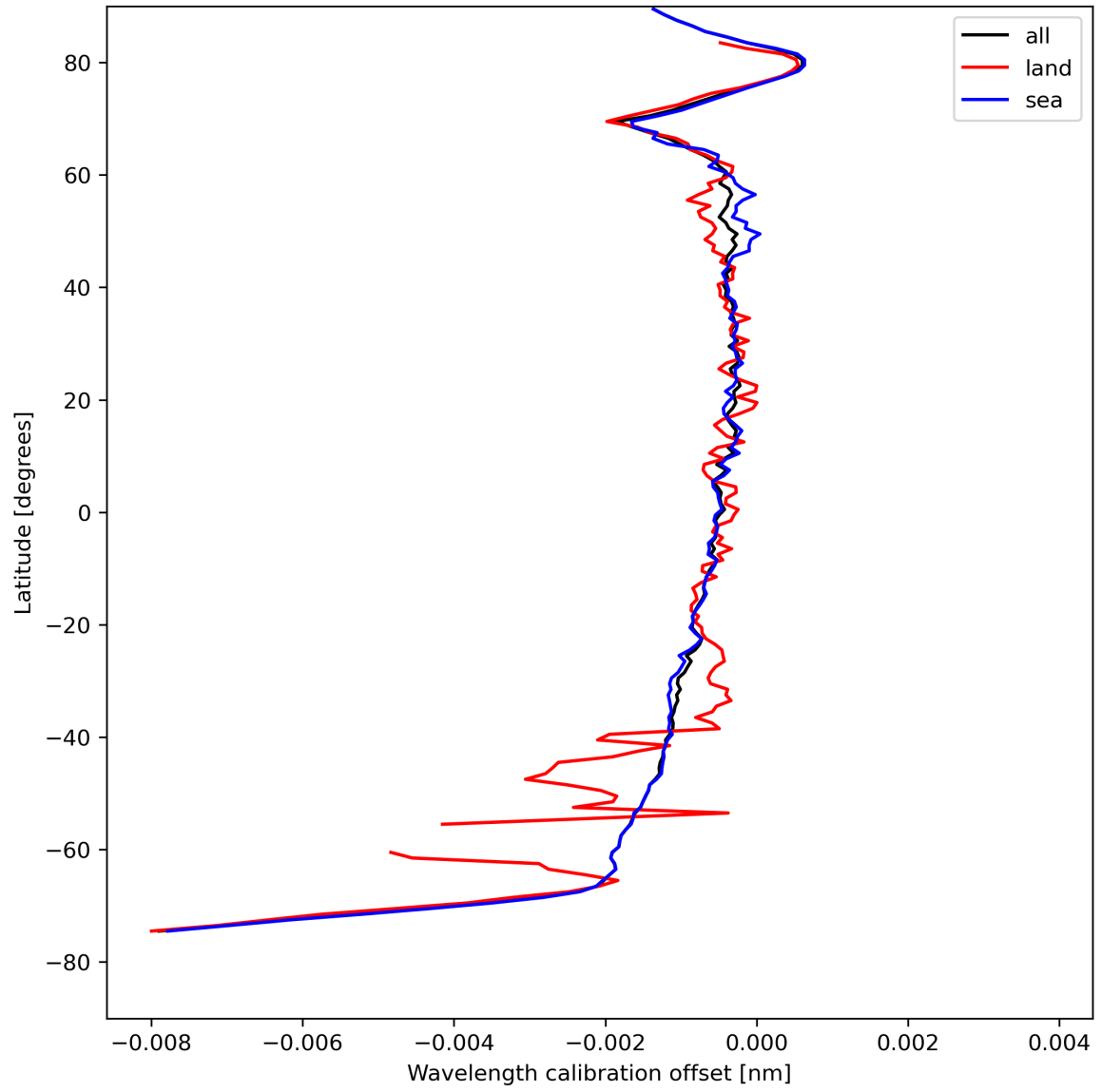
Figure 18: Zonal average of “Wavelength calibration offset” for 2024-08-14 to 2024-08-16.
