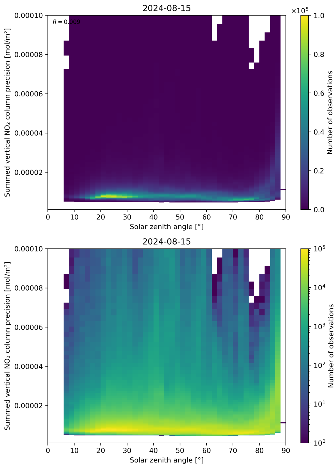
Figure 152: Scatter density plot of “Solar zenith angle” against “Summed vertical NO 2 column precision” for 2024-08-14 to 2024-08-16.
