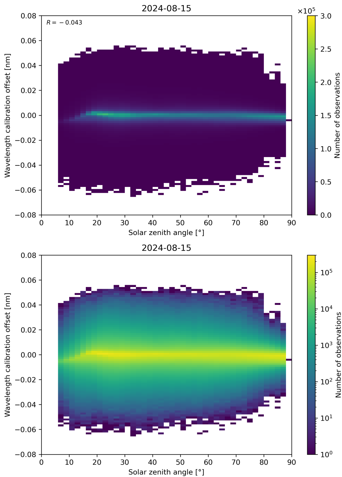
Figure 158: Scatter density plot of “Solar zenith angle” against “Wavelength calibration offset” for 2024-08-14 to 2024-08-16.
