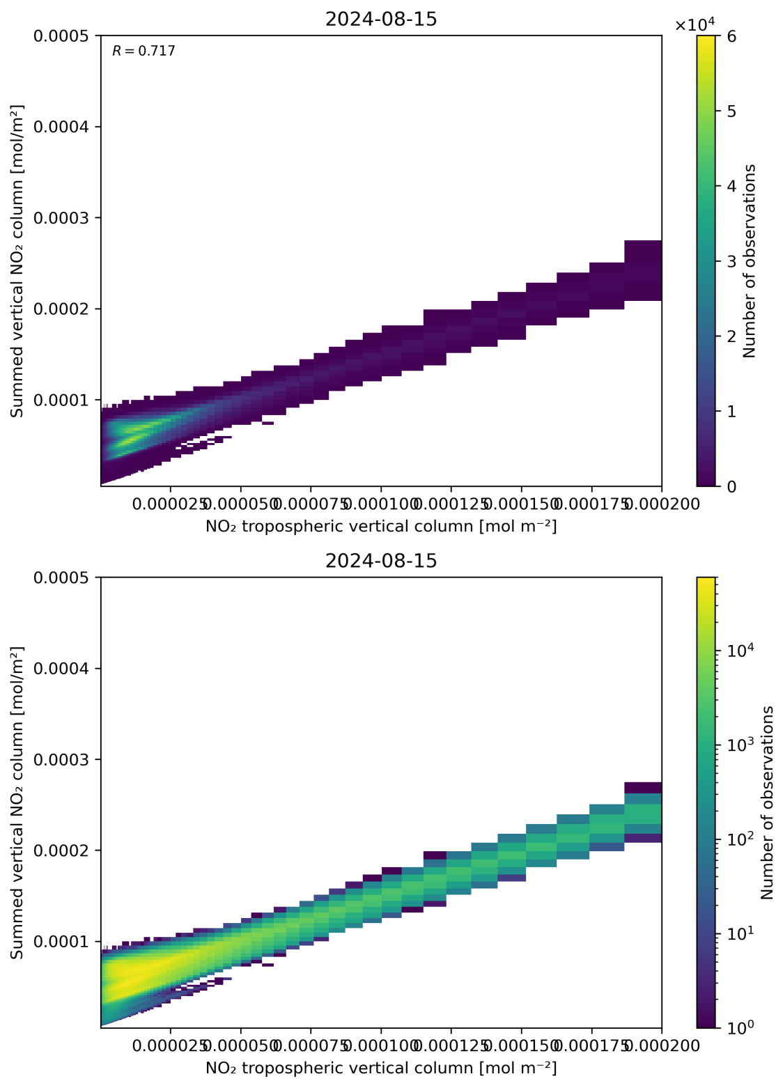
Figure 126: Scatter density plot of “NO 2 tropospheric vertical column” against “Summed vertical NO 2 column” for 2024-08-14 to 2024-08-16.
