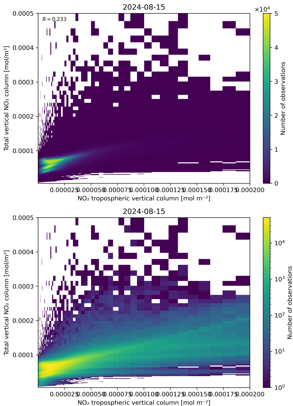
Figure 128: Scatter density plot of “NO 2 tropospheric vertical column” against “Total vertical NO 2 column” for 2024-08-14 to 2024-08-16.
