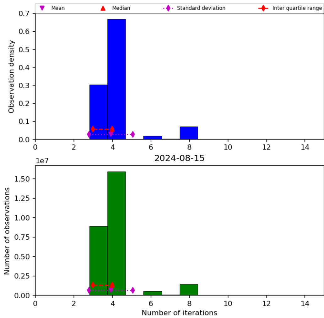
Figure 34: Histogram of “Number of iterations” for 2024-08-14 to 2024-08-16
