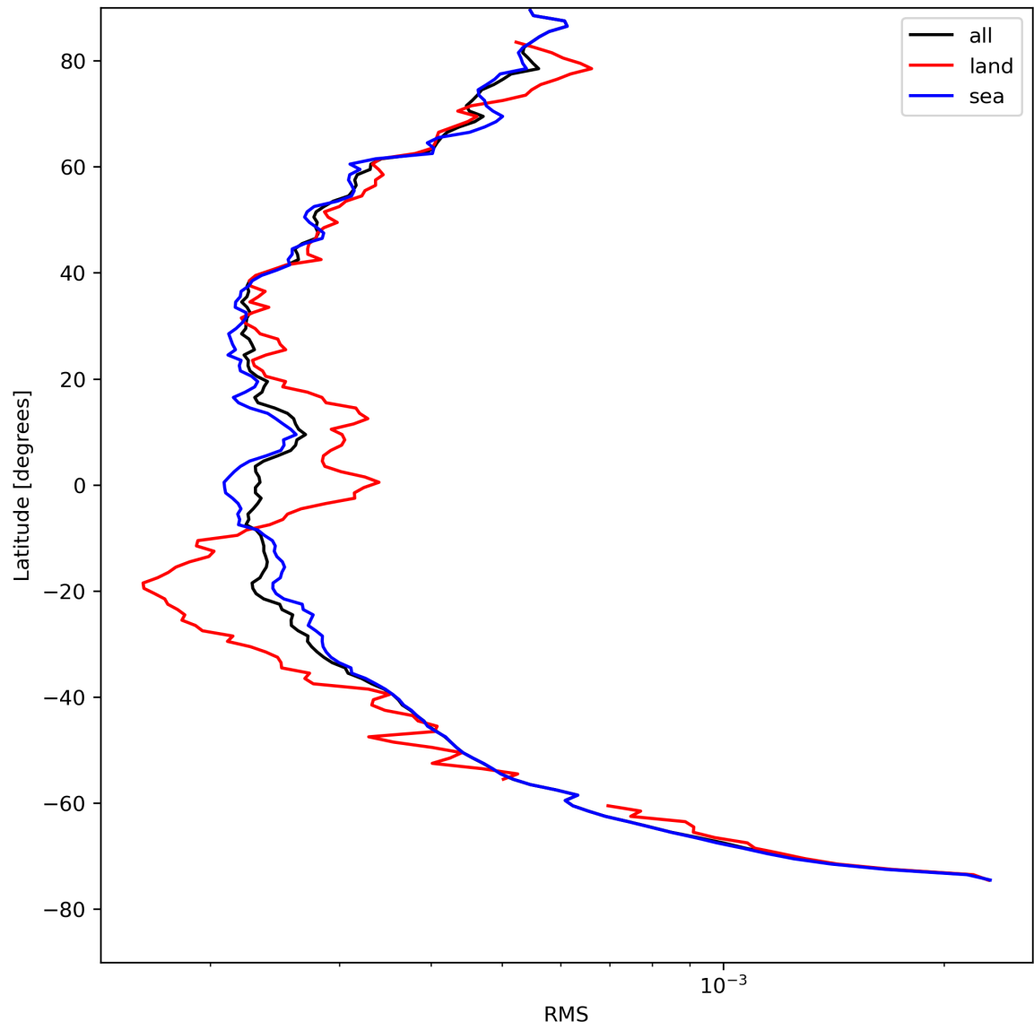
Figure 26: Zonal average of “RMS” for 2024-08-14 to 2024-08-16.
