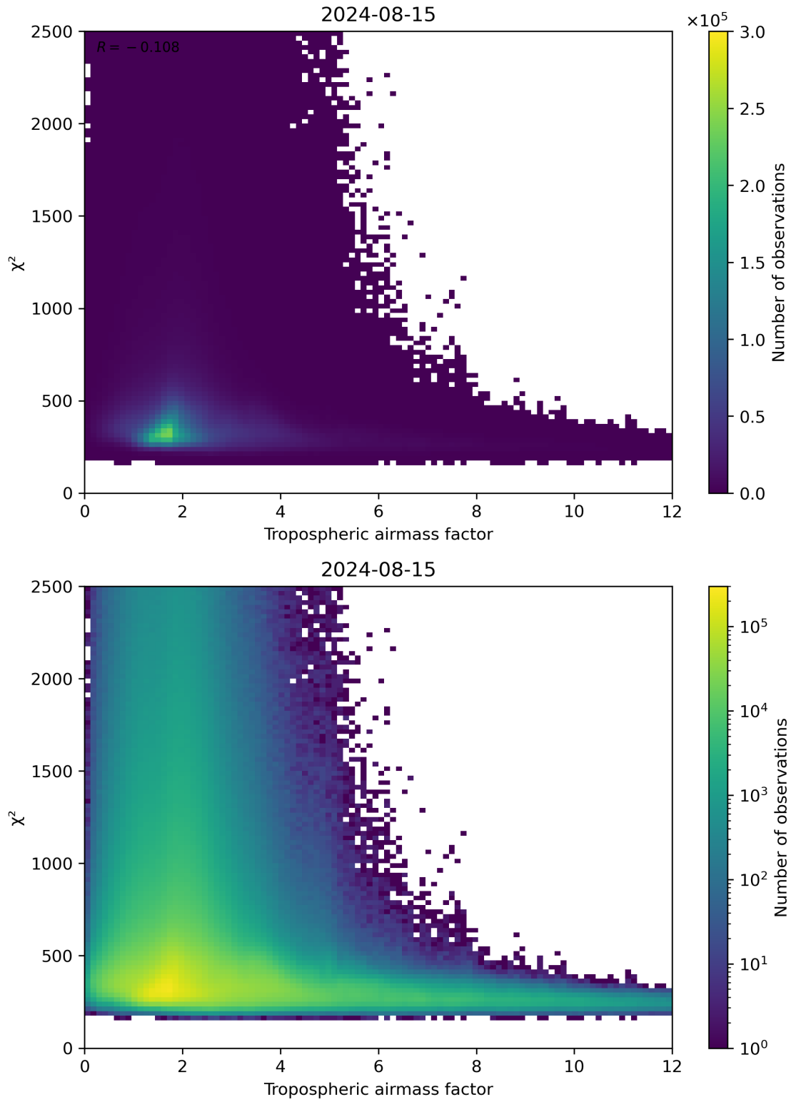
Figure 73: Scatter density plot of “Tropospheric airmass factor” against “ \chi^2 ” for 2024-08-14 to 2024-08-16.
