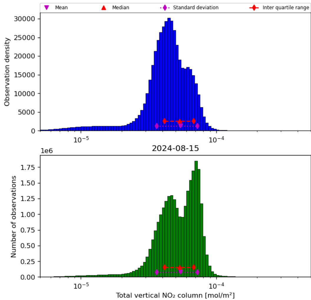
Figure 38: Histogram of “Total vertical NO 2 column” for 2024-08-14 to 2024-08-16
