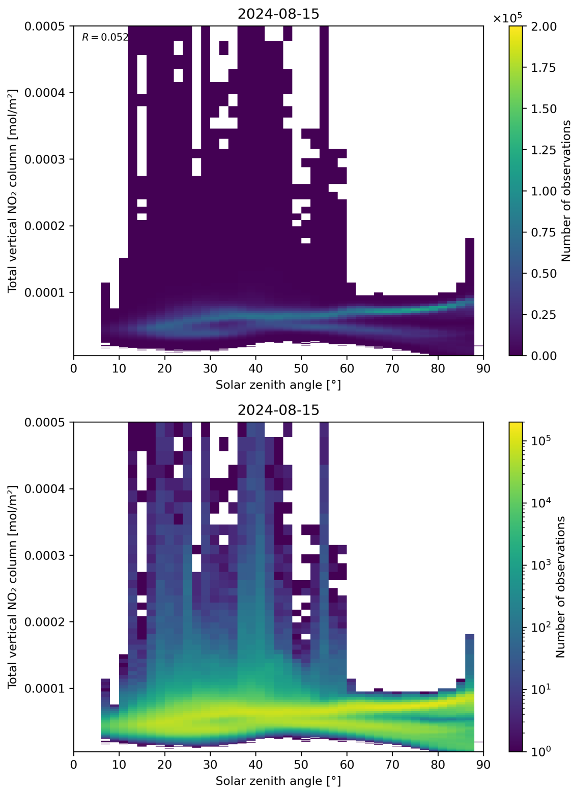
Figure 153: Scatter density plot of “Solar zenith angle” against “Total vertical NO 2 column” for 2024-08-14 to 2024-08-16.
