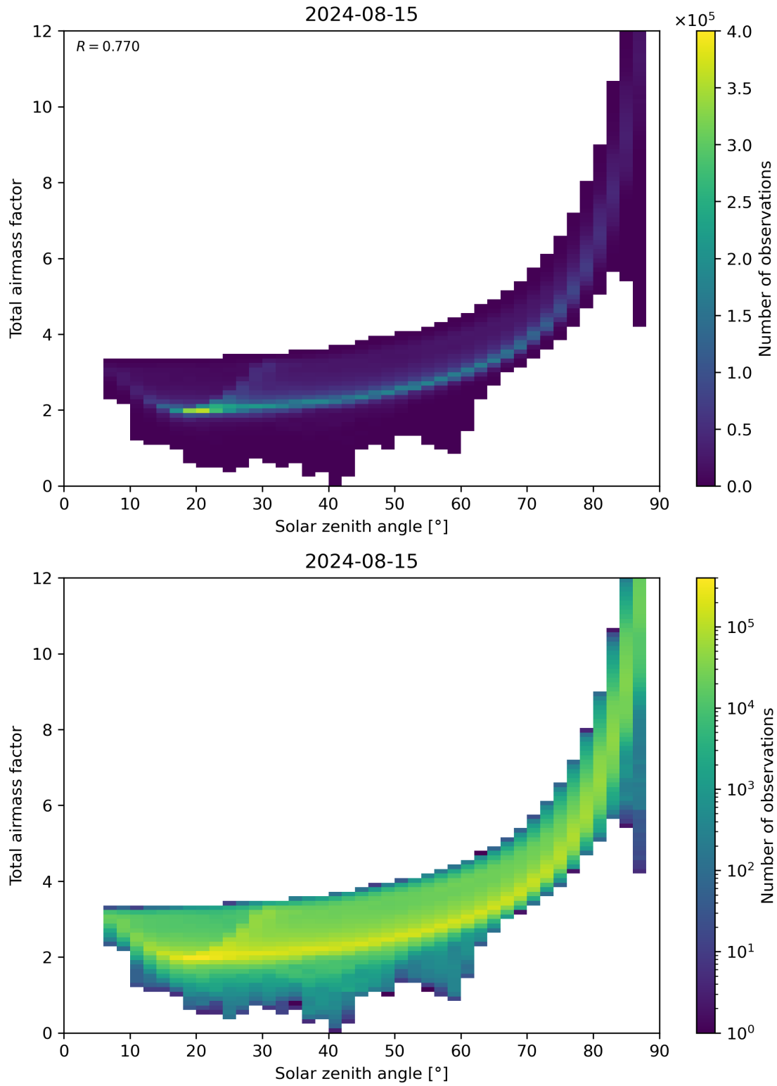
Figure 146: Scatter density plot of “Solar zenith angle” against “Total air mass factor” for 2024-08-14 to 2024-08-16.
