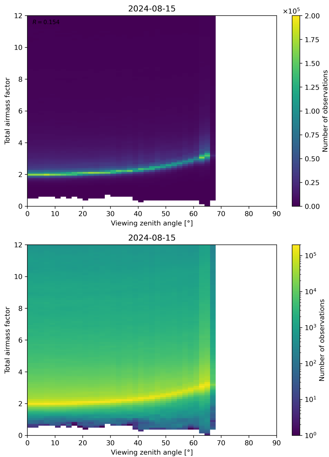
Figure 160: Scatter density plot of “Viewing zenith angle” against “Total airmass factor” for 2024-08-14 to 2024-08-16.
