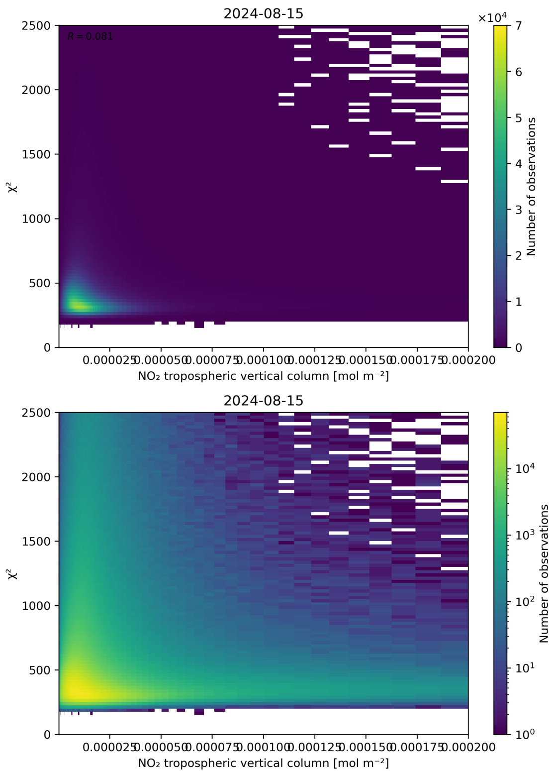
Figure 124: Scatter density plot of “NO 2 tropospheric vertical column” against “ \chi^2 ” for 2024-08-14 to 2024-08-16.
