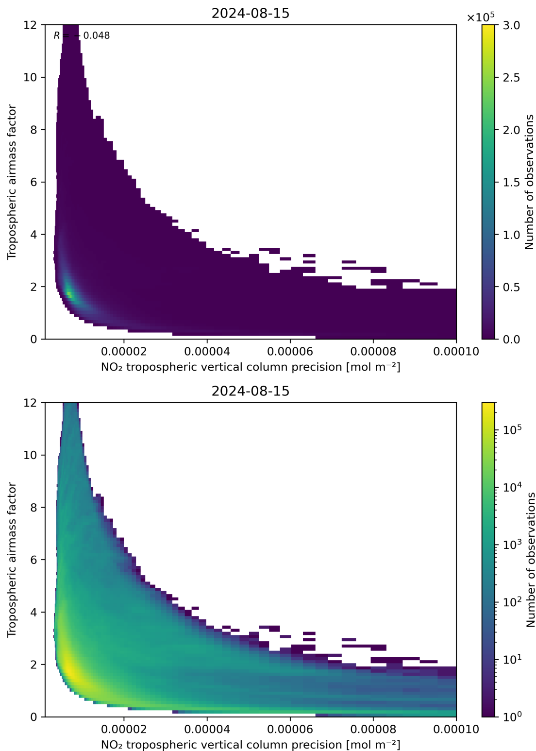
Figure 133: Scatter density plot of “NO 2 tropospheric vertical column precision” against “Tropospheric airmass factor” for 2024-08-14 to 2024-08-16.
