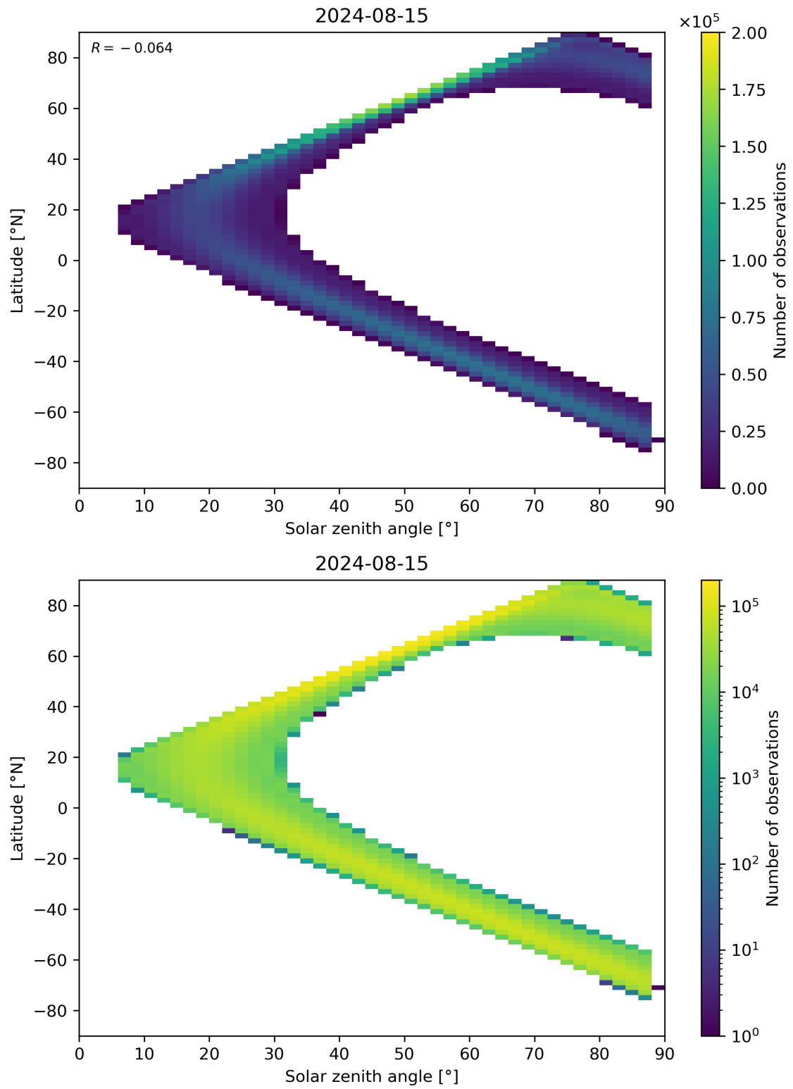
Figure 149: Scatter density plot of “Solar zenith angle” against “Latitude” for 2024-08-14 to 2024-08-16.
