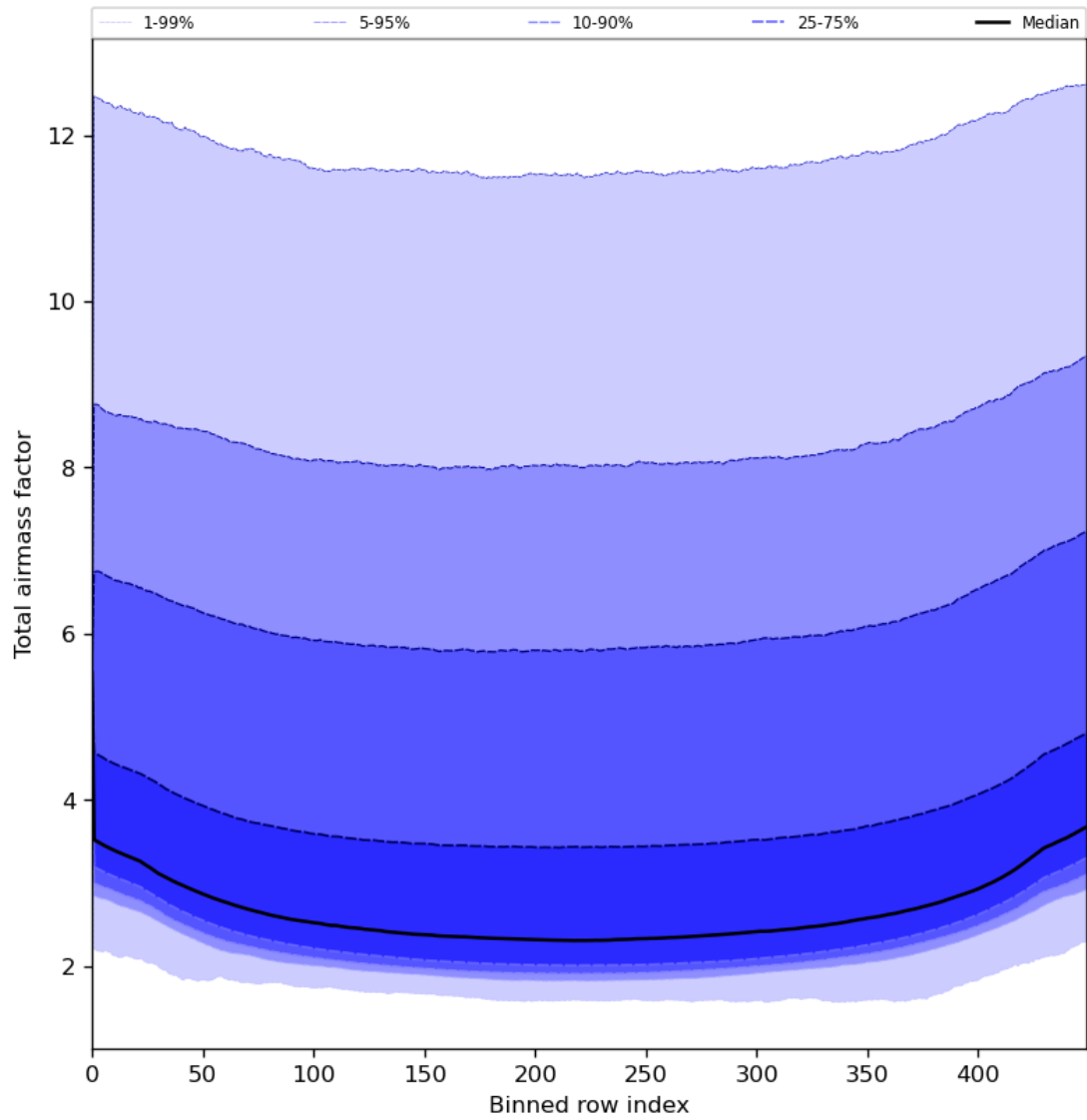
Figure 49: Along track statistics of “Total airmass factor” for 2024-08-14 to 2024-08-16
