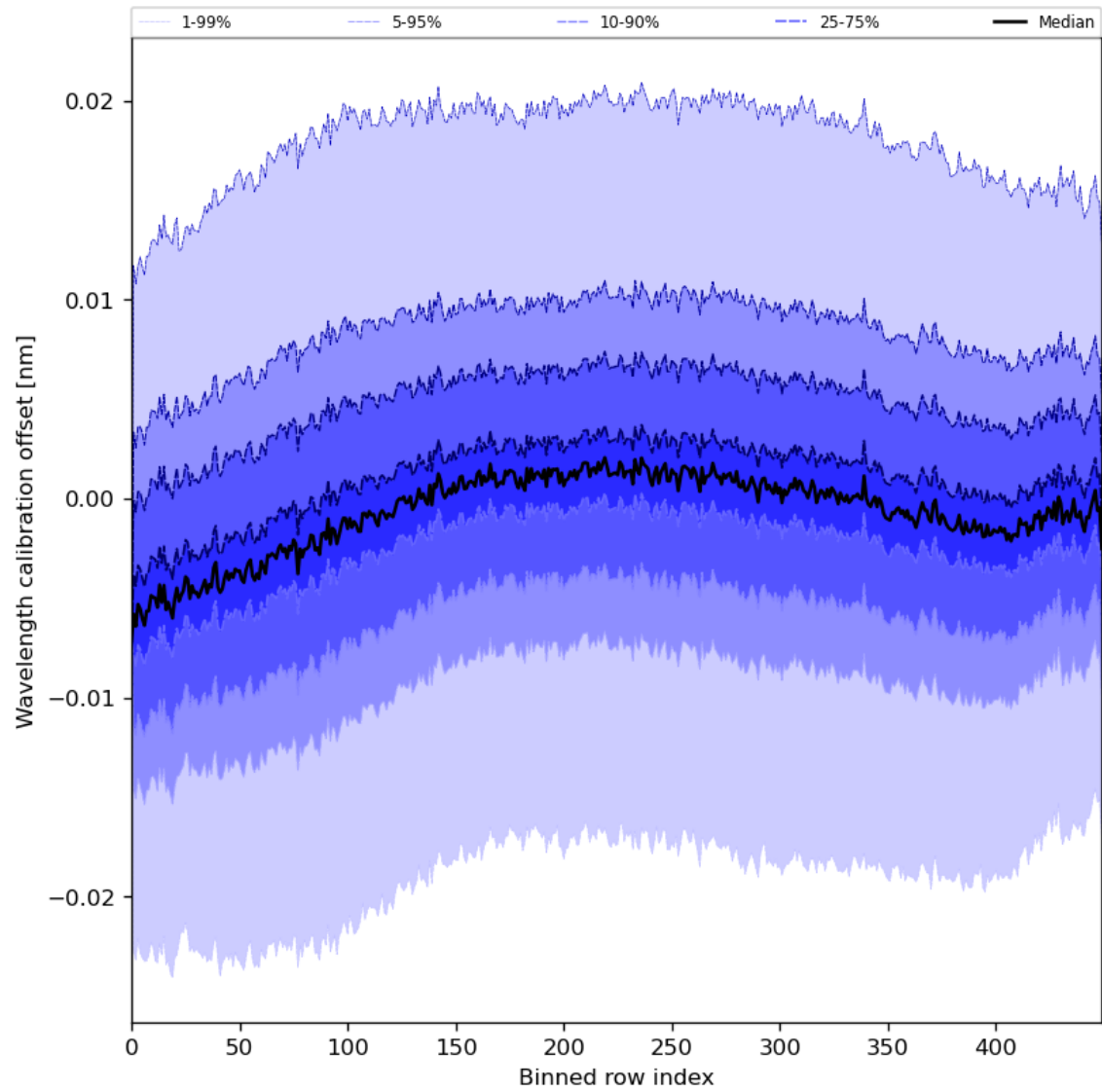
Figure 52: Along track statistics of “Wavelength calibration offset” for 2024-08-14 to 2024-08-16
