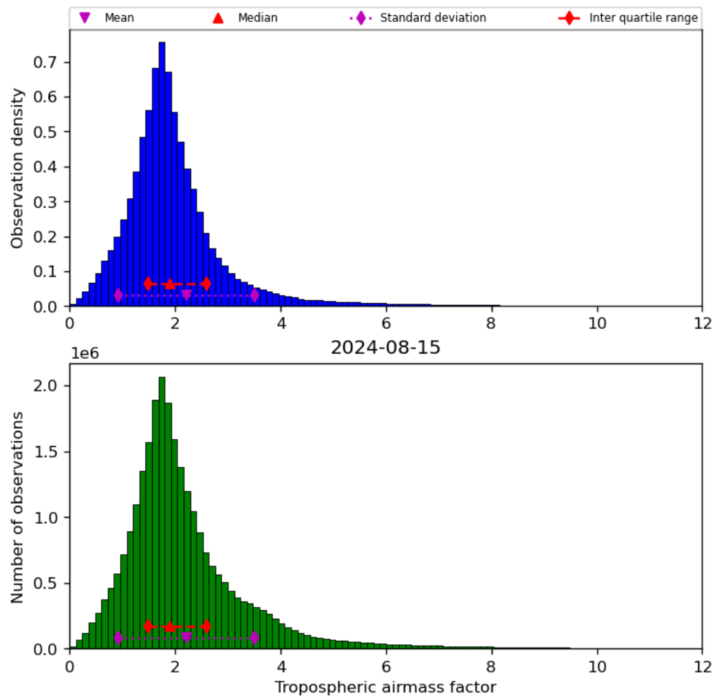
Figure 31: Histogram of “Tropospheric airmass factor” for 2024-08-14 to 2024-08-16
