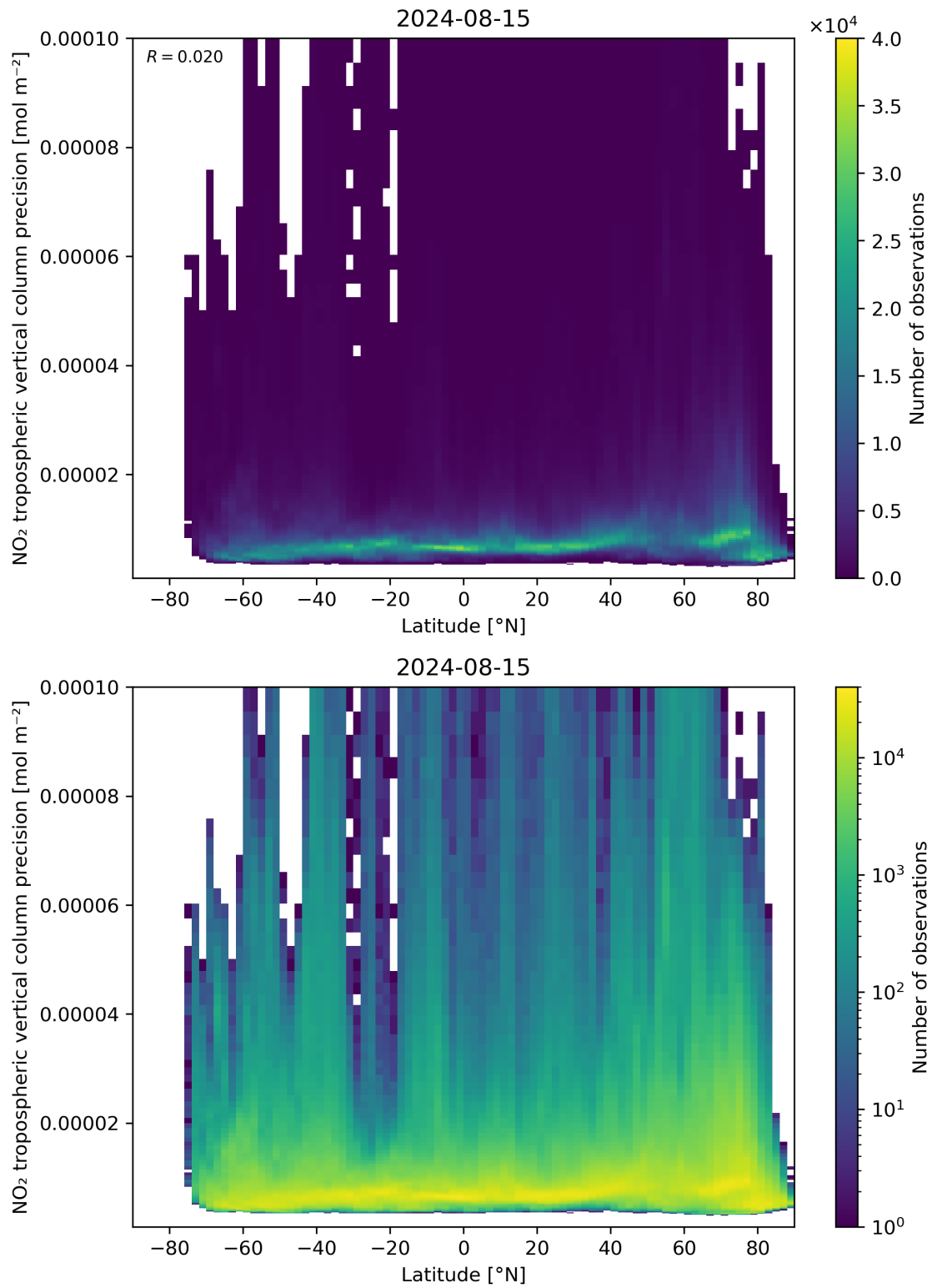
Figure 93: Scatter density plot of “Latitude” against “NO 2 tropospheric vertical column precision” for 2024-08-14 to 2024-08-16.
