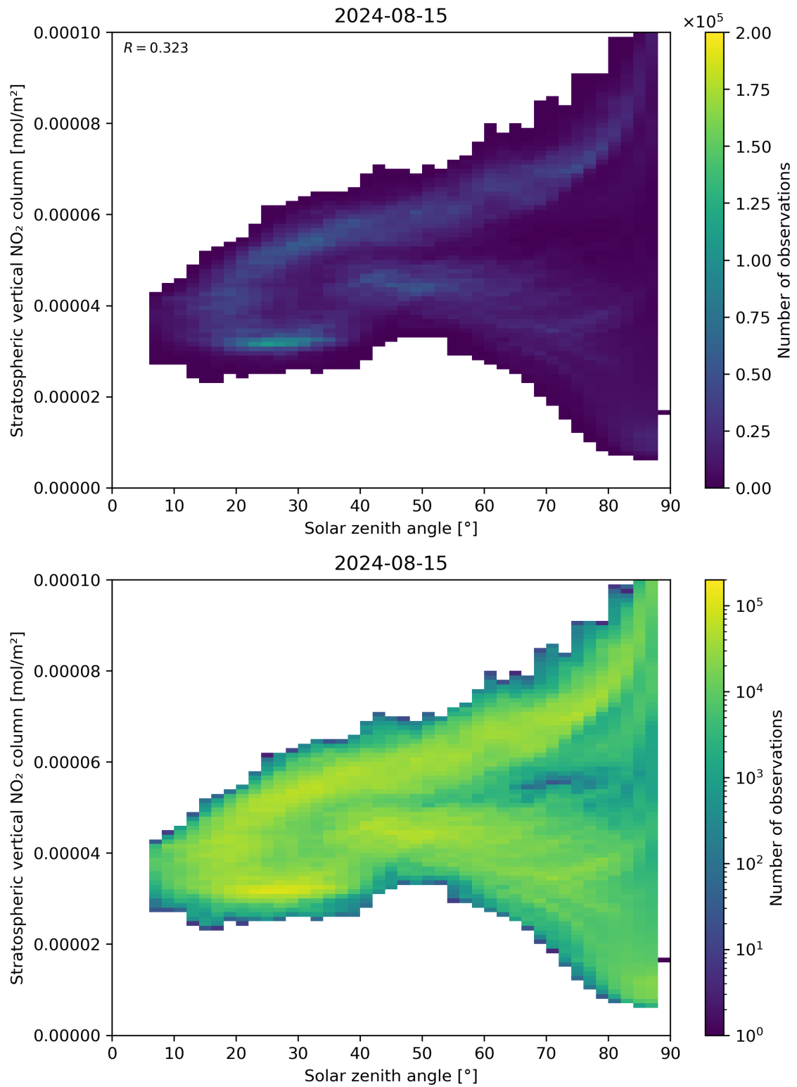
Figure 150: Scatter density plot of “Solar zenith angle” against “Stratospheric vertical NO 2 column” for 2024-08-14 to 2024-08-16.
