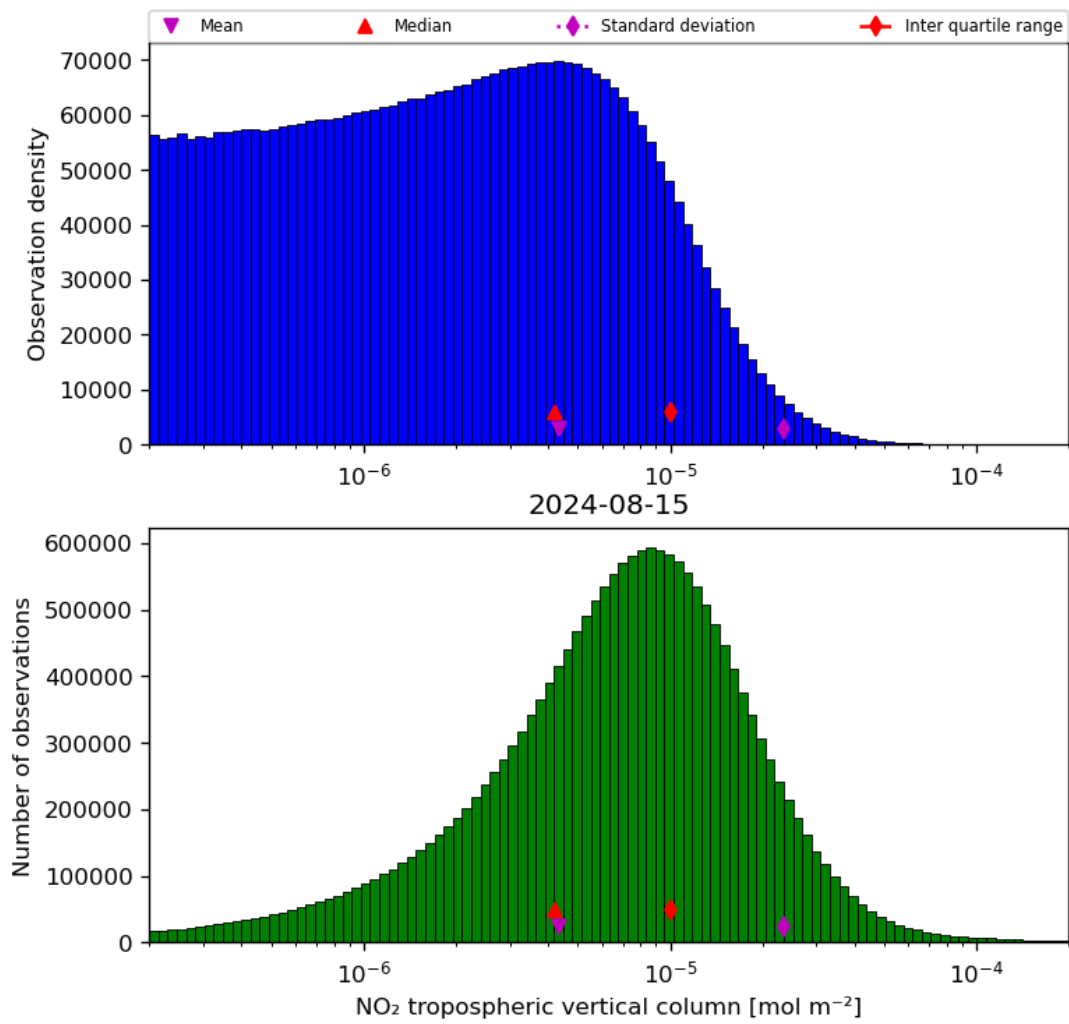
Figure 29: Histogram of “NO 2 tropospheric vertical column” for 2024-08-14 to 2024-08-16
