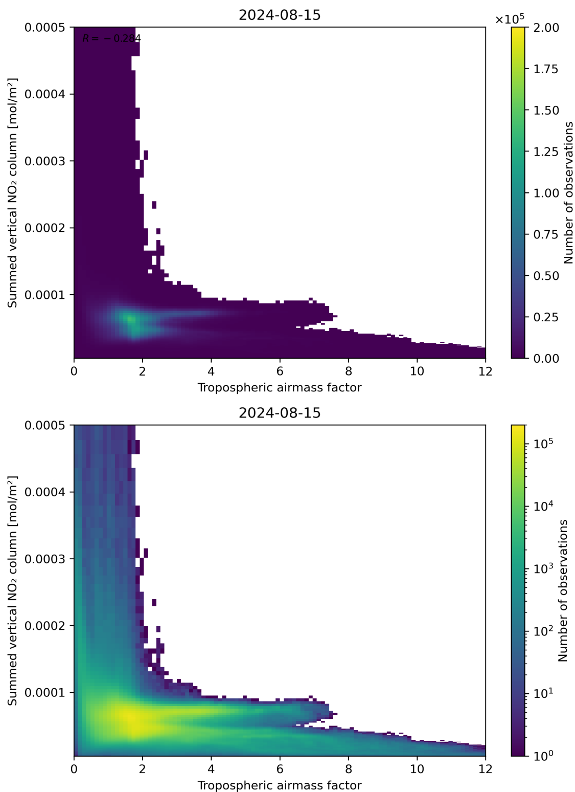
Figure 75: Scatter density plot of “Tropospheric airmass factor” against “Summed vertical NO 2 column” for 2024-08-14 to 2024-08-16.
