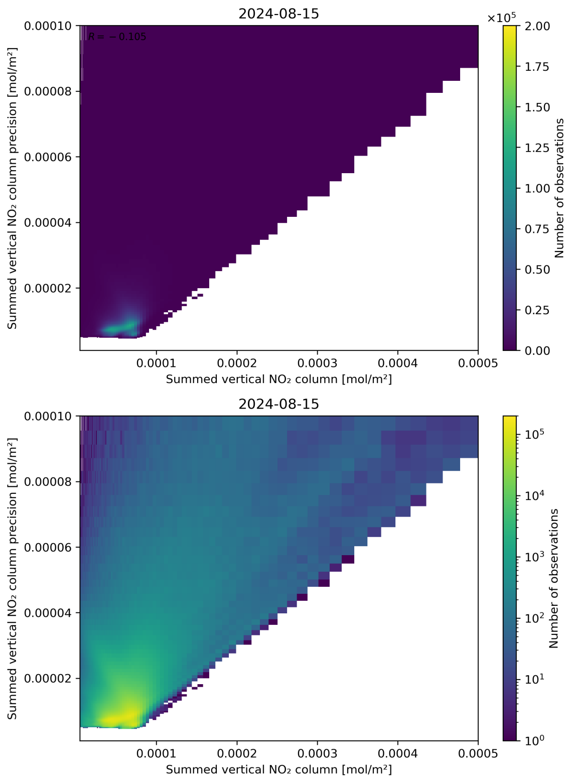
Figure 105: Scatter density plot of “Summed vertical NO 2 column” against “Summed vertical NO 2 column precision” for 2024-08-14 to 2024-08-16.
