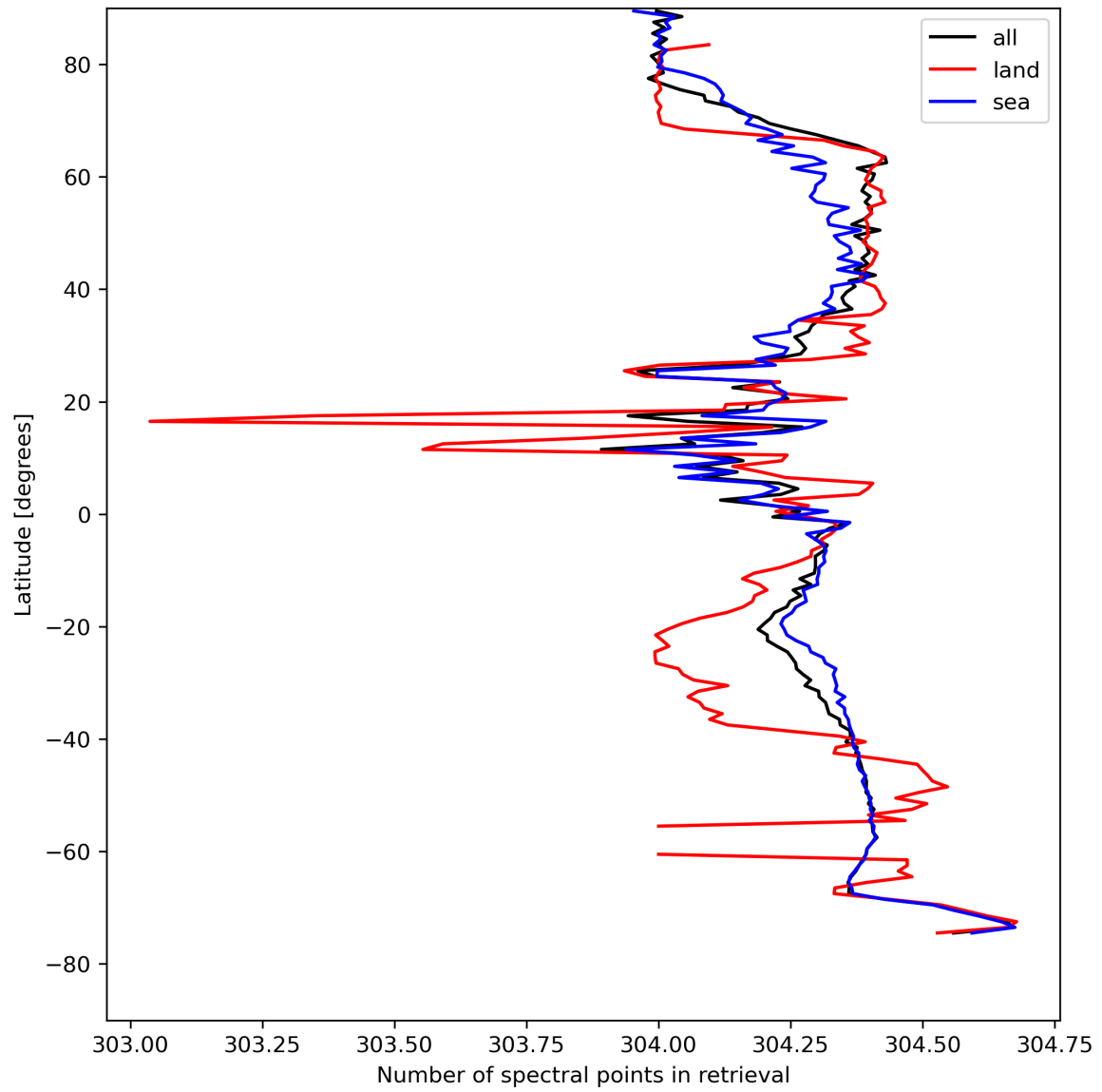
Figure 16: Zonal average of “Number of spectral points in retrieval” for 2024-08-14 to 2024-08-16.
