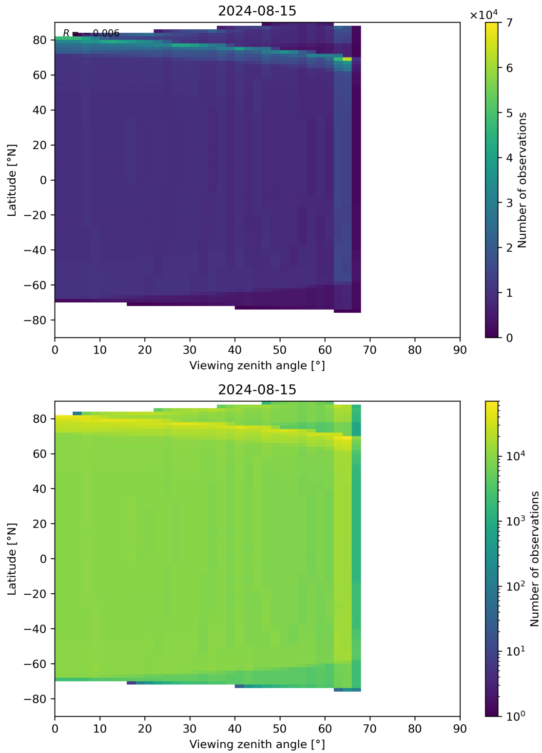
Figure 163: Scatter density plot of “Viewing zenith angle” against “Latitude” for 2024-08-14 to 2024-08-16.
