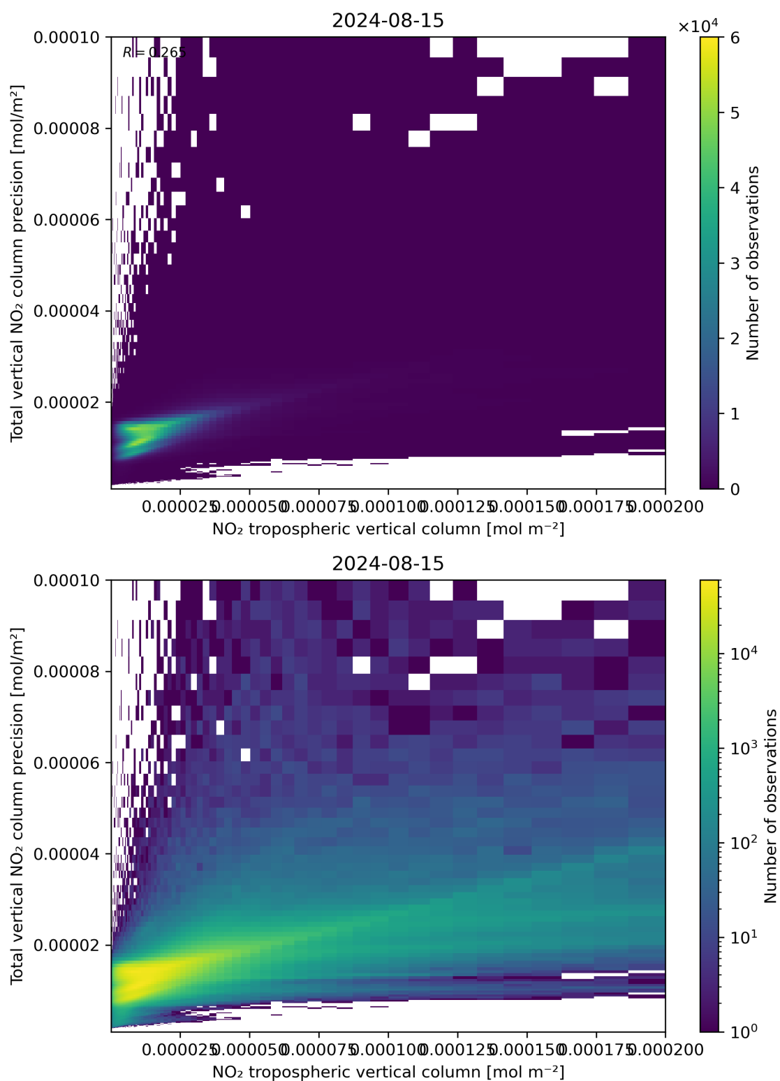
Figure 129: Scatter density plot of “NO 2 tropospheric vertical column” against “Total vertical NO 2 column precision” for 2024-08-14 to 2024-08-16.
