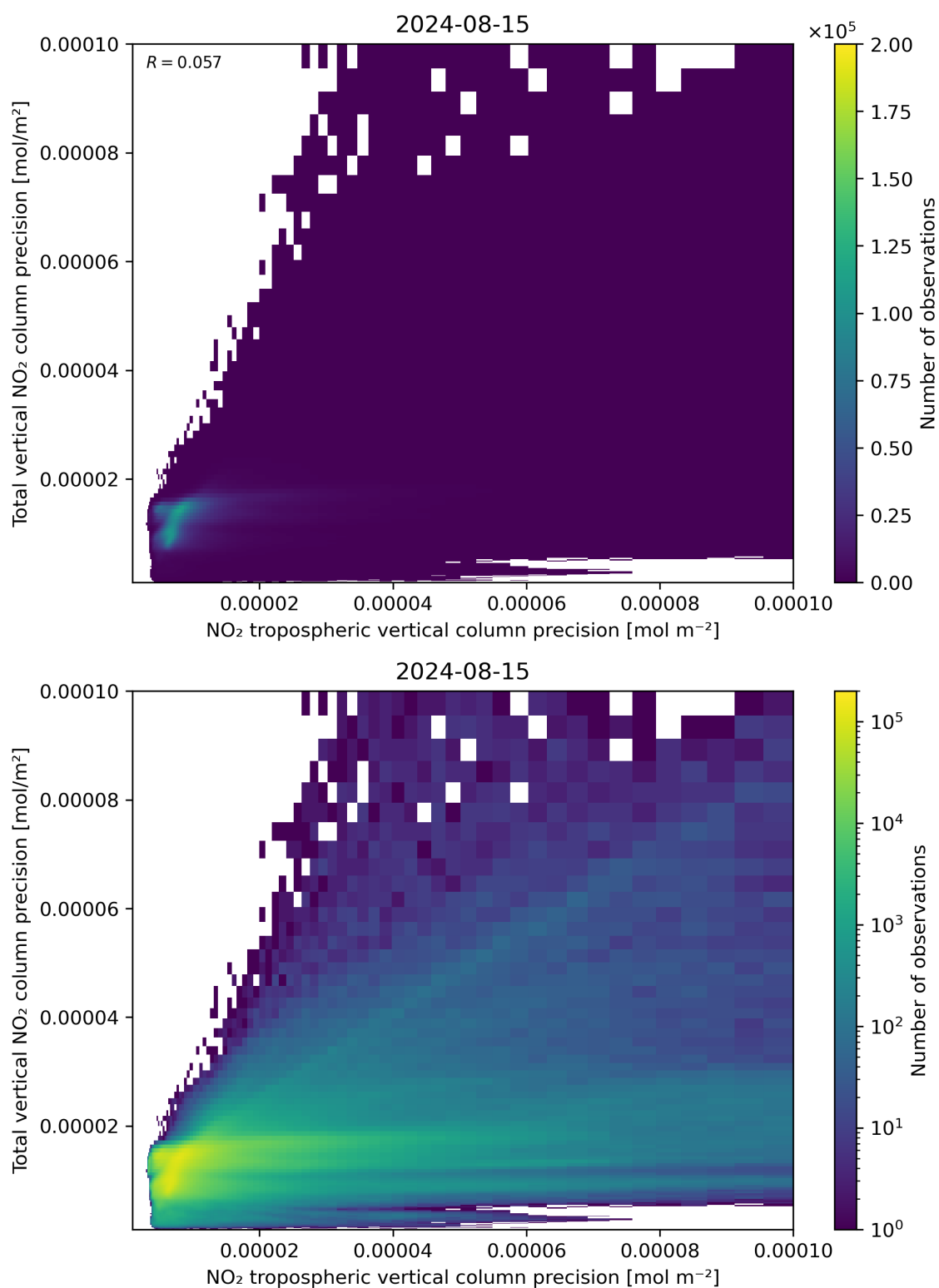
Figure 139: Scatter density plot of “NO 2 tropospheric vertical column precision” against “Total vertical NO 2 column precision” for 2024-08-14 to 2024-08-16.
