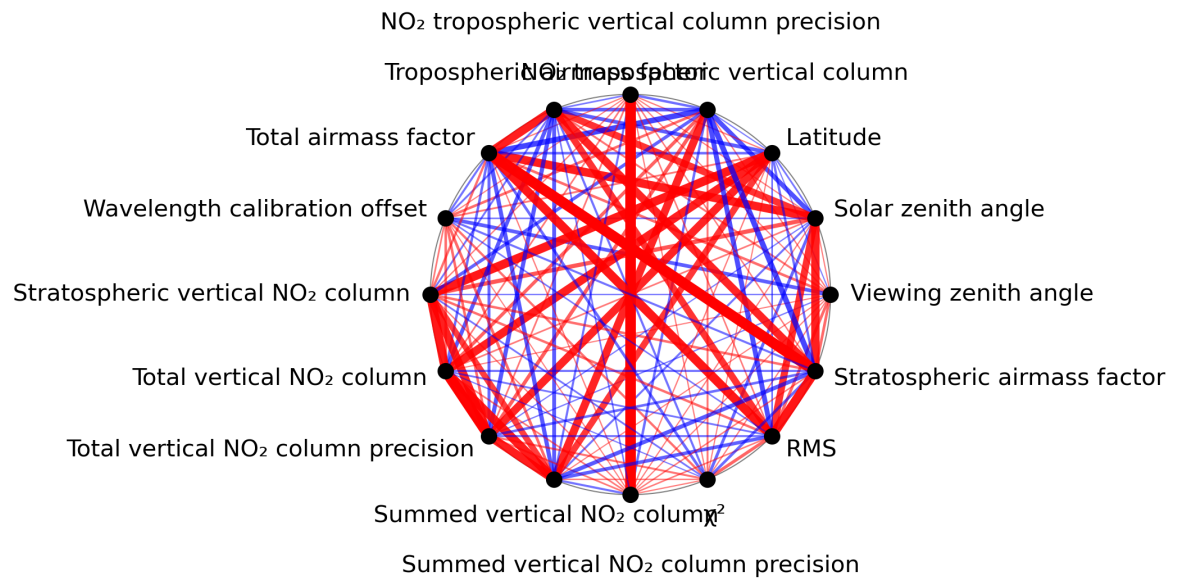
Figure 1: Map of correlation graph for 2024-08-14 to 2024-08-16.
