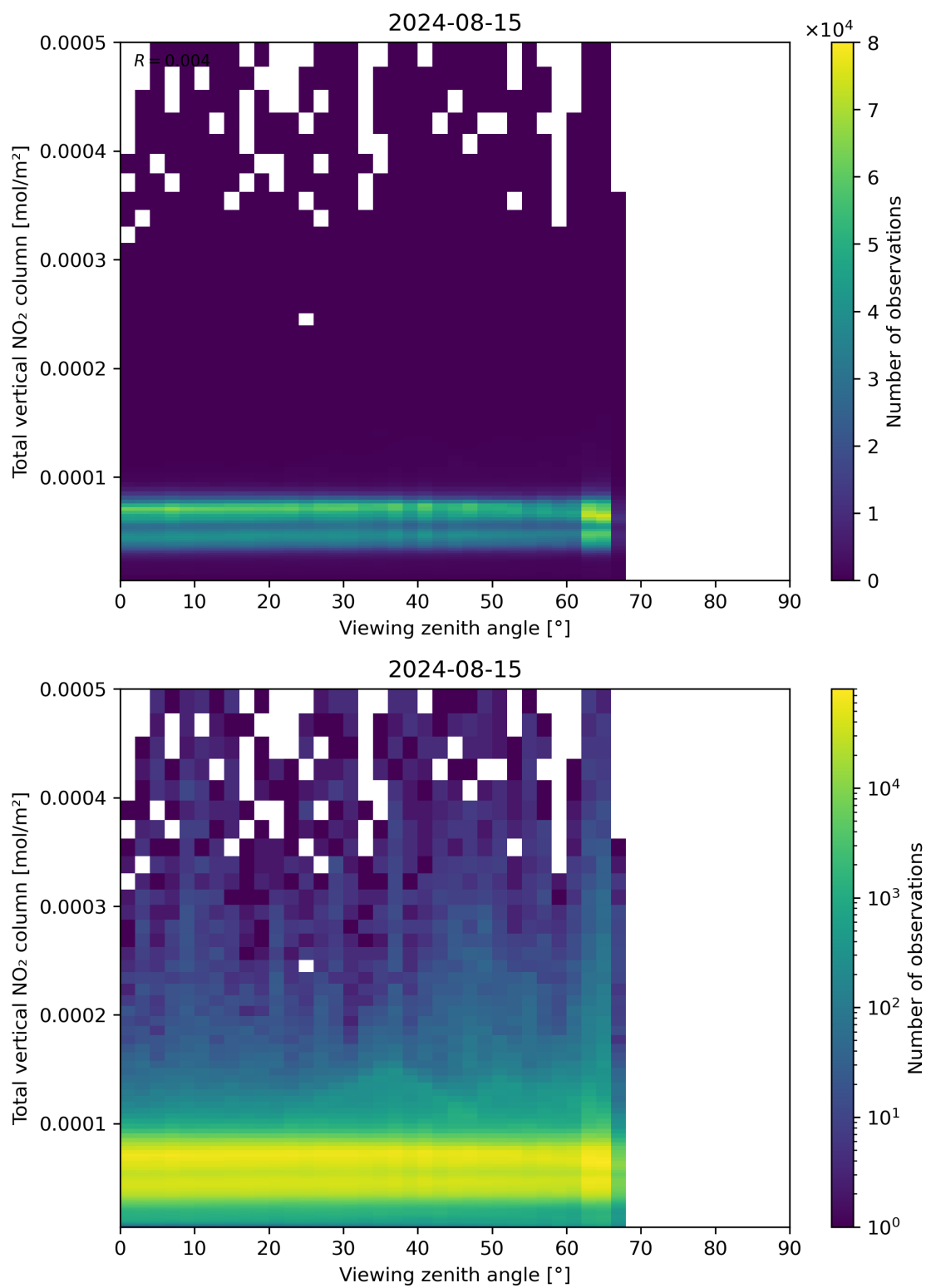
Figure 167: Scatter density plot of “Viewing zenith angle” against “Total vertical NO 2 column” for 2024-08-14 to 2024-08-16.
