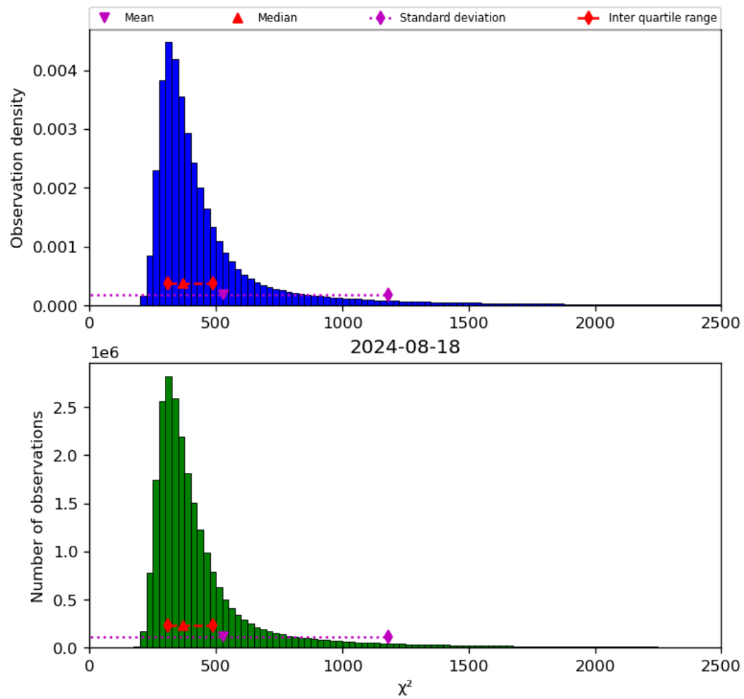
Figure 42: Histogram of “ \chi^2 ” for 2024-08-17 to 2024-08-19
