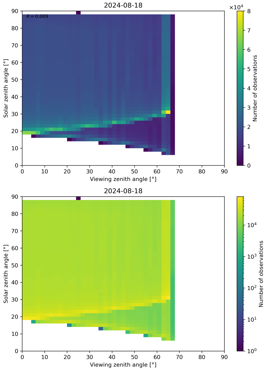
Figure 172: Scatter density plot of “Viewing zenith angle” against “Solar zenith angle” for 2024-08-17 to 2024-08-19.
