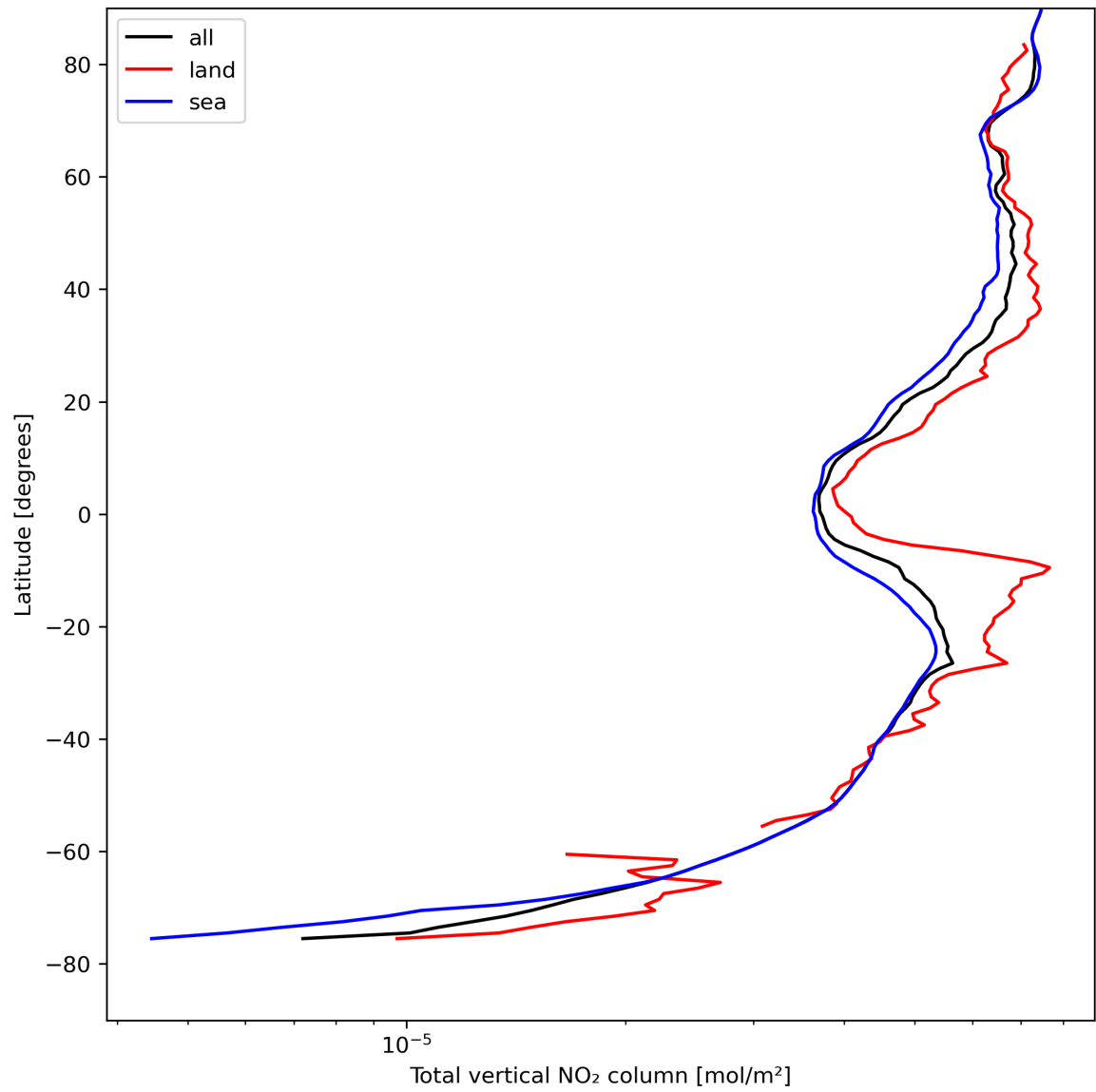
Figure 21: Zonal average of “Total vertical NO 2 column” for 2024-08-17 to 2024-08-19.
