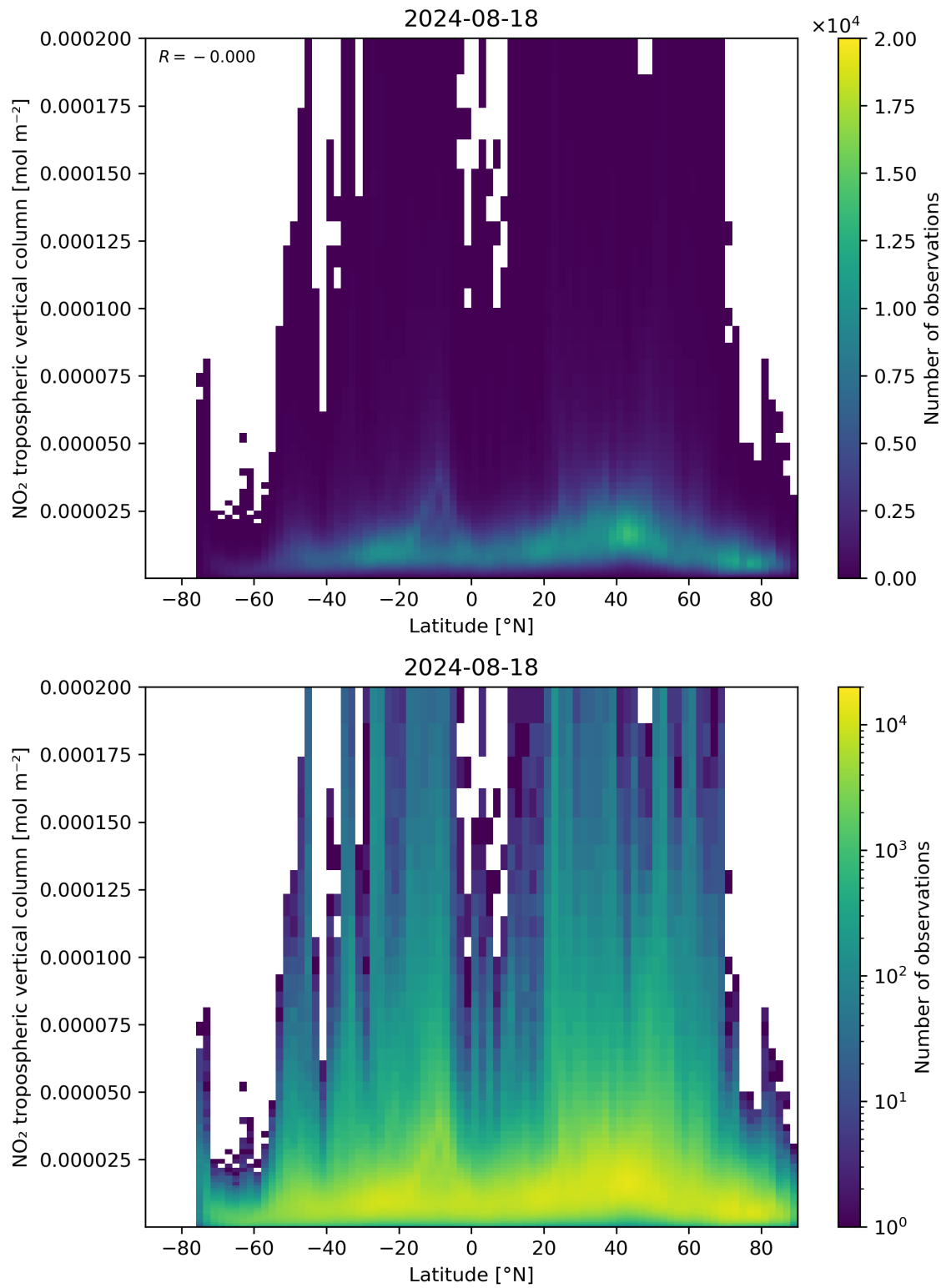
Figure 92: Scatter density plot of “Latitude” against “NO 2 tropospheric vertical column” for 2024-08-17 to 2024-08-19.
