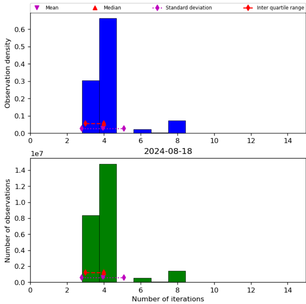
Figure 34: Histogram of “Number of iterations” for 2024-08-17 to 2024-08-19
