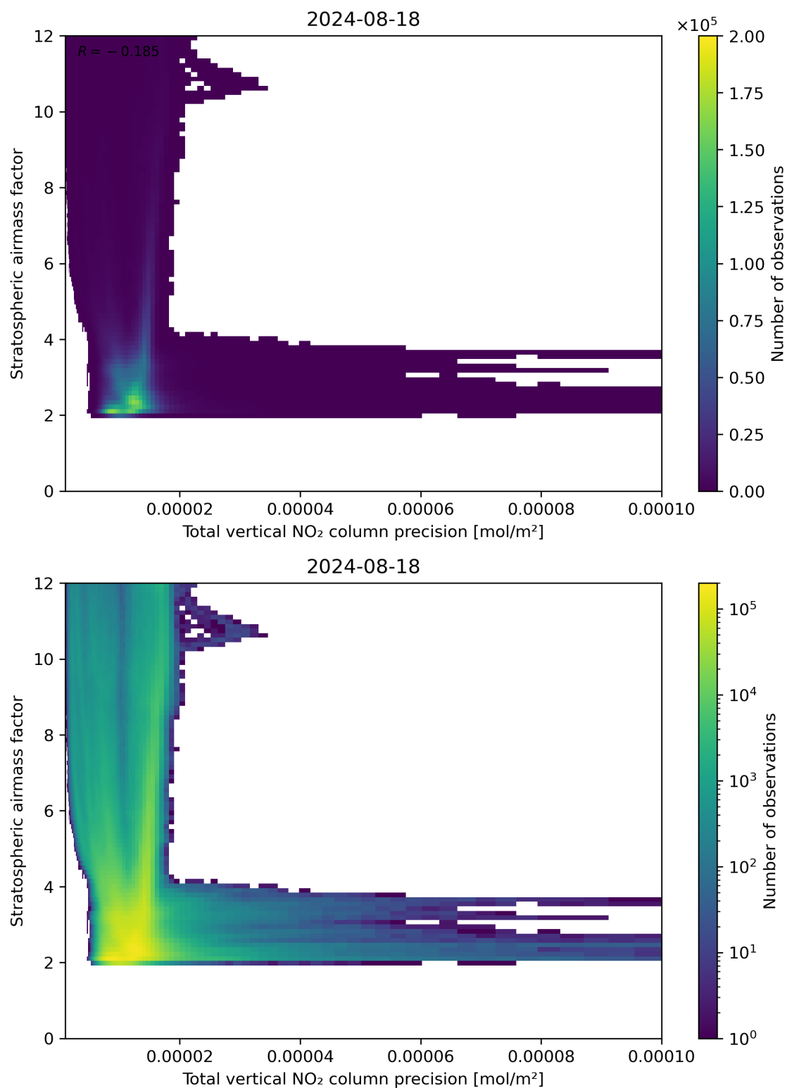
Figure 115: Scatter density plot of “Total vertical NO 2 column precision” against “Stratospheric airmass factor” for 2024-08-17 to 2024-08-19.
