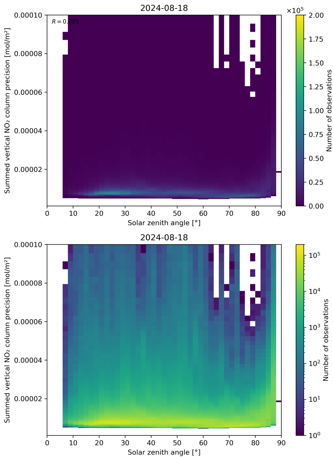
Figure 152: Scatter density plot of “Solar zenith angle” against “Summed vertical NO 2 column precision” for 2024-08-17 to 2024-08-19.
