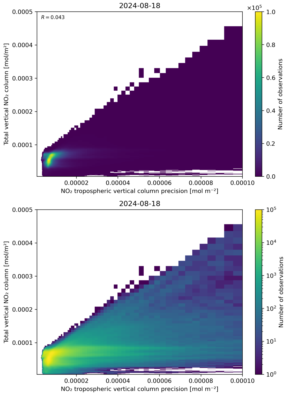
Figure 138: Scatter density plot of “NO 2 tropospheric vertical column precision” against “Total vertical NO 2 column” for 2024-08-17 to 2024-08-19.
