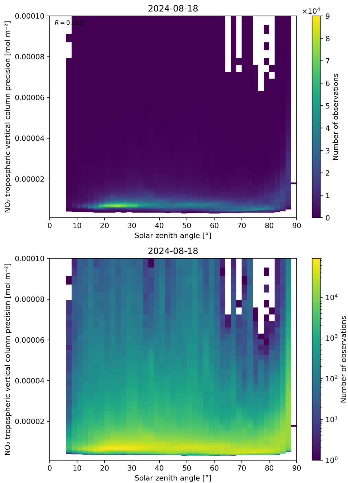
Figure 156: Scatter density plot of “Solar zenith angle” against “NO 2 tropospheric vertical column precision” for 2024-08-17 to 2024-08-19.
