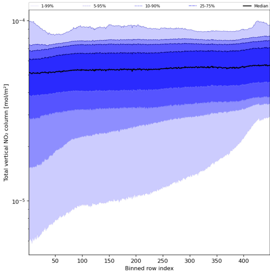
Figure 55: Along track statistics of “Total vertical NO 2 column” for 2024-08-17 to 2024-08-19
