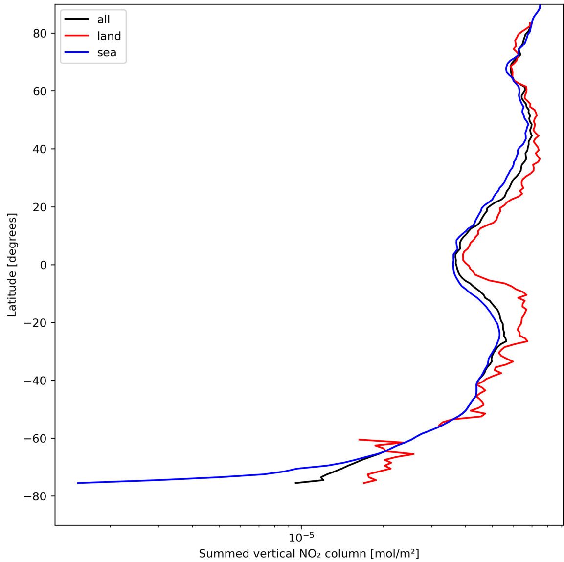
Figure 23: Zonal average of “Summed vertical NO 2 column” for 2024-08-17 to 2024-08-19.
