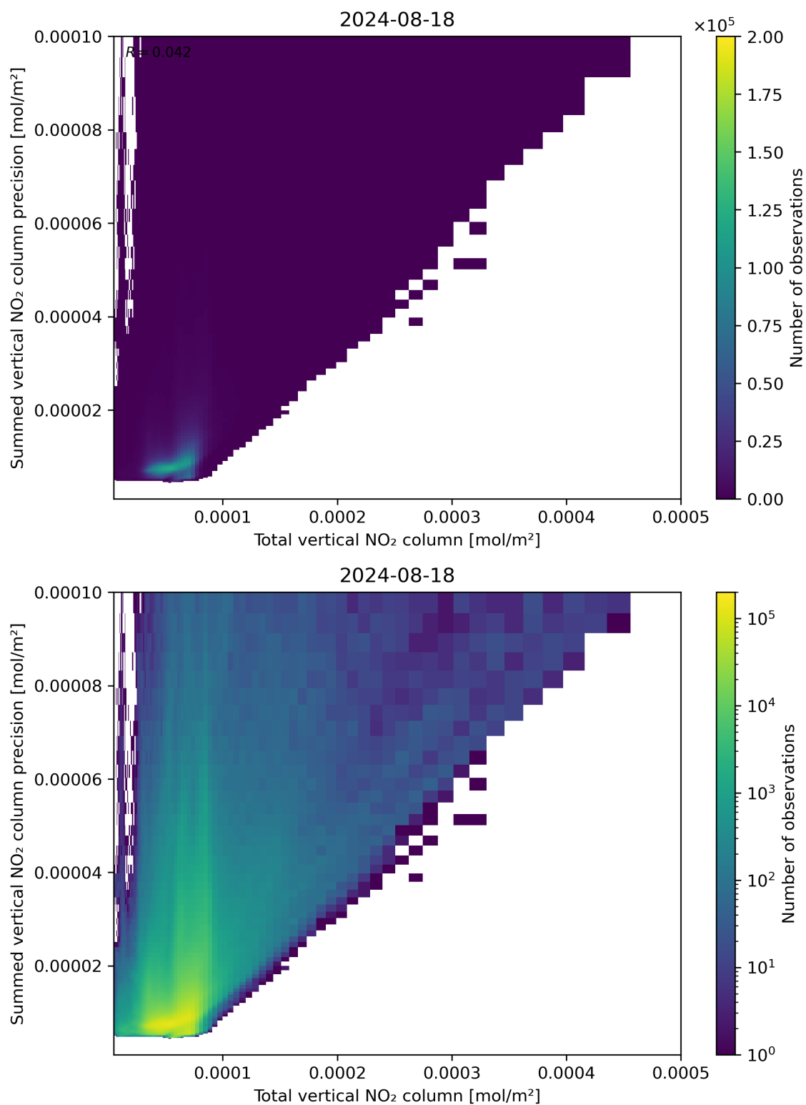
Figure 113: Scatter density plot of “Total vertical NO 2 column” against “Summed vertical NO 2 column precision” for 2024-08-17 to 2024-08-19.
