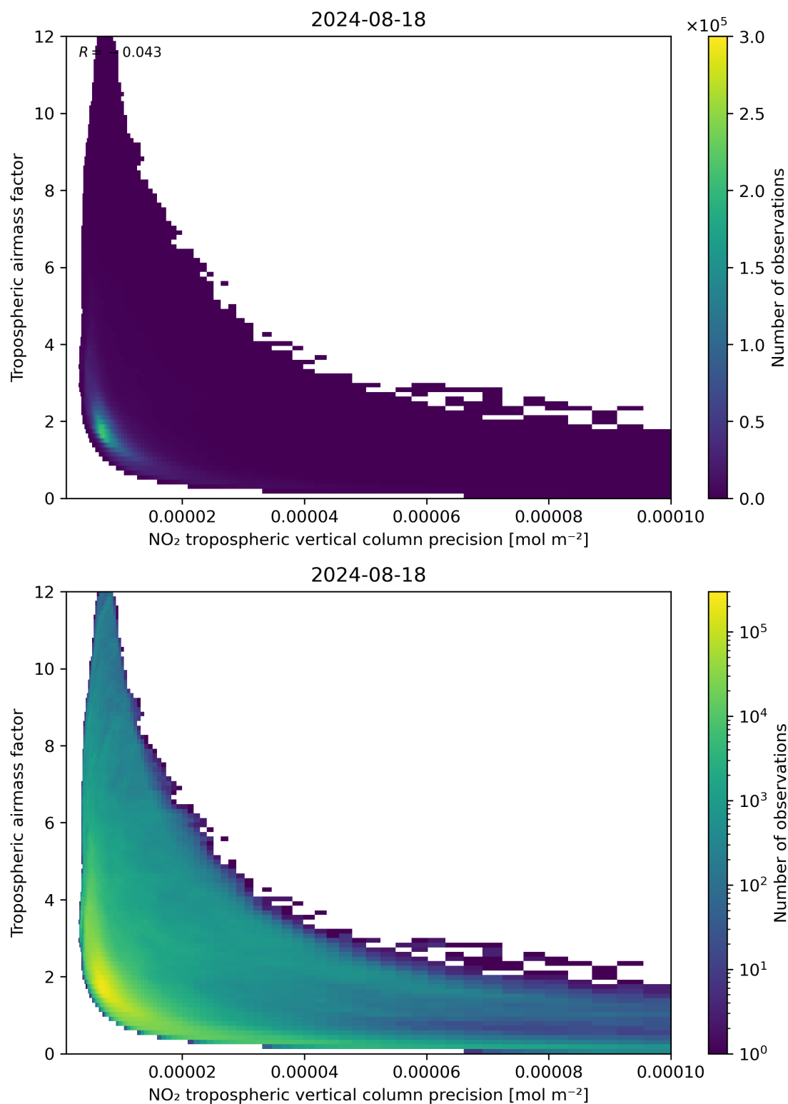
Figure 133: Scatter density plot of “NO 2 tropospheric vertical column precision” against “Tropospheric airmass factor” for 2024-08-17 to 2024-08-19.
