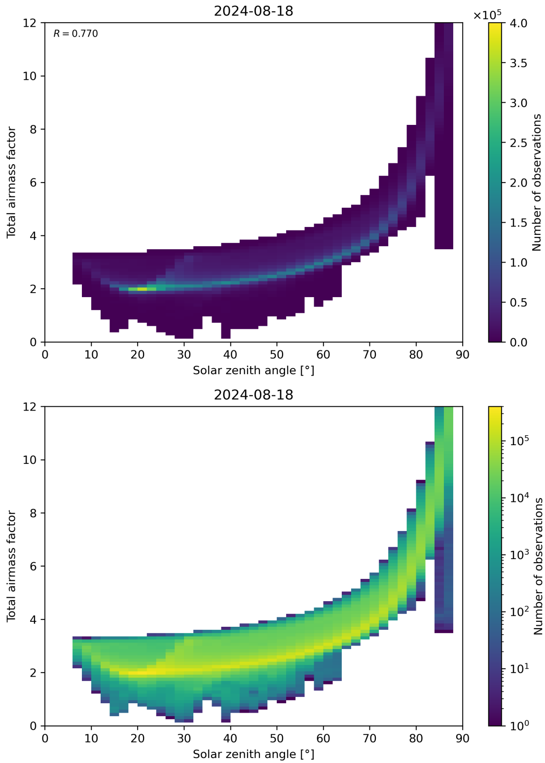
Figure 146: Scatter density plot of “Solar zenith angle” against “Total air mass factor” for 2024-08-17 to 2024-08-19.
