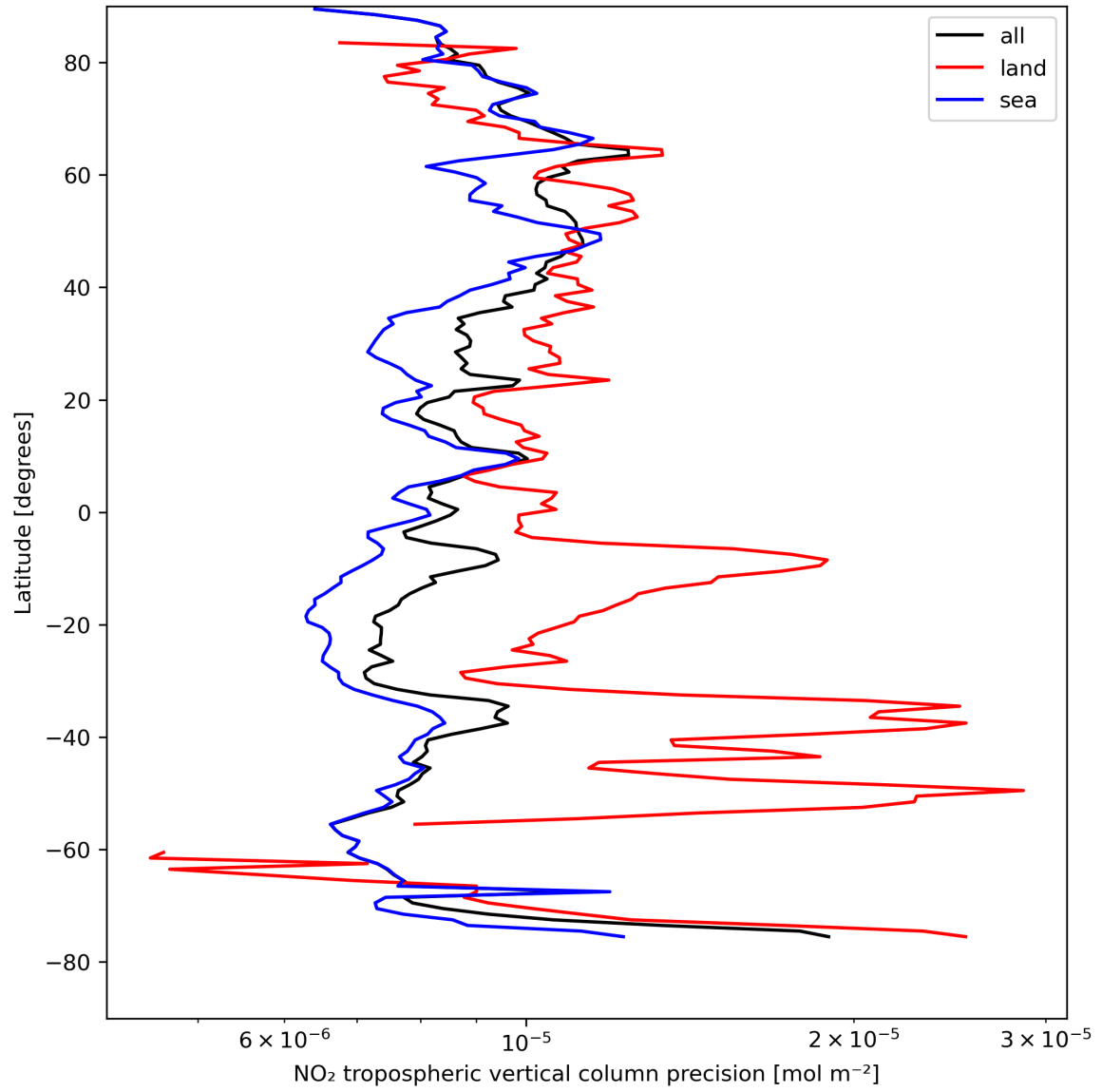
Figure 13: Zonal average of “NO 2 tropospheric vertical column precision” for 2024-08-17 to 2024-08-19.
