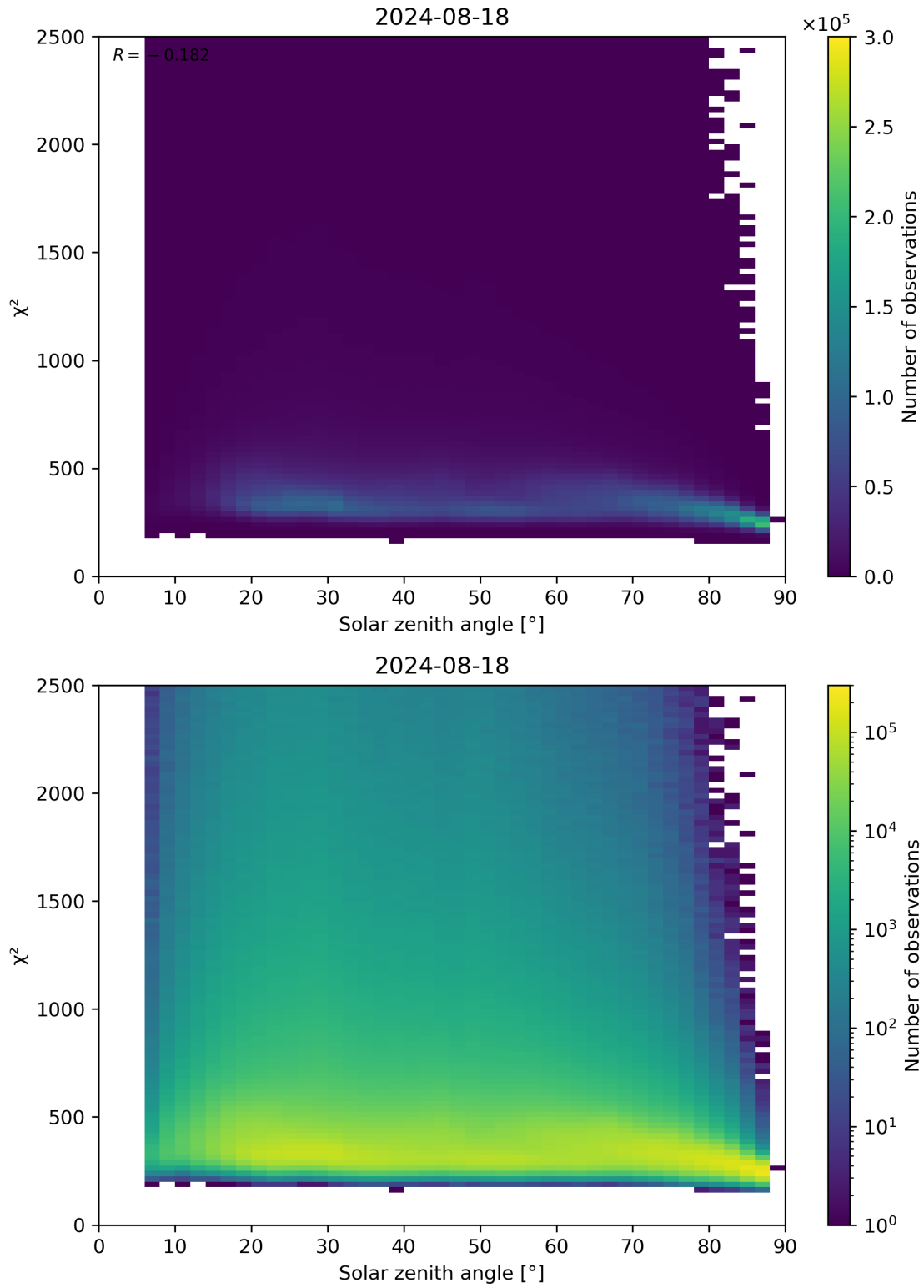
Figure 148: Scatter density plot of “Solar zenith angle” against “ \chi^2 ” for 2024-08-17 to 2024-08-19.
