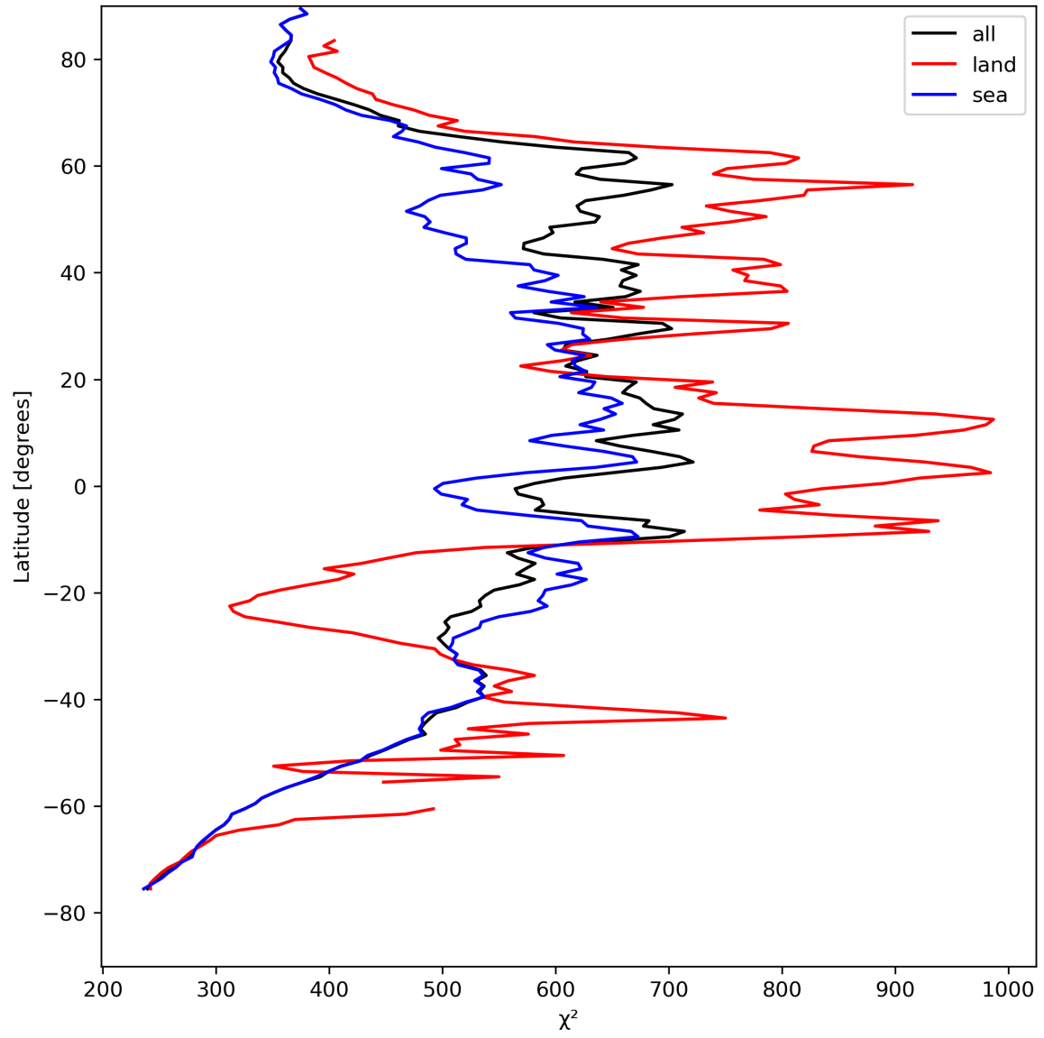
Figure 25: Zonal average of “ \chi^2 ” for 2024-08-17 to 2024-08-19.
