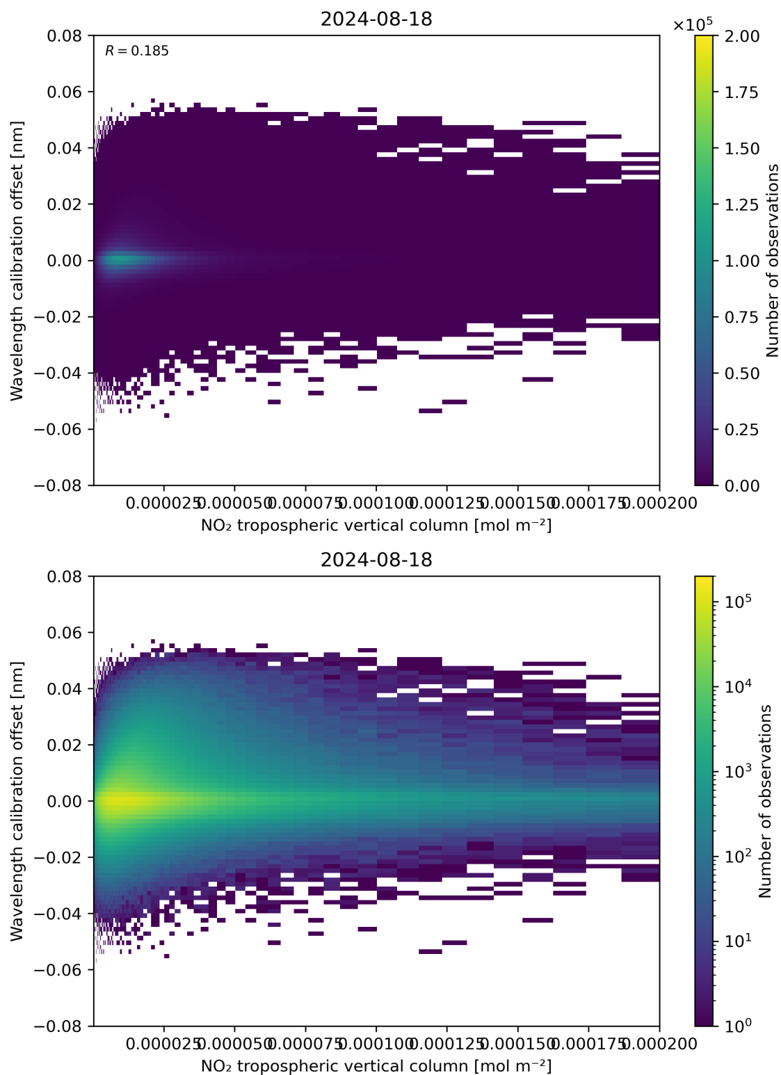
Figure 143: Scatter density plot of “NO 2 tropospheric vertical column” against “Wavelength calibration offset” for 2024-08-17 to 2024-08-19.
