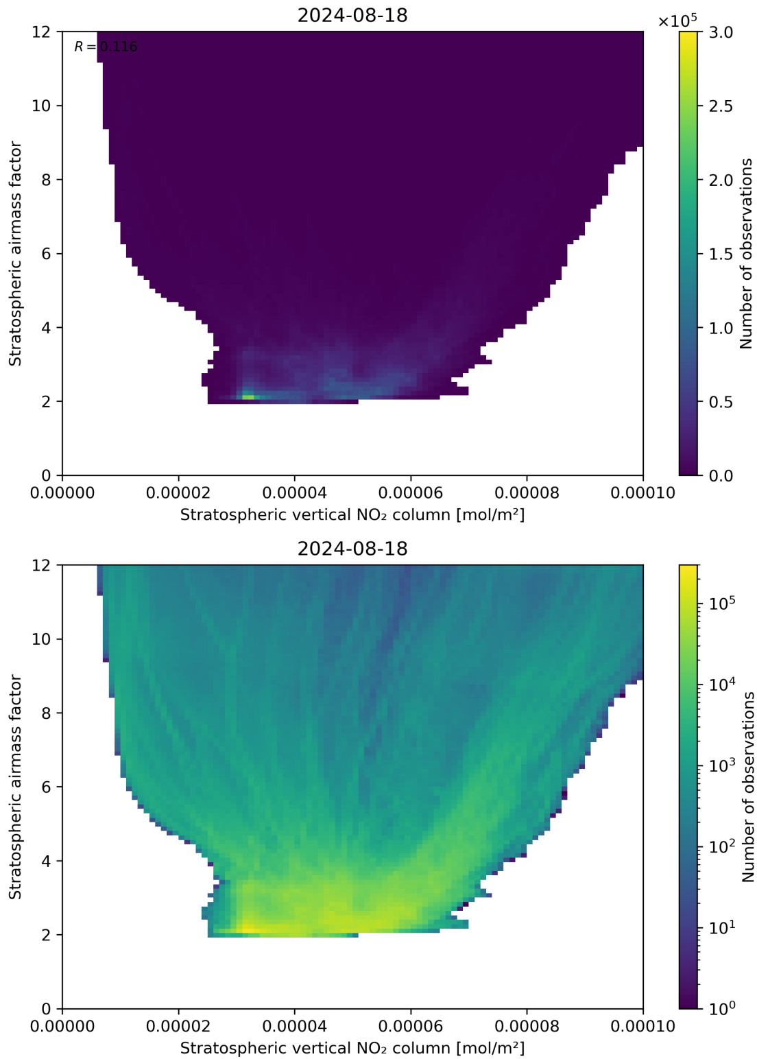
Figure 96: Scatter density plot of “Stratospheric vertical NO 2 column” against “Stratospheric airmass factor” for 2024-08-17 to 2024-08-19.
