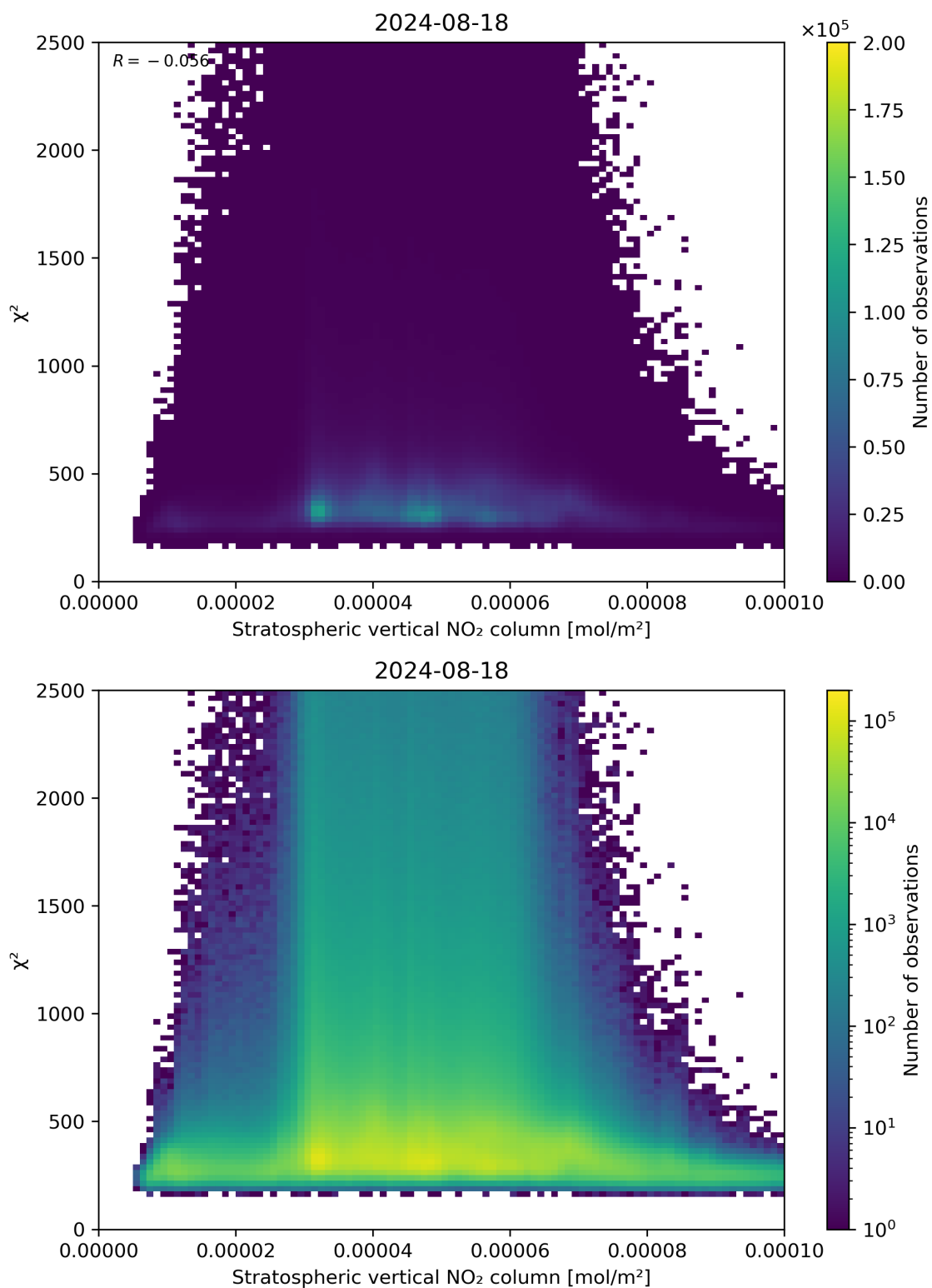
Figure 97: Scatter density plot of “Stratospheric vertical NO 2 column” against “ \chi^2 ” for 2024-08-17 to 2024-08-19.
