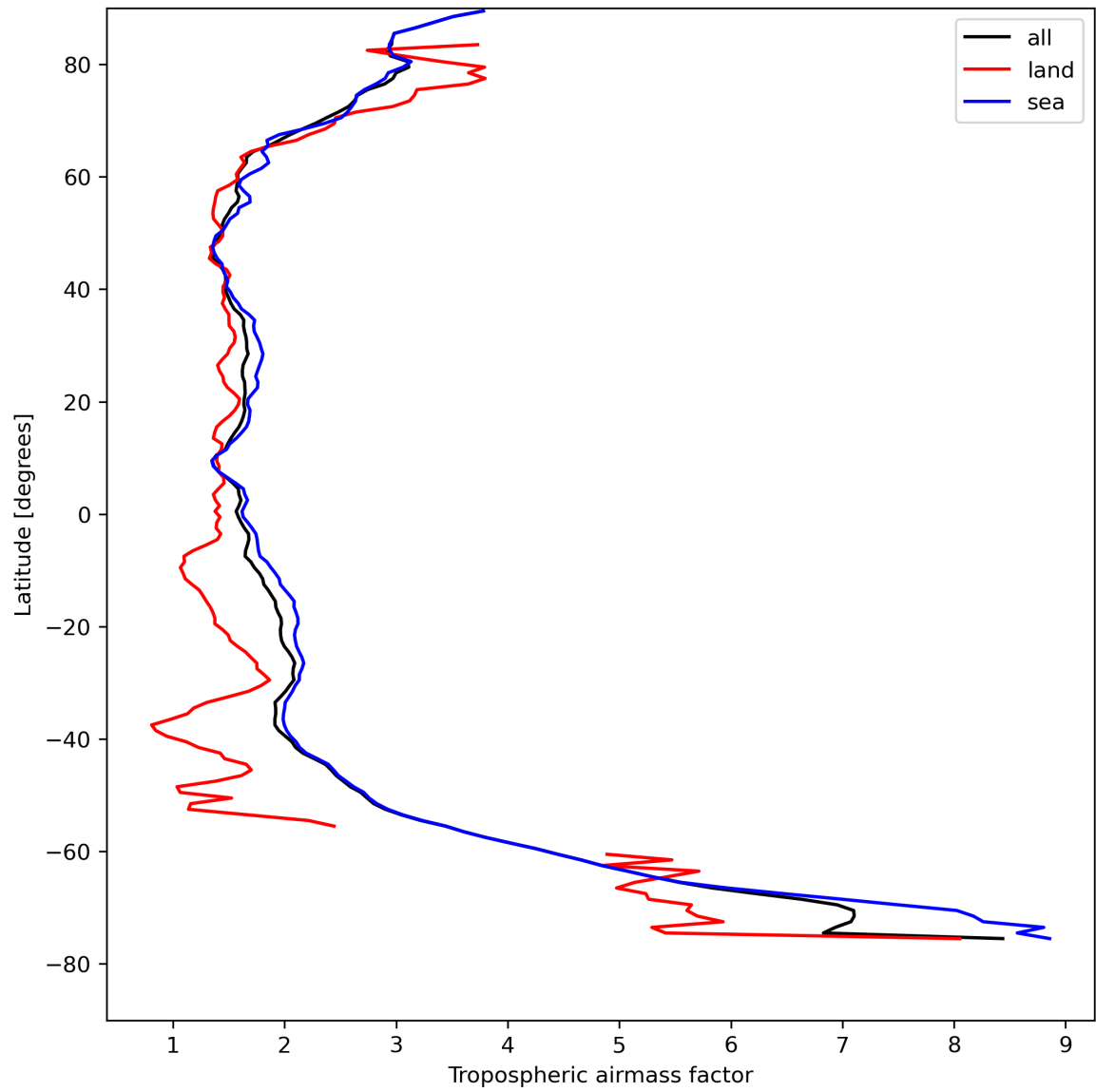
Figure 14: Zonal average of “Tropospheric air mass factor” for 2024-08-17 to 2024-08-19.
