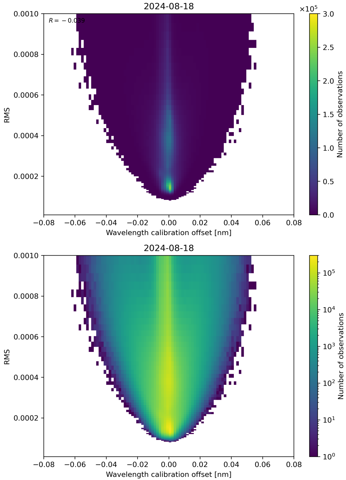
Figure 181: Scatter density plot of “Wavelength calibration offset” against “RMS” for 2024-08-17 to 2024-08-19.
