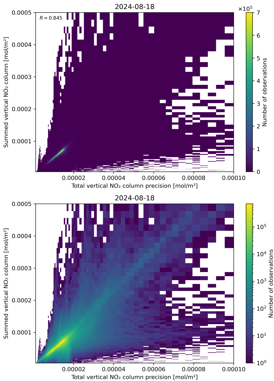
Figure 117: Scatter density plot of “Total vertical NO 2 column precision” against “Summed vertical NO 2 column” for 2024-08-17 to 2024-08-19.
