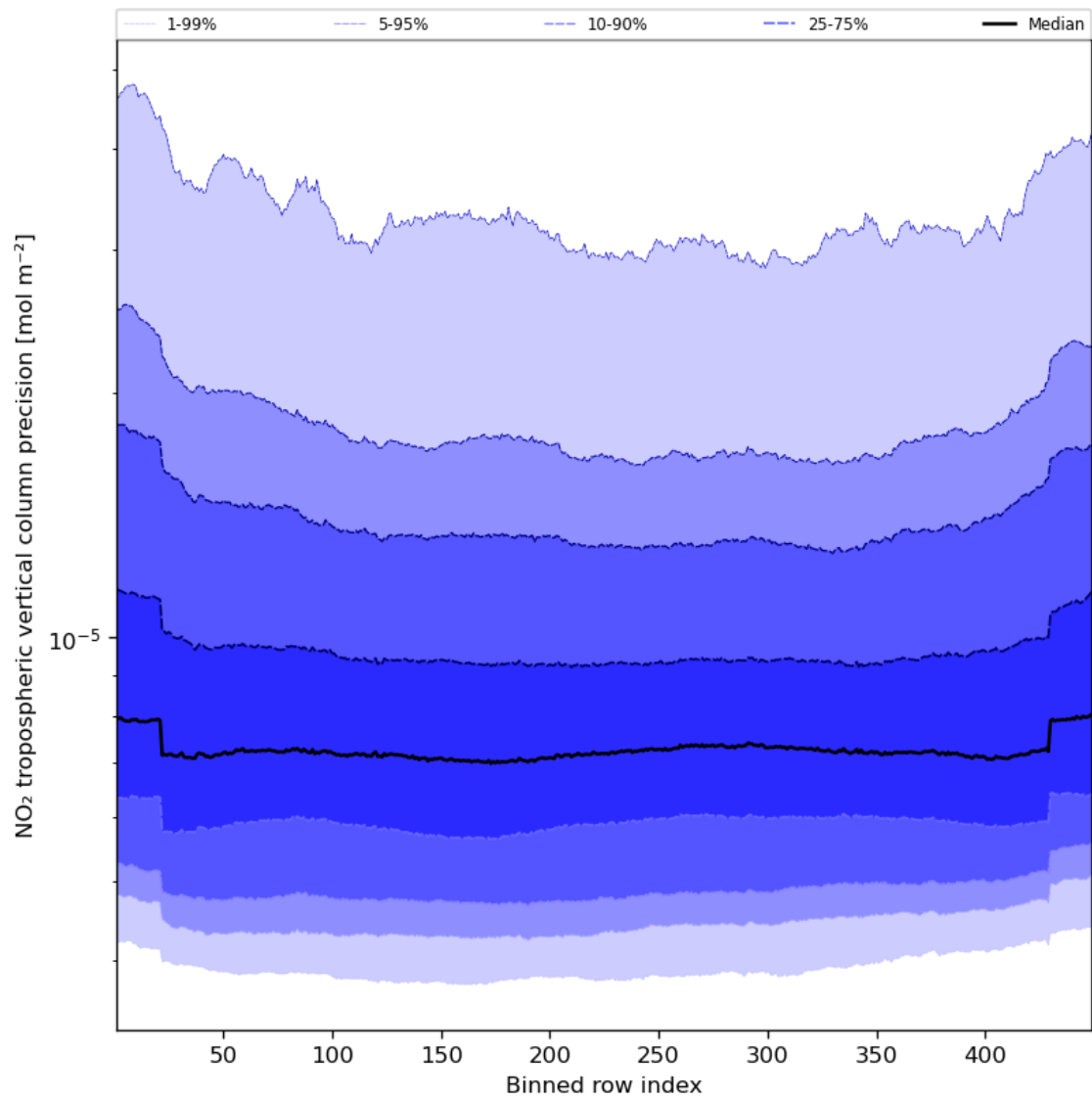
Figure 47: Along track statistics of “NO 2 tropospheric vertical column precision” for 2024-08-17 to 2024-08-19
