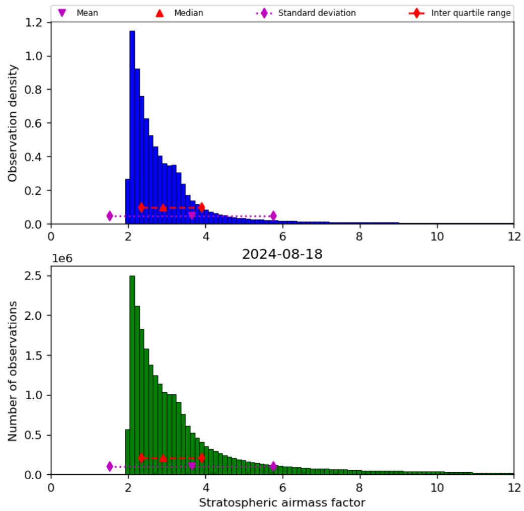
Figure 44: Histogram of “Stratospheric airmass factor” for 2024-08-17 to 2024-08-19
