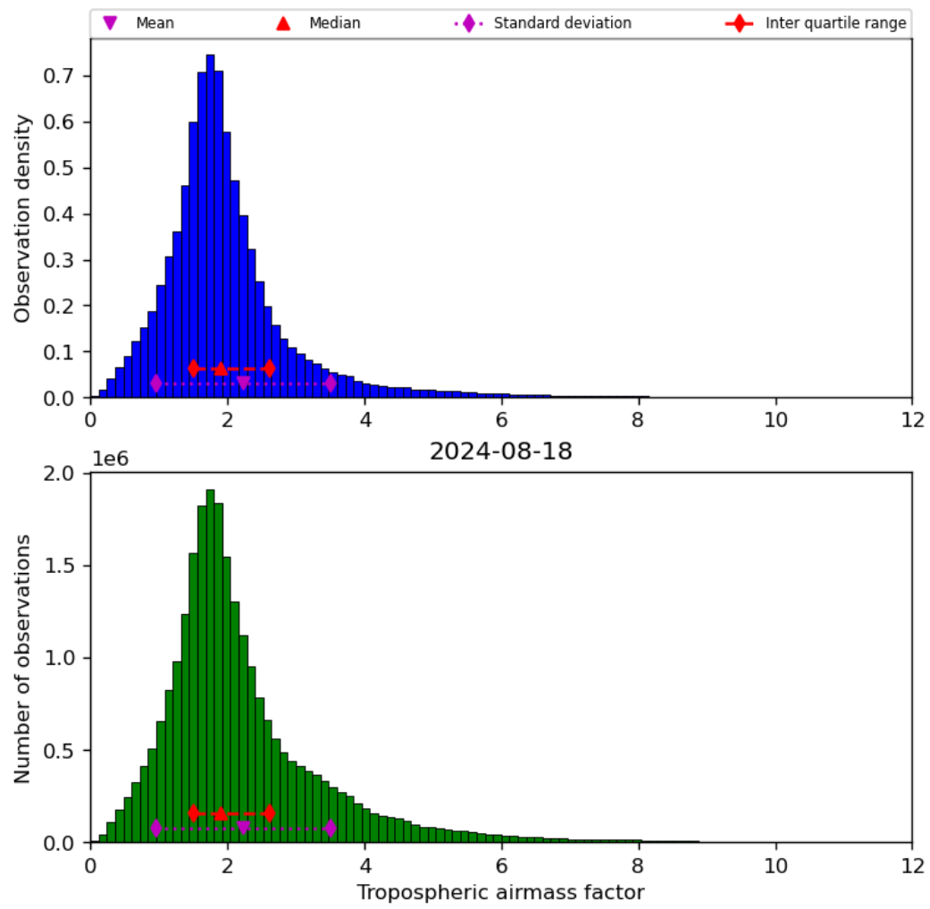
Figure 31: Histogram of “Tropospheric airmass factor” for 2024-08-17 to 2024-08-19
