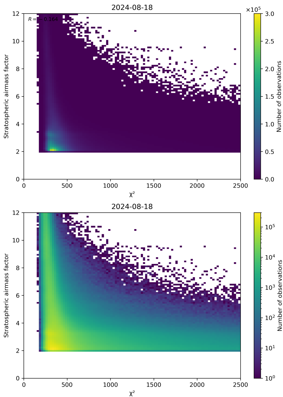
Figure 81: Scatter density plot of “ \chi^2 ” against “Stratospheric airmass factor” for 2024-08-17 to 2024-08-19.
