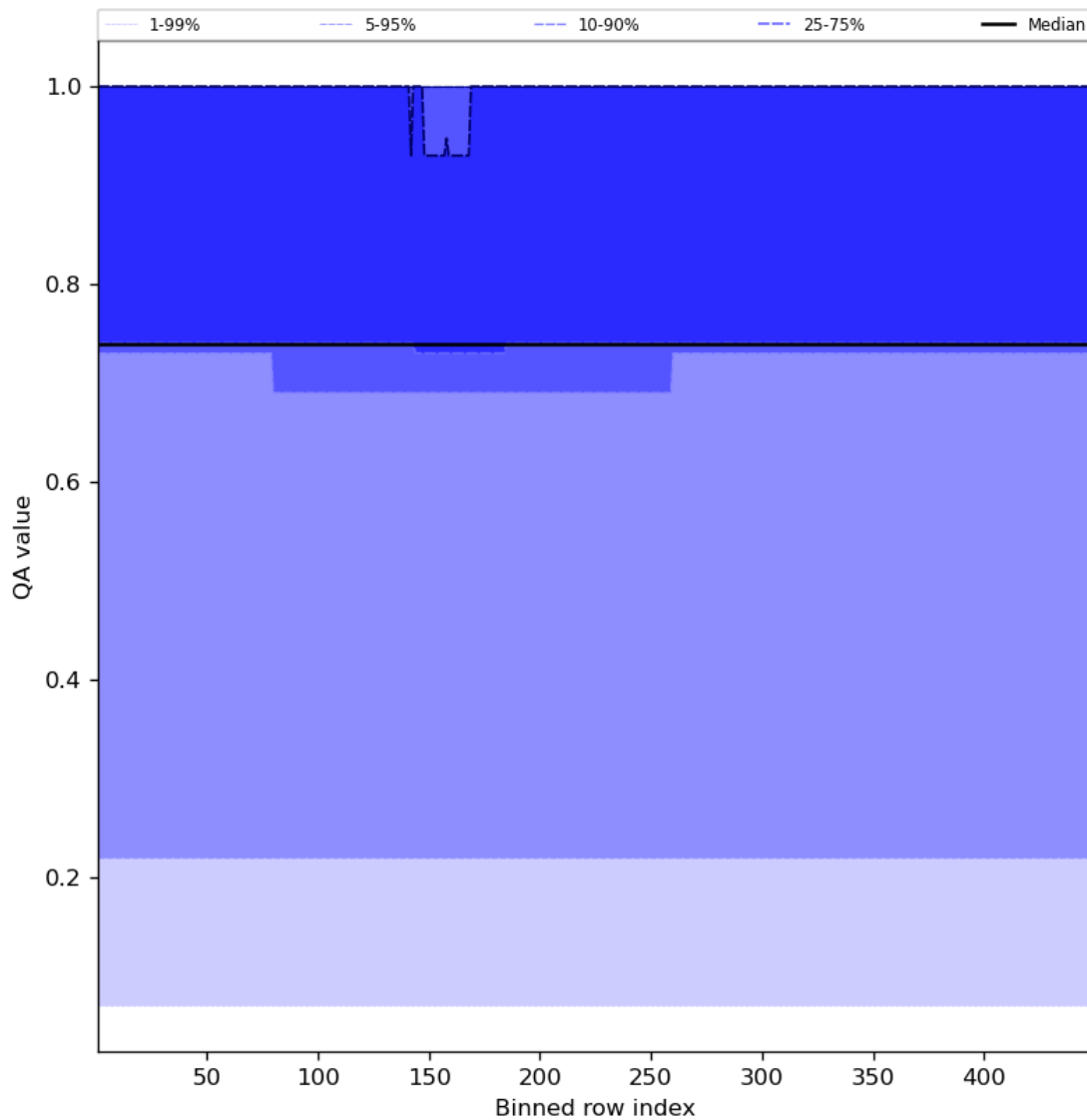
Figure 45: Along track statistics of "QA value" for 2024-08-17 to 2024-08-19
