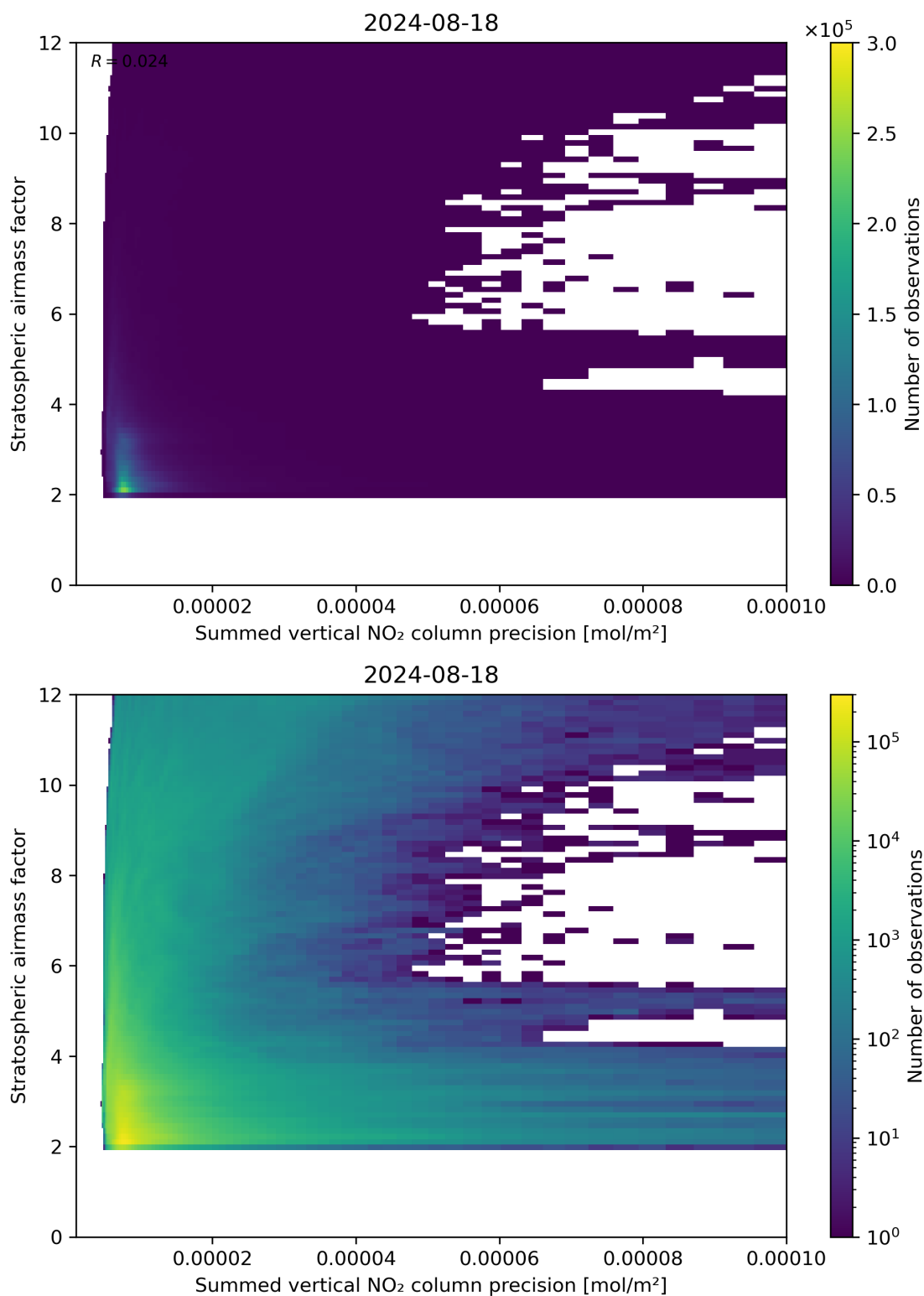
Figure 106: Scatter density plot of “Summed vertical NO 2 column precision” against “Stratospheric airmass factor” for 2024-08-17 to 2024-08-19.
