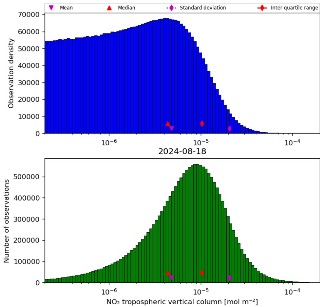
Figure 29: Histogram of “NO 2 tropospheric vertical column” for 2024-08-17 to 2024-08-19
