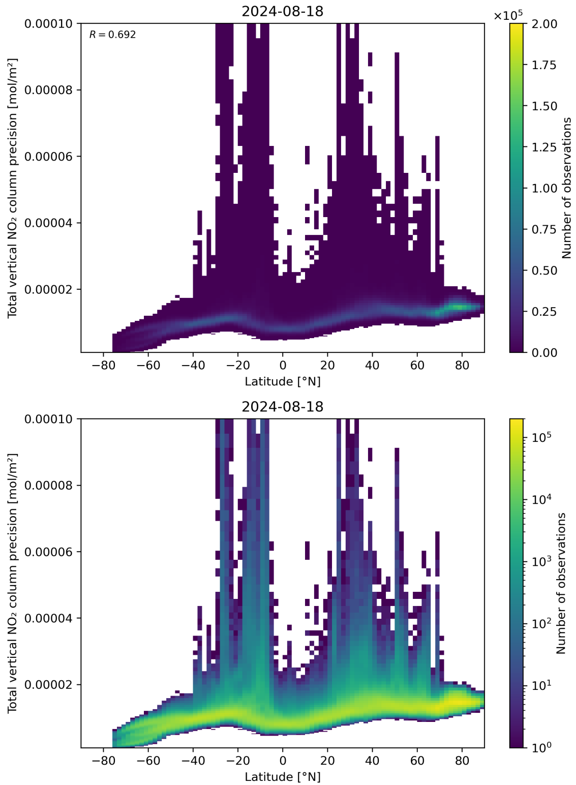
Figure 91: Scatter density plot of “Latitude” against “Total vertical NO 2 column precision” for 2024-08-17 to 2024-08-19.
