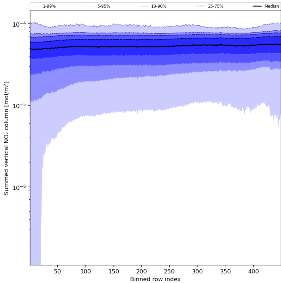
Figure 57: Along track statistics of “Summed vertical NO 2 column” for 2024-08-17 to 2024-08-19
