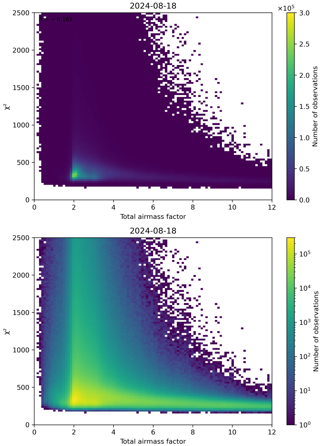
Figure 63: Scatter density plot of “Total airmass factor” against “ \chi^2 ” for 2024-08-17 to 2024-08-19.
