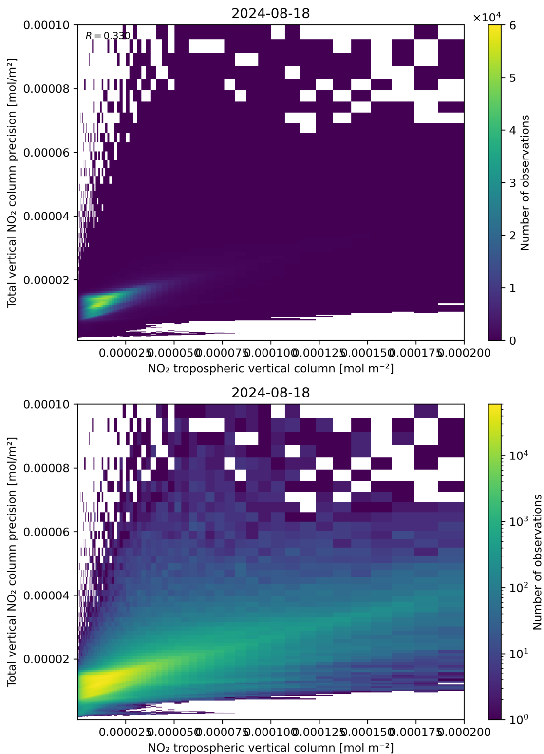
Figure 129: Scatter density plot of “NO 2 tropospheric vertical column” against “Total vertical NO 2 column precision” for 2024-08-17 to 2024-08-19.
