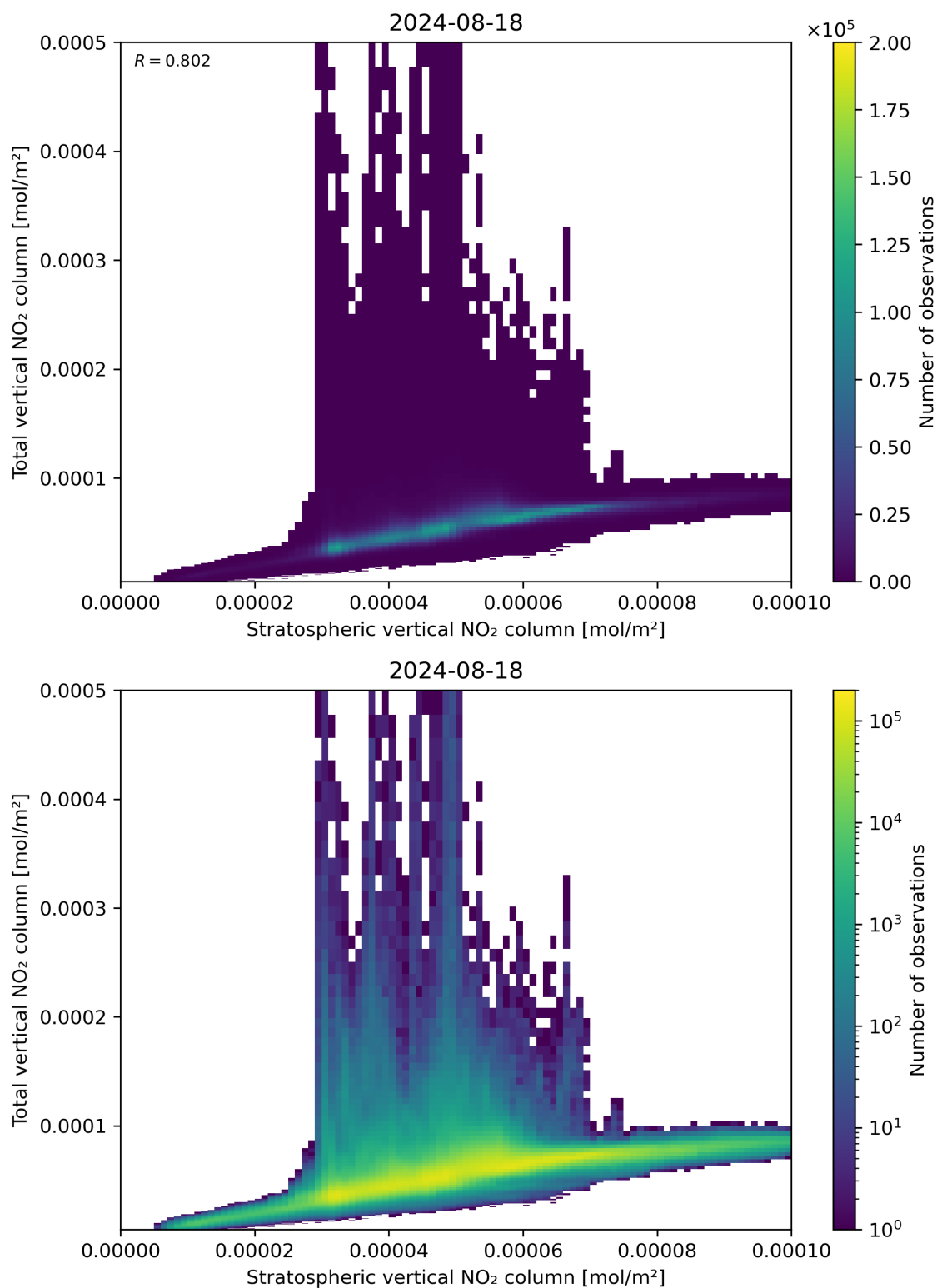
Figure 100: Scatter density plot of “Stratospheric vertical NO 2 column” against “Total vertical NO 2 column” for 2024-08-17 to 2024-08-19.
