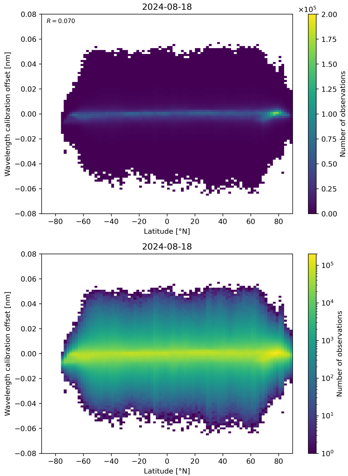
Figure 95: Scatter density plot of “Latitude” against “Wavelength calibration offset” for 2024-08-17 to 2024-08-19.
