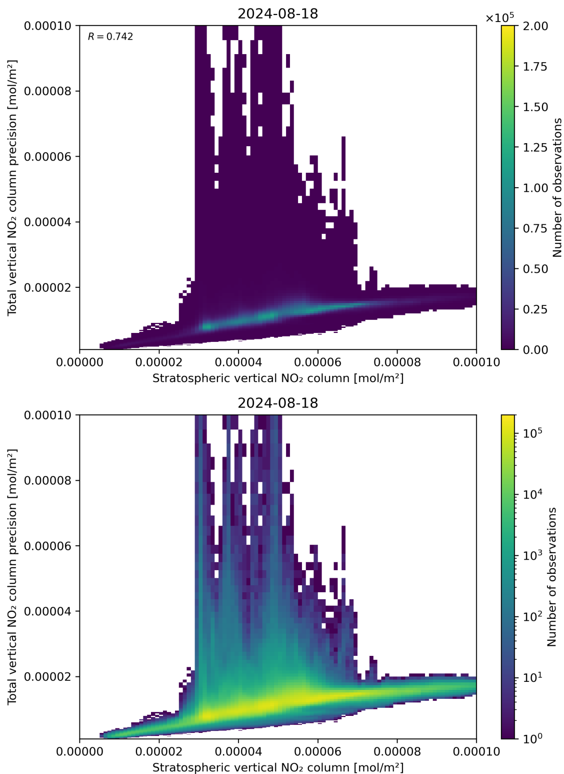
Figure 101: Scatter density plot of “Stratospheric vertical NO 2 column” against “Total vertical NO 2 column precision” for 2024-08-17 to 2024-08-19.
