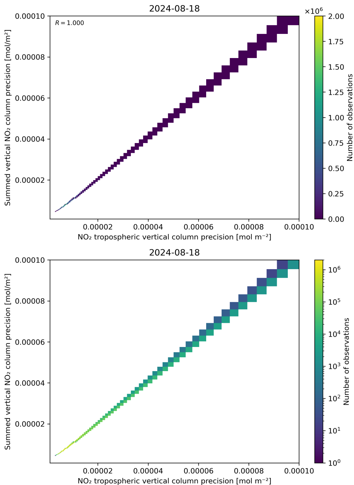
Figure 137: Scatter density plot of “NO 2 tropospheric vertical column precision” against “Summed vertical NO 2 column precision” for 2024-08-17 to 2024-08-19.
