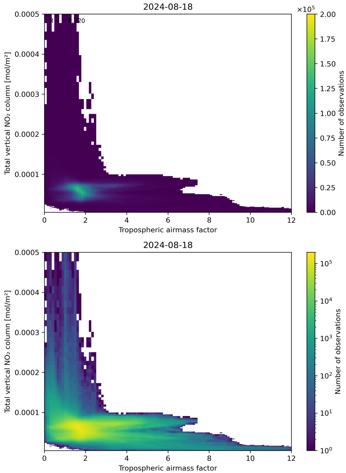
Figure 77: Scatter density plot of “Tropospheric airmass factor” against “Total vertical NO 2 column” for 2024-08-17 to 2024-08-19.
