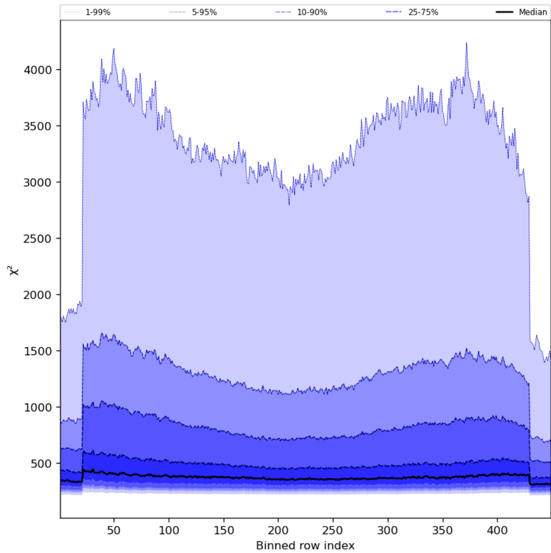
Figure 59: Along track statistics of “ \chi^2 ” for 2024-08-17 to 2024-08-19
