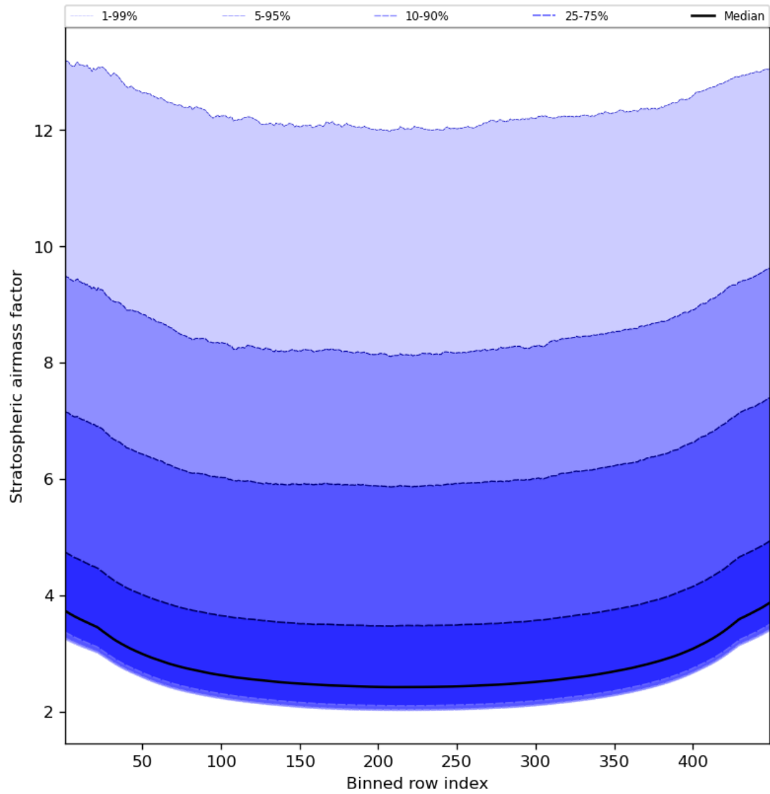
Figure 61: Along track statistics of “Stratospheric airmass factor” for 2024-08-17 to 2024-08-19
