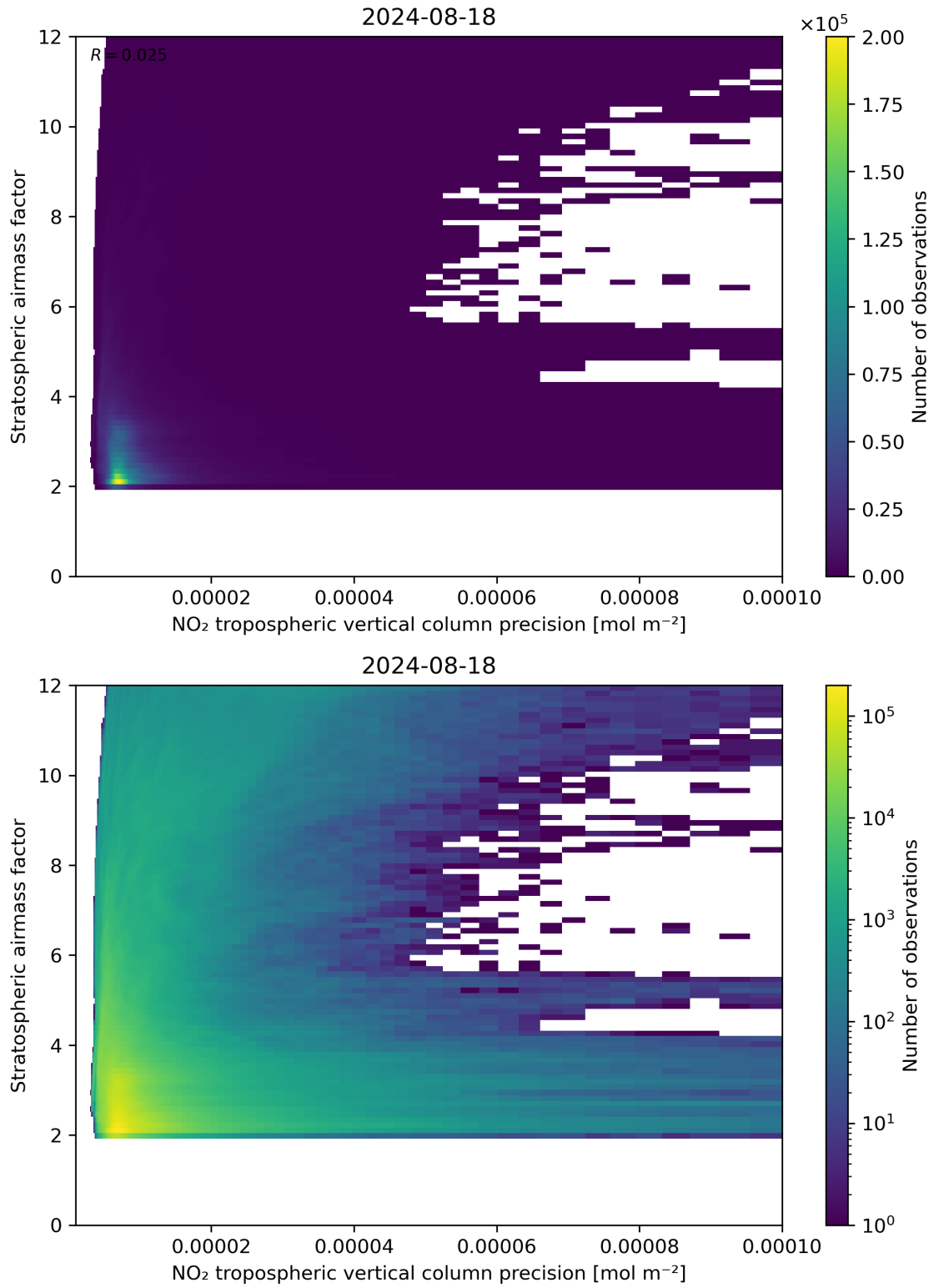
Figure 131: Scatter density plot of “NO 2 tropospheric vertical column precision” against “Stratospheric airmass factor” for 2024-08-17 to 2024-08-19.
