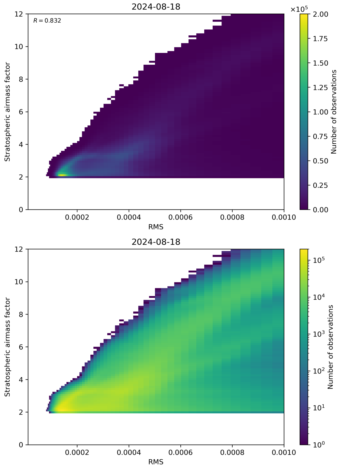
Figure 144: Scatter density plot of “RMS” against “Stratospheric airmass factor” for 2024-08-17 to 2024-08-19.
