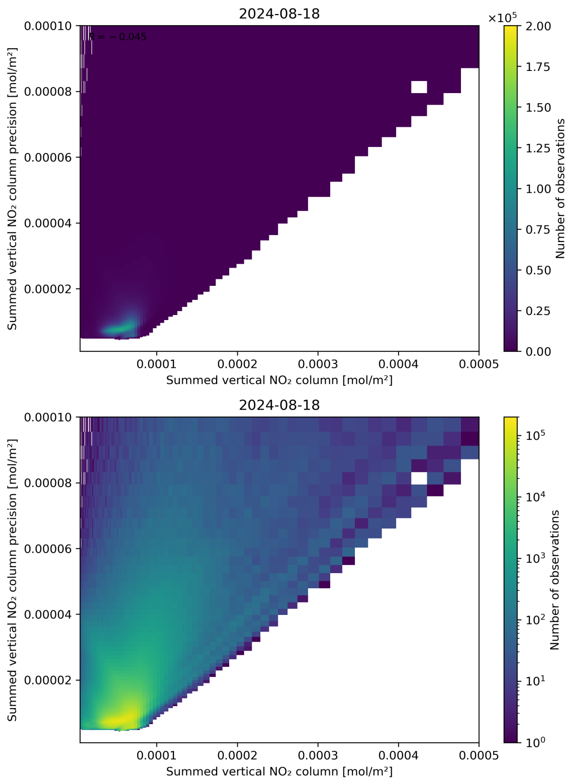
Figure 105: Scatter density plot of “Summed vertical NO 2 column” against “Summed vertical NO 2 column precision” for 2024-08-17 to 2024-08-19.
