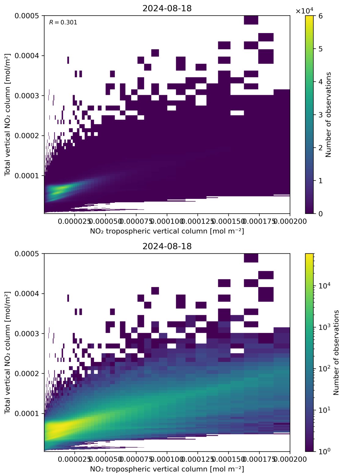
Figure 128: Scatter density plot of “NO 2 tropospheric vertical column” against “Total vertical NO 2 column” for 2024-08-17 to 2024-08-19.
