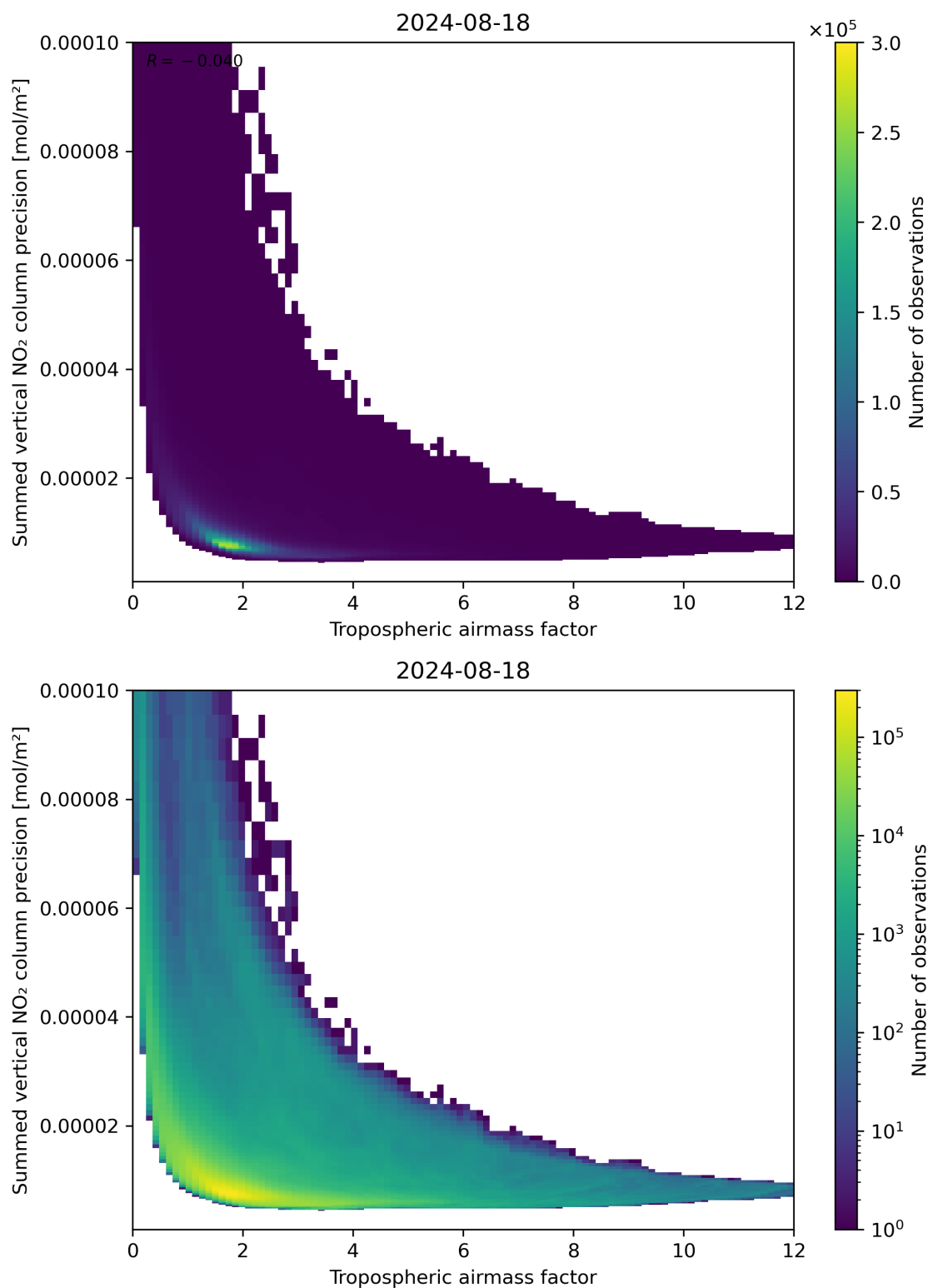
Figure 76: Scatter density plot of “Tropospheric air mass factor” against “Summed vertical NO 2 column precision” for 2024-08-17 to 2024-08-19.
