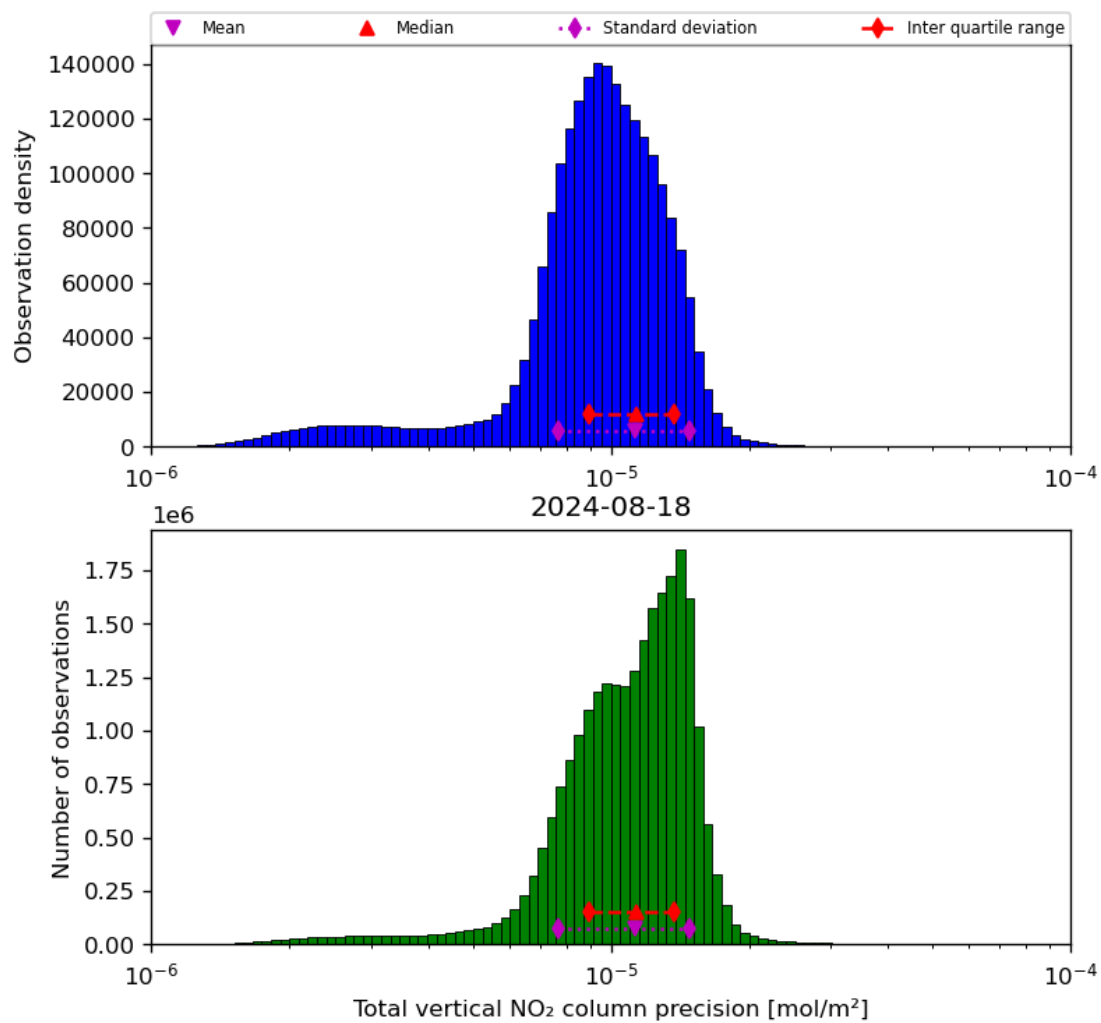
Figure 39: Histogram of “Total vertical NO 2 column precision” for 2024-08-17 to 2024-08-19
