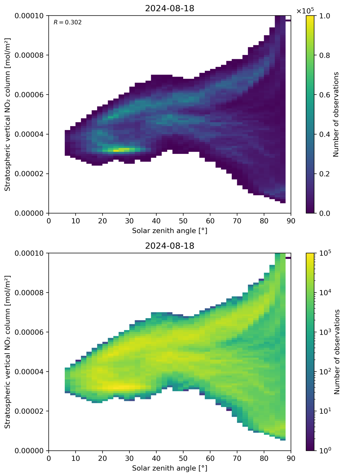
Figure 150: Scatter density plot of “Solar zenith angle” against “Stratospheric vertical NO 2 column” for 2024-08-17 to 2024-08-19.
