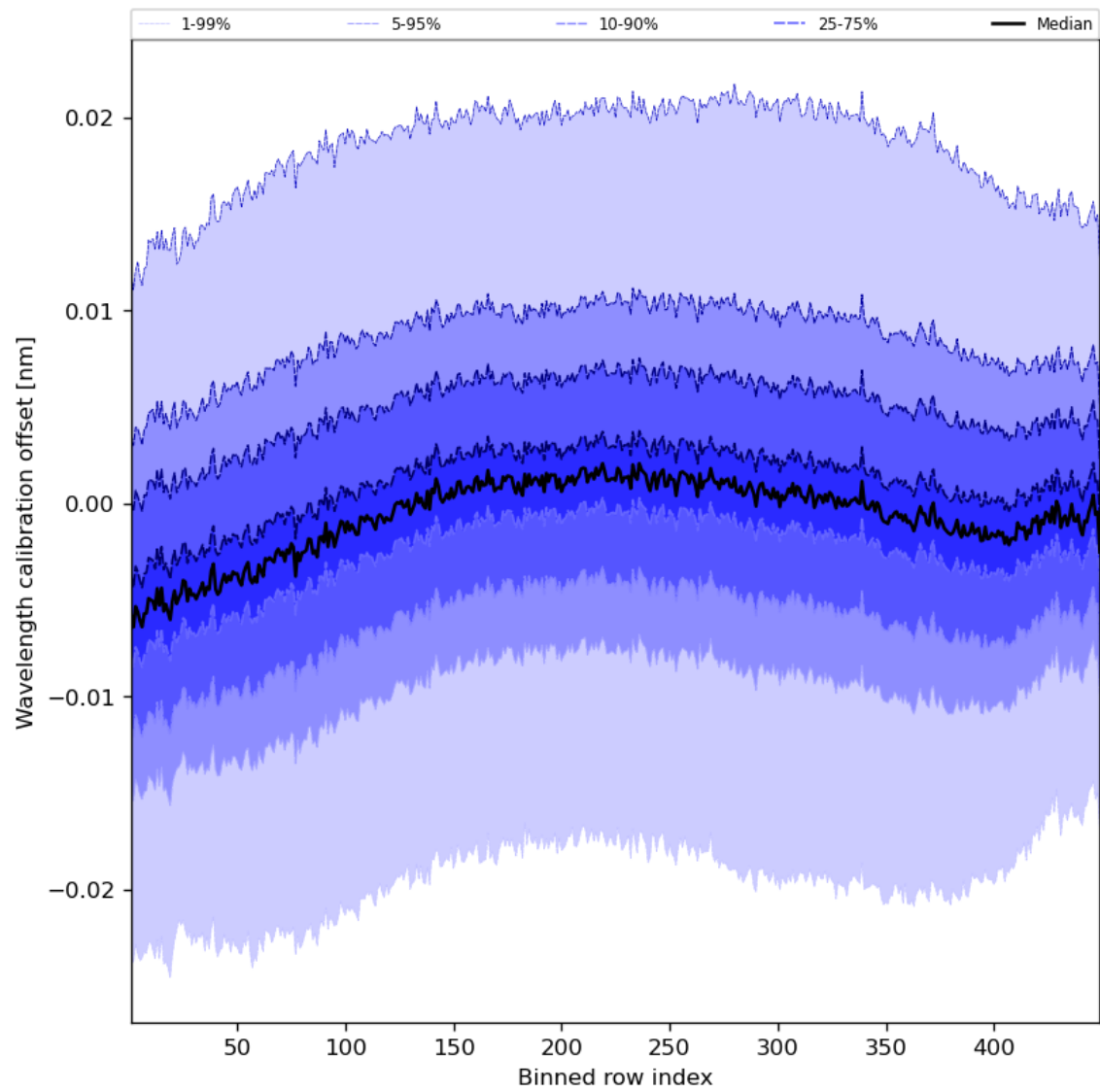
Figure 52: Along track statistics of “Wavelength calibration offset” for 2024-08-17 to 2024-08-19
