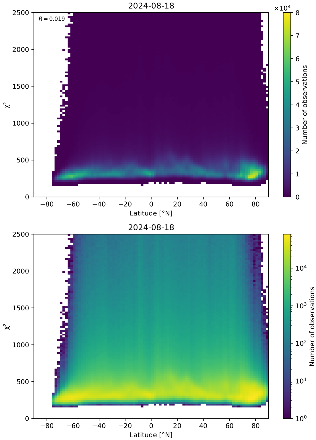
Figure 86: Scatter density plot of “Latitude” against “ \chi^2 ” for 2024-08-17 to 2024-08-19.
