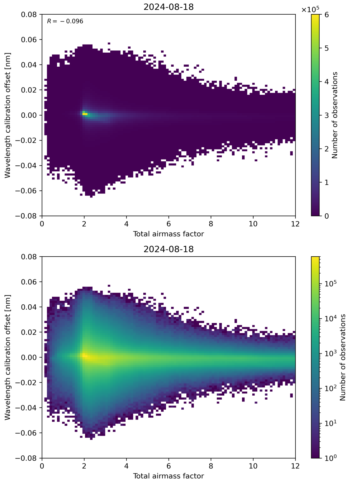
Figure 70: Scatter density plot of “Total airmass factor” against “Wavelength calibration offset” for 2024-08-17 to 2024-08-19.
