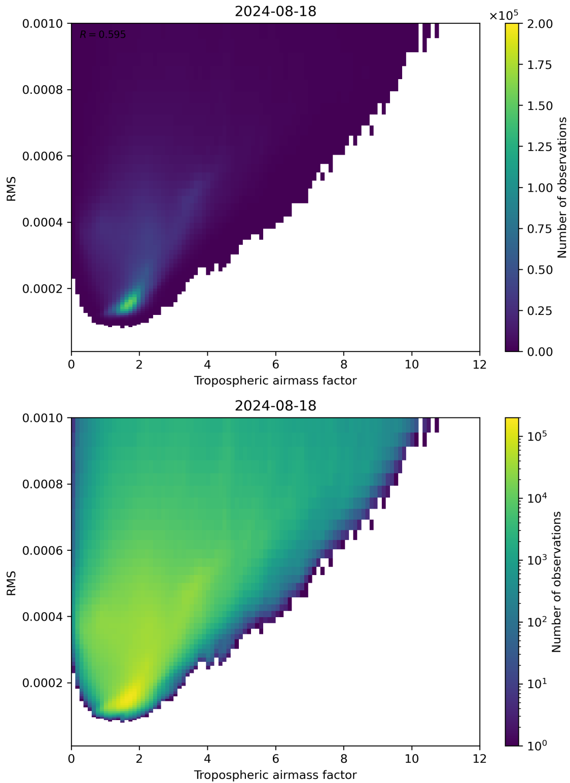
Figure 79: Scatter density plot of “Tropospheric airmass factor” against “RMS” for 2024-08-17 to 2024-08-19.
