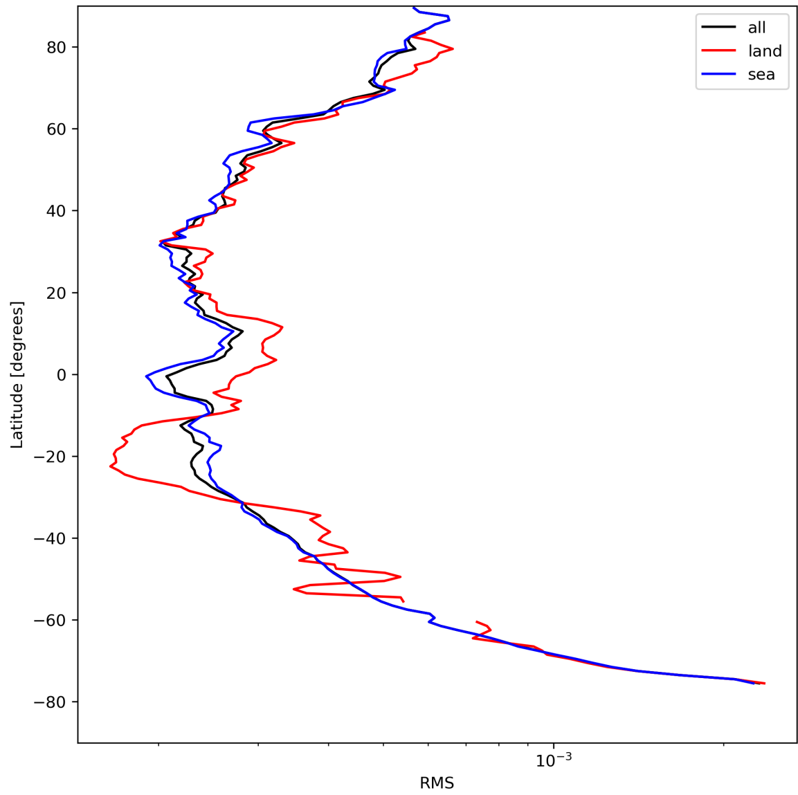
Figure 26: Zonal average of “RMS” for 2024-08-17 to 2024-08-19.
