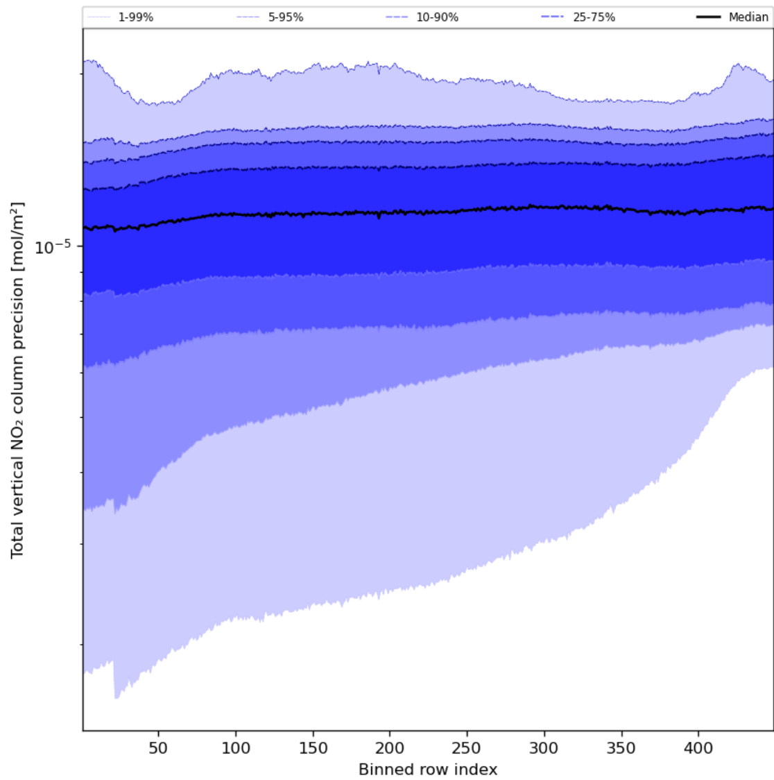
Figure 56: Along track statistics of “Total vertical NO 2 column precision” for 2024-08-17 to 2024-08-19
