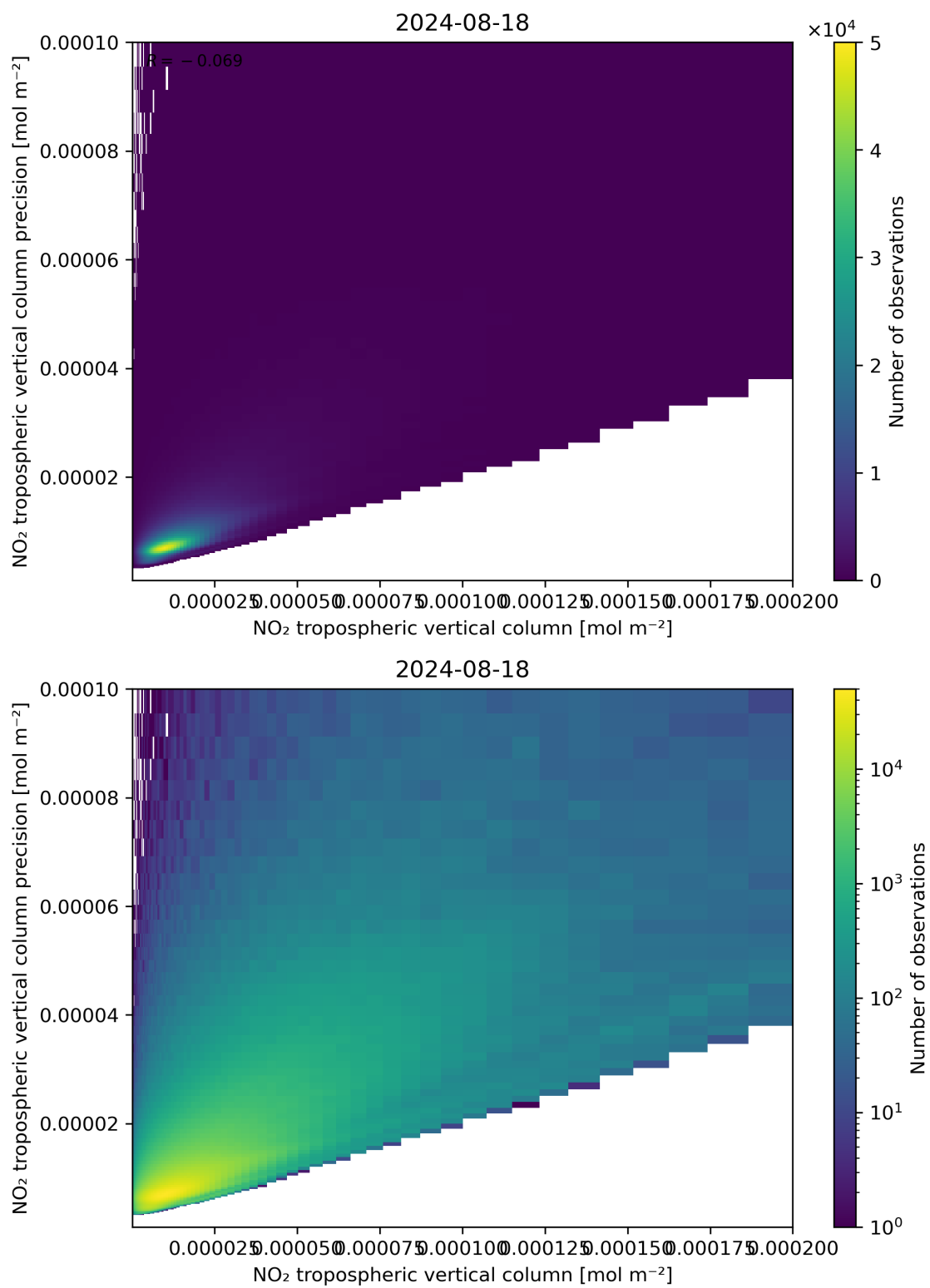
Figure 130: Scatter density plot of “NO 2 tropospheric vertical column” against “NO 2 tropospheric vertical column precision” for 2024-08-17 to 2024-08-19.
