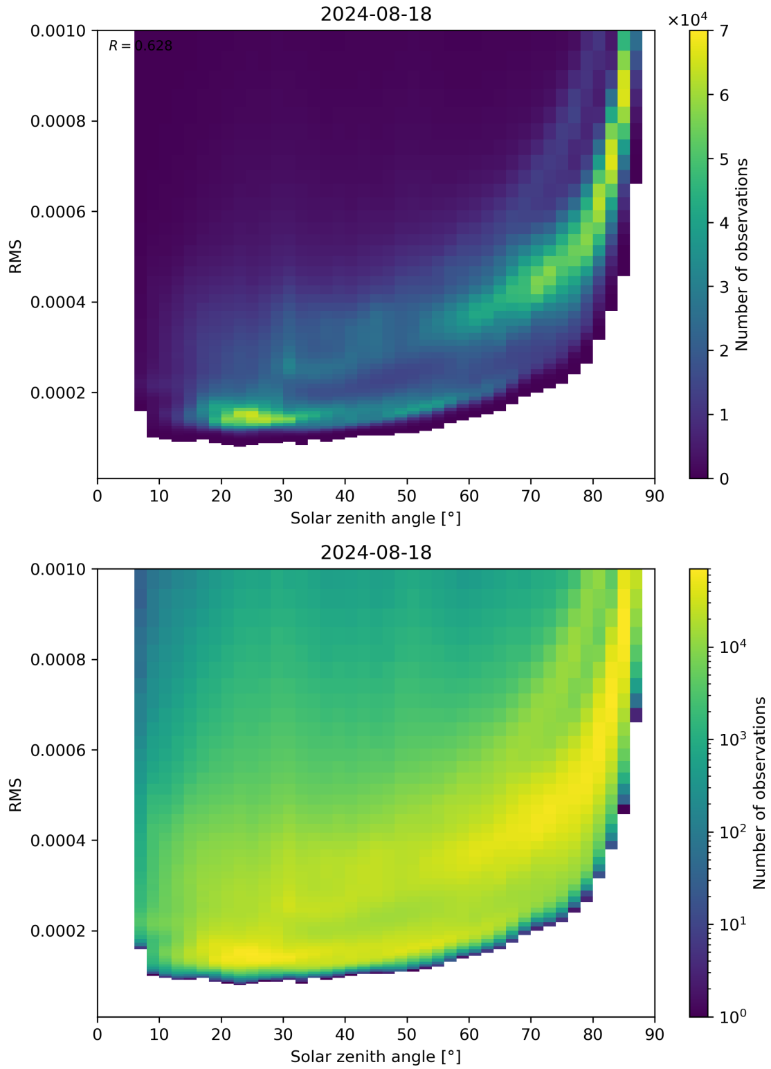
Figure 157: Scatter density plot of “Solar zenith angle” against “RMS” for 2024-08-17 to 2024-08-19.
