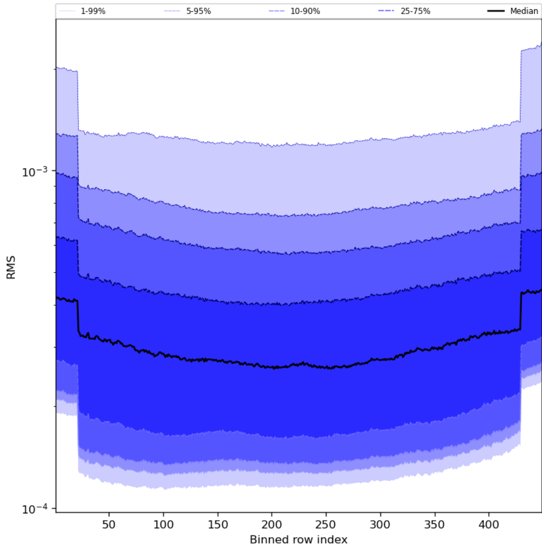
Figure 60: Along track statistics of “RMS” for 2024-08-17 to 2024-08-19
