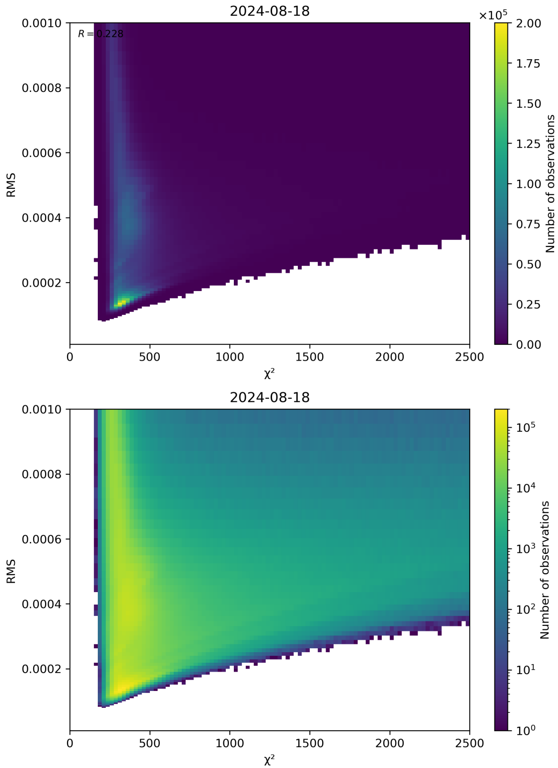
Figure 82: Scatter density plot of “ \chi^2 ” against “RMS” for 2024-08-17 to 2024-08-19.
