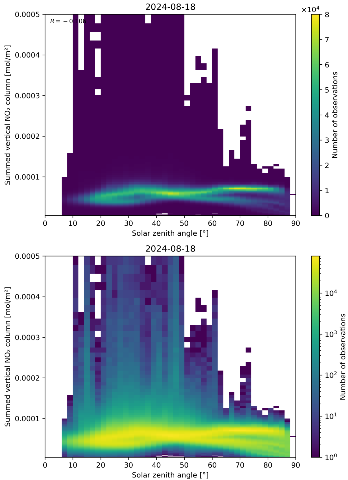
Figure 151: Scatter density plot of “Solar zenith angle” against “Summed vertical NO 2 column” for 2024-08-17 to 2024-08-19.
