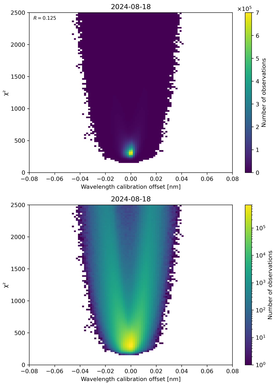
Figure 175: Scatter density plot of “Wavelength calibration offset” against “ \chi^2 ” for 2024-08-17 to 2024-08-19.
