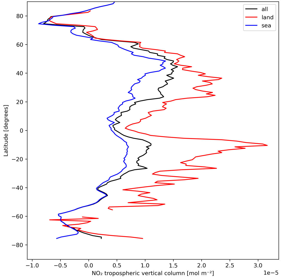
Figure 12: Zonal average of “NO 2 tropospheric vertical column” for 2024-08-17 to 2024-08-19.
