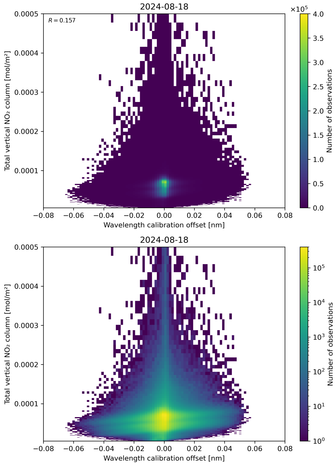
Figure 179: Scatter density plot of “Wavelength calibration offset” against “Total vertical NO 2 column” for 2024-08-17 to 2024-08-19.
