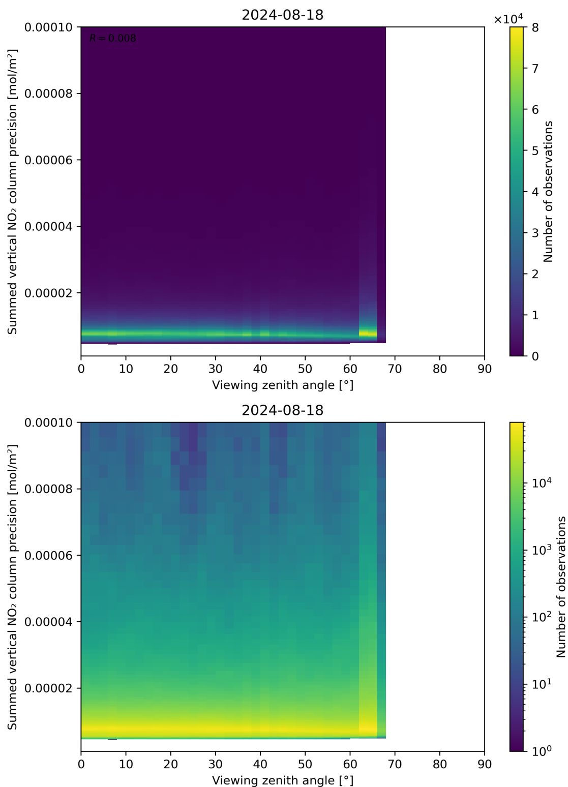
Figure 166: Scatter density plot of “Viewing zenith angle” against “Summed vertical NO 2 column precision” for 2024-08-17 to 2024-08-19.
