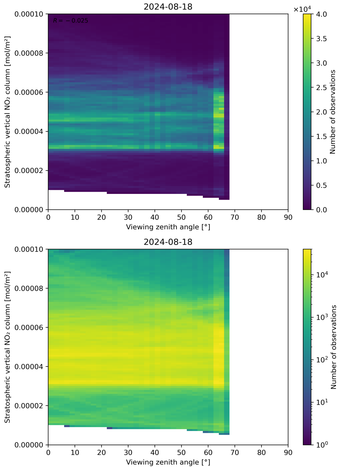
Figure 164: Scatter density plot of “Viewing zenith angle” against “Stratospheric vertical NO 2 column” for 2024-08-17 to 2024-08-19.
