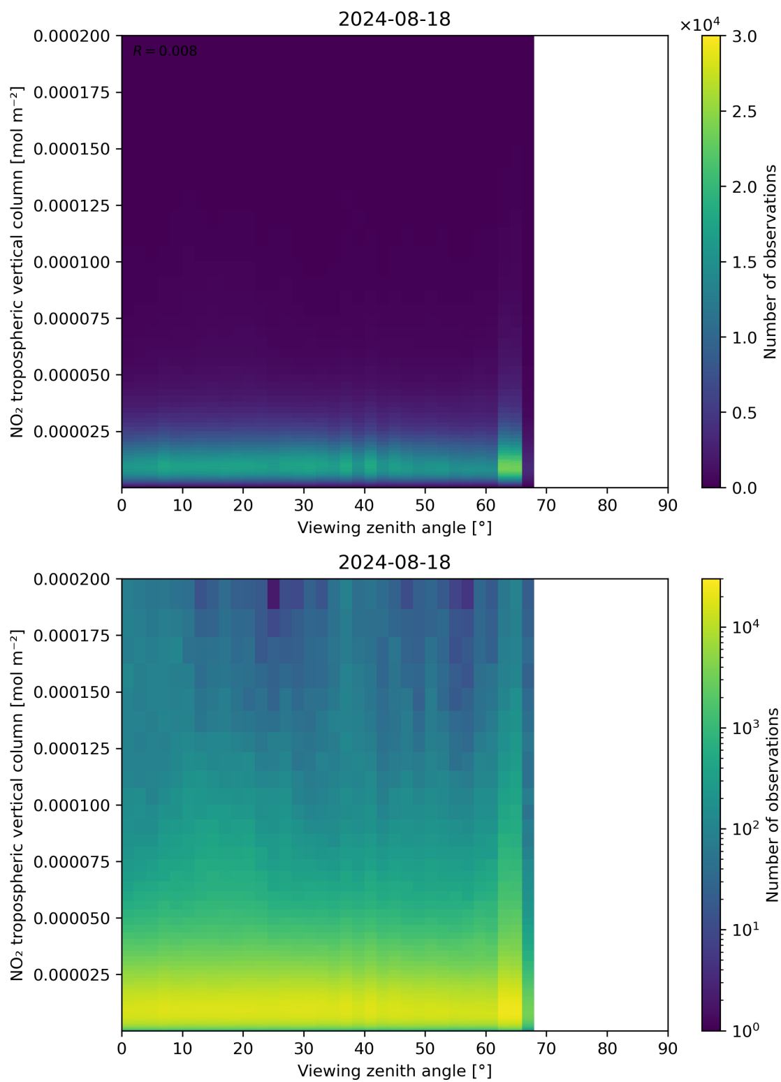
Figure 169: Scatter density plot of “Viewing zenith angle” against “NO 2 tropospheric vertical column” for 2024-08-17 to 2024-08-19.
