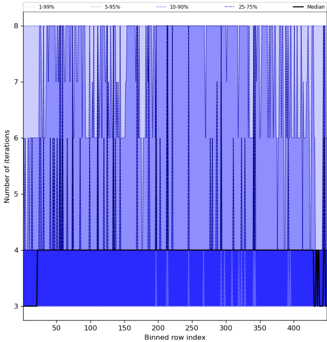
Figure 51: Along track statistics of “Number of iterations” for 2024-08-17 to 2024-08-19
