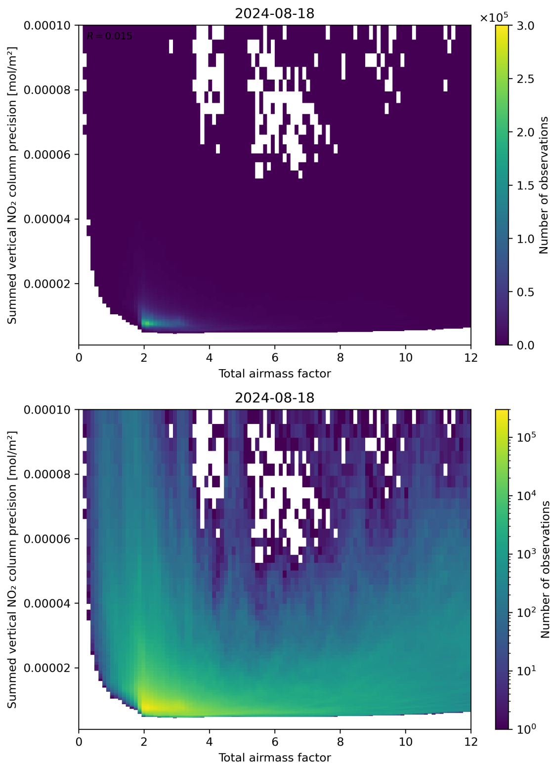
Figure 66: Scatter density plot of “Total airmass factor” against “Summed vertical NO 2 column precision” for 2024-08-17 to 2024-08-19.
