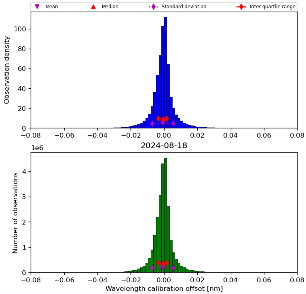
Figure 35: Histogram of “Wavelength calibration offset” for 2024-08-17 to 2024-08-19
