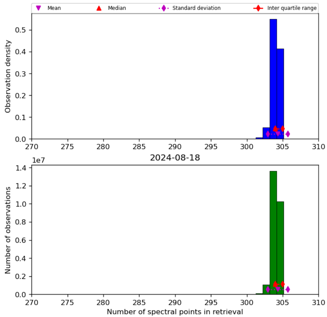
Figure 33: Histogram of “Number of spectral points in retrieval” for 2024-08-17 to 2024-08-19
