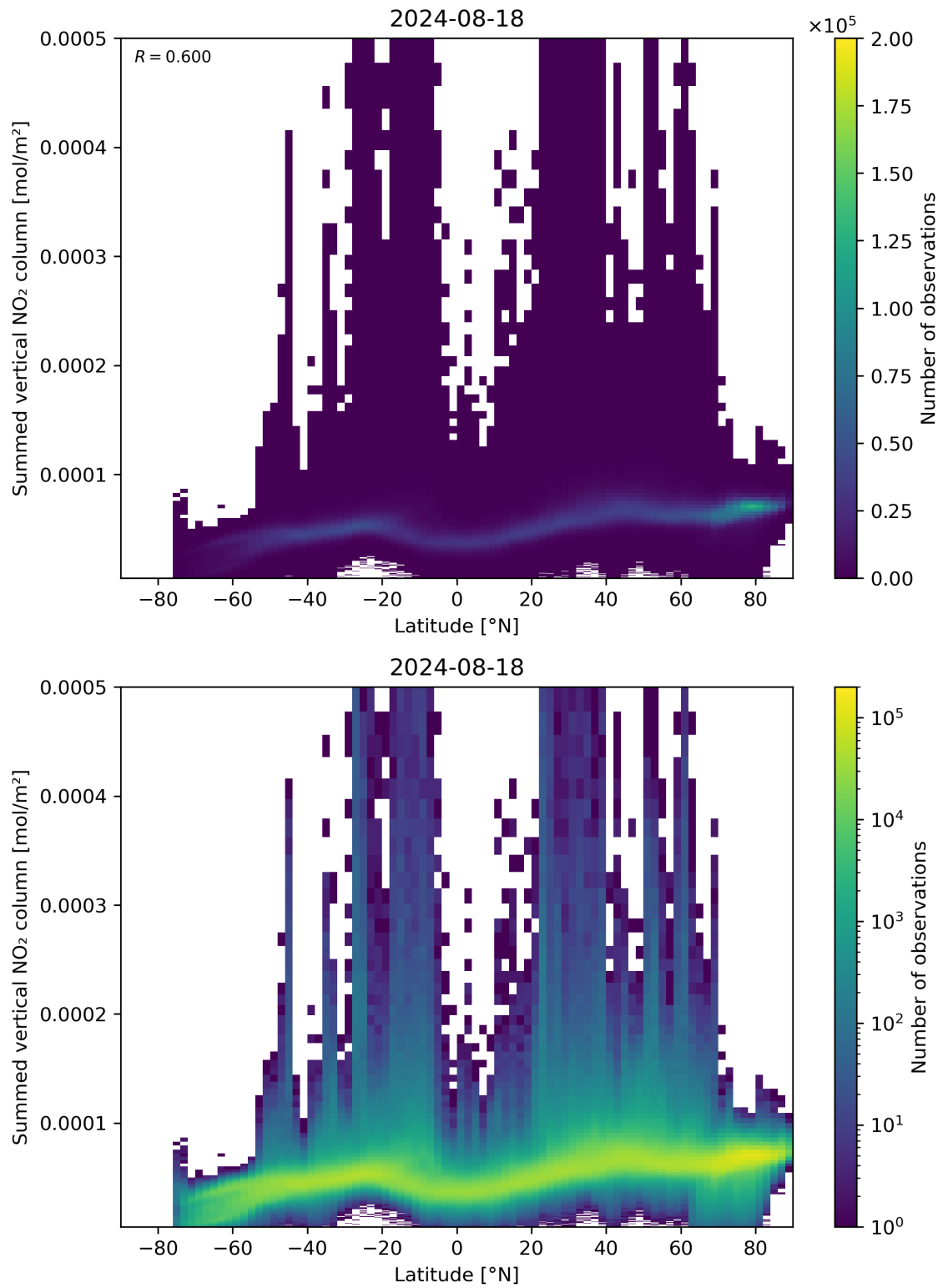
Figure 88: Scatter density plot of “Latitude” against “Summed vertical NO 2 column” for 2024-08-17 to 2024-08-19.
