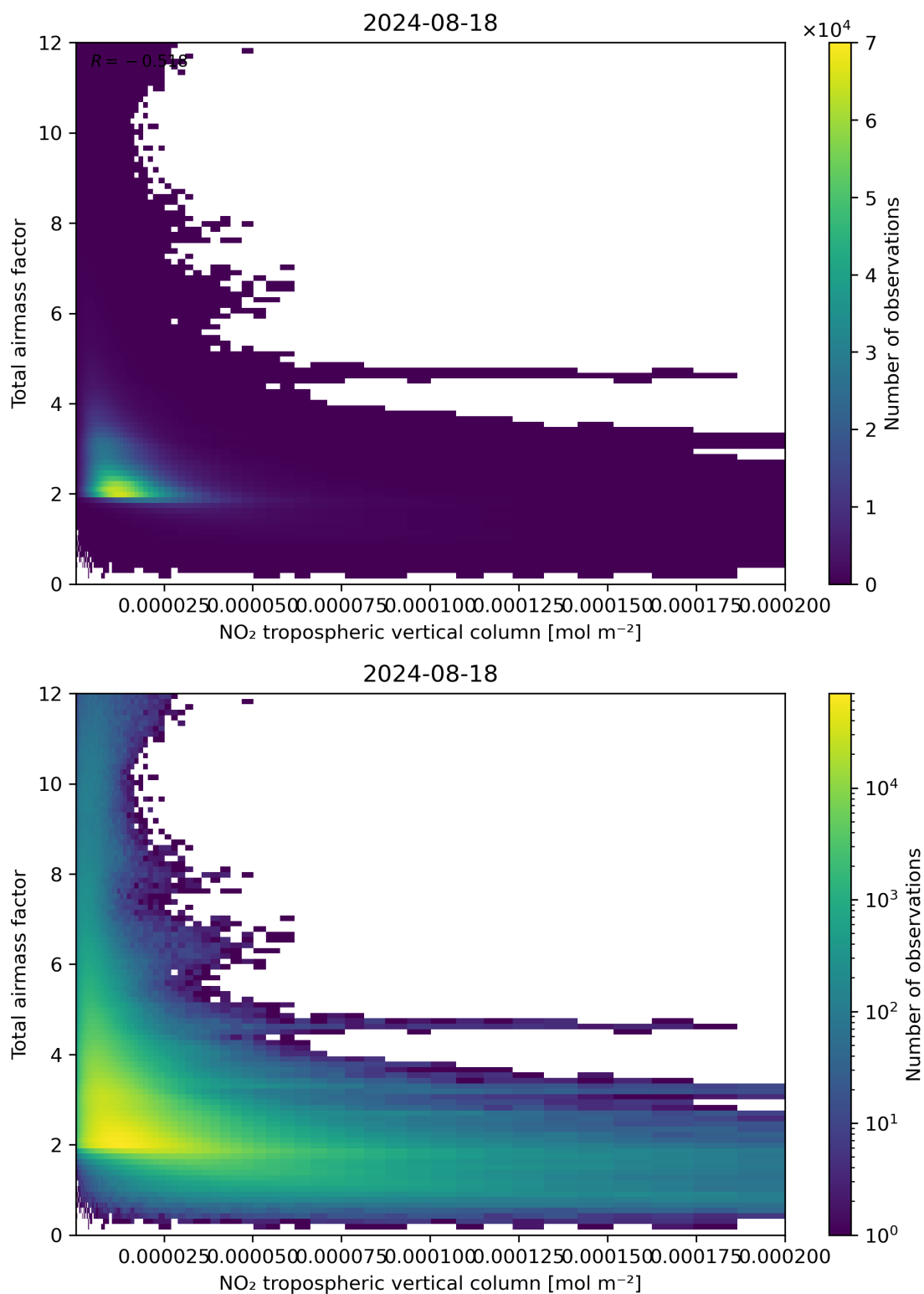
Figure 122: Scatter density plot of “NO 2 tropospheric vertical column” against “Total airmass factor” for 2024-08-17 to 2024-08-19.
