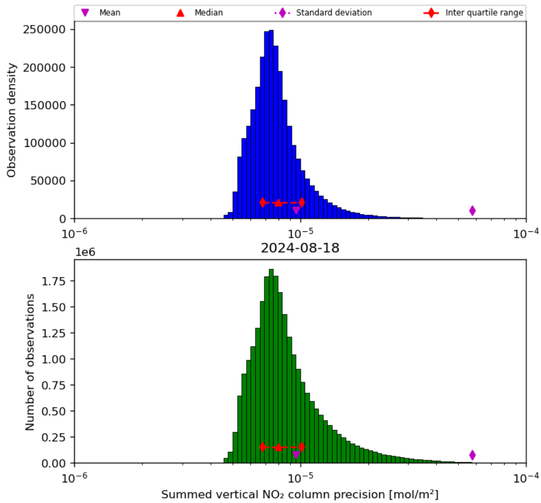
Figure 41: Histogram of "Summed vertical NO 2 column precision" for 2024-08-17 to 2024-08-19
