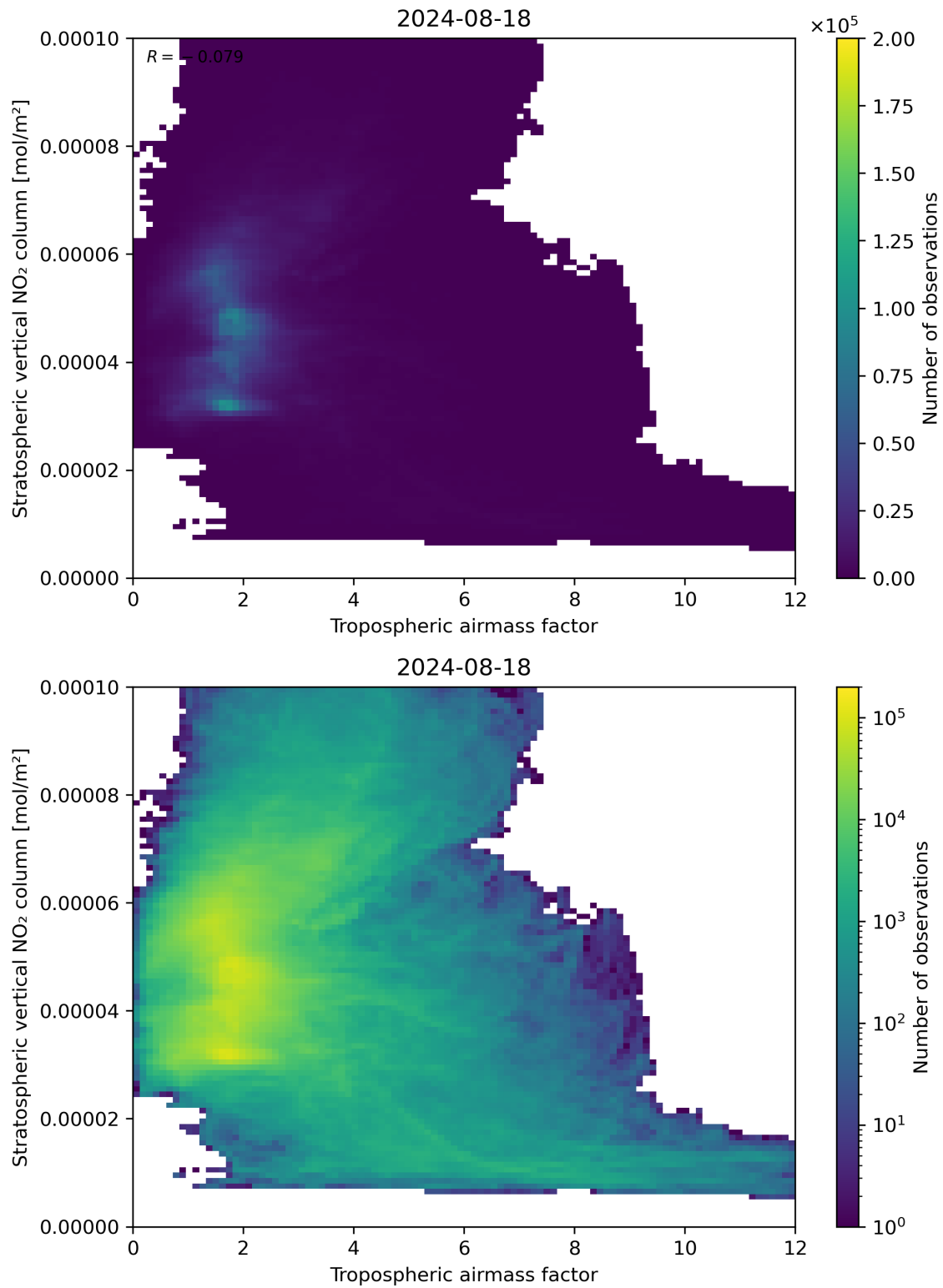
Figure 74: Scatter density plot of “Tropospheric air mass factor” against “Stratospheric vertical NO 2 column” for 2024-08-17 to 2024-08-19.
