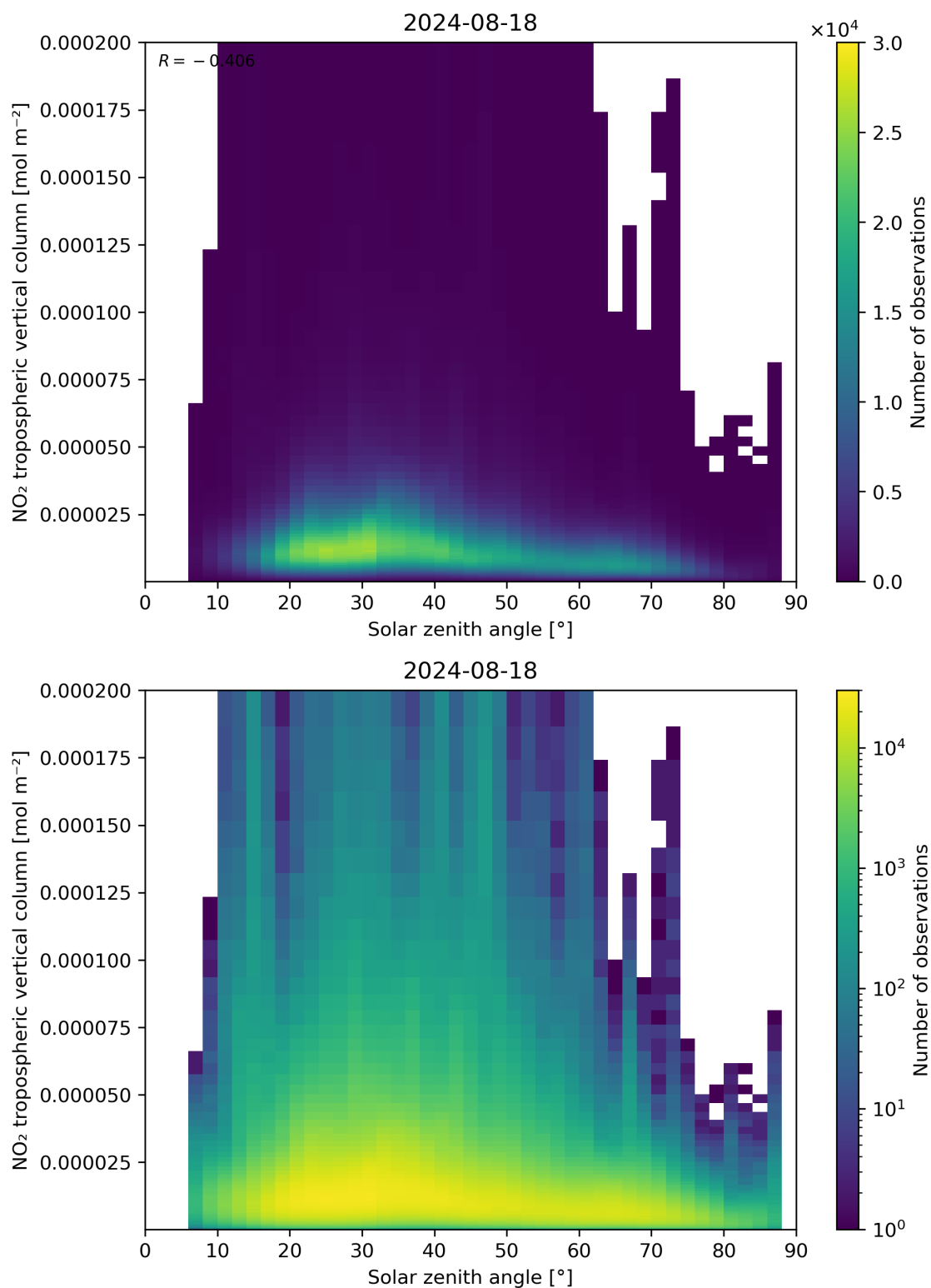
Figure 155: Scatter density plot of “Solar zenith angle” against “NO 2 tropospheric vertical column” for 2024-08-17 to 2024-08-19.
