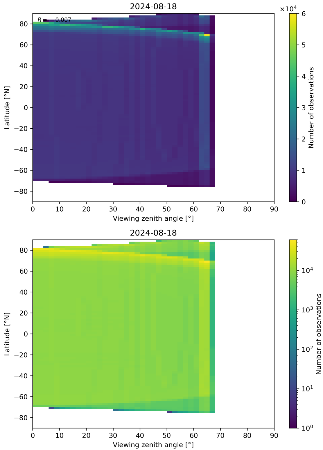
Figure 163: Scatter density plot of “Viewing zenith angle” against “Latitude” for 2024-08-17 to 2024-08-19.
