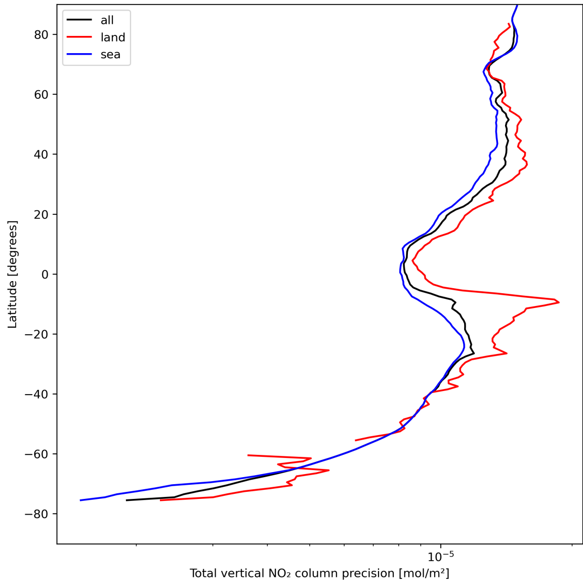
Figure 22: Zonal average of “Total vertical NO 2 column precision” for 2024-08-17 to 2024-08-19.
