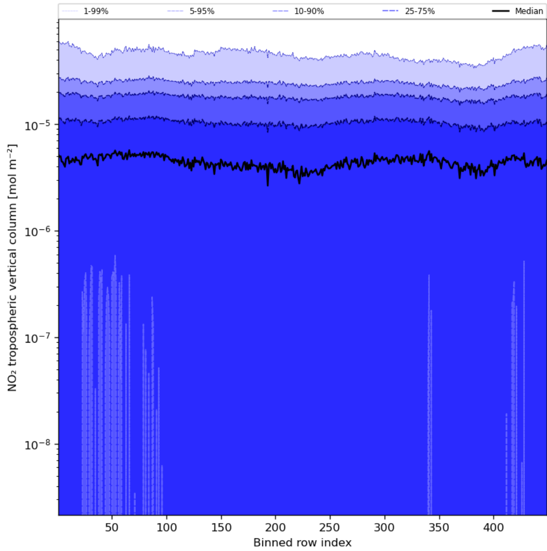
Figure 46: Along track statistics of “NO 2 tropospheric vertical column” for 2024-08-17 to 2024-08-19
