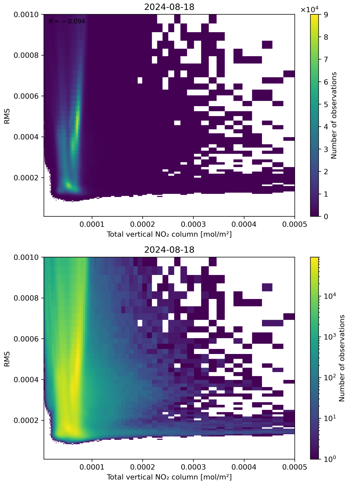
Figure 120: Scatter density plot of “Total vertical NO 2 column” against “RMS” for 2024-08-17 to 2024-08-19.
