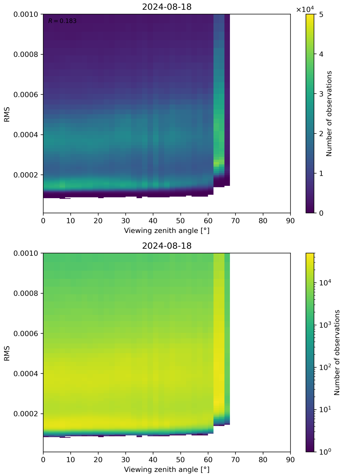
Figure 171: Scatter density plot of “Viewing zenith angle” against “RMS” for 2024-08-17 to 2024-08-19.
