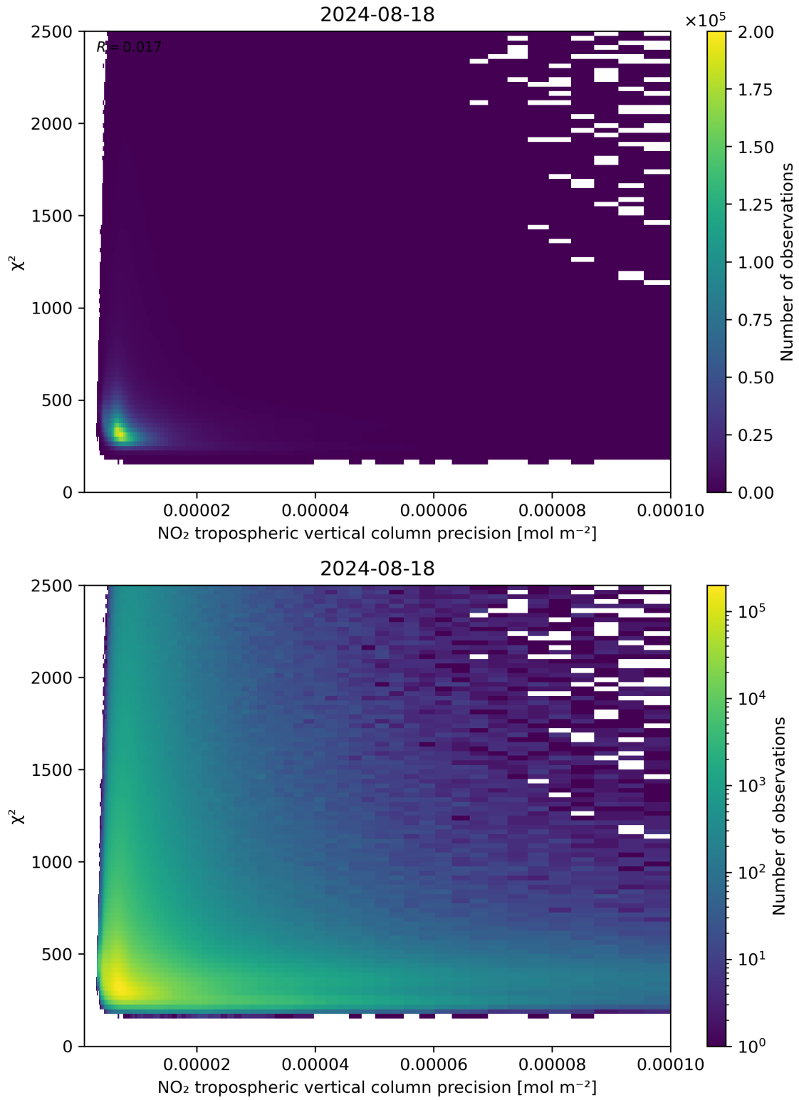
Figure 134: Scatter density plot of “NO 2 tropospheric vertical column precision” against “ \chi^2 ” for 2024-08-17 to 2024-08-19.
