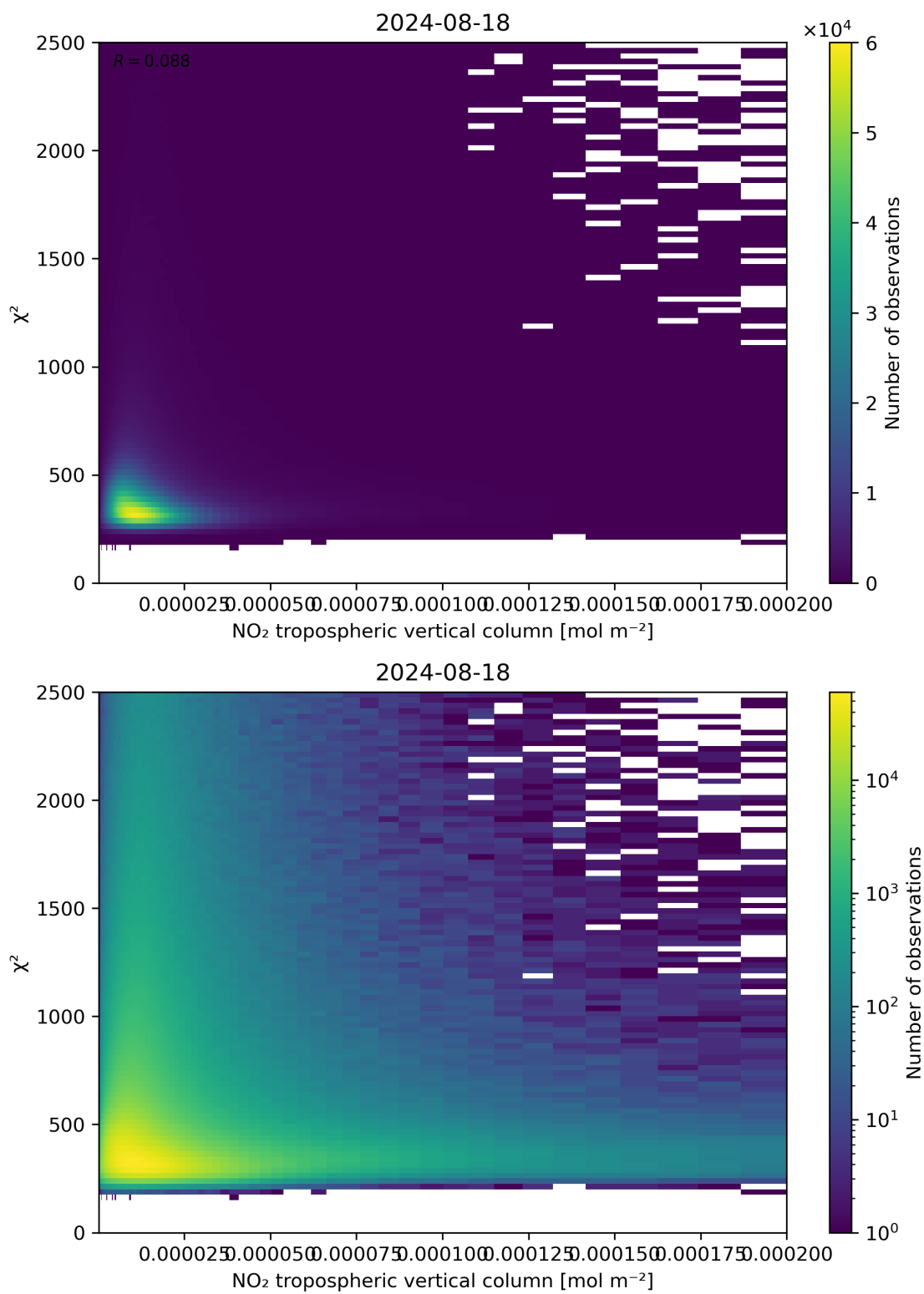
Figure 124: Scatter density plot of “NO 2 tropospheric vertical column” against “ \chi^2 ” for 2024-08-17 to 2024-08-19.
