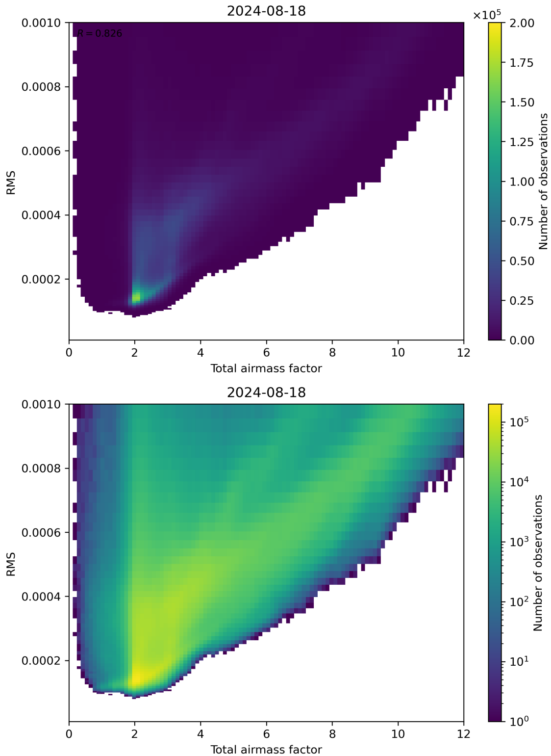
Figure 69: Scatter density plot of “Total airmass factor” against “RMS” for 2024-08-17 to 2024-08-19.
