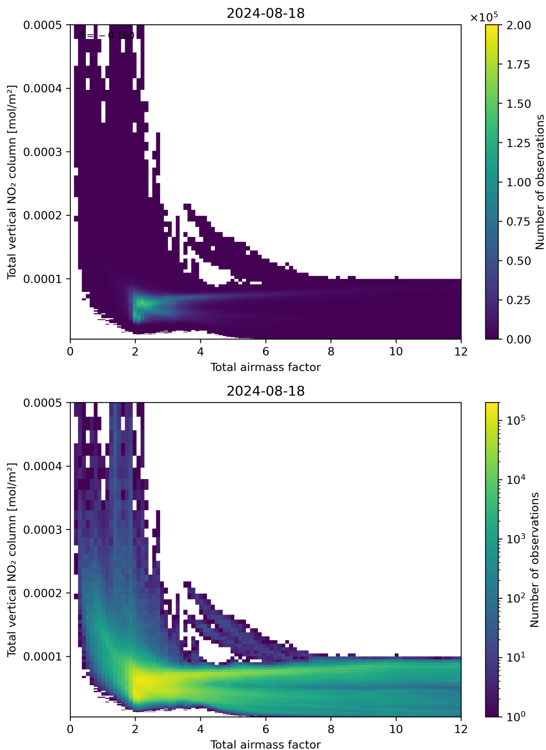
Figure 67: Scatter density plot of “Total airmass factor” against “Total vertical NO 2 column” for 2024-08-17 to 2024-08-19.
