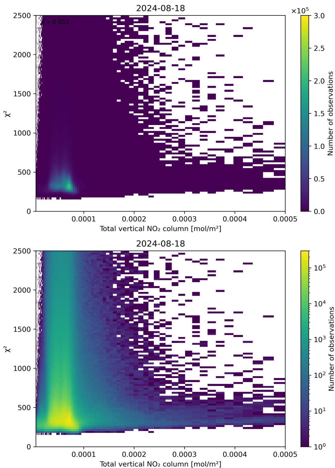
Figure 111: Scatter density plot of “Total vertical NO 2 column” against “ \chi^2 ” for 2024-08-17 to 2024-08-19.
