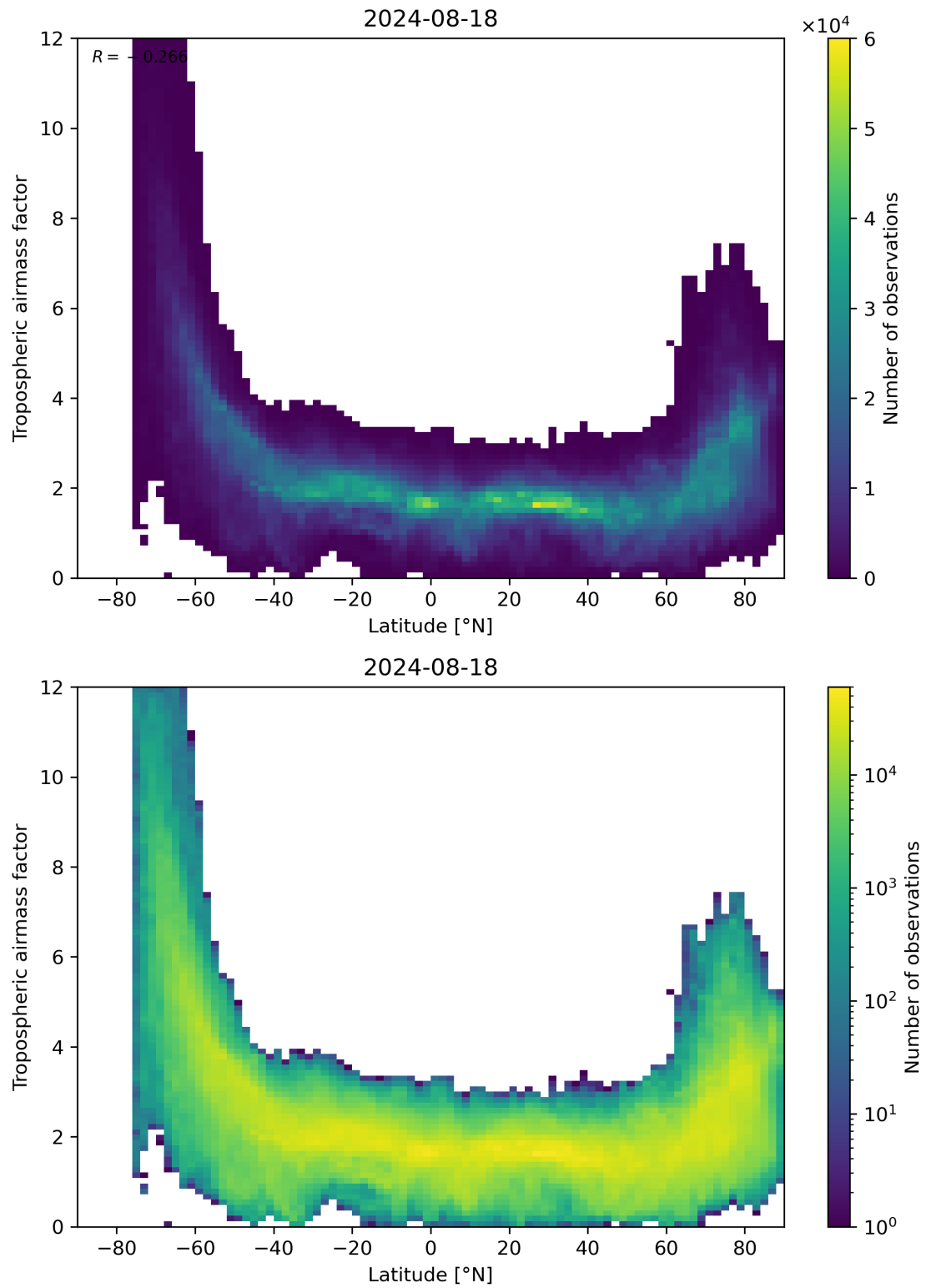
Figure 85: Scatter density plot of “Latitude” against “Tropospheric air mass factor” for 2024-08-17 to 2024-08-19.
