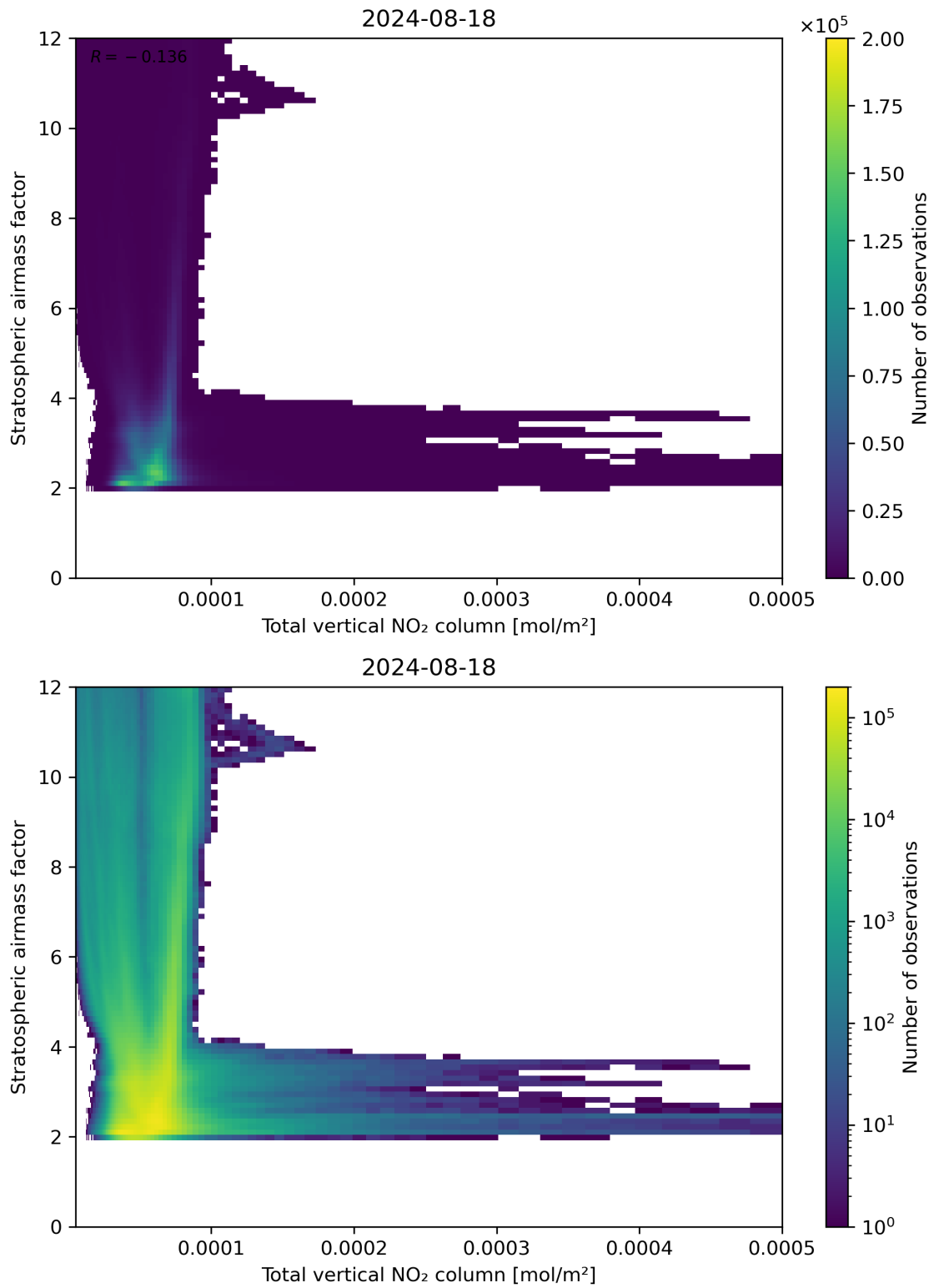
Figure 110: Scatter density plot of “Total vertical NO 2 column” against “Stratospheric airmass factor” for 2024-08-17 to 2024-08-19.
