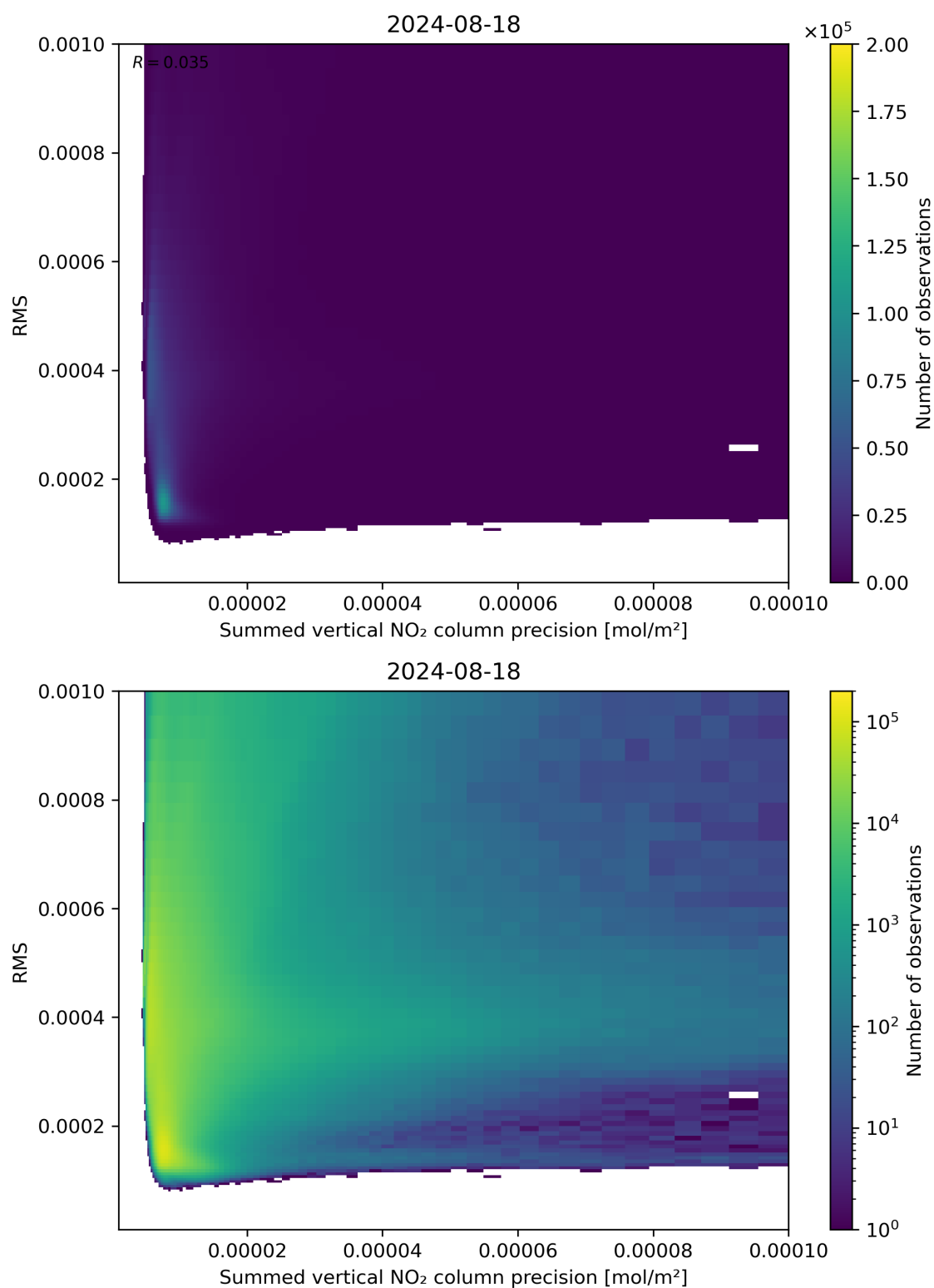
Figure 108: Scatter density plot of “Summed vertical NO 2 column precision” against “RMS” for 2024-08-17 to 2024-08-19.
