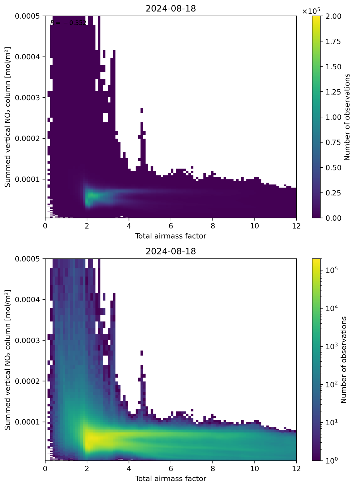
Figure 65: Scatter density plot of “Total airmass factor” against “Summed vertical NO 2 column” for 2024-08-17 to 2024-08-19.
