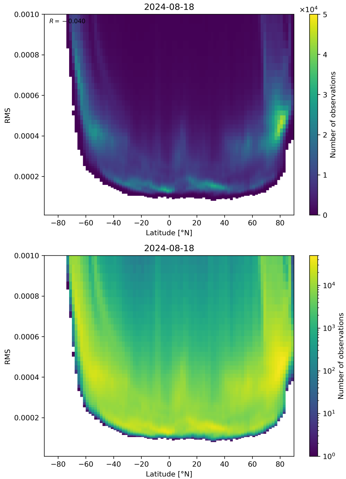
Figure 94: Scatter density plot of “Latitude” against “RMS” for 2024-08-17 to 2024-08-19.
