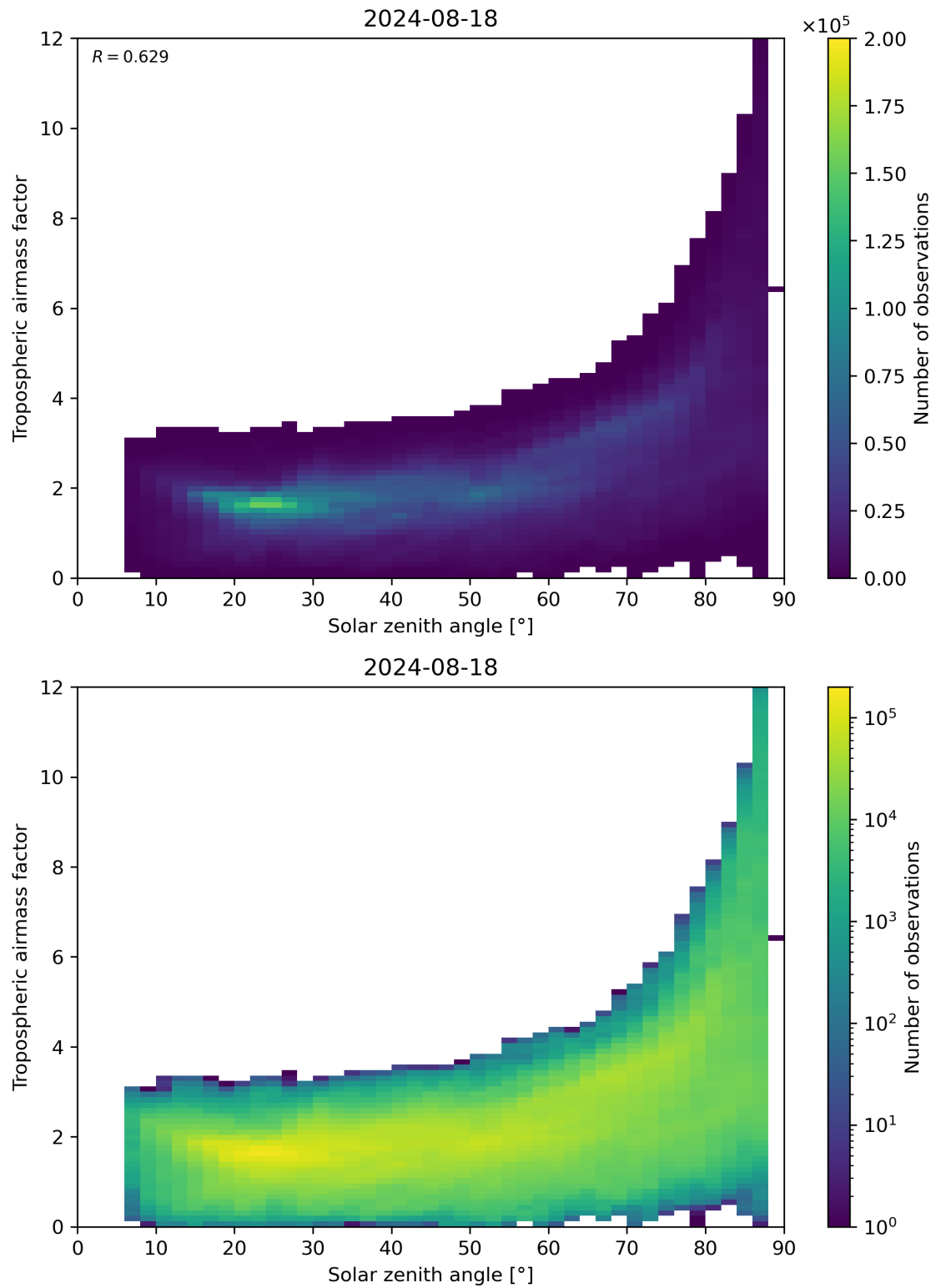
Figure 147: Scatter density plot of “Solar zenith angle” against “Tropospheric airmass factor” for 2024-08-17 to 2024-08-19.
