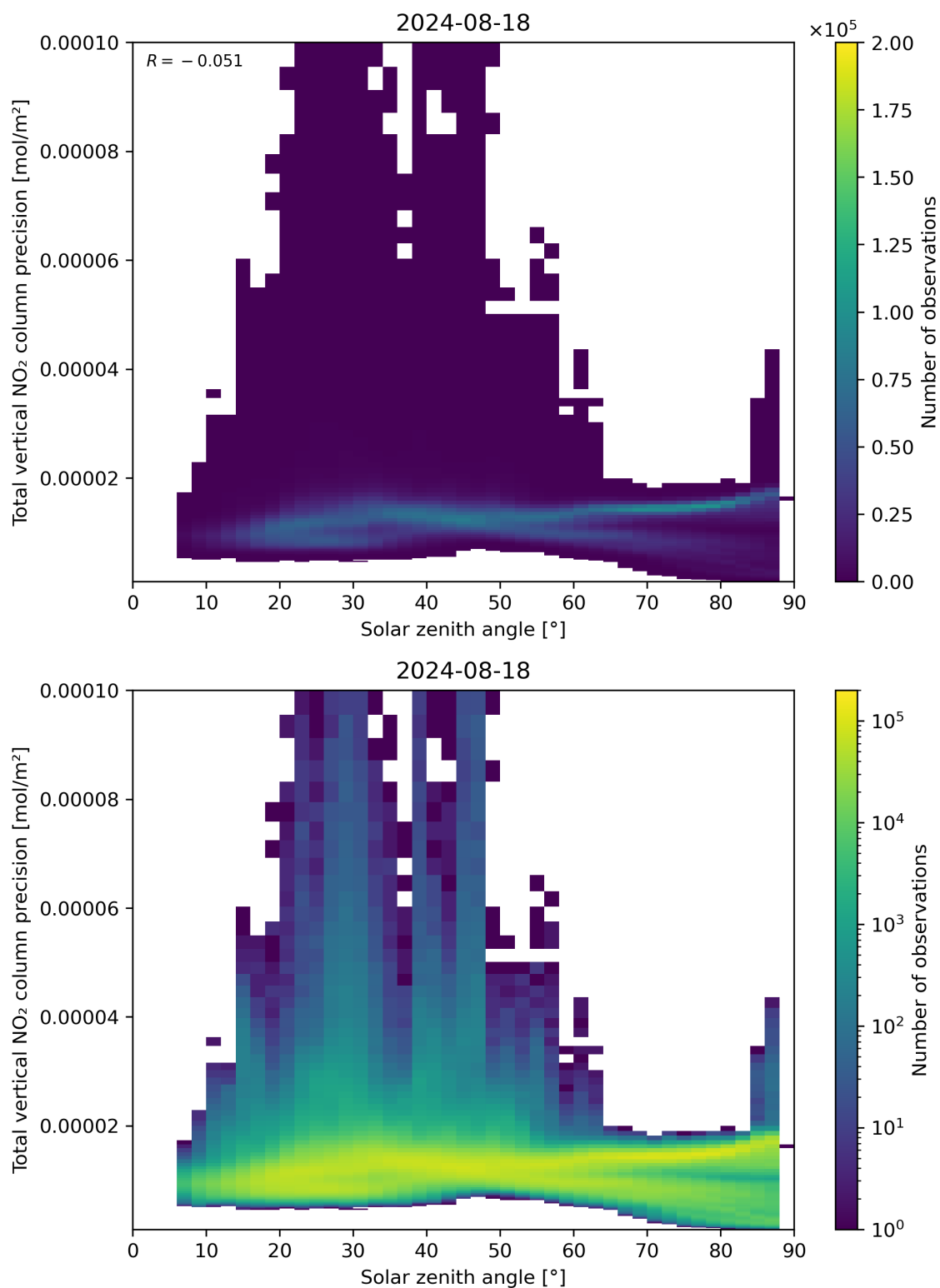
Figure 154: Scatter density plot of “Solar zenith angle” against “Total vertical NO 2 column precision” for 2024-08-17 to 2024-08-19.
