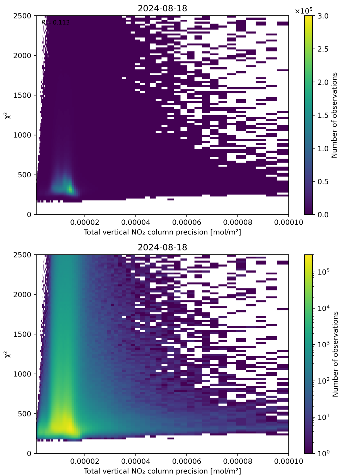
Figure 116: Scatter density plot of “Total vertical NO 2 column precision” against “ \chi^2 ” for 2024-08-17 to 2024-08-19.
