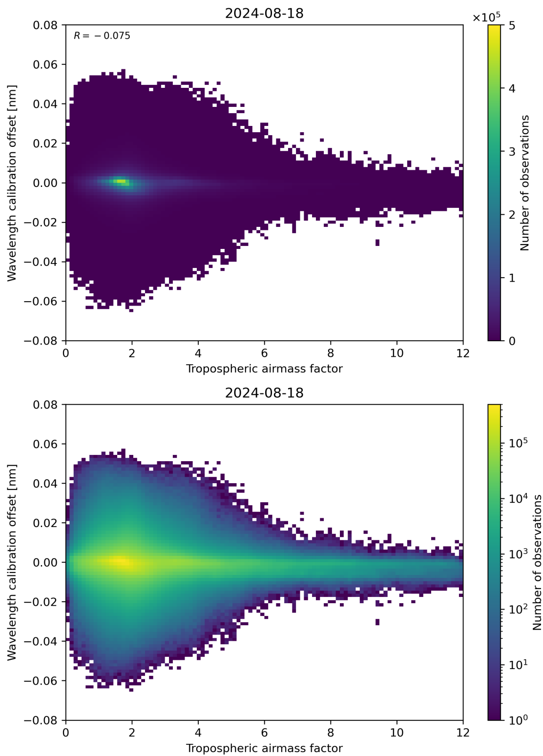
Figure 80: Scatter density plot of “Tropospheric air mass factor” against “Wavelength calibration offset” for 2024-08-17 to 2024-08-19.
