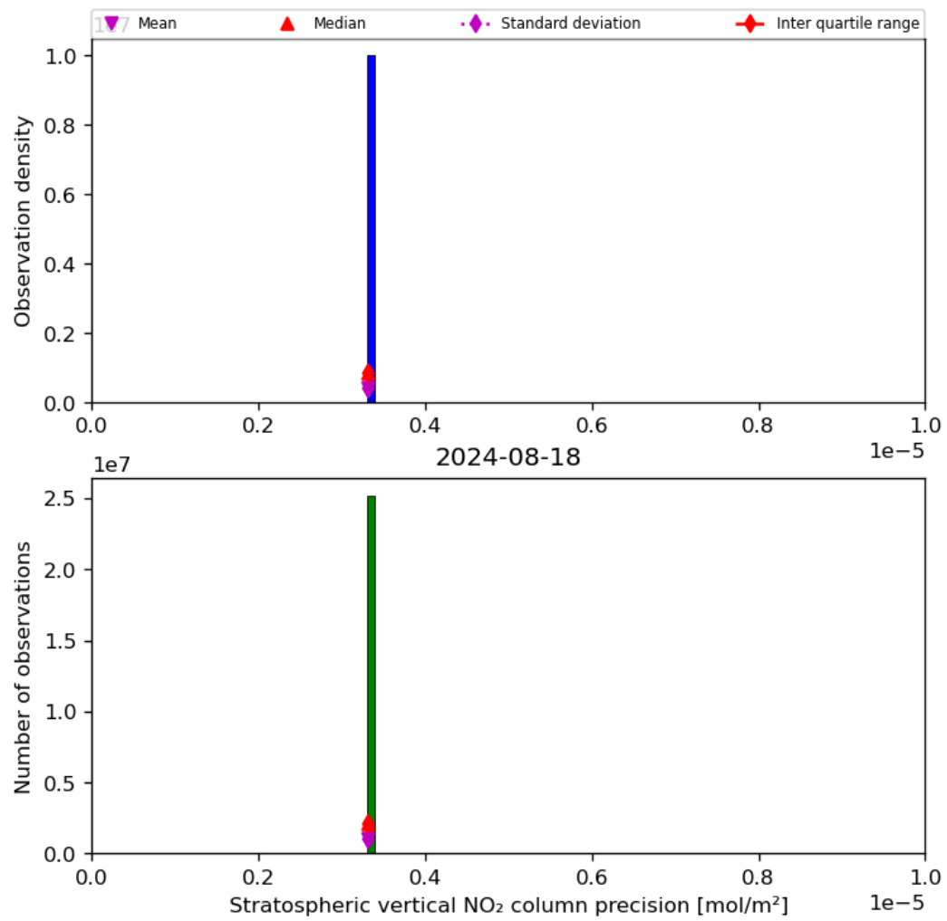
Figure 37: Histogram of “Stratospheric vertical NO 2 column precision” for 2024-08-17 to 2024-08-19
