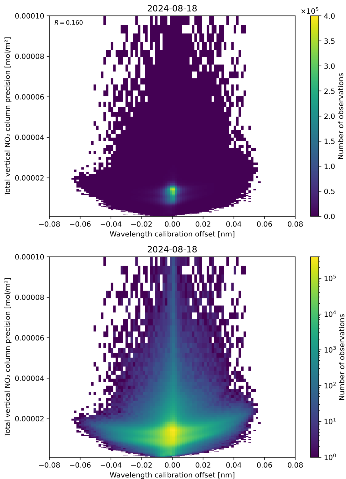
Figure 180: Scatter density plot of “Wavelength calibration offset” against “Total vertical NO 2 column precision” for 2024-08-17 to 2024-08-19.
