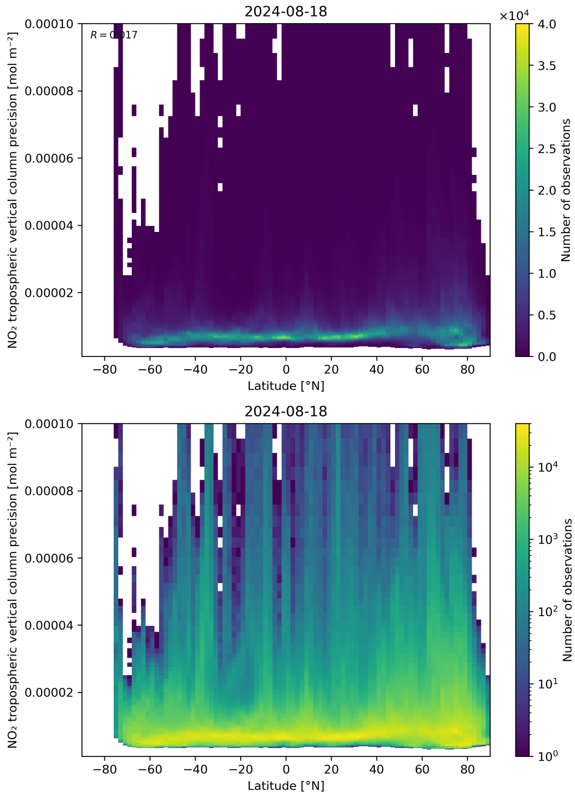
Figure 93: Scatter density plot of “Latitude” against “NO 2 tropospheric vertical column precision” for 2024-08-17 to 2024-08-19.
