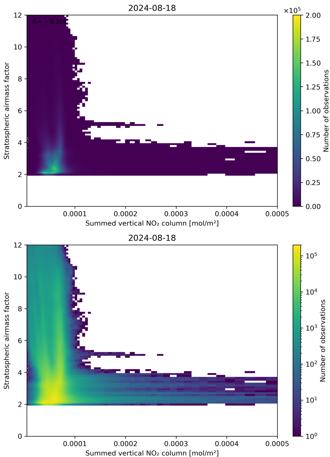
Figure 103: Scatter density plot of “Summed vertical NO 2 column” against “Stratospheric airmass factor” for 2024-08-17 to 2024-08-19.
