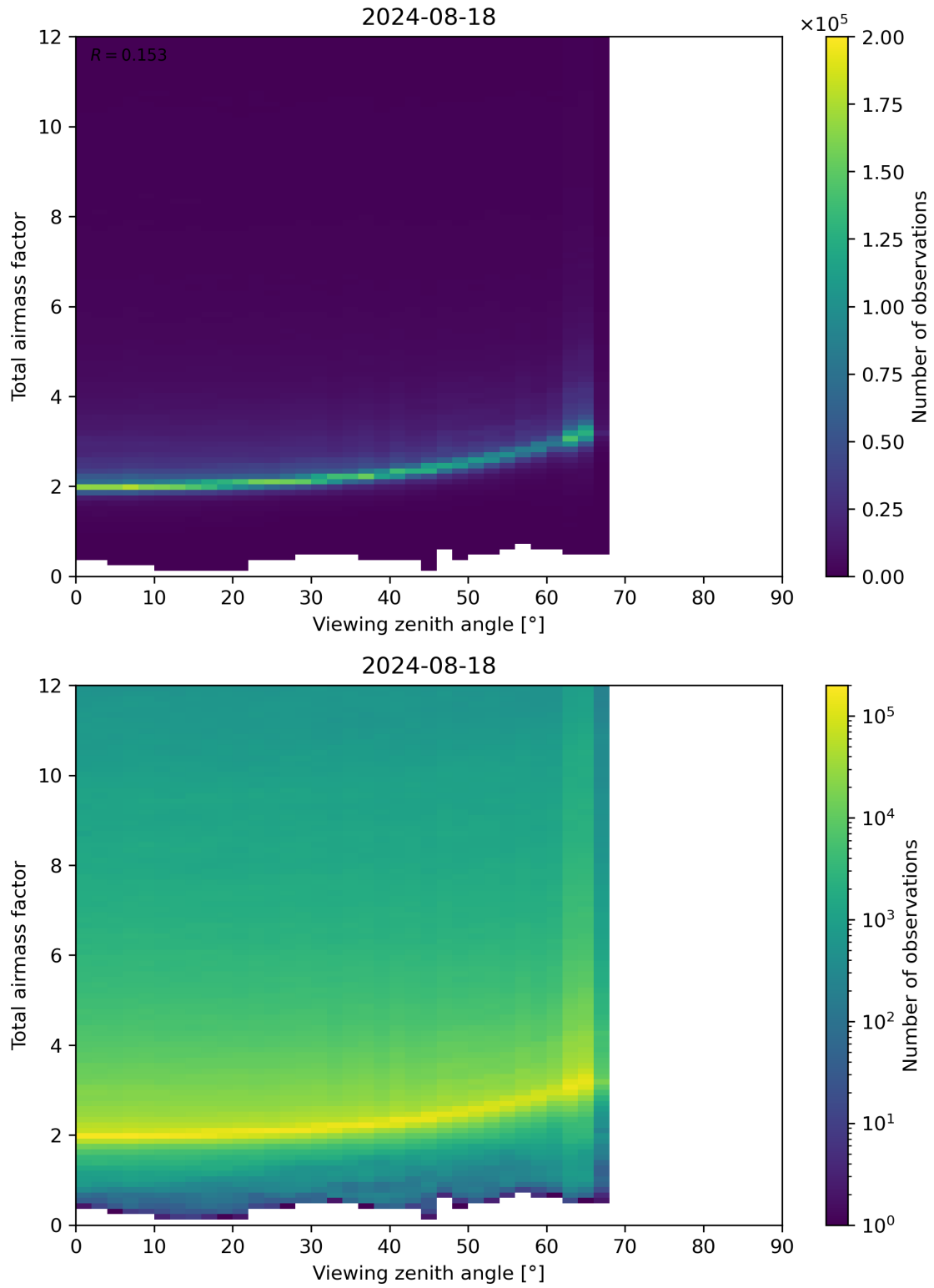
Figure 160: Scatter density plot of “Viewing zenith angle” against “Total airmass factor” for 2024-08-17 to 2024-08-19.
