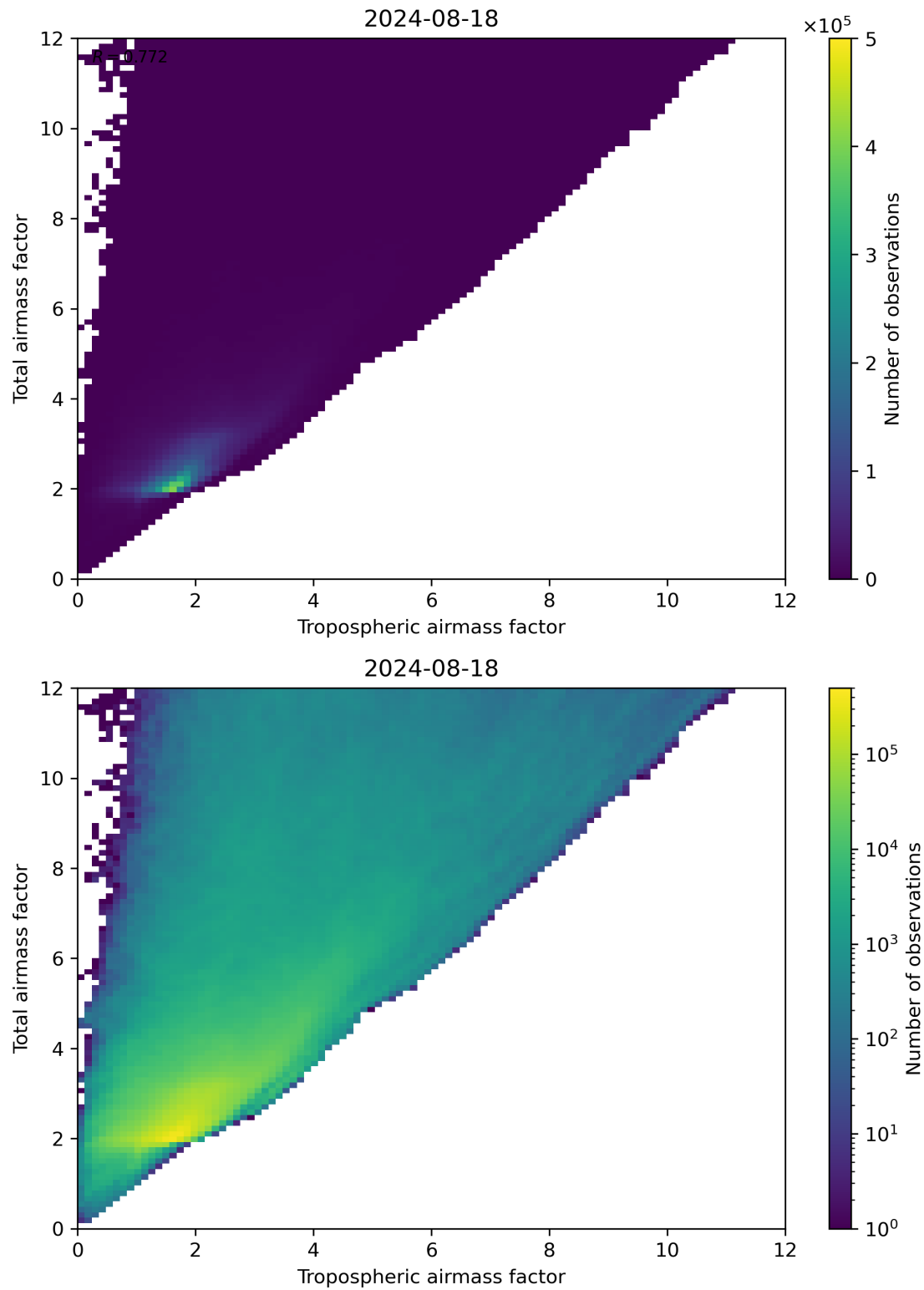
Figure 72: Scatter density plot of “Tropospheric airmass factor” against “Total airmass factor” for 2024-08-17 to 2024-08-19.
