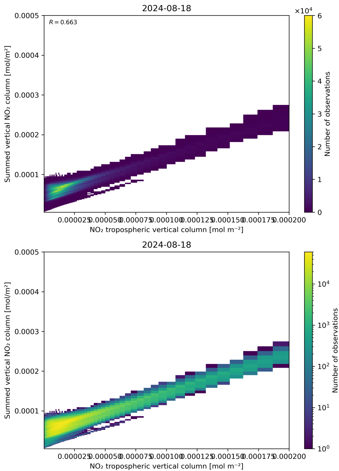
Figure 126: Scatter density plot of “NO 2 tropospheric vertical column” against “Summed vertical NO 2 column” for 2024-08-17 to 2024-08-19.
