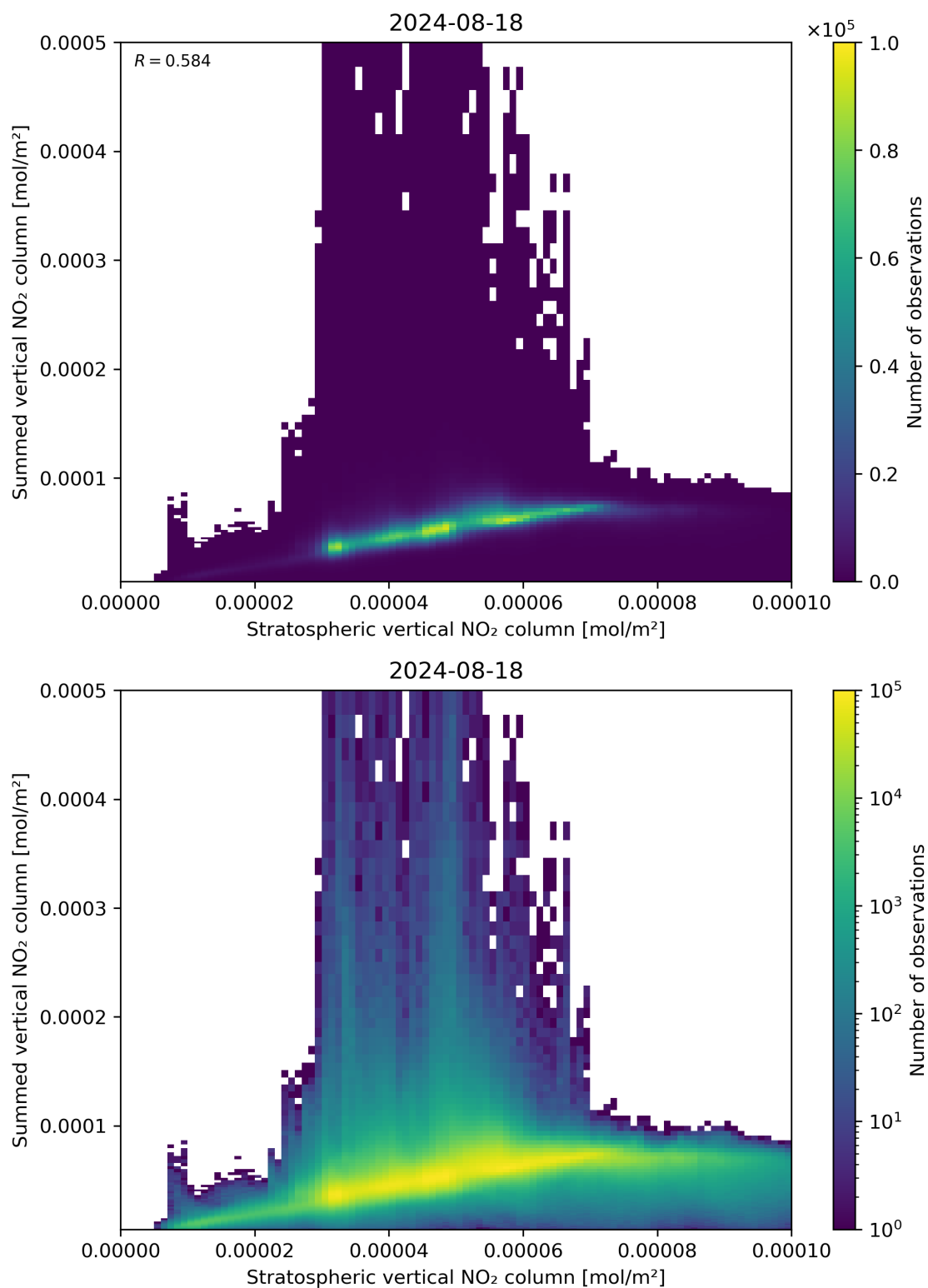
Figure 98: Scatter density plot of “Stratospheric vertical NO 2 column” against “Summed vertical NO 2 column” for 2024-08-17 to 2024-08-19.
