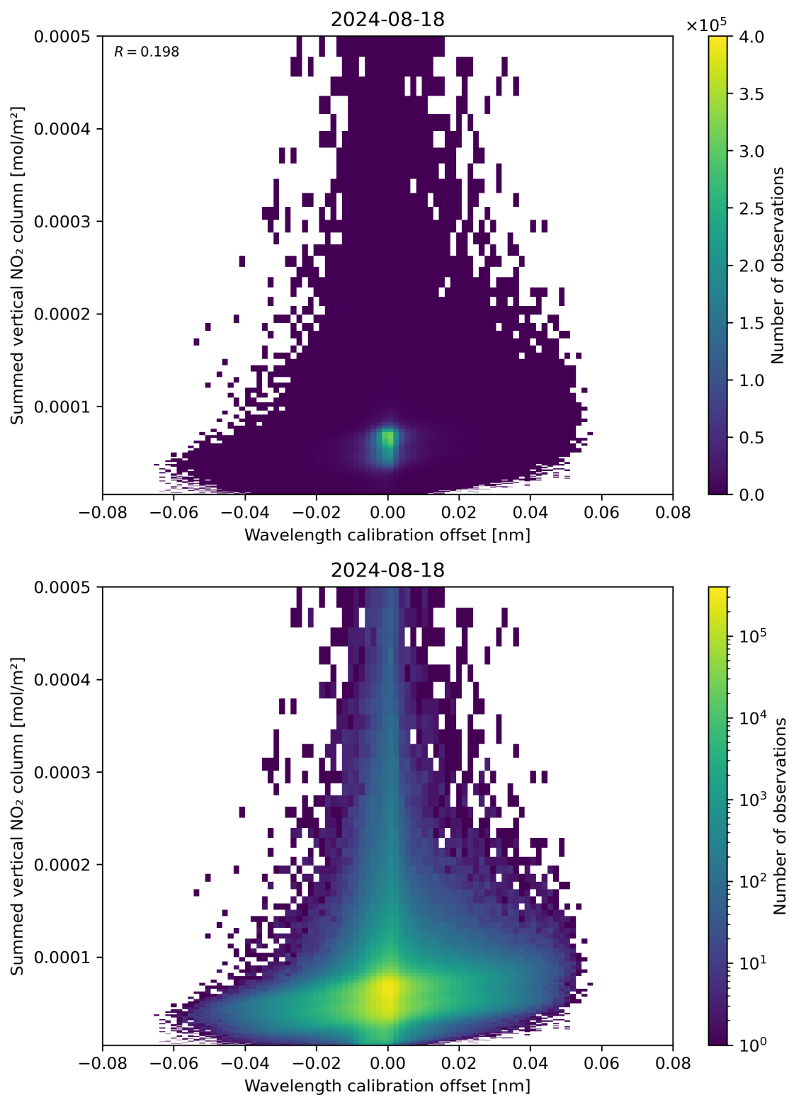
Figure 177: Scatter density plot of “Wavelength calibration offset” against “Summed vertical NO 2 column” for 2024-08-17 to 2024-08-19.
