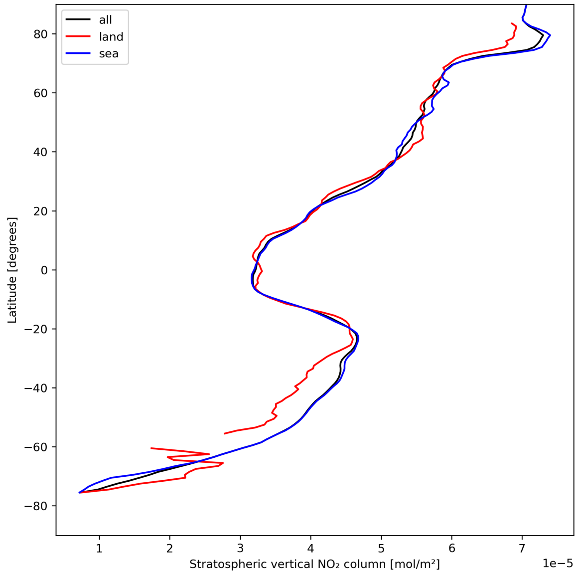
Figure 19: Zonal average of “Stratospheric vertical NO 2 column” for 2024-08-17 to 2024-08-19.
