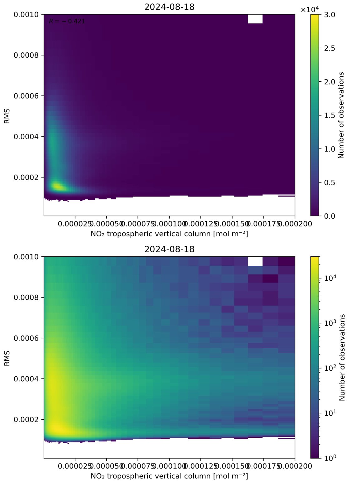
Figure 142: Scatter density plot of “NO 2 tropospheric vertical column” against “RMS” for 2024-08-17 to 2024-08-19.
