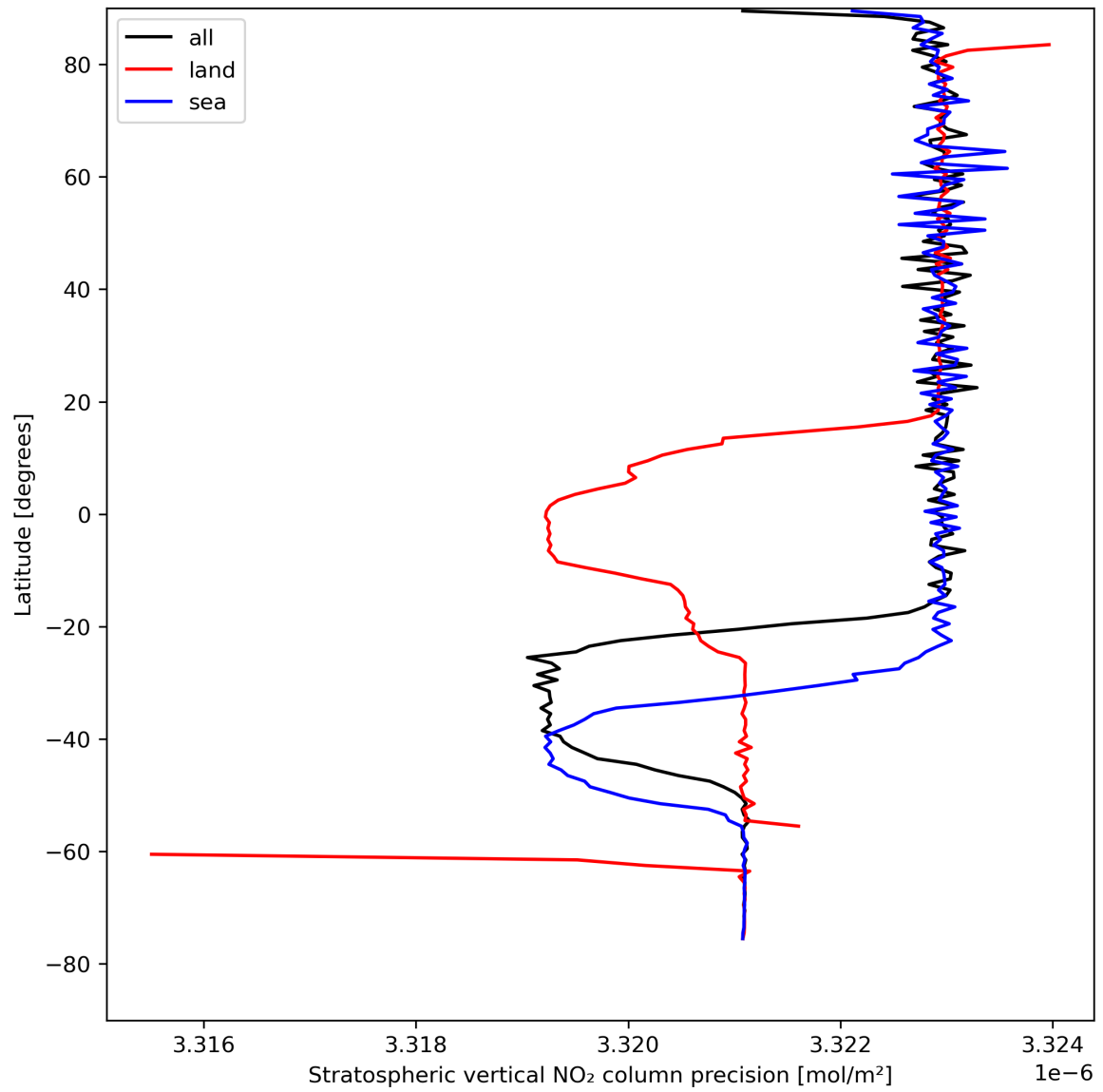
Figure 20: Zonal average of “Stratospheric vertical NO 2 column precision” for 2024-08-17 to 2024-08-19.
