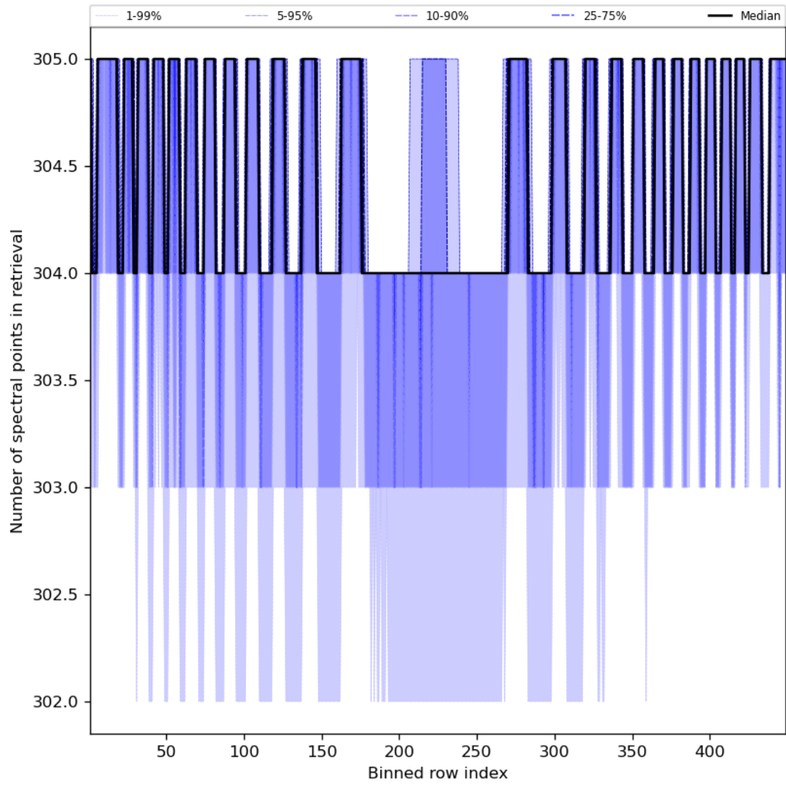
Figure 50: Along track statistics of “Number of spectral points in retrieval” for 2024-08-17 to 2024-08-19
