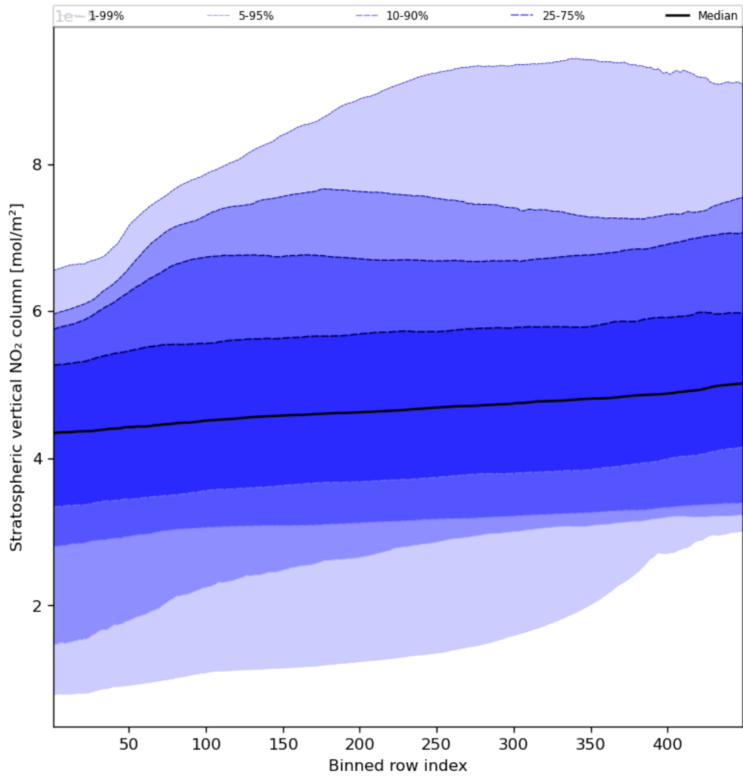
Figure 53: Along track statistics of “Stratospheric vertical NO 2 column” for 2024-08-17 to 2024-08-19
