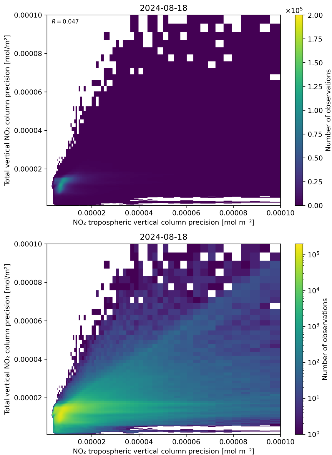
Figure 139: Scatter density plot of “NO 2 tropospheric vertical column precision” against “Total vertical NO 2 column precision” for 2024-08-17 to 2024-08-19.
