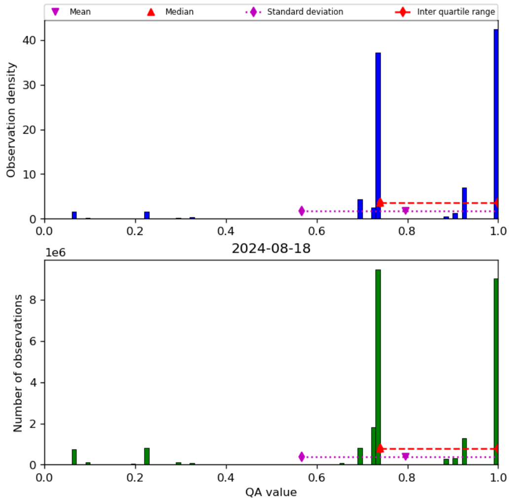
Figure 28: Histogram of “QA value” for 2024-08-17 to 2024-08-19
