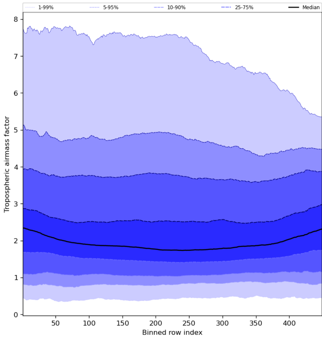
Figure 48: Along track statistics of “Tropospheric airmass factor” for 2024-08-17 to 2024-08-19
