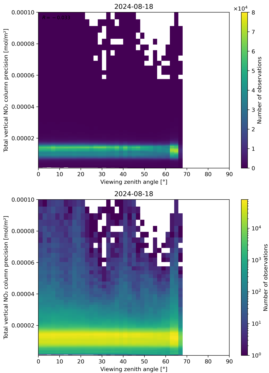
Figure 168: Scatter density plot of “Viewing zenith angle” against “Total vertical NO 2 column precision” for 2024-08-17 to 2024-08-19.
