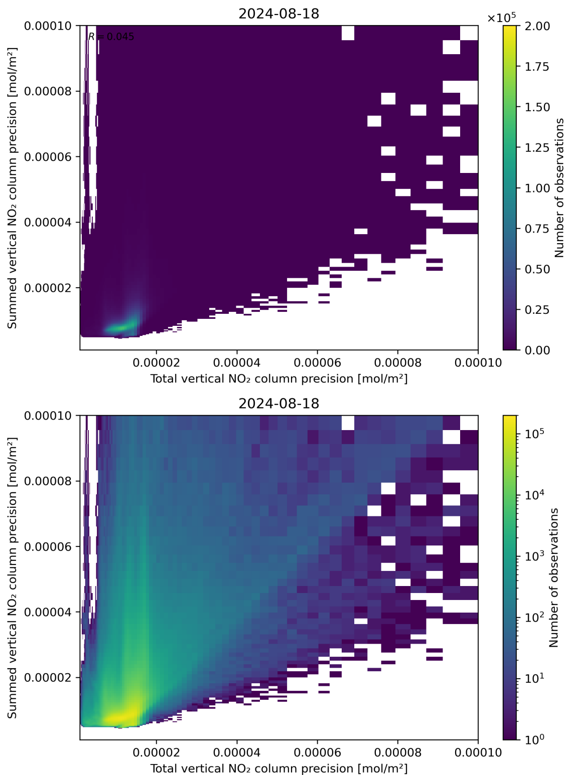
Figure 118: Scatter density plot of “Total vertical NO 2 column precision” against “Summed vertical NO 2 column precision” for 2024-08-17 to 2024-08-19.
