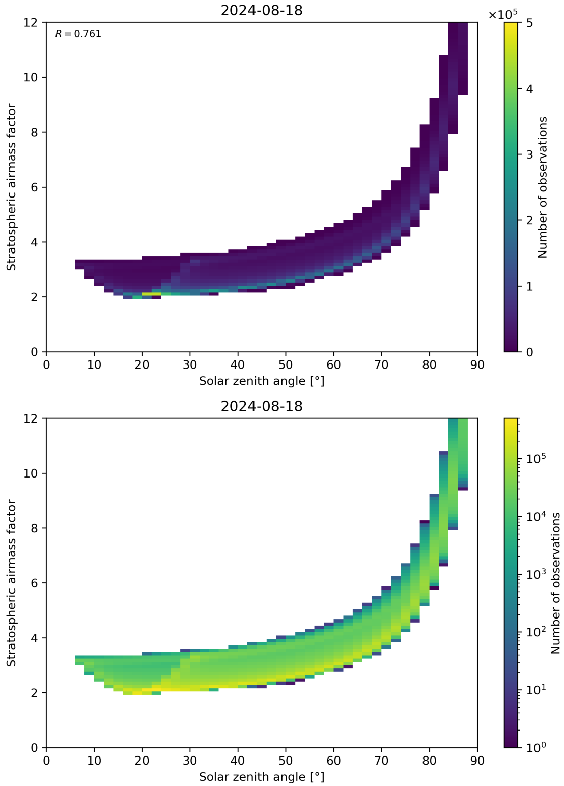
Figure 145: Scatter density plot of “Solar zenith angle” against “Stratospheric airmass factor” for 2024-08-17 to 2024-08-19.
