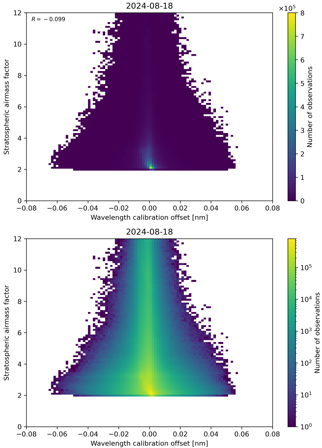
Figure 174: Scatter density plot of “Wavelength calibration offset” against “Stratospheric airmass factor” for 2024-08-17 to 2024-08-19.
