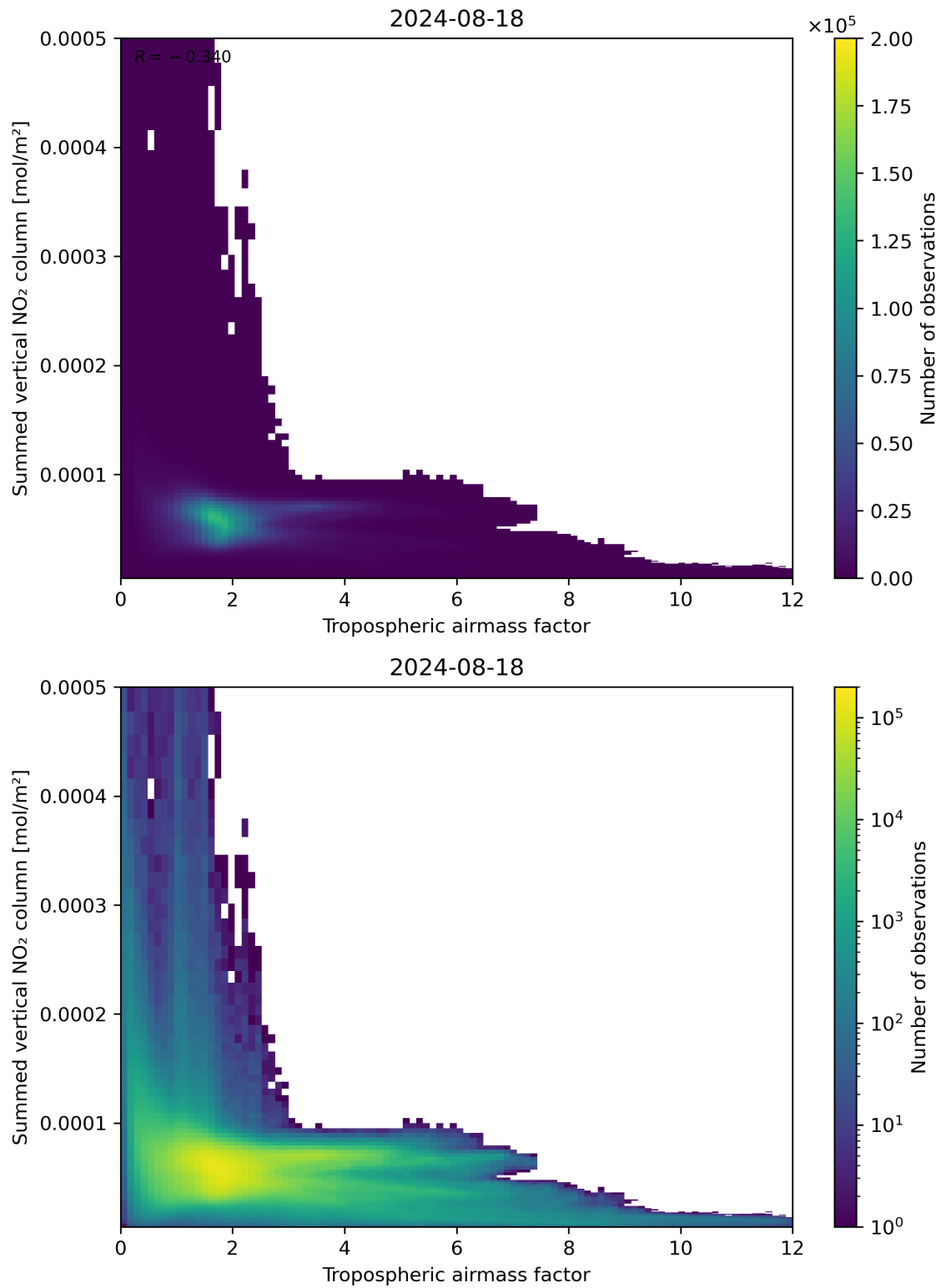
Figure 75: Scatter density plot of “Tropospheric airmass factor” against “Summed vertical NO 2 column” for 2024-08-17 to 2024-08-19.
