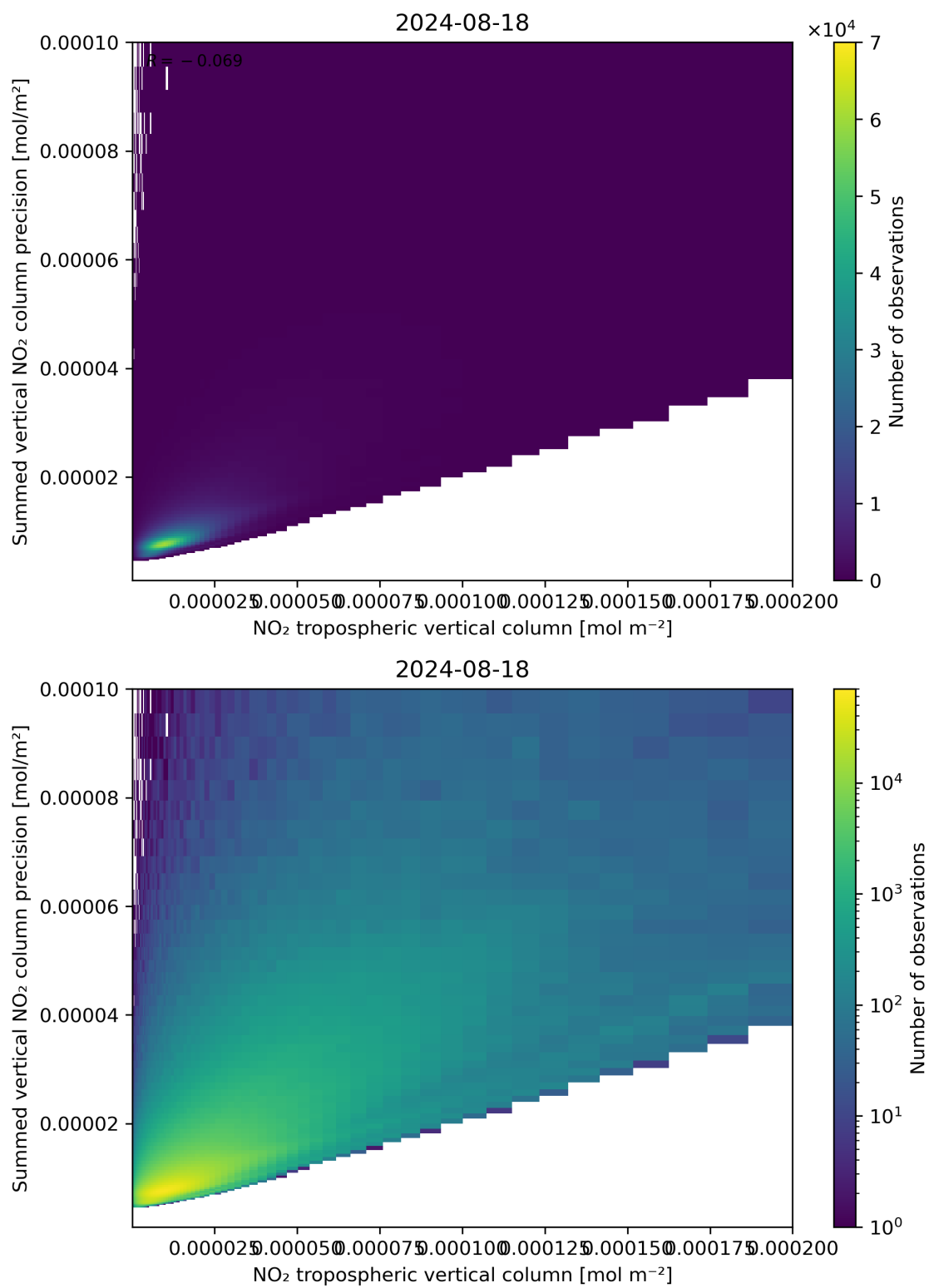
Figure 127: Scatter density plot of “NO 2 tropospheric vertical column” against “Summed vertical NO 2 column precision” for 2024-08-17 to 2024-08-19.
