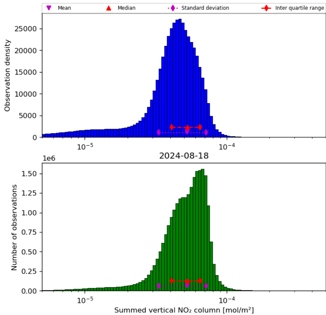
Figure 40: Histogram of “Summed vertical NO 2 column” for 2024-08-17 to 2024-08-19
