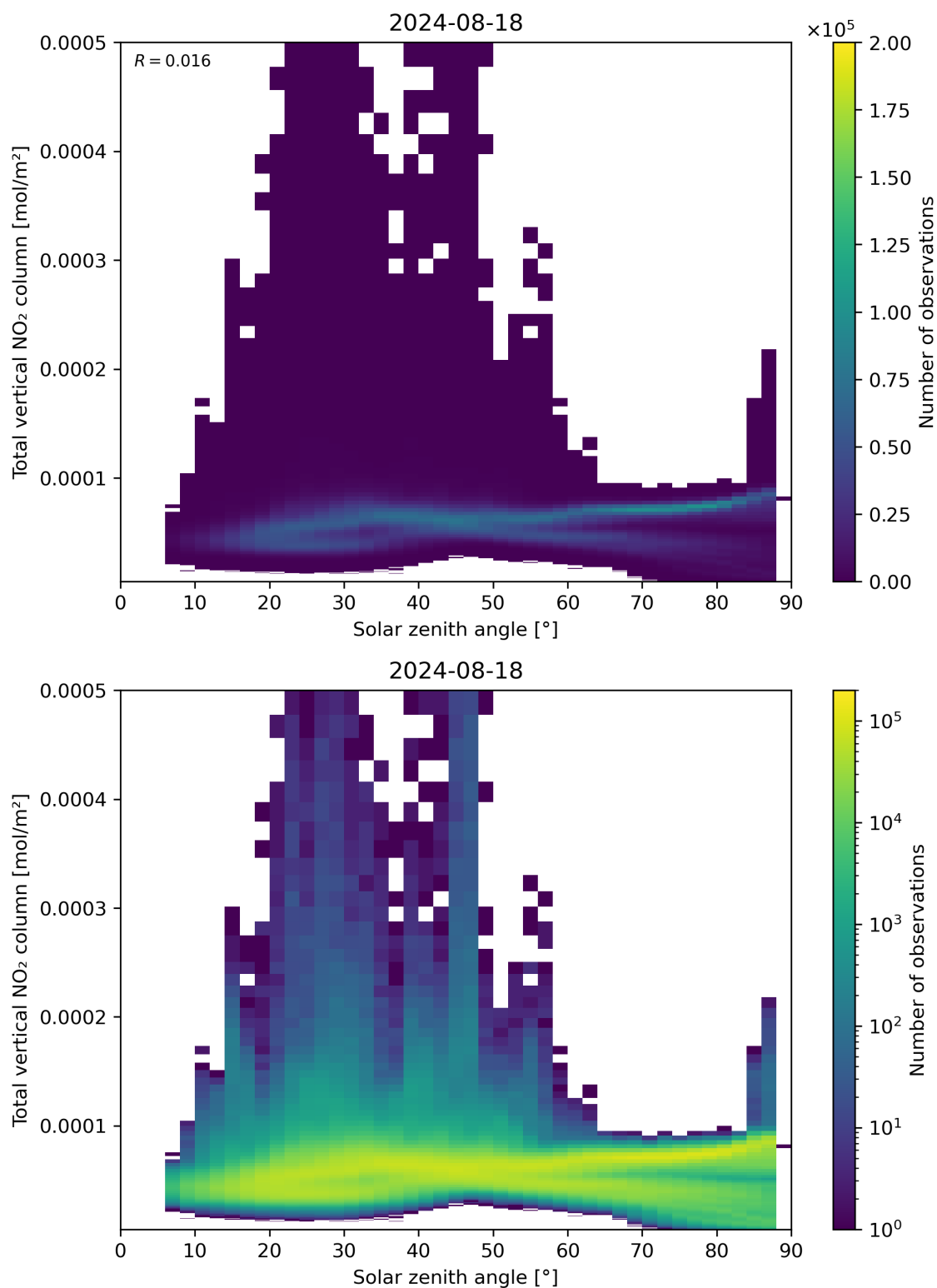
Figure 153: Scatter density plot of “Solar zenith angle” against “Total vertical NO 2 column” for 2024-08-17 to 2024-08-19.
