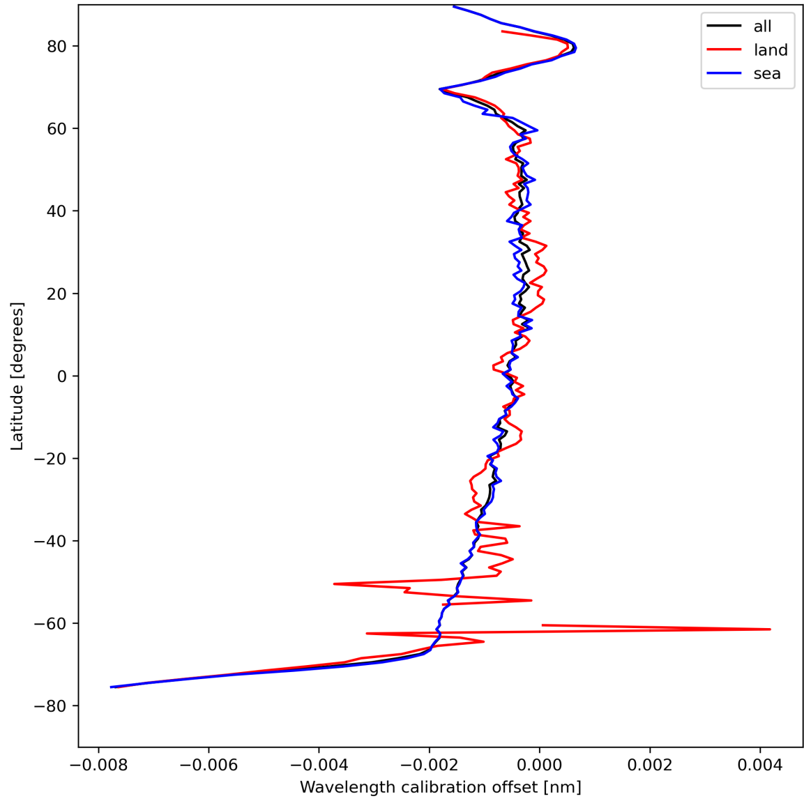
Figure 18: Zonal average of “Wavelength calibration offset” for 2024-08-17 to 2024-08-19.
