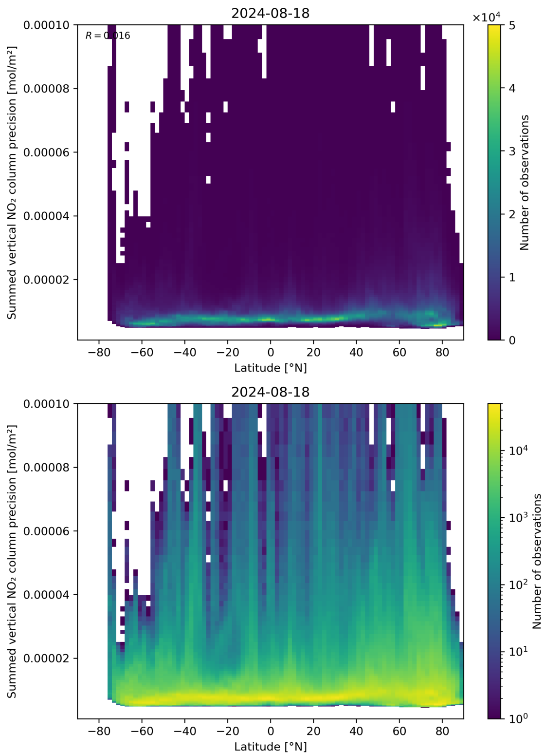
Figure 89: Scatter density plot of “Latitude” against “Summed vertical NO 2 column precision” for 2024-08-17 to 2024-08-19.
