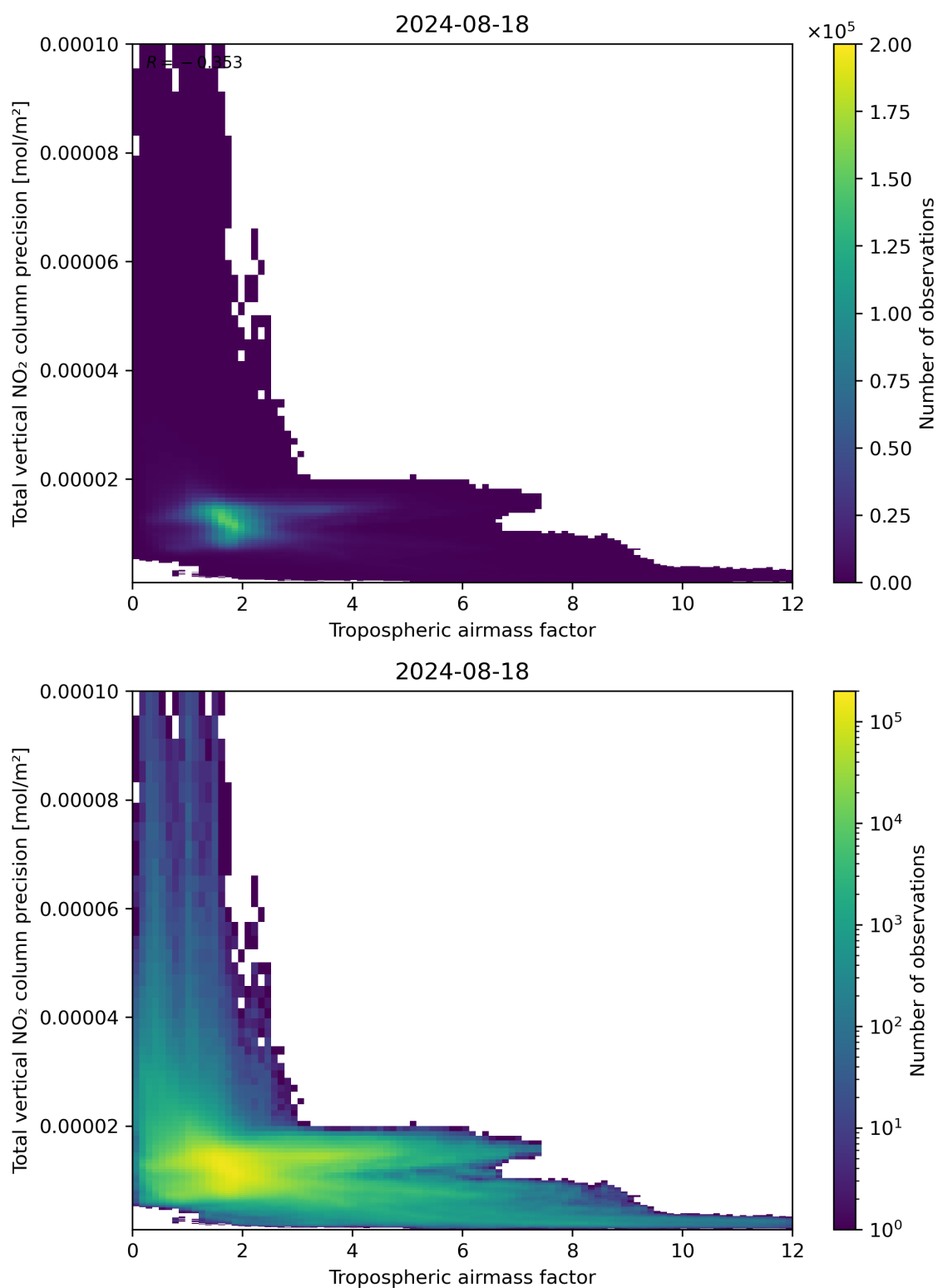
Figure 78: Scatter density plot of “Tropospheric air mass factor” against “Total vertical NO 2 column precision” for 2024-08-17 to 2024-08-19.
