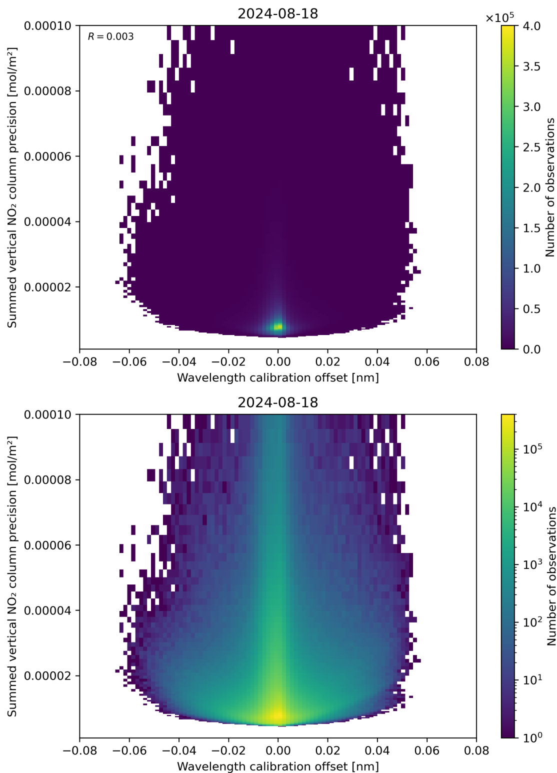
Figure 178: Scatter density plot of “Wavelength calibration offset” against “Summed vertical NO 2 column precision” for 2024-08-17 to 2024-08-19.
