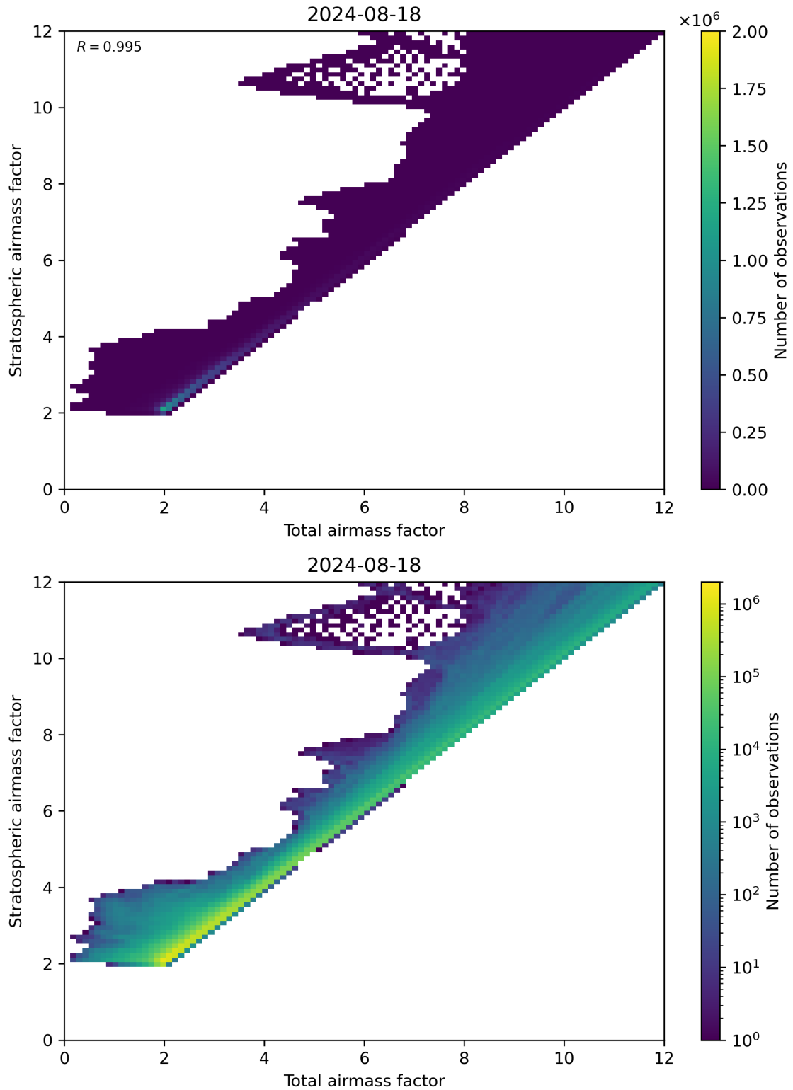
Figure 62: Scatter density plot of “Total airmass factor” against “Stratospheric airmass factor” for 2024-08-17 to 2024-08-19.
