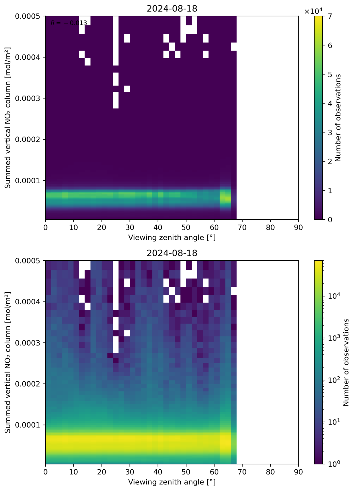
Figure 165: Scatter density plot of “Viewing zenith angle” against “Summed vertical NO 2 column” for 2024-08-17 to 2024-08-19.
