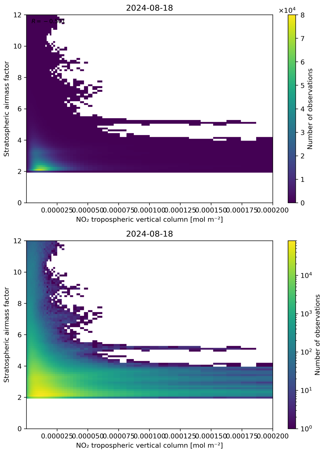
Figure 121: Scatter density plot of “NO 2 tropospheric vertical column” against “Stratospheric airmass factor” for 2024-08-17 to 2024-08-19.
