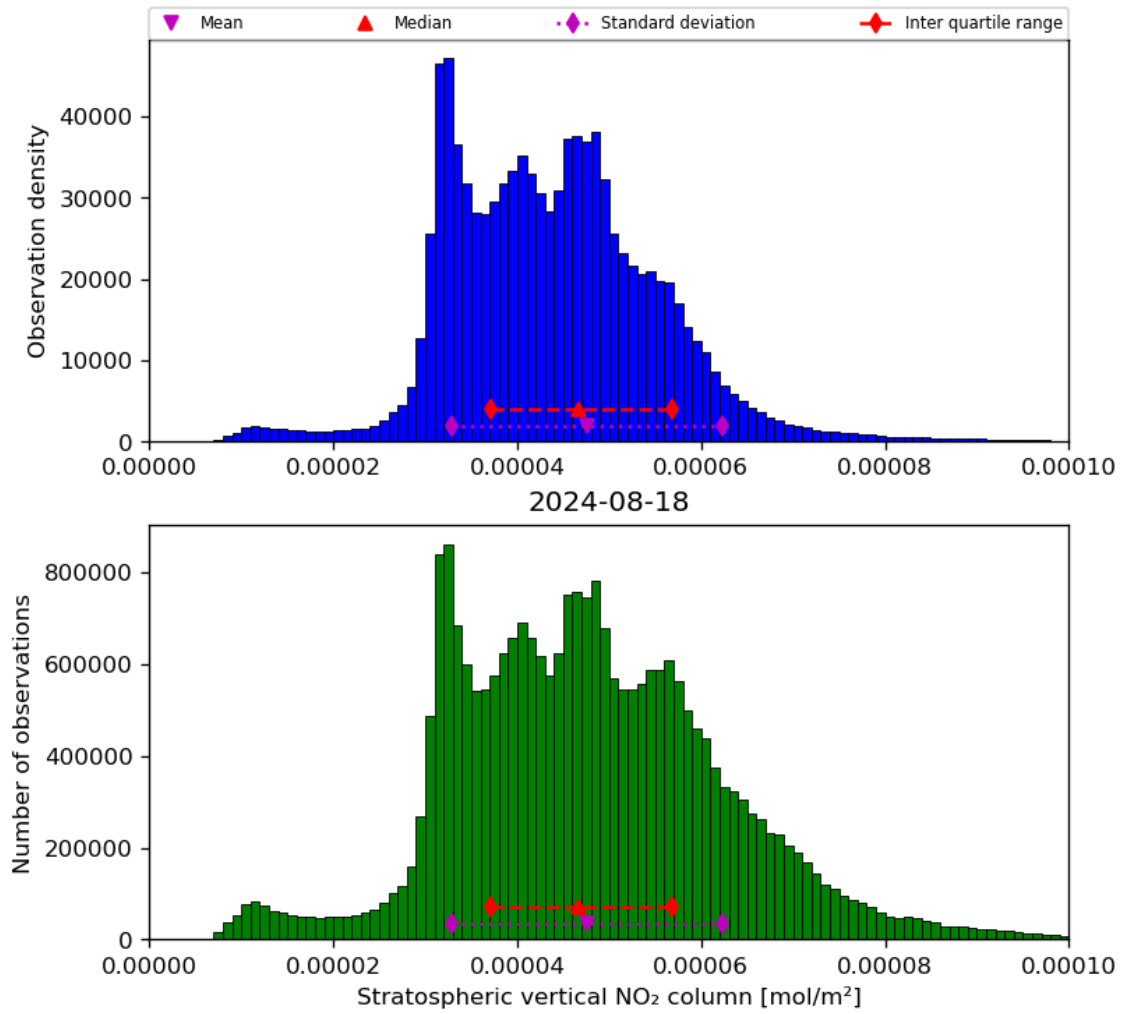
Figure 36: Histogram of “Stratospheric vertical NO 2 column” for 2024-08-17 to 2024-08-19
