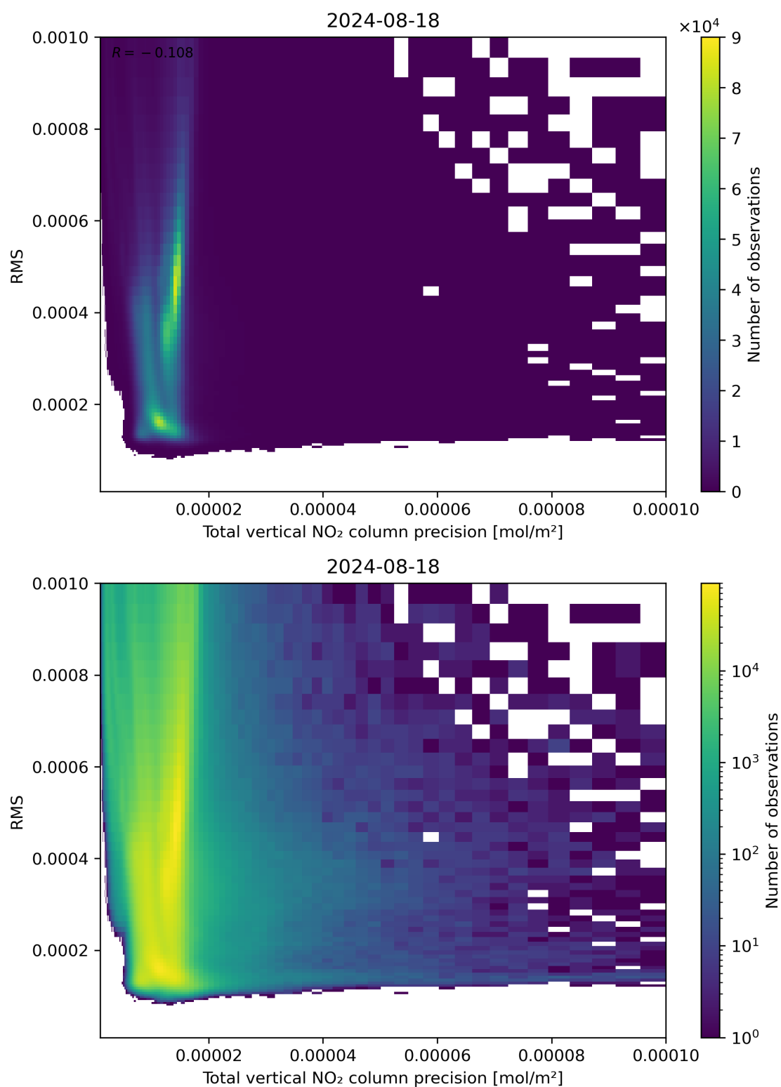
Figure 119: Scatter density plot of “Total vertical NO 2 column precision” against “RMS” for 2024-08-17 to 2024-08-19.
