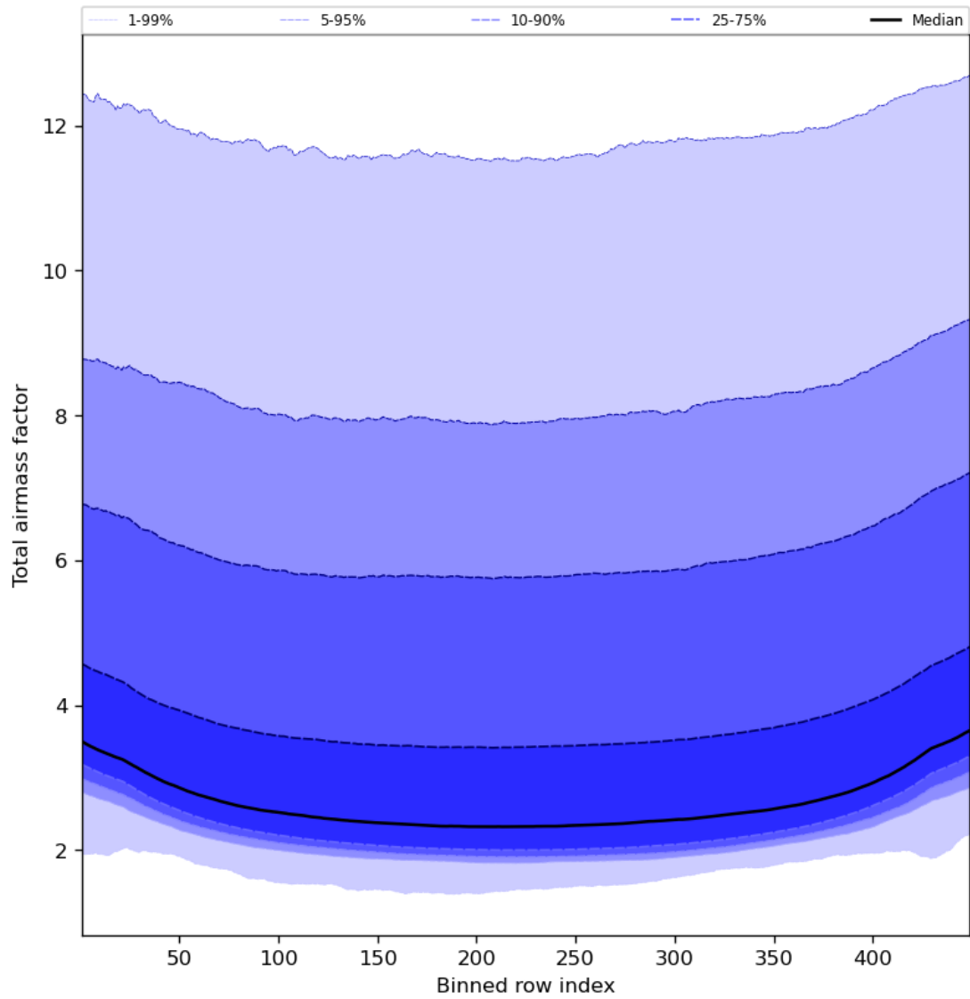
Figure 49: Along track statistics of “Total airmass factor” for 2024-08-17 to 2024-08-19
