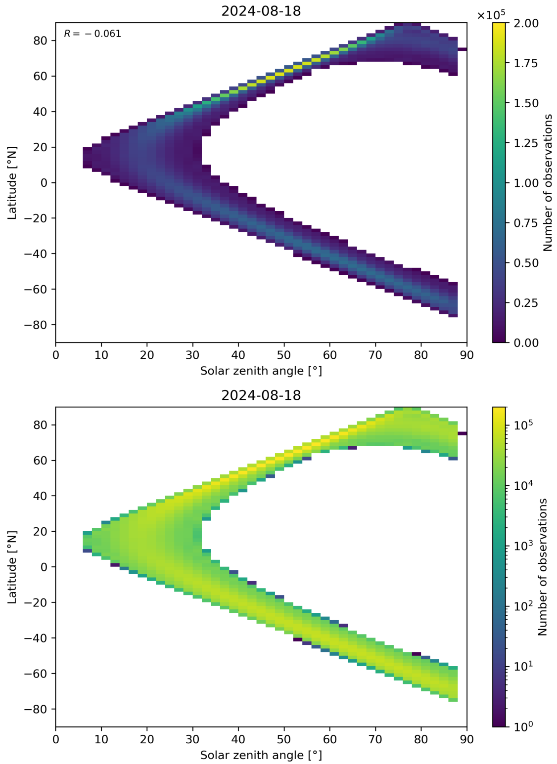
Figure 149: Scatter density plot of “Solar zenith angle” against “Latitude” for 2024-08-17 to 2024-08-19.
