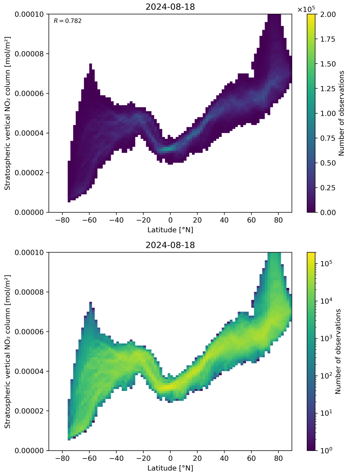
Figure 87: Scatter density plot of “Latitude” against “Stratospheric vertical NO 2 column” for 2024-08-17 to 2024-08-19.
