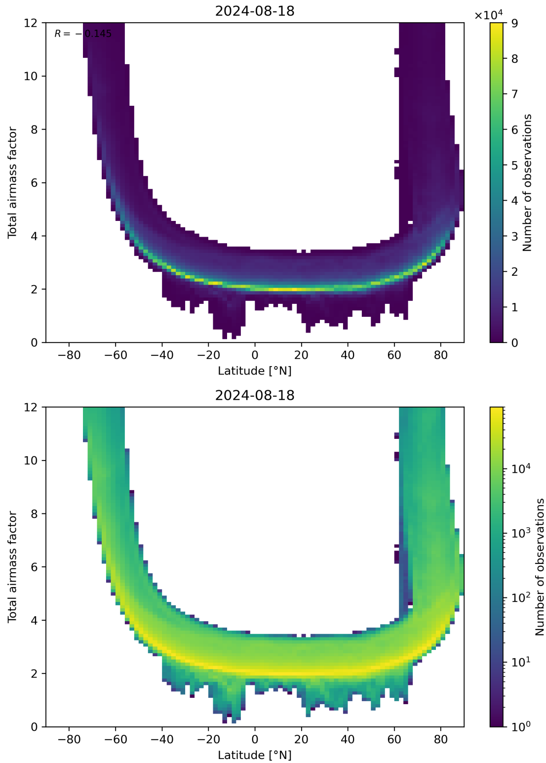
Figure 84: Scatter density plot of “Latitude” against “Total airmass factor” for 2024-08-17 to 2024-08-19.
