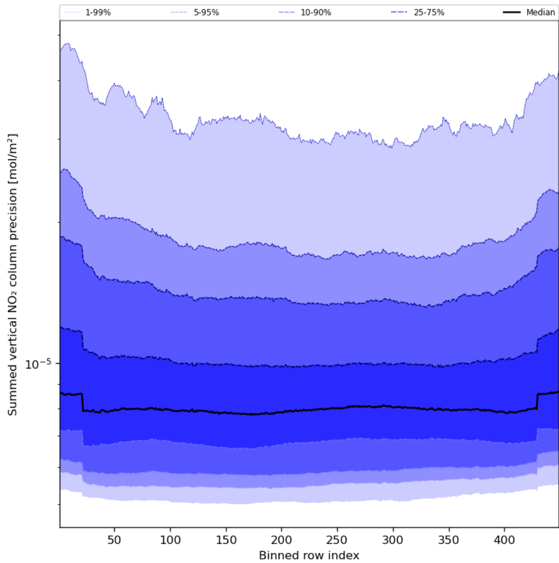
Figure 58: Along track statistics of “Summed vertical NO 2 column precision” for 2024-08-17 to 2024-08-19
