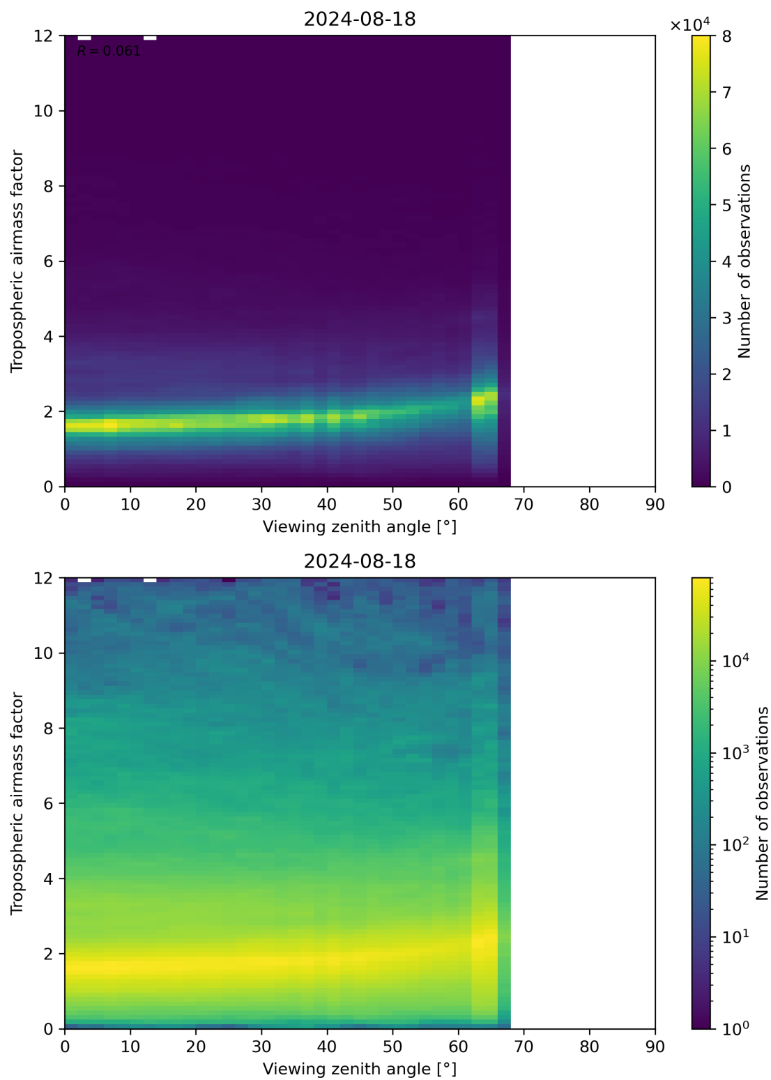
Figure 161: Scatter density plot of “Viewing zenith angle” against “Tropospheric airmass factor” for 2024-08-17 to 2024-08-19.
