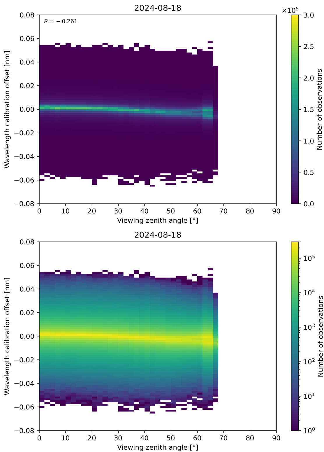
Figure 173: Scatter density plot of “Viewing zenith angle” against “Wavelength calibration offset” for 2024-08-17 to 2024-08-19.
