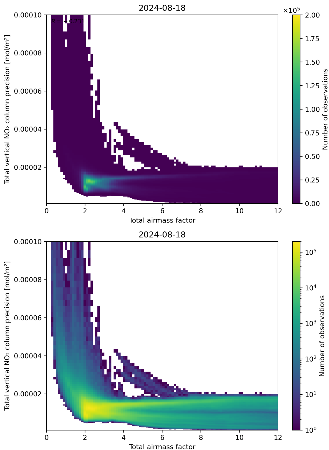
Figure 68: Scatter density plot of “Total airmass factor” against “Total vertical NO 2 column precision” for 2024-08-17 to 2024-08-19.
