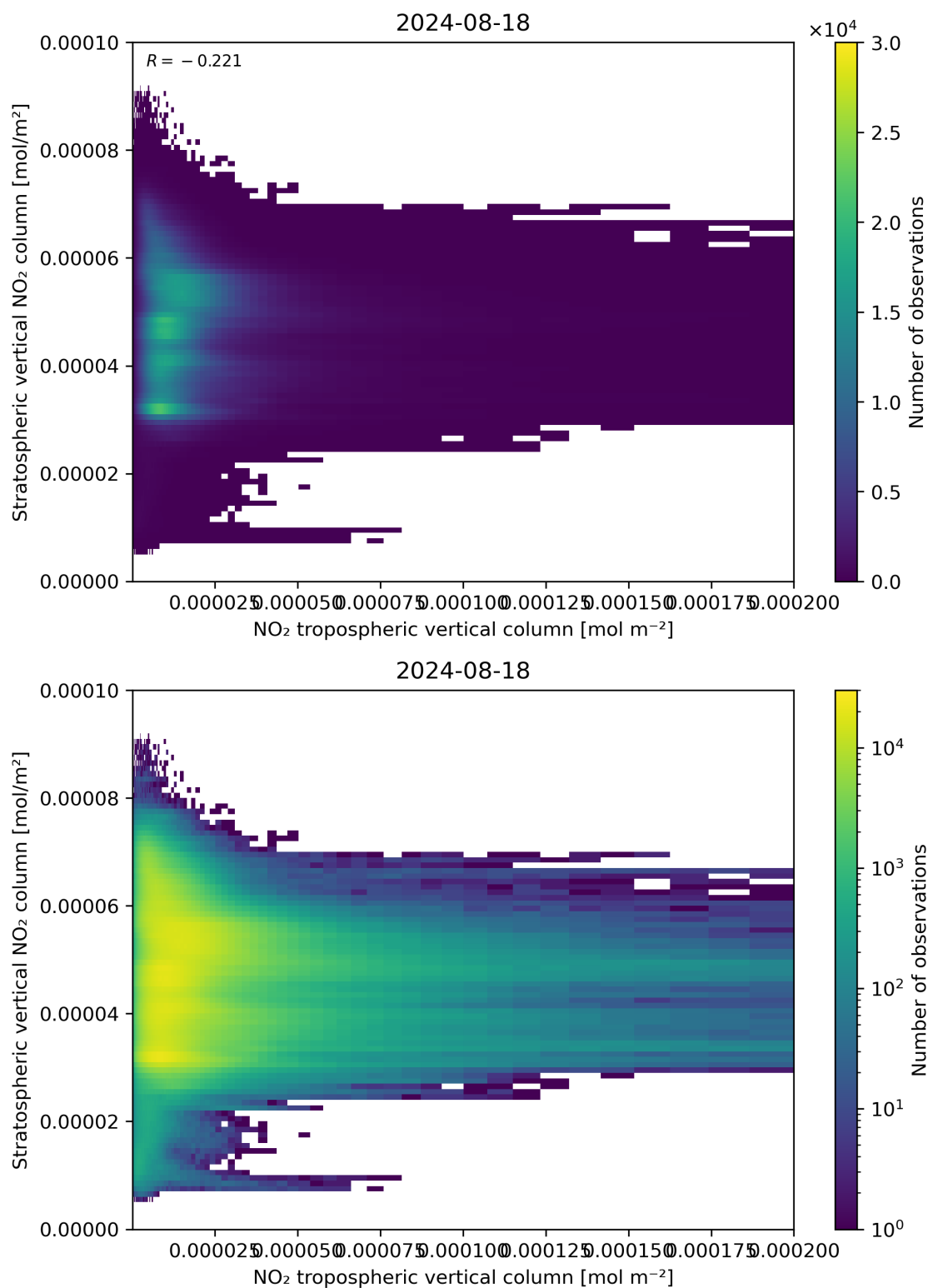
Figure 125: Scatter density plot of “NO 2 tropospheric vertical column” against “Stratospheric vertical NO 2 column” for 2024-08-17 to 2024-08-19.
