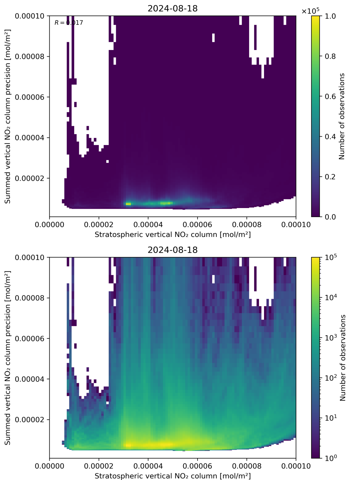
Figure 99: Scatter density plot of “Stratospheric vertical NO 2 column” against “Summed vertical NO 2 column precision” for 2024-08-17 to 2024-08-19.
