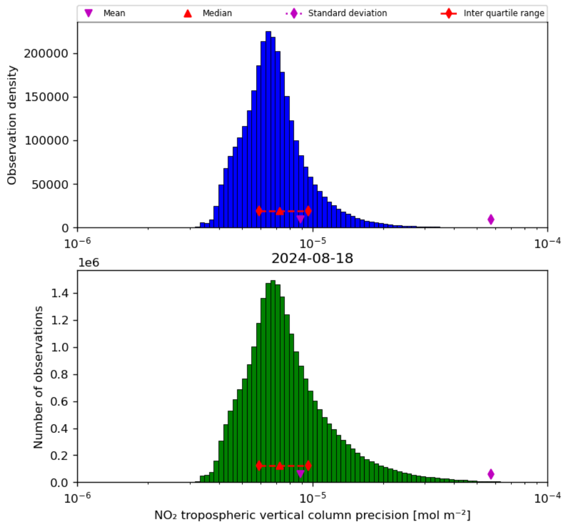
Figure 30: Histogram of “NO 2 tropospheric vertical column precision” for 2024-08-17 to 2024-08-19
