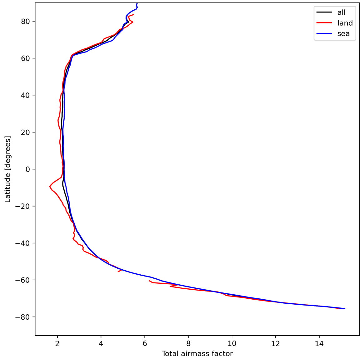
Figure 15: Zonal average of “Total airmass factor” for 2024-08-17 to 2024-08-19.
