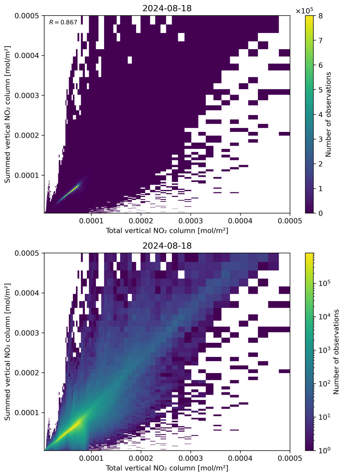
Figure 112: Scatter density plot of “Total vertical NO 2 column” against “Summed vertical NO 2 column” for 2024-08-17 to 2024-08-19.
