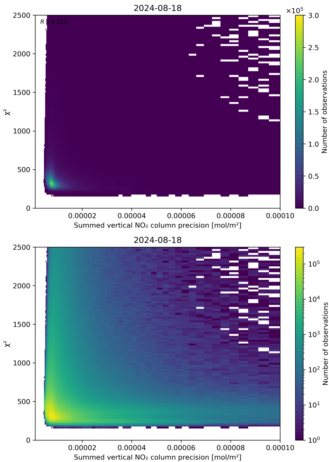
Figure 107: Scatter density plot of “Summed vertical NO 2 column precision” against “ \chi^2 ” for 2024-08-17 to 2024-08-19.
