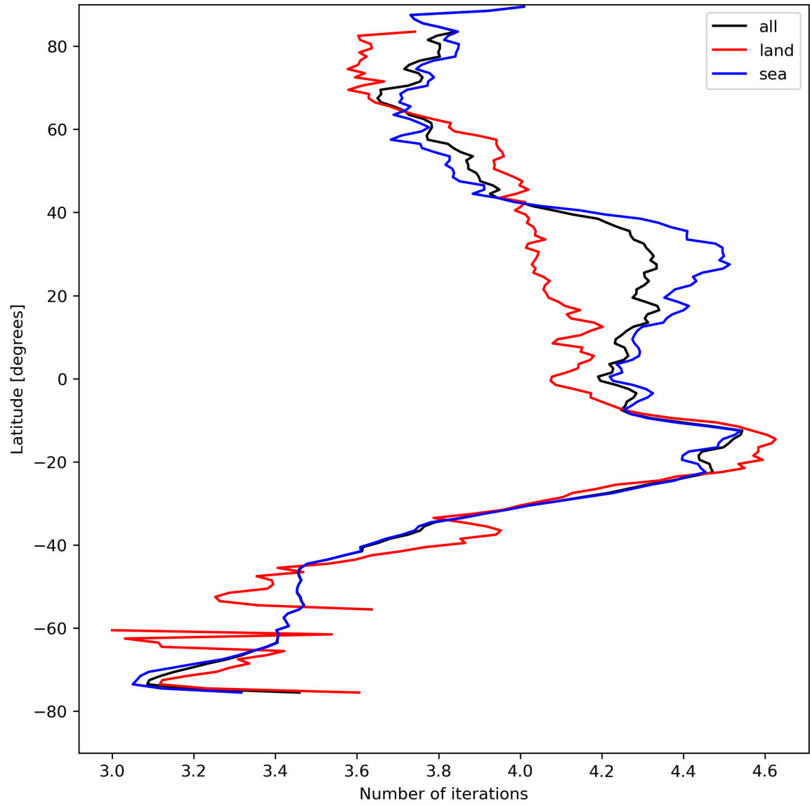
Figure 17: Zonal average of “Number of iterations” for 2024-08-17 to 2024-08-19.
