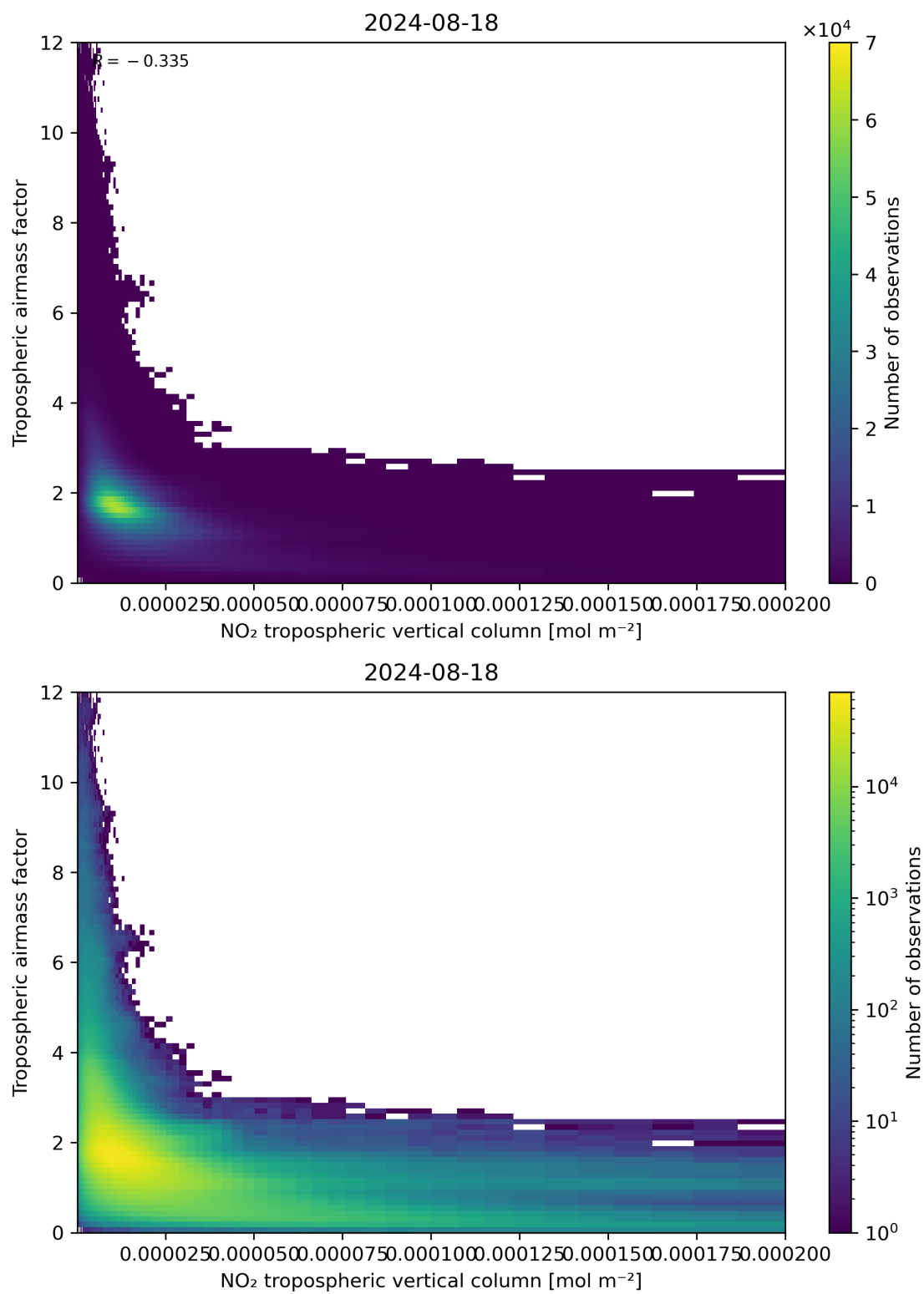
Figure 123: Scatter density plot of “NO 2 tropospheric vertical column” against “Tropospheric air mass factor” for 2024-08-17 to 2024-08-19.
