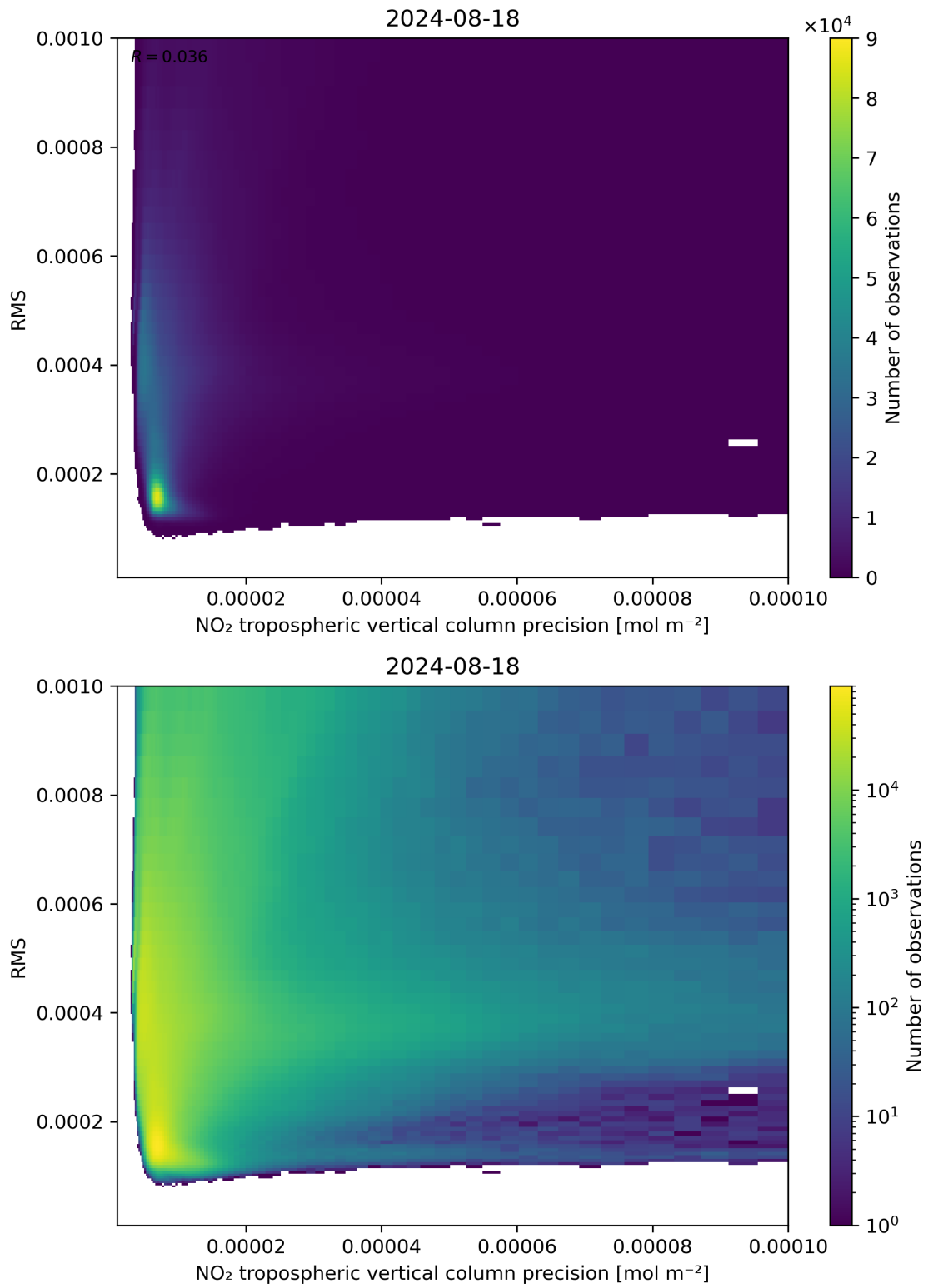
Figure 140: Scatter density plot of “NO 2 tropospheric vertical column precision” against “RMS” for 2024-08-17 to 2024-08-19.
