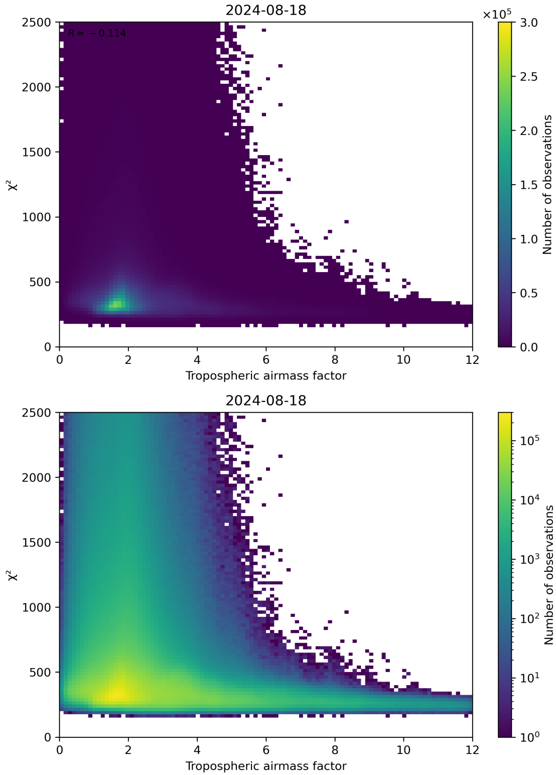
Figure 73: Scatter density plot of “Tropospheric airmass factor” against “ \chi^2 ” for 2024-08-17 to 2024-08-19.
