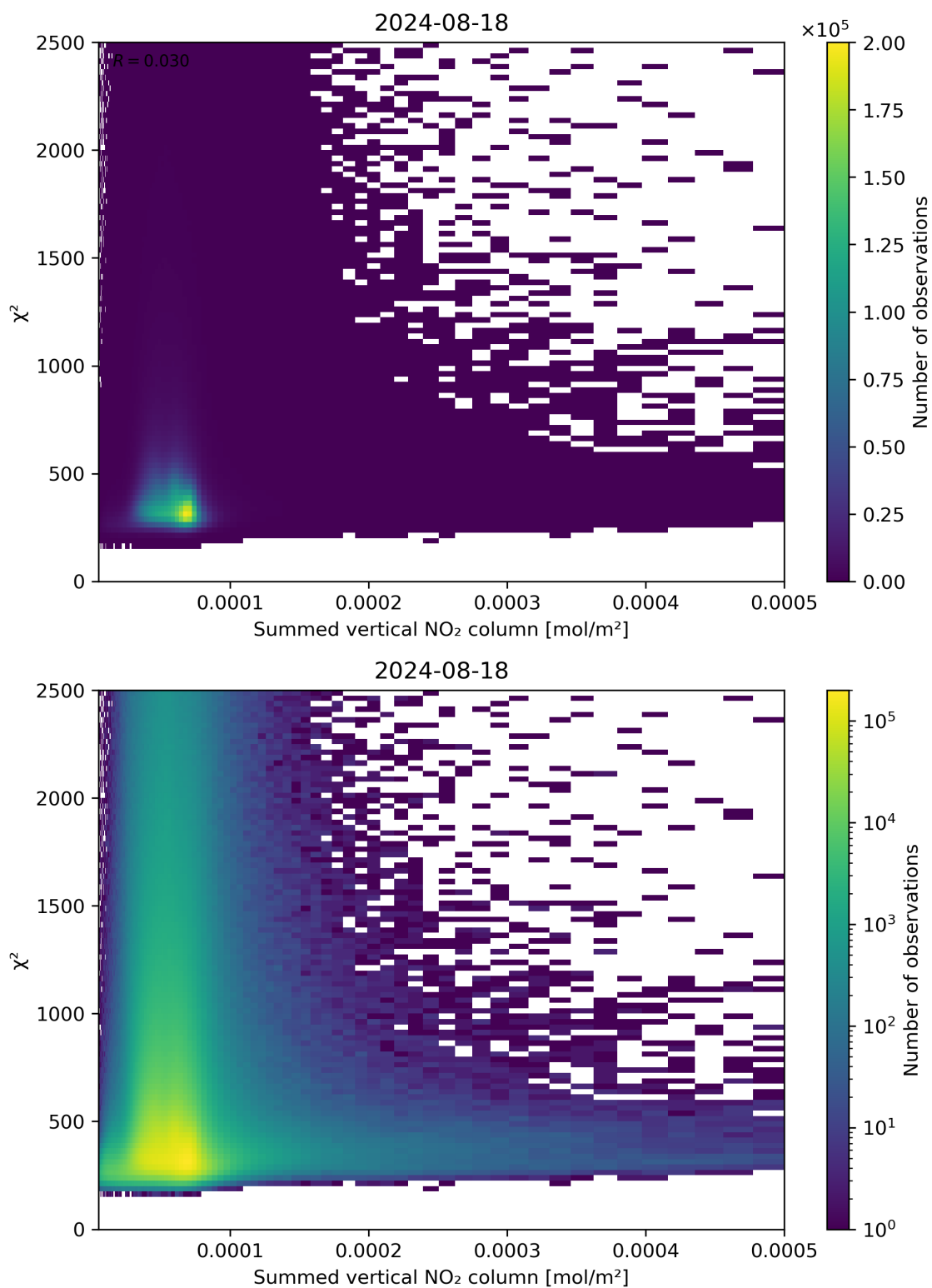
Figure 104: Scatter density plot of “Summed vertical NO 2 column” against “ \chi^2 ” for 2024-08-17 to 2024-08-19.
