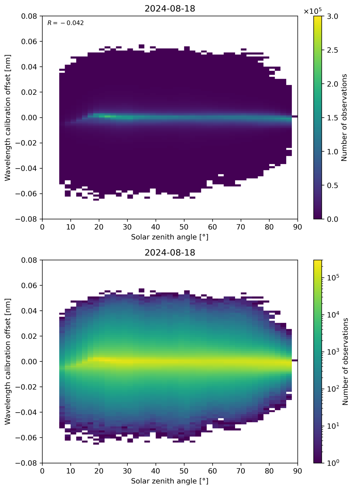
Figure 158: Scatter density plot of “Solar zenith angle” against “Wavelength calibration offset” for 2024-08-17 to 2024-08-19.
