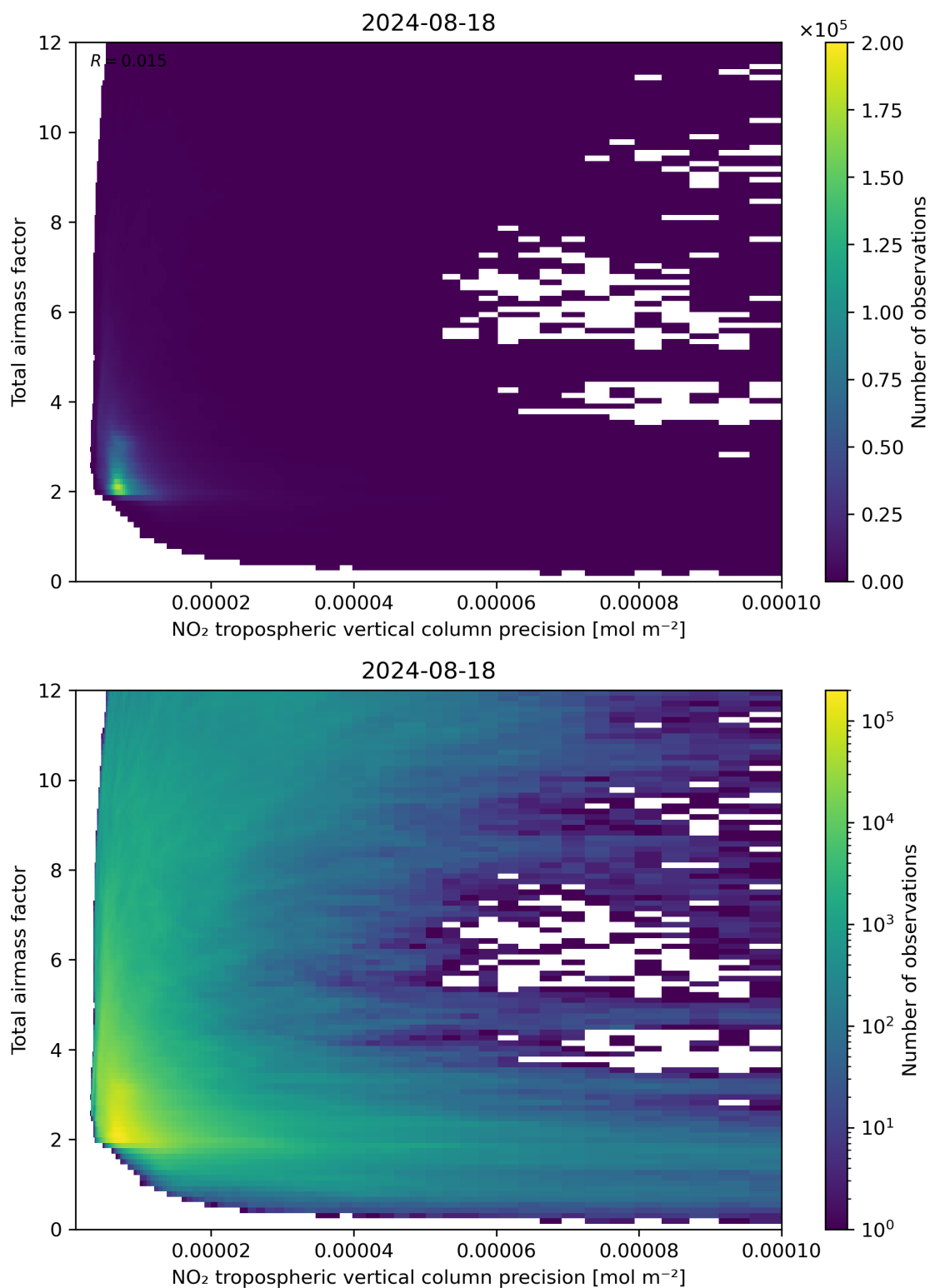
Figure 132: Scatter density plot of “NO 2 tropospheric vertical column precision” against “Total air mass factor” for 2024-08-17 to 2024-08-19.
