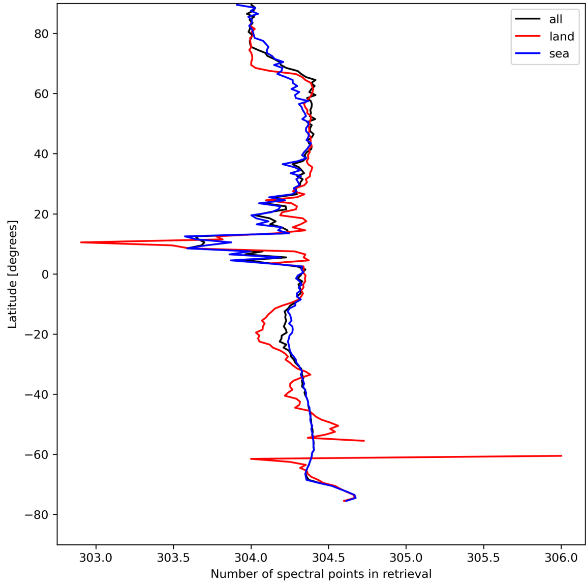
Figure 16: Zonal average of “Number of spectral points in retrieval” for 2024-08-17 to 2024-08-19.
