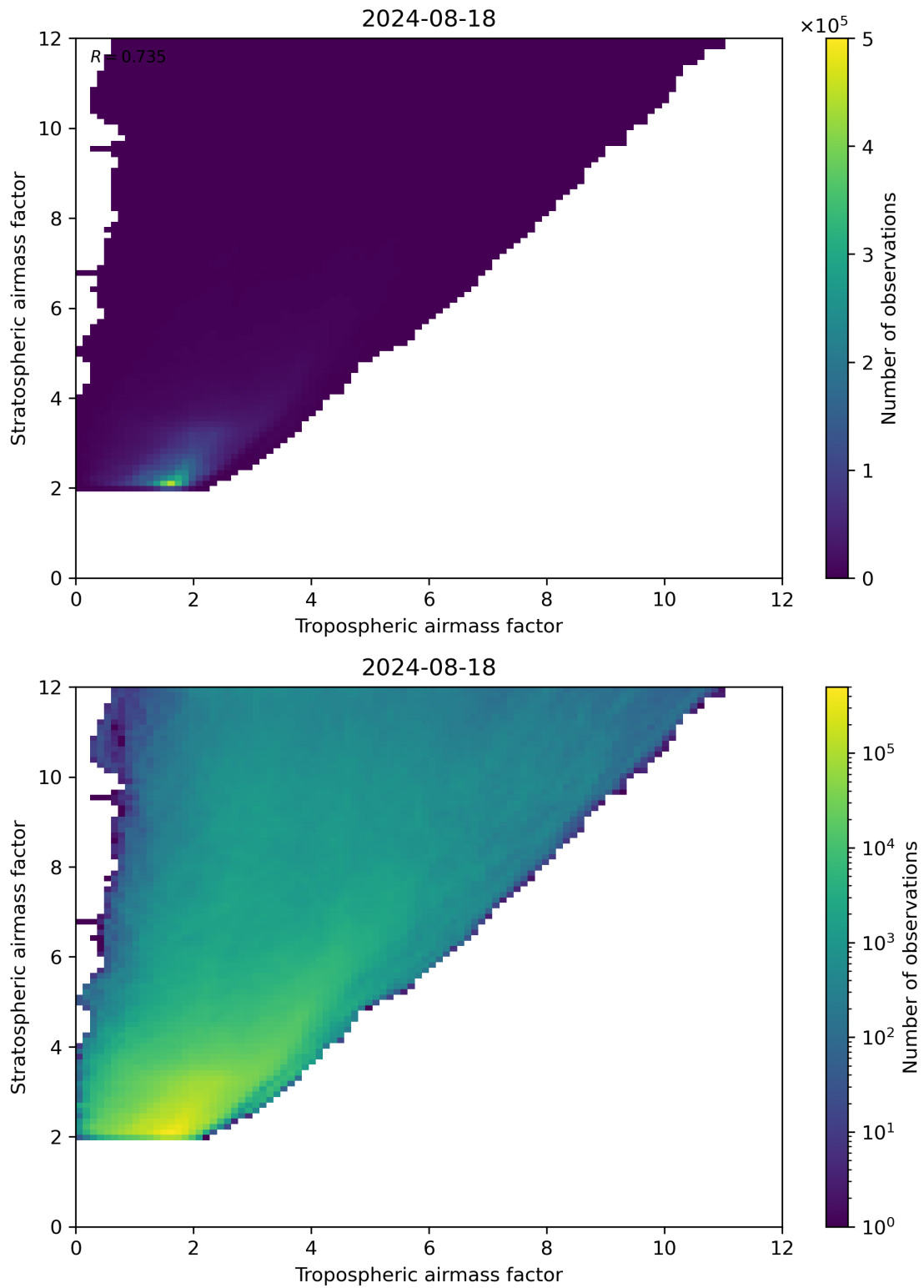
Figure 71: Scatter density plot of “Tropospheric airmass factor” against “Stratospheric airmass factor” for 2024-08-17 to 2024-08-19.
