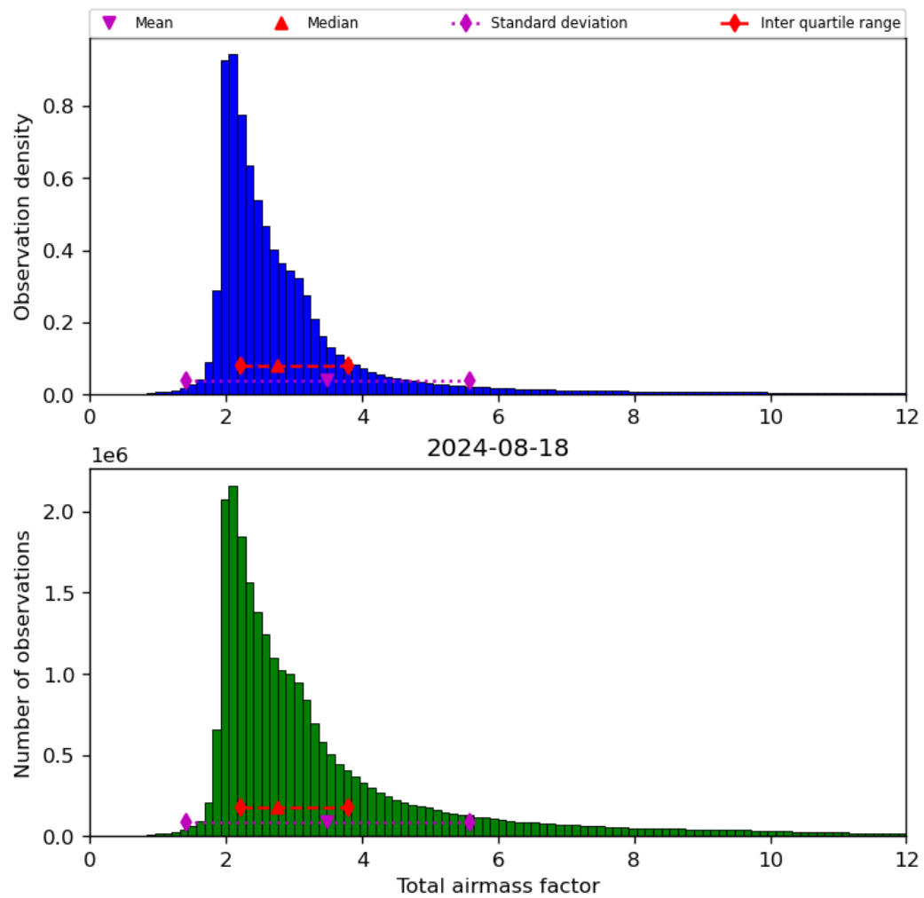
Figure 32: Histogram of “Total airmass factor” for 2024-08-17 to 2024-08-19
