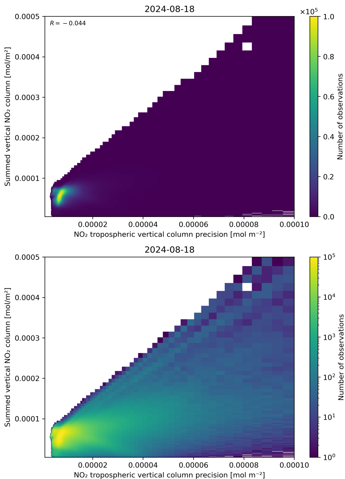
Figure 136: Scatter density plot of “NO 2 tropospheric vertical column precision” against “Summed vertical NO 2 column” for 2024-08-17 to 2024-08-19.
