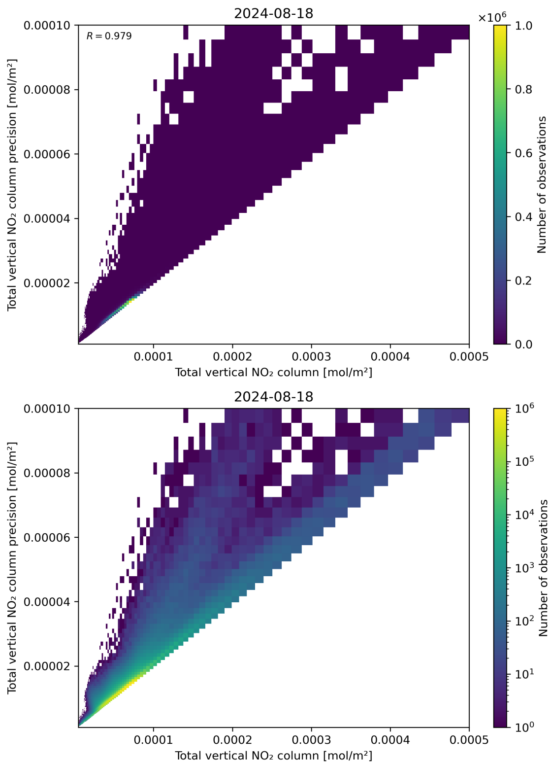
Figure 114: Scatter density plot of “Total vertical NO 2 column” against “Total vertical NO 2 column precision” for 2024-08-17 to 2024-08-19.
