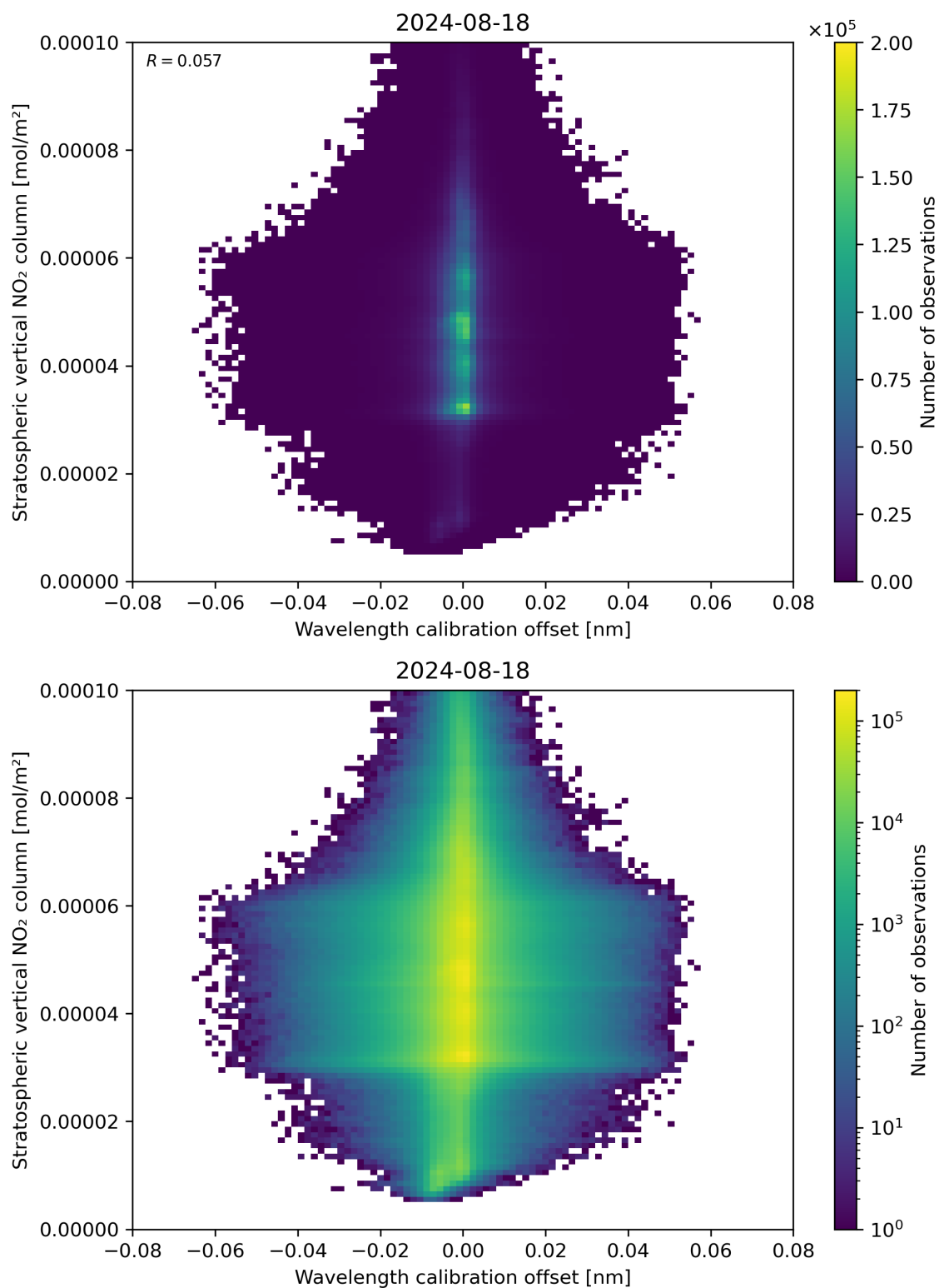
Figure 176: Scatter density plot of “Wavelength calibration offset” against “Stratospheric vertical NO 2 column” for 2024-08-17 to 2024-08-19.
