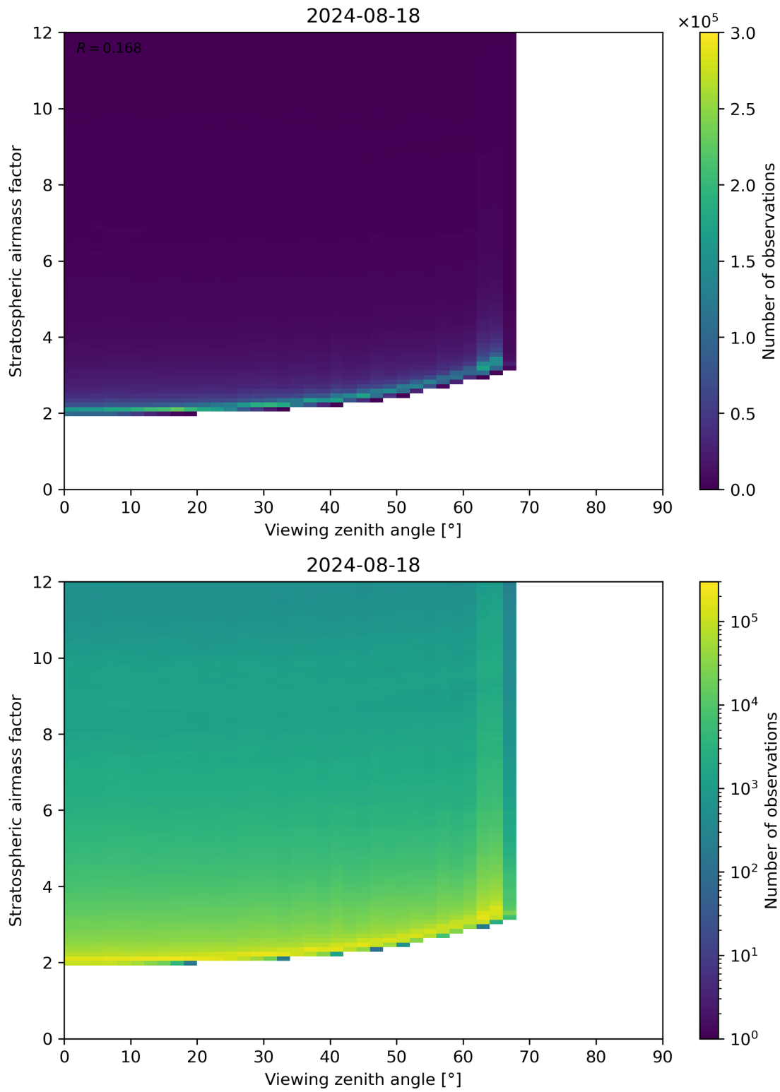
Figure 159: Scatter density plot of “Viewing zenith angle” against “Stratospheric airmass factor” for 2024-08-17 to 2024-08-19.
