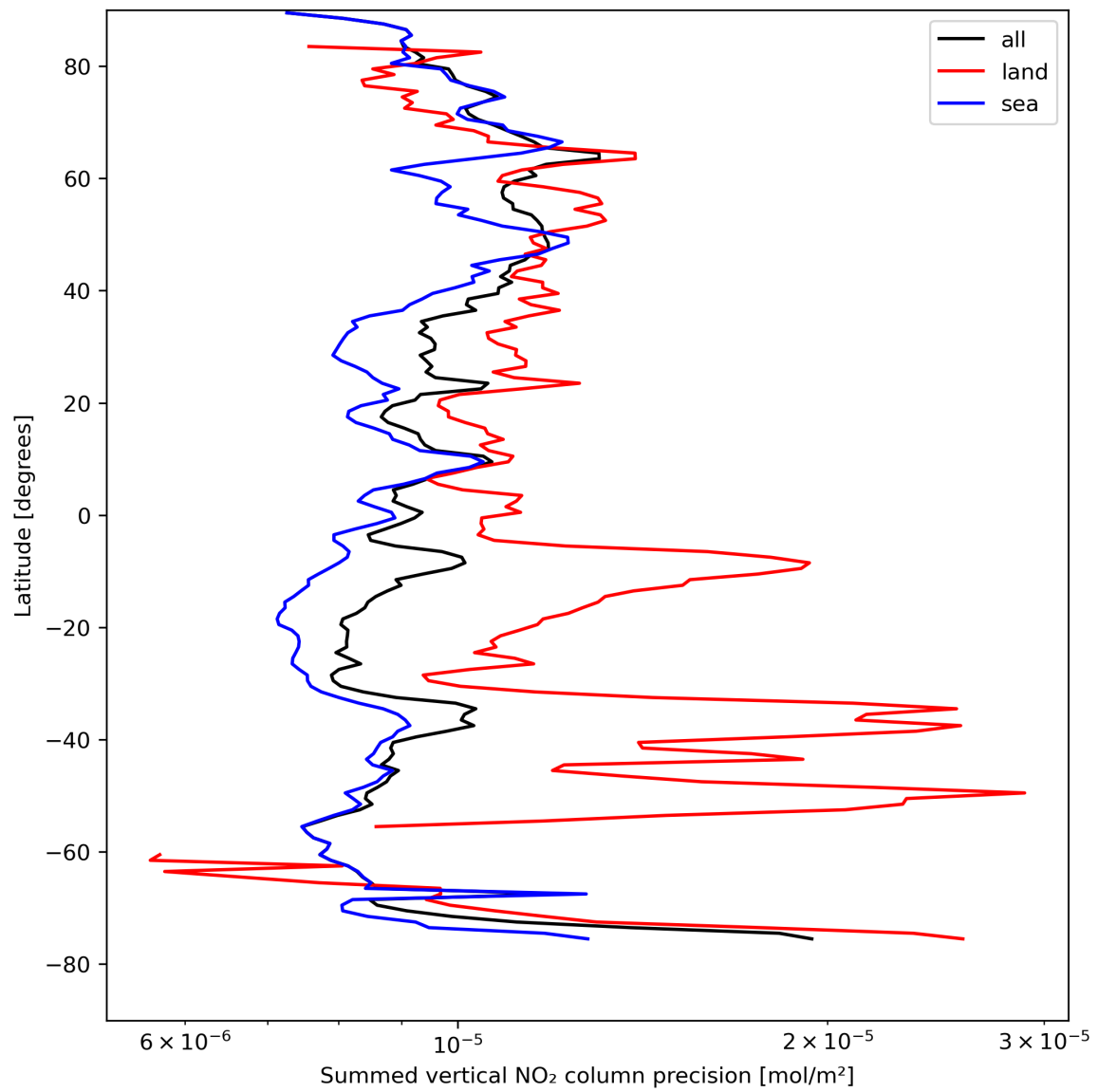
Figure 24: Zonal average of “Summed vertical NO 2 column precision” for 2024-08-17 to 2024-08-19.
