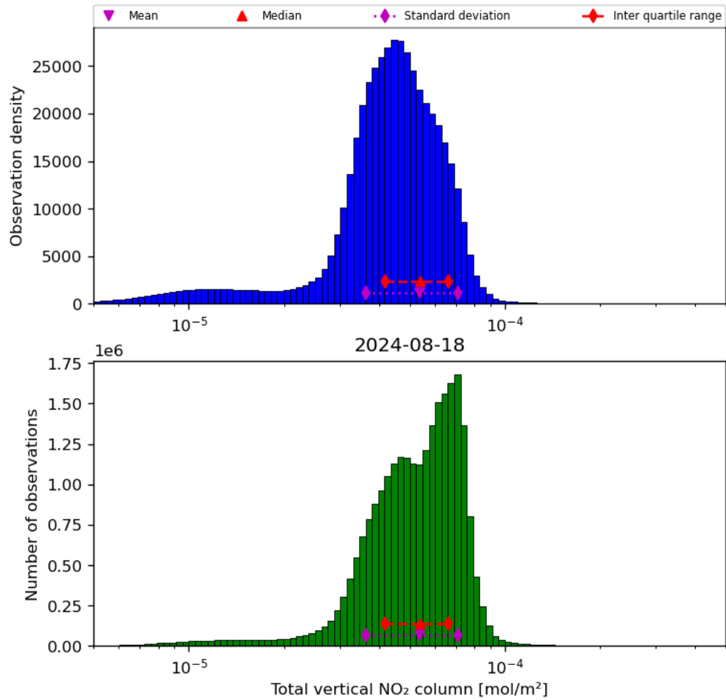
Figure 38: Histogram of “Total vertical NO 2 column” for 2024-08-17 to 2024-08-19
