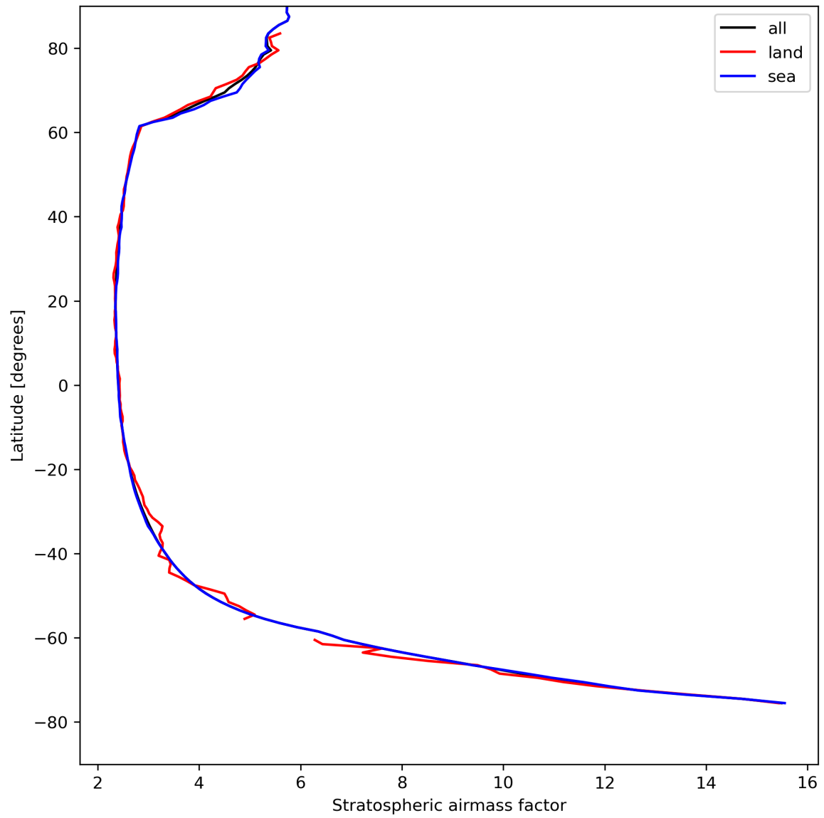
Figure 27: Zonal average of “Stratospheric airmass factor” for 2024-08-17 to 2024-08-19.
