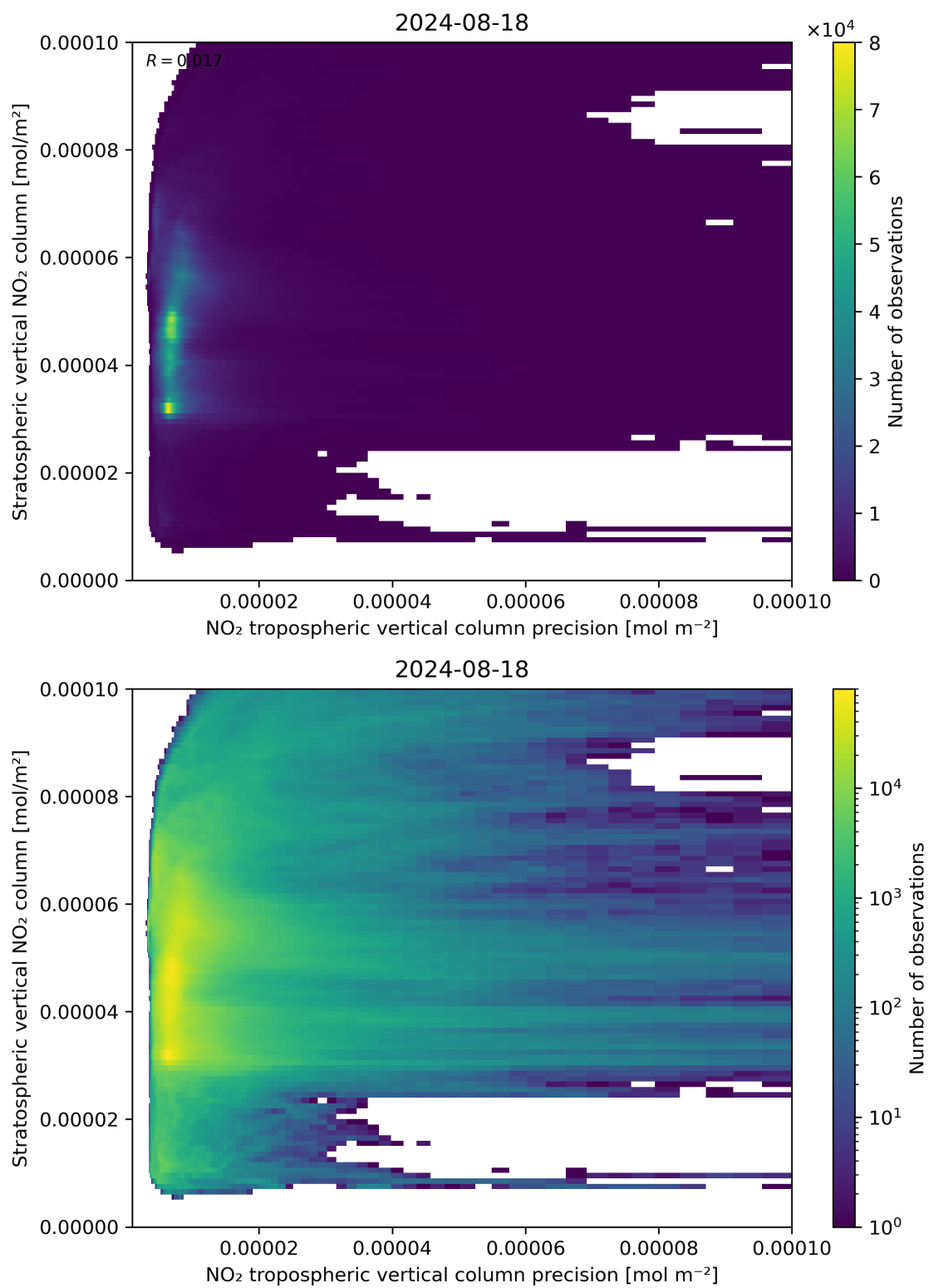
Figure 135: Scatter density plot of “NO 2 tropospheric vertical column precision” against “Stratospheric vertical NO 2 column” for 2024-08-17 to 2024-08-19.
