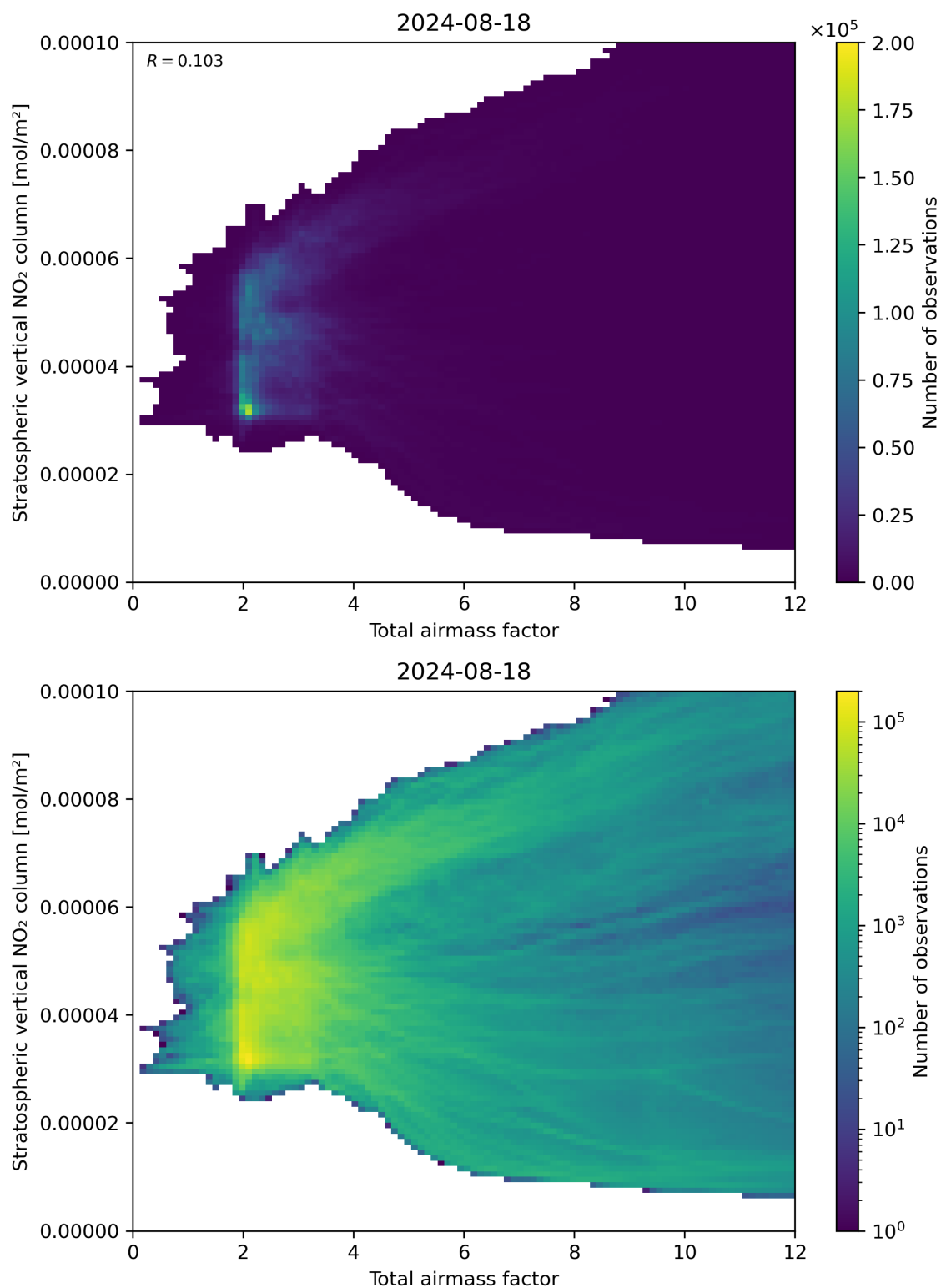
Figure 64: Scatter density plot of “Total airmass factor” against “Stratospheric vertical \text{NO}_2 column” for 2024-08-17 to 2024-08-19.
