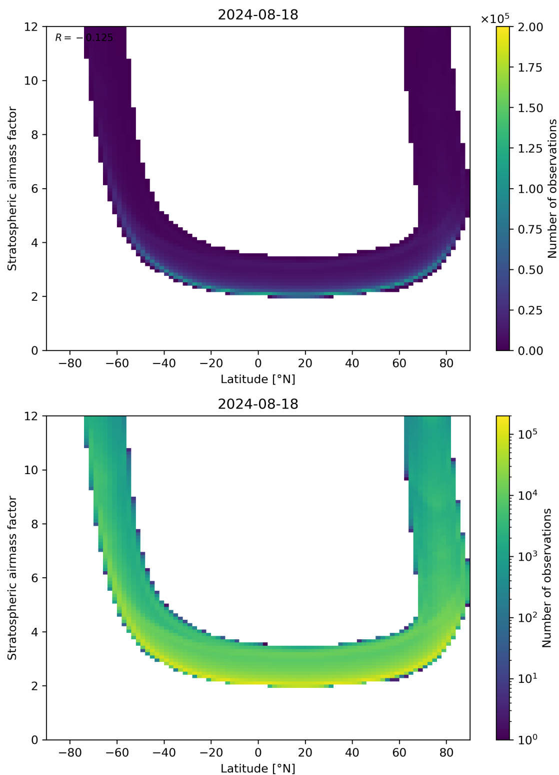
Figure 83: Scatter density plot of “Latitude” against “Stratospheric air mass factor” for 2024-08-17 to 2024-08-19.
