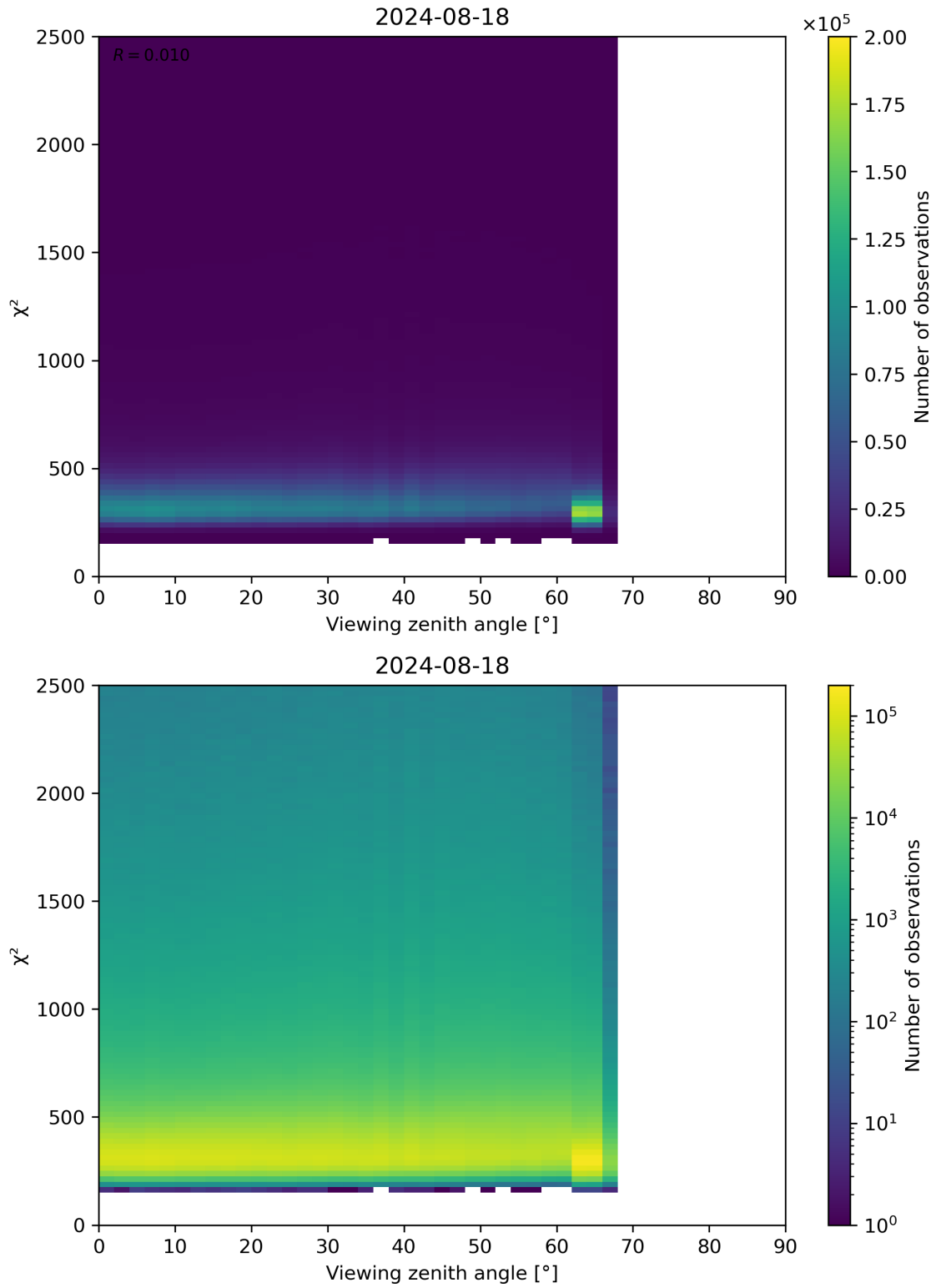
Figure 162: Scatter density plot of “Viewing zenith angle” against “ \chi^2 ” for 2024-08-17 to 2024-08-19.
