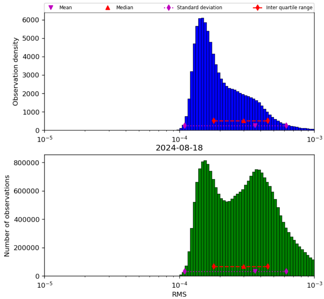
Figure 43: Histogram of “RMS” for 2024-08-17 to 2024-08-19
