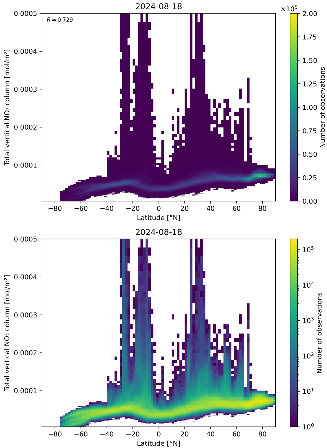
Figure 90: Scatter density plot of “Latitude” against “Total vertical NO 2 column” for 2024-08-17 to 2024-08-19.
