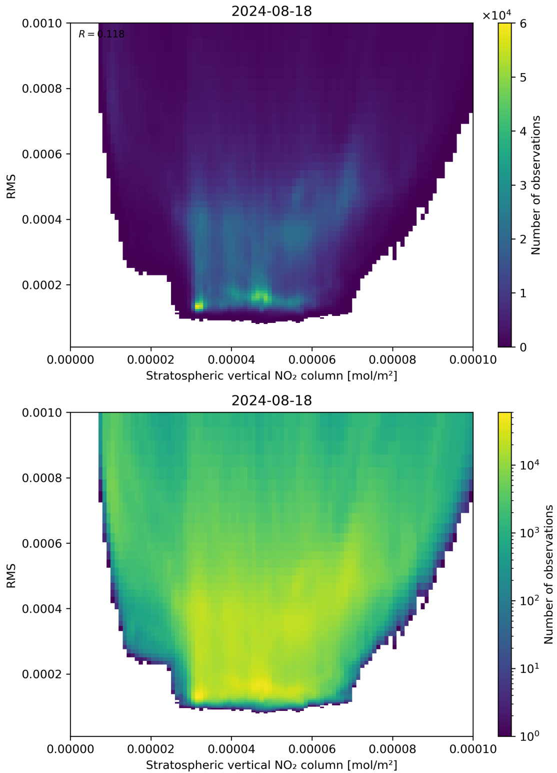
Figure 102: Scatter density plot of “Stratospheric vertical NO 2 column” against “RMS” for 2024-08-17 to 2024-08-19.
