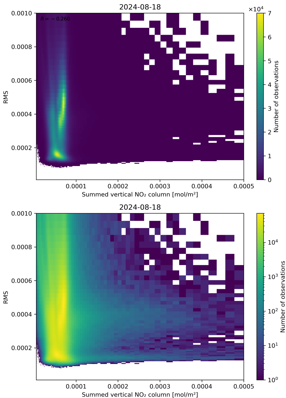
Figure 109: Scatter density plot of “Summed vertical NO 2 column” against “RMS” for 2024-08-17 to 2024-08-19.
