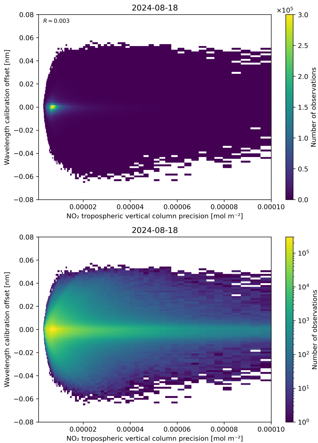
Figure 141: Scatter density plot of “NO 2 tropospheric vertical column precision” against “Wavelength calibration offset” for 2024-08-17 to 2024-08-19.
