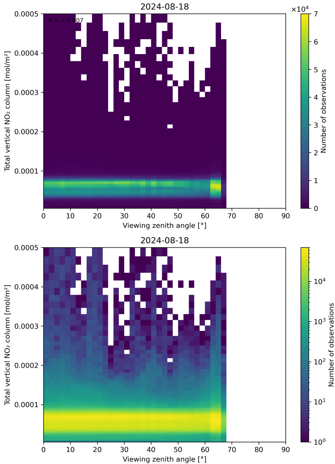
Figure 167: Scatter density plot of “Viewing zenith angle” against “Total vertical NO 2 column” for 2024-08-17 to 2024-08-19.
