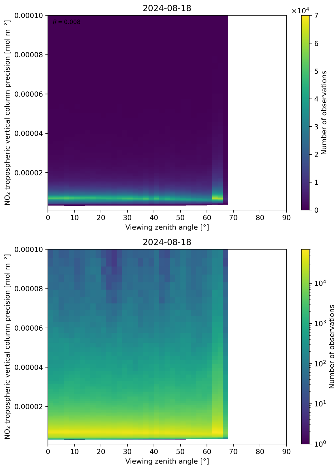
Figure 170: Scatter density plot of “Viewing zenith angle” against “NO 2 tropospheric vertical column precision” for 2024-08-17 to 2024-08-19.
