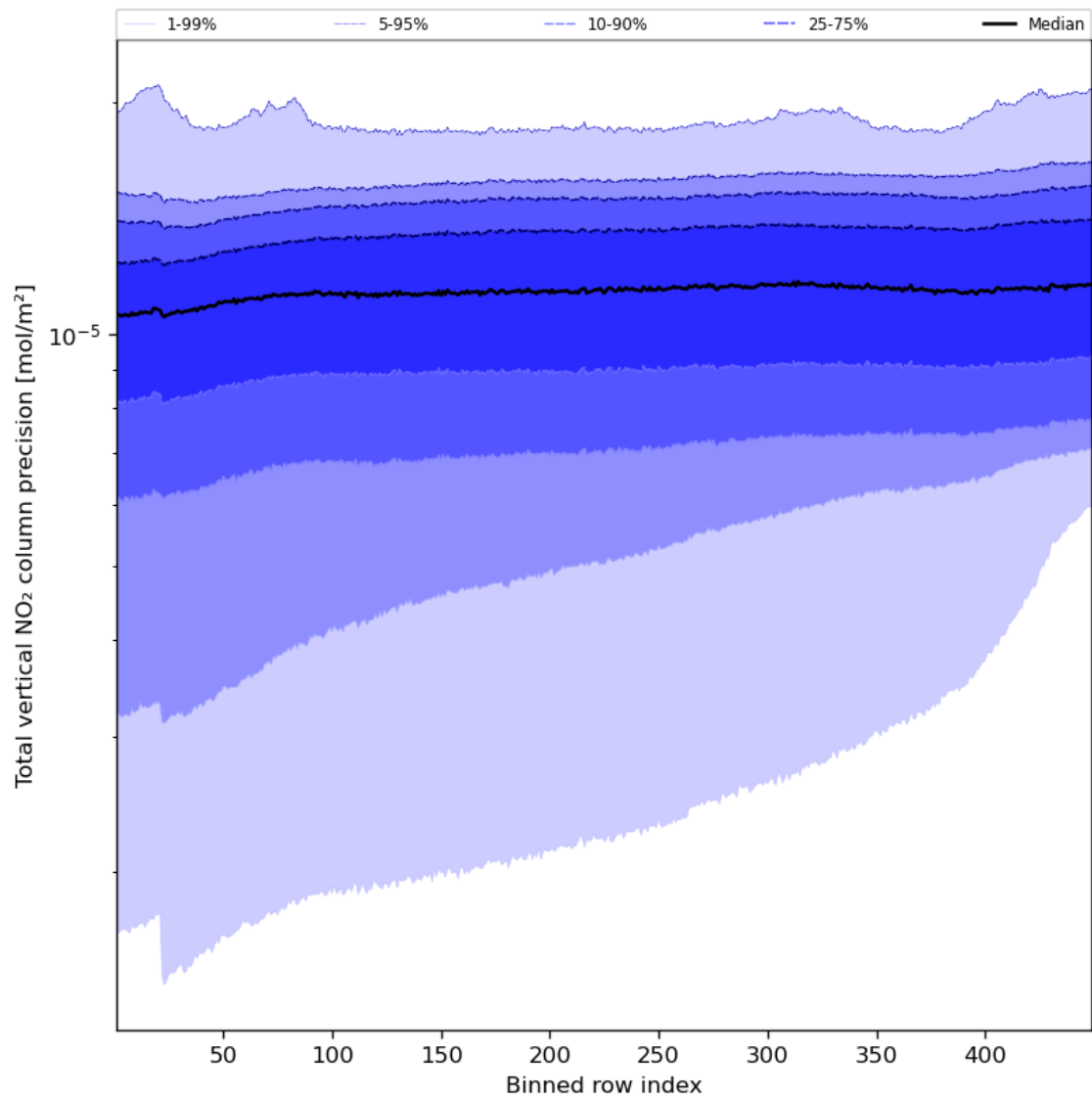
Figure 56: Along track statistics of “Total vertical NO 2 column precision” for 2024-08-19 to 2024-08-21
