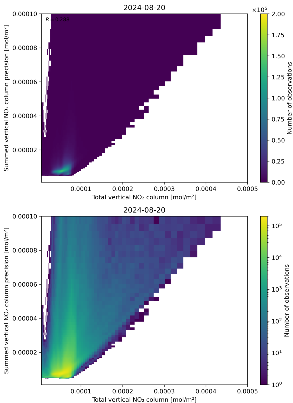
Figure 113: Scatter density plot of “Total vertical NO 2 column” against “Summed vertical NO 2 column precision” for 2024-08-19 to 2024-08-21.
