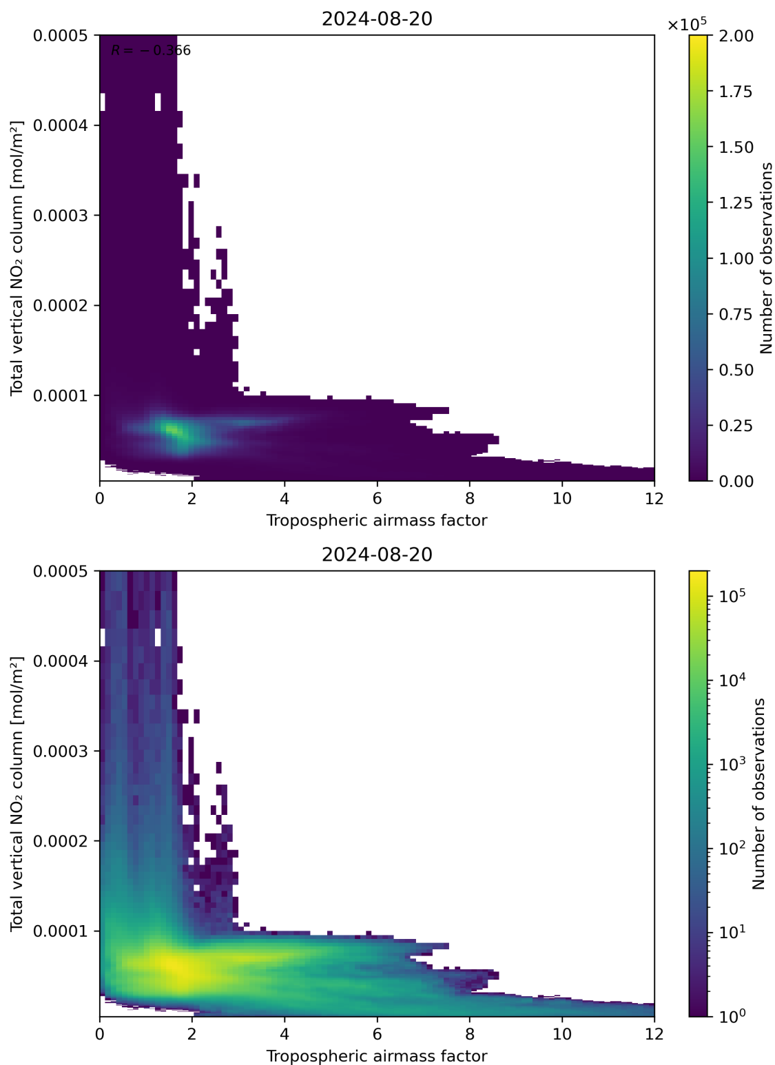
Figure 77: Scatter density plot of “Tropospheric airmass factor” against “Total vertical NO 2 column” for 2024-08-19 to 2024-08-21.
