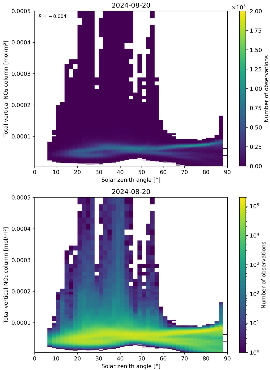
Figure 153: Scatter density plot of “Solar zenith angle” against “Total vertical NO 2 column” for 2024-08-19 to 2024-08-21.
