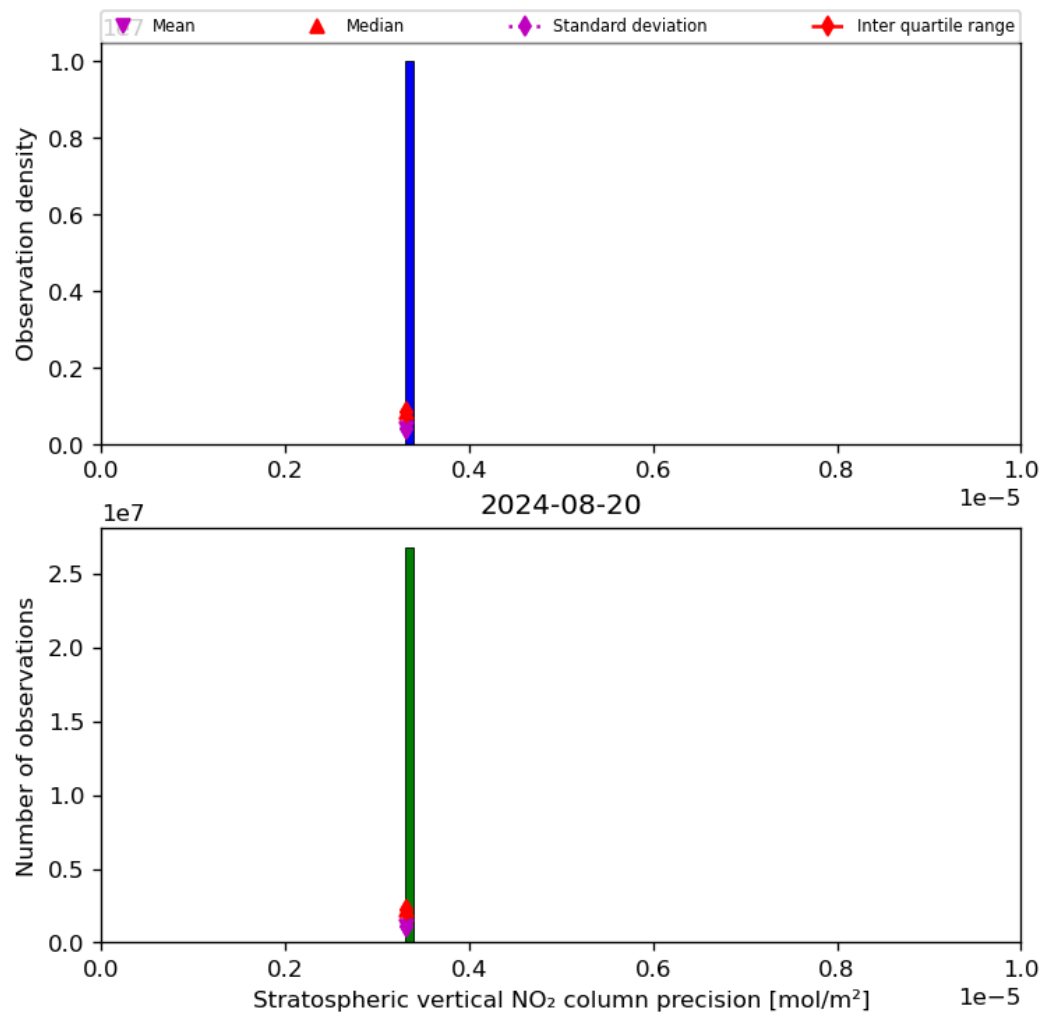
Figure 37: Histogram of “Stratospheric vertical NO 2 column precision” for 2024-08-19 to 2024-08-21
