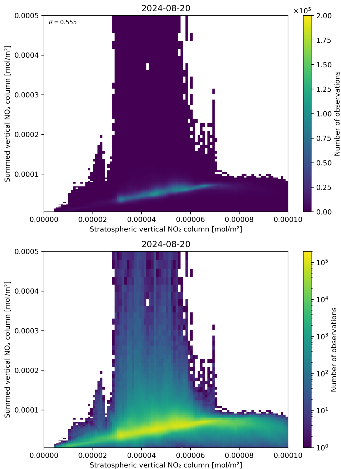
Figure 98: Scatter density plot of “Stratospheric vertical NO 2 column” against “Summed vertical NO 2 column” for 2024-08-19 to 2024-08-21.
