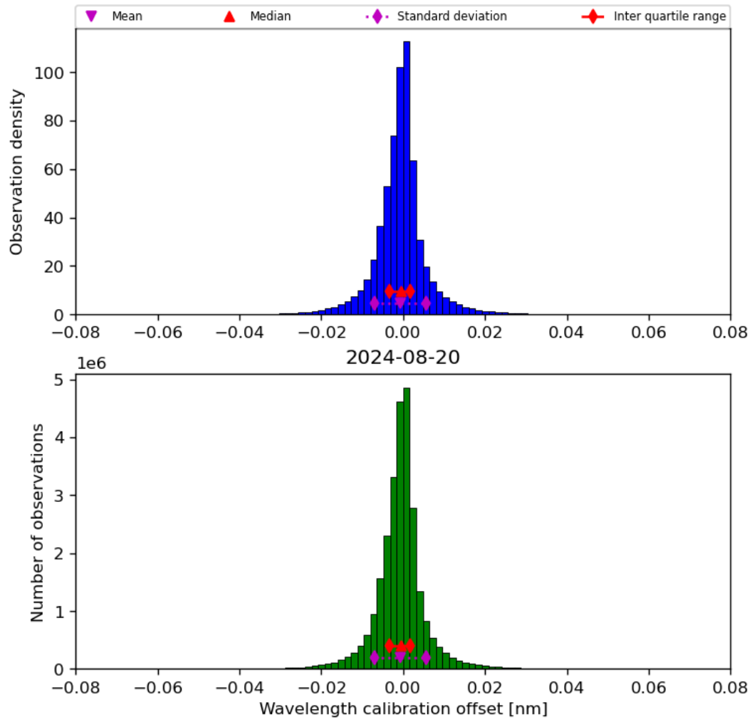
Figure 35: Histogram of “Wavelength calibration offset” for 2024-08-19 to 2024-08-21
