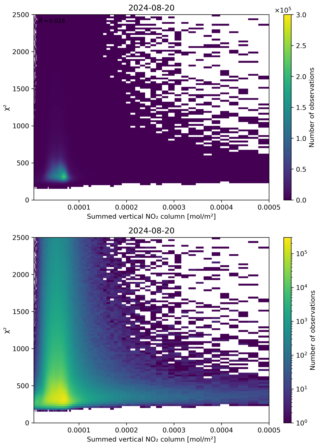
Figure 104: Scatter density plot of “Summed vertical NO 2 column” against “ \chi^2 ” for 2024-08-19 to 2024-08-21.
