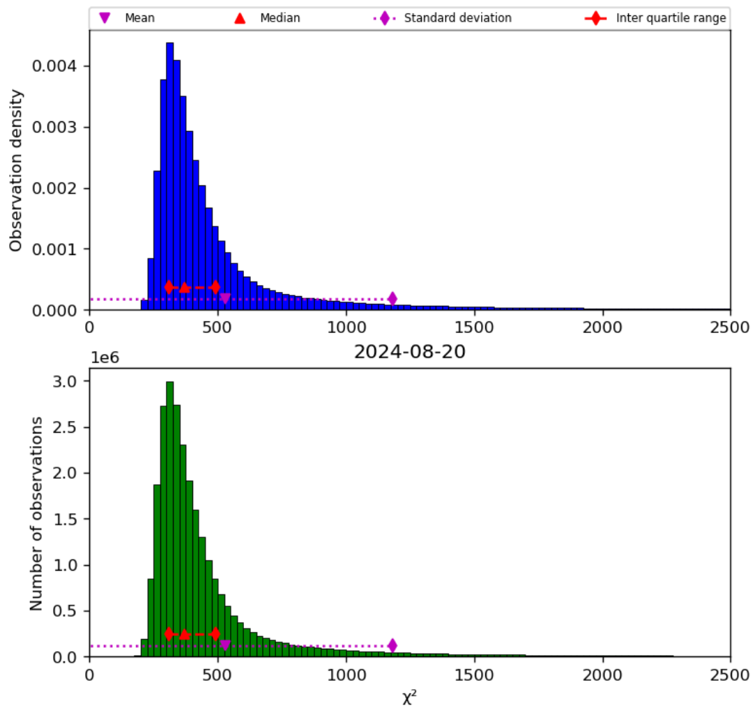
Figure 42: Histogram of " \chi^2 " for 2024-08-19 to 2024-08-21
