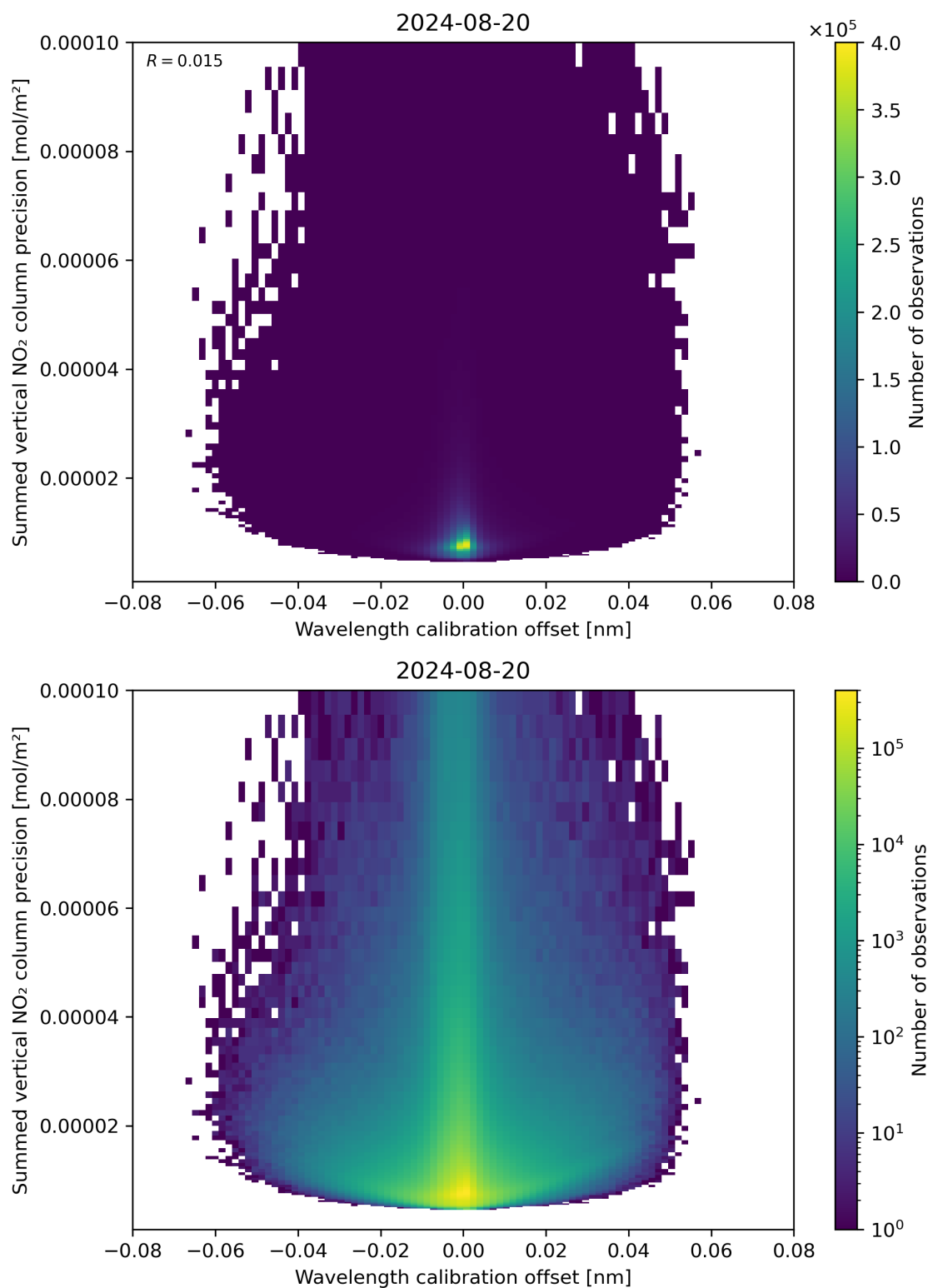
Figure 178: Scatter density plot of “Wavelength calibration offset” against “Summed vertical NO 2 column precision” for 2024-08-19 to 2024-08-21.
