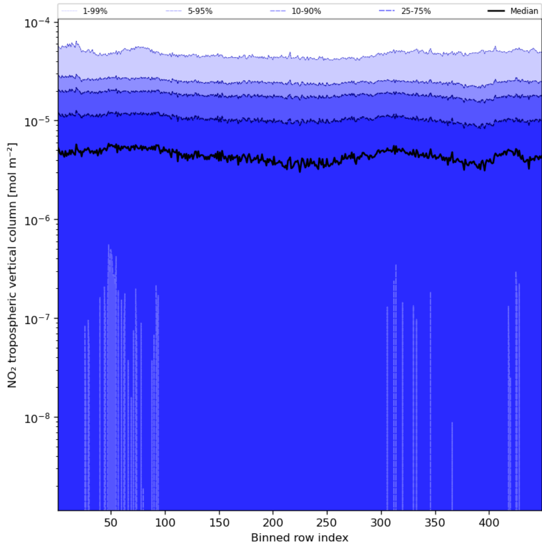
Figure 46: Along track statistics of “NO 2 tropospheric vertical column” for 2024-08-19 to 2024-08-21
