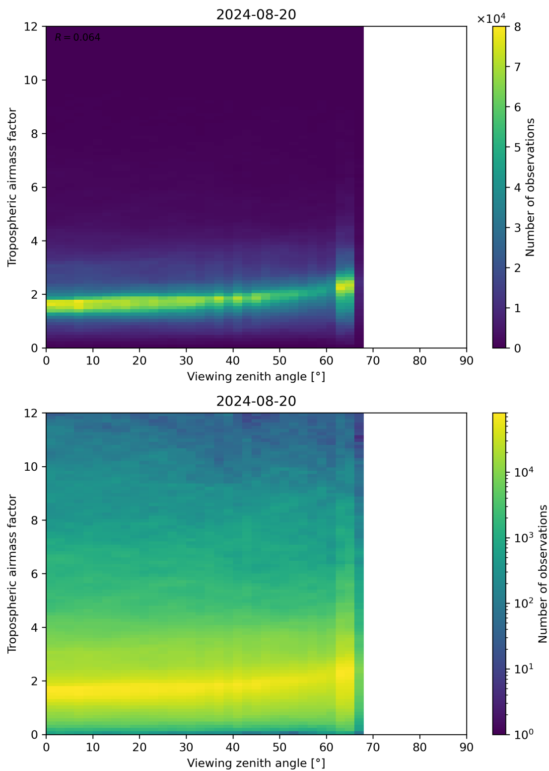
Figure 161: Scatter density plot of “Viewing zenith angle” against “Tropospheric airmass factor” for 2024-08-19 to 2024-08-21.
