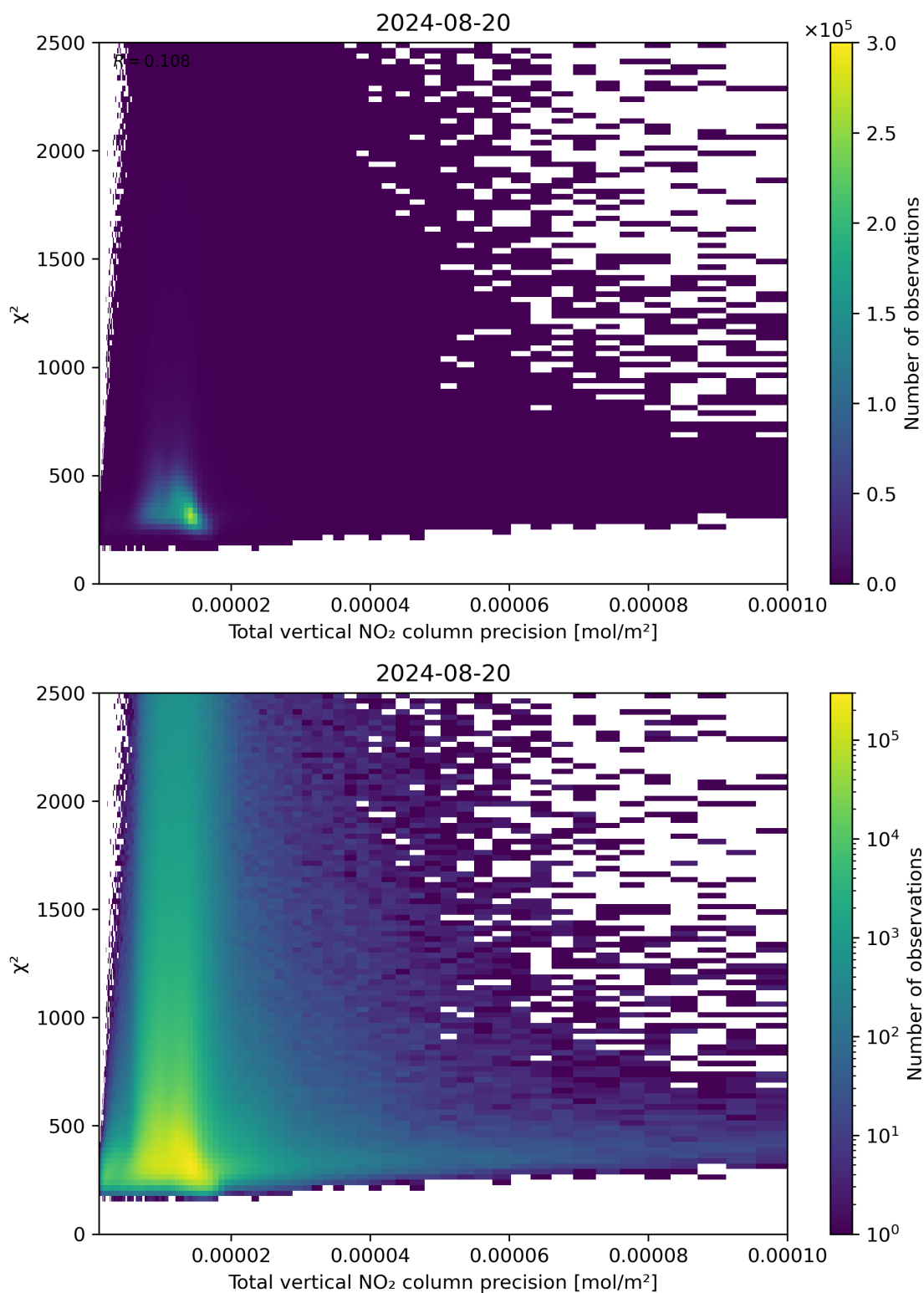
Figure 116: Scatter density plot of “Total vertical NO 2 column precision” against “ \chi^2 ” for 2024-08-19 to 2024-08-21.
