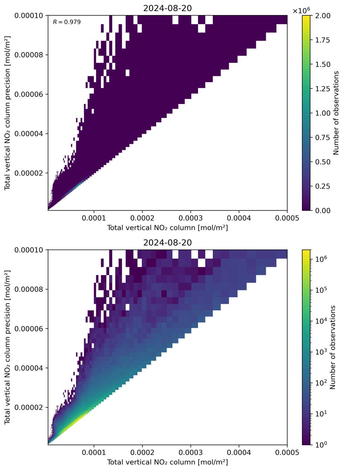
Figure 114: Scatter density plot of “Total vertical NO 2 column” against “Total vertical NO 2 column precision” for 2024-08-19 to 2024-08-21.
