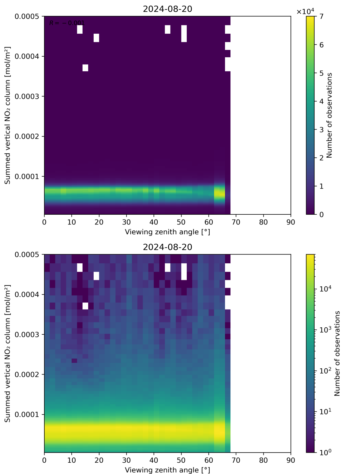
Figure 165: Scatter density plot of “Viewing zenith angle” against “Summed vertical NO 2 column” for 2024-08-19 to 2024-08-21.
