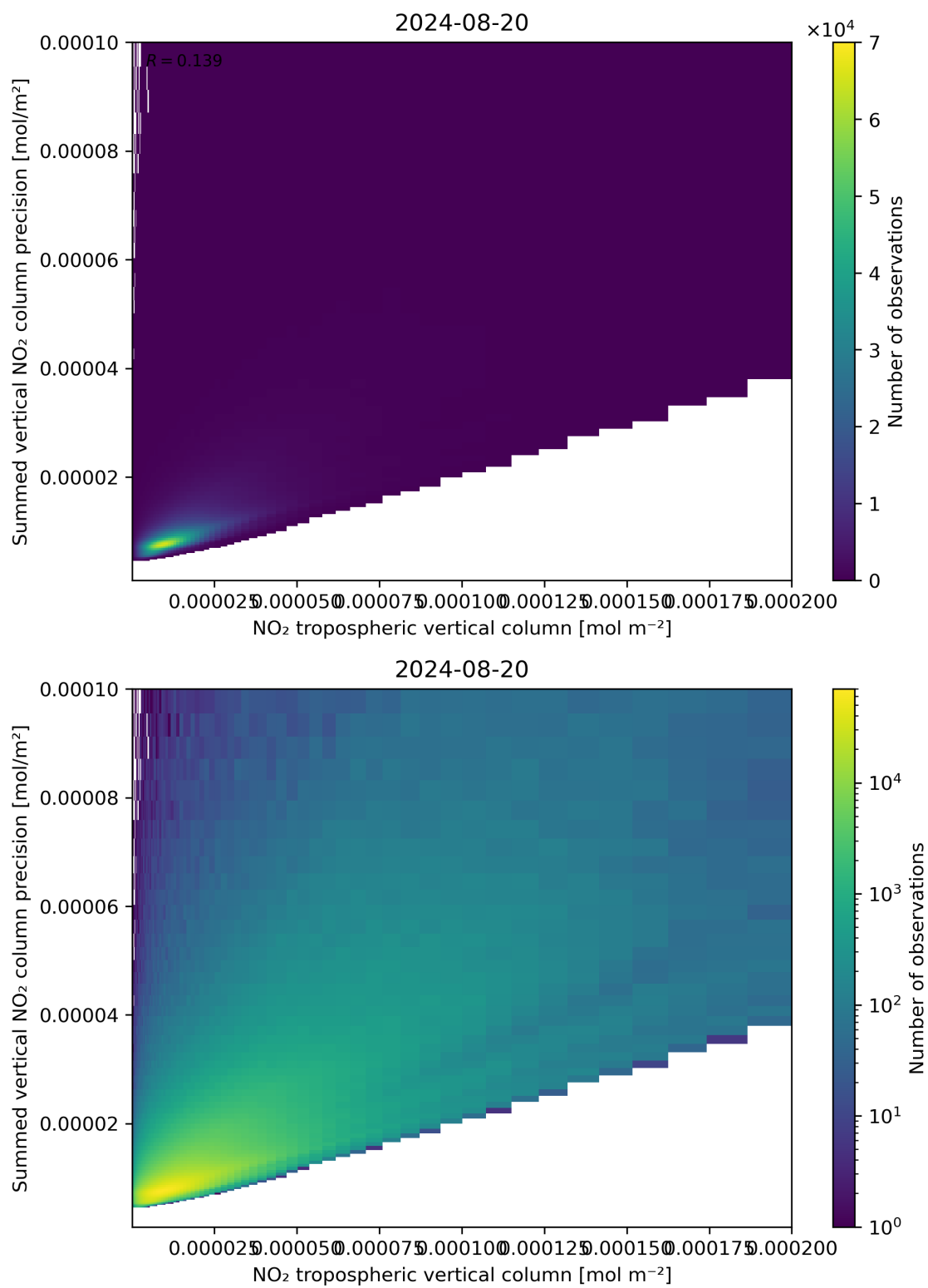
Figure 127: Scatter density plot of “NO 2 tropospheric vertical column” against “Summed vertical NO 2 column precision” for 2024-08-19 to 2024-08-21.
