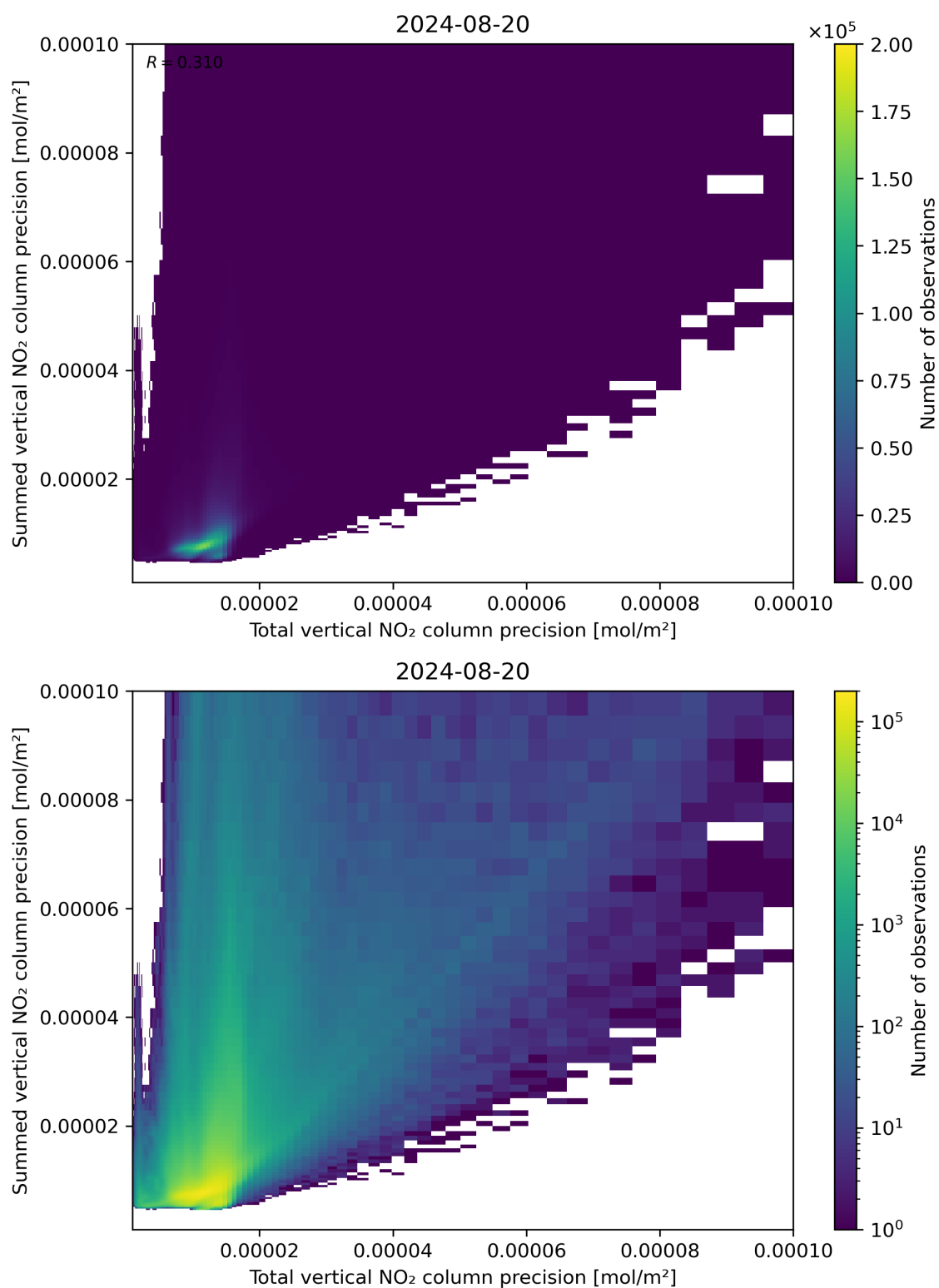
Figure 118: Scatter density plot of “Total vertical NO 2 column precision” against “Summed vertical NO 2 column precision” for 2024-08-19 to 2024-08-21.
