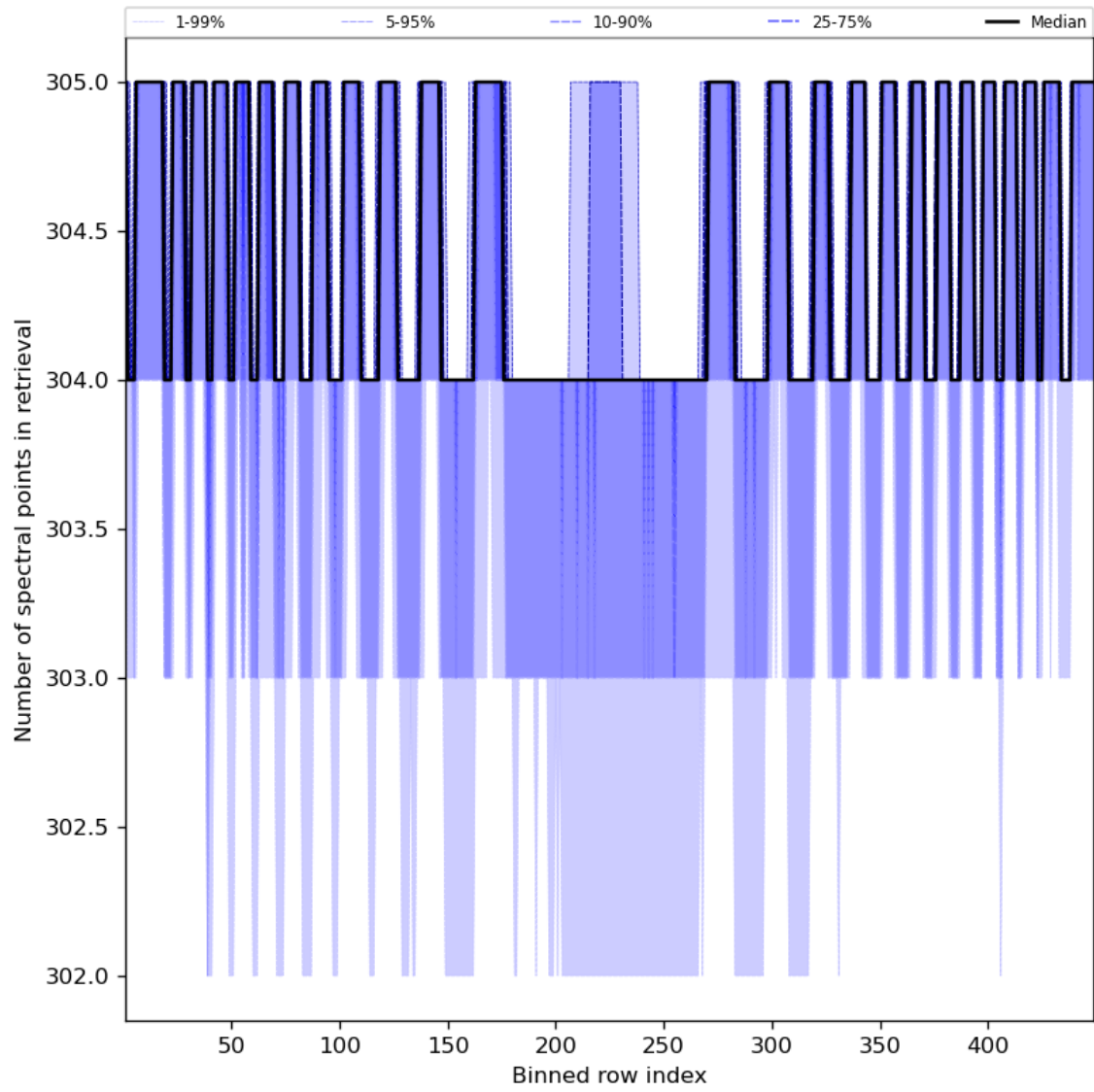
Figure 50: Along track statistics of “Number of spectral points in retrieval” for 2024-08-19 to 2024-08-21
