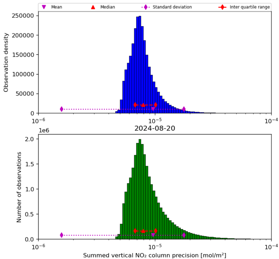
Figure 41: Histogram of “Summed vertical NO 2 column precision” for 2024-08-19 to 2024-08-21
