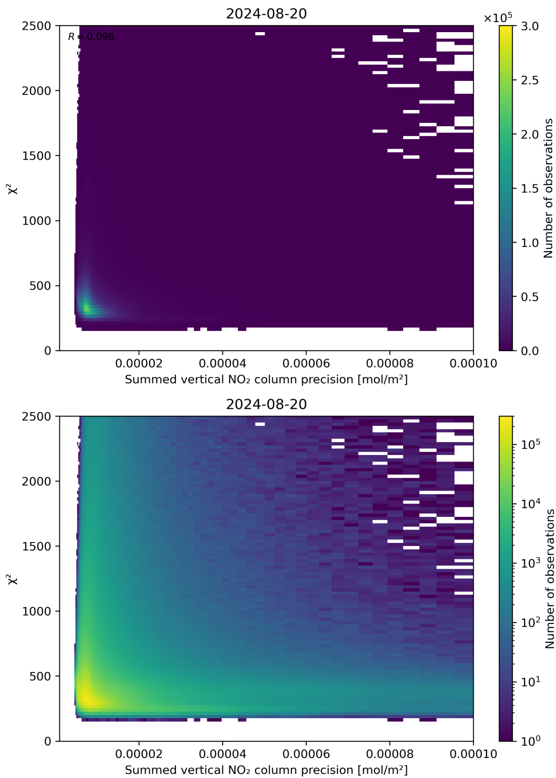
Figure 107: Scatter density plot of “Summed vertical NO 2 column precision” against “ \chi^2 ” for 2024-08-19 to 2024-08-21.
