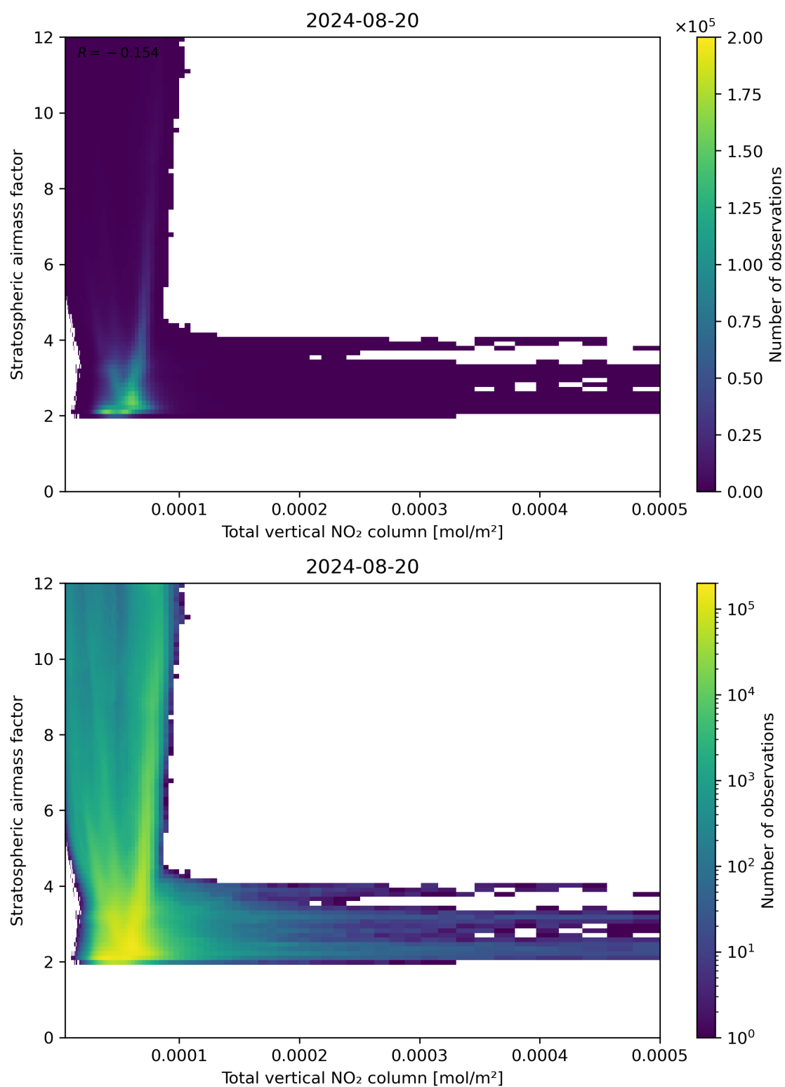
Figure 110: Scatter density plot of “Total vertical NO 2 column” against “Stratospheric airmass factor” for 2024-08-19 to 2024-08-21.
