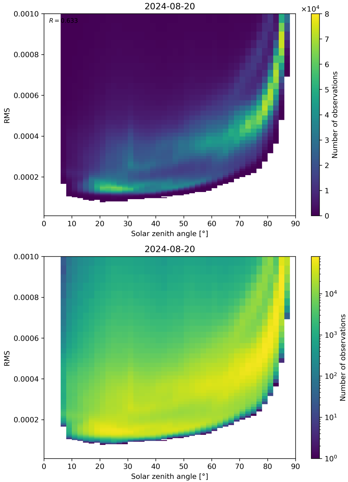
Figure 157: Scatter density plot of “Solar zenith angle” against “RMS” for 2024-08-19 to 2024-08-21.
