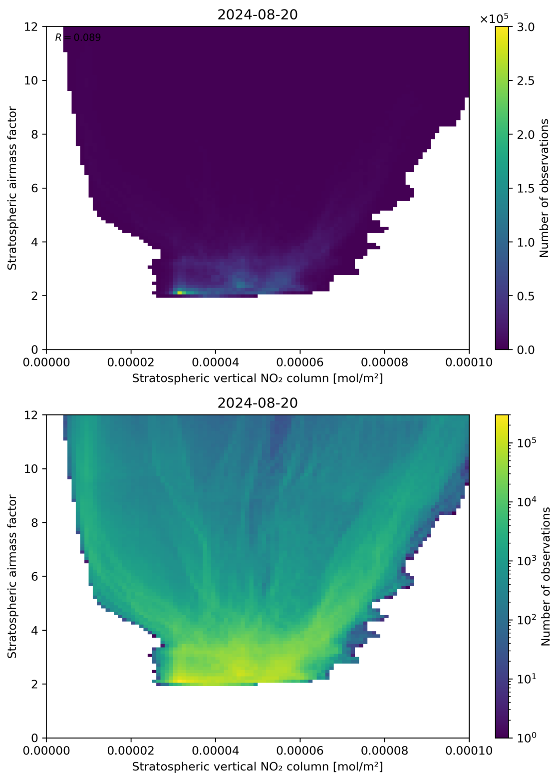
Figure 96: Scatter density plot of “Stratospheric vertical NO 2 column” against “Stratospheric airmass factor” for 2024-08-19 to 2024-08-21.
