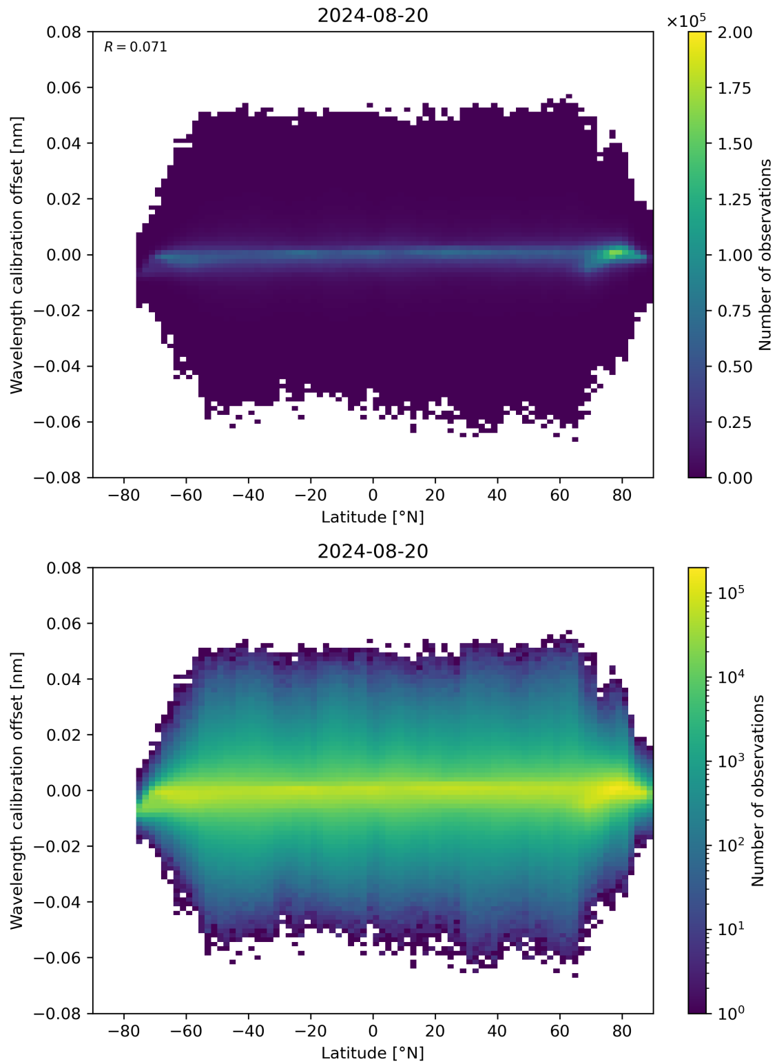
Figure 95: Scatter density plot of “Latitude” against “Wavelength calibration offset” for 2024-08-19 to 2024-08-21.
