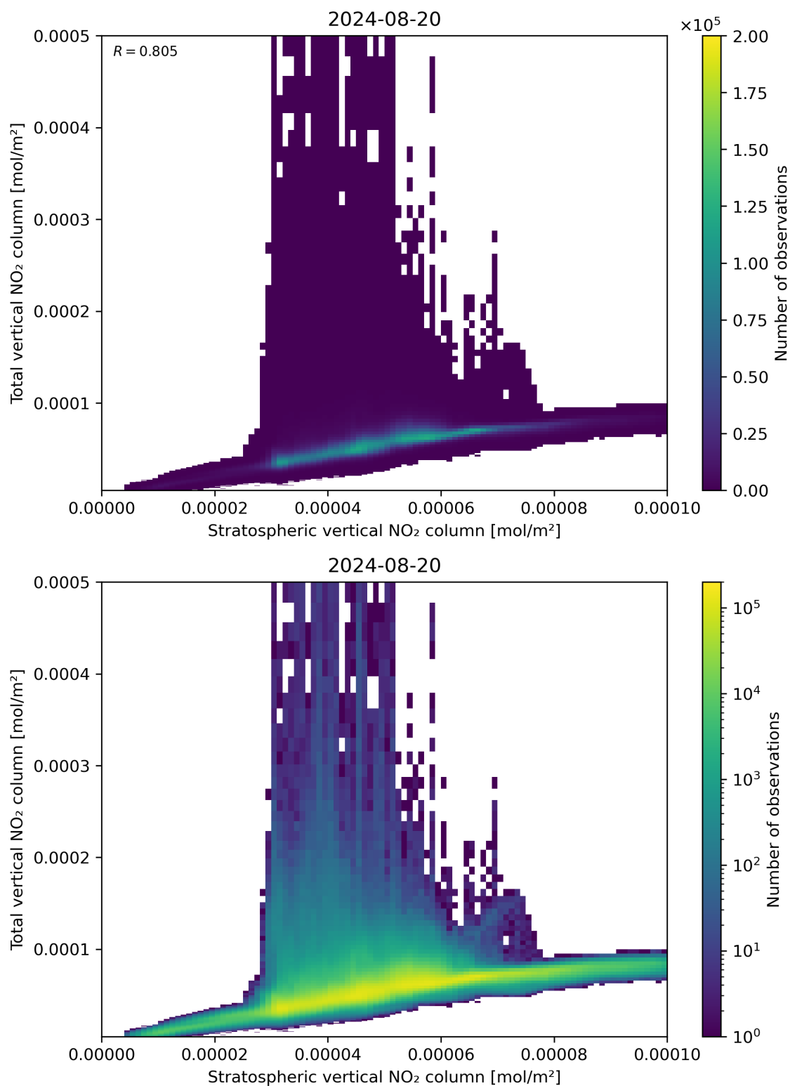
Figure 100: Scatter density plot of “Stratospheric vertical NO 2 column” against “Total vertical NO 2 column” for 2024-08-19 to 2024-08-21.
