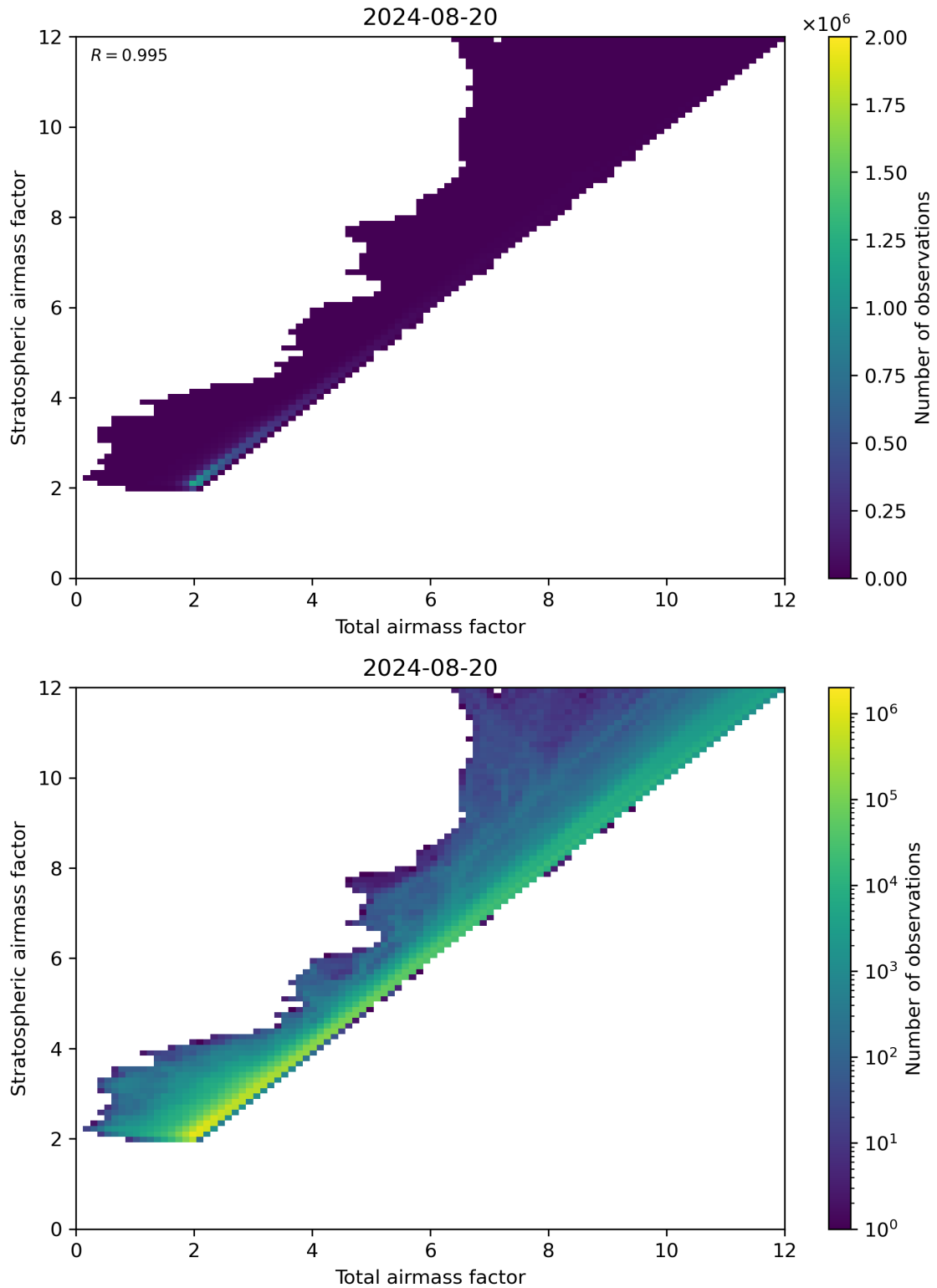
Figure 62: Scatter density plot of “Total airmass factor” against “Stratospheric airmass factor” for 2024-08-19 to 2024-08-21.
