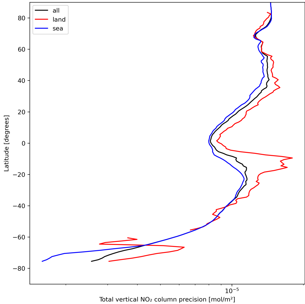
Figure 22: Zonal average of “Total vertical NO 2 column precision” for 2024-08-19 to 2024-08-21.
