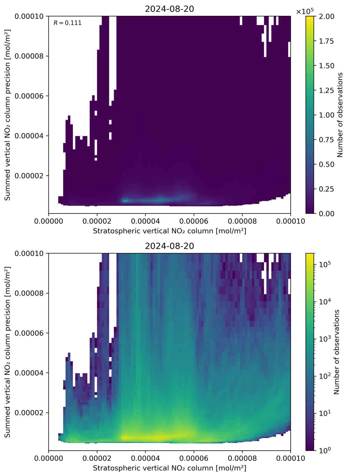
Figure 99: Scatter density plot of “Stratospheric vertical NO 2 column” against “Summed vertical NO 2 column precision” for 2024-08-19 to 2024-08-21.
