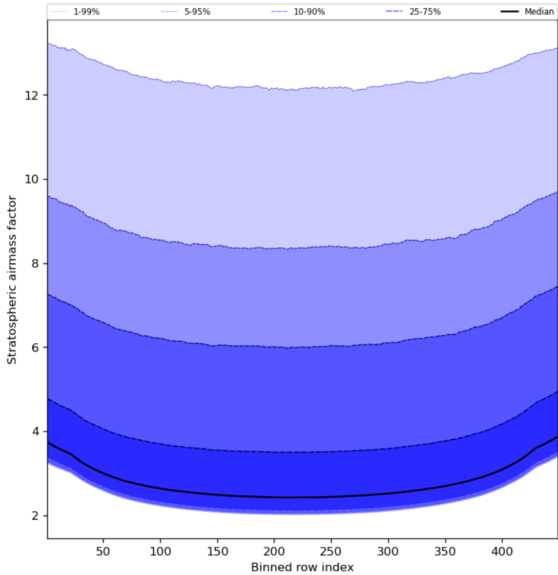
Figure 61: Along track statistics of “Stratospheric airmass factor” for 2024-08-19 to 2024-08-21
