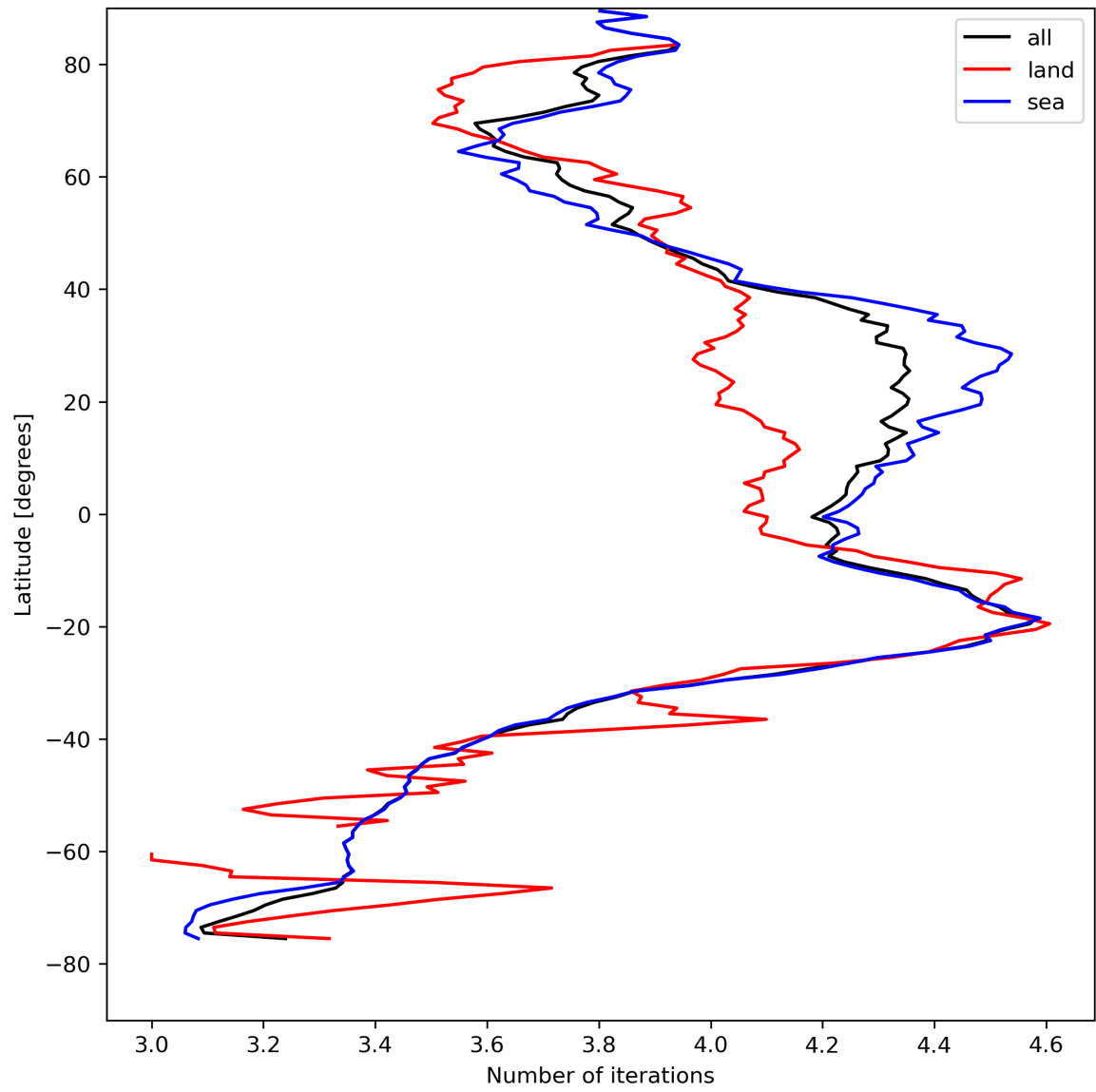
Figure 17: Zonal average of “Number of iterations” for 2024-08-19 to 2024-08-21.
