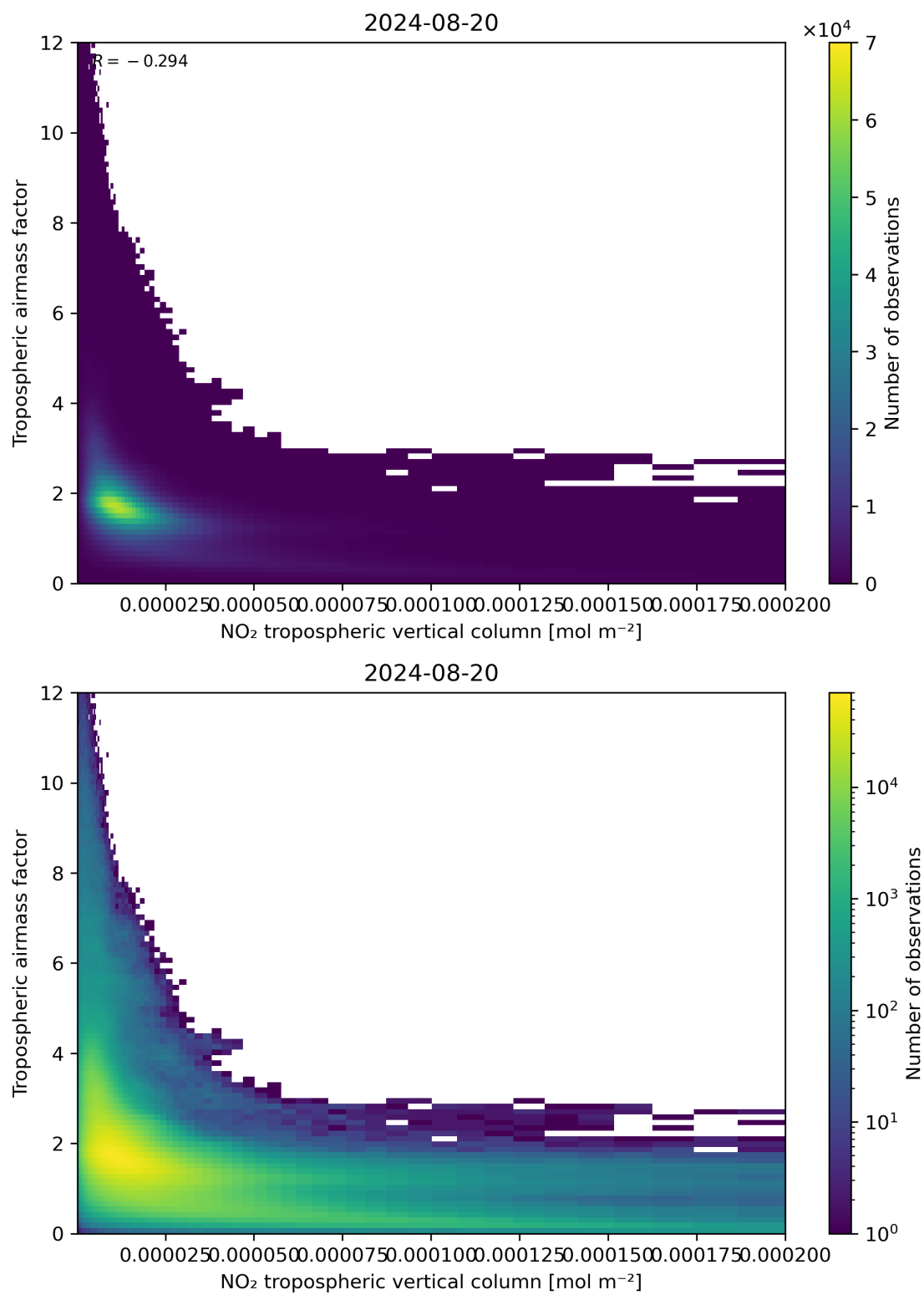
Figure 123: Scatter density plot of “NO 2 tropospheric vertical column” against “Tropospheric air mass factor” for 2024-08-19 to 2024-08-21.
