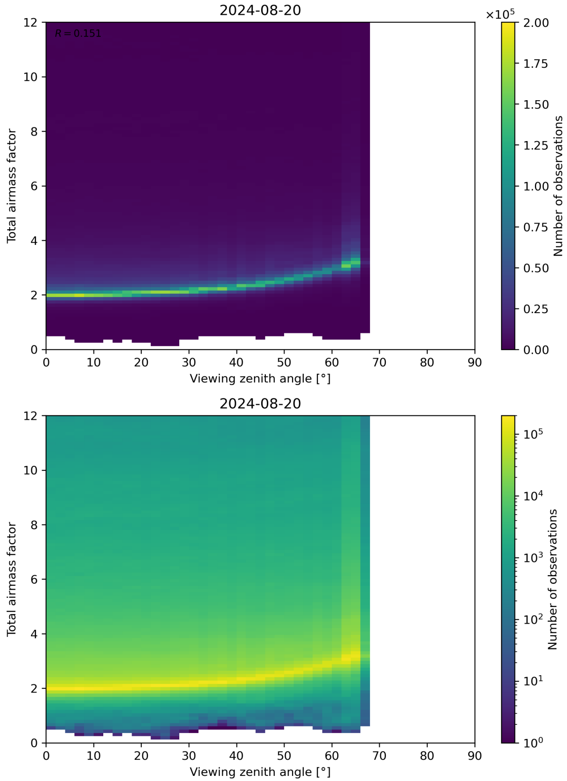
Figure 160: Scatter density plot of “Viewing zenith angle” against “Total airmass factor” for 2024-08-19 to 2024-08-21.
