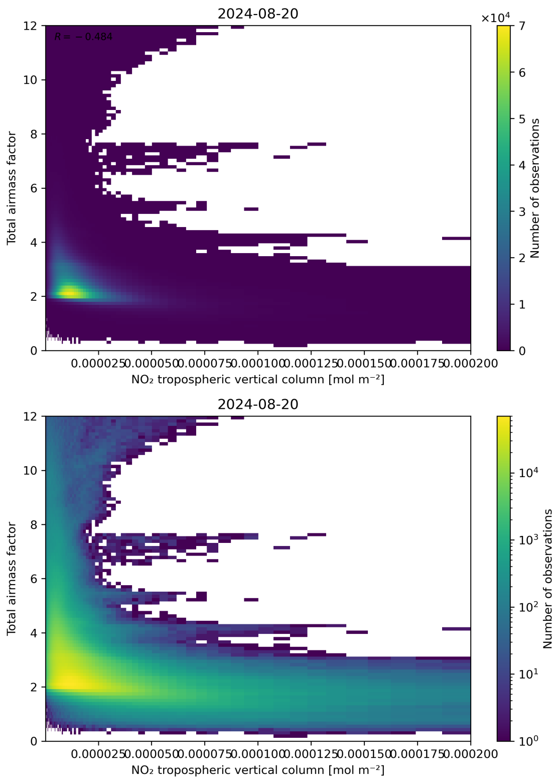
Figure 122: Scatter density plot of “NO 2 tropospheric vertical column” against “Total air mass factor” for 2024-08-19 to 2024-08-21.
