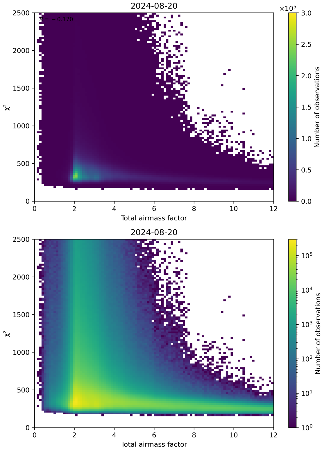
Figure 63: Scatter density plot of “Total airmass factor” against “ \chi^2 ” for 2024-08-19 to 2024-08-21.
