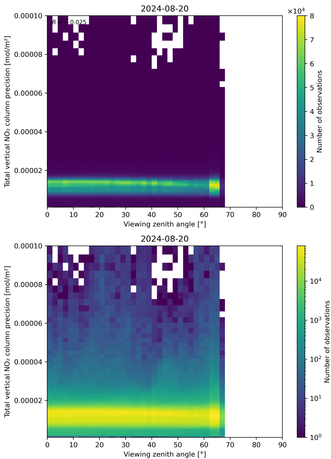
Figure 168: Scatter density plot of “Viewing zenith angle” against “Total vertical NO 2 column precision” for 2024-08-19 to 2024-08-21.
