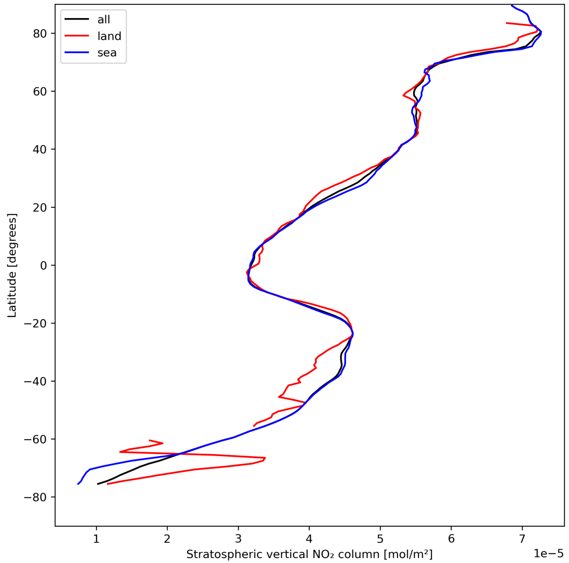
Figure 19: Zonal average of “Stratospheric vertical NO 2 column” for 2024-08-19 to 2024-08-21.
