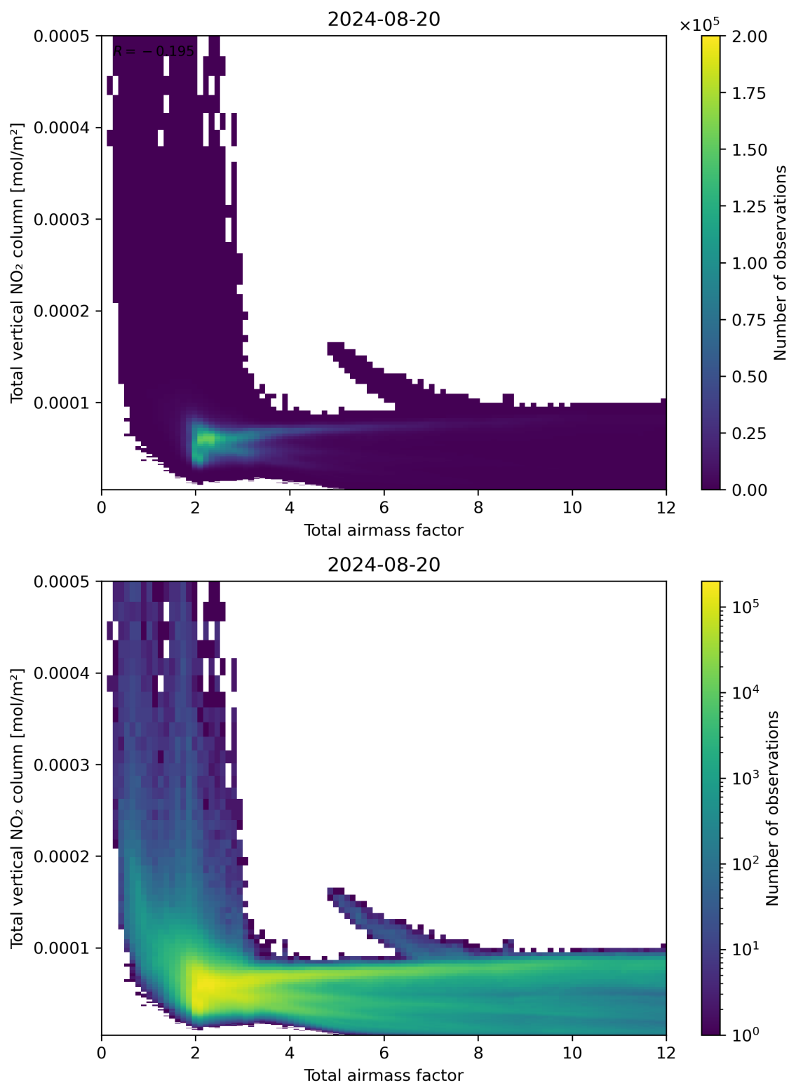
Figure 67: Scatter density plot of “Total airmass factor” against “Total vertical NO 2 column” for 2024-08-19 to 2024-08-21.
