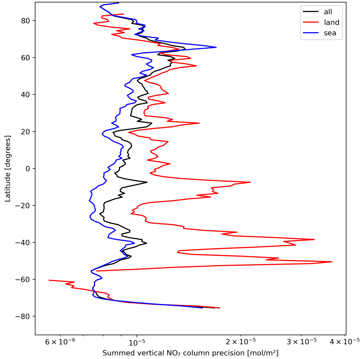
Figure 24: Zonal average of “Summed vertical NO 2 column precision” for 2024-08-19 to 2024-08-21.
