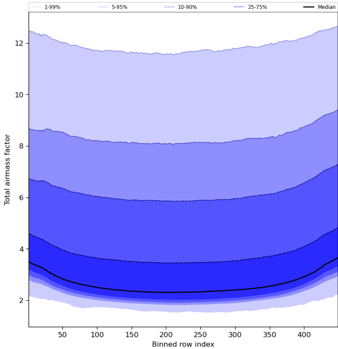
Figure 49: Along track statistics of “Total airmass factor” for 2024-08-19 to 2024-08-21
