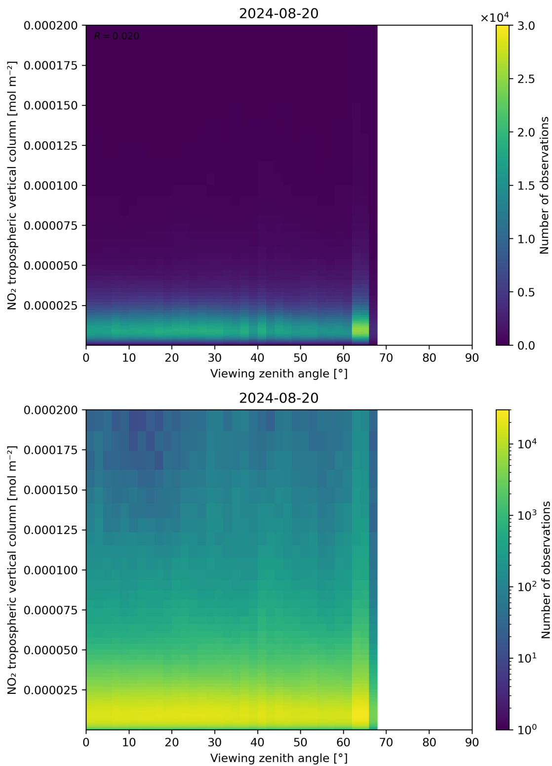
Figure 169: Scatter density plot of “Viewing zenith angle” against “NO 2 tropospheric vertical column” for 2024-08-19 to 2024-08-21.
