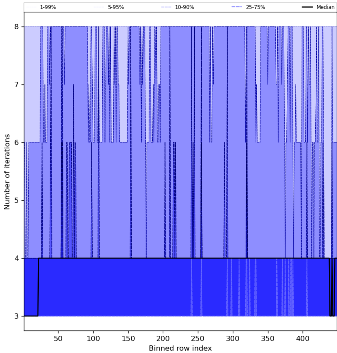
Figure 51: Along track statistics of “Number of iterations” for 2024-08-19 to 2024-08-21
