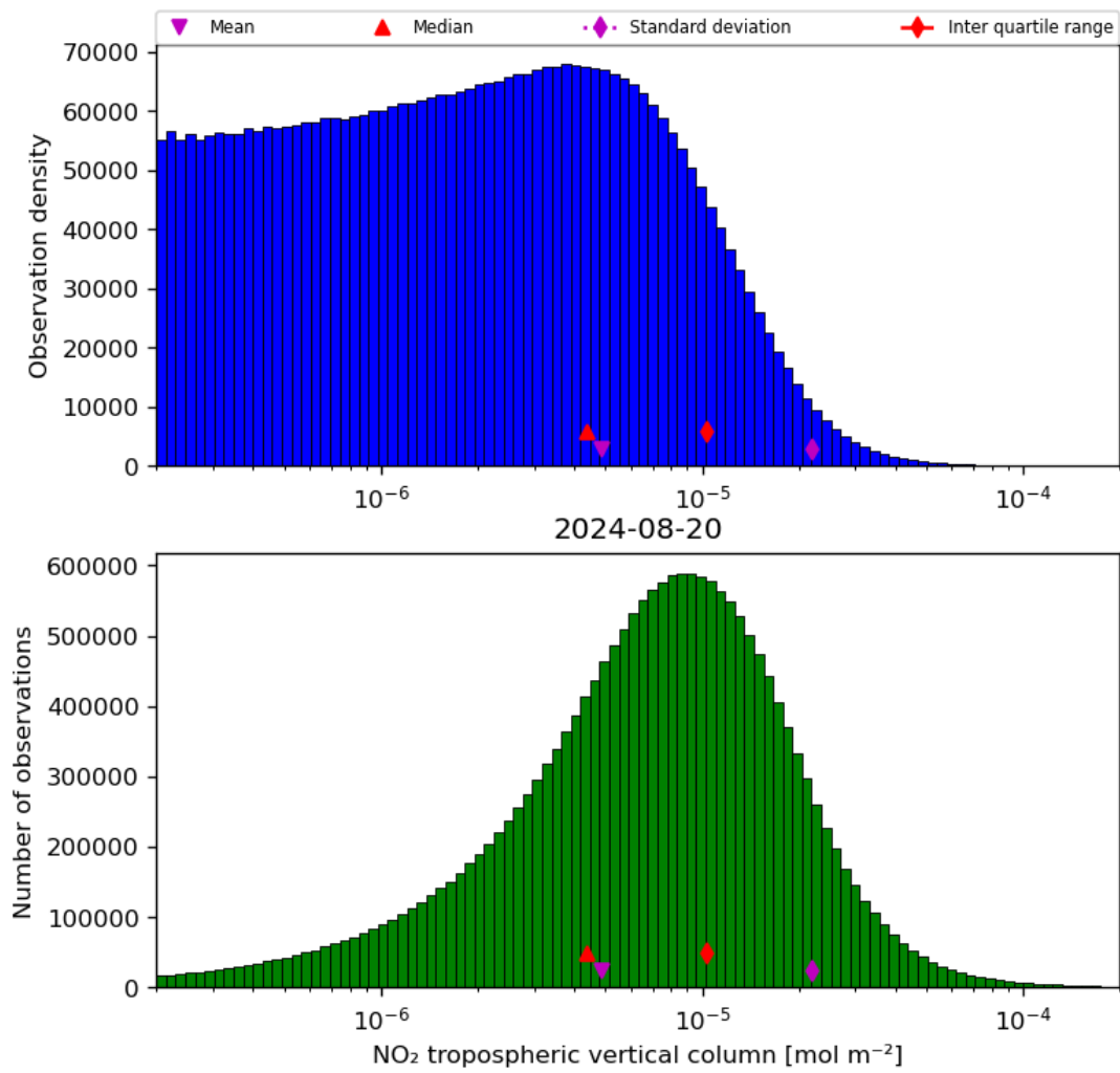
Figure 29: Histogram of “NO 2 tropospheric vertical column” for 2024-08-19 to 2024-08-21
