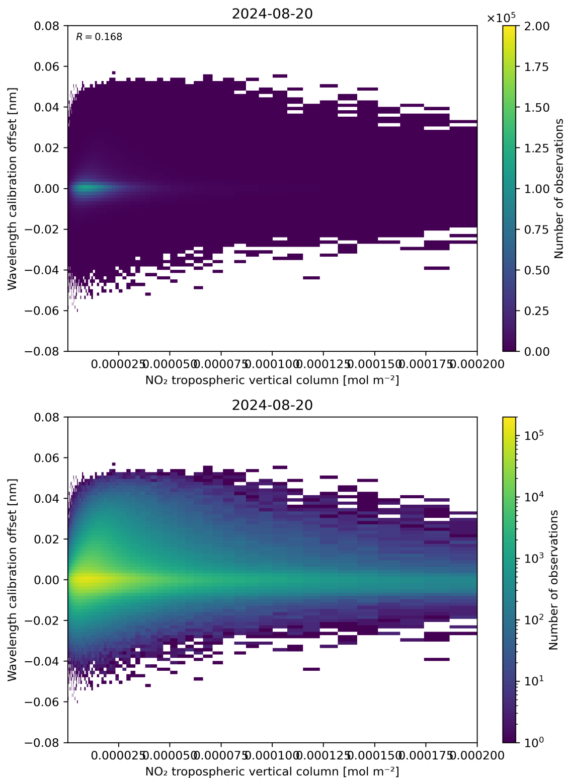
Figure 143: Scatter density plot of “NO 2 tropospheric vertical column” against “Wavelength calibration offset” for 2024-08-19 to 2024-08-21.
