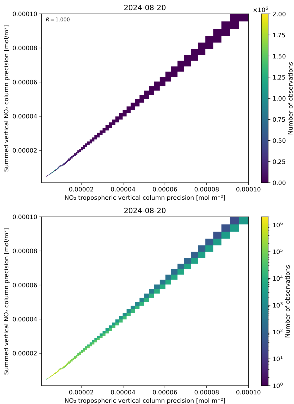
Figure 137: Scatter density plot of “NO 2 tropospheric vertical column precision” against “Summed vertical NO 2 column precision” for 2024-08-19 to 2024-08-21.
