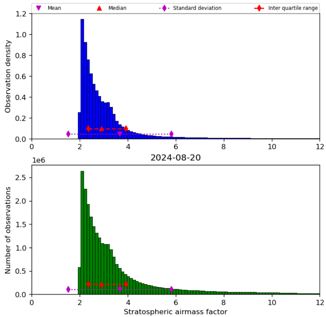
Figure 44: Histogram of “Stratospheric airmass factor” for 2024-08-19 to 2024-08-21
