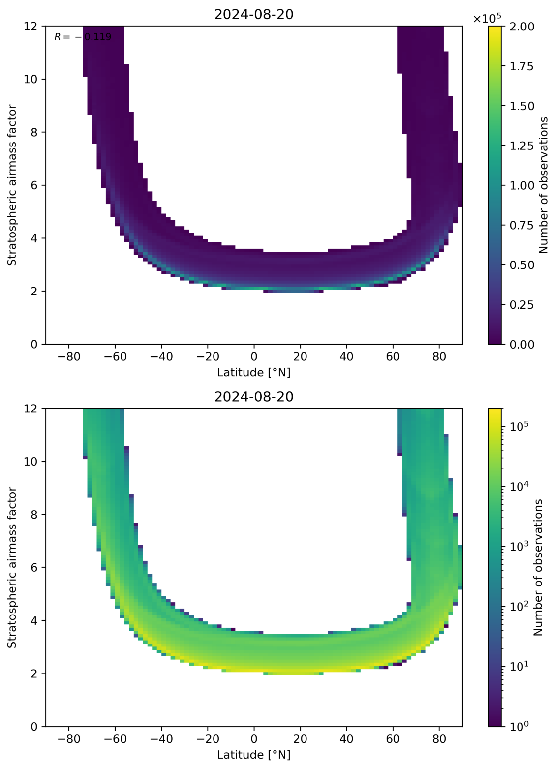
Figure 83: Scatter density plot of “Latitude” against “Stratospheric air mass factor” for 2024-08-19 to 2024-08-21.
