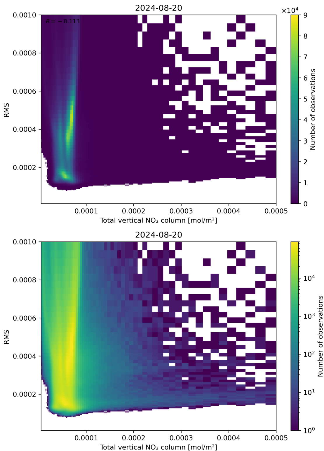
Figure 120: Scatter density plot of “Total vertical NO 2 column” against “RMS” for 2024-08-19 to 2024-08-21.
