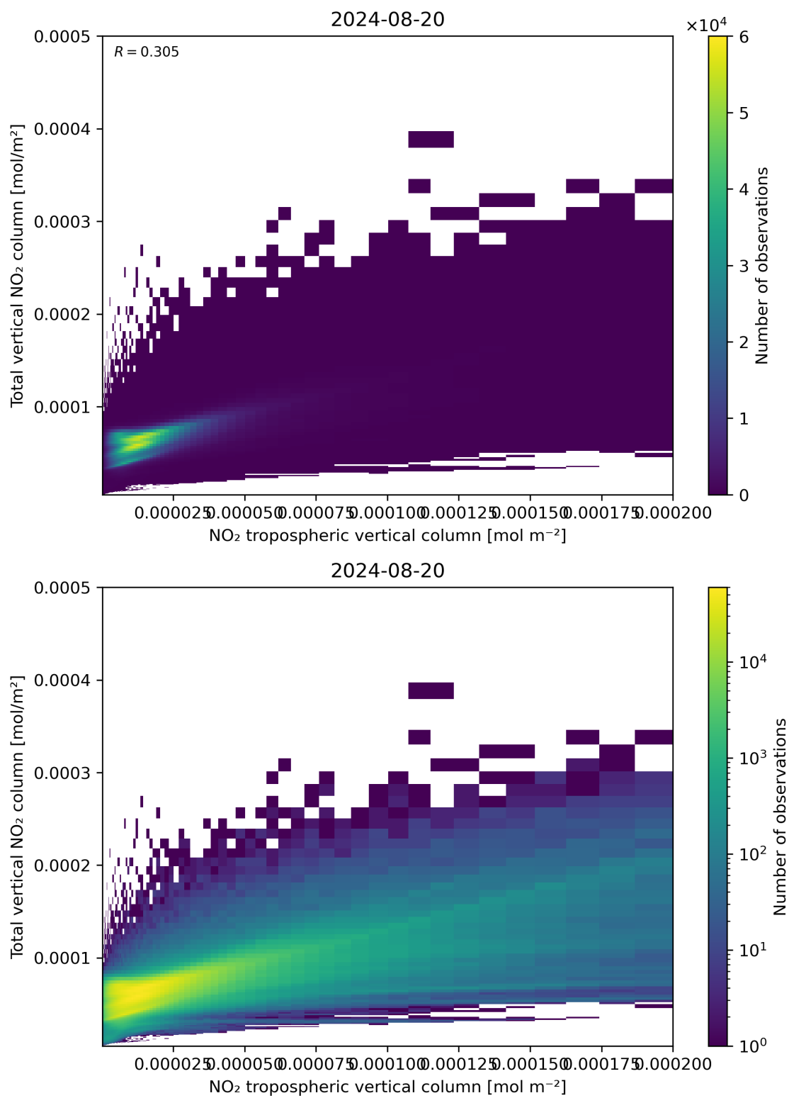
Figure 128: Scatter density plot of “NO 2 tropospheric vertical column” against “Total vertical NO 2 column” for 2024-08-19 to 2024-08-21.
