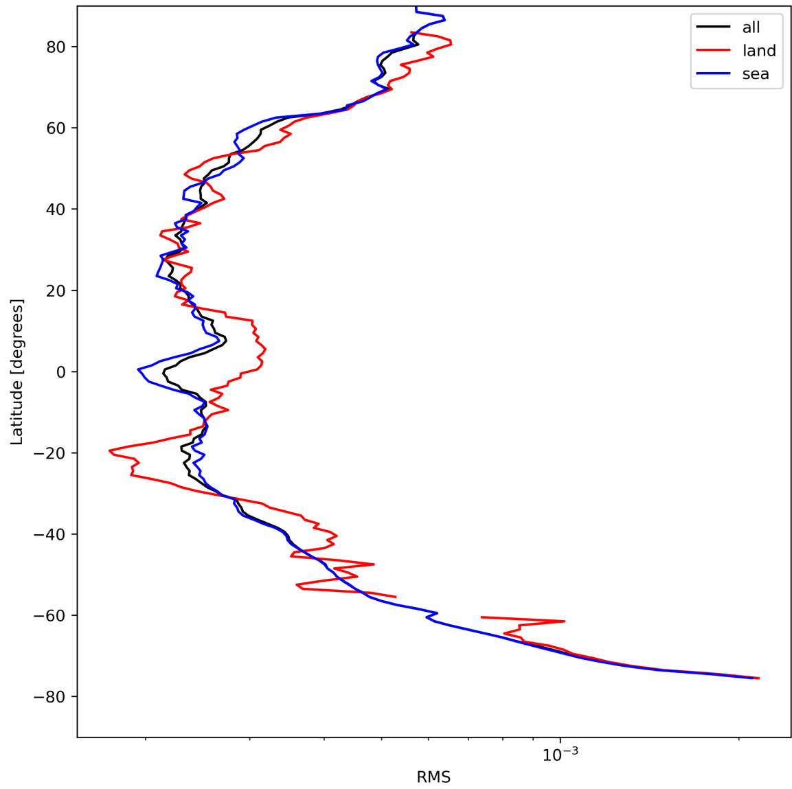
Figure 26: Zonal average of “RMS” for 2024-08-19 to 2024-08-21.
