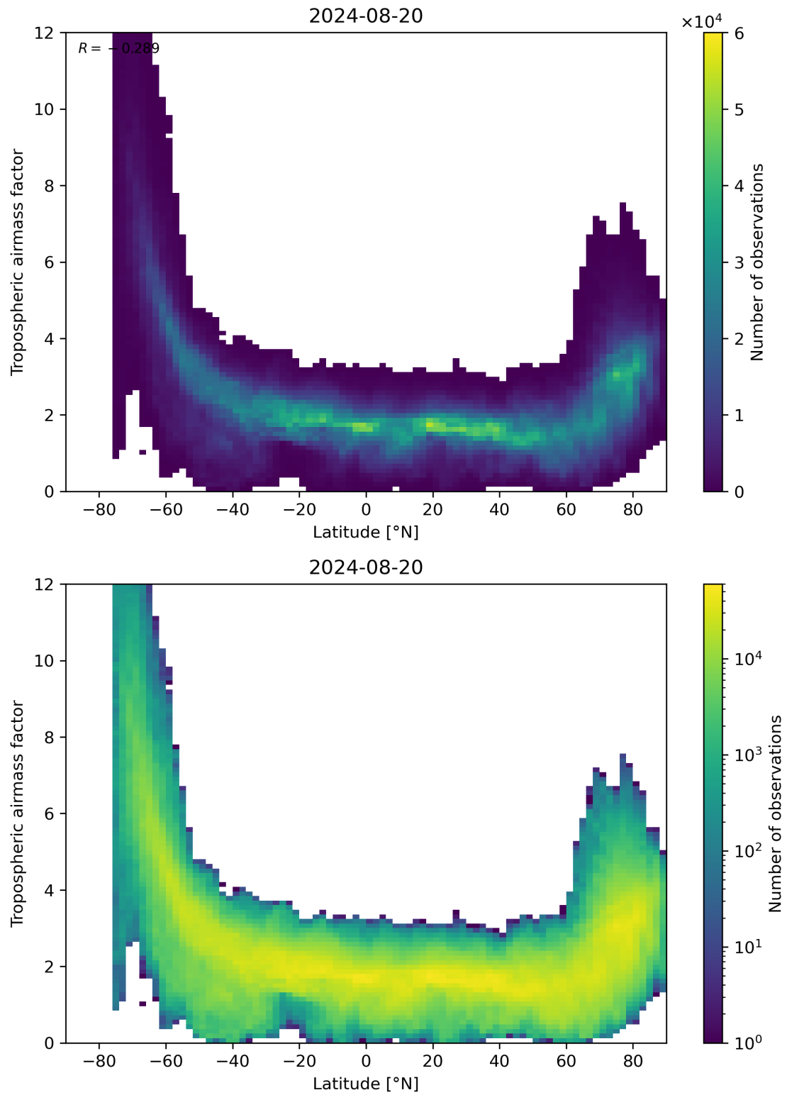
Figure 85: Scatter density plot of “Latitude” against “Tropospheric airmass factor” for 2024-08-19 to 2024-08-21.
