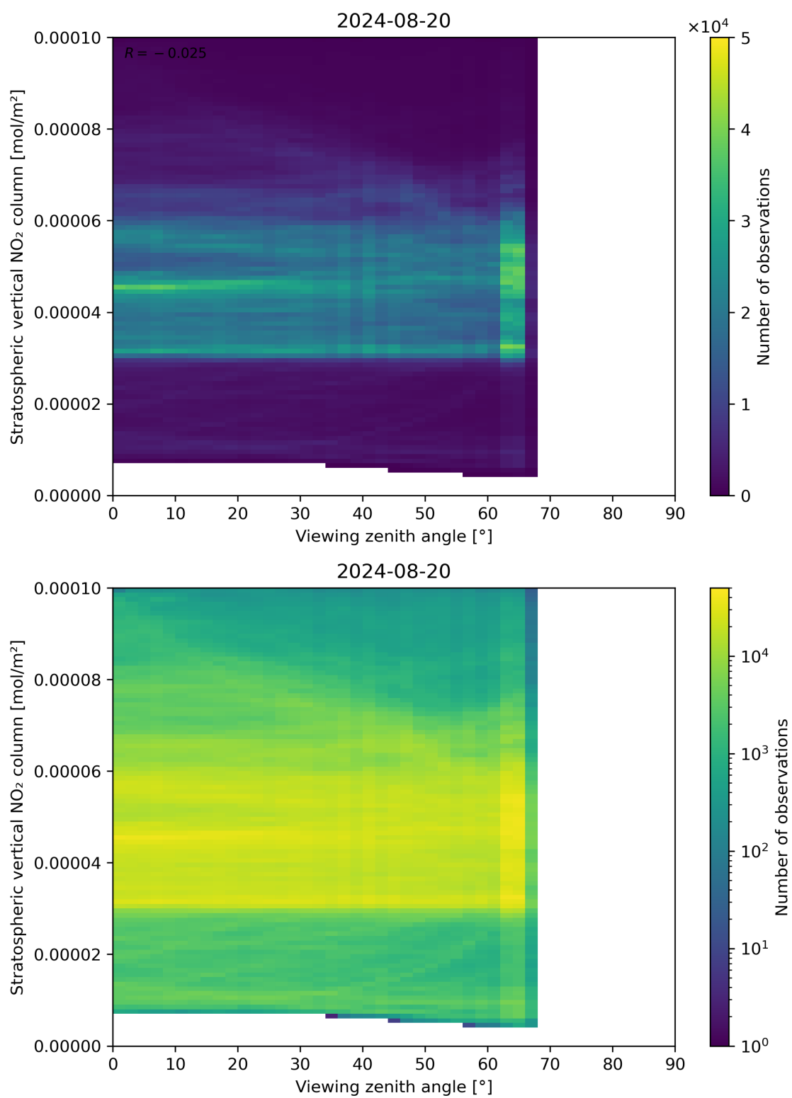
Figure 164: Scatter density plot of “Viewing zenith angle” against “Stratospheric vertical NO 2 column” for 2024-08-19 to 2024-08-21.
