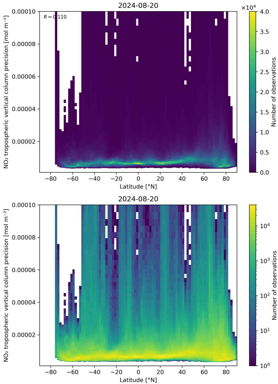
Figure 93: Scatter density plot of “Latitude” against “NO 2 tropospheric vertical column precision” for 2024-08-19 to 2024-08-21.
