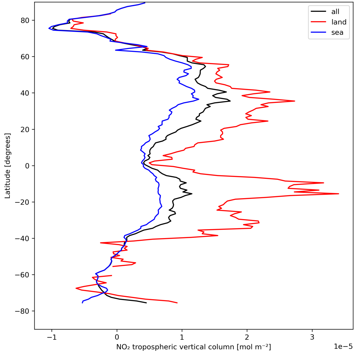
Figure 12: Zonal average of “NO 2 tropospheric vertical column” for 2024-08-19 to 2024-08-21.
