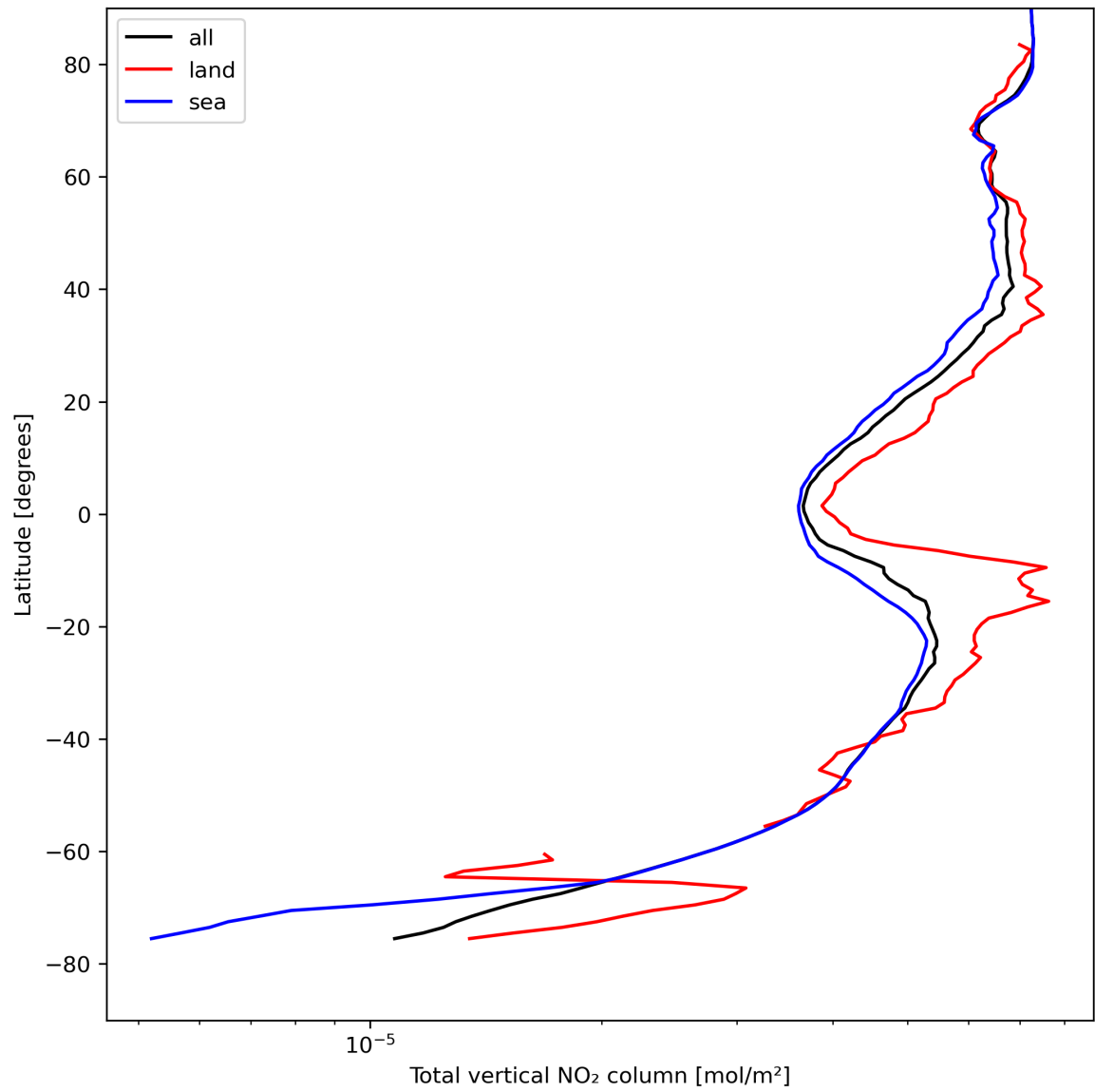
Figure 21: Zonal average of “Total vertical NO 2 column” for 2024-08-19 to 2024-08-21.
