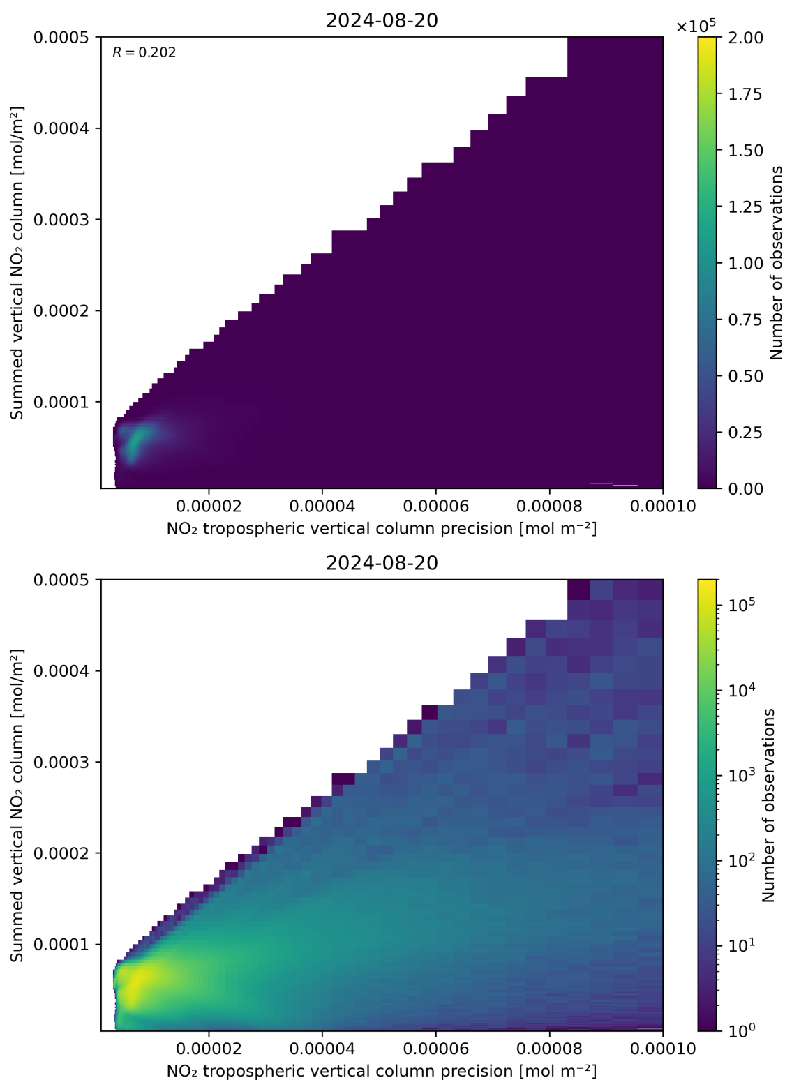
Figure 136: Scatter density plot of “NO 2 tropospheric vertical column precision” against “Summed vertical NO 2 column” for 2024-08-19 to 2024-08-21.
