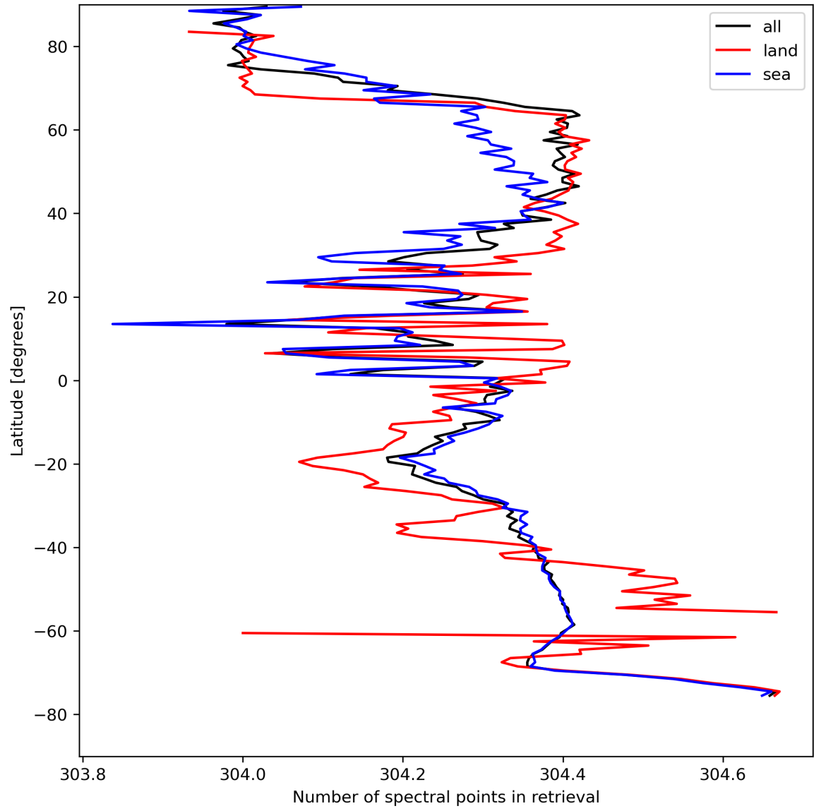
Figure 16: Zonal average of “Number of spectral points in retrieval” for 2024-08-19 to 2024-08-21.
