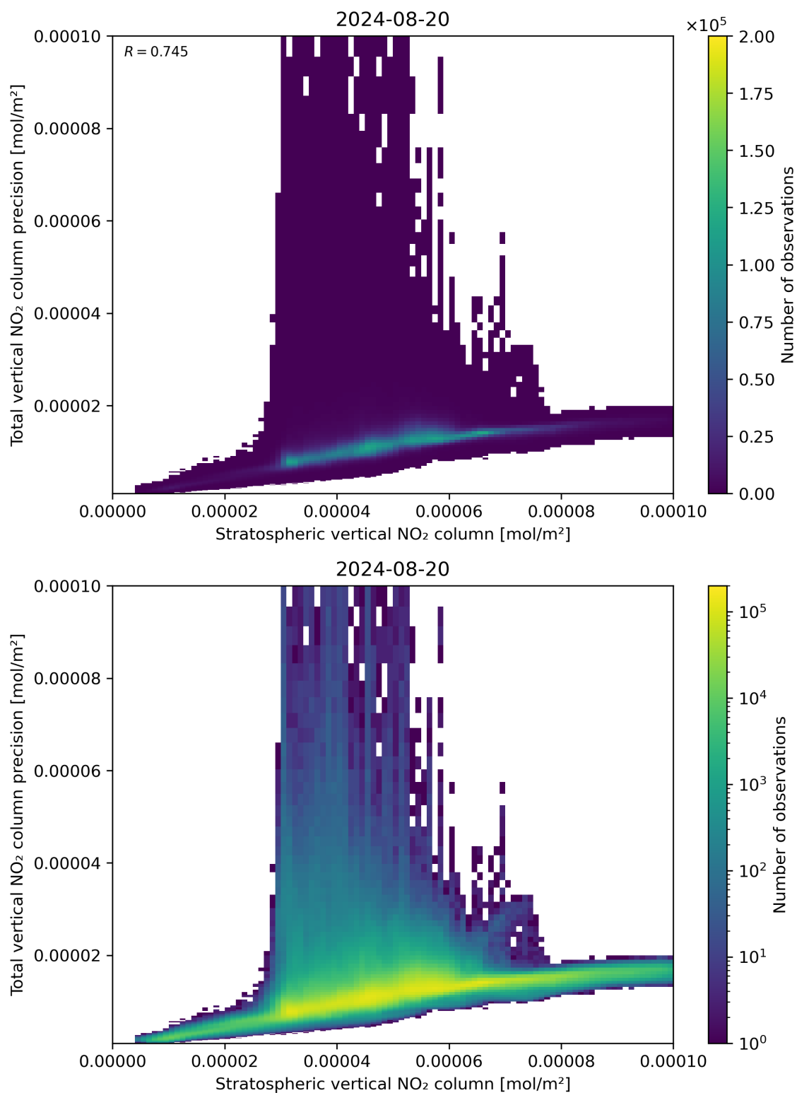
Figure 101: Scatter density plot of “Stratospheric vertical NO 2 column” against “Total vertical NO 2 column precision” for 2024-08-19 to 2024-08-21.
