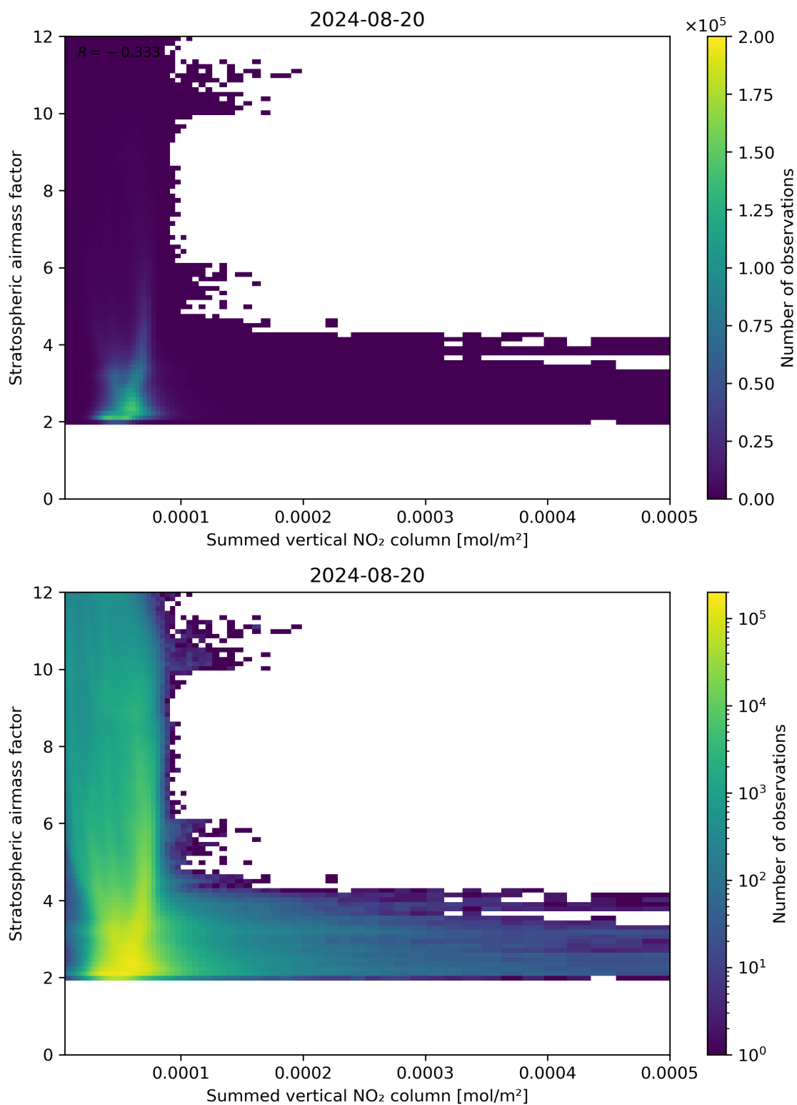
Figure 103: Scatter density plot of “Summed vertical NO 2 column” against “Stratospheric airmass factor” for 2024-08-19 to 2024-08-21.
