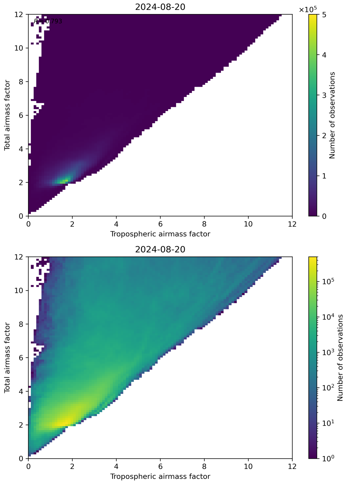
Figure 72: Scatter density plot of “Tropospheric airmass factor” against “Total airmass factor” for 2024-08-19 to 2024-08-21.
