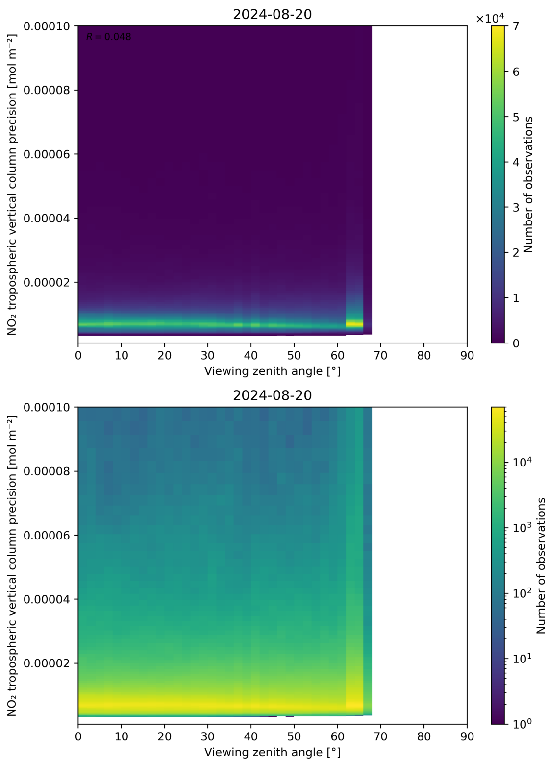
Figure 170: Scatter density plot of “Viewing zenith angle” against “NO 2 tropospheric vertical column precision” for 2024-08-19 to 2024-08-21.
