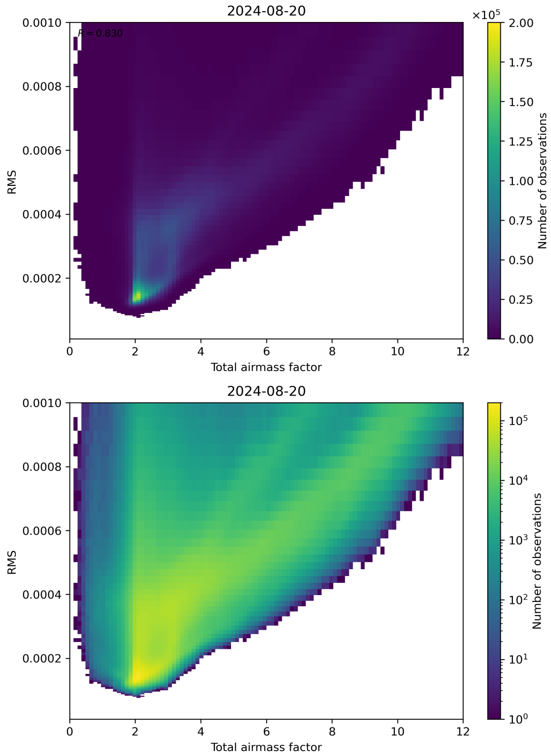
Figure 69: Scatter density plot of “Total airmass factor” against “RMS” for 2024-08-19 to 2024-08-21.
