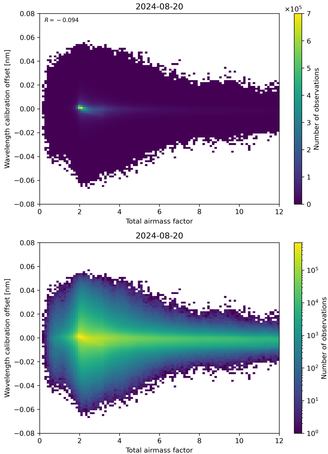
Figure 70: Scatter density plot of “Total airmass factor” against “Wavelength calibration offset” for 2024-08-19 to 2024-08-21.
