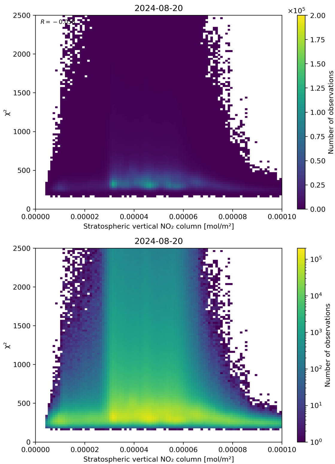
Figure 97: Scatter density plot of “Stratospheric vertical NO 2 column” against “ \chi^2 ” for 2024-08-19 to 2024-08-21.
