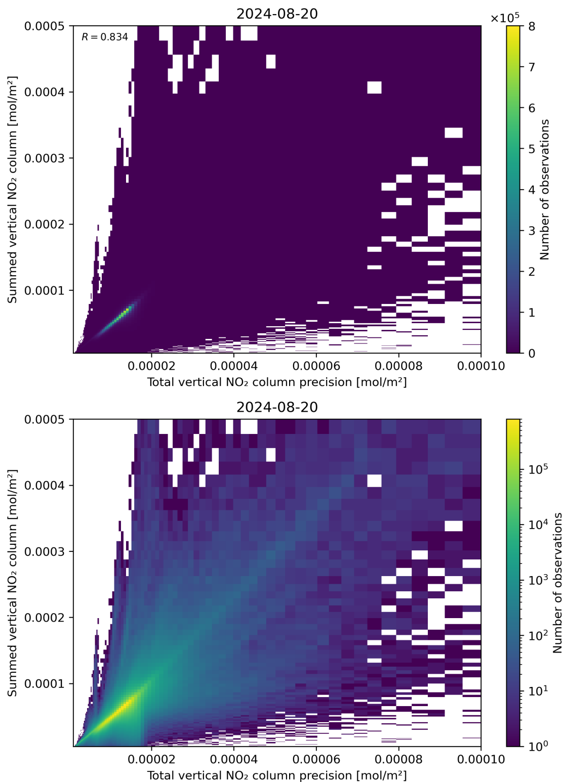
Figure 117: Scatter density plot of “Total vertical NO 2 column precision” against “Summed vertical NO 2 column” for 2024-08-19 to 2024-08-21.
