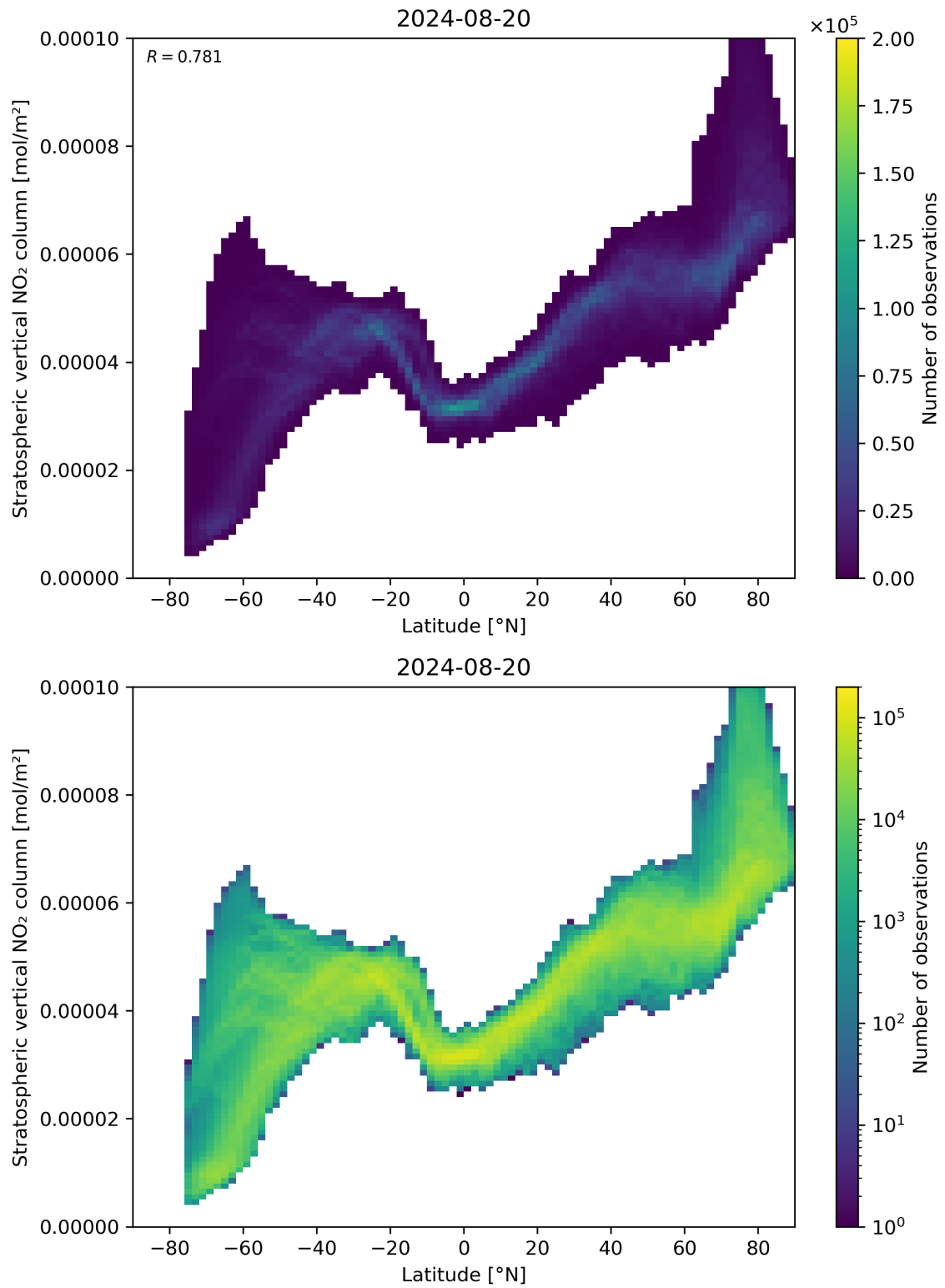
Figure 87: Scatter density plot of “Latitude” against “Stratospheric vertical NO 2 column” for 2024-08-19 to 2024-08-21.
