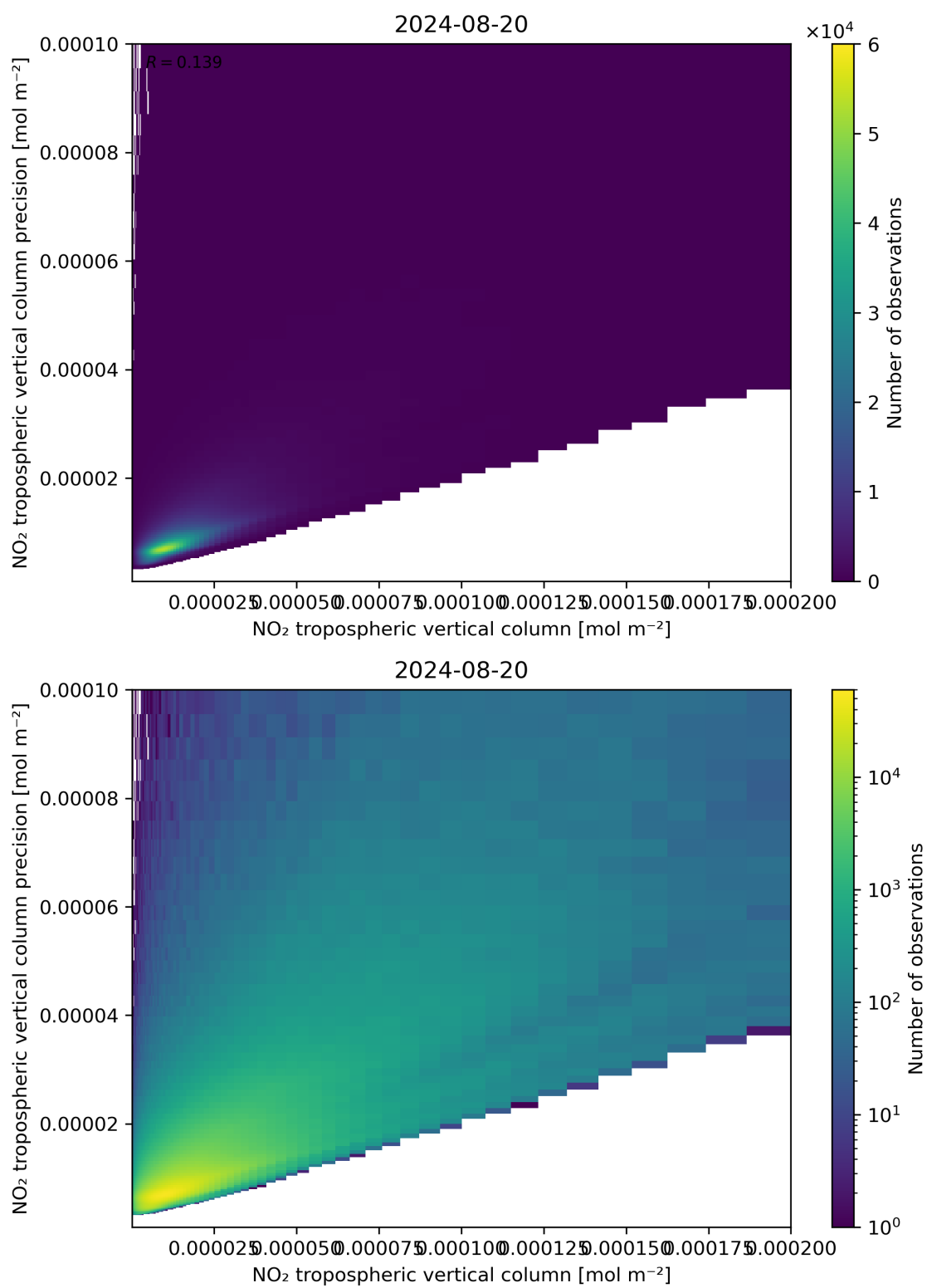
Figure 130: Scatter density plot of “NO 2 tropospheric vertical column” against “NO 2 tropospheric vertical column precision” for 2024-08-19 to 2024-08-21.
