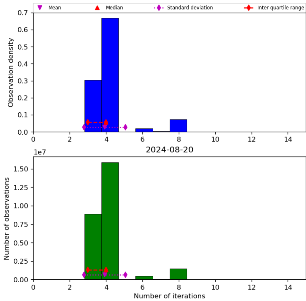
Figure 34: Histogram of “Number of iterations” for 2024-08-19 to 2024-08-21
