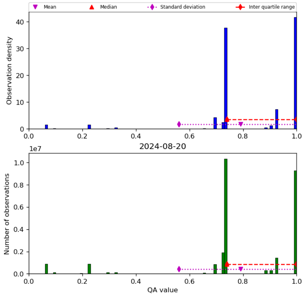
Figure 28: Histogram of “QA value” for 2024-08-19 to 2024-08-21
