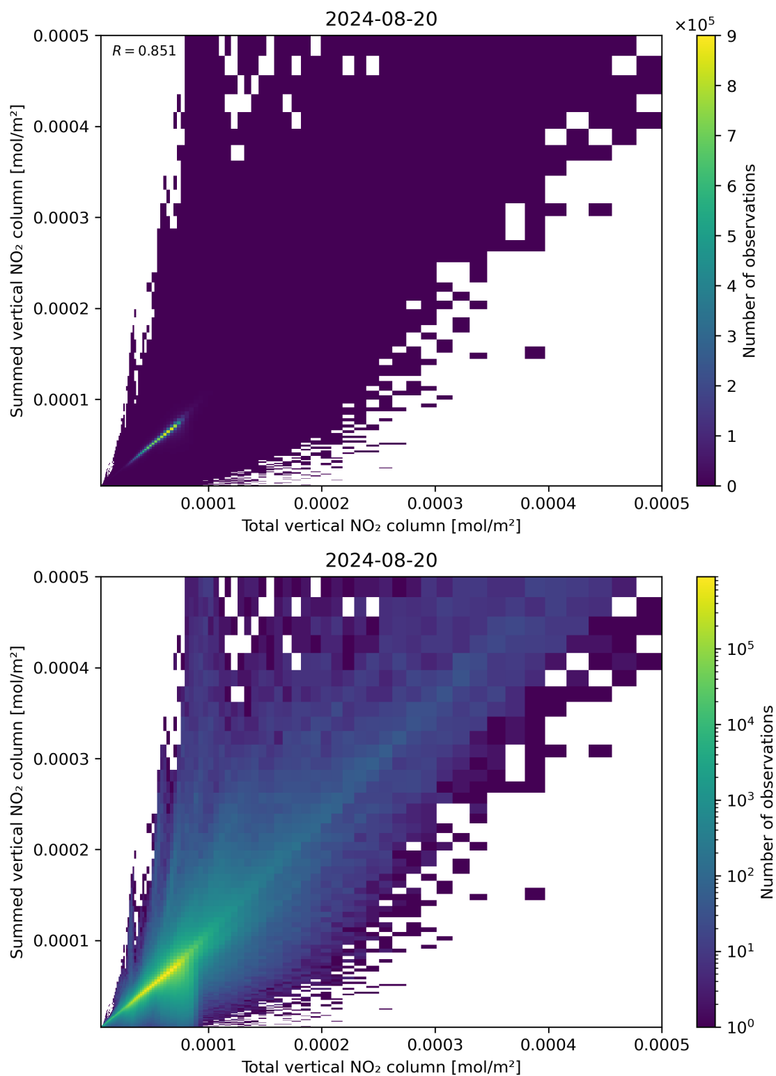
Figure 112: Scatter density plot of “Total vertical NO 2 column” against “Summed vertical NO 2 column” for 2024-08-19 to 2024-08-21.
