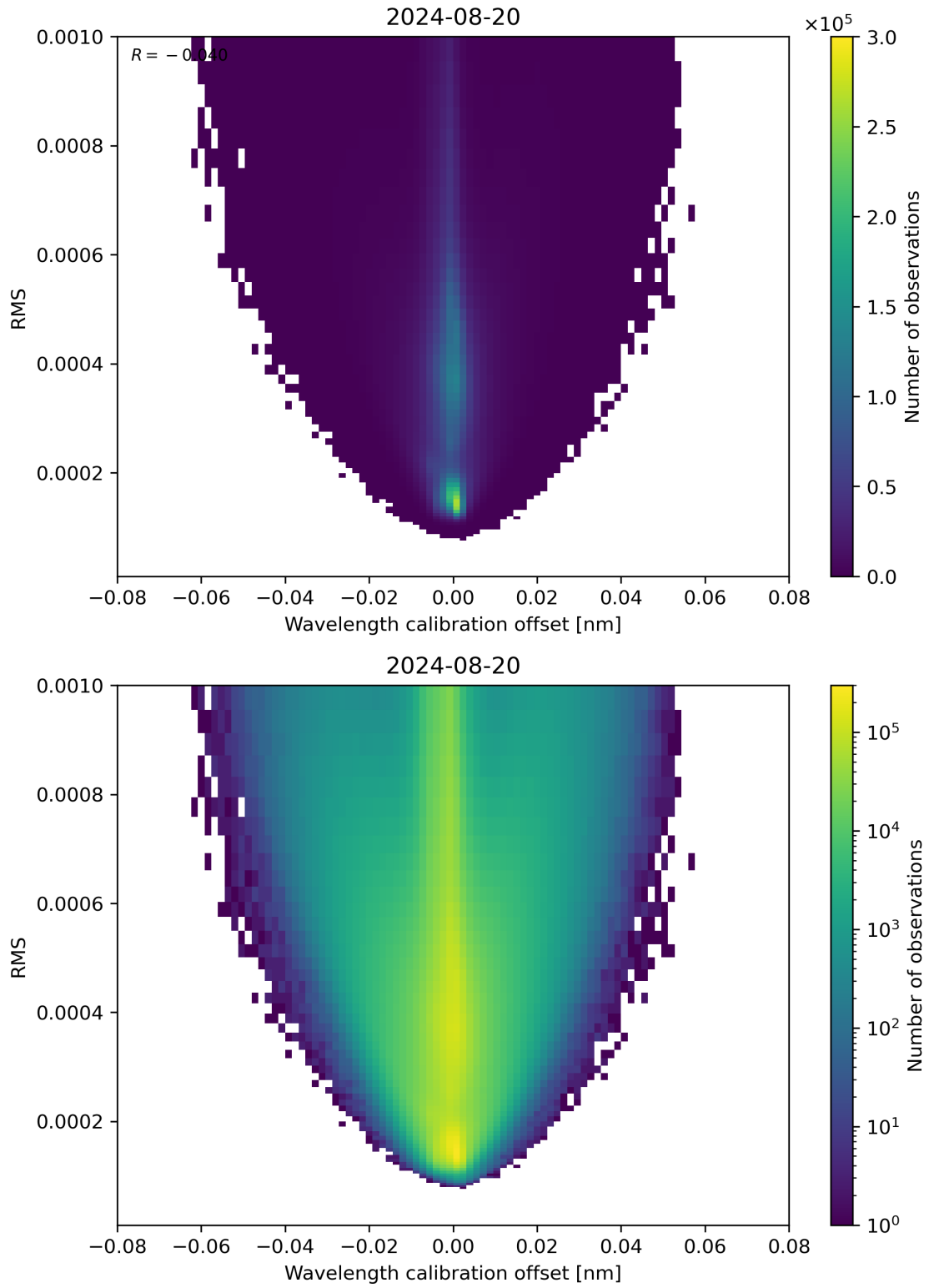
Figure 181: Scatter density plot of “Wavelength calibration offset” against “RMS” for 2024-08-19 to 2024-08-21.
