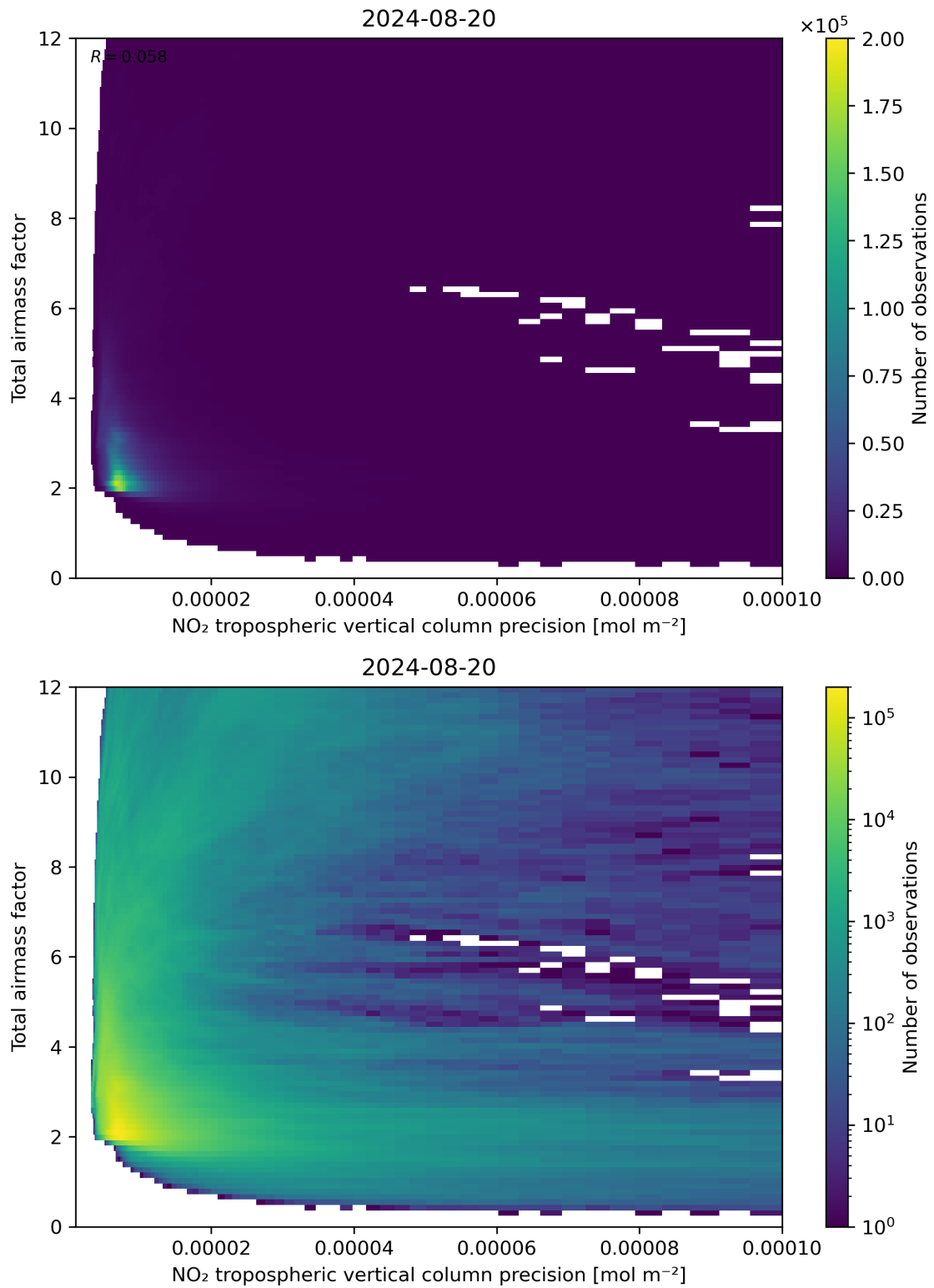
Figure 132: Scatter density plot of “NO 2 tropospheric vertical column precision” against “Total air mass factor” for 2024-08-19 to 2024-08-21.
