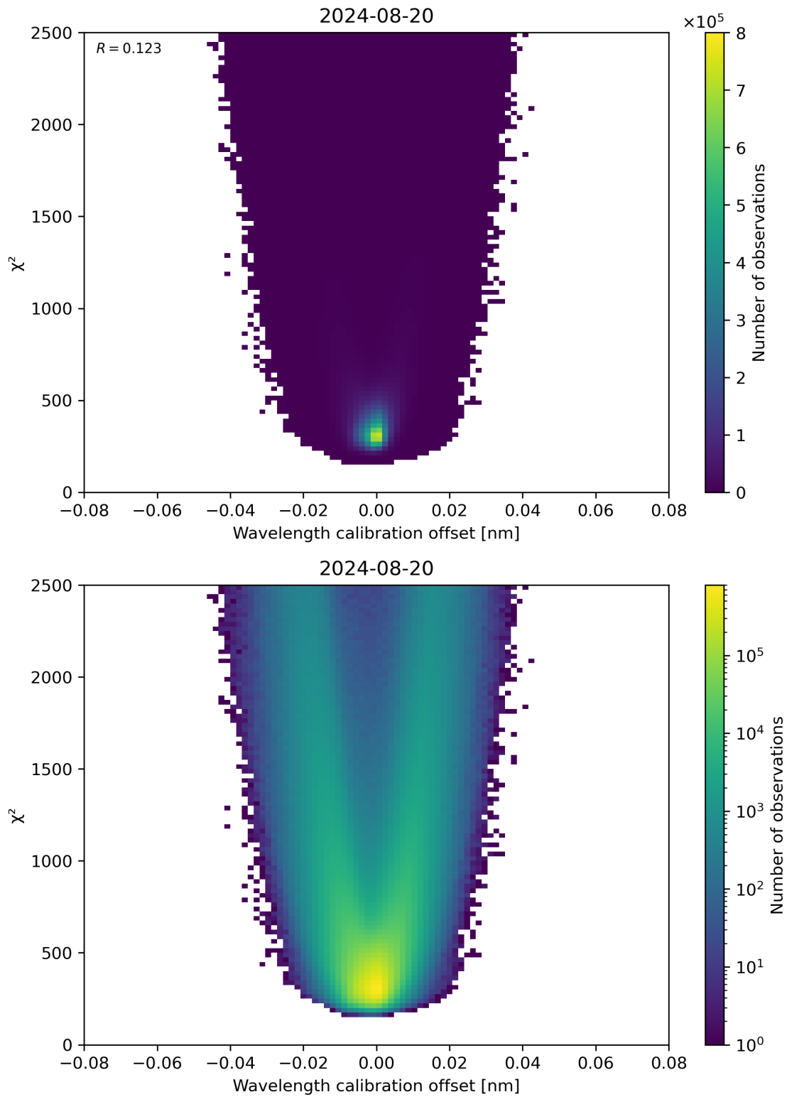
Figure 175: Scatter density plot of “Wavelength calibration offset” against “ \chi^2 ” for 2024-08-19 to 2024-08-21.
