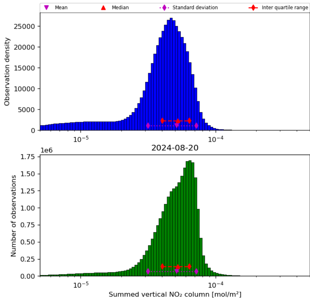
Figure 40: Histogram of “Summed vertical NO 2 column” for 2024-08-19 to 2024-08-21
