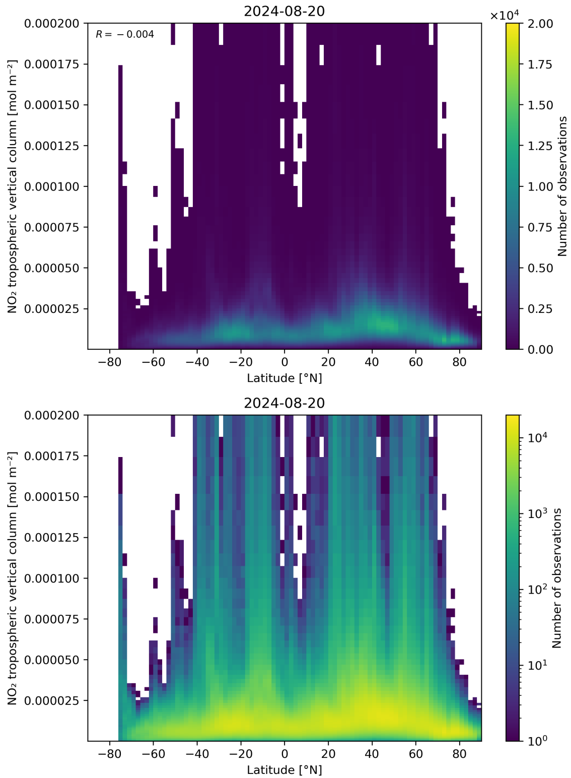
Figure 92: Scatter density plot of “Latitude” against “NO 2 tropospheric vertical column” for 2024-08-19 to 2024-08-21.
