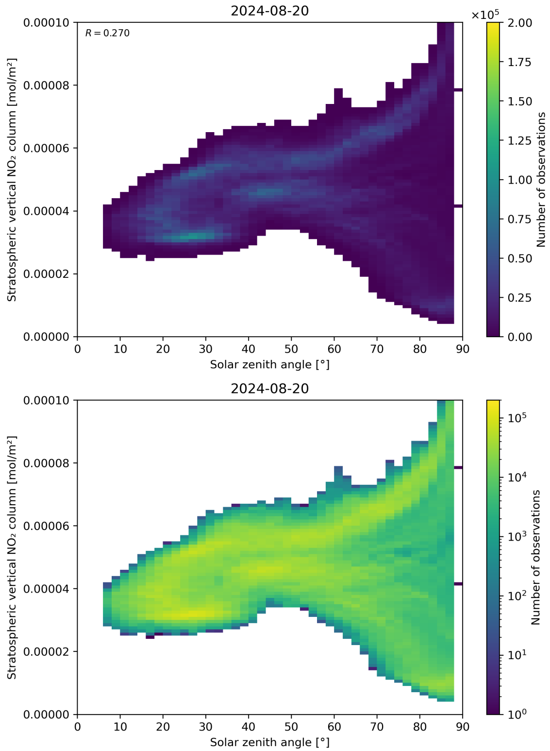
Figure 150: Scatter density plot of “Solar zenith angle” against “Stratospheric vertical \text{NO}_2 column” for 2024-08-19 to 2024-08-21.
