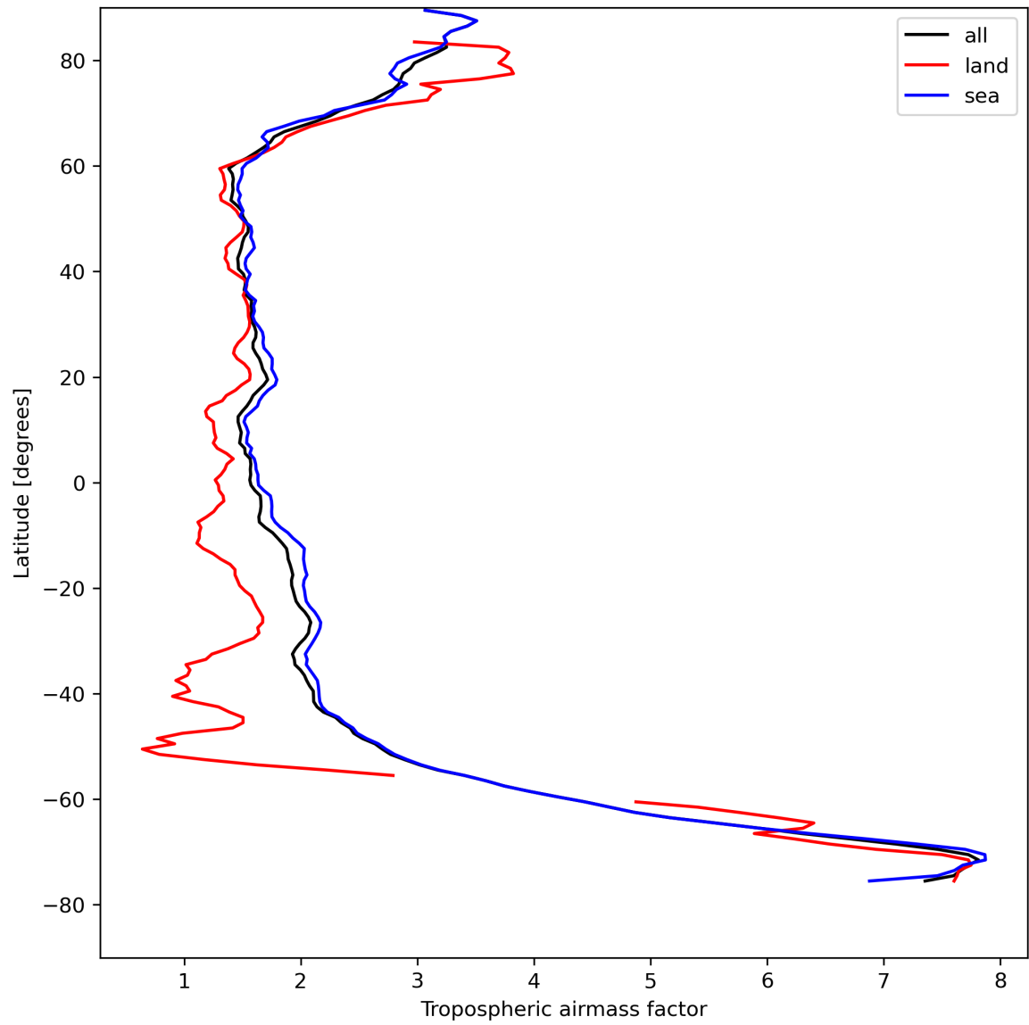
Figure 14: Zonal average of “Tropospheric airmass factor” for 2024-08-19 to 2024-08-21.
