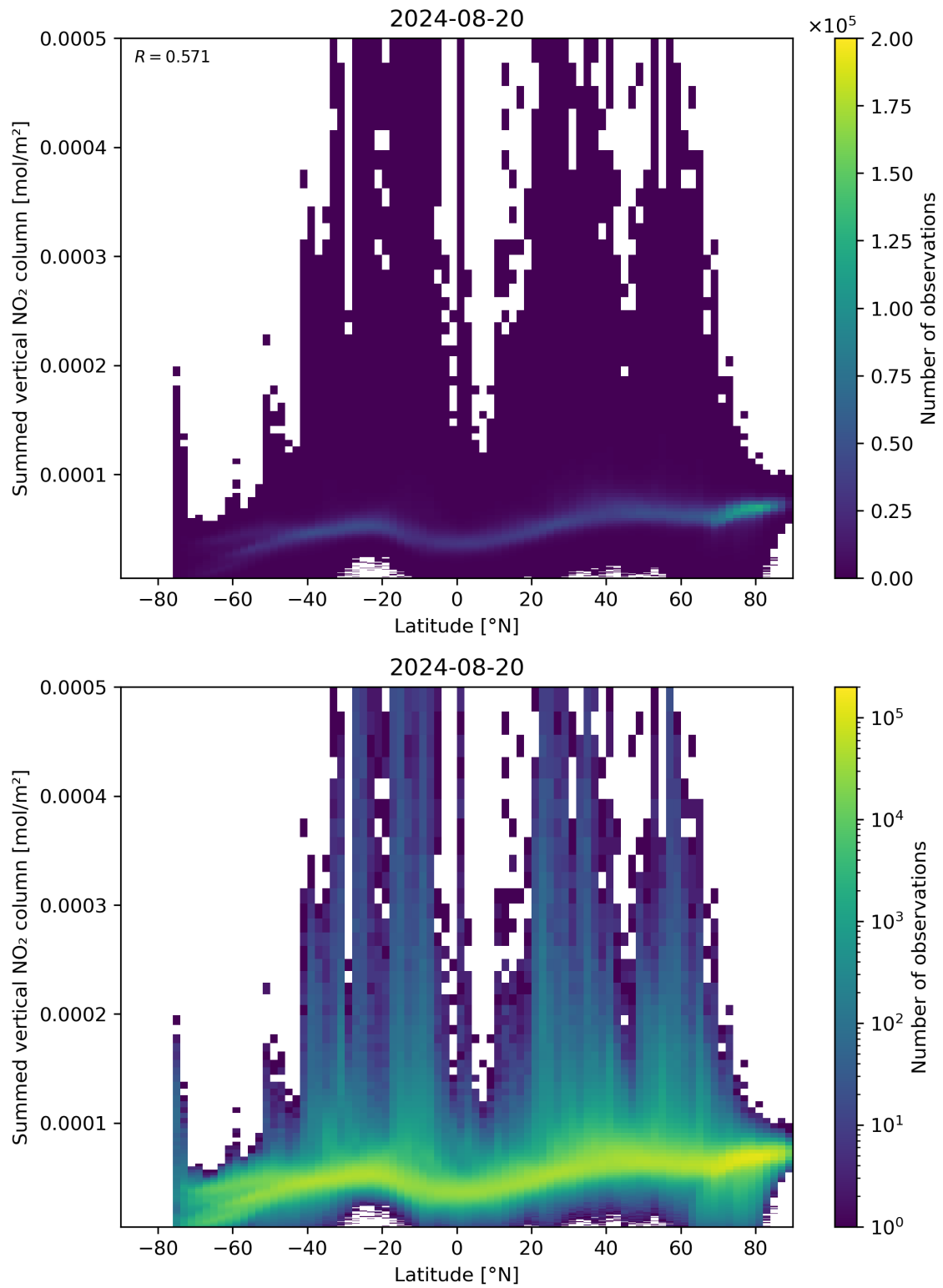
Figure 88: Scatter density plot of “Latitude” against “Summed vertical NO 2 column” for 2024-08-19 to 2024-08-21.
