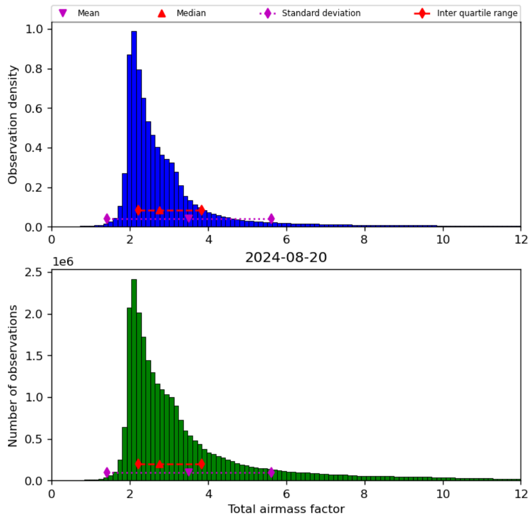
Figure 32: Histogram of “Total airmass factor” for 2024-08-19 to 2024-08-21
