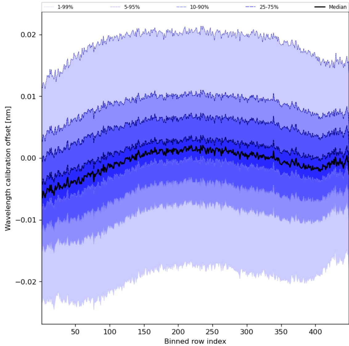
Figure 52: Along track statistics of “Wavelength calibration offset” for 2024-08-19 to 2024-08-21
