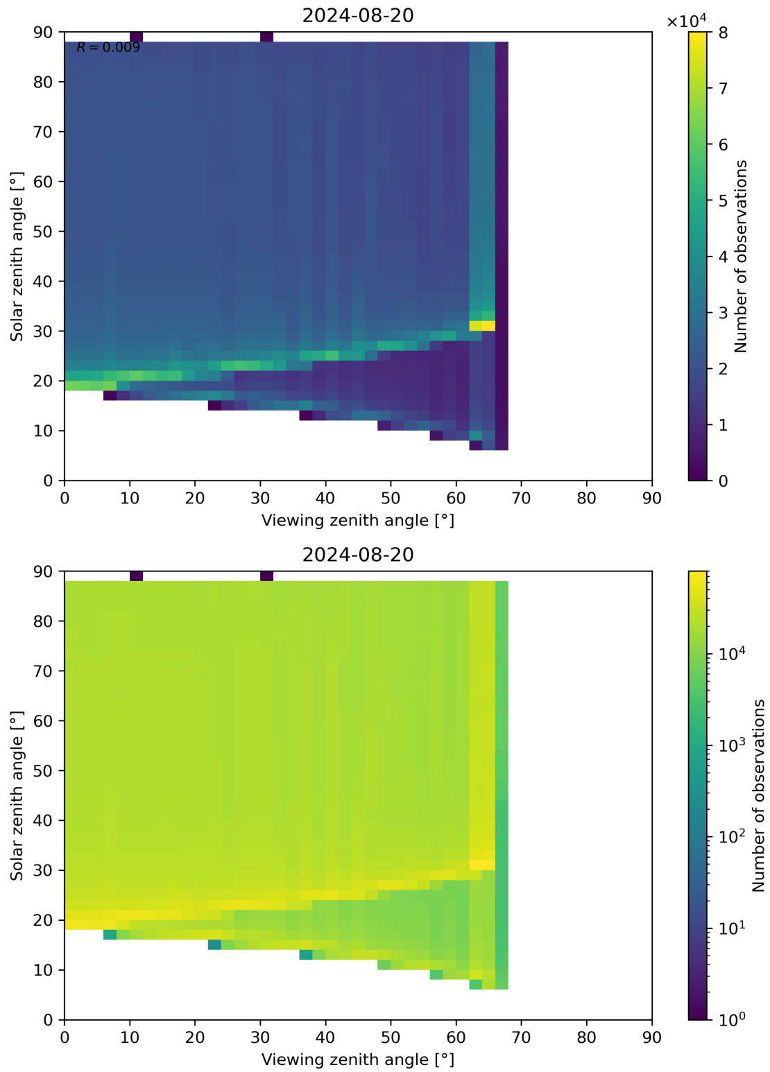
Figure 172: Scatter density plot of “Viewing zenith angle” against “Solar zenith angle” for 2024-08-19 to 2024-08-21.
