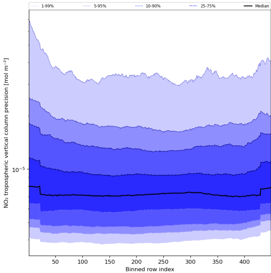
Figure 47: Along track statistics of “NO 2 tropospheric vertical column precision” for 2024-08-19 to 2024-08-21
