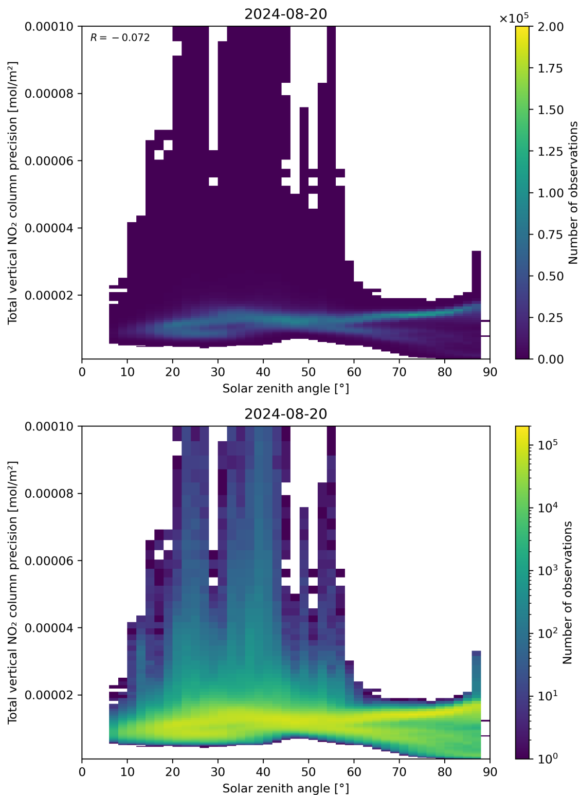
Figure 154: Scatter density plot of “Solar zenith angle” against “Total vertical NO 2 column precision” for 2024-08-19 to 2024-08-21.
