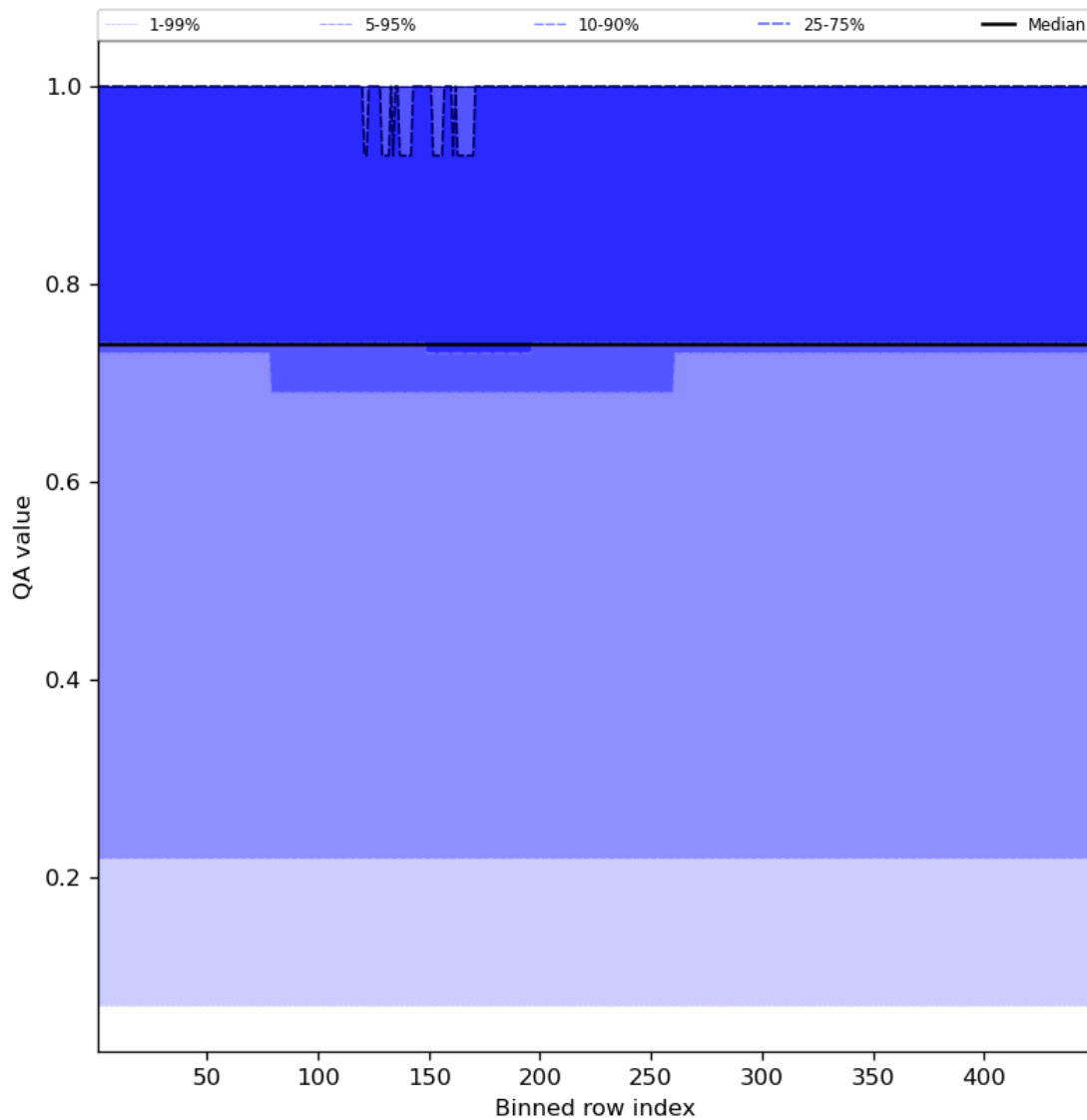
Figure 45: Along track statistics of “QA value” for 2024-08-19 to 2024-08-21
