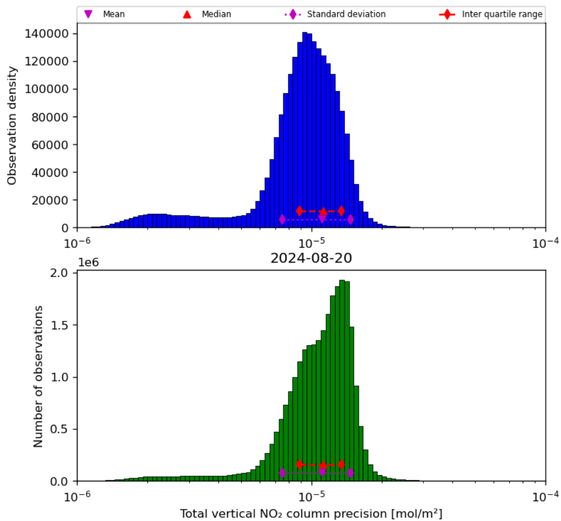
Figure 39: Histogram of "Total vertical NO 2 column precision" for 2024-08-19 to 2024-08-21
