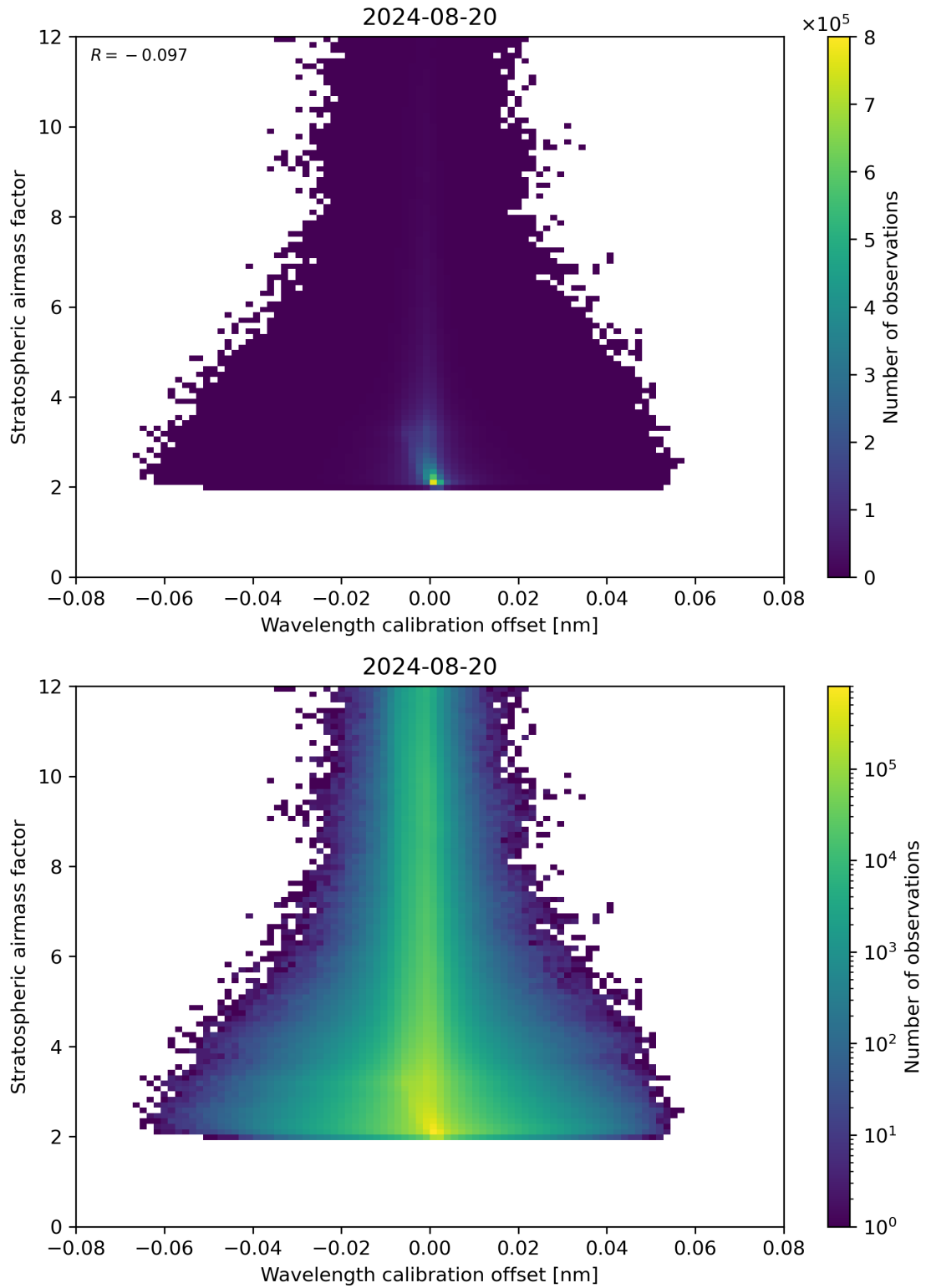
Figure 174: Scatter density plot of “Wavelength calibration offset” against “Stratospheric airmass factor” for 2024-08-19 to 2024-08-21.
