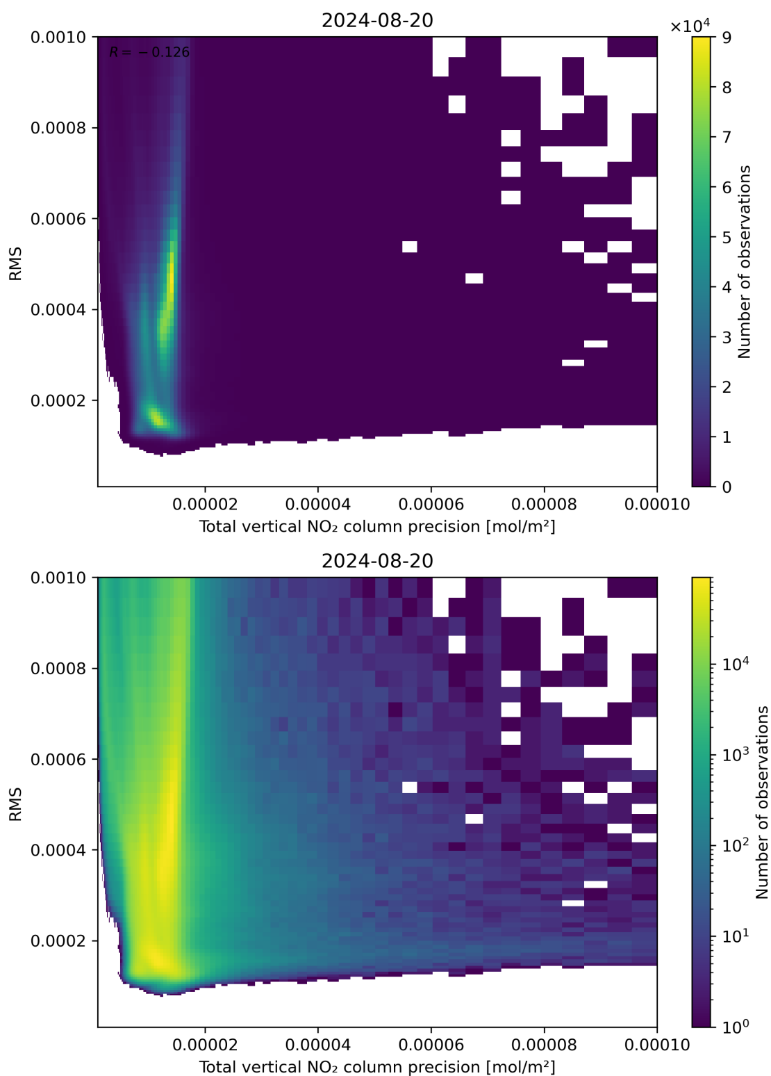
Figure 119: Scatter density plot of “Total vertical NO 2 column precision” against “RMS” for 2024-08-19 to 2024-08-21.
