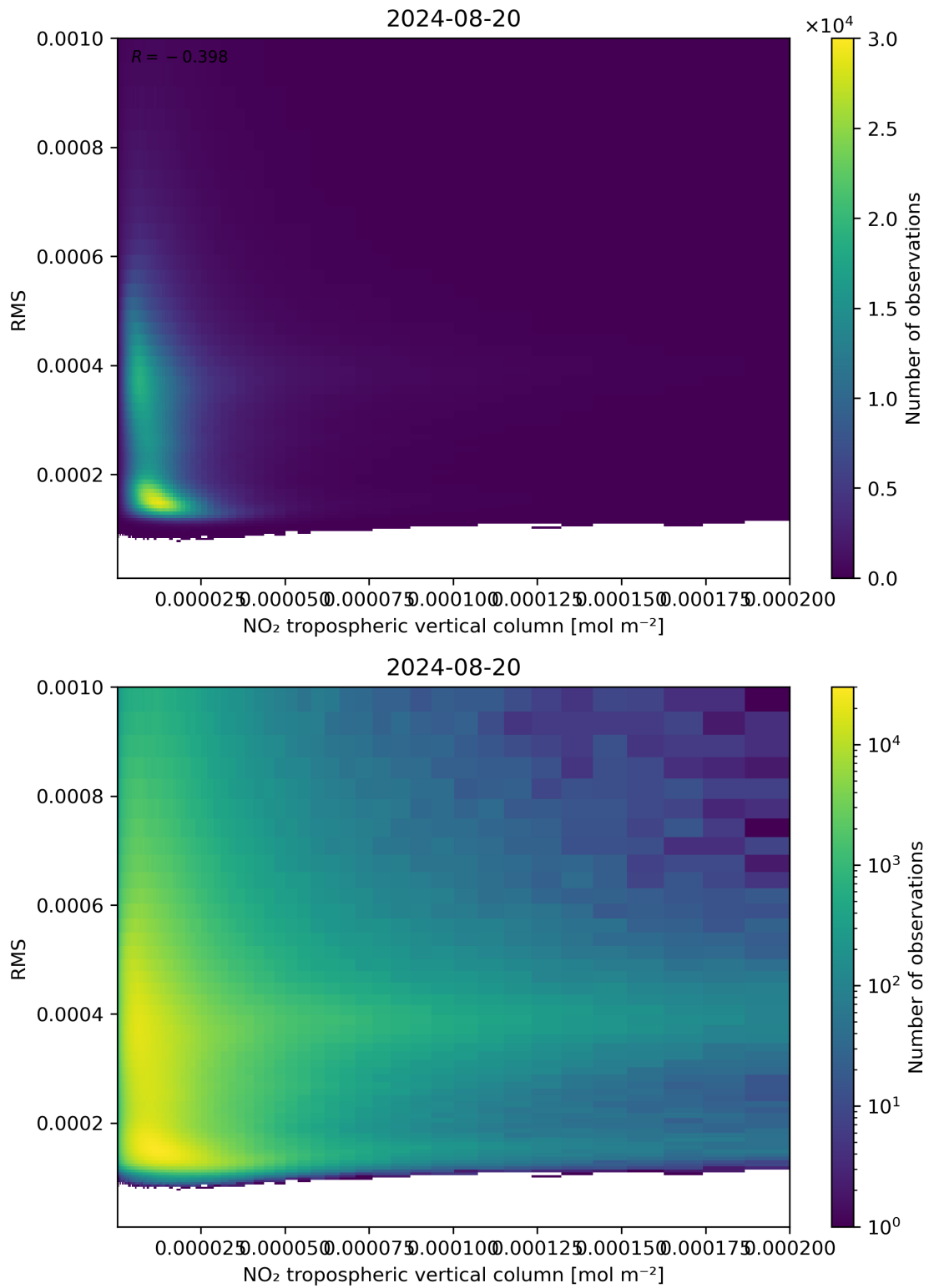
Figure 142: Scatter density plot of “NO 2 tropospheric vertical column” against “RMS” for 2024-08-19 to 2024-08-21.
