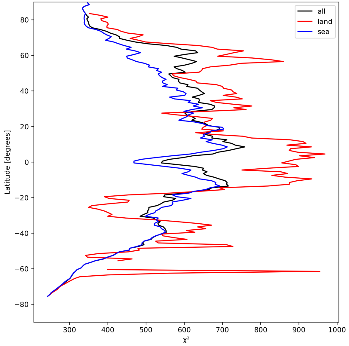
Figure 25: Zonal average of “ \chi^2 ” for 2024-08-19 to 2024-08-21.
