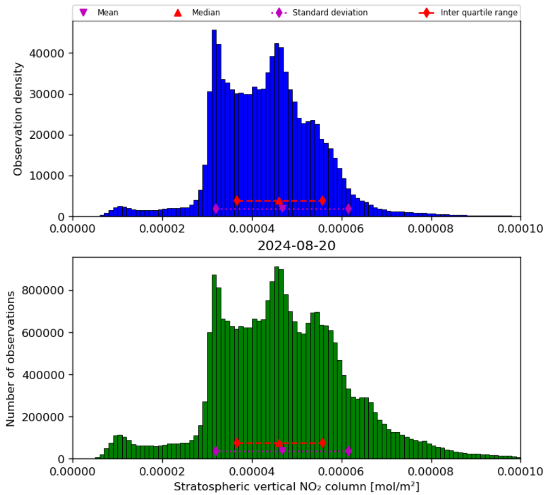
Figure 36: Histogram of “Stratospheric vertical NO 2 column” for 2024-08-19 to 2024-08-21
