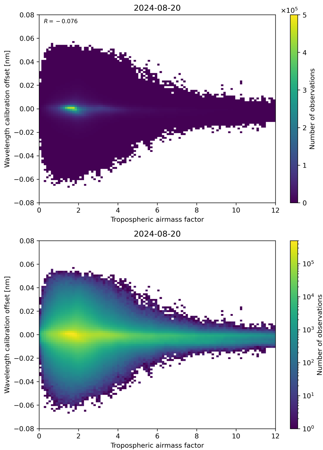
Figure 80: Scatter density plot of “Tropospheric airmass factor” against “Wavelength calibration offset” for 2024-08-19 to 2024-08-21.
