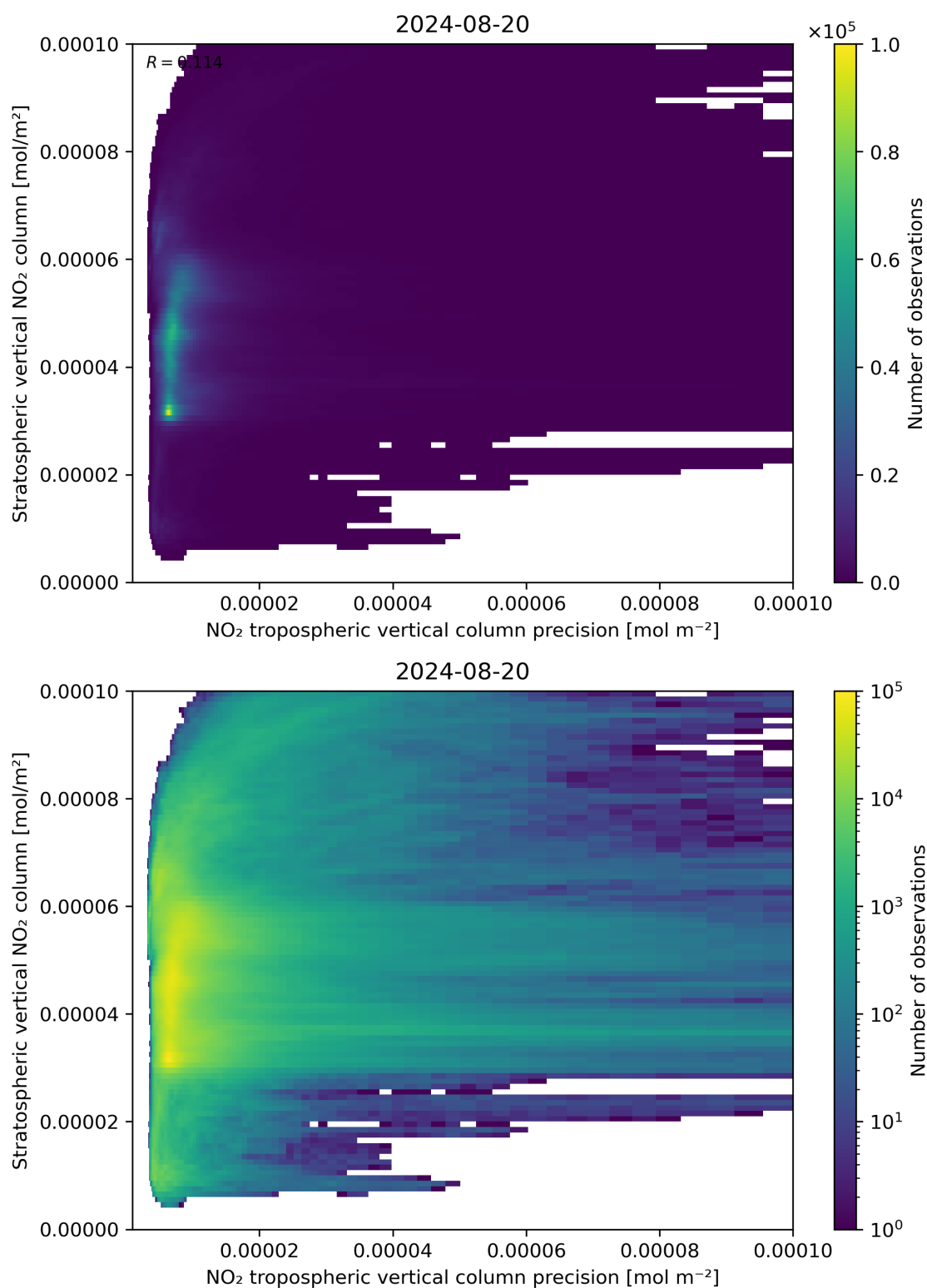
Figure 135: Scatter density plot of “NO 2 tropospheric vertical column precision” against “Stratospheric vertical NO 2 column” for 2024-08-19 to 2024-08-21.
