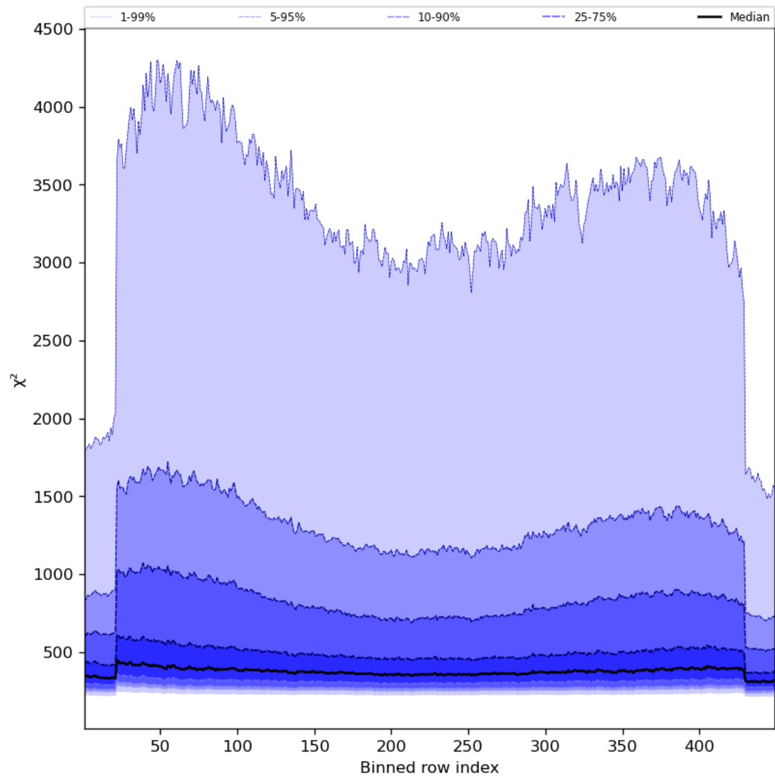
Figure 59: Along track statistics of “ \chi^2 ” for 2024-08-19 to 2024-08-21
