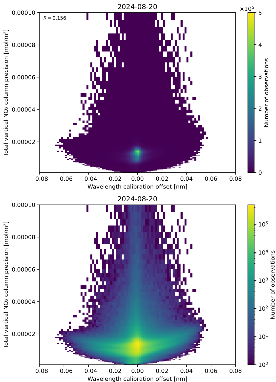
Figure 180: Scatter density plot of “Wavelength calibration offset” against “Total vertical NO 2 column precision” for 2024-08-19 to 2024-08-21.
