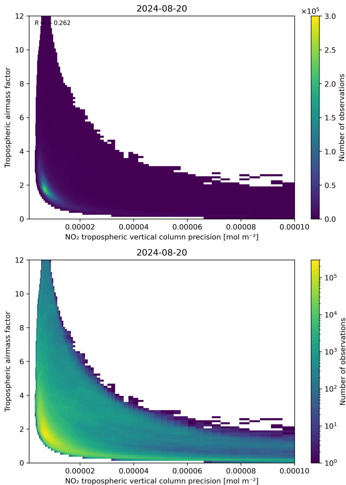
Figure 133: Scatter density plot of “NO 2 tropospheric vertical column precision” against “Tropospheric airmass factor” for 2024-08-19 to 2024-08-21.
