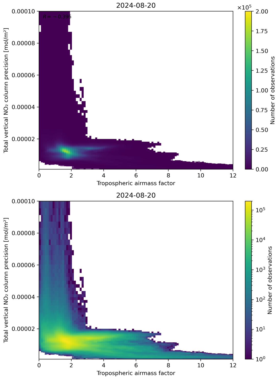
Figure 78: Scatter density plot of “Tropospheric air mass factor” against “Total vertical NO 2 column precision” for 2024-08-19 to 2024-08-21.
