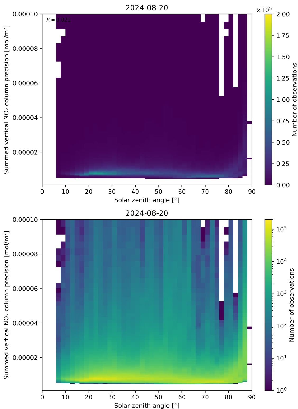
Figure 152: Scatter density plot of “Solar zenith angle” against “Summed vertical NO 2 column precision” for 2024-08-19 to 2024-08-21.
