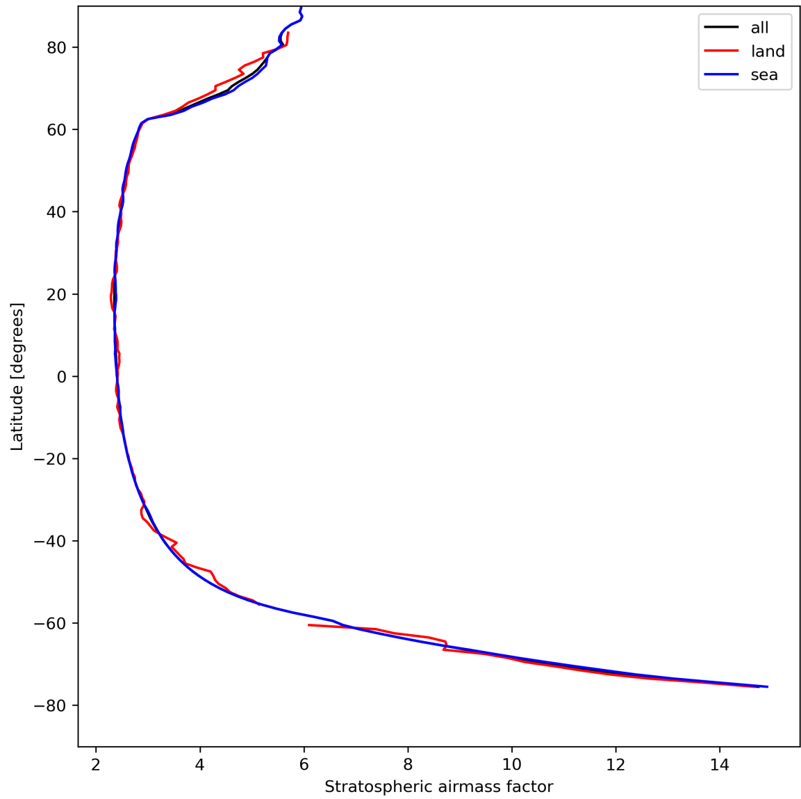
Figure 27: Zonal average of “Stratospheric airmass factor” for 2024-08-19 to 2024-08-21.
