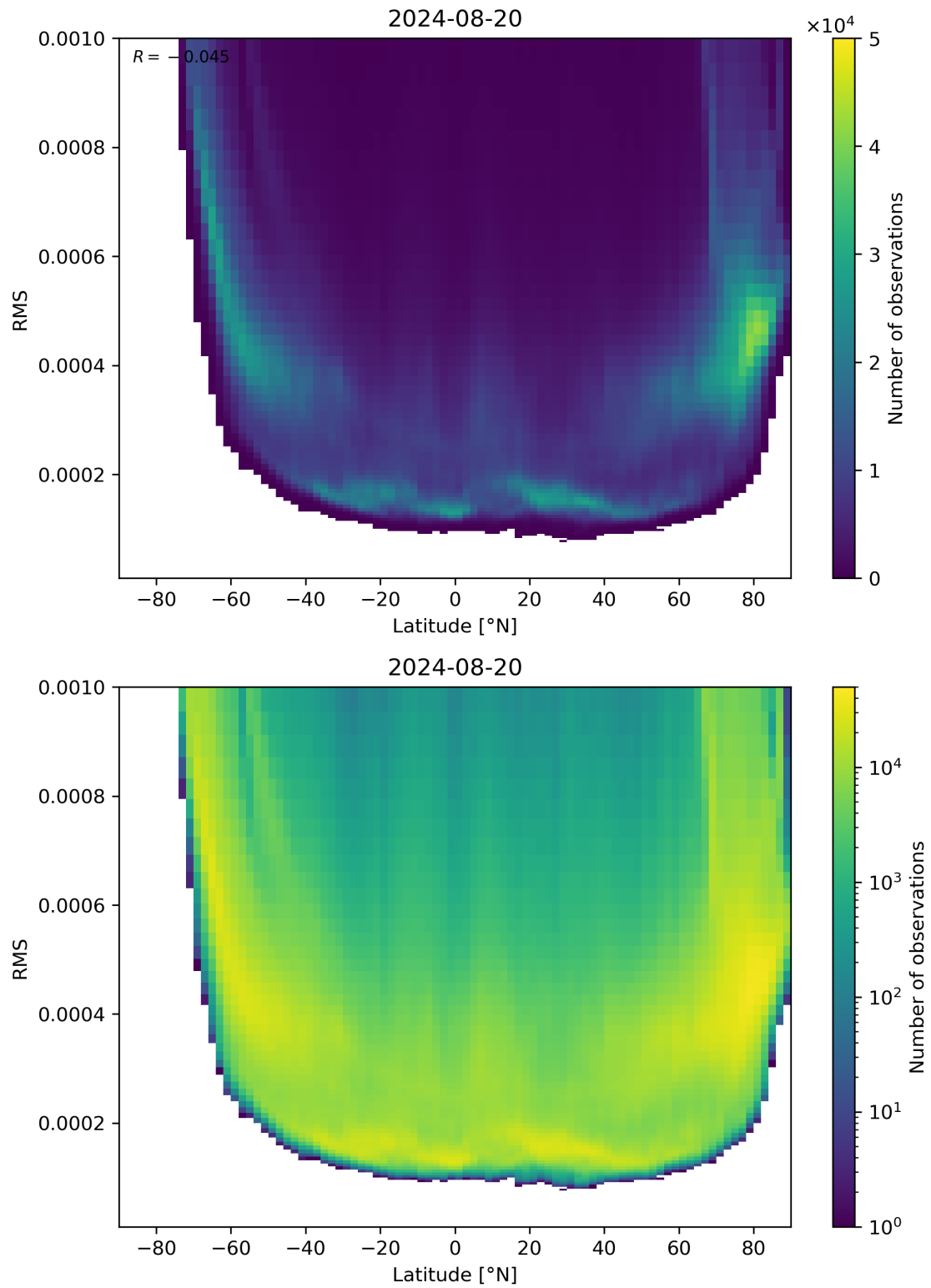
Figure 94: Scatter density plot of “Latitude” against “RMS” for 2024-08-19 to 2024-08-21.
