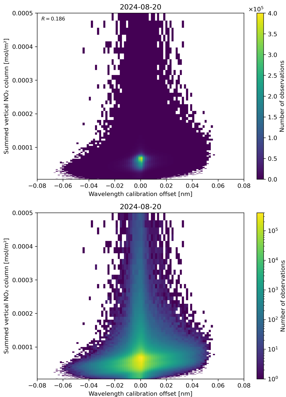
Figure 177: Scatter density plot of “Wavelength calibration offset” against “Summed vertical NO 2 column” for 2024-08-19 to 2024-08-21.
