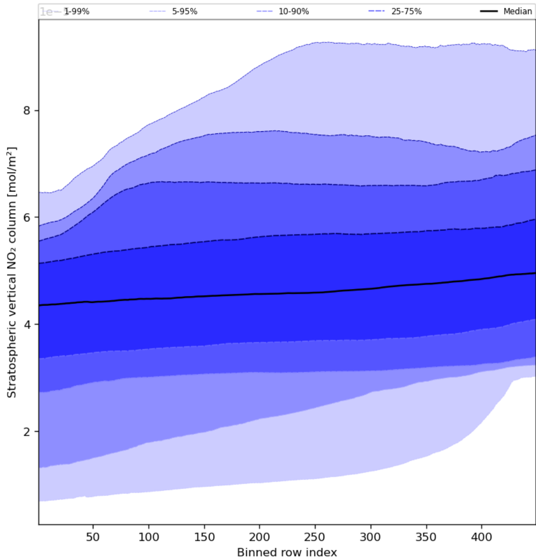
Figure 53: Along track statistics of “Stratospheric vertical NO 2 column” for 2024-08-19 to 2024-08-21
