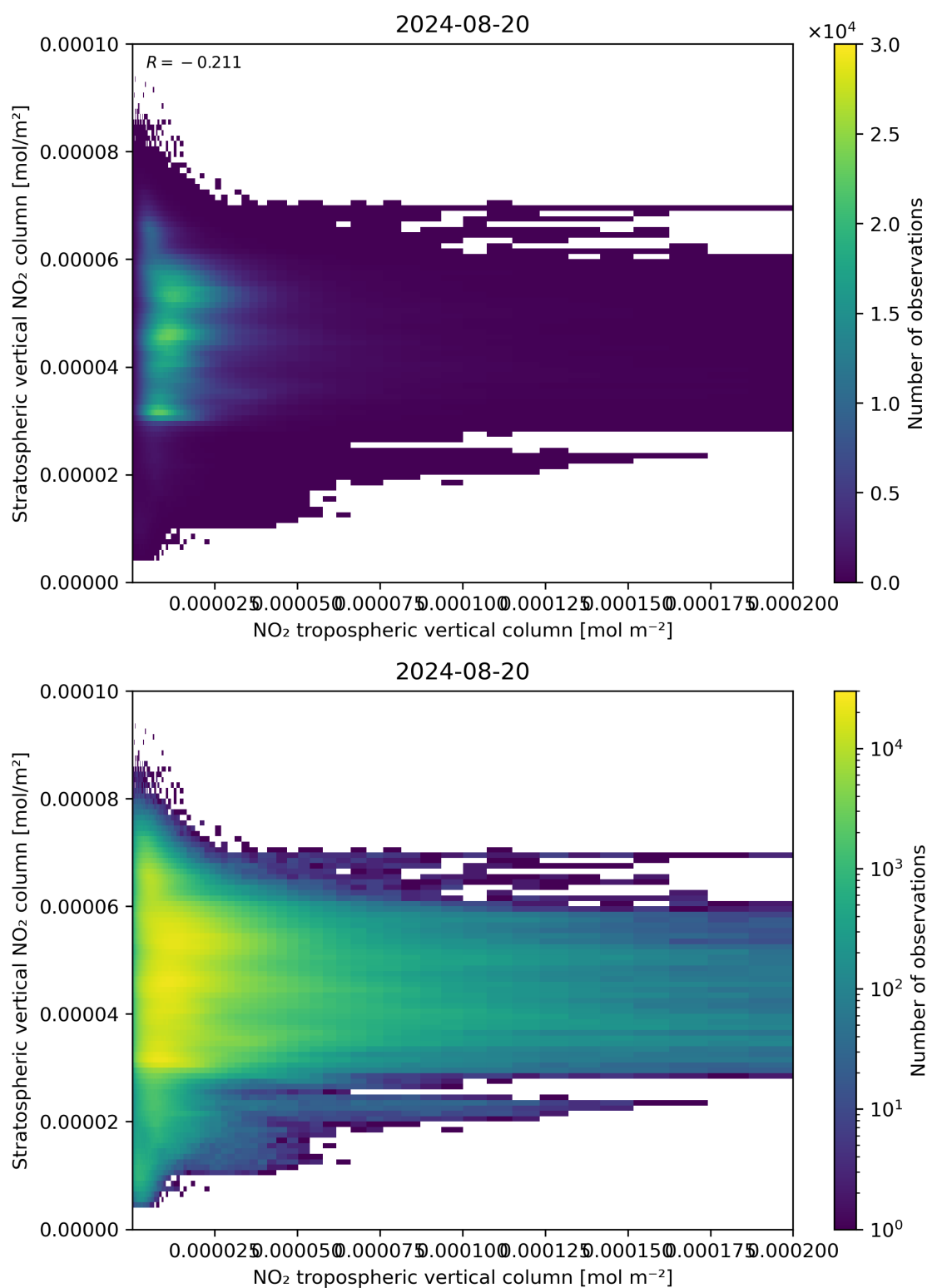
Figure 125: Scatter density plot of “NO 2 tropospheric vertical column” against “Stratospheric vertical NO 2 column” for 2024-08-19 to 2024-08-21.
