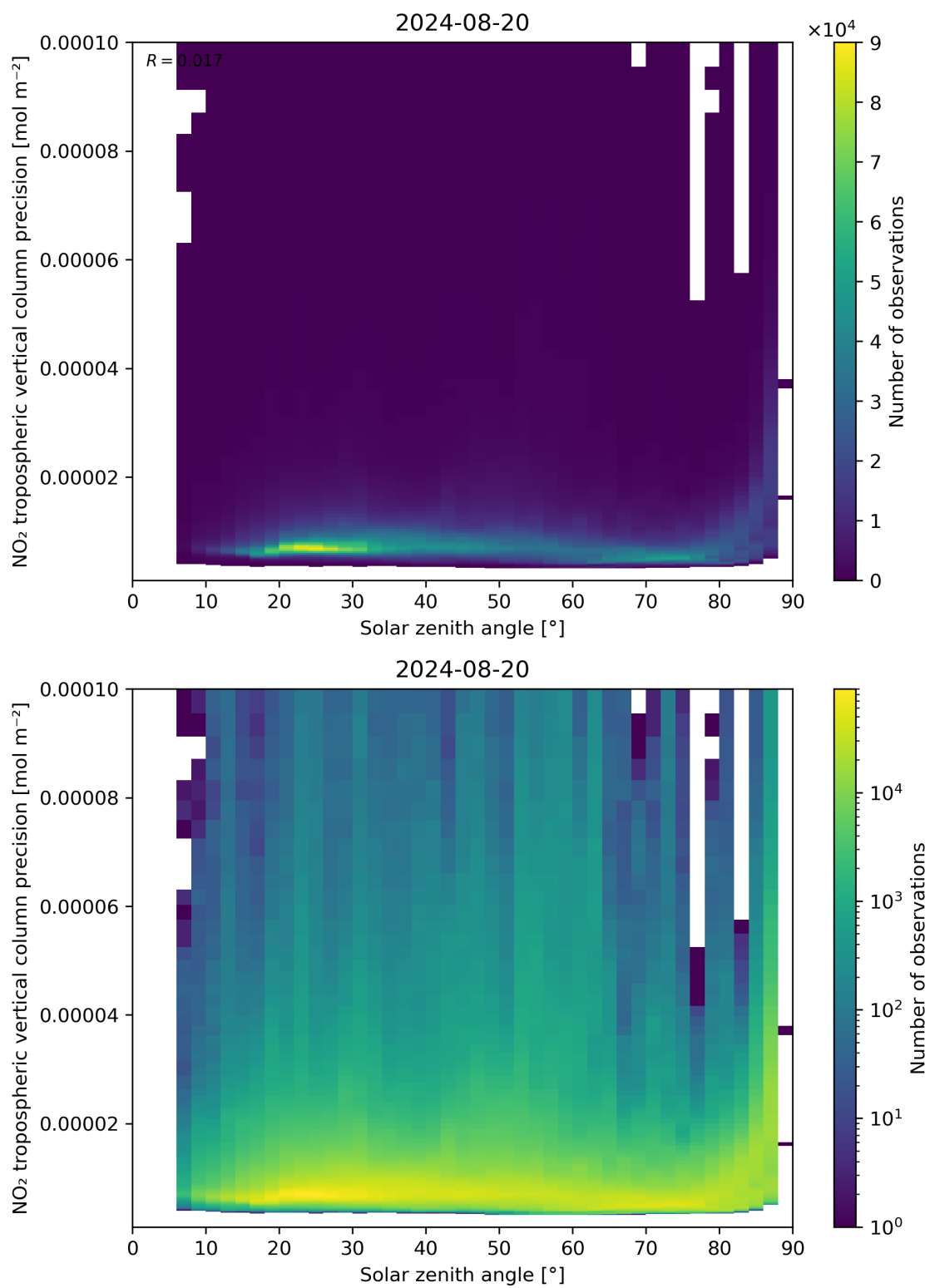
Figure 156: Scatter density plot of “Solar zenith angle” against “NO 2 tropospheric vertical column precision” for 2024-08-19 to 2024-08-21.
