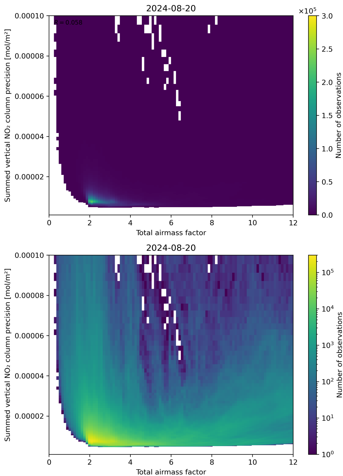
Figure 66: Scatter density plot of “Total airmass factor” against “Summed vertical NO 2 column precision” for 2024-08-19 to 2024-08-21.
