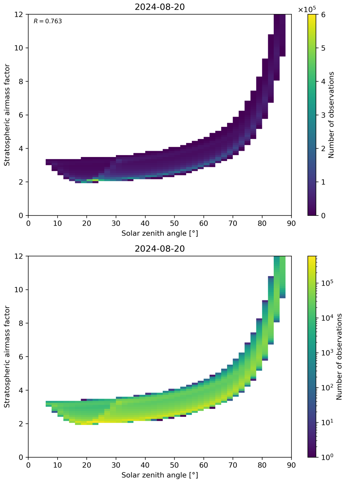
Figure 145: Scatter density plot of “Solar zenith angle” against “Stratospheric airmass factor” for 2024-08-19 to 2024-08-21.
