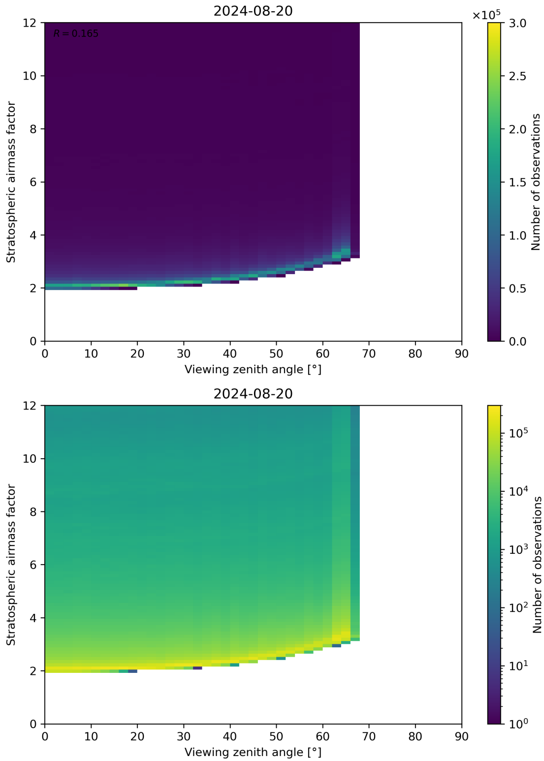
Figure 159: Scatter density plot of “Viewing zenith angle” against “Stratospheric airmass factor” for 2024-08-19 to 2024-08-21.
