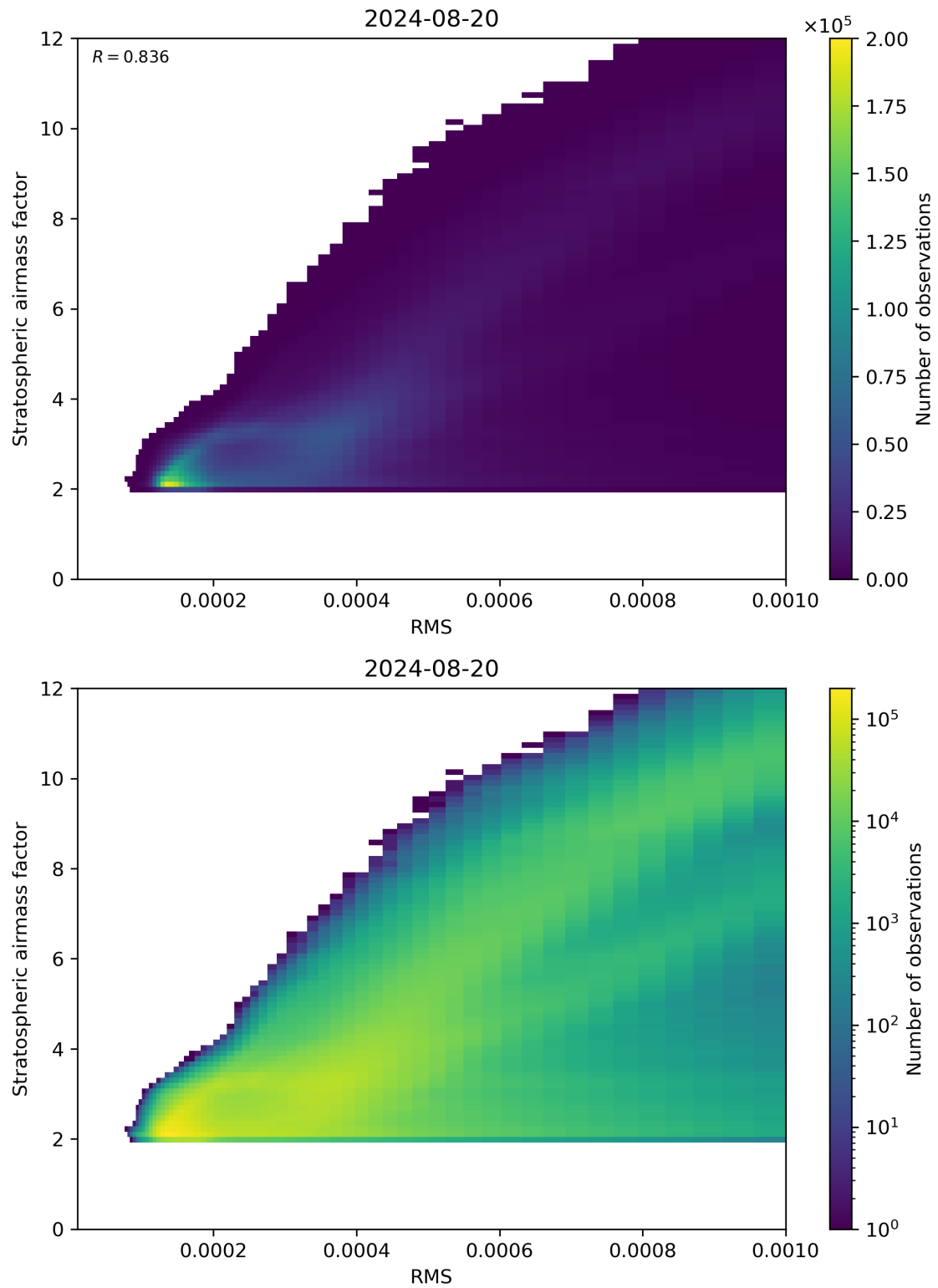
Figure 144: Scatter density plot of “RMS” against “Stratospheric airmass factor” for 2024-08-19 to 2024-08-21.
