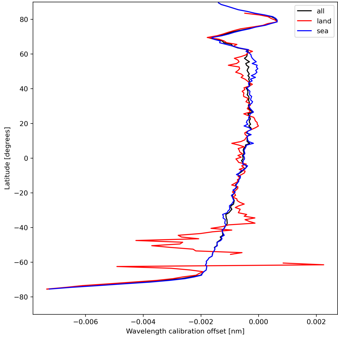
Figure 18: Zonal average of “Wavelength calibration offset” for 2024-08-19 to 2024-08-21.
