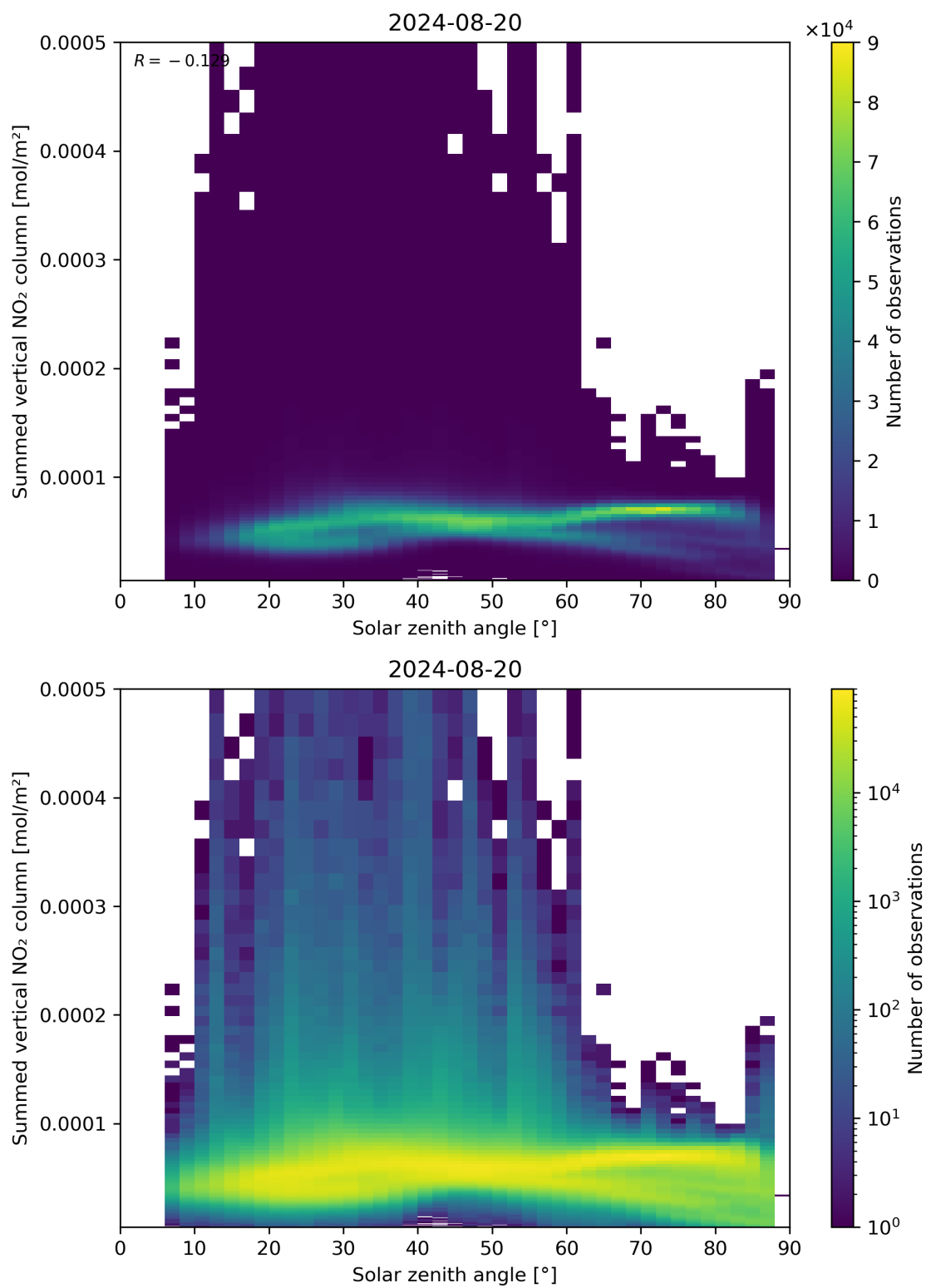
Figure 151: Scatter density plot of “Solar zenith angle” against “Summed vertical NO 2 column” for 2024-08-19 to 2024-08-21.
