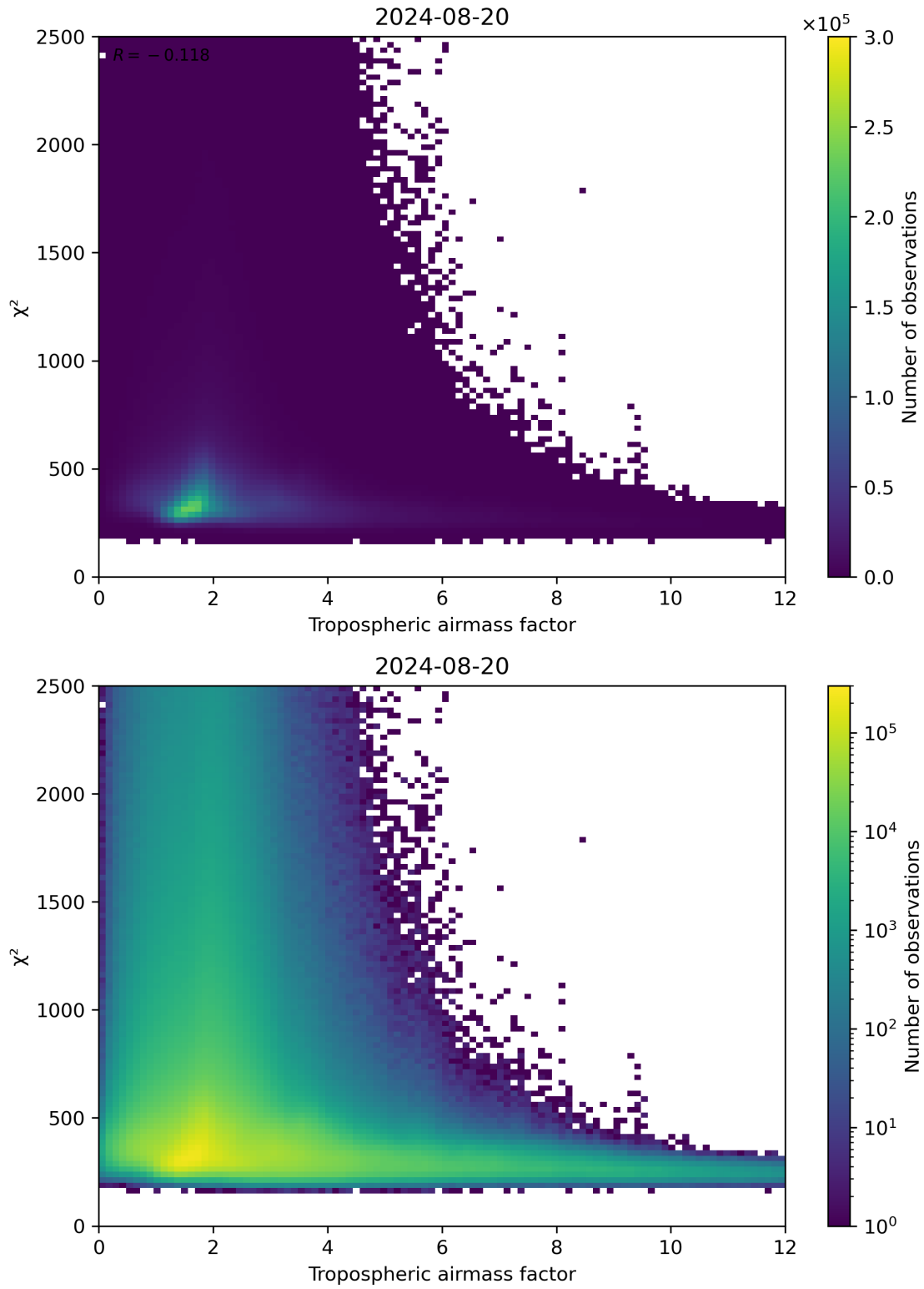
Figure 73: Scatter density plot of “Tropospheric airmass factor” against “ \chi^2 ” for 2024-08-19 to 2024-08-21.
