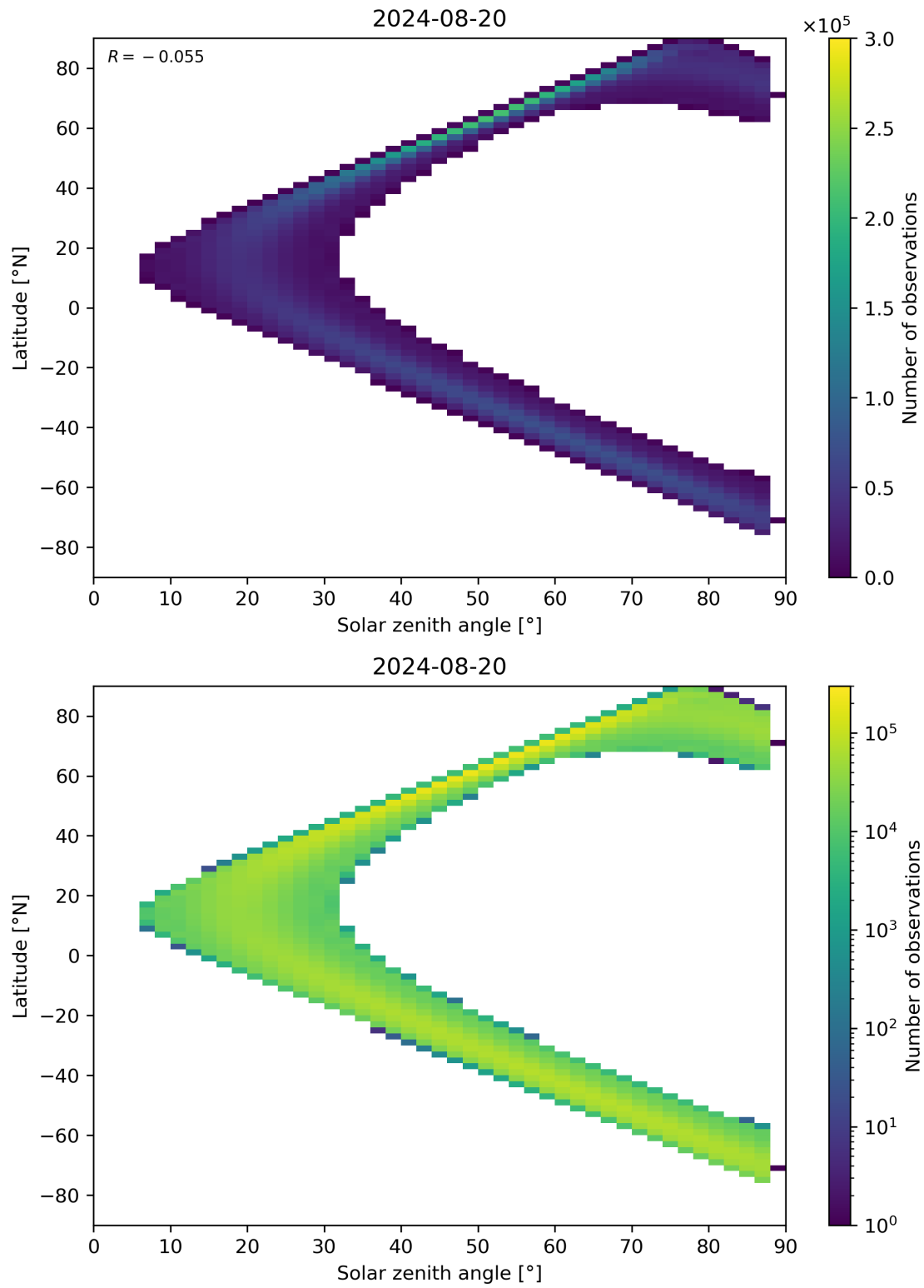
Figure 149: Scatter density plot of “Solar zenith angle” against “Latitude” for 2024-08-19 to 2024-08-21.
