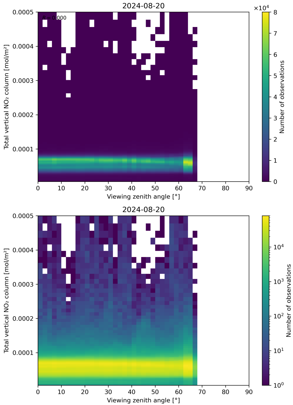
Figure 167: Scatter density plot of “Viewing zenith angle” against “Total vertical NO 2 column” for 2024-08-19 to 2024-08-21.
