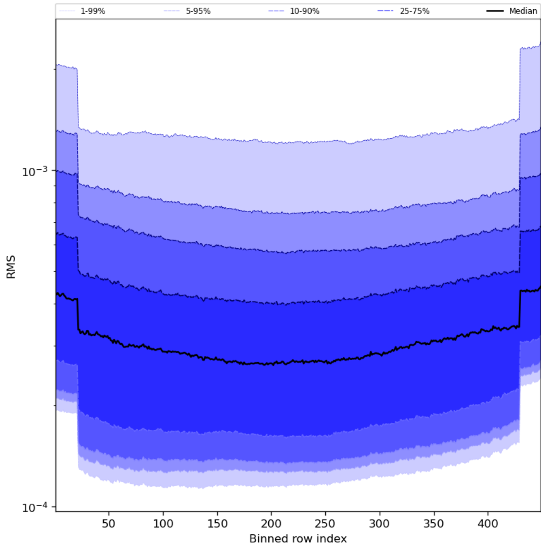
Figure 60: Along track statistics of “RMS” for 2024-08-19 to 2024-08-21
