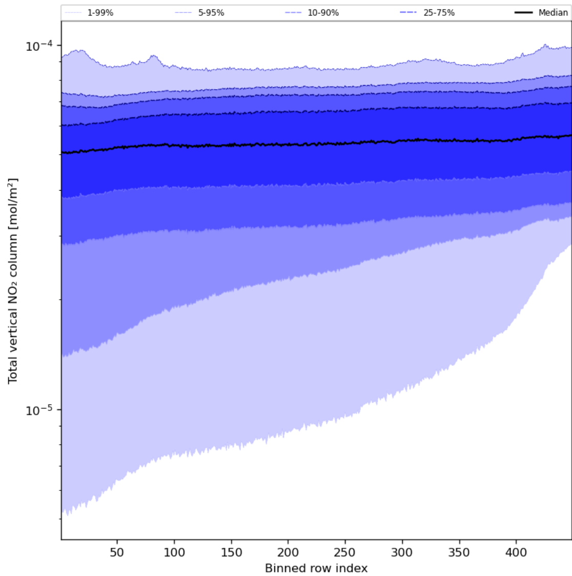
Figure 55: Along track statistics of “Total vertical NO 2 column” for 2024-08-19 to 2024-08-21
