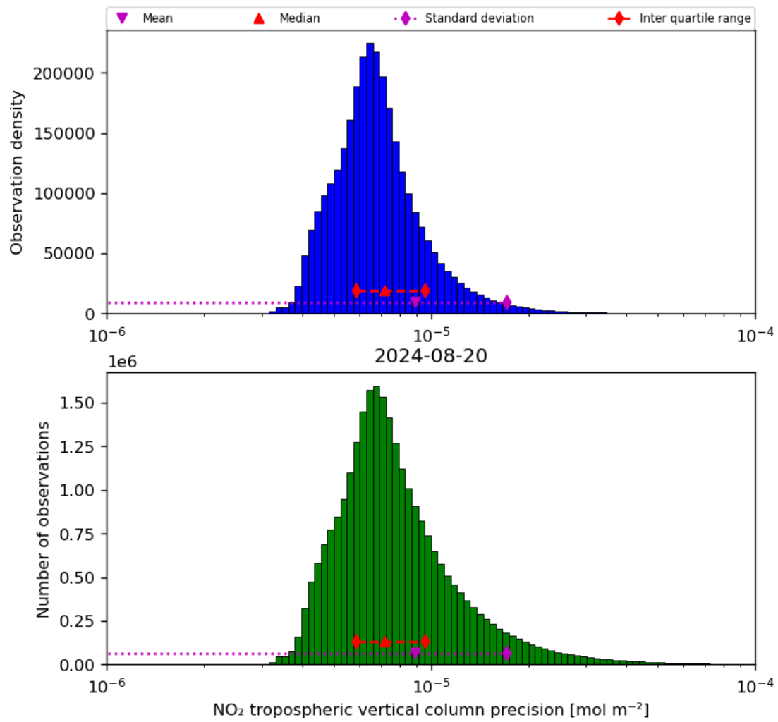
Figure 30: Histogram of “NO 2 tropospheric vertical column precision” for 2024-08-19 to 2024-08-21
