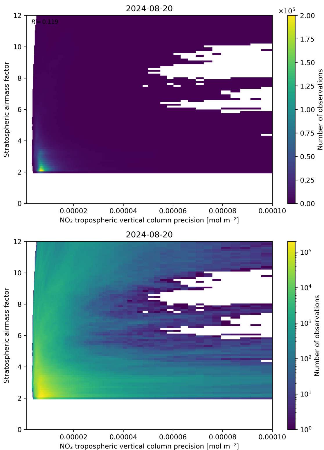
Figure 131: Scatter density plot of “NO 2 tropospheric vertical column precision” against “Stratospheric airmass factor” for 2024-08-19 to 2024-08-21.
