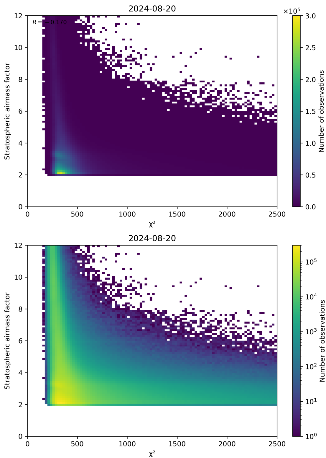
Figure 81: Scatter density plot of “ \chi^2 ” against “Stratospheric airmass factor” for 2024-08-19 to 2024-08-21.
