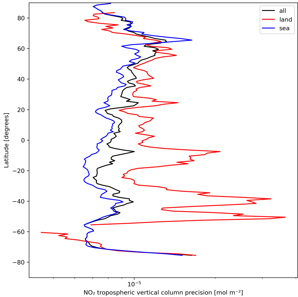
Figure 13: Zonal average of “NO 2 tropospheric vertical column precision” for 2024-08-19 to 2024-08-21.
