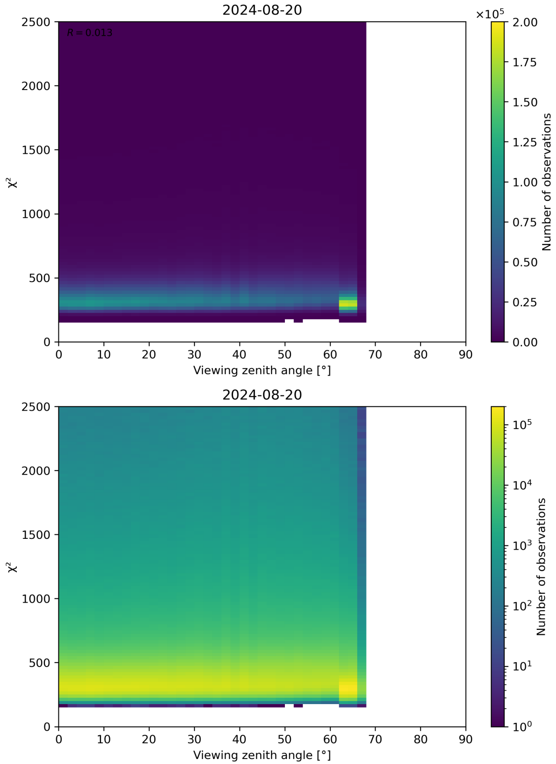
Figure 162: Scatter density plot of “Viewing zenith angle” against “ \chi^2 ” for 2024-08-19 to 2024-08-21.
