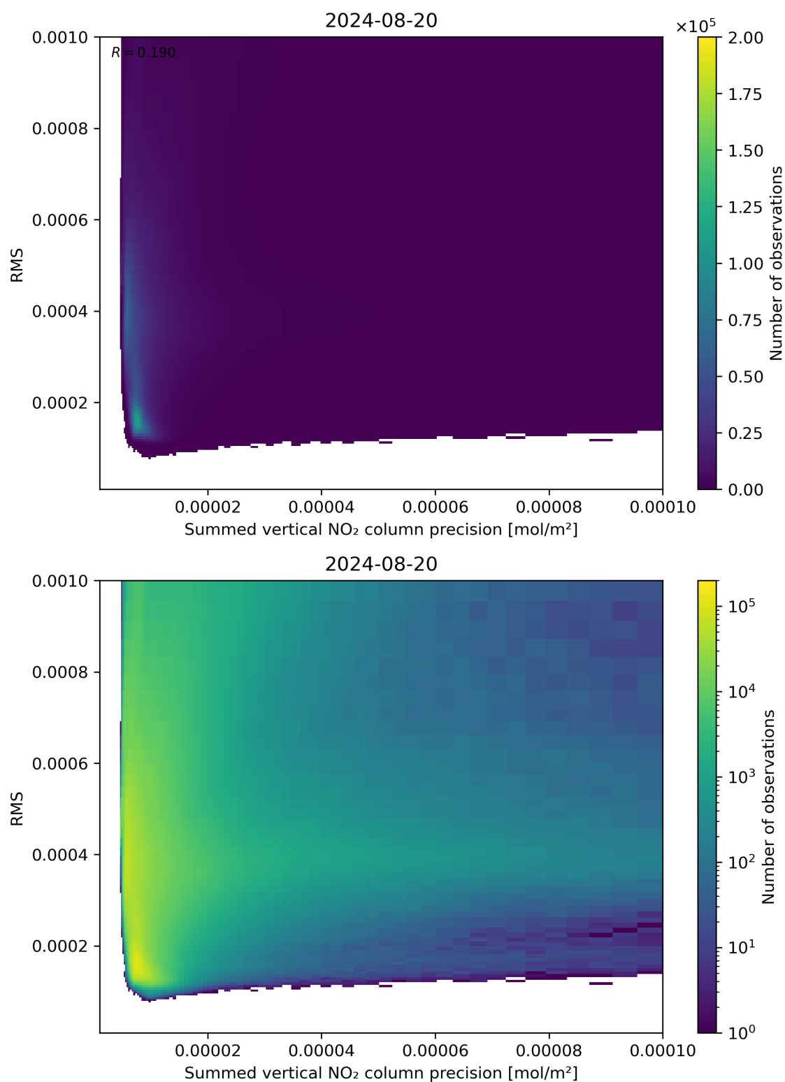
Figure 108: Scatter density plot of “Summed vertical NO 2 column precision” against “RMS” for 2024-08-19 to 2024-08-21.
