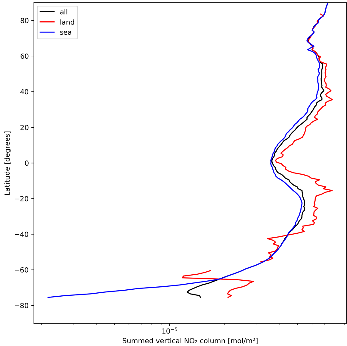
Figure 23: Zonal average of “Summed vertical NO 2 column” for 2024-08-19 to 2024-08-21.
