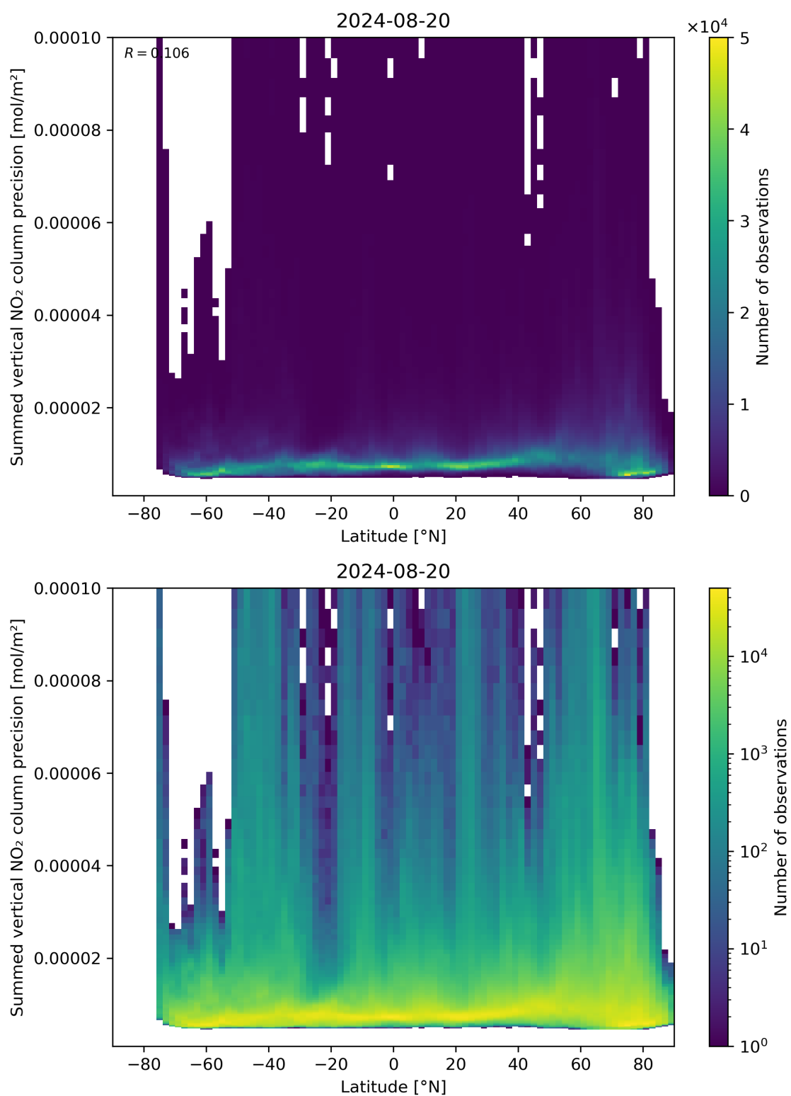
Figure 89: Scatter density plot of “Latitude” against “Summed vertical NO 2 column precision” for 2024-08-19 to 2024-08-21.
