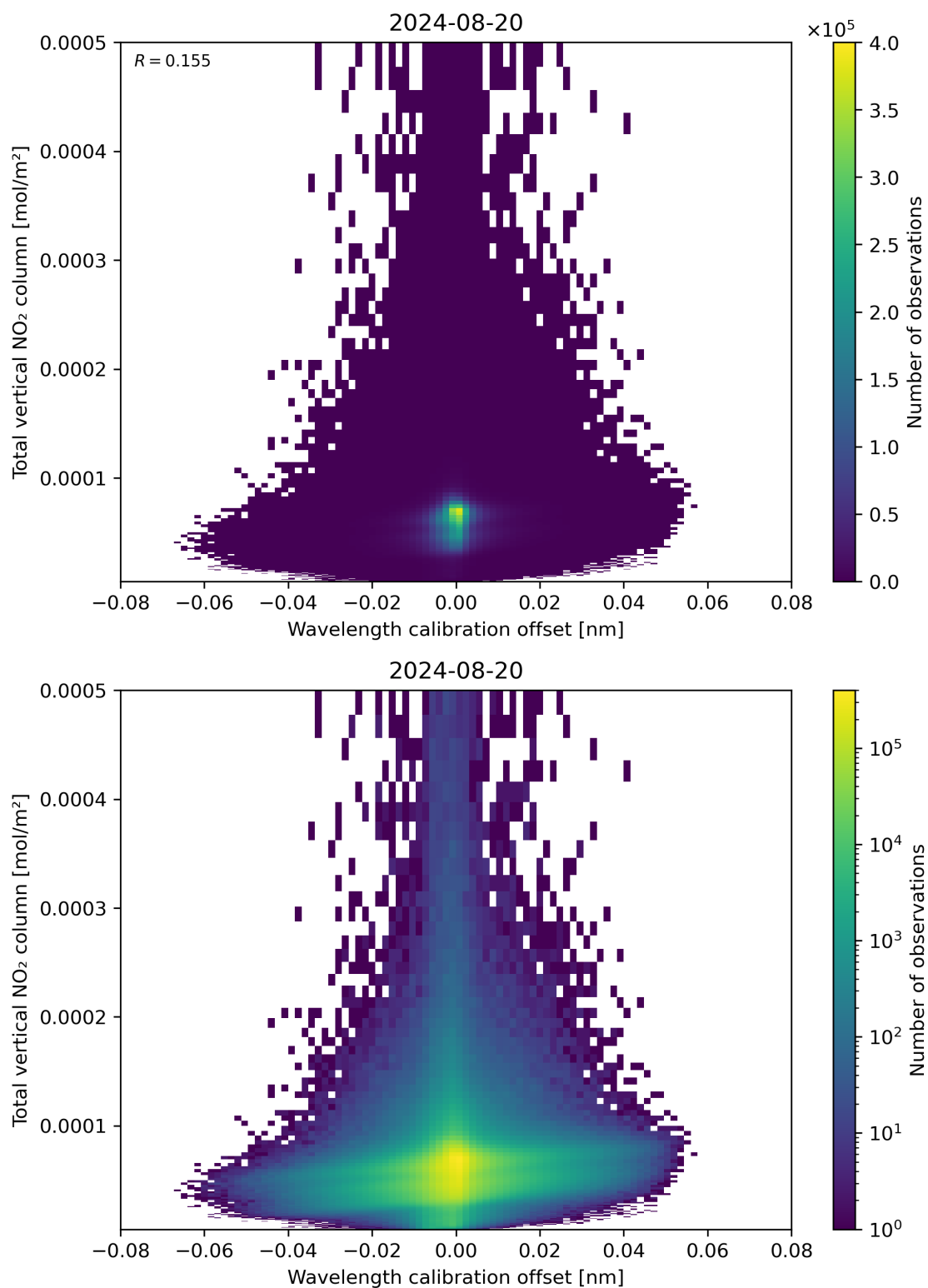
Figure 179: Scatter density plot of “Wavelength calibration offset” against “Total vertical NO 2 column” for 2024-08-19 to 2024-08-21.
