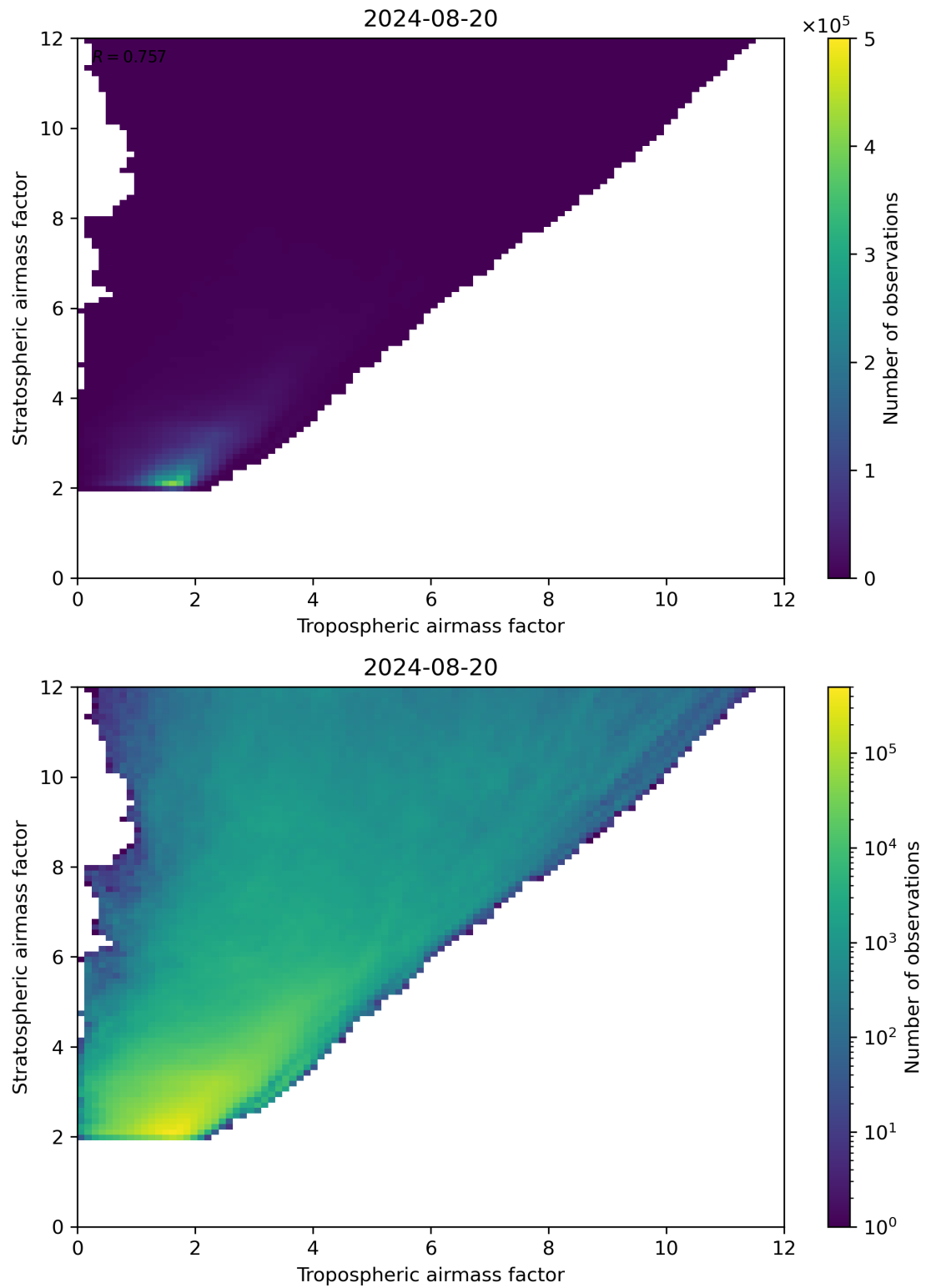
Figure 71: Scatter density plot of “Tropospheric airmass factor” against “Stratospheric airmass factor” for 2024-08-19 to 2024-08-21.
