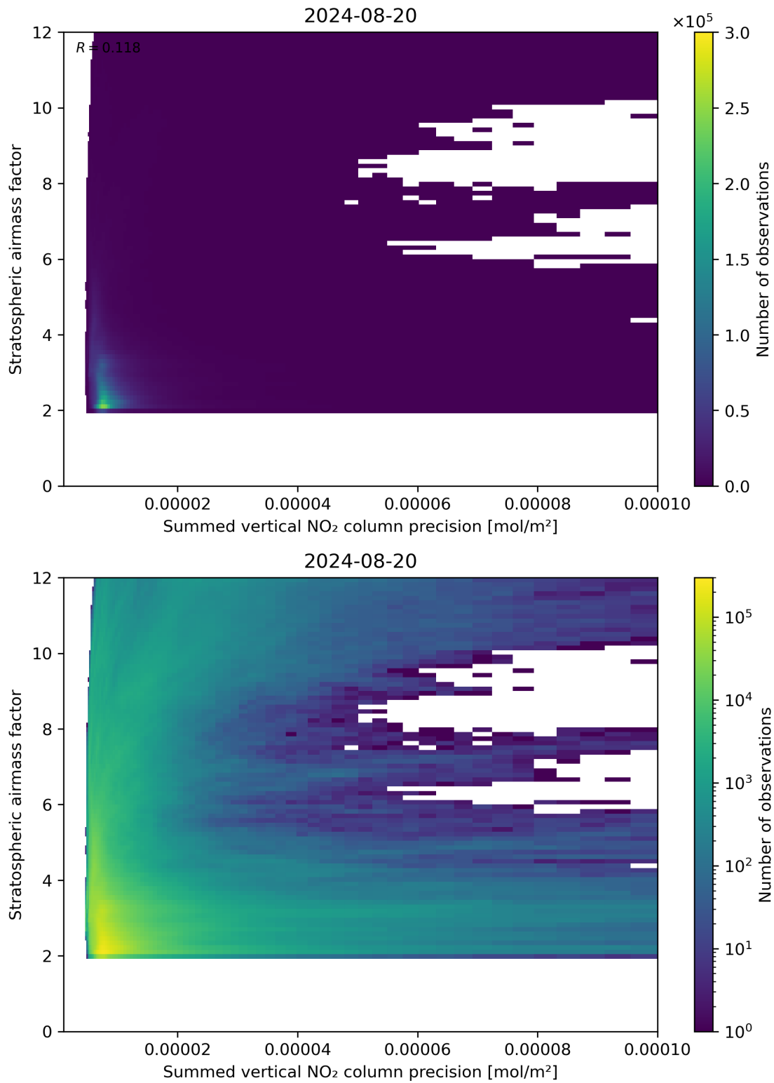
Figure 106: Scatter density plot of “Summed vertical NO 2 column precision” against “Stratospheric airmass factor” for 2024-08-19 to 2024-08-21.
