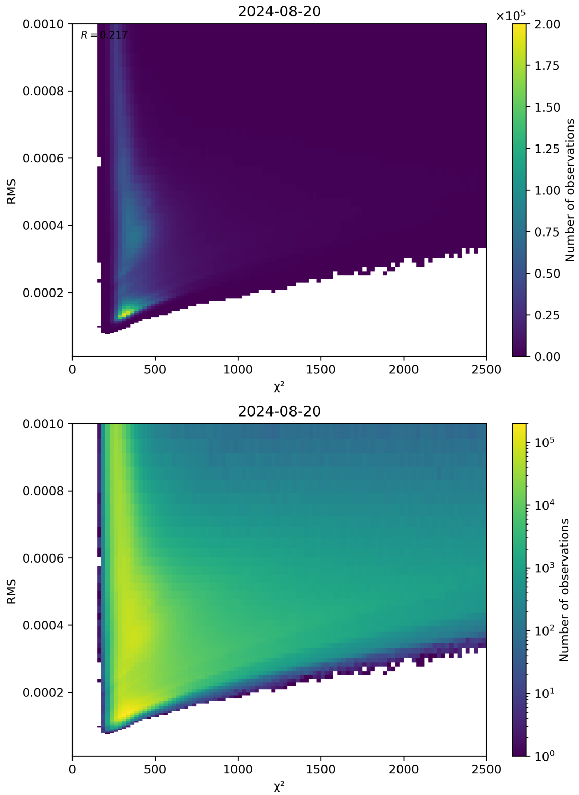
Figure 82: Scatter density plot of “ \chi^2 ” against “RMS” for 2024-08-19 to 2024-08-21.
