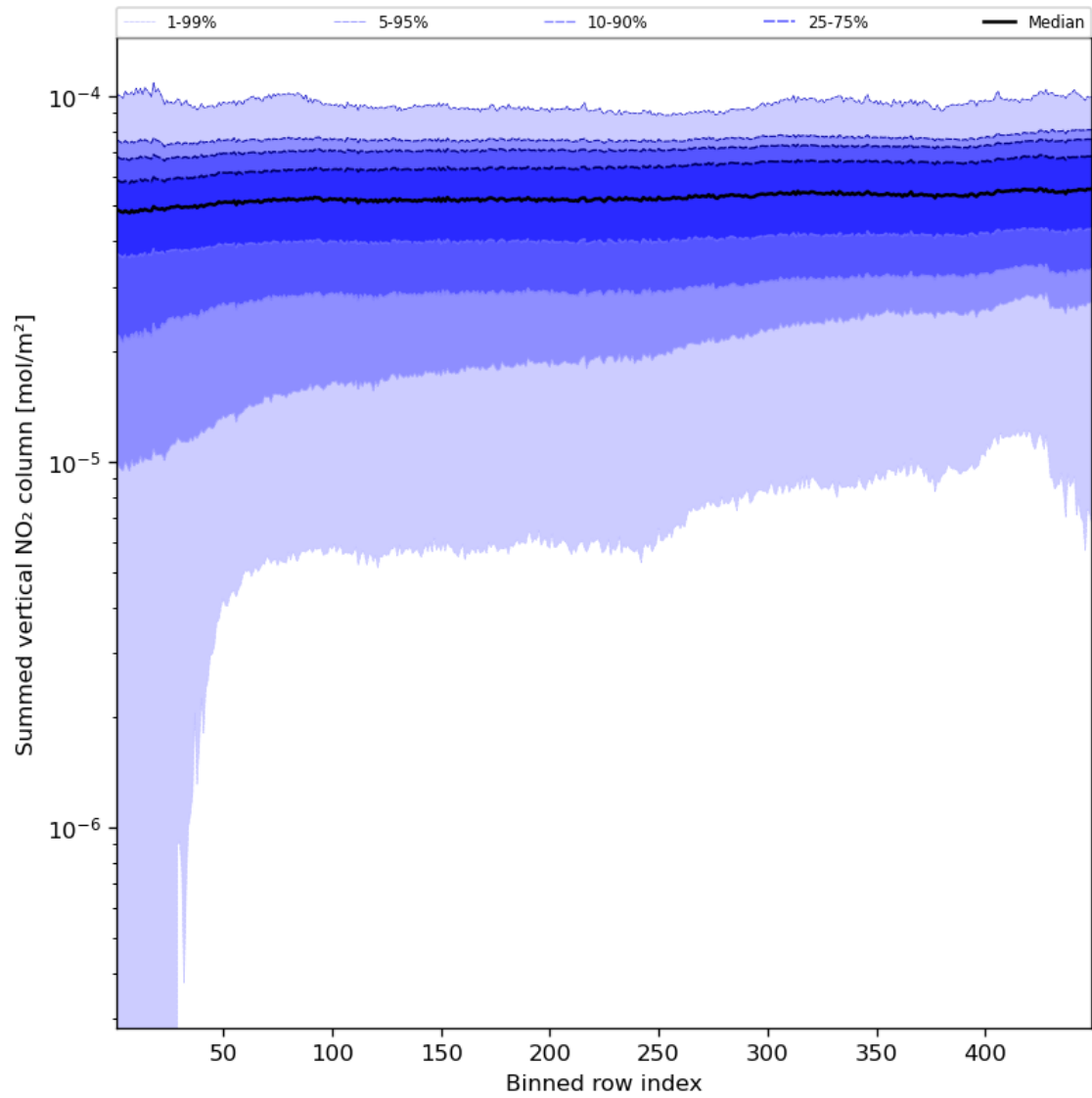
Figure 57: Along track statistics of “Summed vertical NO 2 column” for 2024-08-19 to 2024-08-21
