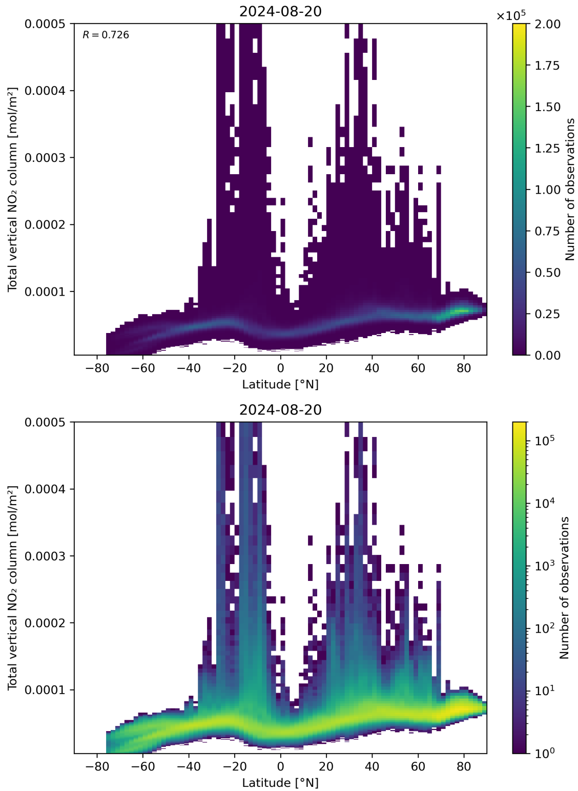
Figure 90: Scatter density plot of “Latitude” against “Total vertical NO 2 column” for 2024-08-19 to 2024-08-21.
