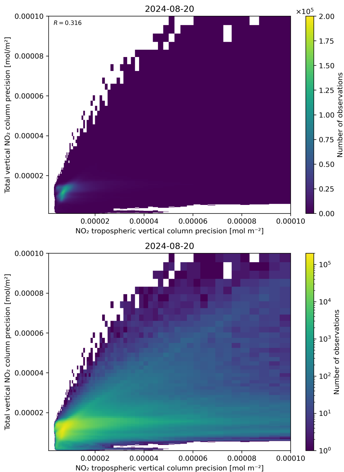
Figure 139: Scatter density plot of “NO 2 tropospheric vertical column precision” against “Total vertical NO 2 column precision” for 2024-08-19 to 2024-08-21.
