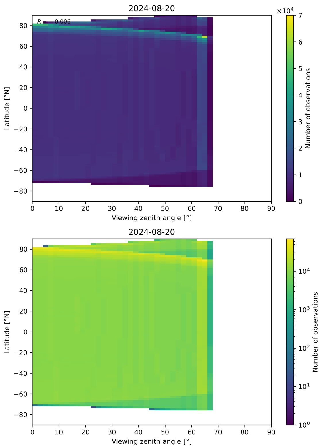
Figure 163: Scatter density plot of “Viewing zenith angle” against “Latitude” for 2024-08-19 to 2024-08-21.
