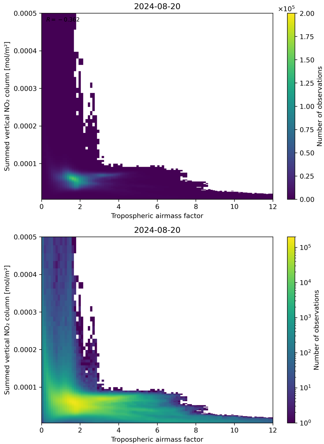
Figure 75: Scatter density plot of “Tropospheric air mass factor” against “Summed vertical NO 2 column” for 2024-08-19 to 2024-08-21.
