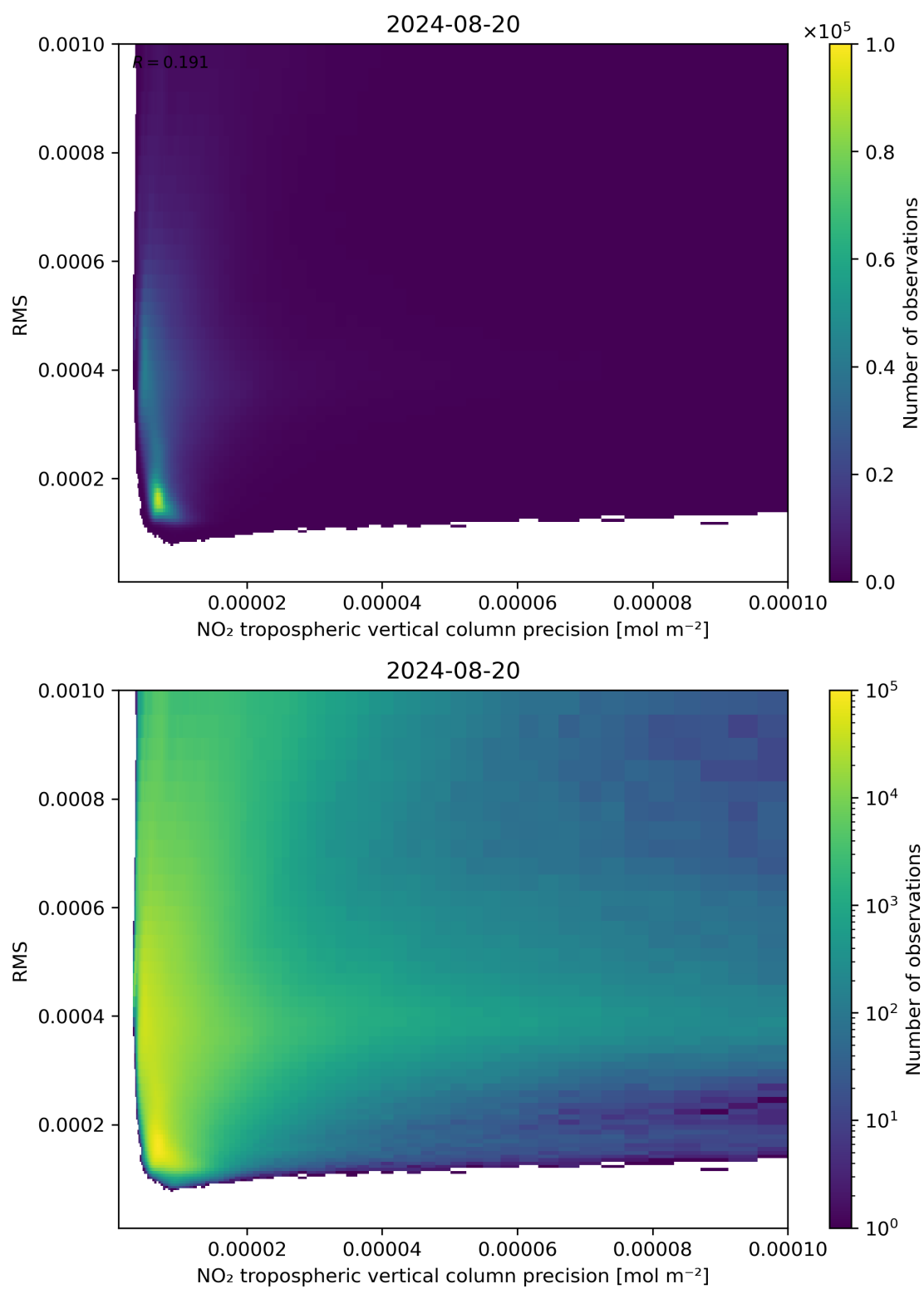
Figure 140: Scatter density plot of “NO 2 tropospheric vertical column precision” against “RMS” for 2024-08-19 to 2024-08-21.
