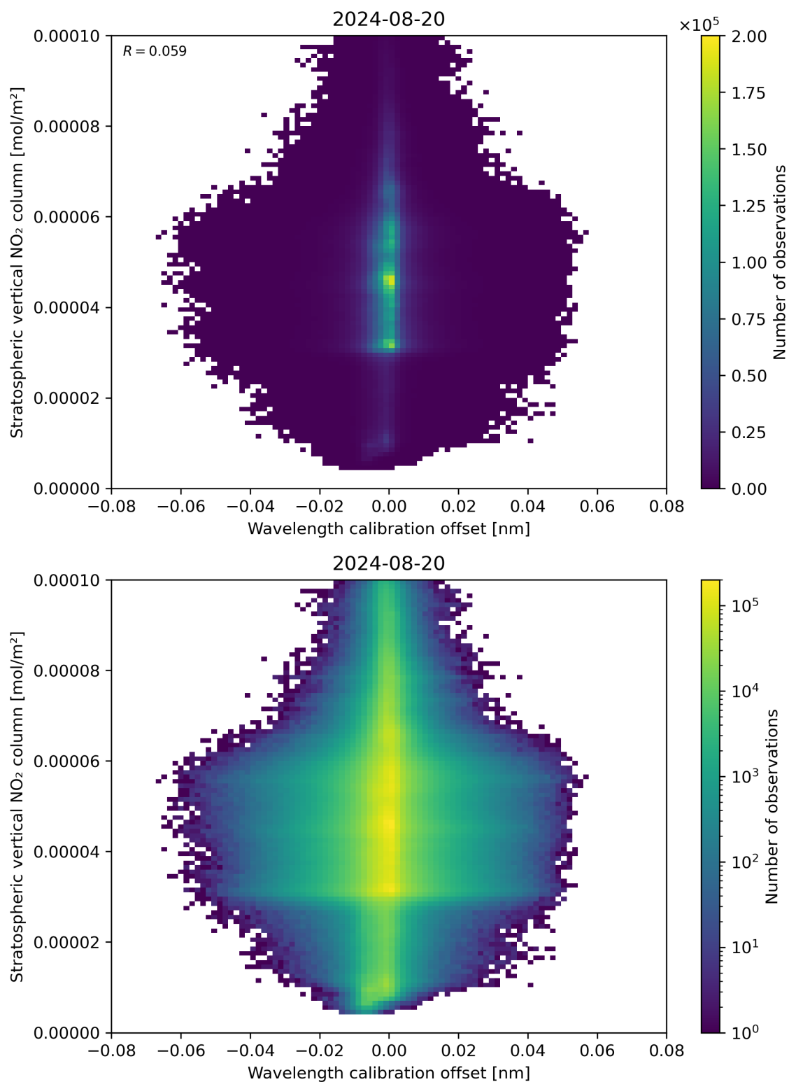
Figure 176: Scatter density plot of “Wavelength calibration offset” against “Stratospheric vertical NO 2 column” for 2024-08-19 to 2024-08-21.
