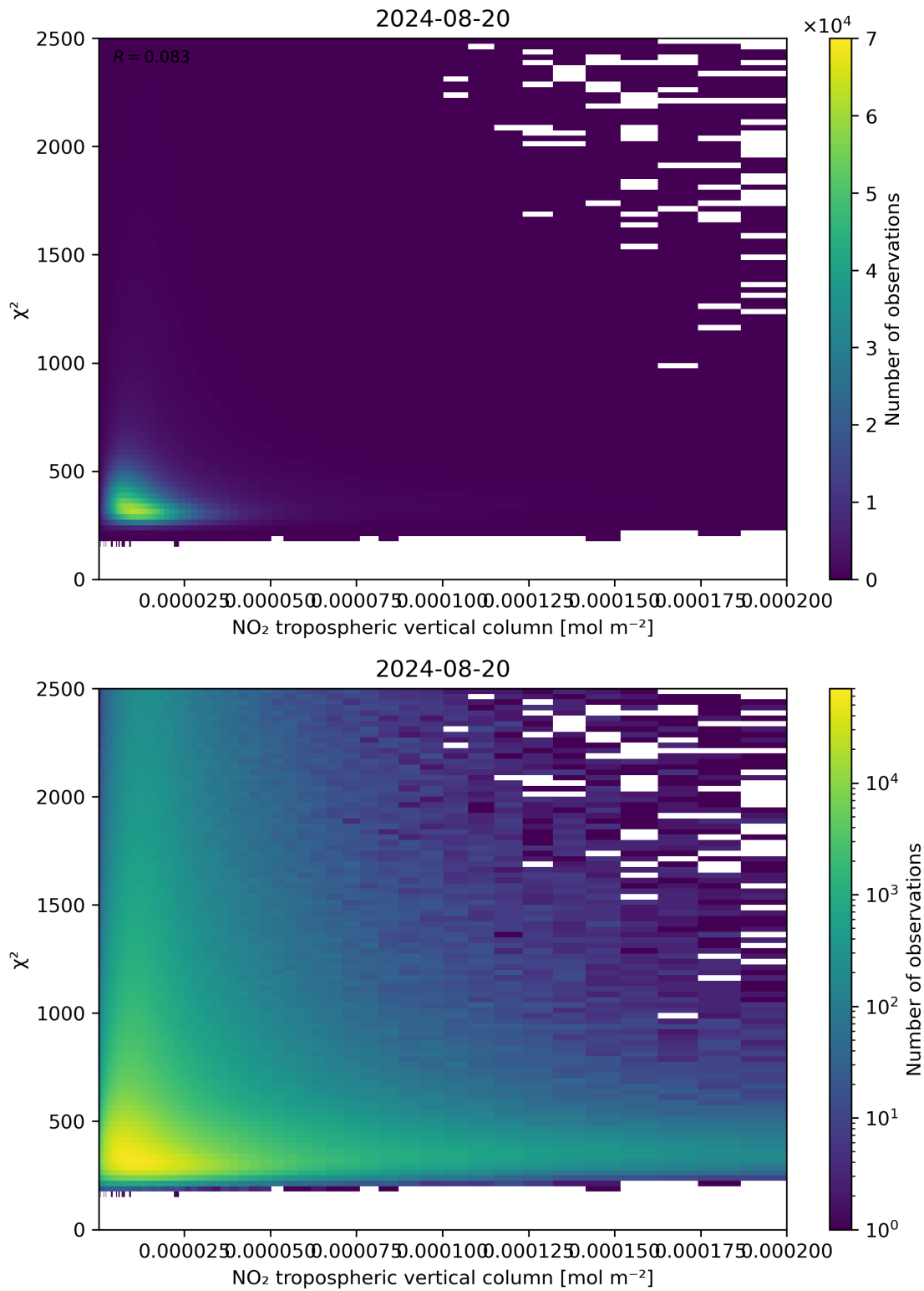
Figure 124: Scatter density plot of “NO 2 tropospheric vertical column” against “ \chi^2 ” for 2024-08-19 to 2024-08-21.
