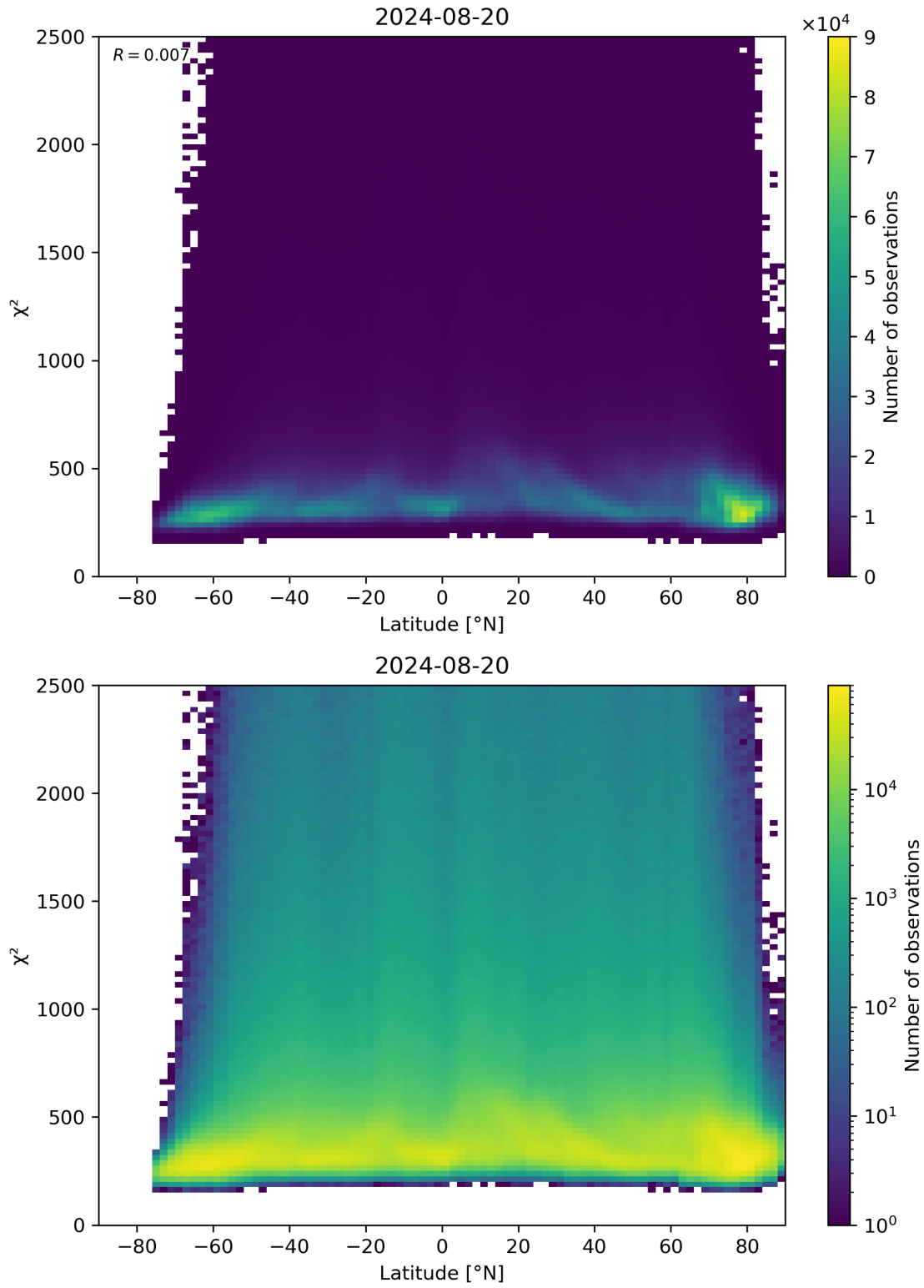
Figure 86: Scatter density plot of “Latitude” against “ \chi^2 ” for 2024-08-19 to 2024-08-21.
