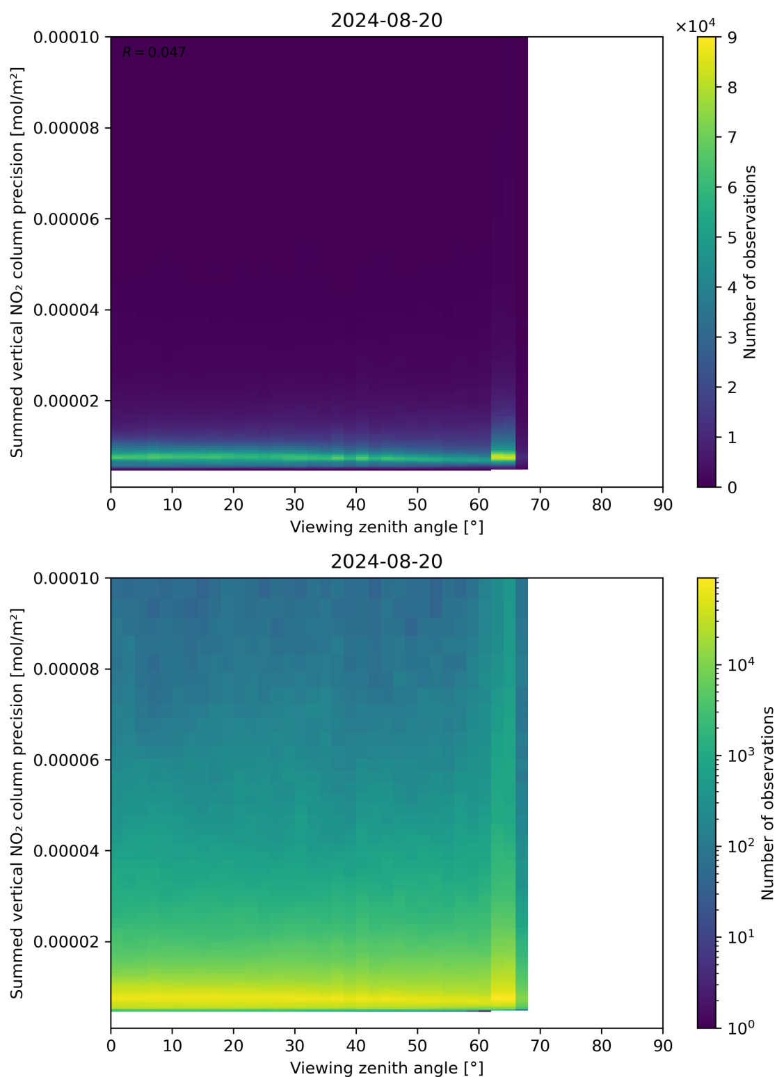
Figure 166: Scatter density plot of “Viewing zenith angle” against “Summed vertical NO 2 column precision” for 2024-08-19 to 2024-08-21.
