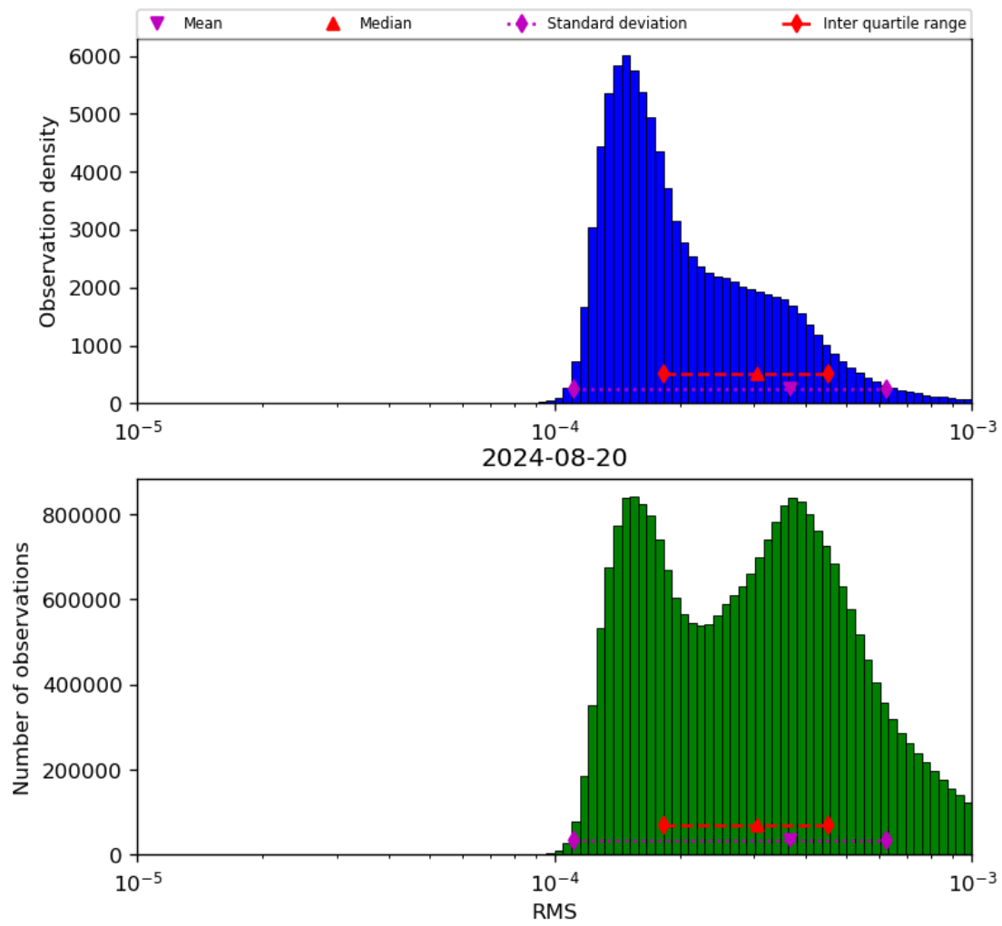
Figure 43: Histogram of “RMS” for 2024-08-19 to 2024-08-21
