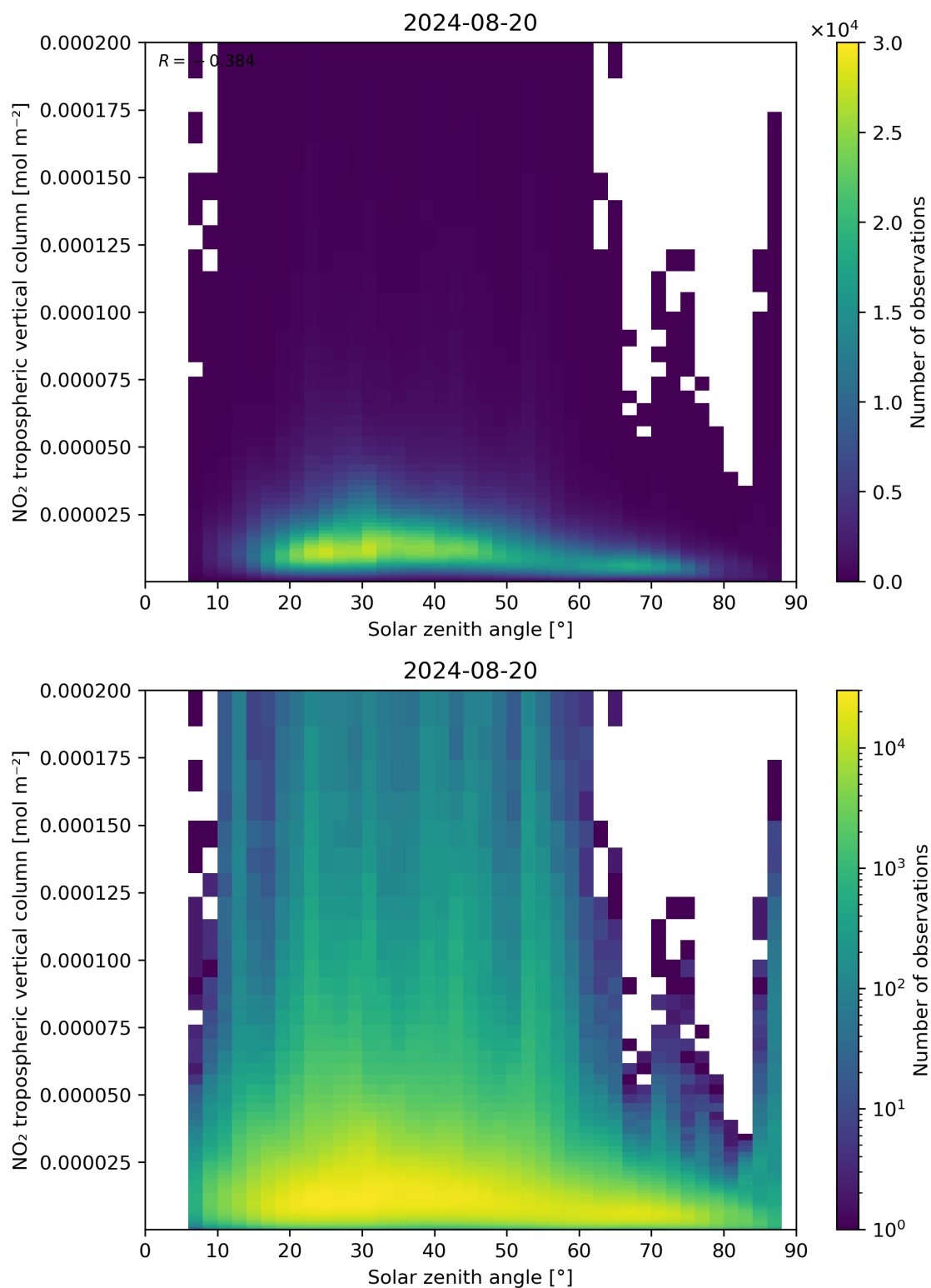
Figure 155: Scatter density plot of “Solar zenith angle” against “NO 2 tropospheric vertical column” for 2024-08-19 to 2024-08-21.
