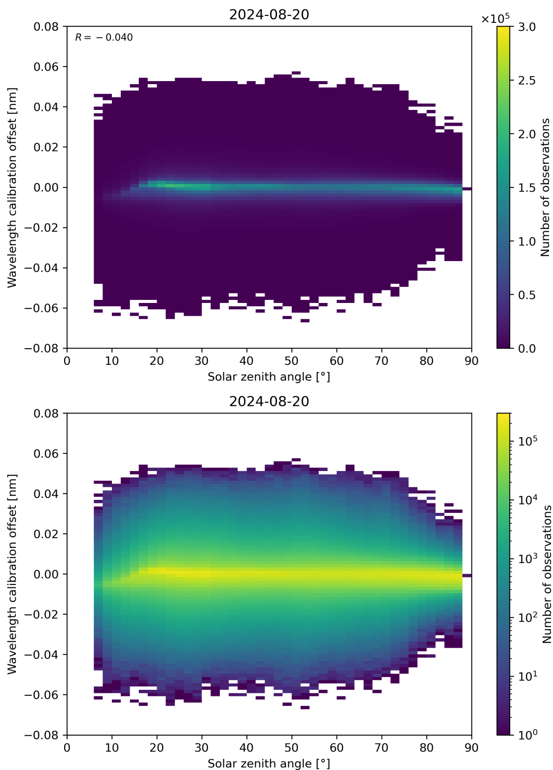
Figure 158: Scatter density plot of “Solar zenith angle” against “Wavelength calibration offset” for 2024-08-19 to 2024-08-21.
