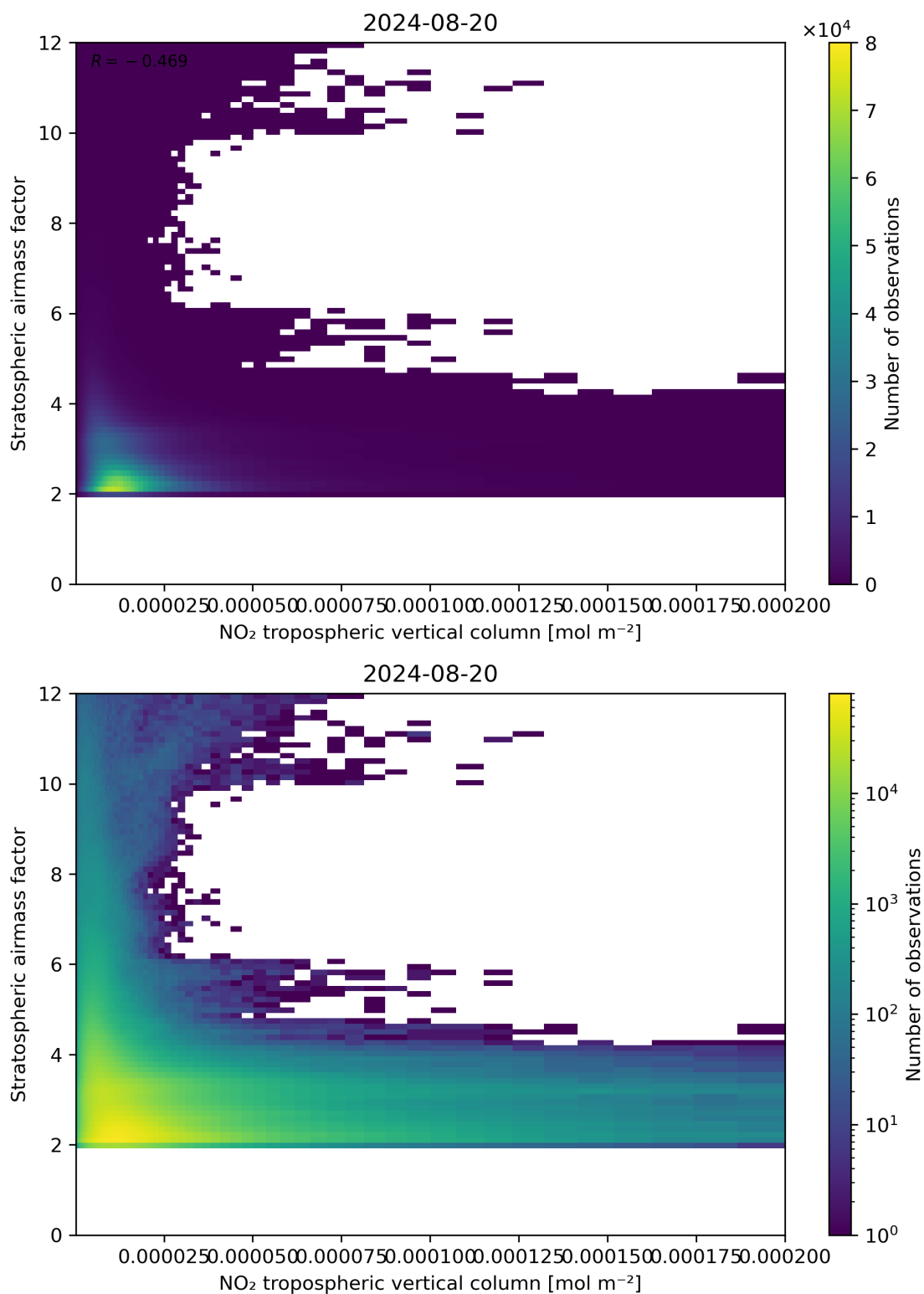
Figure 121: Scatter density plot of “NO 2 tropospheric vertical column” against “Stratospheric air mass factor” for 2024-08-19 to 2024-08-21.
