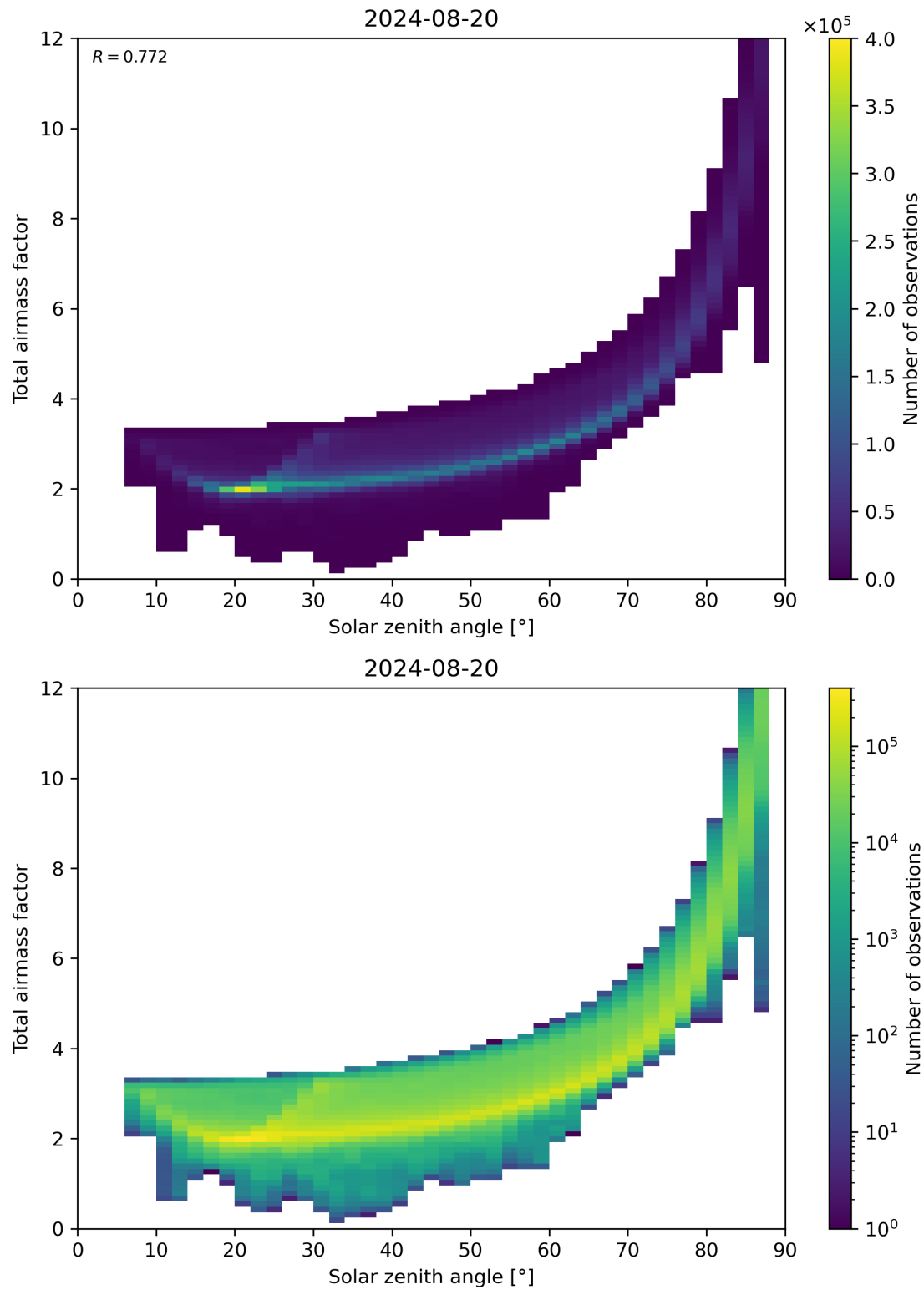
Figure 146: Scatter density plot of “Solar zenith angle” against “Total air mass factor” for 2024-08-19 to 2024-08-21.
