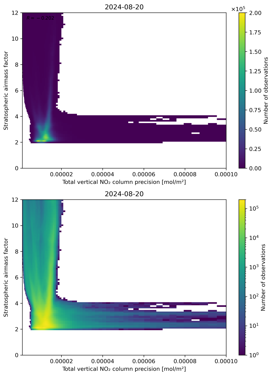
Figure 115: Scatter density plot of “Total vertical NO 2 column precision” against “Stratospheric air mass factor” for 2024-08-19 to 2024-08-21.
