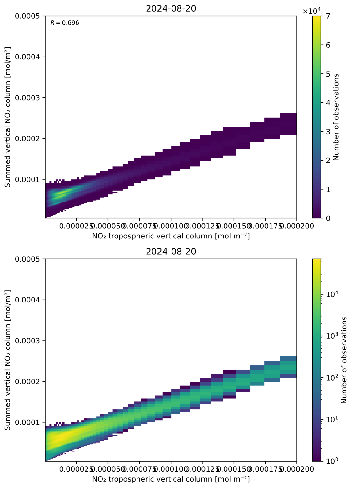
Figure 126: Scatter density plot of “NO 2 tropospheric vertical column” against “Summed vertical NO 2 column” for 2024-08-19 to 2024-08-21.
