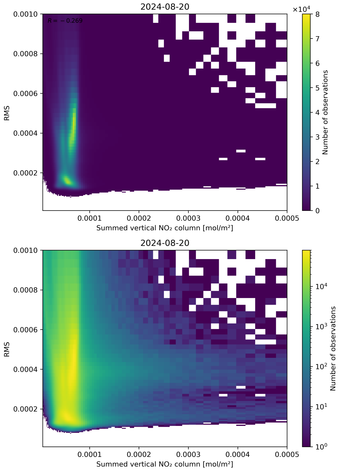
Figure 109: Scatter density plot of “Summed vertical NO 2 column” against “RMS” for 2024-08-19 to 2024-08-21.
