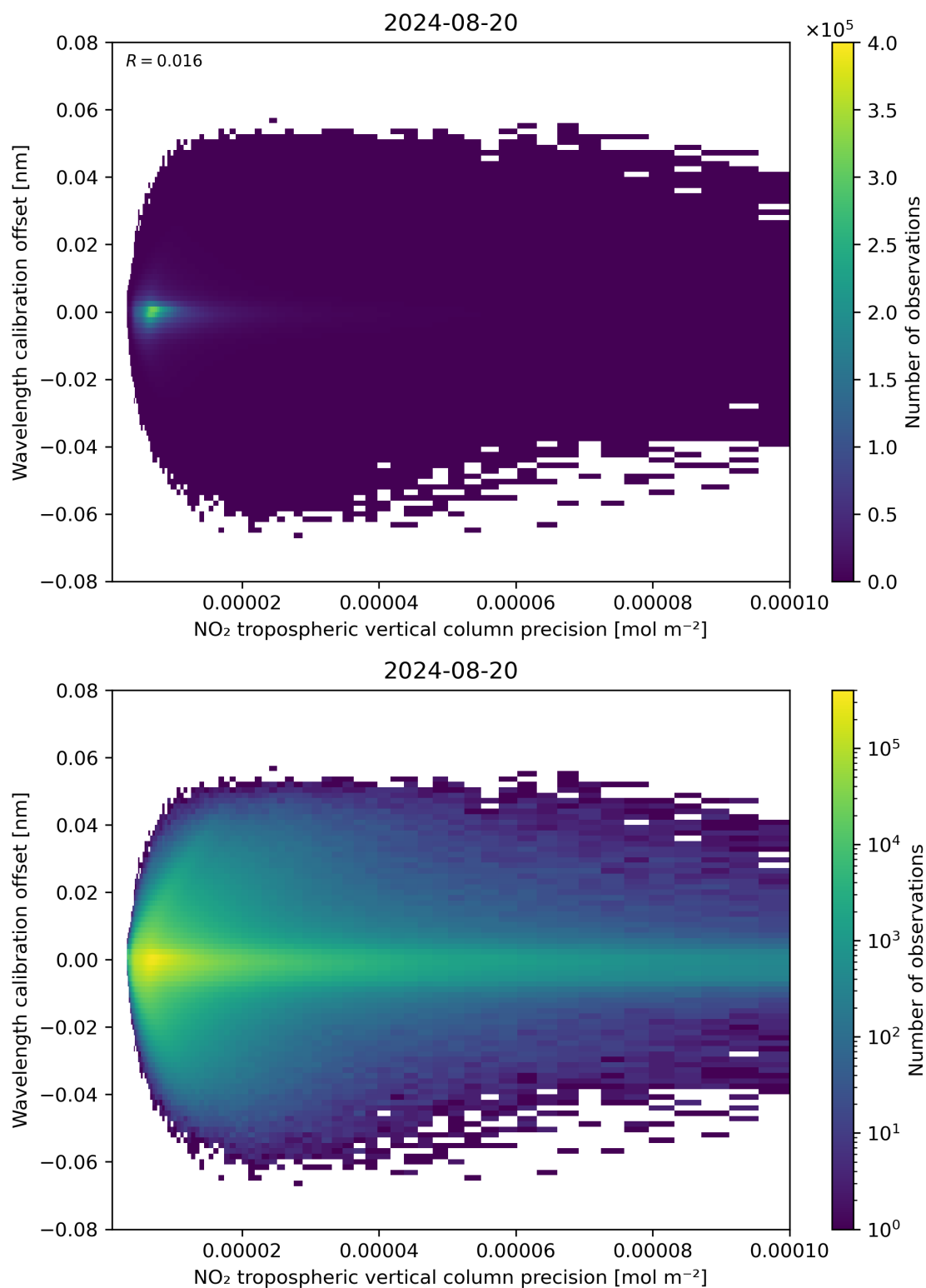
Figure 141: Scatter density plot of “NO 2 tropospheric vertical column precision” against “Wavelength calibration offset” for 2024-08-19 to 2024-08-21.
