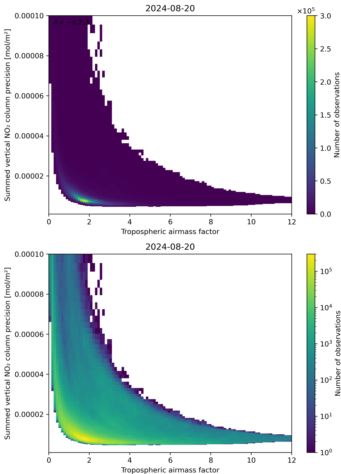
Figure 76: Scatter density plot of “Tropospheric air mass factor” against “Summed vertical NO 2 column precision” for 2024-08-19 to 2024-08-21.
