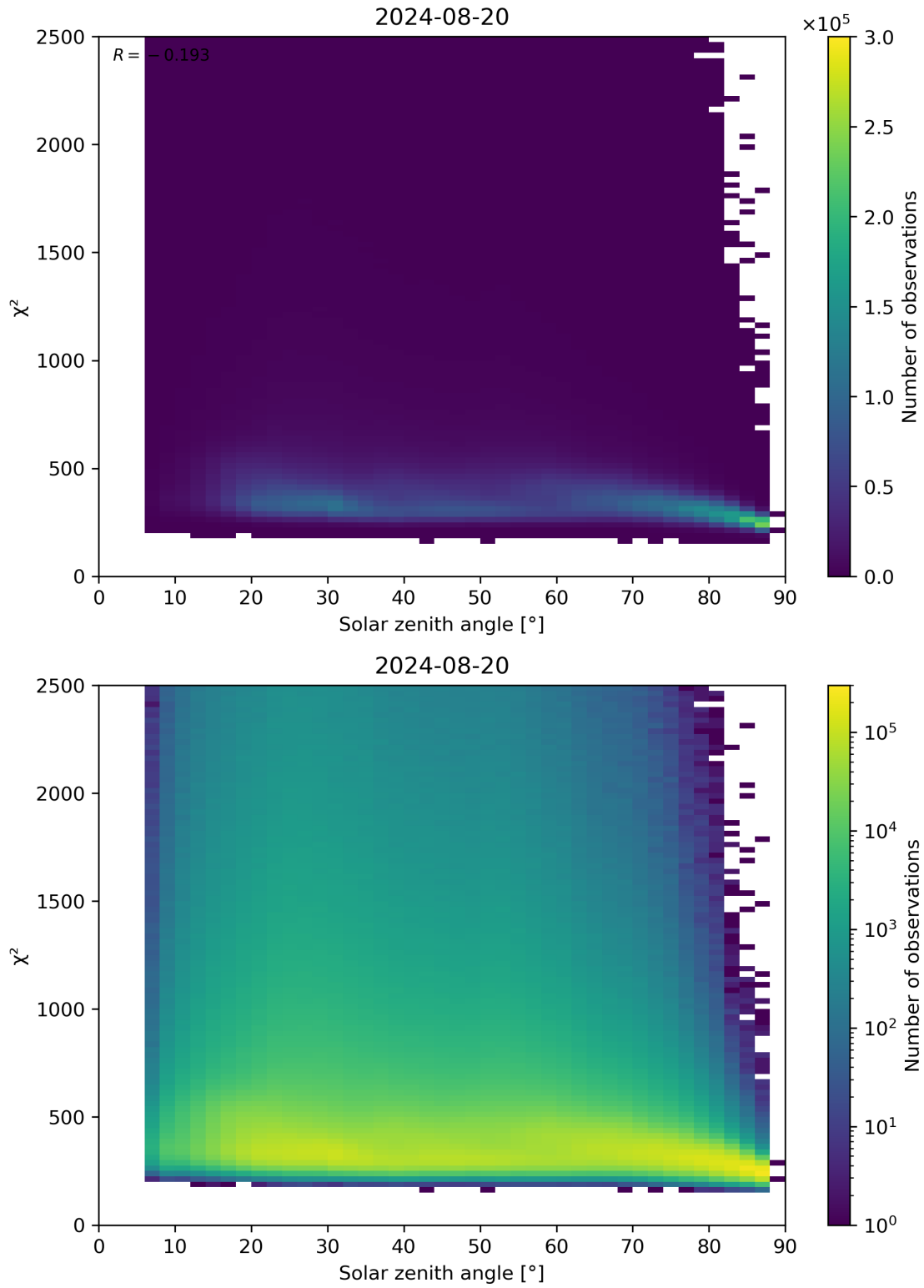
Figure 148: Scatter density plot of “Solar zenith angle” against “ \chi^2 ” for 2024-08-19 to 2024-08-21.
