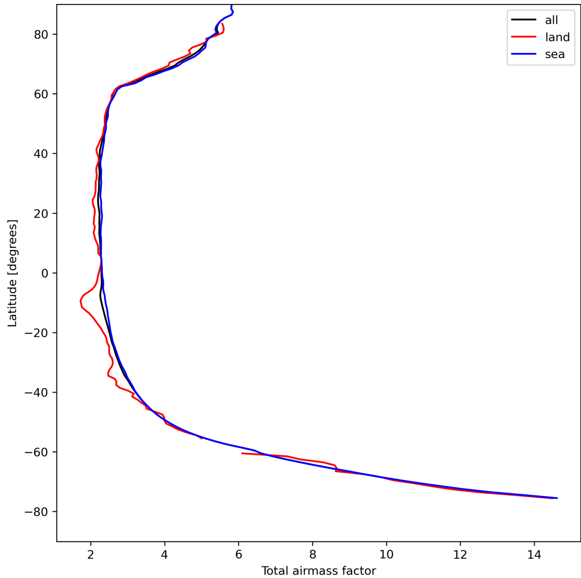
Figure 15: Zonal average of “Total airmass factor” for 2024-08-19 to 2024-08-21.
