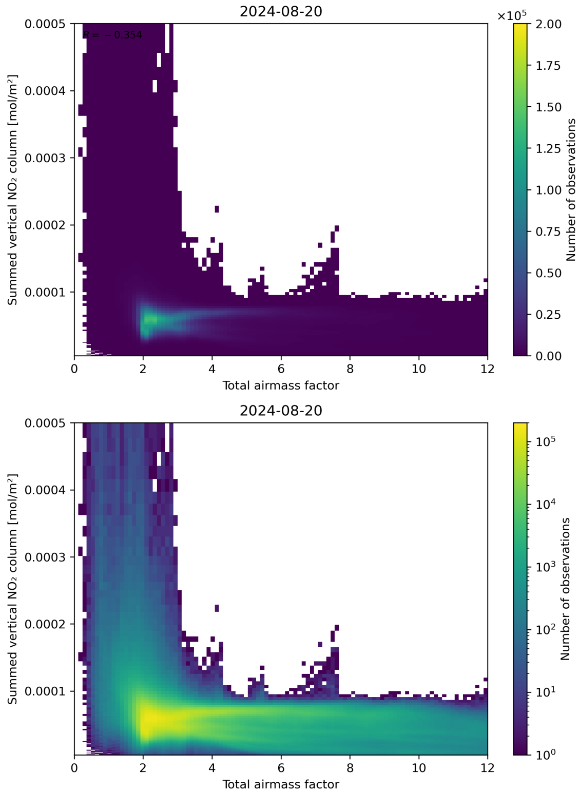
Figure 65: Scatter density plot of “Total airmass factor” against “Summed vertical NO 2 column” for 2024-08-19 to 2024-08-21.
