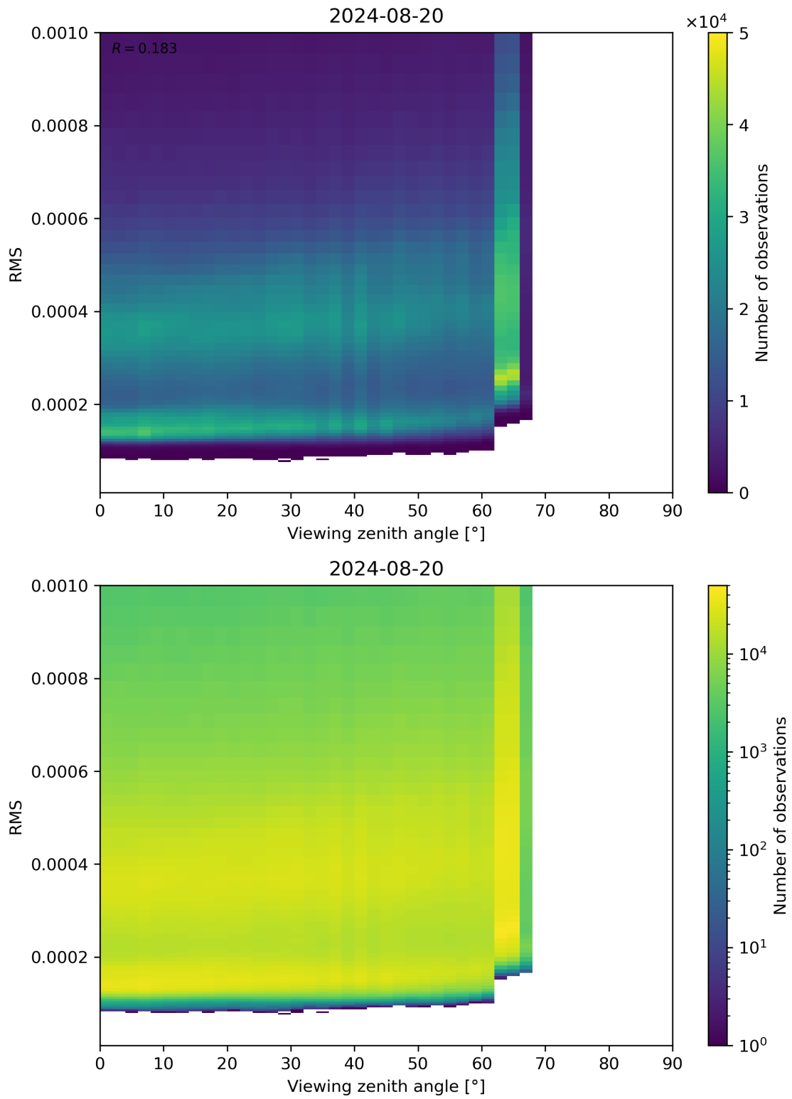
Figure 171: Scatter density plot of “Viewing zenith angle” against “RMS” for 2024-08-19 to 2024-08-21.
