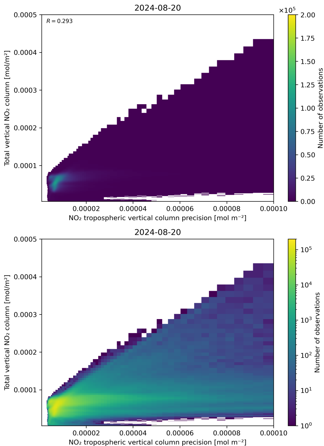
Figure 138: Scatter density plot of “NO 2 tropospheric vertical column precision” against “Total vertical NO 2 column” for 2024-08-19 to 2024-08-21.
