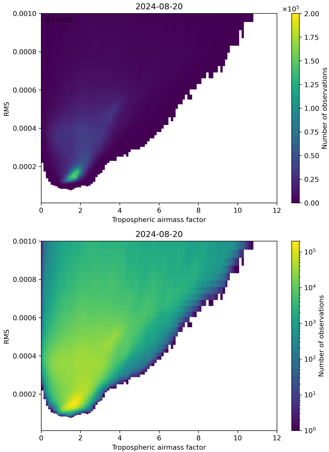
Figure 79: Scatter density plot of “Tropospheric airmass factor” against “RMS” for 2024-08-19 to 2024-08-21.
