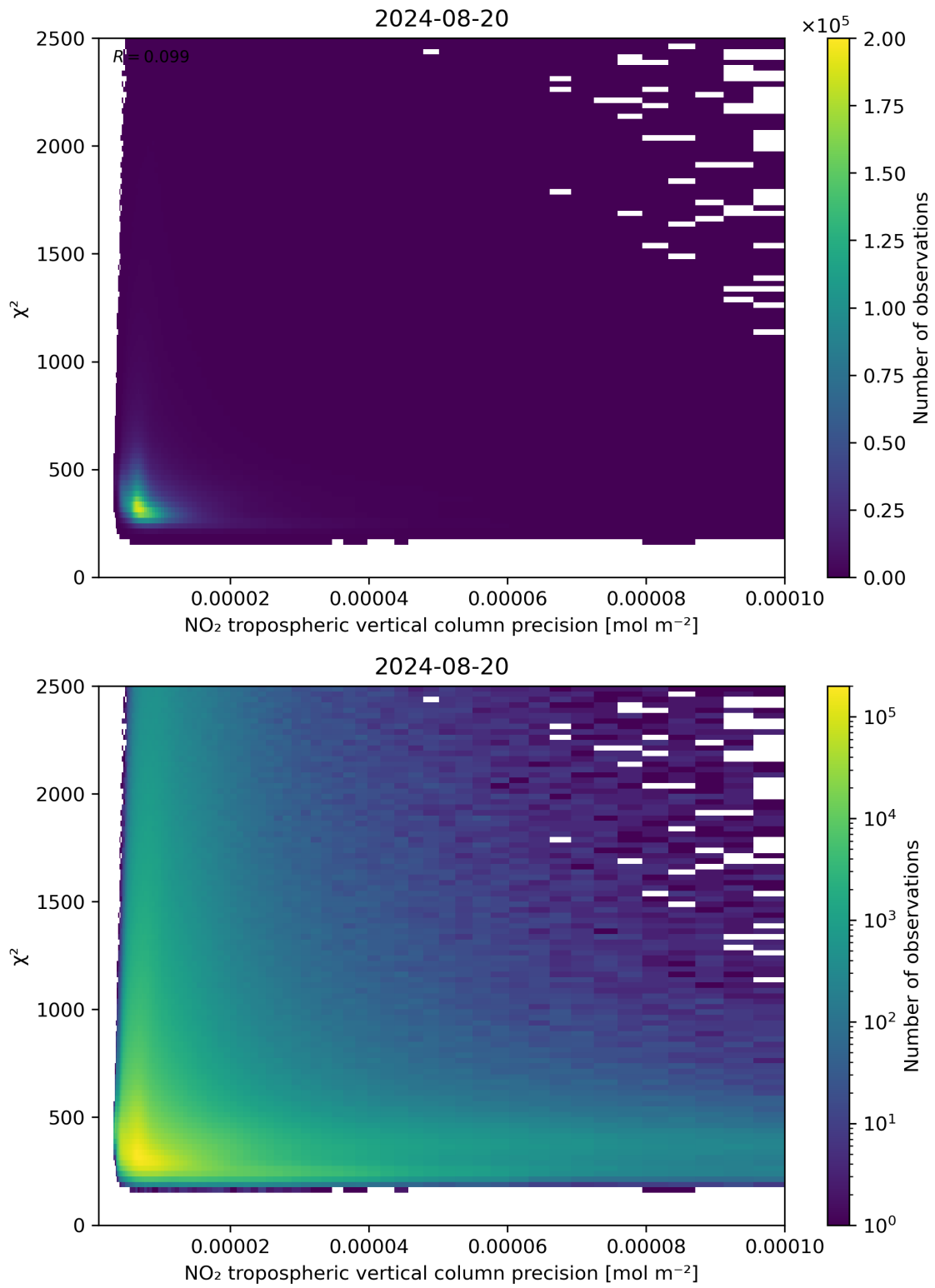
Figure 134: Scatter density plot of “NO 2 tropospheric vertical column precision” against “ \chi^2 ” for 2024-08-19 to 2024-08-21.
