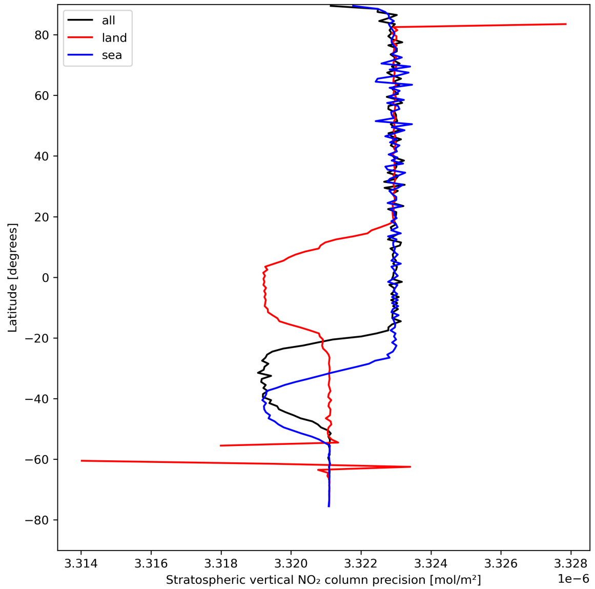
Figure 20: Zonal average of “Stratospheric vertical NO 2 column precision” for 2024-08-19 to 2024-08-21.
