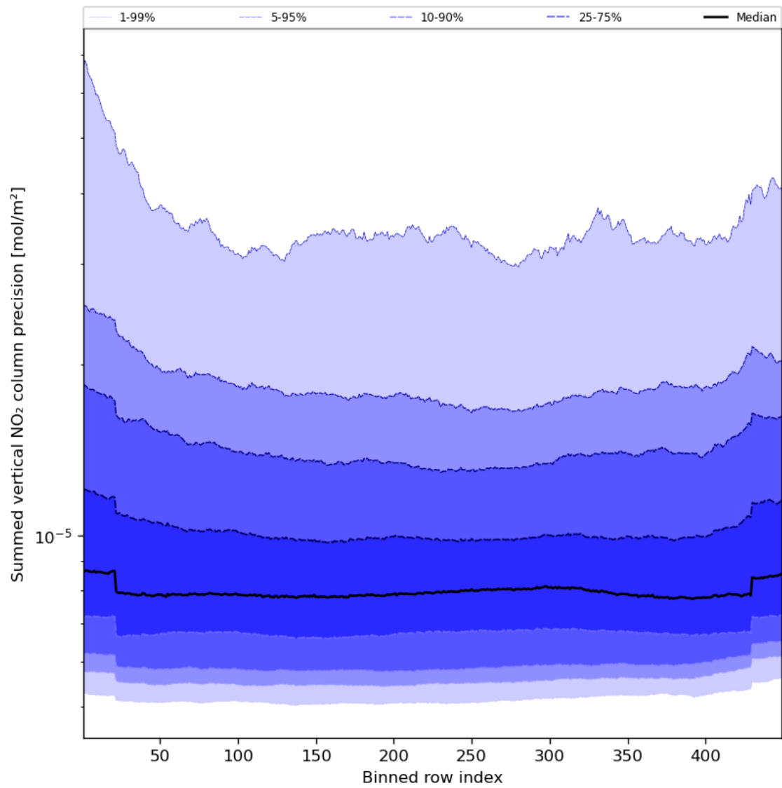
Figure 58: Along track statistics of “Summed vertical NO 2 column precision” for 2024-08-19 to 2024-08-21
