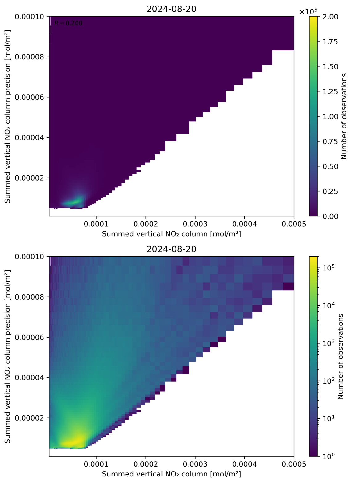
Figure 105: Scatter density plot of “Summed vertical NO 2 column” against “Summed vertical NO 2 column precision” for 2024-08-19 to 2024-08-21.
