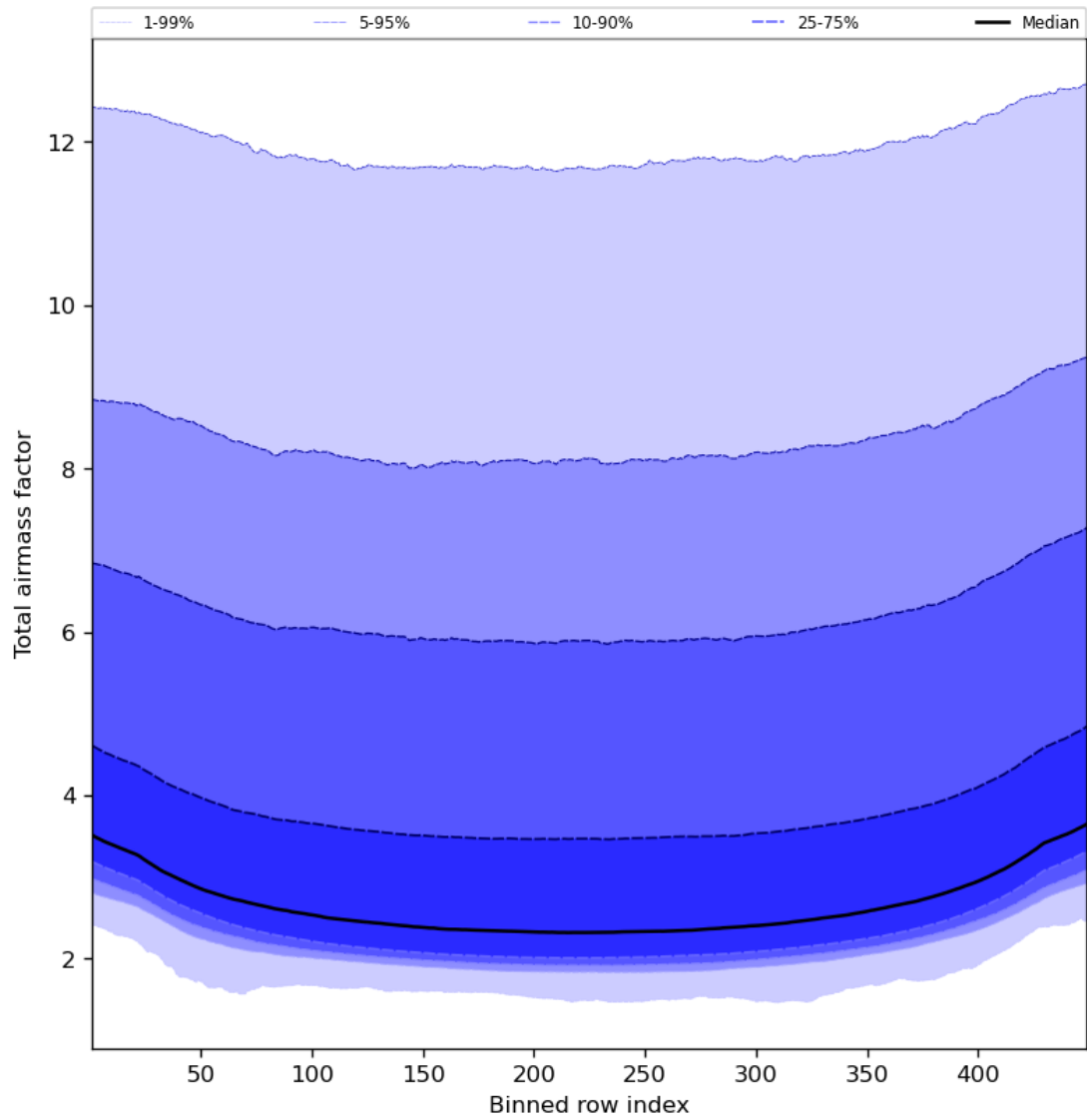
Figure 49: Along track statistics of “Total airmass factor” for 2024-08-22 to 2024-08-23
