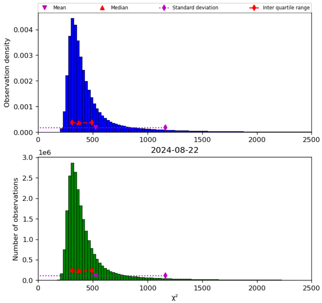
Figure 42: Histogram of “ \chi^2 ” for 2024-08-22 to 2024-08-23
