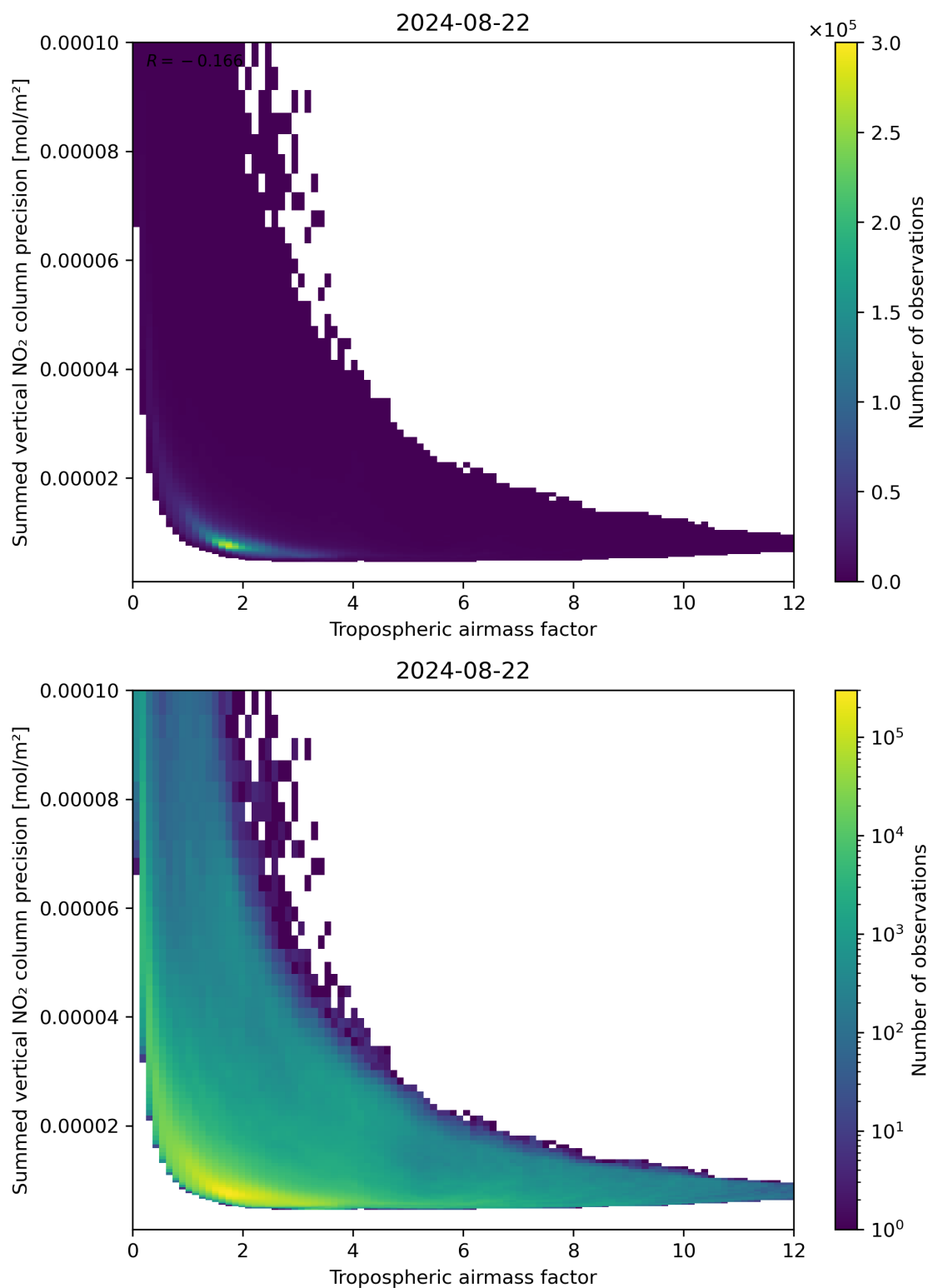
Figure 76: Scatter density plot of “Tropospheric air mass factor” against “Summed vertical NO 2 column precision” for 2024-08-22 to 2024-08-23.
