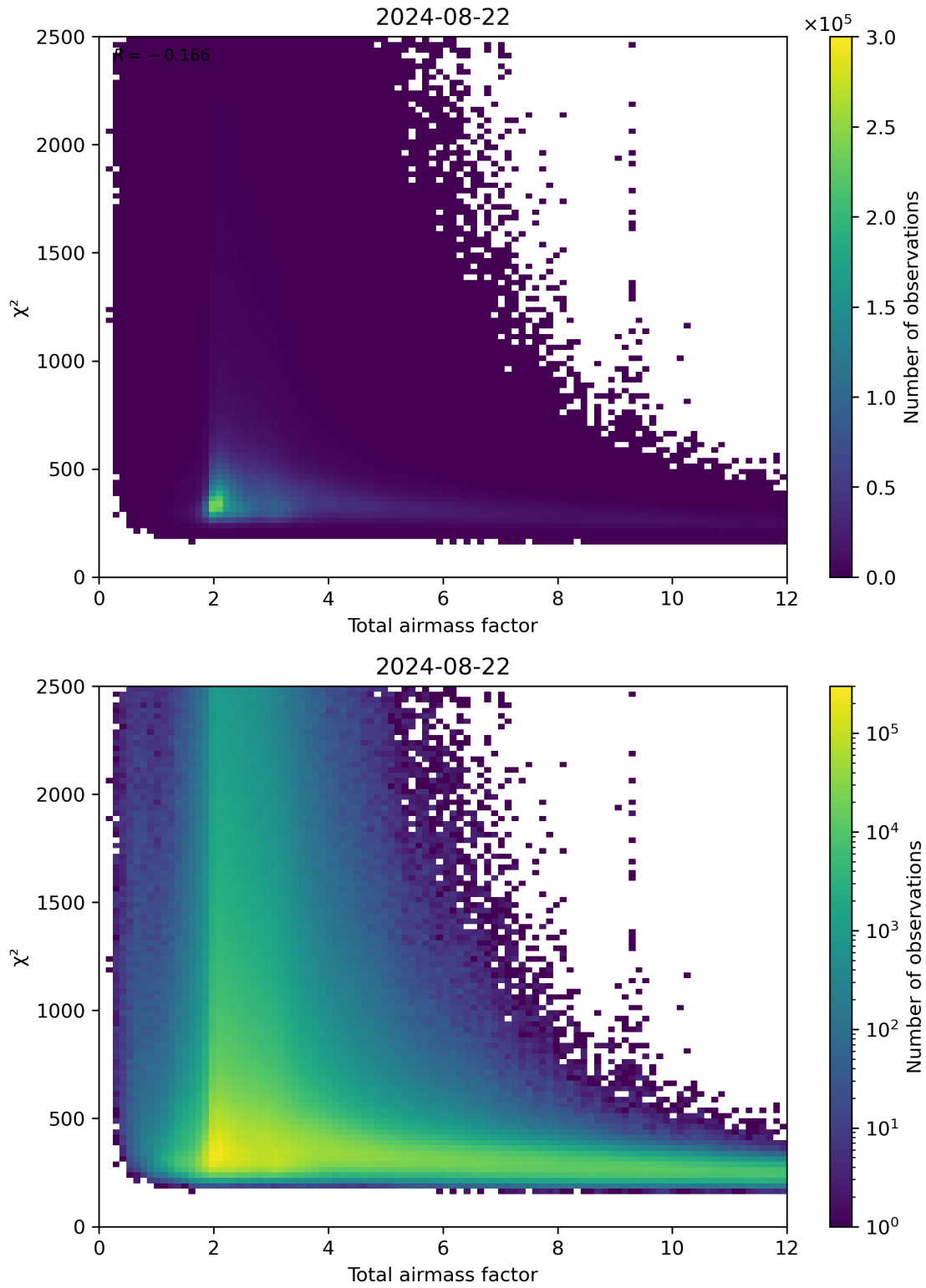
Figure 63: Scatter density plot of “Total airmass factor” against “ \chi^2 ” for 2024-08-22 to 2024-08-23.
