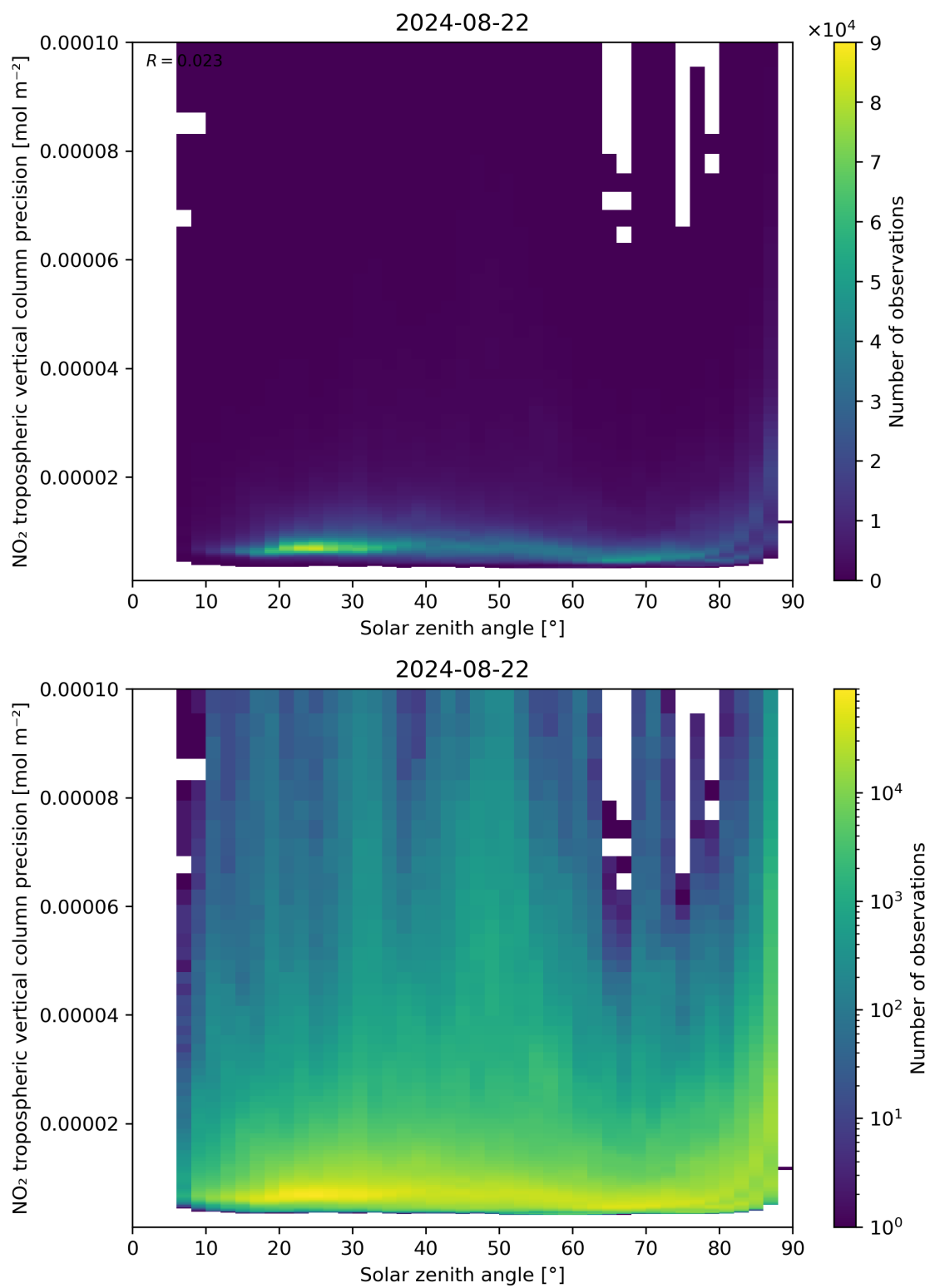
Figure 156: Scatter density plot of “Solar zenith angle” against “NO 2 tropospheric vertical column precision” for 2024-08-22 to 2024-08-23.
