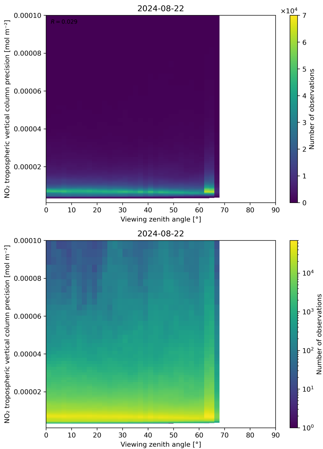
Figure 170: Scatter density plot of “Viewing zenith angle” against “NO 2 tropospheric vertical column precision” for 2024-08-22 to 2024-08-23.
