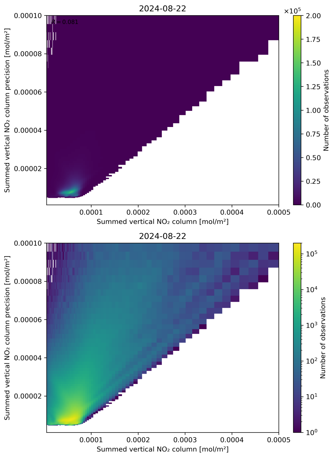
Figure 105: Scatter density plot of “Summed vertical NO 2 column” against “Summed vertical NO 2 column precision” for 2024-08-22 to 2024-08-23.
