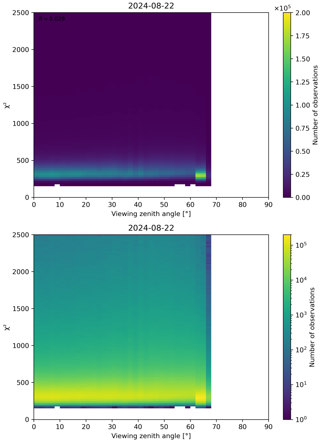
Figure 162: Scatter density plot of “Viewing zenith angle” against “ \chi^2 ” for 2024-08-22 to 2024-08-23.
