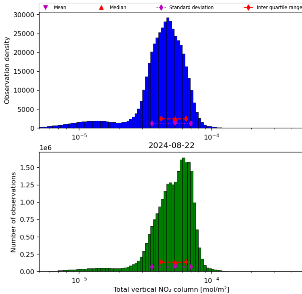
Figure 38: Histogram of “Total vertical NO 2 column” for 2024-08-22 to 2024-08-23
