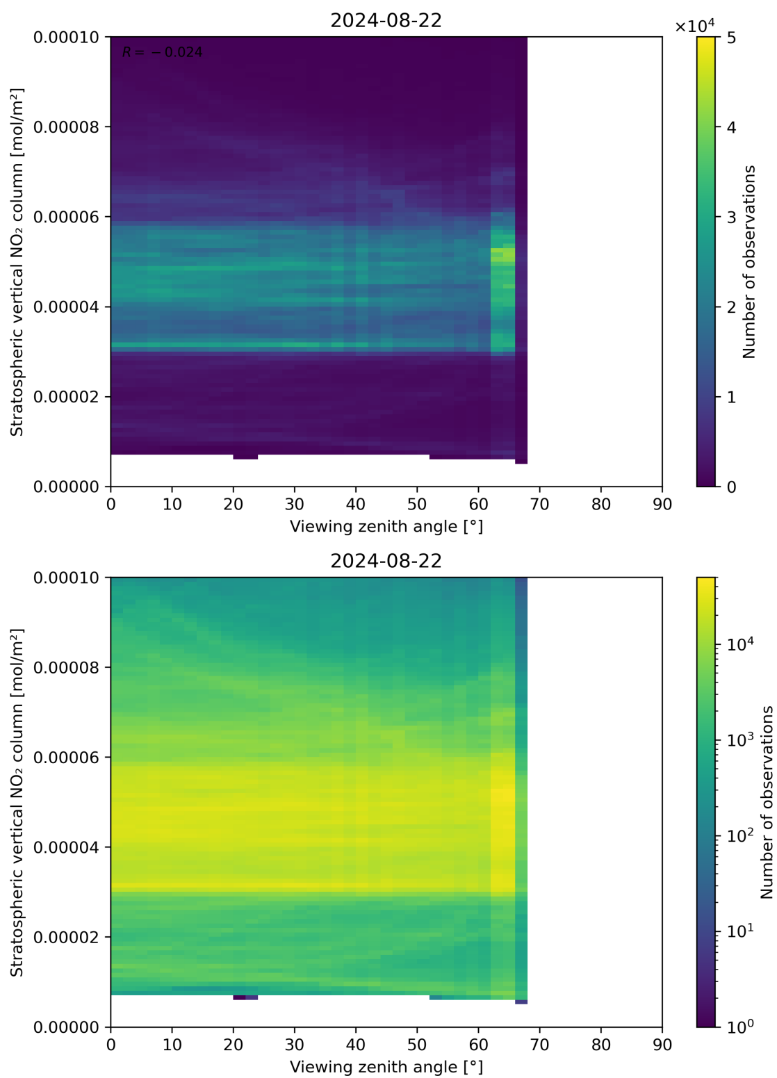
Figure 164: Scatter density plot of “Viewing zenith angle” against “Stratospheric vertical NO 2 column” for 2024-08-22 to 2024-08-23.
