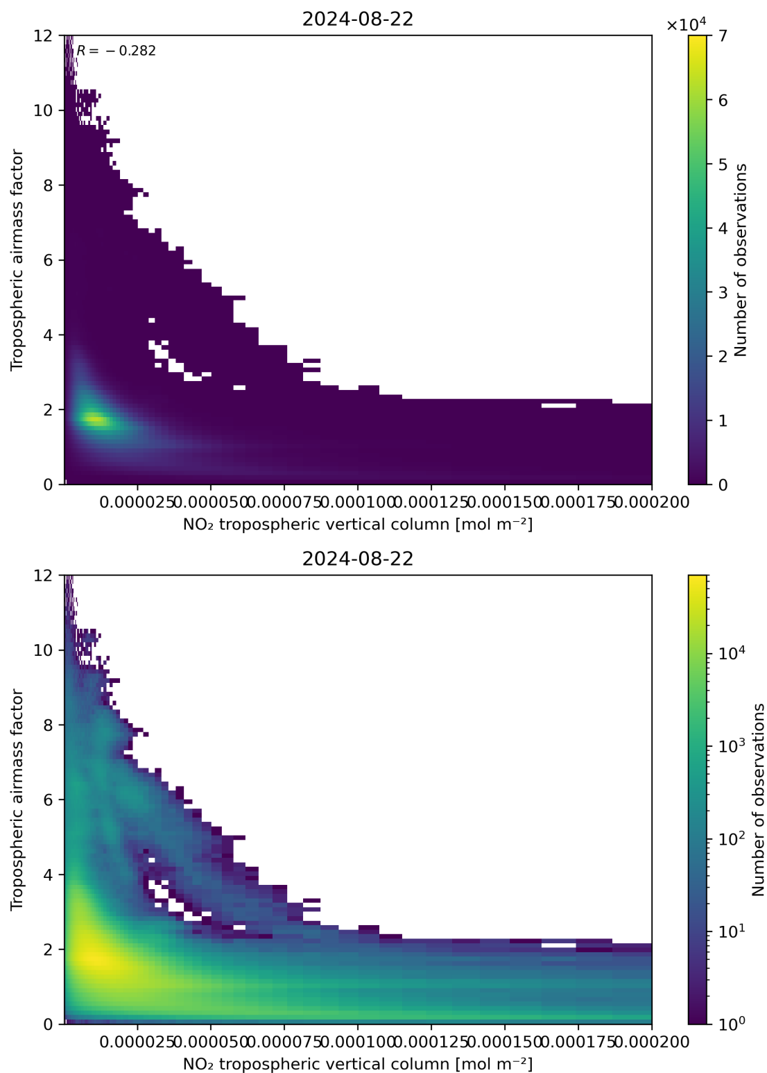
Figure 123: Scatter density plot of “NO 2 tropospheric vertical column” against “Tropospheric air mass factor” for 2024-08-22 to 2024-08-23.
