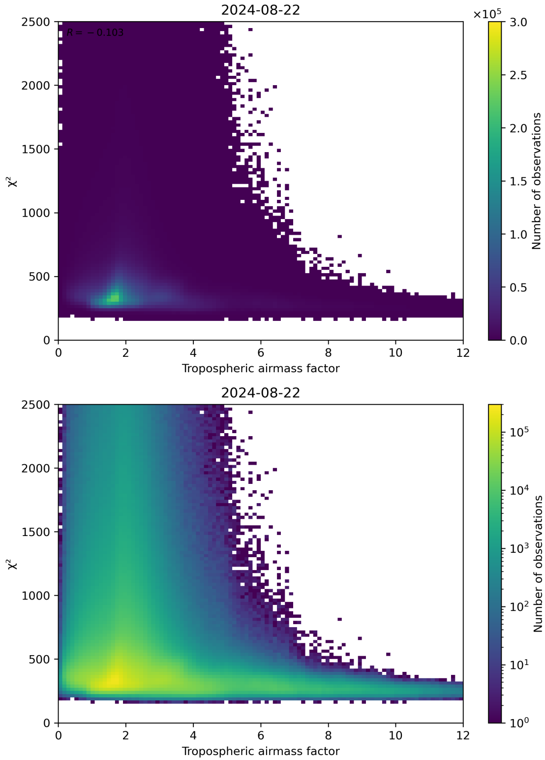
Figure 73: Scatter density plot of “Tropospheric airmass factor” against “ \chi^2 ” for 2024-08-22 to 2024-08-23.
