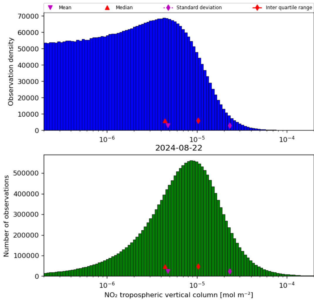
Figure 29: Histogram of “NO 2 tropospheric vertical column” for 2024-08-22 to 2024-08-23
