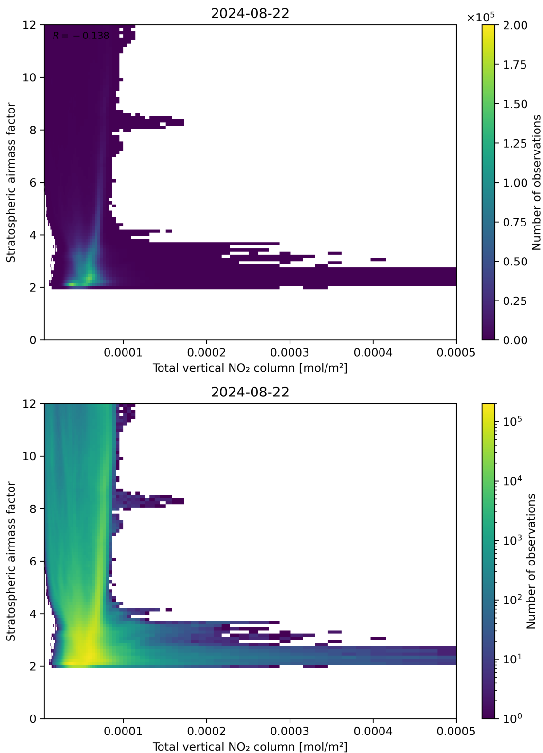
Figure 110: Scatter density plot of “Total vertical NO 2 column” against “Stratospheric airmass factor” for 2024-08-22 to 2024-08-23.
