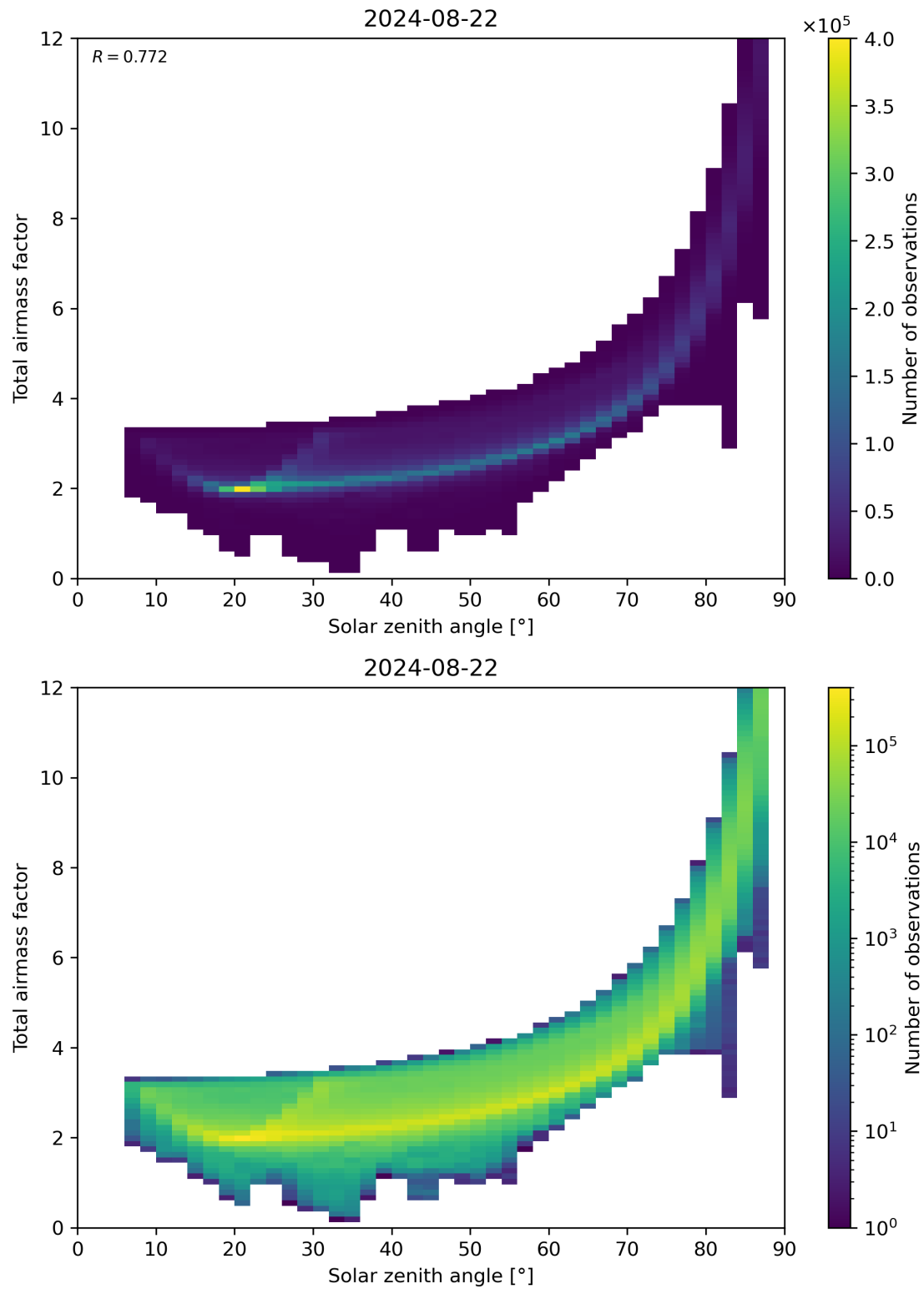
Figure 146: Scatter density plot of “Solar zenith angle” against “Total air mass factor” for 2024-08-22 to 2024-08-23.
