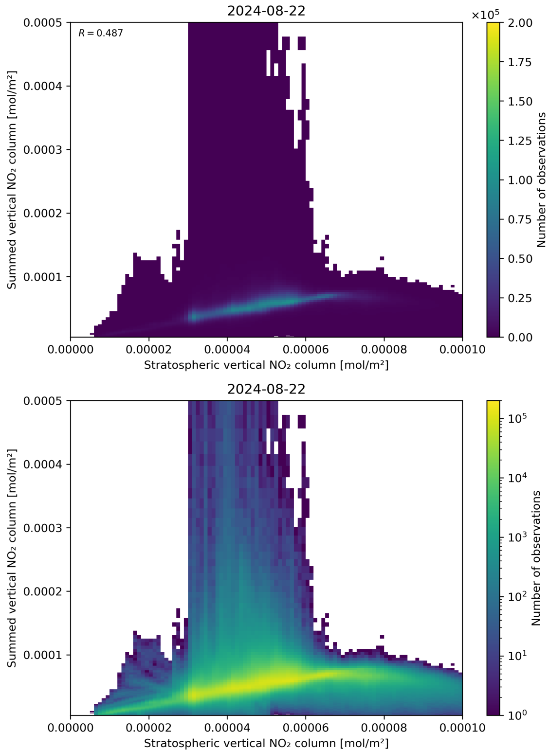
Figure 98: Scatter density plot of “Stratospheric vertical NO 2 column” against “Summed vertical NO 2 column” for 2024-08-22 to 2024-08-23.
