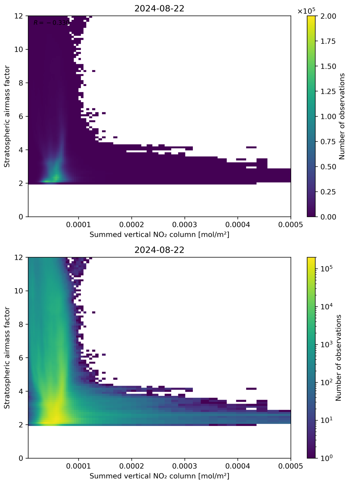
Figure 103: Scatter density plot of “Summed vertical NO 2 column” against “Stratospheric air mass factor” for 2024-08-22 to 2024-08-23.
