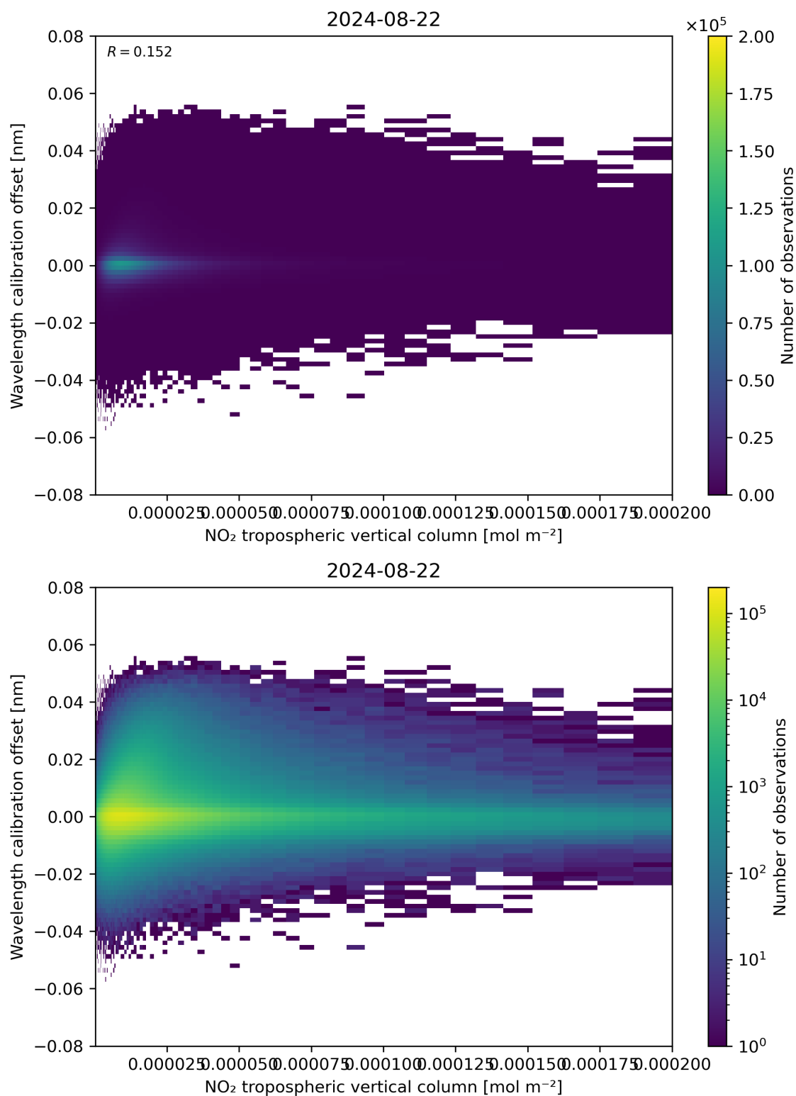
Figure 143: Scatter density plot of “NO 2 tropospheric vertical column” against “Wavelength calibration offset” for 2024-08-22 to 2024-08-23.
