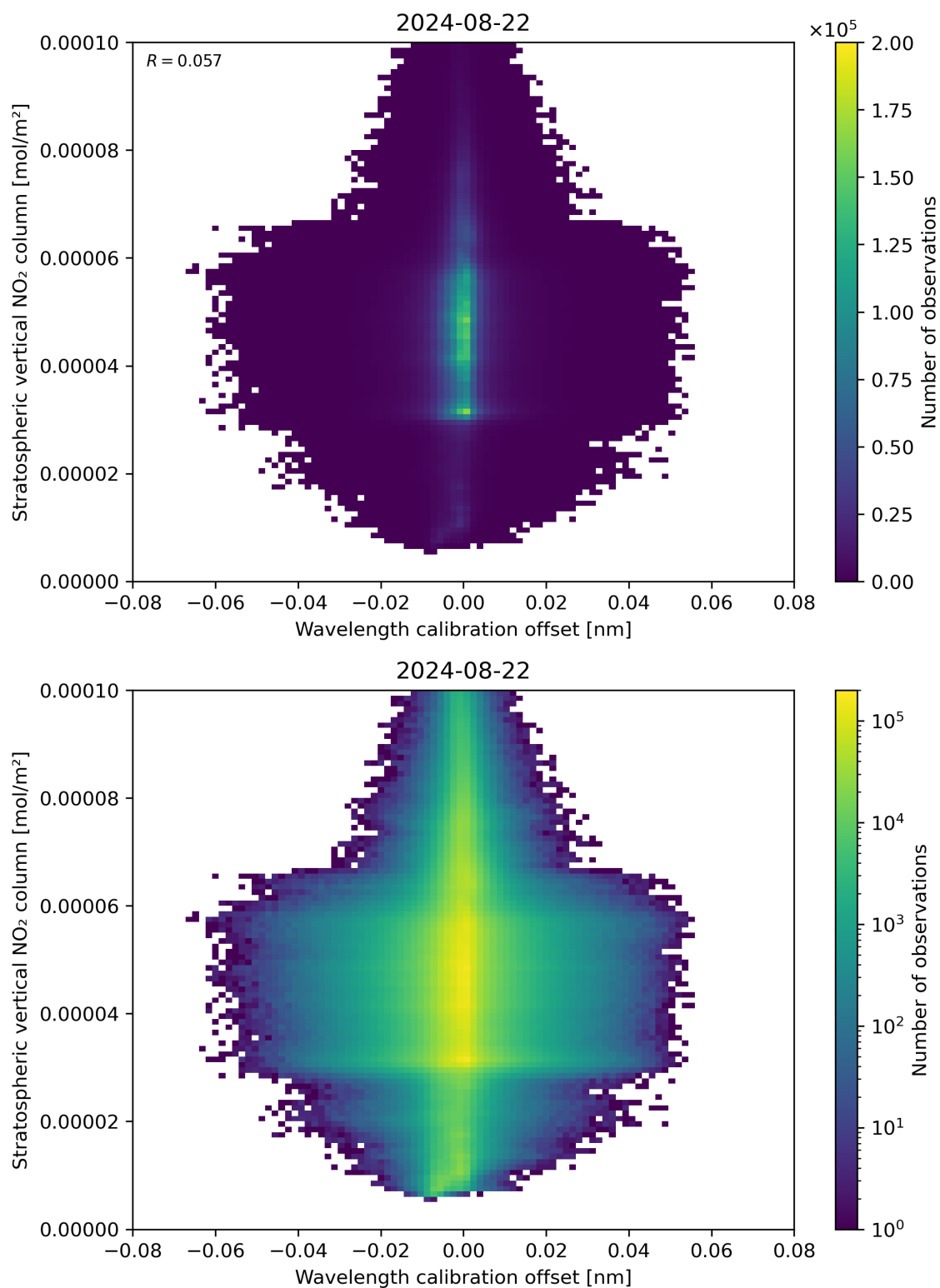
Figure 176: Scatter density plot of “Wavelength calibration offset” against “Stratospheric vertical NO 2 column” for 2024-08-22 to 2024-08-23.
