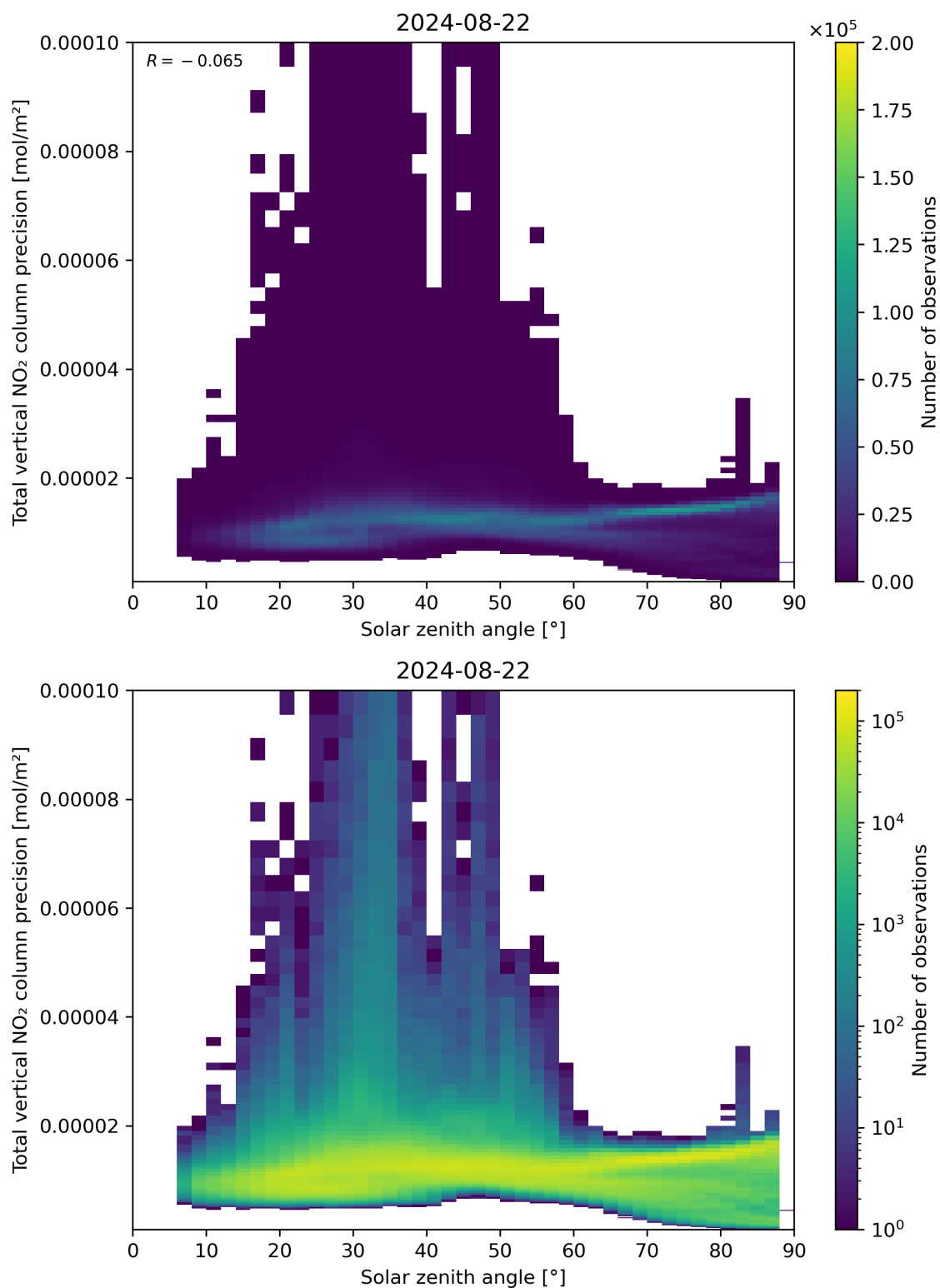
Figure 154: Scatter density plot of “Solar zenith angle” against “Total vertical NO 2 column precision” for 2024-08-22 to 2024-08-23.
