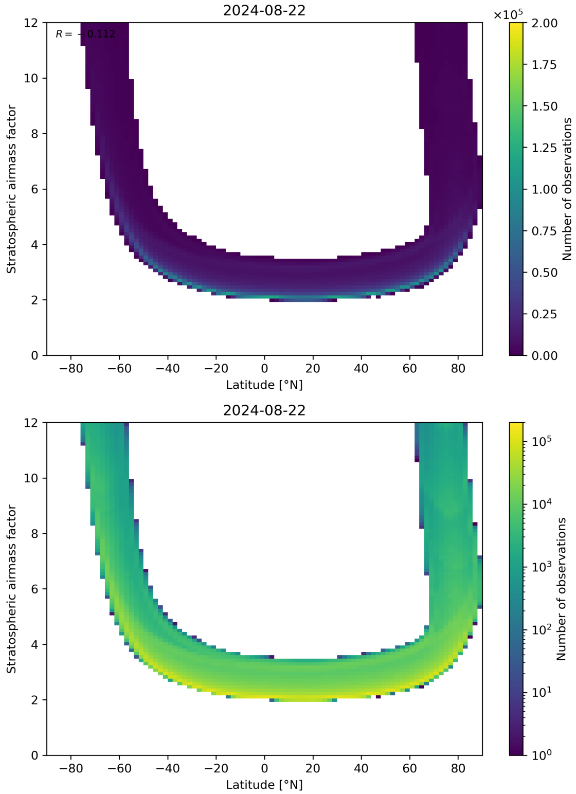
Figure 83: Scatter density plot of “Latitude” against “Stratospheric air mass factor” for 2024-08-22 to 2024-08-23.
