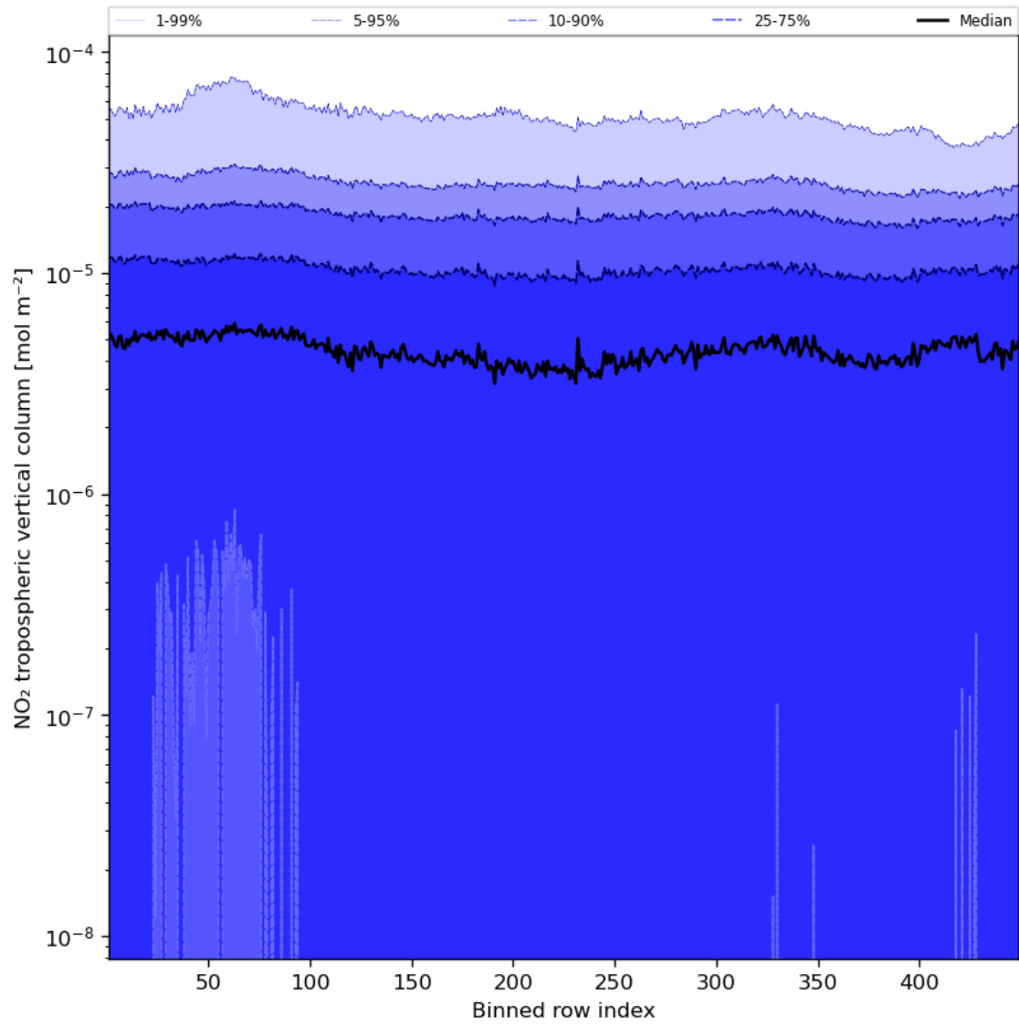
Figure 46: Along track statistics of “NO 2 tropospheric vertical column” for 2024-08-22 to 2024-08-23
