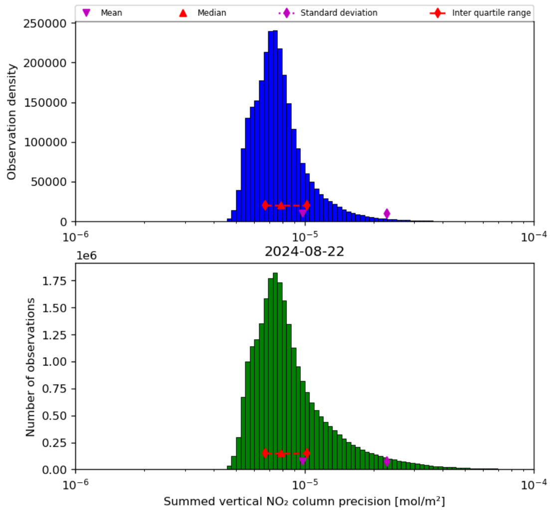
Figure 41: Histogram of “Summed vertical NO 2 column precision” for 2024-08-22 to 2024-08-23
