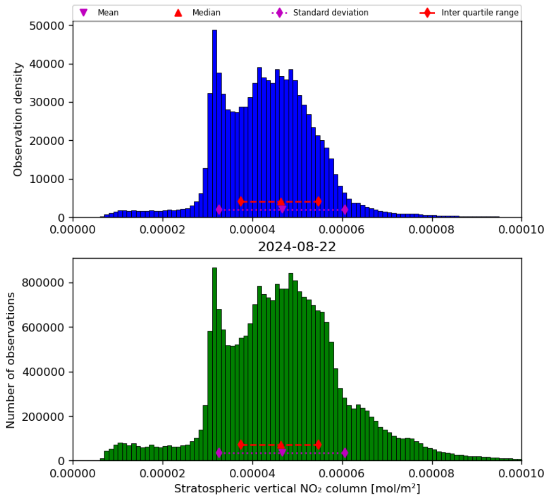
Figure 36: Histogram of “Stratospheric vertical NO 2 column” for 2024-08-22 to 2024-08-23
