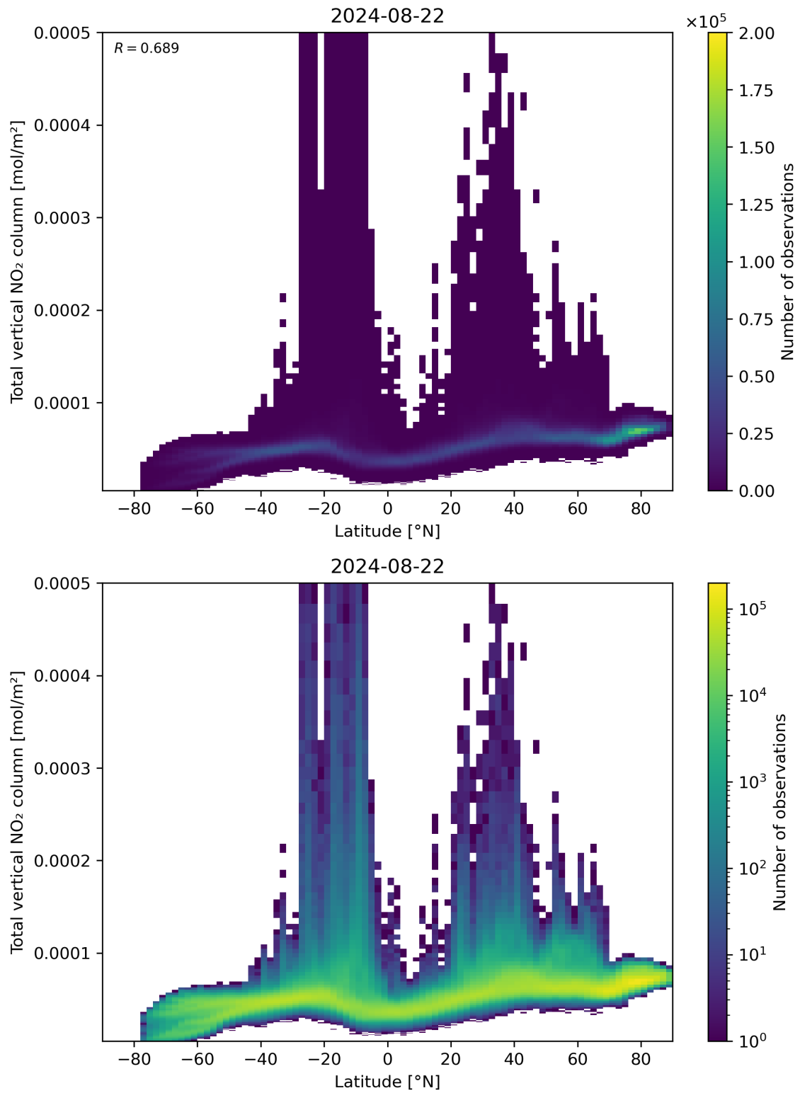
Figure 90: Scatter density plot of “Latitude” against “Total vertical NO 2 column” for 2024-08-22 to 2024-08-23.
