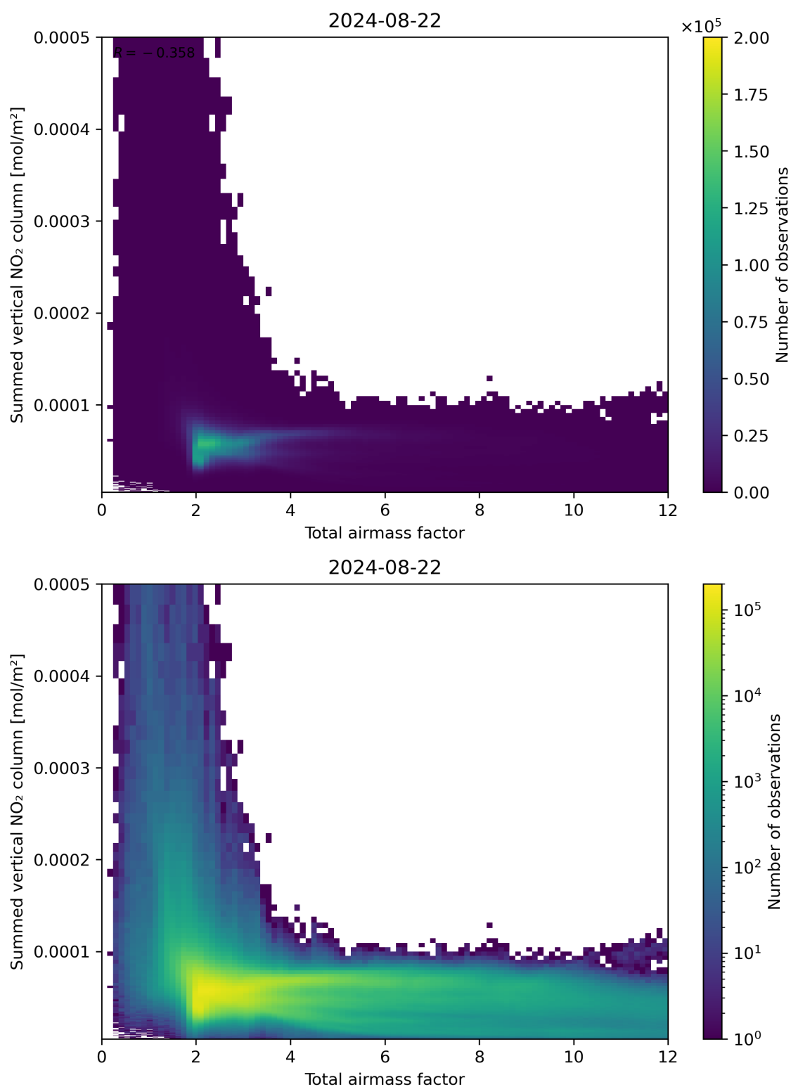
Figure 65: Scatter density plot of “Total airmass factor” against “Summed vertical NO 2 column” for 2024-08-22 to 2024-08-23.
