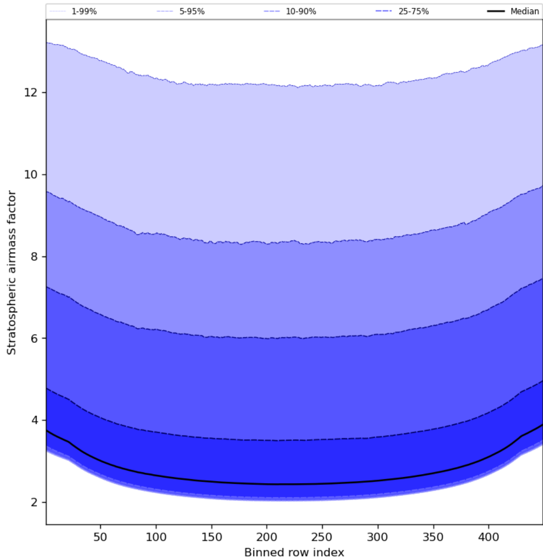
Figure 61: Along track statistics of “Stratospheric airmass factor” for 2024-08-22 to 2024-08-23
