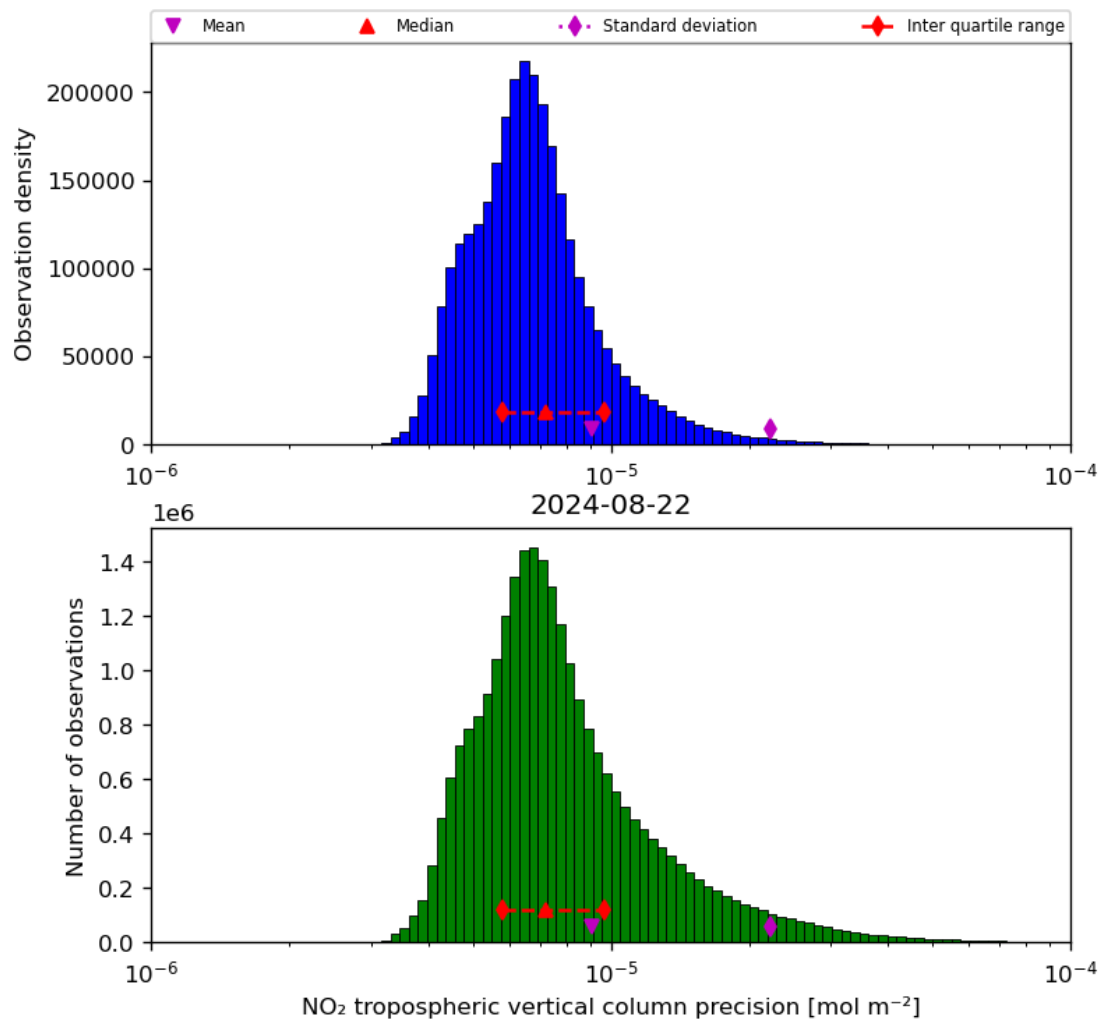
Figure 30: Histogram of “NO 2 tropospheric vertical column precision” for 2024-08-22 to 2024-08-23
