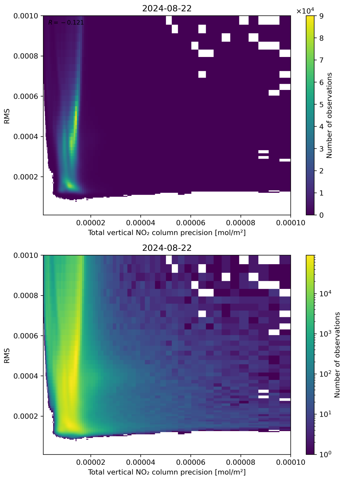
Figure 119: Scatter density plot of “Total vertical NO 2 column precision” against “RMS” for 2024-08-22 to 2024-08-23.
