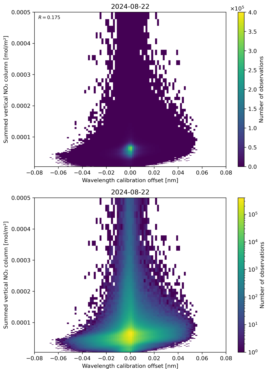
Figure 177: Scatter density plot of “Wavelength calibration offset” against “Summed vertical NO 2 column” for 2024-08-22 to 2024-08-23.
