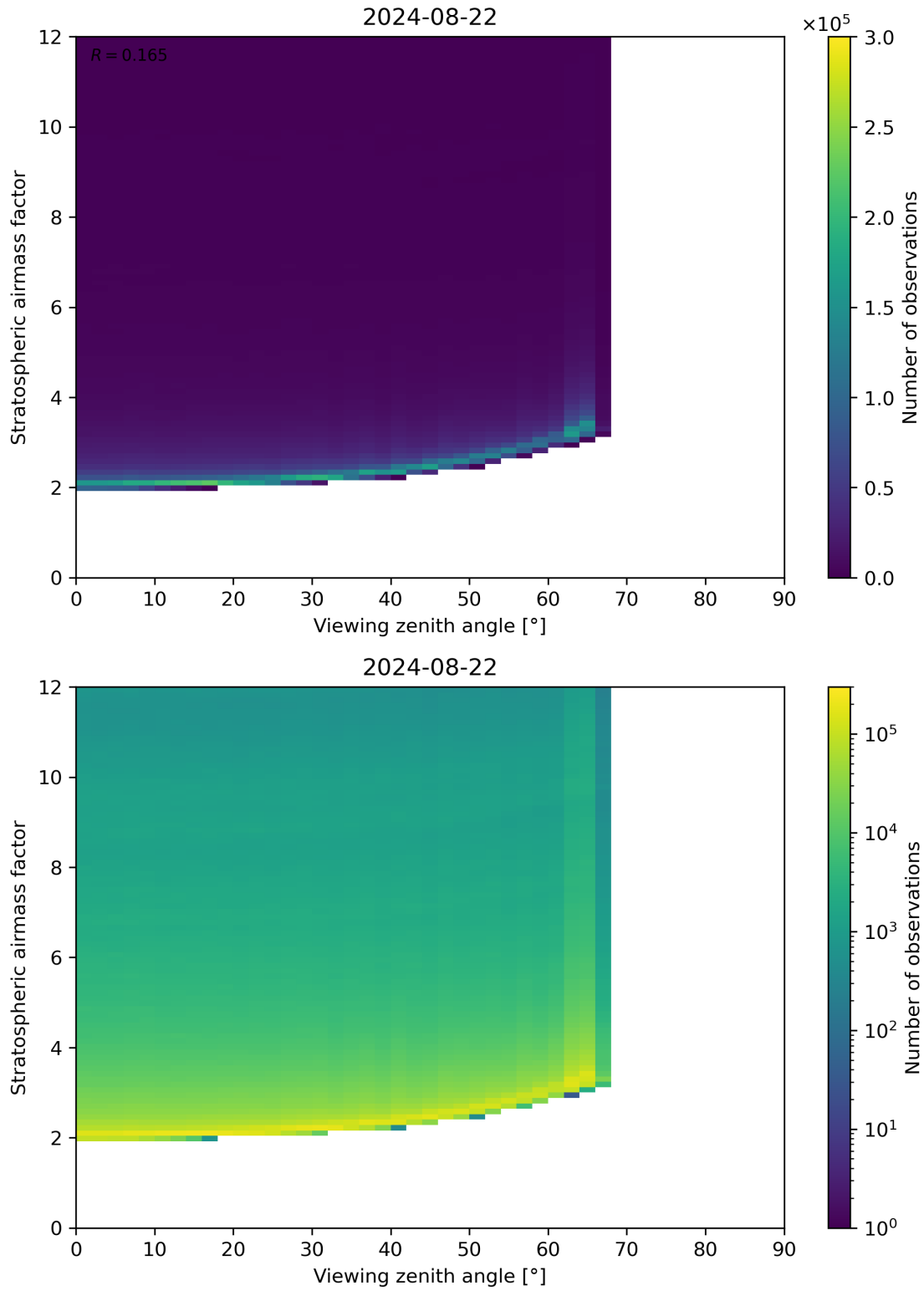
Figure 159: Scatter density plot of “Viewing zenith angle” against “Stratospheric airmass factor” for 2024-08-22 to 2024-08-23.
