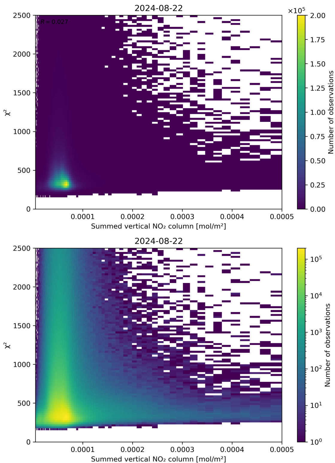
Figure 104: Scatter density plot of “Summed vertical NO 2 column” against “ \chi^2 ” for 2024-08-22 to 2024-08-23.
