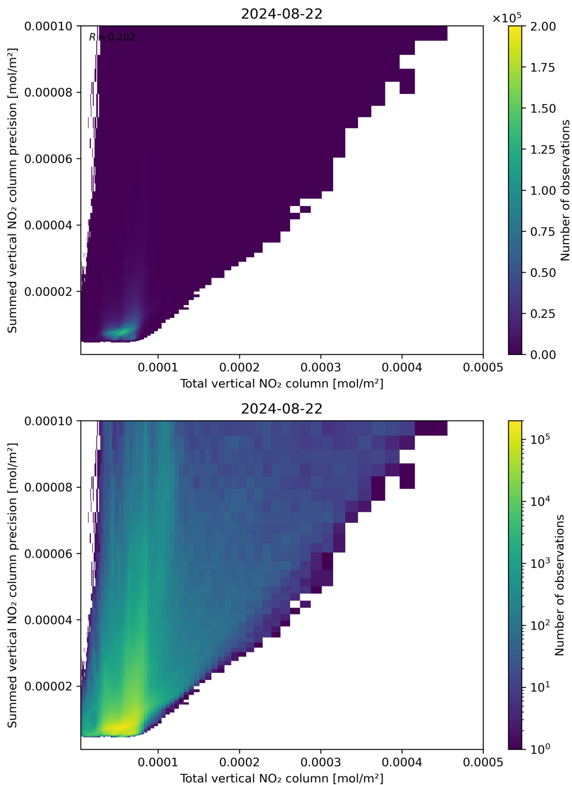
Figure 113: Scatter density plot of “Total vertical NO 2 column” against “Summed vertical NO 2 column precision” for 2024-08-22 to 2024-08-23.
