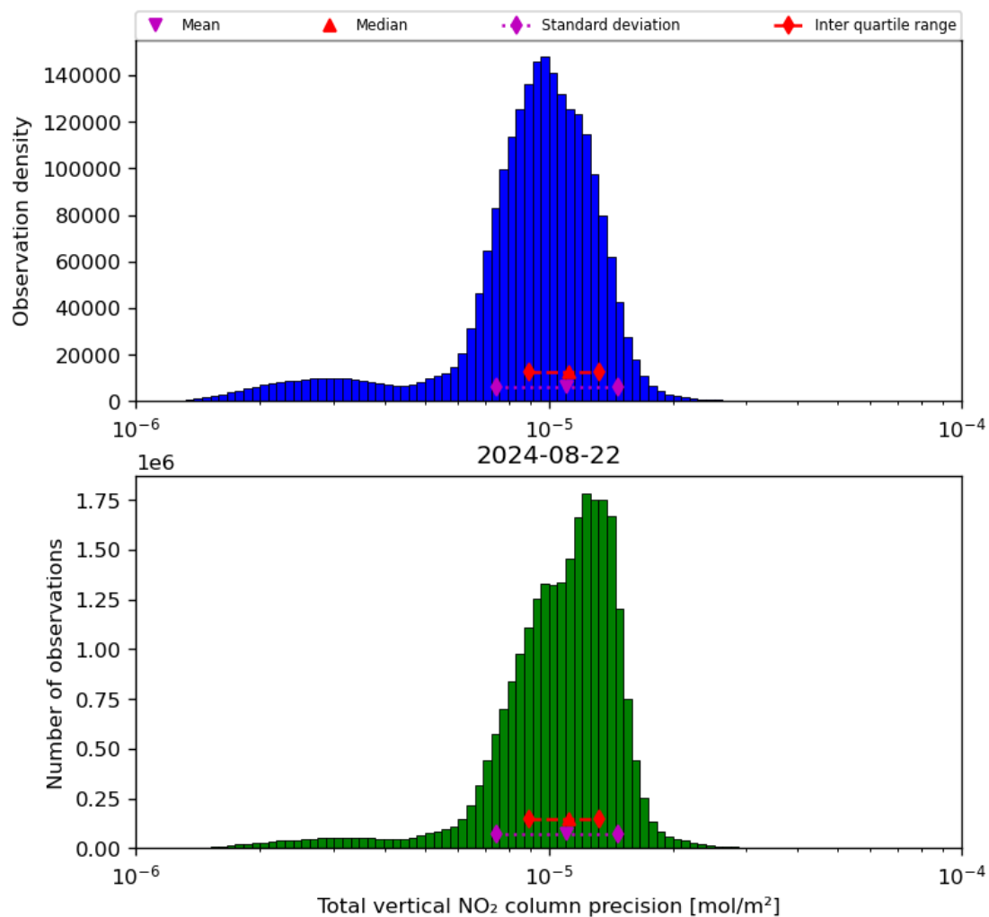
Figure 39: Histogram of “Total vertical NO 2 column precision” for 2024-08-22 to 2024-08-23
