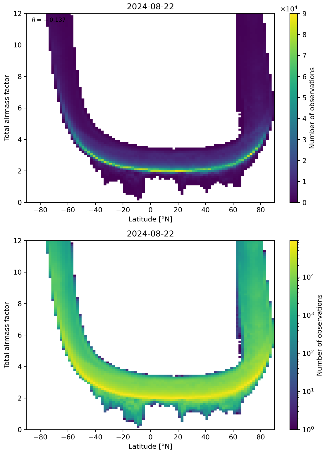
Figure 84: Scatter density plot of “Latitude” against “Total airmass factor” for 2024-08-22 to 2024-08-23.
