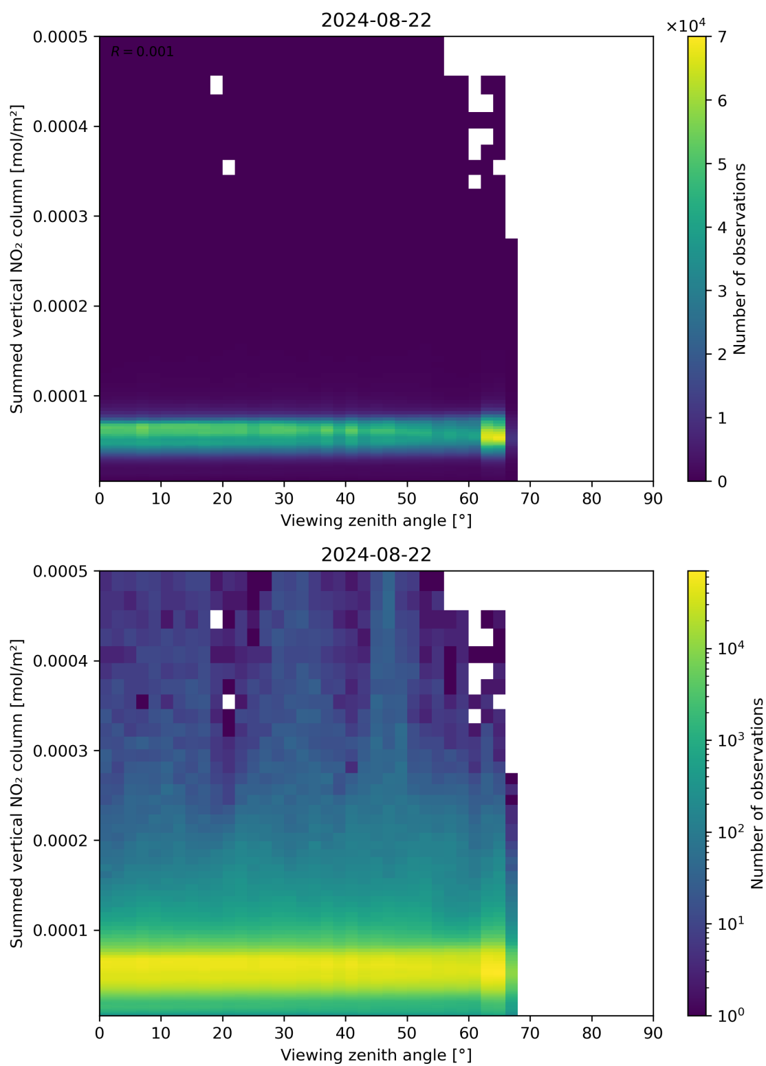
Figure 165: Scatter density plot of “Viewing zenith angle” against “Summed vertical NO 2 column” for 2024-08-22 to 2024-08-23.
