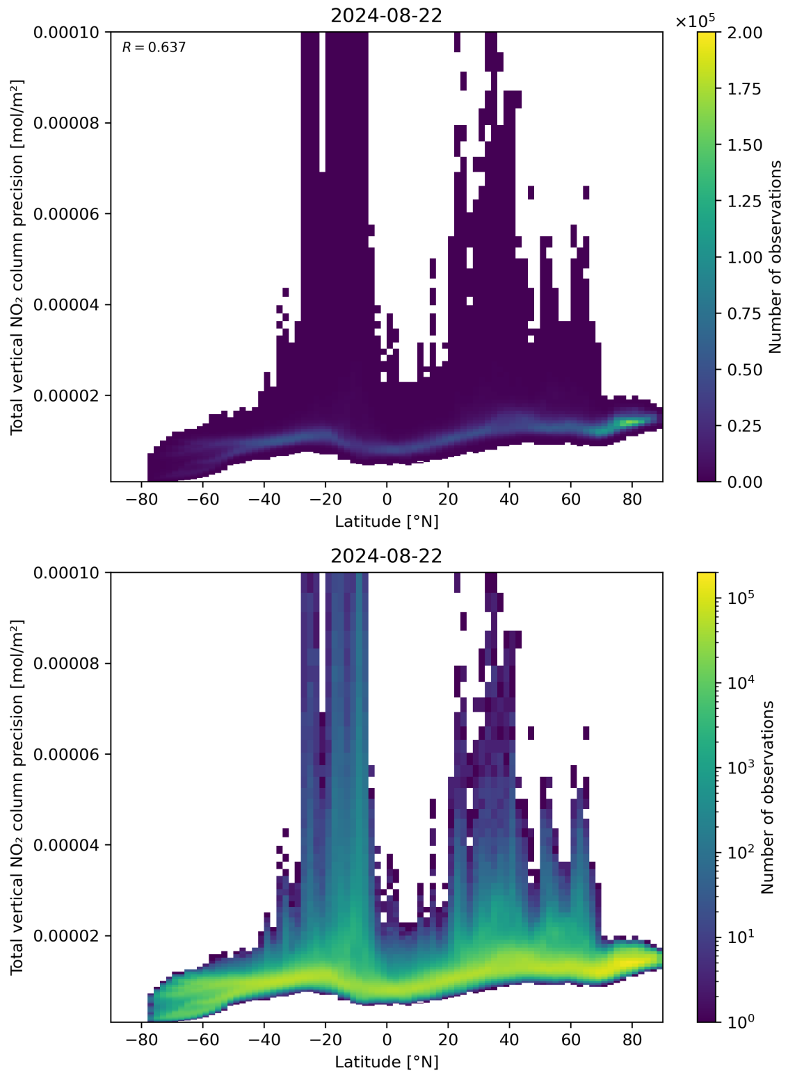
Figure 91: Scatter density plot of “Latitude” against “Total vertical NO 2 column precision” for 2024-08-22 to 2024-08-23.
