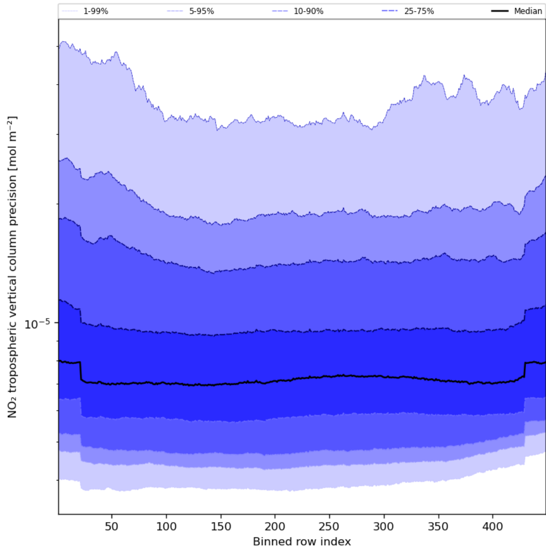
Figure 47: Along track statistics of “NO 2 tropospheric vertical column precision” for 2024-08-22 to 2024-08-23
