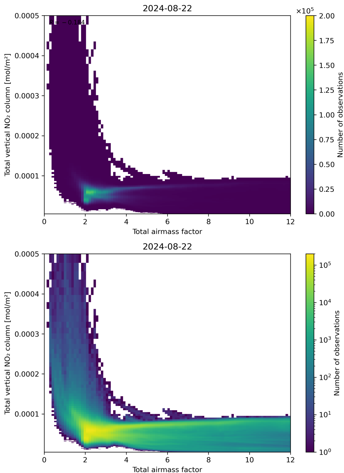
Figure 67: Scatter density plot of “Total airmass factor” against “Total vertical NO 2 column” for 2024-08-22 to 2024-08-23.
