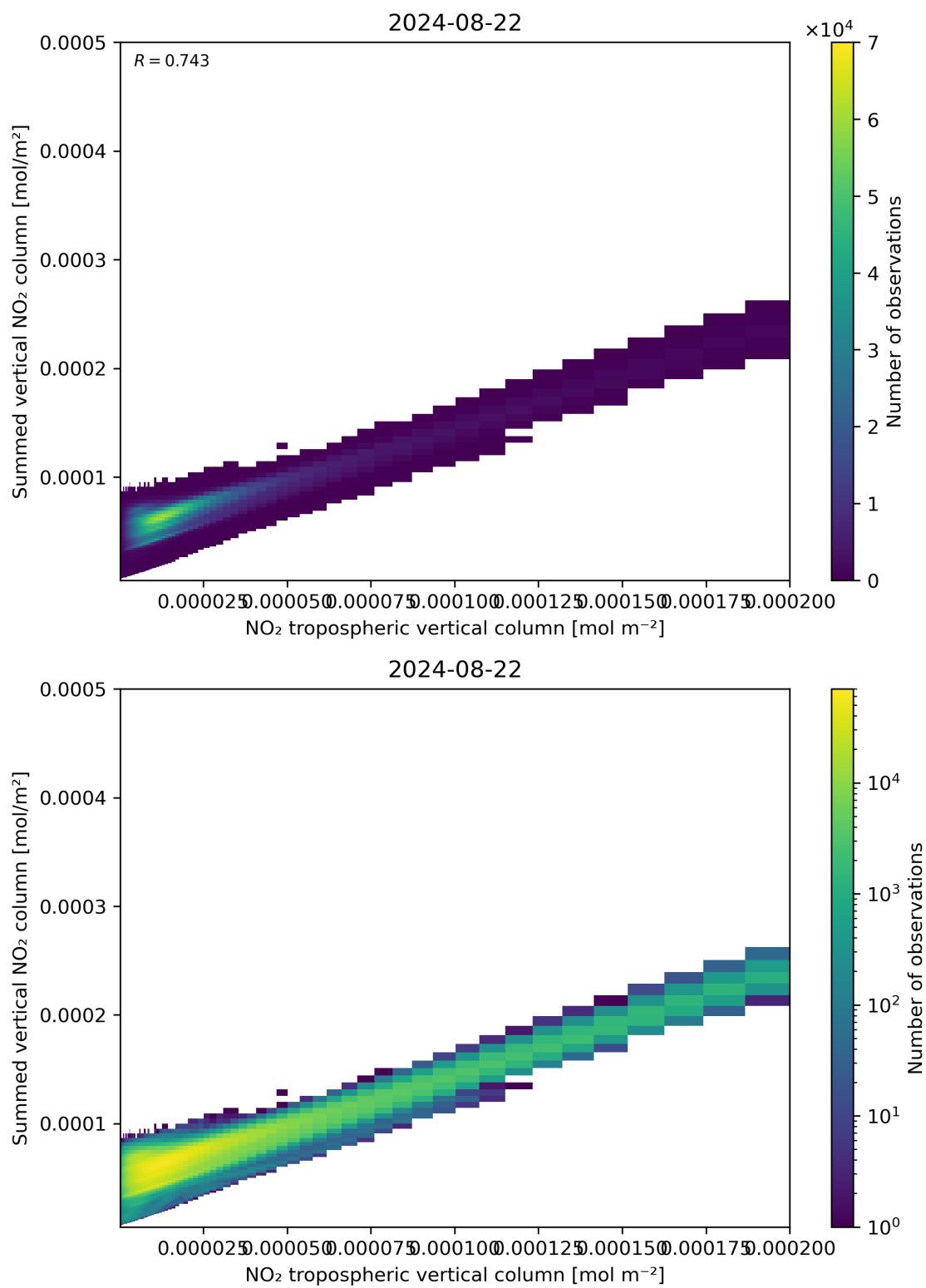
Figure 126: Scatter density plot of “NO 2 tropospheric vertical column” against “Summed vertical NO 2 column” for 2024-08-22 to 2024-08-23.
