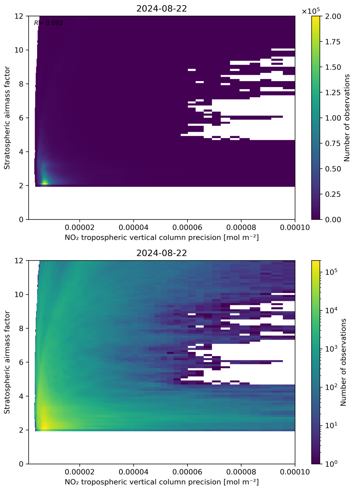
Figure 131: Scatter density plot of “NO 2 tropospheric vertical column precision” against “Stratospheric airmass factor” for 2024-08-22 to 2024-08-23.
