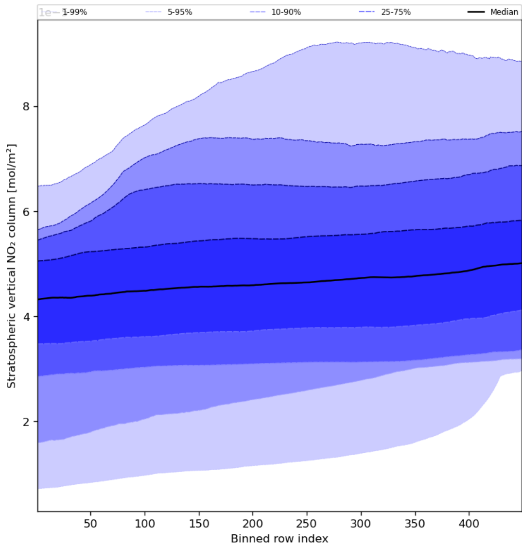
Figure 53: Along track statistics of “Stratospheric vertical NO 2 column” for 2024-08-22 to 2024-08-23
