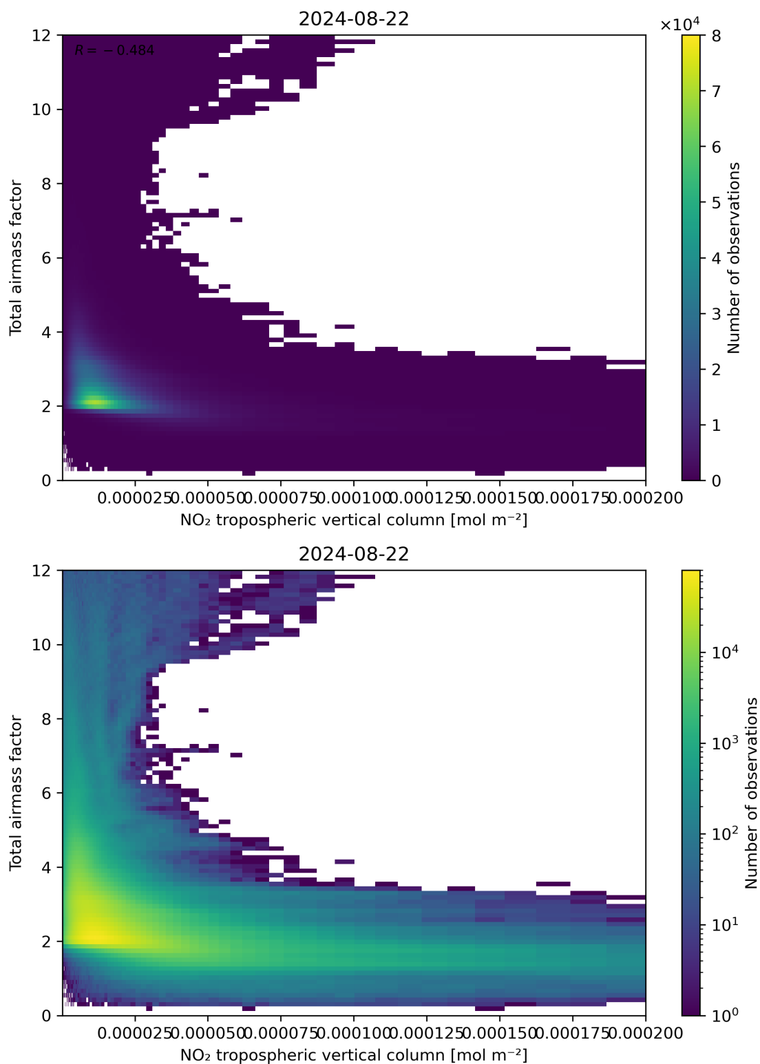
Figure 122: Scatter density plot of “NO 2 tropospheric vertical column” against “Total air mass factor” for 2024-08-22 to 2024-08-23.
