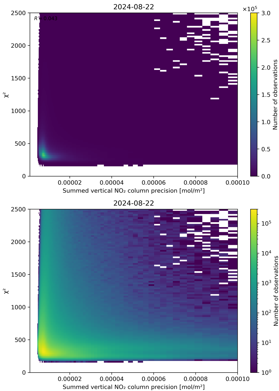
Figure 107: Scatter density plot of “Summed vertical NO 2 column precision” against “ \chi^2 ” for 2024-08-22 to 2024-08-23.
