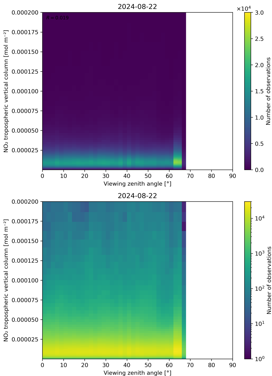
Figure 169: Scatter density plot of “Viewing zenith angle” against “NO 2 tropospheric vertical column” for 2024-08-22 to 2024-08-23.
