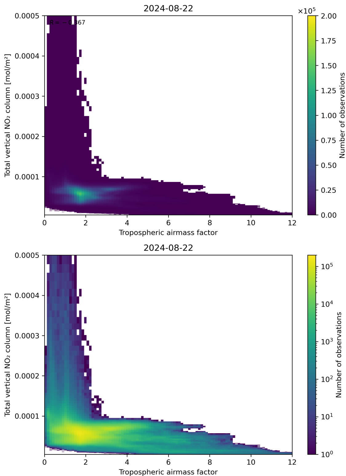
Figure 77: Scatter density plot of “Tropospheric airmass factor” against “Total vertical NO 2 column” for 2024-08-22 to 2024-08-23.
