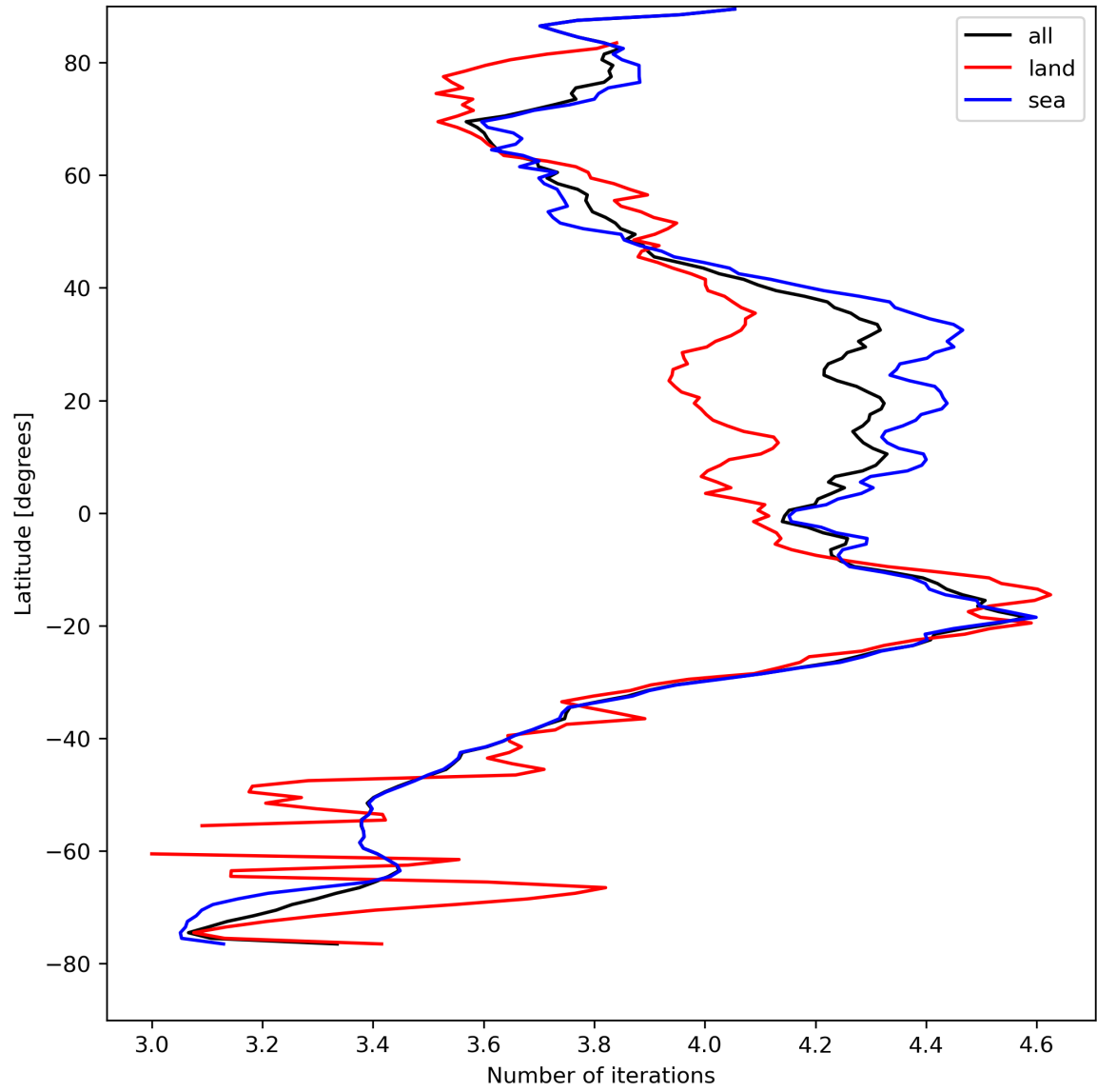
Figure 17: Zonal average of “Number of iterations” for 2024-08-22 to 2024-08-23.
