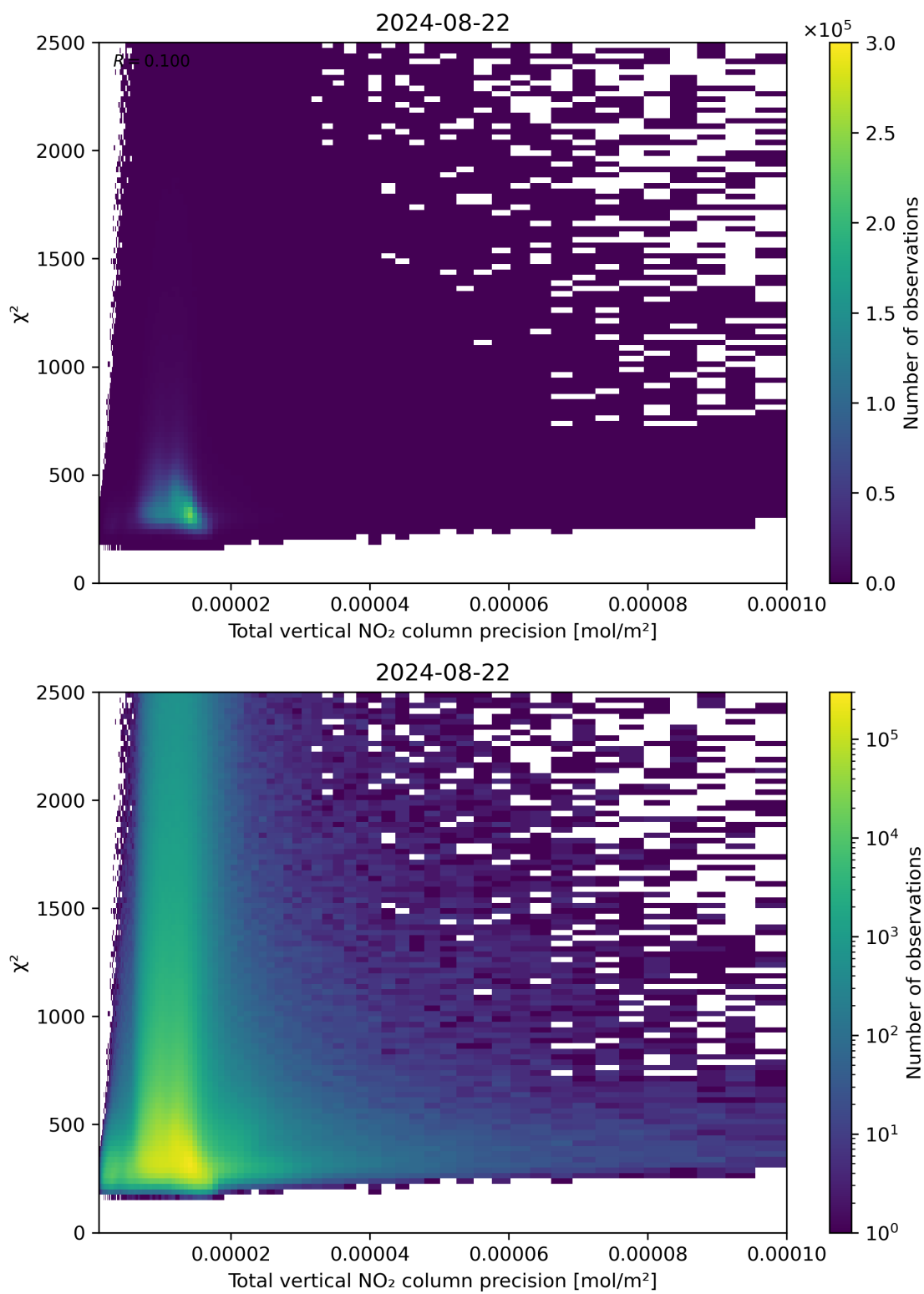
Figure 116: Scatter density plot of “Total vertical NO 2 column precision” against “ \chi^2 ” for 2024-08-22 to 2024-08-23.
