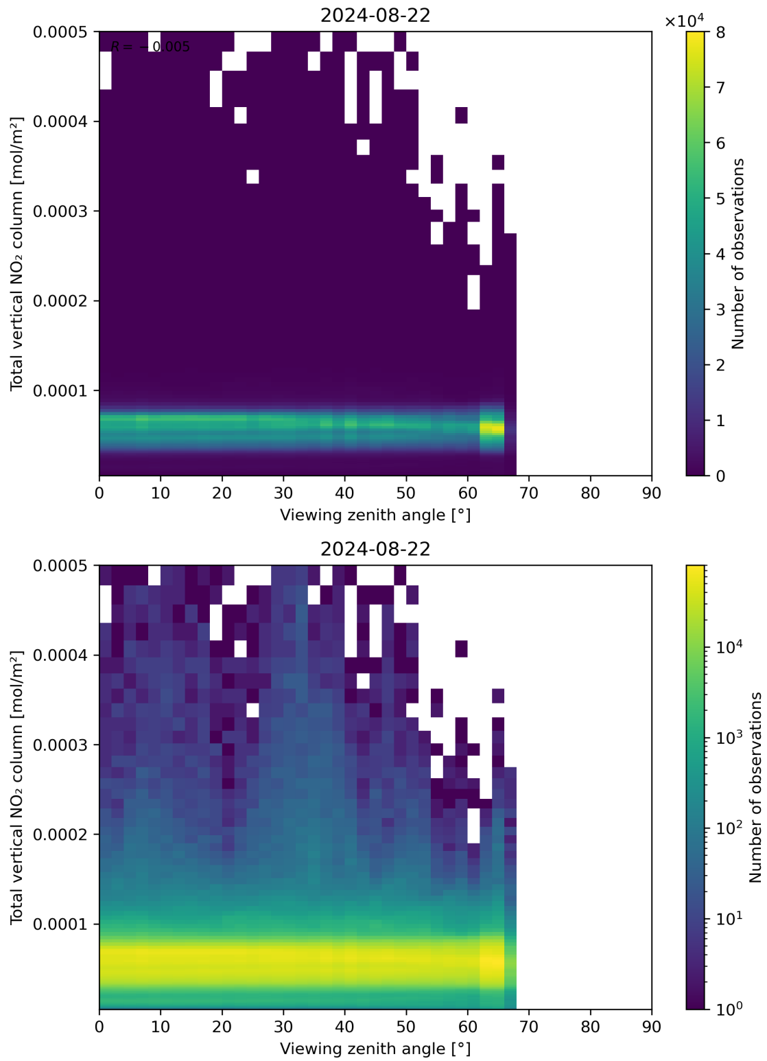
Figure 167: Scatter density plot of “Viewing zenith angle” against “Total vertical NO 2 column” for 2024-08-22 to 2024-08-23.
