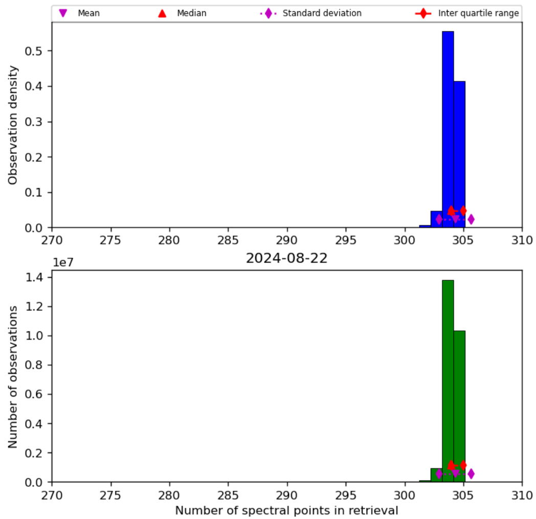
Figure 33: Histogram of “Number of spectral points in retrieval” for 2024-08-22 to 2024-08-23
