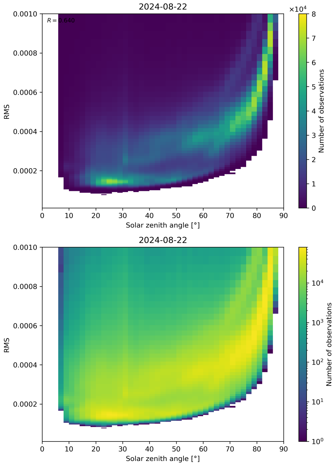
Figure 157: Scatter density plot of “Solar zenith angle” against “RMS” for 2024-08-22 to 2024-08-23.
