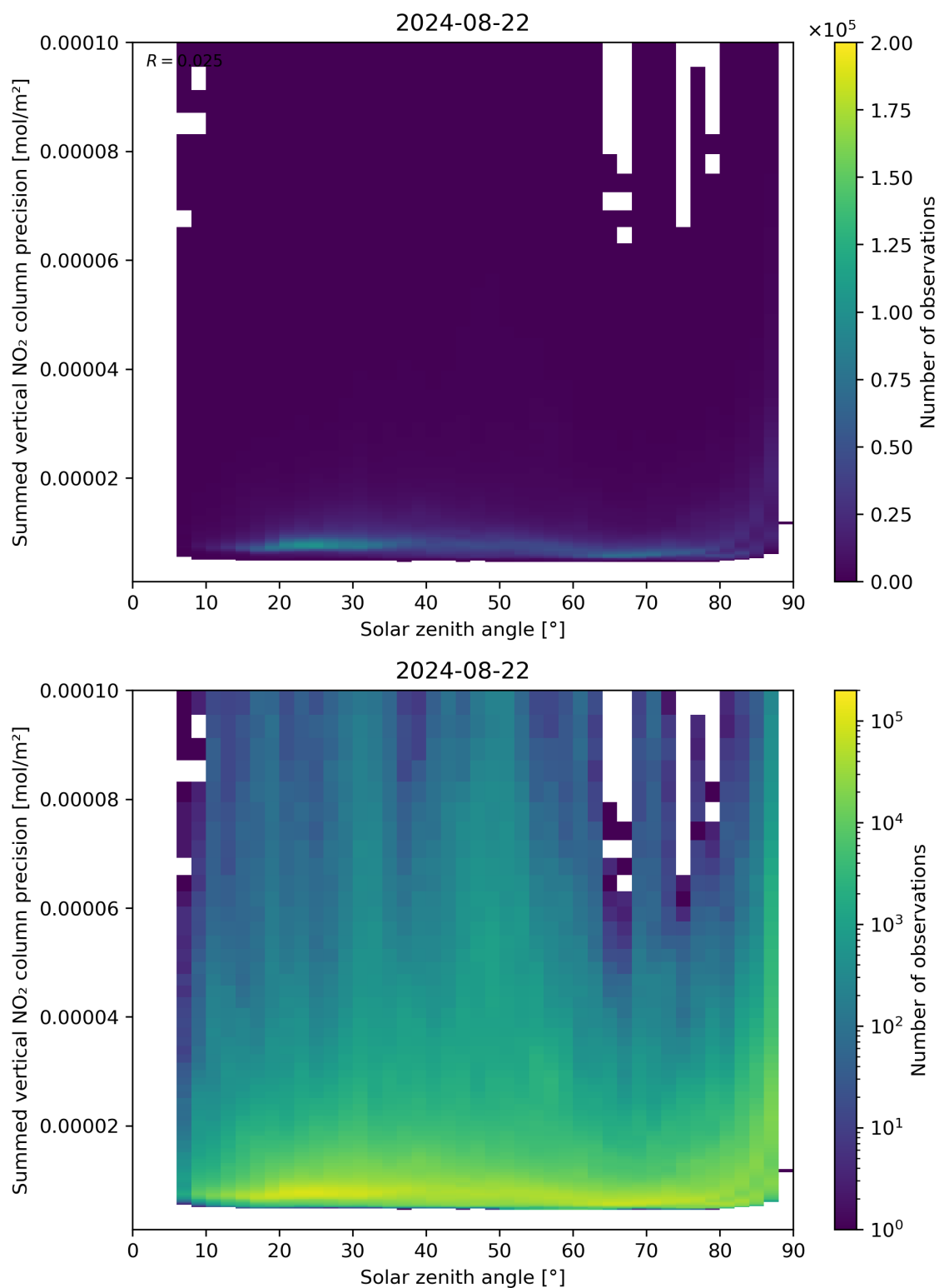
Figure 152: Scatter density plot of “Solar zenith angle” against “Summed vertical NO 2 column precision” for 2024-08-22 to 2024-08-23.
