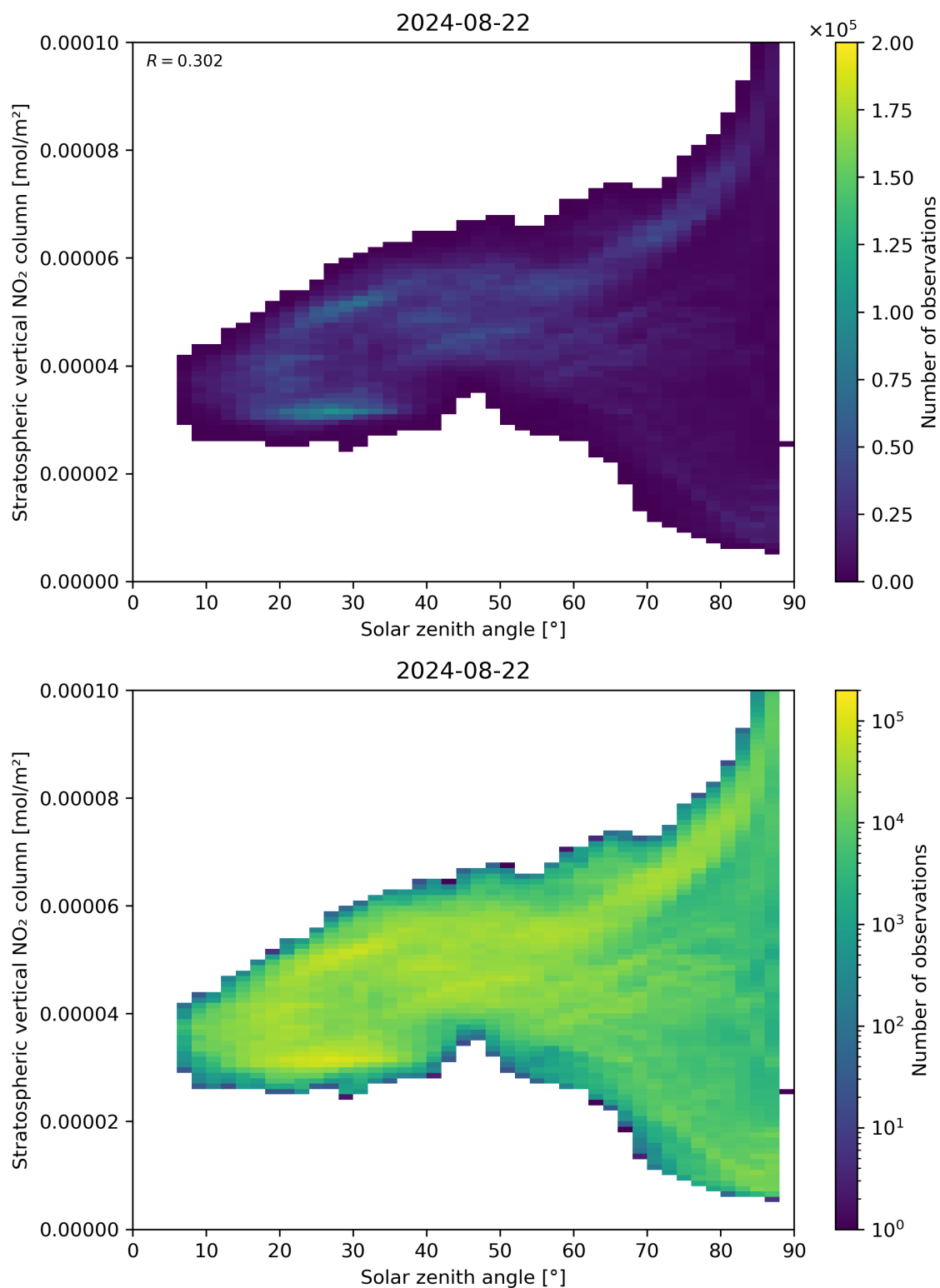
Figure 150: Scatter density plot of “Solar zenith angle” against “Stratospheric vertical NO 2 column” for 2024-08-22 to 2024-08-23.
