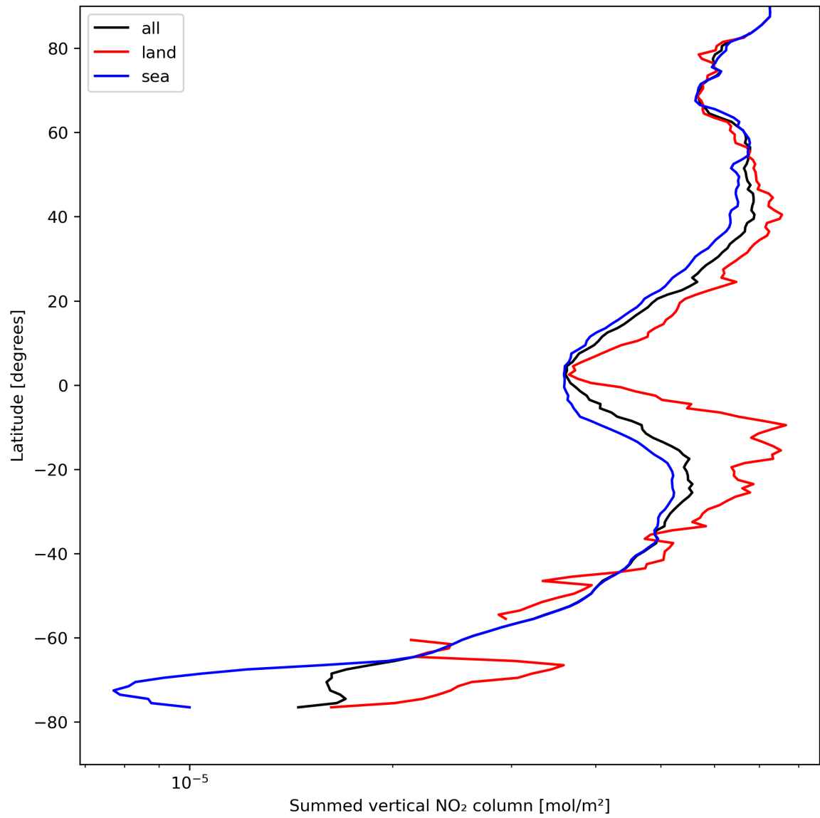
Figure 23: Zonal average of “Summed vertical NO 2 column” for 2024-08-22 to 2024-08-23.
