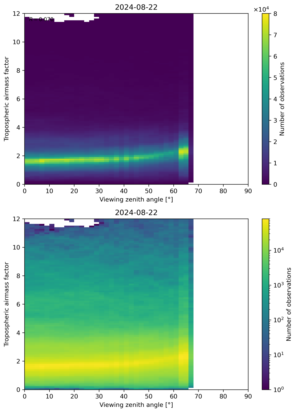
Figure 161: Scatter density plot of “Viewing zenith angle” against “Tropospheric airmass factor” for 2024-08-22 to 2024-08-23.
