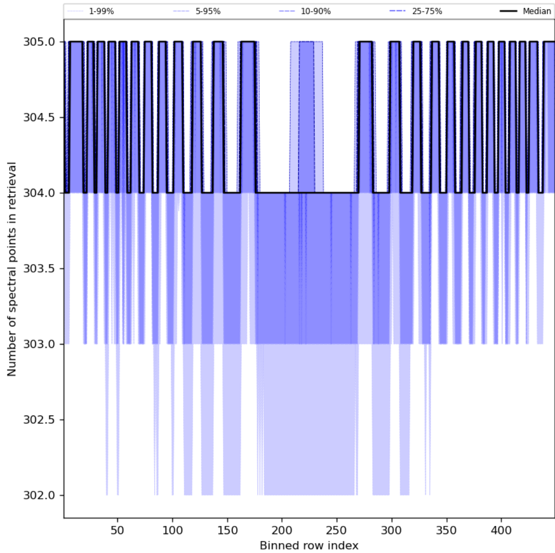
Figure 50: Along track statistics of “Number of spectral points in retrieval” for 2024-08-22 to 2024-08-23
