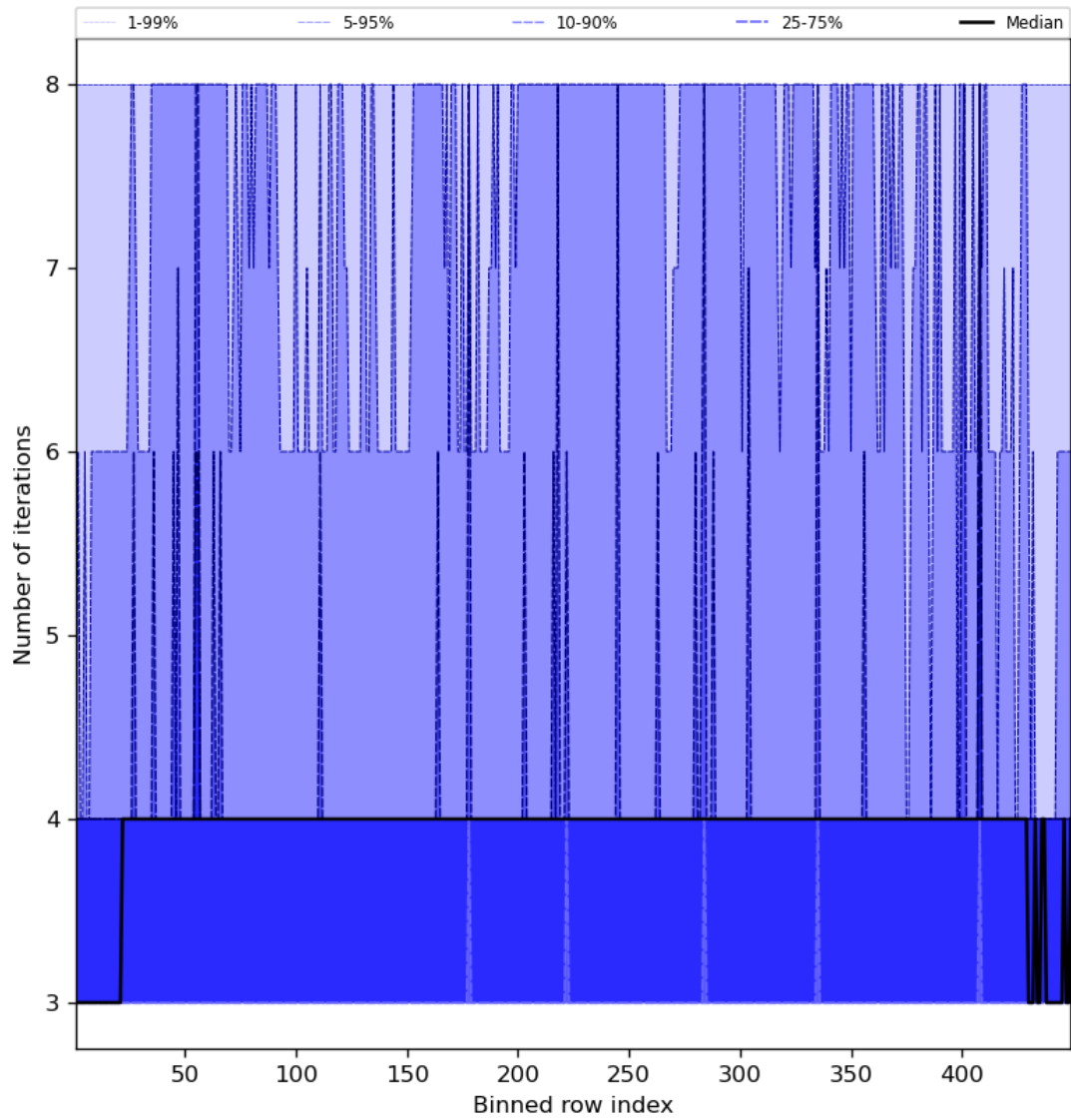
Figure 51: Along track statistics of “Number of iterations” for 2024-08-22 to 2024-08-23
