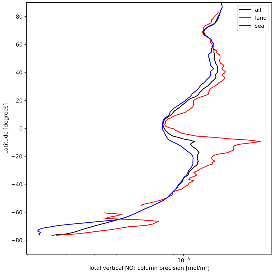
Figure 22: Zonal average of “Total vertical NO 2 column precision” for 2024-08-22 to 2024-08-23.
