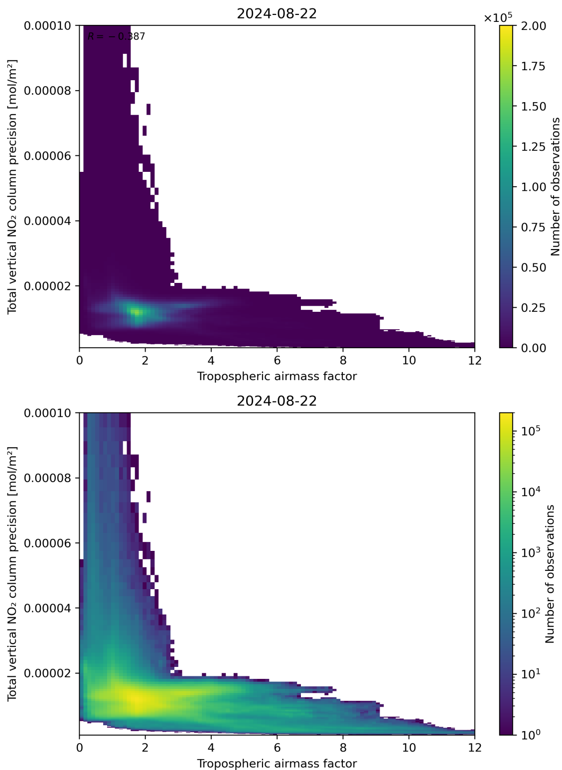
Figure 78: Scatter density plot of “Tropospheric air mass factor” against “Total vertical NO 2 column precision” for 2024-08-22 to 2024-08-23.
