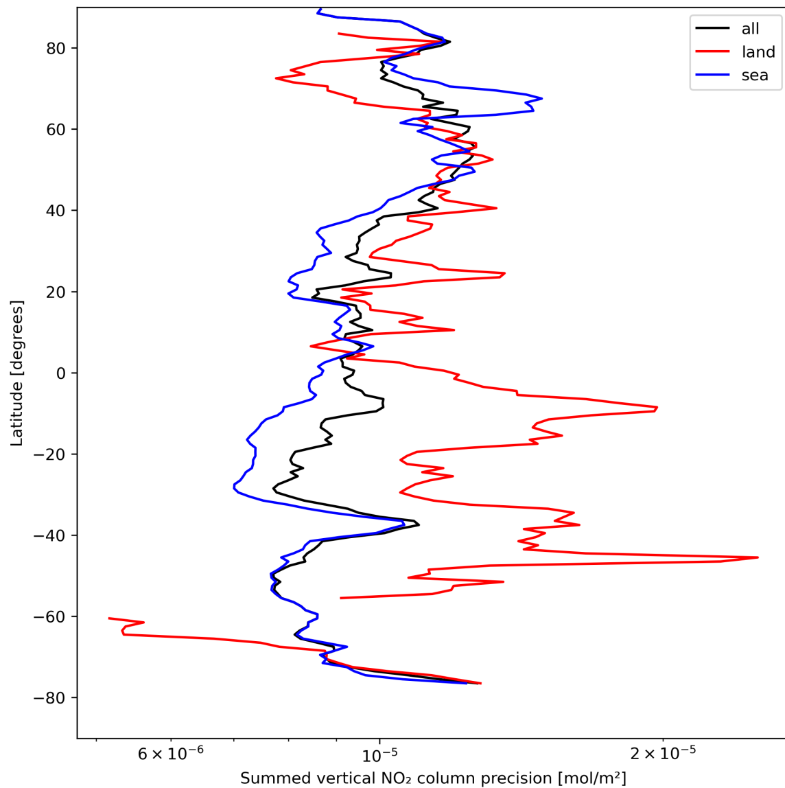
Figure 24: Zonal average of “Summed vertical NO 2 column precision” for 2024-08-22 to 2024-08-23.
