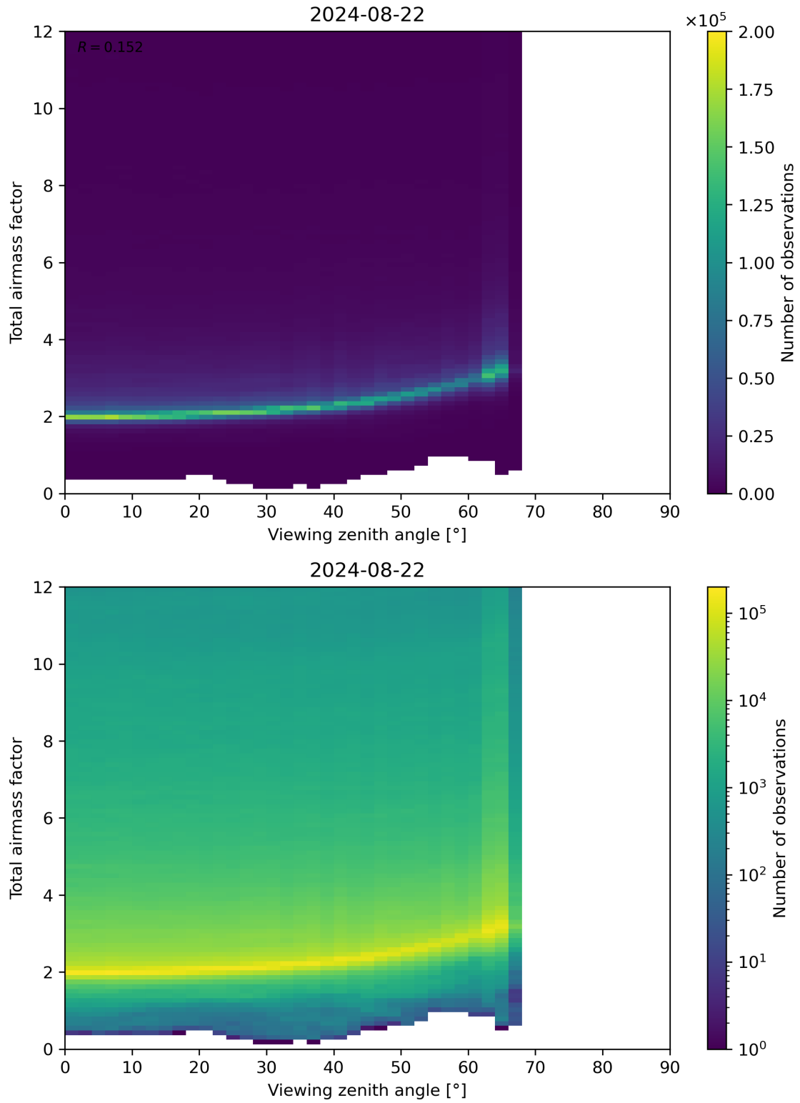
Figure 160: Scatter density plot of “Viewing zenith angle” against “Total airmass factor” for 2024-08-22 to 2024-08-23.
