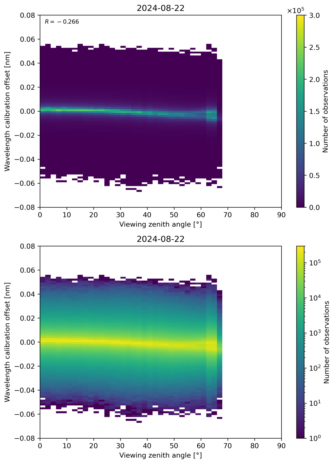
Figure 173: Scatter density plot of “Viewing zenith angle” against “Wavelength calibration offset” for 2024-08-22 to 2024-08-23.
