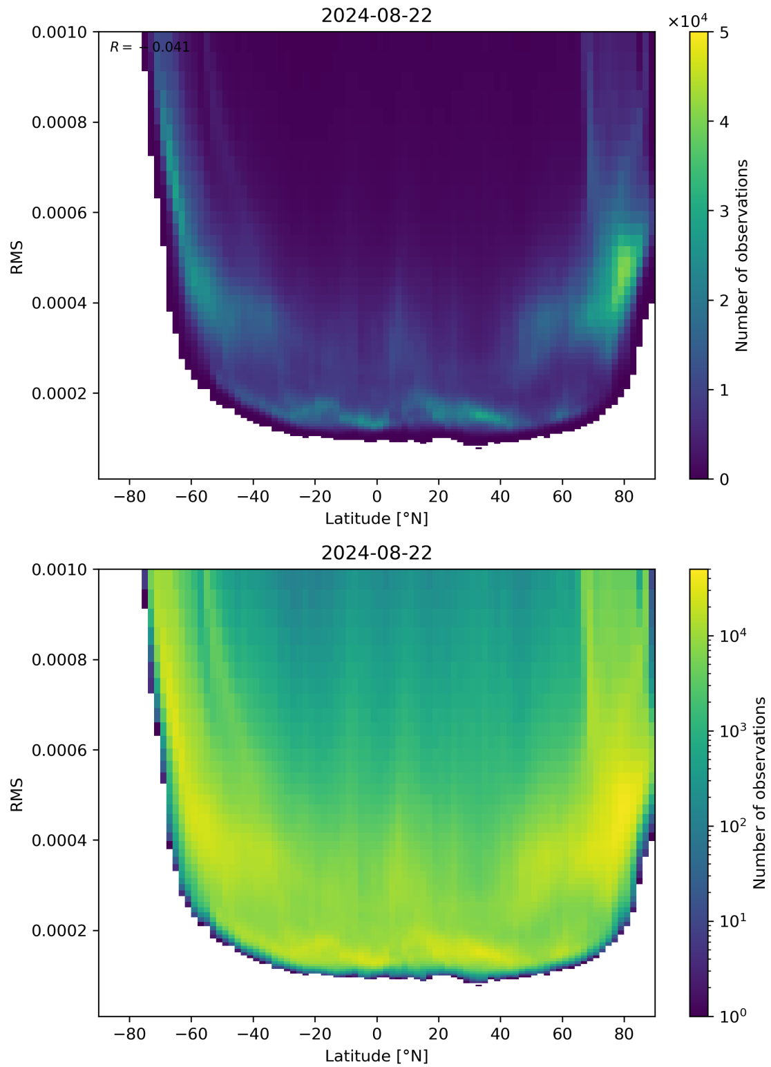
Figure 94: Scatter density plot of “Latitude” against “RMS” for 2024-08-22 to 2024-08-23.
