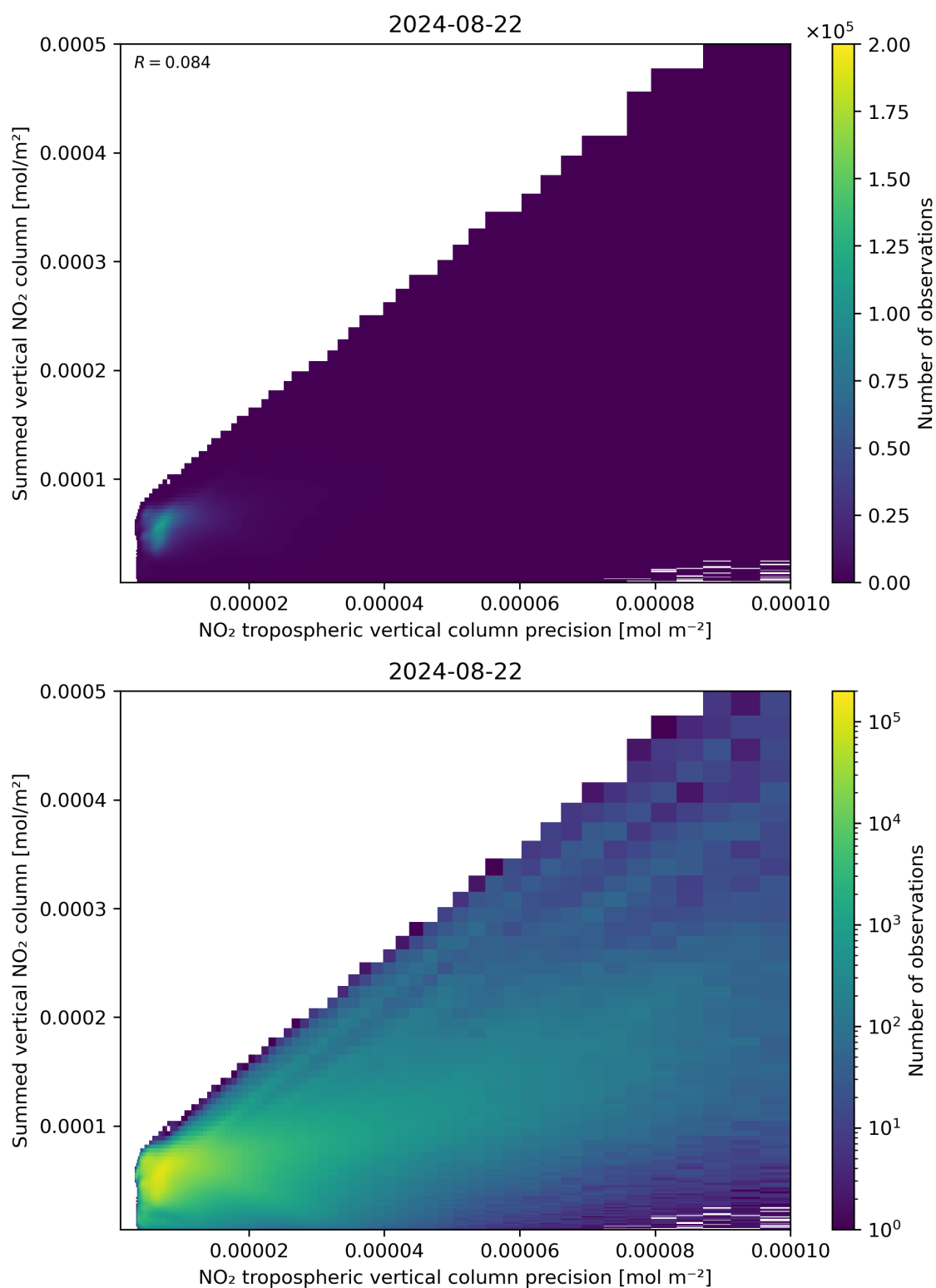
Figure 136: Scatter density plot of “NO 2 tropospheric vertical column precision” against “Summed vertical NO 2 column” for 2024-08-22 to 2024-08-23.
