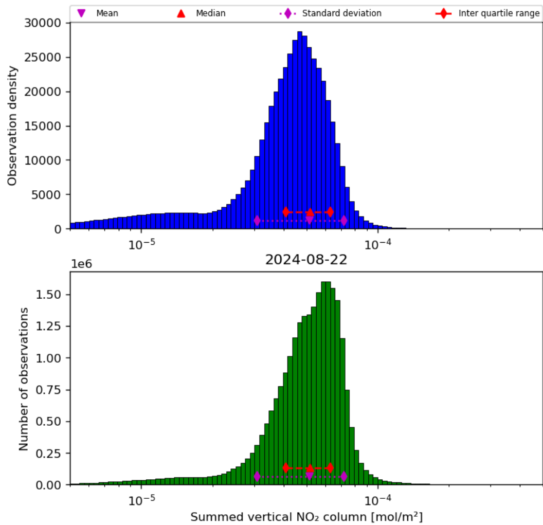
Figure 40: Histogram of “Summed vertical NO 2 column” for 2024-08-22 to 2024-08-23
