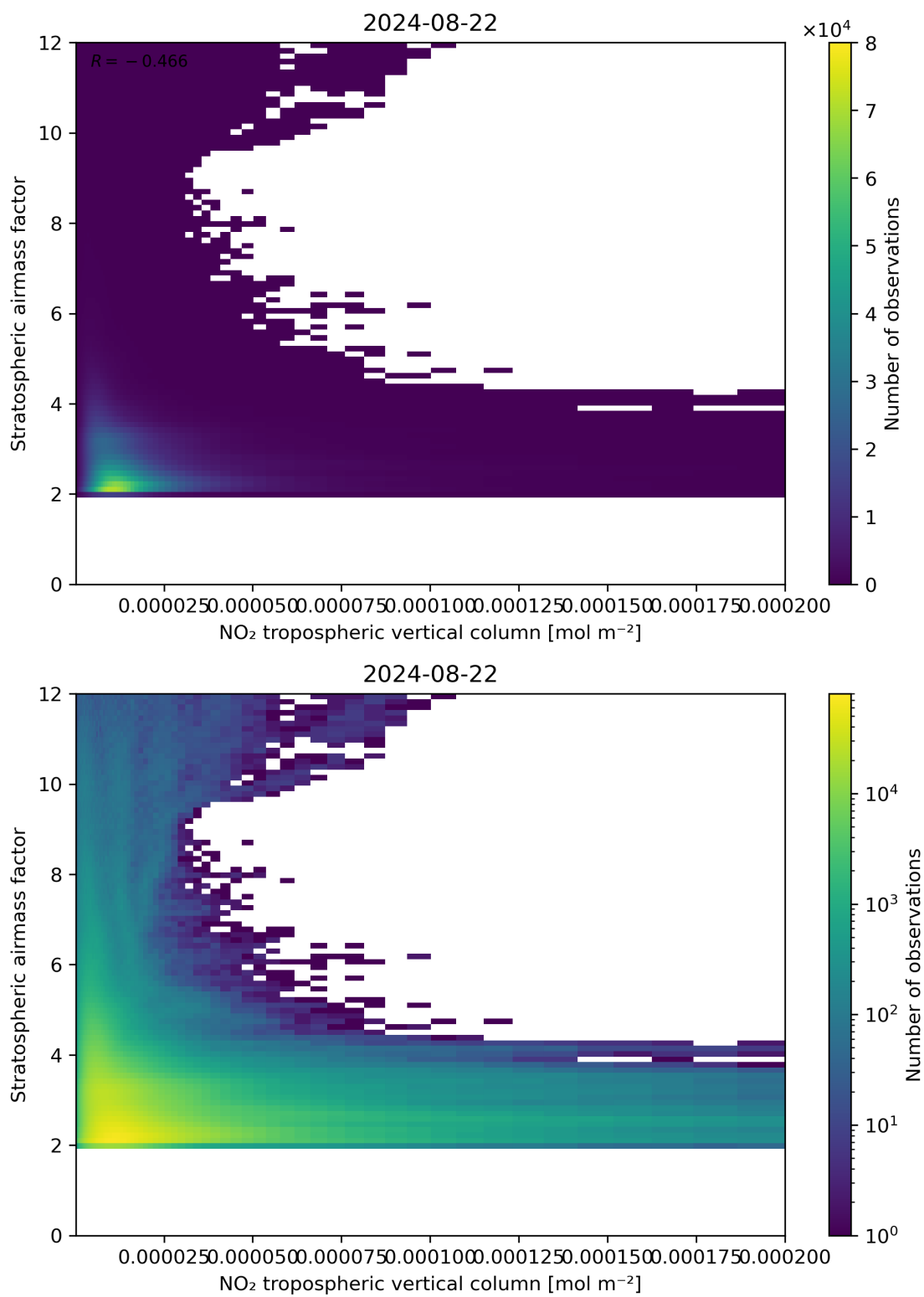
Figure 121: Scatter density plot of “NO 2 tropospheric vertical column” against “Stratospheric air mass factor” for 2024-08-22 to 2024-08-23.
