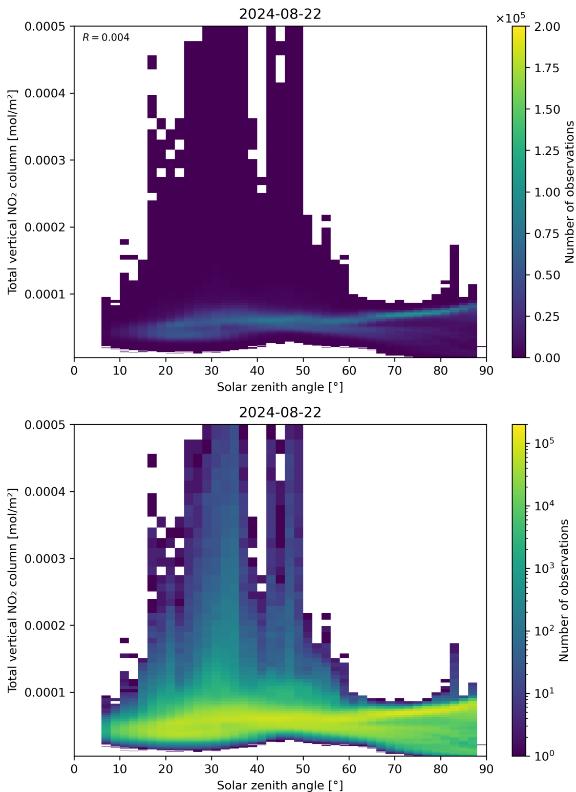
Figure 153: Scatter density plot of “Solar zenith angle” against “Total vertical NO 2 column” for 2024-08-22 to 2024-08-23.
