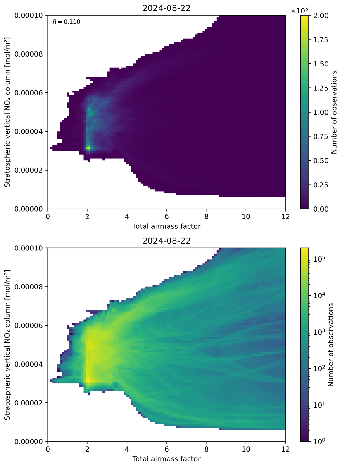
Figure 64: Scatter density plot of “Total airmass factor” against “Stratospheric vertical NO 2 column” for 2024-08-22 to 2024-08-23.
