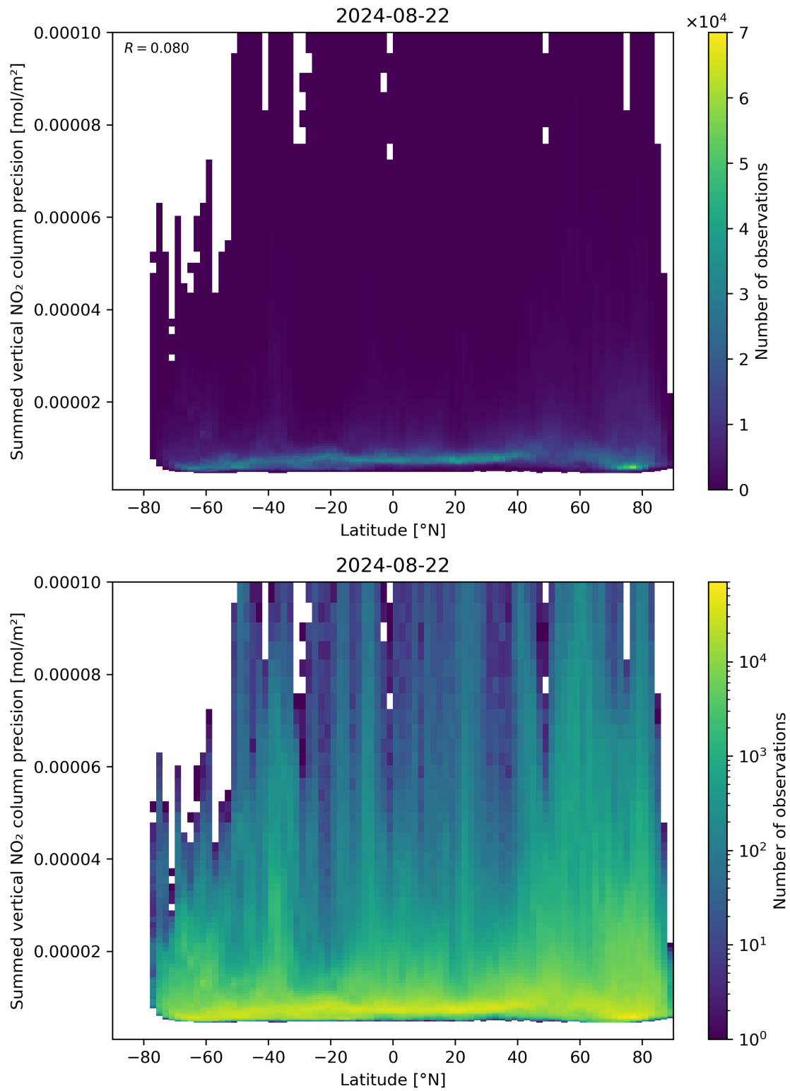
Figure 89: Scatter density plot of “Latitude” against “Summed vertical NO 2 column precision” for 2024-08-22 to 2024-08-23.
