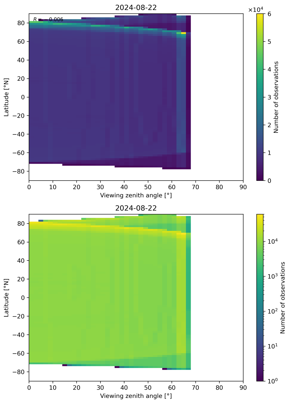
Figure 163: Scatter density plot of “Viewing zenith angle” against “Latitude” for 2024-08-22 to 2024-08-23.
