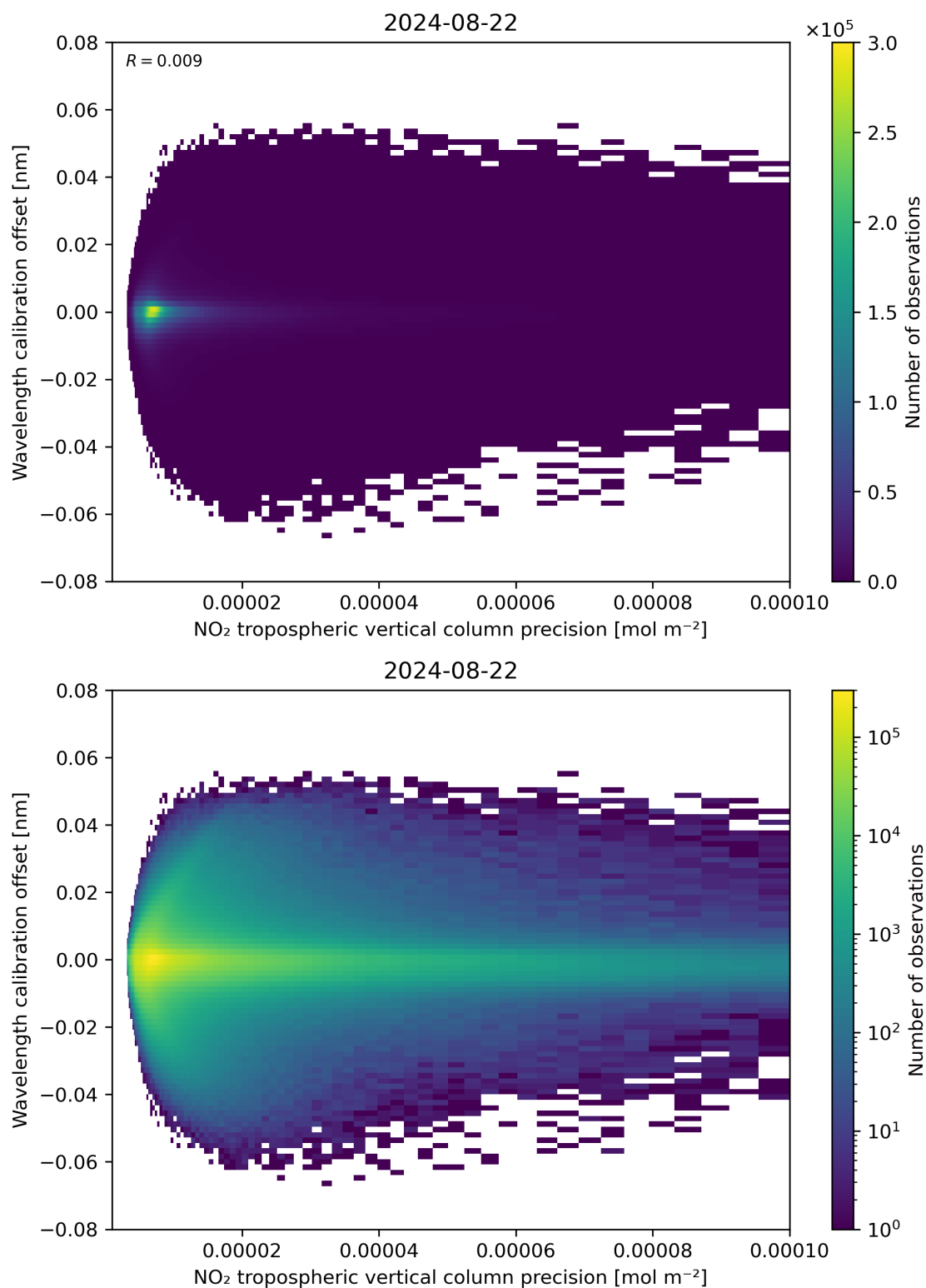
Figure 141: Scatter density plot of “NO 2 tropospheric vertical column precision” against “Wavelength calibration offset” for 2024-08-22 to 2024-08-23.
