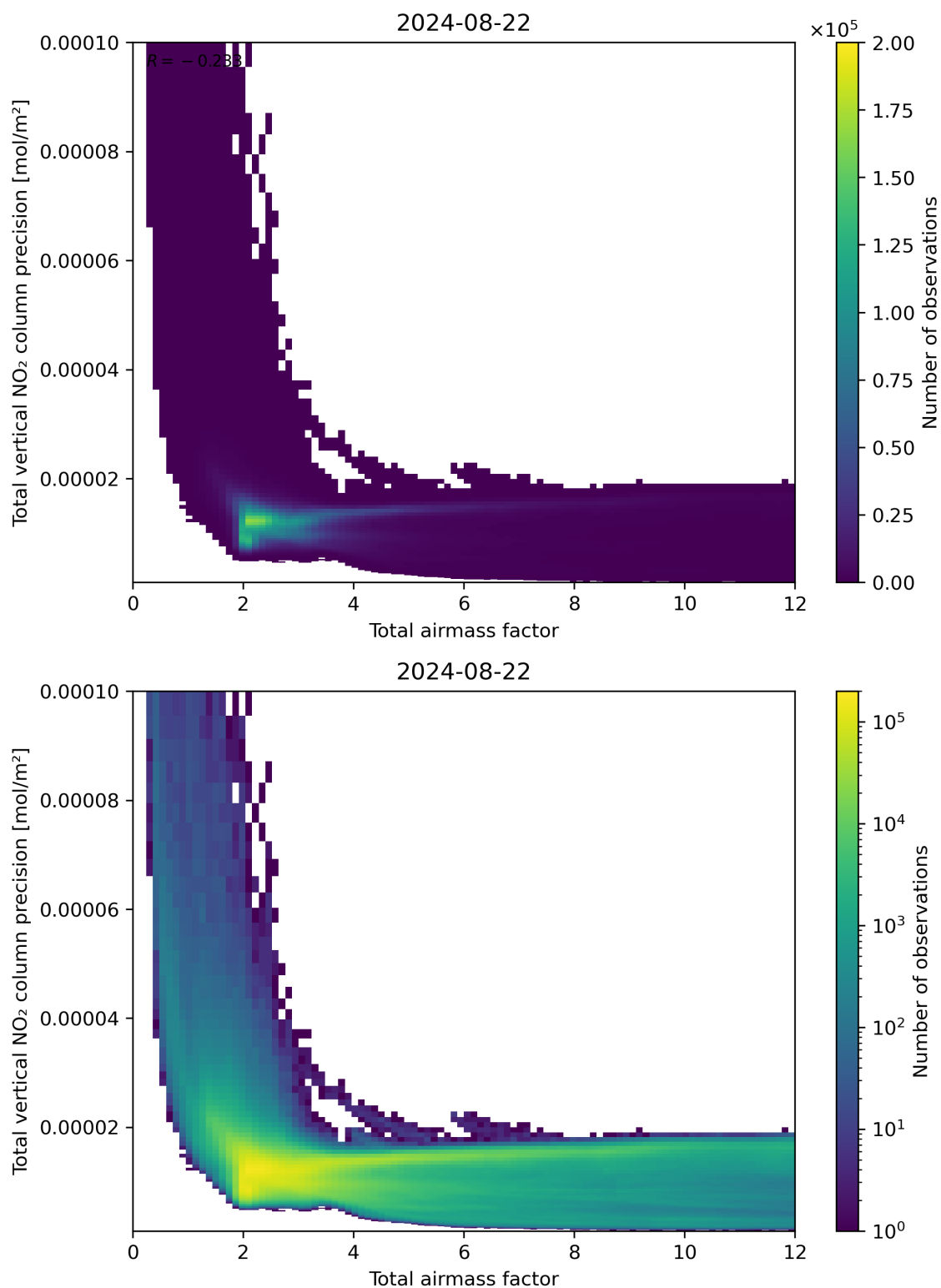
Figure 68: Scatter density plot of “Total airmass factor” against “Total vertical NO 2 column precision” for 2024-08-22 to 2024-08-23.
