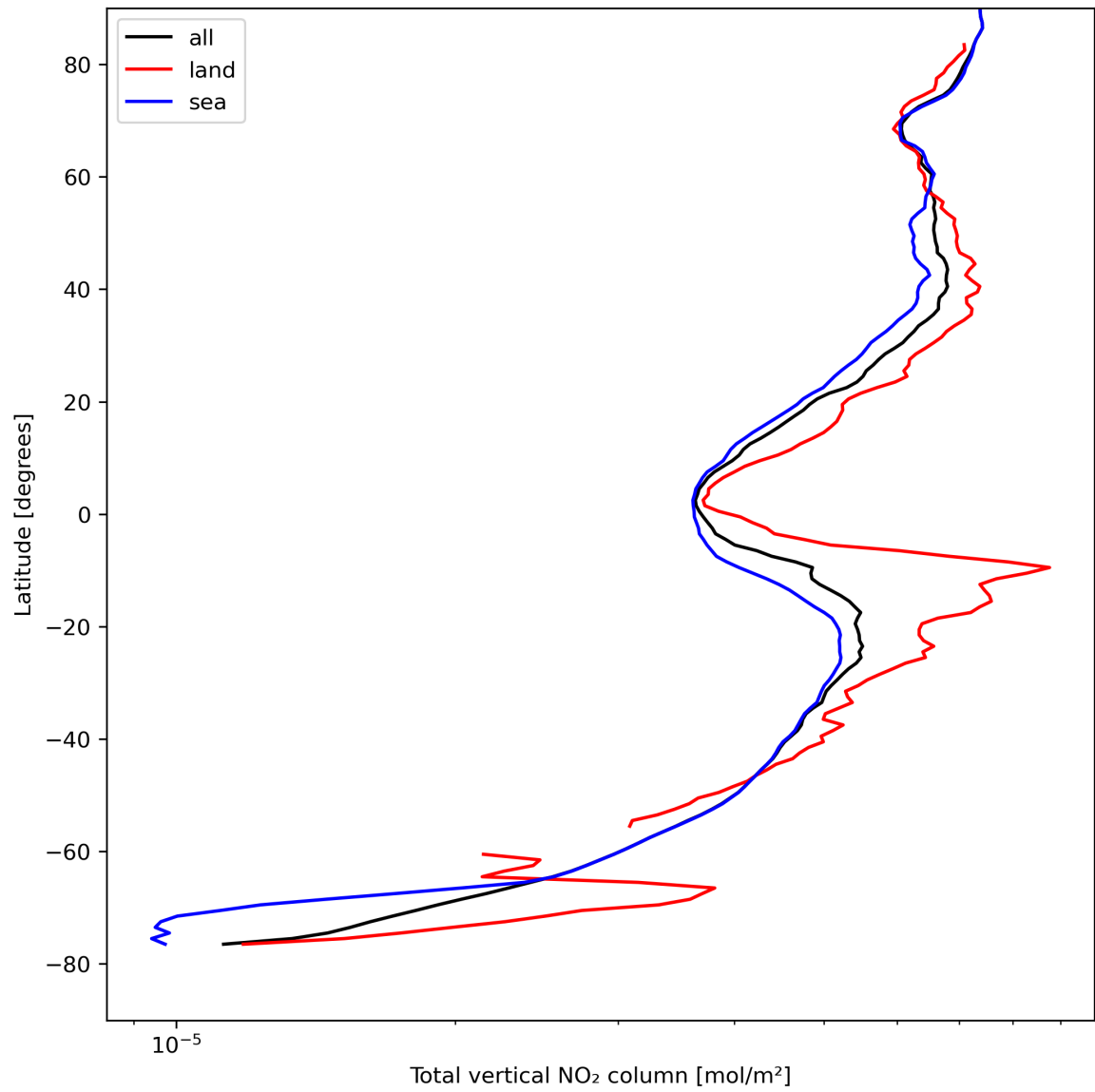
Figure 21: Zonal average of “Total vertical NO 2 column” for 2024-08-22 to 2024-08-23.
