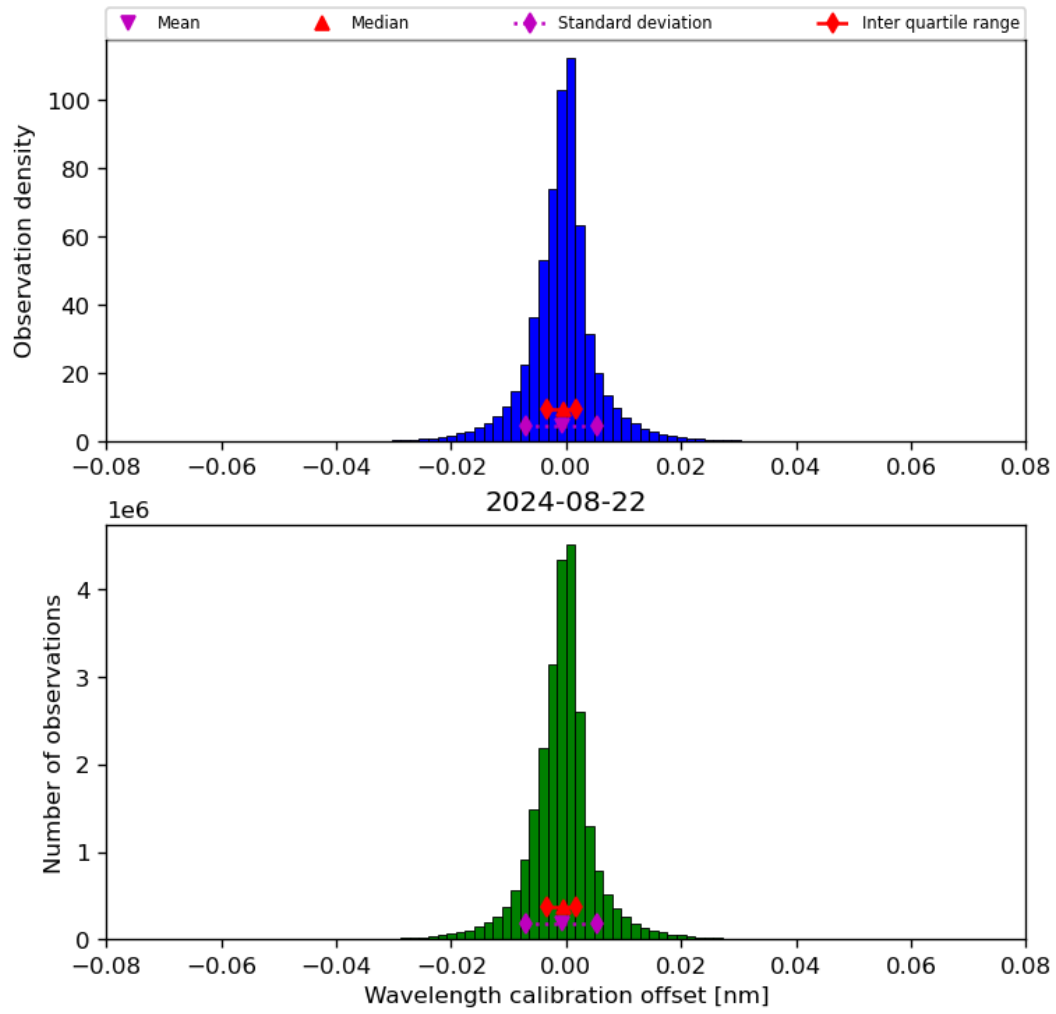
Figure 35: Histogram of “Wavelength calibration offset” for 2024-08-22 to 2024-08-23
