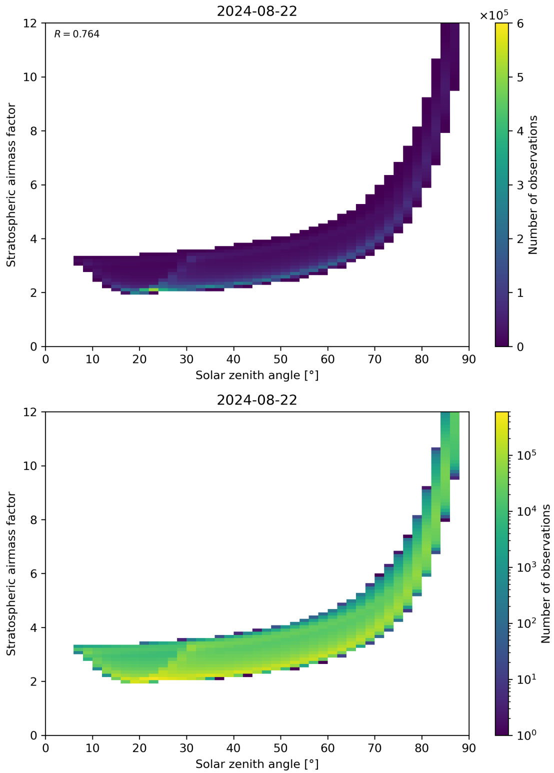
Figure 145: Scatter density plot of “Solar zenith angle” against “Stratospheric airmass factor” for 2024-08-22 to 2024-08-23.
