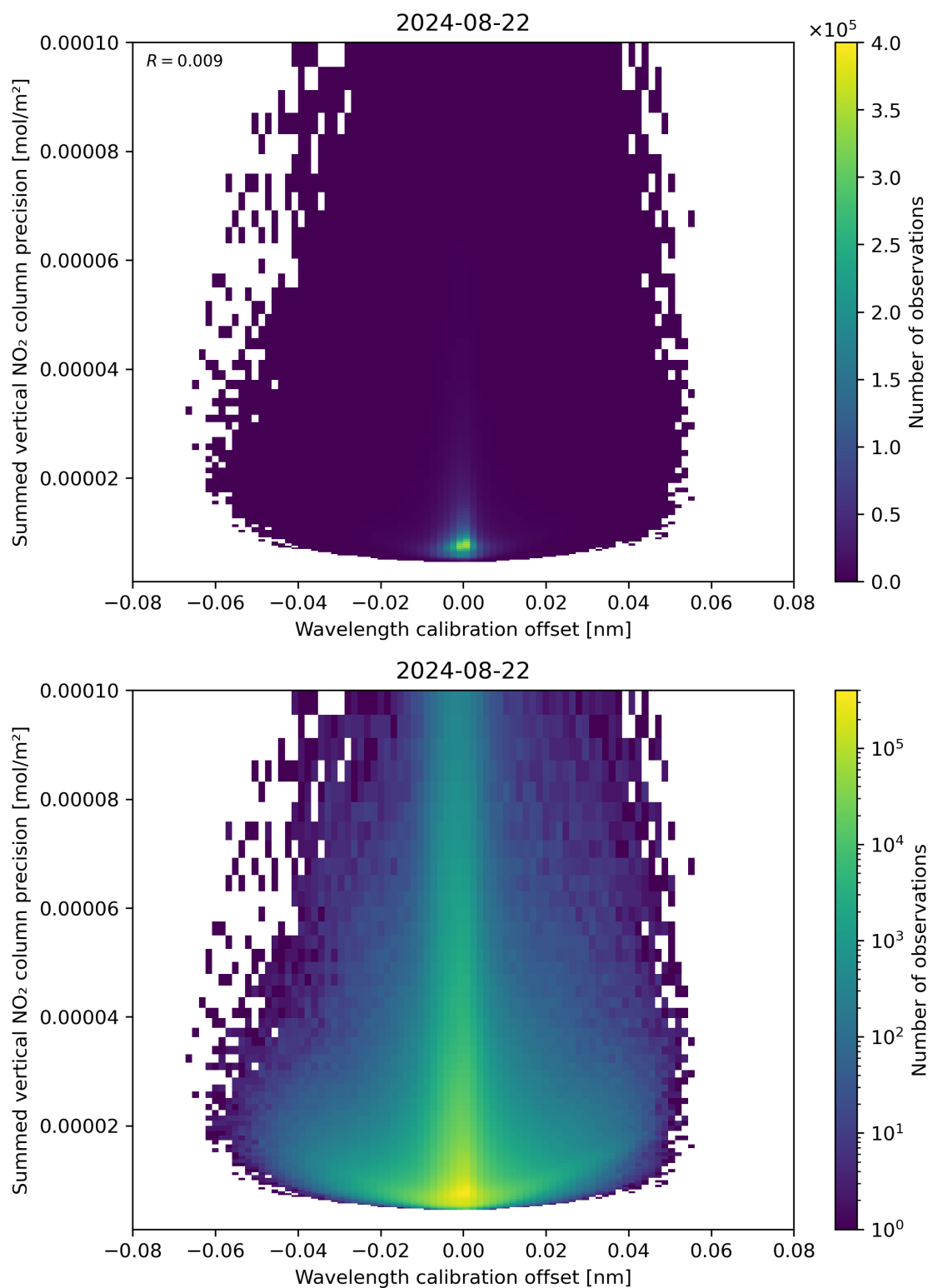
Figure 178: Scatter density plot of “Wavelength calibration offset” against “Summed vertical NO 2 column precision” for 2024-08-22 to 2024-08-23.
