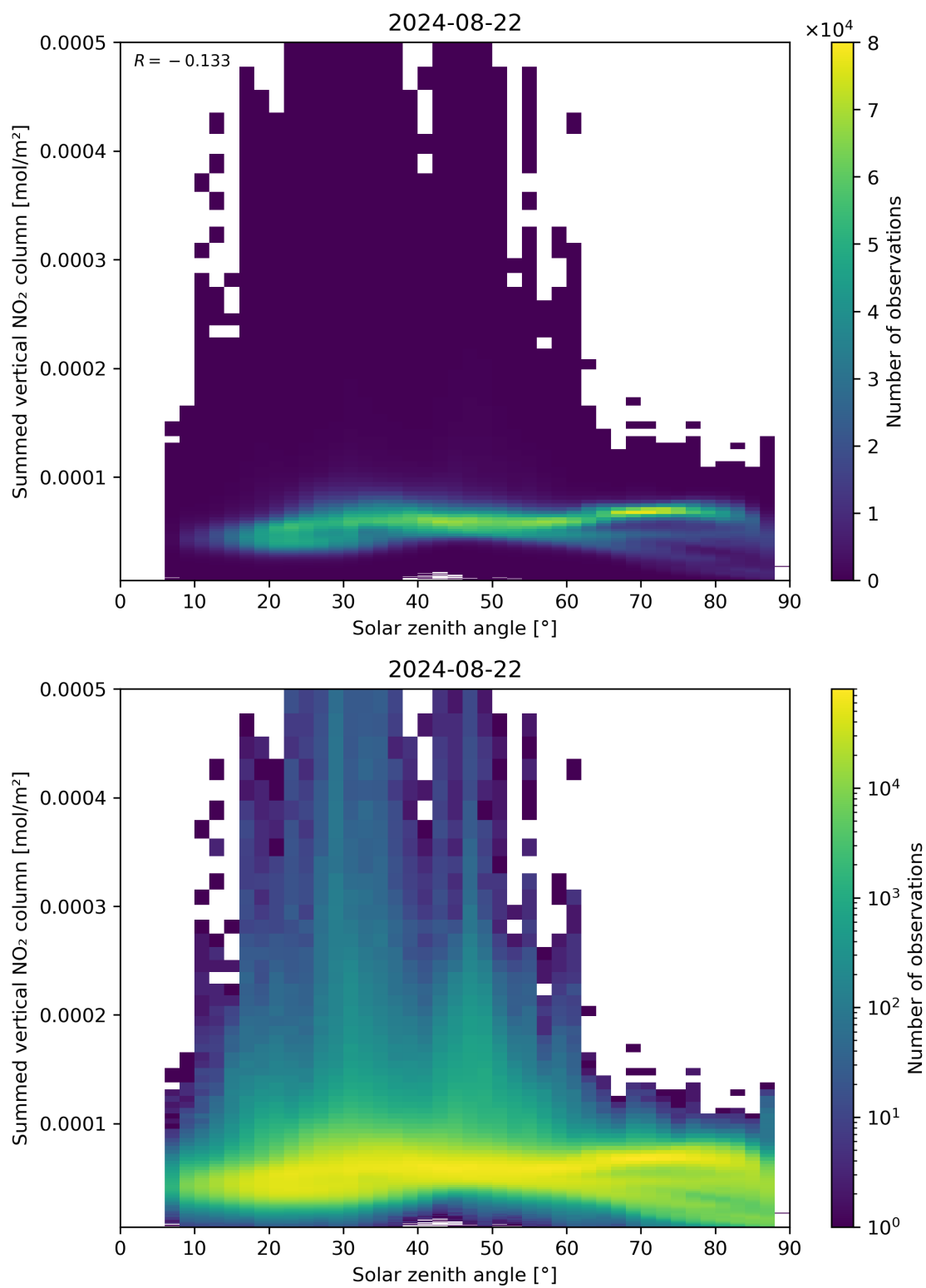
Figure 151: Scatter density plot of “Solar zenith angle” against “Summed vertical NO 2 column” for 2024-08-22 to 2024-08-23.
