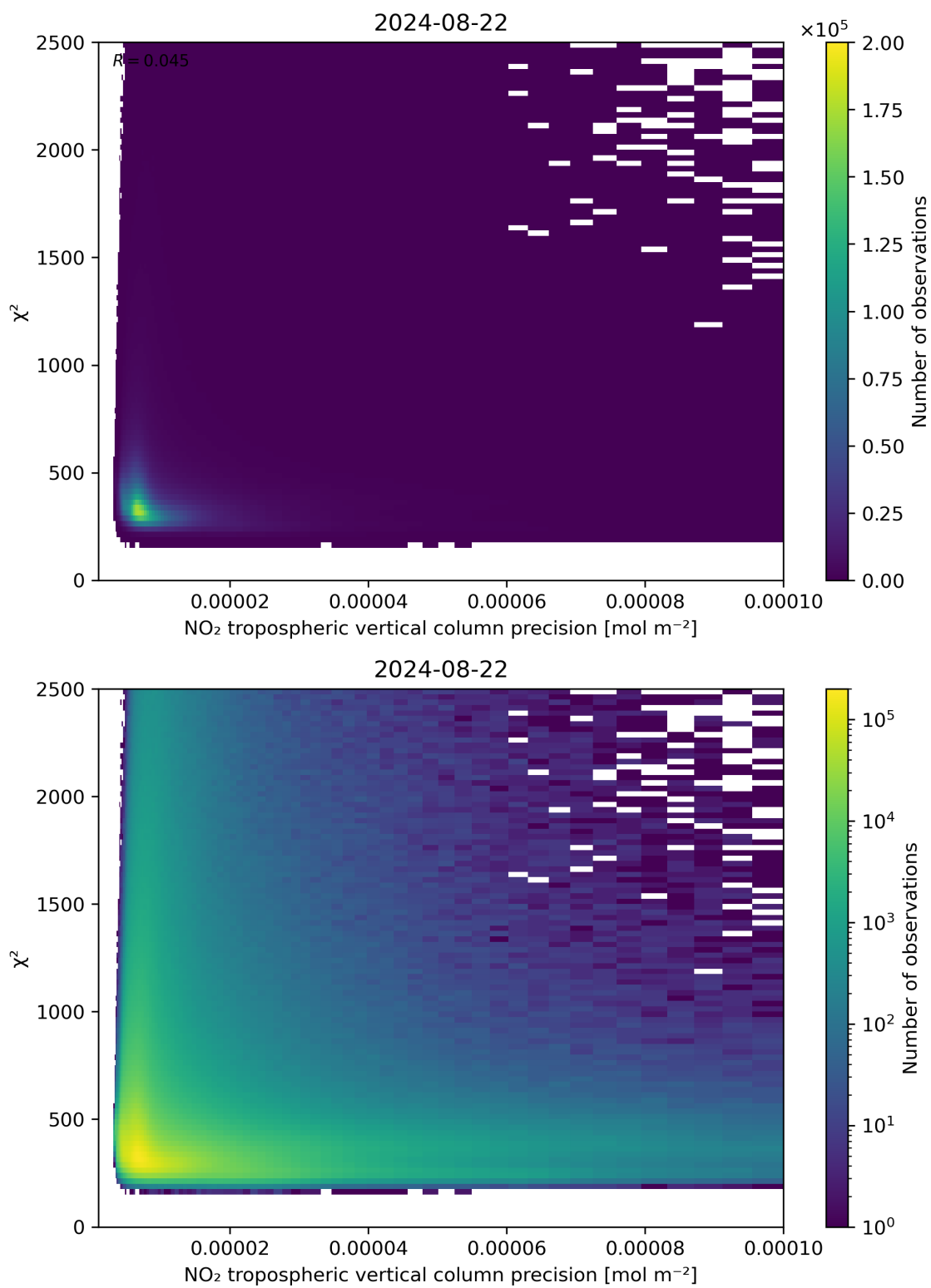
Figure 134: Scatter density plot of “NO 2 tropospheric vertical column precision” against “ \chi^2 ” for 2024-08-22 to 2024-08-23.
