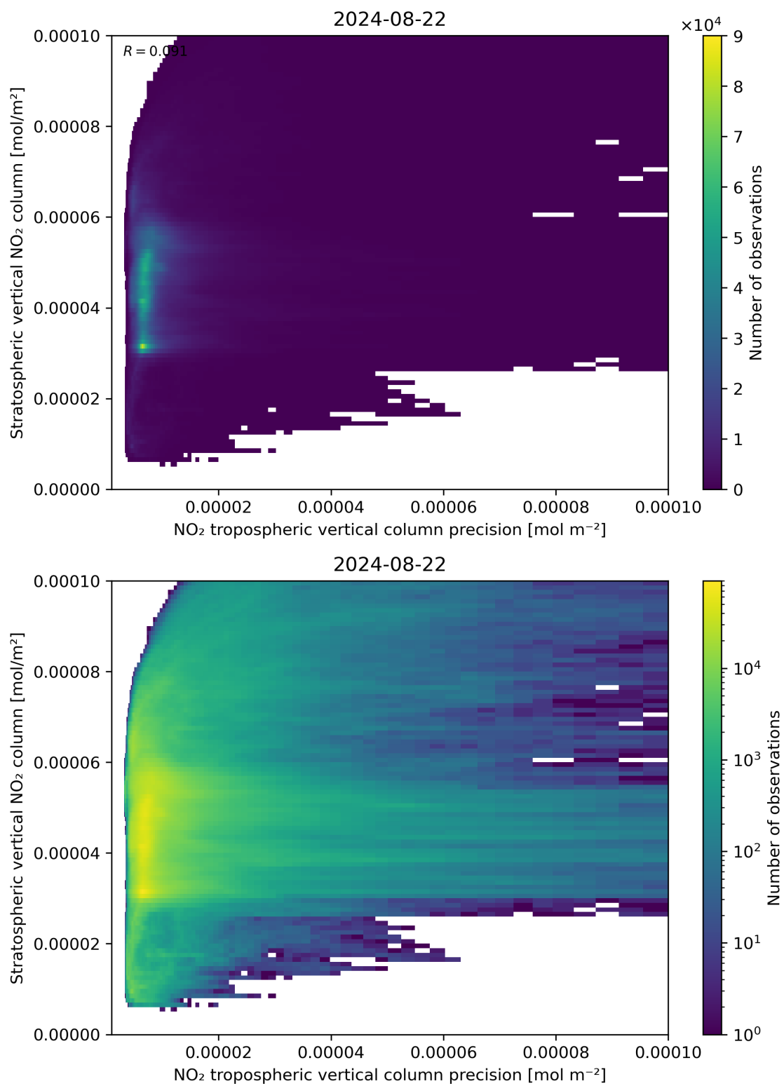
Figure 135: Scatter density plot of “NO 2 tropospheric vertical column precision” against “Stratospheric vertical NO 2 column” for 2024-08-22 to 2024-08-23.
