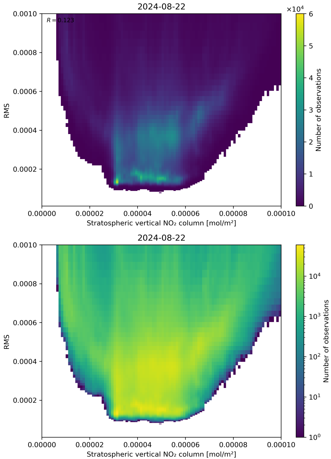
Figure 102: Scatter density plot of “Stratospheric vertical NO 2 column” against “RMS” for 2024-08-22 to 2024-08-23.
