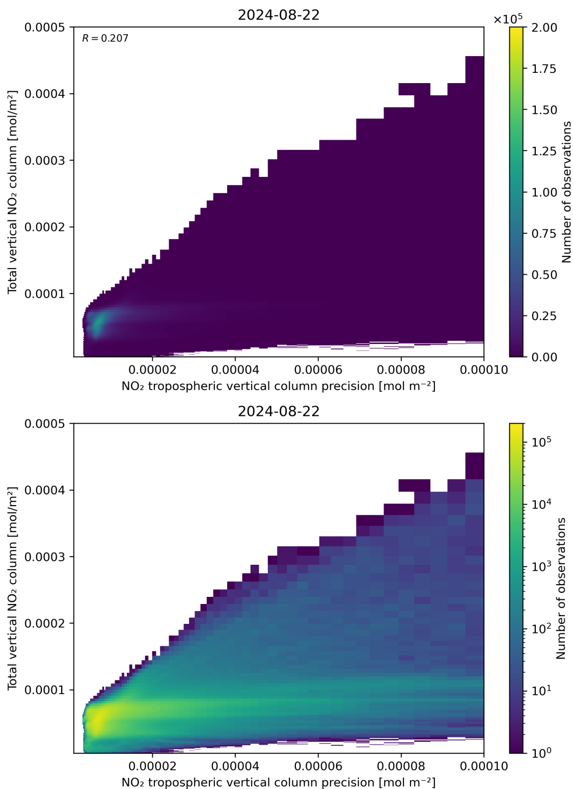
Figure 138: Scatter density plot of “NO 2 tropospheric vertical column precision” against “Total vertical NO 2 column” for 2024-08-22 to 2024-08-23.
