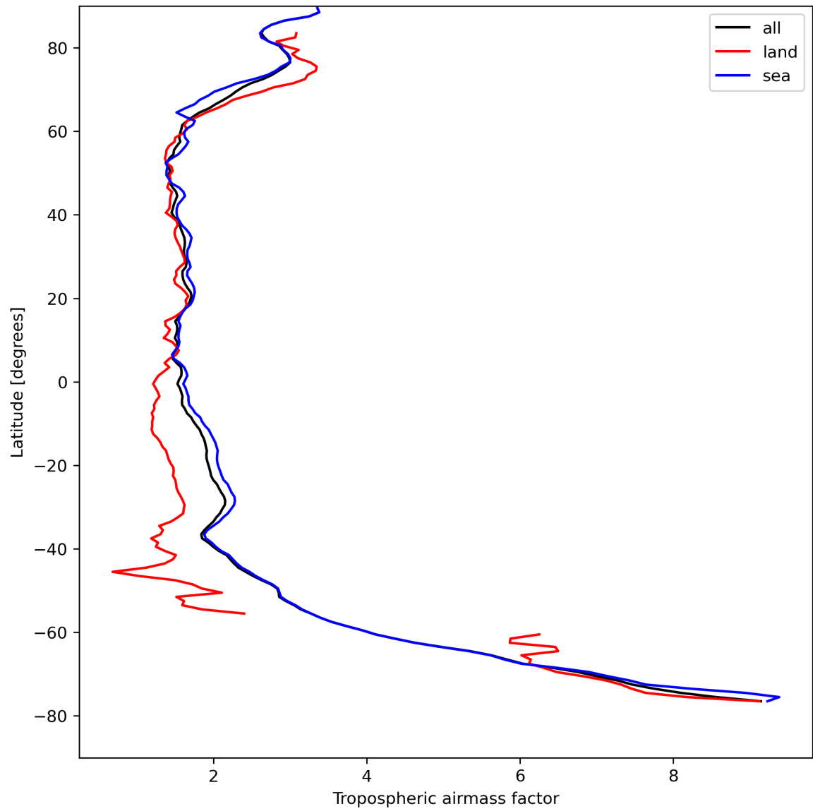
Figure 14: Zonal average of “Tropospheric airmass factor” for 2024-08-22 to 2024-08-23.
