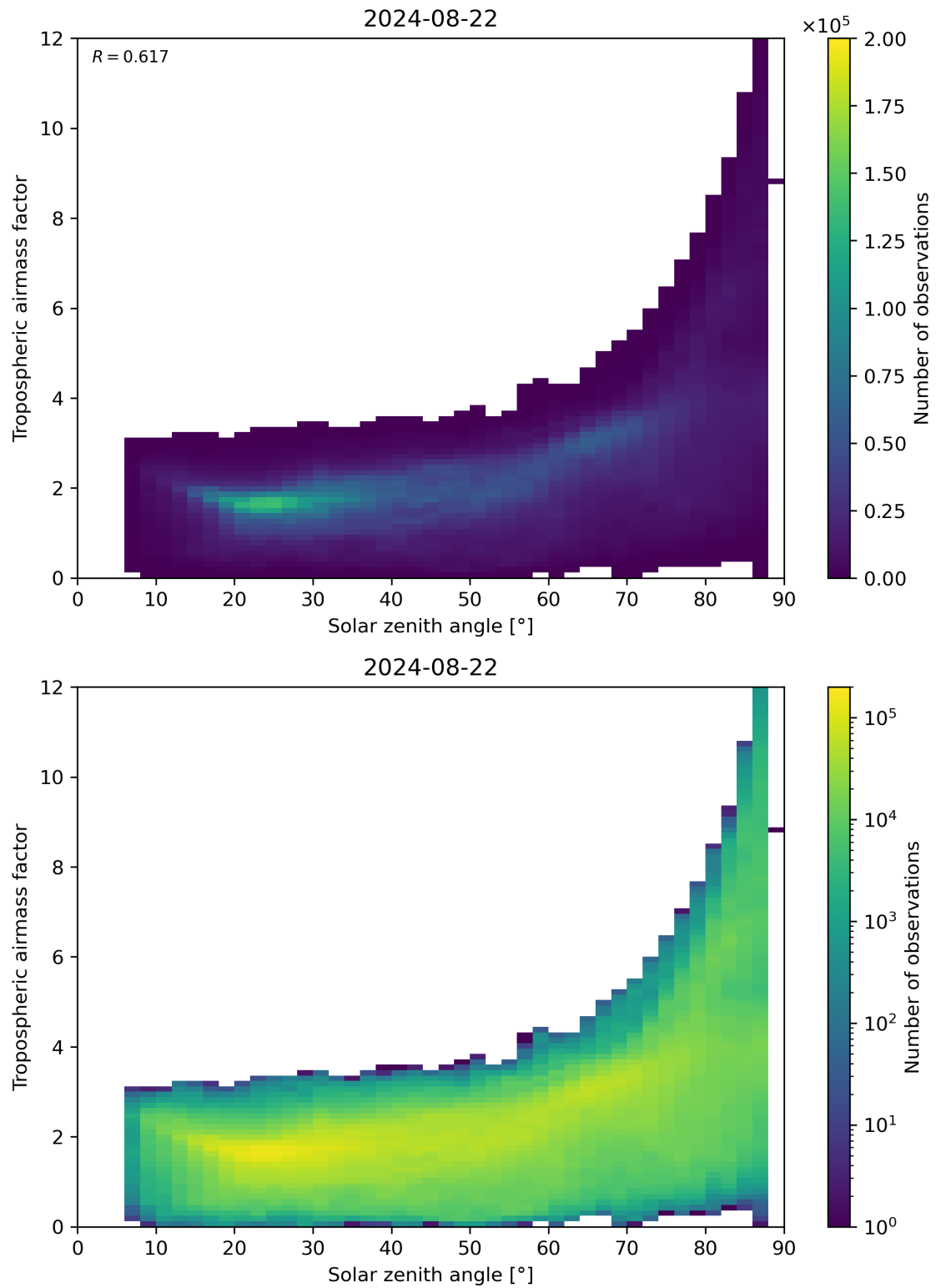
Figure 147: Scatter density plot of “Solar zenith angle” against “Tropospheric airmass factor” for 2024-08-22 to 2024-08-23.
