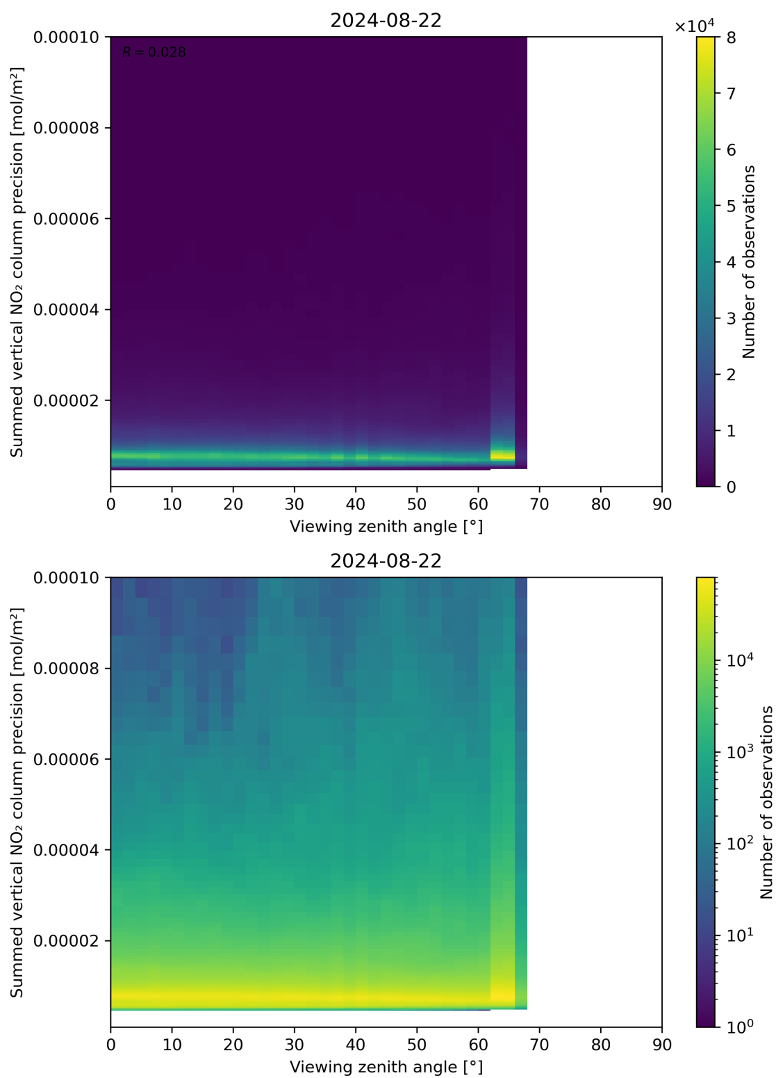
Figure 166: Scatter density plot of “Viewing zenith angle” against “Summed vertical NO 2 column precision” for 2024-08-22 to 2024-08-23.
