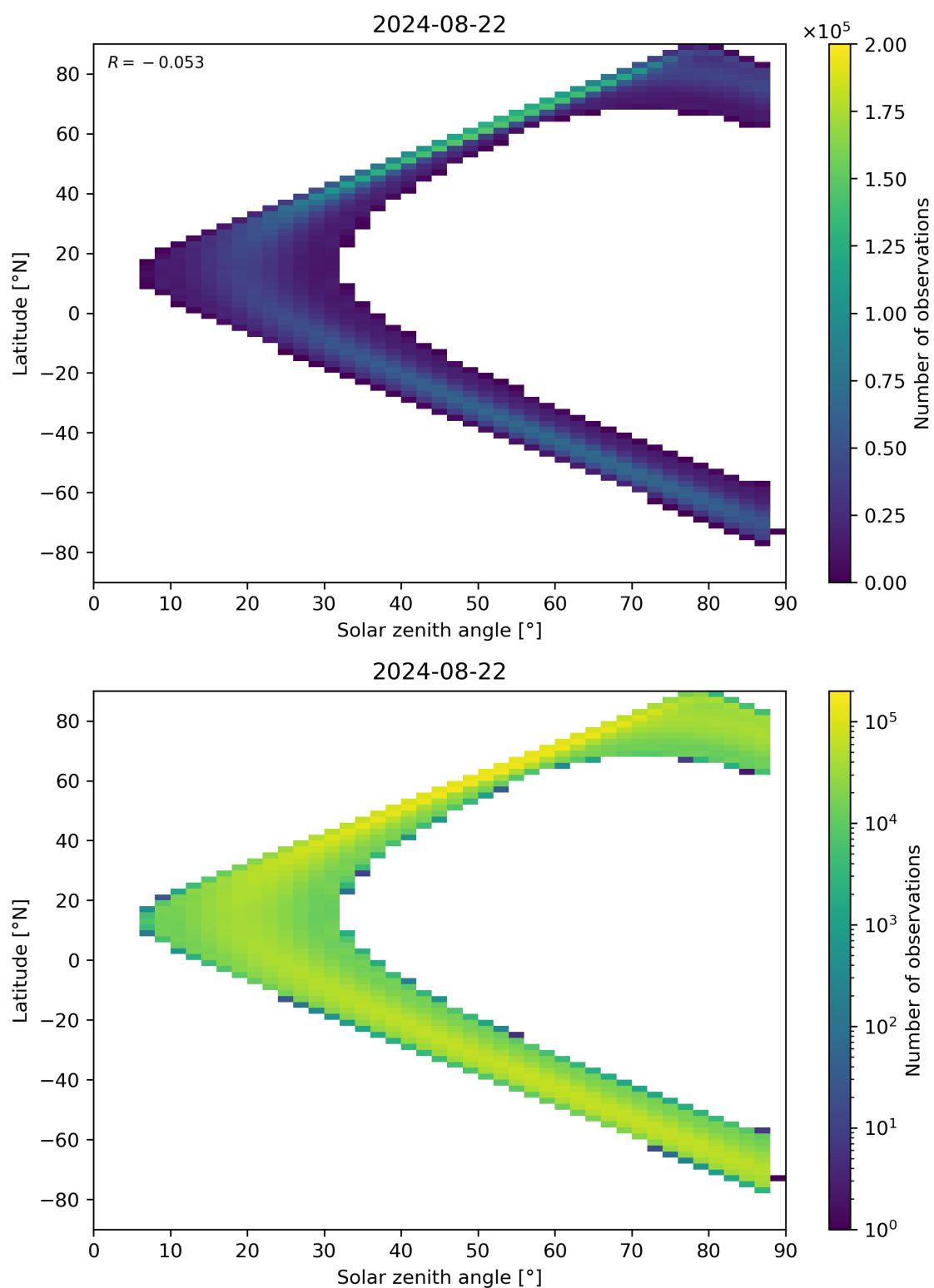
Figure 149: Scatter density plot of “Solar zenith angle” against “Latitude” for 2024-08-22 to 2024-08-23.
