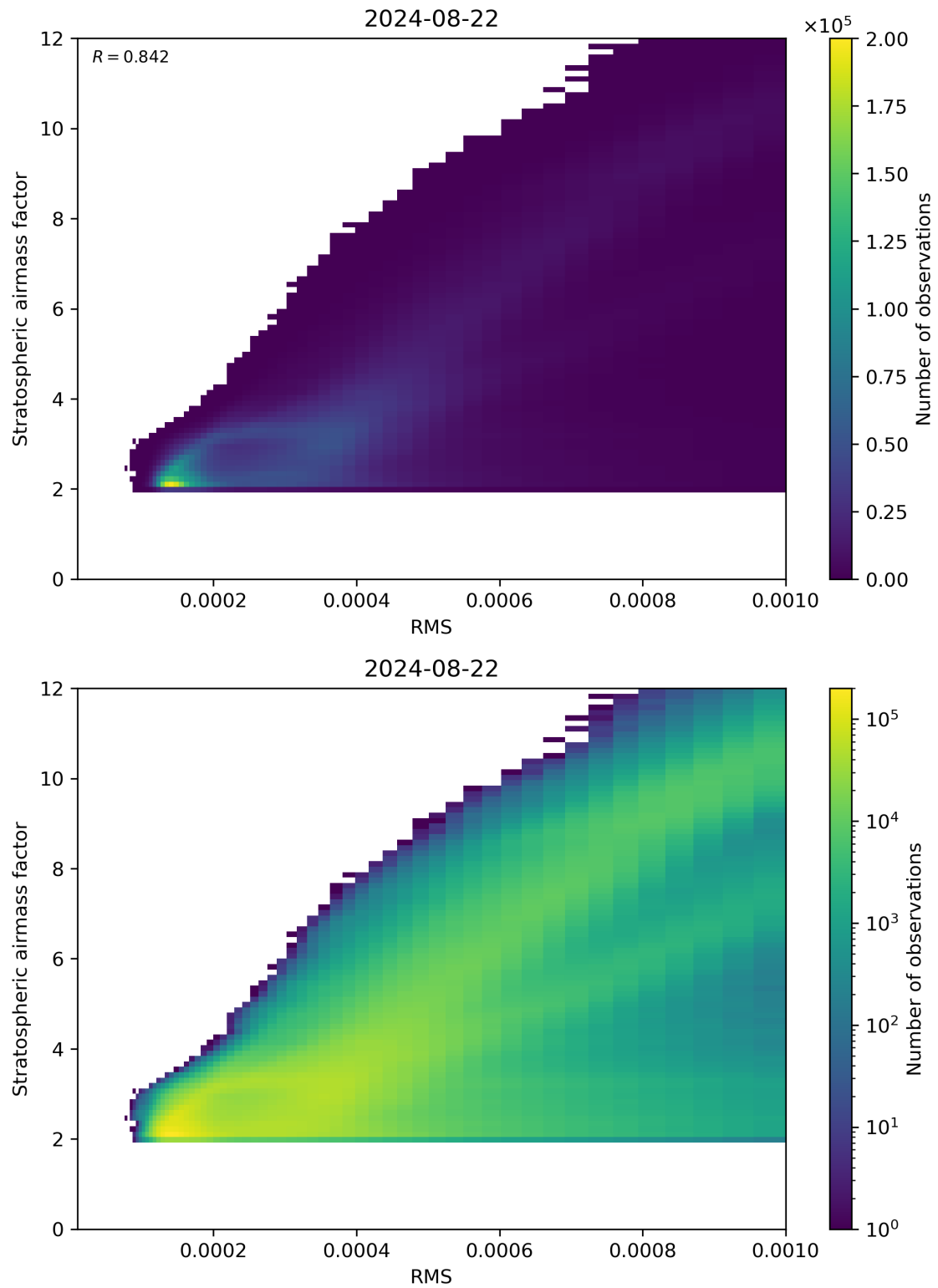
Figure 144: Scatter density plot of “RMS” against “Stratospheric airmass factor” for 2024-08-22 to 2024-08-23.
