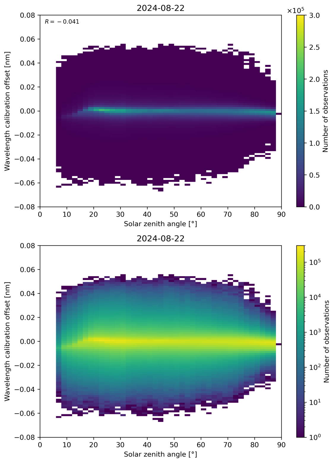
Figure 158: Scatter density plot of “Solar zenith angle” against “Wavelength calibration offset” for 2024-08-22 to 2024-08-23.
