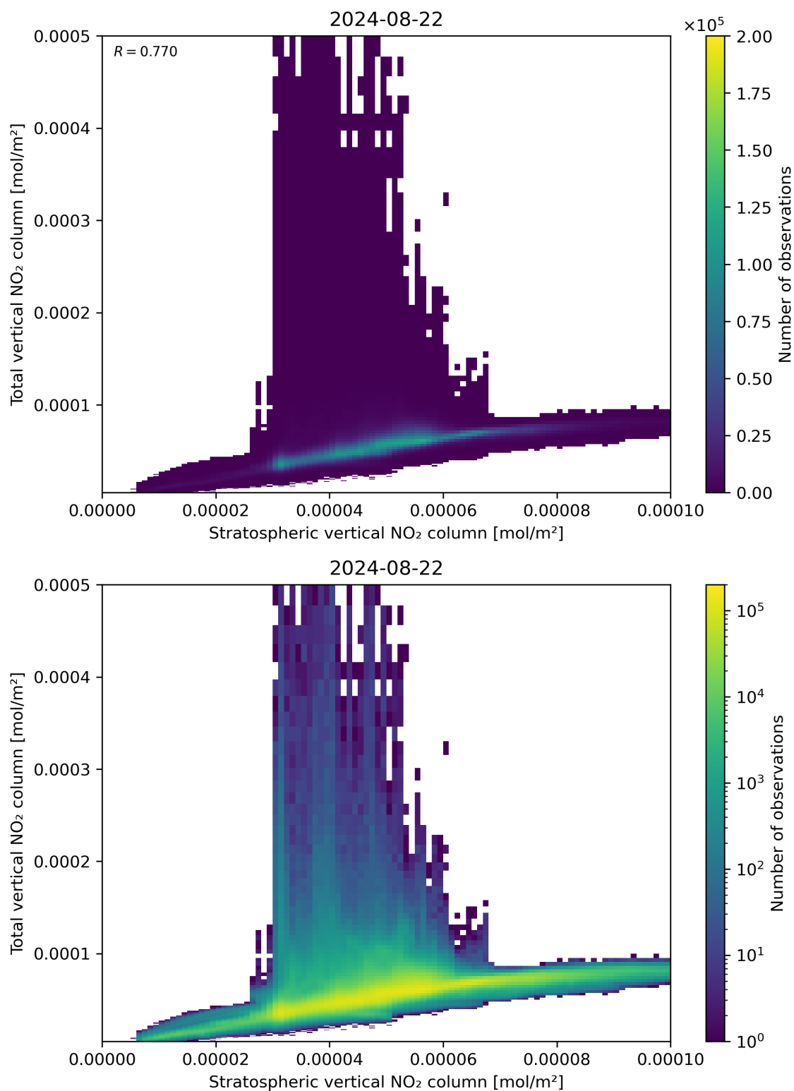
Figure 100: Scatter density plot of “Stratospheric vertical NO 2 column” against “Total vertical NO 2 column” for 2024-08-22 to 2024-08-23.
