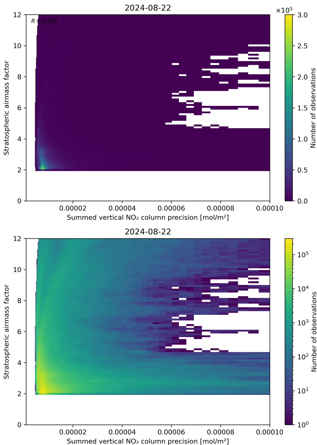
Figure 106: Scatter density plot of “Summed vertical NO 2 column precision” against “Stratospheric airmass factor” for 2024-08-22 to 2024-08-23.
