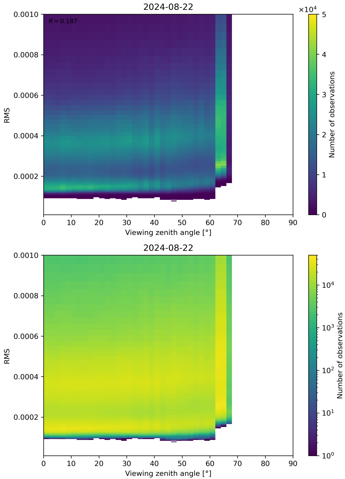
Figure 171: Scatter density plot of “Viewing zenith angle” against “RMS” for 2024-08-22 to 2024-08-23.
