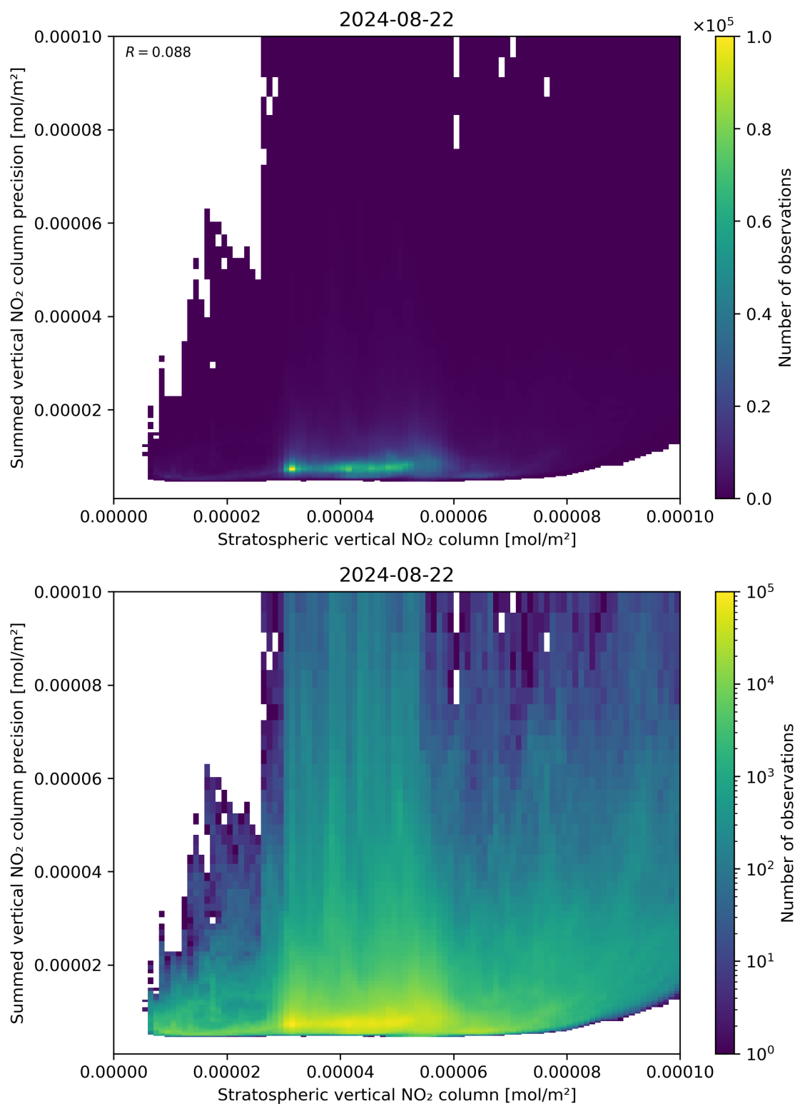
Figure 99: Scatter density plot of “Stratospheric vertical NO 2 column” against “Summed vertical NO 2 column precision” for 2024-08-22 to 2024-08-23.
