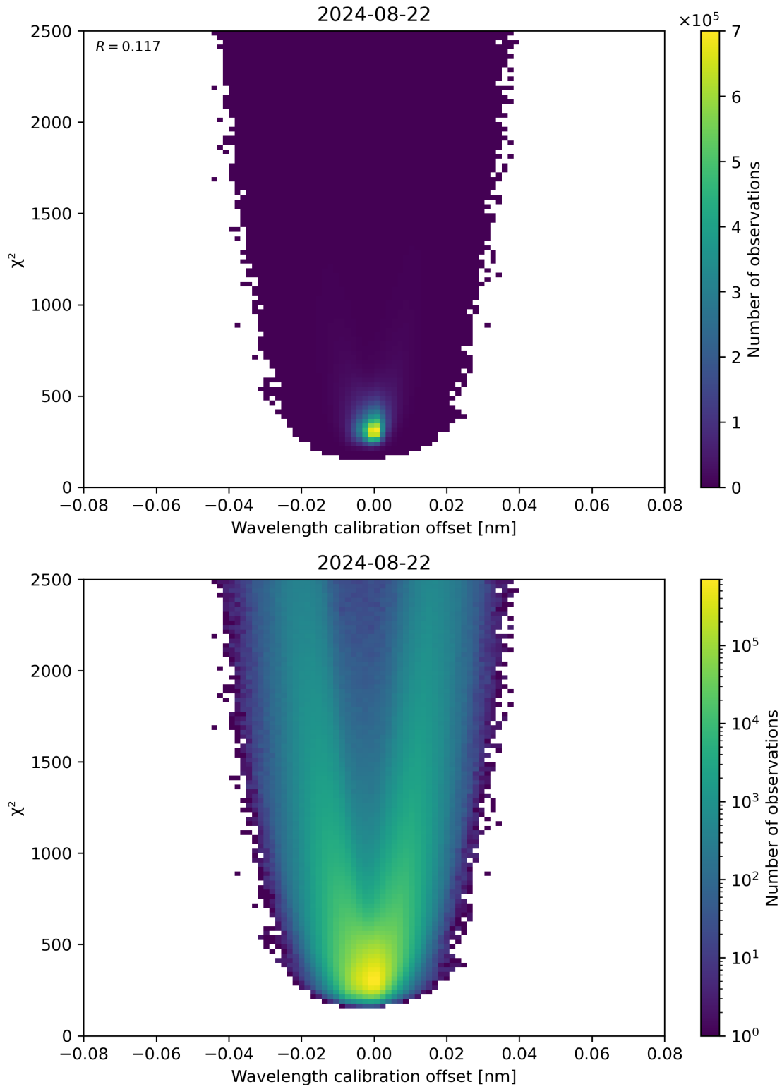
Figure 175: Scatter density plot of “Wavelength calibration offset” against “ \chi^2 ” for 2024-08-22 to 2024-08-23.
