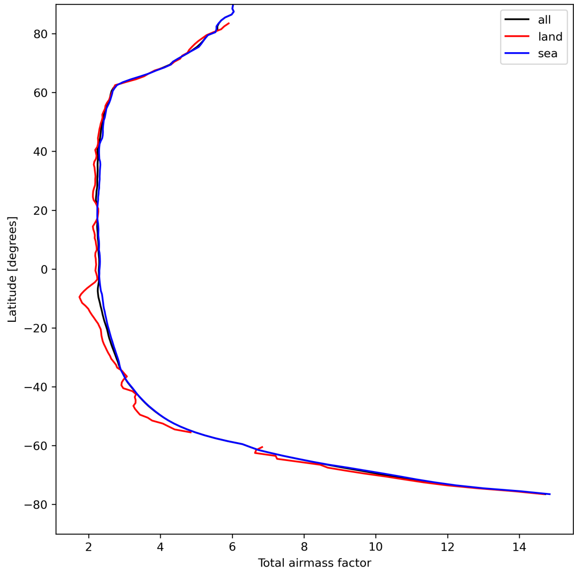
Figure 15: Zonal average of “Total airmass factor” for 2024-08-22 to 2024-08-23.
