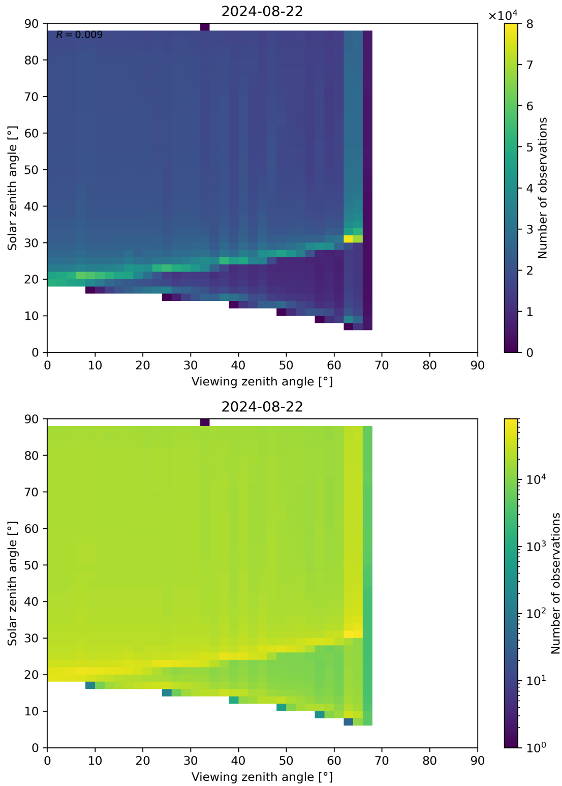
Figure 172: Scatter density plot of “Viewing zenith angle” against “Solar zenith angle” for 2024-08-22 to 2024-08-23.
