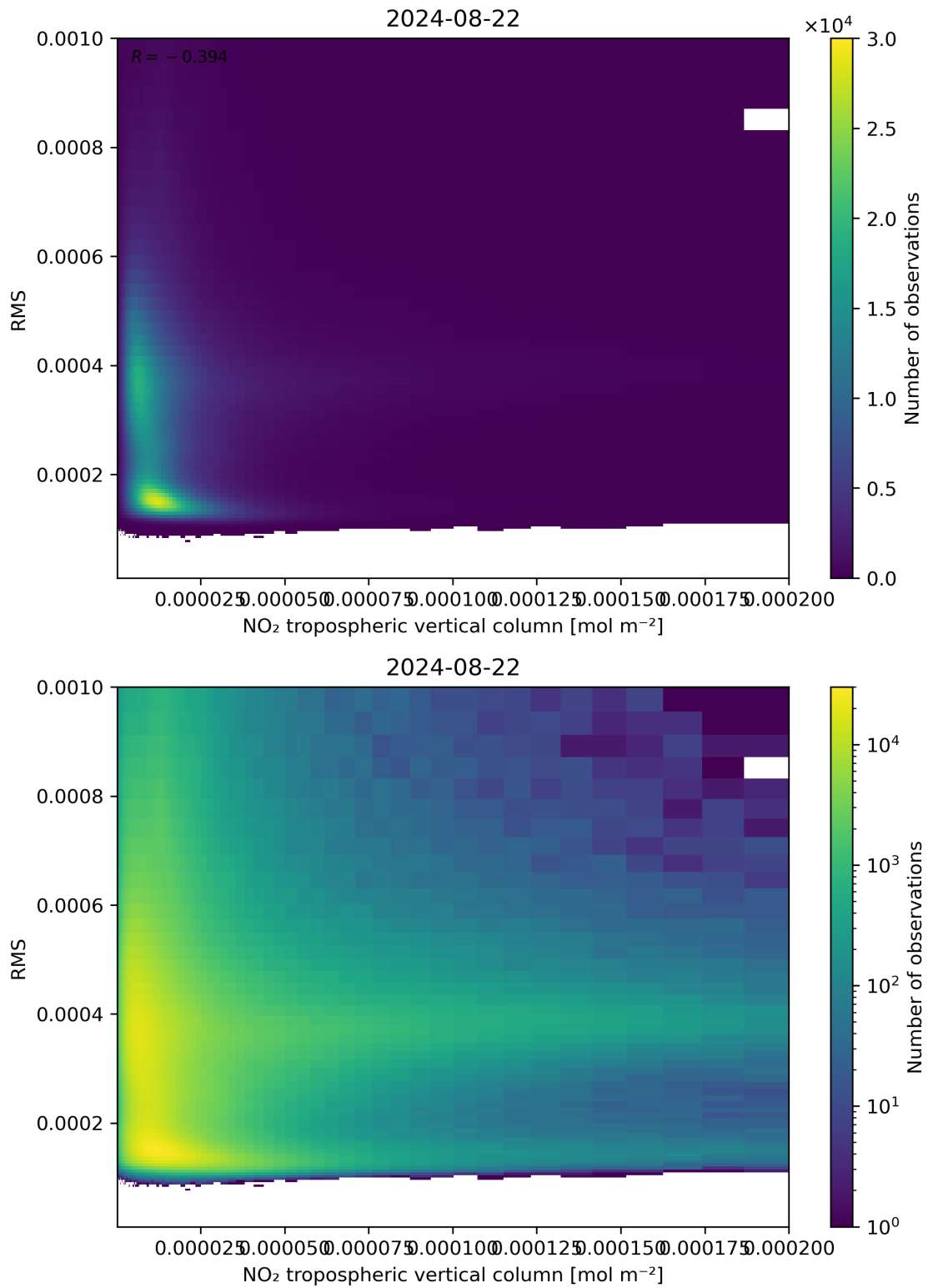
Figure 142: Scatter density plot of “NO 2 tropospheric vertical column” against “RMS” for 2024-08-22 to 2024-08-23.
