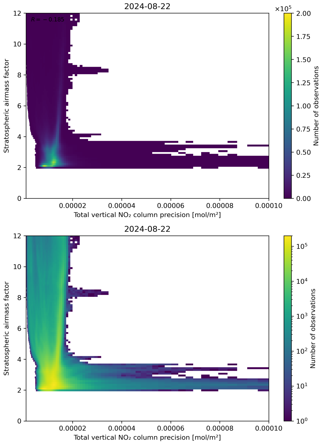
Figure 115: Scatter density plot of “Total vertical NO 2 column precision” against “Stratospheric air mass factor” for 2024-08-22 to 2024-08-23.
