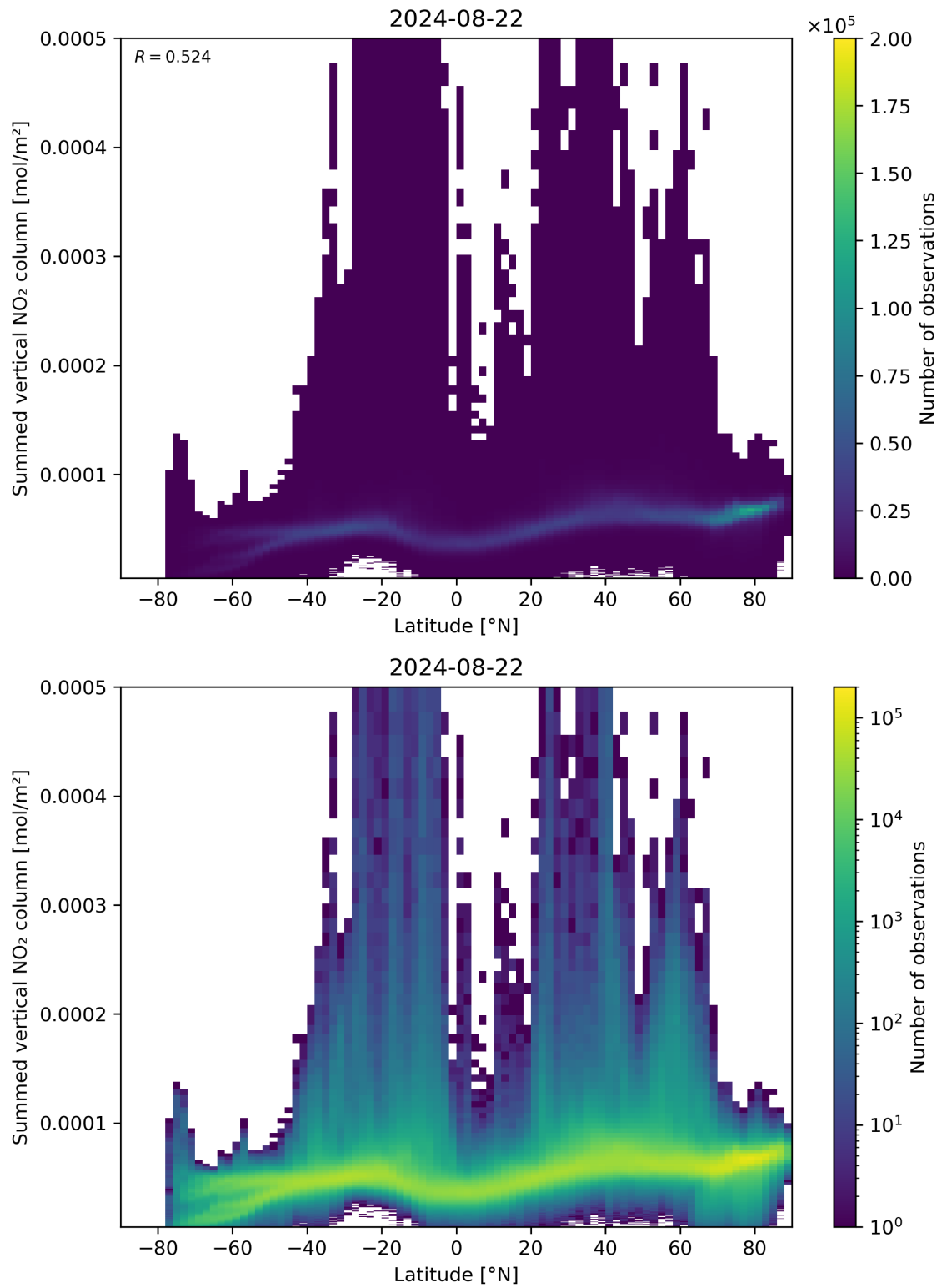
Figure 88: Scatter density plot of “Latitude” against “Summed vertical NO 2 column” for 2024-08-22 to 2024-08-23.
