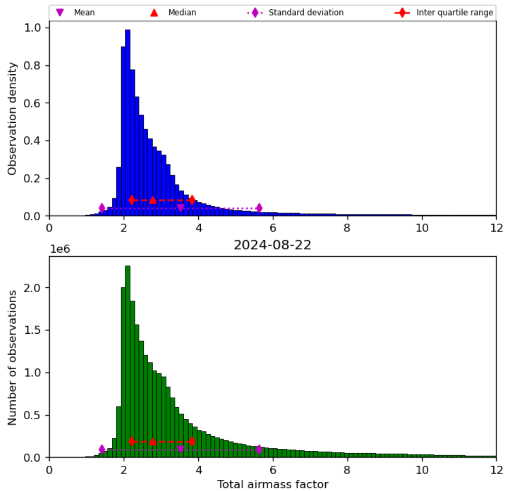
Figure 32: Histogram of “Total airmass factor” for 2024-08-22 to 2024-08-23
