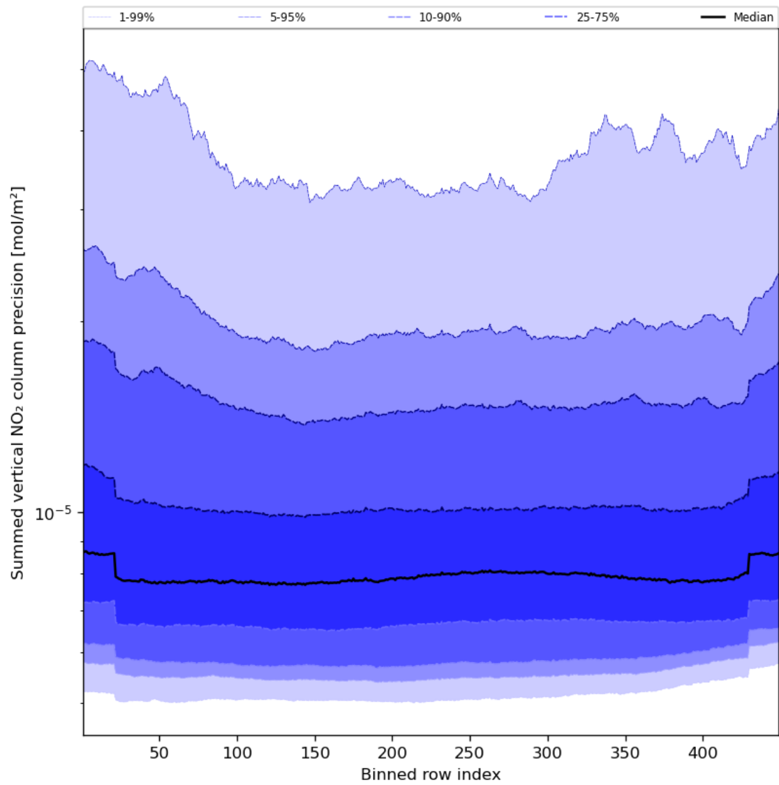
Figure 58: Along track statistics of “Summed vertical NO 2 column precision” for 2024-08-22 to 2024-08-23
