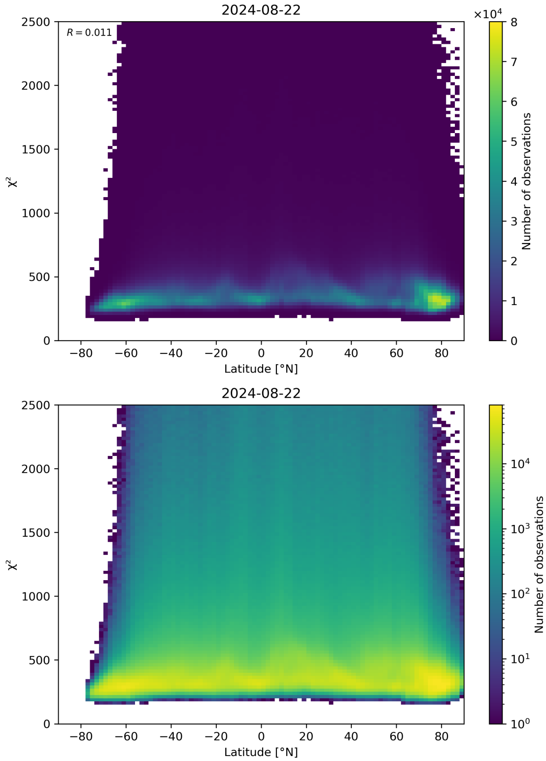
Figure 86: Scatter density plot of “Latitude” against “ \chi^2 ” for 2024-08-22 to 2024-08-23.
