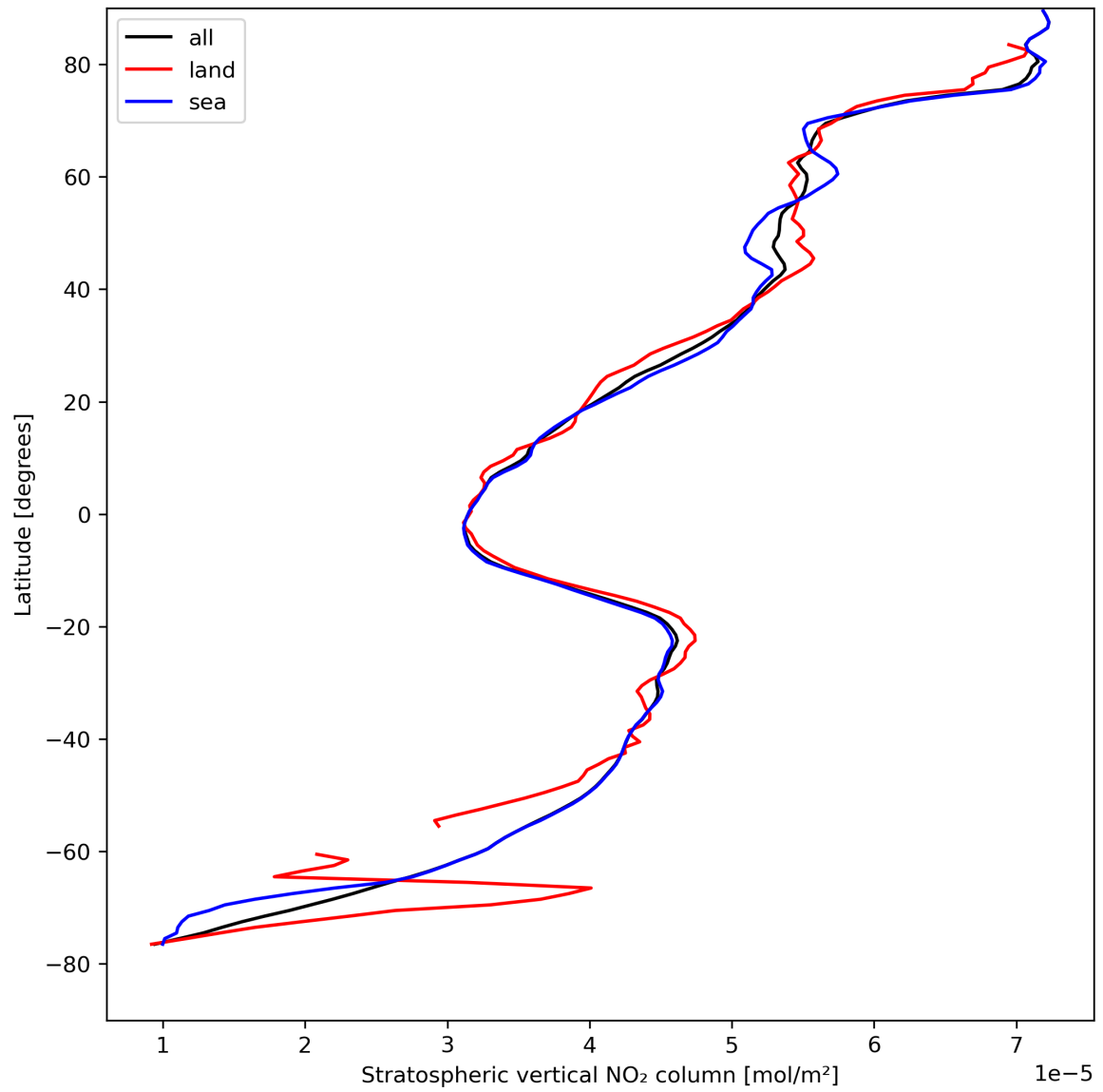
Figure 19: Zonal average of “Stratospheric vertical NO 2 column” for 2024-08-22 to 2024-08-23.
