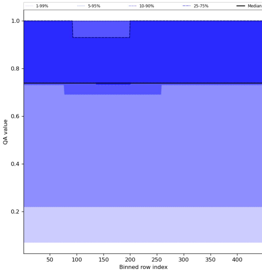
Figure 45: Along track statistics of “QA value” for 2024-08-22 to 2024-08-23
