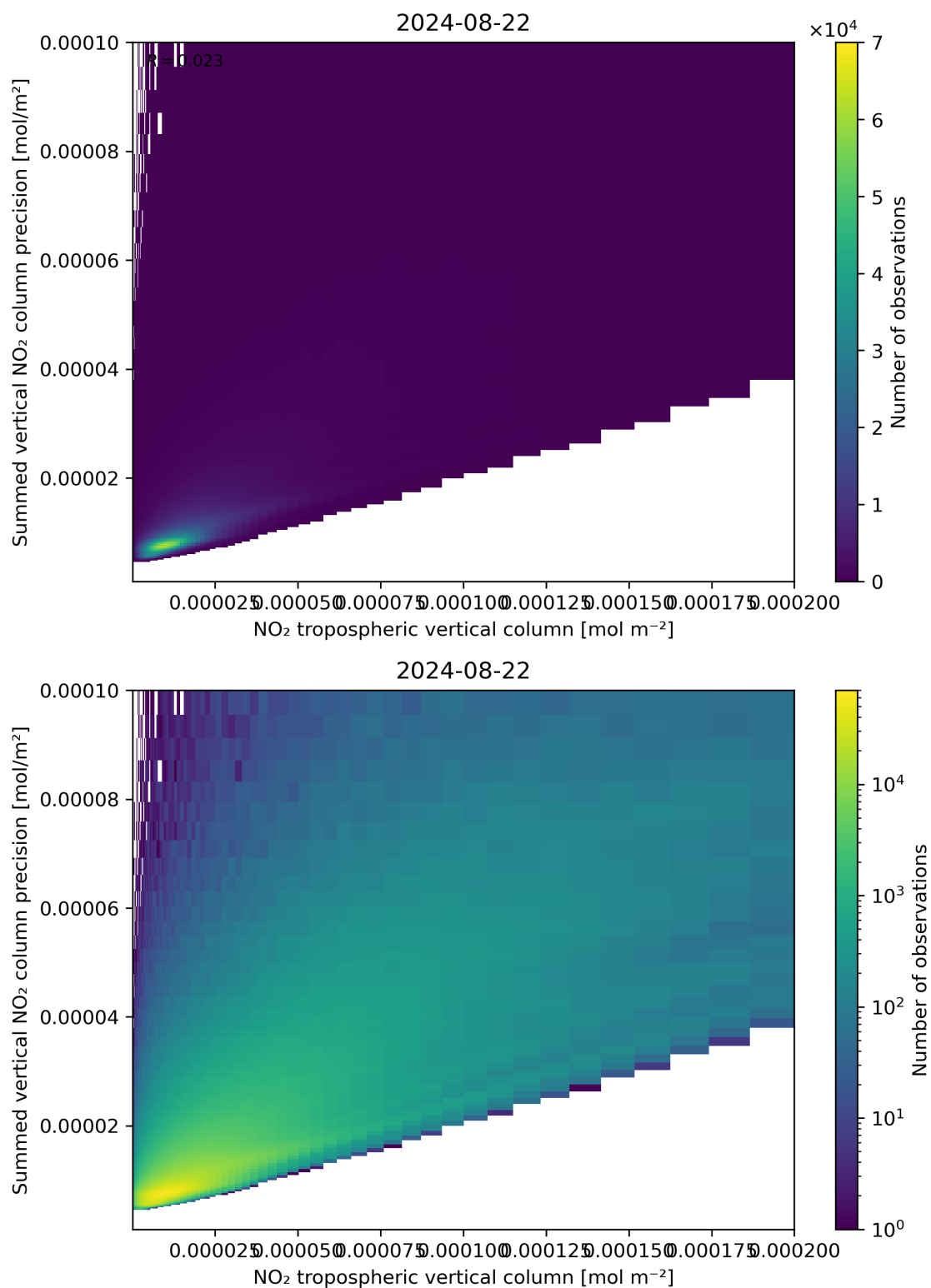
Figure 127: Scatter density plot of “NO 2 tropospheric vertical column” against “Summed vertical NO 2 column precision” for 2024-08-22 to 2024-08-23.
