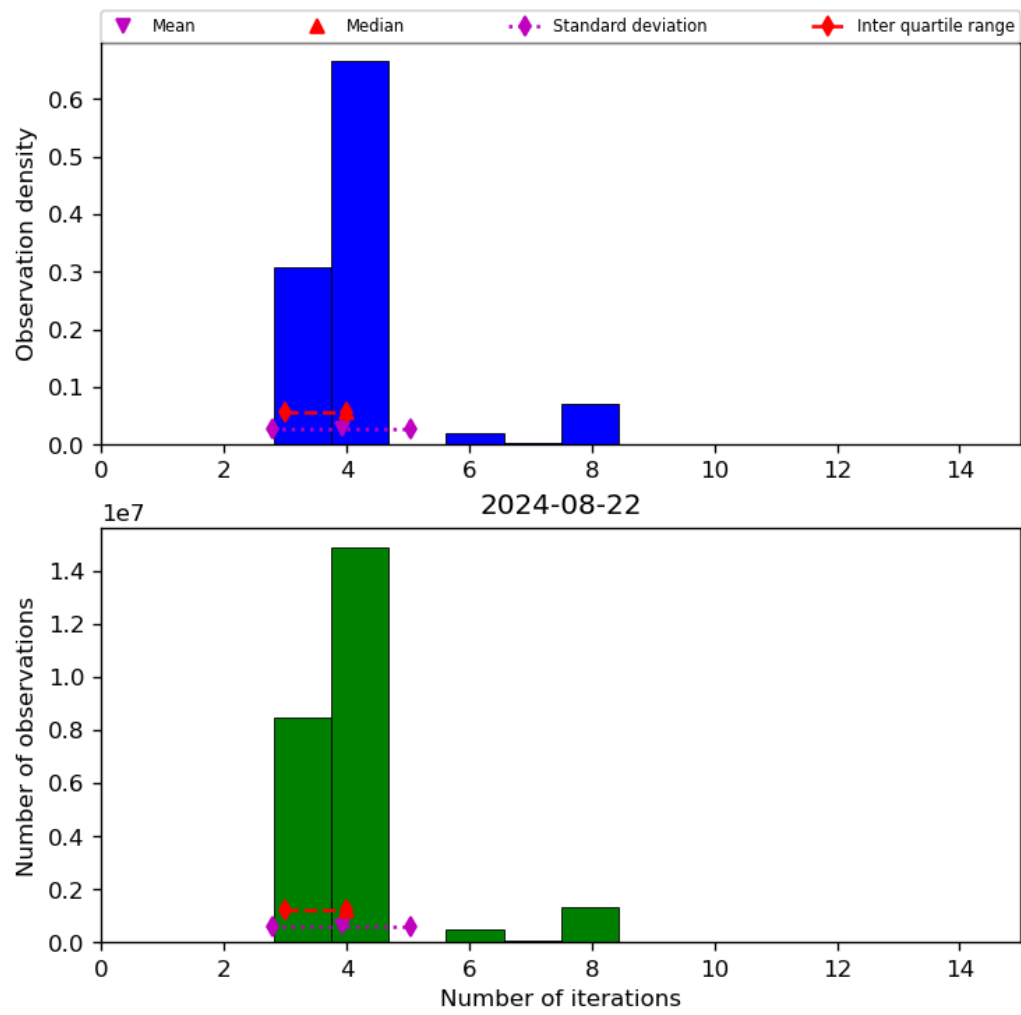
Figure 34: Histogram of “Number of iterations” for 2024-08-22 to 2024-08-23
