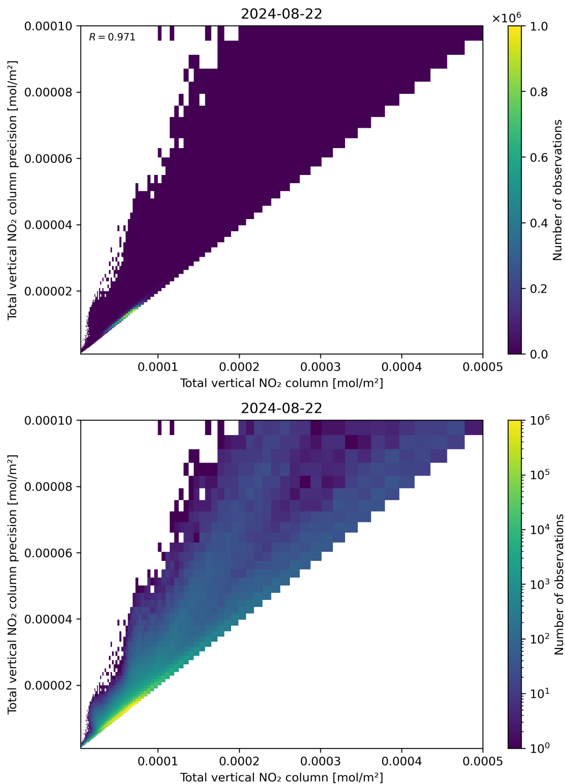
Figure 114: Scatter density plot of “Total vertical NO 2 column” against “Total vertical NO 2 column precision” for 2024-08-22 to 2024-08-23.
