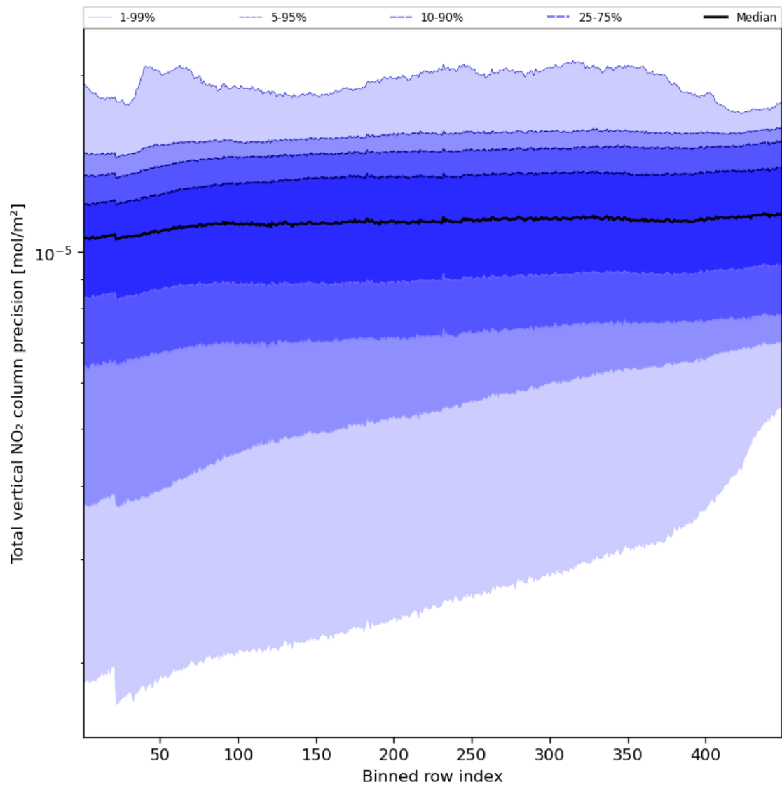
Figure 56: Along track statistics of “Total vertical NO 2 column precision” for 2024-08-22 to 2024-08-23
