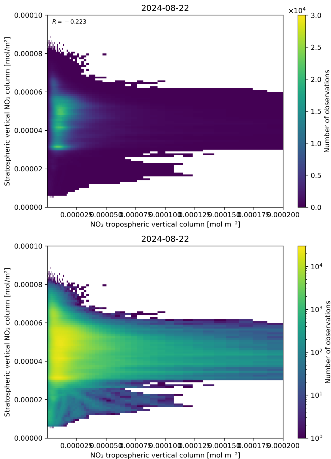
Figure 125: Scatter density plot of “NO 2 tropospheric vertical column” against “Stratospheric vertical NO 2 column” for 2024-08-22 to 2024-08-23.
