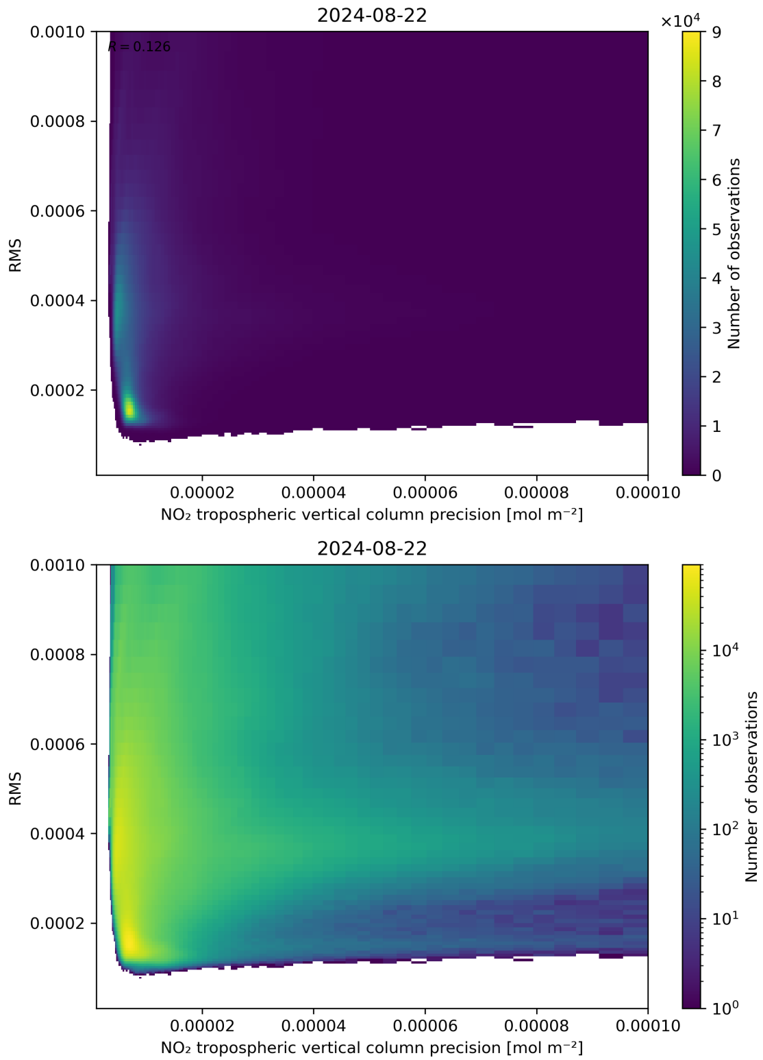
Figure 140: Scatter density plot of “NO 2 tropospheric vertical column precision” against “RMS” for 2024-08-22 to 2024-08-23.
