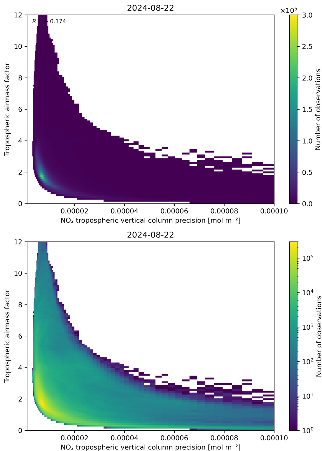
Figure 133: Scatter density plot of “NO 2 tropospheric vertical column precision” against “Tropospheric airmass factor” for 2024-08-22 to 2024-08-23.
