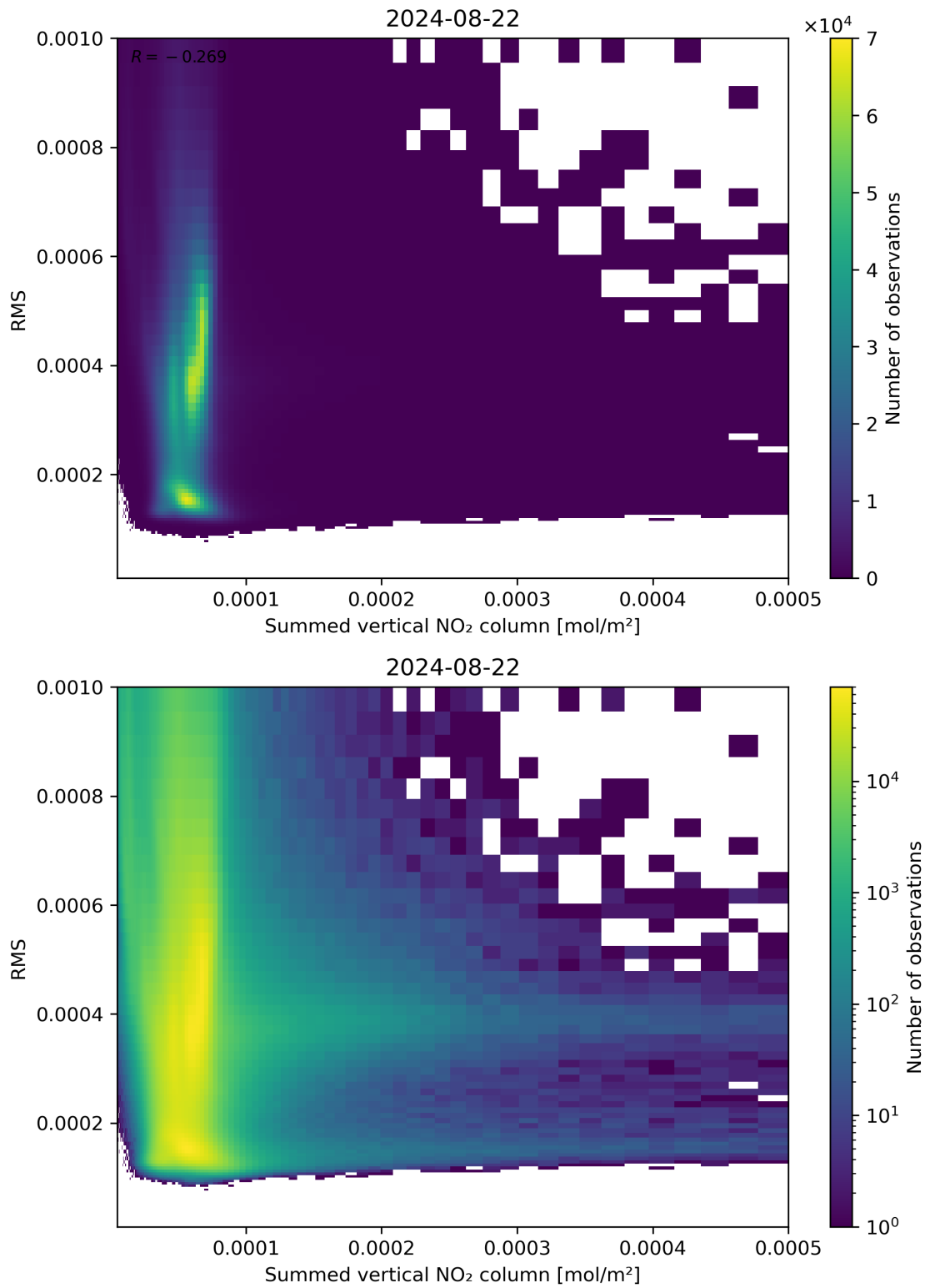
Figure 109: Scatter density plot of “Summed vertical NO 2 column” against “RMS” for 2024-08-22 to 2024-08-23.
