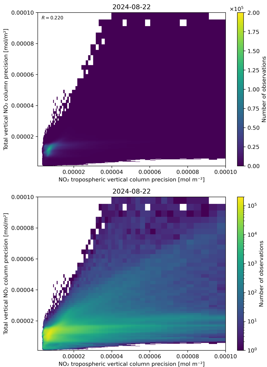
Figure 139: Scatter density plot of “NO 2 tropospheric vertical column precision” against “Total vertical NO 2 column precision” for 2024-08-22 to 2024-08-23.
