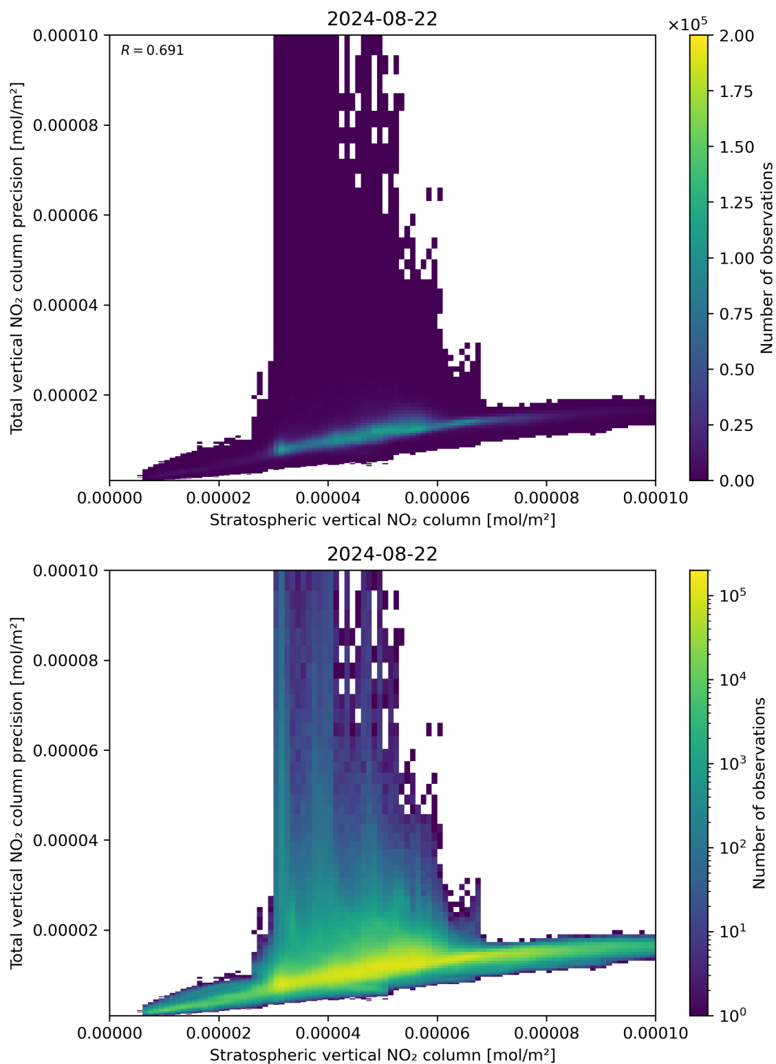
Figure 101: Scatter density plot of “Stratospheric vertical NO 2 column” against “Total vertical NO 2 column precision” for 2024-08-22 to 2024-08-23.
