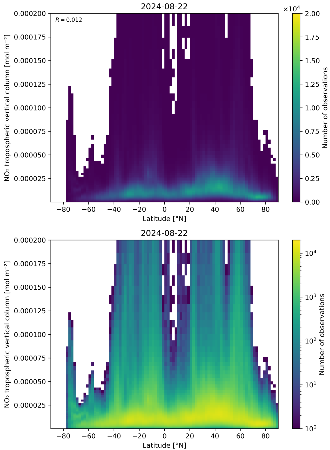
Figure 92: Scatter density plot of “Latitude” against “NO 2 tropospheric vertical column” for 2024-08-22 to 2024-08-23.
