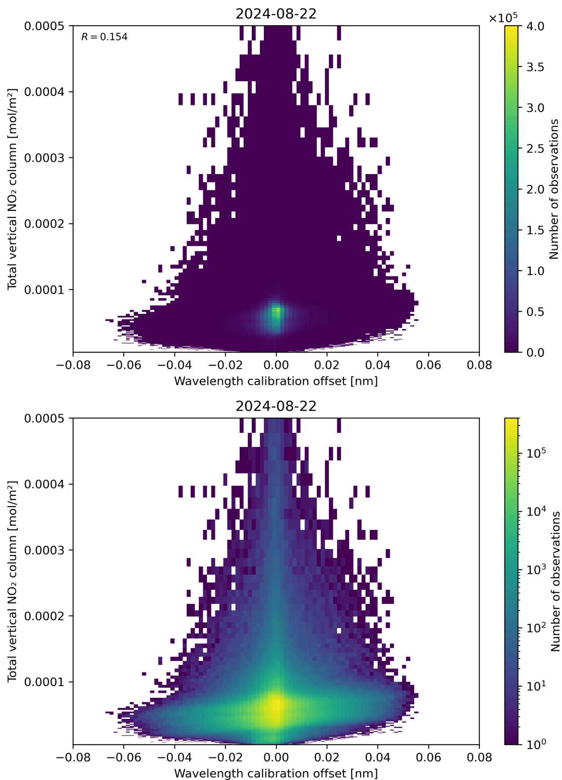
Figure 179: Scatter density plot of “Wavelength calibration offset” against “Total vertical NO 2 column” for 2024-08-22 to 2024-08-23.
