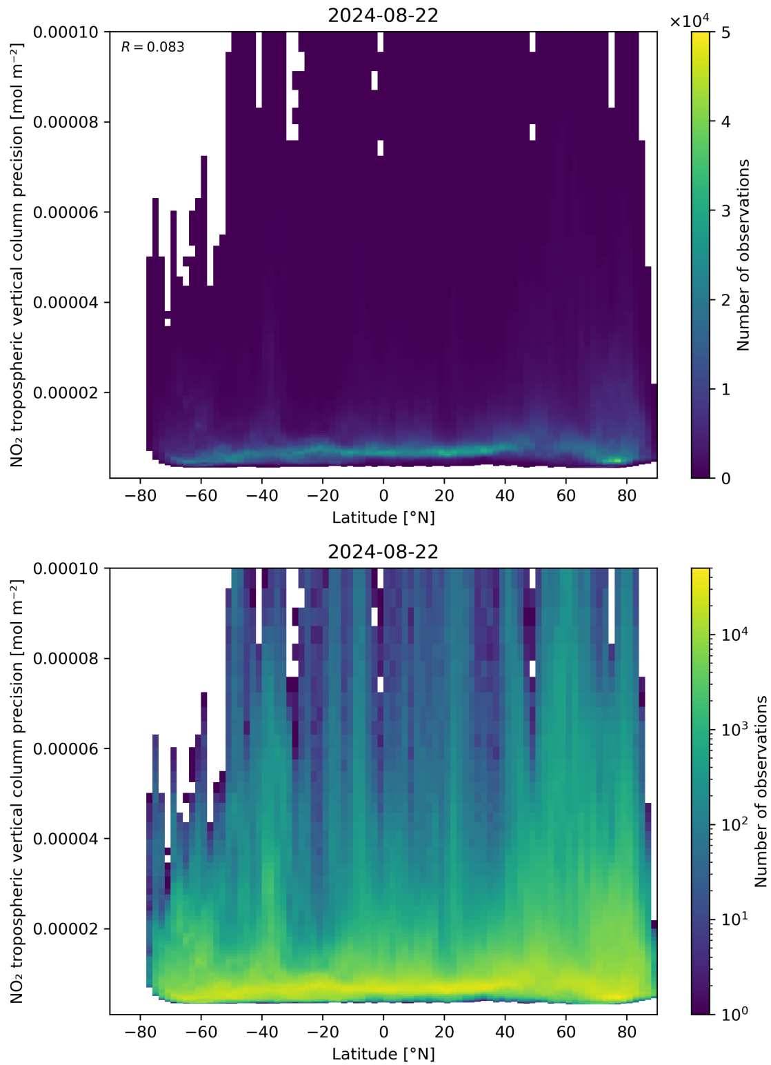
Figure 93: Scatter density plot of “Latitude” against “NO 2 tropospheric vertical column precision” for 2024-08-22 to 2024-08-23.
