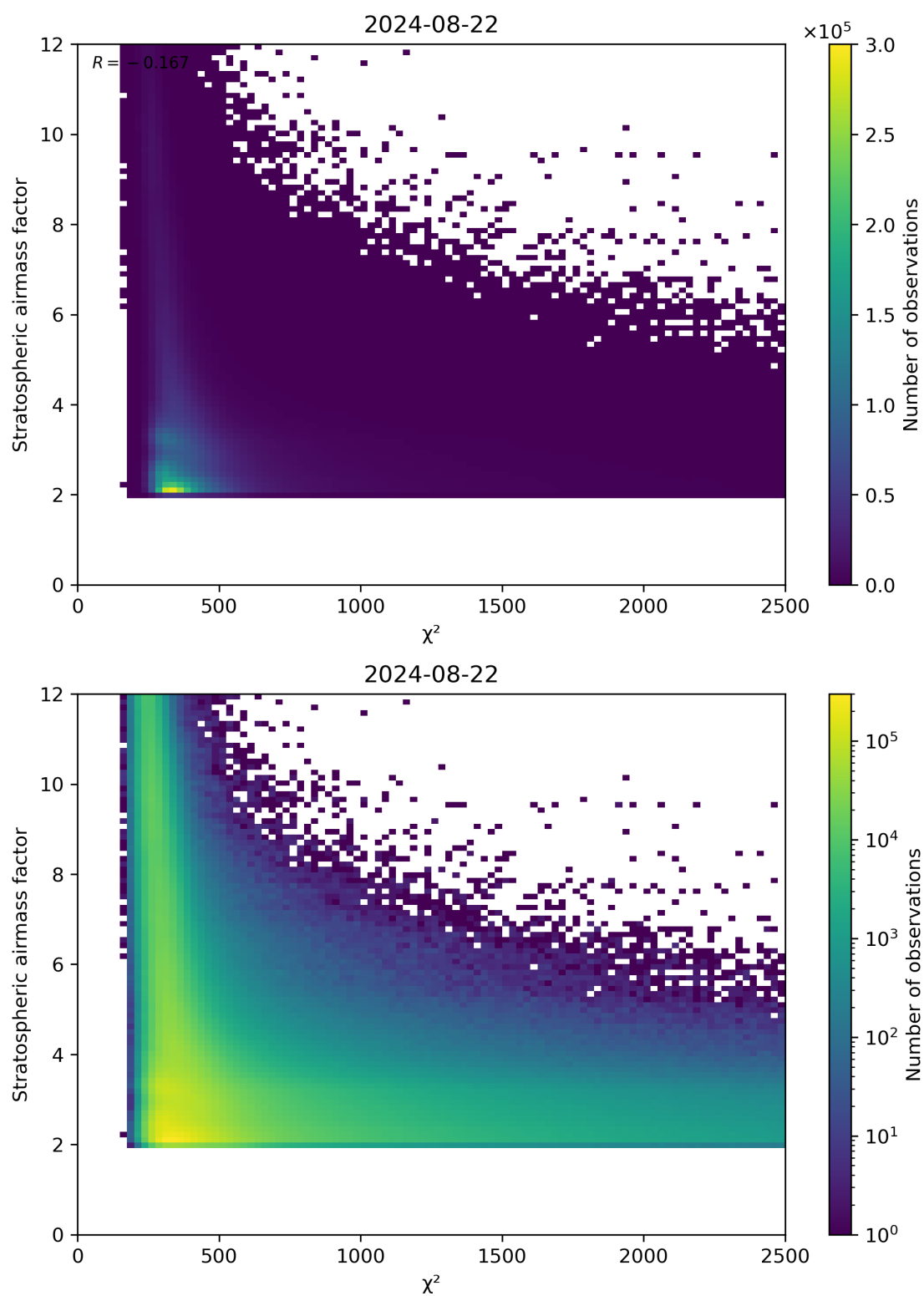
Figure 81: Scatter density plot of “ \chi^2 ” against “Stratospheric airmass factor” for 2024-08-22 to 2024-08-23.
