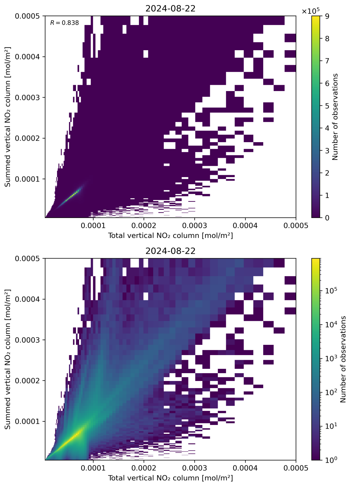
Figure 112: Scatter density plot of “Total vertical NO 2 column” against “Summed vertical NO 2 column” for 2024-08-22 to 2024-08-23.
