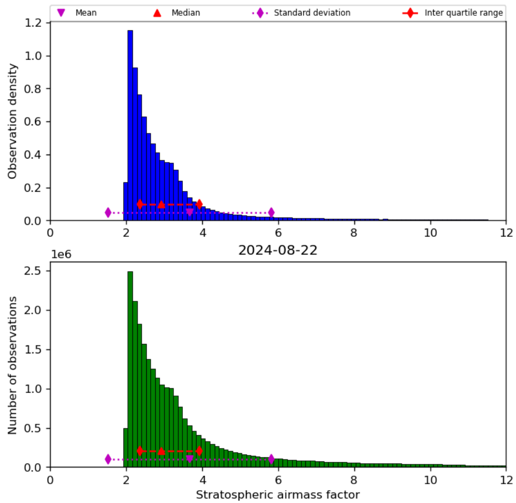
Figure 44: Histogram of “Stratospheric airmass factor” for 2024-08-22 to 2024-08-23
