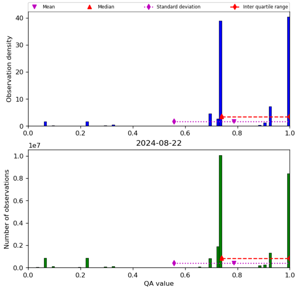
Figure 28: Histogram of “QA value” for 2024-08-22 to 2024-08-23
