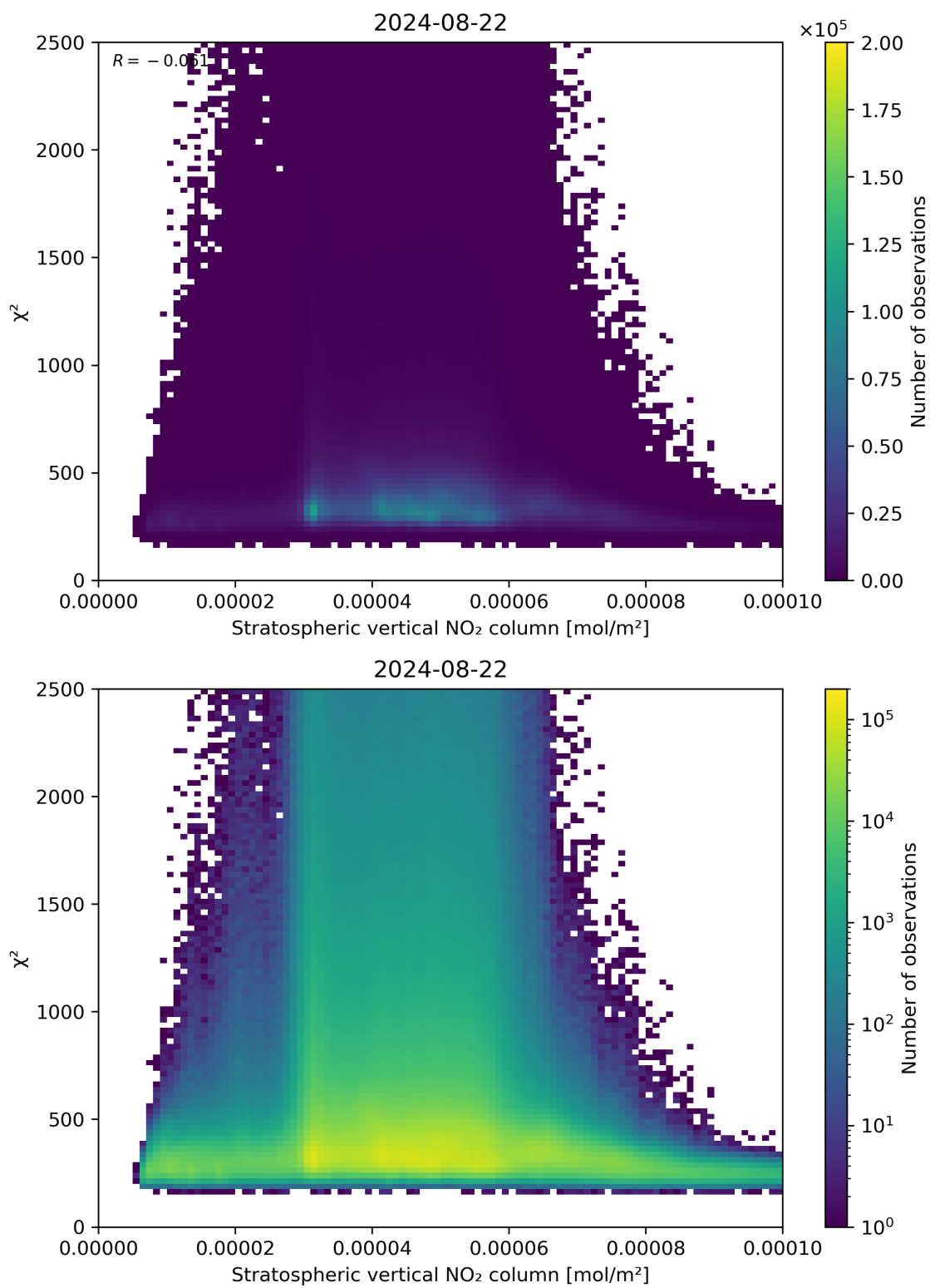
Figure 97: Scatter density plot of “Stratospheric vertical NO 2 column” against “ \chi^2 ” for 2024-08-22 to 2024-08-23.
