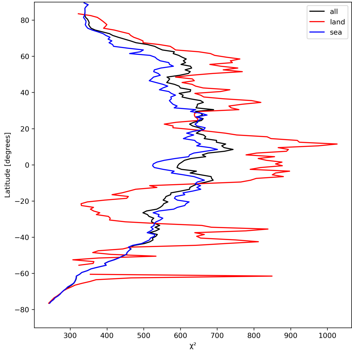
Figure 25: Zonal average of “ \chi^2 ” for 2024-08-22 to 2024-08-23.
