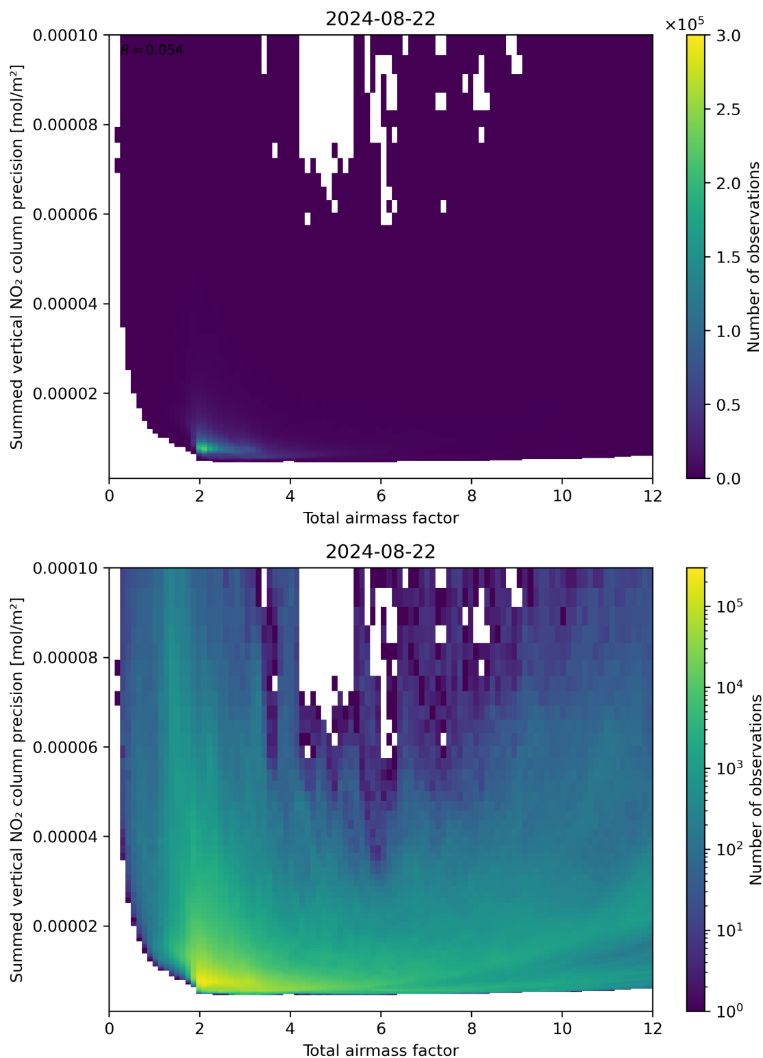
Figure 66: Scatter density plot of “Total airmass factor” against “Summed vertical NO 2 column precision” for 2024-08-22 to 2024-08-23.
