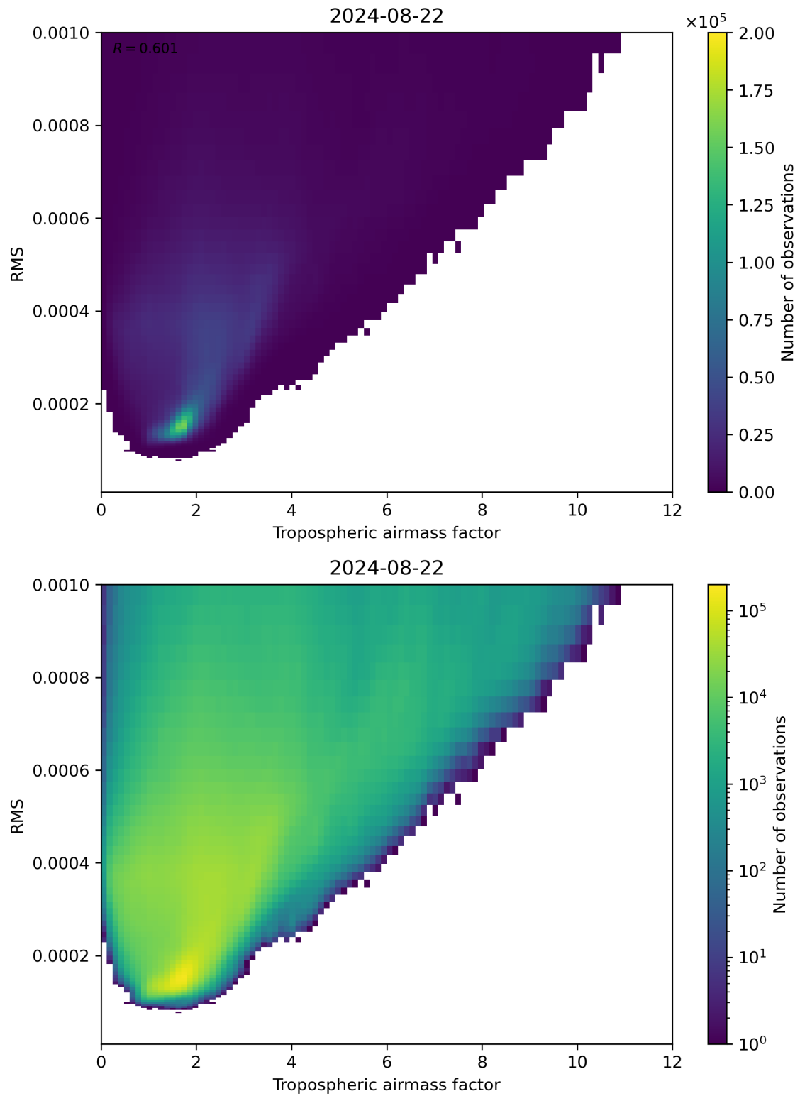
Figure 79: Scatter density plot of “Tropospheric airmass factor” against “RMS” for 2024-08-22 to 2024-08-23.
