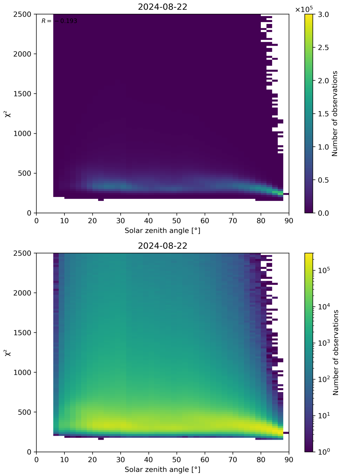
Figure 148: Scatter density plot of “Solar zenith angle” against “ \chi^2 ” for 2024-08-22 to 2024-08-23.
