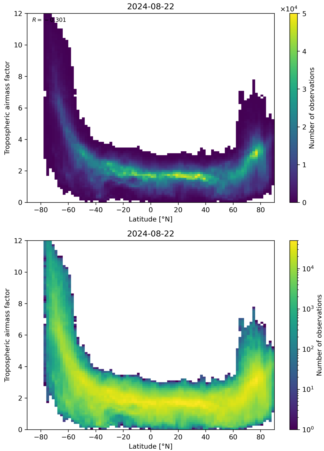
Figure 85: Scatter density plot of “Latitude” against “Tropospheric airmass factor” for 2024-08-22 to 2024-08-23.
