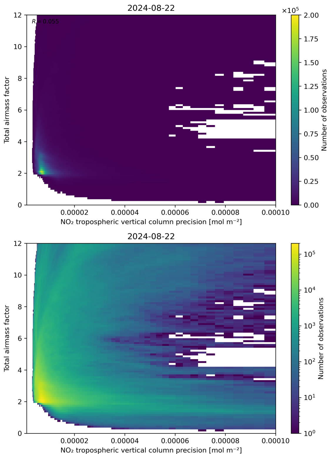
Figure 132: Scatter density plot of “NO 2 tropospheric vertical column precision” against “Total air mass factor” for 2024-08-22 to 2024-08-23.
