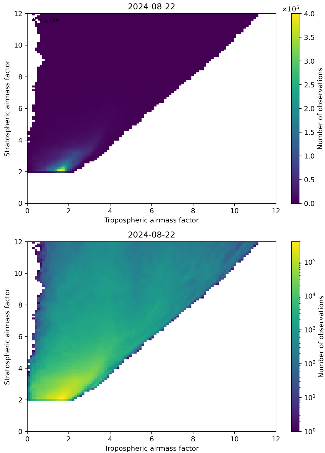
Figure 71: Scatter density plot of “Tropospheric airmass factor” against “Stratospheric airmass factor” for 2024-08-22 to 2024-08-23.
