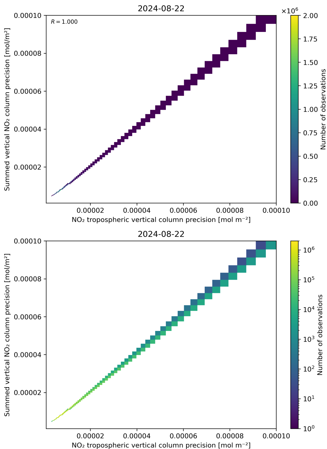
Figure 137: Scatter density plot of “NO 2 tropospheric vertical column precision” against “Summed vertical NO 2 column precision” for 2024-08-22 to 2024-08-23.
