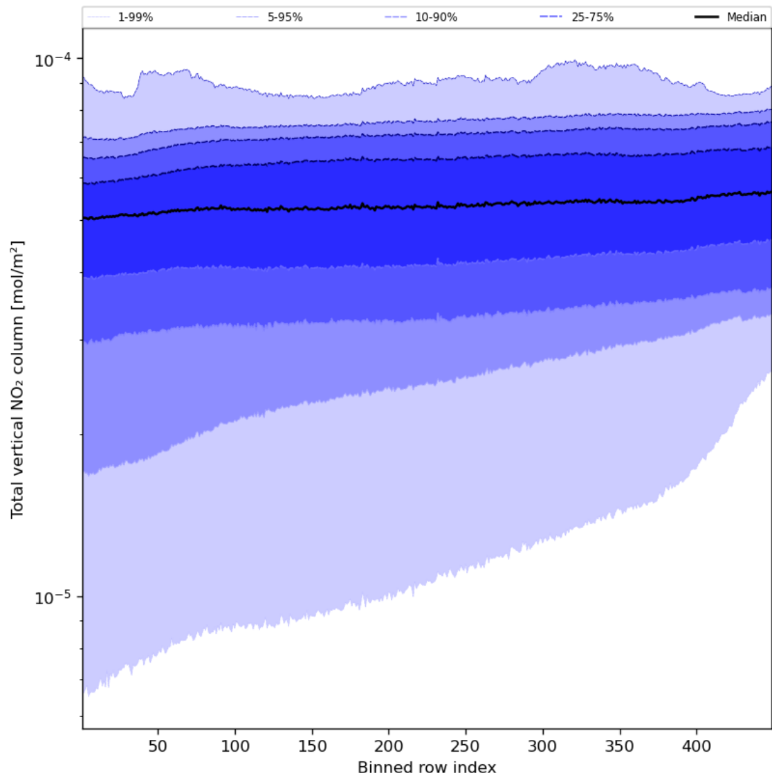
Figure 55: Along track statistics of “Total vertical NO 2 column” for 2024-08-22 to 2024-08-23
