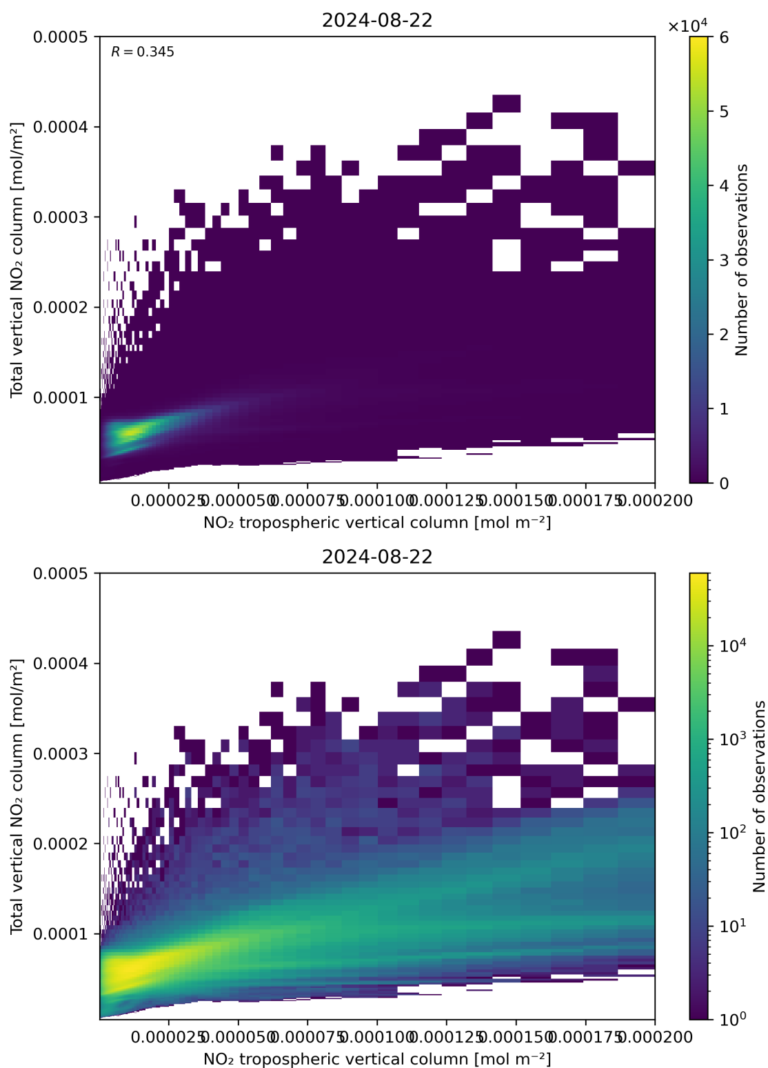
Figure 128: Scatter density plot of “NO 2 tropospheric vertical column” against “Total vertical NO 2 column” for 2024-08-22 to 2024-08-23.
