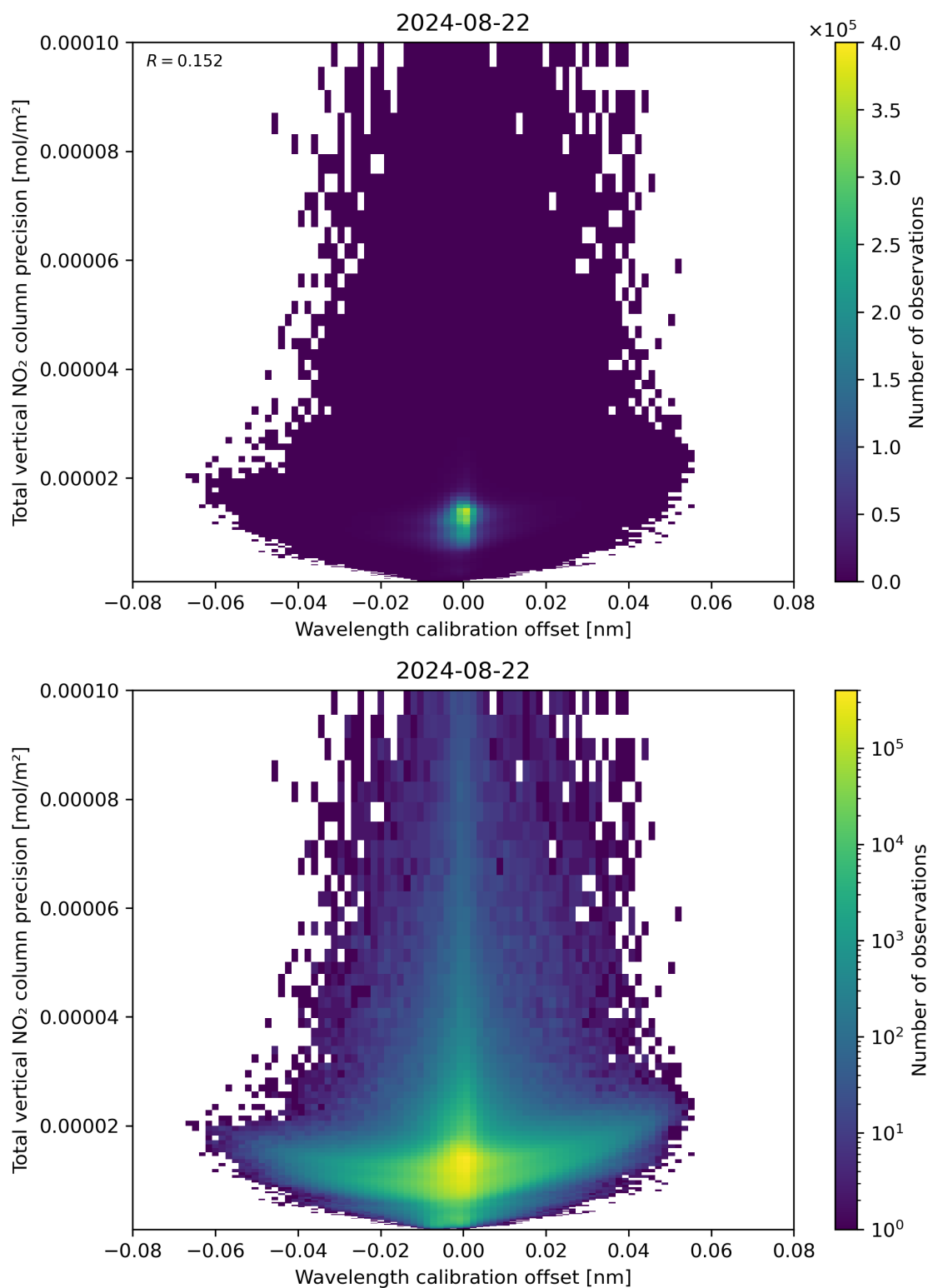
Figure 180: Scatter density plot of “Wavelength calibration offset” against “Total vertical NO 2 column precision” for 2024-08-22 to 2024-08-23.
