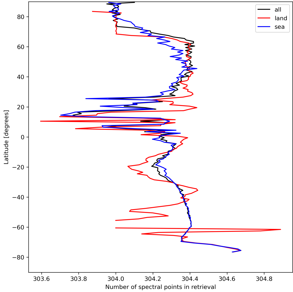
Figure 16: Zonal average of “Number of spectral points in retrieval” for 2024-08-22 to 2024-08-23.
