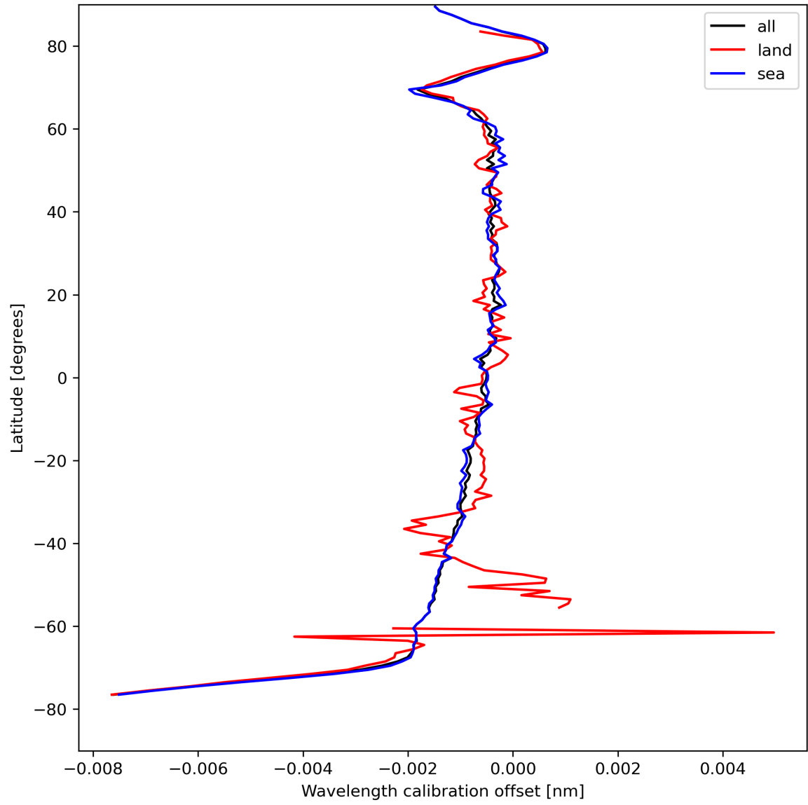
Figure 18: Zonal average of “Wavelength calibration offset” for 2024-08-22 to 2024-08-23.
