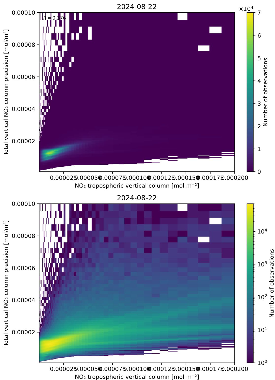
Figure 129: Scatter density plot of “NO 2 tropospheric vertical column” against “Total vertical NO 2 column precision” for 2024-08-22 to 2024-08-23.
