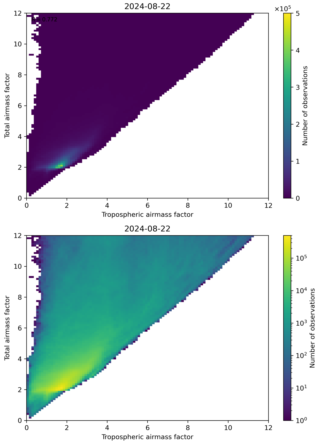
Figure 72: Scatter density plot of “Tropospheric airmass factor” against “Total airmass factor” for 2024-08-22 to 2024-08-23.
