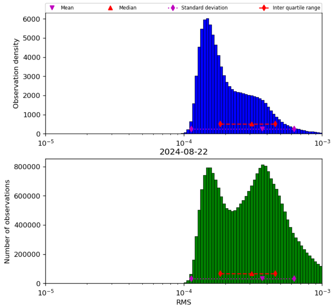
Figure 43: Histogram of “RMS” for 2024-08-22 to 2024-08-23
