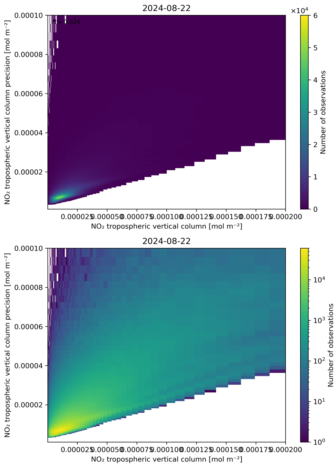
Figure 130: Scatter density plot of “NO 2 tropospheric vertical column” against “NO 2 tropospheric vertical column precision” for 2024-08-22 to 2024-08-23.
