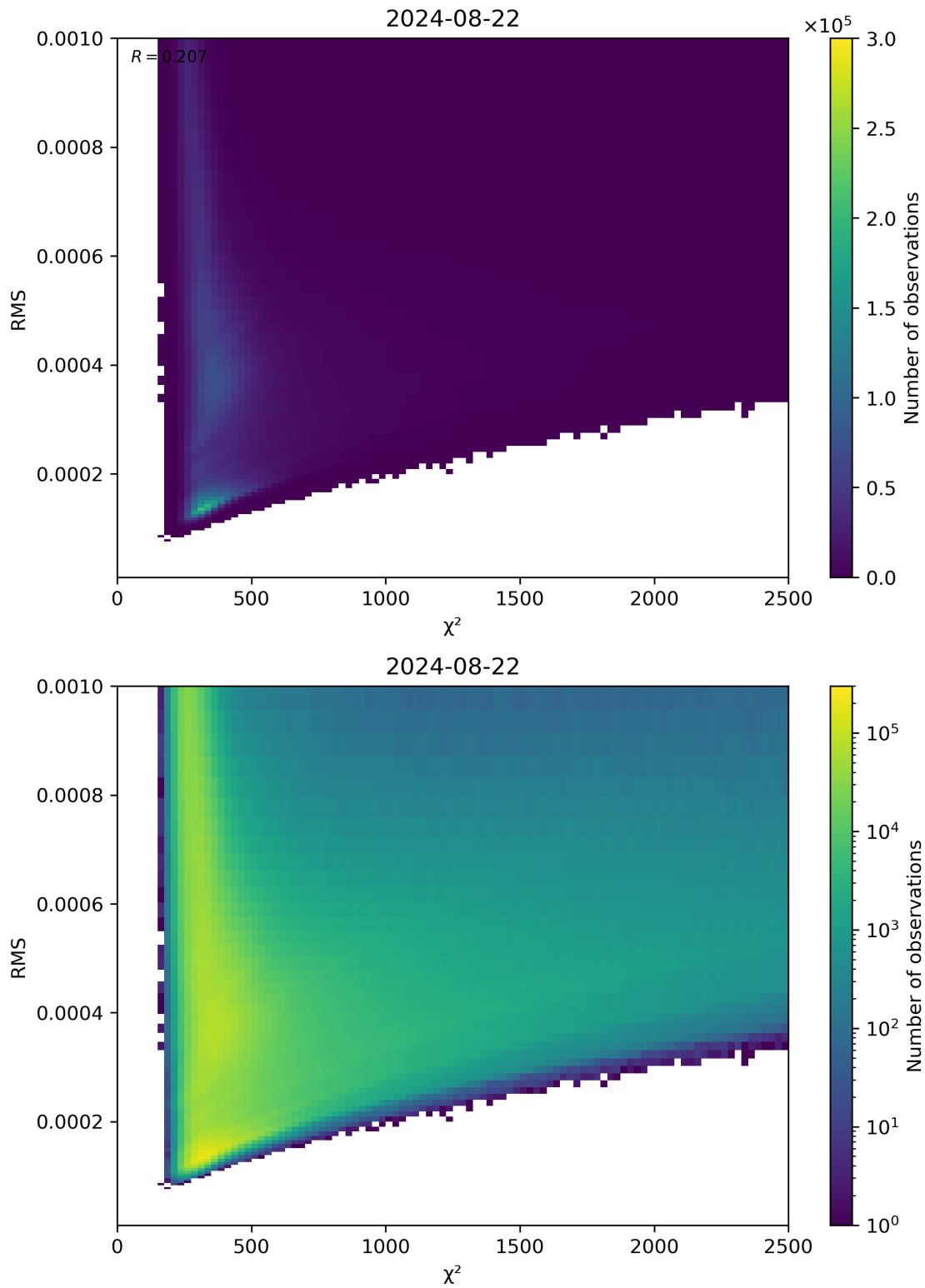
Figure 82: Scatter density plot of “ \chi^2 ” against “RMS” for 2024-08-22 to 2024-08-23.
