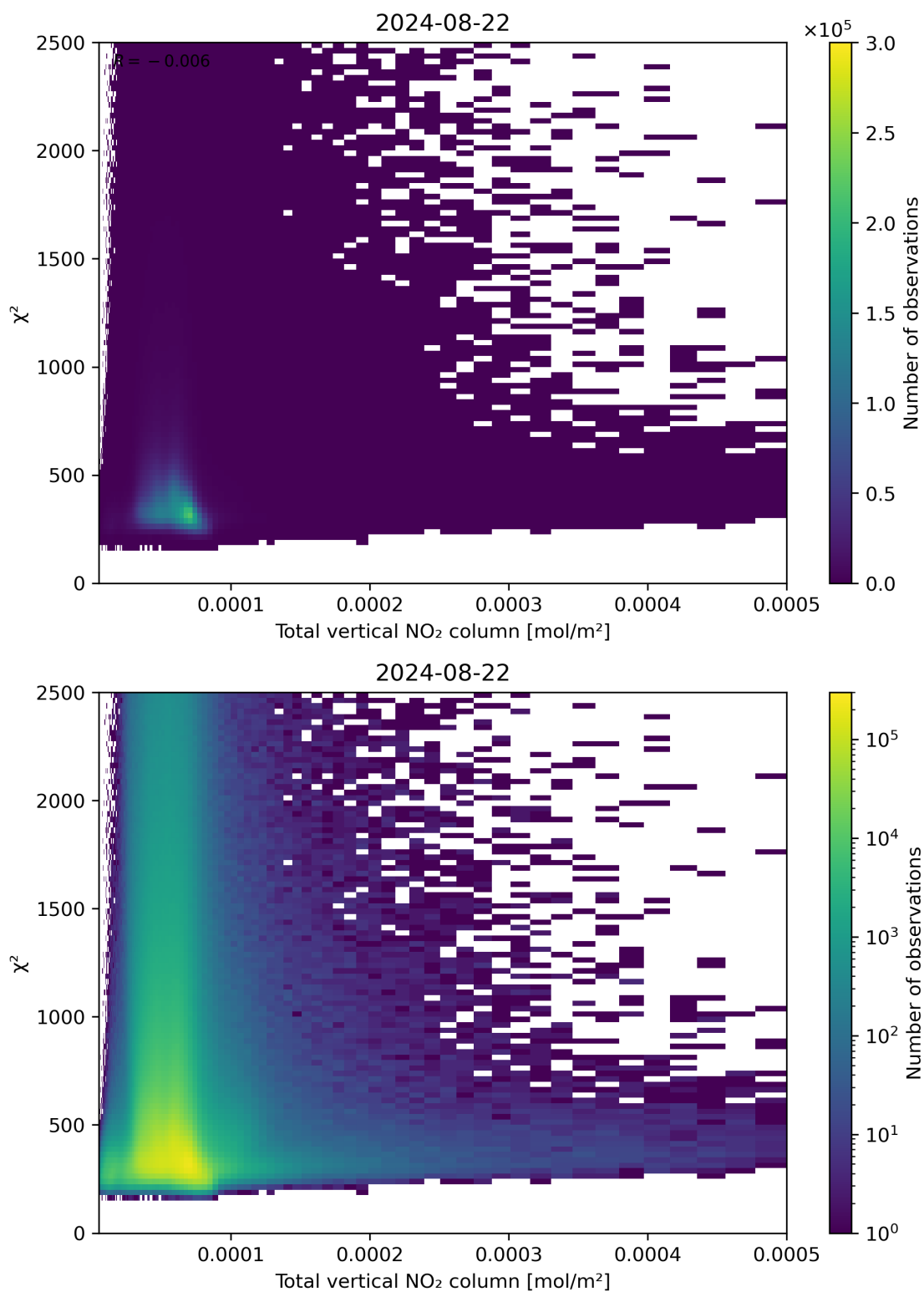
Figure 111: Scatter density plot of “Total vertical NO 2 column” against “ \chi^2 ” for 2024-08-22 to 2024-08-23.
