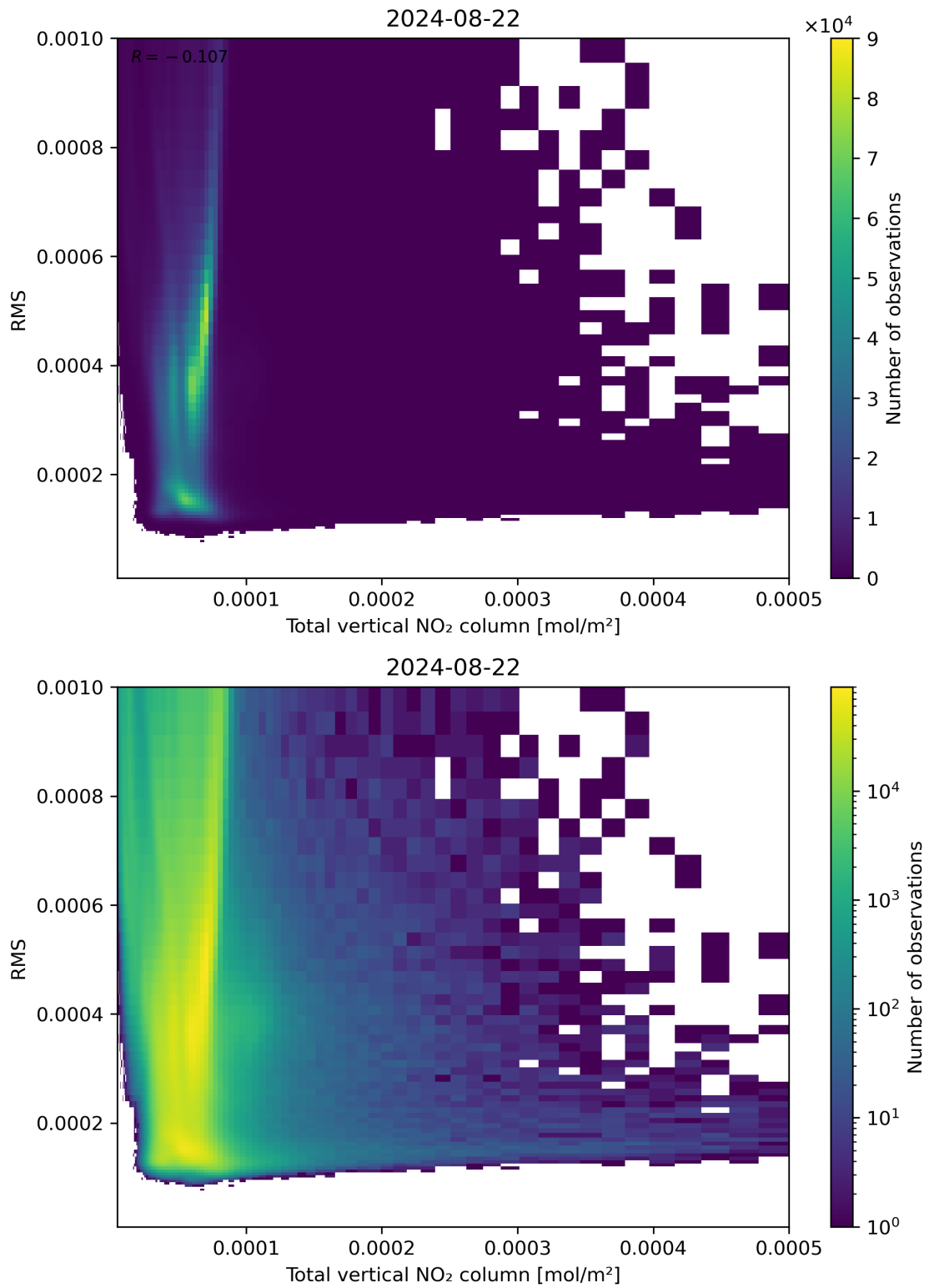
Figure 120: Scatter density plot of “Total vertical NO 2 column” against “RMS” for 2024-08-22 to 2024-08-23.
