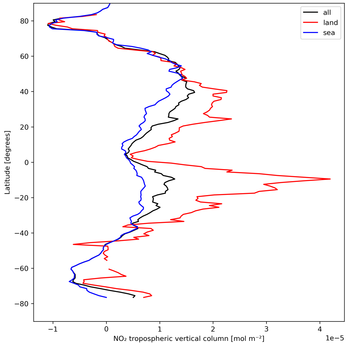
Figure 12: Zonal average of “NO 2 tropospheric vertical column” for 2024-08-22 to 2024-08-23.
