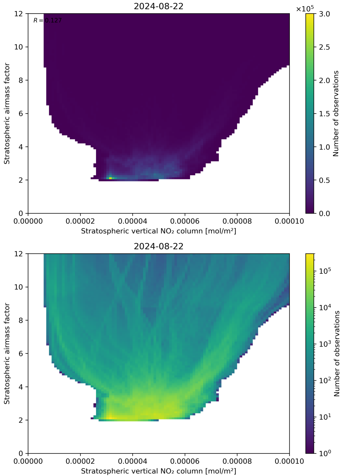
Figure 96: Scatter density plot of “Stratospheric vertical NO 2 column” against “Stratospheric airmass factor” for 2024-08-22 to 2024-08-23.
