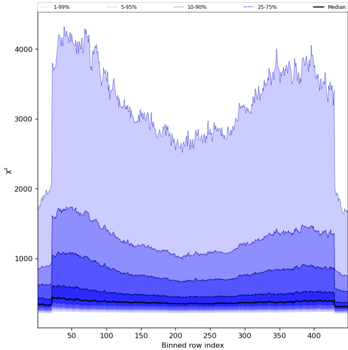
Figure 59: Along track statistics of “ \chi^2 ” for 2024-08-22 to 2024-08-23
