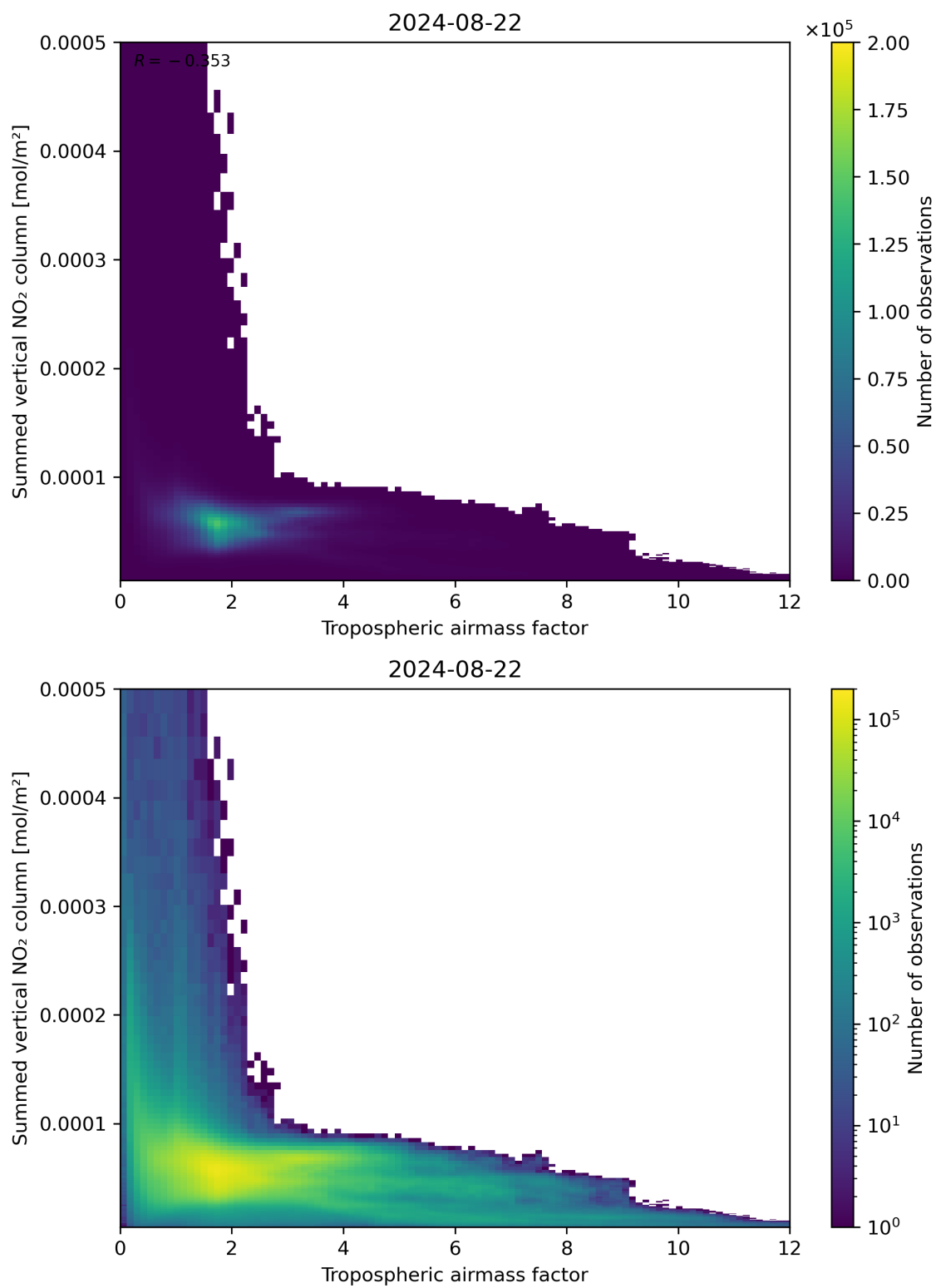
Figure 75: Scatter density plot of “Tropospheric air mass factor” against “Summed vertical NO 2 column” for 2024-08-22 to 2024-08-23.
