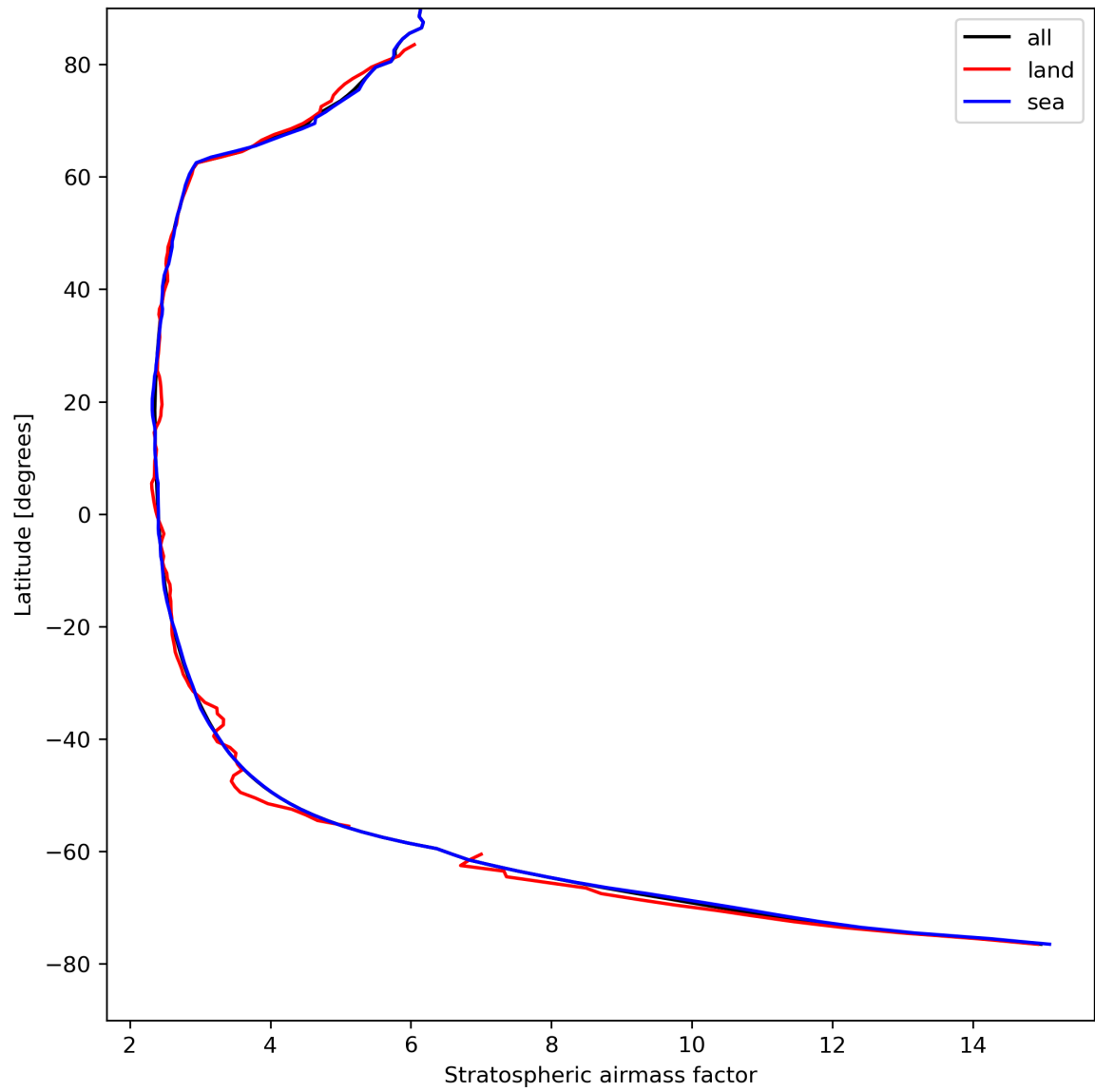
Figure 27: Zonal average of “Stratospheric air mass factor” for 2024-08-22 to 2024-08-23.
