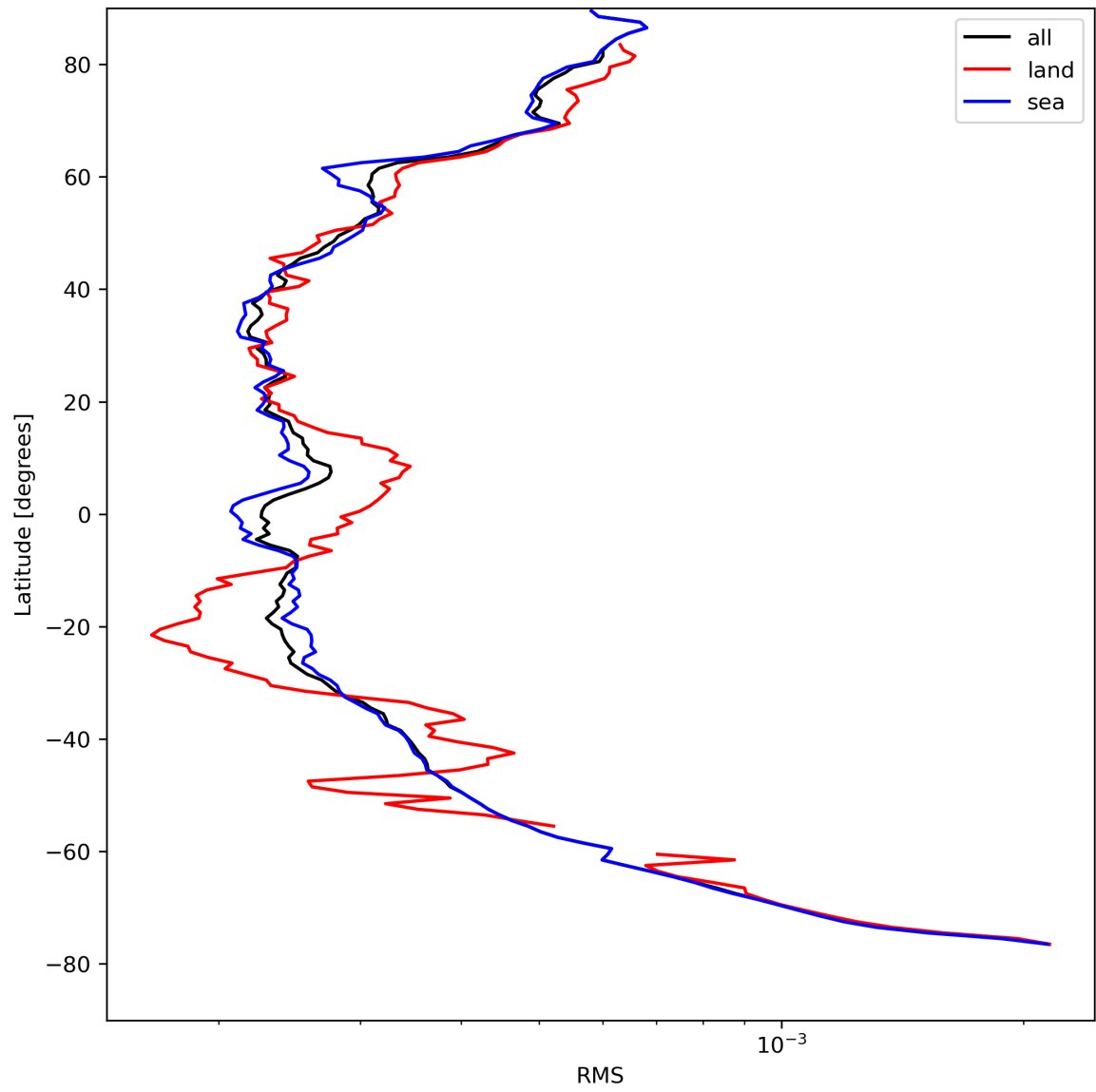
Figure 26: Zonal average of “RMS” for 2024-08-22 to 2024-08-23.
