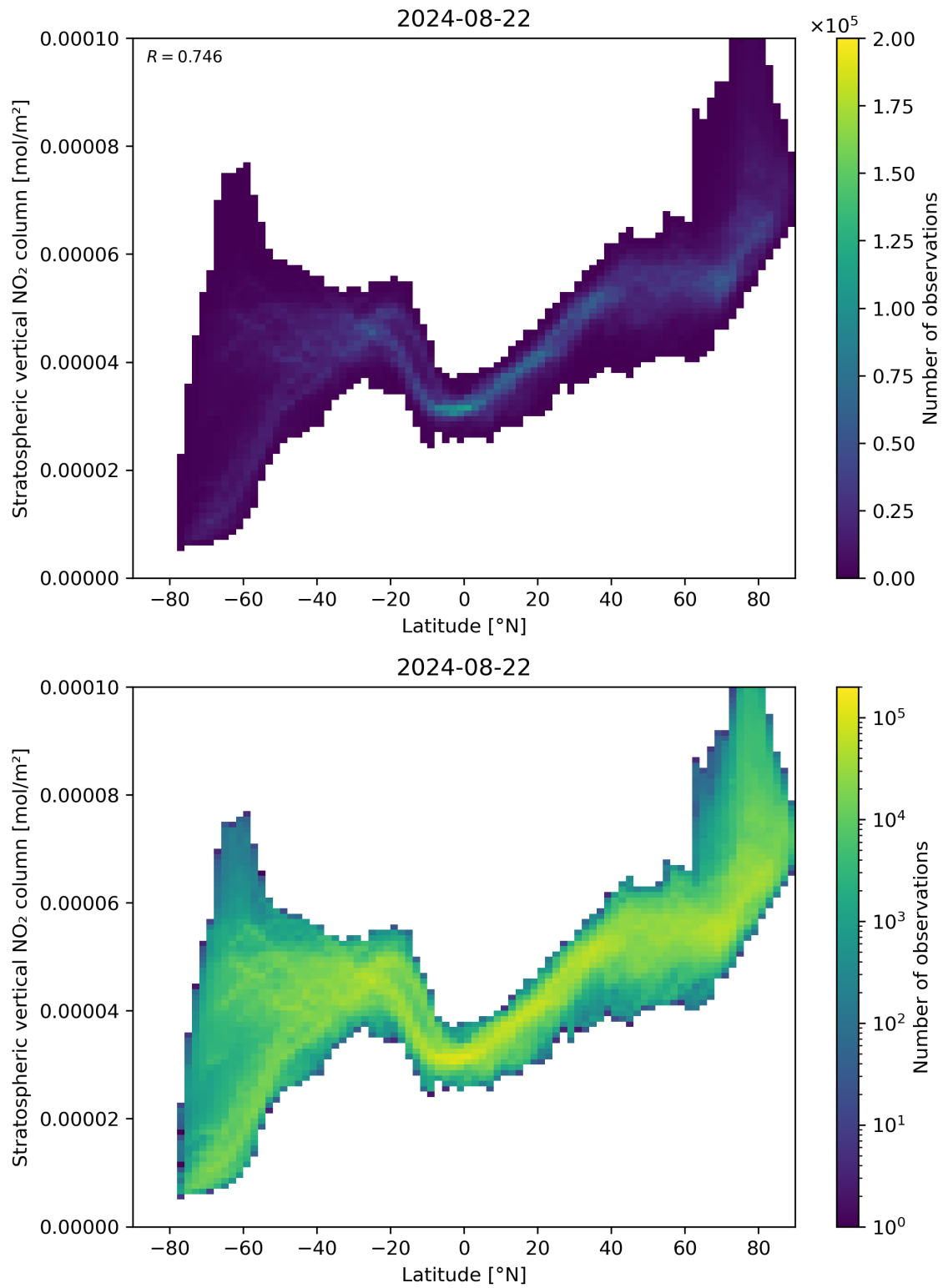
Figure 87: Scatter density plot of “Latitude” against “Stratospheric vertical NO 2 column” for 2024-08-22 to 2024-08-23.
