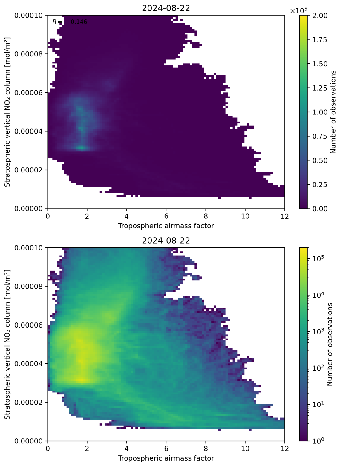
Figure 74: Scatter density plot of “Tropospheric air mass factor” against “Stratospheric vertical NO 2 column” for 2024-08-22 to 2024-08-23.
