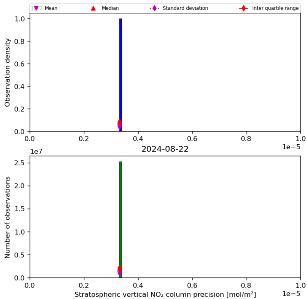
Figure 37: Histogram of “Stratospheric vertical NO 2 column precision” for 2024-08-22 to 2024-08-23
