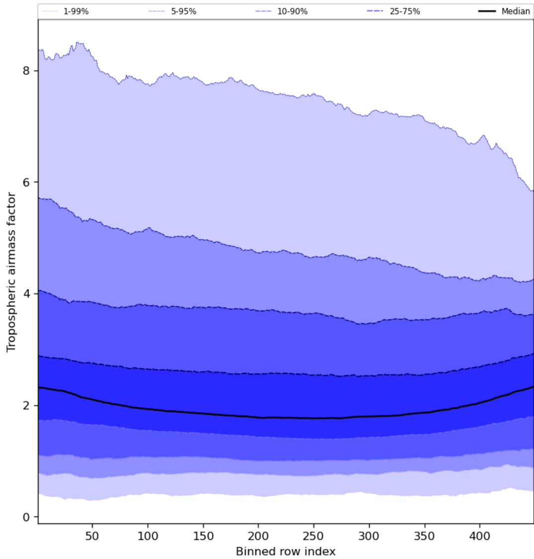
Figure 48: Along track statistics of “Tropospheric airmass factor” for 2024-08-22 to 2024-08-23
