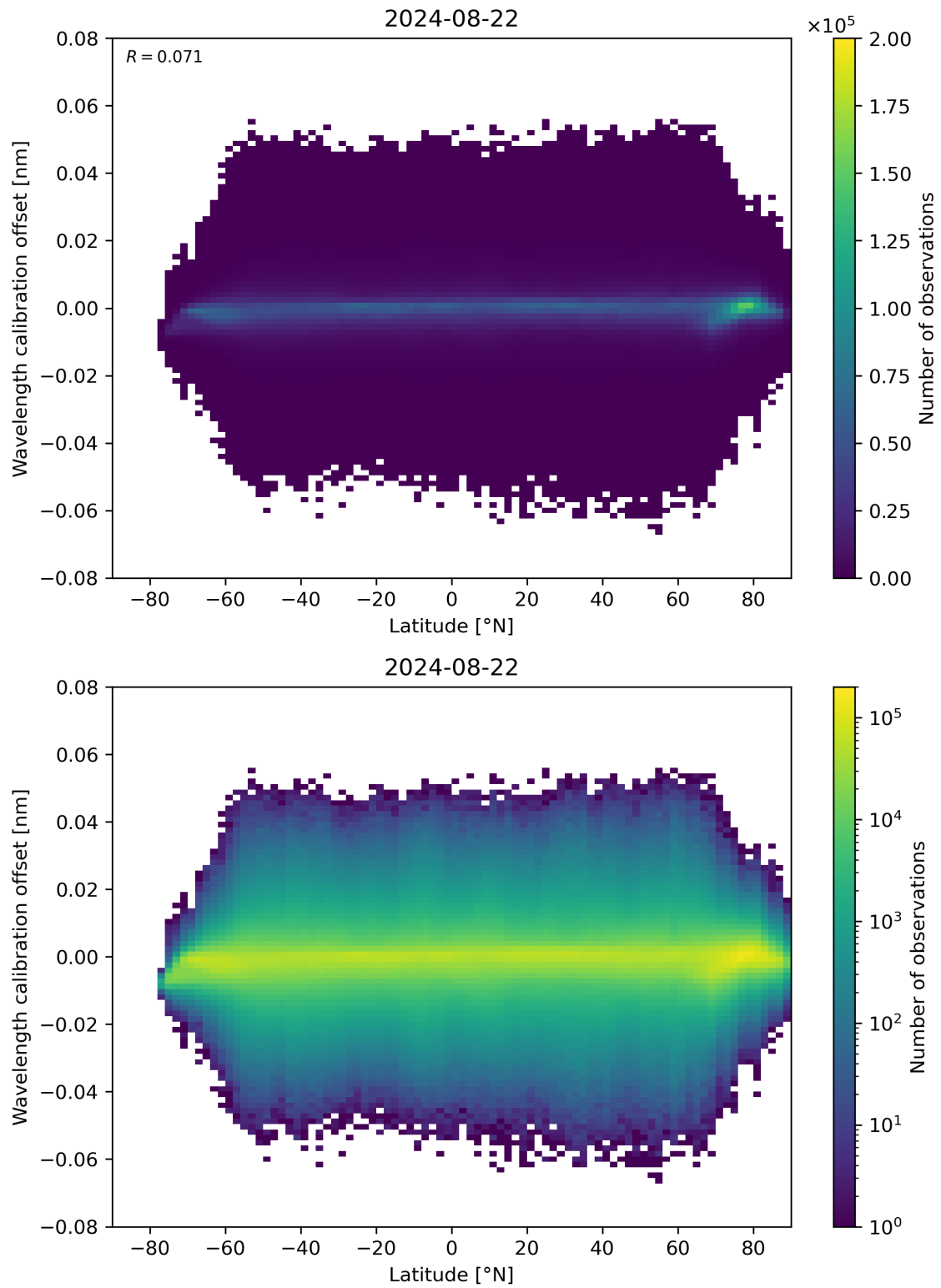
Figure 95: Scatter density plot of “Latitude” against “Wavelength calibration offset” for 2024-08-22 to 2024-08-23.
