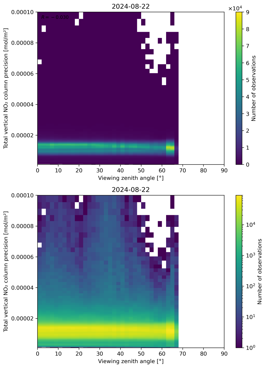
Figure 168: Scatter density plot of “Viewing zenith angle” against “Total vertical NO 2 column precision” for 2024-08-22 to 2024-08-23.
