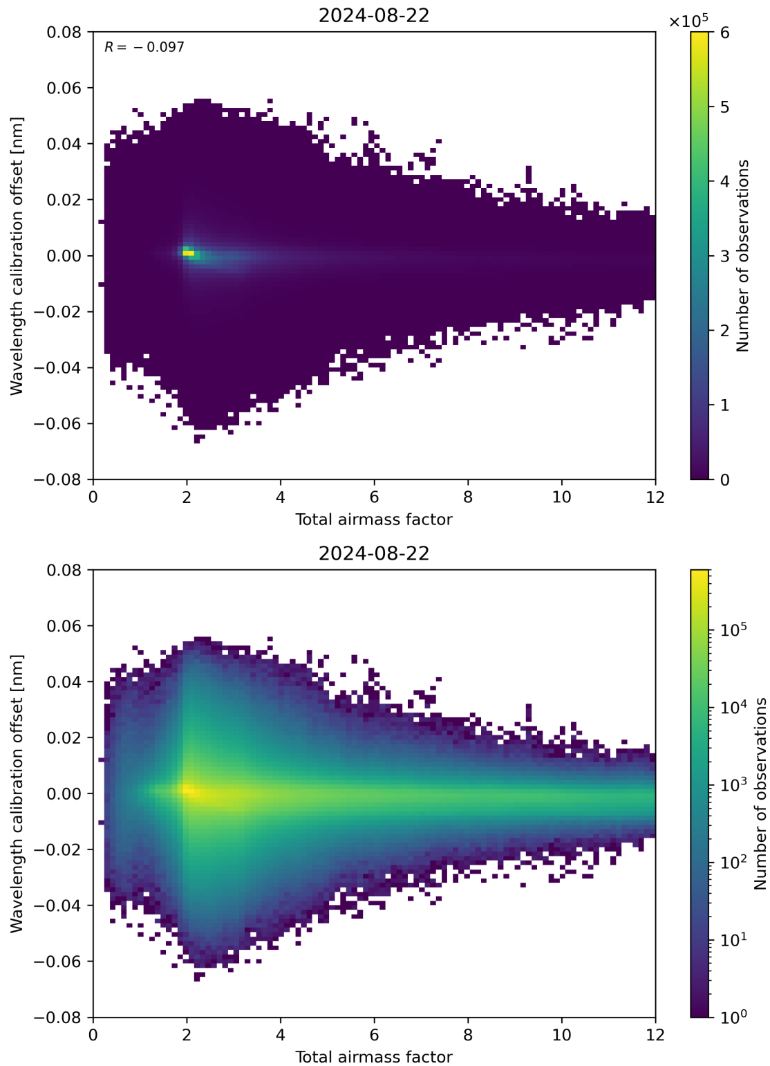
Figure 70: Scatter density plot of “Total airmass factor” against “Wavelength calibration offset” for 2024-08-22 to 2024-08-23.
