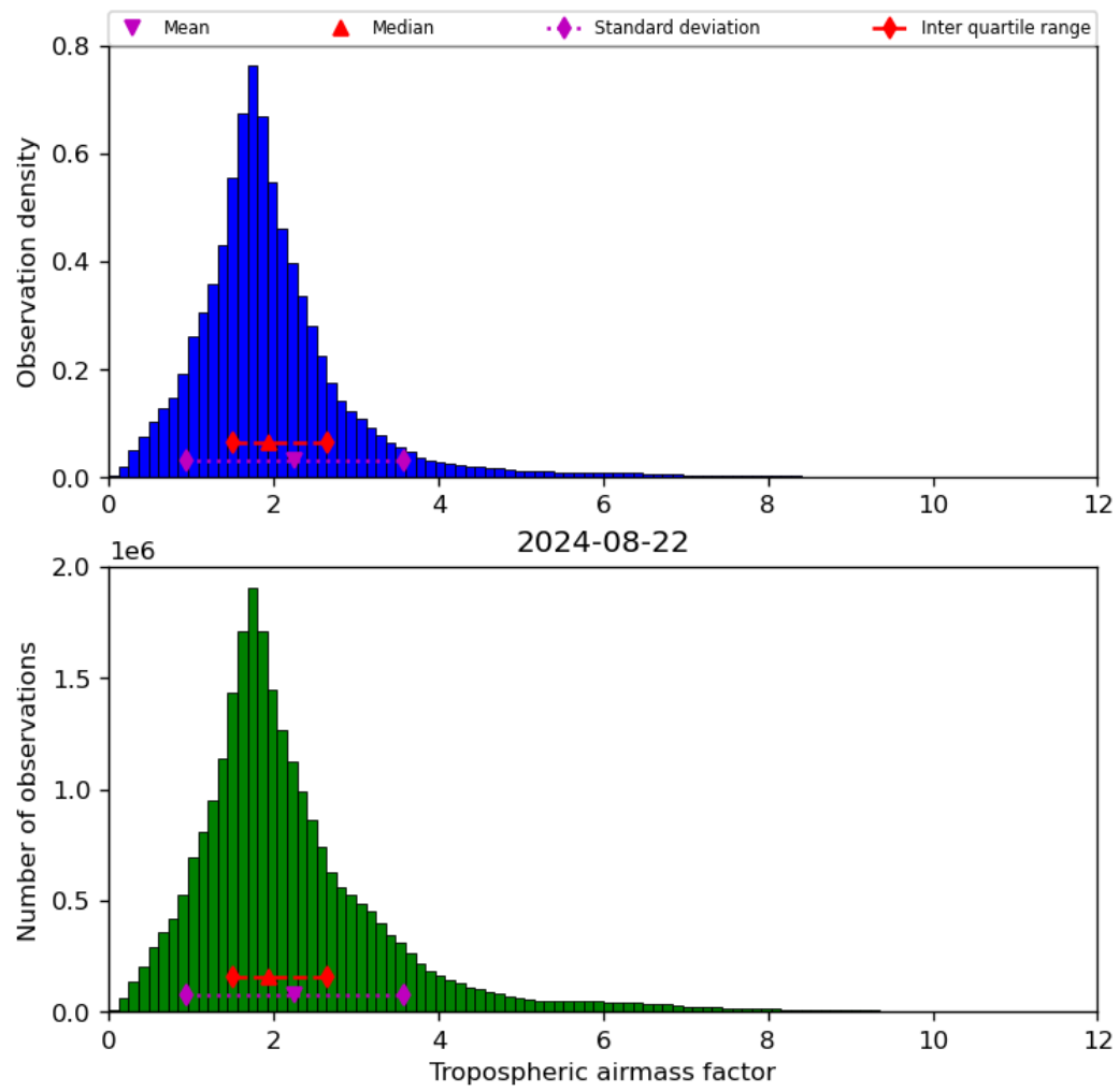
Figure 31: Histogram of “Tropospheric airmass factor” for 2024-08-22 to 2024-08-23
