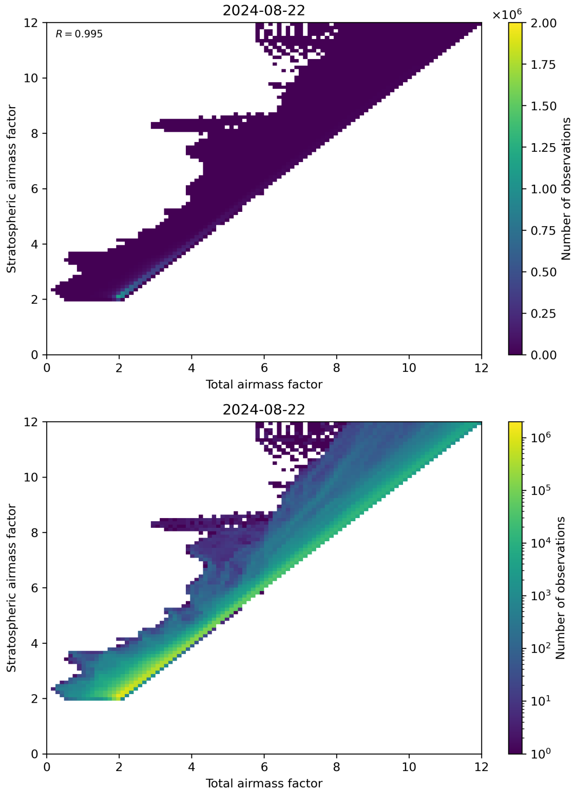
Figure 62: Scatter density plot of “Total airmass factor” against “Stratospheric airmass factor” for 2024-08-22 to 2024-08-23.
