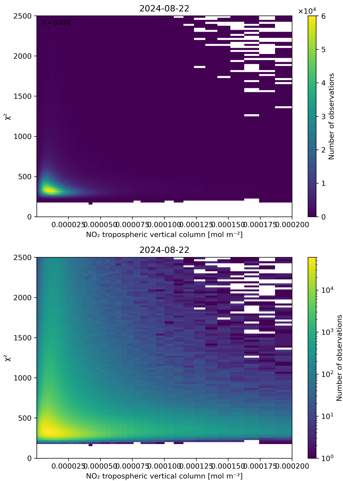
Figure 124: Scatter density plot of “NO 2 tropospheric vertical column” against “ \chi^2 ” for 2024-08-22 to 2024-08-23.
