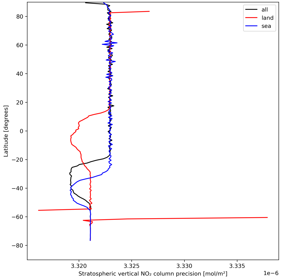
Figure 20: Zonal average of “Stratospheric vertical NO 2 column precision” for 2024-08-22 to 2024-08-23.
