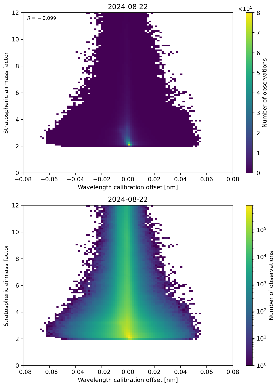
Figure 174: Scatter density plot of “Wavelength calibration offset” against “Stratospheric airmass factor” for 2024-08-22 to 2024-08-23.
