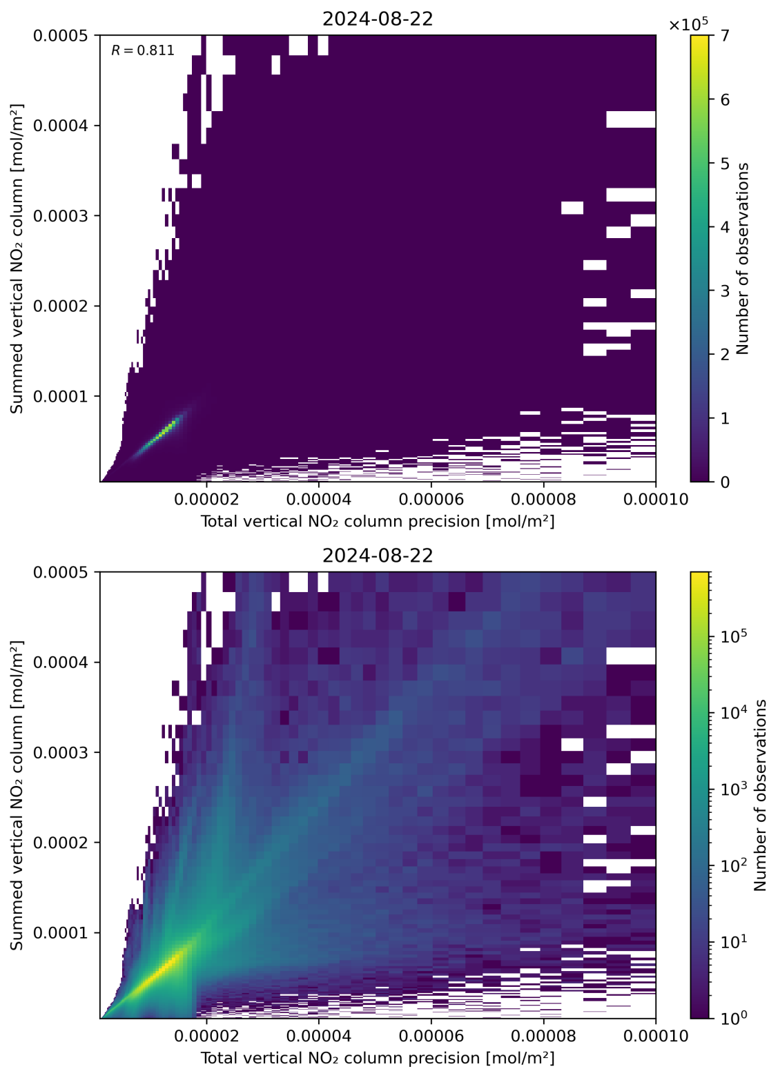
Figure 117: Scatter density plot of “Total vertical NO 2 column precision” against “Summed vertical NO 2 column” for 2024-08-22 to 2024-08-23.
