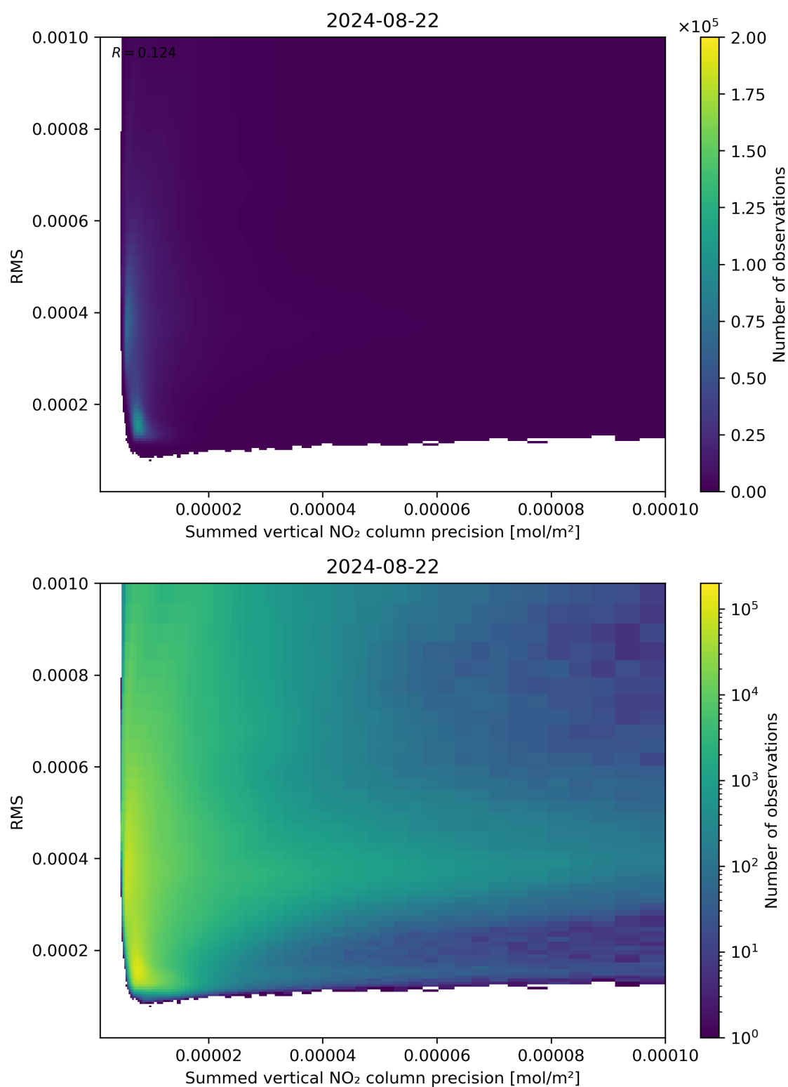
Figure 108: Scatter density plot of “Summed vertical NO 2 column precision” against “RMS” for 2024-08-22 to 2024-08-23.
