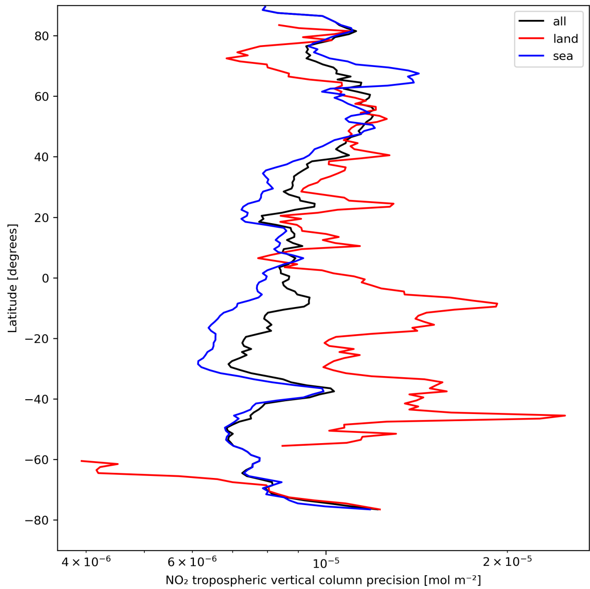
Figure 13: Zonal average of “NO 2 tropospheric vertical column precision” for 2024-08-22 to 2024-08-23.
