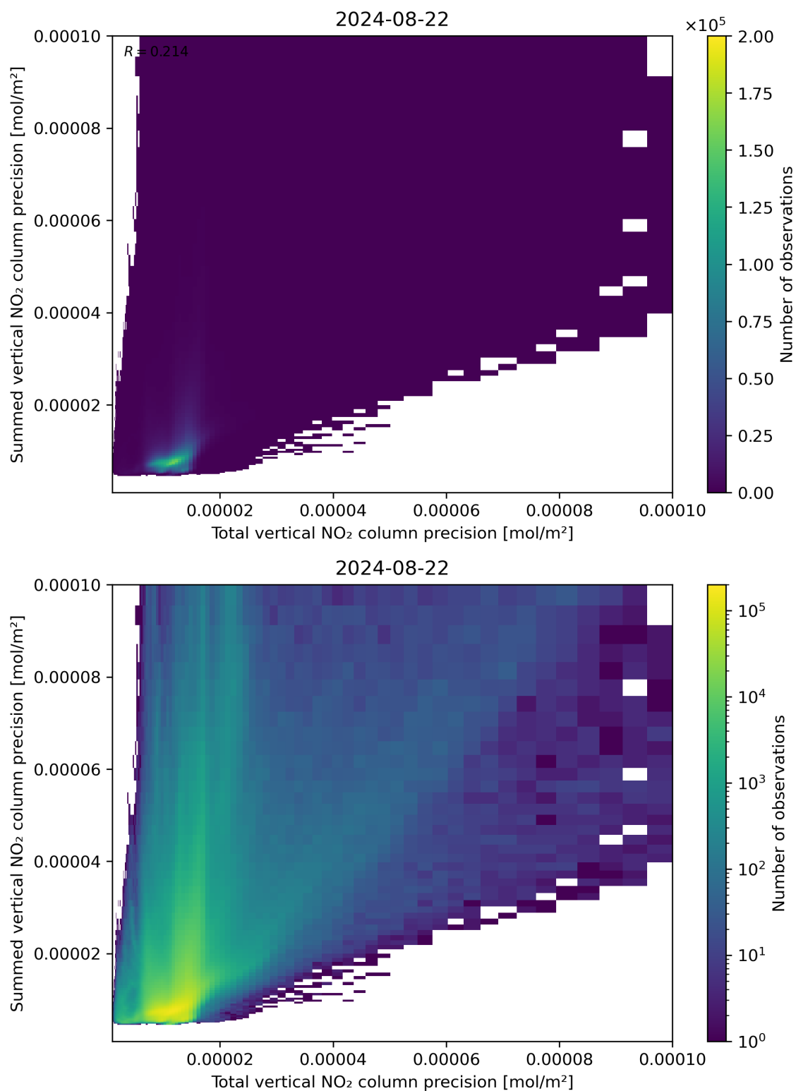
Figure 118: Scatter density plot of “Total vertical NO 2 column precision” against “Summed vertical NO 2 column precision” for 2024-08-22 to 2024-08-23.
