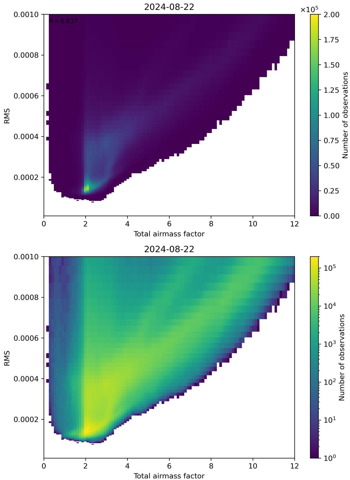
Figure 69: Scatter density plot of “Total airmass factor” against “RMS” for 2024-08-22 to 2024-08-23.
