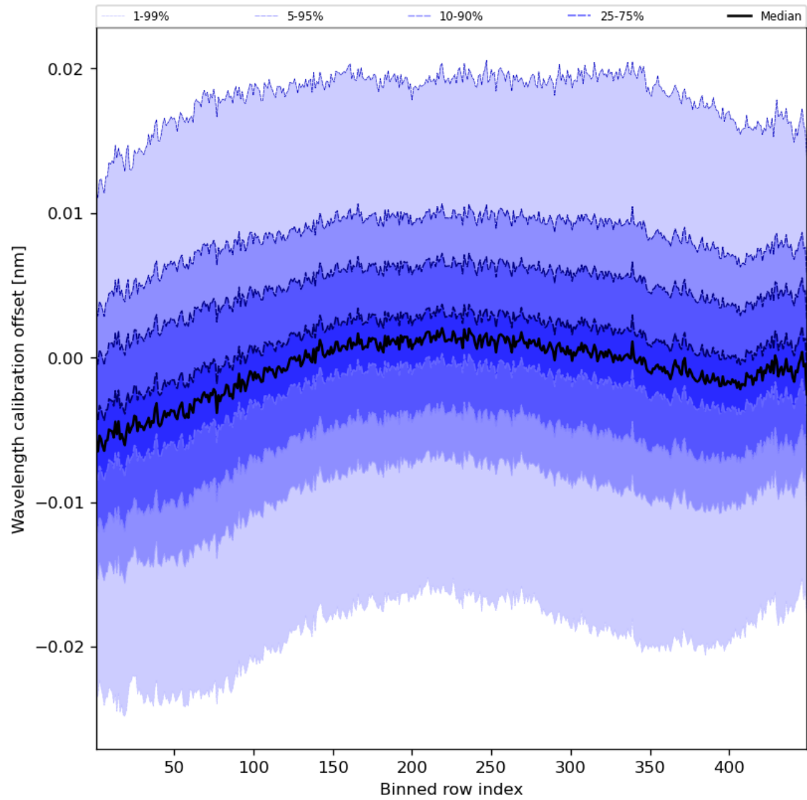
Figure 52: Along track statistics of “Wavelength calibration offset” for 2024-08-22 to 2024-08-23
