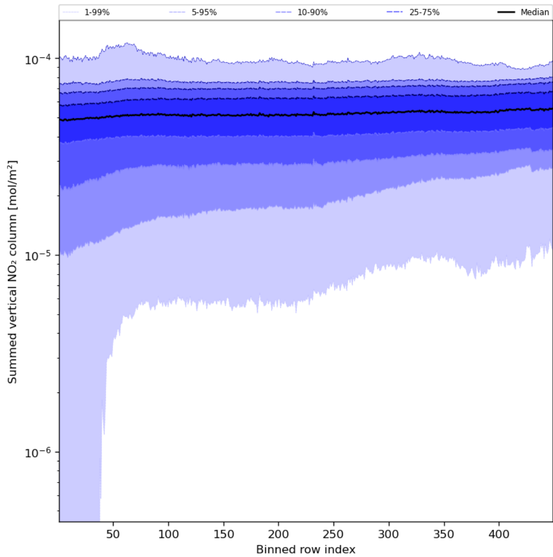
Figure 57: Along track statistics of “Summed vertical NO 2 column” for 2024-08-22 to 2024-08-23
