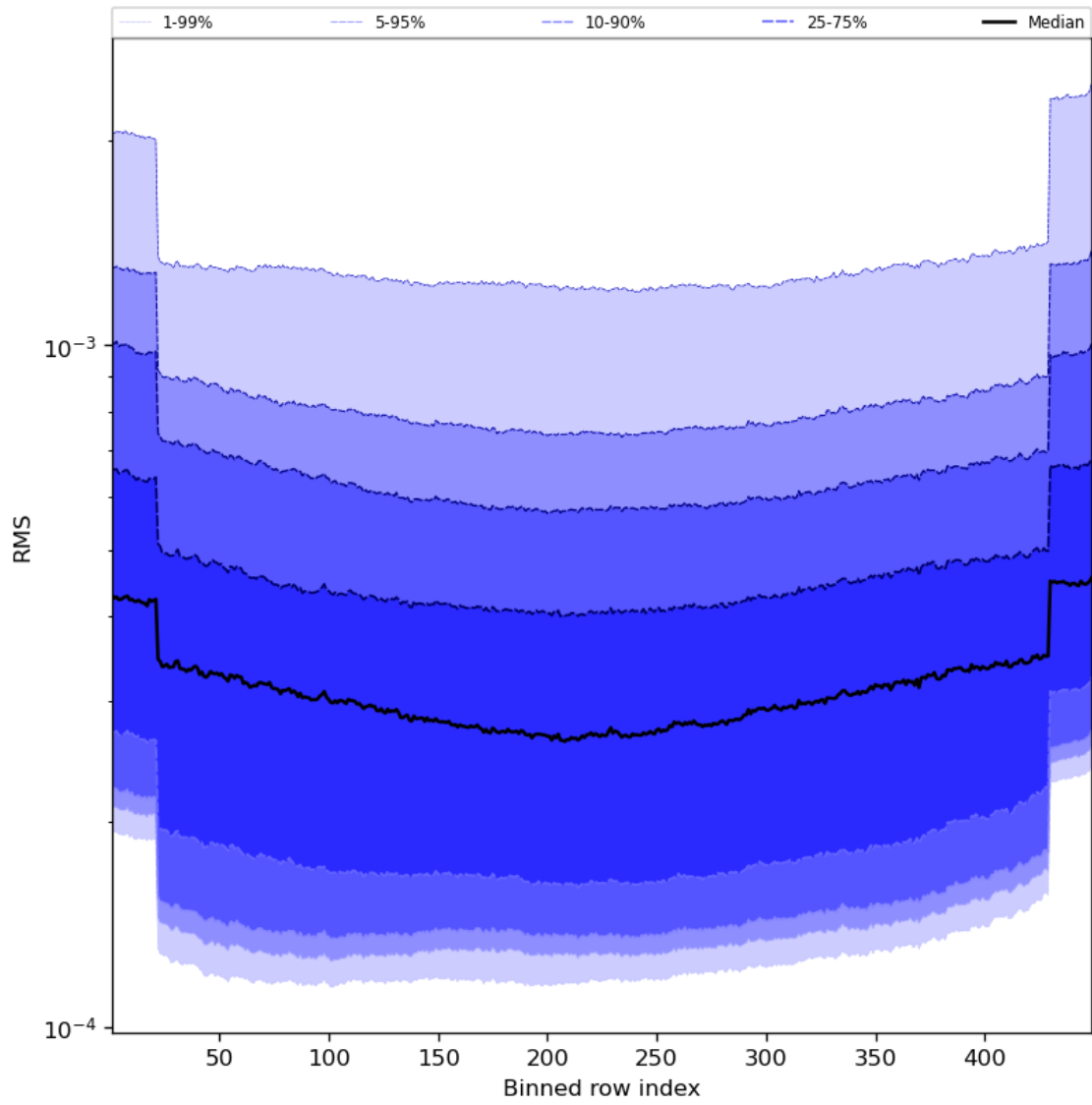
Figure 60: Along track statistics of “RMS” for 2024-08-22 to 2024-08-23
