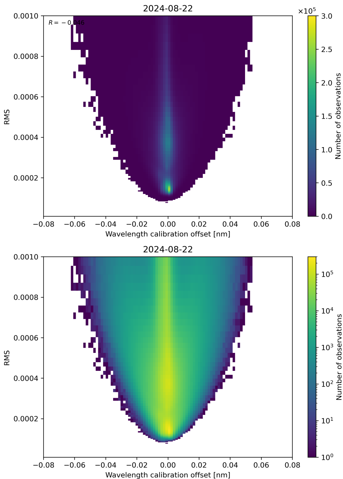
Figure 181: Scatter density plot of “Wavelength calibration offset” against “RMS” for 2024-08-22 to 2024-08-23.
