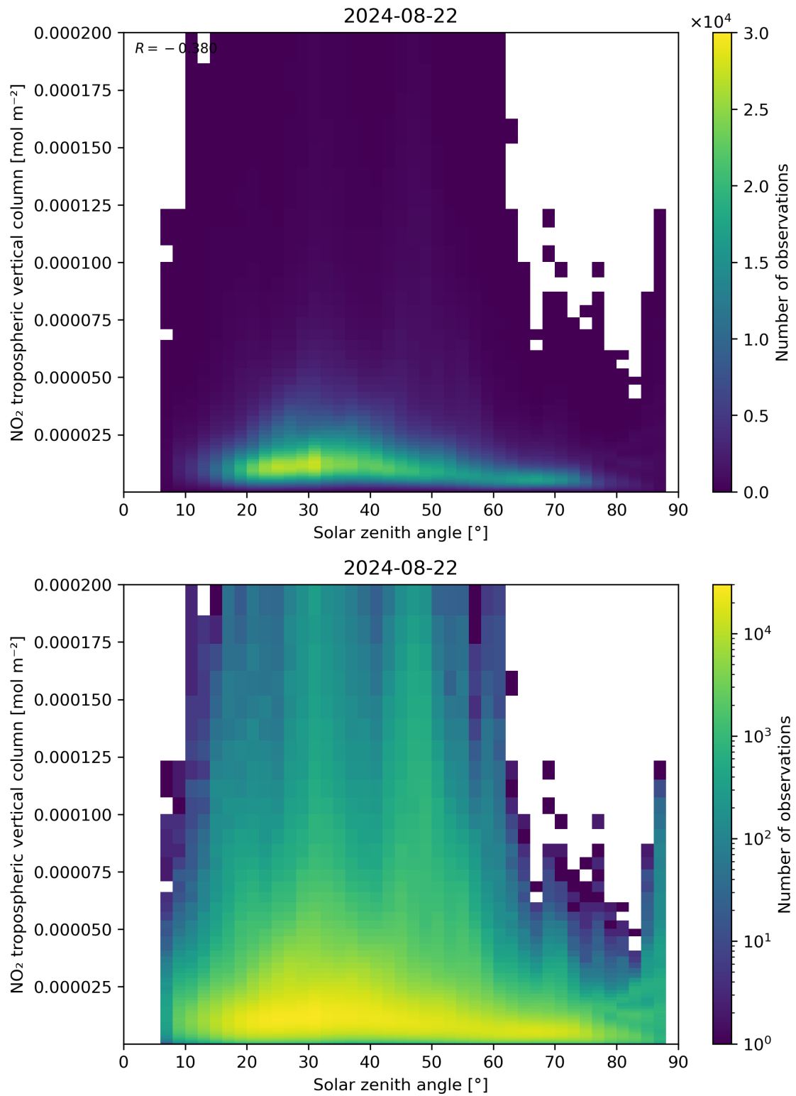
Figure 155: Scatter density plot of “Solar zenith angle” against “NO 2 tropospheric vertical column” for 2024-08-22 to 2024-08-23.
