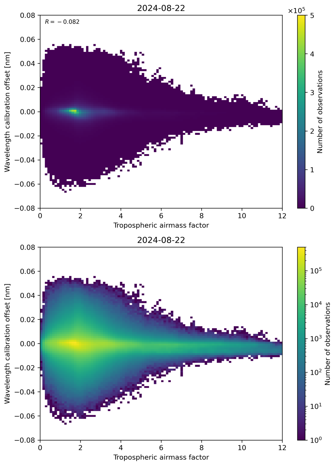
Figure 80: Scatter density plot of “Tropospheric airmass factor” against “Wavelength calibration offset” for 2024-08-22 to 2024-08-23.
