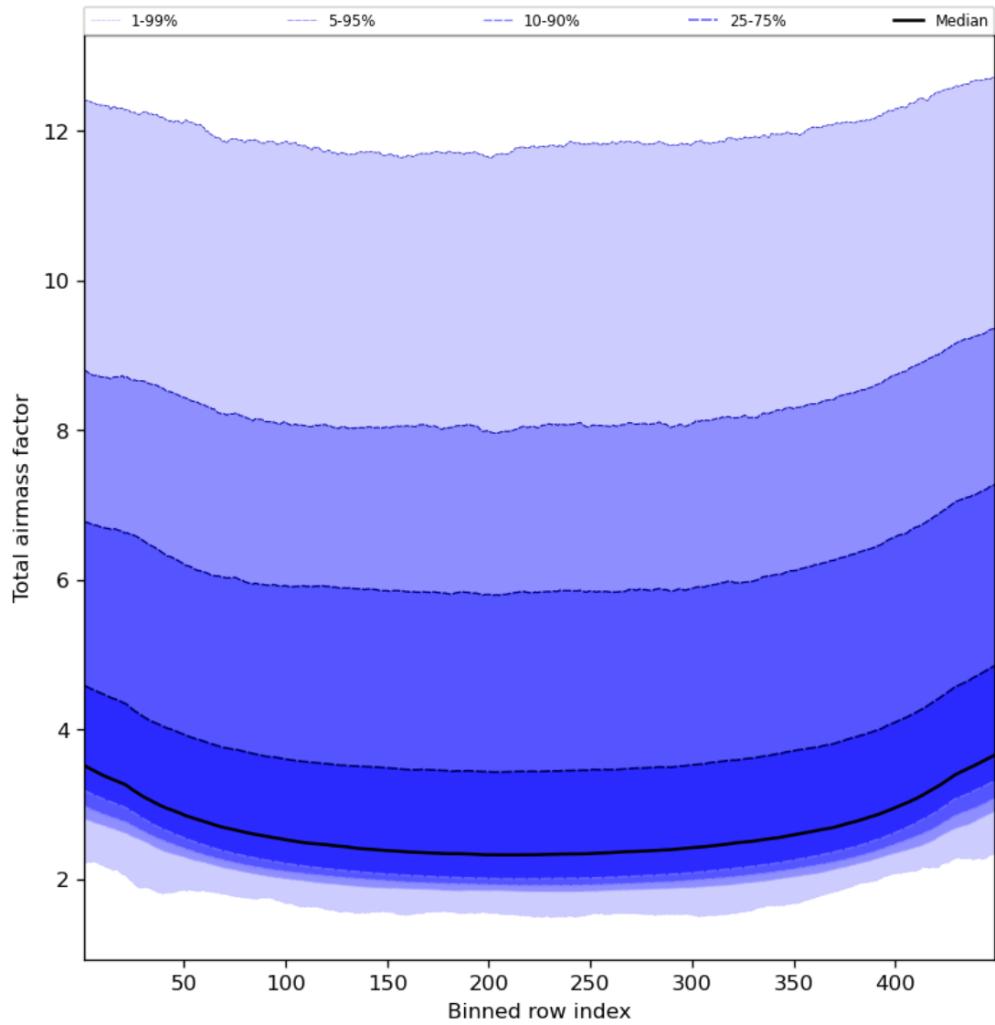
Figure 49: Along track statistics of “Total airmass factor” for 2024-08-22 to 2024-08-24
