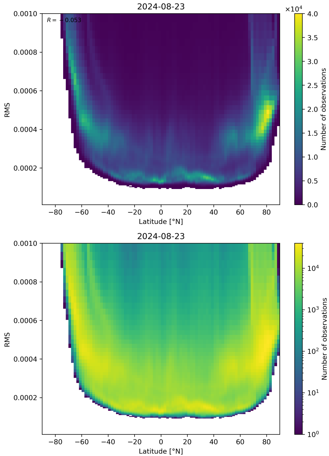
Figure 94: Scatter density plot of “Latitude” against “RMS” for 2024-08-22 to 2024-08-24.
