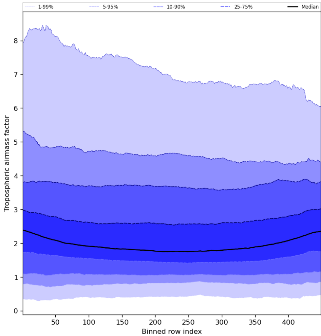
Figure 48: Along track statistics of “Tropospheric airmass factor” for 2024-08-22 to 2024-08-24
