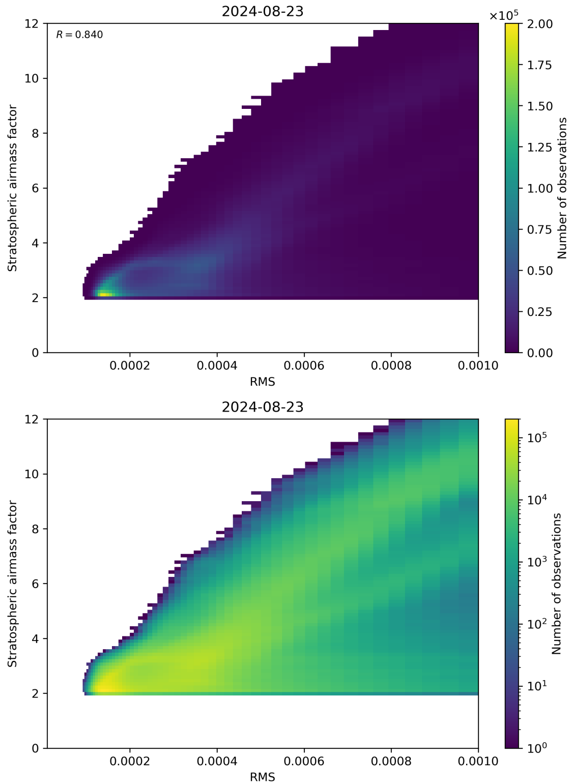
Figure 144: Scatter density plot of “RMS” against “Stratospheric airmass factor” for 2024-08-22 to 2024-08-24.
