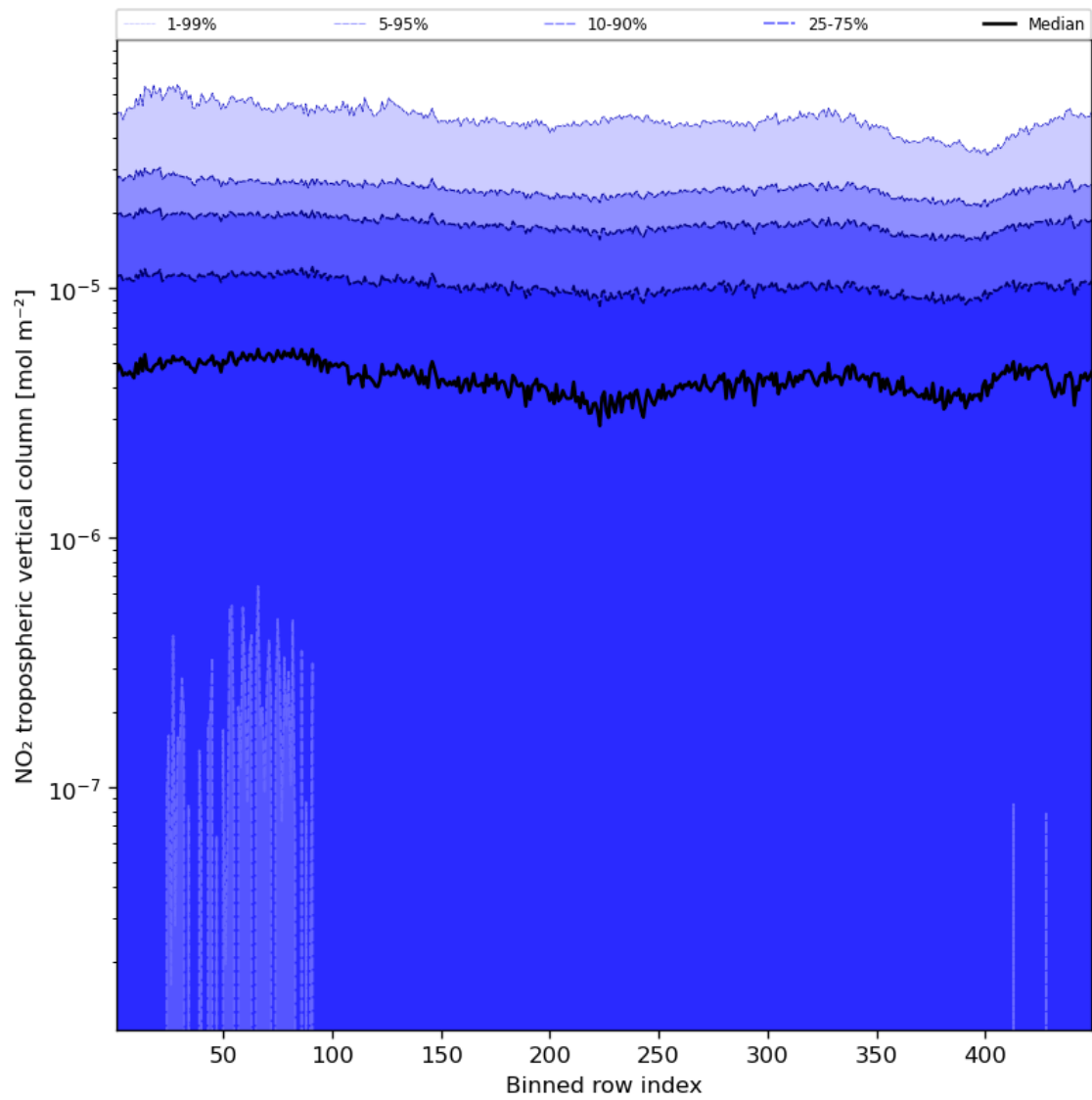
Figure 46: Along track statistics of “NO 2 tropospheric vertical column” for 2024-08-22 to 2024-08-24
