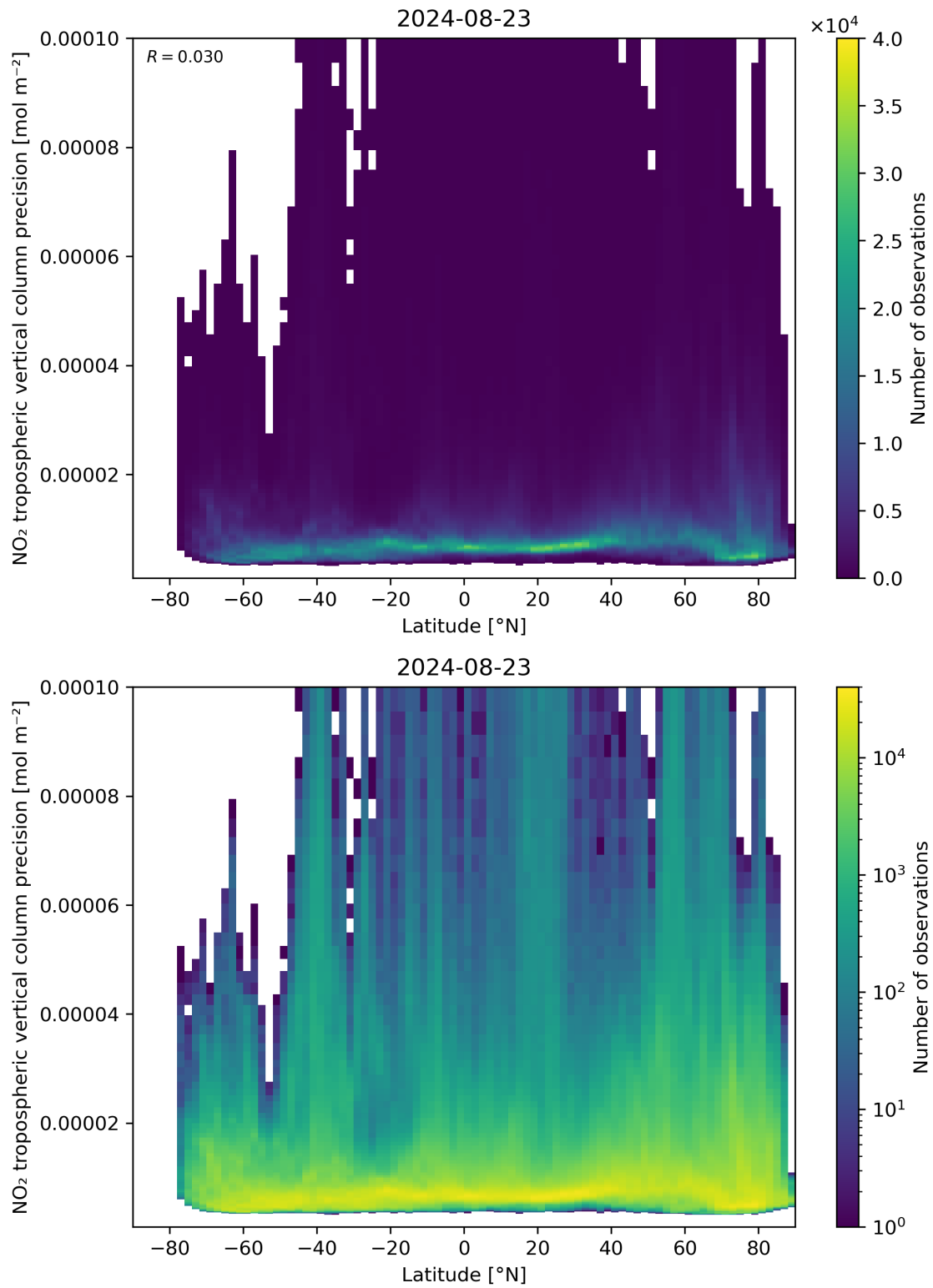
Figure 93: Scatter density plot of “Latitude” against “NO 2 tropospheric vertical column precision” for 2024-08-22 to 2024-08-24.
