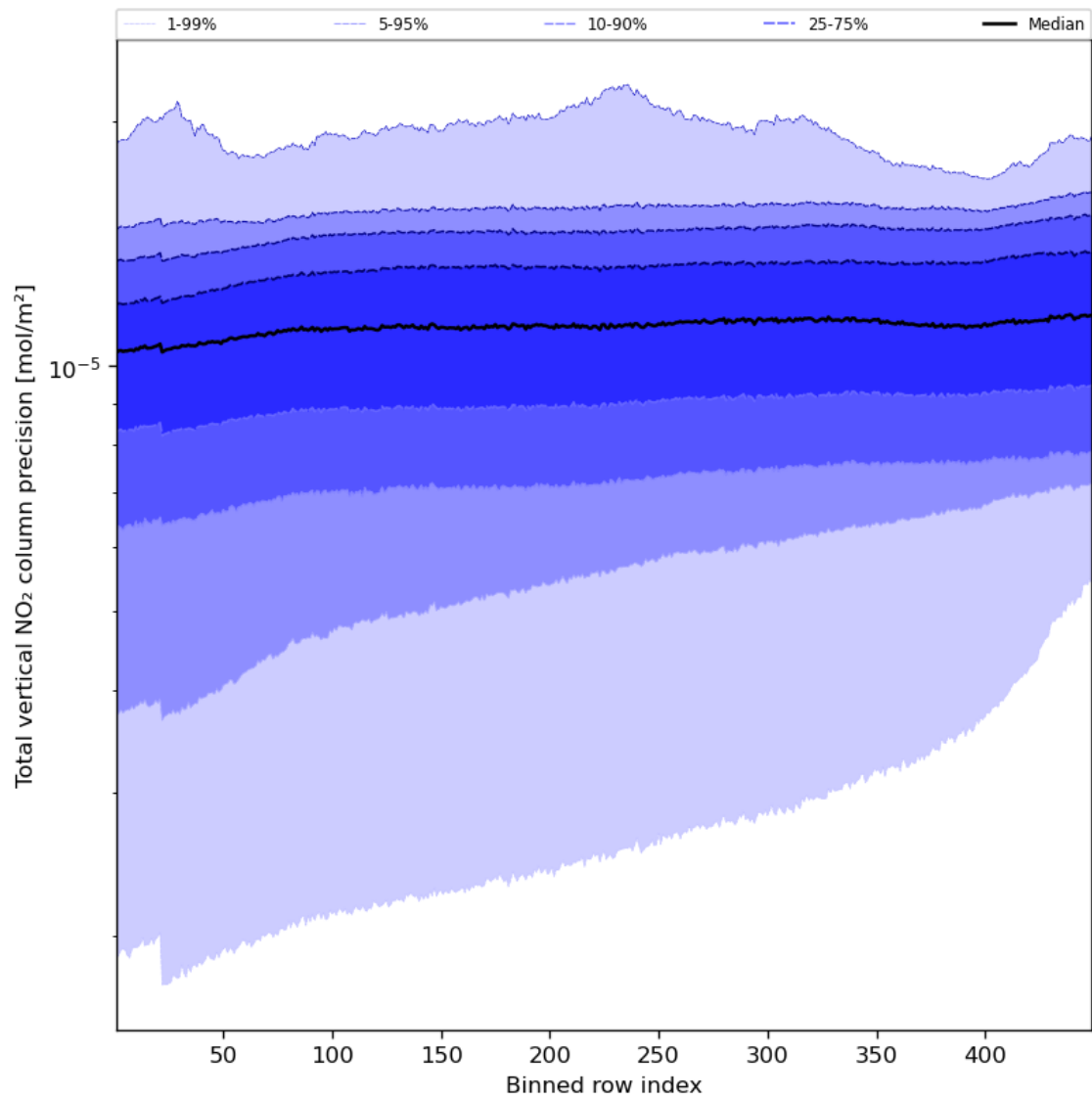
Figure 56: Along track statistics of “Total vertical NO 2 column precision” for 2024-08-22 to 2024-08-24
