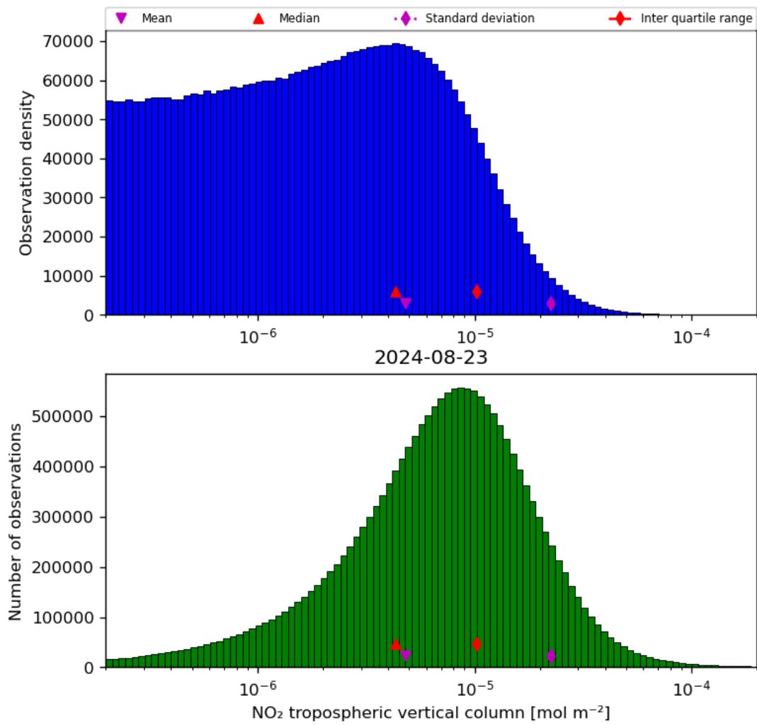
Figure 29: Histogram of “NO 2 tropospheric vertical column” for 2024-08-22 to 2024-08-24
