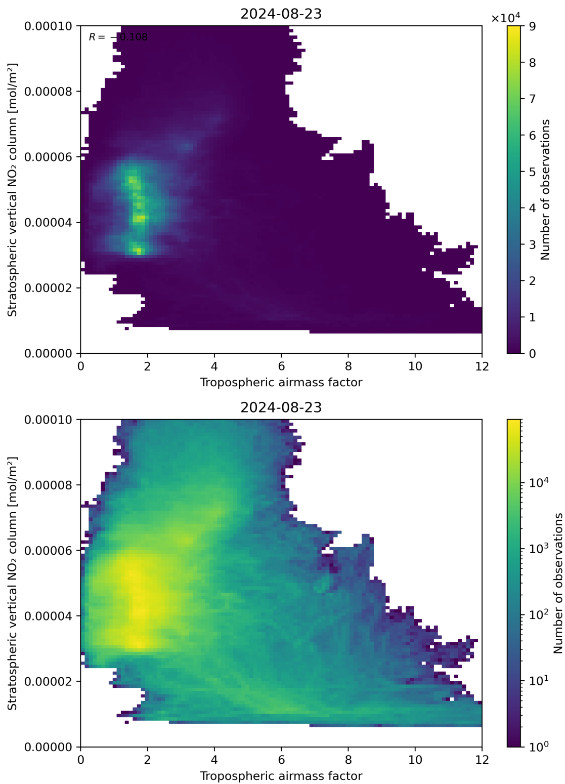
Figure 74: Scatter density plot of “Tropospheric air mass factor” against “Stratospheric vertical NO 2 column” for 2024-08-22 to 2024-08-24.
