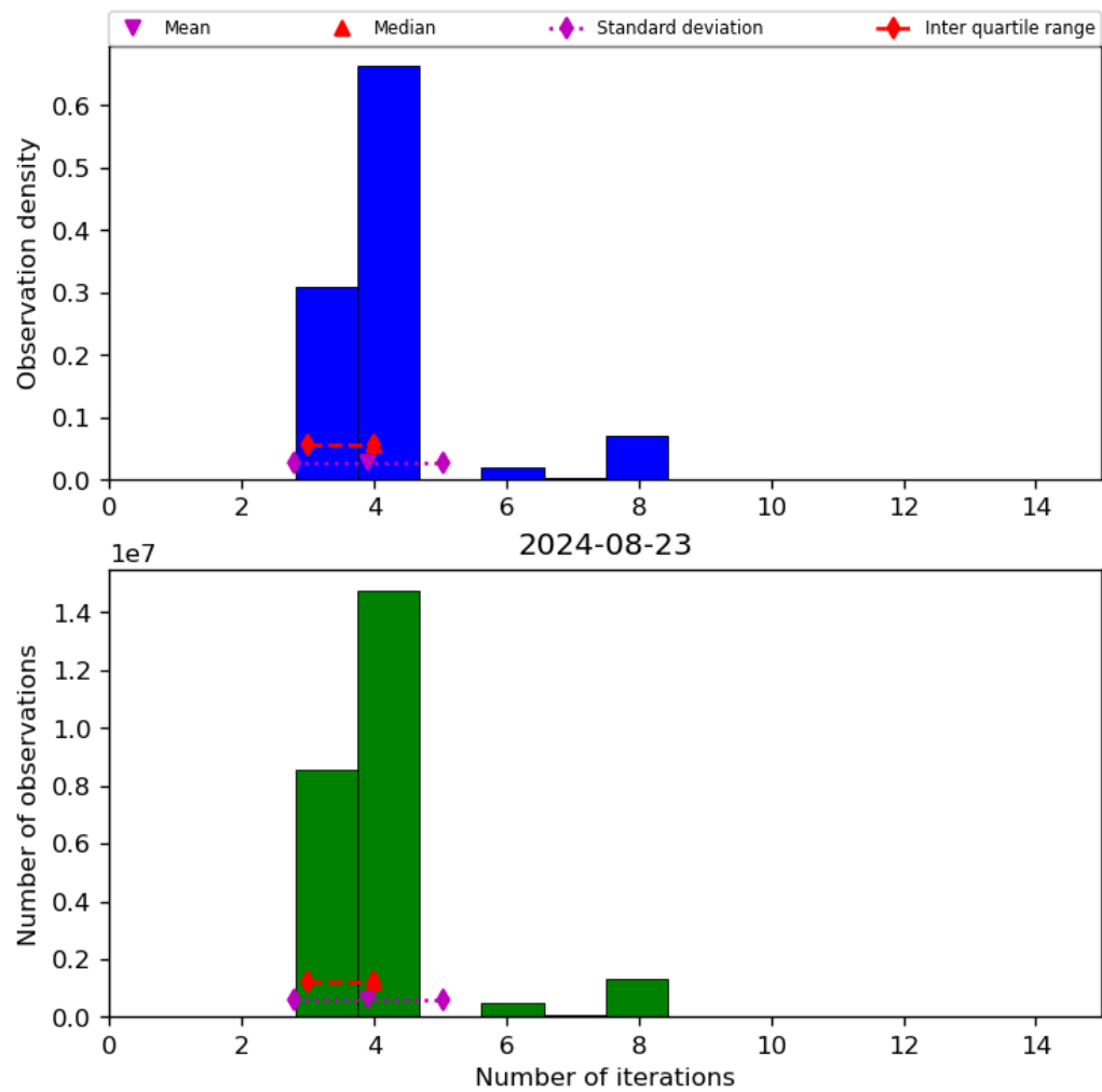
Figure 34: Histogram of “Number of iterations” for 2024-08-22 to 2024-08-24
