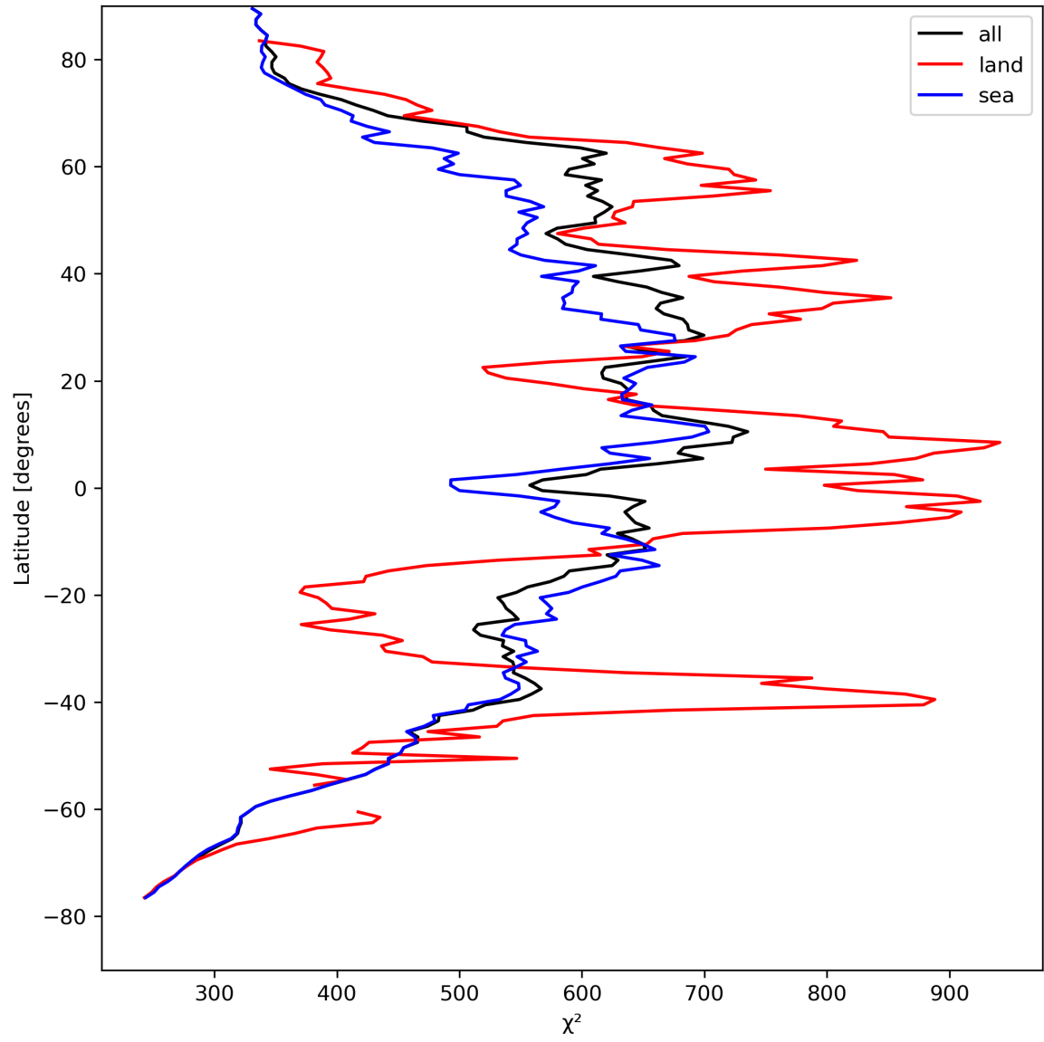
Figure 25: Zonal average of “ \chi^2 ” for 2024-08-22 to 2024-08-24.
