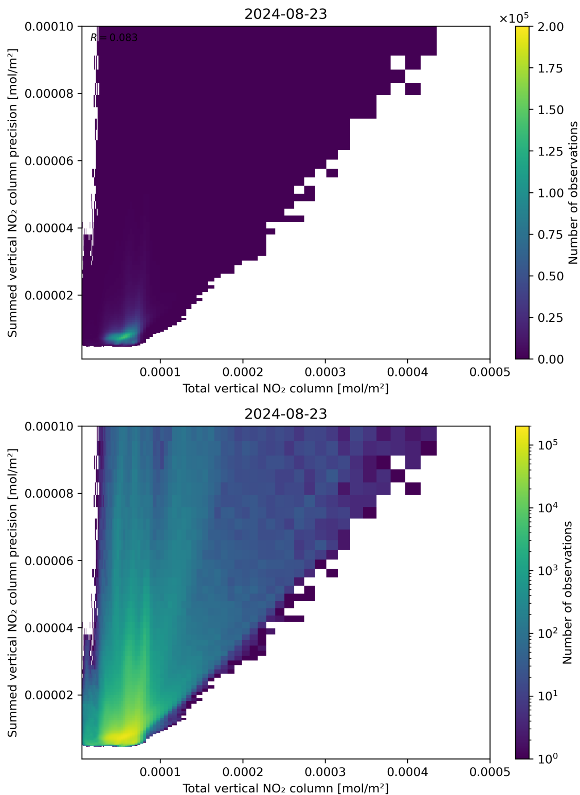
Figure 113: Scatter density plot of “Total vertical NO 2 column” against “Summed vertical NO 2 column precision” for 2024-08-22 to 2024-08-24.
