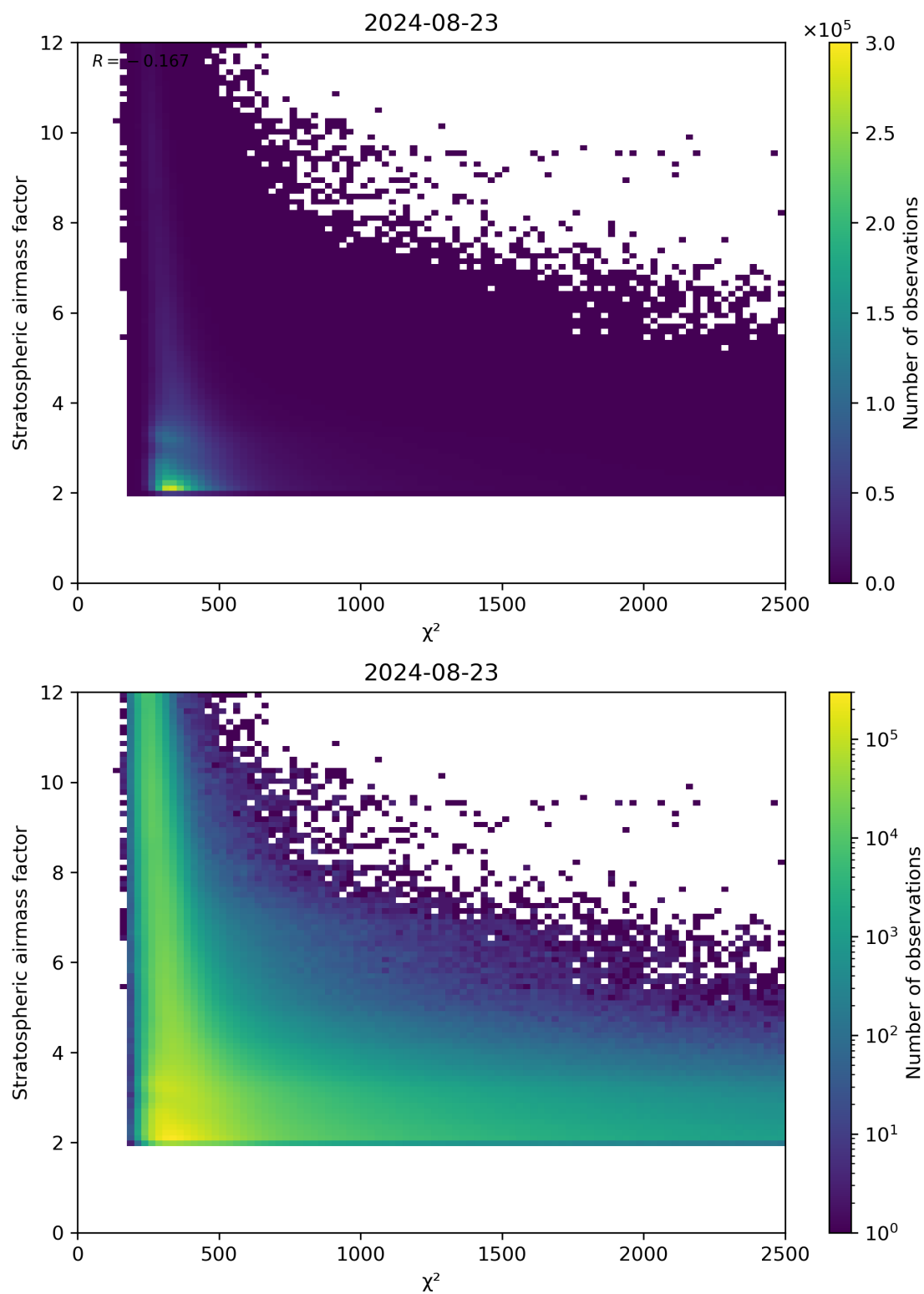
Figure 81: Scatter density plot of “ \chi^2 ” against “Stratospheric airmass factor” for 2024-08-22 to 2024-08-24.
