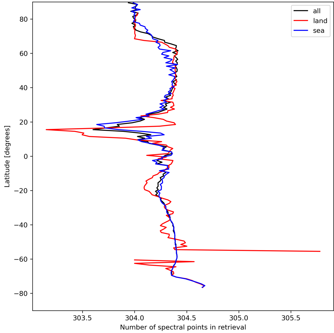
Figure 16: Zonal average of “Number of spectral points in retrieval” for 2024-08-22 to 2024-08-24.
