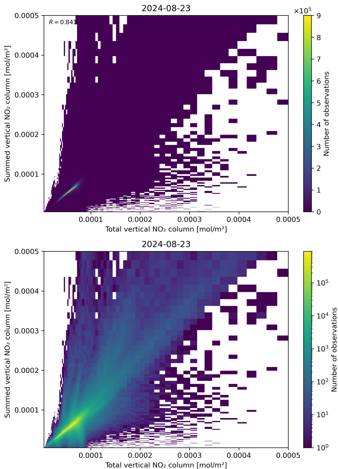
Figure 112: Scatter density plot of “Total vertical NO 2 column” against “Summed vertical NO 2 column” for 2024-08-22 to 2024-08-24.
