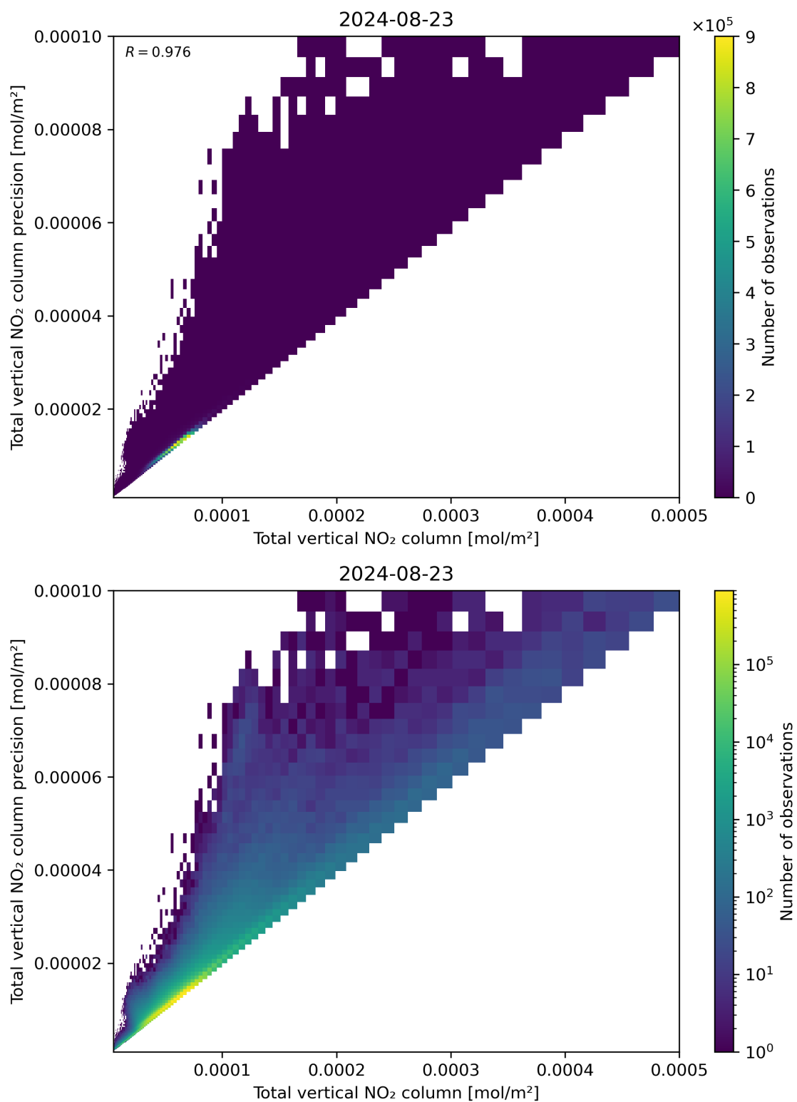
Figure 114: Scatter density plot of “Total vertical NO 2 column” against “Total vertical NO 2 column precision” for 2024-08-22 to 2024-08-24.
