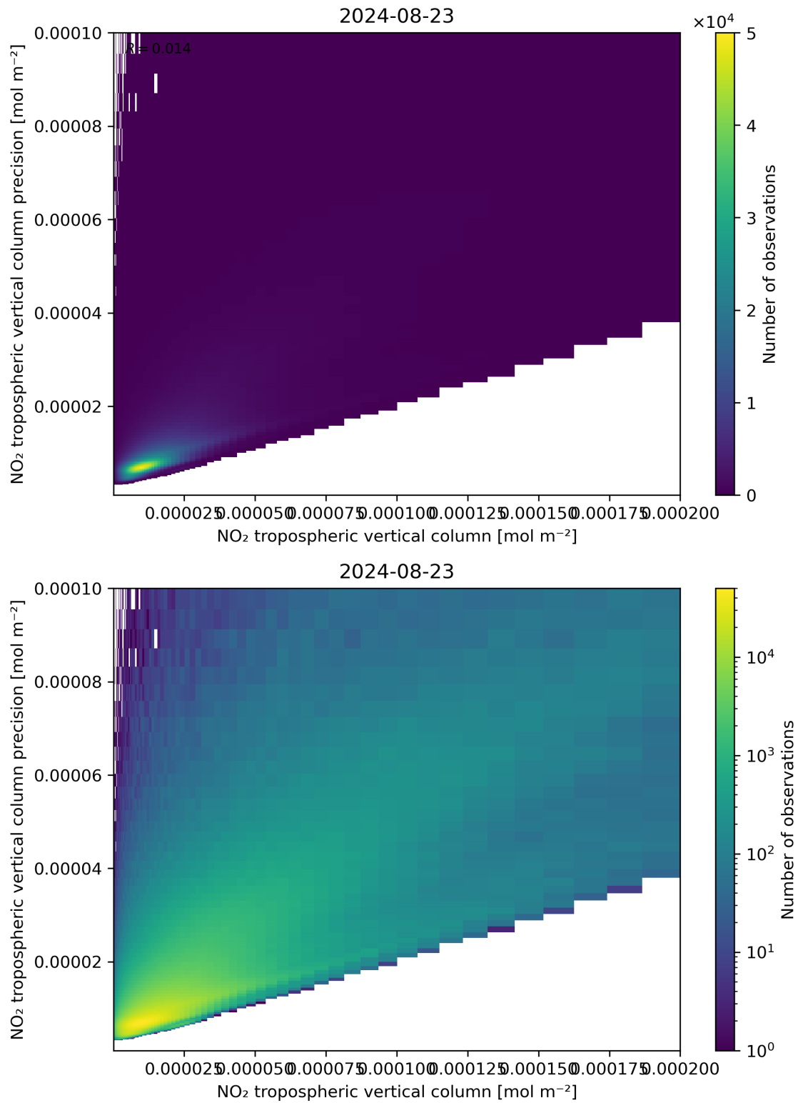
Figure 130: Scatter density plot of “NO 2 tropospheric vertical column” against “NO 2 tropospheric vertical column precision” for 2024-08-22 to 2024-08-24.
