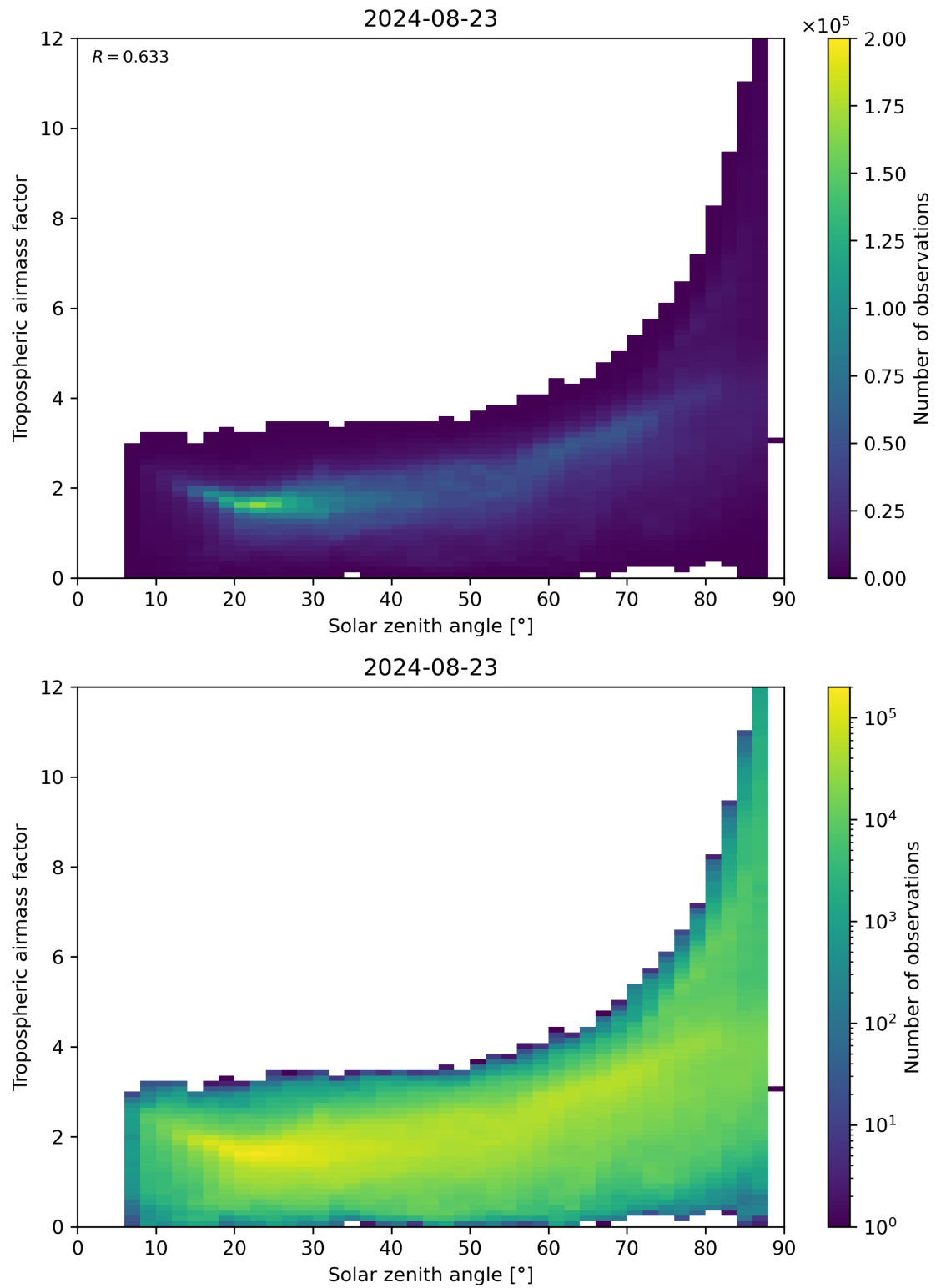
Figure 147: Scatter density plot of “Solar zenith angle” against “Tropospheric airmass factor” for 2024-08-22 to 2024-08-24.
