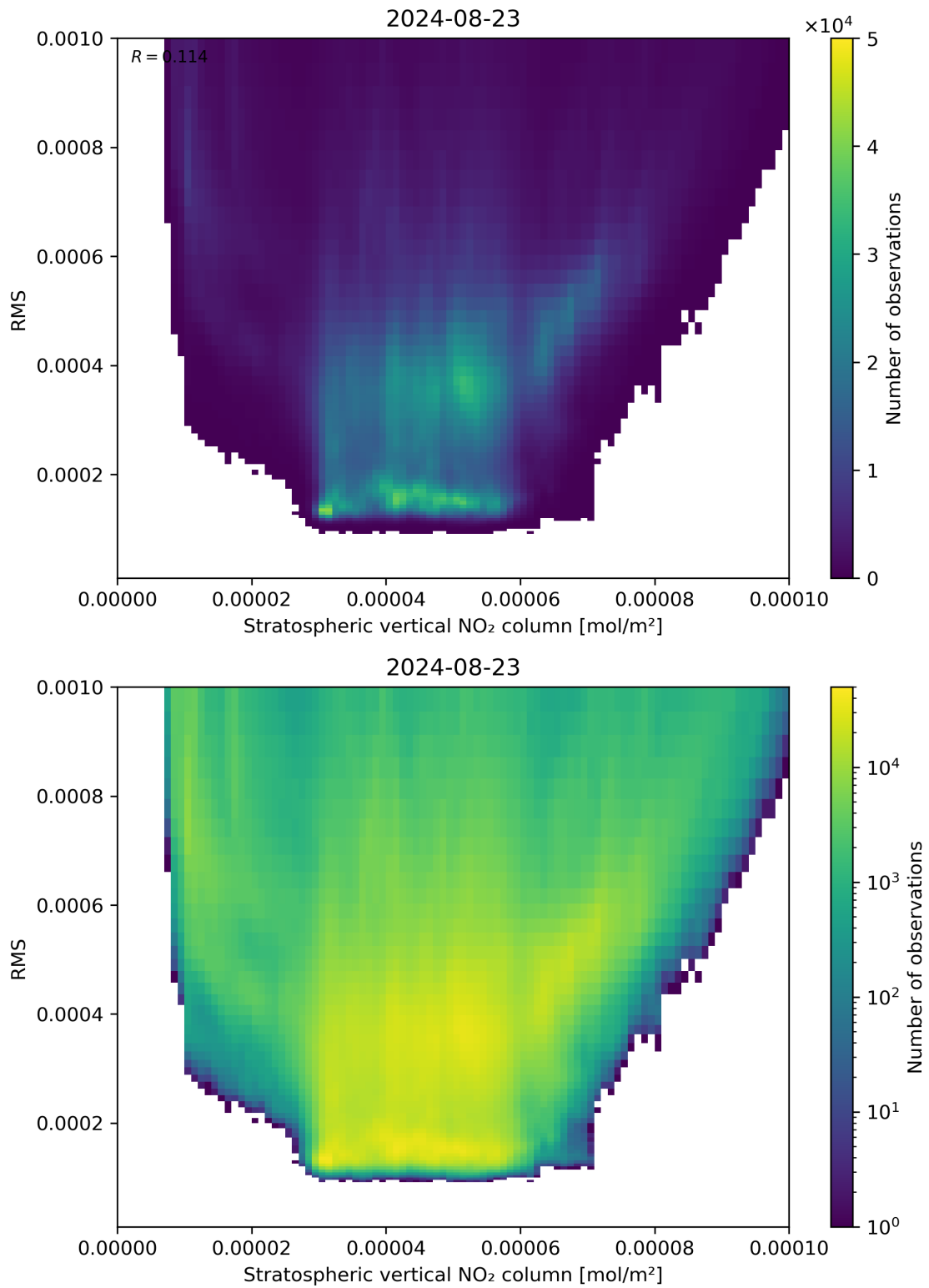
Figure 102: Scatter density plot of “Stratospheric vertical NO 2 column” against “RMS” for 2024-08-22 to 2024-08-24.
