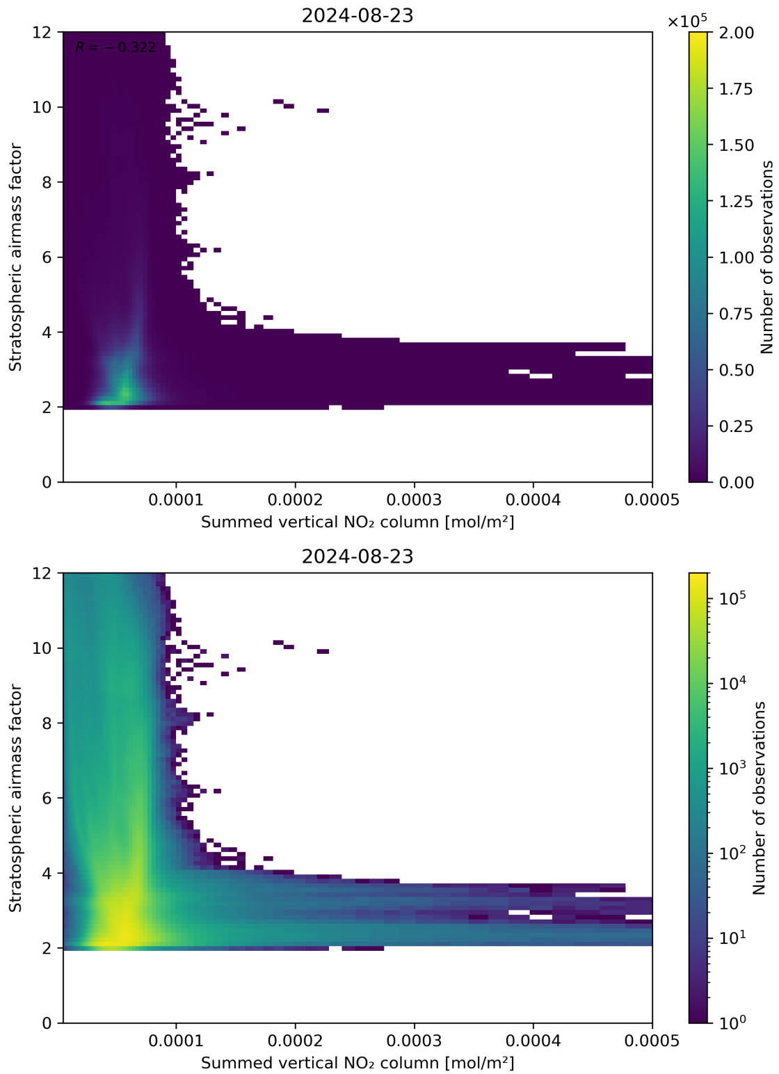
Figure 103: Scatter density plot of “Summed vertical NO 2 column” against “Stratospheric airmass factor” for 2024-08-22 to 2024-08-24.
