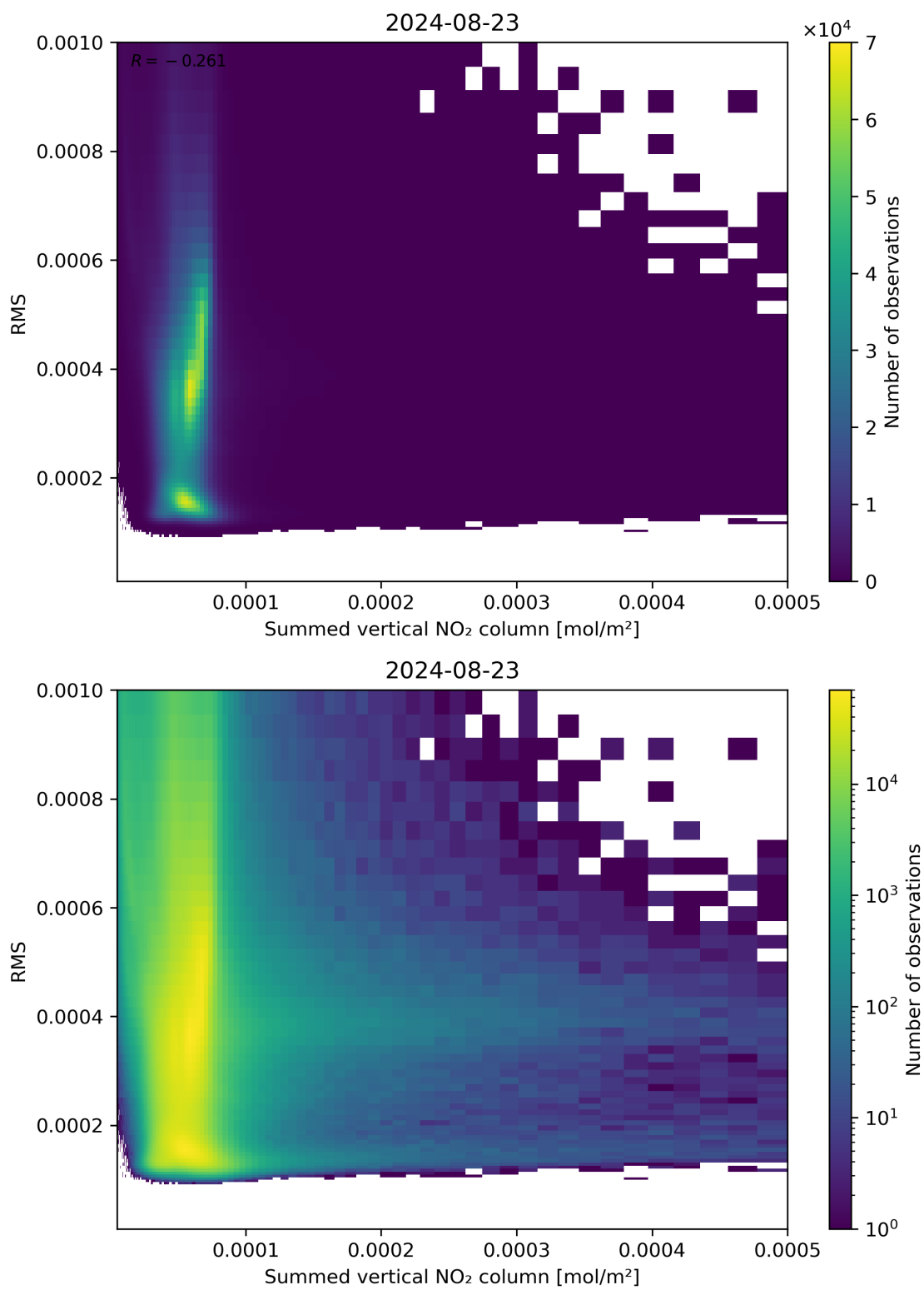
Figure 109: Scatter density plot of “Summed vertical NO 2 column” against “RMS” for 2024-08-22 to 2024-08-24.
