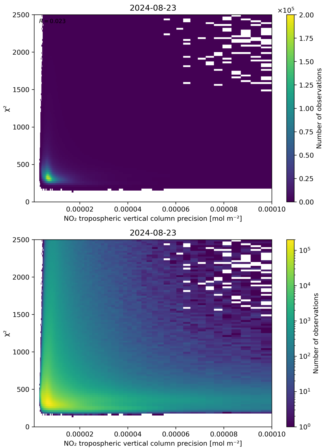
Figure 134: Scatter density plot of “NO 2 tropospheric vertical column precision” against “ \chi^2 ” for 2024-08-22 to 2024-08-24.
