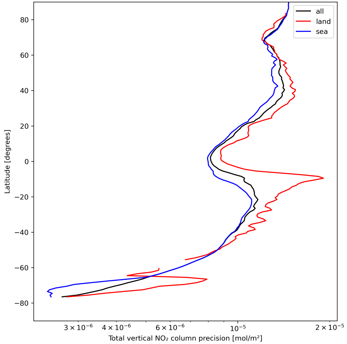
Figure 22: Zonal average of “Total vertical NO 2 column precision” for 2024-08-22 to 2024-08-24.
