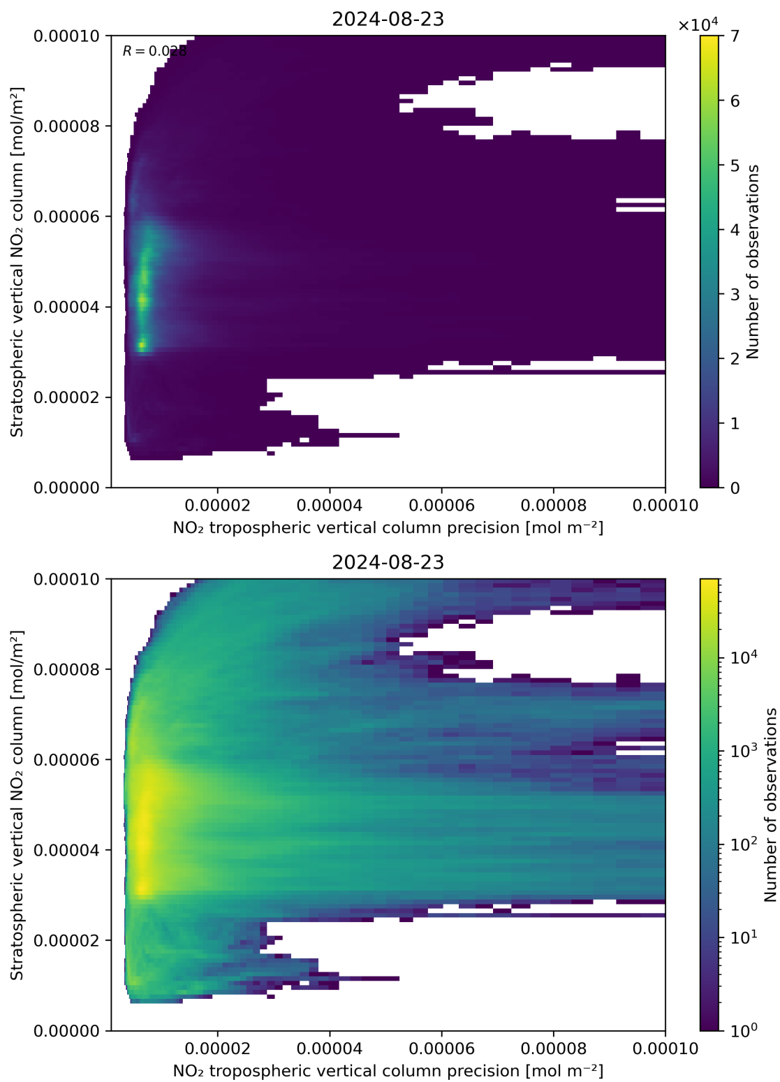
Figure 135: Scatter density plot of “NO 2 tropospheric vertical column precision” against “Stratospheric vertical NO 2 column” for 2024-08-22 to 2024-08-24.
