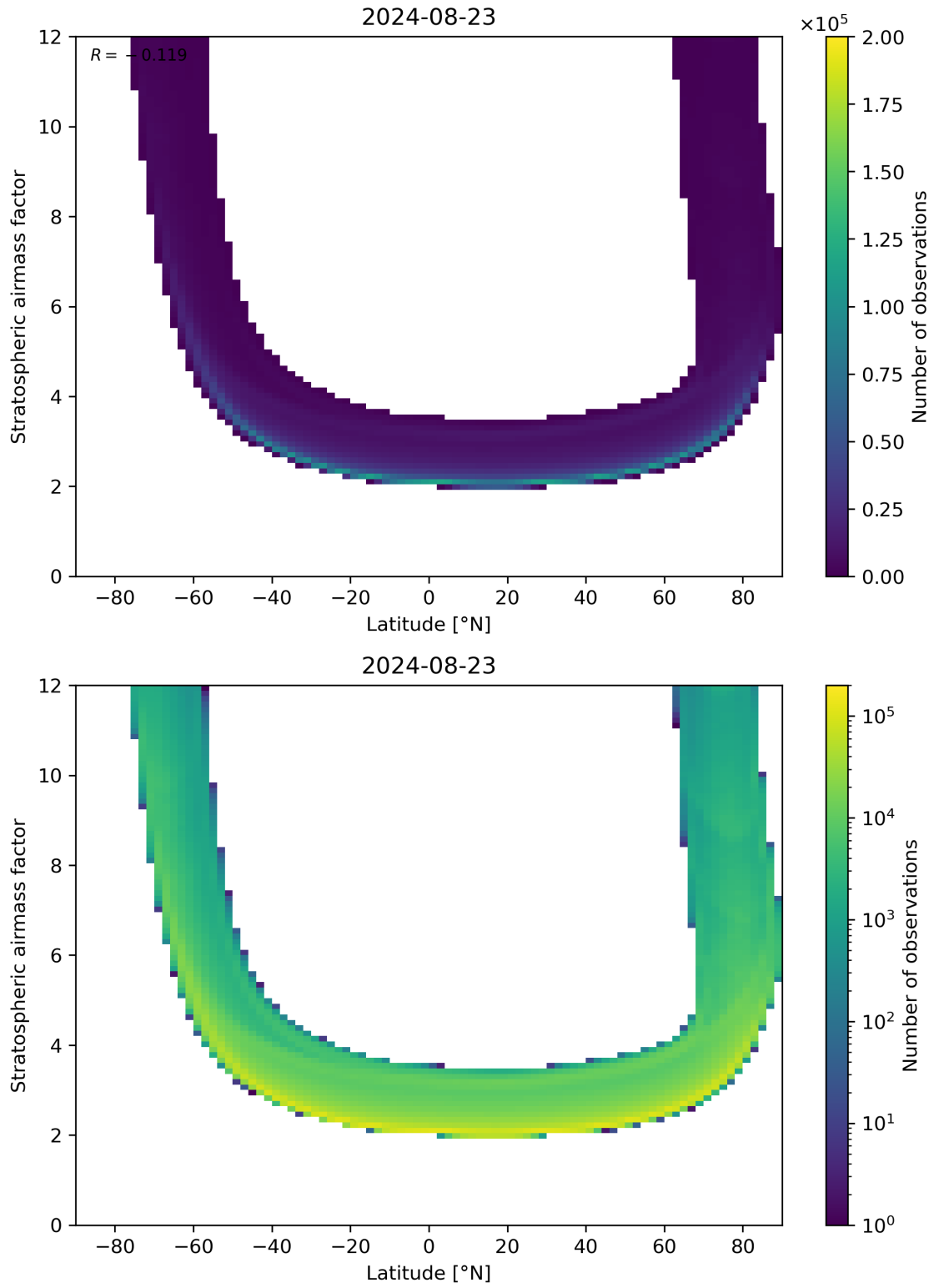
Figure 83: Scatter density plot of “Latitude” against “Stratospheric air mass factor” for 2024-08-22 to 2024-08-24.
