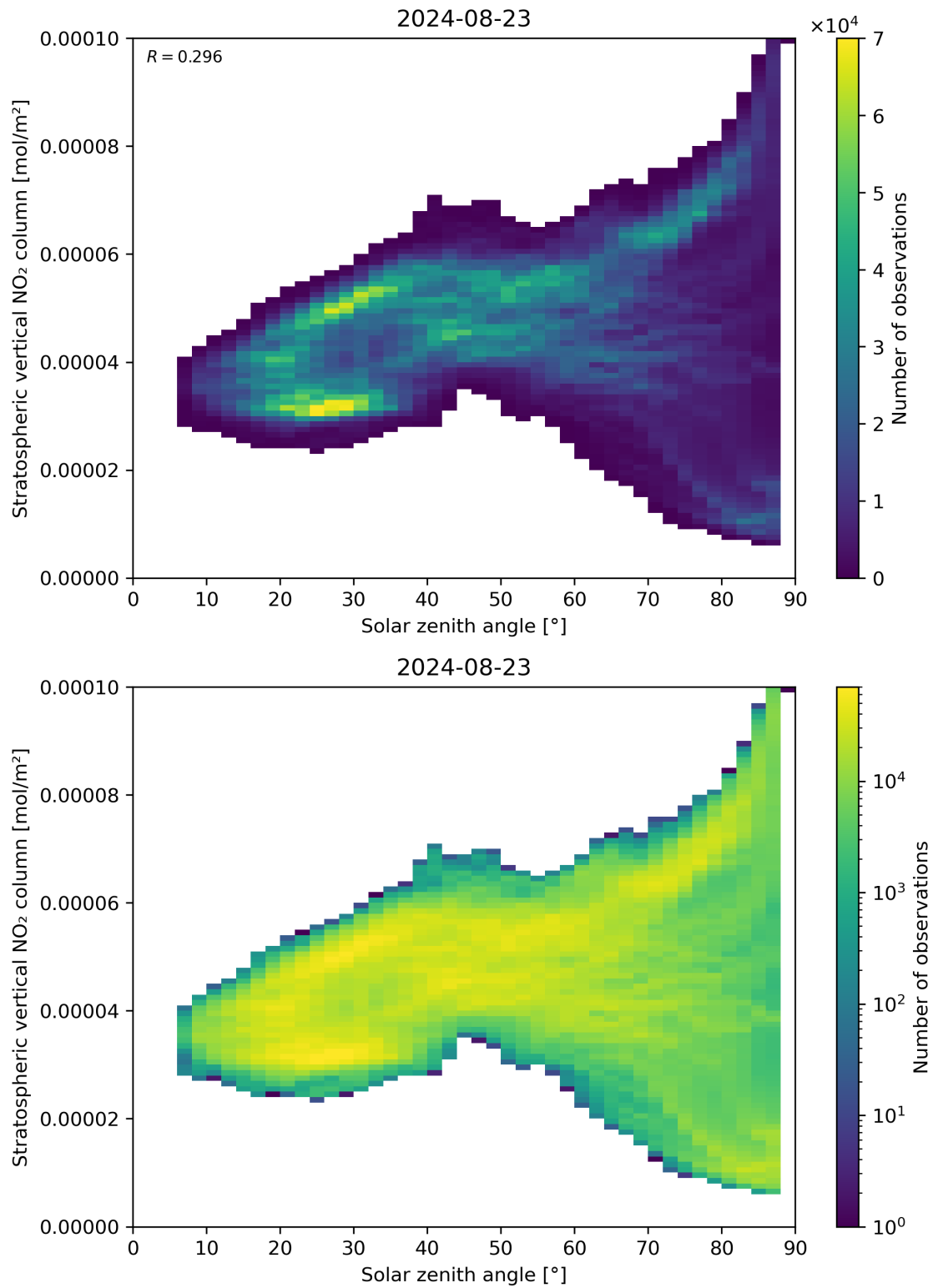
Figure 150: Scatter density plot of “Solar zenith angle” against “Stratospheric vertical NO 2 column” for 2024-08-22 to 2024-08-24.
