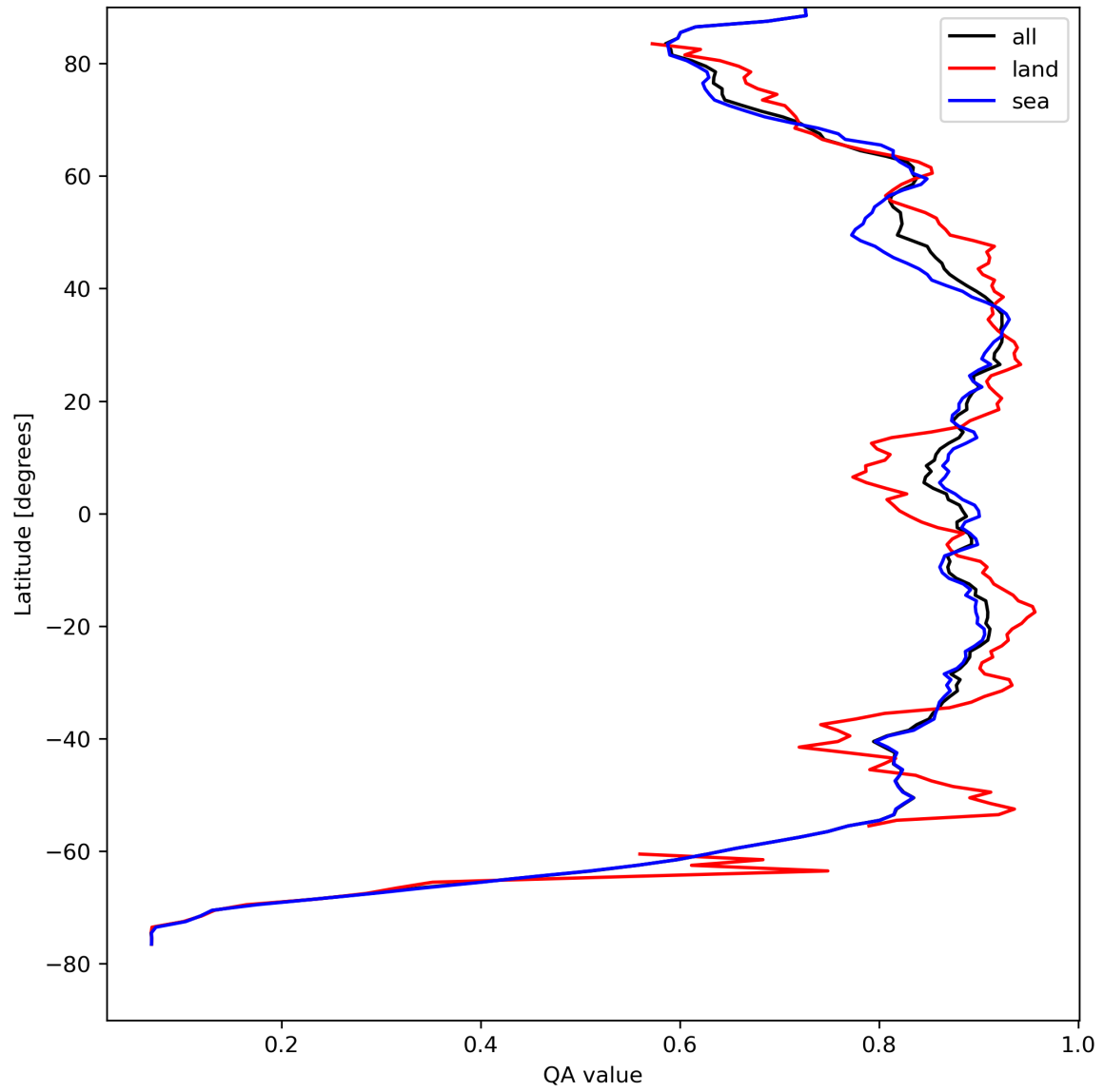
Figure 11: Zonal average of “QA value” for 2024-08-22 to 2024-08-24.
