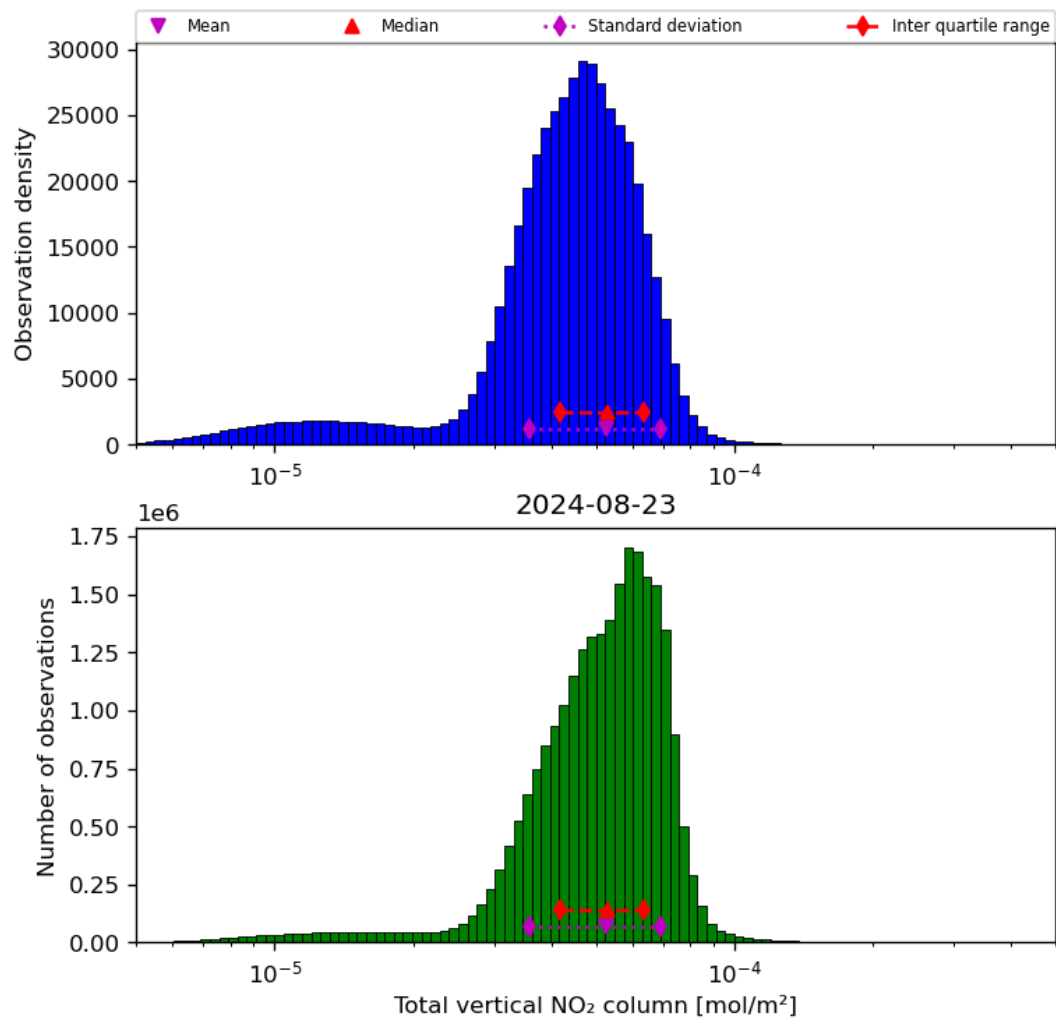
Figure 38: Histogram of “Total vertical NO 2 column” for 2024-08-22 to 2024-08-24
