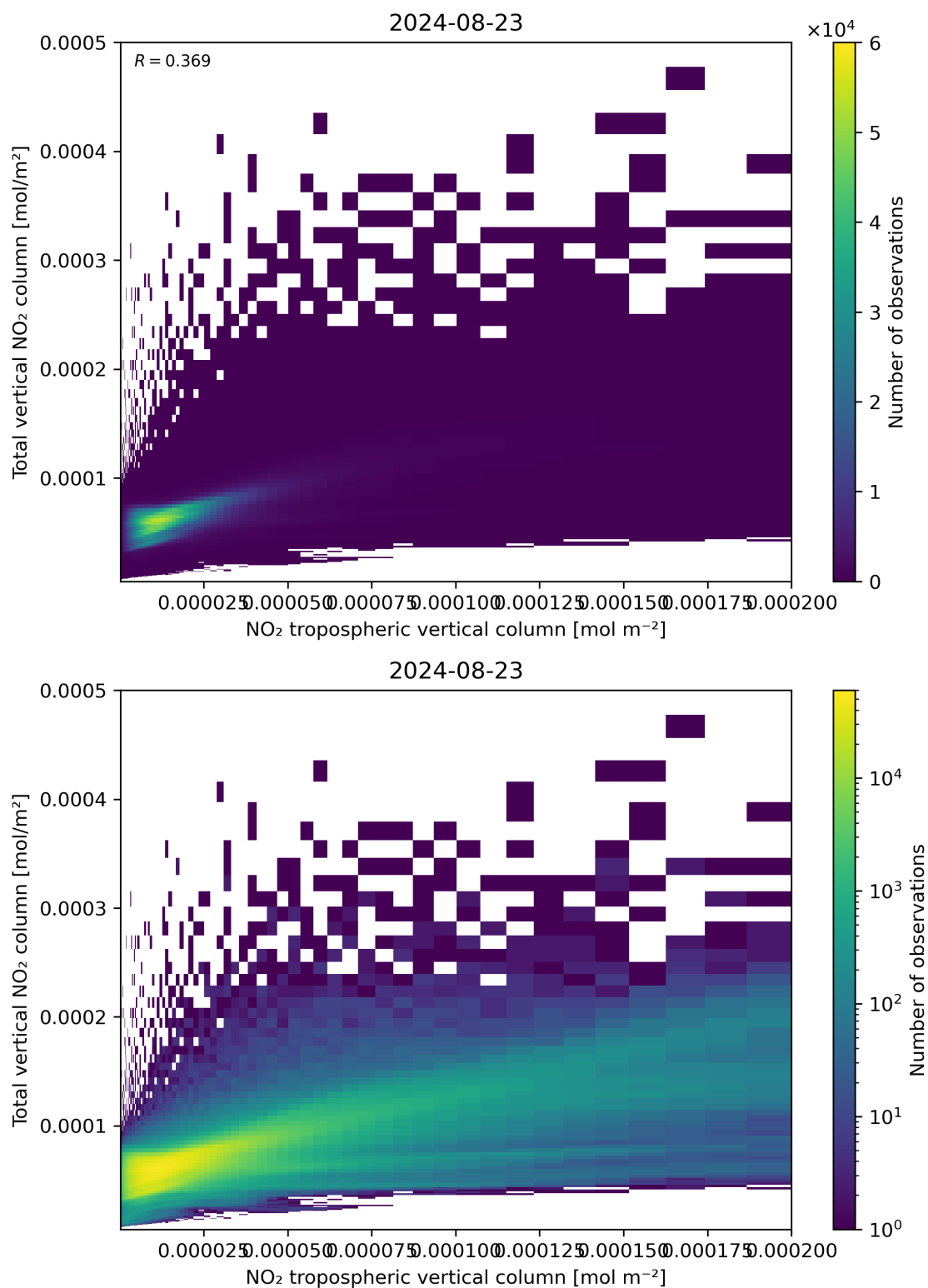
Figure 128: Scatter density plot of “NO 2 tropospheric vertical column” against “Total vertical NO 2 column” for 2024-08-22 to 2024-08-24.
