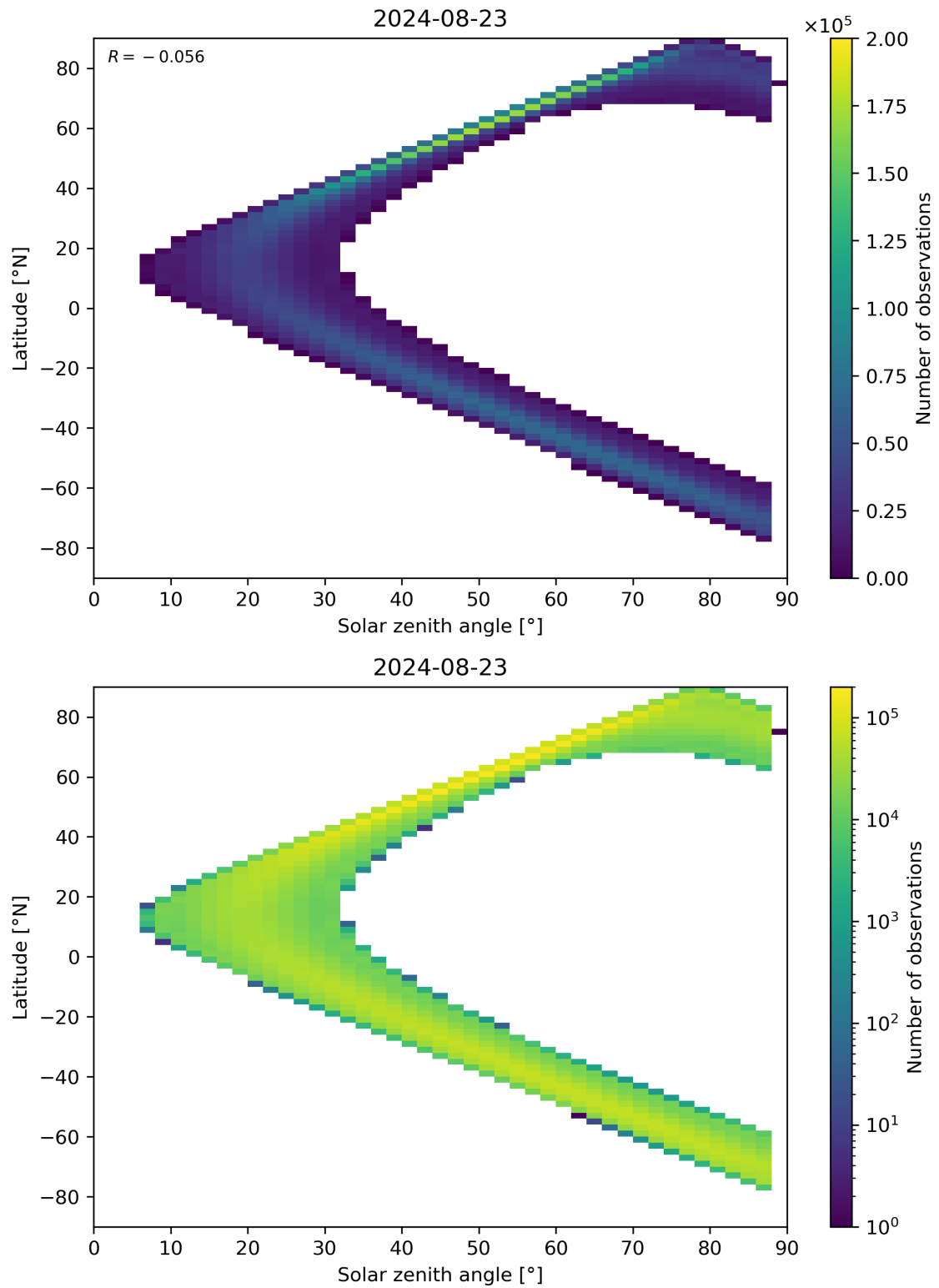
Figure 149: Scatter density plot of “Solar zenith angle” against “Latitude” for 2024-08-22 to 2024-08-24.
