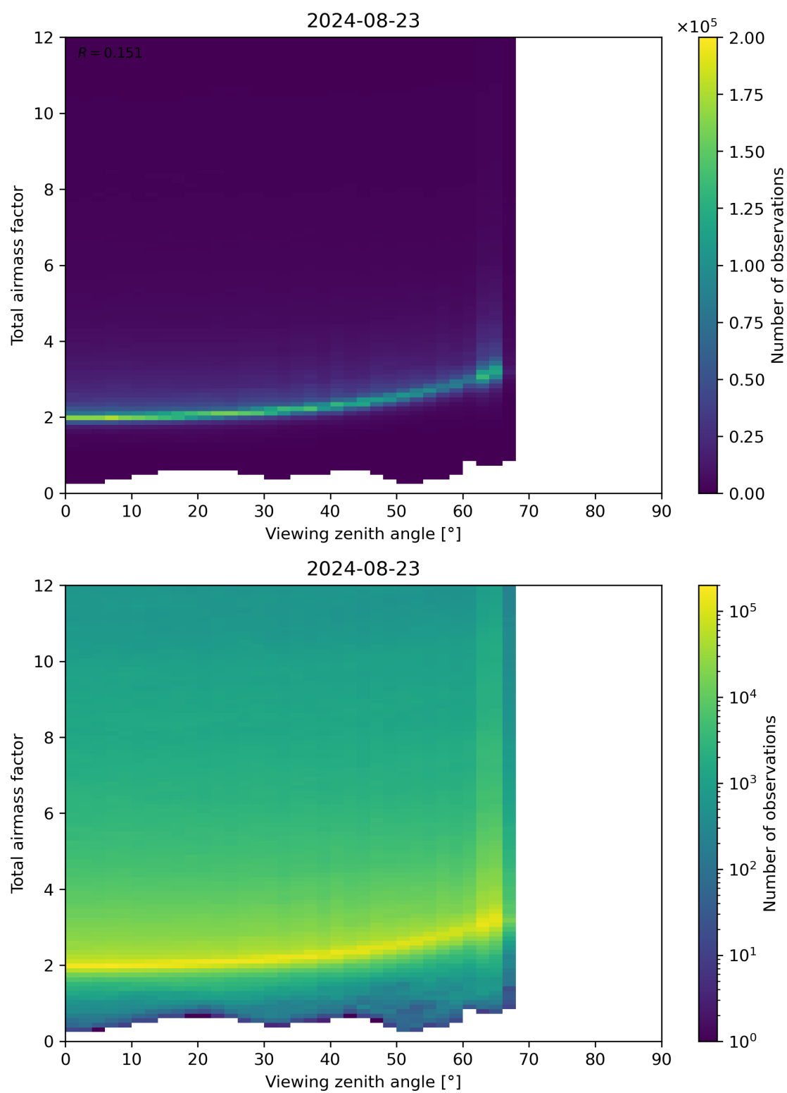
Figure 160: Scatter density plot of “Viewing zenith angle” against “Total airmass factor” for 2024-08-22 to 2024-08-24.
