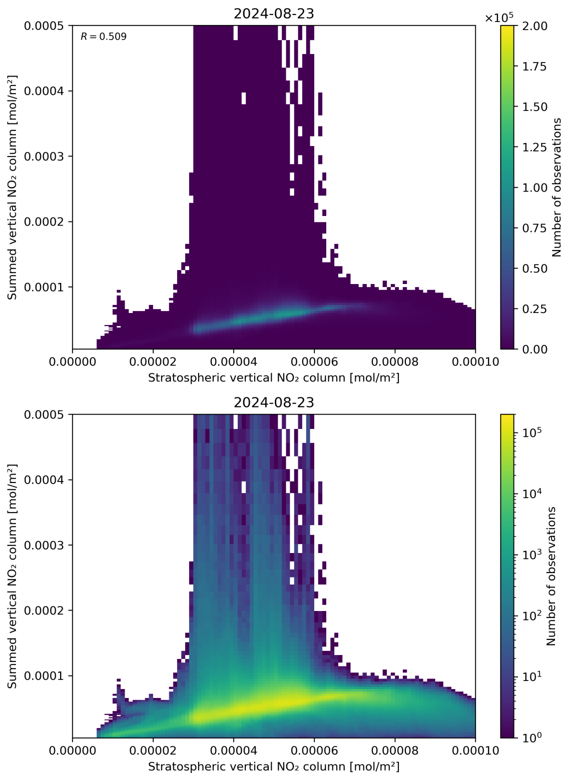
Figure 98: Scatter density plot of “Stratospheric vertical NO 2 column” against “Summed vertical NO 2 column” for 2024-08-22 to 2024-08-24.
