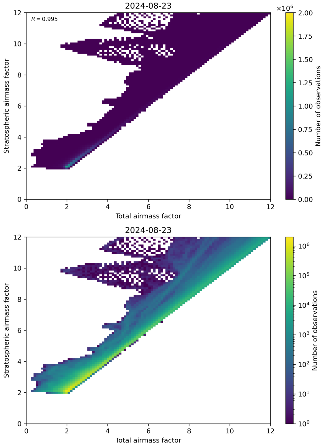
Figure 62: Scatter density plot of “Total airmass factor” against “Stratospheric airmass factor” for 2024-08-22 to 2024-08-24.
