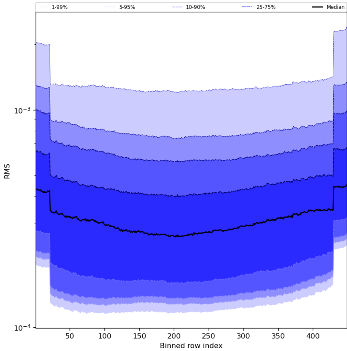
Figure 60: Along track statistics of “RMS” for 2024-08-22 to 2024-08-24
