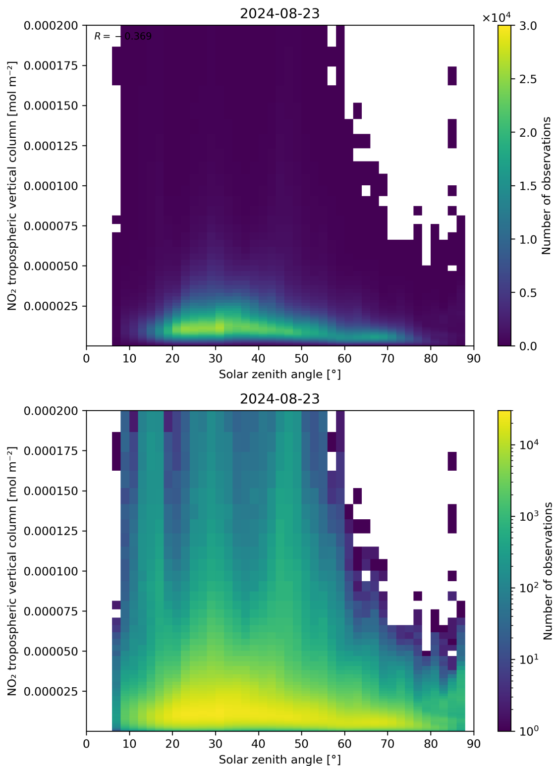
Figure 155: Scatter density plot of “Solar zenith angle” against “NO 2 tropospheric vertical column” for 2024-08-22 to 2024-08-24.
