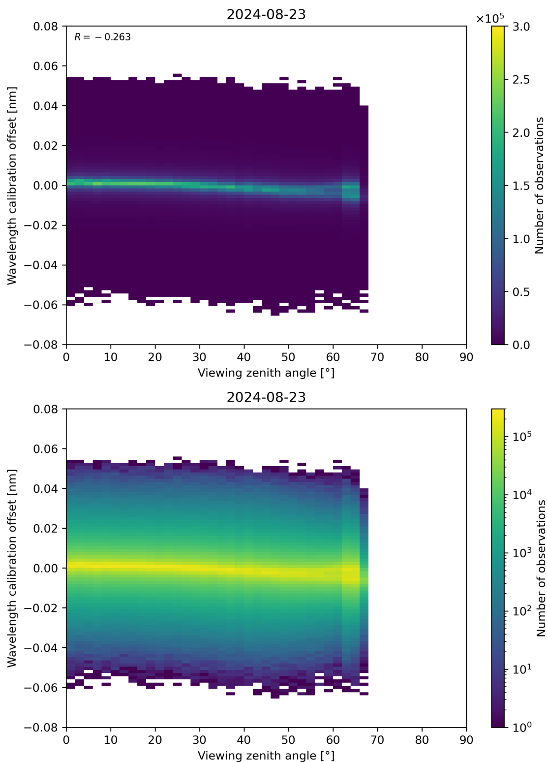
Figure 173: Scatter density plot of “Viewing zenith angle” against “Wavelength calibration offset” for 2024-08-22 to 2024-08-24.
