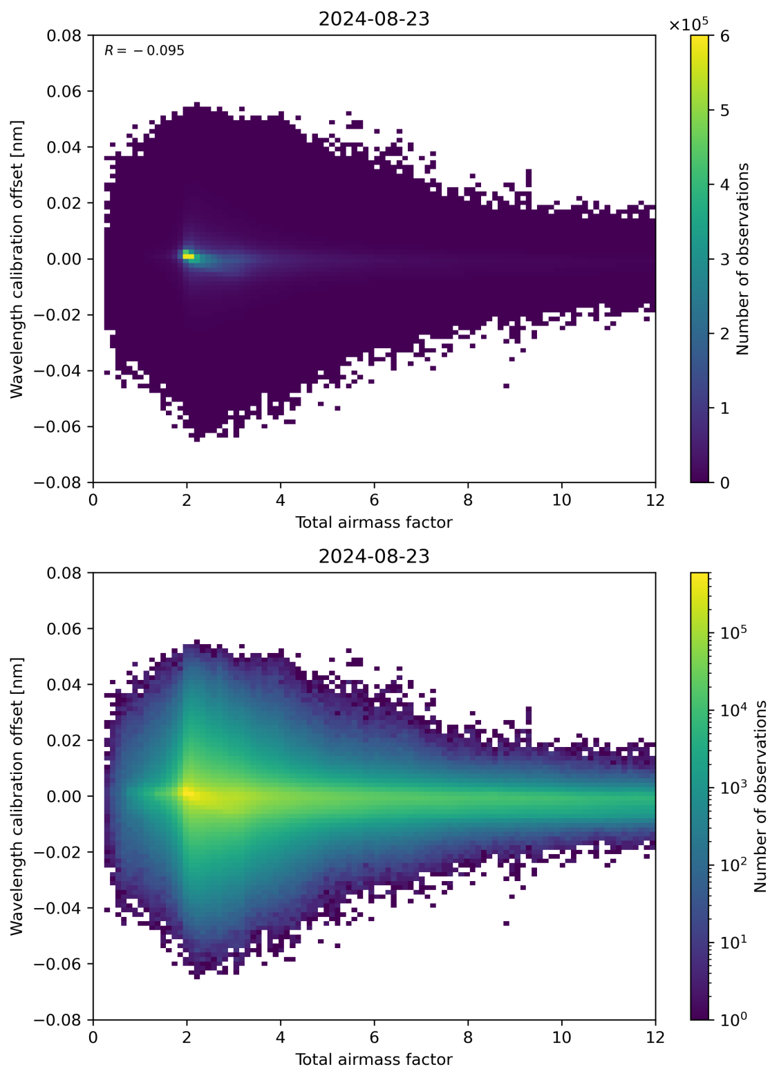
Figure 70: Scatter density plot of “Total airmass factor” against “Wavelength calibration offset” for 2024-08-22 to 2024-08-24.
