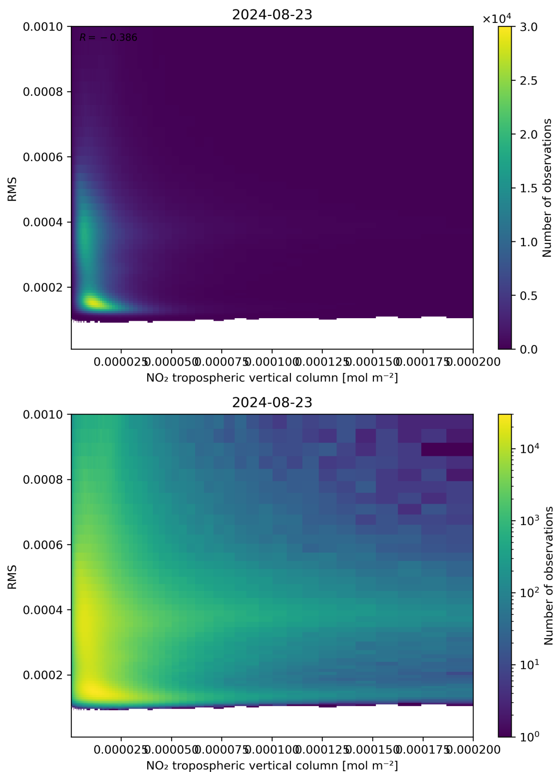
Figure 142: Scatter density plot of “NO 2 tropospheric vertical column” against “RMS” for 2024-08-22 to 2024-08-24.
