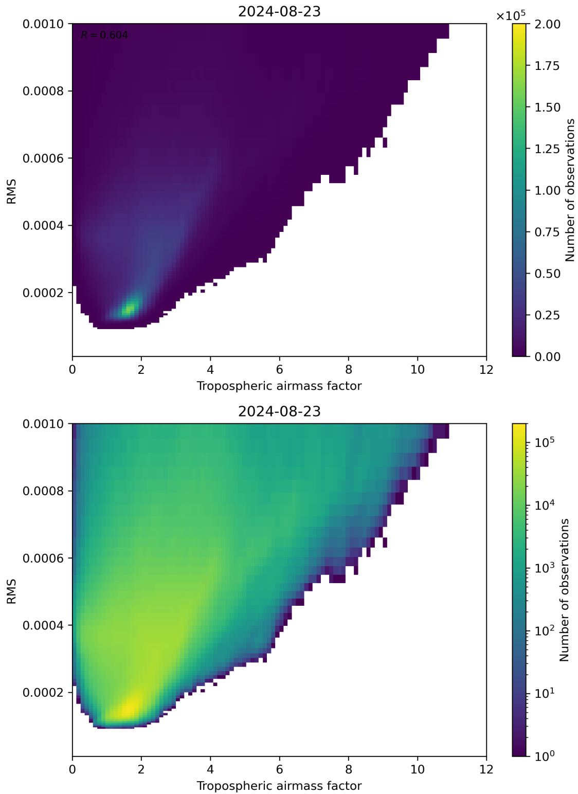
Figure 79: Scatter density plot of “Tropospheric airmass factor” against “RMS” for 2024-08-22 to 2024-08-24.
