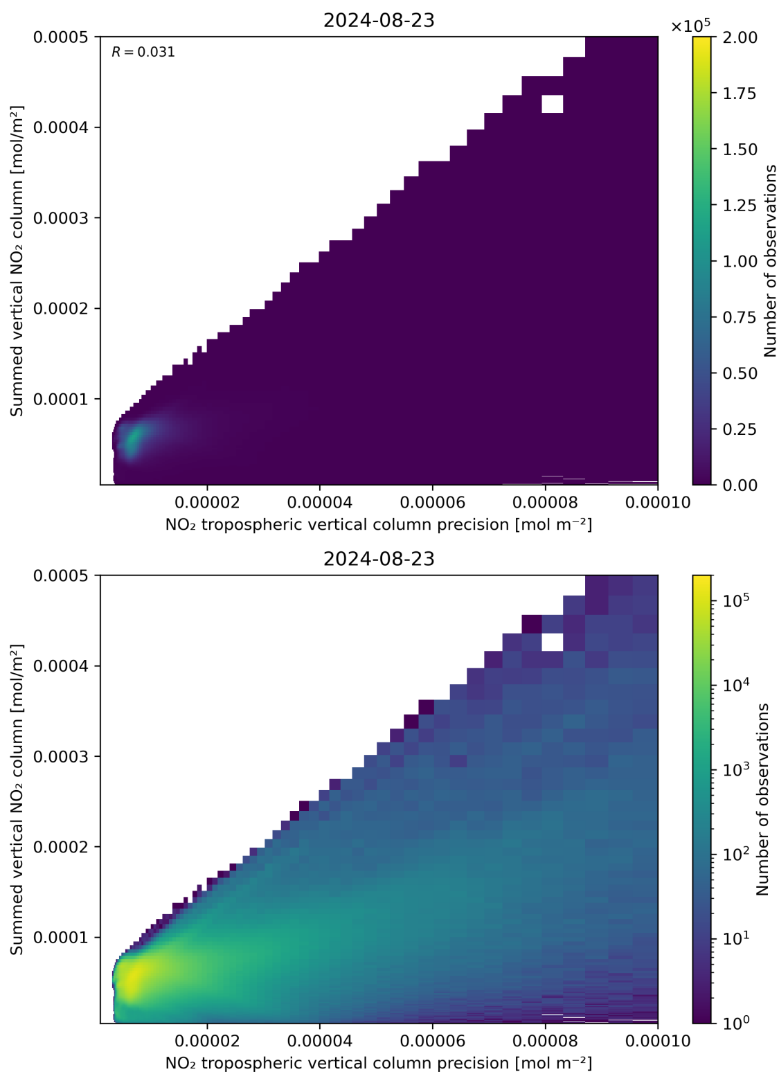
Figure 136: Scatter density plot of “NO 2 tropospheric vertical column precision” against “Summed vertical NO 2 column” for 2024-08-22 to 2024-08-24.
