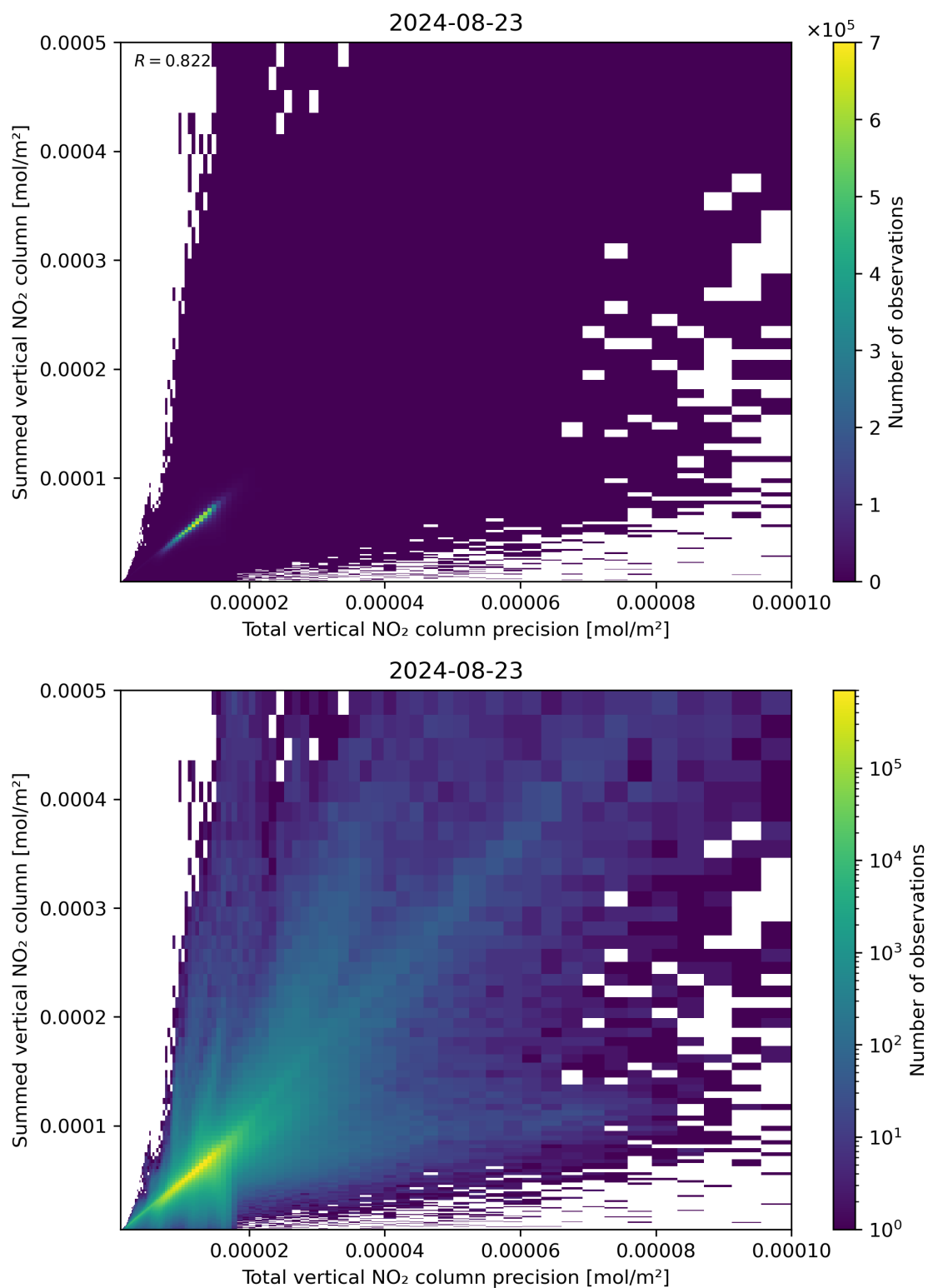
Figure 117: Scatter density plot of “Total vertical NO 2 column precision” against “Summed vertical NO 2 column” for 2024-08-22 to 2024-08-24.
