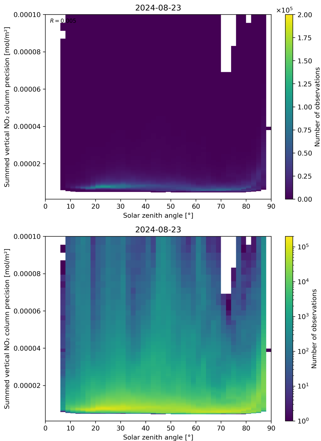
Figure 152: Scatter density plot of “Solar zenith angle” against “Summed vertical NO 2 column precision” for 2024-08-22 to 2024-08-24.
