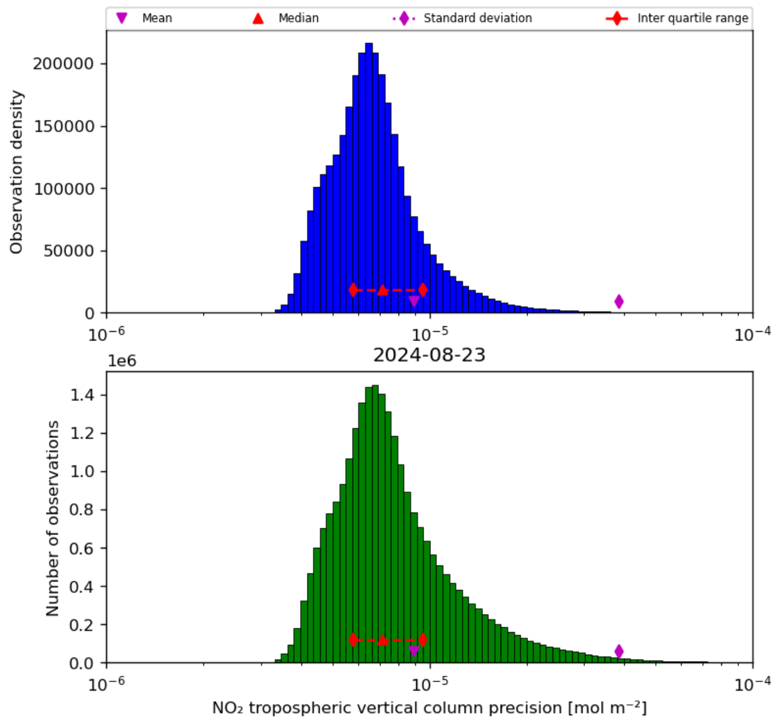
Figure 30: Histogram of “NO 2 tropospheric vertical column precision” for 2024-08-22 to 2024-08-24
