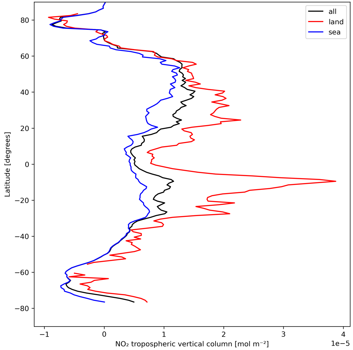
Figure 12: Zonal average of “NO 2 tropospheric vertical column” for 2024-08-22 to 2024-08-24.
