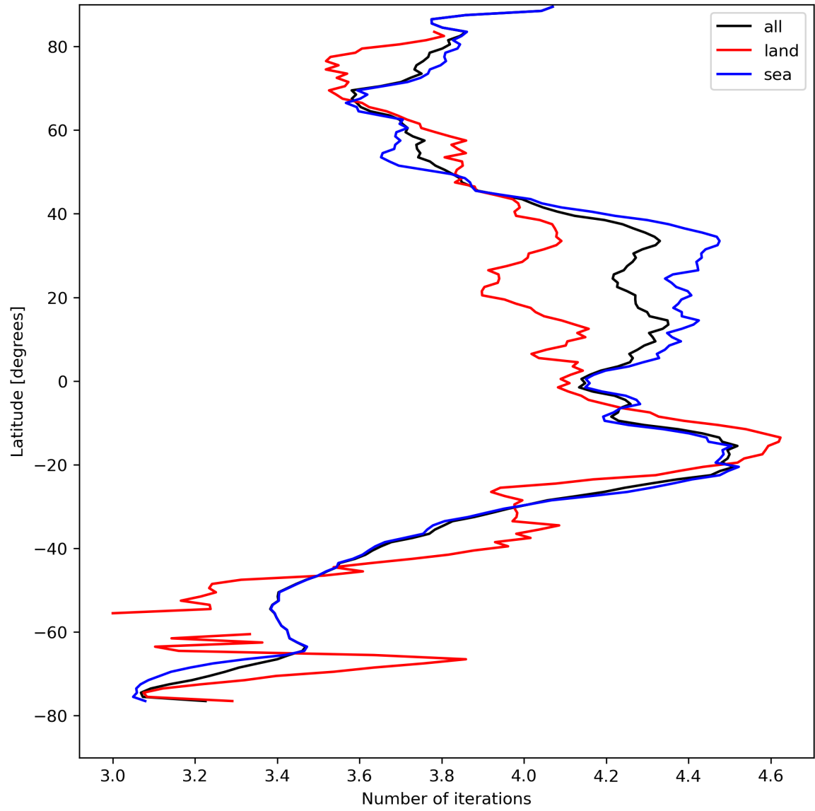
Figure 17: Zonal average of “Number of iterations” for 2024-08-22 to 2024-08-24.
