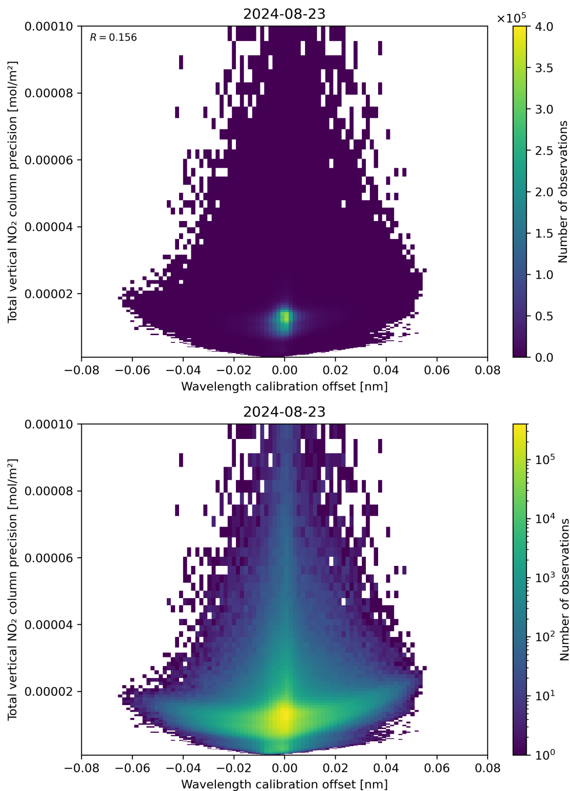
Figure 180: Scatter density plot of “Wavelength calibration offset” against “Total vertical NO 2 column precision” for 2024-08-22 to 2024-08-24.
