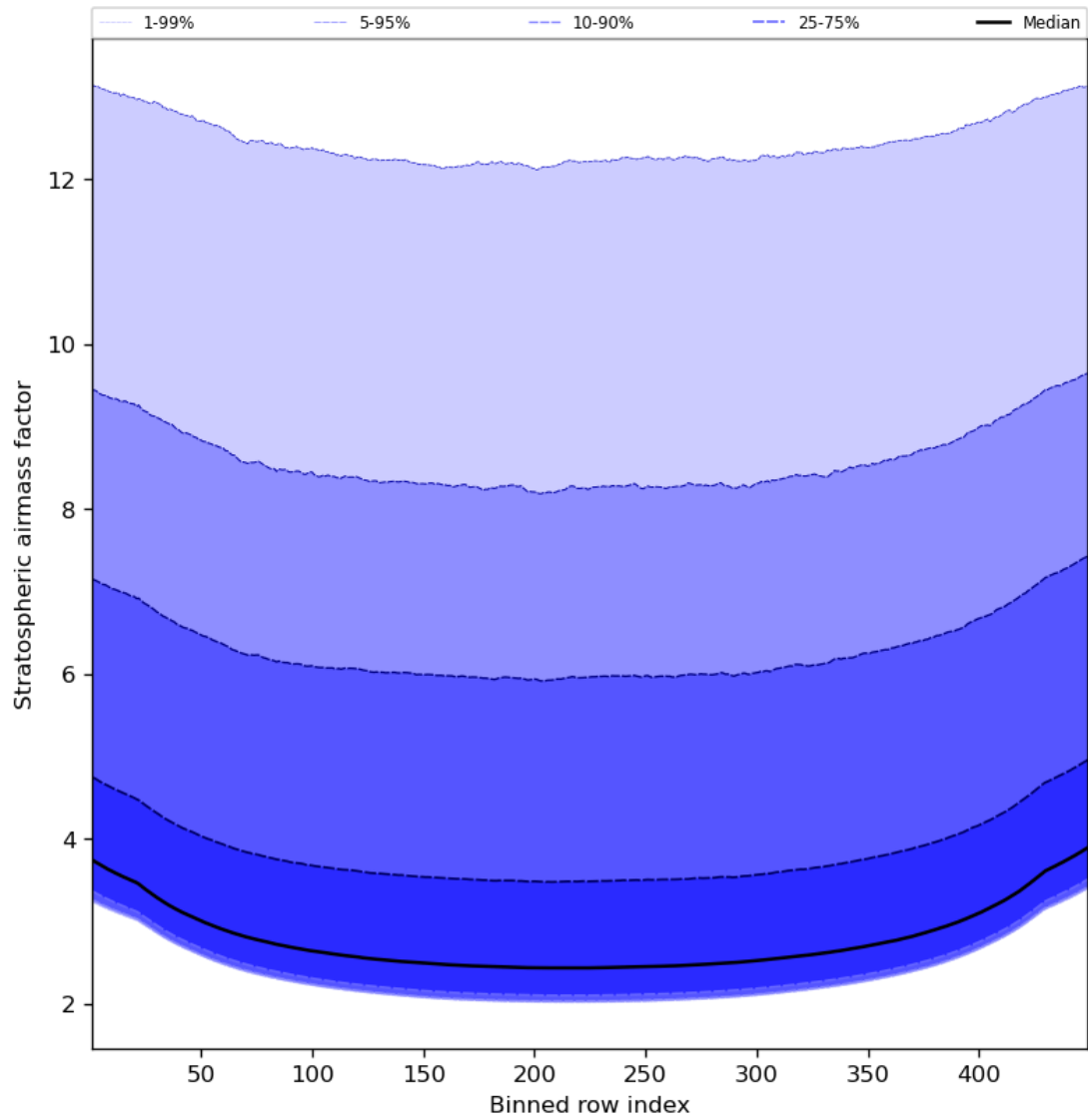
Figure 61: Along track statistics of “Stratospheric airmass factor” for 2024-08-22 to 2024-08-24
