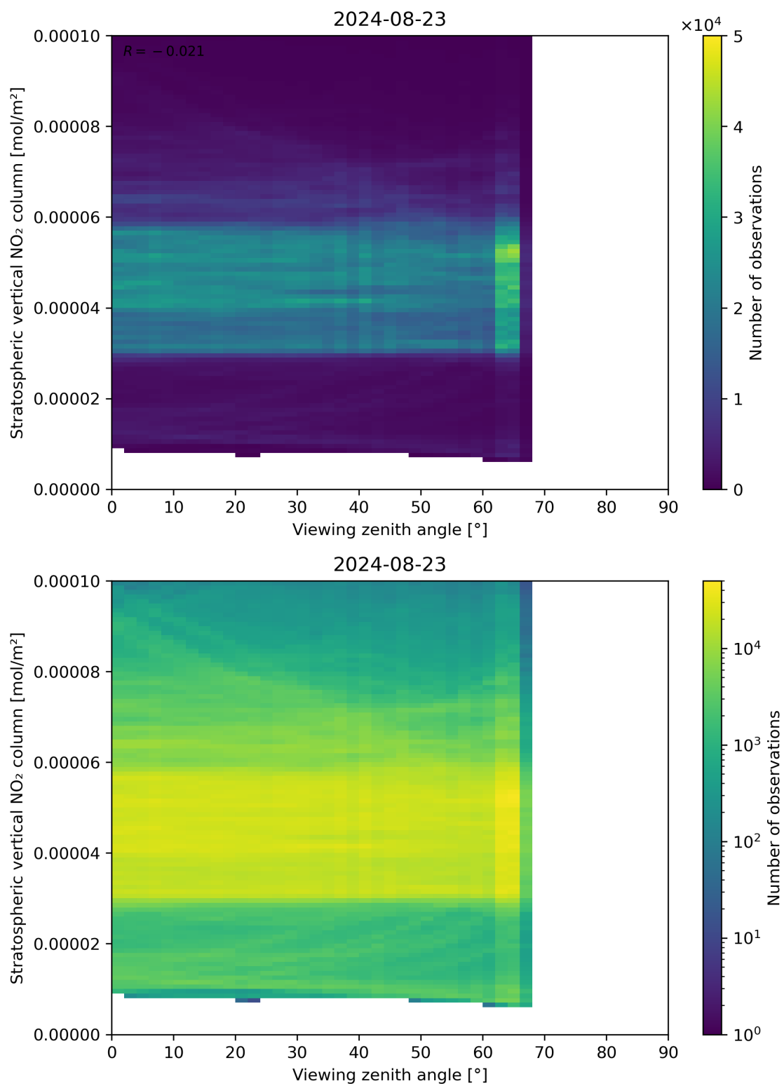
Figure 164: Scatter density plot of “Viewing zenith angle” against “Stratospheric vertical NO 2 column” for 2024-08-22 to 2024-08-24.
