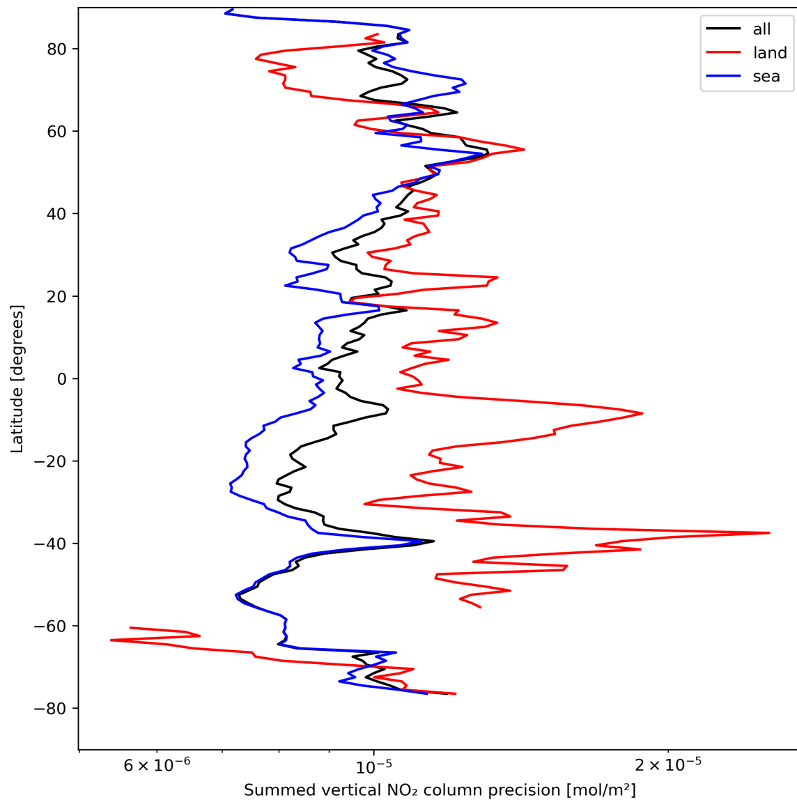
Figure 24: Zonal average of “Summed vertical NO 2 column precision” for 2024-08-22 to 2024-08-24.
