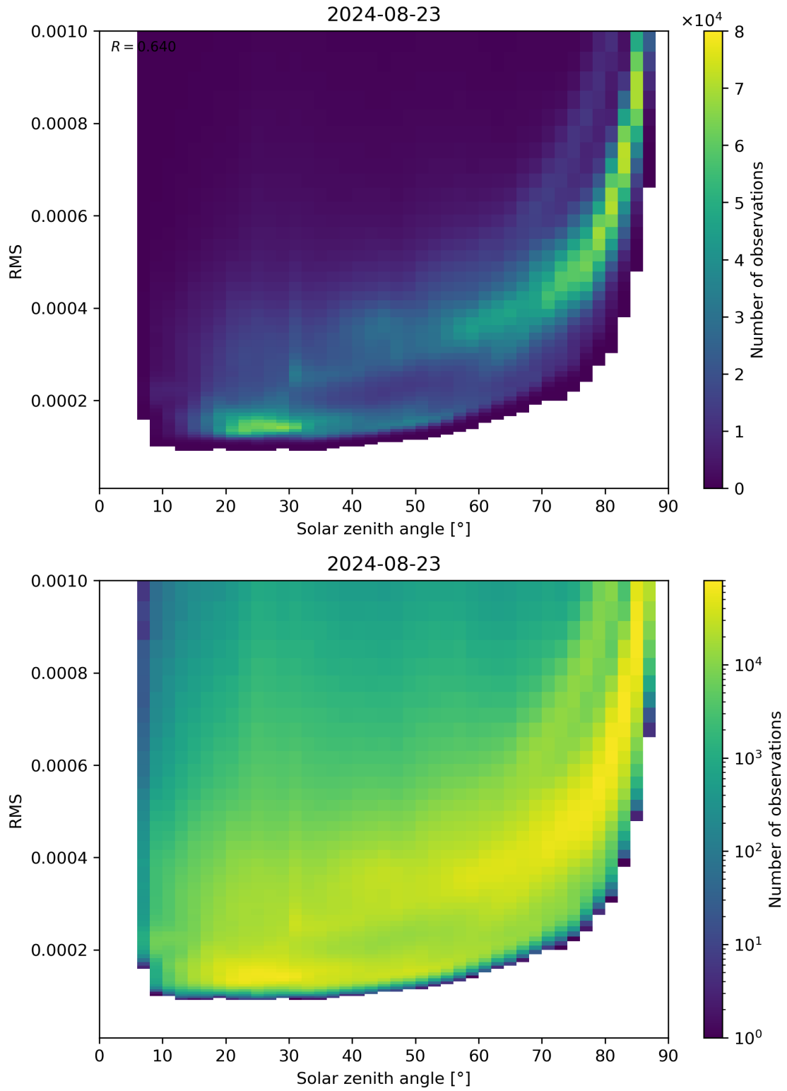
Figure 157: Scatter density plot of “Solar zenith angle” against “RMS” for 2024-08-22 to 2024-08-24.
