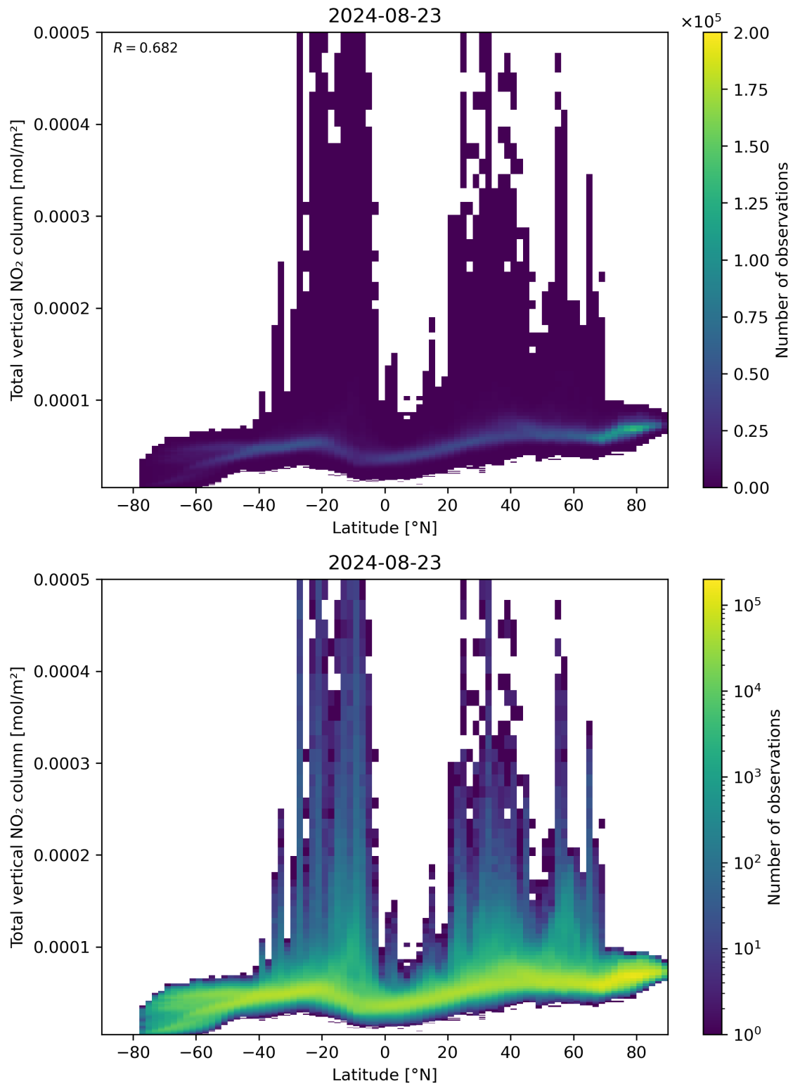
Figure 90: Scatter density plot of “Latitude” against “Total vertical NO 2 column” for 2024-08-22 to 2024-08-24.
