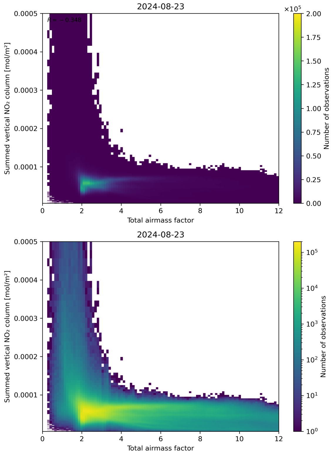
Figure 65: Scatter density plot of “Total airmass factor” against “Summed vertical NO 2 column” for 2024-08-22 to 2024-08-24.
