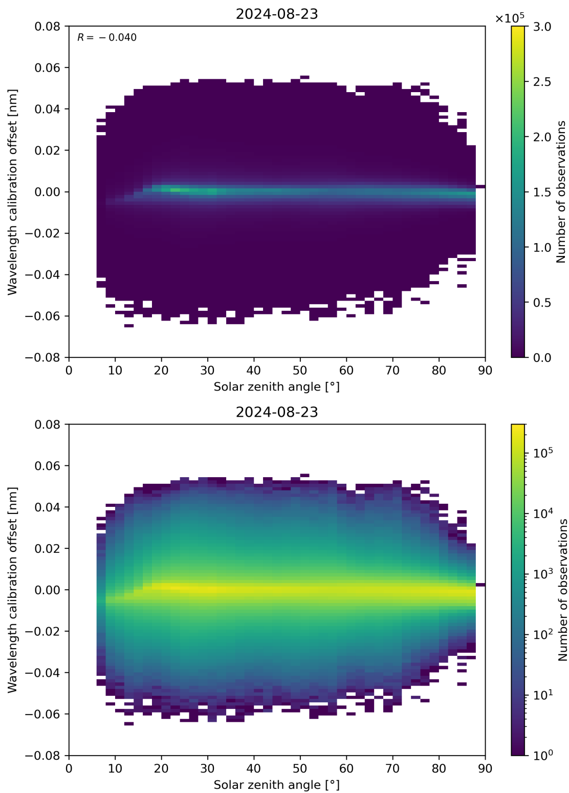
Figure 158: Scatter density plot of “Solar zenith angle” against “Wavelength calibration offset” for 2024-08-22 to 2024-08-24.
