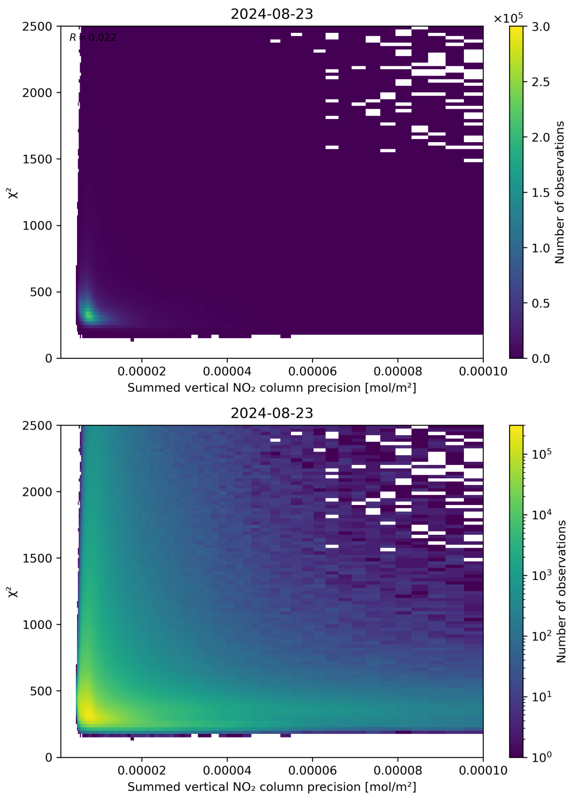
Figure 107: Scatter density plot of “Summed vertical NO 2 column precision” against “ \chi^2 ” for 2024-08-22 to 2024-08-24.
