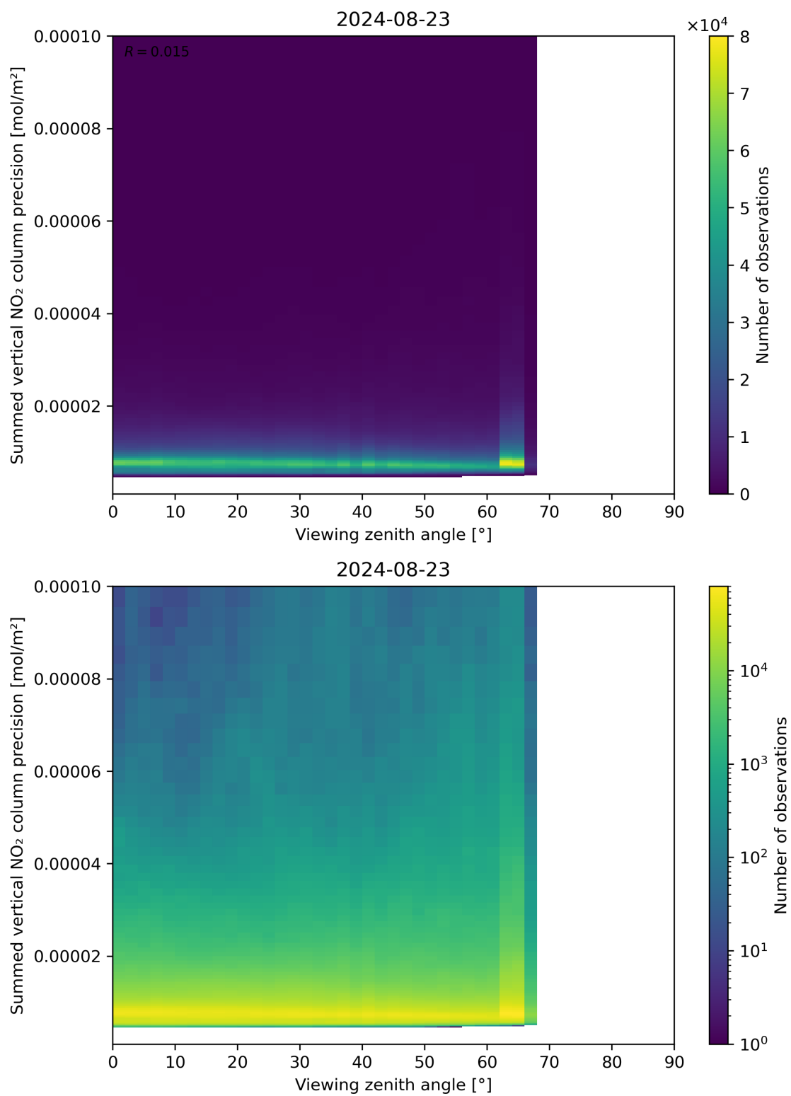
Figure 166: Scatter density plot of “Viewing zenith angle” against “Summed vertical NO 2 column precision” for 2024-08-22 to 2024-08-24.
