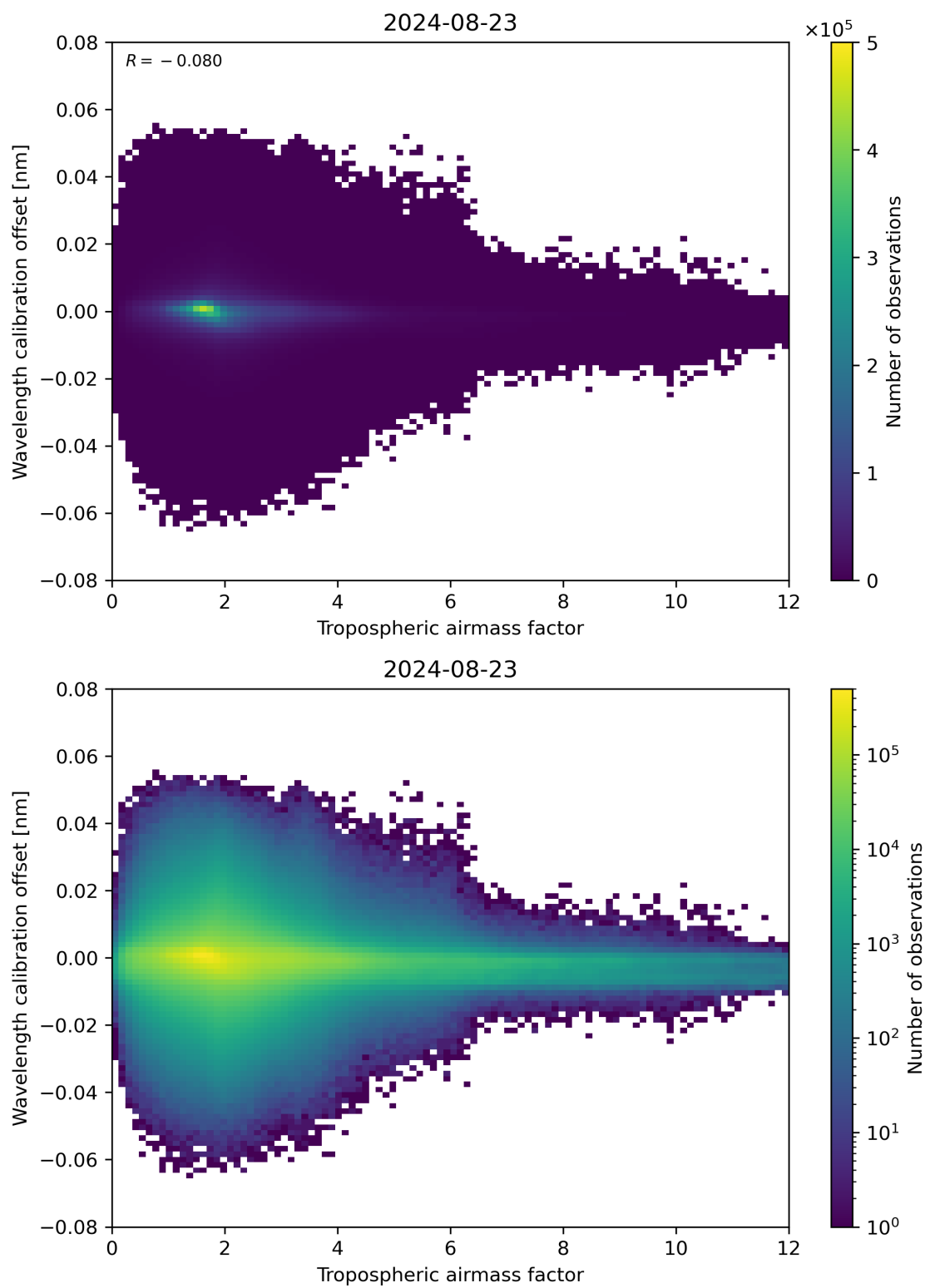
Figure 80: Scatter density plot of “Tropospheric airmass factor” against “Wavelength calibration offset” for 2024-08-22 to 2024-08-24.
