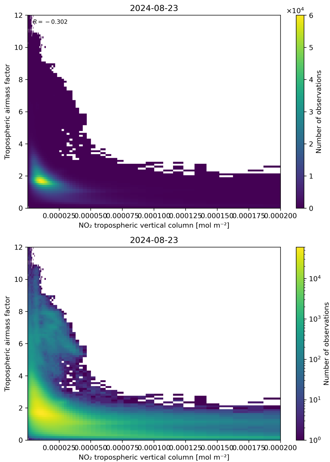
Figure 123: Scatter density plot of “NO 2 tropospheric vertical column” against “Tropospheric air mass factor” for 2024-08-22 to 2024-08-24.
