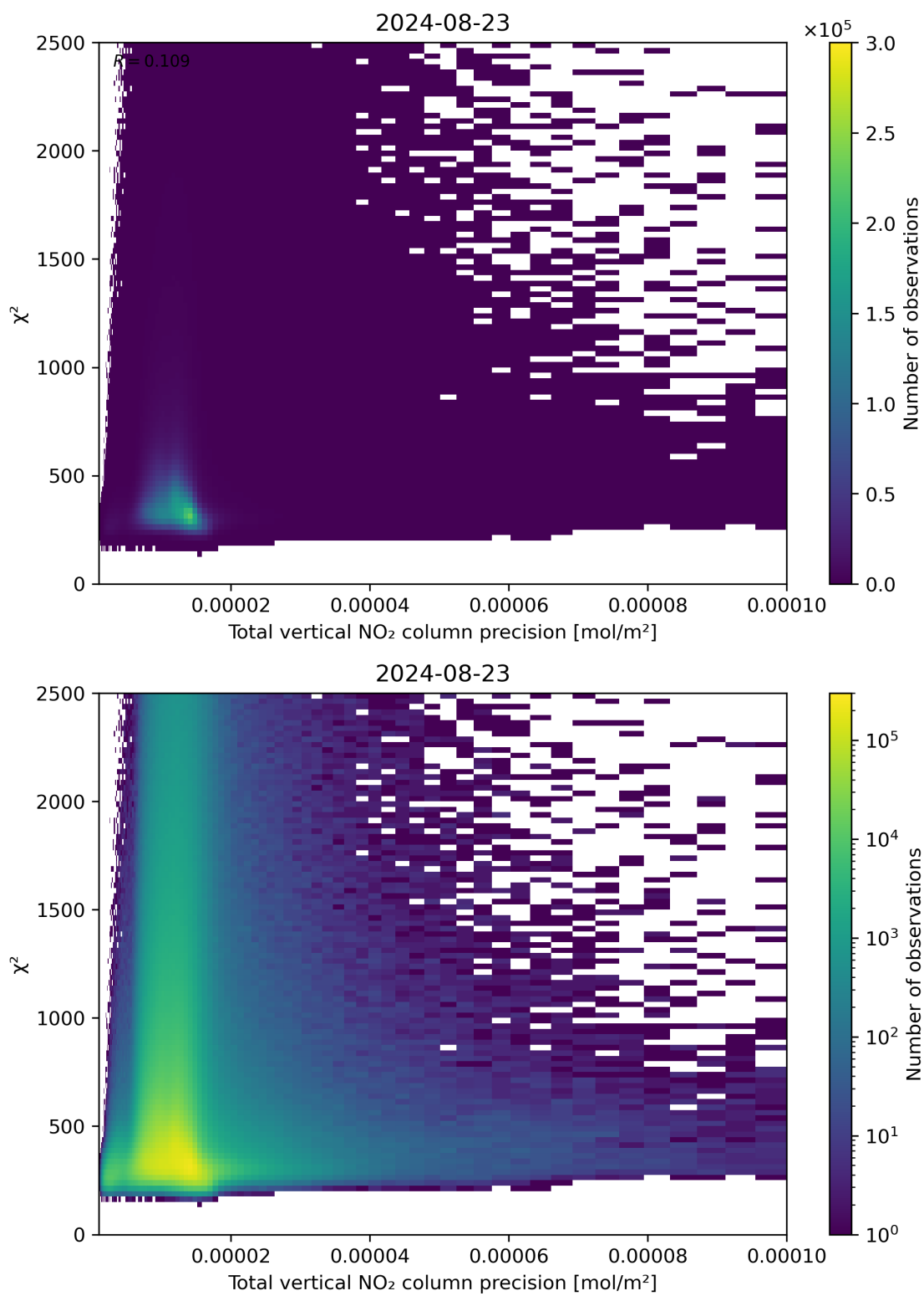
Figure 116: Scatter density plot of “Total vertical NO 2 column precision” against “ \chi^2 ” for 2024-08-22 to 2024-08-24.
