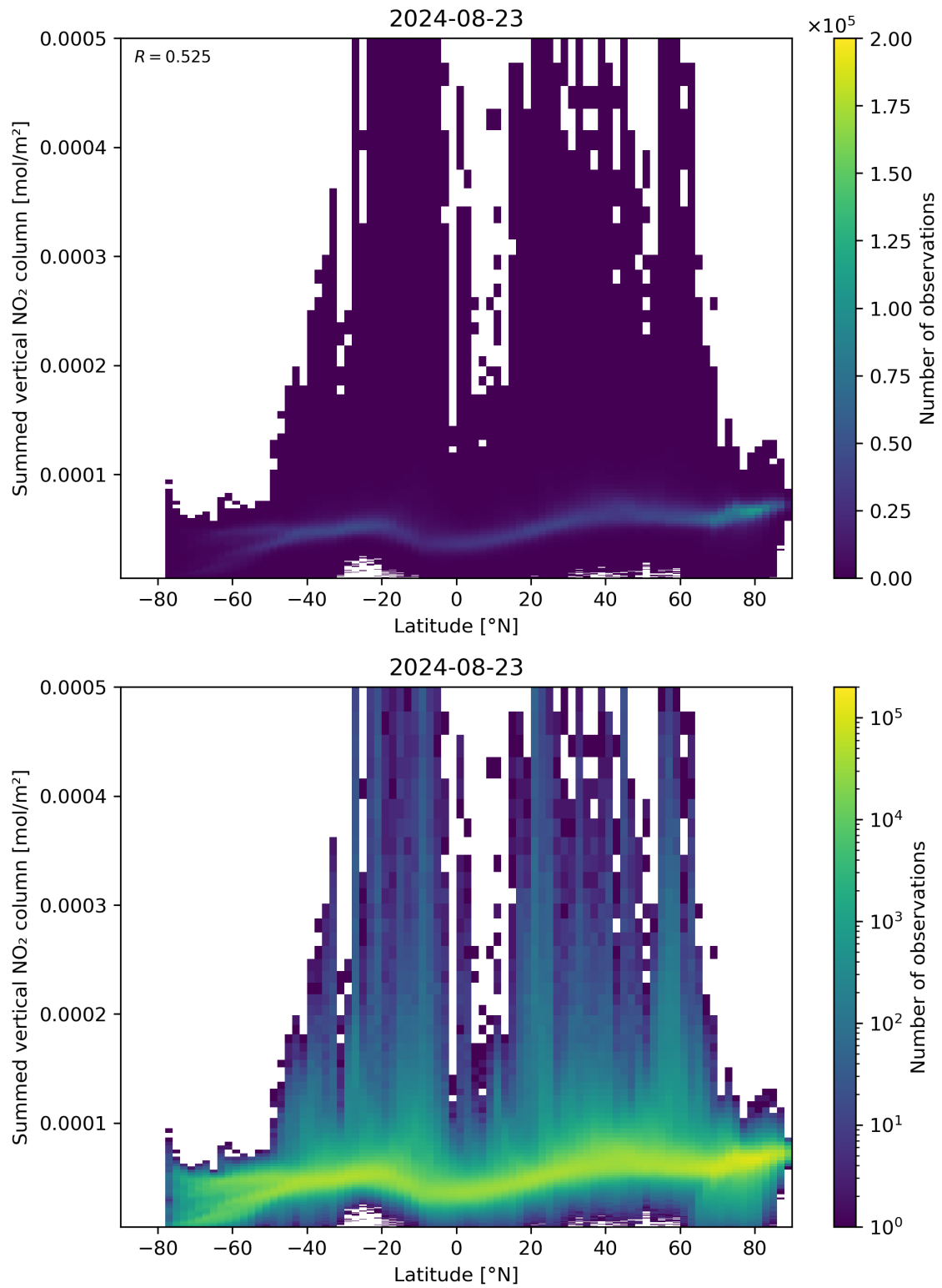
Figure 88: Scatter density plot of “Latitude” against “Summed vertical NO 2 column” for 2024-08-22 to 2024-08-24.
