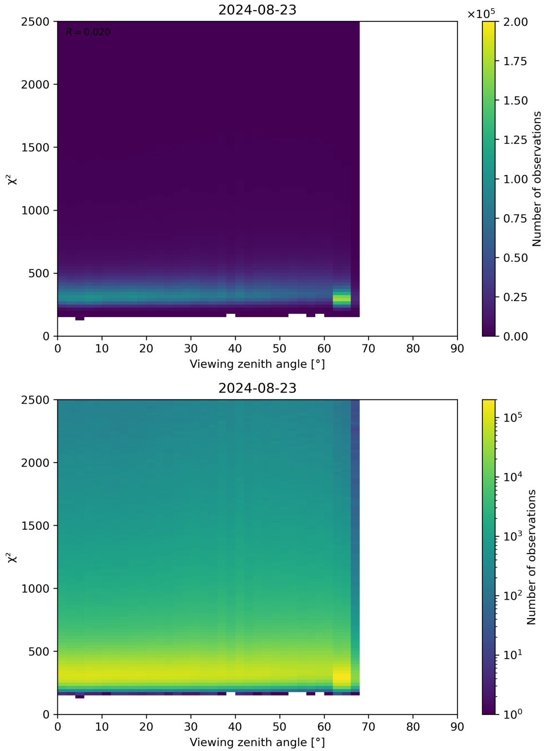
Figure 162: Scatter density plot of “Viewing zenith angle” against “ \chi^2 ” for 2024-08-22 to 2024-08-24.
