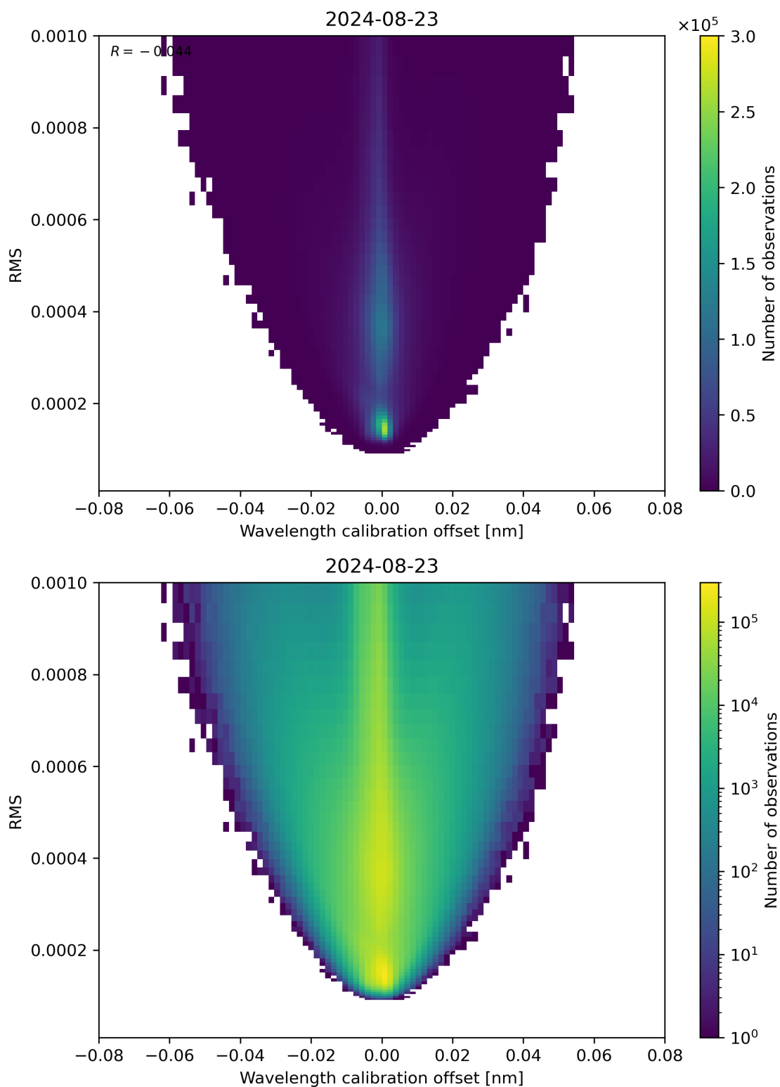
Figure 181: Scatter density plot of “Wavelength calibration offset” against “RMS” for 2024-08-22 to 2024-08-24.
