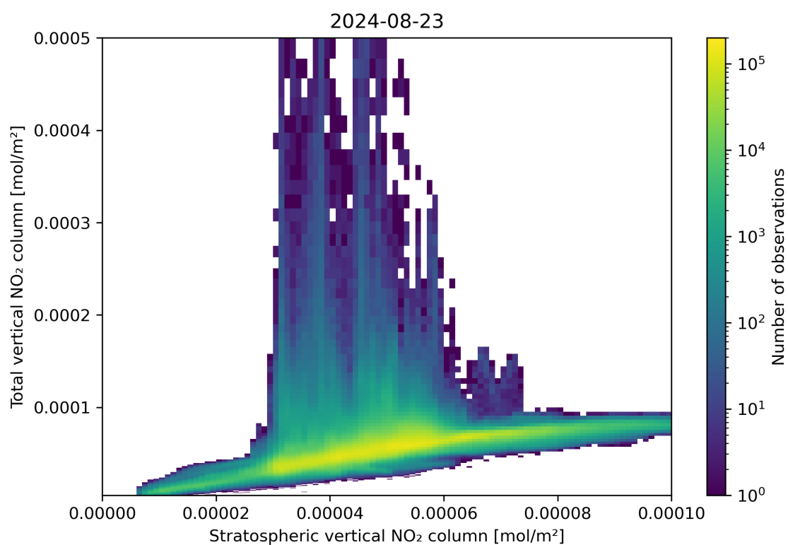
Figure 100: Scatter density plot of “Stratospheric vertical NO 2 column” against “Total vertical NO 2 column” for 2024-08-22 to 2024-08-24.
