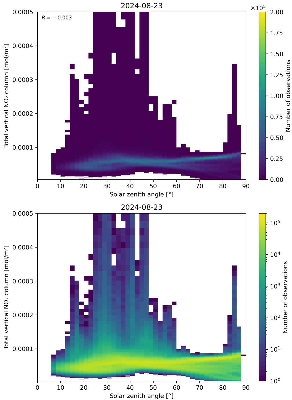
Figure 153: Scatter density plot of “Solar zenith angle” against “Total vertical NO 2 column” for 2024-08-22 to 2024-08-24.
