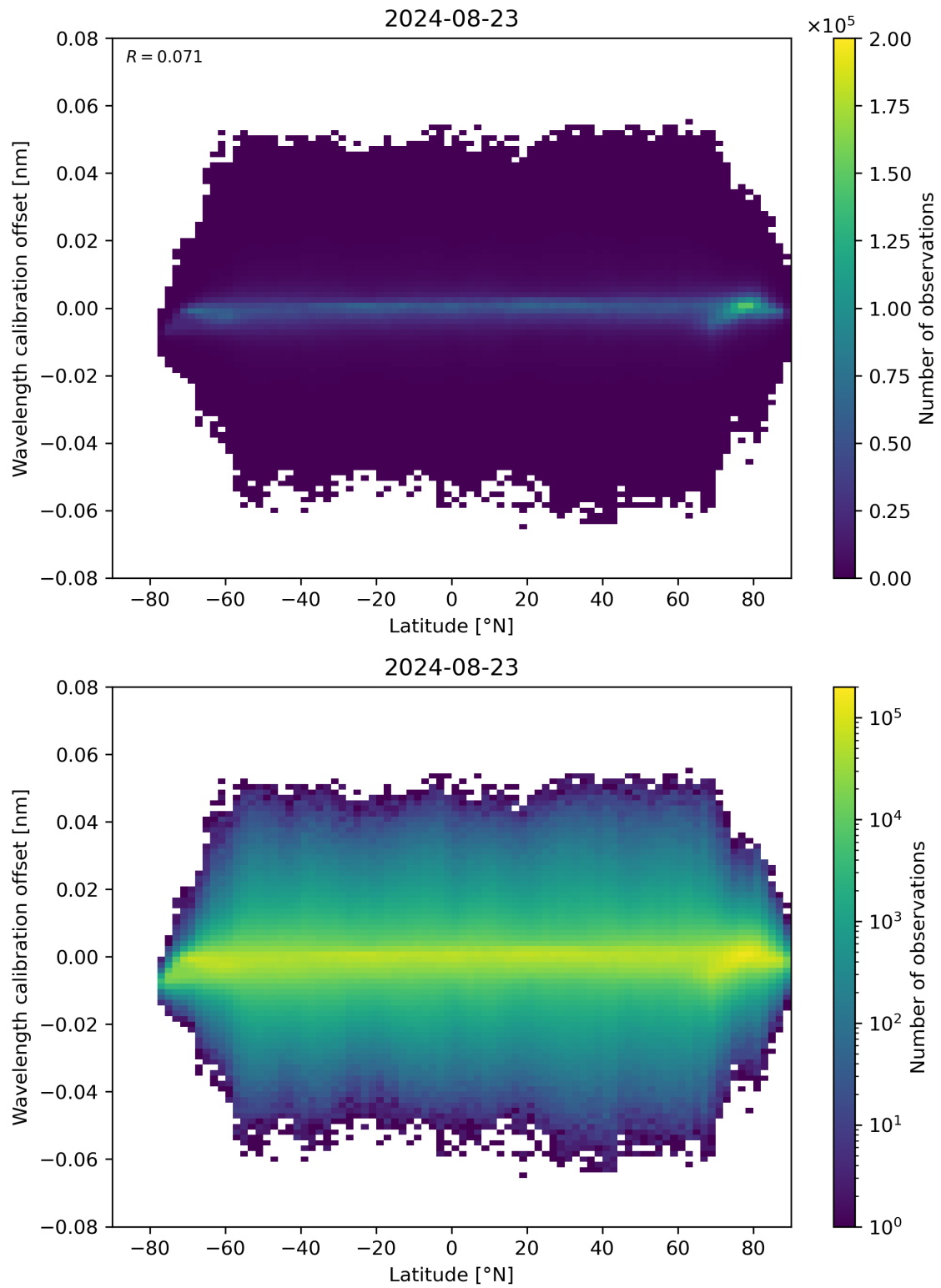
Figure 95: Scatter density plot of “Latitude” against “Wavelength calibration offset” for 2024-08-22 to 2024-08-24.
