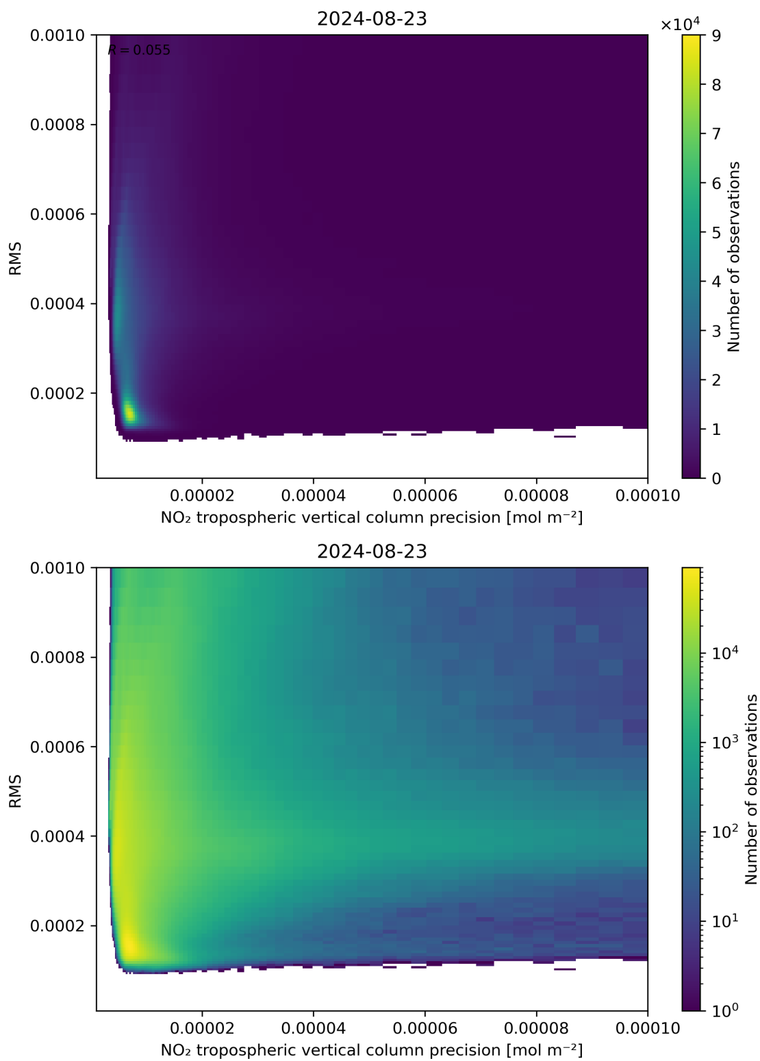
Figure 140: Scatter density plot of “NO 2 tropospheric vertical column precision” against “RMS” for 2024-08-22 to 2024-08-24.
