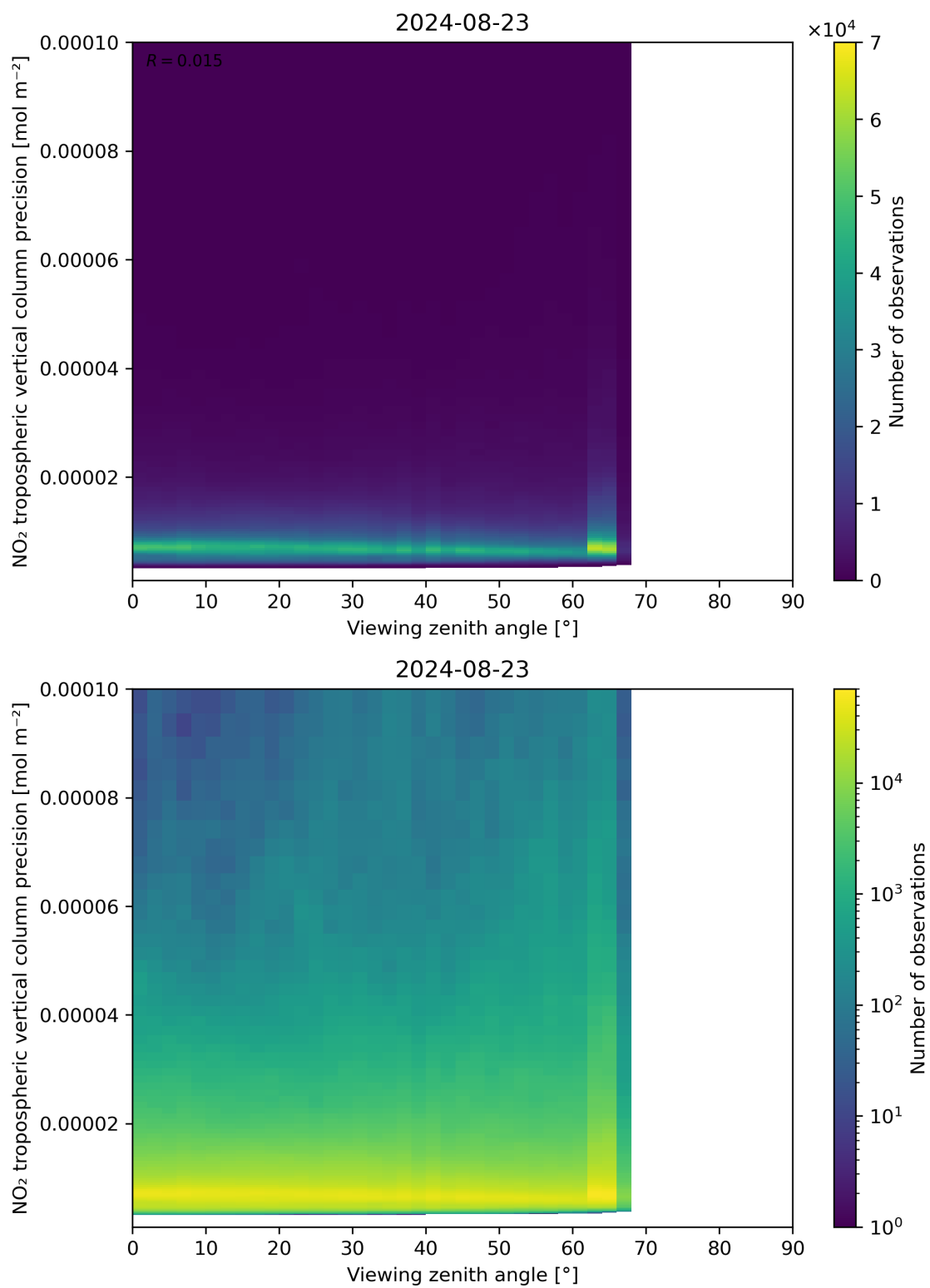
Figure 170: Scatter density plot of “Viewing zenith angle” against “NO 2 tropospheric vertical column precision” for 2024-08-22 to 2024-08-24.
