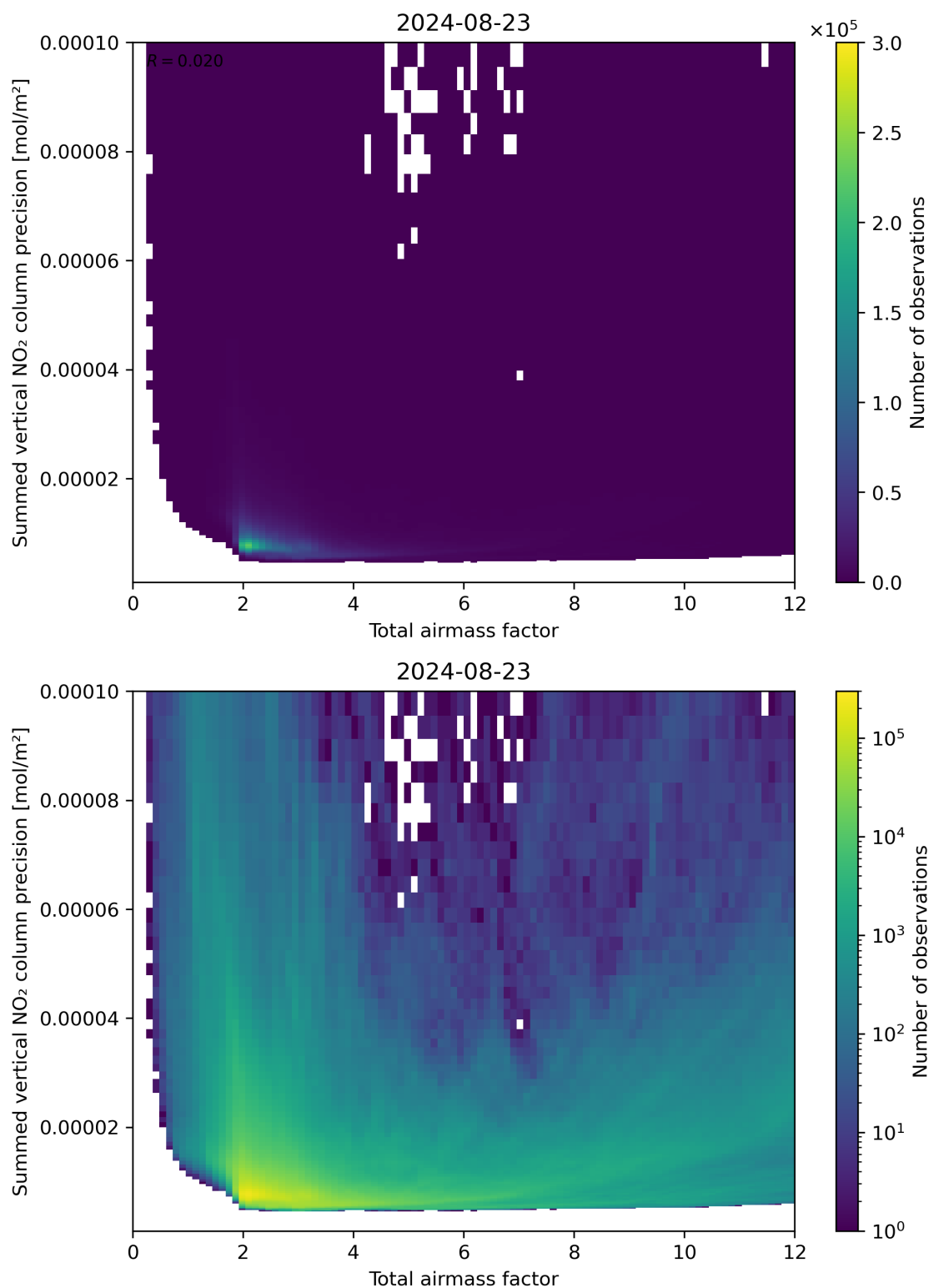
Figure 66: Scatter density plot of “Total airmass factor” against “Summed vertical NO 2 column precision” for 2024-08-22 to 2024-08-24.
