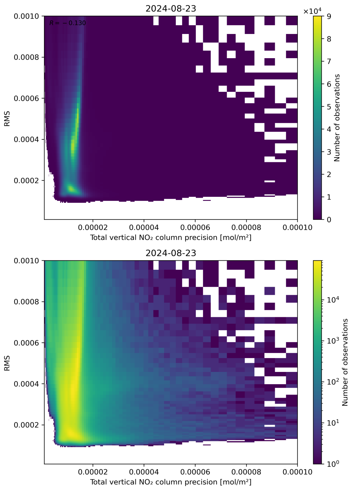
Figure 119: Scatter density plot of “Total vertical NO 2 column precision” against “RMS” for 2024-08-22 to 2024-08-24.
