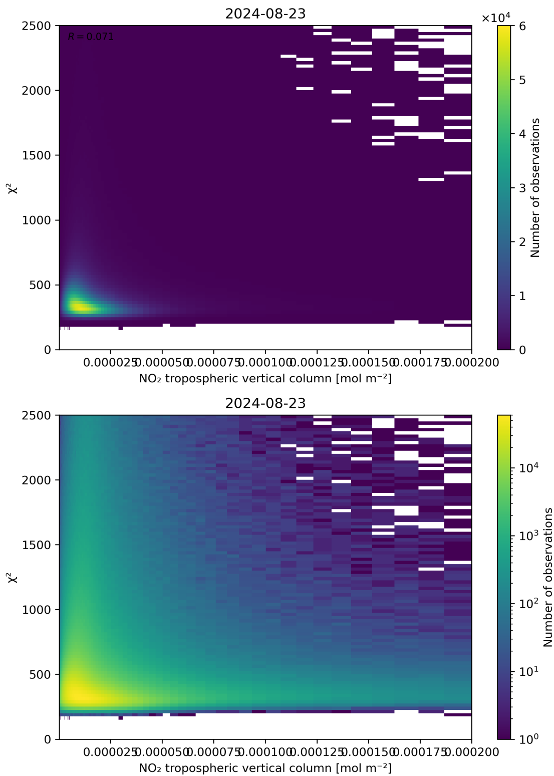
Figure 124: Scatter density plot of “NO 2 tropospheric vertical column” against “ \chi^2 ” for 2024-08-22 to 2024-08-24.
