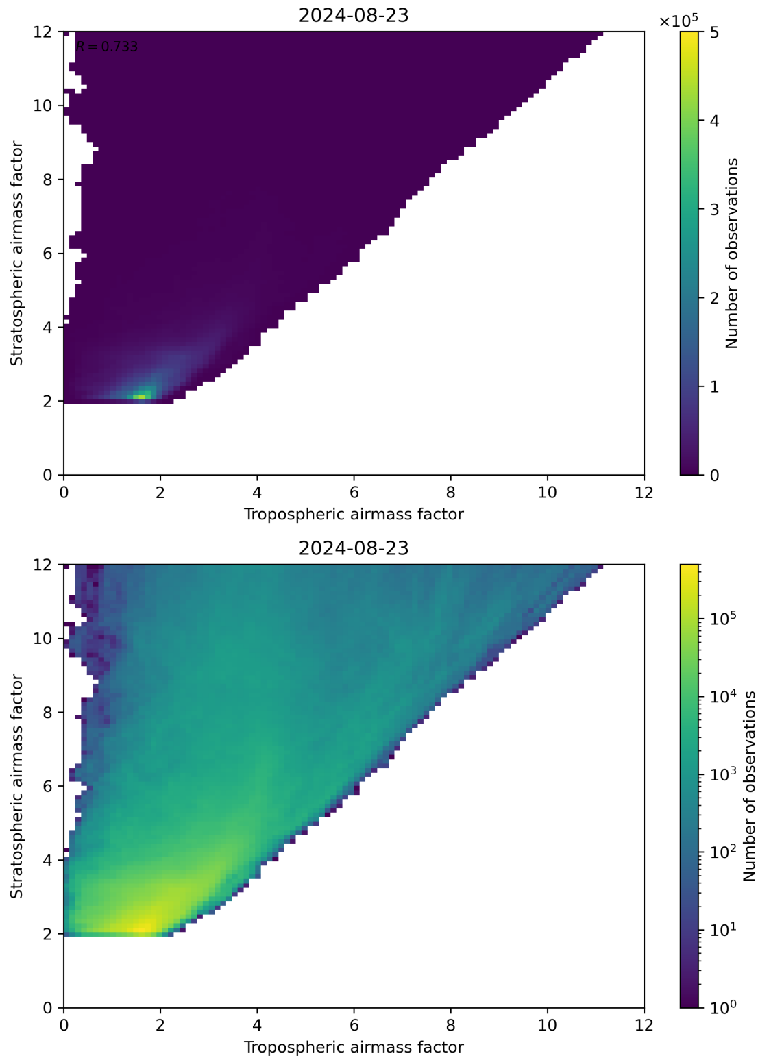
Figure 71: Scatter density plot of “Tropospheric airmass factor” against “Stratospheric airmass factor” for 2024-08-22 to 2024-08-24.
