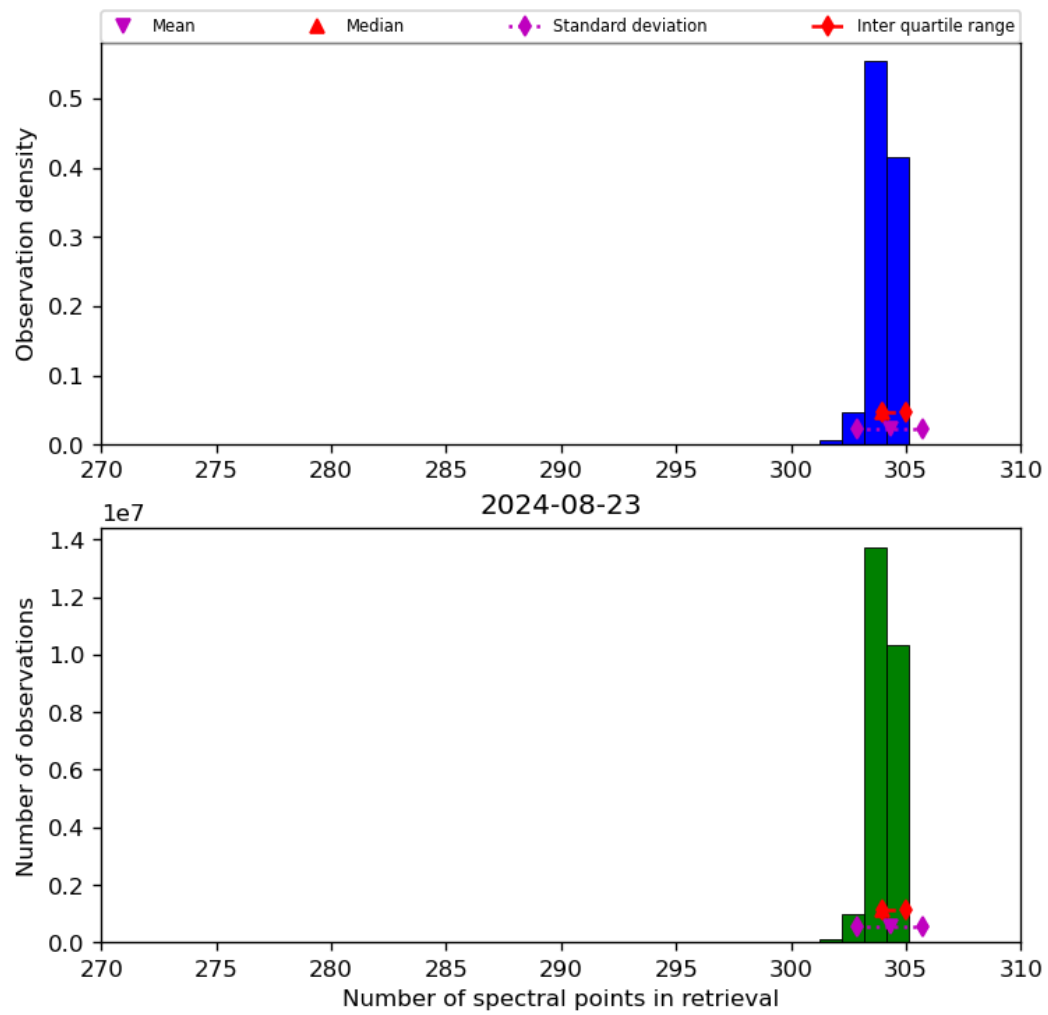
Figure 33: Histogram of “Number of spectral points in retrieval” for 2024-08-22 to 2024-08-24
