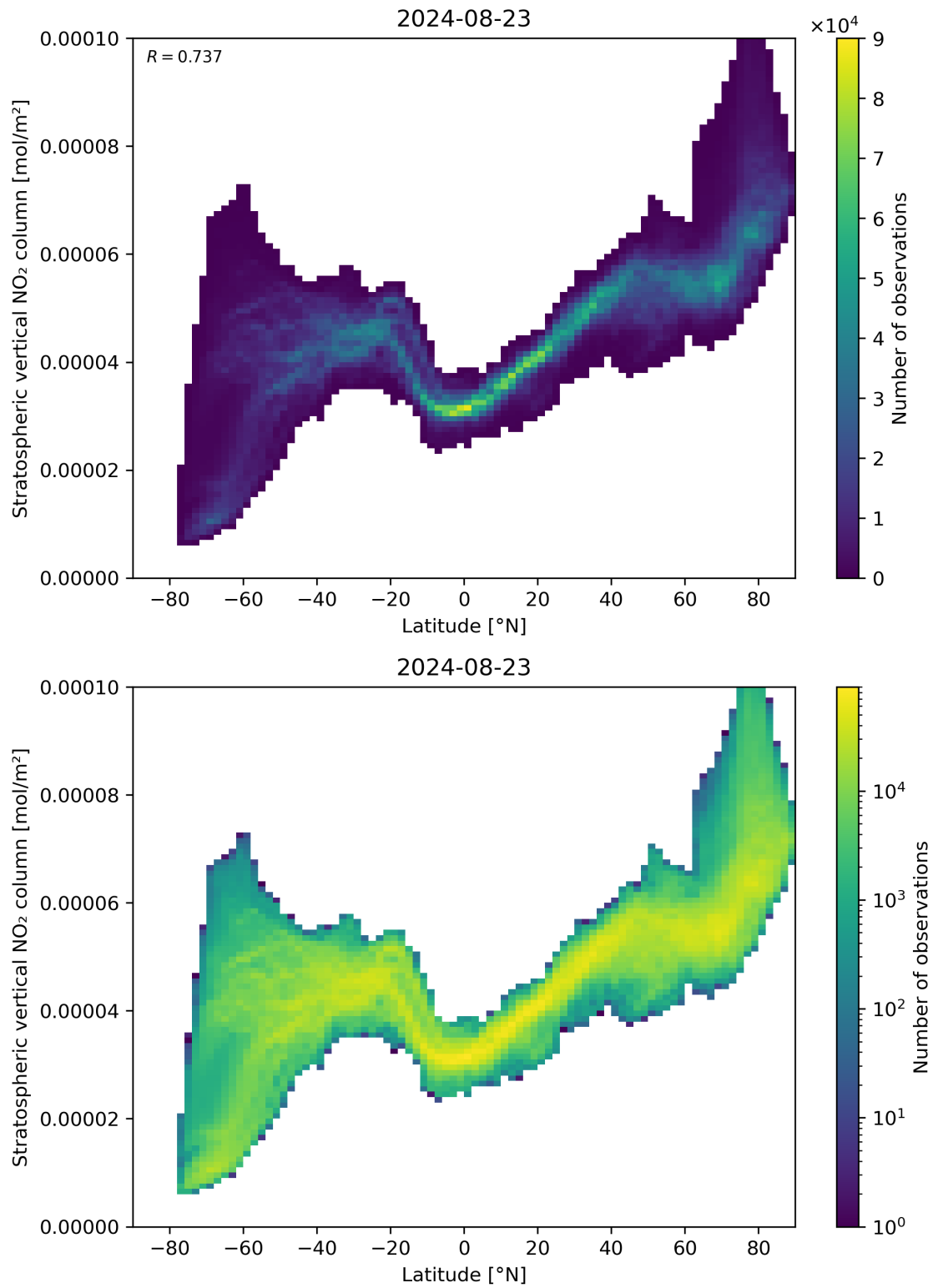
Figure 87: Scatter density plot of “Latitude” against “Stratospheric vertical NO 2 column” for 2024-08-22 to 2024-08-24.
