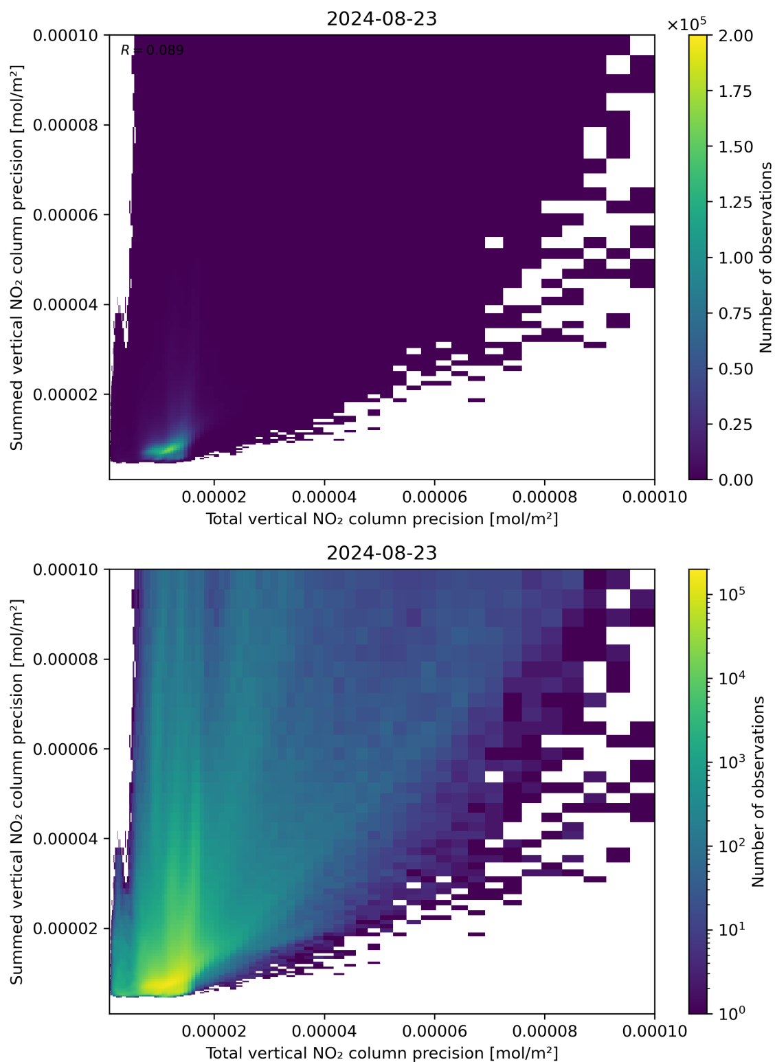
Figure 118: Scatter density plot of “Total vertical NO 2 column precision” against “Summed vertical NO 2 column precision” for 2024-08-22 to 2024-08-24.
