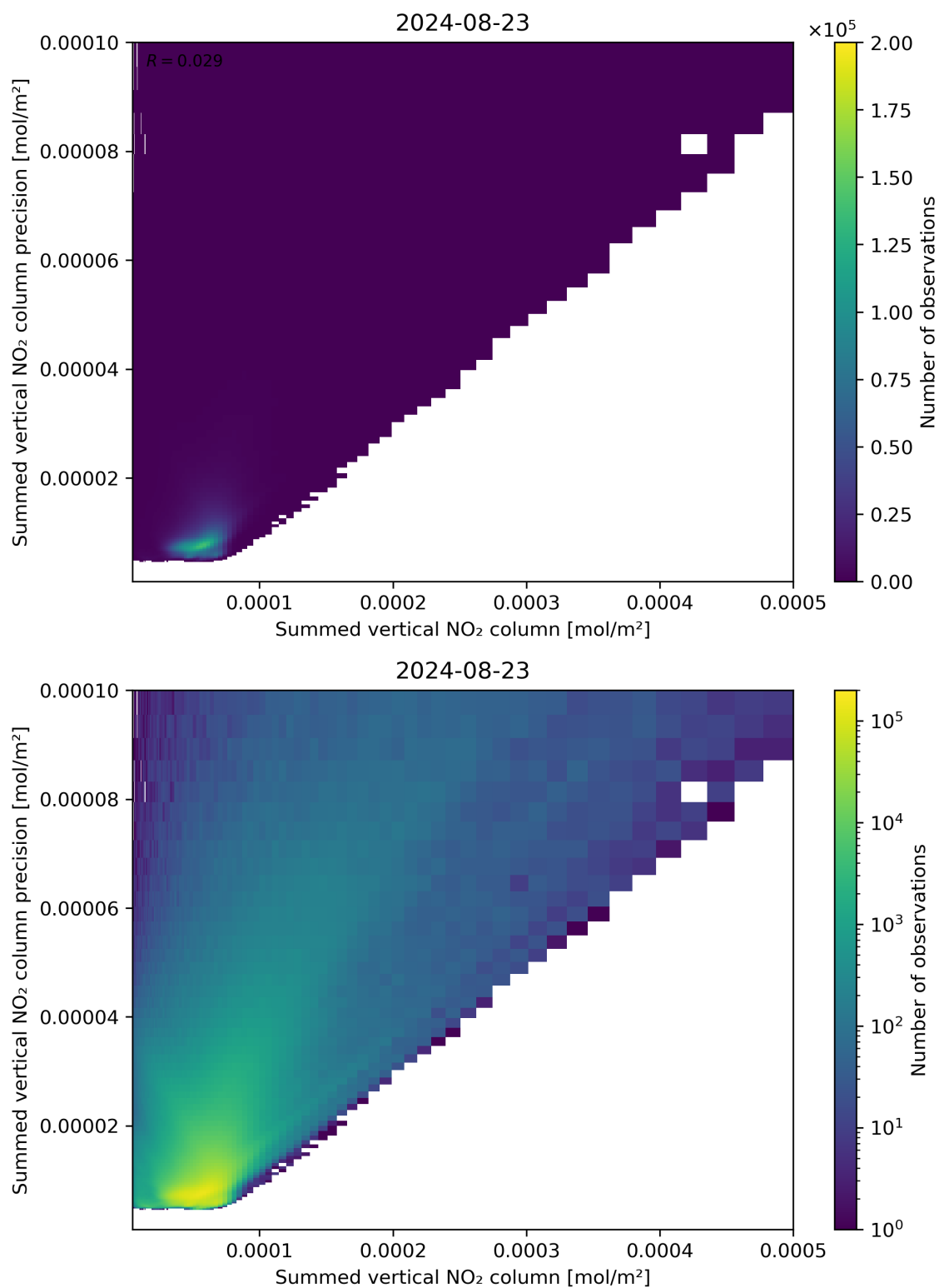
Figure 105: Scatter density plot of “Summed vertical NO 2 column” against “Summed vertical NO 2 column precision” for 2024-08-22 to 2024-08-24.
