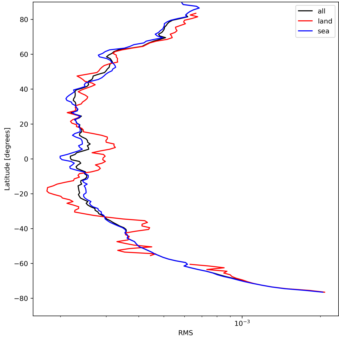
Figure 26: Zonal average of “RMS” for 2024-08-22 to 2024-08-24.
