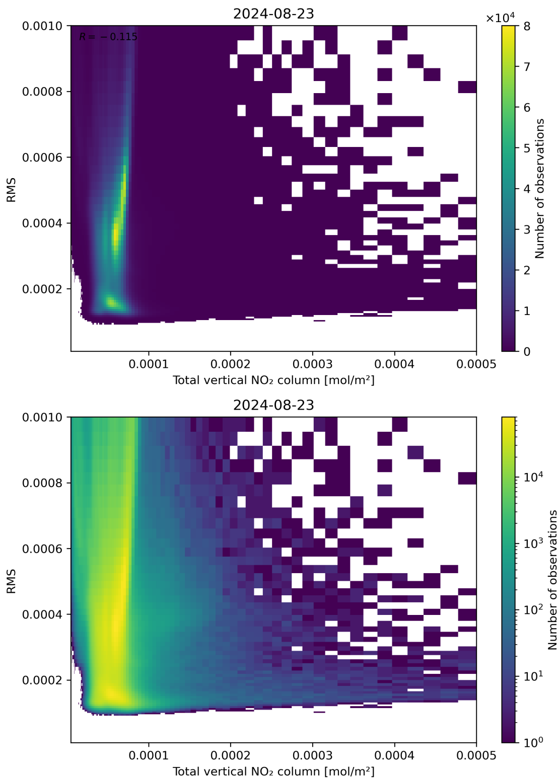
Figure 120: Scatter density plot of “Total vertical NO 2 column” against “RMS” for 2024-08-22 to 2024-08-24.
