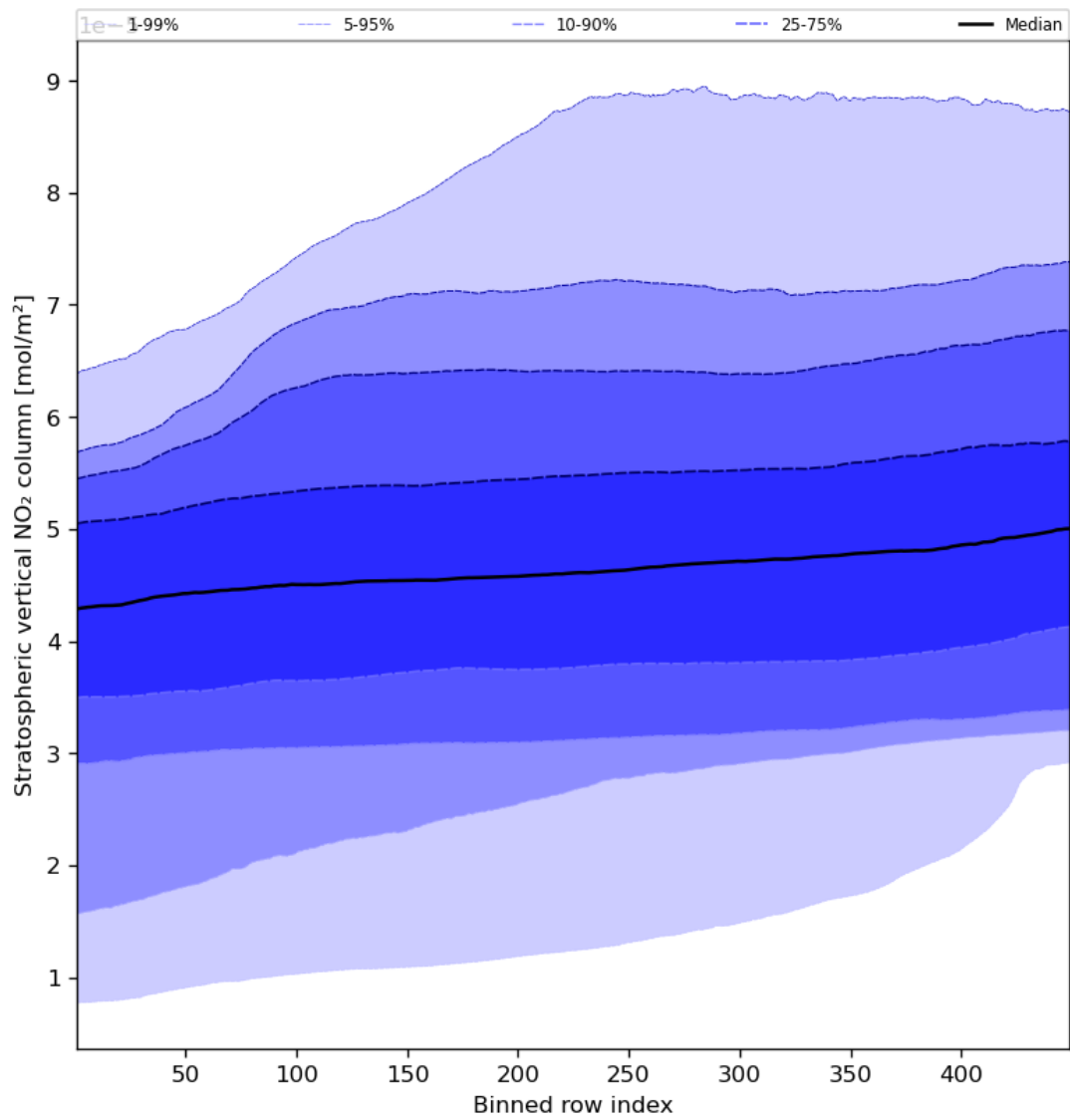
Figure 53: Along track statistics of “Stratospheric vertical NO 2 column” for 2024-08-22 to 2024-08-24
