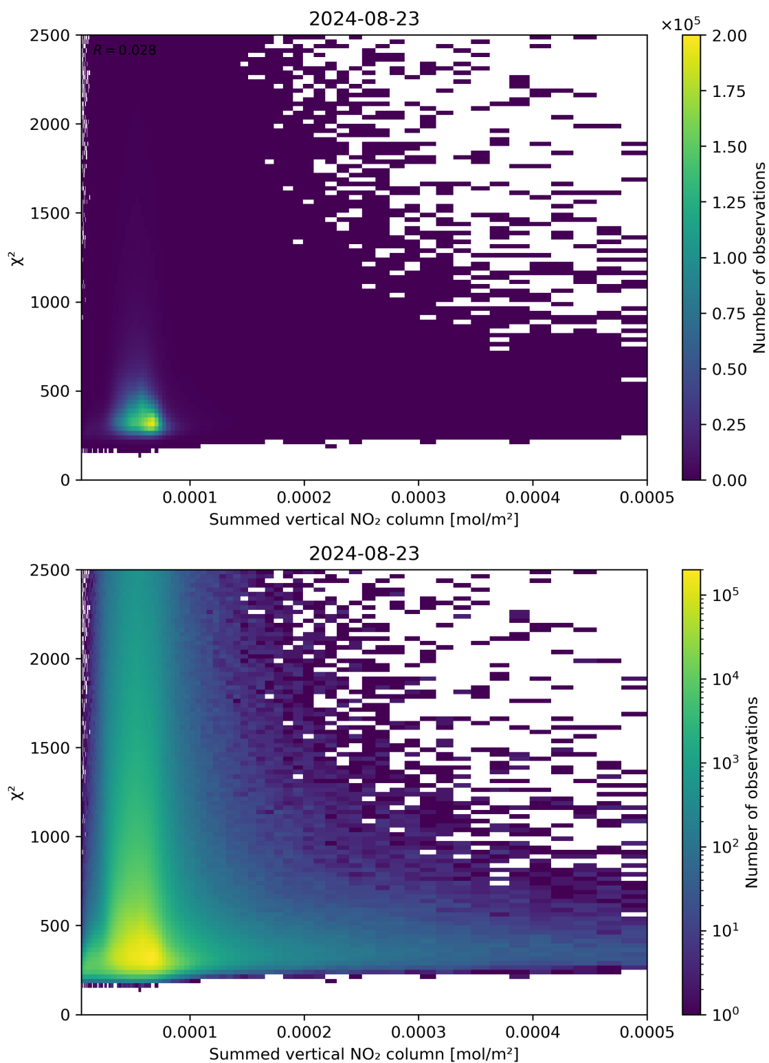
Figure 104: Scatter density plot of “Summed vertical NO 2 column” against “ \chi^2 ” for 2024-08-22 to 2024-08-24.
