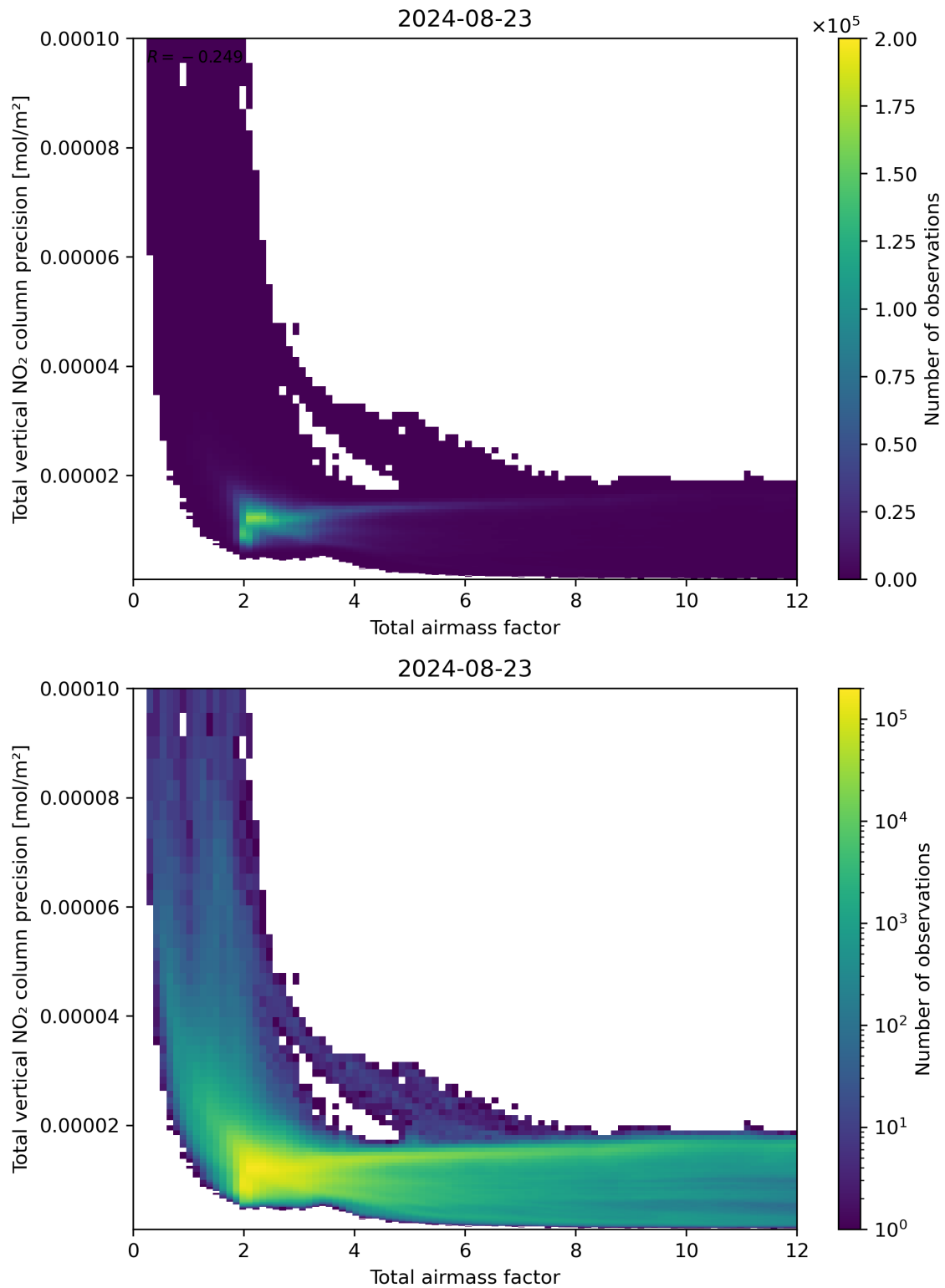
Figure 68: Scatter density plot of “Total airmass factor” against “Total vertical NO 2 column precision” for 2024-08-22 to 2024-08-24.
