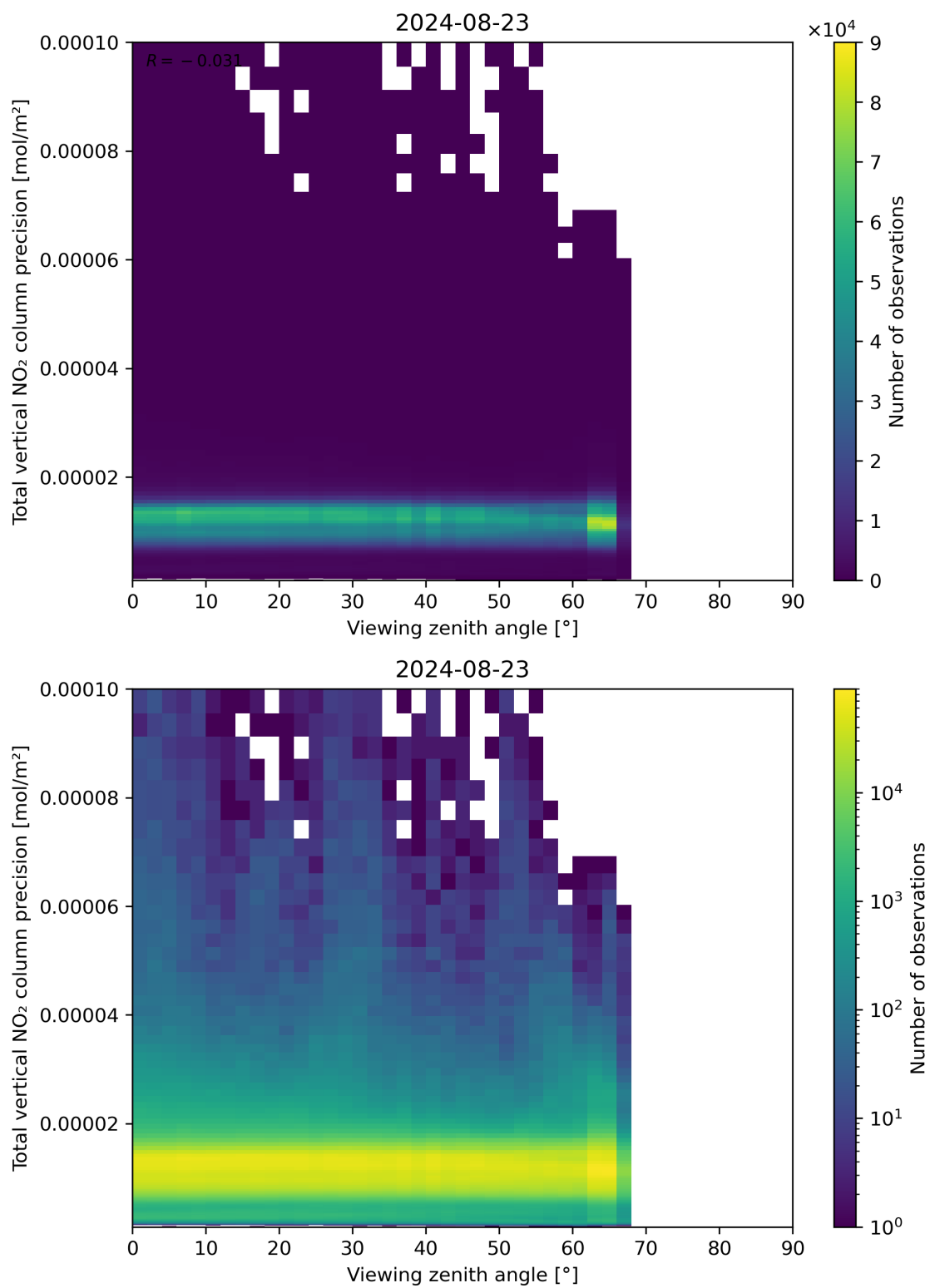
Figure 168: Scatter density plot of “Viewing zenith angle” against “Total vertical NO 2 column precision” for 2024-08-22 to 2024-08-24.
