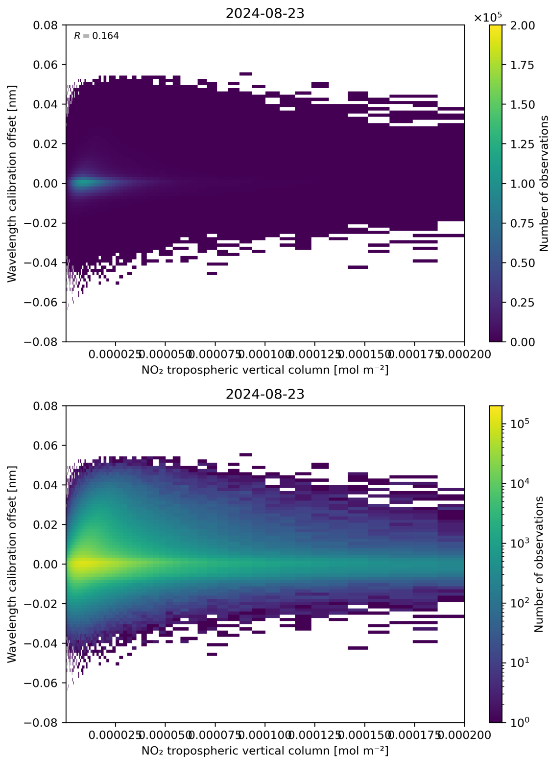
Figure 143: Scatter density plot of “NO 2 tropospheric vertical column” against “Wavelength calibration offset” for 2024-08-22 to 2024-08-24.
