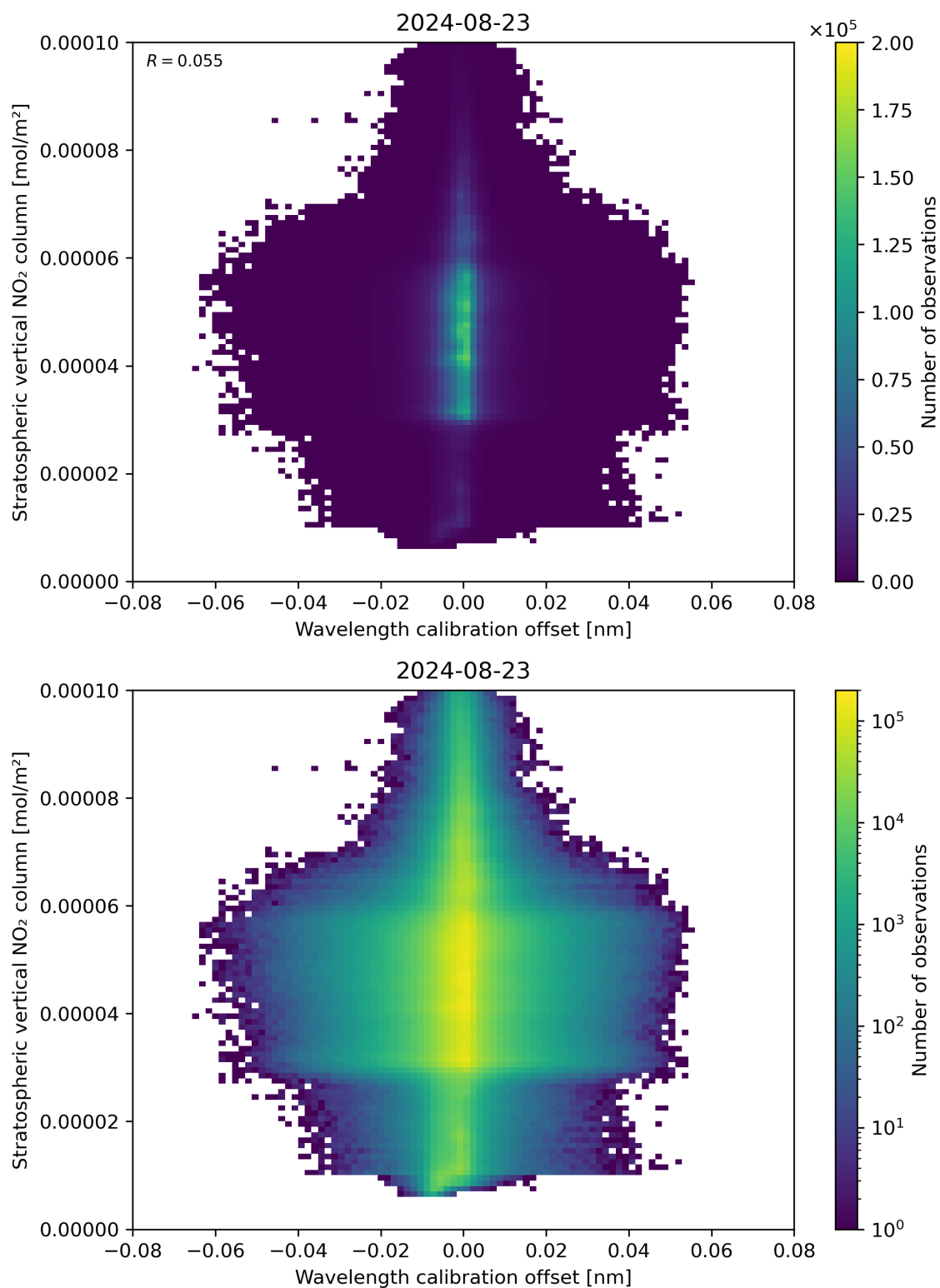
Figure 176: Scatter density plot of “Wavelength calibration offset” against “Stratospheric vertical NO 2 column” for 2024-08-22 to 2024-08-24.
