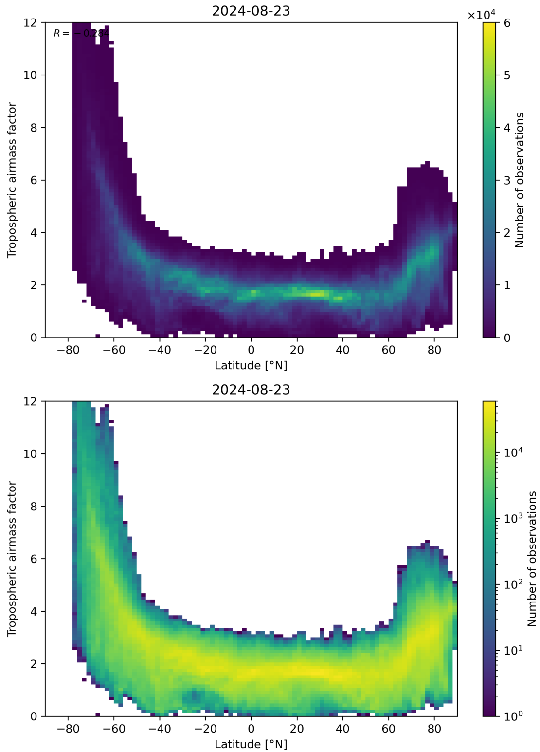
Figure 85: Scatter density plot of “Latitude” against “Tropospheric airmass factor” for 2024-08-22 to 2024-08-24.
