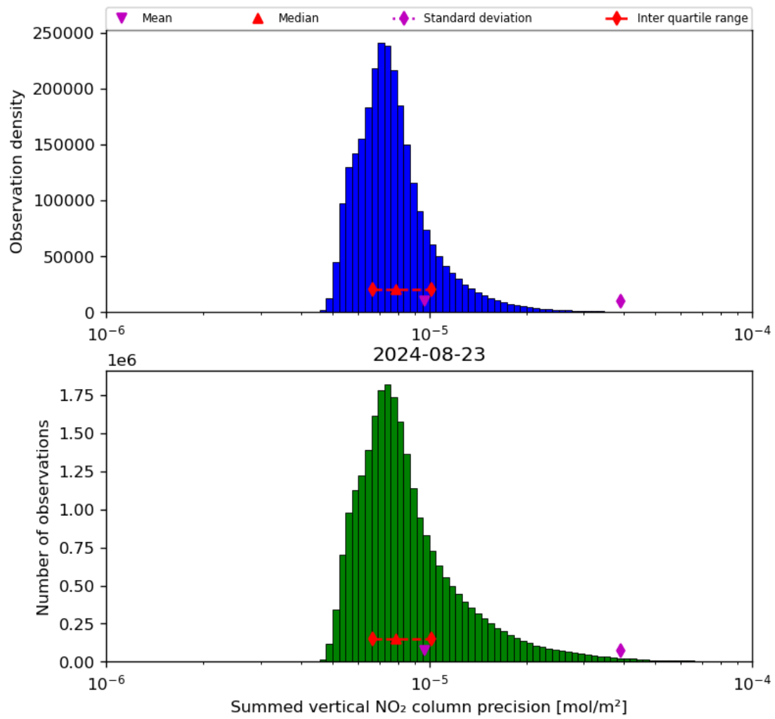
Figure 41: Histogram of “Summed vertical NO 2 column precision” for 2024-08-22 to 2024-08-24
