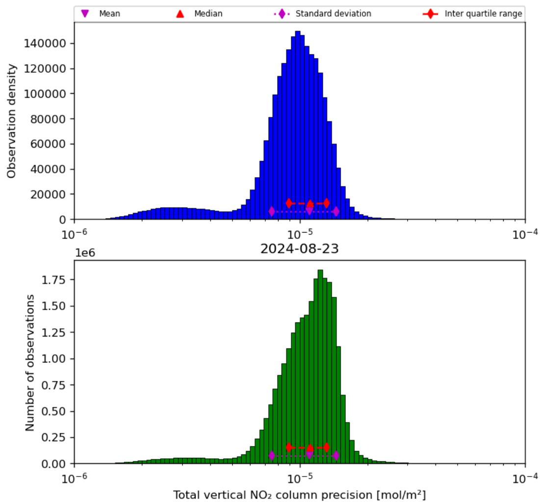
Figure 39: Histogram of “Total vertical NO 2 column precision” for 2024-08-22 to 2024-08-24
