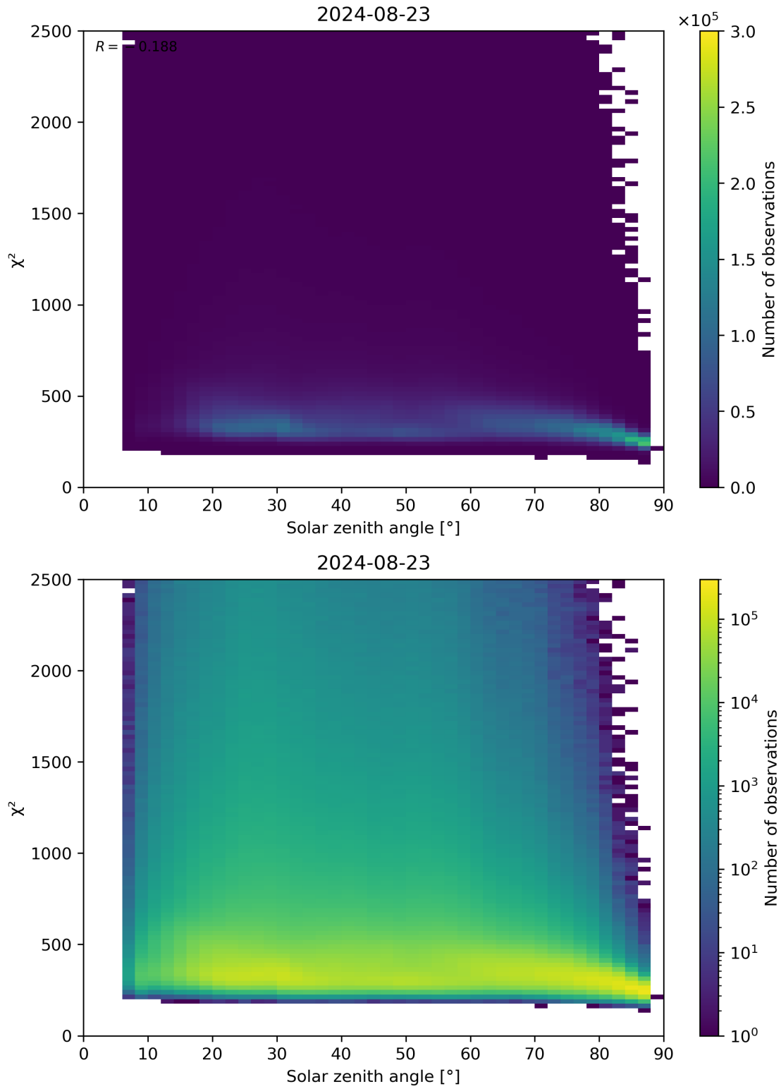
Figure 148: Scatter density plot of “Solar zenith angle” against “ \chi^2 ” for 2024-08-22 to 2024-08-24.
