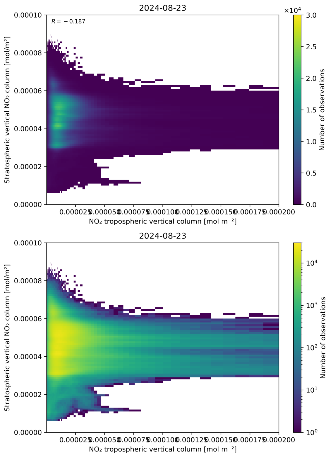
Figure 125: Scatter density plot of “NO 2 tropospheric vertical column” against “Stratospheric vertical NO 2 column” for 2024-08-22 to 2024-08-24.
