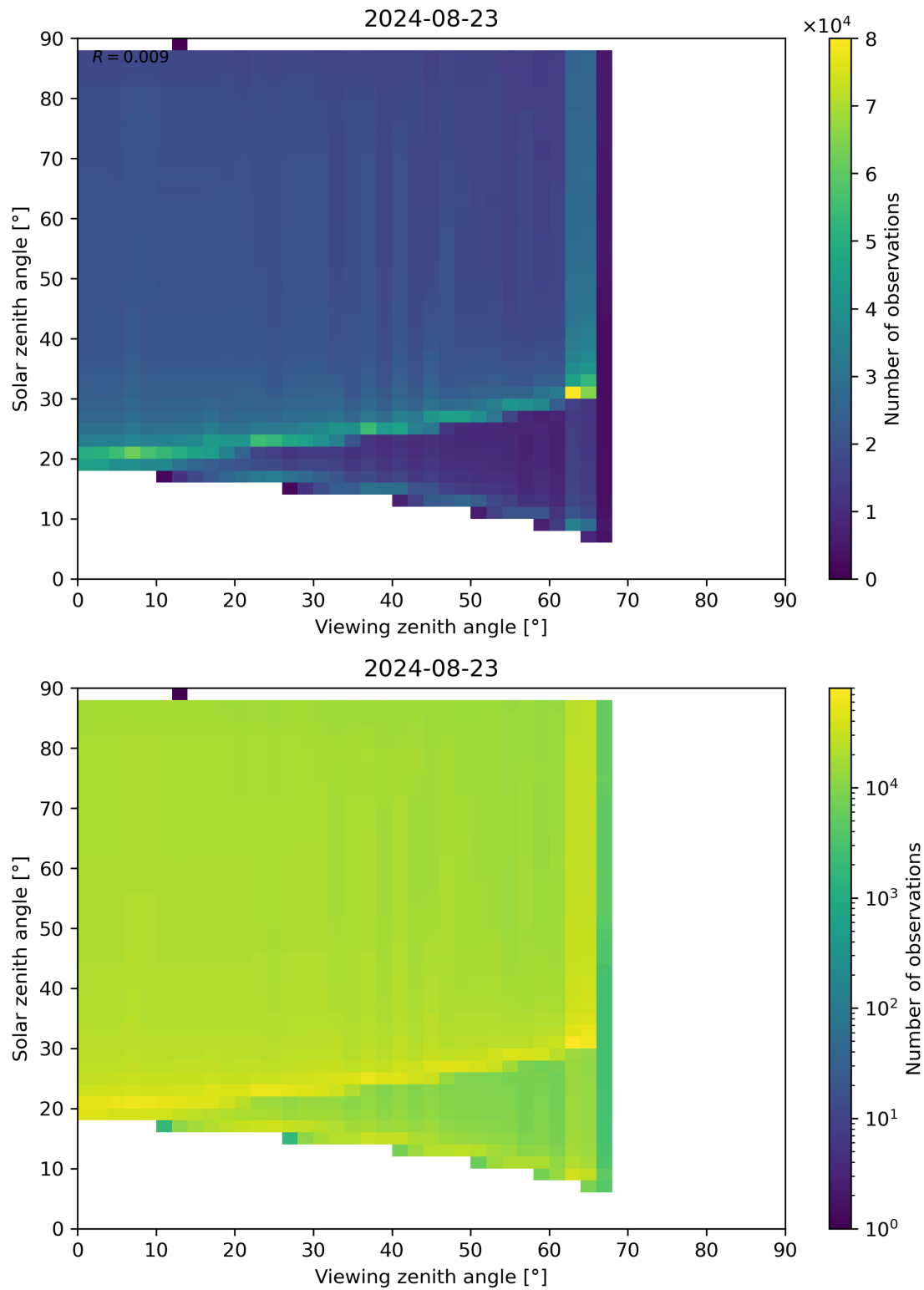
Figure 172: Scatter density plot of “Viewing zenith angle” against “Solar zenith angle” for 2024-08-22 to 2024-08-24.
