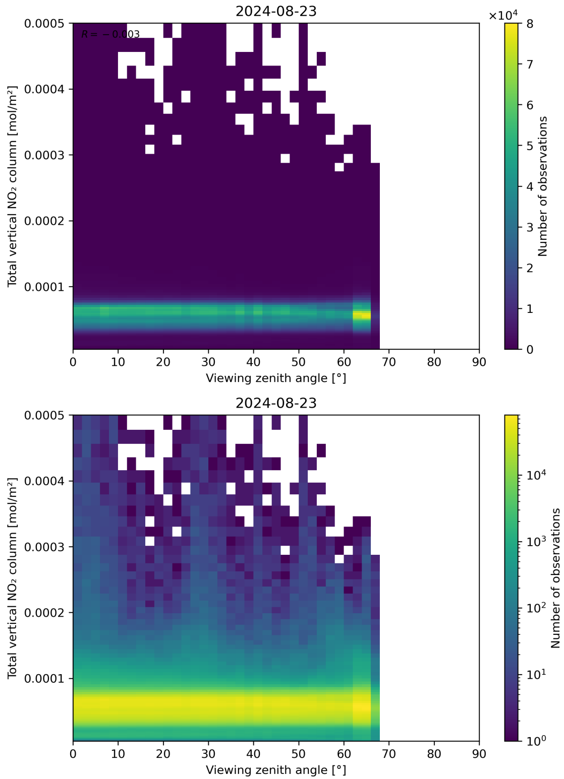
Figure 167: Scatter density plot of “Viewing zenith angle” against “Total vertical NO 2 column” for 2024-08-22 to 2024-08-24.
