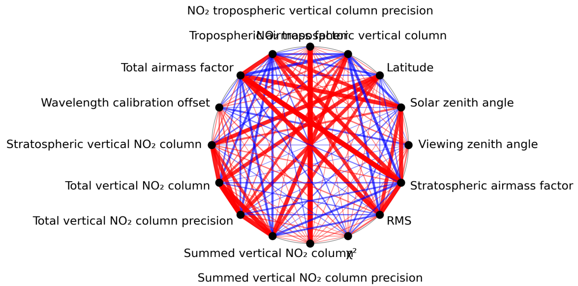
Figure 1: Map of correlation graph for 2024-08-22 to 2024-08-24.
