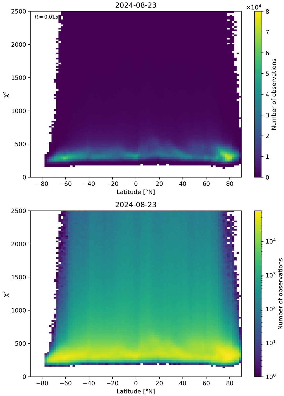
Figure 86: Scatter density plot of “Latitude” against “ \chi^2 ” for 2024-08-22 to 2024-08-24.
