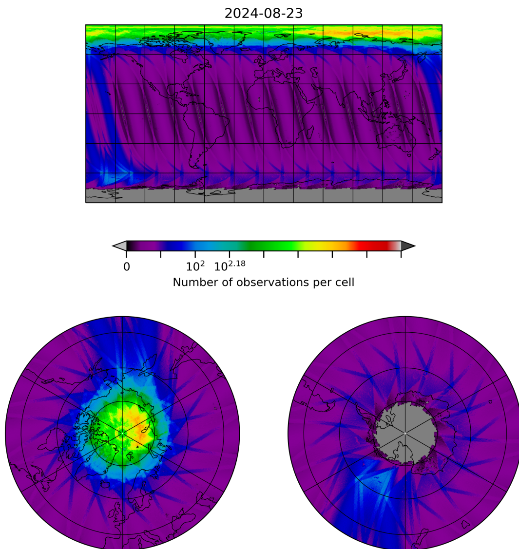
Figure 10: Map of the number of observations for 2024-08-22 to 2024-08-24
