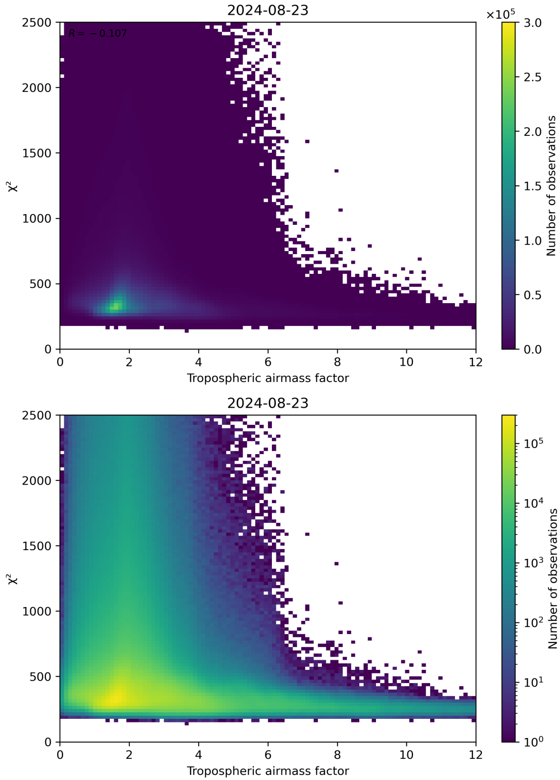
Figure 73: Scatter density plot of “Tropospheric airmass factor” against “ \chi^2 ” for 2024-08-22 to 2024-08-24.
