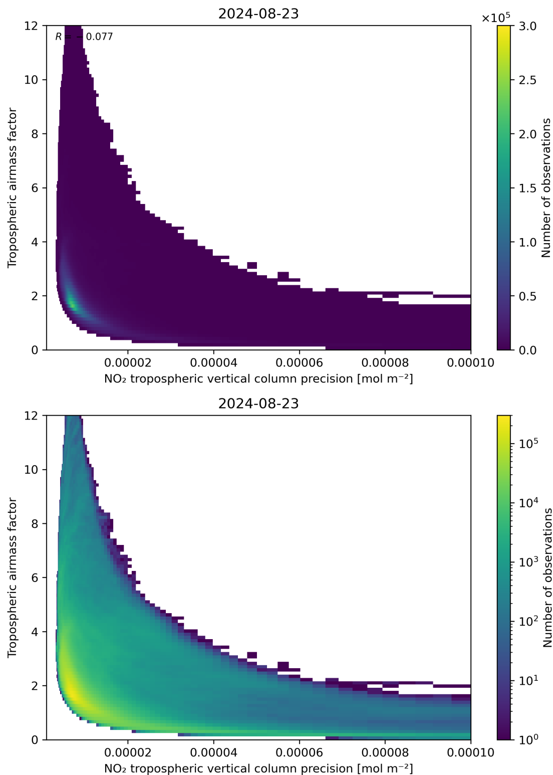
Figure 133: Scatter density plot of “NO 2 tropospheric vertical column precision” against “Tropospheric airmass factor” for 2024-08-22 to 2024-08-24.
