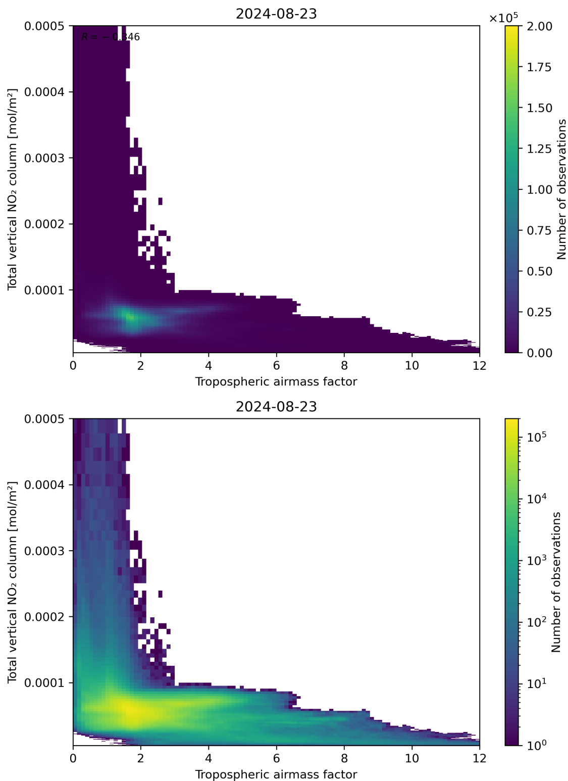
Figure 77: Scatter density plot of “Tropospheric airmass factor” against “Total vertical NO 2 column” for 2024-08-22 to 2024-08-24.
