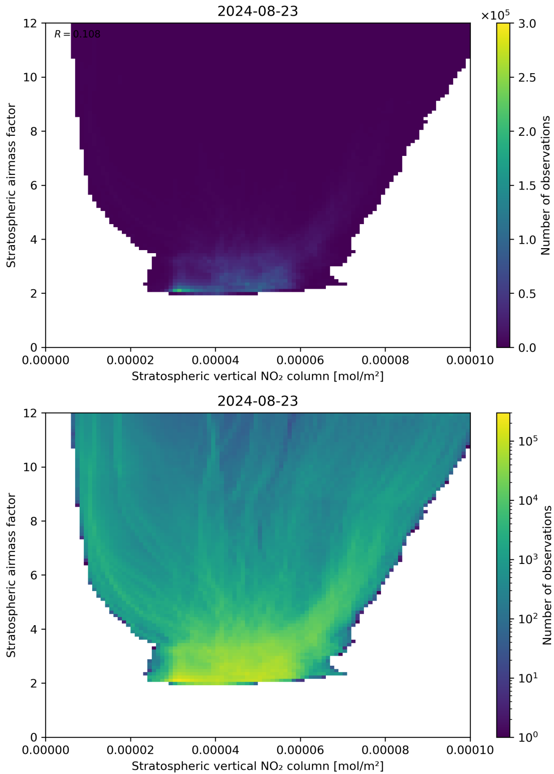
Figure 96: Scatter density plot of “Stratospheric vertical NO 2 column” against “Stratospheric airmass factor” for 2024-08-22 to 2024-08-24.
