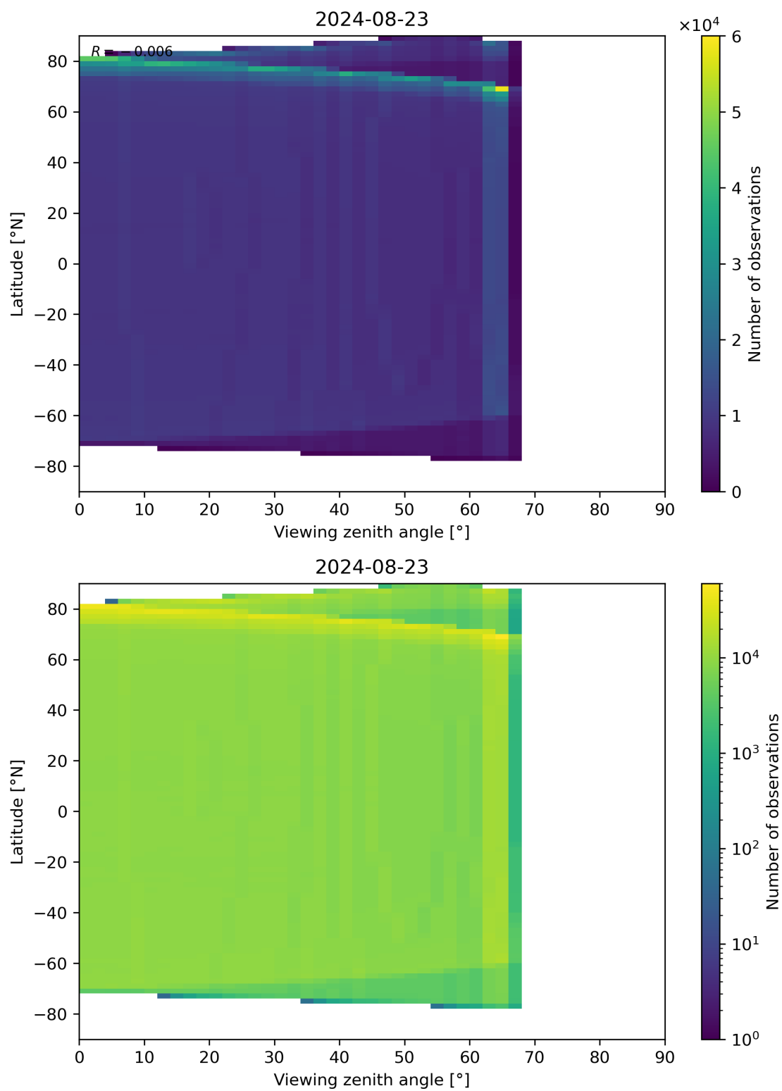
Figure 163: Scatter density plot of “Viewing zenith angle” against “Latitude” for 2024-08-22 to 2024-08-24.
