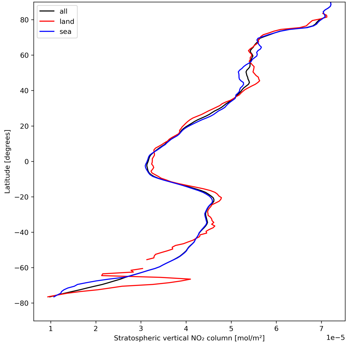
Figure 19: Zonal average of “Stratospheric vertical NO 2 column” for 2024-08-22 to 2024-08-24.
