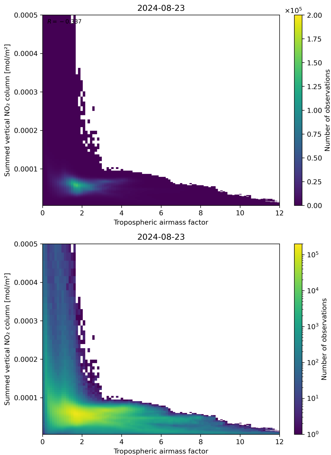
Figure 75: Scatter density plot of “Tropospheric airmass factor” against “Summed vertical NO 2 column” for 2024-08-22 to 2024-08-24.
