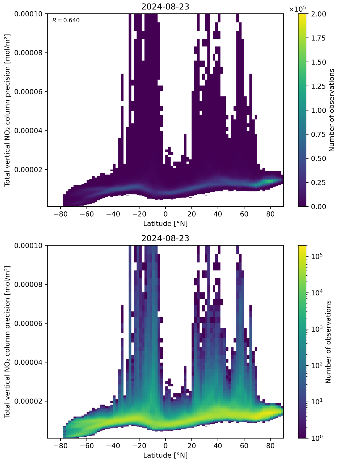
Figure 91: Scatter density plot of “Latitude” against “Total vertical NO 2 column precision” for 2024-08-22 to 2024-08-24.
