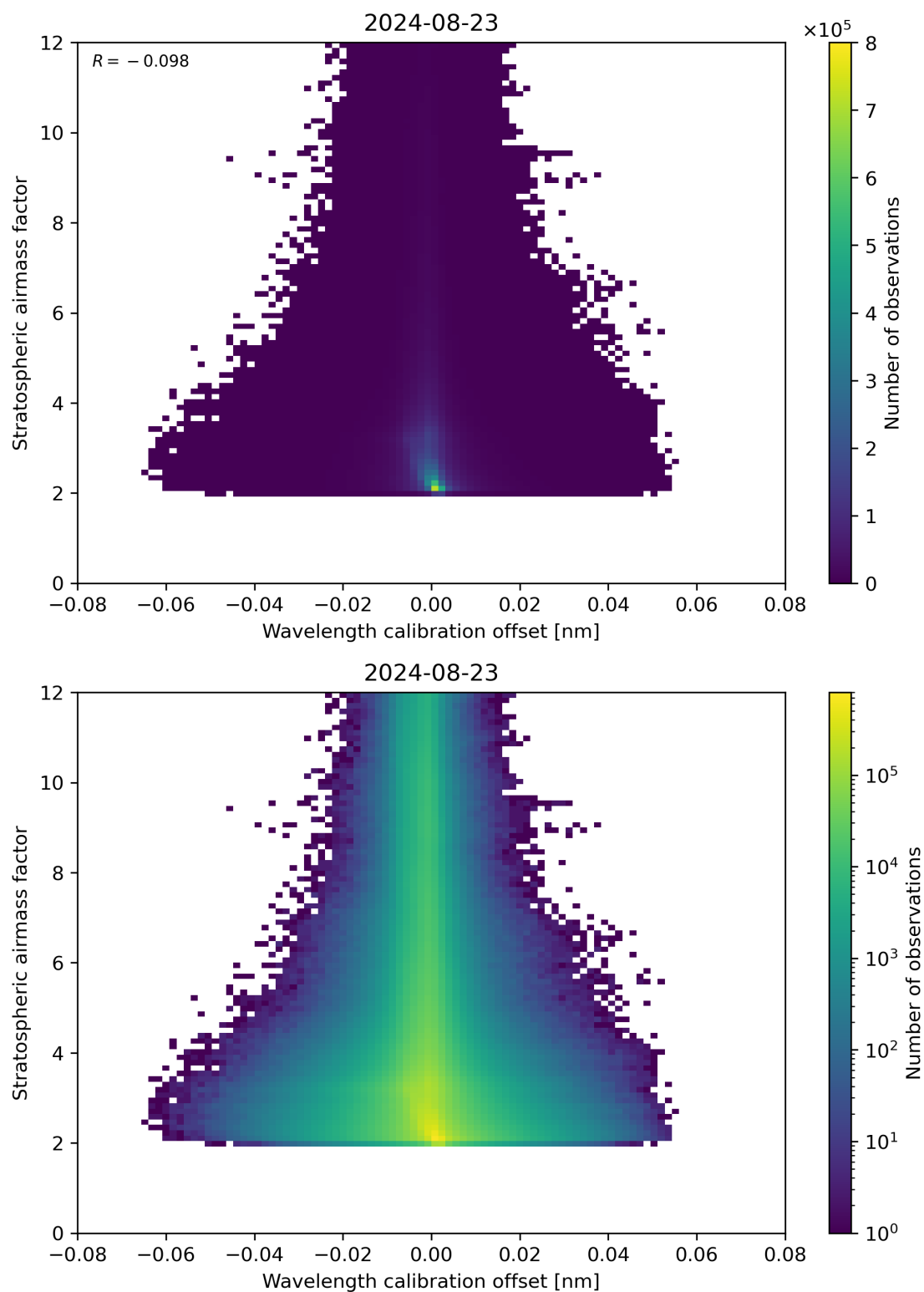
Figure 174: Scatter density plot of “Wavelength calibration offset” against “Stratospheric airmass factor” for 2024-08-22 to 2024-08-24.
