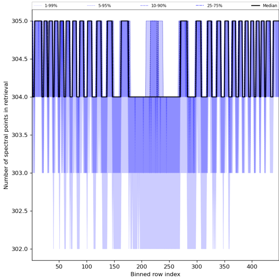
Figure 50: Along track statistics of “Number of spectral points in retrieval” for 2024-08-22 to 2024-08-24
