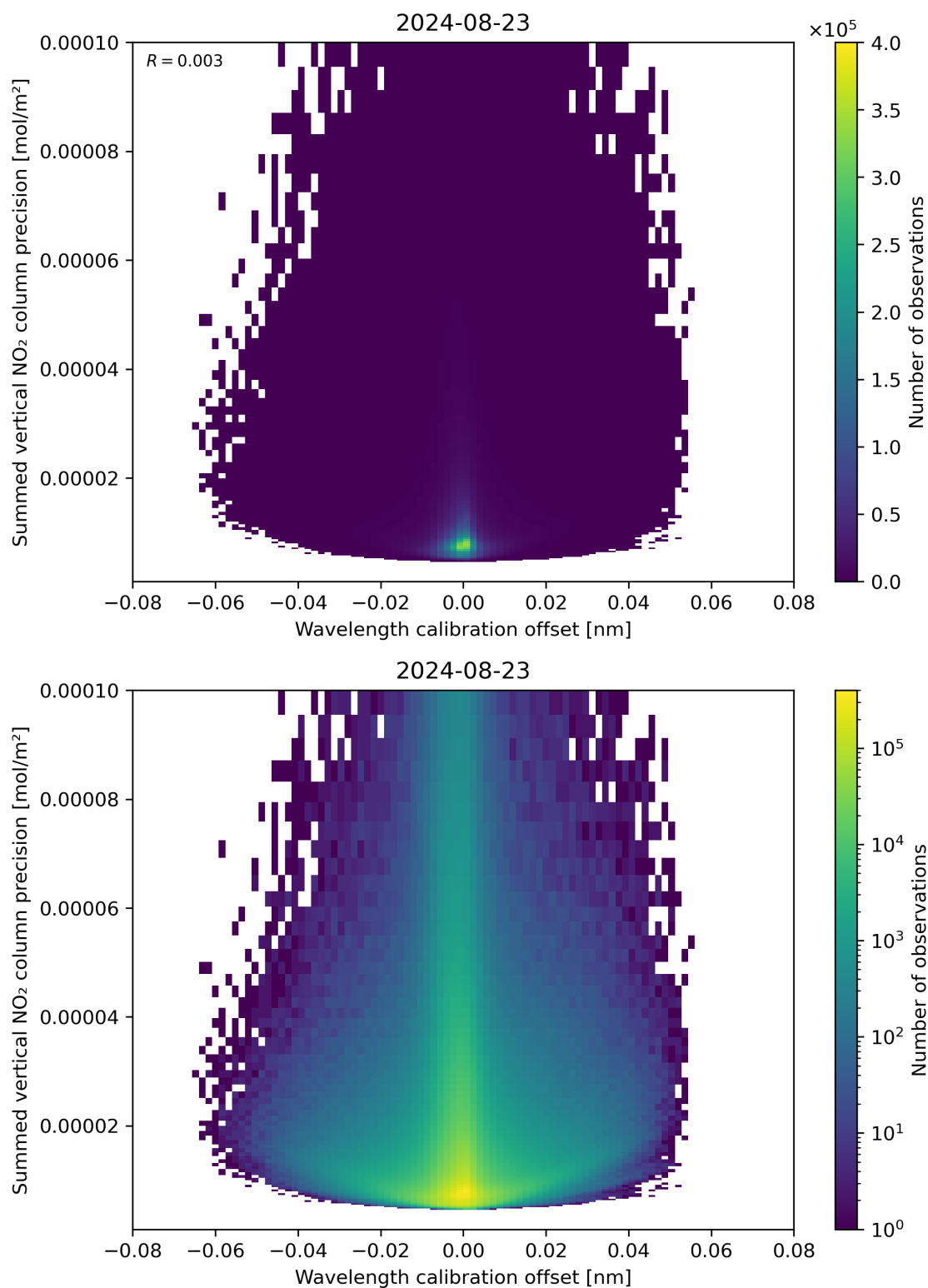
Figure 178: Scatter density plot of “Wavelength calibration offset” against “Summed vertical NO 2 column precision” for 2024-08-22 to 2024-08-24.
