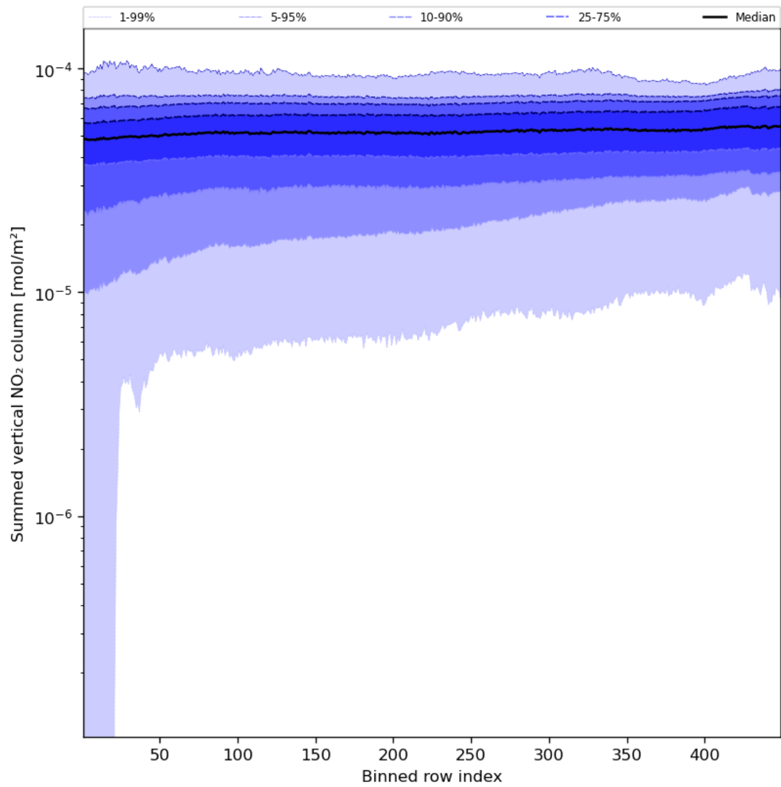
Figure 57: Along track statistics of “Summed vertical NO 2 column” for 2024-08-22 to 2024-08-24
