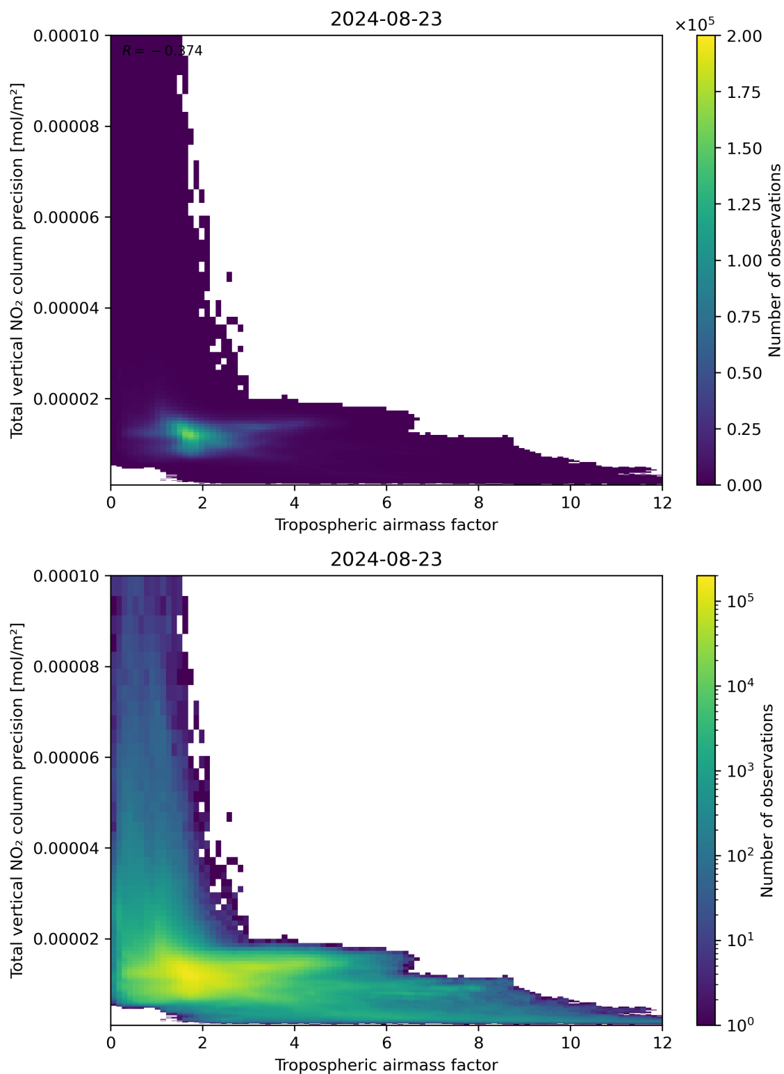
Figure 78: Scatter density plot of “Tropospheric air mass factor” against “Total vertical NO 2 column precision” for 2024-08-22 to 2024-08-24.
