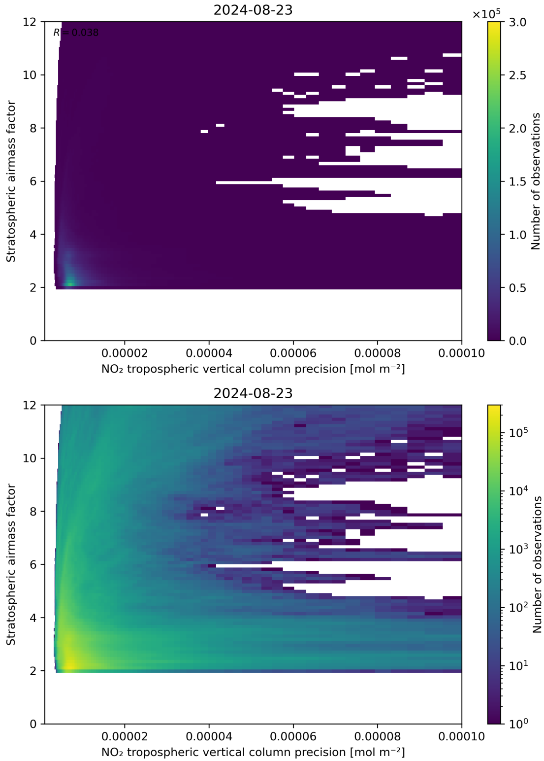
Figure 131: Scatter density plot of “NO 2 tropospheric vertical column precision” against “Stratospheric airmass factor” for 2024-08-22 to 2024-08-24.
