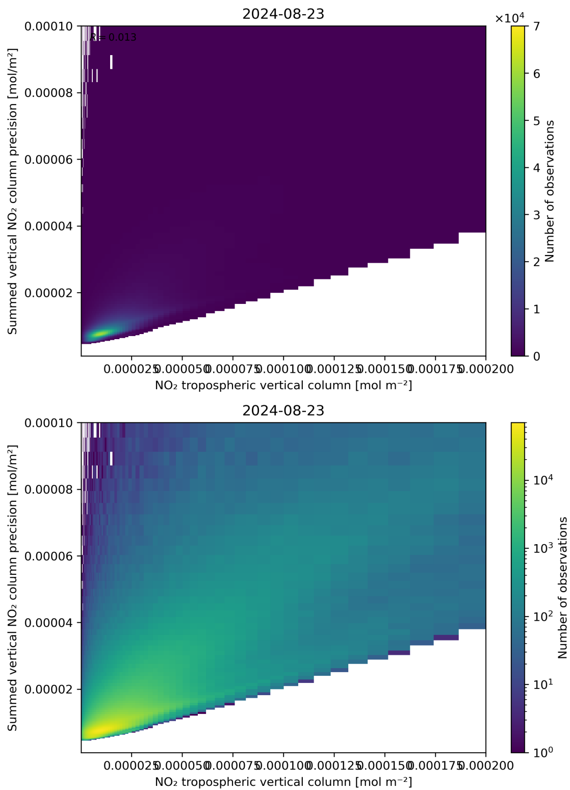
Figure 127: Scatter density plot of “NO 2 tropospheric vertical column” against “Summed vertical NO 2 column precision” for 2024-08-22 to 2024-08-24.
