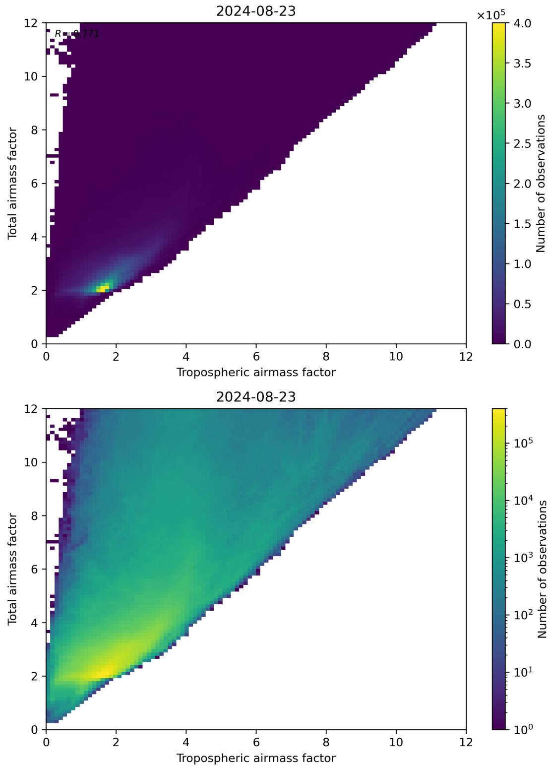
Figure 72: Scatter density plot of “Tropospheric airmass factor” against “Total airmass factor” for 2024-08-22 to 2024-08-24.
