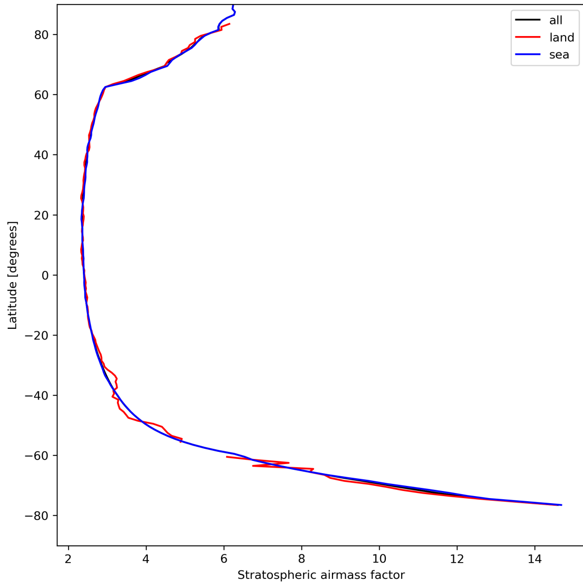
Figure 27: Zonal average of “Stratospheric air mass factor” for 2024-08-22 to 2024-08-24.
