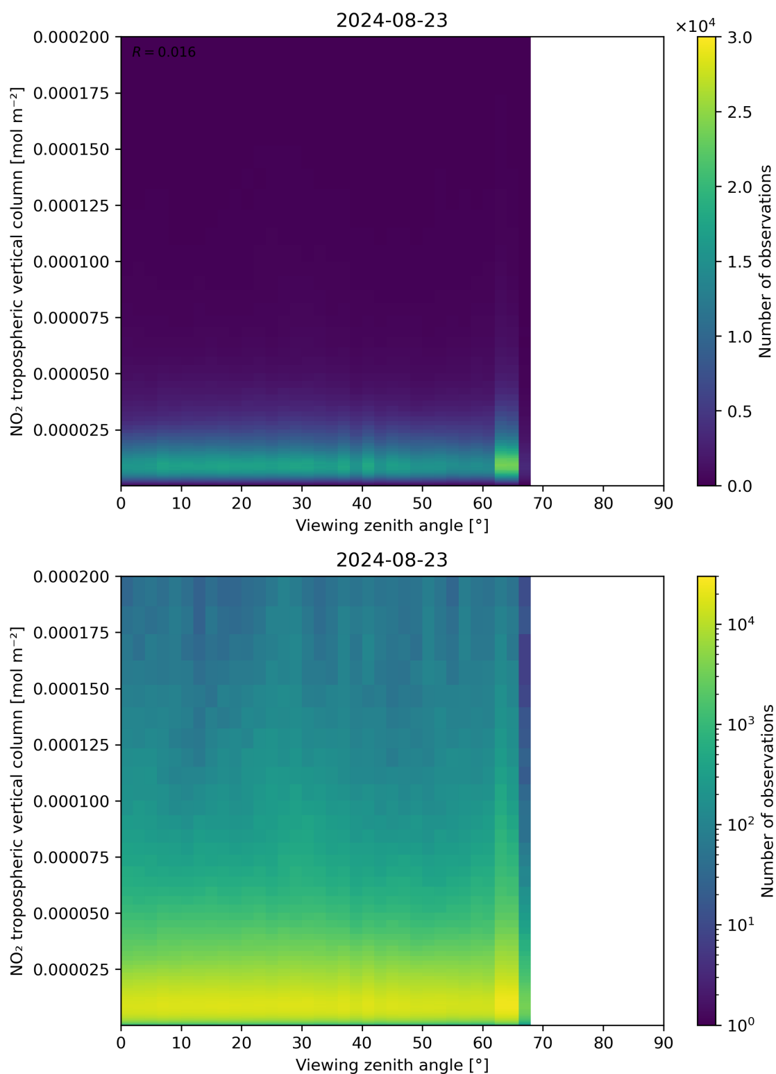
Figure 169: Scatter density plot of “Viewing zenith angle” against “NO 2 tropospheric vertical column” for 2024-08-22 to 2024-08-24.
