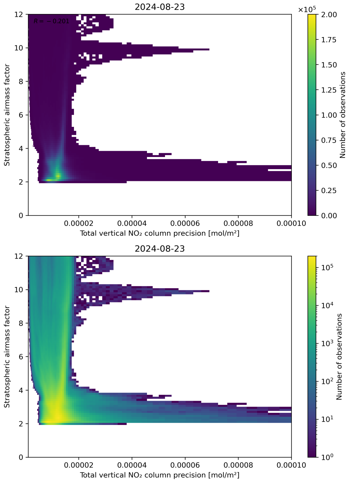
Figure 115: Scatter density plot of “Total vertical NO 2 column precision” against “Stratospheric air mass factor” for 2024-08-22 to 2024-08-24.
