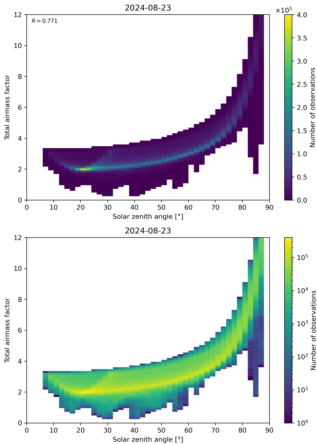
Figure 146: Scatter density plot of “Solar zenith angle” against “Total air mass factor” for 2024-08-22 to 2024-08-24.
