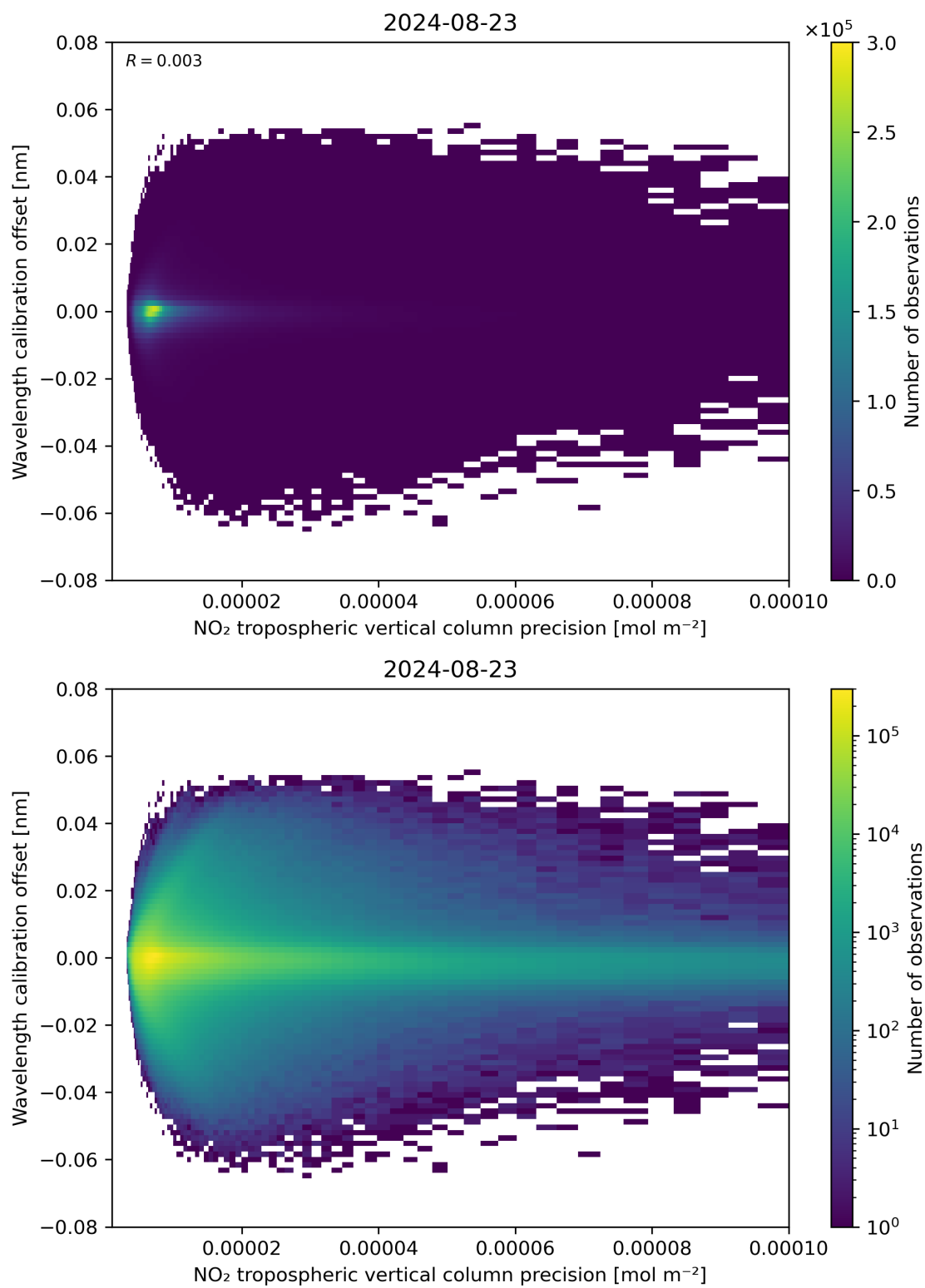
Figure 141: Scatter density plot of “NO 2 tropospheric vertical column precision” against “Wavelength calibration offset” for 2024-08-22 to 2024-08-24.
