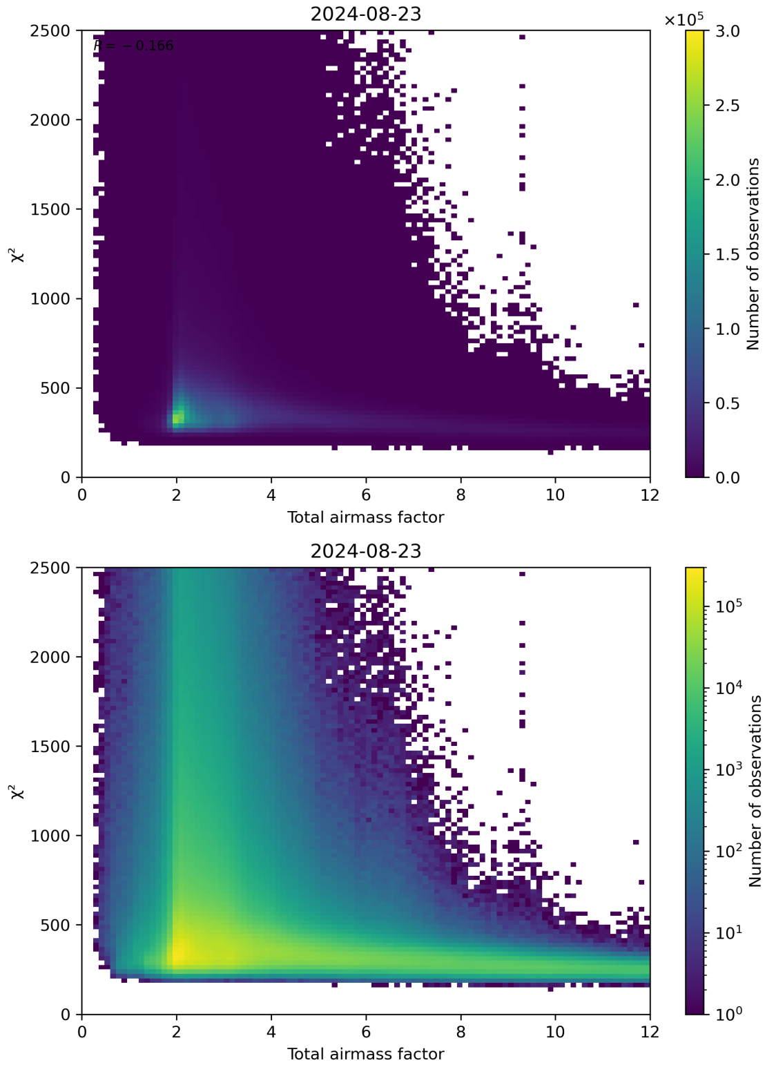
Figure 63: Scatter density plot of “Total airmass factor” against “ \chi^2 ” for 2024-08-22 to 2024-08-24.
