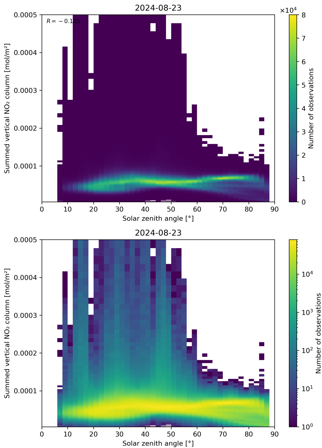
Figure 151: Scatter density plot of “Solar zenith angle” against “Summed vertical NO 2 column” for 2024-08-22 to 2024-08-24.
