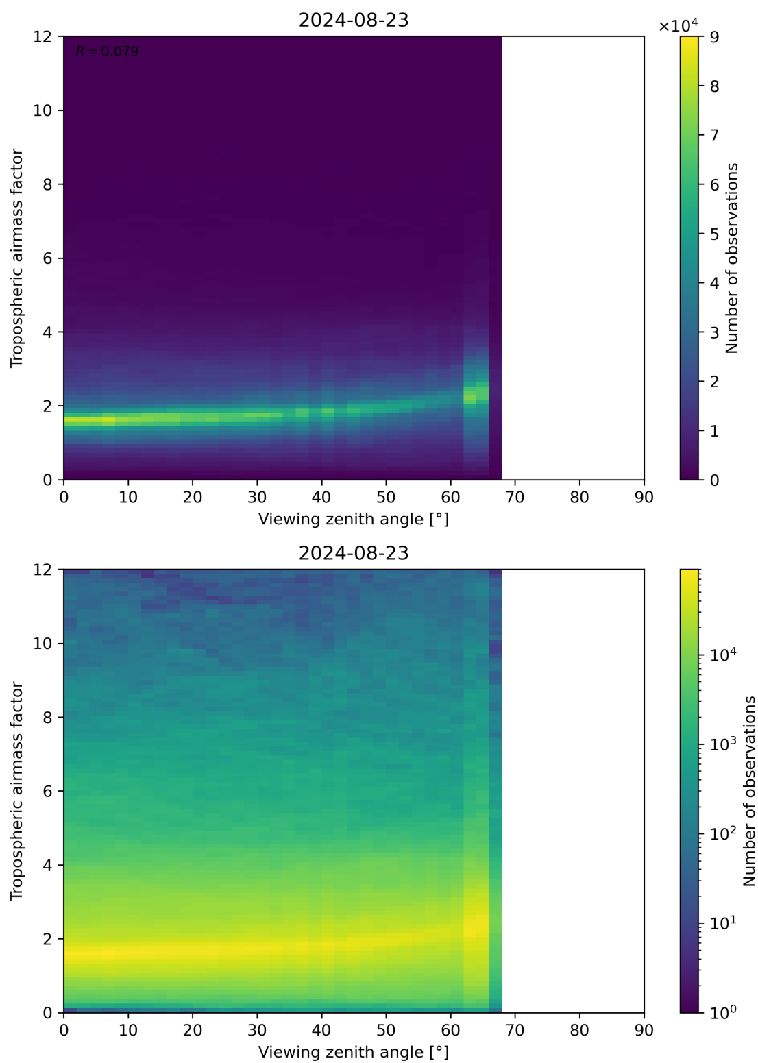
Figure 161: Scatter density plot of “Viewing zenith angle” against “Tropospheric airmass factor” for 2024-08-22 to 2024-08-24.
