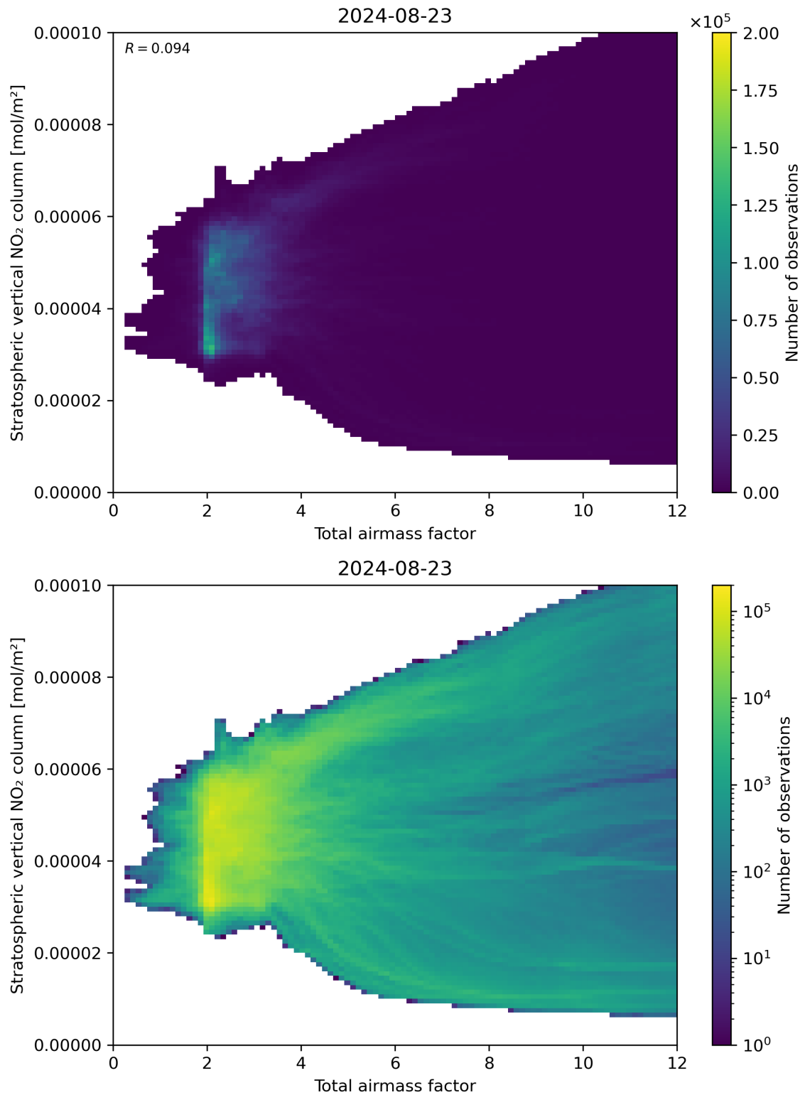
Figure 64: Scatter density plot of “Total airmass factor” against “Stratospheric vertical \text{NO}_2 column” for 2024-08-22 to 2024-08-24.
