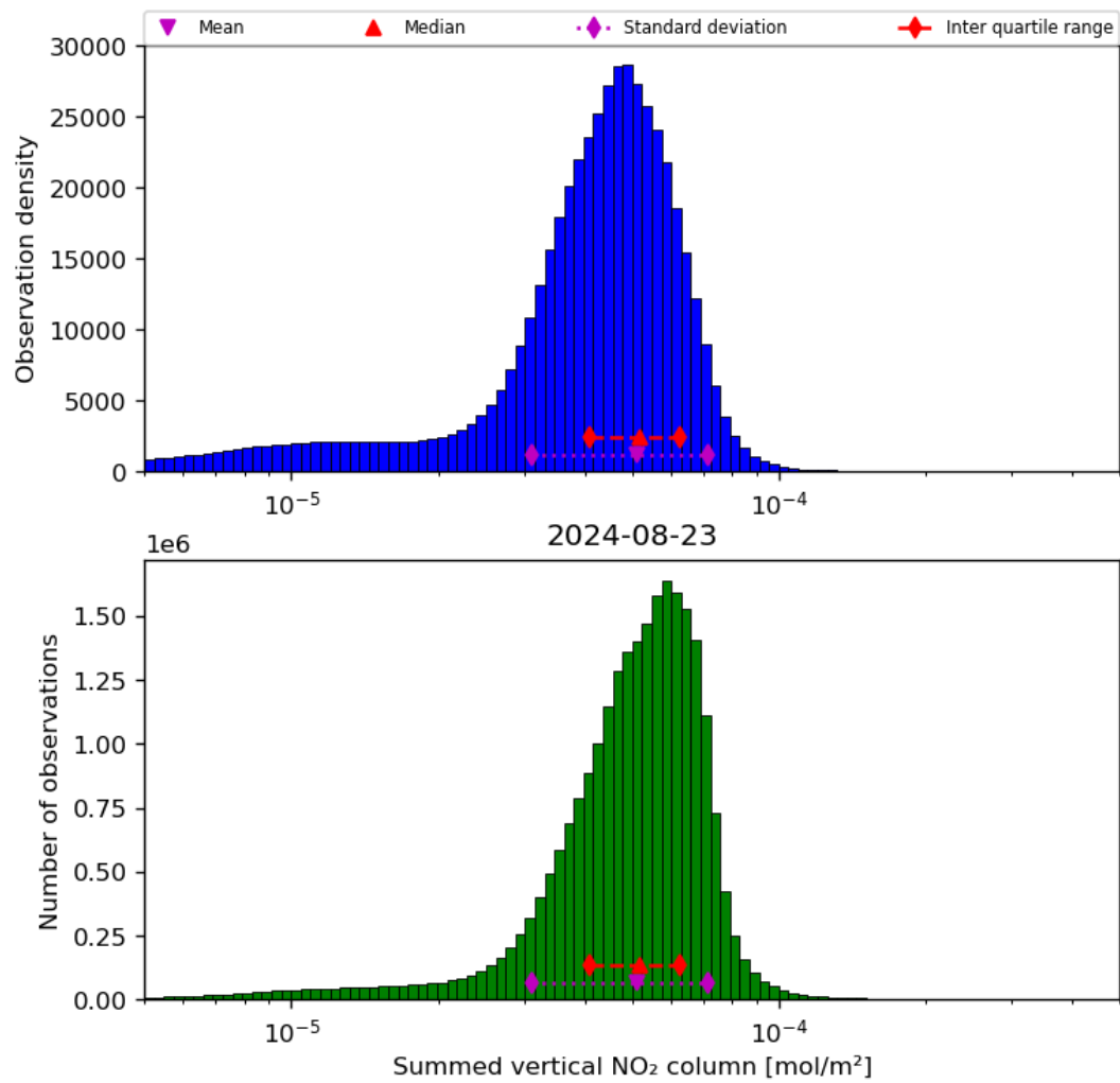
Figure 40: Histogram of “Summed vertical NO 2 column” for 2024-08-22 to 2024-08-24
