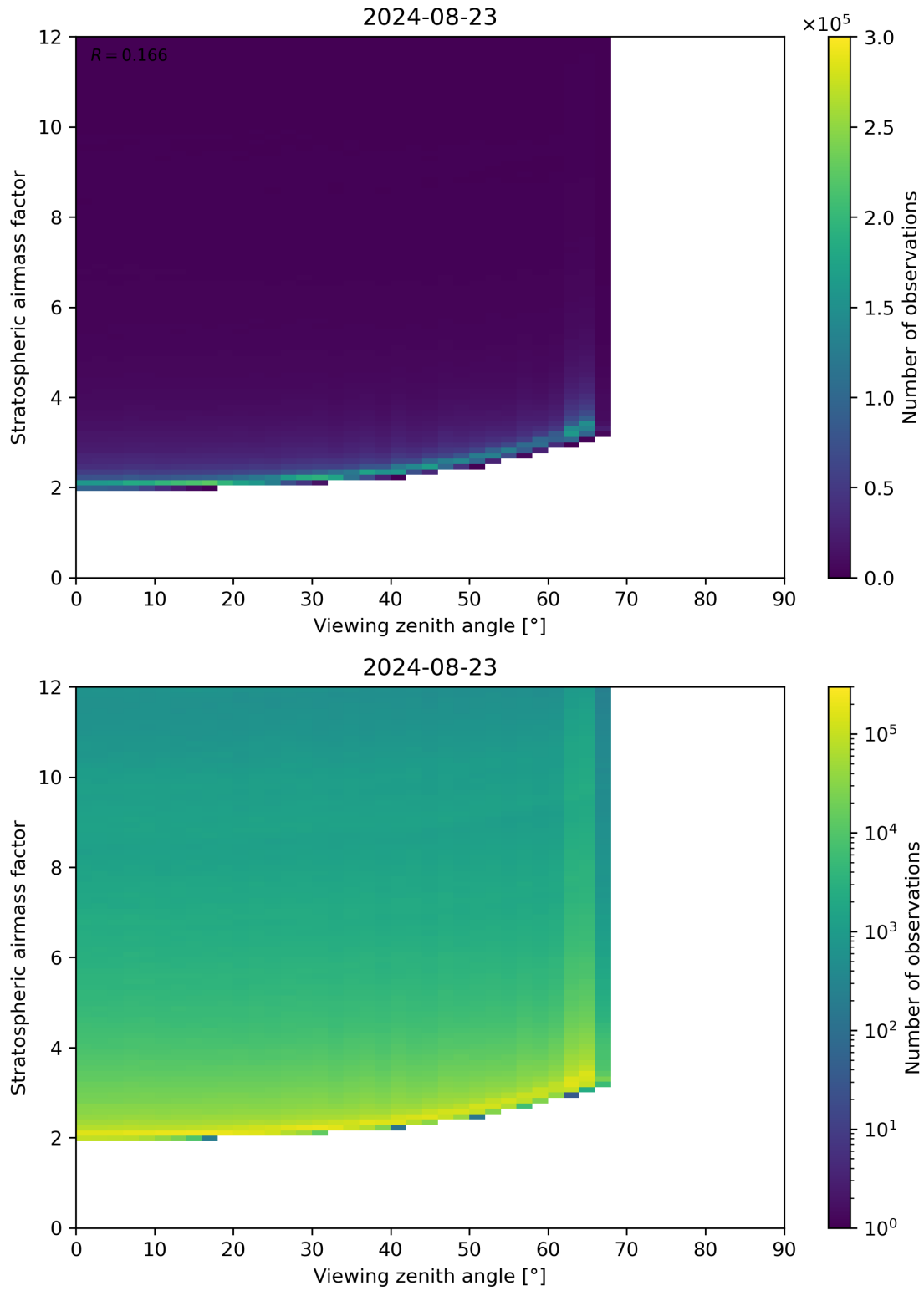
Figure 159: Scatter density plot of “Viewing zenith angle” against “Stratospheric airmass factor” for 2024-08-22 to 2024-08-24.
