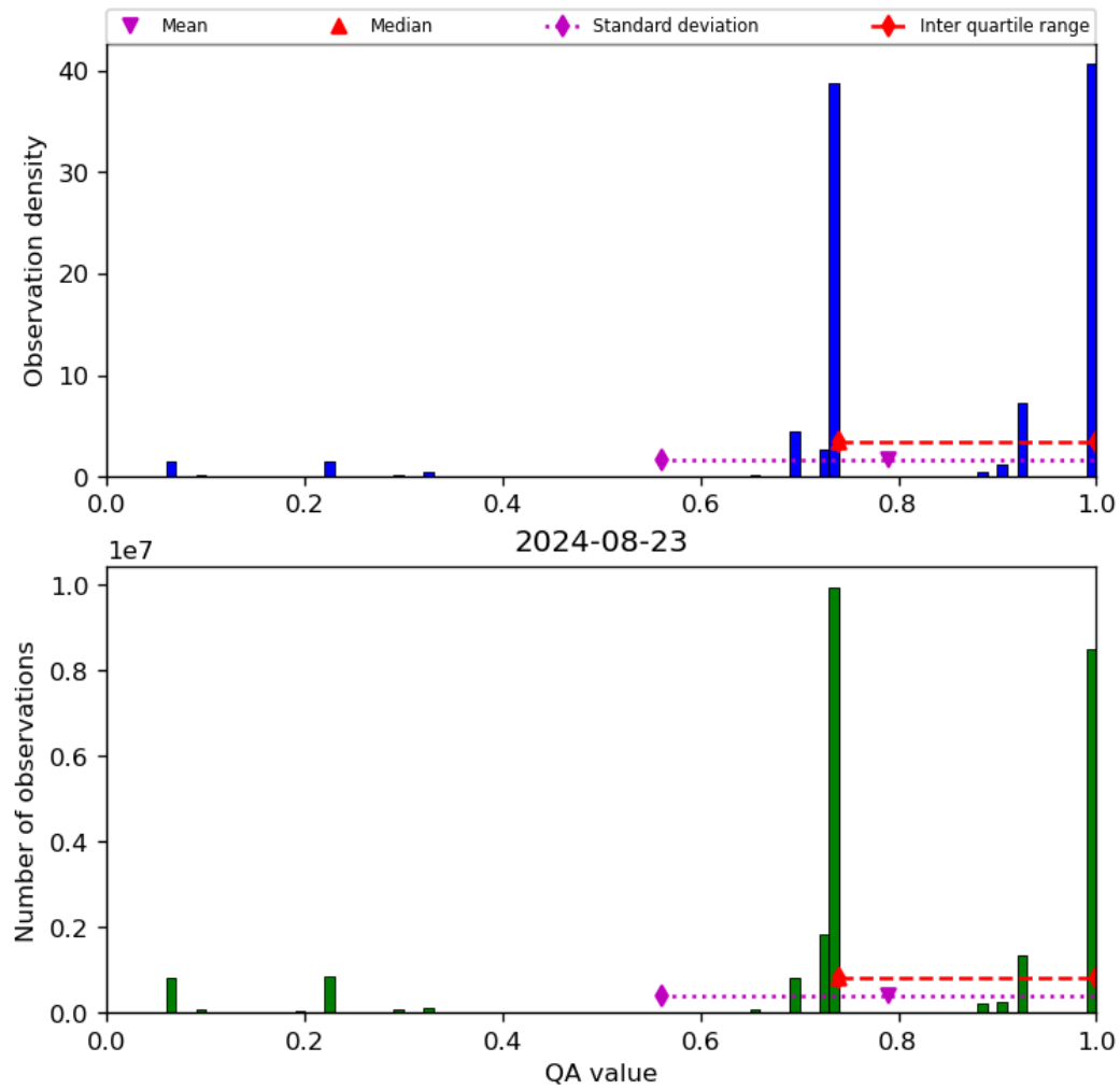
Figure 28: Histogram of “QA value” for 2024-08-22 to 2024-08-24
