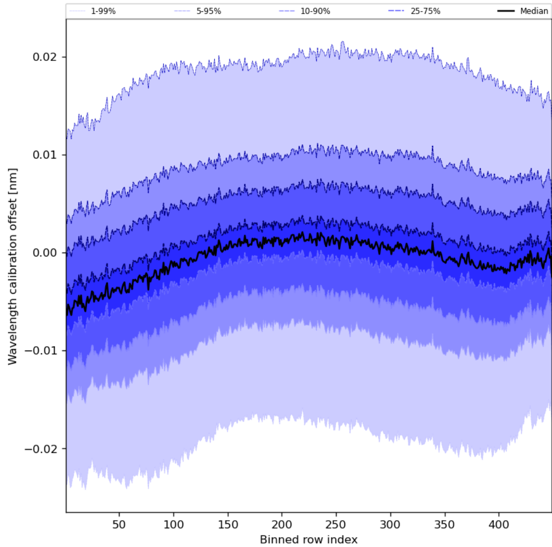
Figure 52: Along track statistics of “Wavelength calibration offset” for 2024-08-22 to 2024-08-24
