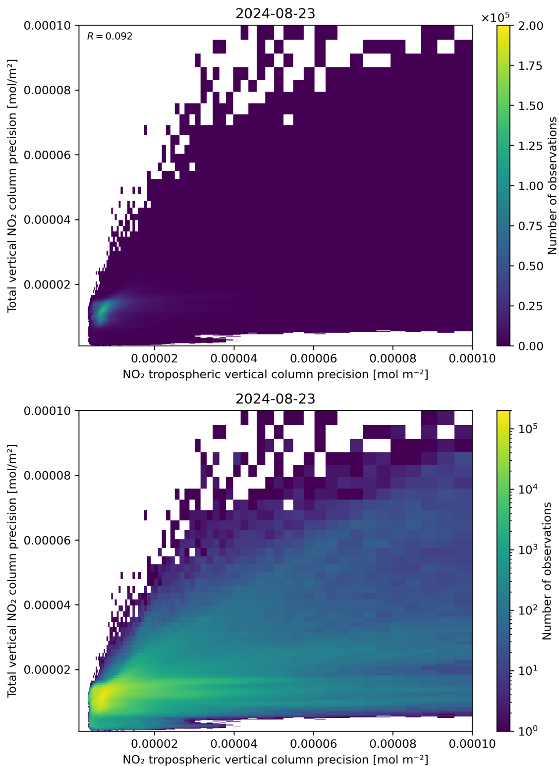
Figure 139: Scatter density plot of “NO 2 tropospheric vertical column precision” against “Total vertical NO 2 column precision” for 2024-08-22 to 2024-08-24.
