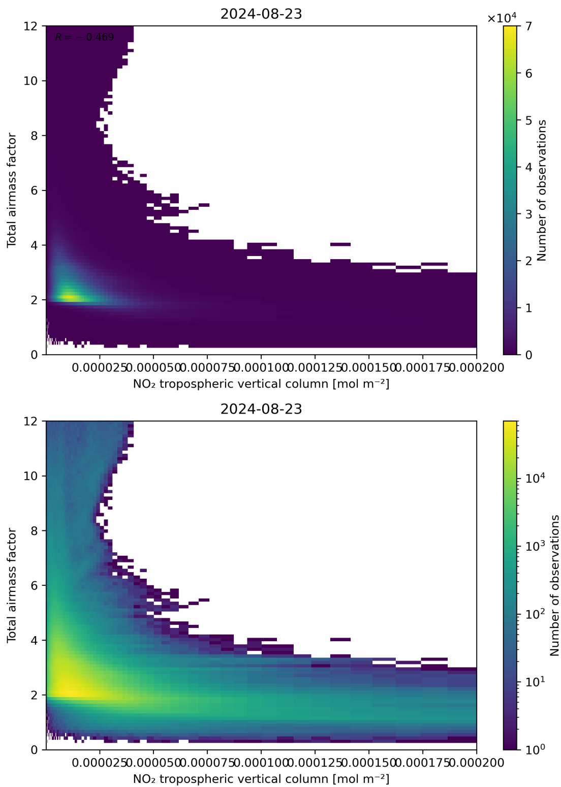
Figure 122: Scatter density plot of “NO 2 tropospheric vertical column” against “Total air mass factor” for 2024-08-22 to 2024-08-24.
