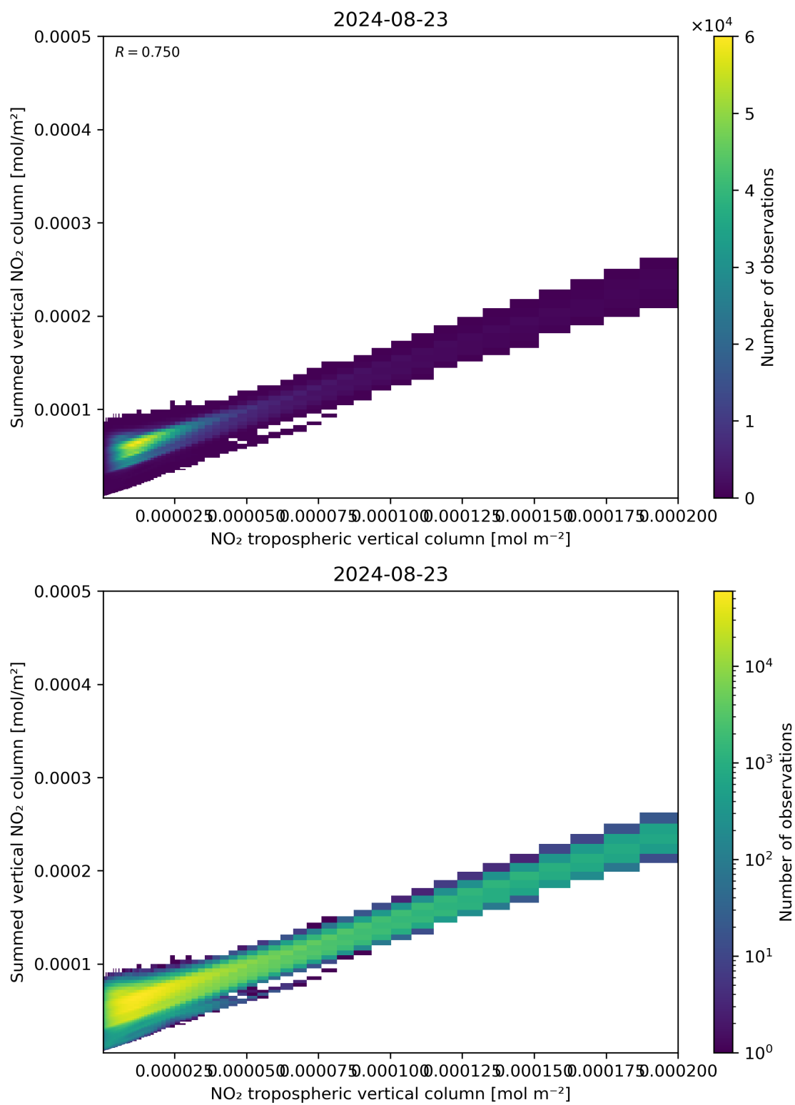
Figure 126: Scatter density plot of “NO 2 tropospheric vertical column” against “Summed vertical NO 2 column” for 2024-08-22 to 2024-08-24.
