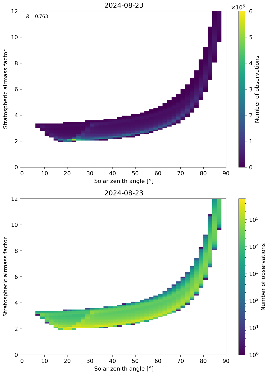
Figure 145: Scatter density plot of “Solar zenith angle” against “Stratospheric airmass factor” for 2024-08-22 to 2024-08-24.
