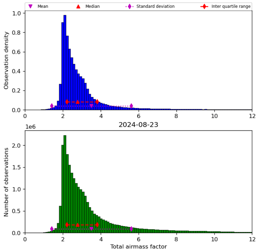
Figure 32: Histogram of “Total airmass factor” for 2024-08-22 to 2024-08-24
