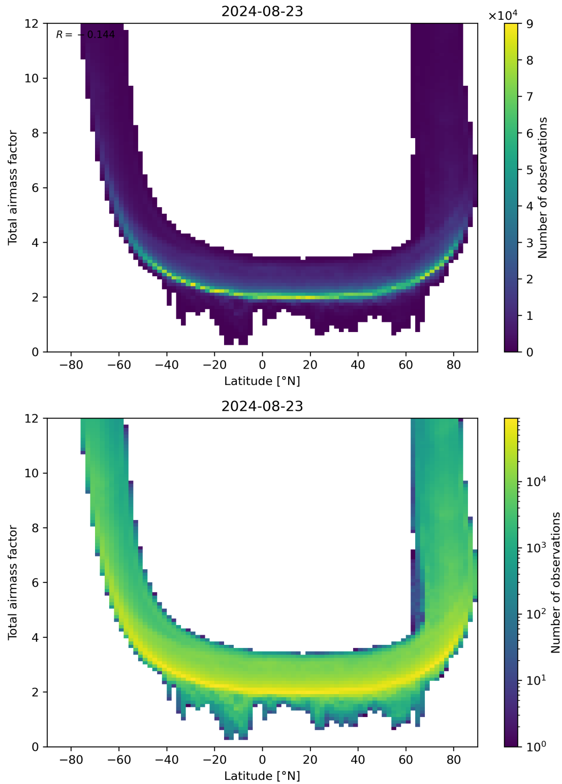
Figure 84: Scatter density plot of “Latitude” against “Total airmass factor” for 2024-08-22 to 2024-08-24.
