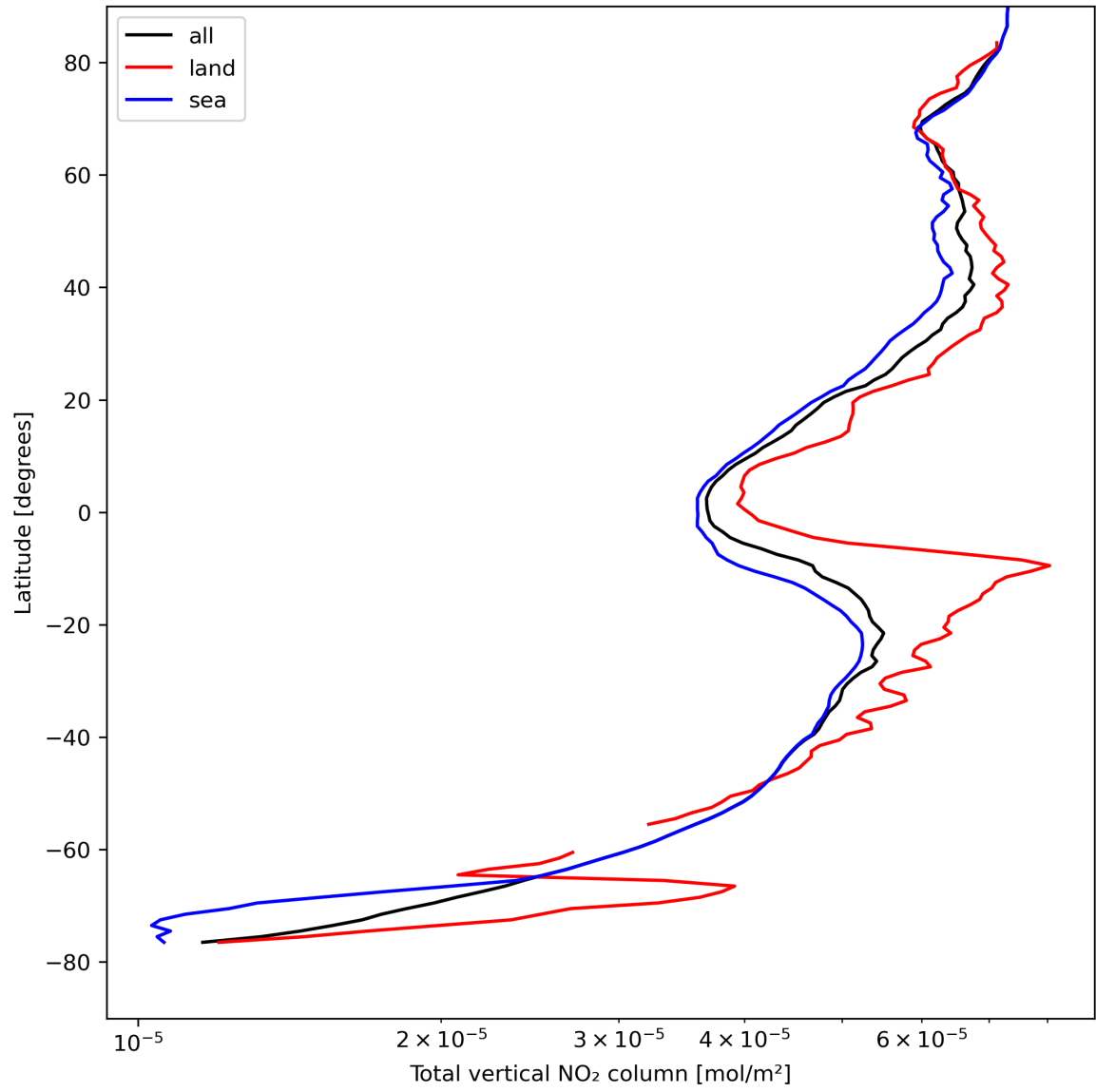
Figure 21: Zonal average of “Total vertical NO 2 column” for 2024-08-22 to 2024-08-24.
