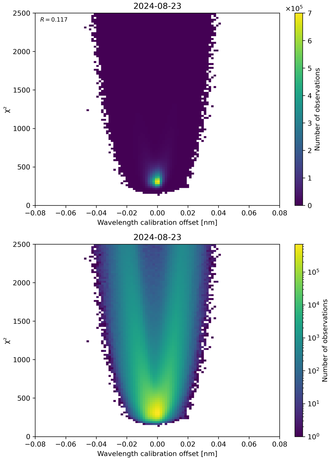
Figure 175: Scatter density plot of “Wavelength calibration offset” against “ \chi^2 ” for 2024-08-22 to 2024-08-24.
