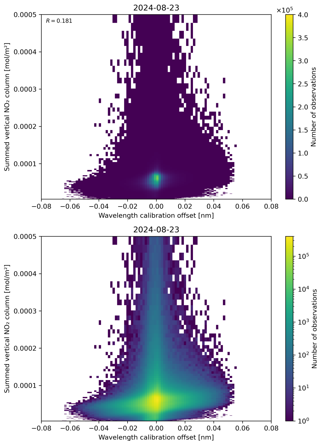
Figure 177: Scatter density plot of “Wavelength calibration offset” against “Summed vertical NO 2 column” for 2024-08-22 to 2024-08-24.
