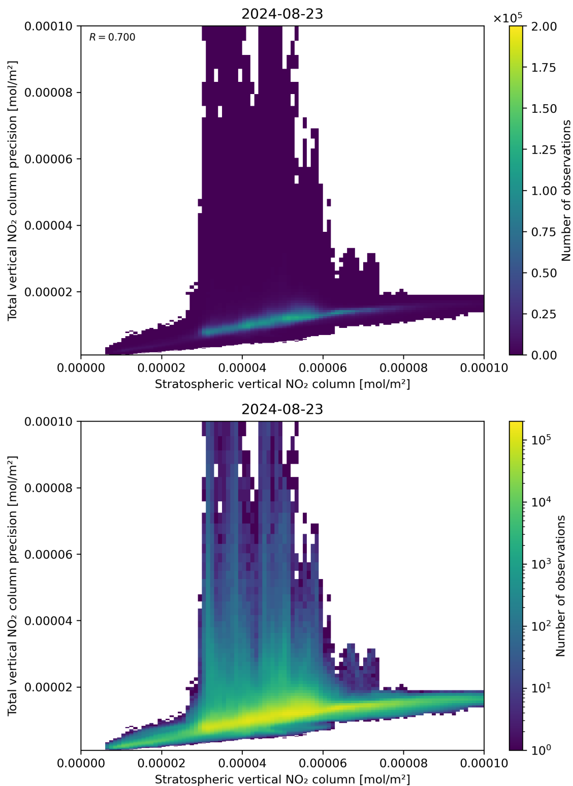
Figure 101: Scatter density plot of “Stratospheric vertical NO 2 column” against “Total vertical NO 2 column precision” for 2024-08-22 to 2024-08-24.
