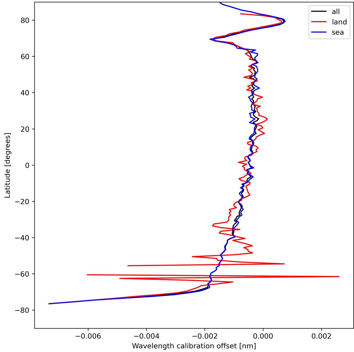
Figure 18: Zonal average of “Wavelength calibration offset” for 2024-08-22 to 2024-08-24.
