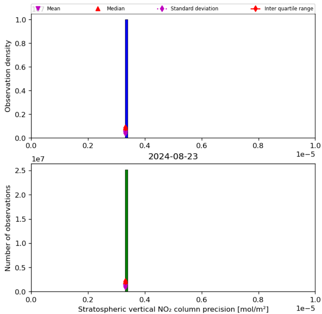
Figure 37: Histogram of “Stratospheric vertical NO 2 column precision” for 2024-08-22 to 2024-08-24
