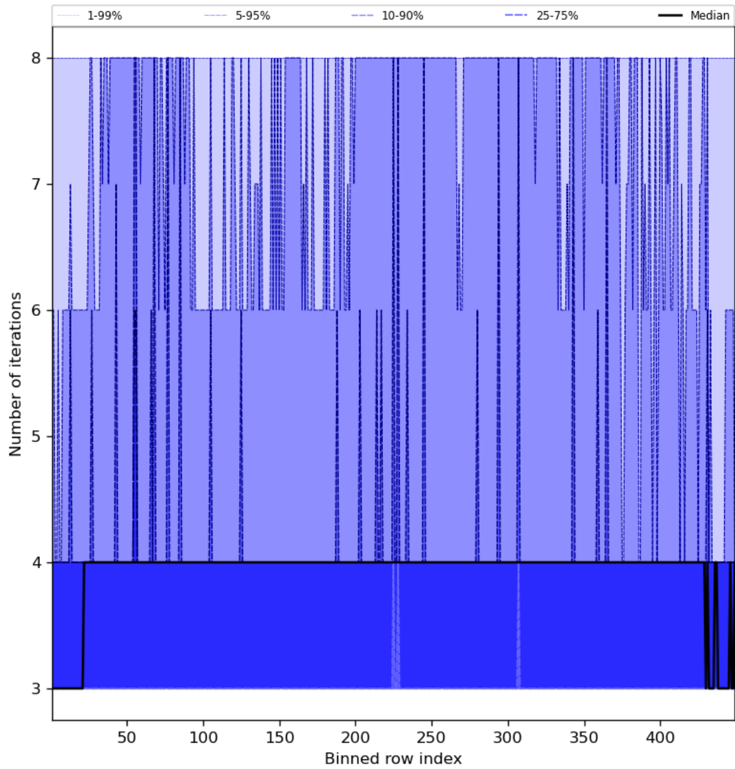
Figure 51: Along track statistics of “Number of iterations” for 2024-08-22 to 2024-08-24
