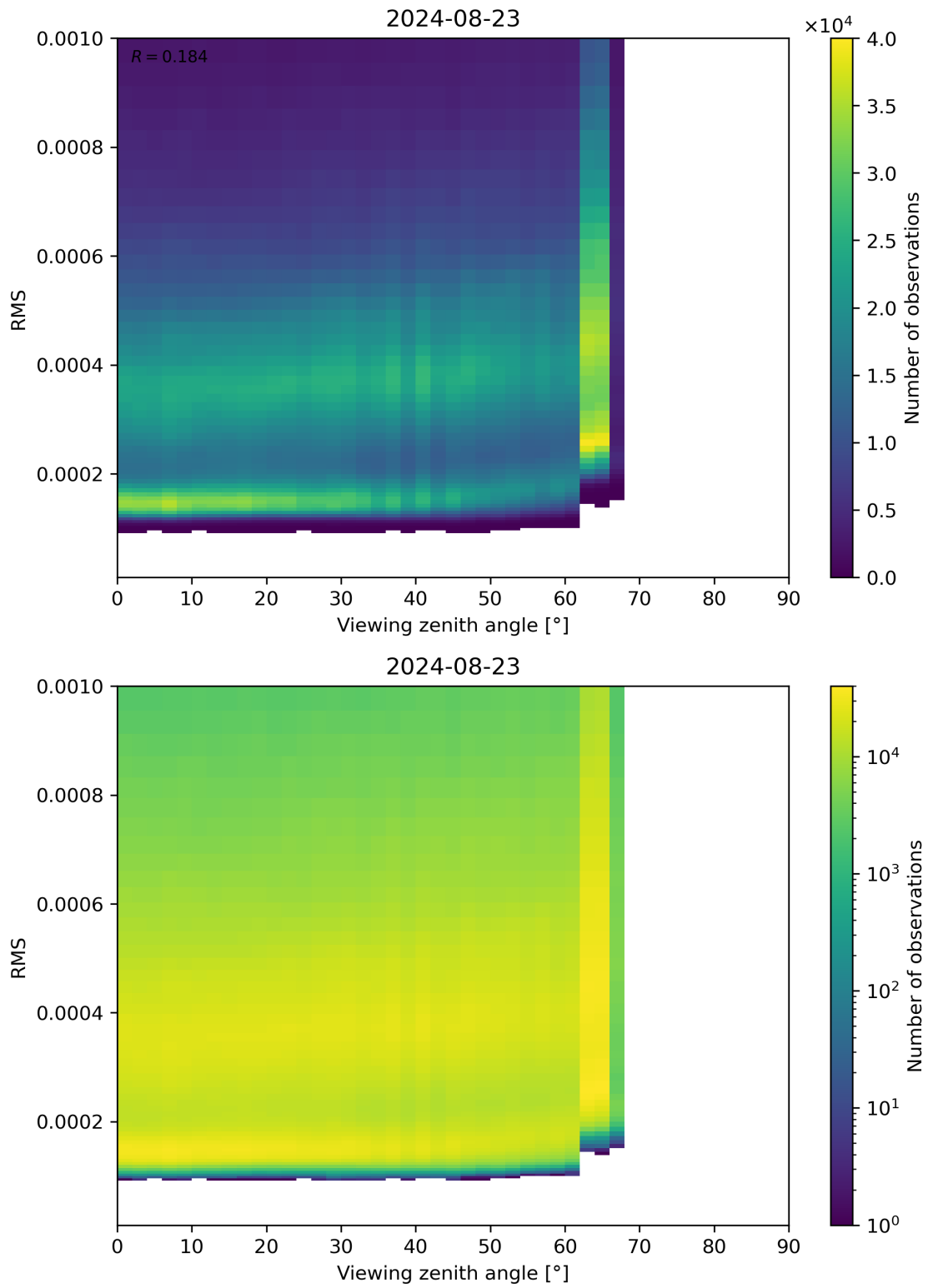
Figure 171: Scatter density plot of “Viewing zenith angle” against “RMS” for 2024-08-22 to 2024-08-24.
