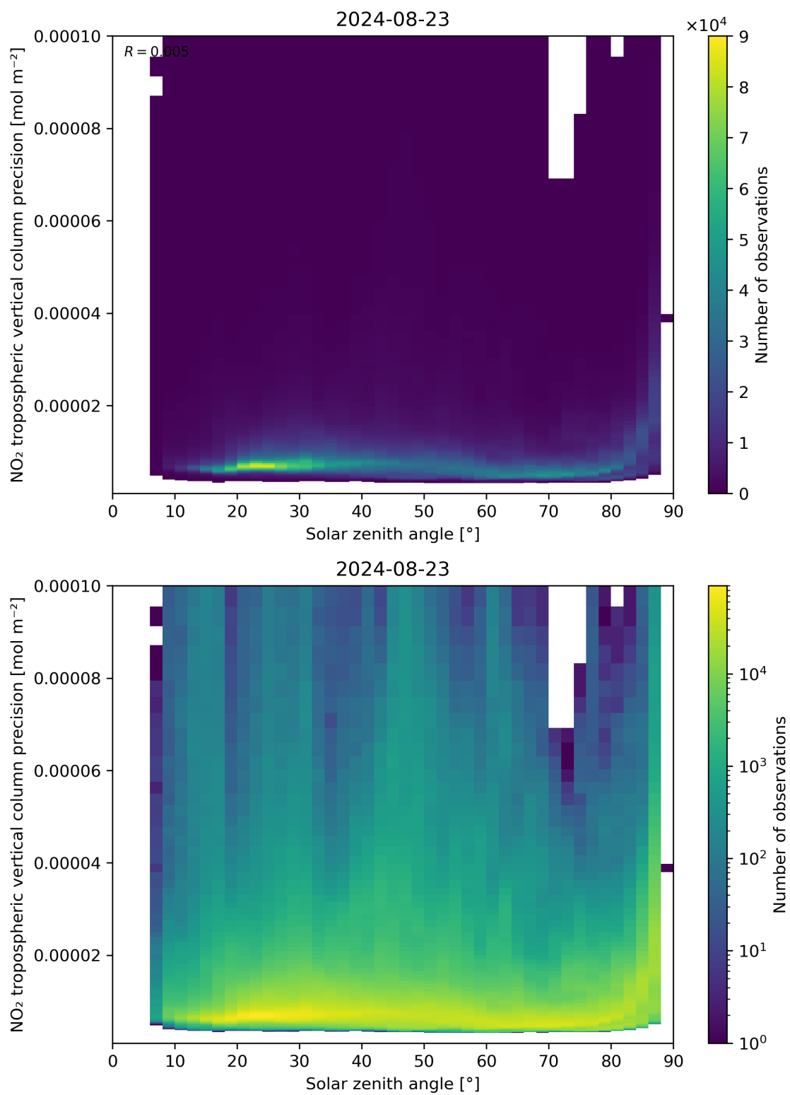
Figure 156: Scatter density plot of “Solar zenith angle” against “NO 2 tropospheric vertical column precision” for 2024-08-22 to 2024-08-24.
