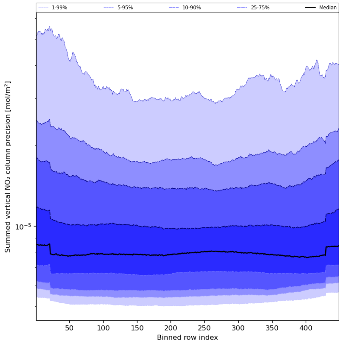
Figure 58: Along track statistics of “Summed vertical NO 2 column precision” for 2024-08-22 to 2024-08-24
