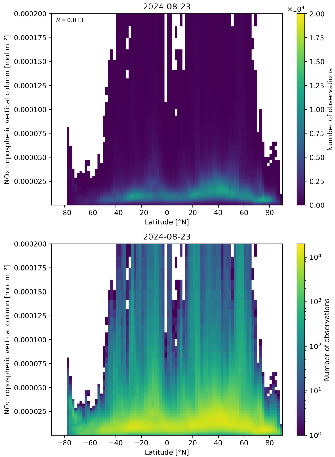
Figure 92: Scatter density plot of “Latitude” against “NO 2 tropospheric vertical column” for 2024-08-22 to 2024-08-24.
