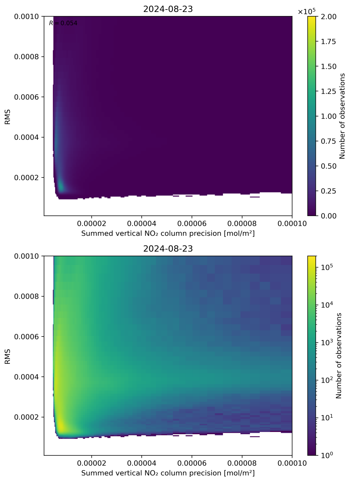
Figure 108: Scatter density plot of “Summed vertical NO 2 column precision” against “RMS” for 2024-08-22 to 2024-08-24.
