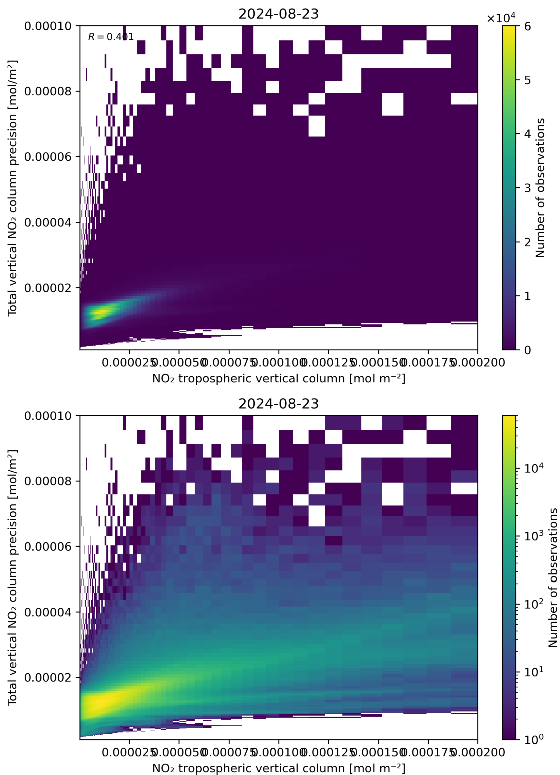
Figure 129: Scatter density plot of “NO 2 tropospheric vertical column” against “Total vertical NO 2 column precision” for 2024-08-22 to 2024-08-24.
