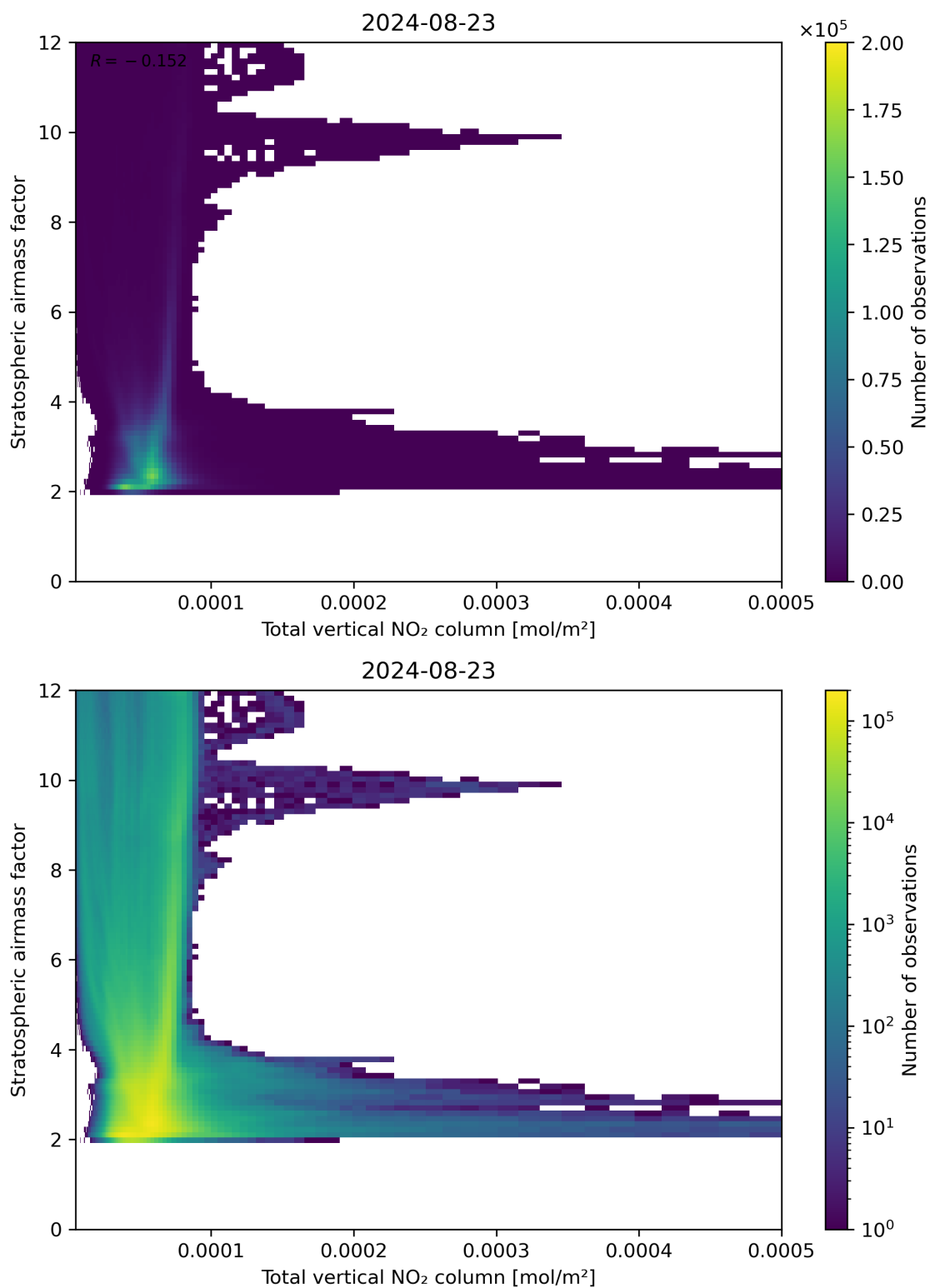
Figure 110: Scatter density plot of “Total vertical NO 2 column” against “Stratospheric airmass factor” for 2024-08-22 to 2024-08-24.
