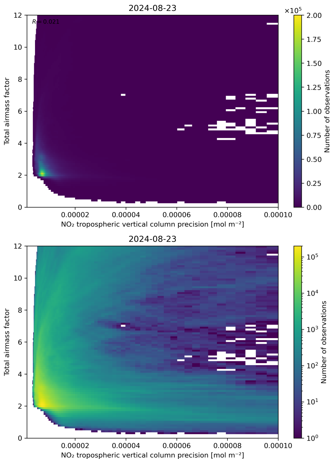
Figure 132: Scatter density plot of “NO 2 tropospheric vertical column precision” against “Total air mass factor” for 2024-08-22 to 2024-08-24.
