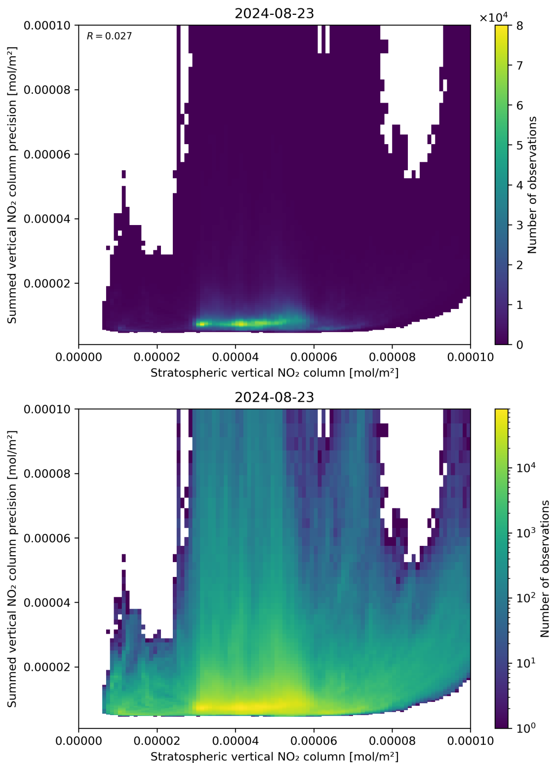
Figure 99: Scatter density plot of “Stratospheric vertical NO 2 column” against “Summed vertical NO 2 column precision” for 2024-08-22 to 2024-08-24.
