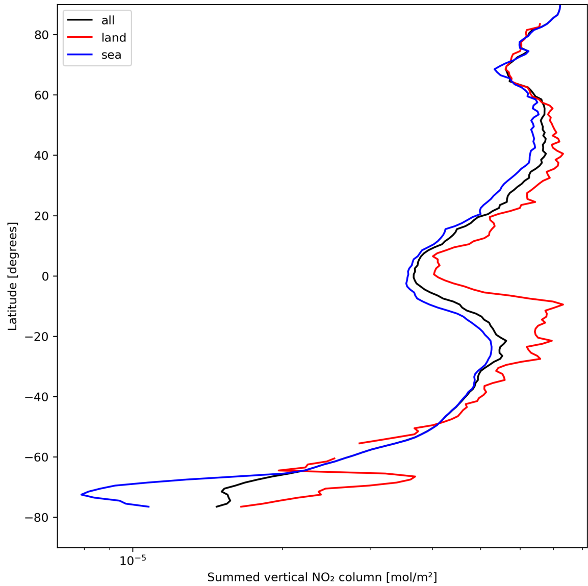
Figure 23: Zonal average of “Summed vertical NO 2 column” for 2024-08-22 to 2024-08-24.
