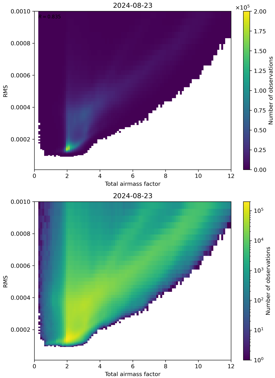
Figure 69: Scatter density plot of “Total airmass factor” against “RMS” for 2024-08-22 to 2024-08-24.
