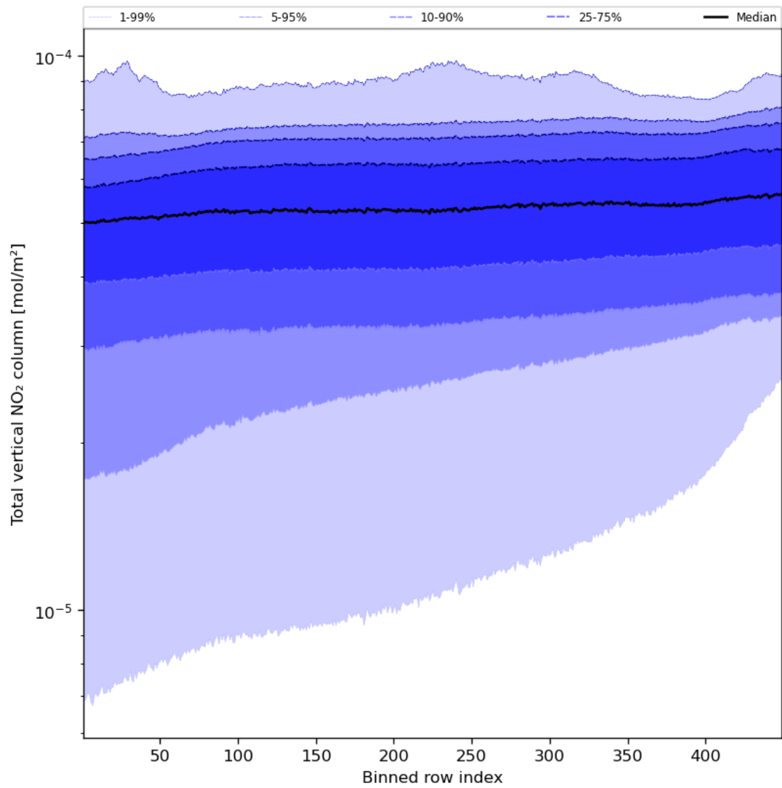
Figure 55: Along track statistics of “Total vertical NO 2 column” for 2024-08-22 to 2024-08-24
