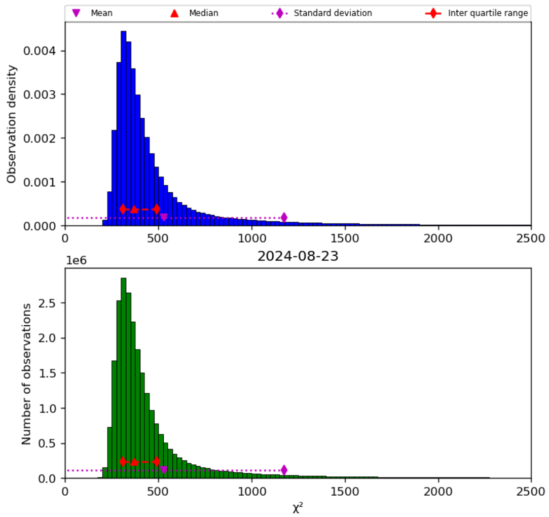
Figure 42: Histogram of “ \chi^2 ” for 2024-08-22 to 2024-08-24
