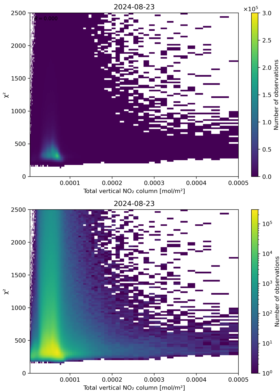
Figure 111: Scatter density plot of “Total vertical NO 2 column” against “ \chi^2 ” for 2024-08-22 to 2024-08-24.
