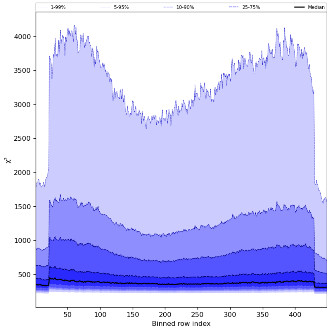
Figure 59: Along track statistics of “ \chi^2 ” for 2024-08-22 to 2024-08-24
