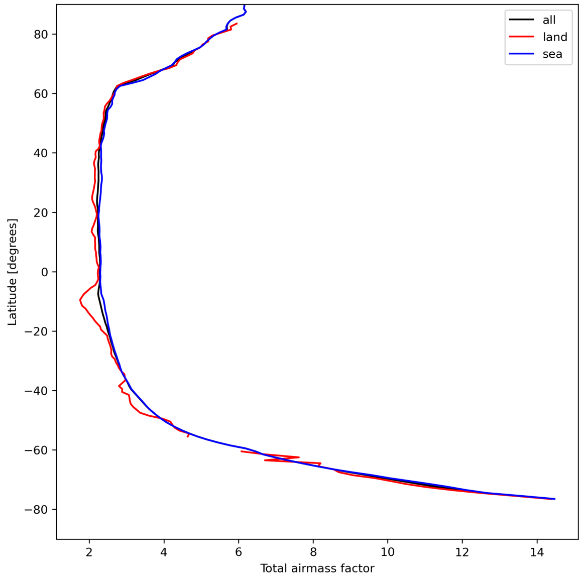
Figure 15: Zonal average of “Total airmass factor” for 2024-08-22 to 2024-08-24.
