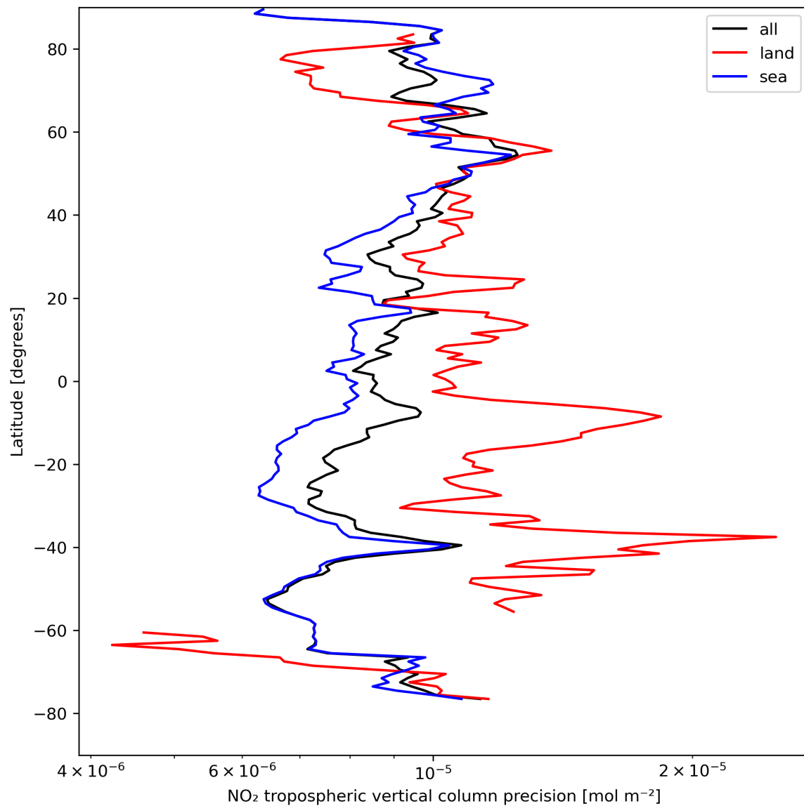
Figure 13: Zonal average of “NO 2 tropospheric vertical column precision” for 2024-08-22 to 2024-08-24.
