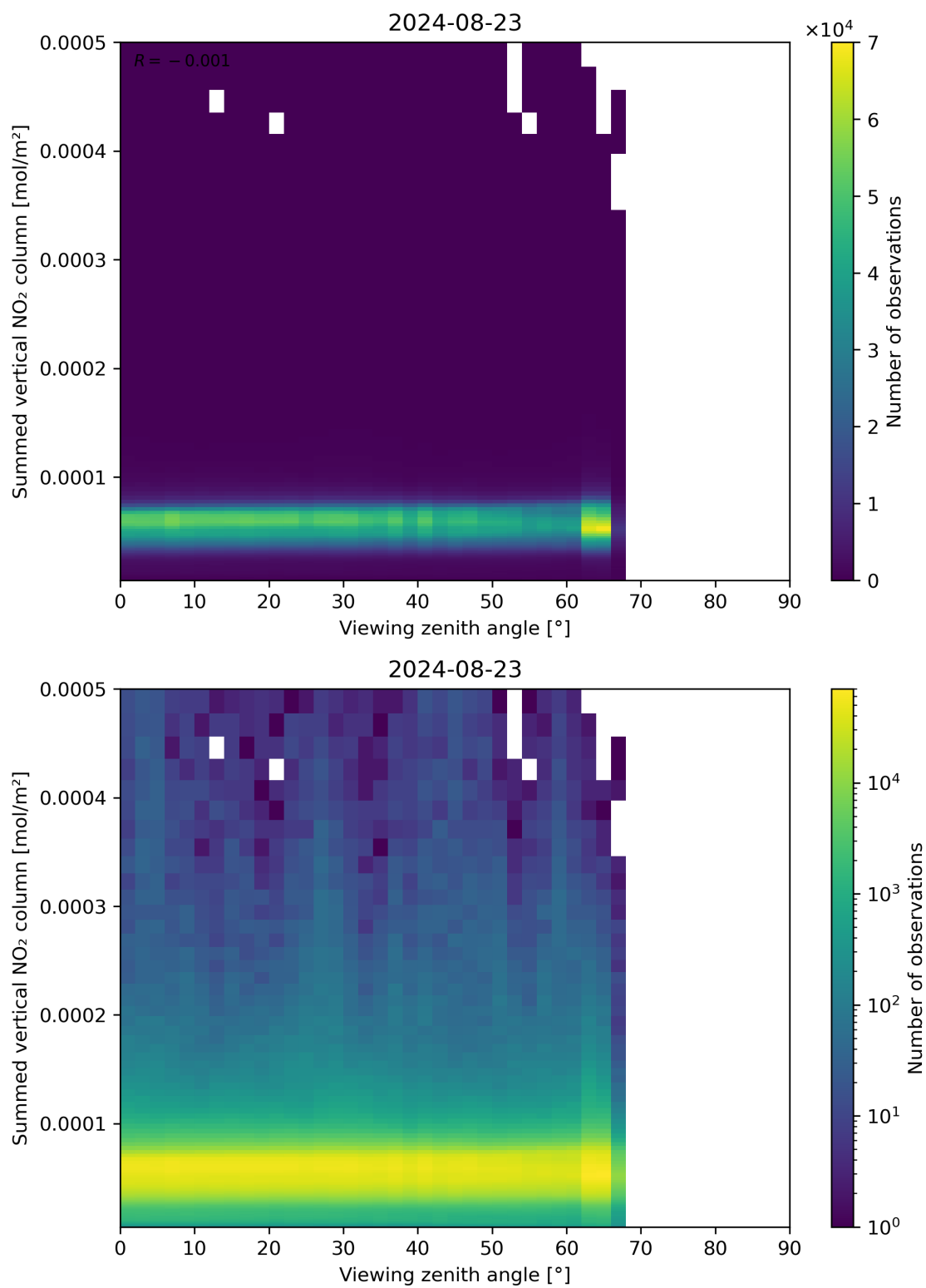
Figure 165: Scatter density plot of “Viewing zenith angle” against “Summed vertical NO 2 column” for 2024-08-22 to 2024-08-24.
