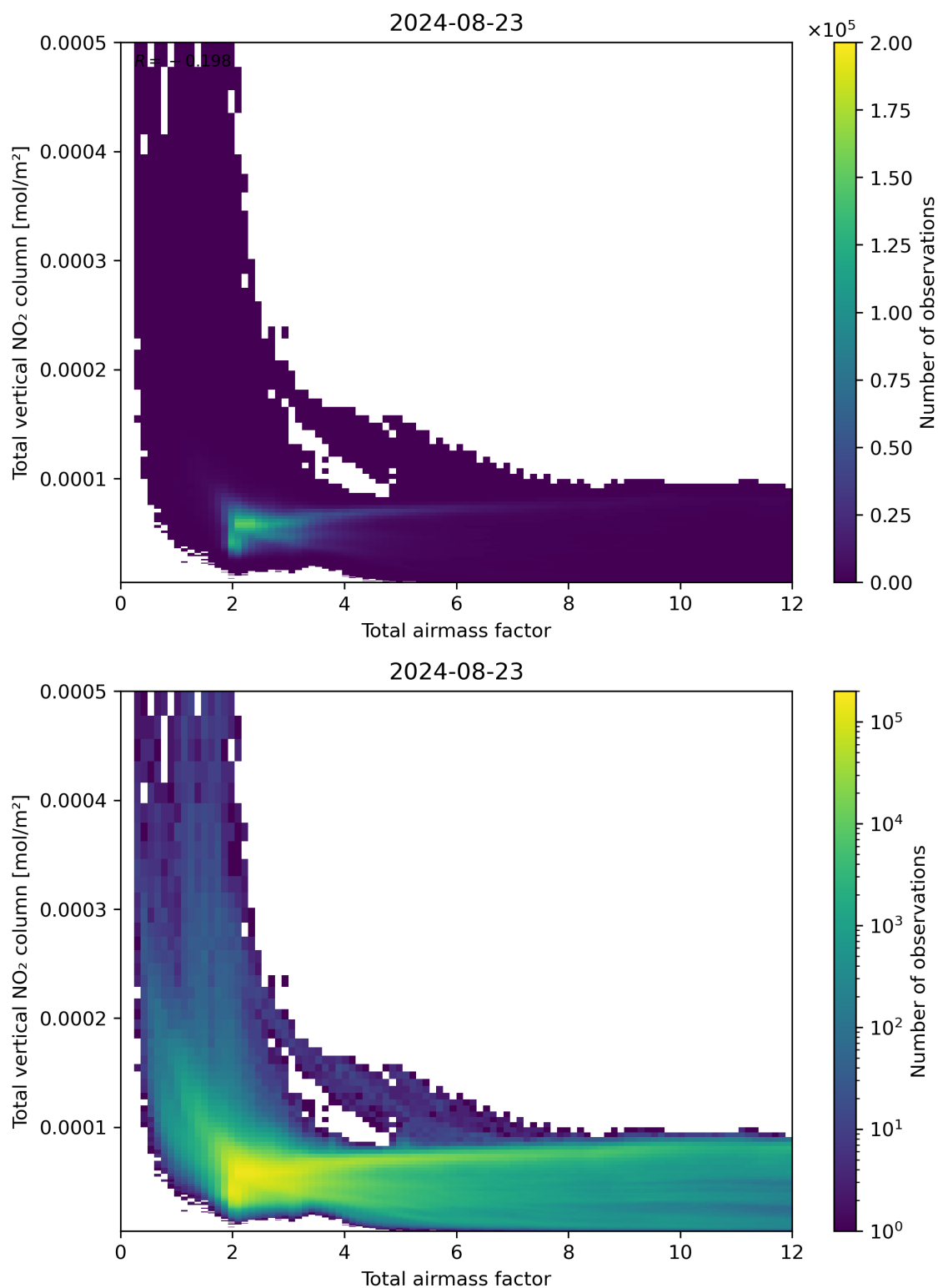
Figure 67: Scatter density plot of “Total airmass factor” against “Total vertical NO 2 column” for 2024-08-22 to 2024-08-24.
