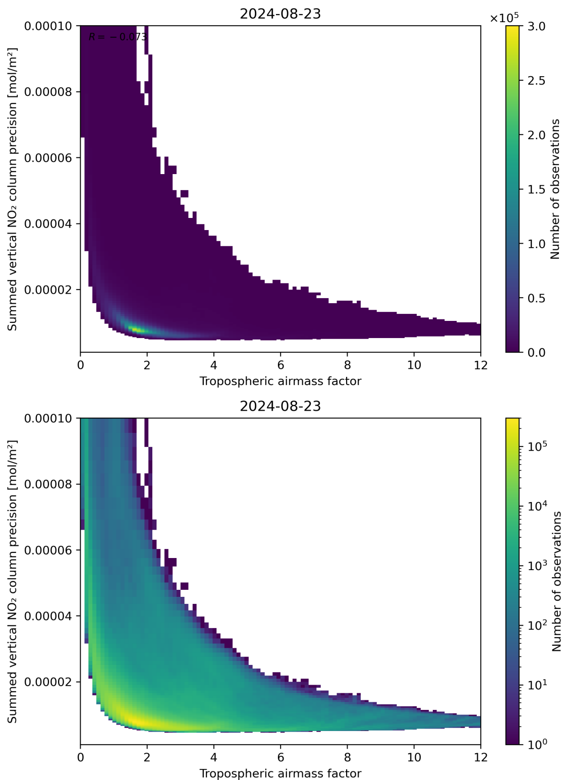
Figure 76: Scatter density plot of “Tropospheric air mass factor” against “Summed vertical NO 2 column precision” for 2024-08-22 to 2024-08-24.
