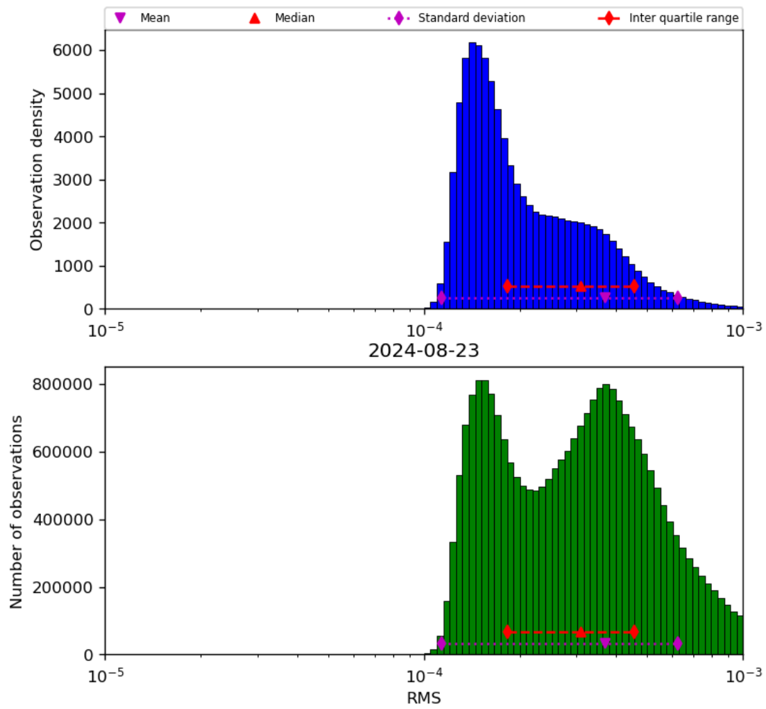
Figure 43: Histogram of “RMS” for 2024-08-22 to 2024-08-24
