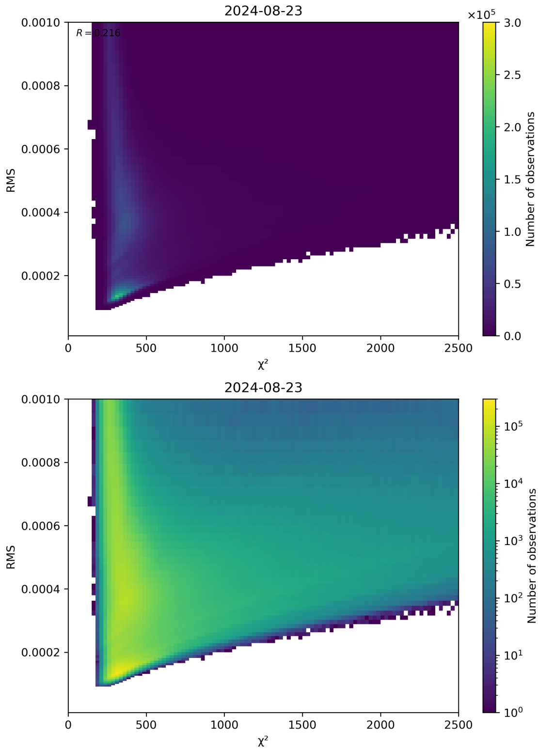
Figure 82: Scatter density plot of “ \chi^2 ” against “RMS” for 2024-08-22 to 2024-08-24.
