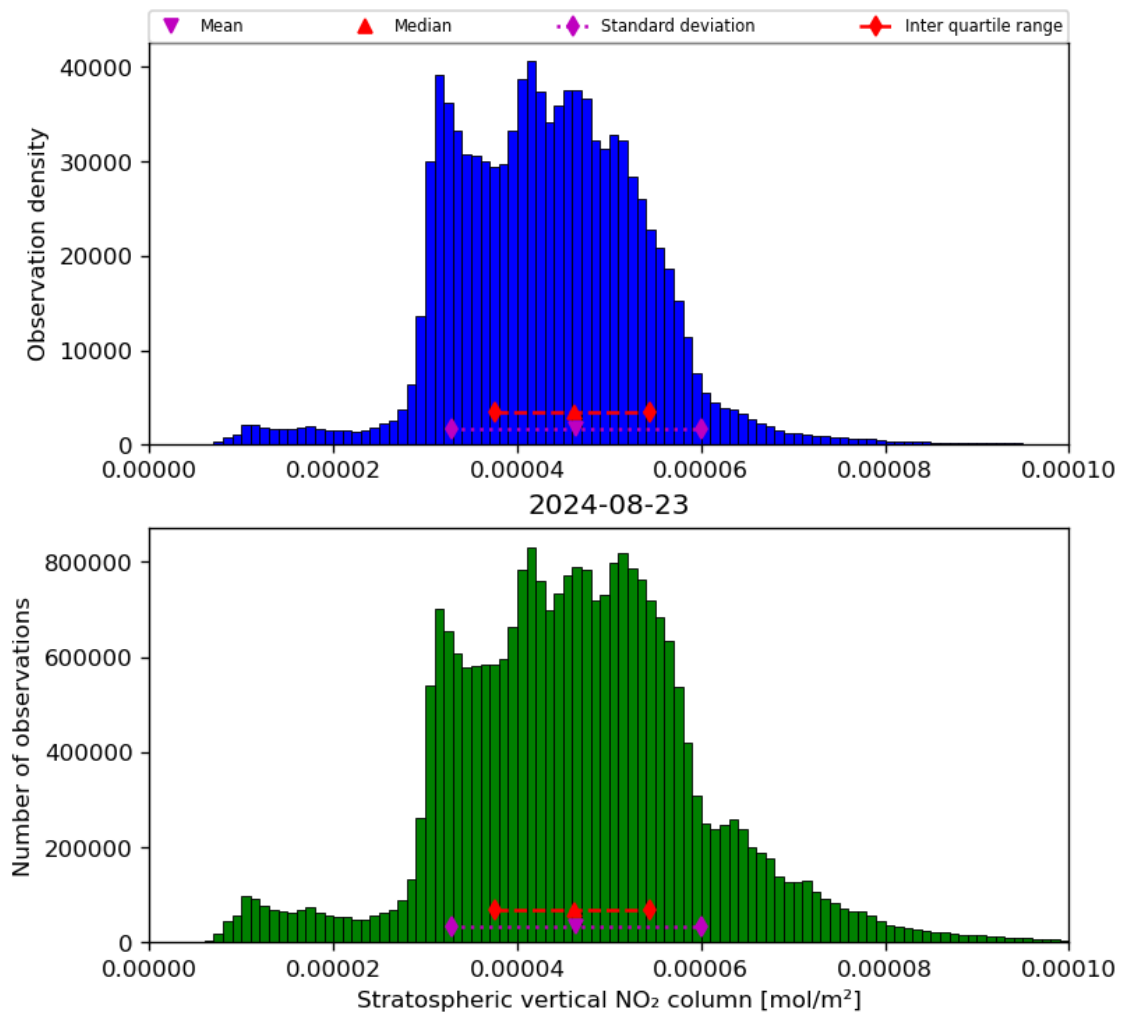
Figure 36: Histogram of “Stratospheric vertical NO 2 column” for 2024-08-22 to 2024-08-24
