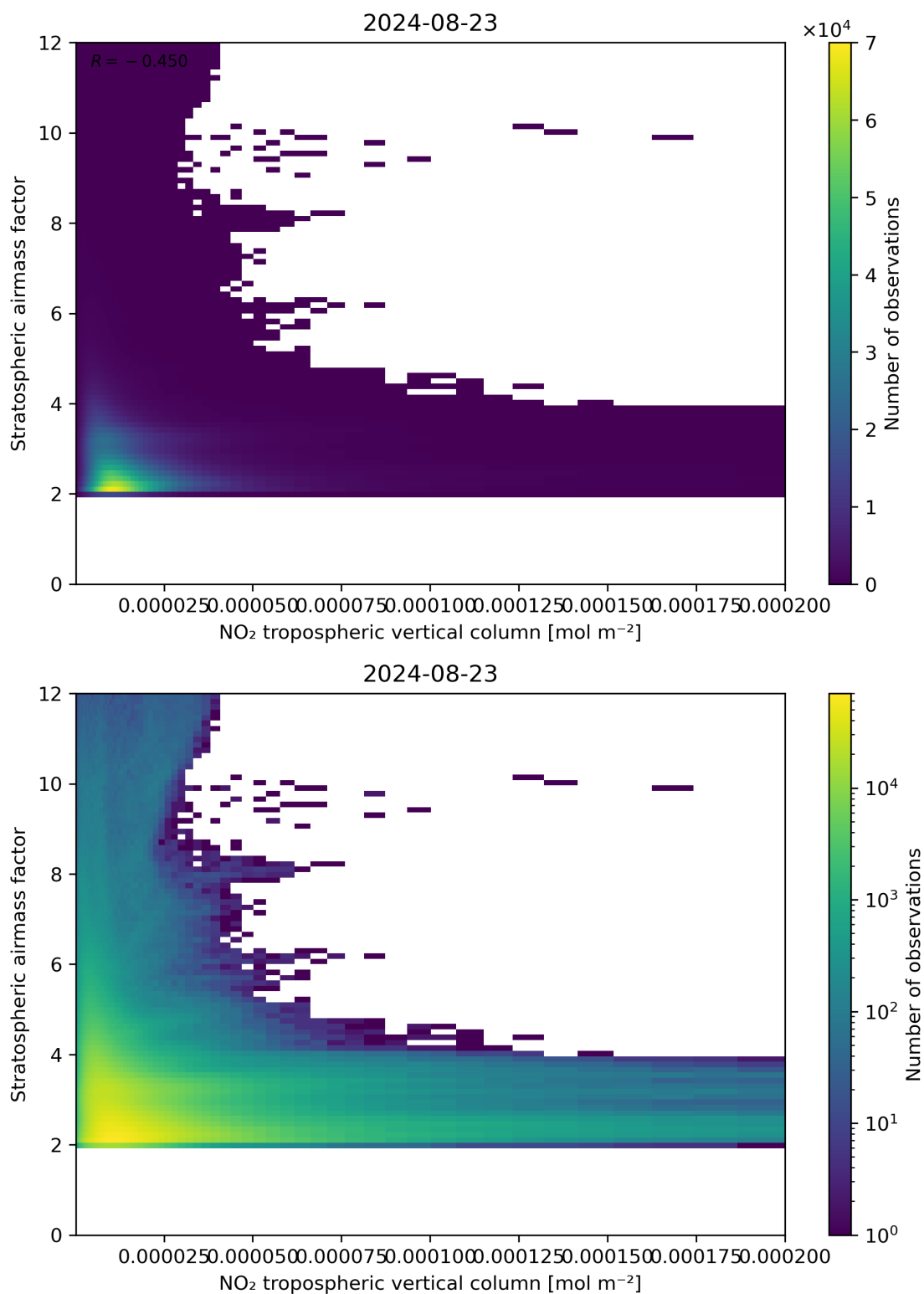
Figure 121: Scatter density plot of “NO 2 tropospheric vertical column” against “Stratospheric air mass factor” for 2024-08-22 to 2024-08-24.
