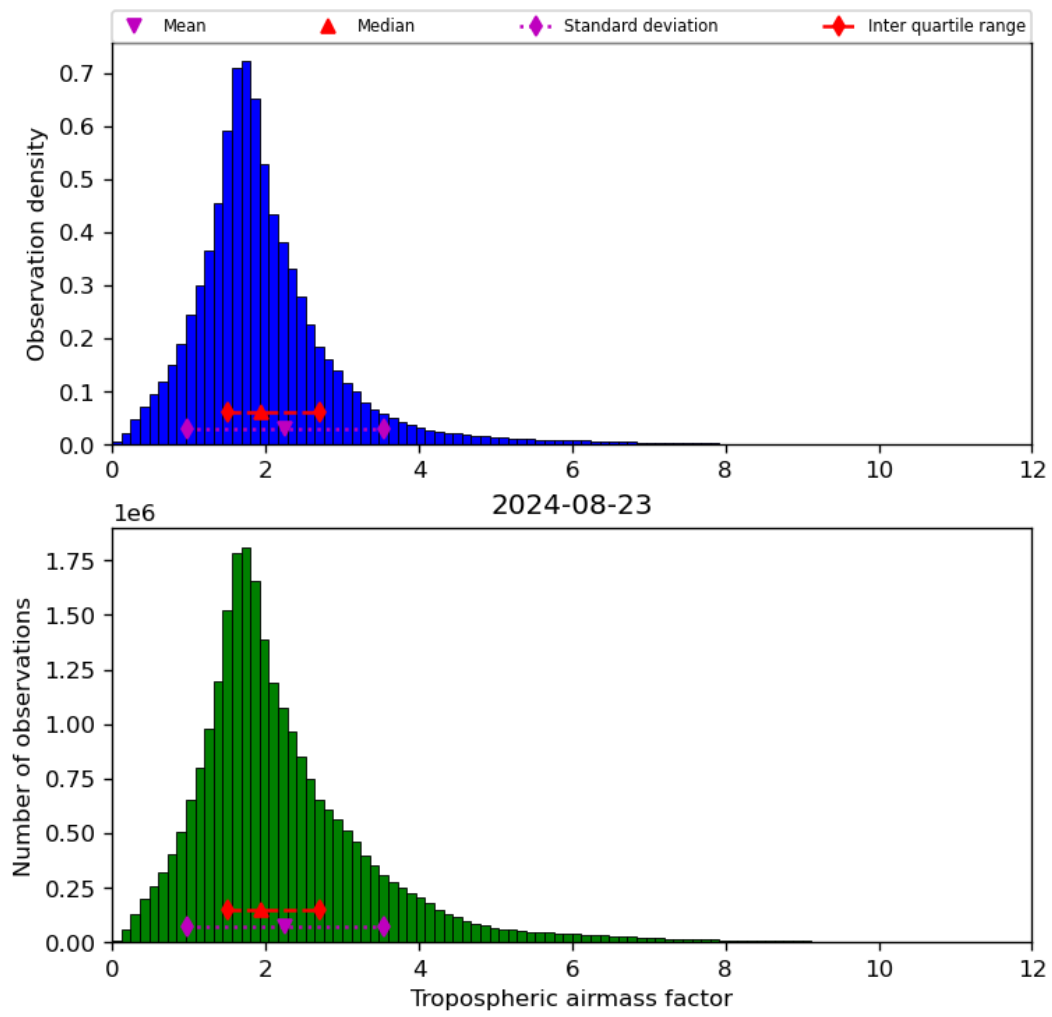
Figure 31: Histogram of “Tropospheric airmass factor” for 2024-08-22 to 2024-08-24
