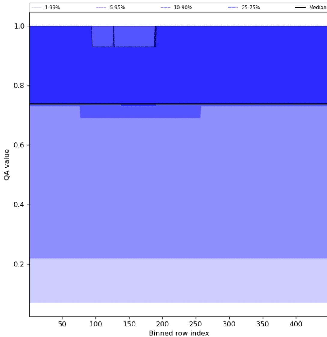
Figure 45: Along track statistics of “QA value” for 2024-08-22 to 2024-08-24
