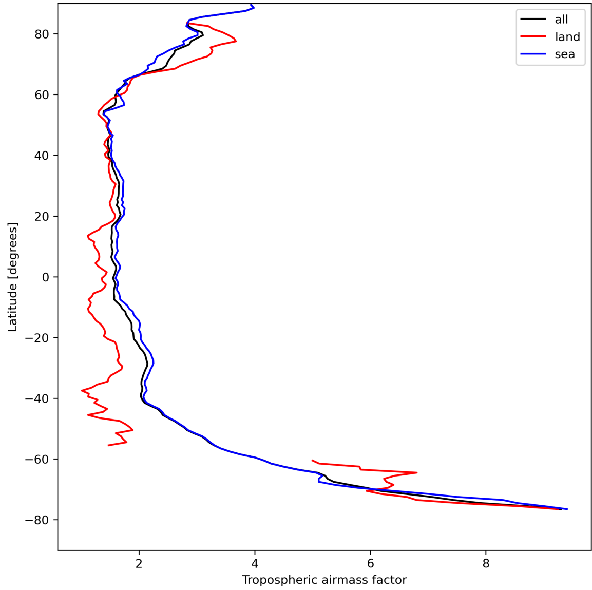
Figure 14: Zonal average of “Tropospheric airmass factor” for 2024-08-22 to 2024-08-24.
