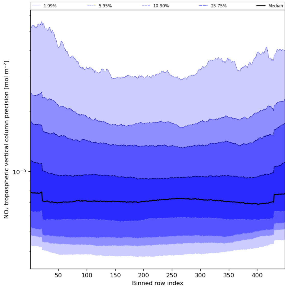
Figure 47: Along track statistics of “NO 2 tropospheric vertical column precision” for 2024-08-22 to 2024-08-24
