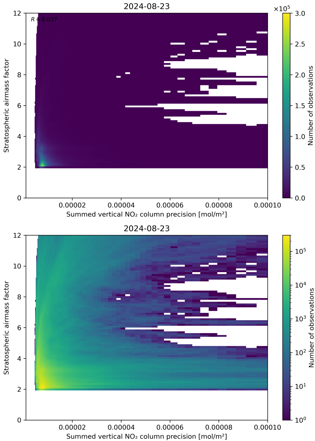
Figure 106: Scatter density plot of “Summed vertical NO 2 column precision” against “Stratospheric airmass factor” for 2024-08-22 to 2024-08-24.
