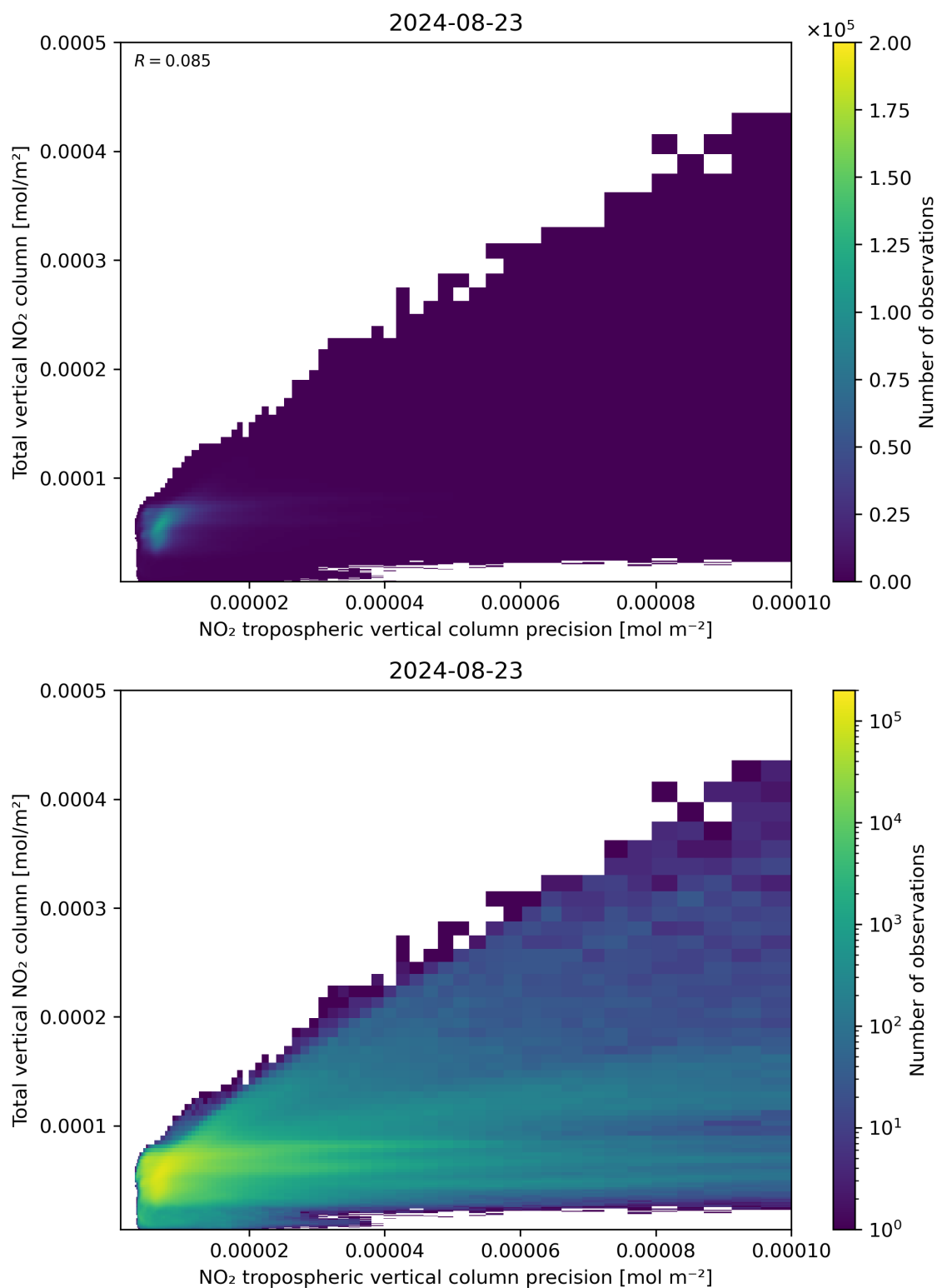
Figure 138: Scatter density plot of “NO 2 tropospheric vertical column precision” against “Total vertical NO 2 column” for 2024-08-22 to 2024-08-24.
