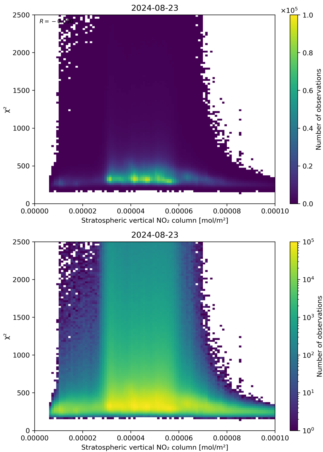
Figure 97: Scatter density plot of “Stratospheric vertical NO 2 column” against “ \chi^2 ” for 2024-08-22 to 2024-08-24.
