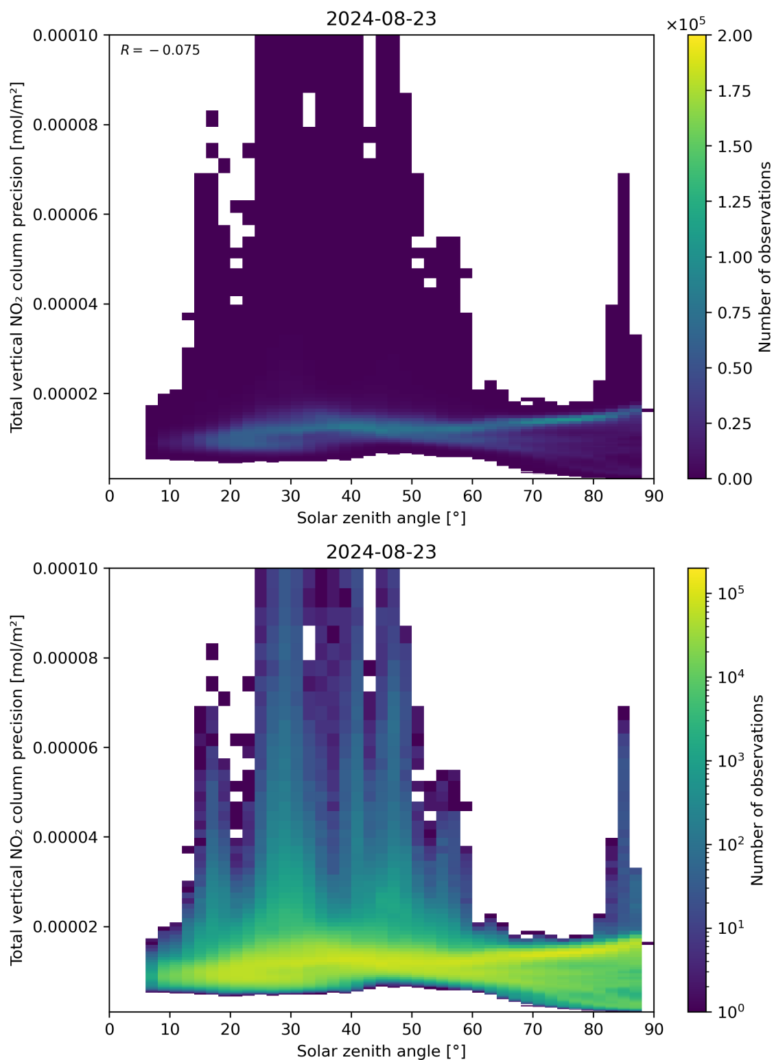
Figure 154: Scatter density plot of “Solar zenith angle” against “Total vertical NO 2 column precision” for 2024-08-22 to 2024-08-24.
