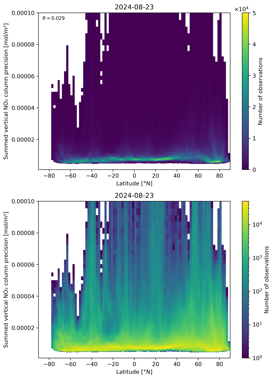
Figure 89: Scatter density plot of “Latitude” against “Summed vertical NO 2 column precision” for 2024-08-22 to 2024-08-24.
