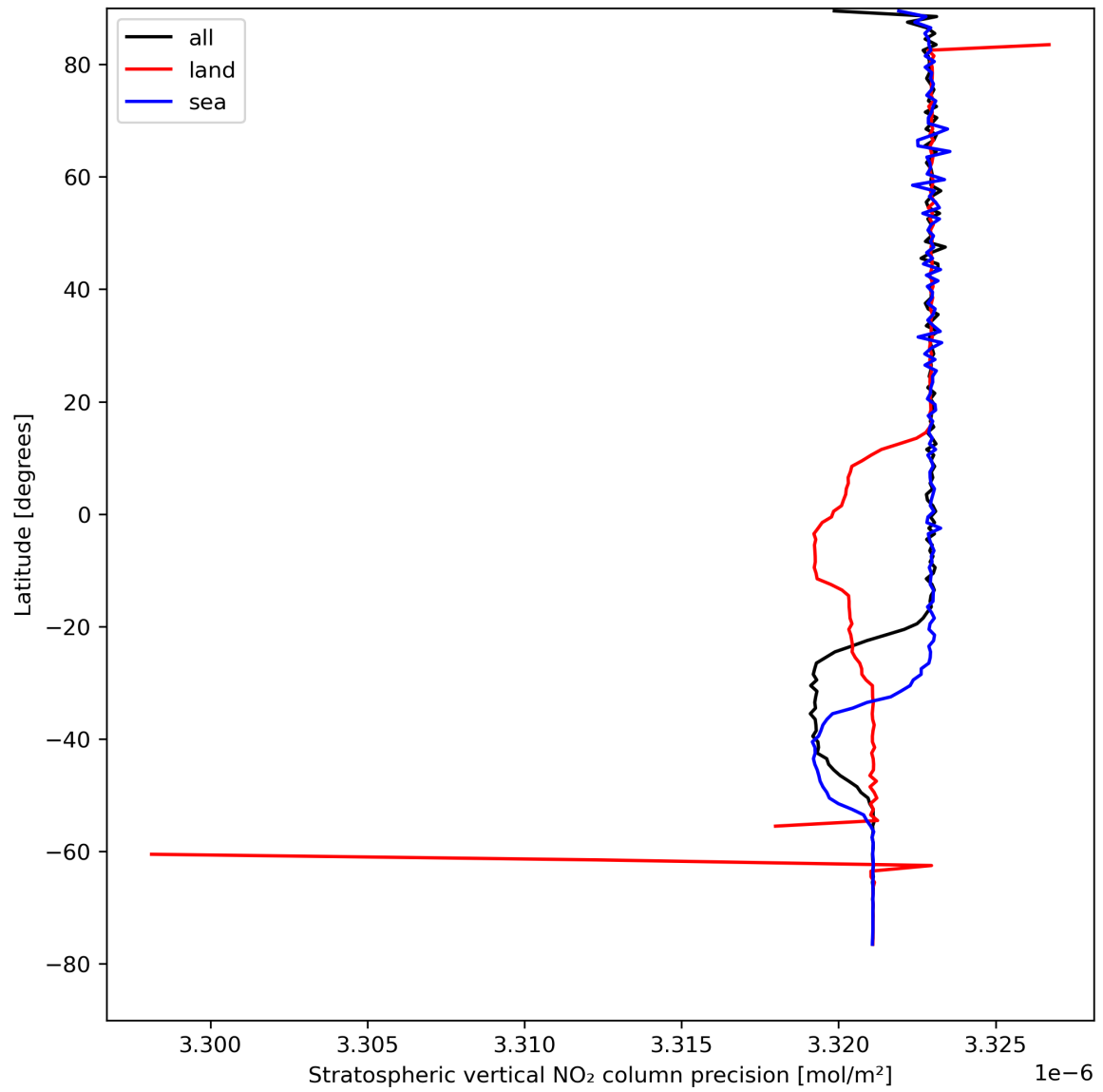
Figure 20: Zonal average of “Stratospheric vertical NO 2 column precision” for 2024-08-22 to 2024-08-24.
