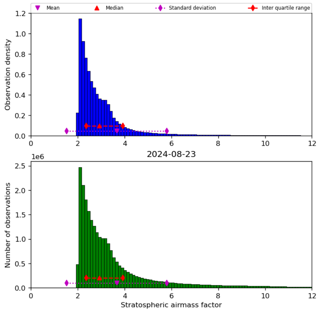
Figure 44: Histogram of “Stratospheric airmass factor” for 2024-08-22 to 2024-08-24
