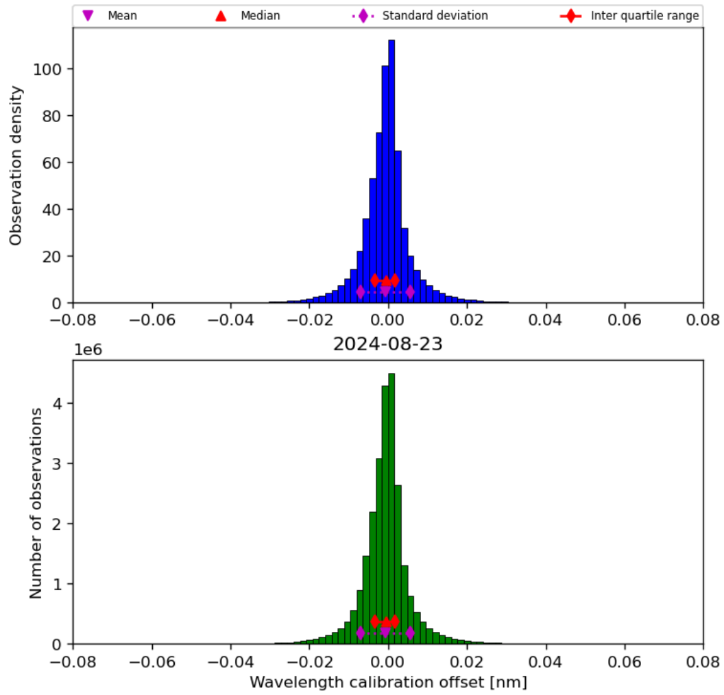
Figure 35: Histogram of “Wavelength calibration offset” for 2024-08-22 to 2024-08-24
