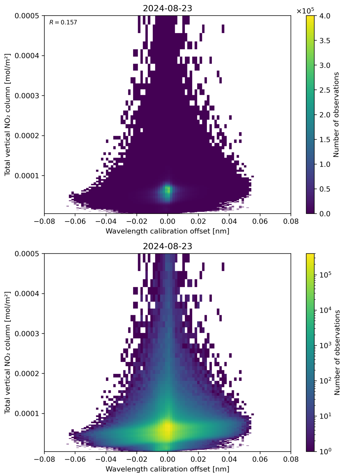
Figure 179: Scatter density plot of “Wavelength calibration offset” against “Total vertical NO 2 column” for 2024-08-22 to 2024-08-24.
