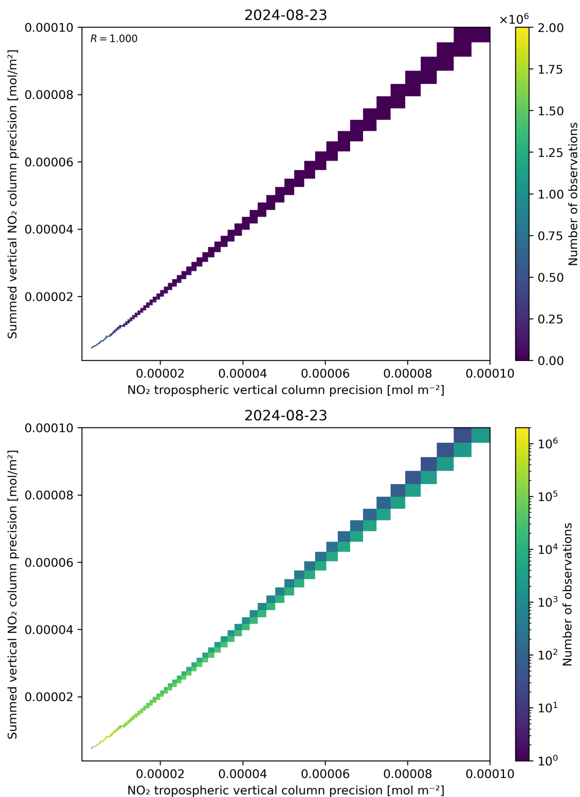
Figure 137: Scatter density plot of “NO 2 tropospheric vertical column precision” against “Summed vertical NO 2 column precision” for 2024-08-22 to 2024-08-24.
