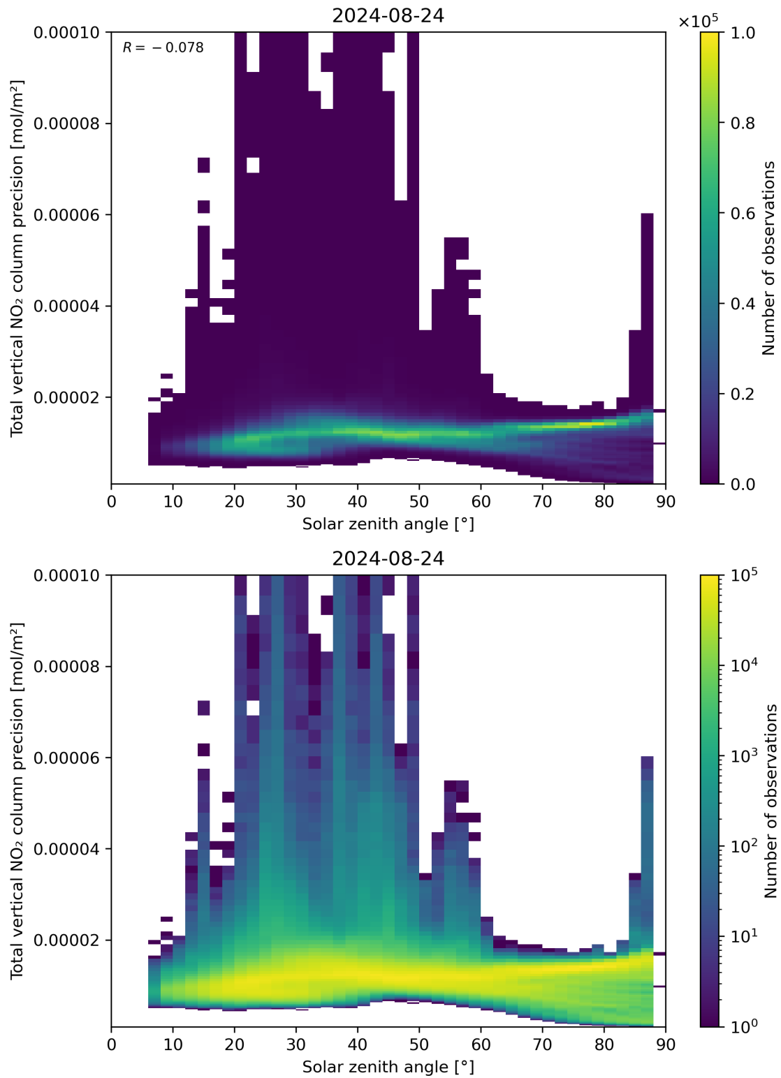
Figure 154: Scatter density plot of “Solar zenith angle” against “Total vertical NO 2 column precision” for 2024-08-23 to 2024-08-25.
