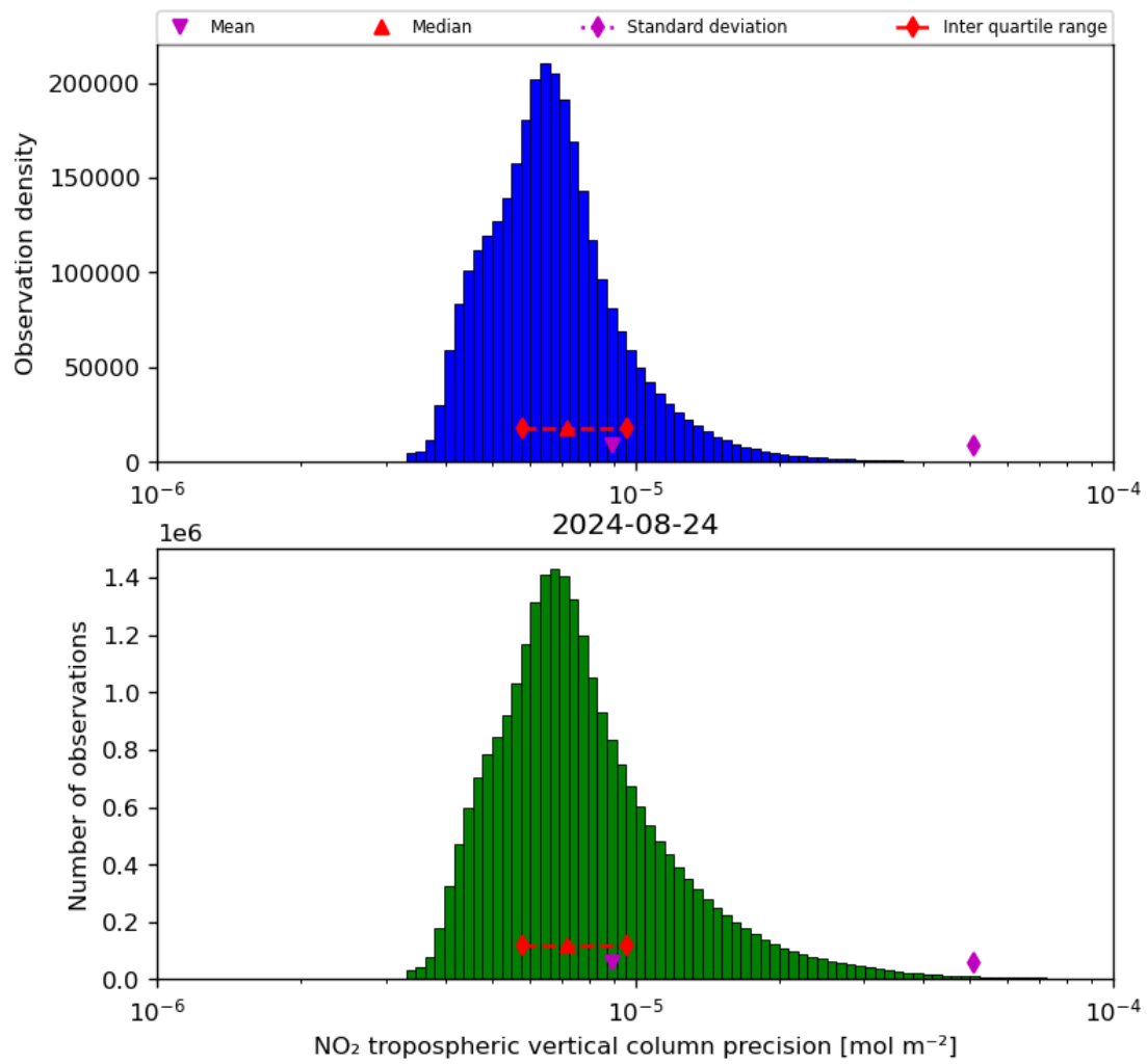
Figure 30: Histogram of “NO 2 tropospheric vertical column precision” for 2024-08-23 to 2024-08-25
