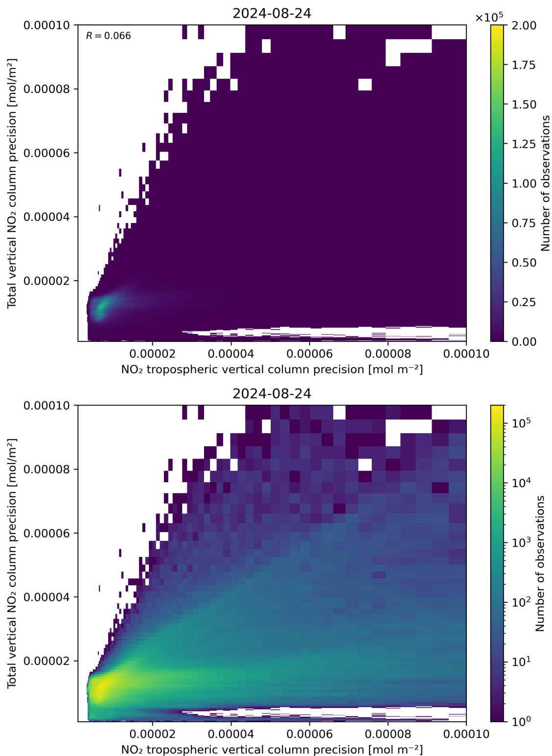
Figure 139: Scatter density plot of “NO 2 tropospheric vertical column precision” against “Total vertical NO 2 column precision” for 2024-08-23 to 2024-08-25.
