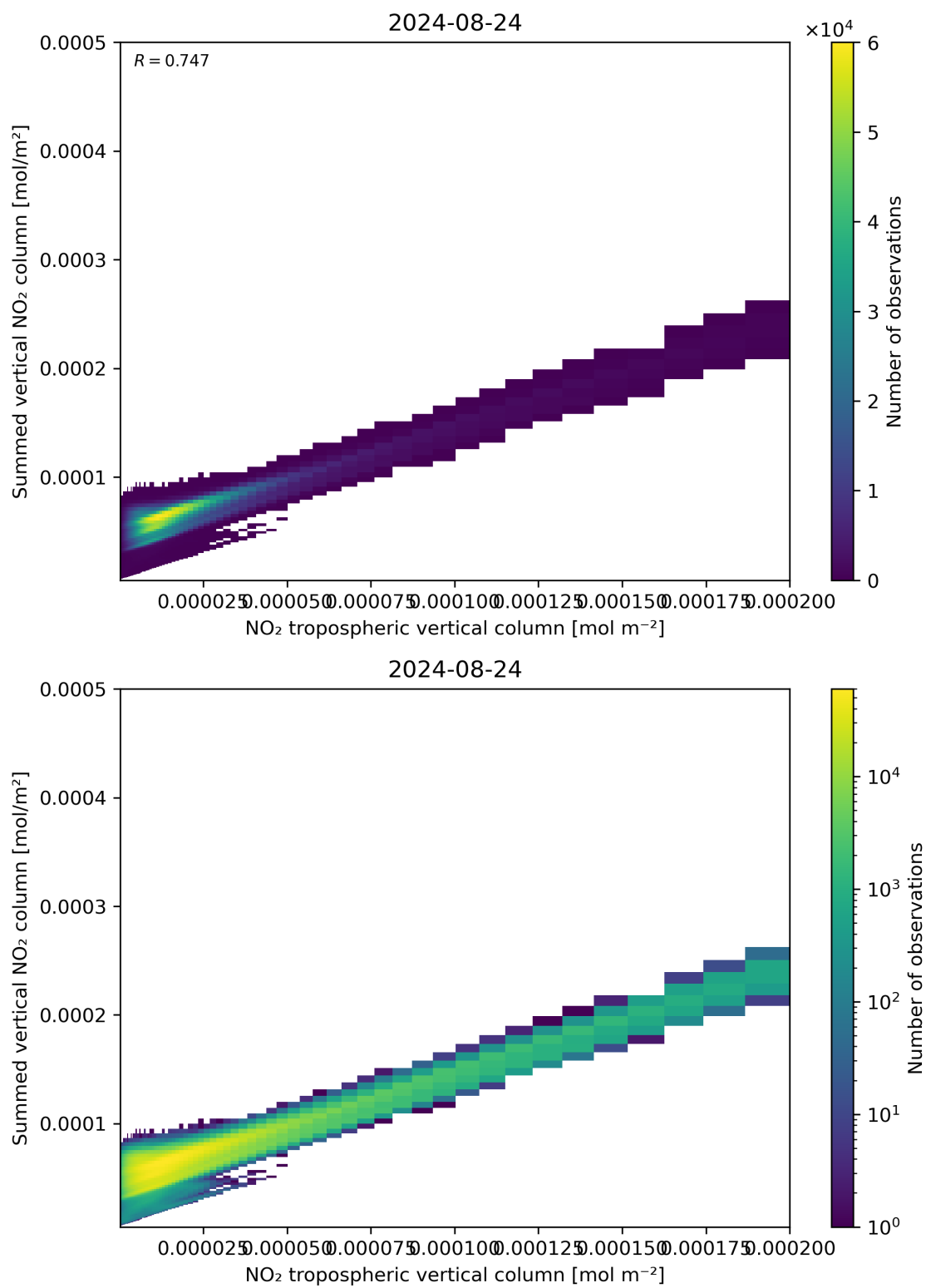
Figure 126: Scatter density plot of “NO 2 tropospheric vertical column” against “Summed vertical NO 2 column” for 2024-08-23 to 2024-08-25.
