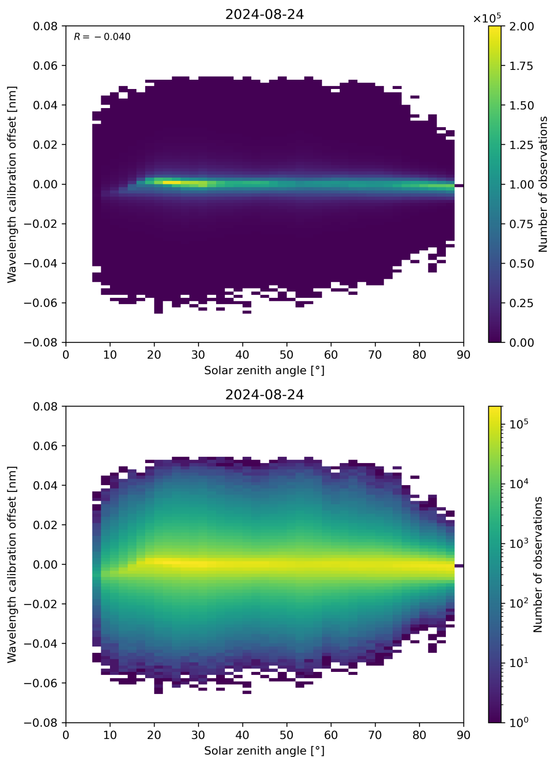
Figure 158: Scatter density plot of “Solar zenith angle” against “Wavelength calibration offset” for 2024-08-23 to 2024-08-25.
