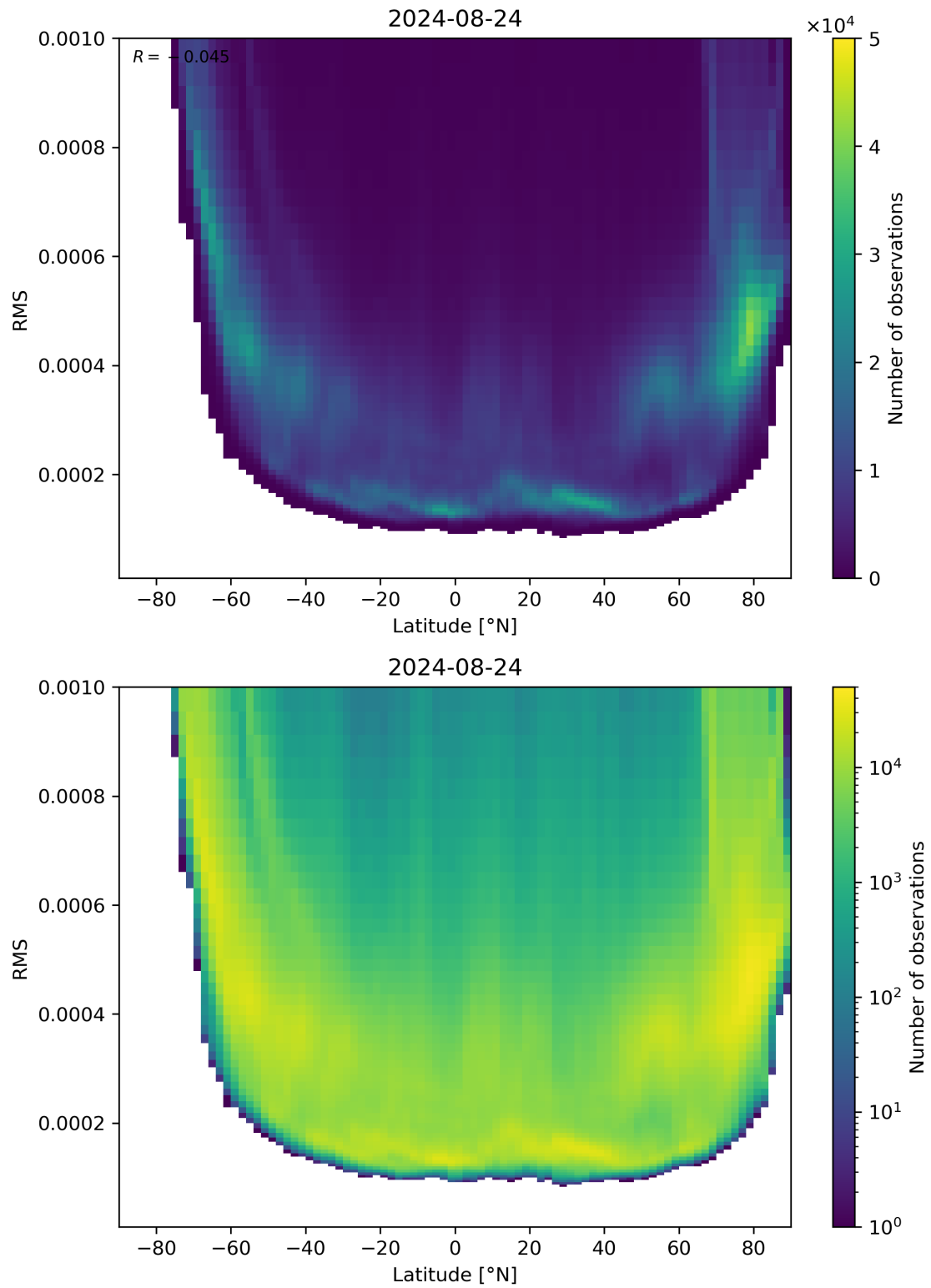
Figure 94: Scatter density plot of “Latitude” against “RMS” for 2024-08-23 to 2024-08-25.
