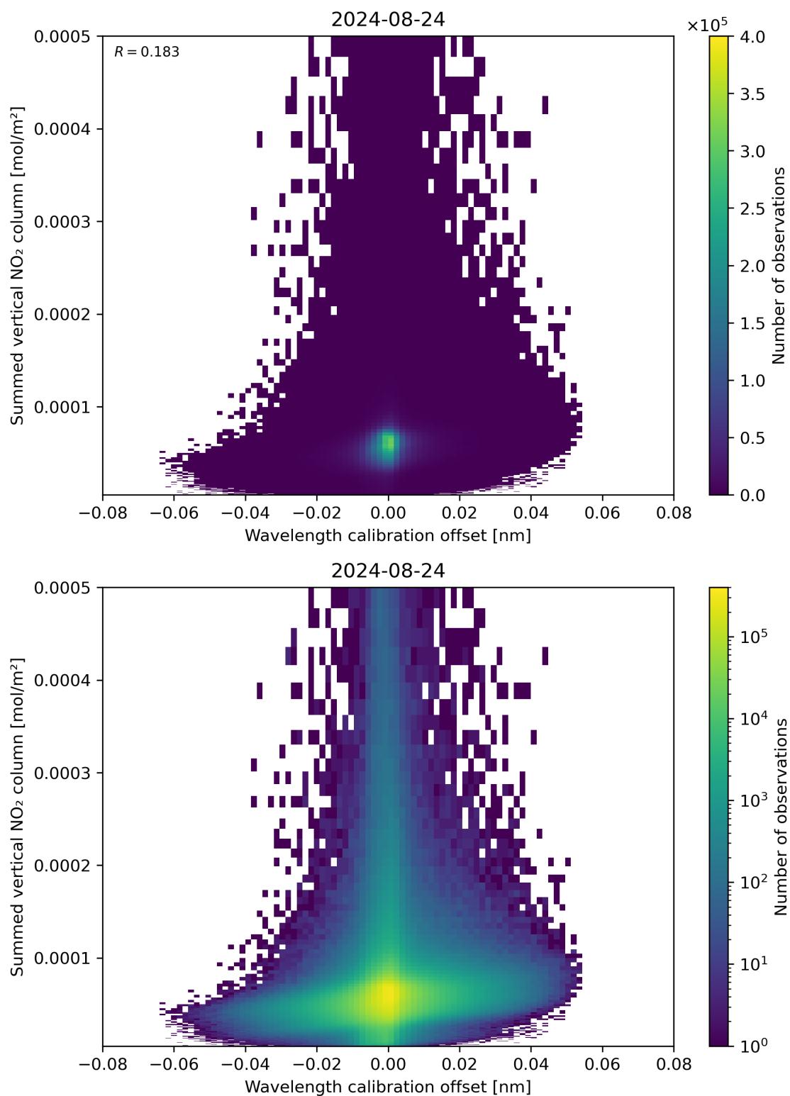
Figure 177: Scatter density plot of “Wavelength calibration offset” against “Summed vertical NO 2 column” for 2024-08-23 to 2024-08-25.
