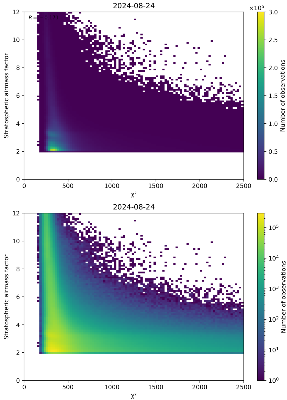
Figure 81: Scatter density plot of “ \chi^2 ” against “Stratospheric airmass factor” for 2024-08-23 to 2024-08-25.
