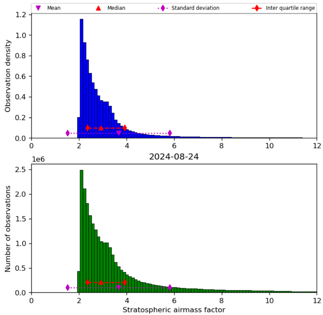
Figure 44: Histogram of “Stratospheric airmass factor” for 2024-08-23 to 2024-08-25
