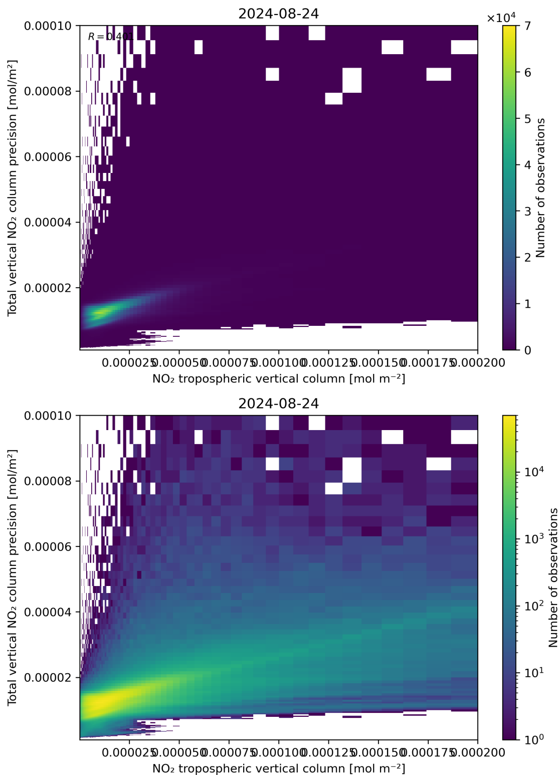
Figure 129: Scatter density plot of “NO 2 tropospheric vertical column” against “Total vertical NO 2 column precision” for 2024-08-23 to 2024-08-25.
