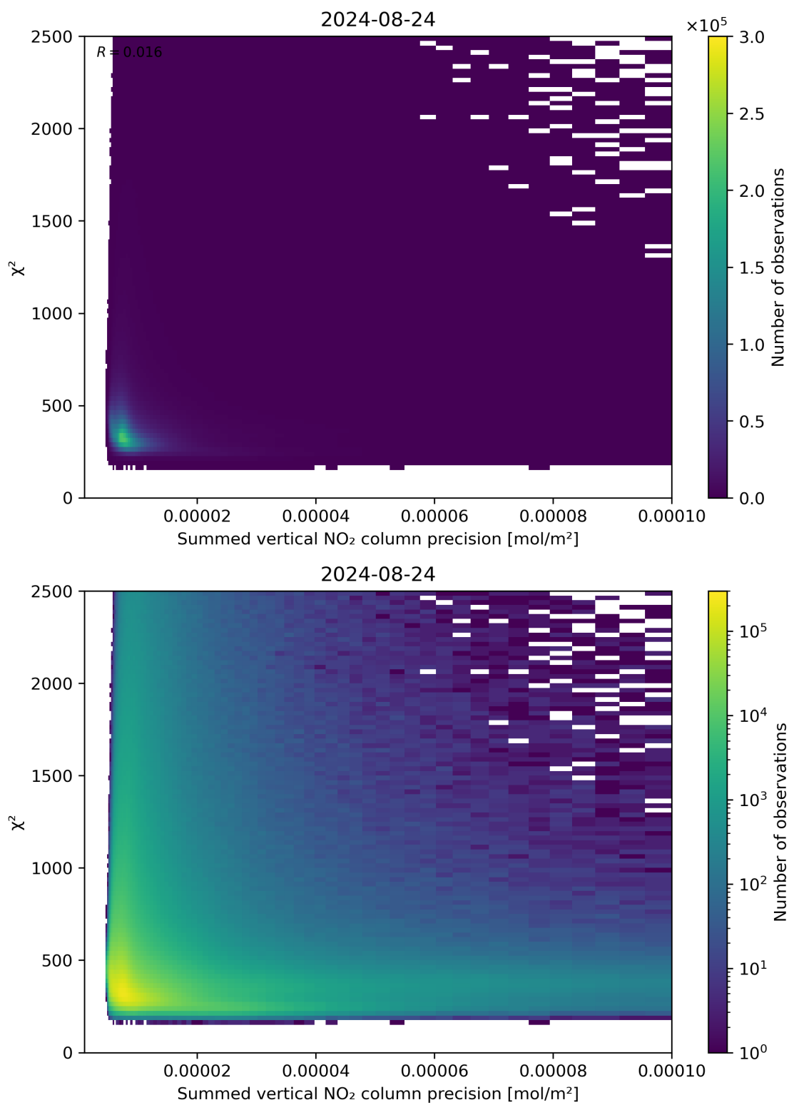
Figure 107: Scatter density plot of “Summed vertical NO 2 column precision” against “ \chi^2 ” for 2024-08-23 to 2024-08-25.
