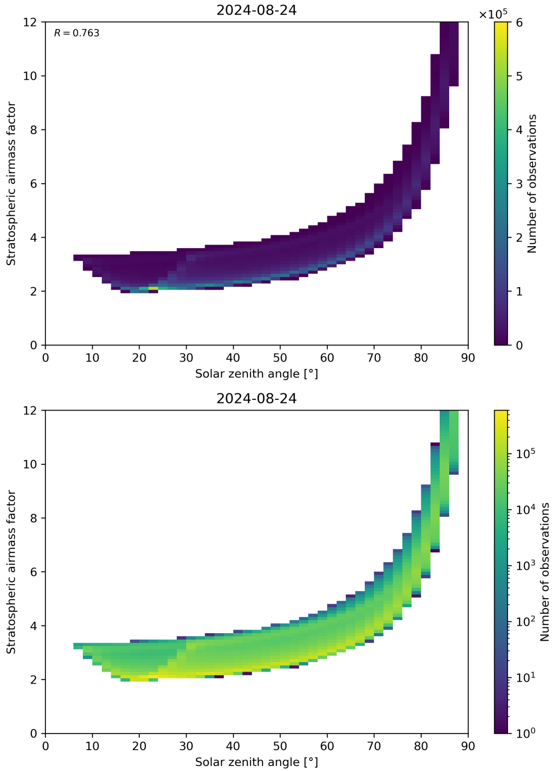
Figure 145: Scatter density plot of “Solar zenith angle” against “Stratospheric airmass factor” for 2024-08-23 to 2024-08-25.
