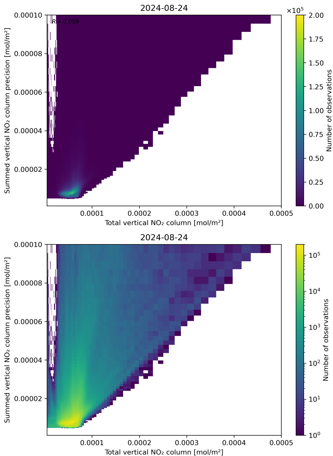
Figure 113: Scatter density plot of “Total vertical NO 2 column” against “Summed vertical NO 2 column precision” for 2024-08-23 to 2024-08-25.
