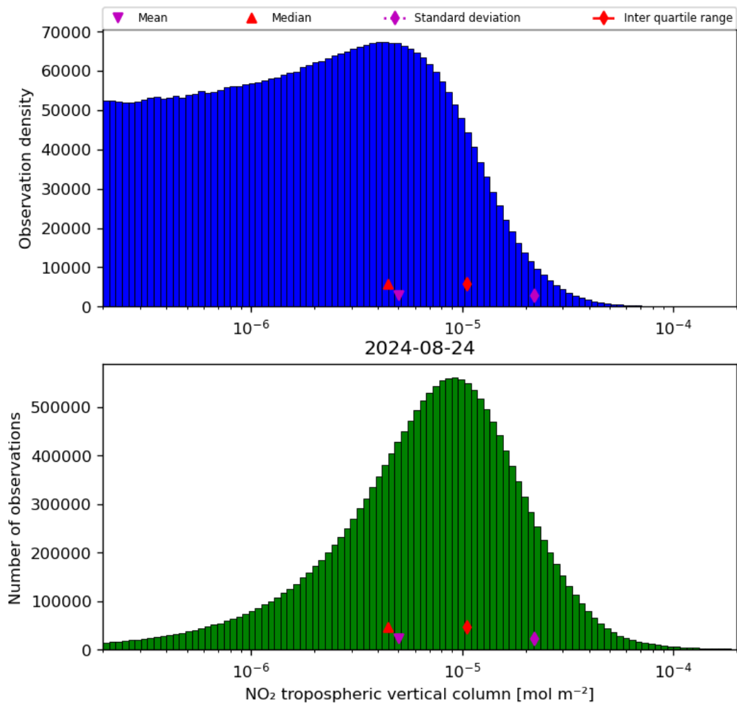
Figure 29: Histogram of “NO 2 tropospheric vertical column” for 2024-08-23 to 2024-08-25
