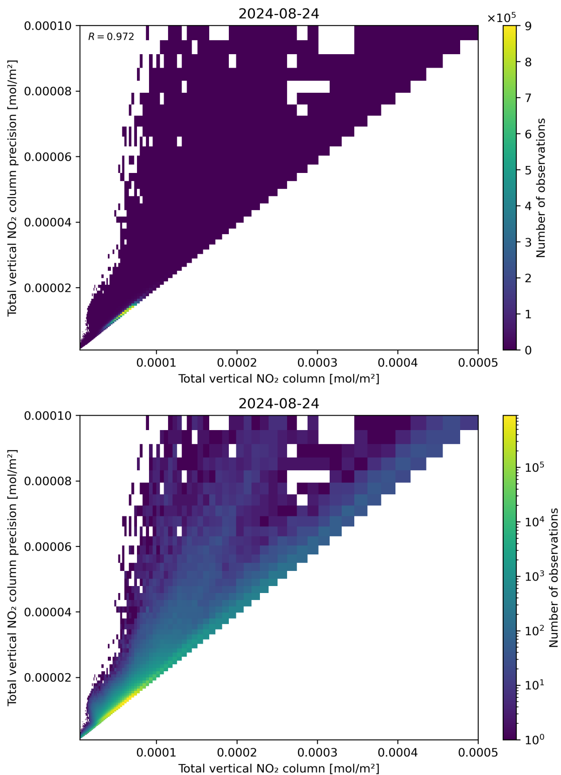
Figure 114: Scatter density plot of “Total vertical NO 2 column” against “Total vertical NO 2 column precision” for 2024-08-23 to 2024-08-25.
