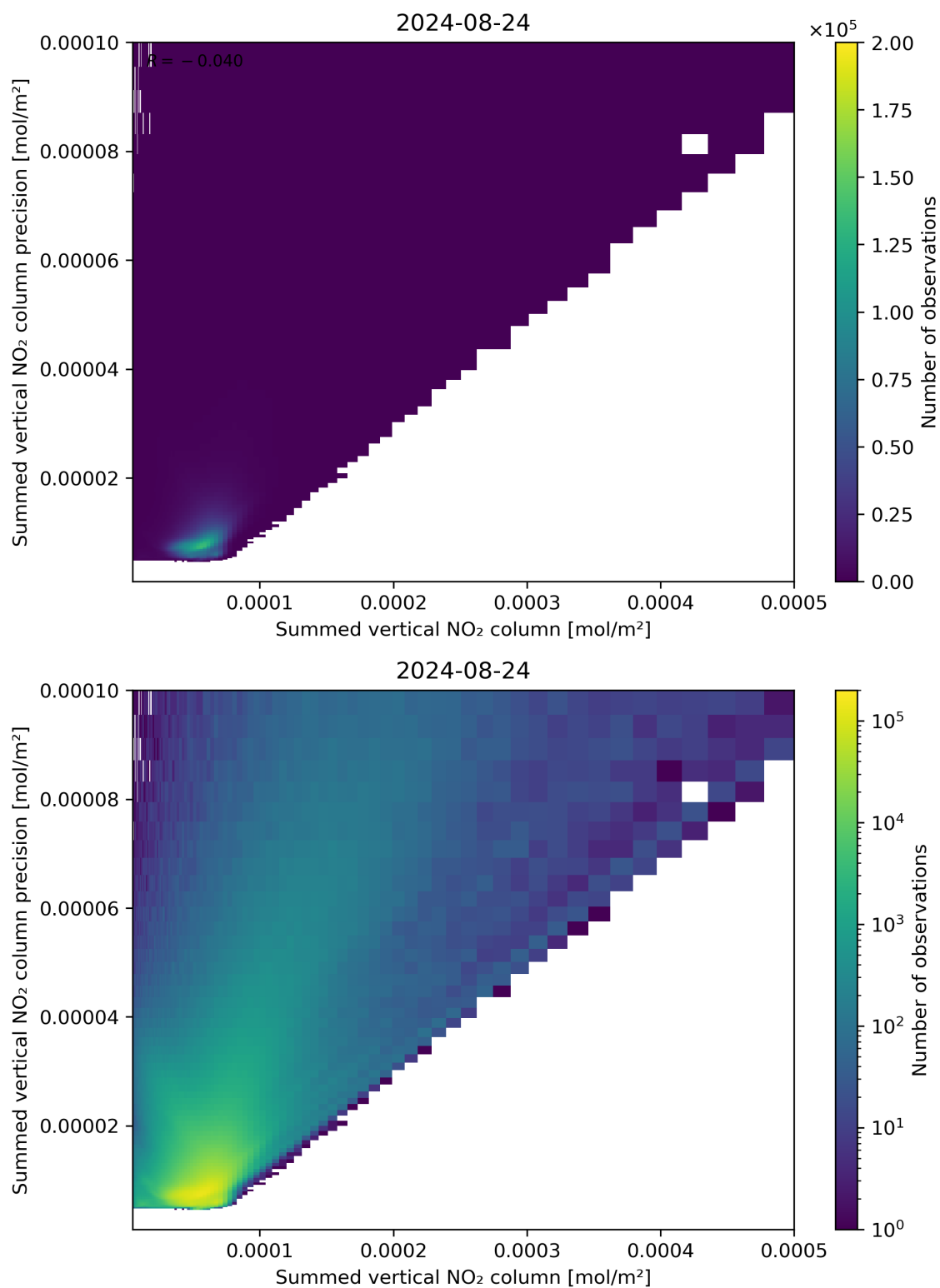
Figure 105: Scatter density plot of “Summed vertical NO 2 column” against “Summed vertical NO 2 column precision” for 2024-08-23 to 2024-08-25.
