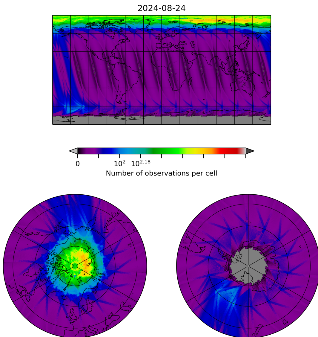
Figure 10: Map of the number of observations for 2024-08-23 to 2024-08-25
