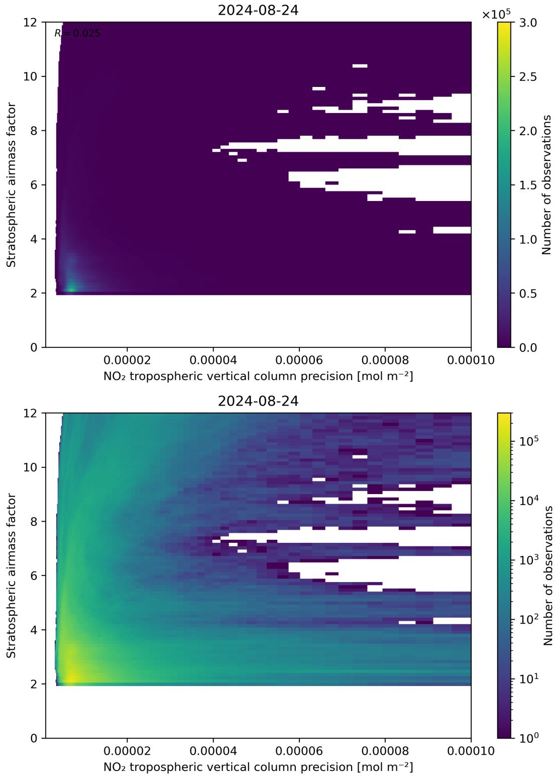
Figure 131: Scatter density plot of “NO 2 tropospheric vertical column precision” against “Stratospheric airmass factor” for 2024-08-23 to 2024-08-25.
