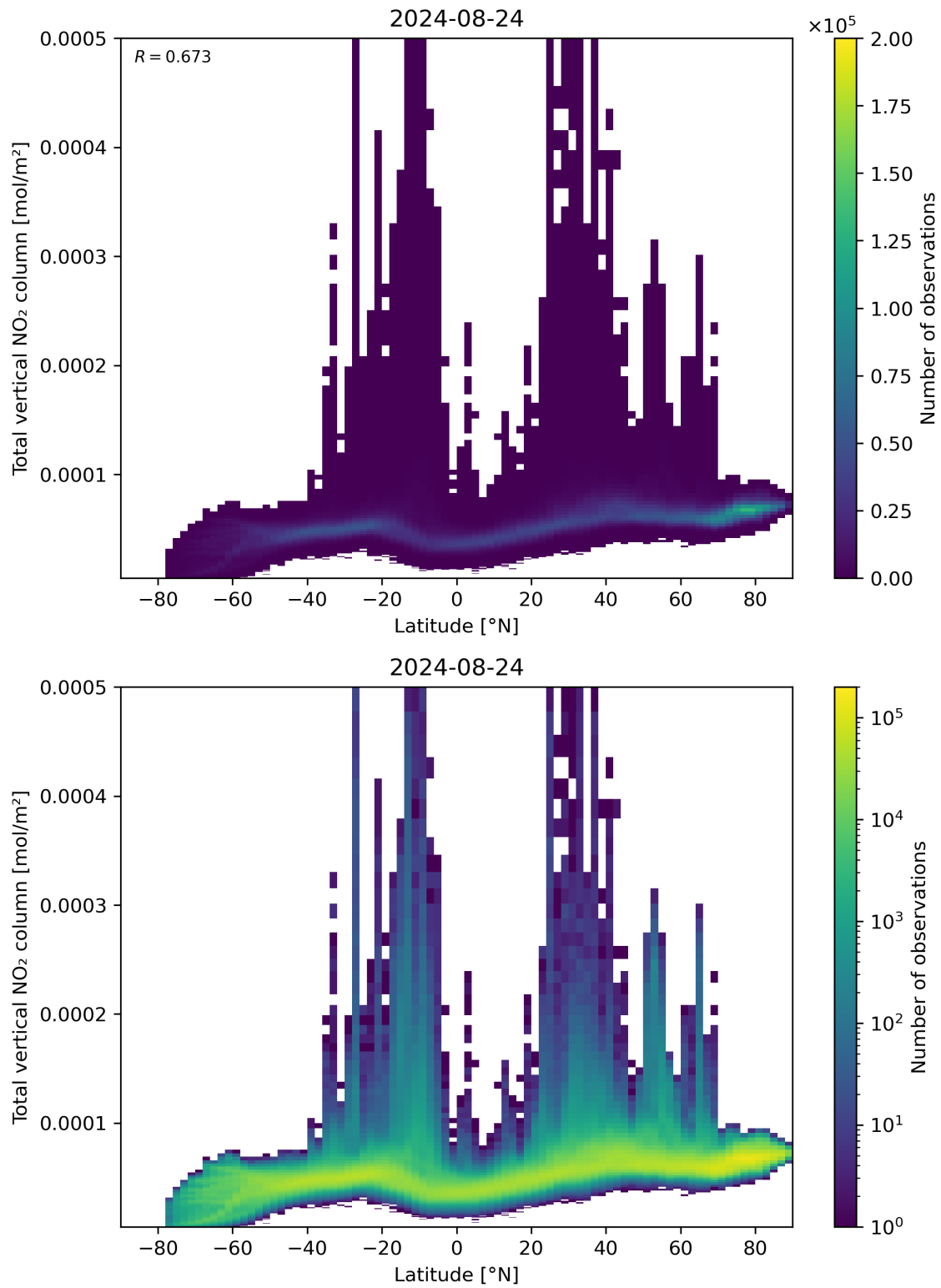
Figure 90: Scatter density plot of “Latitude” against “Total vertical NO 2 column” for 2024-08-23 to 2024-08-25.
