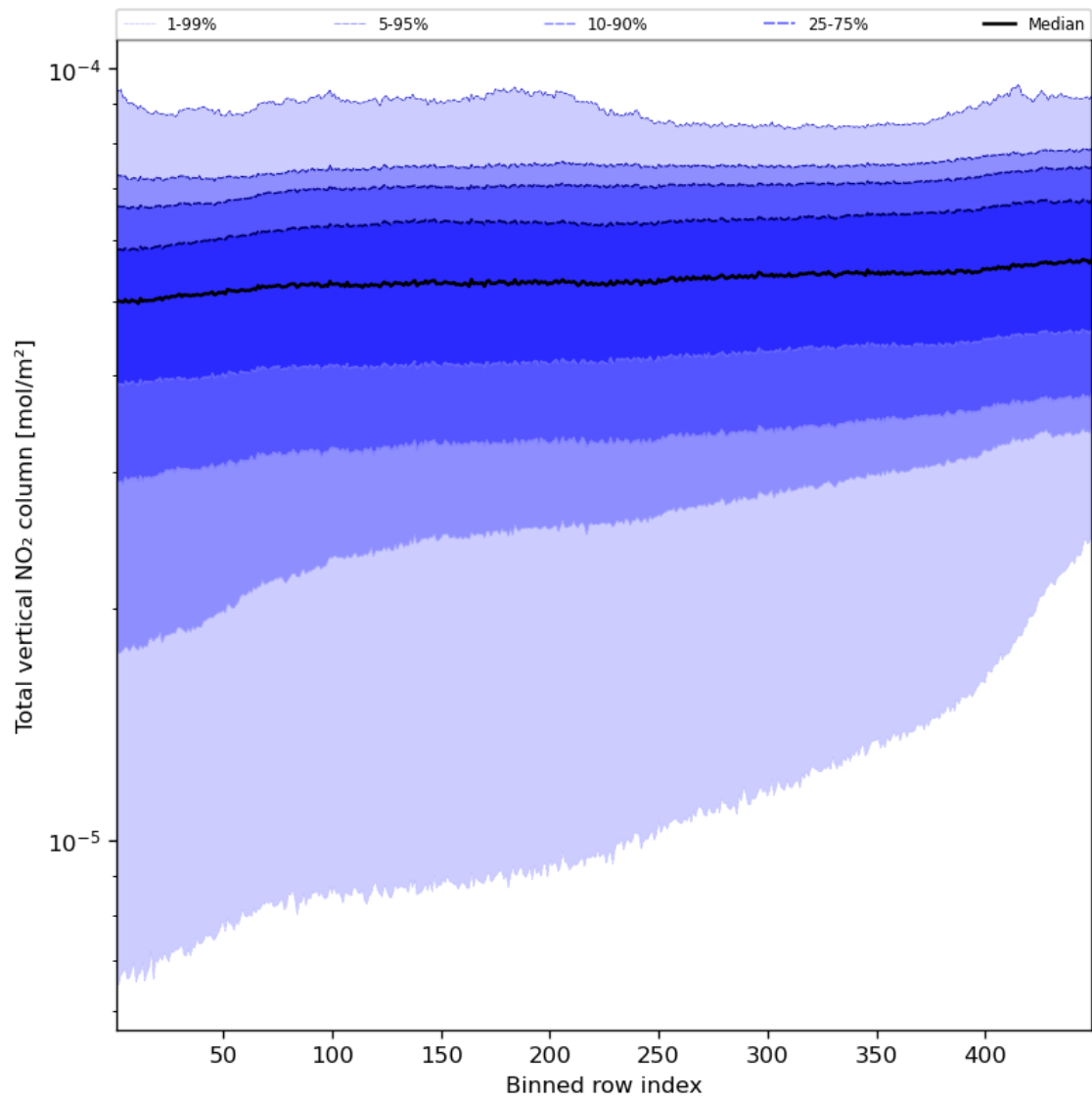
Figure 55: Along track statistics of “Total vertical NO 2 column” for 2024-08-23 to 2024-08-25
