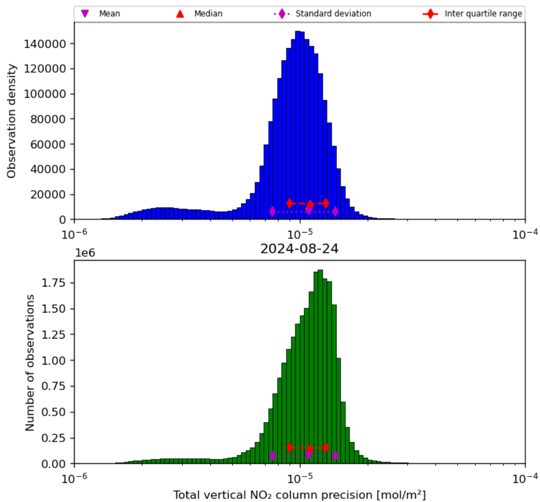
Figure 39: Histogram of “Total vertical NO 2 column precision” for 2024-08-23 to 2024-08-25
