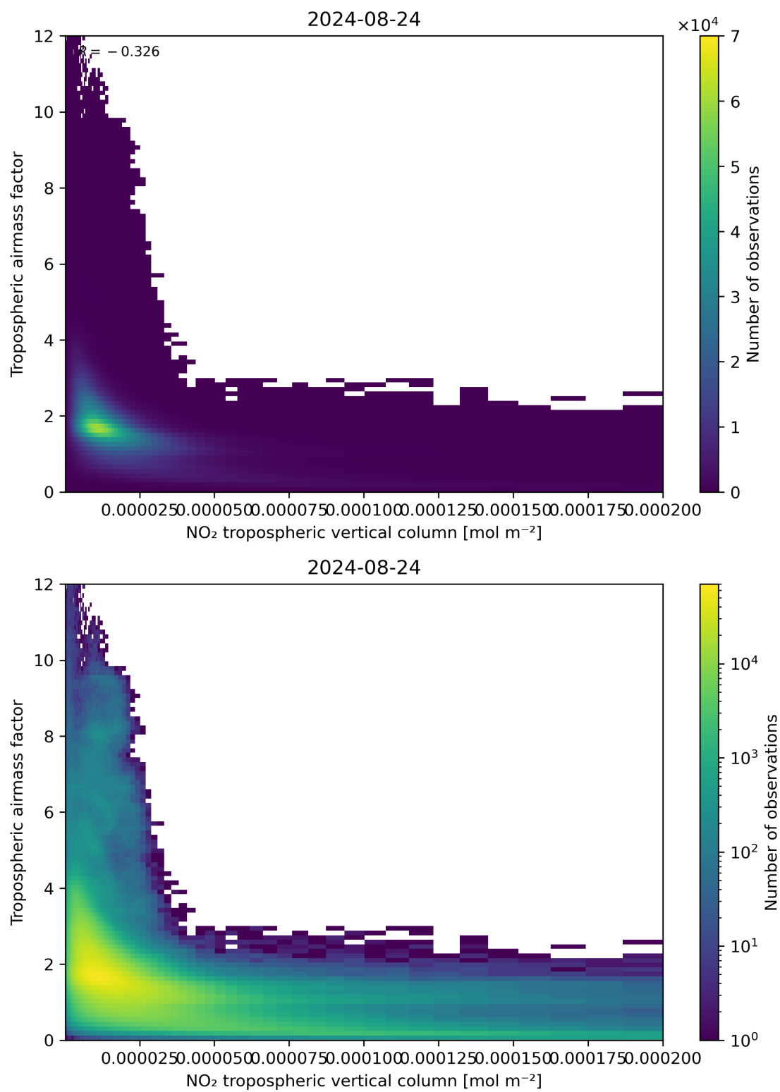
Figure 123: Scatter density plot of “NO 2 tropospheric vertical column” against “Tropospheric air mass factor” for 2024-08-23 to 2024-08-25.
