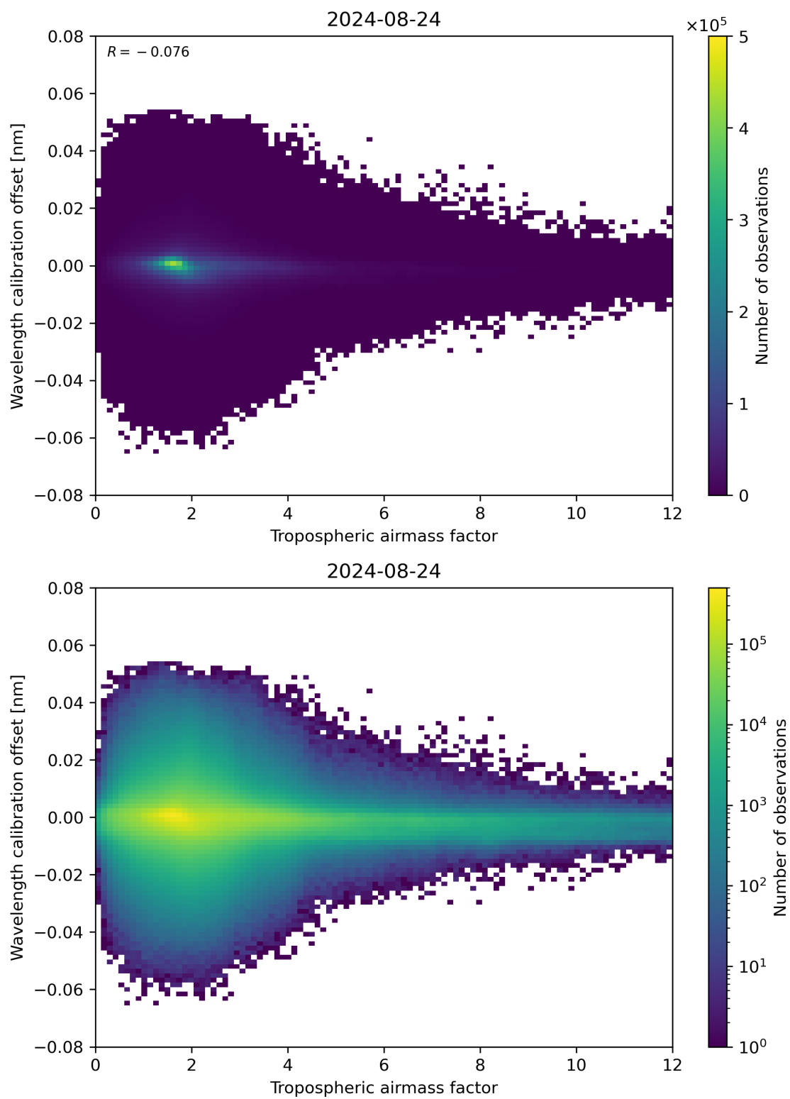
Figure 80: Scatter density plot of “Tropospheric airmass factor” against “Wavelength calibration offset” for 2024-08-23 to 2024-08-25.
