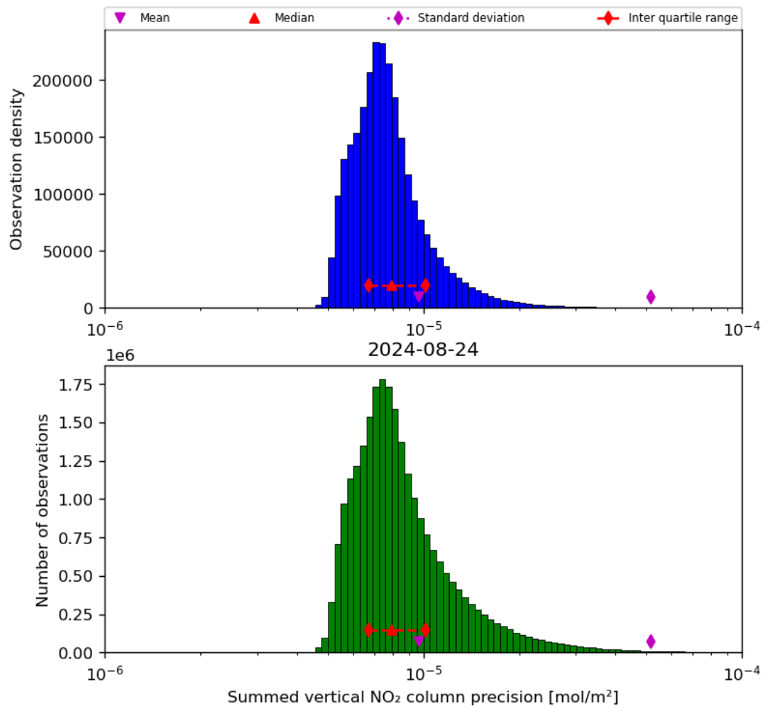
Figure 41: Histogram of “Summed vertical NO 2 column precision” for 2024-08-23 to 2024-08-25
