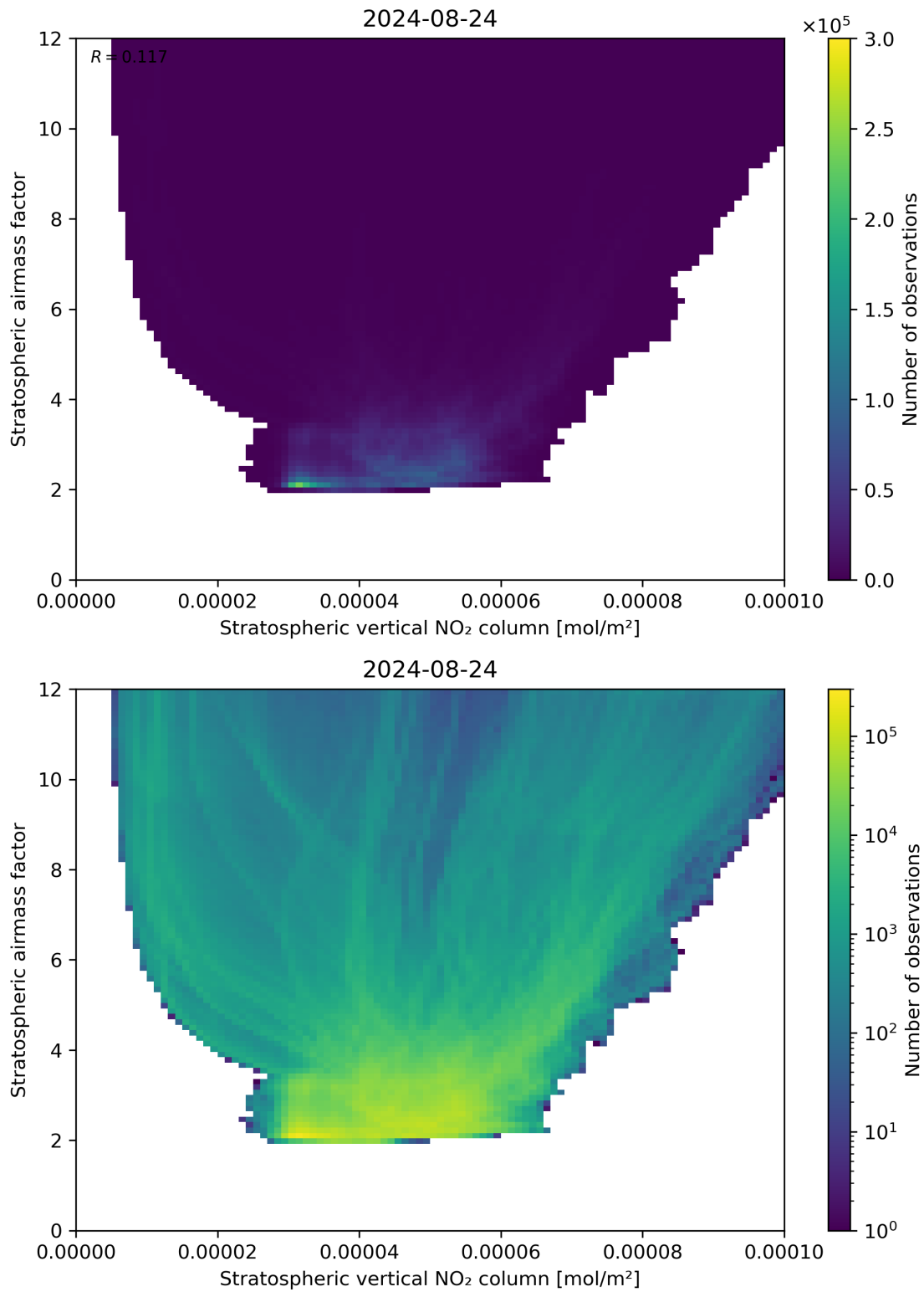
Figure 96: Scatter density plot of “Stratospheric vertical NO 2 column” against “Stratospheric airmass factor” for 2024-08-23 to 2024-08-25.
