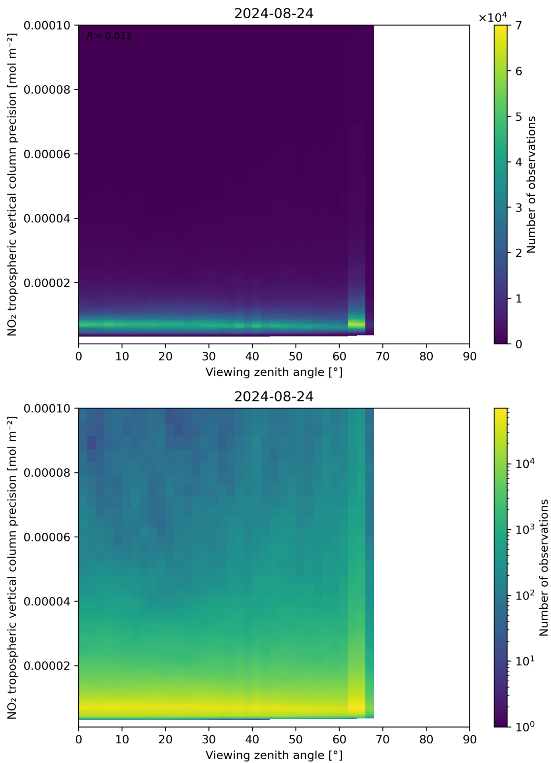
Figure 170: Scatter density plot of “Viewing zenith angle” against “NO 2 tropospheric vertical column precision” for 2024-08-23 to 2024-08-25.
