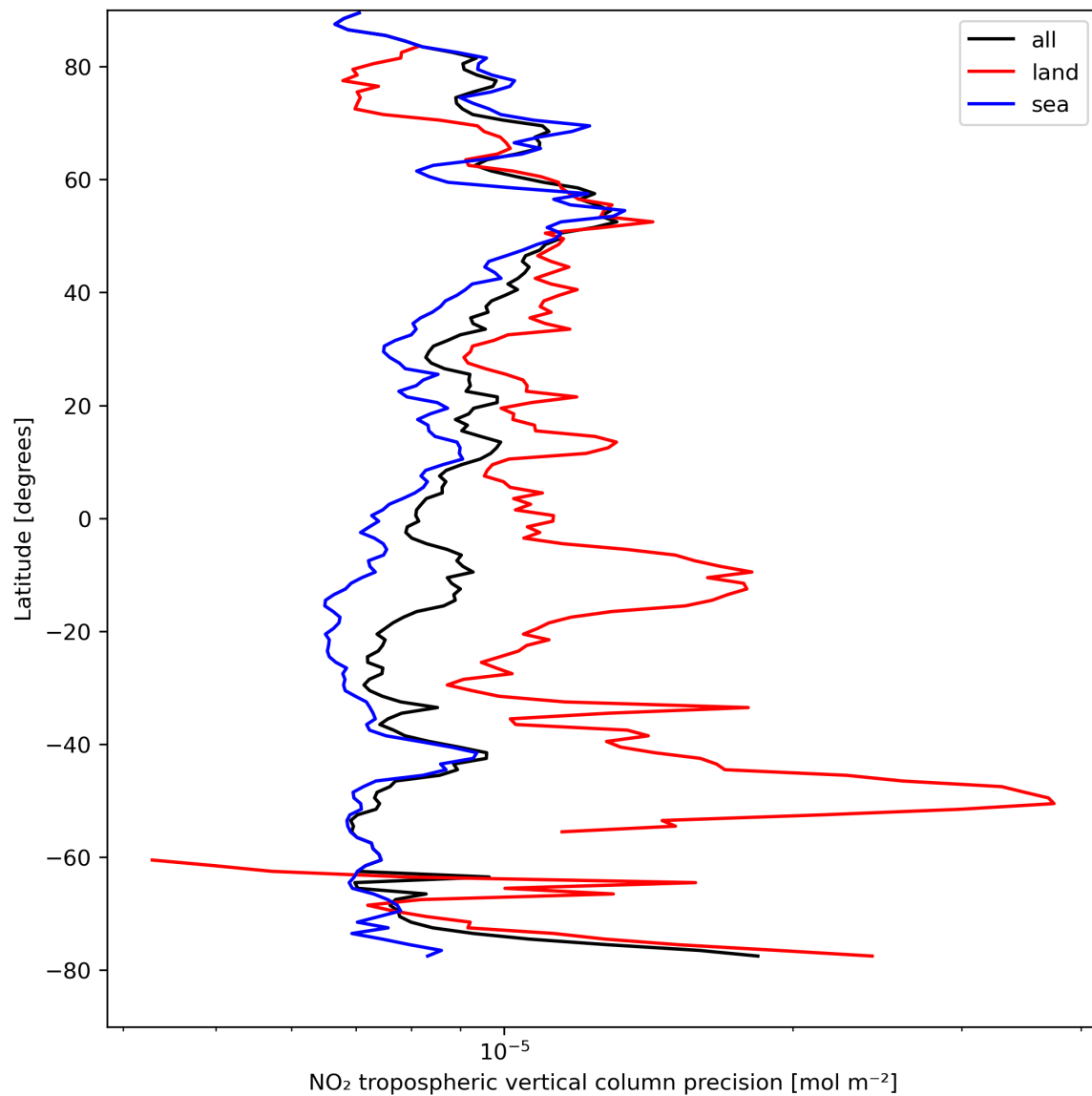
Figure 13: Zonal average of “NO 2 tropospheric vertical column precision” for 2024-08-23 to 2024-08-25.
