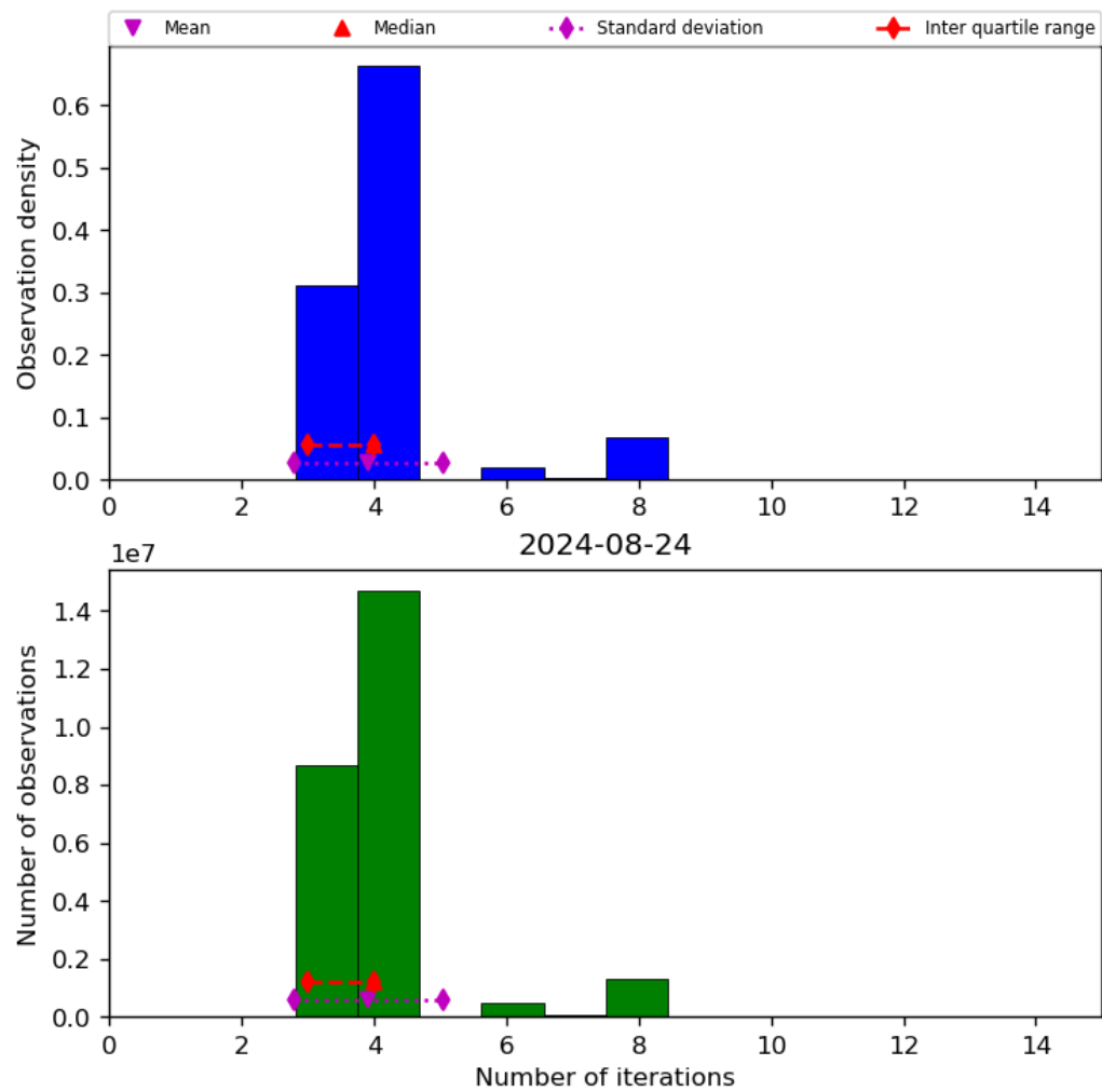
Figure 34: Histogram of “Number of iterations” for 2024-08-23 to 2024-08-25
