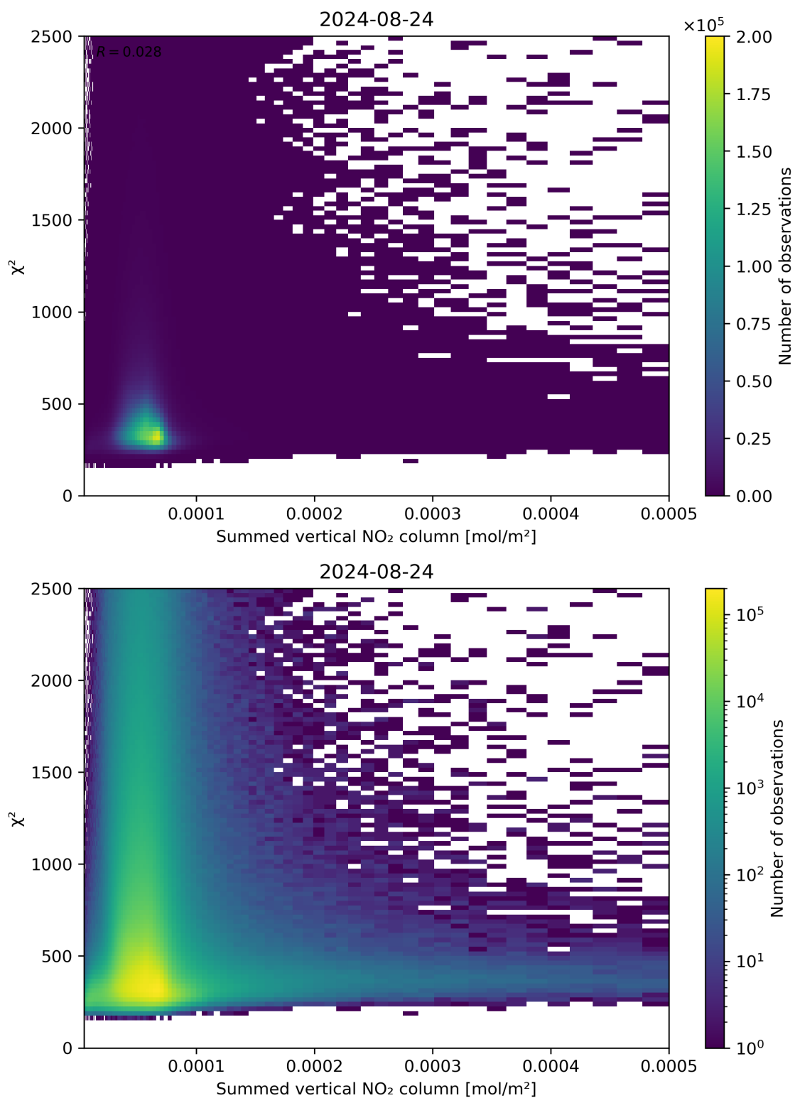
Figure 104: Scatter density plot of “Summed vertical NO 2 column” against “ \chi^2 ” for 2024-08-23 to 2024-08-25.
