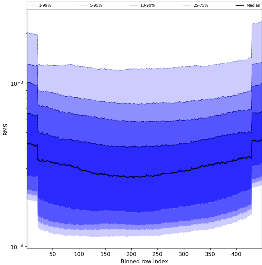
Figure 60: Along track statistics of “RMS” for 2024-08-23 to 2024-08-25
