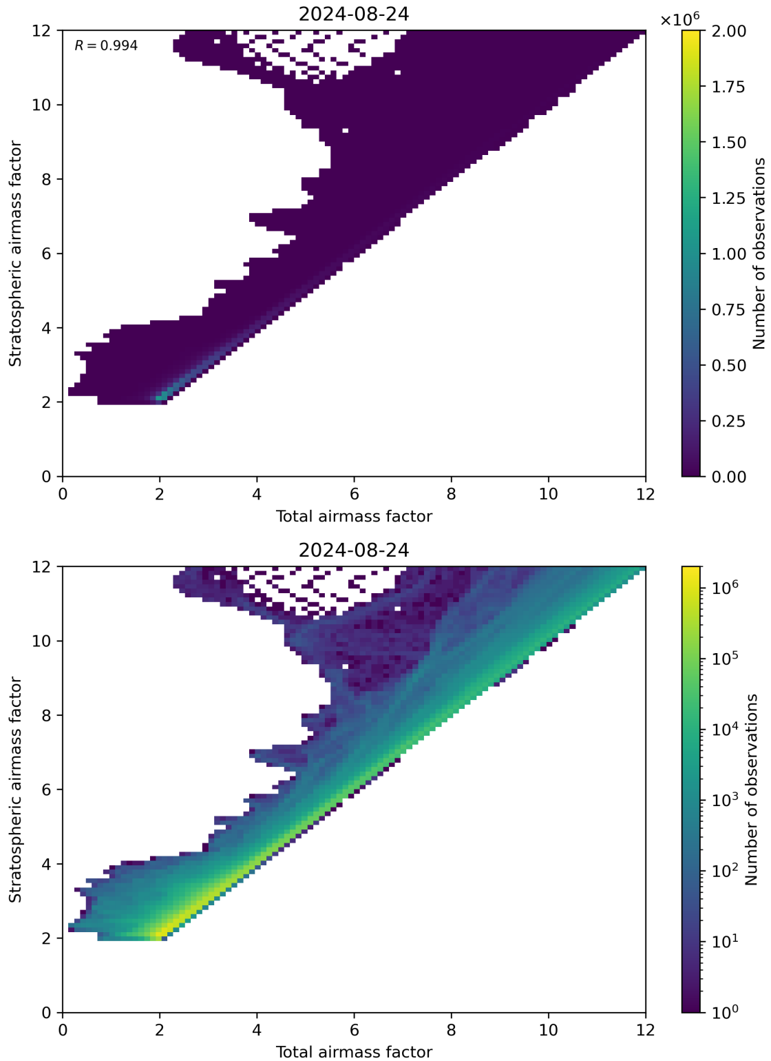
Figure 62: Scatter density plot of “Total airmass factor” against “Stratospheric airmass factor” for 2024-08-23 to 2024-08-25.
