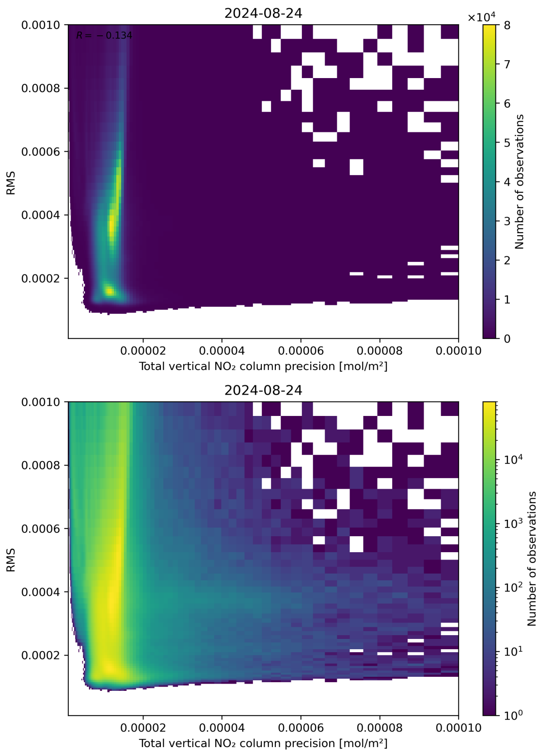
Figure 119: Scatter density plot of “Total vertical NO 2 column precision” against “RMS” for 2024-08-23 to 2024-08-25.
