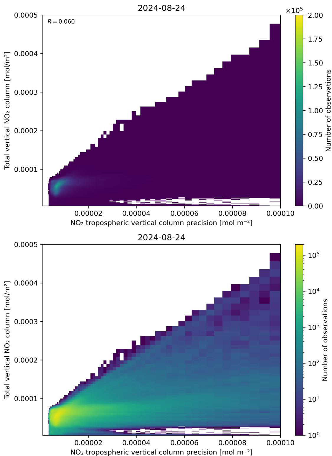
Figure 138: Scatter density plot of “NO 2 tropospheric vertical column precision” against “Total vertical NO 2 column” for 2024-08-23 to 2024-08-25.
