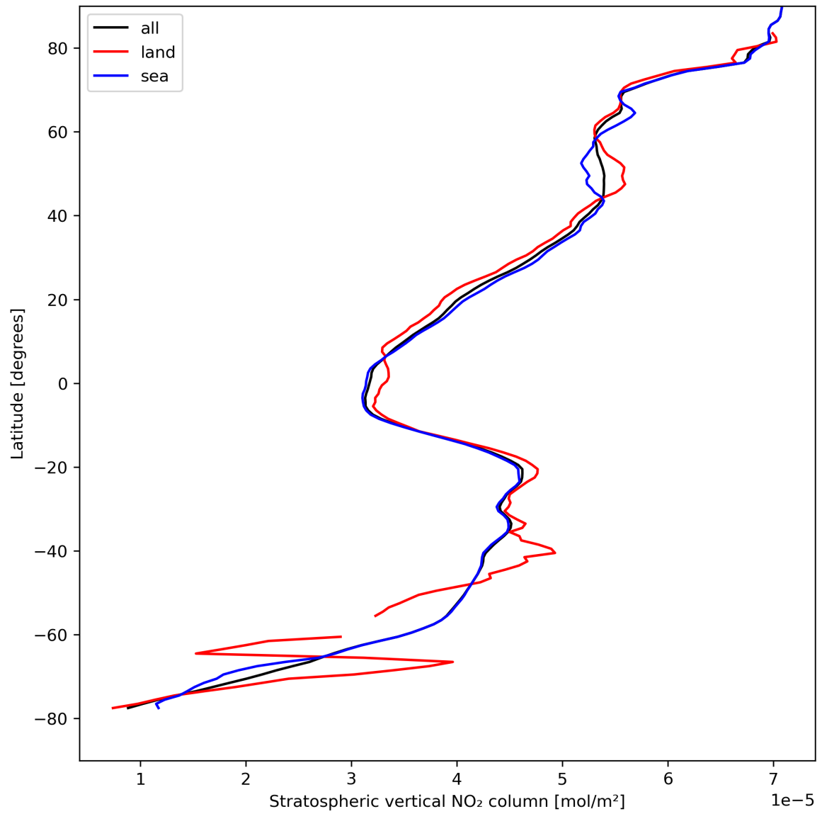
Figure 19: Zonal average of “Stratospheric vertical NO 2 column” for 2024-08-23 to 2024-08-25.
