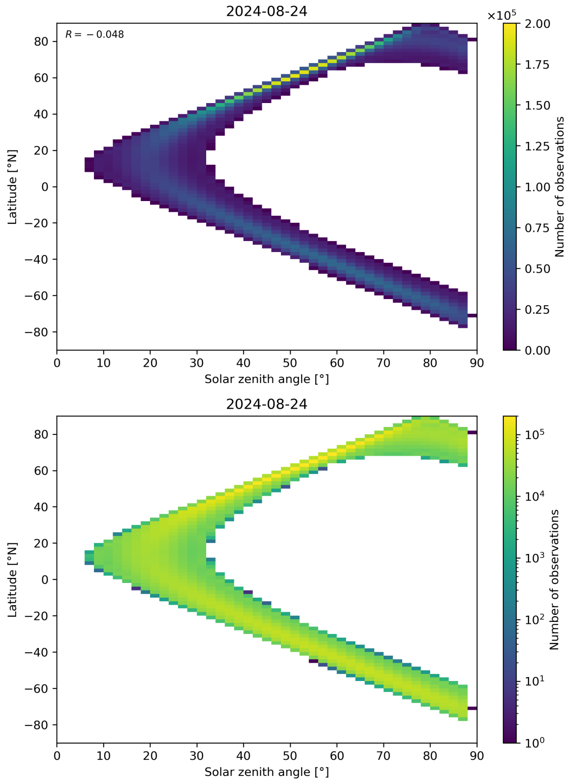
Figure 149: Scatter density plot of “Solar zenith angle” against “Latitude” for 2024-08-23 to 2024-08-25.
