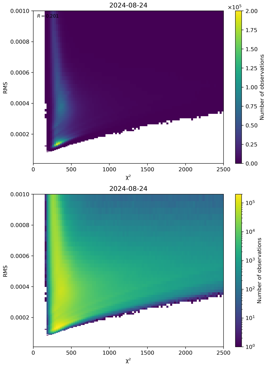
Figure 82: Scatter density plot of “ \chi^2 ” against “RMS” for 2024-08-23 to 2024-08-25.
