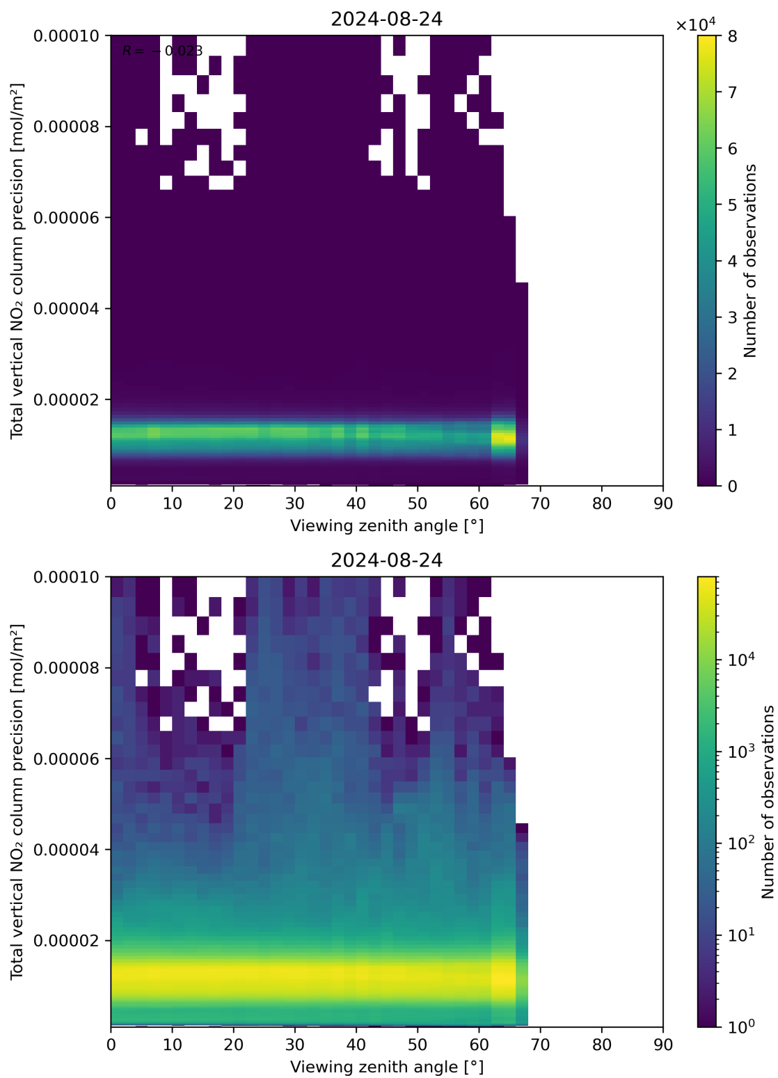
Figure 168: Scatter density plot of “Viewing zenith angle” against “Total vertical NO 2 column precision” for 2024-08-23 to 2024-08-25.
