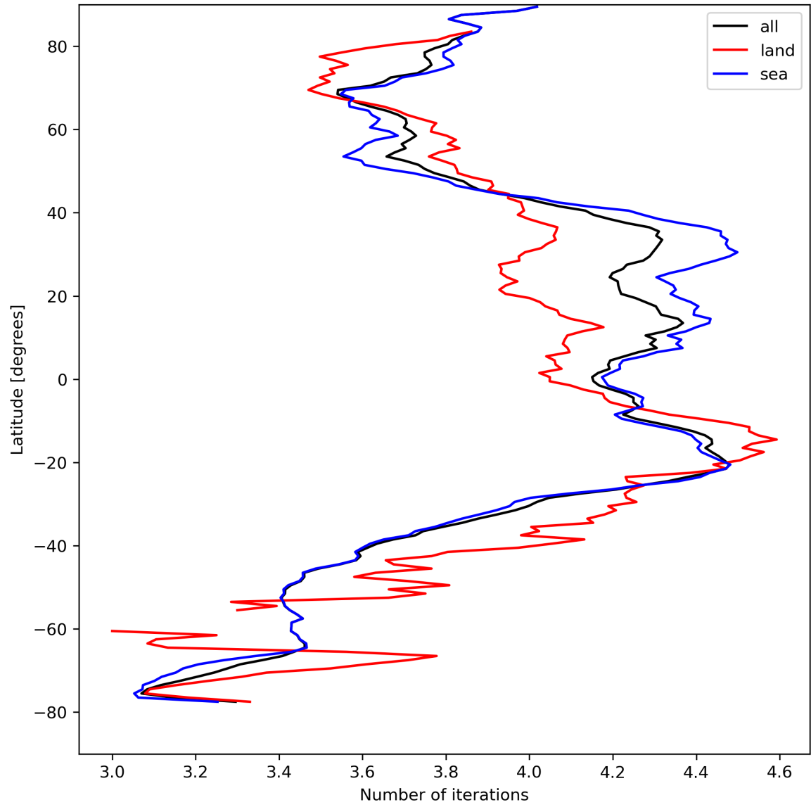
Figure 17: Zonal average of “Number of iterations” for 2024-08-23 to 2024-08-25.
