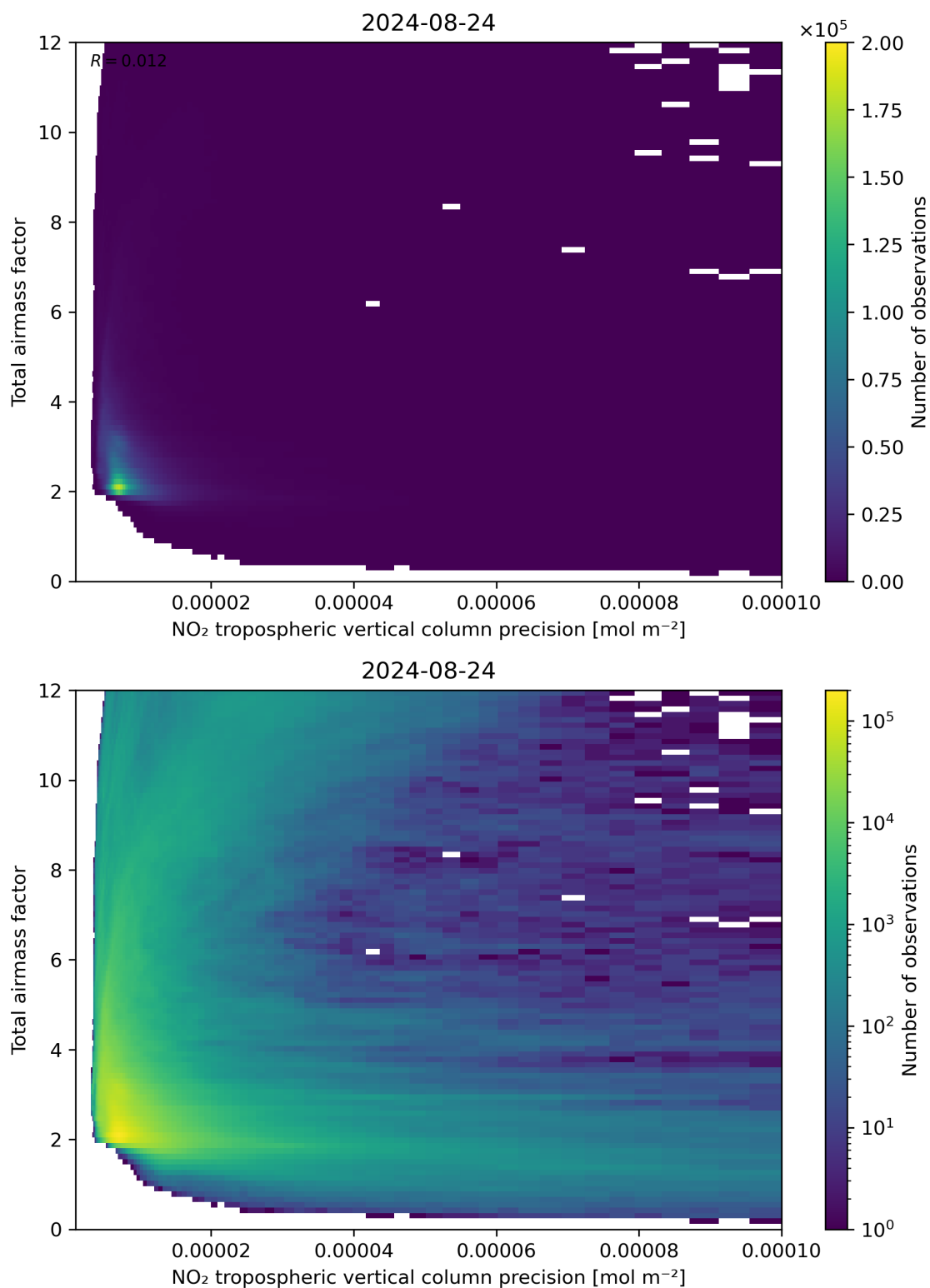
Figure 132: Scatter density plot of “NO 2 tropospheric vertical column precision” against “Total air mass factor” for 2024-08-23 to 2024-08-25.
