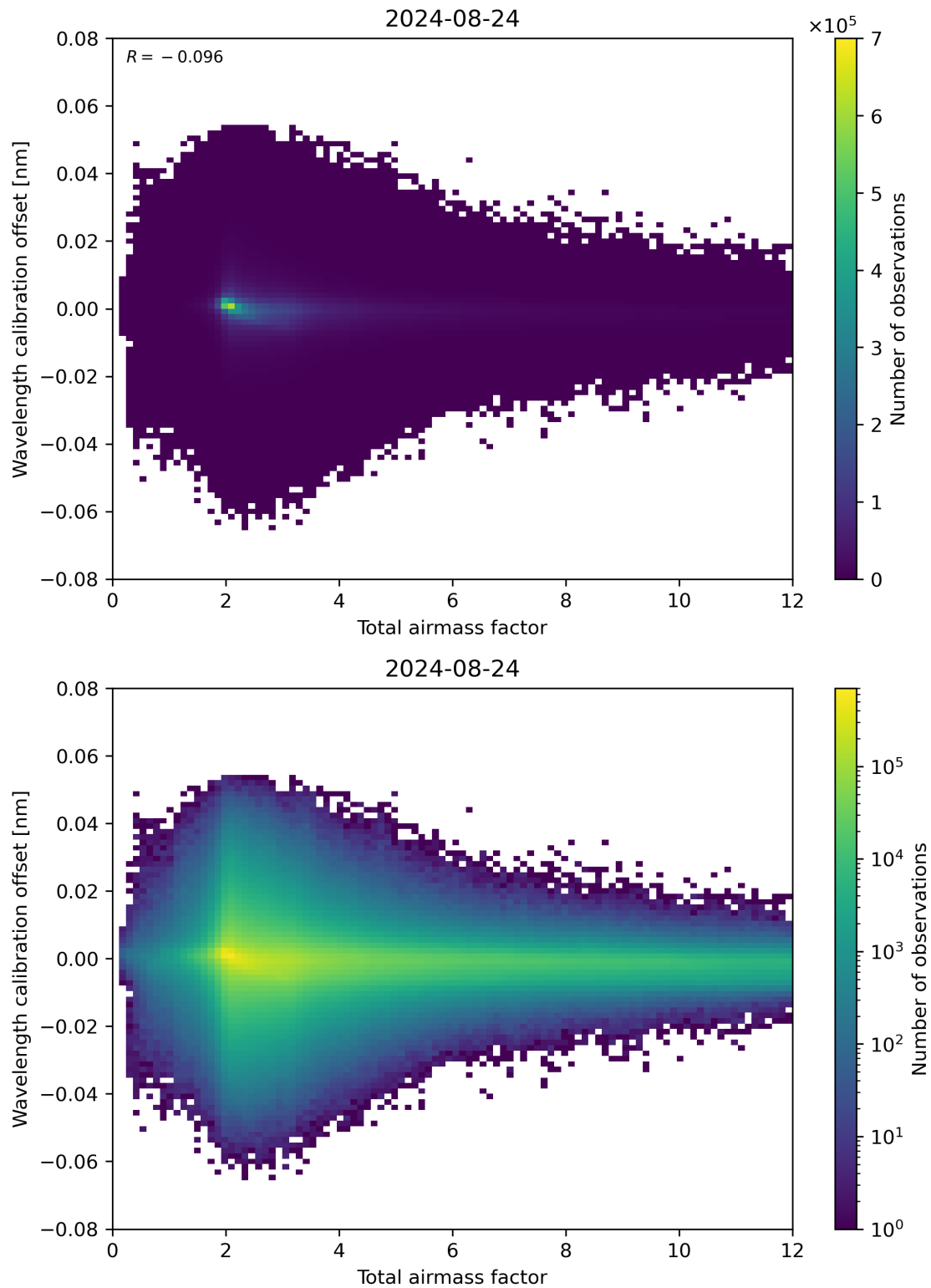
Figure 70: Scatter density plot of “Total airmass factor” against “Wavelength calibration offset” for 2024-08-23 to 2024-08-25.
