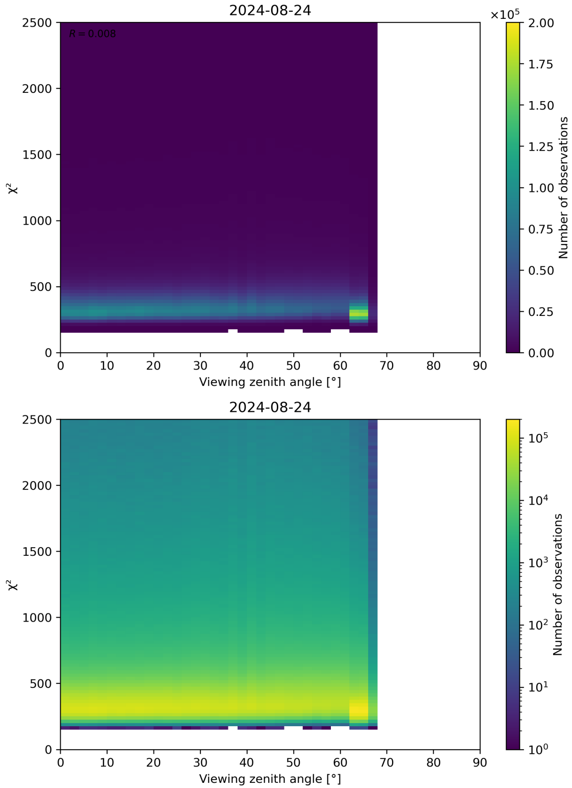
Figure 162: Scatter density plot of “Viewing zenith angle” against “ \chi^2 ” for 2024-08-23 to 2024-08-25.
