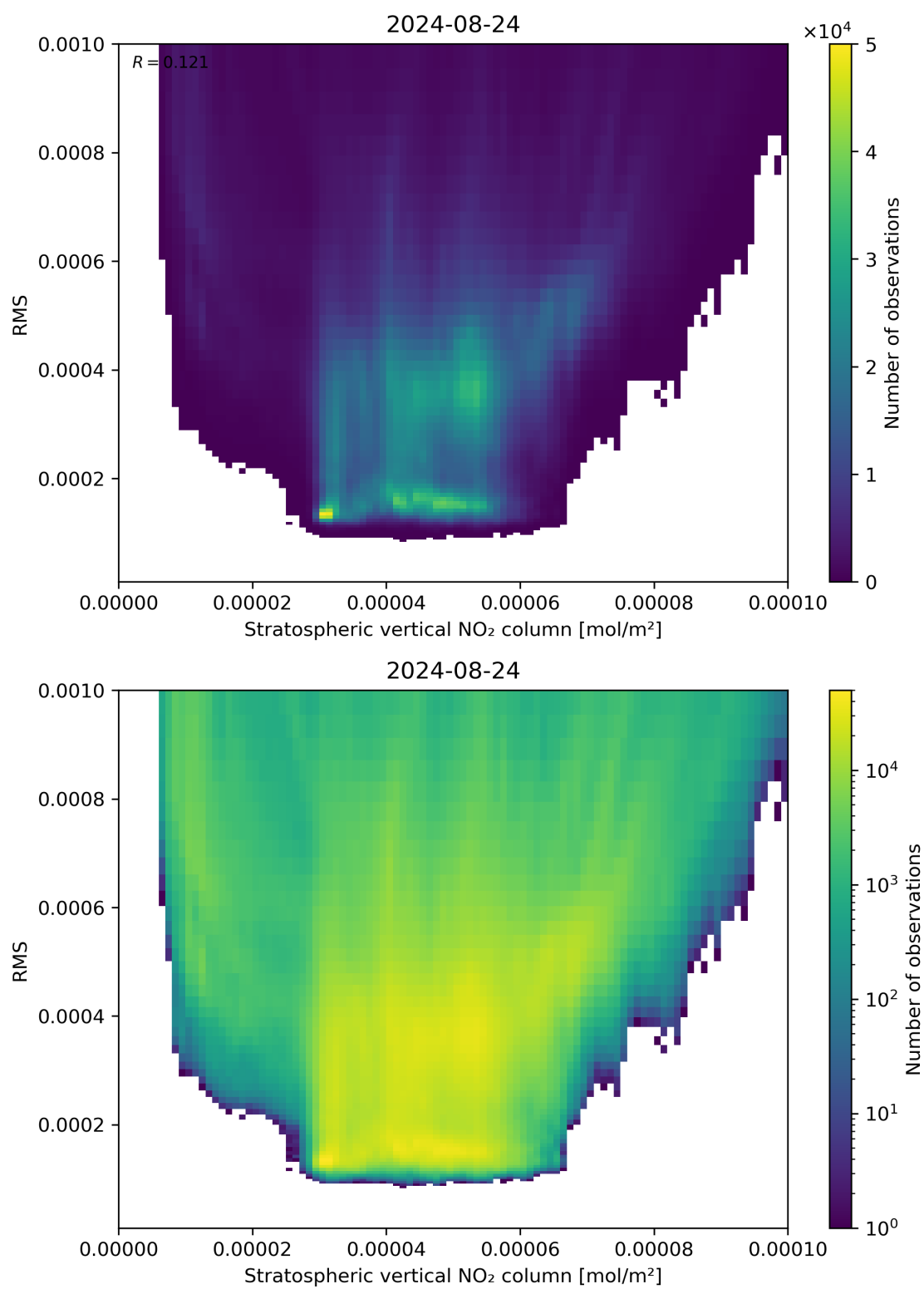
Figure 102: Scatter density plot of “Stratospheric vertical NO 2 column” against “RMS” for 2024-08-23 to 2024-08-25.
