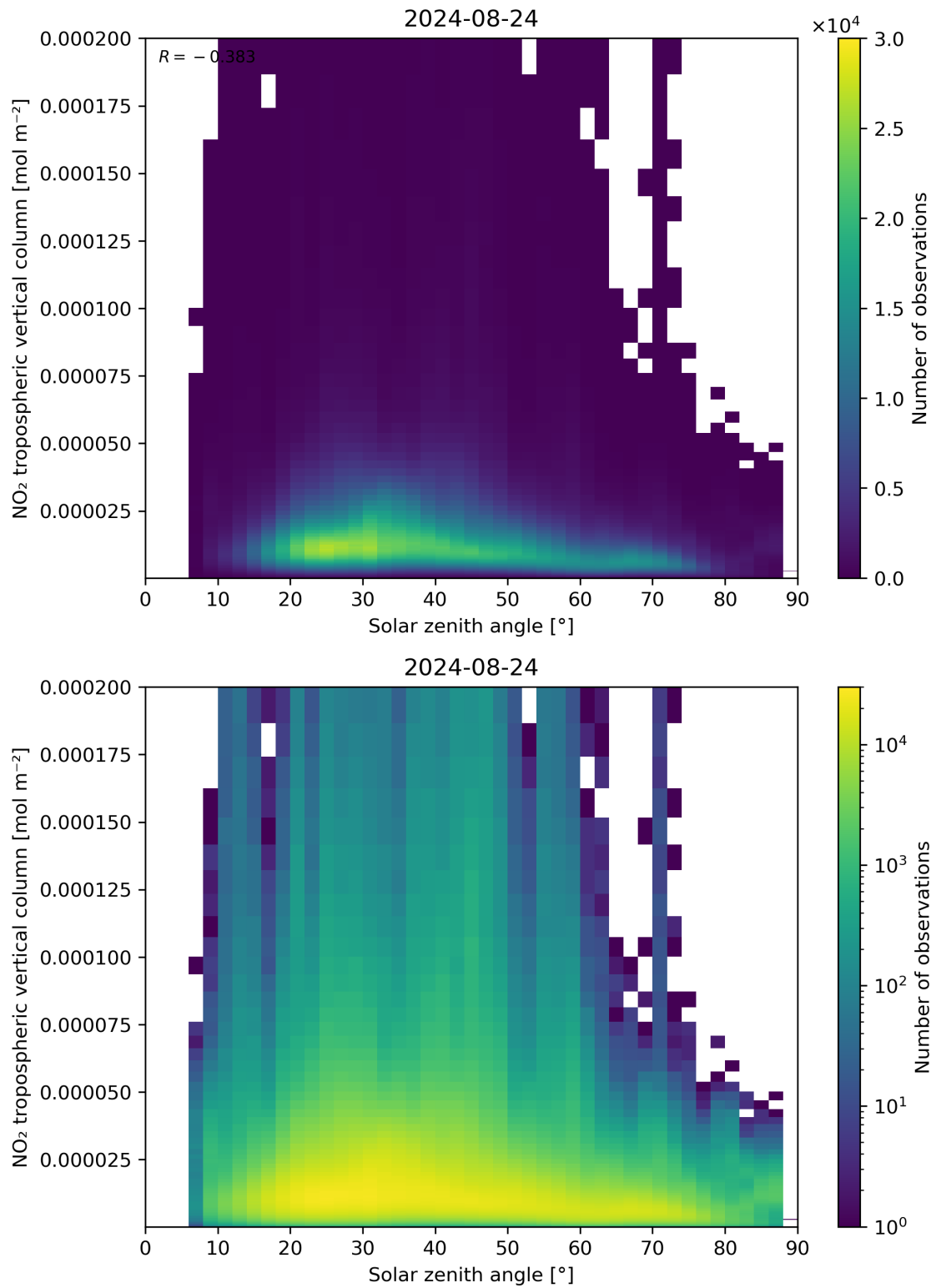
Figure 155: Scatter density plot of “Solar zenith angle” against “NO 2 tropospheric vertical column” for 2024-08-23 to 2024-08-25.
