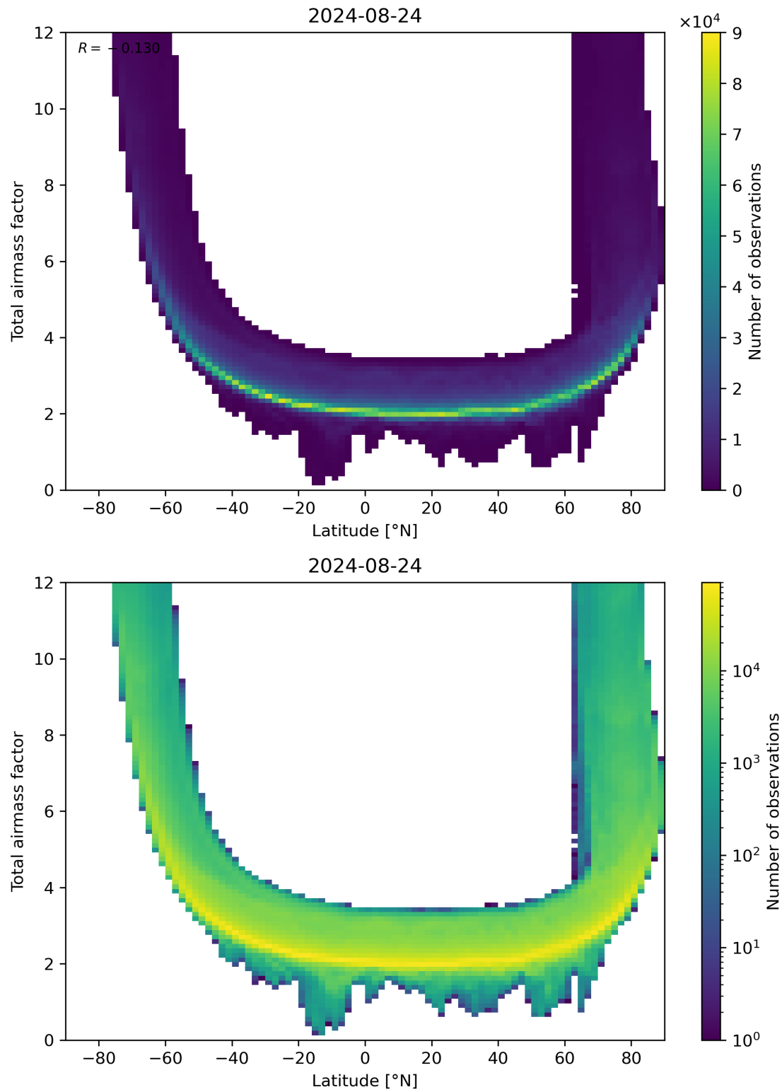
Figure 84: Scatter density plot of “Latitude” against “Total airmass factor” for 2024-08-23 to 2024-08-25.
