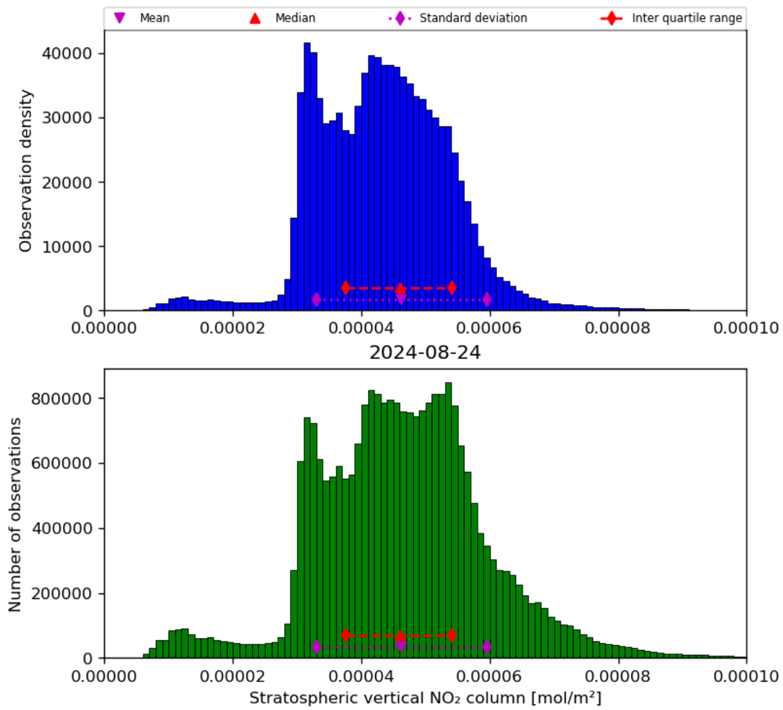
Figure 36: Histogram of “Stratospheric vertical NO 2 column” for 2024-08-23 to 2024-08-25
