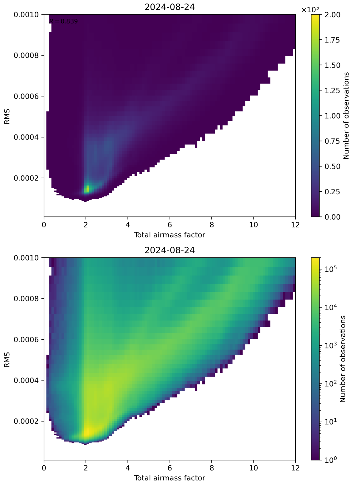
Figure 69: Scatter density plot of “Total airmass factor” against “RMS” for 2024-08-23 to 2024-08-25.
