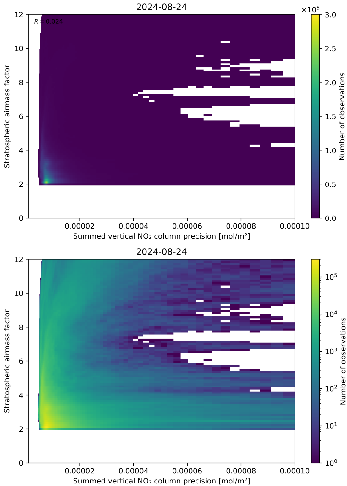
Figure 106: Scatter density plot of “Summed vertical NO 2 column precision” against “Stratospheric airmass factor” for 2024-08-23 to 2024-08-25.
