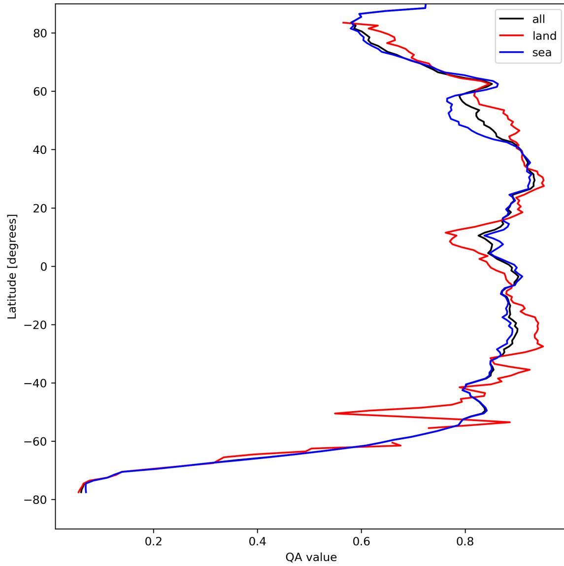
Figure 11: Zonal average of “QA value” for 2024-08-23 to 2024-08-25.
