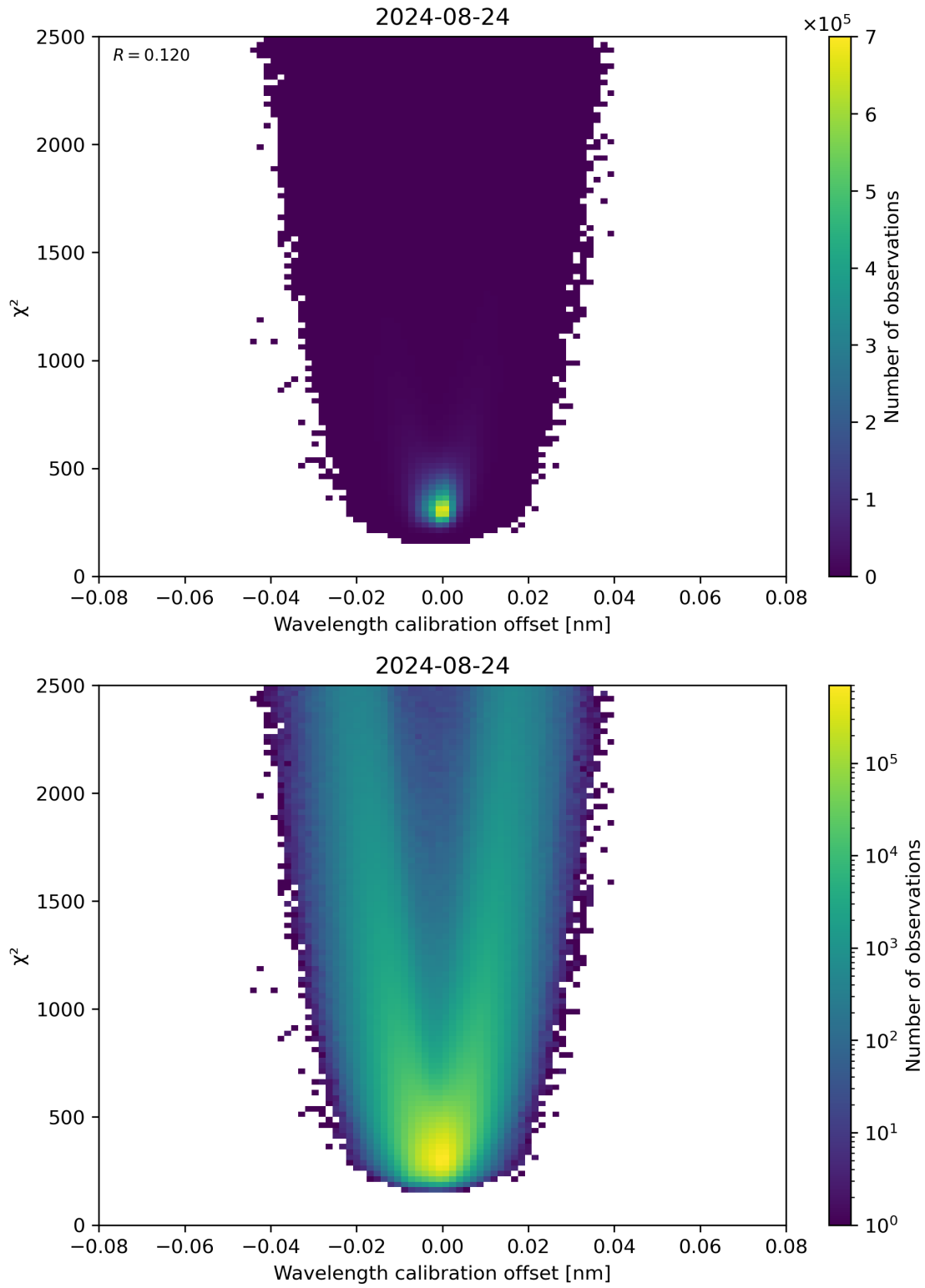
Figure 175: Scatter density plot of “Wavelength calibration offset” against “ \chi^2 ” for 2024-08-23 to 2024-08-25.
