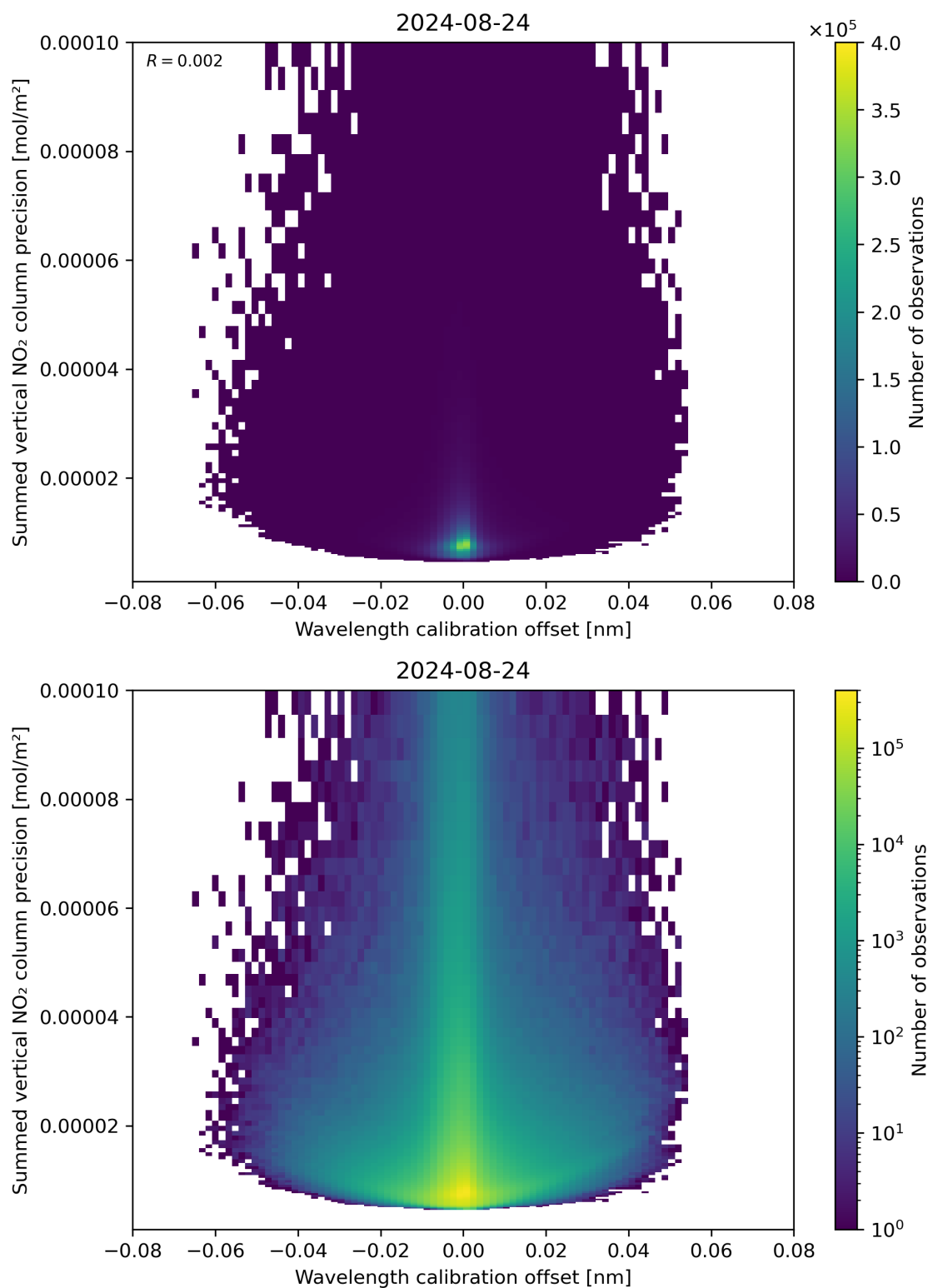
Figure 178: Scatter density plot of “Wavelength calibration offset” against “Summed vertical NO 2 column precision” for 2024-08-23 to 2024-08-25.
