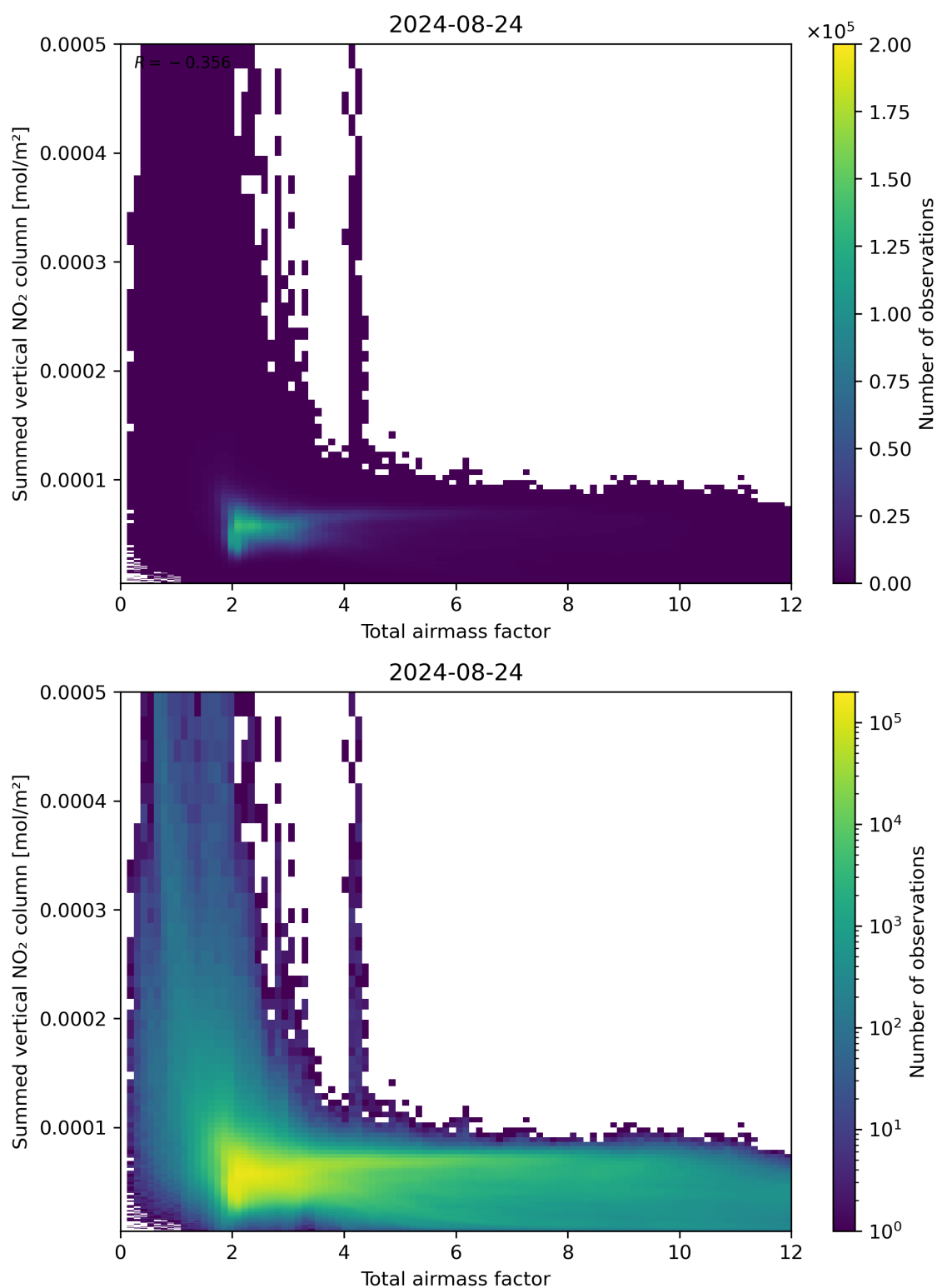
Figure 65: Scatter density plot of “Total airmass factor” against “Summed vertical NO 2 column” for 2024-08-23 to 2024-08-25.
