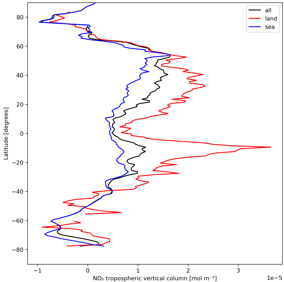
Figure 12: Zonal average of “NO 2 tropospheric vertical column” for 2024-08-23 to 2024-08-25.
