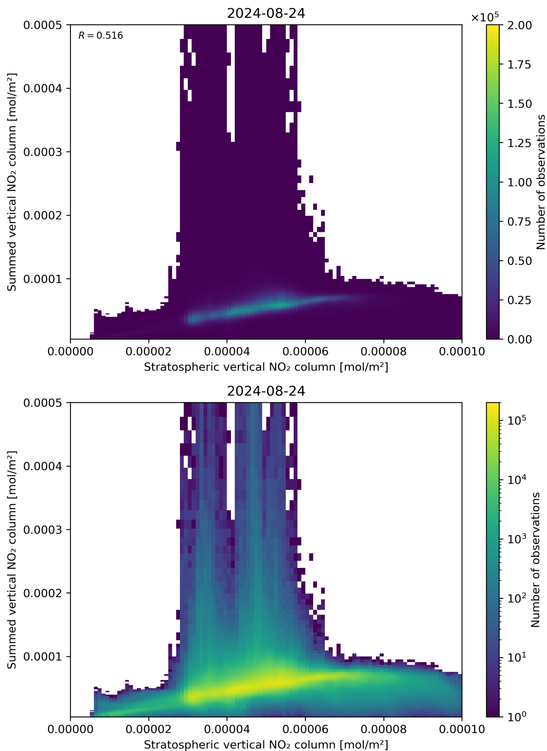
Figure 98: Scatter density plot of “Stratospheric vertical NO 2 column” against “Summed vertical NO 2 column” for 2024-08-23 to 2024-08-25.
