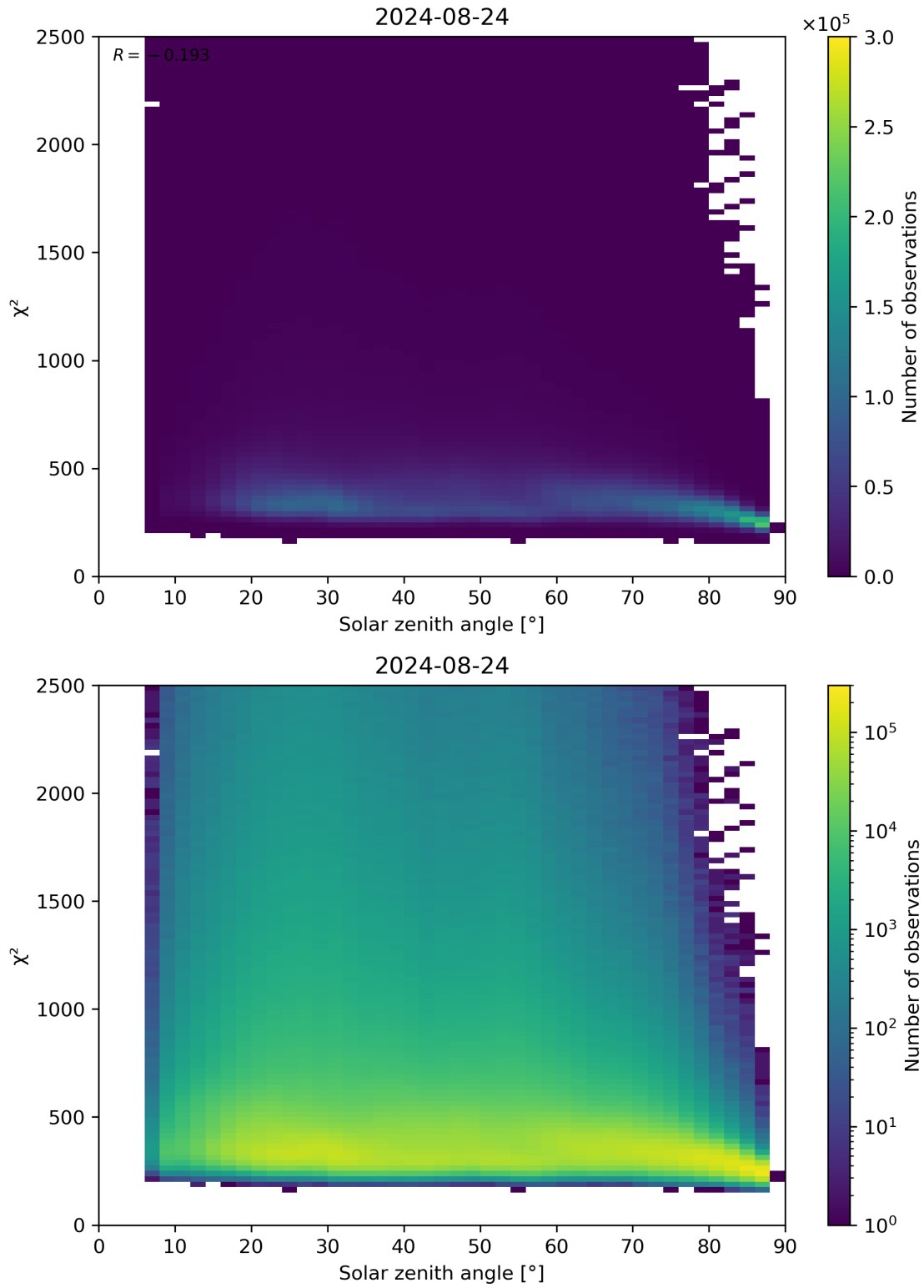
Figure 148: Scatter density plot of “Solar zenith angle” against “ \chi^2 ” for 2024-08-23 to 2024-08-25.
