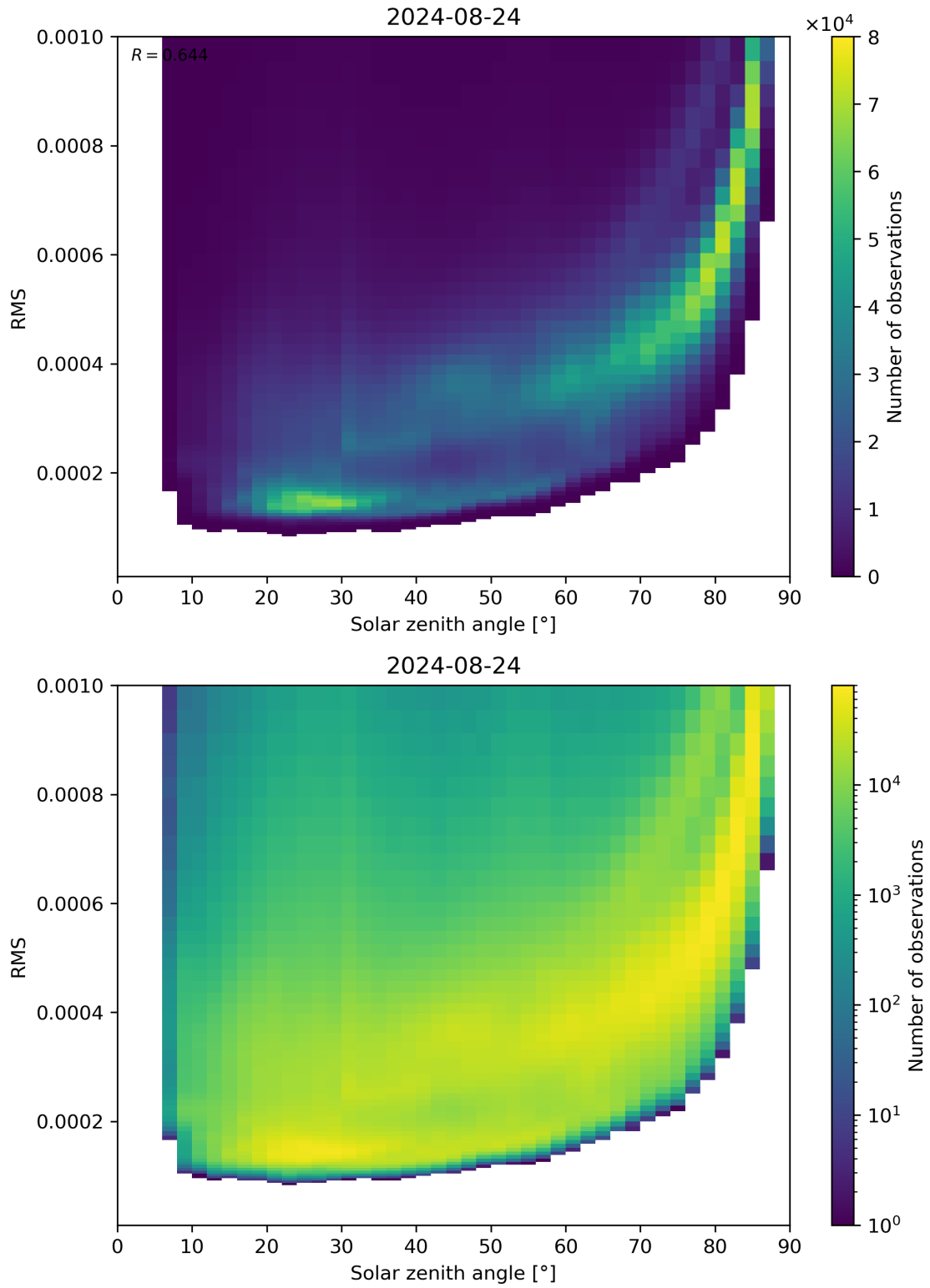
Figure 157: Scatter density plot of “Solar zenith angle” against “RMS” for 2024-08-23 to 2024-08-25.
