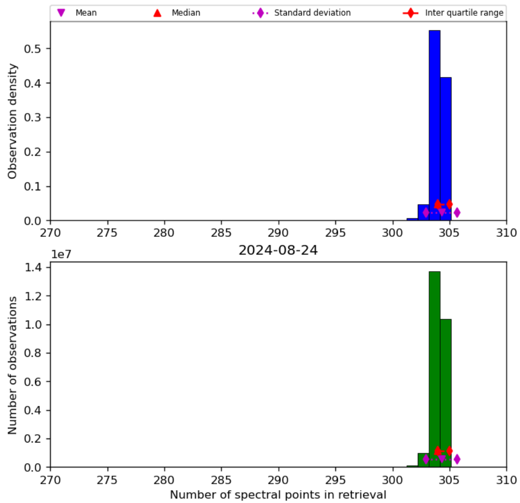
Figure 33: Histogram of “Number of spectral points in retrieval” for 2024-08-23 to 2024-08-25
