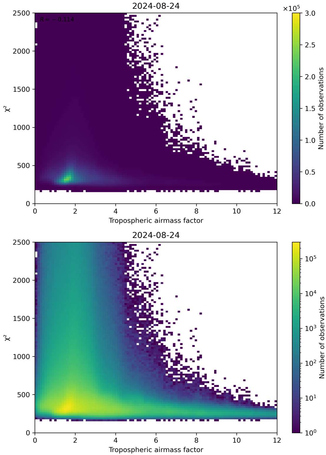
Figure 73: Scatter density plot of “Tropospheric airmass factor” against “ \chi^2 ” for 2024-08-23 to 2024-08-25.
