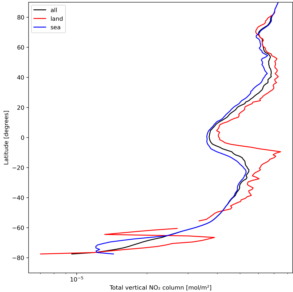
Figure 21: Zonal average of “Total vertical NO 2 column” for 2024-08-23 to 2024-08-25.
