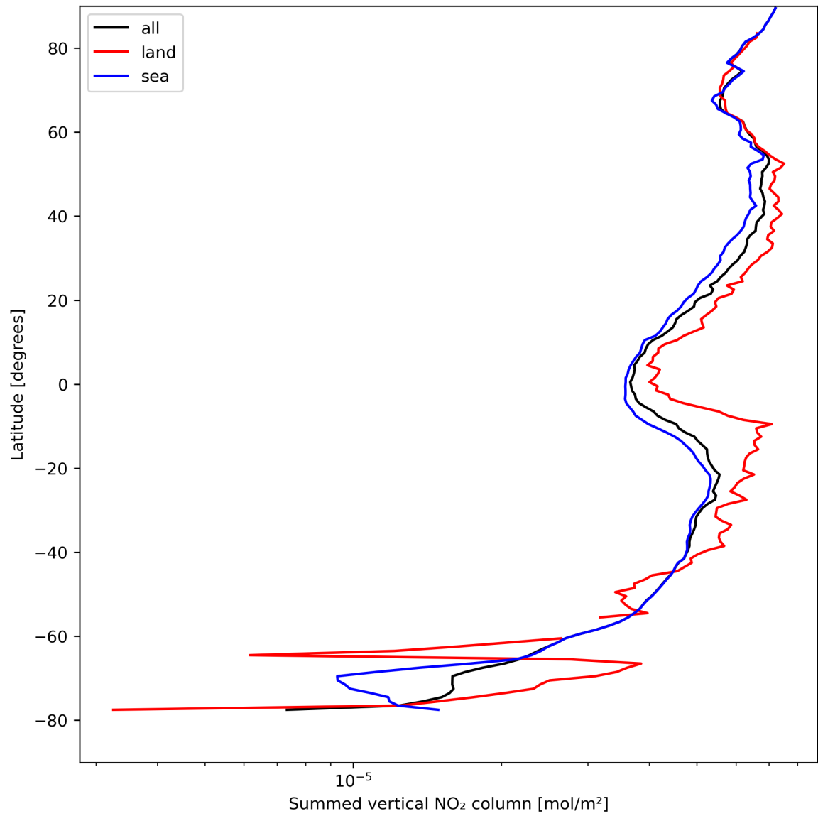
Figure 23: Zonal average of “Summed vertical NO 2 column” for 2024-08-23 to 2024-08-25.
