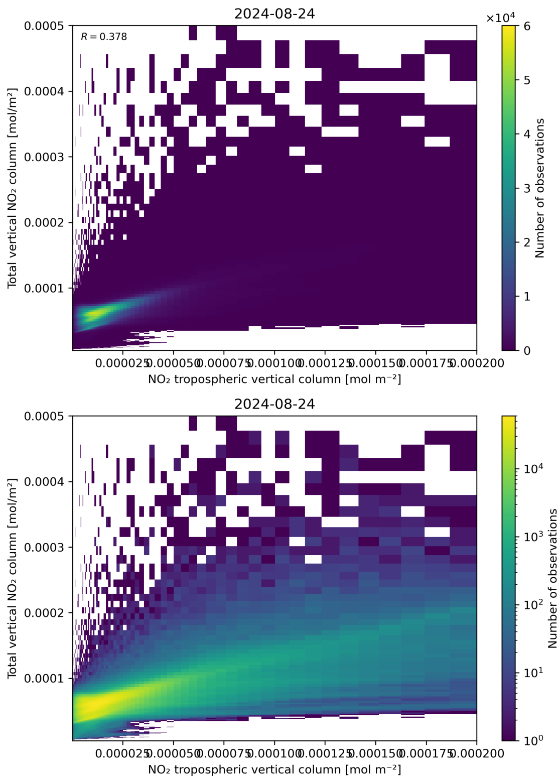
Figure 128: Scatter density plot of “NO 2 tropospheric vertical column” against “Total vertical NO 2 column” for 2024-08-23 to 2024-08-25.
