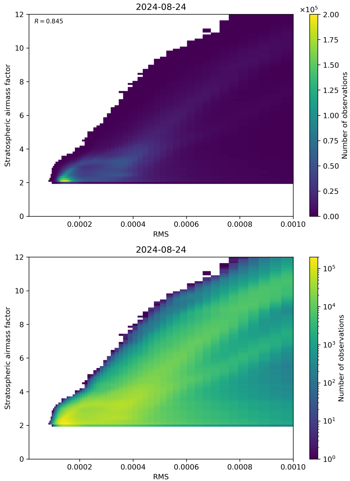
Figure 144: Scatter density plot of “RMS” against “Stratospheric airmass factor” for 2024-08-23 to 2024-08-25.
