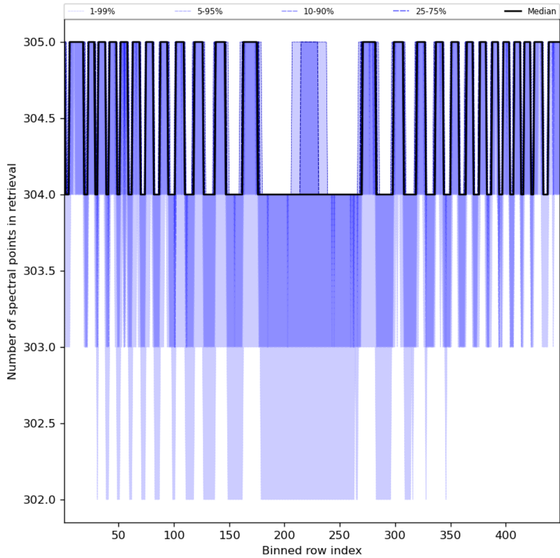
Figure 50: Along track statistics of “Number of spectral points in retrieval” for 2024-08-23 to 2024-08-25
