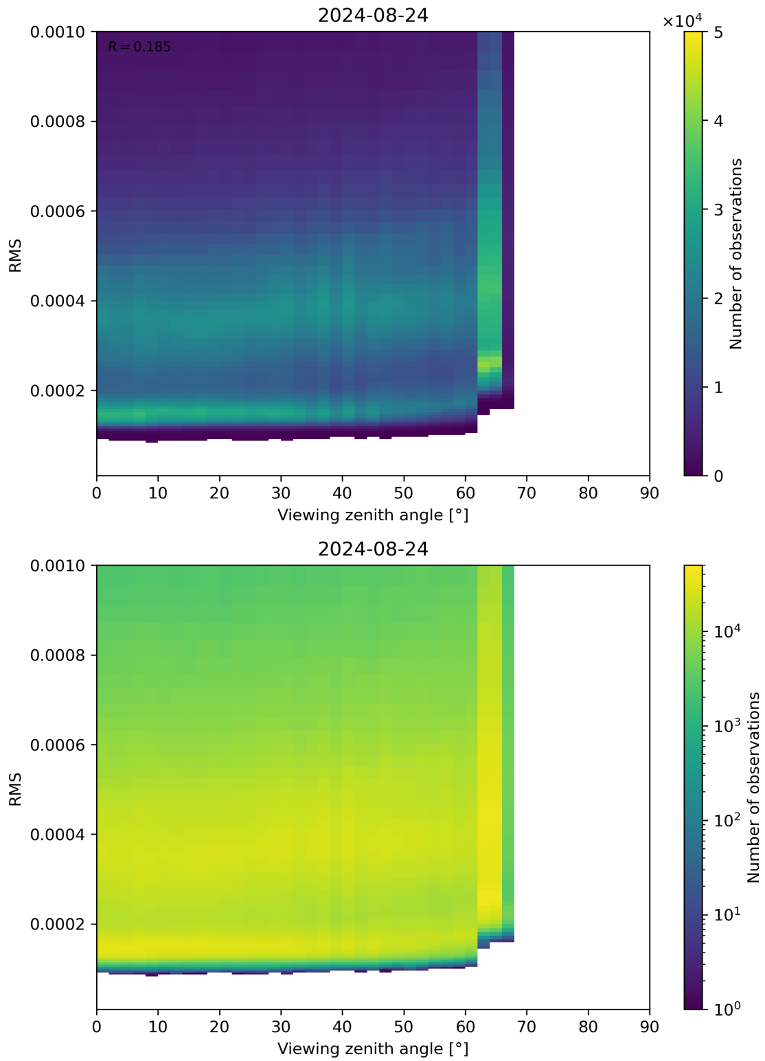
Figure 171: Scatter density plot of “Viewing zenith angle” against “RMS” for 2024-08-23 to 2024-08-25.
