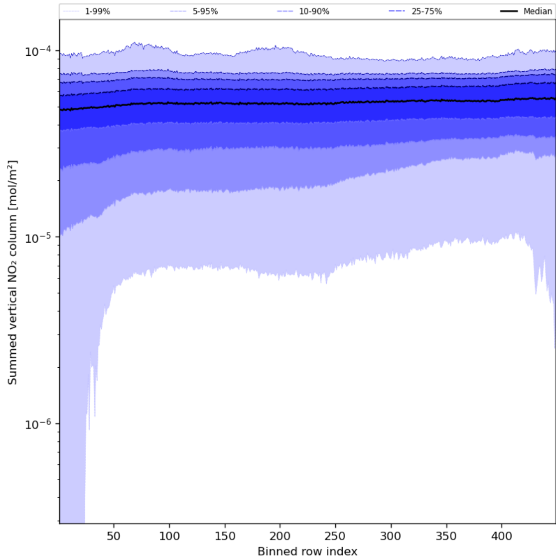
Figure 57: Along track statistics of “Summed vertical NO 2 column” for 2024-08-23 to 2024-08-25
