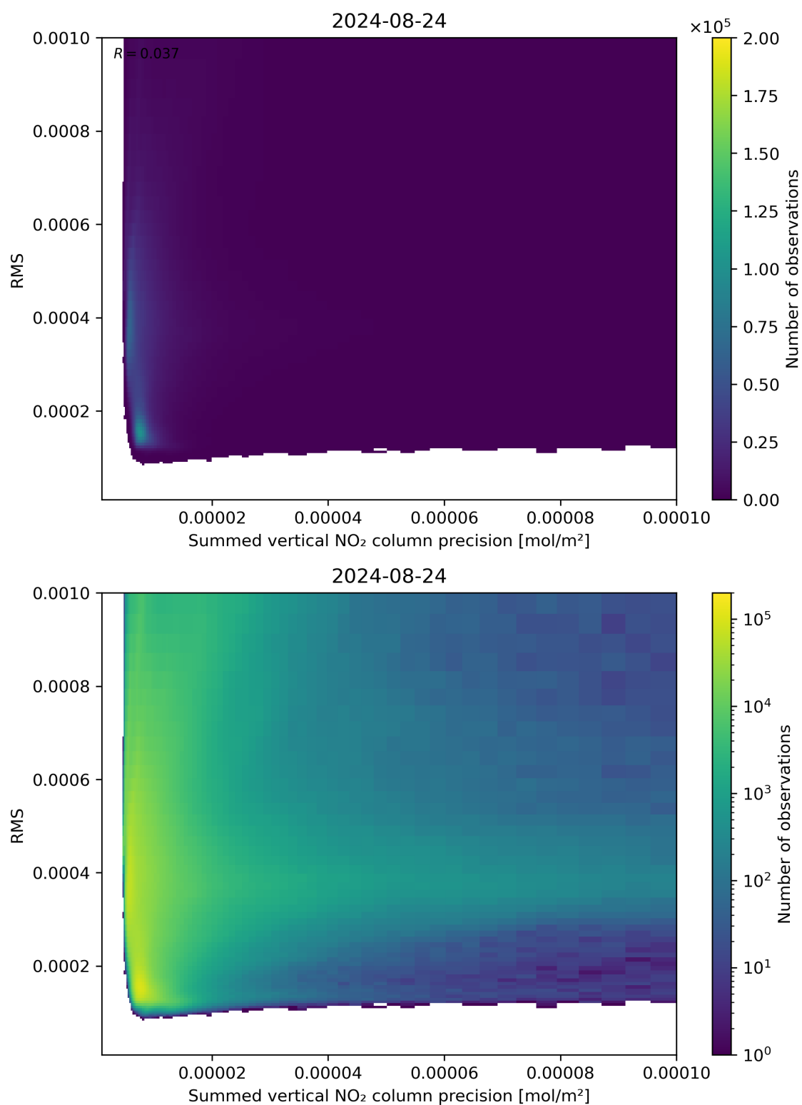
Figure 108: Scatter density plot of “Summed vertical NO 2 column precision” against “RMS” for 2024-08-23 to 2024-08-25.
