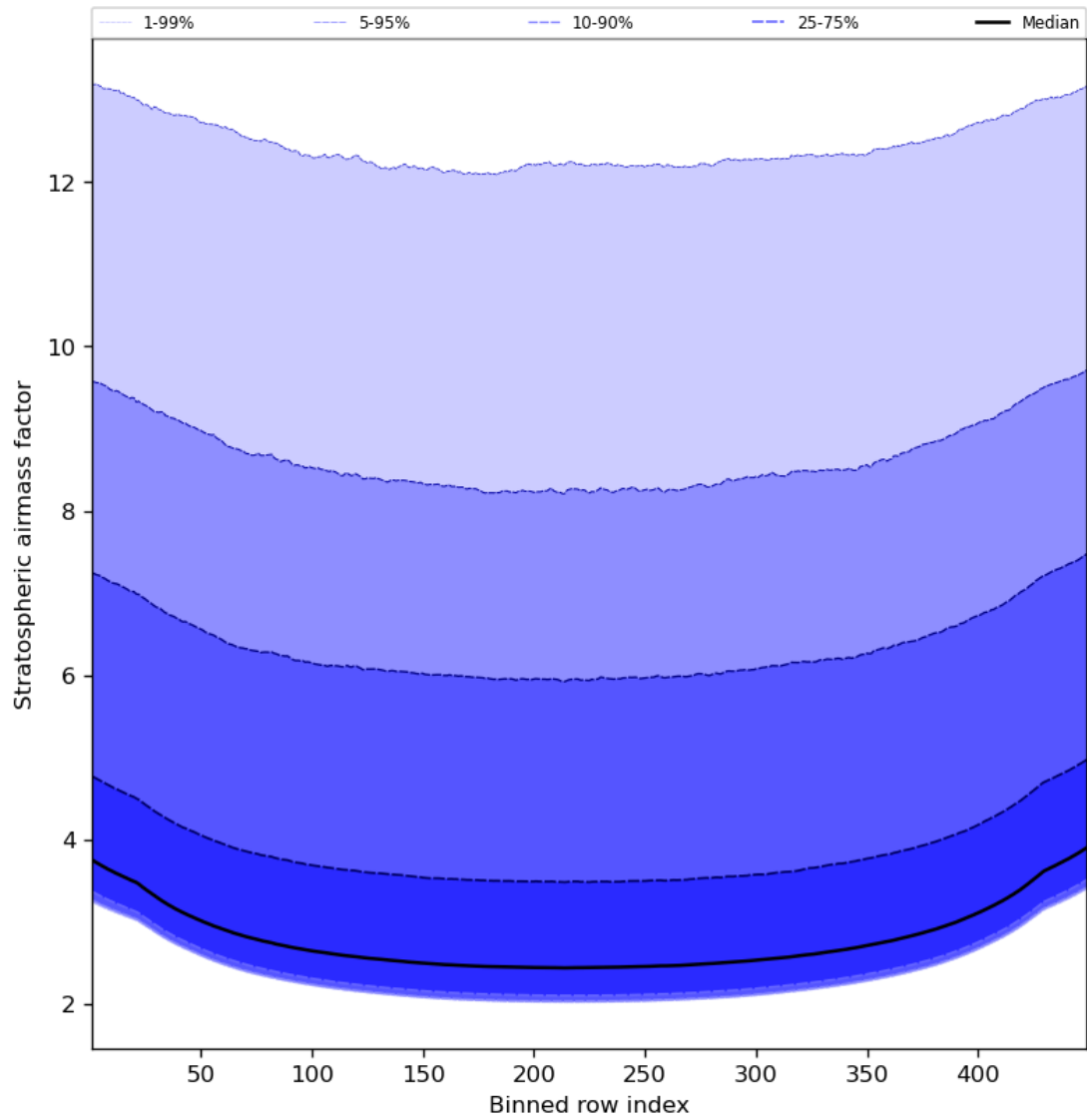
Figure 61: Along track statistics of “Stratospheric airmass factor” for 2024-08-23 to 2024-08-25
