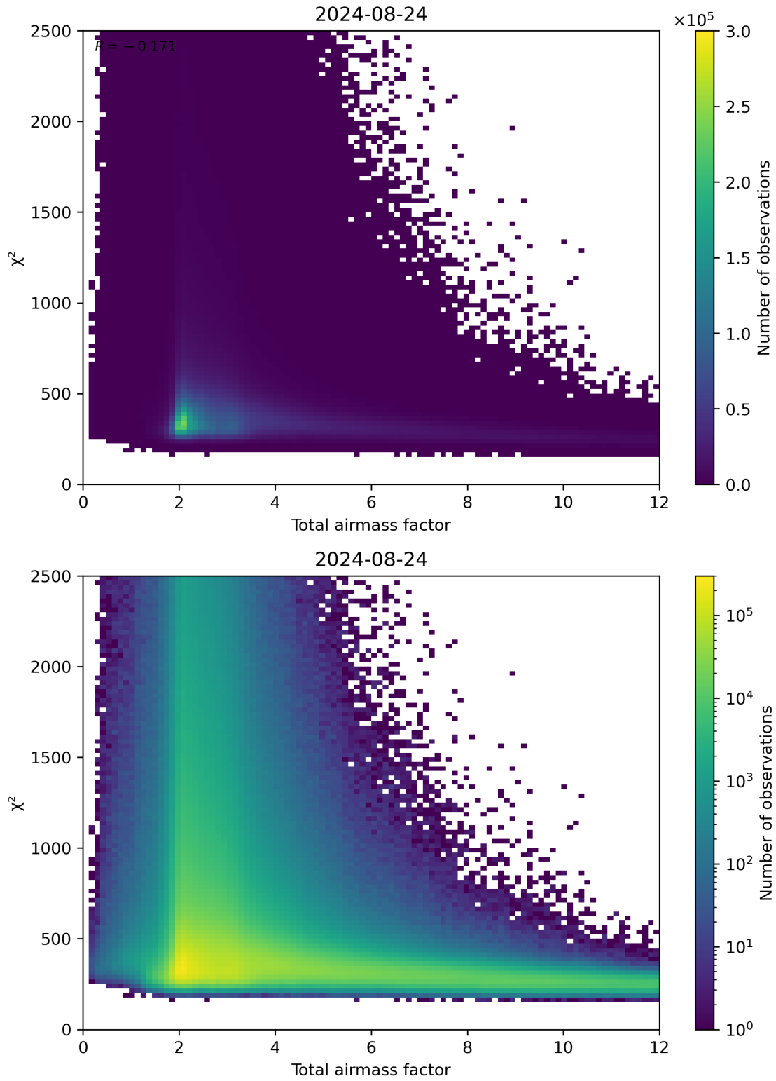
Figure 63: Scatter density plot of “Total airmass factor” against “ \chi^2 ” for 2024-08-23 to 2024-08-25.
