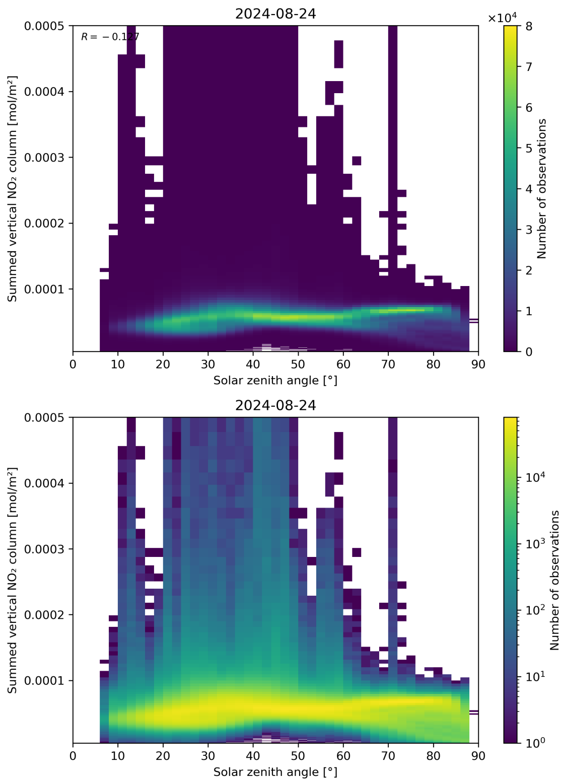
Figure 151: Scatter density plot of “Solar zenith angle” against “Summed vertical NO 2 column” for 2024-08-23 to 2024-08-25.
