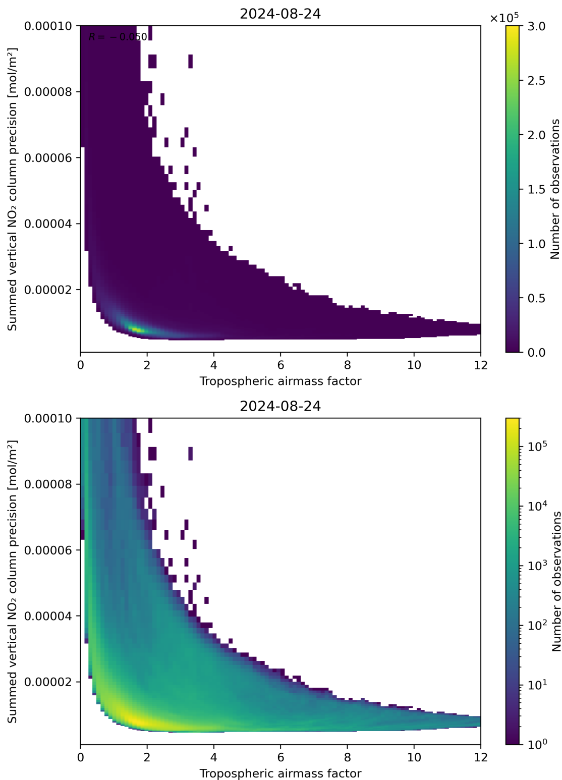
Figure 76: Scatter density plot of “Tropospheric air mass factor” against “Summed vertical NO 2 column precision” for 2024-08-23 to 2024-08-25.
