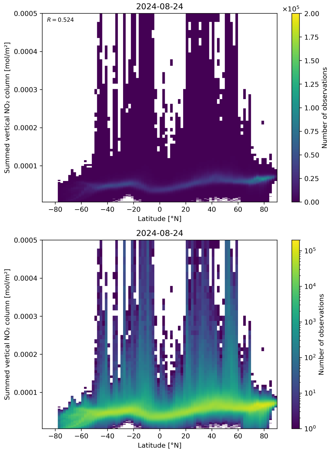
Figure 88: Scatter density plot of “Latitude” against “Summed vertical NO 2 column” for 2024-08-23 to 2024-08-25.
