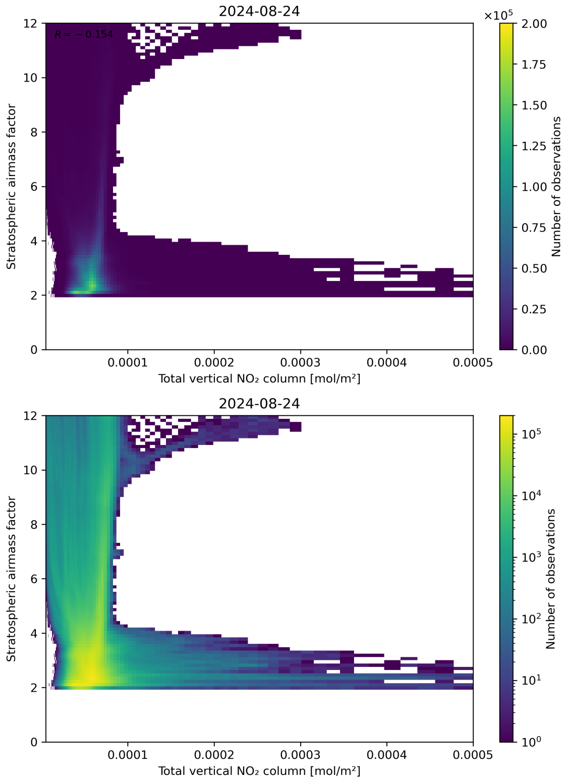
Figure 110: Scatter density plot of “Total vertical NO 2 column” against “Stratospheric airmass factor” for 2024-08-23 to 2024-08-25.
