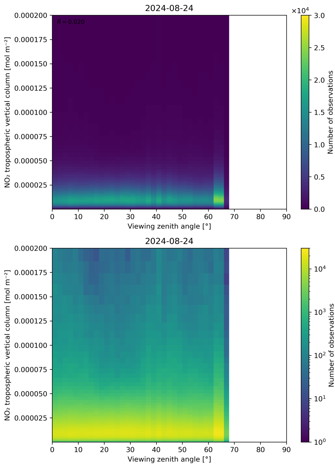
Figure 169: Scatter density plot of “Viewing zenith angle” against “NO 2 tropospheric vertical column” for 2024-08-23 to 2024-08-25.
