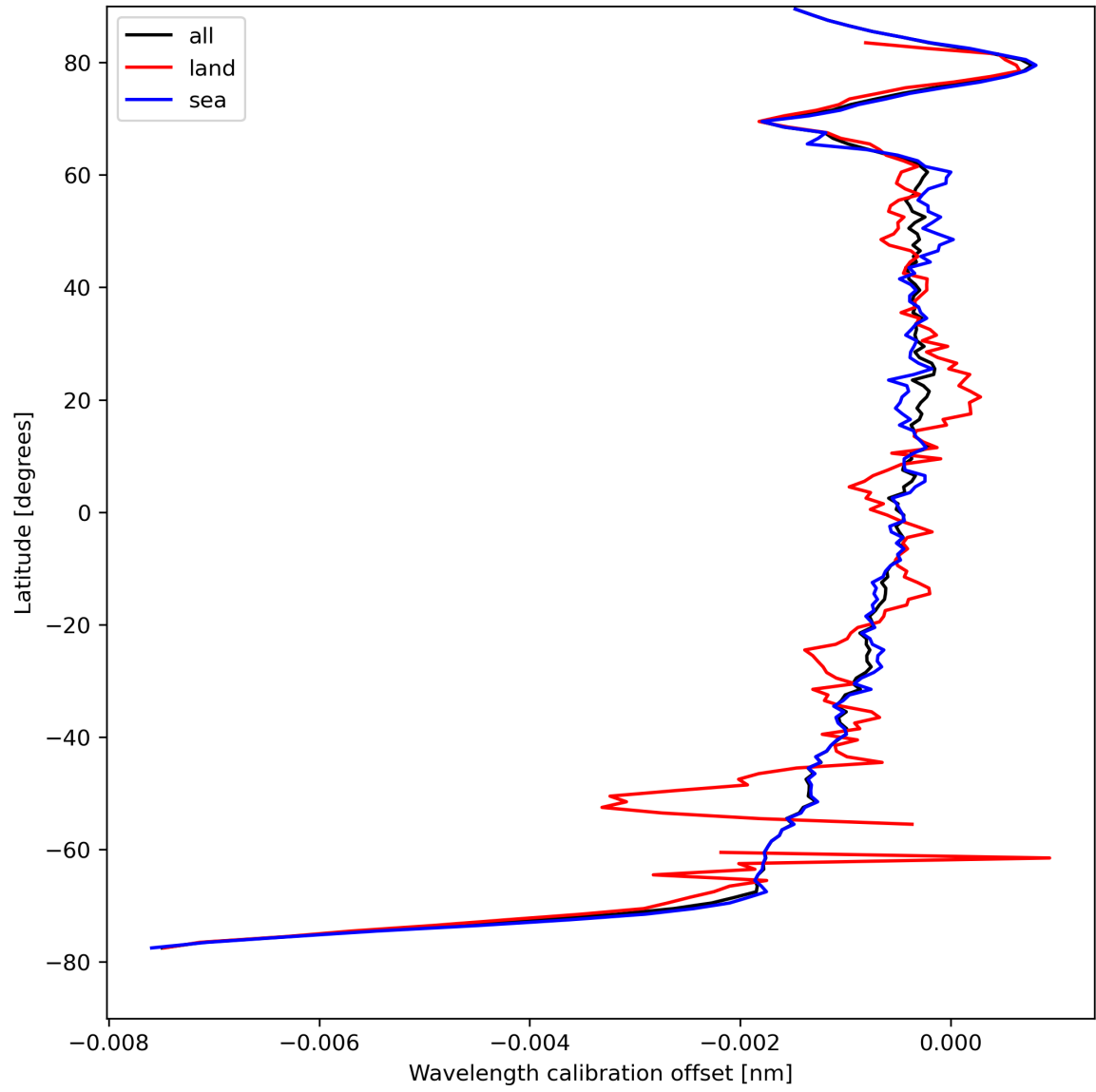
Figure 18: Zonal average of “Wavelength calibration offset” for 2024-08-23 to 2024-08-25.
