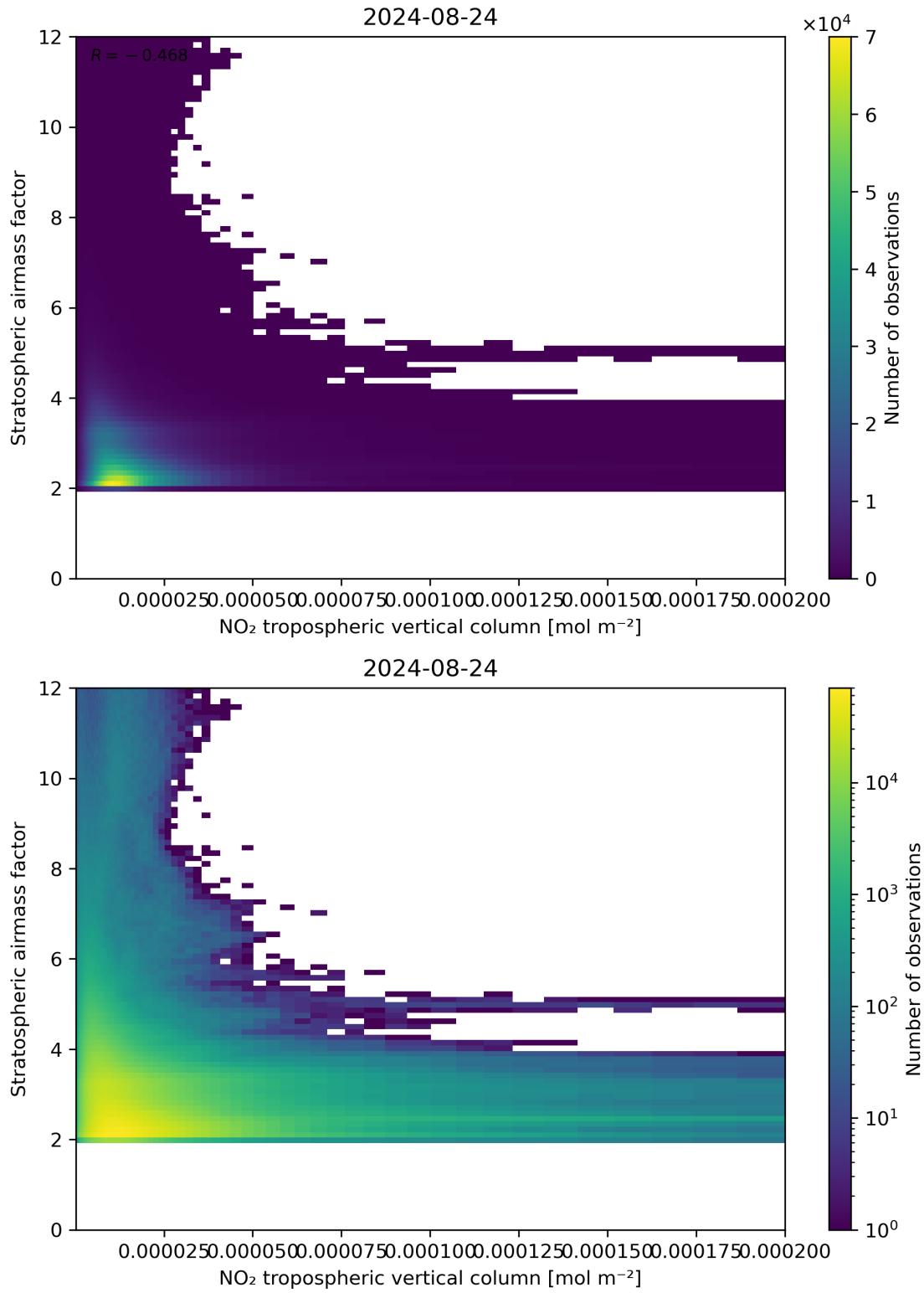
Figure 121: Scatter density plot of “NO 2 tropospheric vertical column” against “Stratospheric air mass factor” for 2024-08-23 to 2024-08-25.
