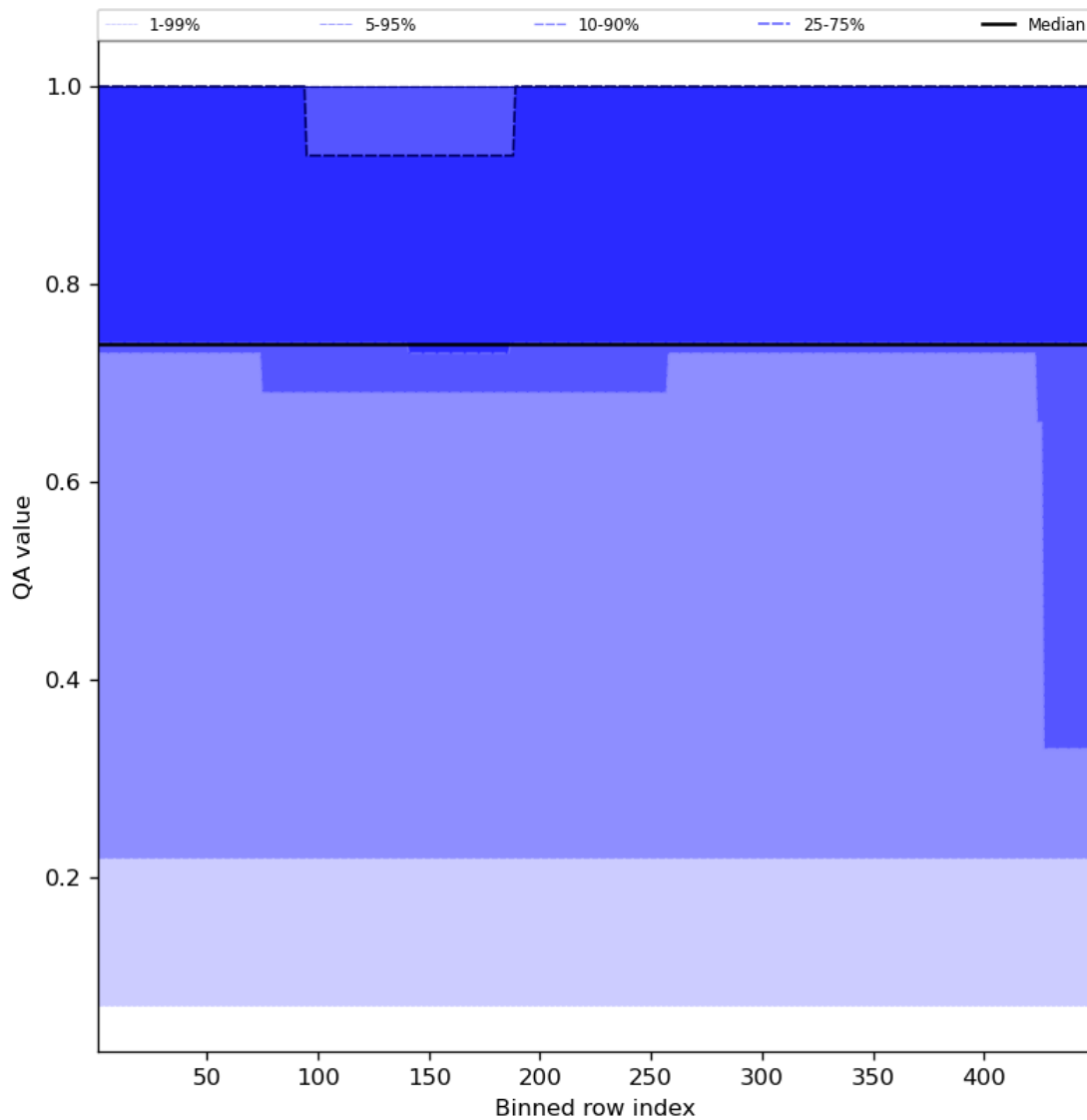
Figure 45: Along track statistics of “QA value” for 2024-08-23 to 2024-08-25
