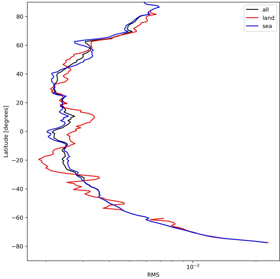
Figure 26: Zonal average of “RMS” for 2024-08-23 to 2024-08-25.
