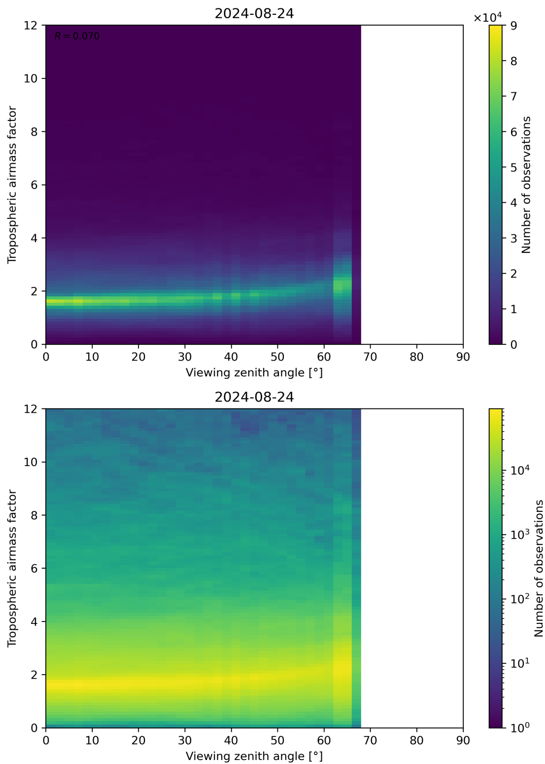
Figure 161: Scatter density plot of “Viewing zenith angle” against “Tropospheric airmass factor” for 2024-08-23 to 2024-08-25.
