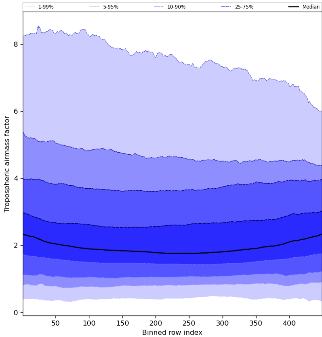
Figure 48: Along track statistics of “Tropospheric air mass factor” for 2024-08-23 to 2024-08-25
