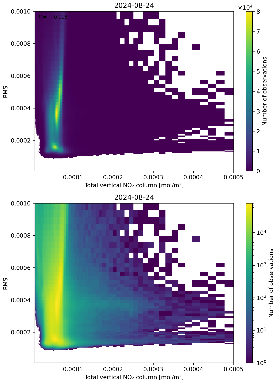
Figure 120: Scatter density plot of “Total vertical NO 2 column” against “RMS” for 2024-08-23 to 2024-08-25.
