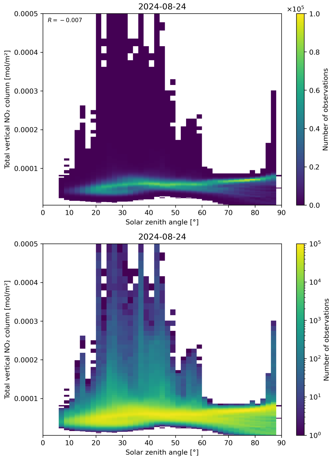
Figure 153: Scatter density plot of “Solar zenith angle” against “Total vertical NO 2 column” for 2024-08-23 to 2024-08-25.
