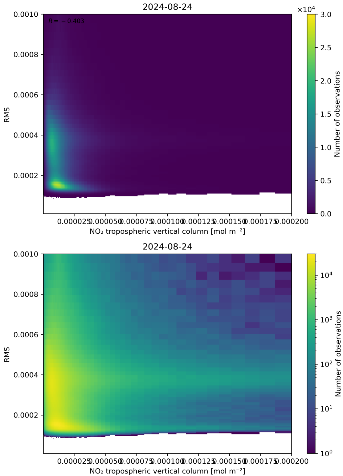
Figure 142: Scatter density plot of “NO 2 tropospheric vertical column” against “RMS” for 2024-08-23 to 2024-08-25.
