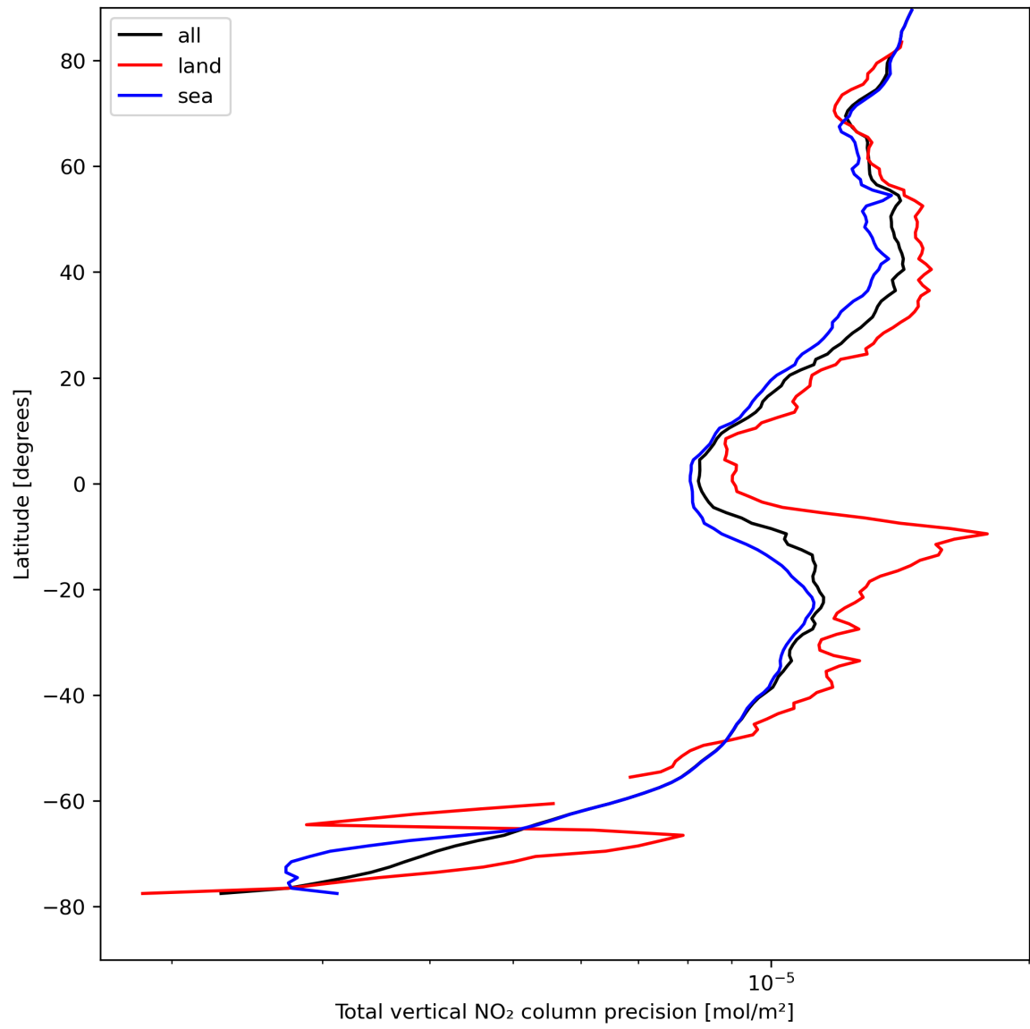
Figure 22: Zonal average of “Total vertical NO 2 column precision” for 2024-08-23 to 2024-08-25.
