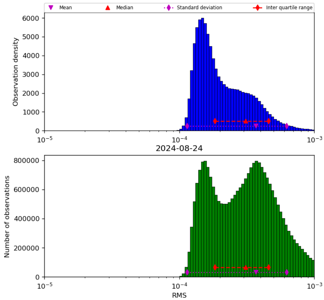
Figure 43: Histogram of “RMS” for 2024-08-23 to 2024-08-25
