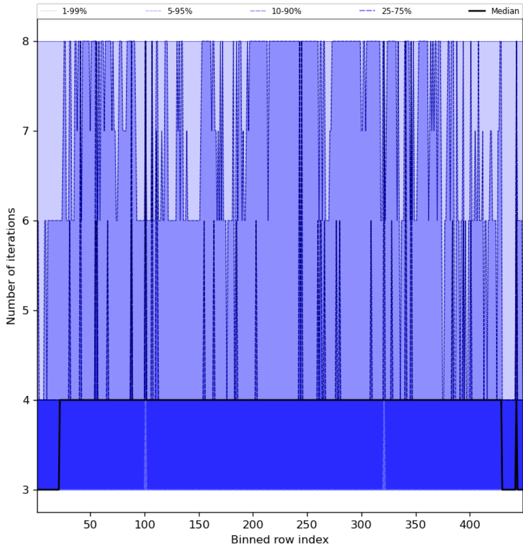
Figure 51: Along track statistics of “Number of iterations” for 2024-08-23 to 2024-08-25
