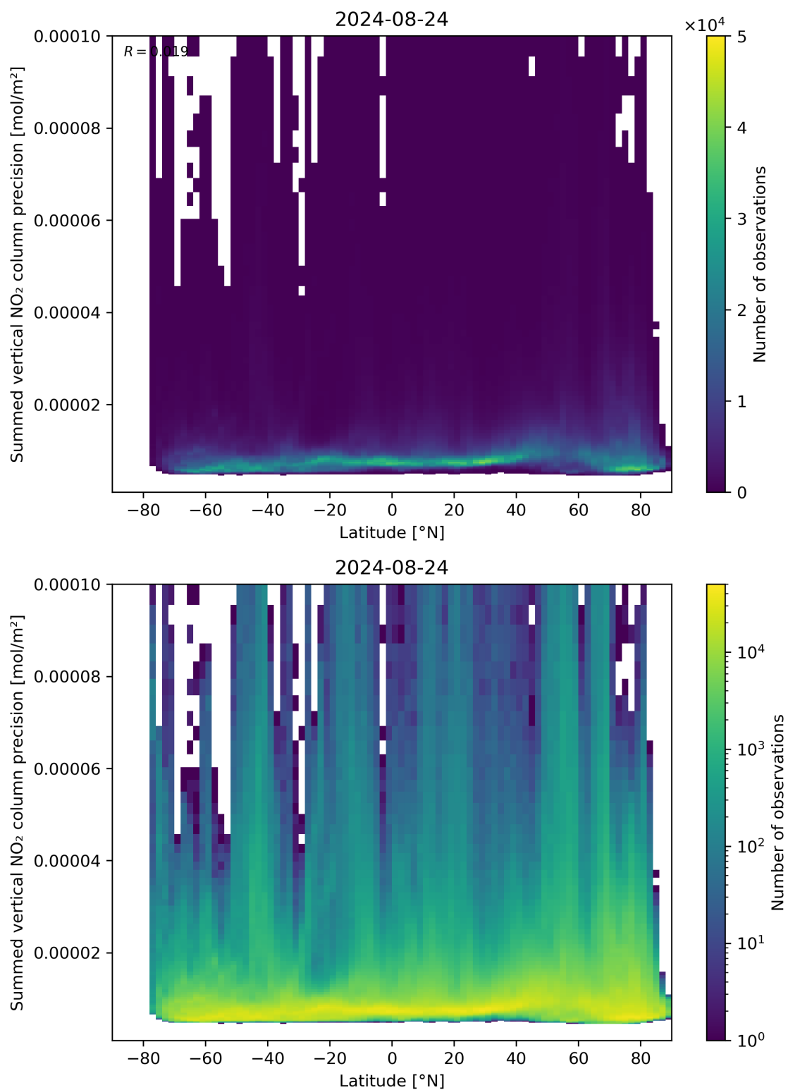
Figure 89: Scatter density plot of “Latitude” against “Summed vertical NO 2 column precision” for 2024-08-23 to 2024-08-25.
