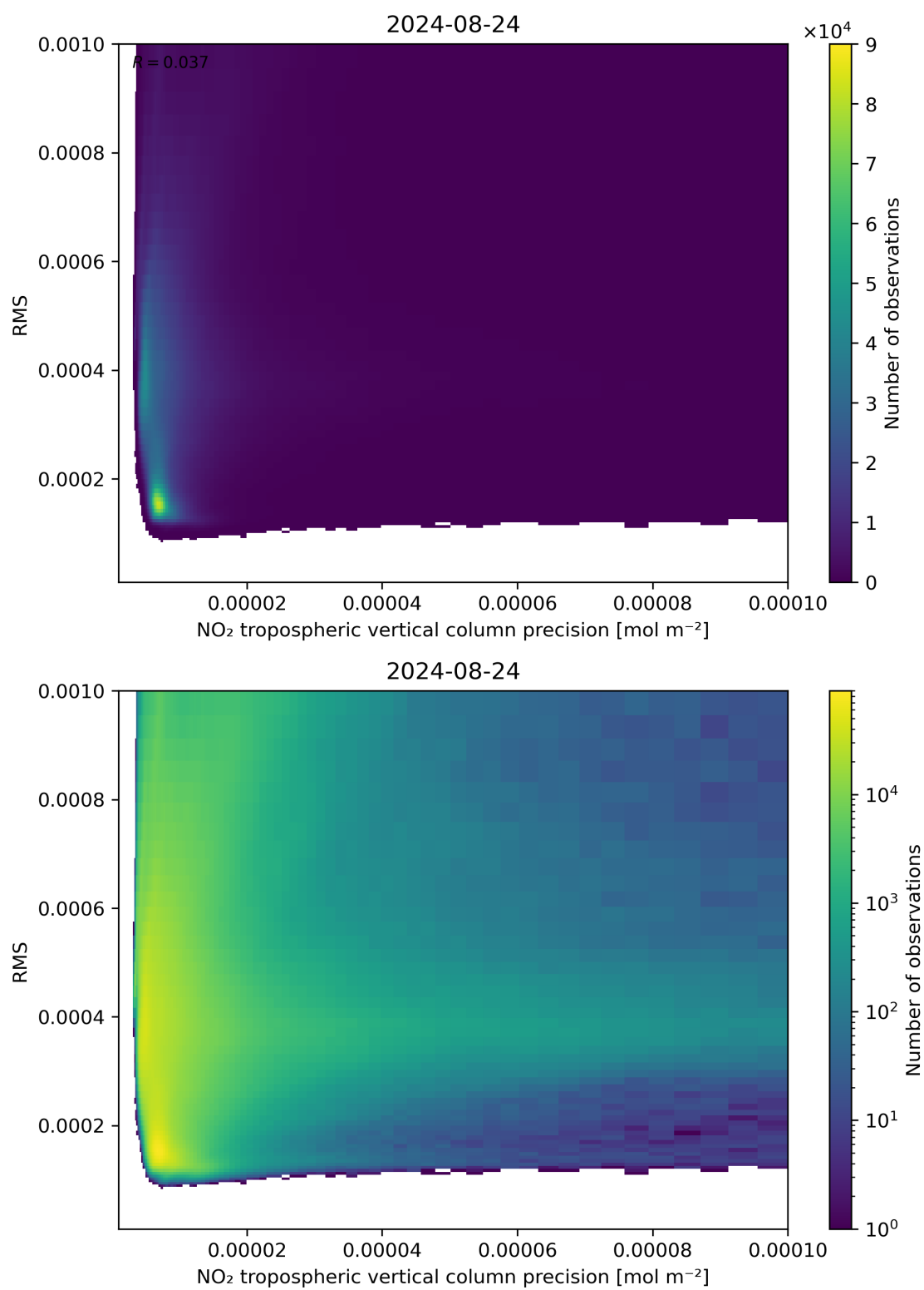
Figure 140: Scatter density plot of “NO 2 tropospheric vertical column precision” against “RMS” for 2024-08-23 to 2024-08-25.
