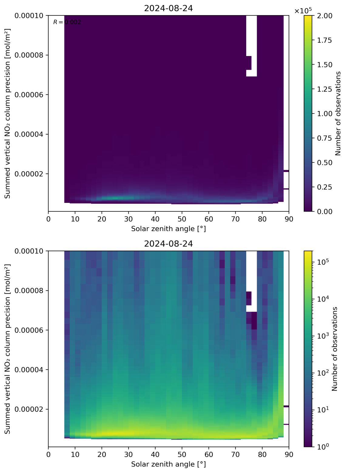
Figure 152: Scatter density plot of “Solar zenith angle” against “Summed vertical NO 2 column precision” for 2024-08-23 to 2024-08-25.
