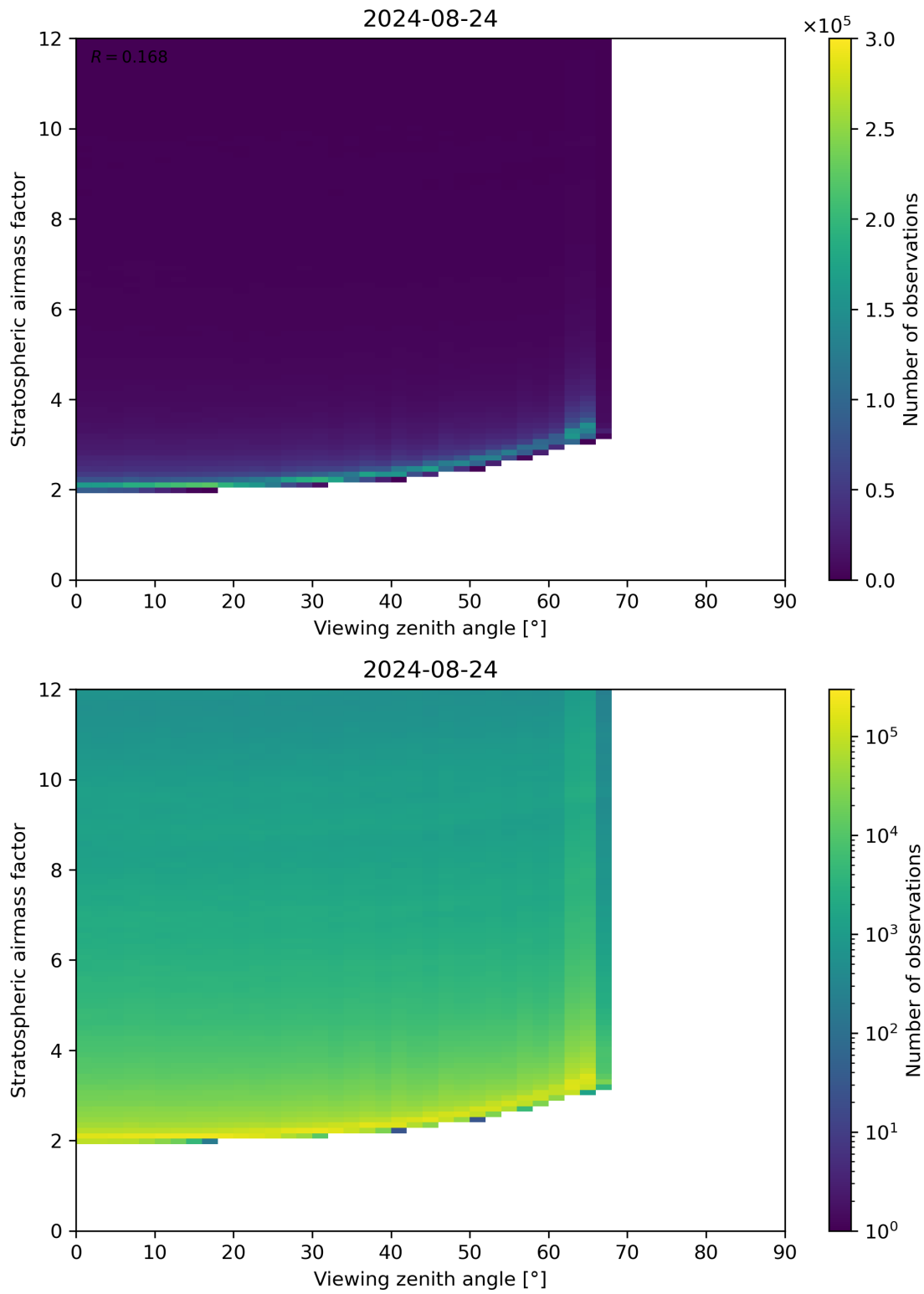
Figure 159: Scatter density plot of “Viewing zenith angle” against “Stratospheric airmass factor” for 2024-08-23 to 2024-08-25.
