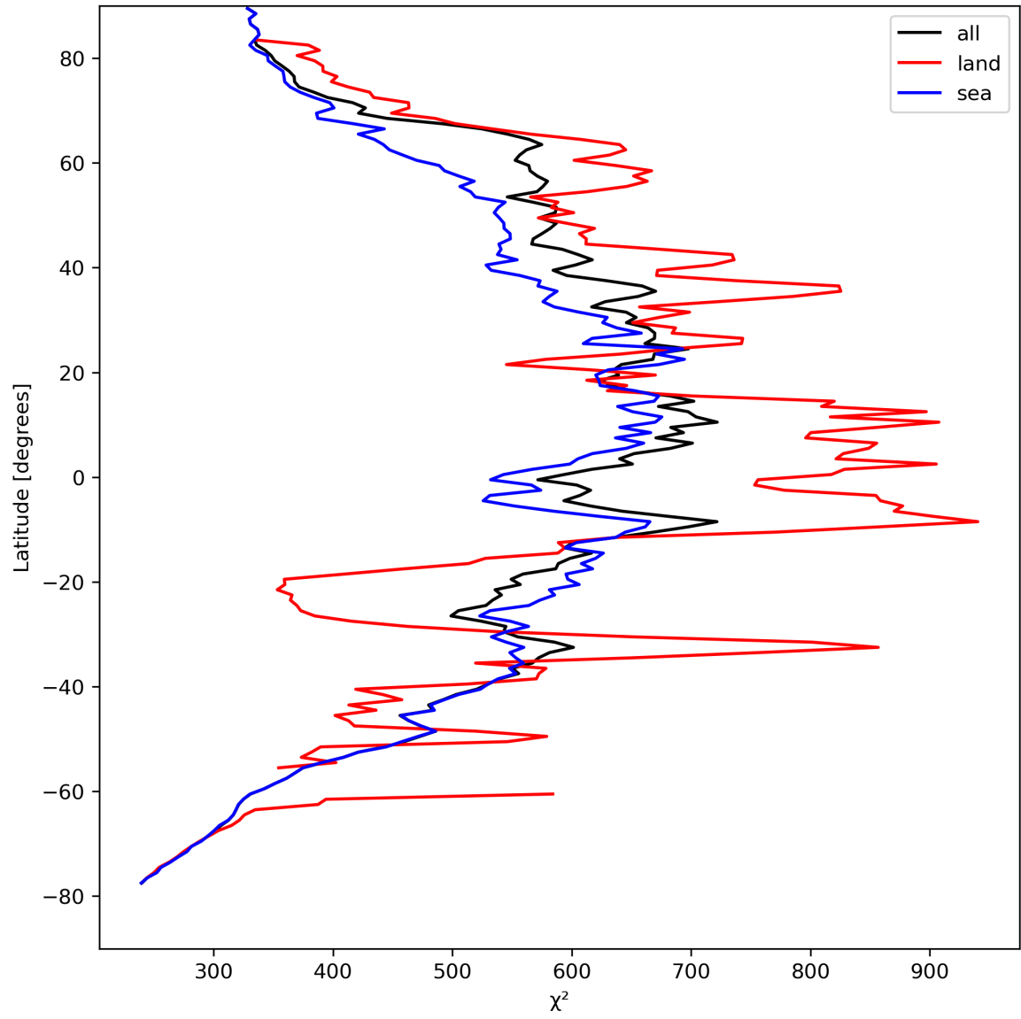
Figure 25: Zonal average of “ \chi^2 ” for 2024-08-23 to 2024-08-25.
