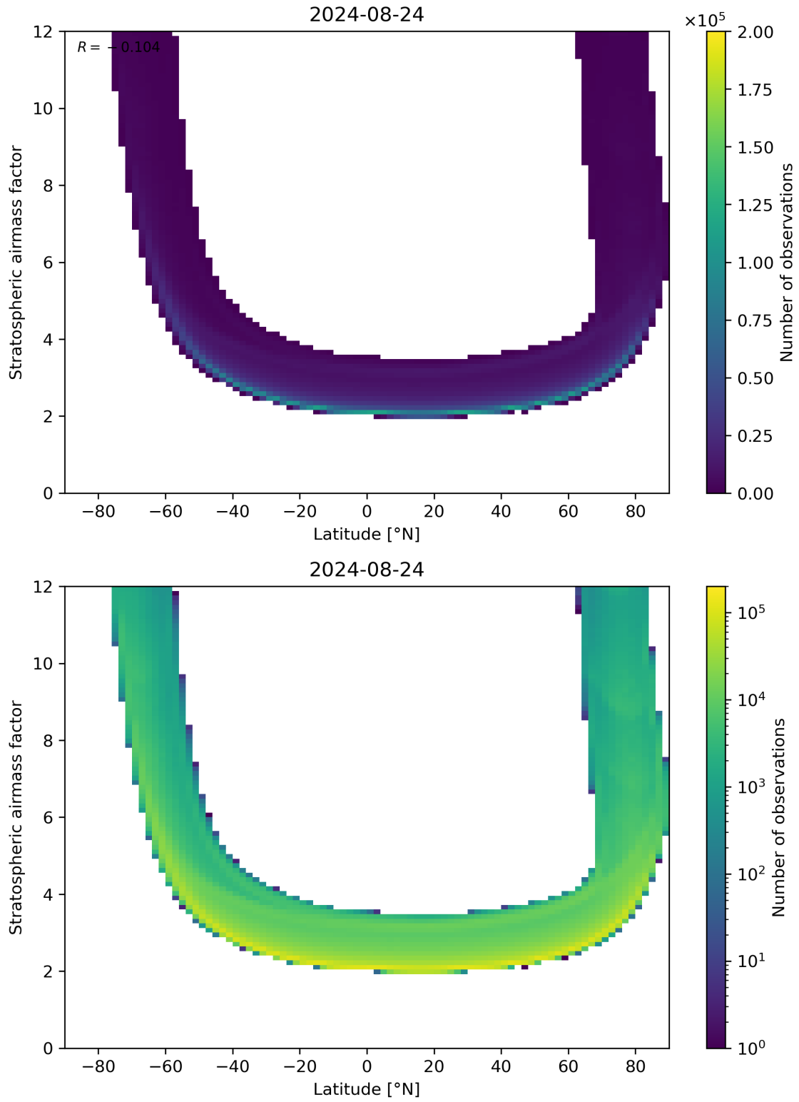
Figure 83: Scatter density plot of “Latitude” against “Stratospheric air mass factor” for 2024-08-23 to 2024-08-25.
