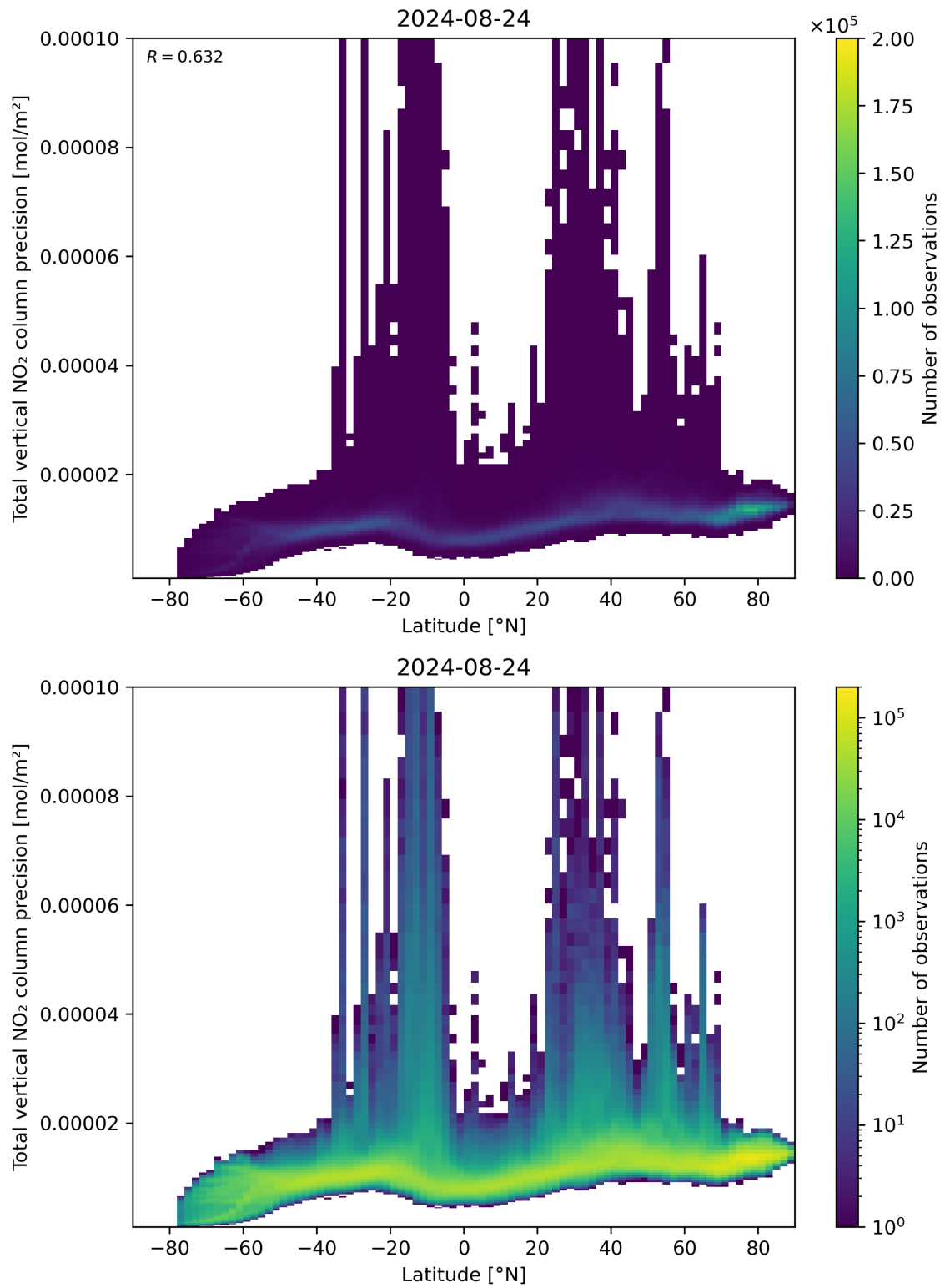
Figure 91: Scatter density plot of “Latitude” against “Total vertical NO 2 column precision” for 2024-08-23 to 2024-08-25.
