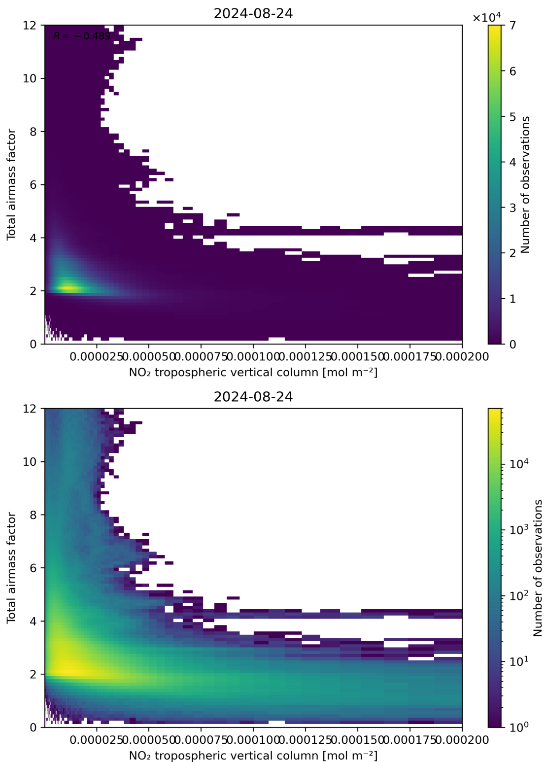
Figure 122: Scatter density plot of “NO 2 tropospheric vertical column” against “Total air mass factor” for 2024-08-23 to 2024-08-25.
