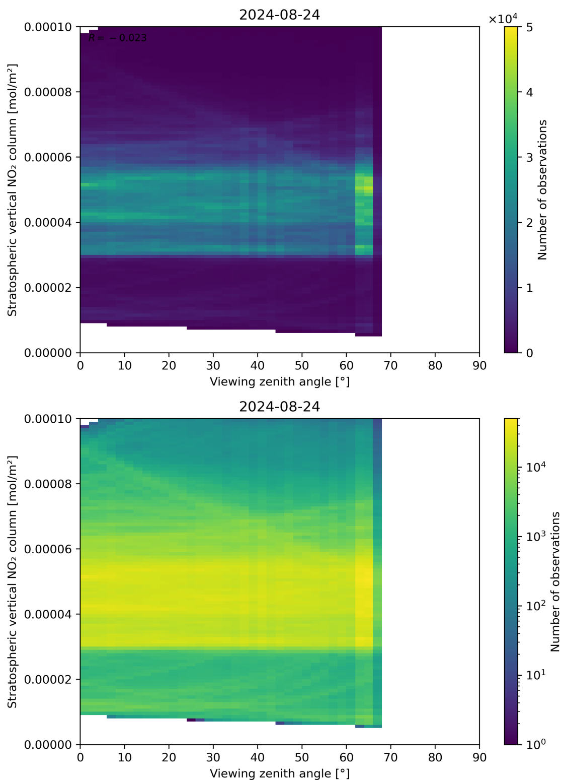
Figure 164: Scatter density plot of “Viewing zenith angle” against “Stratospheric vertical NO 2 column” for 2024-08-23 to 2024-08-25.
