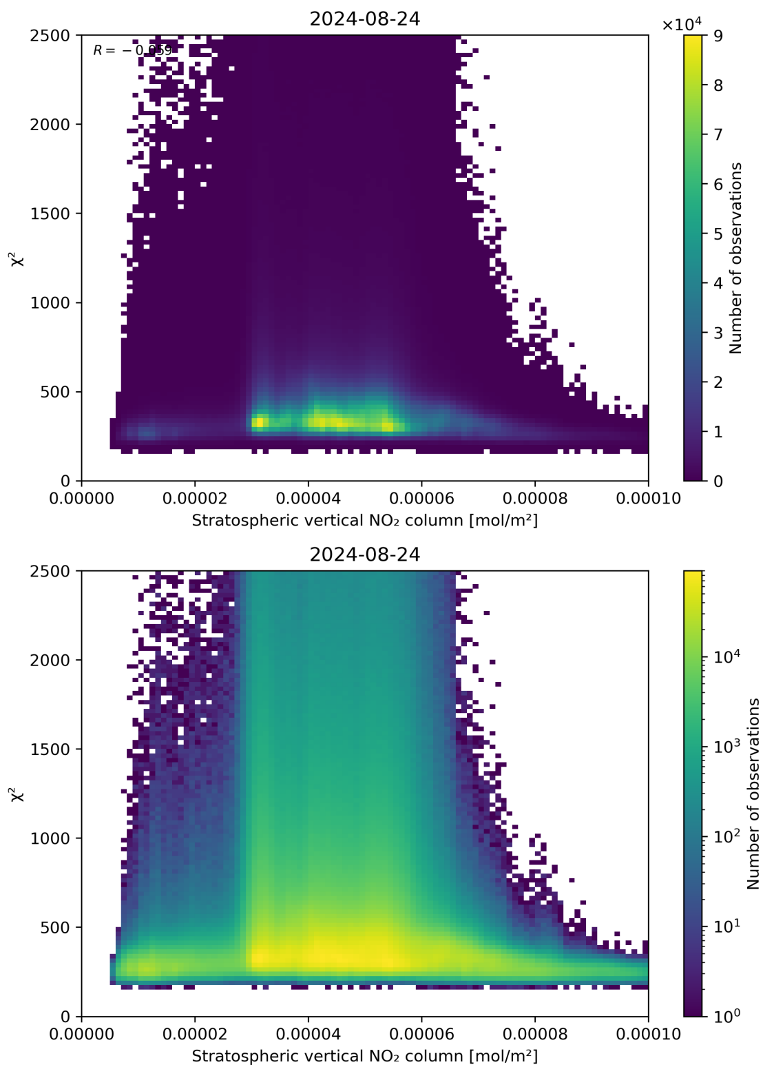
Figure 97: Scatter density plot of “Stratospheric vertical NO 2 column” against “ \chi^2 ” for 2024-08-23 to 2024-08-25.
