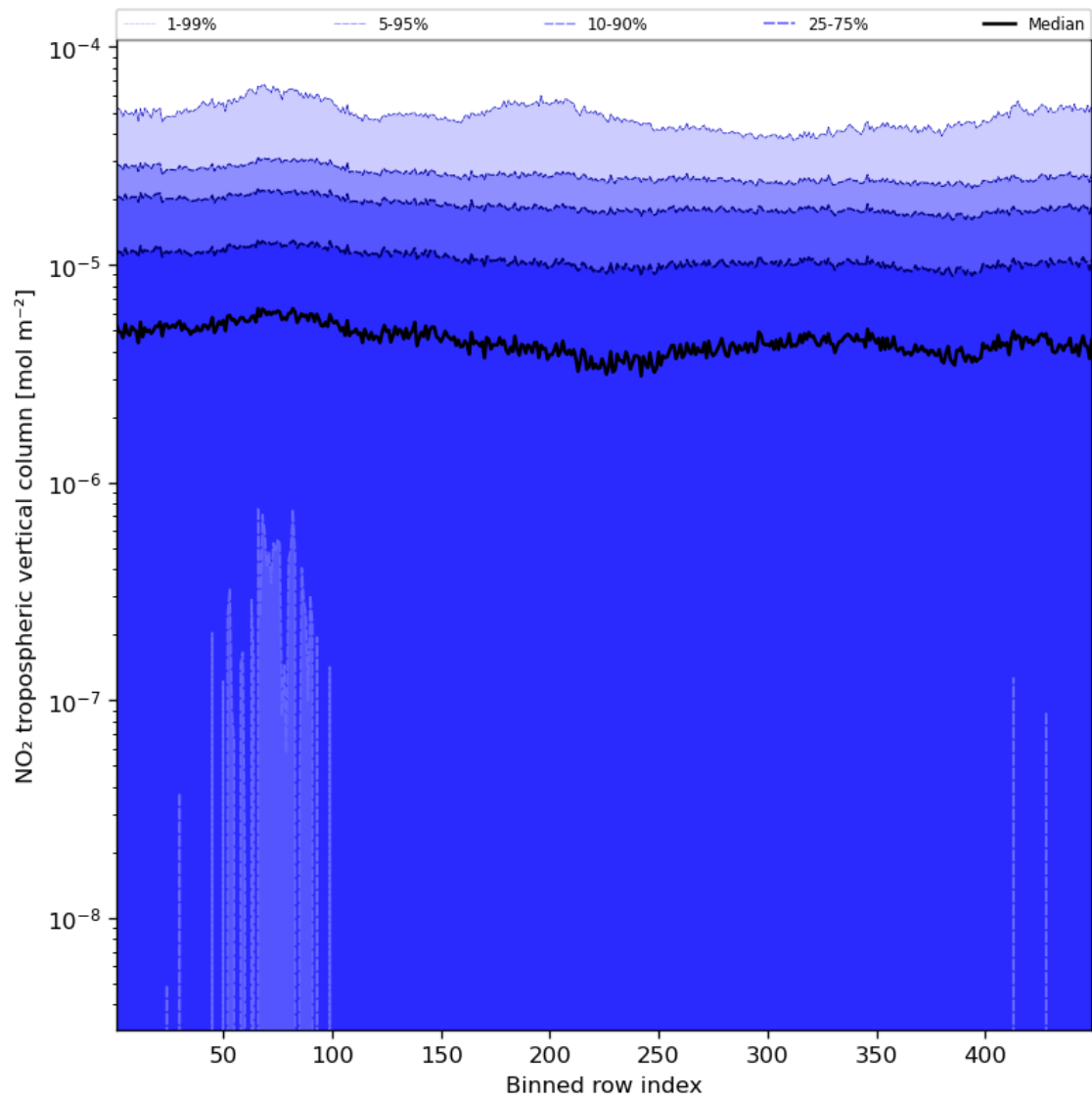
Figure 46: Along track statistics of “NO 2 tropospheric vertical column” for 2024-08-23 to 2024-08-25
