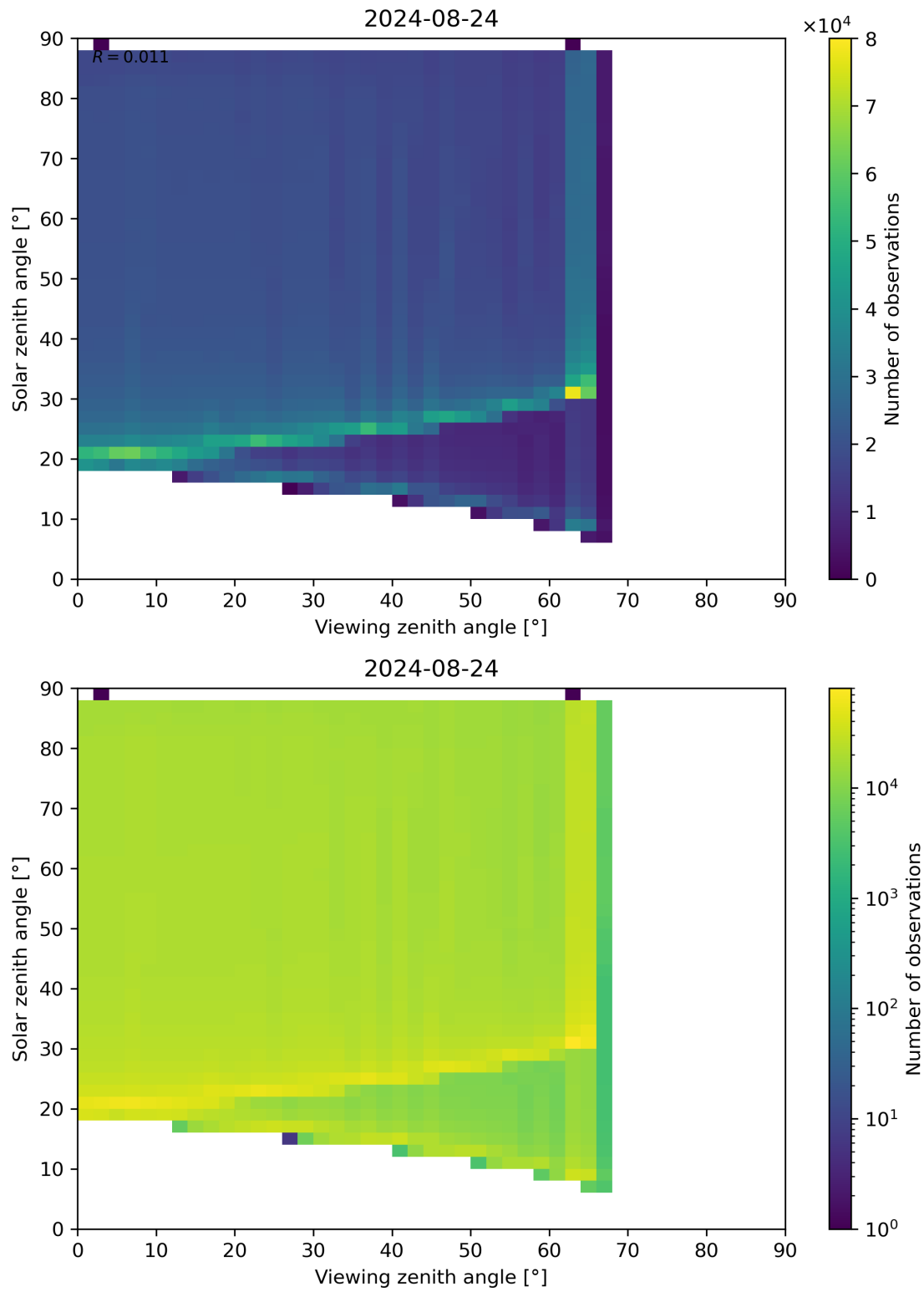
Figure 172: Scatter density plot of “Viewing zenith angle” against “Solar zenith angle” for 2024-08-23 to 2024-08-25.
