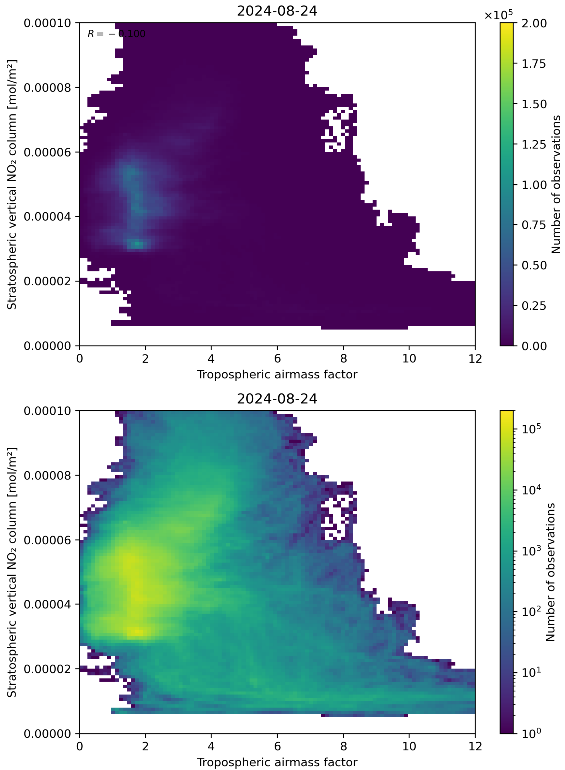
Figure 74: Scatter density plot of “Tropospheric air mass factor” against “Stratospheric vertical NO 2 column” for 2024-08-23 to 2024-08-25.
