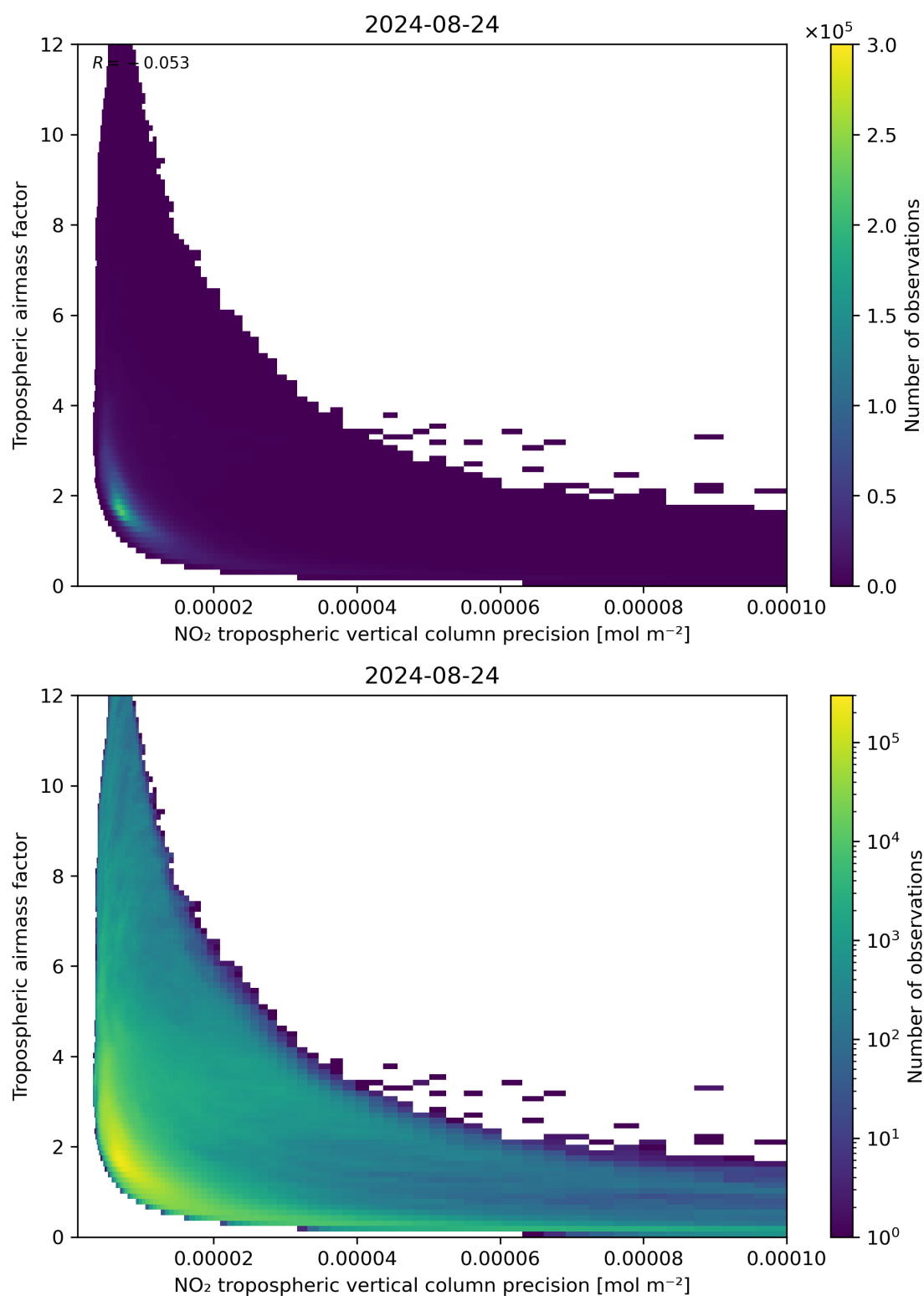
Figure 133: Scatter density plot of “NO 2 tropospheric vertical column precision” against “Tropospheric airmass factor” for 2024-08-23 to 2024-08-25.
