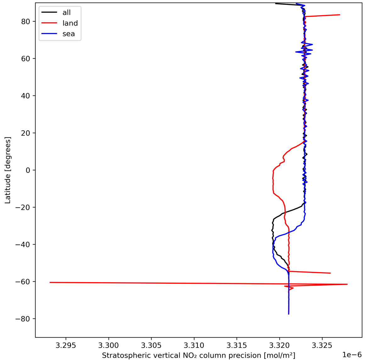
Figure 20: Zonal average of “Stratospheric vertical NO 2 column precision” for 2024-08-23 to 2024-08-25.
