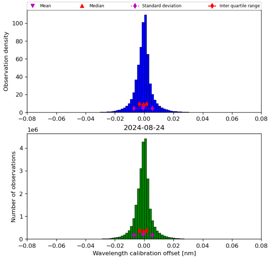
Figure 35: Histogram of “Wavelength calibration offset” for 2024-08-23 to 2024-08-25
