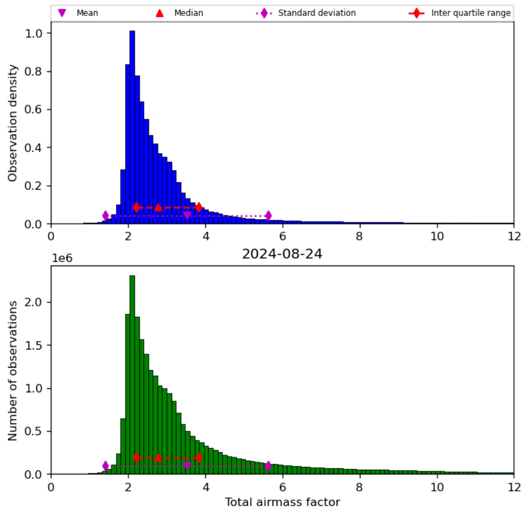
Figure 32: Histogram of “Total airmass factor” for 2024-08-23 to 2024-08-25
