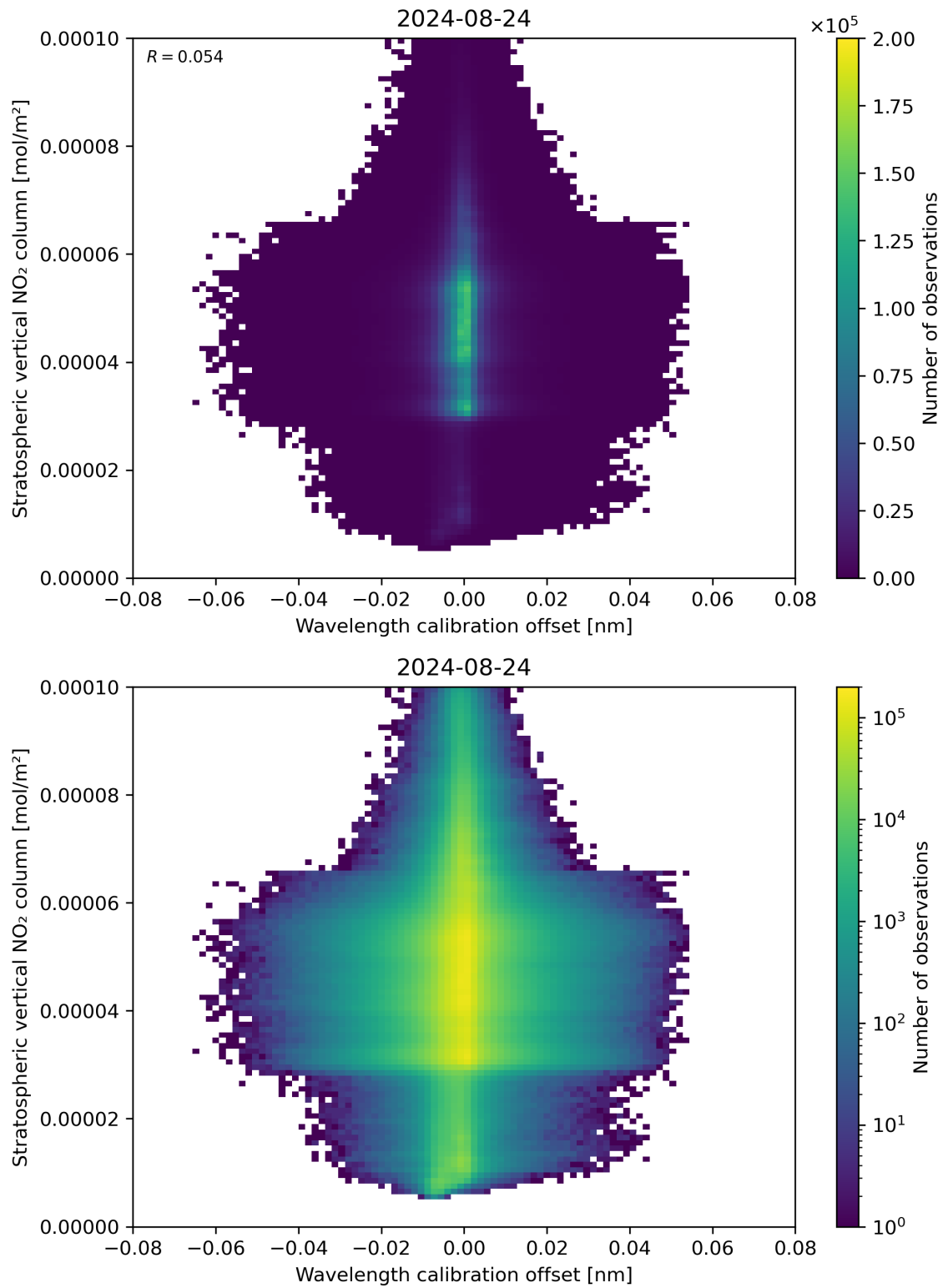
Figure 176: Scatter density plot of “Wavelength calibration offset” against “Stratospheric vertical NO 2 column” for 2024-08-23 to 2024-08-25.
