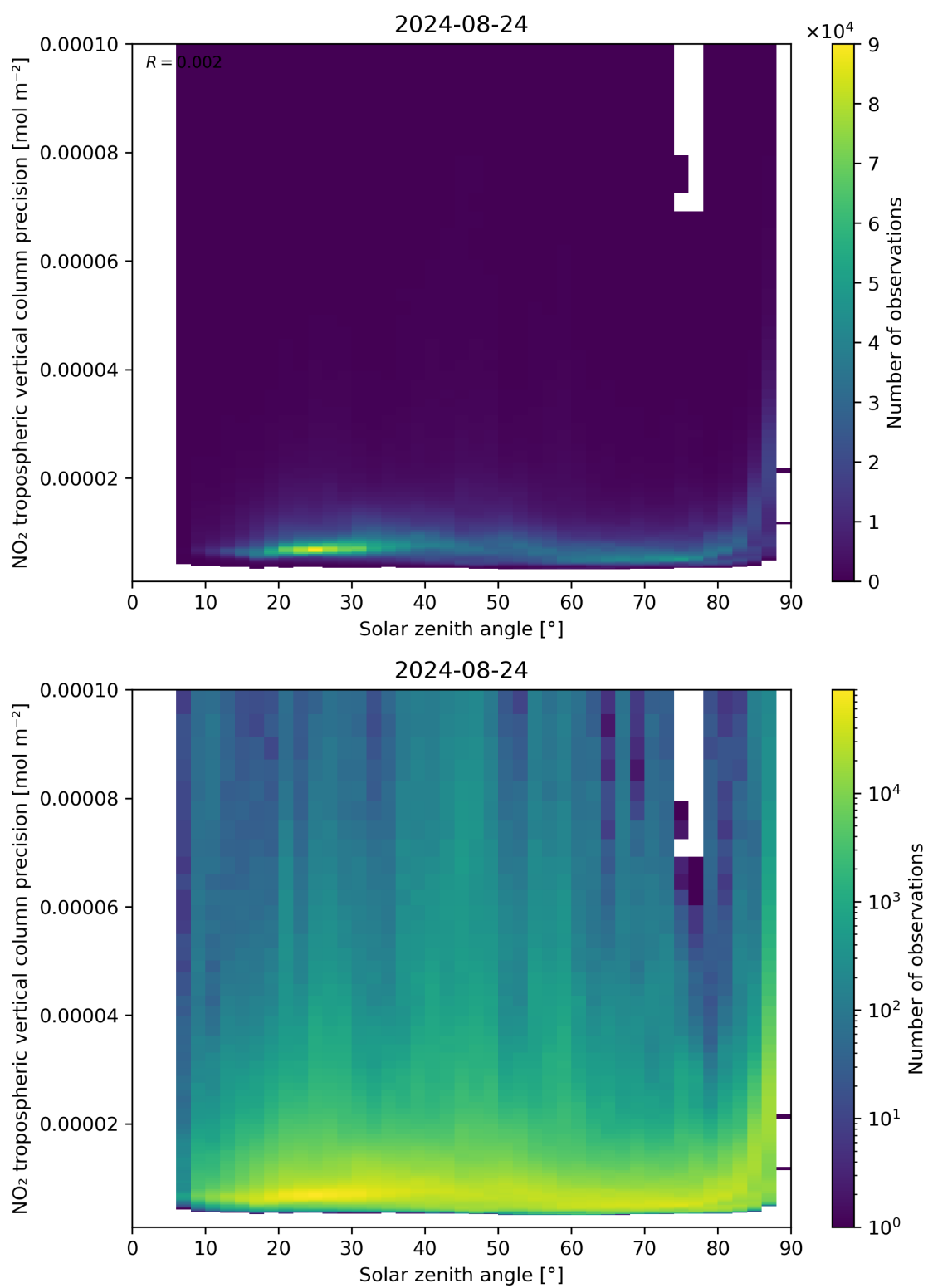
Figure 156: Scatter density plot of “Solar zenith angle” against “NO 2 tropospheric vertical column precision” for 2024-08-23 to 2024-08-25.
