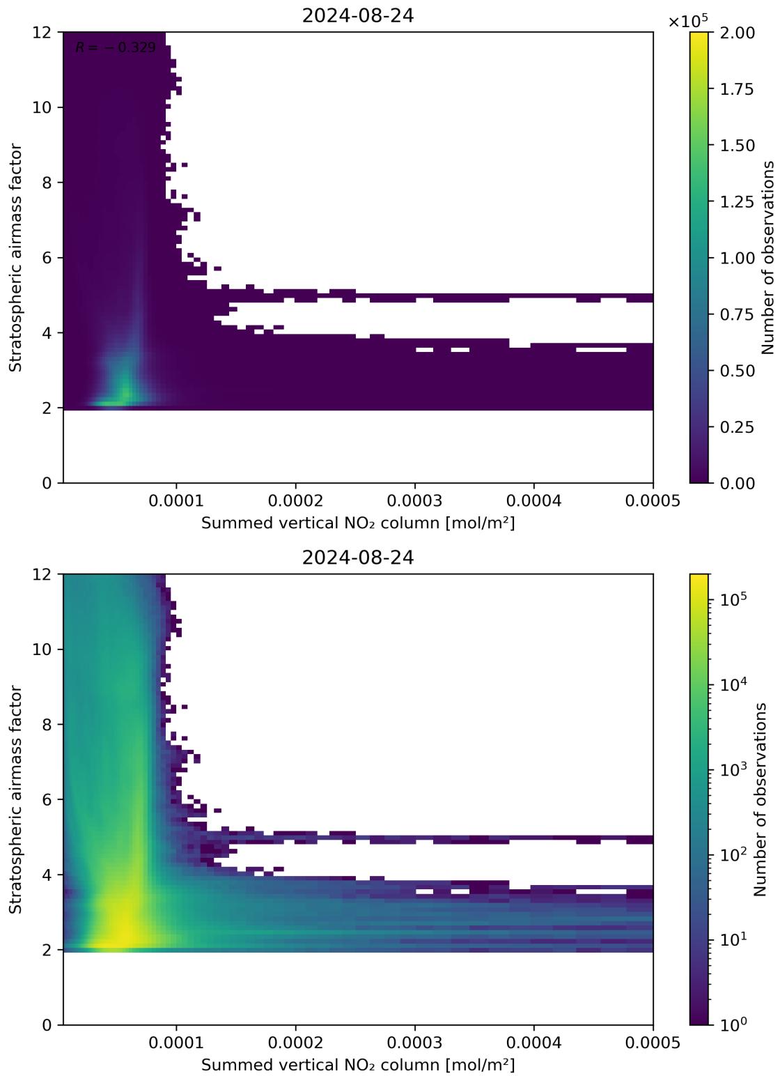
Figure 103: Scatter density plot of “Summed vertical NO 2 column” against “Stratospheric airmass factor” for 2024-08-23 to 2024-08-25.
