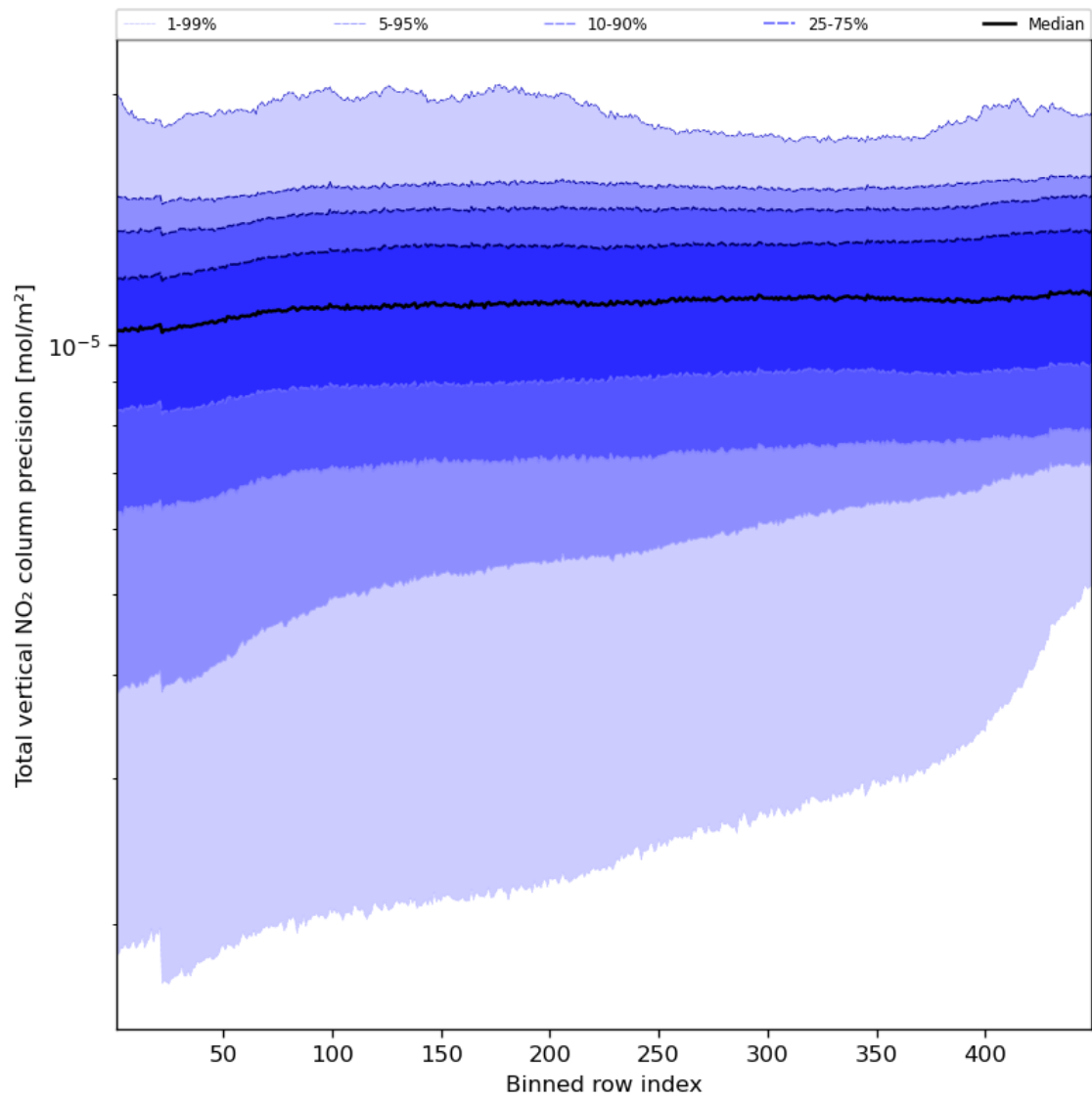
Figure 56: Along track statistics of “Total vertical NO 2 column precision” for 2024-08-23 to 2024-08-25
