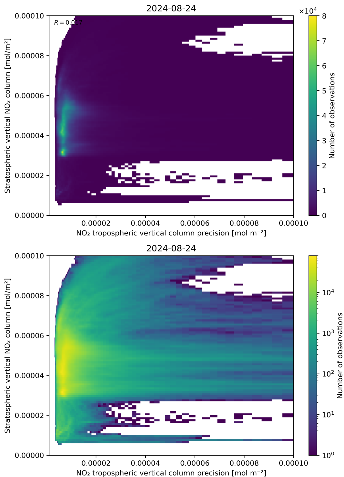
Figure 135: Scatter density plot of “NO 2 tropospheric vertical column precision” against “Stratospheric vertical NO 2 column” for 2024-08-23 to 2024-08-25.
