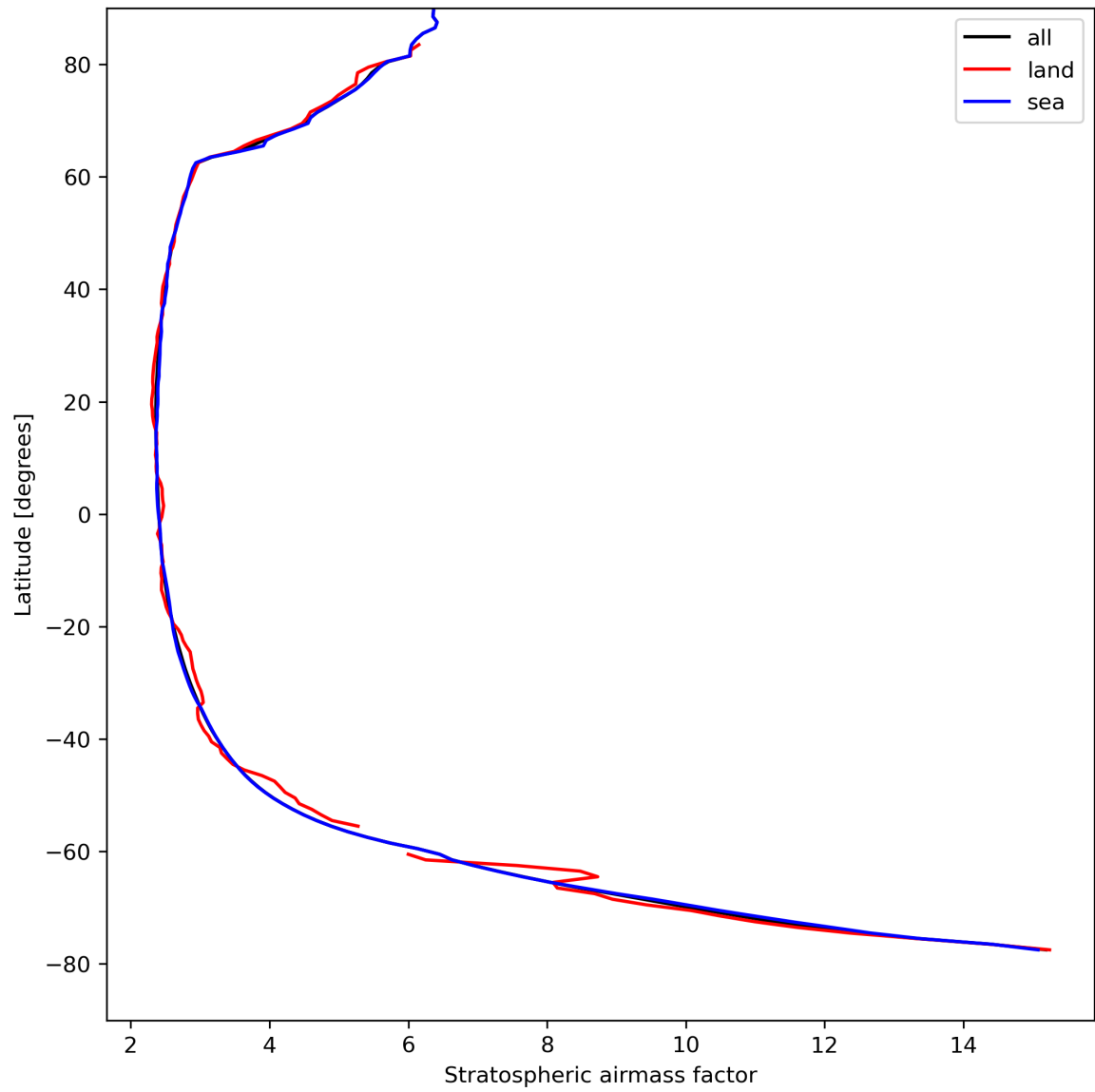
Figure 27: Zonal average of “Stratospheric airmass factor” for 2024-08-23 to 2024-08-25.
