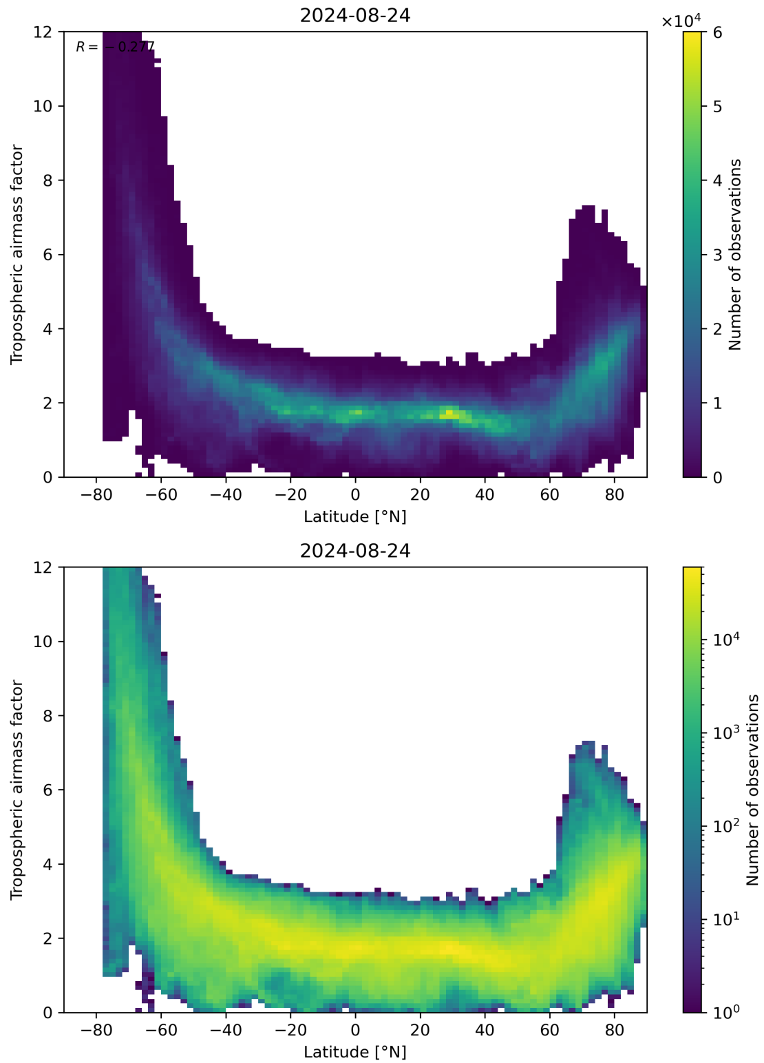
Figure 85: Scatter density plot of “Latitude” against “Tropospheric airmass factor” for 2024-08-23 to 2024-08-25.
