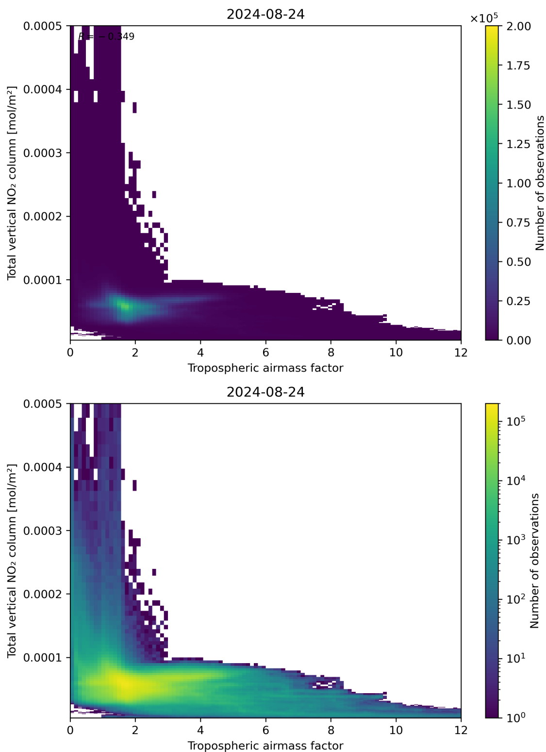
Figure 77: Scatter density plot of “Tropospheric airmass factor” against “Total vertical NO 2 column” for 2024-08-23 to 2024-08-25.
