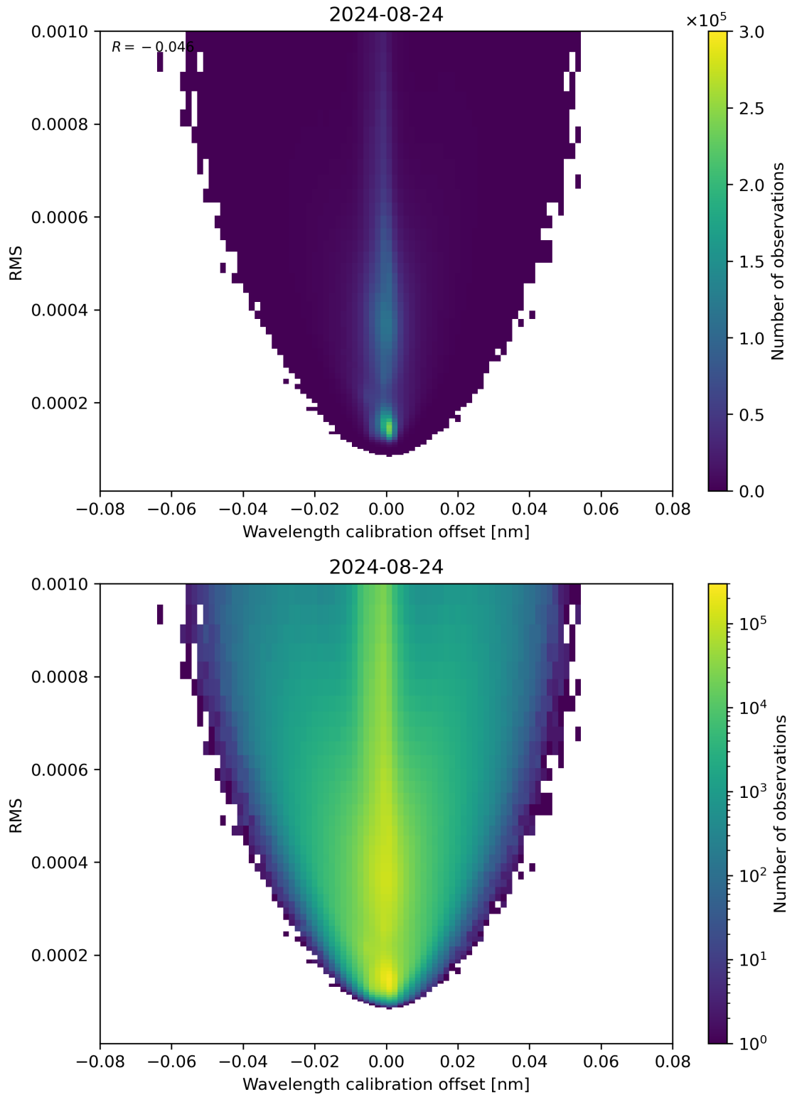
Figure 181: Scatter density plot of “Wavelength calibration offset” against “RMS” for 2024-08-23 to 2024-08-25.
