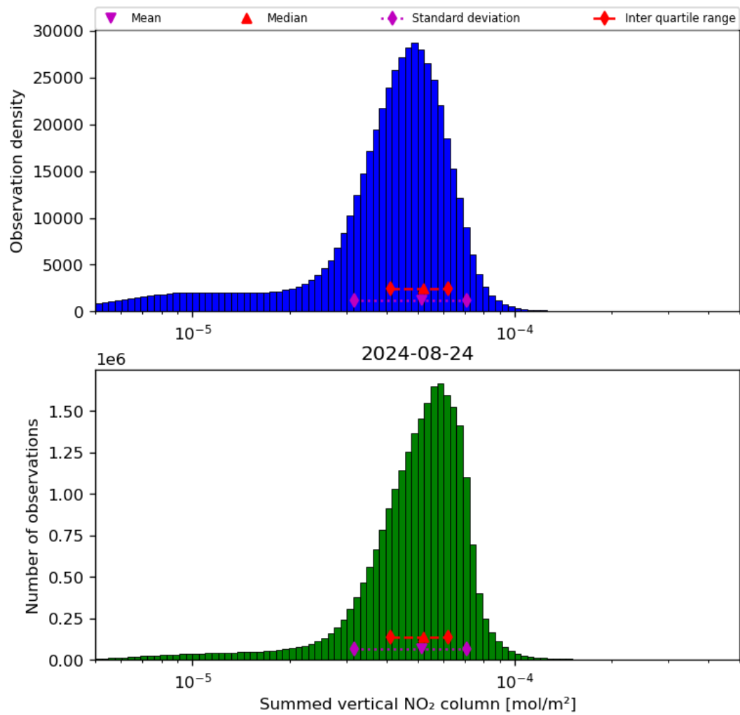
Figure 40: Histogram of “Summed vertical NO 2 column” for 2024-08-23 to 2024-08-25
