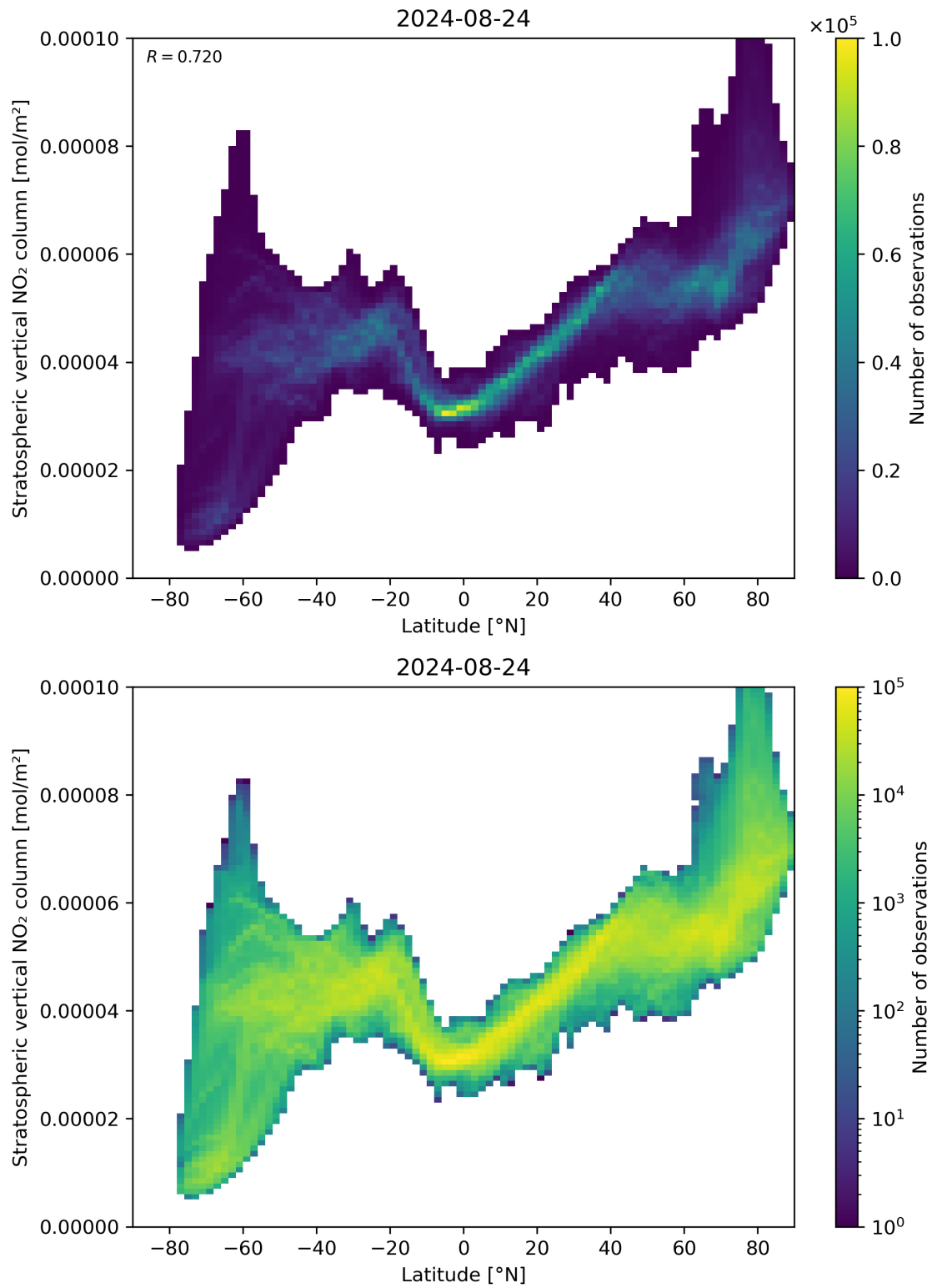
Figure 87: Scatter density plot of “Latitude” against “Stratospheric vertical NO 2 column” for 2024-08-23 to 2024-08-25.
