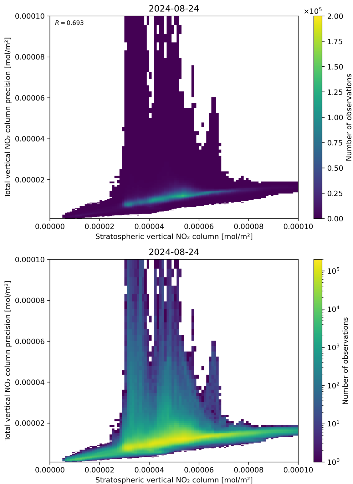
Figure 101: Scatter density plot of “Stratospheric vertical NO 2 column” against “Total vertical NO 2 column precision” for 2024-08-23 to 2024-08-25.
