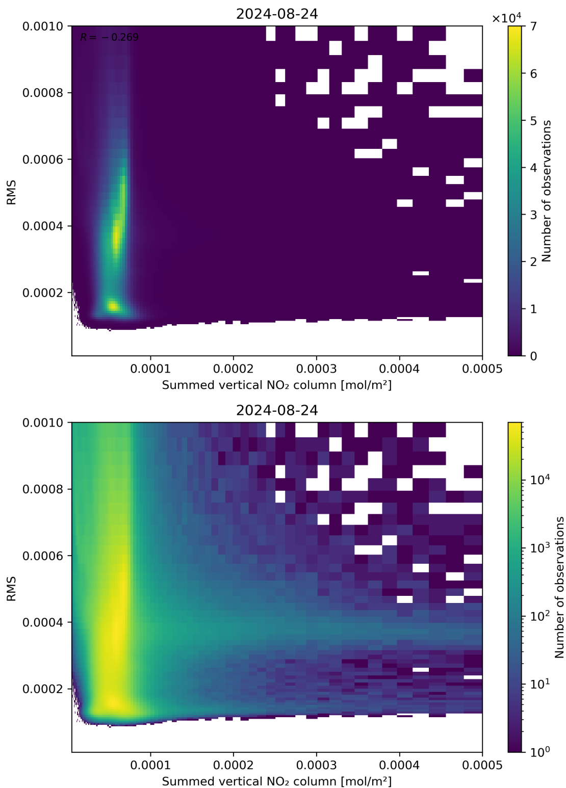
Figure 109: Scatter density plot of “Summed vertical NO 2 column” against “RMS” for 2024-08-23 to 2024-08-25.
