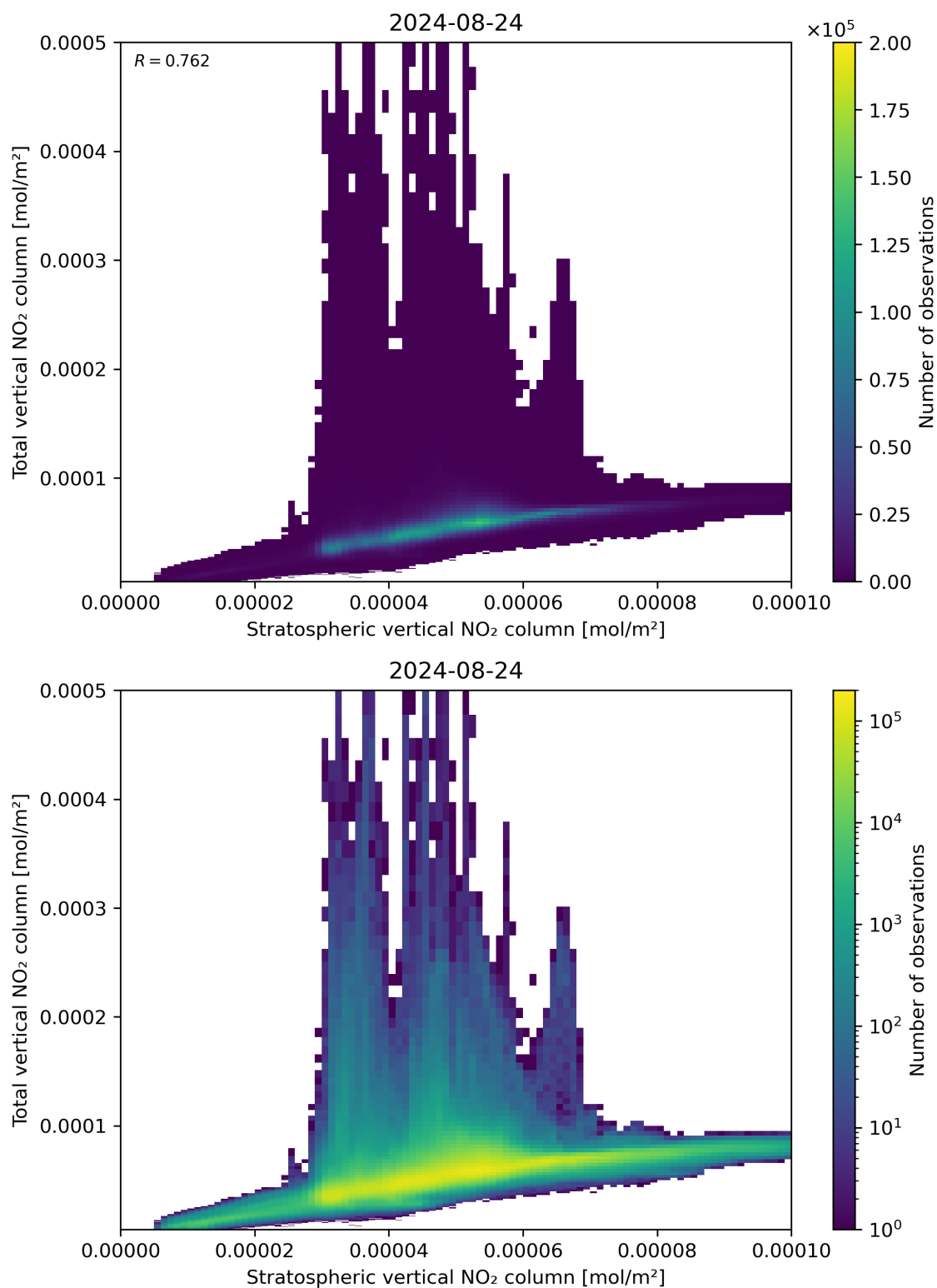
Figure 100: Scatter density plot of “Stratospheric vertical NO 2 column” against “Total vertical NO 2 column” for 2024-08-23 to 2024-08-25.
