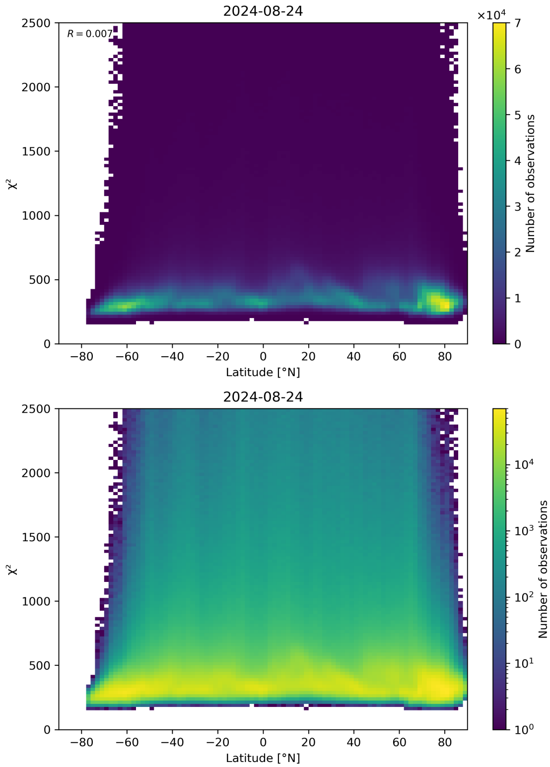
Figure 86: Scatter density plot of “Latitude” against “ \chi^2 ” for 2024-08-23 to 2024-08-25.
