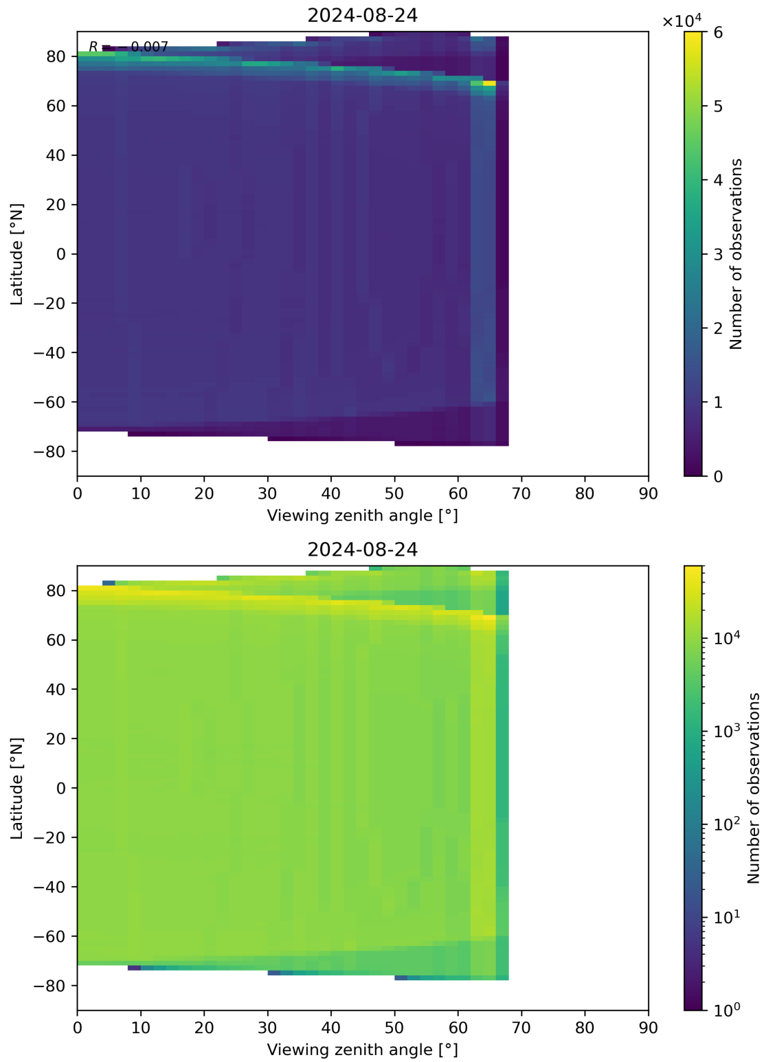
Figure 163: Scatter density plot of “Viewing zenith angle” against “Latitude” for 2024-08-23 to 2024-08-25.
