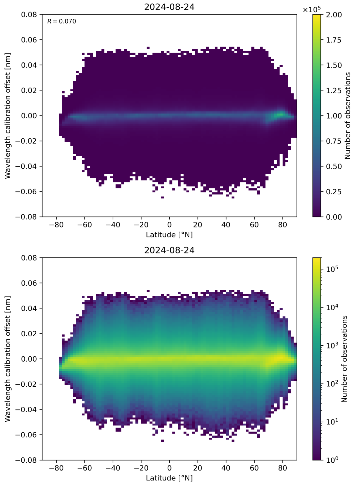
Figure 95: Scatter density plot of “Latitude” against “Wavelength calibration offset” for 2024-08-23 to 2024-08-25.
