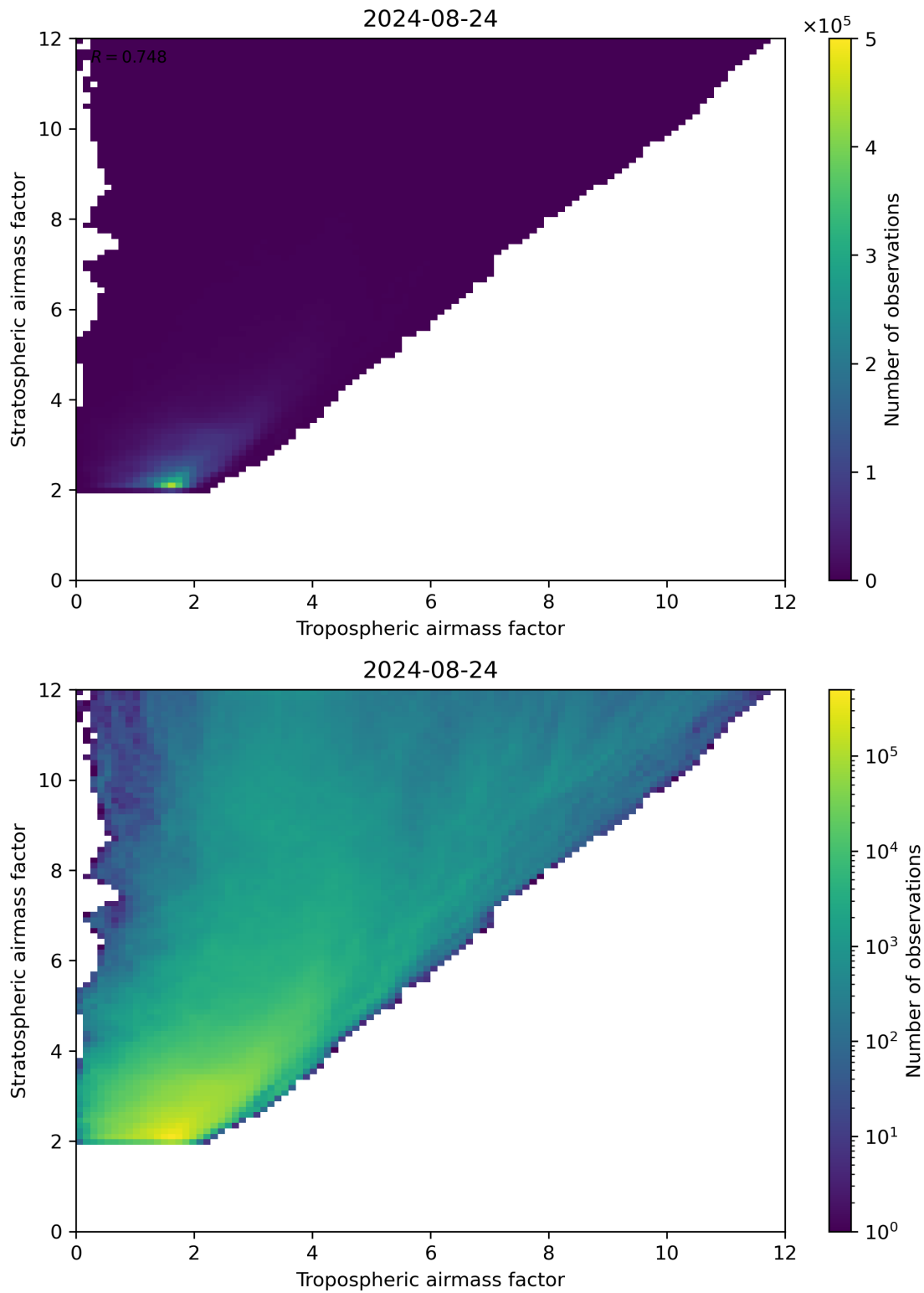
Figure 71: Scatter density plot of “Tropospheric airmass factor” against “Stratospheric airmass factor” for 2024-08-23 to 2024-08-25.
