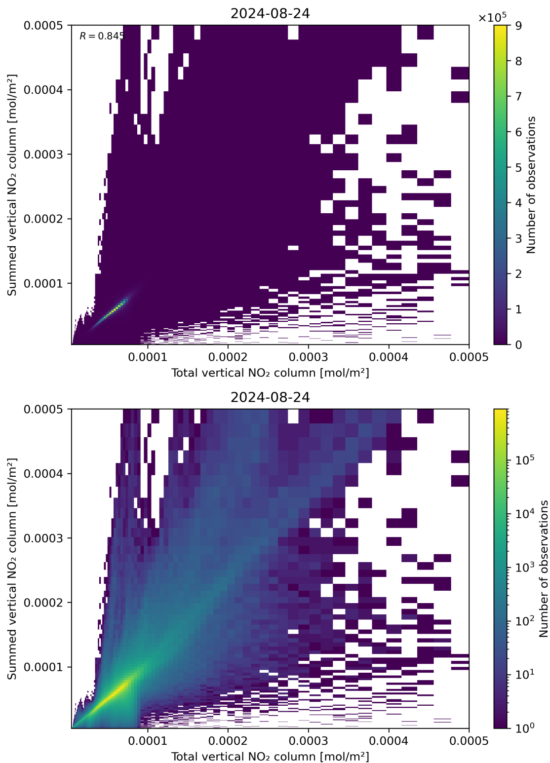
Figure 112: Scatter density plot of “Total vertical NO 2 column” against “Summed vertical NO 2 column” for 2024-08-23 to 2024-08-25.
