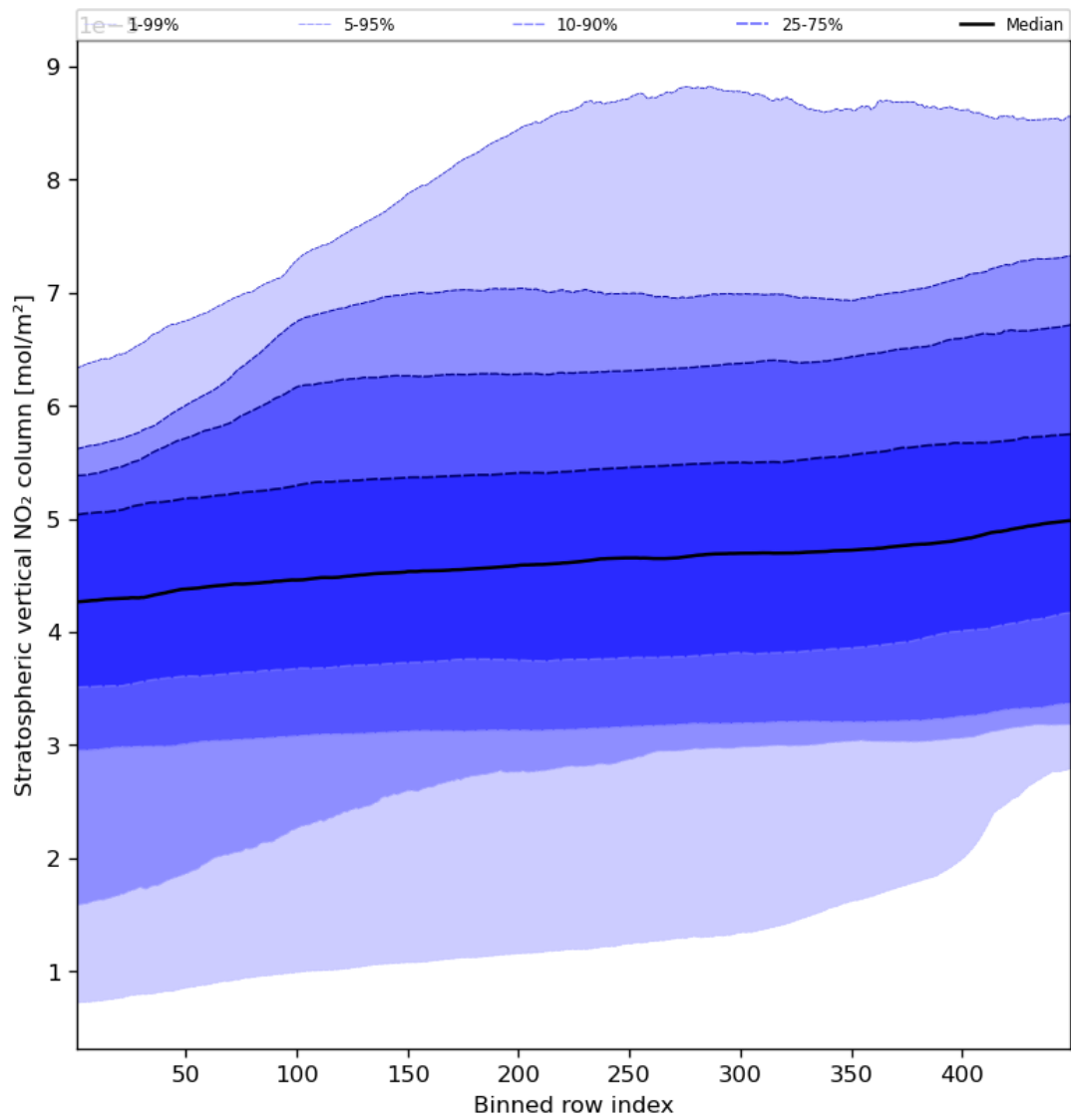
Figure 53: Along track statistics of “Stratospheric vertical NO 2 column” for 2024-08-23 to 2024-08-25
