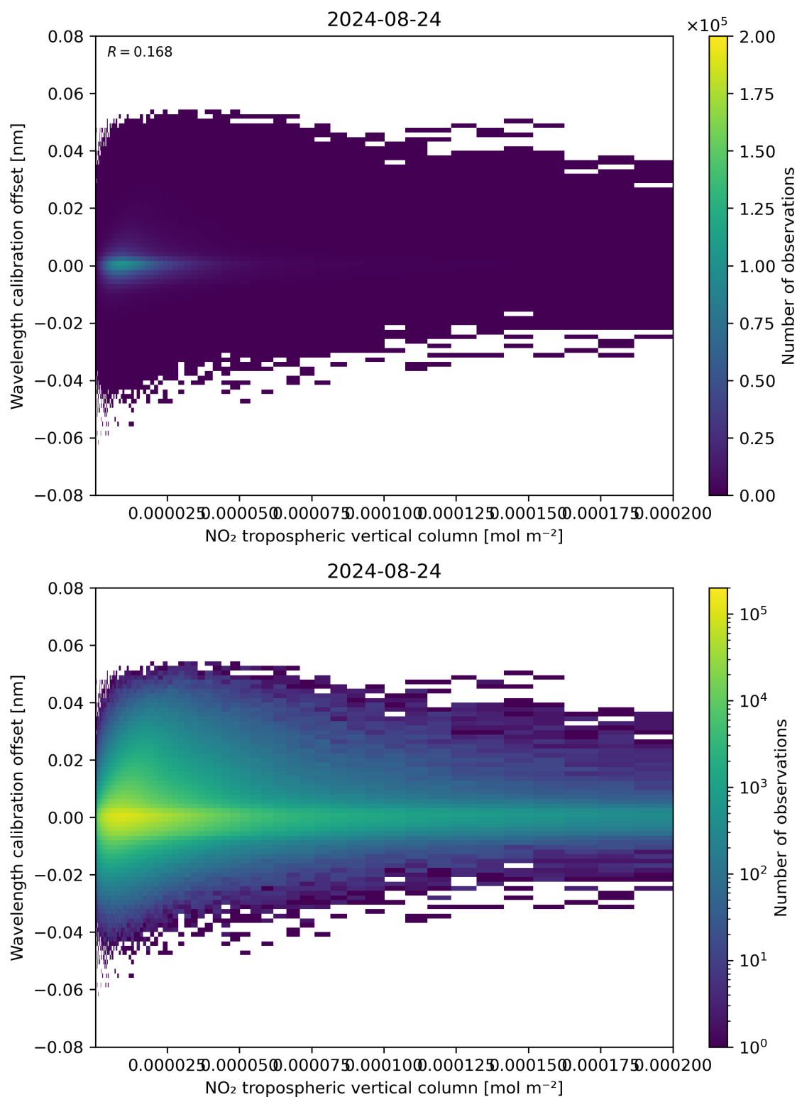
Figure 143: Scatter density plot of “NO 2 tropospheric vertical column” against “Wavelength calibration offset” for 2024-08-23 to 2024-08-25.
