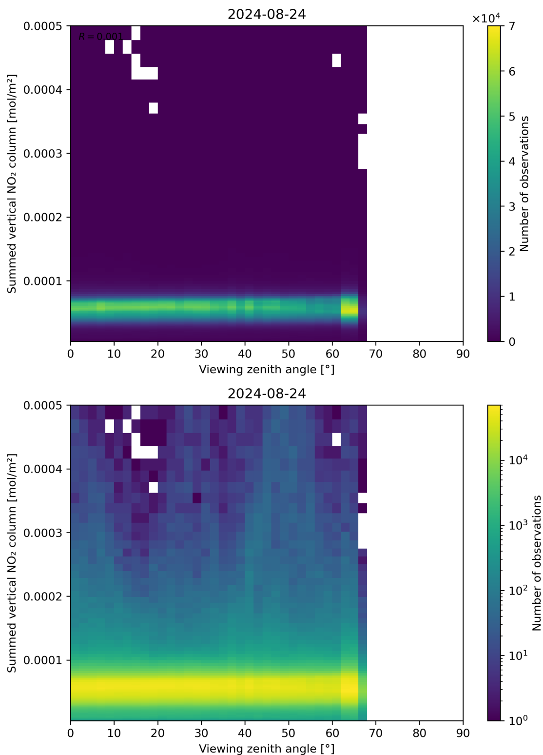
Figure 165: Scatter density plot of “Viewing zenith angle” against “Summed vertical NO 2 column” for 2024-08-23 to 2024-08-25.
