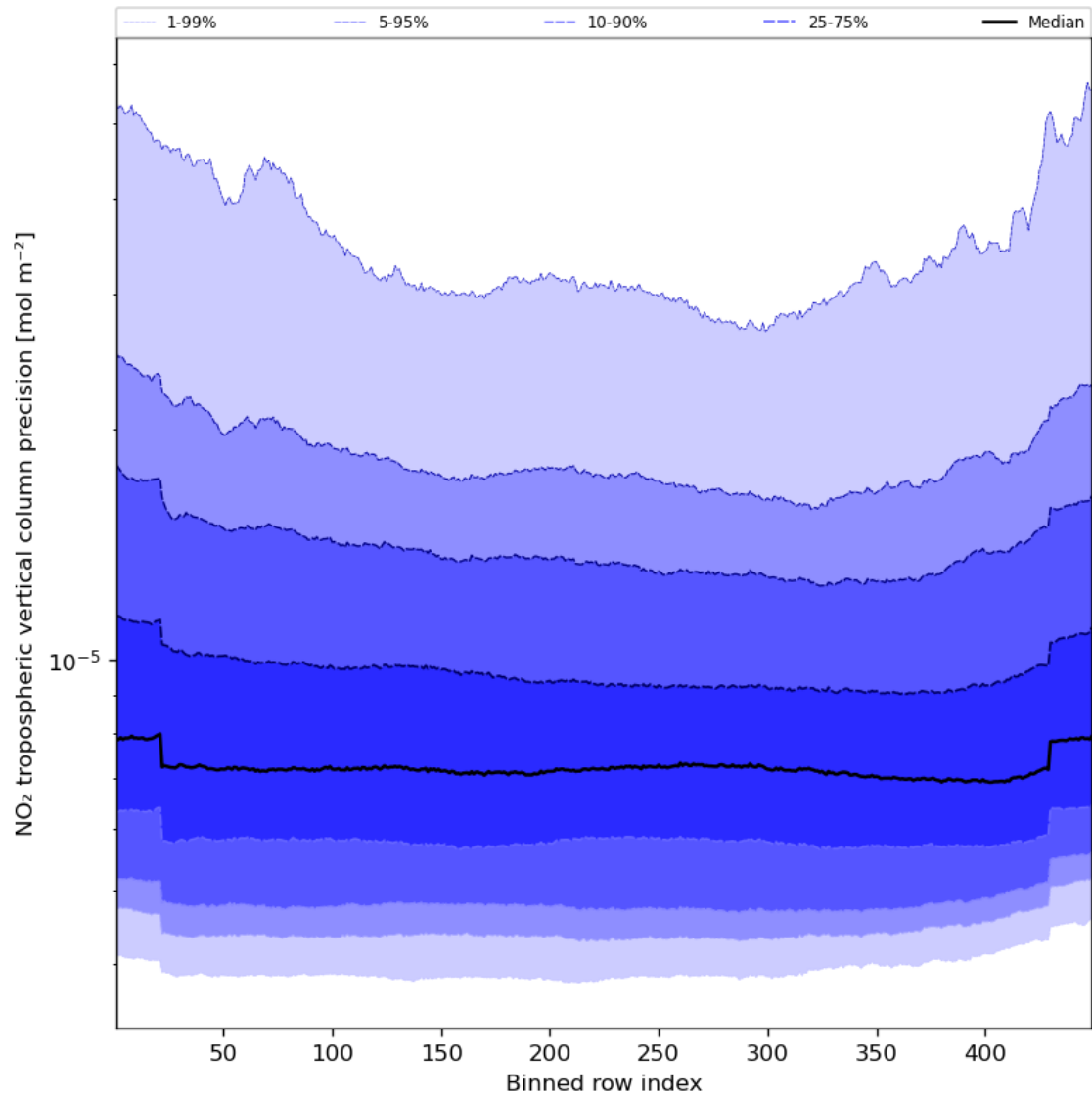
Figure 47: Along track statistics of “NO 2 tropospheric vertical column precision” for 2024-08-23 to 2024-08-25
