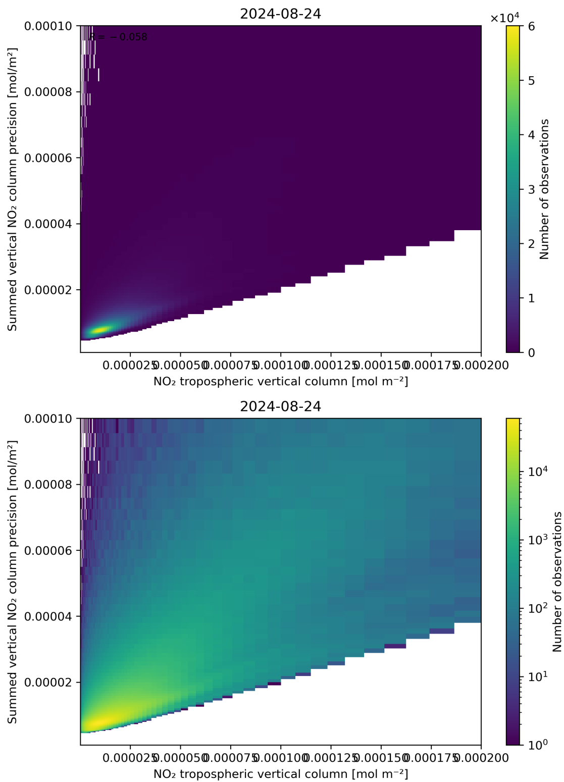
Figure 127: Scatter density plot of “NO 2 tropospheric vertical column” against “Summed vertical NO 2 column precision” for 2024-08-23 to 2024-08-25.
