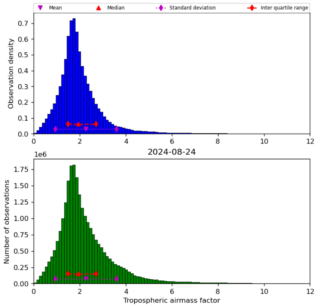
Figure 31: Histogram of “Tropospheric airmass factor” for 2024-08-23 to 2024-08-25
