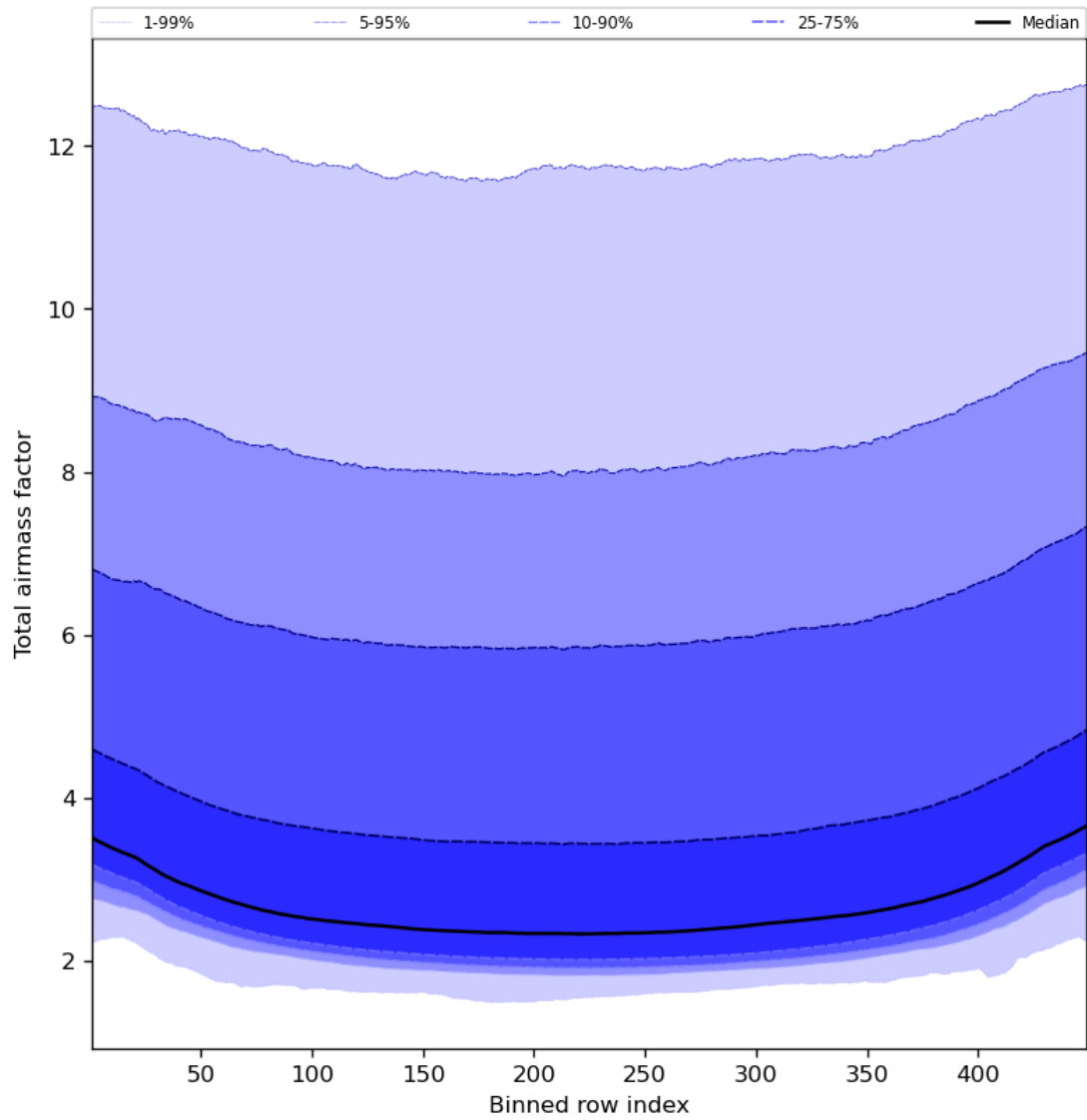
Figure 49: Along track statistics of “Total airmass factor” for 2024-08-23 to 2024-08-25
