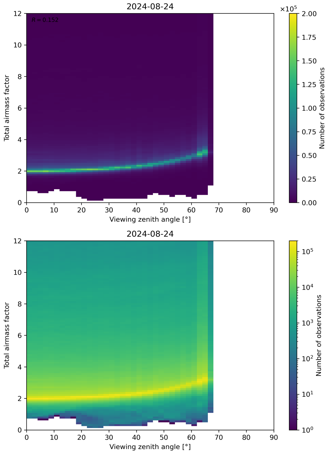
Figure 160: Scatter density plot of “Viewing zenith angle” against “Total airmass factor” for 2024-08-23 to 2024-08-25.
