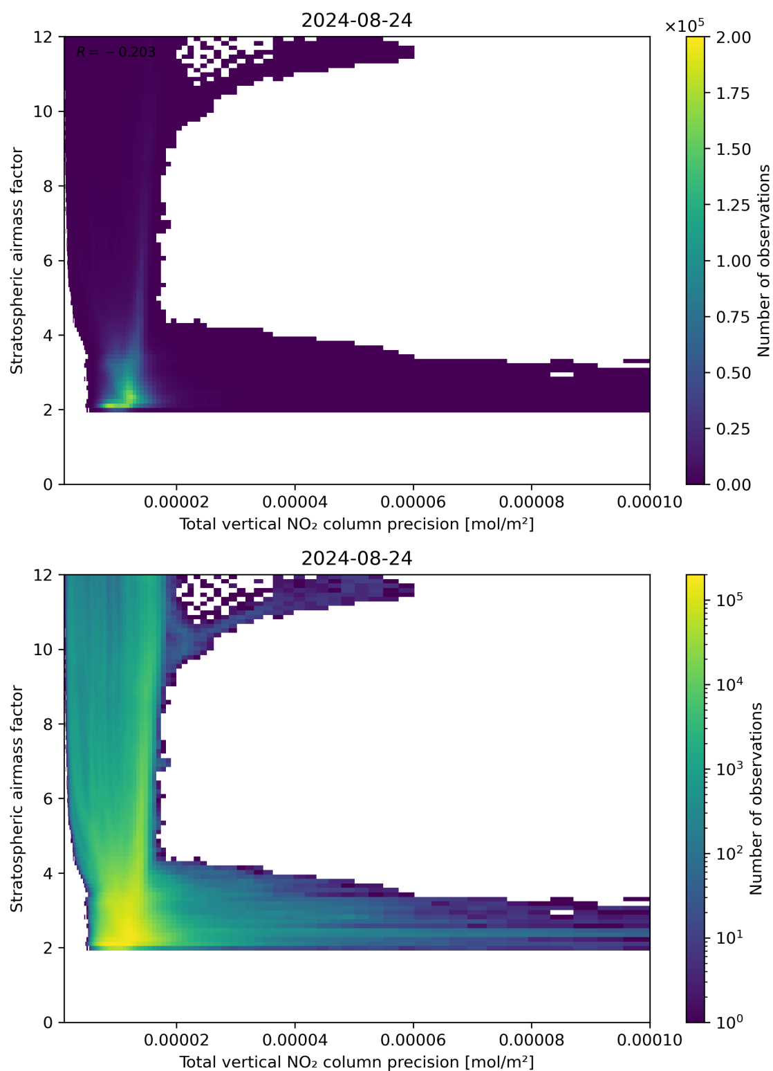
Figure 115: Scatter density plot of “Total vertical NO 2 column precision” against “Stratospheric air mass factor” for 2024-08-23 to 2024-08-25.
