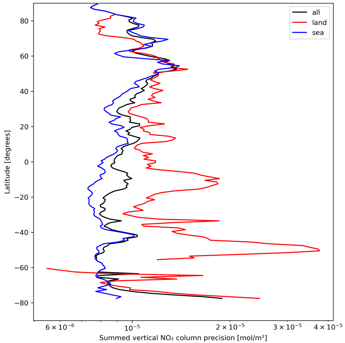
Figure 24: Zonal average of “Summed vertical NO 2 column precision” for 2024-08-23 to 2024-08-25.
