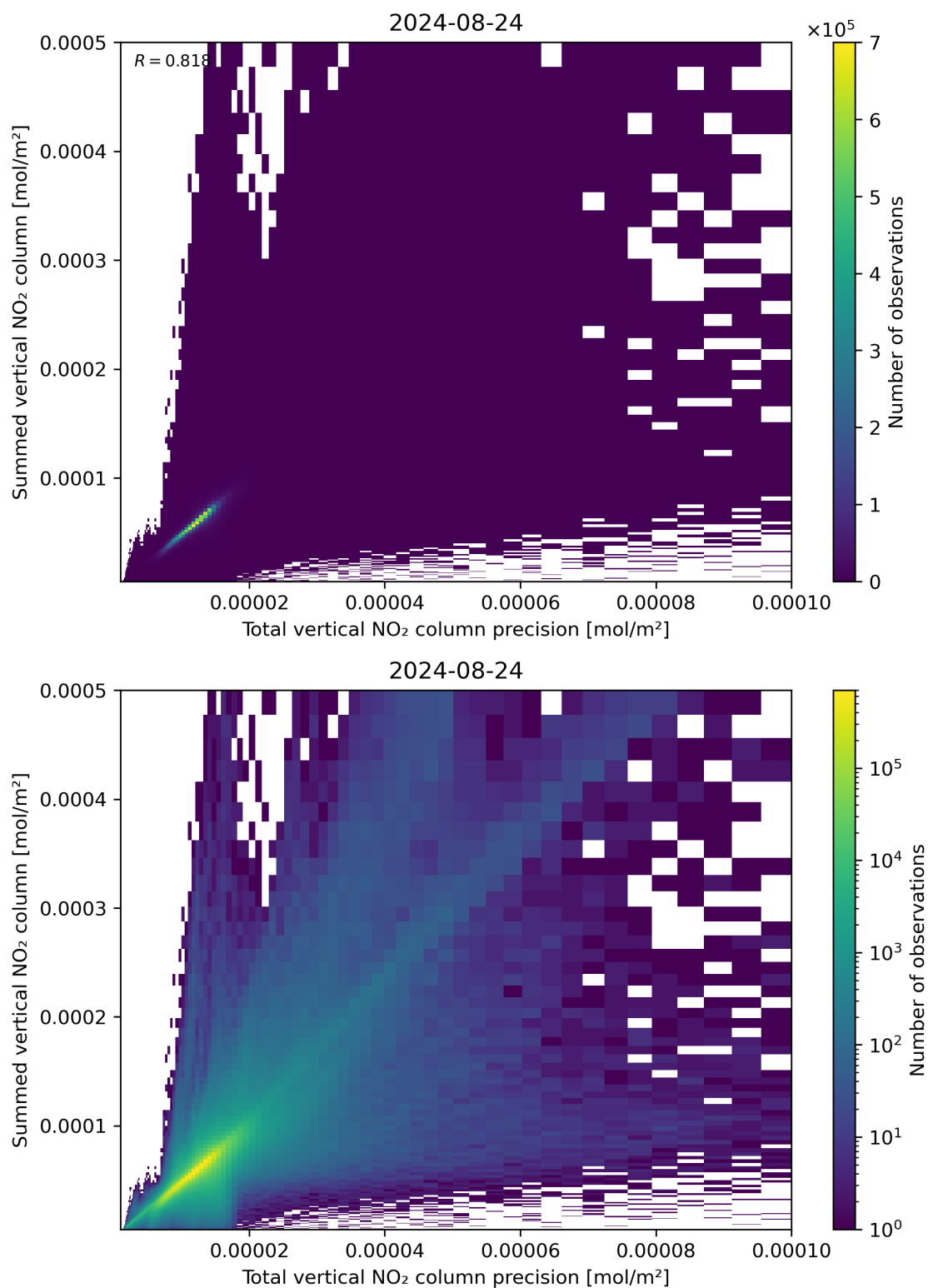
Figure 117: Scatter density plot of “Total vertical NO 2 column precision” against “Summed vertical NO 2 column” for 2024-08-23 to 2024-08-25.
