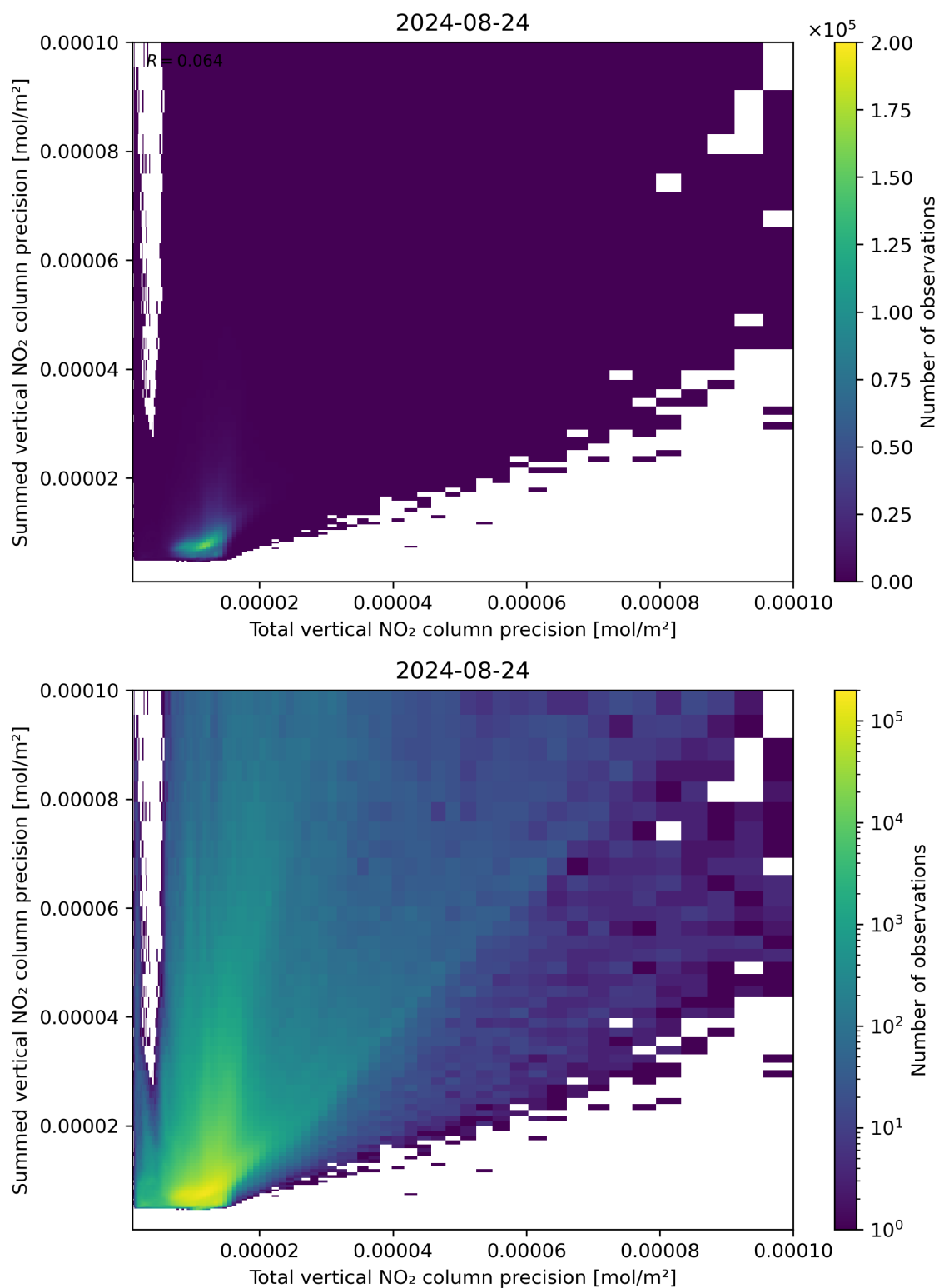
Figure 118: Scatter density plot of “Total vertical NO 2 column precision” against “Summed vertical NO 2 column precision” for 2024-08-23 to 2024-08-25.
