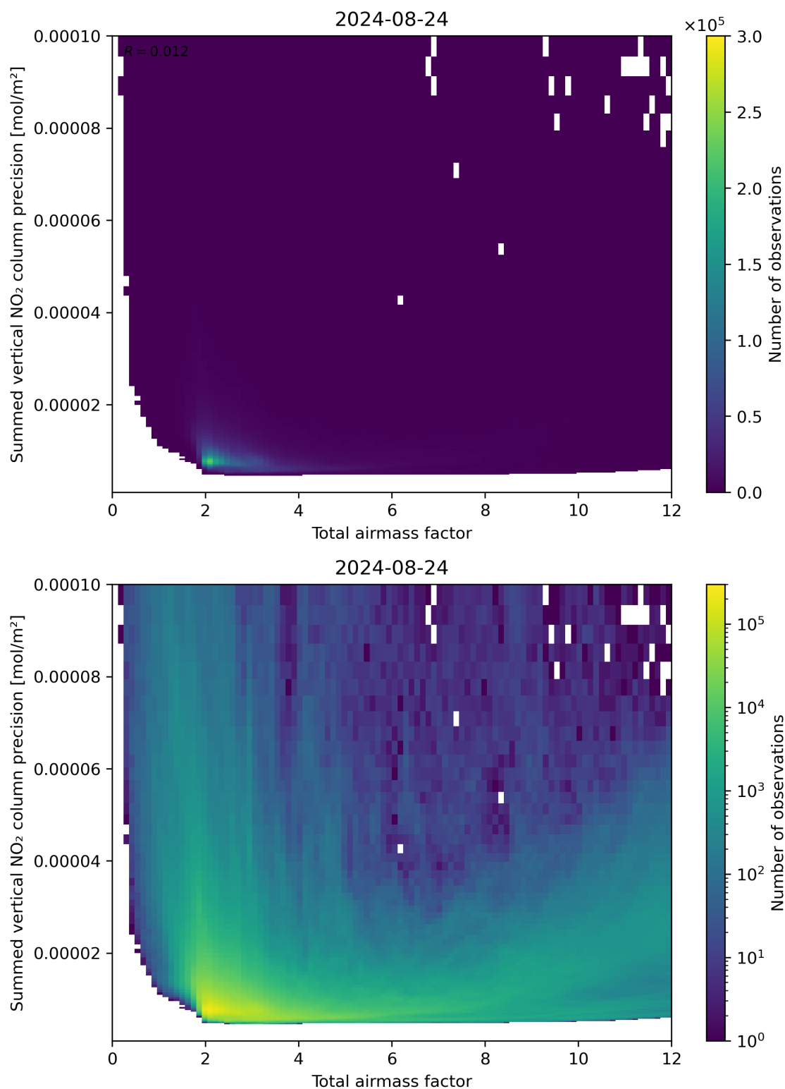
Figure 66: Scatter density plot of “Total airmass factor” against “Summed vertical NO 2 column precision” for 2024-08-23 to 2024-08-25.
