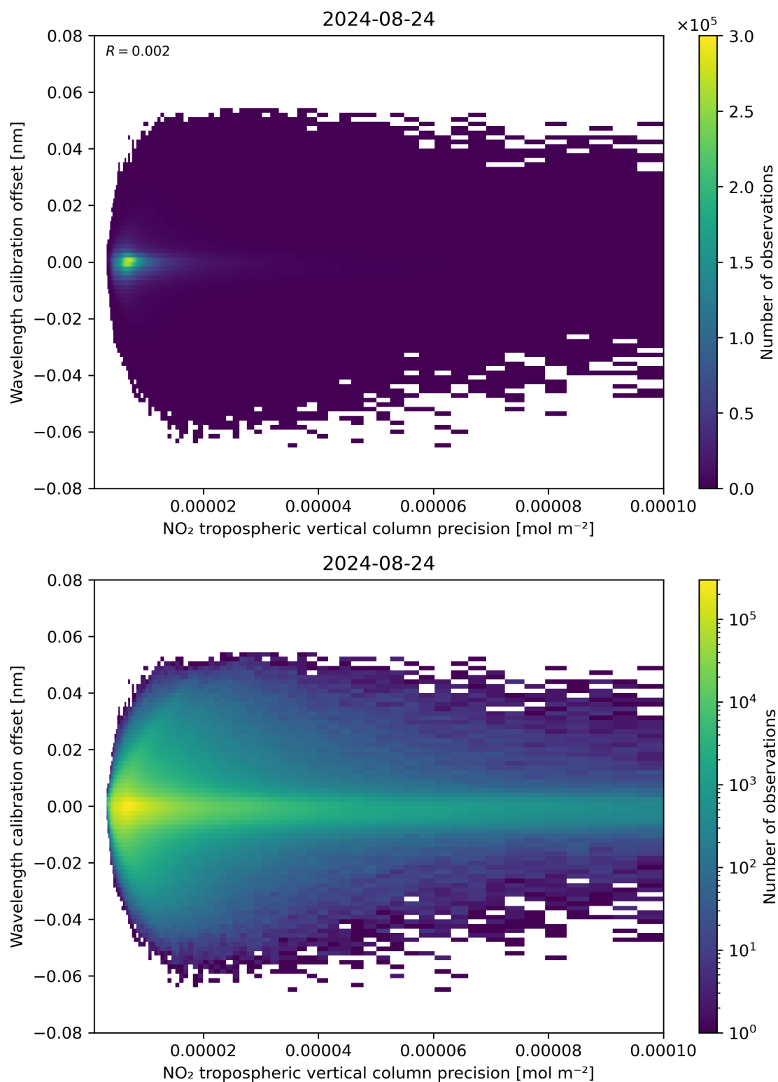
Figure 141: Scatter density plot of “NO 2 tropospheric vertical column precision” against “Wavelength calibration offset” for 2024-08-23 to 2024-08-25.
