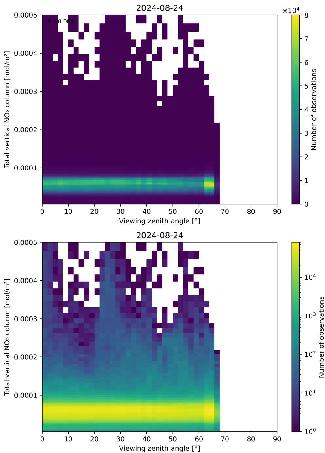
Figure 167: Scatter density plot of “Viewing zenith angle” against “Total vertical NO 2 column” for 2024-08-23 to 2024-08-25.
