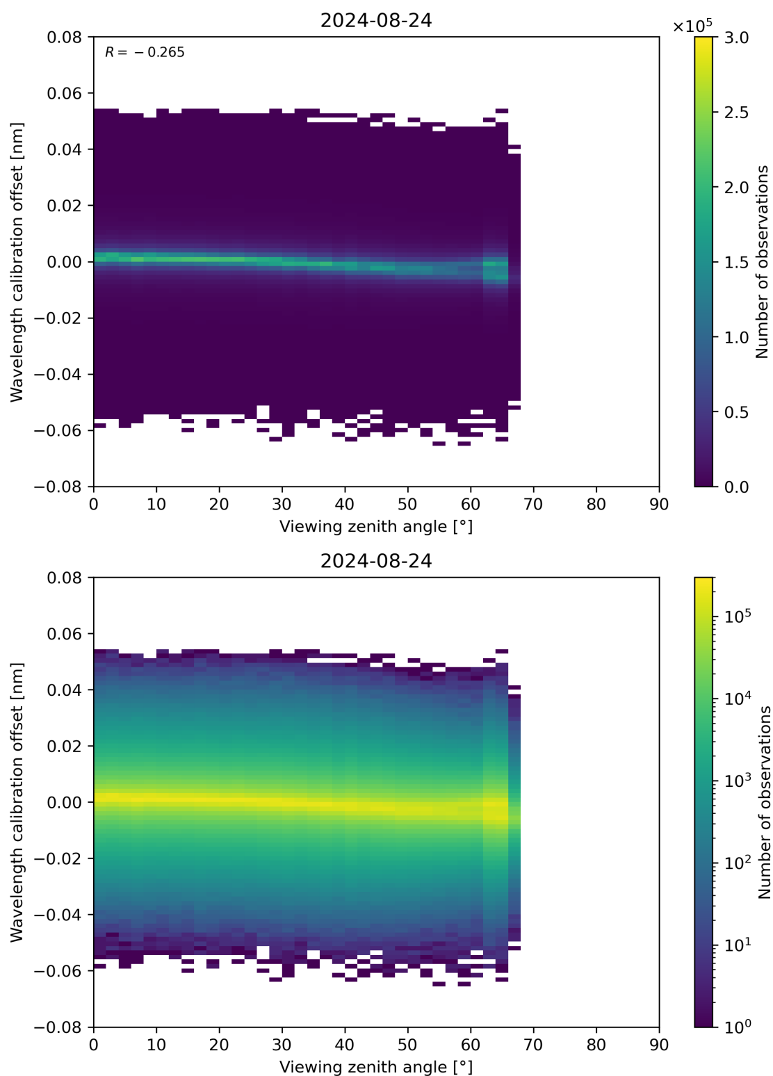
Figure 173: Scatter density plot of “Viewing zenith angle” against “Wavelength calibration offset” for 2024-08-23 to 2024-08-25.
