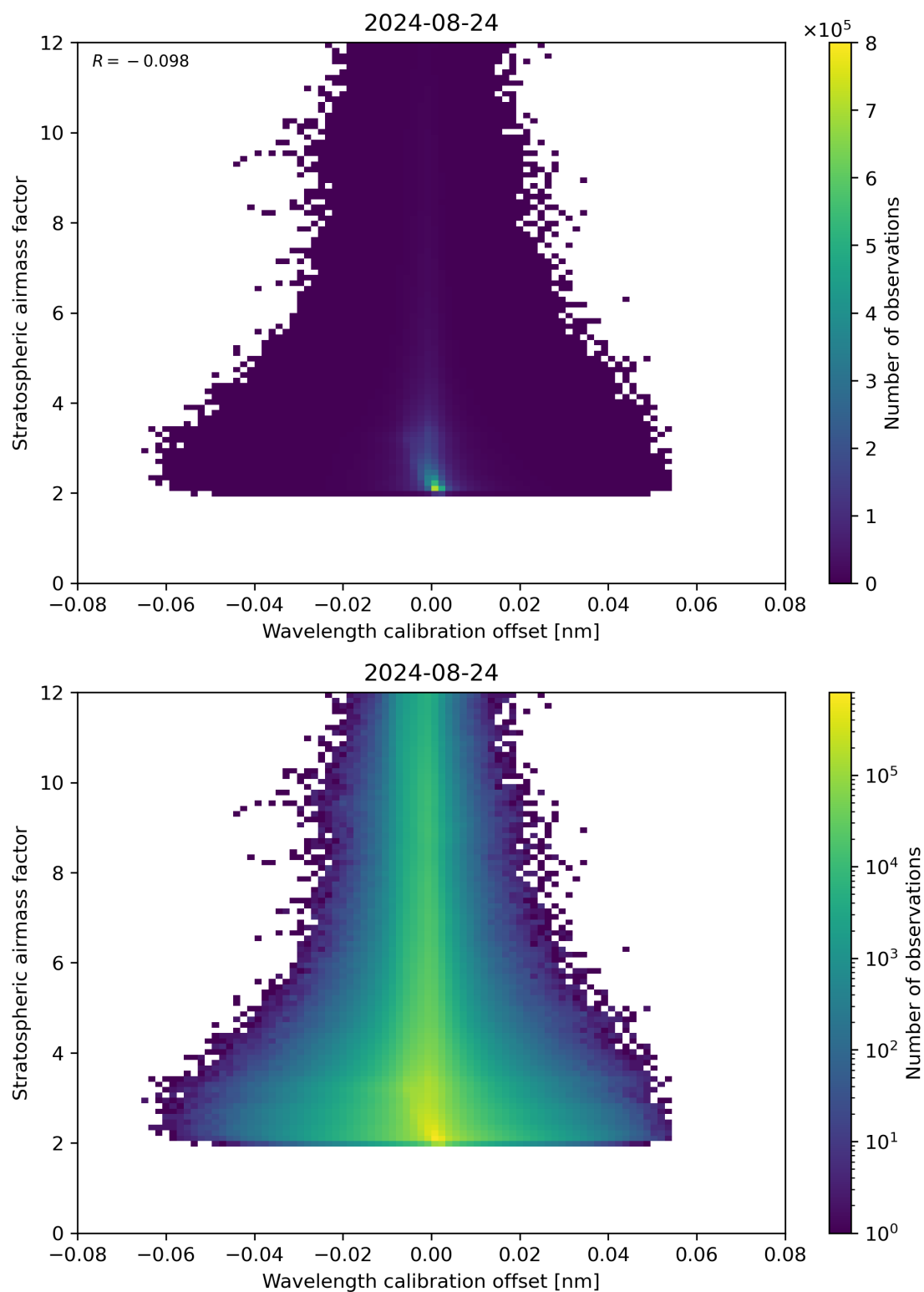
Figure 174: Scatter density plot of “Wavelength calibration offset” against “Stratospheric airmass factor” for 2024-08-23 to 2024-08-25.
