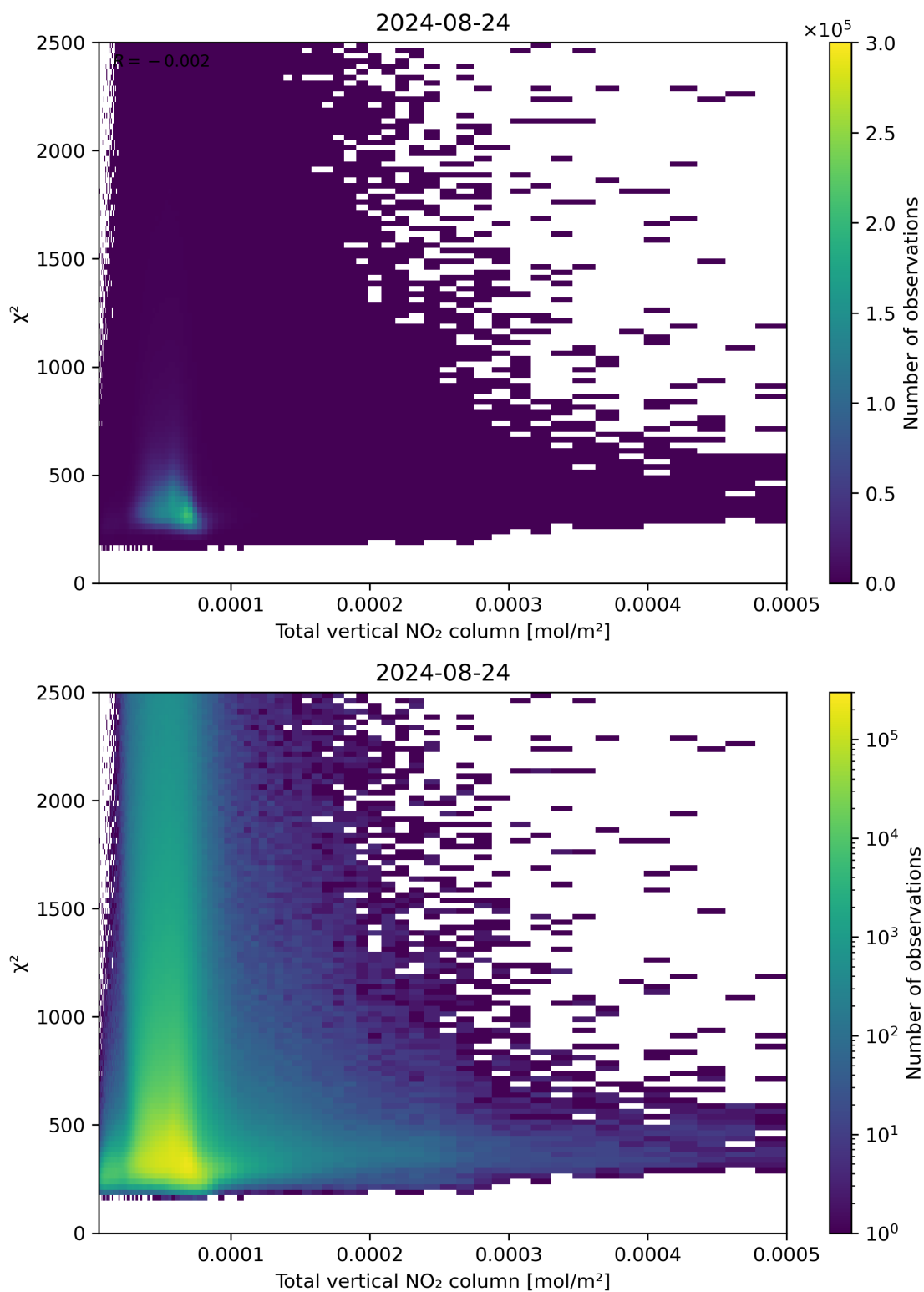
Figure 111: Scatter density plot of “Total vertical NO 2 column” against “ \chi^2 ” for 2024-08-23 to 2024-08-25.
