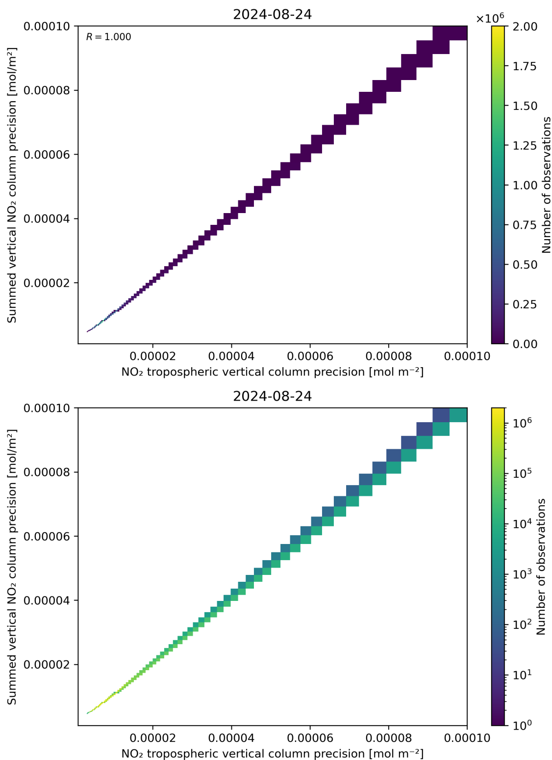
Figure 137: Scatter density plot of “NO 2 tropospheric vertical column precision” against “Summed vertical NO 2 column precision” for 2024-08-23 to 2024-08-25.
