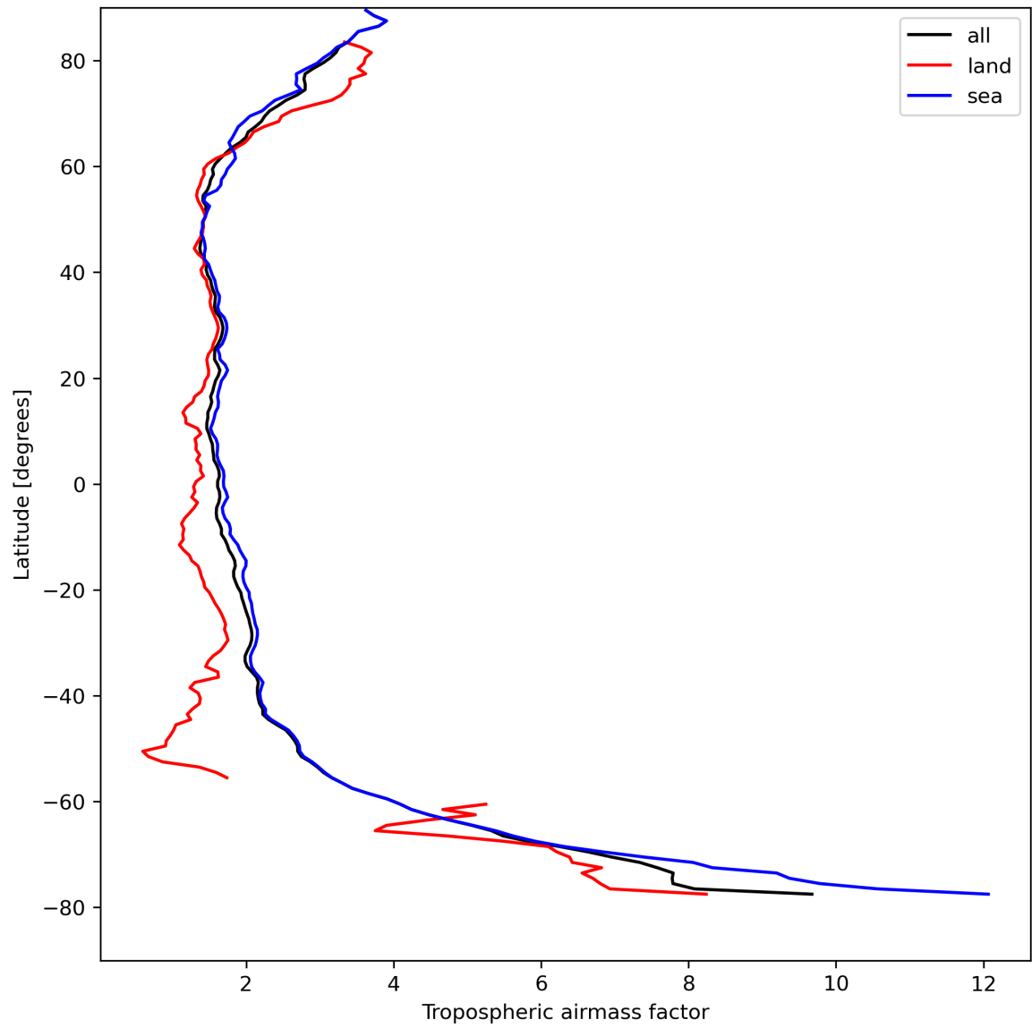
Figure 14: Zonal average of “Tropospheric airmass factor” for 2024-08-23 to 2024-08-25.
