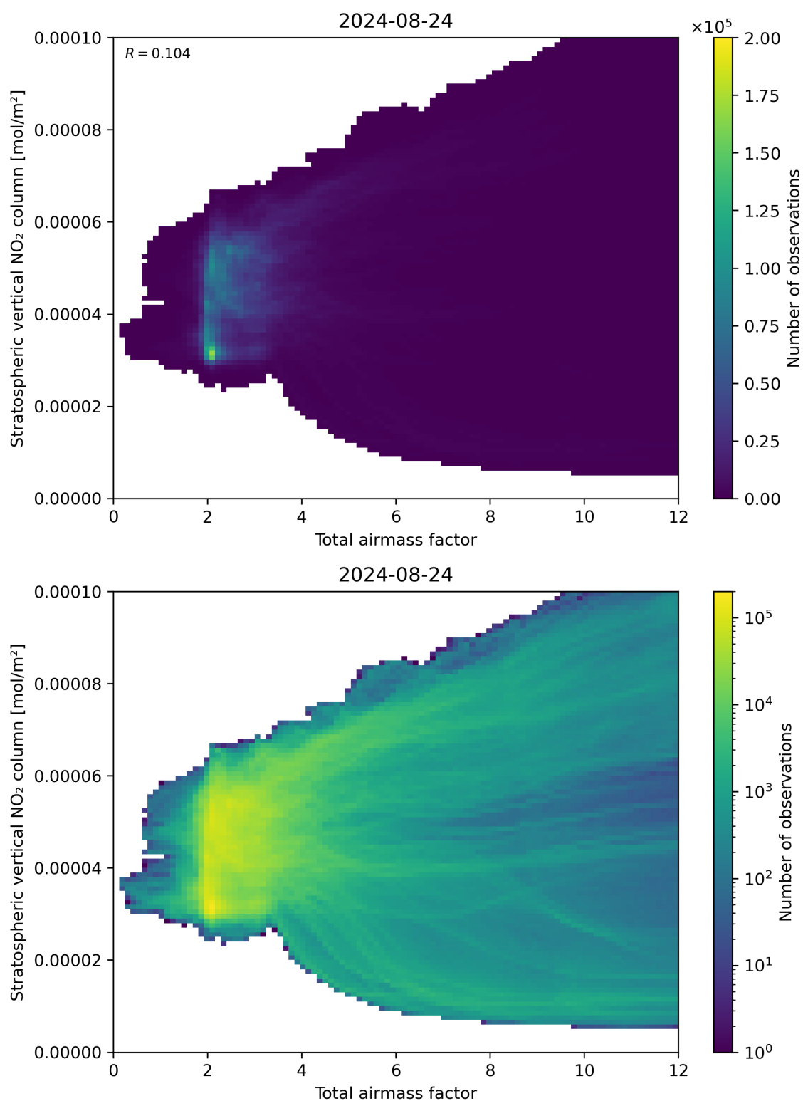
Figure 64: Scatter density plot of “Total airmass factor” against “Stratospheric vertical \text{NO}_2 column” for 2024-08-23 to 2024-08-25.
