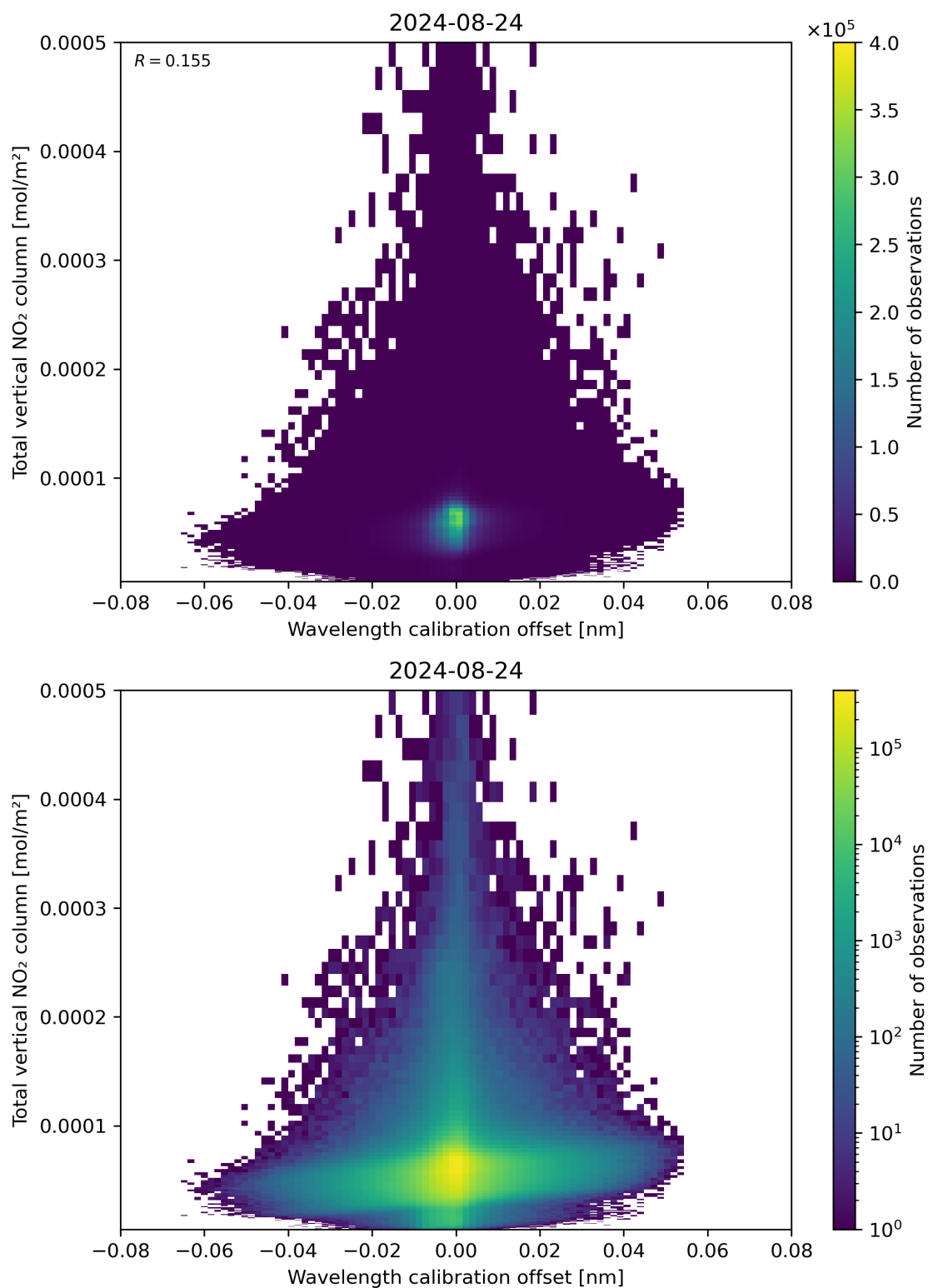
Figure 179: Scatter density plot of “Wavelength calibration offset” against “Total vertical NO 2 column” for 2024-08-23 to 2024-08-25.
