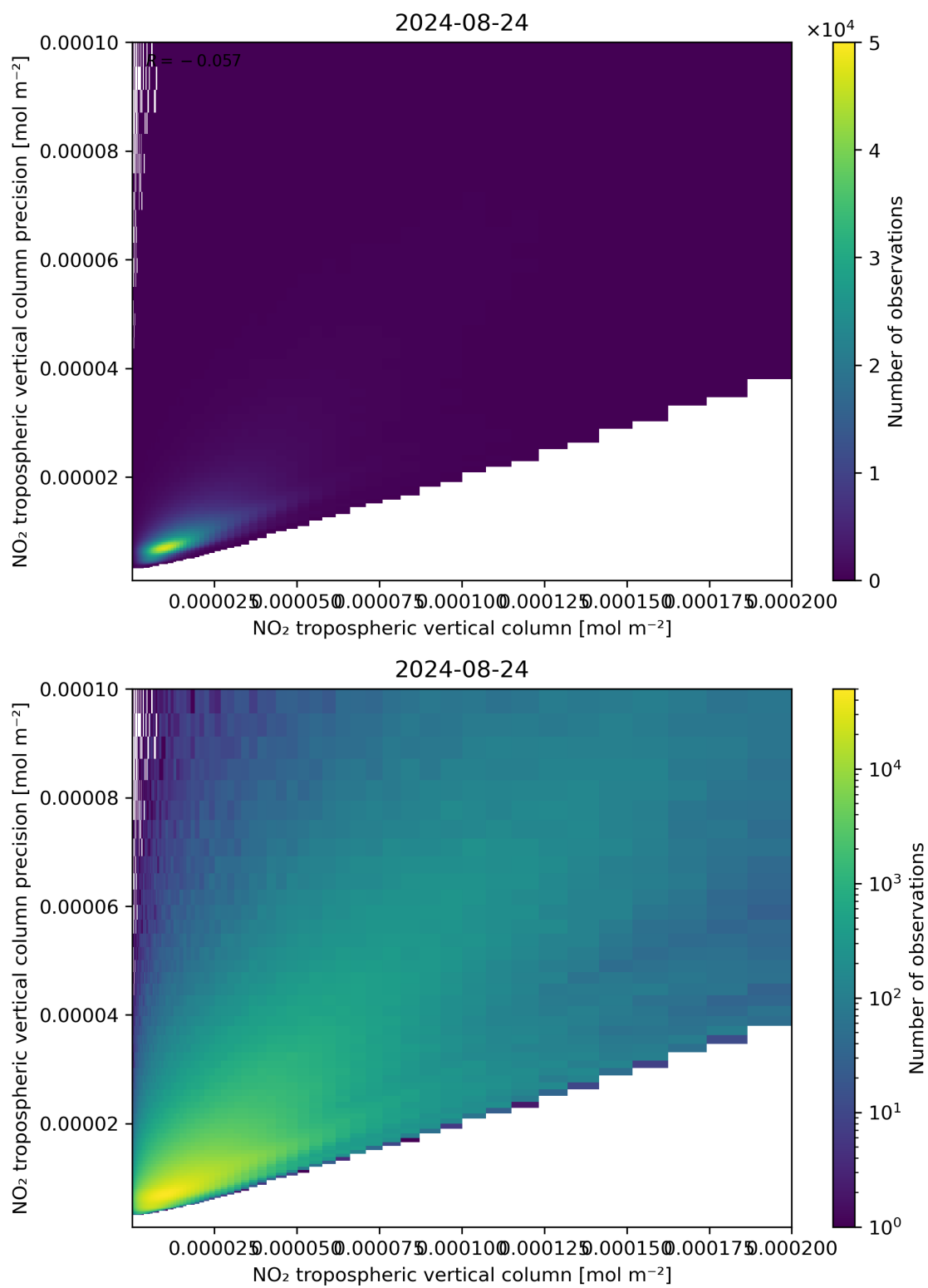
Figure 130: Scatter density plot of “NO 2 tropospheric vertical column” against “NO 2 tropospheric vertical column precision” for 2024-08-23 to 2024-08-25.
