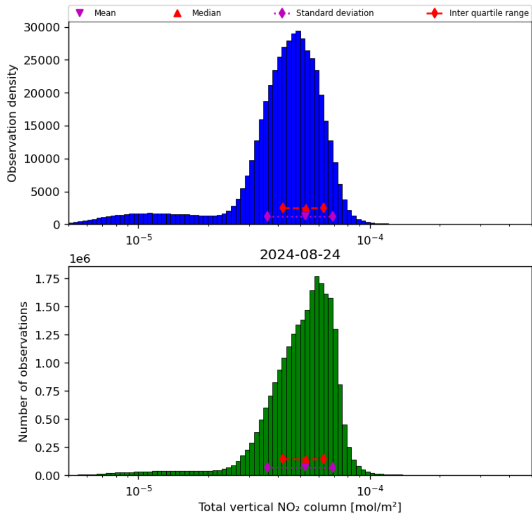
Figure 38: Histogram of “Total vertical NO 2 column” for 2024-08-23 to 2024-08-25
