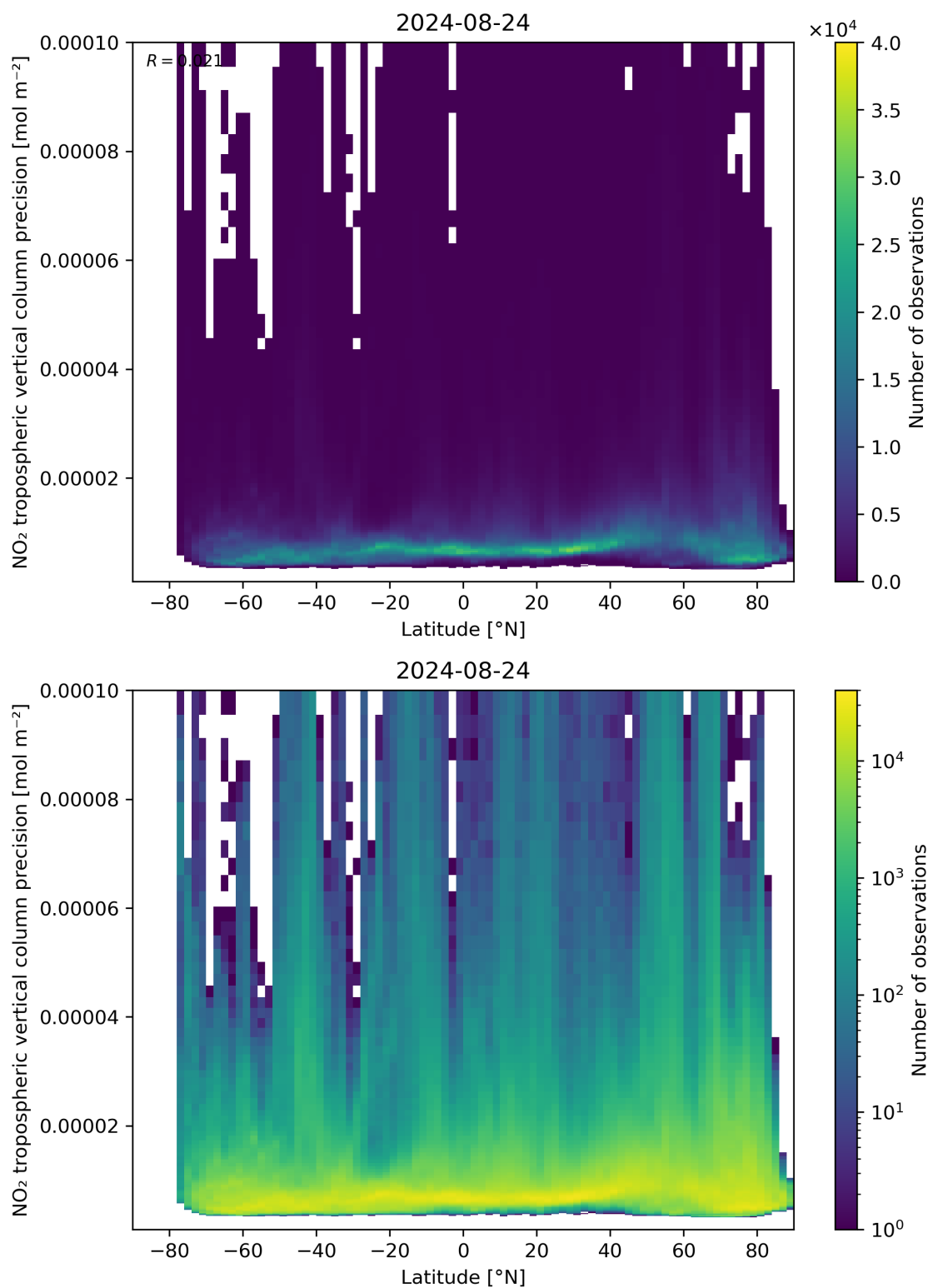
Figure 93: Scatter density plot of “Latitude” against “NO 2 tropospheric vertical column precision” for 2024-08-23 to 2024-08-25.
