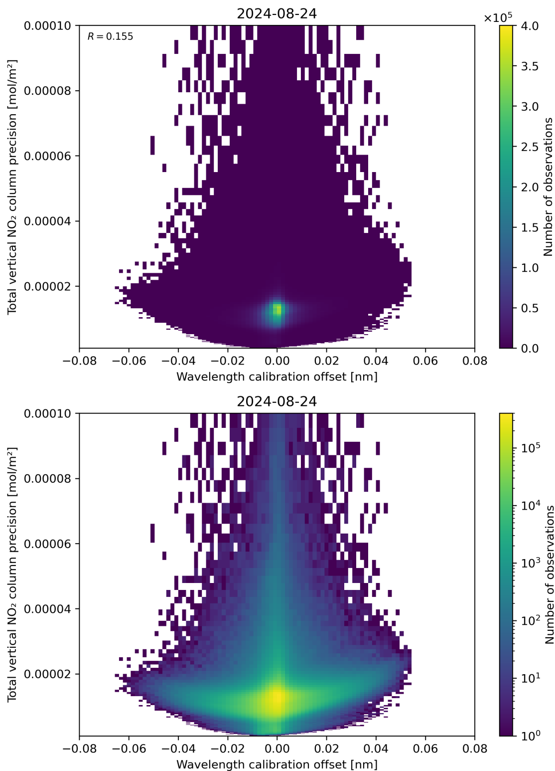
Figure 180: Scatter density plot of “Wavelength calibration offset” against “Total vertical NO 2 column precision” for 2024-08-23 to 2024-08-25.
