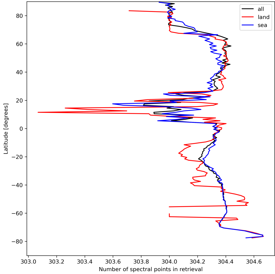
Figure 16: Zonal average of “Number of spectral points in retrieval” for 2024-08-23 to 2024-08-25.
