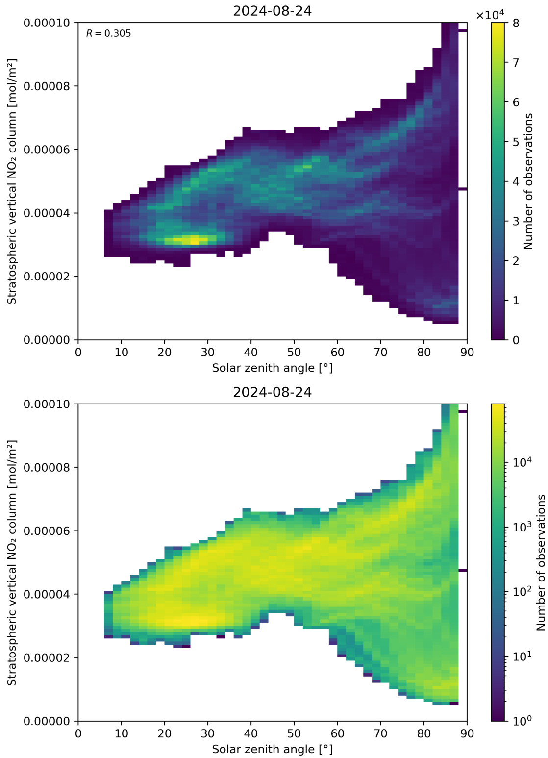
Figure 150: Scatter density plot of “Solar zenith angle” against “Stratospheric vertical NO 2 column” for 2024-08-23 to 2024-08-25.
