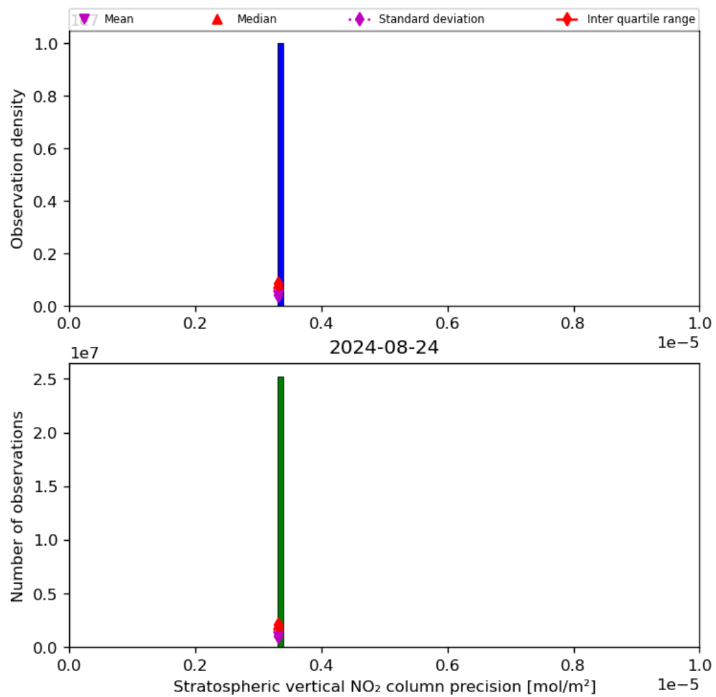
Figure 37: Histogram of “Stratospheric vertical NO 2 column precision” for 2024-08-23 to 2024-08-25
