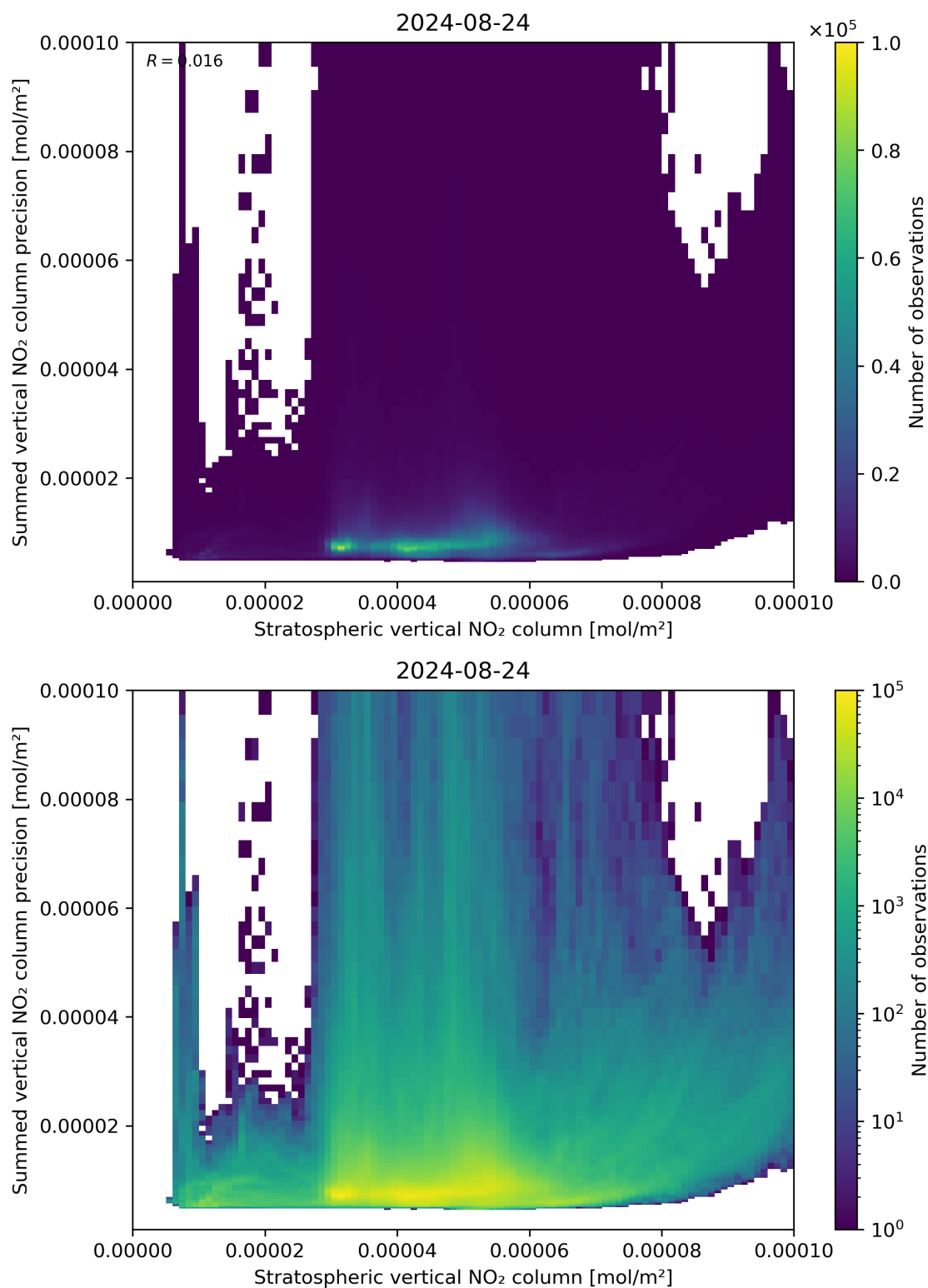
Figure 99: Scatter density plot of “Stratospheric vertical NO 2 column” against “Summed vertical NO 2 column precision” for 2024-08-23 to 2024-08-25.
