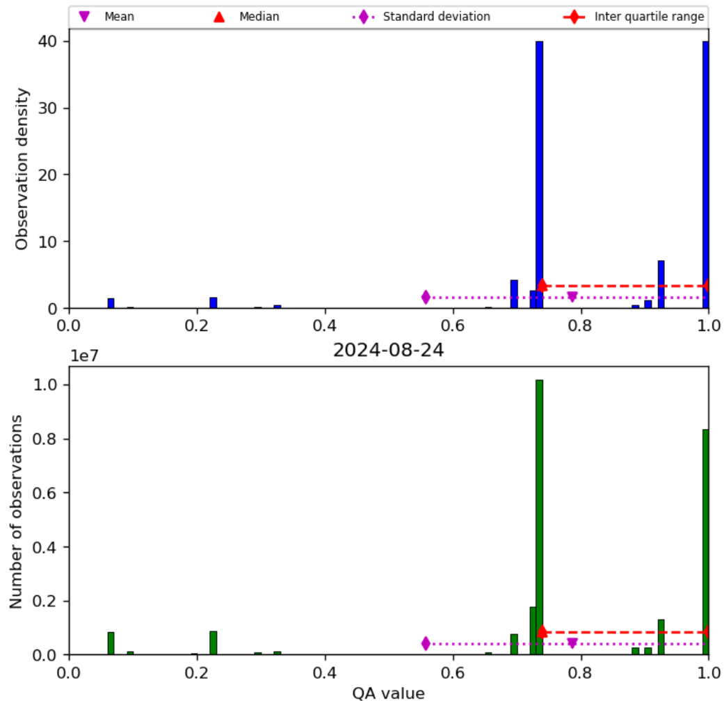
Figure 28: Histogram of “QA value” for 2024-08-23 to 2024-08-25
