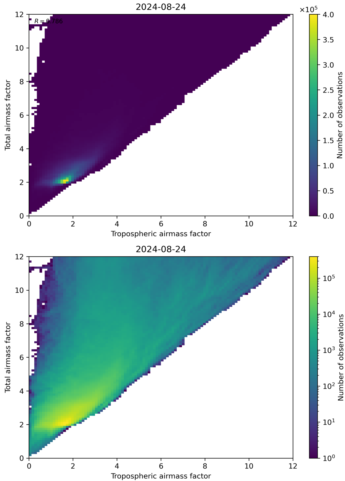
Figure 72: Scatter density plot of “Tropospheric airmass factor” against “Total airmass factor” for 2024-08-23 to 2024-08-25.
