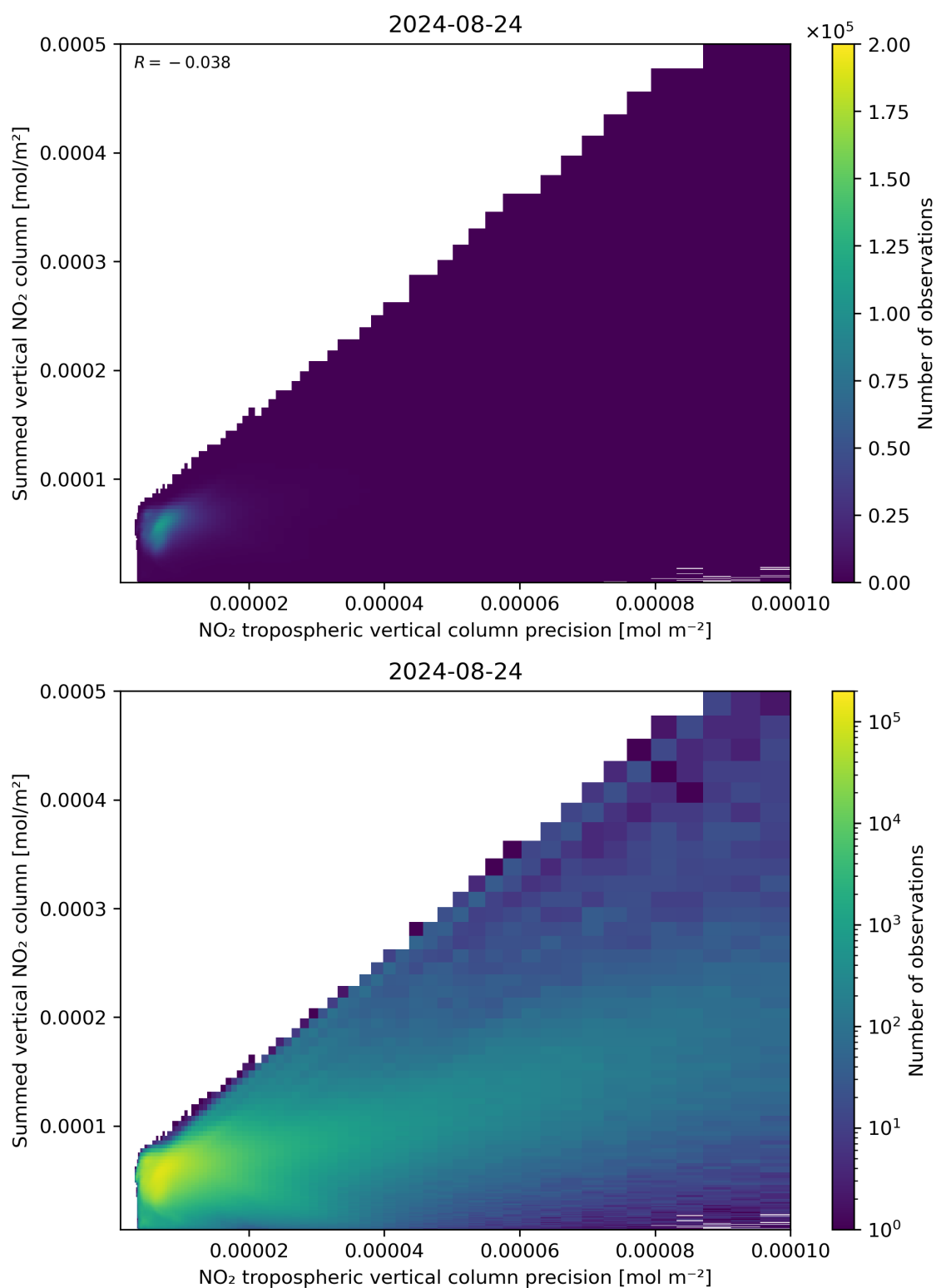
Figure 136: Scatter density plot of “NO 2 tropospheric vertical column precision” against “Summed vertical NO 2 column” for 2024-08-23 to 2024-08-25.
