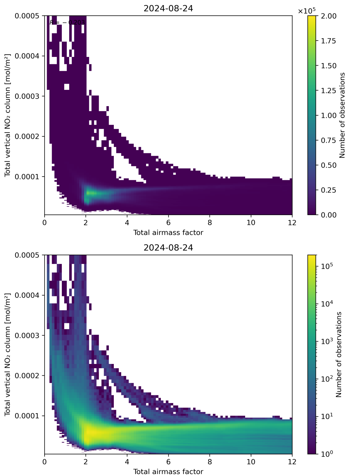
Figure 67: Scatter density plot of “Total airmass factor” against “Total vertical NO 2 column” for 2024-08-23 to 2024-08-25.
