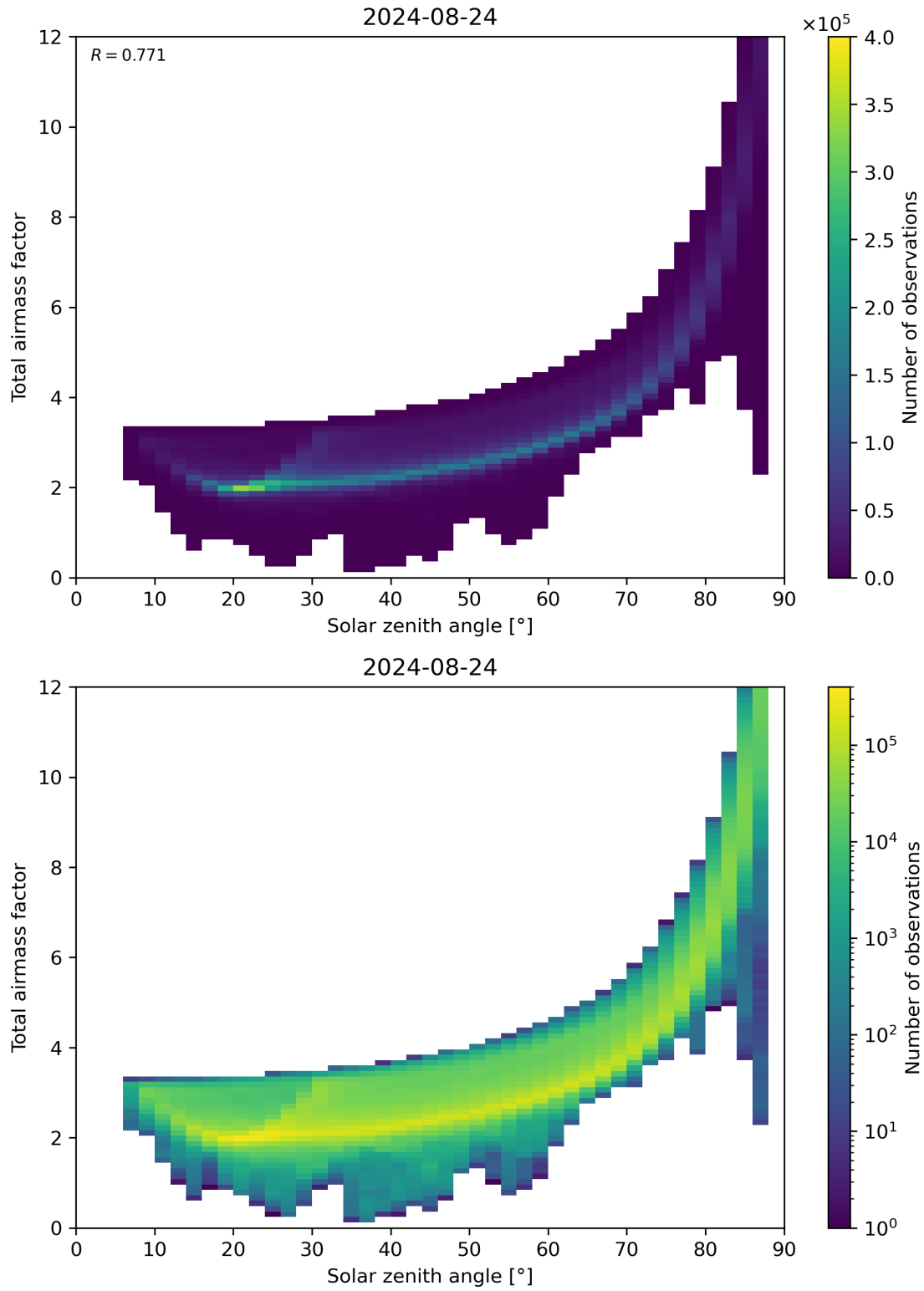
Figure 146: Scatter density plot of “Solar zenith angle” against “Total air mass factor” for 2024-08-23 to 2024-08-25.
