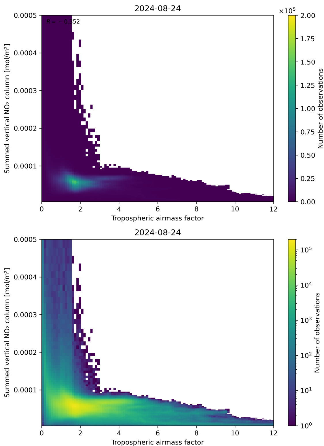
Figure 75: Scatter density plot of “Tropospheric airmass factor” against “Summed vertical NO 2 column” for 2024-08-23 to 2024-08-25.
