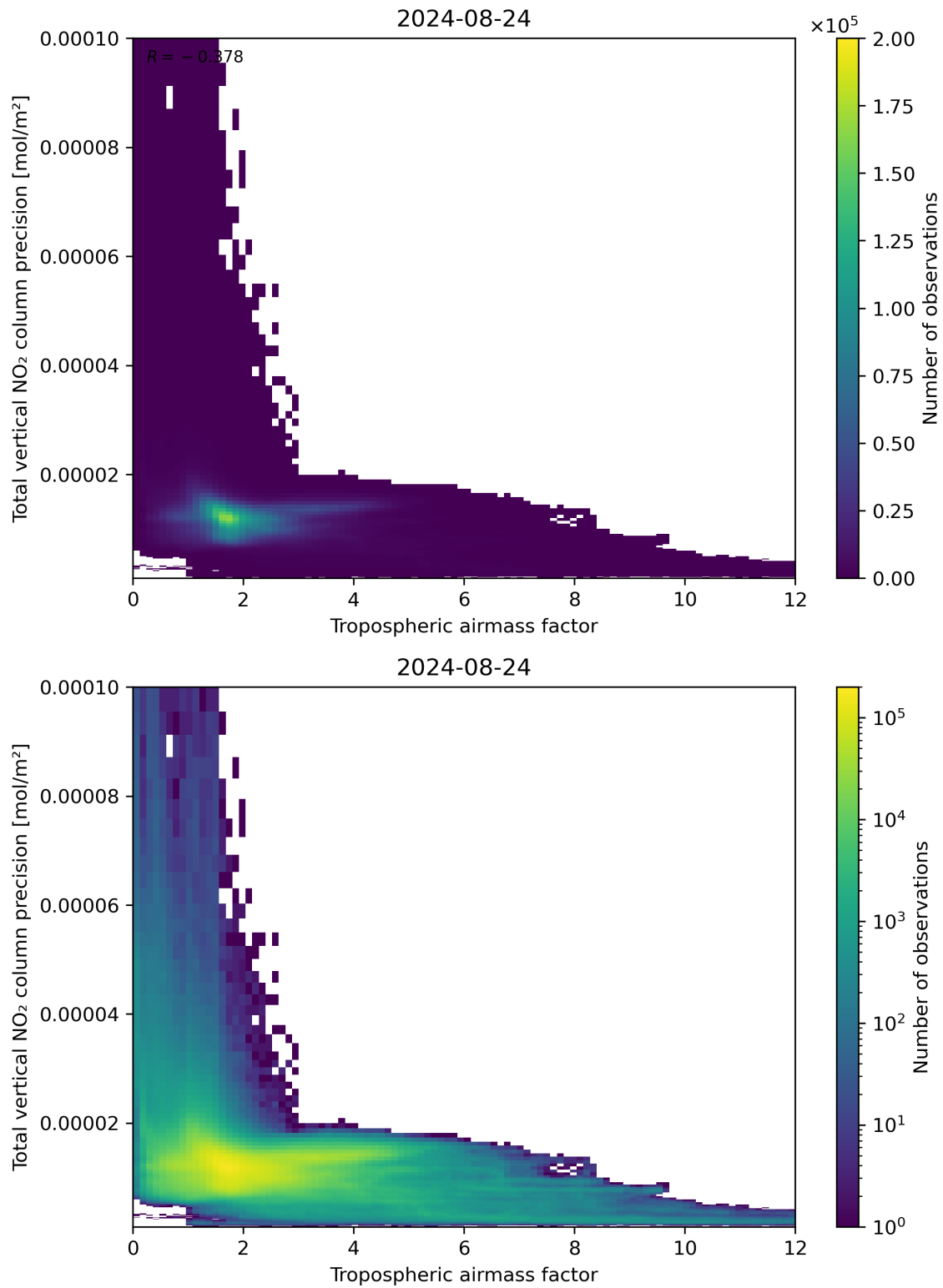
Figure 78: Scatter density plot of “Tropospheric air mass factor” against “Total vertical NO 2 column precision” for 2024-08-23 to 2024-08-25.
