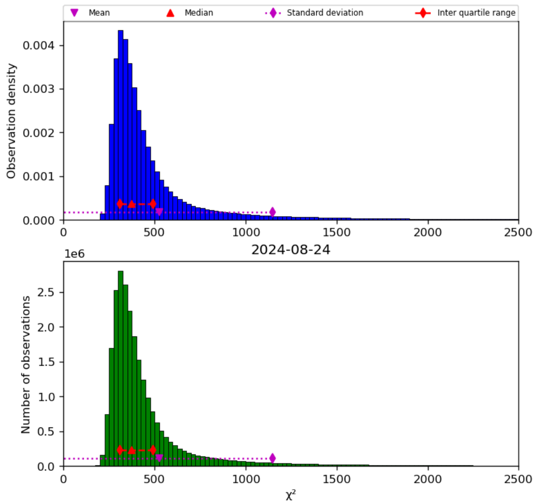
Figure 42: Histogram of " \chi^2 " for 2024-08-23 to 2024-08-25
