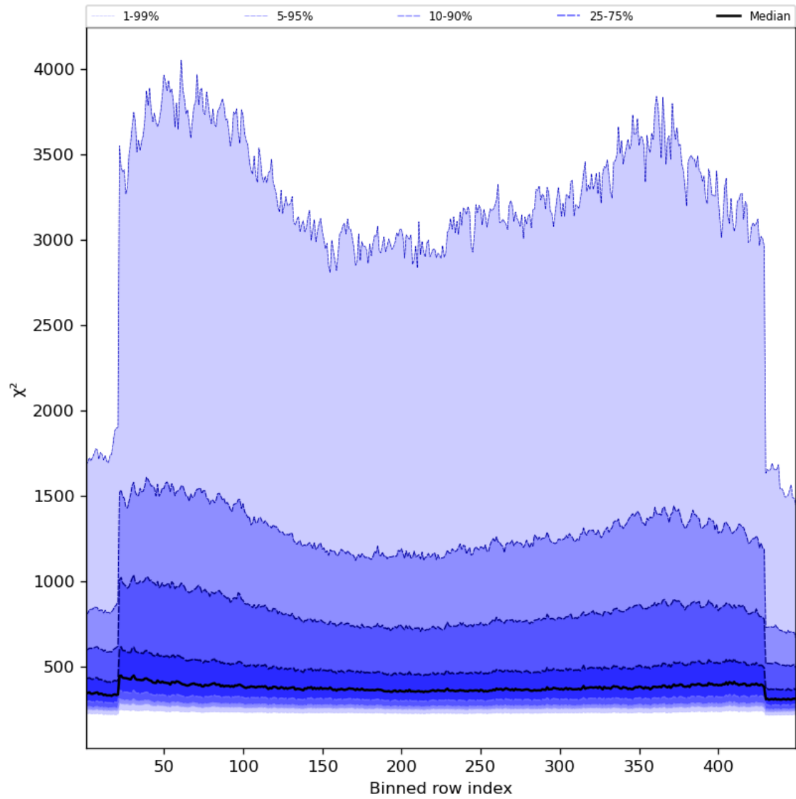
Figure 59: Along track statistics of “ \chi^2 ” for 2024-08-23 to 2024-08-25
