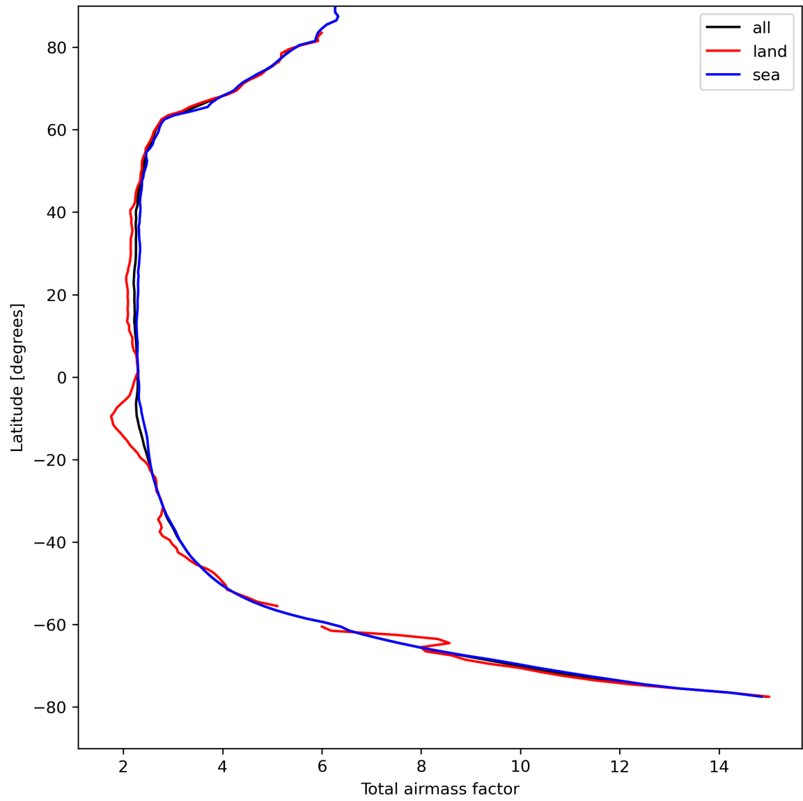
Figure 15: Zonal average of “Total airmass factor” for 2024-08-23 to 2024-08-25.
