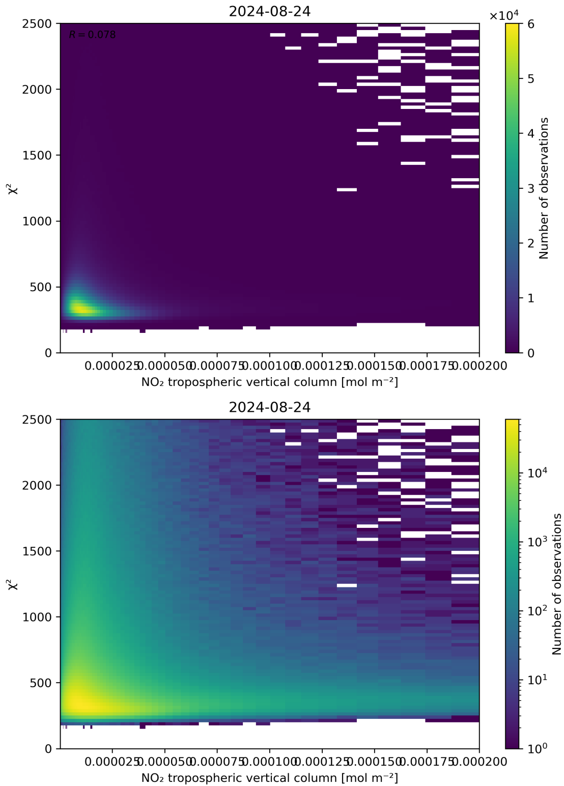
Figure 124: Scatter density plot of “NO 2 tropospheric vertical column” against “ \chi^2 ” for 2024-08-23 to 2024-08-25.
