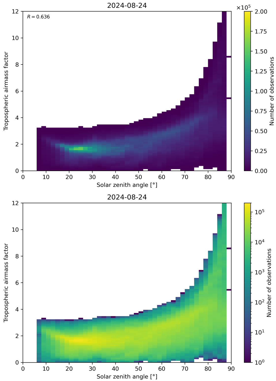
Figure 147: Scatter density plot of “Solar zenith angle” against “Tropospheric airmass factor” for 2024-08-23 to 2024-08-25.
