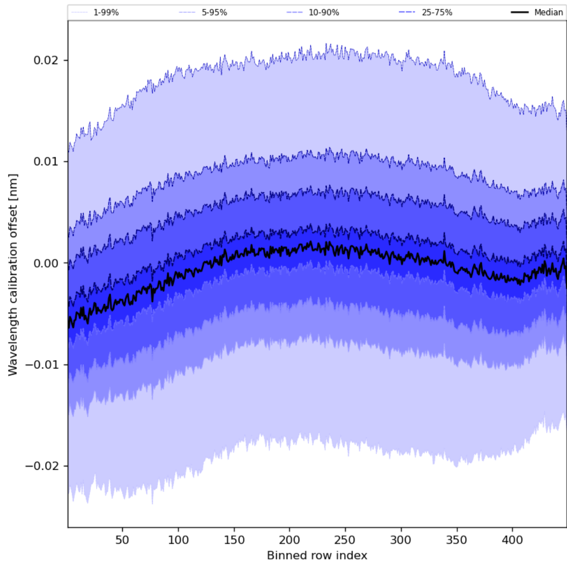
Figure 52: Along track statistics of “Wavelength calibration offset” for 2024-08-23 to 2024-08-25
