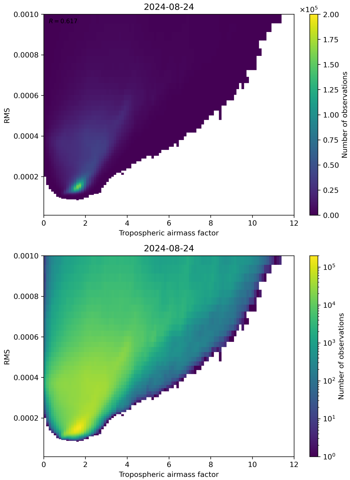
Figure 79: Scatter density plot of “Tropospheric airmass factor” against “RMS” for 2024-08-23 to 2024-08-25.
