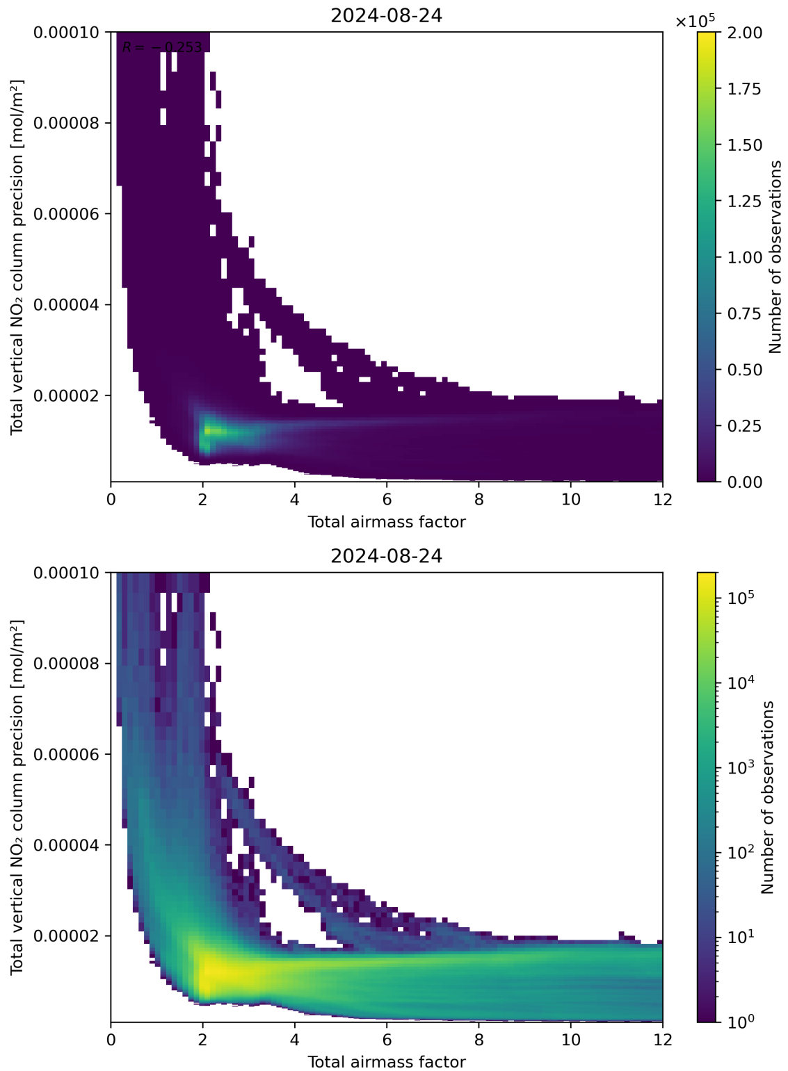
Figure 68: Scatter density plot of “Total airmass factor” against “Total vertical NO 2 column precision” for 2024-08-23 to 2024-08-25.
