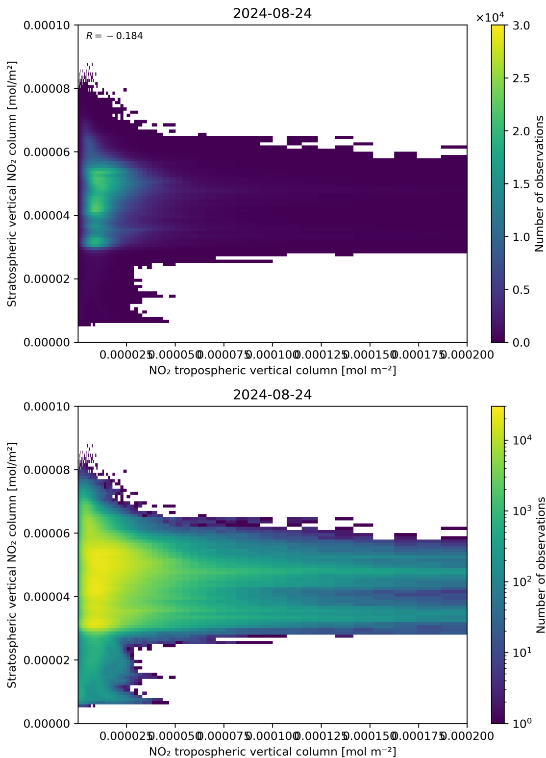
Figure 125: Scatter density plot of “NO 2 tropospheric vertical column” against “Stratospheric vertical NO 2 column” for 2024-08-23 to 2024-08-25.
