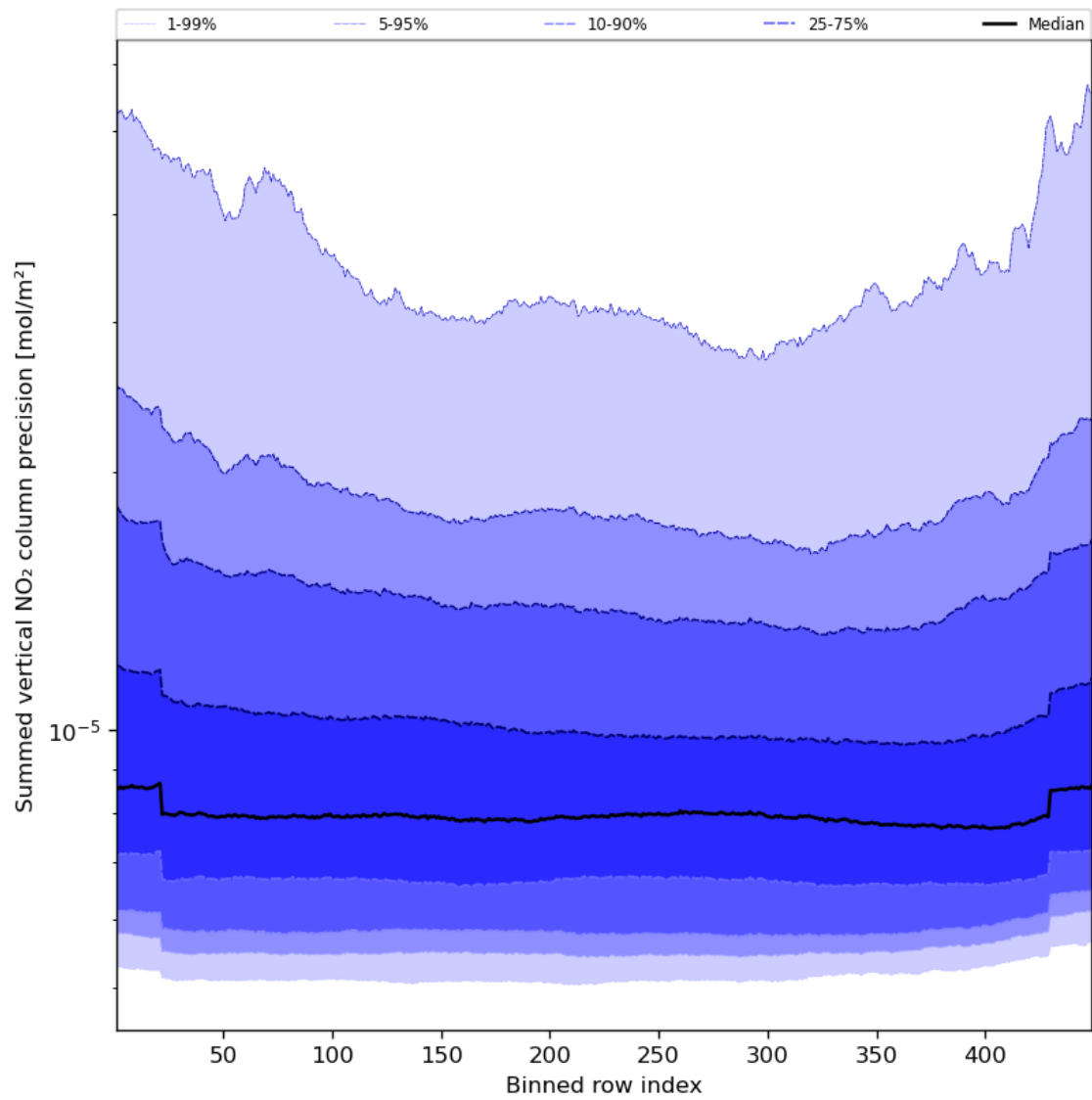
Figure 58: Along track statistics of “Summed vertical NO 2 column precision” for 2024-08-23 to 2024-08-25
