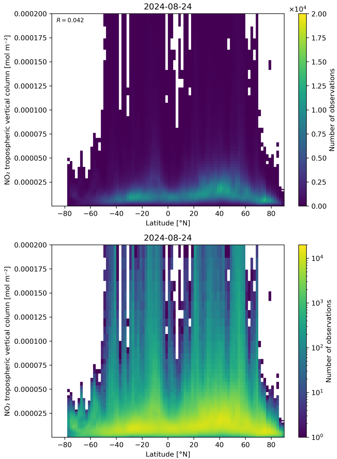
Figure 92: Scatter density plot of “Latitude” against “NO 2 tropospheric vertical column” for 2024-08-23 to 2024-08-25.
