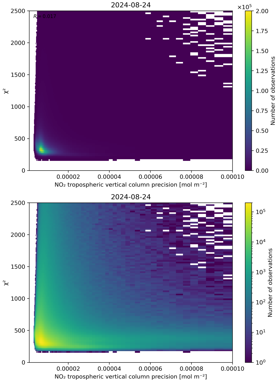
Figure 134: Scatter density plot of “NO 2 tropospheric vertical column precision” against “ \chi^2 ” for 2024-08-23 to 2024-08-25.
