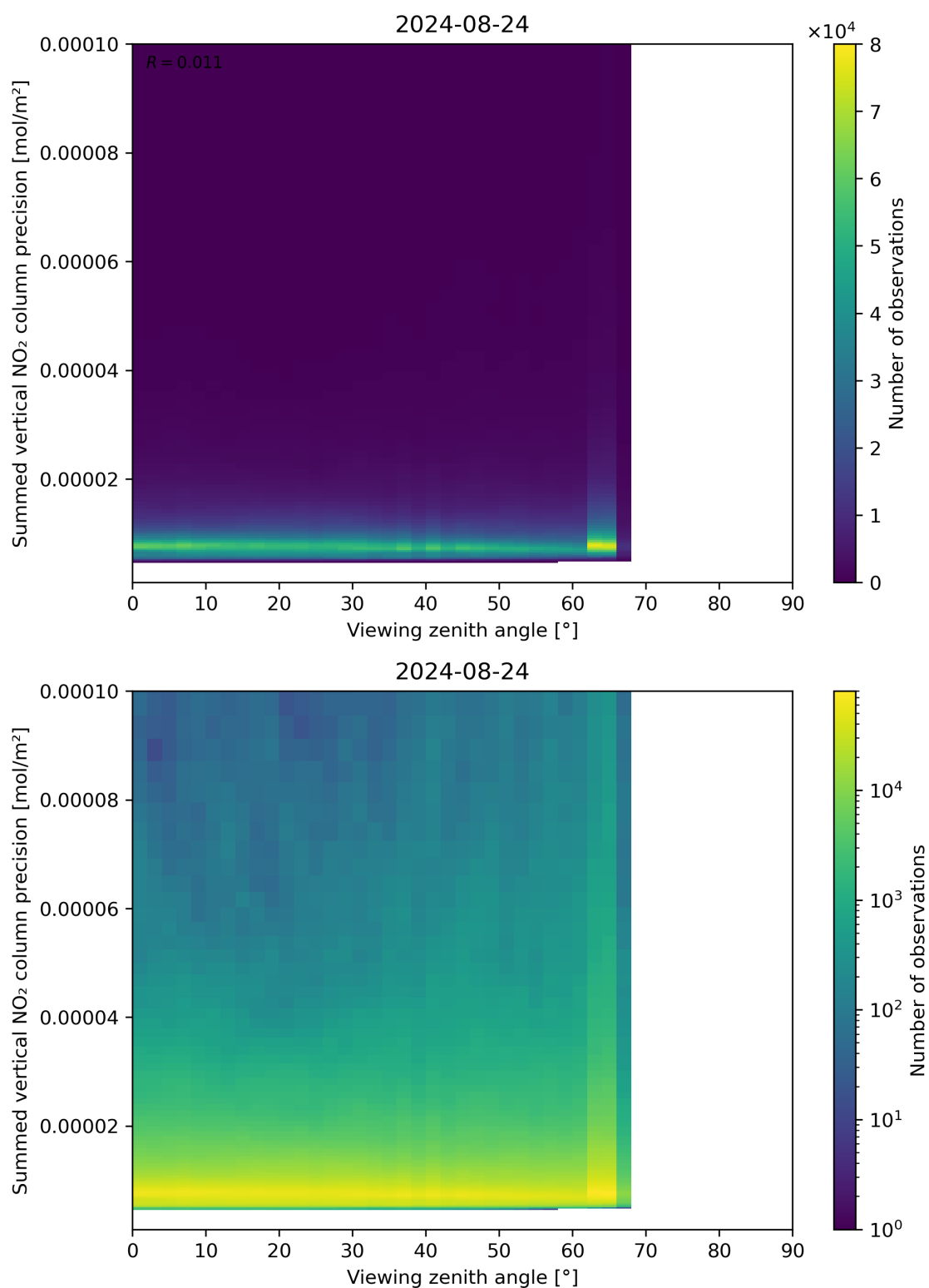
Figure 166: Scatter density plot of “Viewing zenith angle” against “Summed vertical NO 2 column precision” for 2024-08-23 to 2024-08-25.
