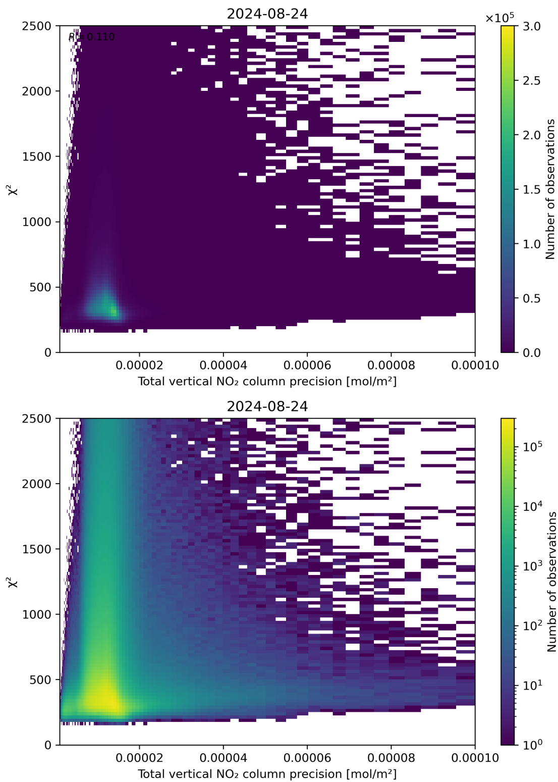
Figure 116: Scatter density plot of “Total vertical NO 2 column precision” against “ \chi^2 ” for 2024-08-23 to 2024-08-25.
