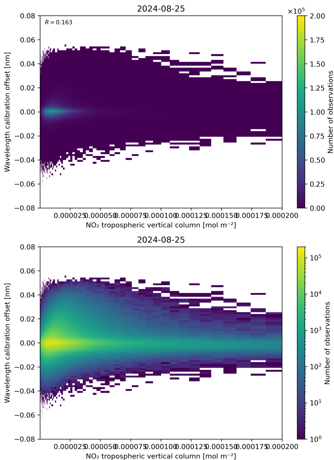
Figure 143: Scatter density plot of “NO 2 tropospheric vertical column” against “Wavelength calibration offset” for 2024-08-24 to 2024-08-26.
