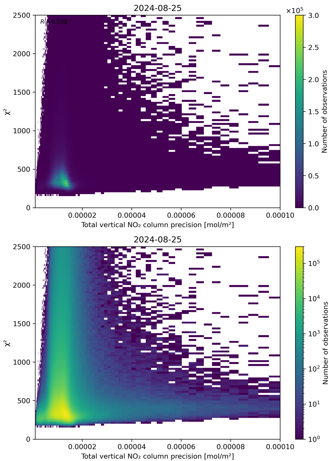
Figure 116: Scatter density plot of “Total vertical NO 2 column precision” against “ \chi^2 ” for 2024-08-24 to 2024-08-26.
