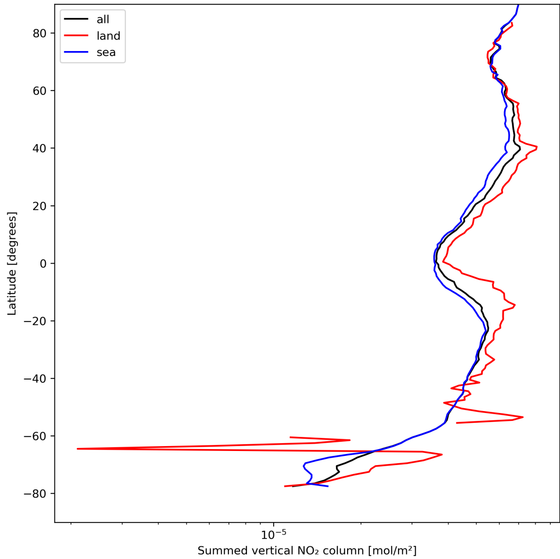
Figure 23: Zonal average of “Summed vertical NO 2 column” for 2024-08-24 to 2024-08-26.
