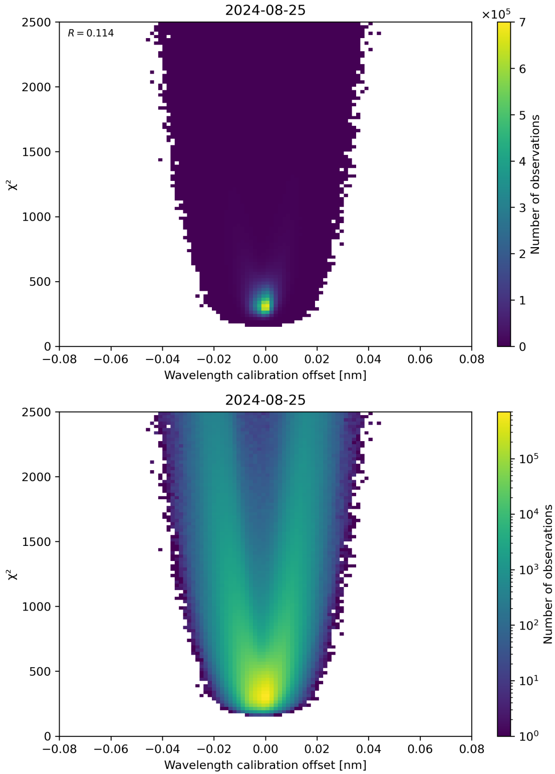
Figure 175: Scatter density plot of “Wavelength calibration offset” against “ \chi^2 ” for 2024-08-24 to 2024-08-26.
