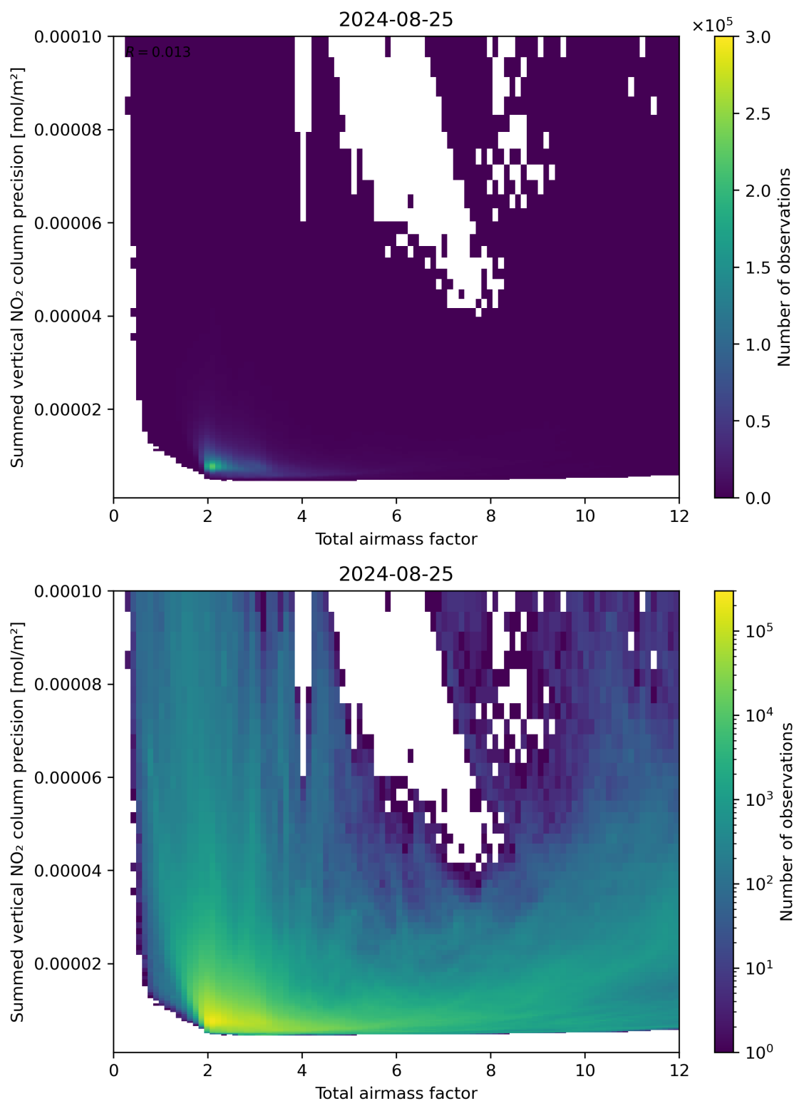
Figure 66: Scatter density plot of “Total airmass factor” against “Summed vertical NO 2 column precision” for 2024-08-24 to 2024-08-26.
