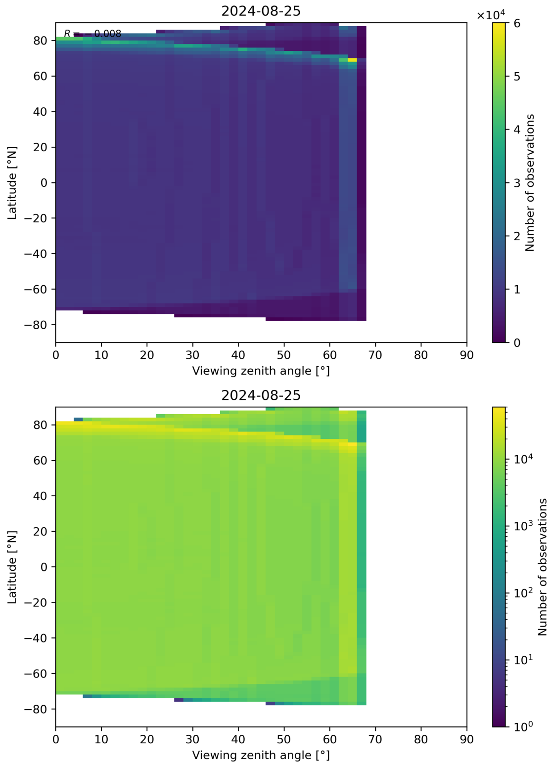
Figure 163: Scatter density plot of “Viewing zenith angle” against “Latitude” for 2024-08-24 to 2024-08-26.
