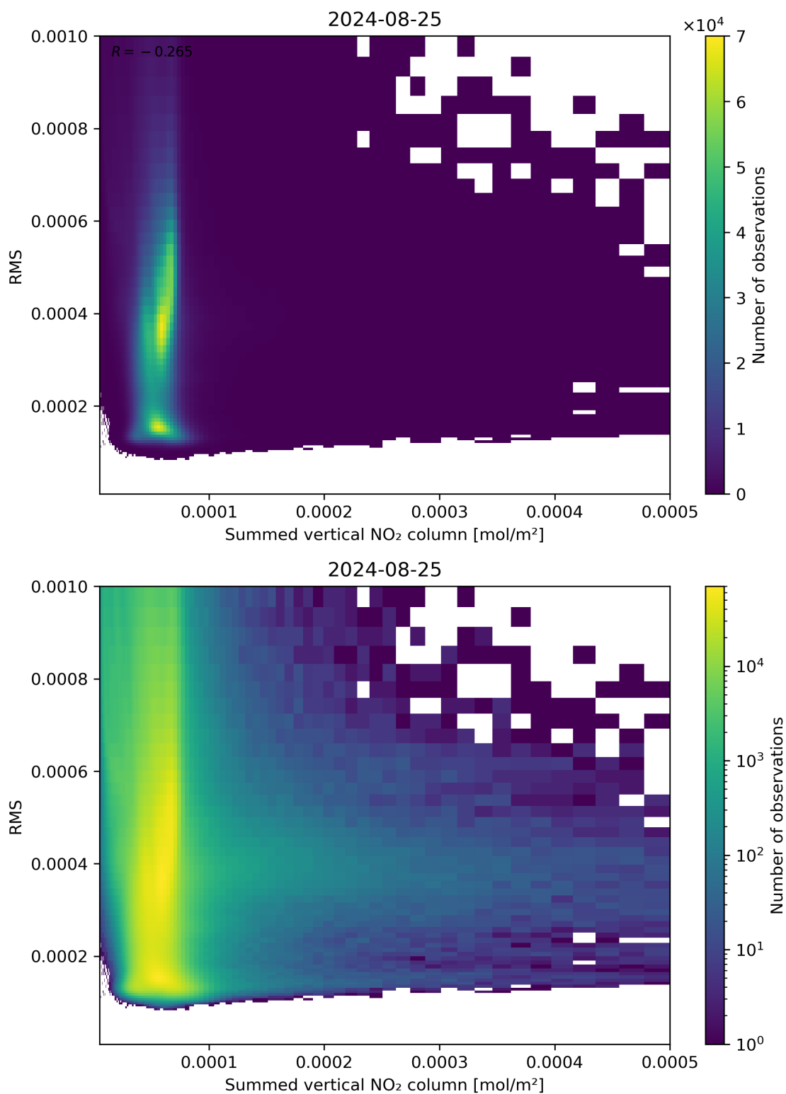
Figure 109: Scatter density plot of “Summed vertical NO 2 column” against “RMS” for 2024-08-24 to 2024-08-26.
