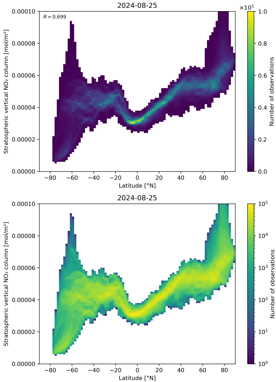
Figure 87: Scatter density plot of “Latitude” against “Stratospheric vertical NO 2 column” for 2024-08-24 to 2024-08-26.
