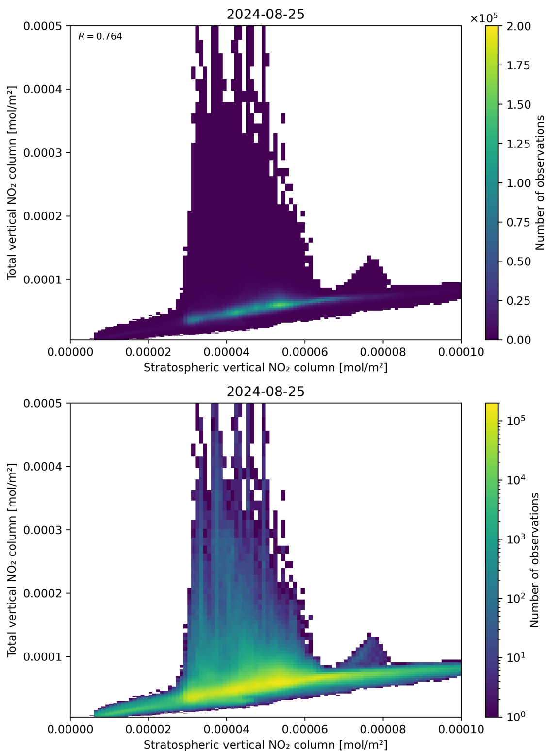
Figure 100: Scatter density plot of “Stratospheric vertical NO 2 column” against “Total vertical NO 2 column” for 2024-08-24 to 2024-08-26.
