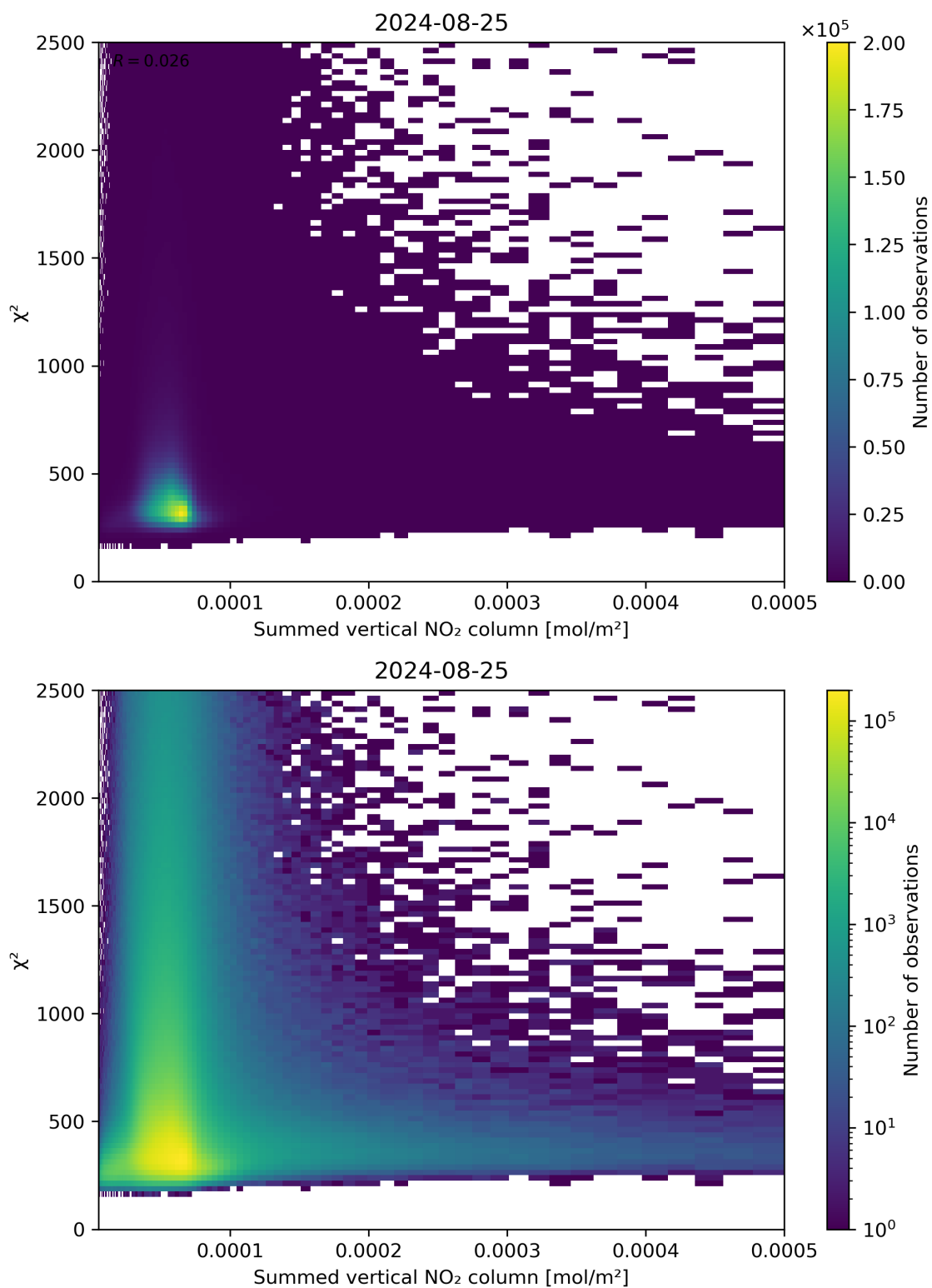
Figure 104: Scatter density plot of “Summed vertical NO 2 column” against “ \chi^2 ” for 2024-08-24 to 2024-08-26.
