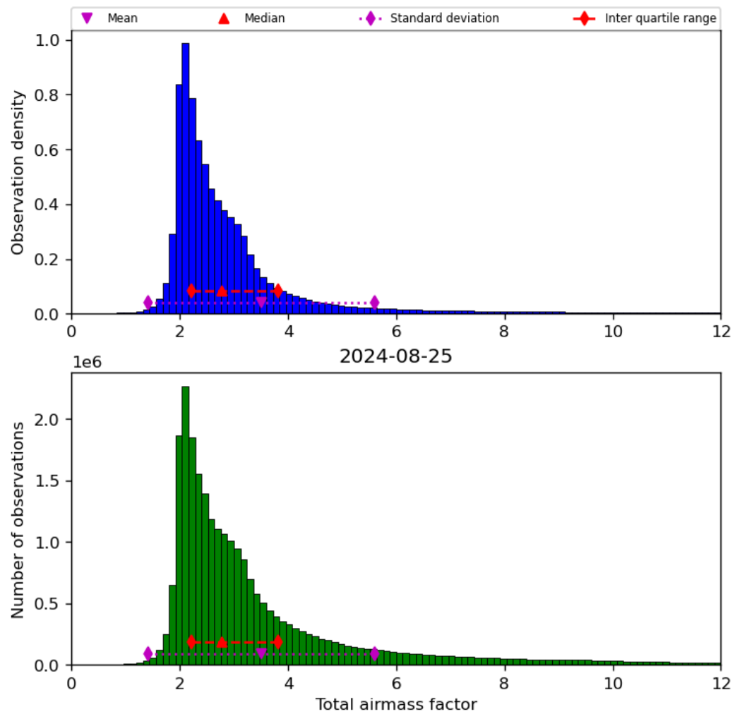
Figure 32: Histogram of “Total airmass factor” for 2024-08-24 to 2024-08-26
