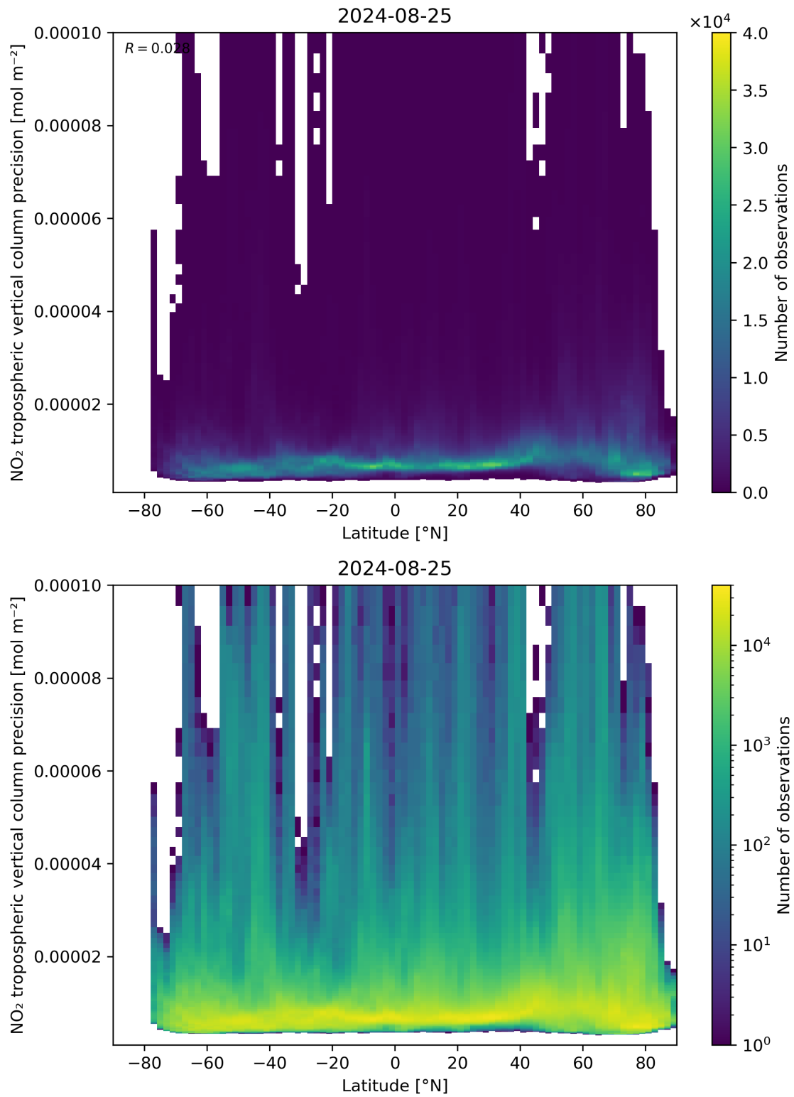
Figure 93: Scatter density plot of “Latitude” against “NO 2 tropospheric vertical column precision” for 2024-08-24 to 2024-08-26.
