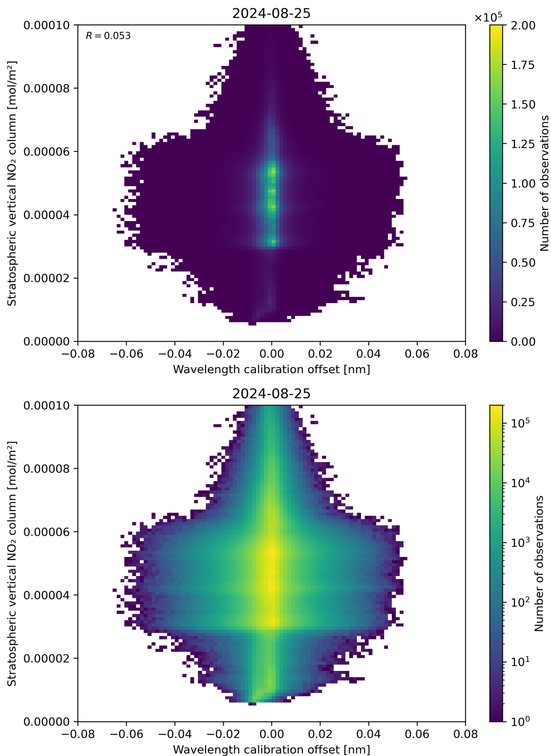
Figure 176: Scatter density plot of “Wavelength calibration offset” against “Stratospheric vertical NO 2 column” for 2024-08-24 to 2024-08-26.
