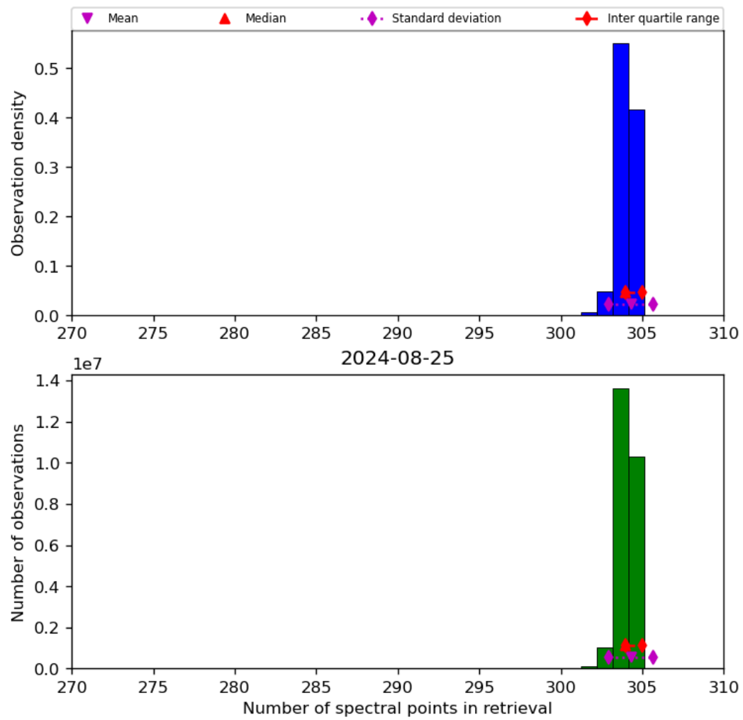
Figure 33: Histogram of “Number of spectral points in retrieval” for 2024-08-24 to 2024-08-26
