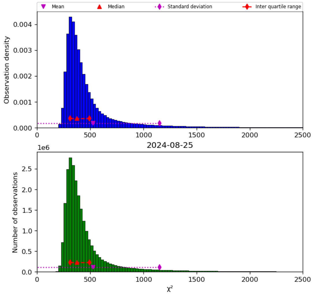
Figure 42: Histogram of " \chi^2 " for 2024-08-24 to 2024-08-26
