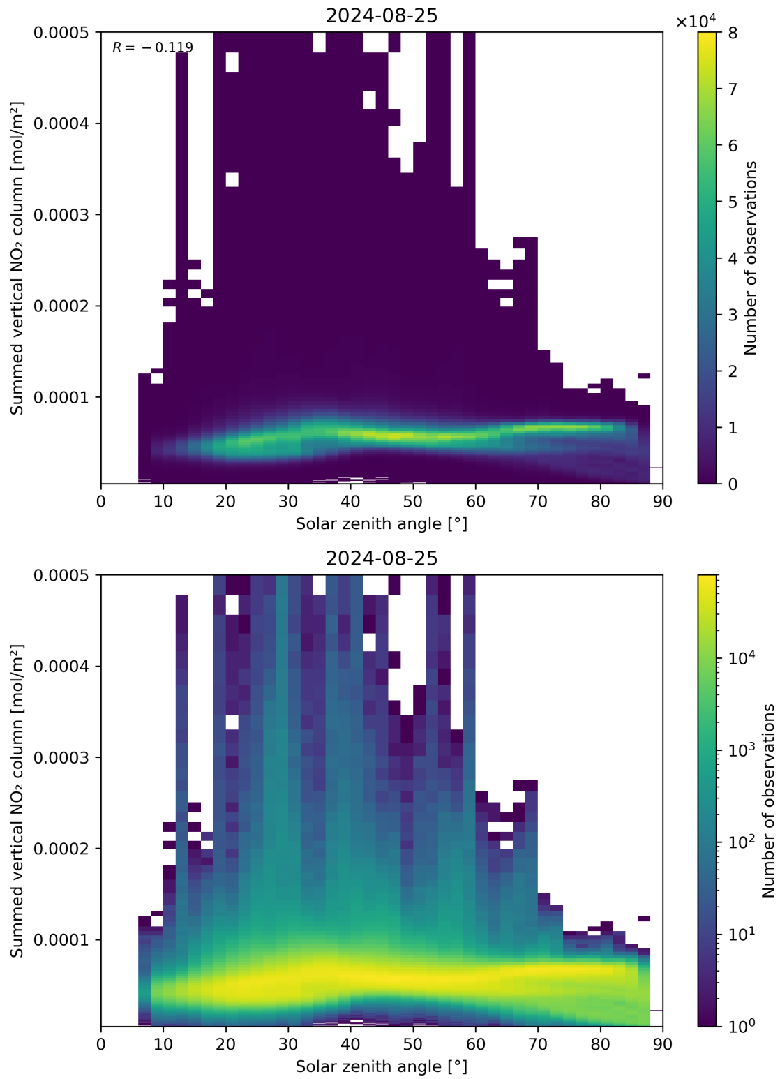
Figure 151: Scatter density plot of “Solar zenith angle” against “Summed vertical NO 2 column” for 2024-08-24 to 2024-08-26.
