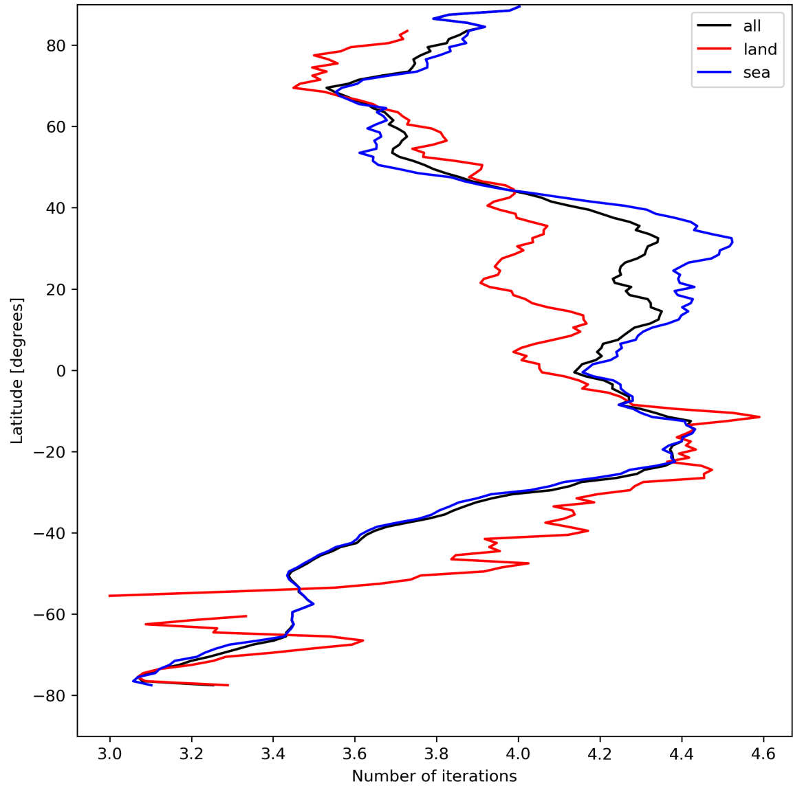
Figure 17: Zonal average of “Number of iterations” for 2024-08-24 to 2024-08-26.
