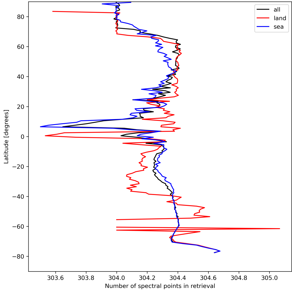
Figure 16: Zonal average of “Number of spectral points in retrieval” for 2024-08-24 to 2024-08-26.
