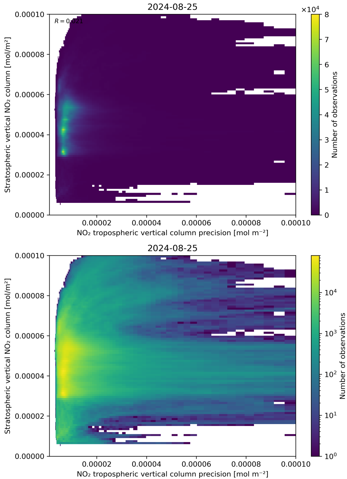
Figure 135: Scatter density plot of “NO 2 tropospheric vertical column precision” against “Stratospheric vertical NO 2 column” for 2024-08-24 to 2024-08-26.
