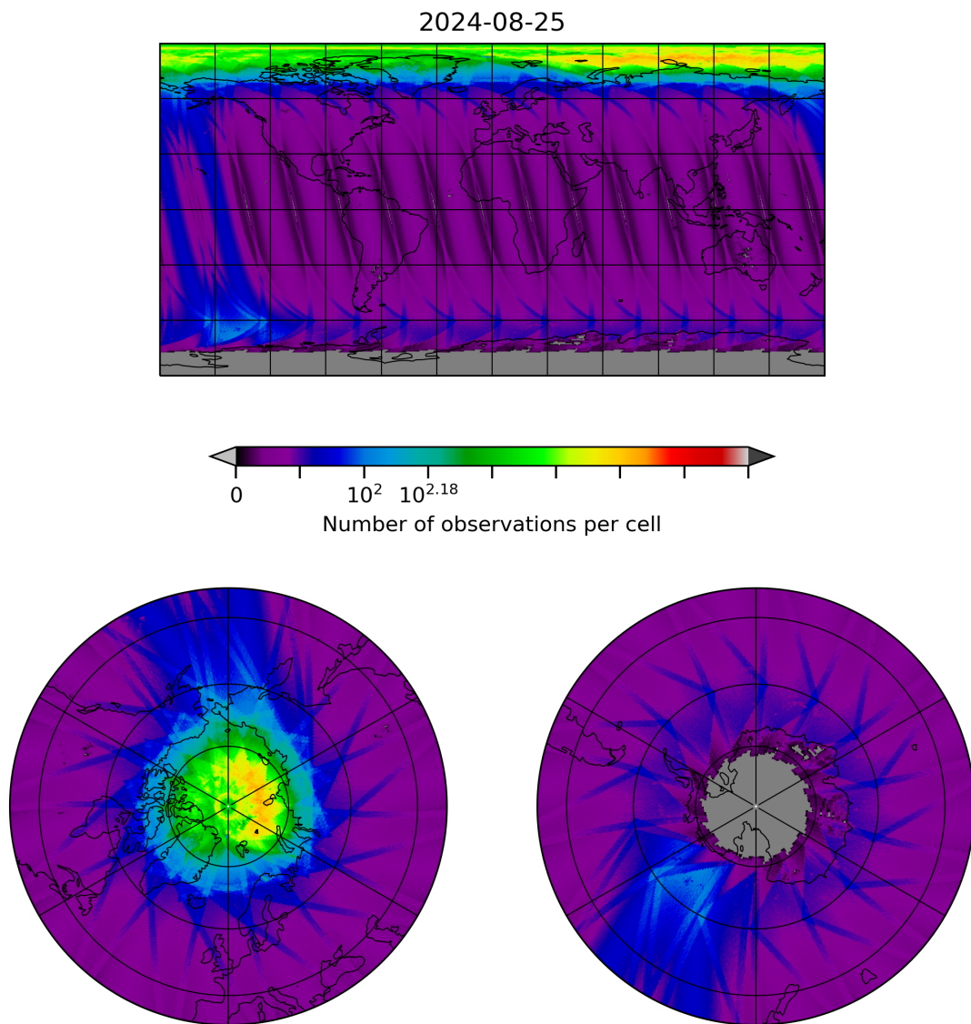
Figure 10: Map of the number of observations for 2024-08-24 to 2024-08-26
