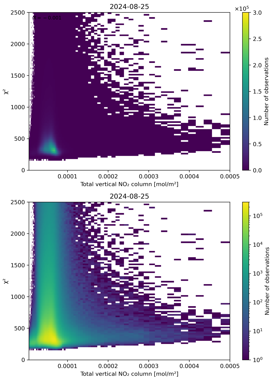
Figure 111: Scatter density plot of “Total vertical NO 2 column” against “ \chi^2 ” for 2024-08-24 to 2024-08-26.
