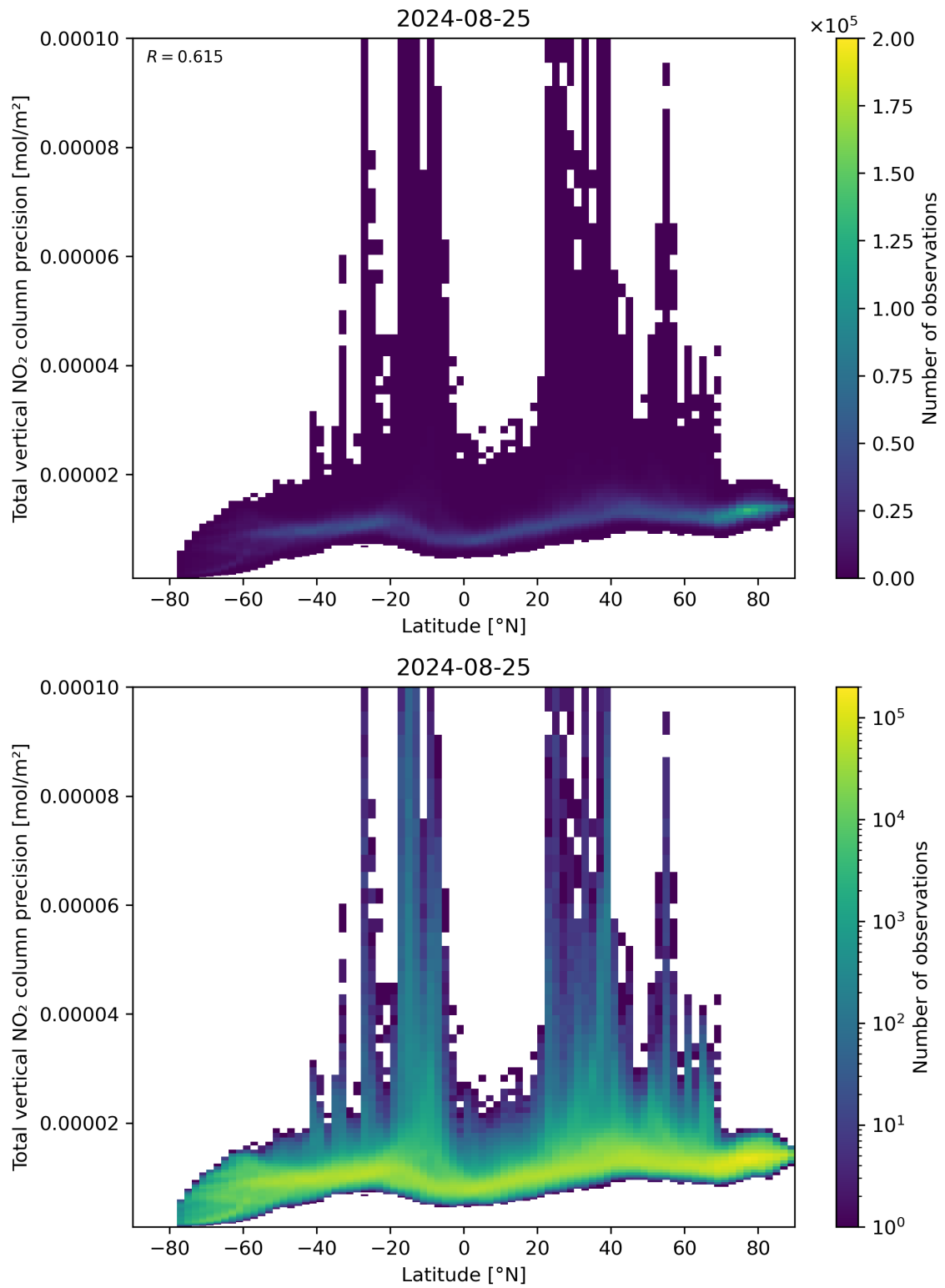
Figure 91: Scatter density plot of “Latitude” against “Total vertical NO 2 column precision” for 2024-08-24 to 2024-08-26.
