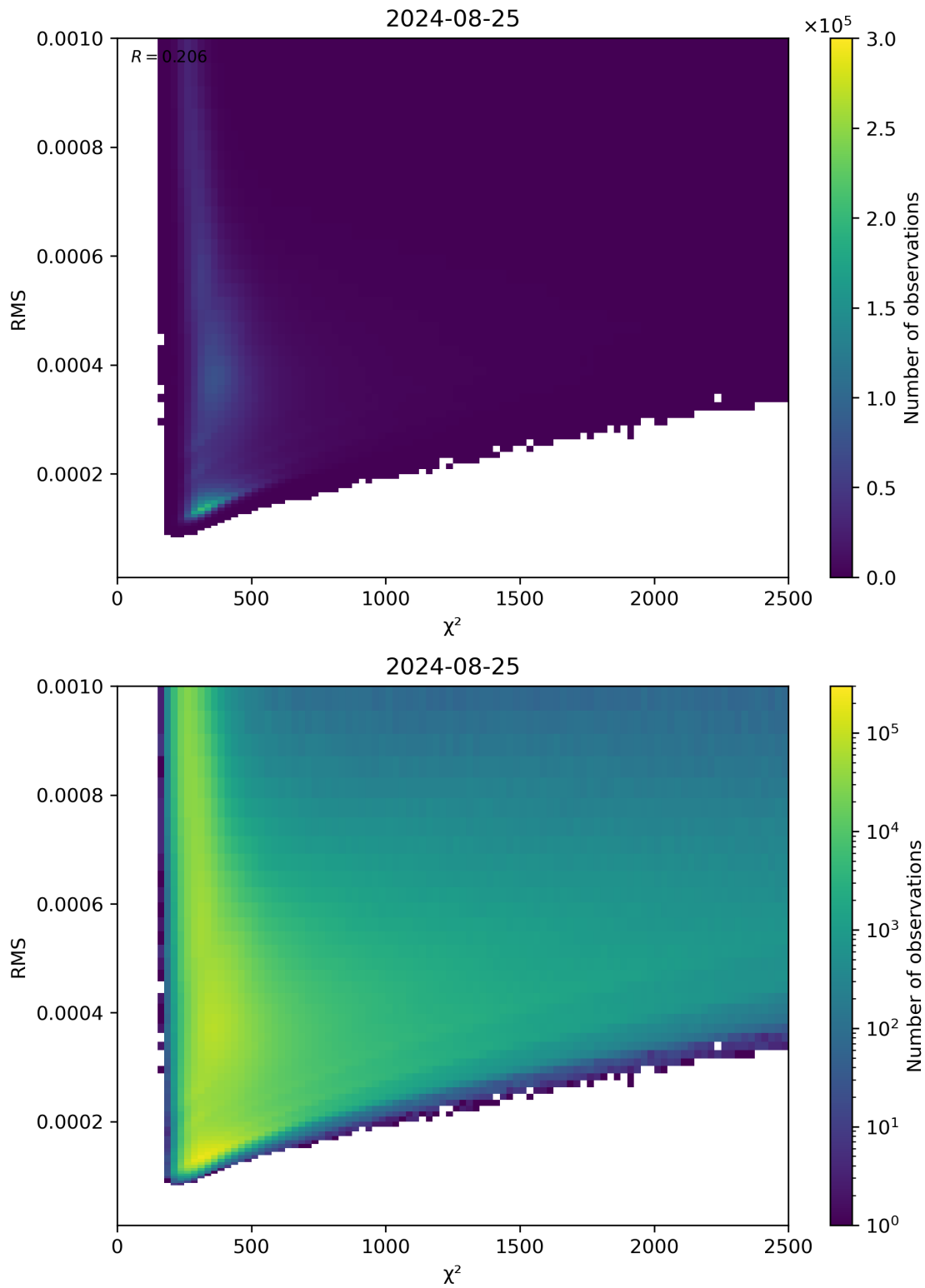
Figure 82: Scatter density plot of “ \chi^2 ” against “RMS” for 2024-08-24 to 2024-08-26.
