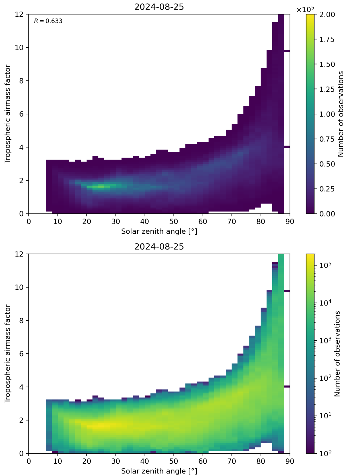
Figure 147: Scatter density plot of “Solar zenith angle” against “Tropospheric airmass factor” for 2024-08-24 to 2024-08-26.
