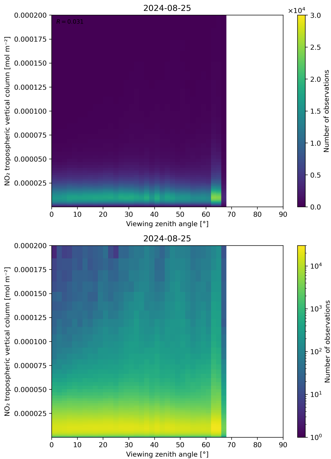
Figure 169: Scatter density plot of “Viewing zenith angle” against “NO 2 tropospheric vertical column” for 2024-08-24 to 2024-08-26.
