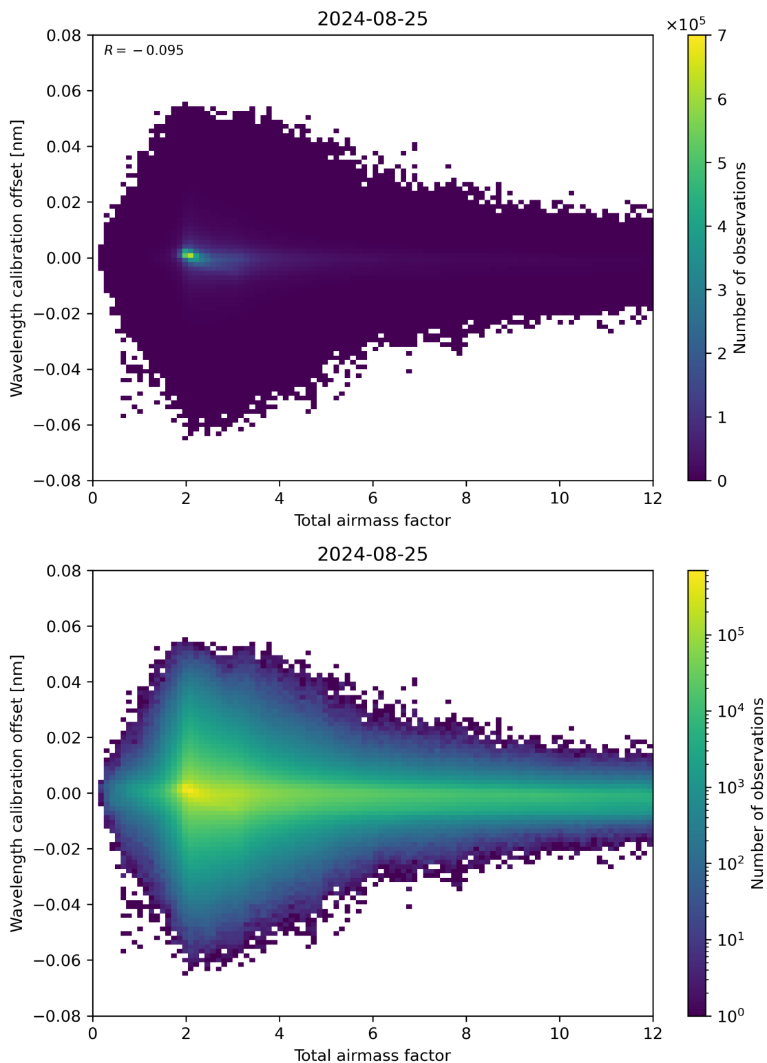
Figure 70: Scatter density plot of “Total airmass factor” against “Wavelength calibration offset” for 2024-08-24 to 2024-08-26.
