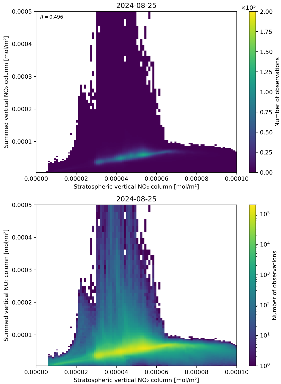
Figure 98: Scatter density plot of “Stratospheric vertical NO 2 column” against “Summed vertical NO 2 column” for 2024-08-24 to 2024-08-26.
