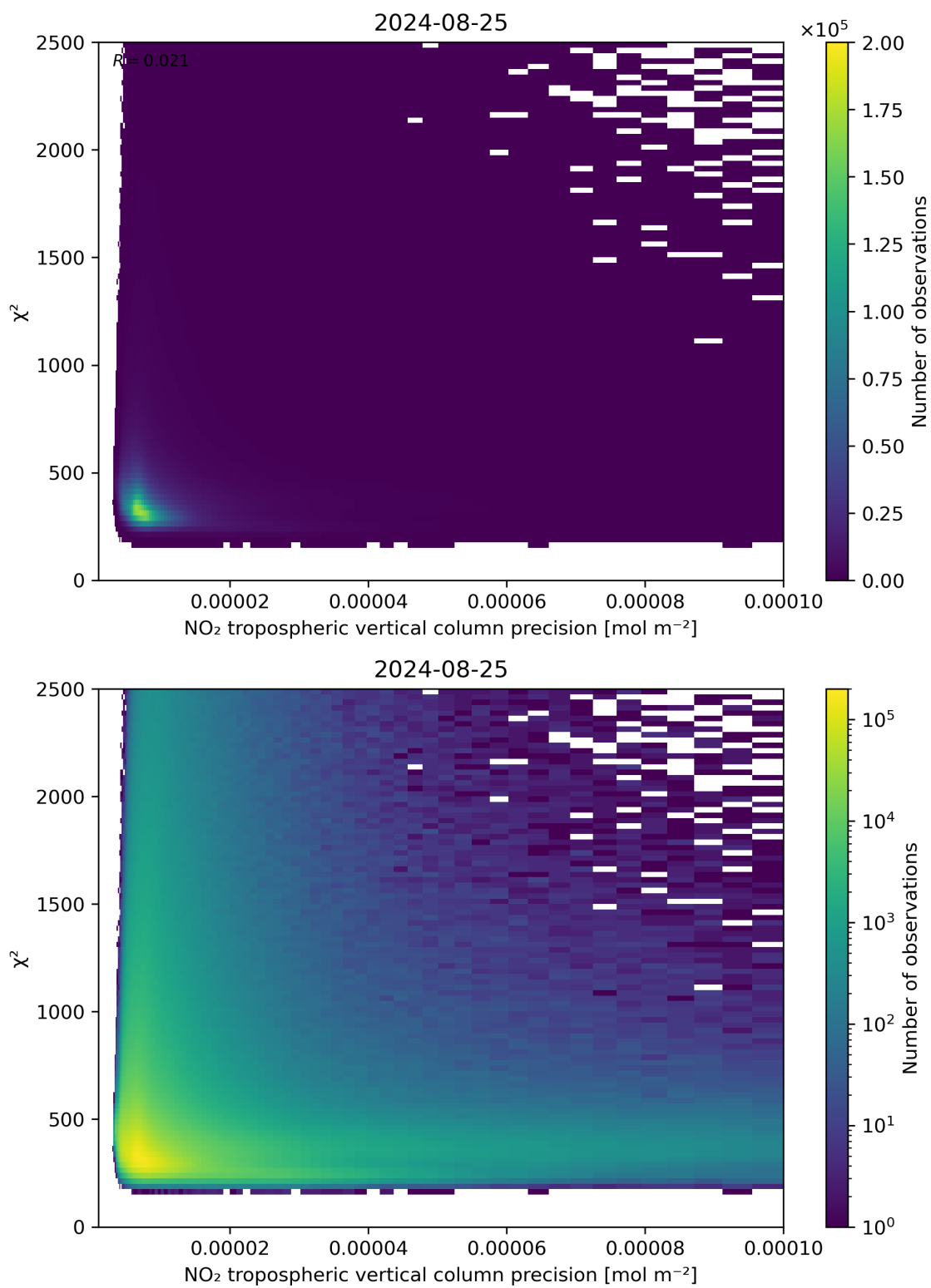
Figure 134: Scatter density plot of “NO 2 tropospheric vertical column precision” against “ \chi^2 ” for 2024-08-24 to 2024-08-26.
