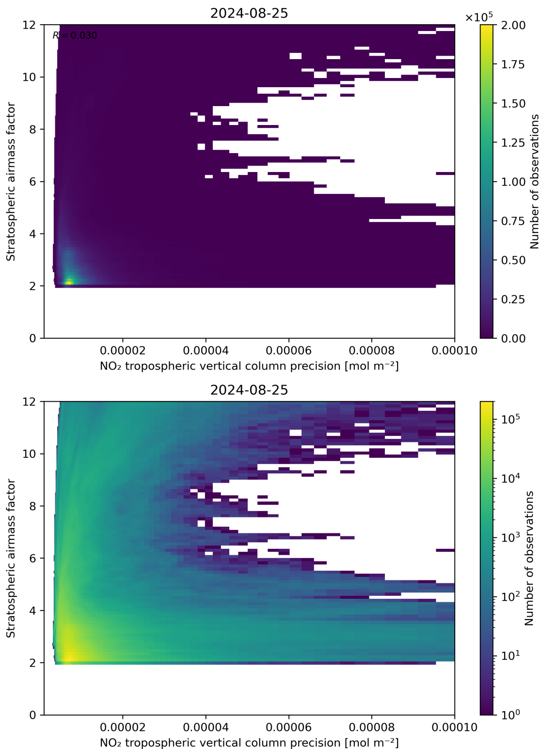
Figure 131: Scatter density plot of “NO 2 tropospheric vertical column precision” against “Stratospheric airmass factor” for 2024-08-24 to 2024-08-26.
