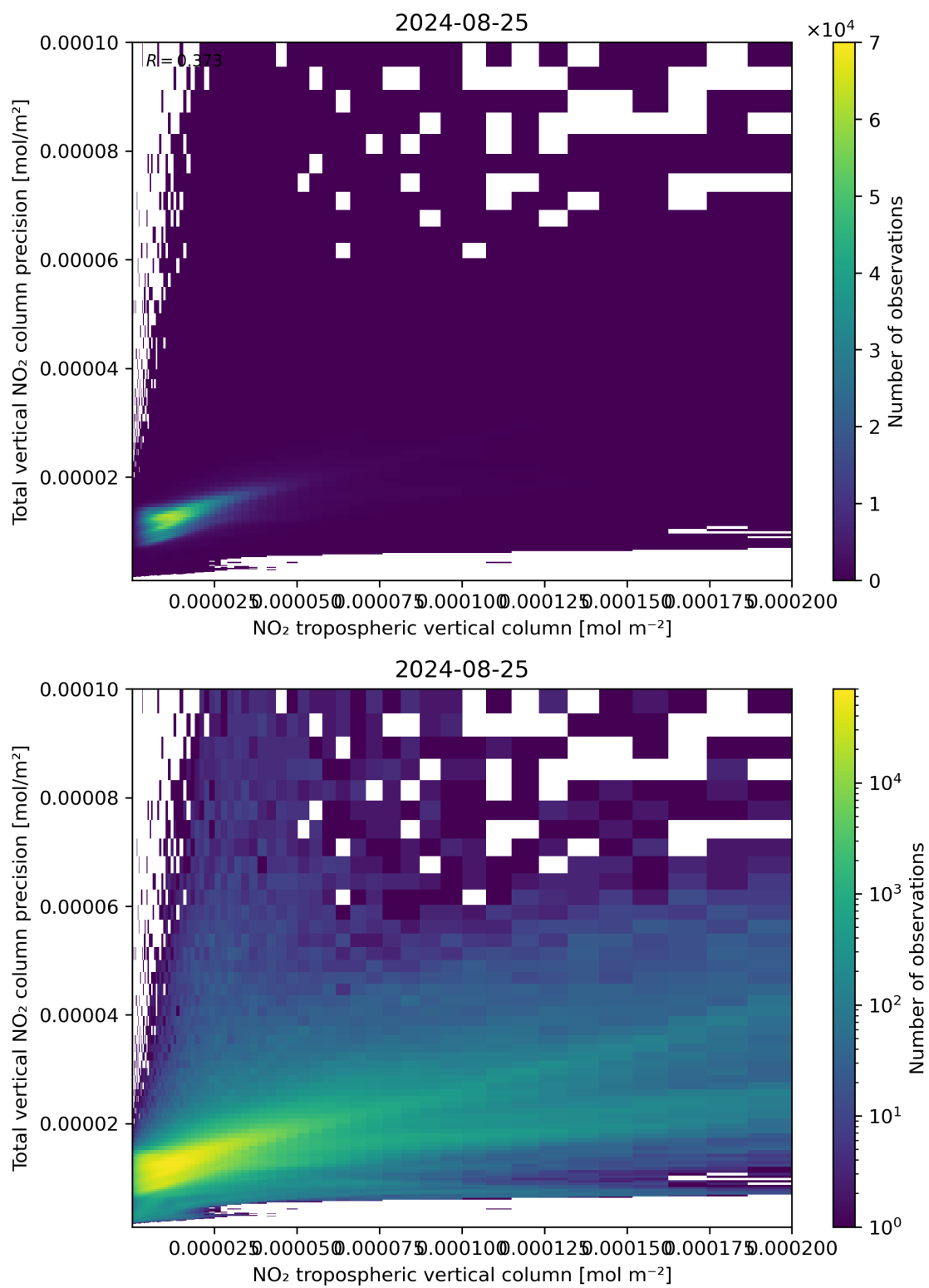
Figure 129: Scatter density plot of “NO 2 tropospheric vertical column” against “Total vertical NO 2 column precision” for 2024-08-24 to 2024-08-26.
