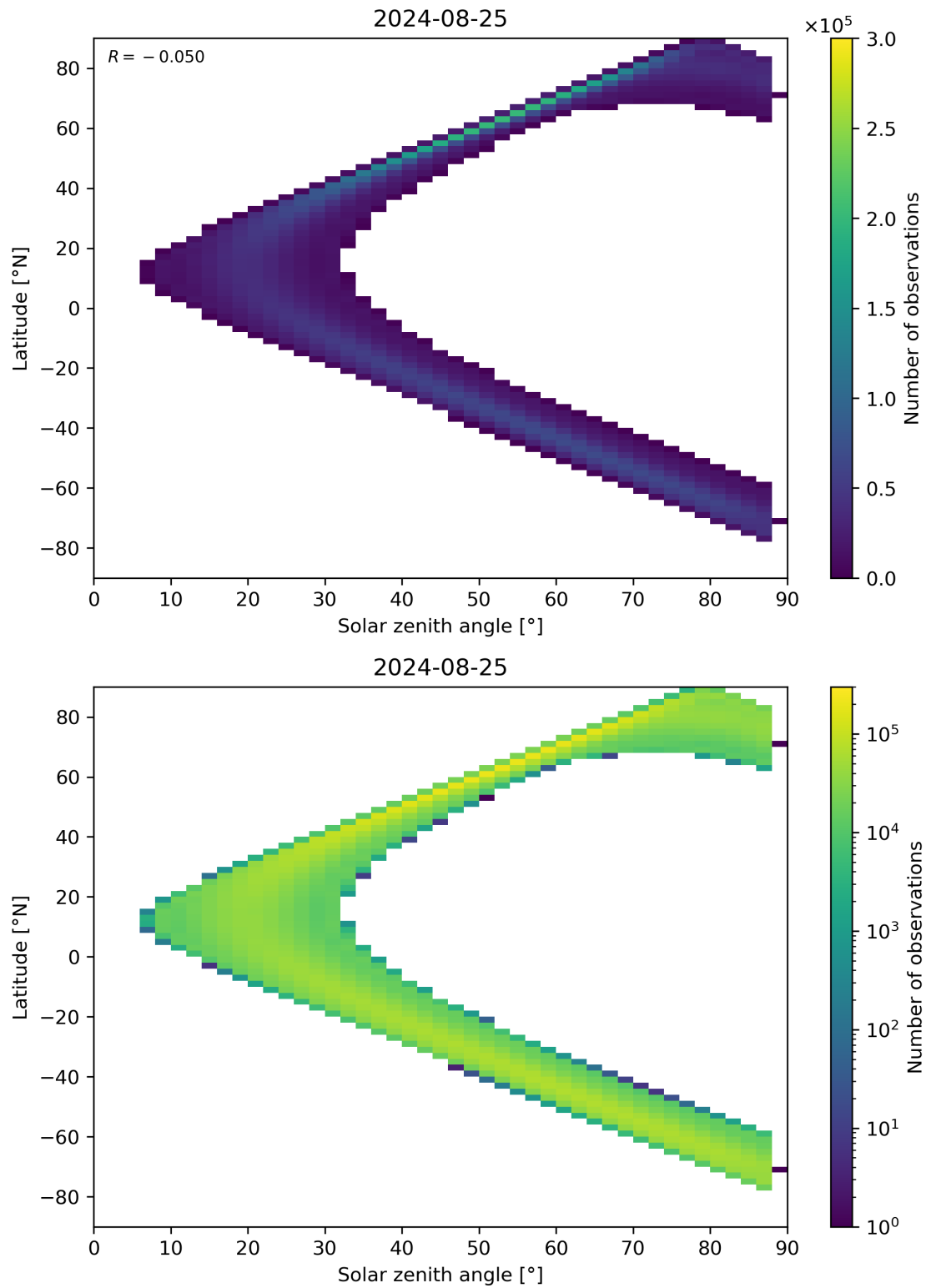
Figure 149: Scatter density plot of “Solar zenith angle” against “Latitude” for 2024-08-24 to 2024-08-26.
