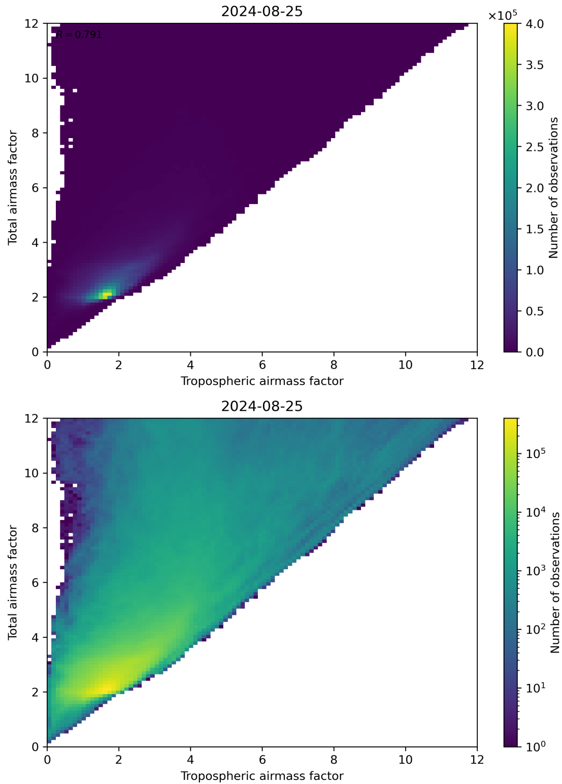
Figure 72: Scatter density plot of “Tropospheric airmass factor” against “Total airmass factor” for 2024-08-24 to 2024-08-26.
