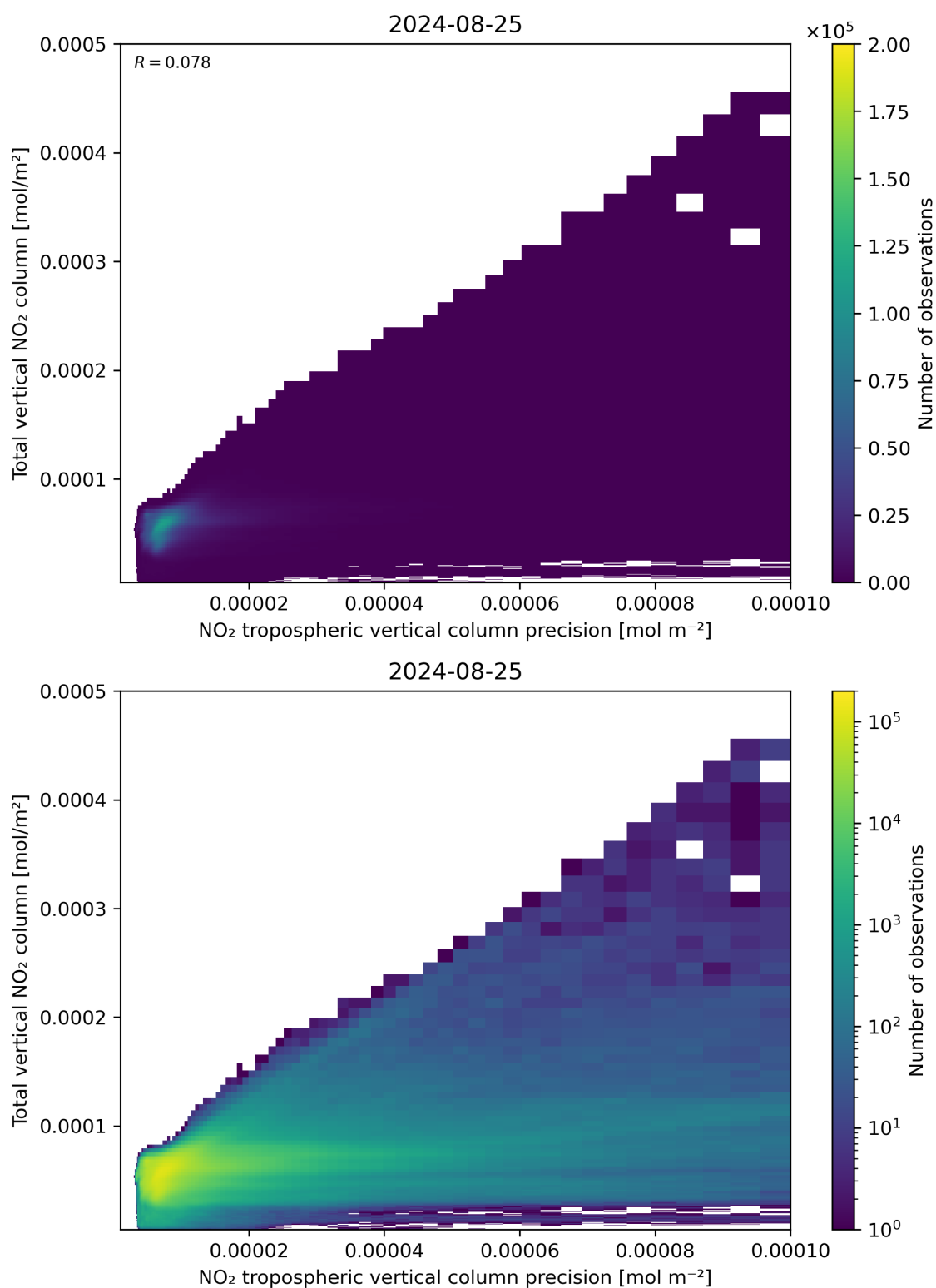
Figure 138: Scatter density plot of “NO 2 tropospheric vertical column precision” against “Total vertical NO 2 column” for 2024-08-24 to 2024-08-26.
