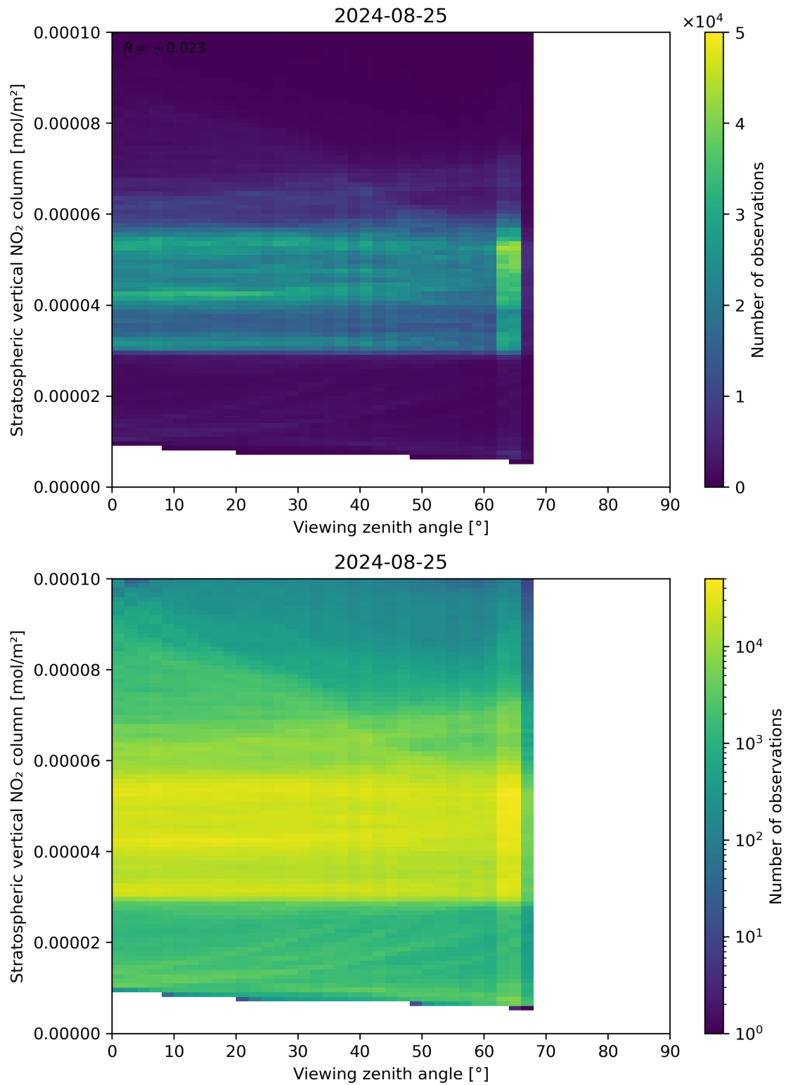
Figure 164: Scatter density plot of “Viewing zenith angle” against “Stratospheric vertical NO 2 column” for 2024-08-24 to 2024-08-26.
