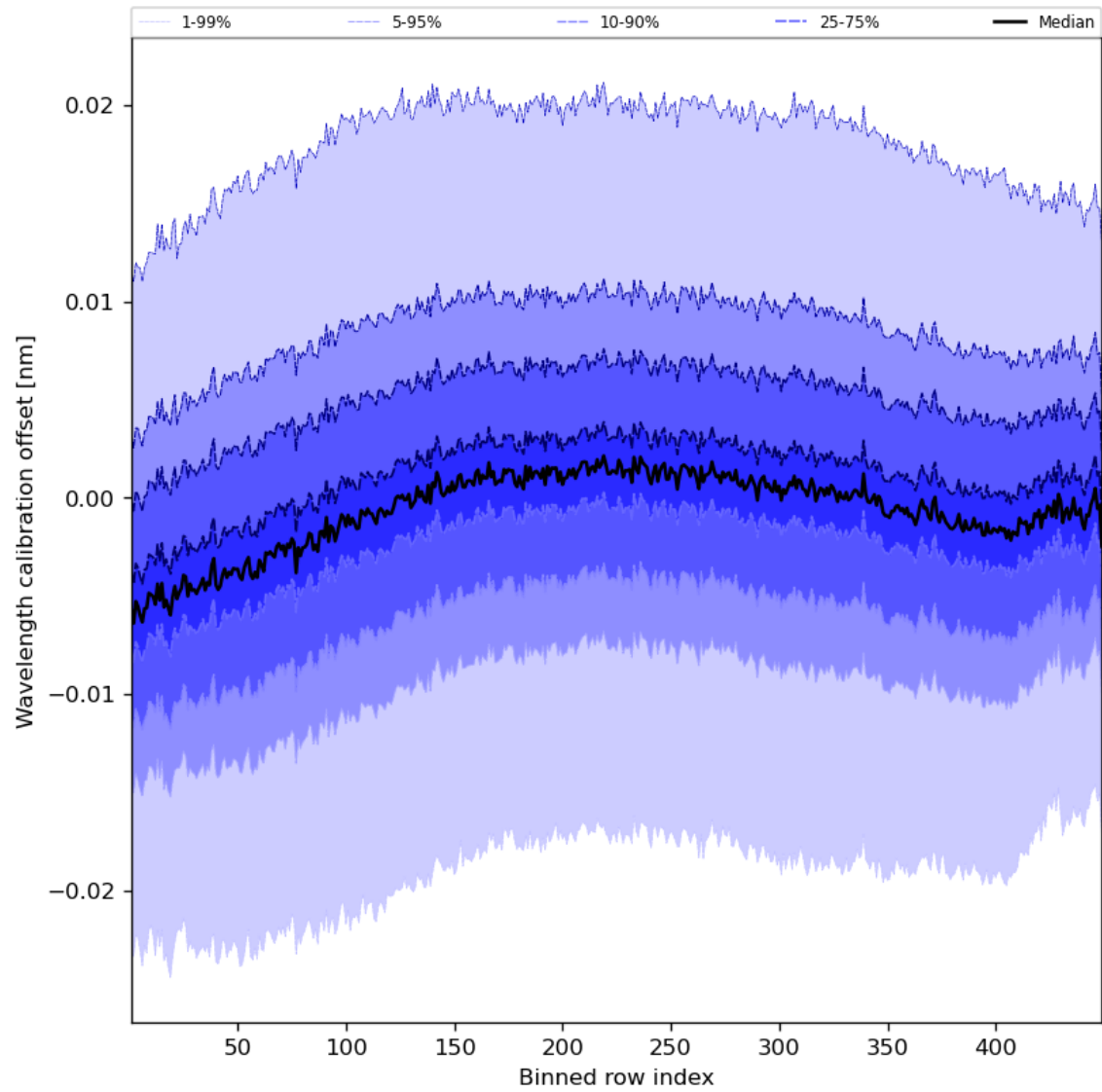
Figure 52: Along track statistics of “Wavelength calibration offset” for 2024-08-24 to 2024-08-26
