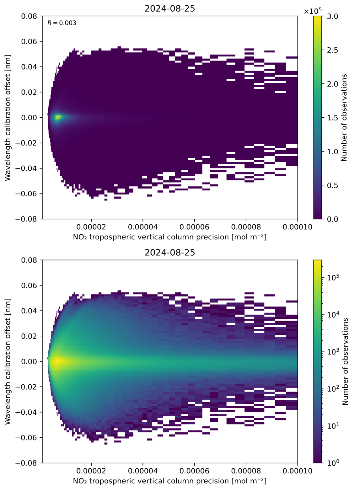
Figure 141: Scatter density plot of “NO 2 tropospheric vertical column precision” against “Wavelength calibration offset” for 2024-08-24 to 2024-08-26.
