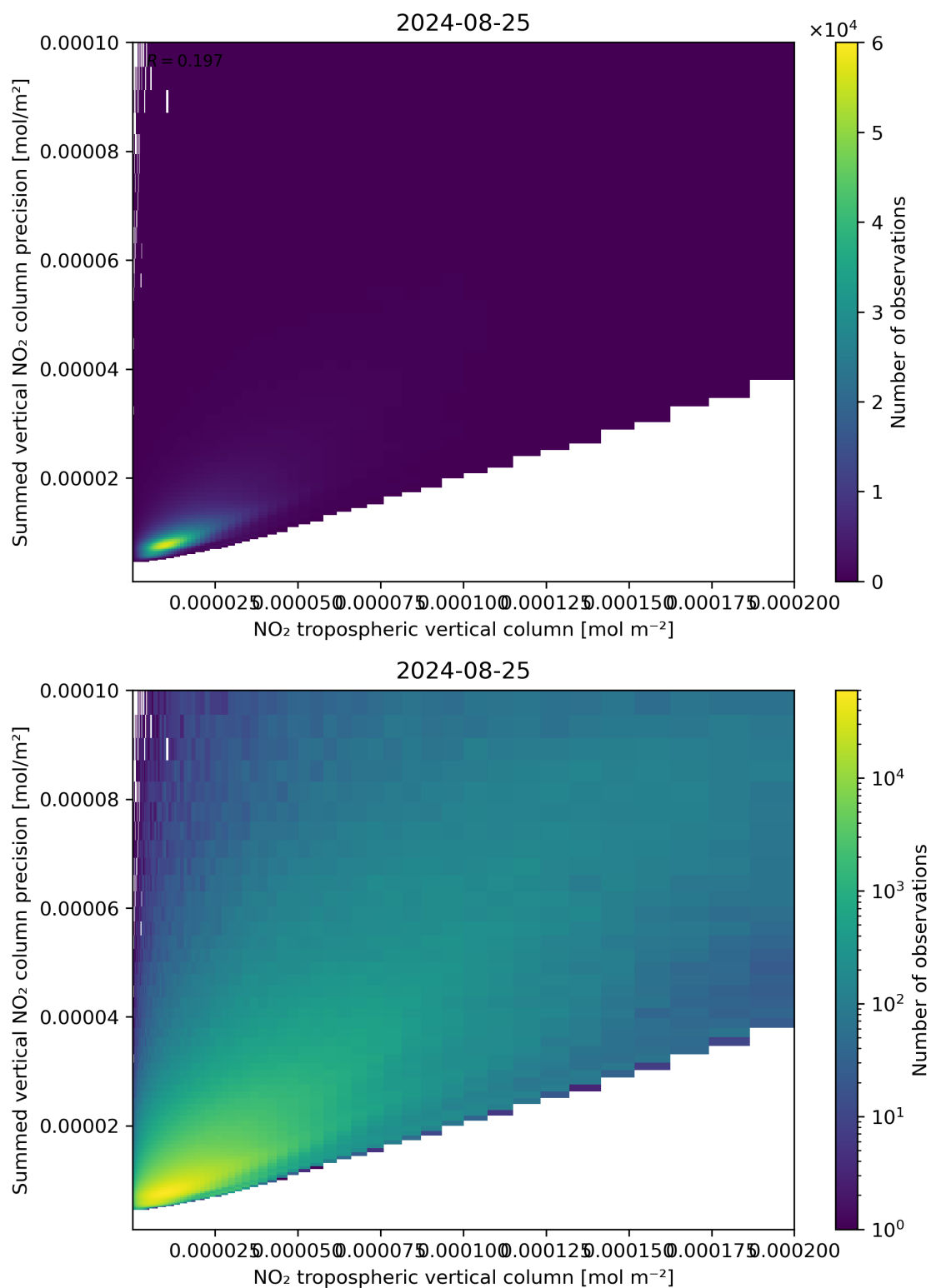
Figure 127: Scatter density plot of “NO 2 tropospheric vertical column” against “Summed vertical NO 2 column precision” for 2024-08-24 to 2024-08-26.
