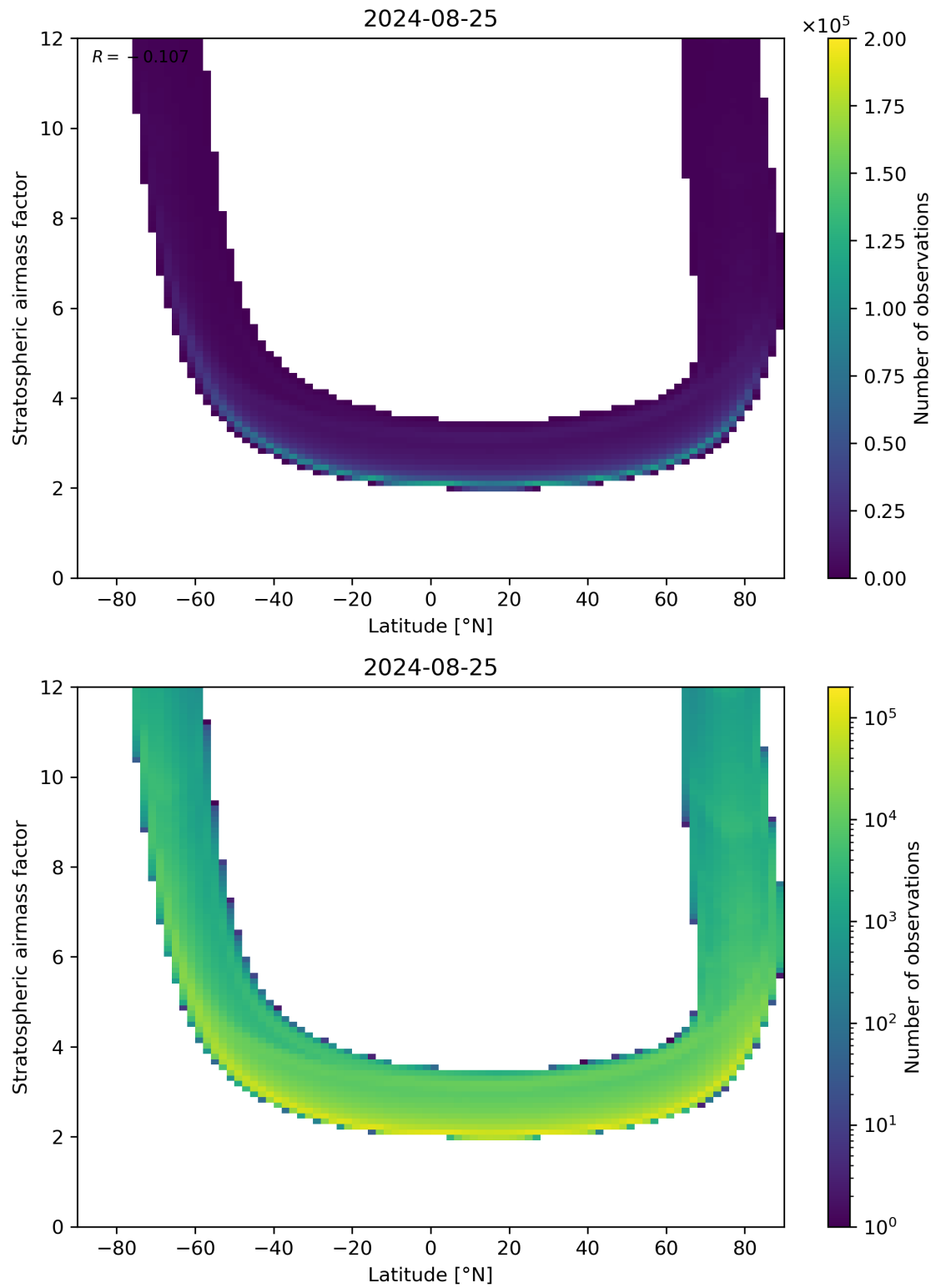
Figure 83: Scatter density plot of “Latitude” against “Stratospheric air mass factor” for 2024-08-24 to 2024-08-26.
