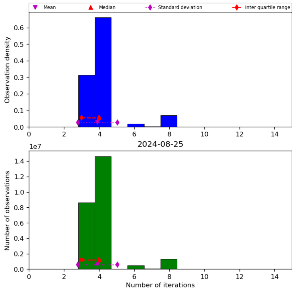
Figure 34: Histogram of “Number of iterations” for 2024-08-24 to 2024-08-26
