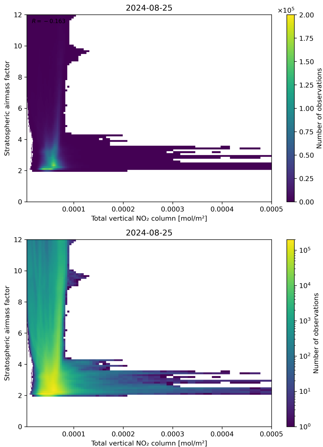
Figure 110: Scatter density plot of “Total vertical NO 2 column” against “Stratospheric airmass factor” for 2024-08-24 to 2024-08-26.
