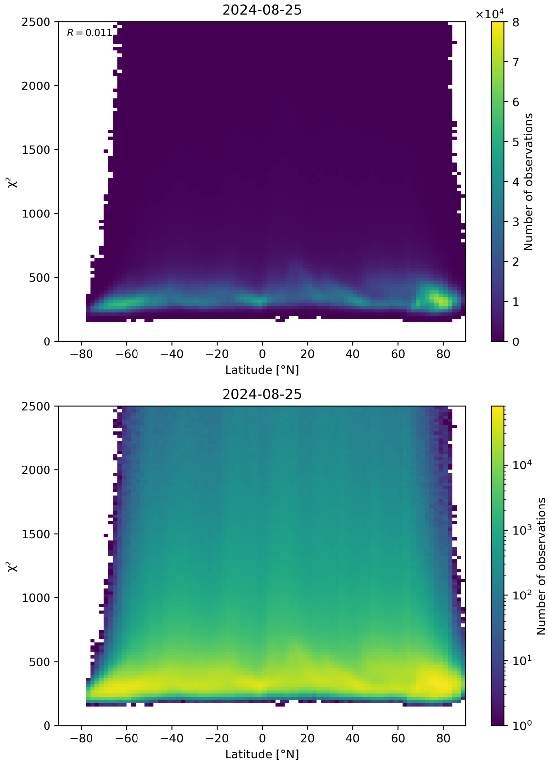
Figure 86: Scatter density plot of “Latitude” against “ \chi^2 ” for 2024-08-24 to 2024-08-26.
