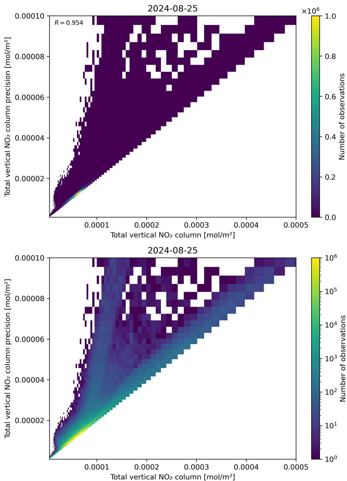
Figure 114: Scatter density plot of “Total vertical NO 2 column” against “Total vertical NO 2 column precision” for 2024-08-24 to 2024-08-26.
