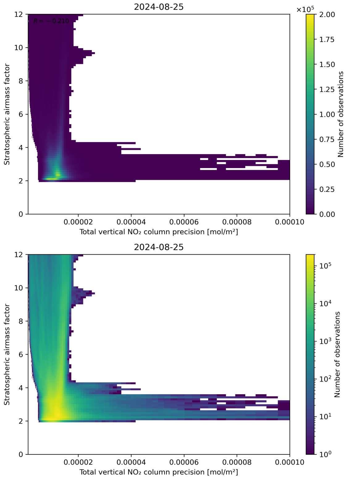
Figure 115: Scatter density plot of “Total vertical NO 2 column precision” against “Stratospheric air mass factor” for 2024-08-24 to 2024-08-26.
