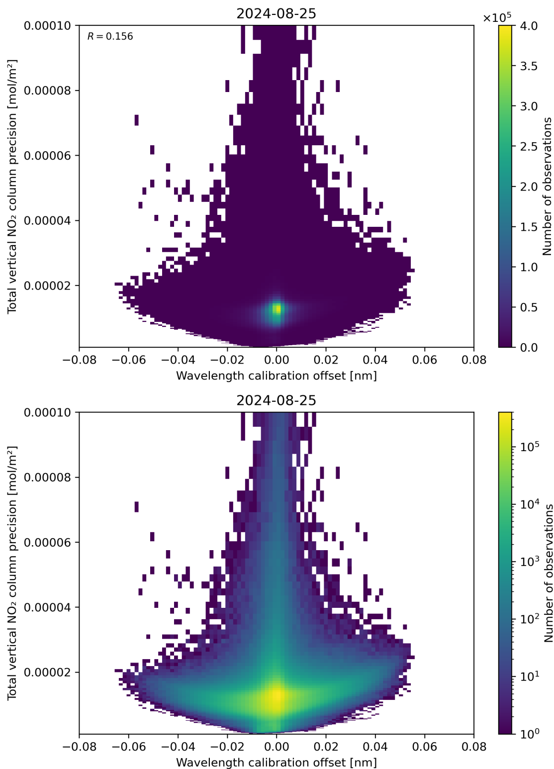
Figure 180: Scatter density plot of “Wavelength calibration offset” against “Total vertical NO 2 column precision” for 2024-08-24 to 2024-08-26.
