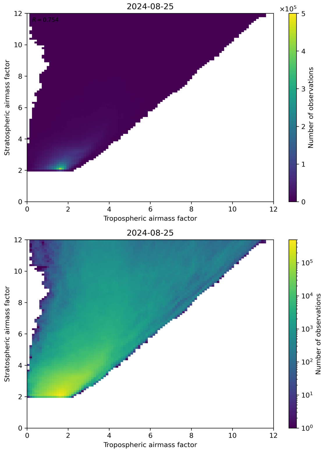
Figure 71: Scatter density plot of “Tropospheric airmass factor” against “Stratospheric airmass factor” for 2024-08-24 to 2024-08-26.
