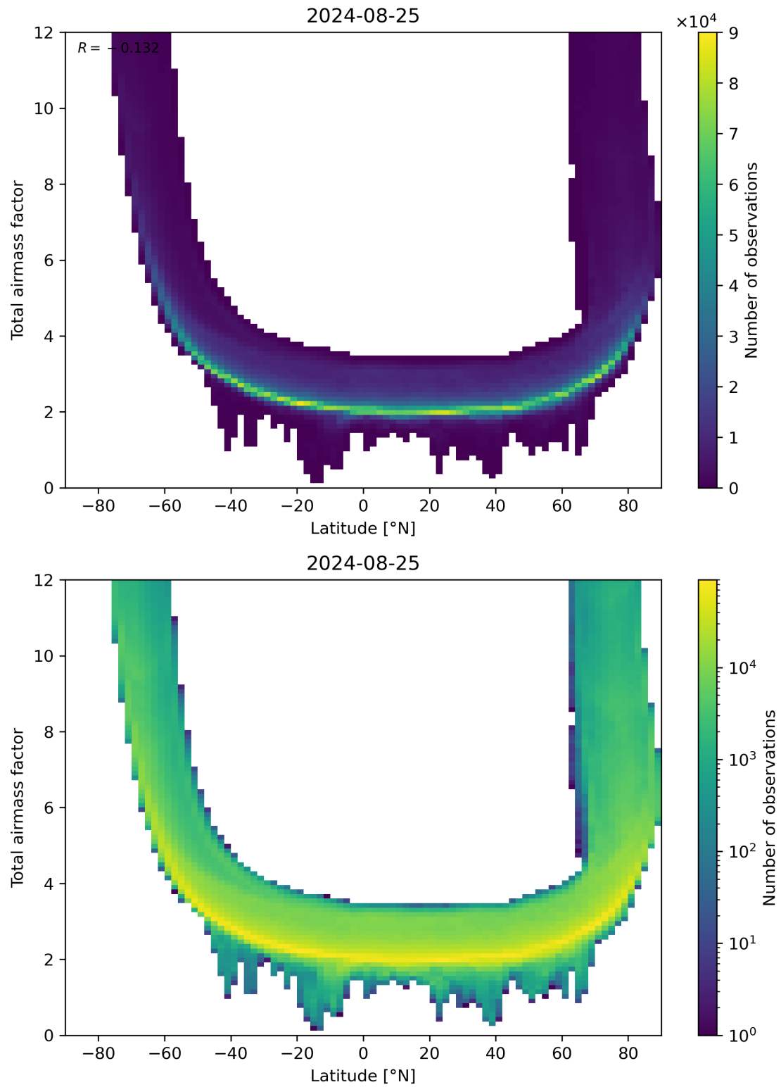
Figure 84: Scatter density plot of “Latitude” against “Total airmass factor” for 2024-08-24 to 2024-08-26.
