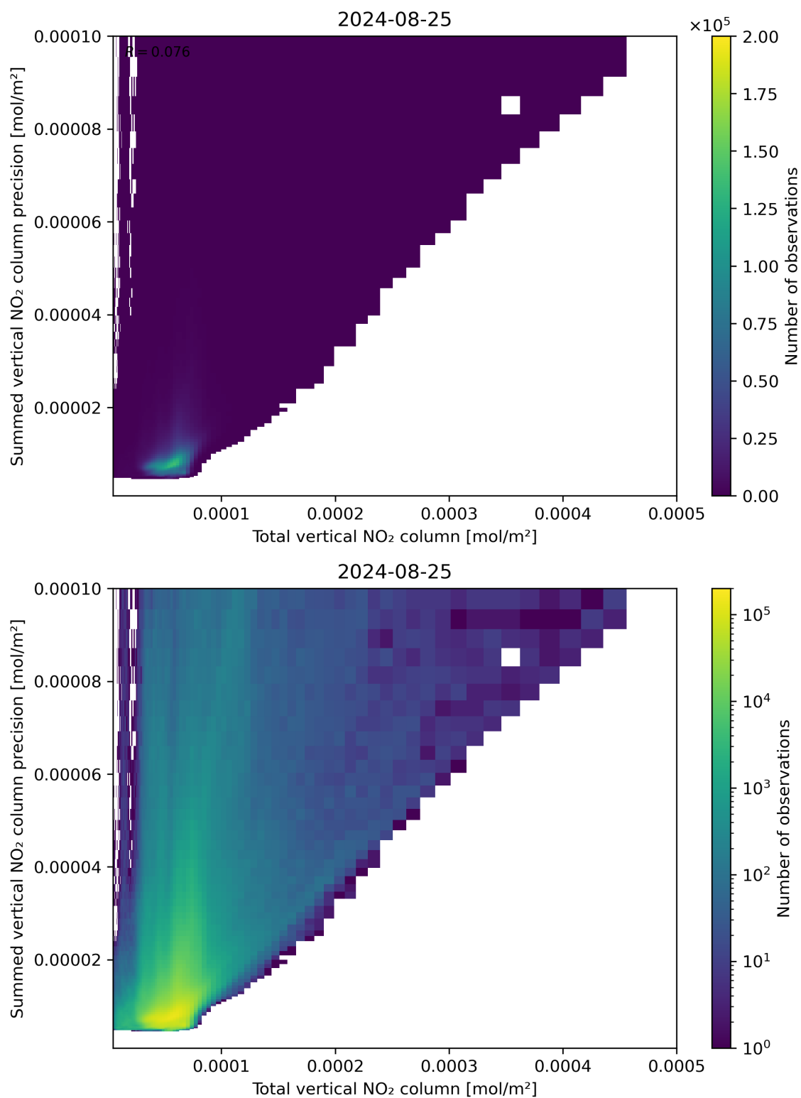
Figure 113: Scatter density plot of “Total vertical NO 2 column” against “Summed vertical NO 2 column precision” for 2024-08-24 to 2024-08-26.
