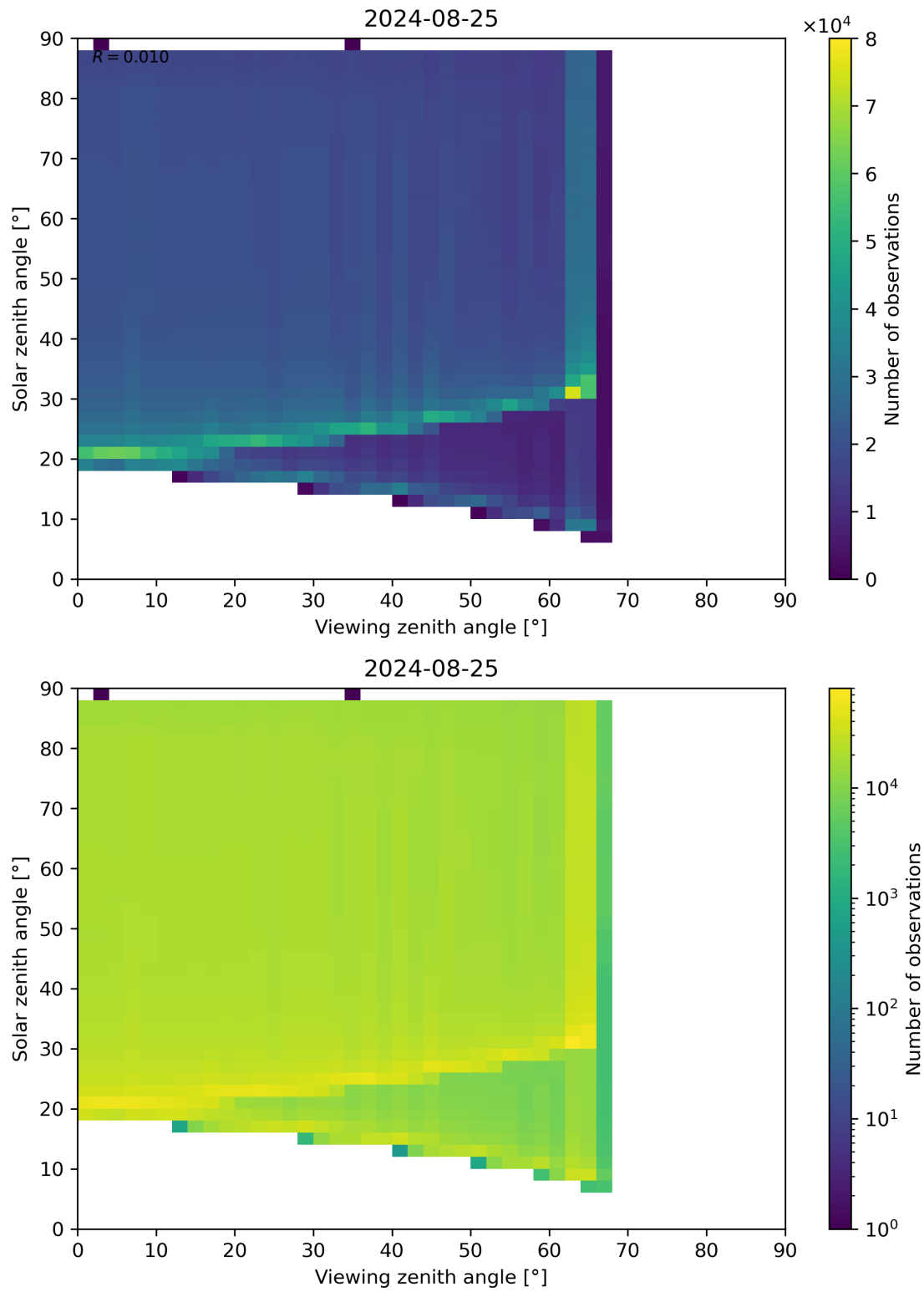
Figure 172: Scatter density plot of “Viewing zenith angle” against “Solar zenith angle” for 2024-08-24 to 2024-08-26.
