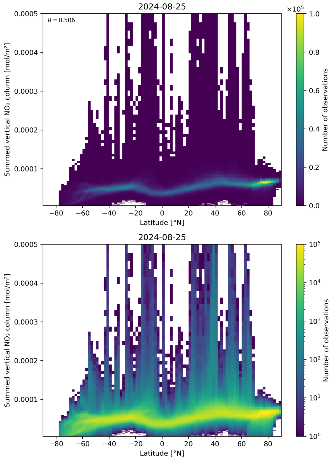
Figure 88: Scatter density plot of “Latitude” against “Summed vertical NO 2 column” for 2024-08-24 to 2024-08-26.
