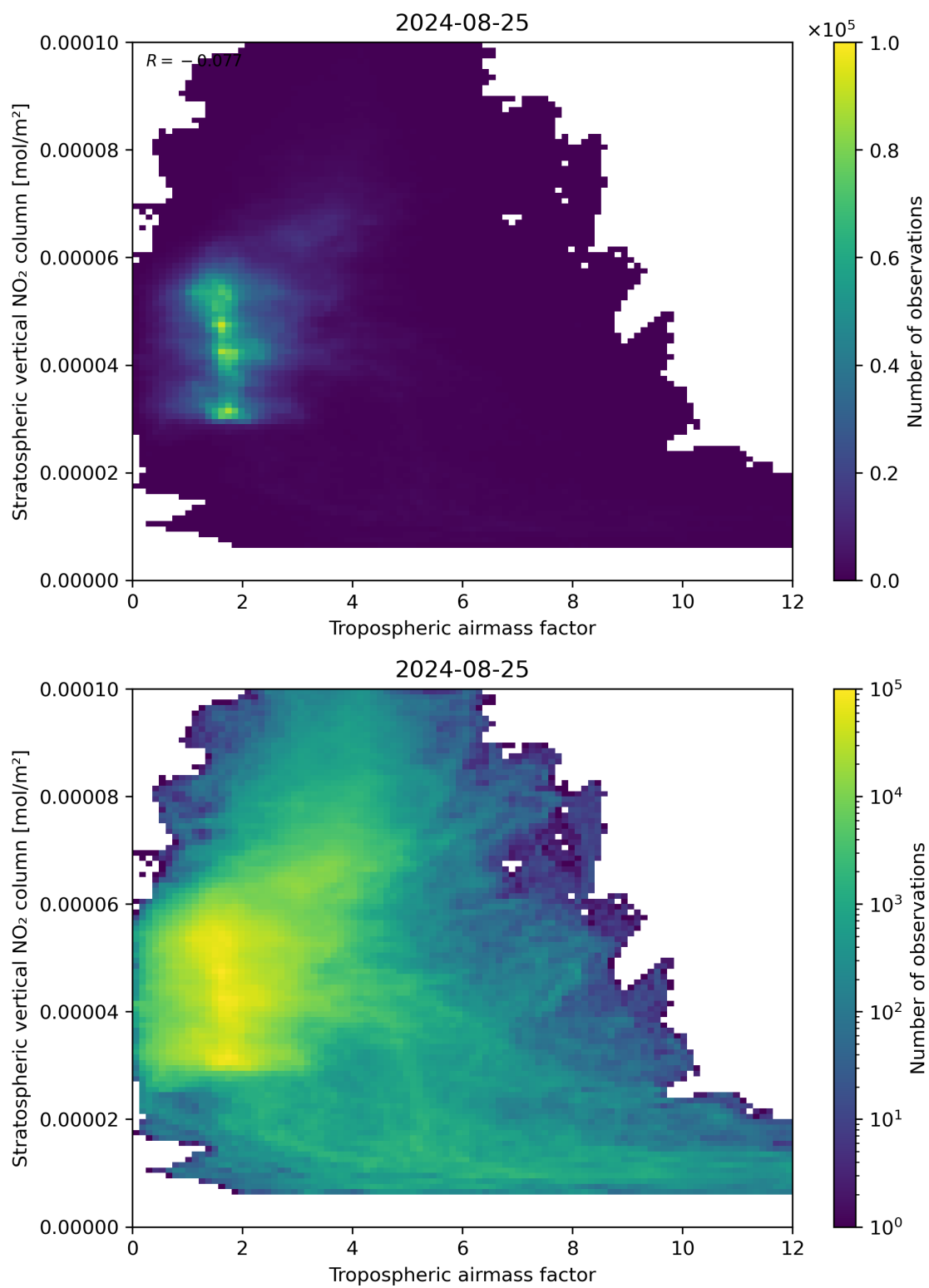
Figure 74: Scatter density plot of “Tropospheric air mass factor” against “Stratospheric vertical NO 2 column” for 2024-08-24 to 2024-08-26.
