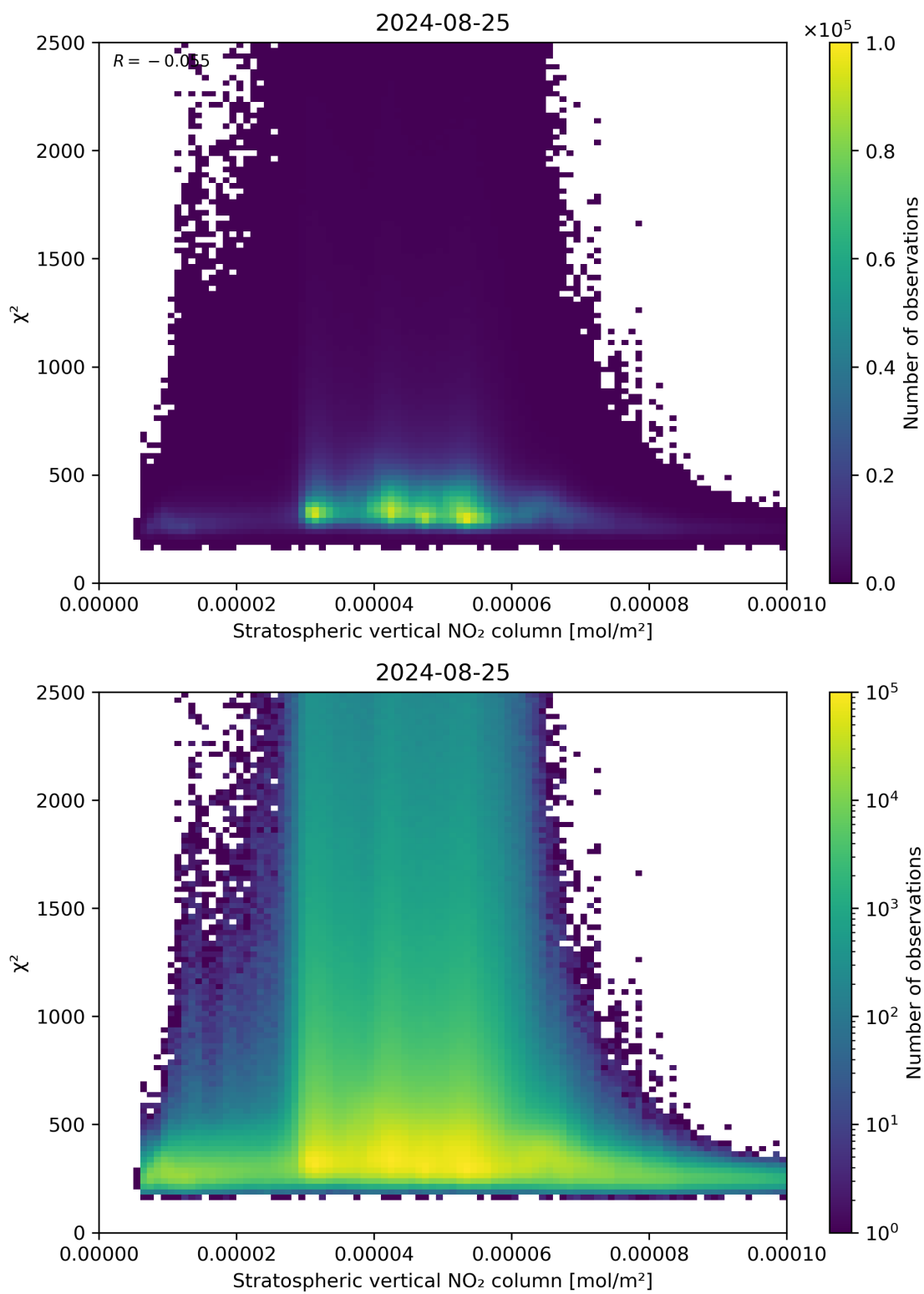
Figure 97: Scatter density plot of “Stratospheric vertical NO 2 column” against “ \chi^2 ” for 2024-08-24 to 2024-08-26.
