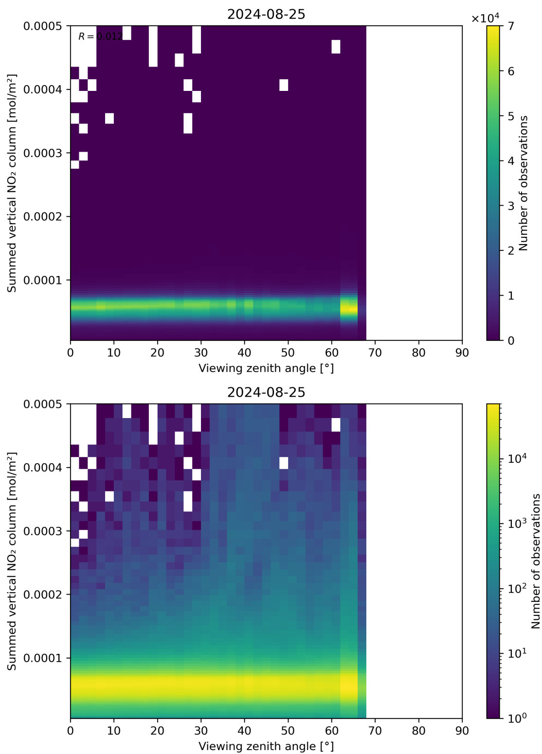
Figure 165: Scatter density plot of “Viewing zenith angle” against “Summed vertical NO 2 column” for 2024-08-24 to 2024-08-26.
