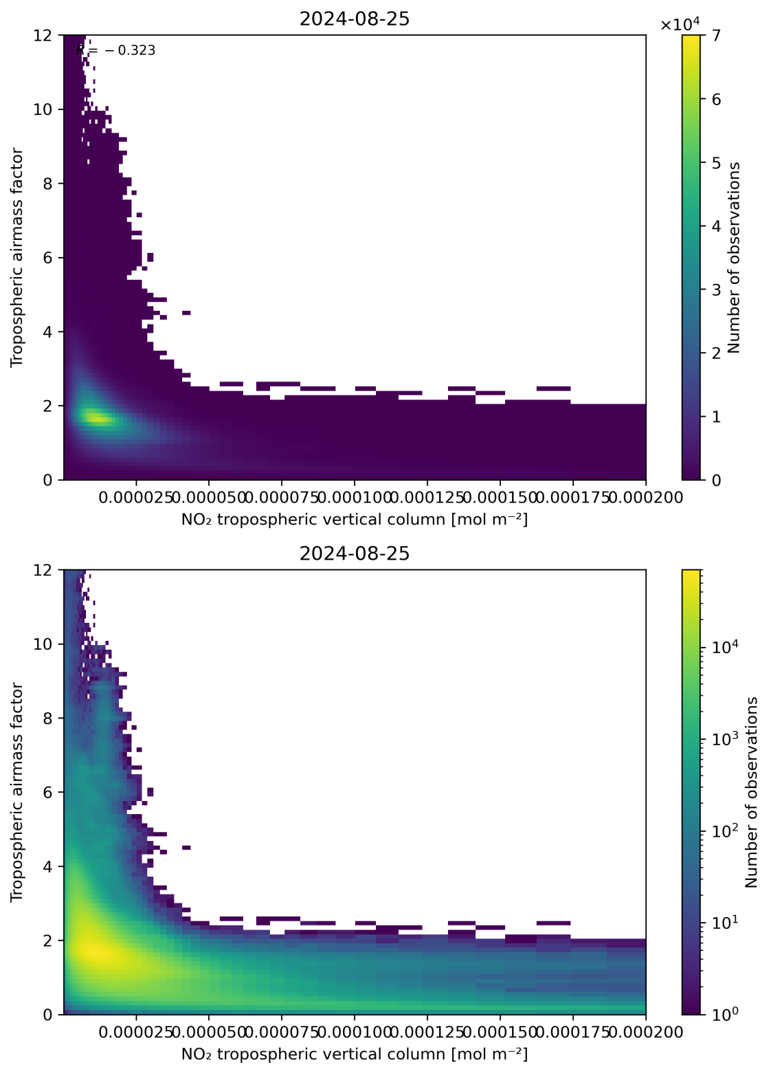
Figure 123: Scatter density plot of “NO 2 tropospheric vertical column” against “Tropospheric air mass factor” for 2024-08-24 to 2024-08-26.
