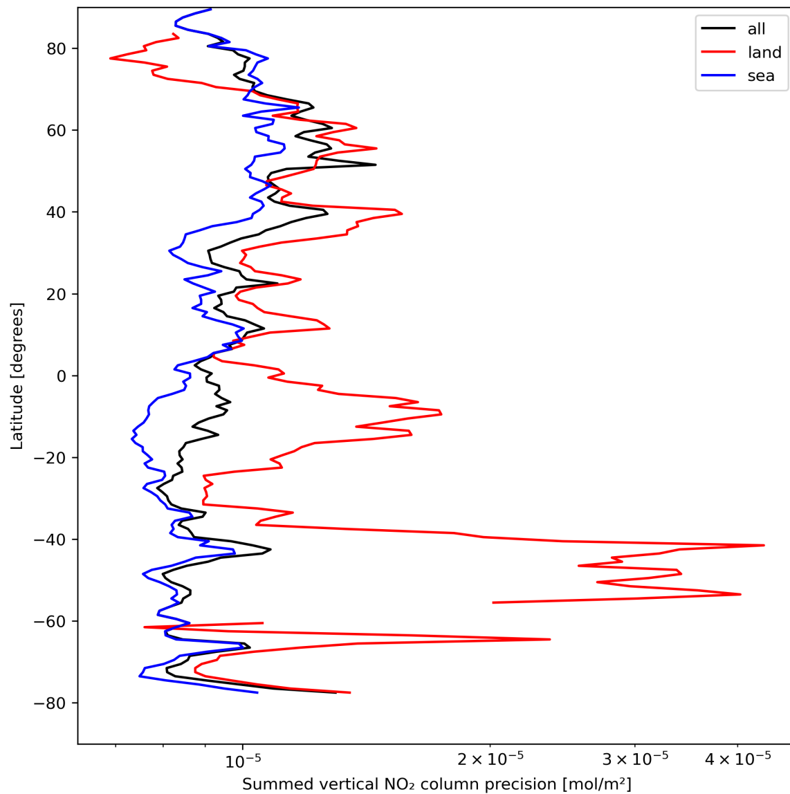
Figure 24: Zonal average of “Summed vertical NO 2 column precision” for 2024-08-24 to 2024-08-26.
