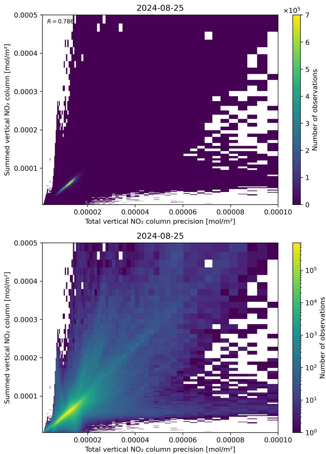
Figure 117: Scatter density plot of “Total vertical NO 2 column precision” against “Summed vertical NO 2 column” for 2024-08-24 to 2024-08-26.
