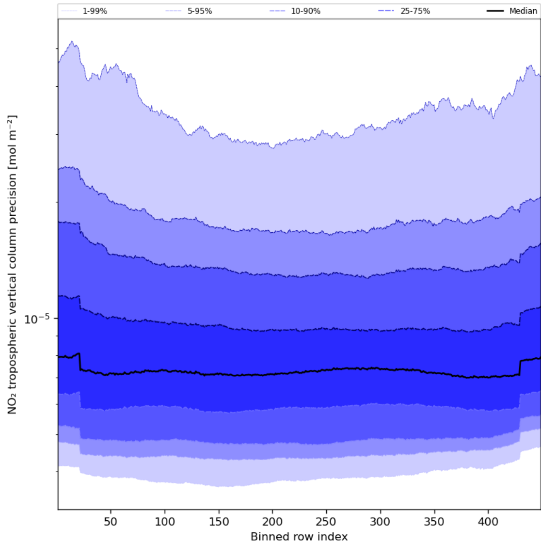
Figure 47: Along track statistics of “NO 2 tropospheric vertical column precision” for 2024-08-24 to 2024-08-26
