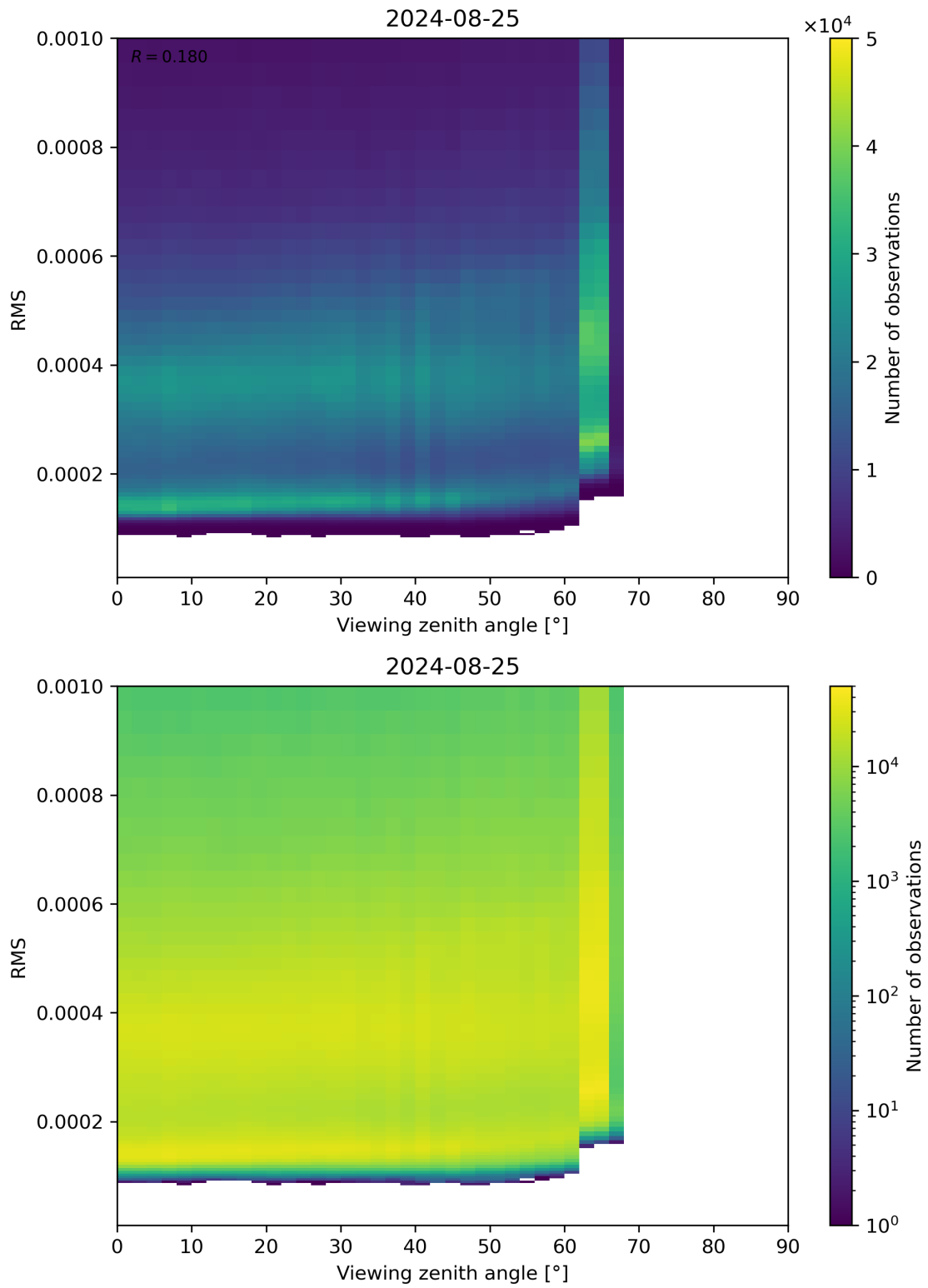
Figure 171: Scatter density plot of “Viewing zenith angle” against “RMS” for 2024-08-24 to 2024-08-26.
