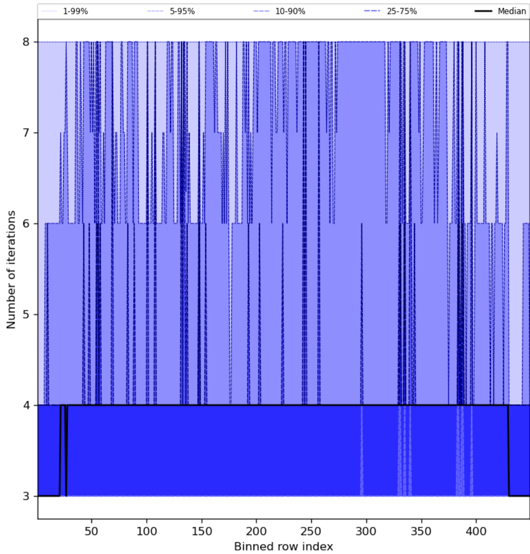
Figure 51: Along track statistics of “Number of iterations” for 2024-08-24 to 2024-08-26
