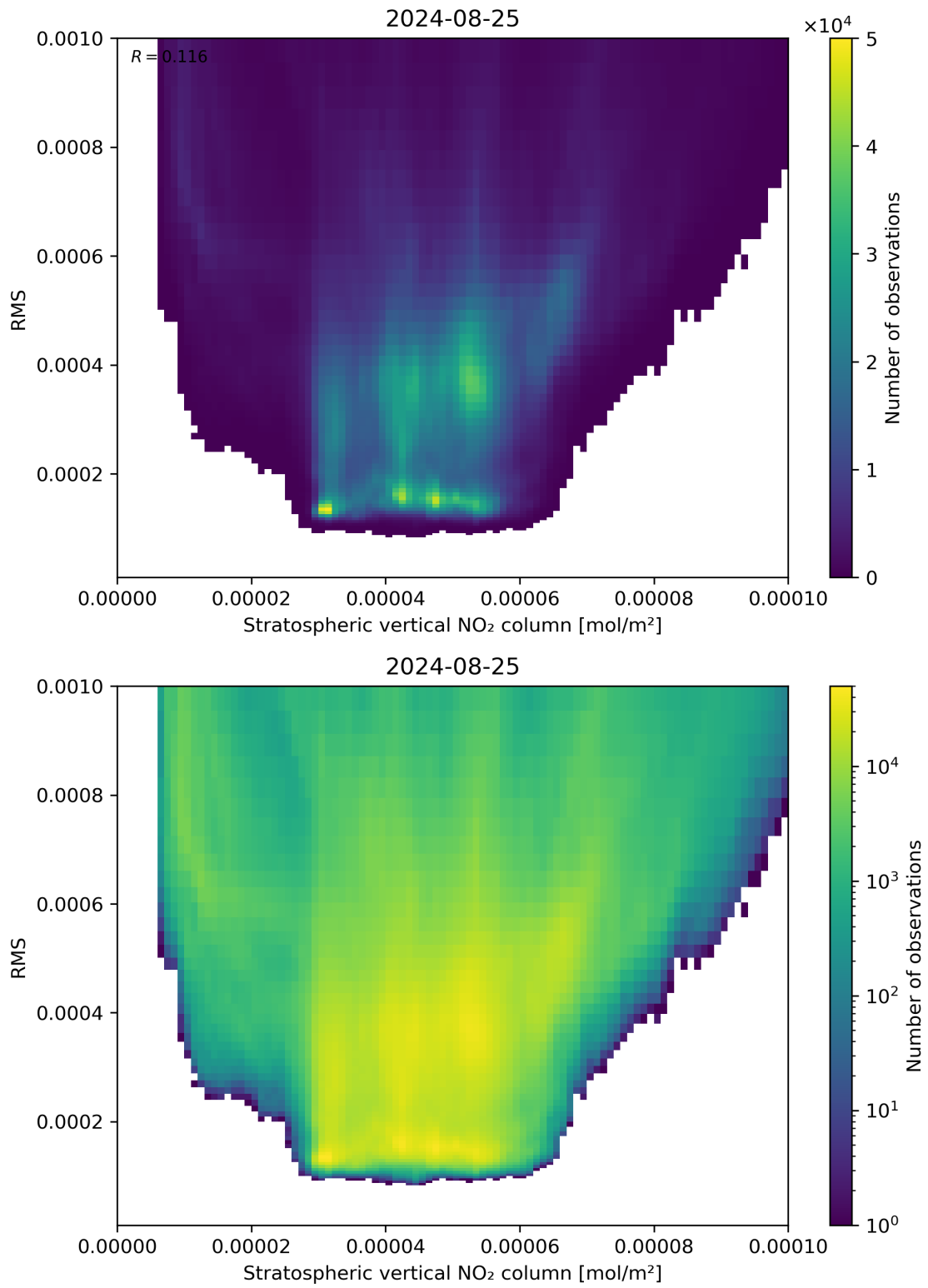
Figure 102: Scatter density plot of “Stratospheric vertical NO 2 column” against “RMS” for 2024-08-24 to 2024-08-26.
