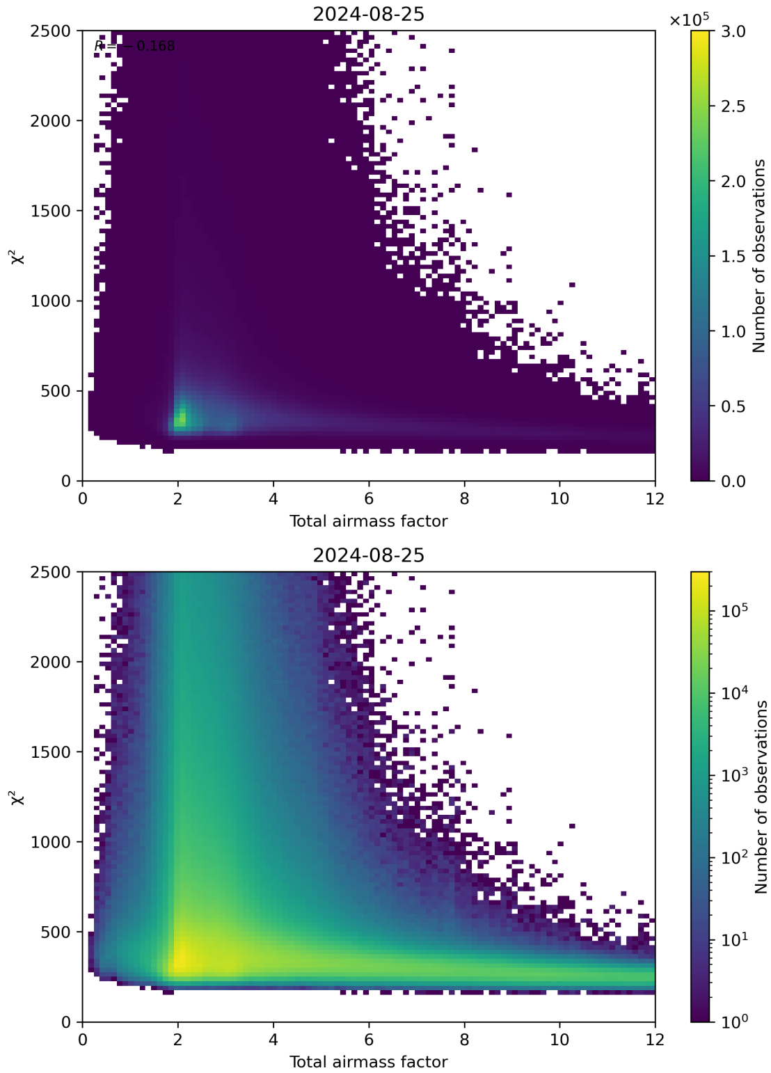
Figure 63: Scatter density plot of “Total airmass factor” against “ \chi^2 ” for 2024-08-24 to 2024-08-26.
