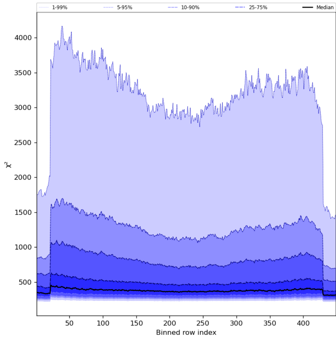
Figure 59: Along track statistics of “ \chi^2 ” for 2024-08-24 to 2024-08-26
