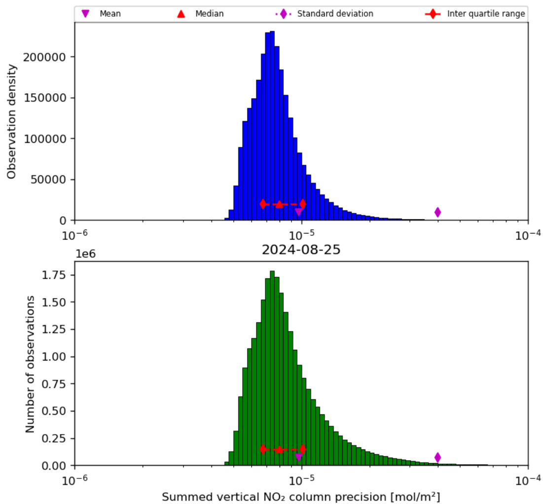
Figure 41: Histogram of "Summed vertical NO 2 column precision" for 2024-08-24 to 2024-08-26
