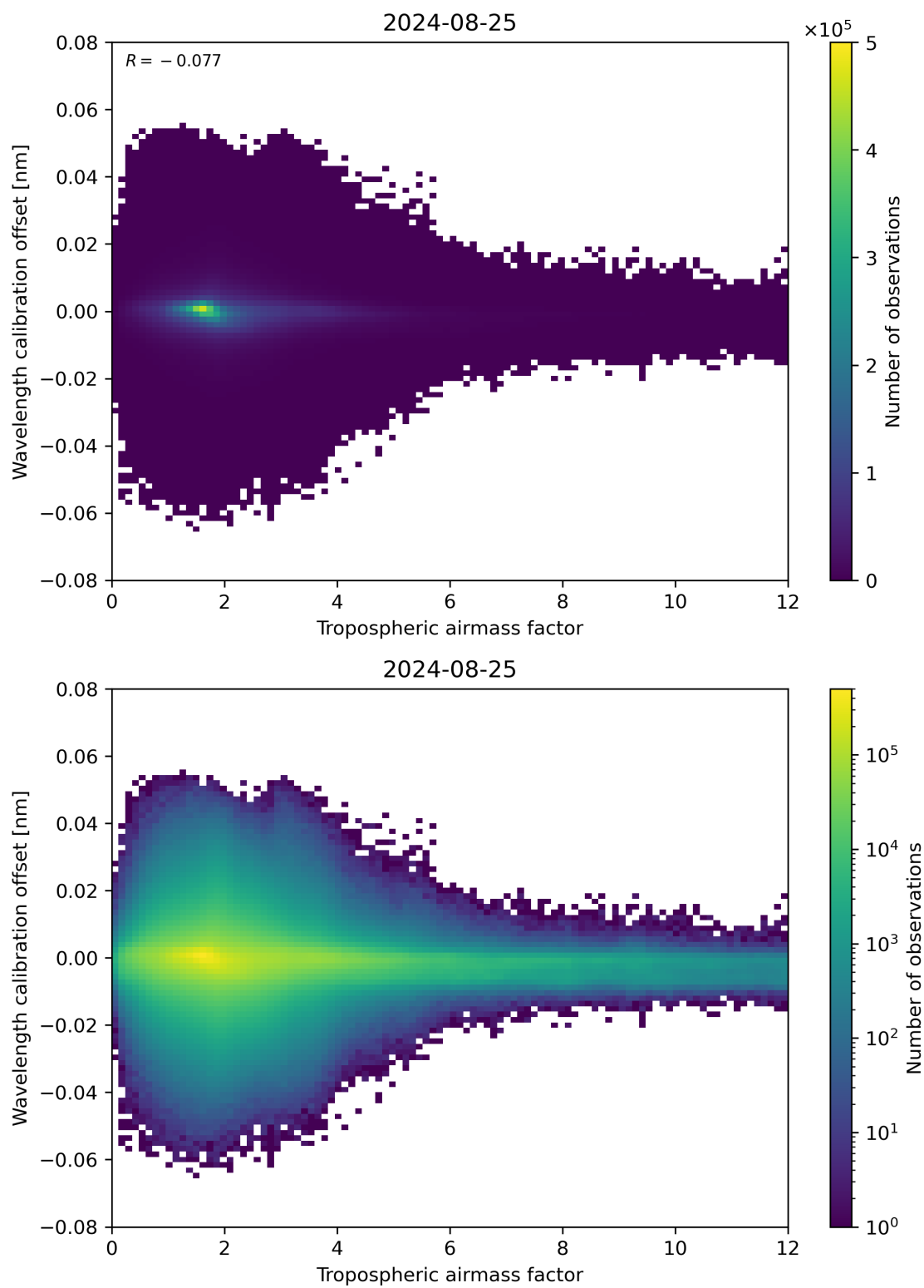
Figure 80: Scatter density plot of “Tropospheric airmass factor” against “Wavelength calibration offset” for 2024-08-24 to 2024-08-26.
