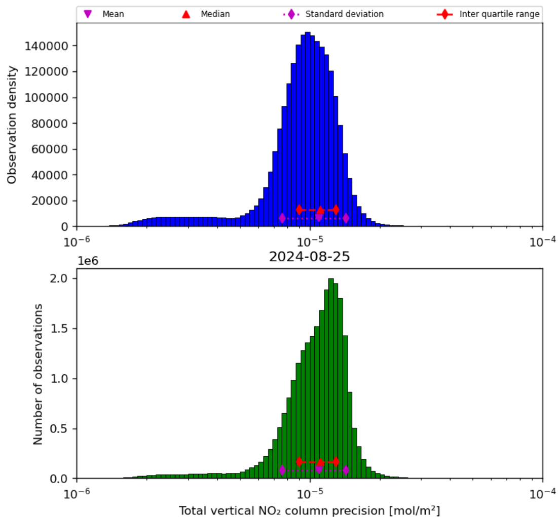
Figure 39: Histogram of “Total vertical NO 2 column precision” for 2024-08-24 to 2024-08-26
