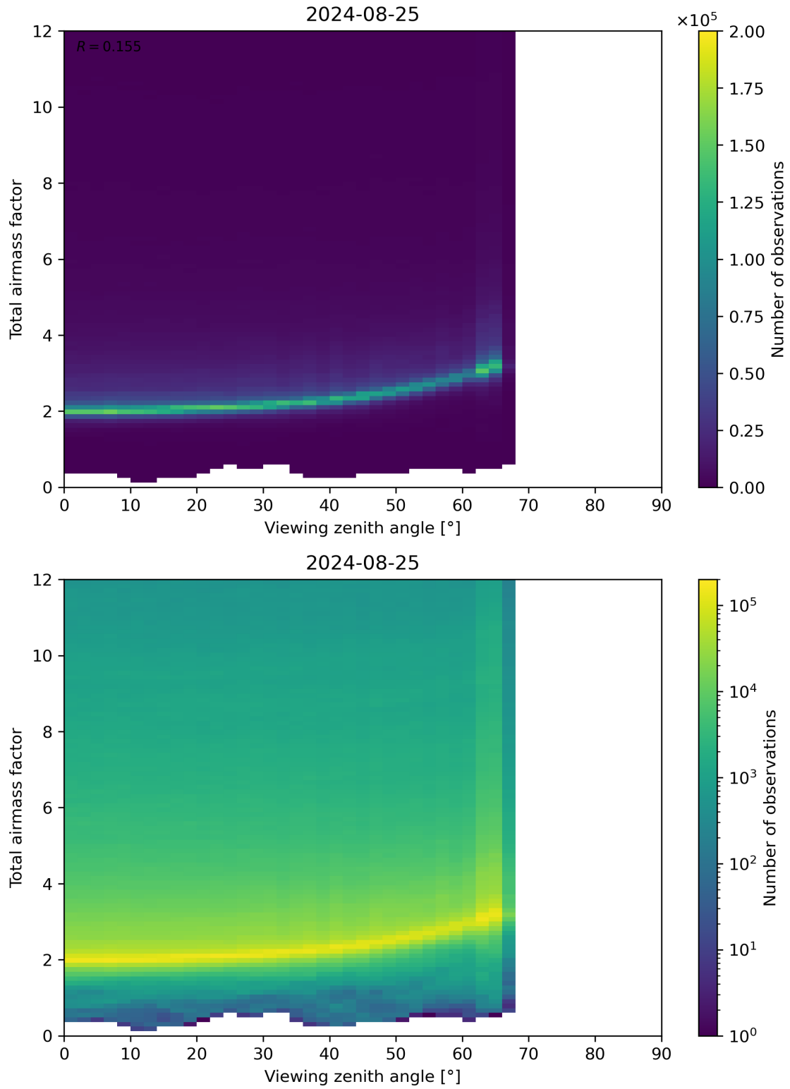
Figure 160: Scatter density plot of “Viewing zenith angle” against “Total airmass factor” for 2024-08-24 to 2024-08-26.
