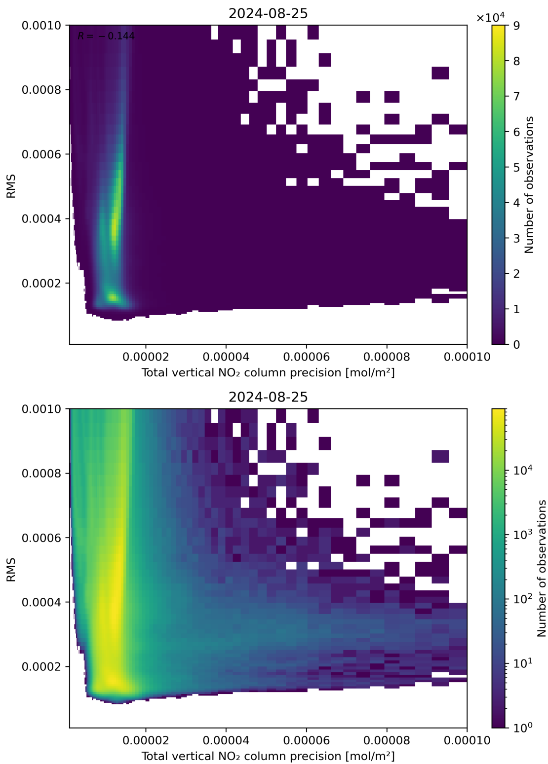
Figure 119: Scatter density plot of “Total vertical NO 2 column precision” against “RMS” for 2024-08-24 to 2024-08-26.
