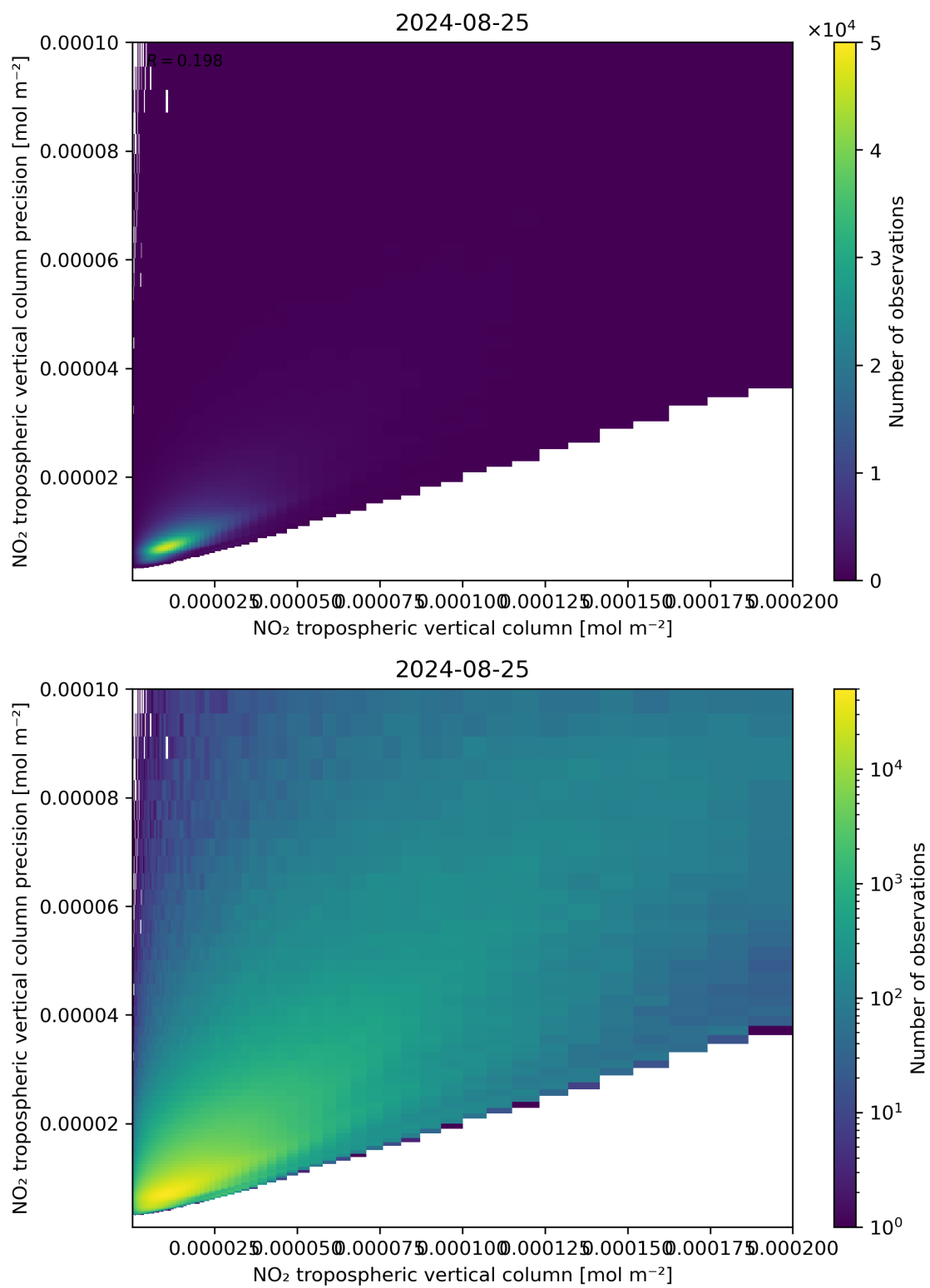
Figure 130: Scatter density plot of “NO 2 tropospheric vertical column” against “NO 2 tropospheric vertical column precision” for 2024-08-24 to 2024-08-26.
