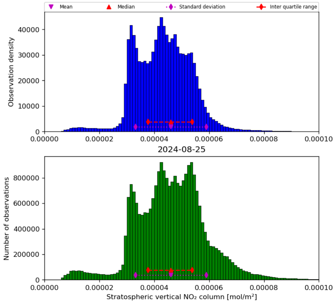
Figure 36: Histogram of “Stratospheric vertical NO 2 column” for 2024-08-24 to 2024-08-26
