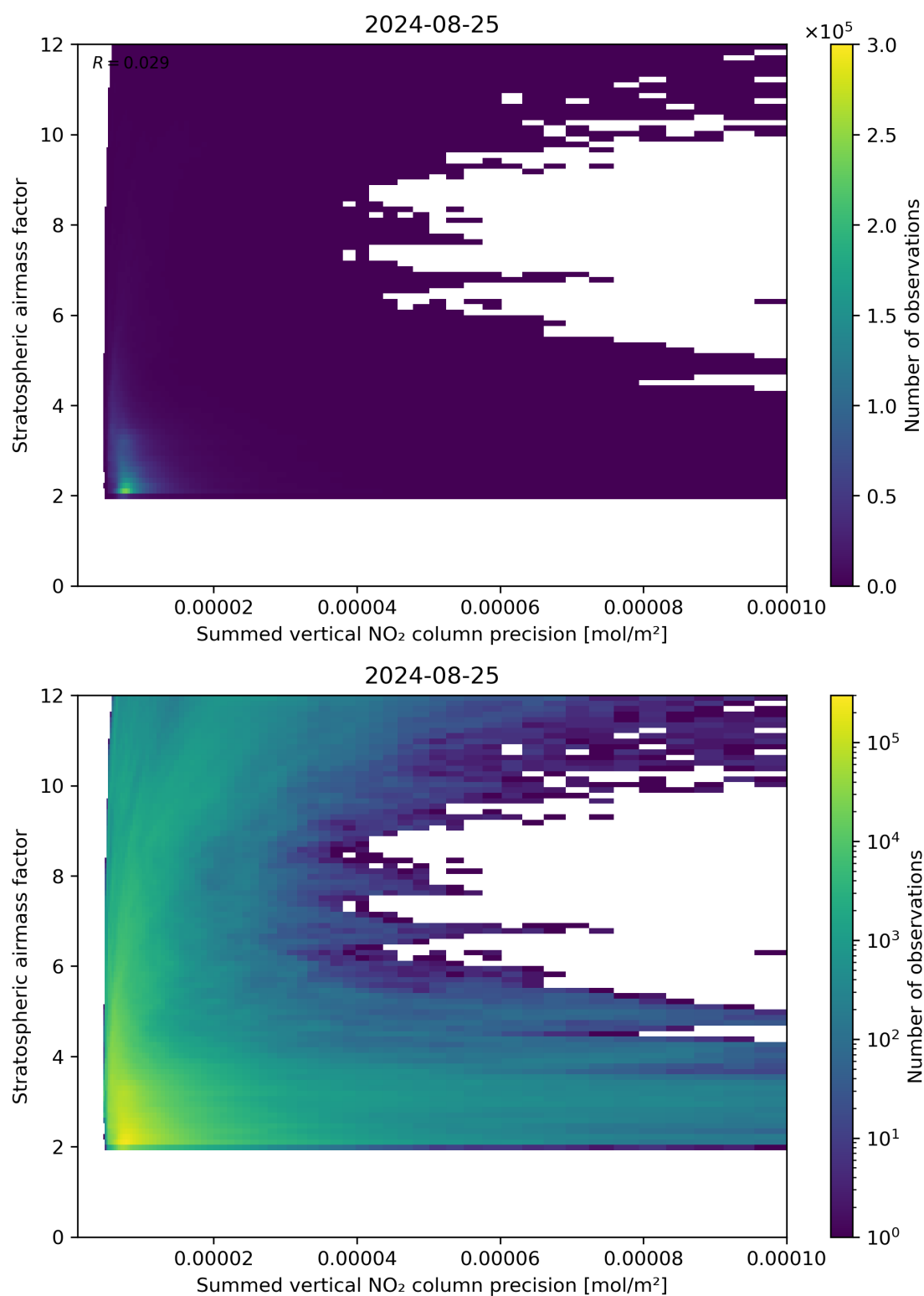
Figure 106: Scatter density plot of “Summed vertical NO 2 column precision” against “Stratospheric airmass factor” for 2024-08-24 to 2024-08-26.
