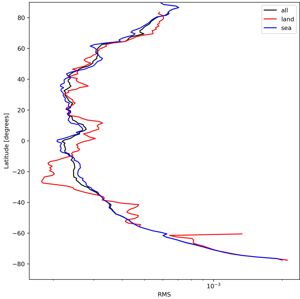
Figure 26: Zonal average of “RMS” for 2024-08-24 to 2024-08-26.
