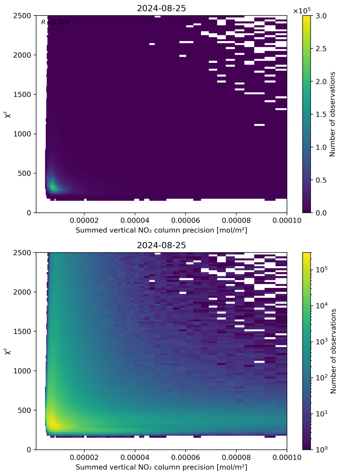
Figure 107: Scatter density plot of “Summed vertical NO 2 column precision” against “ \chi^2 ” for 2024-08-24 to 2024-08-26.
