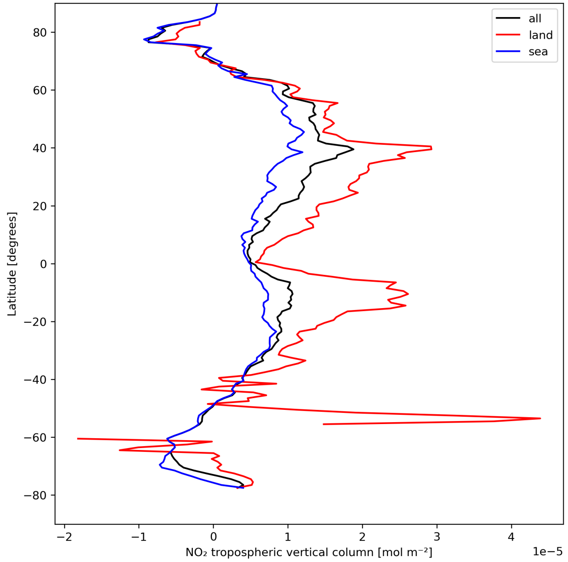
Figure 12: Zonal average of “NO 2 tropospheric vertical column” for 2024-08-24 to 2024-08-26.
