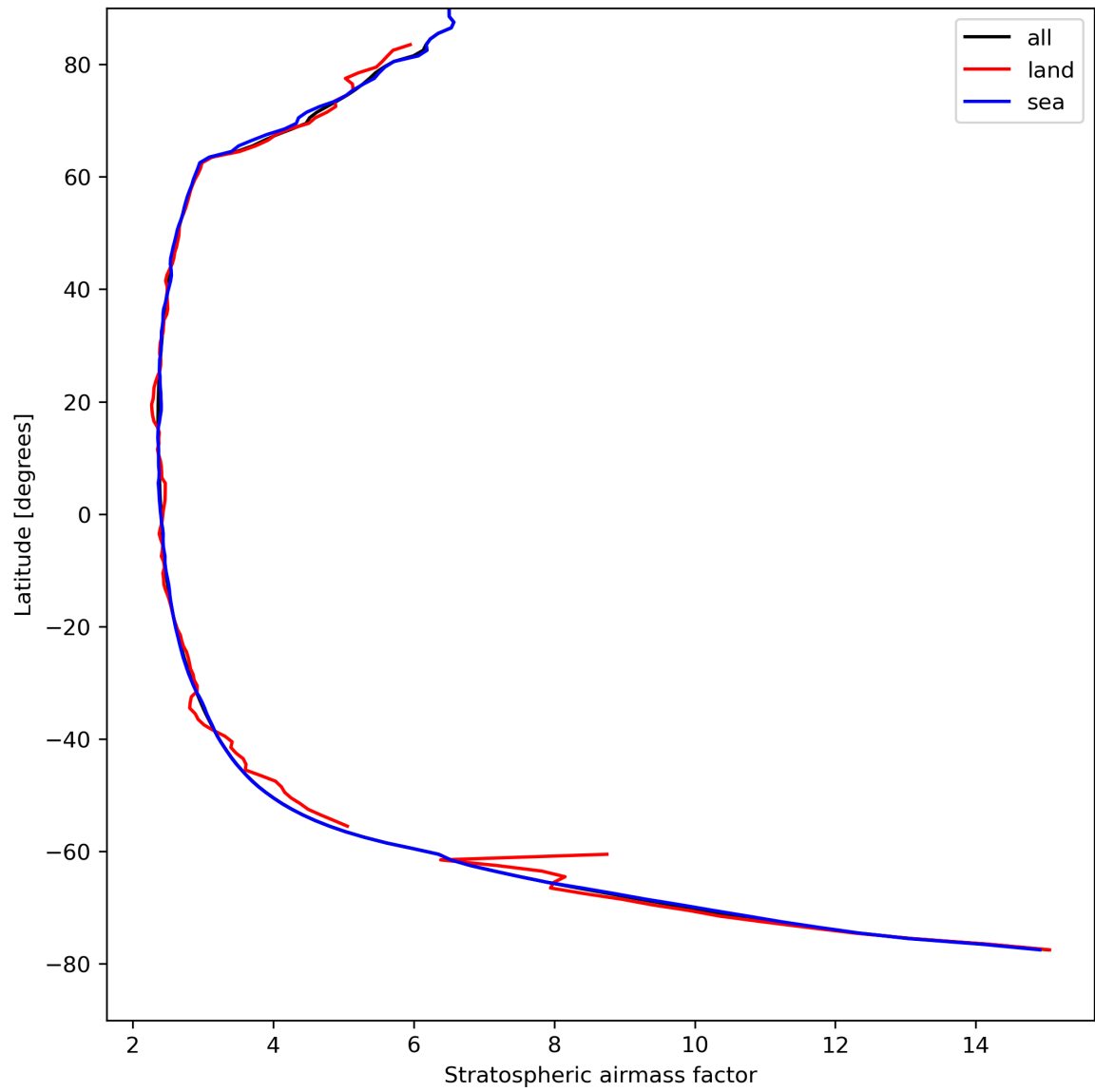
Figure 27: Zonal average of “Stratospheric air mass factor” for 2024-08-24 to 2024-08-26.
