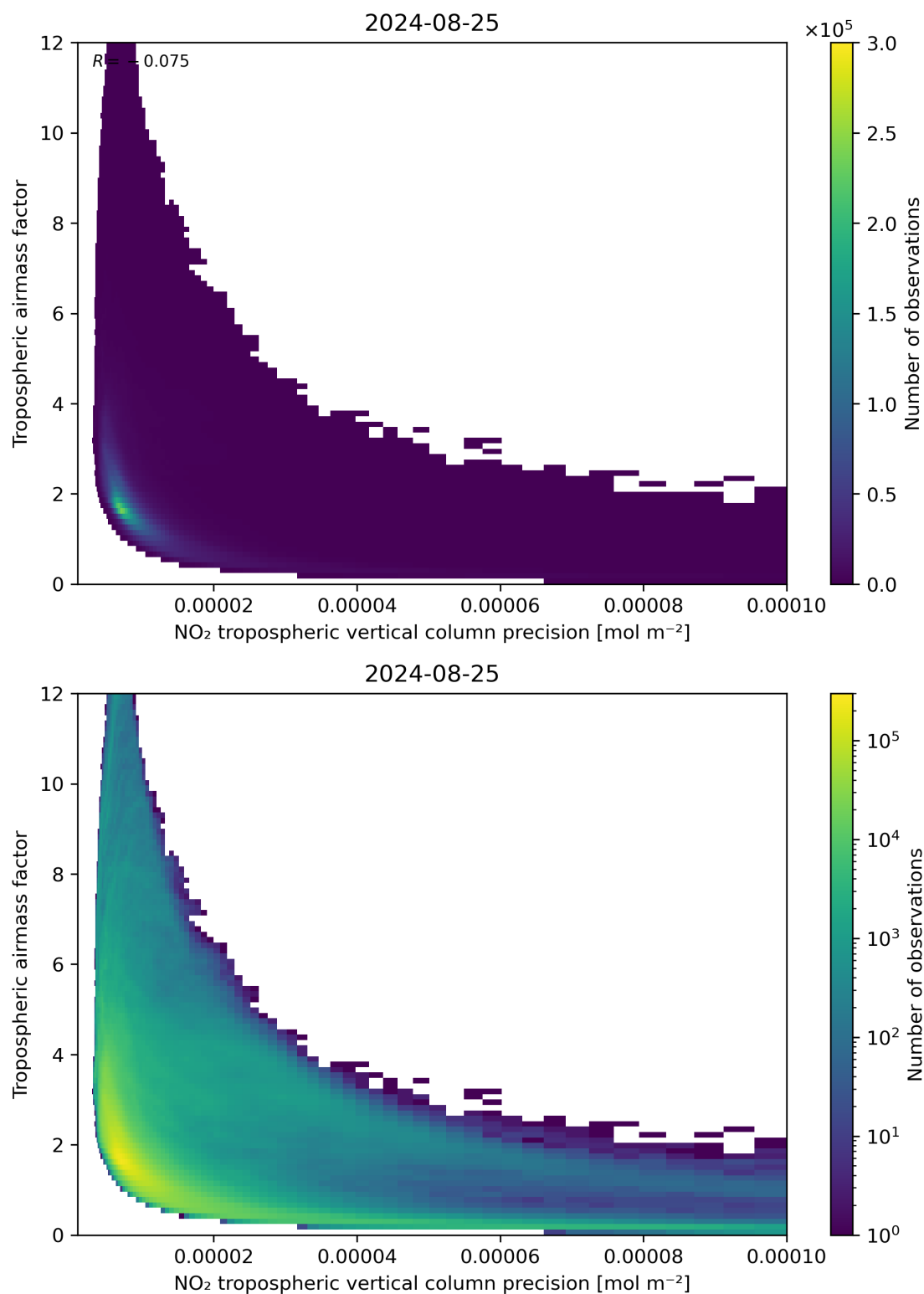
Figure 133: Scatter density plot of “NO 2 tropospheric vertical column precision” against “Tropospheric air mass factor” for 2024-08-24 to 2024-08-26.
