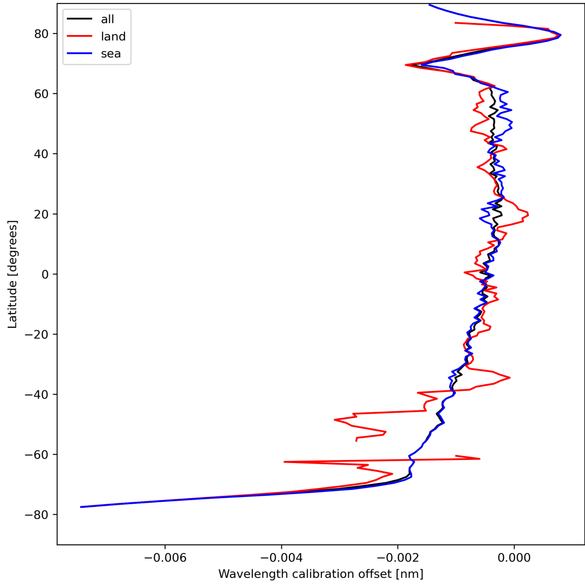
Figure 18: Zonal average of “Wavelength calibration offset” for 2024-08-24 to 2024-08-26.
