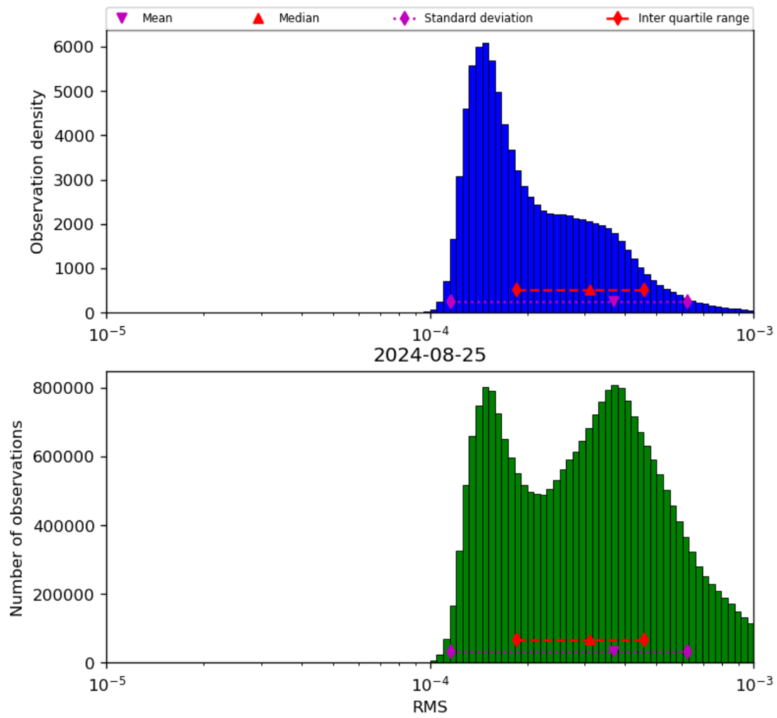
Figure 43: Histogram of “RMS” for 2024-08-24 to 2024-08-26
