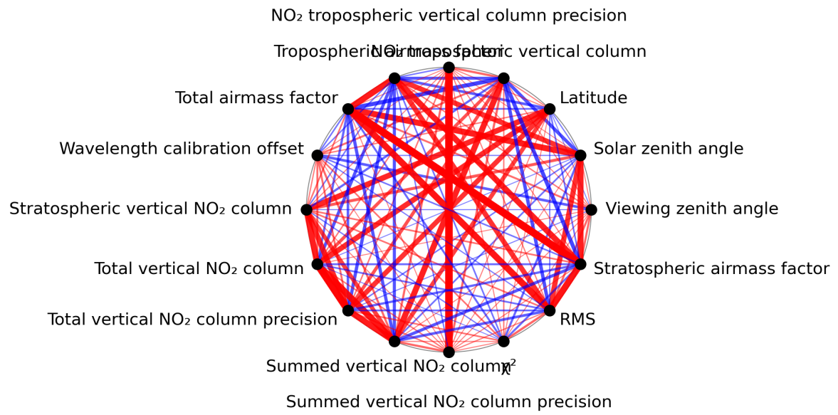
Figure 1: Map of correlation graph for 2024-08-24 to 2024-08-26.
