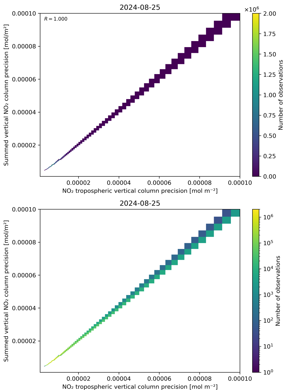
Figure 137: Scatter density plot of “NO 2 tropospheric vertical column precision” against “Summed vertical NO 2 column precision” for 2024-08-24 to 2024-08-26.
