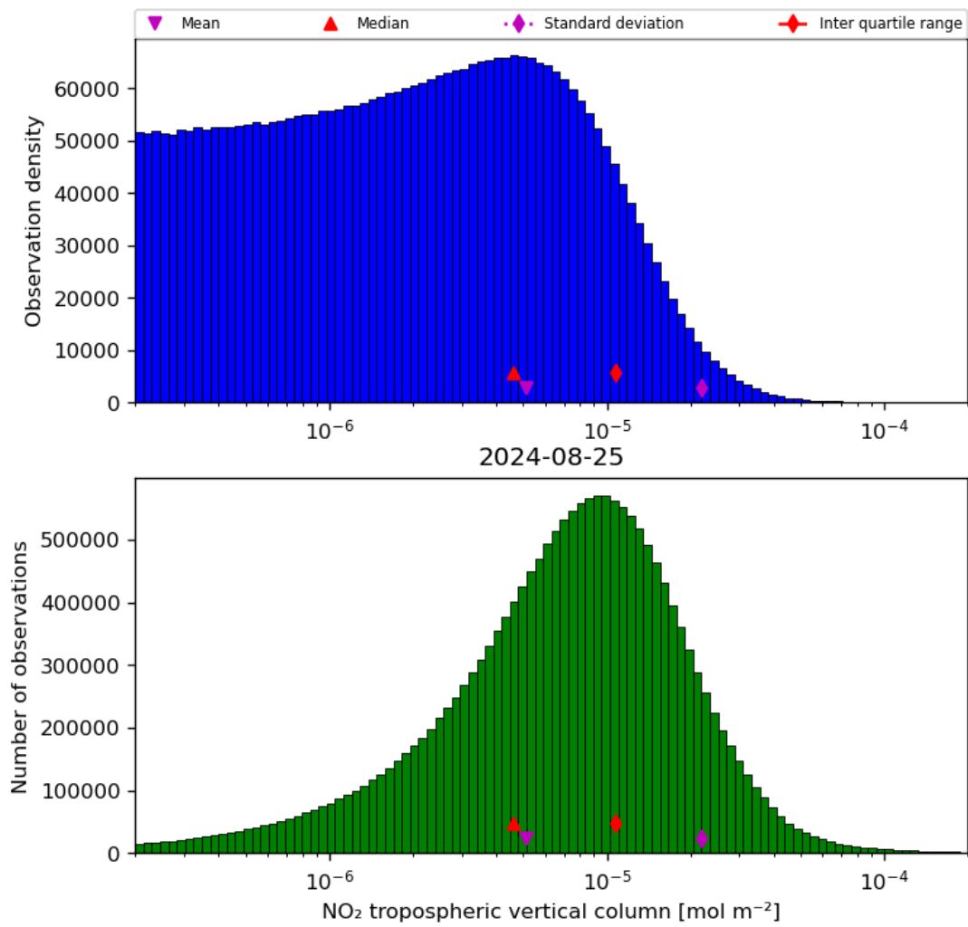
Figure 29: Histogram of “NO 2 tropospheric vertical column” for 2024-08-24 to 2024-08-26
