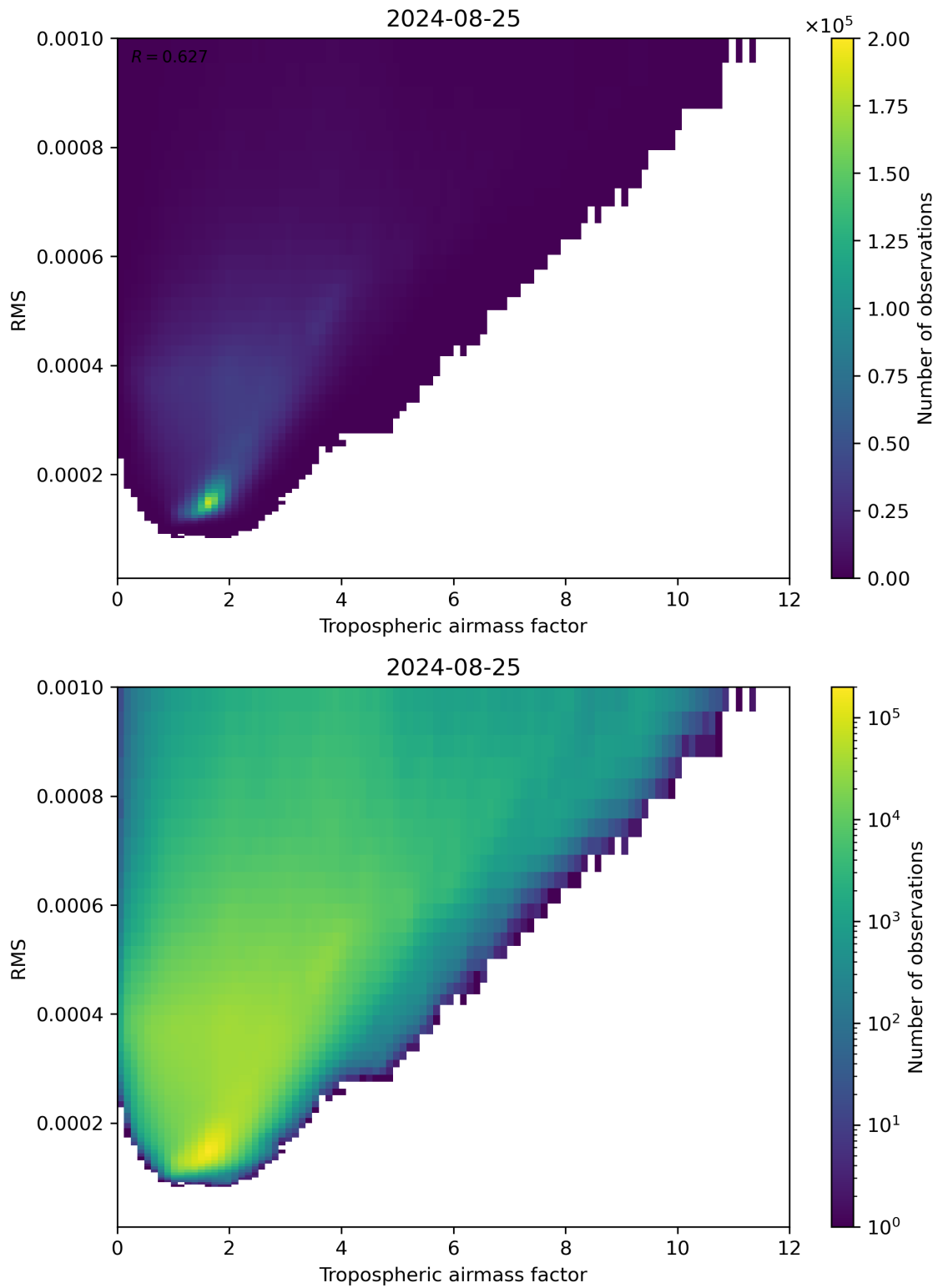
Figure 79: Scatter density plot of “Tropospheric airmass factor” against “RMS” for 2024-08-24 to 2024-08-26.
