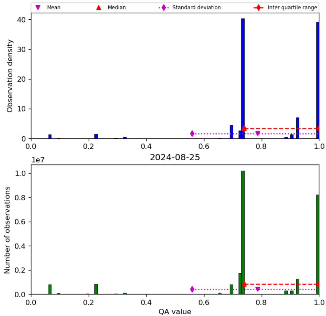
Figure 28: Histogram of “QA value” for 2024-08-24 to 2024-08-26
