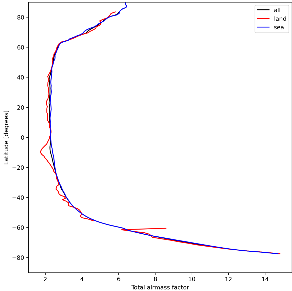
Figure 15: Zonal average of “Total airmass factor” for 2024-08-24 to 2024-08-26.
