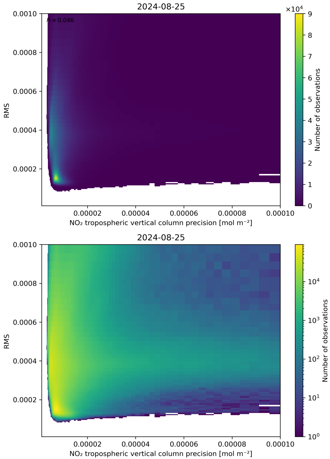
Figure 140: Scatter density plot of “NO 2 tropospheric vertical column precision” against “RMS” for 2024-08-24 to 2024-08-26.
