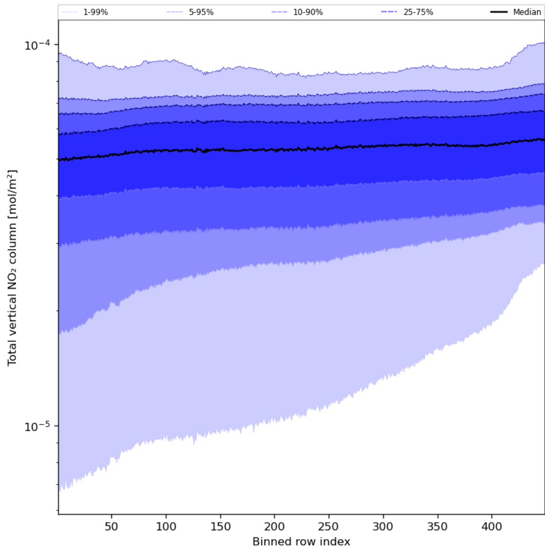
Figure 55: Along track statistics of “Total vertical NO 2 column” for 2024-08-24 to 2024-08-26
