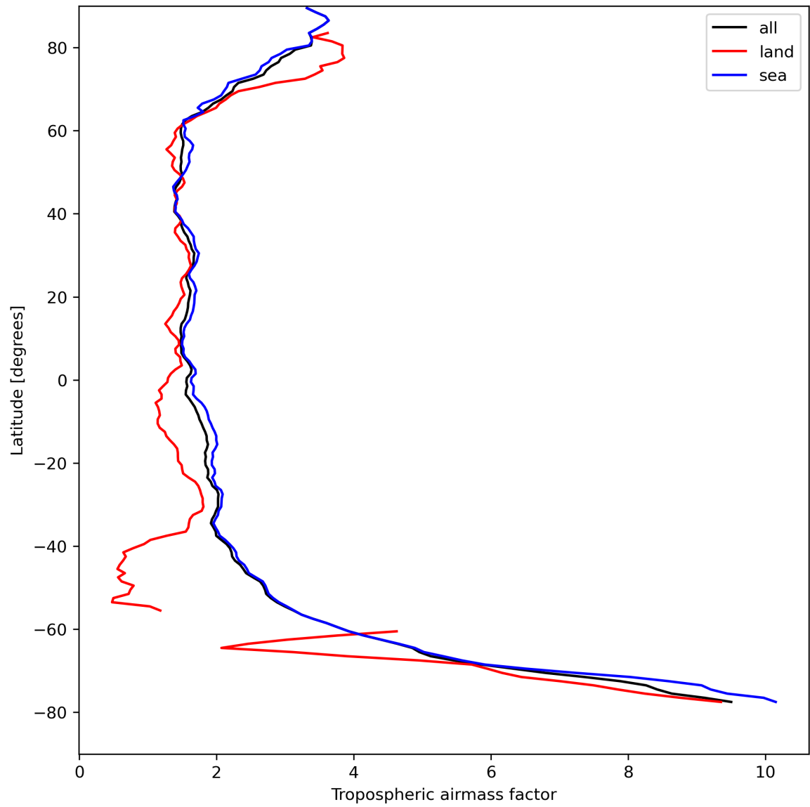
Figure 14: Zonal average of “Tropospheric airmass factor” for 2024-08-24 to 2024-08-26.
