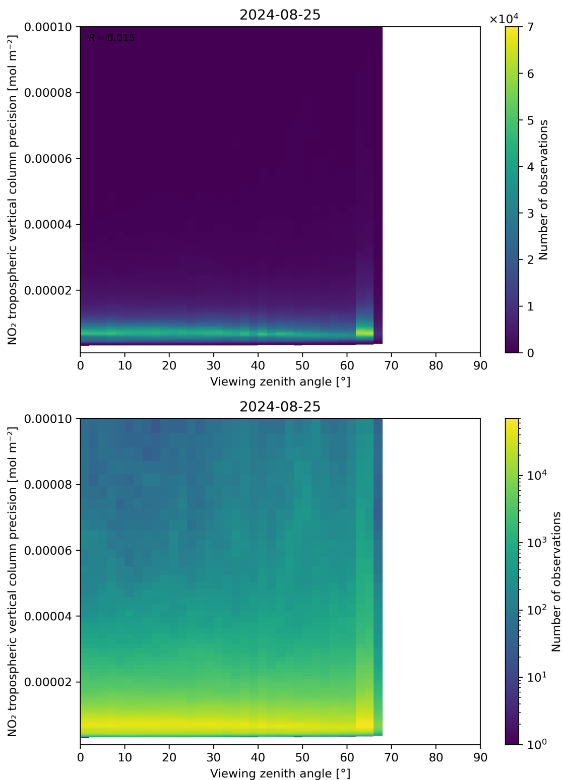
Figure 170: Scatter density plot of “Viewing zenith angle” against “NO 2 tropospheric vertical column precision” for 2024-08-24 to 2024-08-26.
