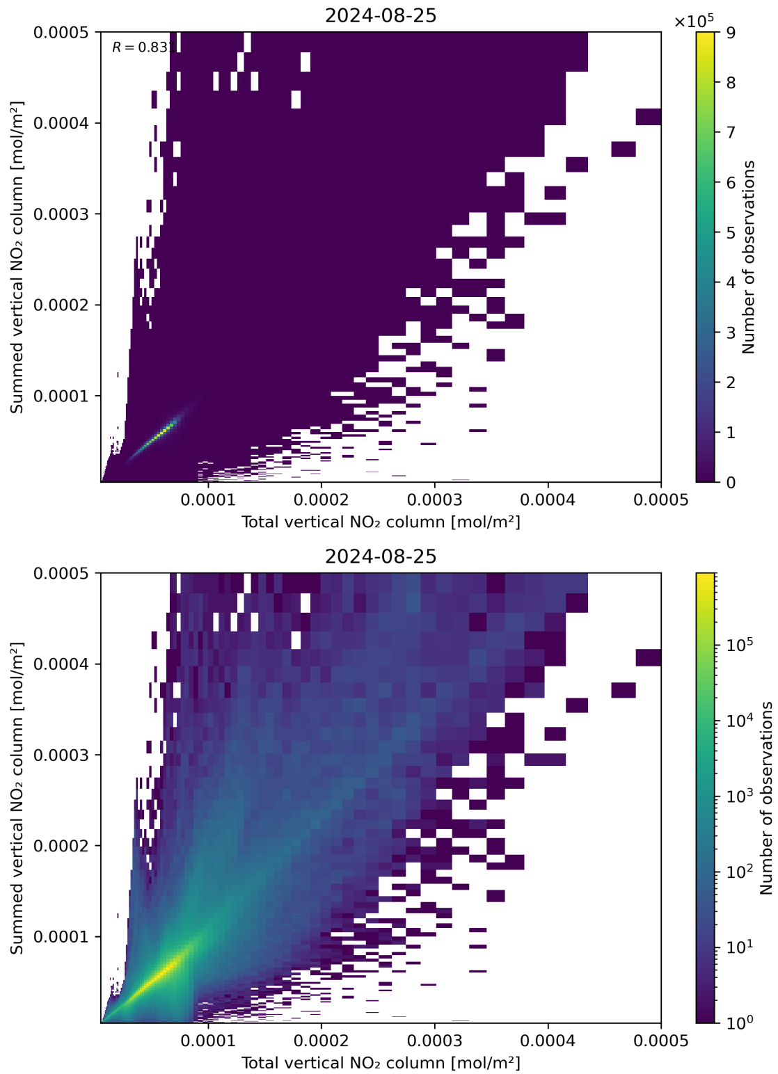
Figure 112: Scatter density plot of “Total vertical NO 2 column” against “Summed vertical NO 2 column” for 2024-08-24 to 2024-08-26.
