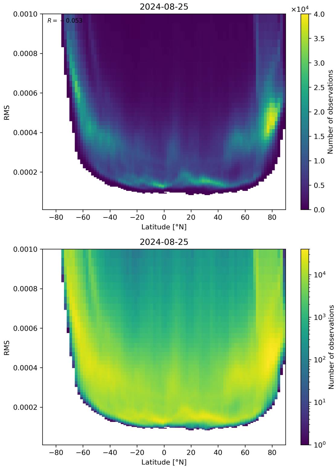
Figure 94: Scatter density plot of “Latitude” against “RMS” for 2024-08-24 to 2024-08-26.
