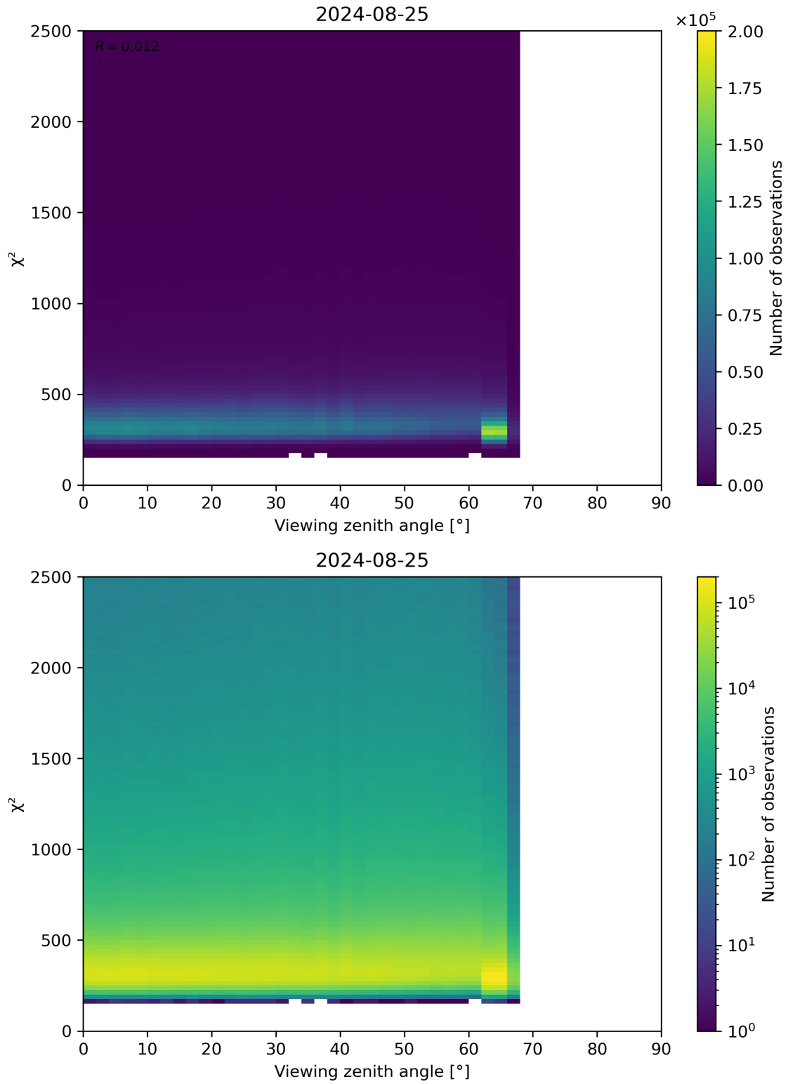
Figure 162: Scatter density plot of “Viewing zenith angle” against “ \chi^2 ” for 2024-08-24 to 2024-08-26.
