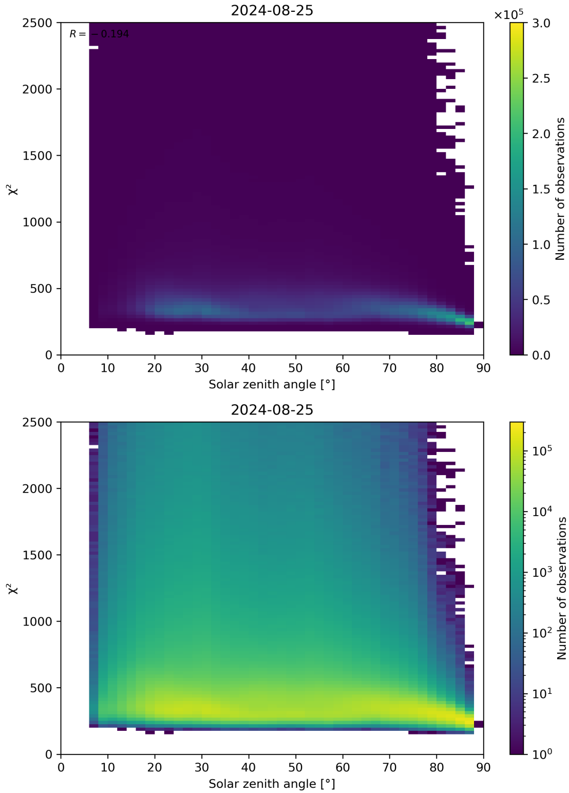
Figure 148: Scatter density plot of “Solar zenith angle” against “ \chi^2 ” for 2024-08-24 to 2024-08-26.
