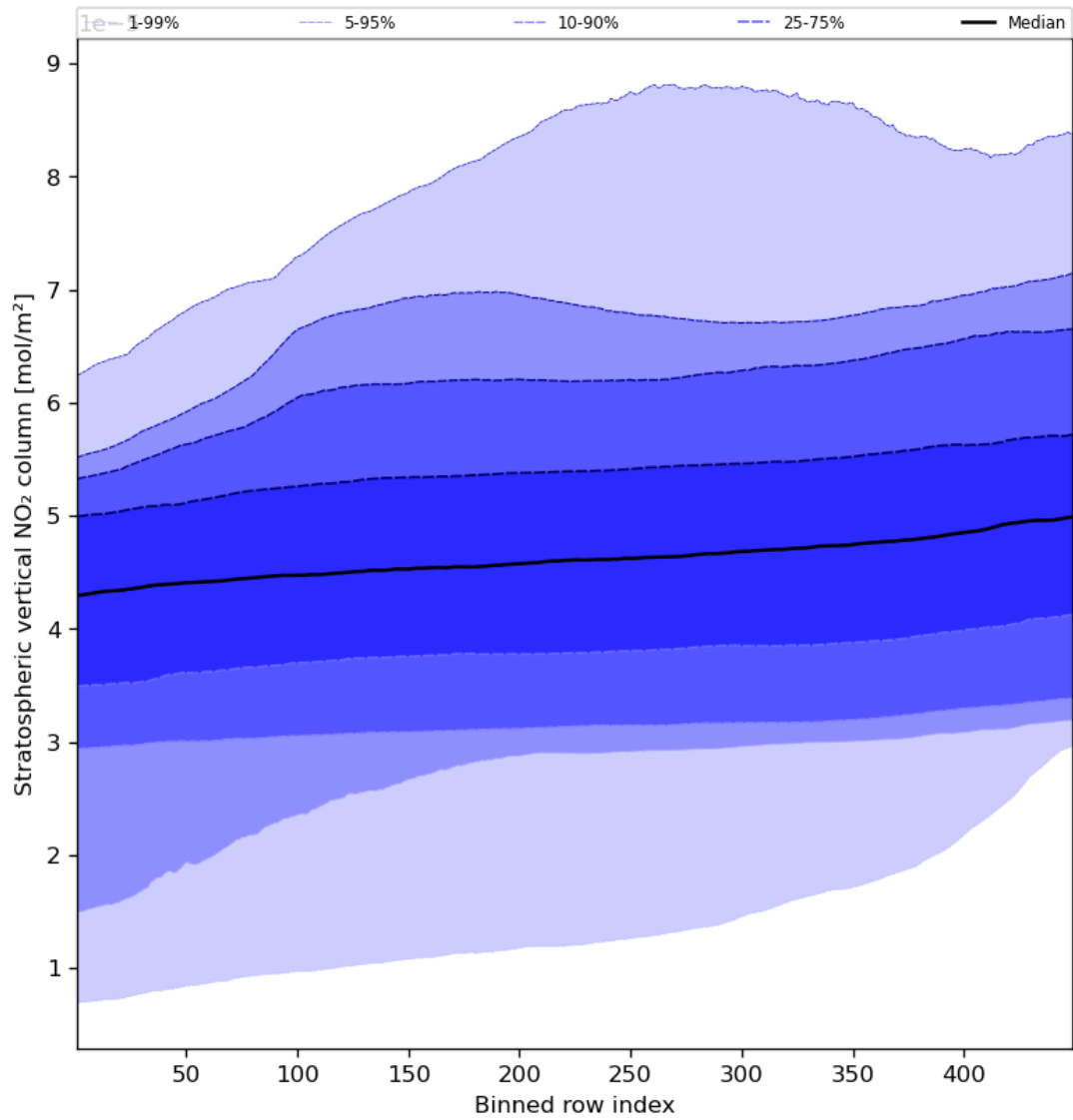
Figure 53: Along track statistics of “Stratospheric vertical NO 2 column” for 2024-08-24 to 2024-08-26
