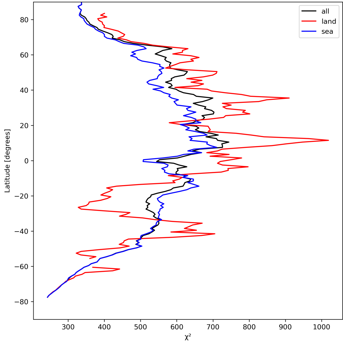
Figure 25: Zonal average of “ \chi^2 ” for 2024-08-24 to 2024-08-26.
