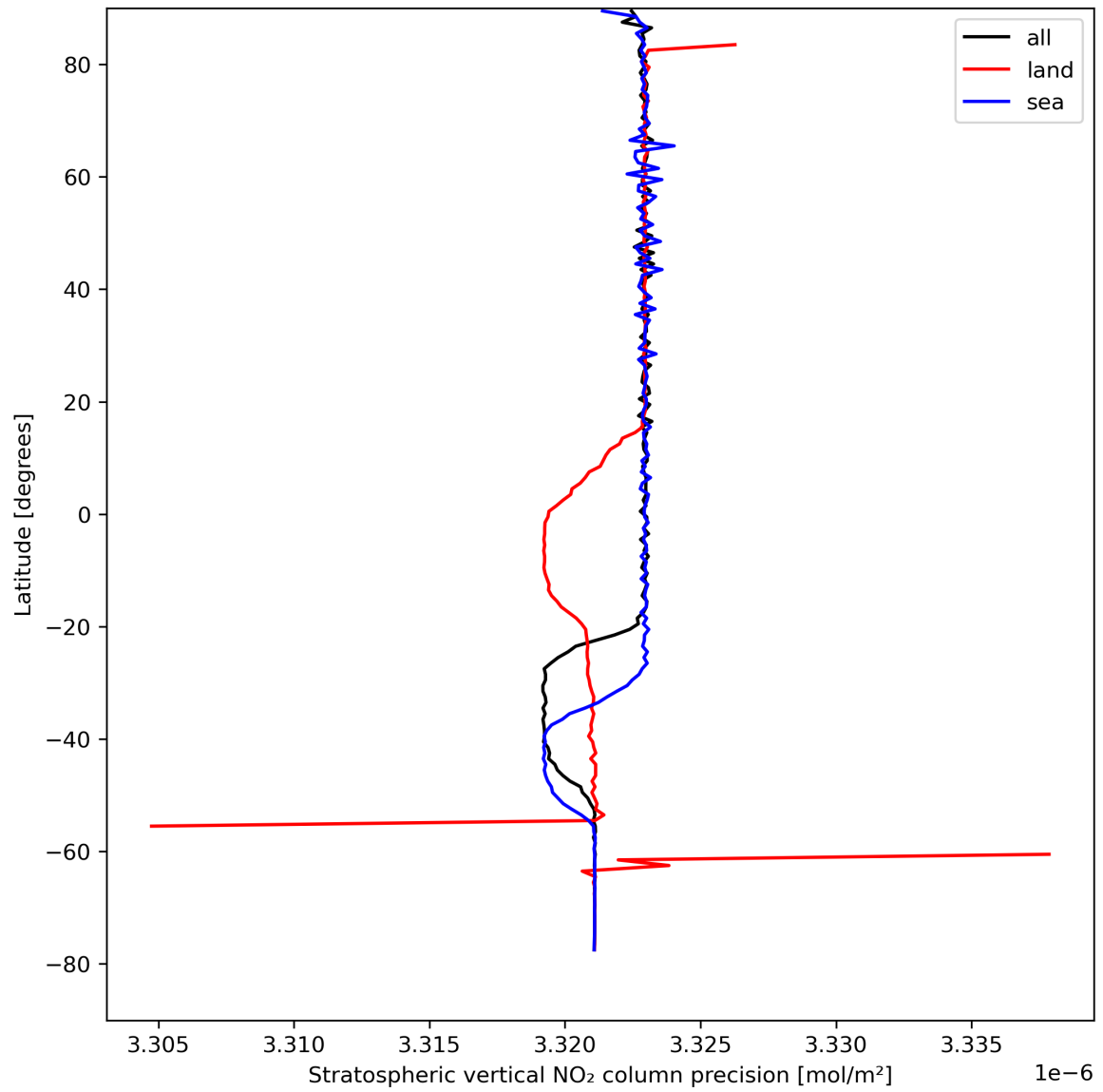
Figure 20: Zonal average of “Stratospheric vertical NO 2 column precision” for 2024-08-24 to 2024-08-26.
