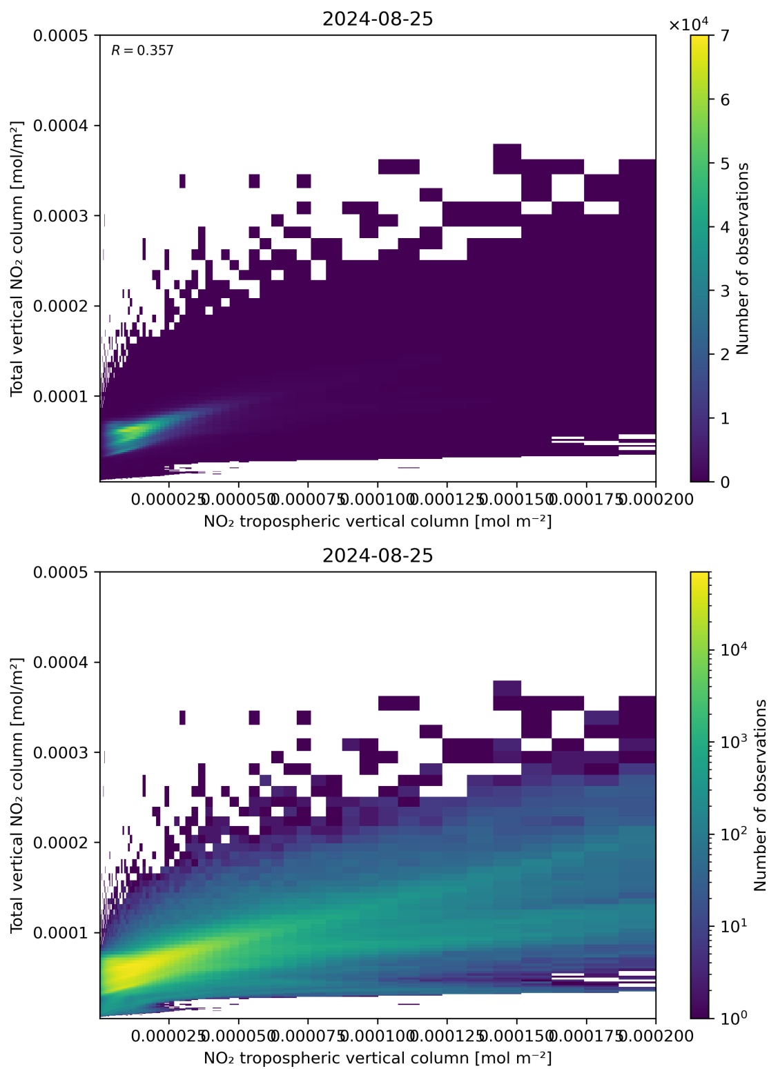
Figure 128: Scatter density plot of “NO 2 tropospheric vertical column” against “Total vertical NO 2 column” for 2024-08-24 to 2024-08-26.
