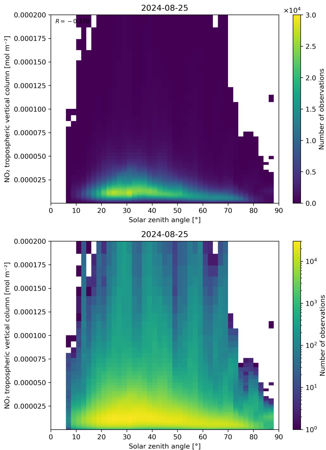
Figure 155: Scatter density plot of “Solar zenith angle” against “NO 2 tropospheric vertical column” for 2024-08-24 to 2024-08-26.
