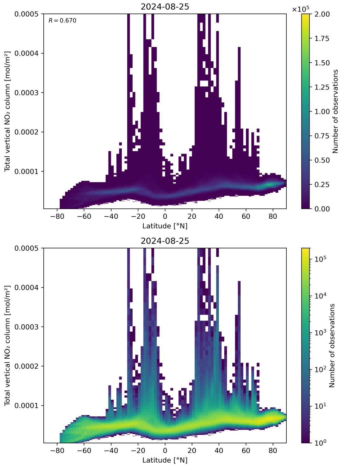
Figure 90: Scatter density plot of “Latitude” against “Total vertical NO 2 column” for 2024-08-24 to 2024-08-26.
