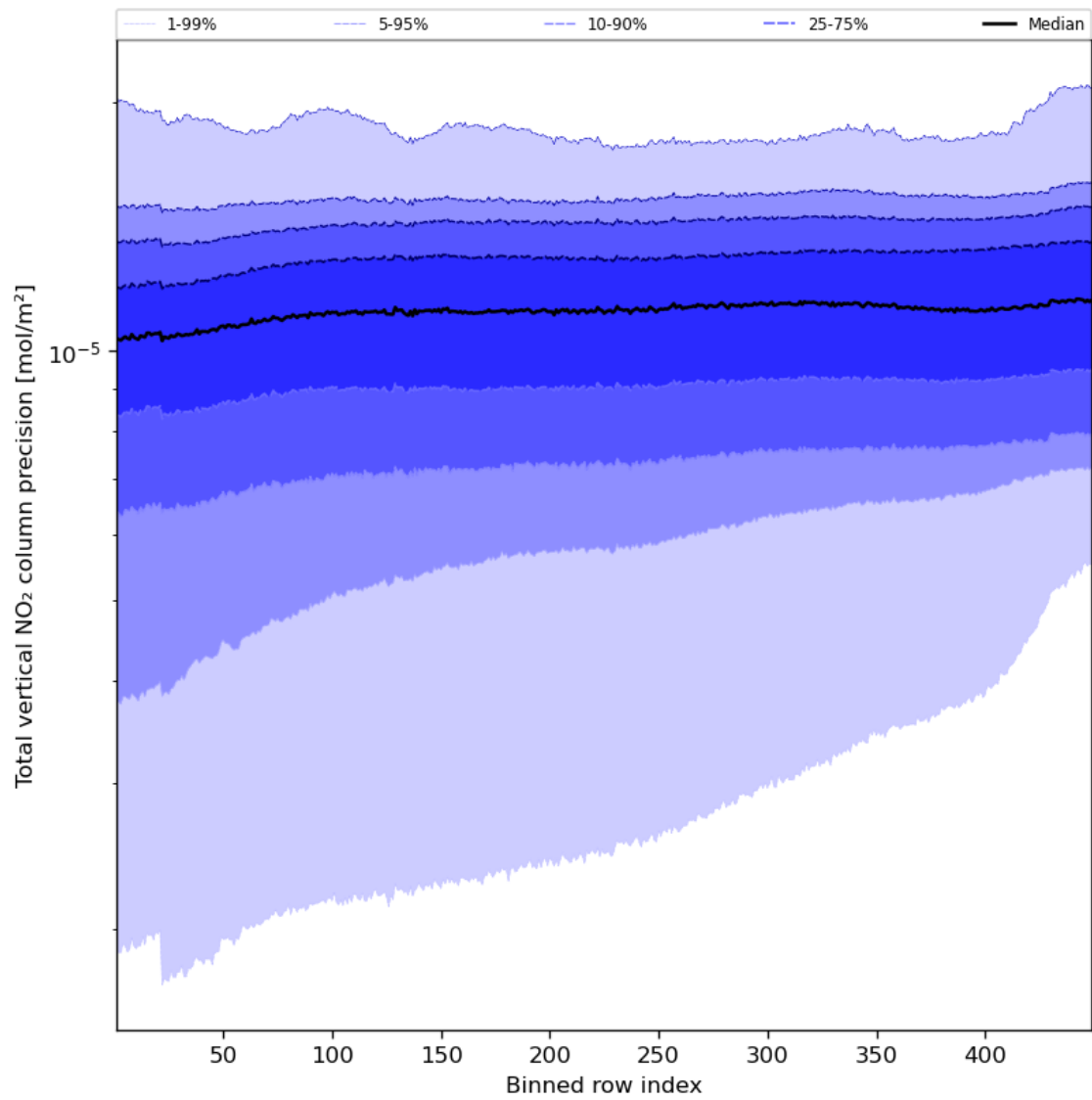
Figure 56: Along track statistics of “Total vertical NO 2 column precision” for 2024-08-24 to 2024-08-26
