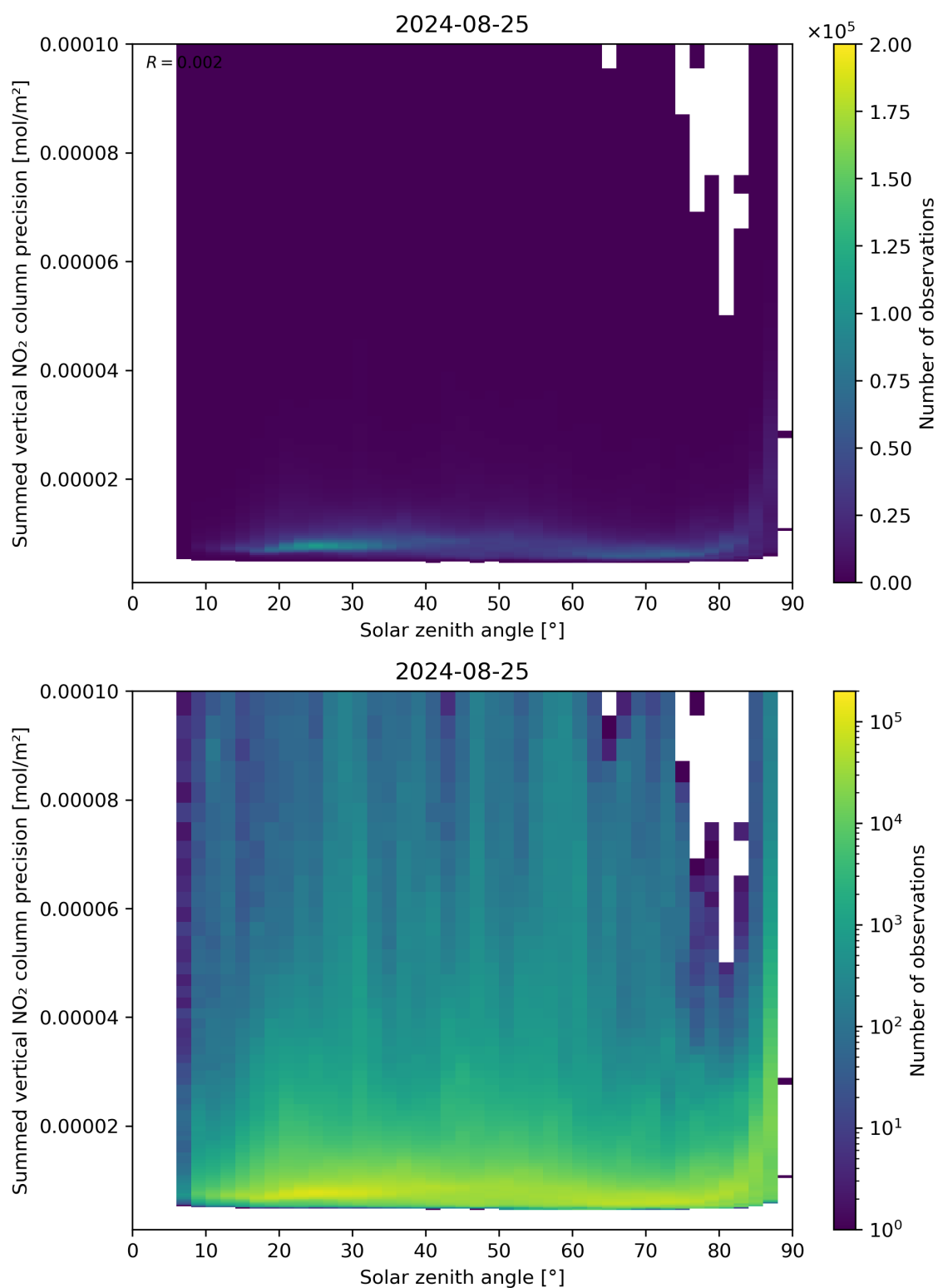
Figure 152: Scatter density plot of “Solar zenith angle” against “Summed vertical NO 2 column precision” for 2024-08-24 to 2024-08-26.
