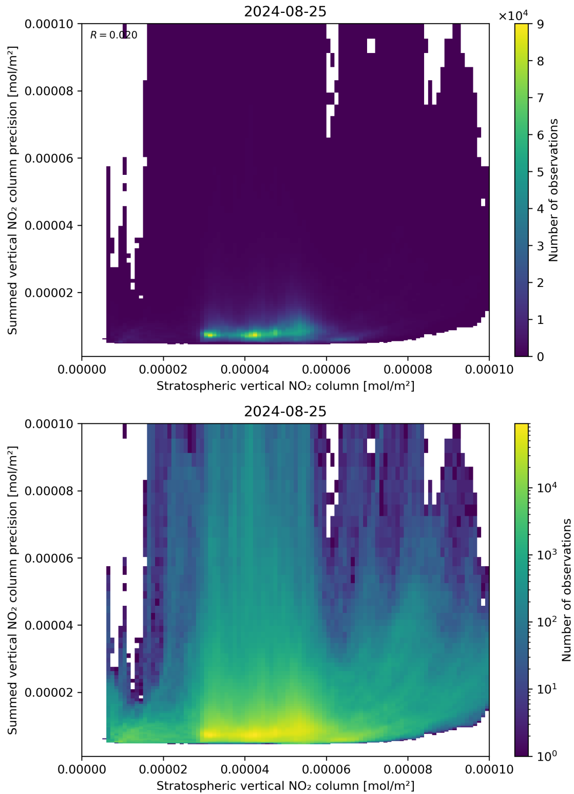
Figure 99: Scatter density plot of “Stratospheric vertical NO 2 column” against “Summed vertical NO 2 column precision” for 2024-08-24 to 2024-08-26.
