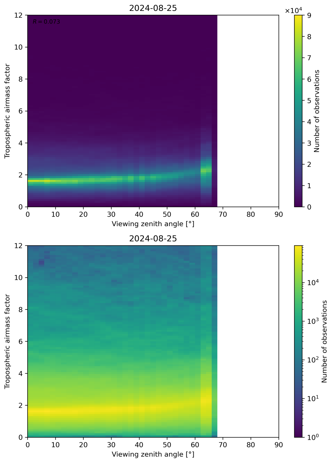
Figure 161: Scatter density plot of “Viewing zenith angle” against “Tropospheric airmass factor” for 2024-08-24 to 2024-08-26.
