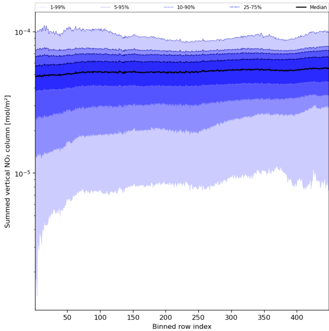
Figure 57: Along track statistics of “Summed vertical NO 2 column” for 2024-08-24 to 2024-08-26
