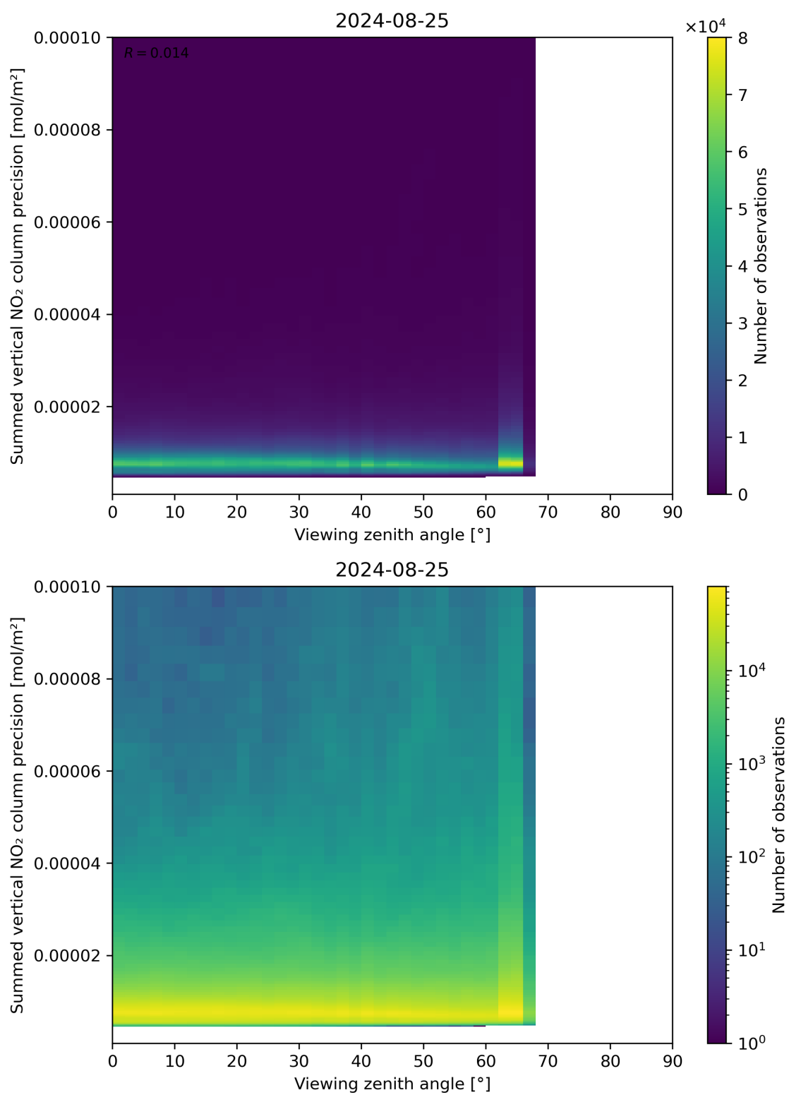
Figure 166: Scatter density plot of “Viewing zenith angle” against “Summed vertical NO 2 column precision” for 2024-08-24 to 2024-08-26.
