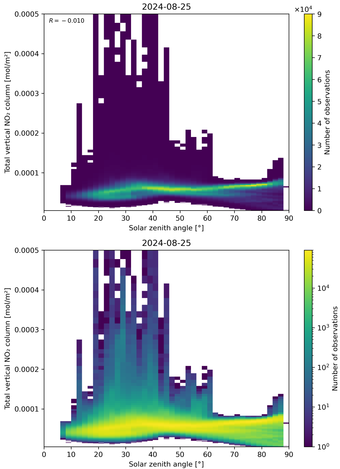
Figure 153: Scatter density plot of “Solar zenith angle” against “Total vertical NO 2 column” for 2024-08-24 to 2024-08-26.
