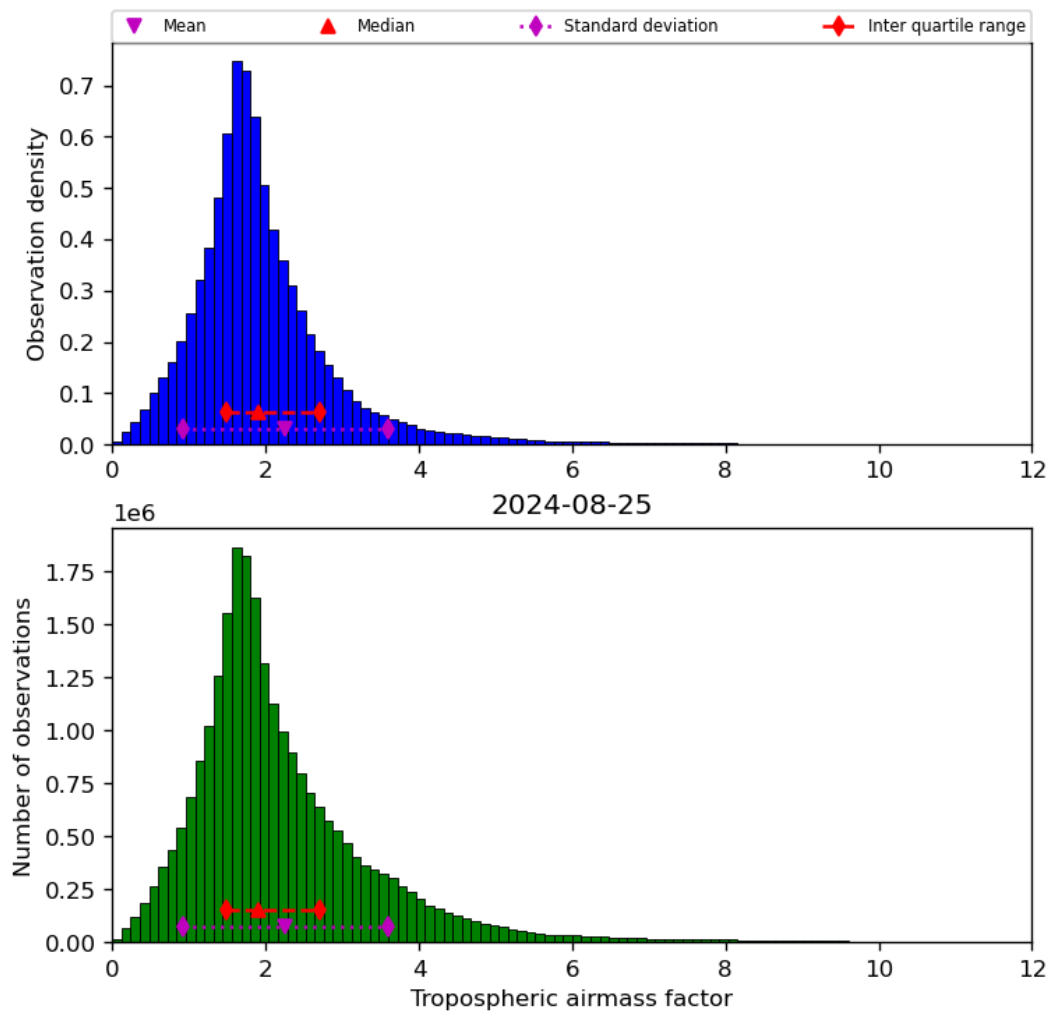
Figure 31: Histogram of “Tropospheric airmass factor” for 2024-08-24 to 2024-08-26
