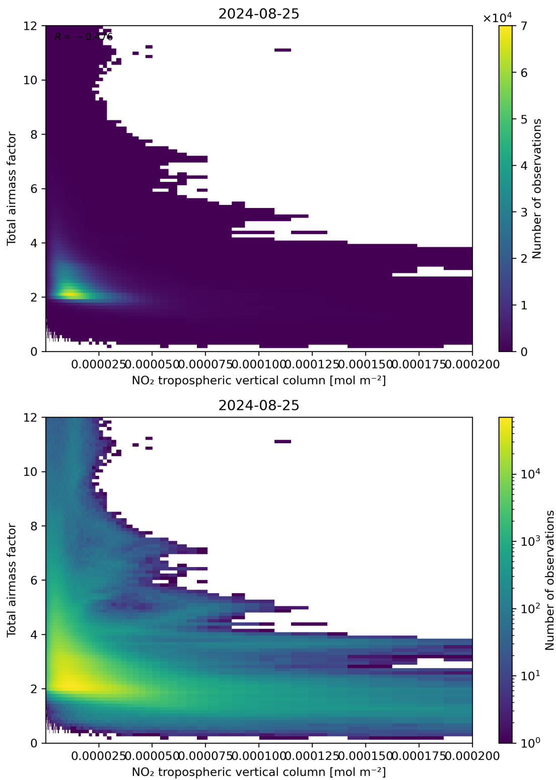
Figure 122: Scatter density plot of “NO 2 tropospheric vertical column” against “Total air mass factor” for 2024-08-24 to 2024-08-26.
