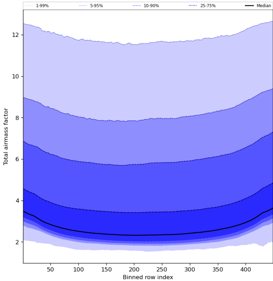
Figure 49: Along track statistics of “Total airmass factor” for 2024-08-24 to 2024-08-26
