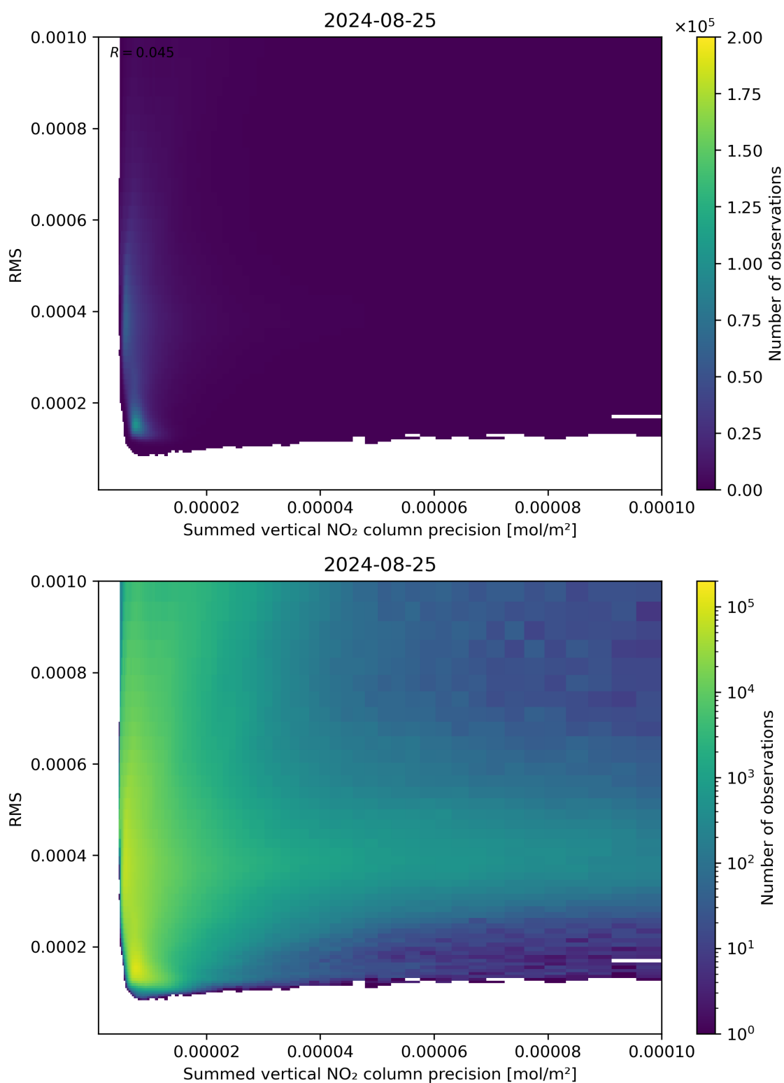
Figure 108: Scatter density plot of “Summed vertical NO 2 column precision” against “RMS” for 2024-08-24 to 2024-08-26.
