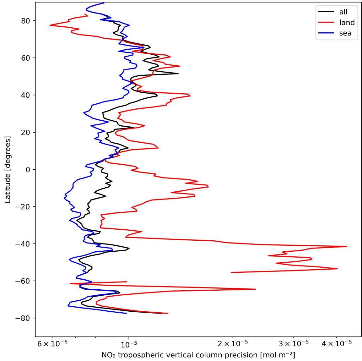
Figure 13: Zonal average of “NO 2 tropospheric vertical column precision” for 2024-08-24 to 2024-08-26.
