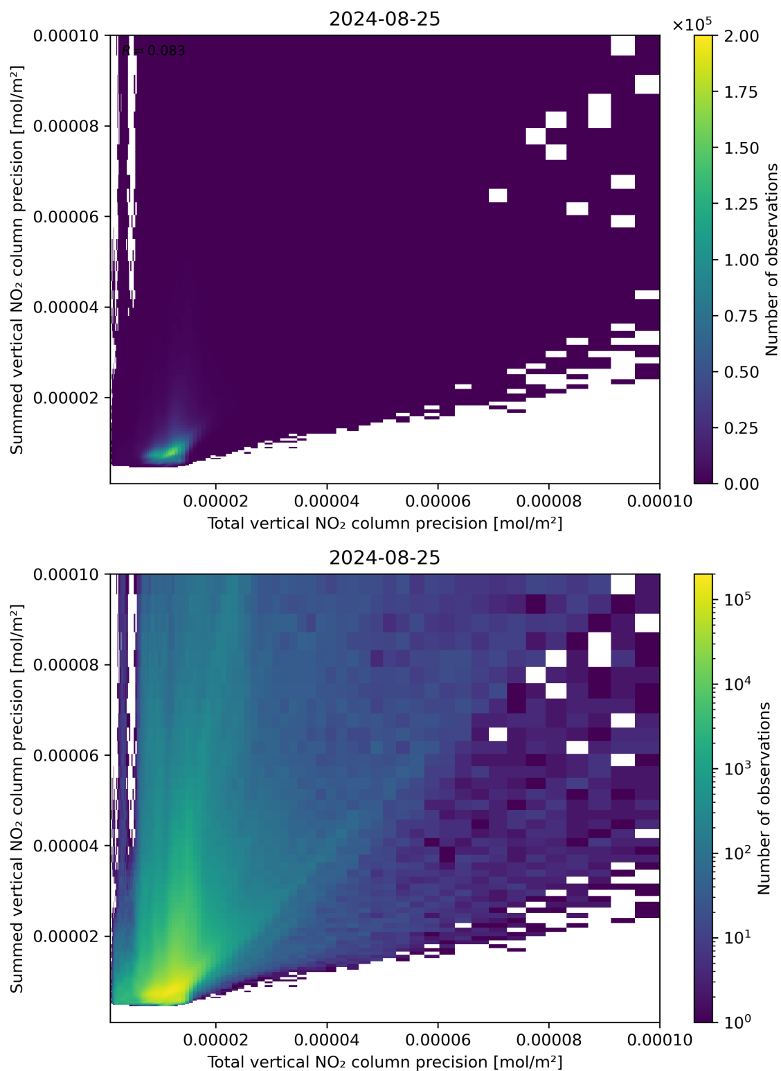
Figure 118: Scatter density plot of “Total vertical NO 2 column precision” against “Summed vertical NO 2 column precision” for 2024-08-24 to 2024-08-26.
