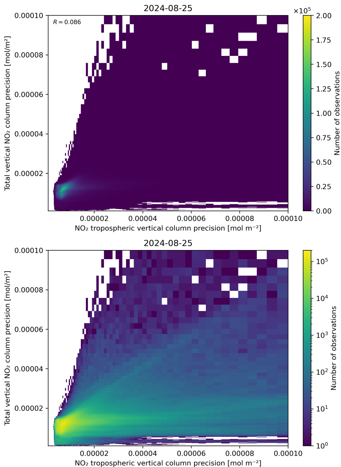
Figure 139: Scatter density plot of “NO 2 tropospheric vertical column precision” against “Total vertical NO 2 column precision” for 2024-08-24 to 2024-08-26.
