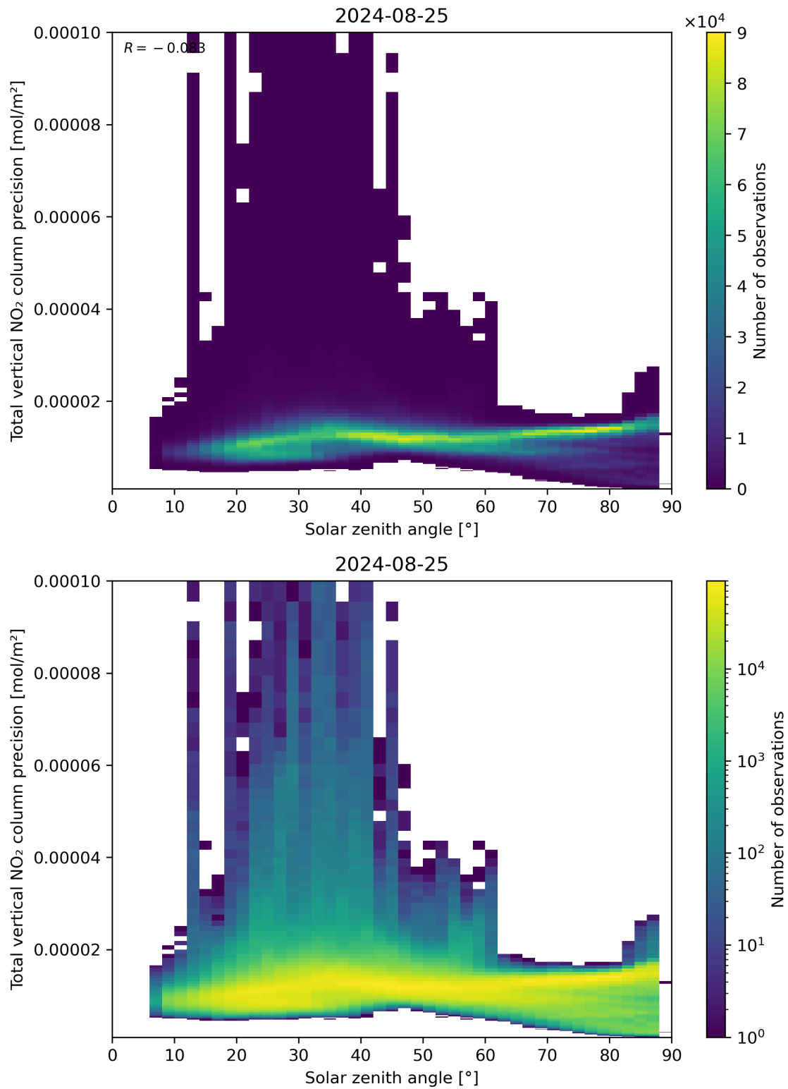
Figure 154: Scatter density plot of “Solar zenith angle” against “Total vertical NO 2 column precision” for 2024-08-24 to 2024-08-26.
