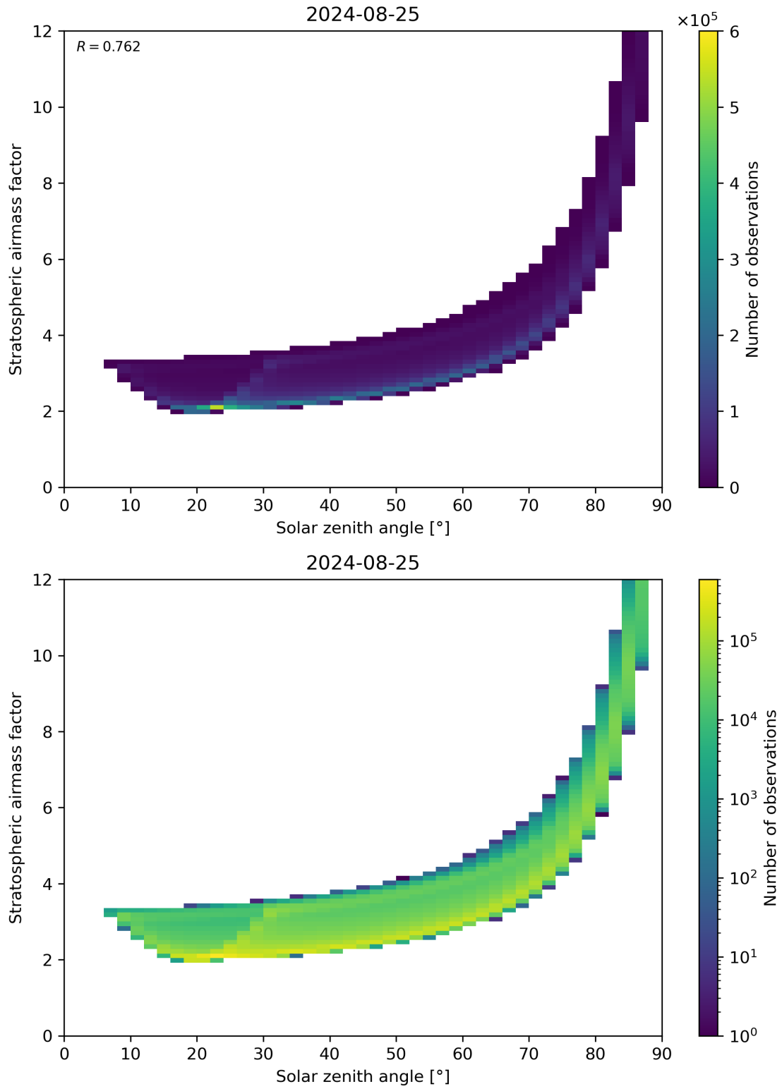
Figure 145: Scatter density plot of “Solar zenith angle” against “Stratospheric airmass factor” for 2024-08-24 to 2024-08-26.
