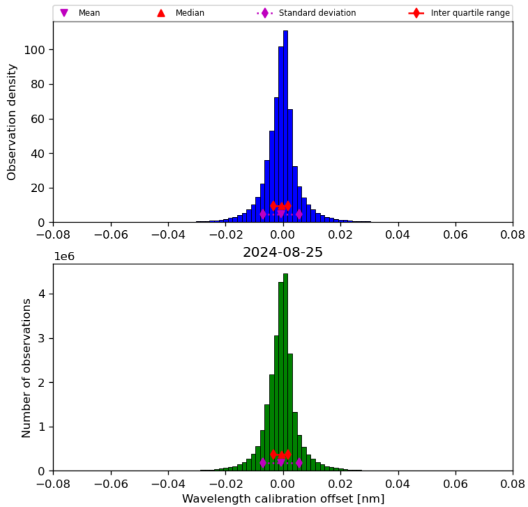
Figure 35: Histogram of “Wavelength calibration offset” for 2024-08-24 to 2024-08-26
