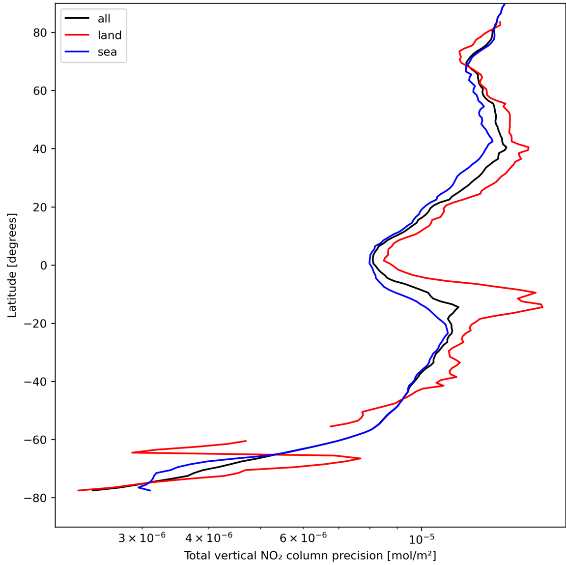
Figure 22: Zonal average of “Total vertical NO 2 column precision” for 2024-08-24 to 2024-08-26.
