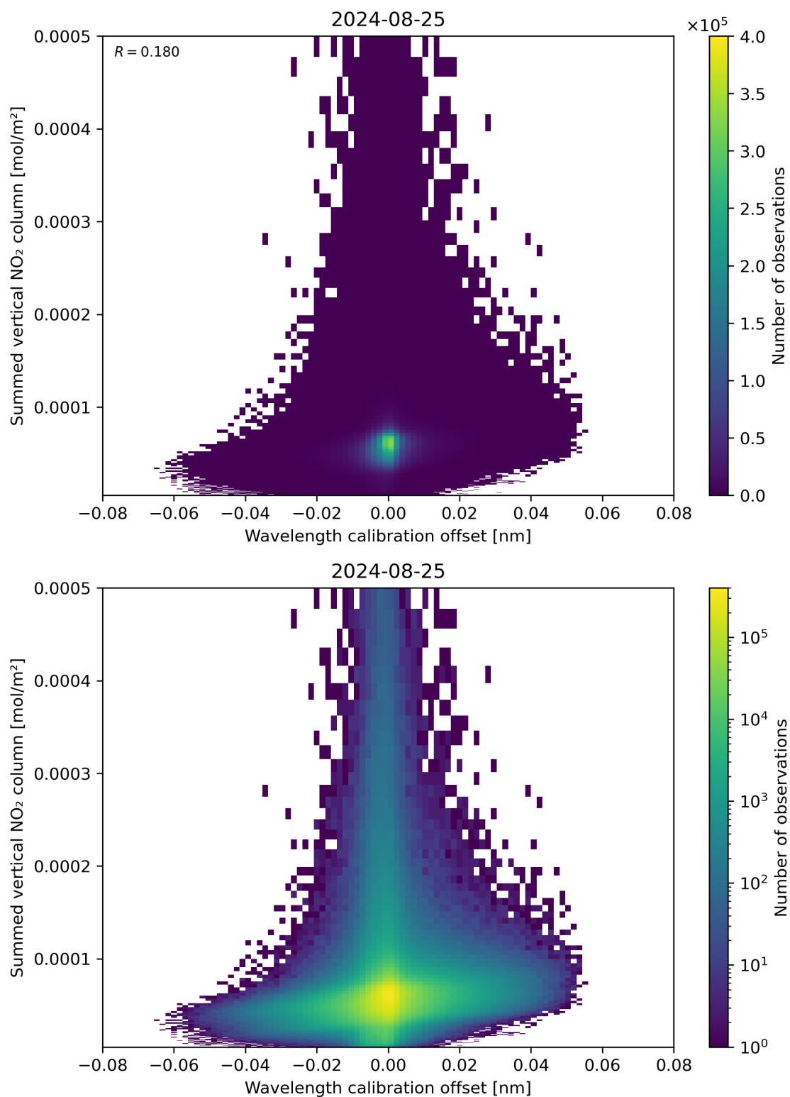
Figure 177: Scatter density plot of “Wavelength calibration offset” against “Summed vertical NO 2 column” for 2024-08-24 to 2024-08-26.
