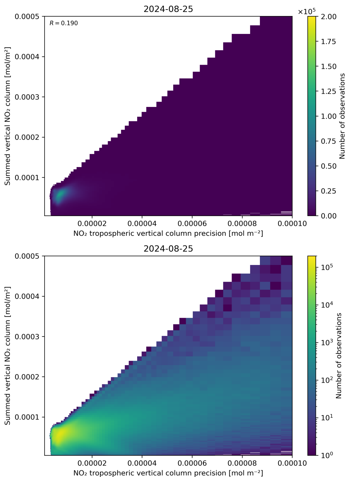
Figure 136: Scatter density plot of “NO 2 tropospheric vertical column precision” against “Summed vertical NO 2 column” for 2024-08-24 to 2024-08-26.
