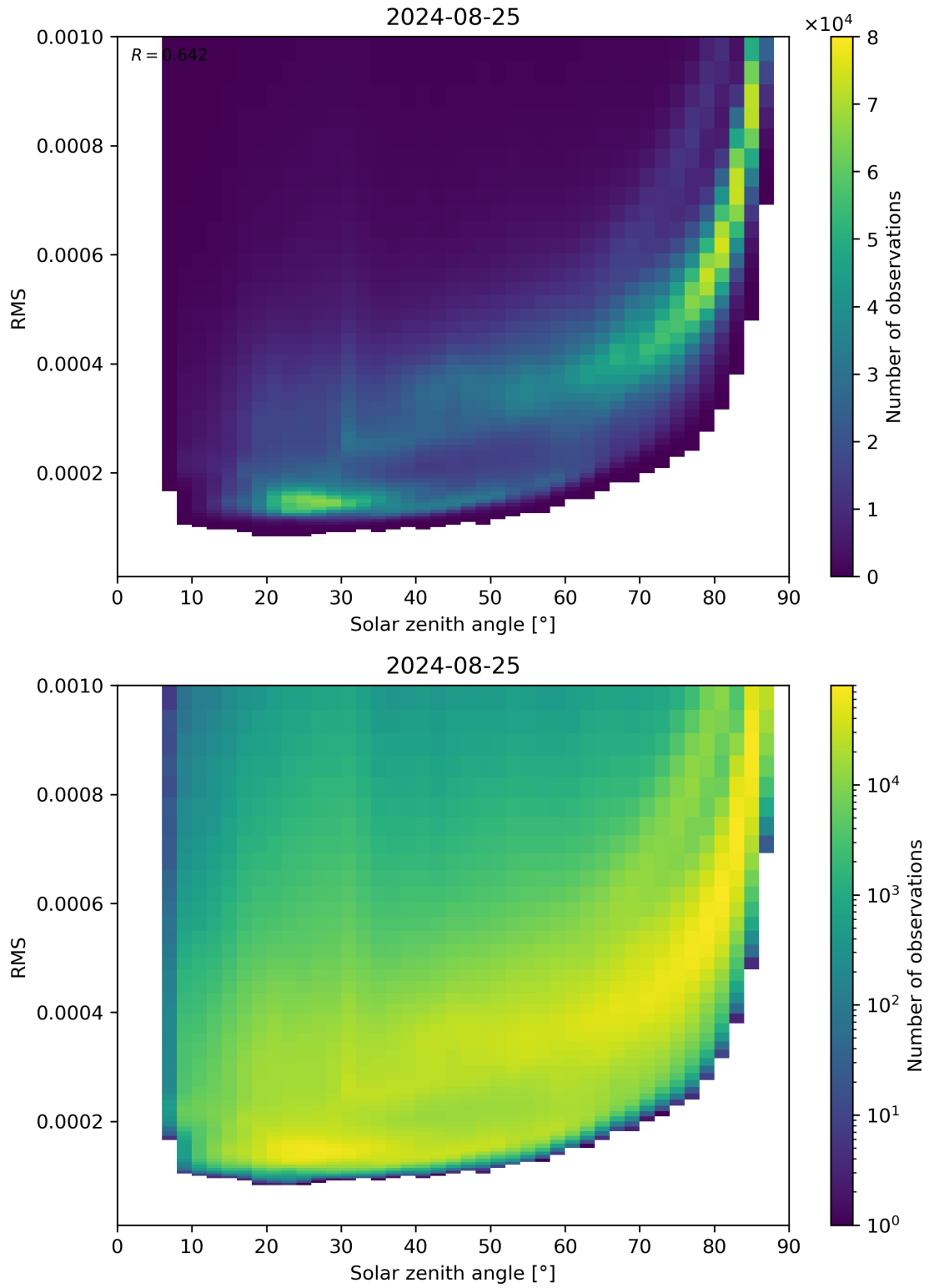
Figure 157: Scatter density plot of “Solar zenith angle” against “RMS” for 2024-08-24 to 2024-08-26.
