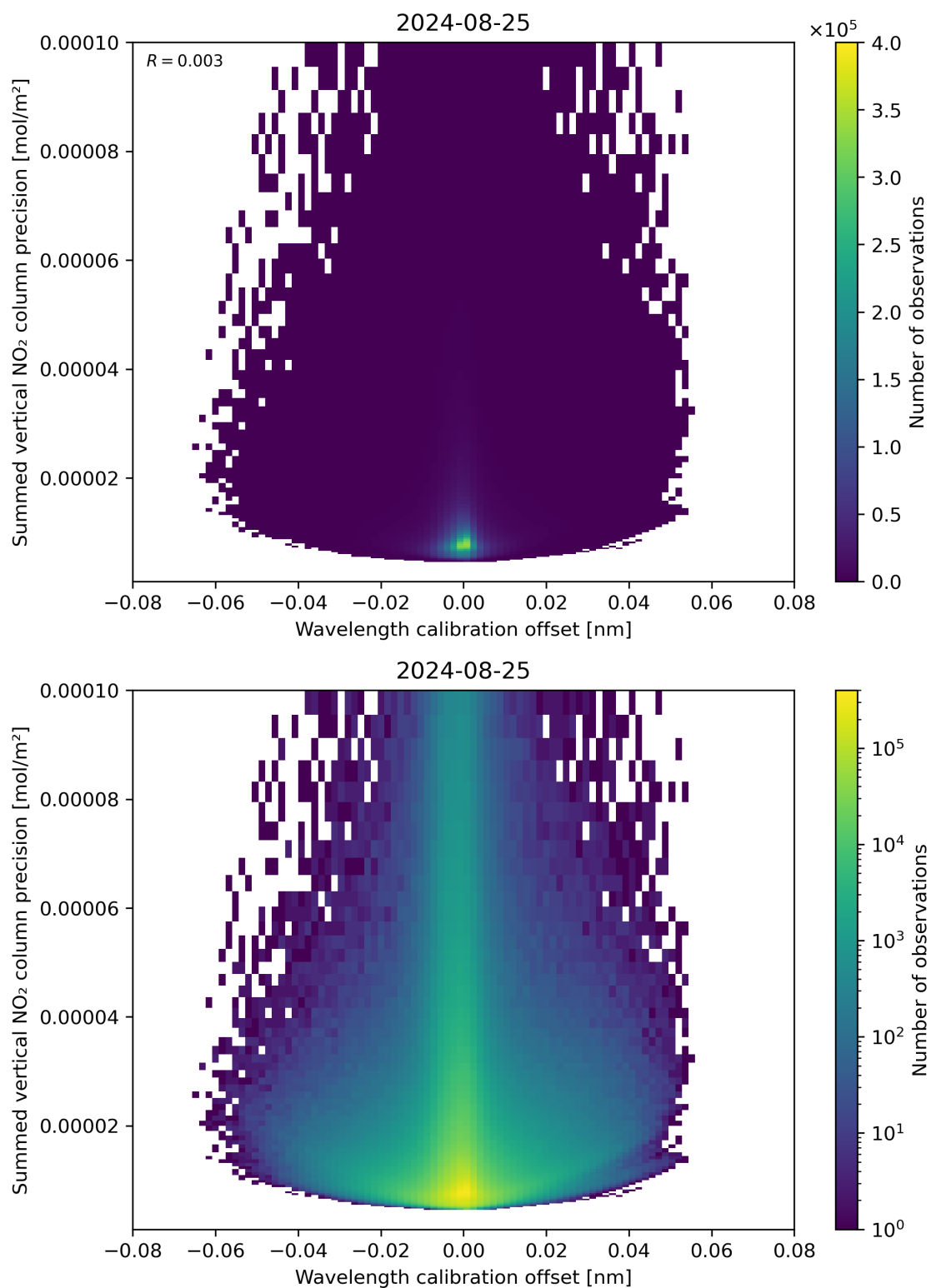
Figure 178: Scatter density plot of “Wavelength calibration offset” against “Summed vertical NO 2 column precision” for 2024-08-24 to 2024-08-26.
