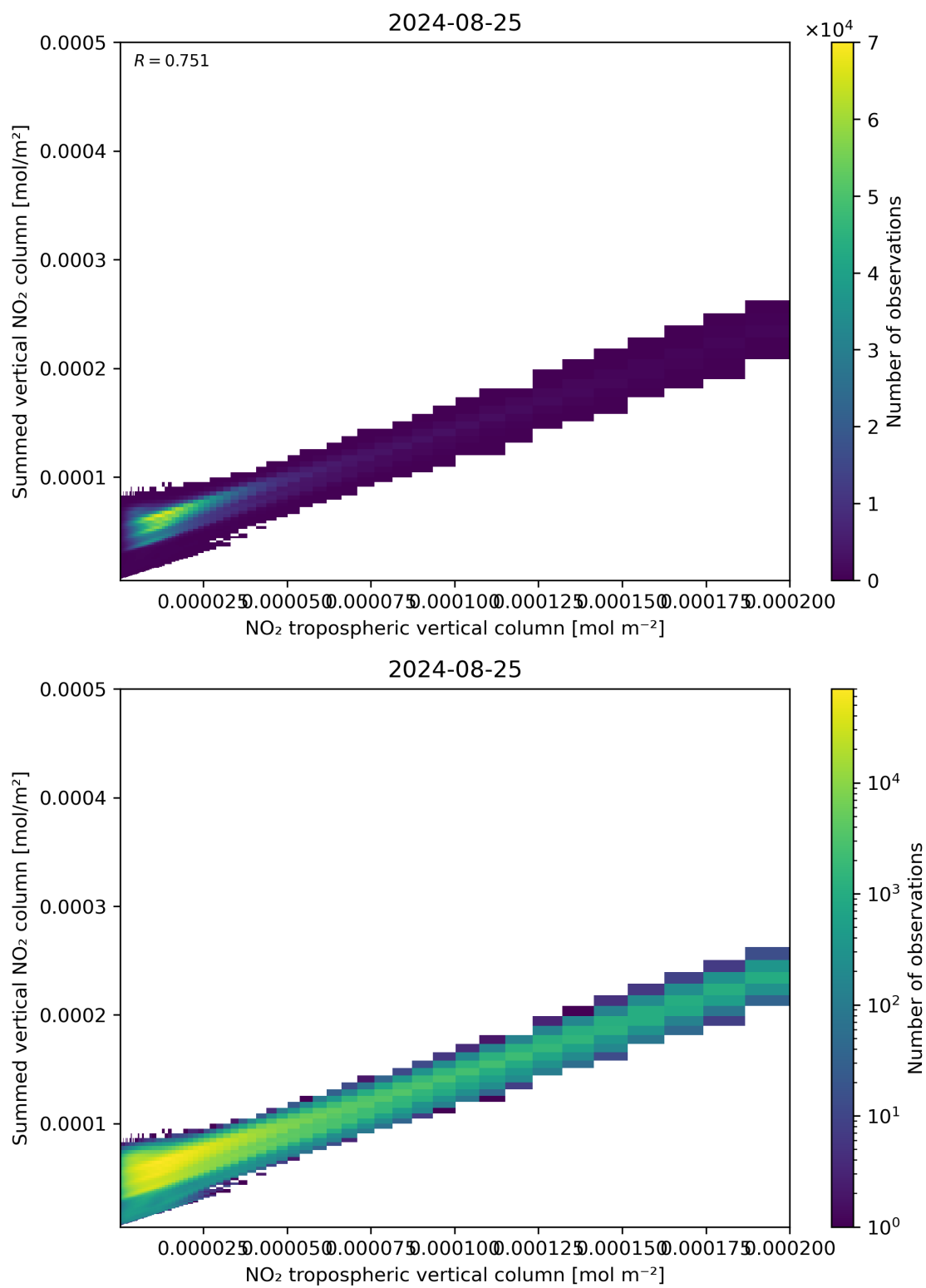
Figure 126: Scatter density plot of “NO 2 tropospheric vertical column” against “Summed vertical NO 2 column” for 2024-08-24 to 2024-08-26.
