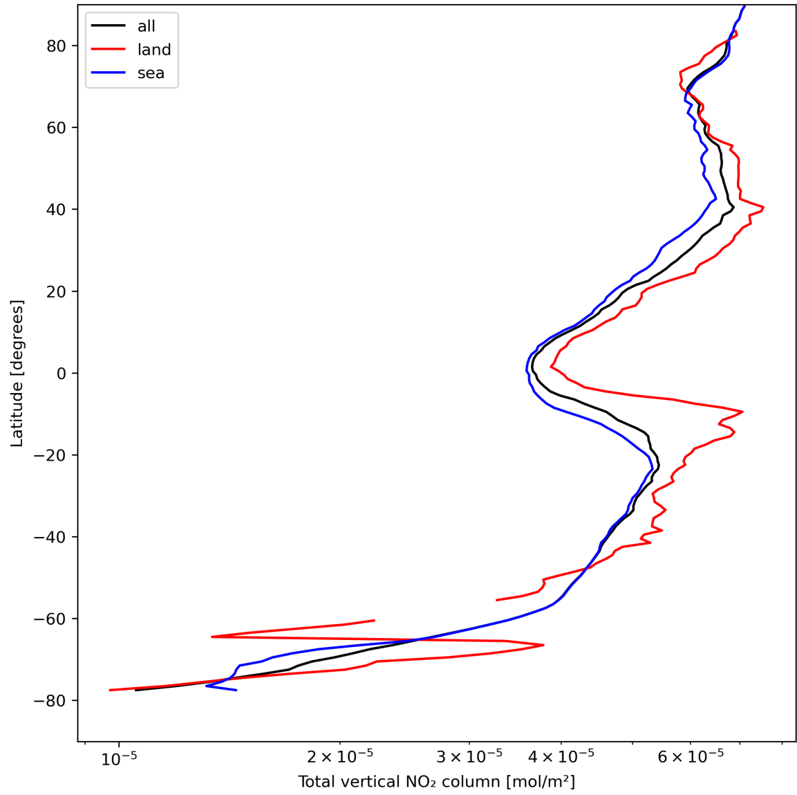
Figure 21: Zonal average of “Total vertical NO 2 column” for 2024-08-24 to 2024-08-26.
