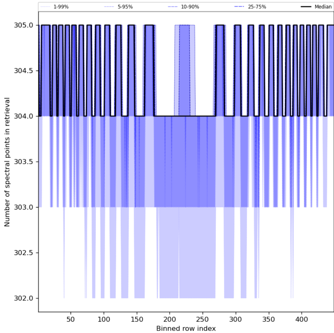
Figure 50: Along track statistics of “Number of spectral points in retrieval” for 2024-08-24 to 2024-08-26
