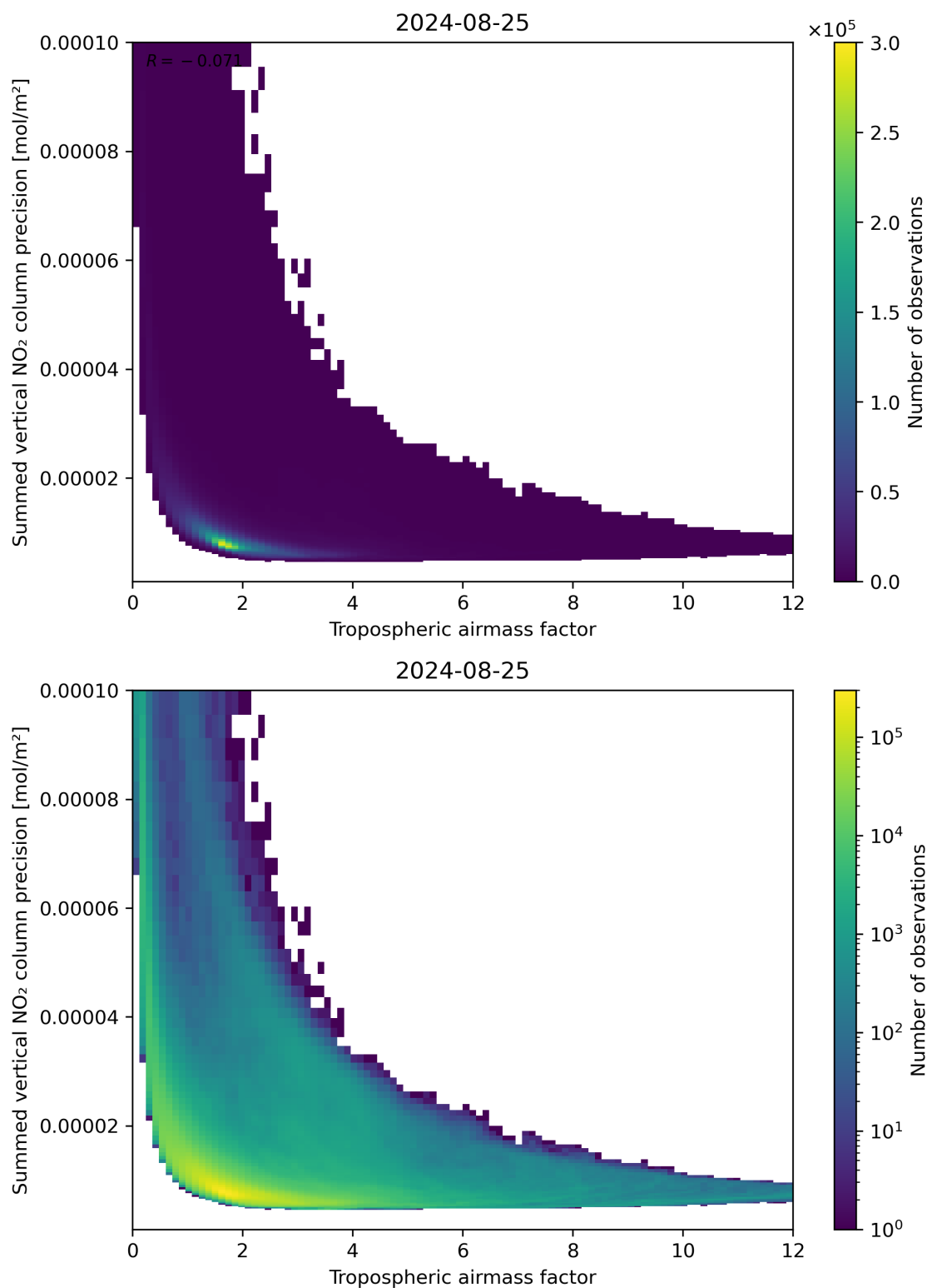
Figure 76: Scatter density plot of “Tropospheric air mass factor” against “Summed vertical NO 2 column precision” for 2024-08-24 to 2024-08-26.
