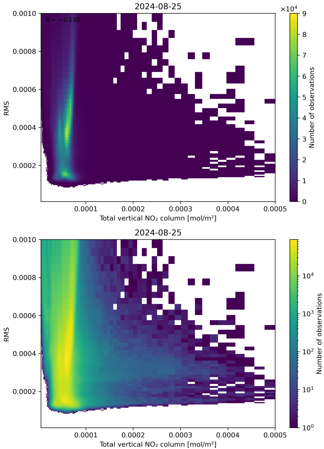
Figure 120: Scatter density plot of “Total vertical NO 2 column” against “RMS” for 2024-08-24 to 2024-08-26.
