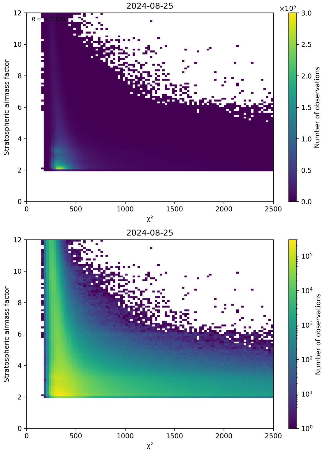
Figure 81: Scatter density plot of “ \chi^2 ” against “Stratospheric airmass factor” for 2024-08-24 to 2024-08-26.
