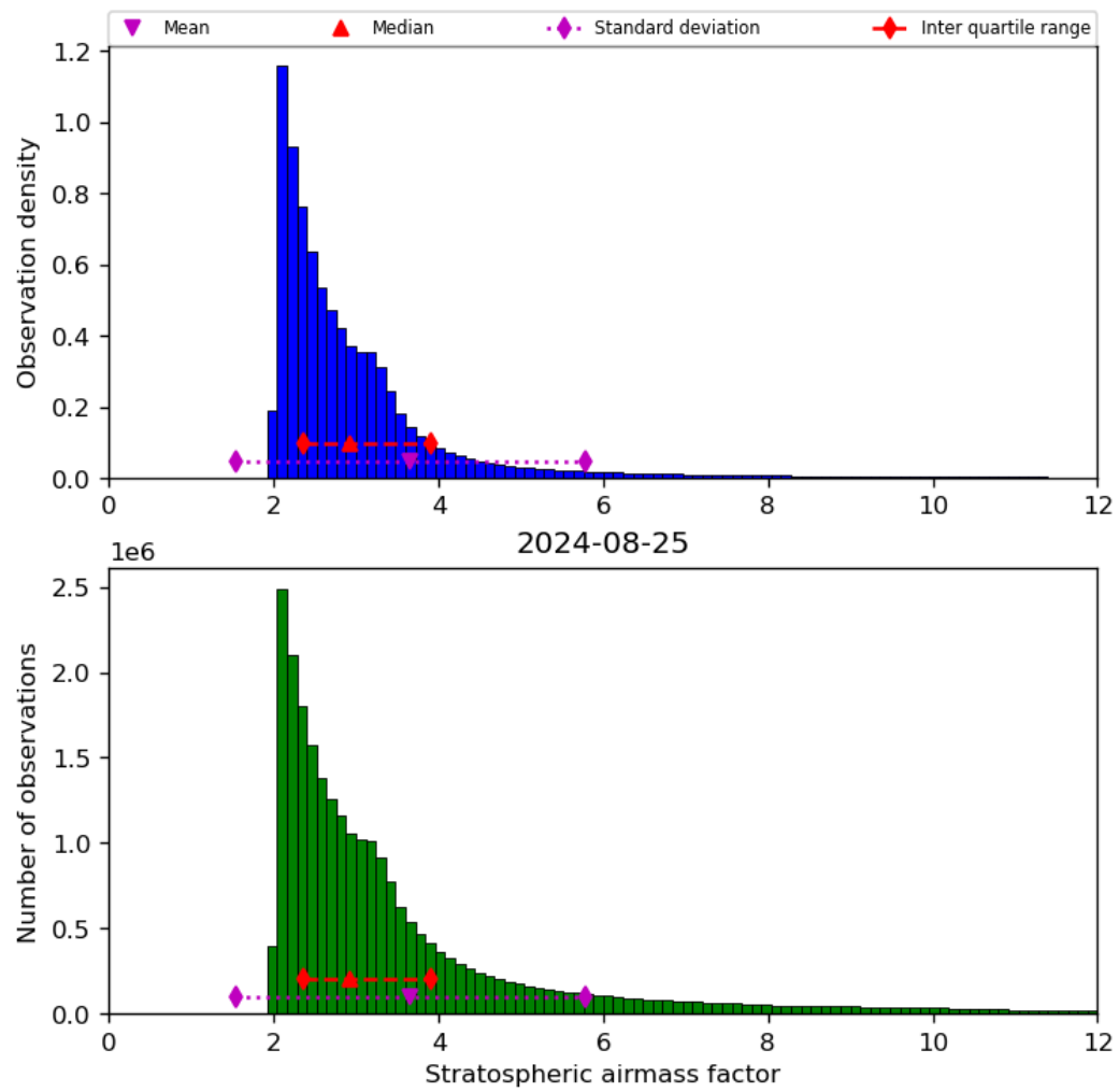
Figure 44: Histogram of “Stratospheric airmass factor” for 2024-08-24 to 2024-08-26
