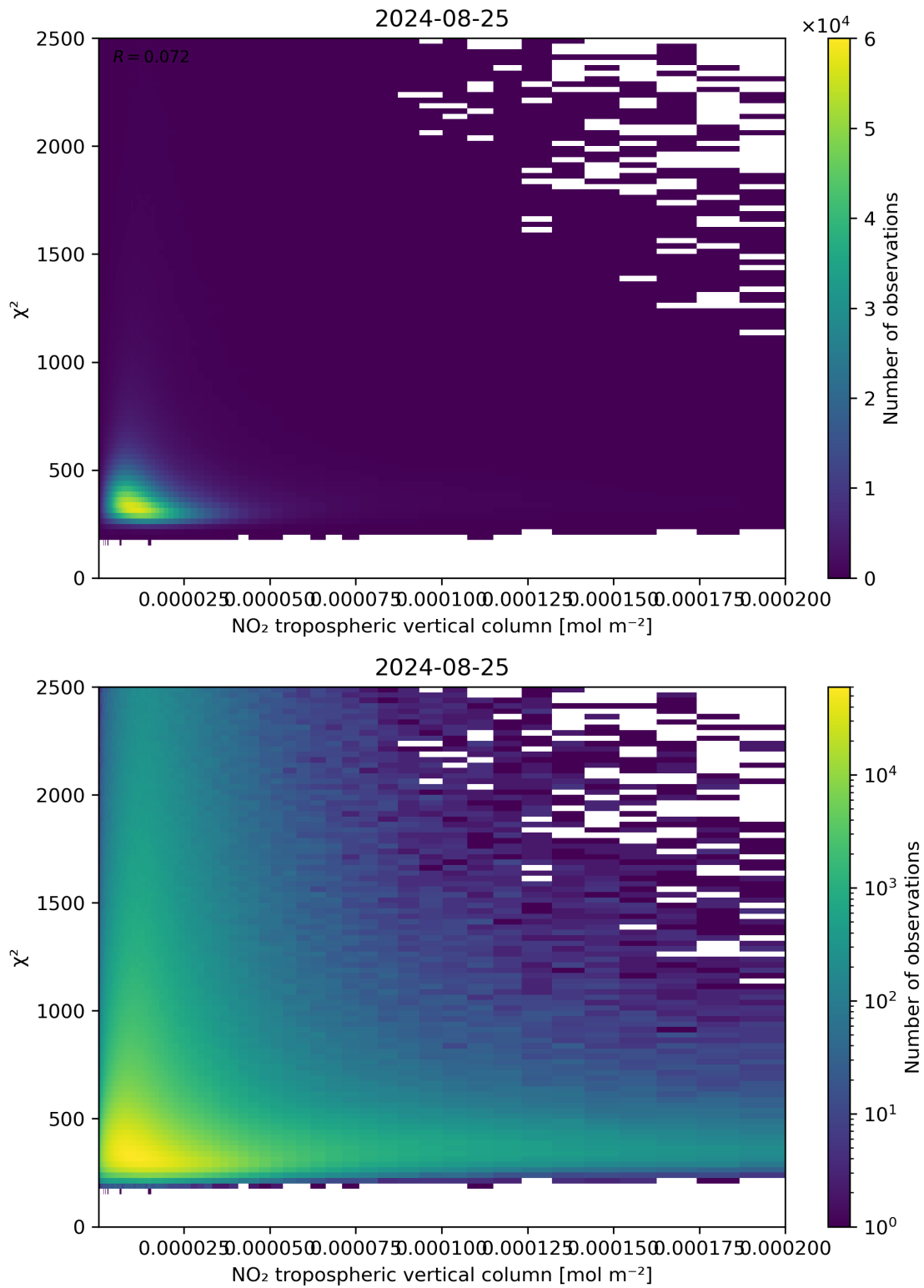
Figure 124: Scatter density plot of “NO 2 tropospheric vertical column” against “ \chi^2 ” for 2024-08-24 to 2024-08-26.
