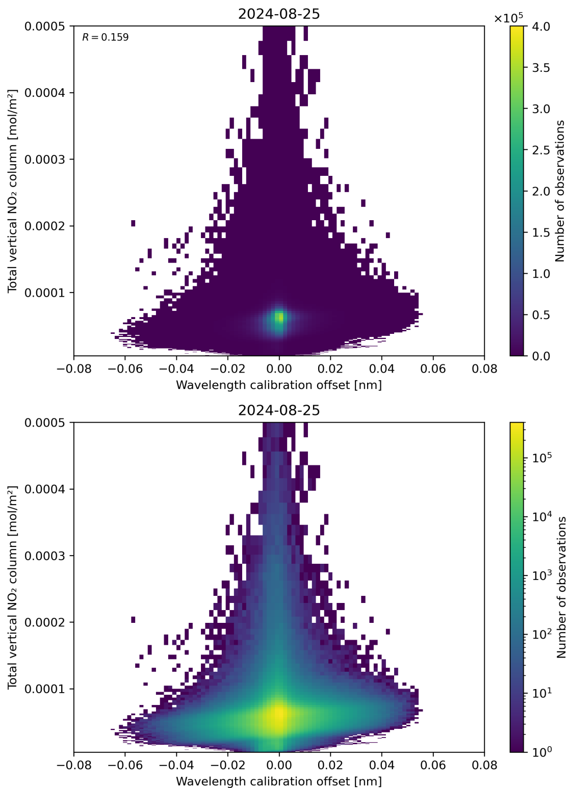
Figure 179: Scatter density plot of “Wavelength calibration offset” against “Total vertical NO 2 column” for 2024-08-24 to 2024-08-26.
