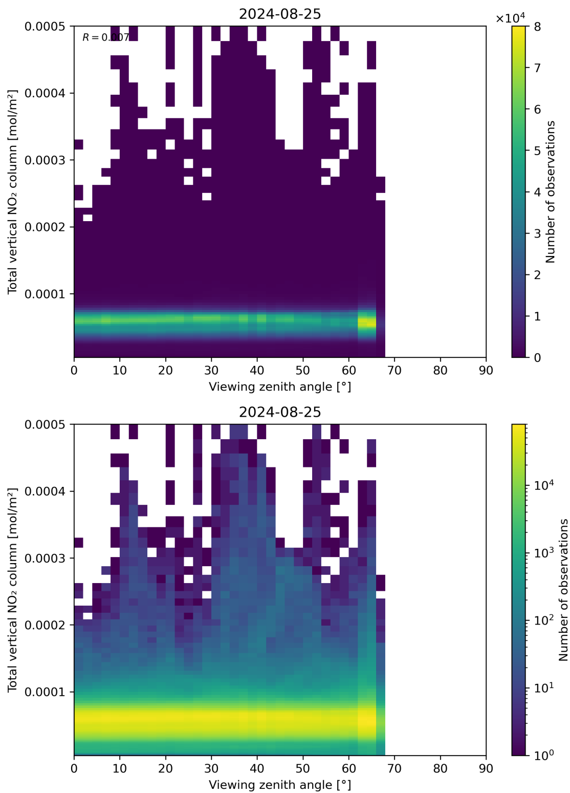
Figure 167: Scatter density plot of “Viewing zenith angle” against “Total vertical NO 2 column” for 2024-08-24 to 2024-08-26.
