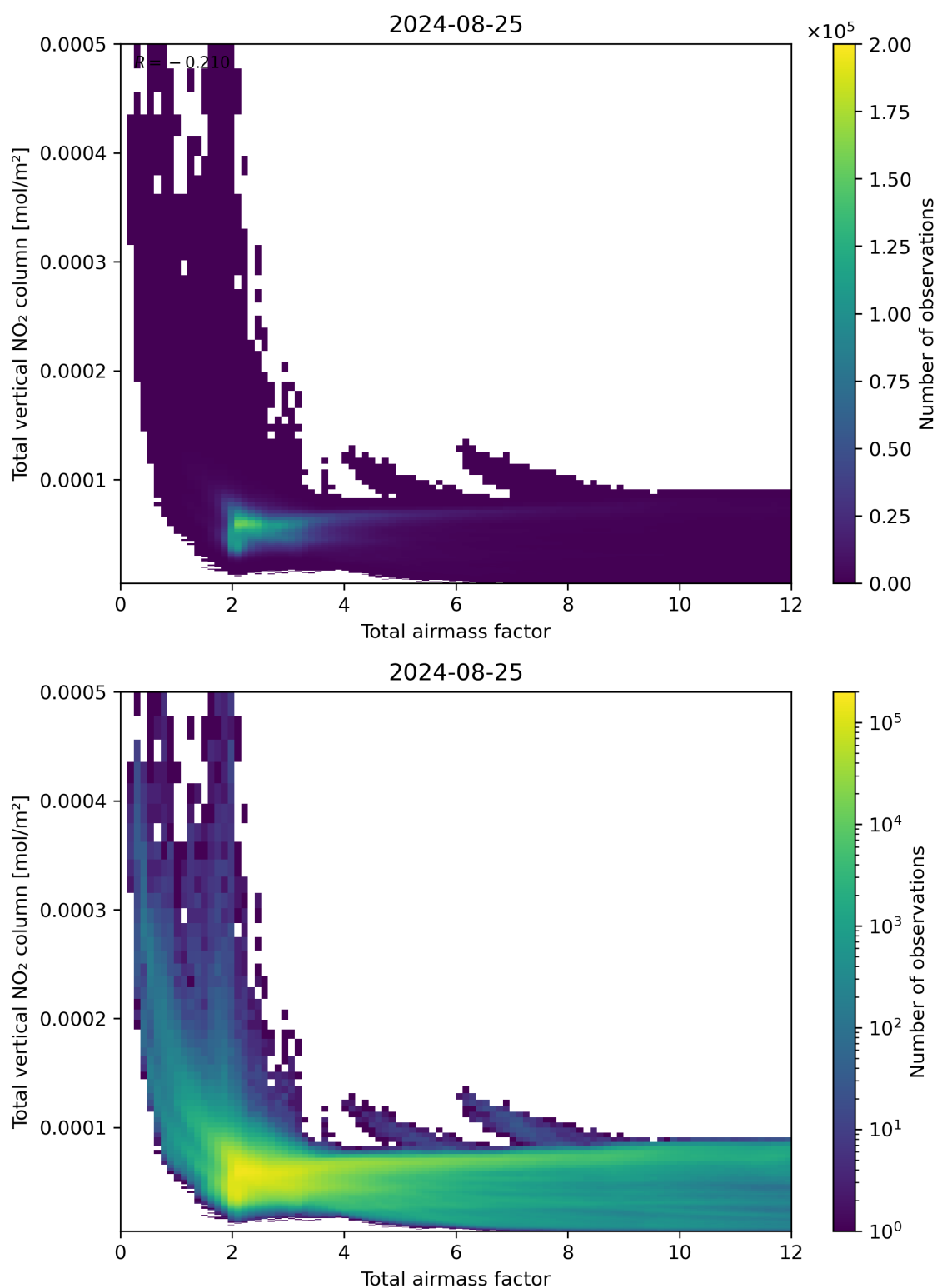
Figure 67: Scatter density plot of “Total airmass factor” against “Total vertical NO 2 column” for 2024-08-24 to 2024-08-26.
