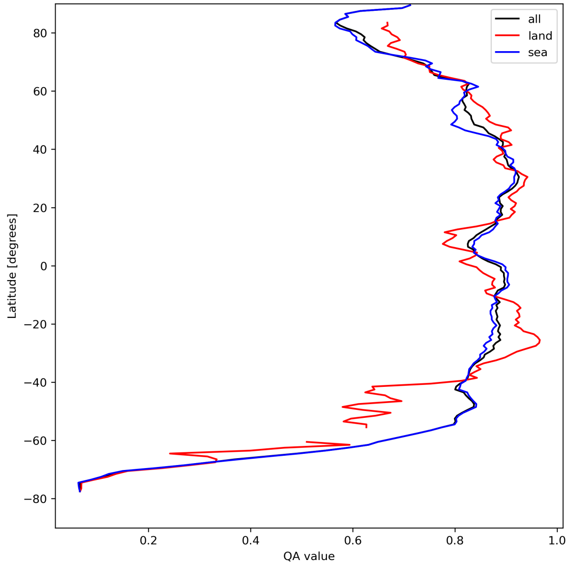
Figure 11: Zonal average of “QA value” for 2024-08-24 to 2024-08-26.
