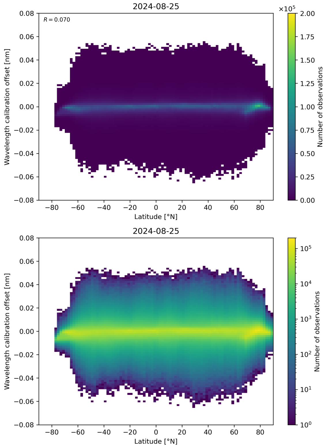
Figure 95: Scatter density plot of “Latitude” against “Wavelength calibration offset” for 2024-08-24 to 2024-08-26.
