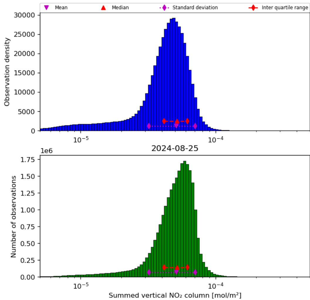
Figure 40: Histogram of “Summed vertical NO 2 column” for 2024-08-24 to 2024-08-26
