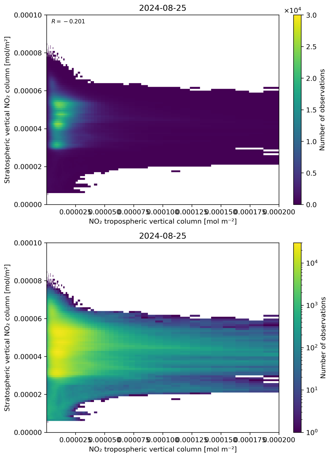
Figure 125: Scatter density plot of “NO 2 tropospheric vertical column” against “Stratospheric vertical NO 2 column” for 2024-08-24 to 2024-08-26.
