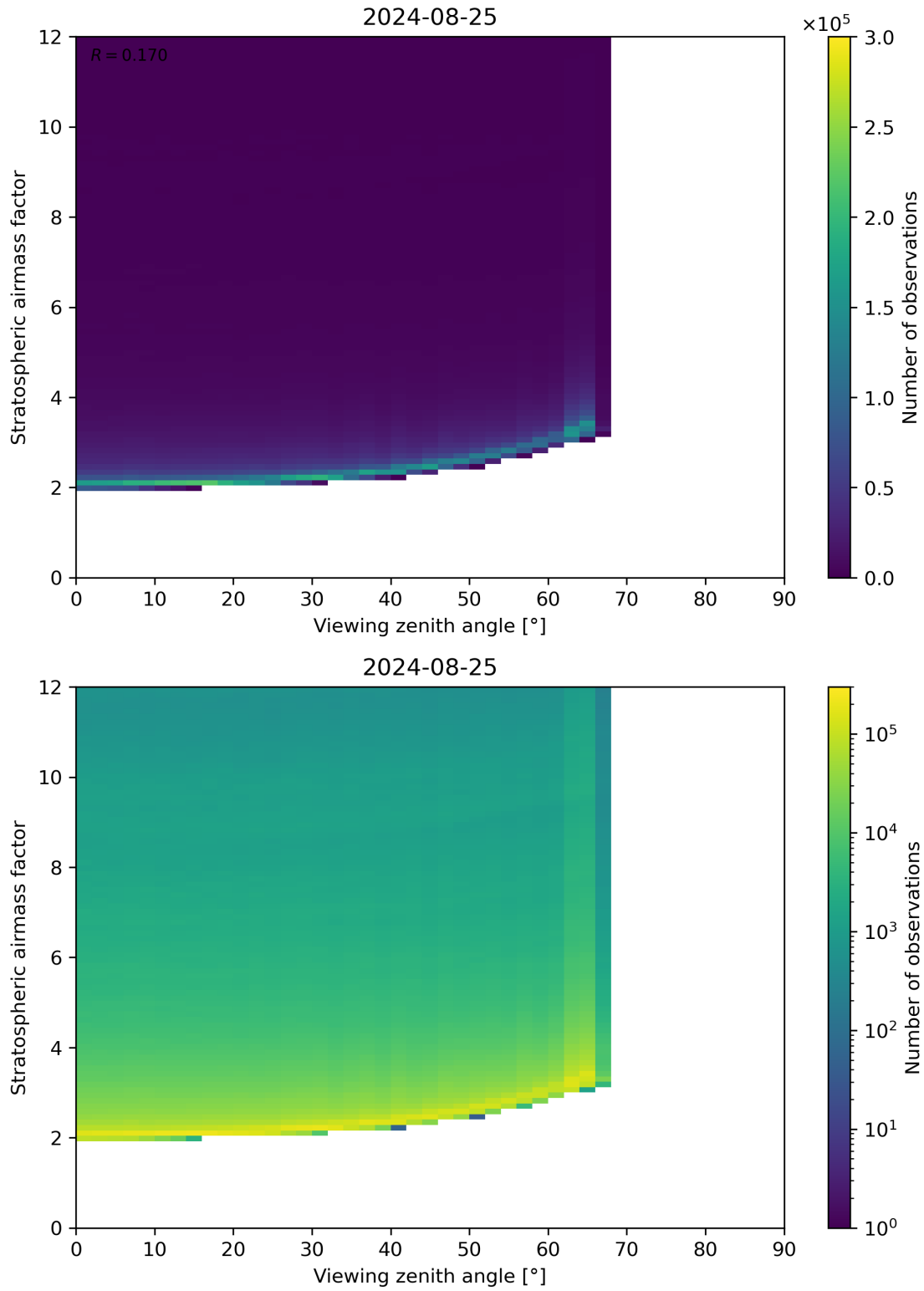
Figure 159: Scatter density plot of “Viewing zenith angle” against “Stratospheric airmass factor” for 2024-08-24 to 2024-08-26.
