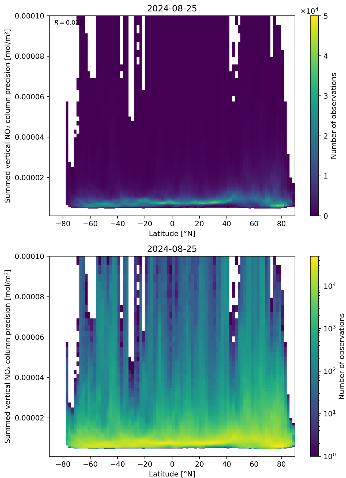
Figure 89: Scatter density plot of “Latitude” against “Summed vertical NO 2 column precision” for 2024-08-24 to 2024-08-26.
