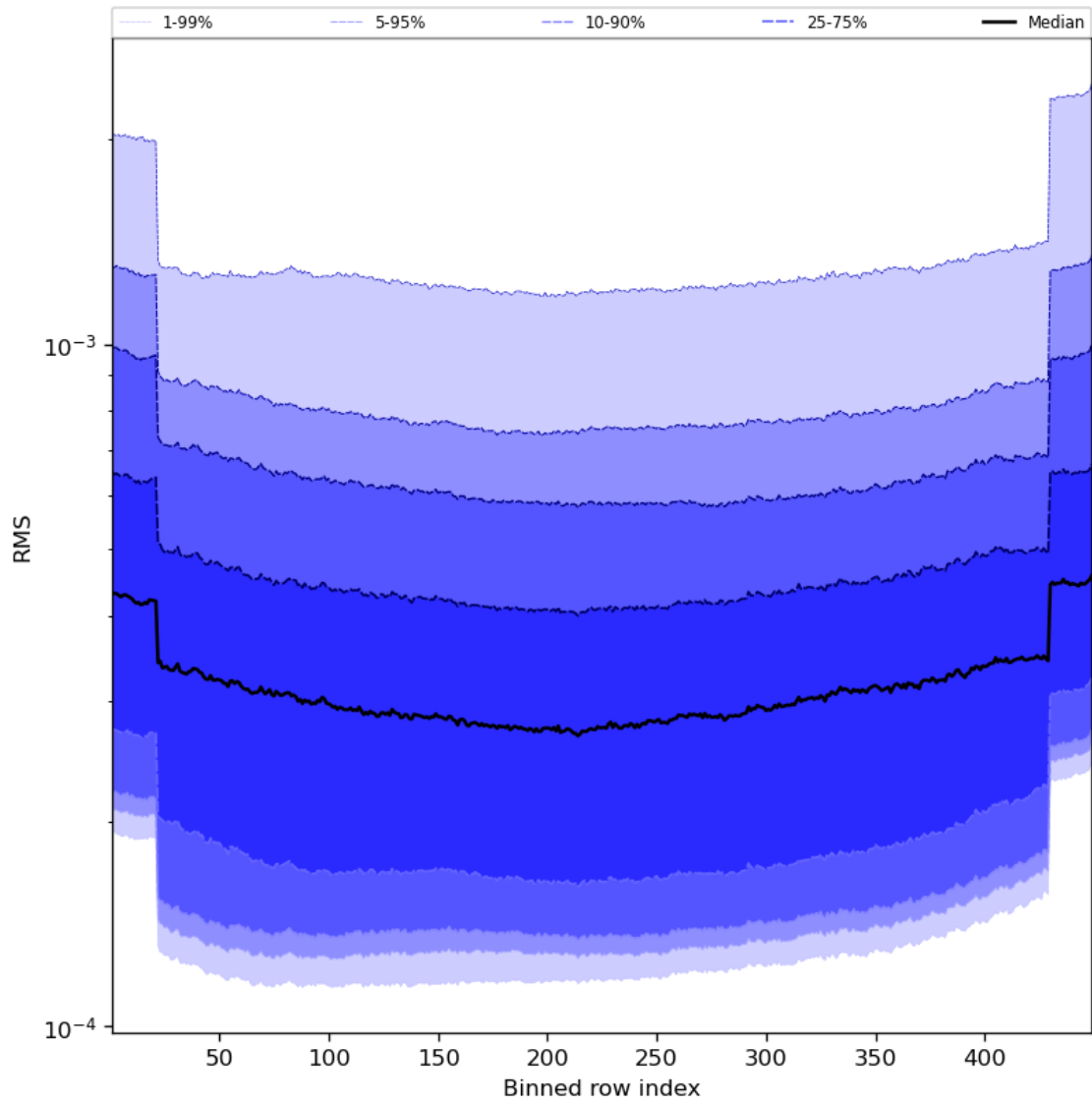
Figure 60: Along track statistics of “RMS” for 2024-08-24 to 2024-08-26
