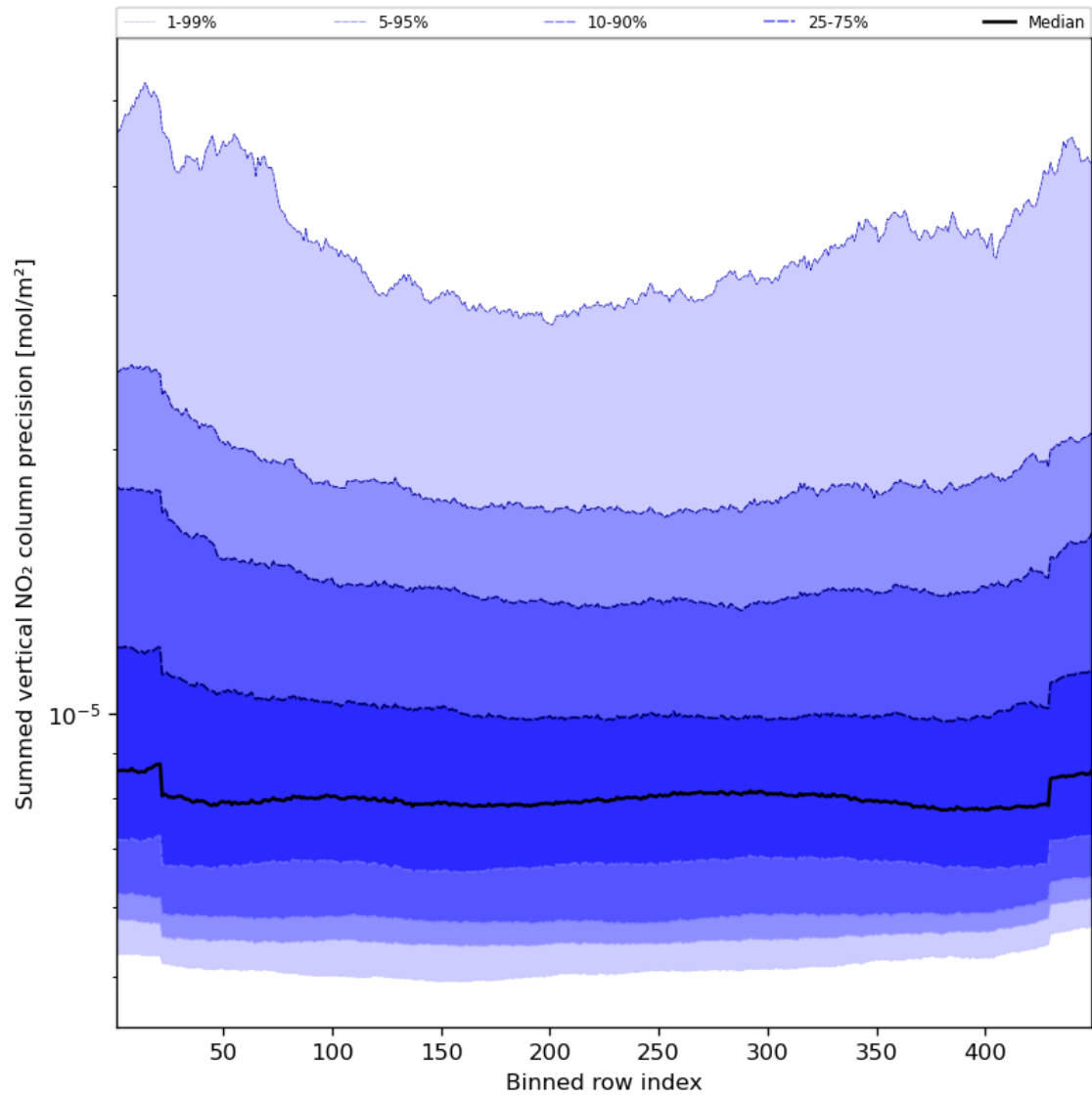
Figure 58: Along track statistics of “Summed vertical NO 2 column precision” for 2024-08-24 to 2024-08-26
