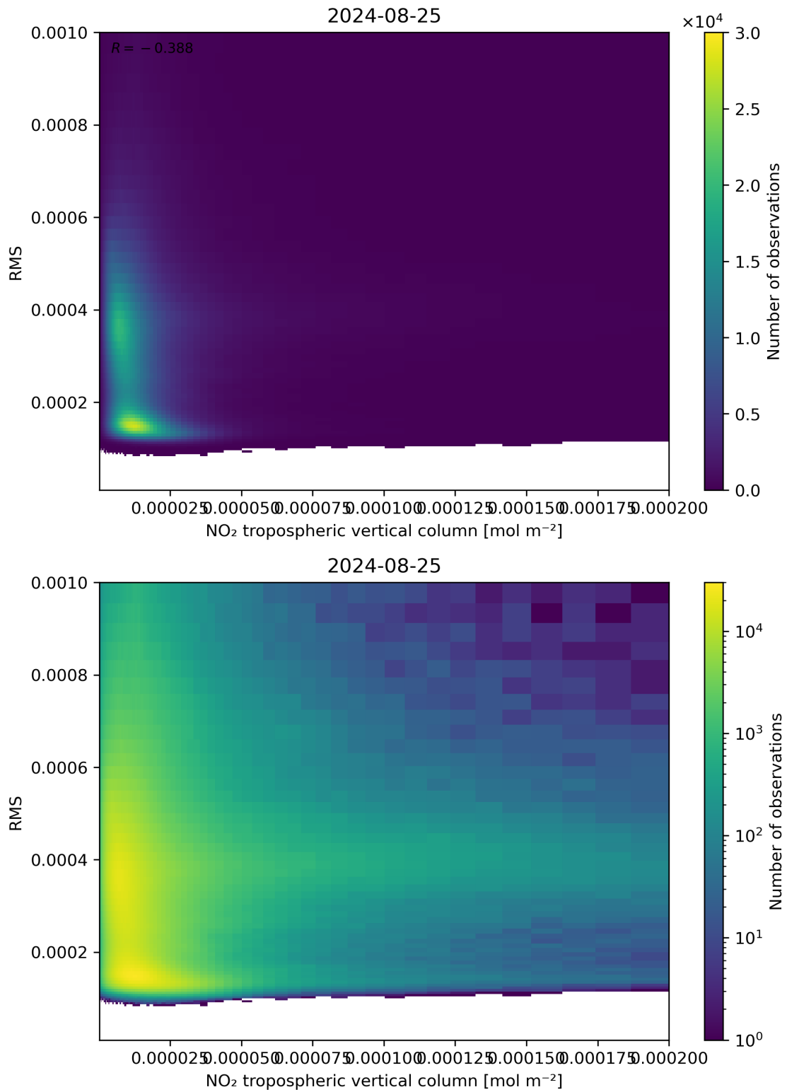
Figure 142: Scatter density plot of “NO 2 tropospheric vertical column” against “RMS” for 2024-08-24 to 2024-08-26.
