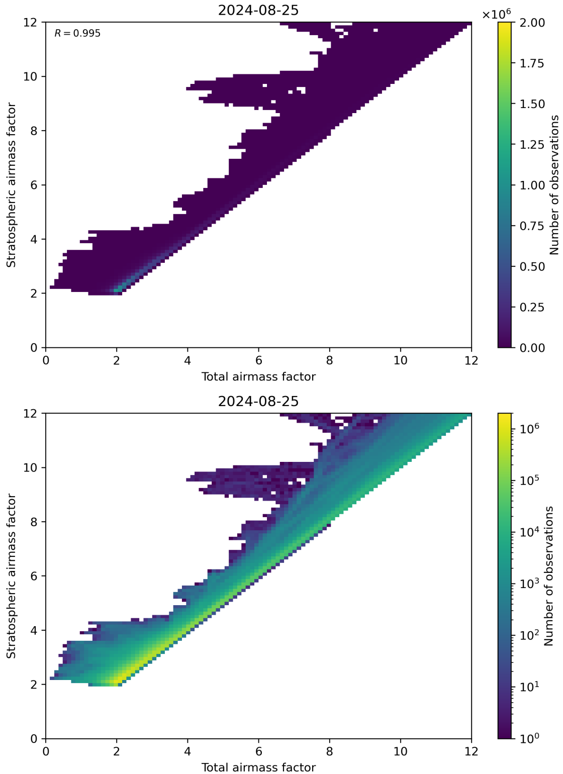
Figure 62: Scatter density plot of “Total airmass factor” against “Stratospheric airmass factor” for 2024-08-24 to 2024-08-26.
