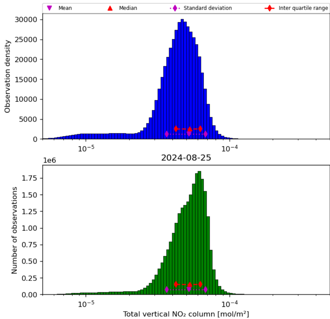
Figure 38: Histogram of “Total vertical NO 2 column” for 2024-08-24 to 2024-08-26
