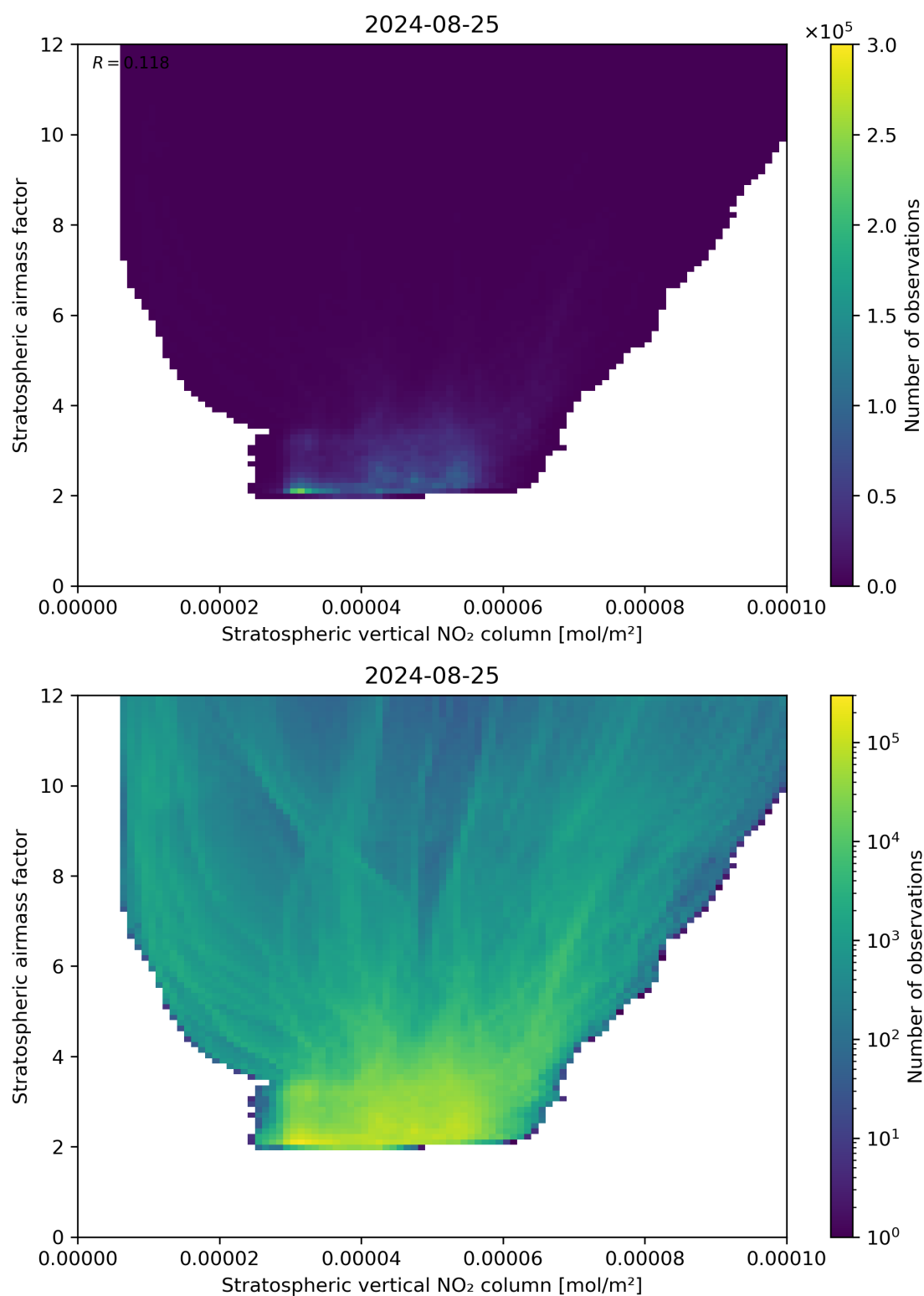
Figure 96: Scatter density plot of “Stratospheric vertical NO 2 column” against “Stratospheric airmass factor” for 2024-08-24 to 2024-08-26.
