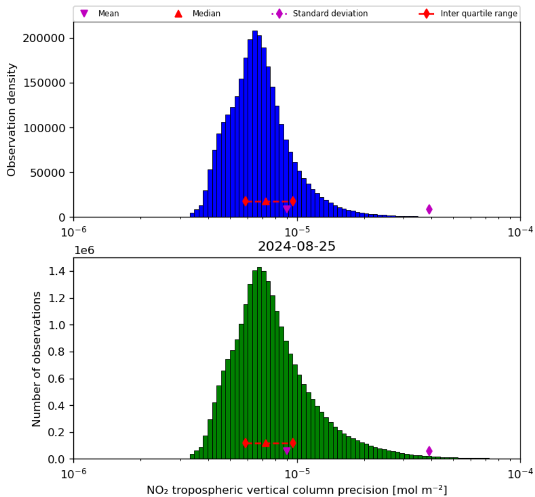
Figure 30: Histogram of “NO 2 tropospheric vertical column precision” for 2024-08-24 to 2024-08-26
