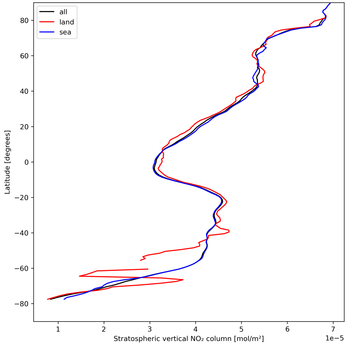
Figure 19: Zonal average of “Stratospheric vertical NO 2 column” for 2024-08-24 to 2024-08-26.
