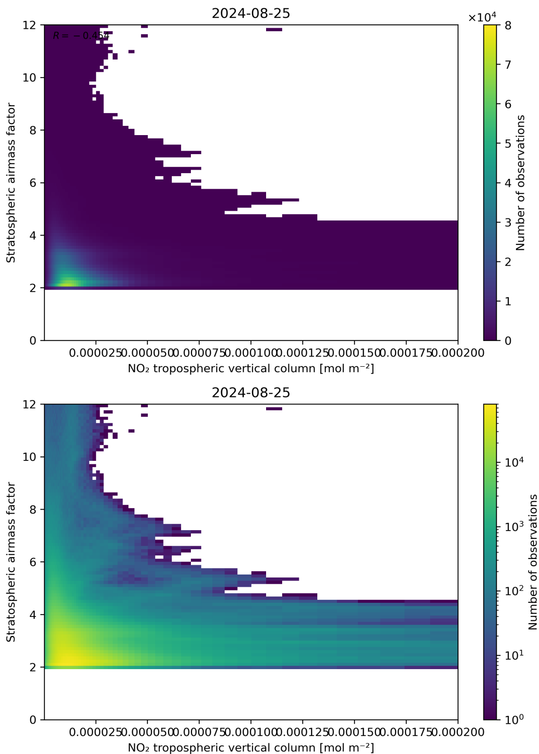
Figure 121: Scatter density plot of “NO 2 tropospheric vertical column” against “Stratospheric airmass factor” for 2024-08-24 to 2024-08-26.
