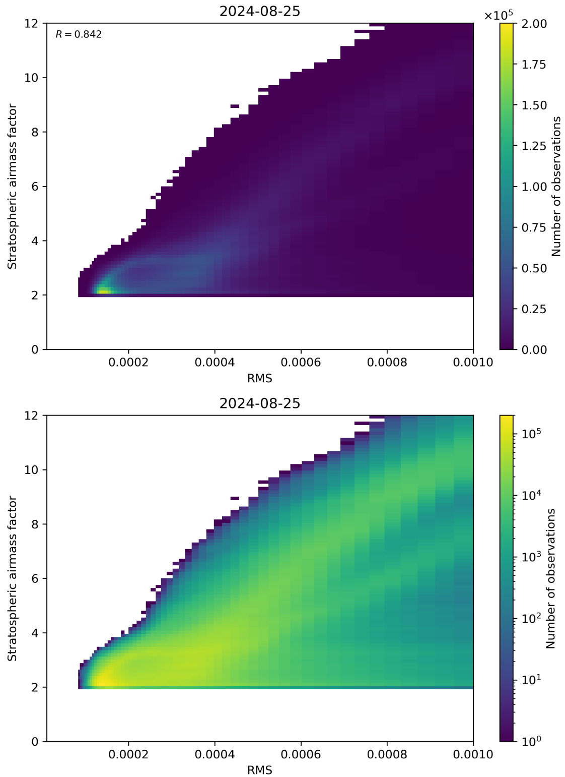
Figure 144: Scatter density plot of “RMS” against “Stratospheric airmass factor” for 2024-08-24 to 2024-08-26.
