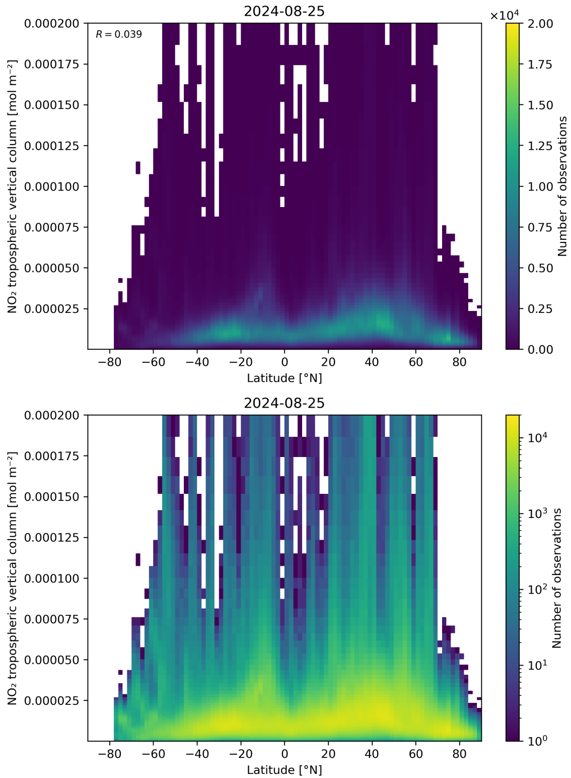
Figure 92: Scatter density plot of “Latitude” against “NO 2 tropospheric vertical column” for 2024-08-24 to 2024-08-26.
