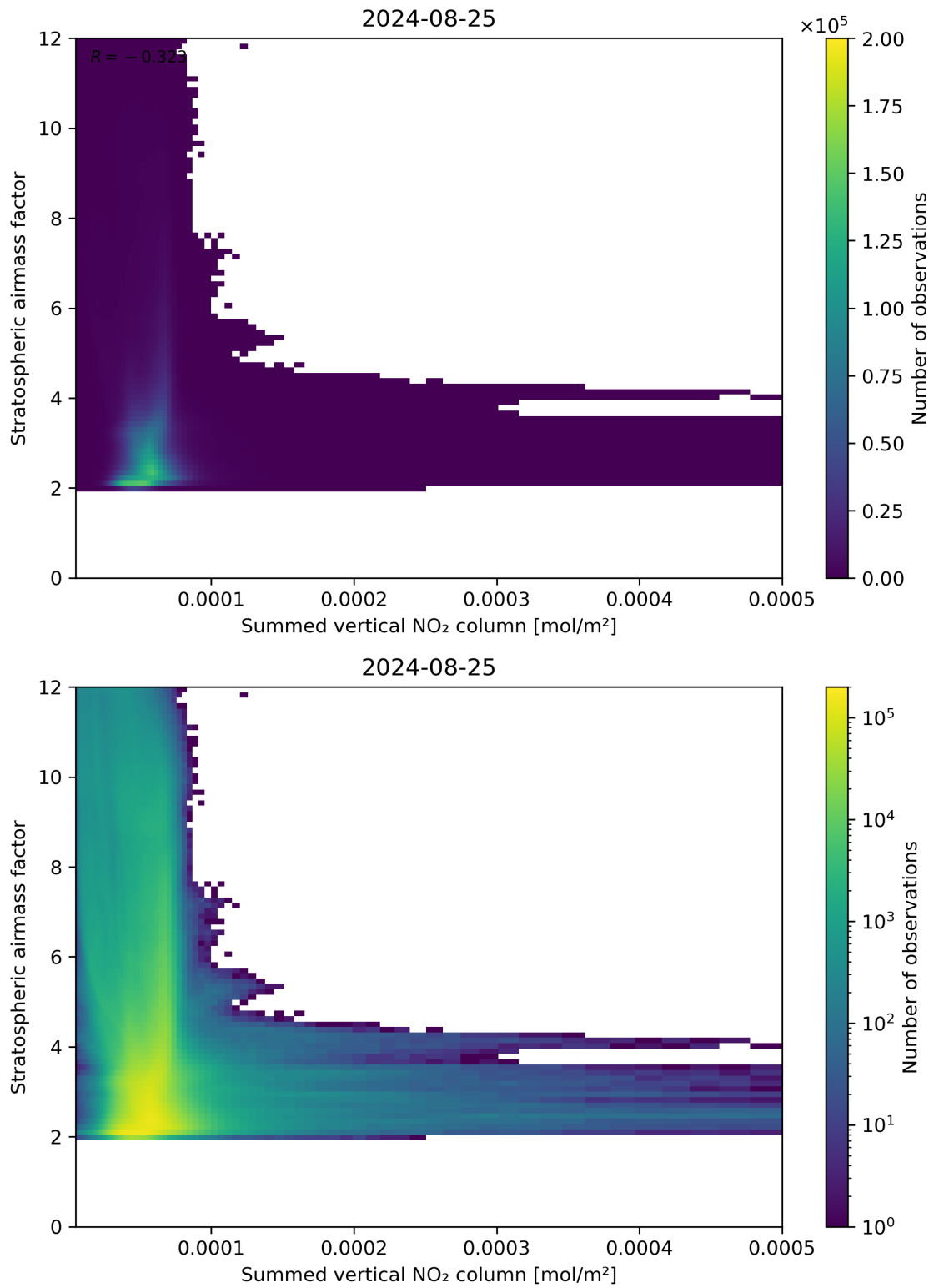
Figure 103: Scatter density plot of “Summed vertical NO 2 column” against “Stratospheric airmass factor” for 2024-08-24 to 2024-08-26.
