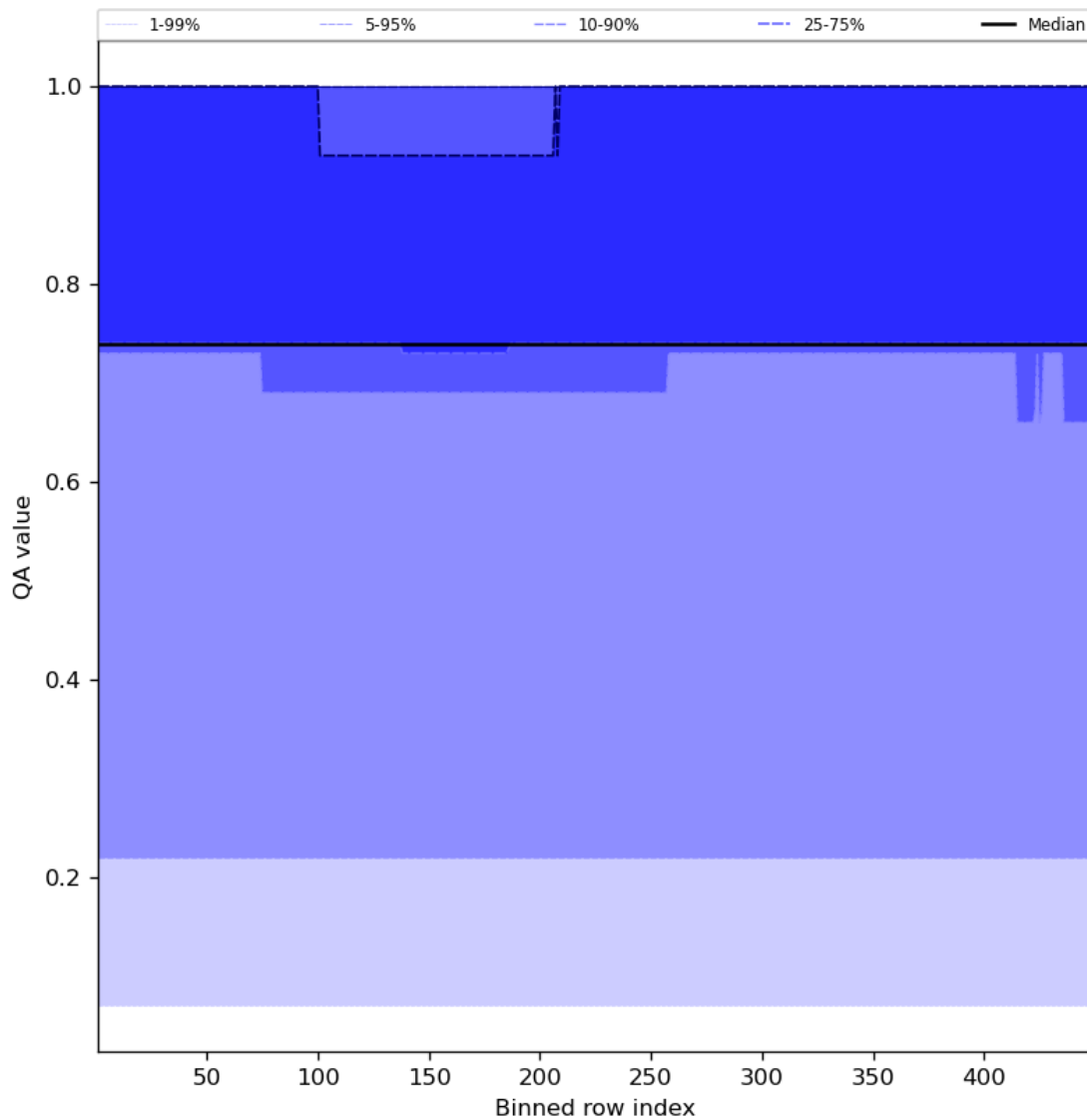
Figure 45: Along track statistics of “QA value” for 2024-08-24 to 2024-08-26
