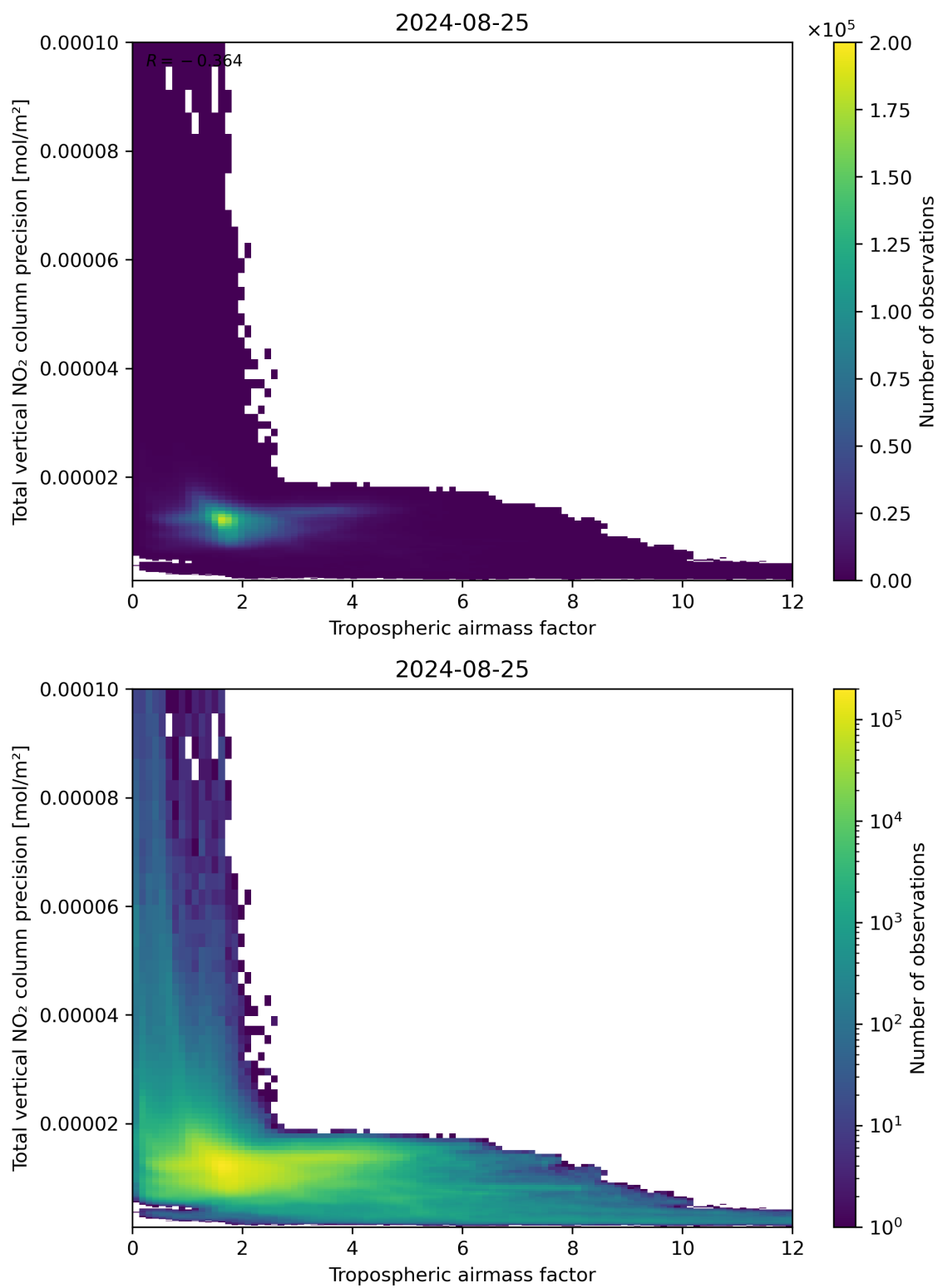
Figure 78: Scatter density plot of “Tropospheric air mass factor” against “Total vertical NO 2 column precision” for 2024-08-24 to 2024-08-26.
