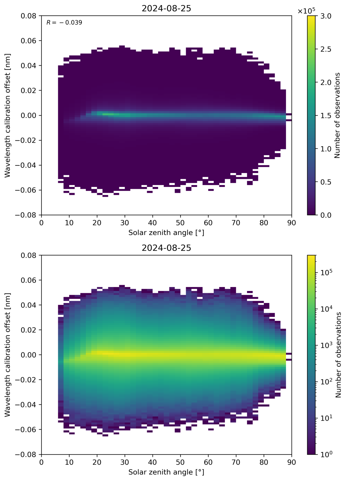
Figure 158: Scatter density plot of “Solar zenith angle” against “Wavelength calibration offset” for 2024-08-24 to 2024-08-26.
