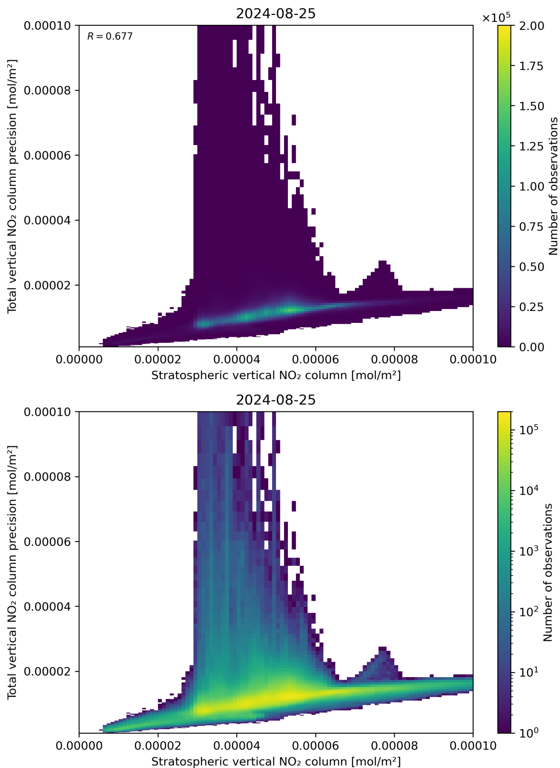
Figure 101: Scatter density plot of “Stratospheric vertical NO 2 column” against “Total vertical NO 2 column precision” for 2024-08-24 to 2024-08-26.
