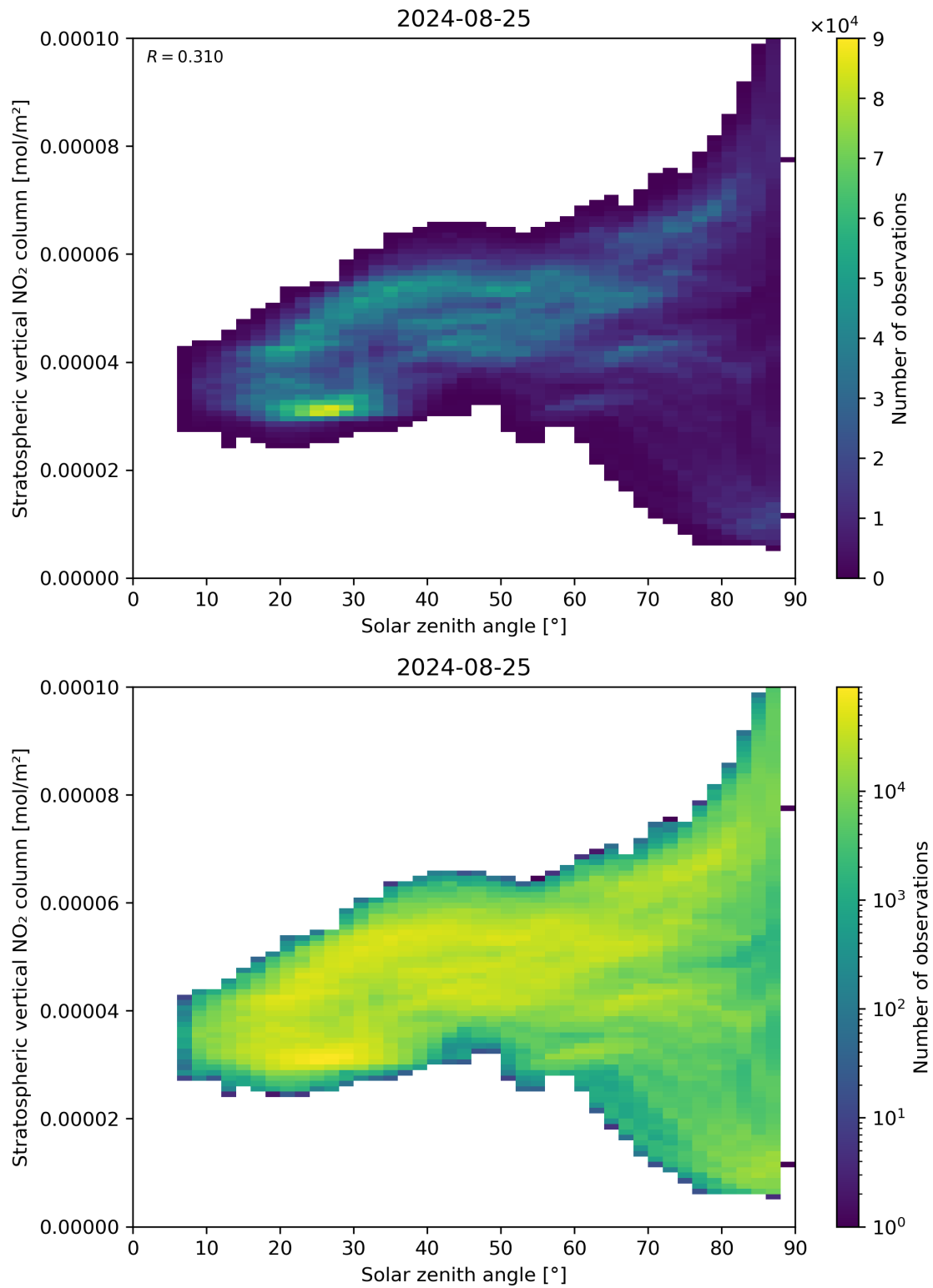
Figure 150: Scatter density plot of “Solar zenith angle” against “Stratospheric vertical NO 2 column” for 2024-08-24 to 2024-08-26.
