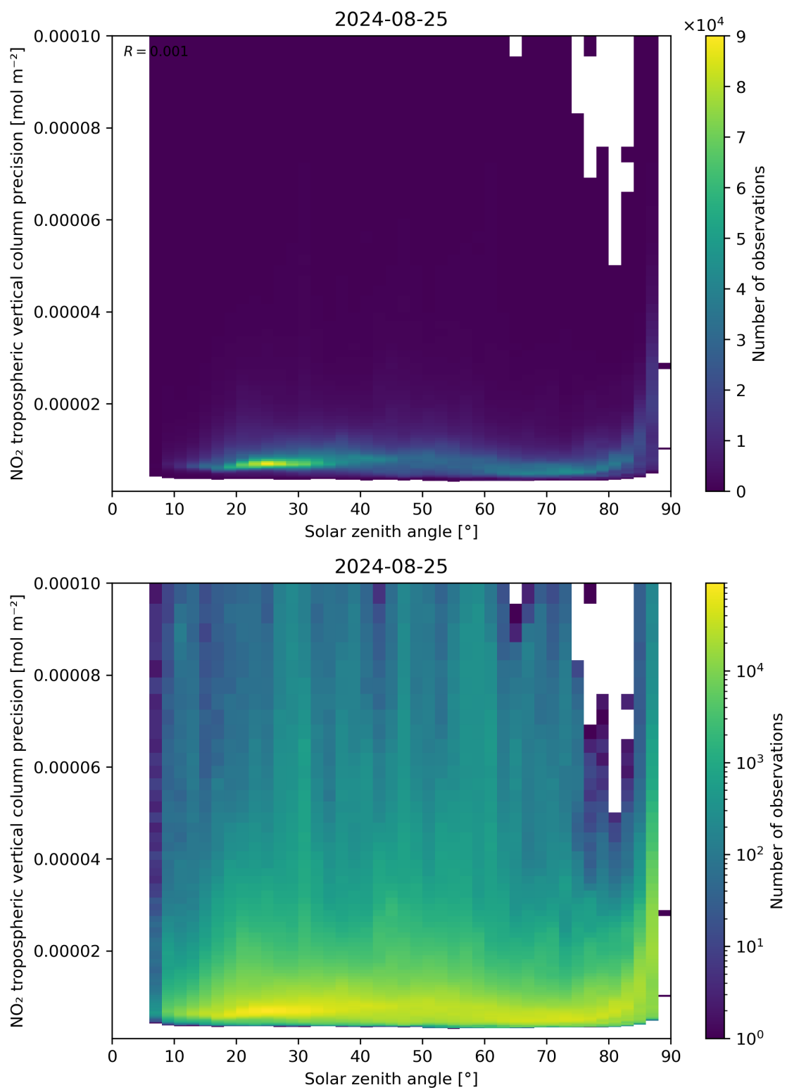
Figure 156: Scatter density plot of “Solar zenith angle” against “NO 2 tropospheric vertical column precision” for 2024-08-24 to 2024-08-26.
