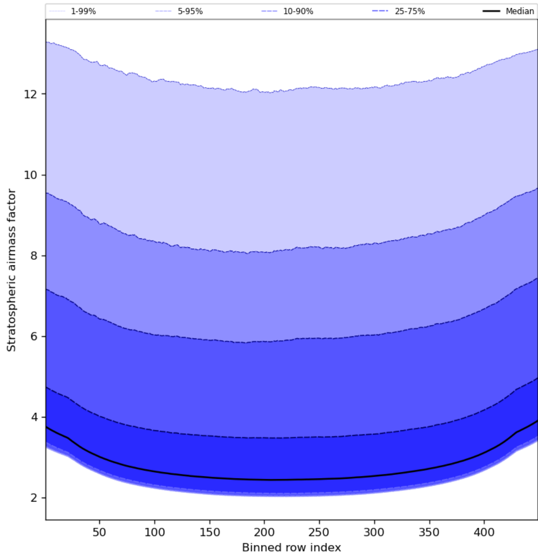
Figure 61: Along track statistics of “Stratospheric airmass factor” for 2024-08-24 to 2024-08-26
