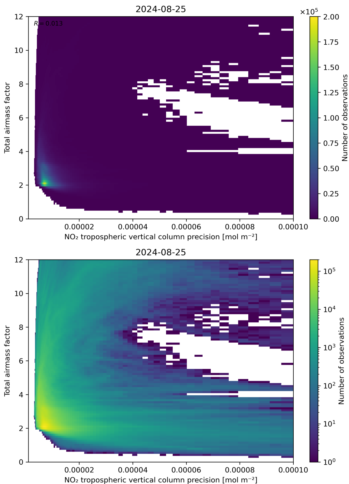
Figure 132: Scatter density plot of “NO 2 tropospheric vertical column precision” against “Total air mass factor” for 2024-08-24 to 2024-08-26.
