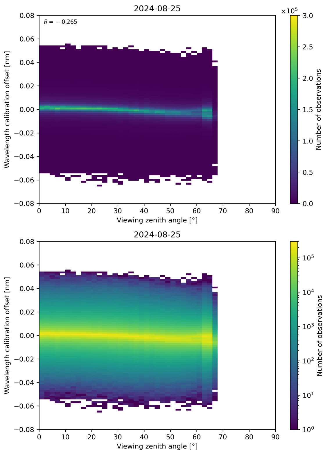
Figure 173: Scatter density plot of “Viewing zenith angle” against “Wavelength calibration offset” for 2024-08-24 to 2024-08-26.
