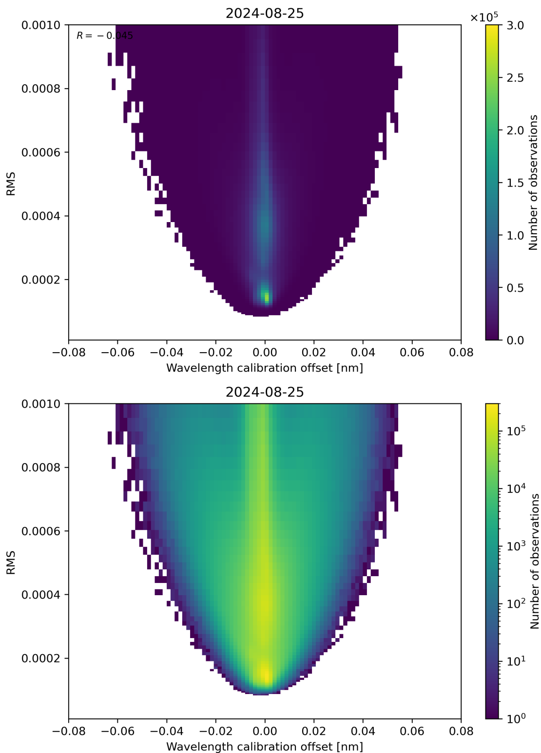
Figure 181: Scatter density plot of “Wavelength calibration offset” against “RMS” for 2024-08-24 to 2024-08-26.
