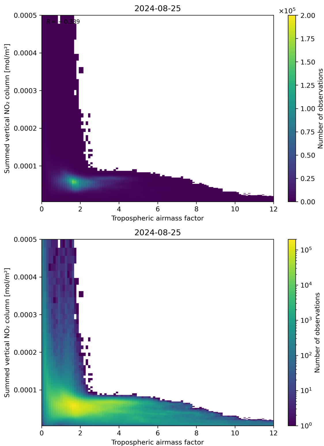
Figure 75: Scatter density plot of “Tropospheric airmass factor” against “Summed vertical NO 2 column” for 2024-08-24 to 2024-08-26.
