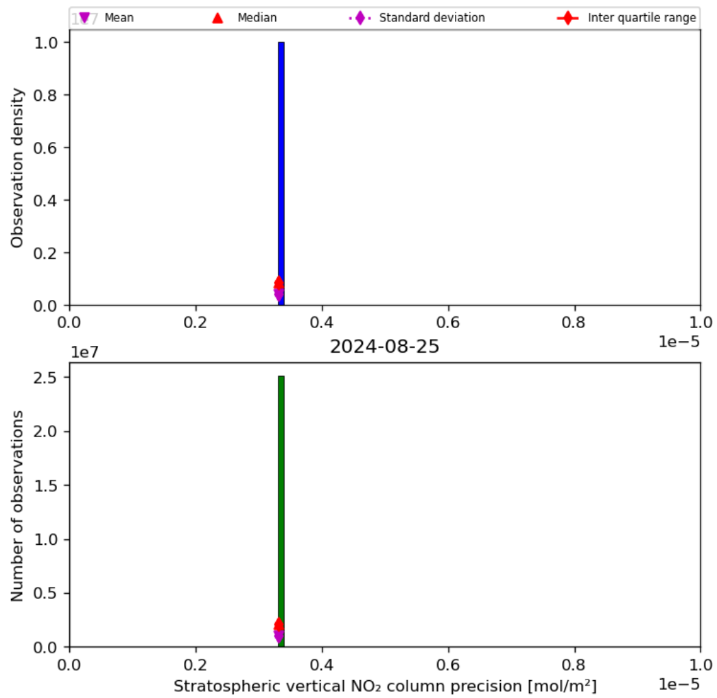
Figure 37: Histogram of “Stratospheric vertical NO 2 column precision” for 2024-08-24 to 2024-08-26
