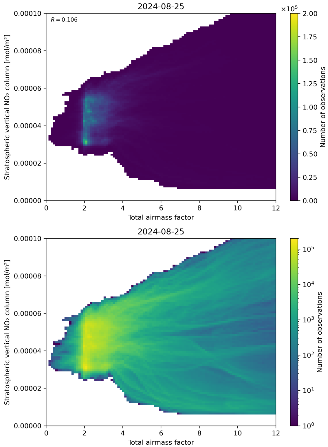
Figure 64: Scatter density plot of “Total airmass factor” against “Stratospheric vertical NO 2 column” for 2024-08-24 to 2024-08-26.
