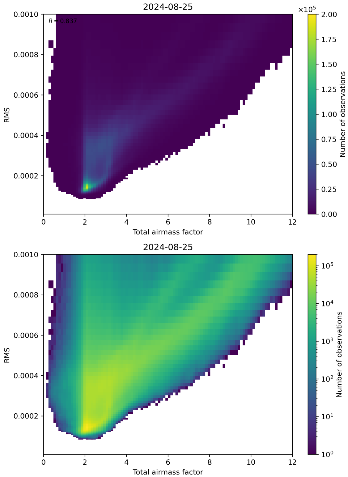
Figure 69: Scatter density plot of “Total airmass factor” against “RMS” for 2024-08-24 to 2024-08-26.
