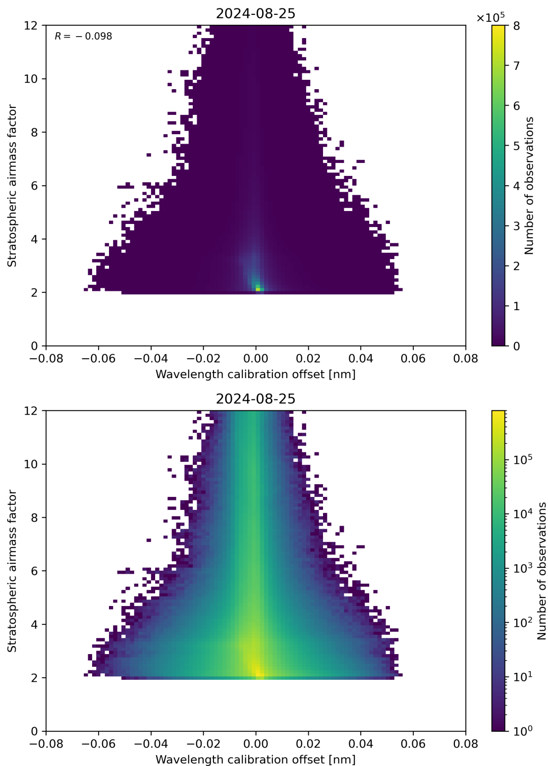
Figure 174: Scatter density plot of “Wavelength calibration offset” against “Stratospheric airmass factor” for 2024-08-24 to 2024-08-26.
