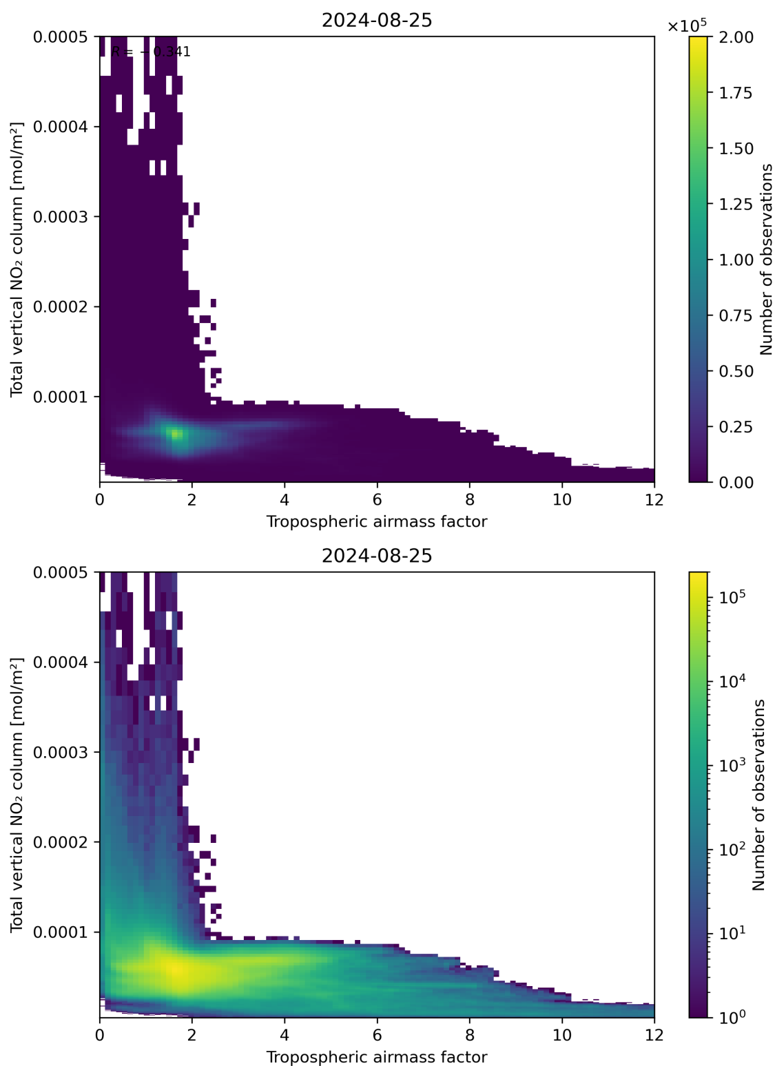
Figure 77: Scatter density plot of “Tropospheric airmass factor” against “Total vertical NO 2 column” for 2024-08-24 to 2024-08-26.
