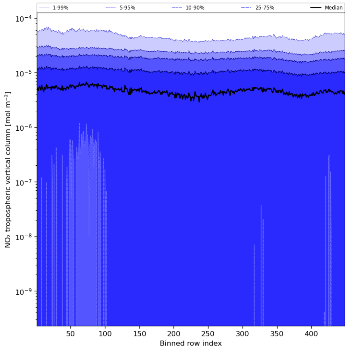
Figure 46: Along track statistics of “NO 2 tropospheric vertical column” for 2024-08-24 to 2024-08-26
