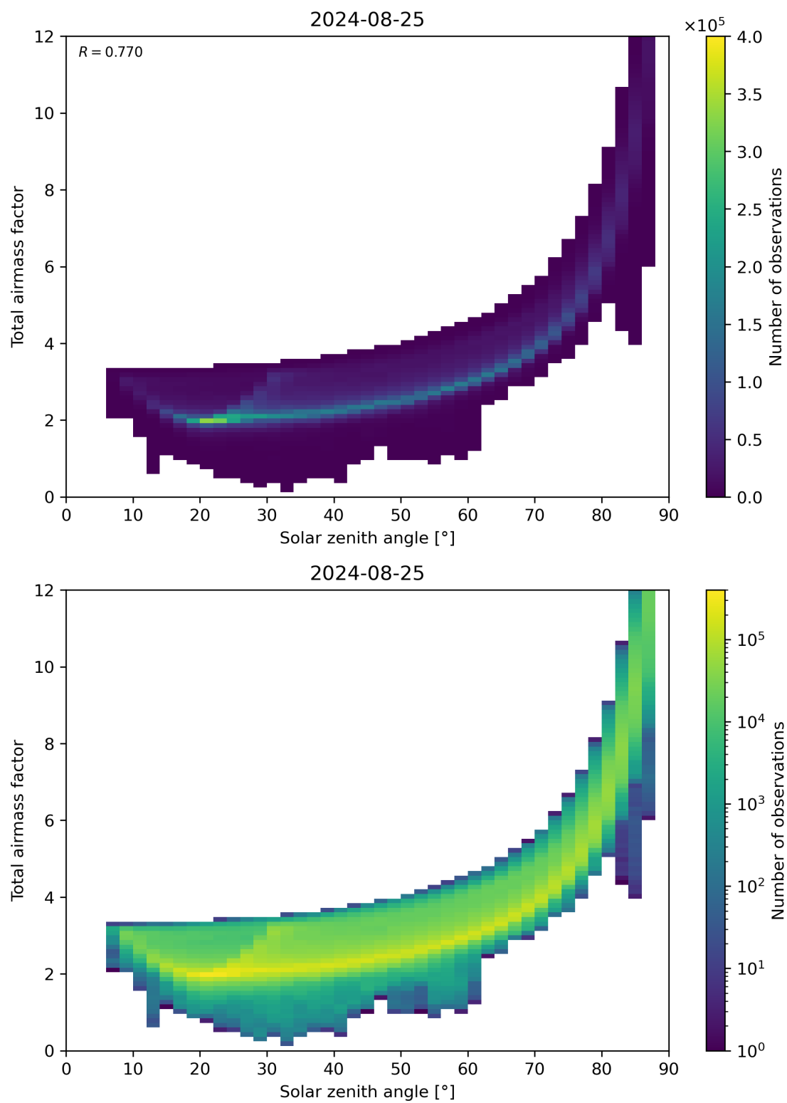
Figure 146: Scatter density plot of “Solar zenith angle” against “Total air mass factor” for 2024-08-24 to 2024-08-26.
