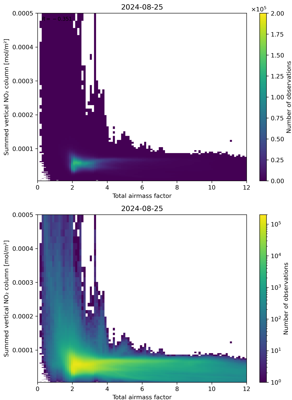
Figure 65: Scatter density plot of “Total airmass factor” against “Summed vertical NO 2 column” for 2024-08-24 to 2024-08-26.
