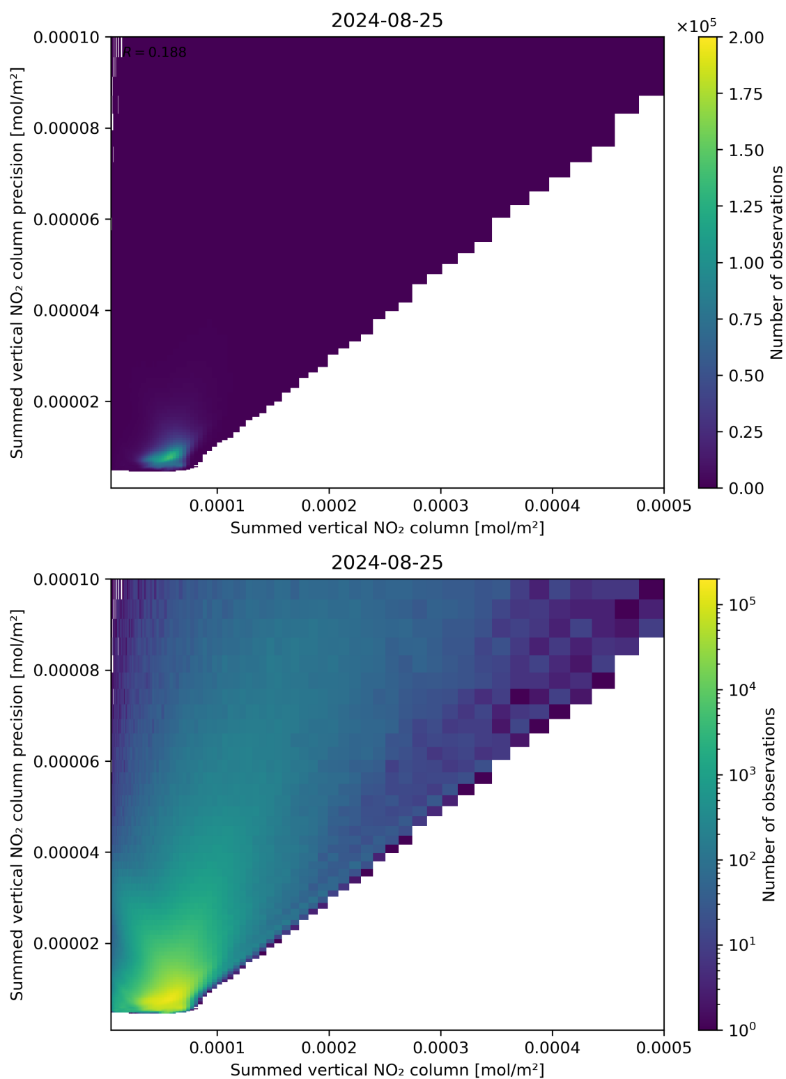
Figure 105: Scatter density plot of “Summed vertical NO 2 column” against “Summed vertical NO 2 column precision” for 2024-08-24 to 2024-08-26.
