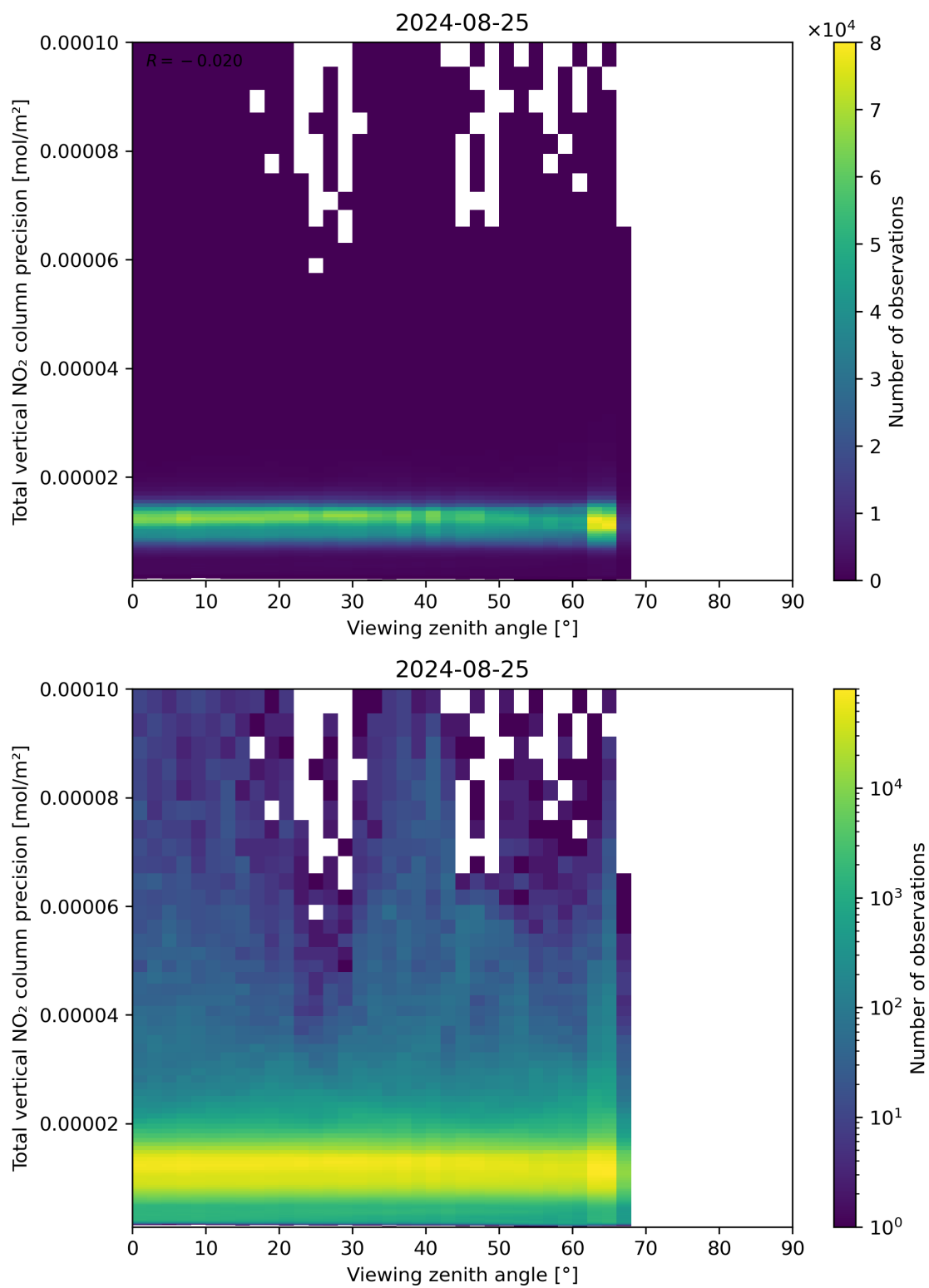
Figure 168: Scatter density plot of “Viewing zenith angle” against “Total vertical NO 2 column precision” for 2024-08-24 to 2024-08-26.
