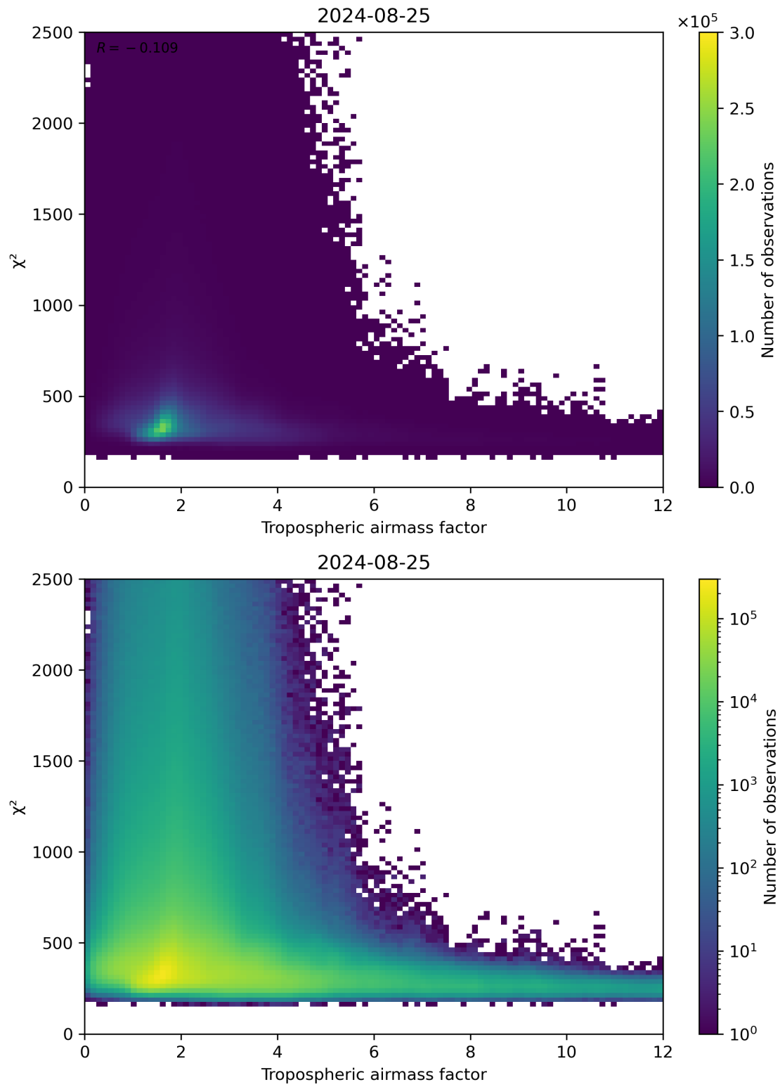
Figure 73: Scatter density plot of “Tropospheric airmass factor” against “ \chi^2 ” for 2024-08-24 to 2024-08-26.
