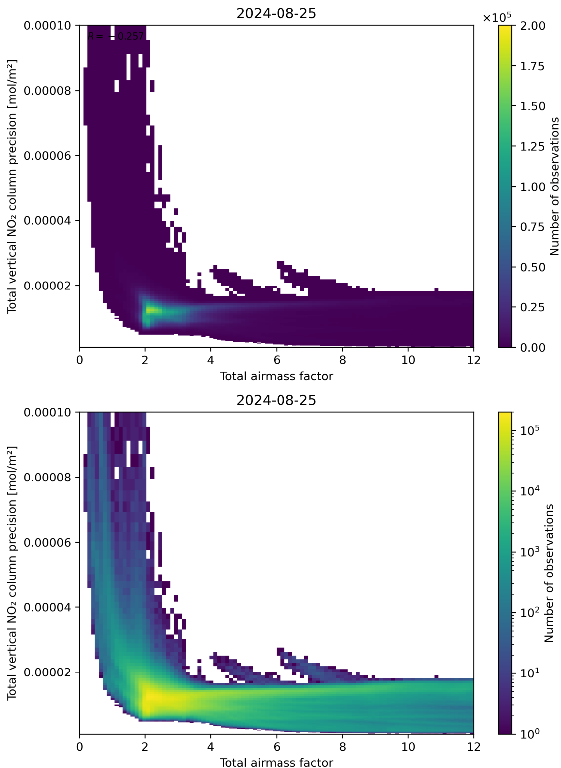
Figure 68: Scatter density plot of “Total airmass factor” against “Total vertical NO 2 column precision” for 2024-08-24 to 2024-08-26.
