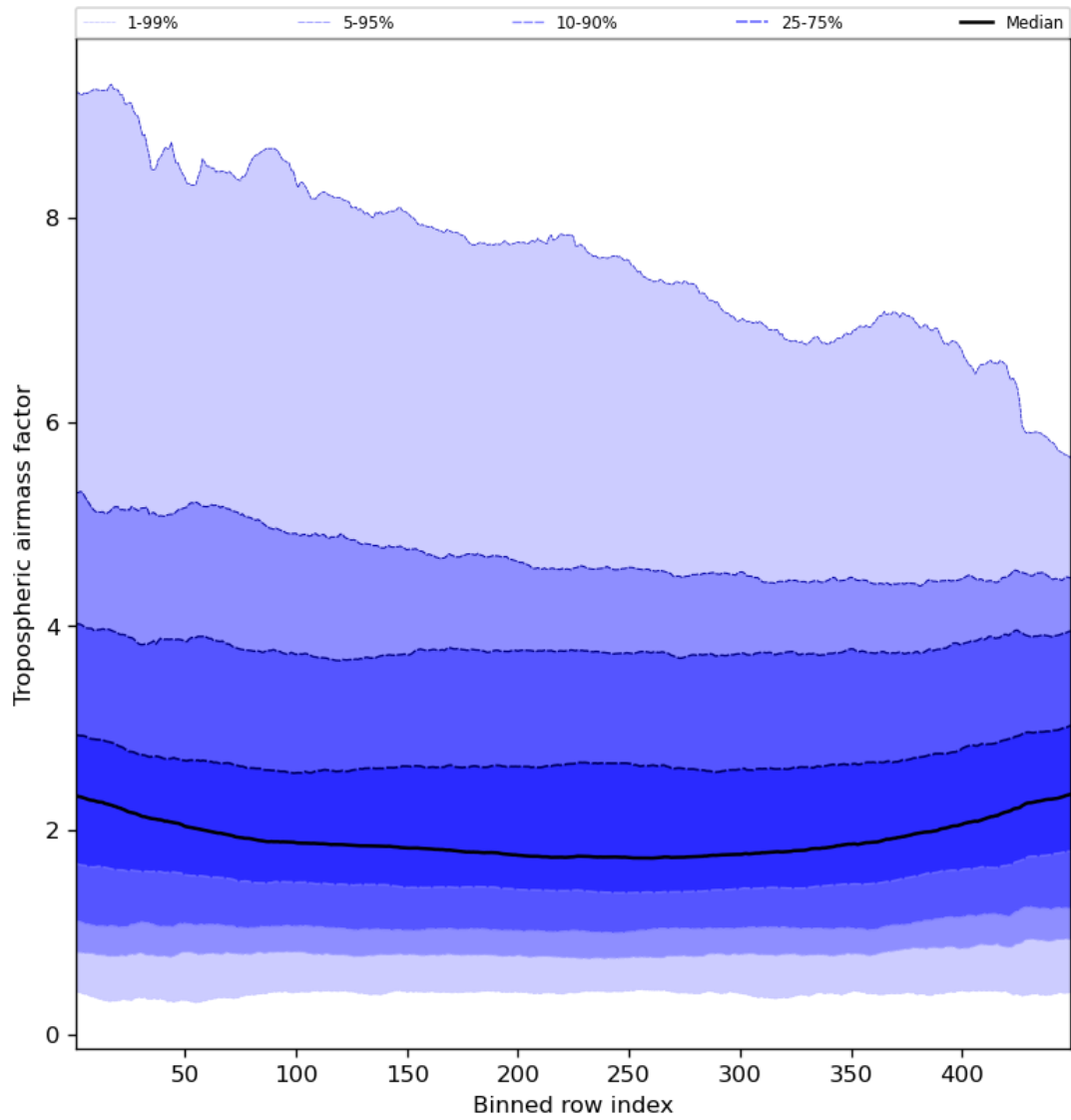
Figure 48: Along track statistics of “Tropospheric air mass factor” for 2024-08-24 to 2024-08-26
