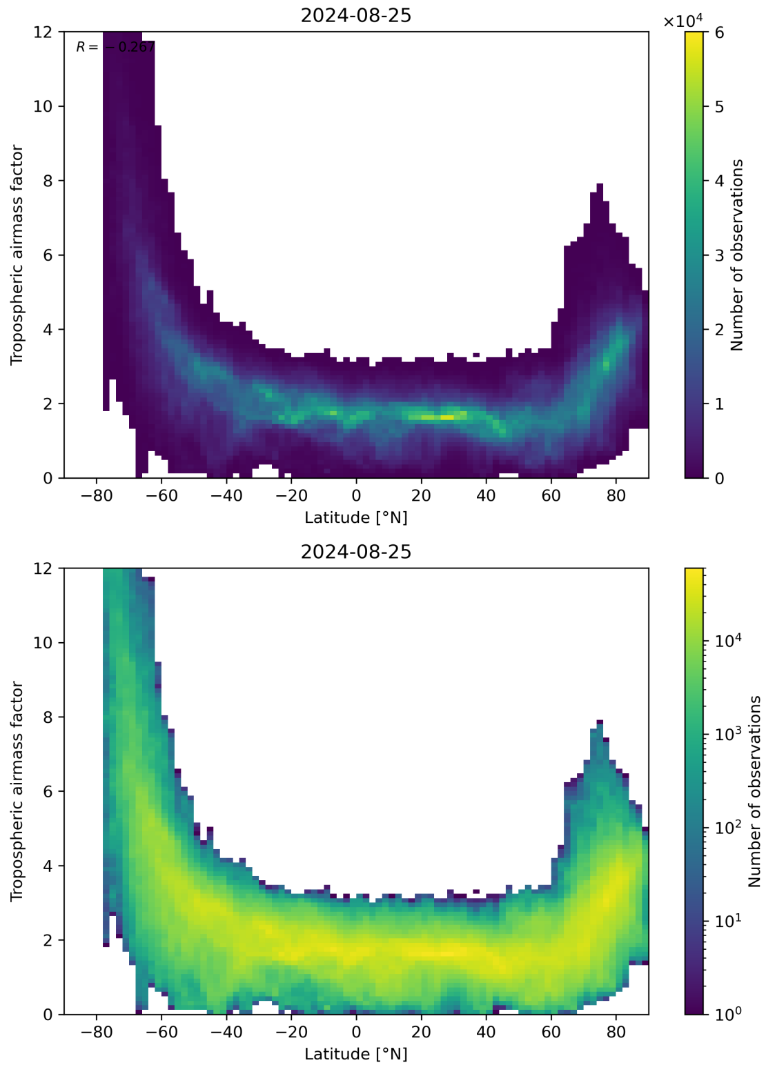
Figure 85: Scatter density plot of “Latitude” against “Tropospheric airmass factor” for 2024-08-24 to 2024-08-26.
