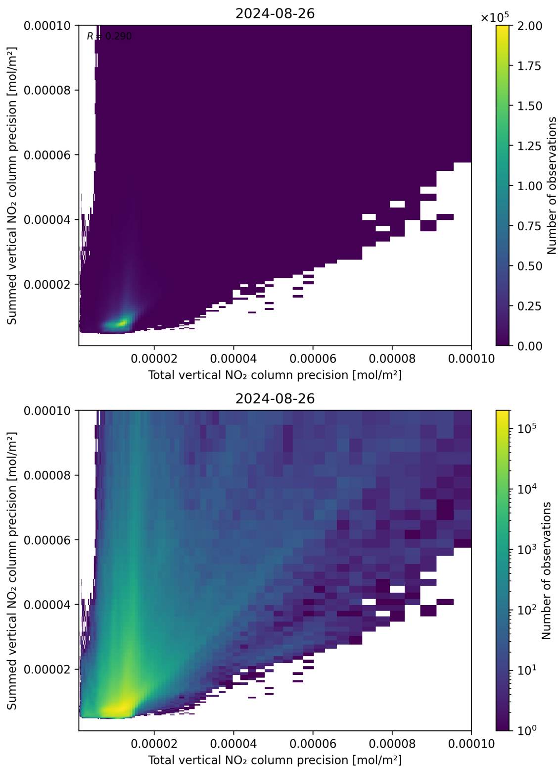
Figure 118: Scatter density plot of “Total vertical NO 2 column precision” against “Summed vertical NO 2 column precision” for 2024-08-25 to 2024-08-27.
