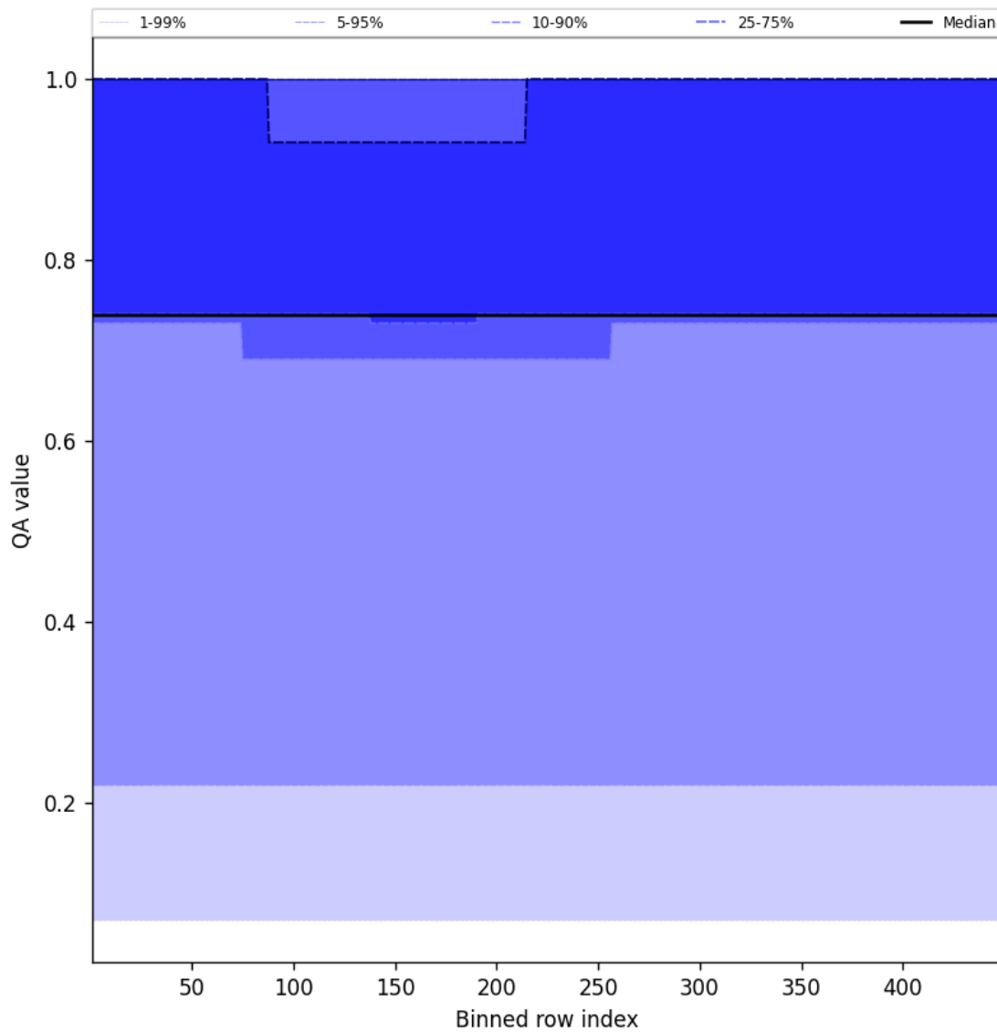
Figure 45: Along track statistics of “QA value” for 2024-08-25 to 2024-08-27
