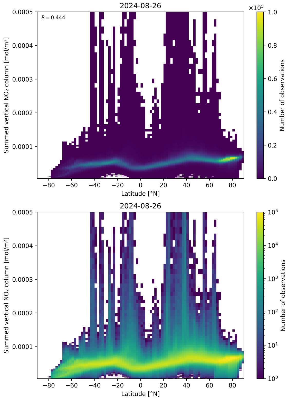
Figure 88: Scatter density plot of “Latitude” against “Summed vertical NO 2 column” for 2024-08-25 to 2024-08-27.
