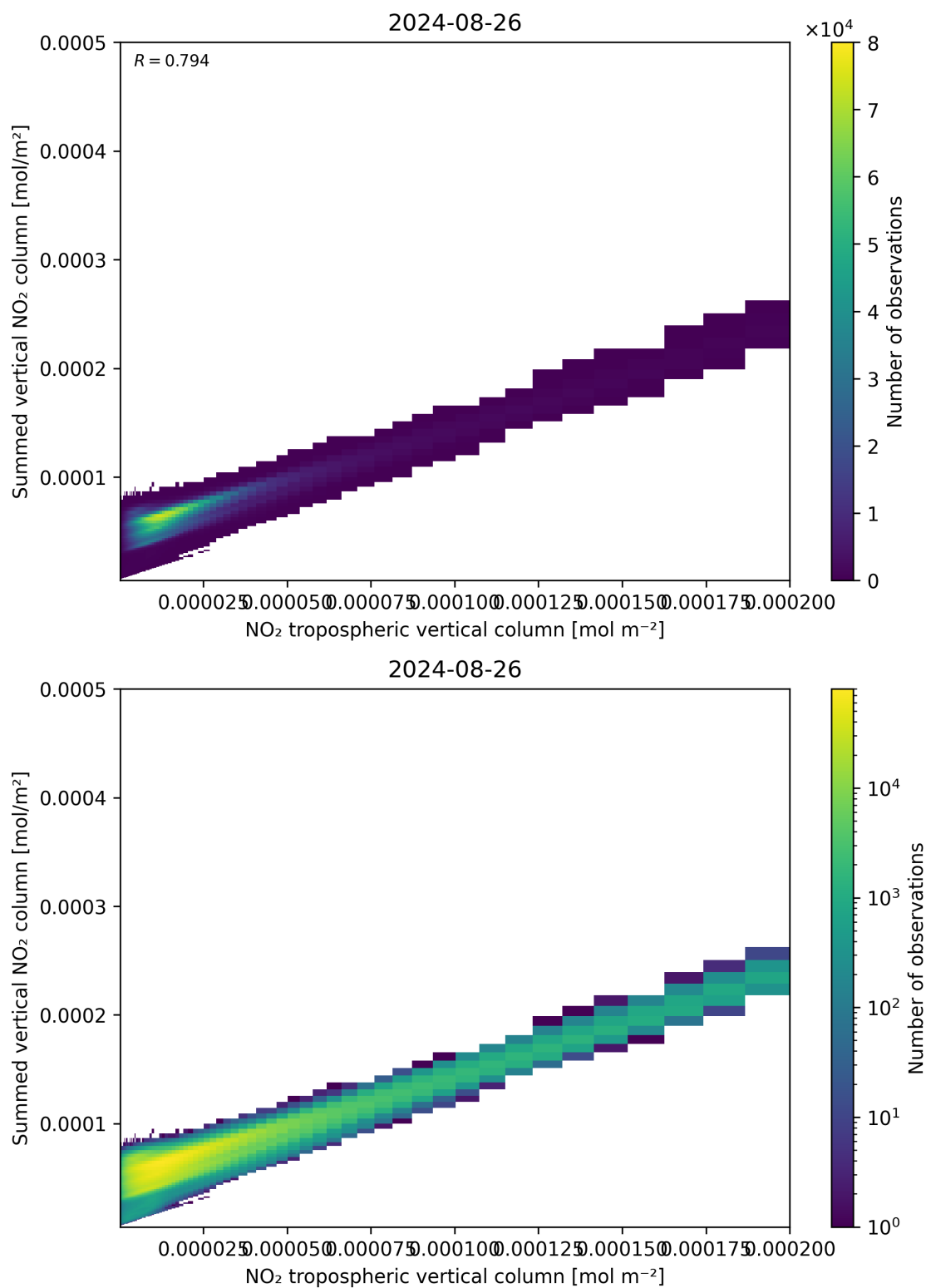
Figure 126: Scatter density plot of “NO 2 tropospheric vertical column” against “Summed vertical NO 2 column” for 2024-08-25 to 2024-08-27.
