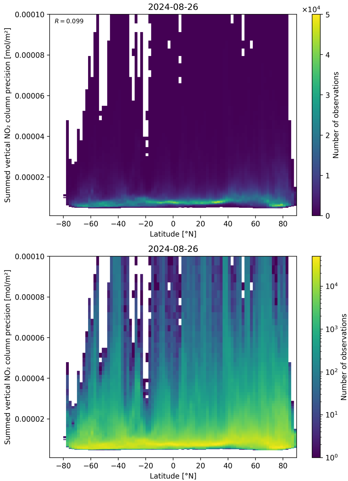
Figure 89: Scatter density plot of “Latitude” against “Summed vertical NO 2 column precision” for 2024-08-25 to 2024-08-27.
