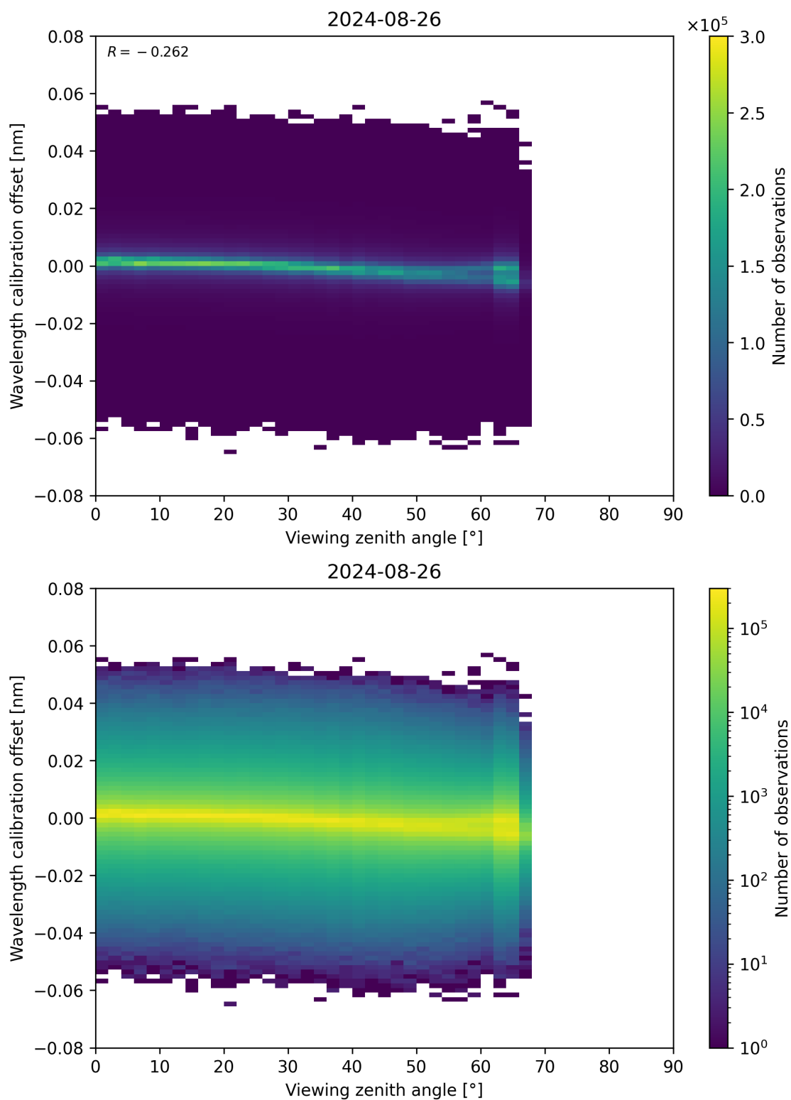
Figure 173: Scatter density plot of “Viewing zenith angle” against “Wavelength calibration offset” for 2024-08-25 to 2024-08-27.
