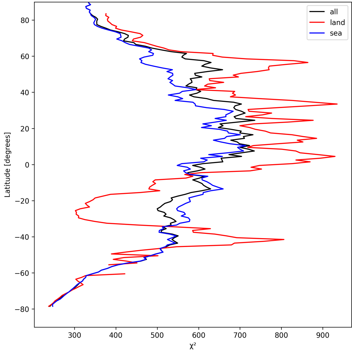
Figure 25: Zonal average of “ \chi^2 ” for 2024-08-25 to 2024-08-27.
