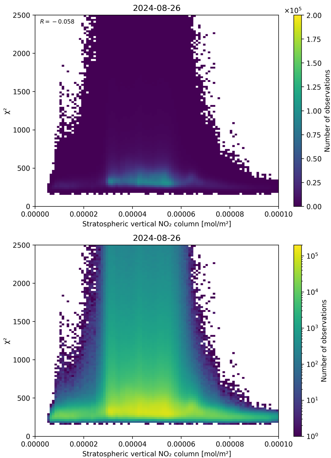
Figure 97: Scatter density plot of “Stratospheric vertical NO 2 column” against “ \chi^2 ” for 2024-08-25 to 2024-08-27.
