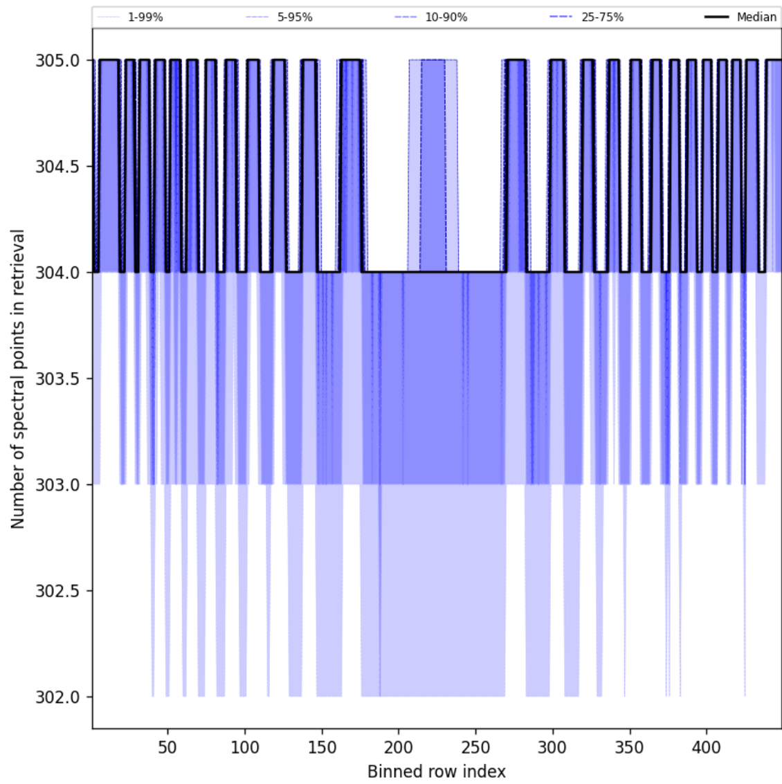
Figure 50: Along track statistics of “Number of spectral points in retrieval” for 2024-08-25 to 2024-08-27
