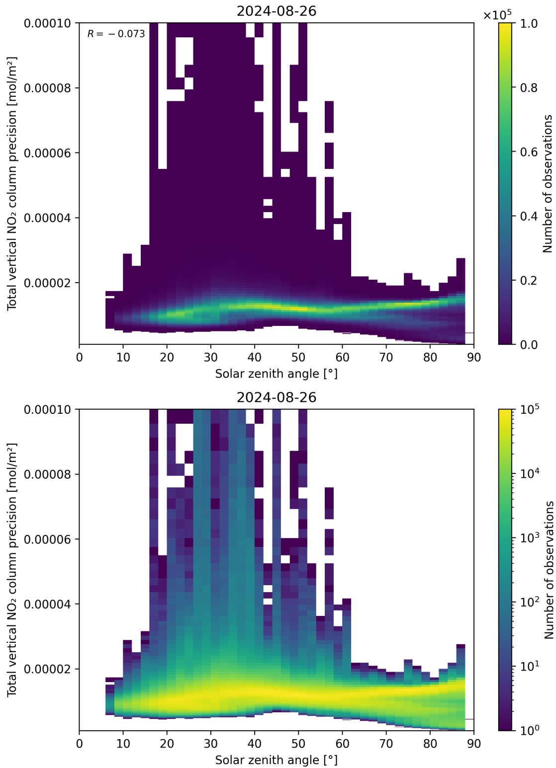
Figure 154: Scatter density plot of “Solar zenith angle” against “Total vertical NO 2 column precision” for 2024-08-25 to 2024-08-27.
