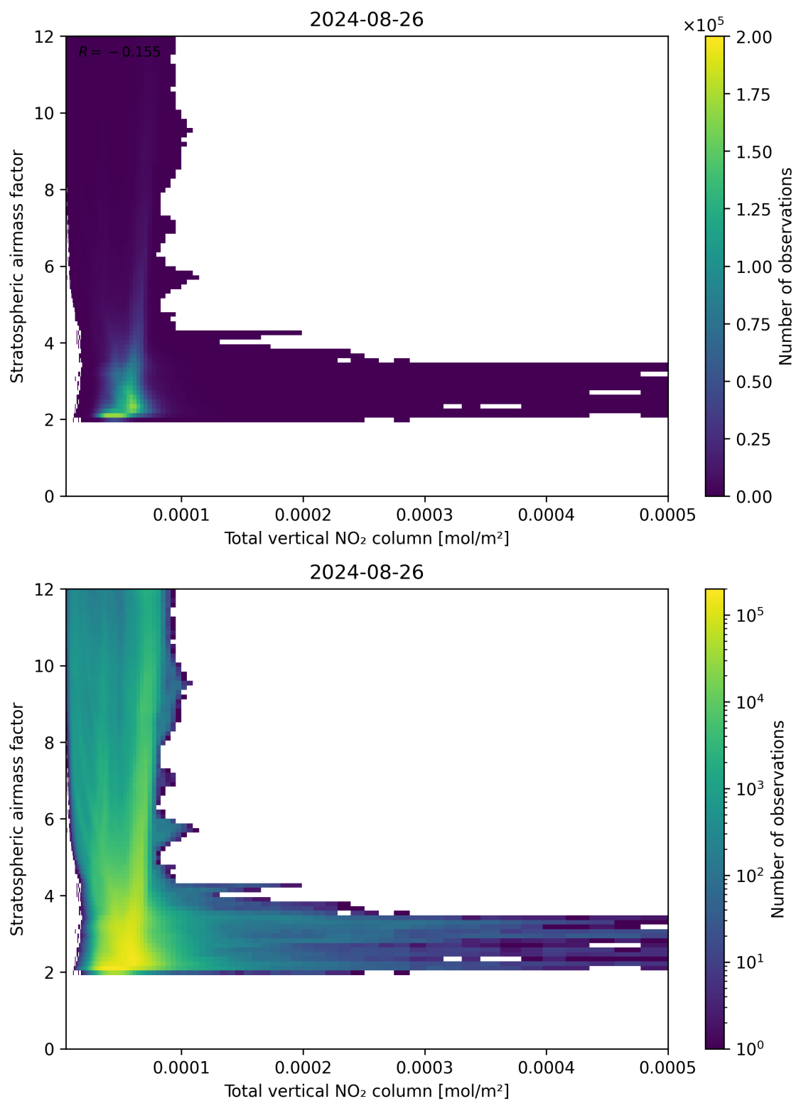
Figure 110: Scatter density plot of “Total vertical NO 2 column” against “Stratospheric airmass factor” for 2024-08-25 to 2024-08-27.
