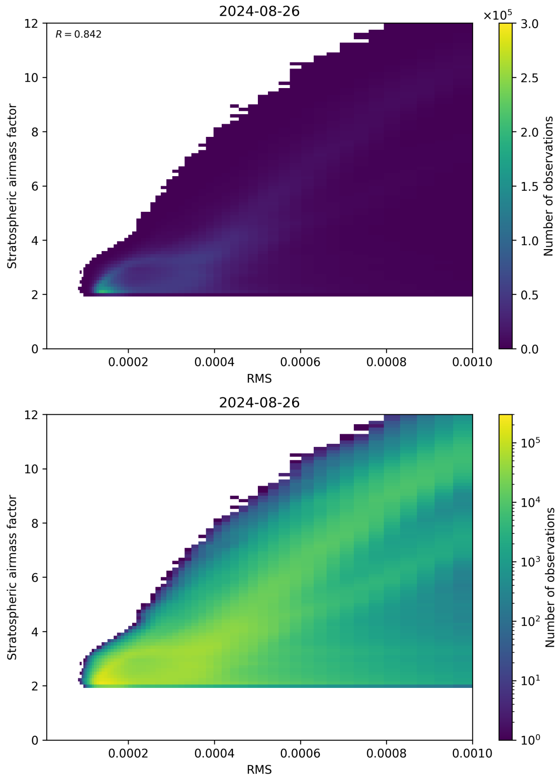
Figure 144: Scatter density plot of “RMS” against “Stratospheric airmass factor” for 2024-08-25 to 2024-08-27.
