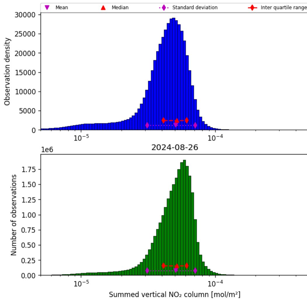
Figure 40: Histogram of “Summed vertical NO 2 column” for 2024-08-25 to 2024-08-27
