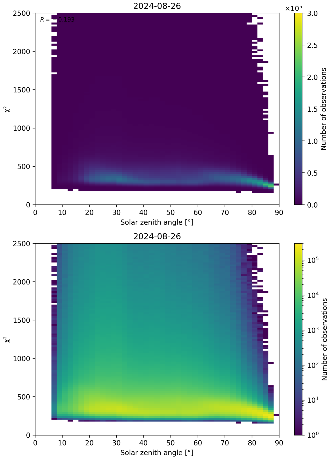
Figure 148: Scatter density plot of “Solar zenith angle” against “ \chi^2 ” for 2024-08-25 to 2024-08-27.
