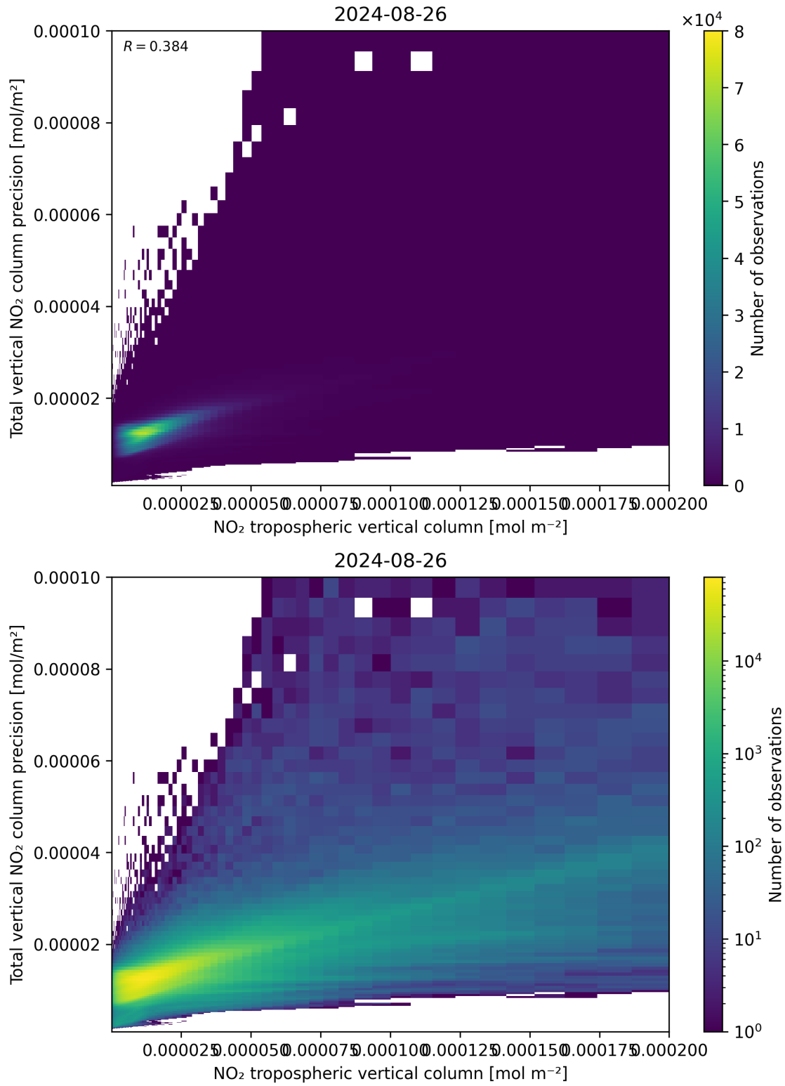
Figure 129: Scatter density plot of “NO 2 tropospheric vertical column” against “Total vertical NO 2 column precision” for 2024-08-25 to 2024-08-27.
