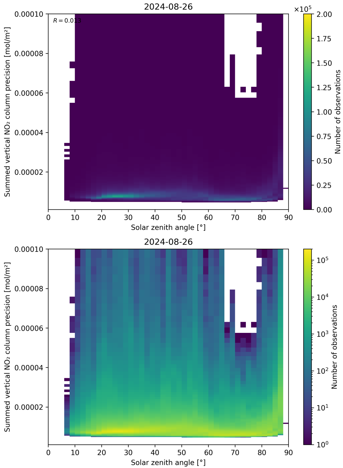
Figure 152: Scatter density plot of “Solar zenith angle” against “Summed vertical NO 2 column precision” for 2024-08-25 to 2024-08-27.
