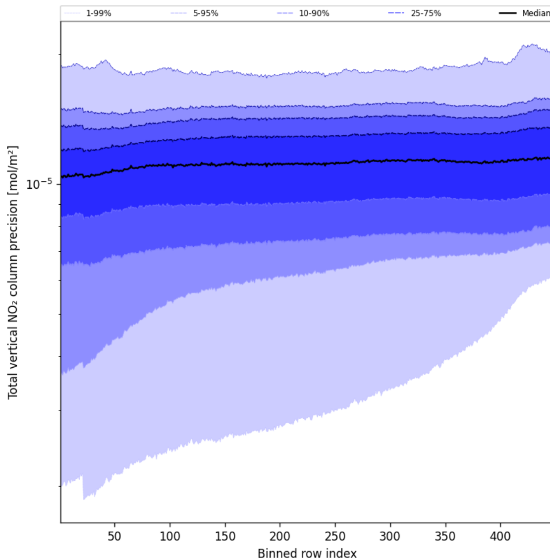
Figure 56: Along track statistics of “Total vertical NO 2 column precision” for 2024-08-25 to 2024-08-27
