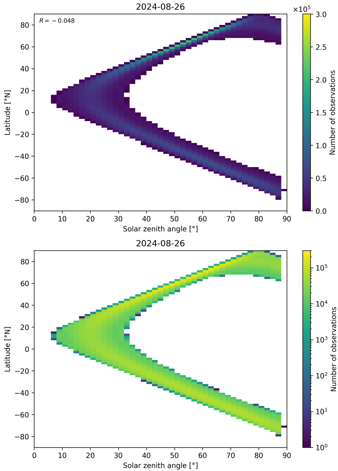
Figure 149: Scatter density plot of “Solar zenith angle” against “Latitude” for 2024-08-25 to 2024-08-27.
