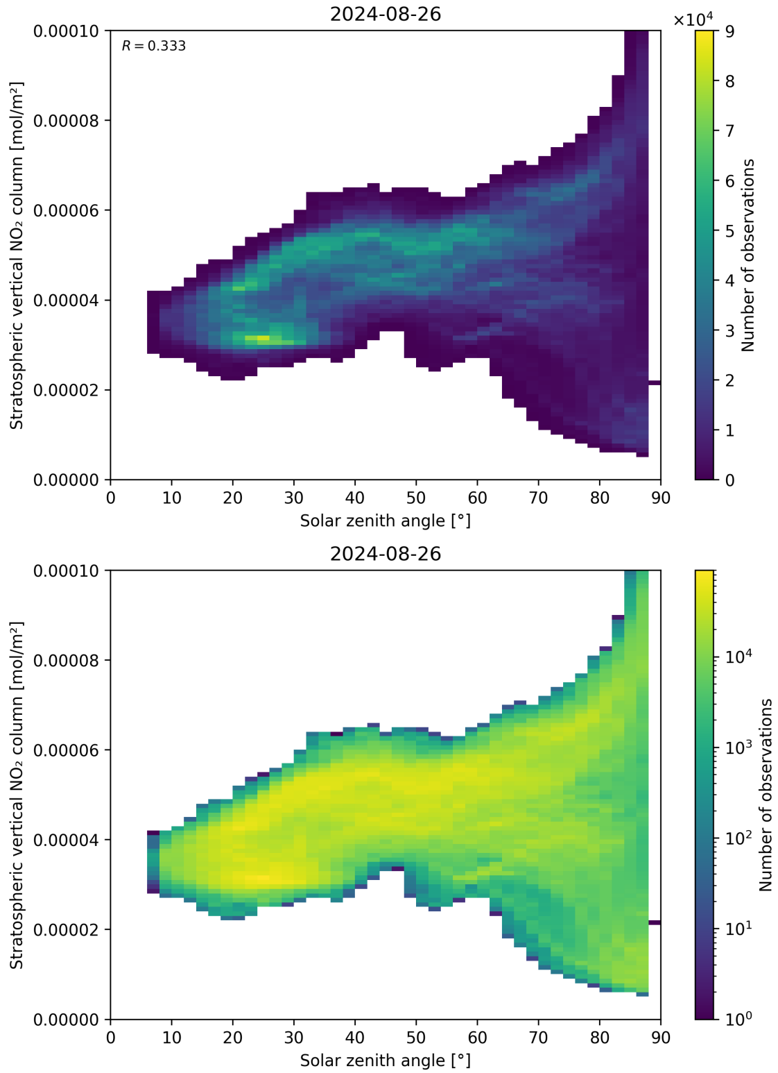
Figure 150: Scatter density plot of “Solar zenith angle” against “Stratospheric vertical NO 2 column” for 2024-08-25 to 2024-08-27.
