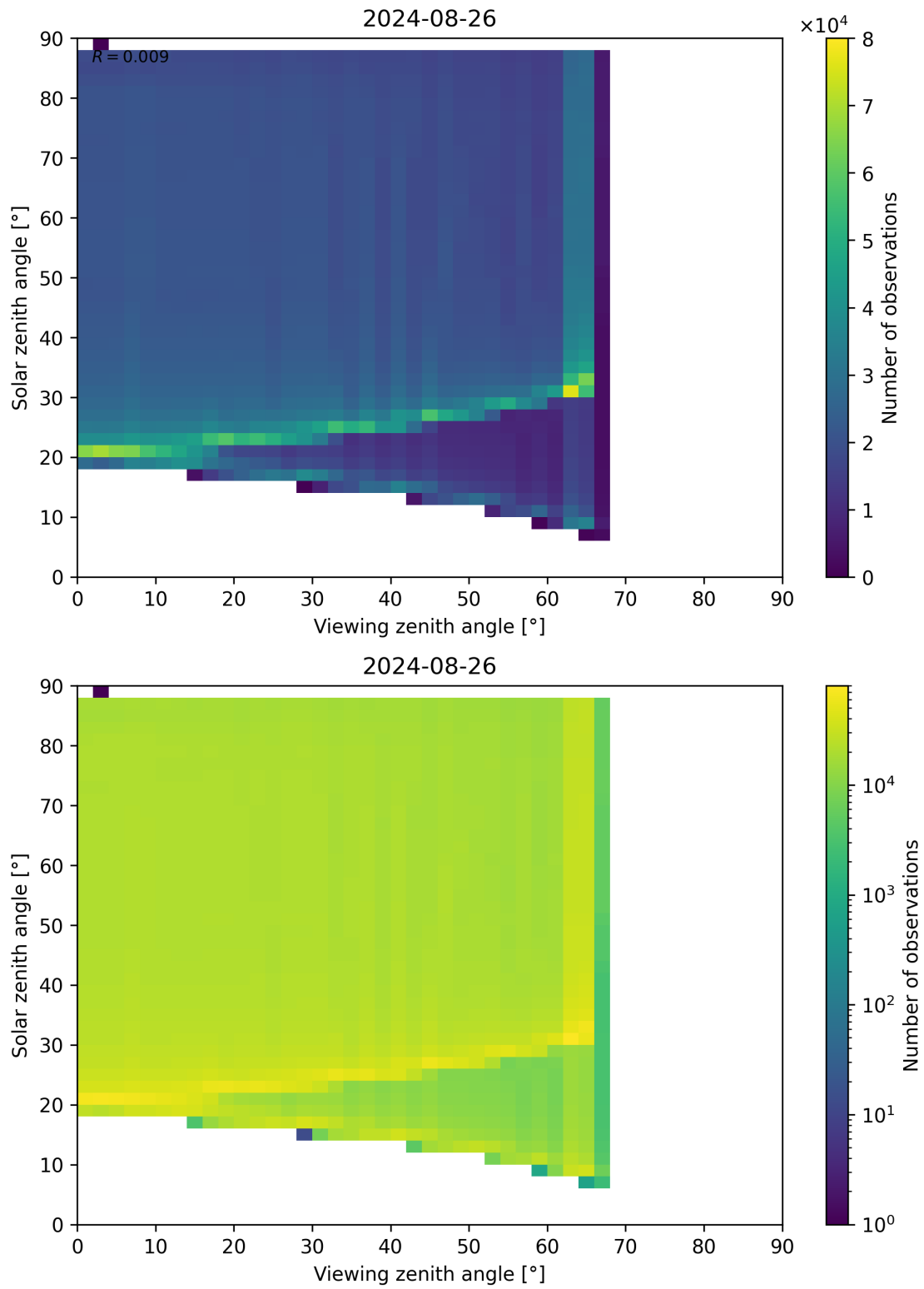
Figure 172: Scatter density plot of “Viewing zenith angle” against “Solar zenith angle” for 2024-08-25 to 2024-08-27.
