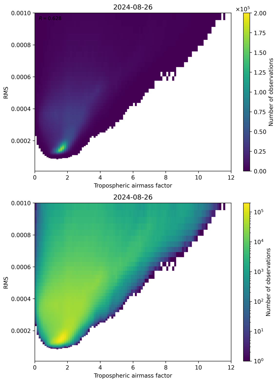
Figure 79: Scatter density plot of “Tropospheric airmass factor” against “RMS” for 2024-08-25 to 2024-08-27.
