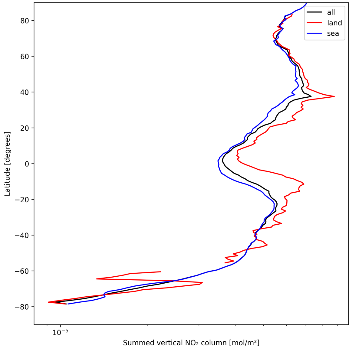
Figure 23: Zonal average of “Summed vertical NO 2 column” for 2024-08-25 to 2024-08-27.
