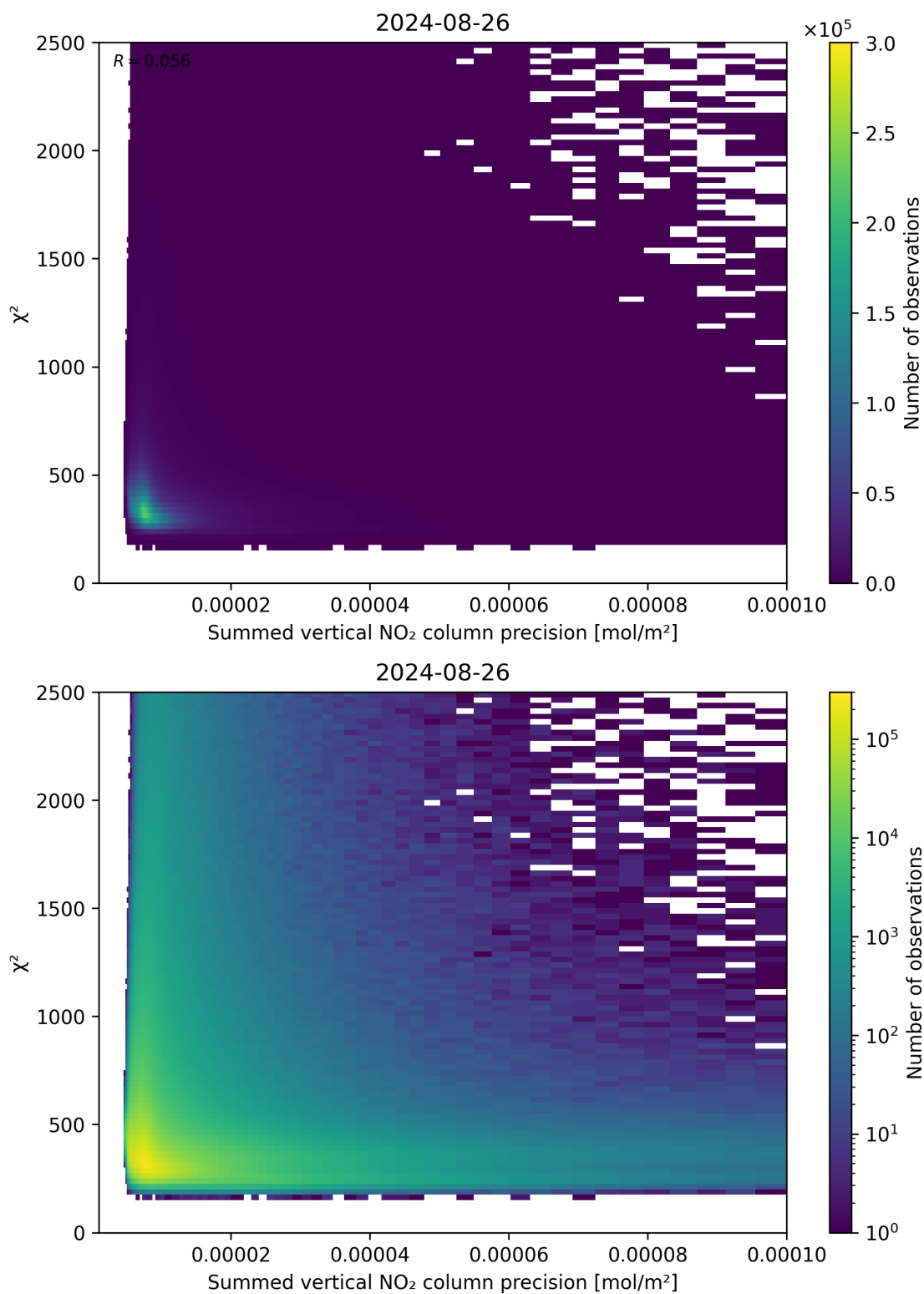
Figure 107: Scatter density plot of “Summed vertical NO 2 column precision” against “ \chi^2 ” for 2024-08-25 to 2024-08-27.
