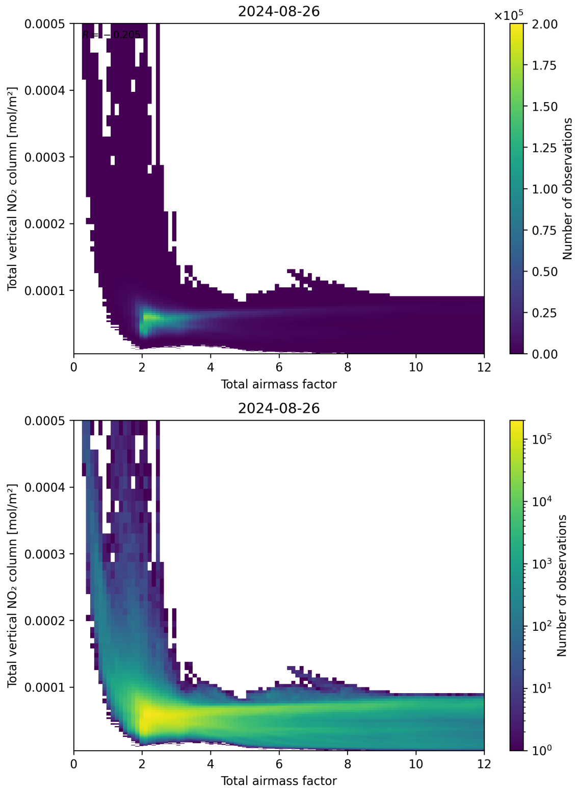
Figure 67: Scatter density plot of “Total airmass factor” against “Total vertical NO 2 column” for 2024-08-25 to 2024-08-27.
