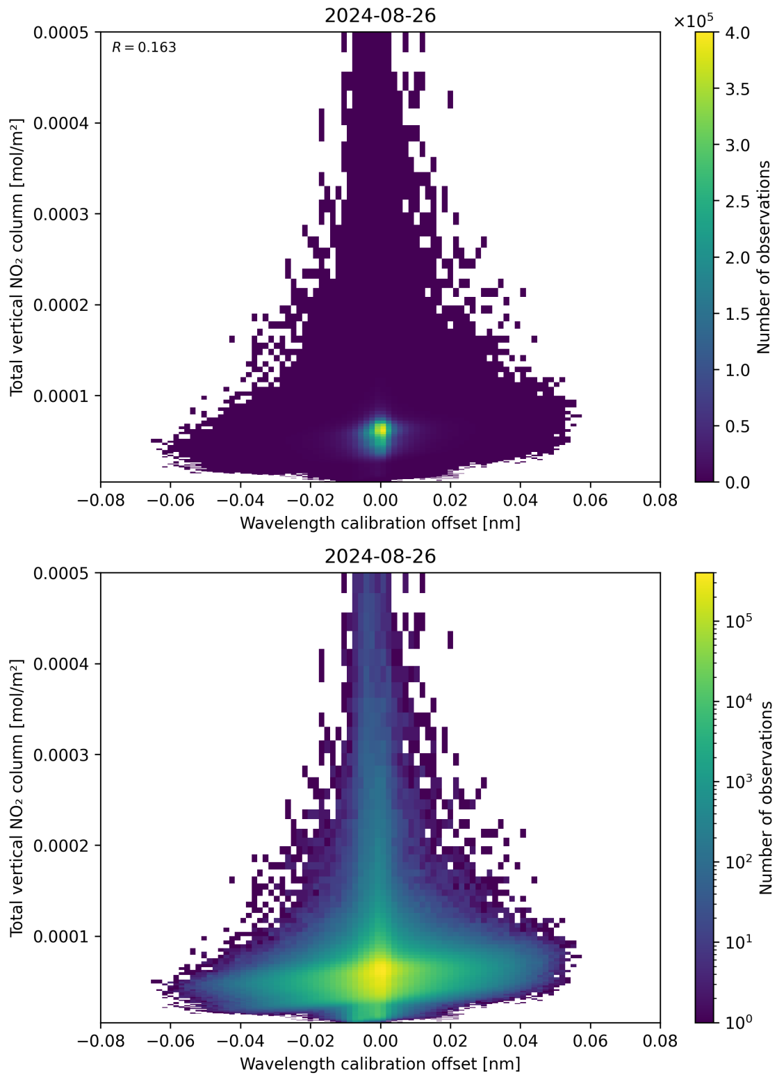
Figure 179: Scatter density plot of “Wavelength calibration offset” against “Total vertical NO 2 column” for 2024-08-25 to 2024-08-27.
