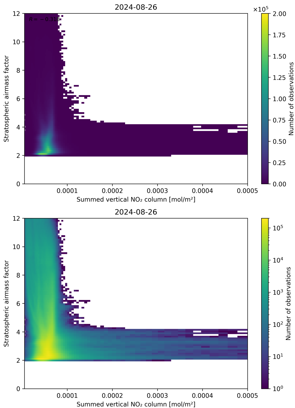
Figure 103: Scatter density plot of “Summed vertical NO 2 column” against “Stratospheric airmass factor” for 2024-08-25 to 2024-08-27.
