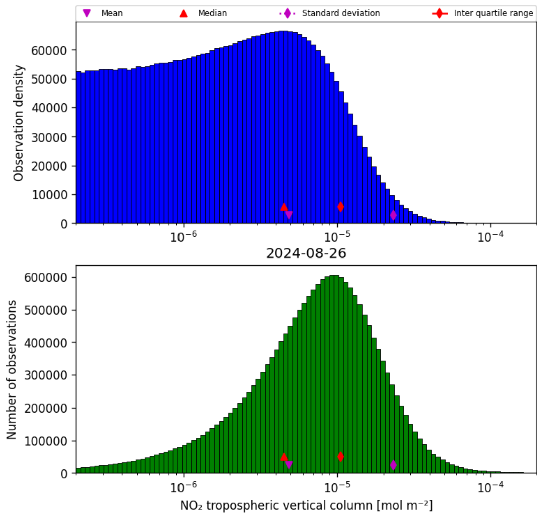
Figure 29: Histogram of “NO 2 tropospheric vertical column” for 2024-08-25 to 2024-08-27
