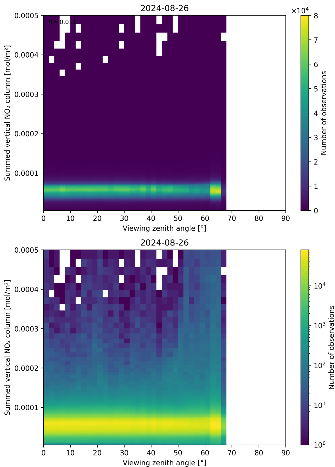
Figure 165: Scatter density plot of “Viewing zenith angle” against “Summed vertical NO 2 column” for 2024-08-25 to 2024-08-27.
