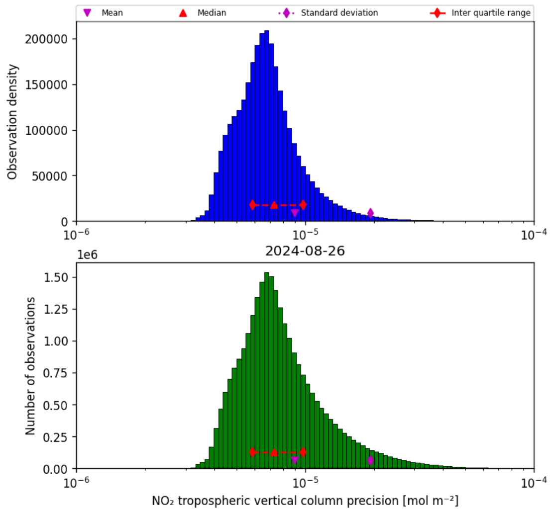
Figure 30: Histogram of “NO 2 tropospheric vertical column precision” for 2024-08-25 to 2024-08-27
