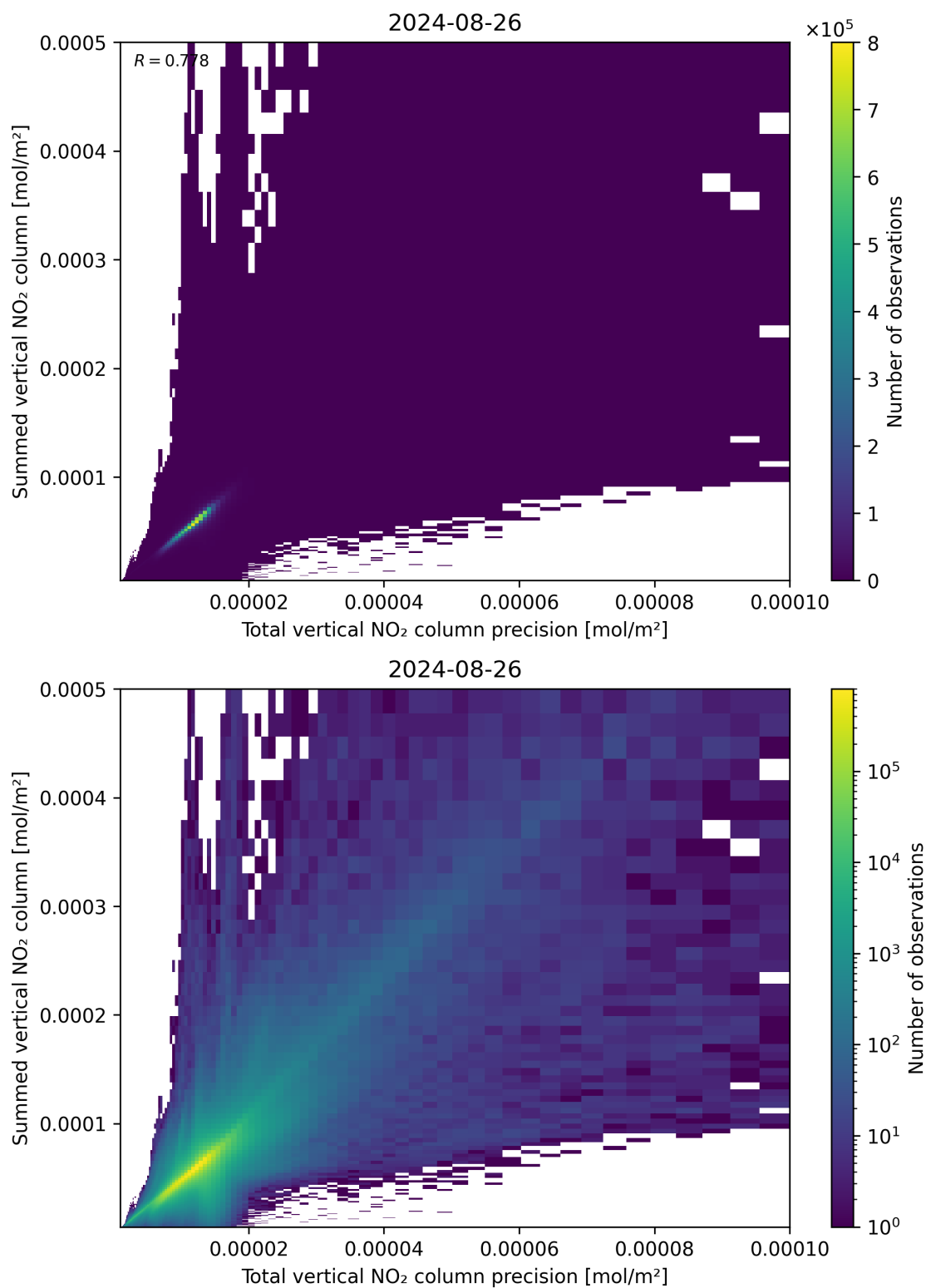
Figure 117: Scatter density plot of “Total vertical NO 2 column precision” against “Summed vertical NO 2 column” for 2024-08-25 to 2024-08-27.
