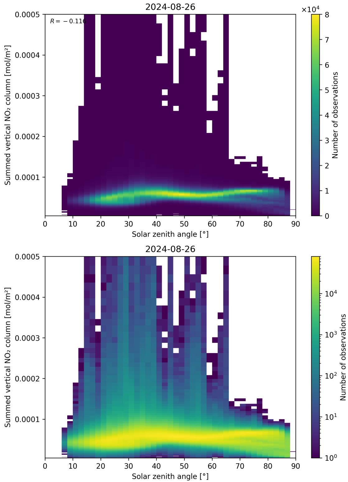
Figure 151: Scatter density plot of “Solar zenith angle” against “Summed vertical NO 2 column” for 2024-08-25 to 2024-08-27.
