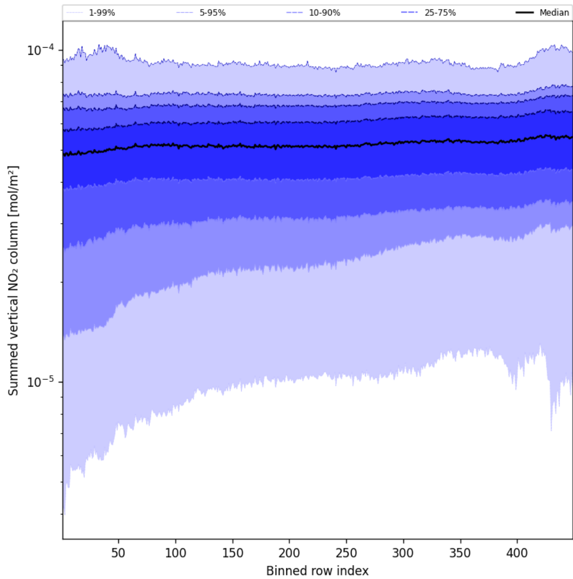
Figure 57: Along track statistics of “Summed vertical NO 2 column” for 2024-08-25 to 2024-08-27
