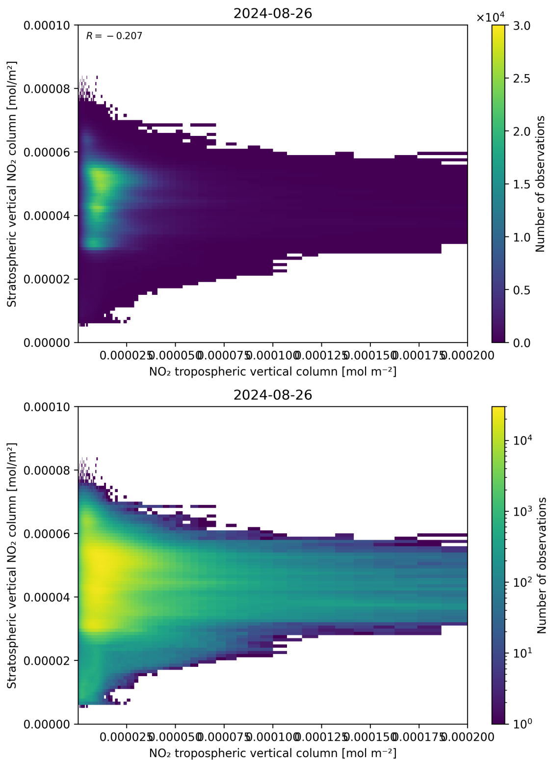
Figure 125: Scatter density plot of “NO 2 tropospheric vertical column” against “Stratospheric vertical NO 2 column” for 2024-08-25 to 2024-08-27.
