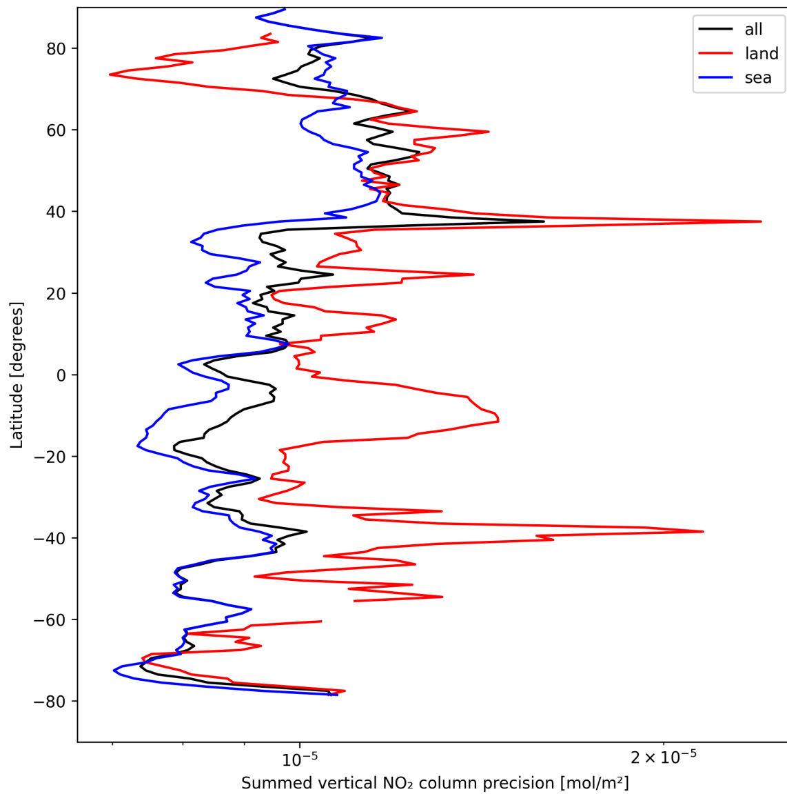
Figure 24: Zonal average of “Summed vertical NO 2 column precision” for 2024-08-25 to 2024-08-27.
