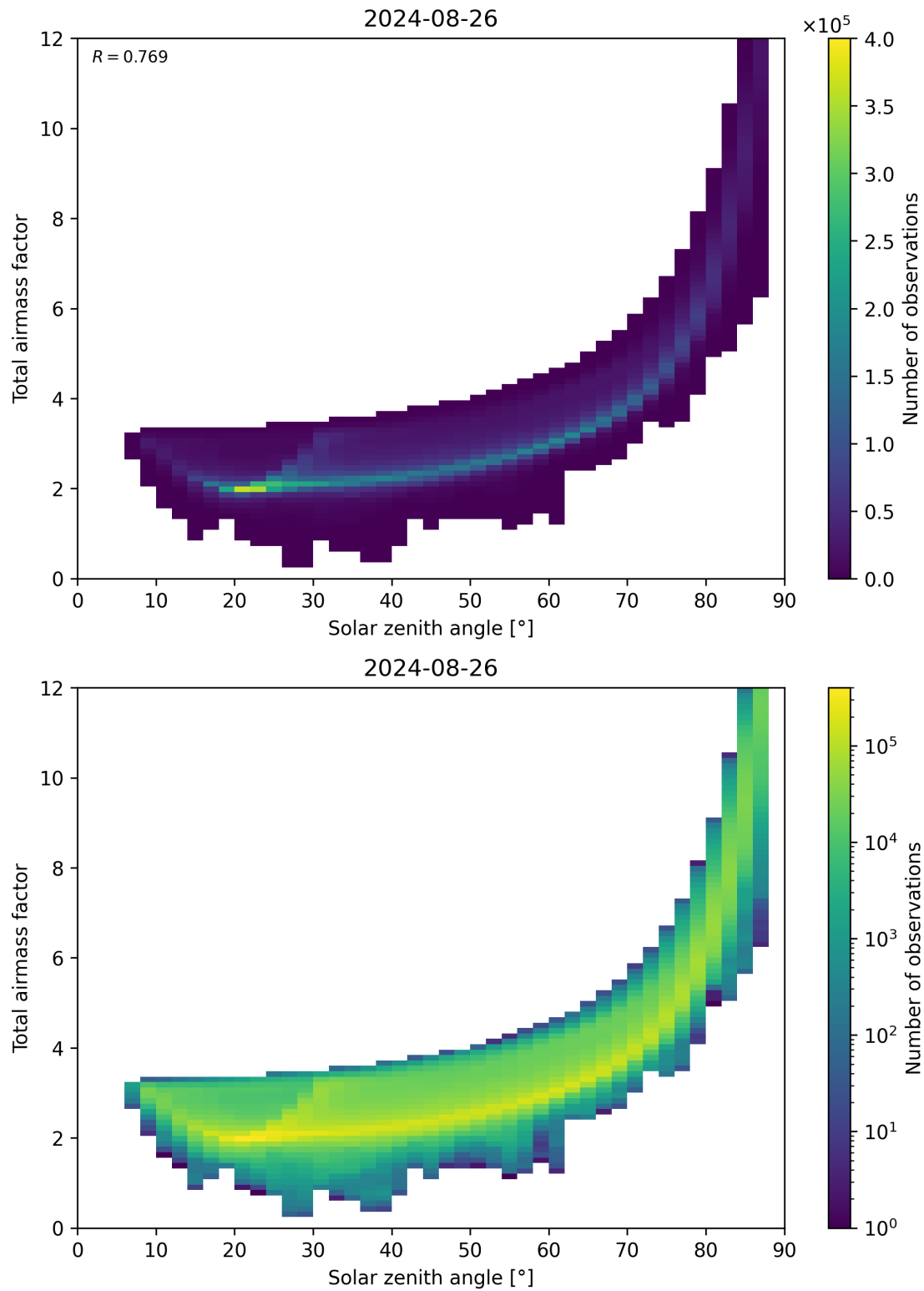
Figure 146: Scatter density plot of “Solar zenith angle” against “Total air mass factor” for 2024-08-25 to 2024-08-27.
