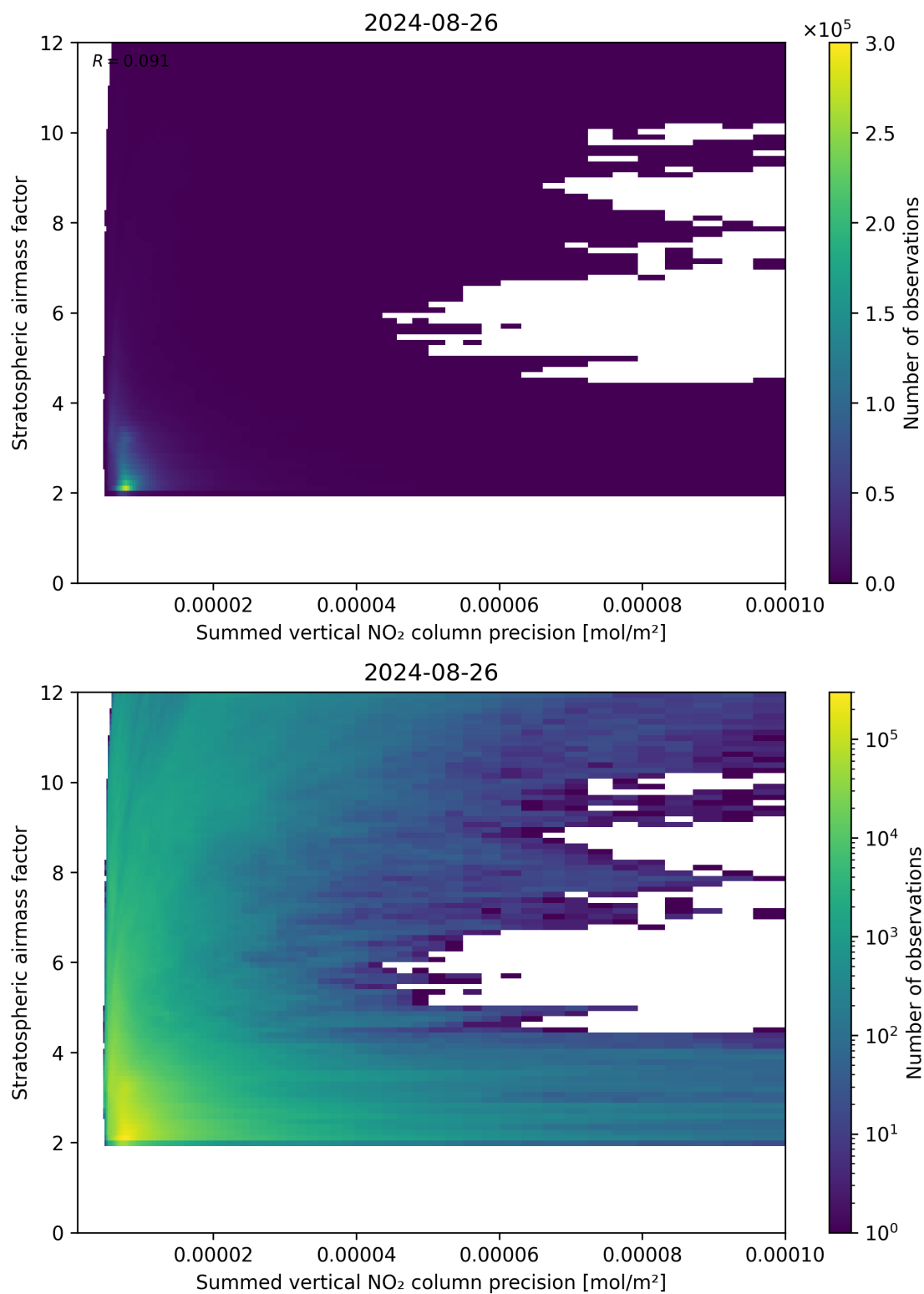
Figure 106: Scatter density plot of “Summed vertical NO 2 column precision” against “Stratospheric airmass factor” for 2024-08-25 to 2024-08-27.
