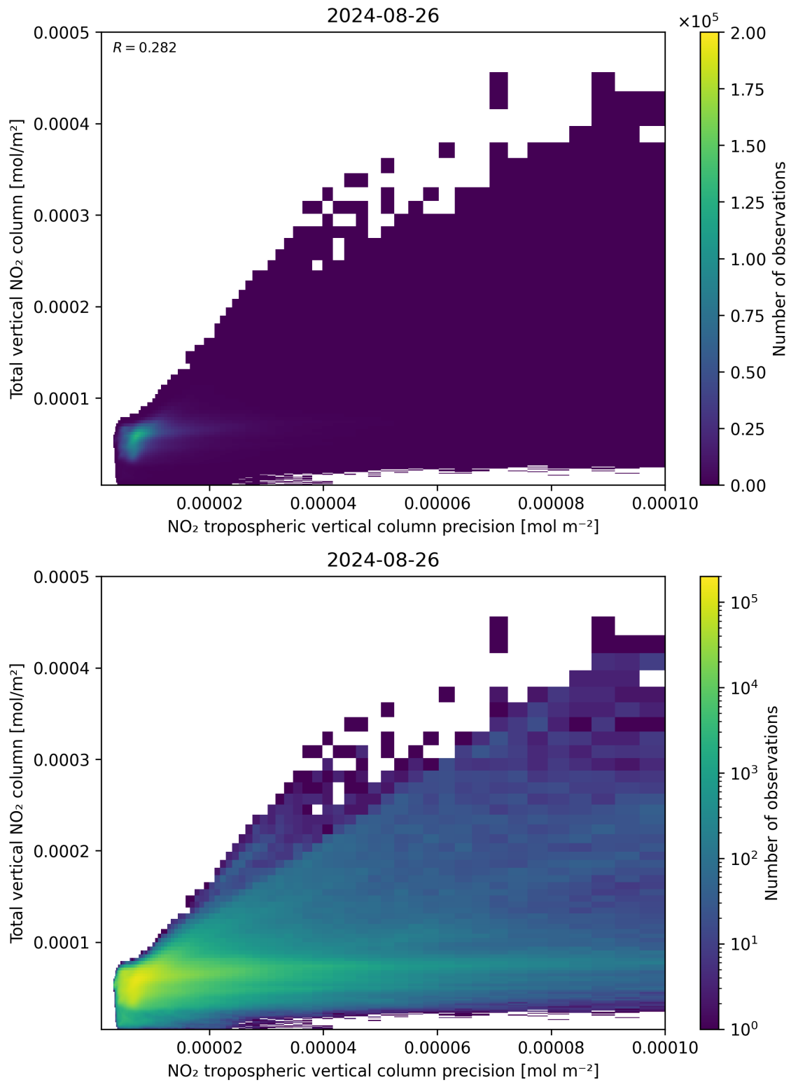
Figure 138: Scatter density plot of “NO 2 tropospheric vertical column precision” against “Total vertical NO 2 column” for 2024-08-25 to 2024-08-27.
