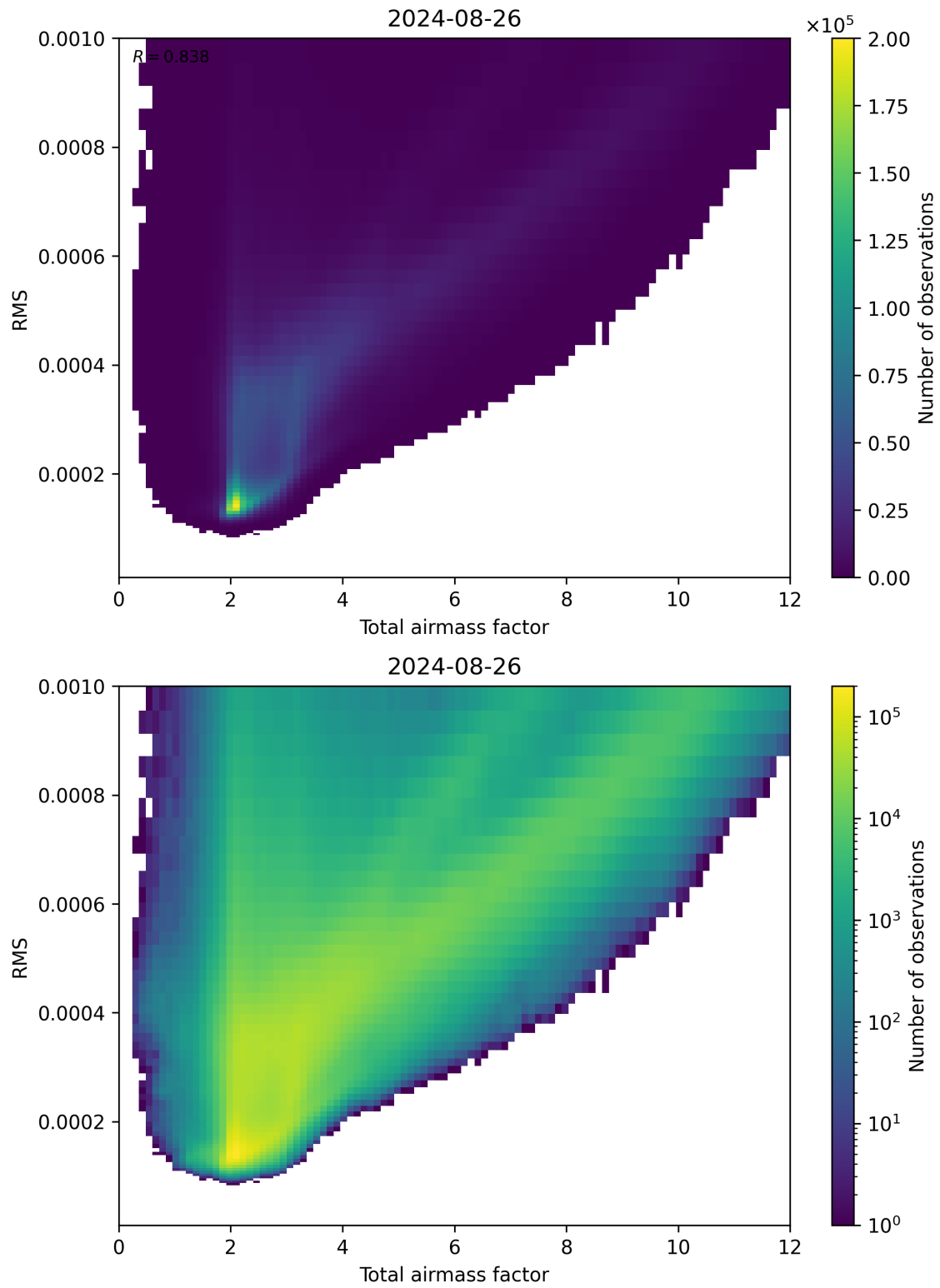
Figure 69: Scatter density plot of “Total airmass factor” against “RMS” for 2024-08-25 to 2024-08-27.
