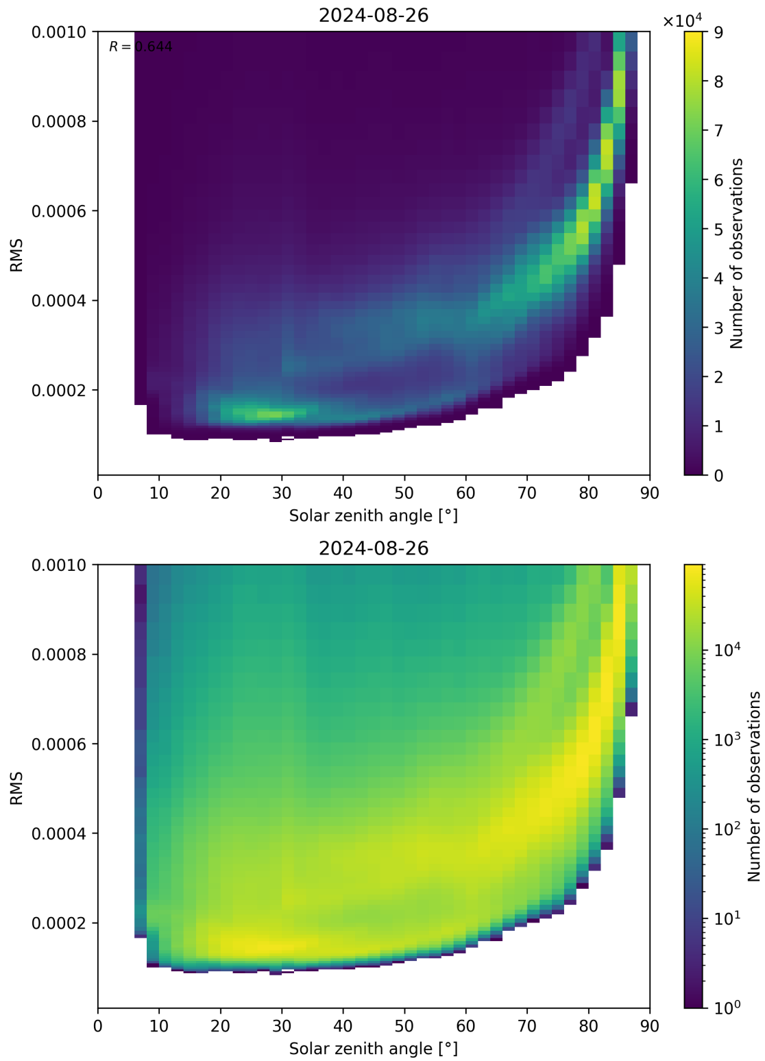
Figure 157: Scatter density plot of “Solar zenith angle” against “RMS” for 2024-08-25 to 2024-08-27.
