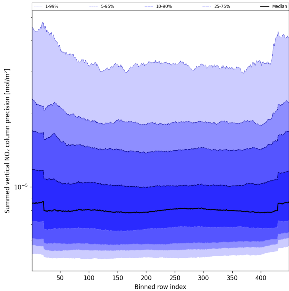
Figure 58: Along track statistics of “Summed vertical NO 2 column precision” for 2024-08-25 to 2024-08-27
