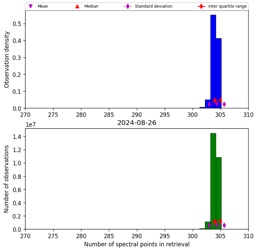
Figure 33: Histogram of “Number of spectral points in retrieval” for 2024-08-25 to 2024-08-27
