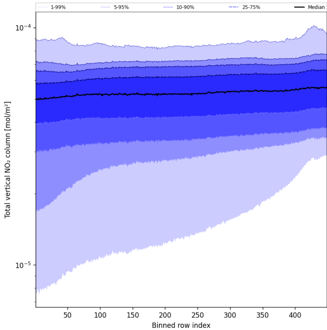
Figure 55: Along track statistics of “Total vertical NO 2 column” for 2024-08-25 to 2024-08-27
