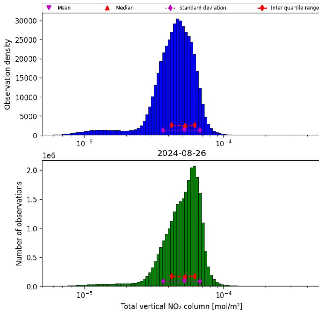
Figure 38: Histogram of “Total vertical NO 2 column” for 2024-08-25 to 2024-08-27
