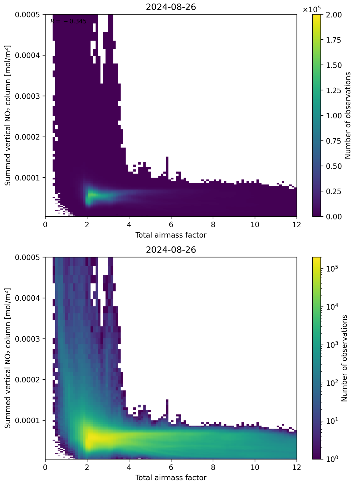
Figure 65: Scatter density plot of “Total airmass factor” against “Summed vertical NO 2 column” for 2024-08-25 to 2024-08-27.
