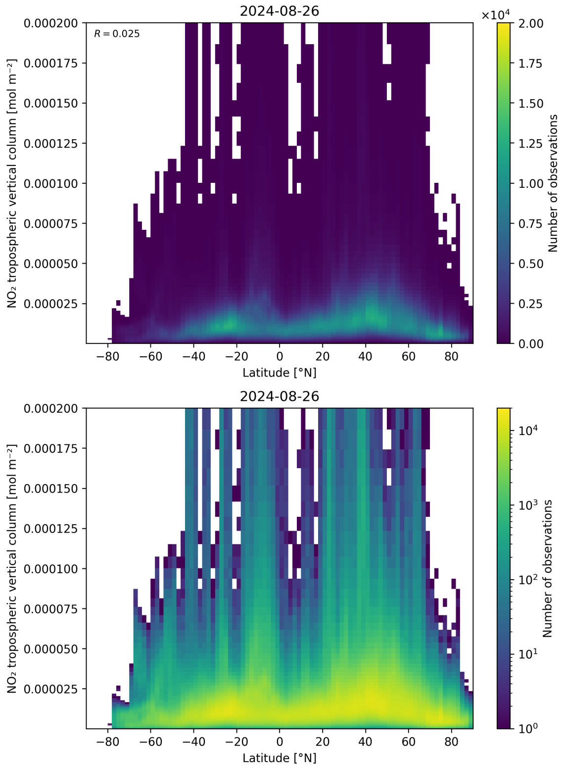
Figure 92: Scatter density plot of “Latitude” against “NO 2 tropospheric vertical column” for 2024-08-25 to 2024-08-27.
