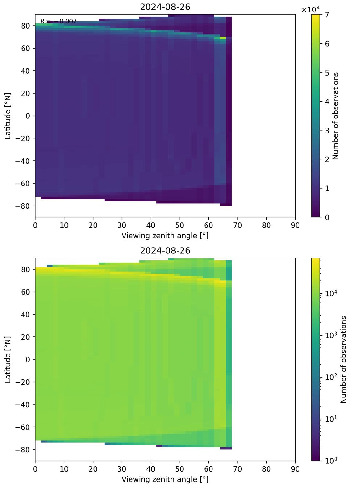
Figure 163: Scatter density plot of “Viewing zenith angle” against “Latitude” for 2024-08-25 to 2024-08-27.
