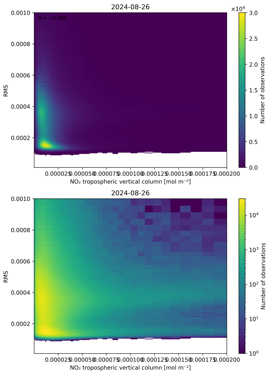
Figure 142: Scatter density plot of “NO 2 tropospheric vertical column” against “RMS” for 2024-08-25 to 2024-08-27.
