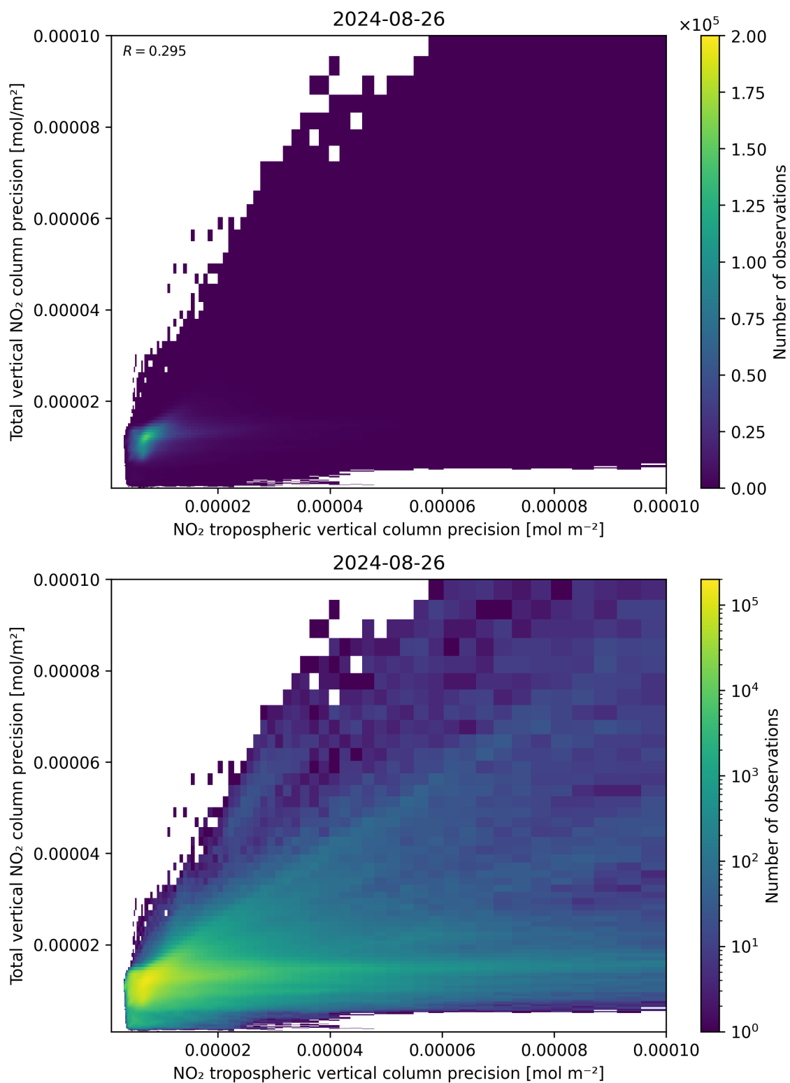
Figure 139: Scatter density plot of “NO 2 tropospheric vertical column precision” against “Total vertical NO 2 column precision” for 2024-08-25 to 2024-08-27.
