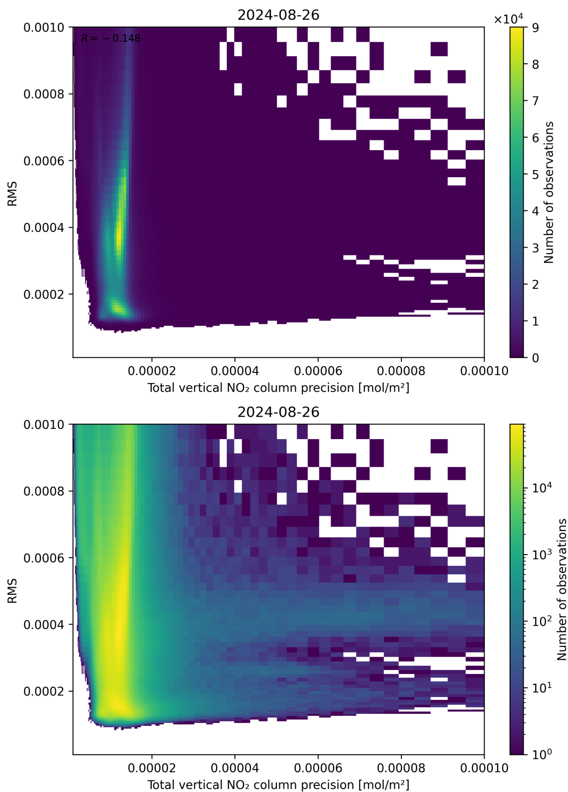
Figure 119: Scatter density plot of “Total vertical NO 2 column precision” against “RMS” for 2024-08-25 to 2024-08-27.
