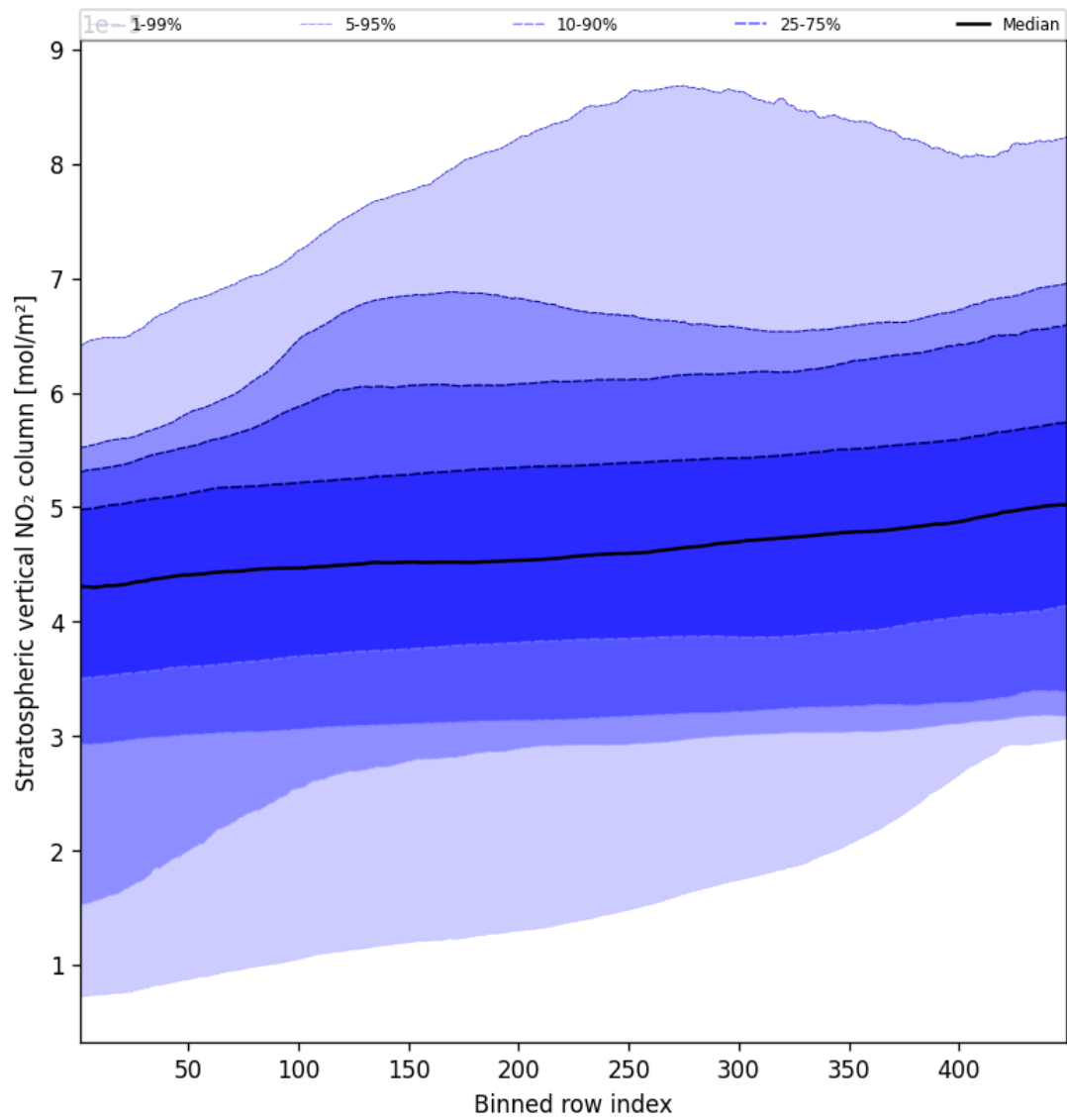
Figure 53: Along track statistics of “Stratospheric vertical NO 2 column” for 2024-08-25 to 2024-08-27
