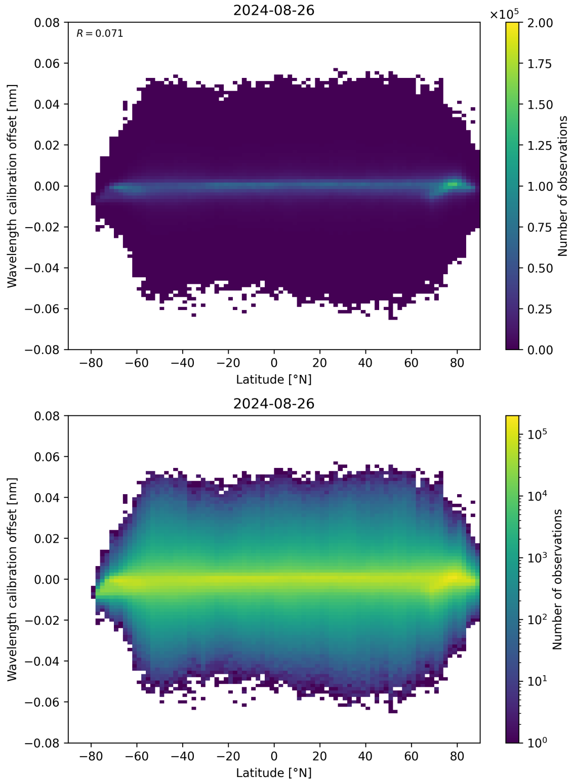
Figure 95: Scatter density plot of “Latitude” against “Wavelength calibration offset” for 2024-08-25 to 2024-08-27.
