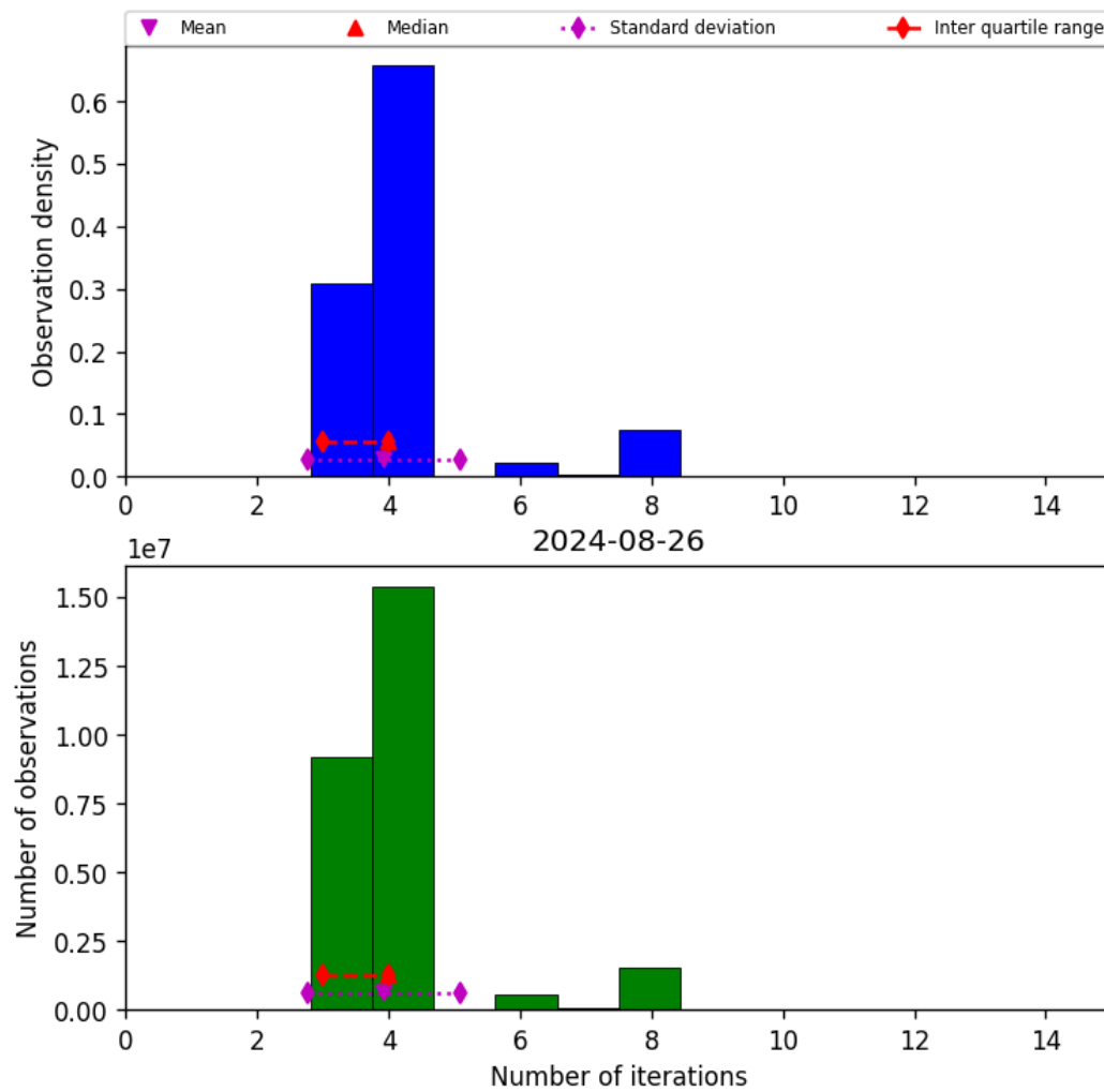
Figure 34: Histogram of “Number of iterations” for 2024-08-25 to 2024-08-27
