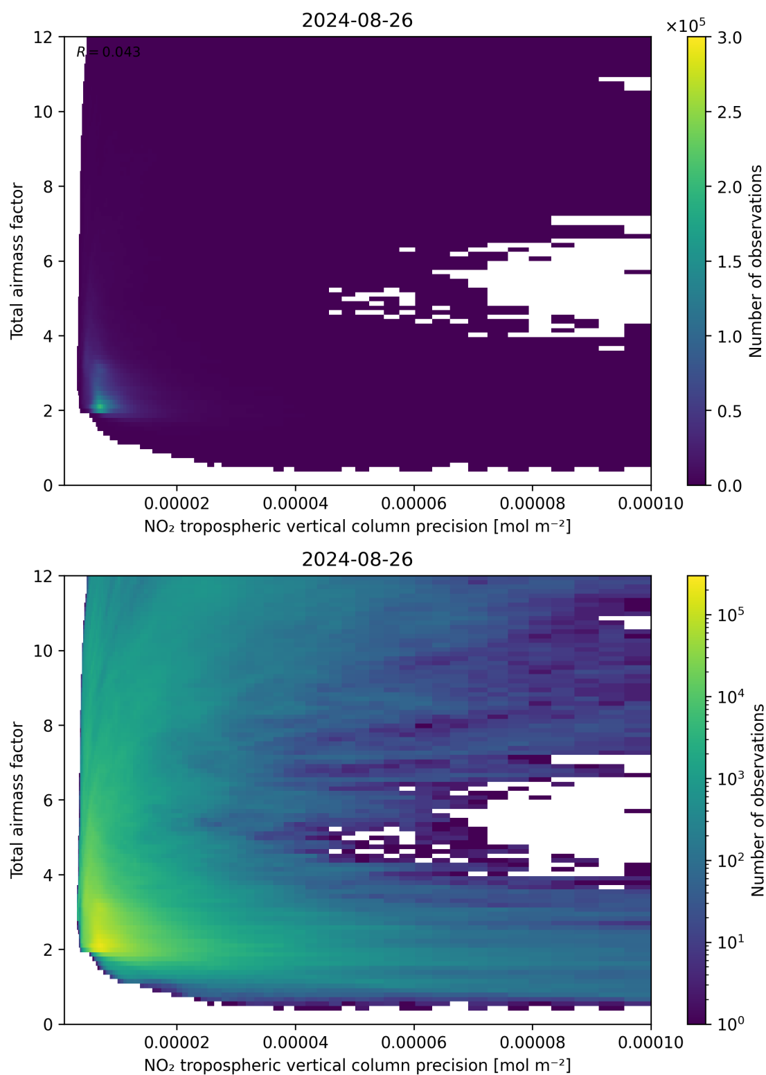
Figure 132: Scatter density plot of “NO 2 tropospheric vertical column precision” against “Total air mass factor” for 2024-08-25 to 2024-08-27.
