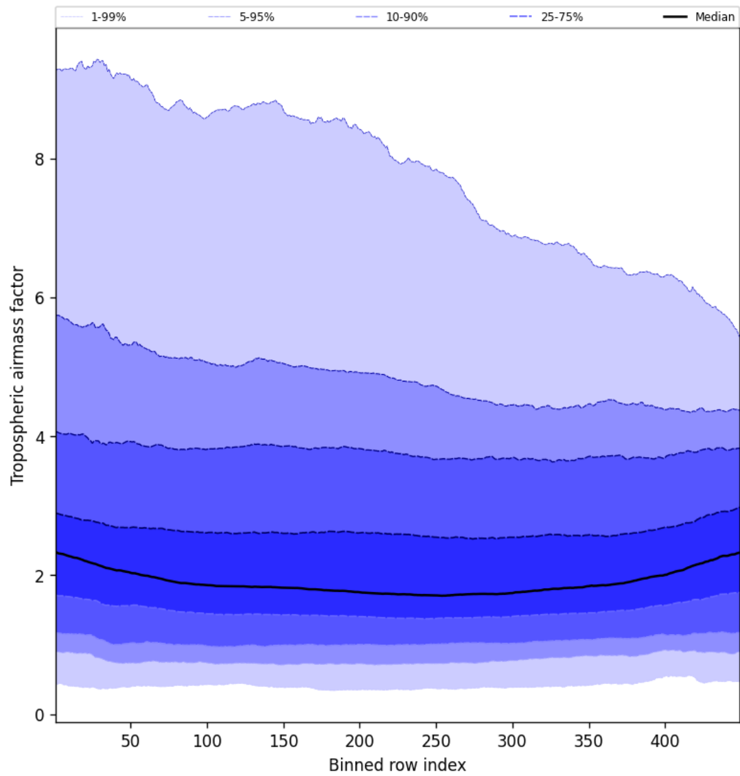
Figure 48: Along track statistics of “Tropospheric air mass factor” for 2024-08-25 to 2024-08-27
