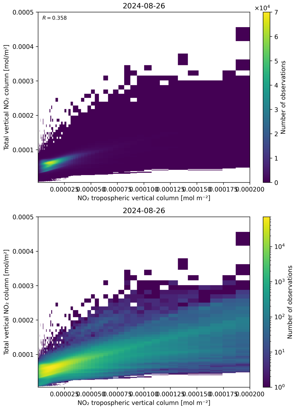
Figure 128: Scatter density plot of “NO 2 tropospheric vertical column” against “Total vertical NO 2 column” for 2024-08-25 to 2024-08-27.
