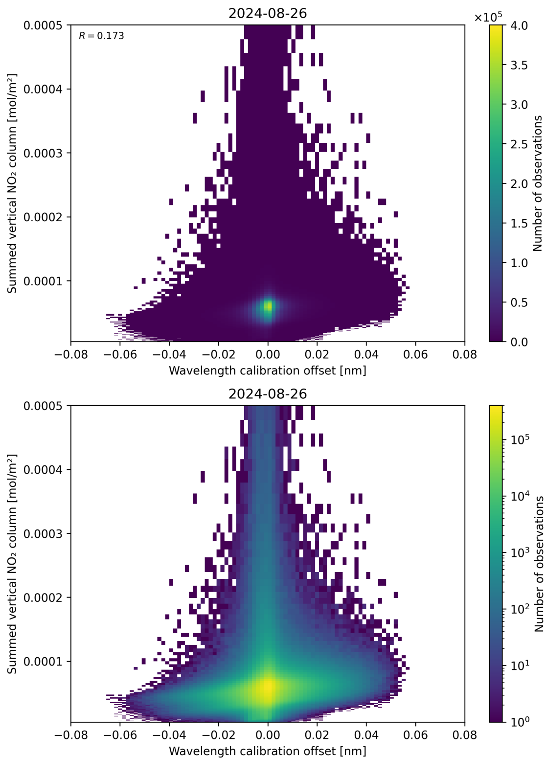
Figure 177: Scatter density plot of “Wavelength calibration offset” against “Summed vertical NO 2 column” for 2024-08-25 to 2024-08-27.
