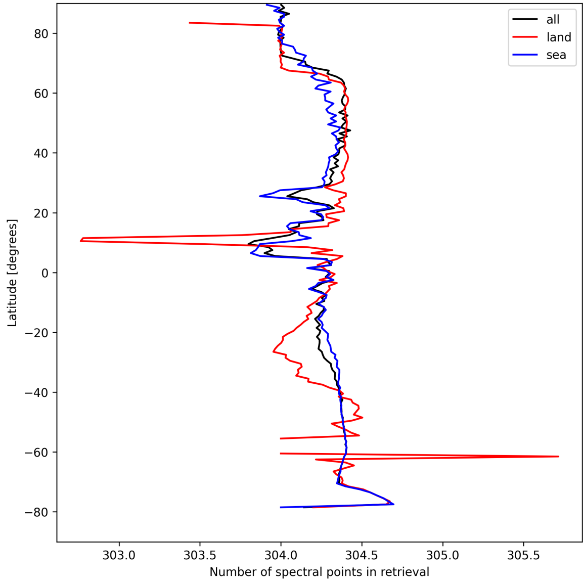
Figure 16: Zonal average of “Number of spectral points in retrieval” for 2024-08-25 to 2024-08-27.
