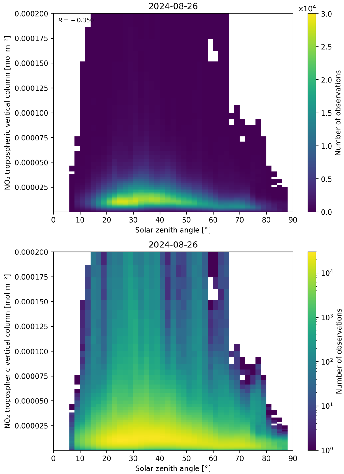
Figure 155: Scatter density plot of “Solar zenith angle” against “NO 2 tropospheric vertical column” for 2024-08-25 to 2024-08-27.
