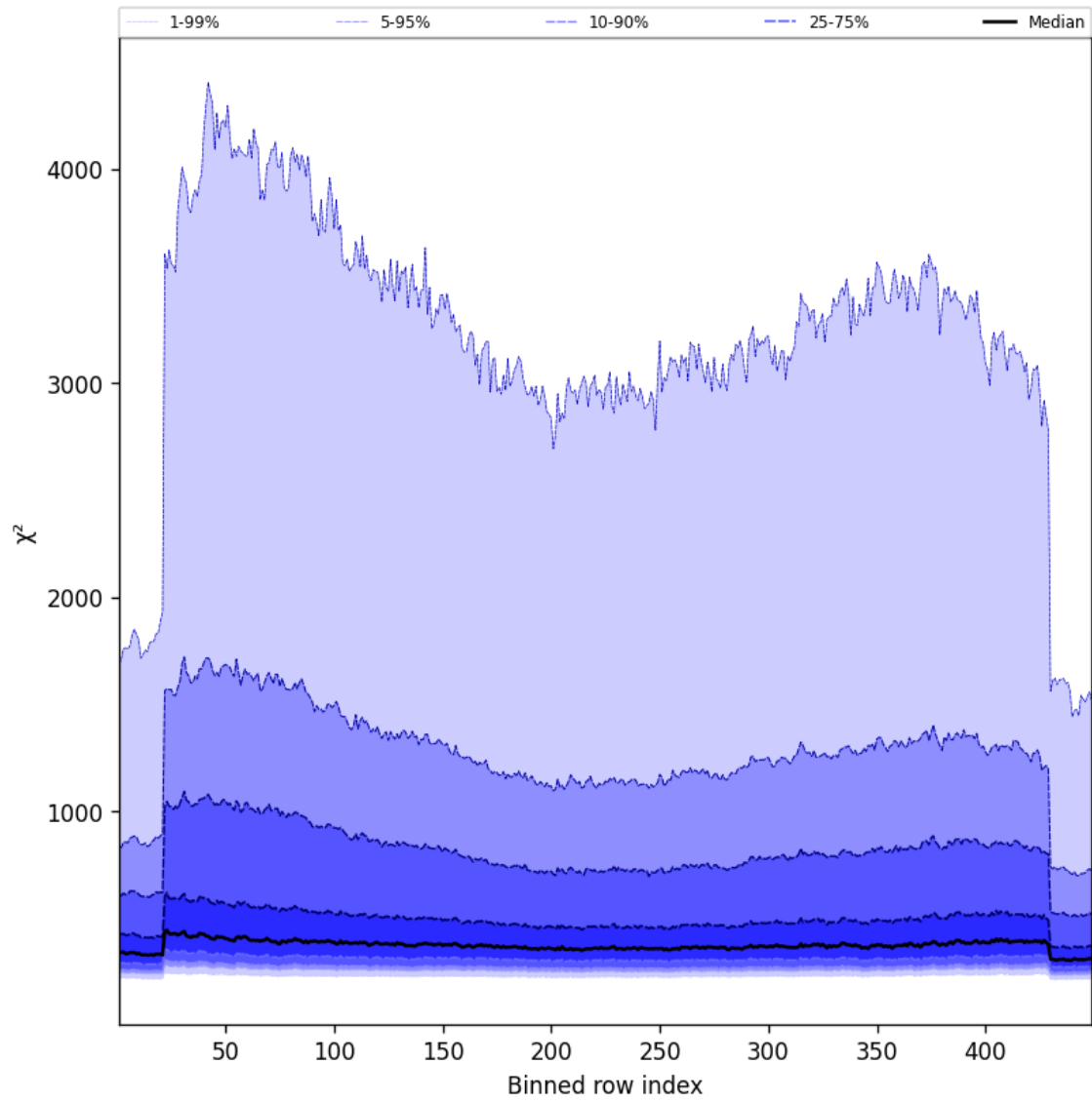
Figure 59: Along track statistics of “ \chi^2 ” for 2024-08-25 to 2024-08-27
