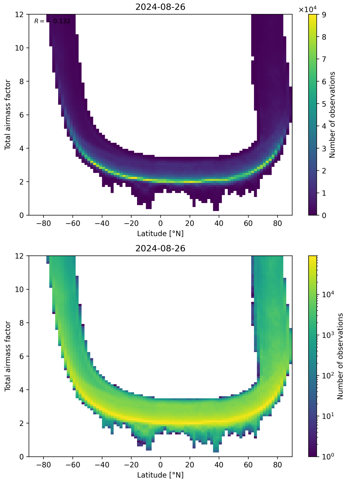
Figure 84: Scatter density plot of “Latitude” against “Total airmass factor” for 2024-08-25 to 2024-08-27.
