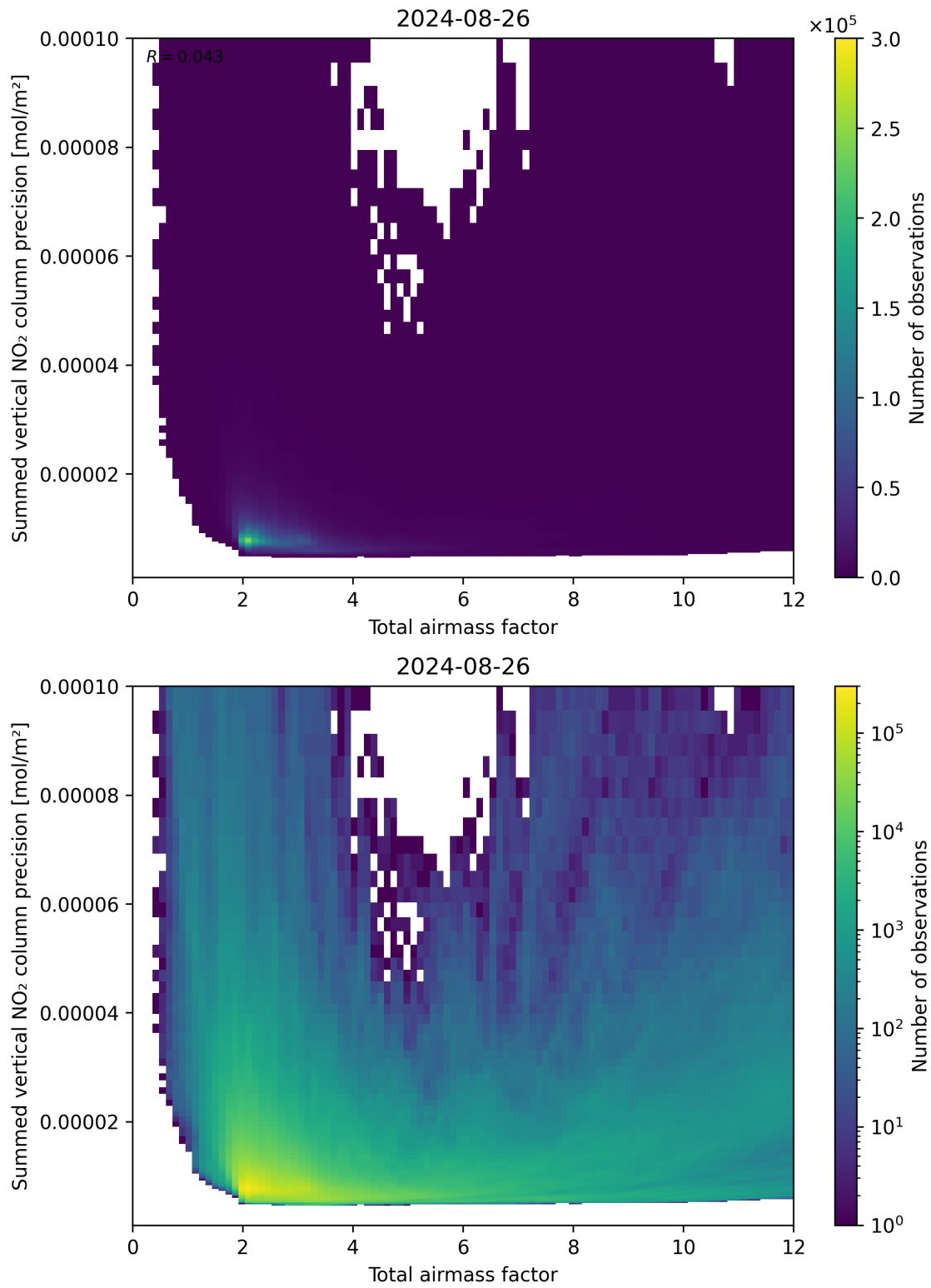
Figure 66: Scatter density plot of “Total airmass factor” against “Summed vertical NO 2 column precision” for 2024-08-25 to 2024-08-27.
