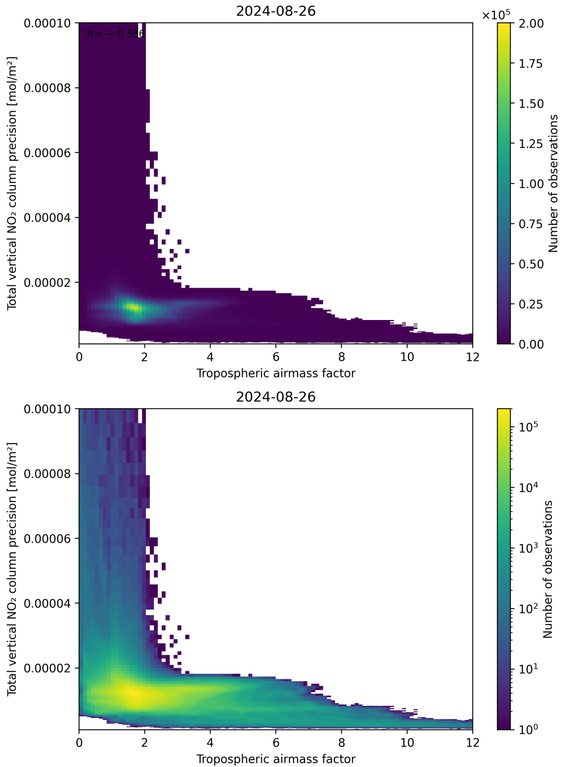
Figure 78: Scatter density plot of “Tropospheric air mass factor” against “Total vertical NO 2 column precision” for 2024-08-25 to 2024-08-27.
