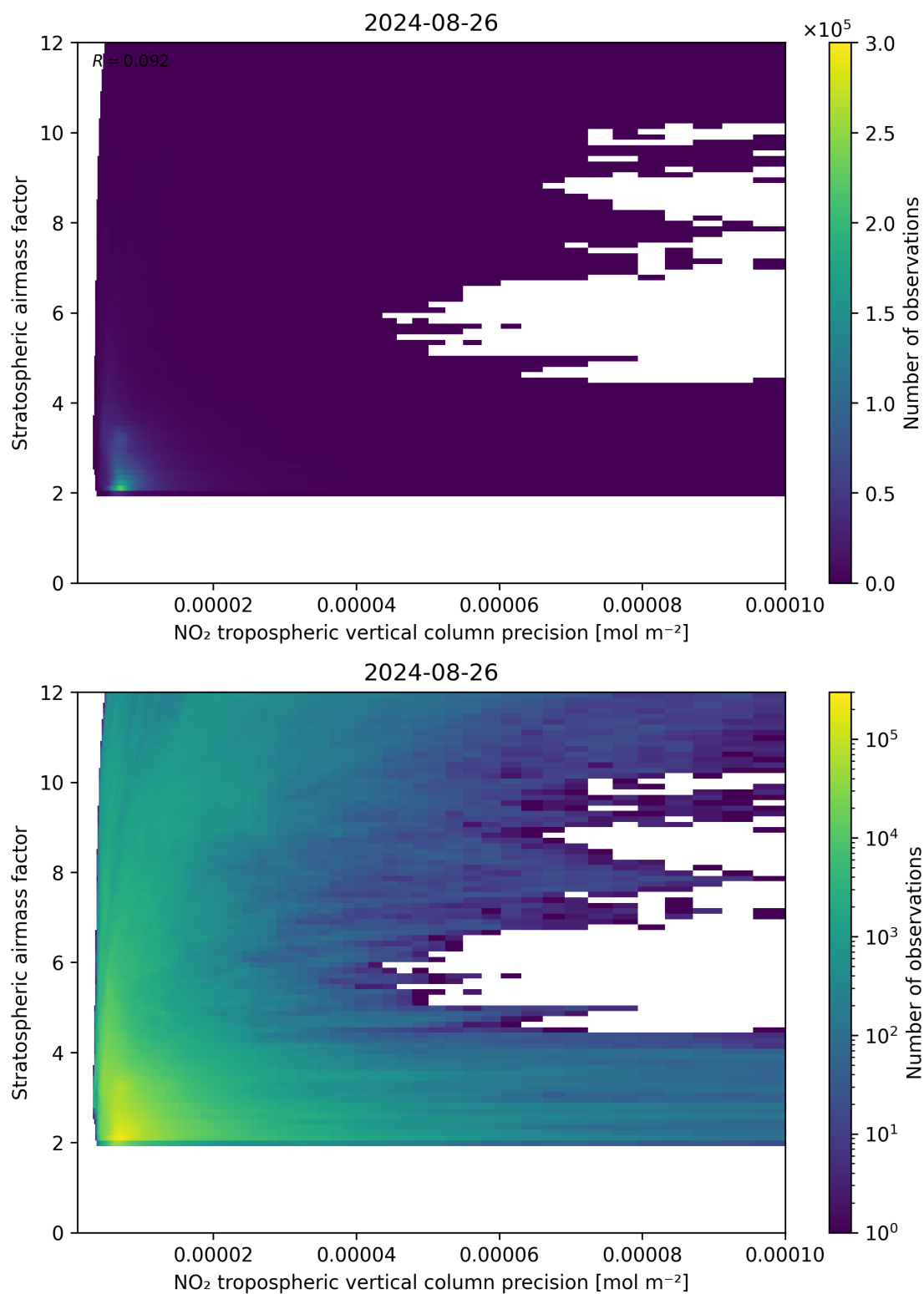
Figure 131: Scatter density plot of “NO 2 tropospheric vertical column precision” against “Stratospheric airmass factor” for 2024-08-25 to 2024-08-27.
