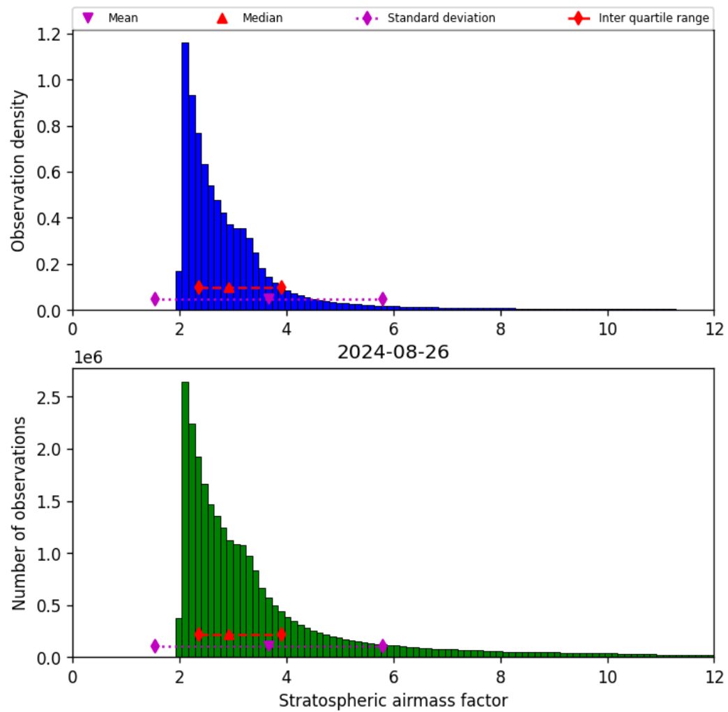
Figure 44: Histogram of “Stratospheric airmass factor” for 2024-08-25 to 2024-08-27
