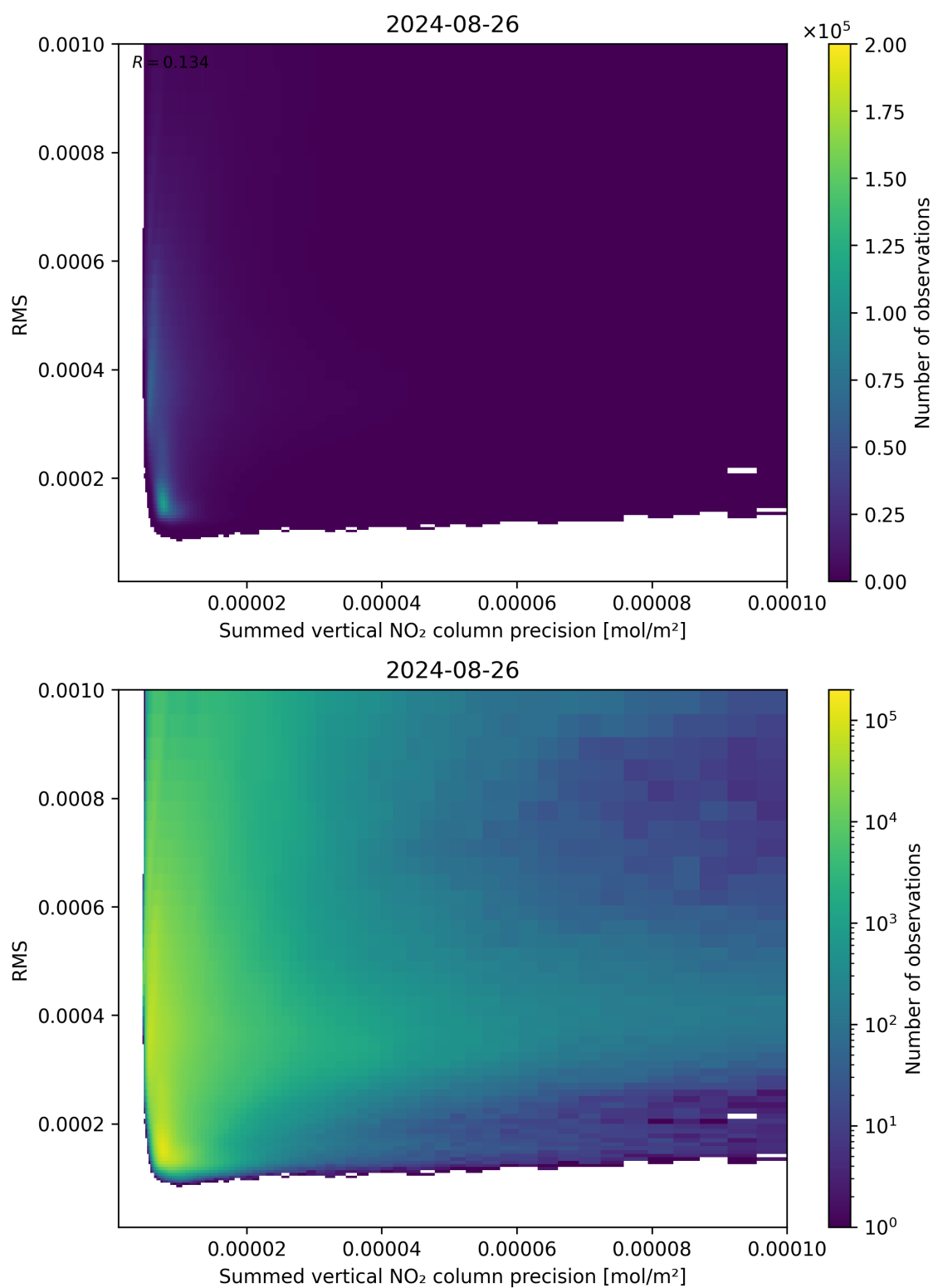
Figure 108: Scatter density plot of “Summed vertical NO 2 column precision” against “RMS” for 2024-08-25 to 2024-08-27.
