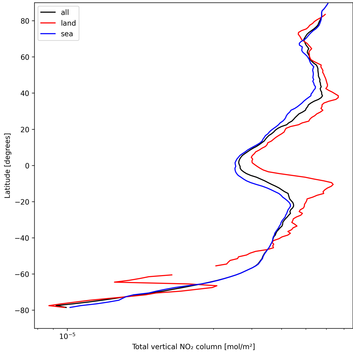
Figure 21: Zonal average of “Total vertical NO 2 column” for 2024-08-25 to 2024-08-27.
