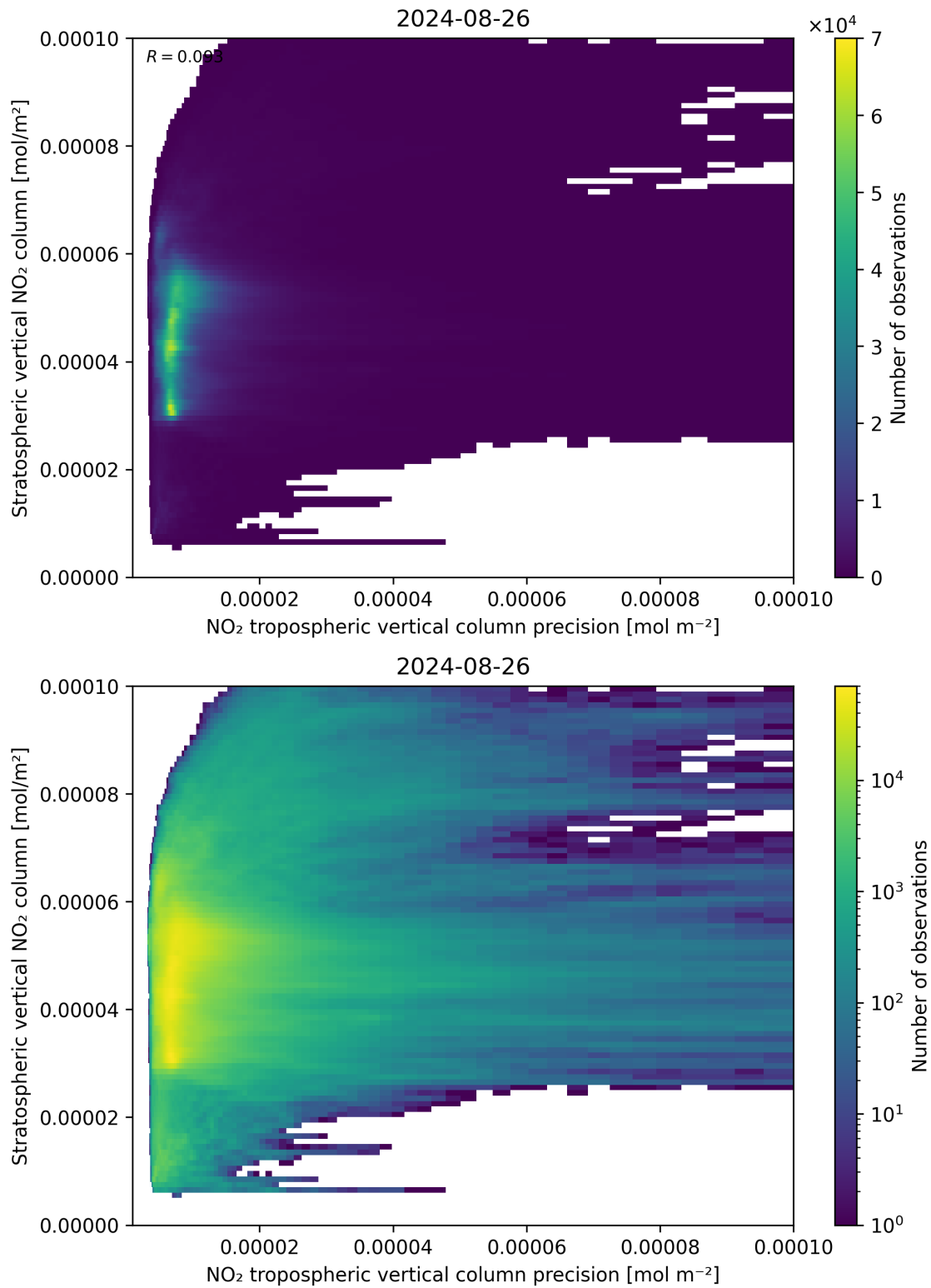
Figure 135: Scatter density plot of “NO 2 tropospheric vertical column precision” against “Stratospheric vertical NO 2 column” for 2024-08-25 to 2024-08-27.
