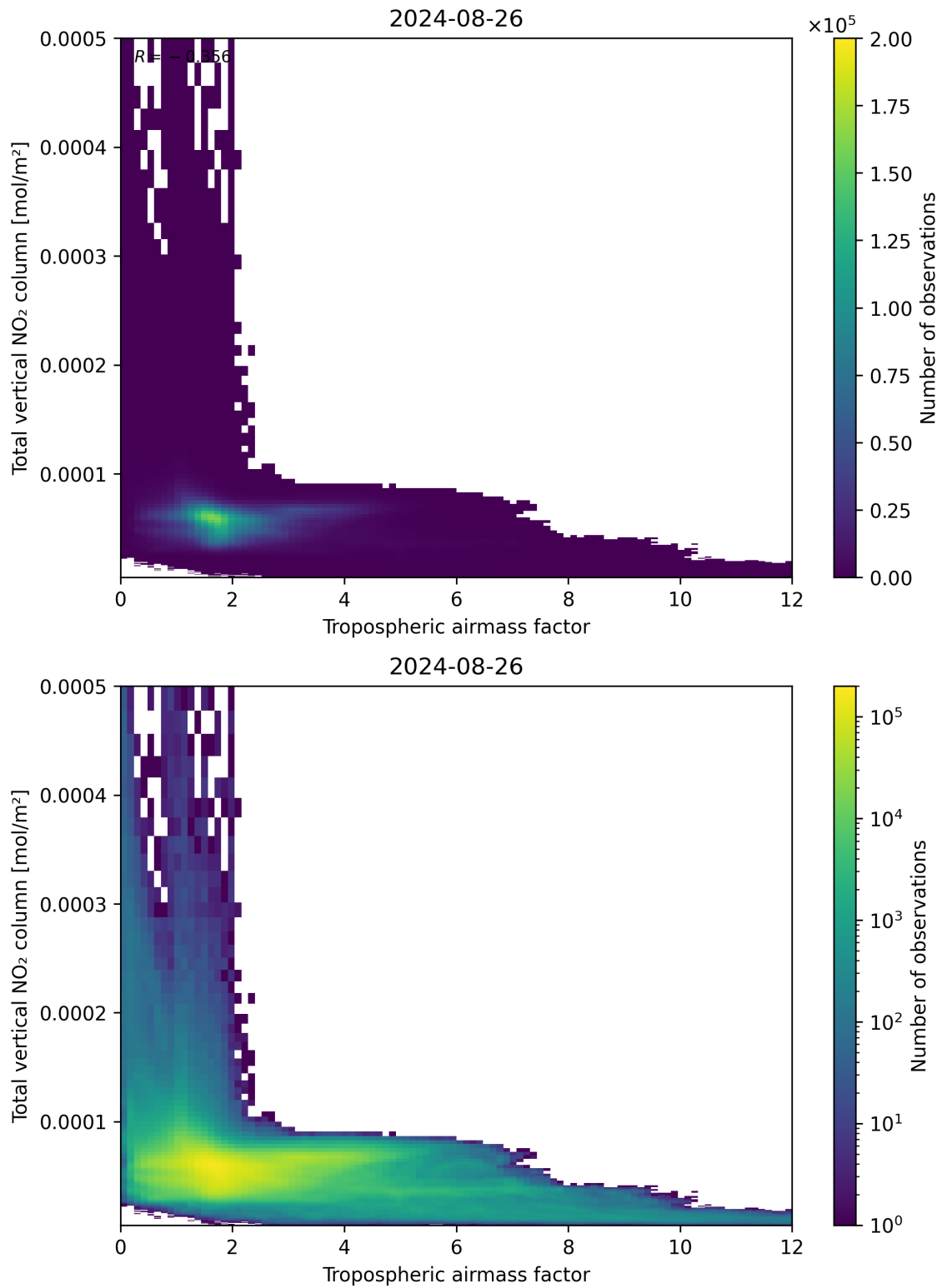
Figure 77: Scatter density plot of “Tropospheric airmass factor” against “Total vertical NO 2 column” for 2024-08-25 to 2024-08-27.
