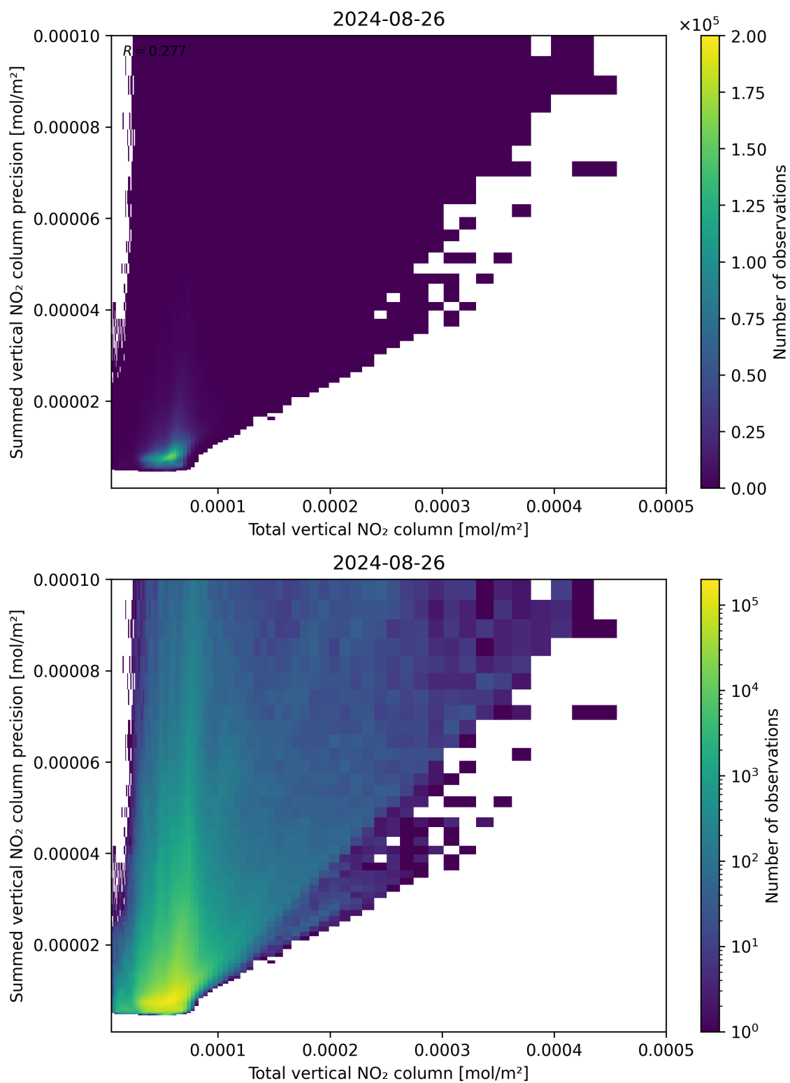
Figure 113: Scatter density plot of “Total vertical NO 2 column” against “Summed vertical NO 2 column precision” for 2024-08-25 to 2024-08-27.
