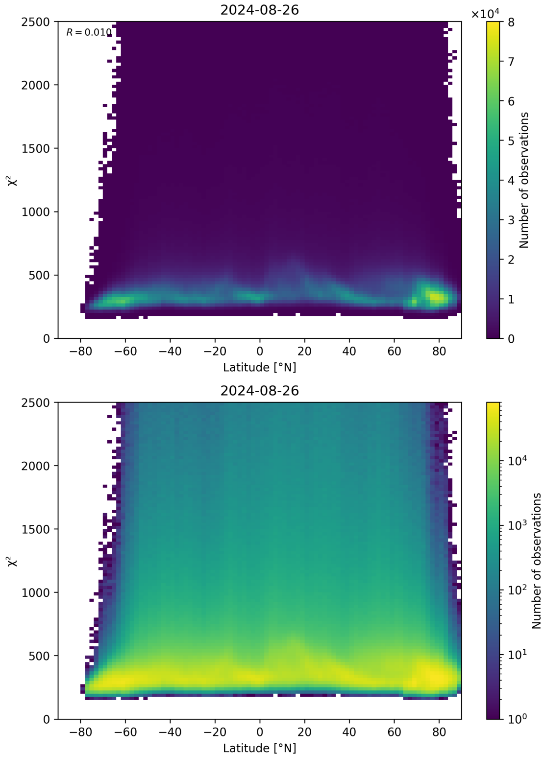
Figure 86: Scatter density plot of “Latitude” against “ \chi^2 ” for 2024-08-25 to 2024-08-27.
