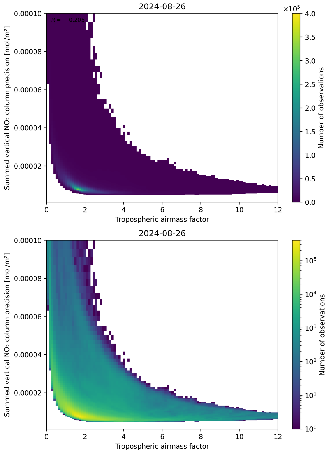
Figure 76: Scatter density plot of “Tropospheric air mass factor” against “Summed vertical NO 2 column precision” for 2024-08-25 to 2024-08-27.
