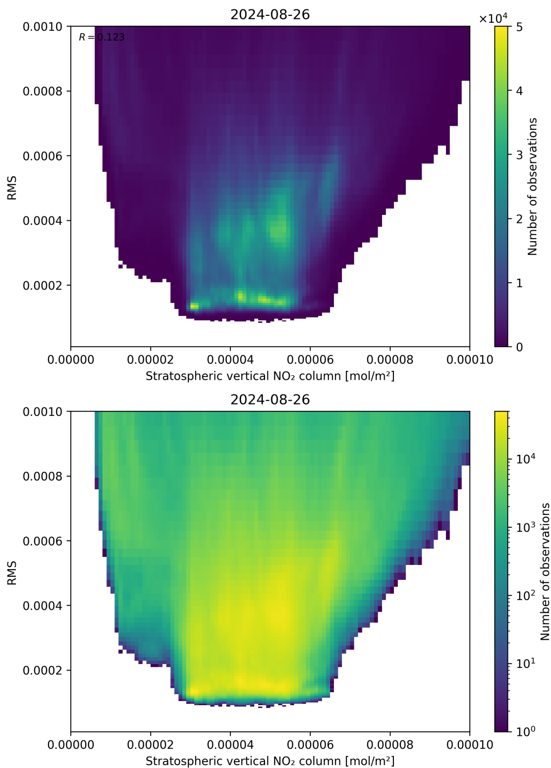
Figure 102: Scatter density plot of “Stratospheric vertical NO 2 column” against “RMS” for 2024-08-25 to 2024-08-27.
