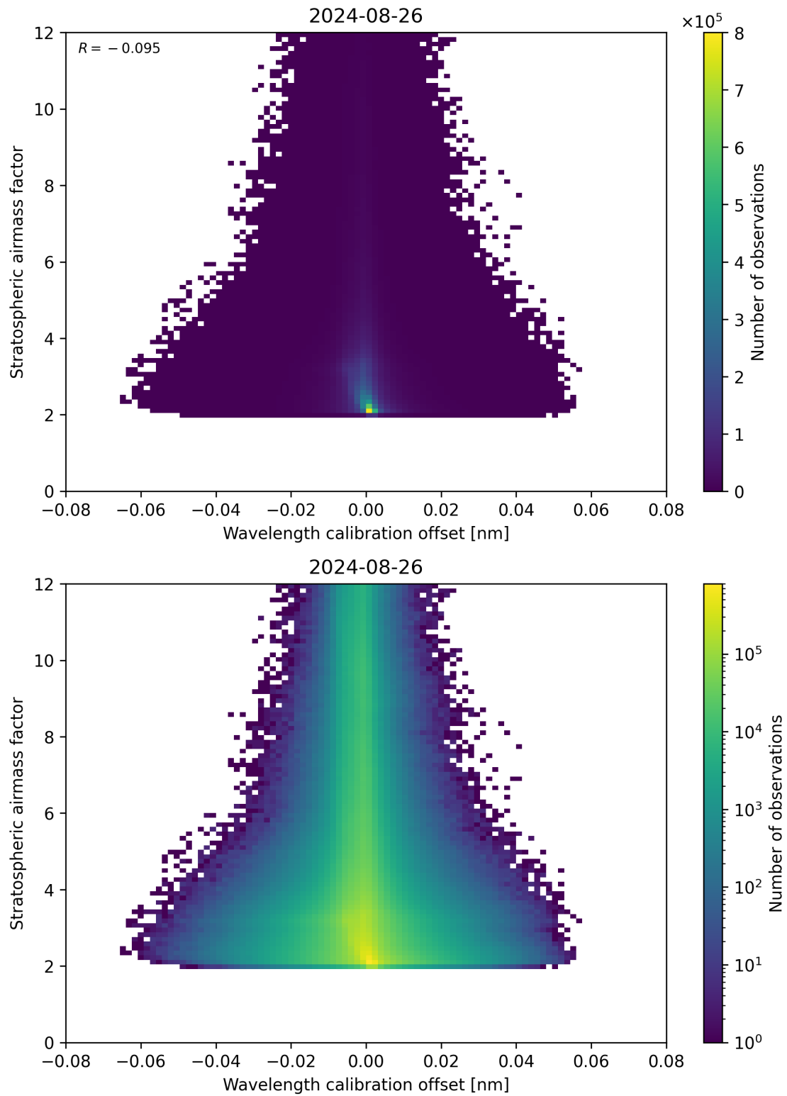
Figure 174: Scatter density plot of “Wavelength calibration offset” against “Stratospheric airmass factor” for 2024-08-25 to 2024-08-27.
