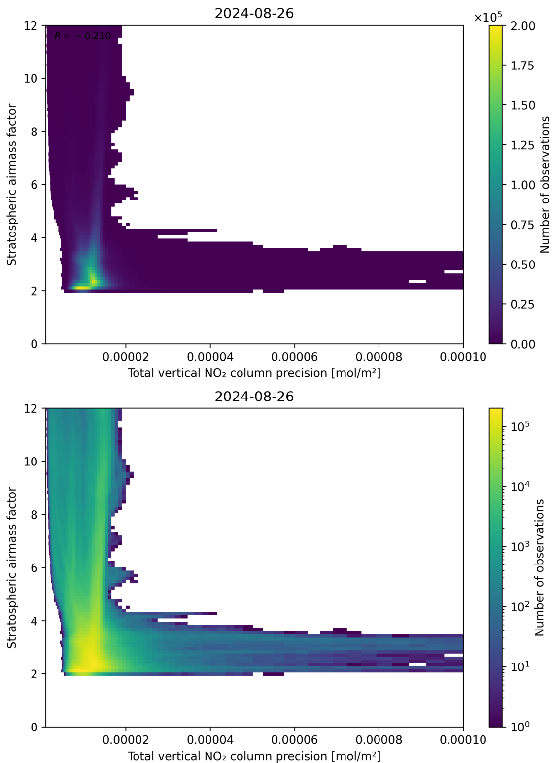
Figure 115: Scatter density plot of “Total vertical NO 2 column precision” against “Stratospheric air mass factor” for 2024-08-25 to 2024-08-27.
