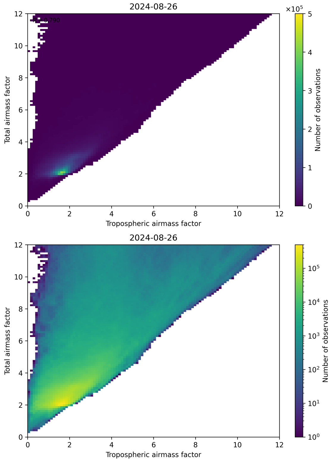
Figure 72: Scatter density plot of “Tropospheric airmass factor” against “Total airmass factor” for 2024-08-25 to 2024-08-27.
