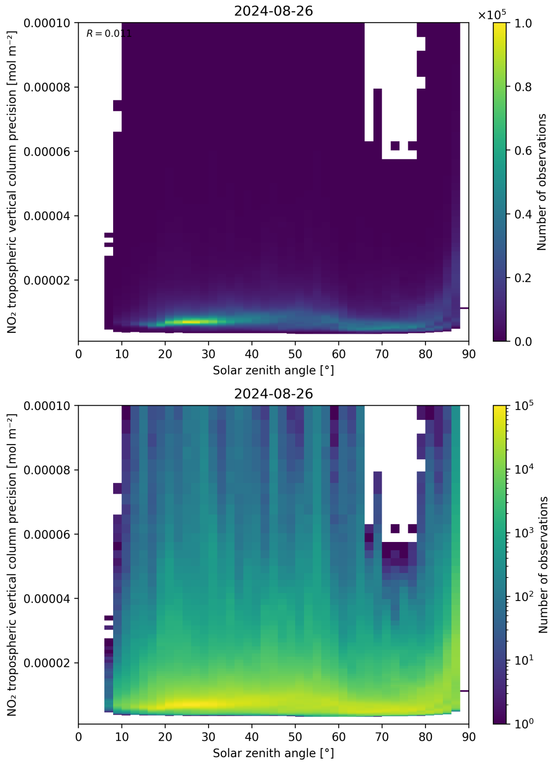
Figure 156: Scatter density plot of “Solar zenith angle” against “NO 2 tropospheric vertical column precision” for 2024-08-25 to 2024-08-27.
