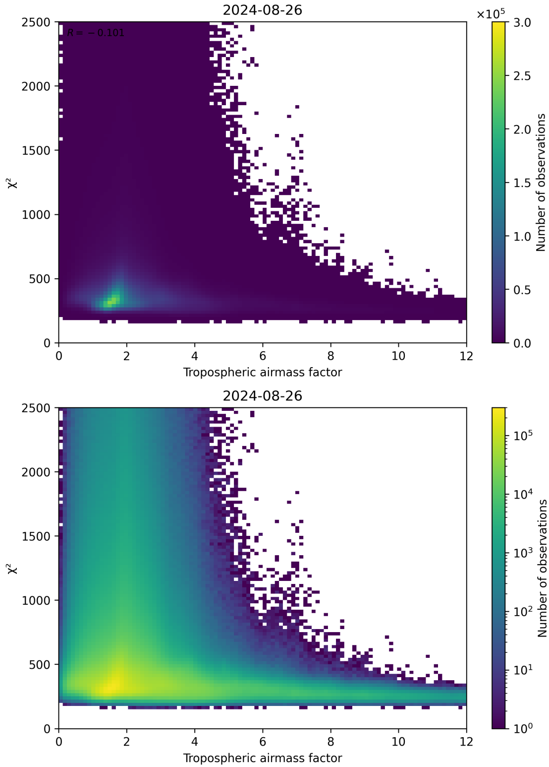
Figure 73: Scatter density plot of “Tropospheric airmass factor” against “ \chi^2 ” for 2024-08-25 to 2024-08-27.
