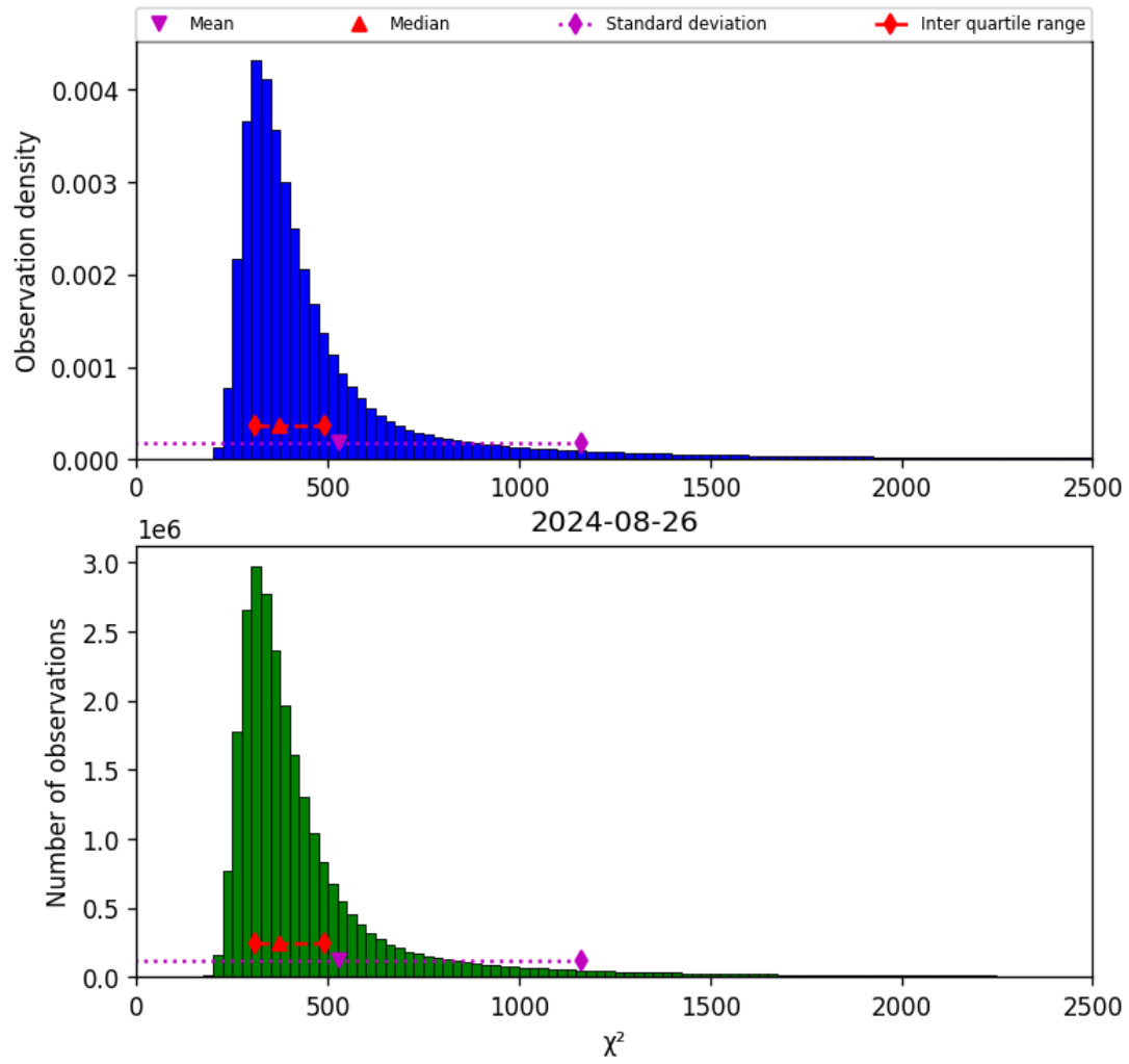
Figure 42: Histogram of “ \chi^2 ” for 2024-08-25 to 2024-08-27
