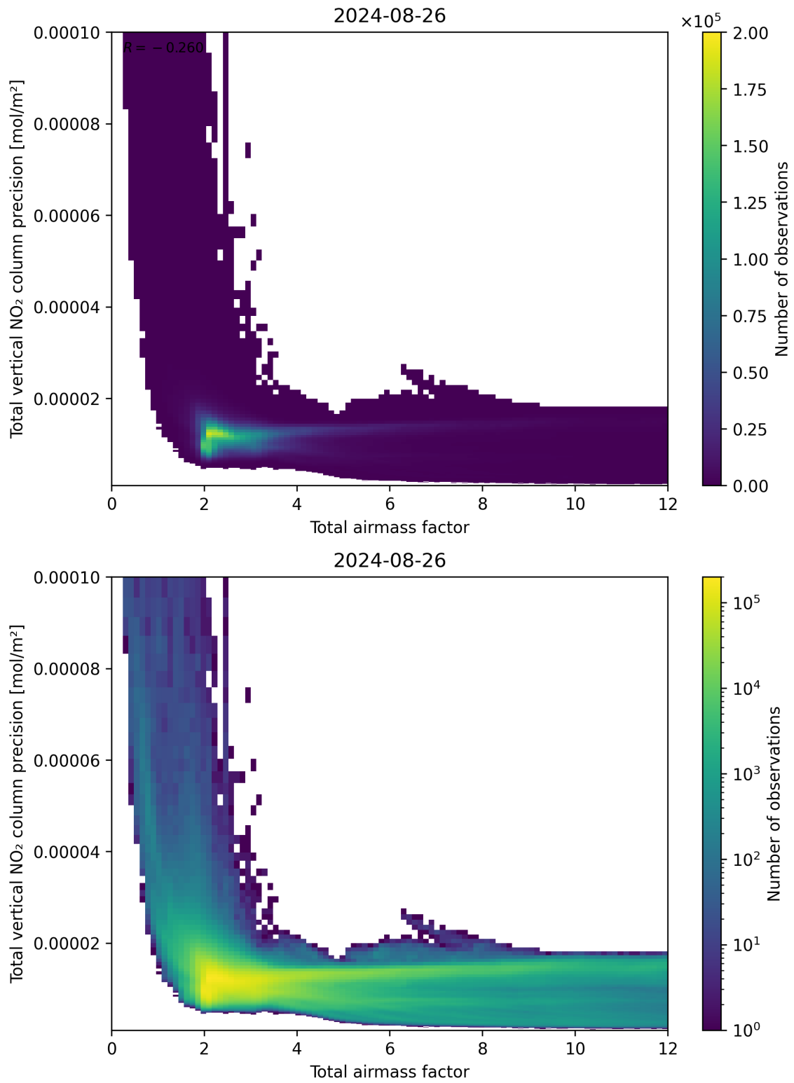
Figure 68: Scatter density plot of “Total airmass factor” against “Total vertical NO 2 column precision” for 2024-08-25 to 2024-08-27.
