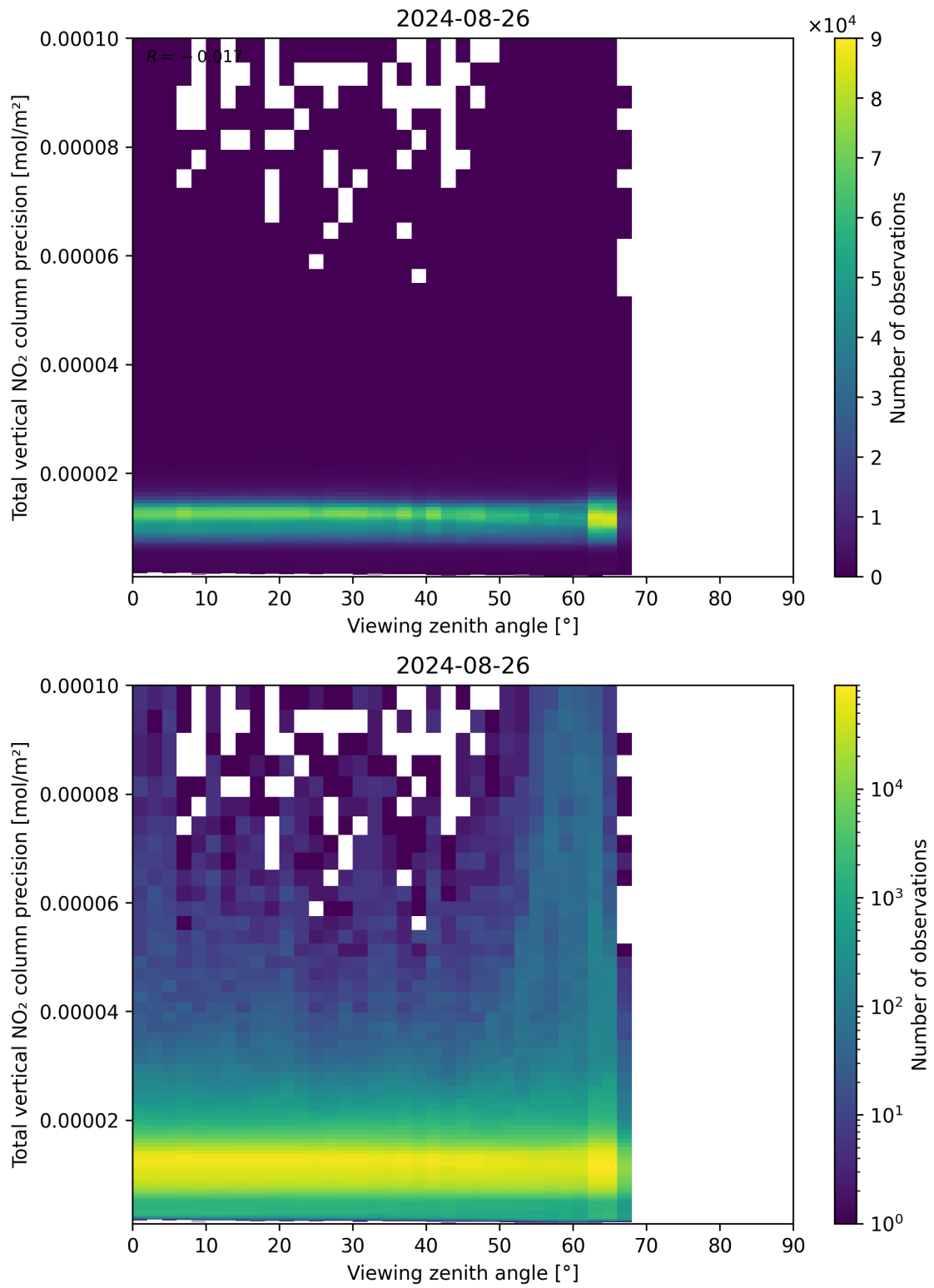
Figure 168: Scatter density plot of “Viewing zenith angle” against “Total vertical NO 2 column precision” for 2024-08-25 to 2024-08-27.
