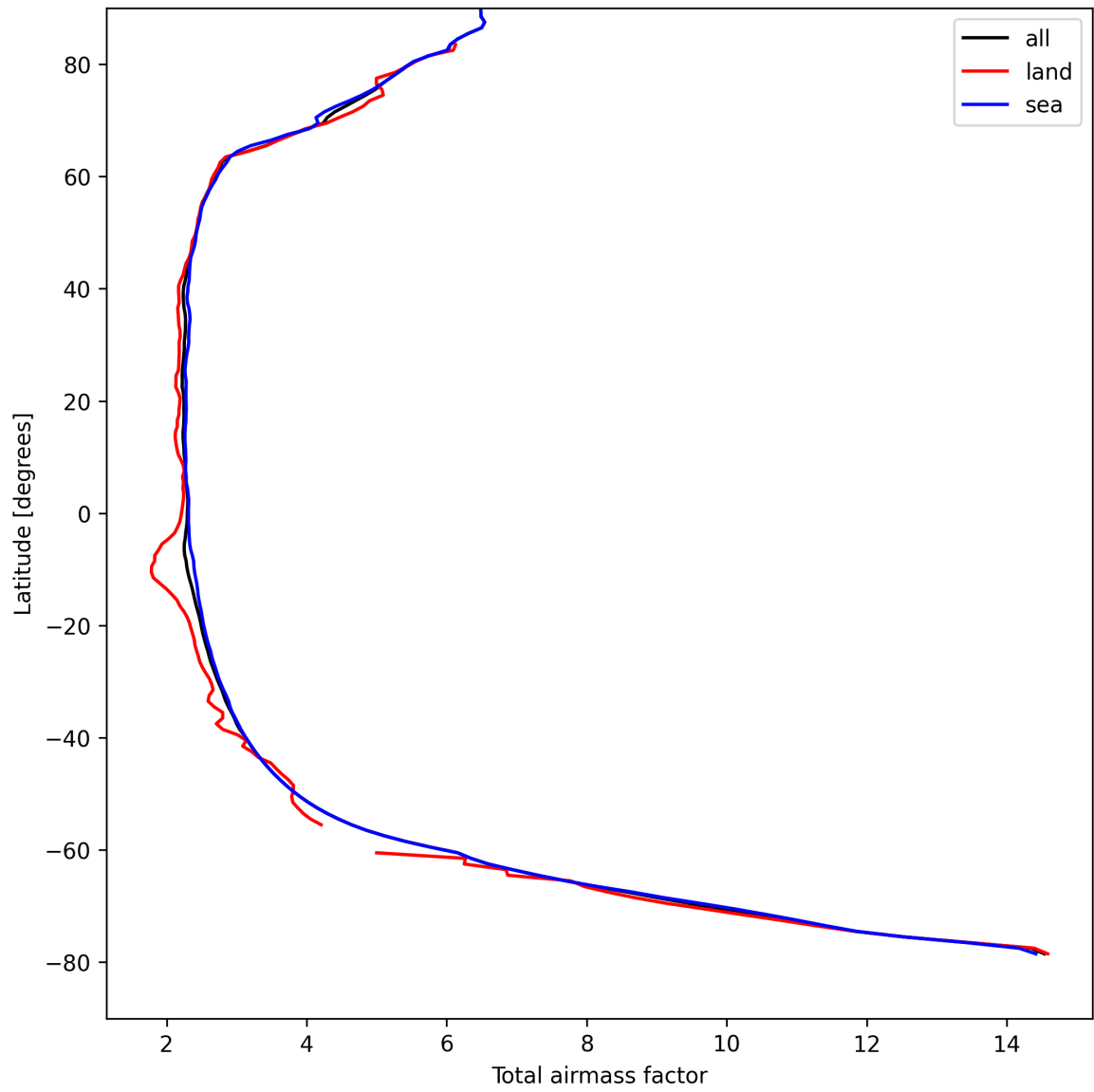
Figure 15: Zonal average of “Total airmass factor” for 2024-08-25 to 2024-08-27.
