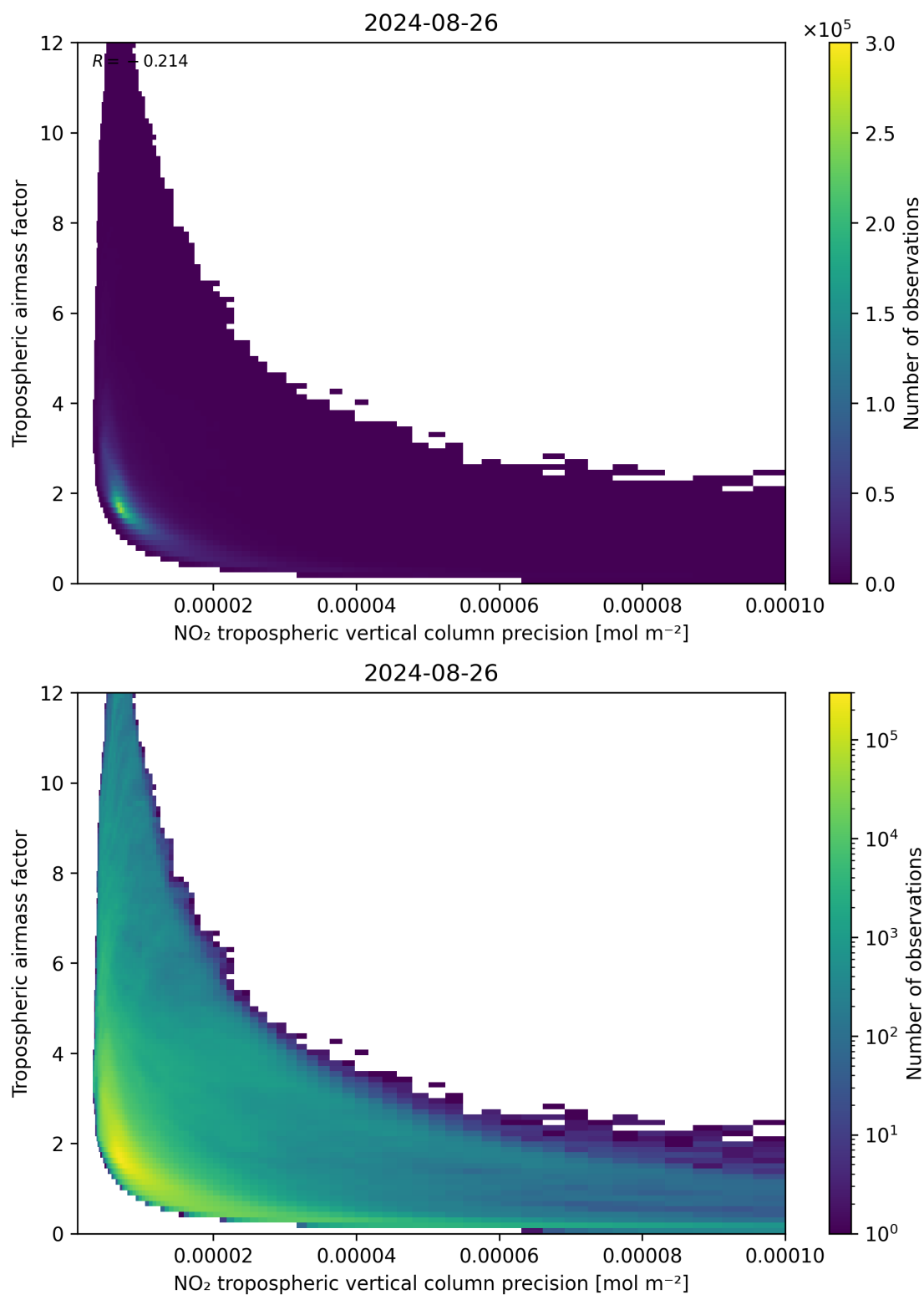
Figure 133: Scatter density plot of “NO 2 tropospheric vertical column precision” against “Tropospheric air mass factor” for 2024-08-25 to 2024-08-27.
