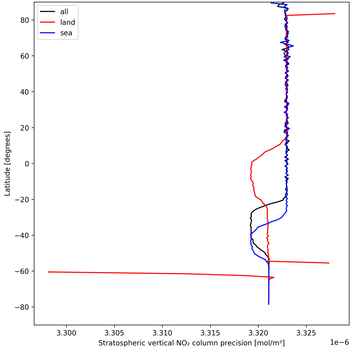
Figure 20: Zonal average of “Stratospheric vertical NO 2 column precision” for 2024-08-25 to 2024-08-27.
