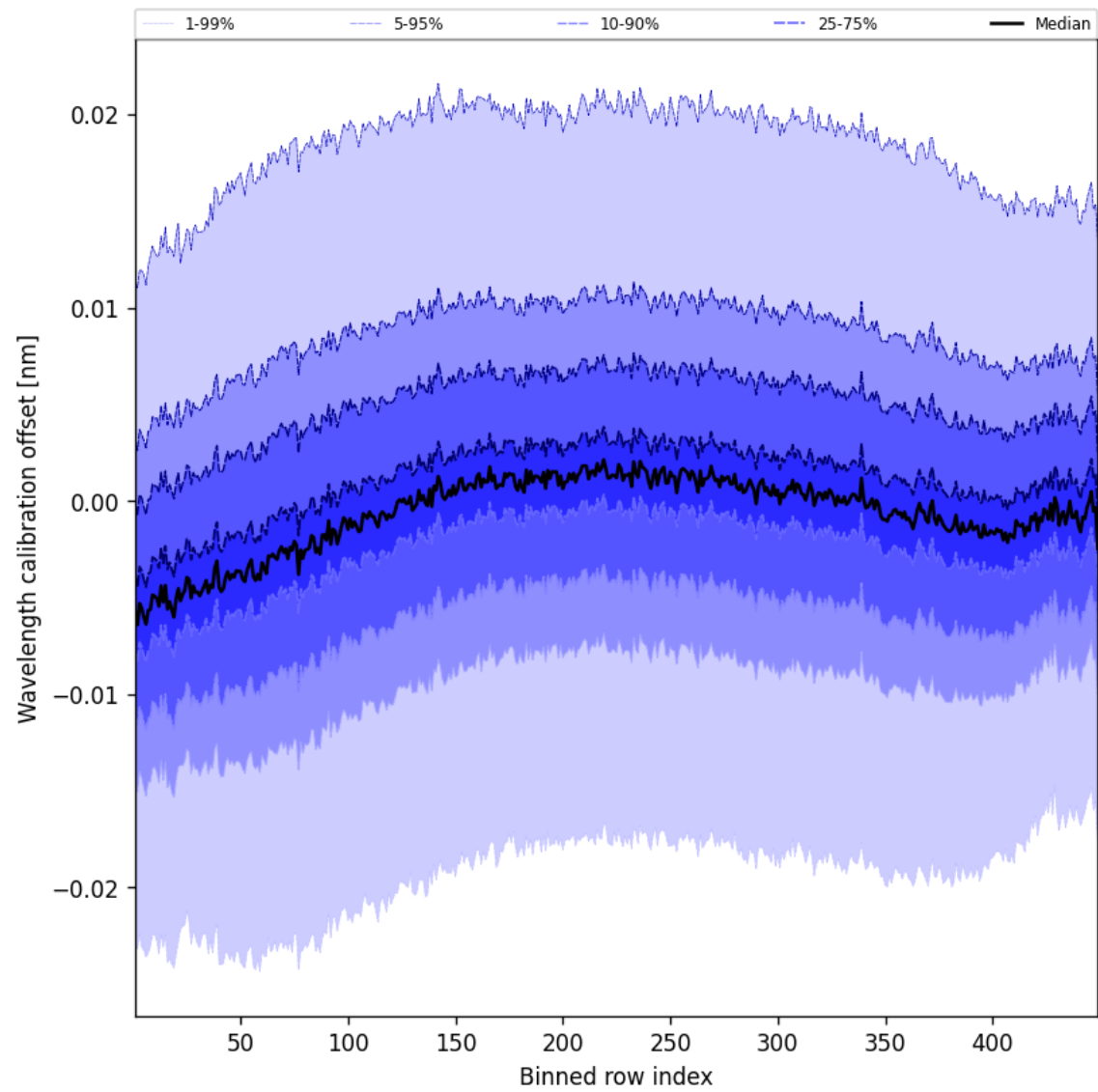
Figure 52: Along track statistics of “Wavelength calibration offset” for 2024-08-25 to 2024-08-27
