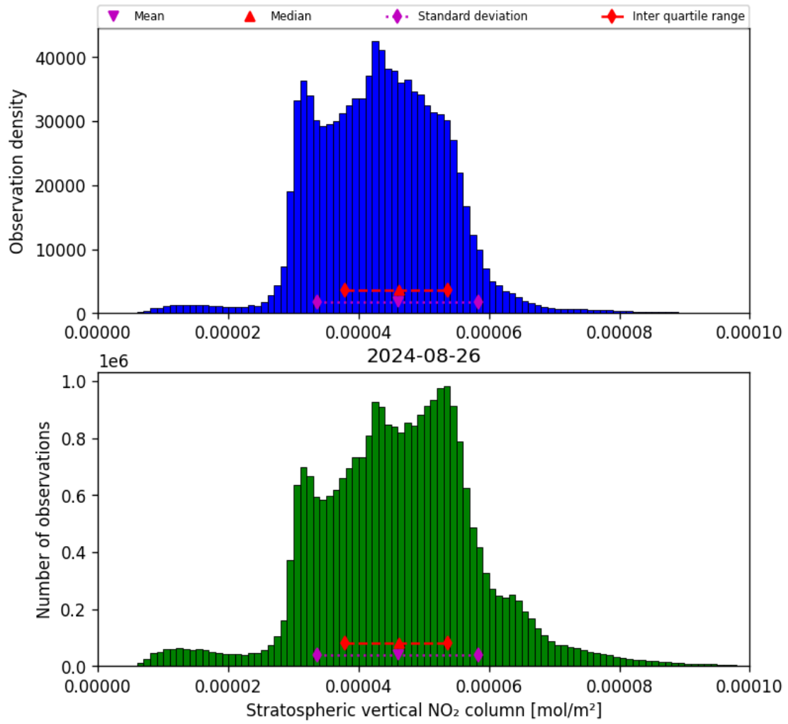
Figure 36: Histogram of “Stratospheric vertical NO 2 column” for 2024-08-25 to 2024-08-27
