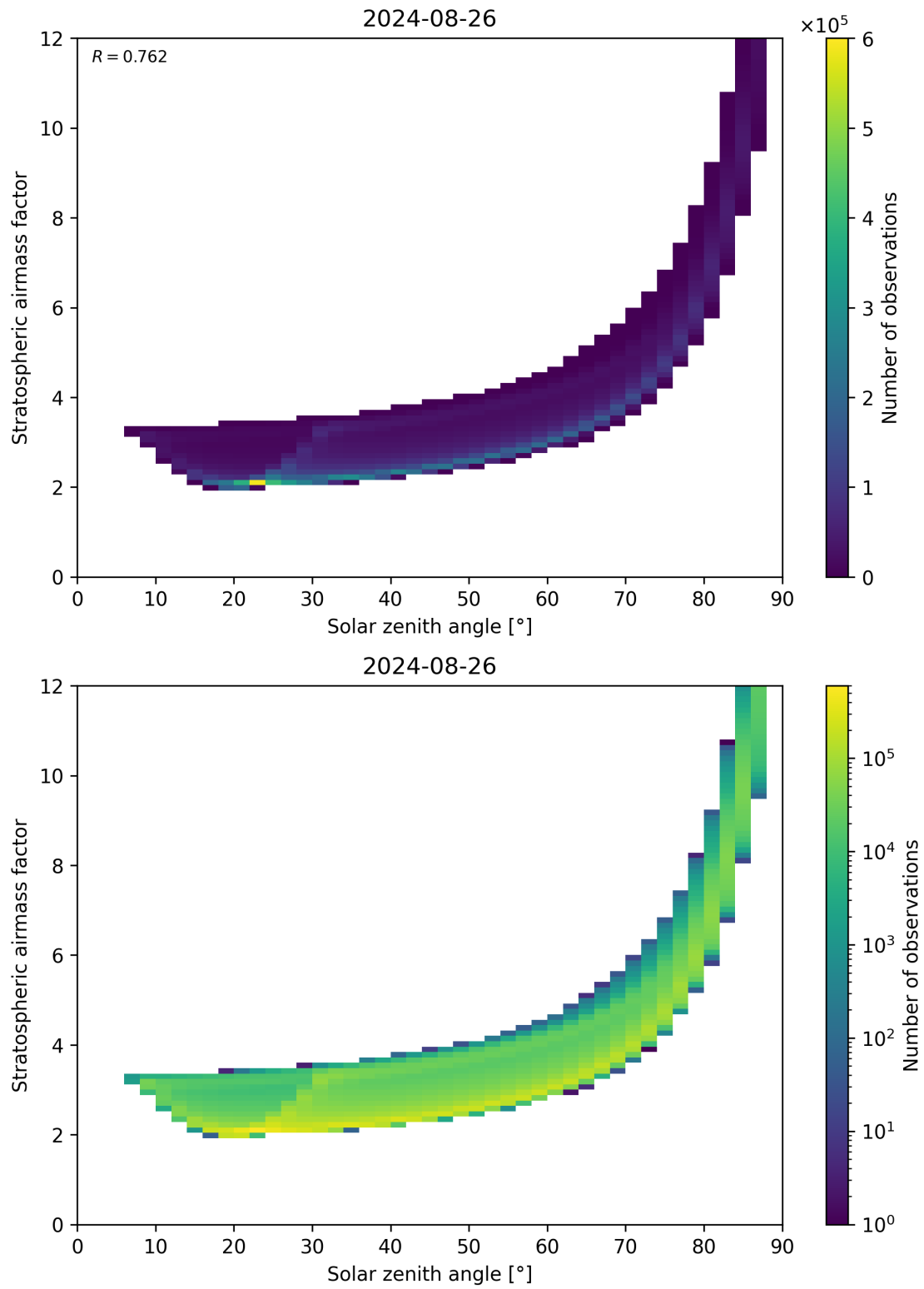
Figure 145: Scatter density plot of “Solar zenith angle” against “Stratospheric airmass factor” for 2024-08-25 to 2024-08-27.
