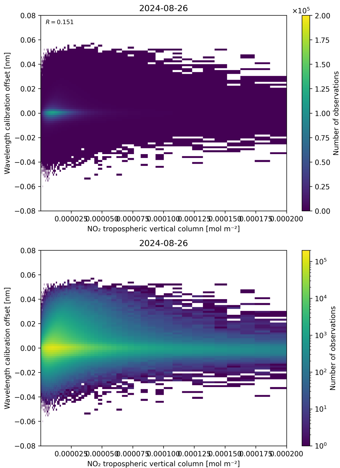
Figure 143: Scatter density plot of “NO 2 tropospheric vertical column” against “Wavelength calibration offset” for 2024-08-25 to 2024-08-27.
