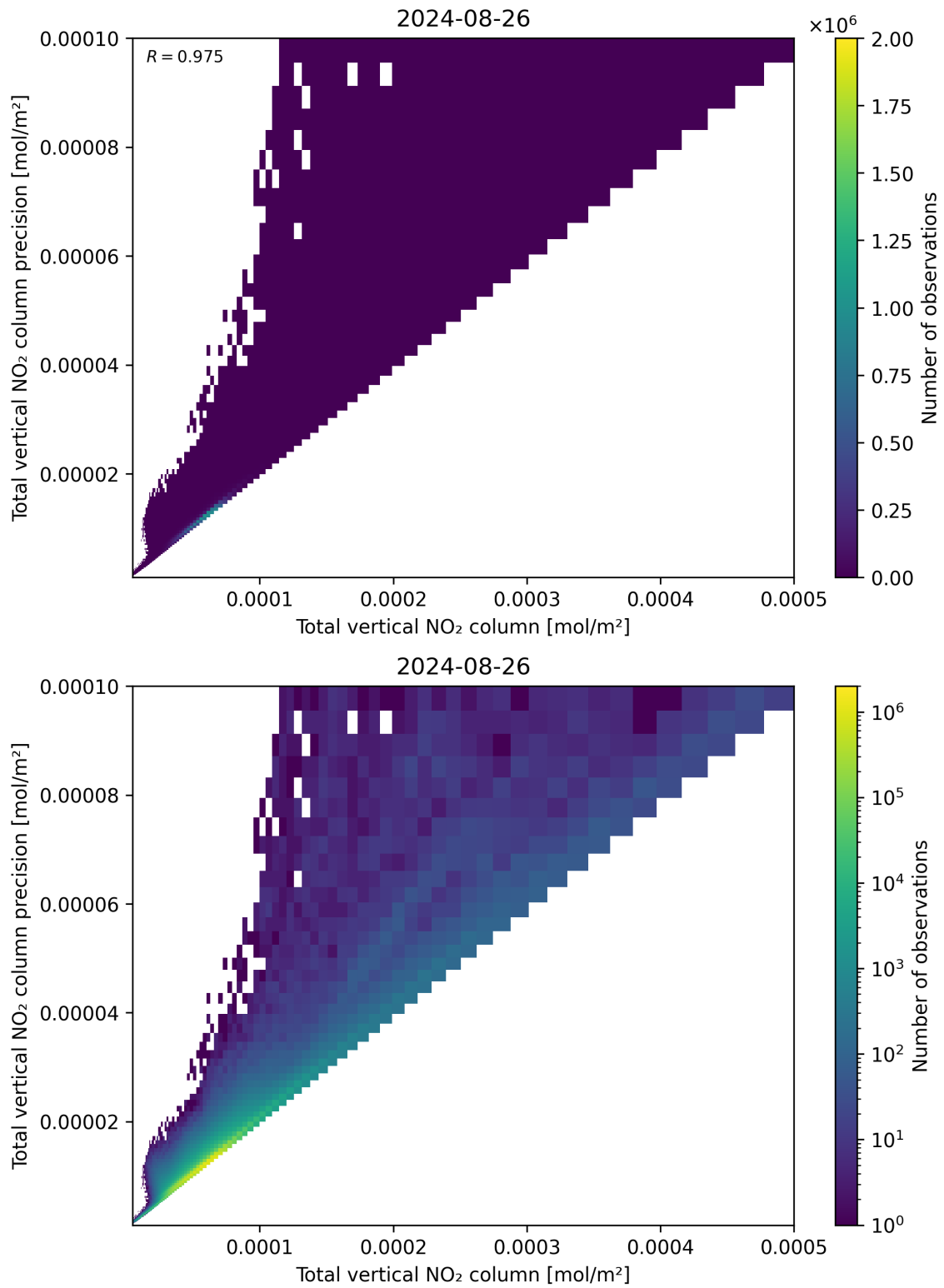
Figure 114: Scatter density plot of “Total vertical NO 2 column” against “Total vertical NO 2 column precision” for 2024-08-25 to 2024-08-27.
