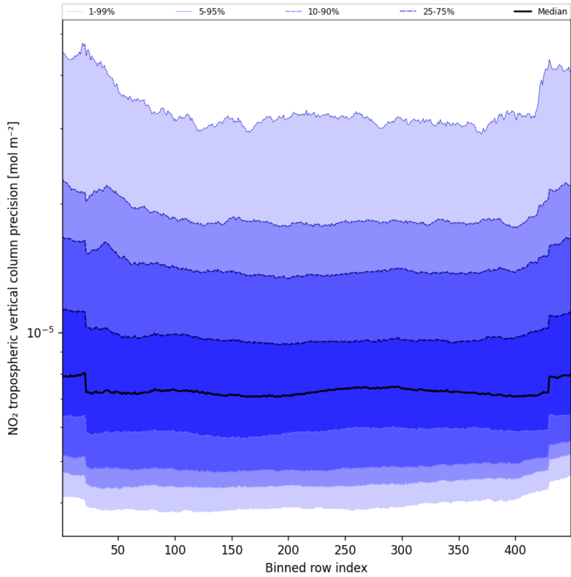
Figure 47: Along track statistics of “NO 2 tropospheric vertical column precision” for 2024-08-25 to 2024-08-27
