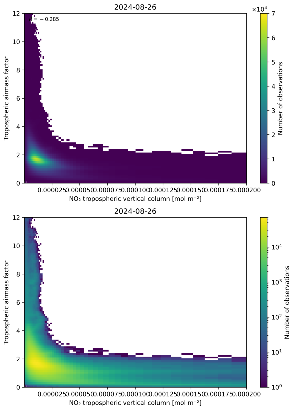
Figure 123: Scatter density plot of “NO 2 tropospheric vertical column” against “Tropospheric air mass factor” for 2024-08-25 to 2024-08-27.
