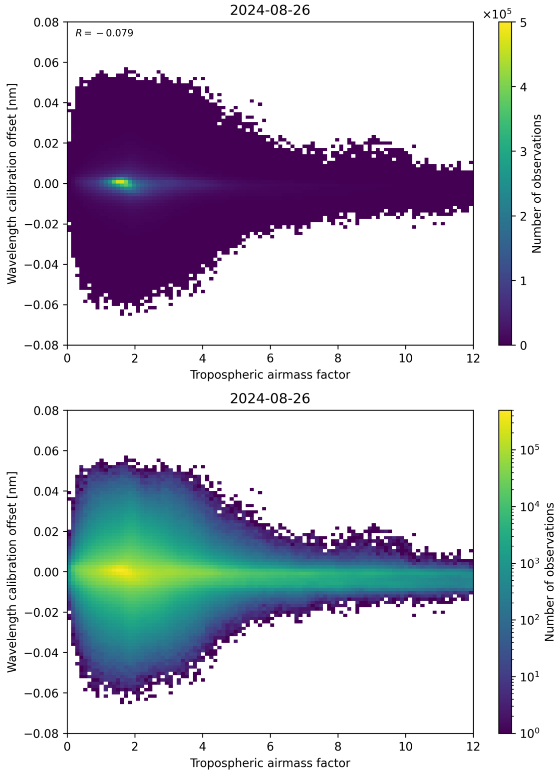
Figure 80: Scatter density plot of “Tropospheric airmass factor” against “Wavelength calibration offset” for 2024-08-25 to 2024-08-27.
