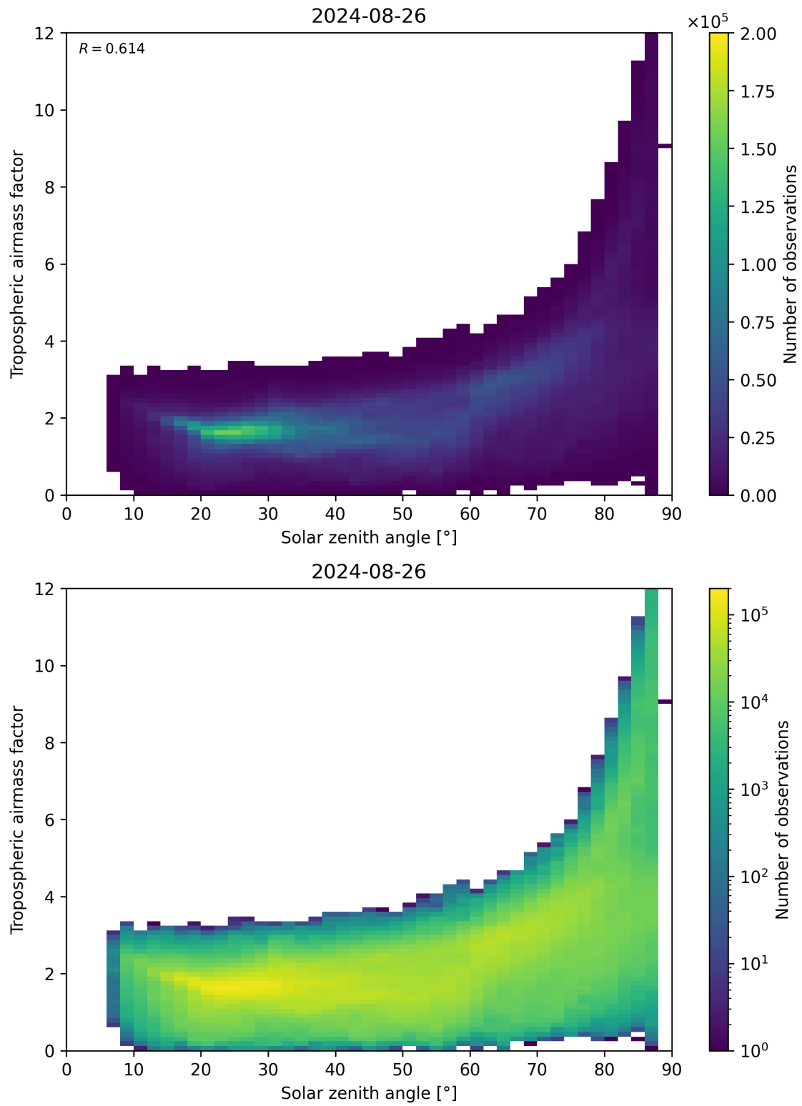
Figure 147: Scatter density plot of “Solar zenith angle” against “Tropospheric airmass factor” for 2024-08-25 to 2024-08-27.
