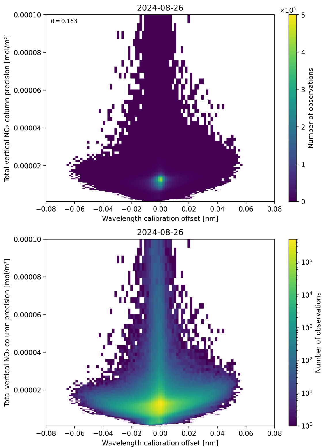
Figure 180: Scatter density plot of “Wavelength calibration offset” against “Total vertical NO 2 column precision” for 2024-08-25 to 2024-08-27.
