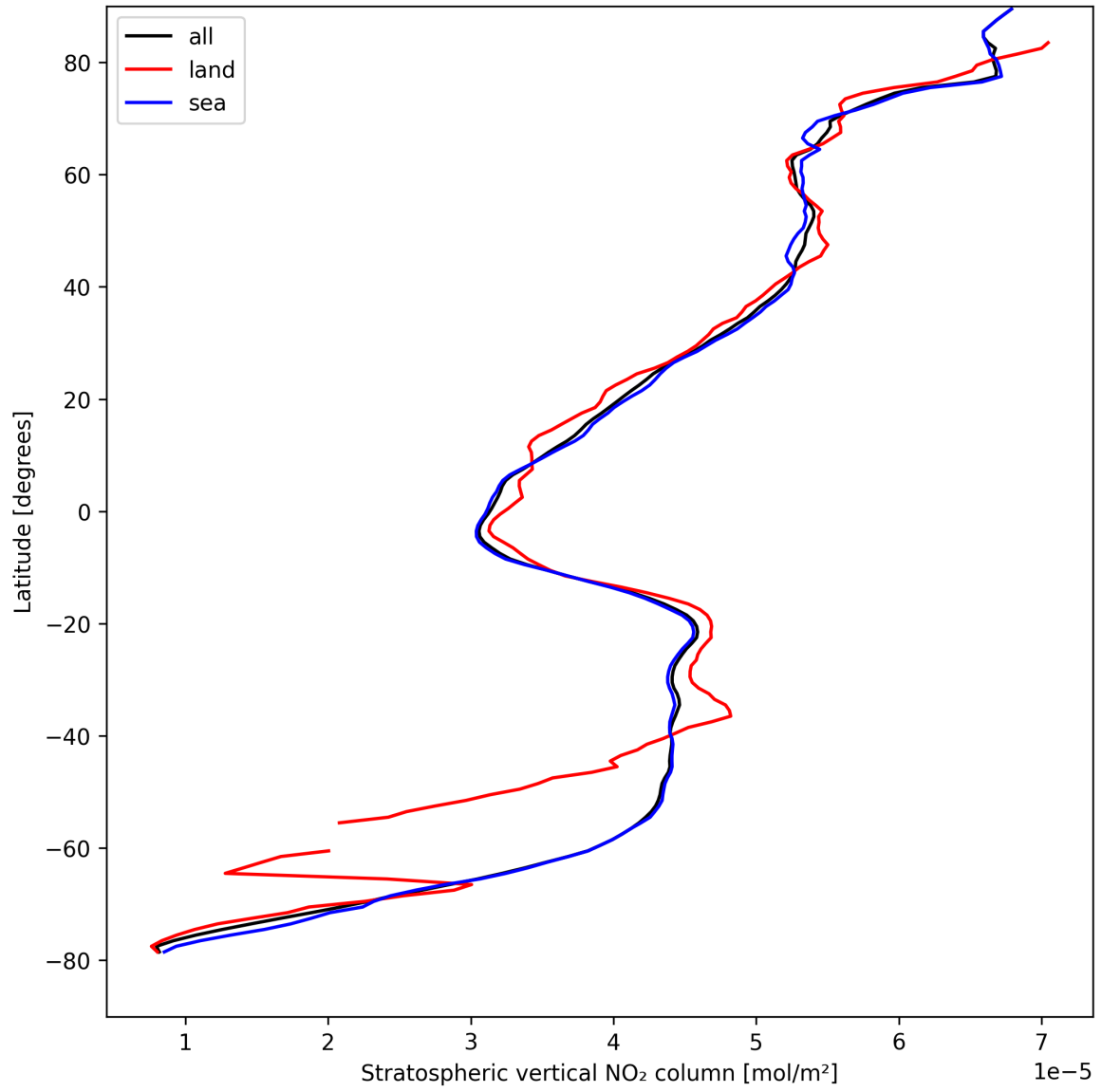
Figure 19: Zonal average of “Stratospheric vertical NO 2 column” for 2024-08-25 to 2024-08-27.
