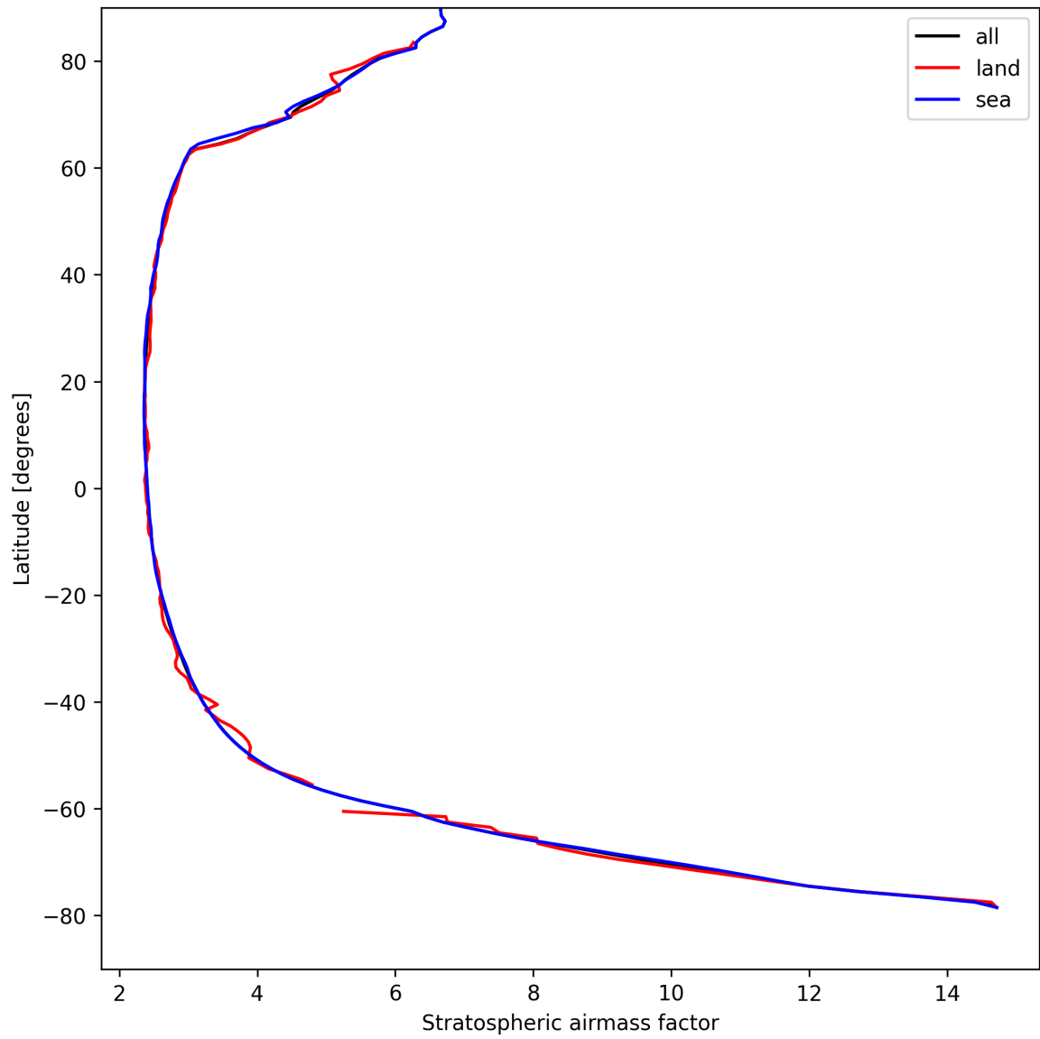
Figure 27: Zonal average of “Stratospheric airmass factor” for 2024-08-25 to 2024-08-27.
