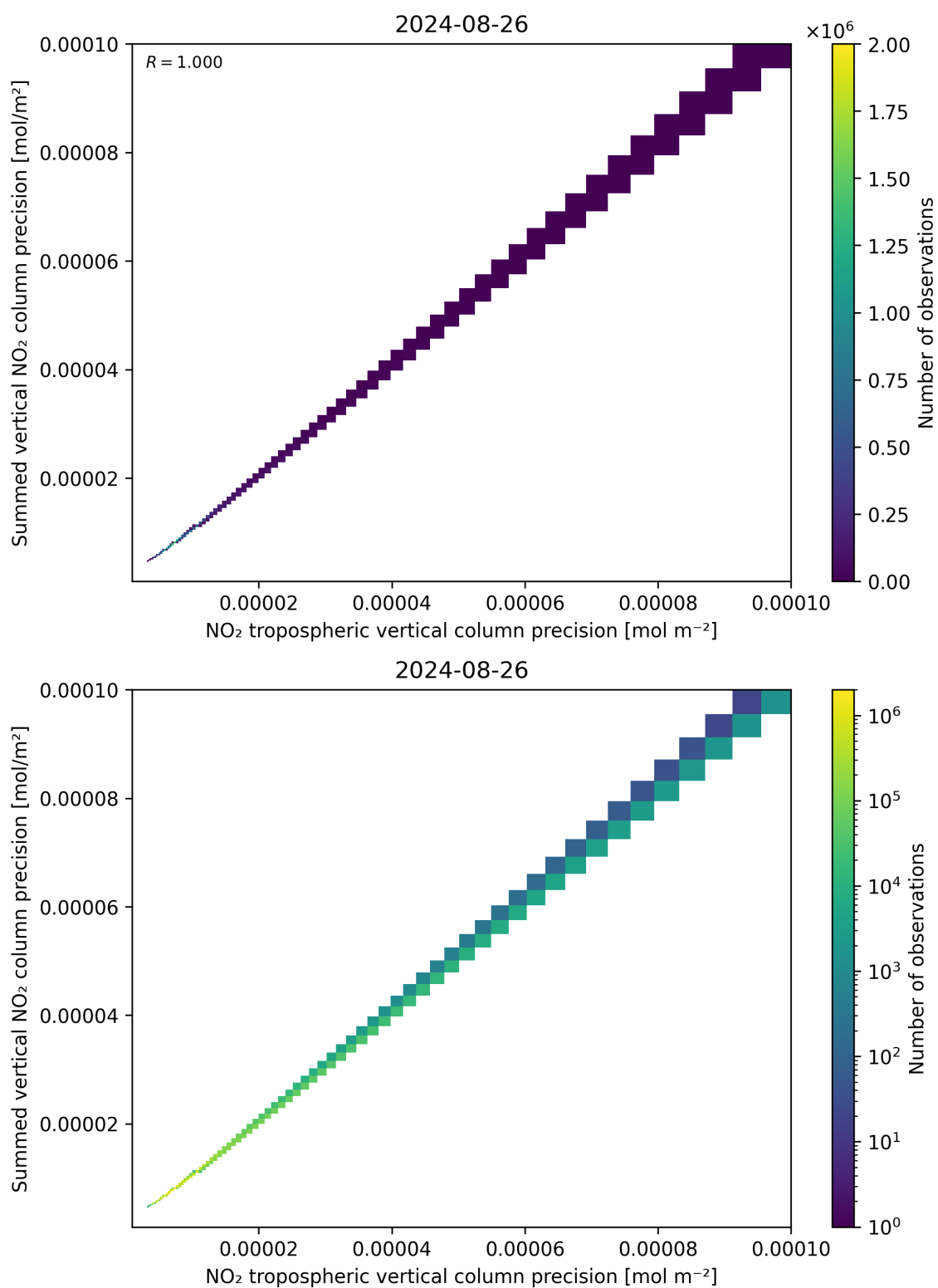
Figure 137: Scatter density plot of “NO 2 tropospheric vertical column precision” against “Summed vertical NO 2 column precision” for 2024-08-25 to 2024-08-27.
