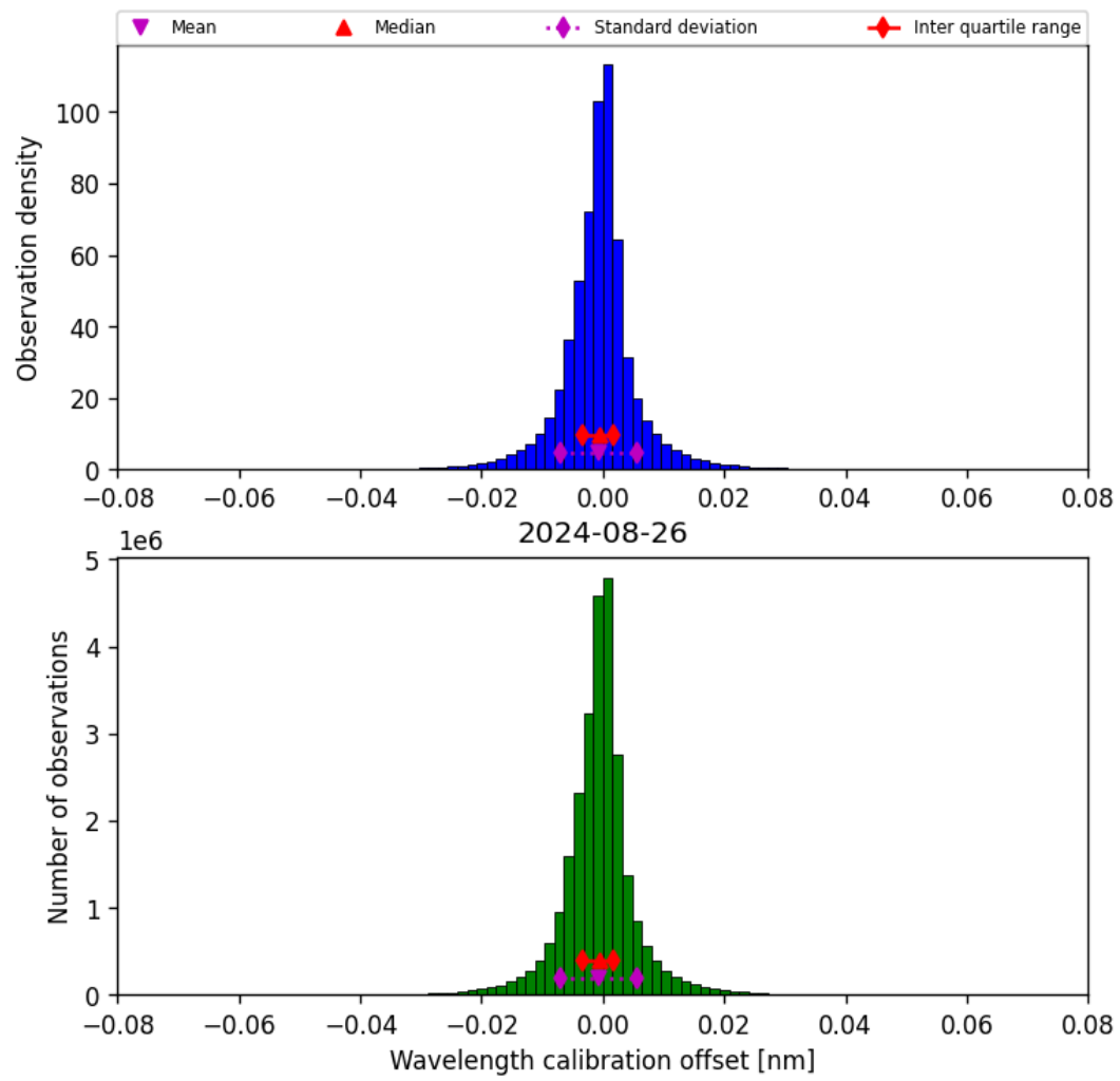
Figure 35: Histogram of “Wavelength calibration offset” for 2024-08-25 to 2024-08-27
