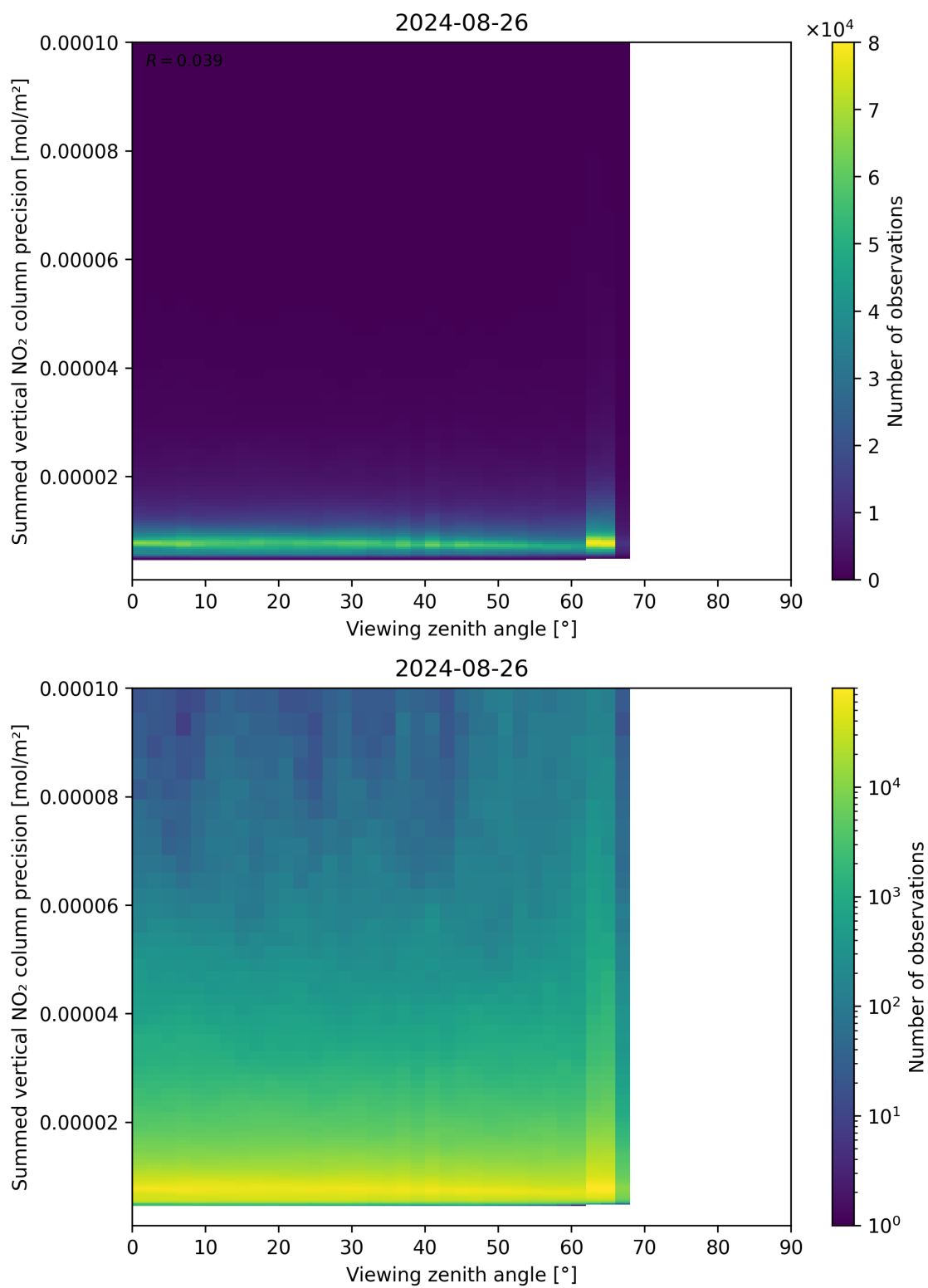
Figure 166: Scatter density plot of “Viewing zenith angle” against “Summed vertical NO 2 column precision” for 2024-08-25 to 2024-08-27.
