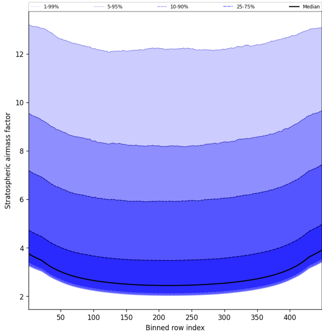
Figure 61: Along track statistics of “Stratospheric airmass factor” for 2024-08-25 to 2024-08-27
