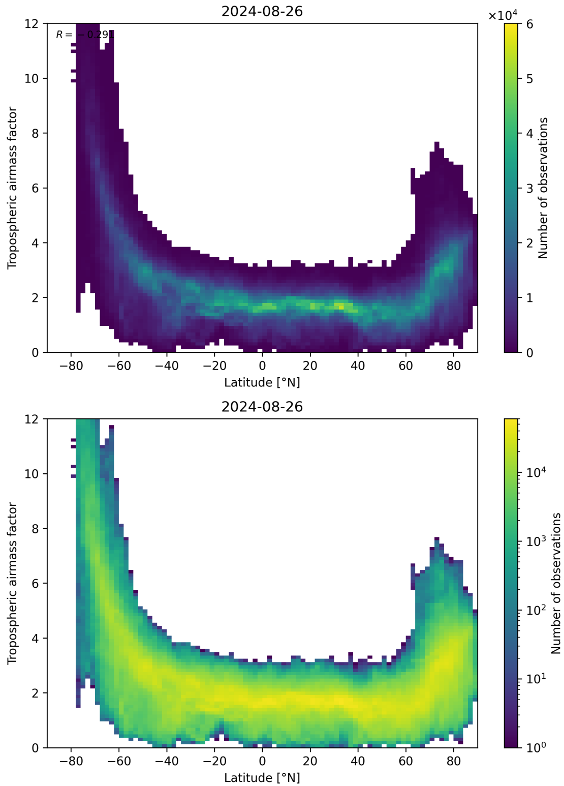
Figure 85: Scatter density plot of “Latitude” against “Tropospheric air mass factor” for 2024-08-25 to 2024-08-27.
