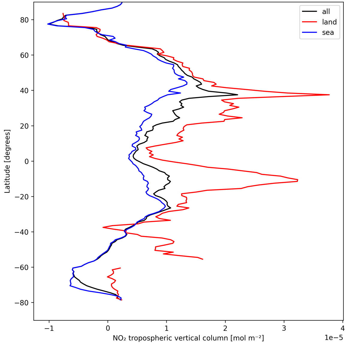
Figure 12: Zonal average of “NO 2 tropospheric vertical column” for 2024-08-25 to 2024-08-27.
