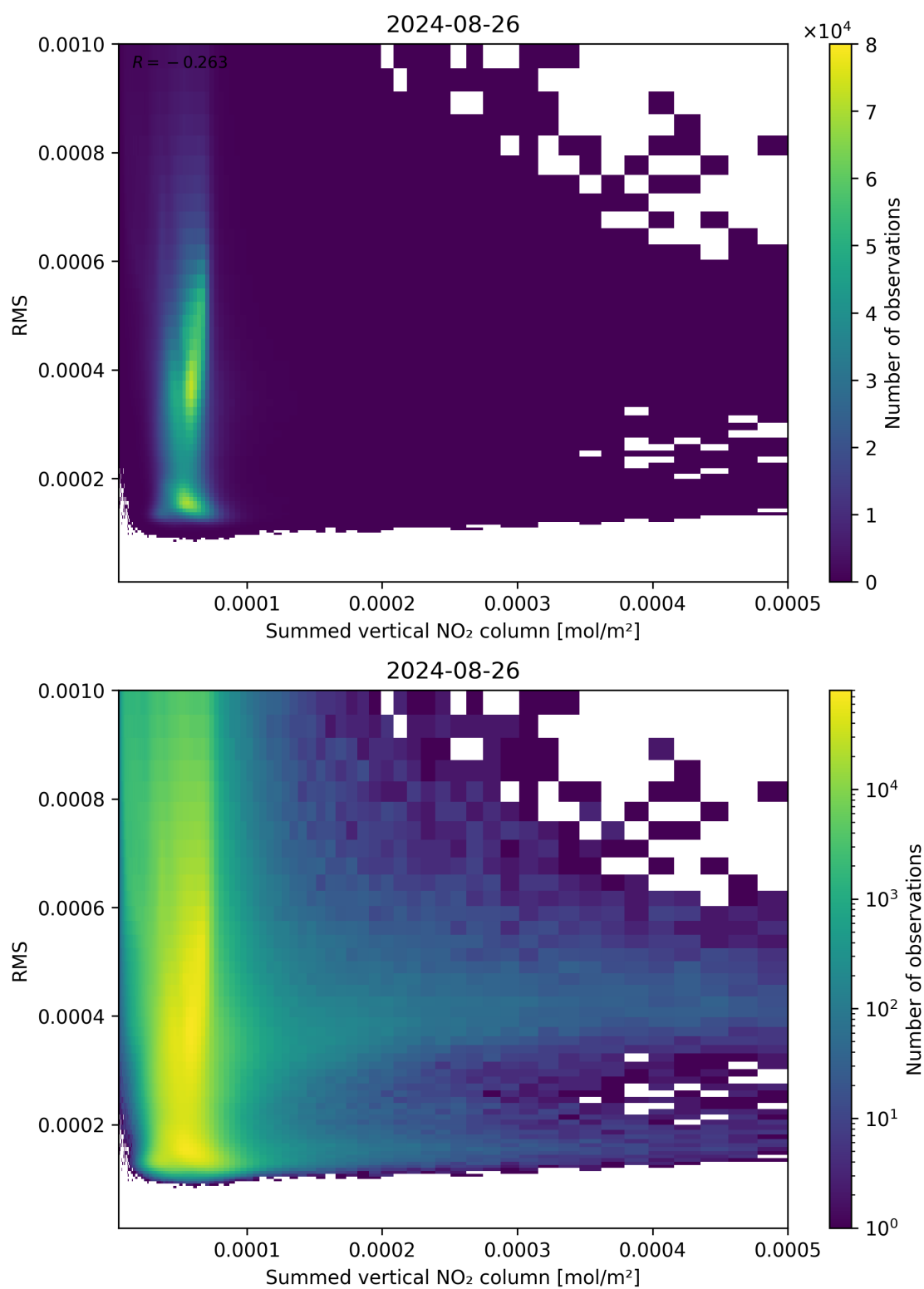
Figure 109: Scatter density plot of “Summed vertical NO 2 column” against “RMS” for 2024-08-25 to 2024-08-27.
