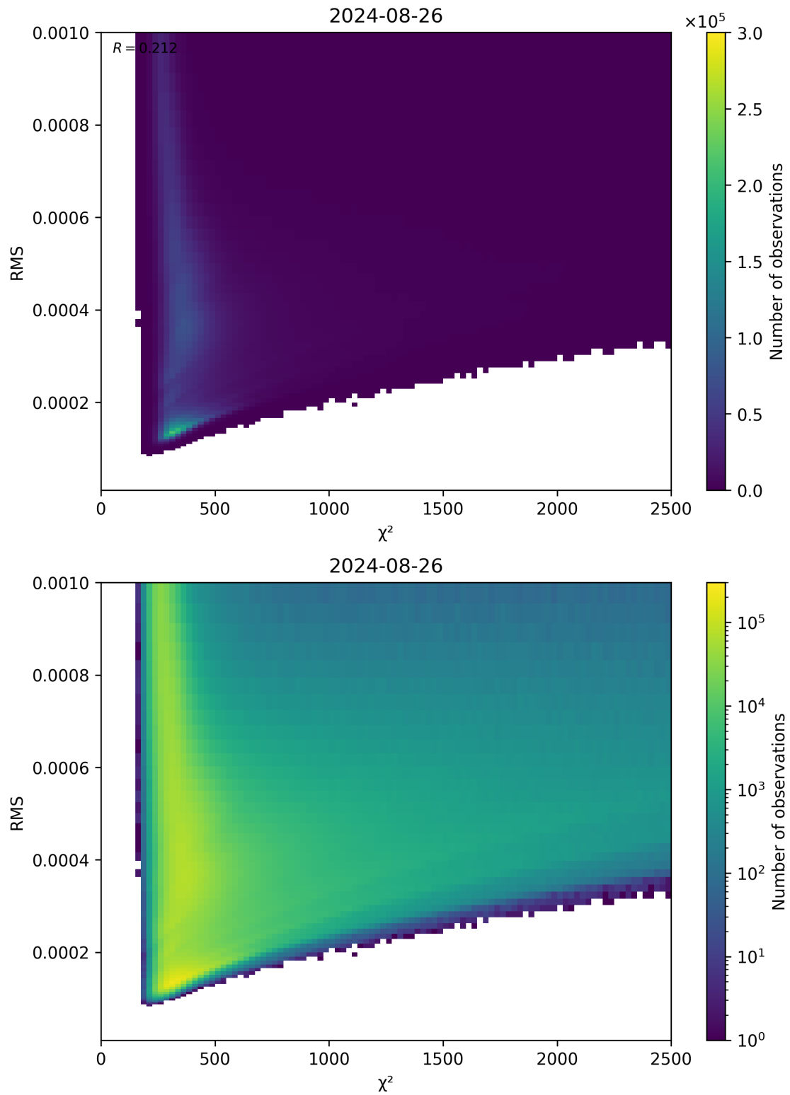
Figure 82: Scatter density plot of “ \chi^2 ” against “RMS” for 2024-08-25 to 2024-08-27.
