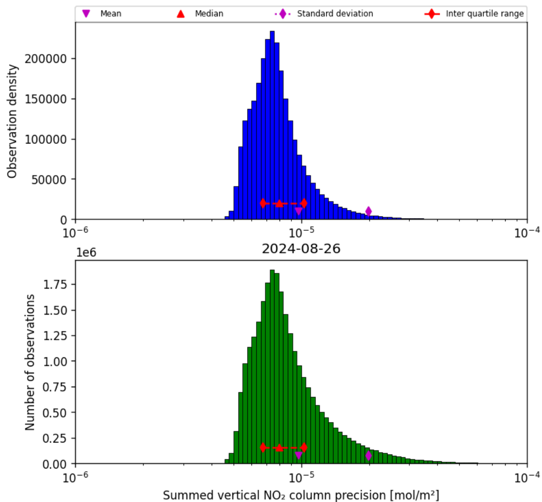
Figure 41: Histogram of “Summed vertical NO 2 column precision” for 2024-08-25 to 2024-08-27
