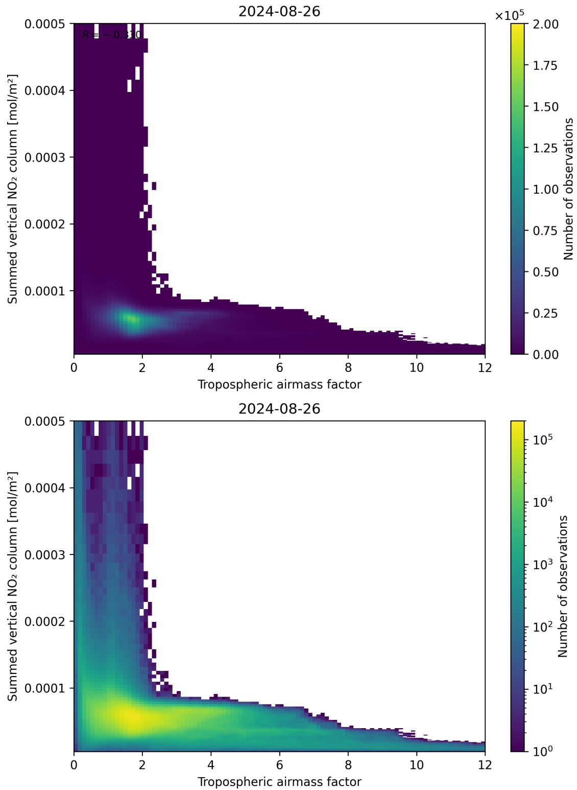
Figure 75: Scatter density plot of “Tropospheric airmass factor” against “Summed vertical NO 2 column” for 2024-08-25 to 2024-08-27.
