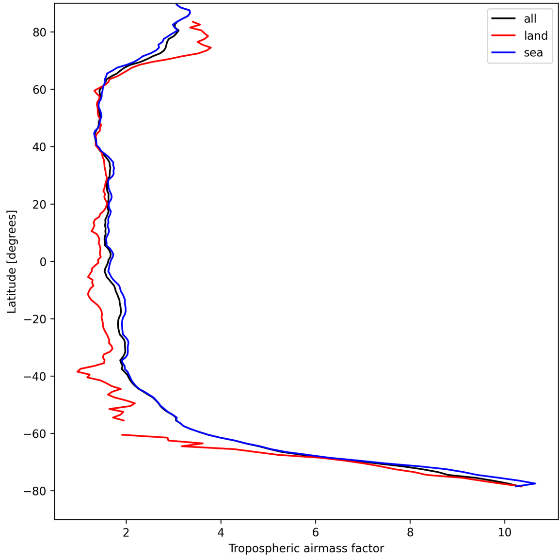
Figure 14: Zonal average of “Tropospheric airmass factor” for 2024-08-25 to 2024-08-27.
