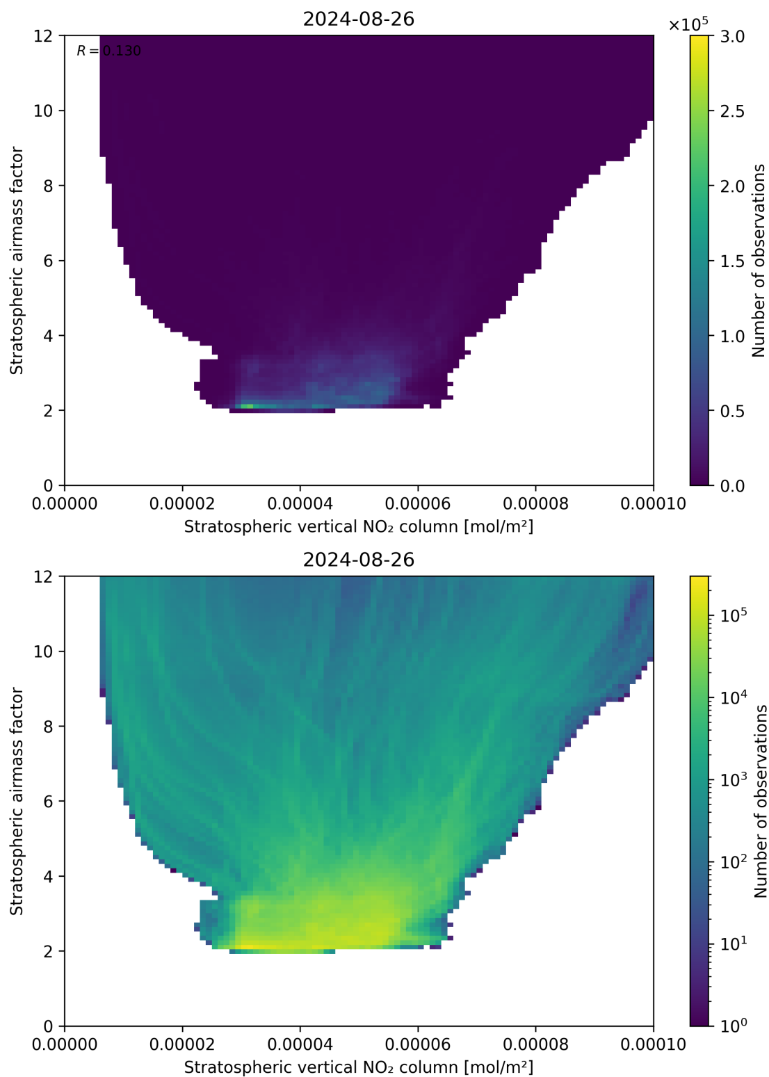
Figure 96: Scatter density plot of “Stratospheric vertical NO 2 column” against “Stratospheric airmass factor” for 2024-08-25 to 2024-08-27.
