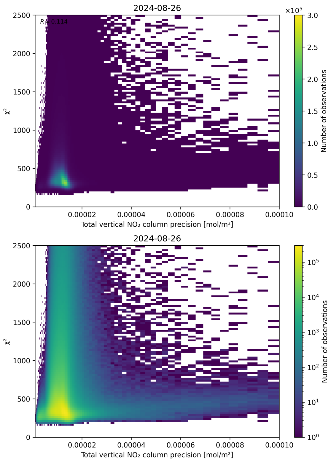
Figure 116: Scatter density plot of “Total vertical NO 2 column precision” against “ \chi^2 ” for 2024-08-25 to 2024-08-27.
