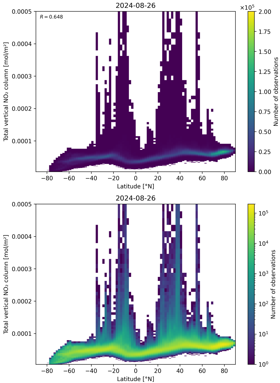
Figure 90: Scatter density plot of “Latitude” against “Total vertical NO 2 column” for 2024-08-25 to 2024-08-27.
