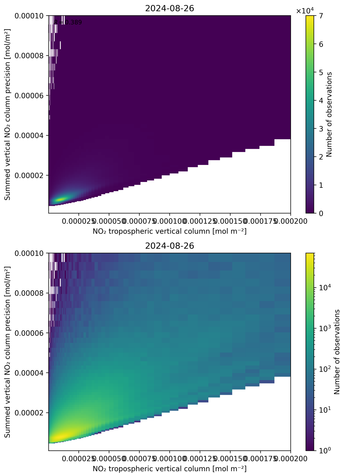
Figure 127: Scatter density plot of “NO 2 tropospheric vertical column” against “Summed vertical NO 2 column precision” for 2024-08-25 to 2024-08-27.
