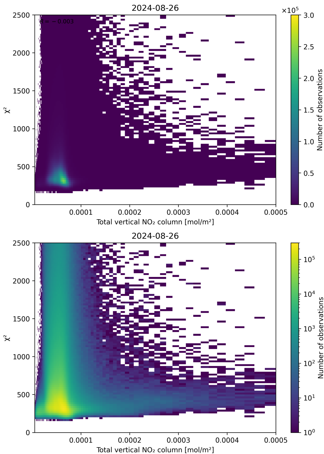
Figure 111: Scatter density plot of “Total vertical NO 2 column” against “ \chi^2 ” for 2024-08-25 to 2024-08-27.
