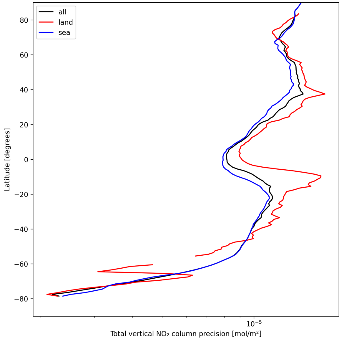
Figure 22: Zonal average of “Total vertical NO 2 column precision” for 2024-08-25 to 2024-08-27.
