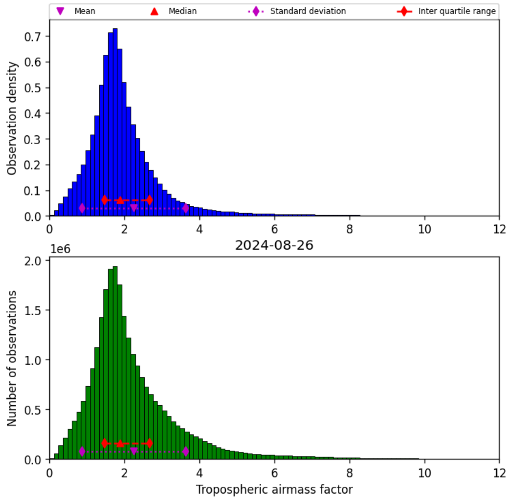
Figure 31: Histogram of “Tropospheric airmass factor” for 2024-08-25 to 2024-08-27
