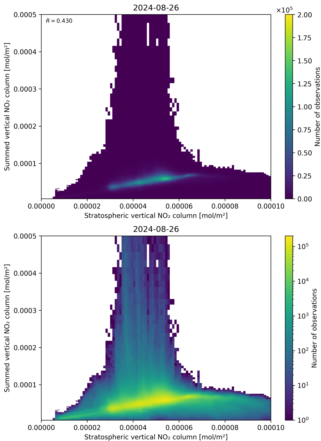
Figure 98: Scatter density plot of “Stratospheric vertical NO 2 column” against “Summed vertical NO 2 column” for 2024-08-25 to 2024-08-27.
