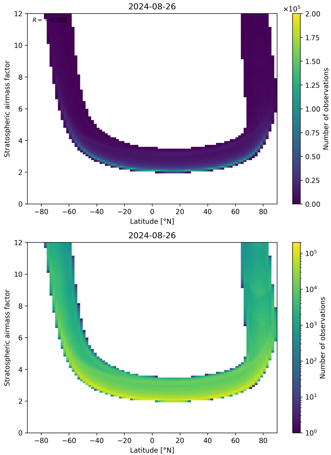
Figure 83: Scatter density plot of “Latitude” against “Stratospheric air mass factor” for 2024-08-25 to 2024-08-27.
