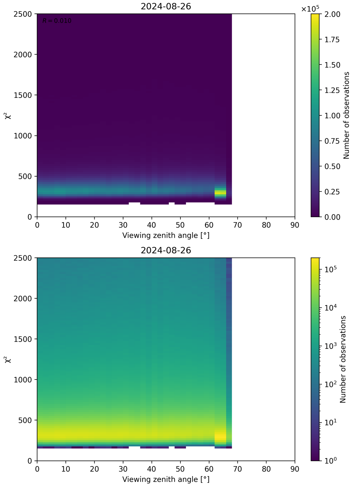
Figure 162: Scatter density plot of “Viewing zenith angle” against “ \chi^2 ” for 2024-08-25 to 2024-08-27.
