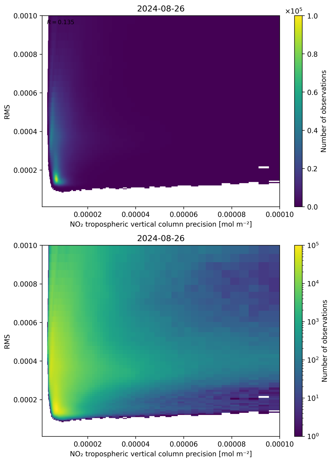
Figure 140: Scatter density plot of “NO 2 tropospheric vertical column precision” against “RMS” for 2024-08-25 to 2024-08-27.
