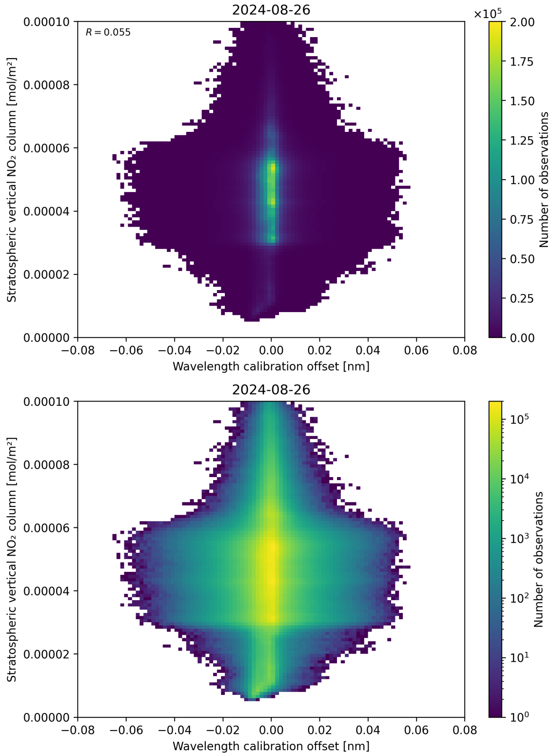
Figure 176: Scatter density plot of “Wavelength calibration offset” against “Stratospheric vertical NO 2 column” for 2024-08-25 to 2024-08-27.
