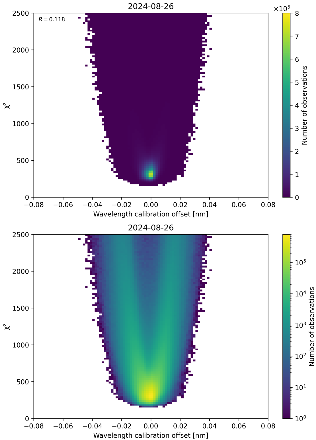
Figure 175: Scatter density plot of “Wavelength calibration offset” against “ \chi^2 ” for 2024-08-25 to 2024-08-27.
