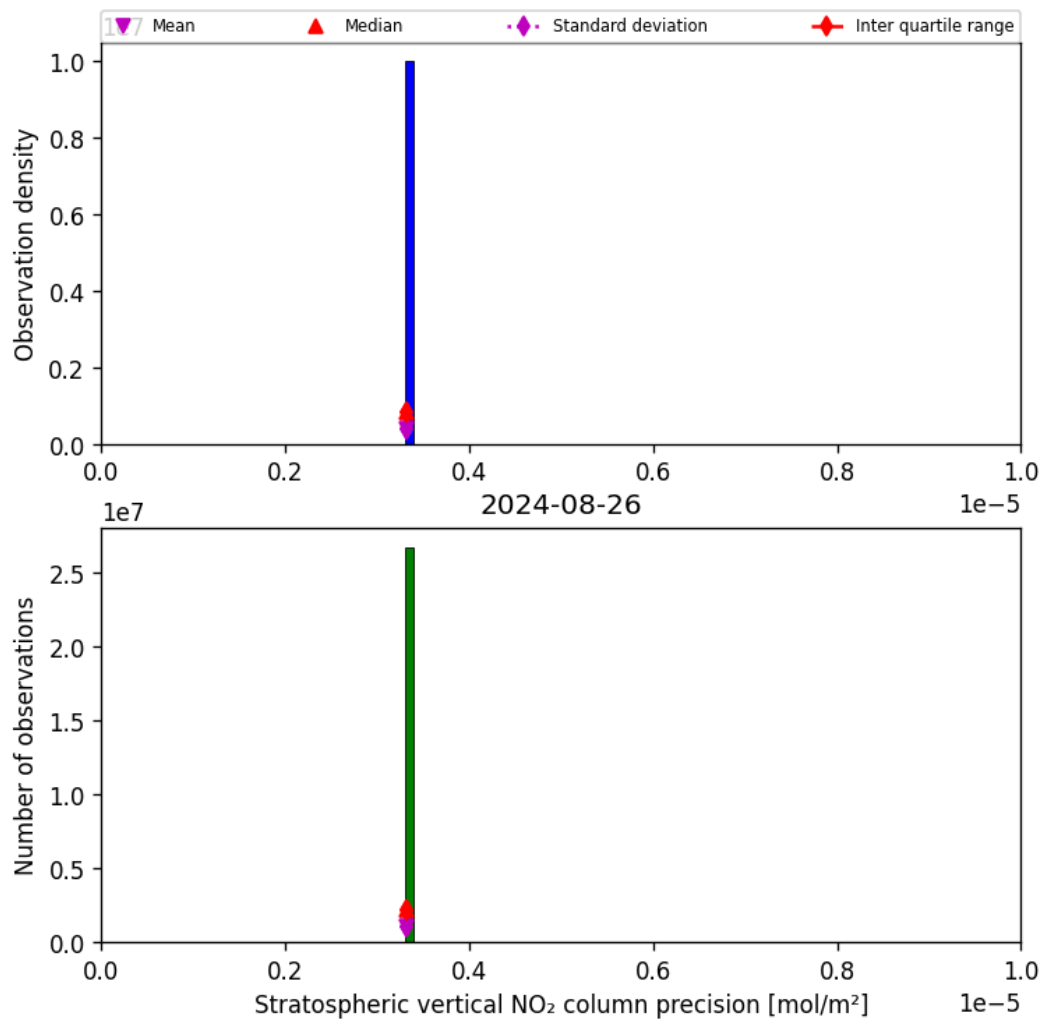
Figure 37: Histogram of “Stratospheric vertical NO 2 column precision” for 2024-08-25 to 2024-08-27
