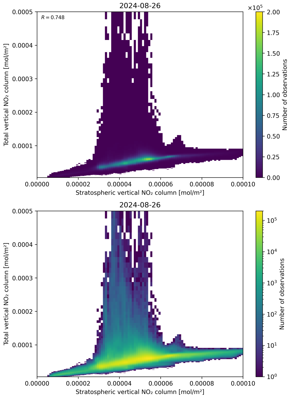
Figure 100: Scatter density plot of “Stratospheric vertical NO 2 column” against “Total vertical NO 2 column” for 2024-08-25 to 2024-08-27.
