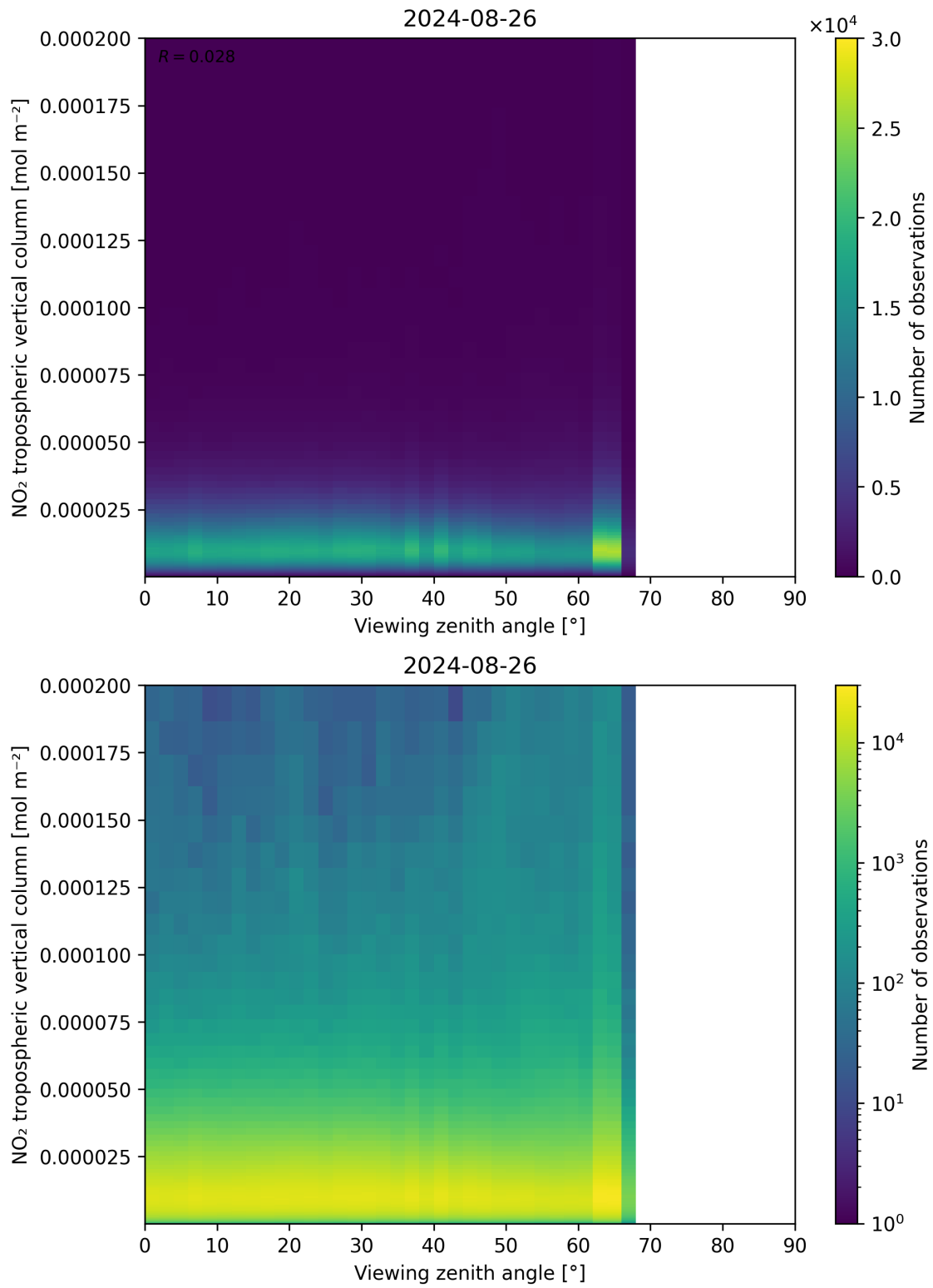
Figure 169: Scatter density plot of “Viewing zenith angle” against “NO 2 tropospheric vertical column” for 2024-08-25 to 2024-08-27.
