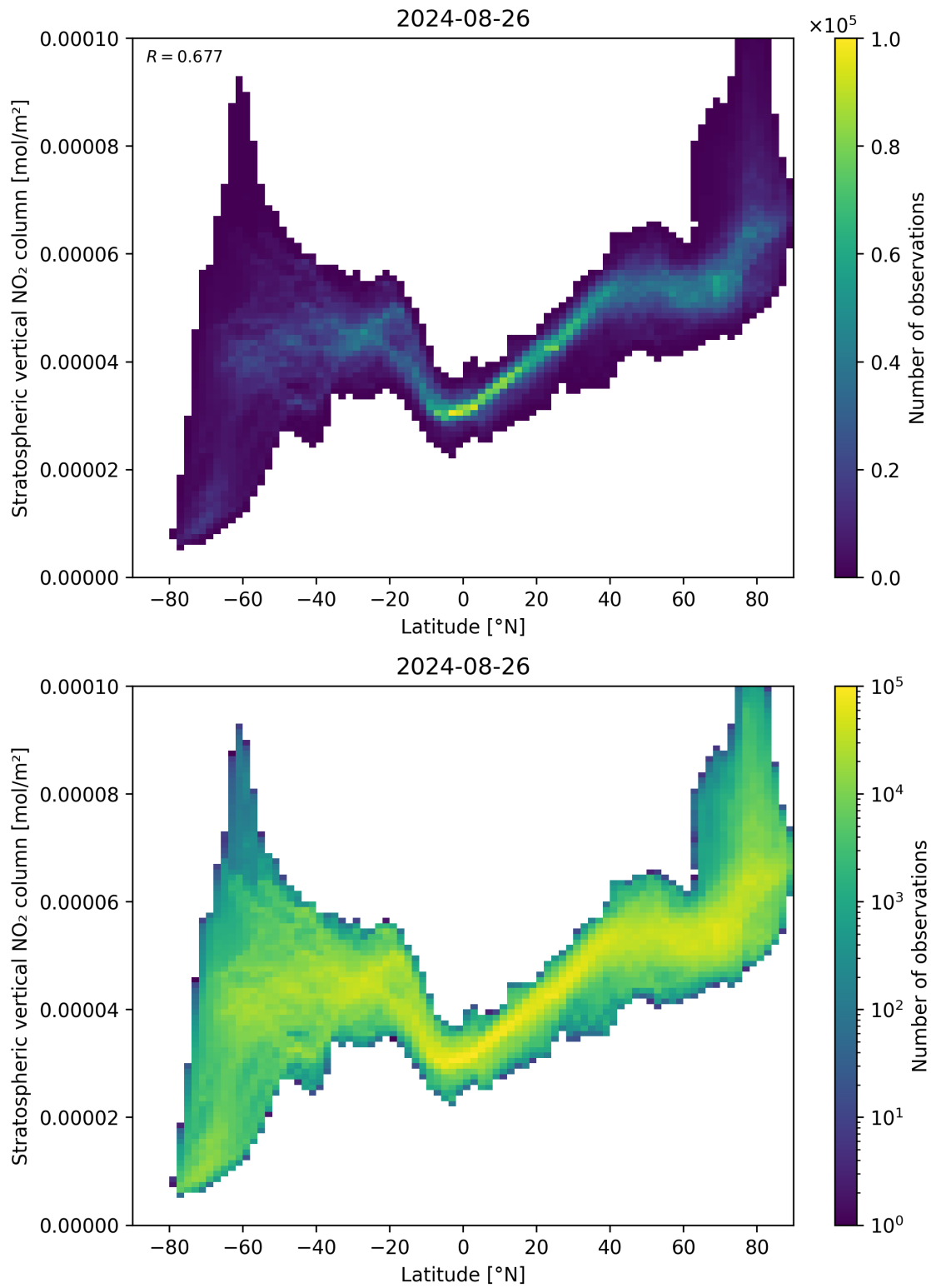
Figure 87: Scatter density plot of “Latitude” against “Stratospheric vertical NO 2 column” for 2024-08-25 to 2024-08-27.
