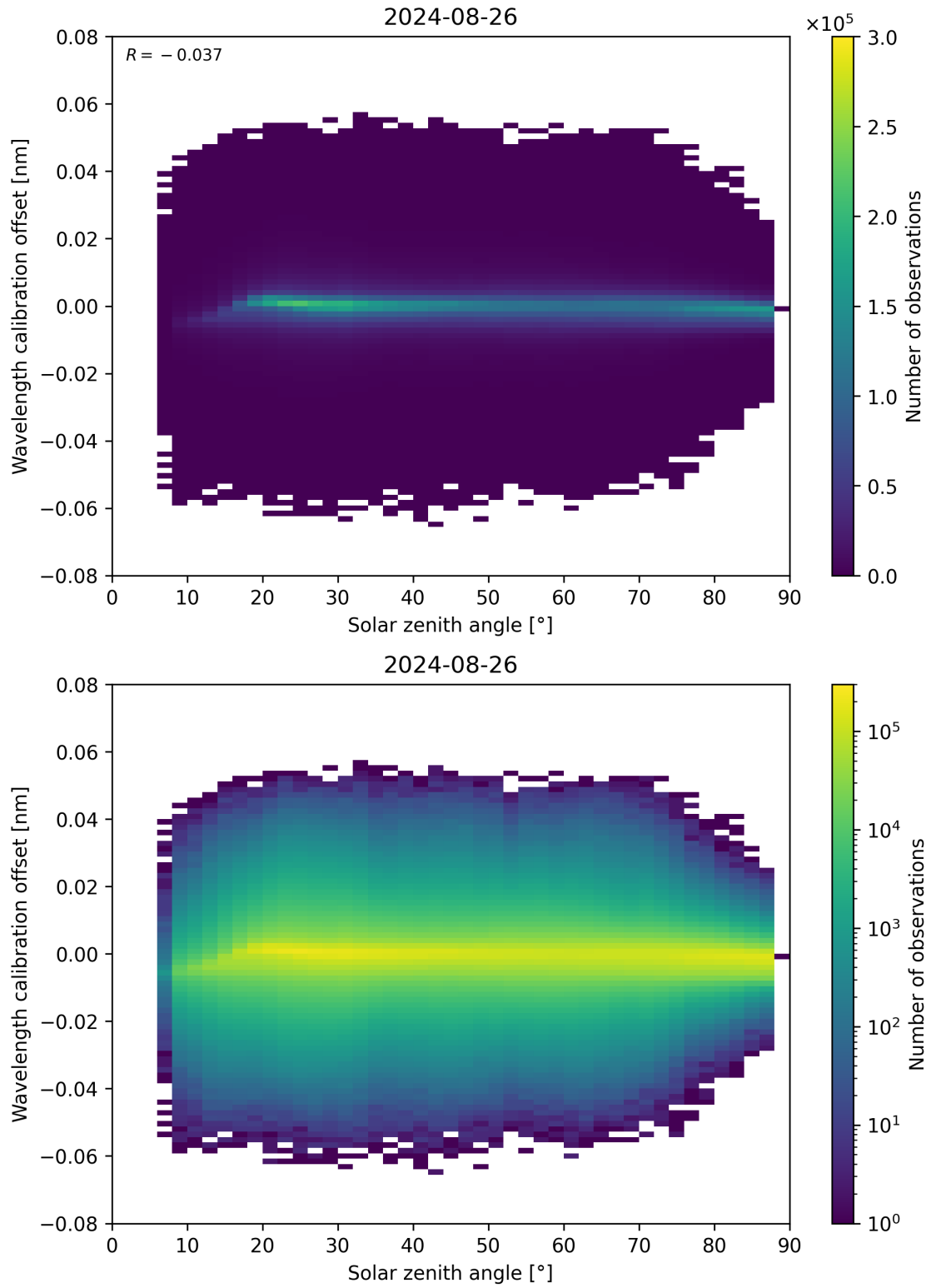
Figure 158: Scatter density plot of “Solar zenith angle” against “Wavelength calibration offset” for 2024-08-25 to 2024-08-27.
