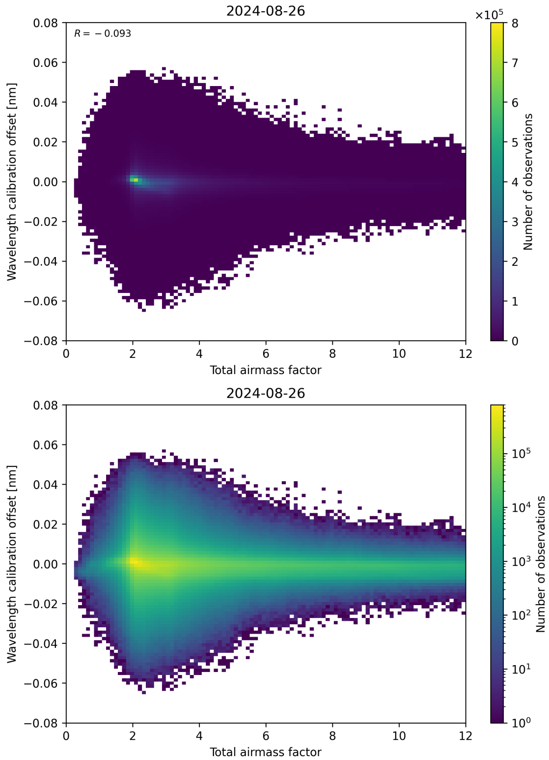
Figure 70: Scatter density plot of “Total airmass factor” against “Wavelength calibration offset” for 2024-08-25 to 2024-08-27.
