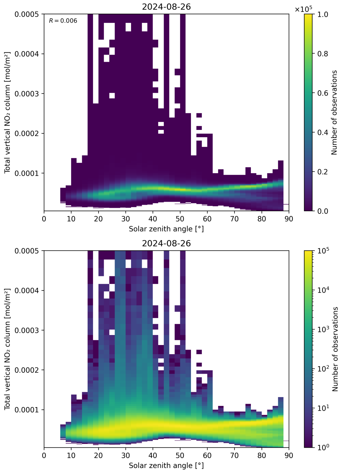
Figure 153: Scatter density plot of “Solar zenith angle” against “Total vertical NO 2 column” for 2024-08-25 to 2024-08-27.
