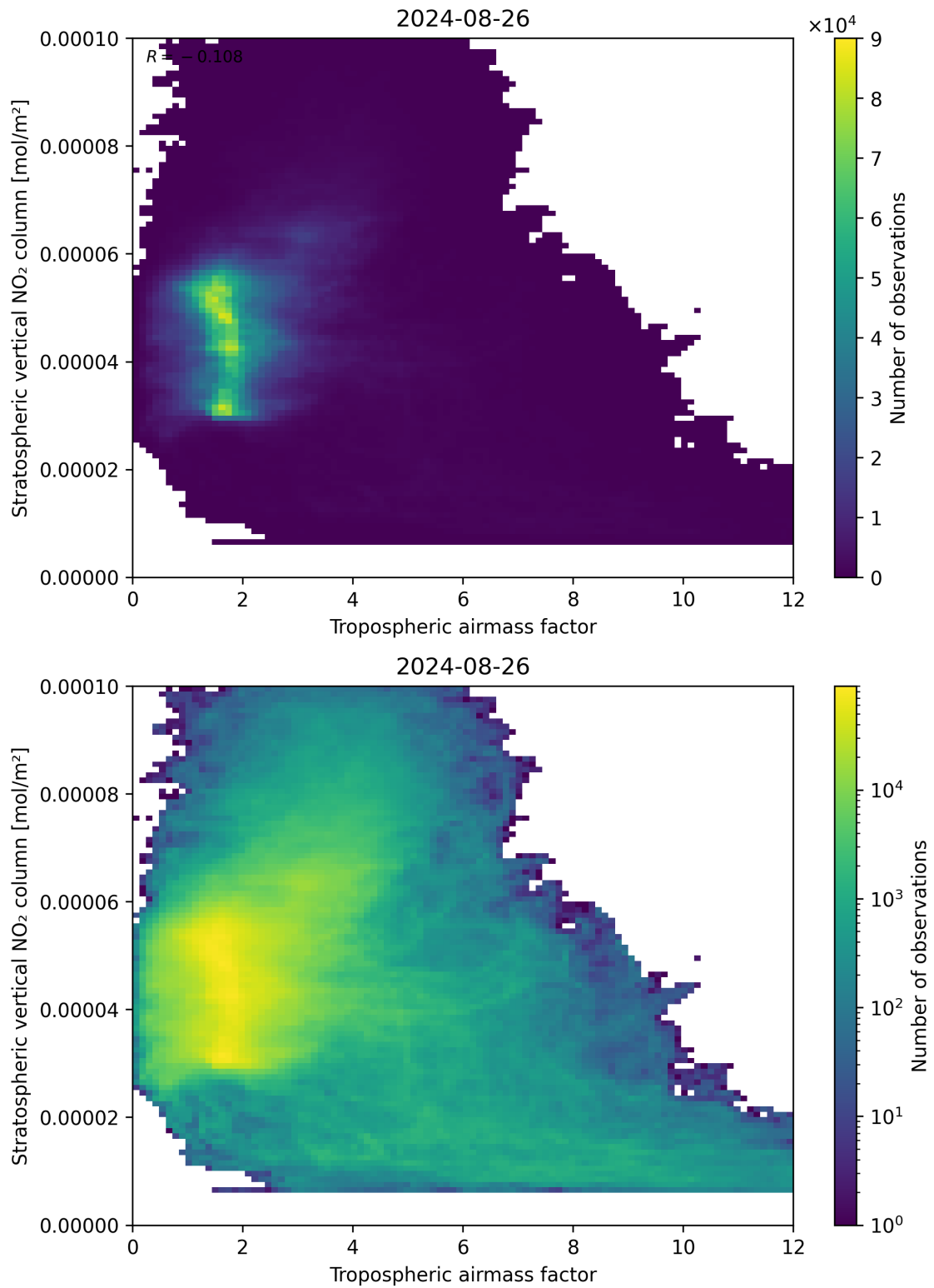
Figure 74: Scatter density plot of “Tropospheric air mass factor” against “Stratospheric vertical NO 2 column” for 2024-08-25 to 2024-08-27.
