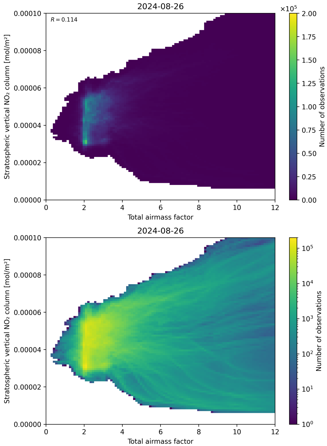
Figure 64: Scatter density plot of “Total airmass factor” against “Stratospheric vertical \text{NO}_2 column” for 2024-08-25 to 2024-08-27.
