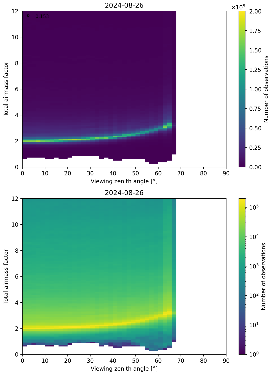
Figure 160: Scatter density plot of “Viewing zenith angle” against “Total airmass factor” for 2024-08-25 to 2024-08-27.
