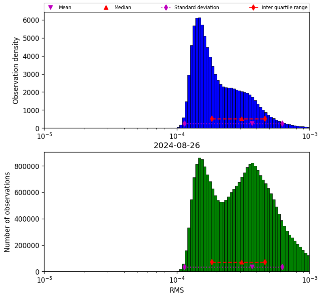
Figure 43: Histogram of “RMS” for 2024-08-25 to 2024-08-27
