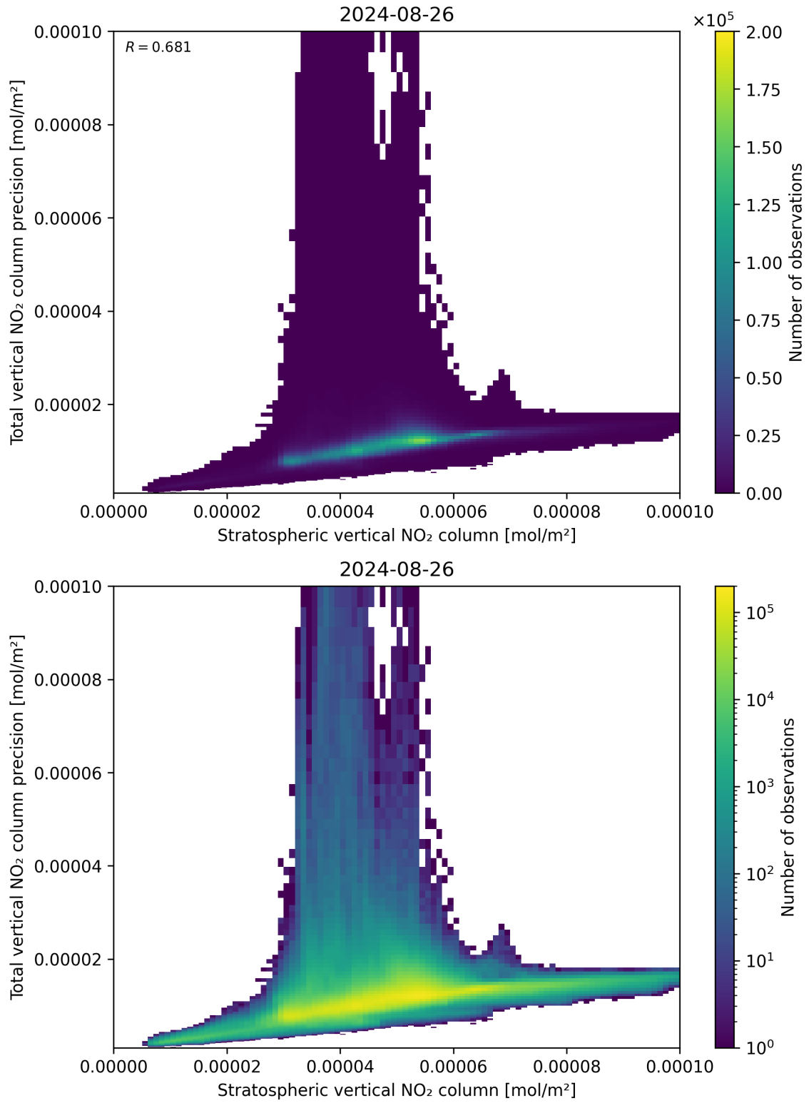
Figure 101: Scatter density plot of “Stratospheric vertical NO 2 column” against “Total vertical NO 2 column precision” for 2024-08-25 to 2024-08-27.
