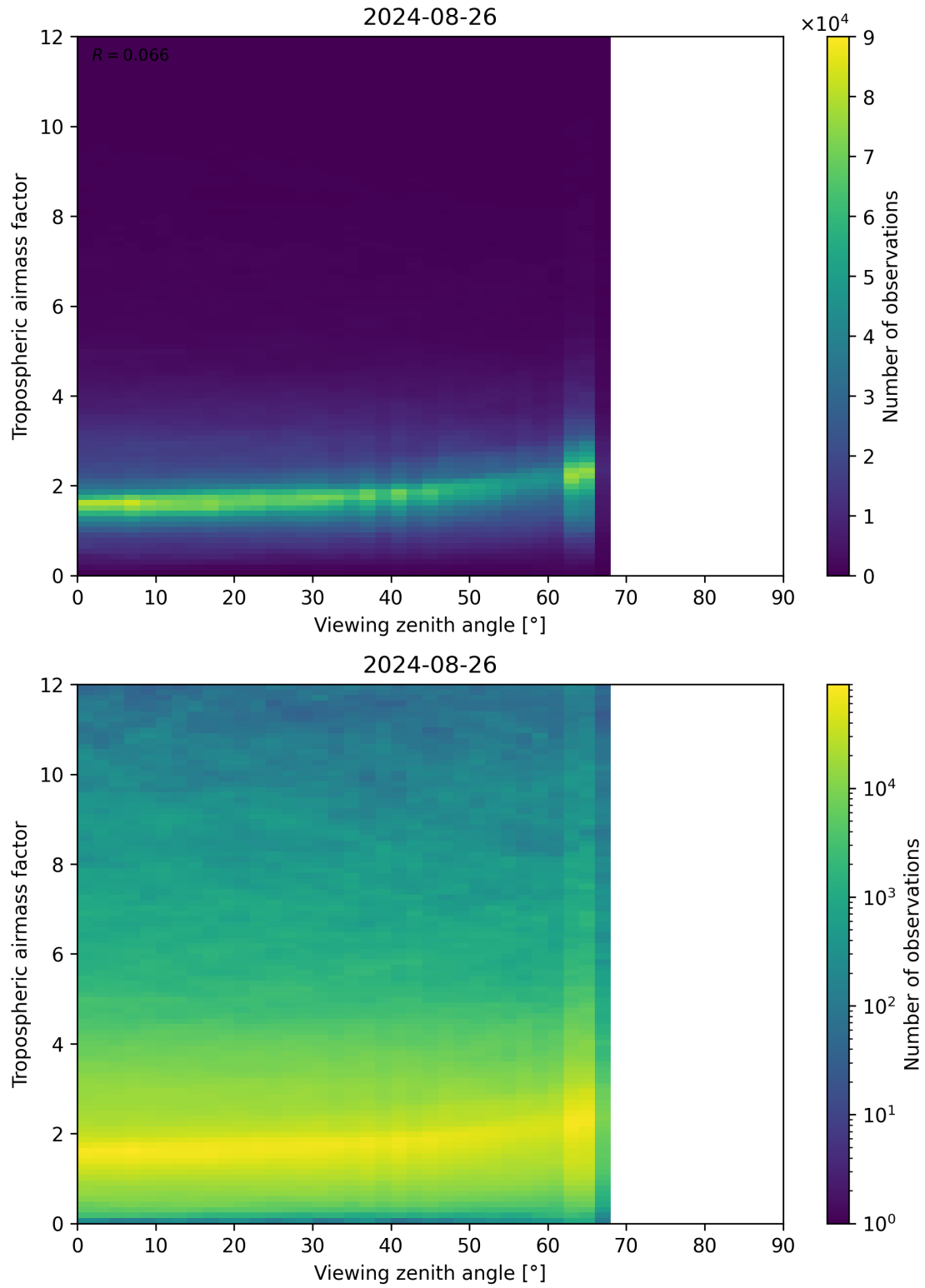
Figure 161: Scatter density plot of “Viewing zenith angle” against “Tropospheric airmass factor” for 2024-08-25 to 2024-08-27.
