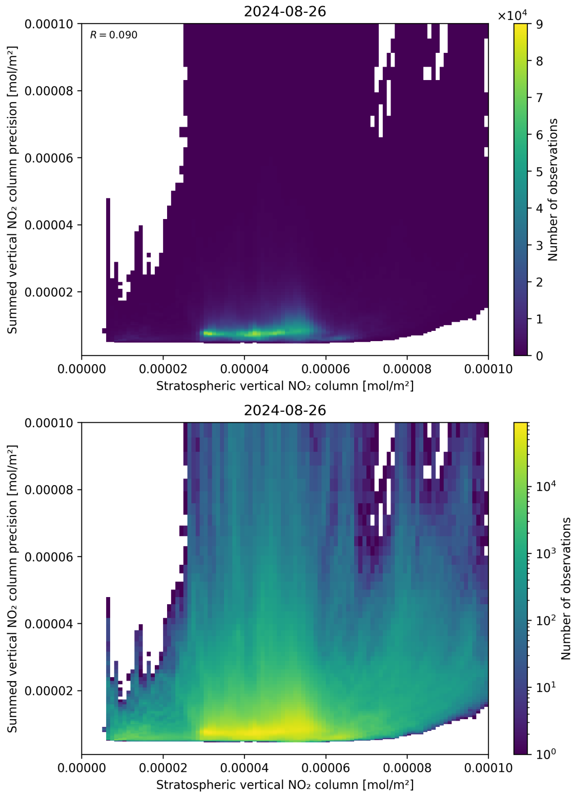
Figure 99: Scatter density plot of “Stratospheric vertical NO 2 column” against “Summed vertical NO 2 column precision” for 2024-08-25 to 2024-08-27.
