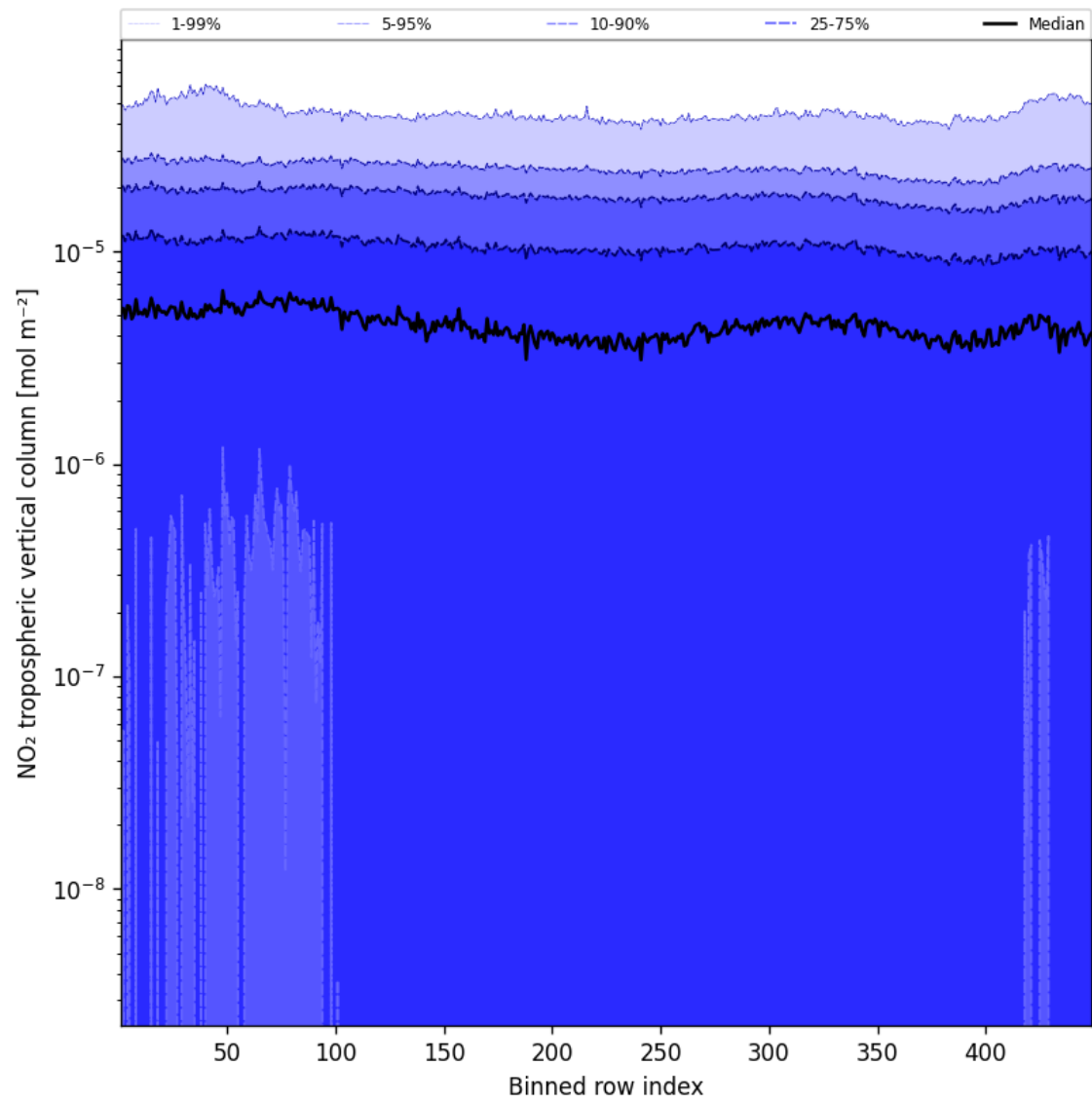
Figure 46: Along track statistics of “NO 2 tropospheric vertical column” for 2024-08-25 to 2024-08-27
