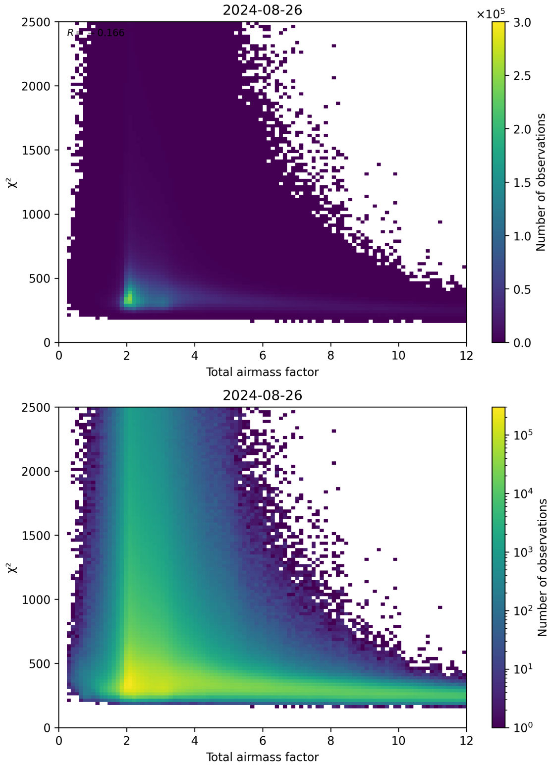
Figure 63: Scatter density plot of “Total airmass factor” against “ \chi^2 ” for 2024-08-25 to 2024-08-27.
