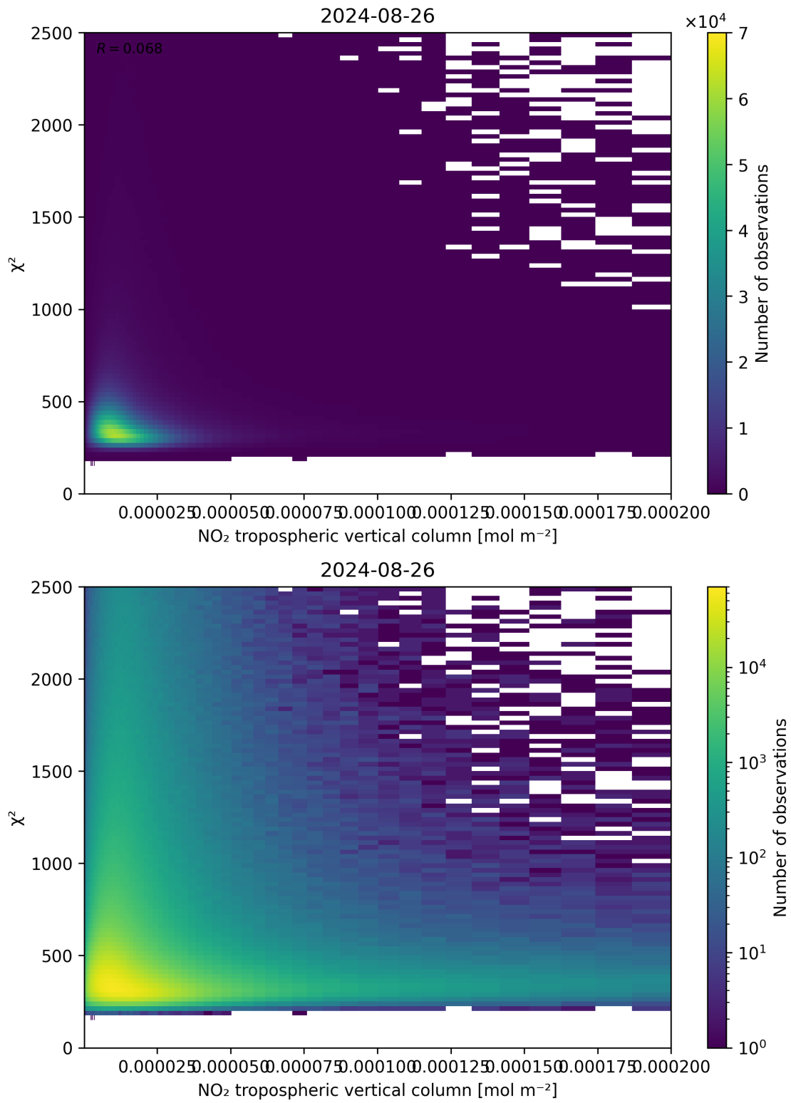
Figure 124: Scatter density plot of “NO 2 tropospheric vertical column” against “ \chi^2 ” for 2024-08-25 to 2024-08-27.
