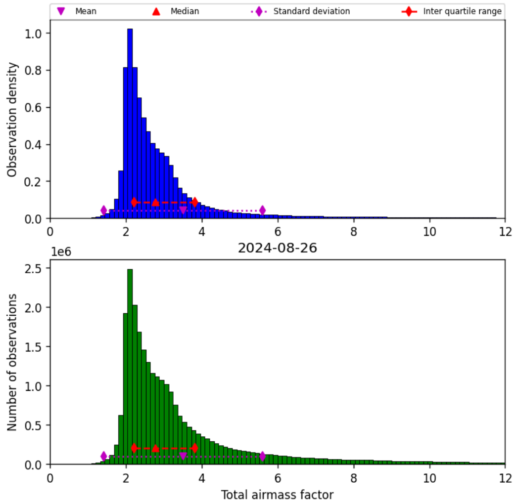
Figure 32: Histogram of “Total airmass factor” for 2024-08-25 to 2024-08-27
