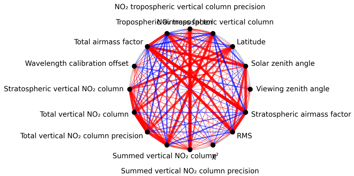
Figure 1: Map of correlation graph for 2024-08-25 to 2024-08-27.
