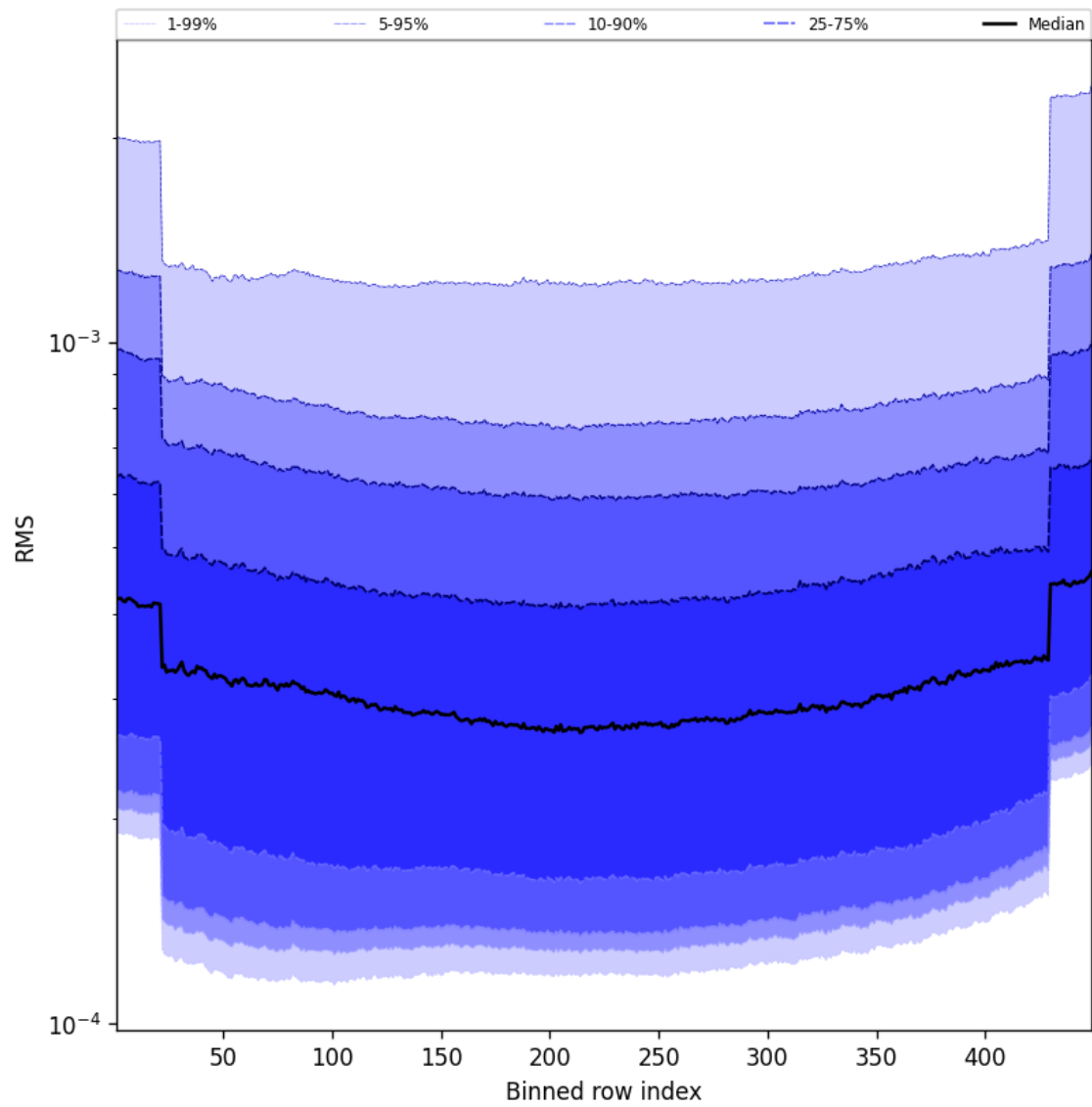
Figure 60: Along track statistics of “RMS” for 2024-08-25 to 2024-08-27
