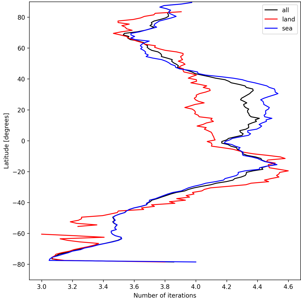
Figure 17: Zonal average of “Number of iterations” for 2024-08-25 to 2024-08-27.
