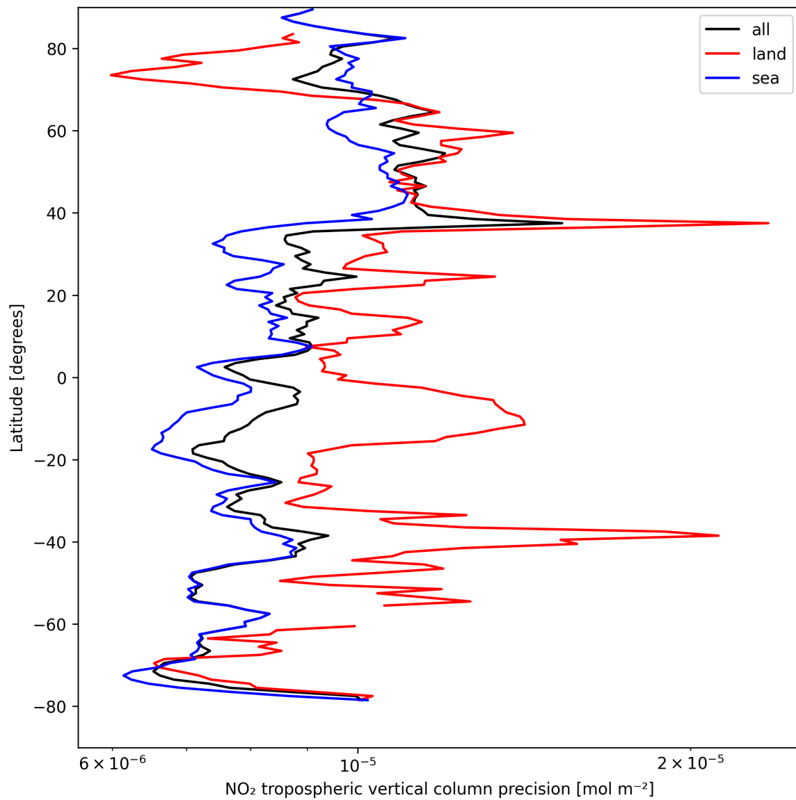
Figure 13: Zonal average of “NO 2 tropospheric vertical column precision” for 2024-08-25 to 2024-08-27.
