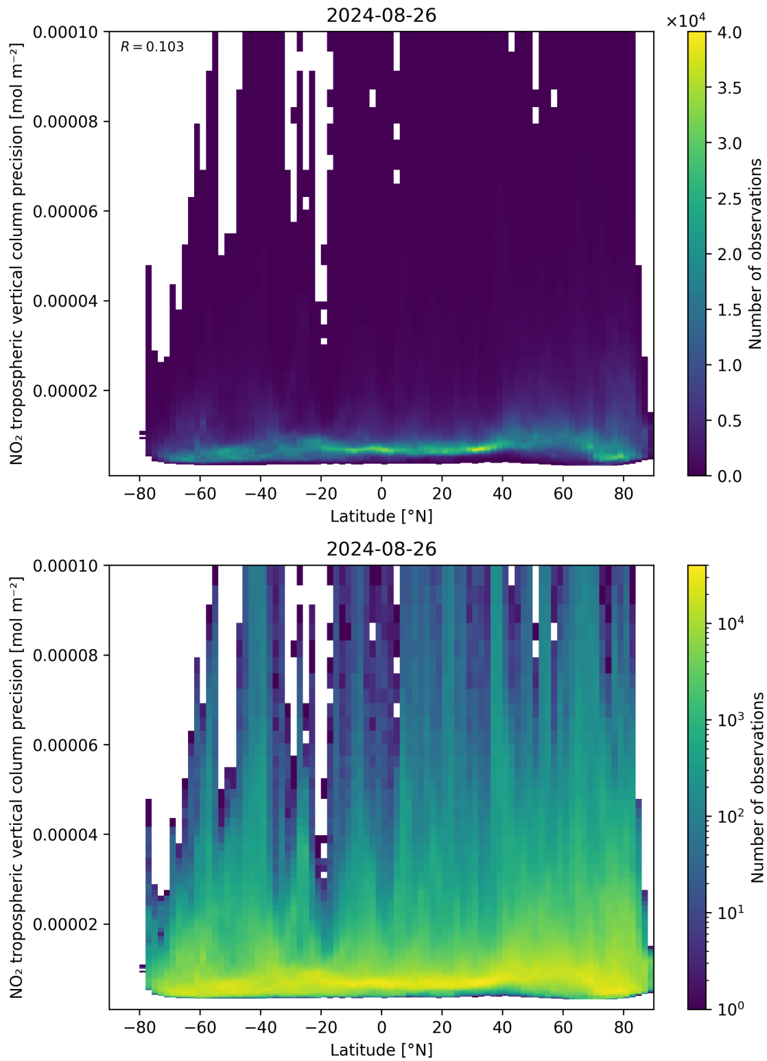
Figure 93: Scatter density plot of “Latitude” against “NO 2 tropospheric vertical column precision” for 2024-08-25 to 2024-08-27.
