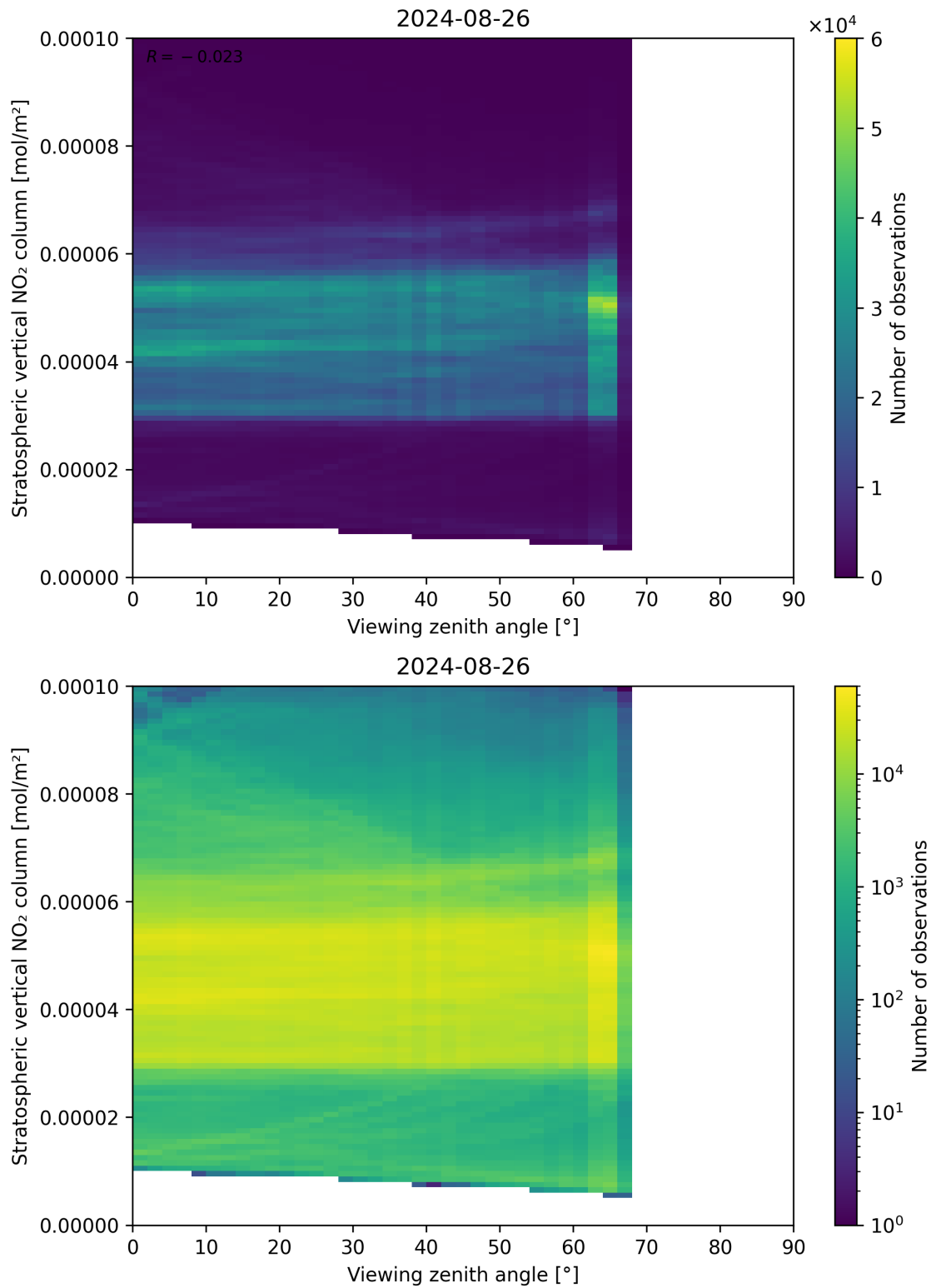
Figure 164: Scatter density plot of “Viewing zenith angle” against “Stratospheric vertical NO 2 column” for 2024-08-25 to 2024-08-27.
