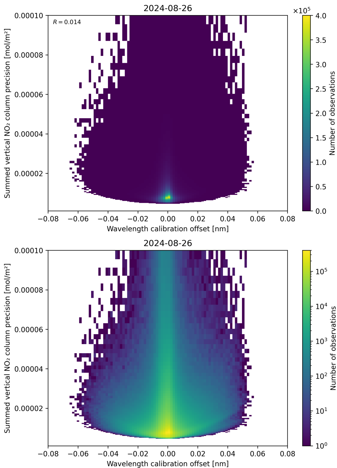
Figure 178: Scatter density plot of “Wavelength calibration offset” against “Summed vertical NO 2 column precision” for 2024-08-25 to 2024-08-27.
