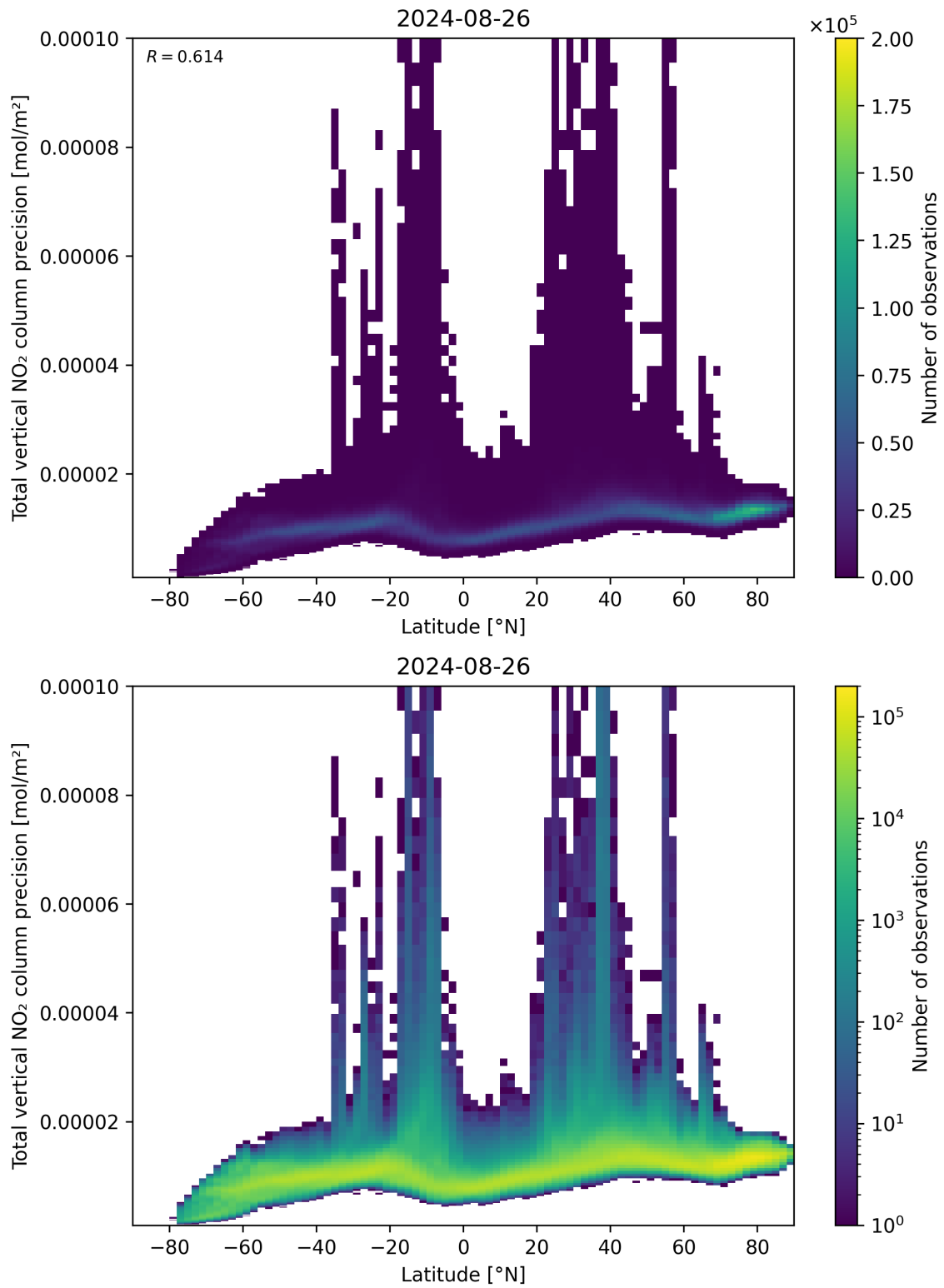
Figure 91: Scatter density plot of “Latitude” against “Total vertical NO 2 column precision” for 2024-08-25 to 2024-08-27.
