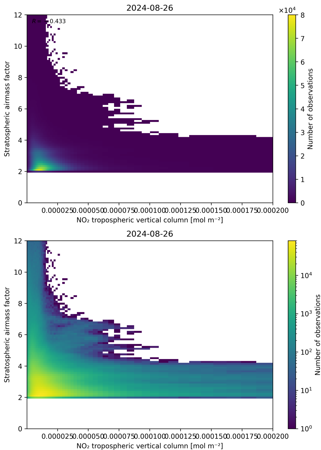
Figure 121: Scatter density plot of “NO 2 tropospheric vertical column” against “Stratospheric air mass factor” for 2024-08-25 to 2024-08-27.
