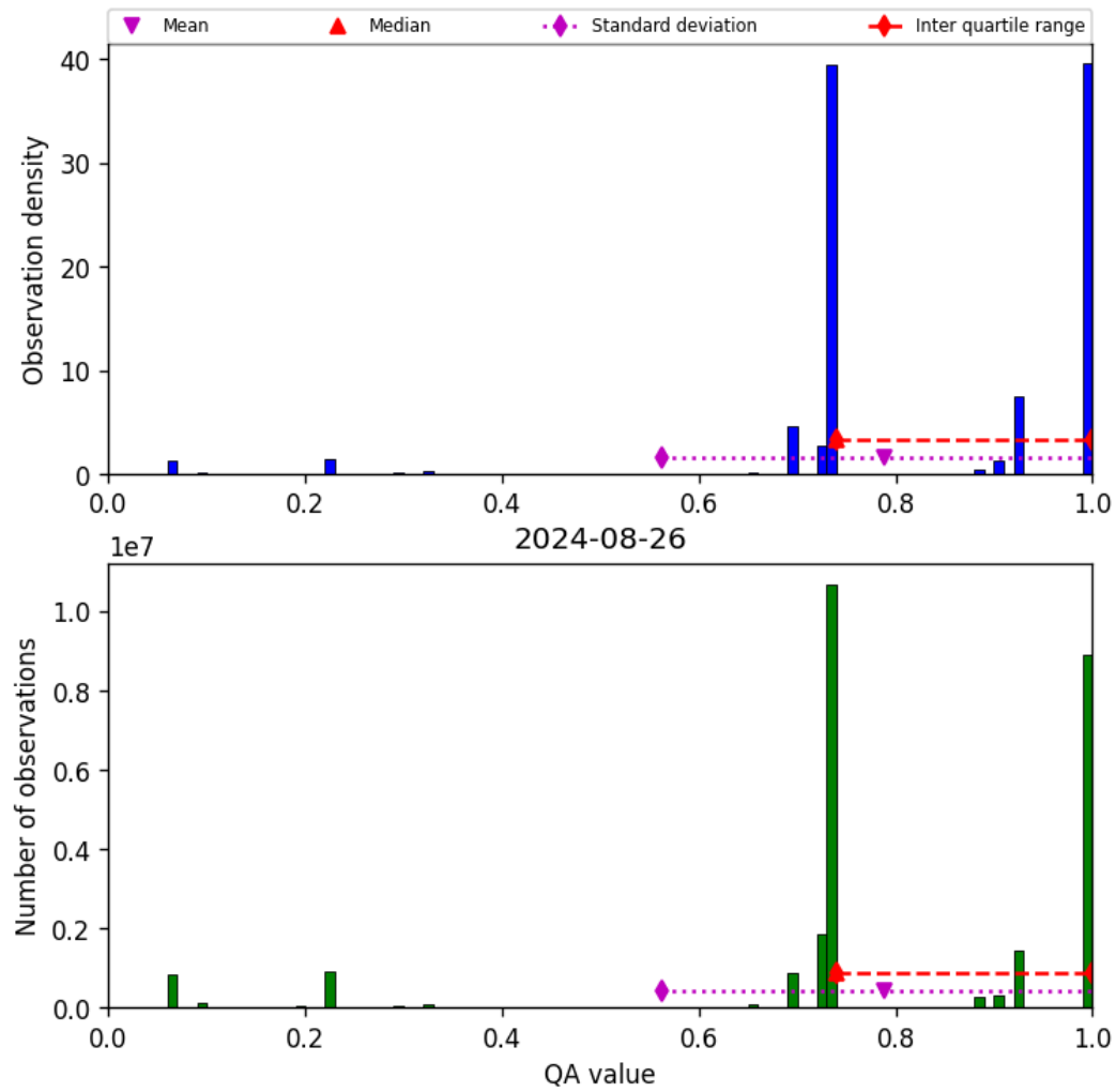
Figure 28: Histogram of “QA value” for 2024-08-25 to 2024-08-27
