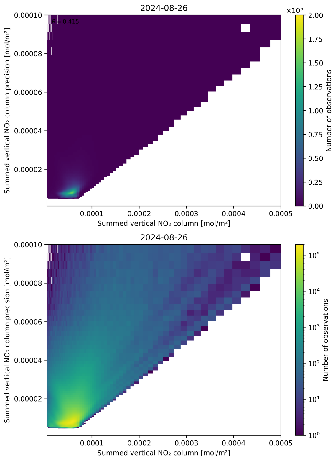
Figure 105: Scatter density plot of “Summed vertical NO 2 column” against “Summed vertical NO 2 column precision” for 2024-08-25 to 2024-08-27.
