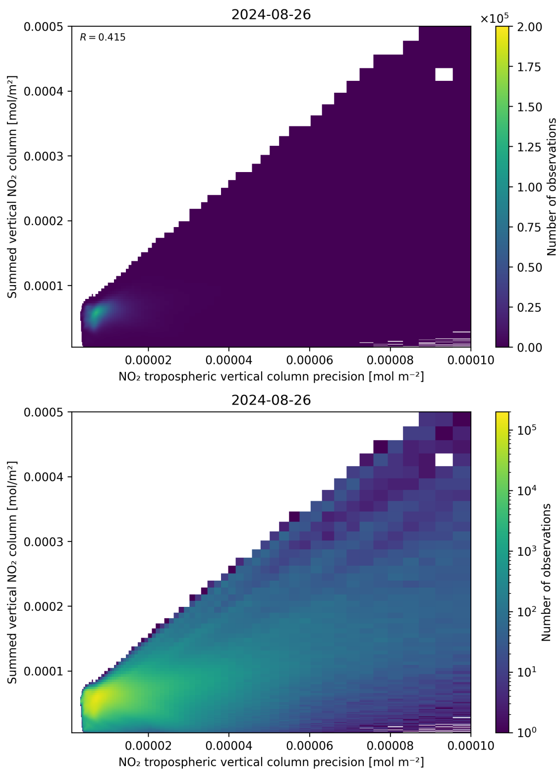
Figure 136: Scatter density plot of “NO 2 tropospheric vertical column precision” against “Summed vertical NO 2 column” for 2024-08-25 to 2024-08-27.
