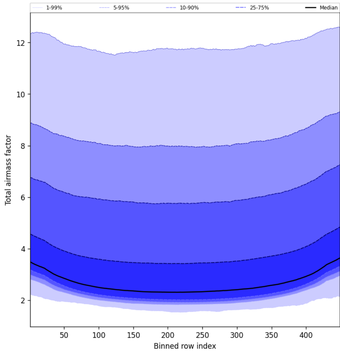
Figure 49: Along track statistics of “Total airmass factor” for 2024-08-25 to 2024-08-27
