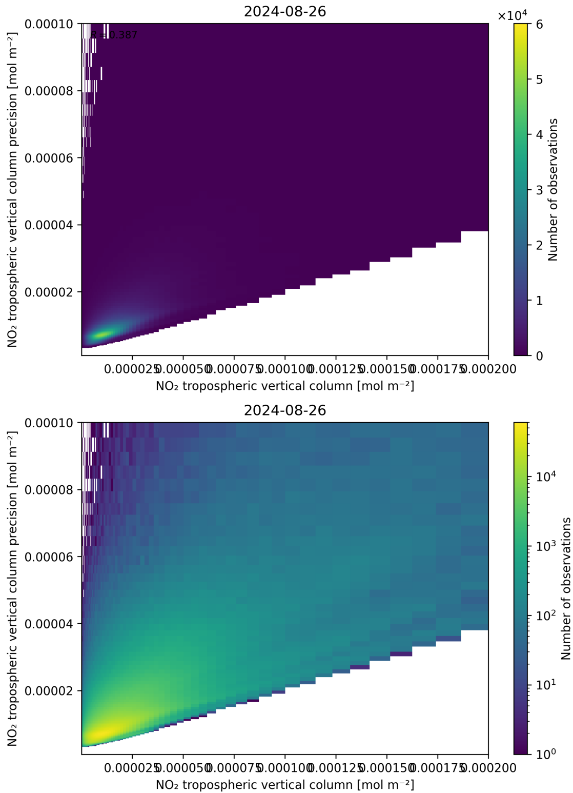
Figure 130: Scatter density plot of “NO 2 tropospheric vertical column” against “NO 2 tropospheric vertical column precision” for 2024-08-25 to 2024-08-27.
