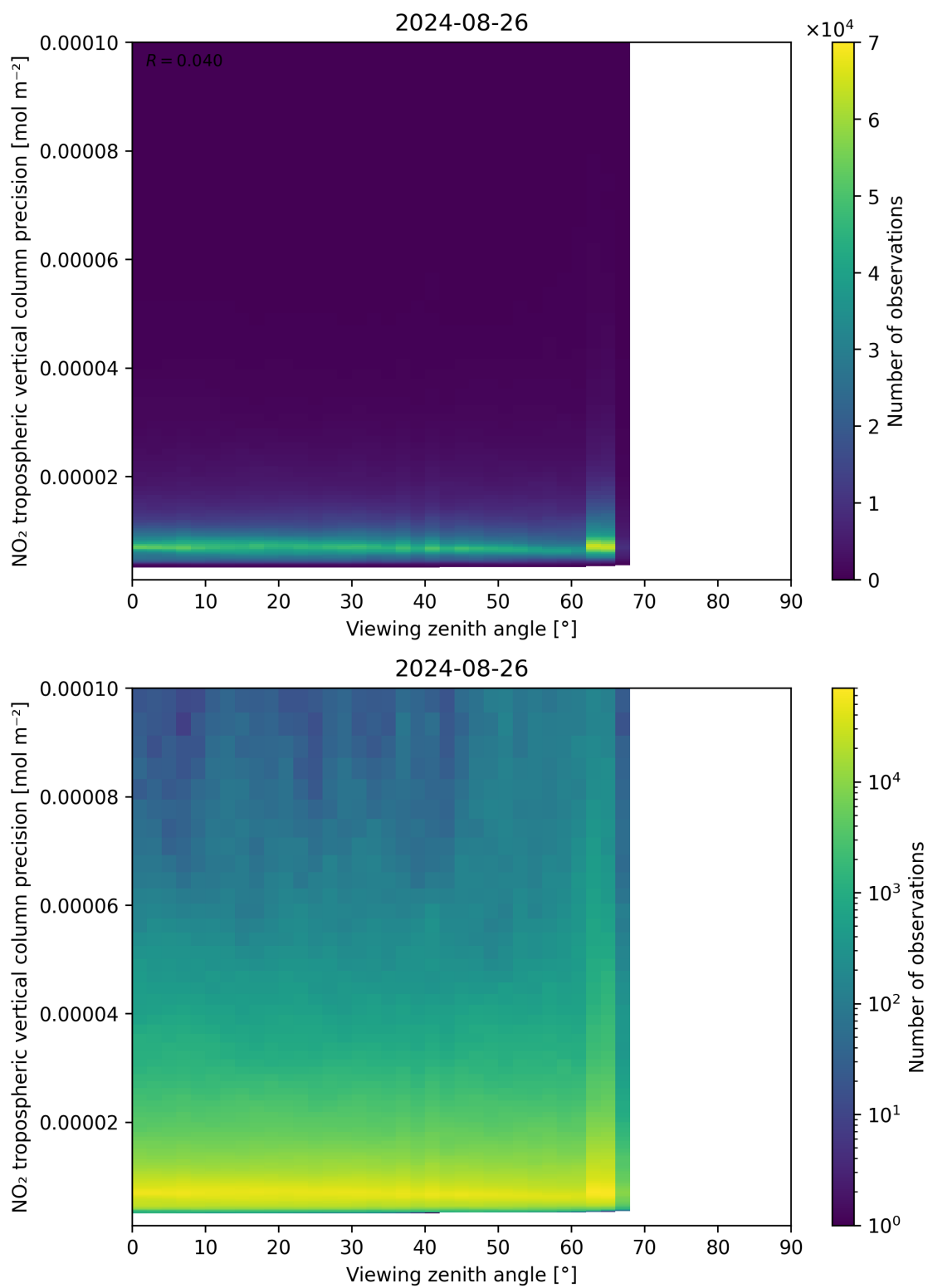
Figure 170: Scatter density plot of “Viewing zenith angle” against “NO 2 tropospheric vertical column precision” for 2024-08-25 to 2024-08-27.
