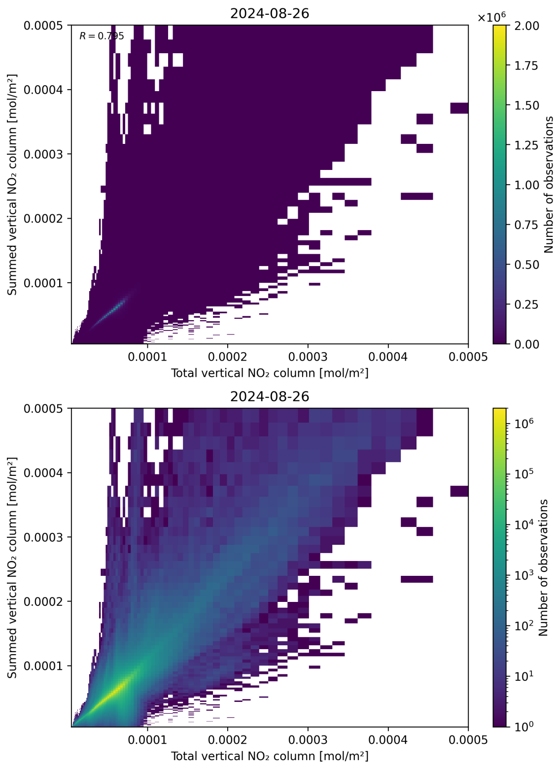
Figure 112: Scatter density plot of “Total vertical NO 2 column” against “Summed vertical NO 2 column” for 2024-08-25 to 2024-08-27.
