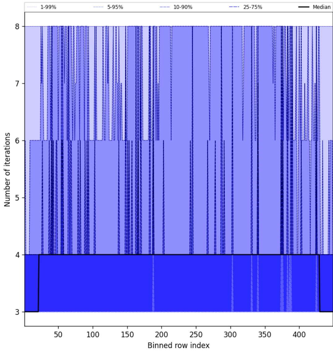
Figure 51: Along track statistics of “Number of iterations” for 2024-08-25 to 2024-08-27
