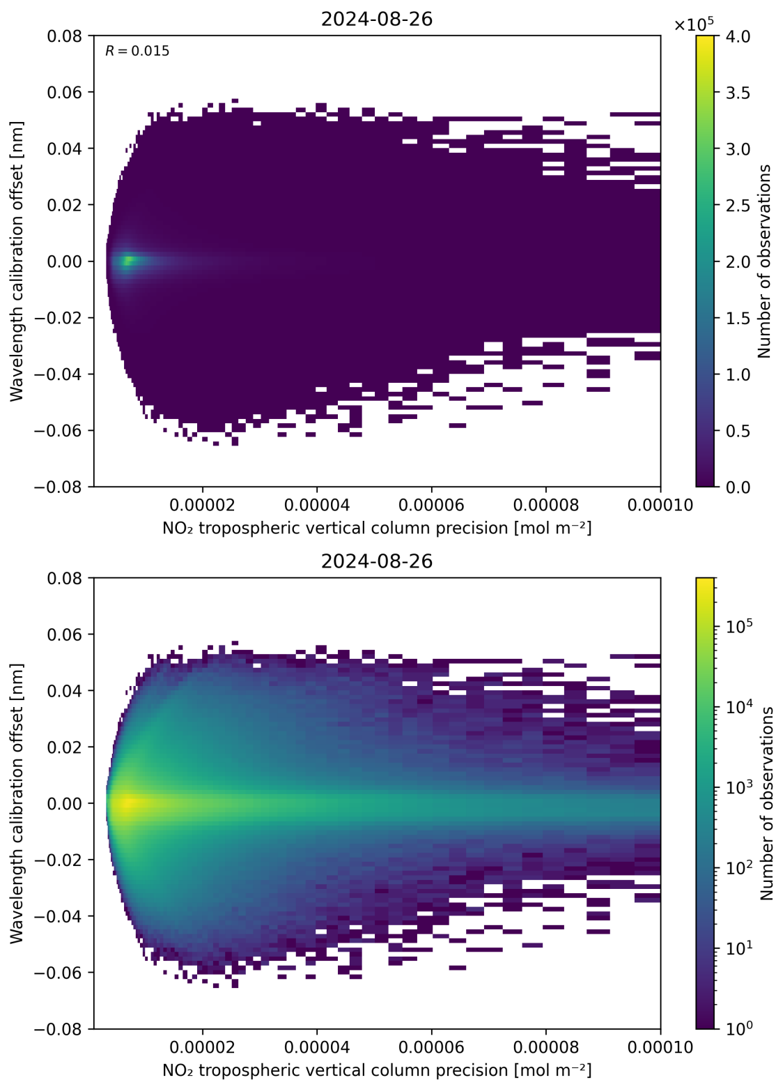
Figure 141: Scatter density plot of “NO 2 tropospheric vertical column precision” against “Wavelength calibration offset” for 2024-08-25 to 2024-08-27.
