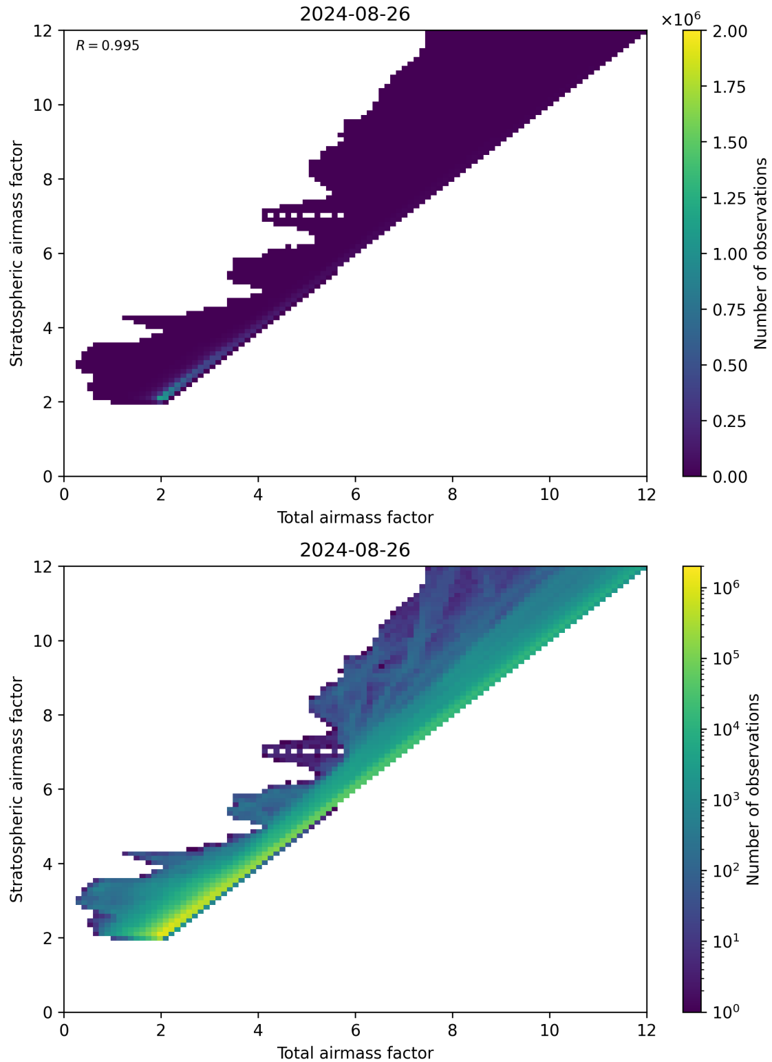
Figure 62: Scatter density plot of “Total airmass factor” against “Stratospheric airmass factor” for 2024-08-25 to 2024-08-27.
