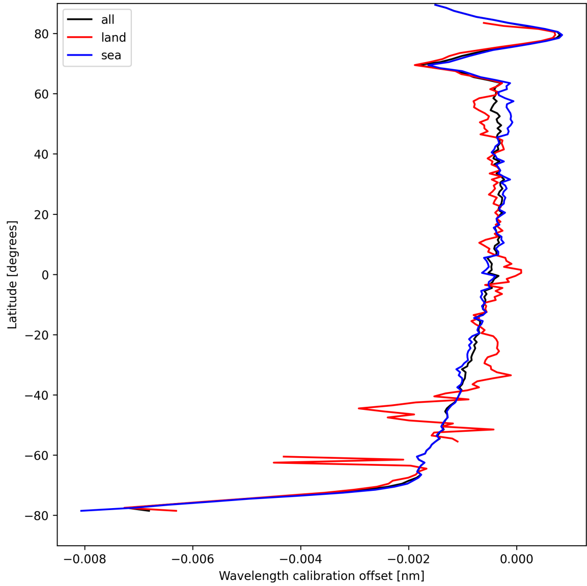
Figure 18: Zonal average of “Wavelength calibration offset” for 2024-08-25 to 2024-08-27.
