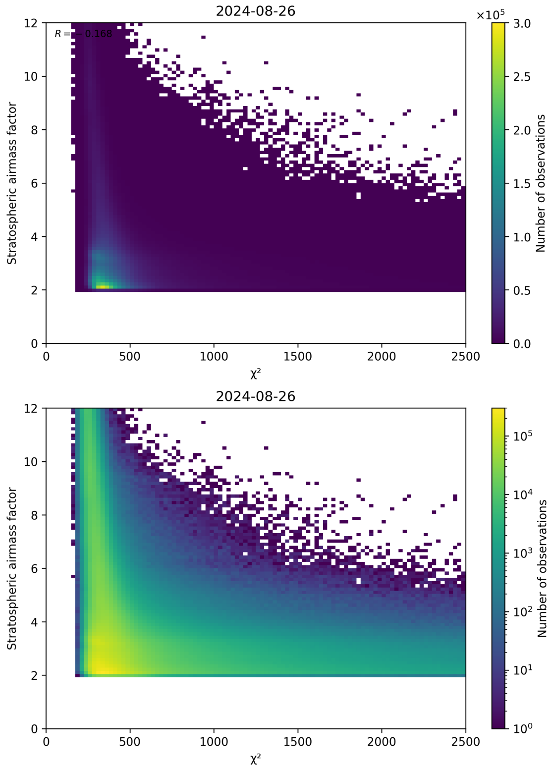
Figure 81: Scatter density plot of “ \chi^2 ” against “Stratospheric airmass factor” for 2024-08-25 to 2024-08-27.
