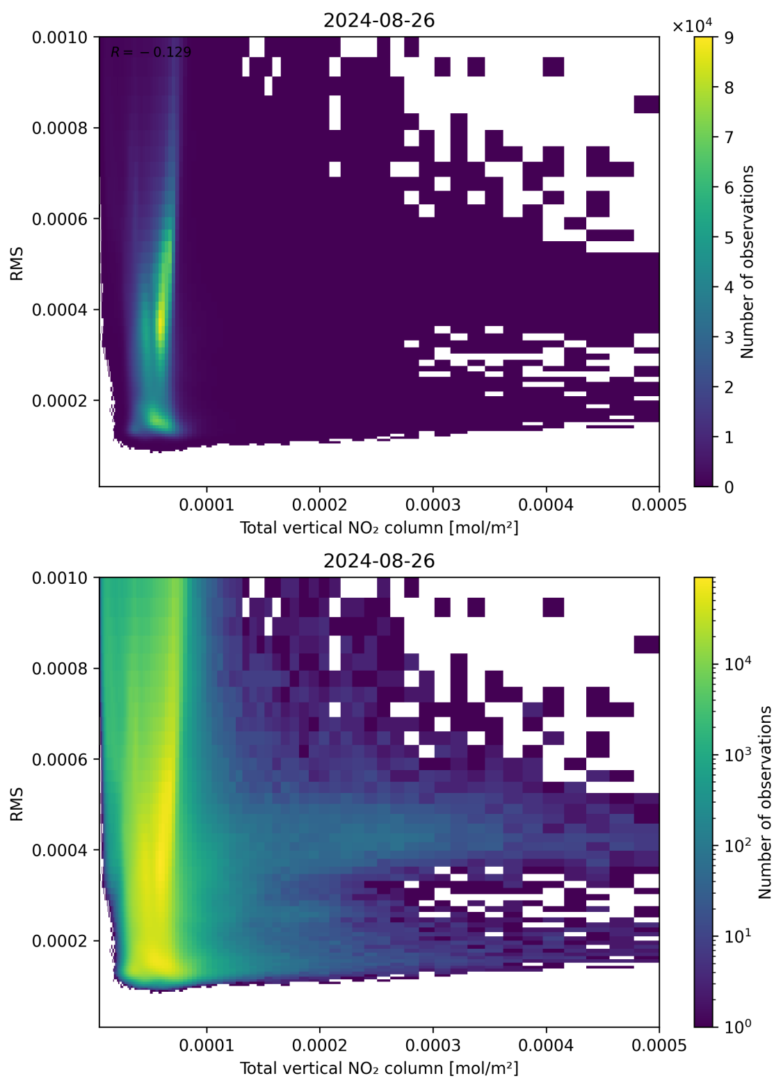
Figure 120: Scatter density plot of “Total vertical NO 2 column” against “RMS” for 2024-08-25 to 2024-08-27.
