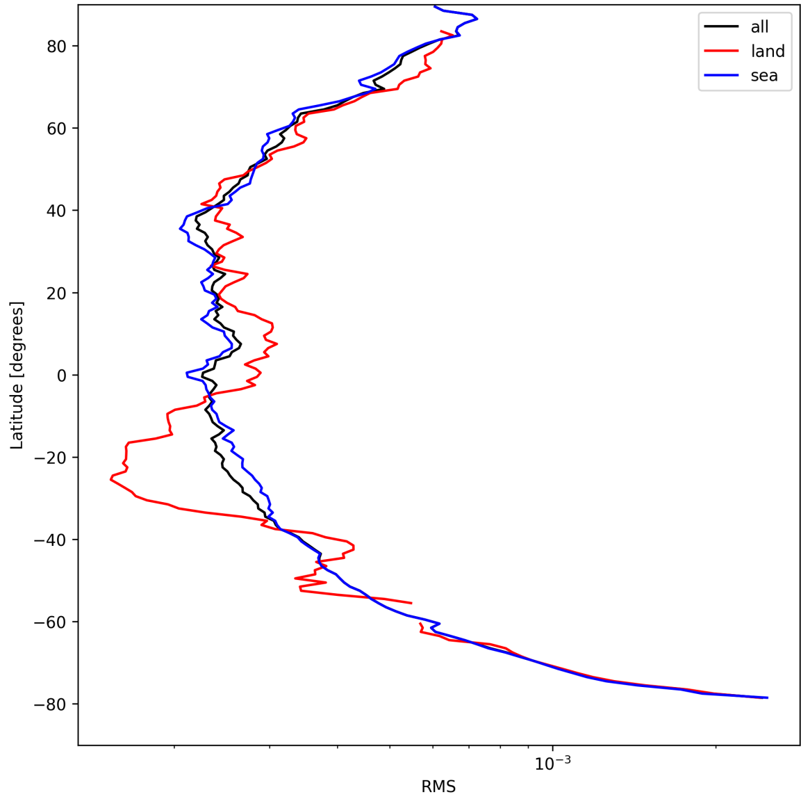
Figure 26: Zonal average of “RMS” for 2024-08-25 to 2024-08-27.
