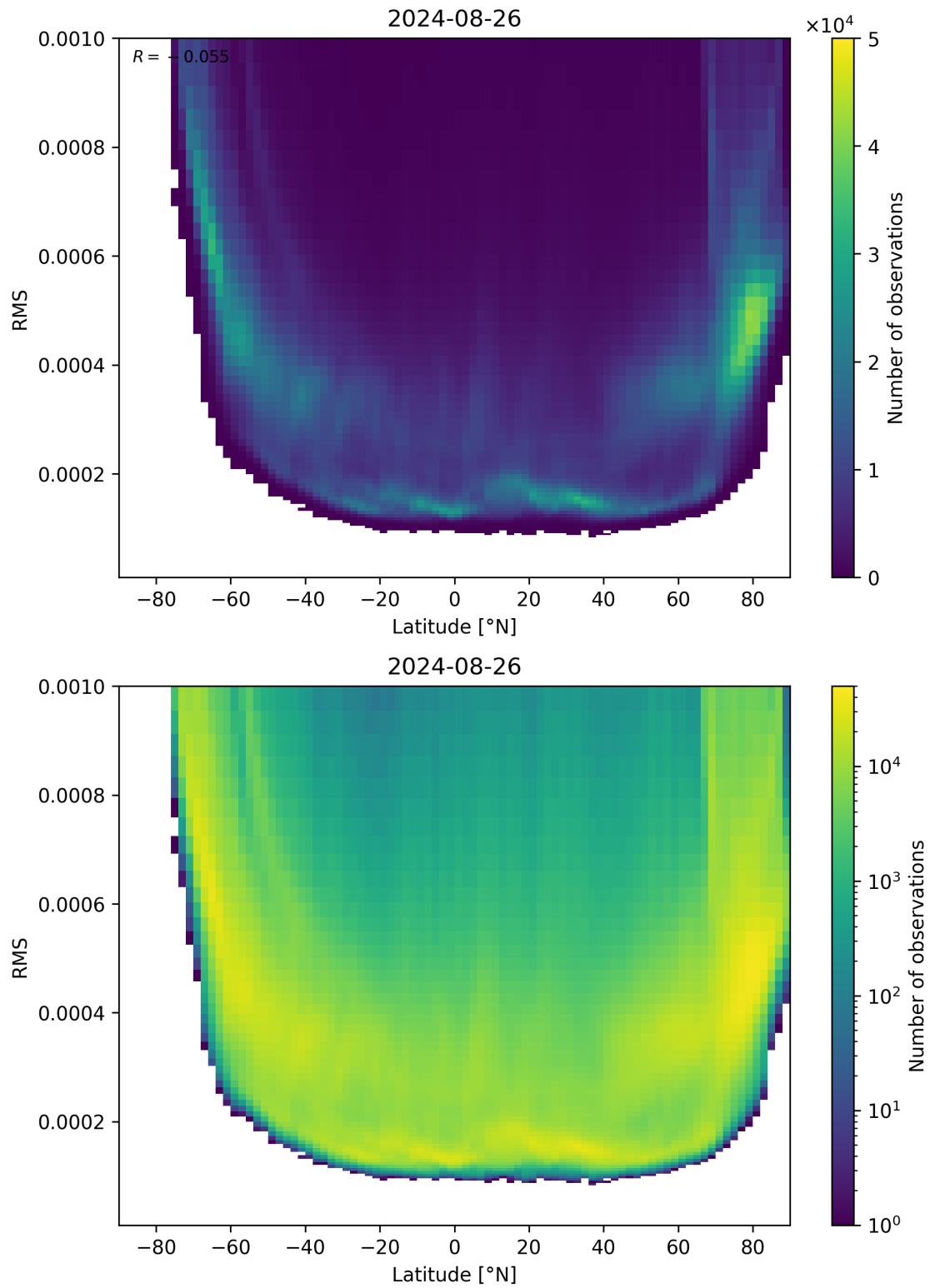
Figure 94: Scatter density plot of “Latitude” against “RMS” for 2024-08-25 to 2024-08-27.
