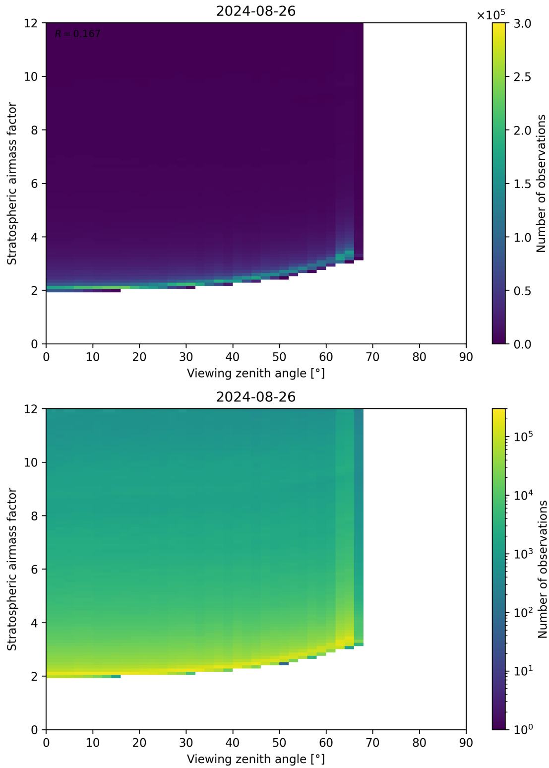
Figure 159: Scatter density plot of “Viewing zenith angle” against “Stratospheric airmass factor” for 2024-08-25 to 2024-08-27.
