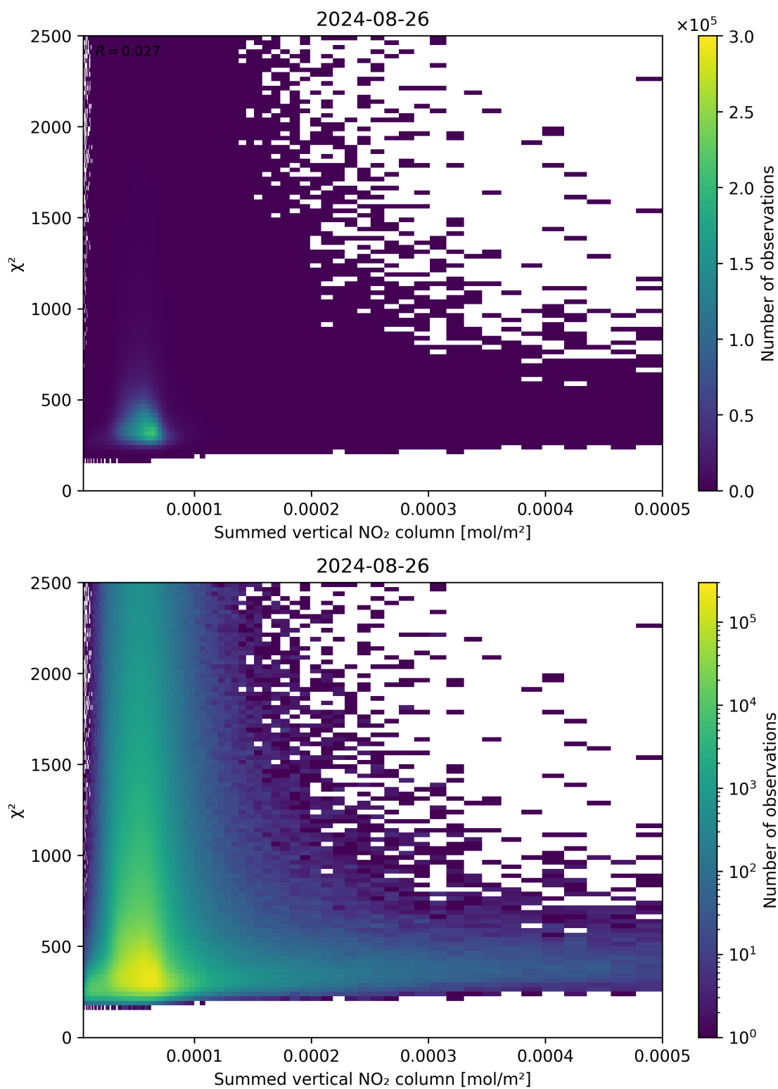
Figure 104: Scatter density plot of “Summed vertical NO 2 column” against “ \chi^2 ” for 2024-08-25 to 2024-08-27.
