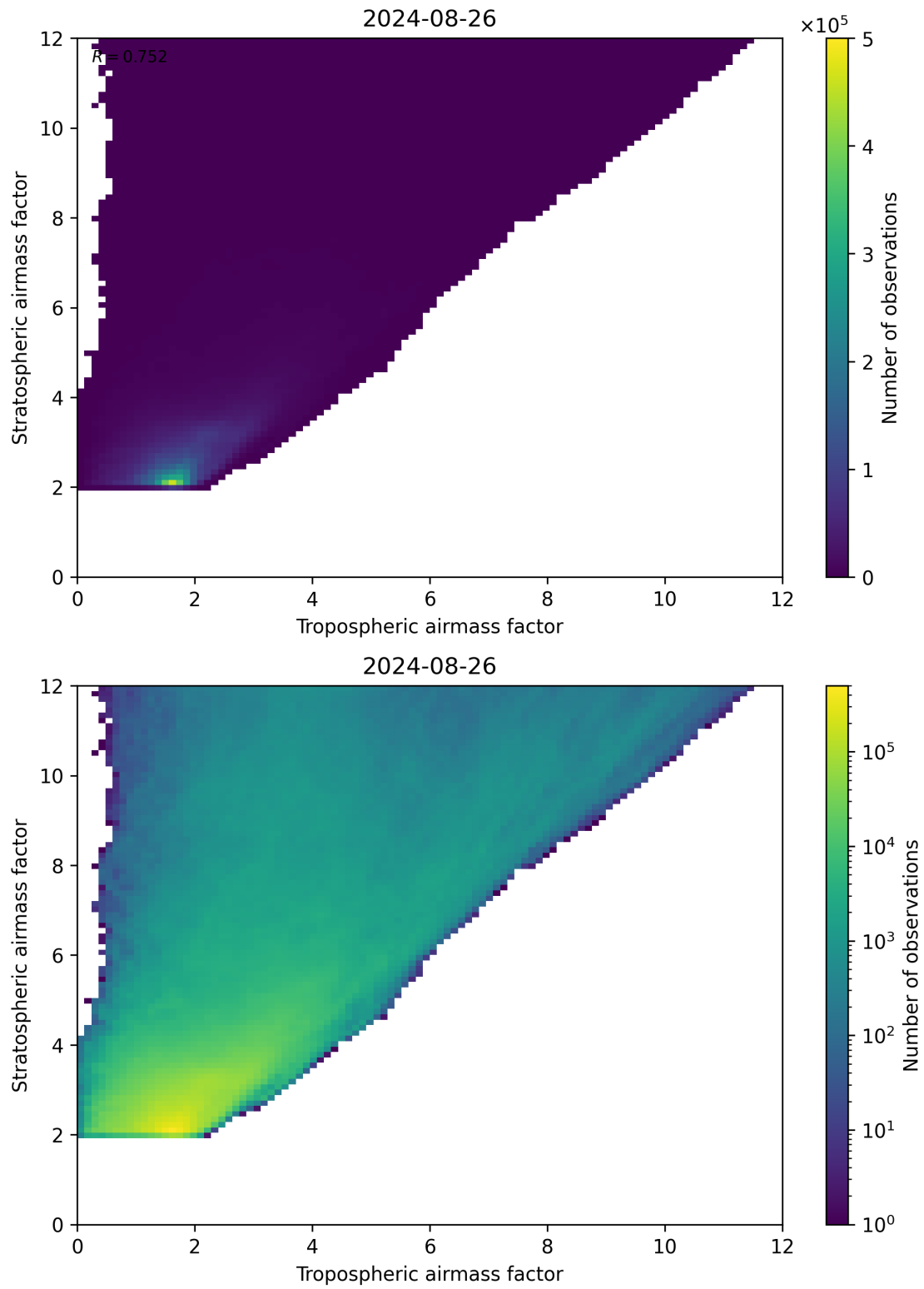
Figure 71: Scatter density plot of “Tropospheric airmass factor” against “Stratospheric airmass factor” for 2024-08-25 to 2024-08-27.
