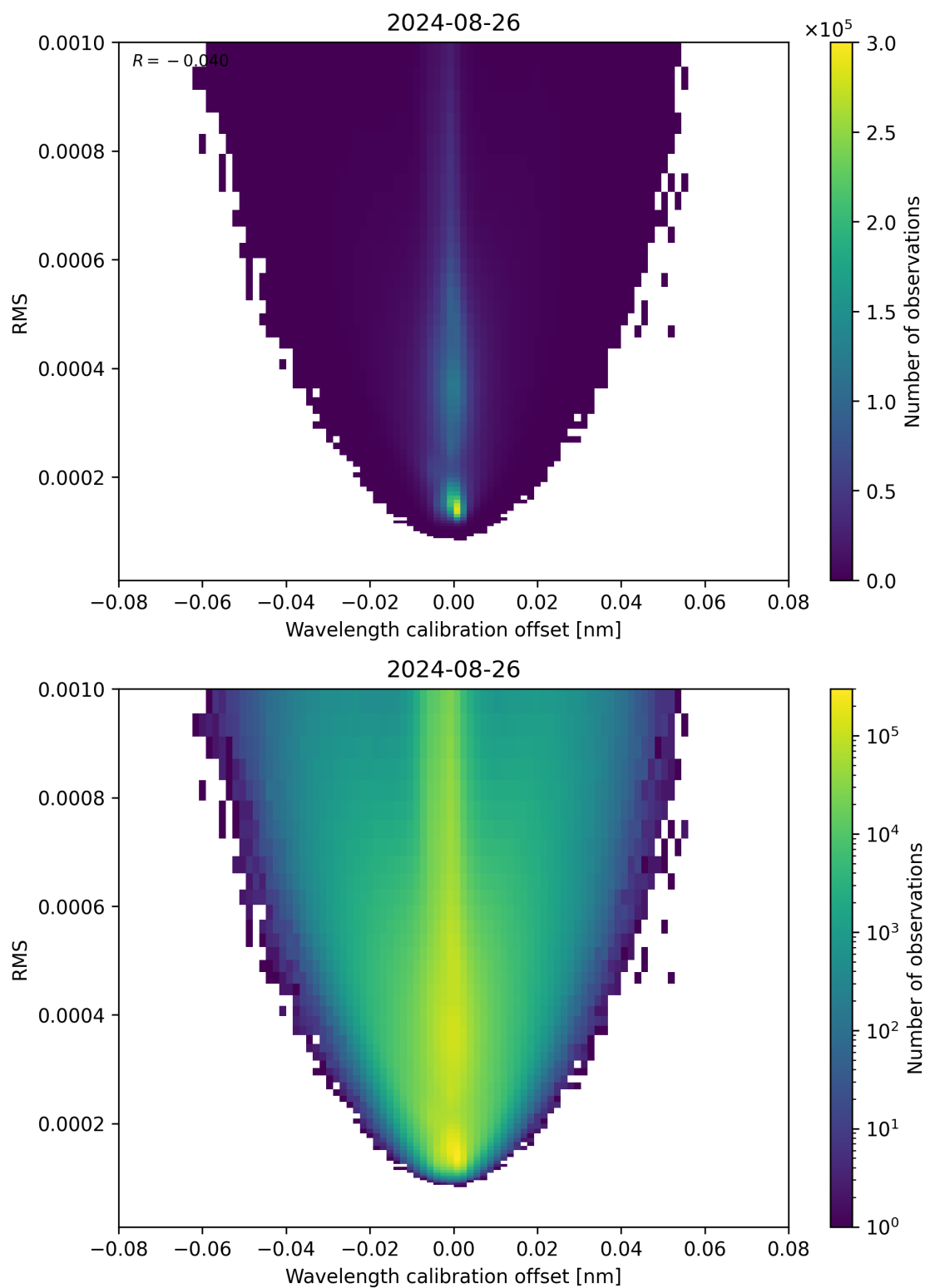
Figure 181: Scatter density plot of “Wavelength calibration offset” against “RMS” for 2024-08-25 to 2024-08-27.
