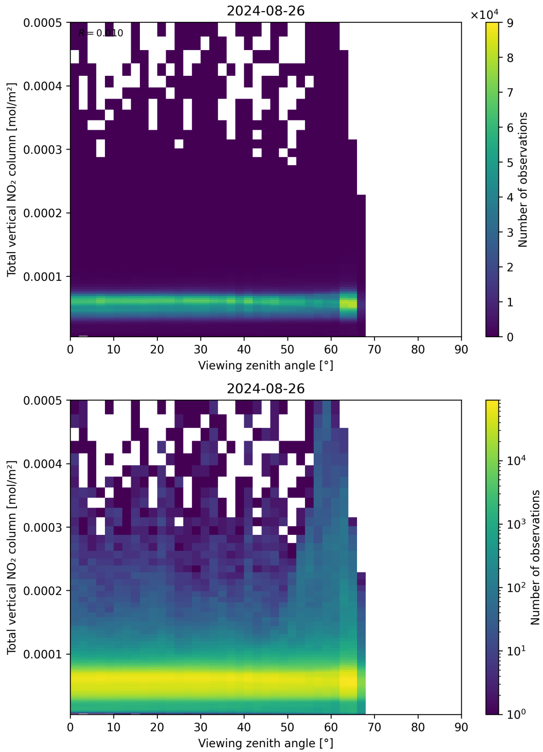
Figure 167: Scatter density plot of “Viewing zenith angle” against “Total vertical NO 2 column” for 2024-08-25 to 2024-08-27.
