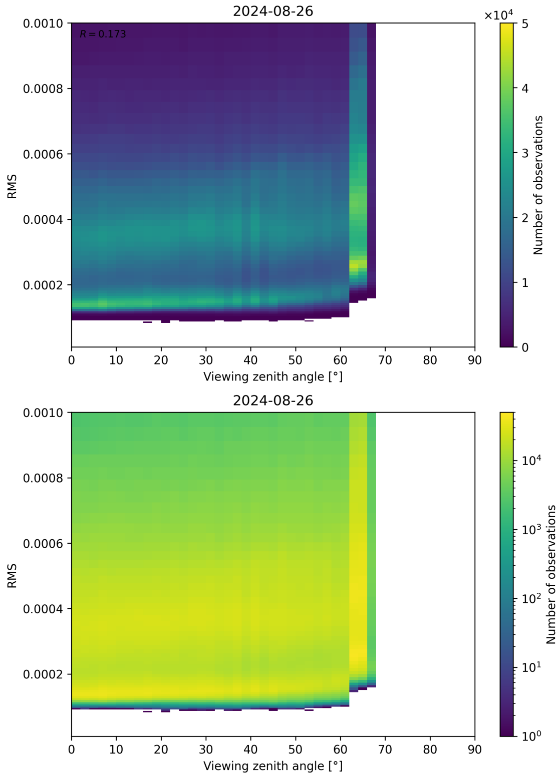
Figure 171: Scatter density plot of “Viewing zenith angle” against “RMS” for 2024-08-25 to 2024-08-27.
