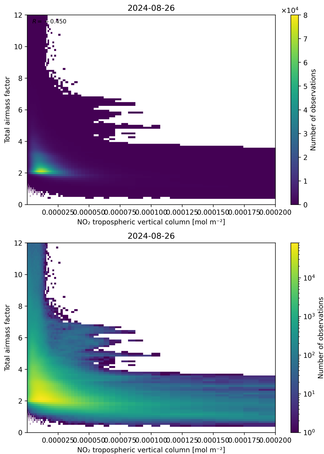
Figure 122: Scatter density plot of “NO 2 tropospheric vertical column” against “Total air mass factor” for 2024-08-25 to 2024-08-27.
