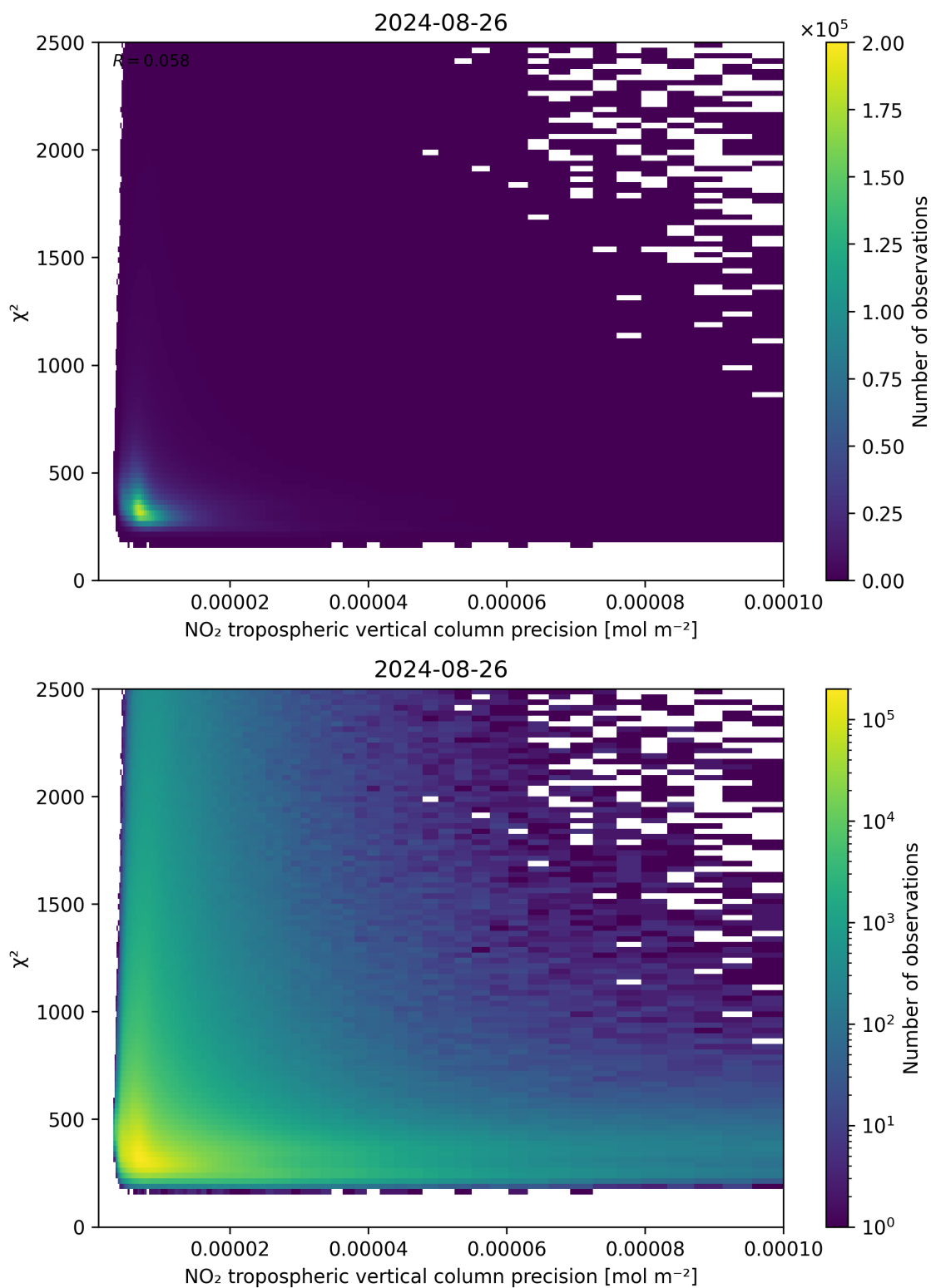
Figure 134: Scatter density plot of “NO 2 tropospheric vertical column precision” against “ \chi^2 ” for 2024-08-25 to 2024-08-27.
