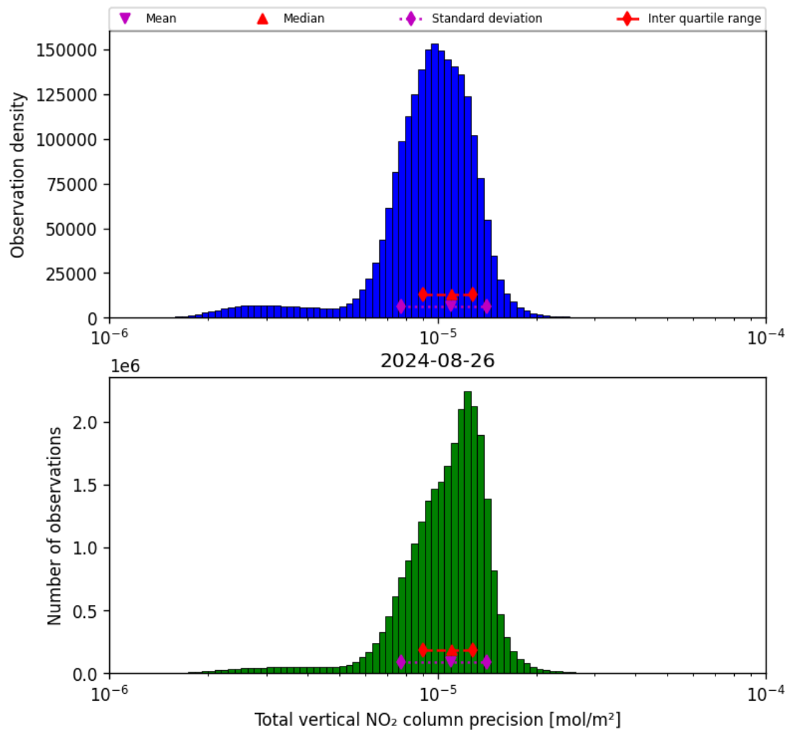
Figure 39: Histogram of “Total vertical NO 2 column precision” for 2024-08-25 to 2024-08-27
